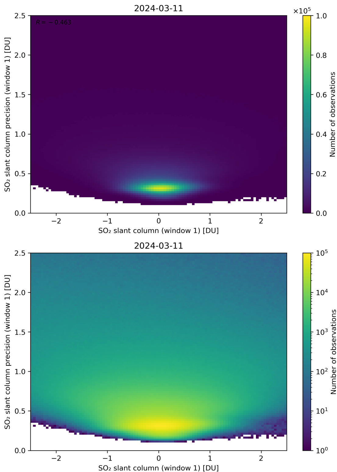
Figure 235: Scatter density plot of “SO 2 slant column (window 1)” against “SO 2 slant column precision (window 1)” for 2024-03-10 to 2024-03-12.
