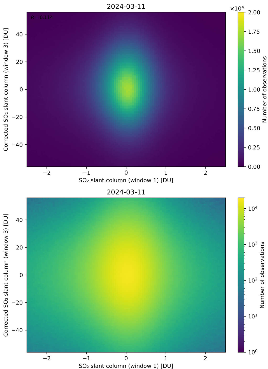
Figure 234: Scatter density plot of “SO 2 slant column (window 1)” against “Corrected SO 2 slant column (window 3)” for 2024-03-10 to 2024-03-12.
