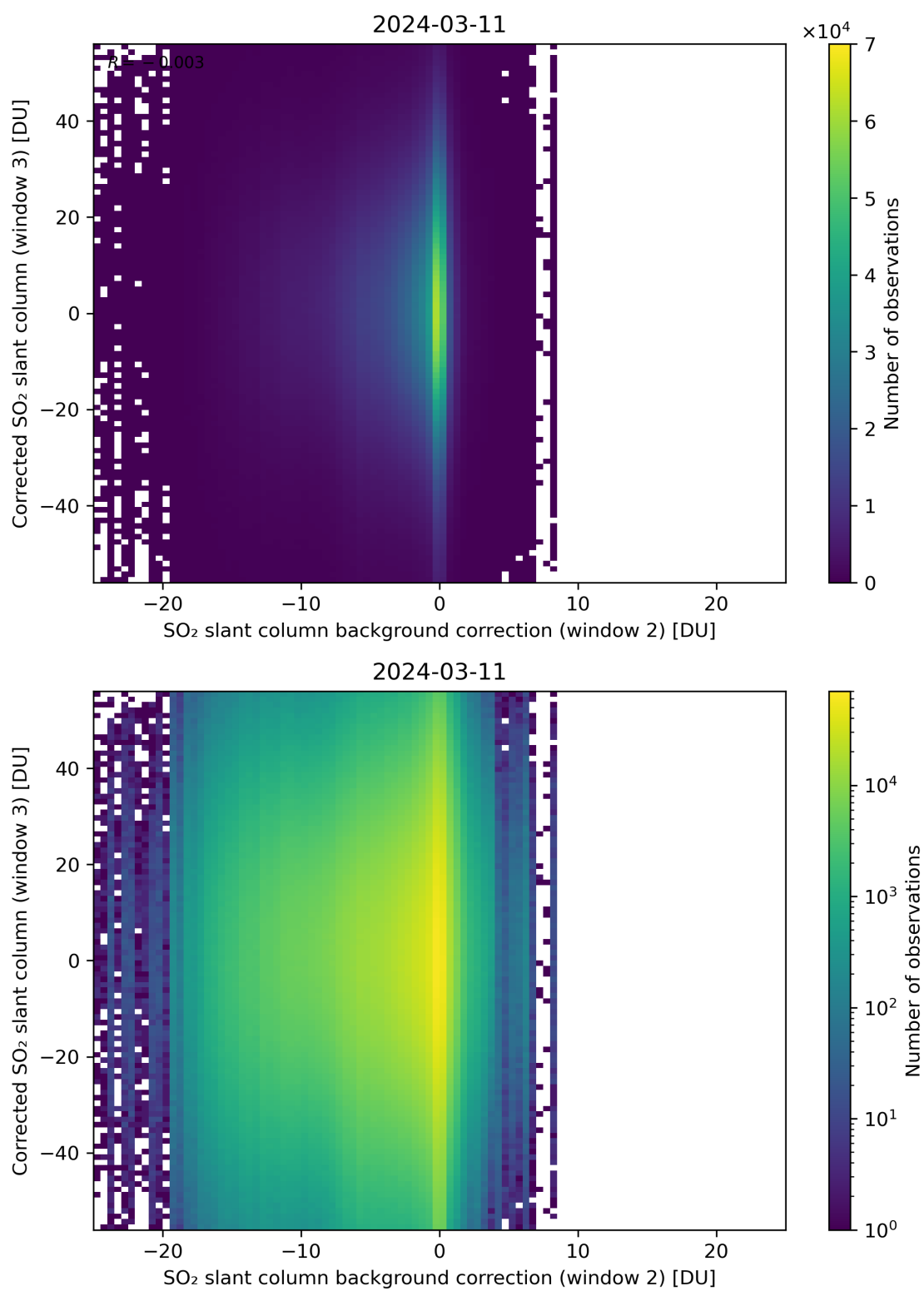
Figure 116: Scatter density plot of “SO 2 slant column background correction (window 2)” against “Corrected SO 2 slant column (window 3)” for 2024-03-10 to 2024-03-12.
