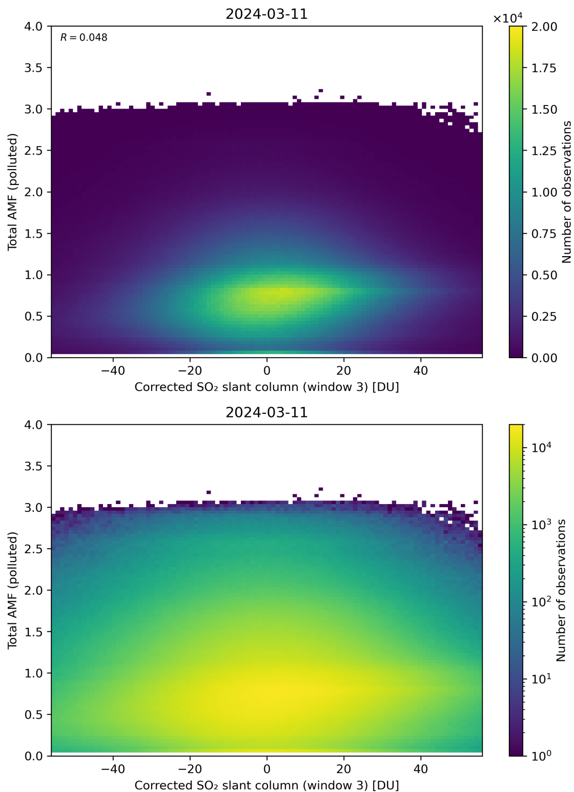
Figure 210: Scatter density plot of “Corrected SO 2 slant column (window 3)” against “Total AMF (polluted)” for 2024-03-10 to 2024-03-12.
