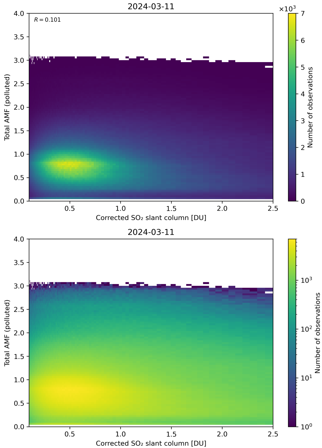
Figure 192: Scatter density plot of “Corrected SO 2 slant column” against “Total AMF (polluted)” for 2024-03-10 to 2024-03-12.
