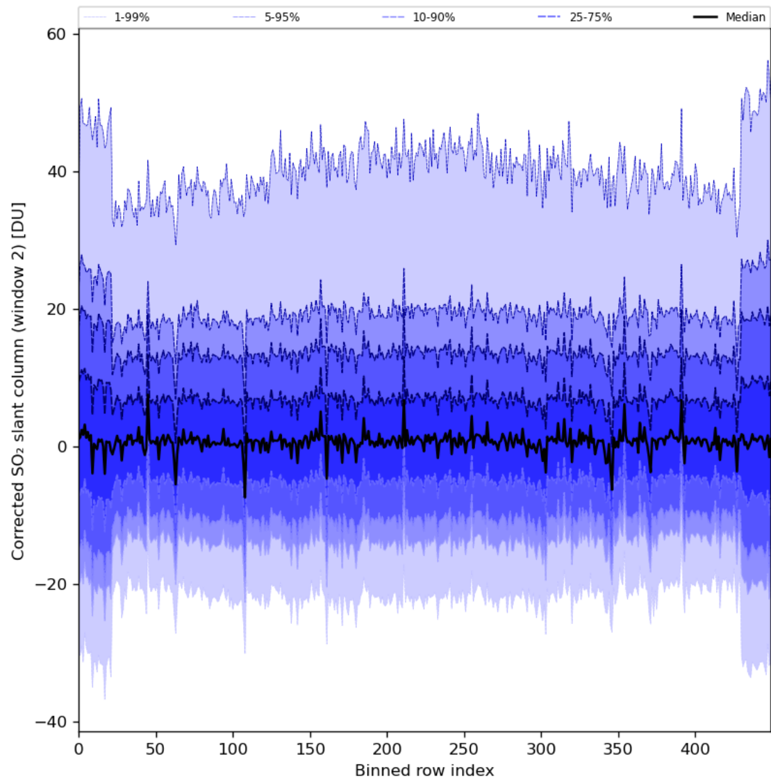
Figure 85: Along track statistics of “Corrected SO 2 slant column (window 2)” for 2024-03-10 to 2024-03-12
