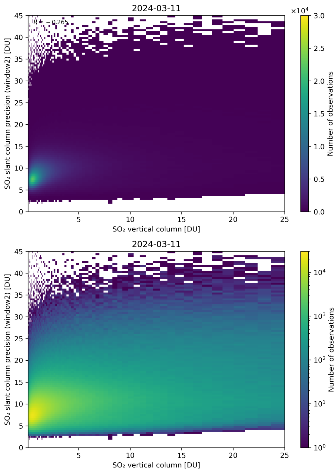
Figure 302: Scatter density plot of “SO 2 vertical column” against “SO 2 slant column precision (window2)” for 2024-03-10 to 2024-03-12.
