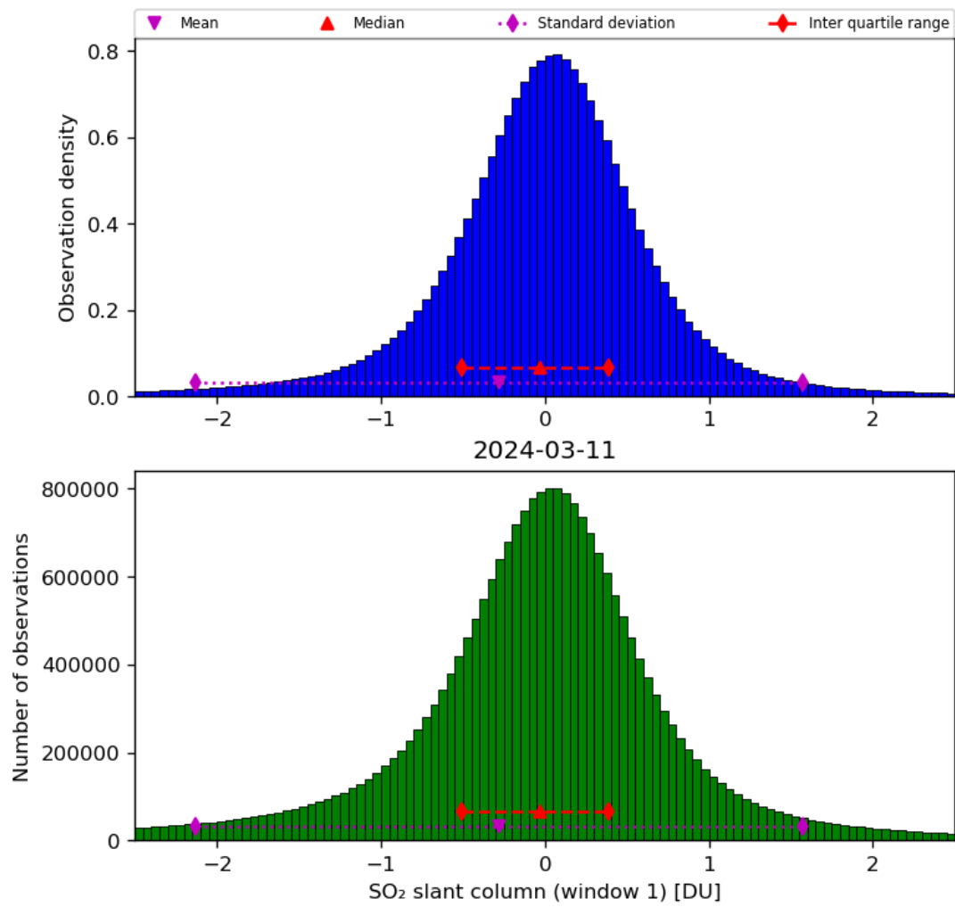
Figure 56: Histogram of “SO 2 slant column (window 1)” for 2024-03-10 to 2024-03-12
