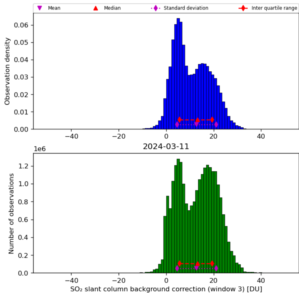
Figure 67: Histogram of “SO 2 slant column background correction (window 3)” for 2024-03-10 to 2024-03-12
