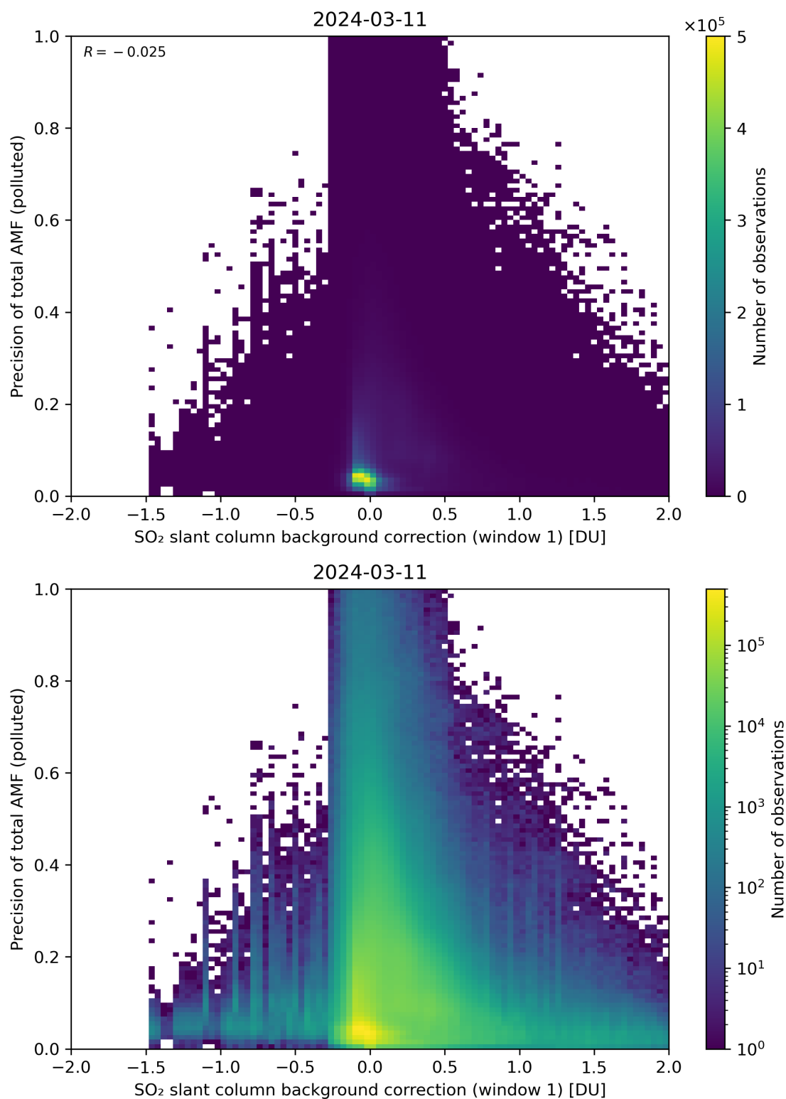
Figure 110: Scatter density plot of “SO 2 slant column background correction (window 1)” against “Precision of total AMF (polluted)” for 2024-03-10 to 2024-03-12.
