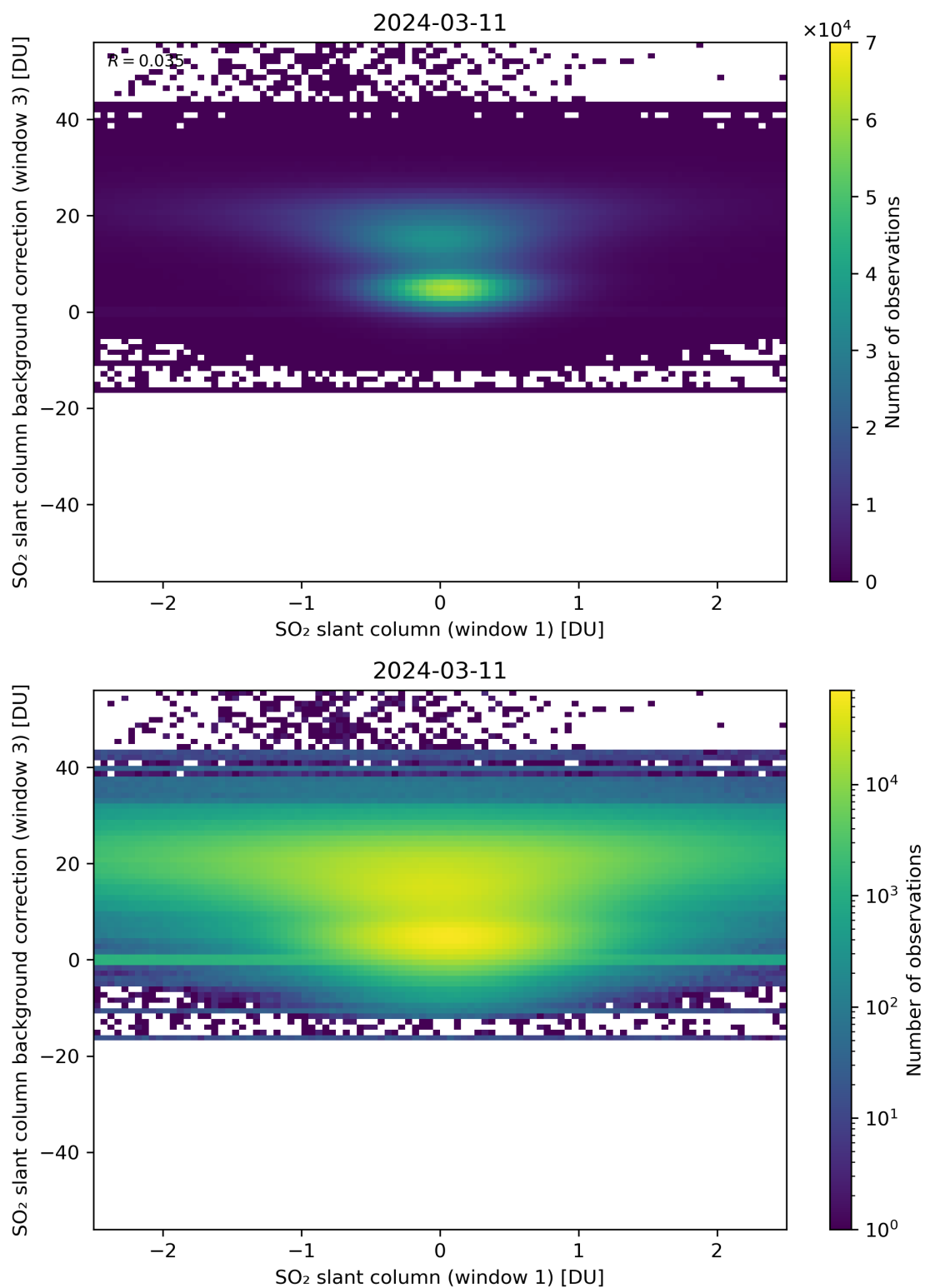
Figure 214: Scatter density plot of “SO 2 slant column (window 1)” against “SO 2 slant column background correction (window 3)” for 2024-03-10 to 2024-03-12.
