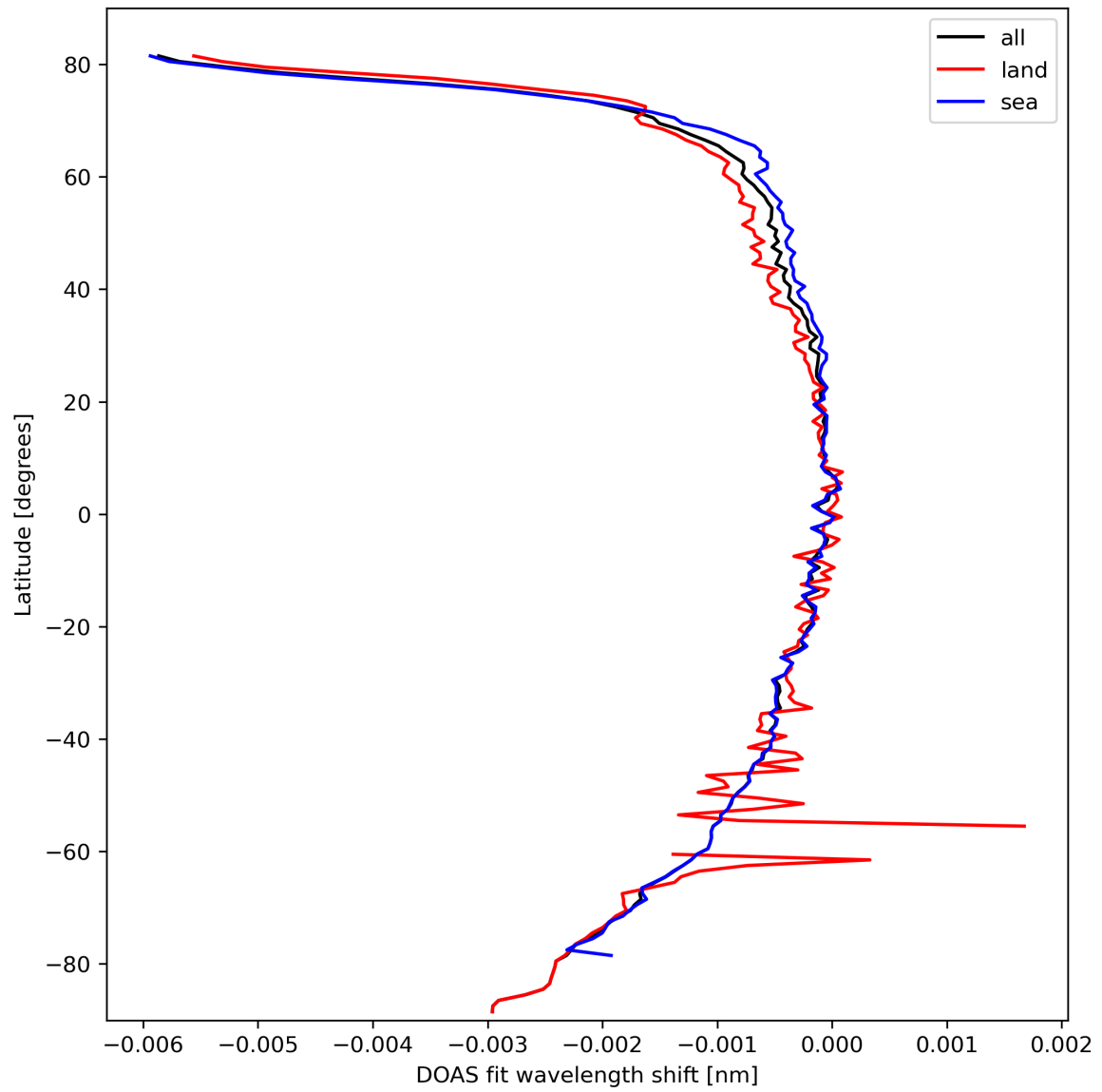
Figure 45: Zonal average of “DOAS fit wavelength shift” for 2024-03-10 to 2024-03-12.
