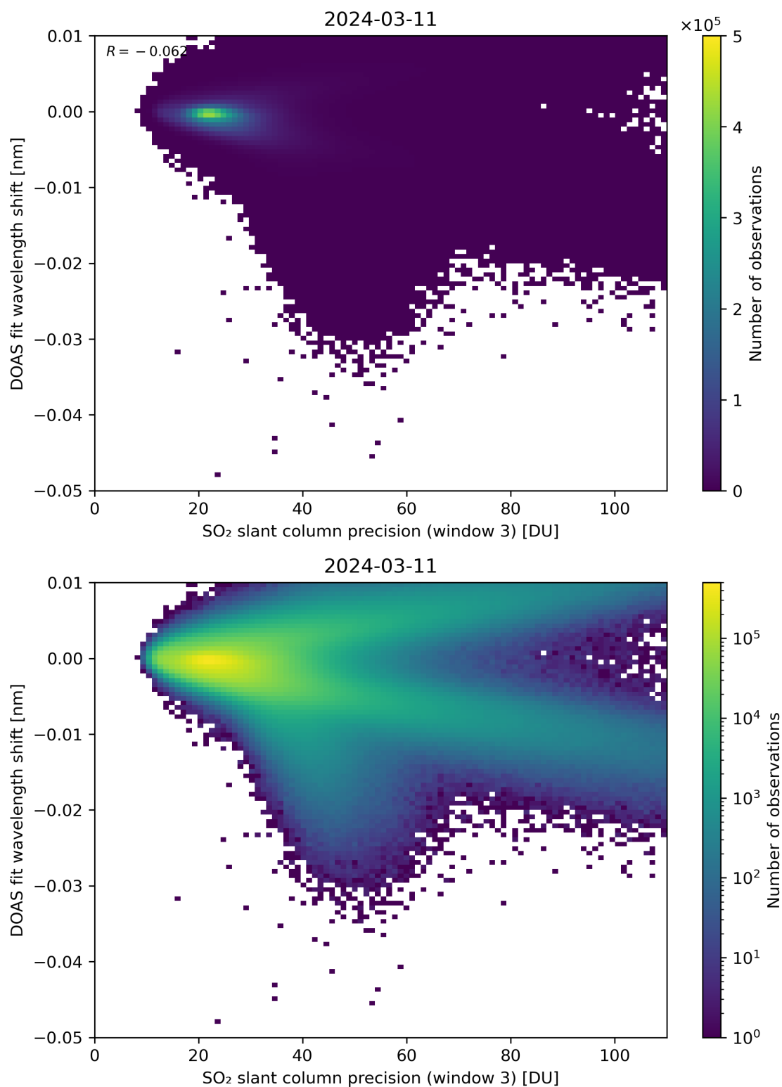
Figure 258: Scatter density plot of “SO 2 slant column precision (window 3)” against “DOAS fit wavelength shift” for 2024-03-10 to 2024-03-12.
