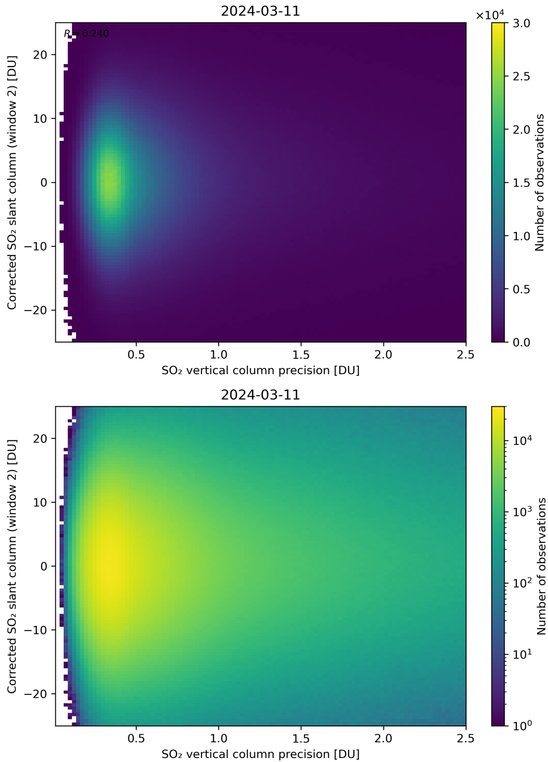
Figure 287: Scatter density plot of “SO 2 vertical column precision” against “Corrected SO 2 slant column (window 2)” for 2024-03-10 to 2024-03-12.
