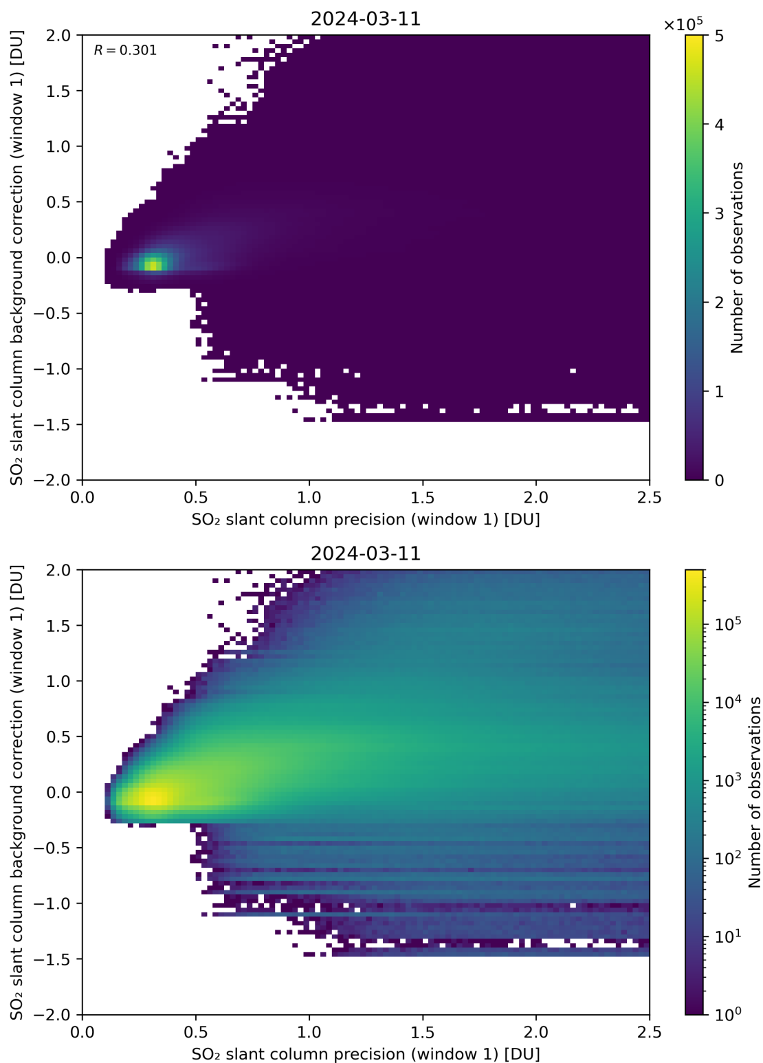
Figure 218: Scatter density plot of “SO 2 slant column precision (window 1)” against “SO 2 slant column background correction (window 1)” for 2024-03-10 to 2024-03-12.
