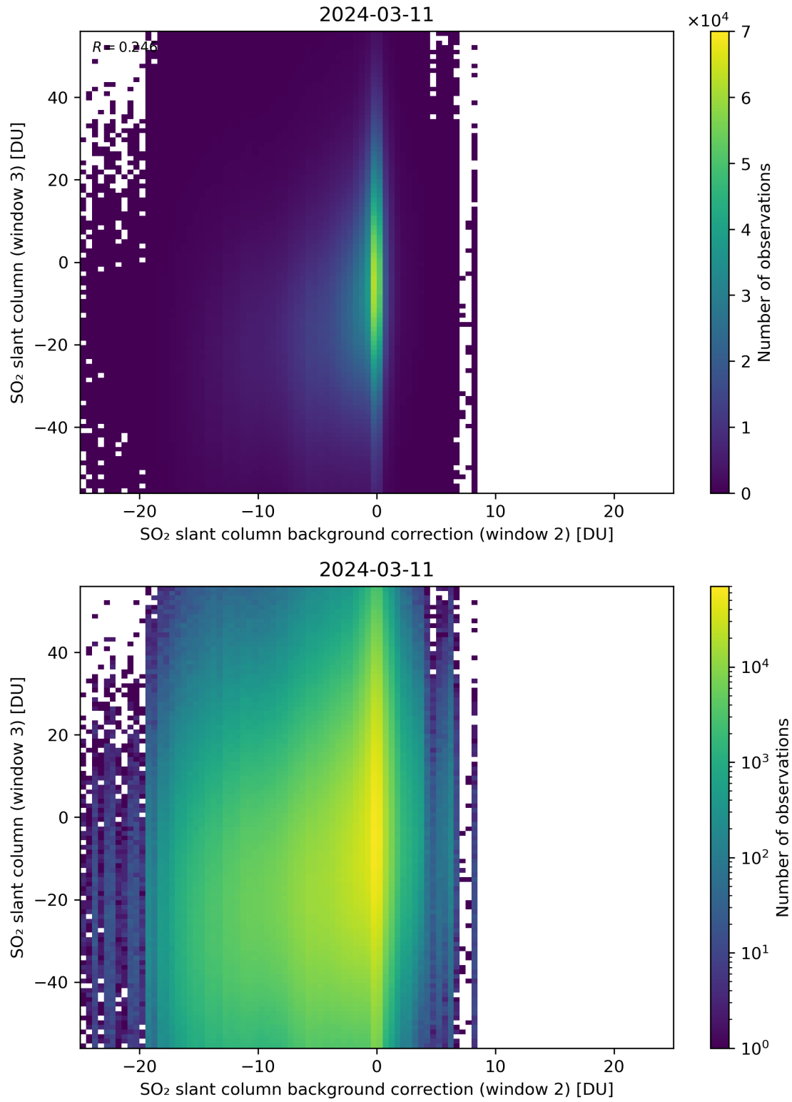
Figure 117: Scatter density plot of “SO 2 slant column background correction (window 2)” against “SO 2 slant column (window 3)” for 2024-03-10 to 2024-03-12.
