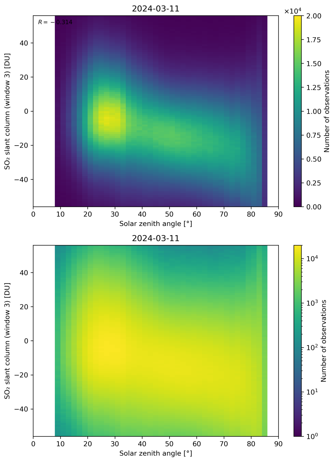
Figure 172: Scatter density plot of “Solar zenith angle” against “SO 2 slant column (window 3)” for 2024-03-10 to 2024-03-12.
