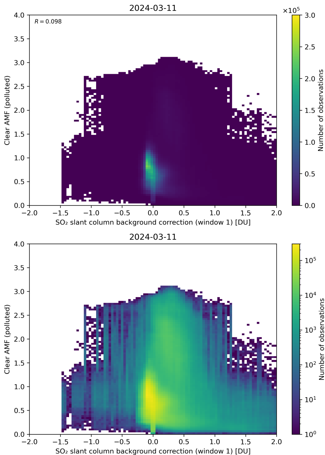
Figure 103: Scatter density plot of “SO 2 slant column background correction (window 1)” against “Clear AMF (polluted)” for 2024-03-10 to 2024-03-12.
