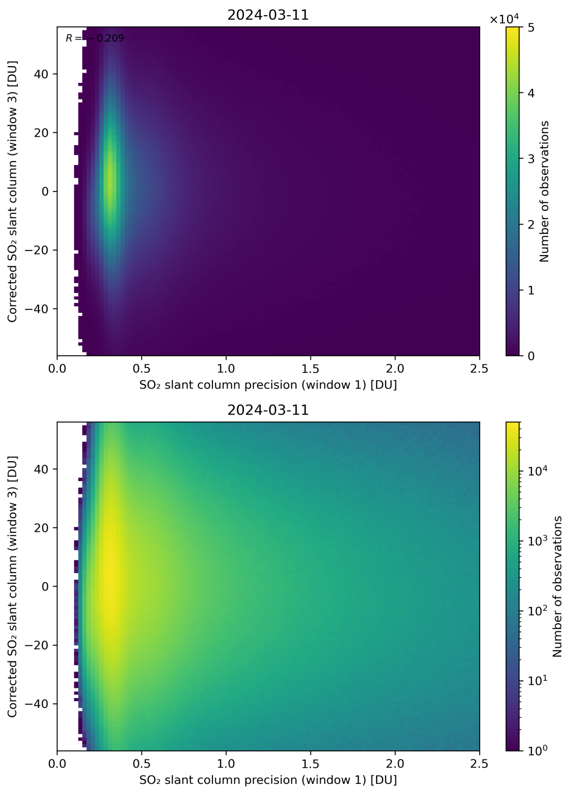
Figure 226: Scatter density plot of “SO 2 slant column precision (window 1)” against “Corrected SO 2 slant column (window 3)” for 2024-03-10 to 2024-03-12.
