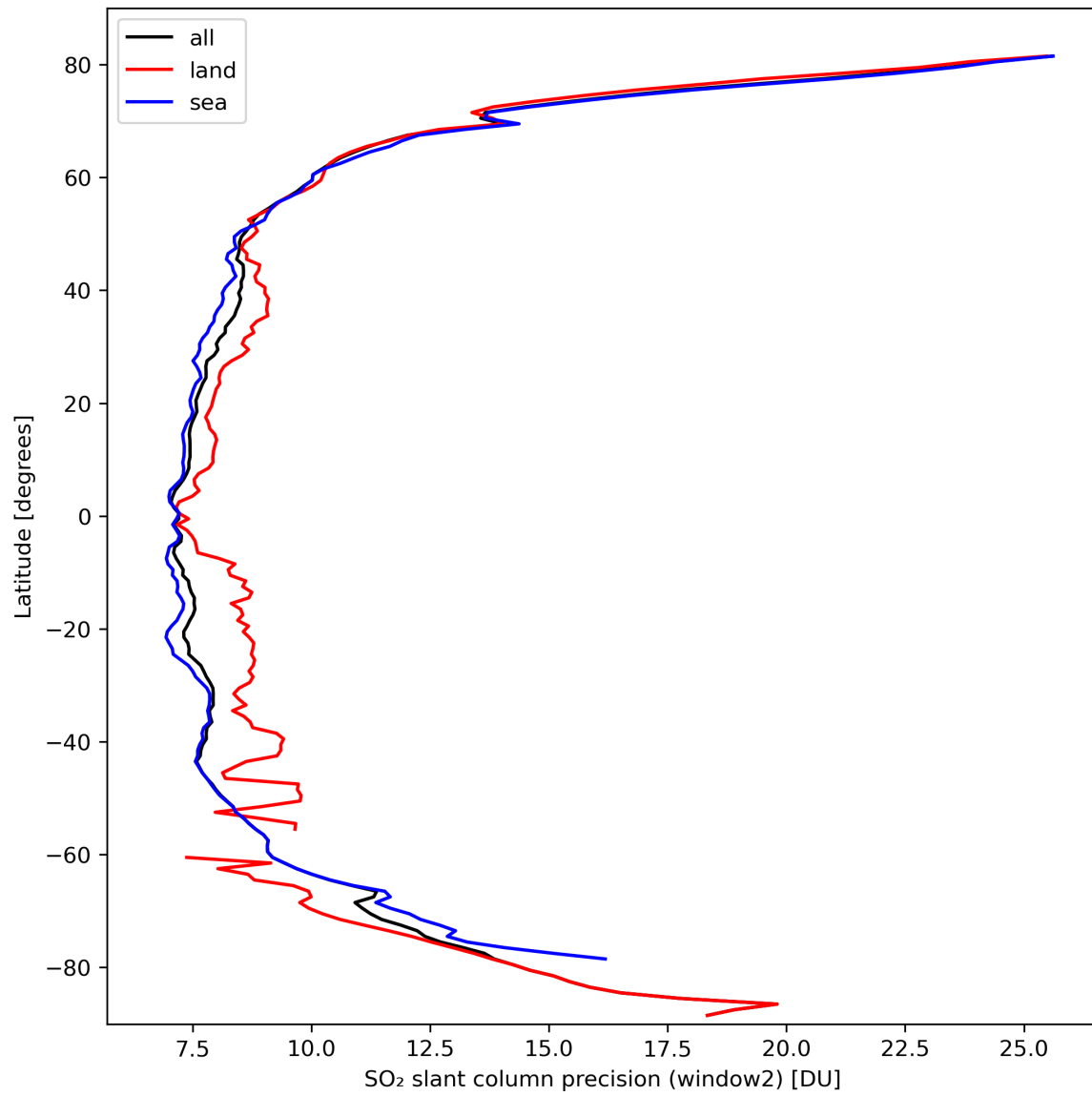
Figure 38: Zonal average of “SO 2 slant column precision (window2)” for 2024-03-10 to 2024-03-12.
