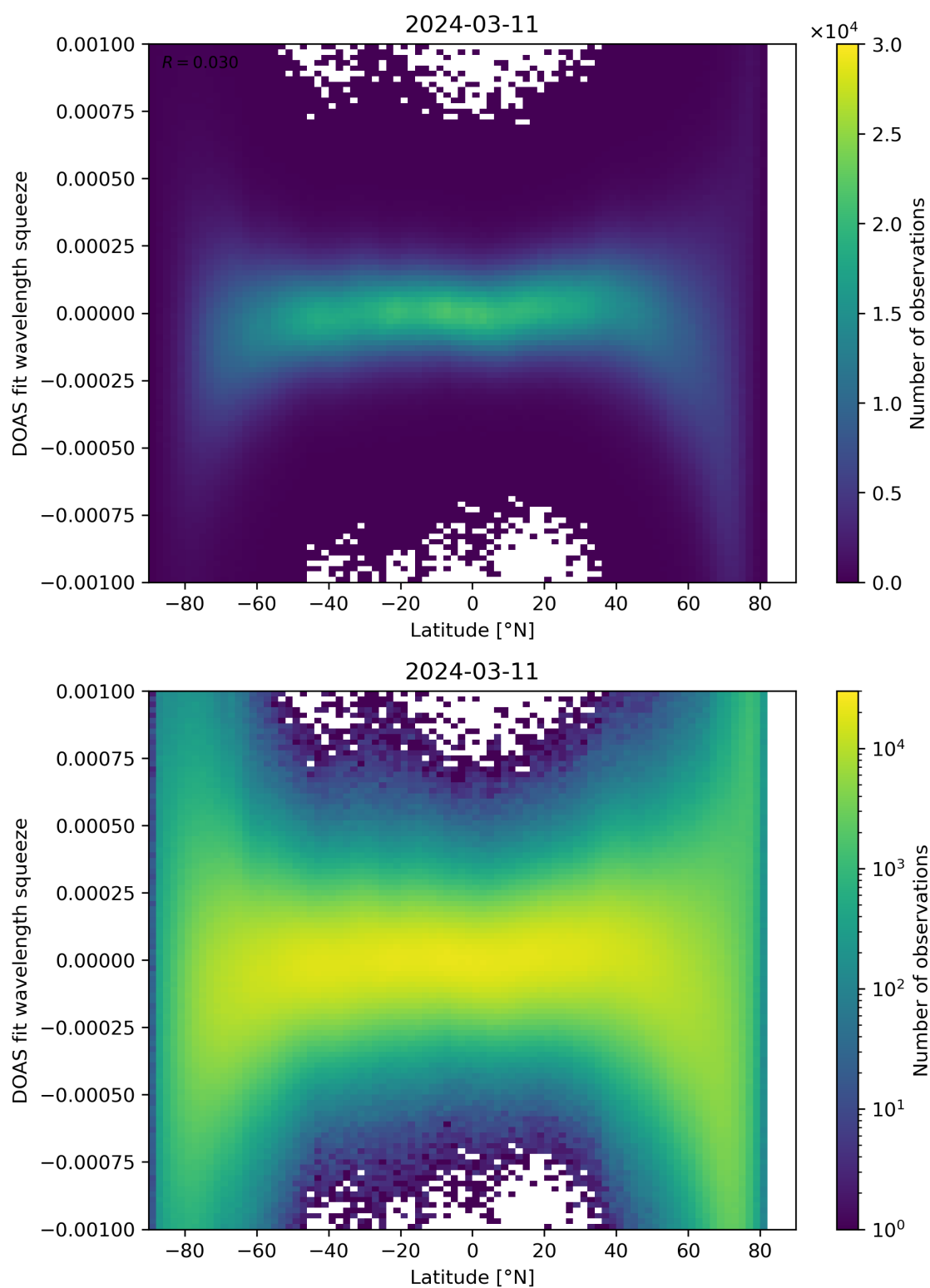
Figure 143: Scatter density plot of “Latitude” against “DOAS fit wavelength squeeze” for 2024-03-10 to 2024-03-12.
