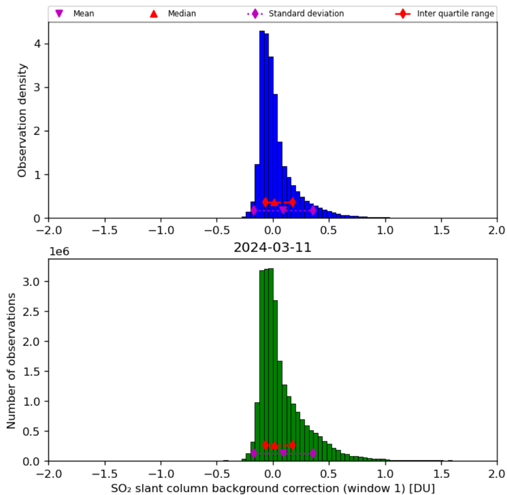
Figure 59: Histogram of “SO 2 slant column background correction (window 1)” for 2024-03-10 to 2024-03-12
