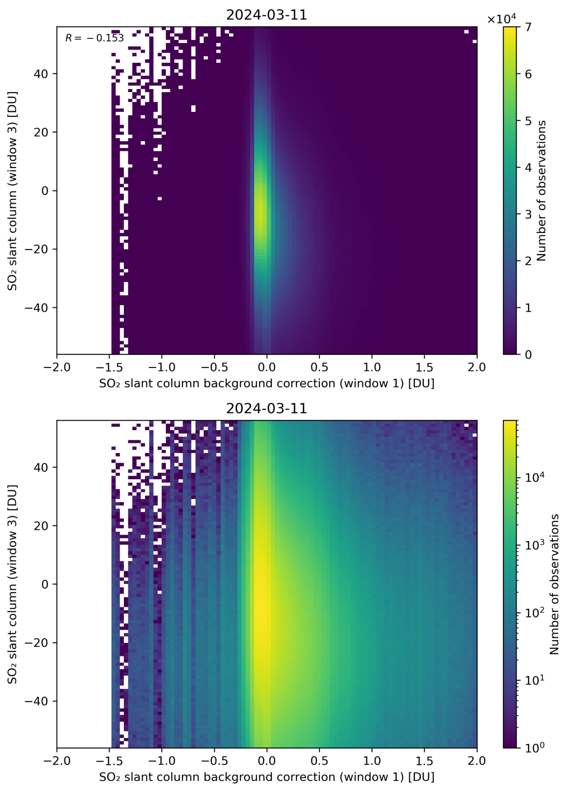
Figure 107: Scatter density plot of “SO 2 slant column background correction (window 1)” against “SO 2 slant column (window 3)” for 2024-03-10 to 2024-03-12.
