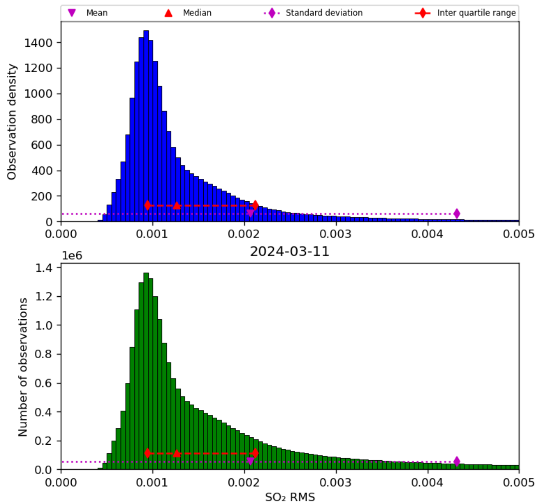
Figure 70: Histogram of “SO 2 RMS” for 2024-03-10 to 2024-03-12
