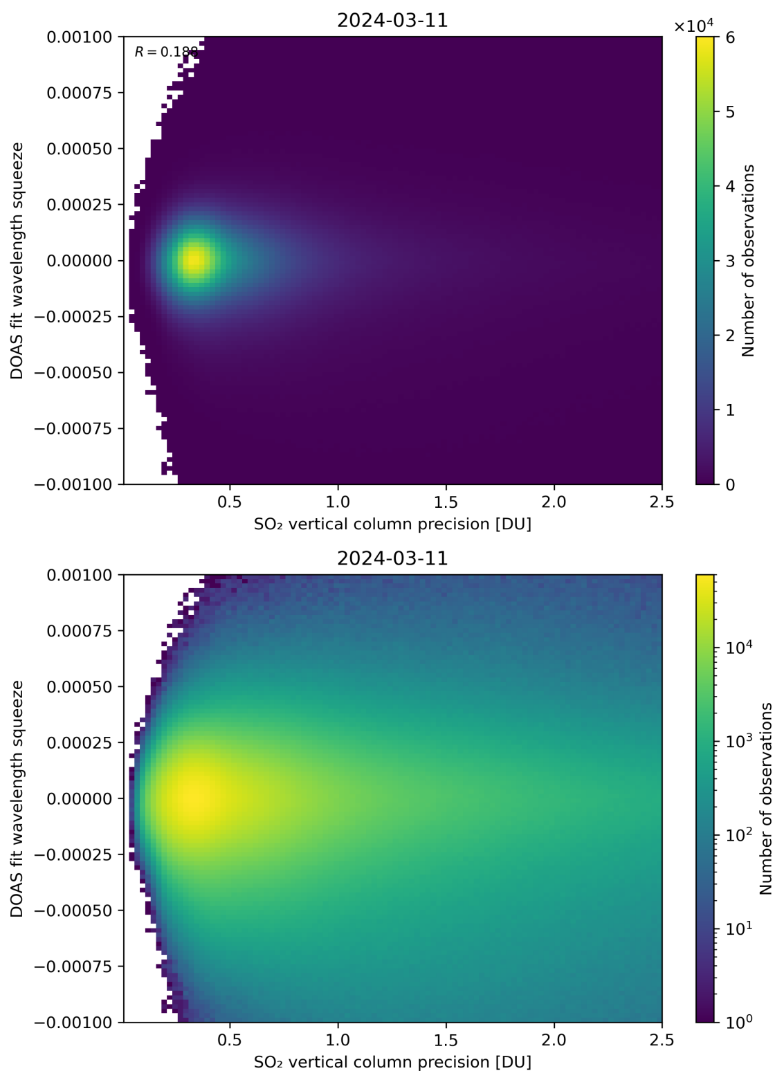
Figure 283: Scatter density plot of “SO 2 vertical column precision” against “DOAS fit wavelength squeeze” for 2024-03-10 to 2024-03-12.
