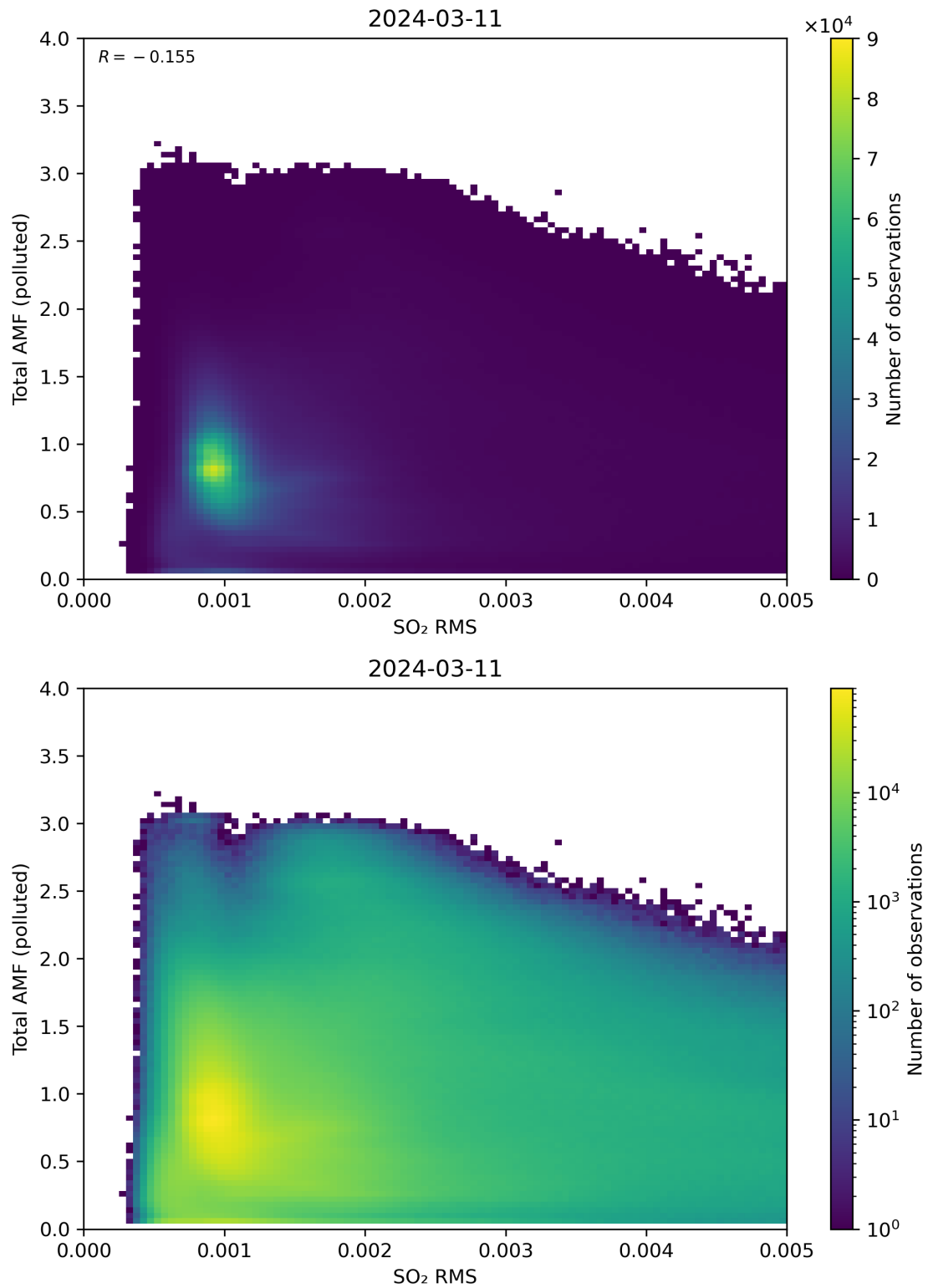
Figure 137: Scatter density plot of “SO 2 RMS” against “Total AMF (polluted)” for 2024-03-10 to 2024-03-12.
