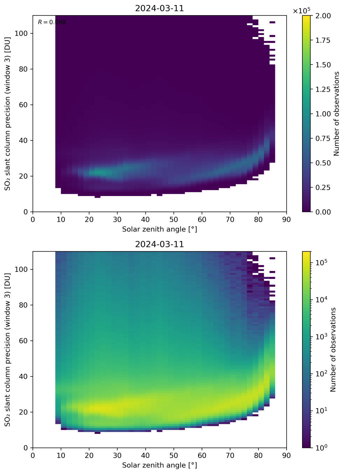
Figure 173: Scatter density plot of “Solar zenith angle” against “SO 2 slant column precision (window 3)” for 2024-03-10 to 2024-03-12.
