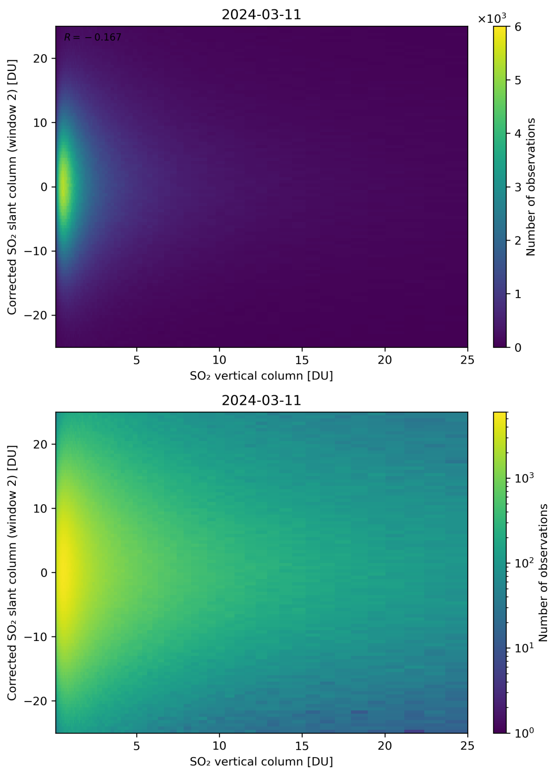
Figure 298: Scatter density plot of “SO 2 vertical column” against “Corrected SO 2 slant column (window 2)” for 2024-03-10 to 2024-03-12.
