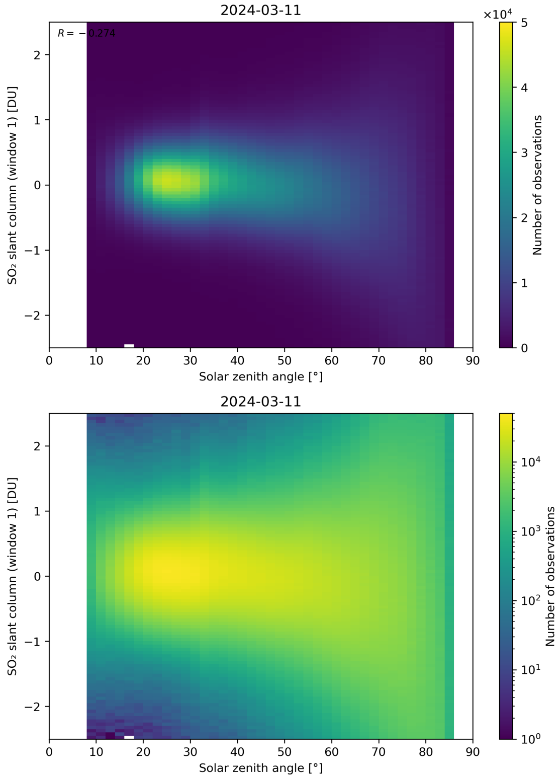
Figure 169: Scatter density plot of “Solar zenith angle” against “SO 2 slant column (window 1)” for 2024-03-10 to 2024-03-12.
