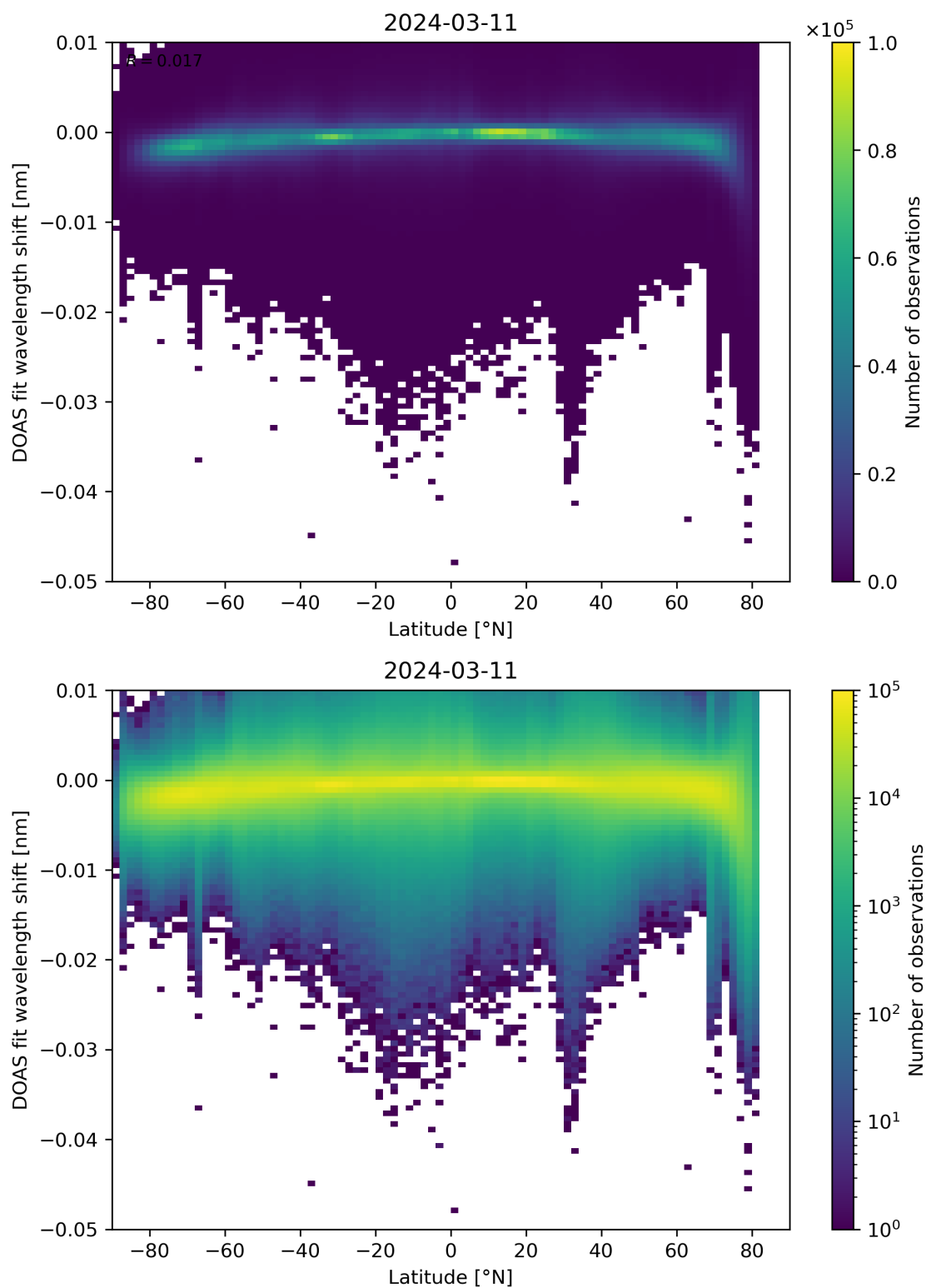
Figure 142: Scatter density plot of “Latitude” against “DOAS fit wavelength shift” for 2024-03-10 to 2024-03-12.
