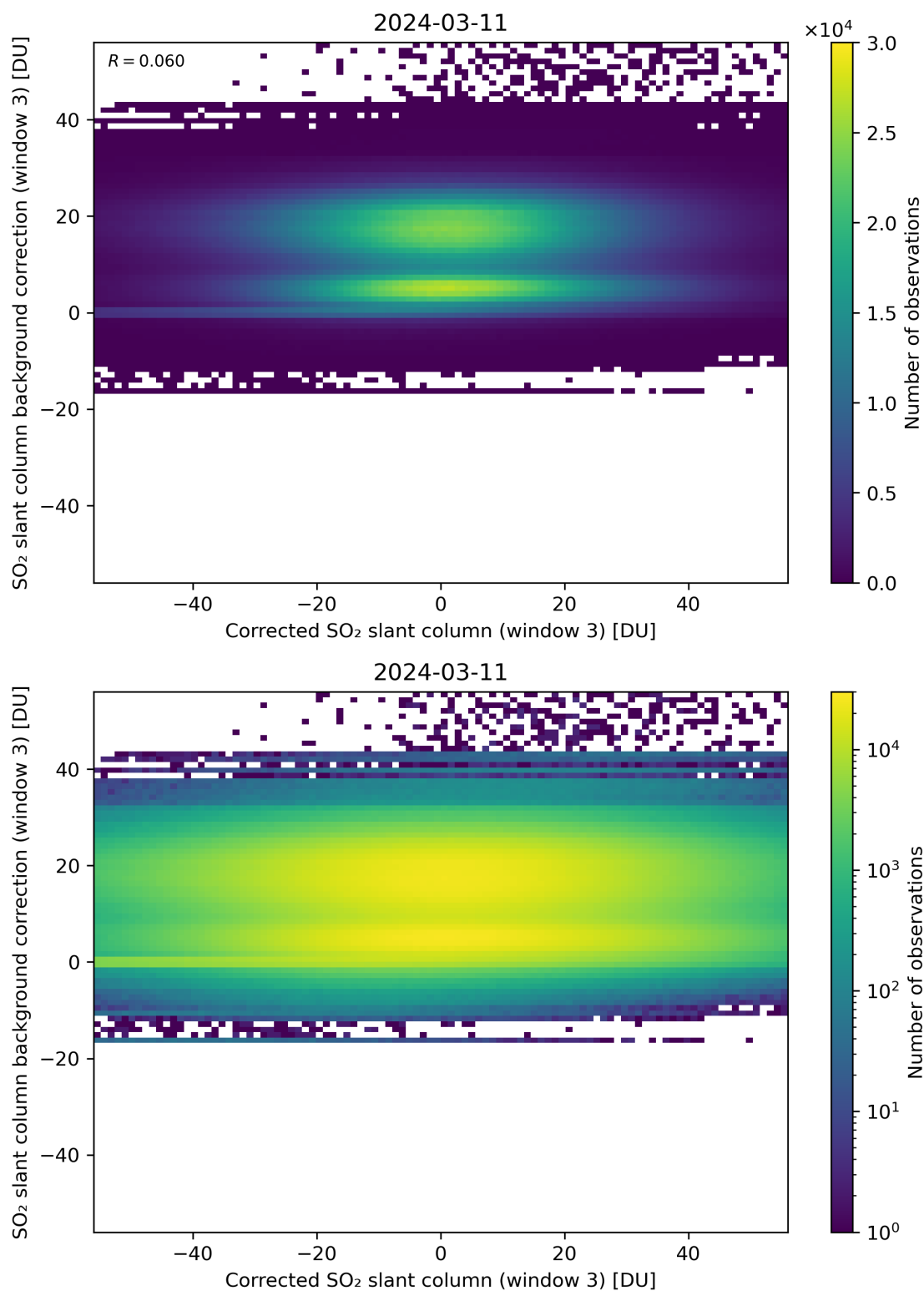
Figure 205: Scatter density plot of “Corrected SO 2 slant column (window 3)” against “SO 2 slant column background correction (window 3)” for 2024-03-10 to 2024-03-12.
