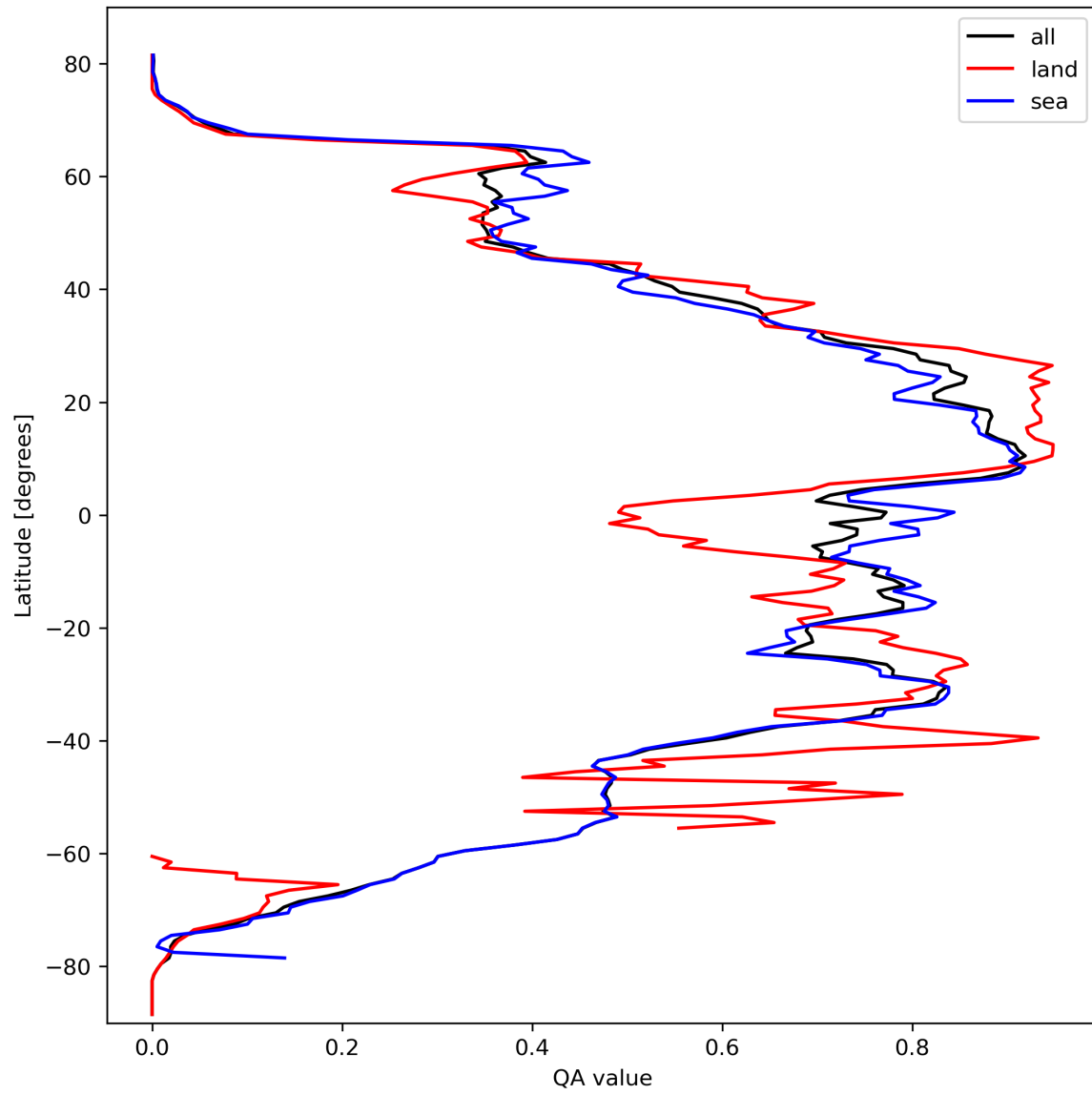
Figure 29: Zonal average of “QA value” for 2024-03-10 to 2024-03-12.
