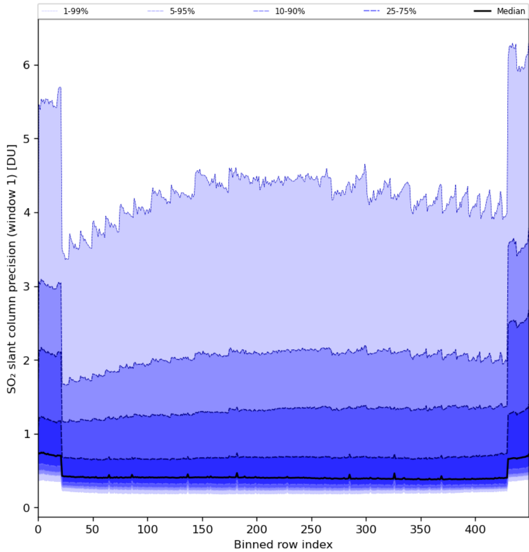
Figure 80: Along track statistics of “SO 2 slant column precision (window 1)” for 2024-03-10 to 2024-03-12
