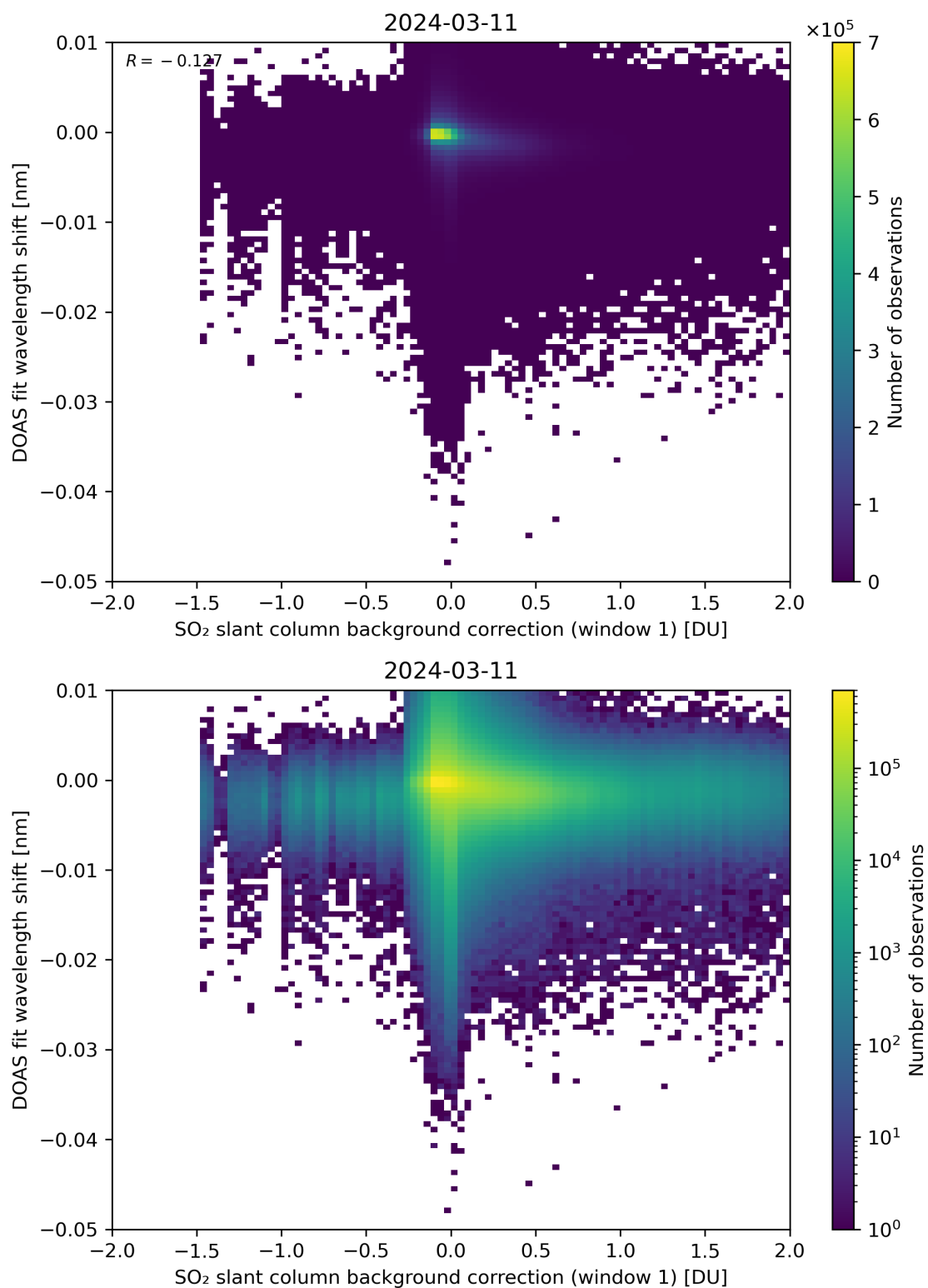
Figure 100: Scatter density plot of “SO 2 slant column background correction (window 1)” against “DOAS fit wavelength shift” for 2024-03-10 to 2024-03-12.
