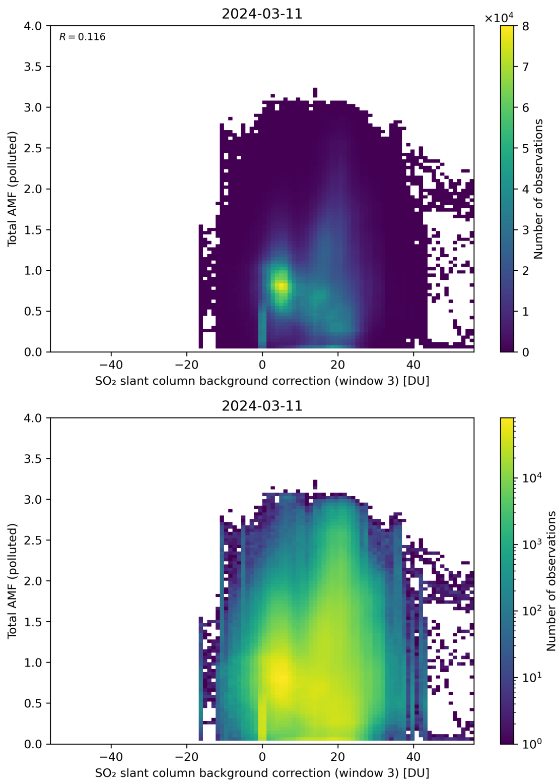
Figure 125: Scatter density plot of “SO 2 slant column background correction (window 3)” against “Total AMF (polluted)” for 2024-03-10 to 2024-03-12.
