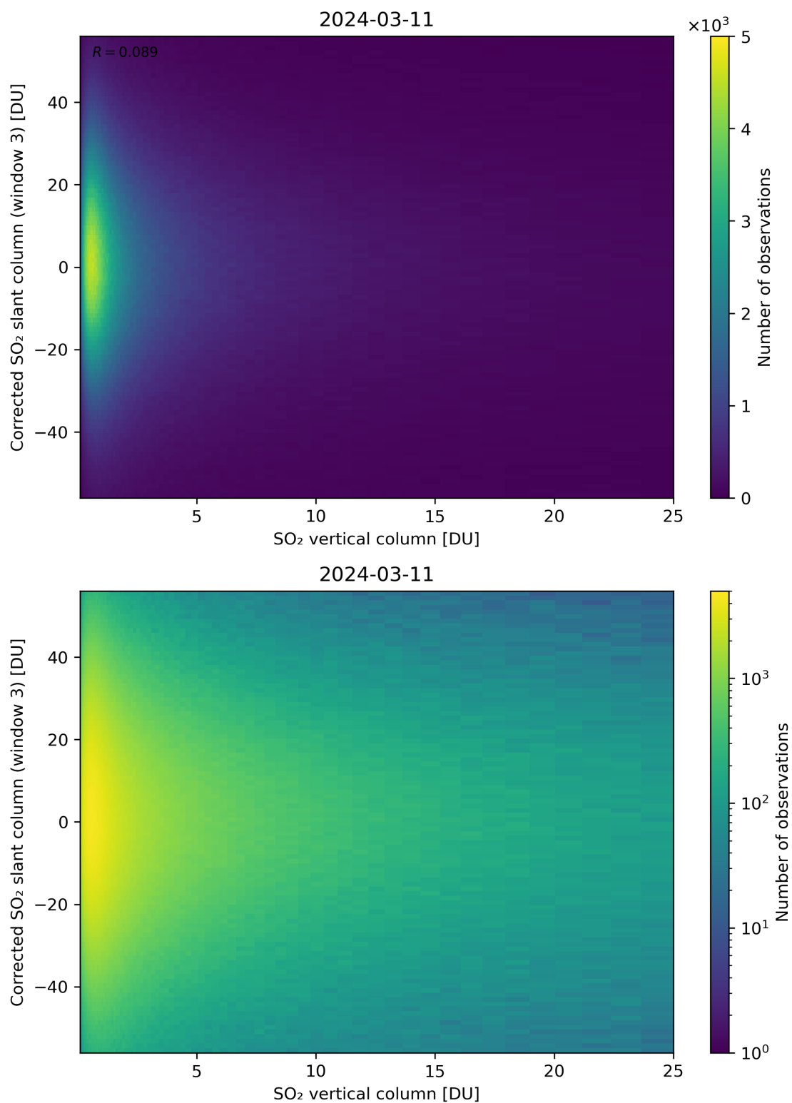
Figure 299: Scatter density plot of “SO 2 vertical column” against “Corrected SO 2 slant column (window 3)” for 2024-03-10 to 2024-03-12.
