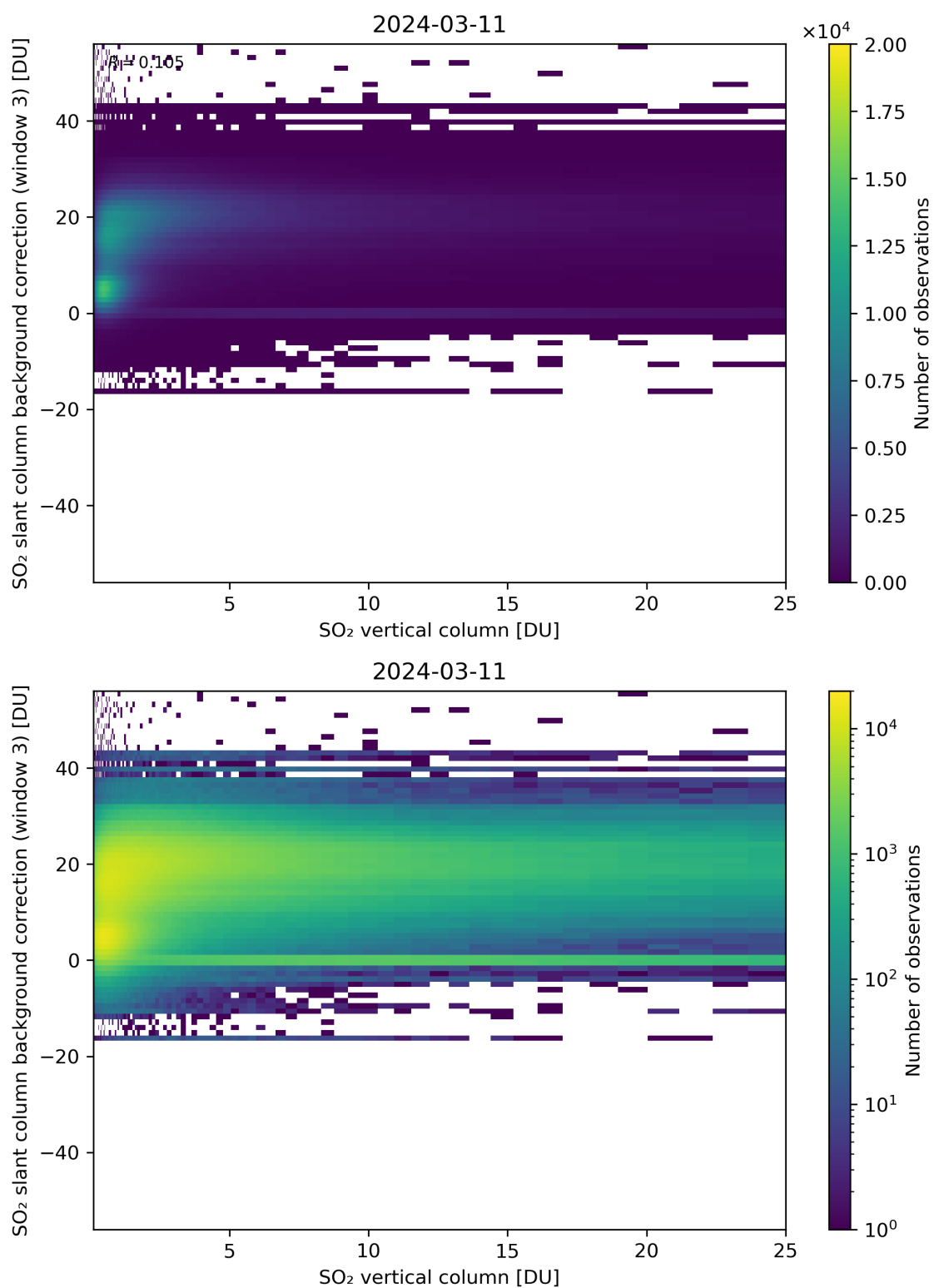
Figure 275: Scatter density plot of “SO 2 vertical column” against “SO 2 slant column background correction (window 3)” for 2024-03-10 to 2024-03-12.
