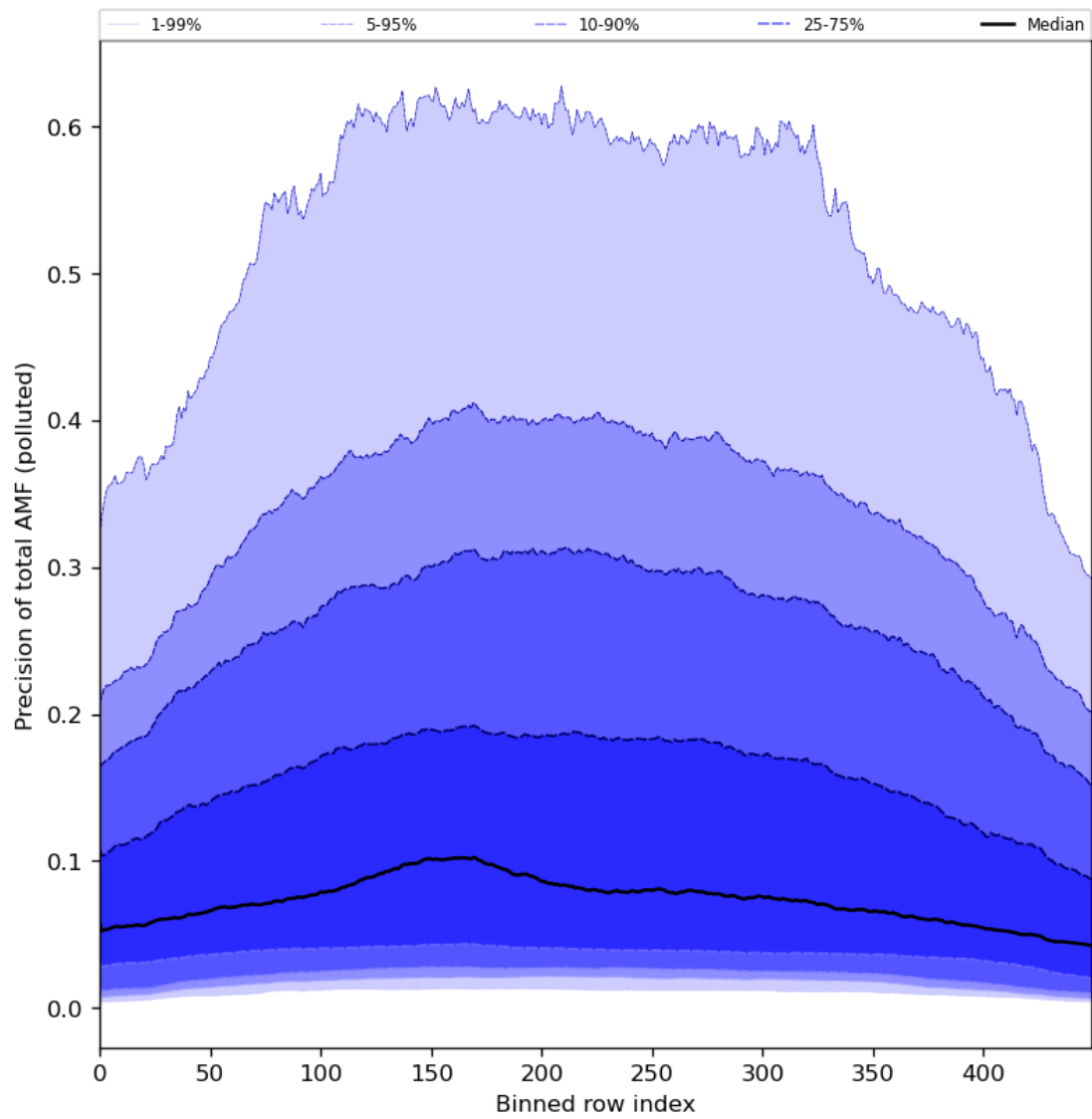
Figure 95: Along track statistics of “Precision of total AMF (polluted)” for 2024-03-10 to 2024-03-12
