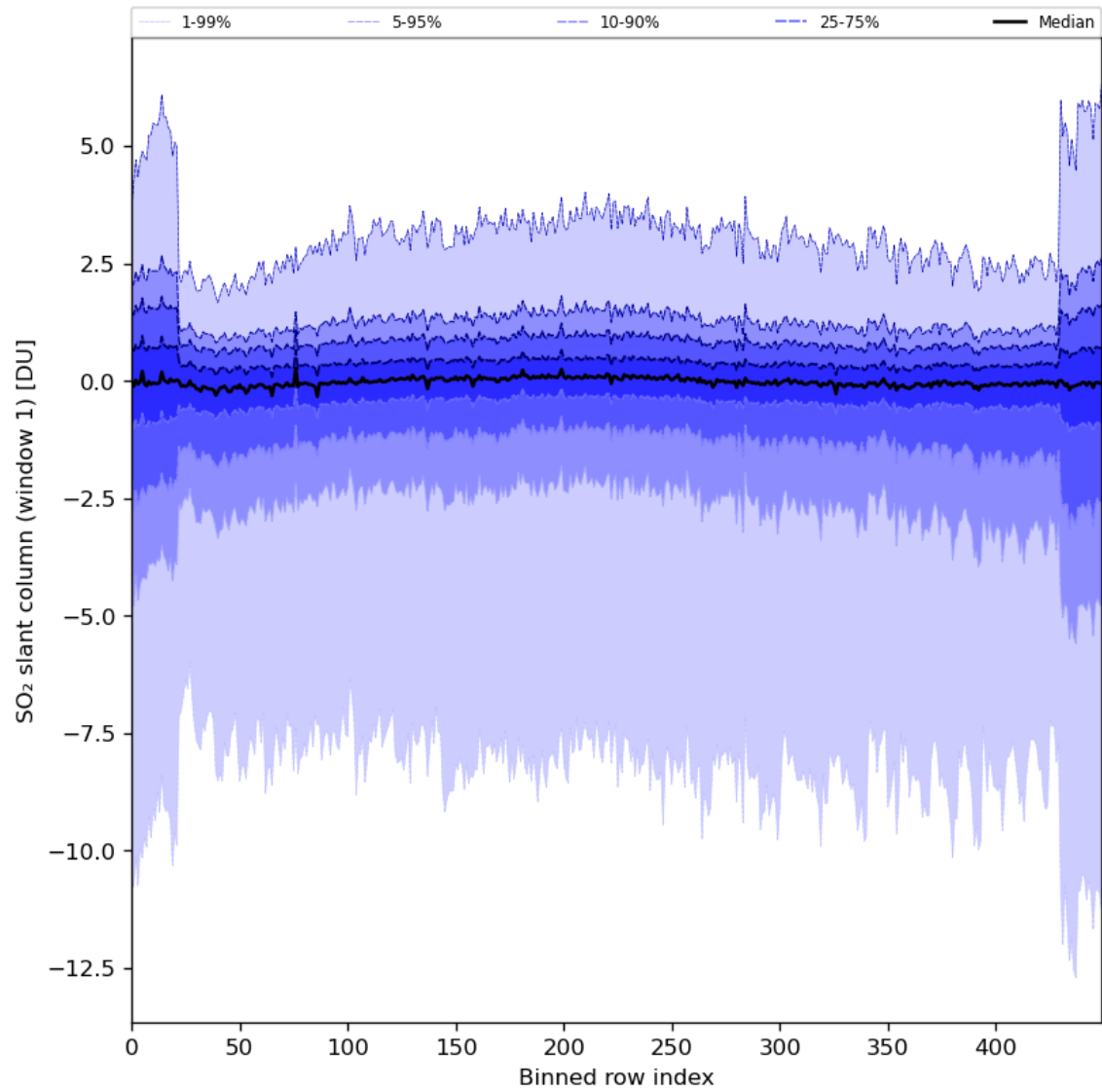
Figure 79: Along track statistics of “SO 2 slant column (window 1)” for 2024-03-10 to 2024-03-12
