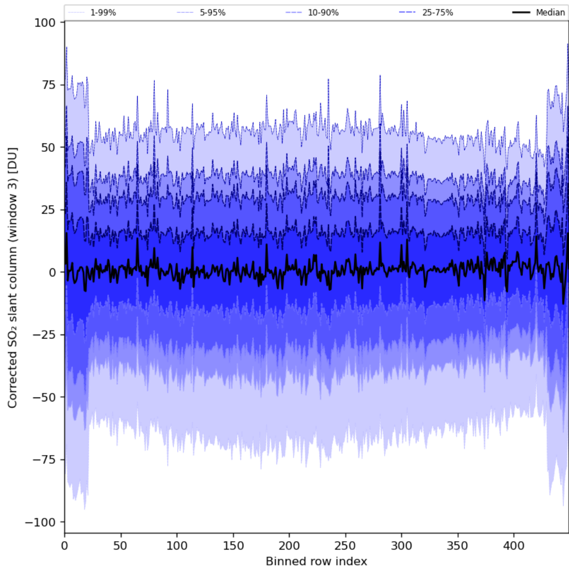
Figure 89: Along track statistics of “Corrected SO 2 slant column (window 3)” for 2024-03-10 to 2024-03-12
