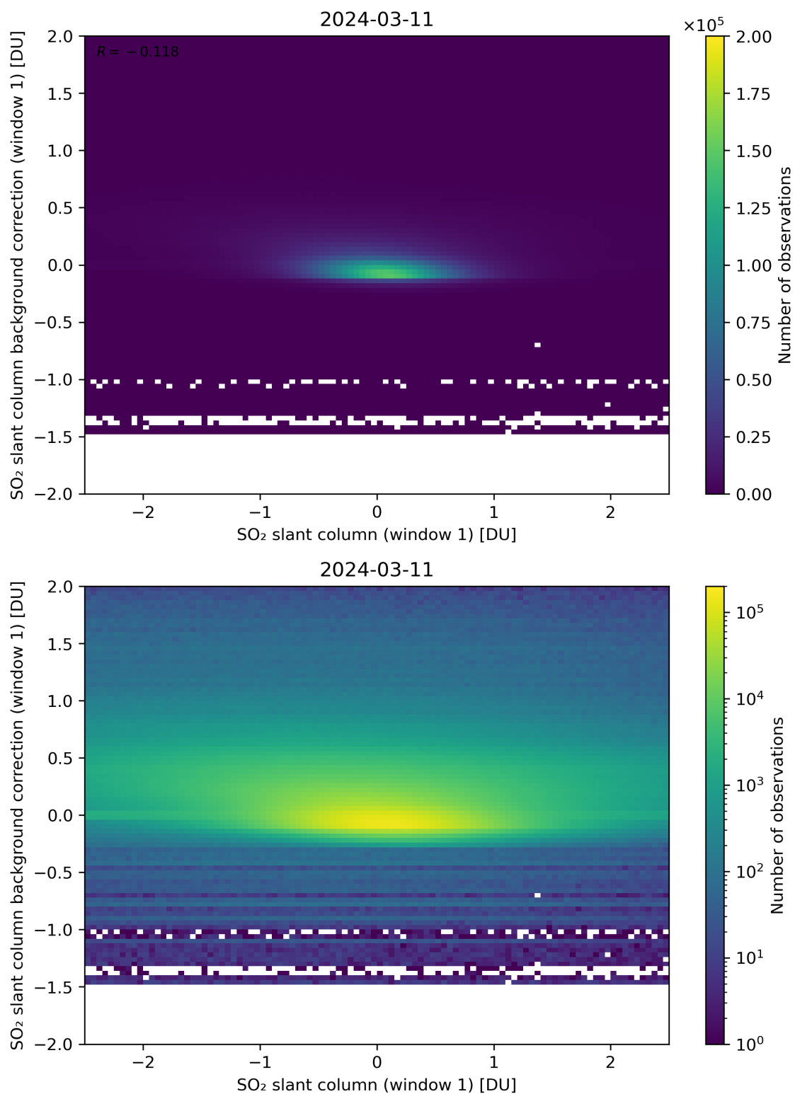
Figure 212: Scatter density plot of “SO 2 slant column (window 1)” against “SO 2 slant column background correction (window 1)” for 2024-03-10 to 2024-03-12.
