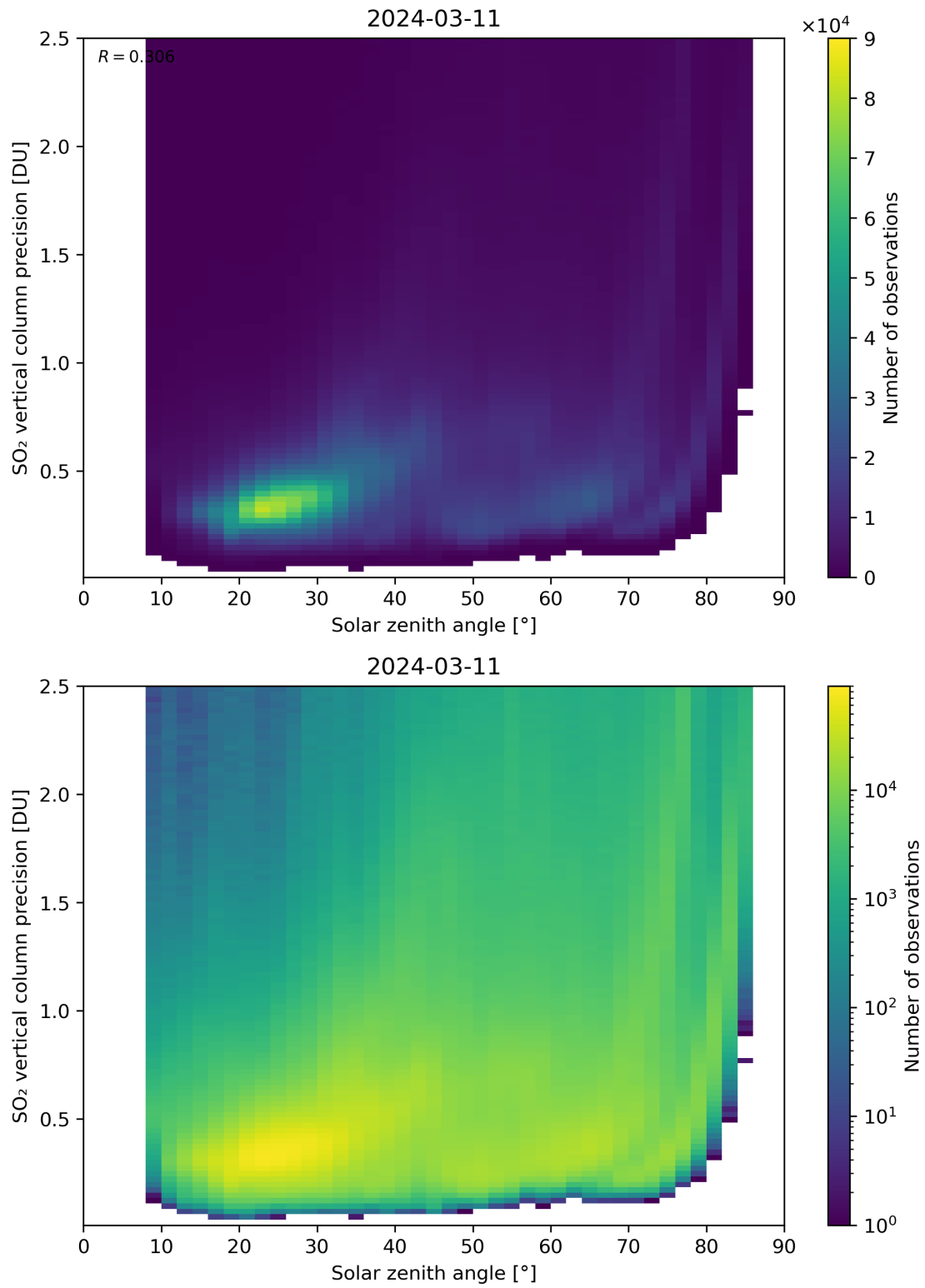
Figure 177: Scatter density plot of “Solar zenith angle” against “SO 2 vertical column precision” for 2024-03-10 to 2024-03-12.
