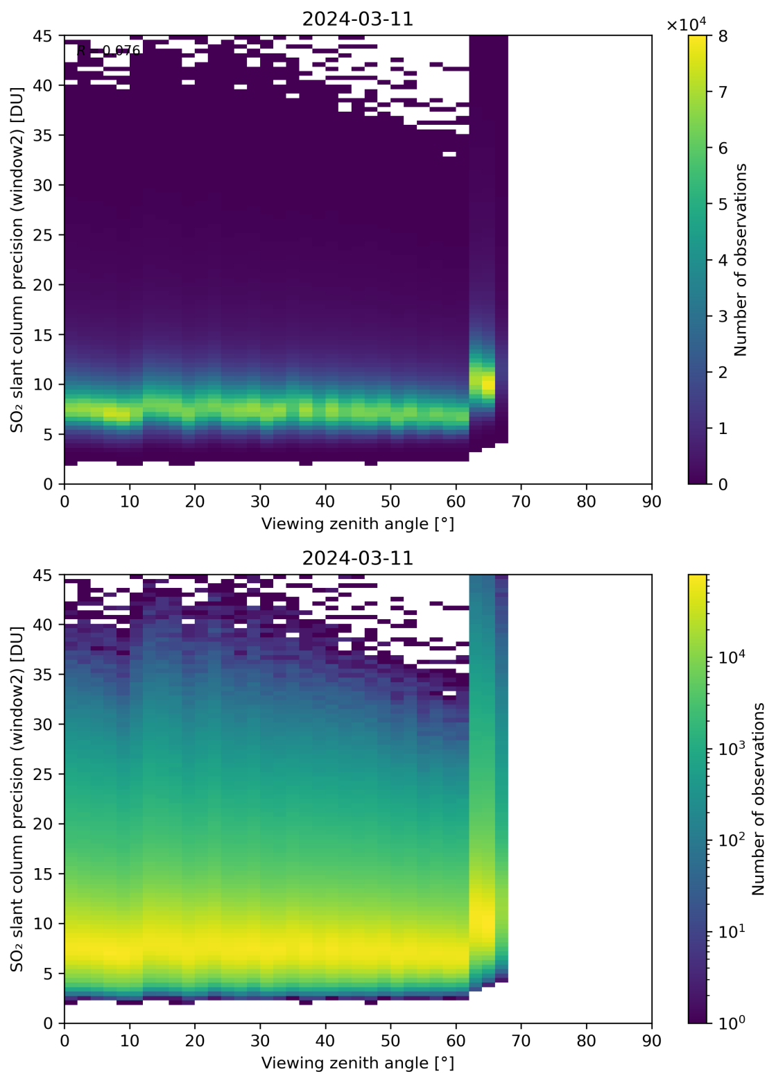
Figure 322: Scatter density plot of “Viewing zenith angle” against “SO 2 slant column precision (window2)” for 2024-03-10 to 2024-03-12.
