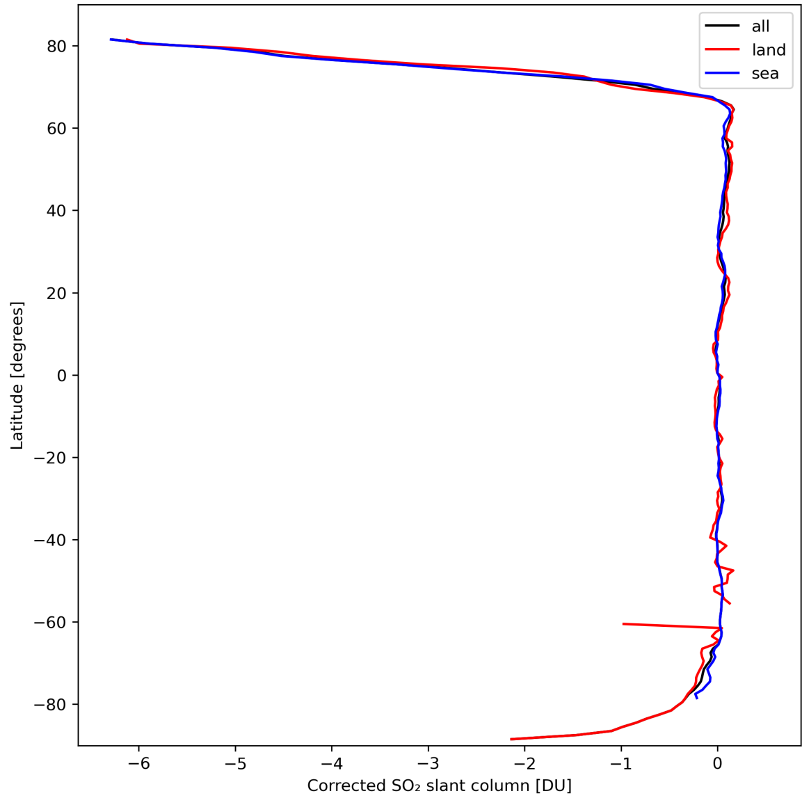
Figure 32: Zonal average of “Corrected SO 2 slant column” for 2024-03-10 to 2024-03-12.
