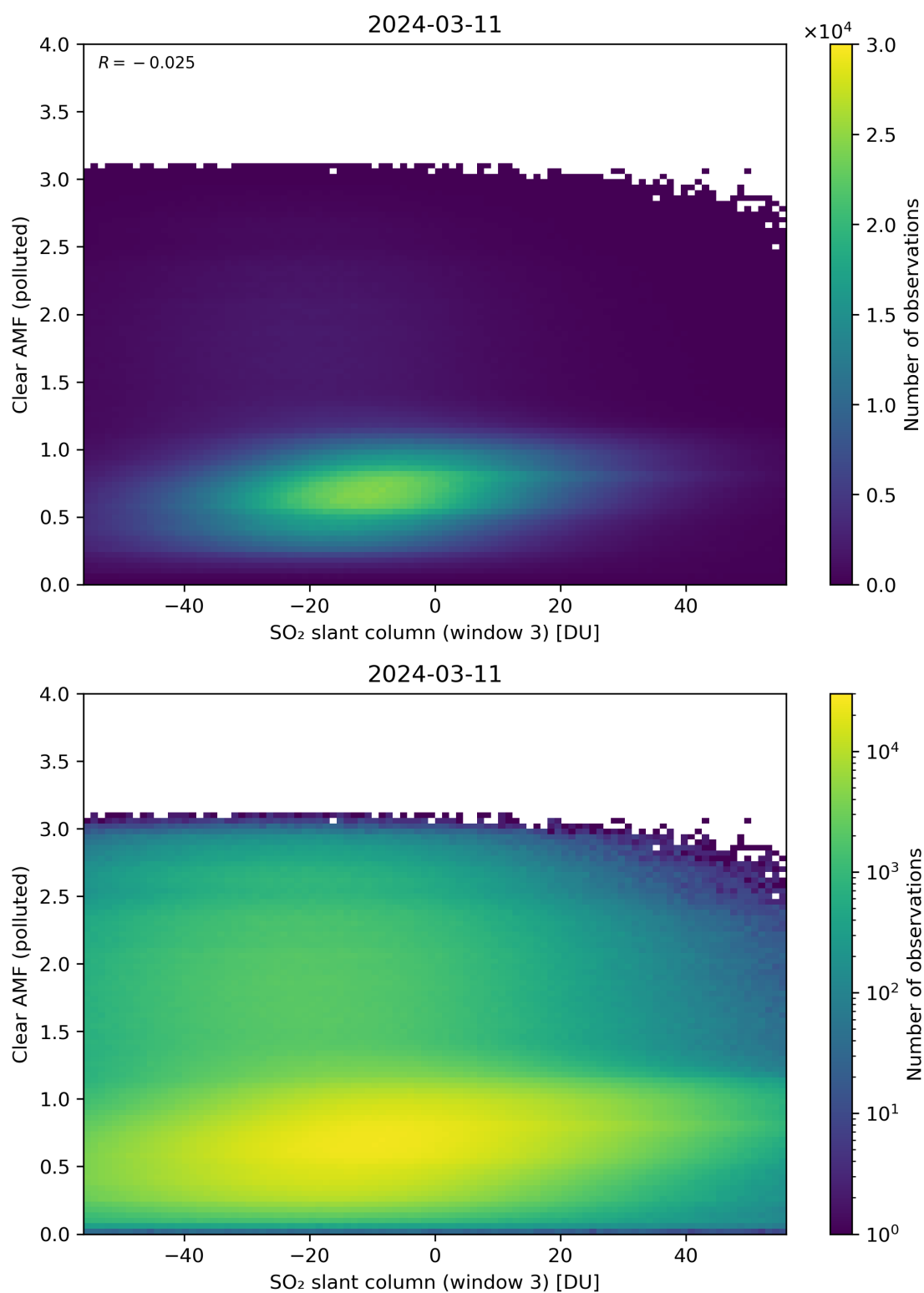
Figure 265: Scatter density plot of “SO 2 slant column (window 3)” against “Clear AMF (polluted)” for 2024-03-10 to 2024-03-12.
