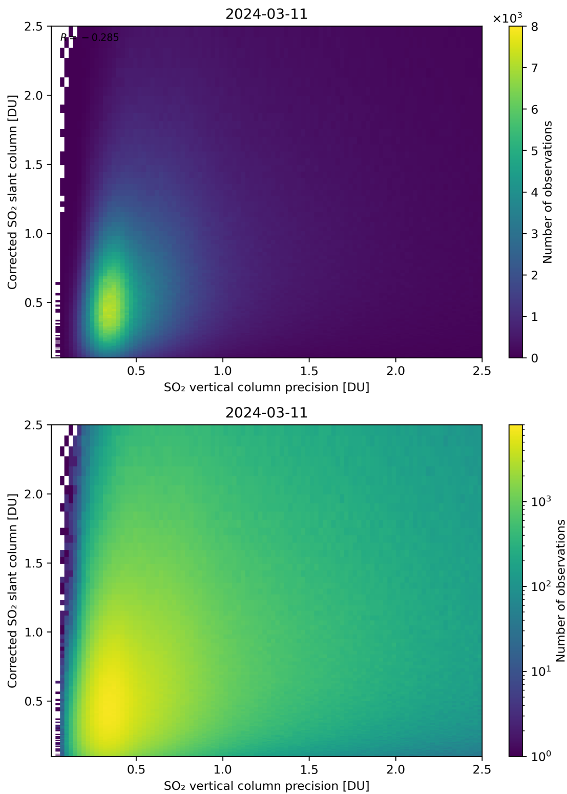
Figure 286: Scatter density plot of “SO 2 vertical column precision” against “Corrected SO 2 slant column” for 2024-03-10 to 2024-03-12.
