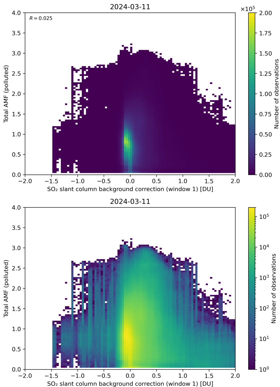
Figure 109: Scatter density plot of “SO 2 slant column background correction (window 1)” against “Total AMF (polluted)” for 2024-03-10 to 2024-03-12.
