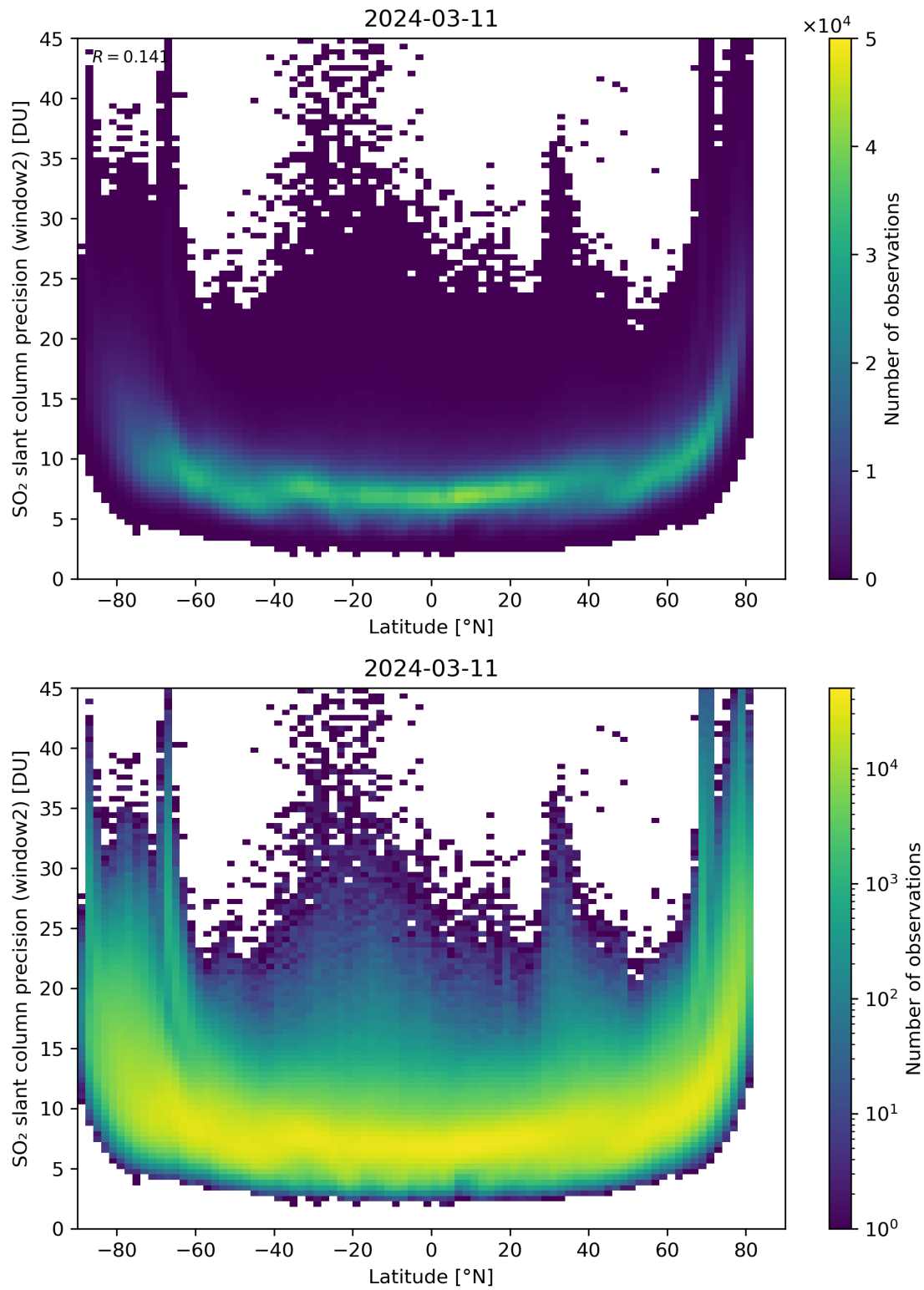
Figure 151: Scatter density plot of “Latitude” against “SO 2 slant column precision (window2)” for 2024-03-10 to 2024-03-12.
