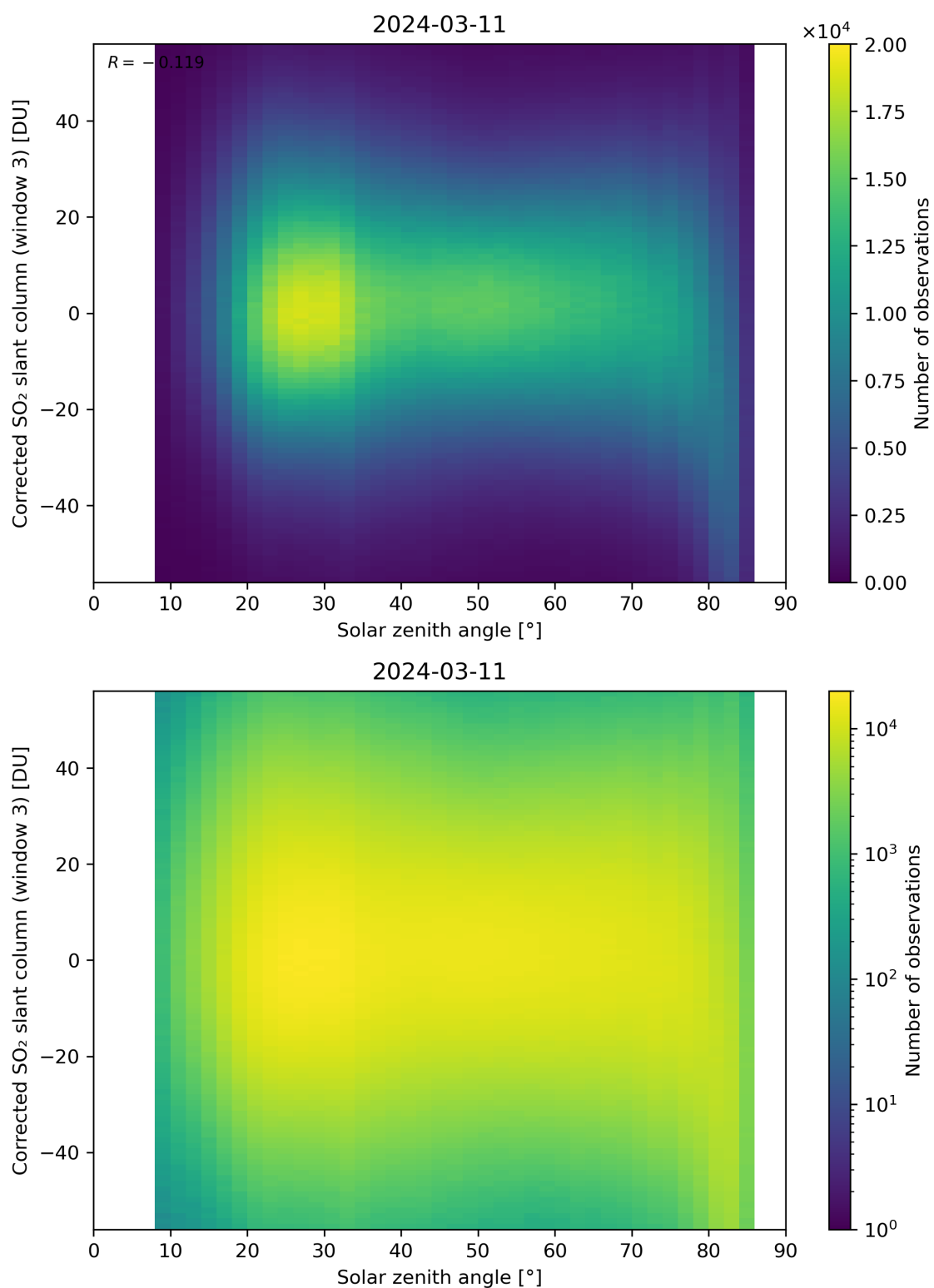
Figure 168: Scatter density plot of “Solar zenith angle” against “Corrected SO 2 slant column (window 3)” for 2024-03-10 to 2024-03-12.
