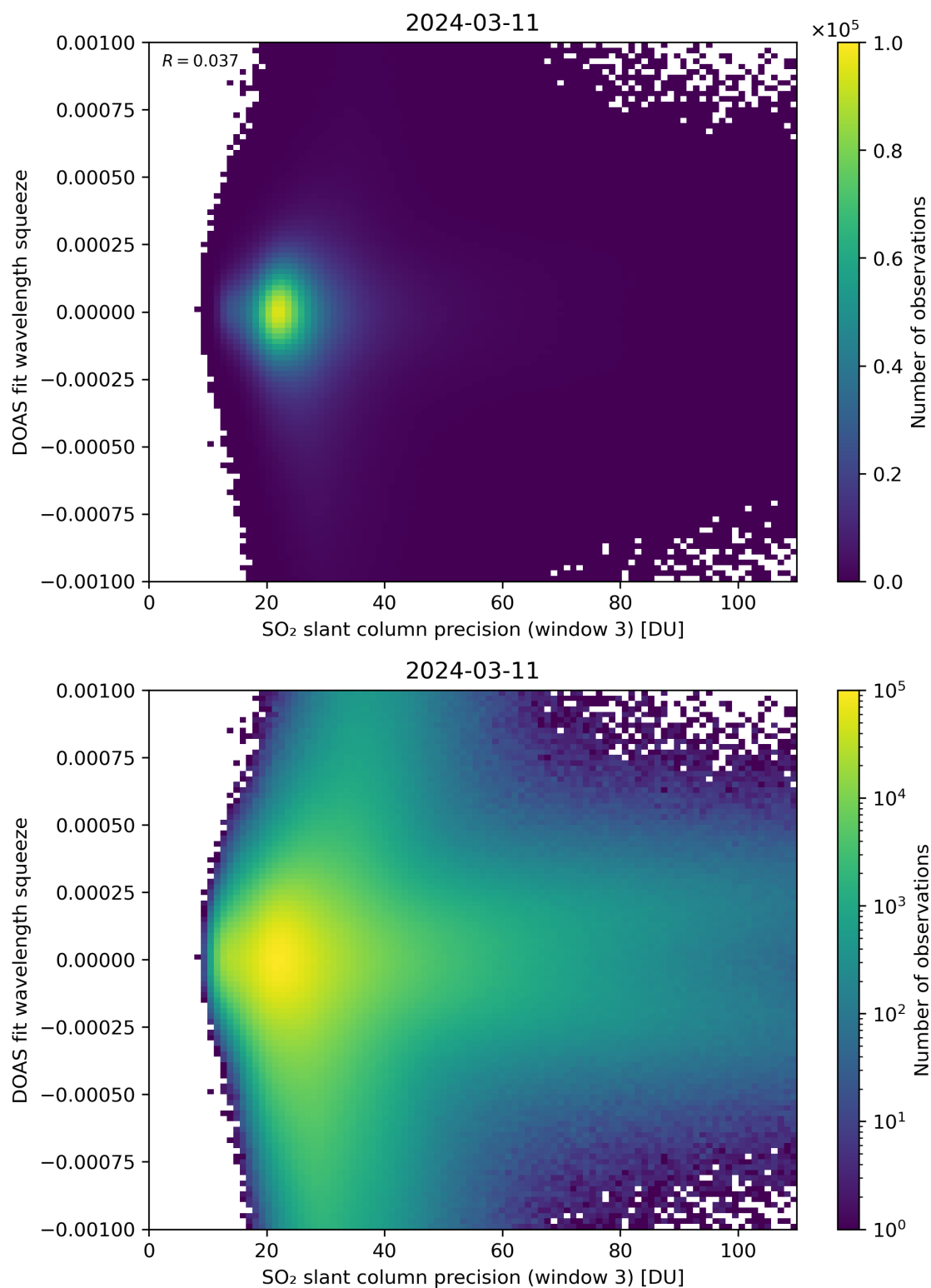
Figure 259: Scatter density plot of “SO 2 slant column precision (window 3)” against “DOAS fit wavelength squeeze” for 2024-03-10 to 2024-03-12.
