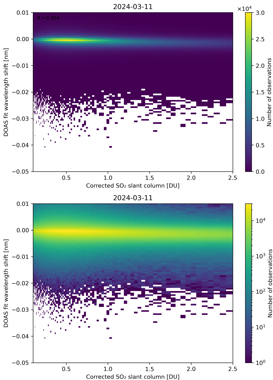
Figure 181: Scatter density plot of “Corrected SO 2 slant column” against “DOAS fit wavelength shift” for 2024-03-10 to 2024-03-12.
