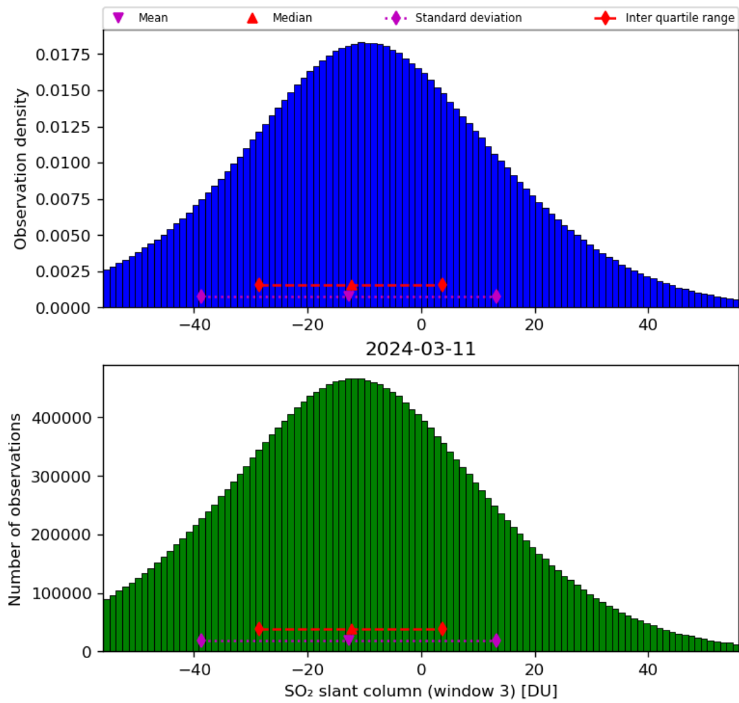
Figure 64: Histogram of “SO 2 slant column (window 3)” for 2024-03-10 to 2024-03-12
