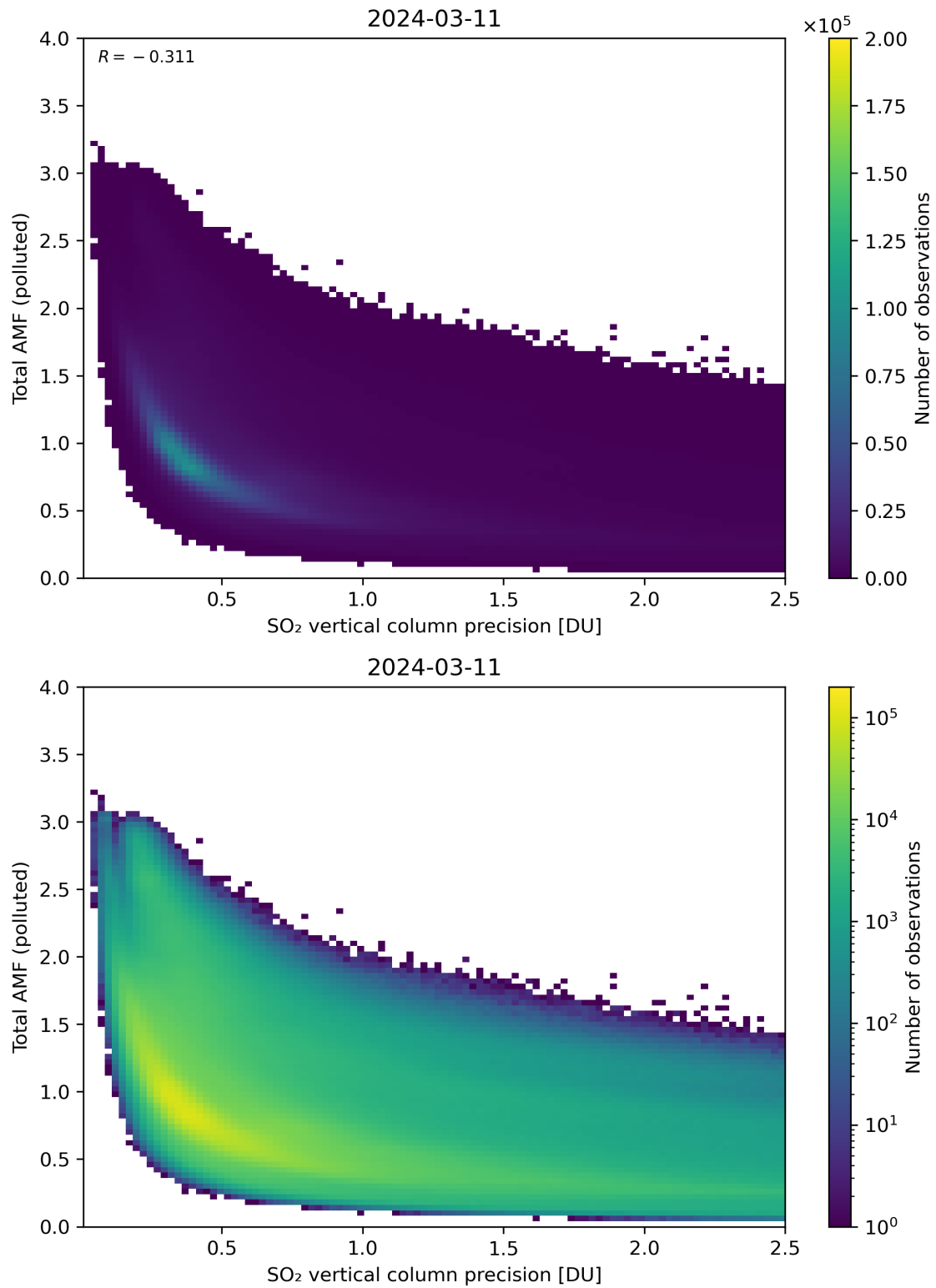
Figure 294: Scatter density plot of “SO 2 vertical column precision” against “Total AMF (polluted)” for 2024-03-10 to 2024-03-12.
