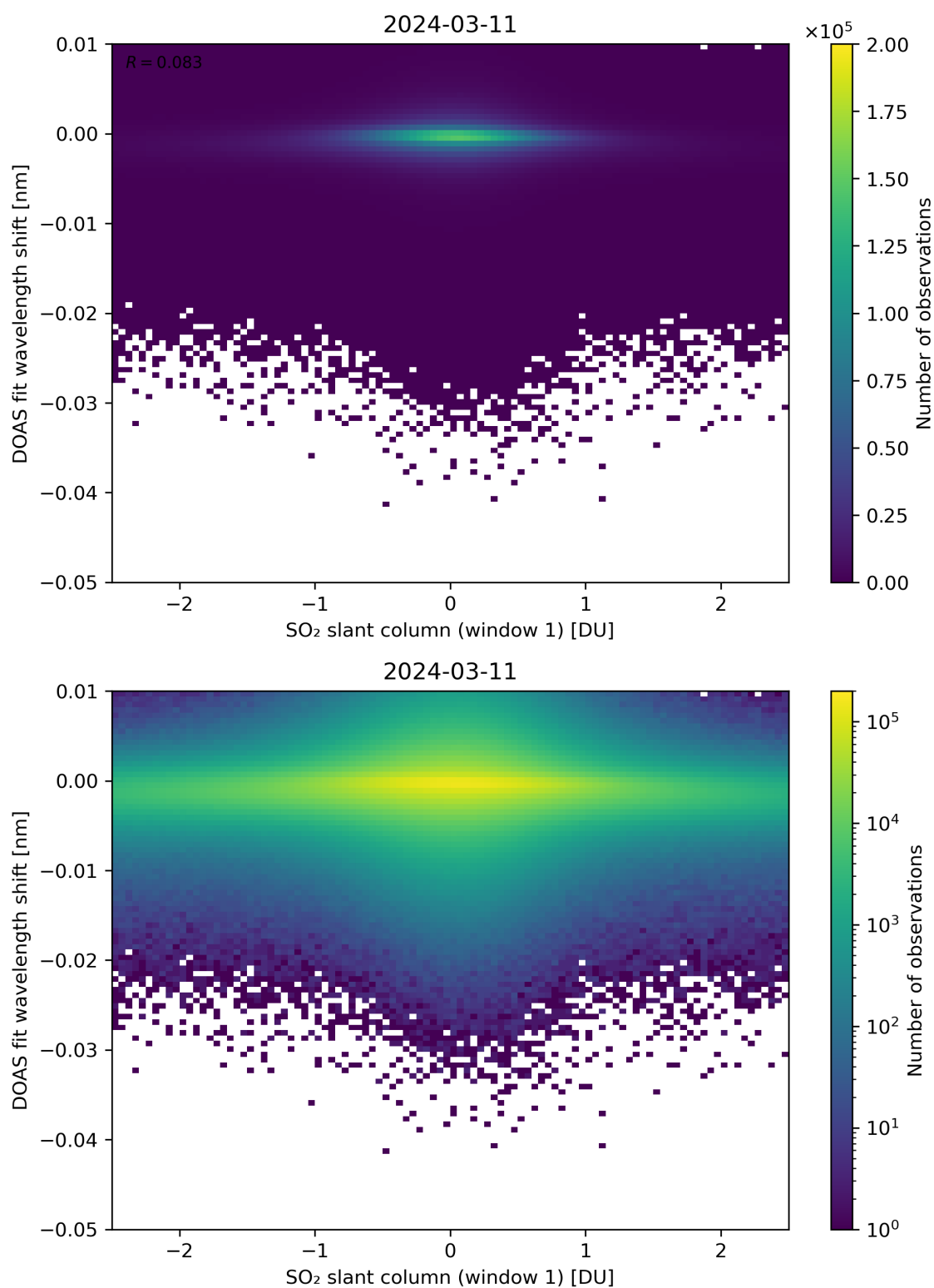
Figure 215: Scatter density plot of “SO 2 slant column (window 1)” against “DOAS fit wavelength shift” for 2024-03-10 to 2024-03-12.
