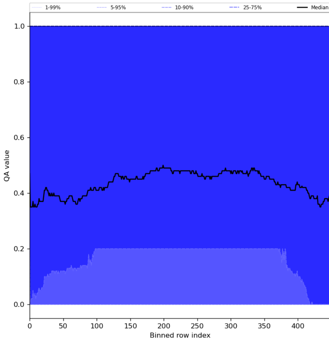
Figure 75: Along track statistics of “QA value” for 2024-03-10 to 2024-03-12
