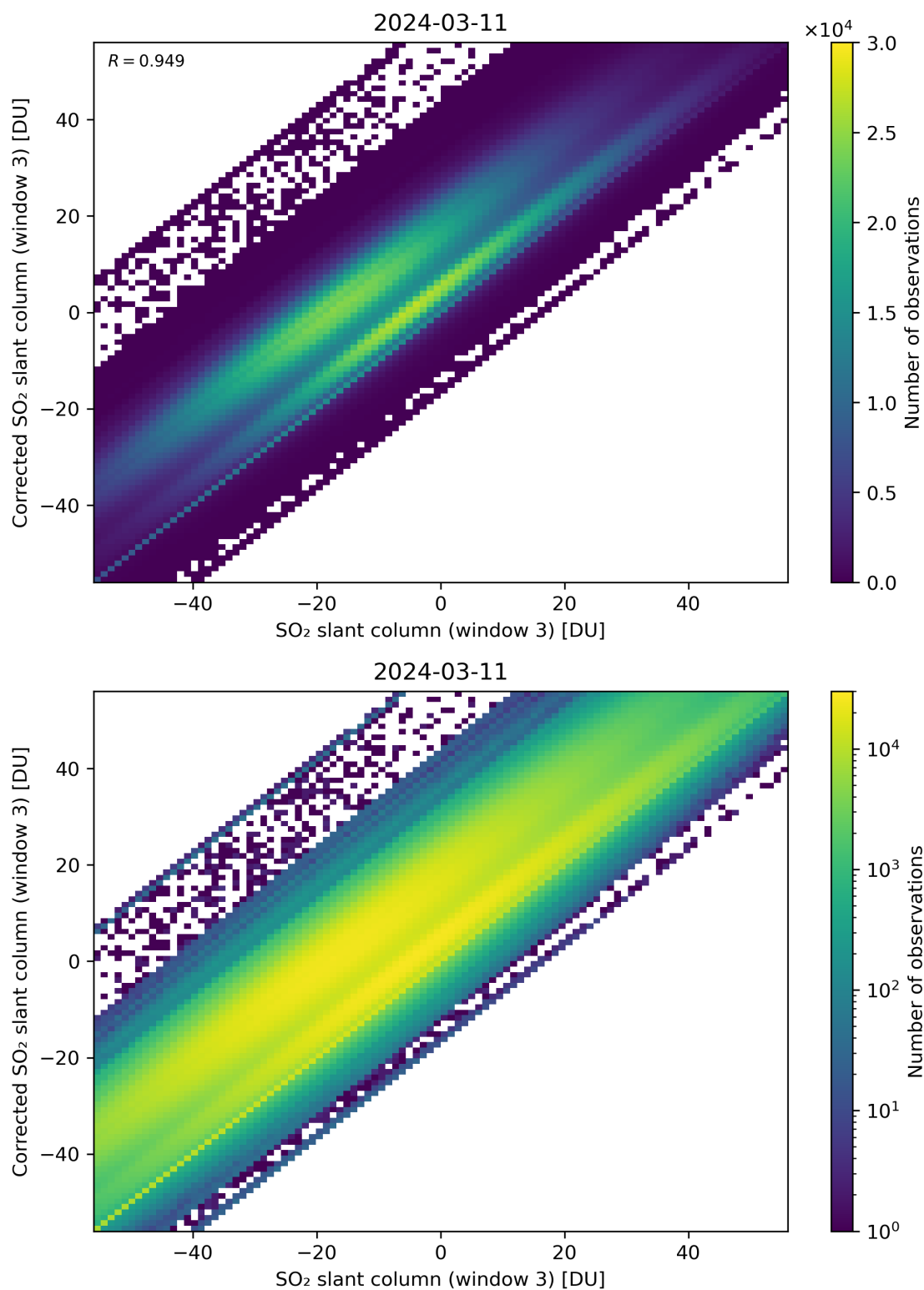
Figure 266: Scatter density plot of “SO 2 slant column (window 3)” against “Corrected SO 2 slant column (window 3)” for 2024-03-10 to 2024-03-12.
