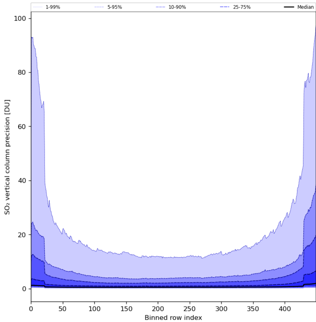
Figure 77: Along track statistics of “SO 2 vertical column precision” for 2024-03-10 to 2024-03-12
