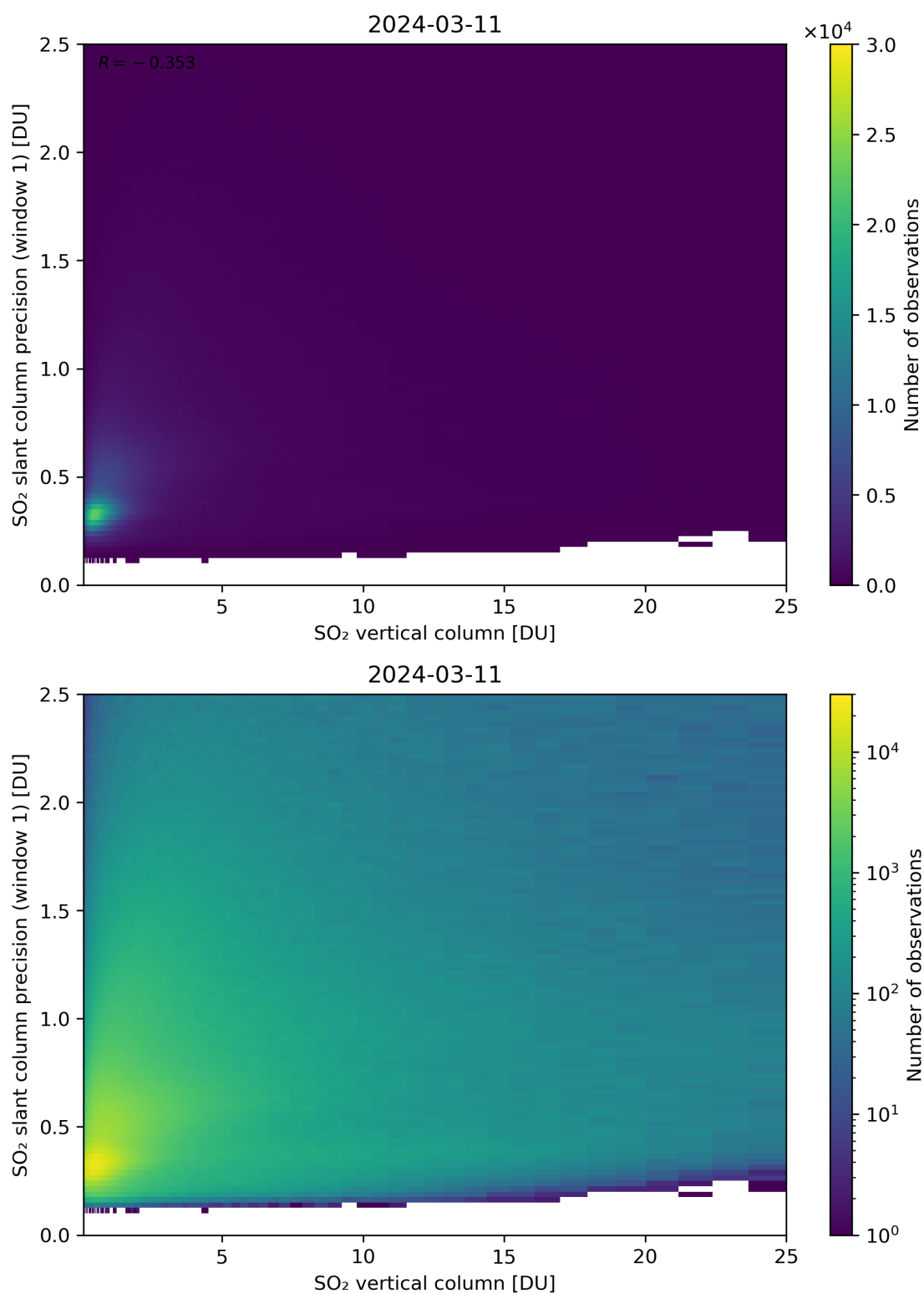
Figure 301: Scatter density plot of “SO 2 vertical column” against “SO 2 slant column precision (window 1)” for 2024-03-10 to 2024-03-12.
