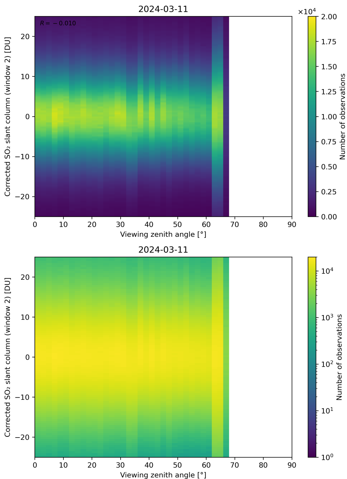
Figure 318: Scatter density plot of “Viewing zenith angle” against “Corrected SO 2 slant column (window 2)” for 2024-03-10 to 2024-03-12.
