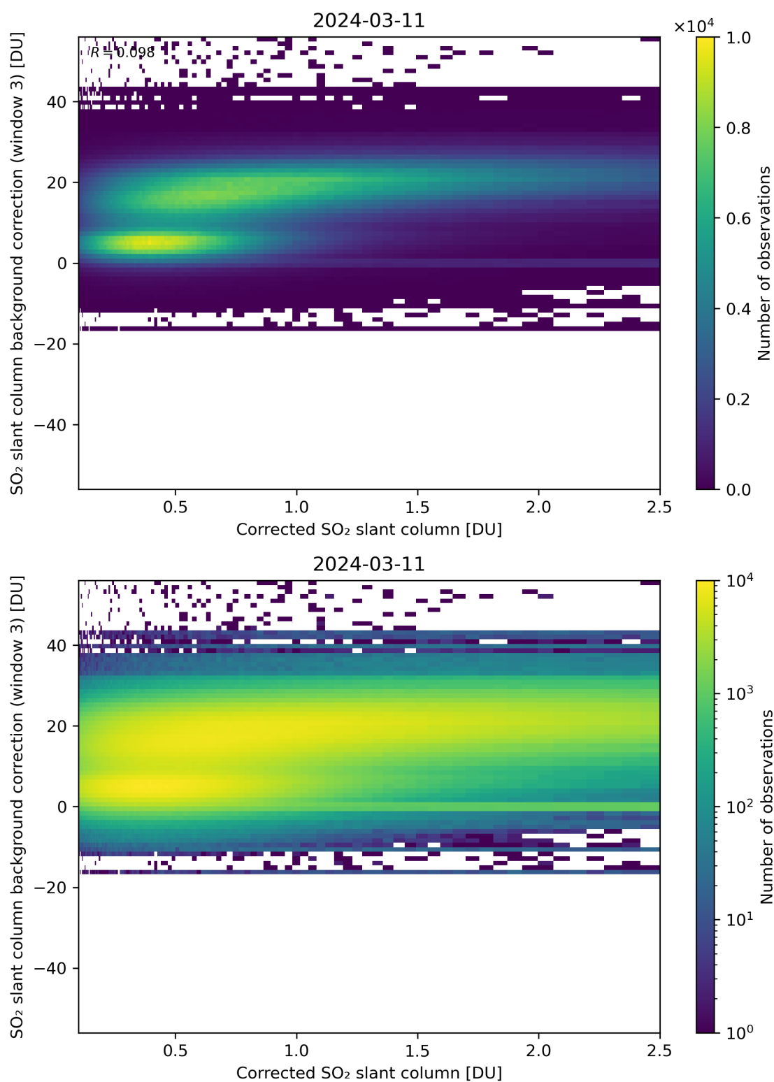
Figure 180: Scatter density plot of “Corrected SO 2 slant column” against “SO 2 slant column background correction (window 3)” for 2024-03-10 to 2024-03-12.
