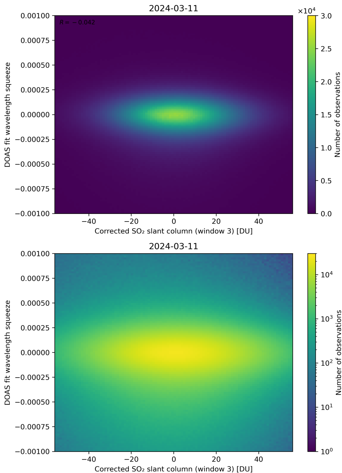
Figure 207: Scatter density plot of “Corrected SO 2 slant column (window 3)” against “DOAS fit wavelength squeeze” for 2024-03-10 to 2024-03-12.
