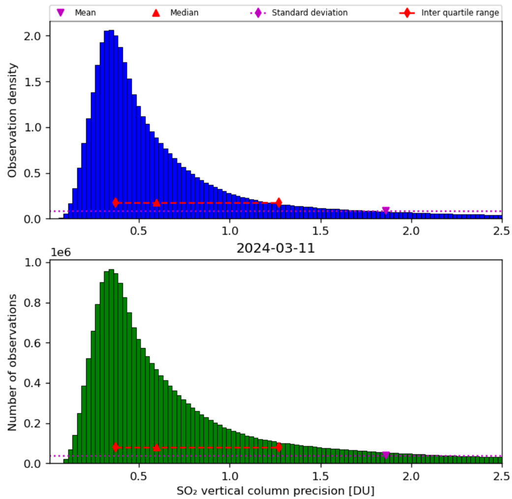
Figure 54: Histogram of “SO 2 vertical column precision” for 2024-03-10 to 2024-03-12
