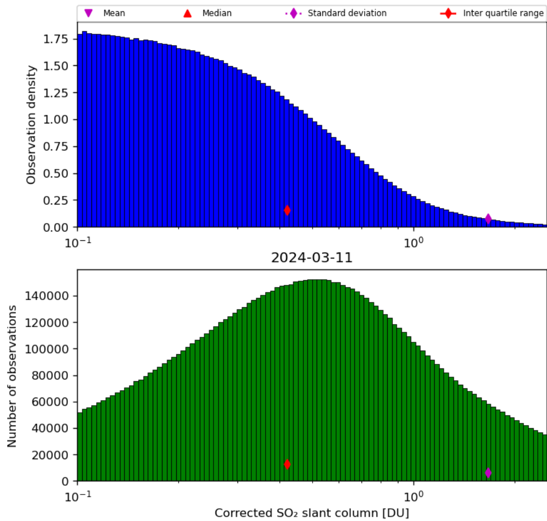
Figure 55: Histogram of “Corrected SO 2 slant column” for 2024-03-10 to 2024-03-12
