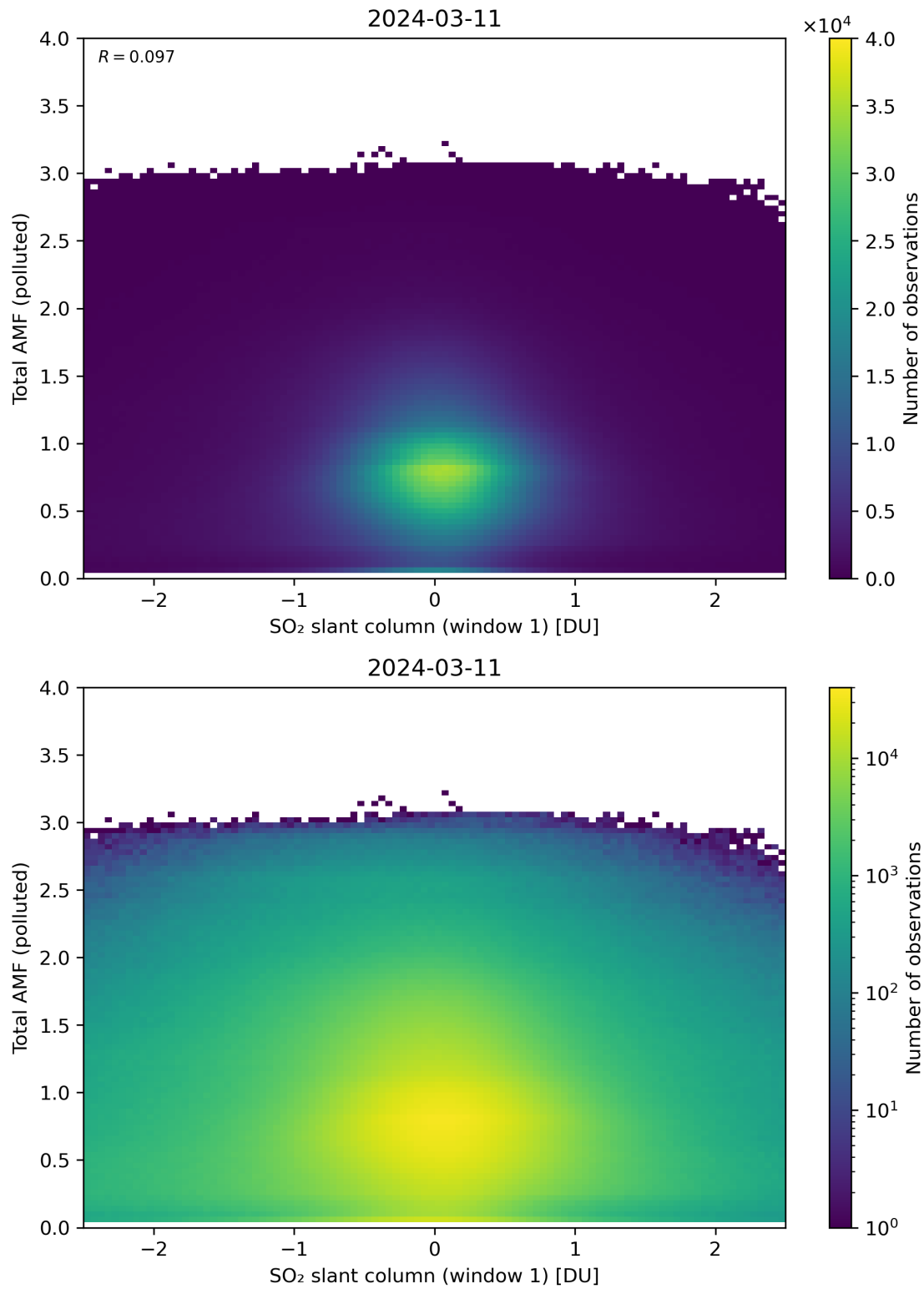
Figure 239: Scatter density plot of “SO 2 slant column (window 1)” against “Total AMF (polluted)” for 2024-03-10 to 2024-03-12.
