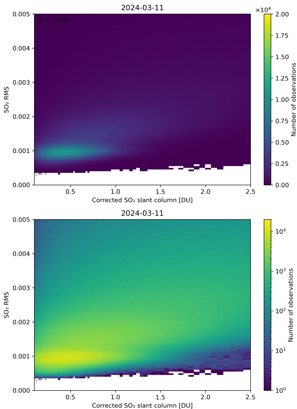
Figure 183: Scatter density plot of “Corrected SO 2 slant column” against “SO 2 RMS” for 2024-03-10 to 2024-03-12.
