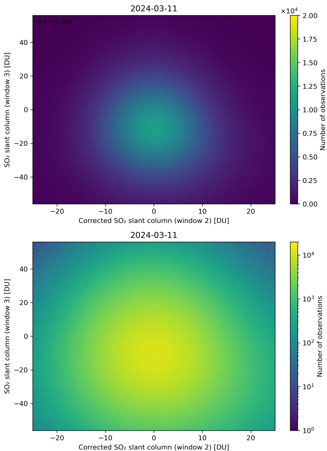
Figure 201: Scatter density plot of “Corrected SO 2 slant column (window 2)” against “SO 2 slant column (window 3)” for 2024-03-10 to 2024-03-12.
