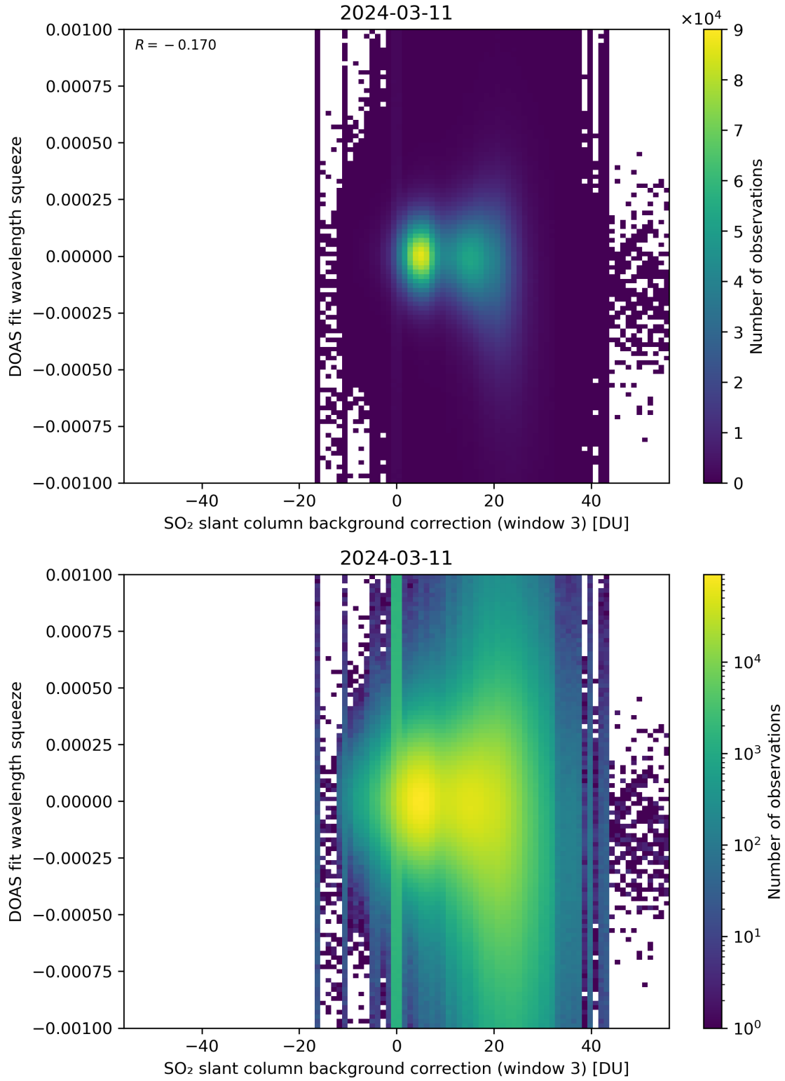
Figure 122: Scatter density plot of “SO 2 slant column background correction (window 3)” against “DOAS fit wavelength squeeze” for 2024-03-10 to 2024-03-12.
