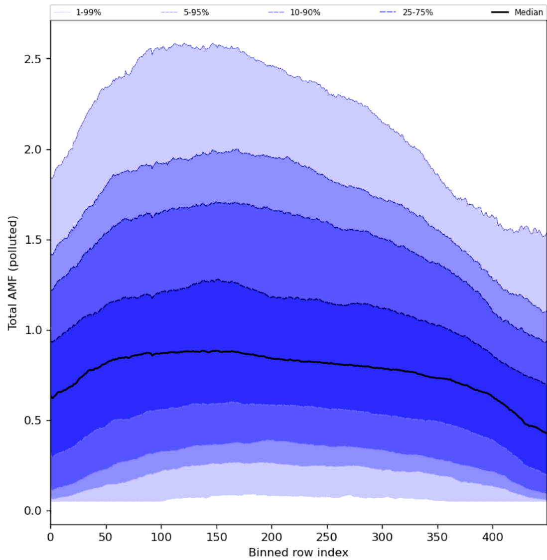
Figure 94: Along track statistics of “Total AMF (polluted)” for 2024-03-10 to 2024-03-12
