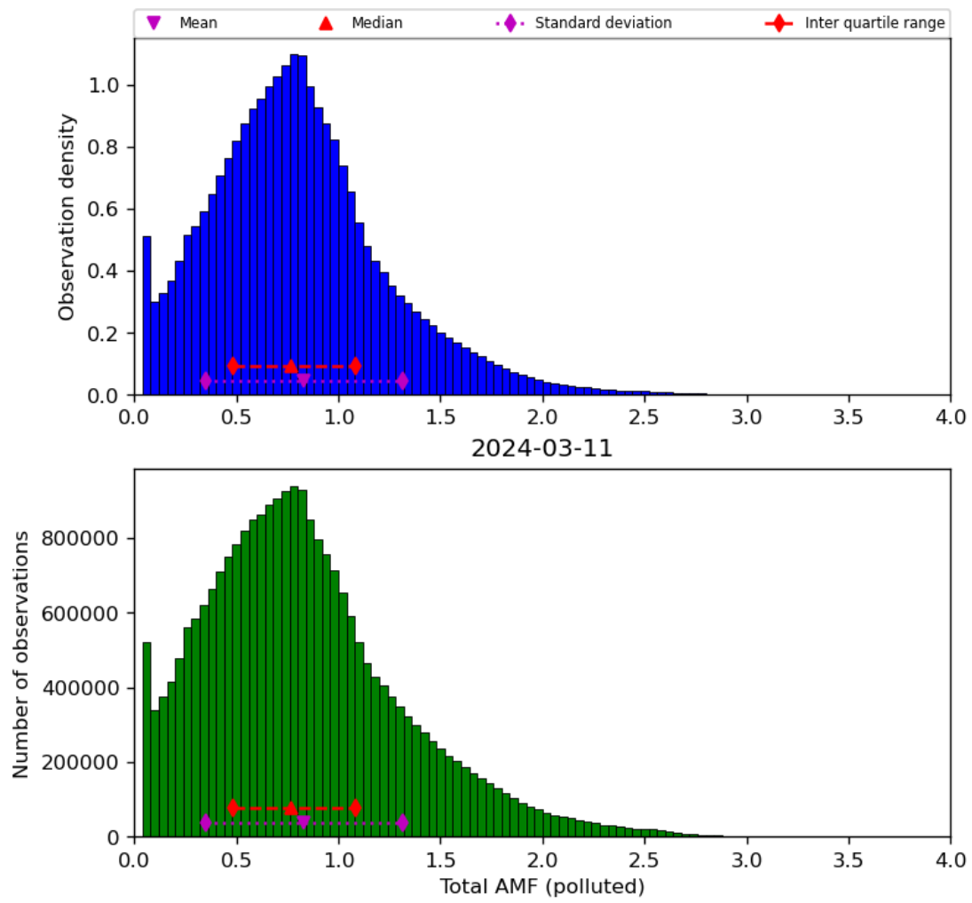
Figure 71: Histogram of “Total AMF (polluted)” for 2024-03-10 to 2024-03-12
