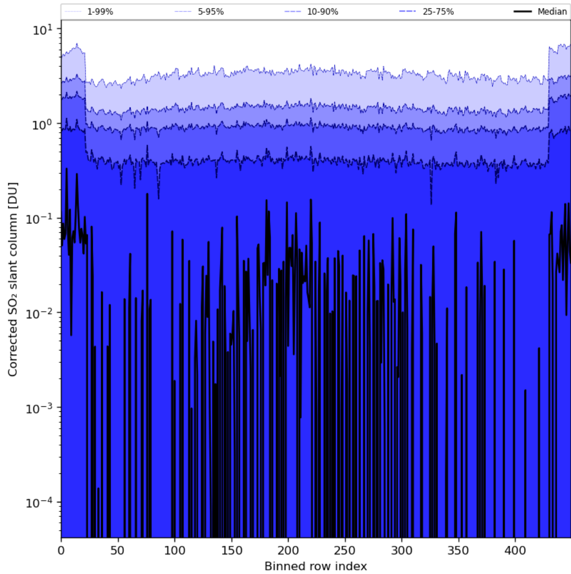
Figure 78: Along track statistics of “Corrected SO 2 slant column” for 2024-03-10 to 2024-03-12
