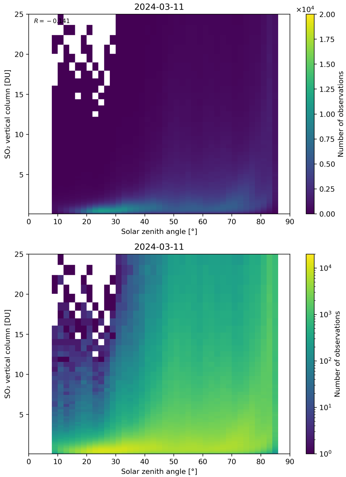
Figure 176: Scatter density plot of “Solar zenith angle” against “SO 2 vertical column” for 2024-03-10 to 2024-03-12.
