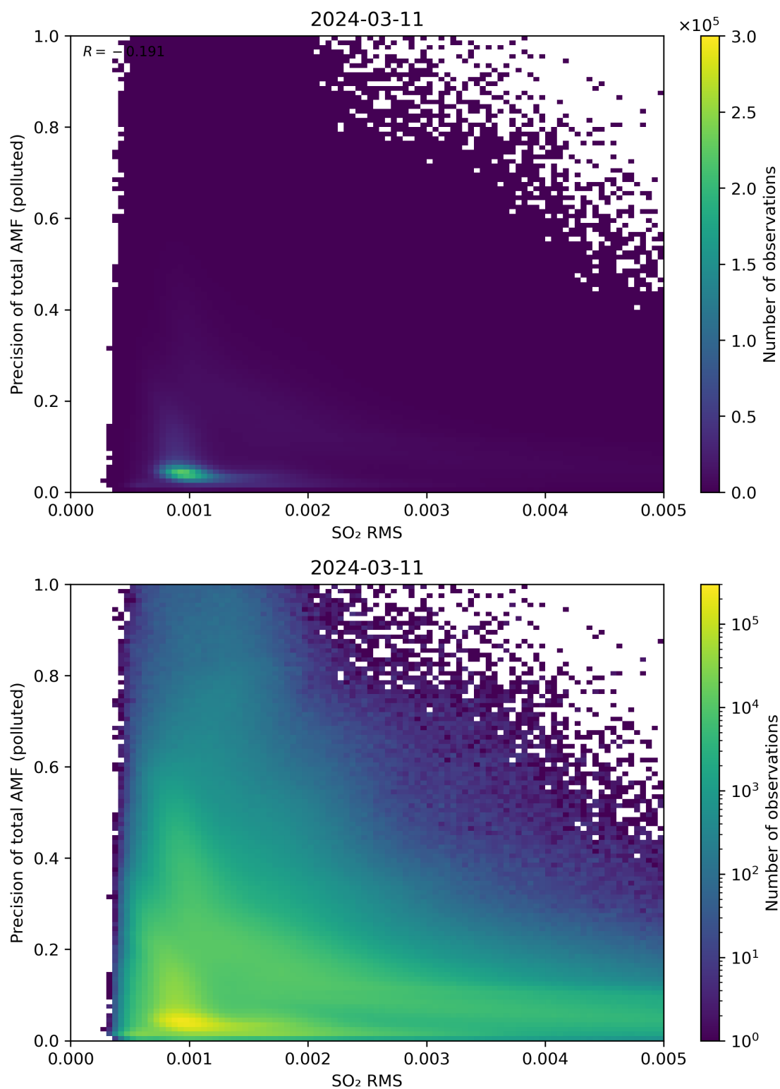
Figure 138: Scatter density plot of “SO 2 RMS” against “Precision of total AMF (polluted)” for 2024-03-10 to 2024-03-12.
