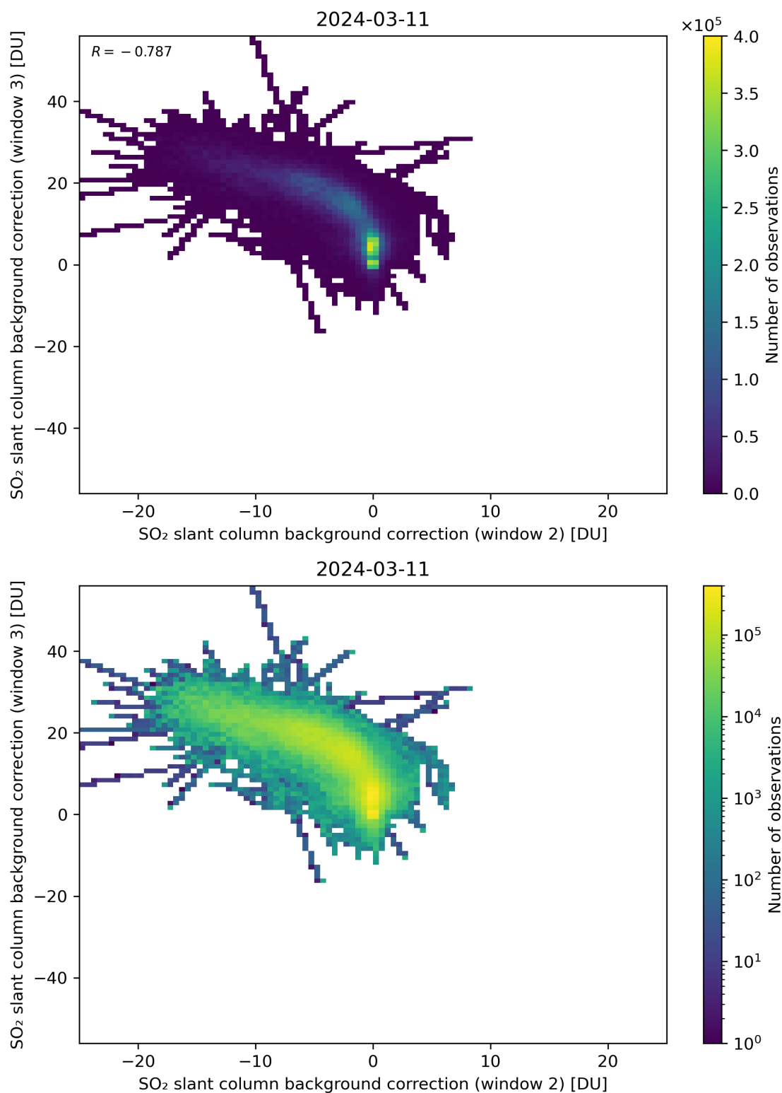
Figure 111: Scatter density plot of “SO 2 slant column background correction (window 2)” against “SO 2 slant column background correction (window 3)” for 2024-03-10 to 2024-03-12.
