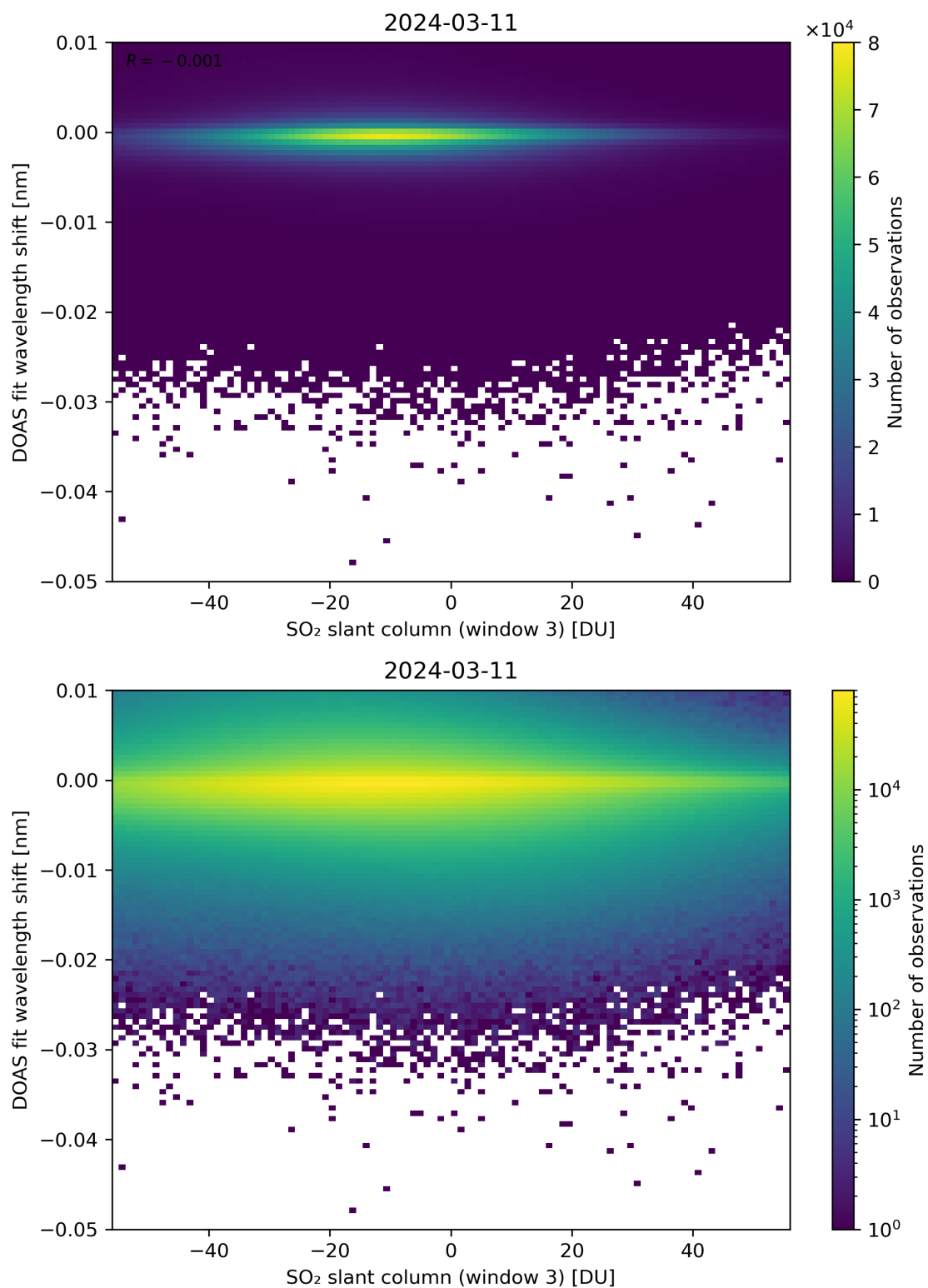
Figure 254: Scatter density plot of “SO 2 slant column (window 3)” against “DOAS fit wavelength shift” for 2024-03-10 to 2024-03-12.
