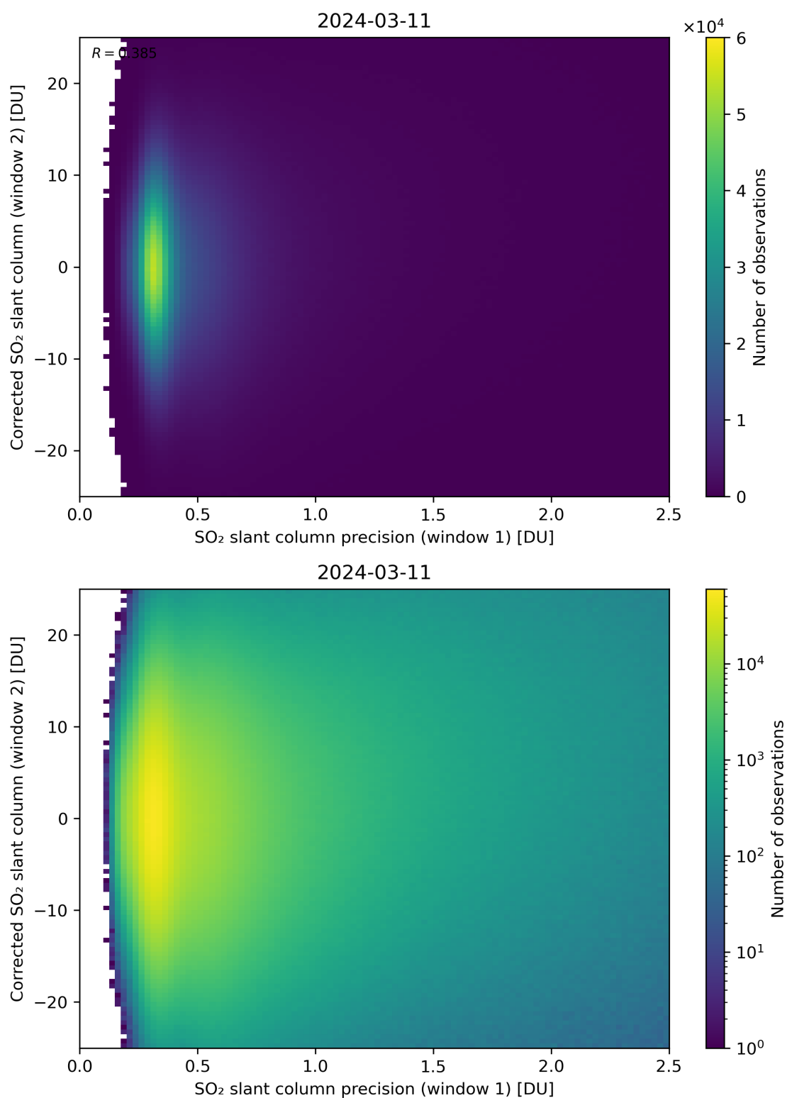
Figure 225: Scatter density plot of “SO 2 slant column precision (window 1)” against “Corrected SO 2 slant column (window 2)” for 2024-03-10 to 2024-03-12.
