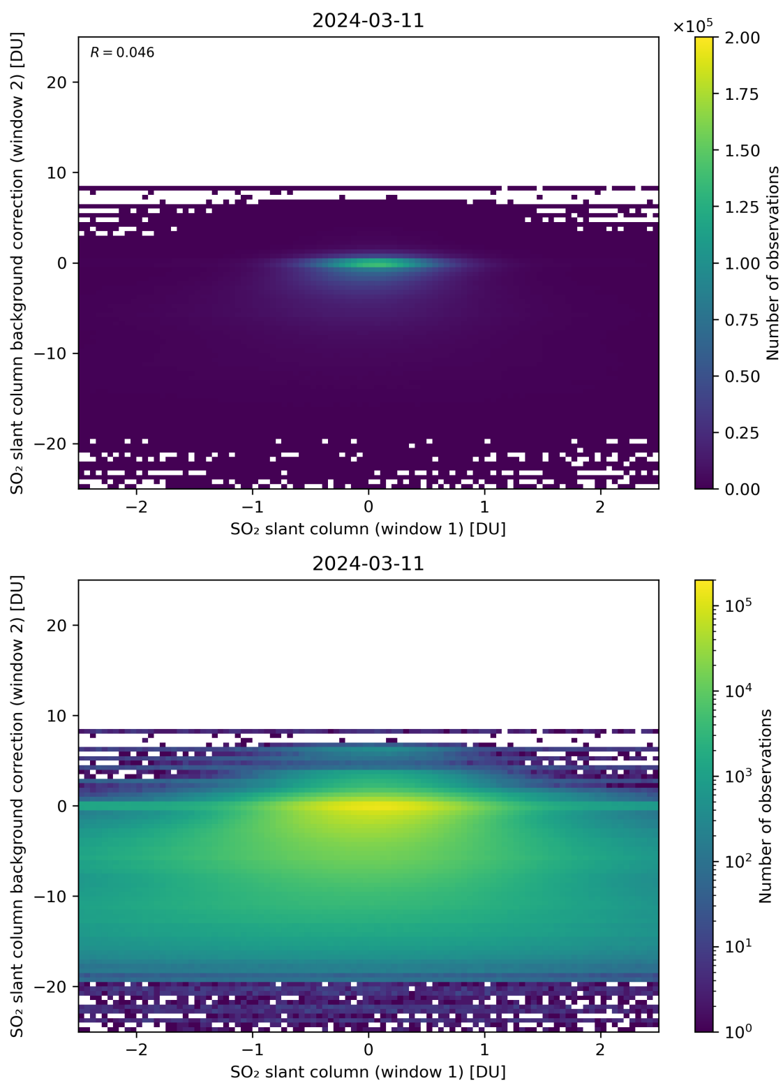
Figure 213: Scatter density plot of “SO 2 slant column (window 1)” against “SO 2 slant column background correction (window 2)” for 2024-03-10 to 2024-03-12.
