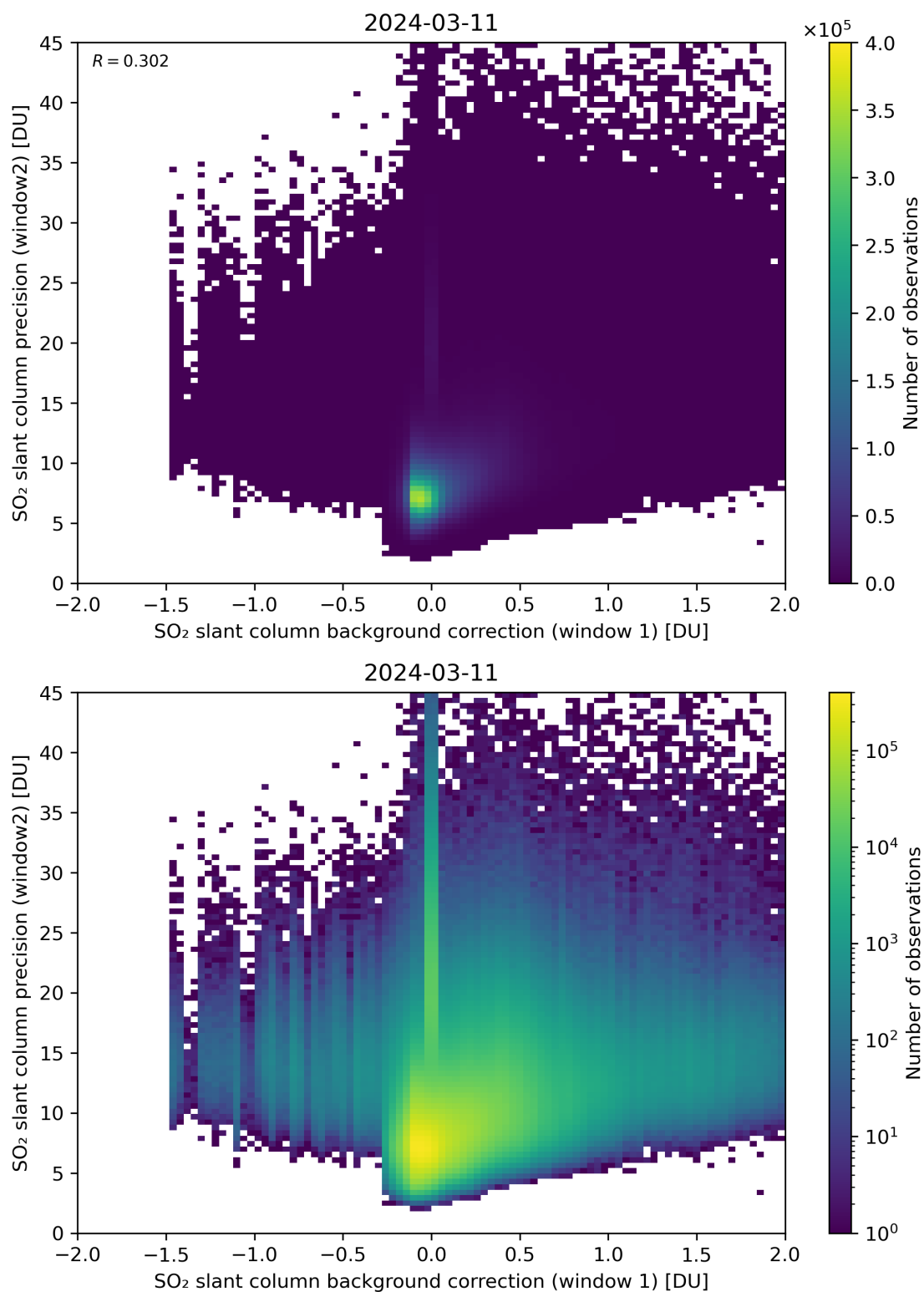
Figure 106: Scatter density plot of “SO 2 slant column background correction (window 1)” against “SO 2 slant column precision (window2)” for 2024-03-10 to 2024-03-12.
