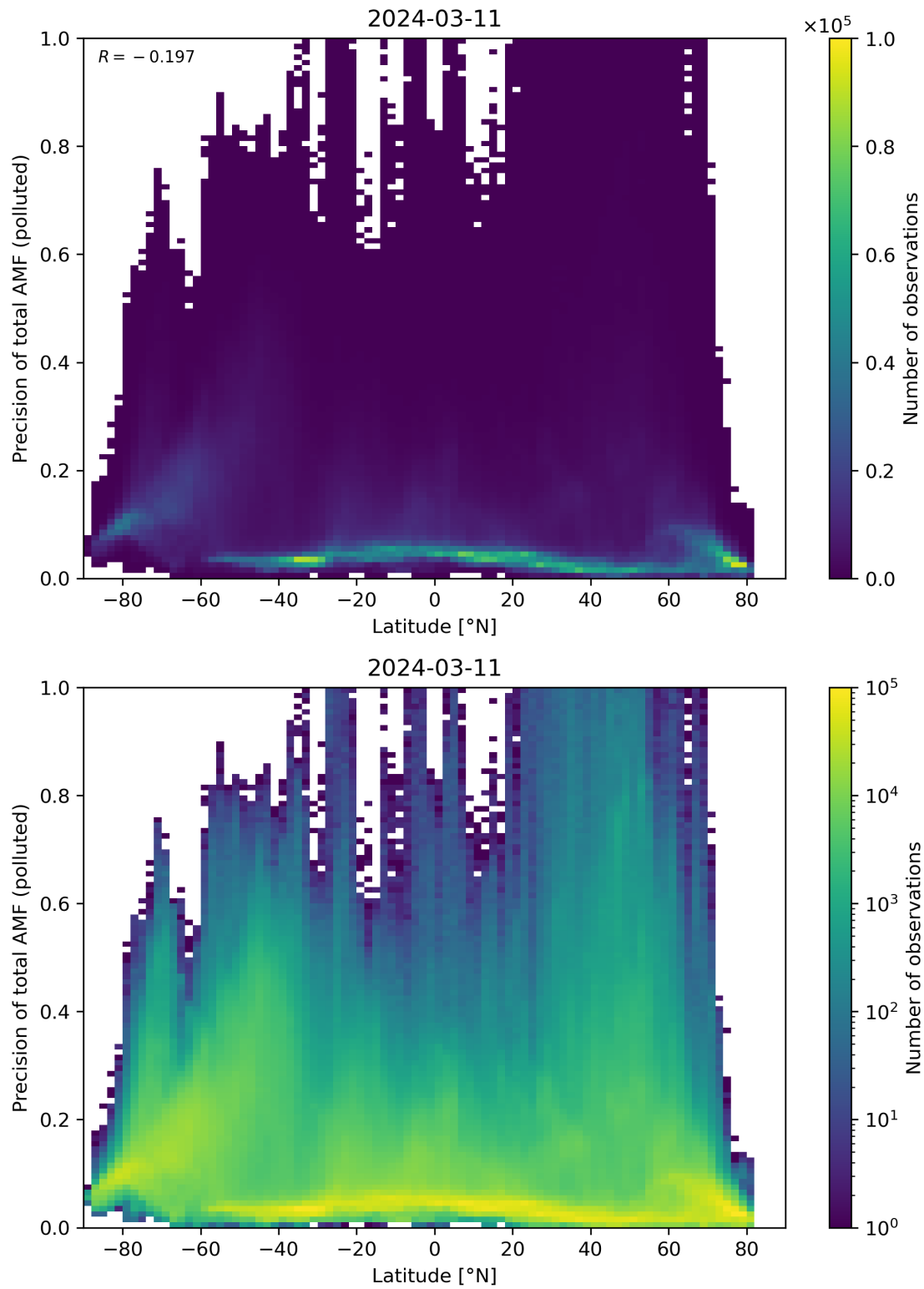
Figure 155: Scatter density plot of “Latitude” against “Precision of total AMF (polluted)” for 2024-03-10 to 2024-03-12.
