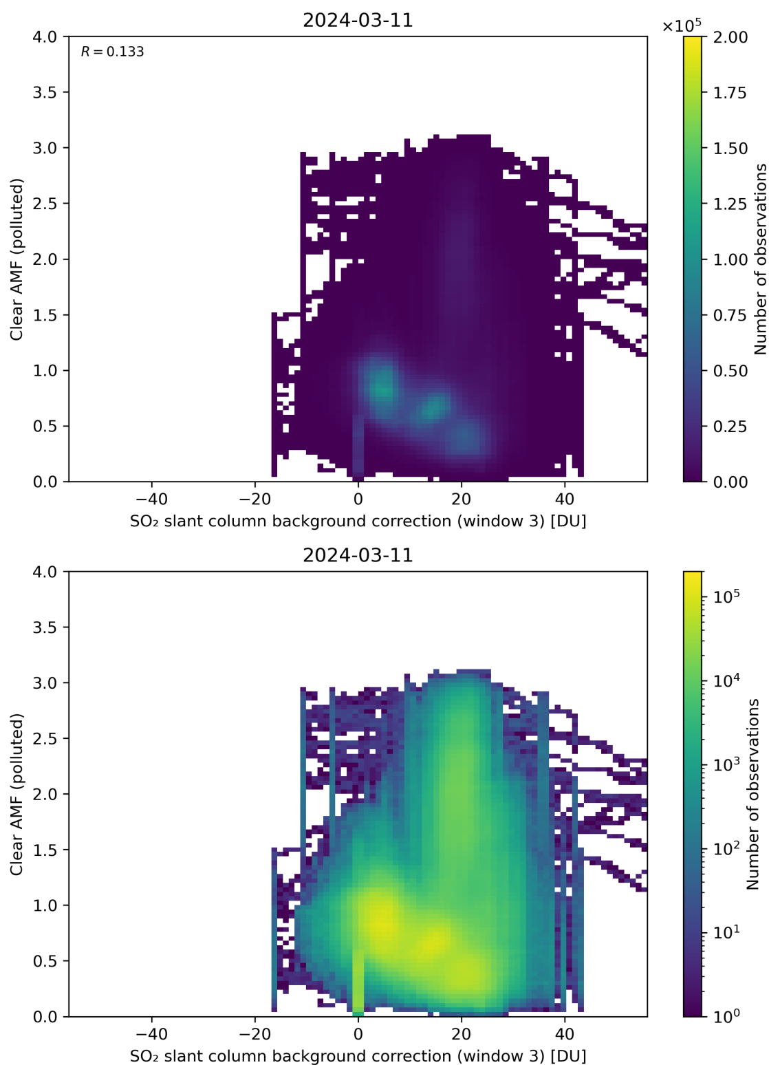
Figure 124: Scatter density plot of “SO 2 slant column background correction (window 3)” against “Clear AMF (polluted)” for 2024-03-10 to 2024-03-12.
