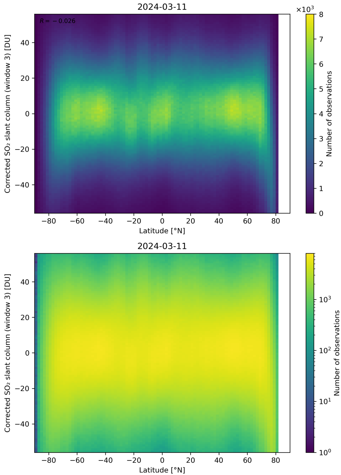
Figure 148: Scatter density plot of “Latitude” against “Corrected SO 2 slant column (window 3)” for 2024-03-10 to 2024-03-12.
