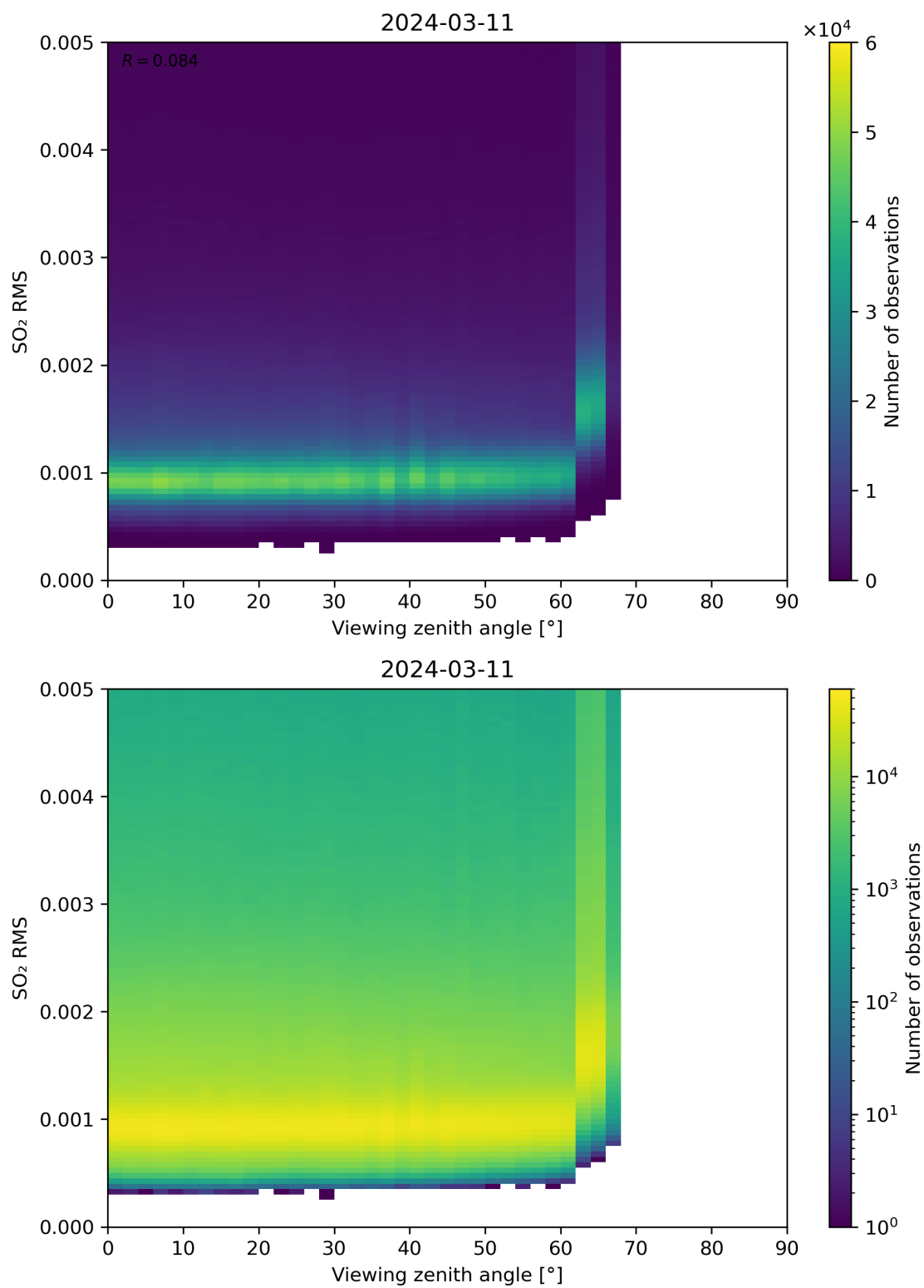
Figure 313: Scatter density plot of “Viewing zenith angle” against “SO 2 RMS” for 2024-03-10 to 2024-03-12.
