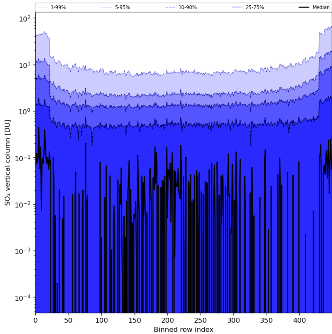
Figure 76: Along track statistics of “SO 2 vertical column” for 2024-03-10 to 2024-03-12
