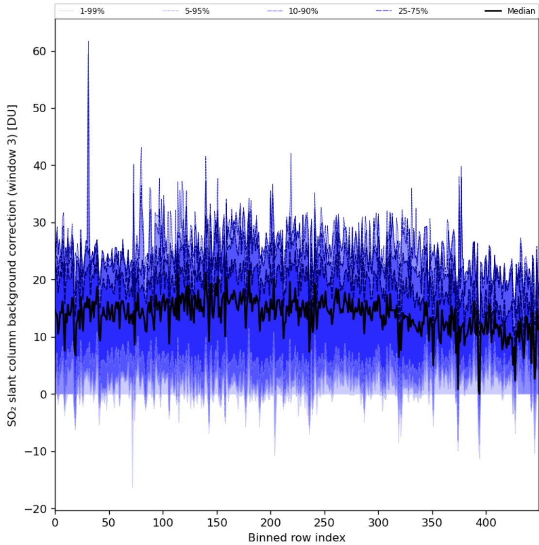
Figure 90: Along track statistics of “SO 2 slant column background correction (window 3)” for 2024-03-10 to 2024-03-12
