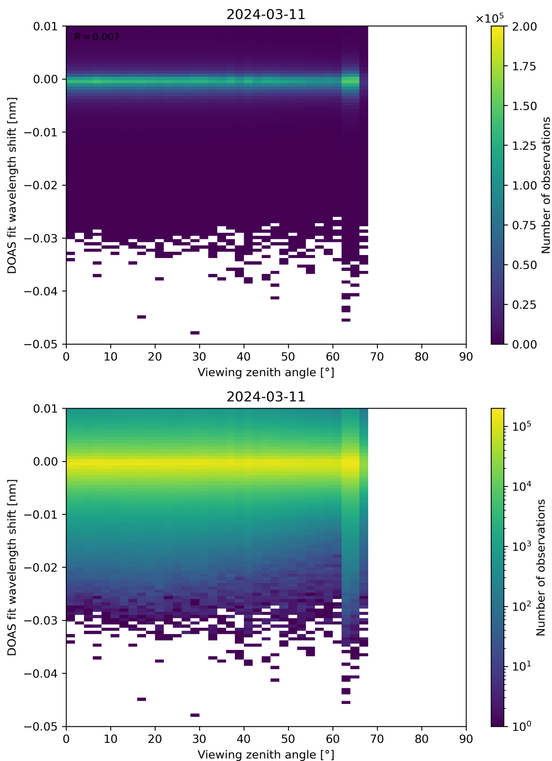
Figure 311: Scatter density plot of “Viewing zenith angle” against “DOAS fit wavelength shift” for 2024-03-10 to 2024-03-12.
