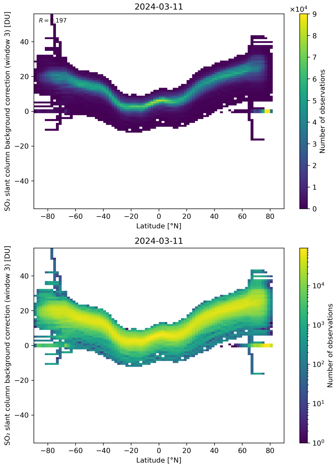
Figure 141: Scatter density plot of “Latitude” against “SO 2 slant column background correction (window 3)” for 2024-03-10 to 2024-03-12.
