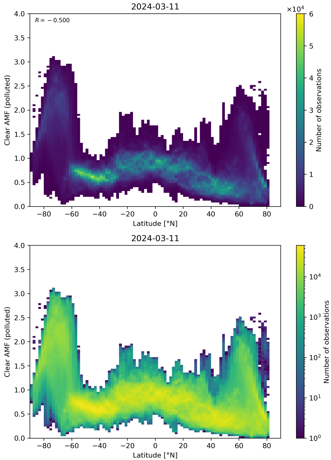
Figure 145: Scatter density plot of “Latitude” against “Clear AMF (polluted)” for 2024-03-10 to 2024-03-12.
