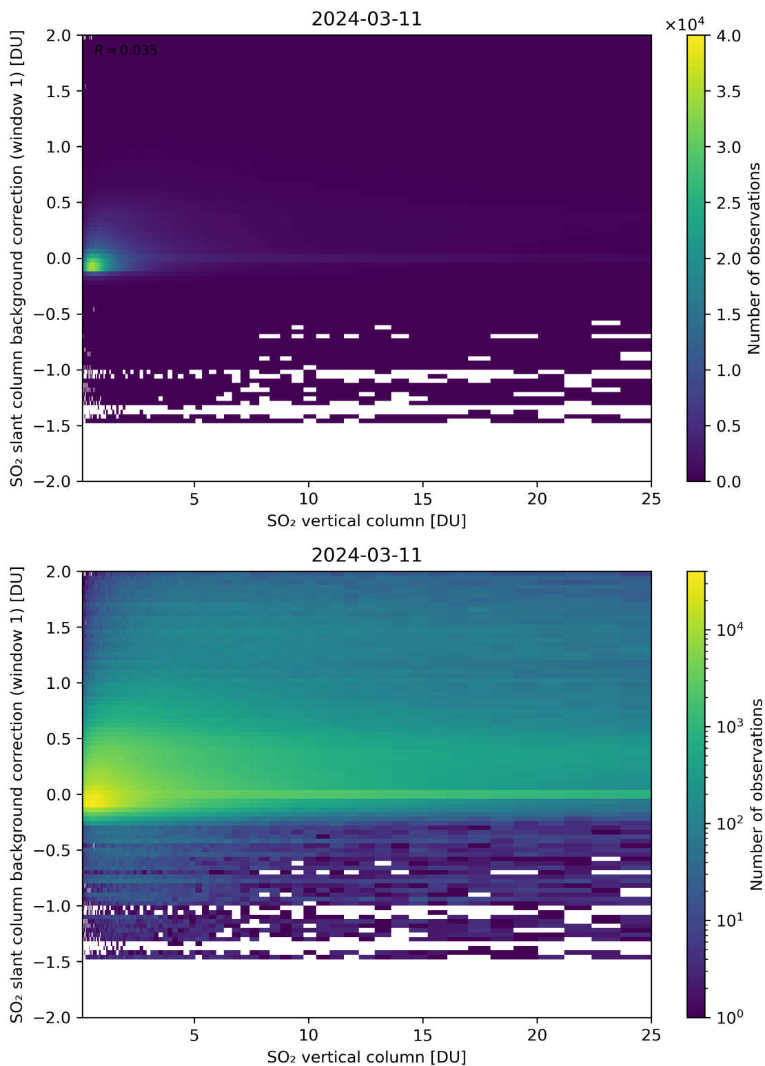
Figure 273: Scatter density plot of “SO 2 vertical column” against “SO 2 slant column background correction (window 1)” for 2024-03-10 to 2024-03-12.
