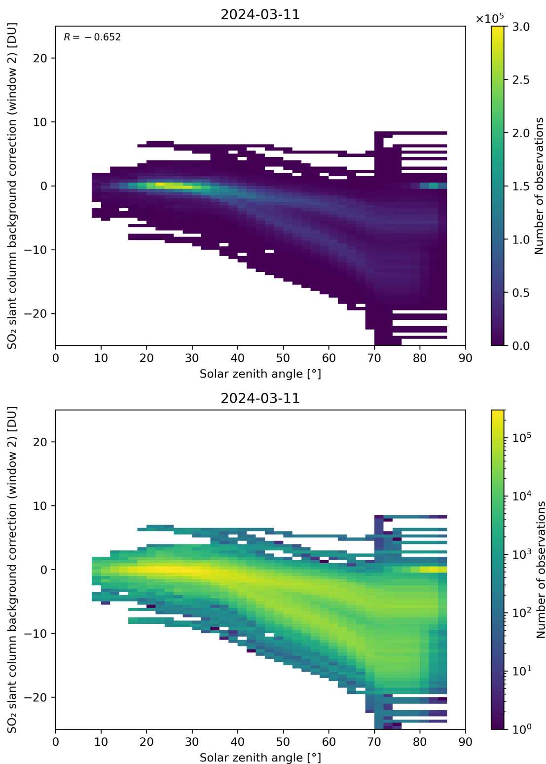
Figure 159: Scatter density plot of “Solar zenith angle” against “SO 2 slant column background correction (window 2)” for 2024-03-10 to 2024-03-12.
