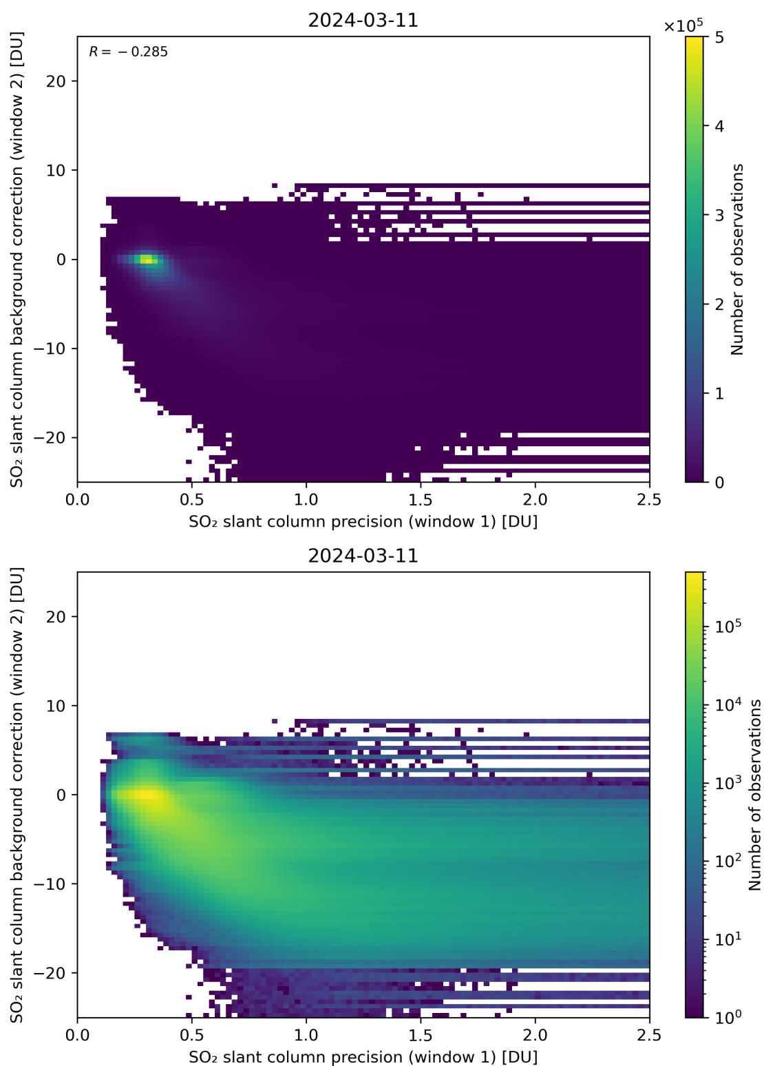
Figure 219: Scatter density plot of “SO 2 slant column precision (window 1)” against “SO 2 slant column background correction (window 2)” for 2024-03-10 to 2024-03-12.
