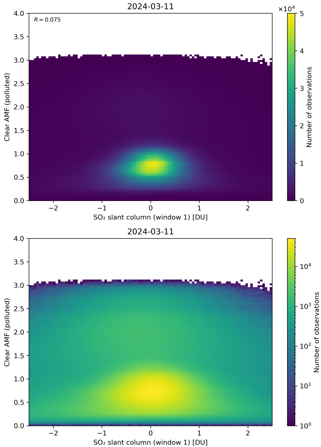
Figure 232: Scatter density plot of “SO 2 slant column (window 1)” against “Clear AMF (polluted)” for 2024-03-10 to 2024-03-12.
