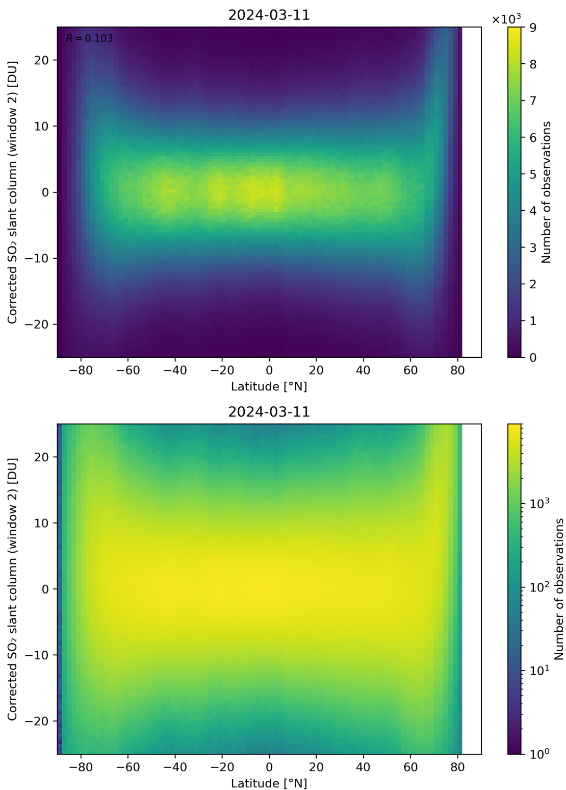
Figure 147: Scatter density plot of “Latitude” against “Corrected SO 2 slant column (window 2)” for 2024-03-10 to 2024-03-12.
