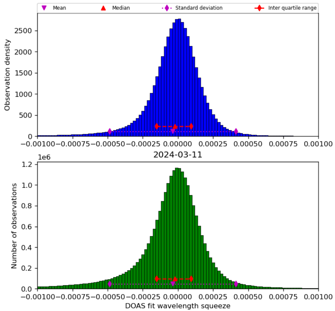
Figure 69: Histogram of “DOAS fit wavelength squeeze” for 2024-03-10 to 2024-03-12
