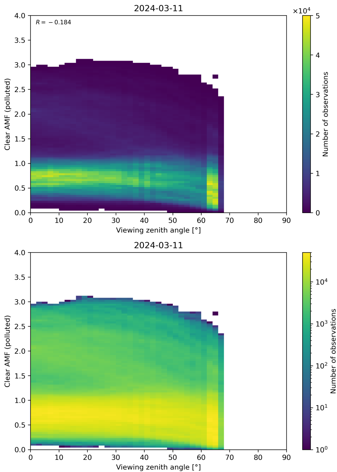
Figure 316: Scatter density plot of “Viewing zenith angle” against “Clear AMF (polluted)” for 2024-03-10 to 2024-03-12.
