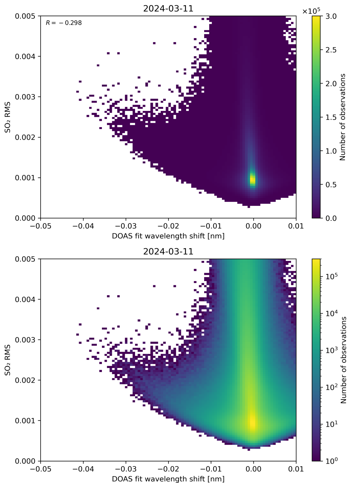
Figure 128: Scatter density plot of “DOAS fit wavelength shift” against “SO 2 RMS” for 2024-03-10 to 2024-03-12.
