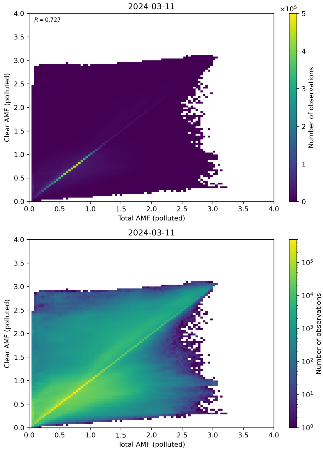
Figure 271: Scatter density plot of “Total AMF (polluted)” against “Clear AMF (polluted)” for 2024-03-10 to 2024-03-12.
