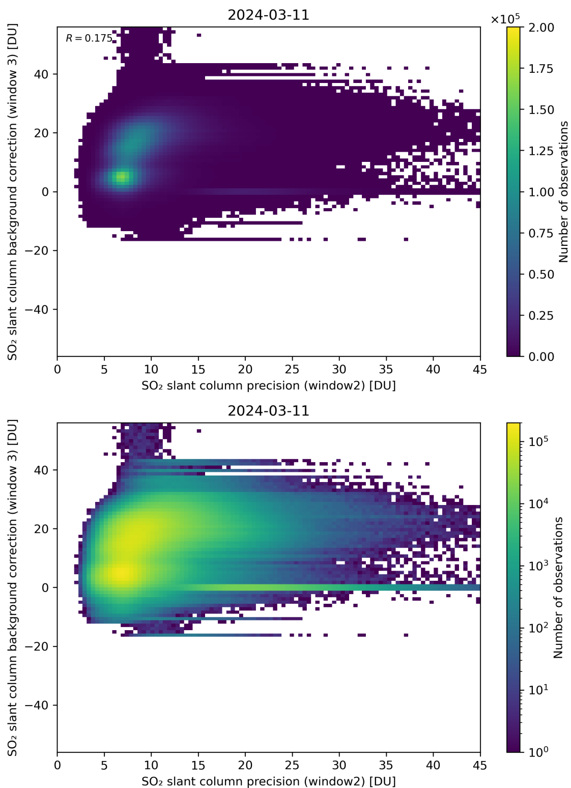
Figure 242: Scatter density plot of “SO 2 slant column precision (window2)” against “SO 2 slant column background correction (window 3)” for 2024-03-10 to 2024-03-12.
