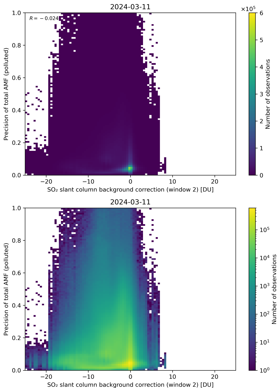
Figure 120: Scatter density plot of “SO 2 slant column background correction (window 2)” against “Precision of total AMF (polluted)” for 2024-03-10 to 2024-03-12.
