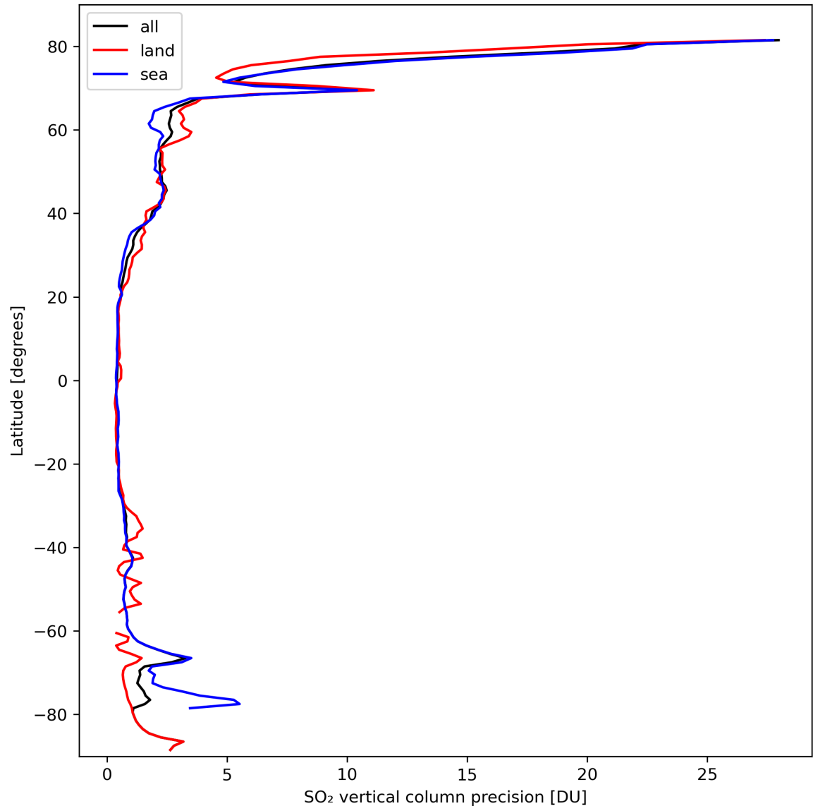
Figure 31: Zonal average of “SO 2 vertical column precision” for 2024-03-10 to 2024-03-12.
