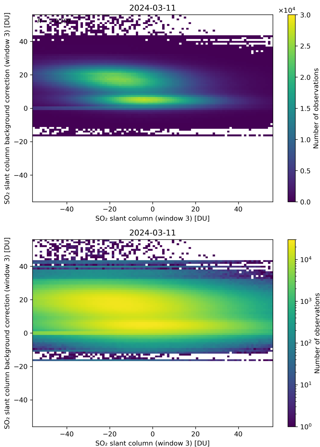
Figure 253: Scatter density plot of “SO 2 slant column (window 3)” against “SO 2 slant column background correction (window 3)” for 2024-03-10 to 2024-03-12.
