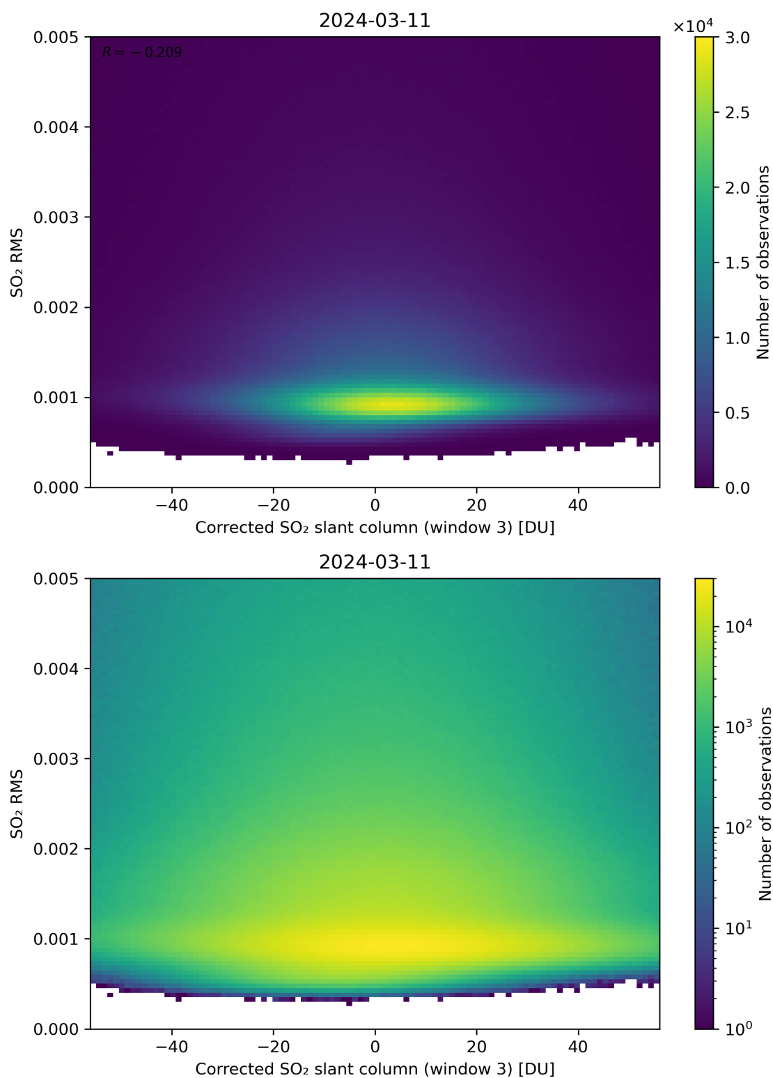
Figure 208: Scatter density plot of “Corrected SO 2 slant column (window 3)” against “SO 2 RMS” for 2024-03-10 to 2024-03-12.
