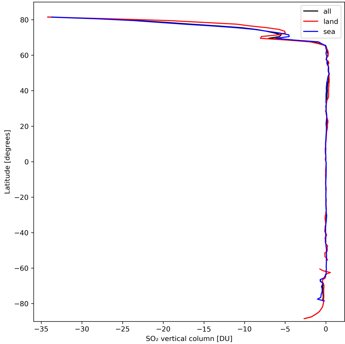
Figure 30: Zonal average of “SO 2 vertical column” for 2024-03-10 to 2024-03-12.
