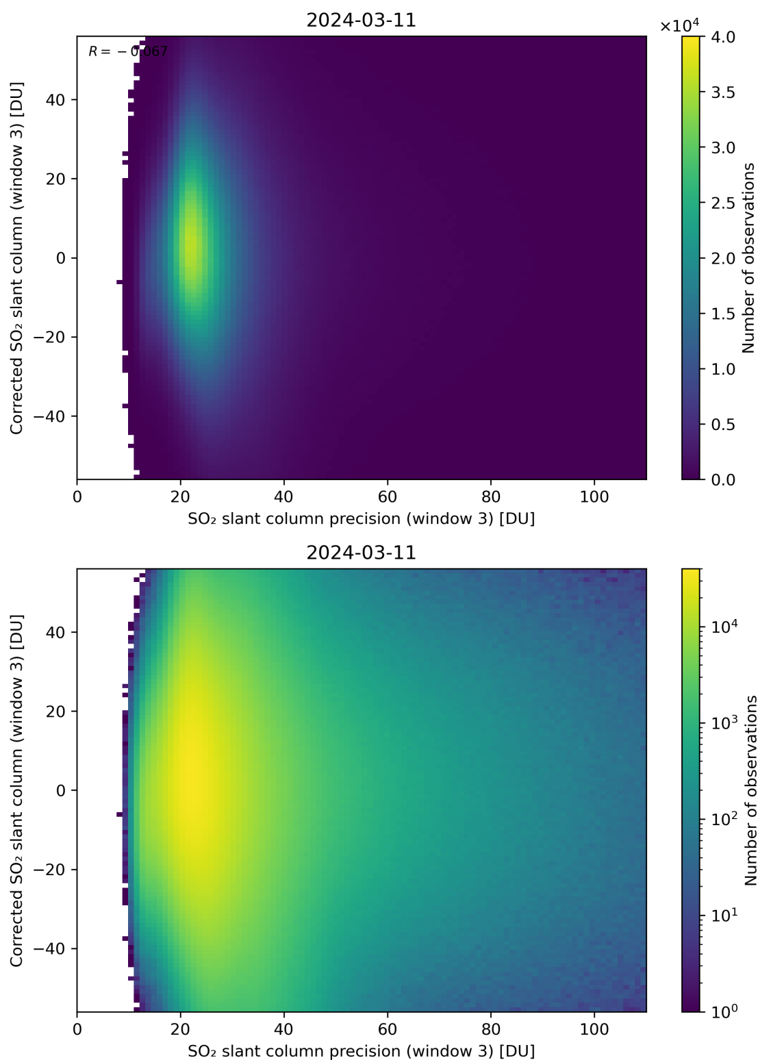
Figure 262: Scatter density plot of “SO 2 slant column precision (window 3)” against “Corrected SO 2 slant column (window 3)” for 2024-03-10 to 2024-03-12.
