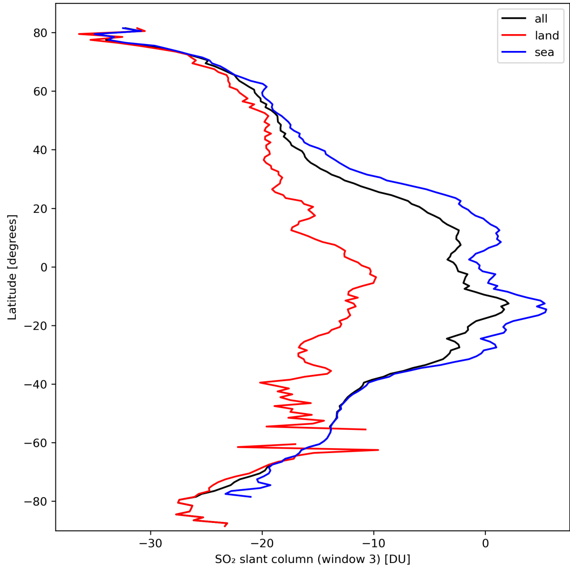
Figure 41: Zonal average of “SO 2 slant column (window 3)” for 2024-03-10 to 2024-03-12.
