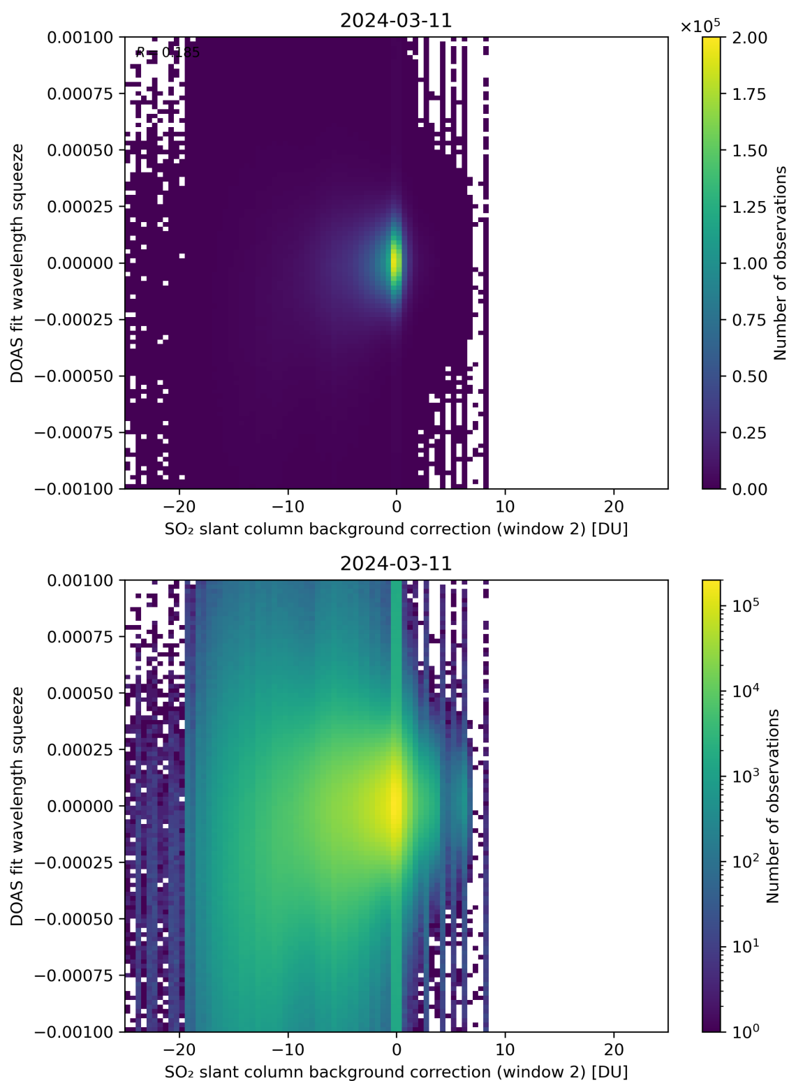
Figure 113: Scatter density plot of “SO 2 slant column background correction (window 2)” against “DOAS fit wavelength squeeze” for 2024-03-10 to 2024-03-12.
