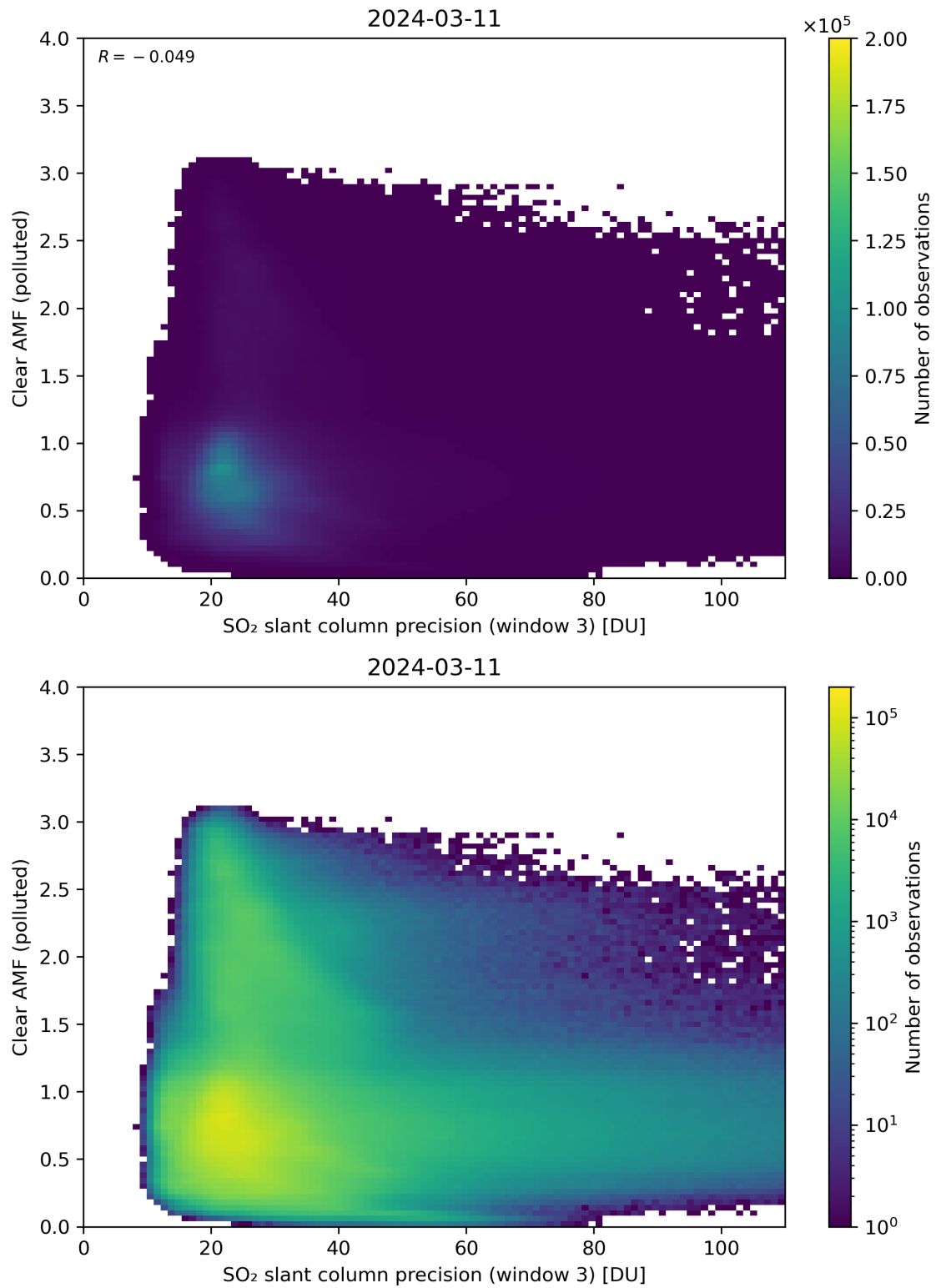
Figure 261: Scatter density plot of “SO 2 slant column precision (window 3)” against “Clear AMF (polluted)” for 2024-03-10 to 2024-03-12.
