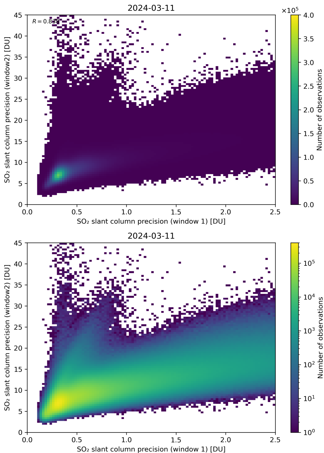
Figure 227: Scatter density plot of “SO 2 slant column precision (window 1)” against “SO 2 slant column precision (window2)” for 2024-03-10 to 2024-03-12.
