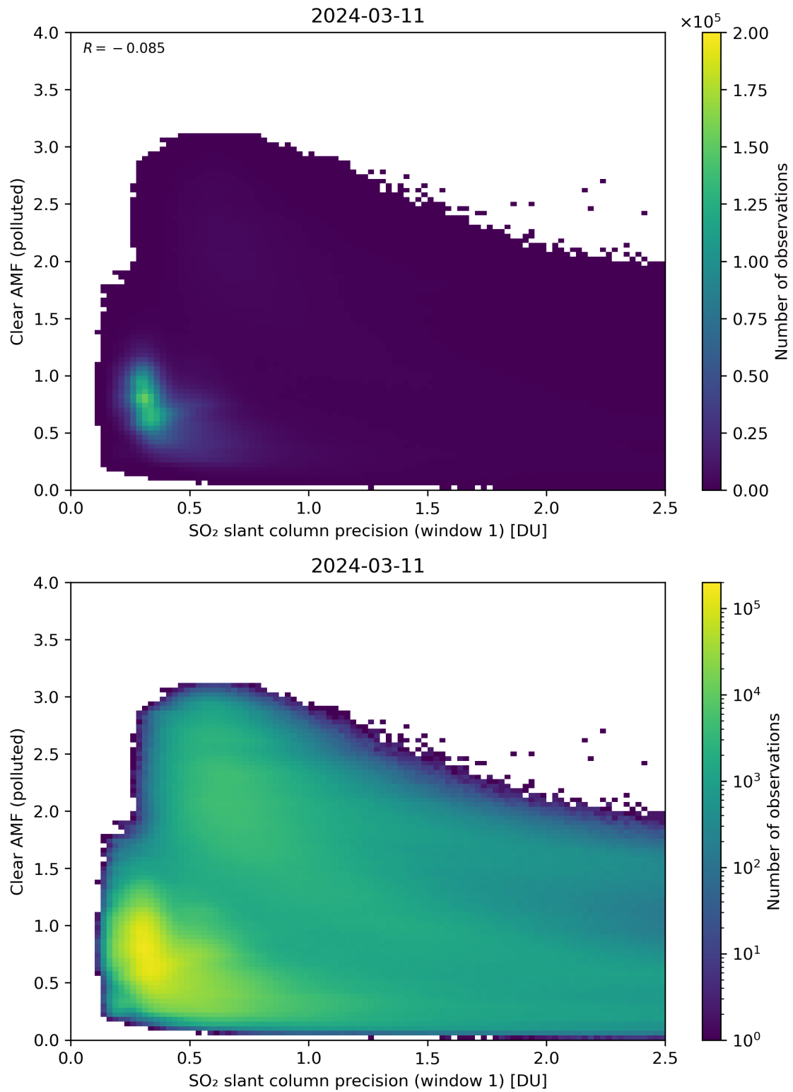
Figure 224: Scatter density plot of “SO 2 slant column precision (window 1)” against “Clear AMF (polluted)” for 2024-03-10 to 2024-03-12.
