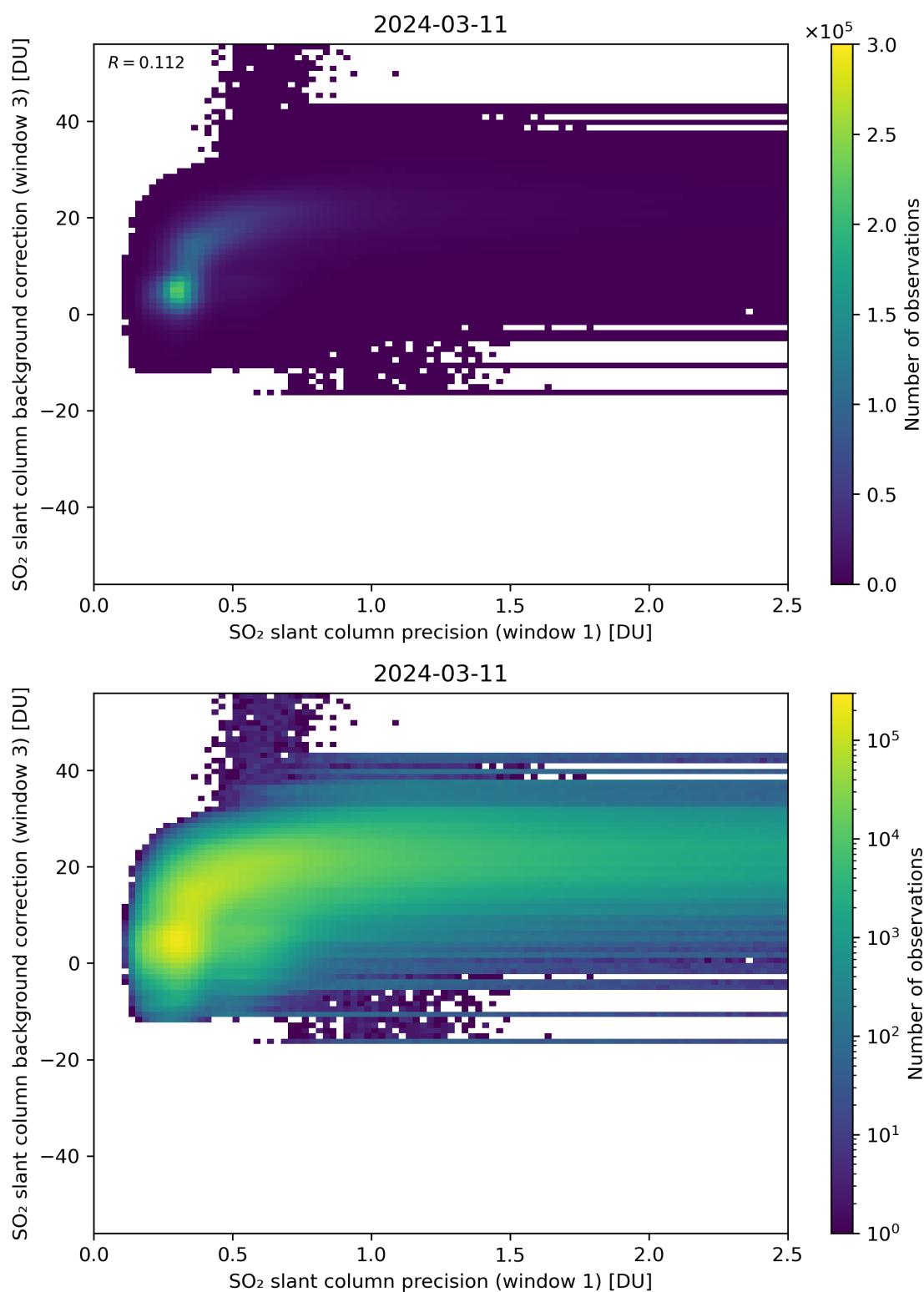
Figure 220: Scatter density plot of “SO 2 slant column precision (window 1)” against “SO 2 slant column background correction (window 3)” for 2024-03-10 to 2024-03-12.
