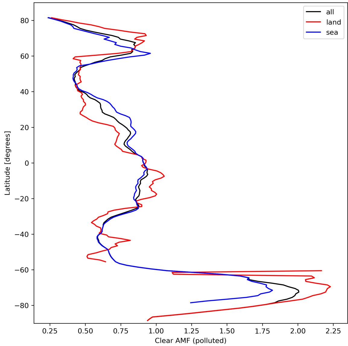
Figure 50: Zonal average of “Clear AMF (polluted)” for 2024-03-10 to 2024-03-12.
