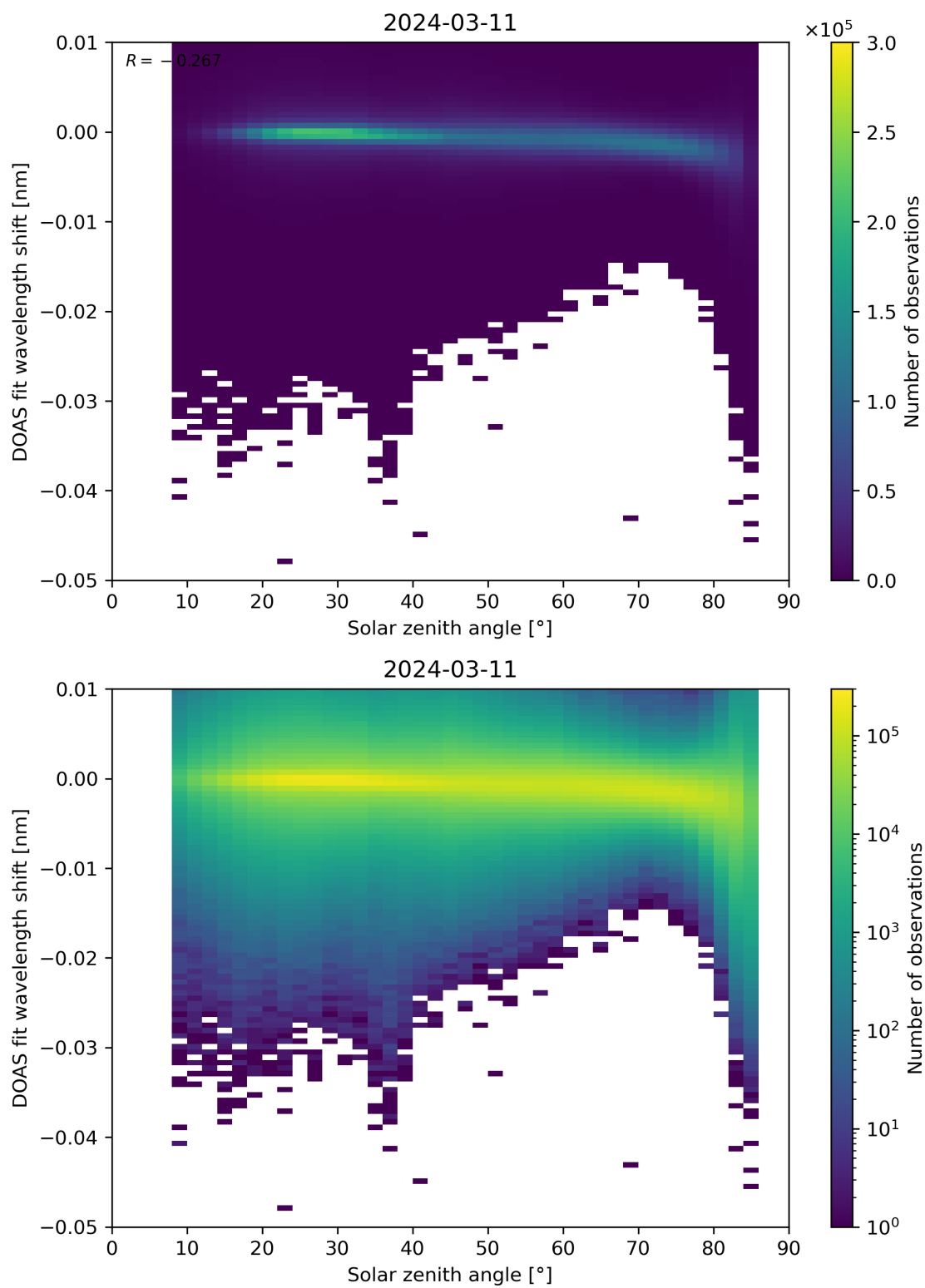
Figure 161: Scatter density plot of “Solar zenith angle” against “DOAS fit wavelength shift” for 2024-03-10 to 2024-03-12.
