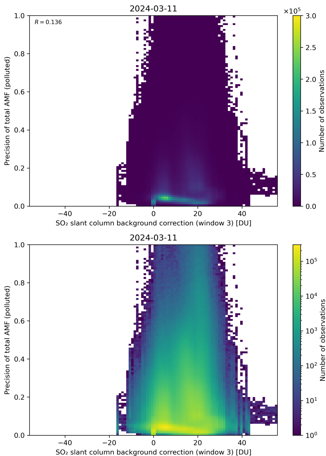
Figure 126: Scatter density plot of “SO 2 slant column background correction (window 3)” against “Precision of total AMF (polluted)” for 2024-03-10 to 2024-03-12.
