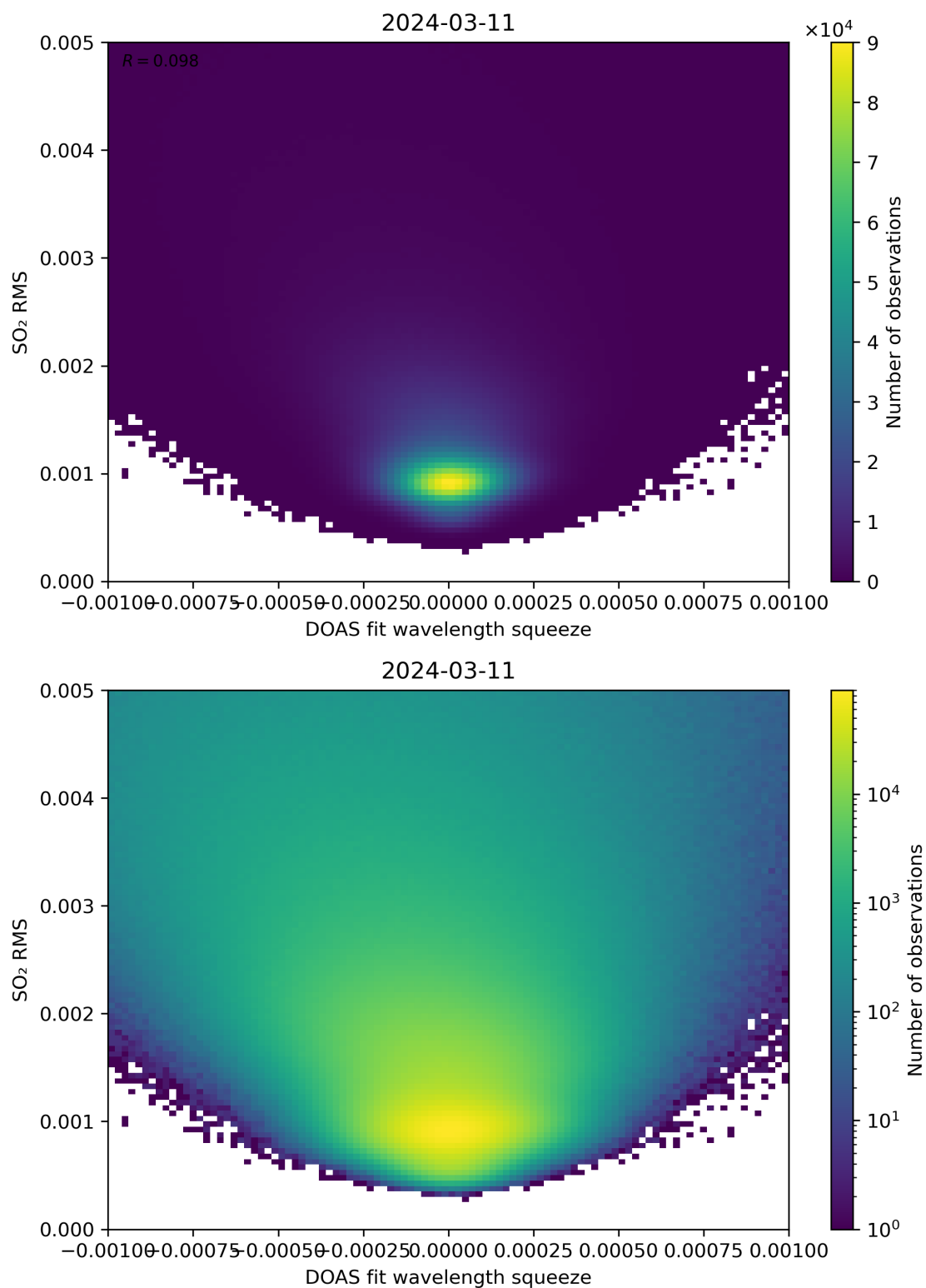
Figure 132: Scatter density plot of “DOAS fit wavelength squeeze” against “SO 2 RMS” for 2024-03-10 to 2024-03-12.
