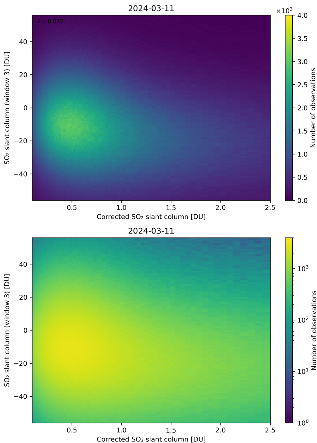
Figure 190: Scatter density plot of “Corrected SO 2 slant column” against “SO 2 slant column (window 3)” for 2024-03-10 to 2024-03-12.
