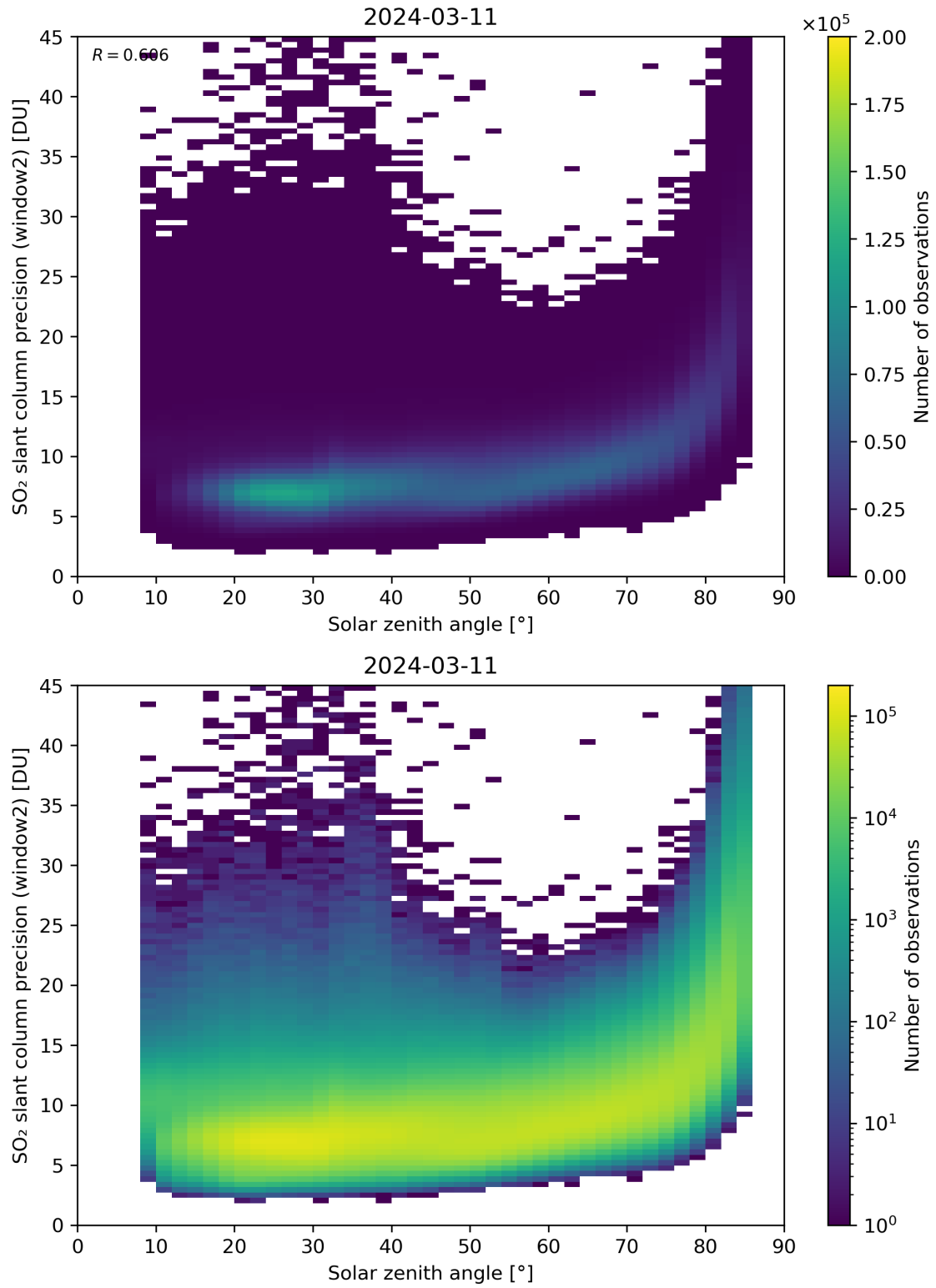
Figure 171: Scatter density plot of “Solar zenith angle” against “SO 2 slant column precision (window2)” for 2024-03-10 to 2024-03-12.
