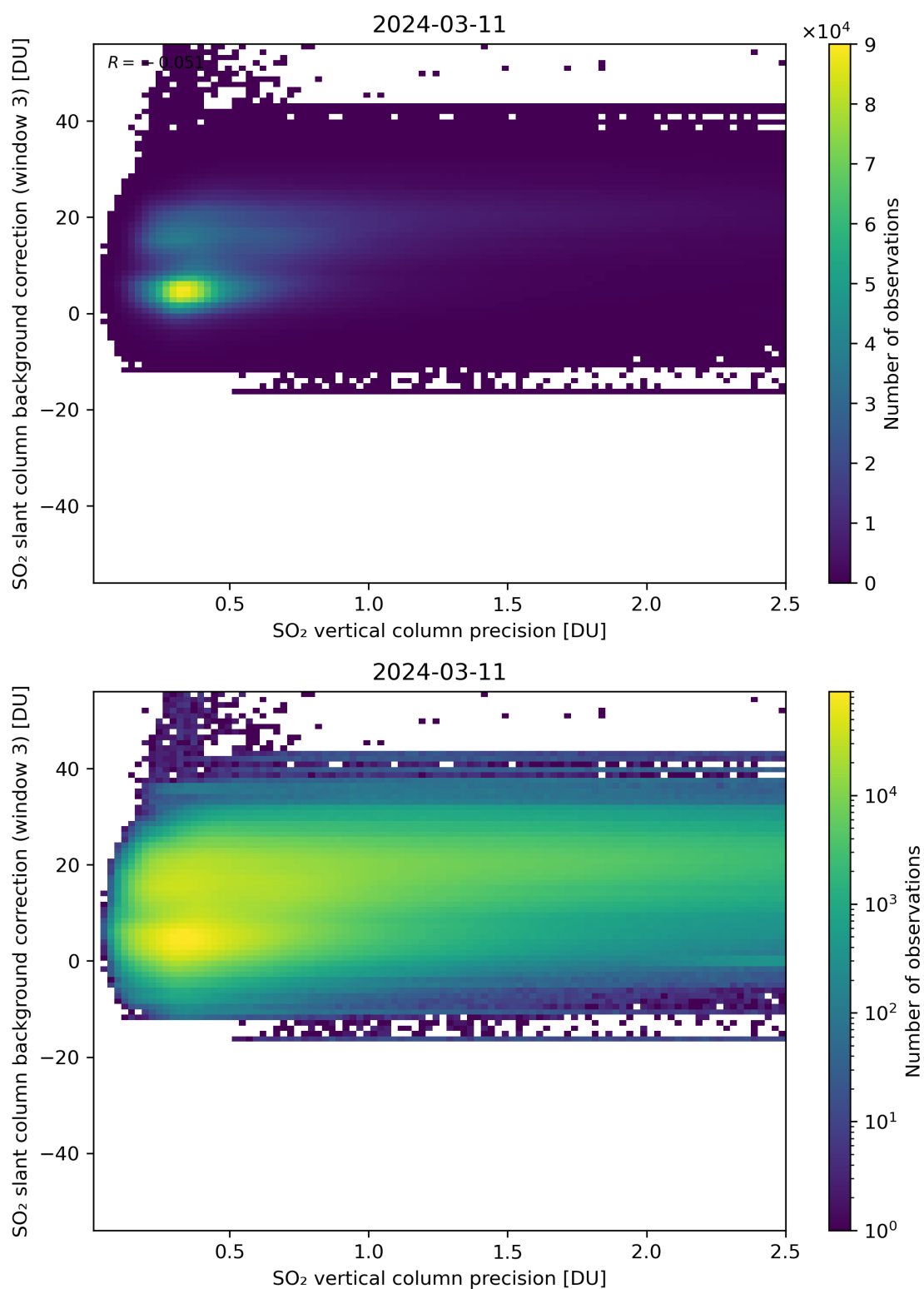
Figure 281: Scatter density plot of “SO 2 vertical column precision” against “SO 2 slant column background correction (window 3)” for 2024-03-10 to 2024-03-12.
