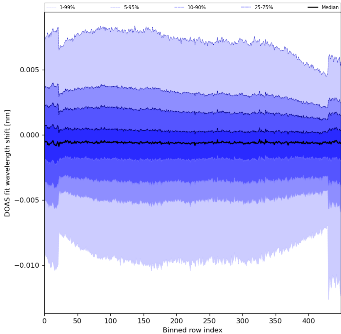
Figure 91: Along track statistics of “DOAS fit wavelength shift” for 2024-03-10 to 2024-03-12
