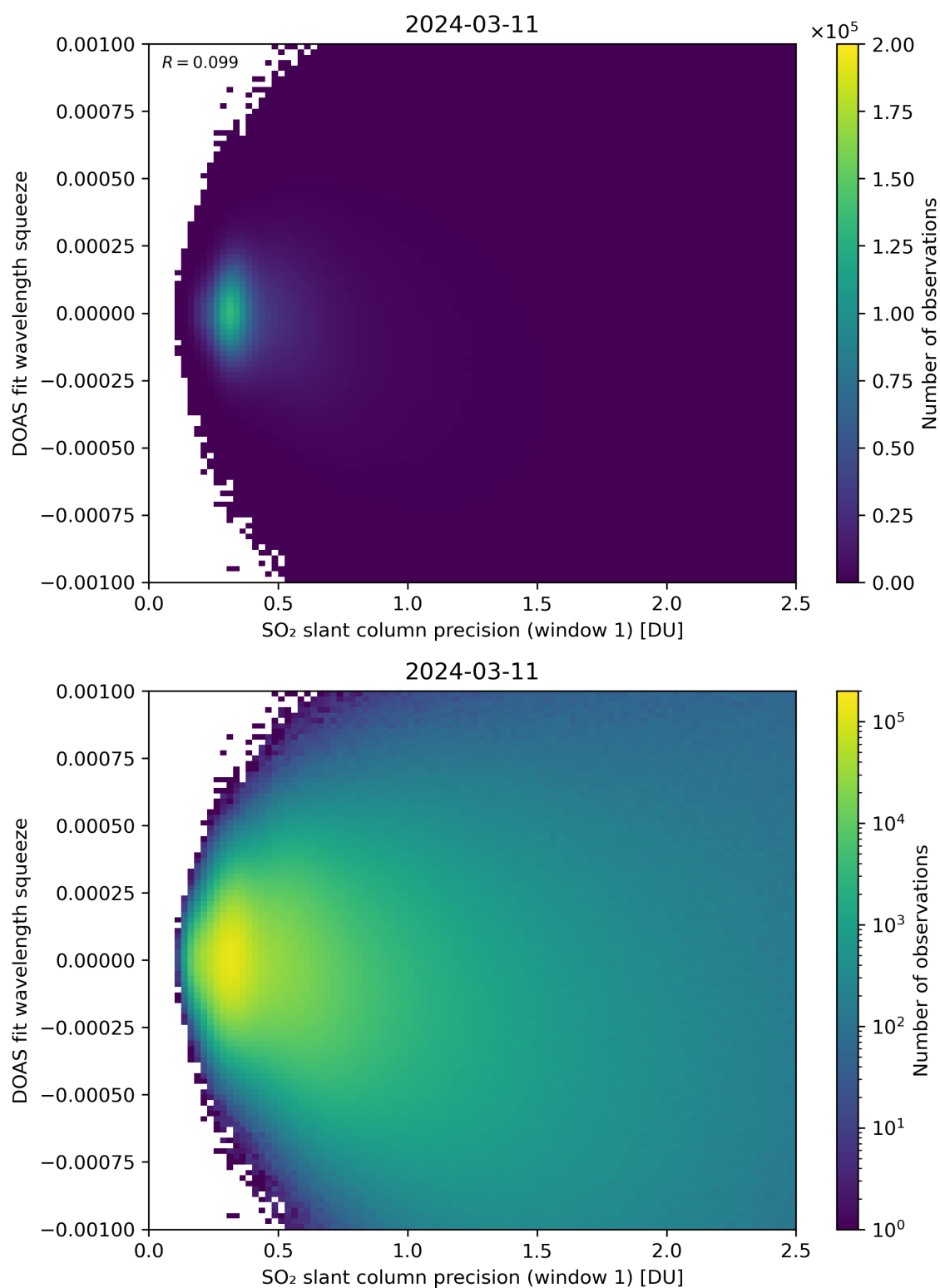
Figure 222: Scatter density plot of “SO 2 slant column precision (window 1)” against “DOAS fit wavelength squeeze” for 2024-03-10 to 2024-03-12.
