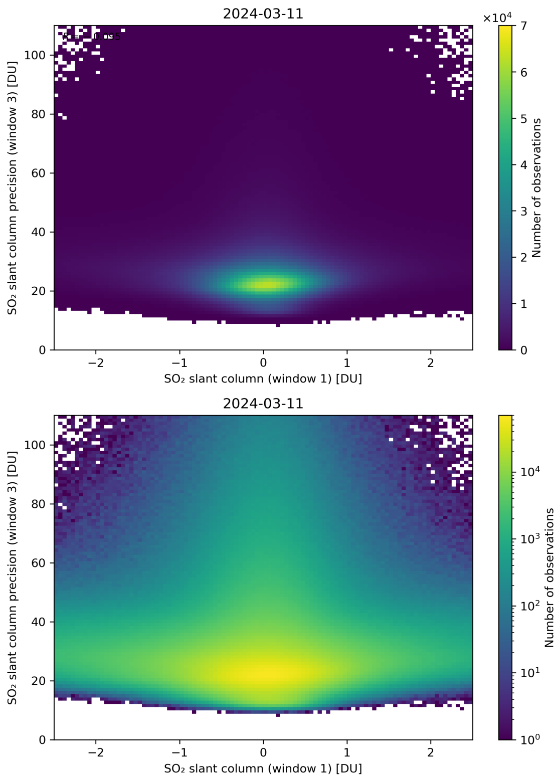
Figure 238: Scatter density plot of “SO 2 slant column (window 1)” against “SO 2 slant column precision (window 3)” for 2024-03-10 to 2024-03-12.
