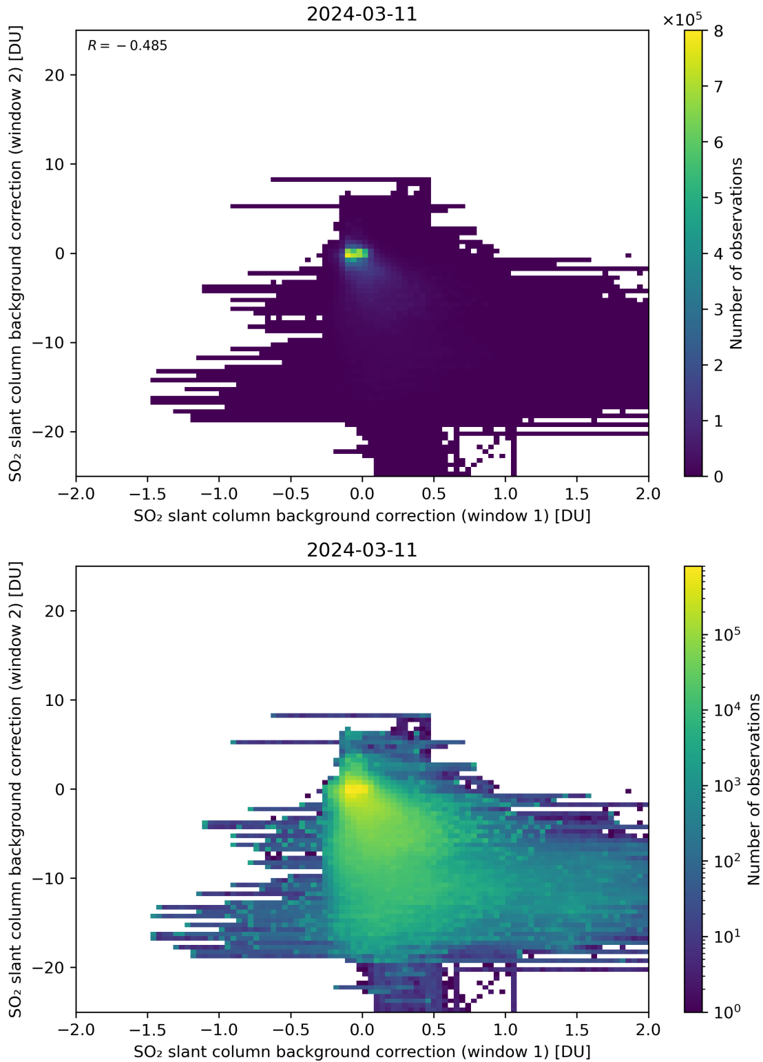
Figure 98: Scatter density plot of “SO 2 slant column background correction (window 1)” against “SO 2 slant column background correction (window 2)” for 2024-03-10 to 2024-03-12.
