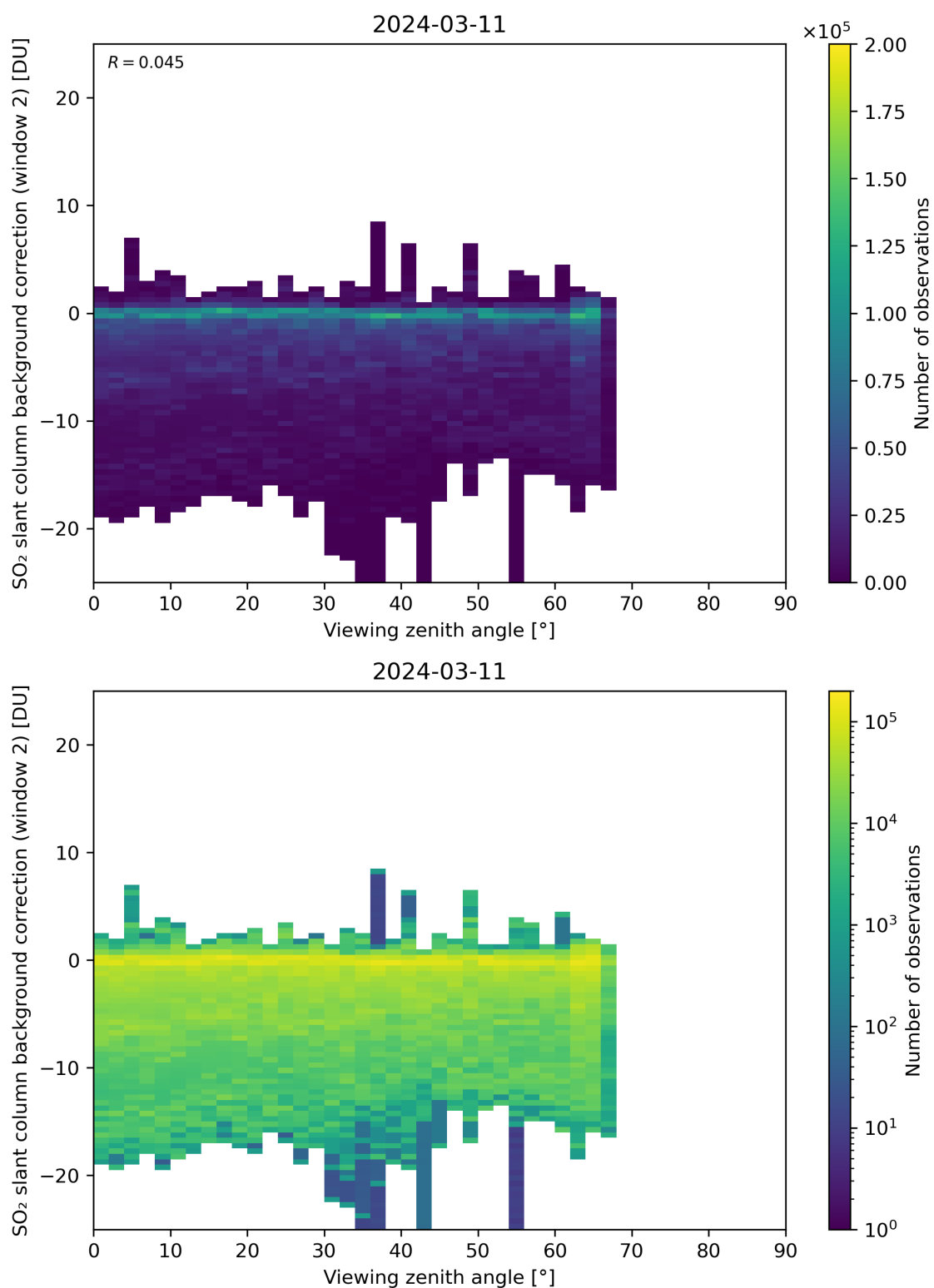
Figure 309: Scatter density plot of “Viewing zenith angle” against “SO 2 slant column background correction (window 2)” for 2024-03-10 to 2024-03-12.
