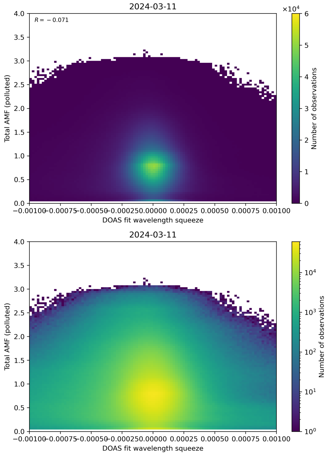
Figure 134: Scatter density plot of “DOAS fit wavelength squeeze” against “Total AMF (polluted)” for 2024-03-10 to 2024-03-12.
