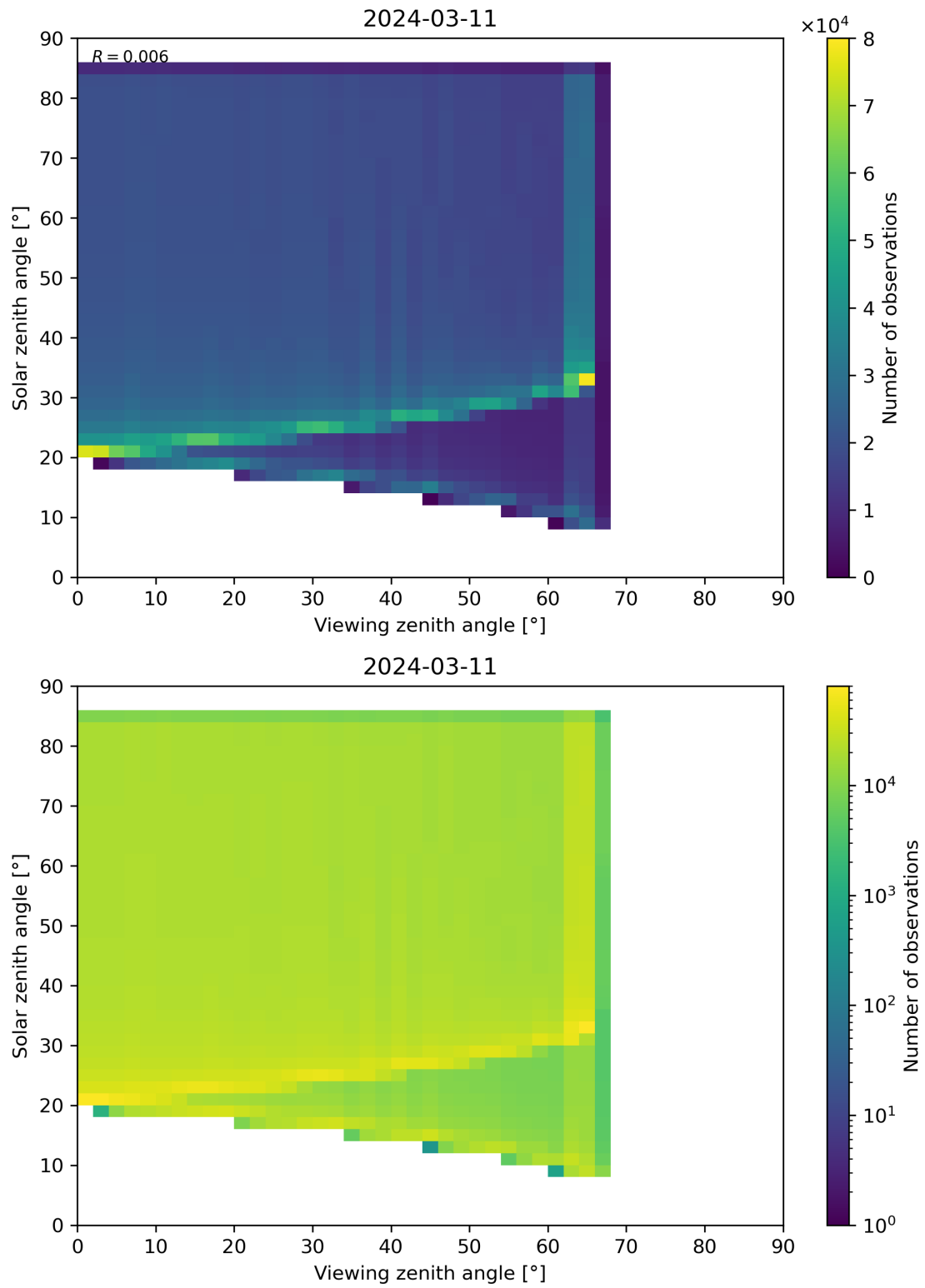
Figure 315: Scatter density plot of “Viewing zenith angle” against “Solar zenith angle” for 2024-03-10 to 2024-03-12.
