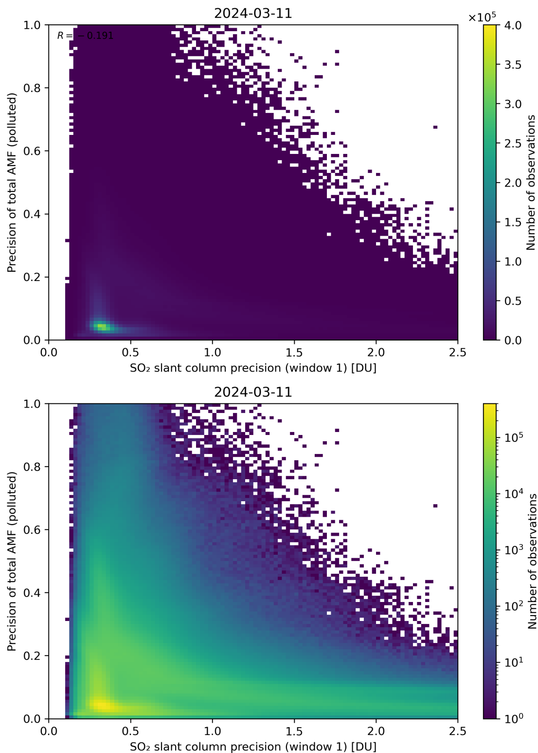
Figure 231: Scatter density plot of “SO 2 slant column precision (window 1)” against “Precision of total AMF (polluted)” for 2024-03-10 to 2024-03-12.
