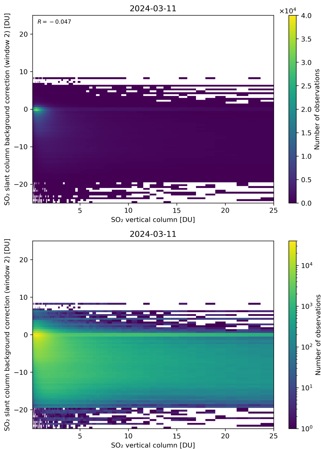
Figure 274: Scatter density plot of “SO 2 vertical column” against “SO 2 slant column background correction (window 2)” for 2024-03-10 to 2024-03-12.
