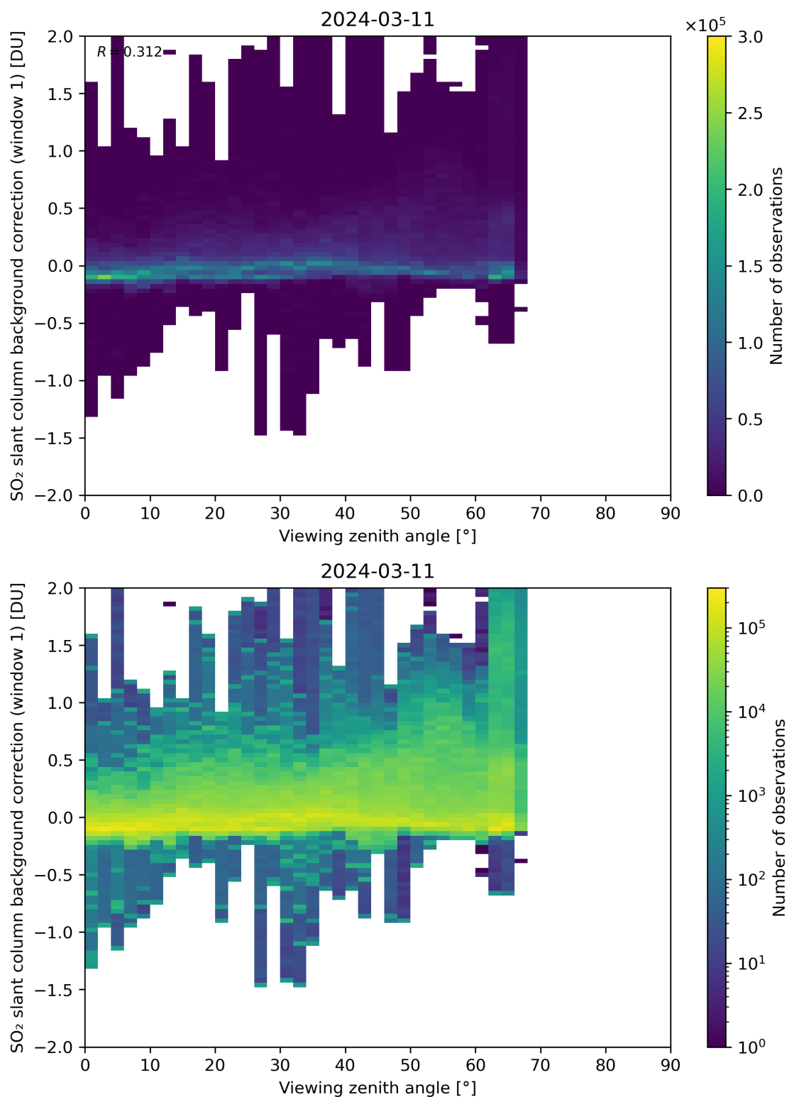
Figure 308: Scatter density plot of “Viewing zenith angle” against “SO 2 slant column background correction (window 1)” for 2024-03-10 to 2024-03-12.
