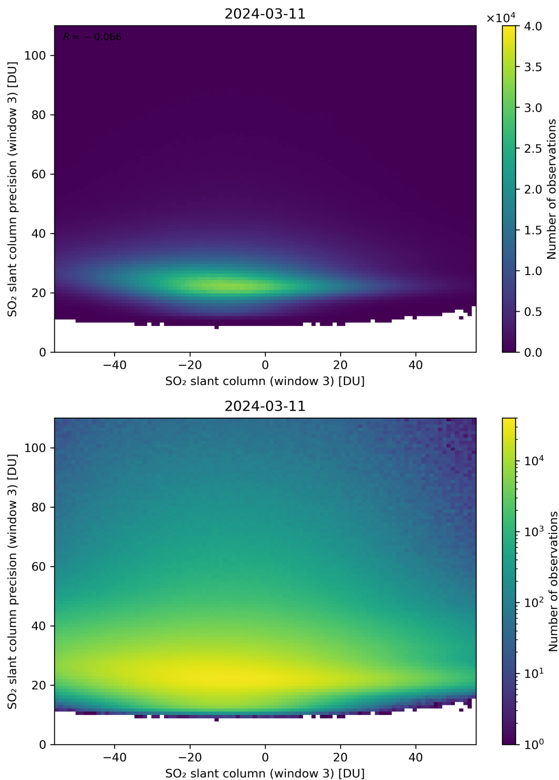
Figure 267: Scatter density plot of “SO 2 slant column (window 3)” against “SO 2 slant column precision (window 3)” for 2024-03-10 to 2024-03-12.
