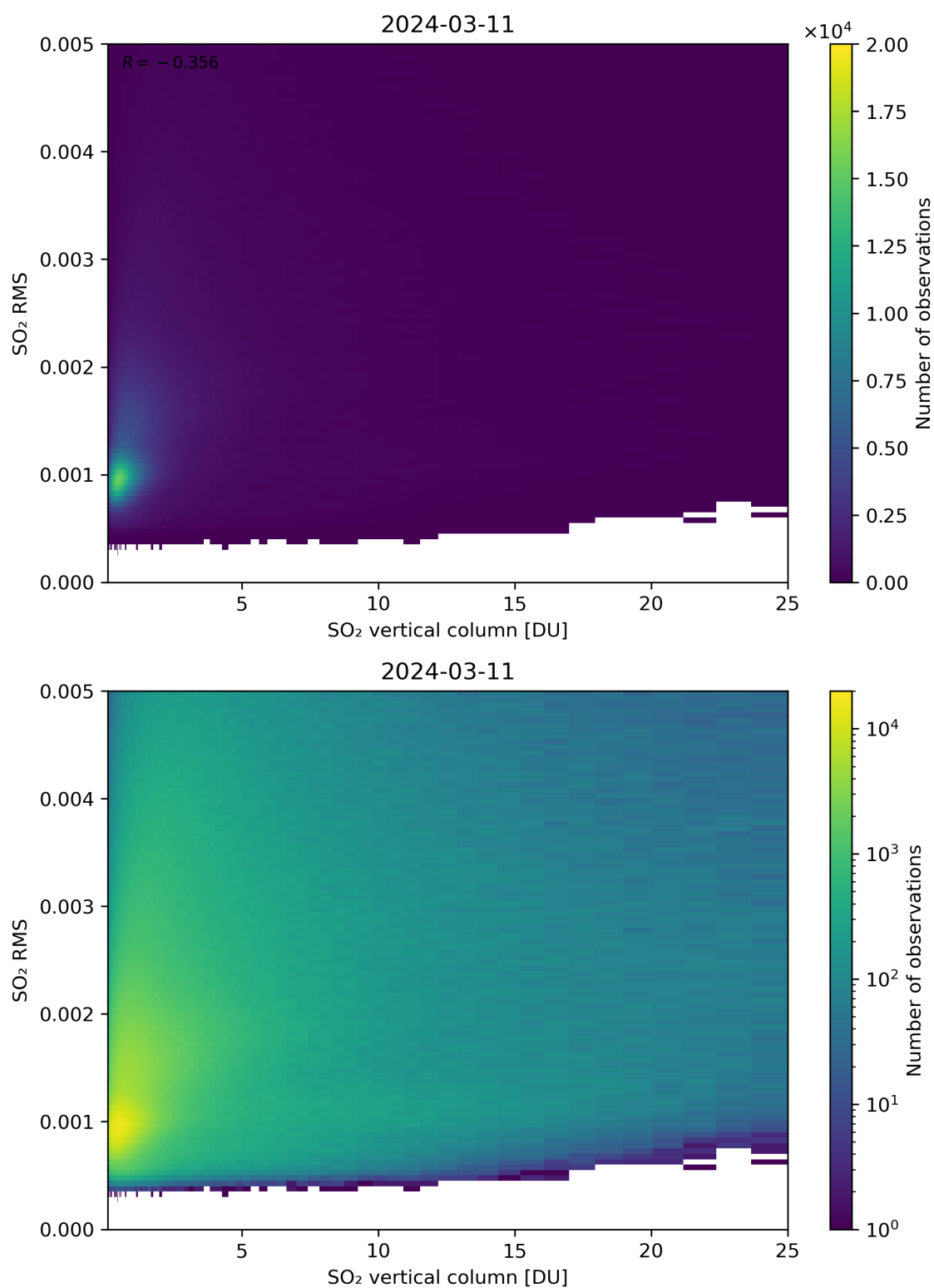
Figure 278: Scatter density plot of “SO 2 vertical column” against “SO 2 RMS” for 2024-03-10 to 2024-03-12.
