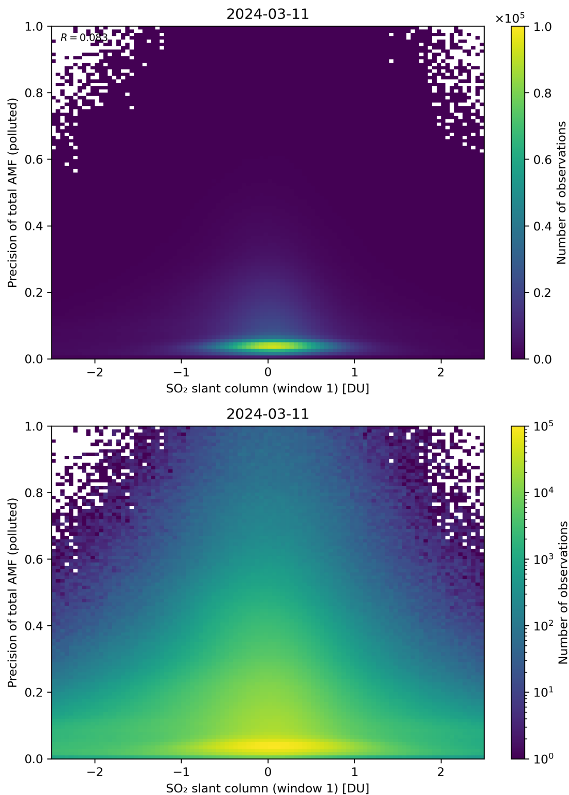
Figure 240: Scatter density plot of “SO 2 slant column (window 1)” against “Precision of total AMF (polluted)” for 2024-03-10 to 2024-03-12.
