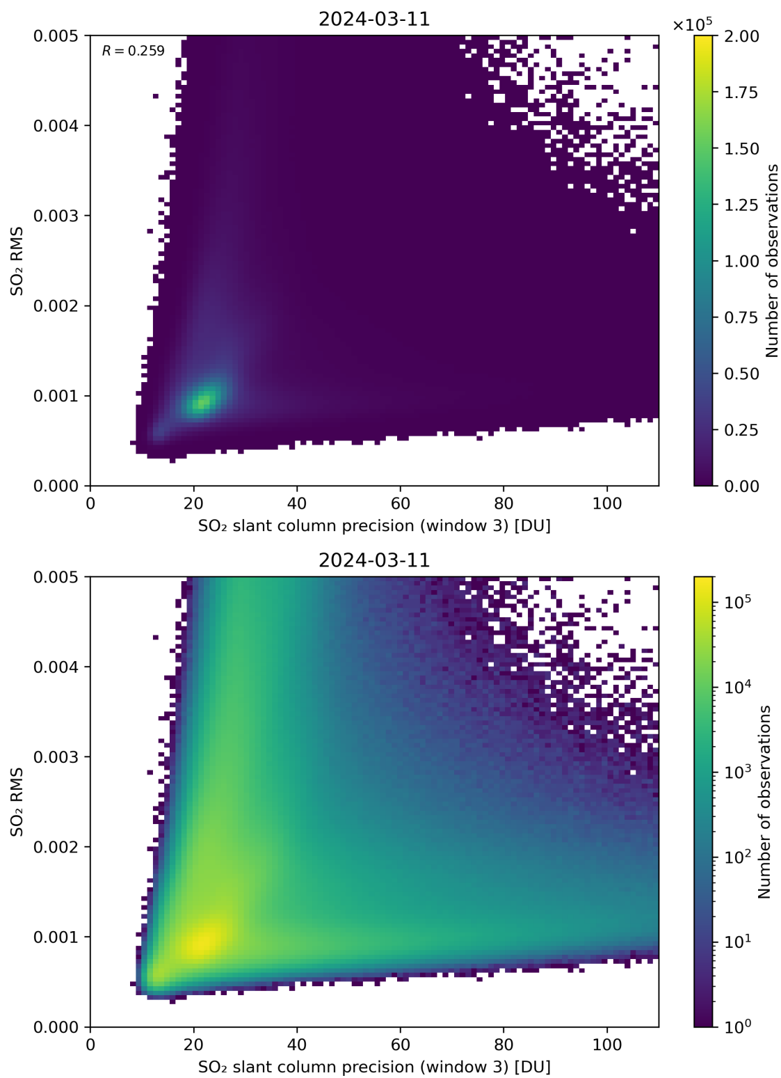
Figure 260: Scatter density plot of “SO 2 slant column precision (window 3)” against “SO 2 RMS” for 2024-03-10 to 2024-03-12.
