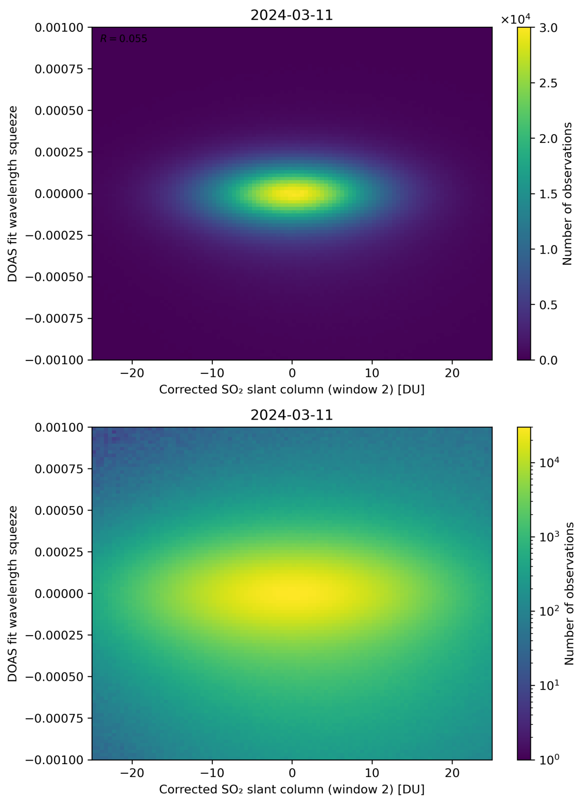
Figure 197: Scatter density plot of “Corrected SO 2 slant column (window 2)” against “DOAS fit wavelength squeeze” for 2024-03-10 to 2024-03-12.
