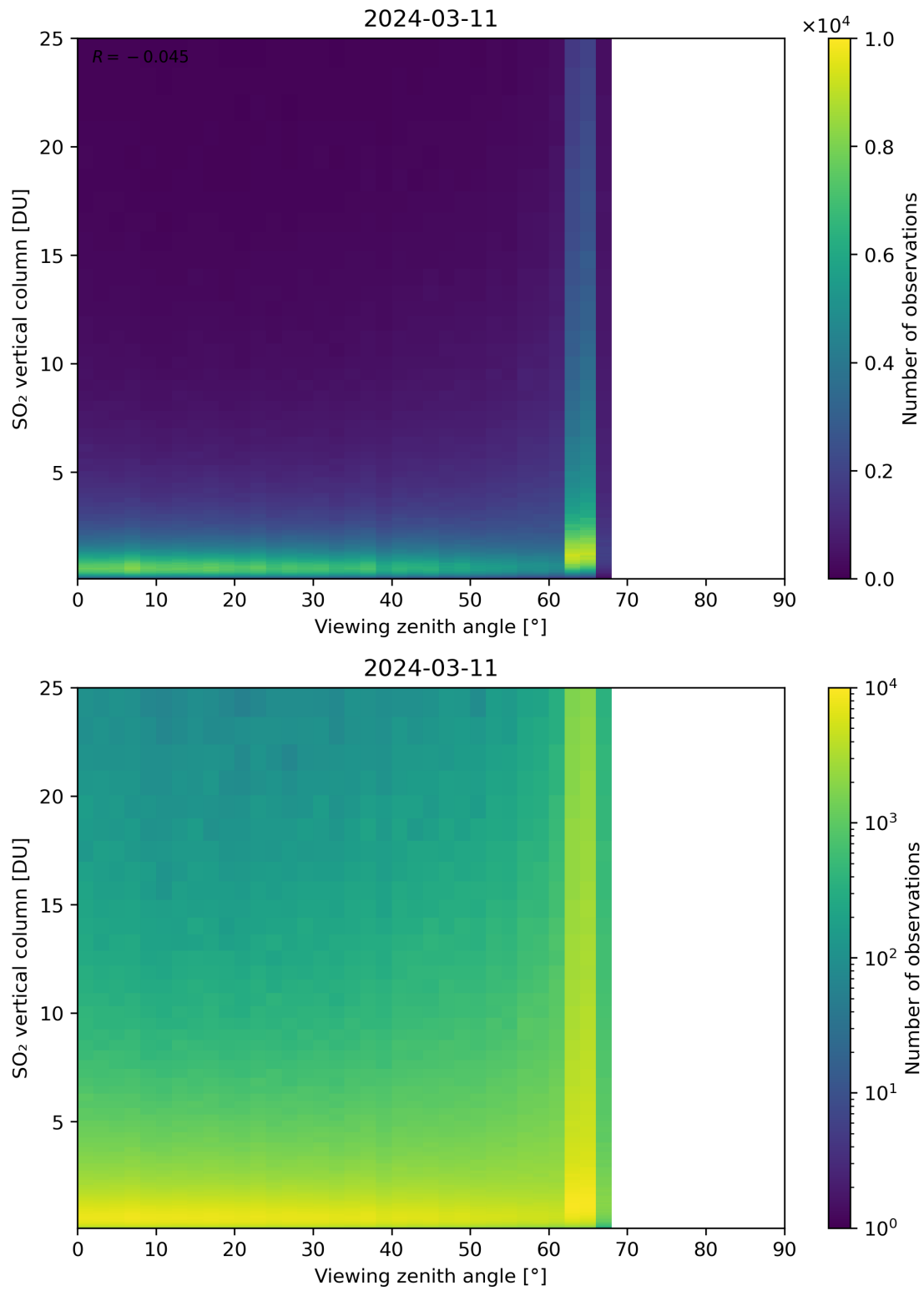
Figure 327: Scatter density plot of “Viewing zenith angle” against “SO 2 vertical column” for 2024-03-10 to 2024-03-12.
