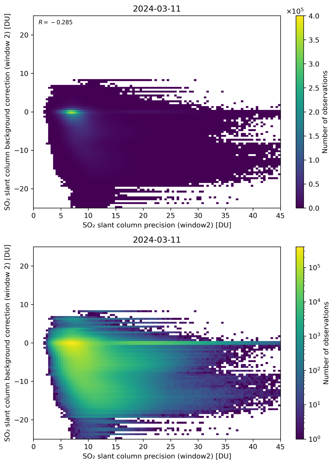
Figure 241: Scatter density plot of “SO 2 slant column precision (window2)” against “SO 2 slant column background correction (window 2)” for 2024-03-10 to 2024-03-12.
