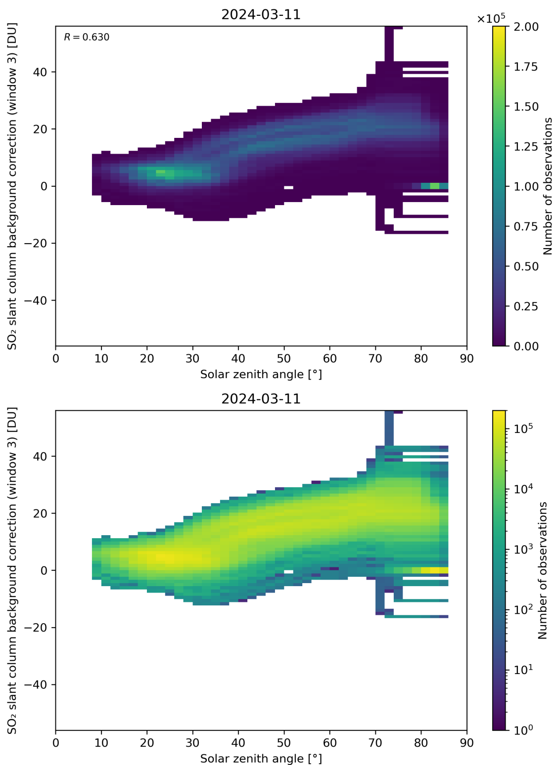
Figure 160: Scatter density plot of “Solar zenith angle” against “SO 2 slant column background correction (window 3)” for 2024-03-10 to 2024-03-12.
