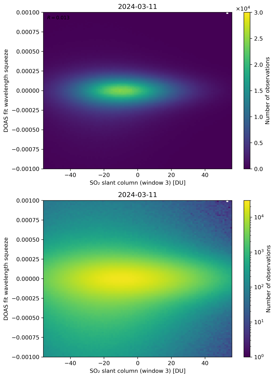
Figure 255: Scatter density plot of “SO 2 slant column (window 3)” against “DOAS fit wavelength squeeze” for 2024-03-10 to 2024-03-12.
