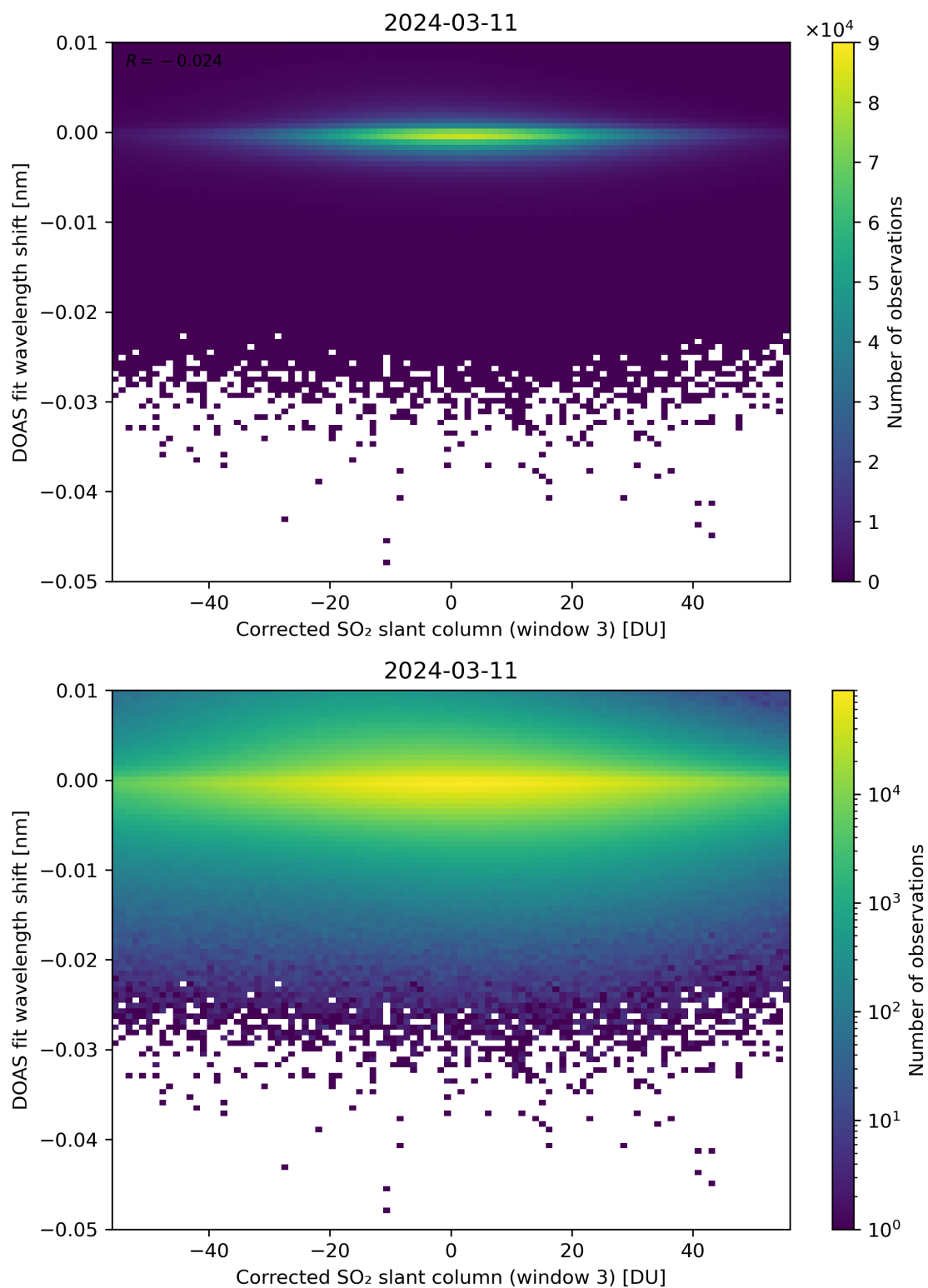
Figure 206: Scatter density plot of “Corrected SO 2 slant column (window 3)” against “DOAS fit wavelength shift” for 2024-03-10 to 2024-03-12.
