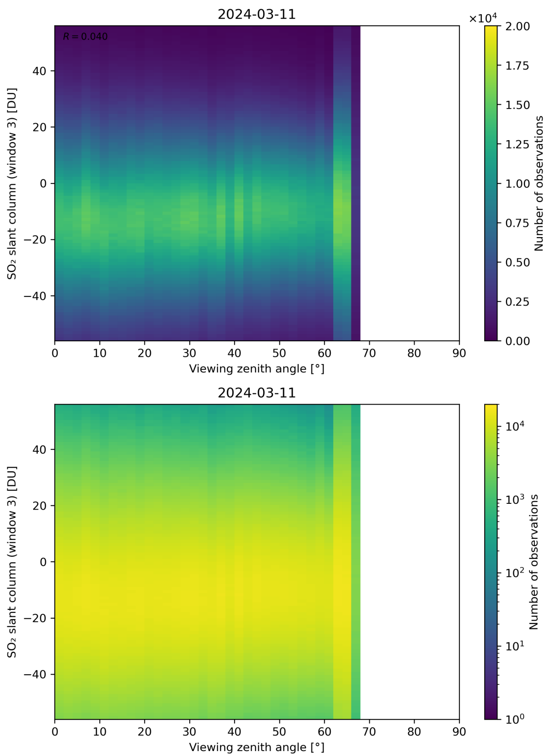
Figure 323: Scatter density plot of “Viewing zenith angle” against “SO 2 slant column (window 3)” for 2024-03-10 to 2024-03-12.
