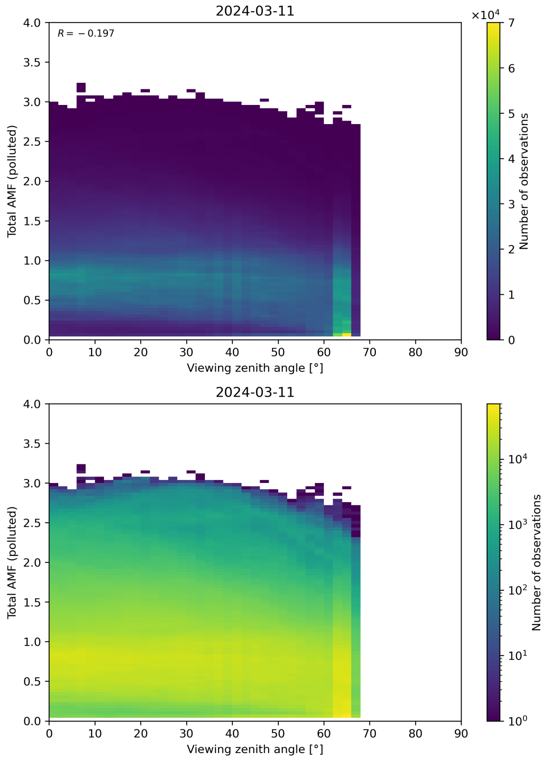
Figure 325: Scatter density plot of “Viewing zenith angle” against “Total AMF (polluted)” for 2024-03-10 to 2024-03-12.
