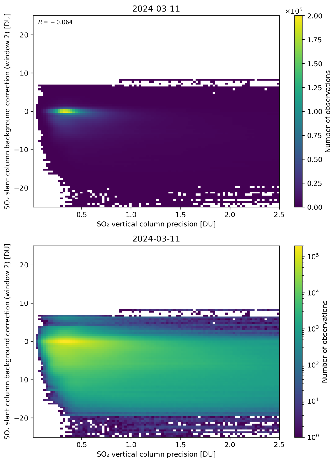
Figure 280: Scatter density plot of “SO 2 vertical column precision” against “SO 2 slant column background correction (window 2)” for 2024-03-10 to 2024-03-12.
