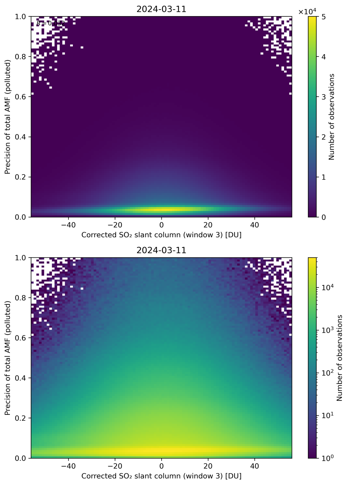
Figure 211: Scatter density plot of “Corrected SO 2 slant column (window 3)” against “Precision of total AMF (polluted)” for 2024-03-10 to 2024-03-12.
