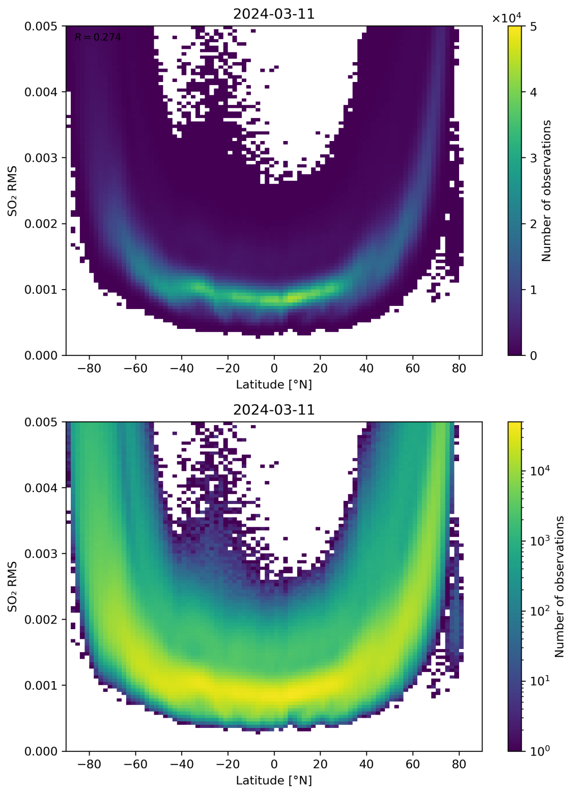
Figure 144: Scatter density plot of “Latitude” against “SO 2 RMS” for 2024-03-10 to 2024-03-12.
