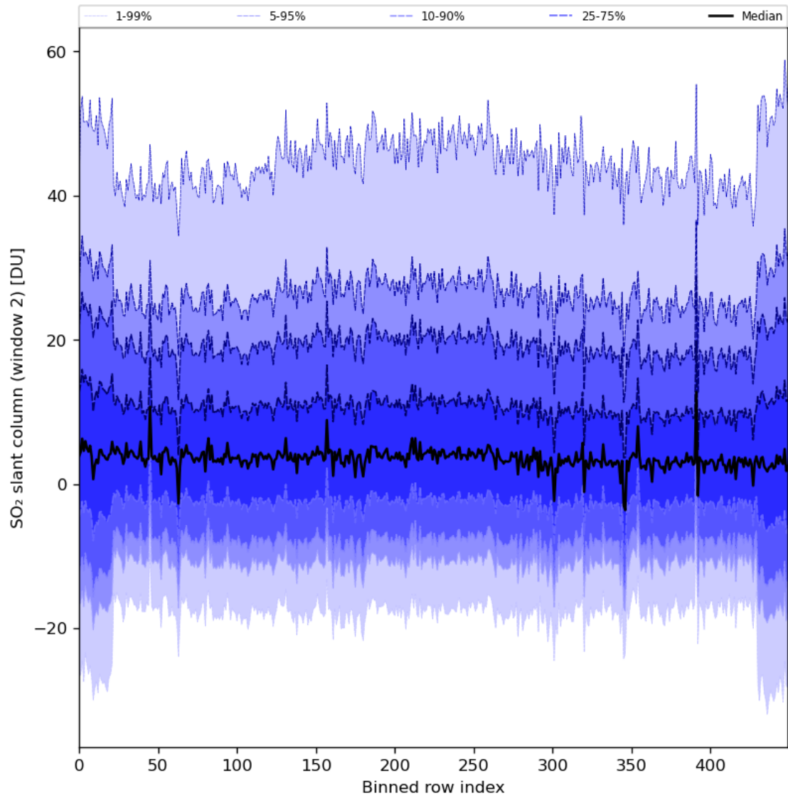
Figure 83: Along track statistics of “SO 2 slant column (window 2)” for 2024-03-10 to 2024-03-12
