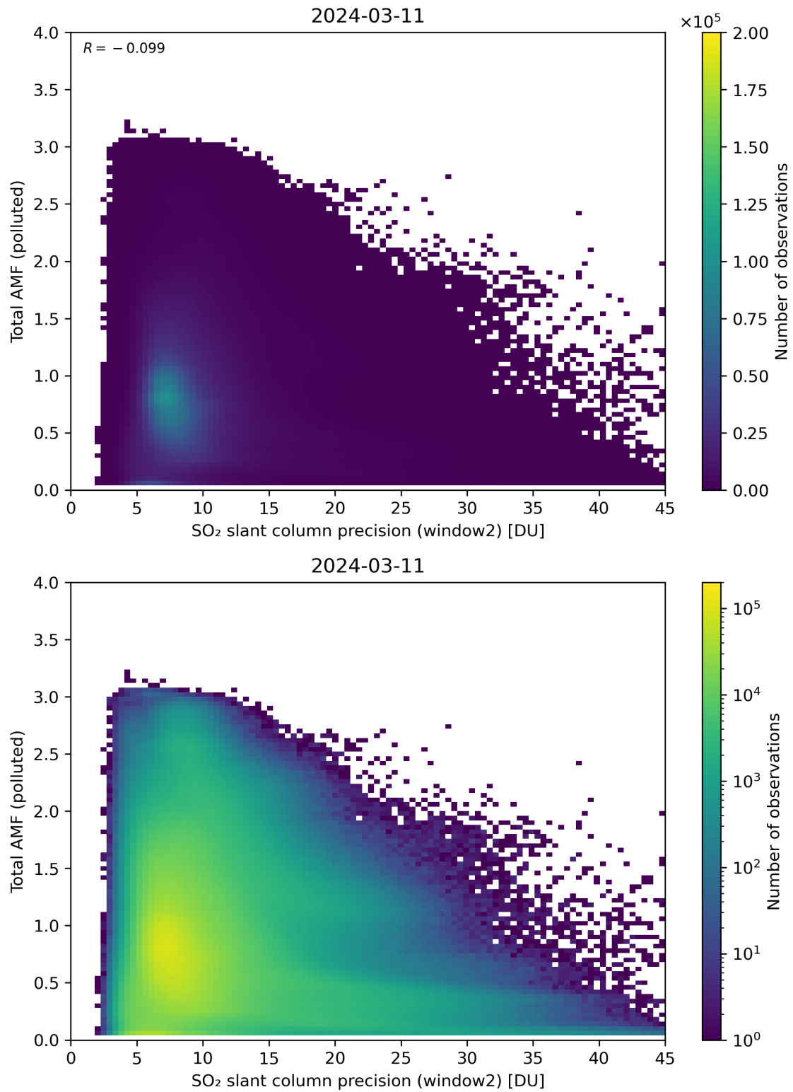
Figure 251: Scatter density plot of “SO 2 slant column precision (window2)” against “Total AMF (polluted)” for 2024-03-10 to 2024-03-12.
