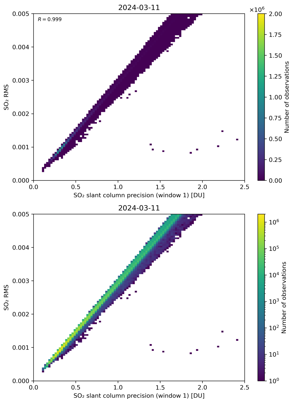
Figure 223: Scatter density plot of “SO 2 slant column precision (window 1)” against “SO 2 RMS” for 2024-03-10 to 2024-03-12.
