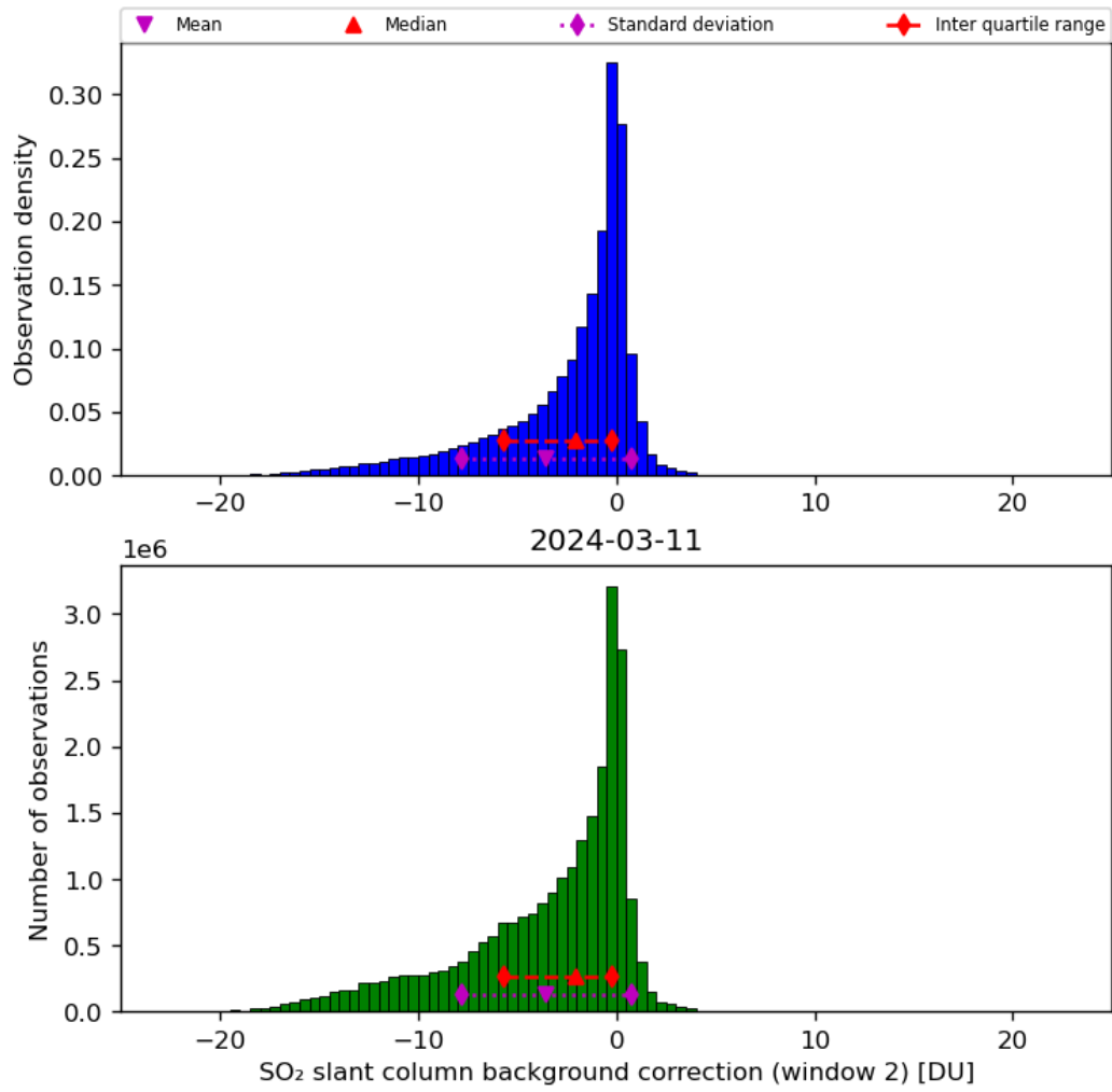
Figure 63: Histogram of “SO 2 slant column background correction (window 2)” for 2024-03-10 to 2024-03-12
