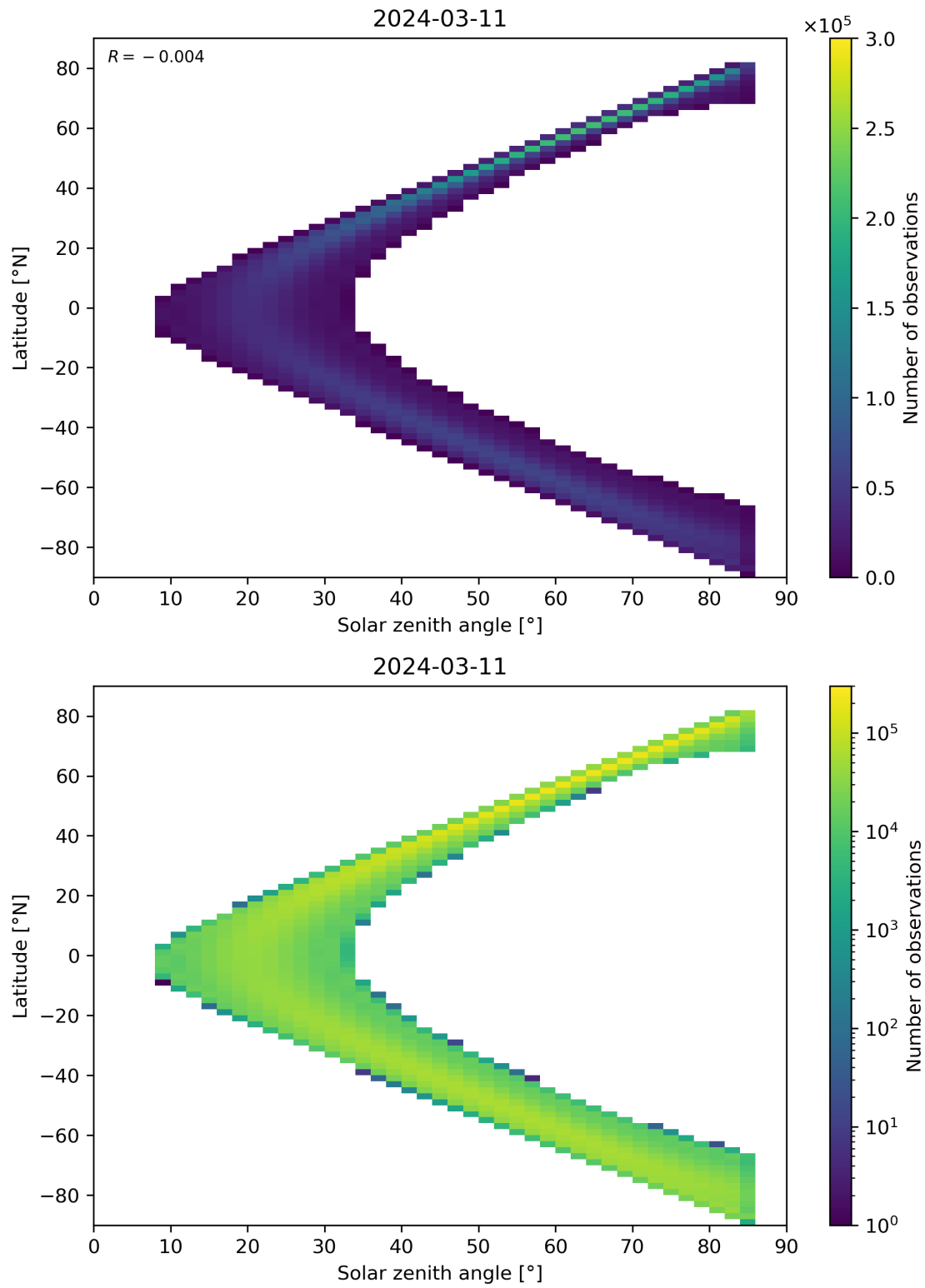
Figure 164: Scatter density plot of “Solar zenith angle” against “Latitude” for 2024-03-10 to 2024-03-12.
