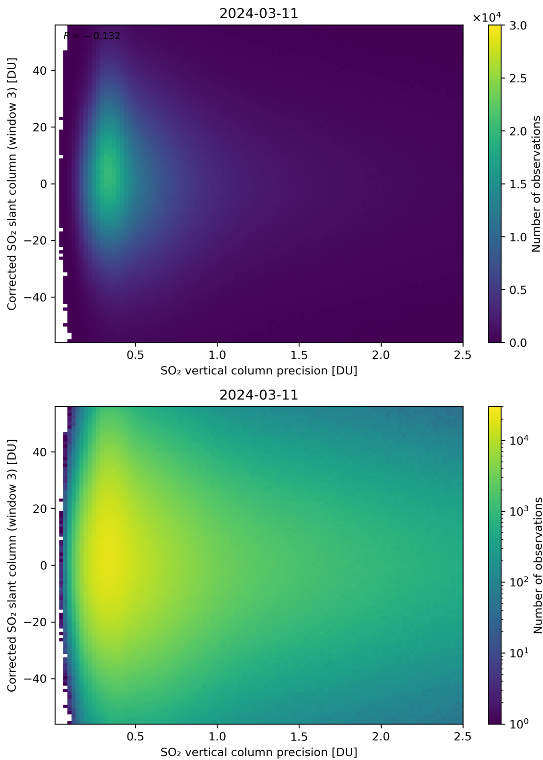
Figure 288: Scatter density plot of “SO 2 vertical column precision” against “Corrected SO 2 slant column (window 3)” for 2024-03-10 to 2024-03-12.
