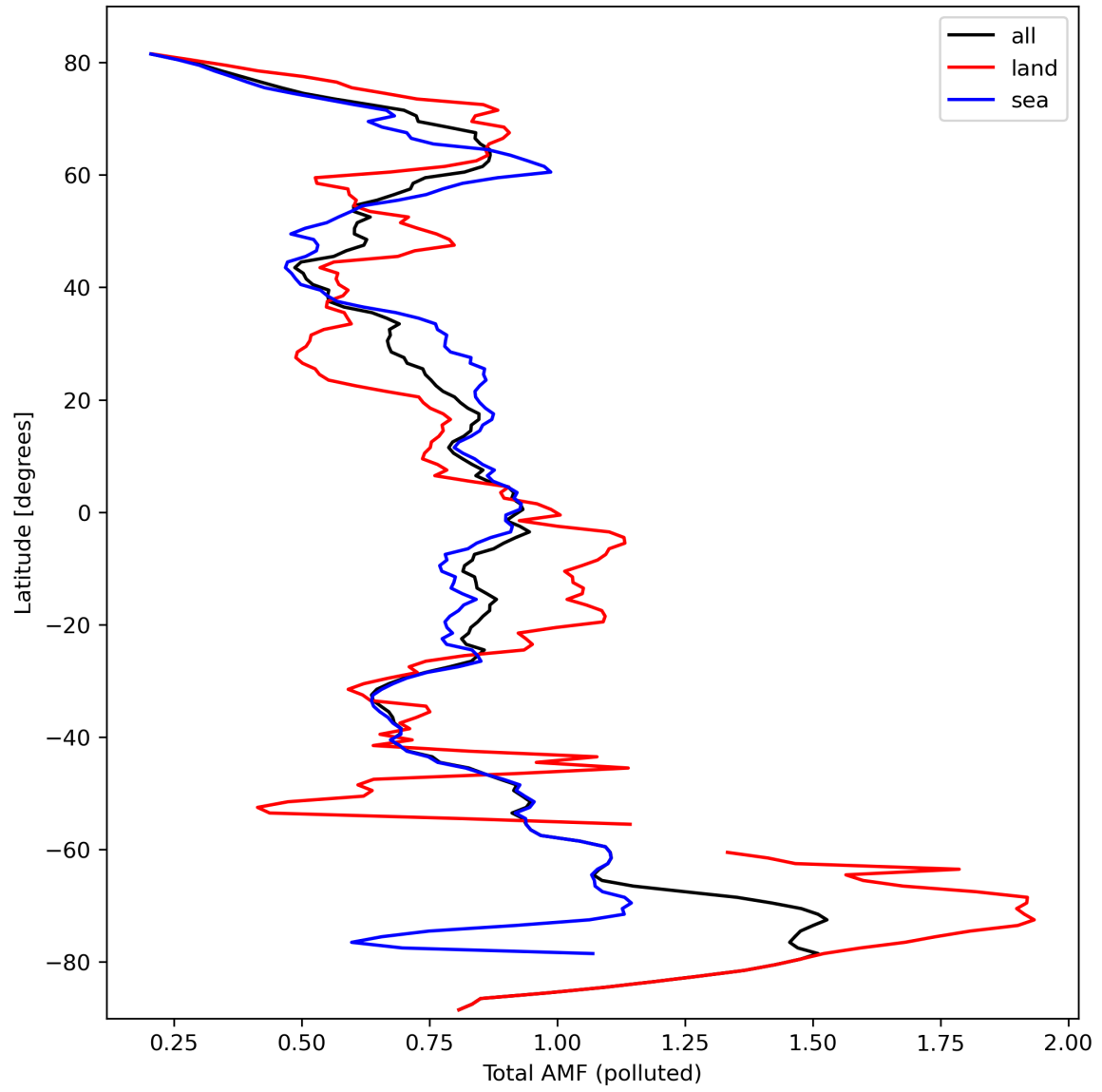
Figure 48: Zonal average of “Total AMF (polluted)” for 2024-03-10 to 2024-03-12.
