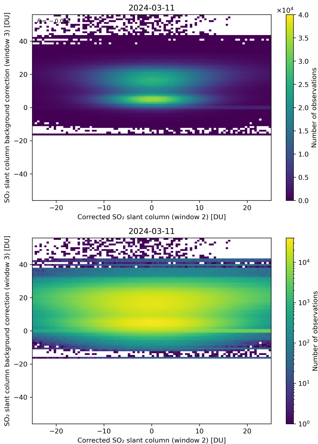
Figure 195: Scatter density plot of “Corrected SO 2 slant column (window 2)” against “SO 2 slant column background correction (window 3)” for 2024-03-10 to 2024-03-12.
