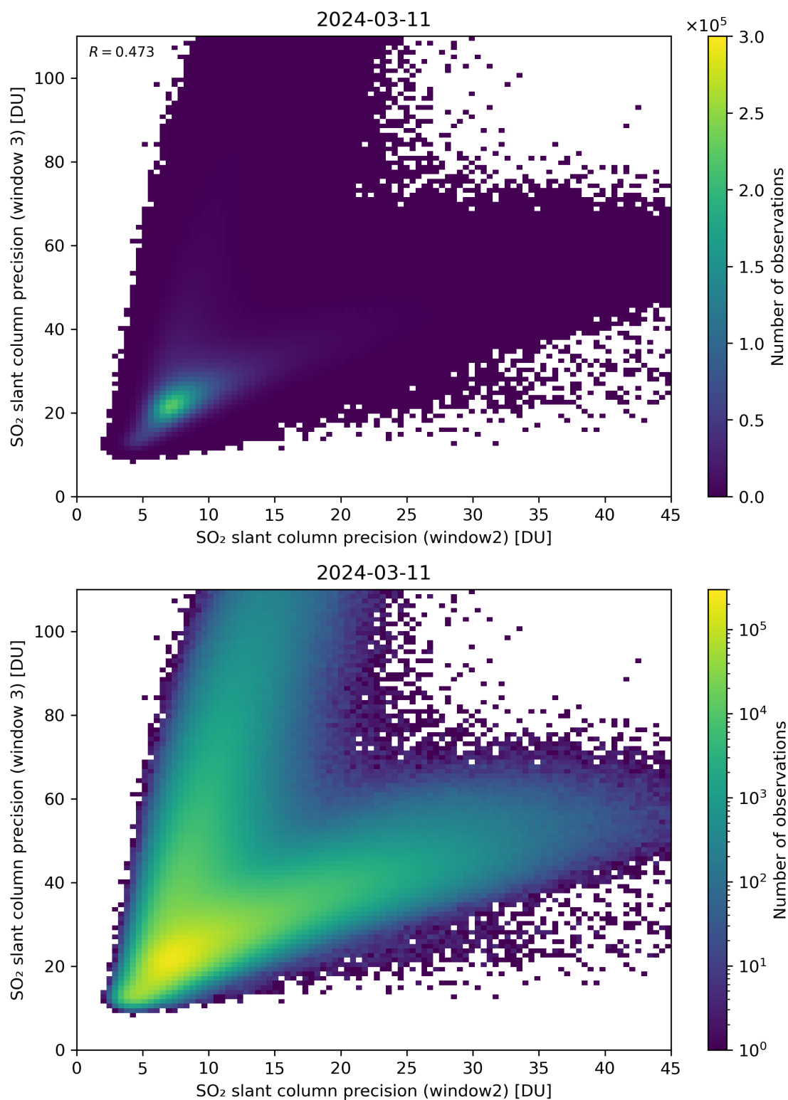
Figure 250: Scatter density plot of “SO 2 slant column precision (window2)” against “SO 2 slant column precision (window 3)” for 2024-03-10 to 2024-03-12.
