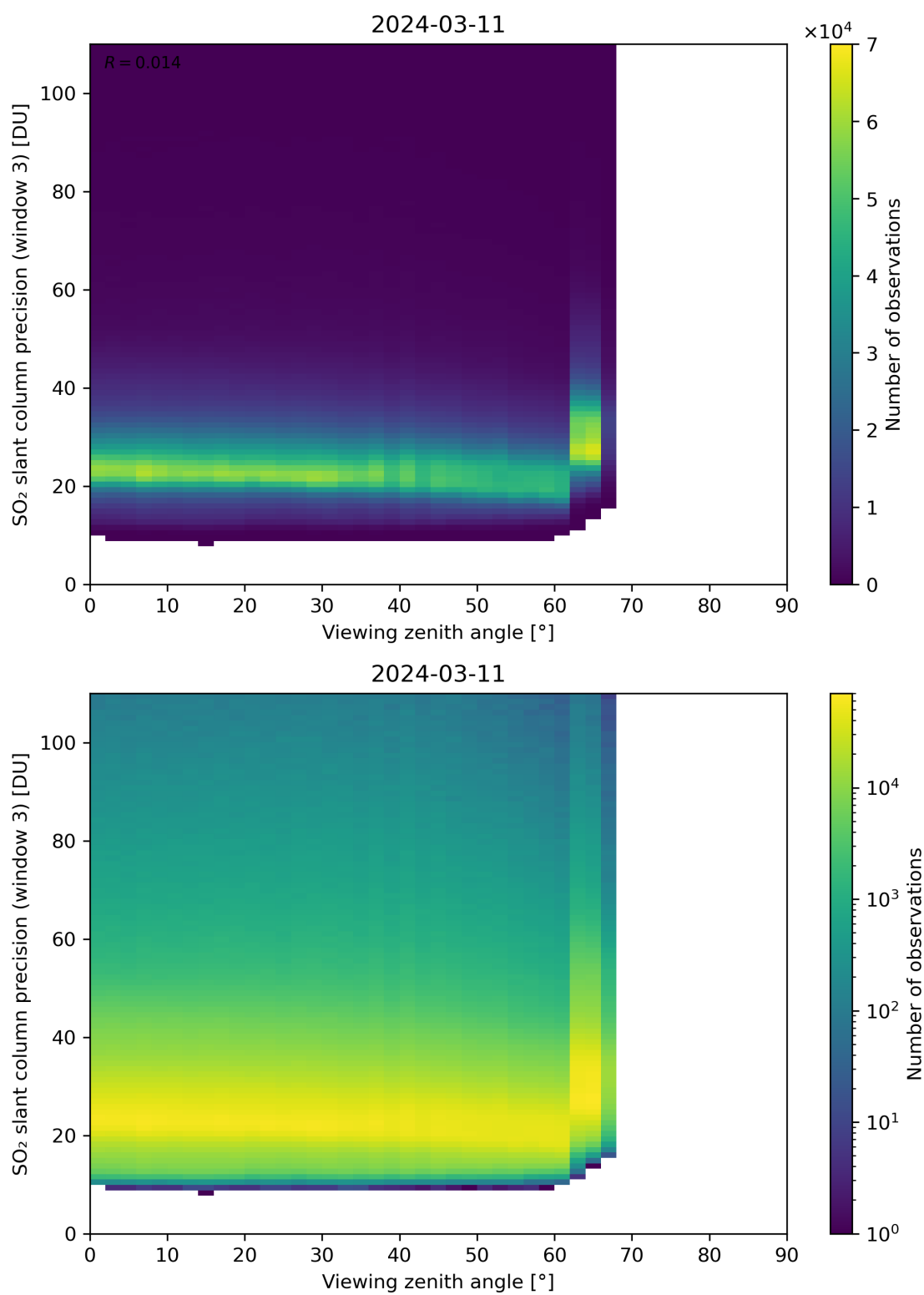
Figure 324: Scatter density plot of “Viewing zenith angle” against “SO 2 slant column precision (window 3)” for 2024-03-10 to 2024-03-12.
