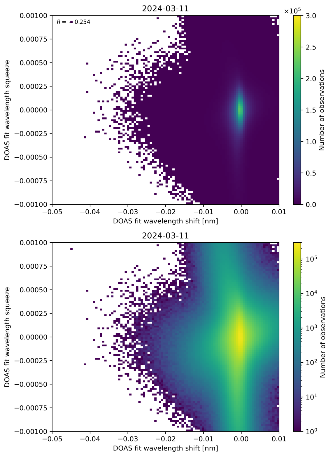
Figure 127: Scatter density plot of “DOAS fit wavelength shift” against “DOAS fit wavelength squeeze” for 2024-03-10 to 2024-03-12.
