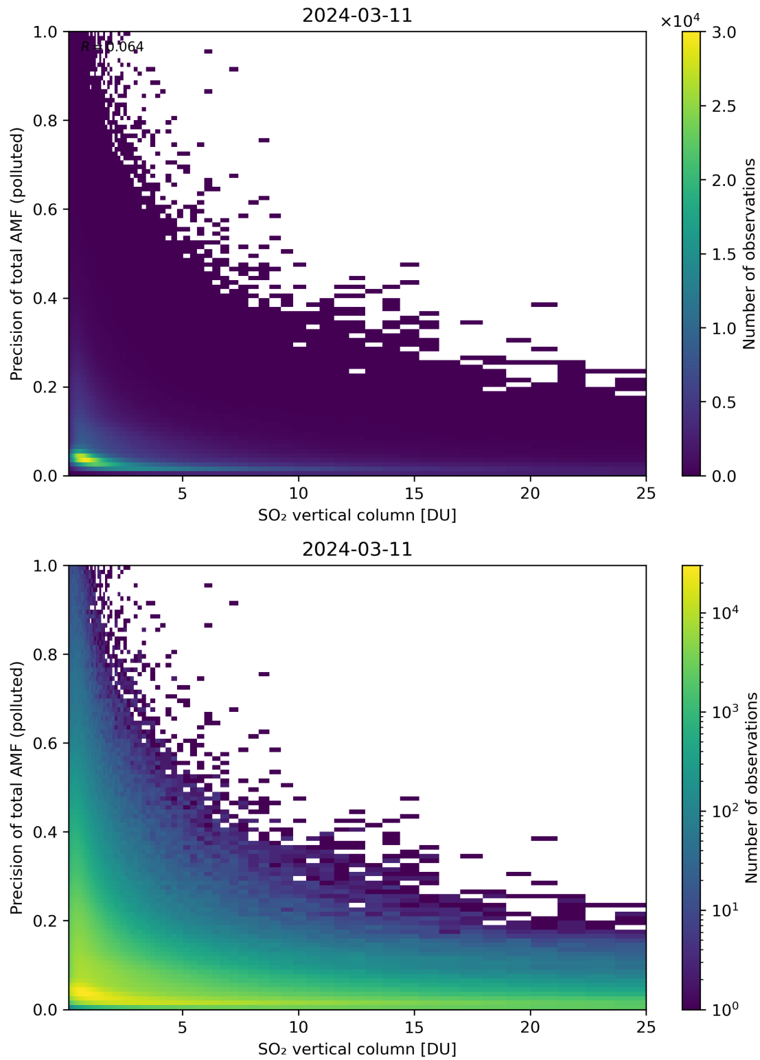
Figure 306: Scatter density plot of “SO 2 vertical column” against “Precision of total AMF (polluted)” for 2024-03-10 to 2024-03-12.
