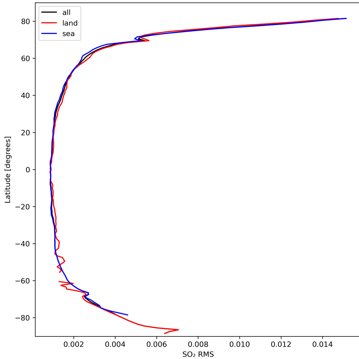
Figure 47: Zonal average of “SO 2 RMS” for 2024-03-10 to 2024-03-12.
