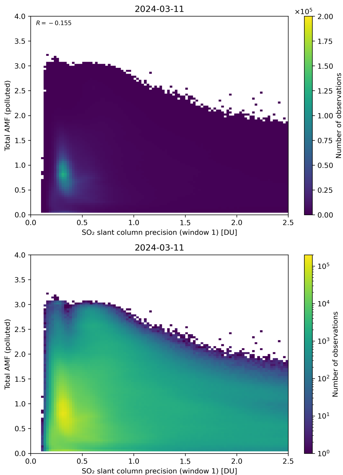
Figure 230: Scatter density plot of “SO 2 slant column precision (window 1)” against “Total AMF (polluted)” for 2024-03-10 to 2024-03-12.
