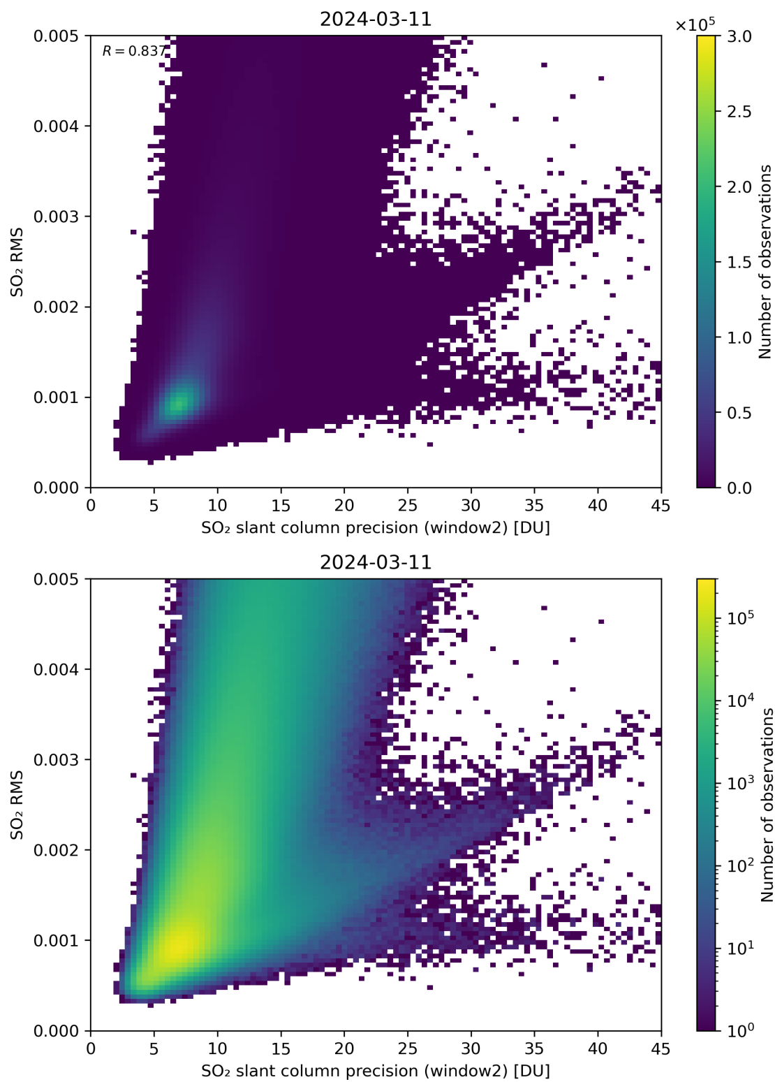
Figure 245: Scatter density plot of “SO 2 slant column precision (window2)” against “SO 2 RMS” for 2024-03-10 to 2024-03-12.
