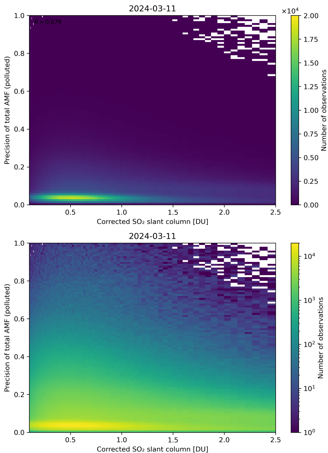
Figure 193: Scatter density plot of “Corrected SO 2 slant column” against “Precision of total AMF (polluted)” for 2024-03-10 to 2024-03-12.
