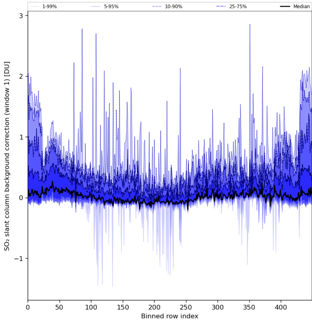
Figure 82: Along track statistics of “SO 2 slant column background correction (window 1)” for 2024-03-10 to 2024-03-12
