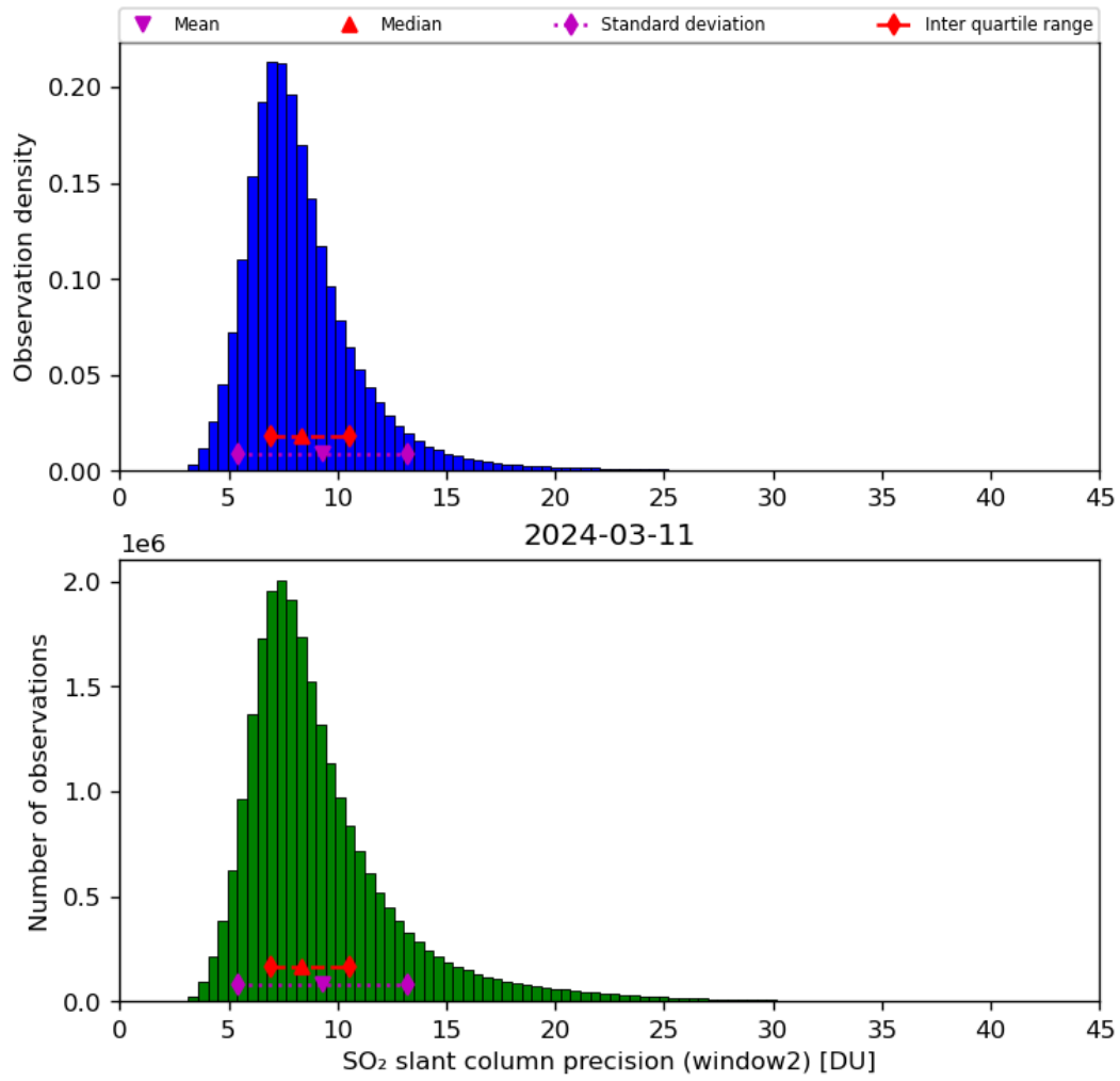
Figure 61: Histogram of “SO 2 slant column precision (window2)” for 2024-03-10 to 2024-03-12
