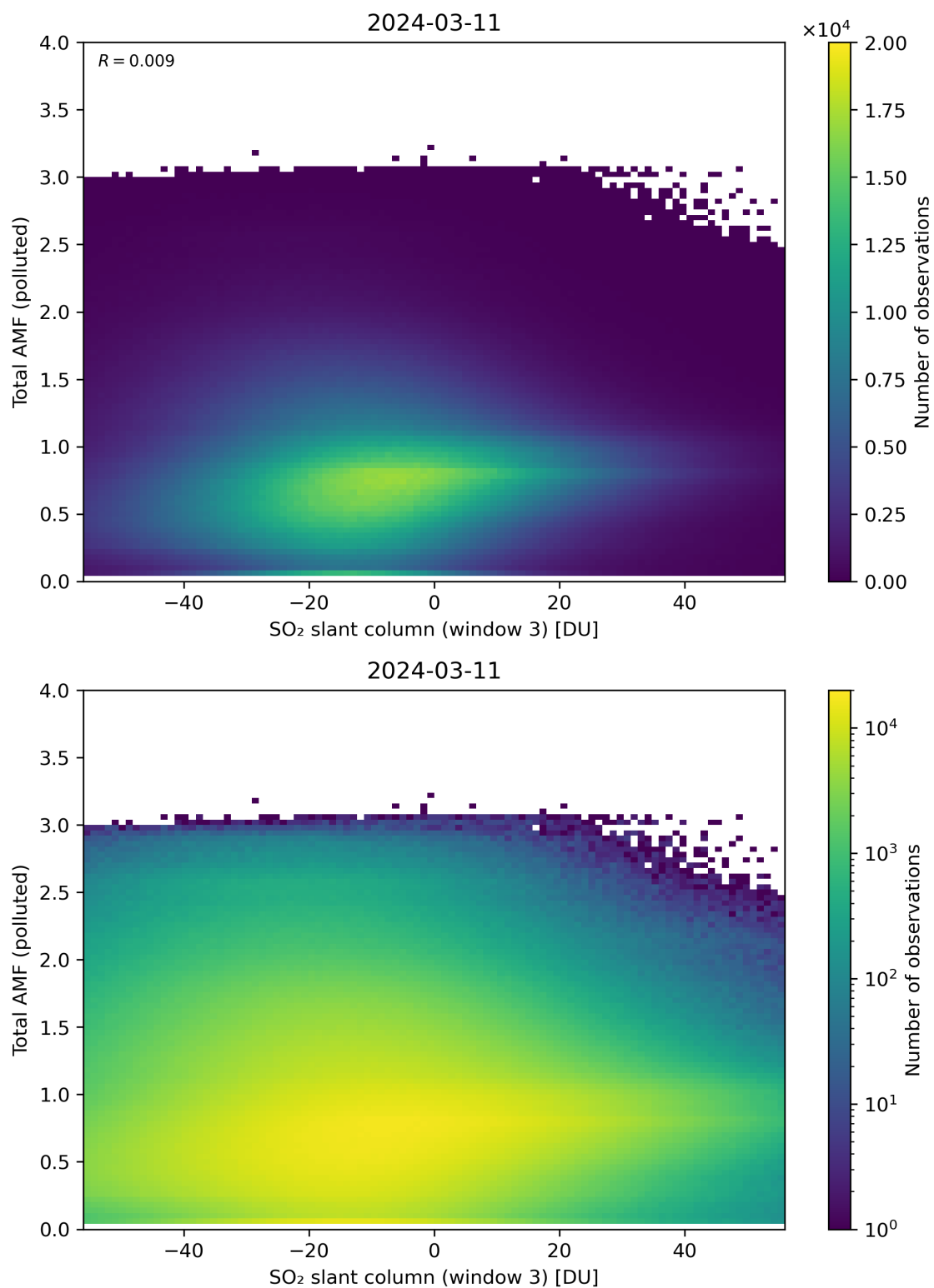
Figure 268: Scatter density plot of “SO 2 slant column (window 3)” against “Total AMF (polluted)” for 2024-03-10 to 2024-03-12.
