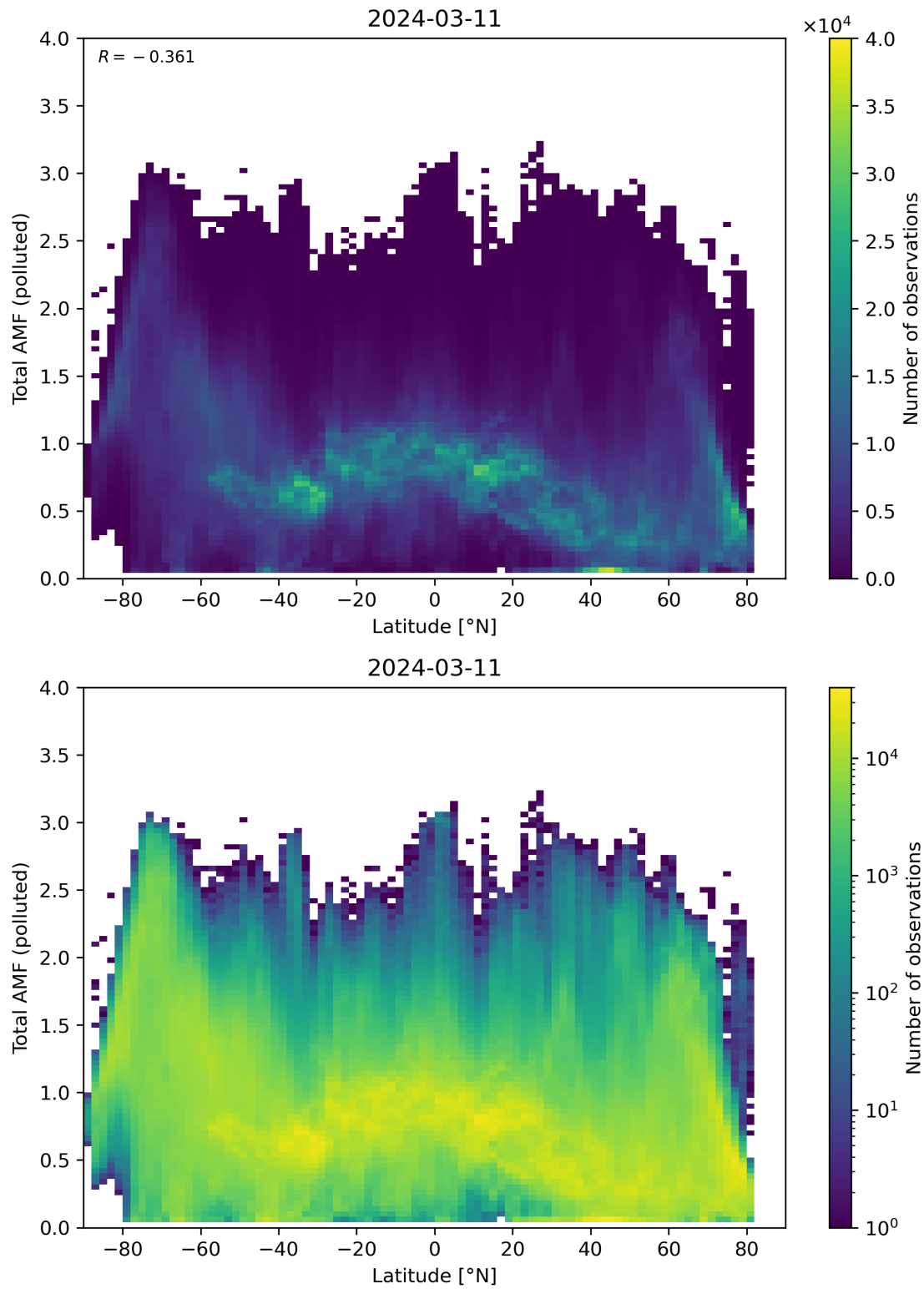
Figure 154: Scatter density plot of “Latitude” against “Total AMF (polluted)” for 2024-03-10 to 2024-03-12.
