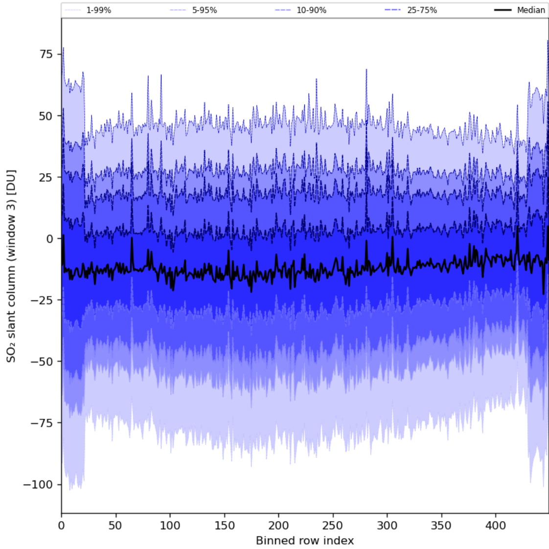
Figure 87: Along track statistics of “SO 2 slant column (window 3)” for 2024-03-10 to 2024-03-12
