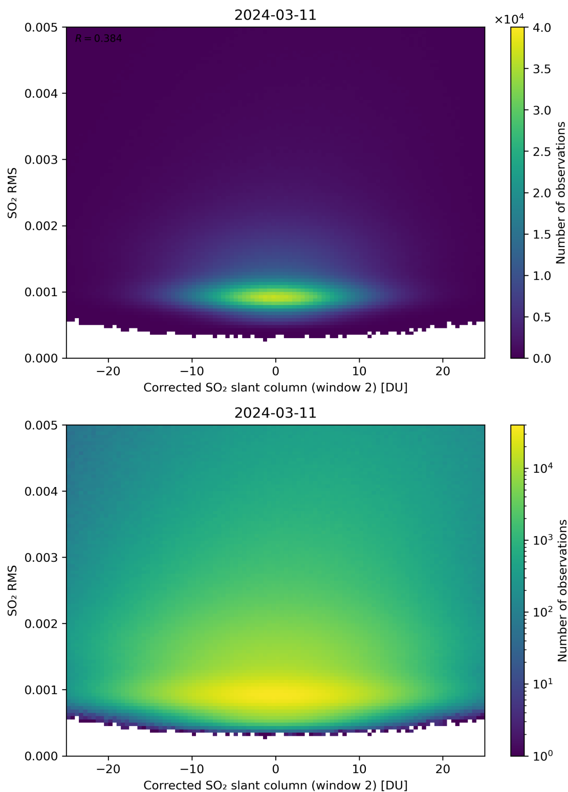
Figure 198: Scatter density plot of “Corrected SO 2 slant column (window 2)” against “SO 2 RMS” for 2024-03-10 to 2024-03-12.
