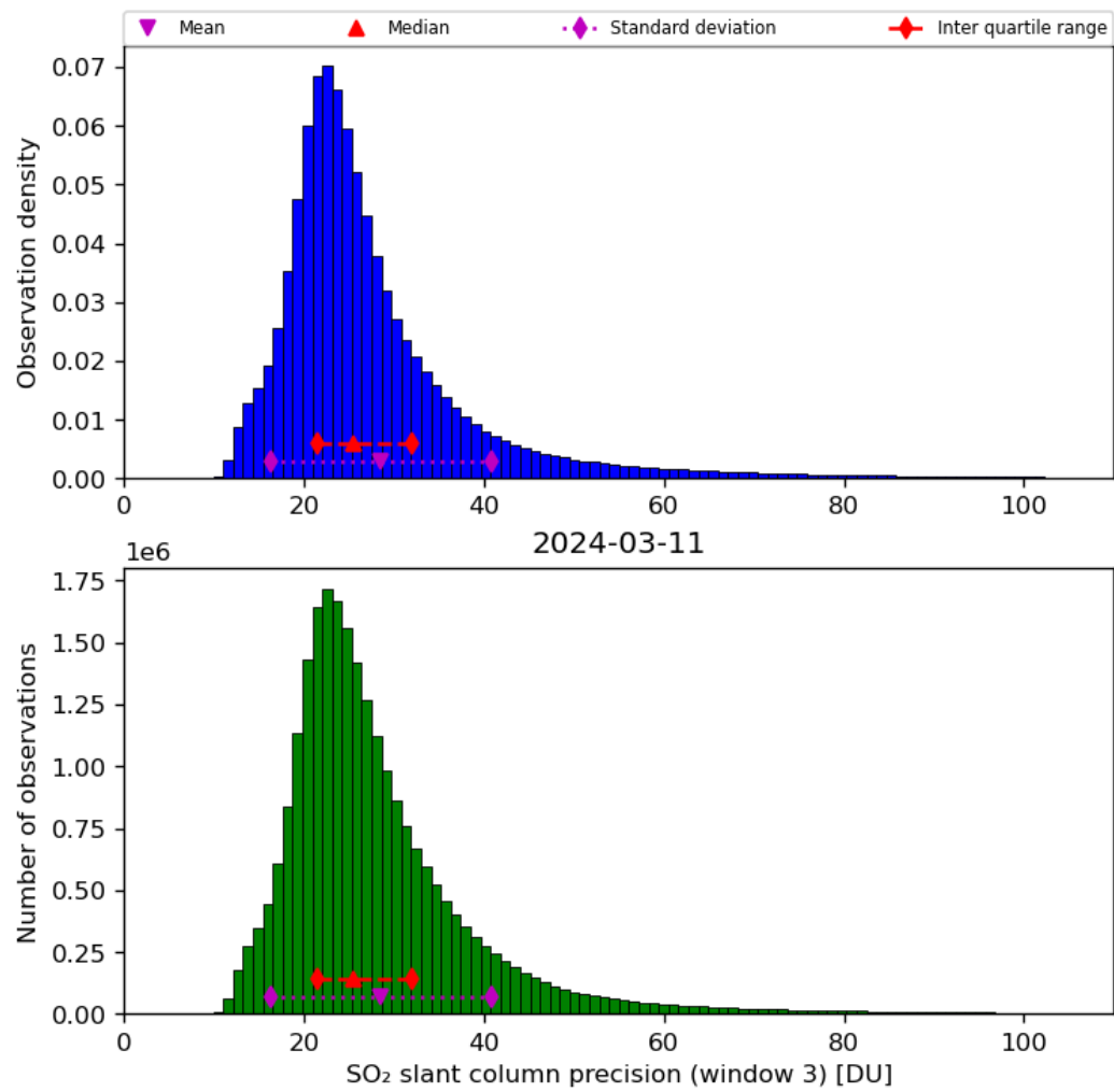
Figure 65: Histogram of “SO 2 slant column precision (window 3)” for 2024-03-10 to 2024-03-12
