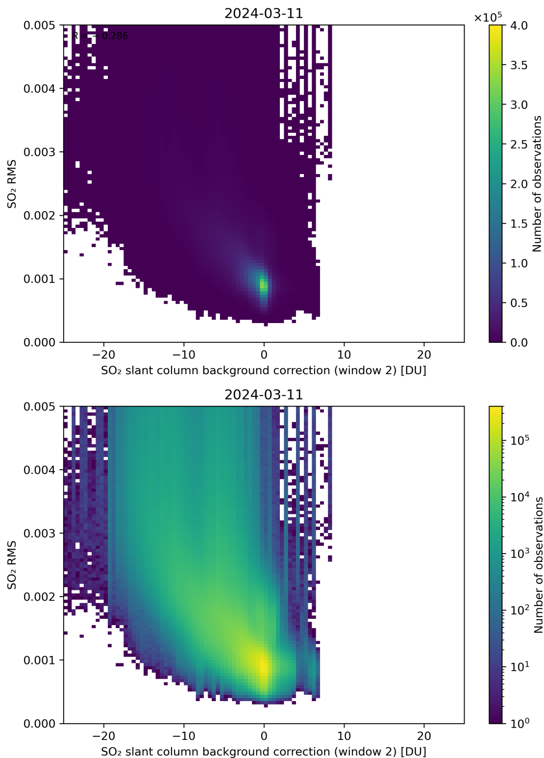
Figure 114: Scatter density plot of “SO 2 slant column background correction (window 2)” against “SO 2 RMS” for 2024-03-10 to 2024-03-12.
