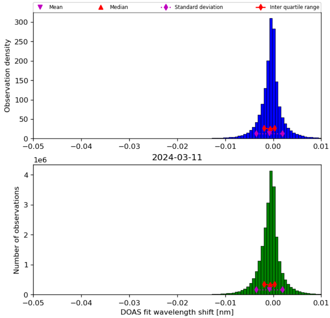
Figure 68: Histogram of “DOAS fit wavelength shift” for 2024-03-10 to 2024-03-12
