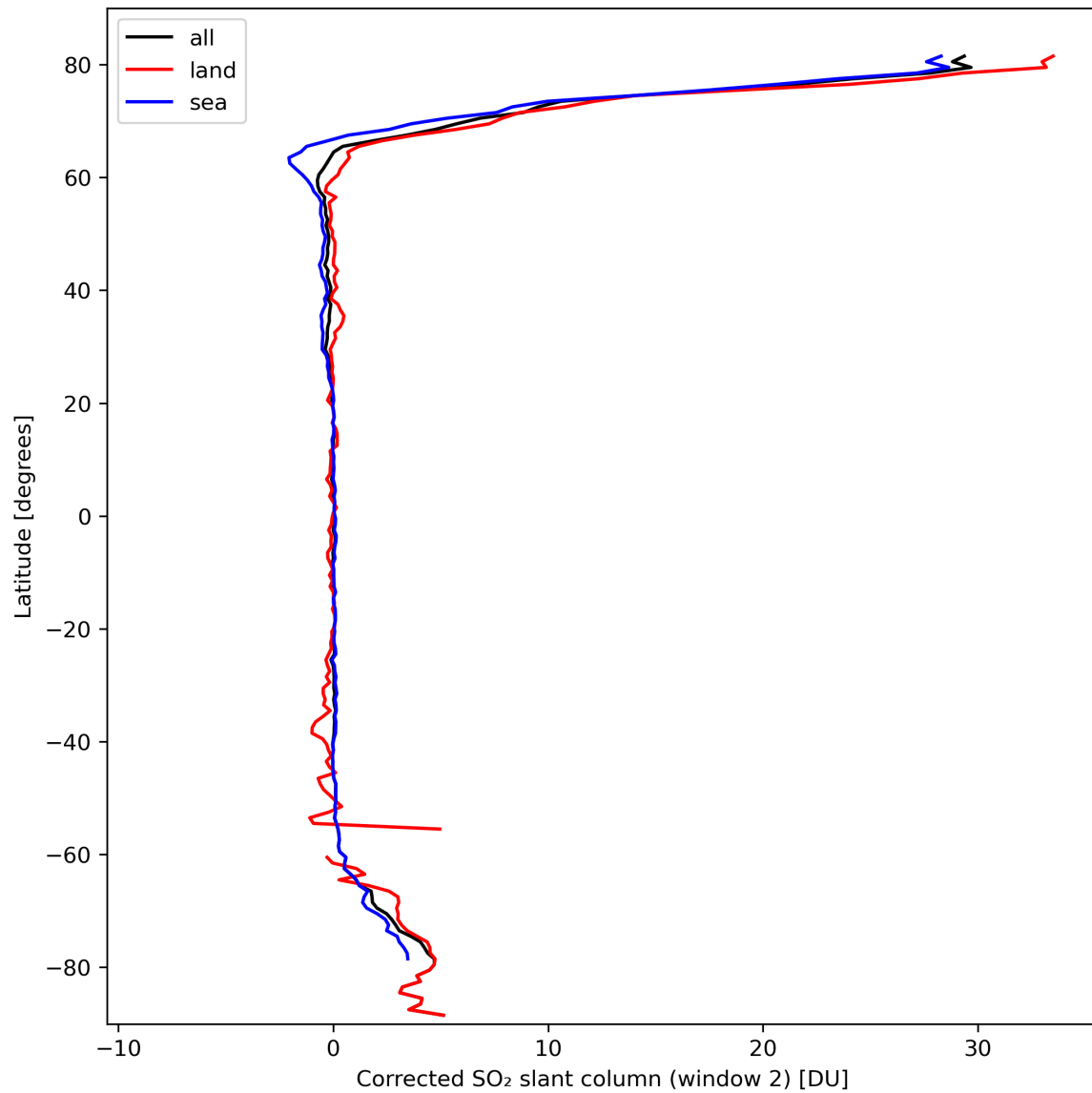
Figure 39: Zonal average of “Corrected SO 2 slant column (window 2)” for 2024-03-10 to 2024-03-12.
