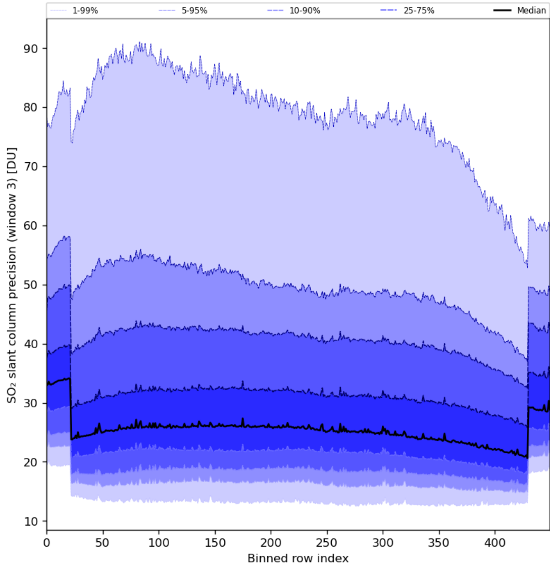
Figure 88: Along track statistics of “SO 2 slant column precision (window 3)” for 2024-03-10 to 2024-03-12
