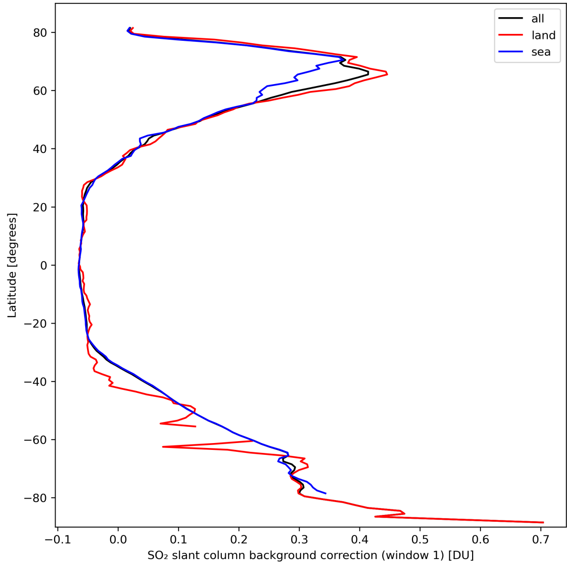
Figure 36: Zonal average of “SO 2 slant column background correction (window 1)” for 2024-03-10 to 2024-03-12.
