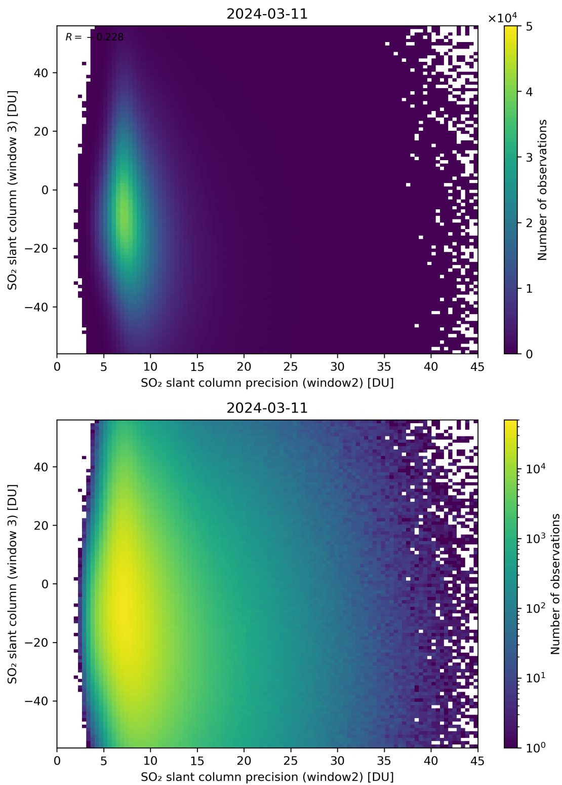
Figure 249: Scatter density plot of “SO 2 slant column precision (window2)” against “SO 2 slant column (window 3)” for 2024-03-10 to 2024-03-12.
