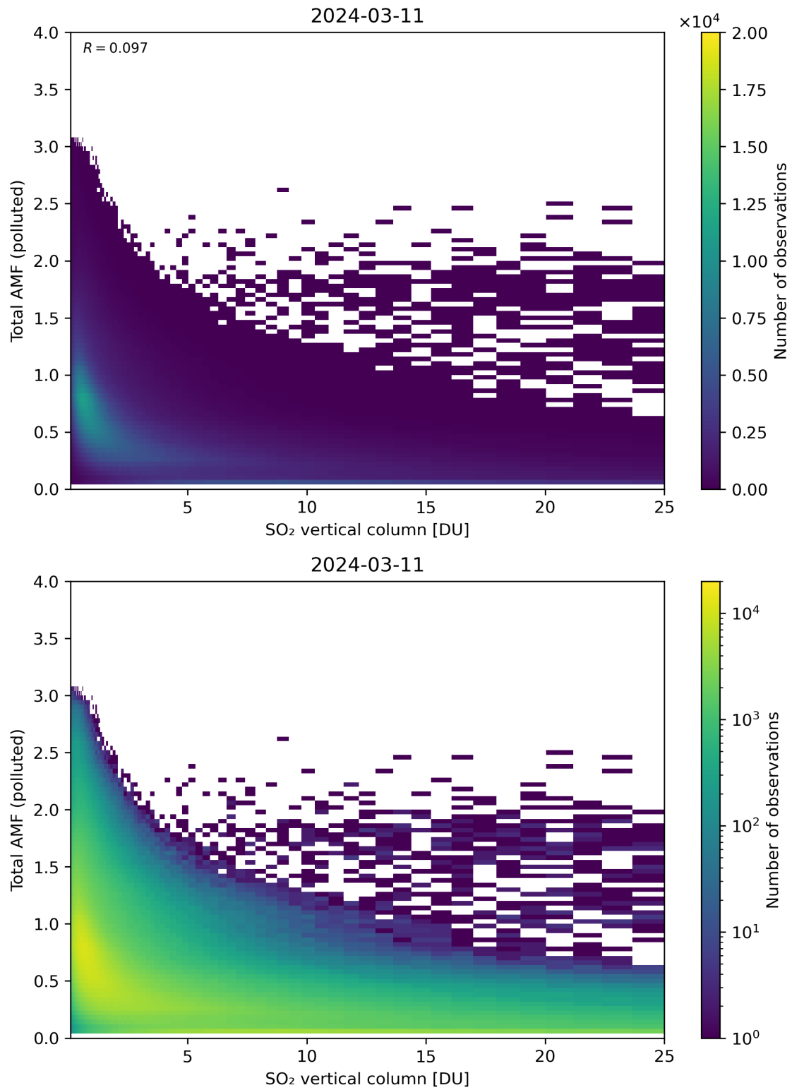
Figure 305: Scatter density plot of “SO 2 vertical column” against “Total AMF (polluted)” for 2024-03-10 to 2024-03-12.
