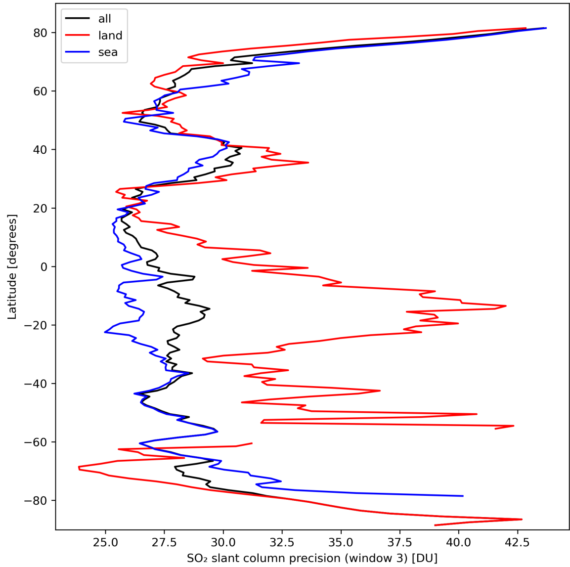
Figure 42: Zonal average of “SO 2 slant column precision (window 3)” for 2024-03-10 to 2024-03-12.
