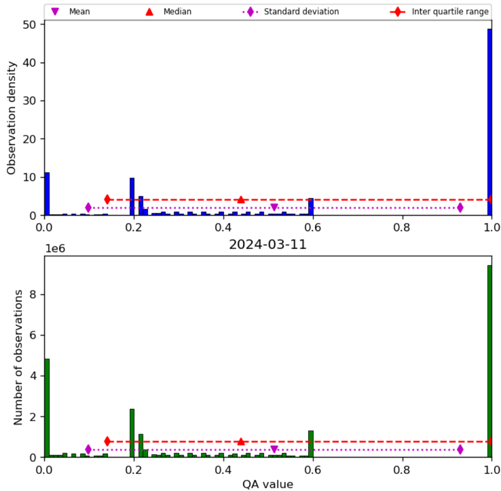
Figure 52: Histogram of “QA value” for 2024-03-10 to 2024-03-12
