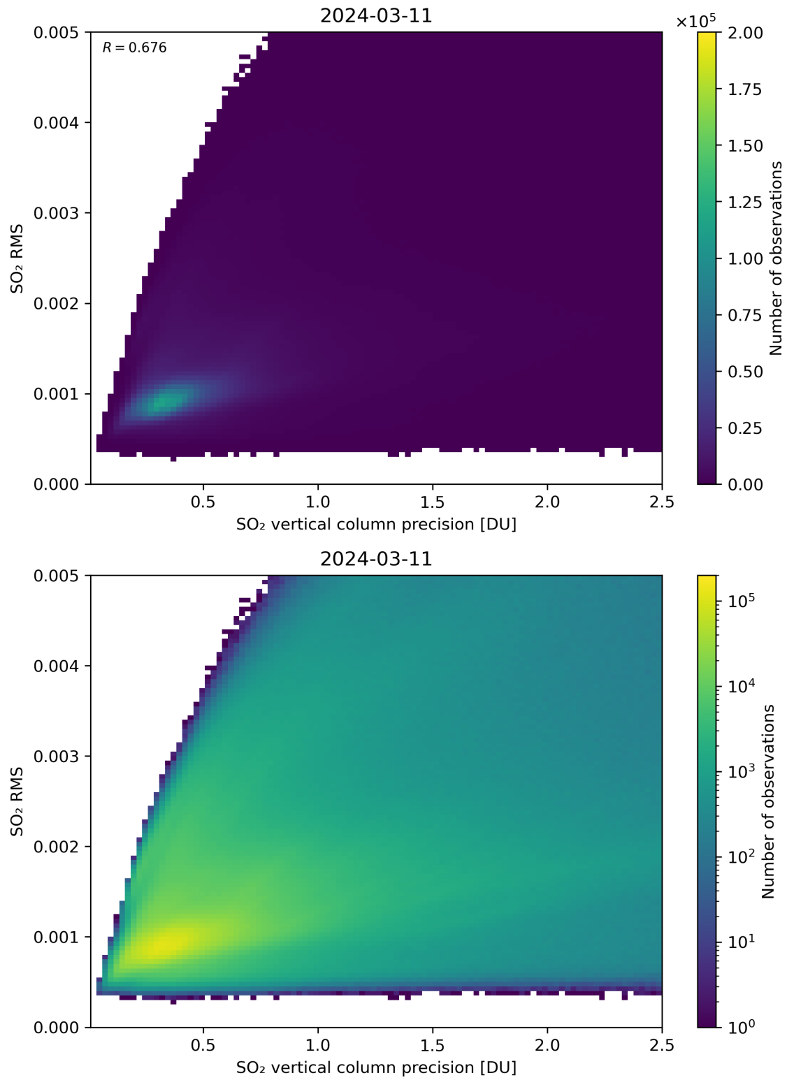
Figure 284: Scatter density plot of “SO 2 vertical column precision” against “SO 2 RMS” for 2024-03-10 to 2024-03-12.
