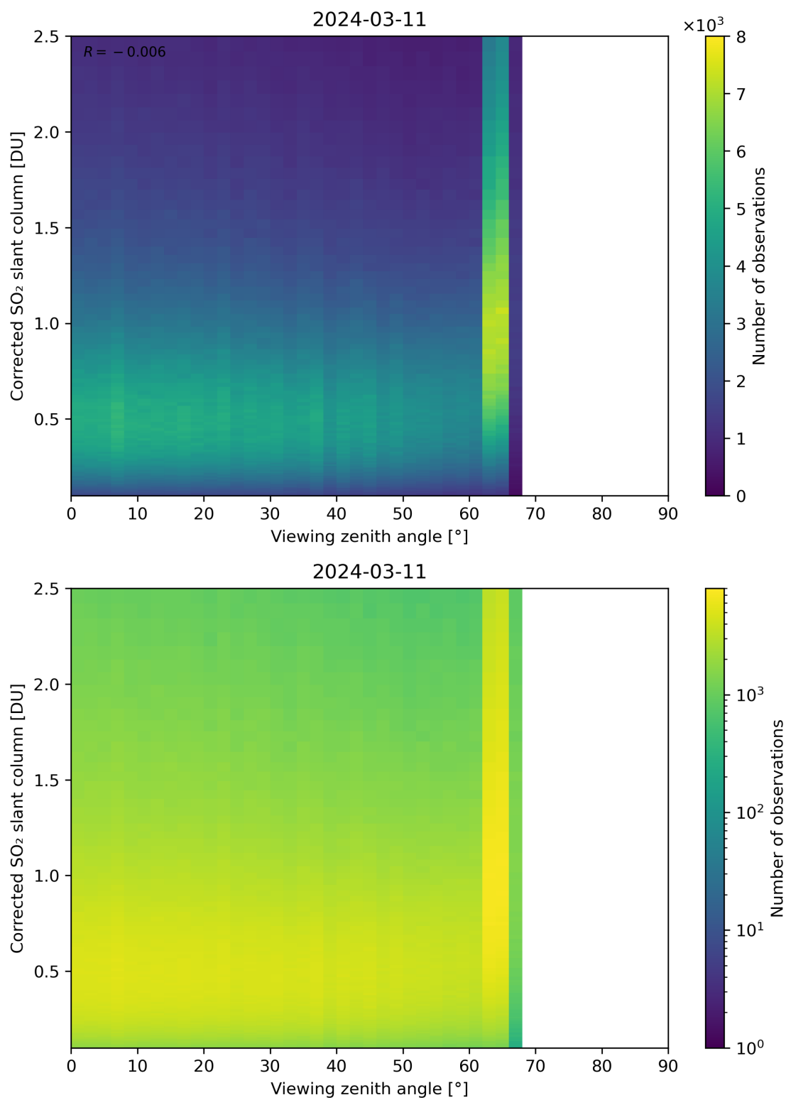
Figure 317: Scatter density plot of “Viewing zenith angle” against “Corrected SO 2 slant column” for 2024-03-10 to 2024-03-12.
