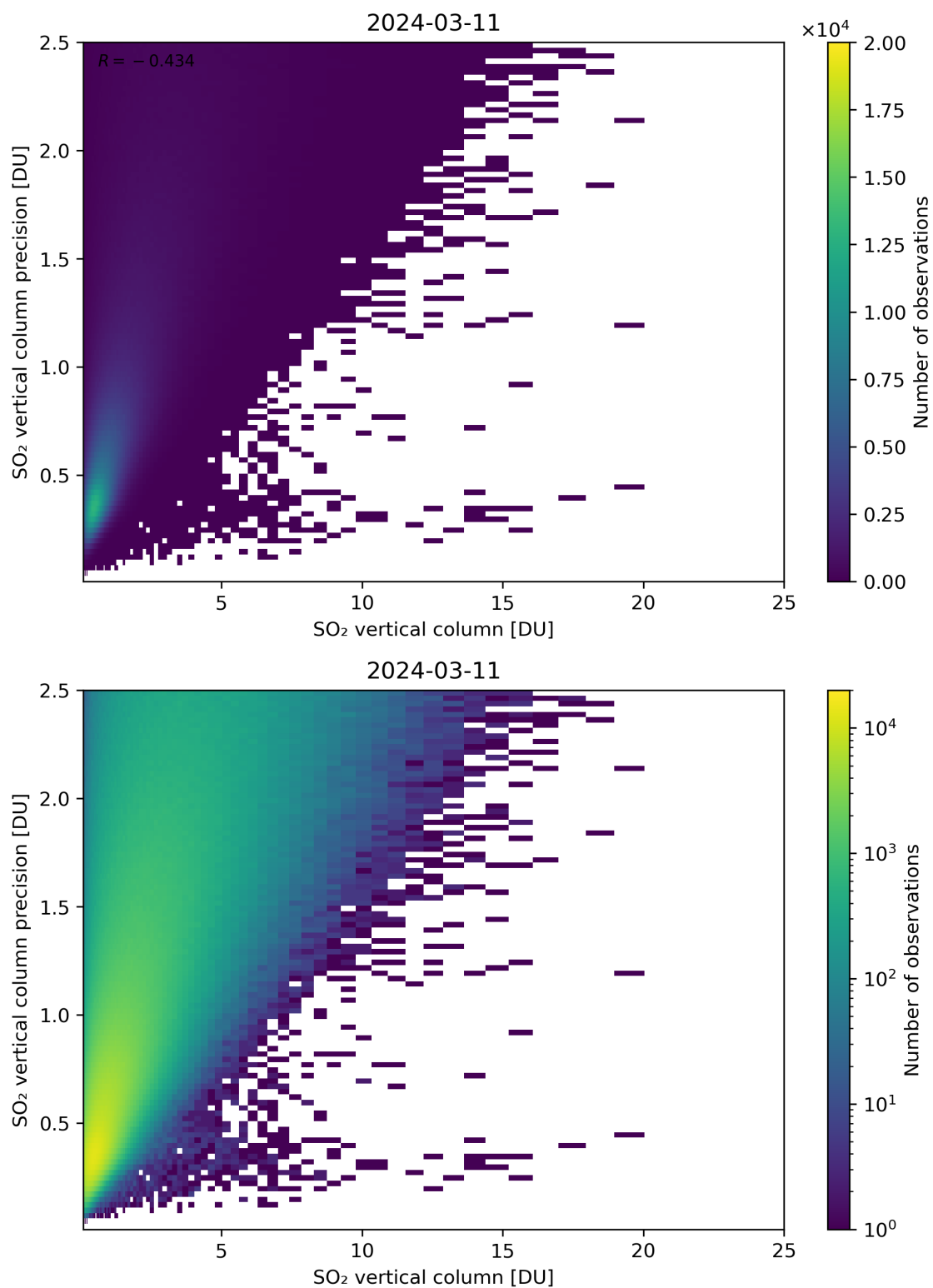
Figure 307: Scatter density plot of “SO 2 vertical column” against “SO 2 vertical column precision” for 2024-03-10 to 2024-03-12.
