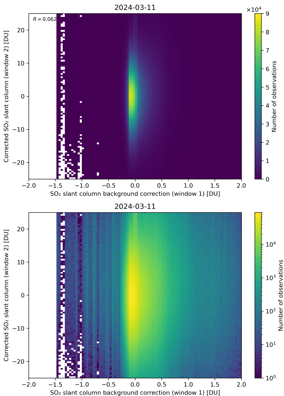
Figure 104: Scatter density plot of “SO 2 slant column background correction (window 1)” against “Corrected SO 2 slant column (window 2)” for 2024-03-10 to 2024-03-12.
