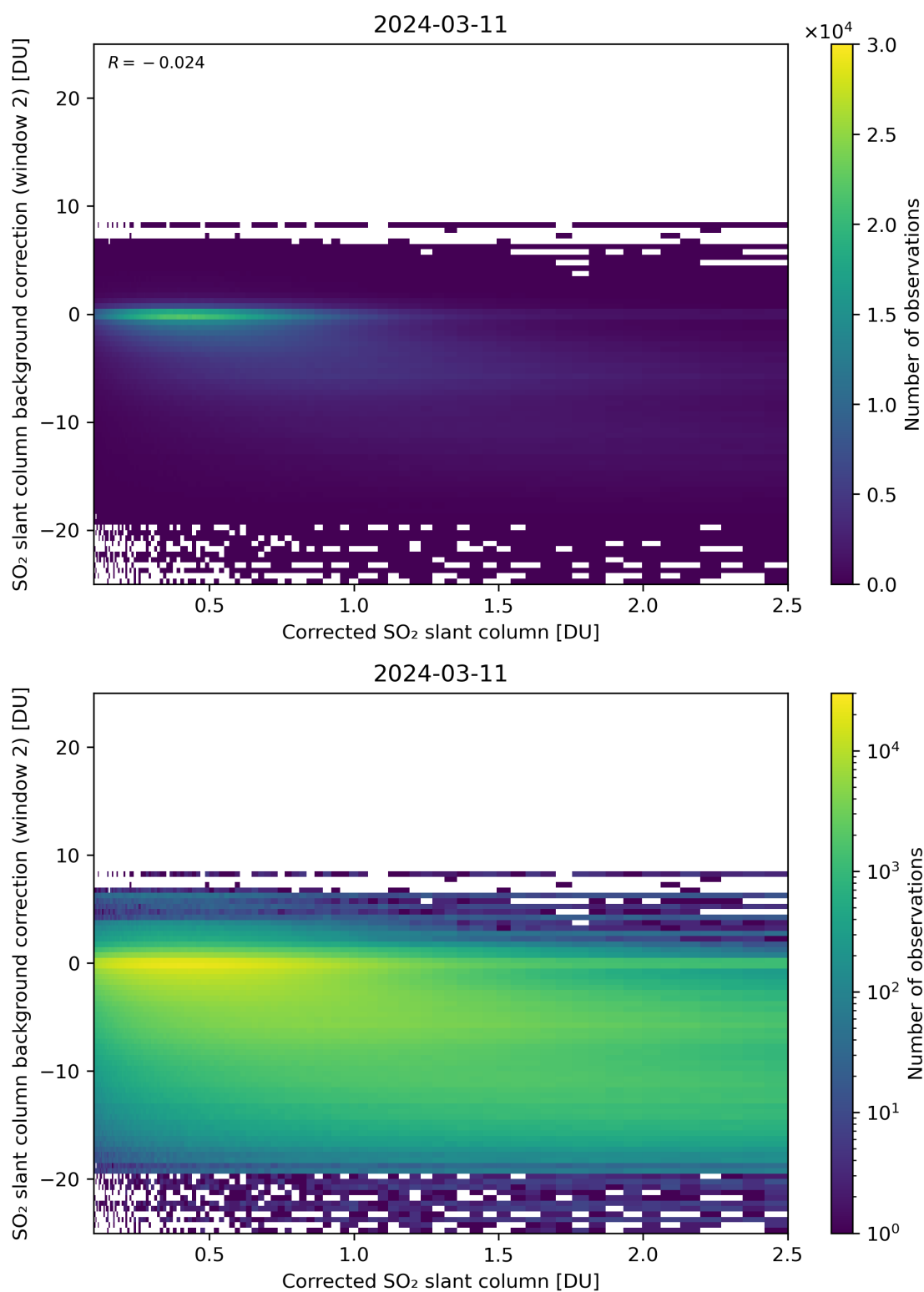
Figure 179: Scatter density plot of “Corrected SO 2 slant column” against “SO 2 slant column background correction (window 2)” for 2024-03-10 to 2024-03-12.
