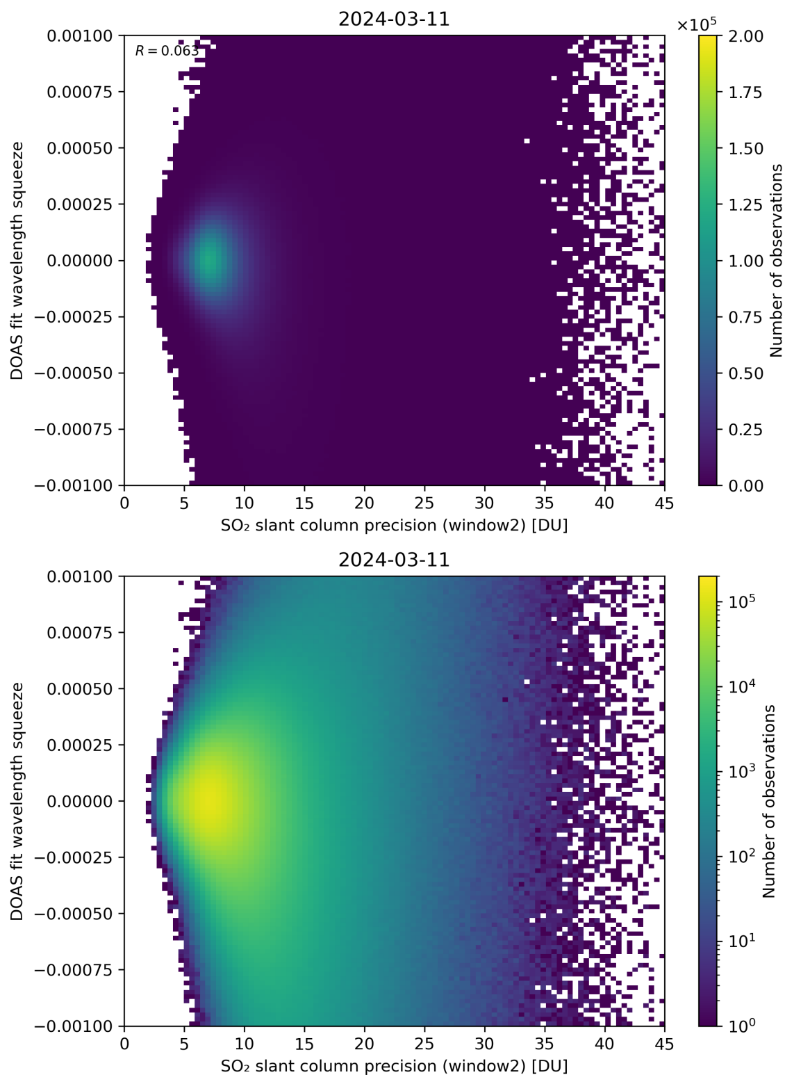
Figure 244: Scatter density plot of “SO 2 slant column precision (window2)” against “DOAS fit wavelength squeeze” for 2024-03-10 to 2024-03-12.
