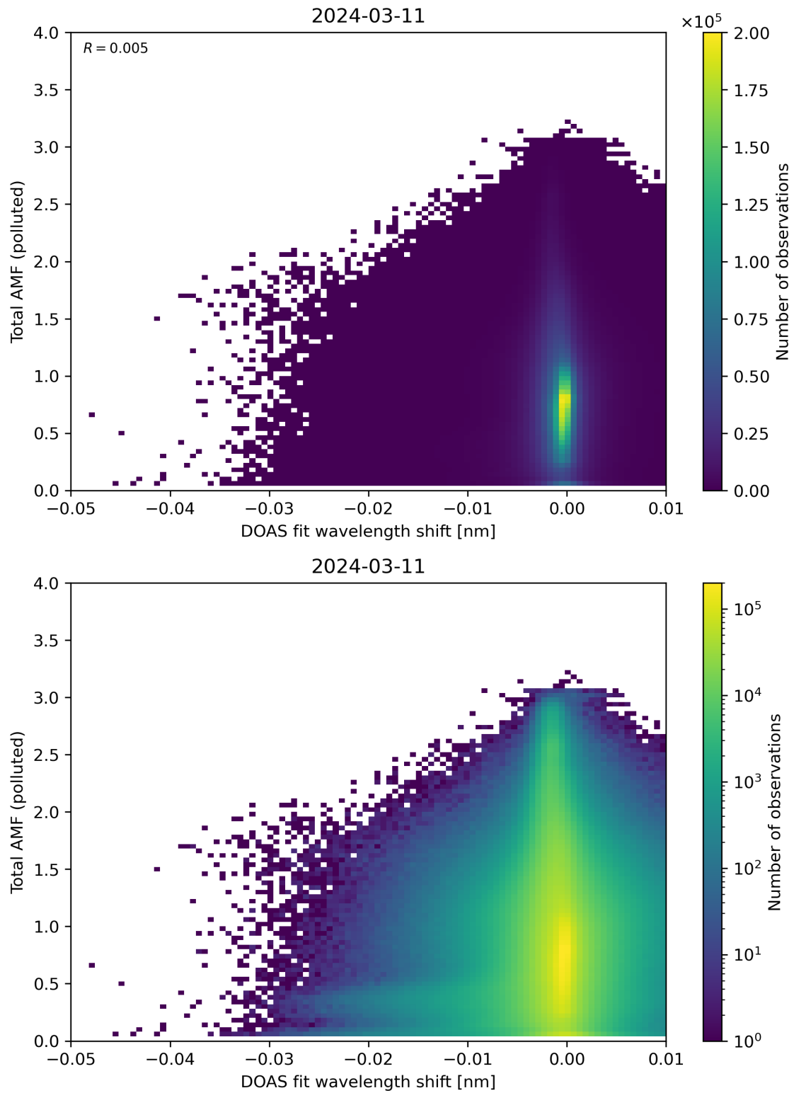
Figure 130: Scatter density plot of “DOAS fit wavelength shift” against “Total AMF (polluted)” for 2024-03-10 to 2024-03-12.
