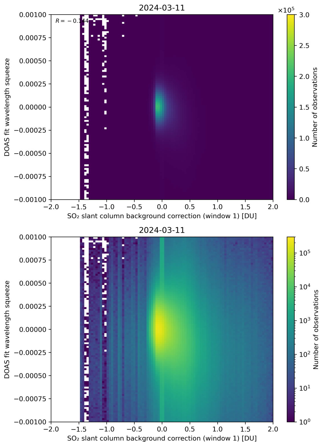
Figure 101: Scatter density plot of “SO 2 slant column background correction (window 1)” against “DOAS fit wavelength squeeze” for 2024-03-10 to 2024-03-12.
