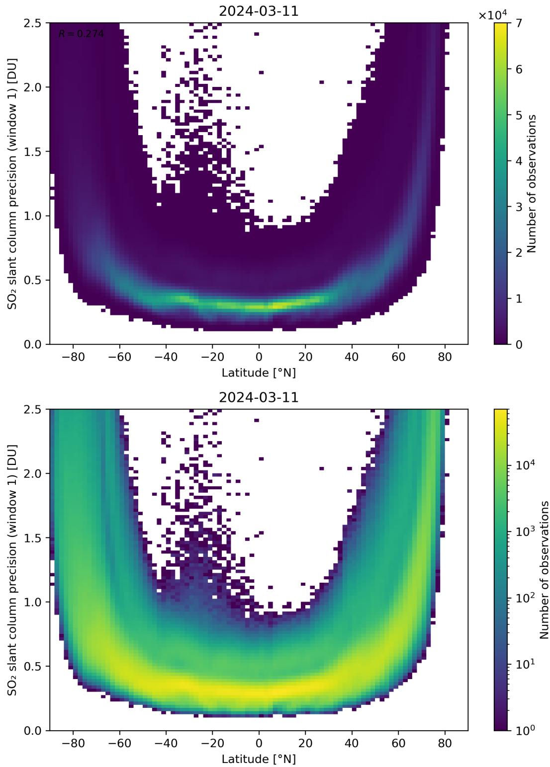
Figure 150: Scatter density plot of “Latitude” against “SO 2 slant column precision (window 1)” for 2024-03-10 to 2024-03-12.
