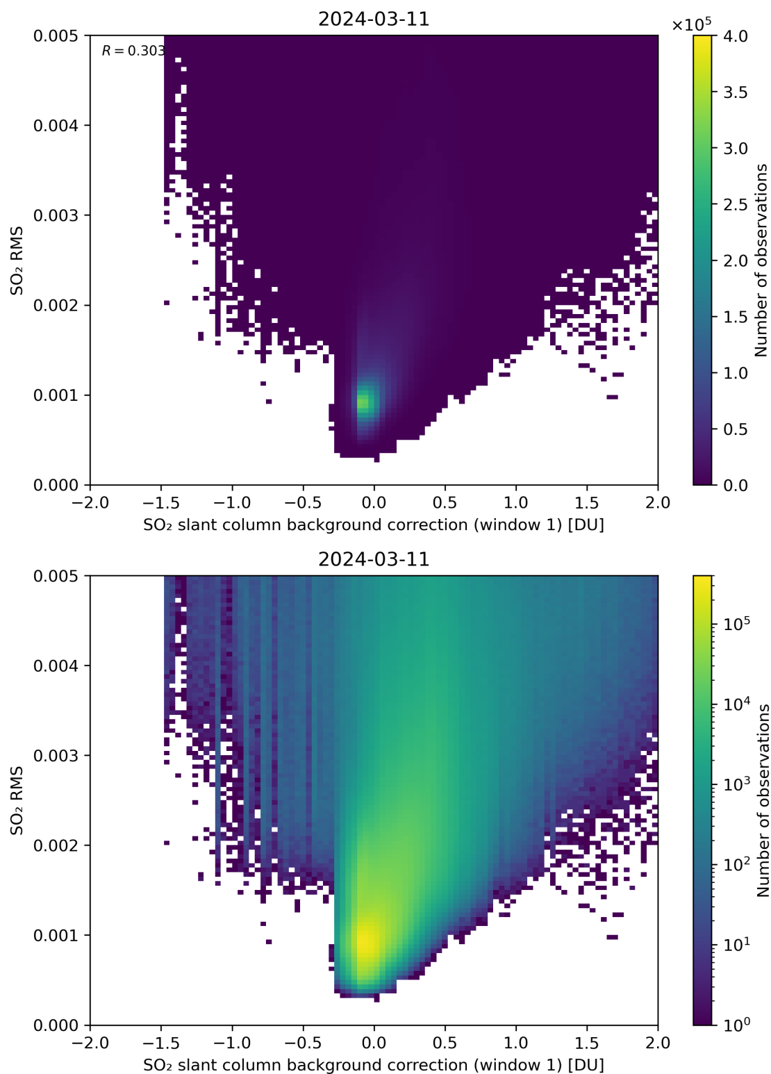
Figure 102: Scatter density plot of “SO 2 slant column background correction (window 1)” against “SO 2 RMS” for 2024-03-10 to 2024-03-12.
