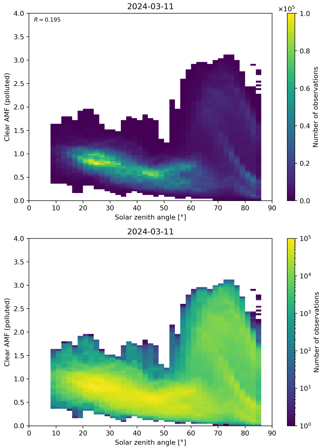
Figure 165: Scatter density plot of “Solar zenith angle” against “Clear AMF (polluted)” for 2024-03-10 to 2024-03-12.
