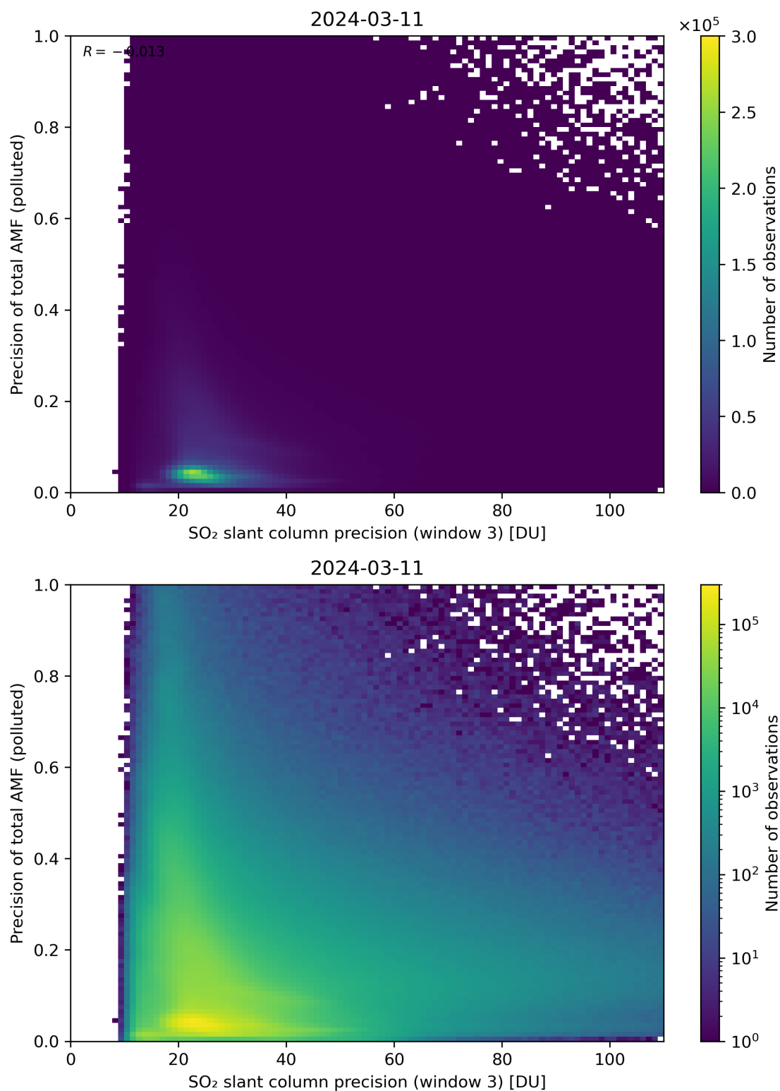
Figure 264: Scatter density plot of “SO 2 slant column precision (window 3)” against “Precision of total AMF (polluted)” for 2024-03-10 to 2024-03-12.
