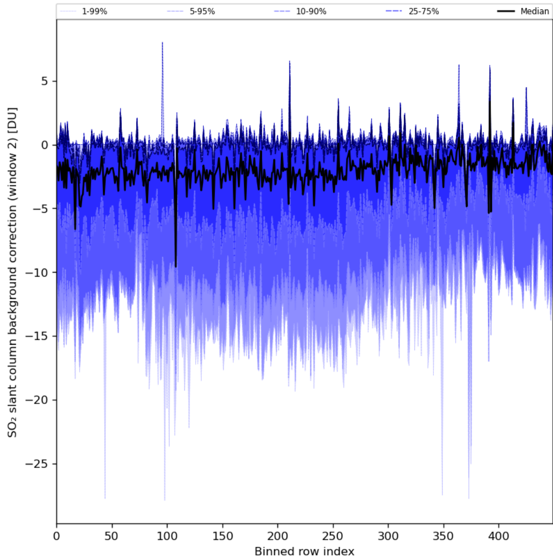
Figure 86: Along track statistics of “SO 2 slant column background correction (window 2)” for 2024-03-10 to 2024-03-12
