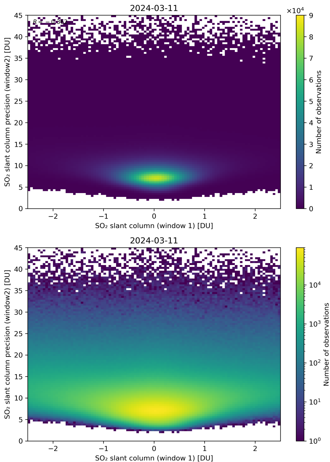
Figure 236: Scatter density plot of “SO 2 slant column (window 1)” against “SO 2 slant column precision (window2)” for 2024-03-10 to 2024-03-12.
