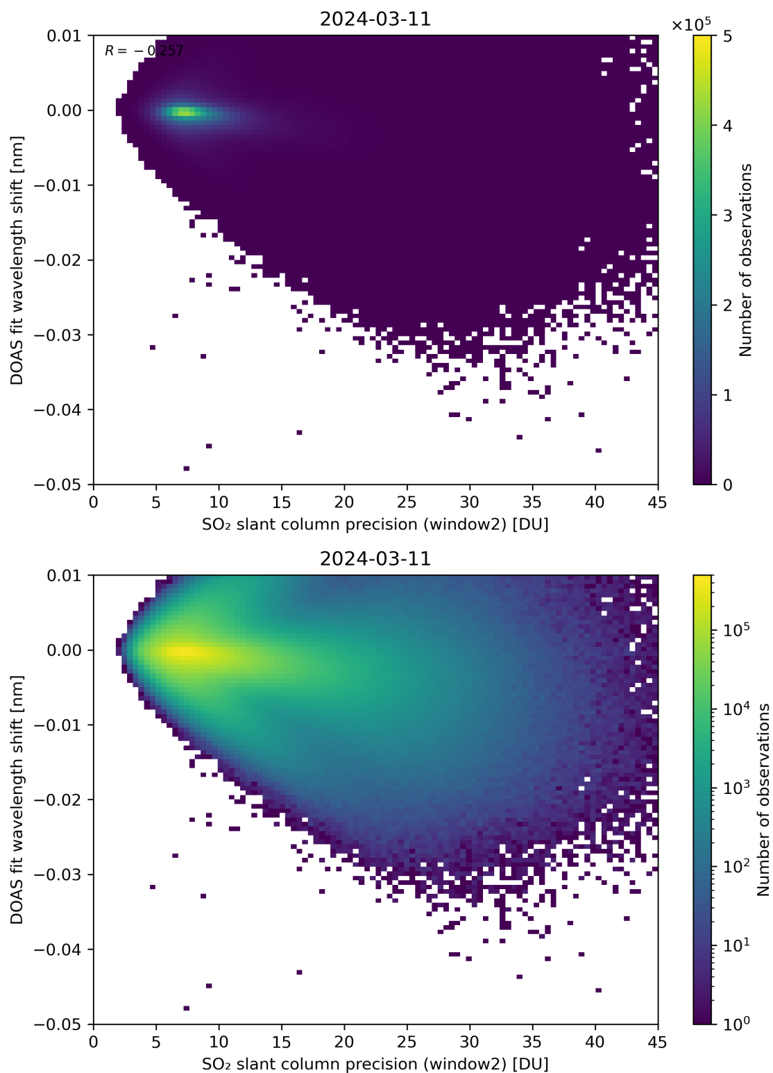
Figure 243: Scatter density plot of “SO 2 slant column precision (window2)” against “DOAS fit wavelength shift” for 2024-03-10 to 2024-03-12.
