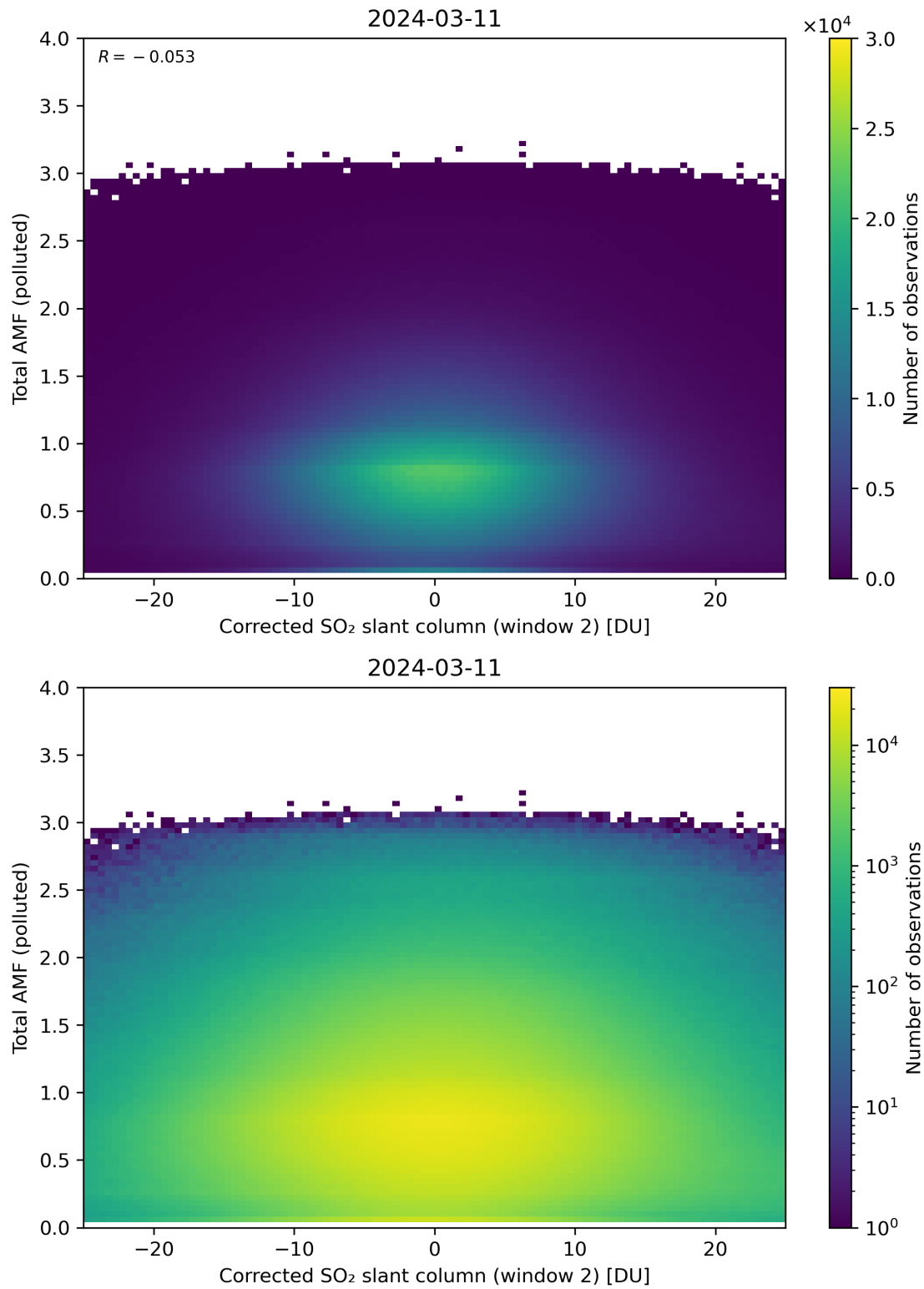
Figure 203: Scatter density plot of “Corrected SO 2 slant column (window 2)” against “Total AMF (polluted)” for 2024-03-10 to 2024-03-12.
