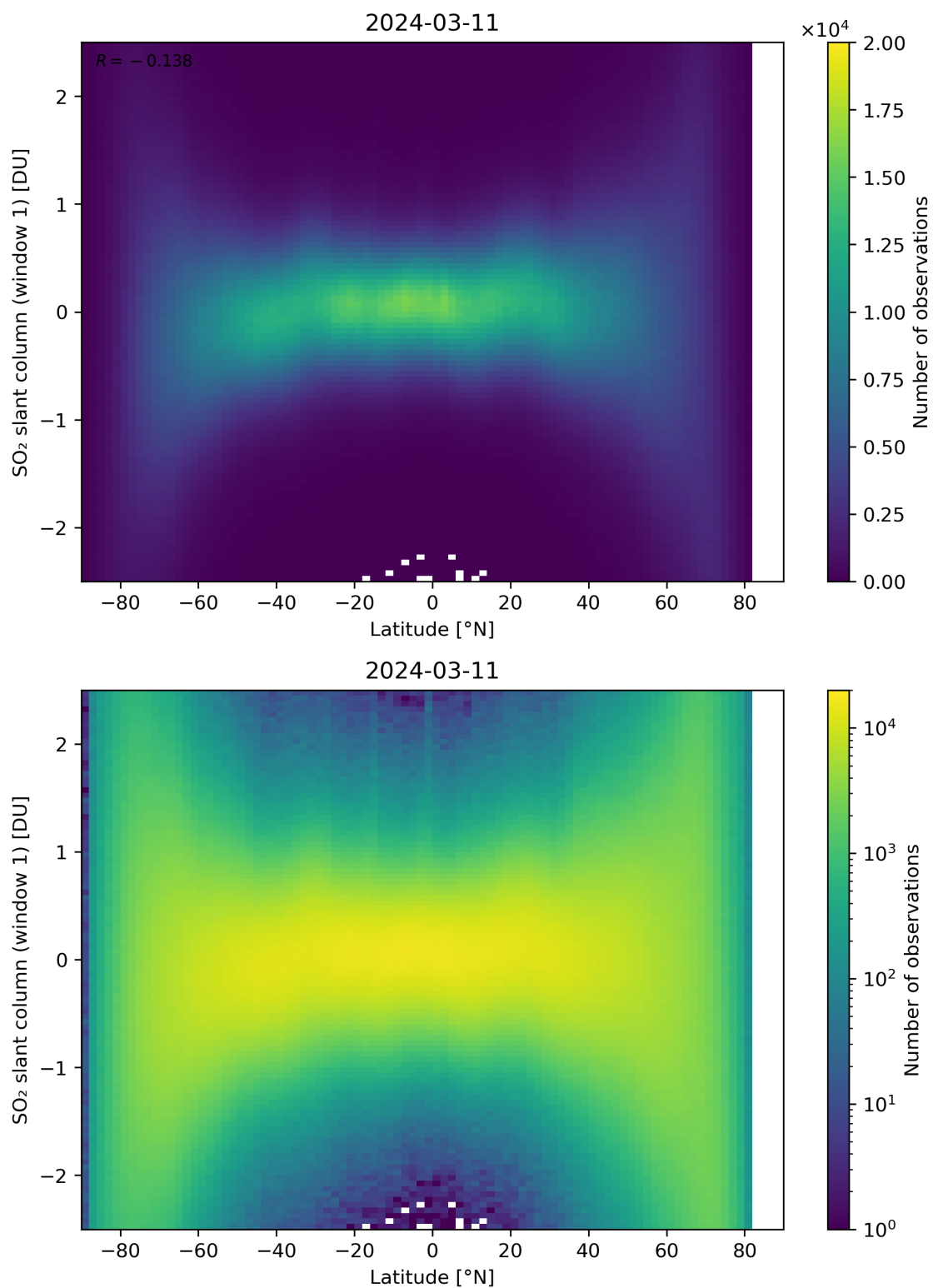
Figure 149: Scatter density plot of “Latitude” against “SO 2 slant column (window 1)” for 2024-03-10 to 2024-03-12.
