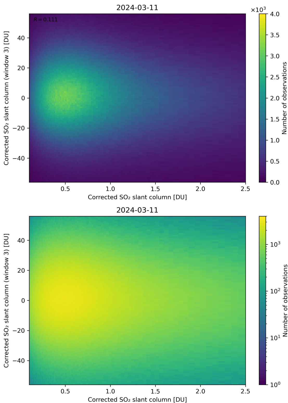
Figure 186: Scatter density plot of “Corrected SO 2 slant column” against “Corrected SO 2 slant column (window 3)” for 2024-03-10 to 2024-03-12.
