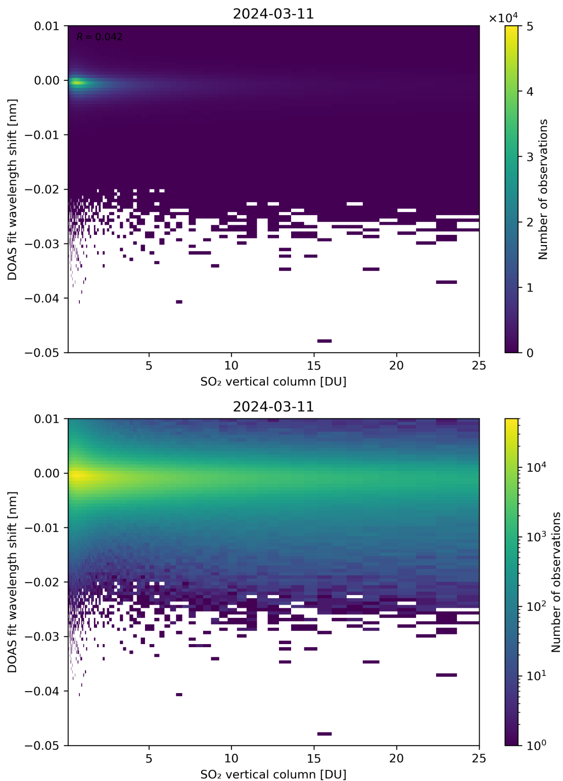
Figure 276: Scatter density plot of “SO 2 vertical column” against “DOAS fit wavelength shift” for 2024-03-10 to 2024-03-12.
