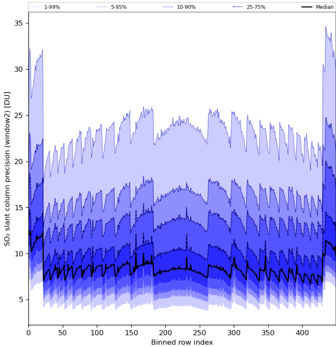
Figure 84: Along track statistics of “SO 2 slant column precision (window2)” for 2024-03-10 to 2024-03-12
