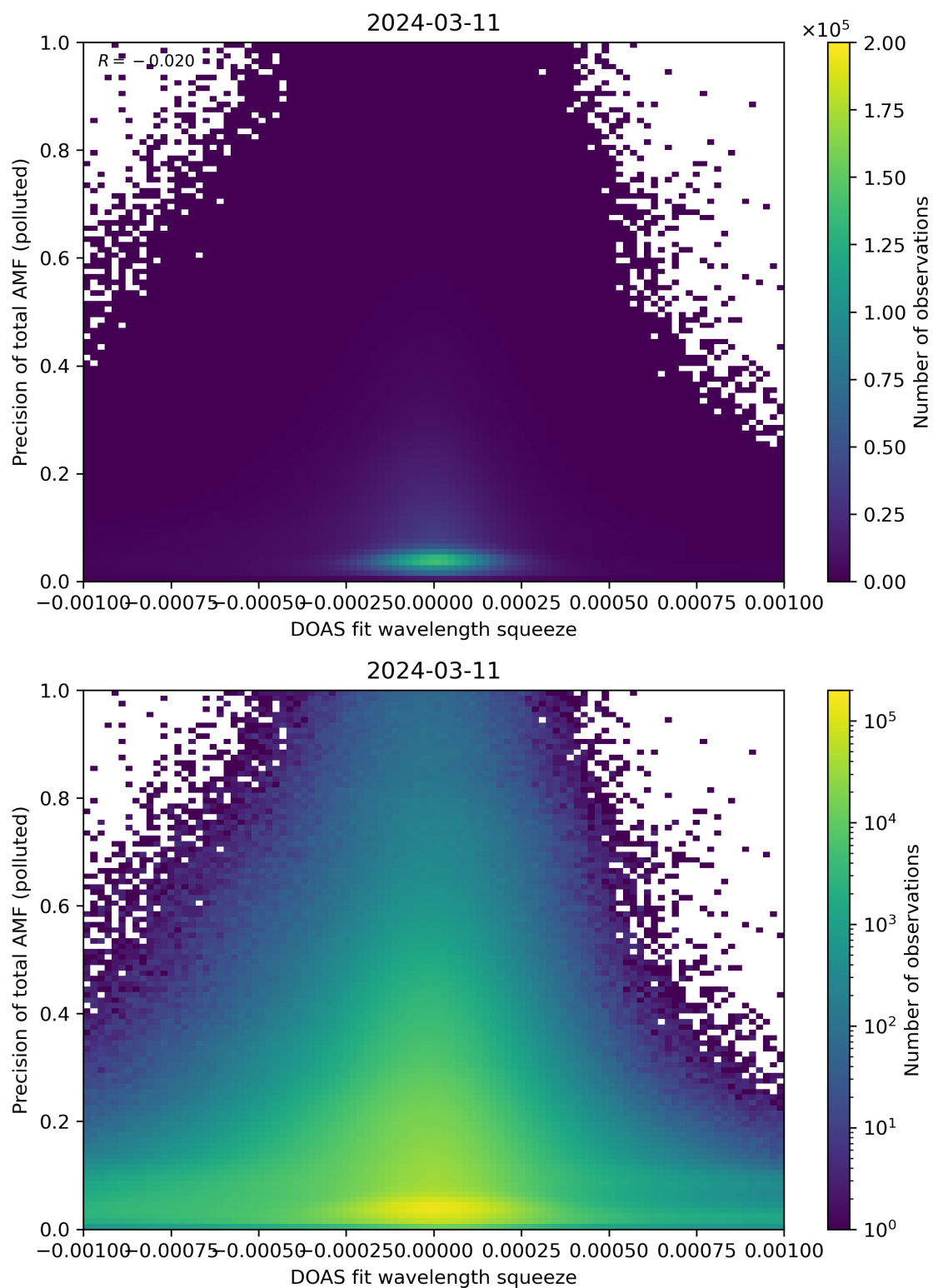
Figure 135: Scatter density plot of “DOAS fit wavelength squeeze” against “Precision of total AMF (polluted)” for 2024-03-10 to 2024-03-12.
