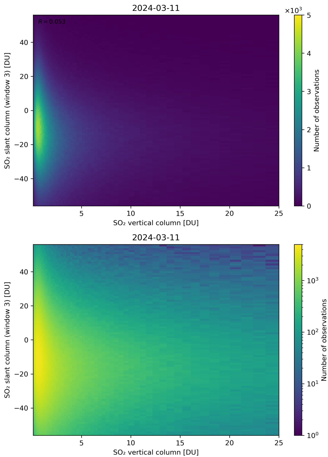
Figure 303: Scatter density plot of “SO 2 vertical column” against “SO 2 slant column (window 3)” for 2024-03-10 to 2024-03-12.
