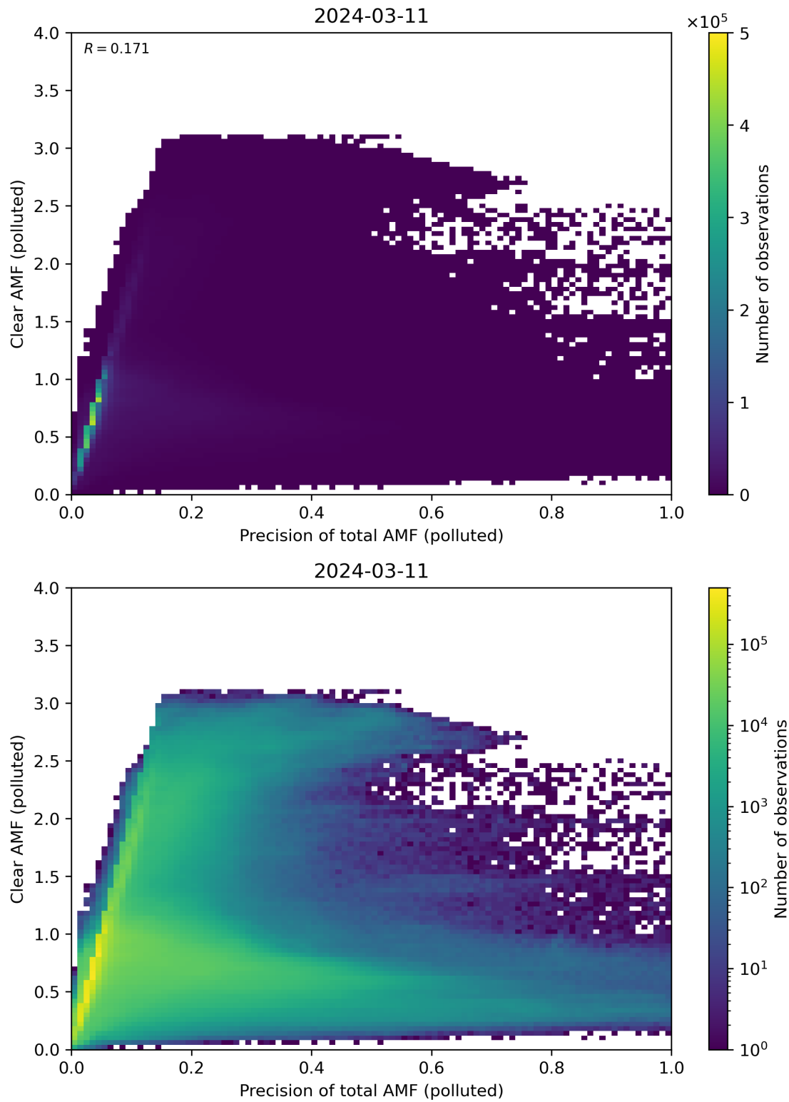
Figure 270: Scatter density plot of “Precision of total AMF (polluted)” against “Clear AMF (polluted)” for 2024-03-10 to 2024-03-12.
