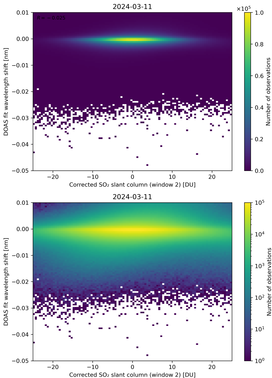
Figure 196: Scatter density plot of “Corrected SO 2 slant column (window 2)” against “DOAS fit wavelength shift” for 2024-03-10 to 2024-03-12.
