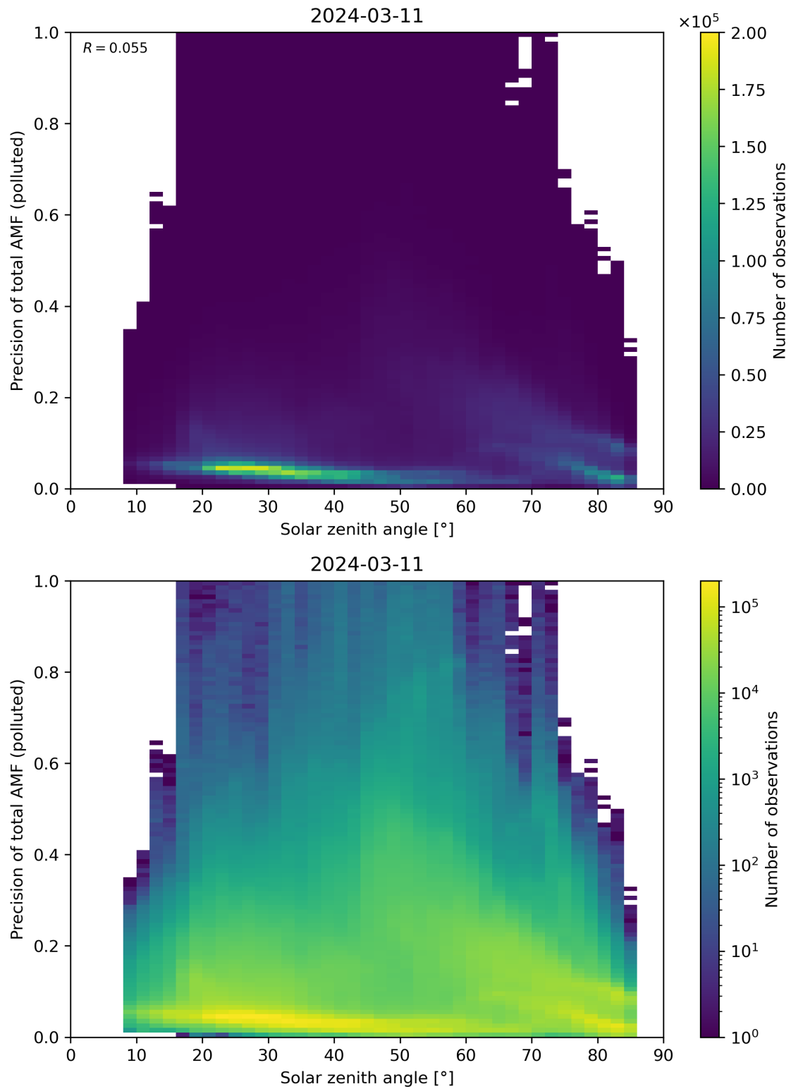
Figure 175: Scatter density plot of “Solar zenith angle” against “Precision of total AMF (polluted)” for 2024-03-10 to 2024-03-12.
