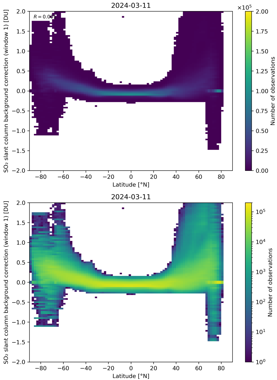
Figure 139: Scatter density plot of “Latitude” against “SO 2 slant column background correction (window 1)” for 2024-03-10 to 2024-03-12.
