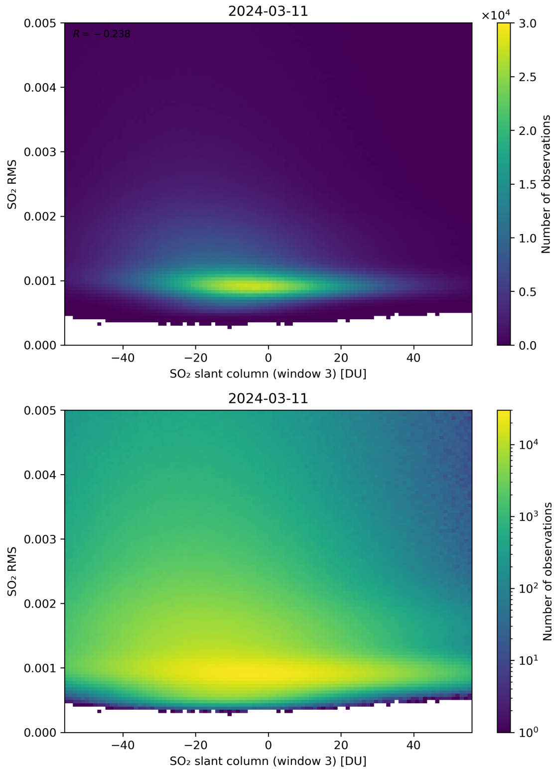
Figure 256: Scatter density plot of “SO 2 slant column (window 3)” against “SO 2 RMS” for 2024-03-10 to 2024-03-12.
