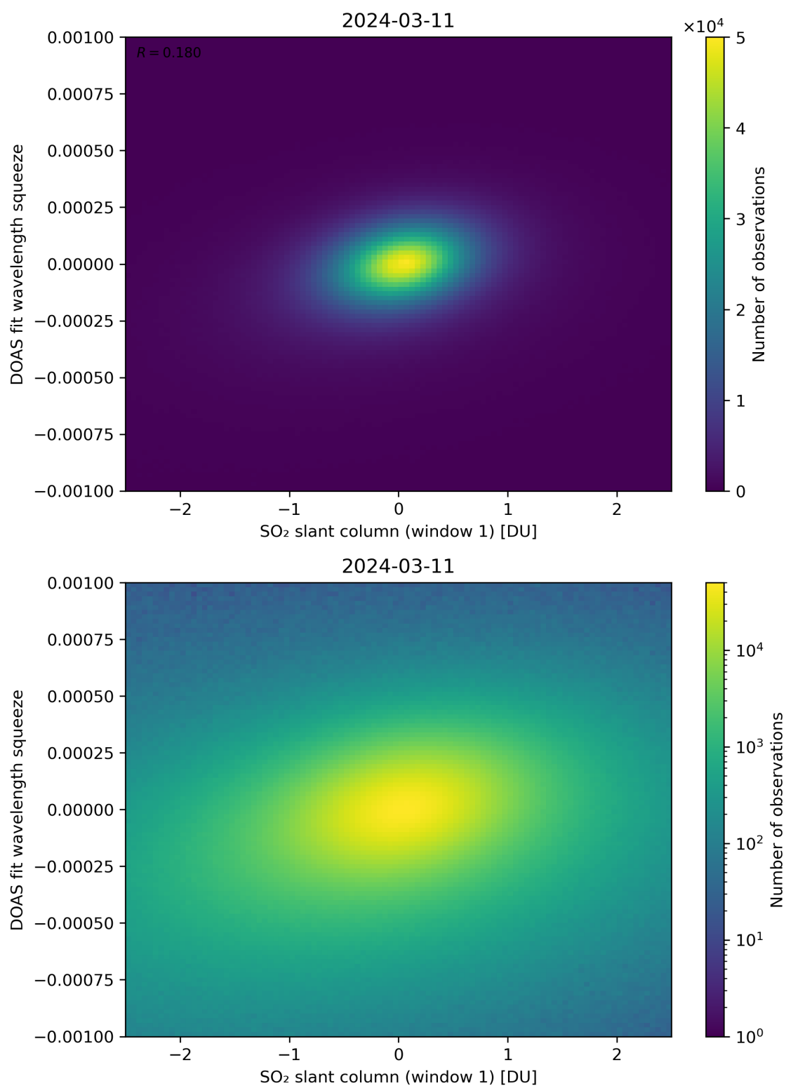
Figure 216: Scatter density plot of “SO 2 slant column (window 1)” against “DOAS fit wavelength squeeze” for 2024-03-10 to 2024-03-12.
