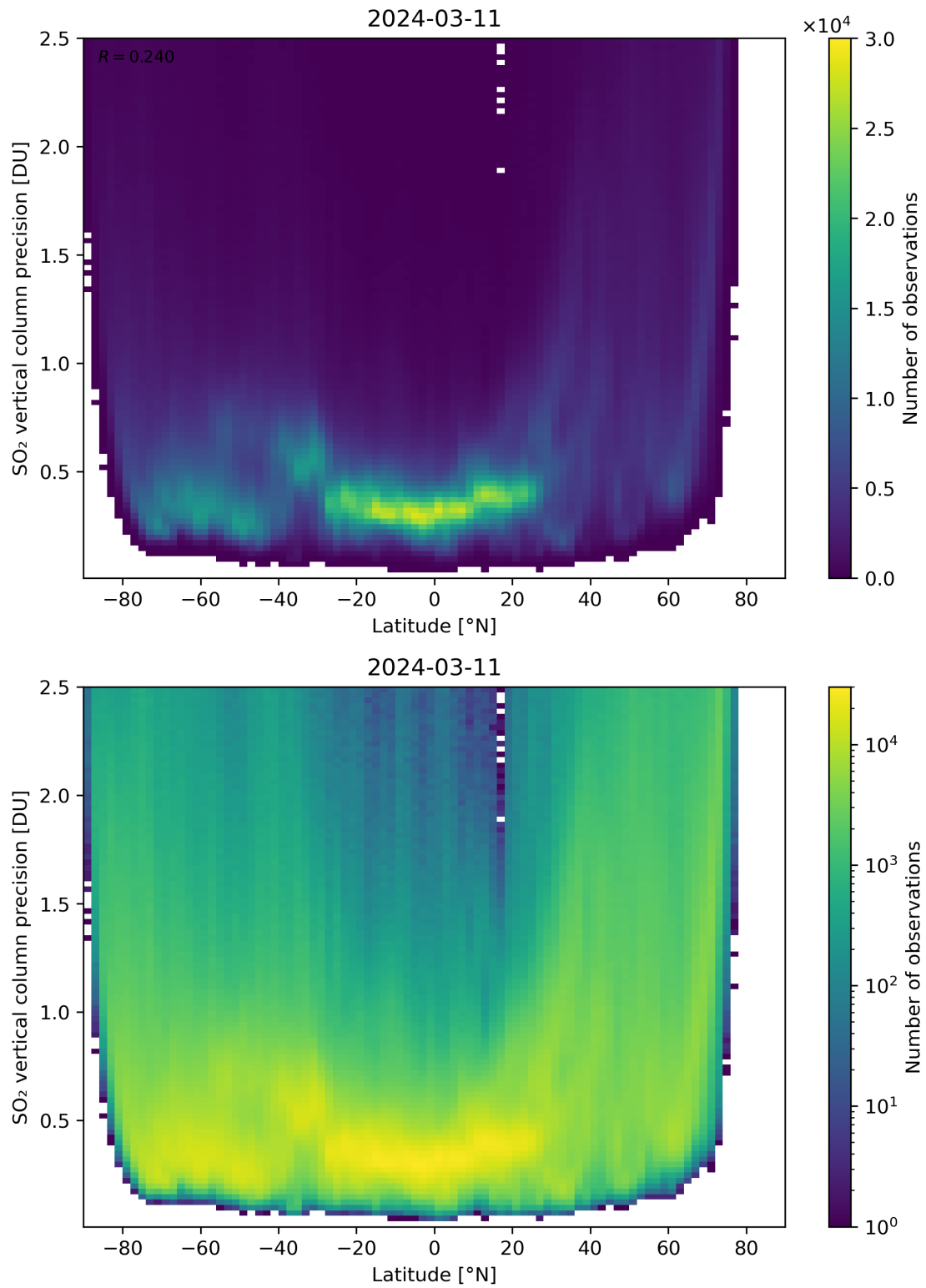
Figure 157: Scatter density plot of “Latitude” against “SO 2 vertical column precision” for 2024-03-10 to 2024-03-12.
