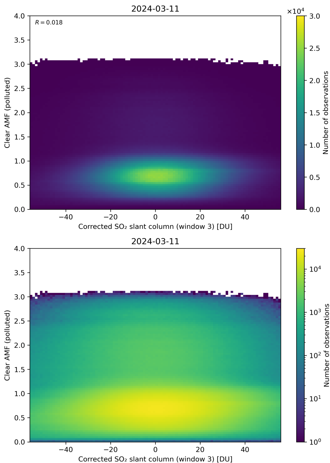
Figure 209: Scatter density plot of “Corrected SO 2 slant column (window 3)” against “Clear AMF (polluted)” for 2024-03-10 to 2024-03-12.
