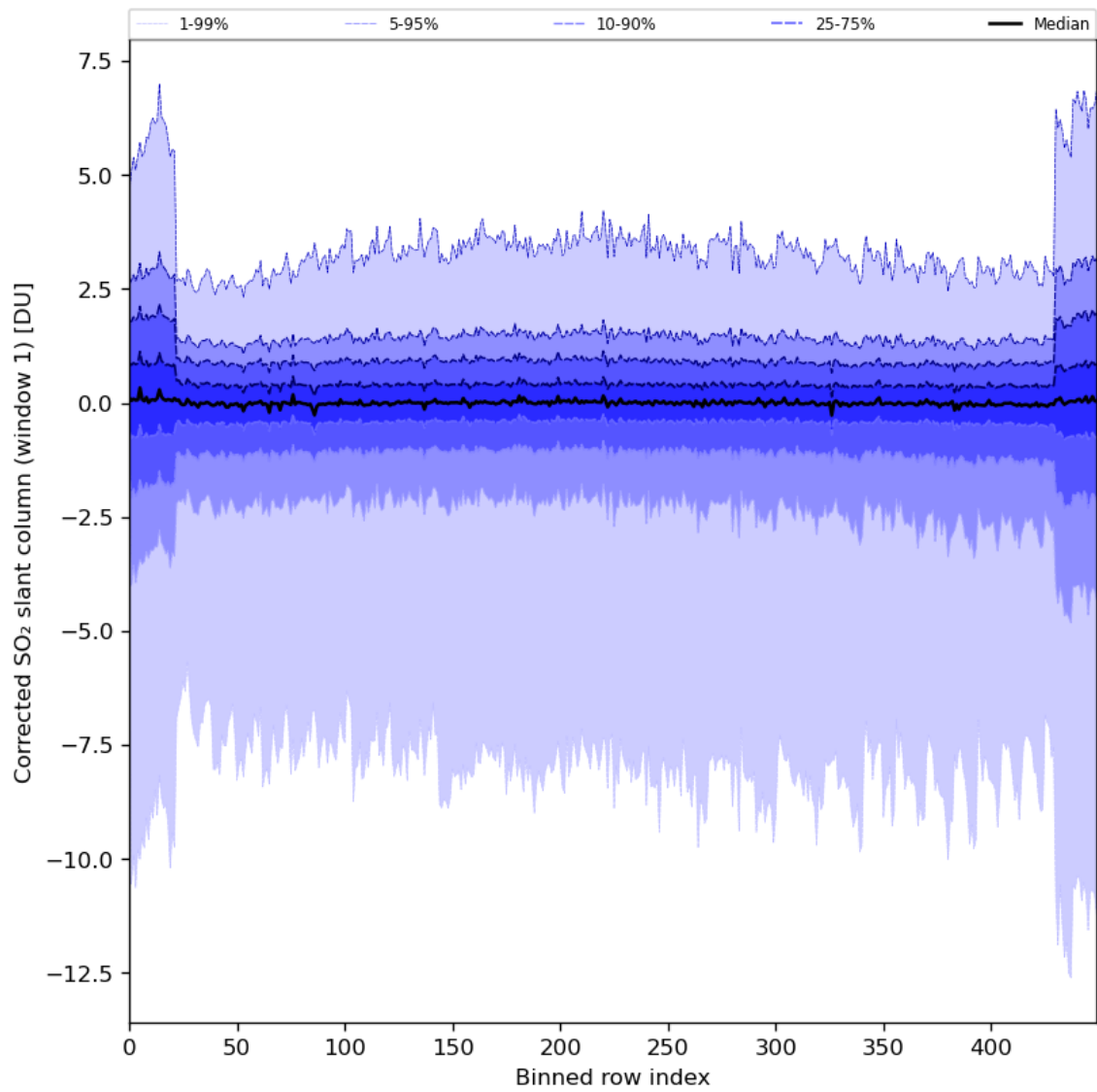
Figure 81: Along track statistics of “Corrected SO 2 slant column (window 1)” for 2024-03-10 to 2024-03-12
