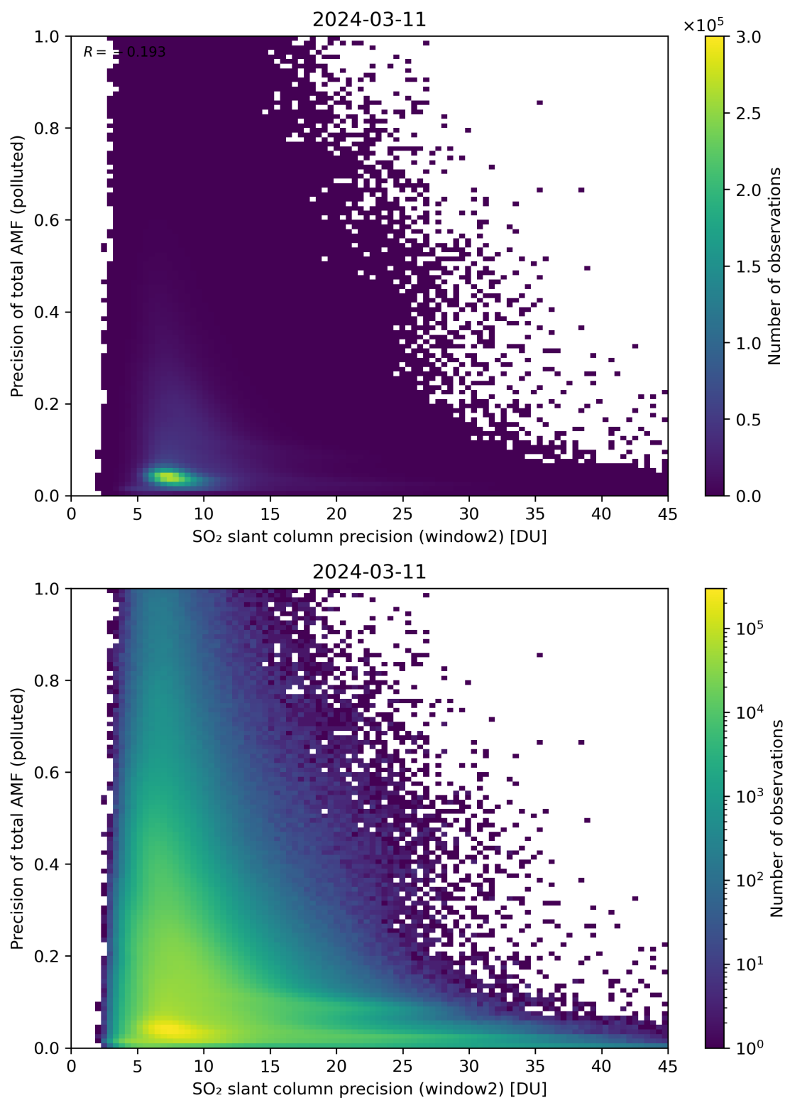
Figure 252: Scatter density plot of “SO 2 slant column precision (window2)” against “Precision of total AMF (polluted)” for 2024-03-10 to 2024-03-12.
