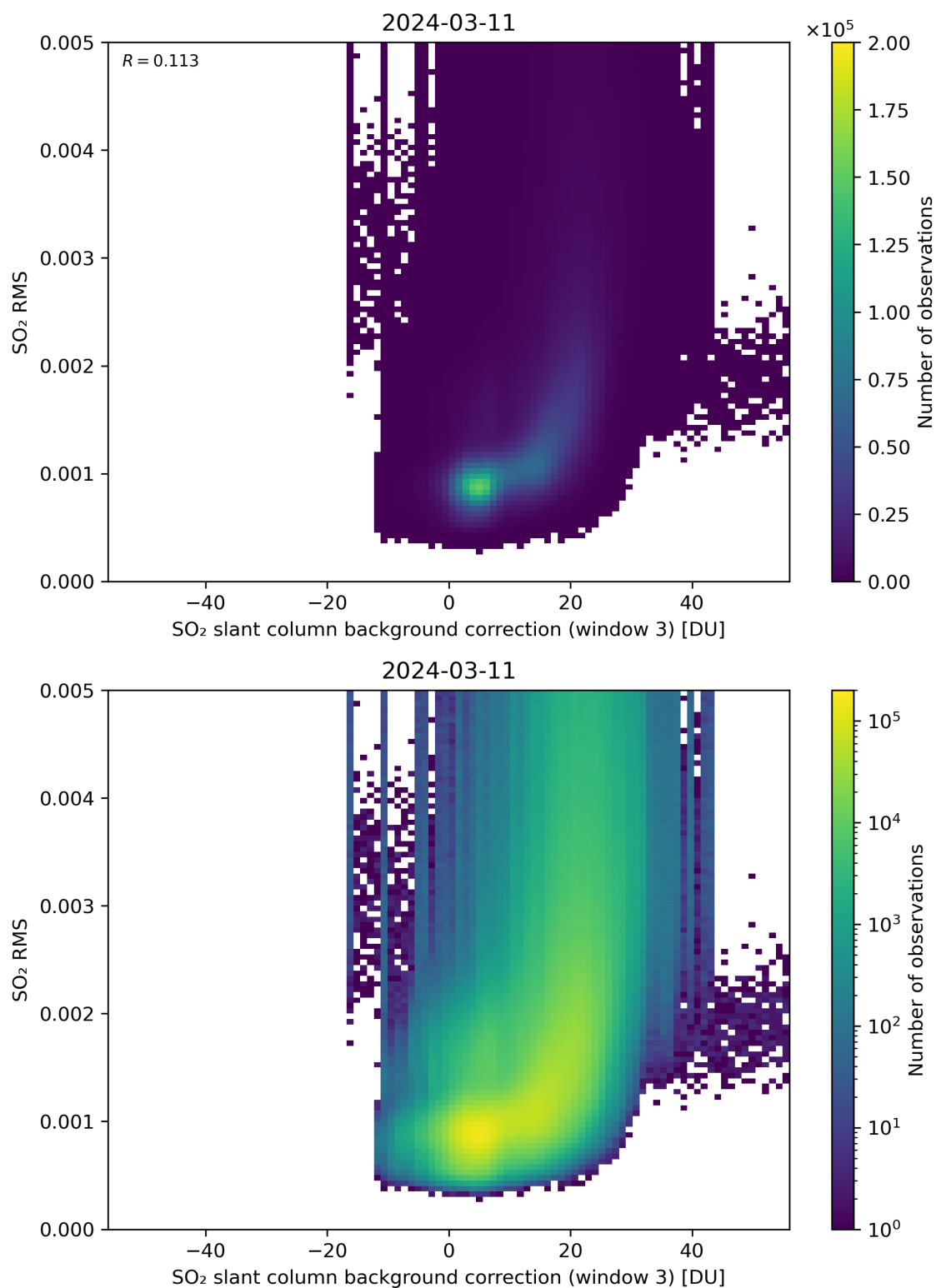
Figure 123: Scatter density plot of “SO 2 slant column background correction (window 3)” against “SO 2 RMS” for 2024-03-10 to 2024-03-12.
