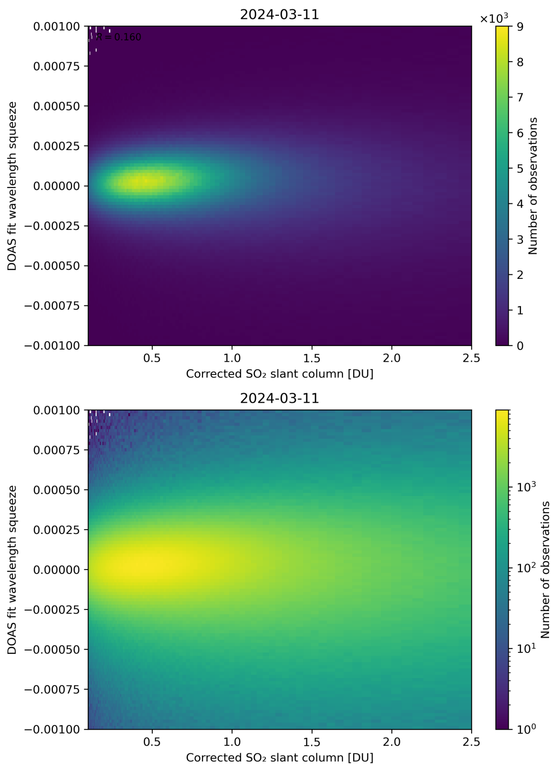
Figure 182: Scatter density plot of “Corrected SO 2 slant column” against “DOAS fit wavelength squeeze” for 2024-03-10 to 2024-03-12.
