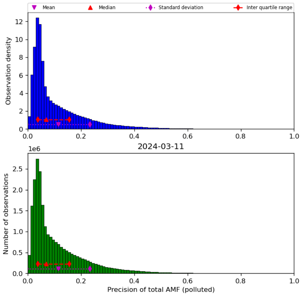
Figure 72: Histogram of “Precision of total AMF (polluted)” for 2024-03-10 to 2024-03-12
