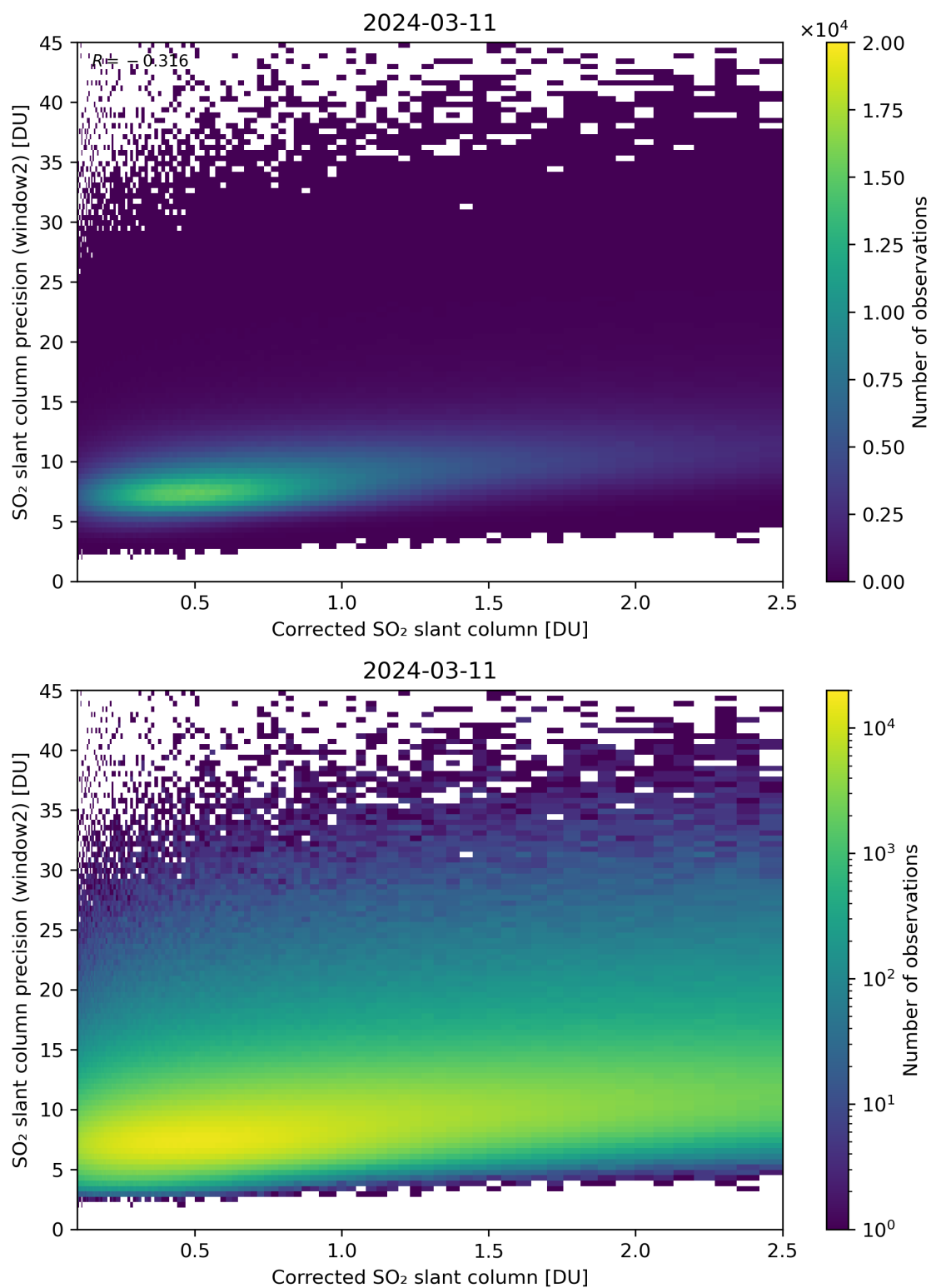
Figure 189: Scatter density plot of “Corrected SO 2 slant column” against “SO 2 slant column precision (window2)” for 2024-03-10 to 2024-03-12.
