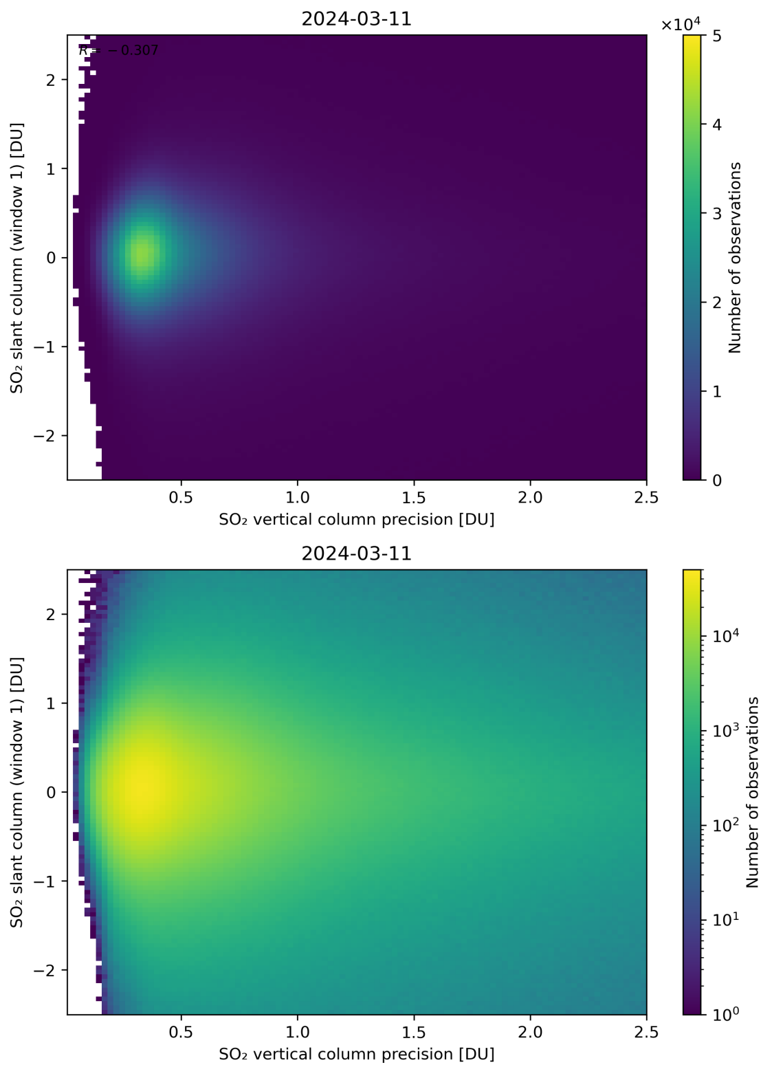
Figure 289: Scatter density plot of “SO 2 vertical column precision” against “SO 2 slant column (window 1)” for 2024-03-10 to 2024-03-12.
