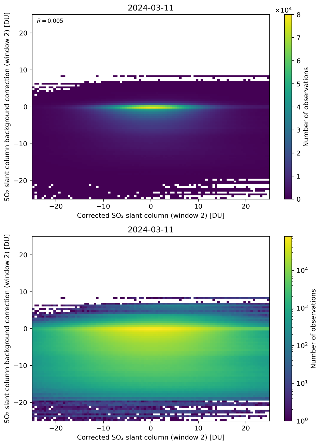
Figure 194: Scatter density plot of “Corrected SO 2 slant column (window 2)” against “SO 2 slant column background correction (window 2)” for 2024-03-10 to 2024-03-12.
