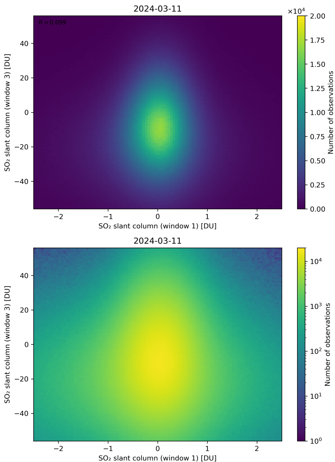
Figure 237: Scatter density plot of “SO 2 slant column (window 1)” against “SO 2 slant column (window 3)” for 2024-03-10 to 2024-03-12.
