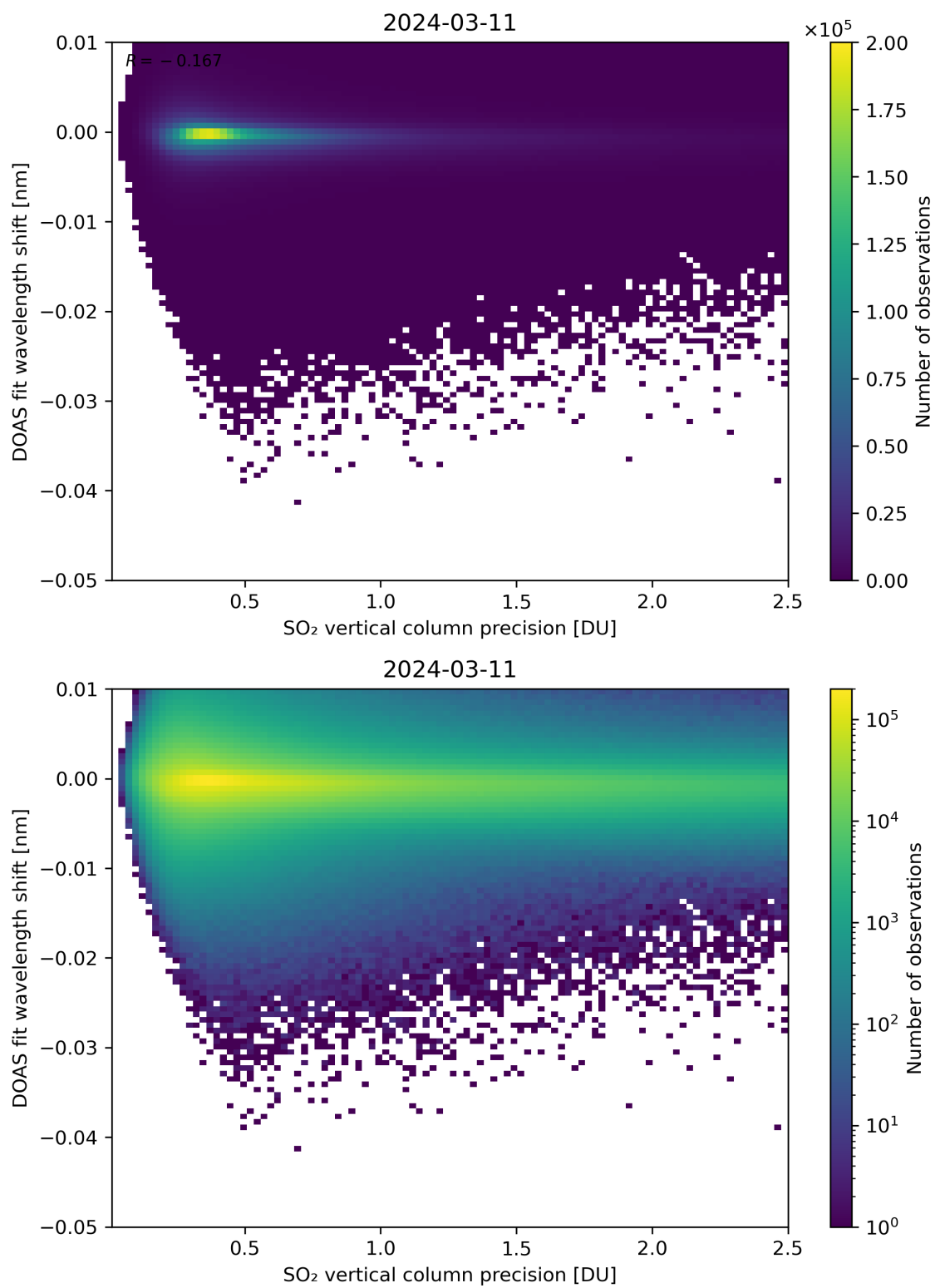
Figure 282: Scatter density plot of “SO 2 vertical column precision” against “DOAS fit wavelength shift” for 2024-03-10 to 2024-03-12.
