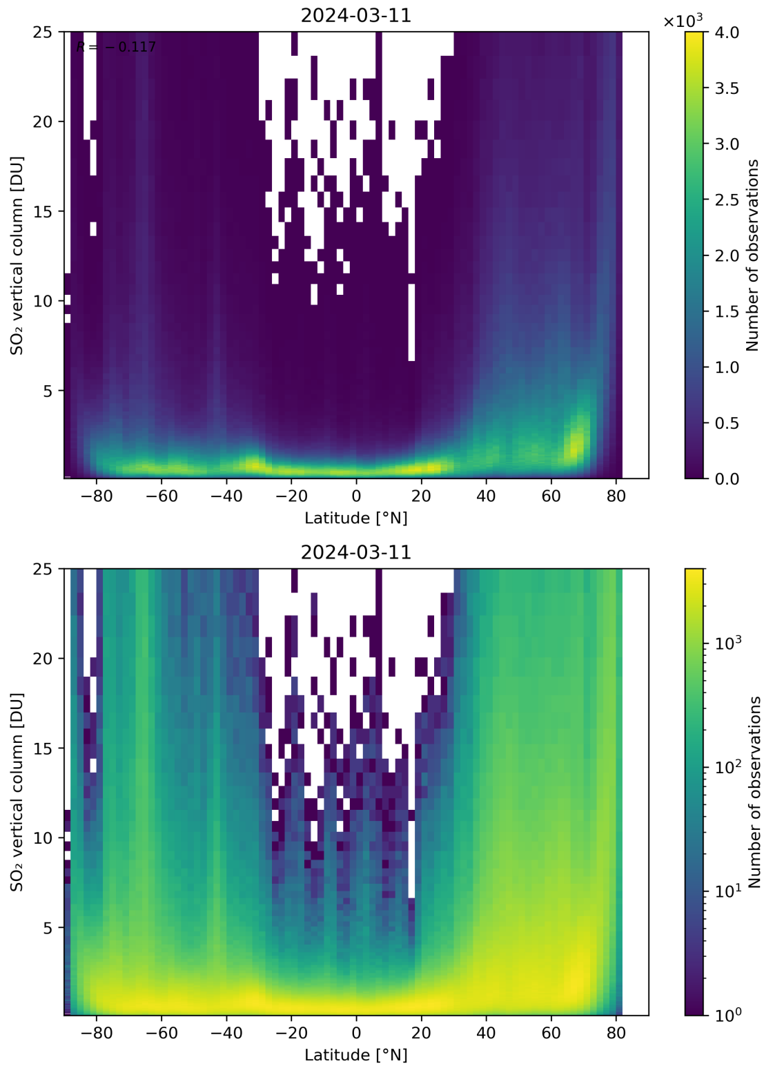
Figure 156: Scatter density plot of “Latitude” against “SO 2 vertical column” for 2024-03-10 to 2024-03-12.
