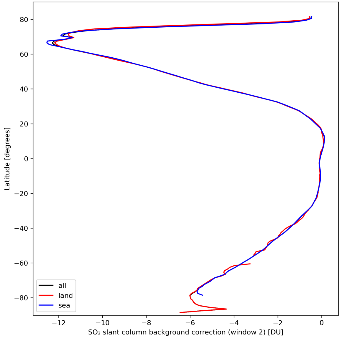
Figure 40: Zonal average of “SO 2 slant column background correction (window 2)” for 2024-03-10 to 2024-03-12.
