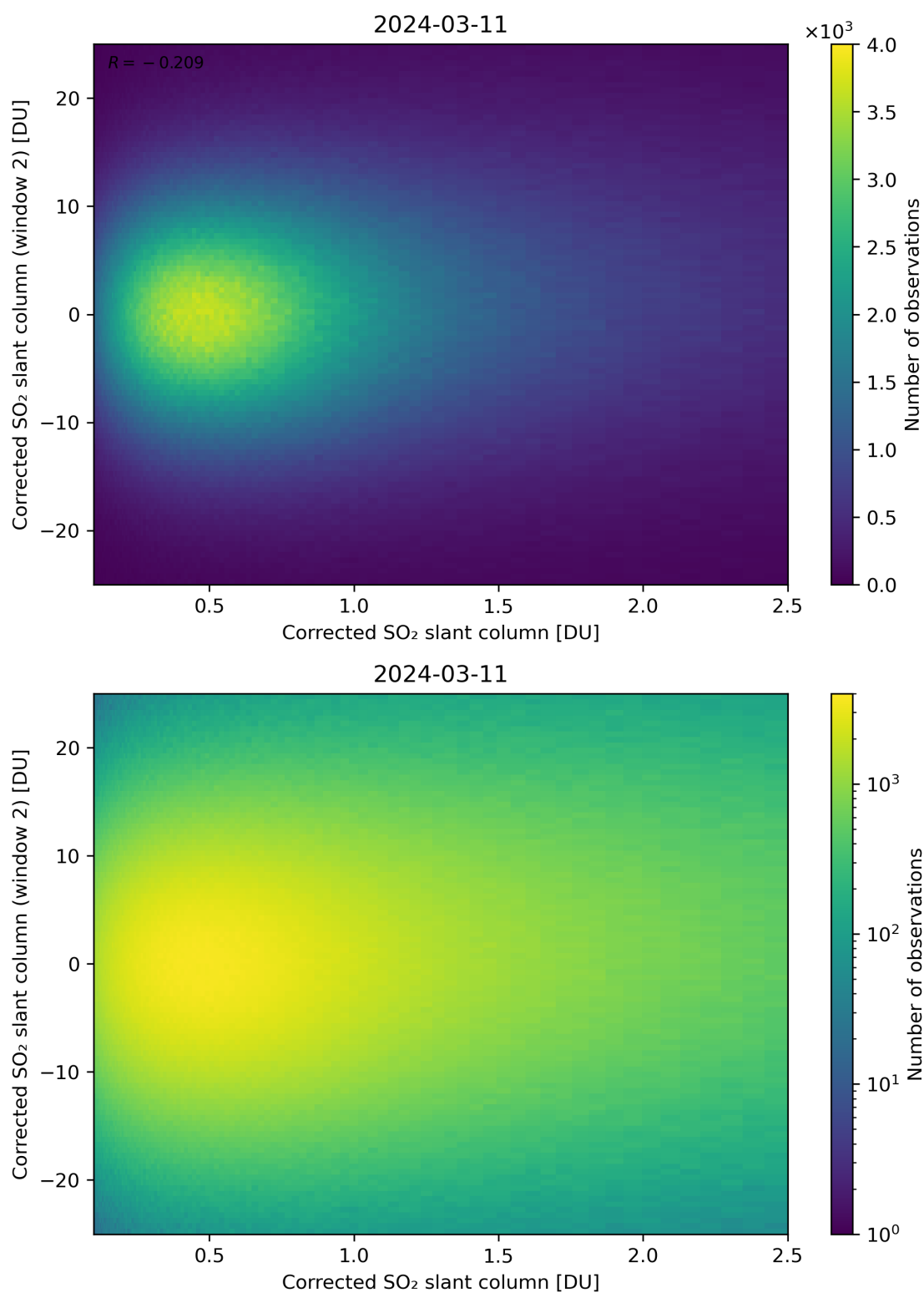
Figure 185: Scatter density plot of “Corrected SO 2 slant column” against “Corrected SO 2 slant column (window 2)” for 2024-03-10 to 2024-03-12.
