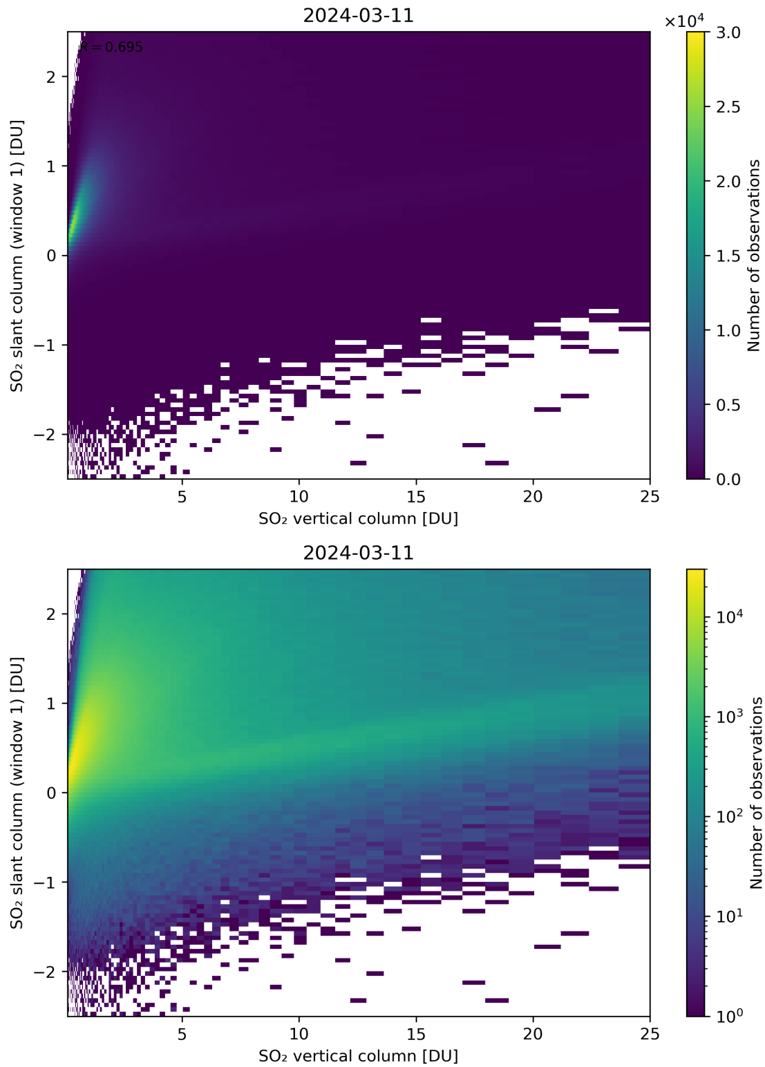
Figure 300: Scatter density plot of “SO 2 vertical column” against “SO 2 slant column (window 1)” for 2024-03-10 to 2024-03-12.
