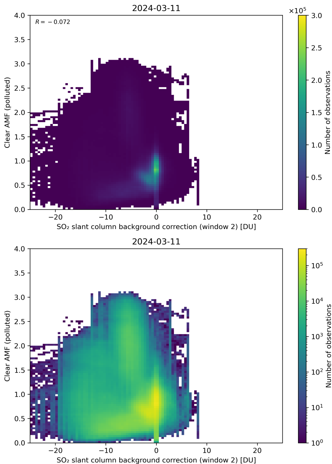
Figure 115: Scatter density plot of “SO 2 slant column background correction (window 2)” against “Clear AMF (polluted)” for 2024-03-10 to 2024-03-12.
