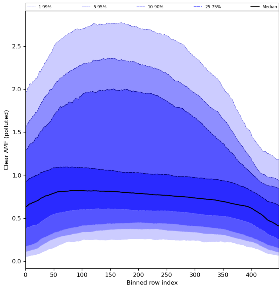
Figure 96: Along track statistics of “Clear AMF (polluted)” for 2024-03-10 to 2024-03-12
