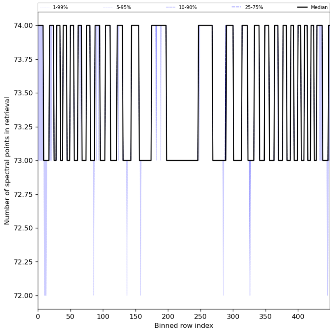
Figure 97: Along track statistics of “Number of spectral points in retrieval” for 2024-03-10 to 2024-03-12
