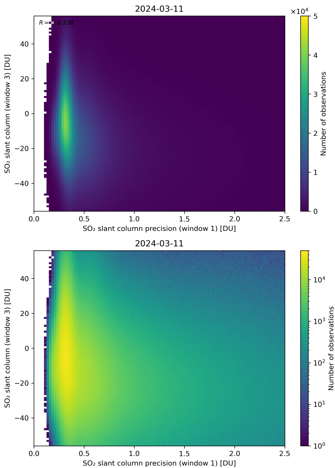
Figure 228: Scatter density plot of “SO 2 slant column precision (window 1)” against “SO 2 slant column (window 3)” for 2024-03-10 to 2024-03-12.
