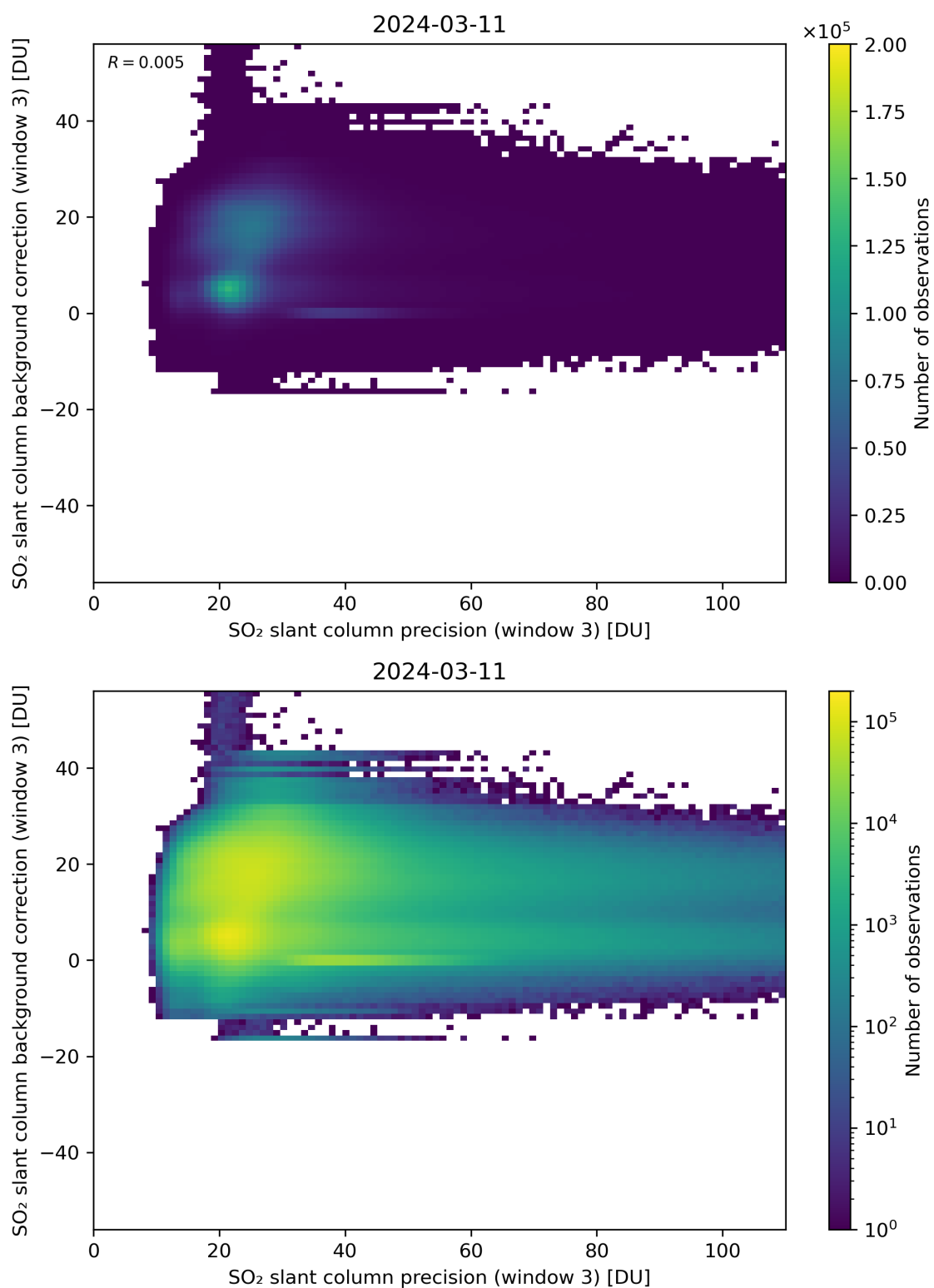
Figure 257: Scatter density plot of “SO 2 slant column precision (window 3)” against “SO 2 slant column background correction (window 3)” for 2024-03-10 to 2024-03-12.
