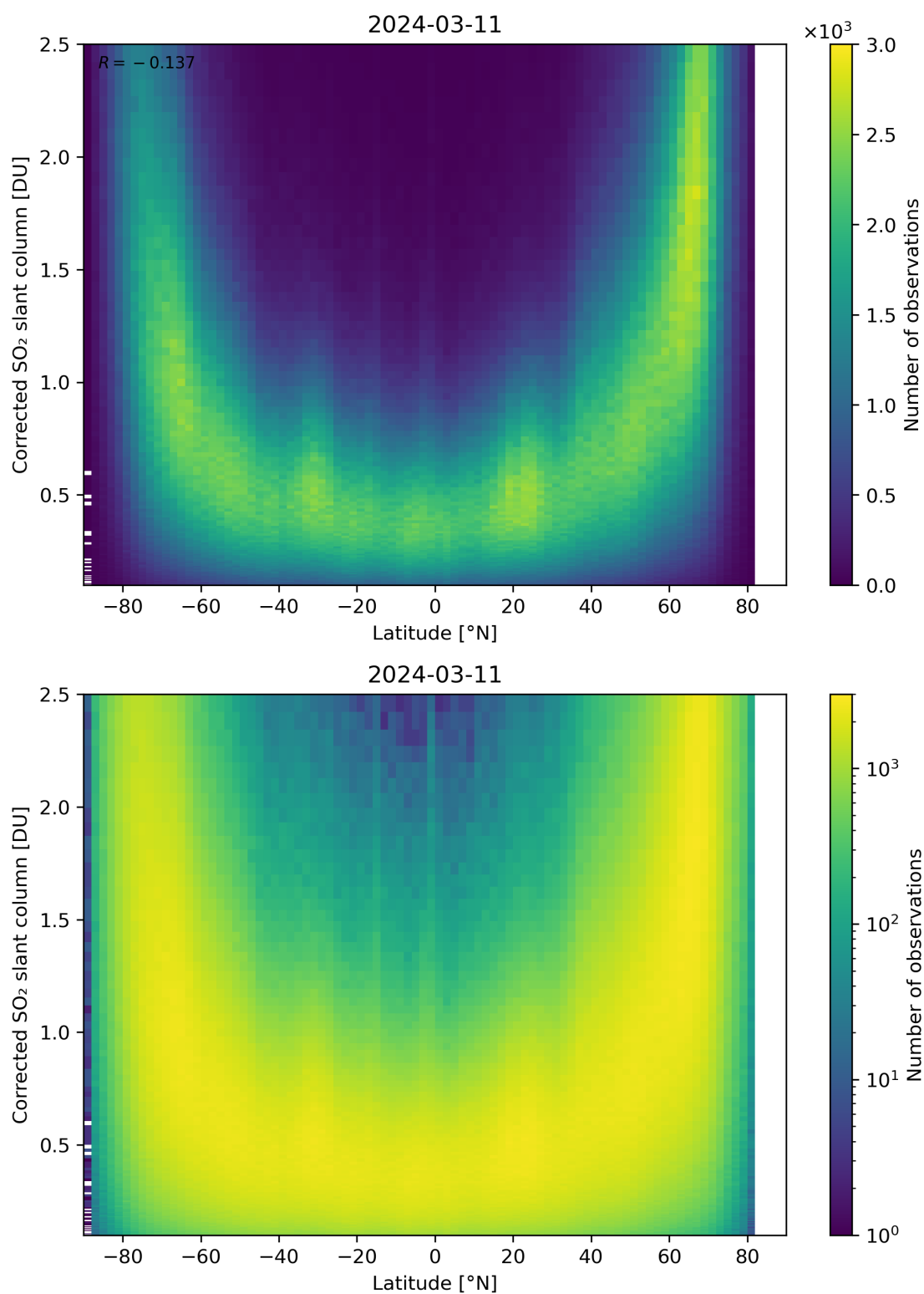
Figure 146: Scatter density plot of “Latitude” against “Corrected SO 2 slant column” for 2024-03-10 to 2024-03-12.
