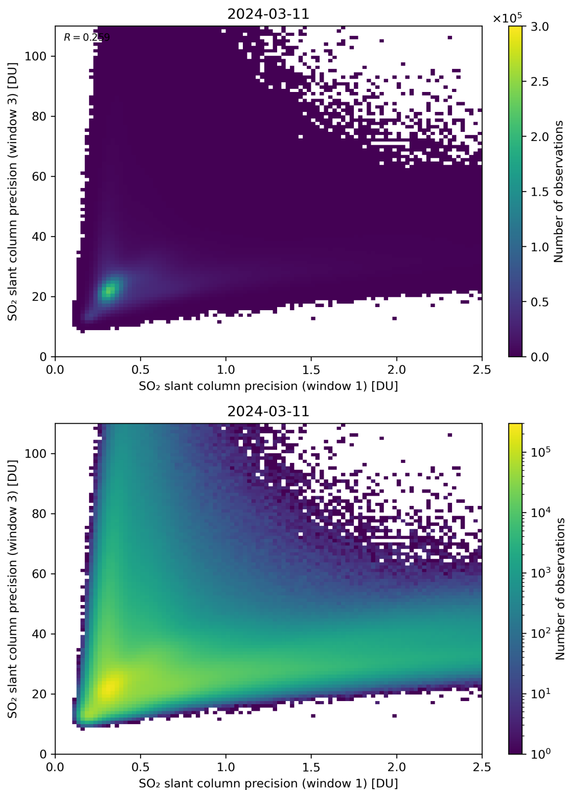
Figure 229: Scatter density plot of “SO 2 slant column precision (window 1)” against “SO 2 slant column precision (window 3)” for 2024-03-10 to 2024-03-12.
