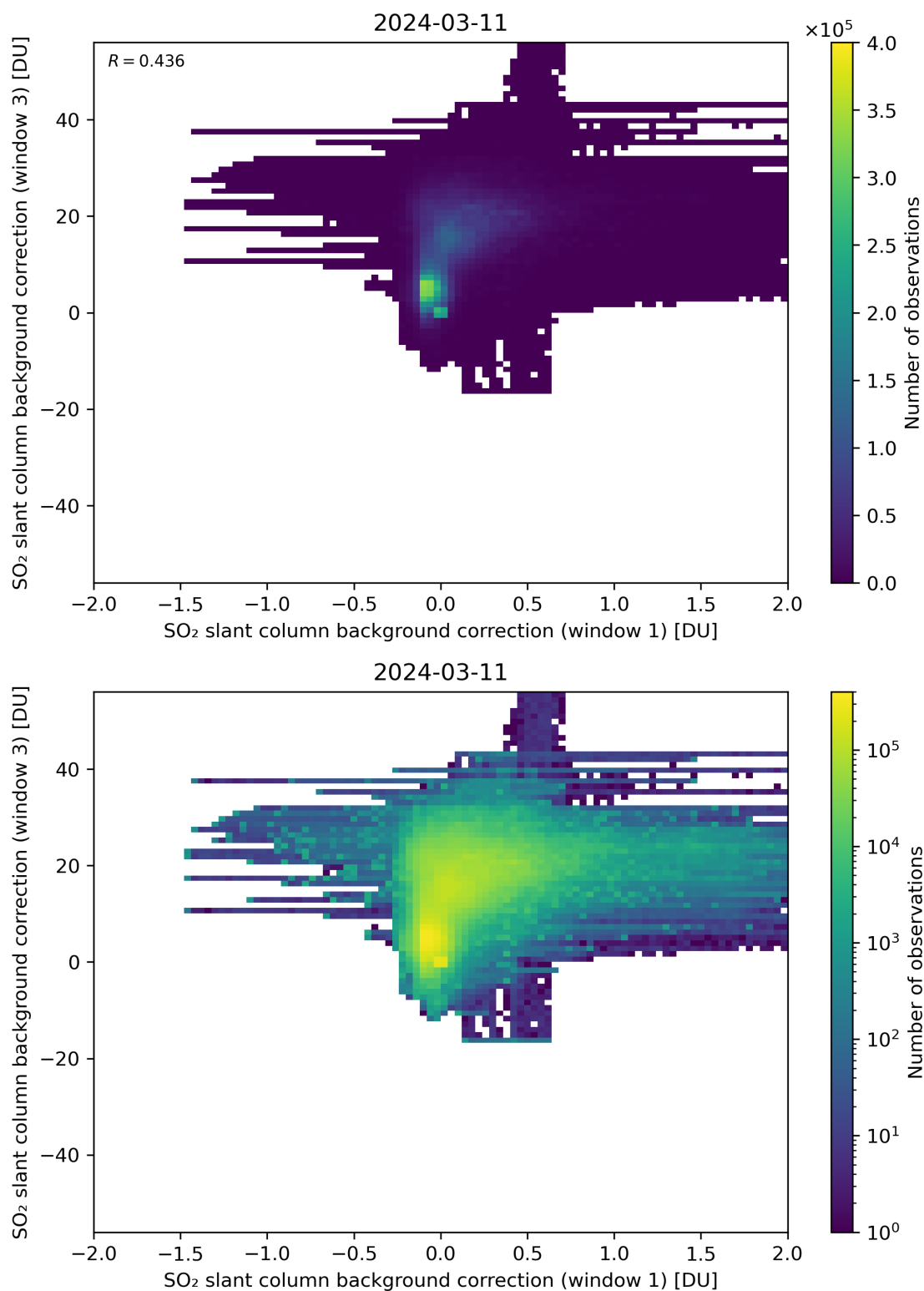
Figure 99: Scatter density plot of “SO 2 slant column background correction (window 1)” against “SO 2 slant column background correction (window 3)” for 2024-03-10 to 2024-03-12.
