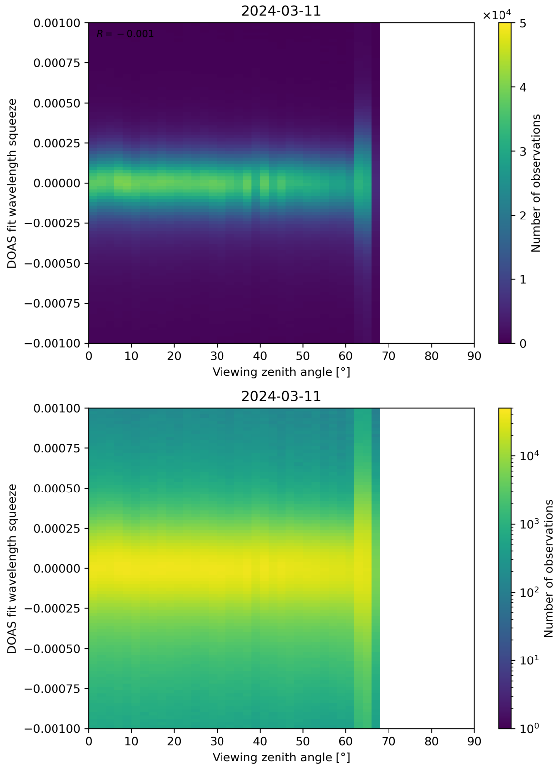
Figure 312: Scatter density plot of “Viewing zenith angle” against “DOAS fit wavelength squeeze” for 2024-03-10 to 2024-03-12.
