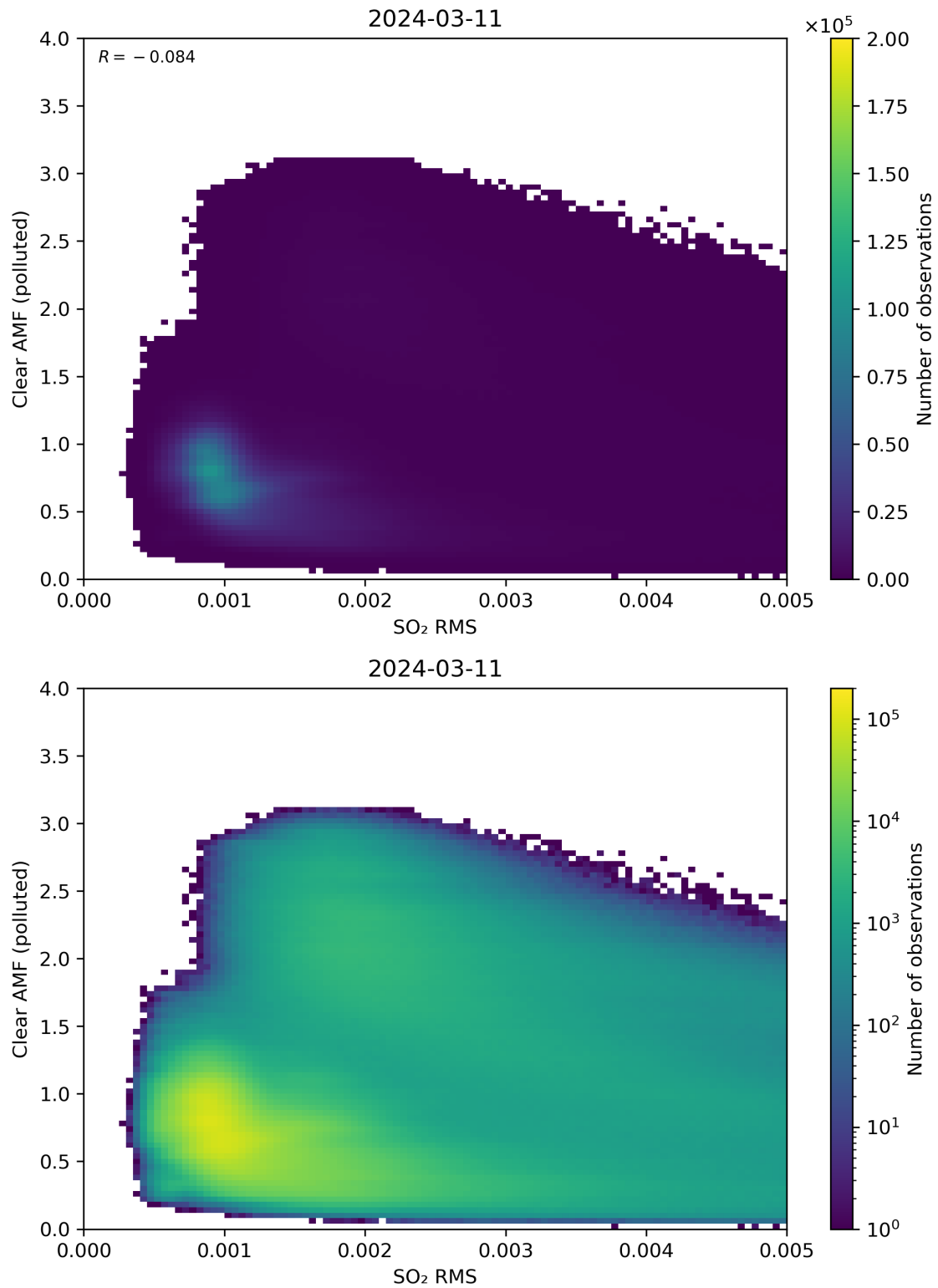
Figure 136: Scatter density plot of “SO 2 RMS” against “Clear AMF (polluted)” for 2024-03-10 to 2024-03-12.
