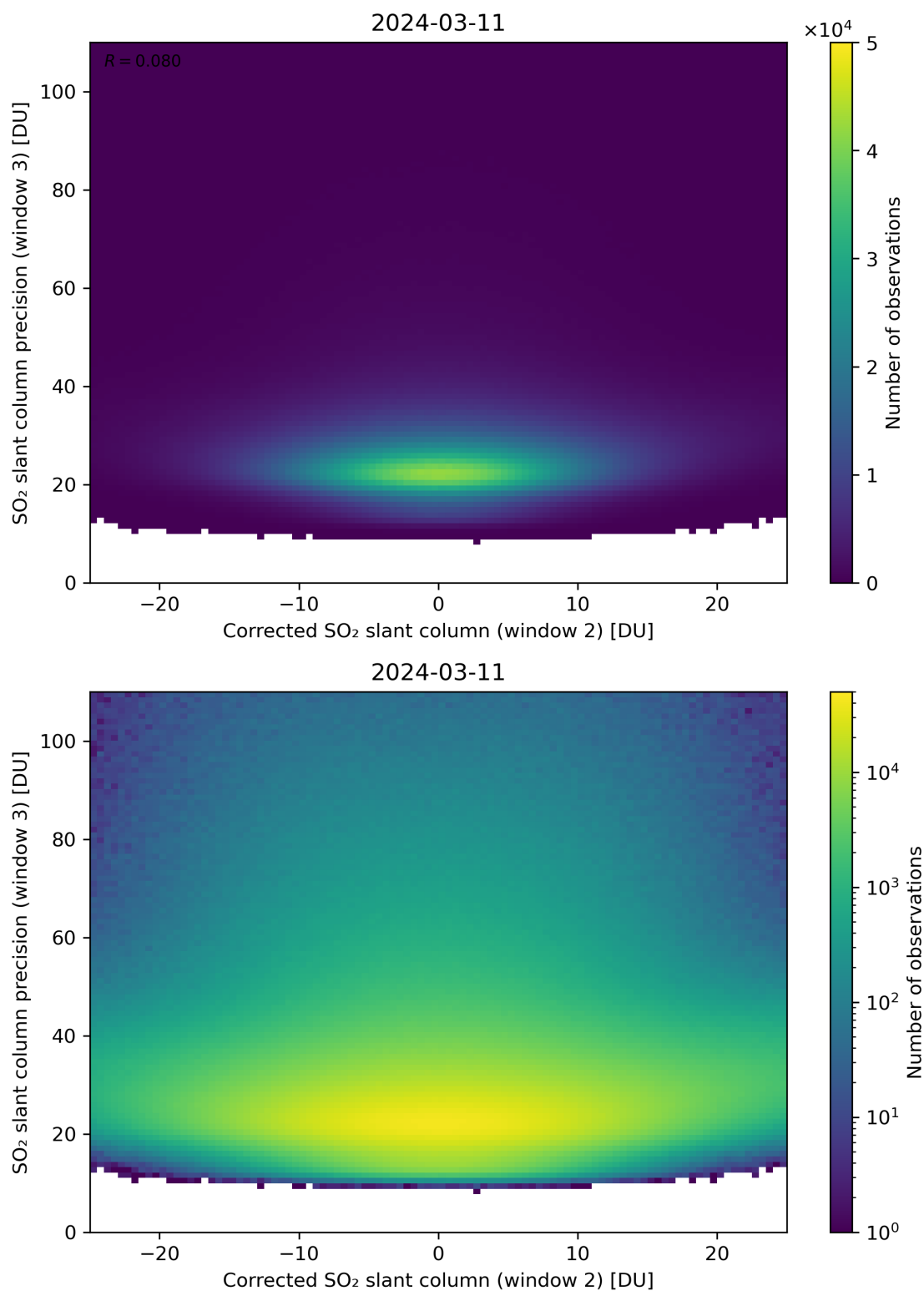
Figure 202: Scatter density plot of “Corrected SO 2 slant column (window 2)” against “SO 2 slant column precision (window 3)” for 2024-03-10 to 2024-03-12.
