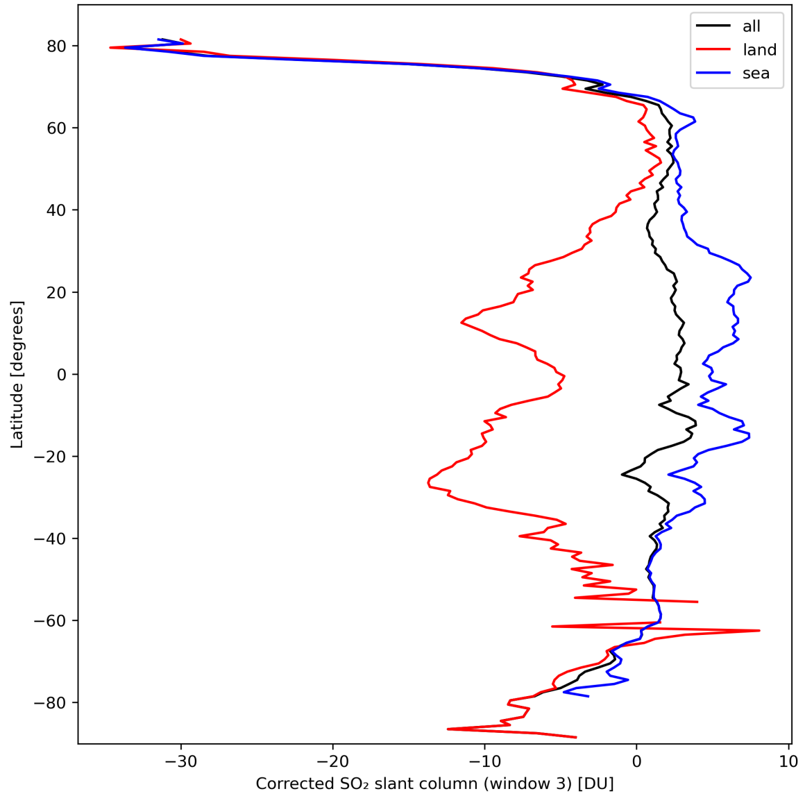
Figure 43: Zonal average of “Corrected SO 2 slant column (window 3)” for 2024-03-10 to 2024-03-12.
