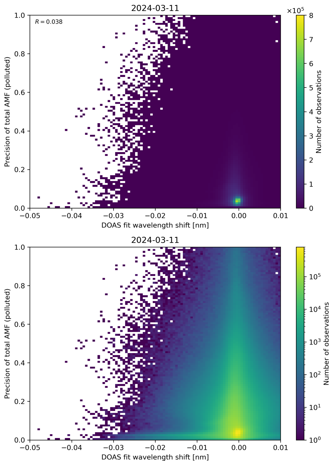
Figure 131: Scatter density plot of “DOAS fit wavelength shift” against “Precision of total AMF (polluted)” for 2024-03-10 to 2024-03-12.
