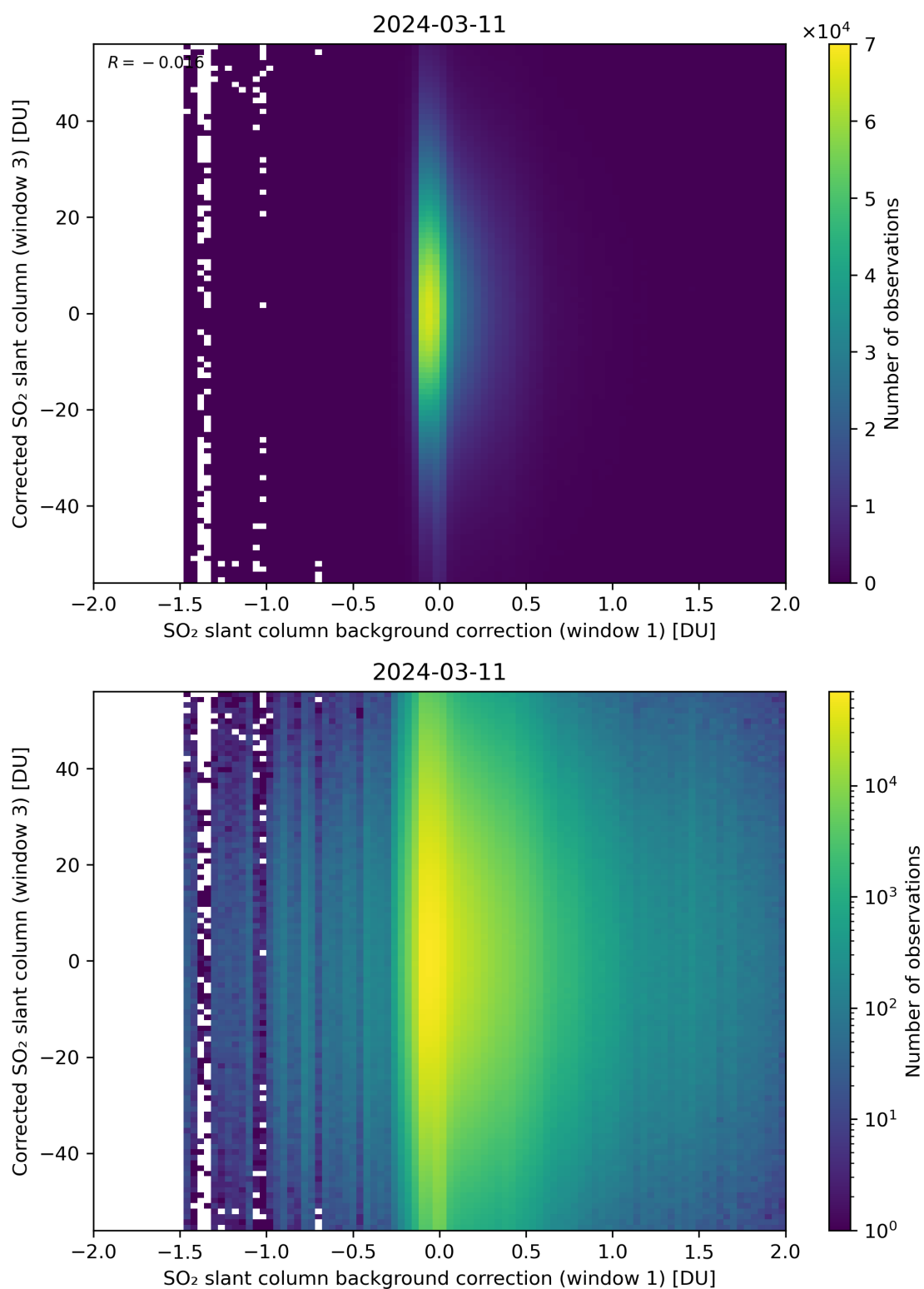
Figure 105: Scatter density plot of “SO 2 slant column background correction (window 1)” against “Corrected SO 2 slant column (window 3)” for 2024-03-10 to 2024-03-12.
