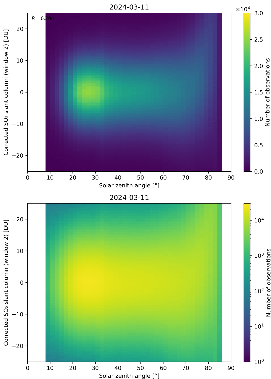
Figure 167: Scatter density plot of “Solar zenith angle” against “Corrected SO 2 slant column (window 2)” for 2024-03-10 to 2024-03-12.
