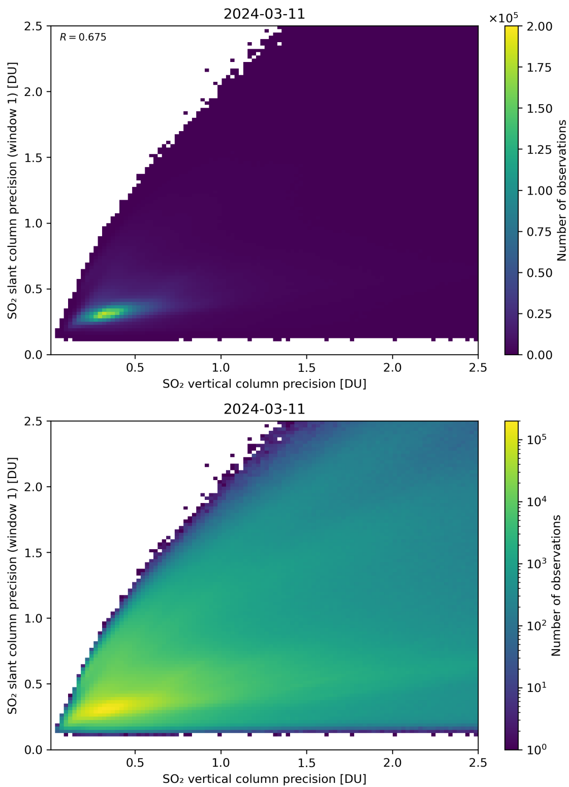
Figure 290: Scatter density plot of “SO 2 vertical column precision” against “SO 2 slant column precision (window 1)” for 2024-03-10 to 2024-03-12.
