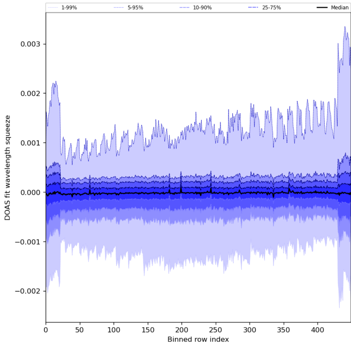
Figure 92: Along track statistics of “DOAS fit wavelength squeeze” for 2024-03-10 to 2024-03-12
