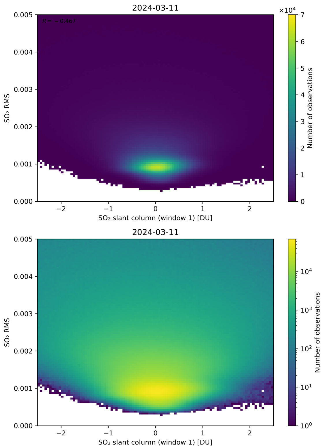
Figure 217: Scatter density plot of “SO 2 slant column (window 1)” against “SO 2 RMS” for 2024-03-10 to 2024-03-12.
