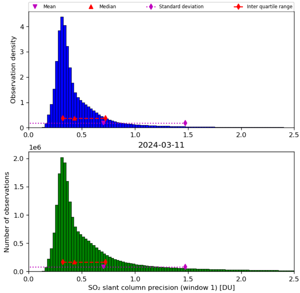
Figure 57: Histogram of “SO 2 slant column precision (window 1)” for 2024-03-10 to 2024-03-12
