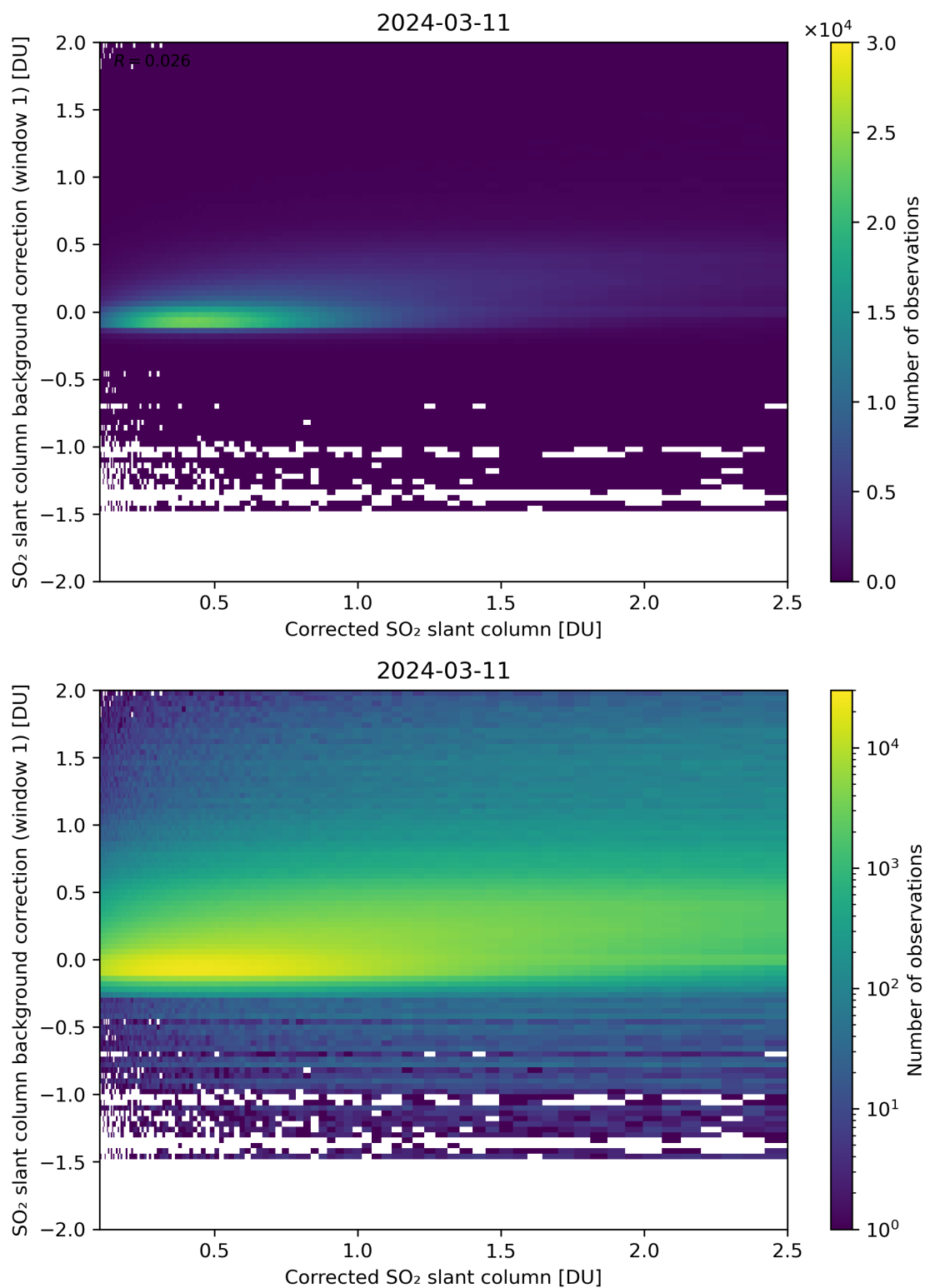
Figure 178: Scatter density plot of “Corrected SO 2 slant column” against “SO 2 slant column background correction (window 1)” for 2024-03-10 to 2024-03-12.
