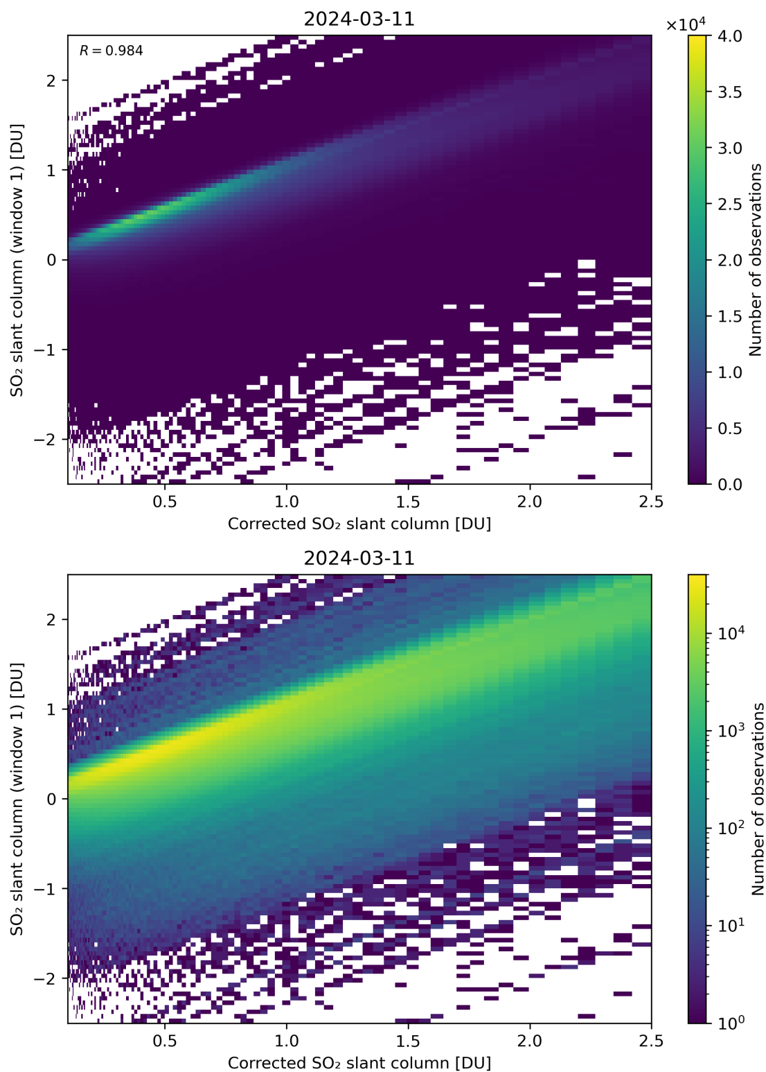
Figure 187: Scatter density plot of “Corrected SO 2 slant column” against “SO 2 slant column (window 1)” for 2024-03-10 to 2024-03-12.
