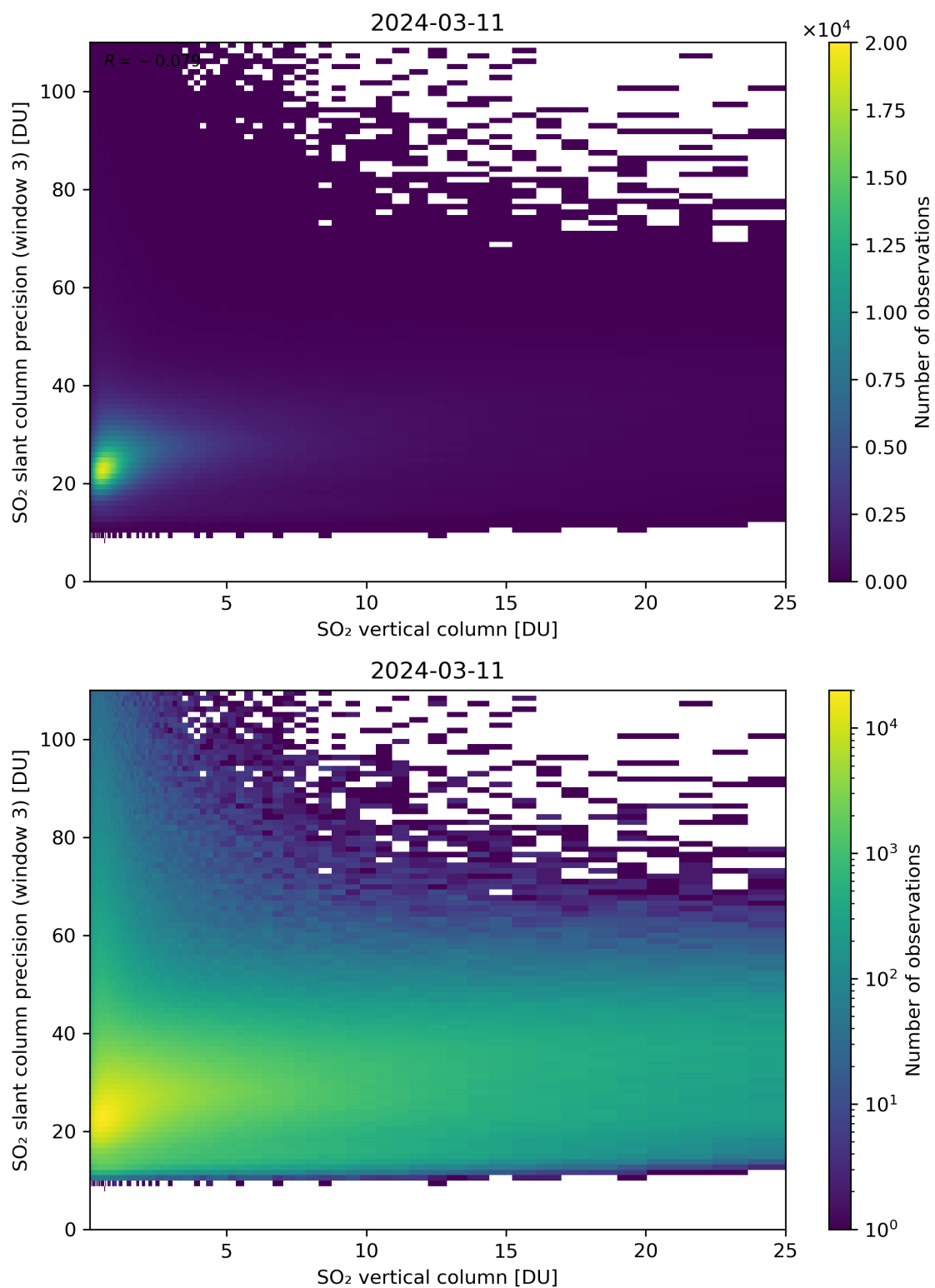
Figure 304: Scatter density plot of “SO 2 vertical column” against “SO 2 slant column precision (window 3)” for 2024-03-10 to 2024-03-12.
