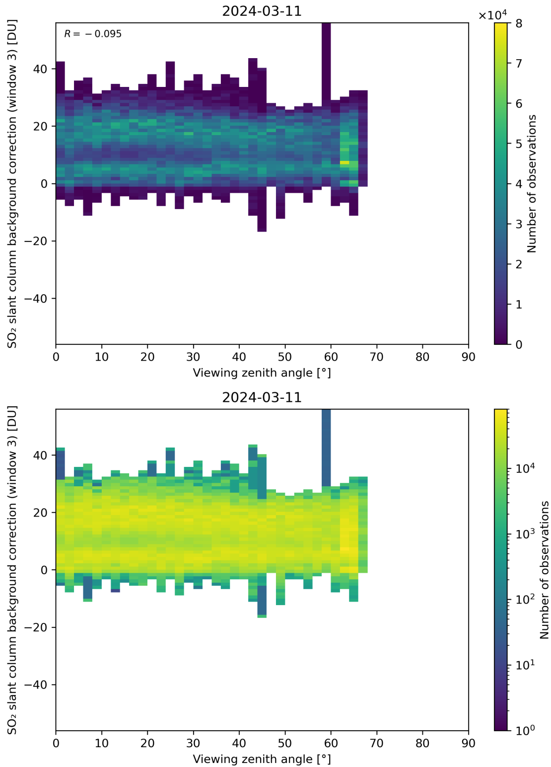
Figure 310: Scatter density plot of “Viewing zenith angle” against “SO 2 slant column background correction (window 3)” for 2024-03-10 to 2024-03-12.
