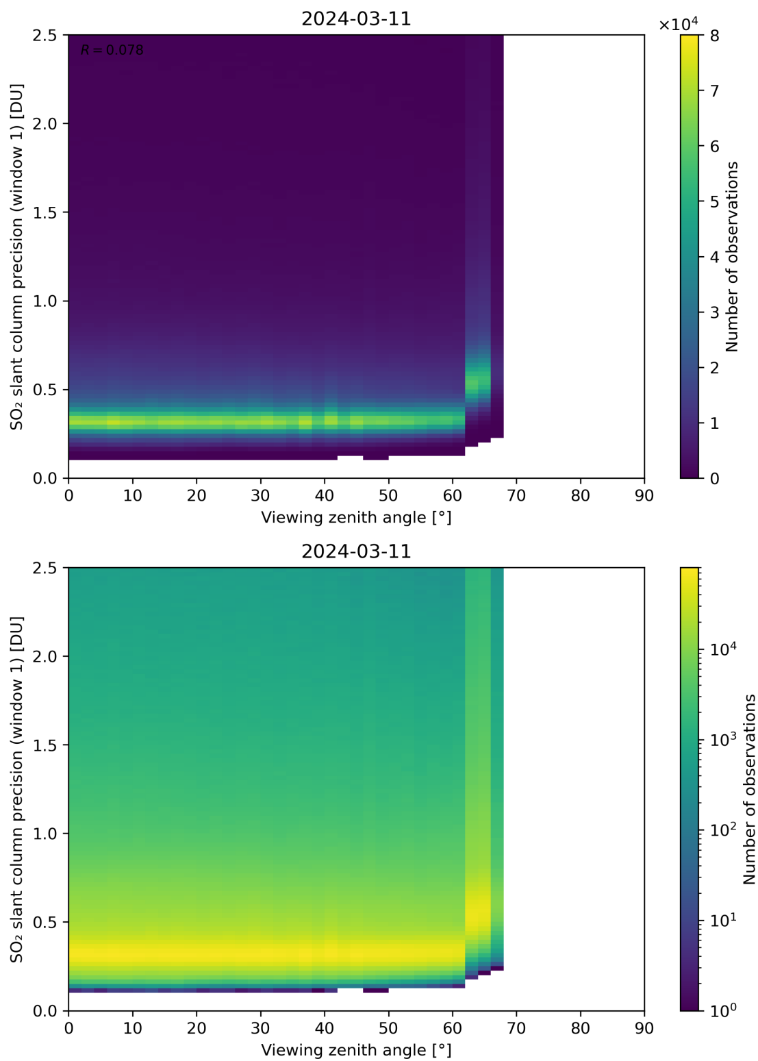
Figure 321: Scatter density plot of “Viewing zenith angle” against “SO 2 slant column precision (window 1)” for 2024-03-10 to 2024-03-12.
