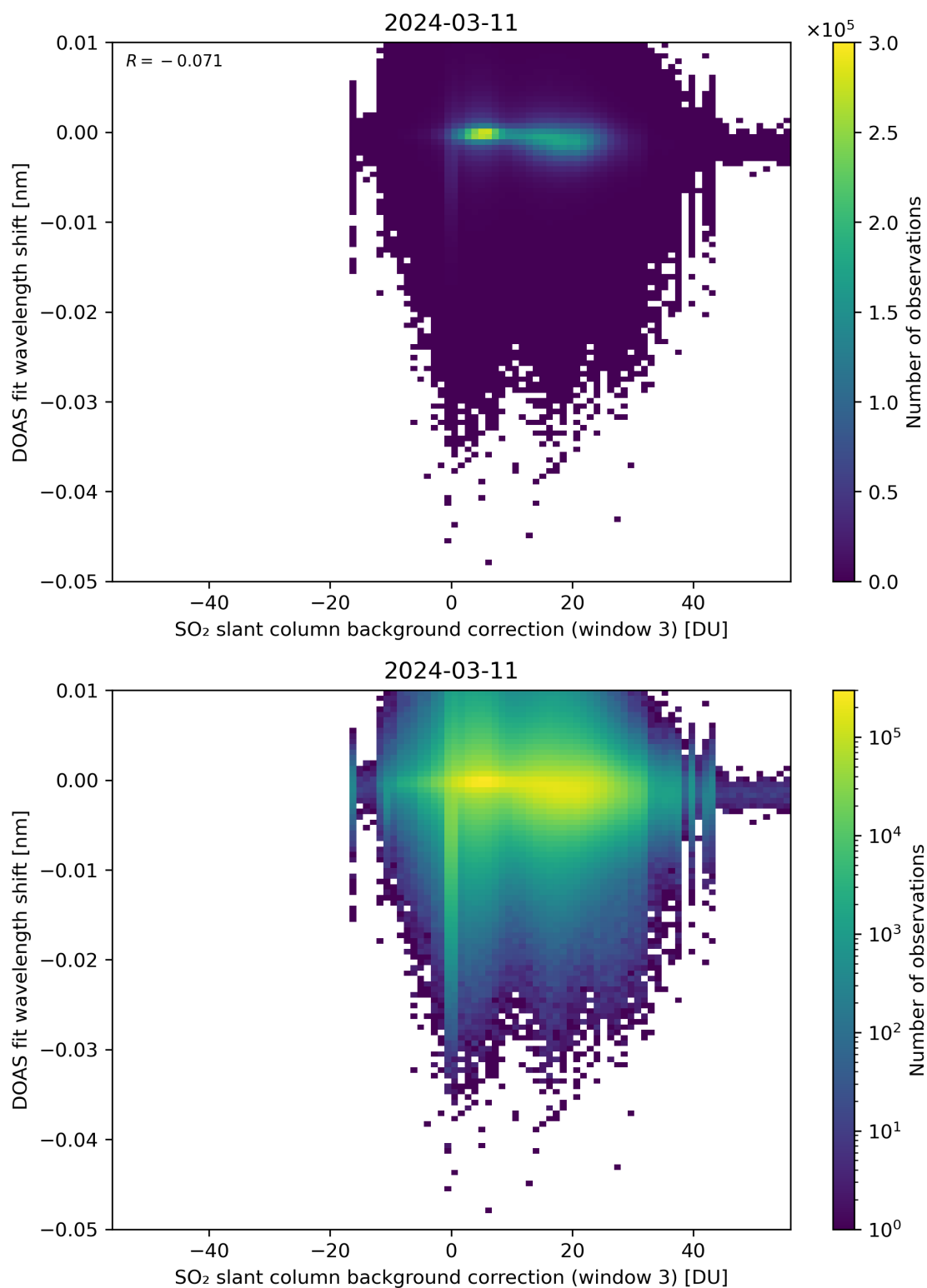
Figure 121: Scatter density plot of “SO 2 slant column background correction (window 3)” against “DOAS fit wavelength shift” for 2024-03-10 to 2024-03-12.
