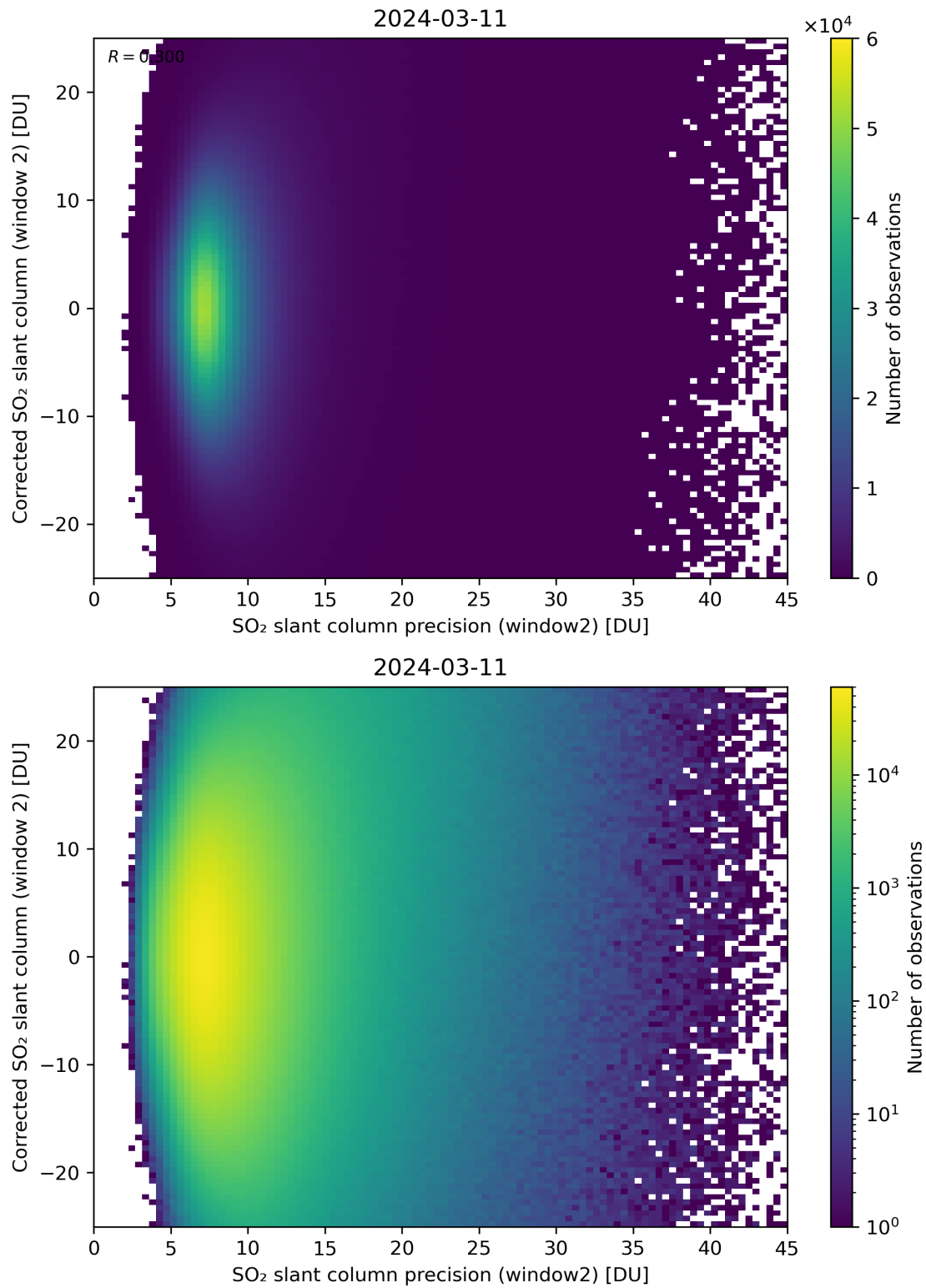
Figure 247: Scatter density plot of “SO 2 slant column precision (window2)” against “Corrected SO 2 slant column (window 2)” for 2024-03-10 to 2024-03-12.
