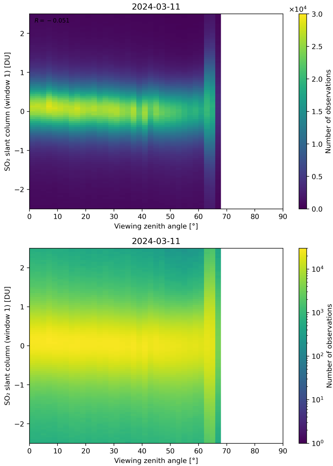
Figure 320: Scatter density plot of “Viewing zenith angle” against “SO 2 slant column (window 1)” for 2024-03-10 to 2024-03-12.
