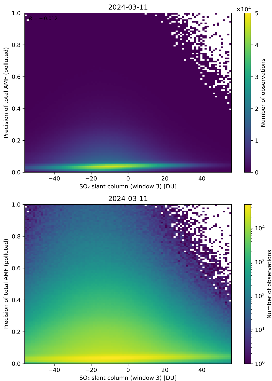
Figure 269: Scatter density plot of “SO 2 slant column (window 3)” against “Precision of total AMF (polluted)” for 2024-03-10 to 2024-03-12.
