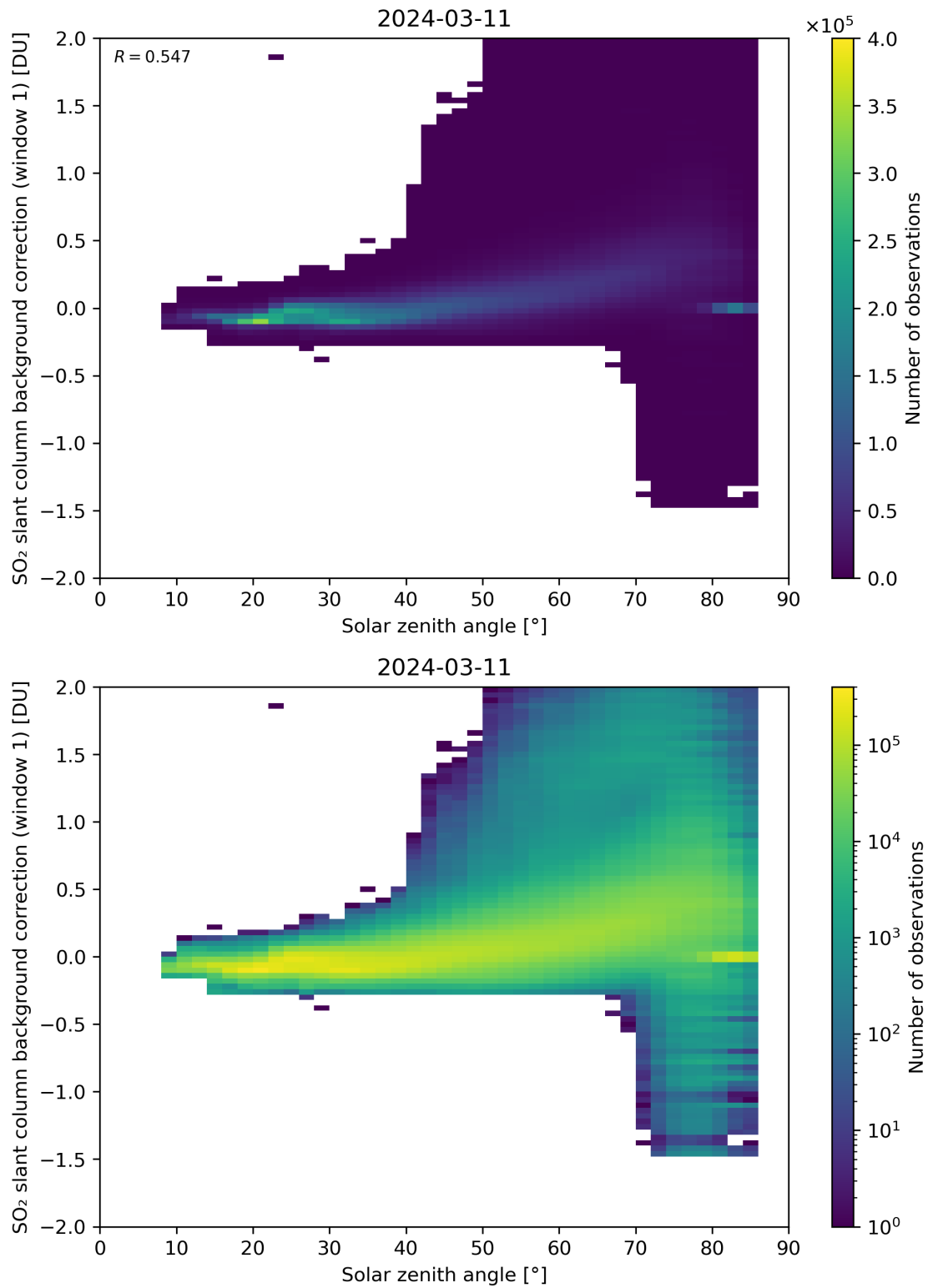
Figure 158: Scatter density plot of “Solar zenith angle” against “SO 2 slant column background correction (window 1)” for 2024-03-10 to 2024-03-12.
