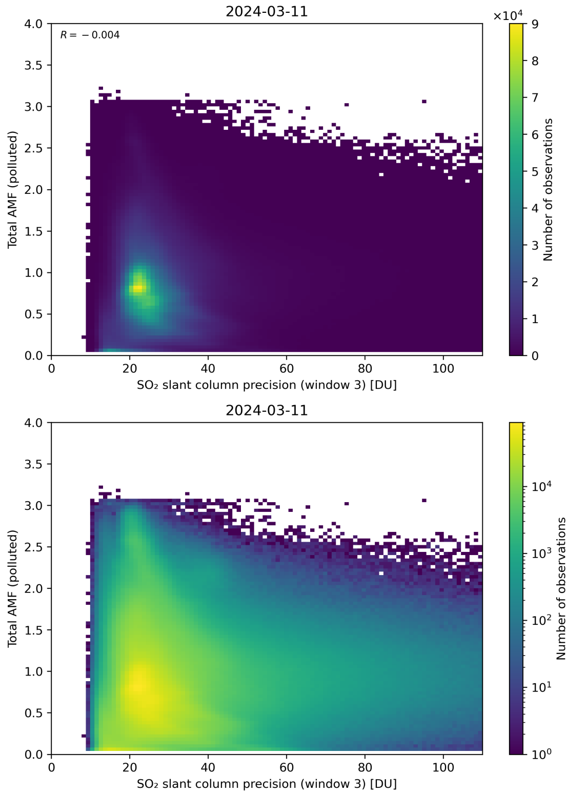
Figure 263: Scatter density plot of “SO 2 slant column precision (window 3)” against “Total AMF (polluted)” for 2024-03-10 to 2024-03-12.
