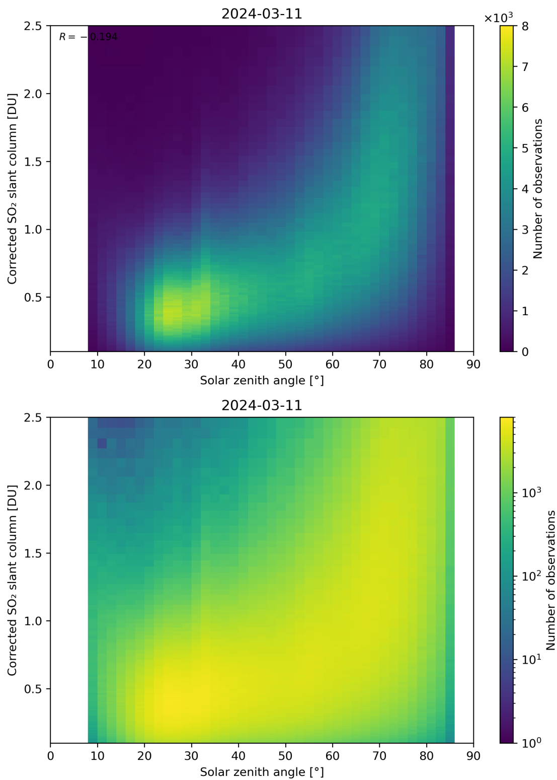
Figure 166: Scatter density plot of “Solar zenith angle” against “Corrected SO 2 slant column” for 2024-03-10 to 2024-03-12.
