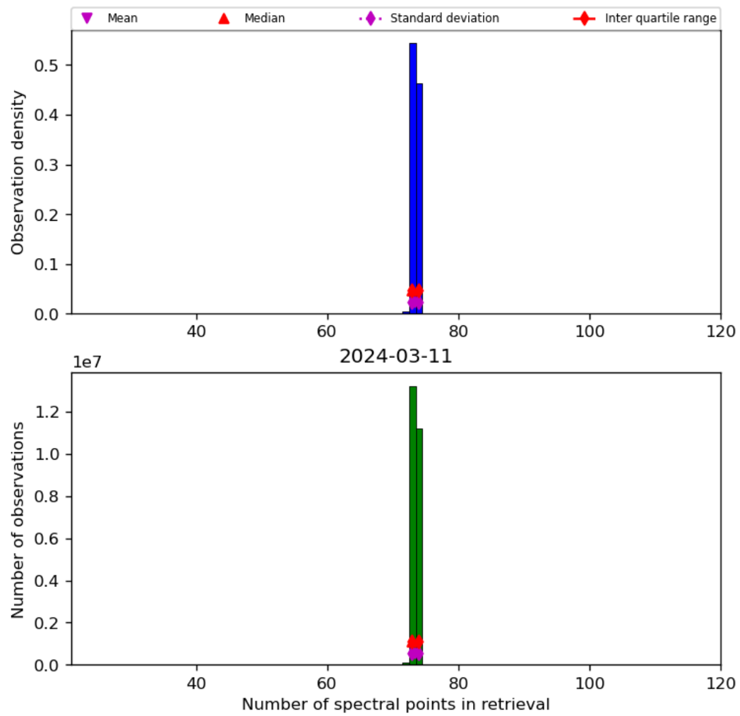
Figure 74: Histogram of “Number of spectral points in retrieval” for 2024-03-10 to 2024-03-12
