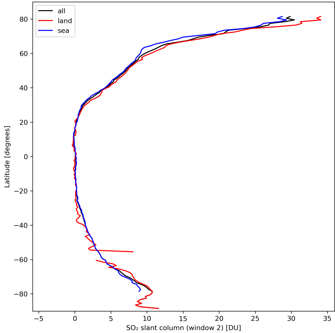
Figure 37: Zonal average of “SO 2 slant column (window 2)” for 2024-03-10 to 2024-03-12.
