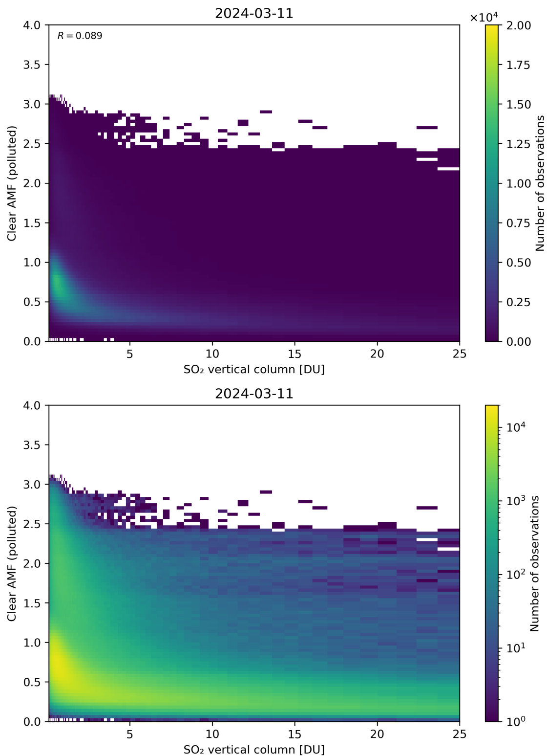
Figure 296: Scatter density plot of “SO 2 vertical column” against “Clear AMF (polluted)” for 2024-03-10 to 2024-03-12.
