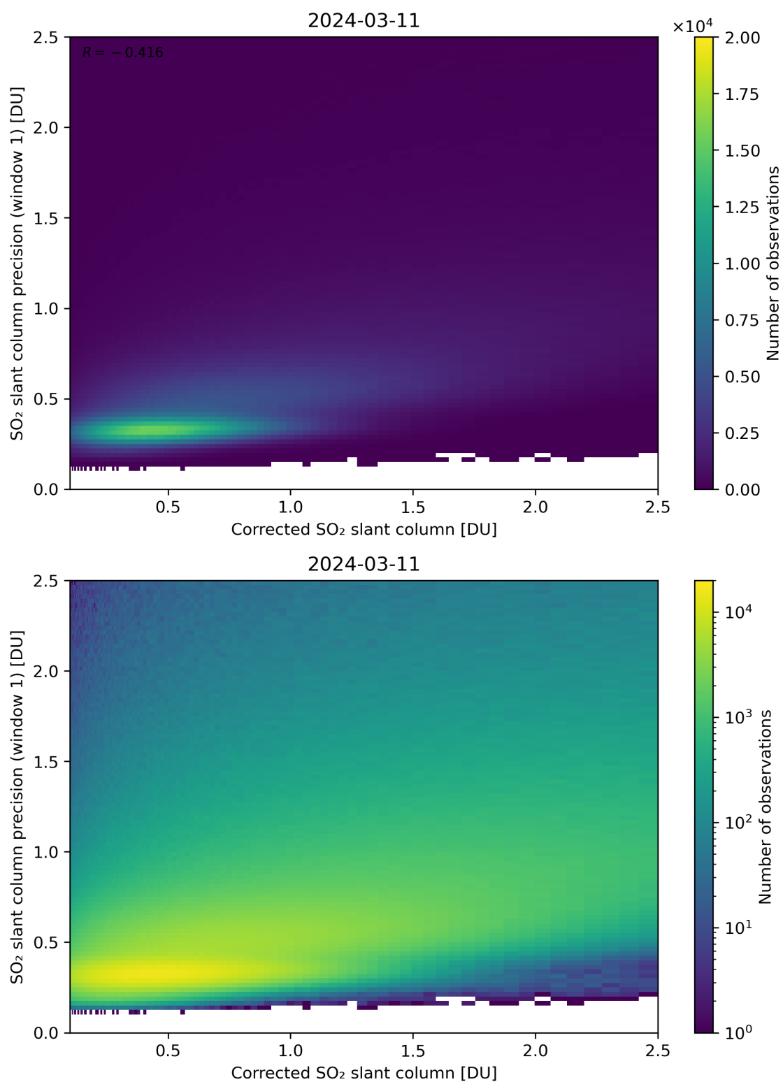
Figure 188: Scatter density plot of “Corrected SO 2 slant column” against “SO 2 slant column precision (window 1)” for 2024-03-10 to 2024-03-12.
