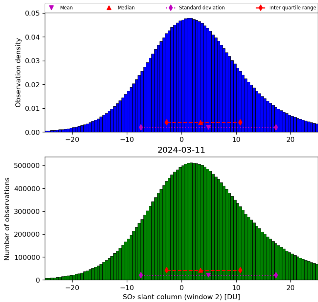
Figure 60: Histogram of “SO 2 slant column (window 2)” for 2024-03-10 to 2024-03-12
