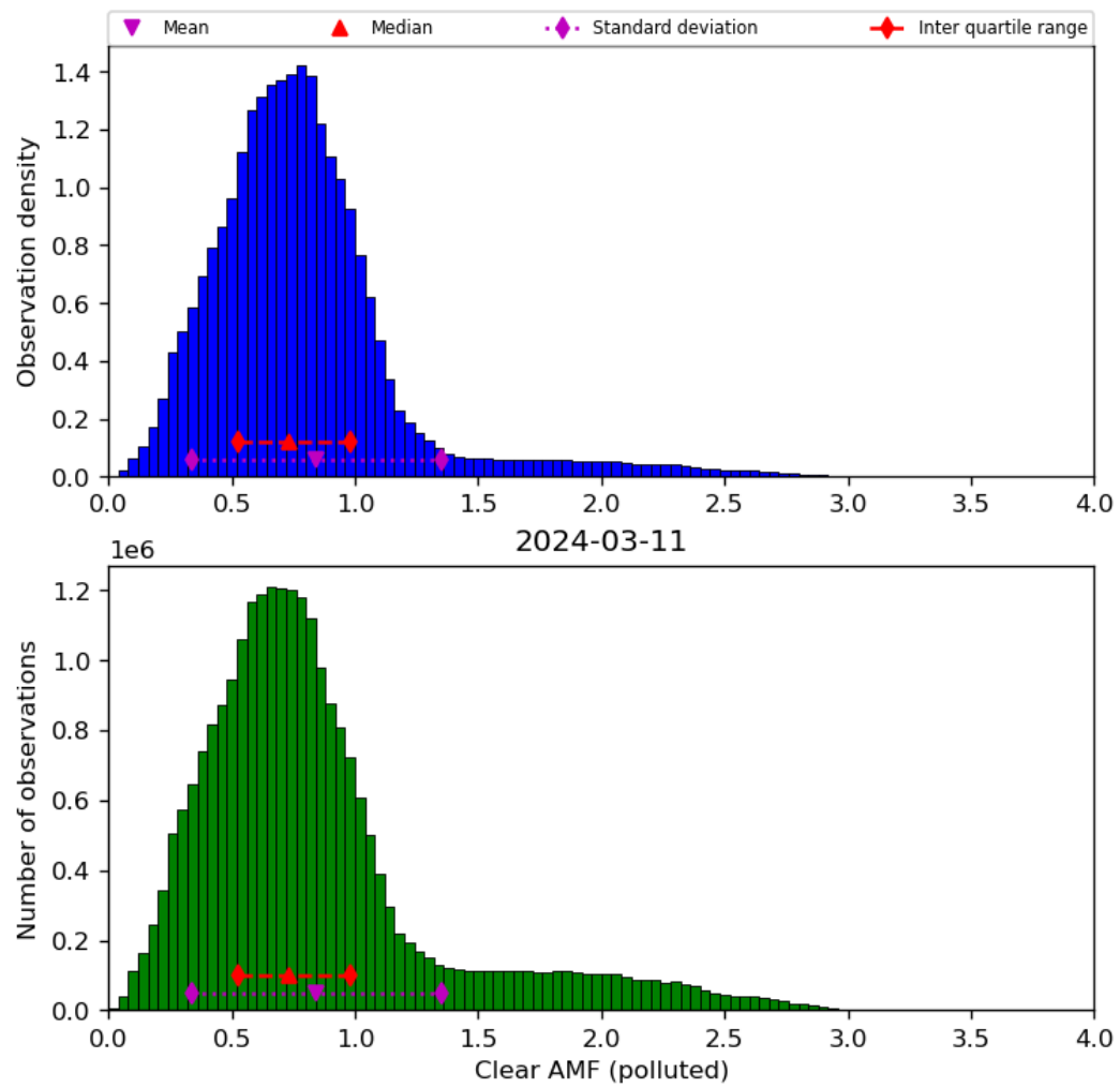
Figure 73: Histogram of “Clear AMF (polluted)” for 2024-03-10 to 2024-03-12
