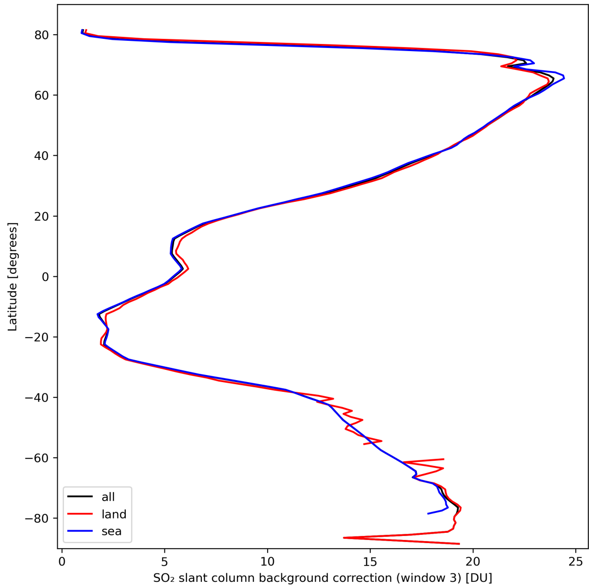
Figure 44: Zonal average of “SO 2 slant column background correction (window 3)” for 2024-03-10 to 2024-03-12.
