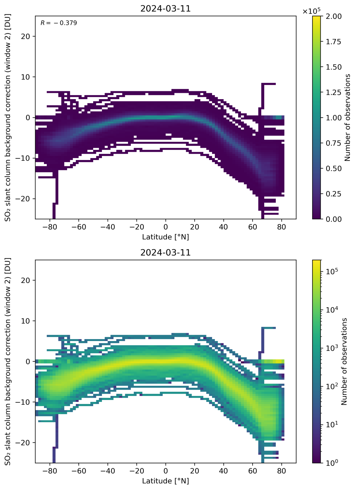
Figure 140: Scatter density plot of “Latitude” against “SO 2 slant column background correction (window 2)” for 2024-03-10 to 2024-03-12.
