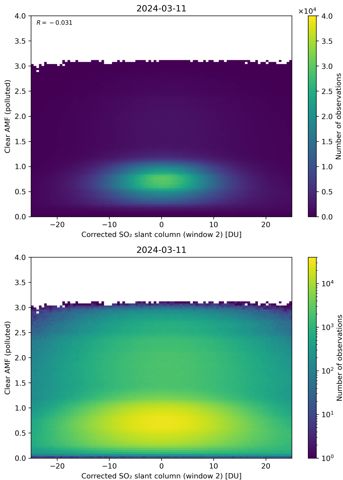
Figure 199: Scatter density plot of “Corrected SO 2 slant column (window 2)” against “Clear AMF (polluted)” for 2024-03-10 to 2024-03-12.
