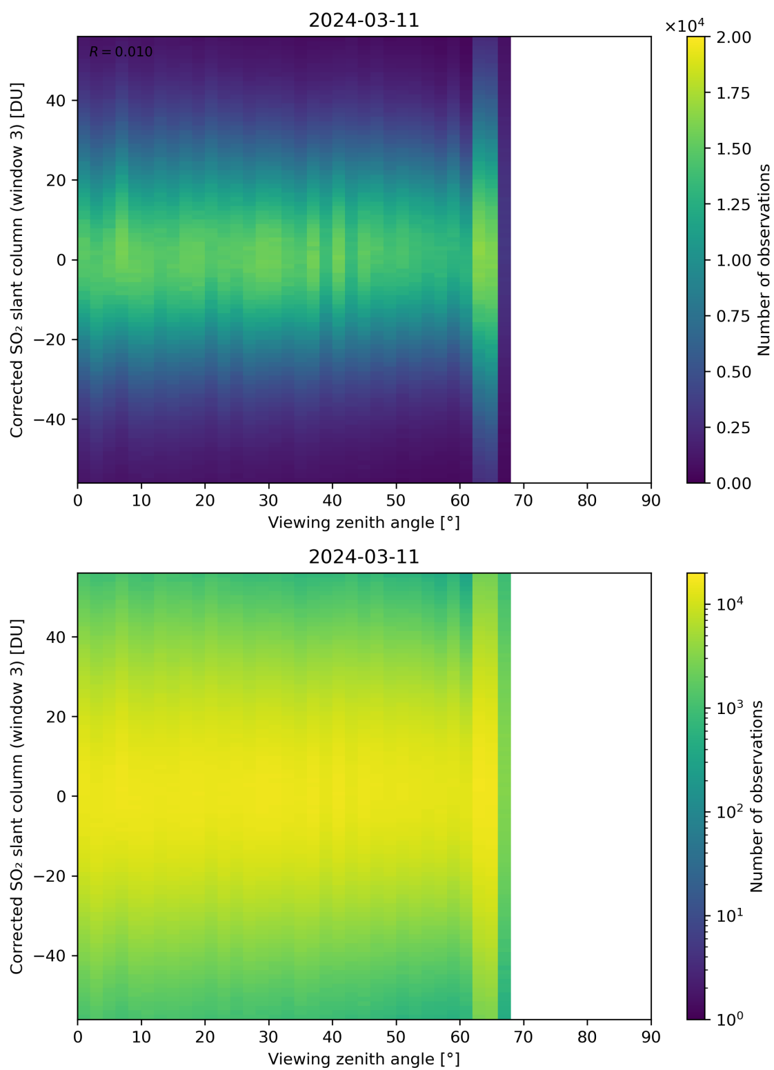
Figure 319: Scatter density plot of “Viewing zenith angle” against “Corrected SO 2 slant column (window 3)” for 2024-03-10 to 2024-03-12.
