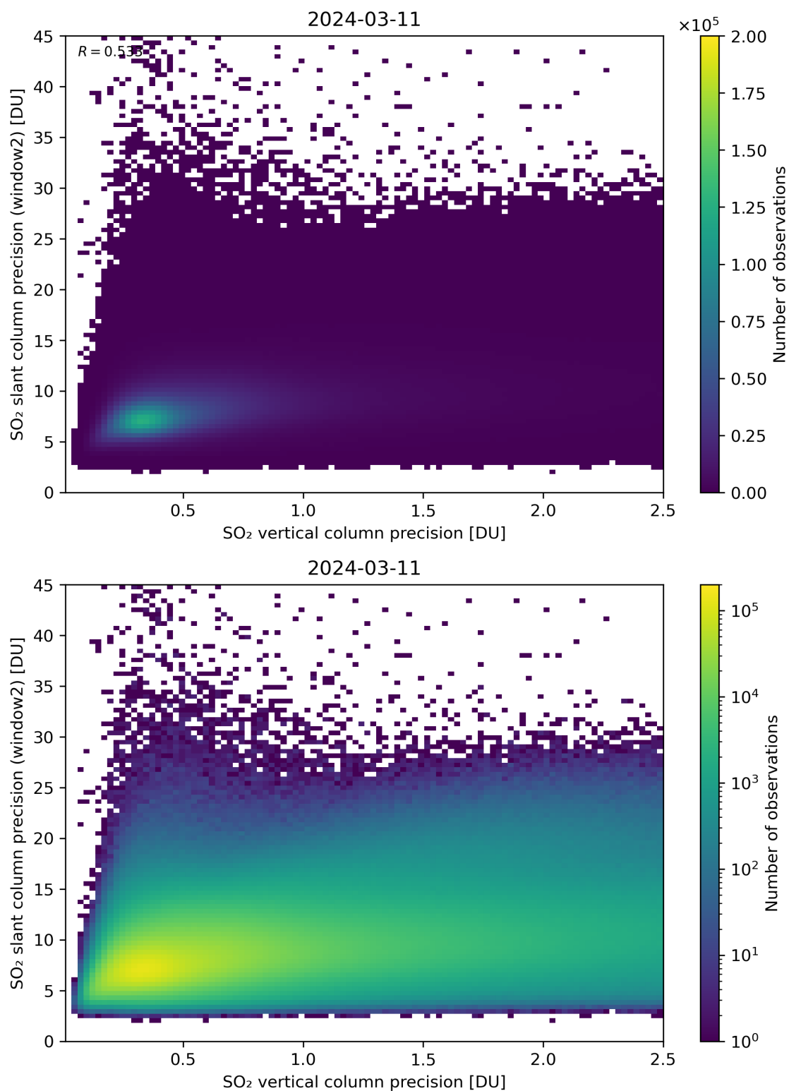
Figure 291: Scatter density plot of “SO 2 vertical column precision” against “SO 2 slant column precision (window2)” for 2024-03-10 to 2024-03-12.
