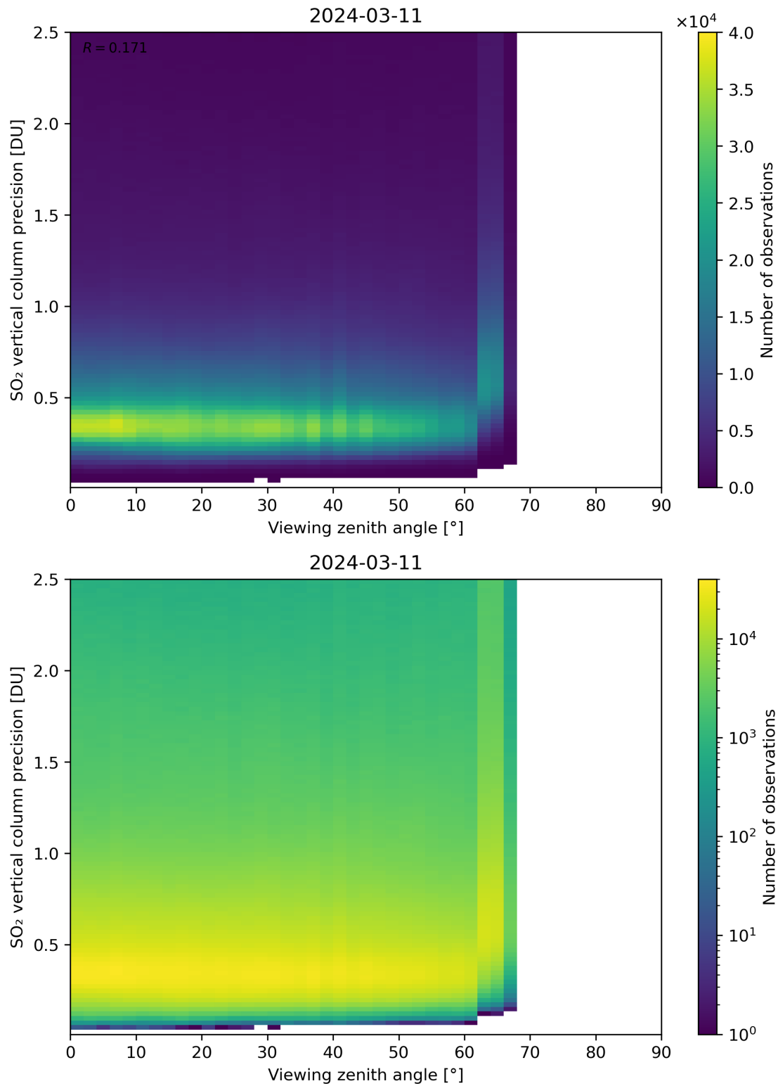
Figure 328: Scatter density plot of “Viewing zenith angle” against “SO 2 vertical column precision” for 2024-03-10 to 2024-03-12.
