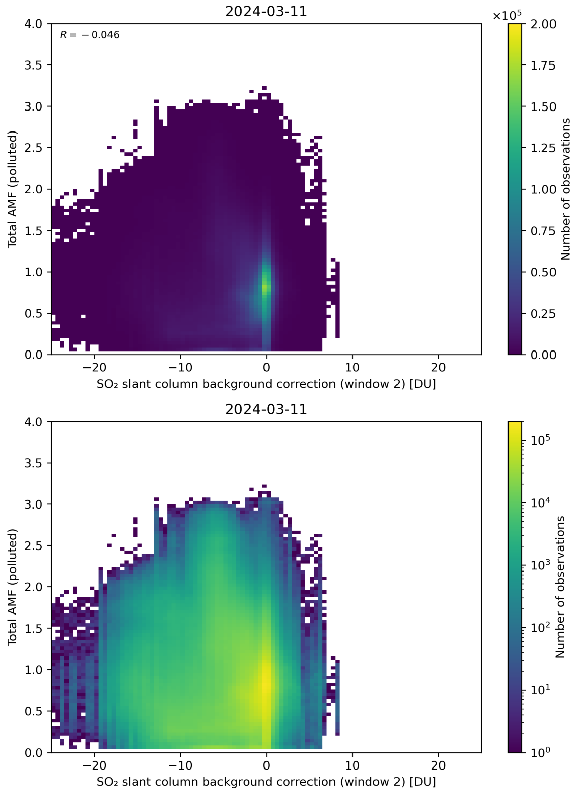
Figure 119: Scatter density plot of “SO 2 slant column background correction (window 2)” against “Total AMF (polluted)” for 2024-03-10 to 2024-03-12.
