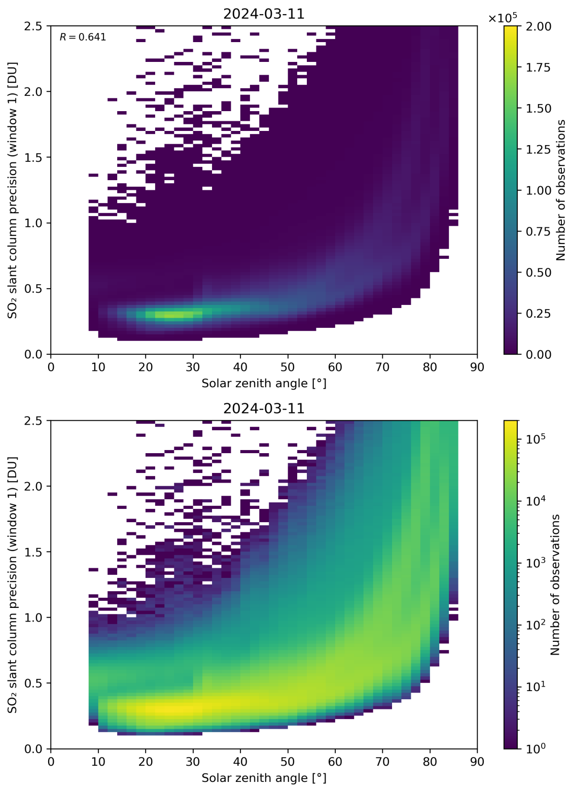
Figure 170: Scatter density plot of “Solar zenith angle” against “SO 2 slant column precision (window 1)” for 2024-03-10 to 2024-03-12.
