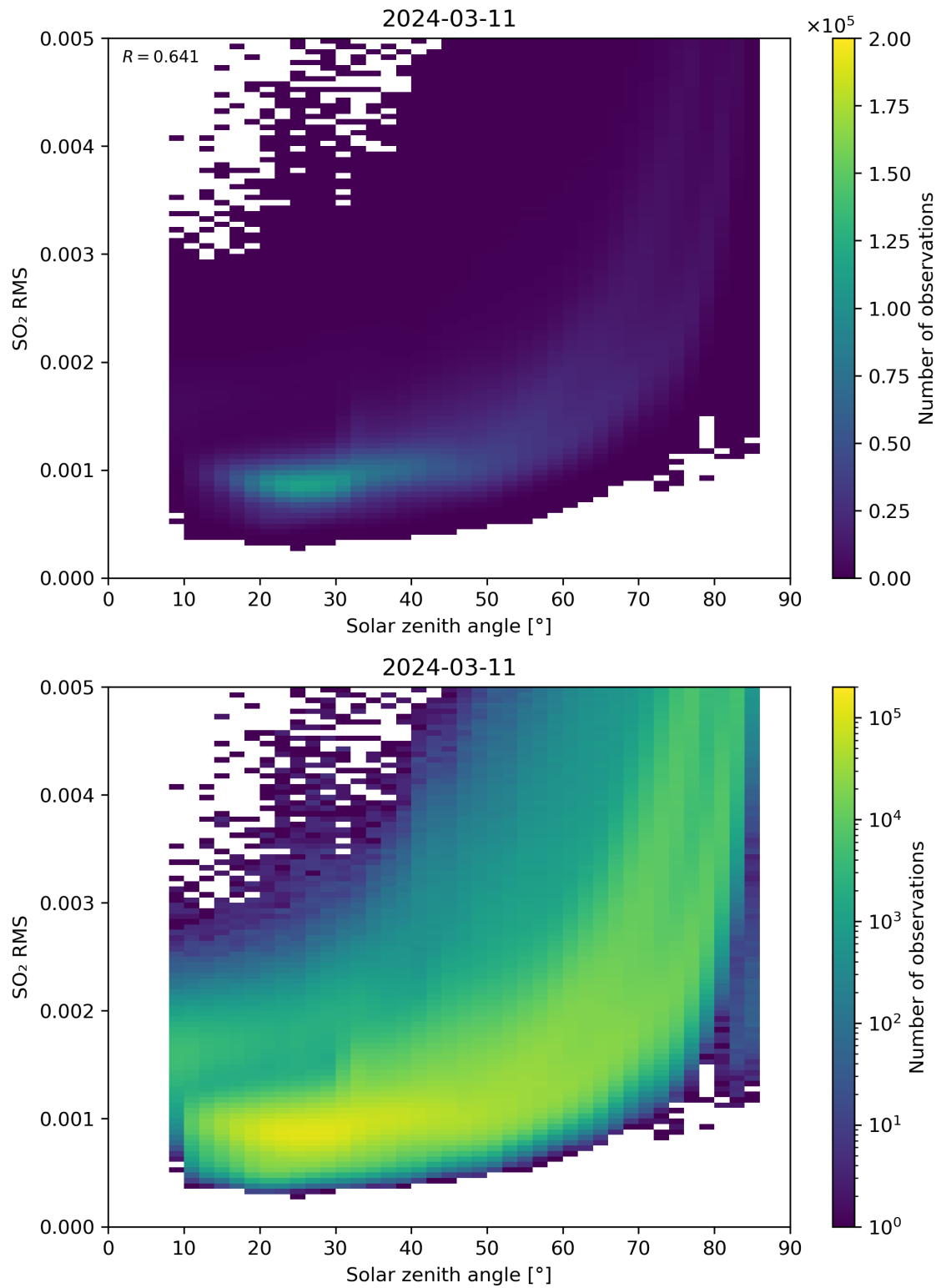
Figure 163: Scatter density plot of “Solar zenith angle” against “SO 2 RMS” for 2024-03-10 to 2024-03-12.
