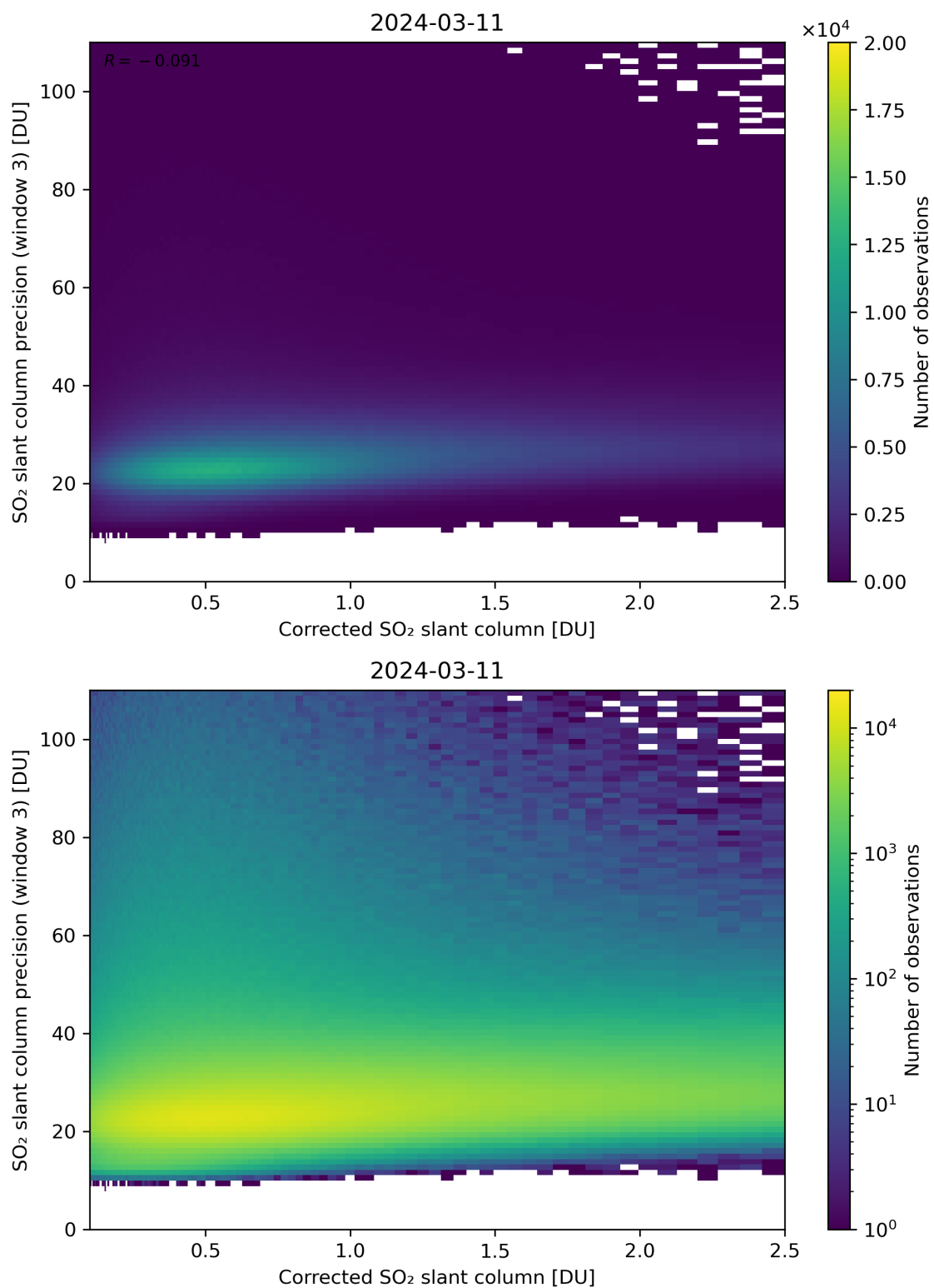
Figure 191: Scatter density plot of “Corrected SO 2 slant column” against “SO 2 slant column precision (window 3)” for 2024-03-10 to 2024-03-12.
