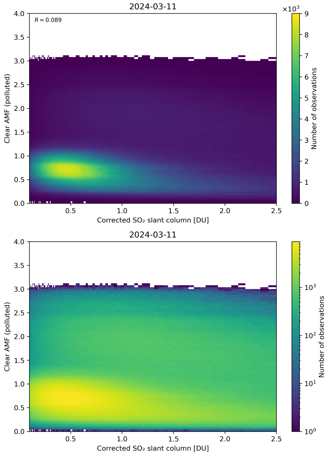
Figure 184: Scatter density plot of “Corrected SO 2 slant column” against “Clear AMF (polluted)” for 2024-03-10 to 2024-03-12.
