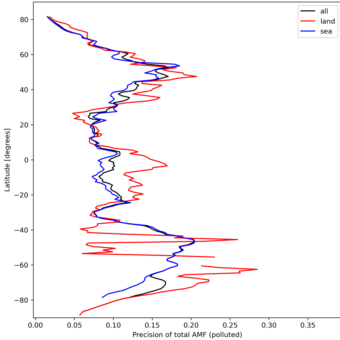
Figure 49: Zonal average of “Precision of total AMF (polluted)” for 2024-03-10 to 2024-03-12.
