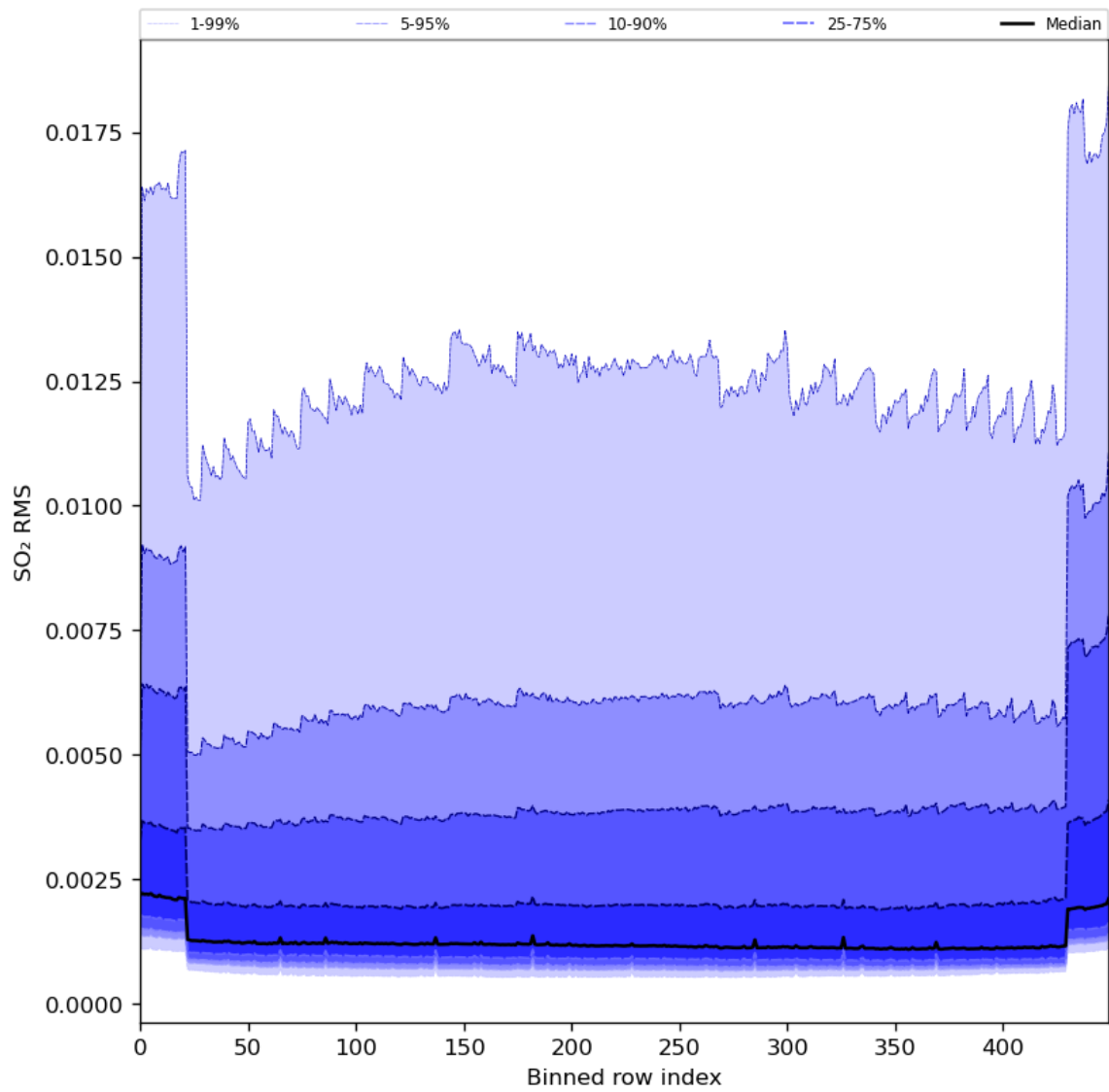
Figure 93: Along track statistics of “SO 2 RMS” for 2024-03-10 to 2024-03-12
