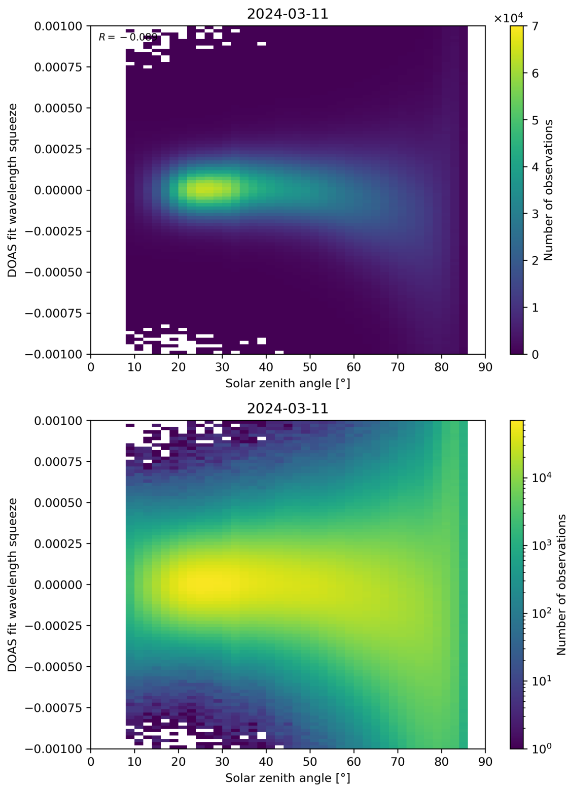
Figure 162: Scatter density plot of “Solar zenith angle” against “DOAS fit wavelength squeeze” for 2024-03-10 to 2024-03-12.
