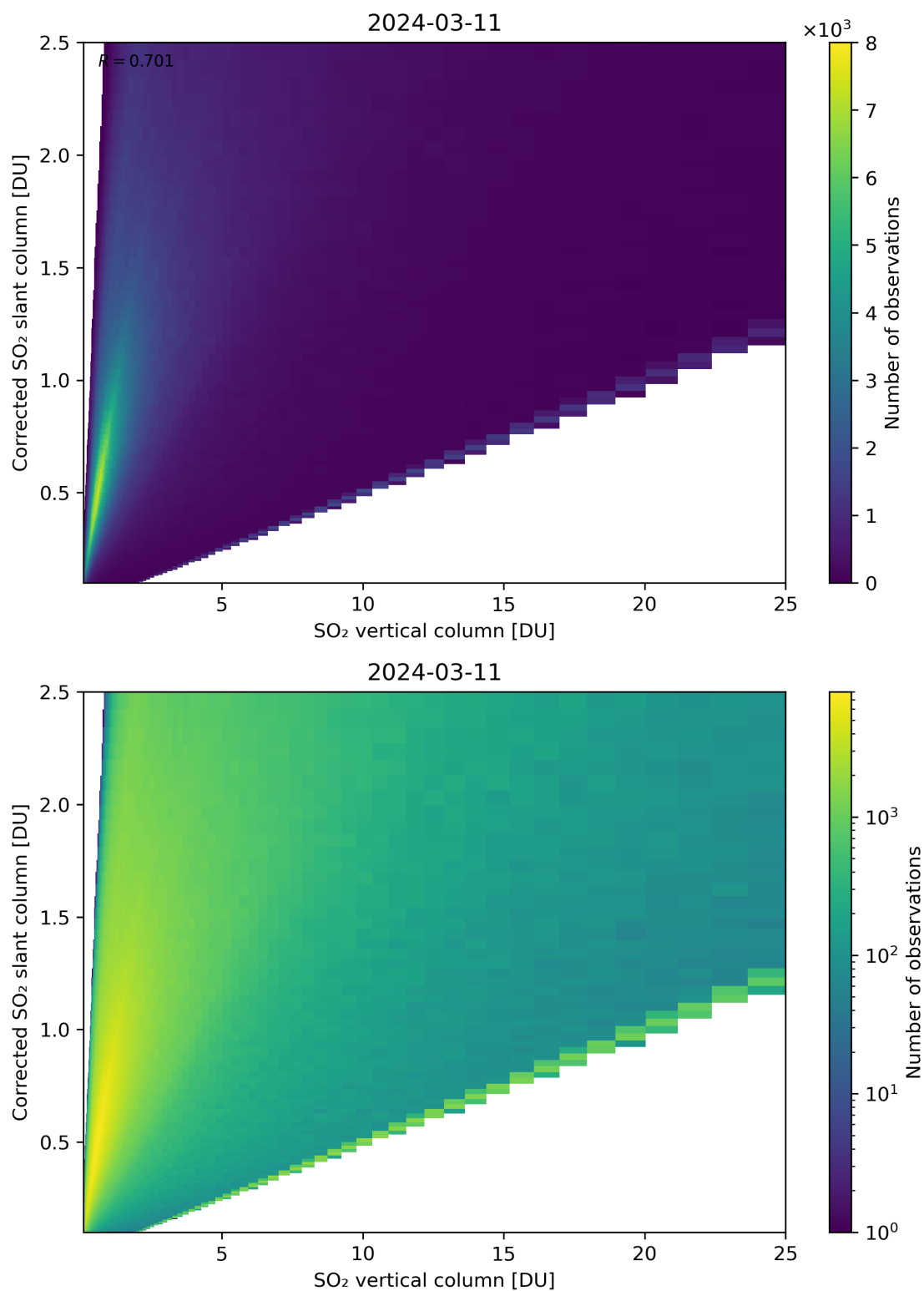
Figure 297: Scatter density plot of “SO 2 vertical column” against “Corrected SO 2 slant column” for 2024-03-10 to 2024-03-12.
