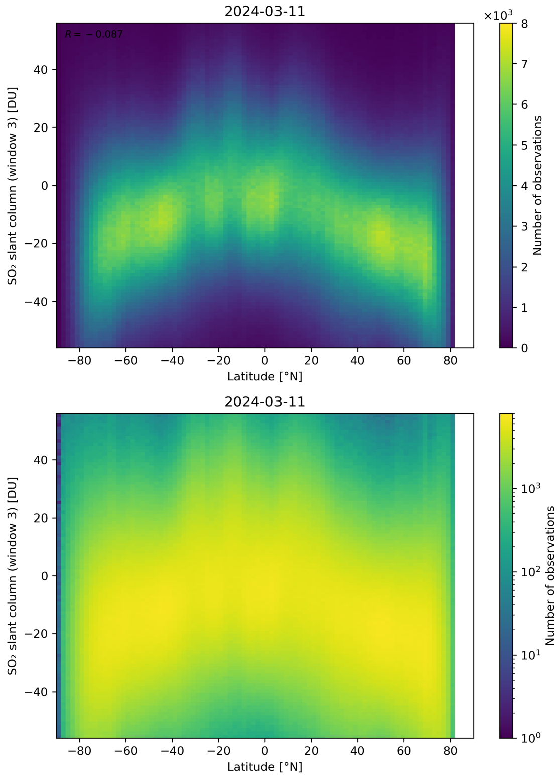
Figure 152: Scatter density plot of “Latitude” against “SO 2 slant column (window 3)” for 2024-03-10 to 2024-03-12.
