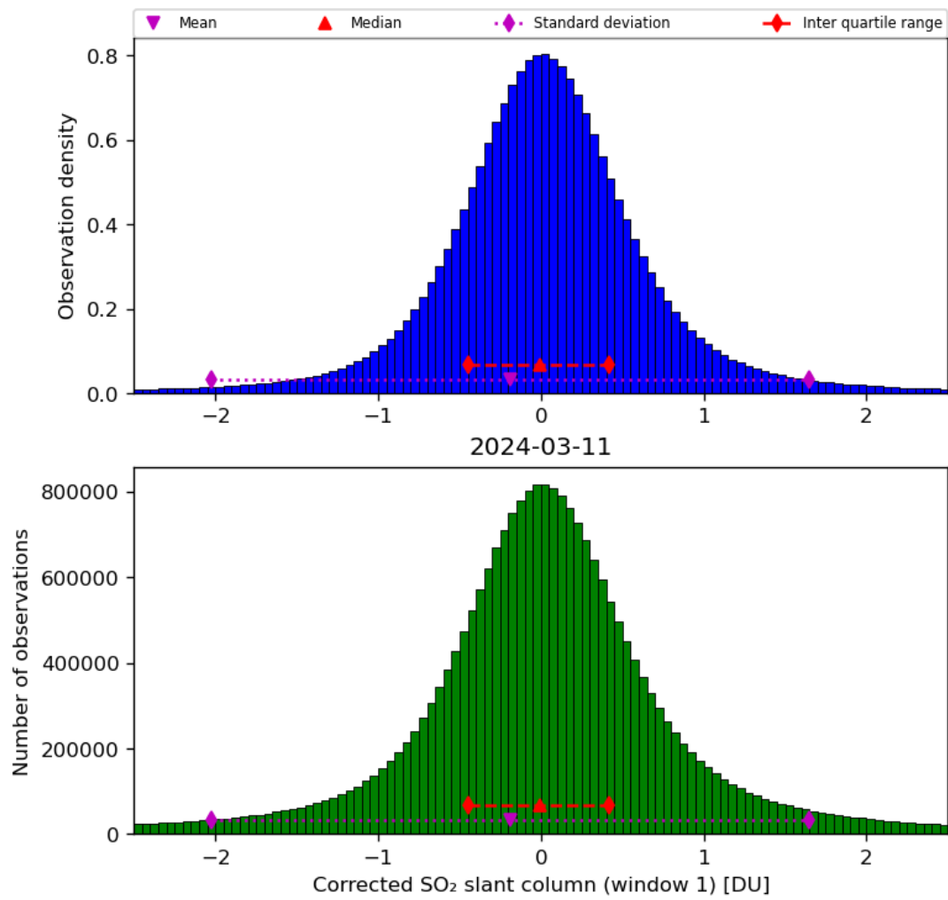
Figure 58: Histogram of “Corrected SO 2 slant column (window 1)” for 2024-03-10 to 2024-03-12
