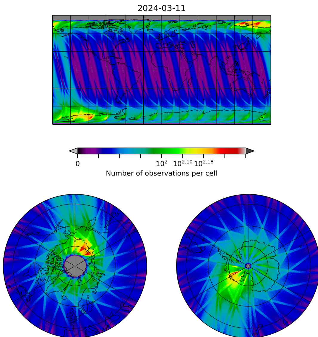
Figure 28: Map of the number of observations for 2024-03-10 to 2024-03-12
