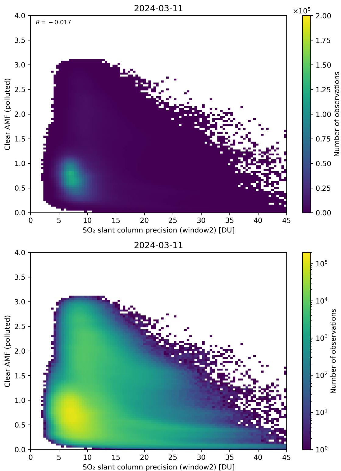
Figure 246: Scatter density plot of “SO 2 slant column precision (window2)” against “Clear AMF (polluted)” for 2024-03-10 to 2024-03-12.
