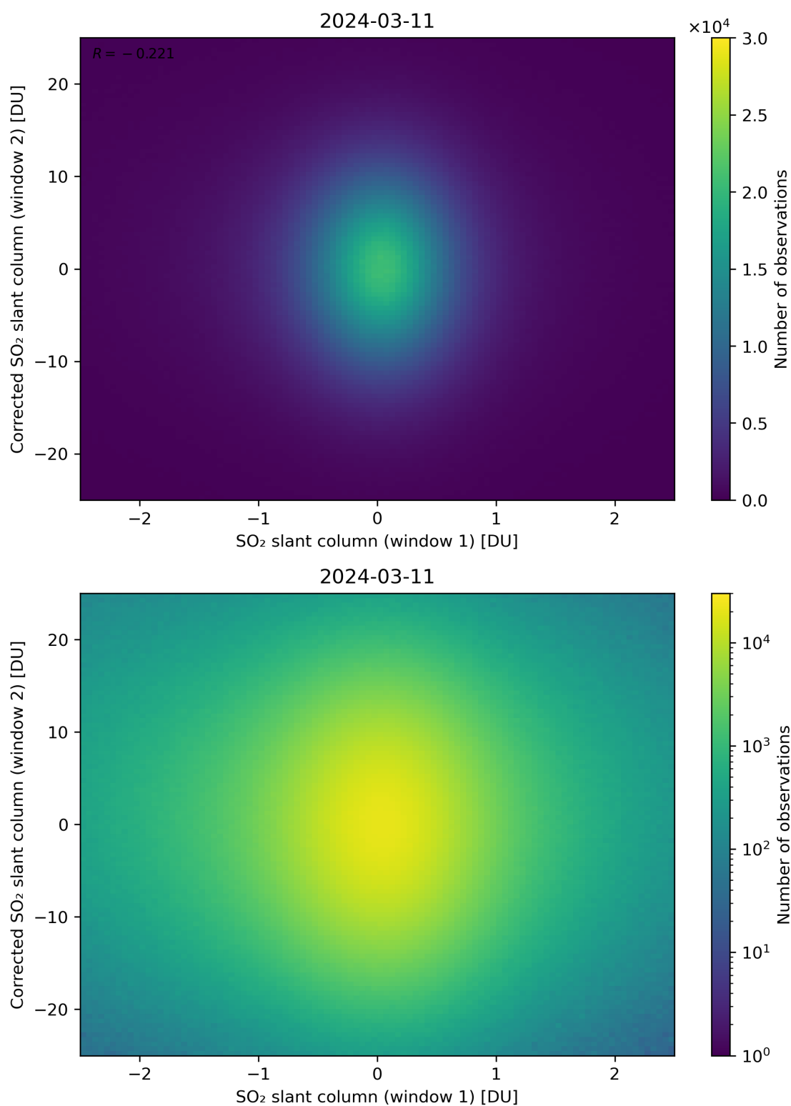
Figure 233: Scatter density plot of “SO 2 slant column (window 1)” against “Corrected SO 2 slant column (window 2)” for 2024-03-10 to 2024-03-12.
