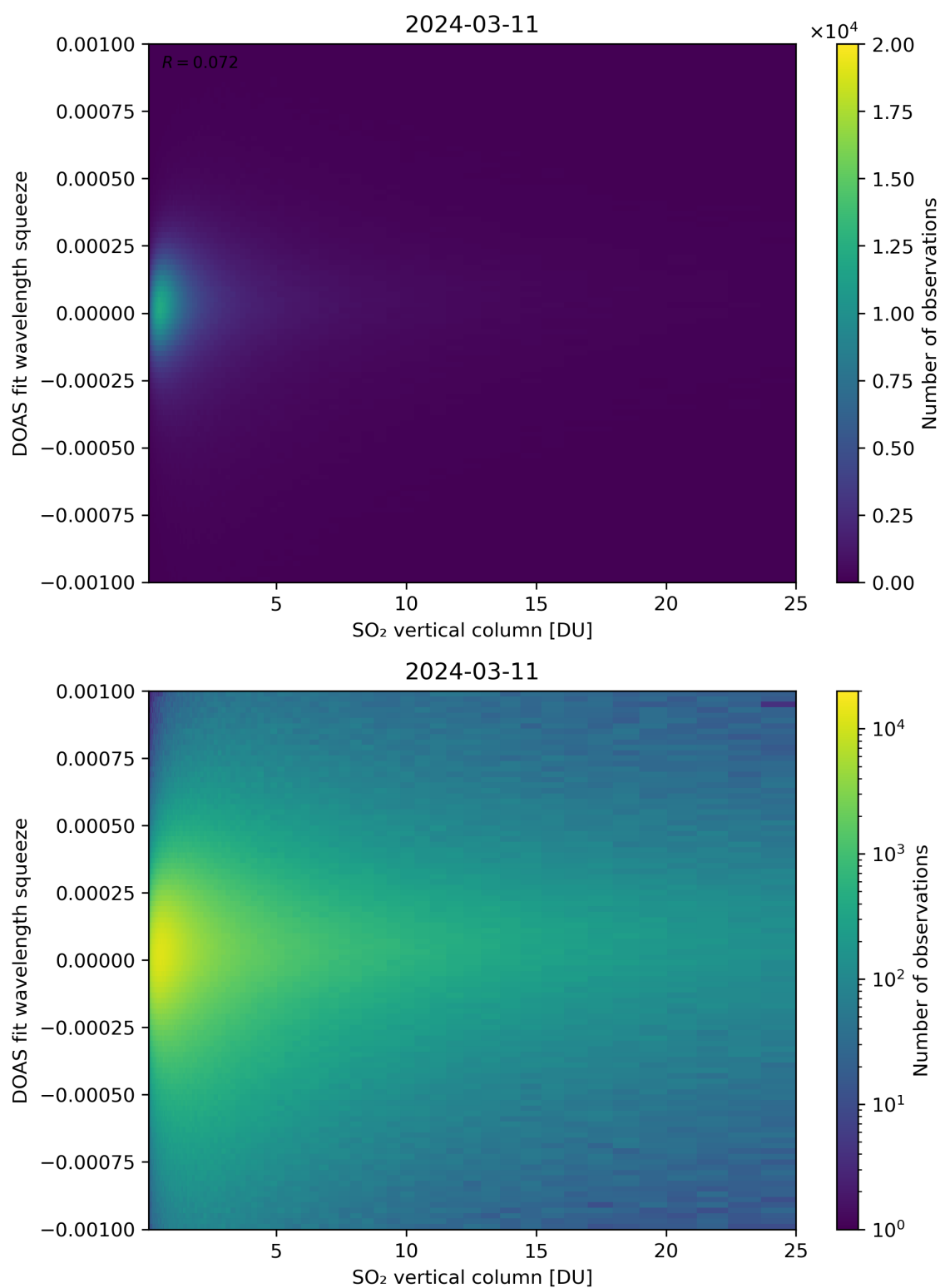
Figure 277: Scatter density plot of “SO 2 vertical column” against “DOAS fit wavelength squeeze” for 2024-03-10 to 2024-03-12.
