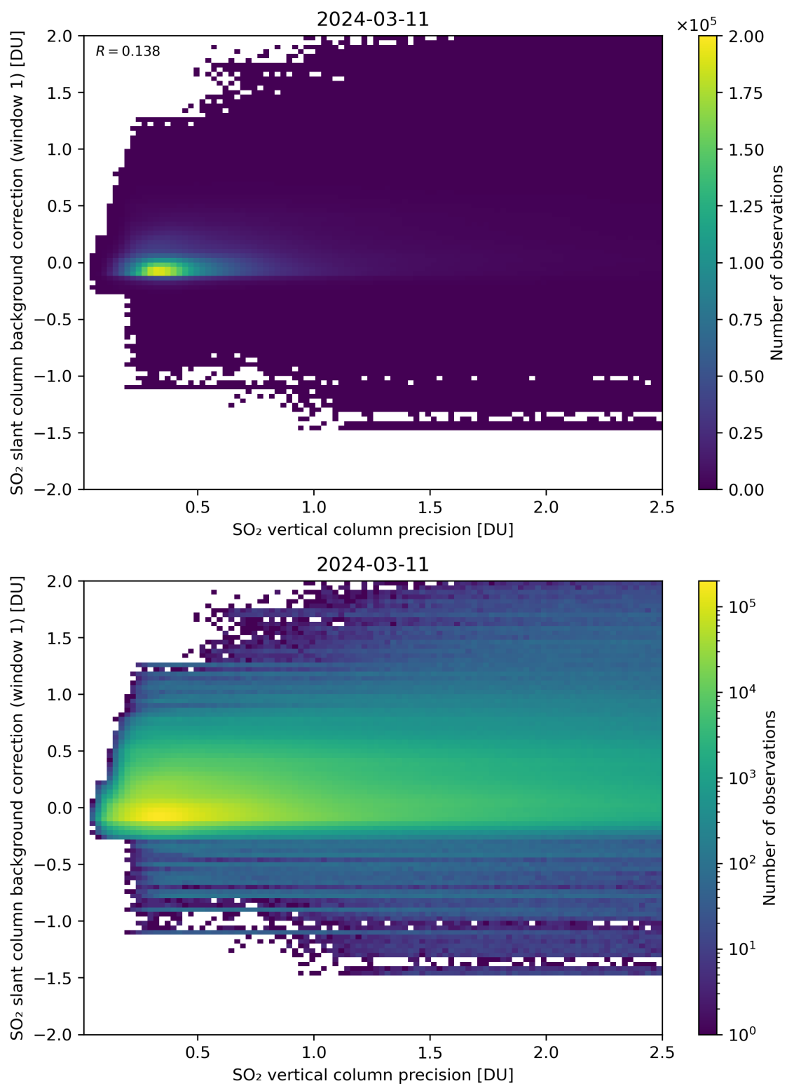
Figure 279: Scatter density plot of “SO 2 vertical column precision” against “SO 2 slant column background correction (window 1)” for 2024-03-10 to 2024-03-12.
