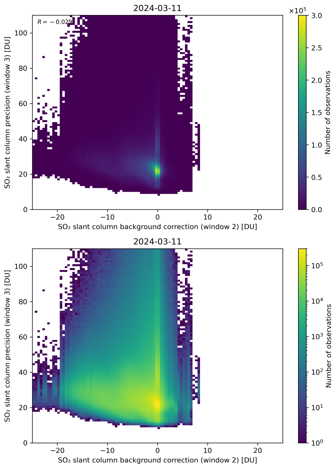
Figure 118: Scatter density plot of “SO 2 slant column background correction (window 2)” against “SO 2 slant column precision (window 3)” for 2024-03-10 to 2024-03-12.
