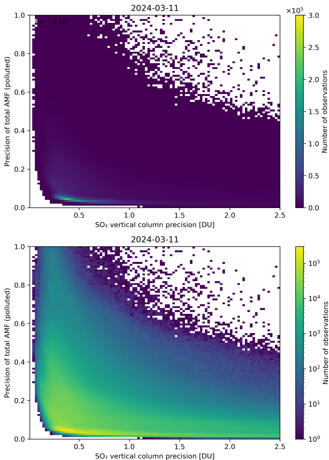
Figure 295: Scatter density plot of “SO 2 vertical column precision” against “Precision of total AMF (polluted)” for 2024-03-10 to 2024-03-12.
