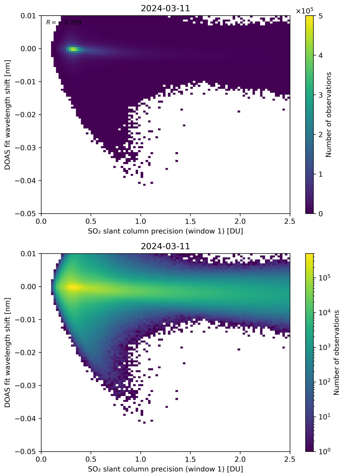
Figure 221: Scatter density plot of “SO 2 slant column precision (window 1)” against “DOAS fit wavelength shift” for 2024-03-10 to 2024-03-12.
