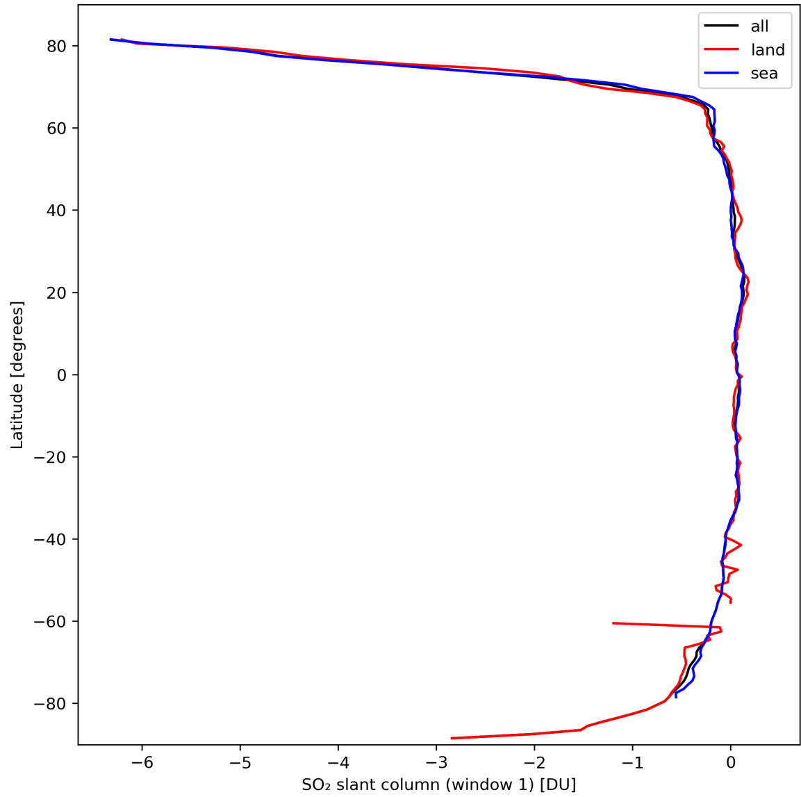
Figure 33: Zonal average of “SO 2 slant column (window 1)” for 2024-03-10 to 2024-03-12.
