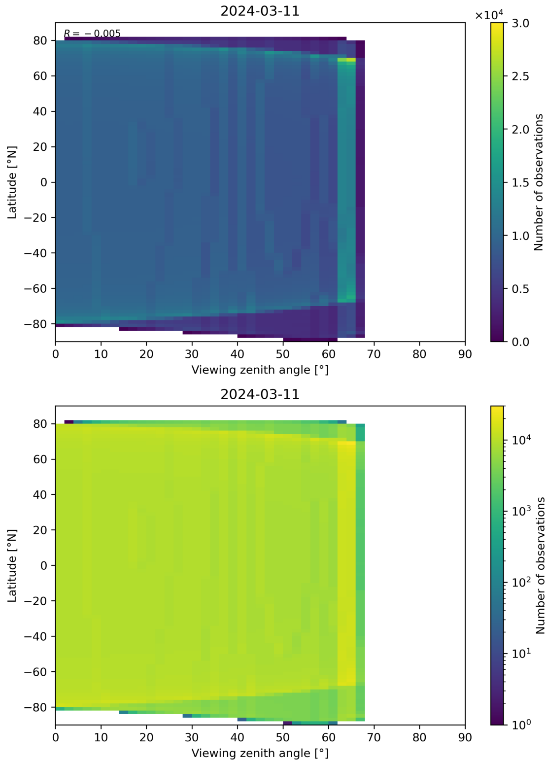
Figure 314: Scatter density plot of “Viewing zenith angle” against “Latitude” for 2024-03-10 to 2024-03-12.
