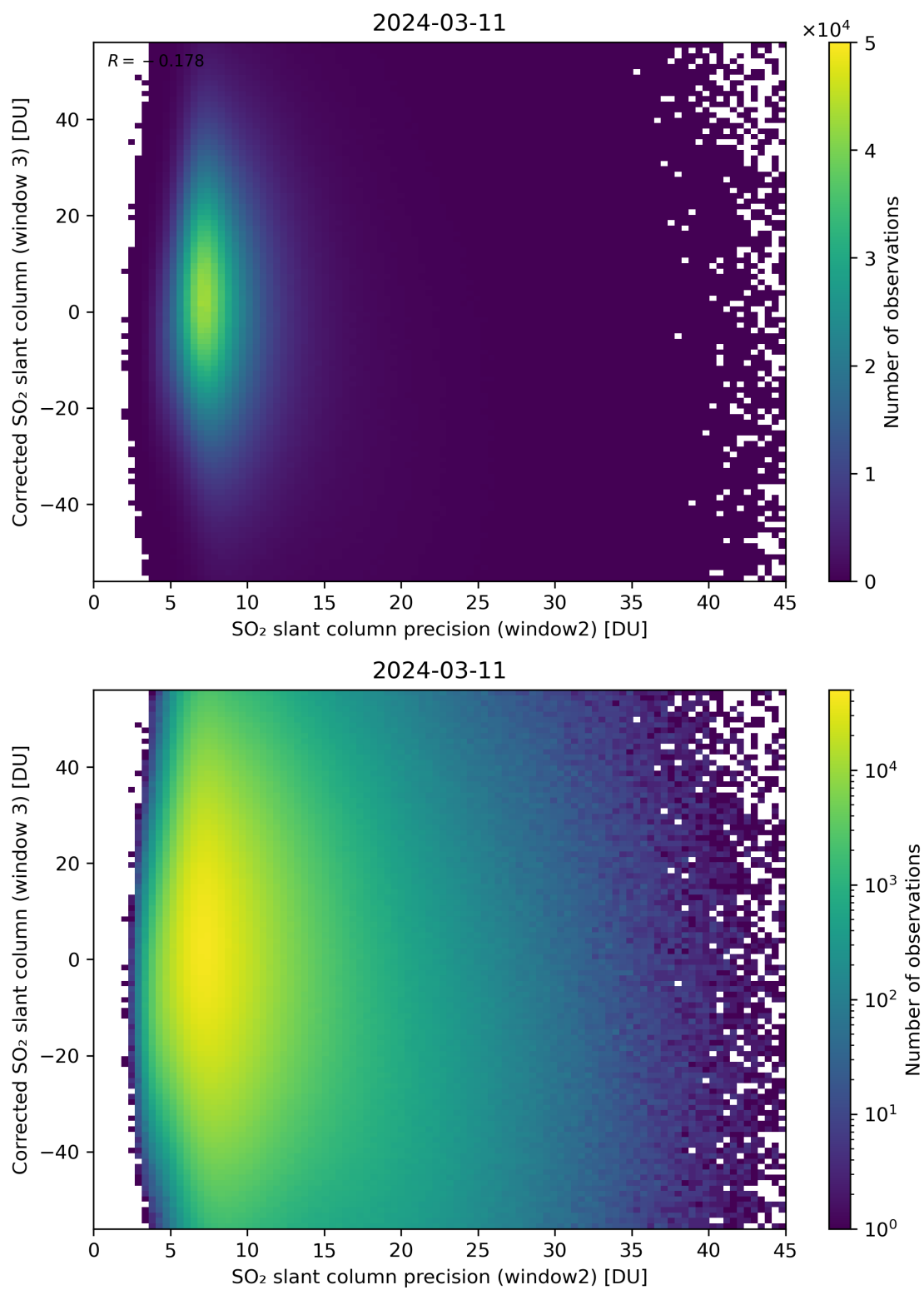
Figure 248: Scatter density plot of “SO 2 slant column precision (window2)” against “Corrected SO 2 slant column (window 3)” for 2024-03-10 to 2024-03-12.
