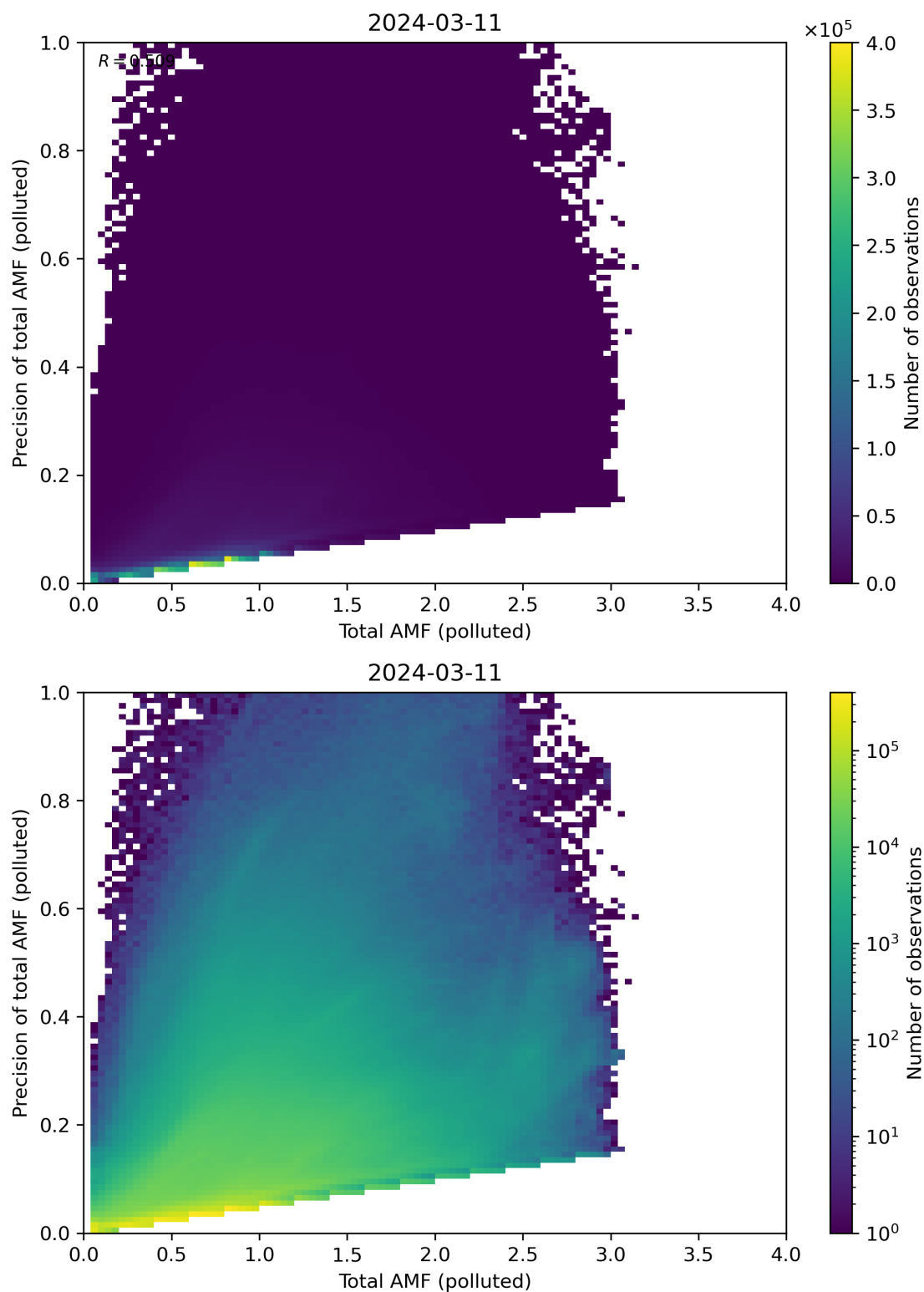
Figure 272: Scatter density plot of “Total AMF (polluted)” against “Precision of total AMF (polluted)” for 2024-03-10 to 2024-03-12.
