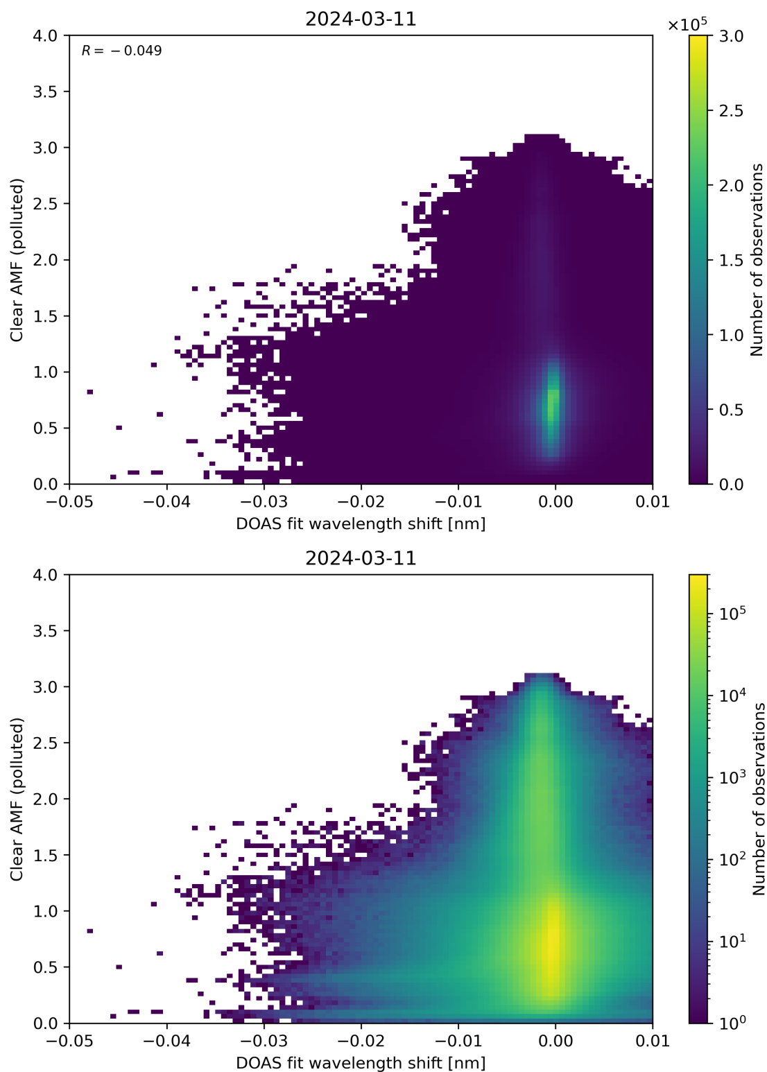
Figure 129: Scatter density plot of “DOAS fit wavelength shift” against “Clear AMF (polluted)” for 2024-03-10 to 2024-03-12.
