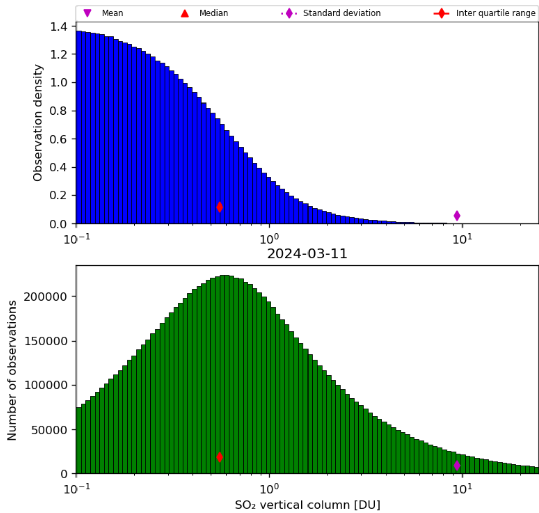
Figure 53: Histogram of “SO 2 vertical column” for 2024-03-10 to 2024-03-12
