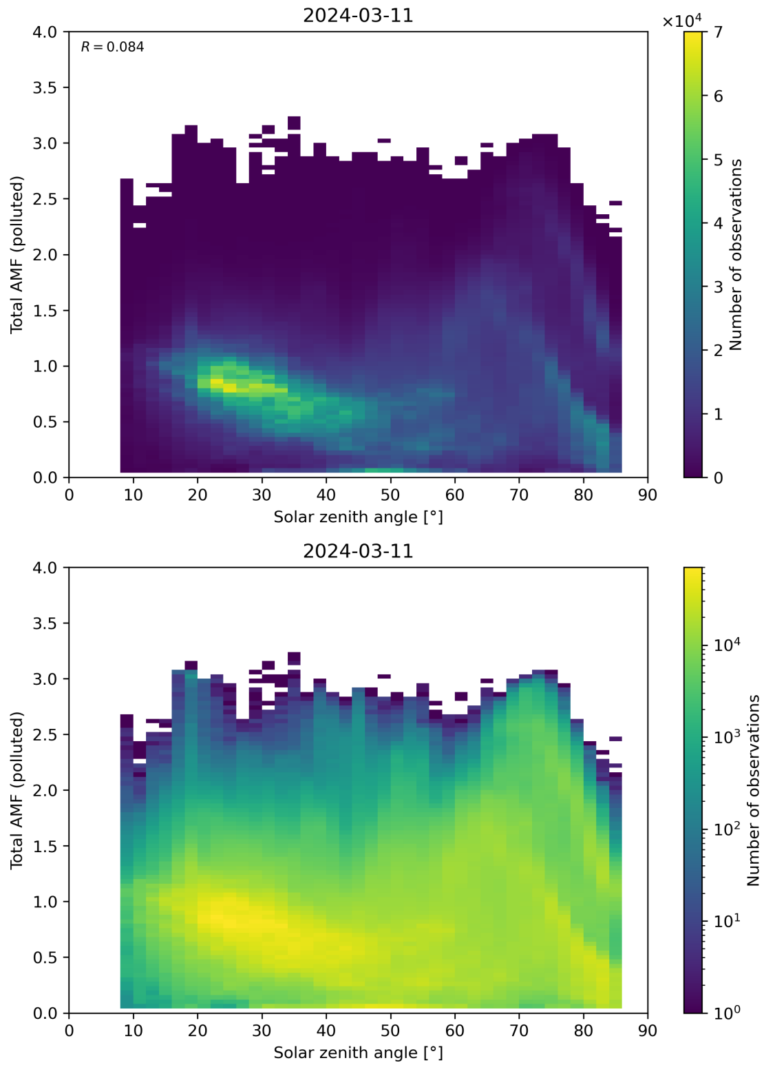
Figure 174: Scatter density plot of “Solar zenith angle” against “Total AMF (polluted)” for 2024-03-10 to 2024-03-12.
