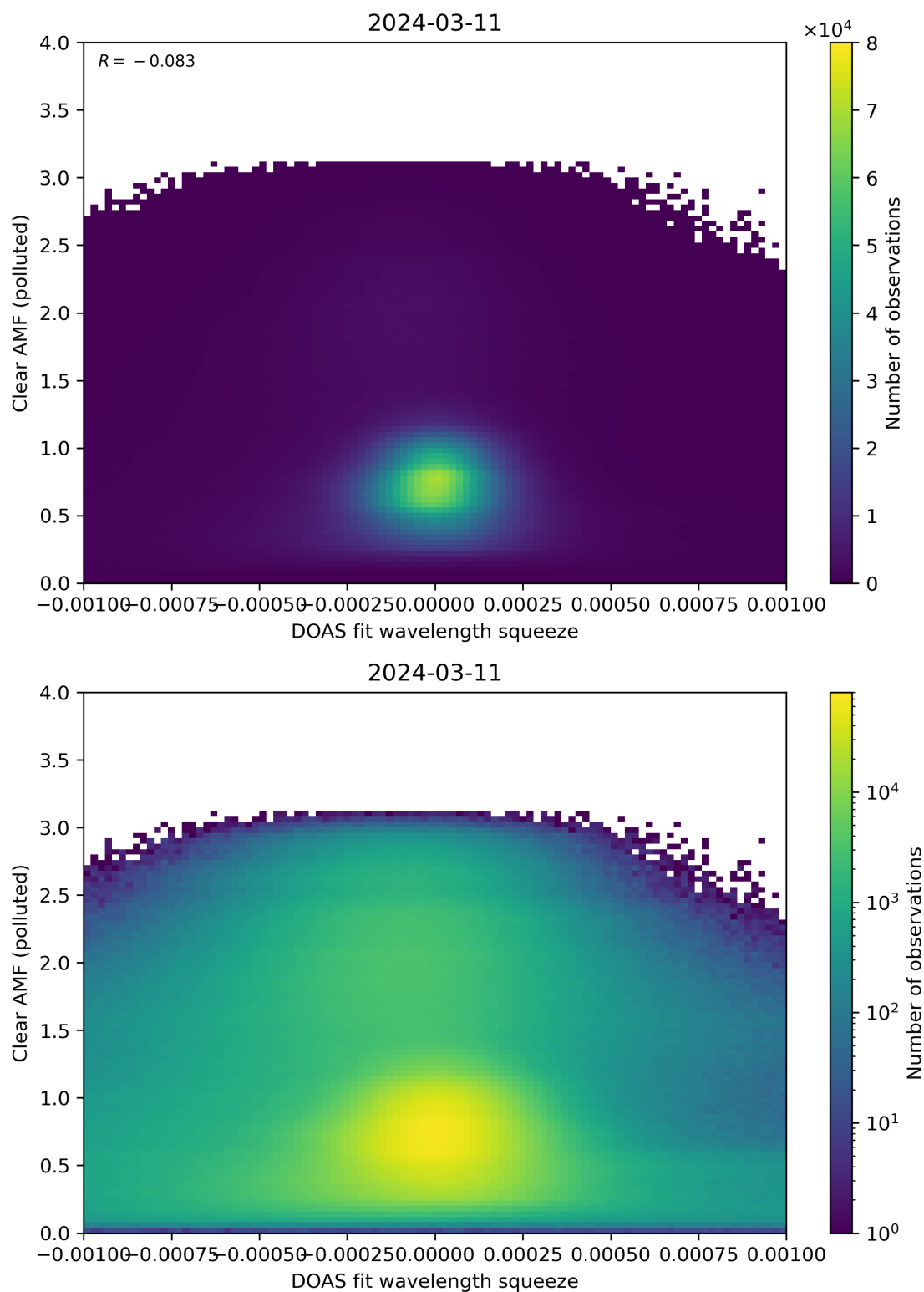
Figure 133: Scatter density plot of “DOAS fit wavelength squeeze” against “Clear AMF (polluted)” for 2024-03-10 to 2024-03-12.
