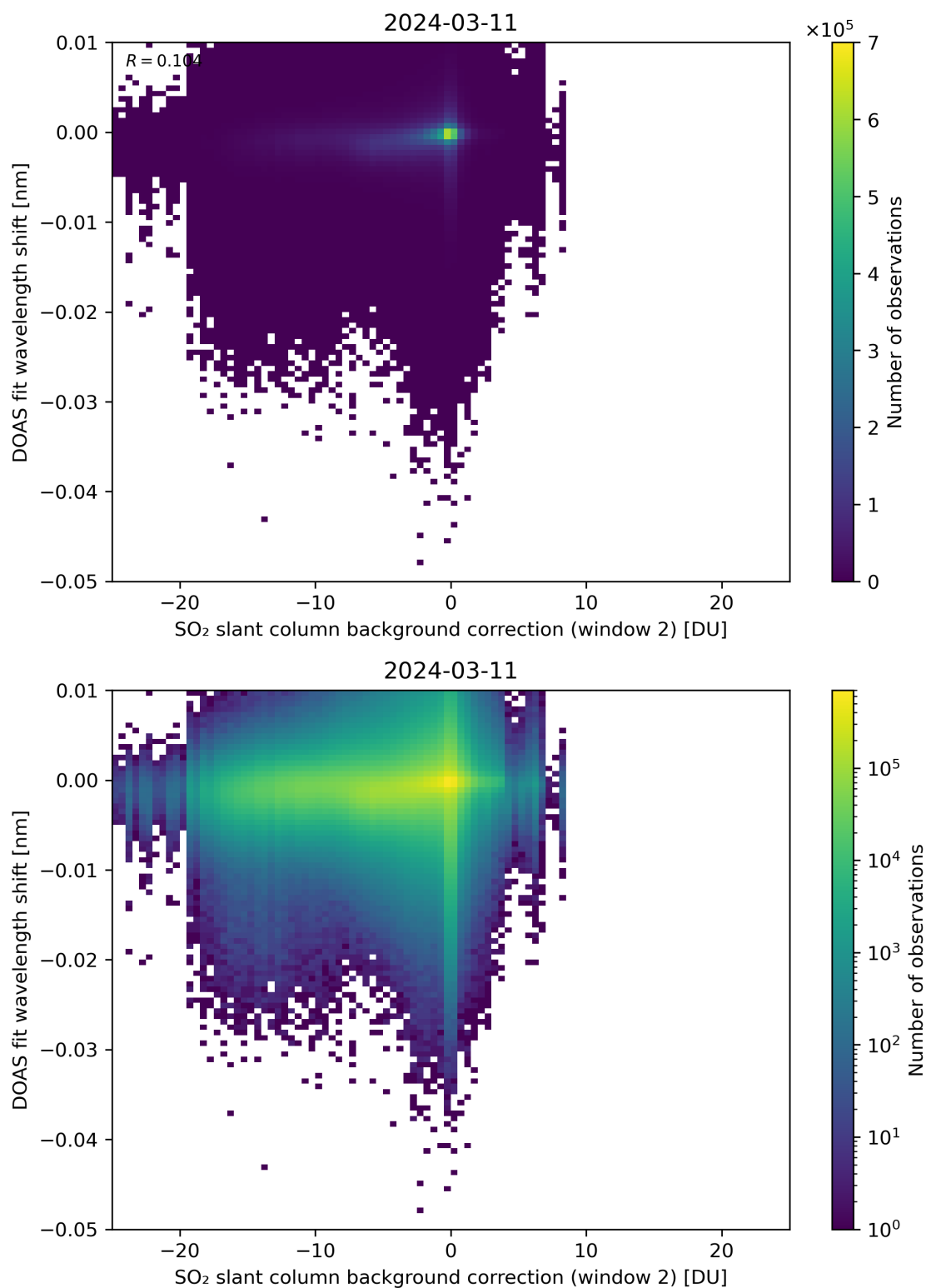
Figure 112: Scatter density plot of “SO 2 slant column background correction (window 2)” against “DOAS fit wavelength shift” for 2024-03-10 to 2024-03-12.
