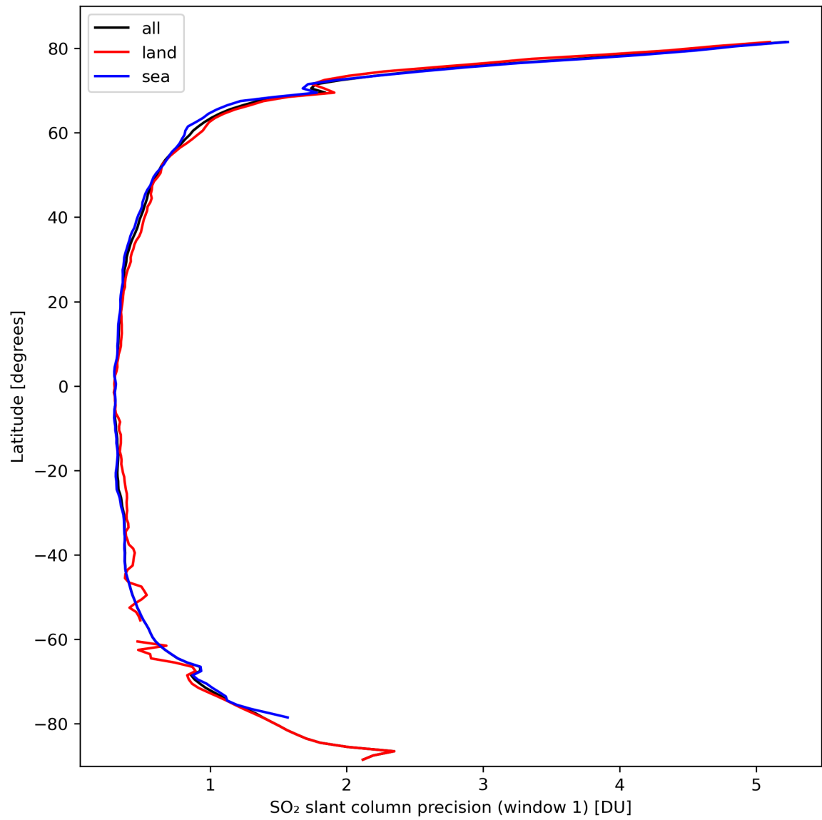
Figure 34: Zonal average of “SO 2 slant column precision (window 1)” for 2024-03-10 to 2024-03-12.
