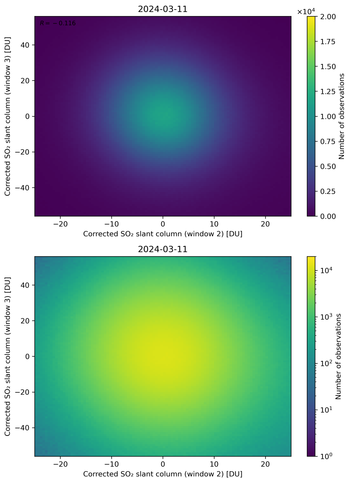
Figure 200: Scatter density plot of “Corrected SO 2 slant column (window 2)” against “Corrected SO 2 slant column (window 3)” for 2024-03-10 to 2024-03-12.
