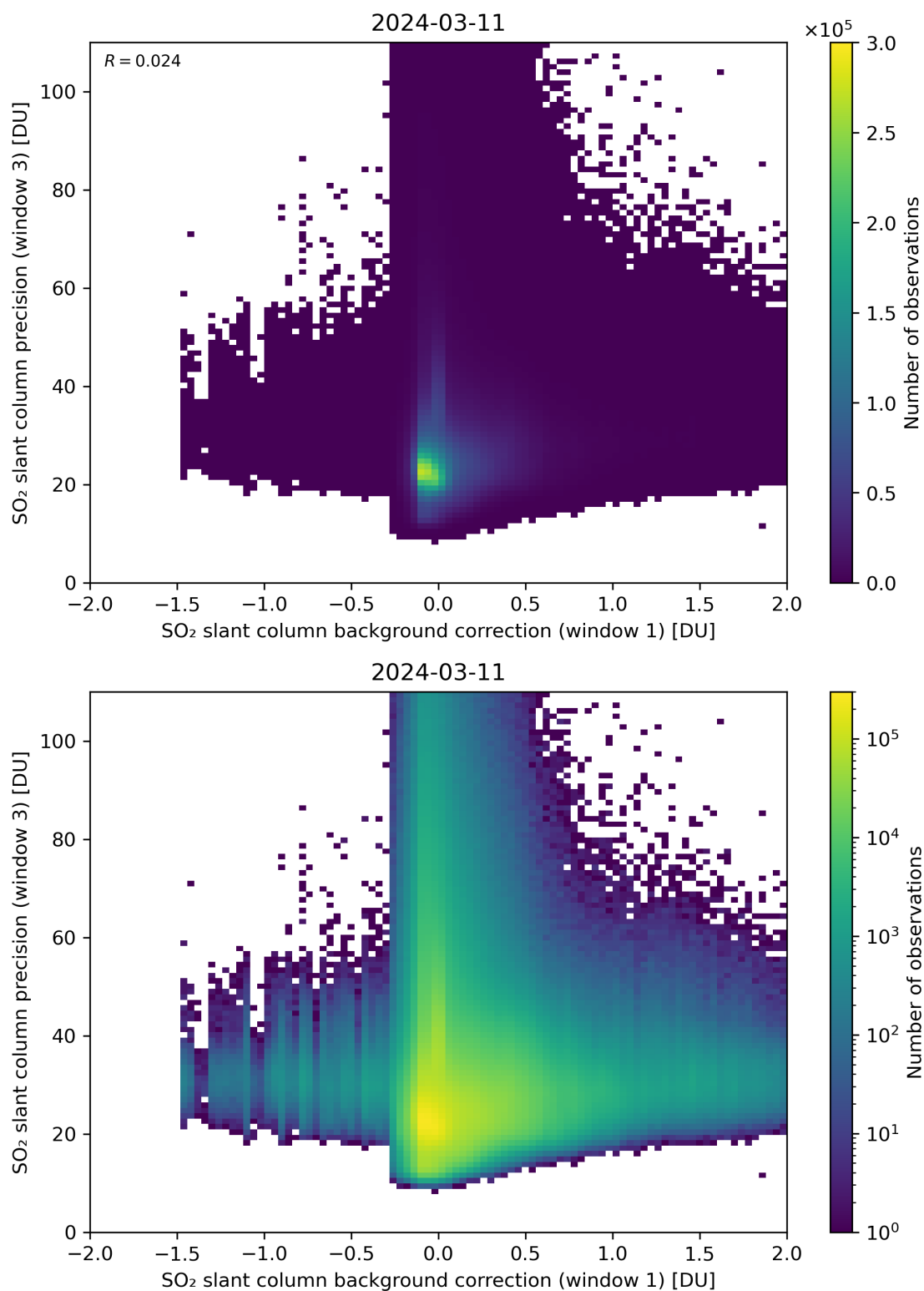
Figure 108: Scatter density plot of “SO 2 slant column background correction (window 1)” against “SO 2 slant column precision (window 3)” for 2024-03-10 to 2024-03-12.
