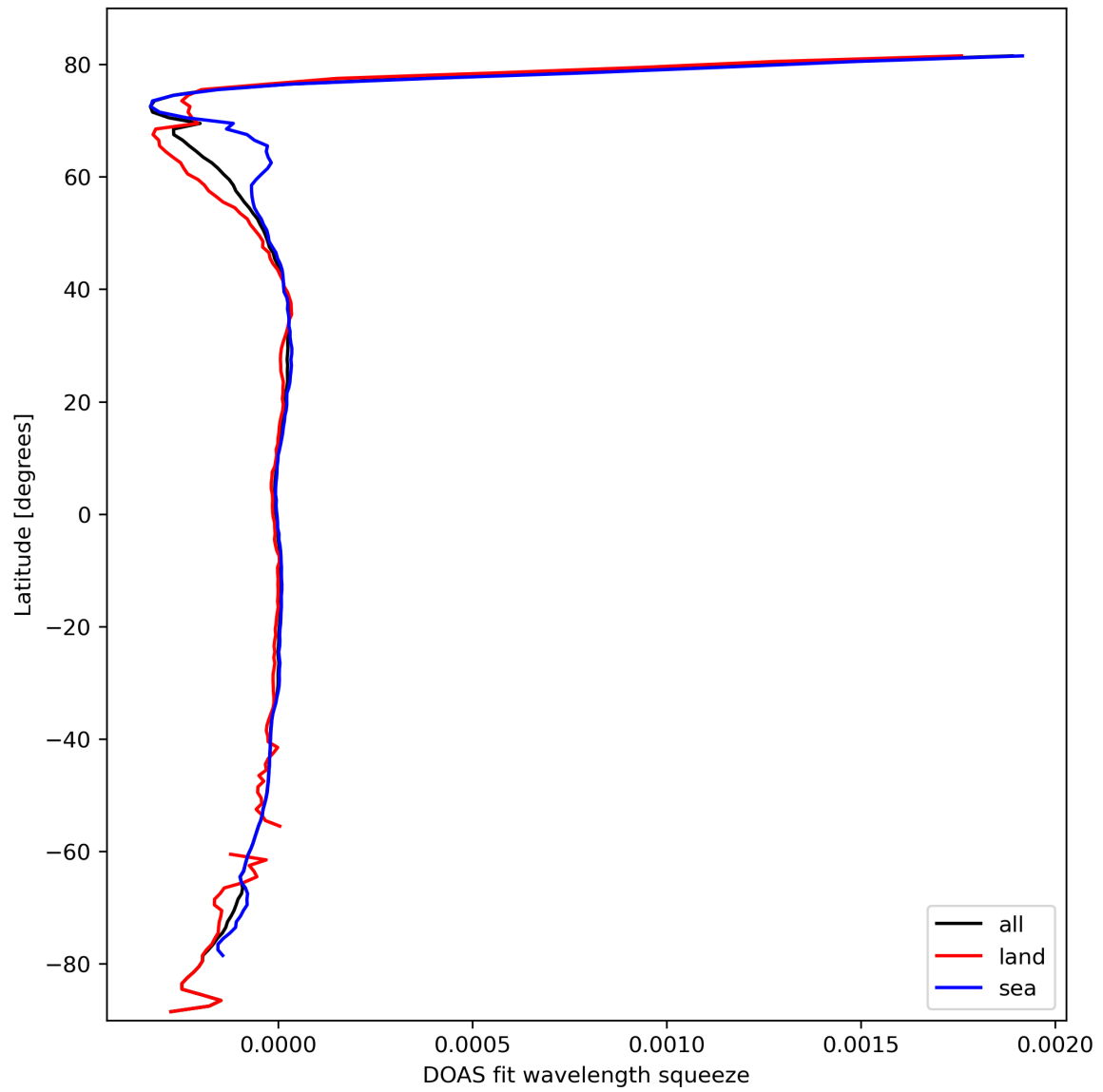
Figure 46: Zonal average of “DOAS fit wavelength squeeze” for 2024-03-10 to 2024-03-12.
