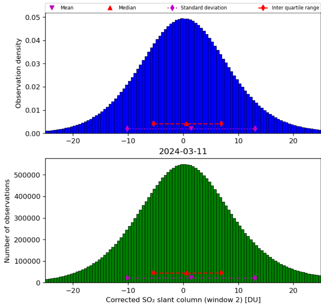
Figure 62: Histogram of “Corrected SO 2 slant column (window 2)” for 2024-03-10 to 2024-03-12
