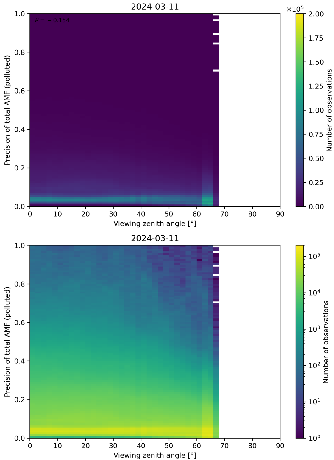
Figure 326: Scatter density plot of “Viewing zenith angle” against “Precision of total AMF (polluted)” for 2024-03-10 to 2024-03-12.
