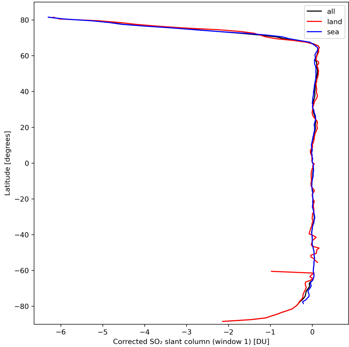
Figure 35: Zonal average of “Corrected SO 2 slant column (window 1)” for 2024-03-10 to 2024-03-12.
