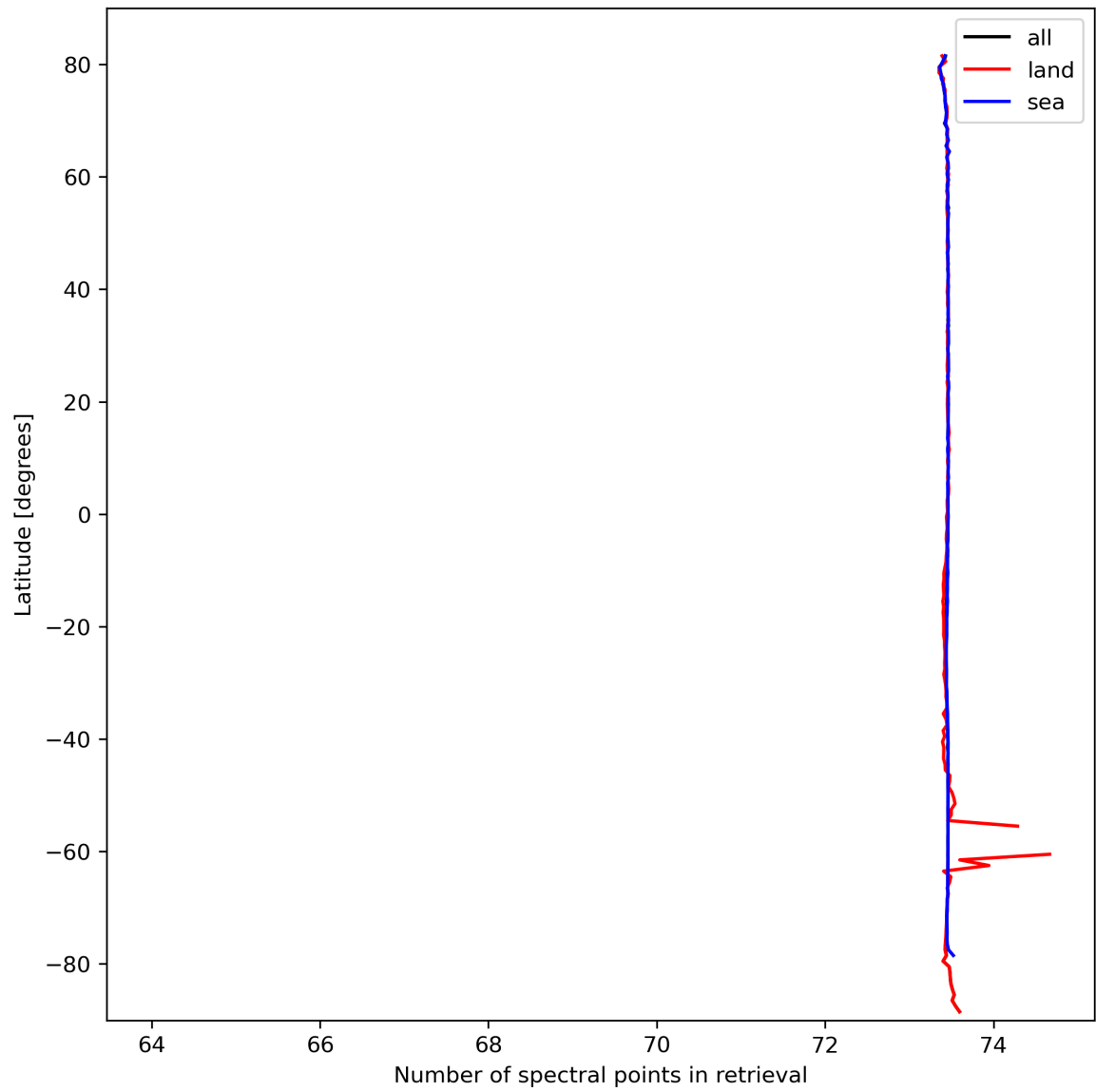
Figure 51: Zonal average of “Number of spectral points in retrieval” for 2024-03-10 to 2024-03-12.
