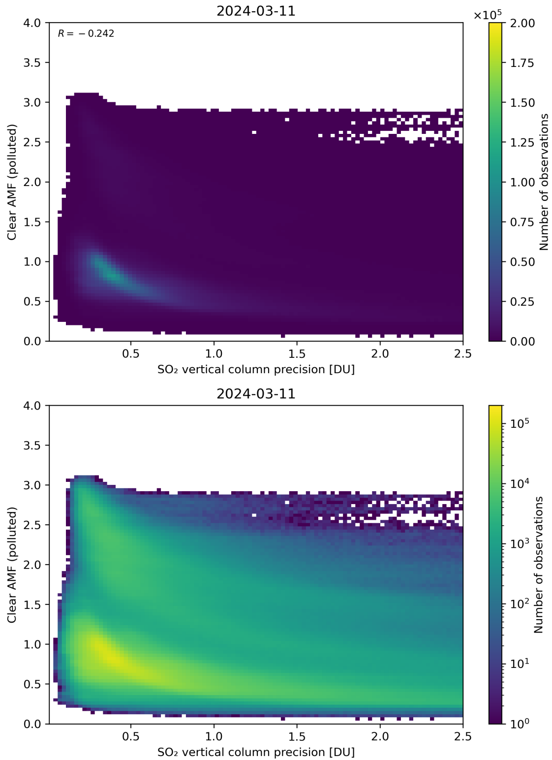
Figure 285: Scatter density plot of “SO 2 vertical column precision” against “Clear AMF (polluted)” for 2024-03-10 to 2024-03-12.
