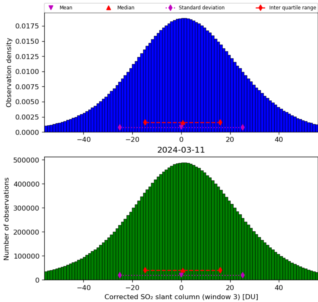
Figure 66: Histogram of "Corrected SO 2 slant column (window 3)" for 2024-03-10 to 2024-03-12
