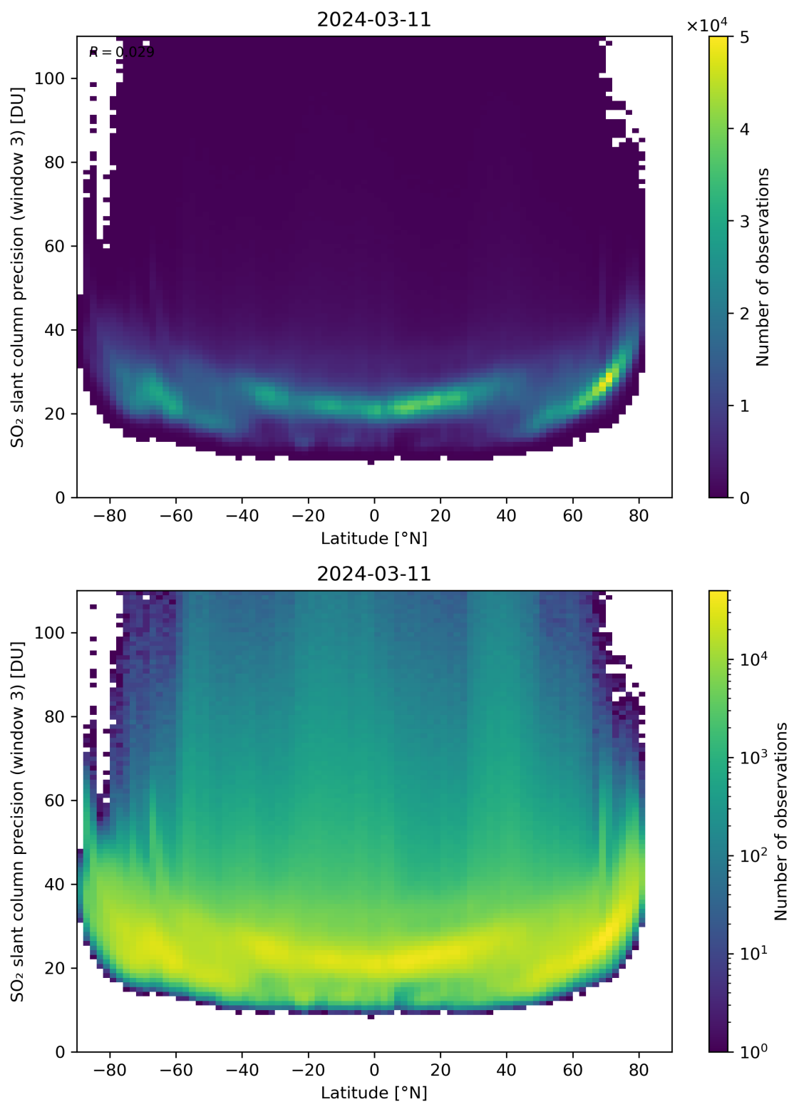
Figure 153: Scatter density plot of “Latitude” against “SO 2 slant column precision (window 3)” for 2024-03-10 to 2024-03-12.
