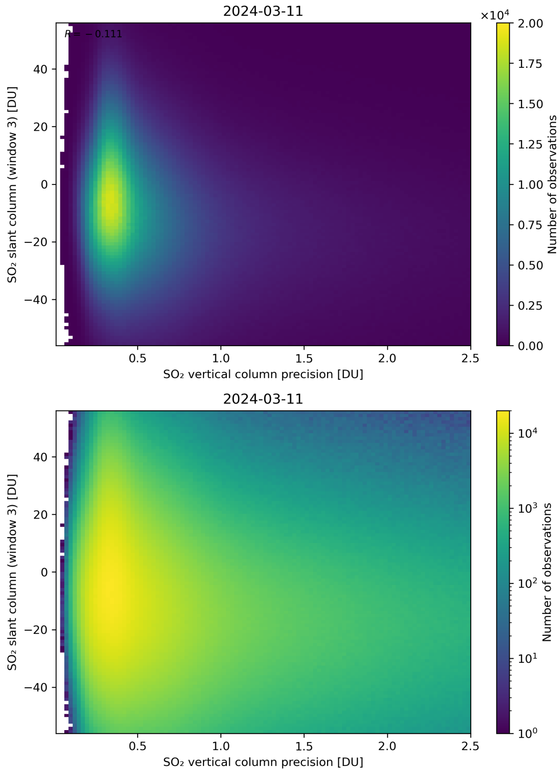
Figure 292: Scatter density plot of “SO 2 vertical column precision” against “SO 2 slant column (window 3)” for 2024-03-10 to 2024-03-12.
