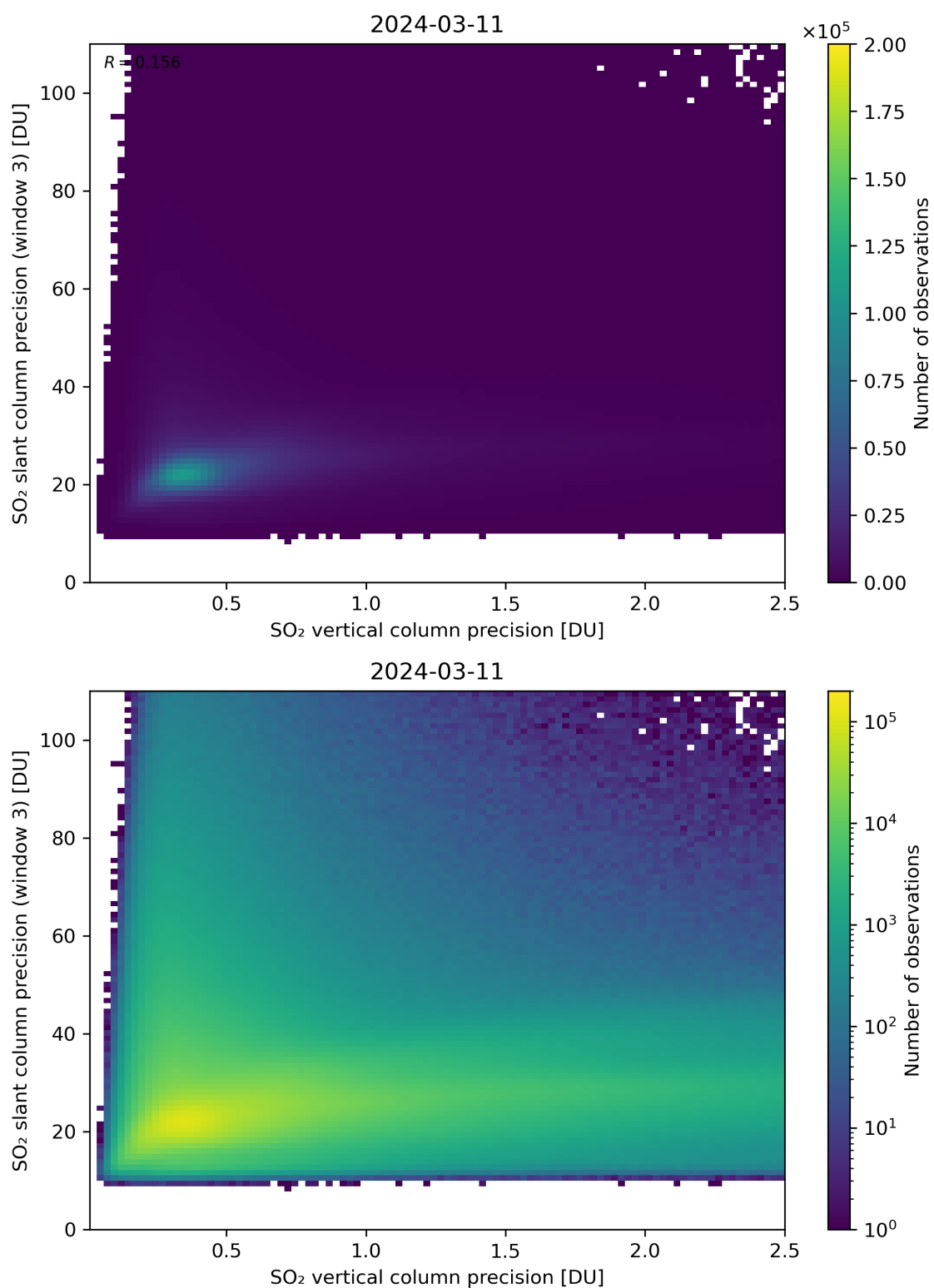
Figure 293: Scatter density plot of “SO 2 vertical column precision” against “SO 2 slant column precision (window 3)” for 2024-03-10 to 2024-03-12.
