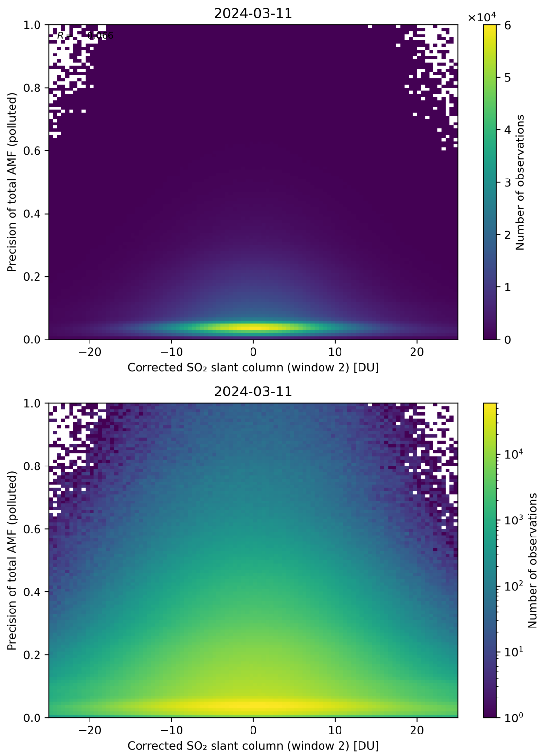
Figure 204: Scatter density plot of “Corrected SO 2 slant column (window 2)” against “Precision of total AMF (polluted)” for 2024-03-10 to 2024-03-12.
