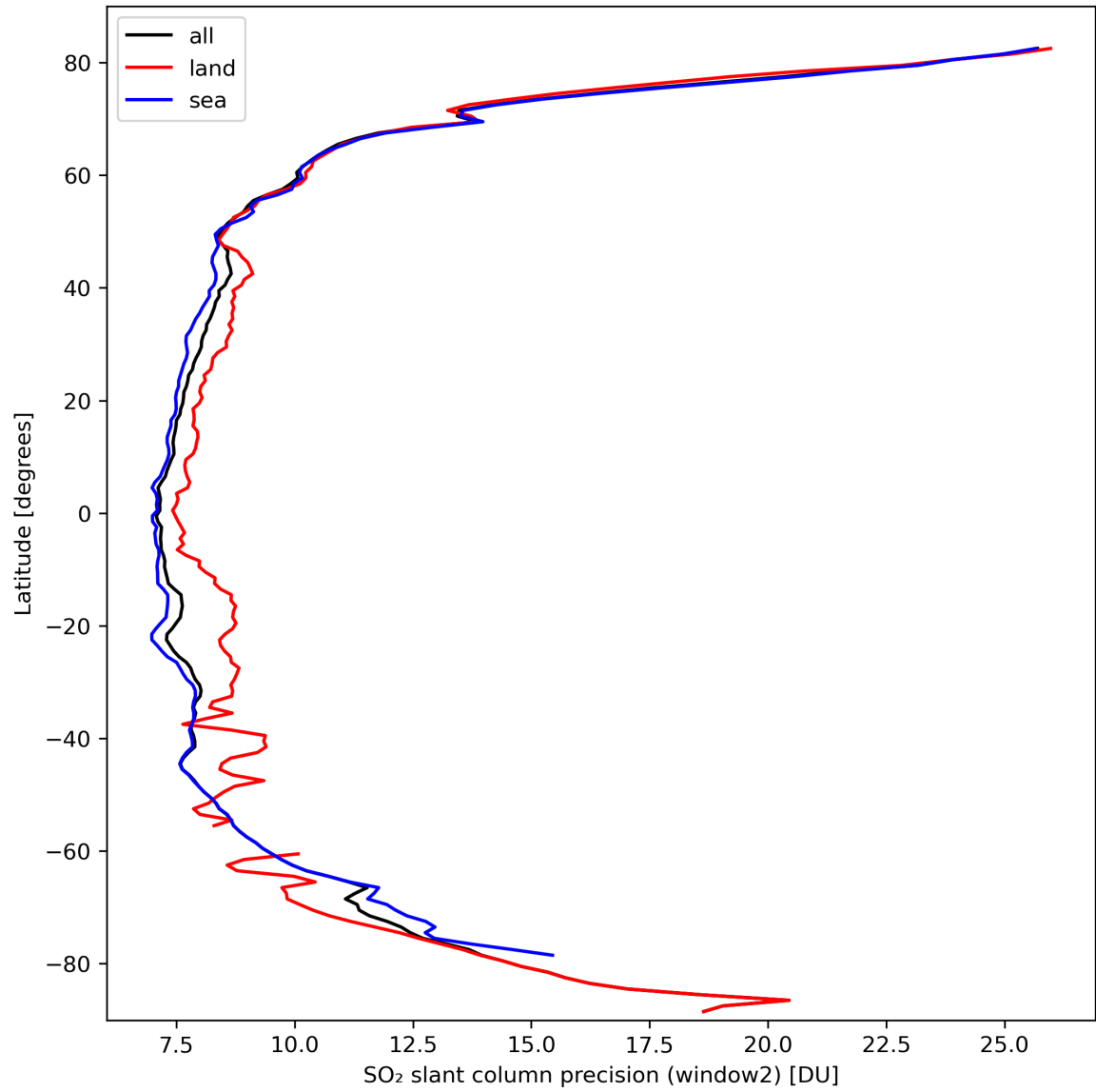
Figure 38: Zonal average of “SO 2 slant column precision (window2)” for 2024-03-11 to 2024-03-13.
