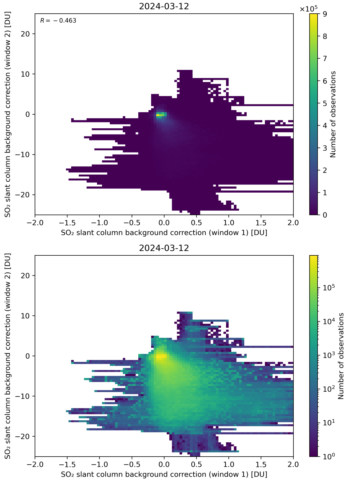
Figure 98: Scatter density plot of “SO 2 slant column background correction (window 1)” against “SO 2 slant column background correction (window 2)” for 2024-03-11 to 2024-03-13.
