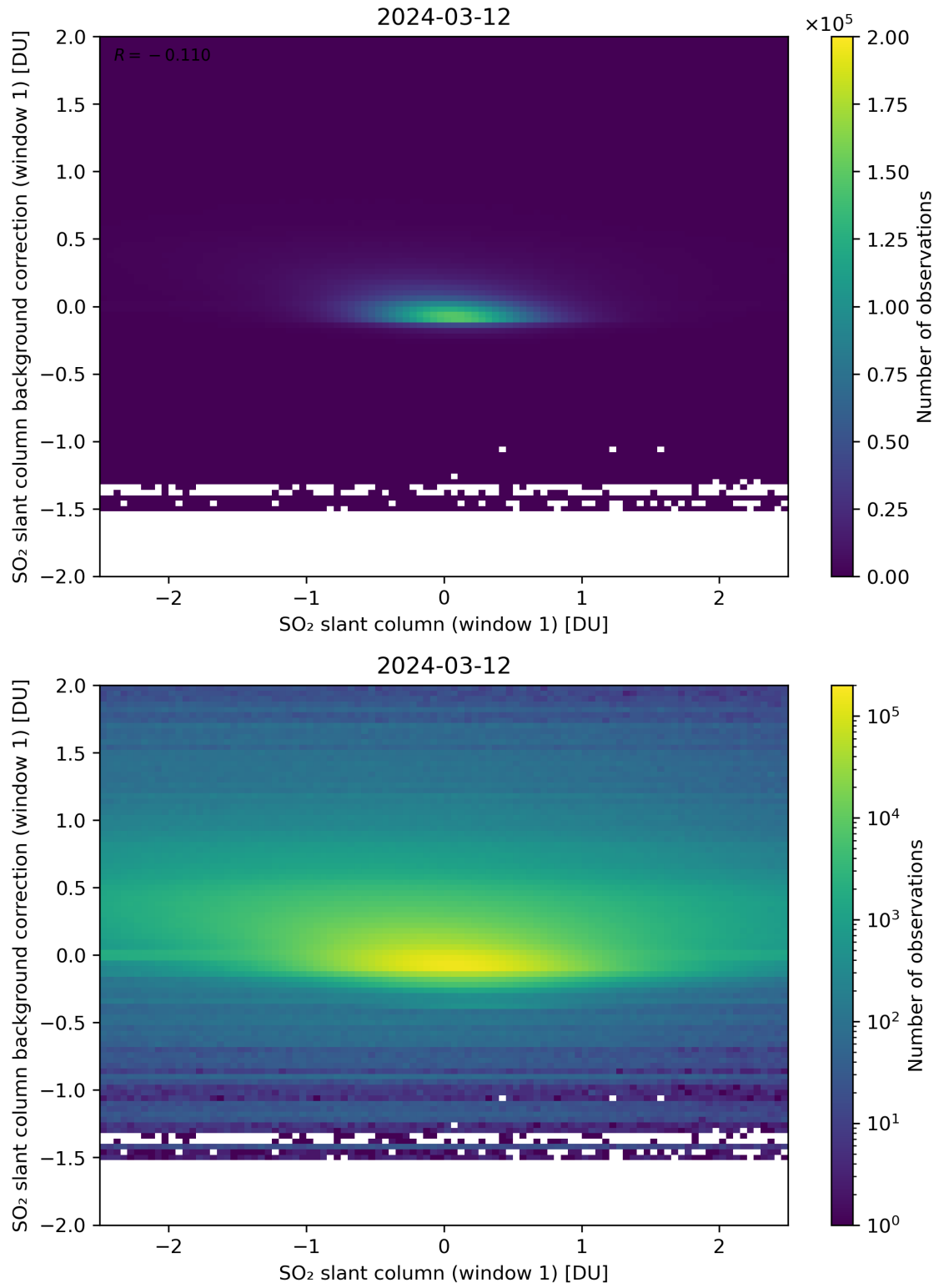
Figure 212: Scatter density plot of “SO 2 slant column (window 1)” against “SO 2 slant column background correction (window 1)” for 2024-03-11 to 2024-03-13.
