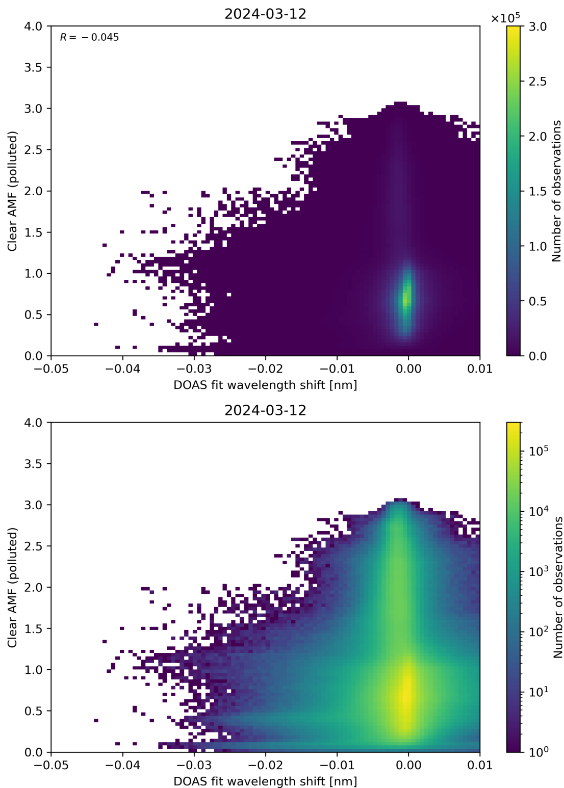
Figure 129: Scatter density plot of “DOAS fit wavelength shift” against “Clear AMF (polluted)” for 2024-03-11 to 2024-03-13.
