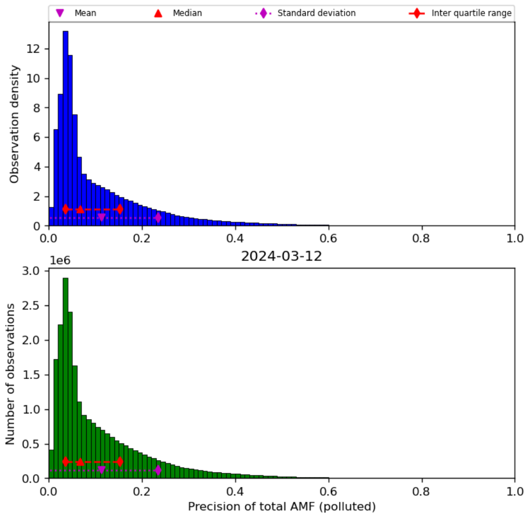
Figure 72: Histogram of “Precision of total AMF (polluted)” for 2024-03-11 to 2024-03-13
