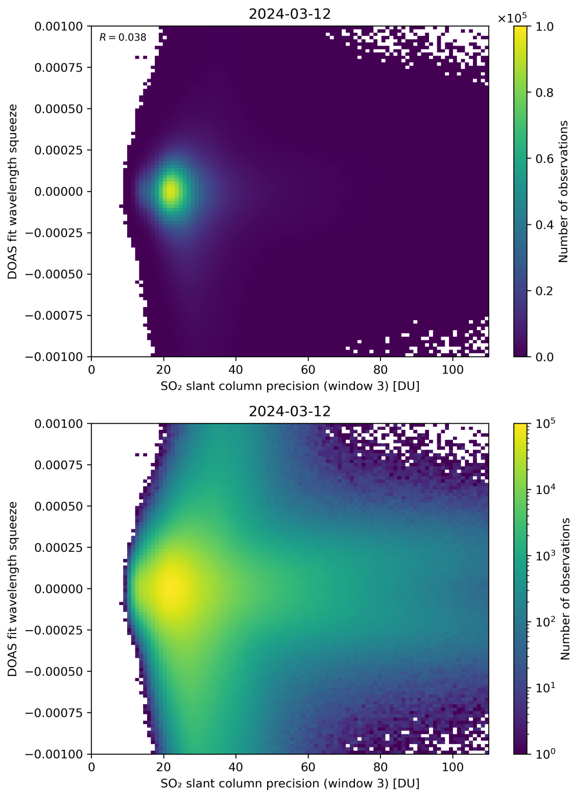
Figure 259: Scatter density plot of “SO 2 slant column precision (window 3)” against “DOAS fit wavelength squeeze” for 2024-03-11 to 2024-03-13.
