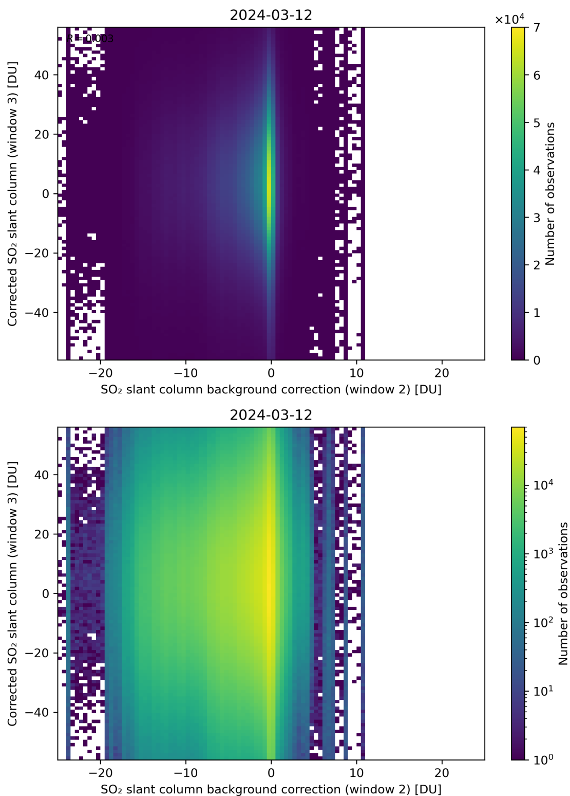
Figure 116: Scatter density plot of “SO 2 slant column background correction (window 2)” against “Corrected SO 2 slant column (window 3)” for 2024-03-11 to 2024-03-13.
