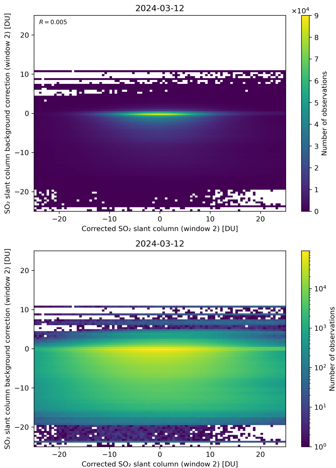
Figure 194: Scatter density plot of “Corrected SO 2 slant column (window 2)” against “SO 2 slant column background correction (window 2)” for 2024-03-11 to 2024-03-13.
