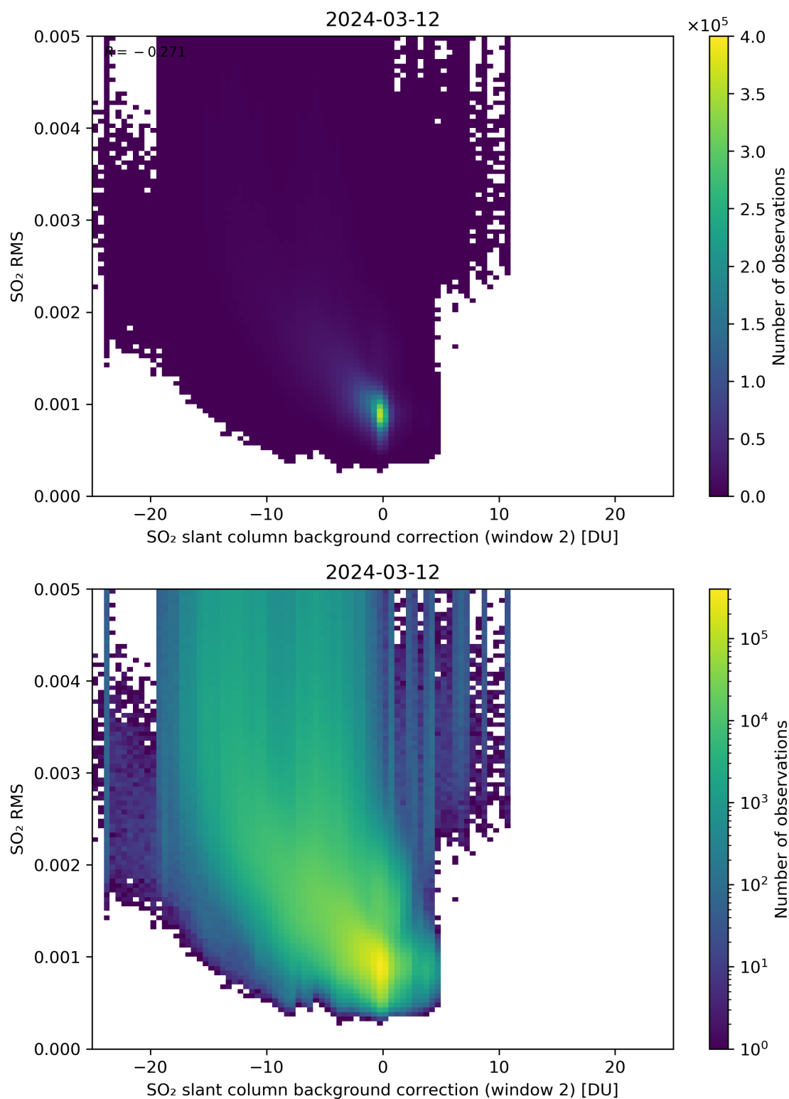
Figure 114: Scatter density plot of “SO 2 slant column background correction (window 2)” against “SO 2 RMS” for 2024-03-11 to 2024-03-13.
