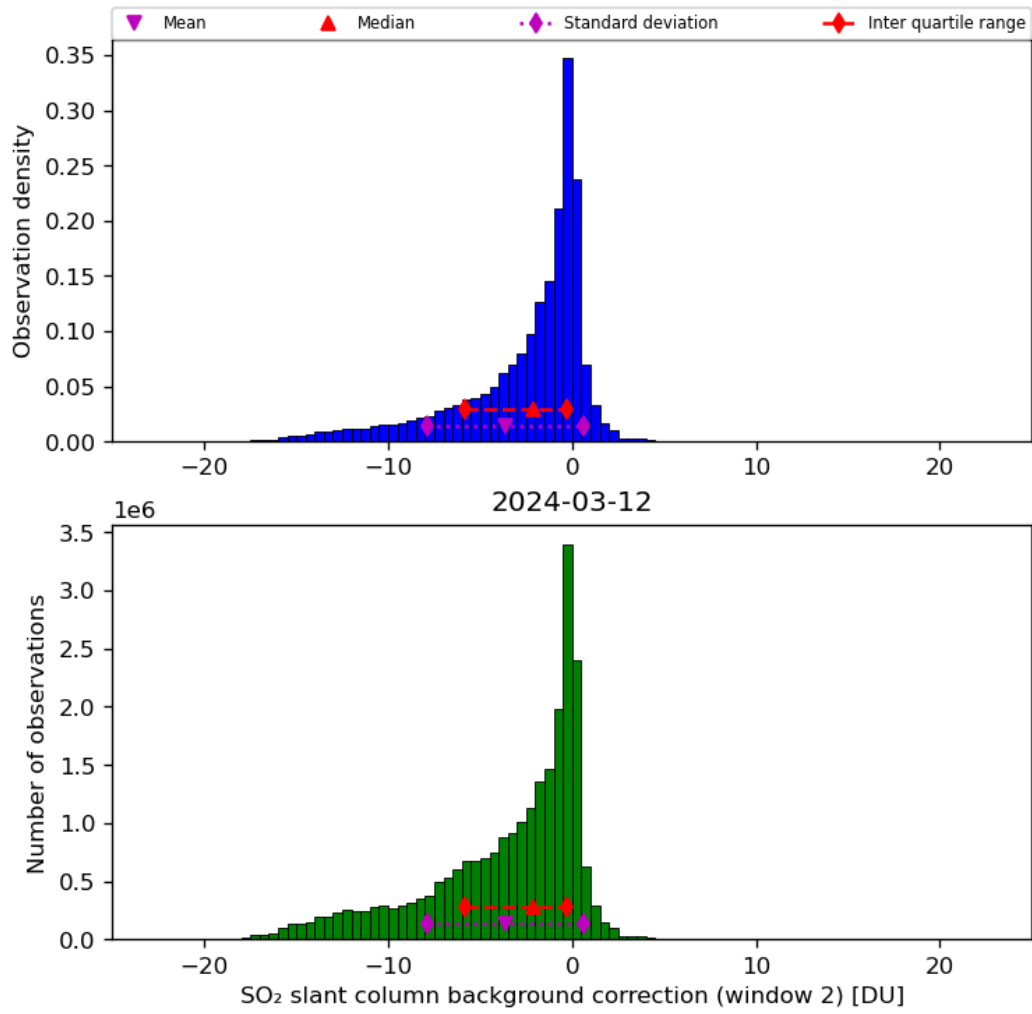
Figure 63: Histogram of “SO 2 slant column background correction (window 2)” for 2024-03-11 to 2024-03-13
