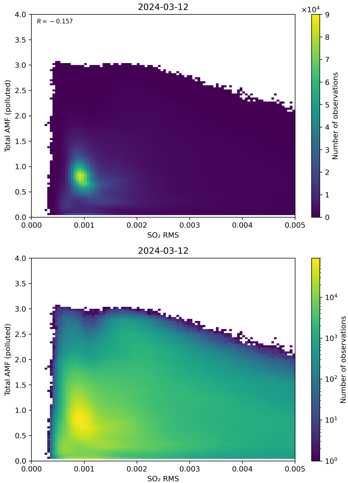
Figure 137: Scatter density plot of “SO 2 RMS” against “Total AMF (polluted)” for 2024-03-11 to 2024-03-13.
