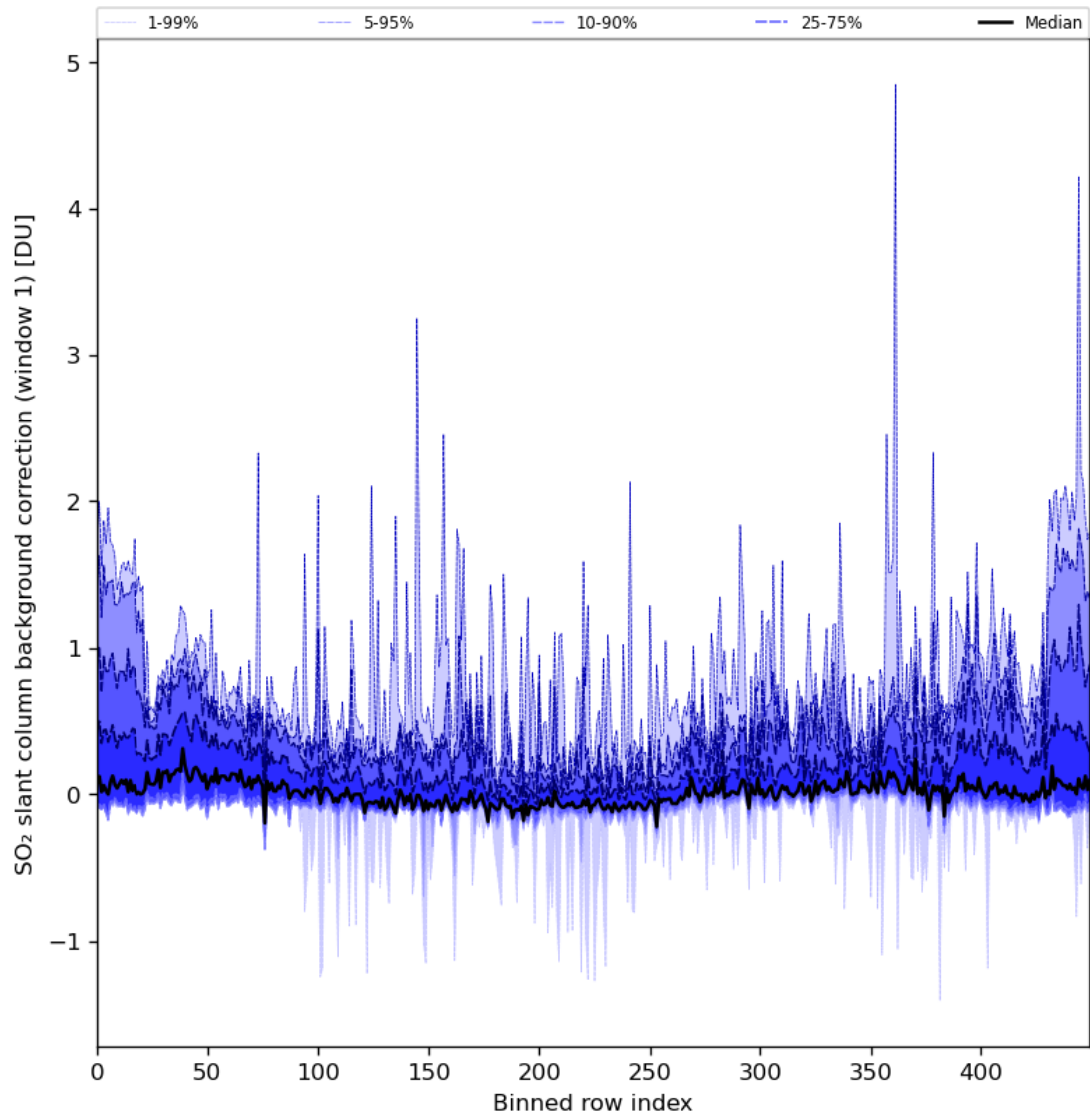
Figure 82: Along track statistics of “SO 2 slant column background correction (window 1)” for 2024-03-11 to 2024-03-13
