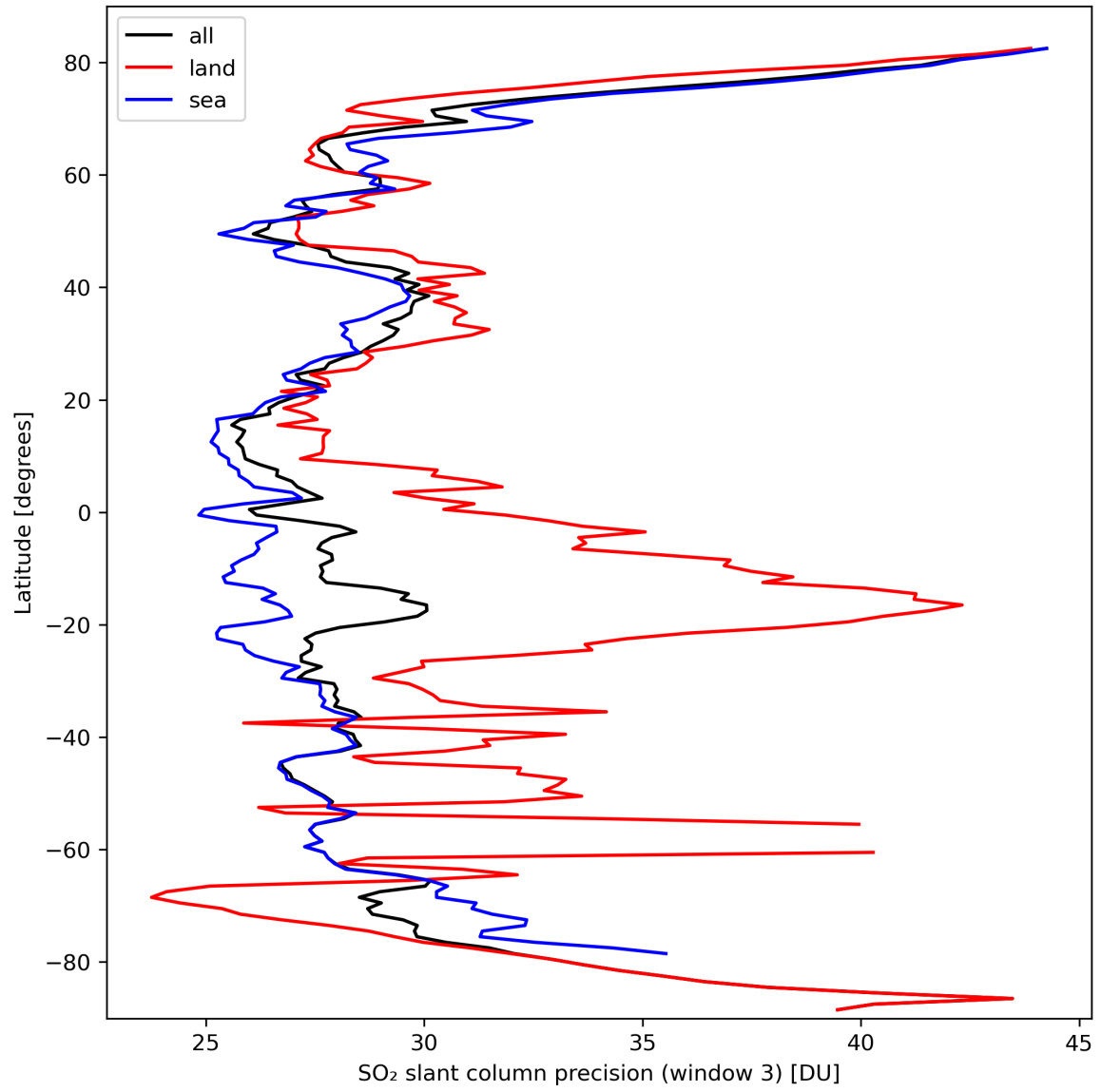
Figure 42: Zonal average of “SO 2 slant column precision (window 3)” for 2024-03-11 to 2024-03-13.
