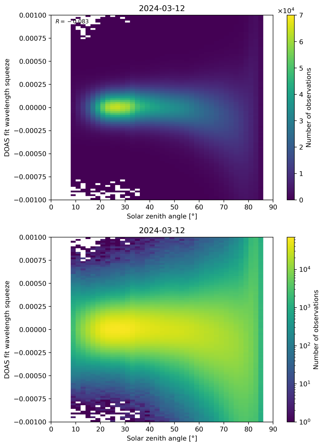
Figure 162: Scatter density plot of “Solar zenith angle” against “DOAS fit wavelength squeeze” for 2024-03-11 to 2024-03-13.
