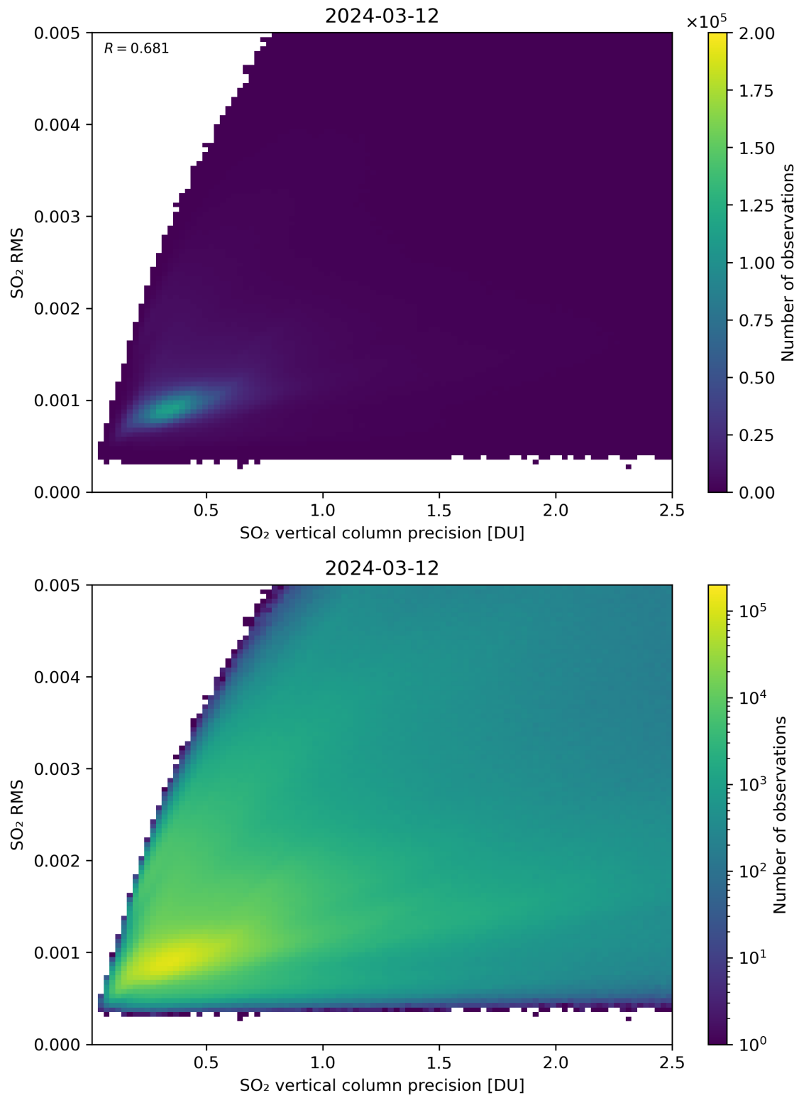
Figure 284: Scatter density plot of “SO 2 vertical column precision” against “SO 2 RMS” for 2024-03-11 to 2024-03-13.
