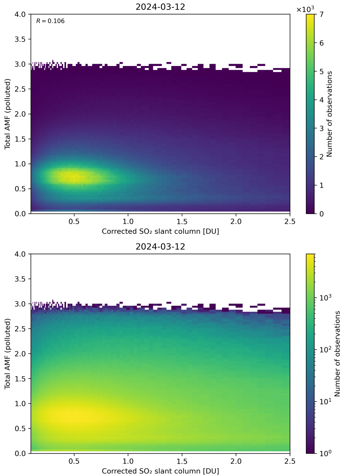
Figure 192: Scatter density plot of “Corrected SO 2 slant column” against “Total AMF (polluted)” for 2024-03-11 to 2024-03-13.
