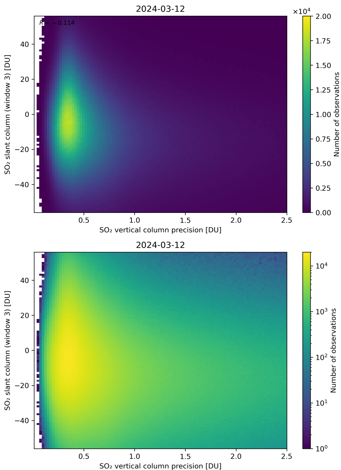
Figure 292: Scatter density plot of “SO 2 vertical column precision” against “SO 2 slant column (window 3)” for 2024-03-11 to 2024-03-13.
