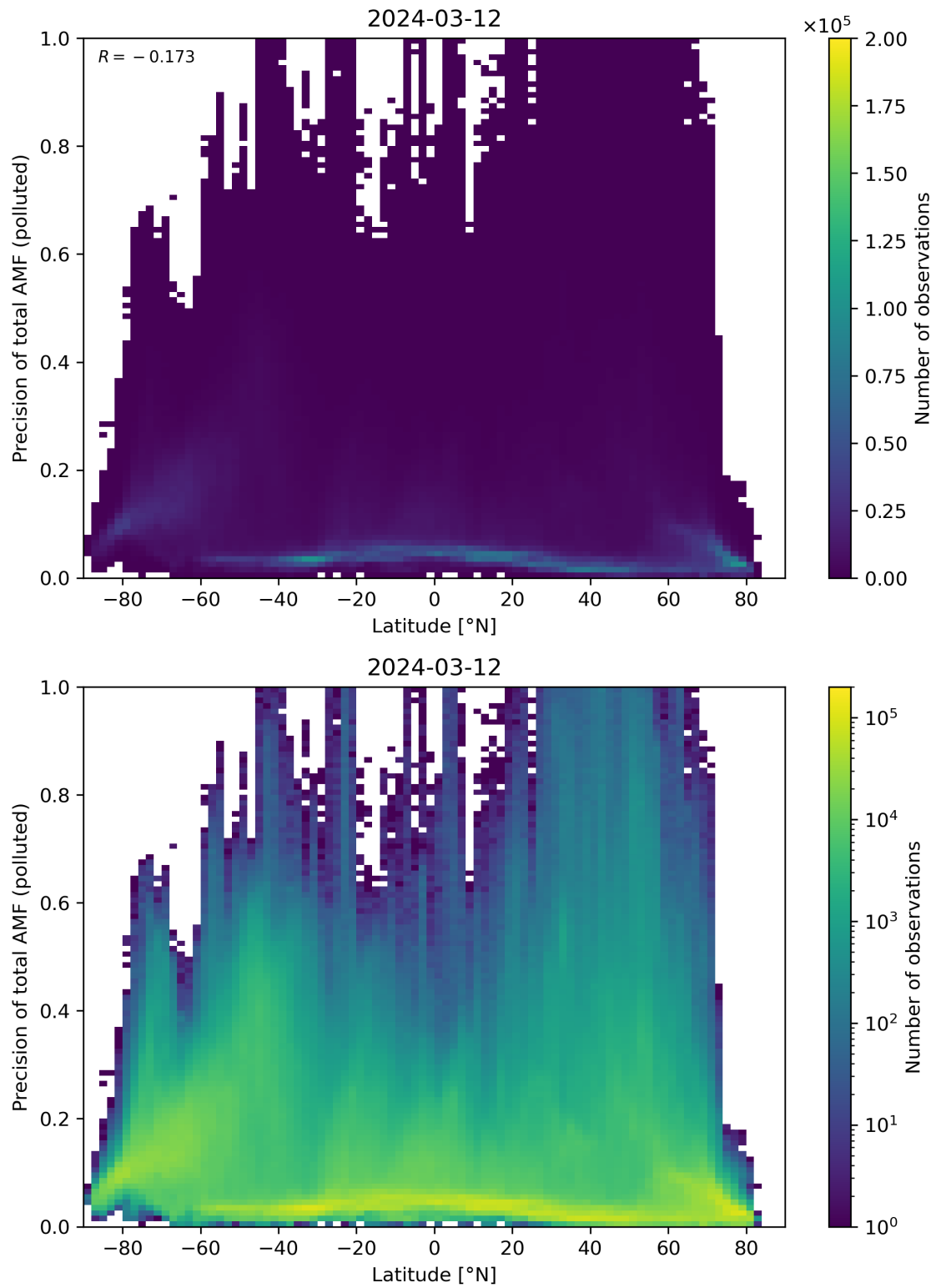
Figure 155: Scatter density plot of “Latitude” against “Precision of total AMF (polluted)” for 2024-03-11 to 2024-03-13.
