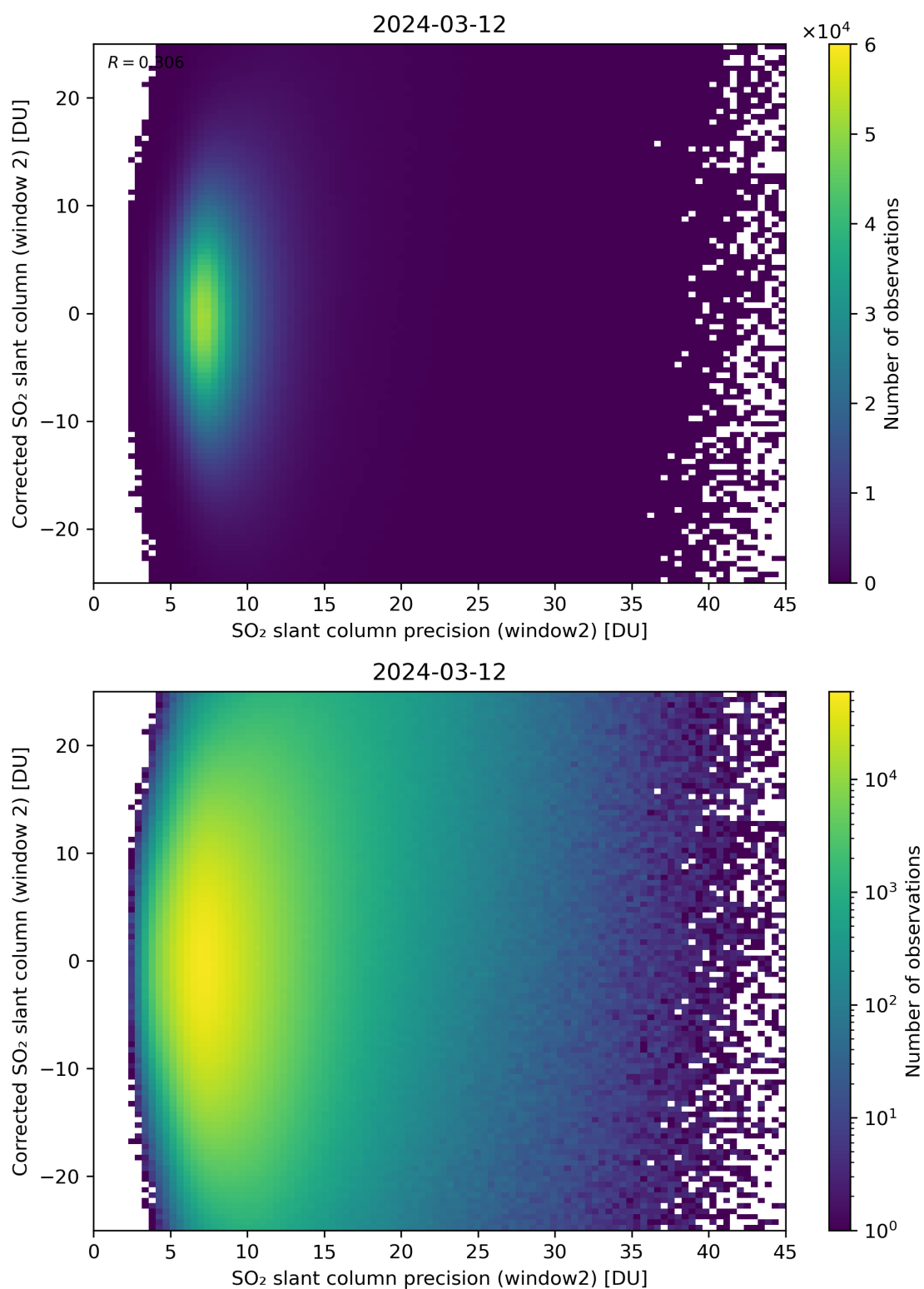
Figure 247: Scatter density plot of “SO 2 slant column precision (window2)” against “Corrected SO 2 slant column (window 2)” for 2024-03-11 to 2024-03-13.
