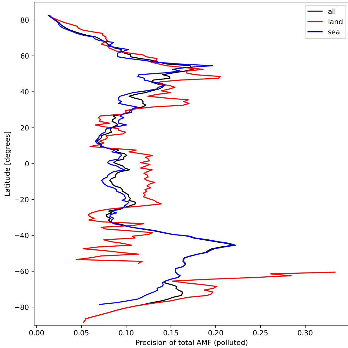
Figure 49: Zonal average of “Precision of total AMF (polluted)” for 2024-03-11 to 2024-03-13.
