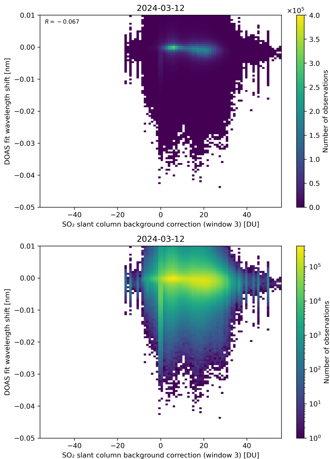
Figure 121: Scatter density plot of “SO 2 slant column background correction (window 3)” against “DOAS fit wavelength shift” for 2024-03-11 to 2024-03-13.
