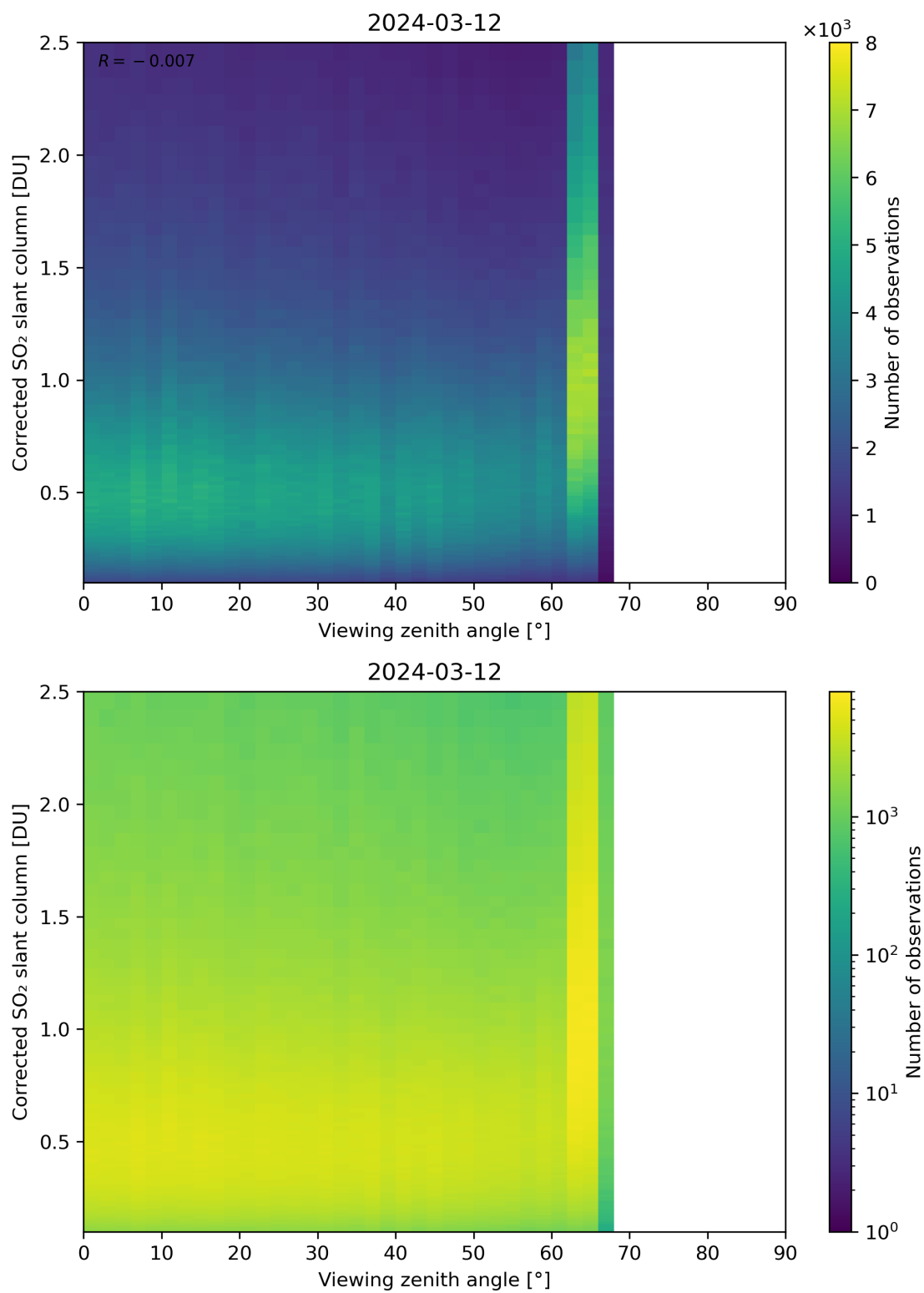
Figure 317: Scatter density plot of “Viewing zenith angle” against “Corrected SO 2 slant column” for 2024-03-11 to 2024-03-13.
