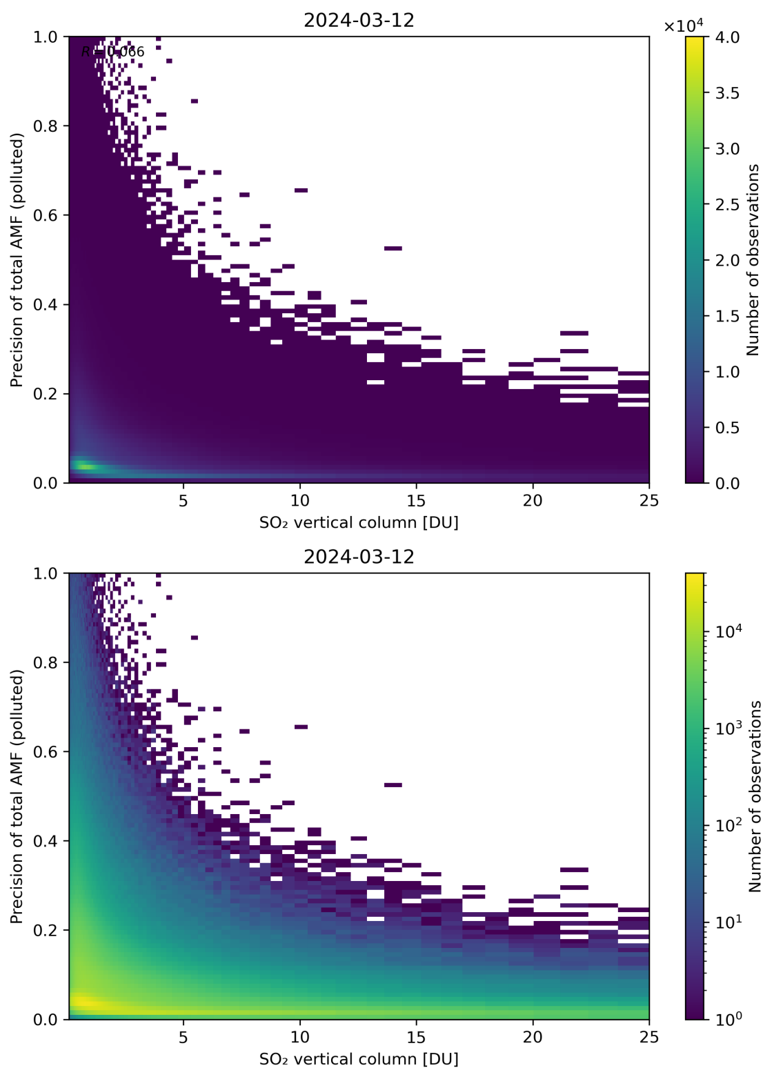
Figure 306: Scatter density plot of “SO 2 vertical column” against “Precision of total AMF (polluted)” for 2024-03-11 to 2024-03-13.
