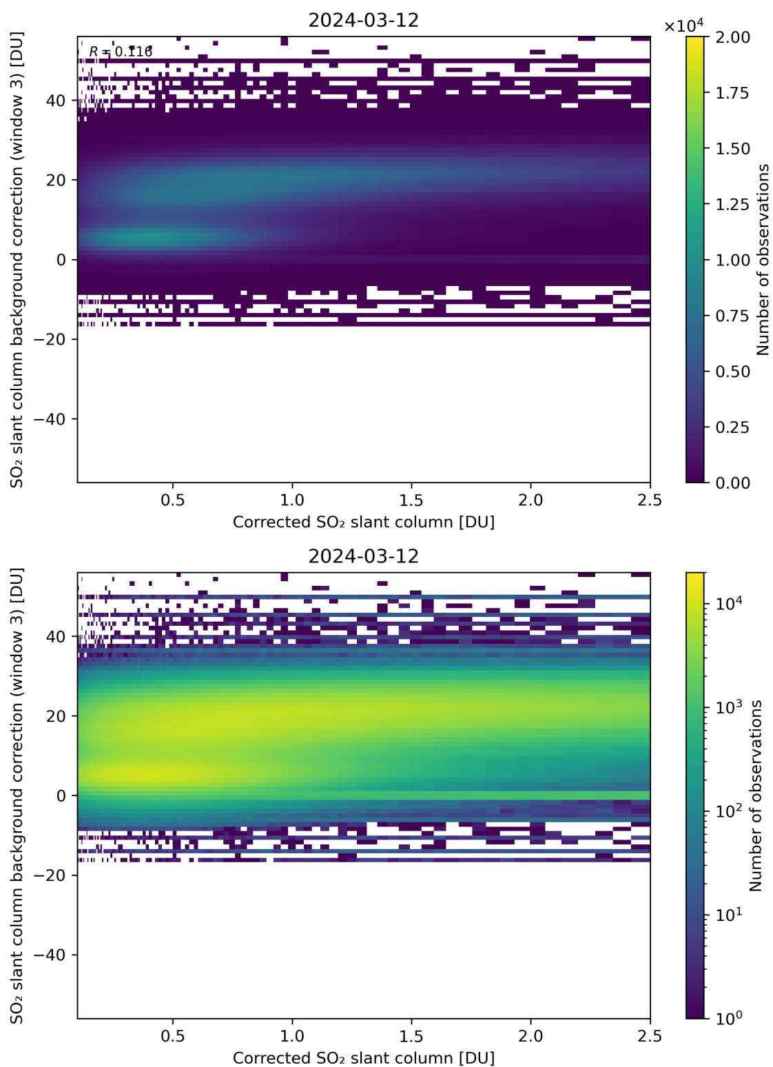
Figure 180: Scatter density plot of “Corrected SO 2 slant column” against “SO 2 slant column background correction (window 3)” for 2024-03-11 to 2024-03-13.
