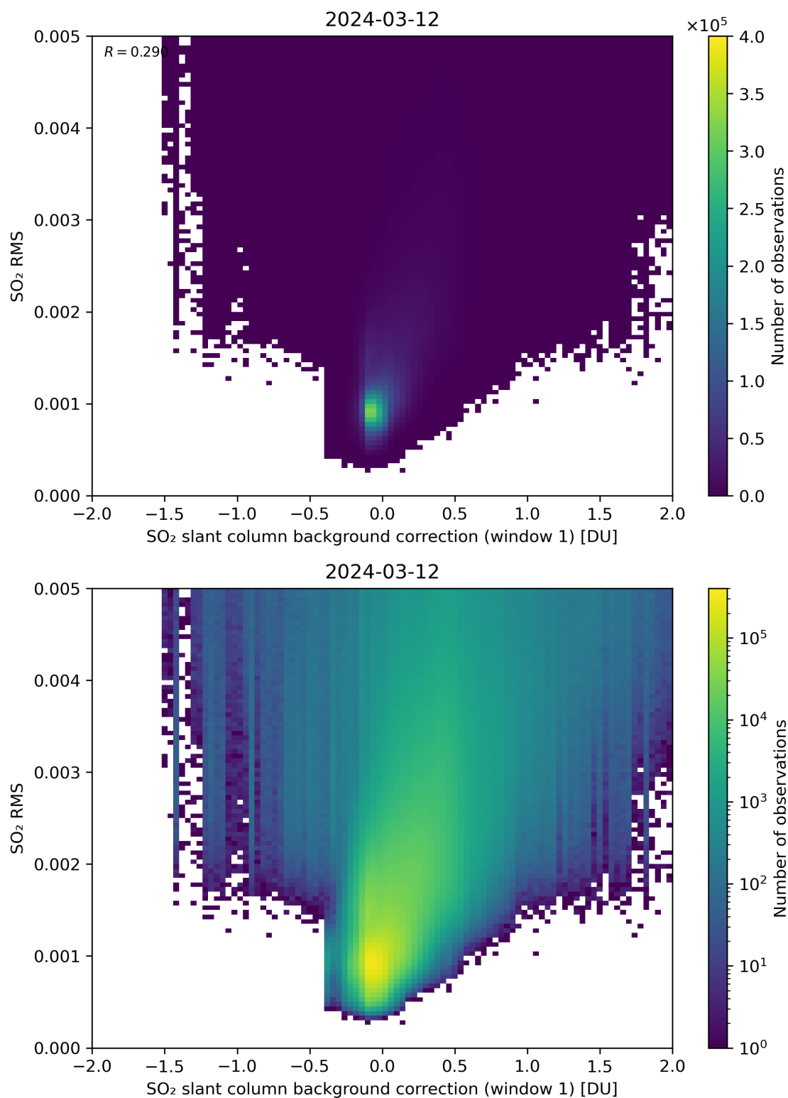
Figure 102: Scatter density plot of “SO 2 slant column background correction (window 1)” against “SO 2 RMS” for 2024-03-11 to 2024-03-13.
