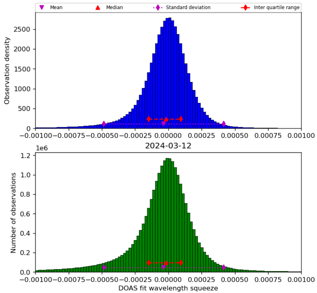
Figure 69: Histogram of “DOAS fit wavelength squeeze” for 2024-03-11 to 2024-03-13
