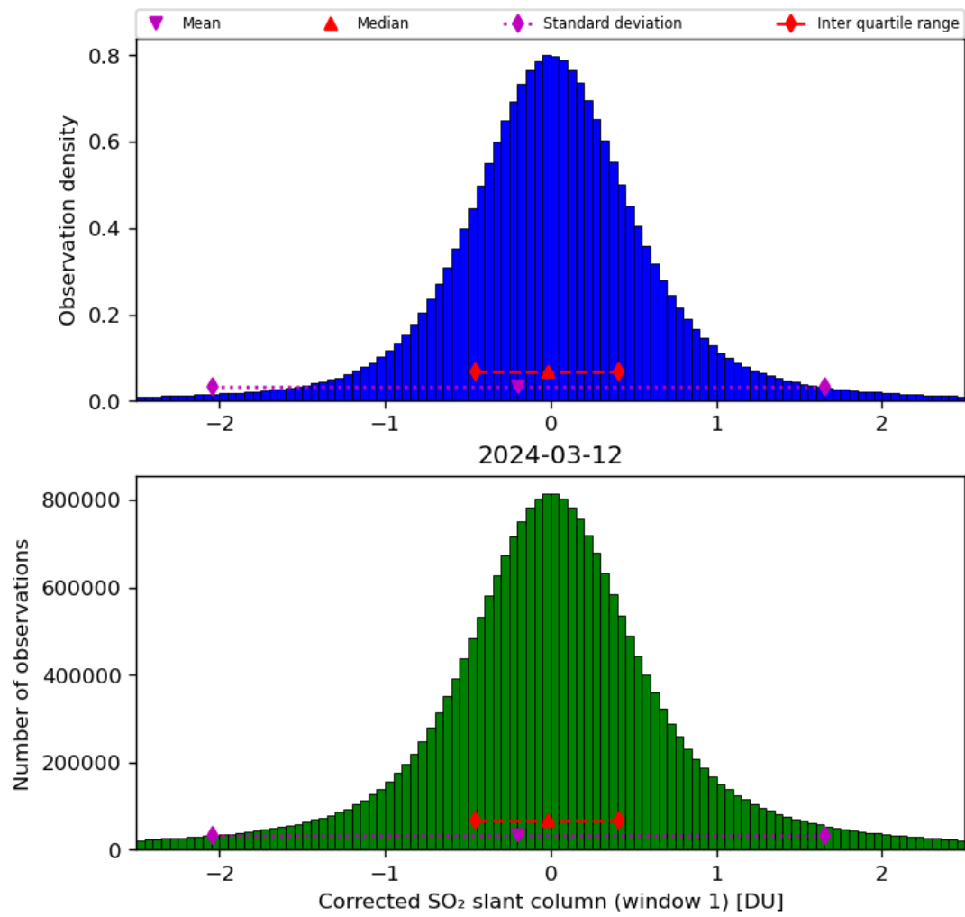
Figure 58: Histogram of “Corrected SO 2 slant column (window 1)” for 2024-03-11 to 2024-03-13
