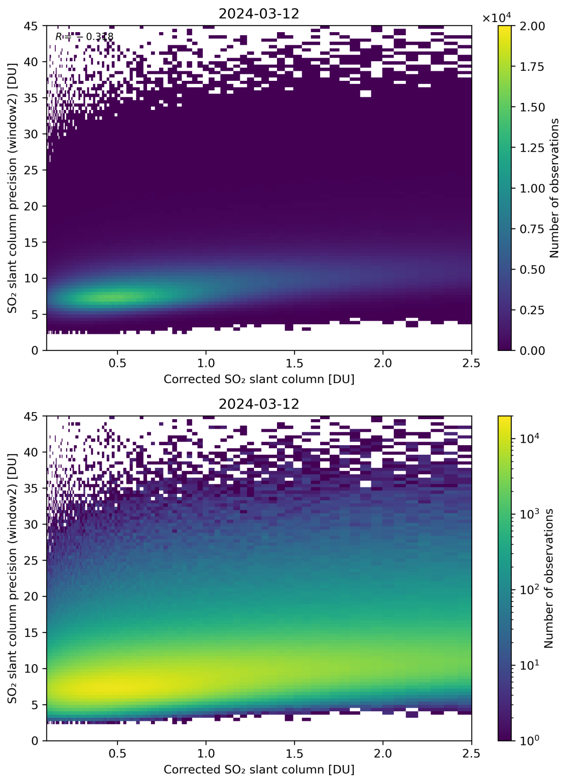
Figure 189: Scatter density plot of “Corrected SO 2 slant column” against “SO 2 slant column precision (window2)” for 2024-03-11 to 2024-03-13.
