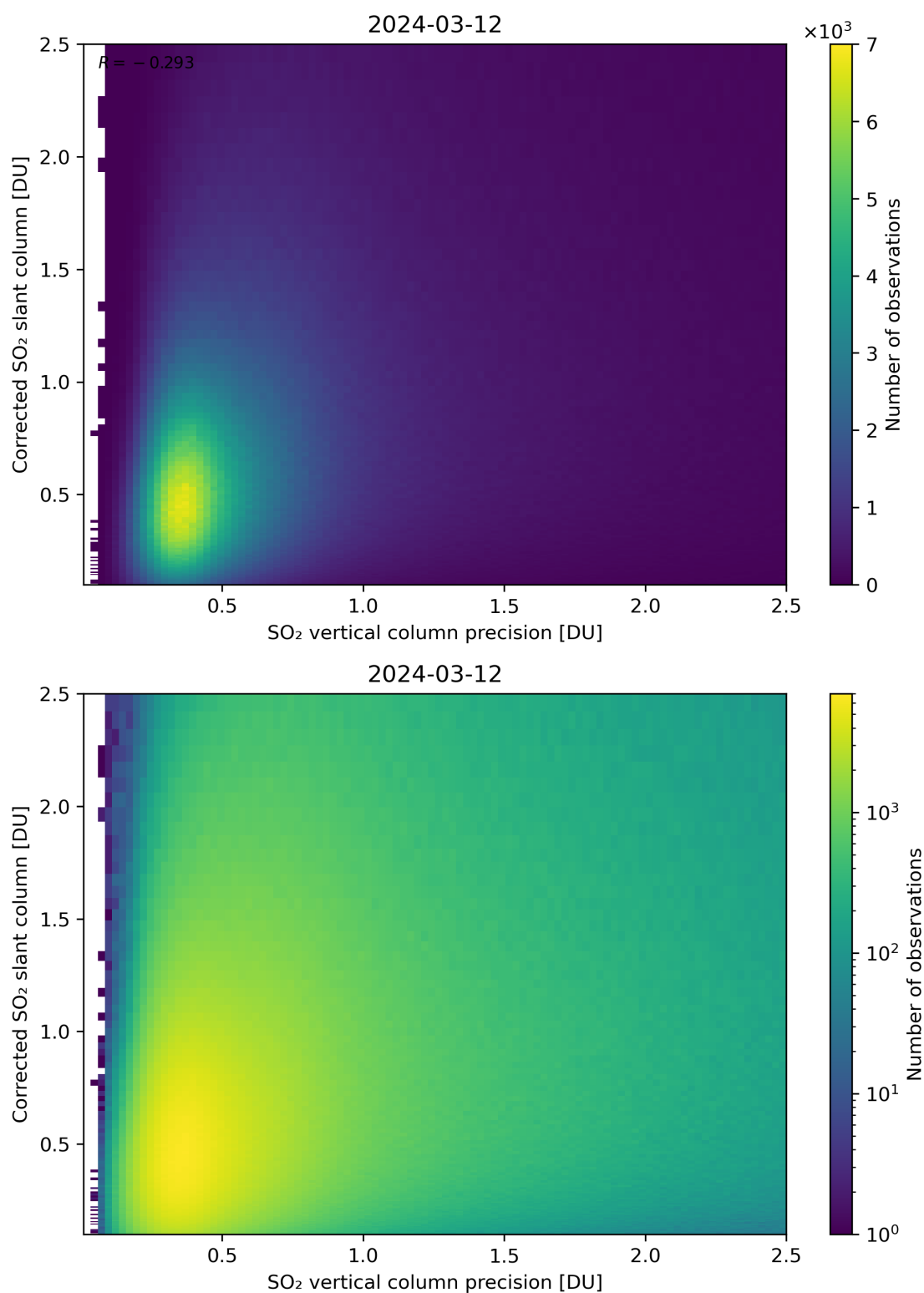
Figure 286: Scatter density plot of “SO 2 vertical column precision” against “Corrected SO 2 slant column” for 2024-03-11 to 2024-03-13.
