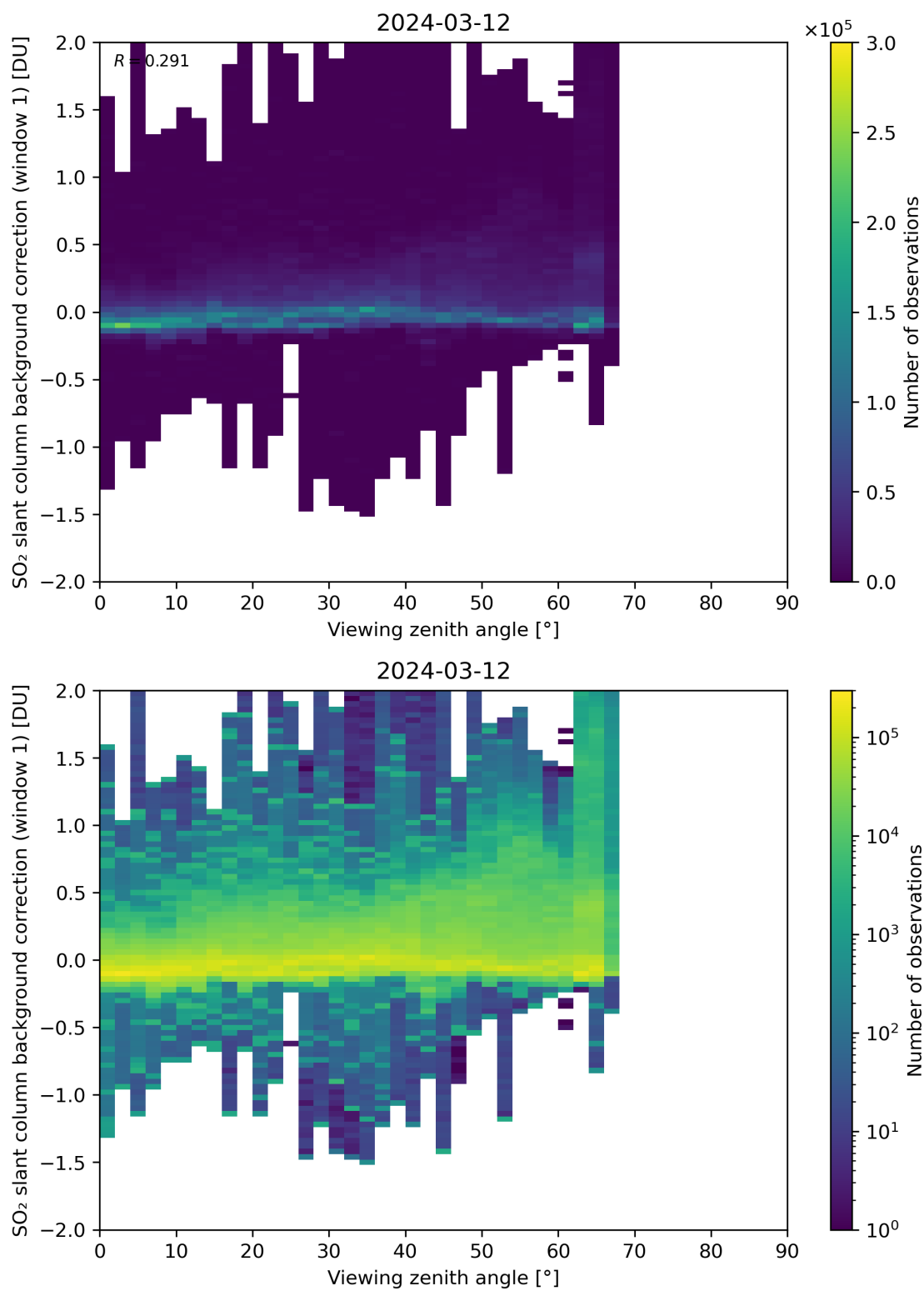
Figure 308: Scatter density plot of “Viewing zenith angle” against “SO 2 slant column background correction (window 1)” for 2024-03-11 to 2024-03-13.
