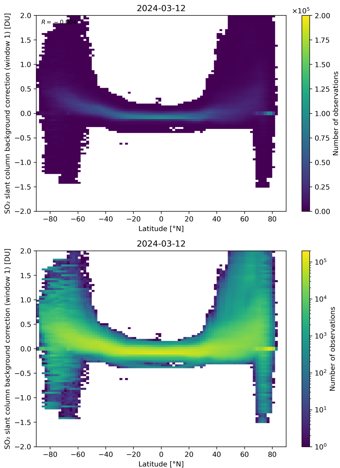
Figure 139: Scatter density plot of “Latitude” against “SO 2 slant column background correction (window 1)” for 2024-03-11 to 2024-03-13.
