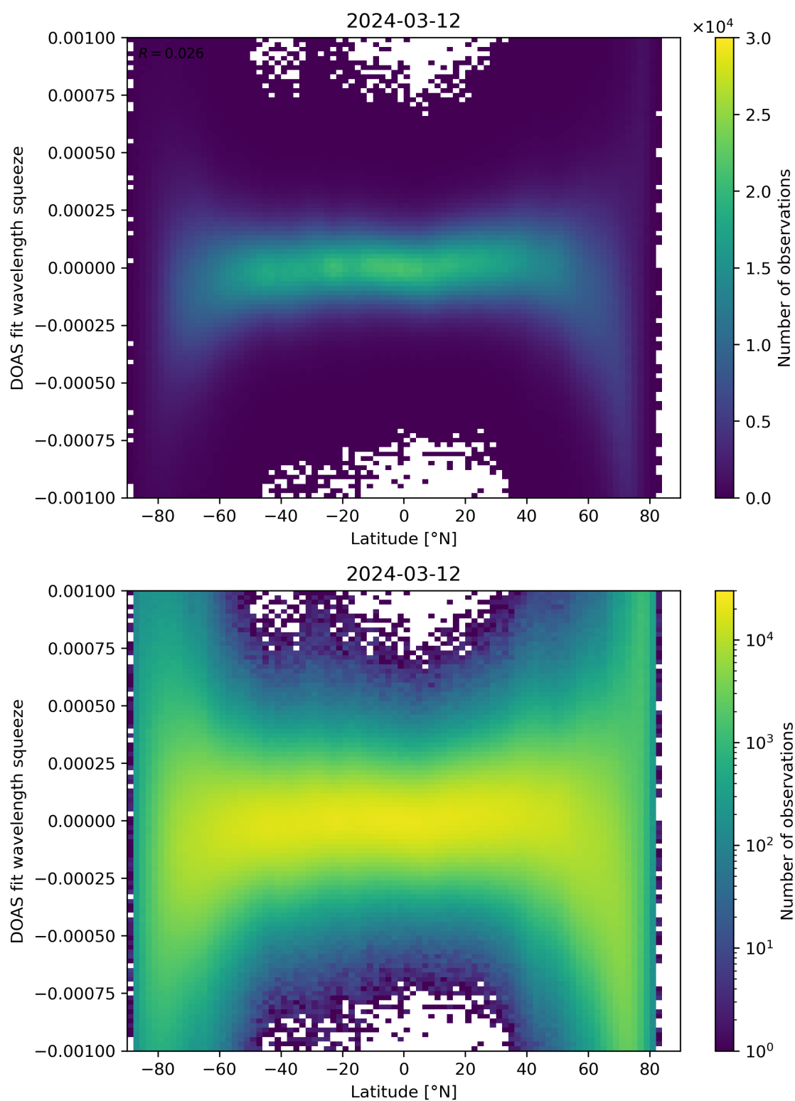
Figure 143: Scatter density plot of “Latitude” against “DOAS fit wavelength squeeze” for 2024-03-11 to 2024-03-13.
