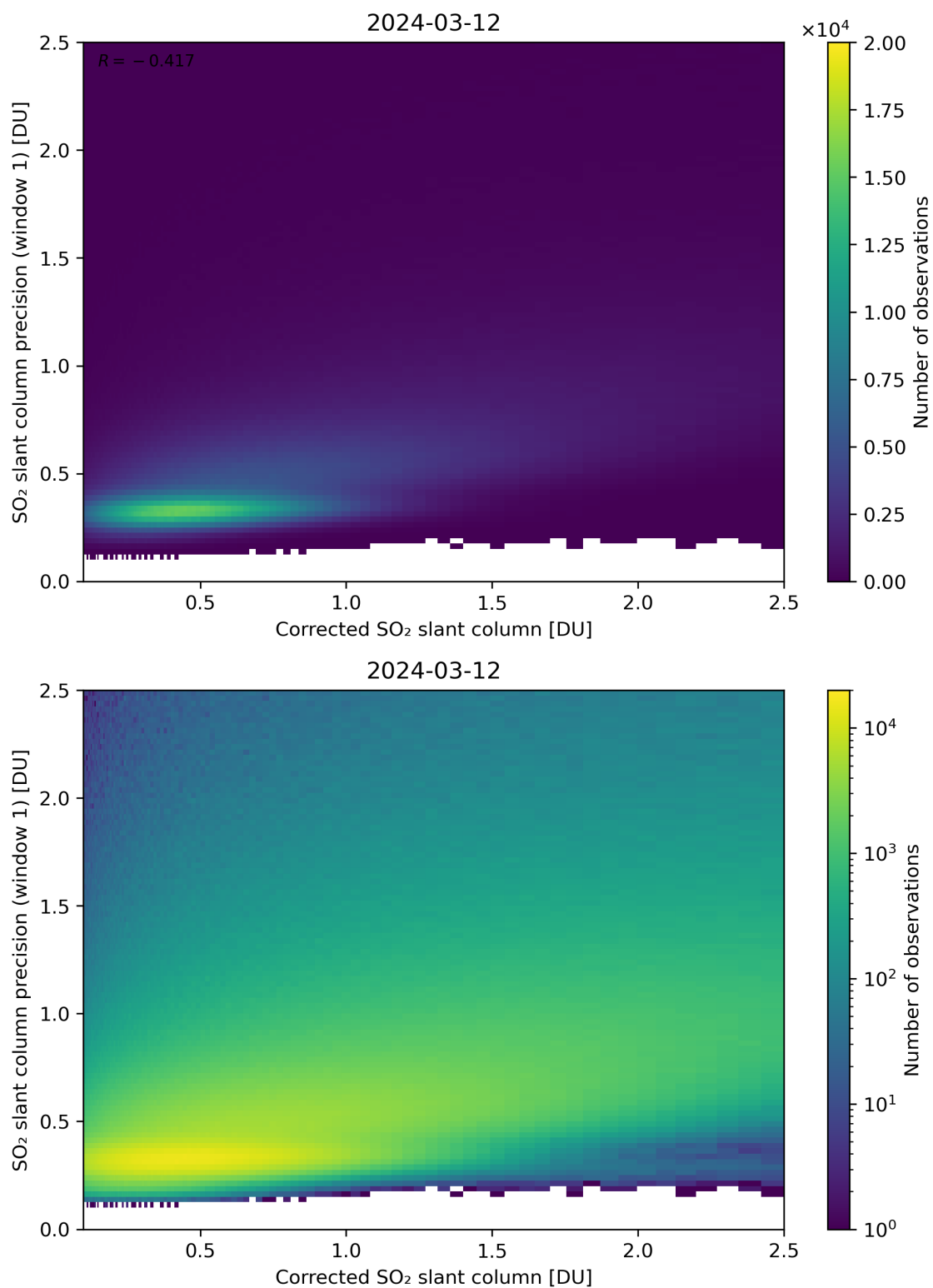
Figure 188: Scatter density plot of “Corrected SO 2 slant column” against “SO 2 slant column precision (window 1)” for 2024-03-11 to 2024-03-13.
