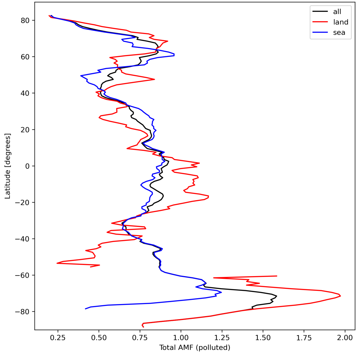
Figure 48: Zonal average of “Total AMF (polluted)” for 2024-03-11 to 2024-03-13.
