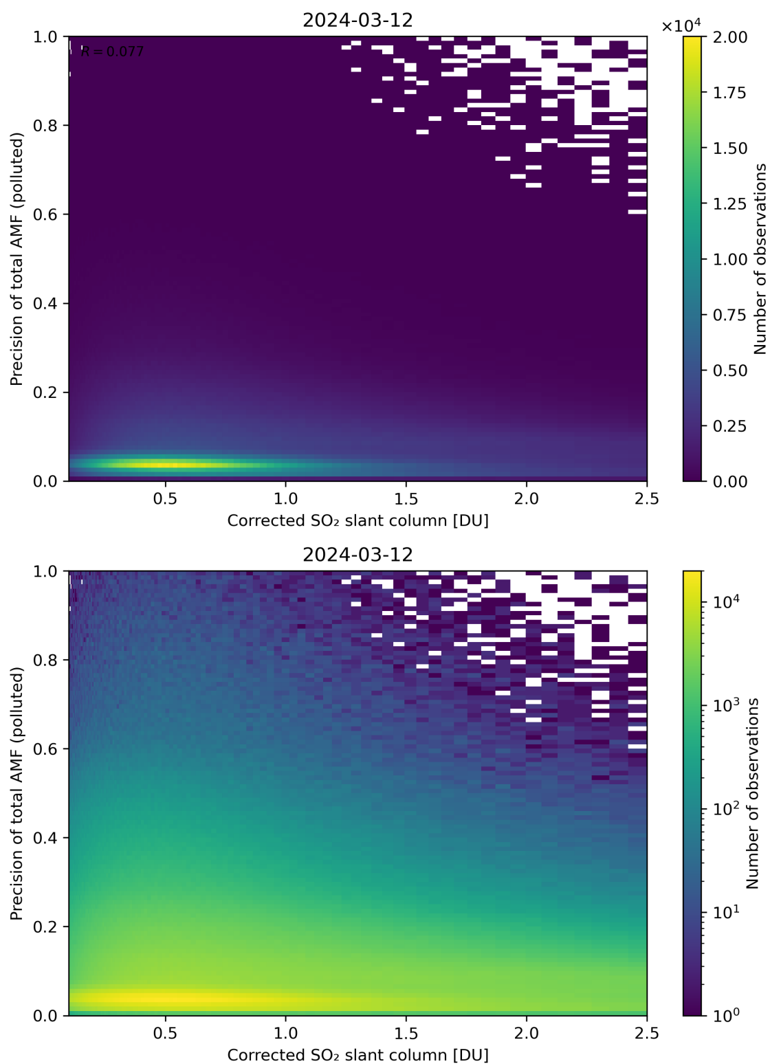
Figure 193: Scatter density plot of “Corrected SO 2 slant column” against “Precision of total AMF (polluted)” for 2024-03-11 to 2024-03-13.
