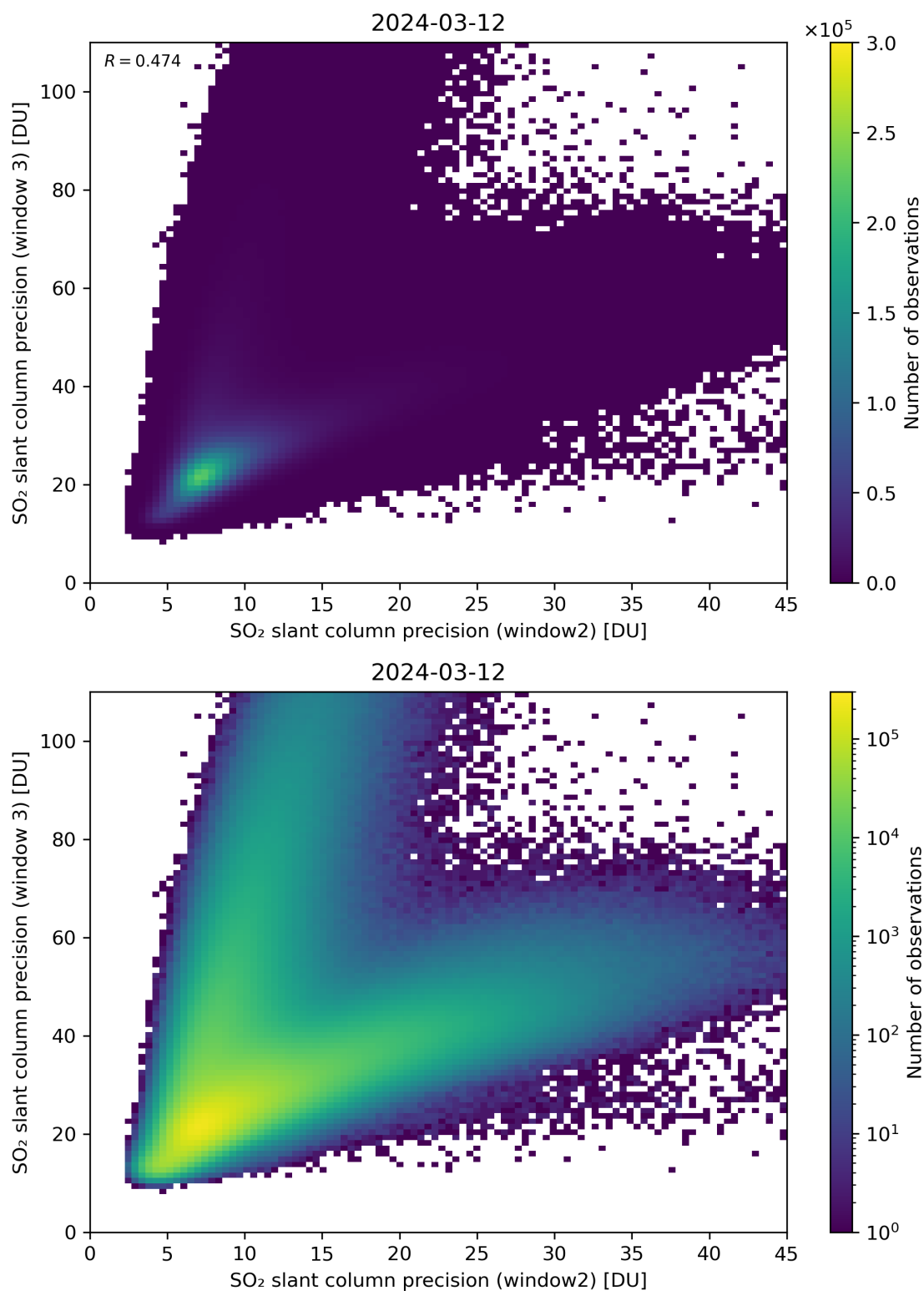
Figure 250: Scatter density plot of “SO 2 slant column precision (window2)” against “SO 2 slant column precision (window 3)” for 2024-03-11 to 2024-03-13.
