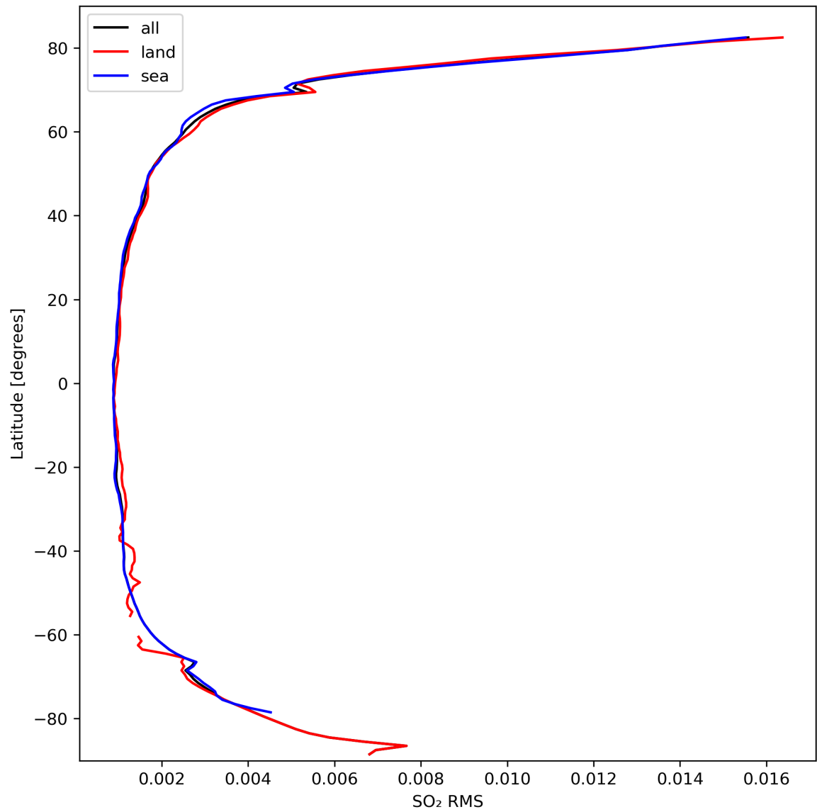
Figure 47: Zonal average of “SO 2 RMS” for 2024-03-11 to 2024-03-13.
