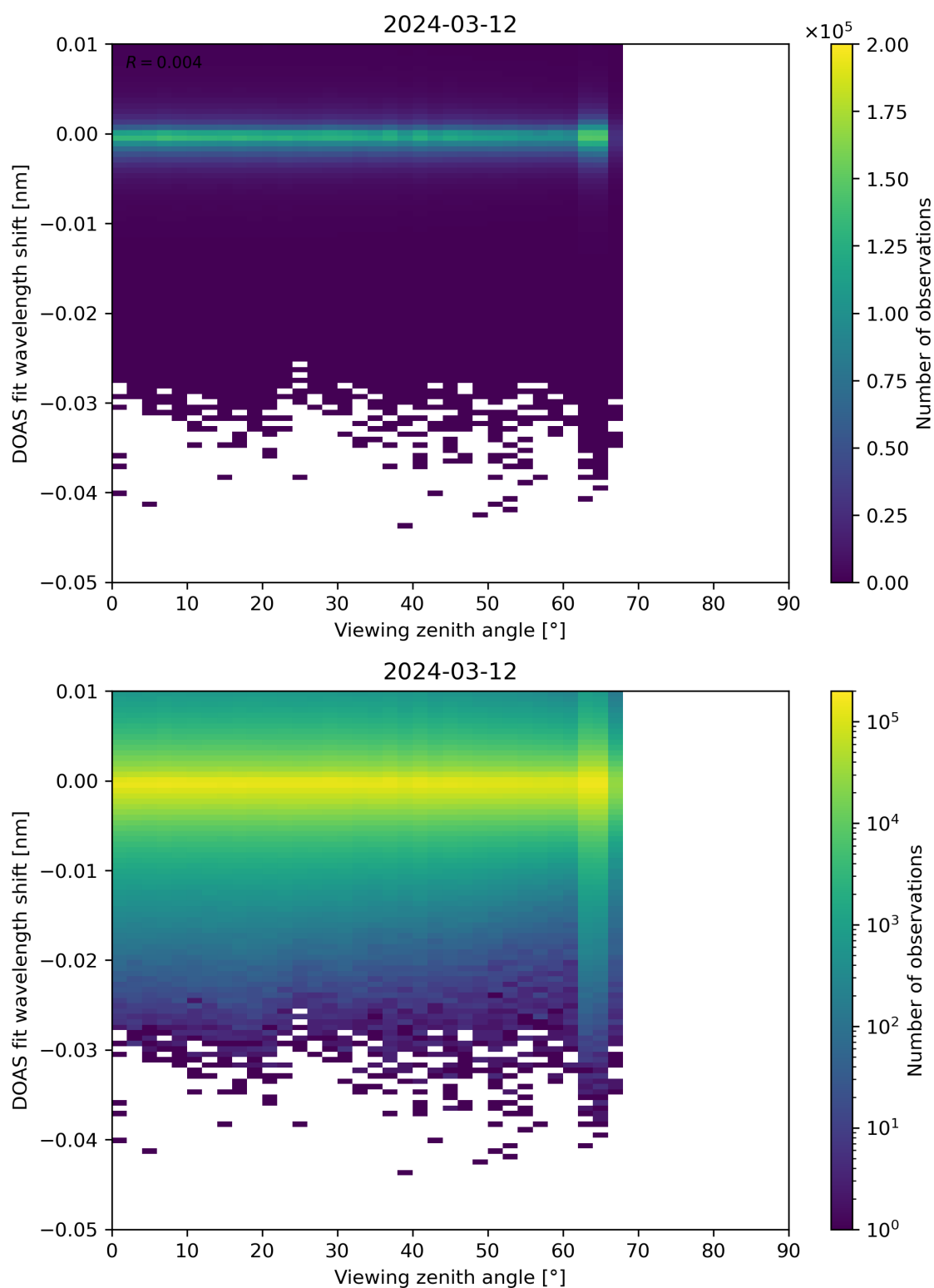
Figure 311: Scatter density plot of “Viewing zenith angle” against “DOAS fit wavelength shift” for 2024-03-11 to 2024-03-13.
