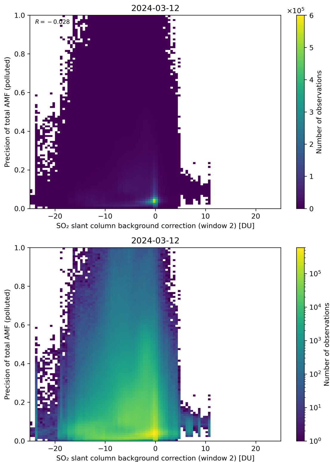
Figure 120: Scatter density plot of “SO 2 slant column background correction (window 2)” against “Precision of total AMF (polluted)” for 2024-03-11 to 2024-03-13.
