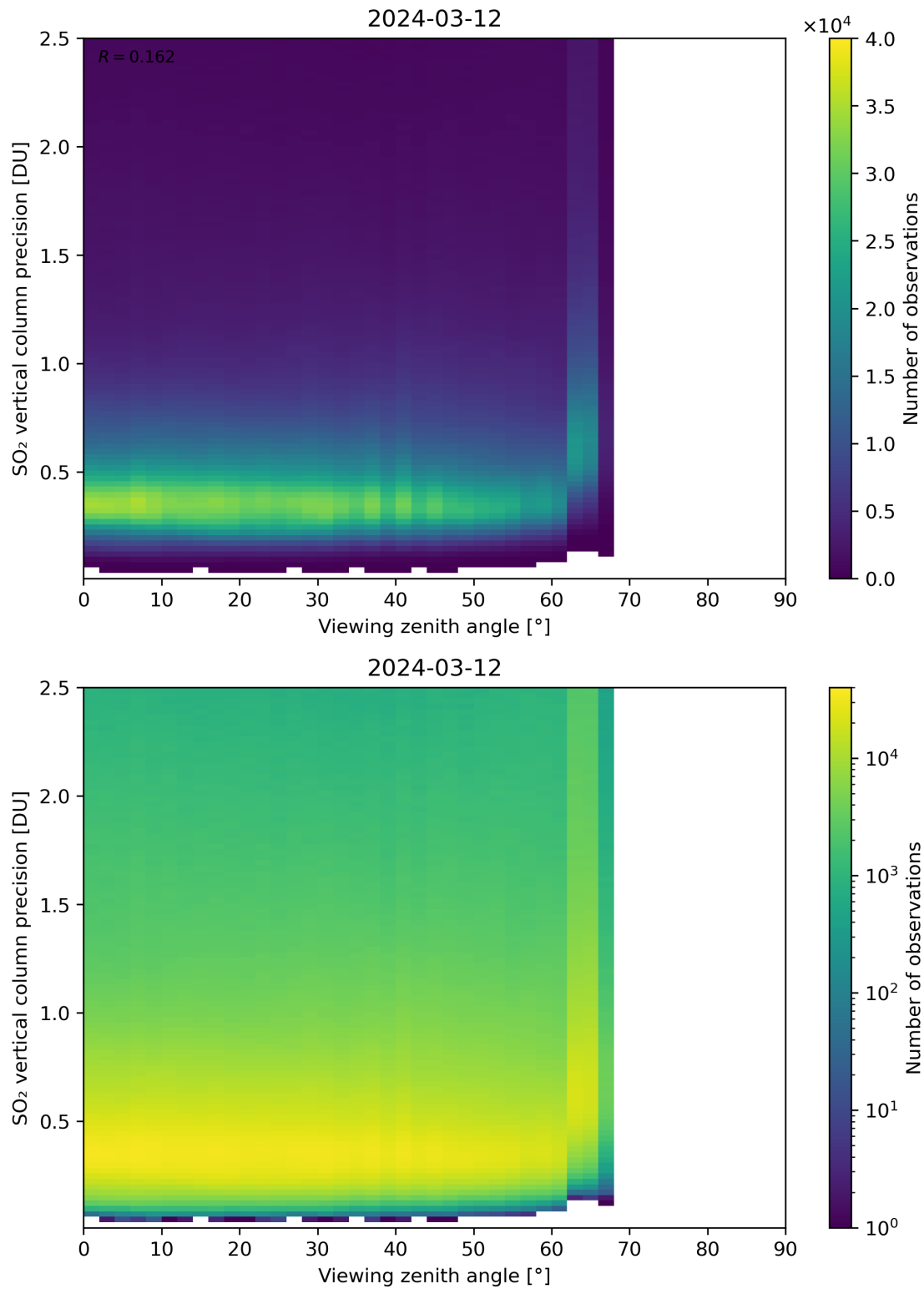
Figure 328: Scatter density plot of “Viewing zenith angle” against “SO 2 vertical column precision” for 2024-03-11 to 2024-03-13.
