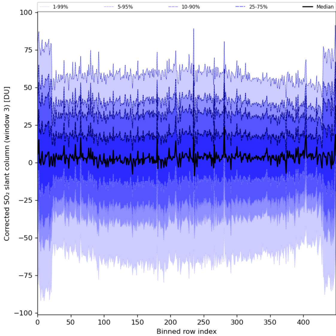
Figure 89: Along track statistics of “Corrected SO 2 slant column (window 3)” for 2024-03-11 to 2024-03-13
