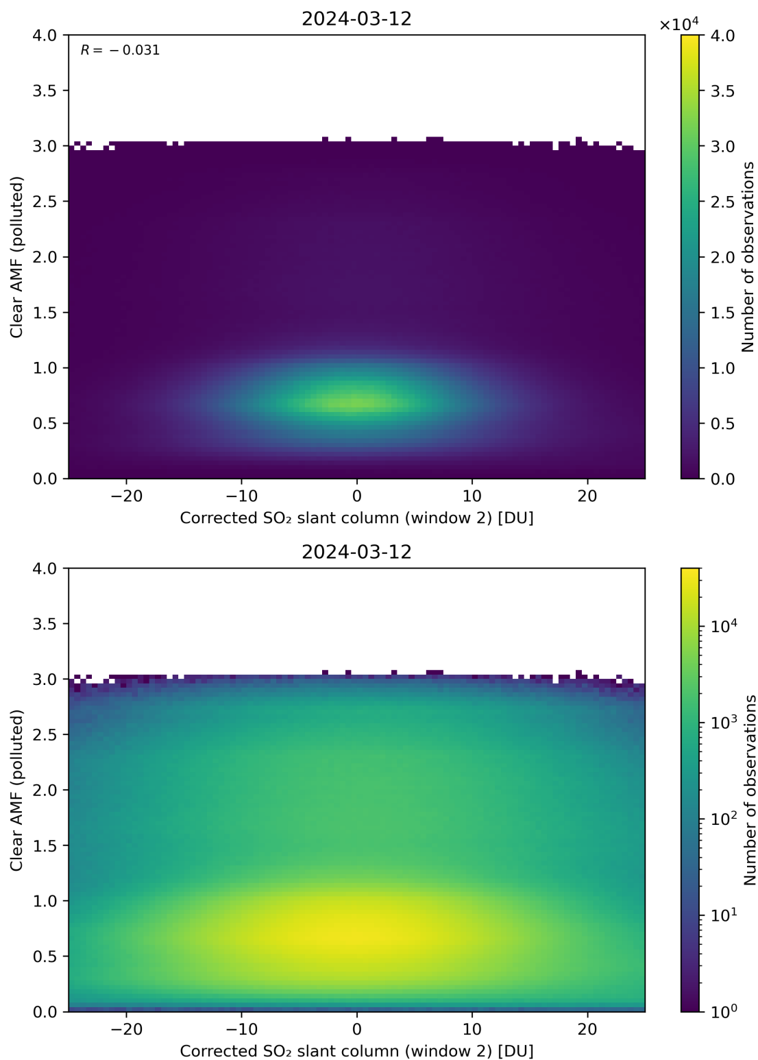
Figure 199: Scatter density plot of “Corrected SO 2 slant column (window 2)” against “Clear AMF (polluted)” for 2024-03-11 to 2024-03-13.
