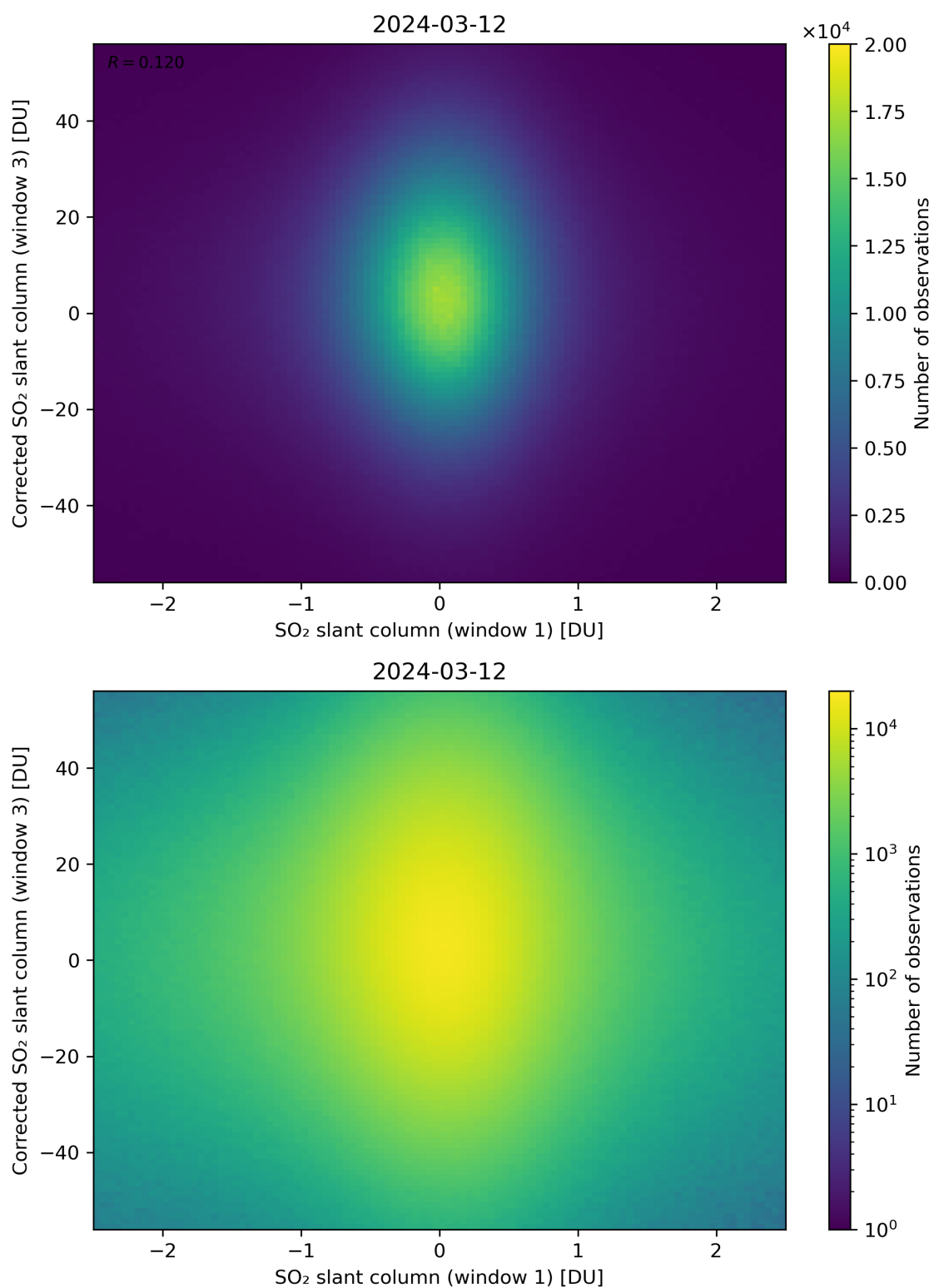
Figure 234: Scatter density plot of “SO 2 slant column (window 1)” against “Corrected SO 2 slant column (window 3)” for 2024-03-11 to 2024-03-13.
