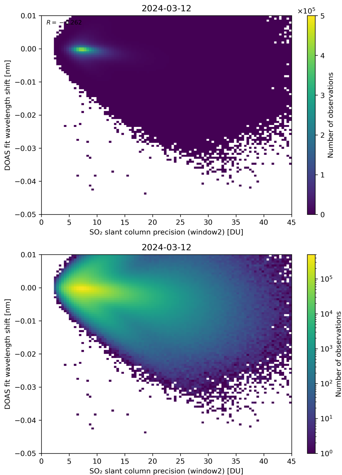
Figure 243: Scatter density plot of “SO 2 slant column precision (window2)” against “DOAS fit wavelength shift” for 2024-03-11 to 2024-03-13.
