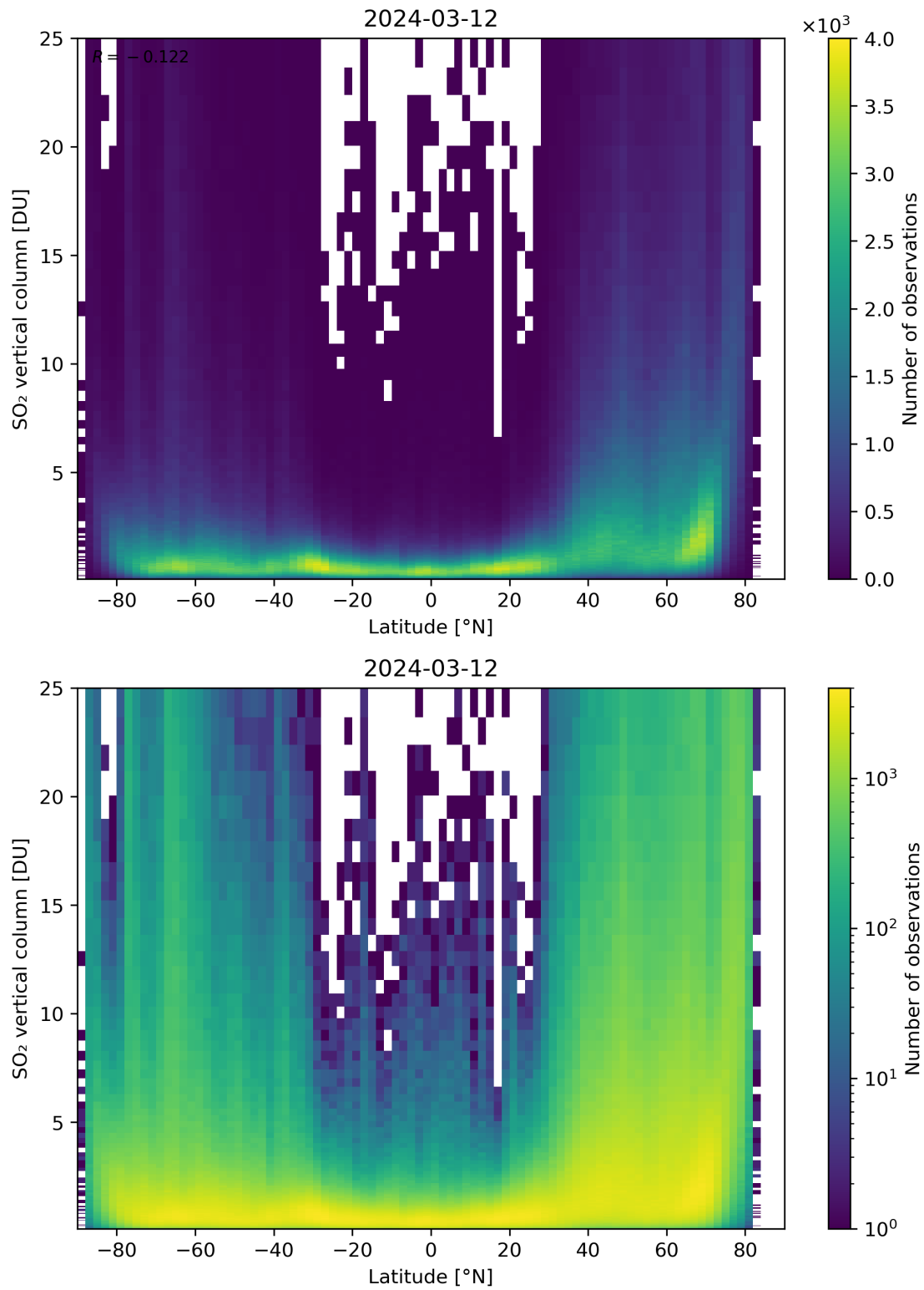
Figure 156: Scatter density plot of “Latitude” against “SO 2 vertical column” for 2024-03-11 to 2024-03-13.
