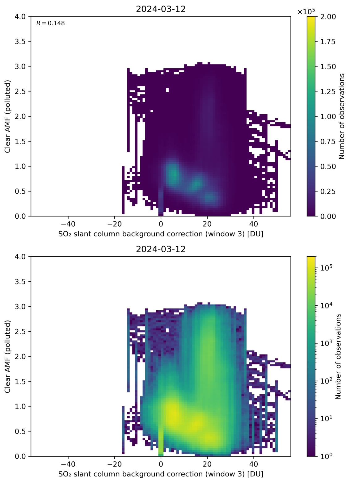
Figure 124: Scatter density plot of “SO 2 slant column background correction (window 3)” against “Clear AMF (polluted)” for 2024-03-11 to 2024-03-13.
