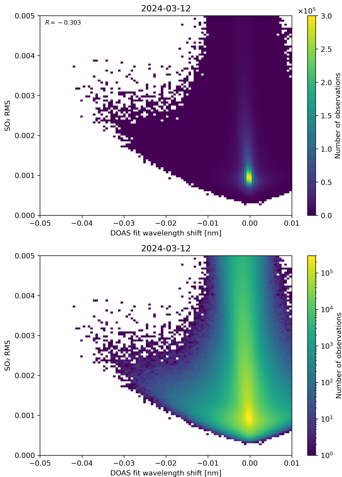
Figure 128: Scatter density plot of “DOAS fit wavelength shift” against “SO 2 RMS” for 2024-03-11 to 2024-03-13.
