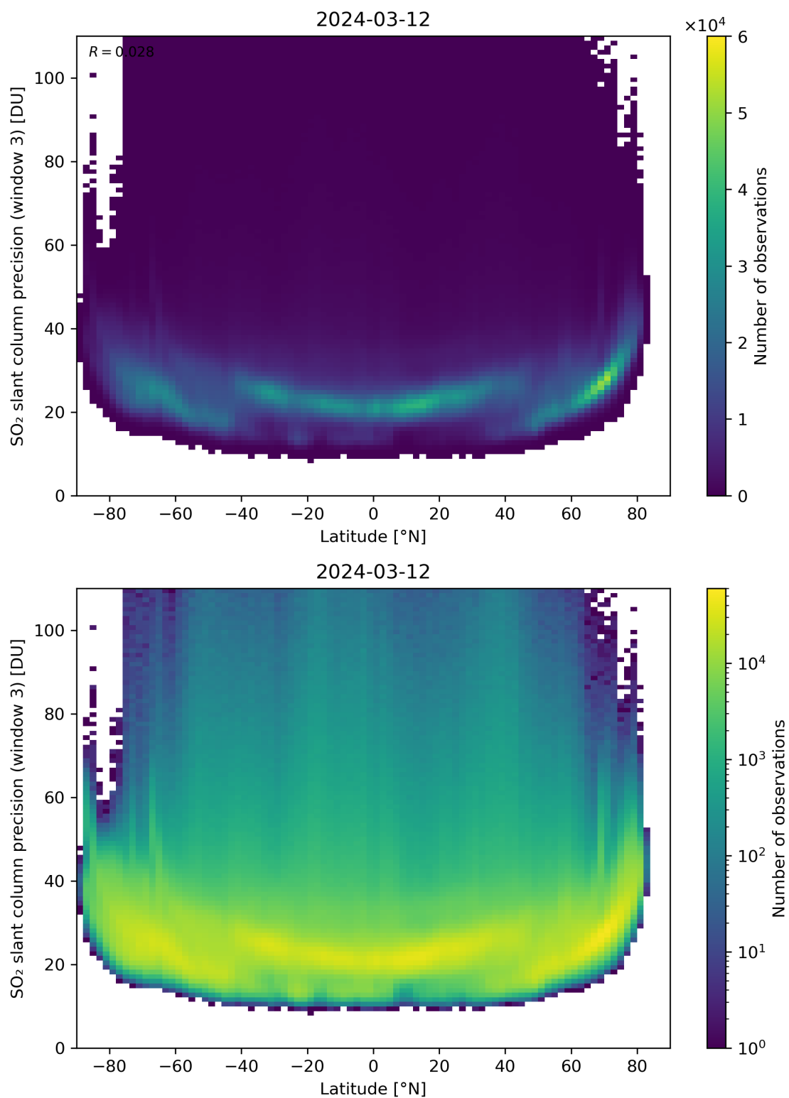
Figure 153: Scatter density plot of “Latitude” against “SO 2 slant column precision (window 3)” for 2024-03-11 to 2024-03-13.
