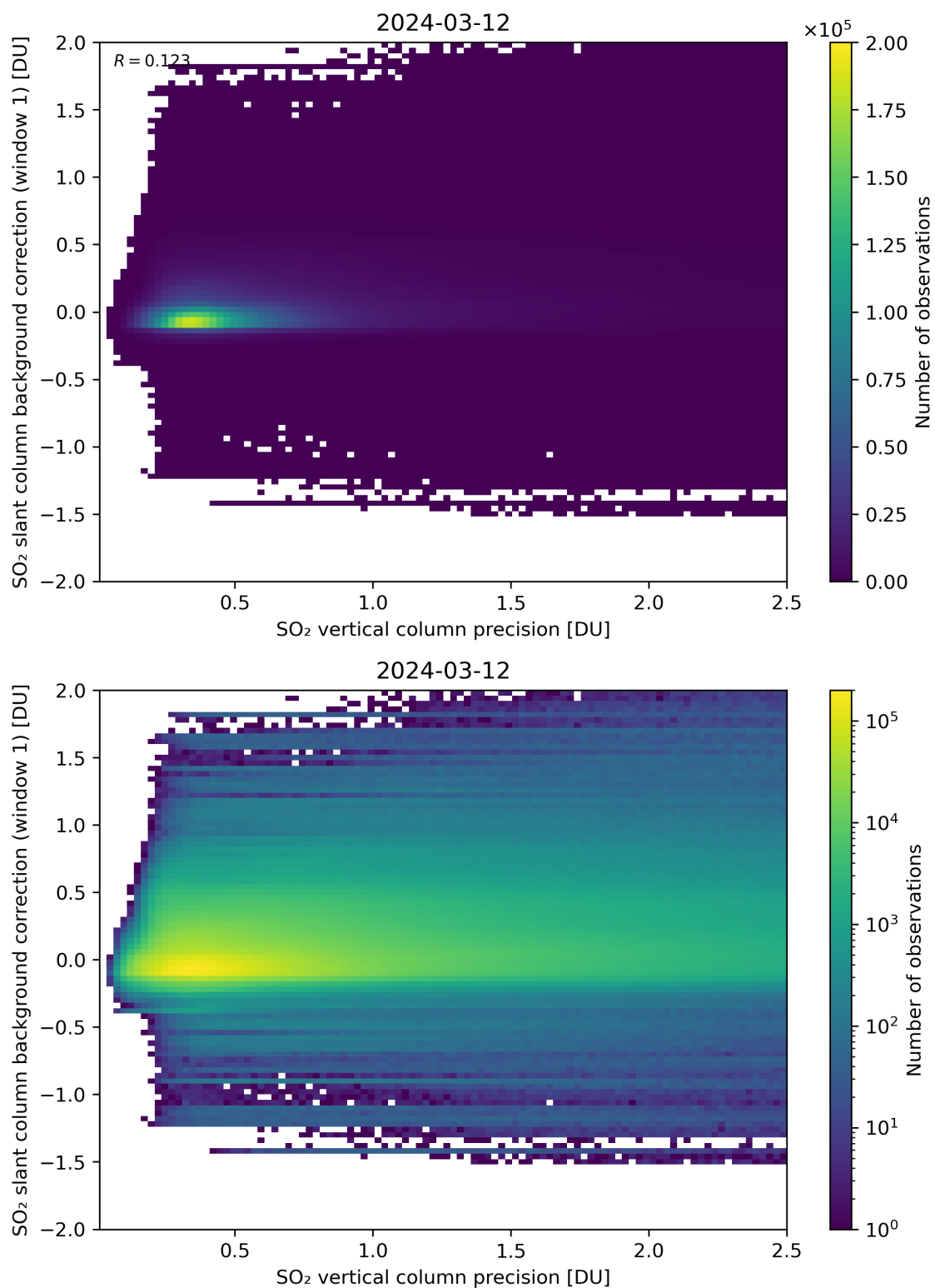
Figure 279: Scatter density plot of “SO 2 vertical column precision” against “SO 2 slant column background correction (window 1)” for 2024-03-11 to 2024-03-13.
