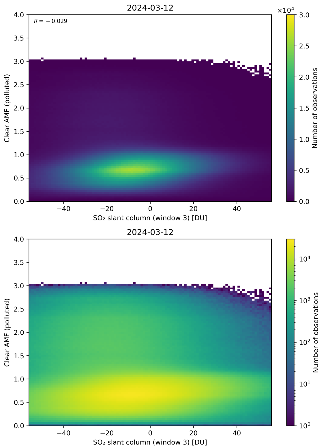
Figure 265: Scatter density plot of “SO 2 slant column (window 3)” against “Clear AMF (polluted)” for 2024-03-11 to 2024-03-13.
