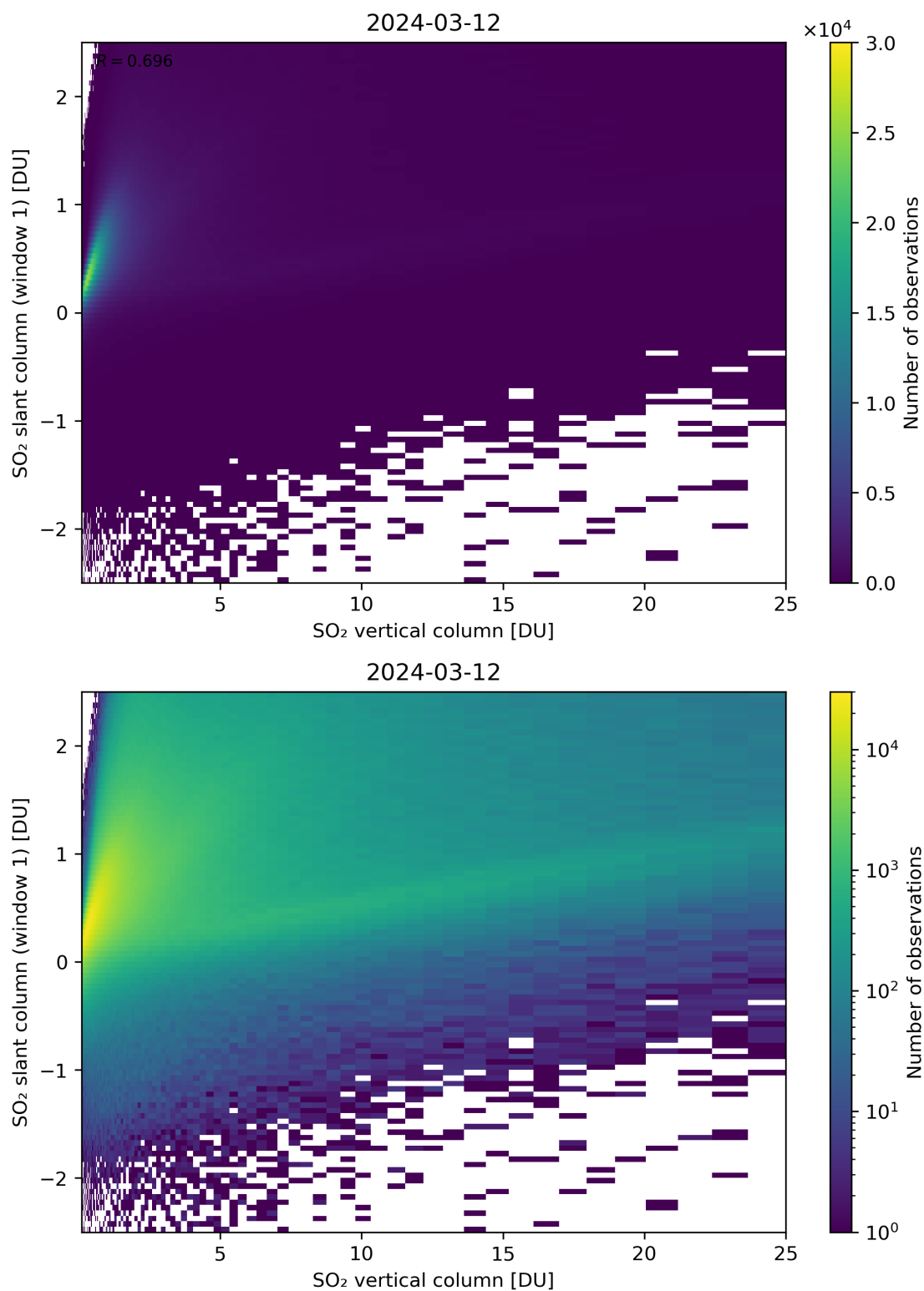
Figure 300: Scatter density plot of “SO 2 vertical column” against “SO 2 slant column (window 1)” for 2024-03-11 to 2024-03-13.
