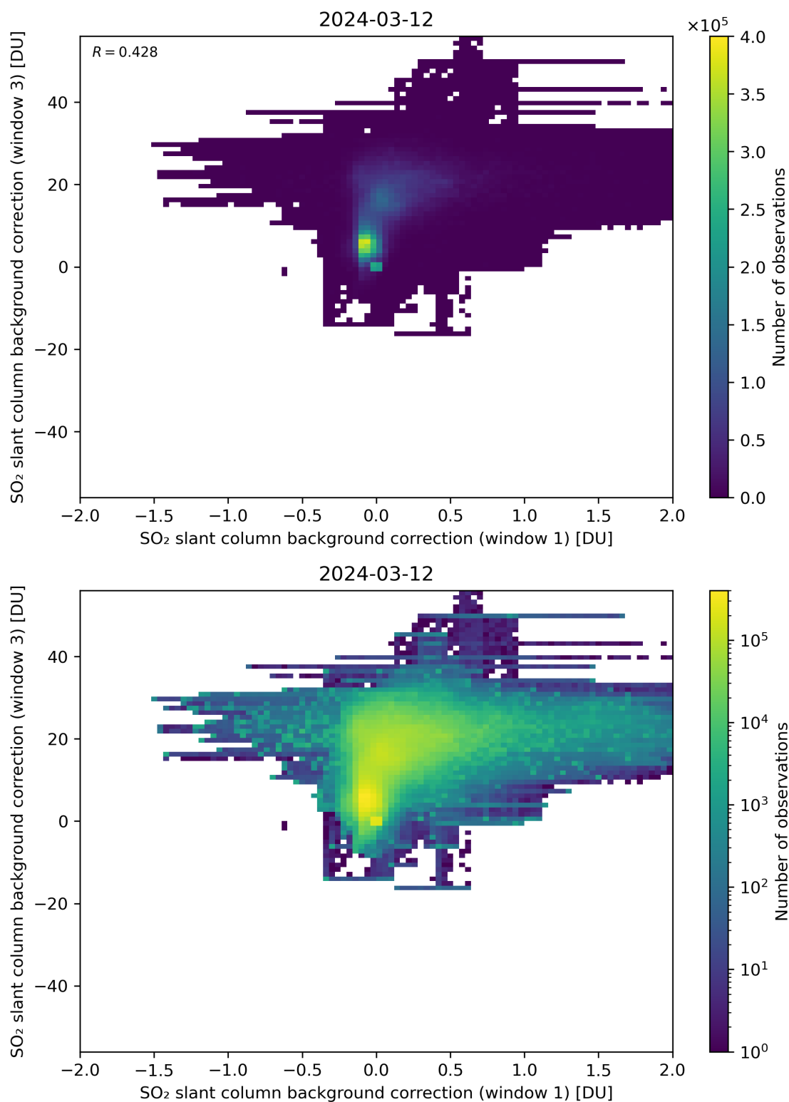
Figure 99: Scatter density plot of “SO 2 slant column background correction (window 1)” against “SO 2 slant column background correction (window 3)” for 2024-03-11 to 2024-03-13.
