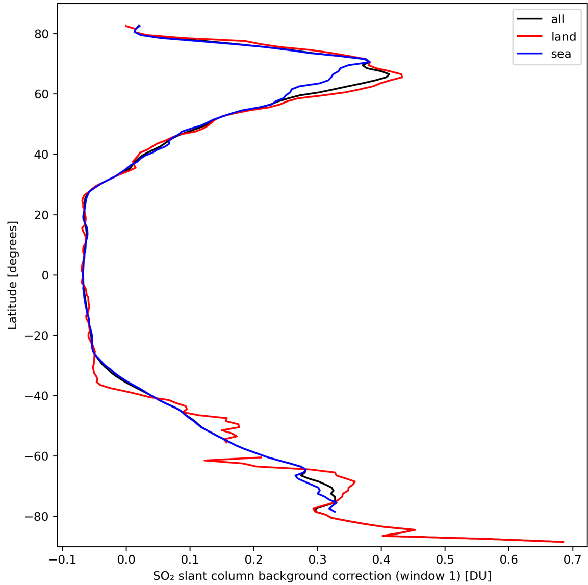
Figure 36: Zonal average of “SO 2 slant column background correction (window 1)” for 2024-03-11 to 2024-03-13.
