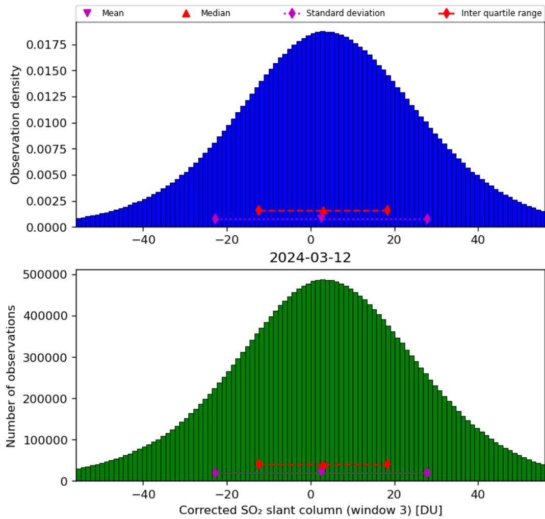
Figure 66: Histogram of “Corrected SO 2 slant column (window 3)” for 2024-03-11 to 2024-03-13
