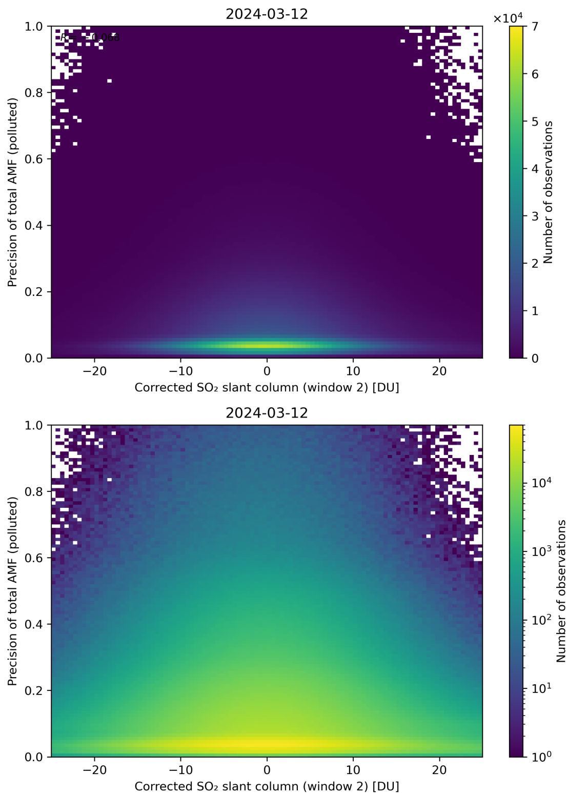
Figure 204: Scatter density plot of “Corrected SO 2 slant column (window 2)” against “Precision of total AMF (polluted)” for 2024-03-11 to 2024-03-13.
