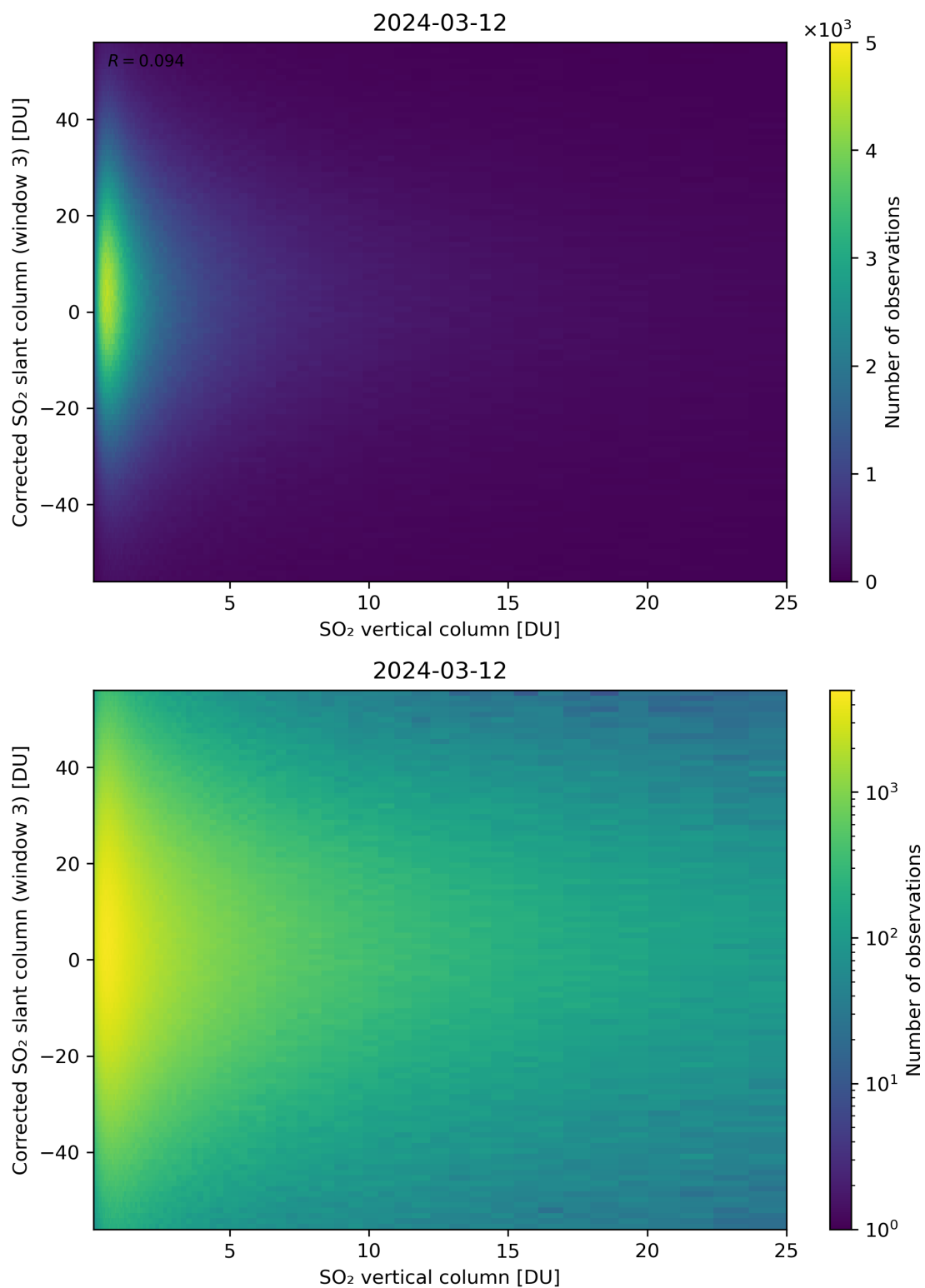
Figure 299: Scatter density plot of “SO 2 vertical column” against “Corrected SO 2 slant column (window 3)” for 2024-03-11 to 2024-03-13.
