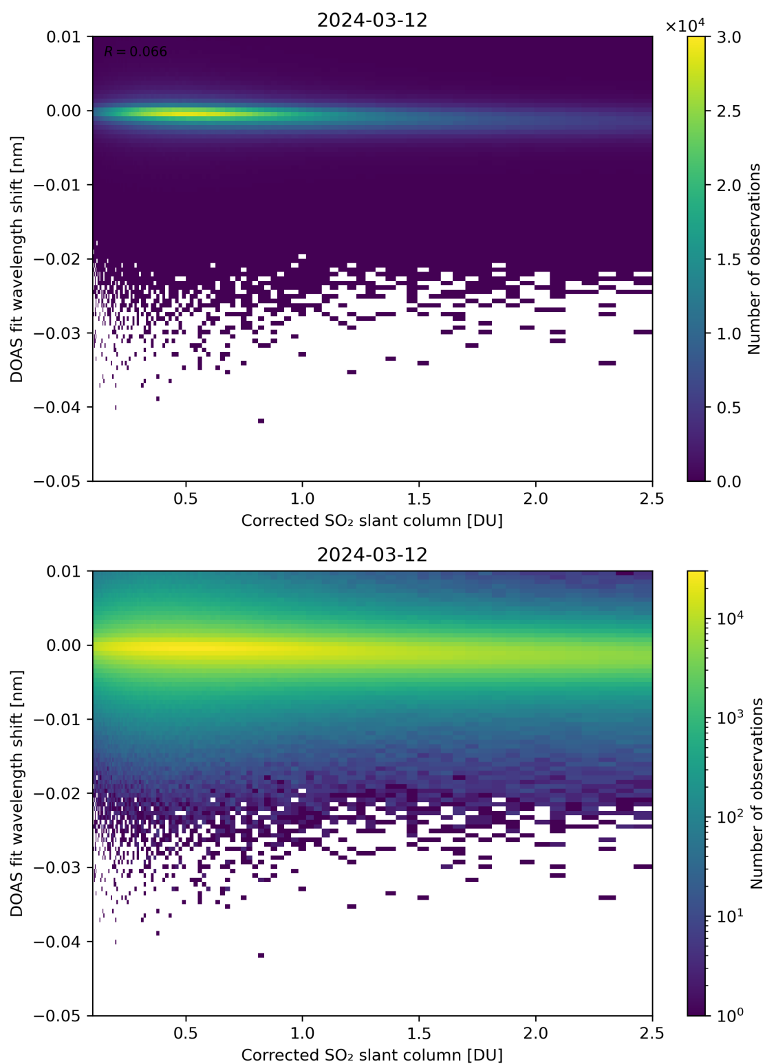
Figure 181: Scatter density plot of “Corrected SO 2 slant column” against “DOAS fit wavelength shift” for 2024-03-11 to 2024-03-13.
