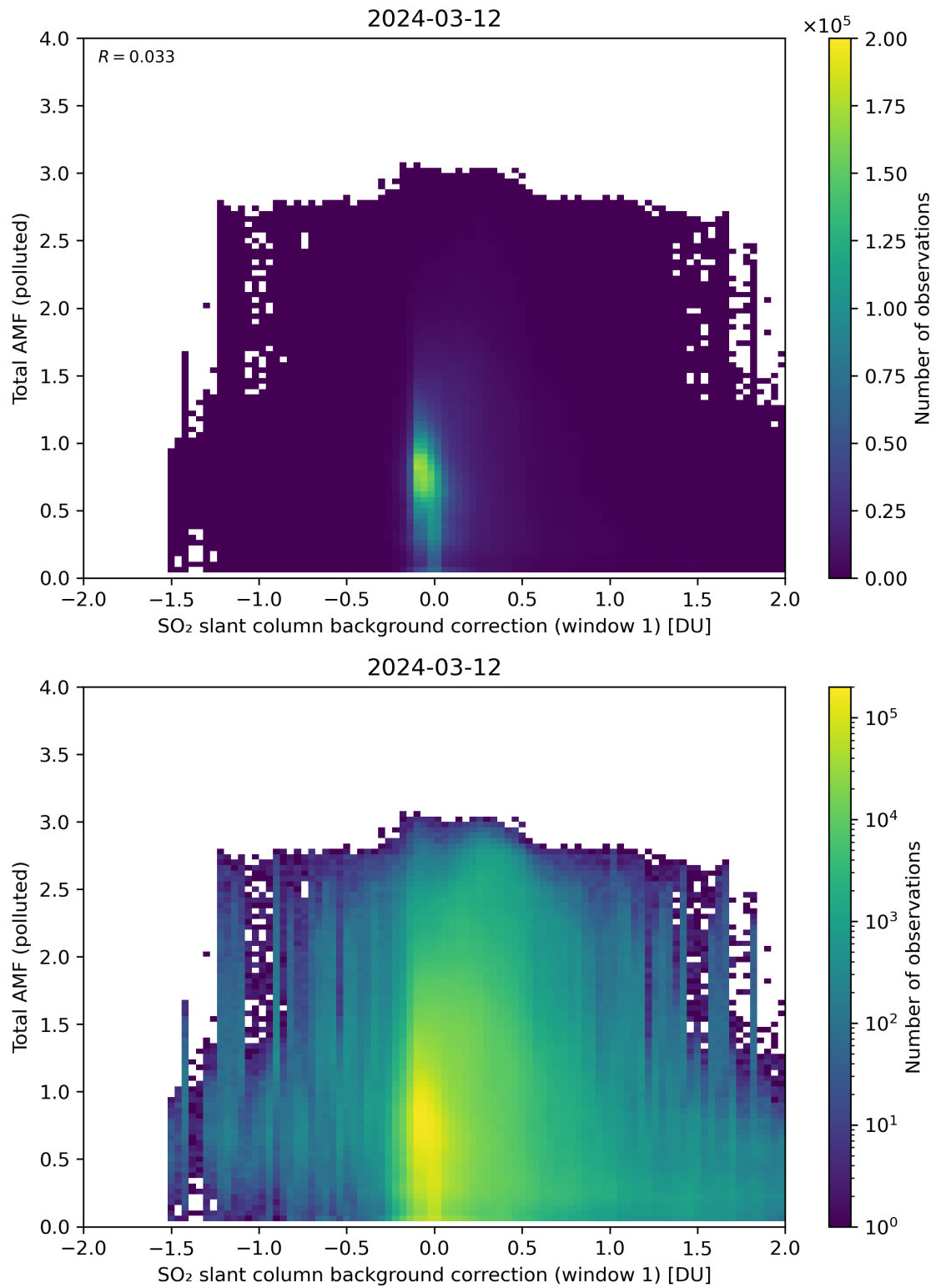
Figure 109: Scatter density plot of “SO 2 slant column background correction (window 1)” against “Total AMF (polluted)” for 2024-03-11 to 2024-03-13.
