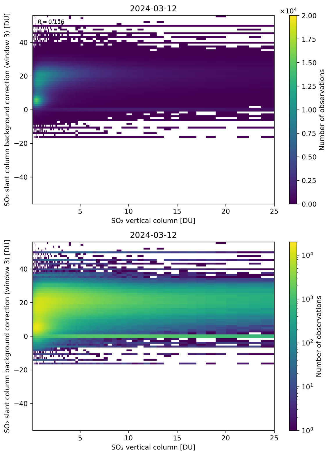
Figure 275: Scatter density plot of “SO 2 vertical column” against “SO 2 slant column background correction (window 3)” for 2024-03-11 to 2024-03-13.
