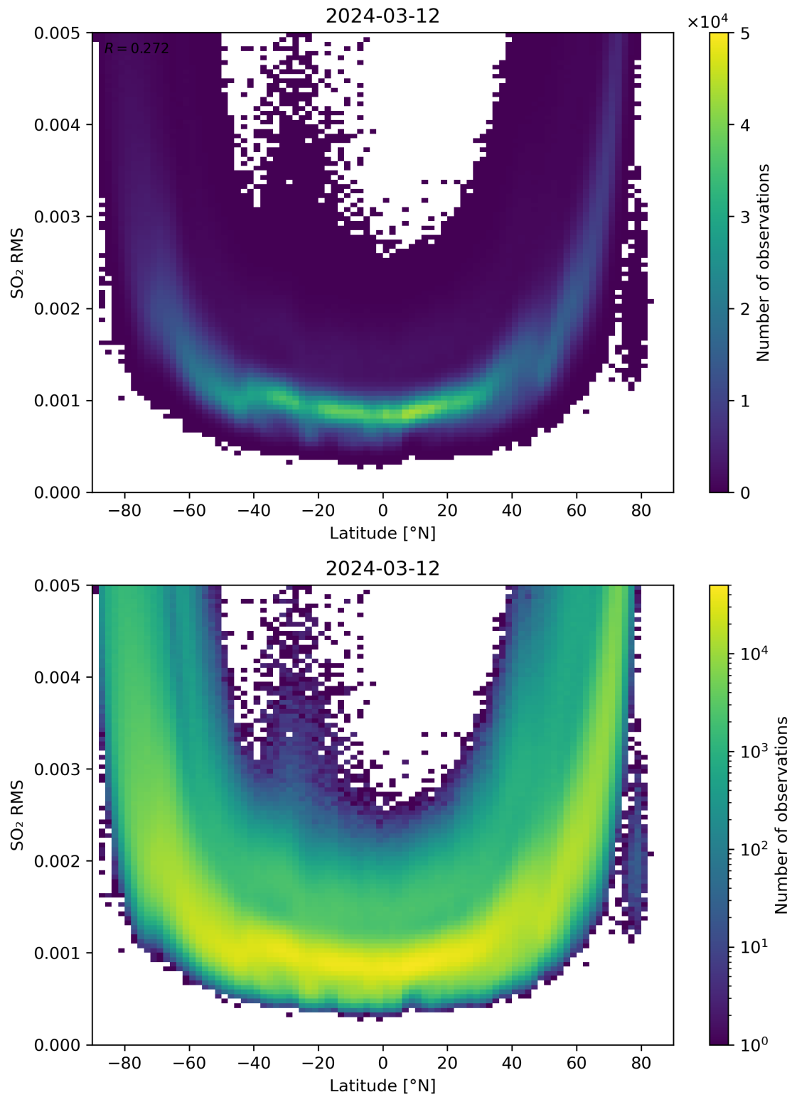
Figure 144: Scatter density plot of “Latitude” against “SO 2 RMS” for 2024-03-11 to 2024-03-13.
