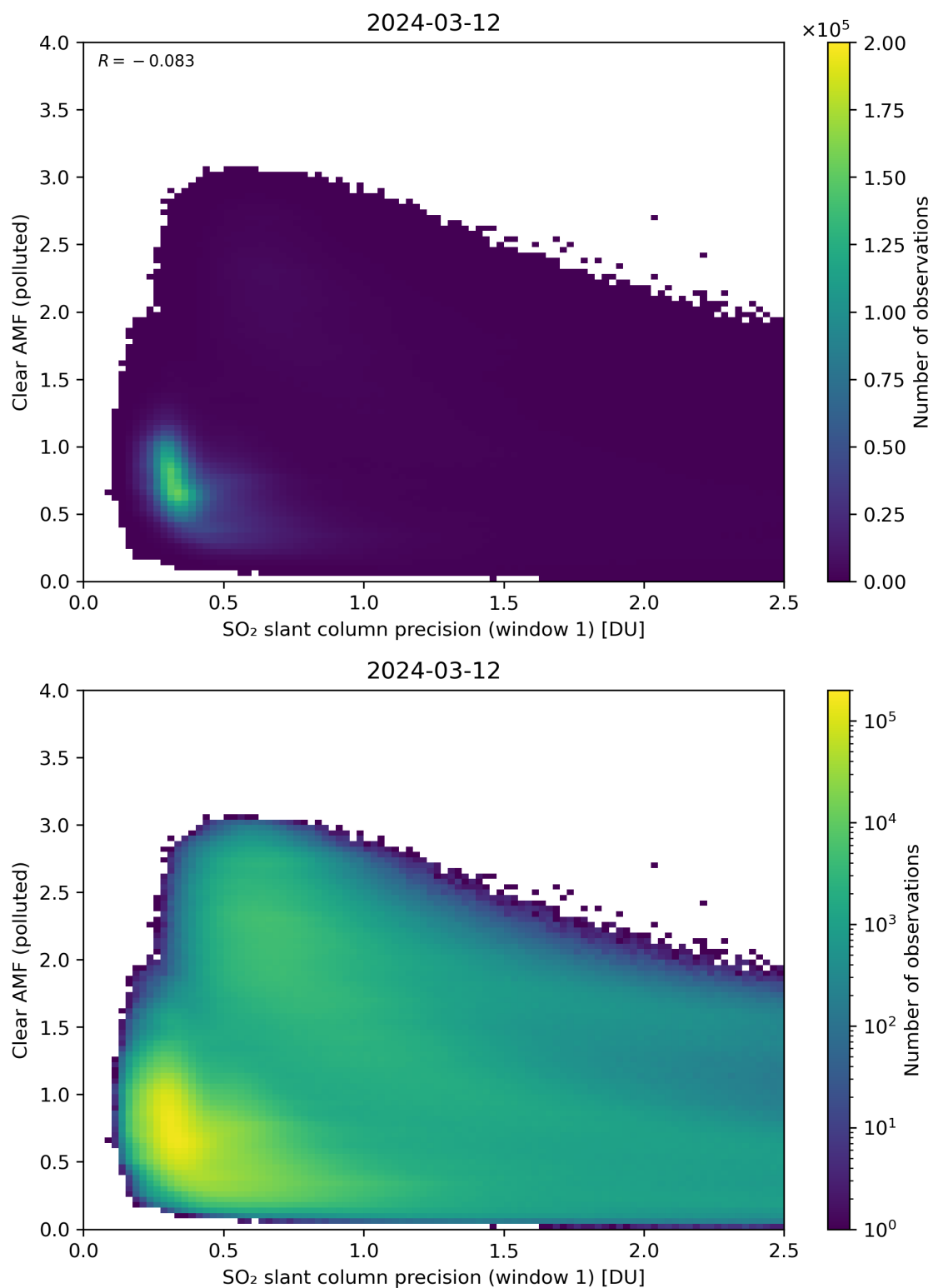
Figure 224: Scatter density plot of “SO 2 slant column precision (window 1)” against “Clear AMF (polluted)” for 2024-03-11 to 2024-03-13.
