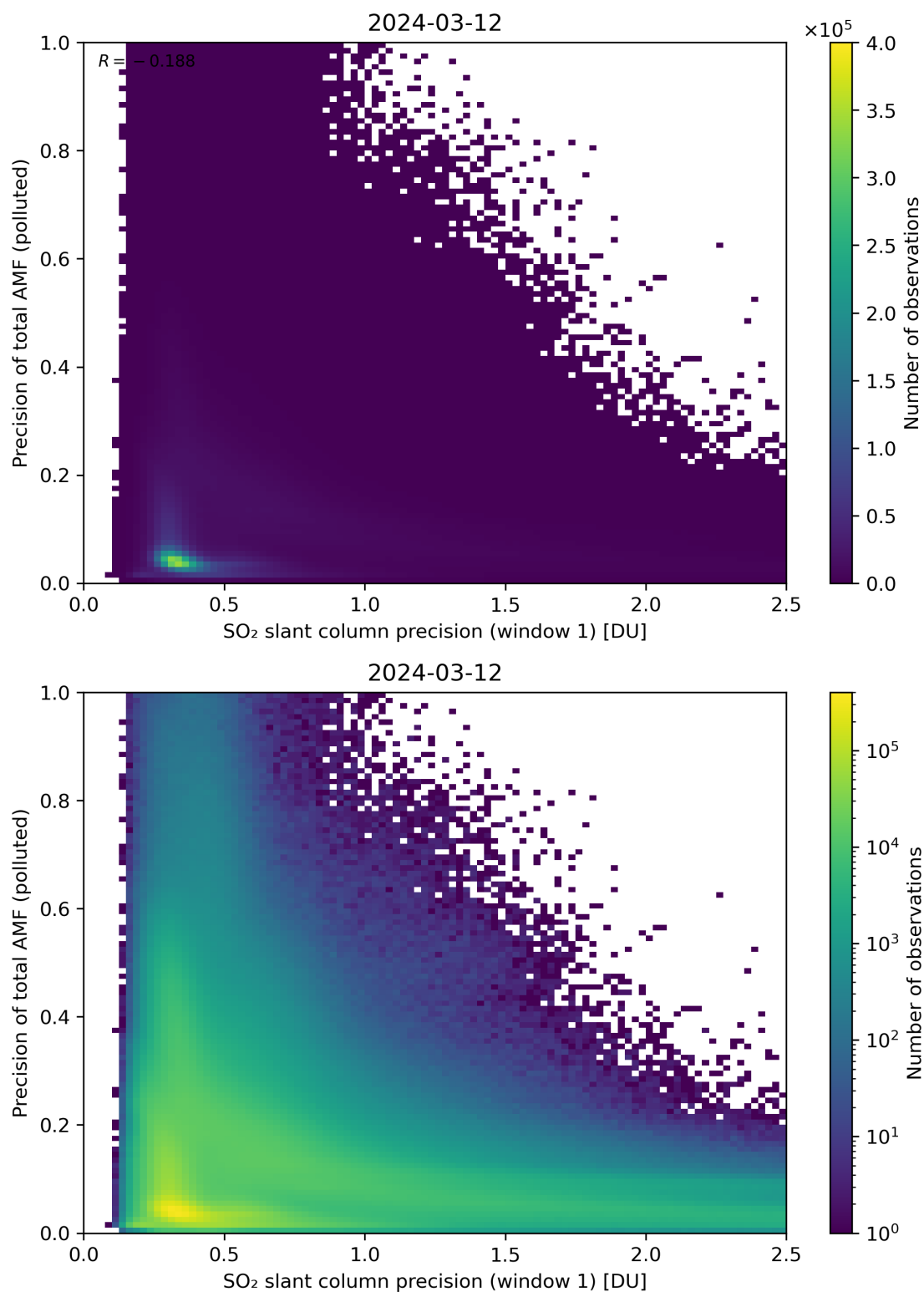
Figure 231: Scatter density plot of “SO 2 slant column precision (window 1)” against “Precision of total AMF (polluted)” for 2024-03-11 to 2024-03-13.
