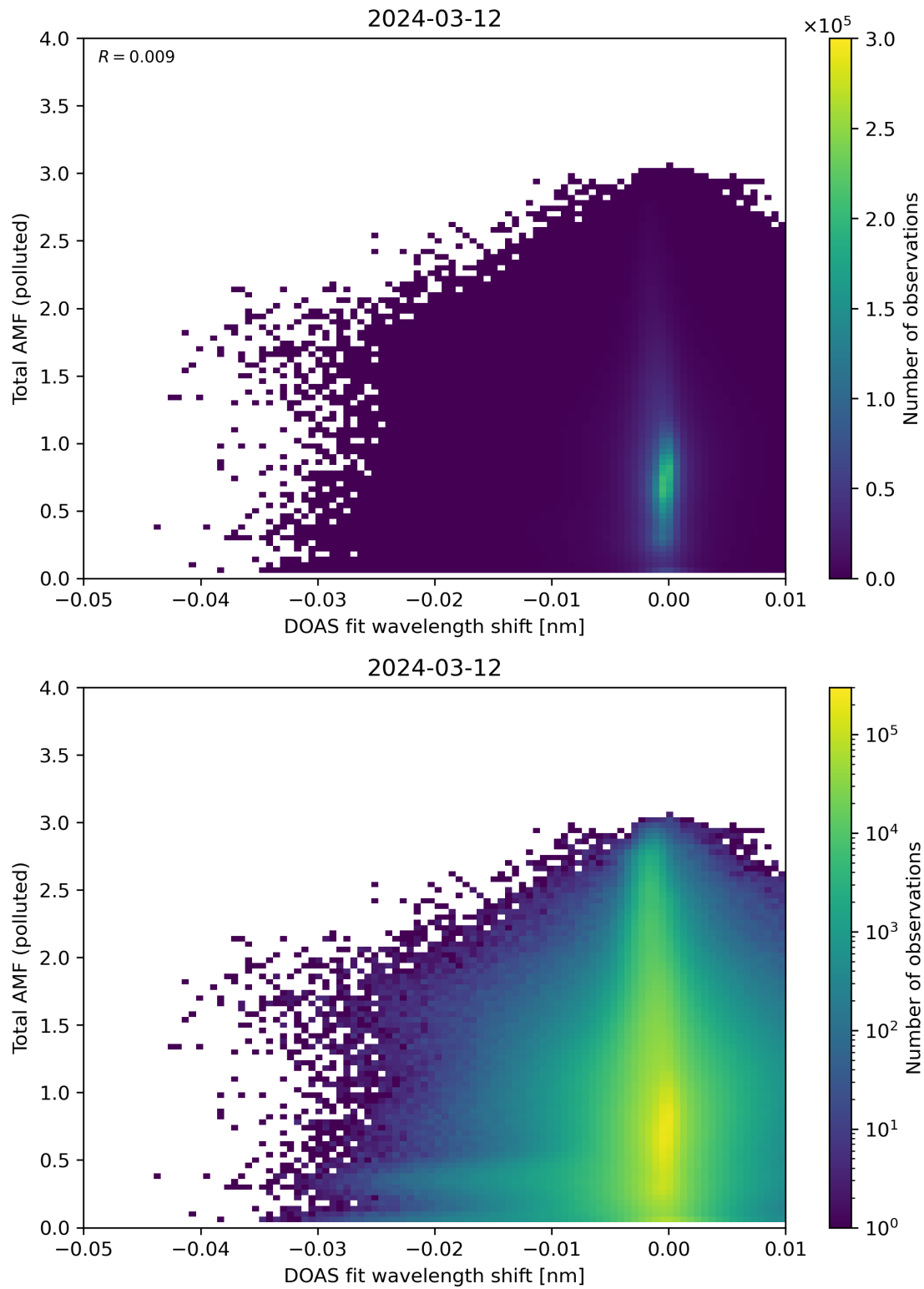
Figure 130: Scatter density plot of “DOAS fit wavelength shift” against “Total AMF (polluted)” for 2024-03-11 to 2024-03-13.
