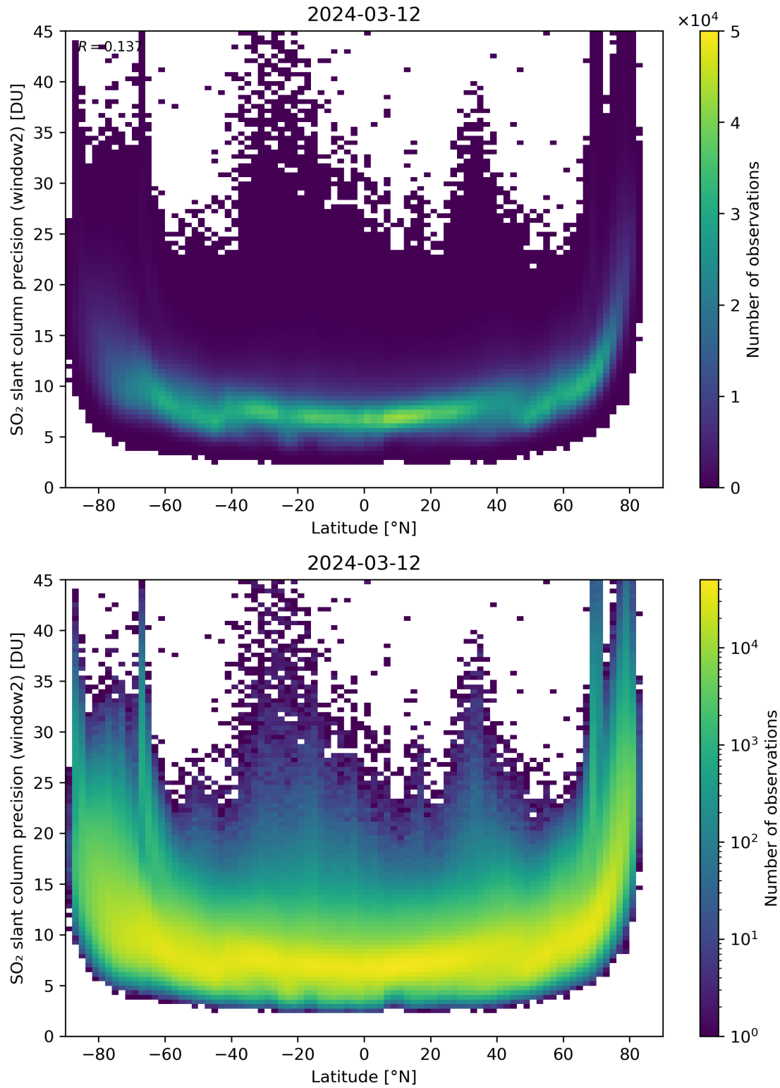
Figure 151: Scatter density plot of “Latitude” against “SO 2 slant column precision (window2)” for 2024-03-11 to 2024-03-13.
