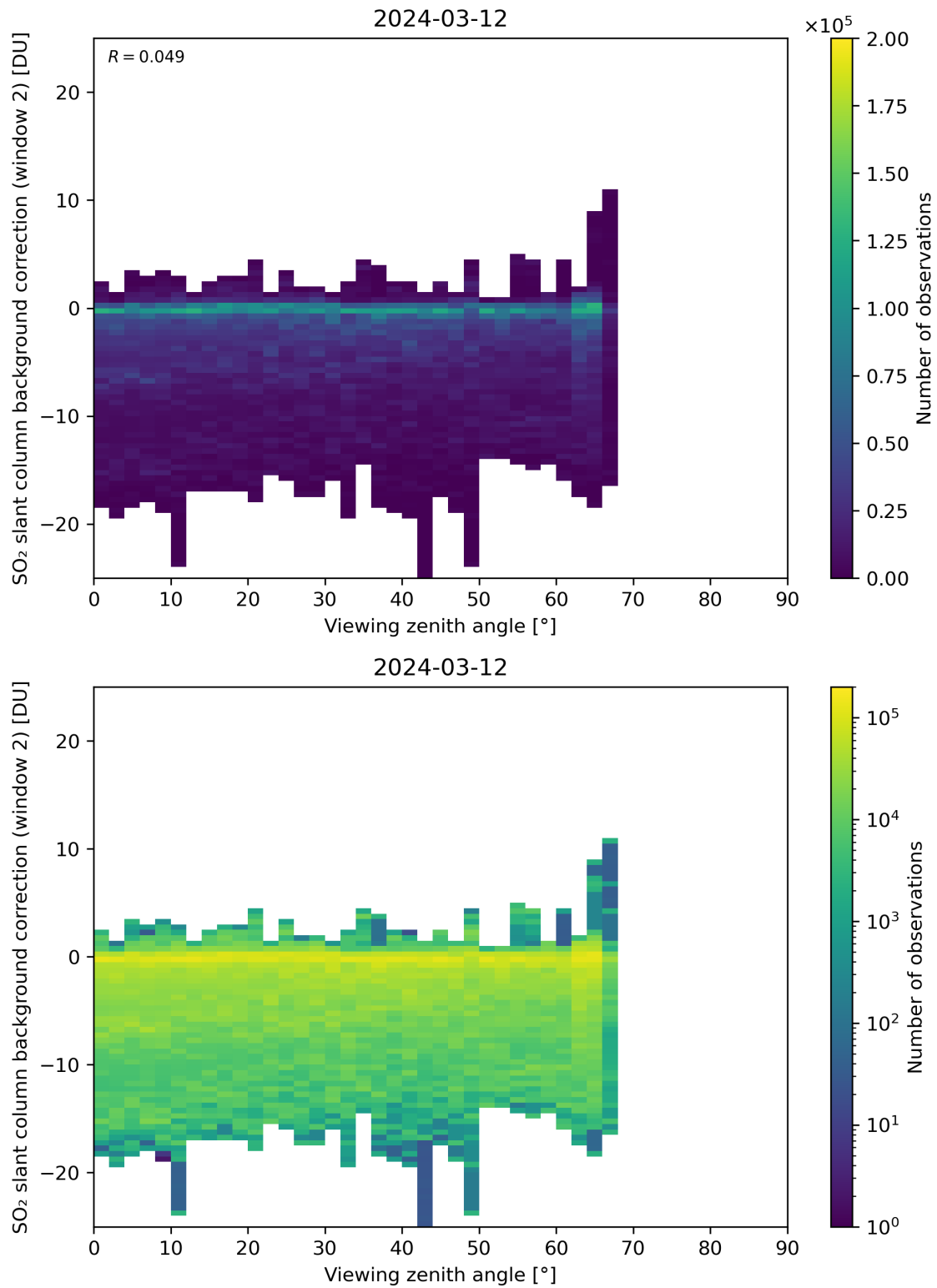
Figure 309: Scatter density plot of “Viewing zenith angle” against “SO 2 slant column background correction (window 2)” for 2024-03-11 to 2024-03-13.
