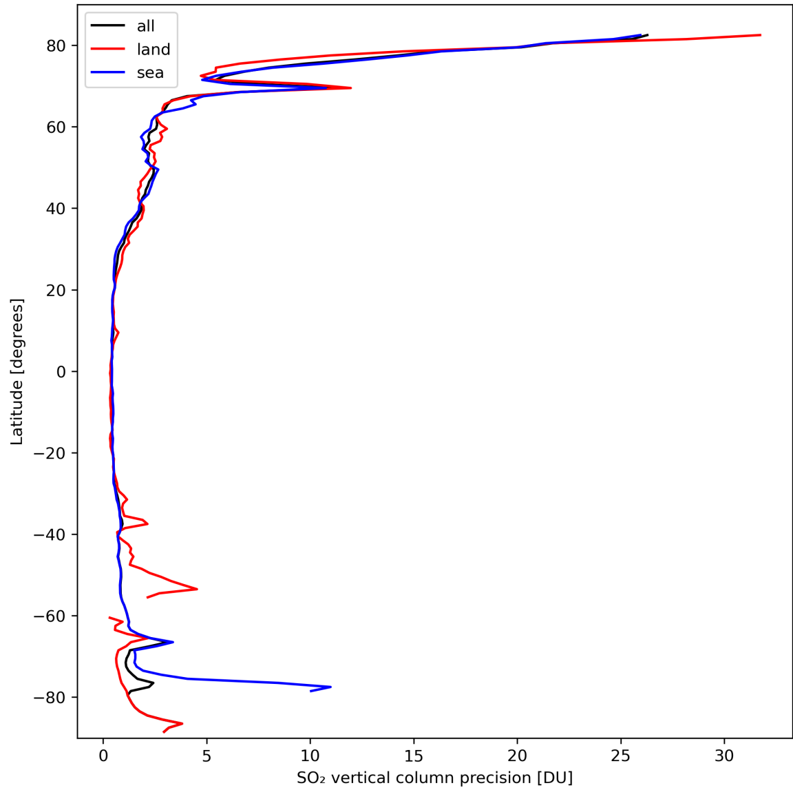
Figure 31: Zonal average of “SO 2 vertical column precision” for 2024-03-11 to 2024-03-13.
