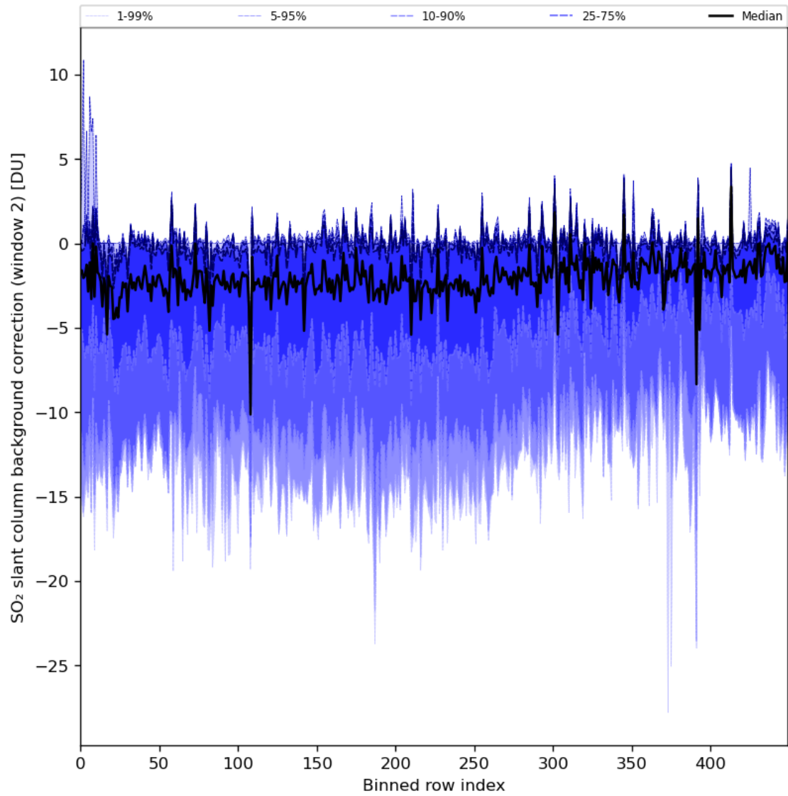
Figure 86: Along track statistics of “SO 2 slant column background correction (window 2)” for 2024-03-11 to 2024-03-13
