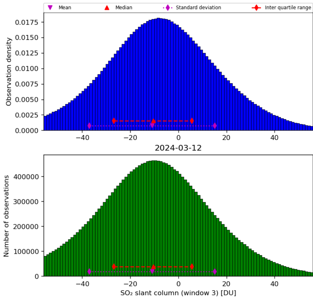
Figure 64: Histogram of “SO 2 slant column (window 3)” for 2024-03-11 to 2024-03-13
