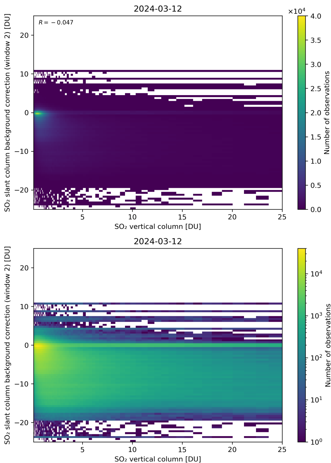
Figure 274: Scatter density plot of “SO 2 vertical column” against “SO 2 slant column background correction (window 2)” for 2024-03-11 to 2024-03-13.
