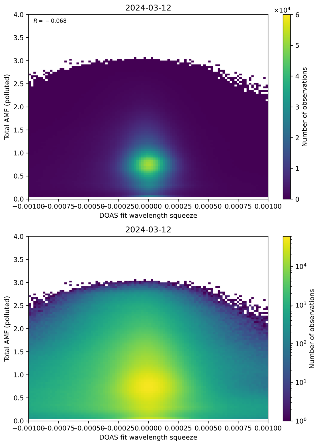
Figure 134: Scatter density plot of “DOAS fit wavelength squeeze” against “Total AMF (polluted)” for 2024-03-11 to 2024-03-13.
