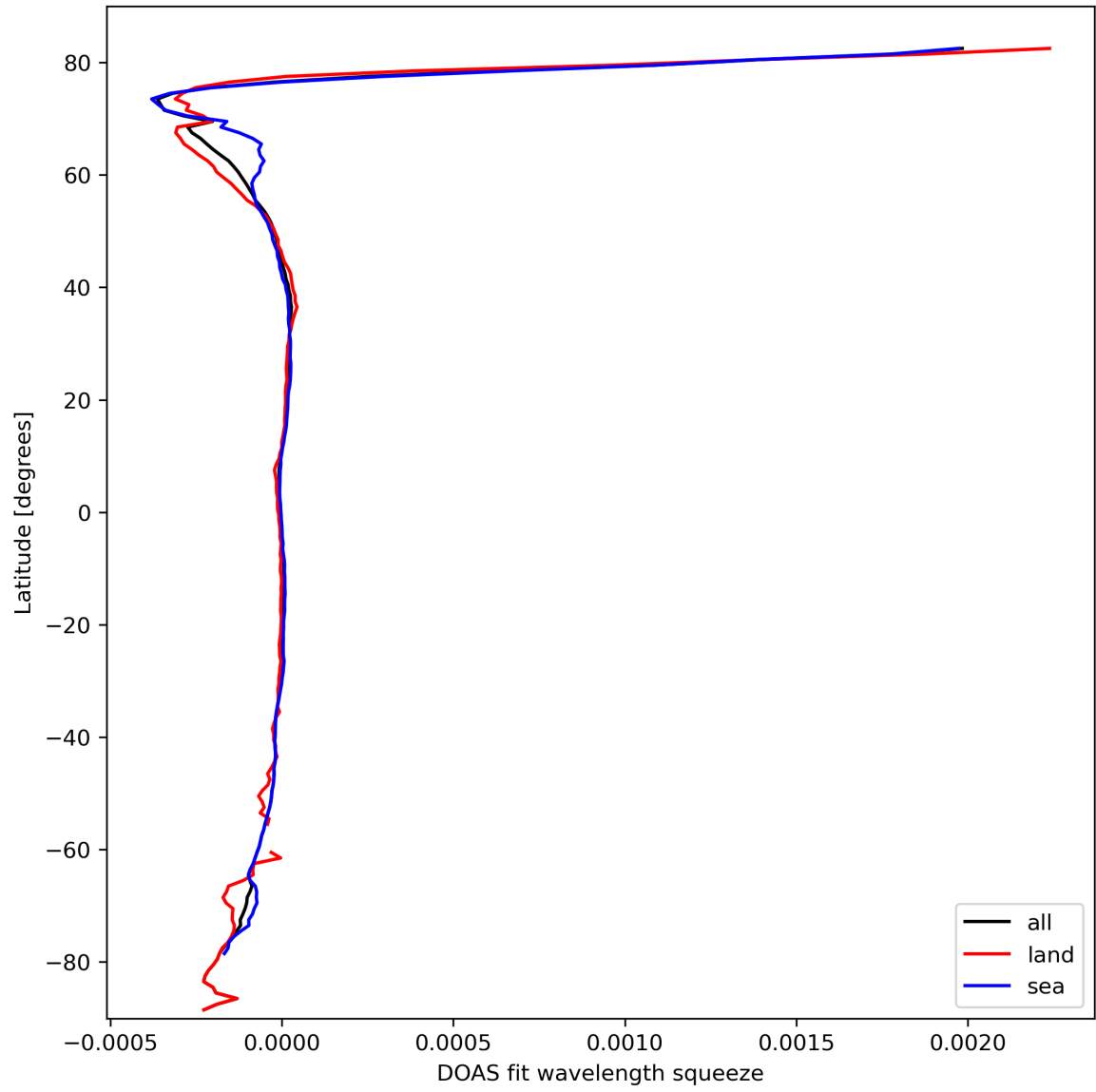
Figure 46: Zonal average of “DOAS fit wavelength squeeze” for 2024-03-11 to 2024-03-13.
