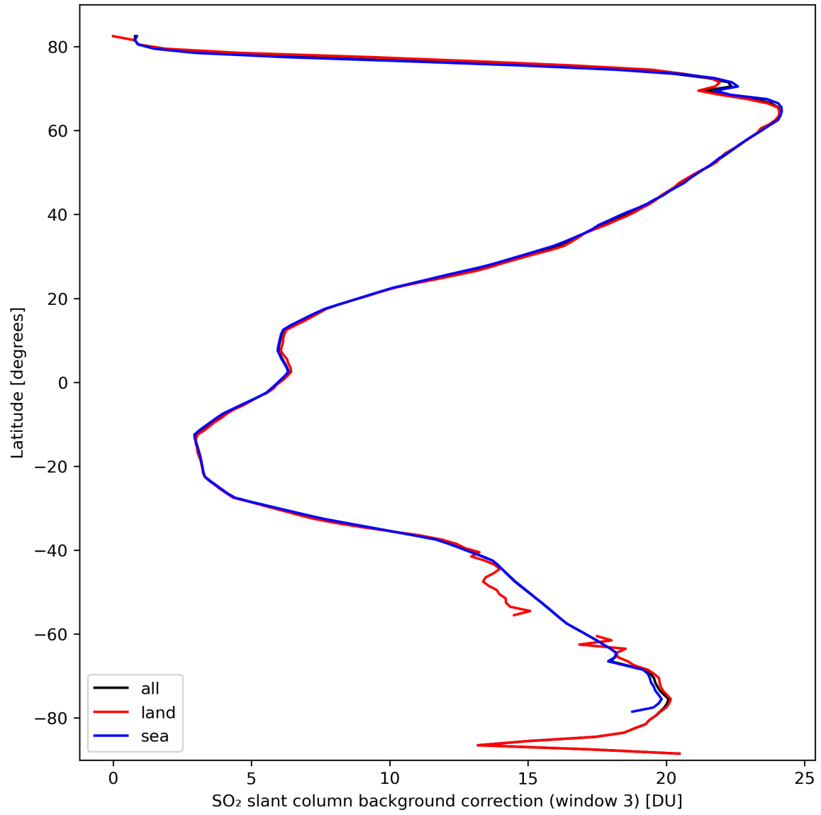
Figure 44: Zonal average of “SO 2 slant column background correction (window 3)” for 2024-03-11 to 2024-03-13.
