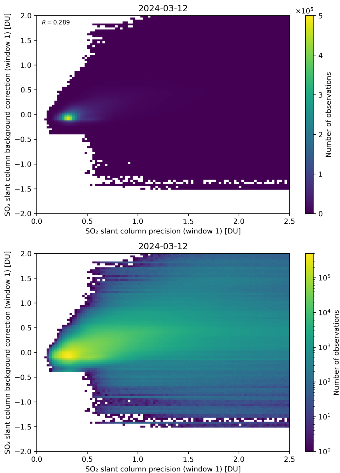
Figure 218: Scatter density plot of “SO 2 slant column precision (window 1)” against “SO 2 slant column background correction (window 1)” for 2024-03-11 to 2024-03-13.
