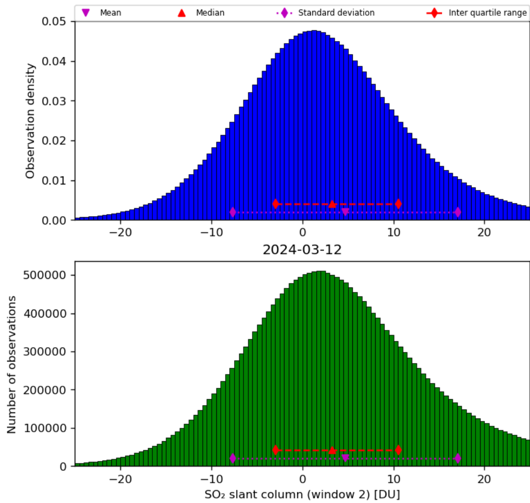
Figure 60: Histogram of “SO 2 slant column (window 2)” for 2024-03-11 to 2024-03-13
