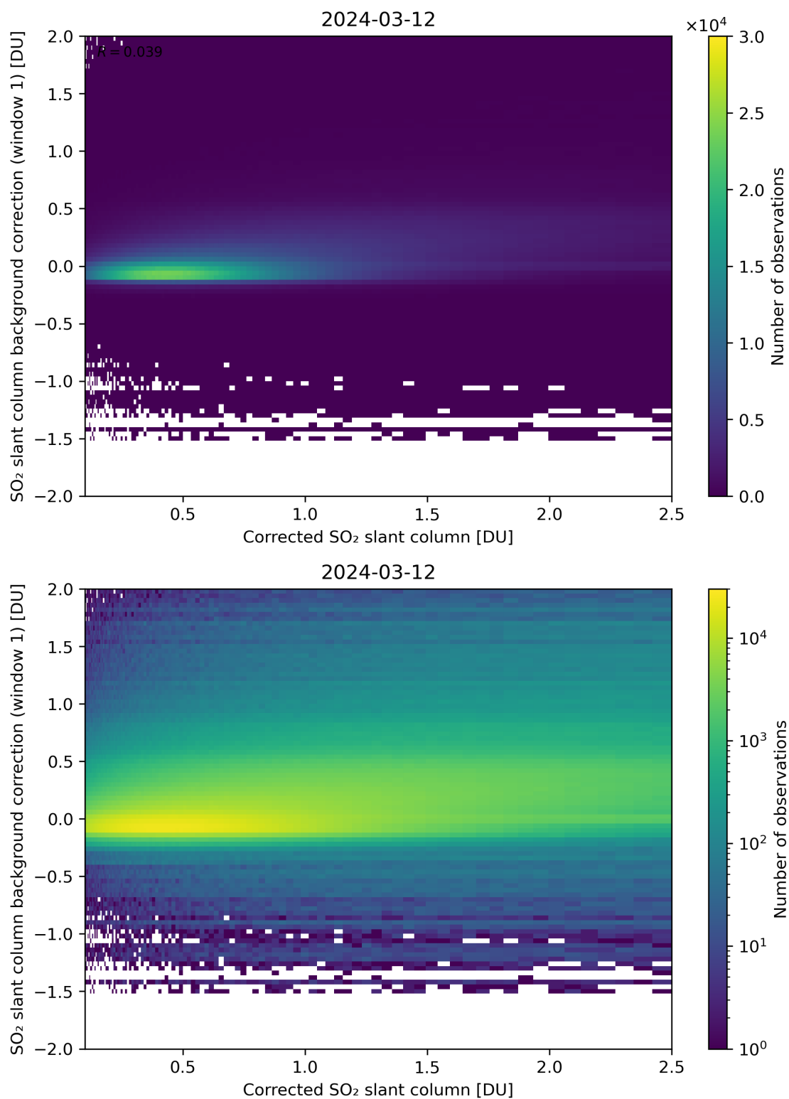
Figure 178: Scatter density plot of “Corrected SO 2 slant column” against “SO 2 slant column background correction (window 1)” for 2024-03-11 to 2024-03-13.
