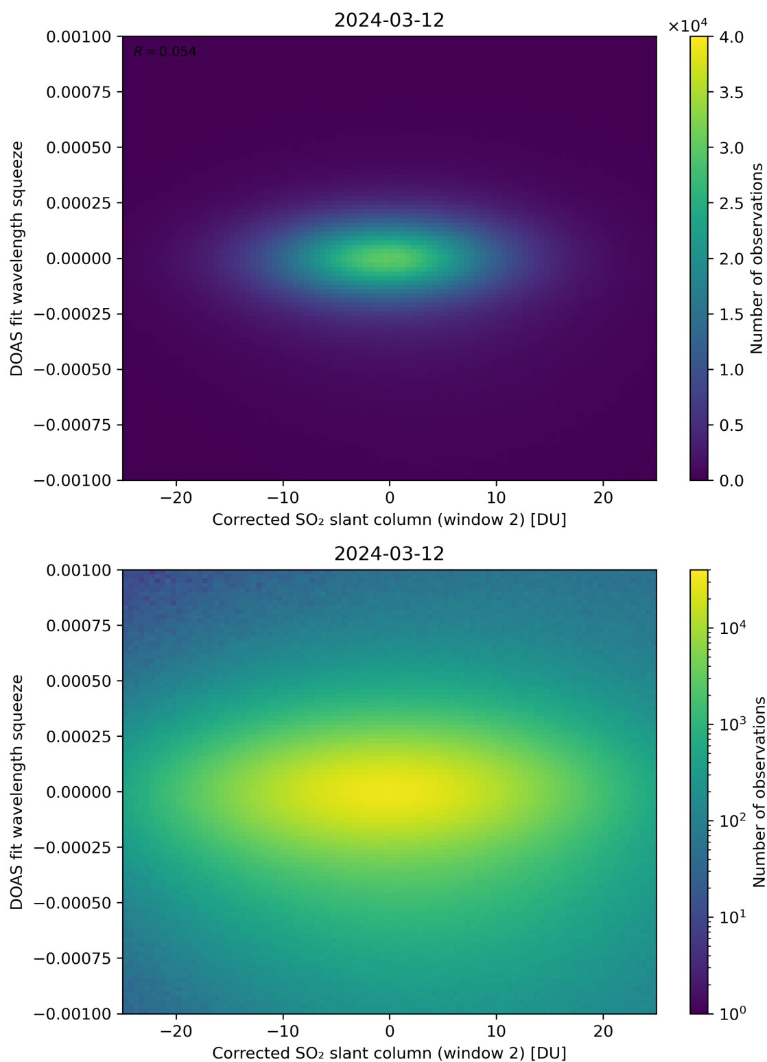
Figure 197: Scatter density plot of “Corrected SO 2 slant column (window 2)” against “DOAS fit wavelength squeeze” for 2024-03-11 to 2024-03-13.
