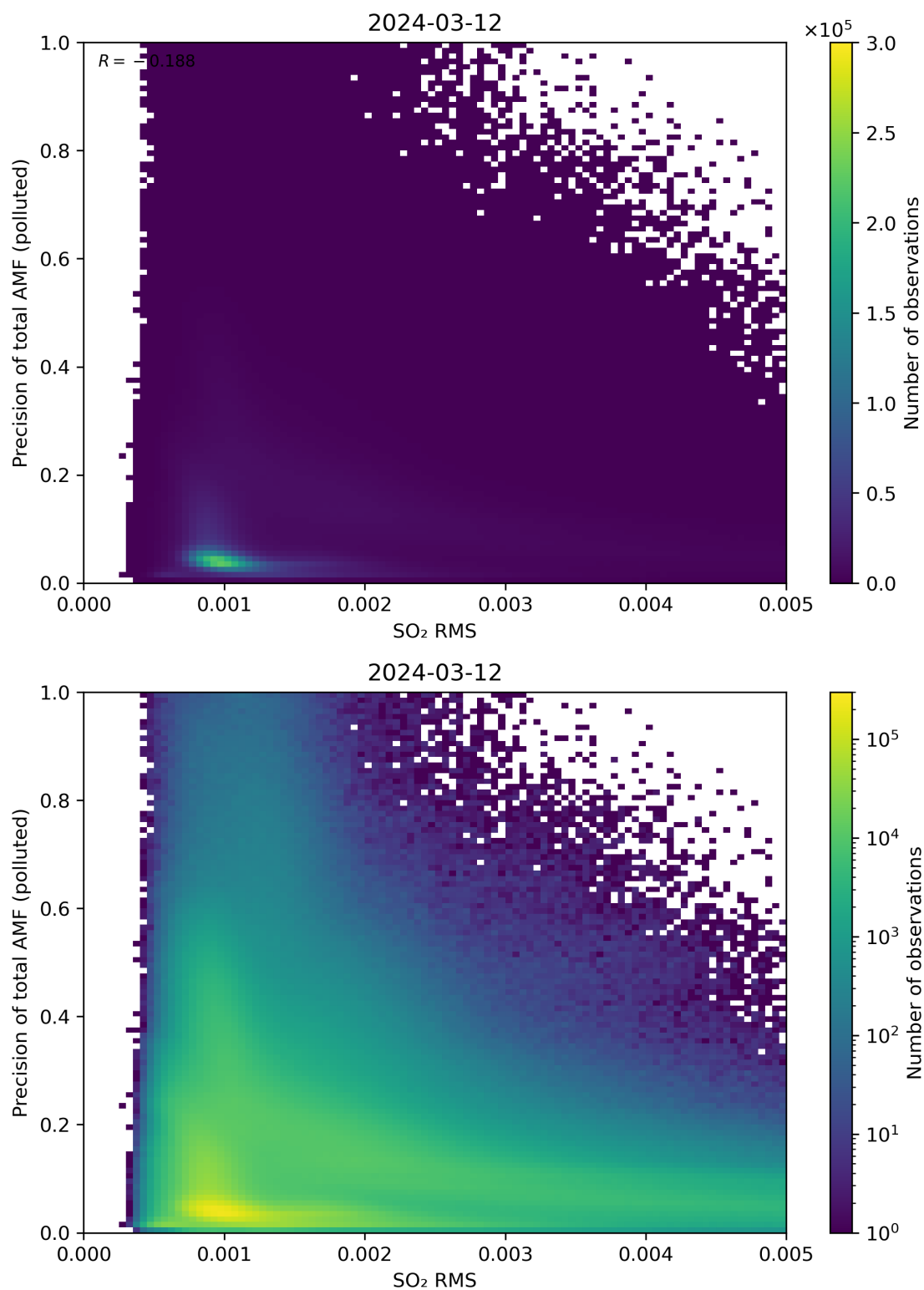
Figure 138: Scatter density plot of “SO 2 RMS” against “Precision of total AMF (polluted)” for 2024-03-11 to 2024-03-13.
