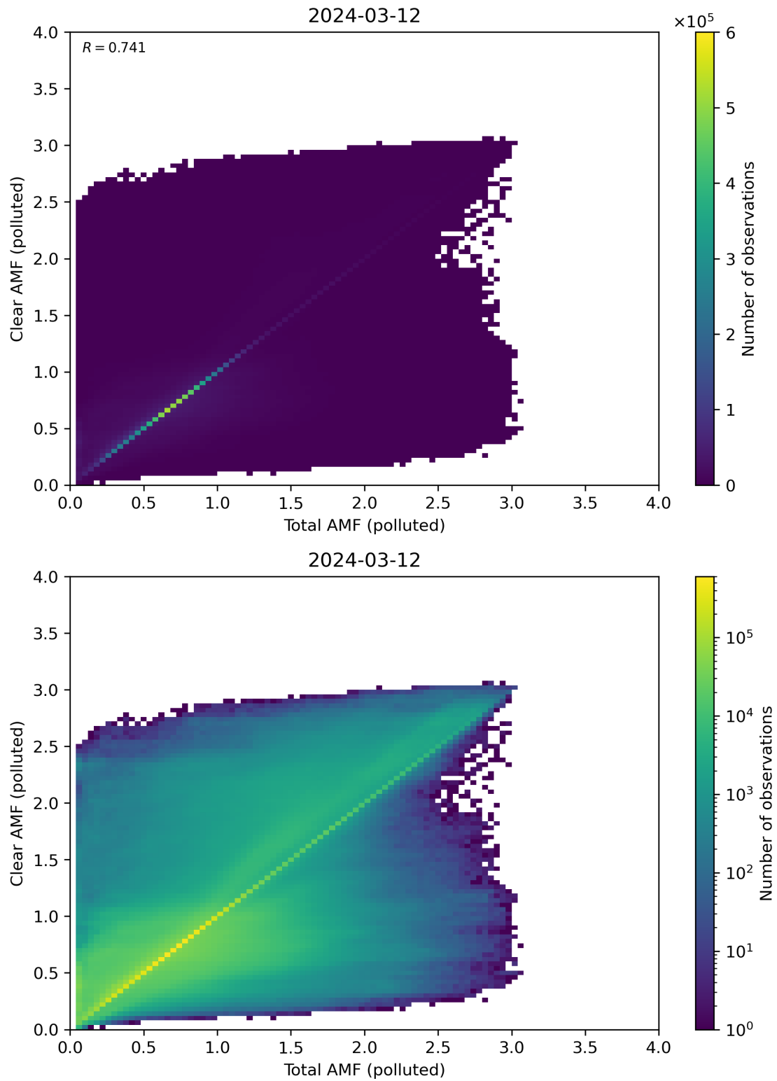
Figure 271: Scatter density plot of “Total AMF (polluted)” against “Clear AMF (polluted)” for 2024-03-11 to 2024-03-13.
