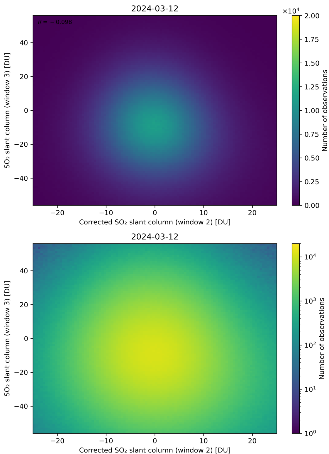
Figure 201: Scatter density plot of “Corrected SO 2 slant column (window 2)” against “SO 2 slant column (window 3)” for 2024-03-11 to 2024-03-13.
