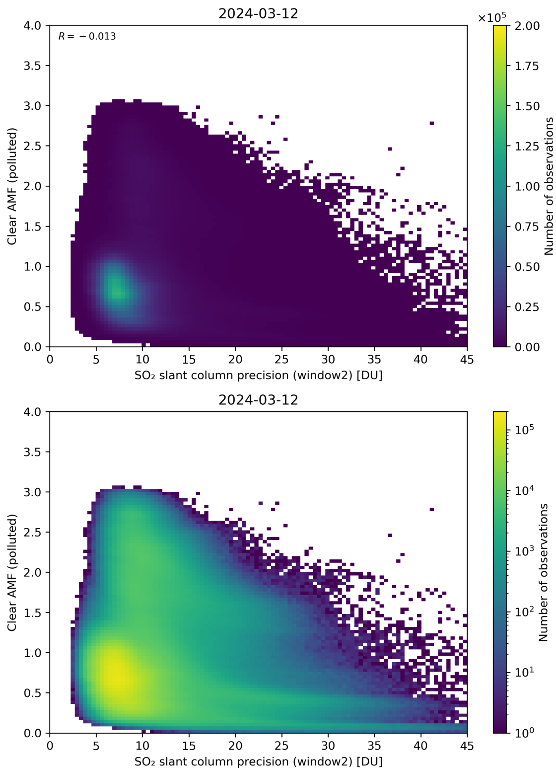
Figure 246: Scatter density plot of “SO 2 slant column precision (window2)” against “Clear AMF (polluted)” for 2024-03-11 to 2024-03-13.
