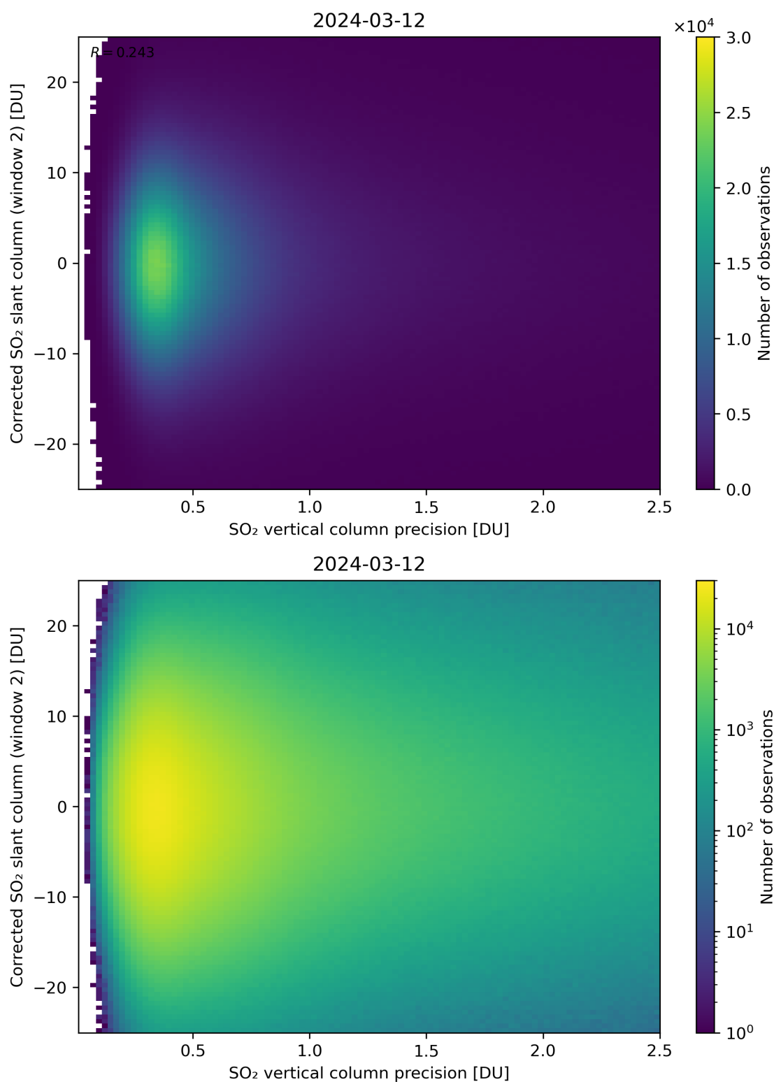
Figure 287: Scatter density plot of “SO 2 vertical column precision” against “Corrected SO 2 slant column (window 2)” for 2024-03-11 to 2024-03-13.
