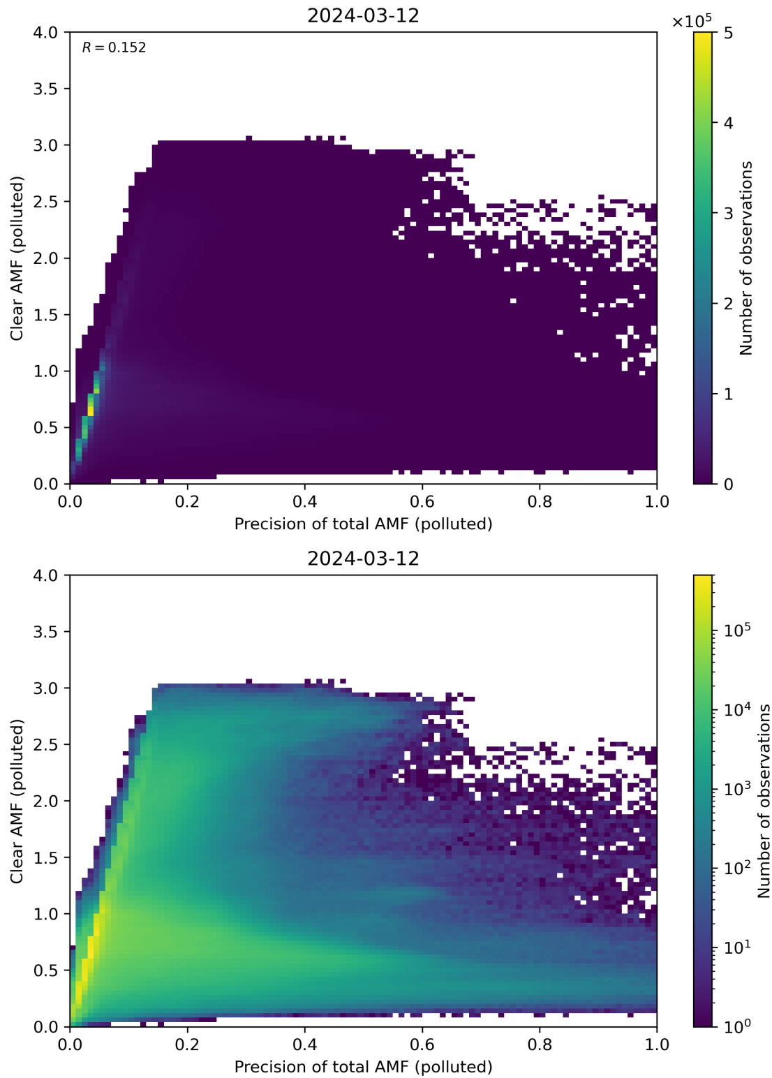
Figure 270: Scatter density plot of “Precision of total AMF (polluted)” against “Clear AMF (polluted)” for 2024-03-11 to 2024-03-13.
