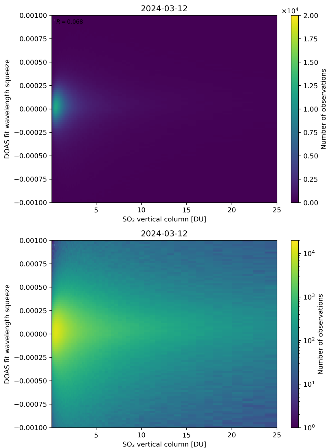
Figure 277: Scatter density plot of “SO 2 vertical column” against “DOAS fit wavelength squeeze” for 2024-03-11 to 2024-03-13.
