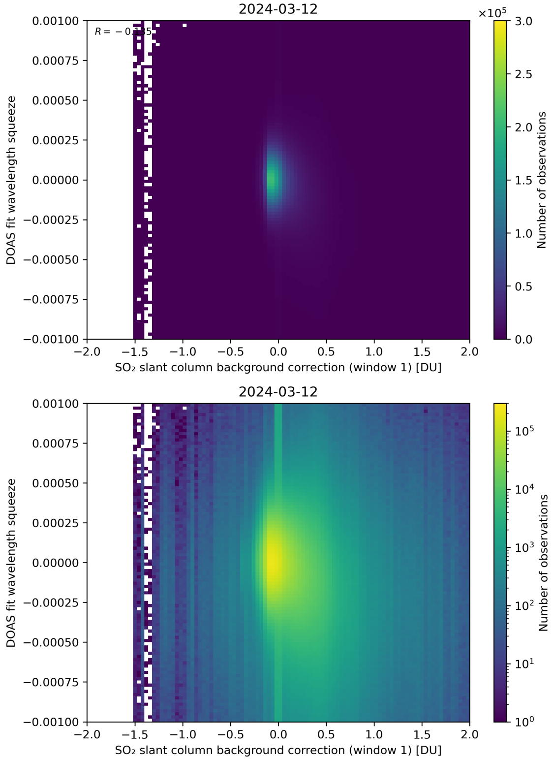
Figure 101: Scatter density plot of “SO 2 slant column background correction (window 1)” against “DOAS fit wavelength squeeze” for 2024-03-11 to 2024-03-13.
