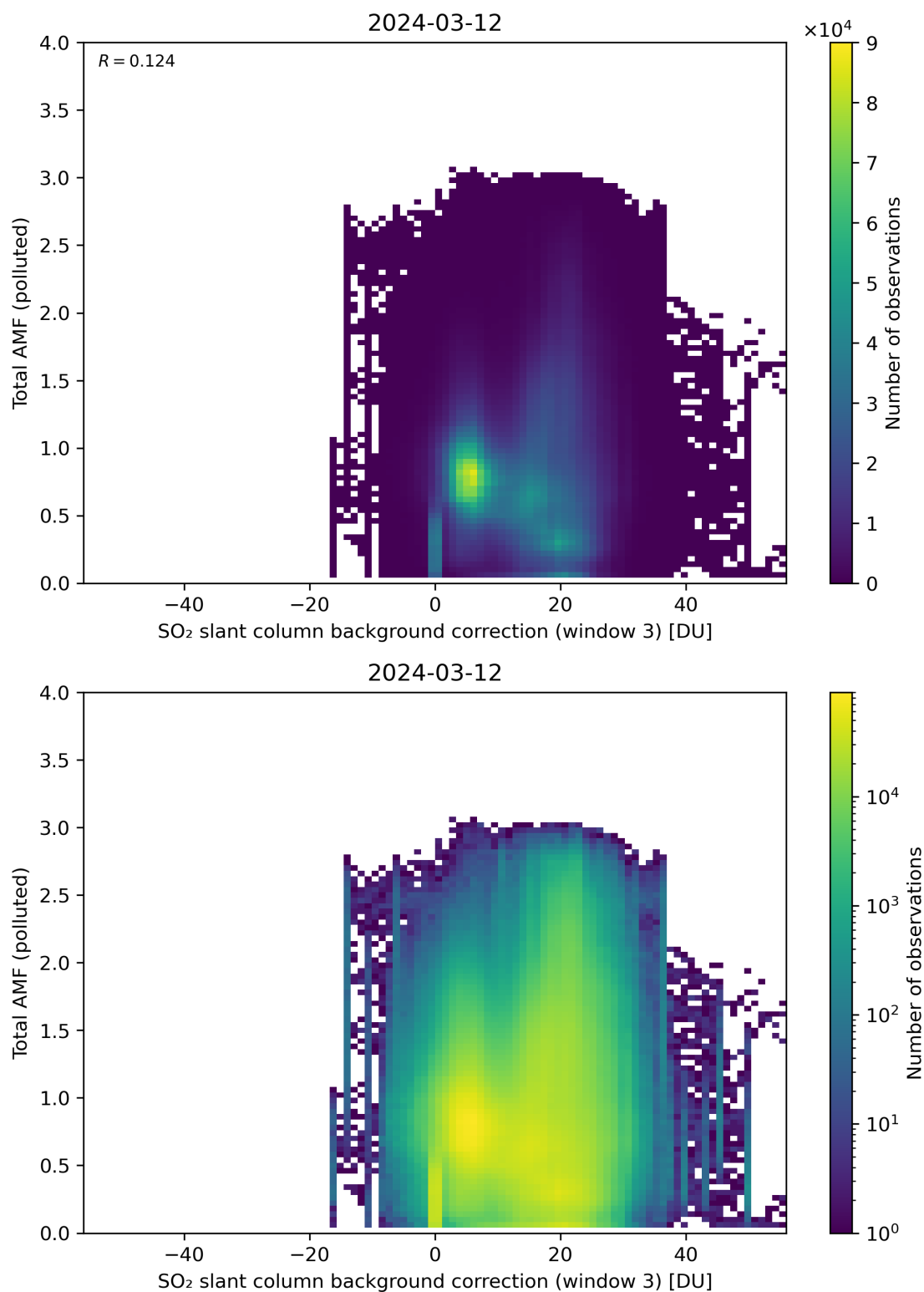
Figure 125: Scatter density plot of “SO 2 slant column background correction (window 3)” against “Total AMF (polluted)” for 2024-03-11 to 2024-03-13.
