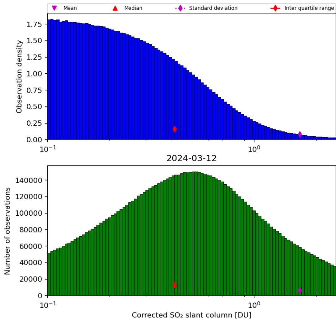
Figure 55: Histogram of “Corrected SO 2 slant column” for 2024-03-11 to 2024-03-13
