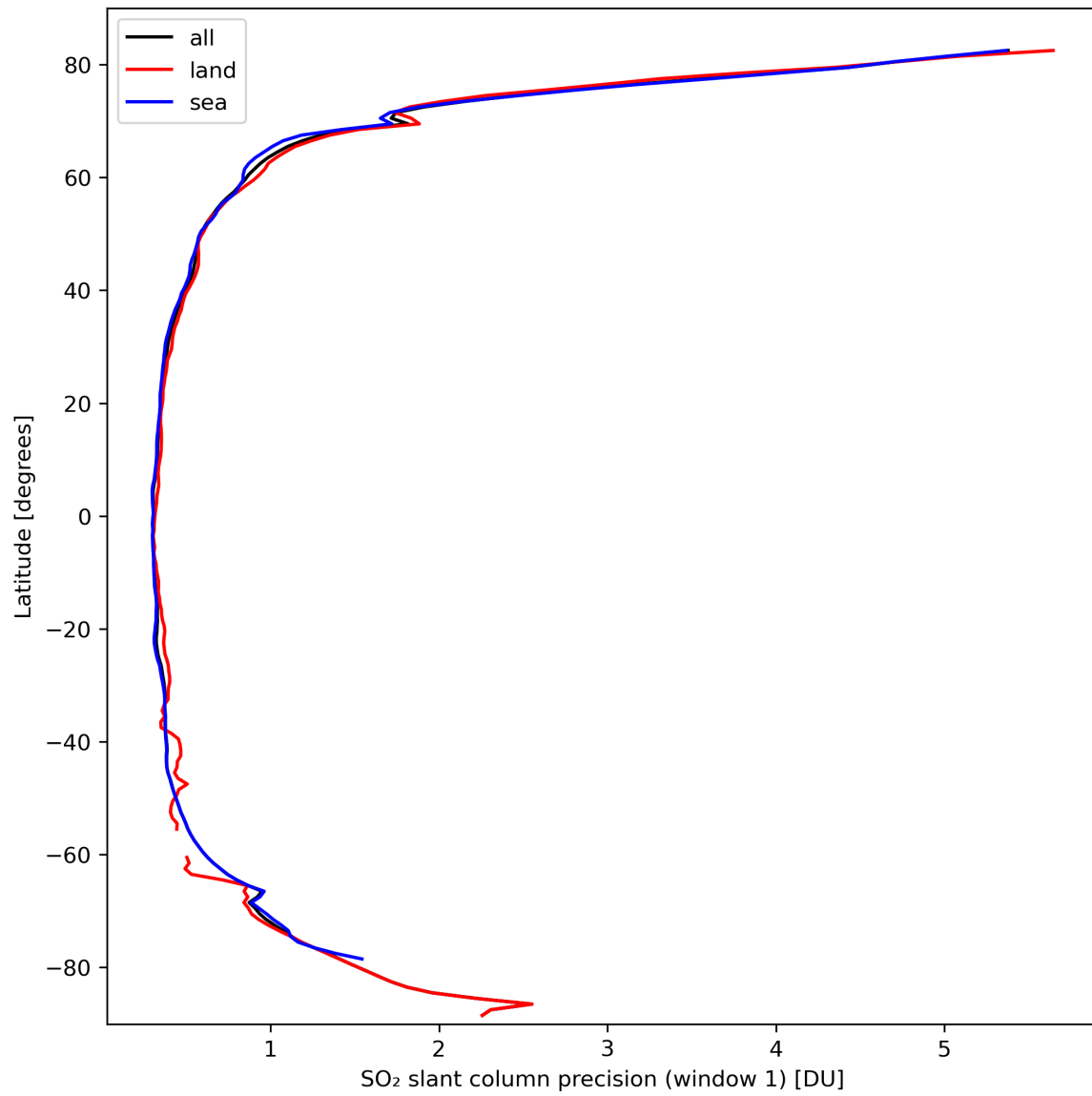
Figure 34: Zonal average of “SO 2 slant column precision (window 1)” for 2024-03-11 to 2024-03-13.
