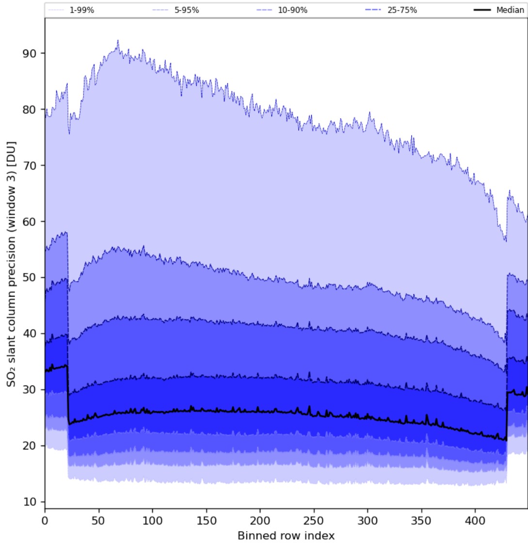
Figure 88: Along track statistics of “SO 2 slant column precision (window 3)” for 2024-03-11 to 2024-03-13
