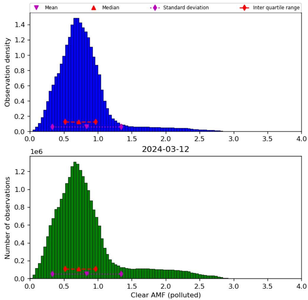
Figure 73: Histogram of “Clear AMF (polluted)” for 2024-03-11 to 2024-03-13
