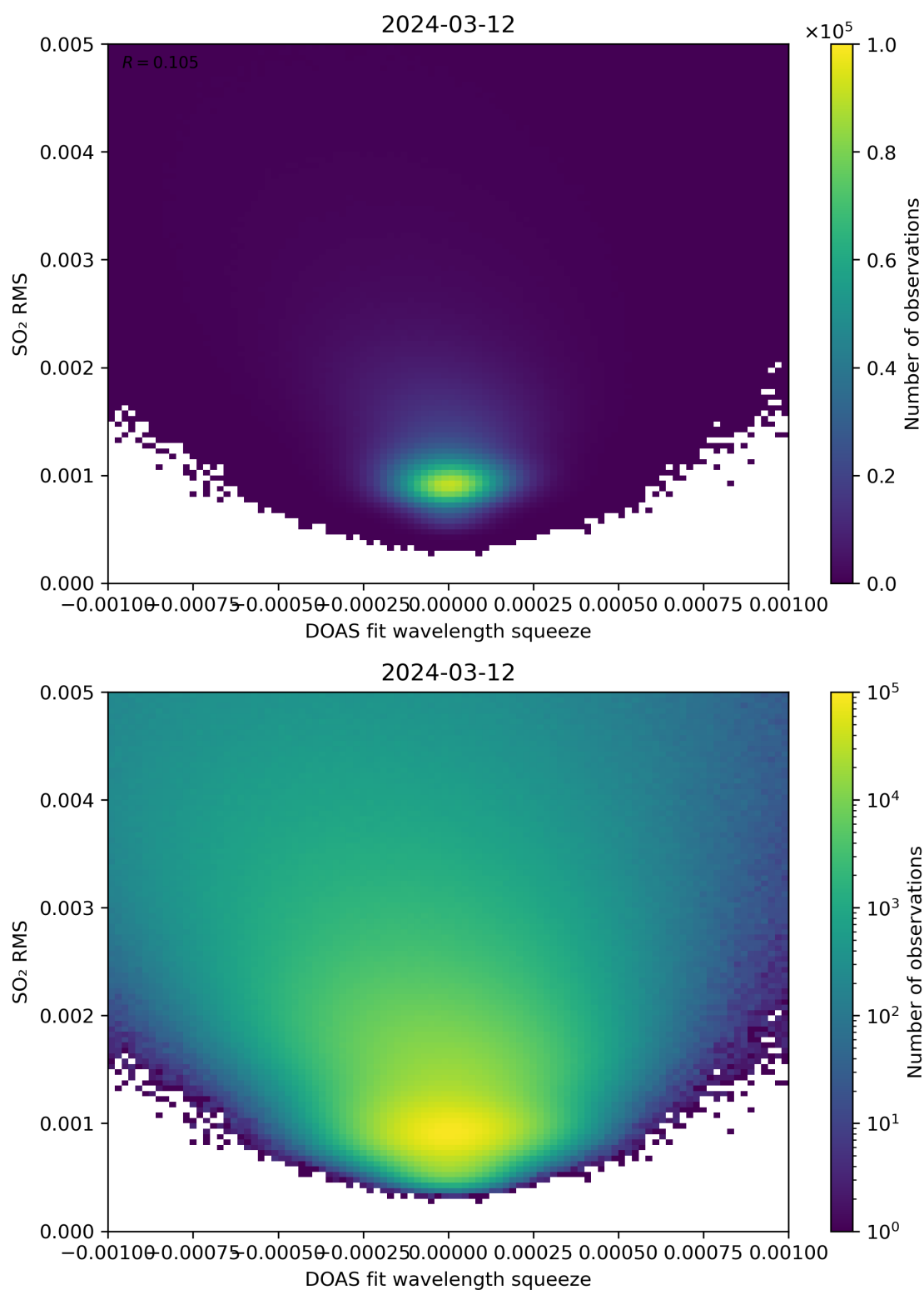
Figure 132: Scatter density plot of “DOAS fit wavelength squeeze” against “SO 2 RMS” for 2024-03-11 to 2024-03-13.
