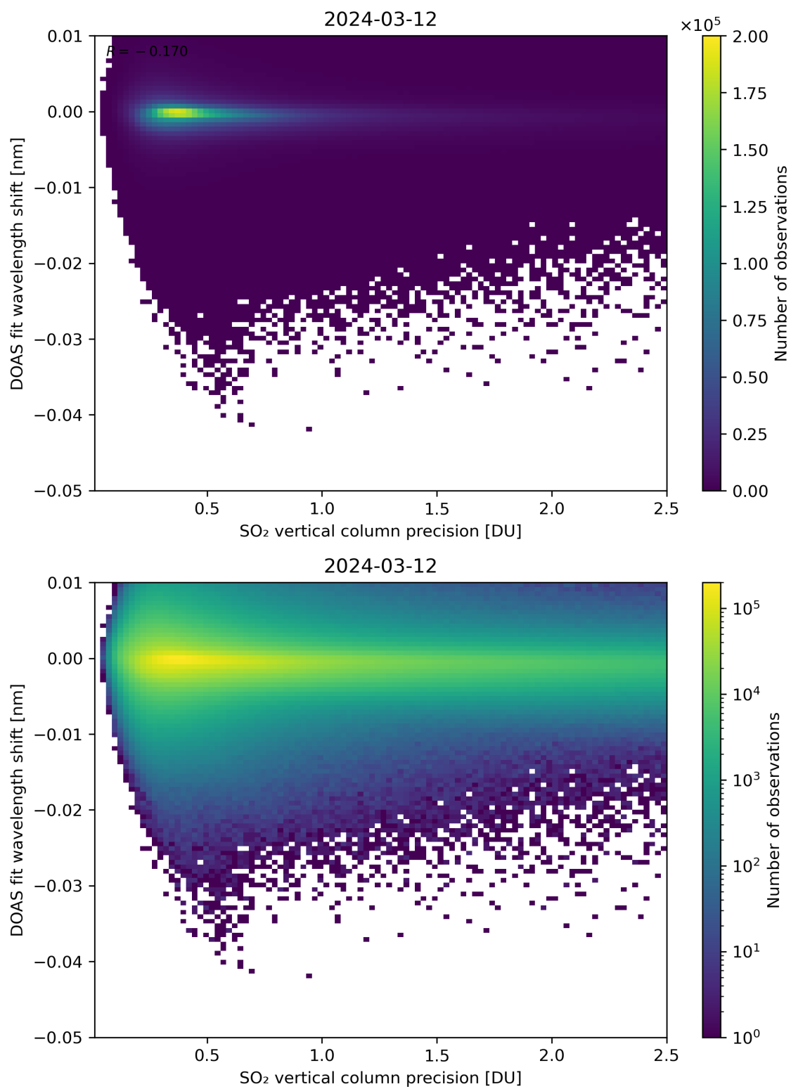
Figure 282: Scatter density plot of “SO 2 vertical column precision” against “DOAS fit wavelength shift” for 2024-03-11 to 2024-03-13.
