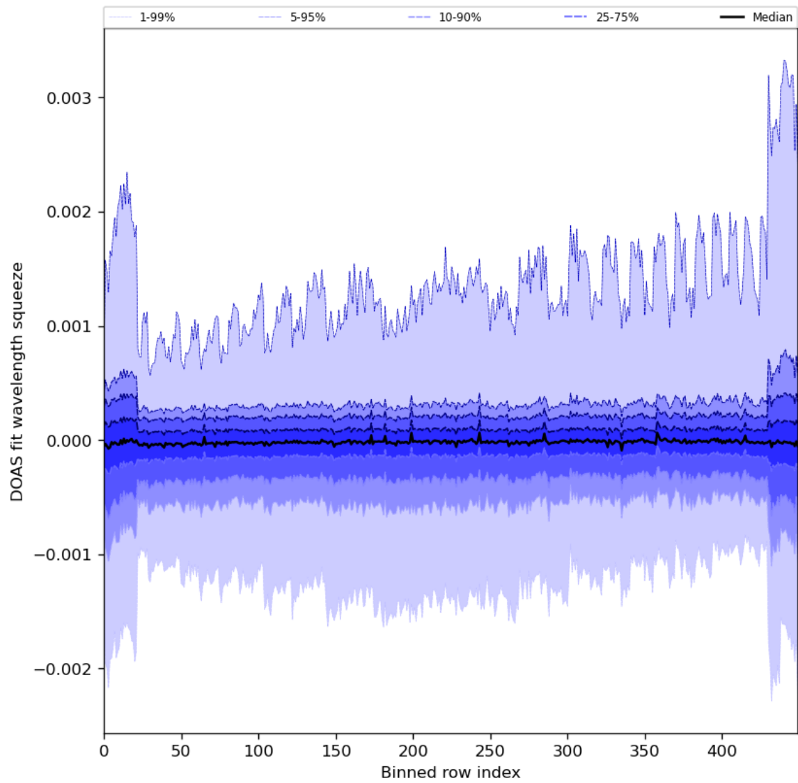
Figure 92: Along track statistics of “DOAS fit wavelength squeeze” for 2024-03-11 to 2024-03-13
