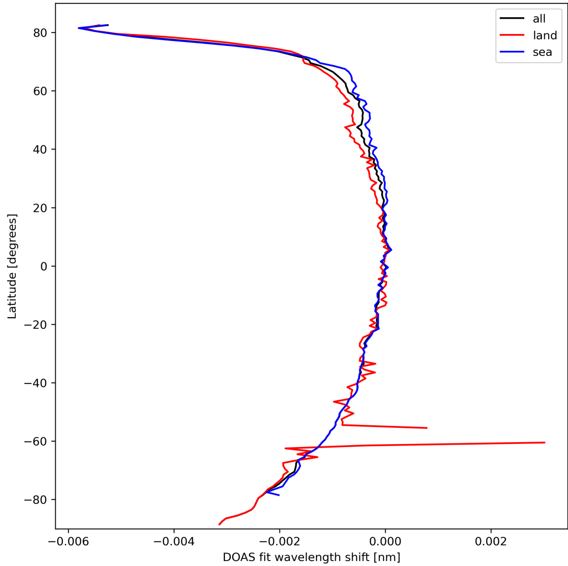
Figure 45: Zonal average of “DOAS fit wavelength shift” for 2024-03-11 to 2024-03-13.
