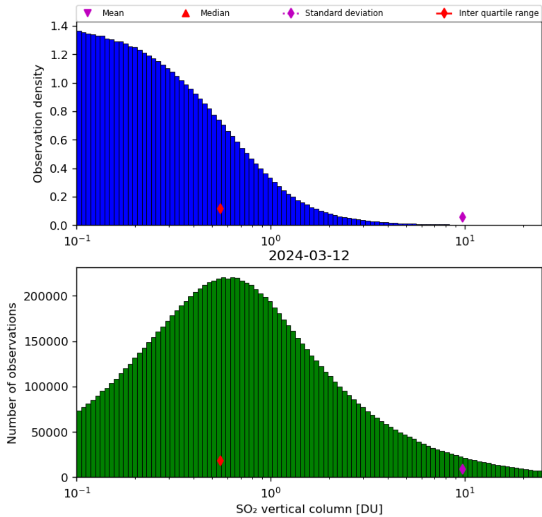
Figure 53: Histogram of “SO 2 vertical column” for 2024-03-11 to 2024-03-13
