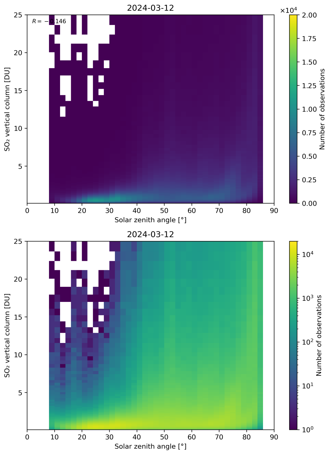
Figure 176: Scatter density plot of “Solar zenith angle” against “SO 2 vertical column” for 2024-03-11 to 2024-03-13.
