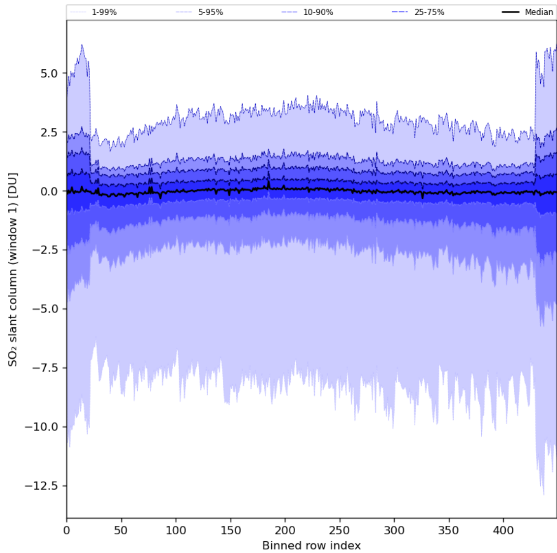
Figure 79: Along track statistics of "SO 2 slant column (window 1)" for 2024-03-11 to 2024-03-13
