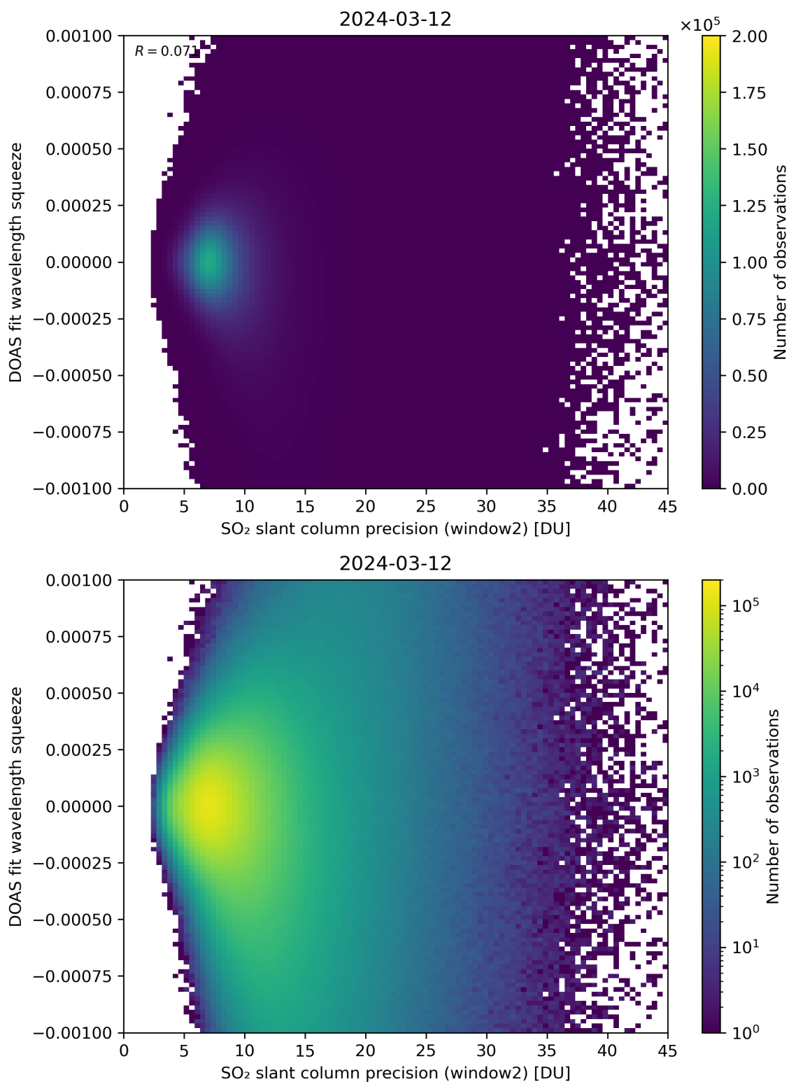
Figure 244: Scatter density plot of “SO 2 slant column precision (window2)” against “DOAS fit wavelength squeeze” for 2024-03-11 to 2024-03-13.
