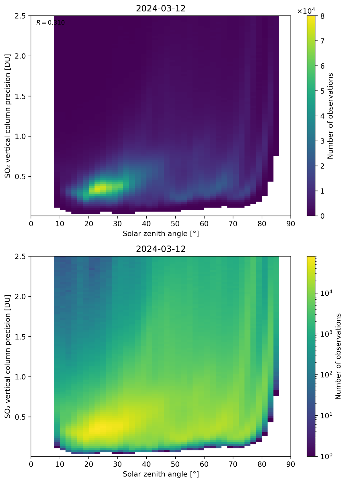
Figure 177: Scatter density plot of “Solar zenith angle” against “SO 2 vertical column precision” for 2024-03-11 to 2024-03-13.
