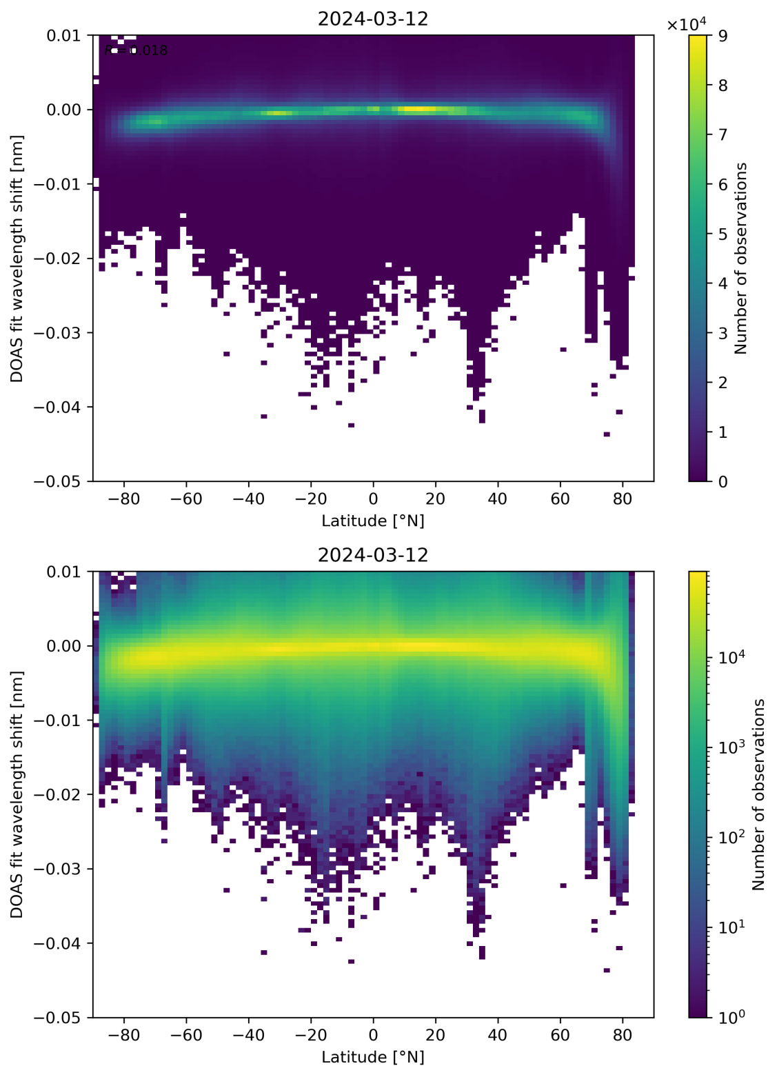
Figure 142: Scatter density plot of “Latitude” against “DOAS fit wavelength shift” for 2024-03-11 to 2024-03-13.
