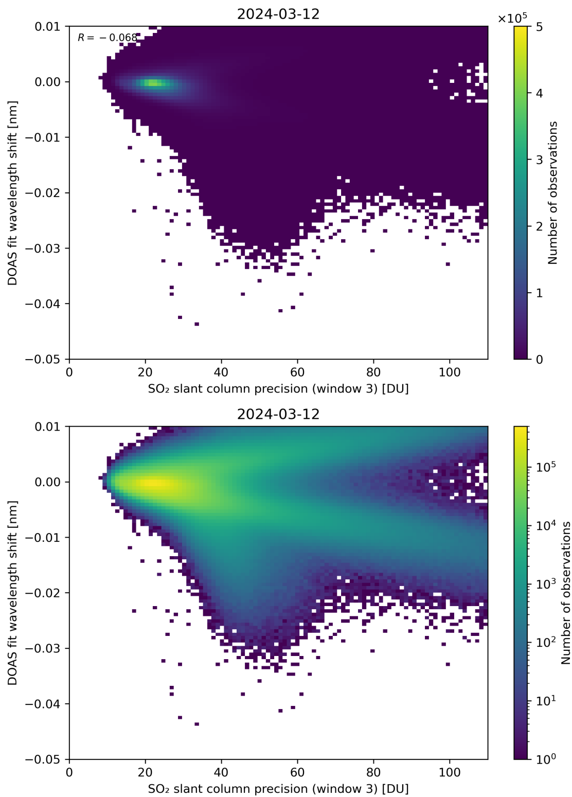
Figure 258: Scatter density plot of “SO 2 slant column precision (window 3)” against “DOAS fit wavelength shift” for 2024-03-11 to 2024-03-13.
