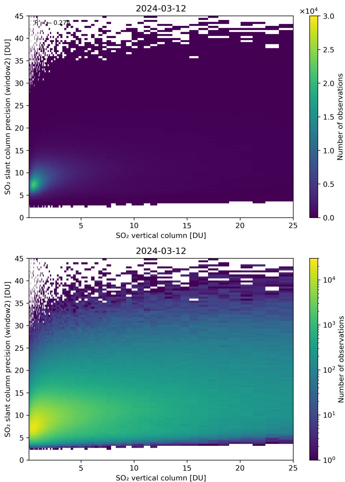
Figure 302: Scatter density plot of “SO 2 vertical column” against “SO 2 slant column precision (window2)” for 2024-03-11 to 2024-03-13.
