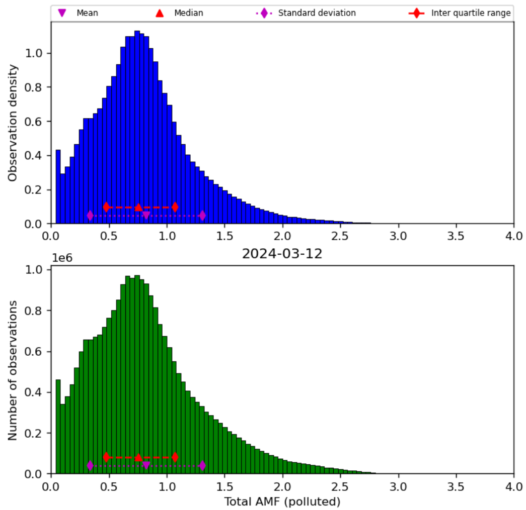
Figure 71: Histogram of “Total AMF (polluted)” for 2024-03-11 to 2024-03-13
