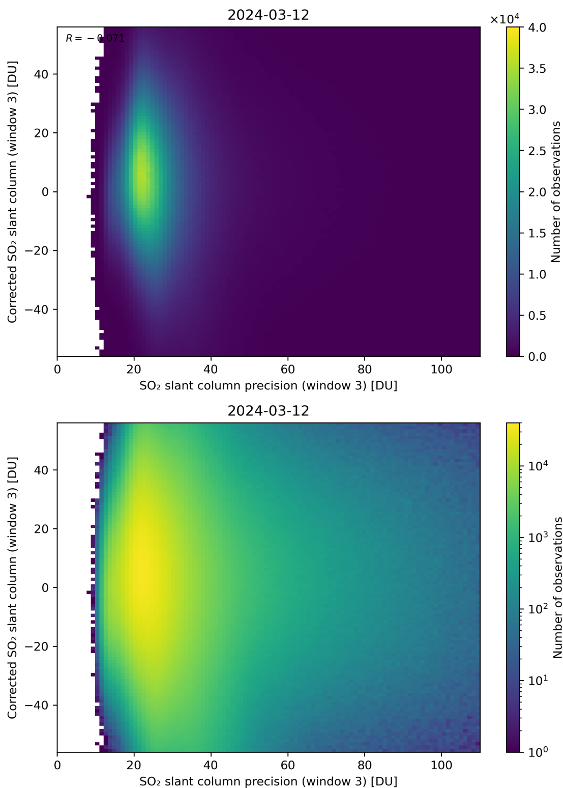
Figure 262: Scatter density plot of “SO 2 slant column precision (window 3)” against “Corrected SO 2 slant column (window 3)” for 2024-03-11 to 2024-03-13.
