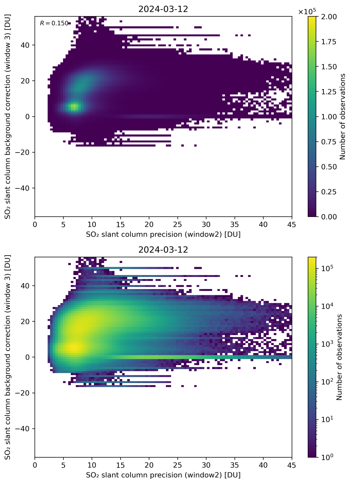
Figure 242: Scatter density plot of “SO 2 slant column precision (window2)” against “SO 2 slant column background correction (window 3)” for 2024-03-11 to 2024-03-13.
