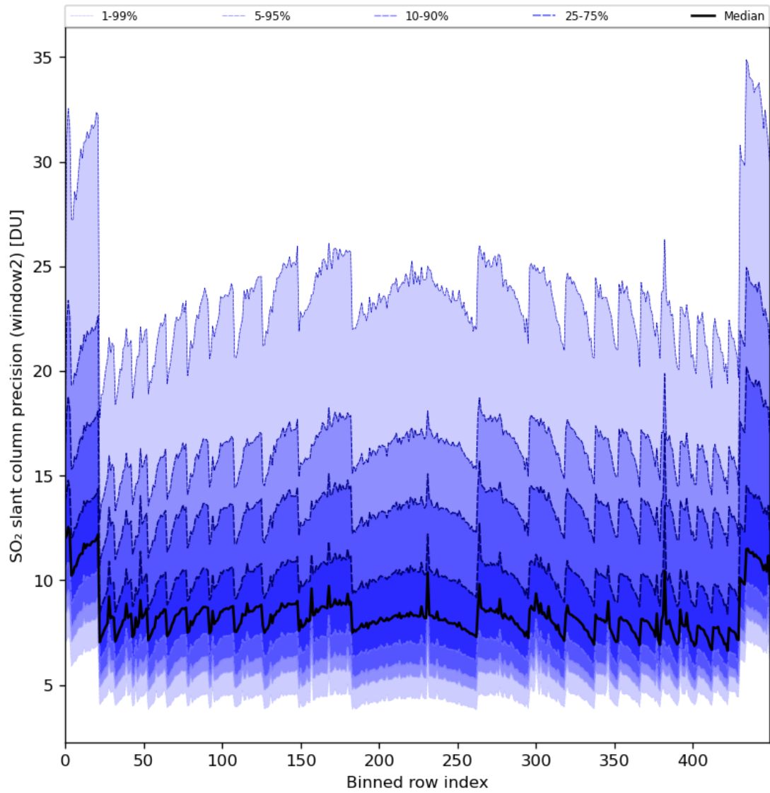
Figure 84: Along track statistics of “SO 2 slant column precision (window2)” for 2024-03-11 to 2024-03-13
