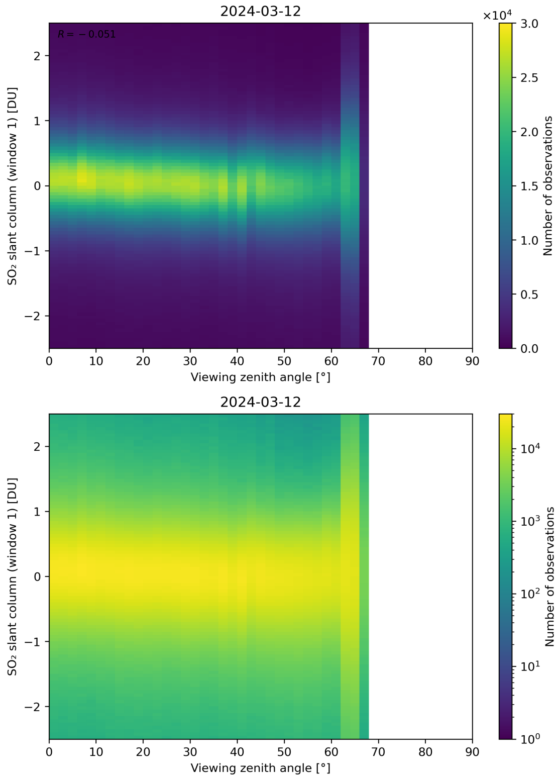
Figure 320: Scatter density plot of “Viewing zenith angle” against “SO 2 slant column (window 1)” for 2024-03-11 to 2024-03-13.
