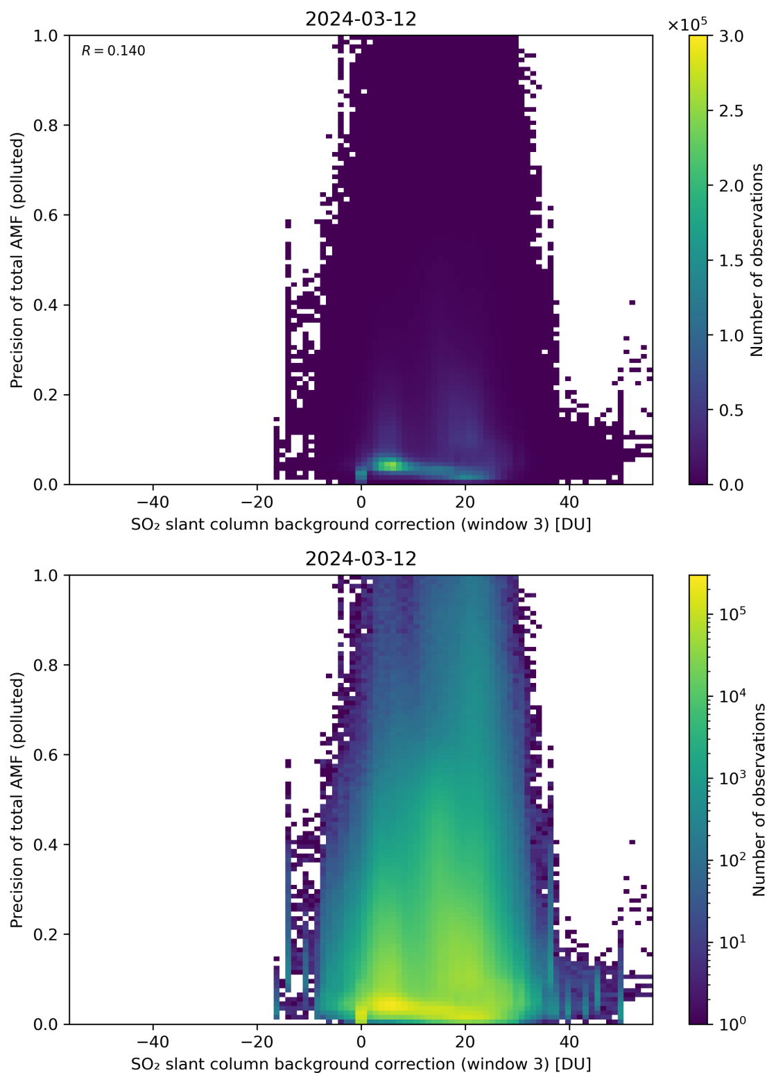
Figure 126: Scatter density plot of “SO 2 slant column background correction (window 3)” against “Precision of total AMF (polluted)” for 2024-03-11 to 2024-03-13.
