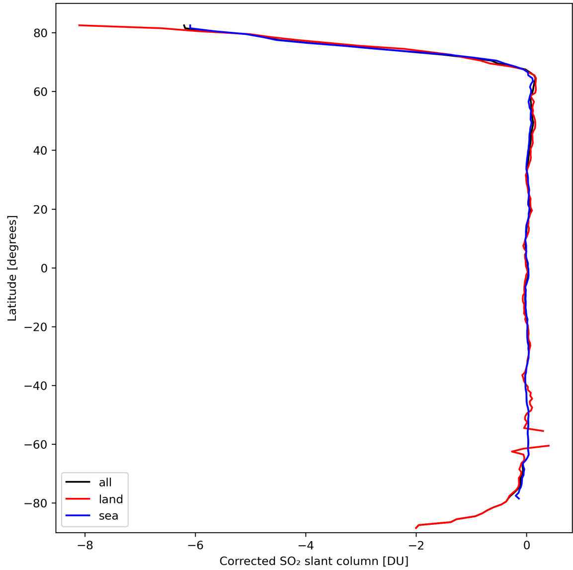
Figure 32: Zonal average of “Corrected SO 2 slant column” for 2024-03-11 to 2024-03-13.
