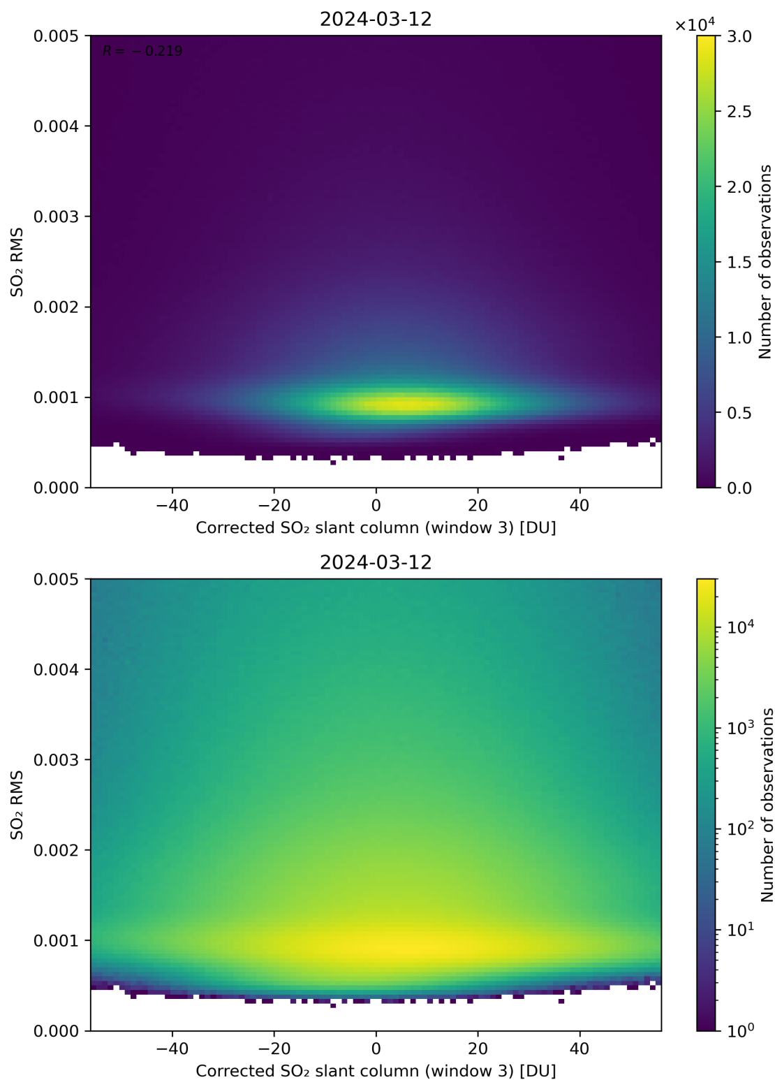
Figure 208: Scatter density plot of “Corrected SO 2 slant column (window 3)” against “SO 2 RMS” for 2024-03-11 to 2024-03-13.
