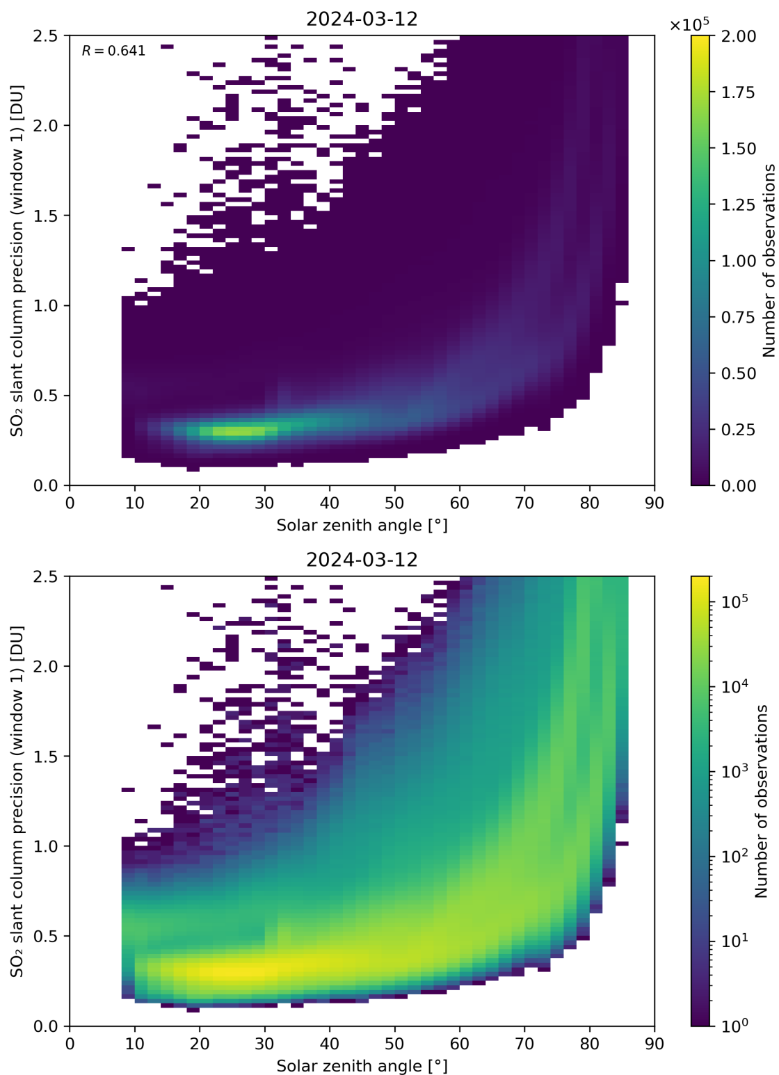
Figure 170: Scatter density plot of “Solar zenith angle” against “SO 2 slant column precision (window 1)” for 2024-03-11 to 2024-03-13.
