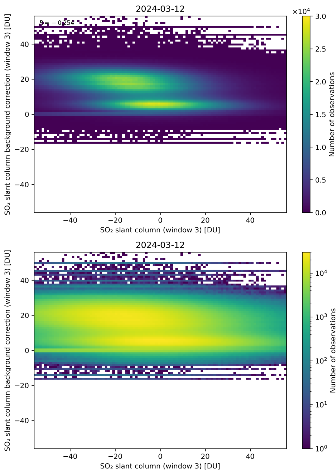
Figure 253: Scatter density plot of “SO 2 slant column (window 3)” against “SO 2 slant column background correction (window 3)” for 2024-03-11 to 2024-03-13.
