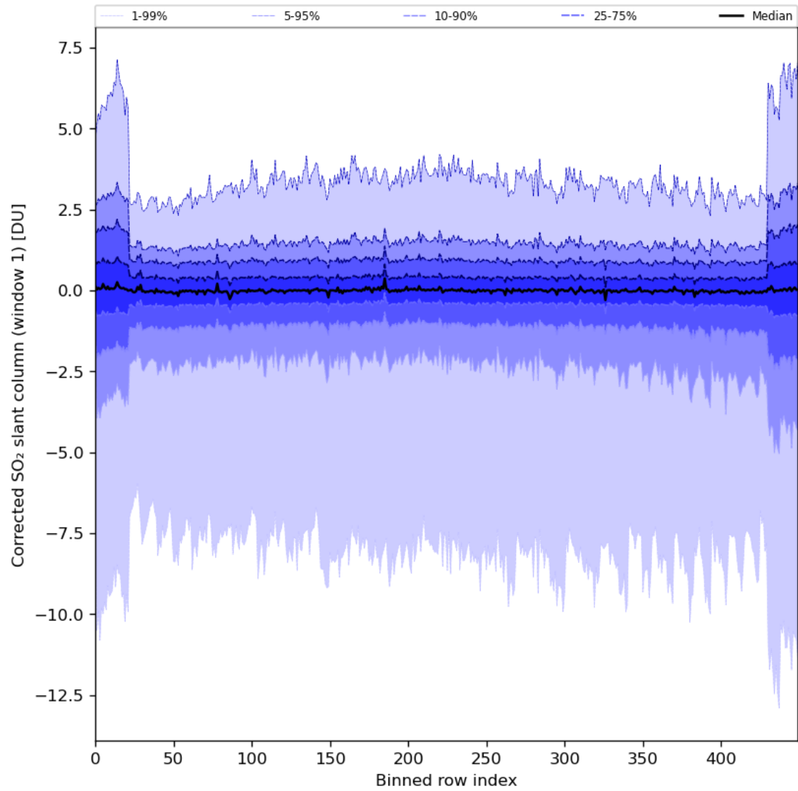
Figure 81: Along track statistics of “Corrected SO 2 slant column (window 1)” for 2024-03-11 to 2024-03-13
