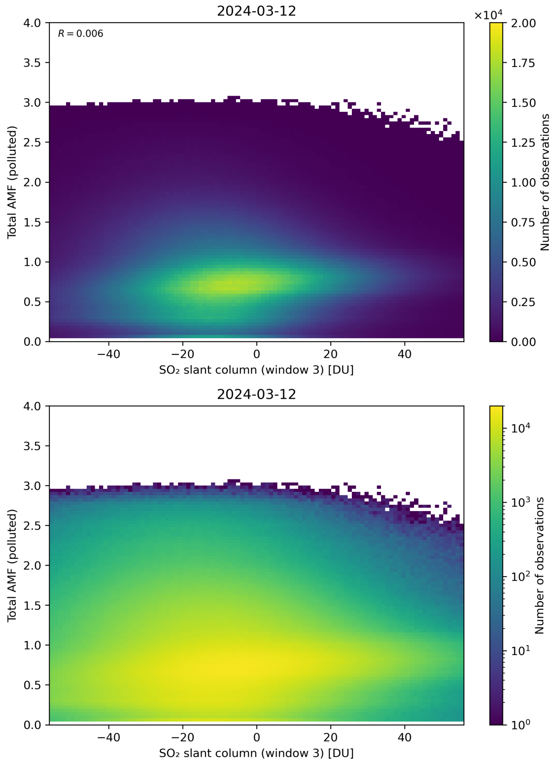
Figure 268: Scatter density plot of “SO 2 slant column (window 3)” against “Total AMF (polluted)” for 2024-03-11 to 2024-03-13.
