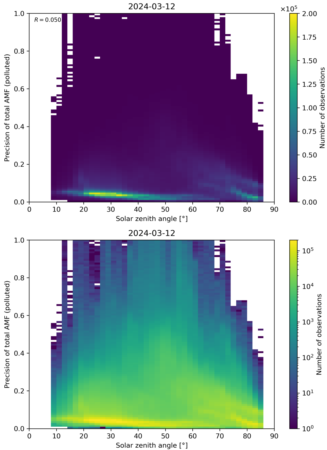
Figure 175: Scatter density plot of “Solar zenith angle” against “Precision of total AMF (polluted)” for 2024-03-11 to 2024-03-13.
