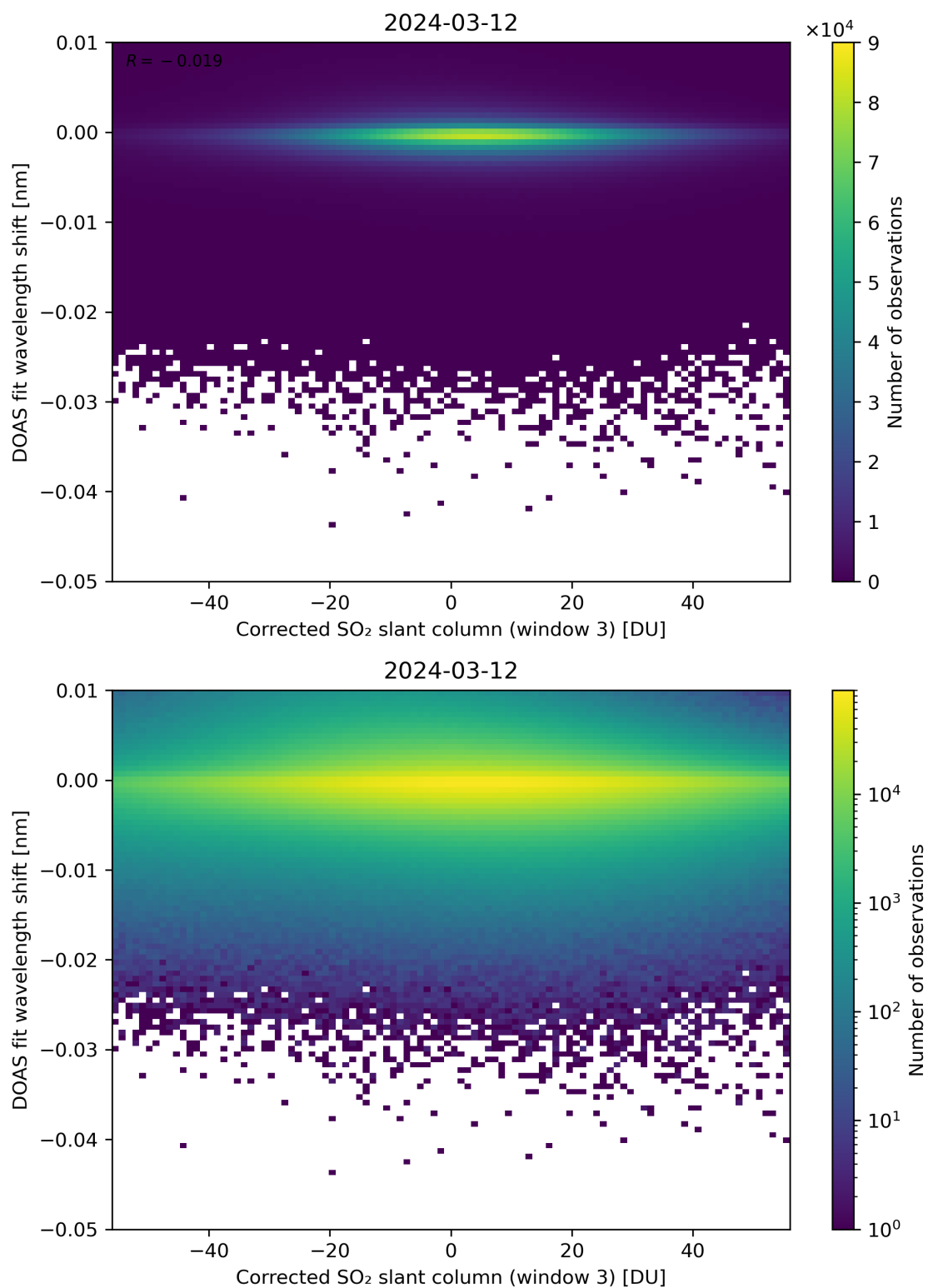
Figure 206: Scatter density plot of “Corrected SO 2 slant column (window 3)” against “DOAS fit wavelength shift” for 2024-03-11 to 2024-03-13.
