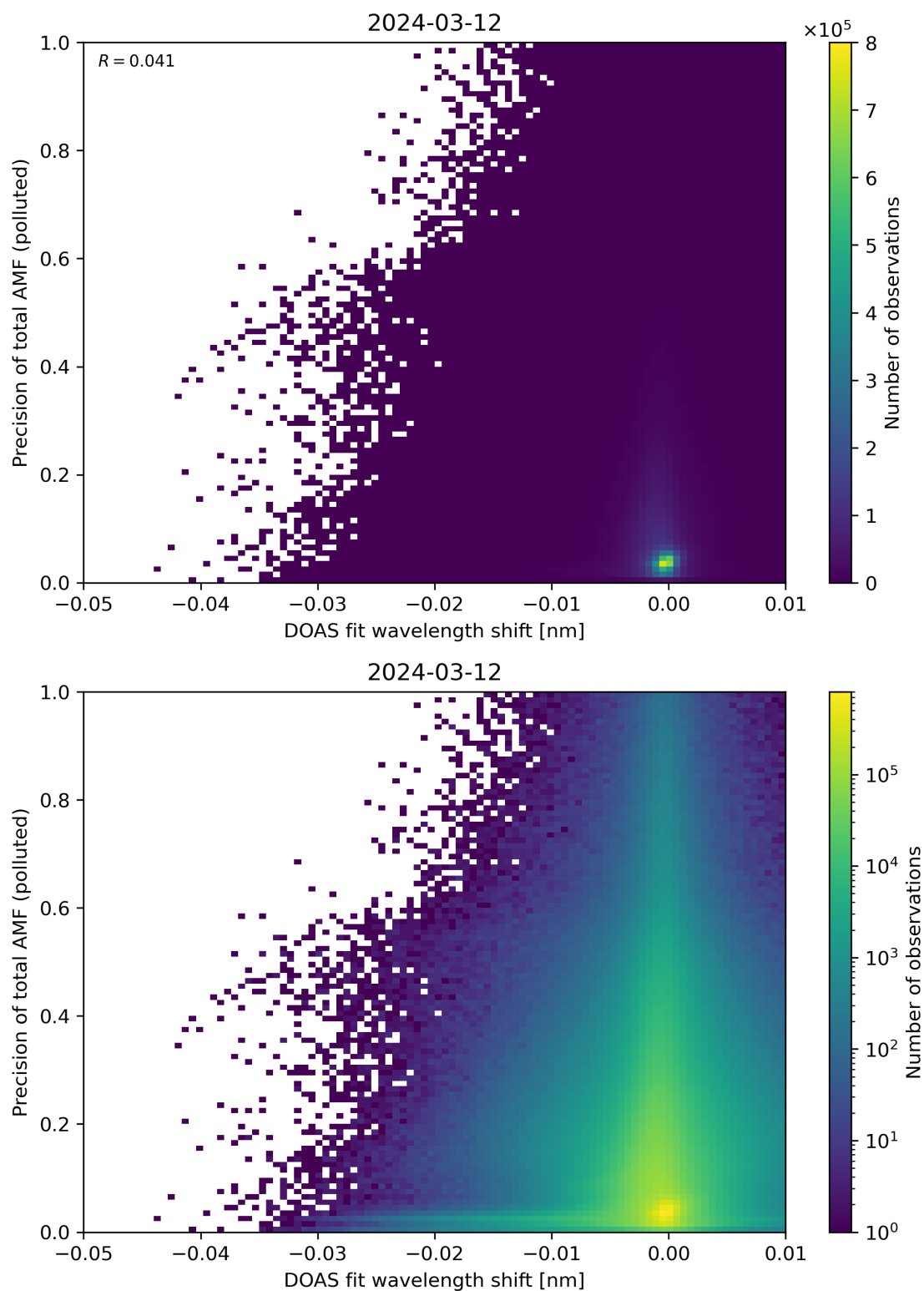
Figure 131: Scatter density plot of “DOAS fit wavelength shift” against “Precision of total AMF (polluted)” for 2024-03-11 to 2024-03-13.
