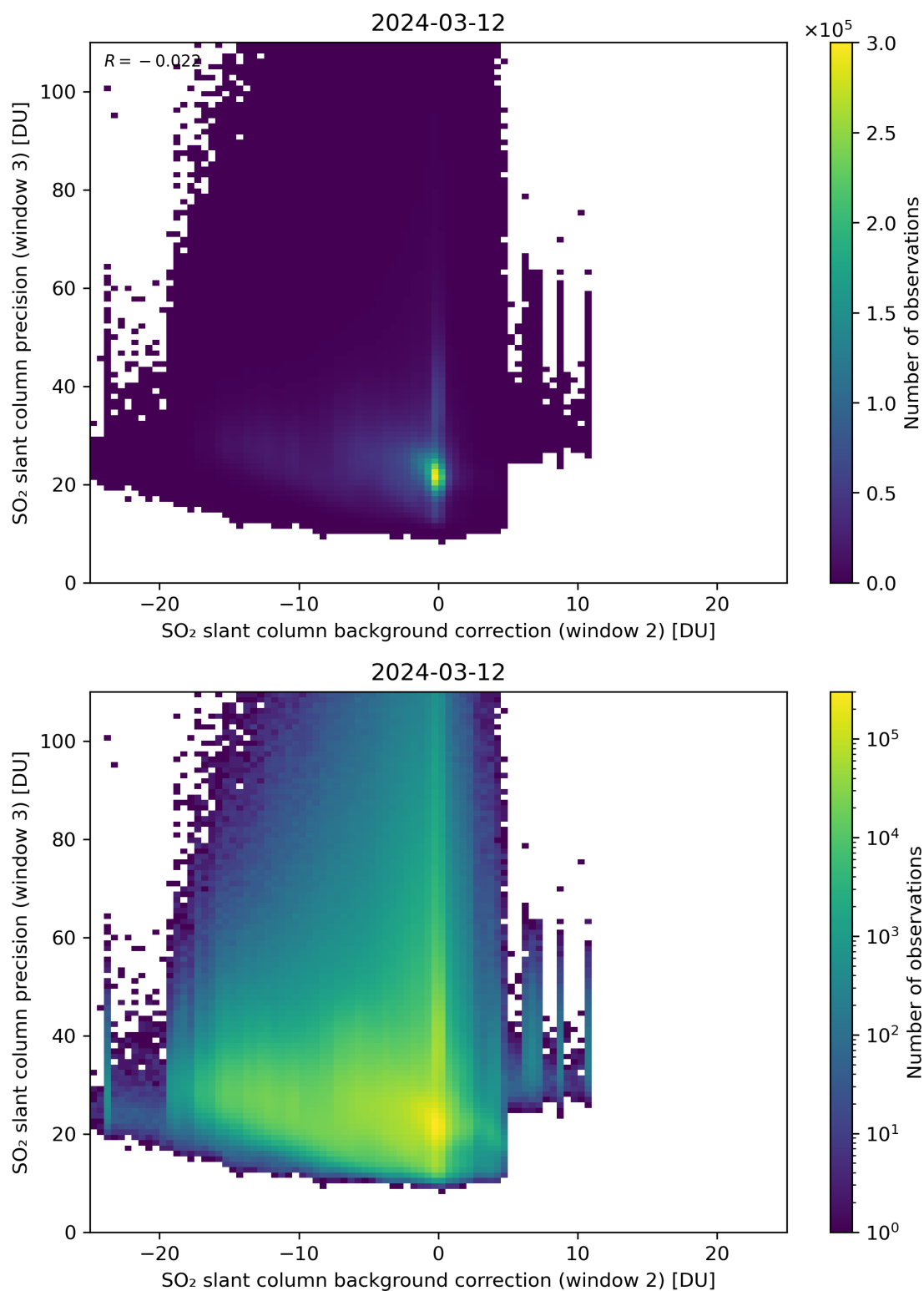
Figure 118: Scatter density plot of “SO 2 slant column background correction (window 2)” against “SO 2 slant column precision (window 3)” for 2024-03-11 to 2024-03-13.
