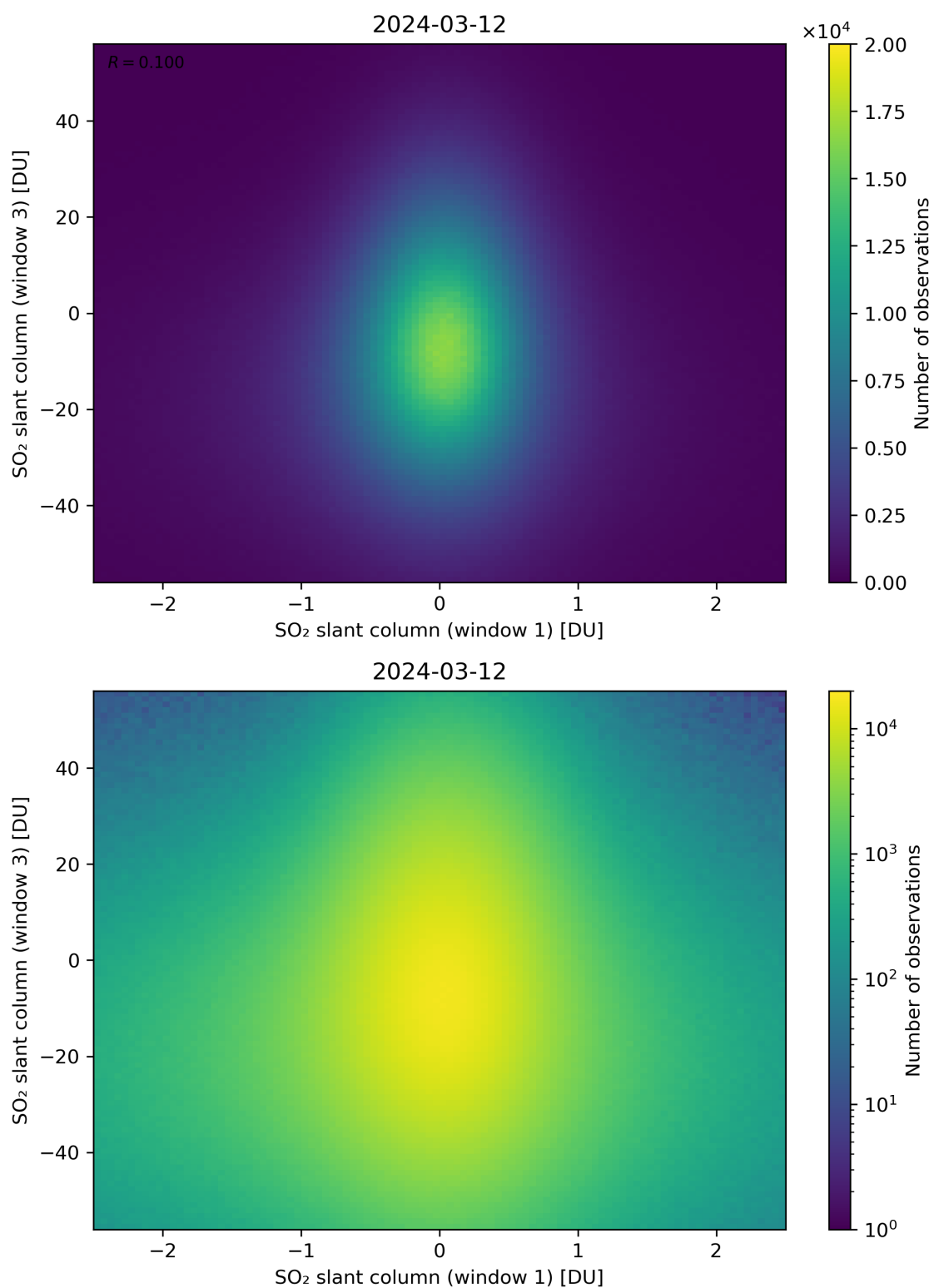
Figure 237: Scatter density plot of “SO 2 slant column (window 1)” against “SO 2 slant column (window 3)” for 2024-03-11 to 2024-03-13.
