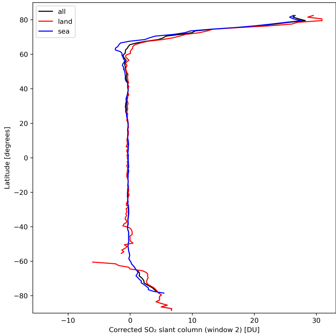
Figure 39: Zonal average of “Corrected SO 2 slant column (window 2)” for 2024-03-11 to 2024-03-13.
