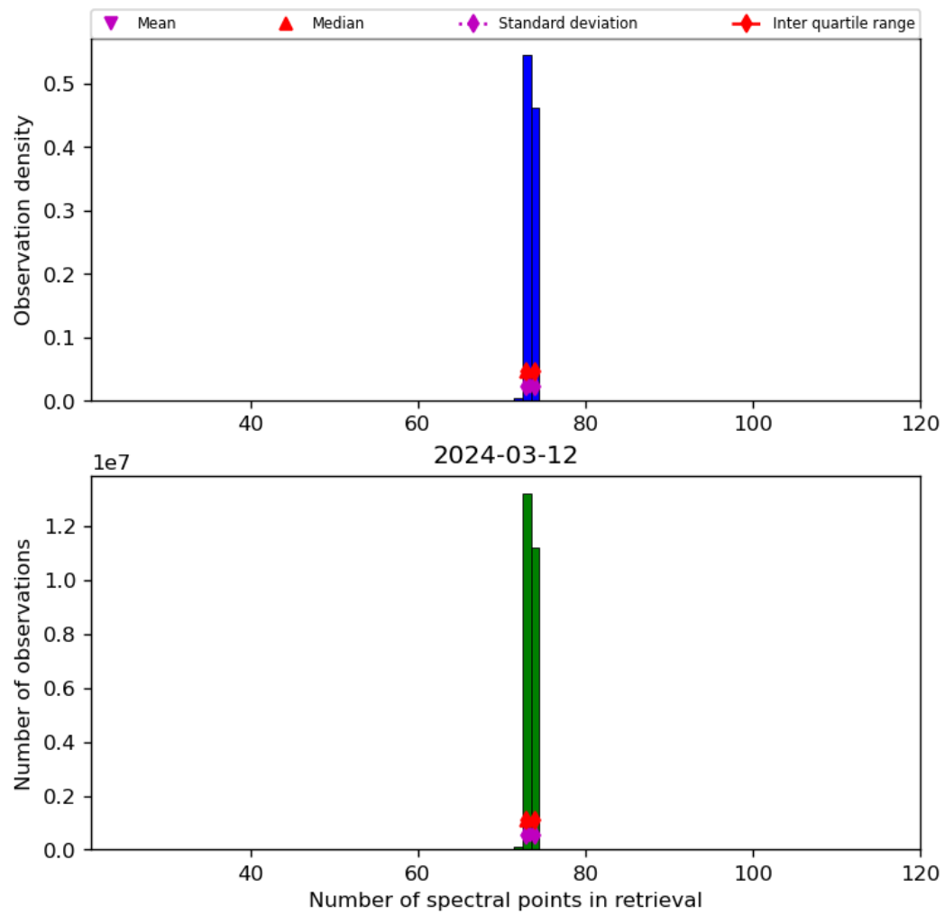
Figure 74: Histogram of “Number of spectral points in retrieval” for 2024-03-11 to 2024-03-13
