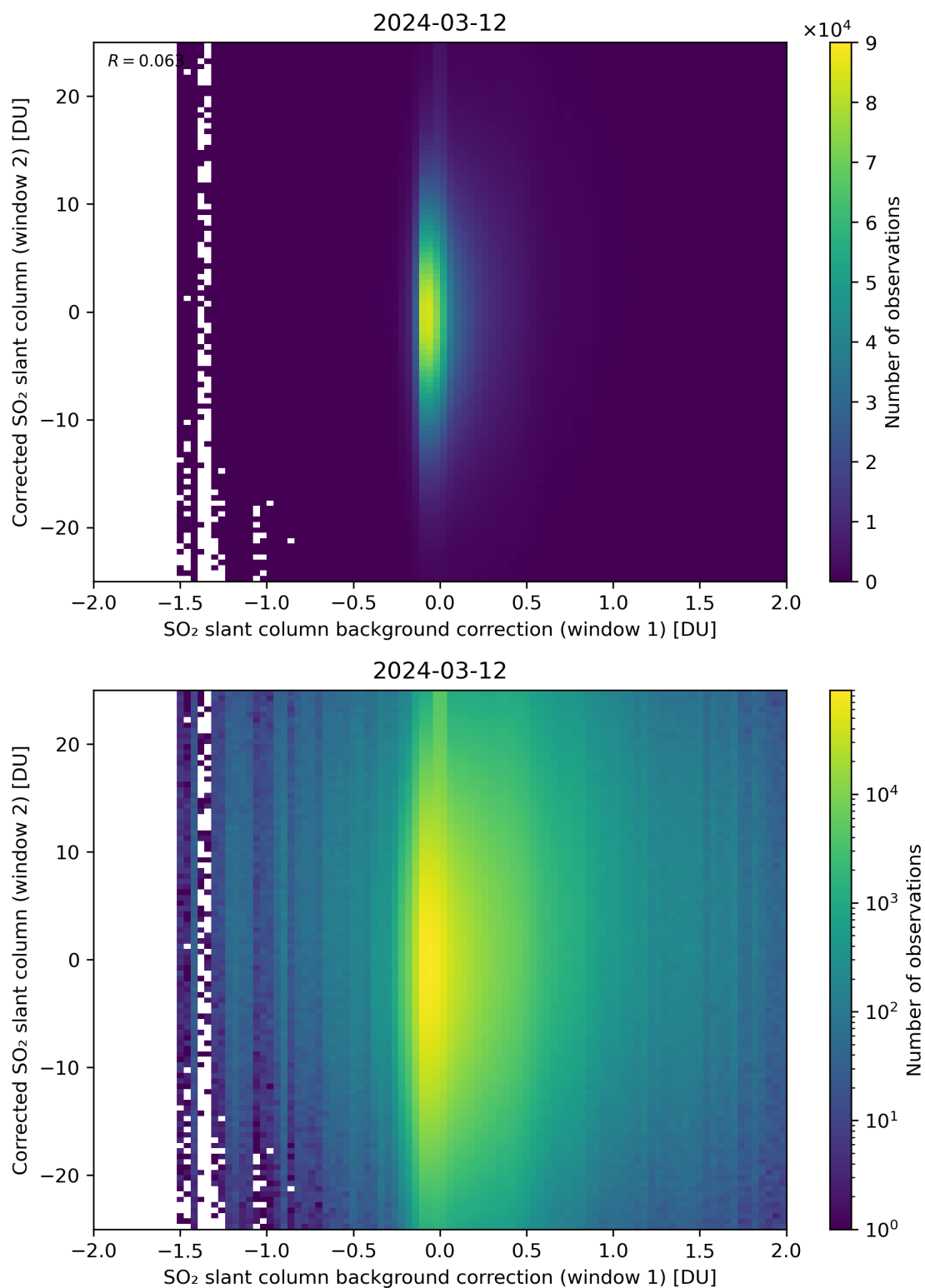
Figure 104: Scatter density plot of “SO 2 slant column background correction (window 1)” against “Corrected SO 2 slant column (window 2)” for 2024-03-11 to 2024-03-13.
