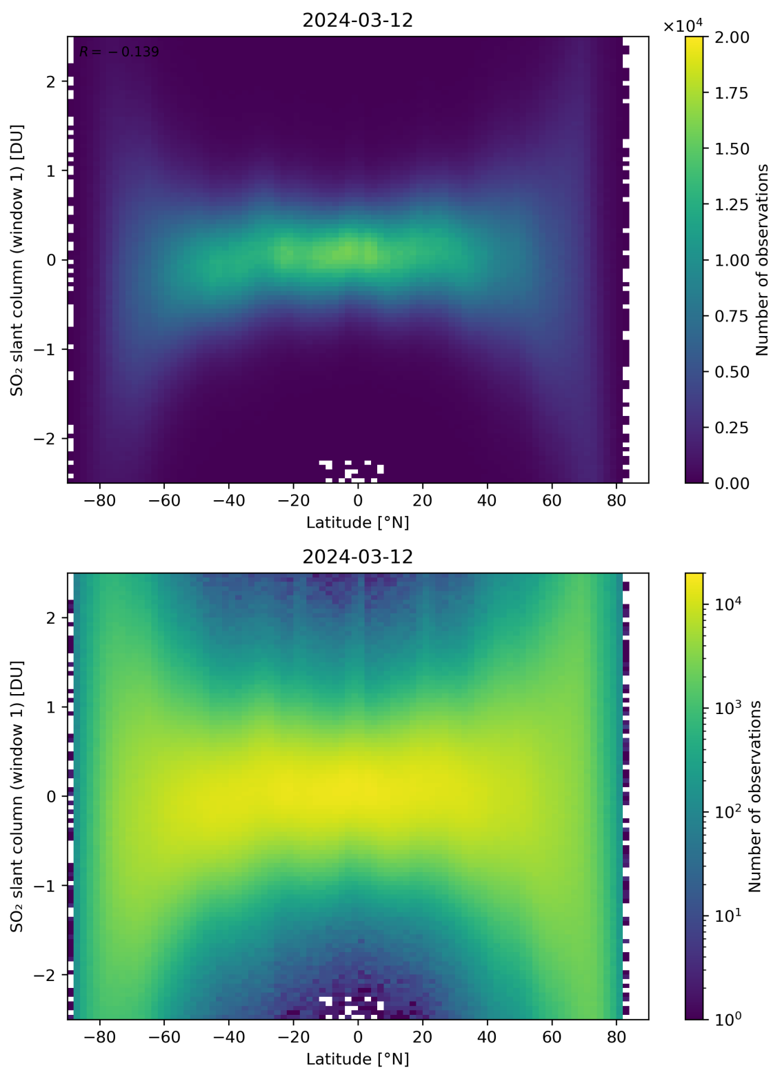
Figure 149: Scatter density plot of “Latitude” against “SO 2 slant column (window 1)” for 2024-03-11 to 2024-03-13.
