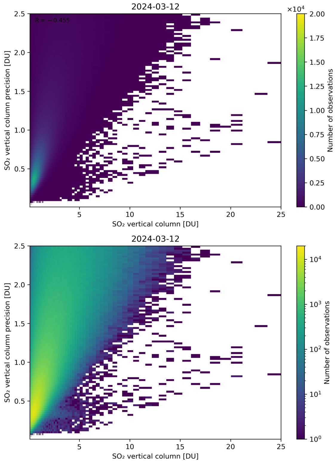
Figure 307: Scatter density plot of “SO 2 vertical column” against “SO 2 vertical column precision” for 2024-03-11 to 2024-03-13.
