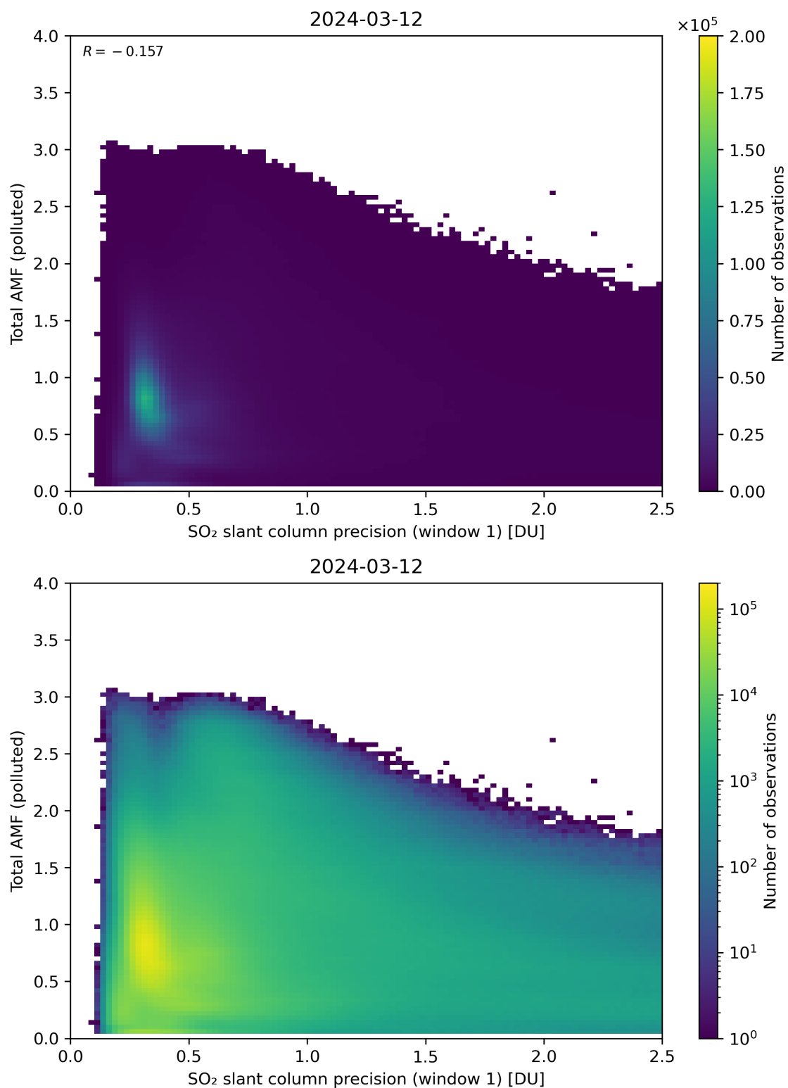
Figure 230: Scatter density plot of “SO 2 slant column precision (window 1)” against “Total AMF (polluted)” for 2024-03-11 to 2024-03-13.
