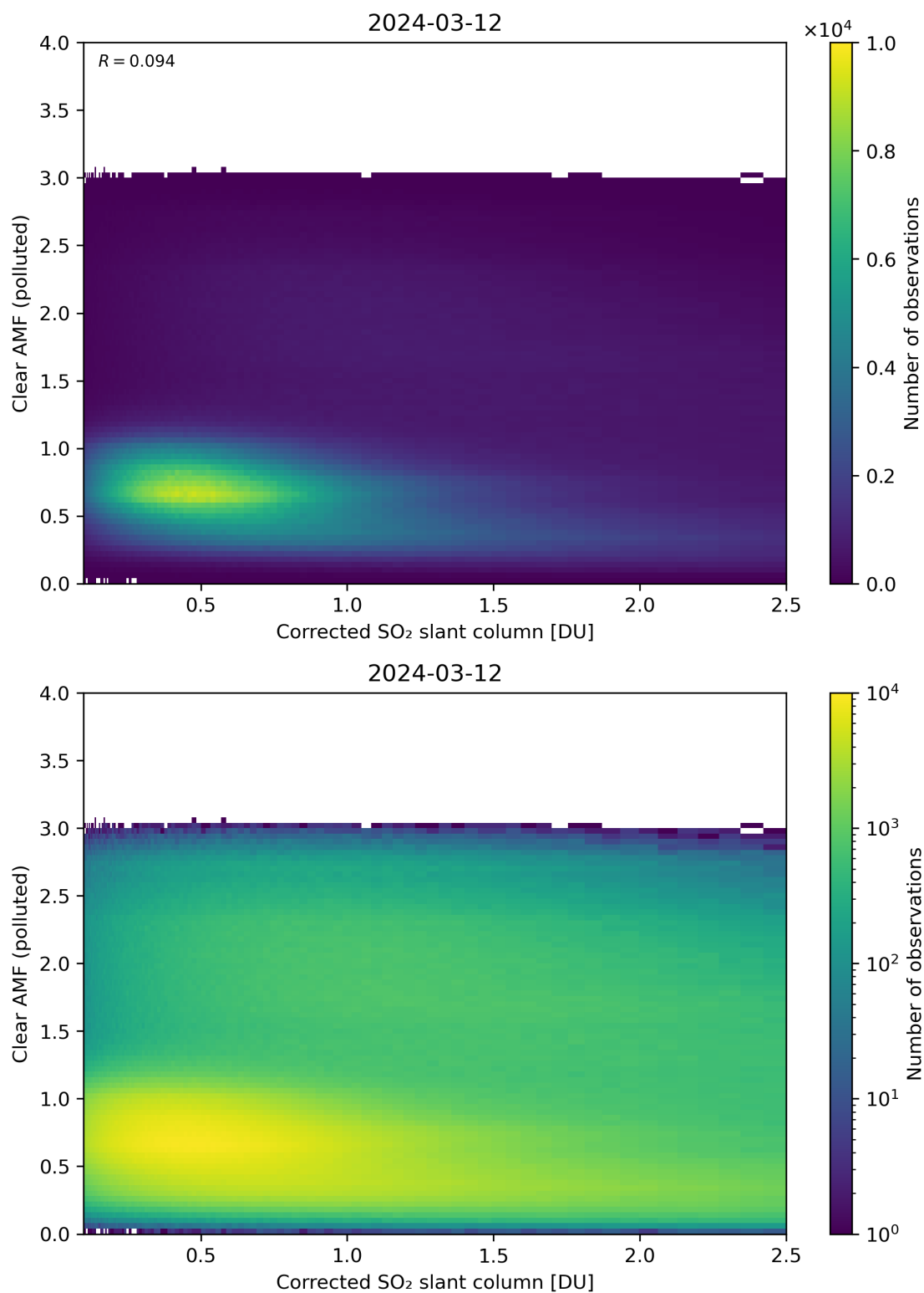
Figure 184: Scatter density plot of “Corrected SO 2 slant column” against “Clear AMF (polluted)” for 2024-03-11 to 2024-03-13.
