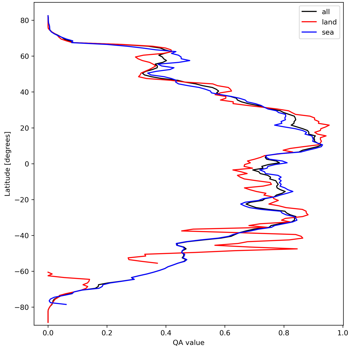
Figure 29: Zonal average of “QA value” for 2024-03-11 to 2024-03-13.
