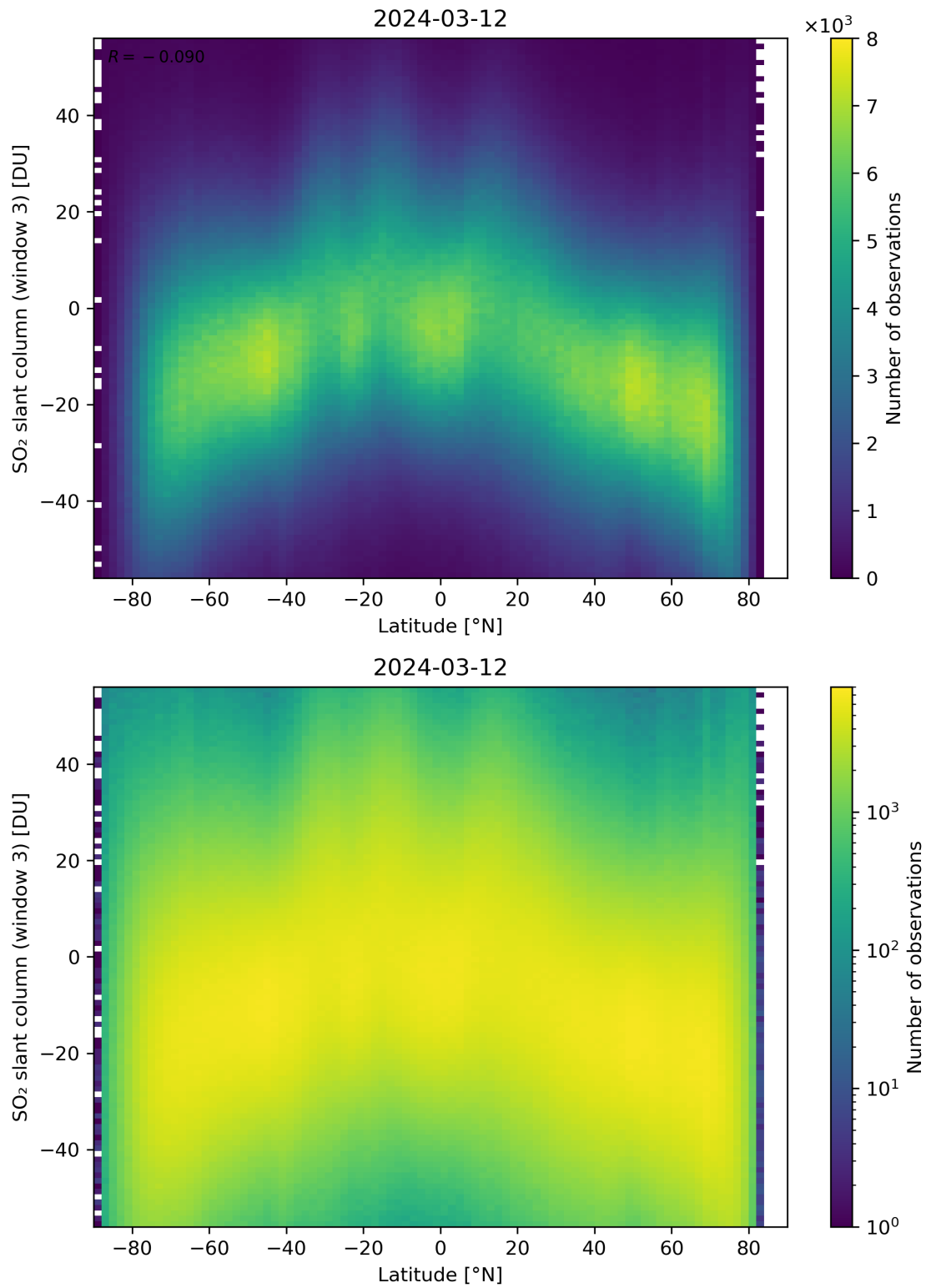
Figure 152: Scatter density plot of “Latitude” against “SO 2 slant column (window 3)” for 2024-03-11 to 2024-03-13.
