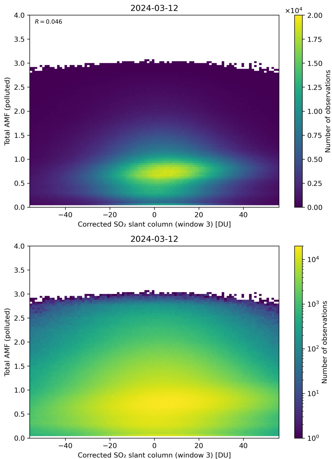
Figure 210: Scatter density plot of “Corrected SO 2 slant column (window 3)” against “Total AMF (polluted)” for 2024-03-11 to 2024-03-13.
