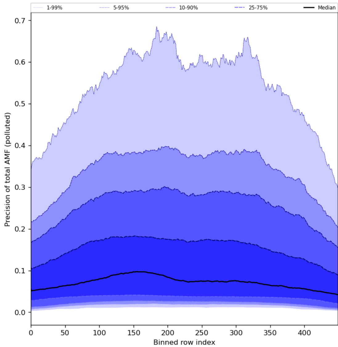
Figure 95: Along track statistics of “Precision of total AMF (polluted)” for 2024-03-11 to 2024-03-13
