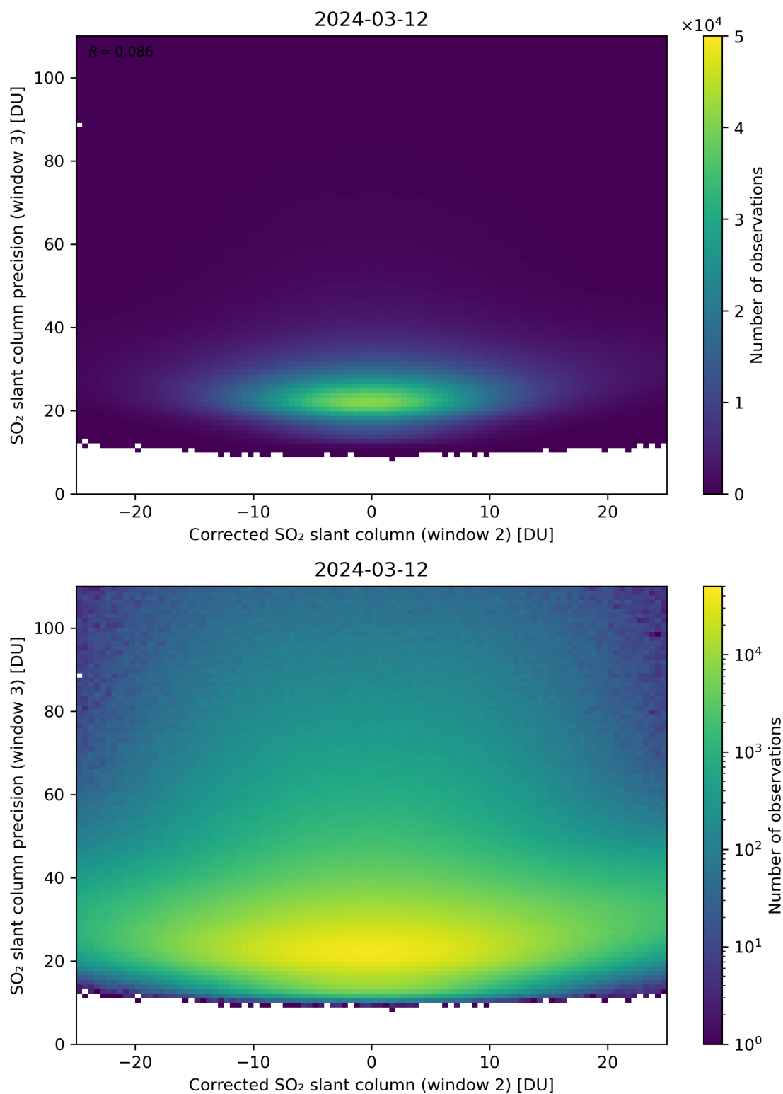
Figure 202: Scatter density plot of “Corrected SO 2 slant column (window 2)” against “SO 2 slant column precision (window 3)” for 2024-03-11 to 2024-03-13.
