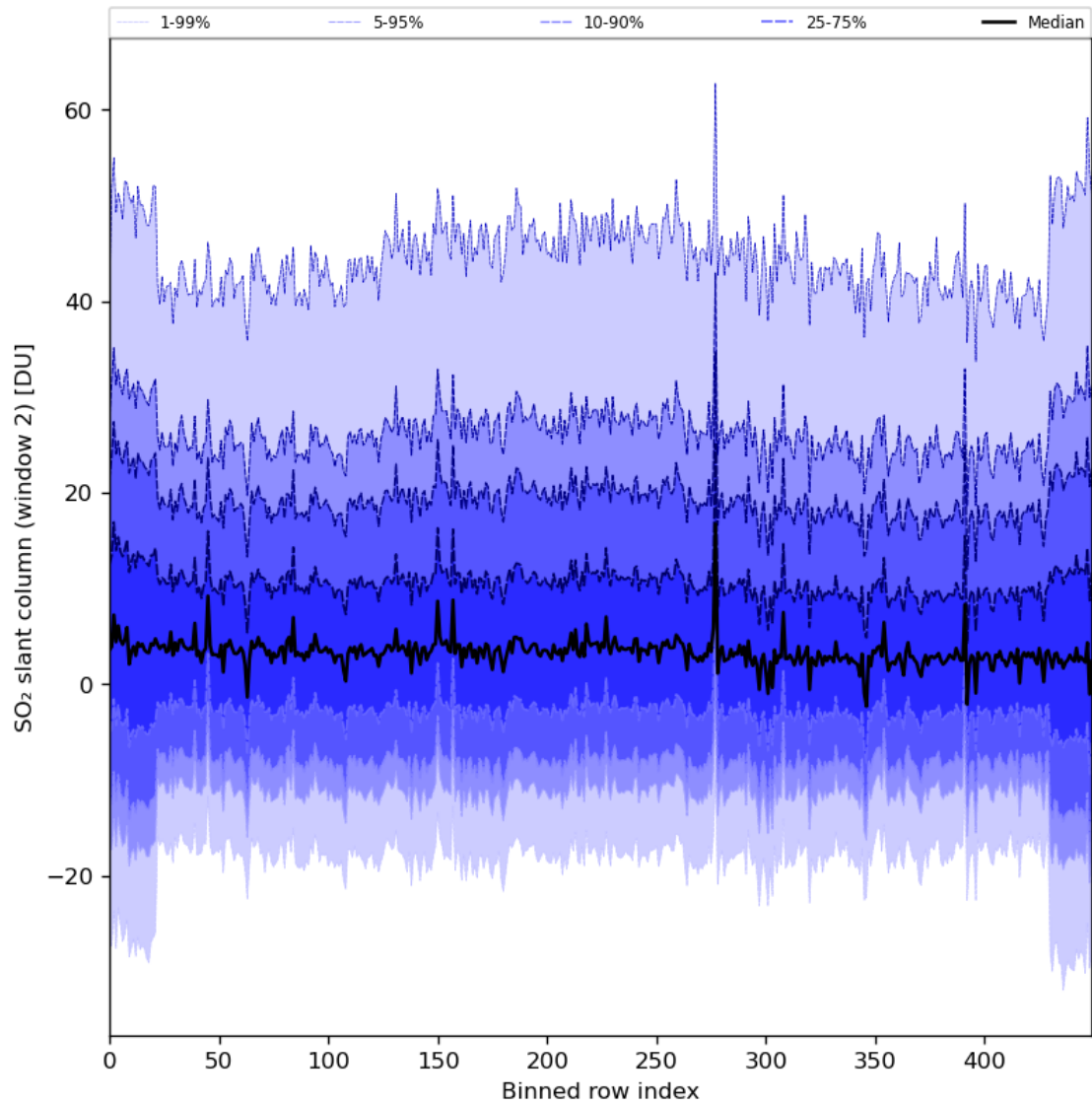
Figure 83: Along track statistics of “SO 2 slant column (window 2)” for 2024-03-11 to 2024-03-13
