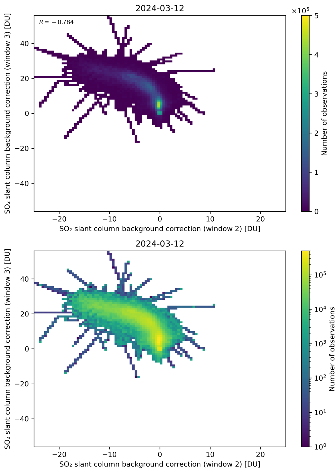
Figure 111: Scatter density plot of “SO 2 slant column background correction (window 2)” against “SO 2 slant column background correction (window 3)” for 2024-03-11 to 2024-03-13.
