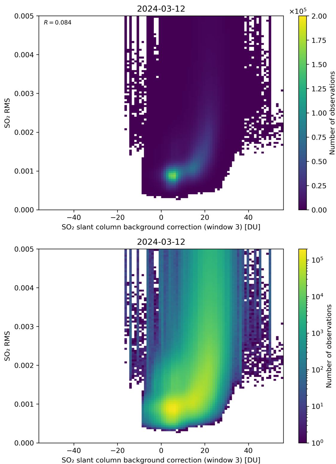
Figure 123: Scatter density plot of “SO 2 slant column background correction (window 3)” against “SO 2 RMS” for 2024-03-11 to 2024-03-13.
