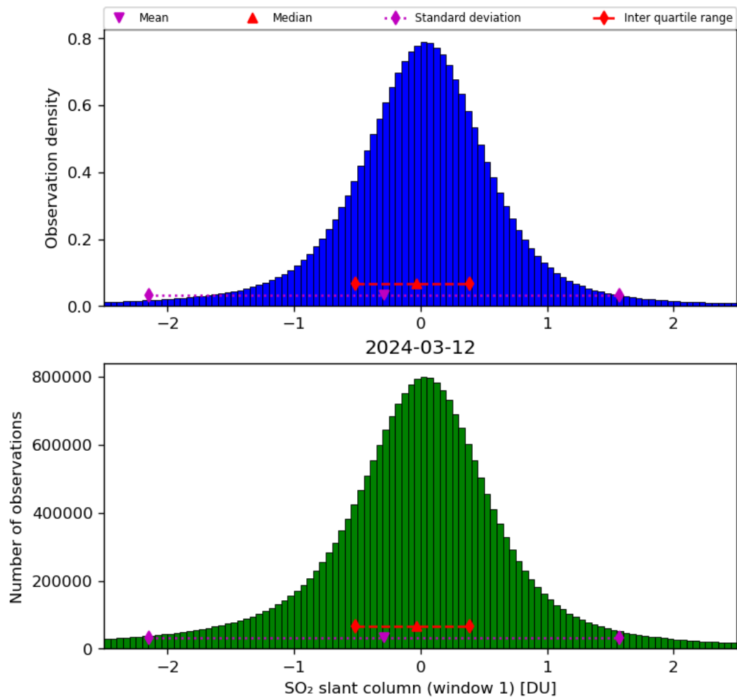
Figure 56: Histogram of “SO 2 slant column (window 1)” for 2024-03-11 to 2024-03-13
