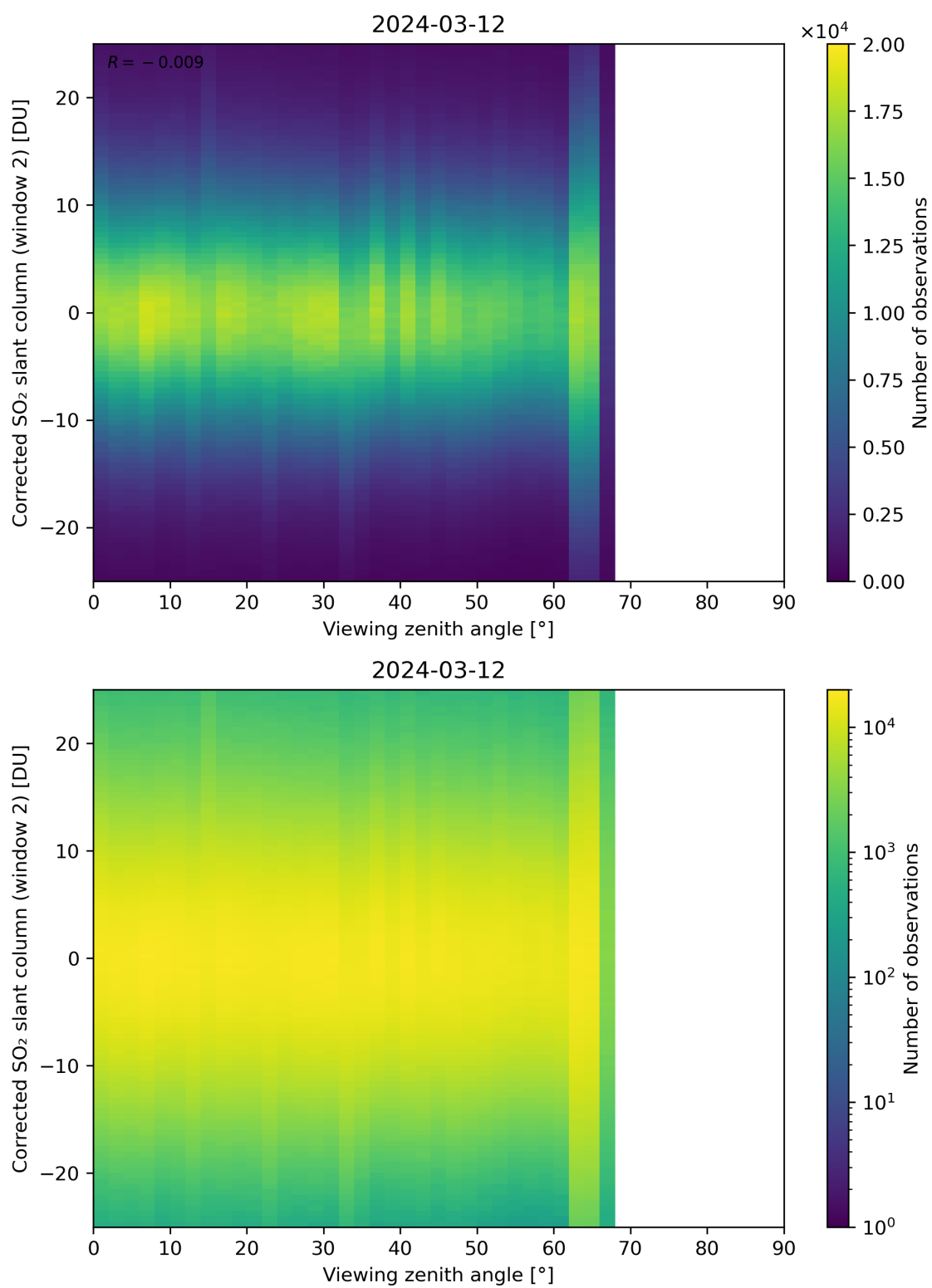
Figure 318: Scatter density plot of “Viewing zenith angle” against “Corrected SO 2 slant column (window 2)” for 2024-03-11 to 2024-03-13.
