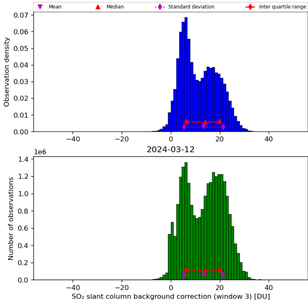
Figure 67: Histogram of "SO 2 slant column background correction (window 3)" for 2024-03-11 to 2024-03-13
