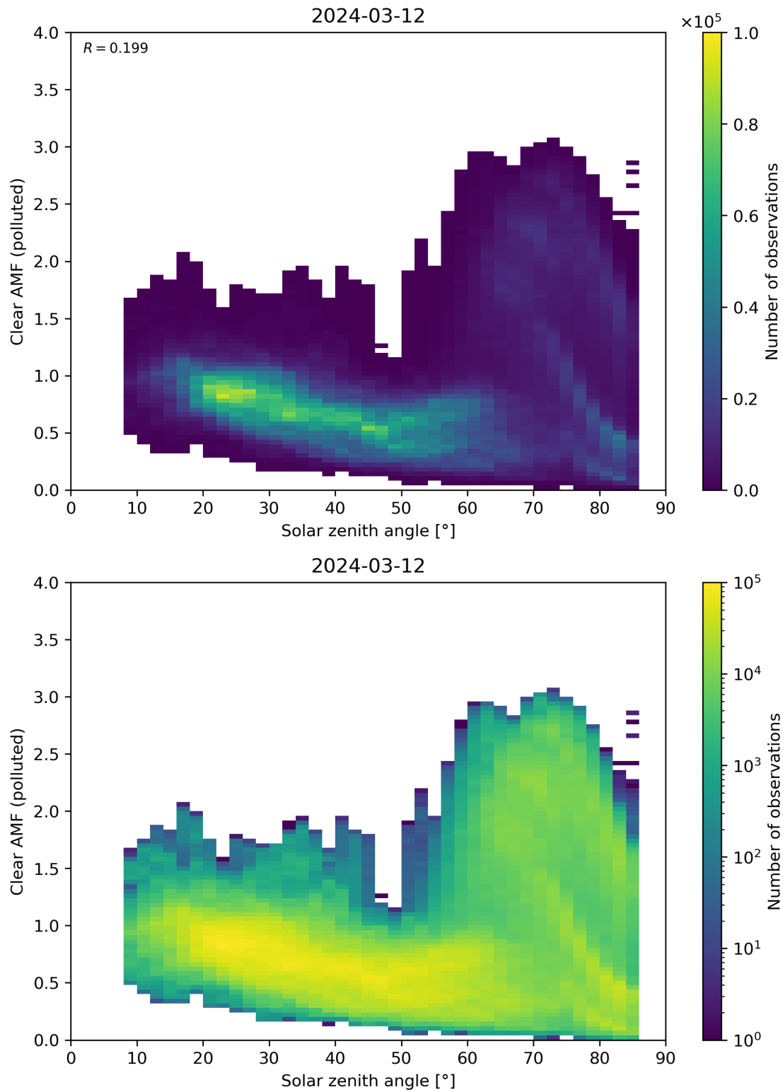
Figure 165: Scatter density plot of “Solar zenith angle” against “Clear AMF (polluted)” for 2024-03-11 to 2024-03-13.
