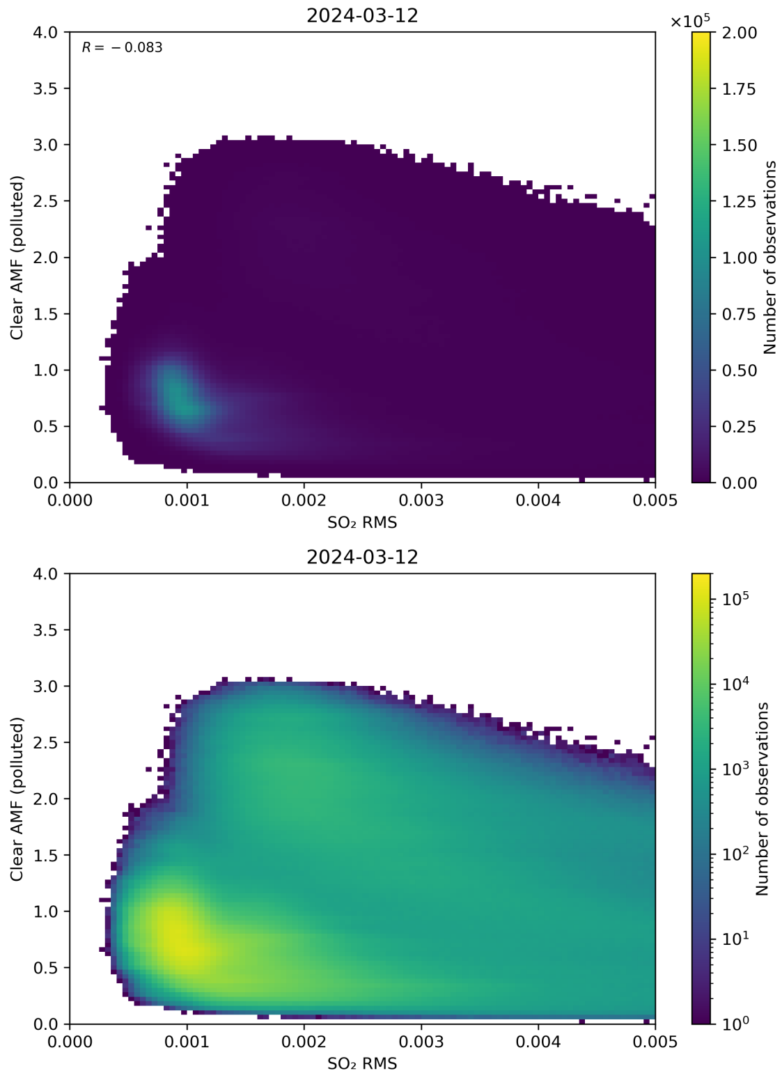
Figure 136: Scatter density plot of “SO 2 RMS” against “Clear AMF (polluted)” for 2024-03-11 to 2024-03-13.
