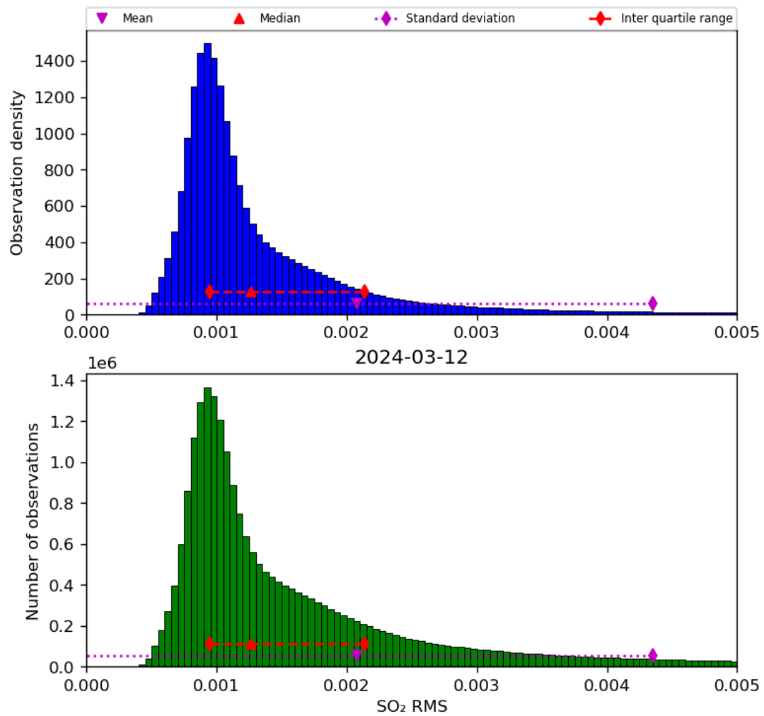
Figure 70: Histogram of “SO 2 RMS” for 2024-03-11 to 2024-03-13
