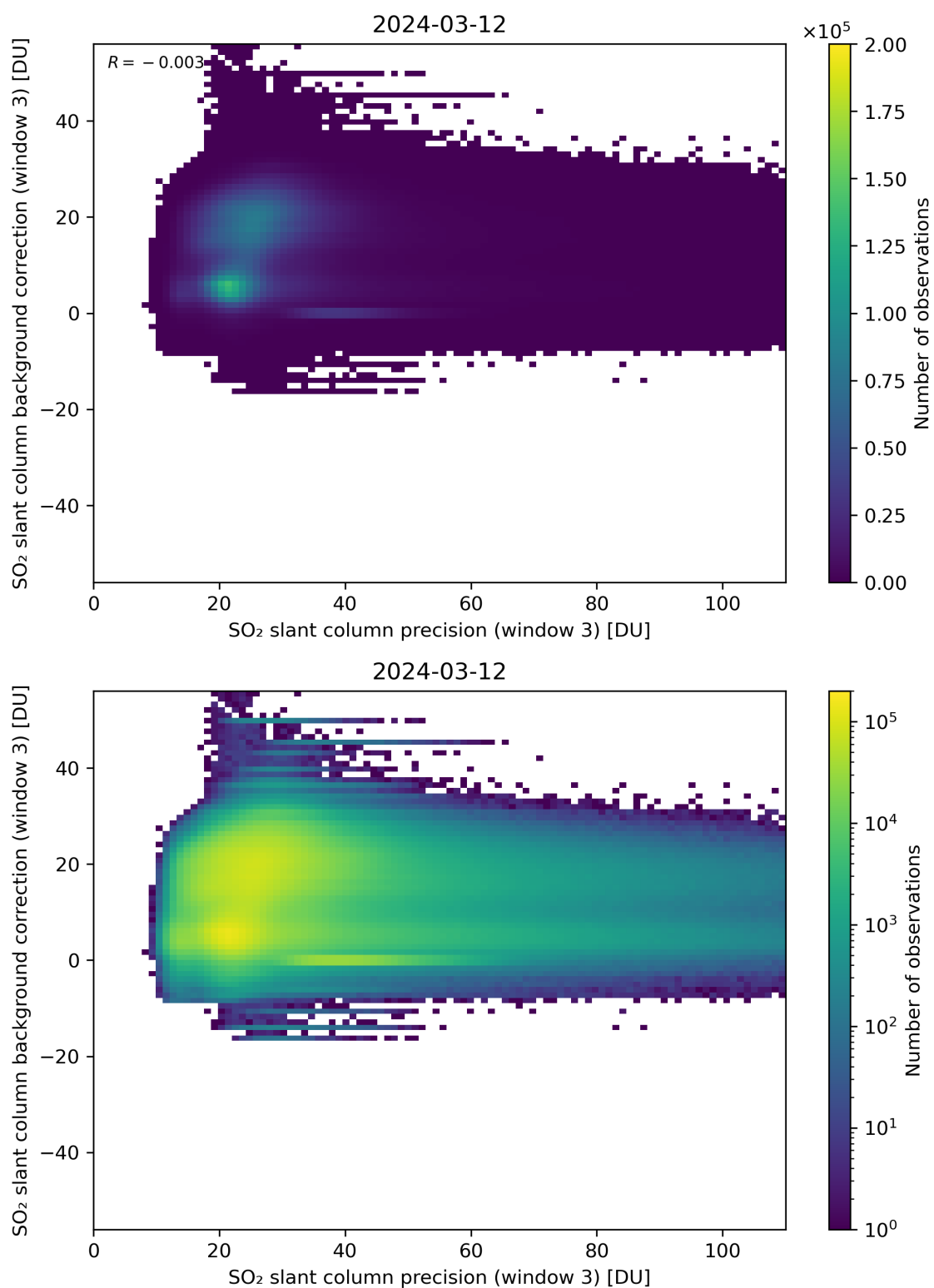
Figure 257: Scatter density plot of “SO 2 slant column precision (window 3)” against “SO 2 slant column background correction (window 3)” for 2024-03-11 to 2024-03-13.
