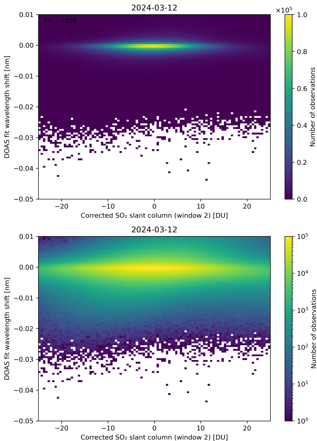
Figure 196: Scatter density plot of “Corrected SO 2 slant column (window 2)” against “DOAS fit wavelength shift” for 2024-03-11 to 2024-03-13.
