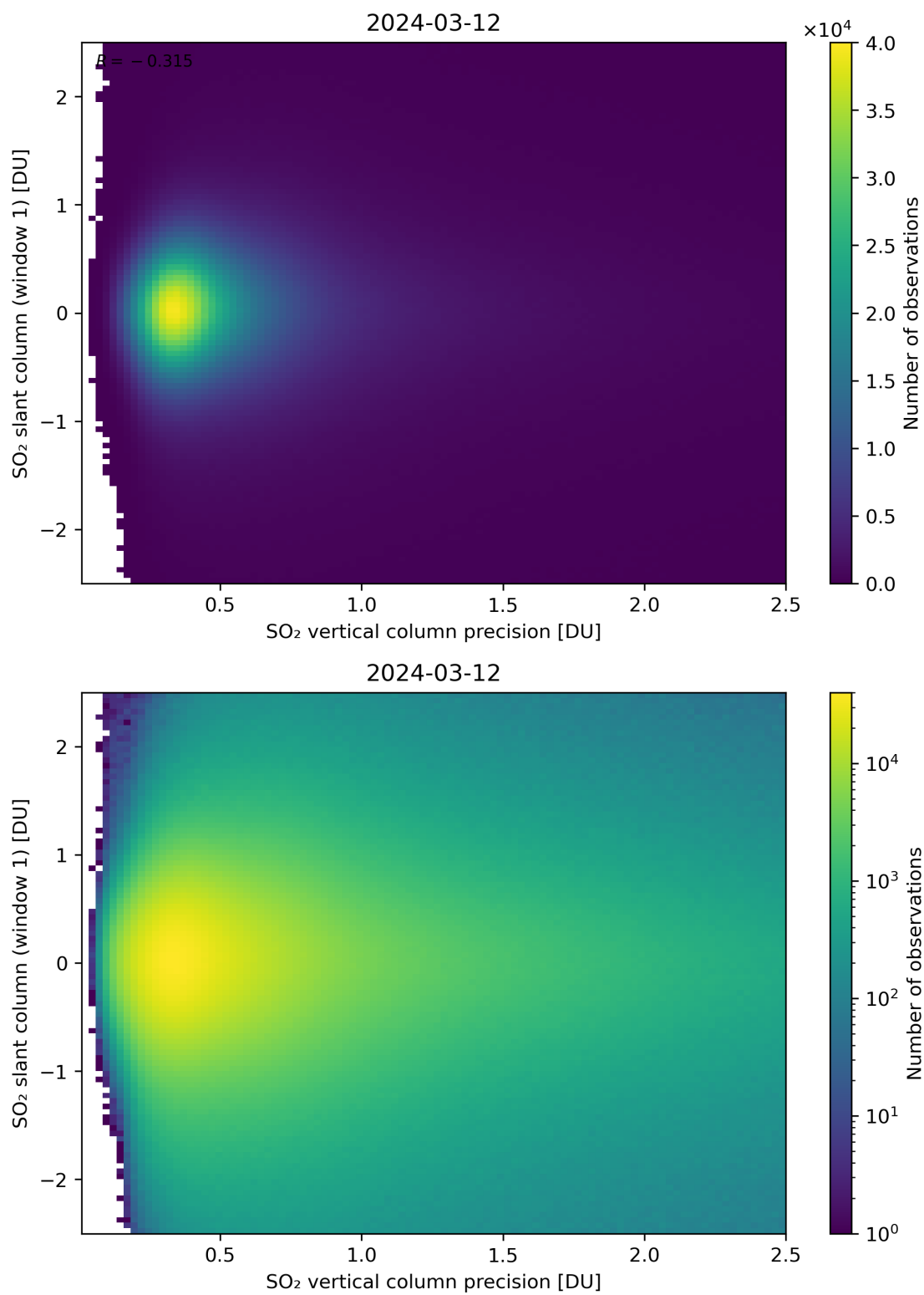
Figure 289: Scatter density plot of “SO 2 vertical column precision” against “SO 2 slant column (window 1)” for 2024-03-11 to 2024-03-13.
