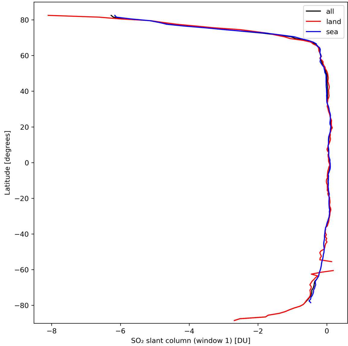
Figure 33: Zonal average of “SO 2 slant column (window 1)” for 2024-03-11 to 2024-03-13.
