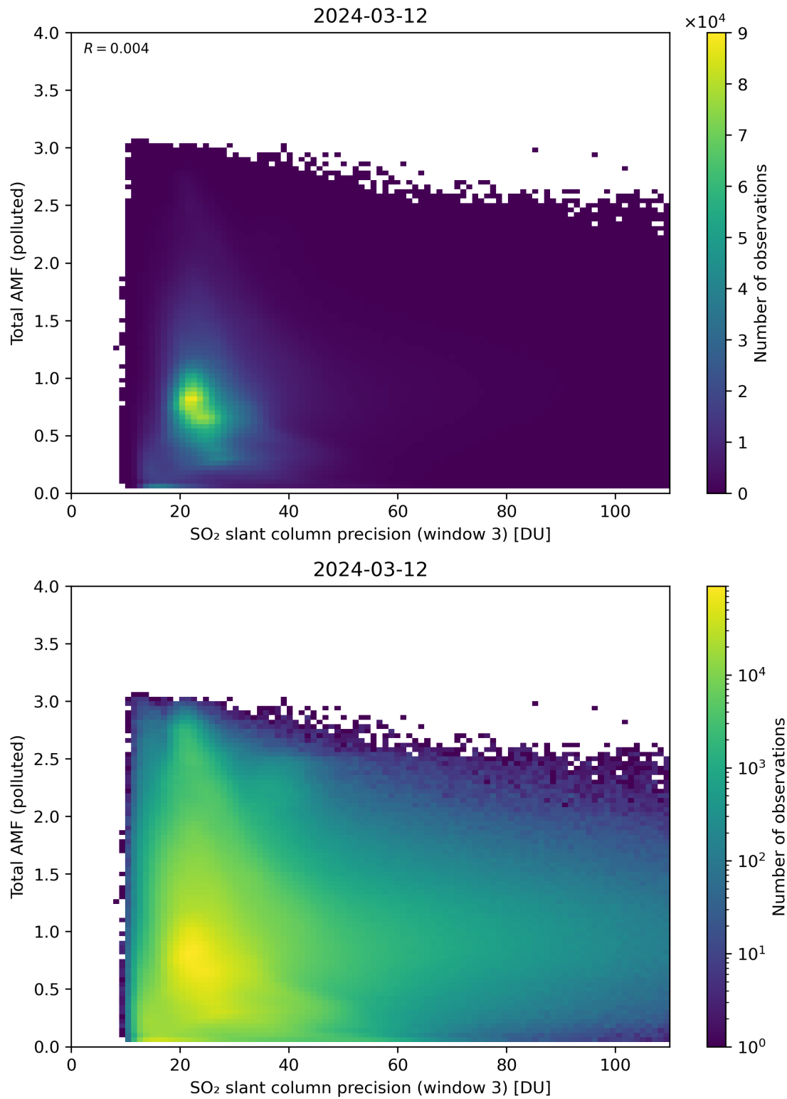
Figure 263: Scatter density plot of “SO 2 slant column precision (window 3)” against “Total AMF (polluted)” for 2024-03-11 to 2024-03-13.
