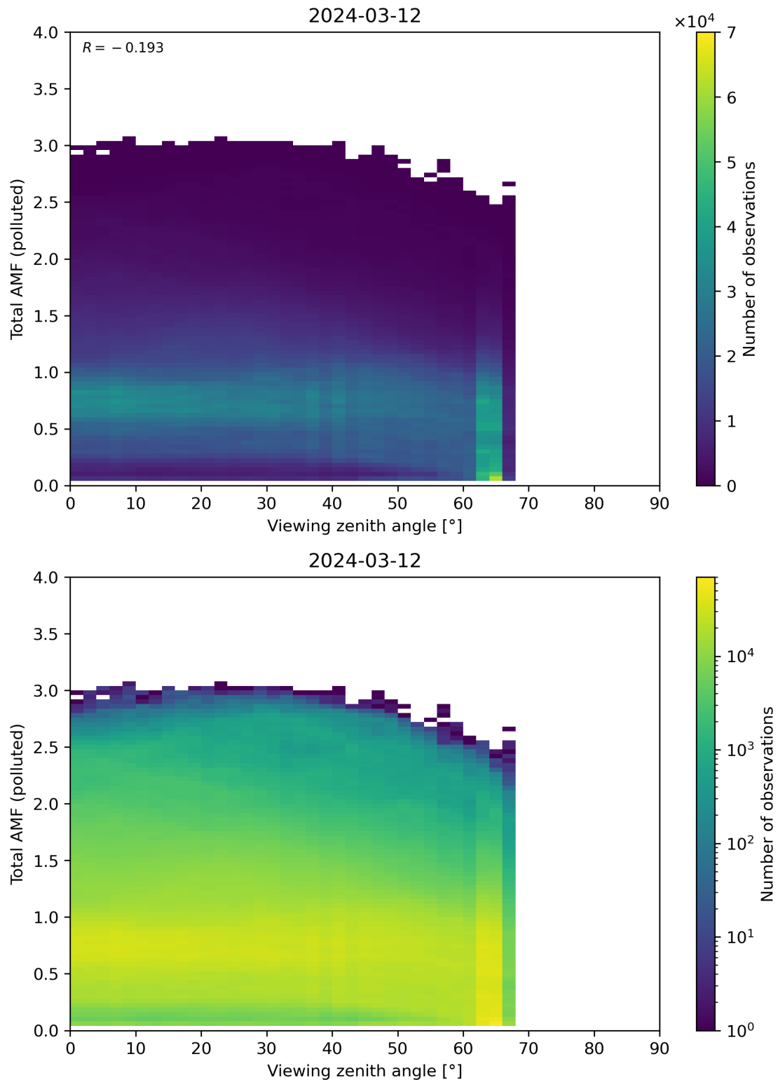
Figure 325: Scatter density plot of “Viewing zenith angle” against “Total AMF (polluted)” for 2024-03-11 to 2024-03-13.
