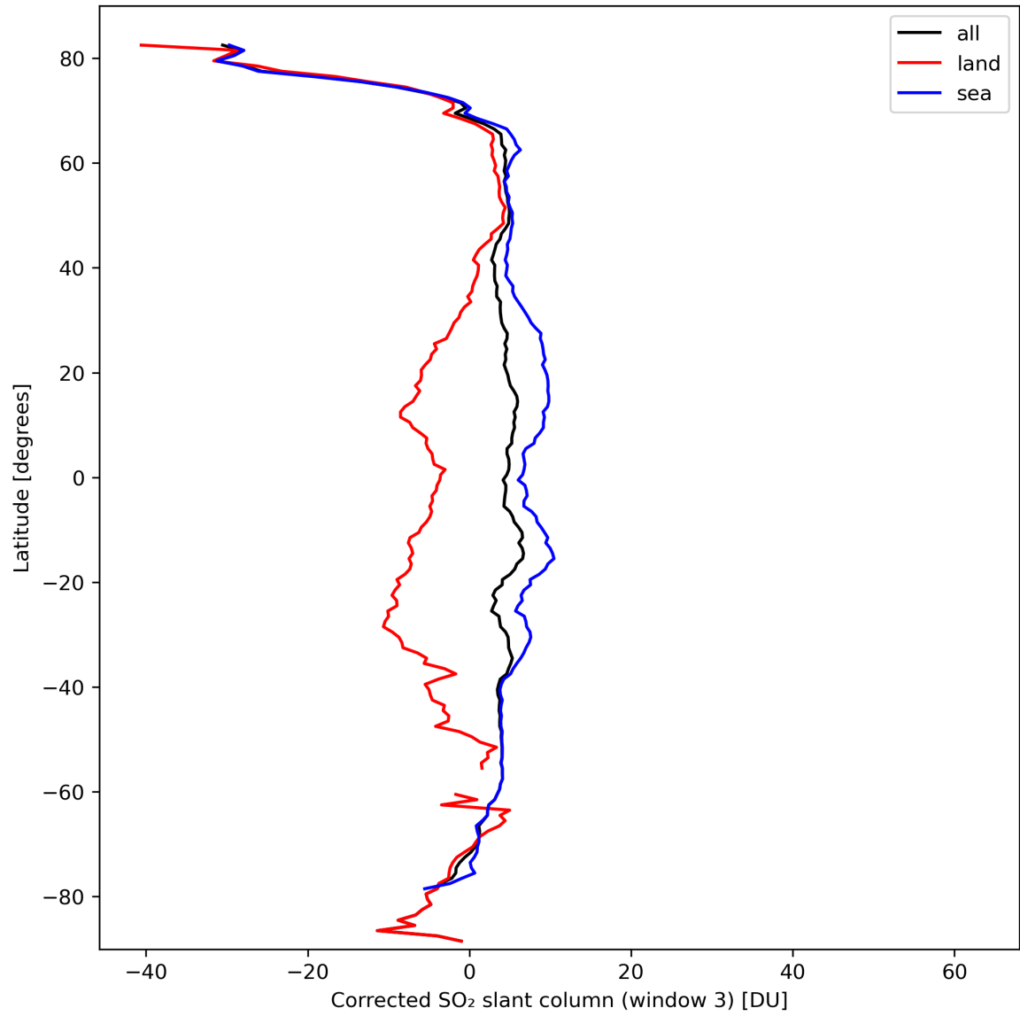
Figure 43: Zonal average of “Corrected SO 2 slant column (window 3)” for 2024-03-11 to 2024-03-13.
