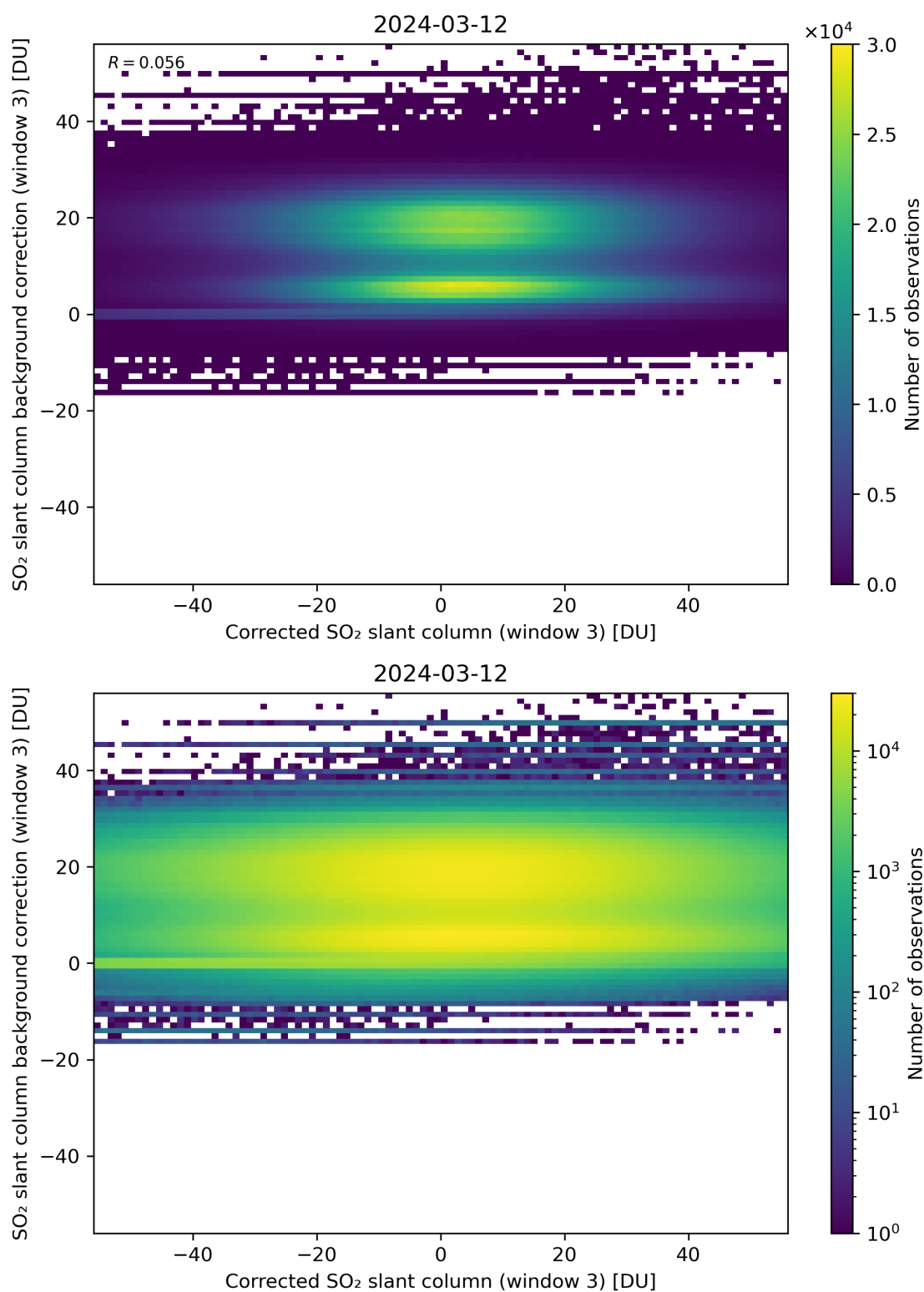
Figure 205: Scatter density plot of “Corrected SO 2 slant column (window 3)” against “SO 2 slant column background correction (window 3)” for 2024-03-11 to 2024-03-13.
