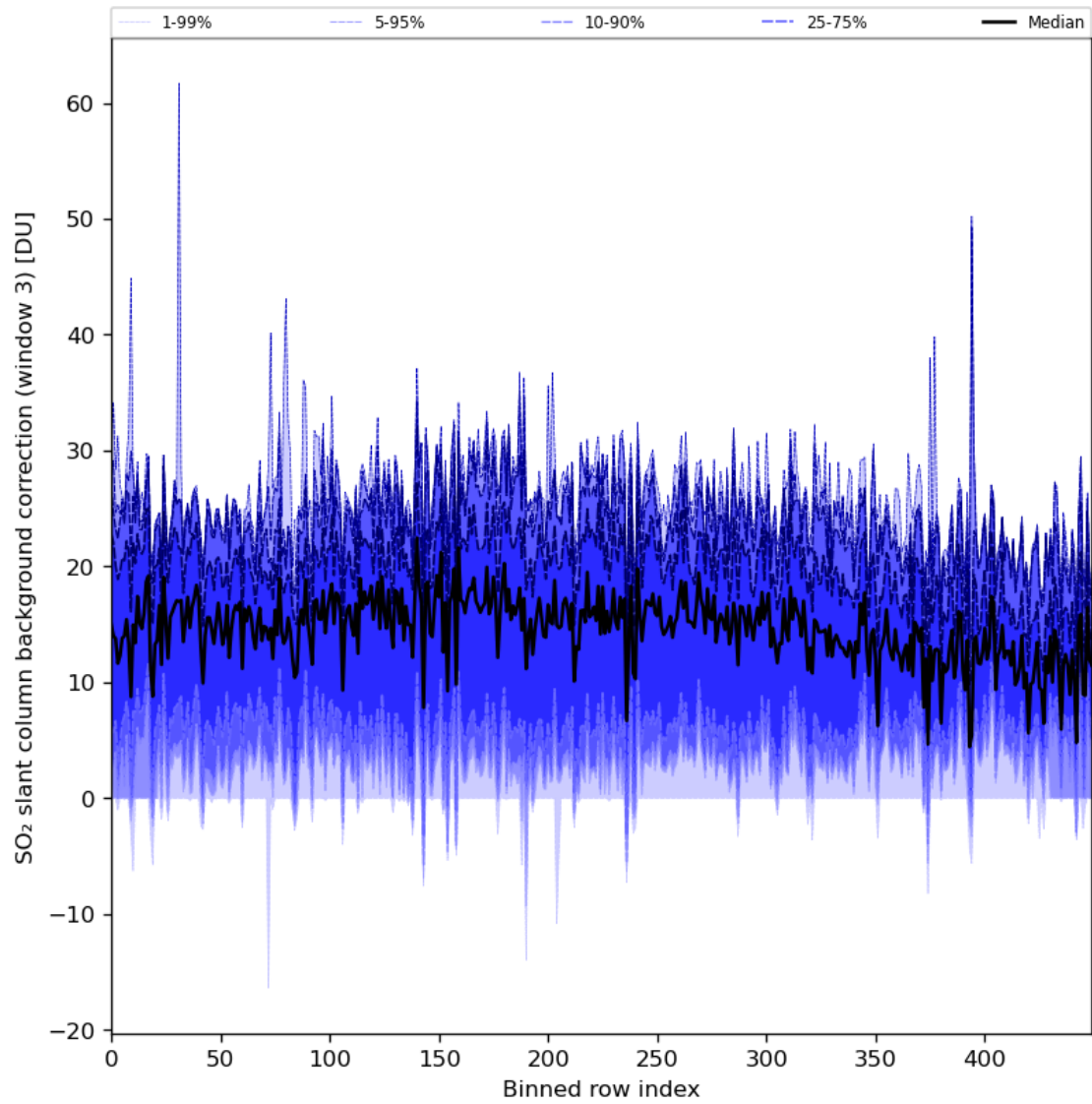
Figure 90: Along track statistics of “SO 2 slant column background correction (window 3)” for 2024-03-11 to 2024-03-13
