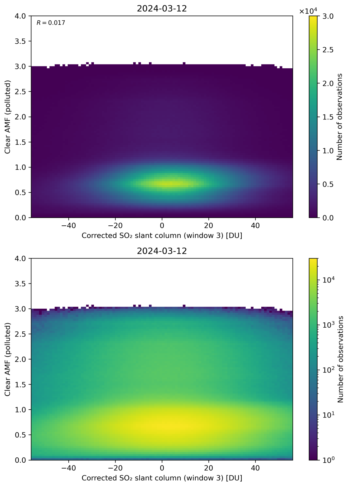
Figure 209: Scatter density plot of “Corrected SO 2 slant column (window 3)” against “Clear AMF (polluted)” for 2024-03-11 to 2024-03-13.
