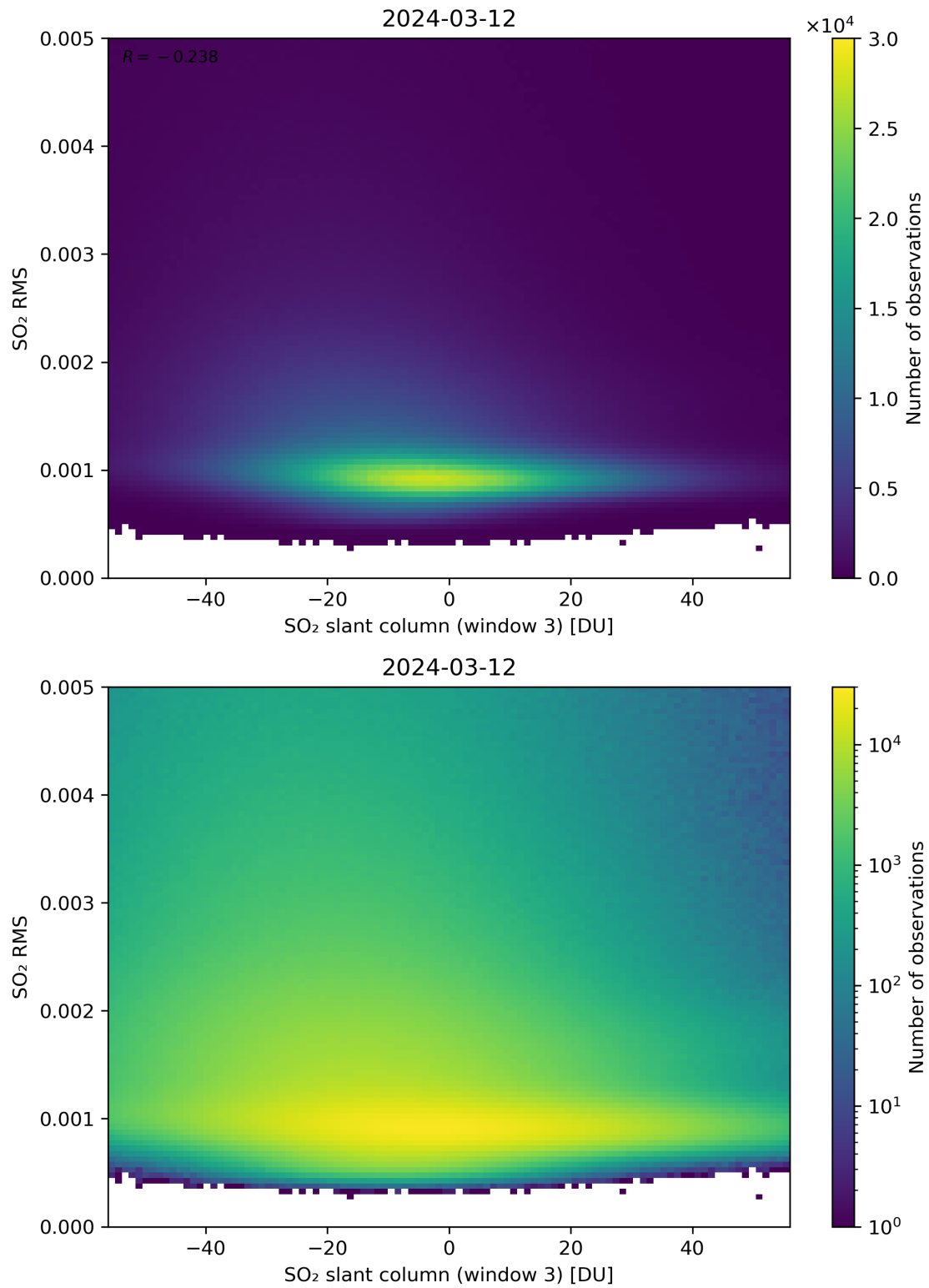
Figure 256: Scatter density plot of “SO 2 slant column (window 3)” against “SO 2 RMS” for 2024-03-11 to 2024-03-13.
