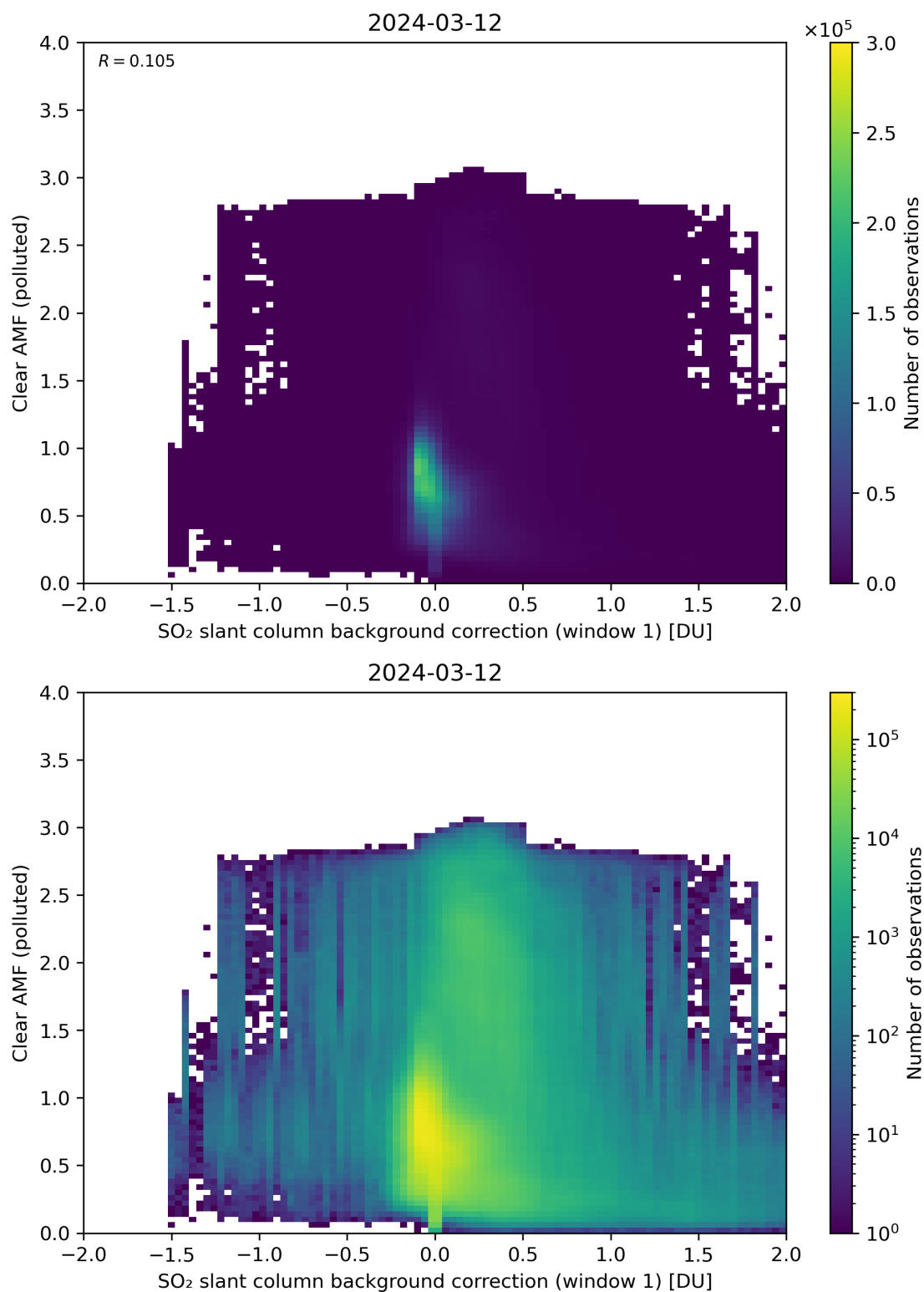
Figure 103: Scatter density plot of “SO 2 slant column background correction (window 1)” against “Clear AMF (polluted)” for 2024-03-11 to 2024-03-13.
