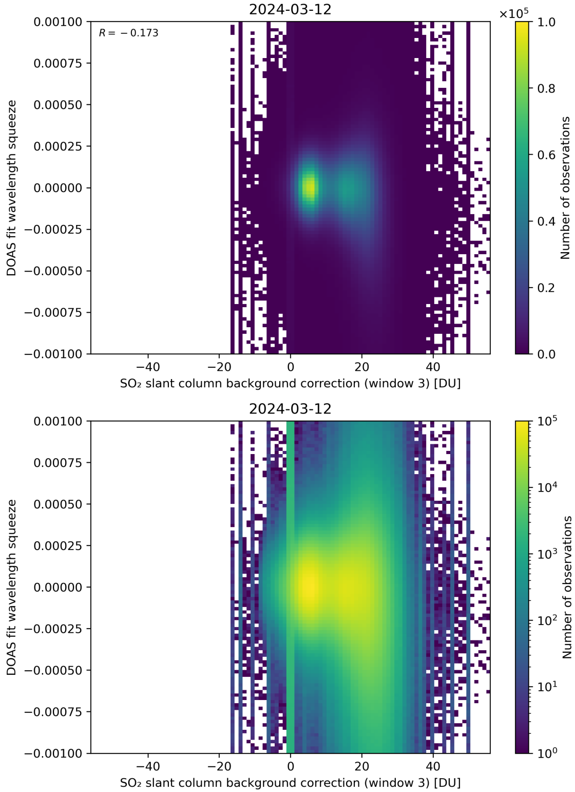
Figure 122: Scatter density plot of “SO 2 slant column background correction (window 3)” against “DOAS fit wavelength squeeze” for 2024-03-11 to 2024-03-13.
