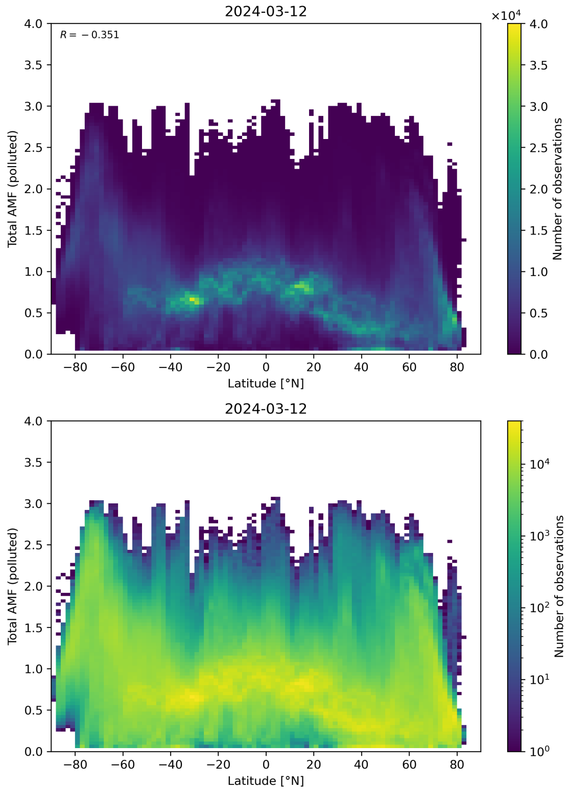
Figure 154: Scatter density plot of “Latitude” against “Total AMF (polluted)” for 2024-03-11 to 2024-03-13.
