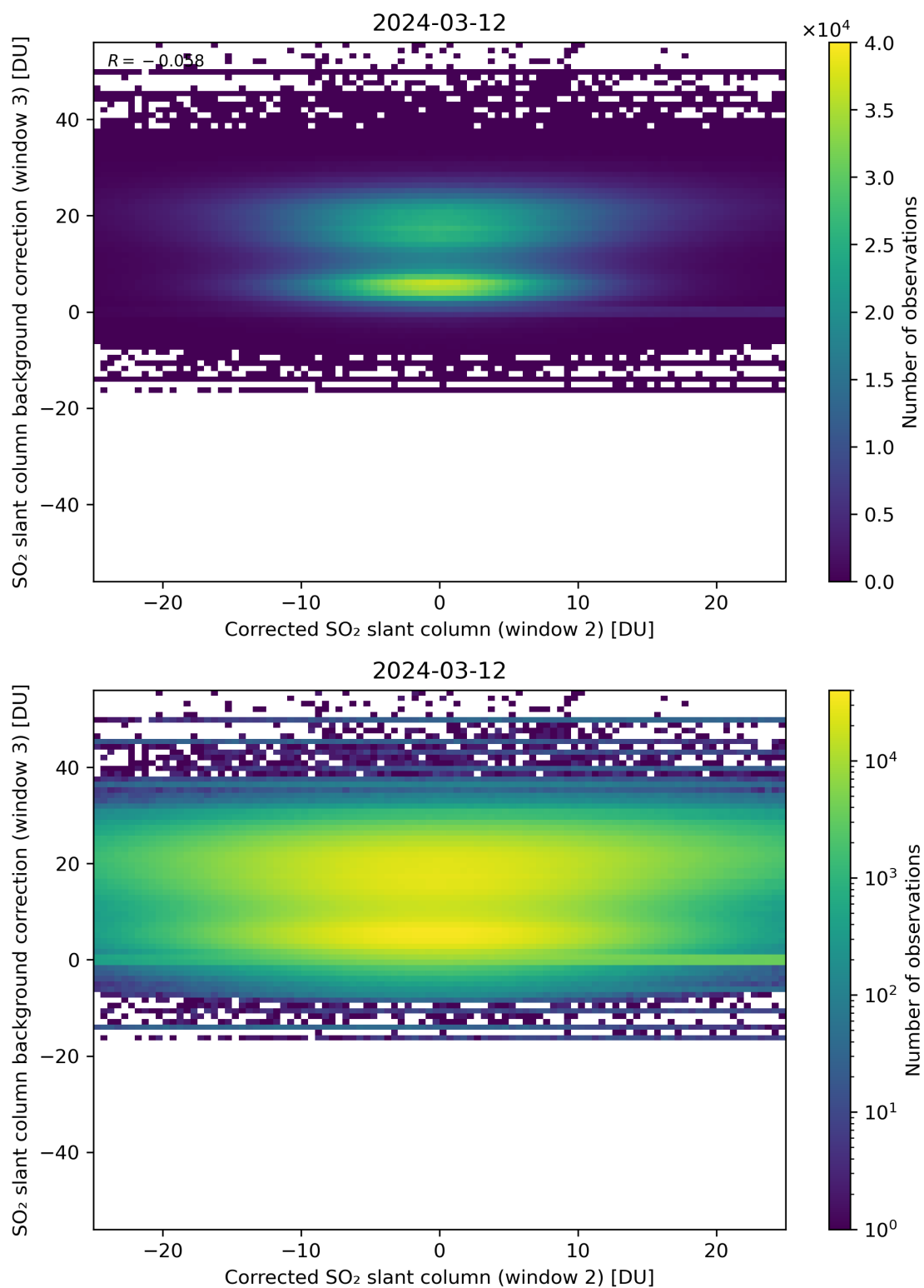
Figure 195: Scatter density plot of “Corrected SO 2 slant column (window 2)” against “SO 2 slant column background correction (window 3)” for 2024-03-11 to 2024-03-13.
