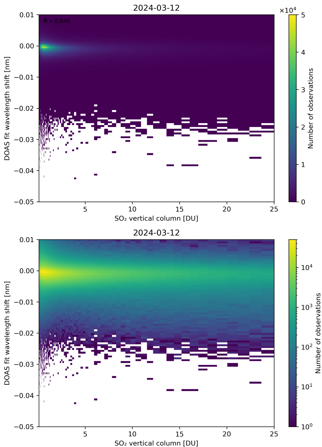
Figure 276: Scatter density plot of “SO 2 vertical column” against “DOAS fit wavelength shift” for 2024-03-11 to 2024-03-13.
