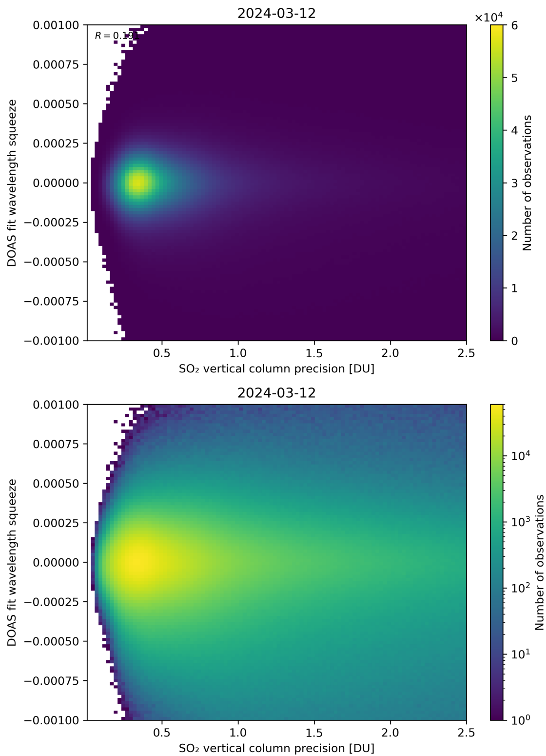
Figure 283: Scatter density plot of “SO 2 vertical column precision” against “DOAS fit wavelength squeeze” for 2024-03-11 to 2024-03-13.
