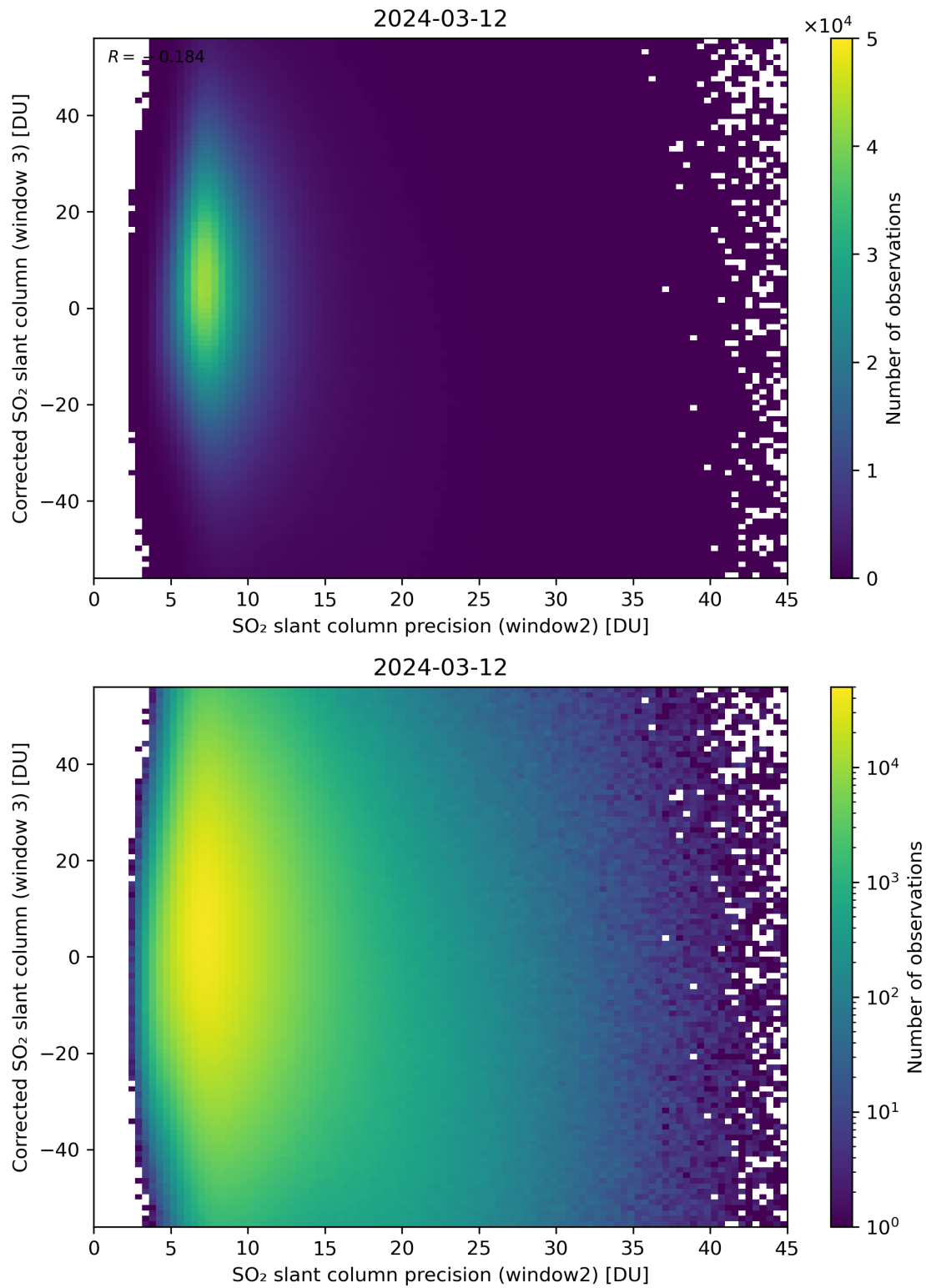
Figure 248: Scatter density plot of “SO 2 slant column precision (window2)” against “Corrected SO 2 slant column (window 3)” for 2024-03-11 to 2024-03-13.
