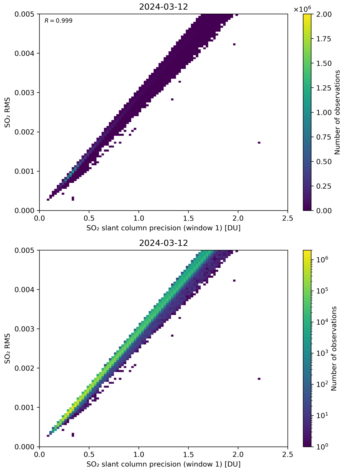
Figure 223: Scatter density plot of “SO 2 slant column precision (window 1)” against “SO 2 RMS” for 2024-03-11 to 2024-03-13.
