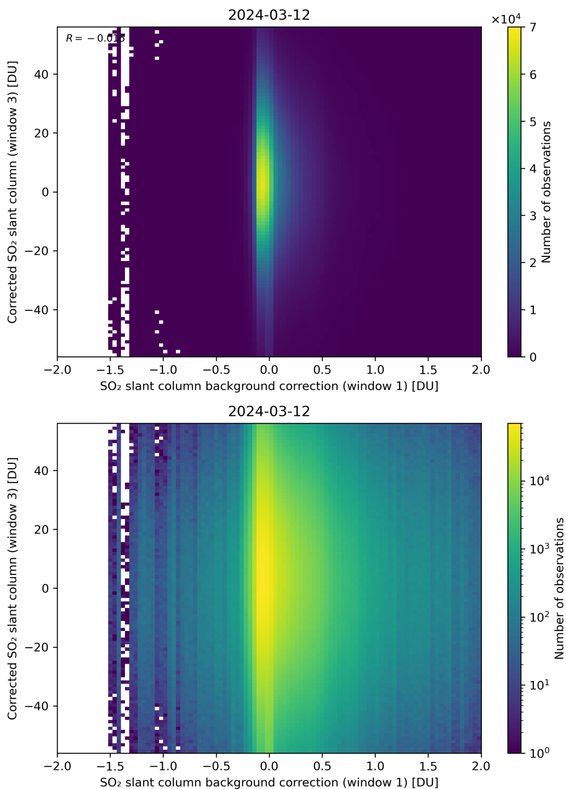
Figure 105: Scatter density plot of “SO 2 slant column background correction (window 1)” against “Corrected SO 2 slant column (window 3)” for 2024-03-11 to 2024-03-13.
