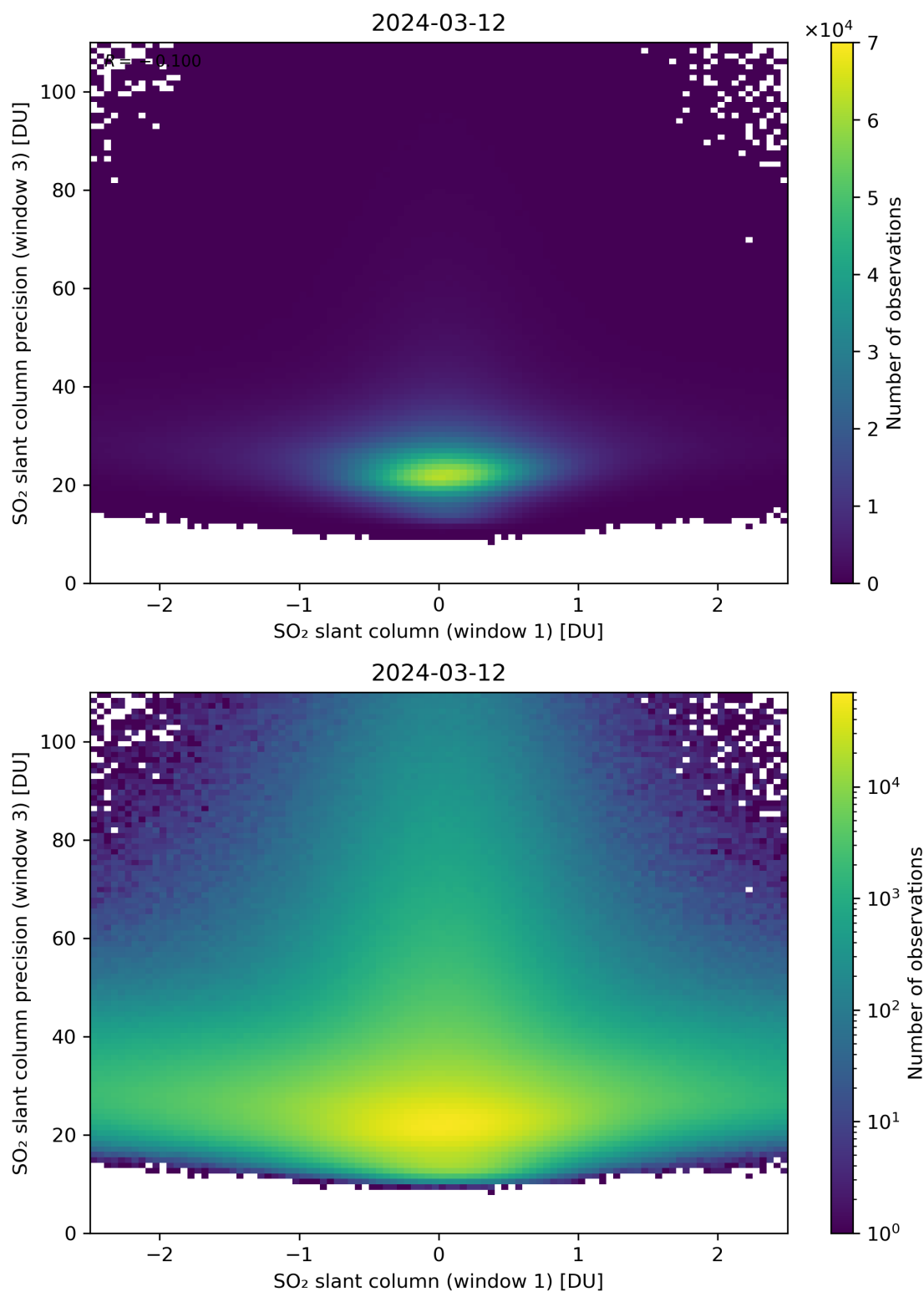
Figure 238: Scatter density plot of “SO 2 slant column (window 1)” against “SO 2 slant column precision (window 3)” for 2024-03-11 to 2024-03-13.
