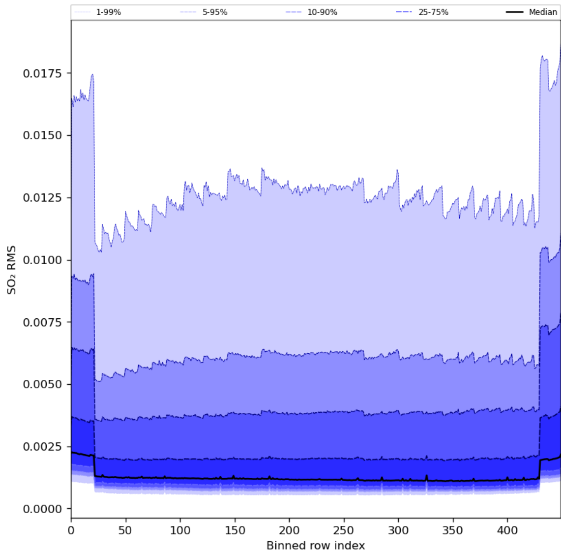
Figure 93: Along track statistics of “SO 2 RMS” for 2024-03-11 to 2024-03-13
