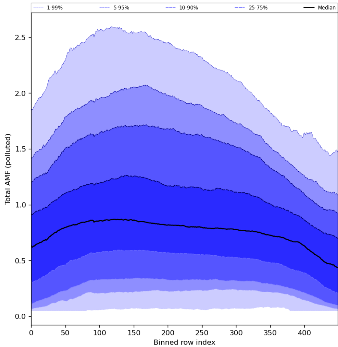
Figure 94: Along track statistics of “Total AMF (polluted)” for 2024-03-11 to 2024-03-13
