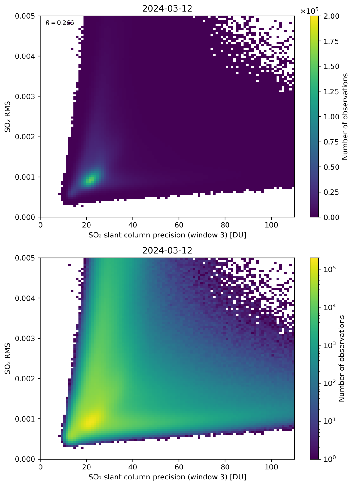
Figure 260: Scatter density plot of “SO 2 slant column precision (window 3)” against “SO 2 RMS” for 2024-03-11 to 2024-03-13.
