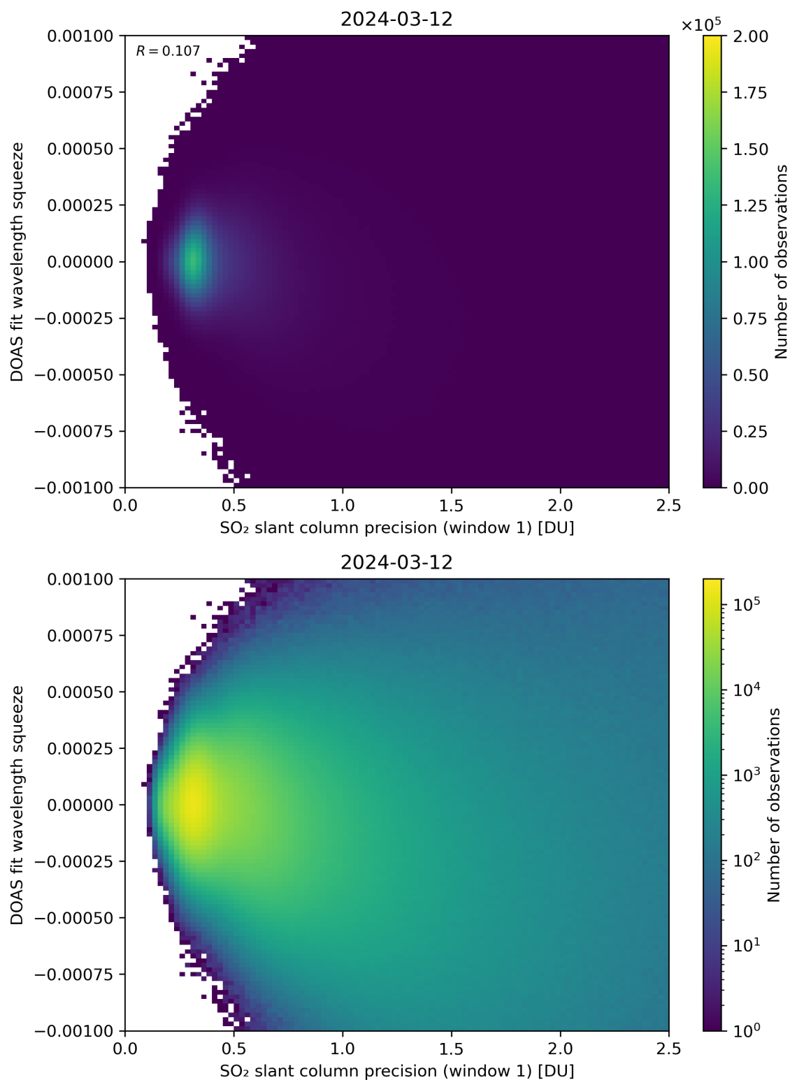
Figure 222: Scatter density plot of “SO 2 slant column precision (window 1)” against “DOAS fit wavelength squeeze” for 2024-03-11 to 2024-03-13.
