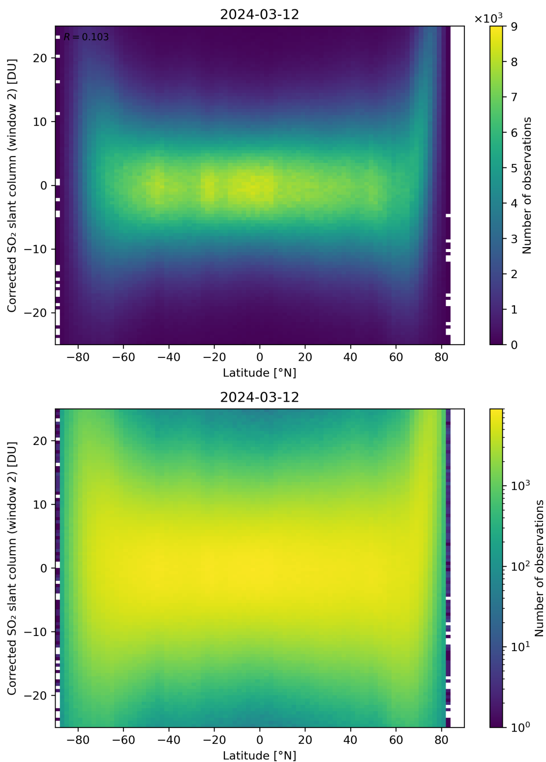
Figure 147: Scatter density plot of “Latitude” against “Corrected SO 2 slant column (window 2)” for 2024-03-11 to 2024-03-13.
