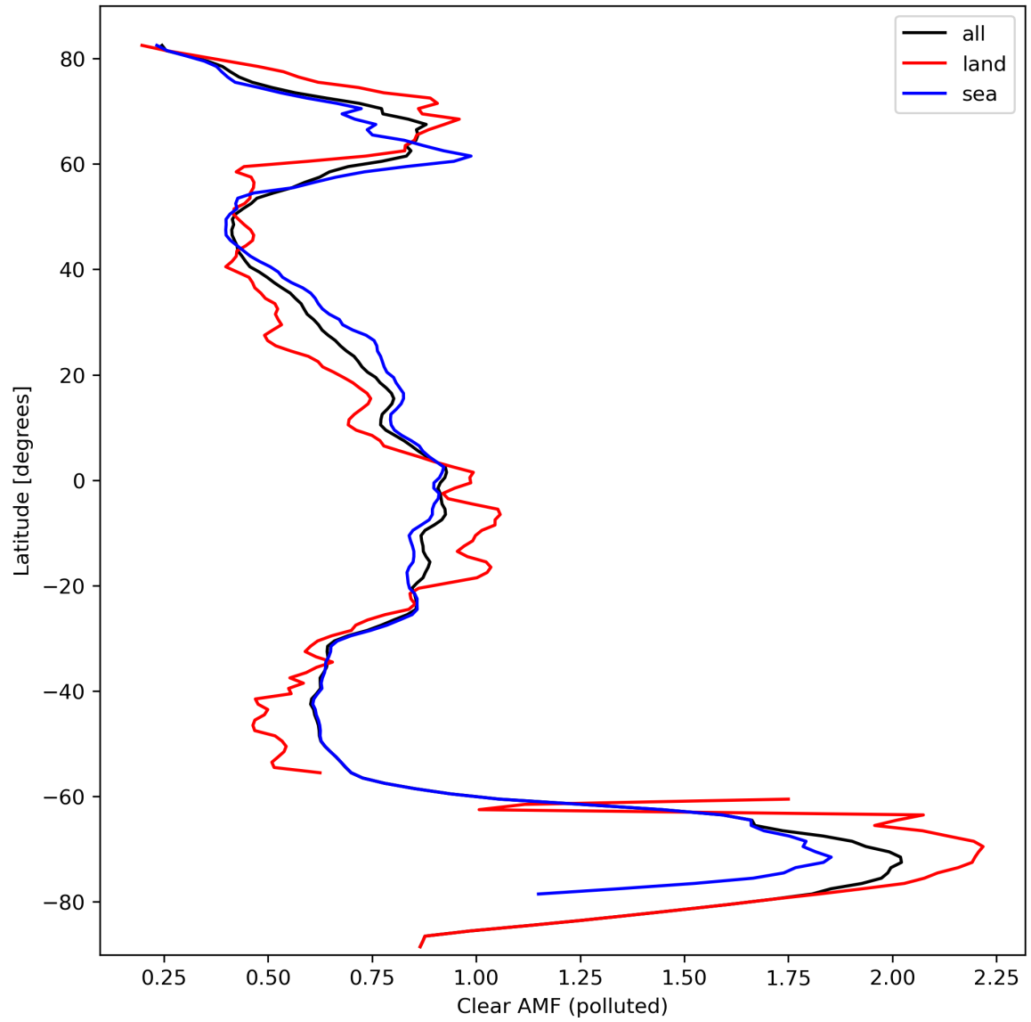
Figure 50: Zonal average of “Clear AMF (polluted)” for 2024-03-11 to 2024-03-13.
