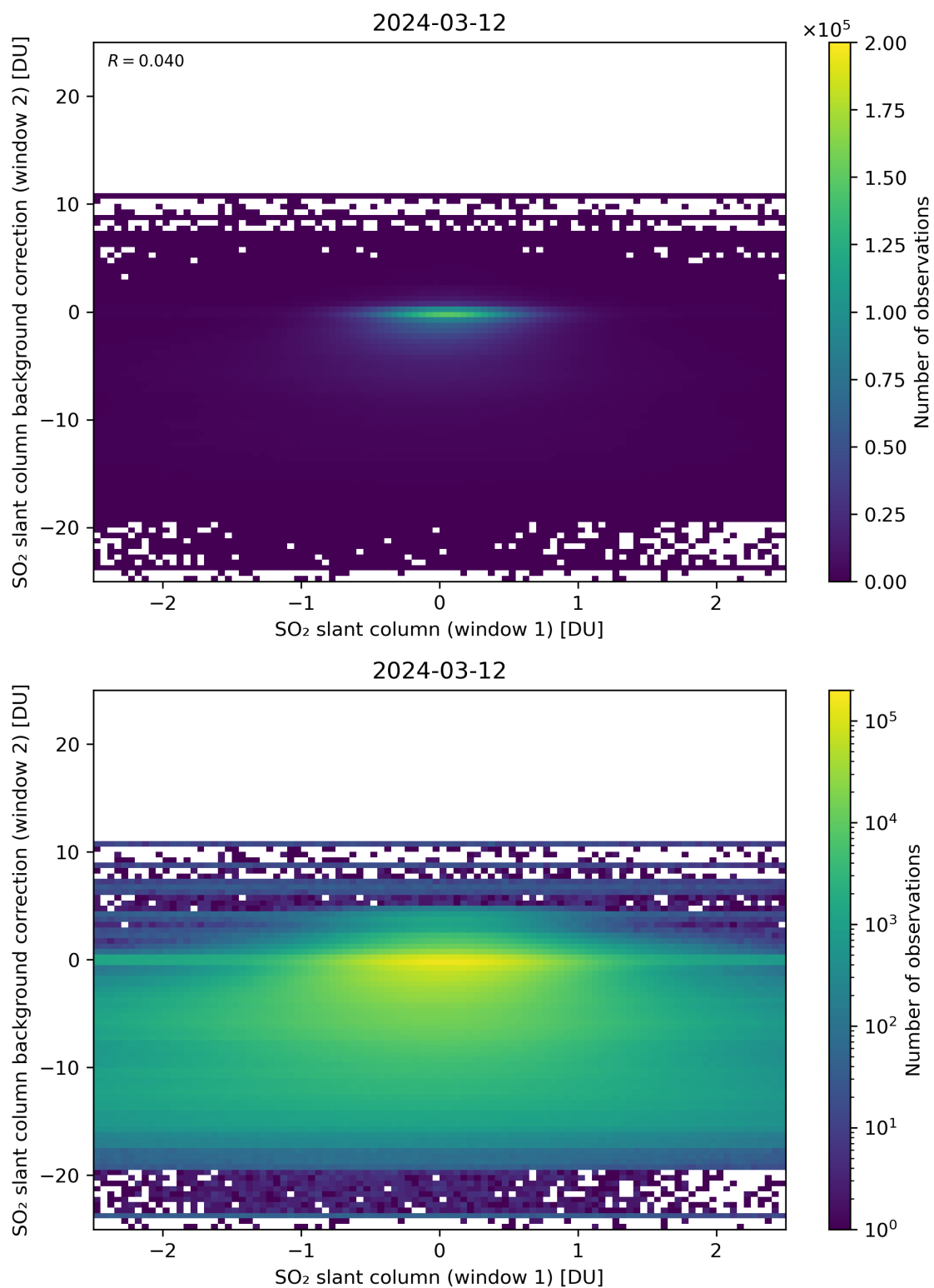
Figure 213: Scatter density plot of “SO 2 slant column (window 1)” against “SO 2 slant column background correction (window 2)” for 2024-03-11 to 2024-03-13.
