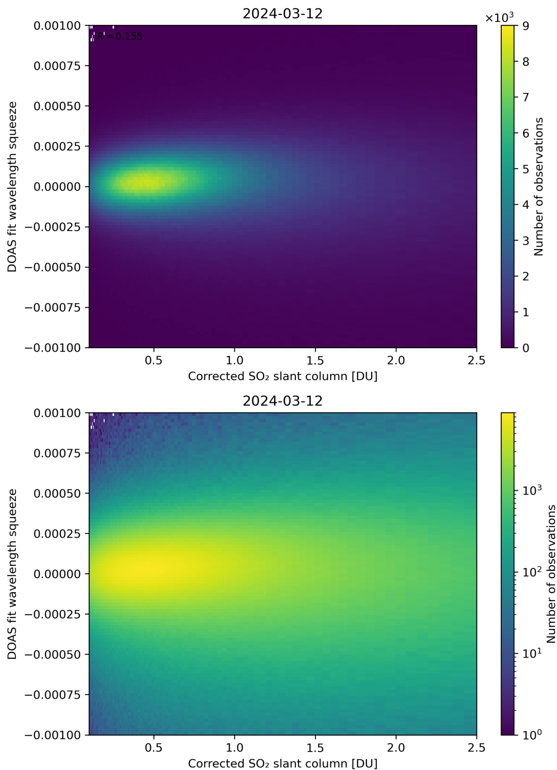
Figure 182: Scatter density plot of “Corrected SO 2 slant column” against “DOAS fit wavelength squeeze” for 2024-03-11 to 2024-03-13.
