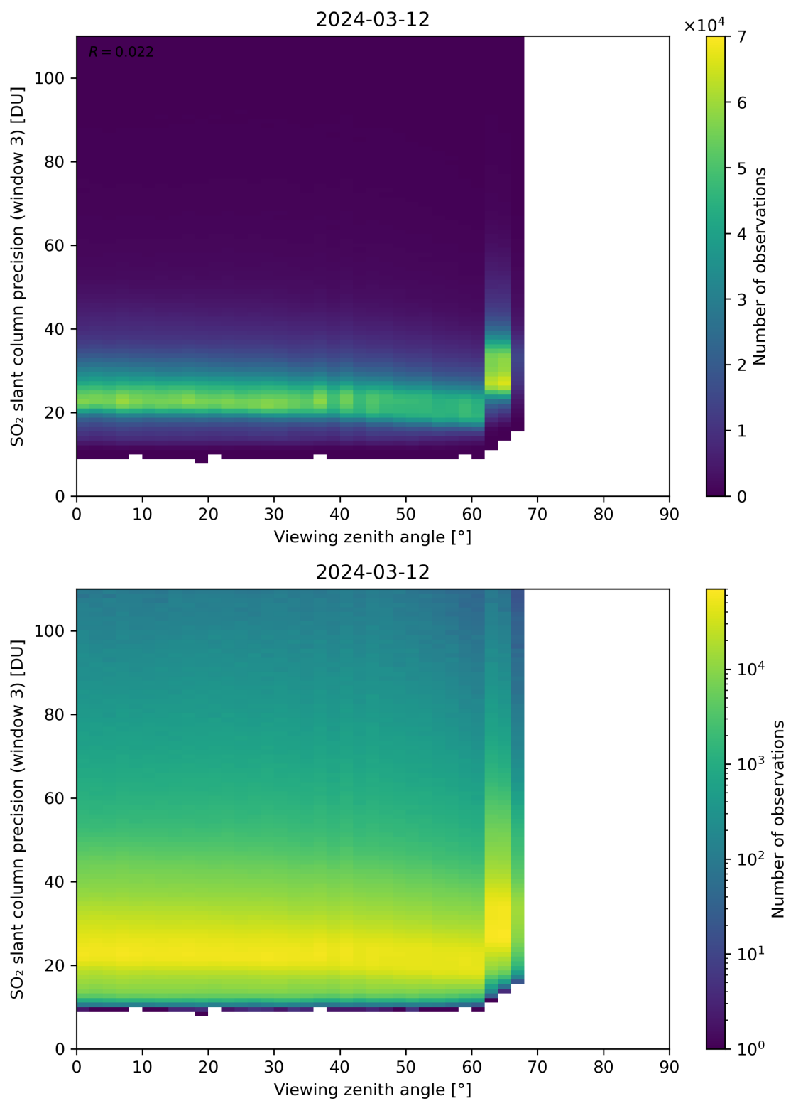
Figure 324: Scatter density plot of “Viewing zenith angle” against “SO 2 slant column precision (window 3)” for 2024-03-11 to 2024-03-13.
