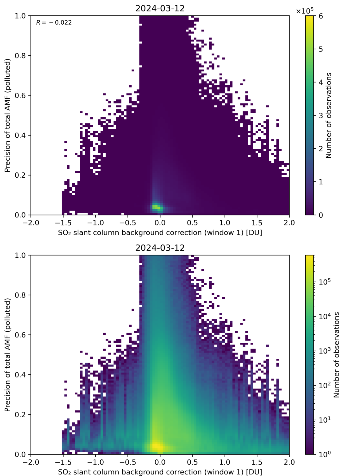
Figure 110: Scatter density plot of “SO 2 slant column background correction (window 1)” against “Precision of total AMF (polluted)” for 2024-03-11 to 2024-03-13.
