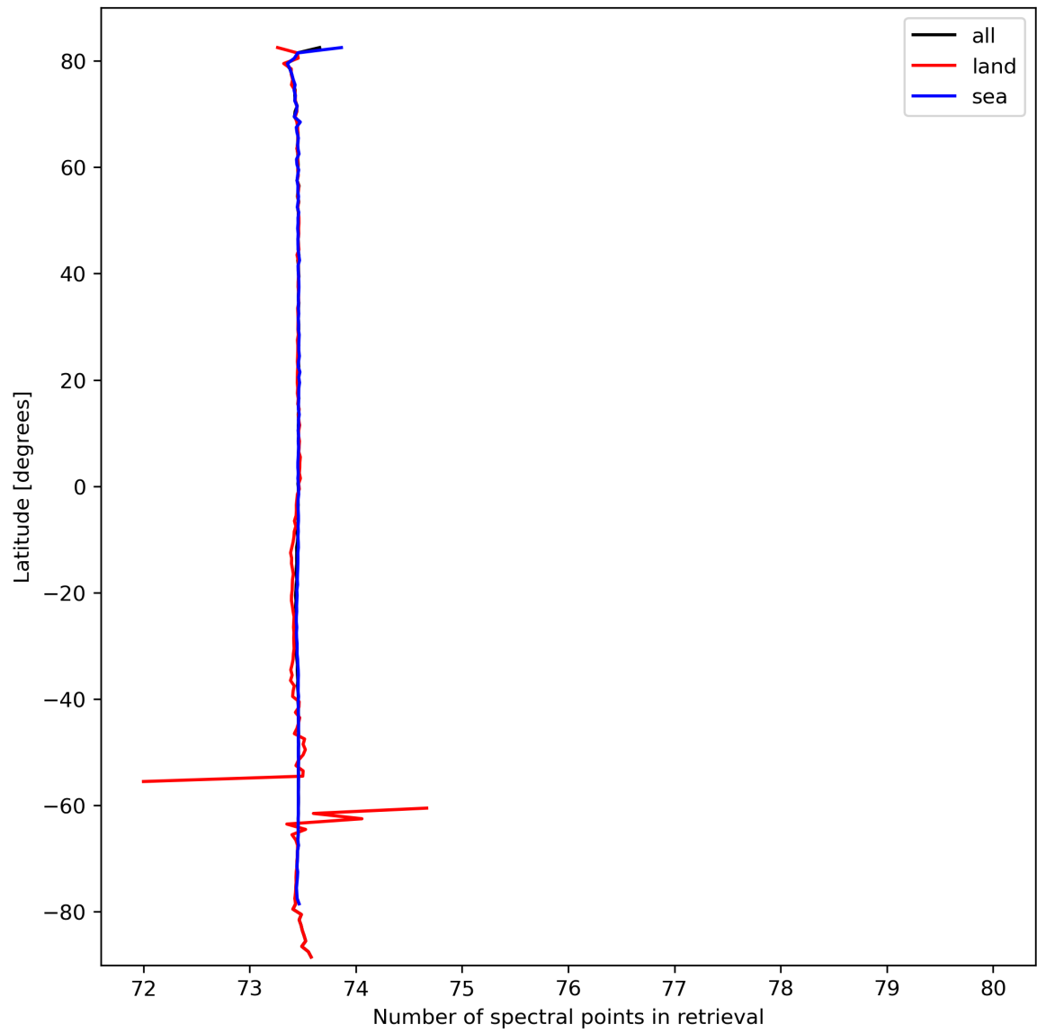
Figure 51: Zonal average of “Number of spectral points in retrieval” for 2024-03-11 to 2024-03-13.
