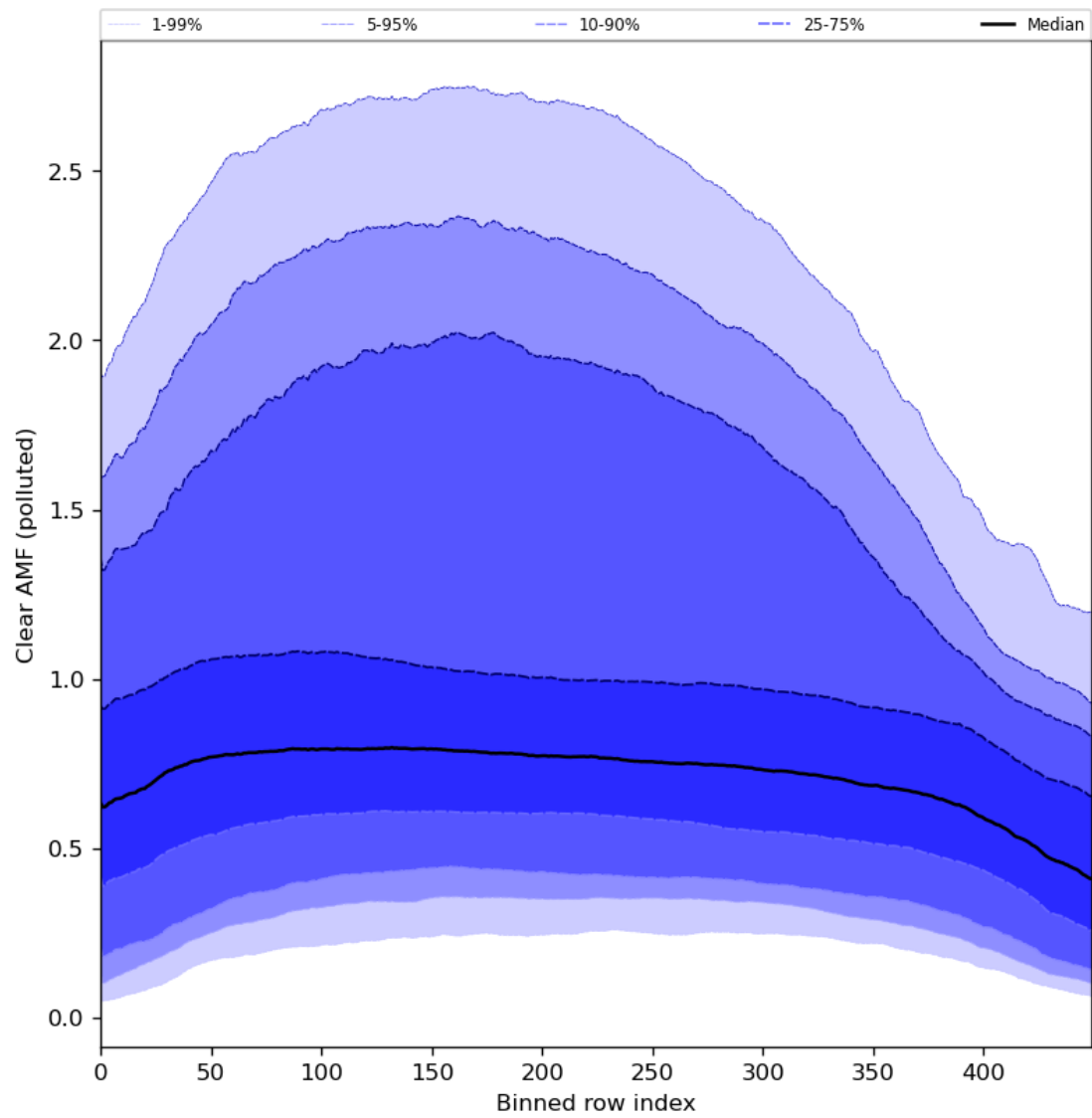
Figure 96: Along track statistics of “Clear AMF (polluted)” for 2024-03-11 to 2024-03-13
