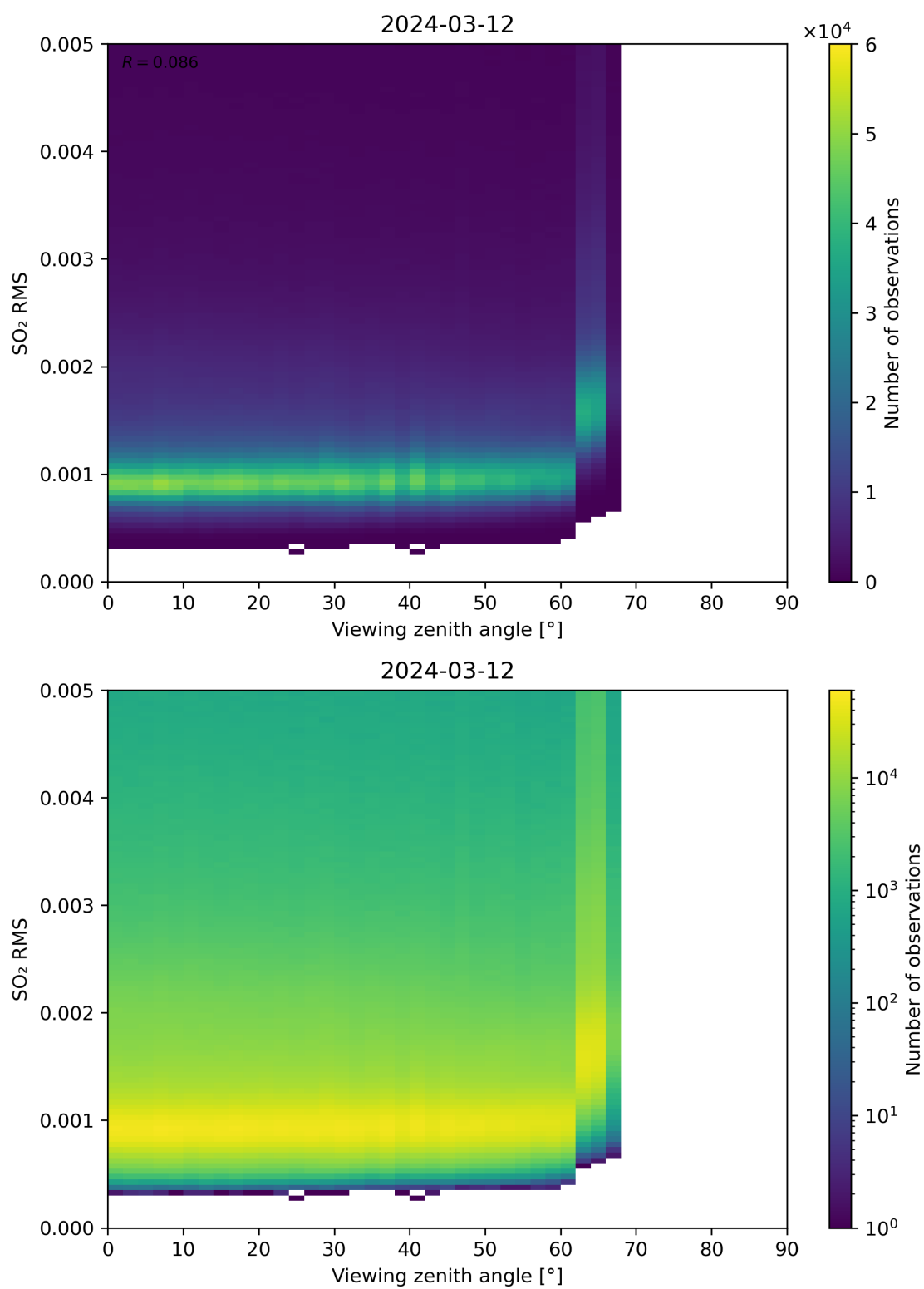
Figure 313: Scatter density plot of “Viewing zenith angle” against “SO 2 RMS” for 2024-03-11 to 2024-03-13.
