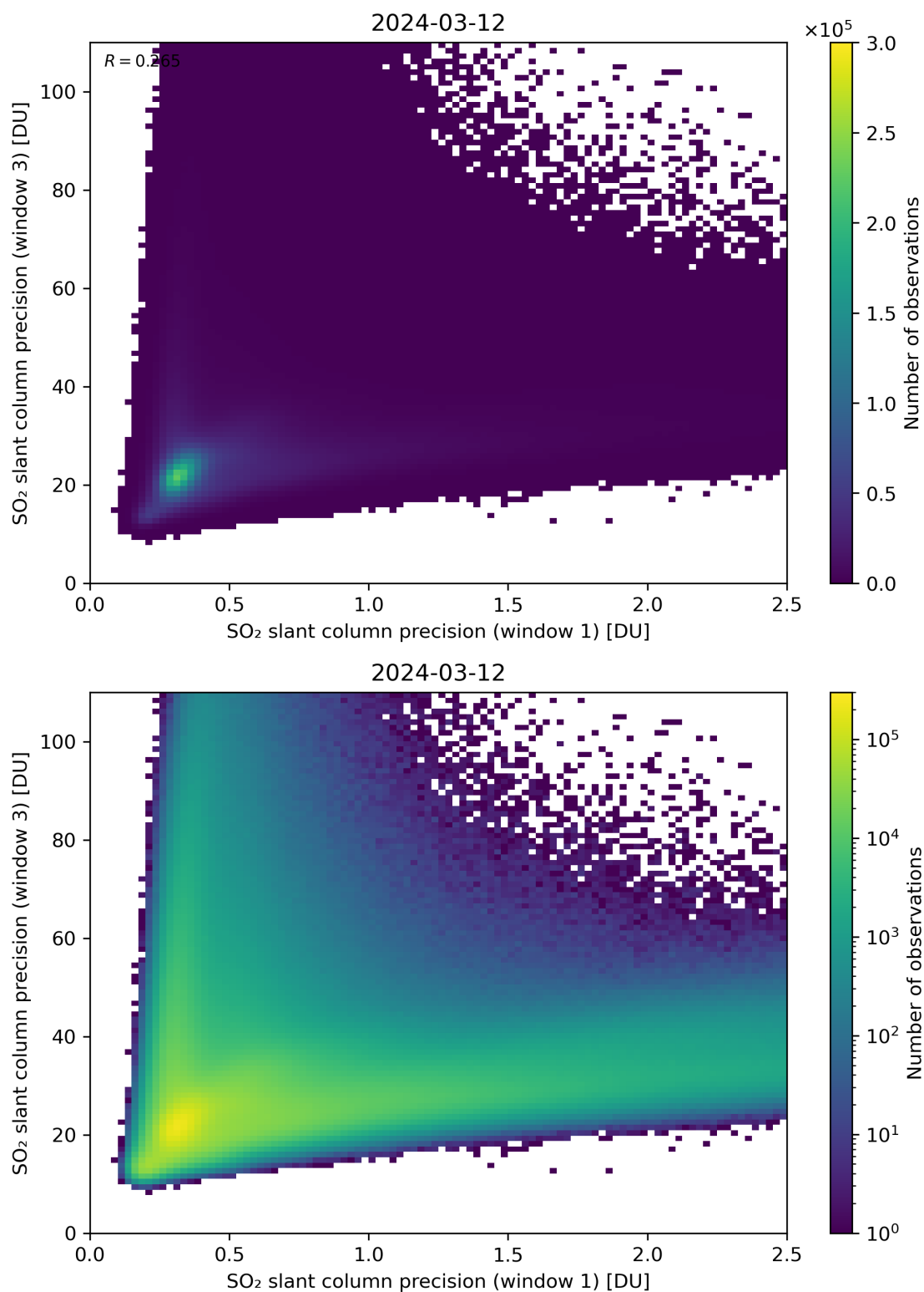
Figure 229: Scatter density plot of “SO 2 slant column precision (window 1)” against “SO 2 slant column precision (window 3)” for 2024-03-11 to 2024-03-13.
