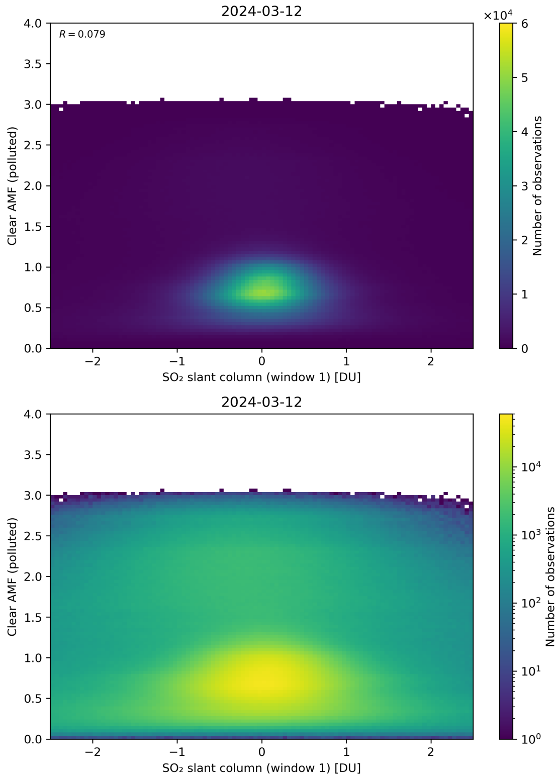
Figure 232: Scatter density plot of “SO 2 slant column (window 1)” against “Clear AMF (polluted)” for 2024-03-11 to 2024-03-13.
