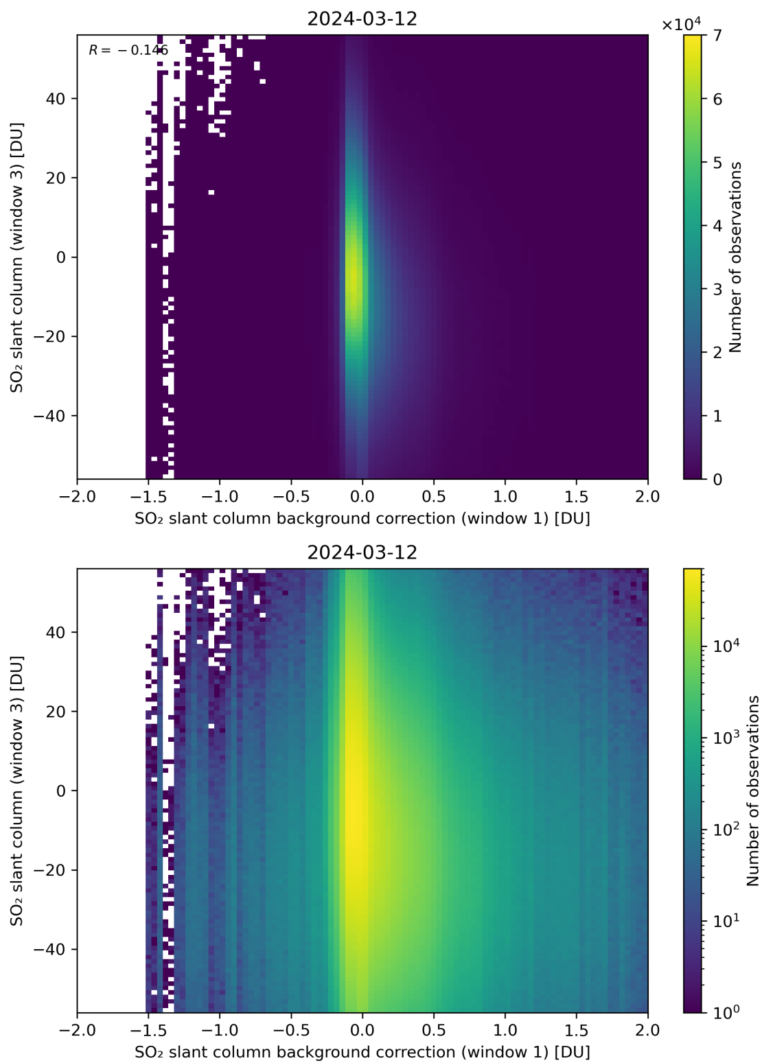
Figure 107: Scatter density plot of “SO 2 slant column background correction (window 1)” against “SO 2 slant column (window 3)” for 2024-03-11 to 2024-03-13.
