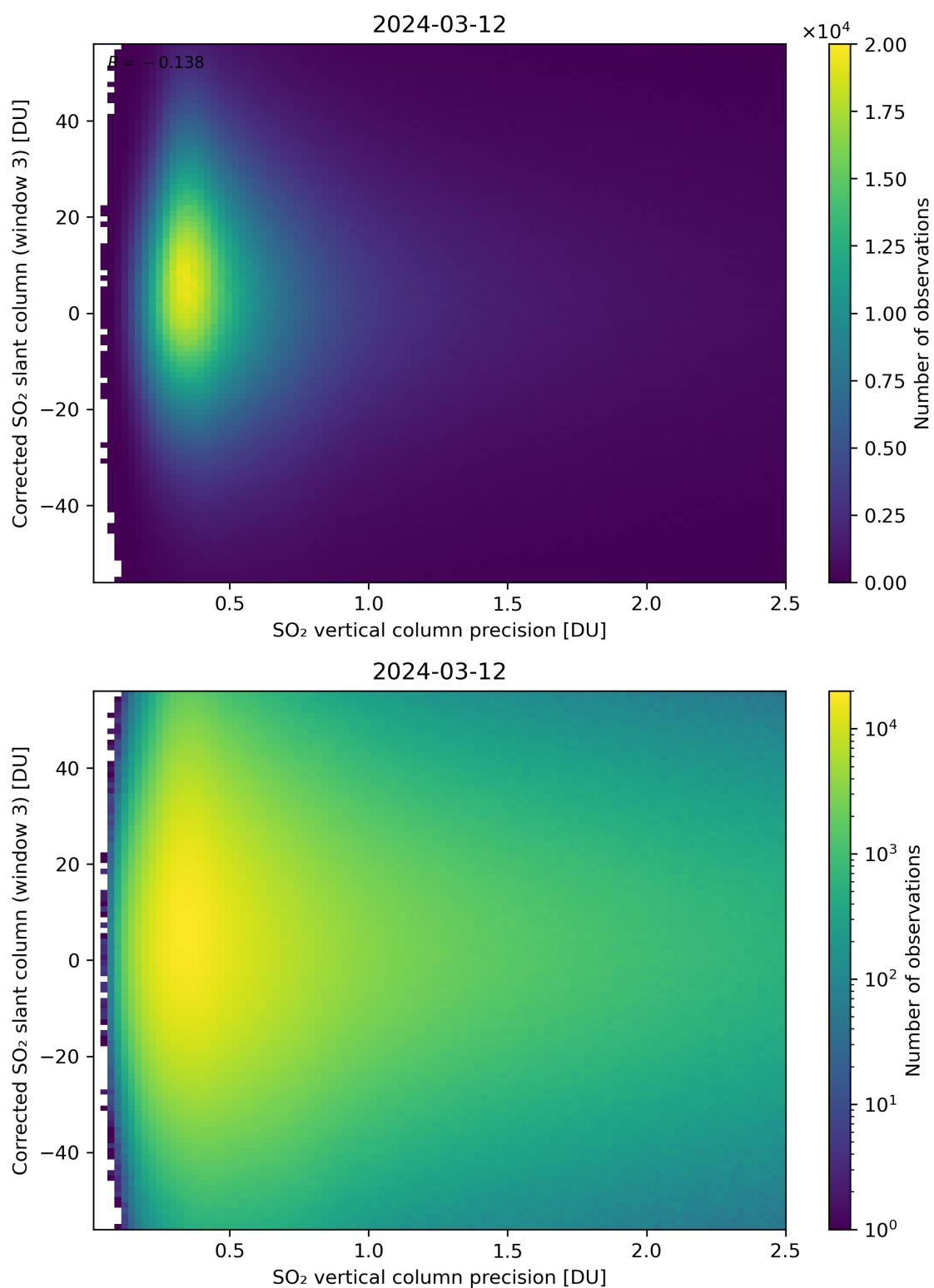
Figure 288: Scatter density plot of “SO 2 vertical column precision” against “Corrected SO 2 slant column (window 3)” for 2024-03-11 to 2024-03-13.
