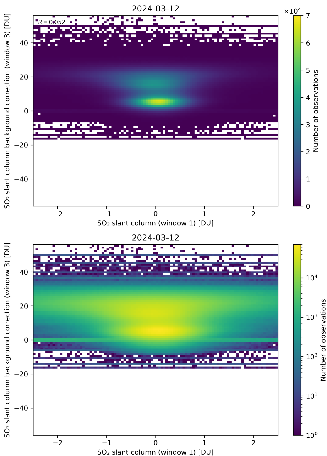
Figure 214: Scatter density plot of “SO 2 slant column (window 1)” against “SO 2 slant column background correction (window 3)” for 2024-03-11 to 2024-03-13.
