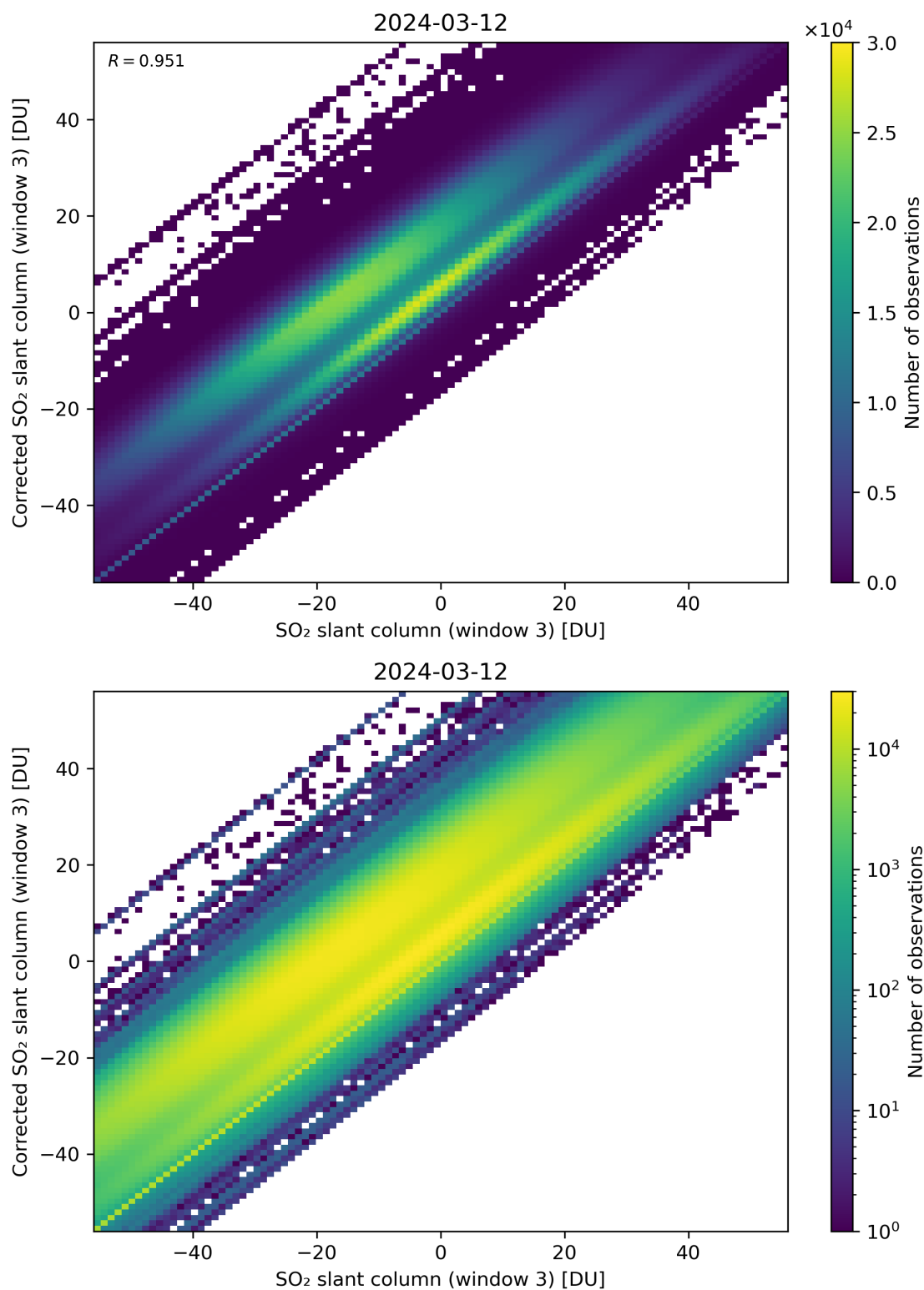
Figure 266: Scatter density plot of “SO 2 slant column (window 3)” against “Corrected SO 2 slant column (window 3)” for 2024-03-11 to 2024-03-13.
