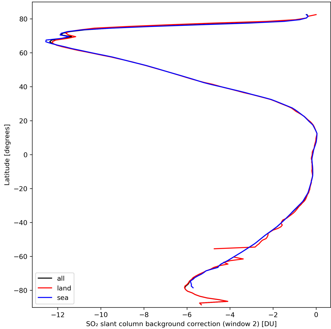
Figure 40: Zonal average of “SO 2 slant column background correction (window 2)” for 2024-03-11 to 2024-03-13.
