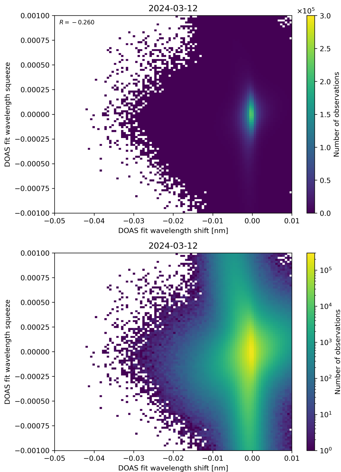
Figure 127: Scatter density plot of “DOAS fit wavelength shift” against “DOAS fit wavelength squeeze” for 2024-03-11 to 2024-03-13.
