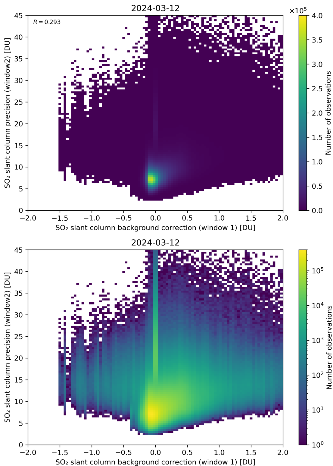
Figure 106: Scatter density plot of “SO 2 slant column background correction (window 1)” against “SO 2 slant column precision (window2)” for 2024-03-11 to 2024-03-13.
