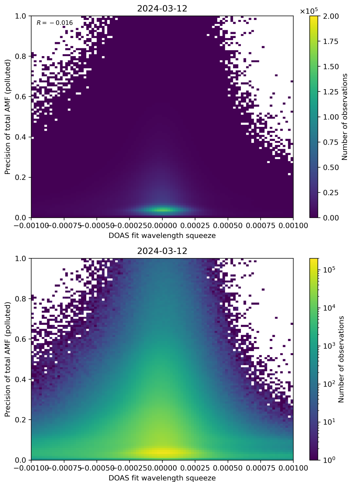
Figure 135: Scatter density plot of “DOAS fit wavelength squeeze” against “Precision of total AMF (polluted)” for 2024-03-11 to 2024-03-13.
