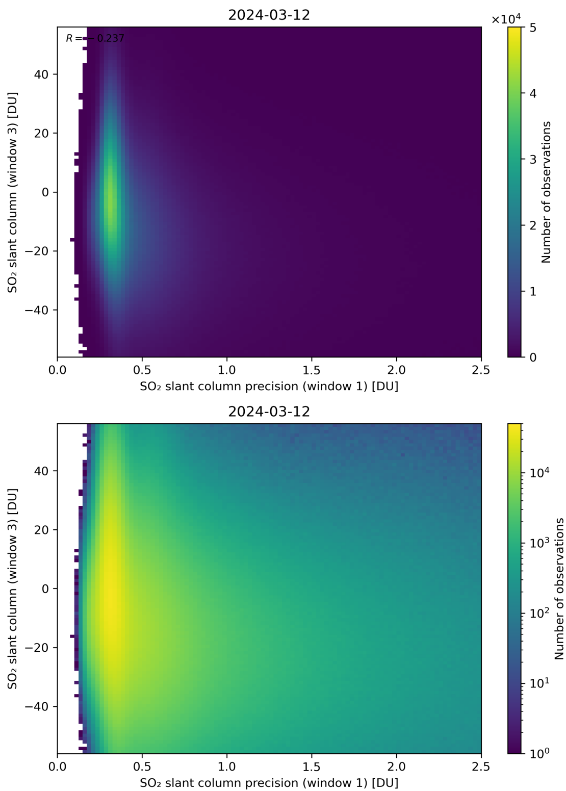
Figure 228: Scatter density plot of “SO 2 slant column precision (window 1)” against “SO 2 slant column (window 3)” for 2024-03-11 to 2024-03-13.
