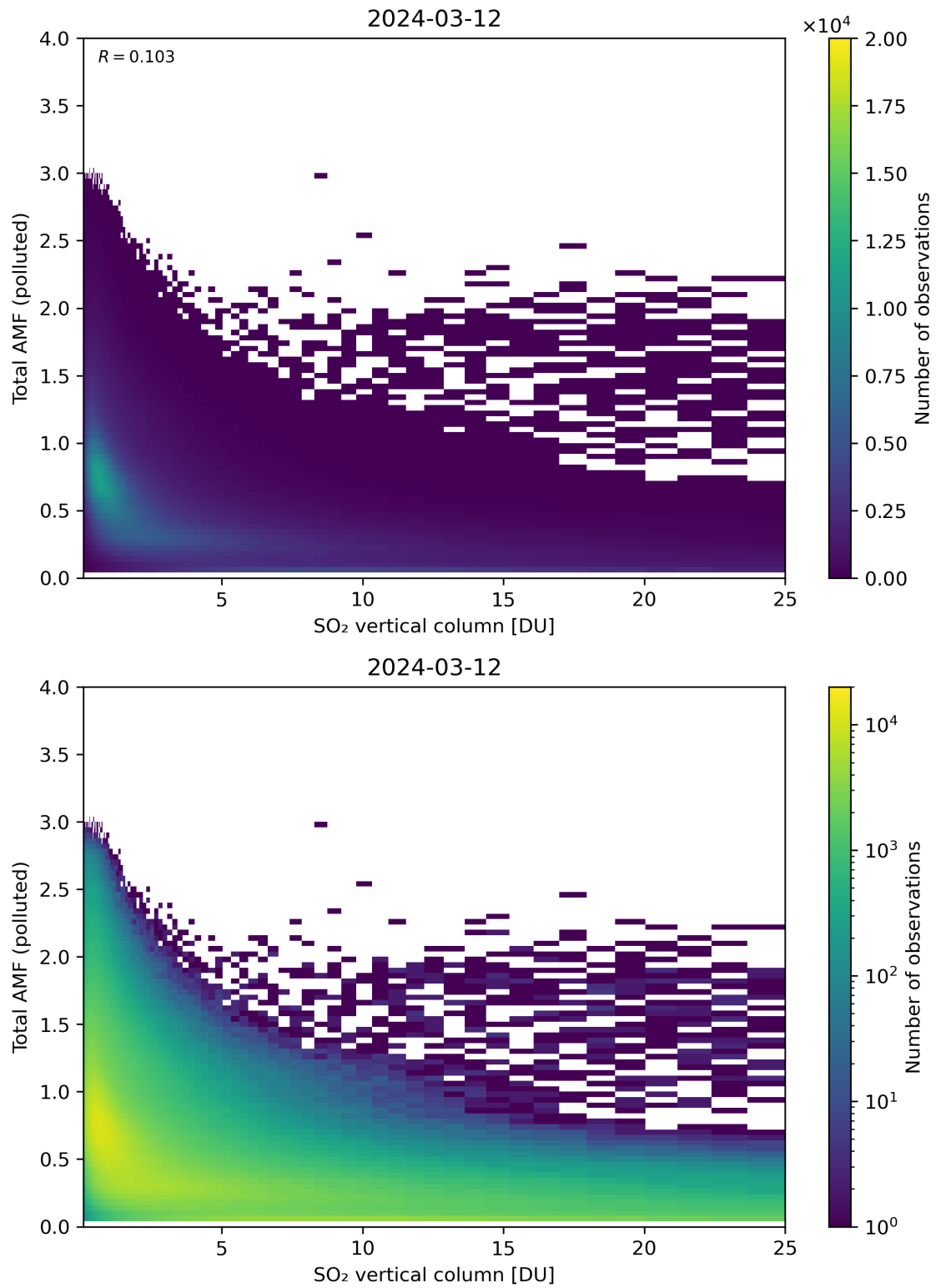
Figure 305: Scatter density plot of “SO 2 vertical column” against “Total AMF (polluted)” for 2024-03-11 to 2024-03-13.
