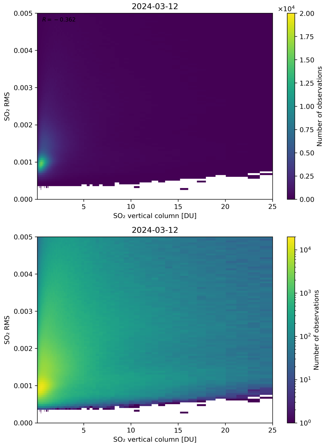
Figure 278: Scatter density plot of “SO 2 vertical column” against “SO 2 RMS” for 2024-03-11 to 2024-03-13.
