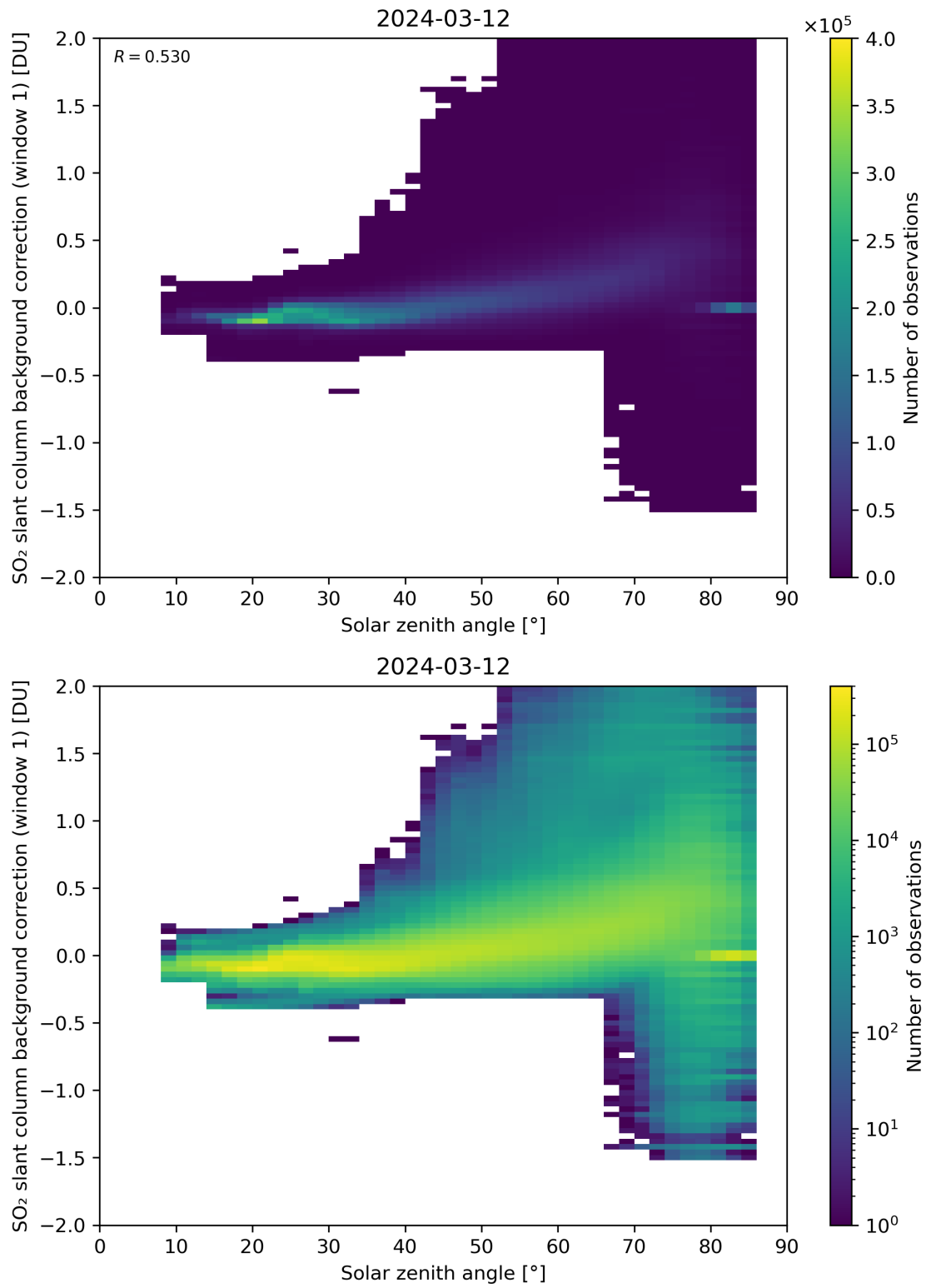
Figure 158: Scatter density plot of “Solar zenith angle” against “SO 2 slant column background correction (window 1)” for 2024-03-11 to 2024-03-13.
