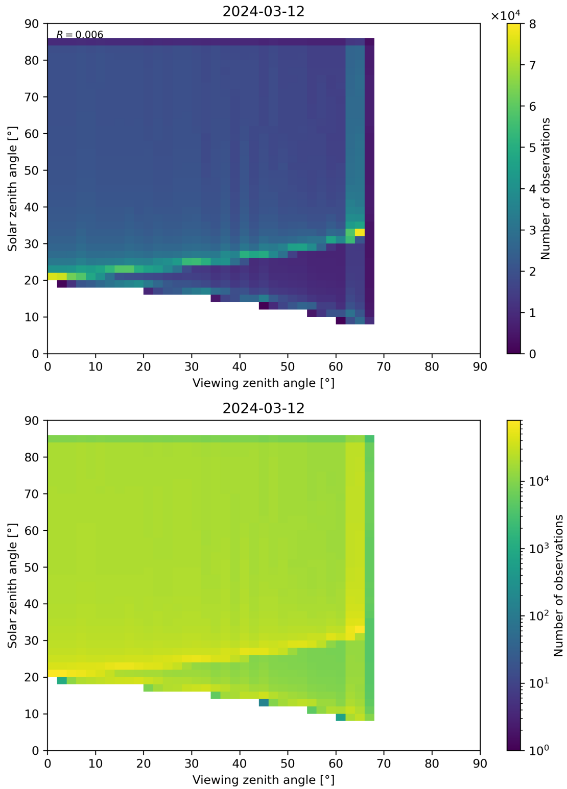
Figure 315: Scatter density plot of “Viewing zenith angle” against “Solar zenith angle” for 2024-03-11 to 2024-03-13.
