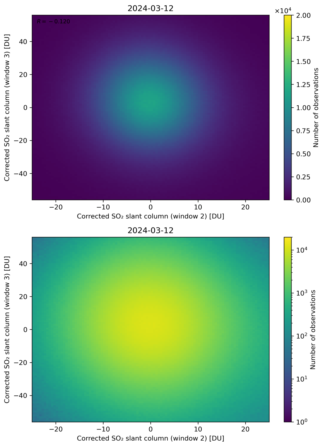
Figure 200: Scatter density plot of “Corrected SO 2 slant column (window 2)” against “Corrected SO 2 slant column (window 3)” for 2024-03-11 to 2024-03-13.
