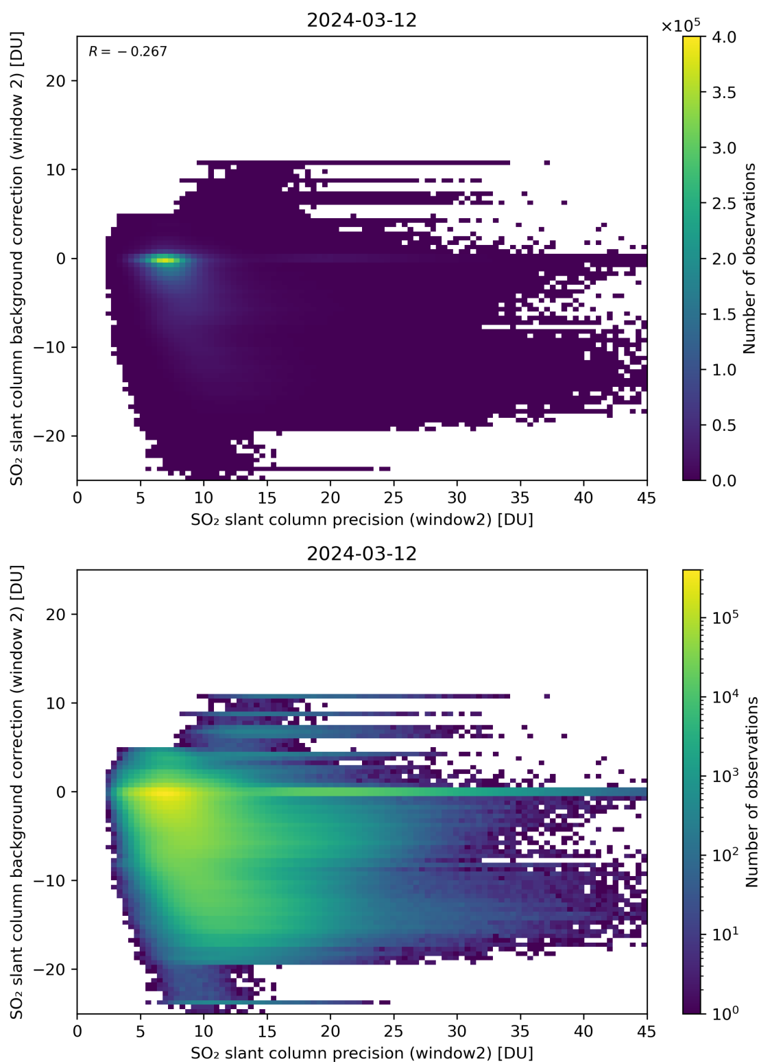
Figure 241: Scatter density plot of “SO 2 slant column precision (window2)” against “SO 2 slant column background correction (window 2)” for 2024-03-11 to 2024-03-13.
