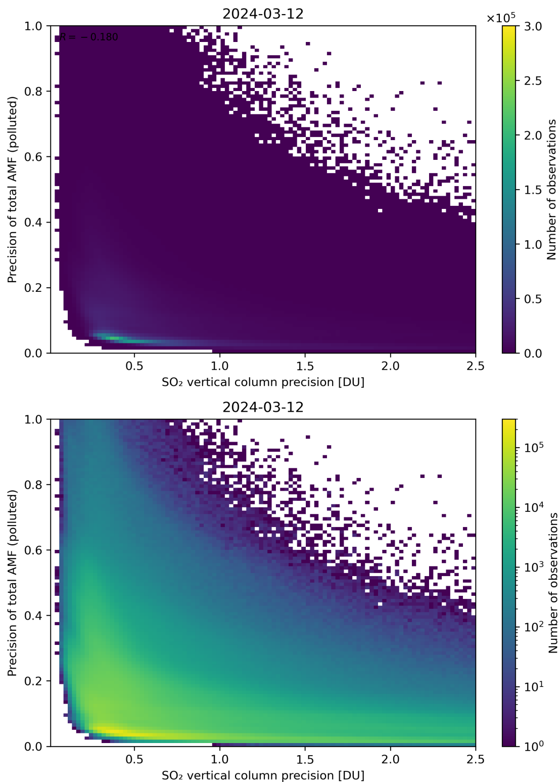
Figure 295: Scatter density plot of “SO 2 vertical column precision” against “Precision of total AMF (polluted)” for 2024-03-11 to 2024-03-13.
