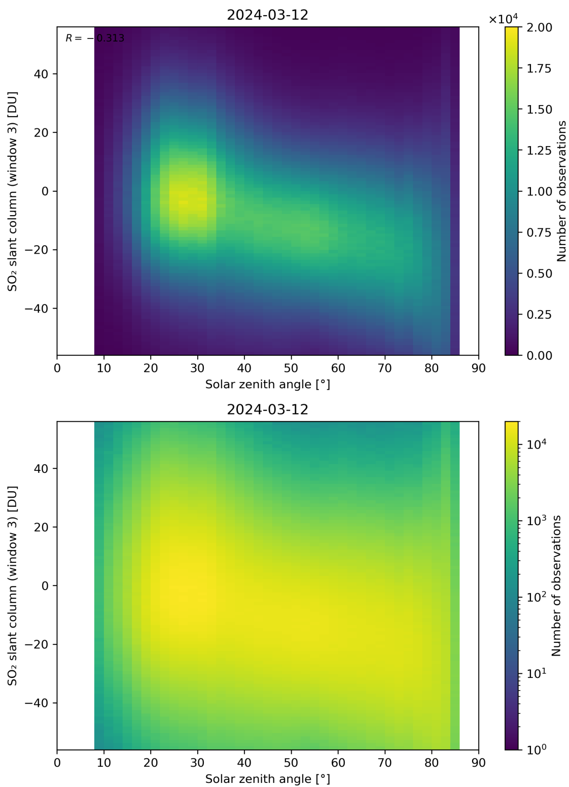
Figure 172: Scatter density plot of “Solar zenith angle” against “SO 2 slant column (window 3)” for 2024-03-11 to 2024-03-13.
