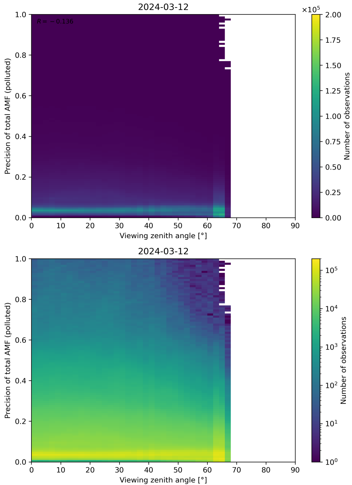
Figure 326: Scatter density plot of “Viewing zenith angle” against “Precision of total AMF (polluted)” for 2024-03-11 to 2024-03-13.
