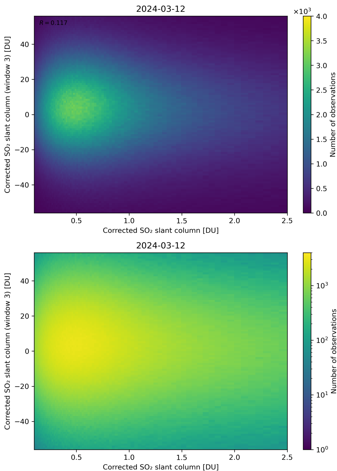
Figure 186: Scatter density plot of “Corrected SO 2 slant column” against “Corrected SO 2 slant column (window 3)” for 2024-03-11 to 2024-03-13.
