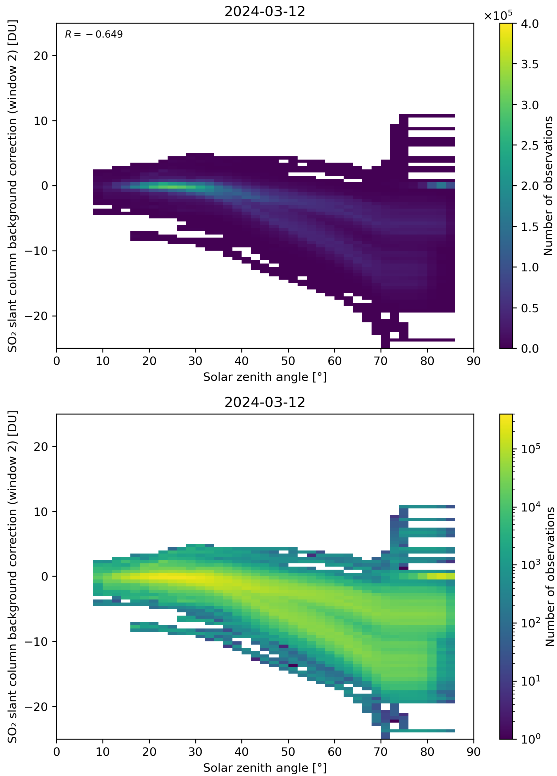
Figure 159: Scatter density plot of “Solar zenith angle” against “SO 2 slant column background correction (window 2)” for 2024-03-11 to 2024-03-13.
