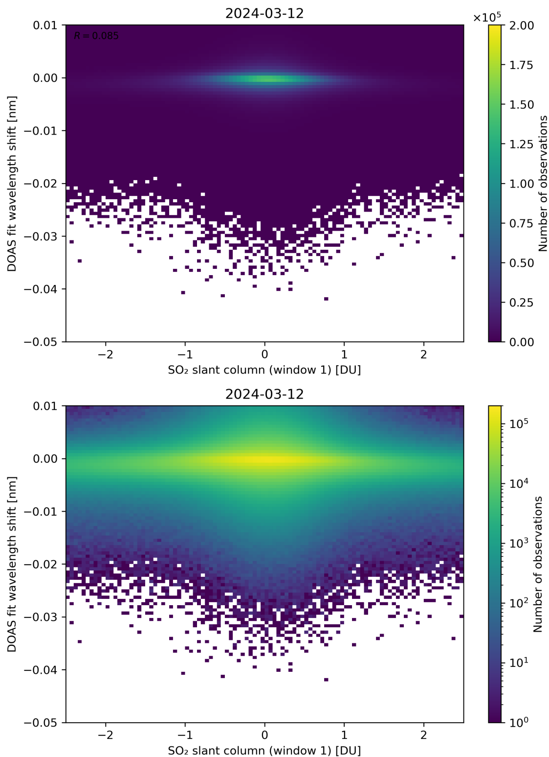
Figure 215: Scatter density plot of “SO 2 slant column (window 1)” against “DOAS fit wavelength shift” for 2024-03-11 to 2024-03-13.
