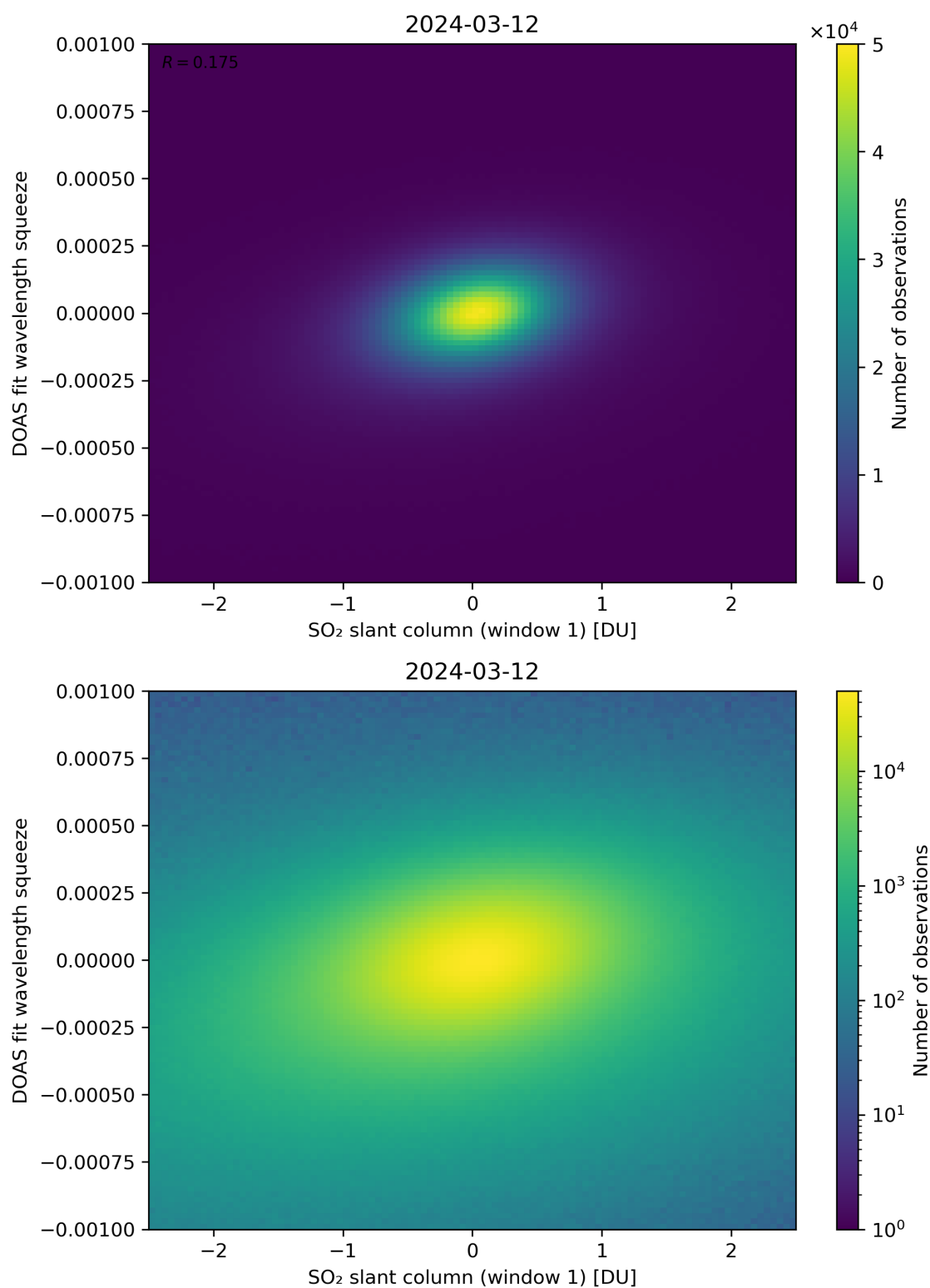
Figure 216: Scatter density plot of “SO 2 slant column (window 1)” against “DOAS fit wavelength squeeze” for 2024-03-11 to 2024-03-13.
