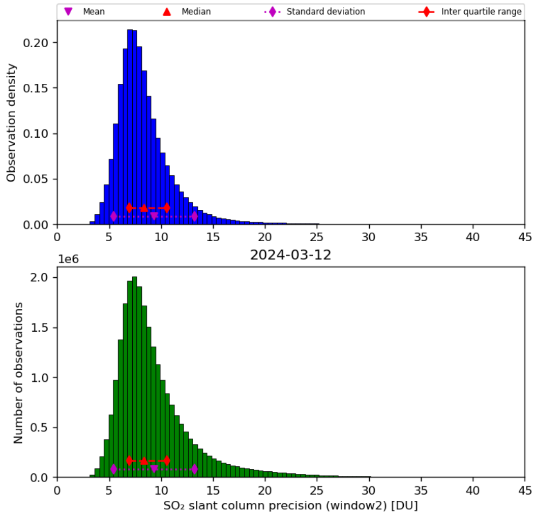
Figure 61: Histogram of “SO 2 slant column precision (window2)” for 2024-03-11 to 2024-03-13
