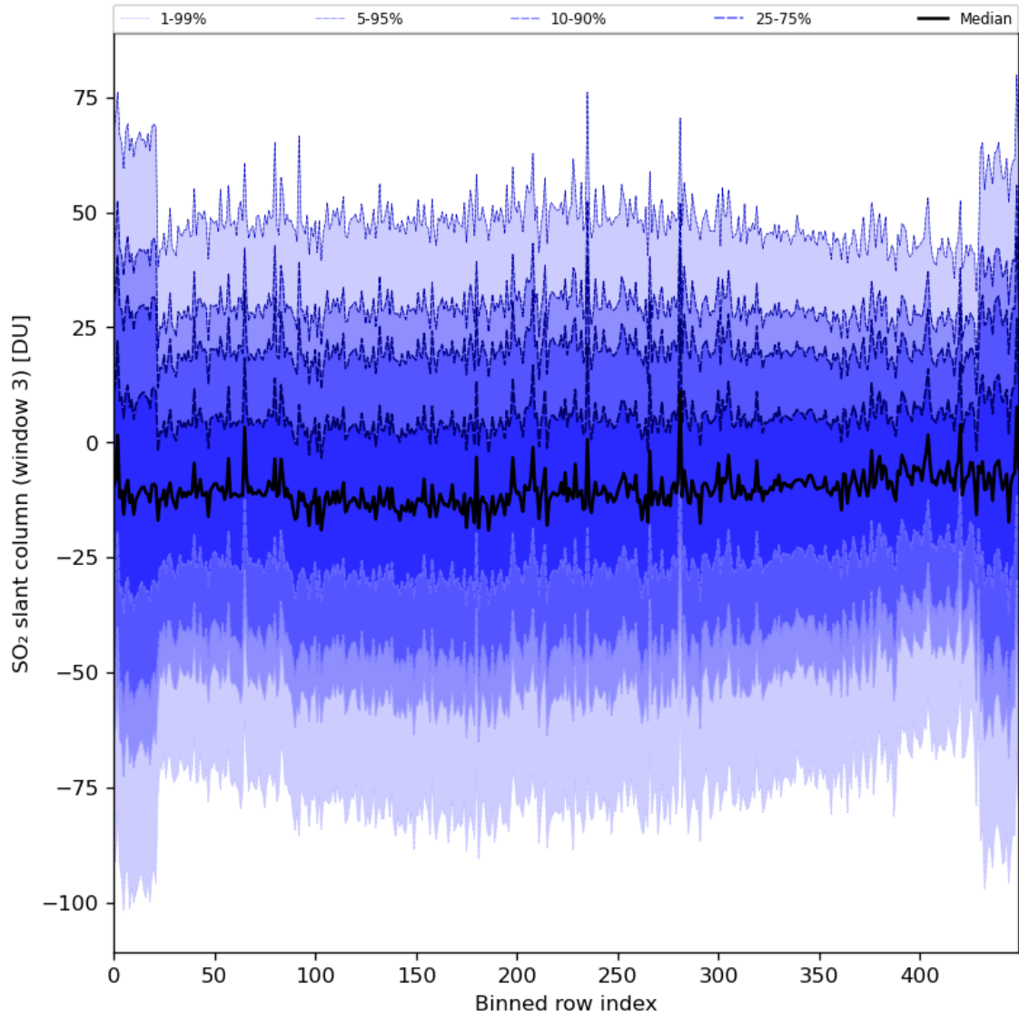
Figure 87: Along track statistics of “SO 2 slant column (window 3)” for 2024-03-11 to 2024-03-13
