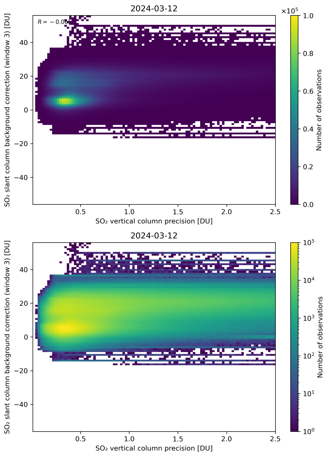
Figure 281: Scatter density plot of “SO 2 vertical column precision” against “SO 2 slant column background correction (window 3)” for 2024-03-11 to 2024-03-13.
