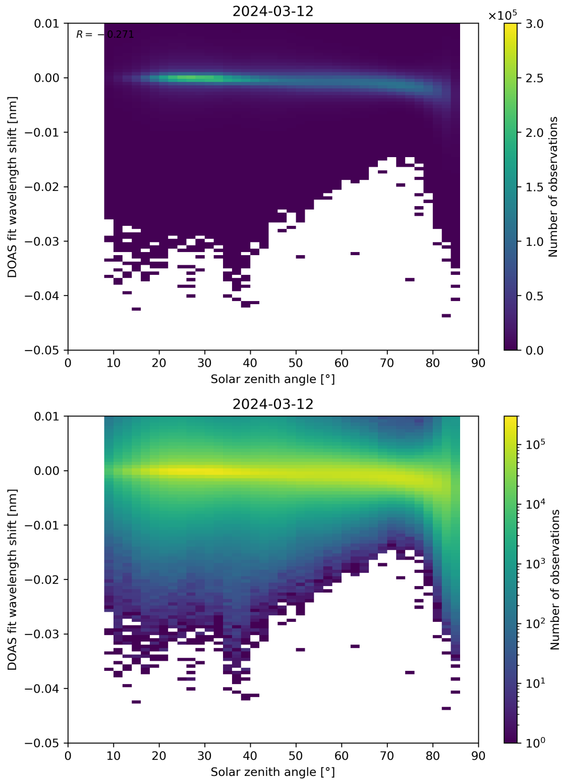
Figure 161: Scatter density plot of “Solar zenith angle” against “DOAS fit wavelength shift” for 2024-03-11 to 2024-03-13.
