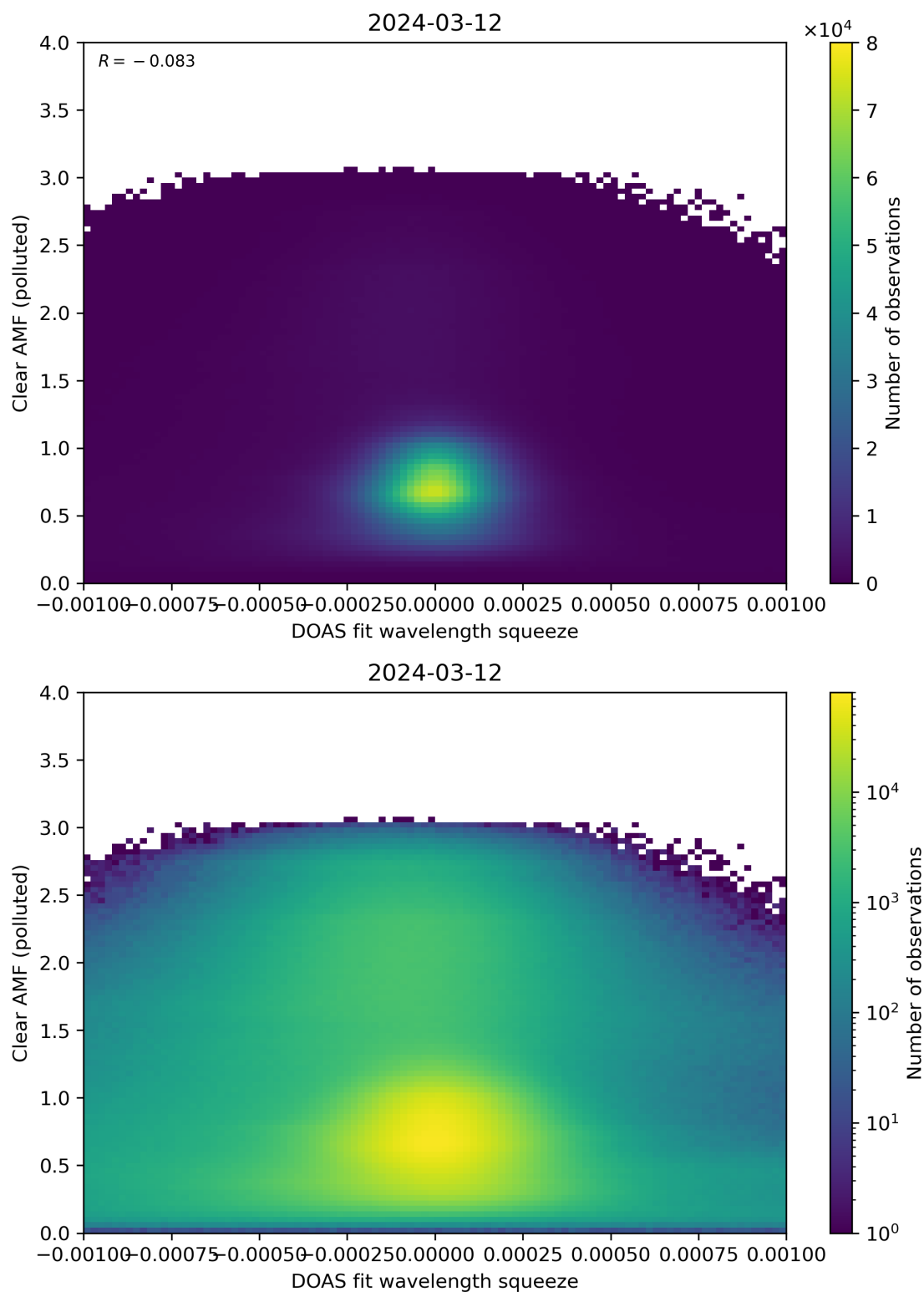
Figure 133: Scatter density plot of “DOAS fit wavelength squeeze” against “Clear AMF (polluted)” for 2024-03-11 to 2024-03-13.
