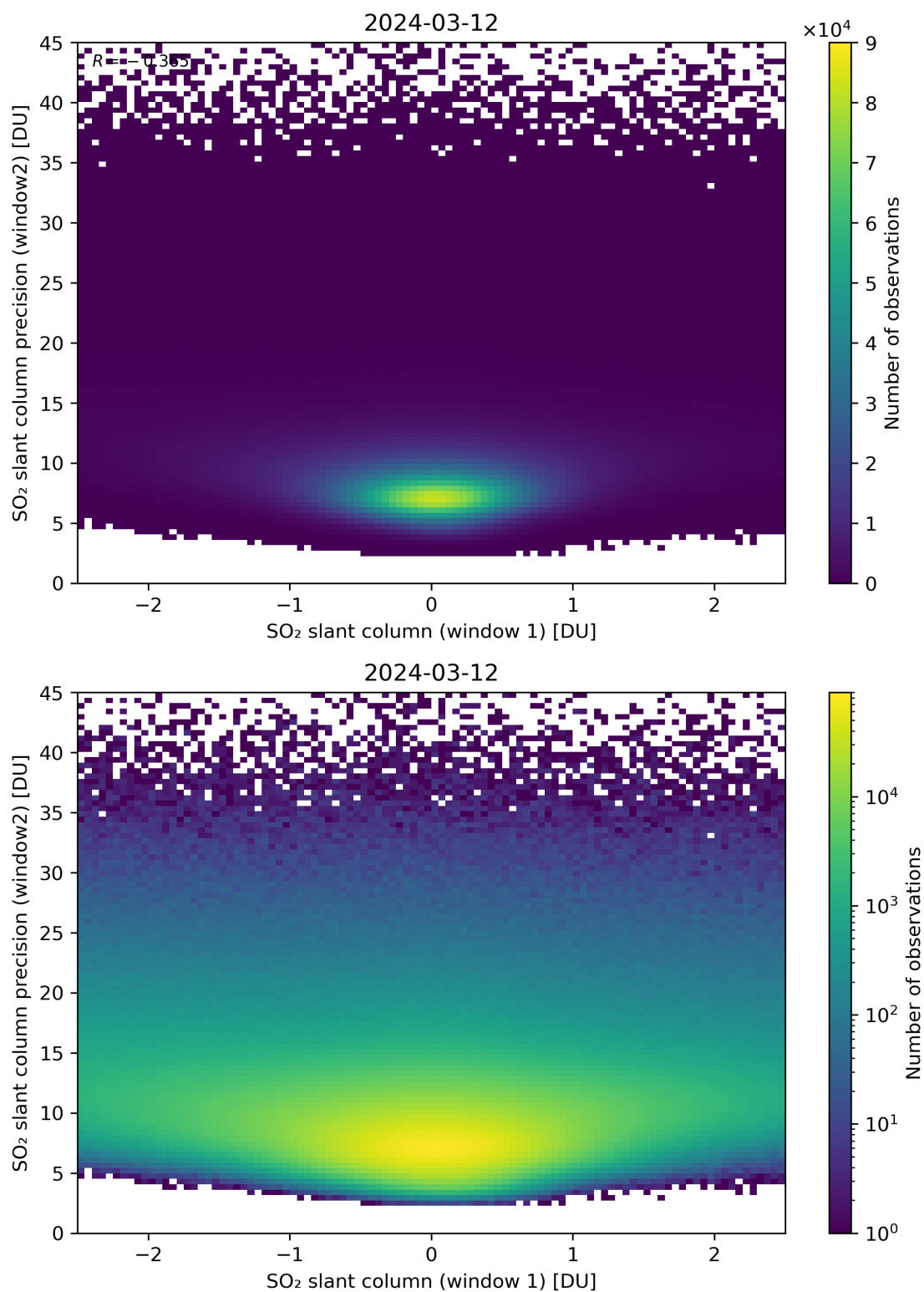
Figure 236: Scatter density plot of “SO 2 slant column (window 1)” against “SO 2 slant column precision (window2)” for 2024-03-11 to 2024-03-13.
