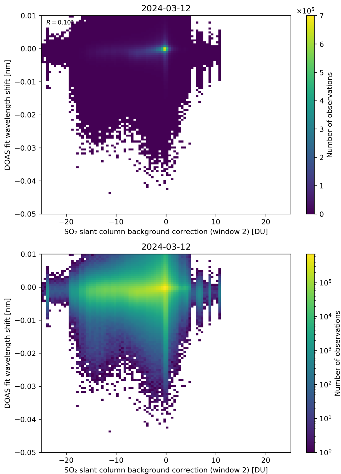
Figure 112: Scatter density plot of “SO 2 slant column background correction (window 2)” against “DOAS fit wavelength shift” for 2024-03-11 to 2024-03-13.
