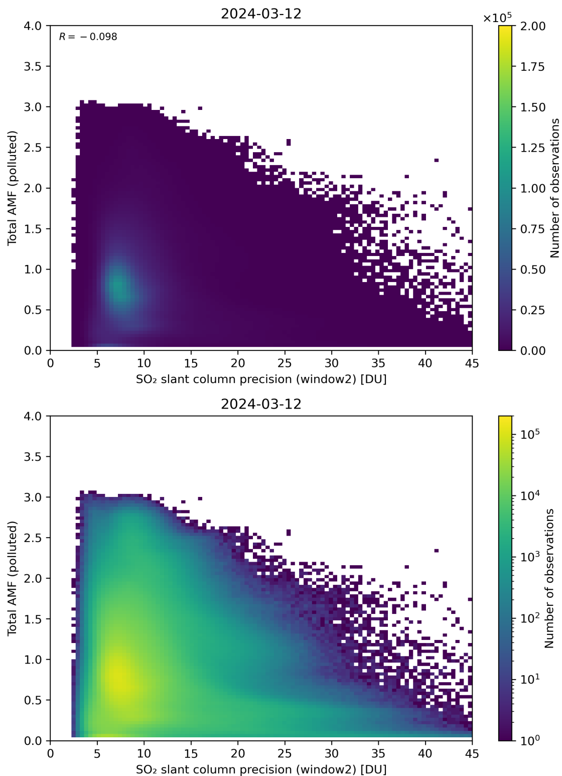
Figure 251: Scatter density plot of “SO 2 slant column precision (window2)” against “Total AMF (polluted)” for 2024-03-11 to 2024-03-13.
