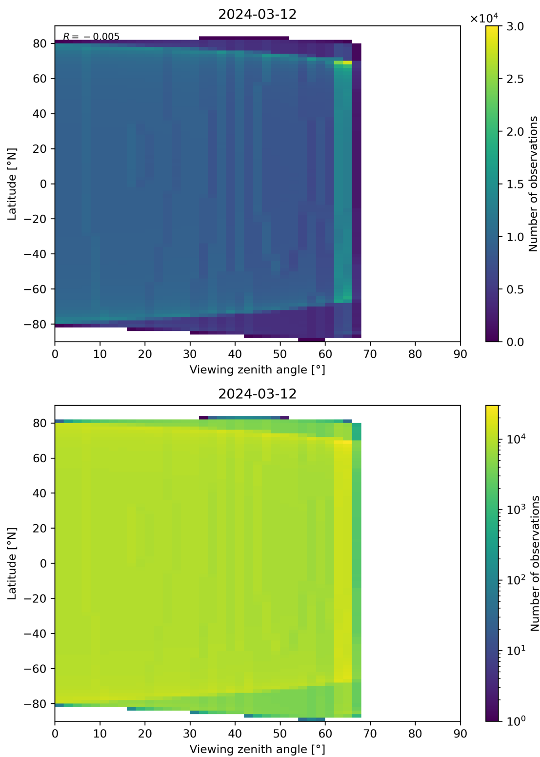
Figure 314: Scatter density plot of “Viewing zenith angle” against “Latitude” for 2024-03-11 to 2024-03-13.
