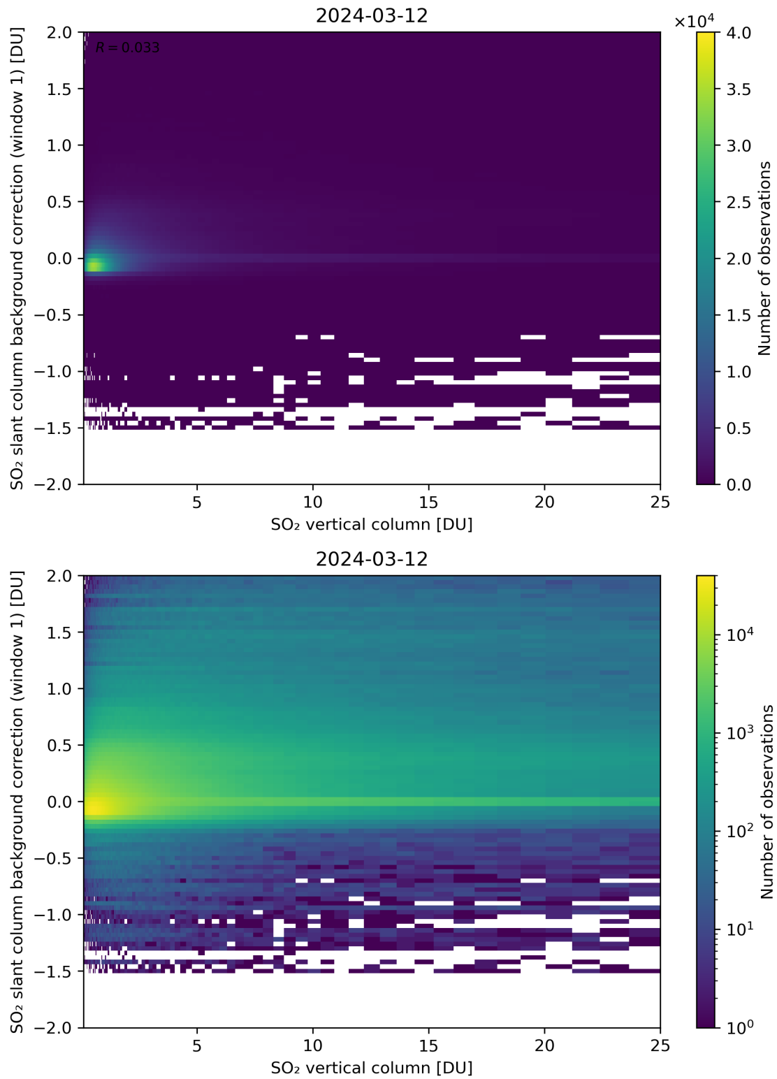
Figure 273: Scatter density plot of “SO 2 vertical column” against “SO 2 slant column background correction (window 1)” for 2024-03-11 to 2024-03-13.
