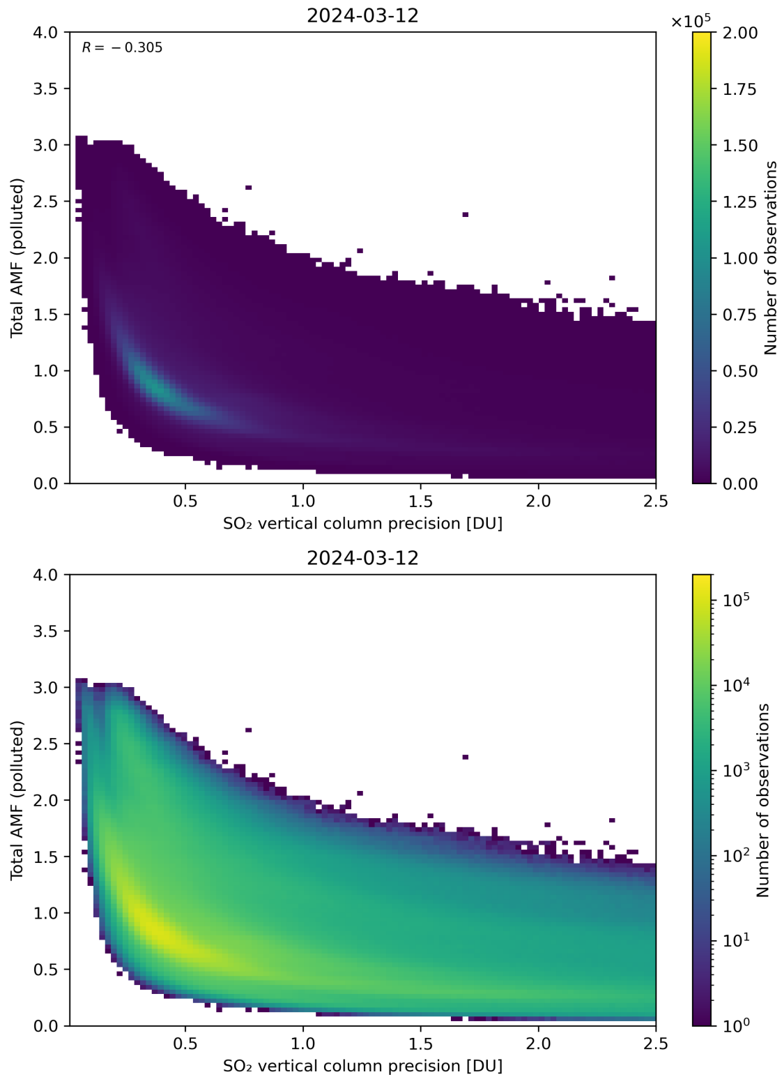
Figure 294: Scatter density plot of “SO 2 vertical column precision” against “Total AMF (polluted)” for 2024-03-11 to 2024-03-13.
