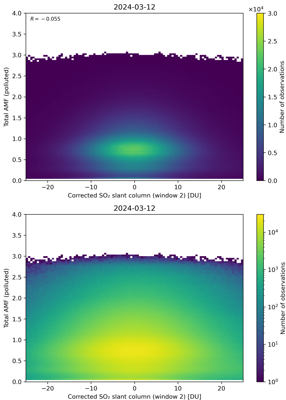
Figure 203: Scatter density plot of “Corrected SO 2 slant column (window 2)” against “Total AMF (polluted)” for 2024-03-11 to 2024-03-13.
