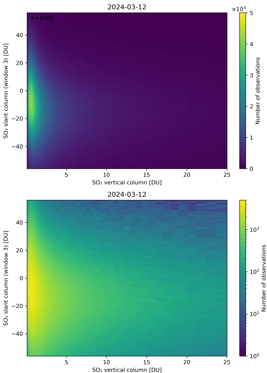
Figure 303: Scatter density plot of “SO 2 vertical column” against “SO 2 slant column (window 3)” for 2024-03-11 to 2024-03-13.
