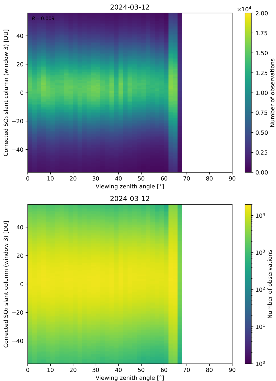
Figure 319: Scatter density plot of “Viewing zenith angle” against “Corrected SO 2 slant column (window 3)” for 2024-03-11 to 2024-03-13.
