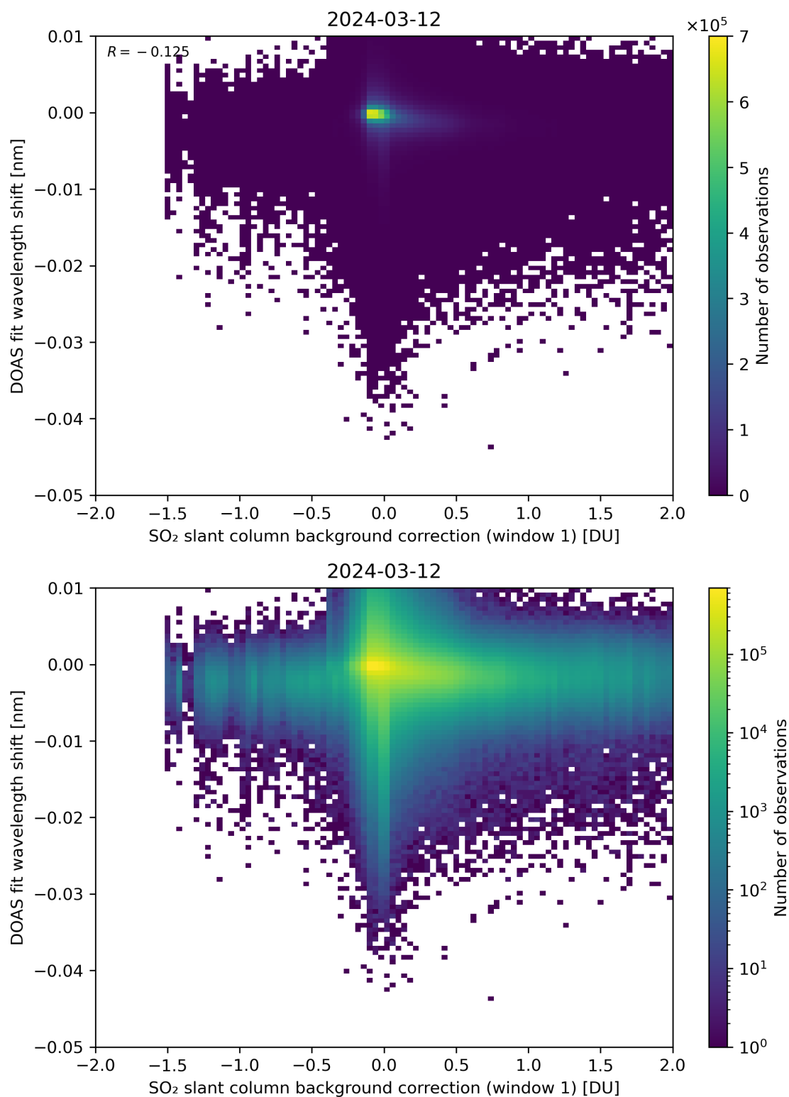
Figure 100: Scatter density plot of “SO 2 slant column background correction (window 1)” against “DOAS fit wavelength shift” for 2024-03-11 to 2024-03-13.
