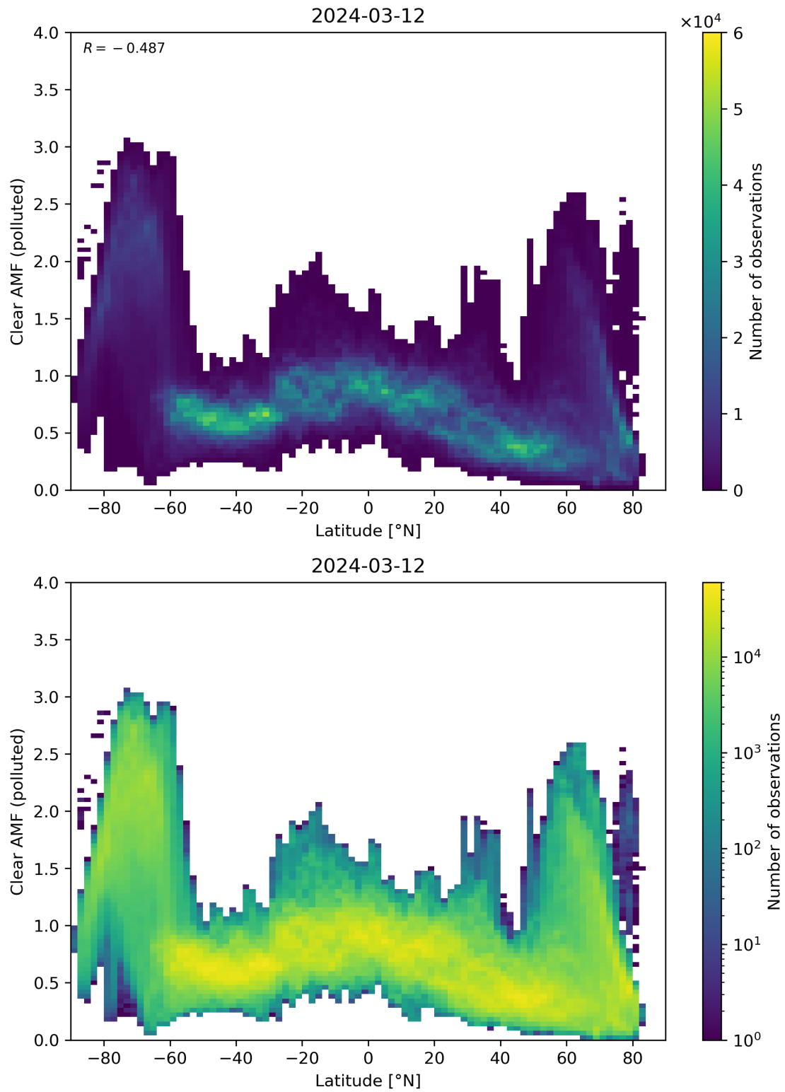
Figure 145: Scatter density plot of “Latitude” against “Clear AMF (polluted)” for 2024-03-11 to 2024-03-13.
