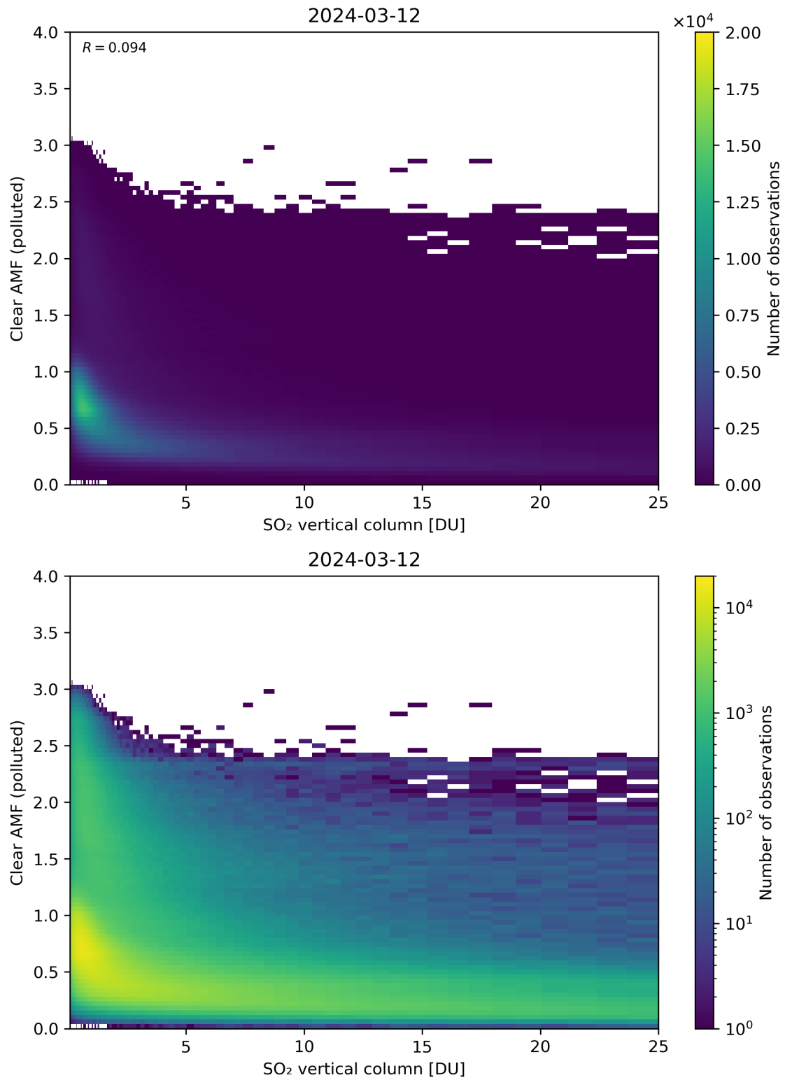
Figure 296: Scatter density plot of “SO 2 vertical column” against “Clear AMF (polluted)” for 2024-03-11 to 2024-03-13.
