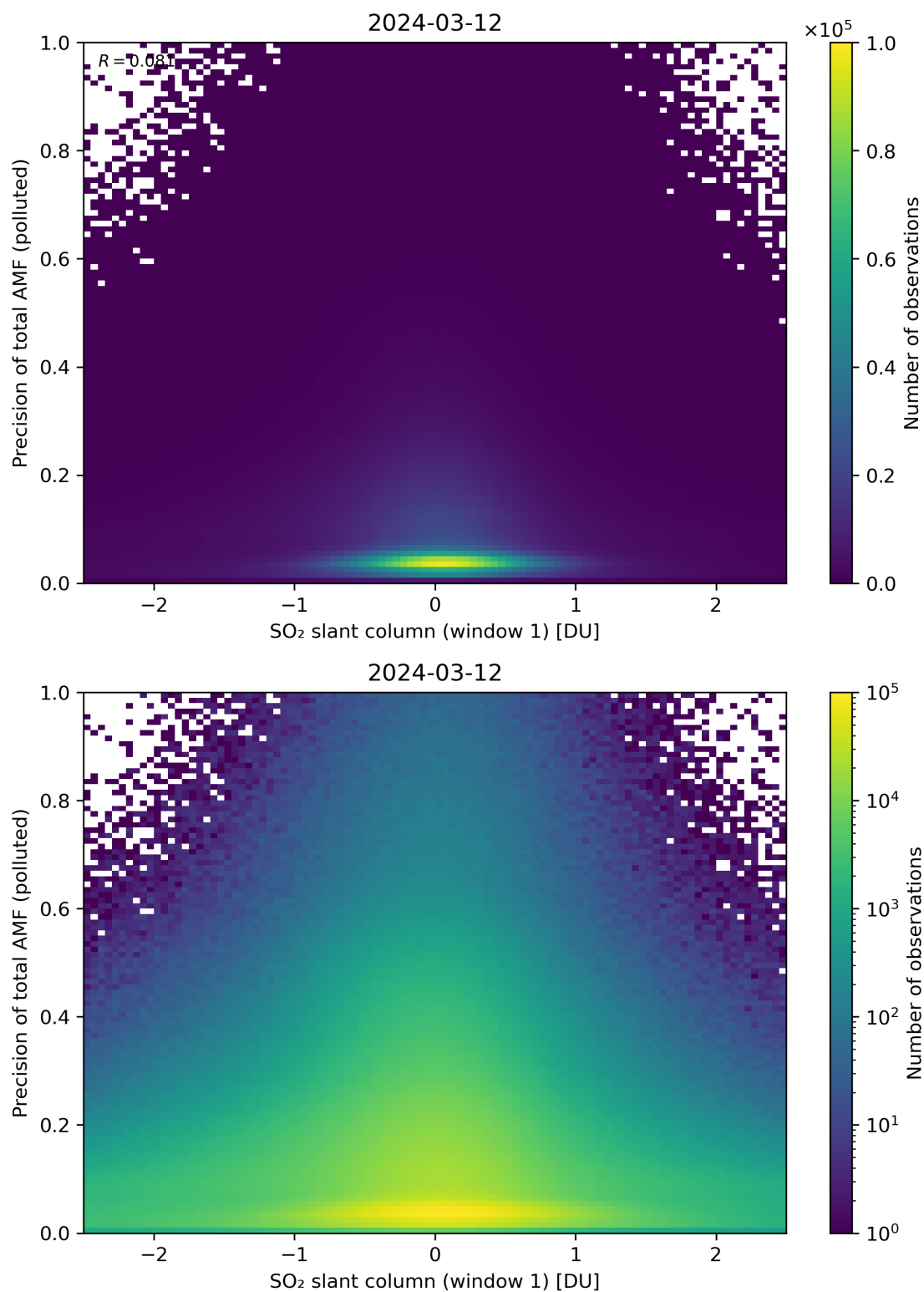
Figure 240: Scatter density plot of “SO 2 slant column (window 1)” against “Precision of total AMF (polluted)” for 2024-03-11 to 2024-03-13.
