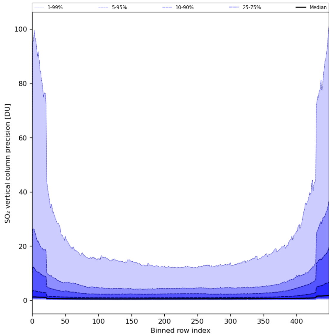
Figure 77: Along track statistics of “SO 2 vertical column precision” for 2024-03-11 to 2024-03-13
