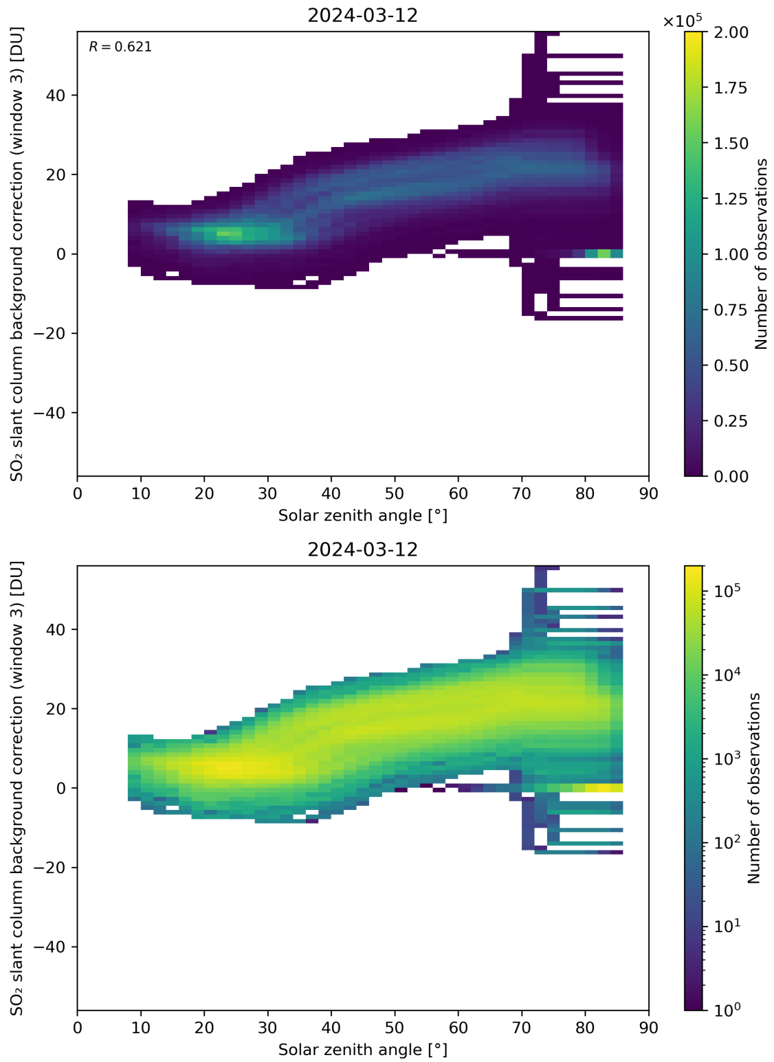
Figure 160: Scatter density plot of “Solar zenith angle” against “SO 2 slant column background correction (window 3)” for 2024-03-11 to 2024-03-13.
