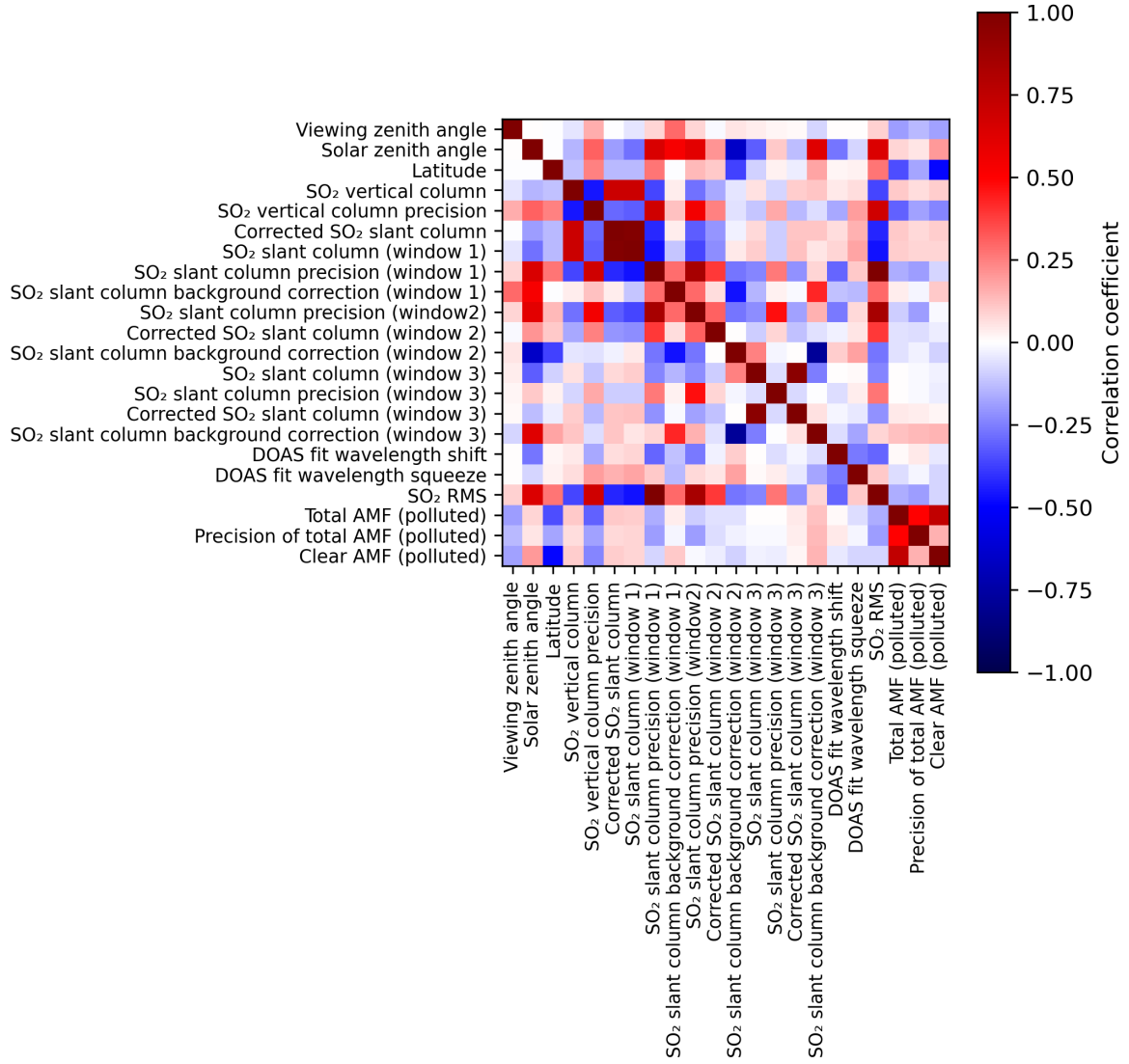
Figure 2: Map of correlation matrix for 2024-03-11 to 2024-03-13.
