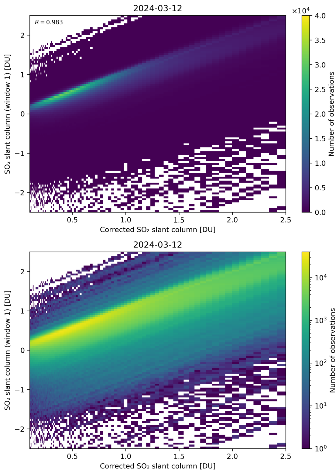
Figure 187: Scatter density plot of “Corrected SO 2 slant column” against “SO 2 slant column (window 1)” for 2024-03-11 to 2024-03-13.
