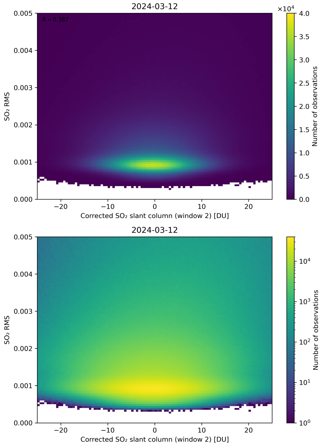
Figure 198: Scatter density plot of “Corrected SO 2 slant column (window 2)” against “SO 2 RMS” for 2024-03-11 to 2024-03-13.
