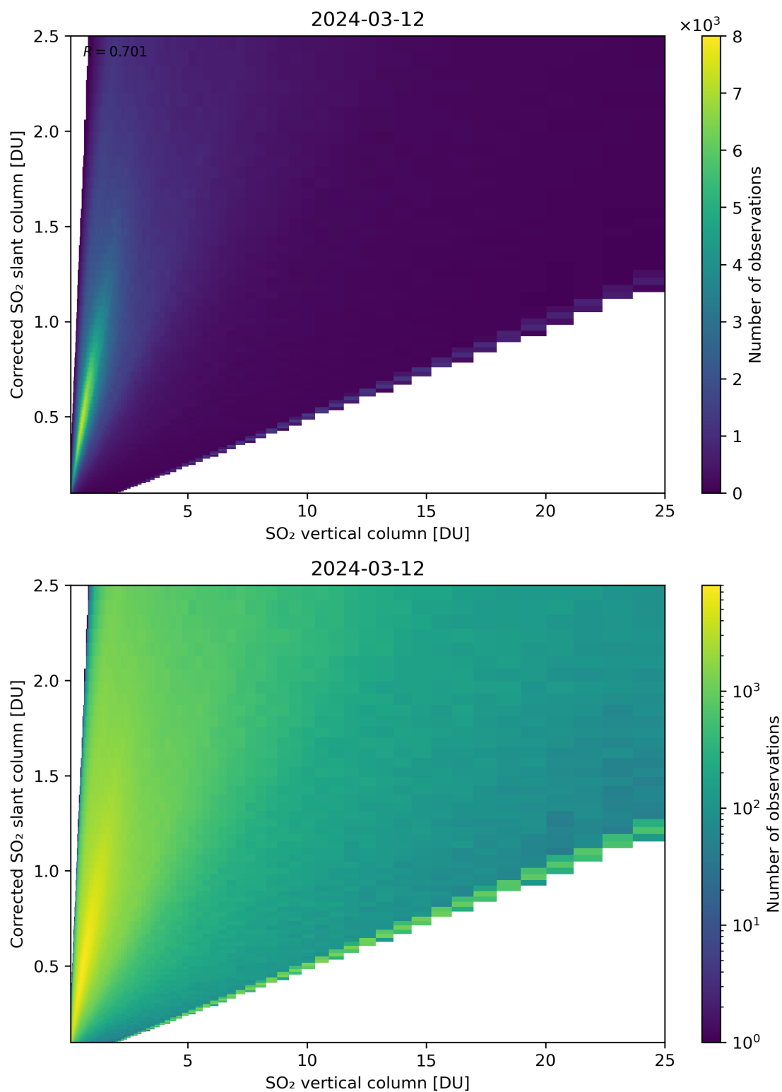
Figure 297: Scatter density plot of “SO 2 vertical column” against “Corrected SO 2 slant column” for 2024-03-11 to 2024-03-13.
