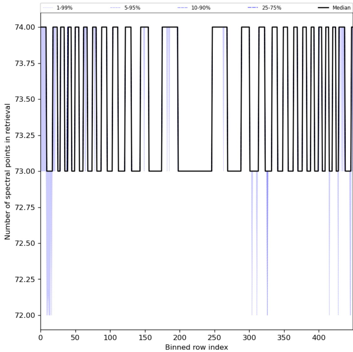
Figure 97: Along track statistics of “Number of spectral points in retrieval” for 2024-03-11 to 2024-03-13
