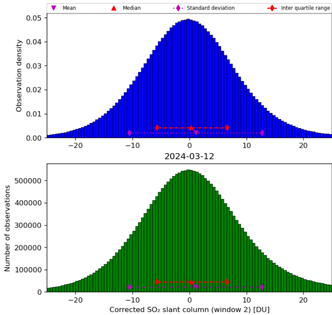
Figure 62: Histogram of “Corrected SO 2 slant column (window 2)” for 2024-03-11 to 2024-03-13
