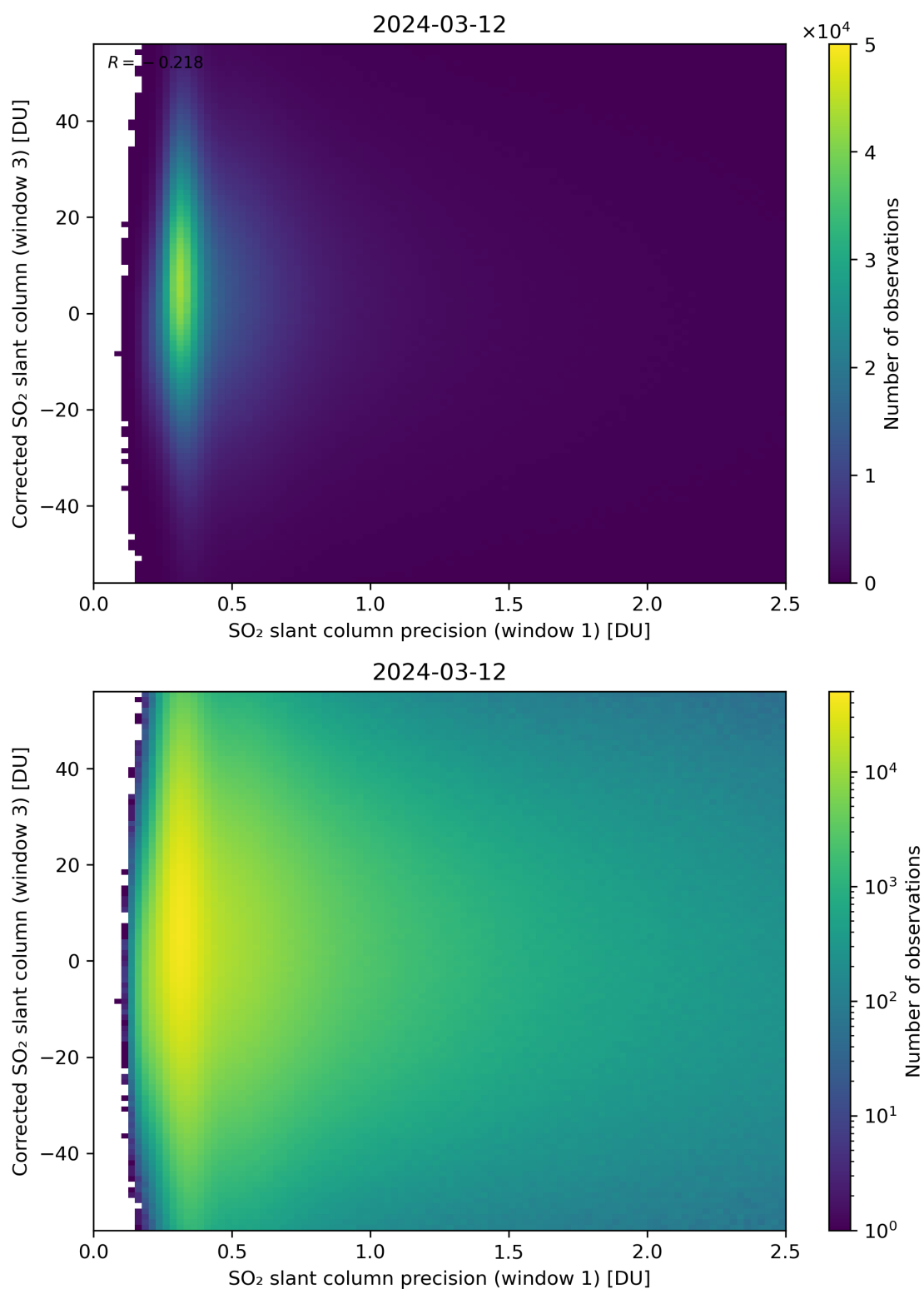
Figure 226: Scatter density plot of “SO 2 slant column precision (window 1)” against “Corrected SO 2 slant column (window 3)” for 2024-03-11 to 2024-03-13.
