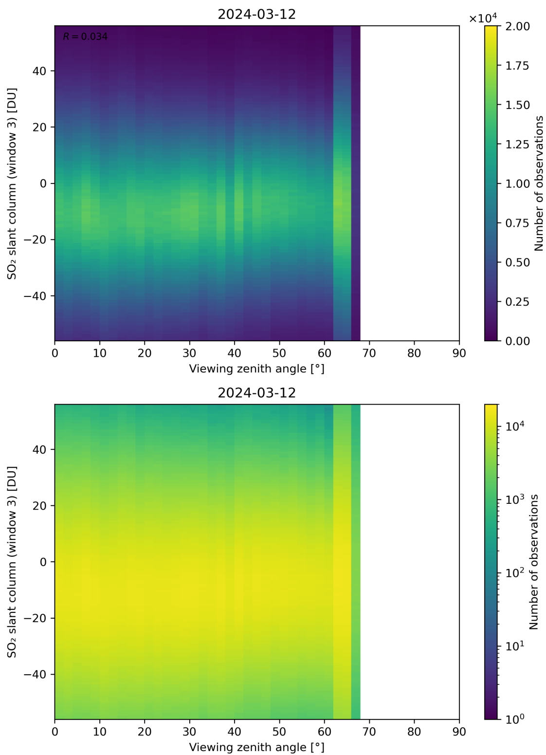
Figure 323: Scatter density plot of “Viewing zenith angle” against “SO 2 slant column (window 3)” for 2024-03-11 to 2024-03-13.
