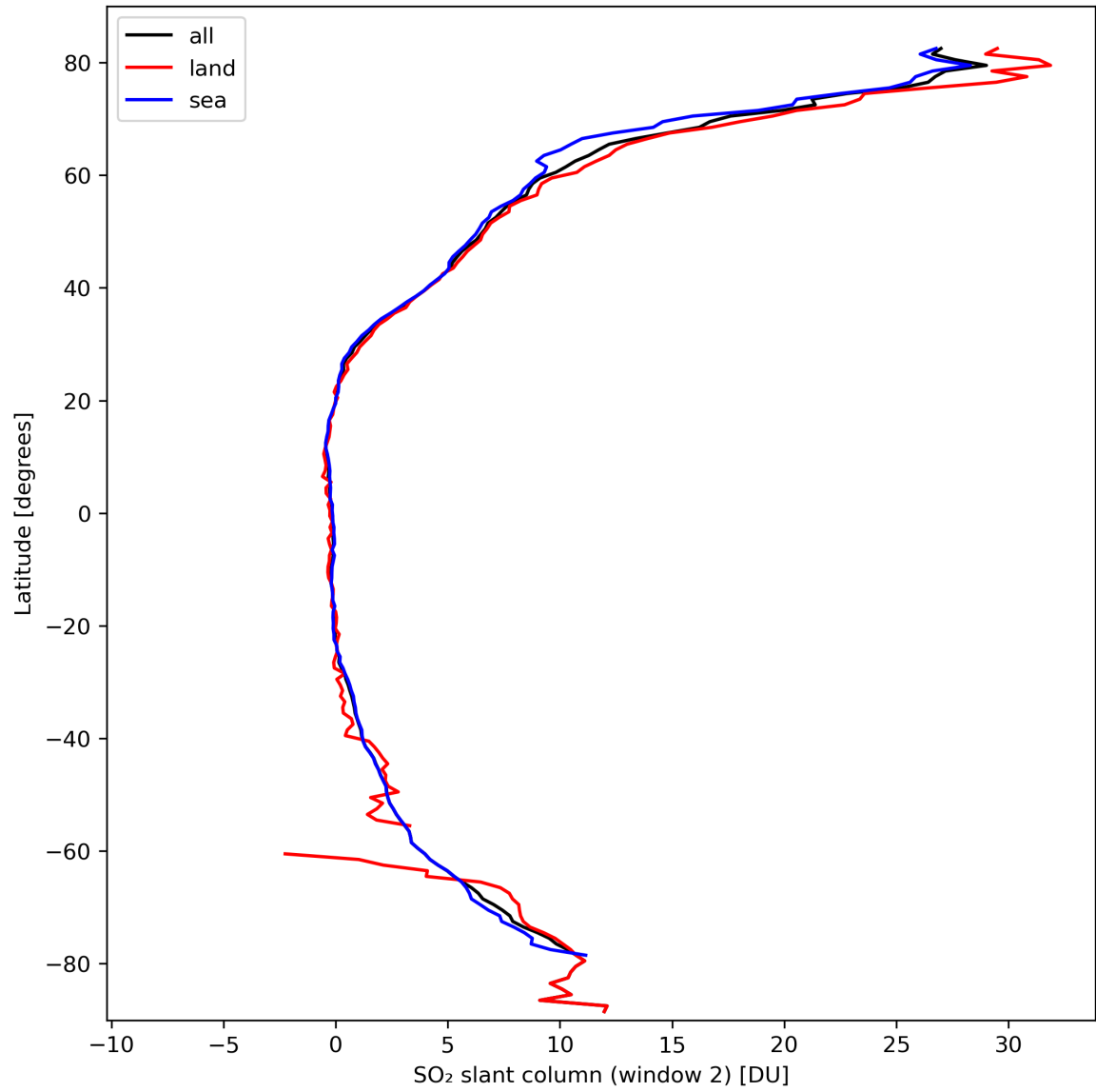
Figure 37: Zonal average of “SO 2 slant column (window 2)” for 2024-03-11 to 2024-03-13.
