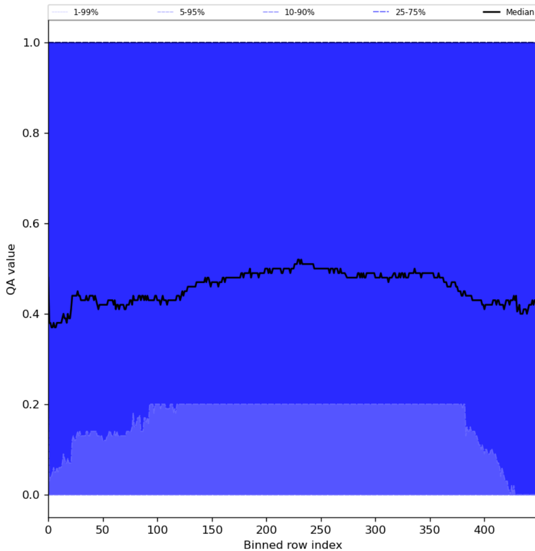
Figure 75: Along track statistics of “QA value” for 2024-03-11 to 2024-03-13
