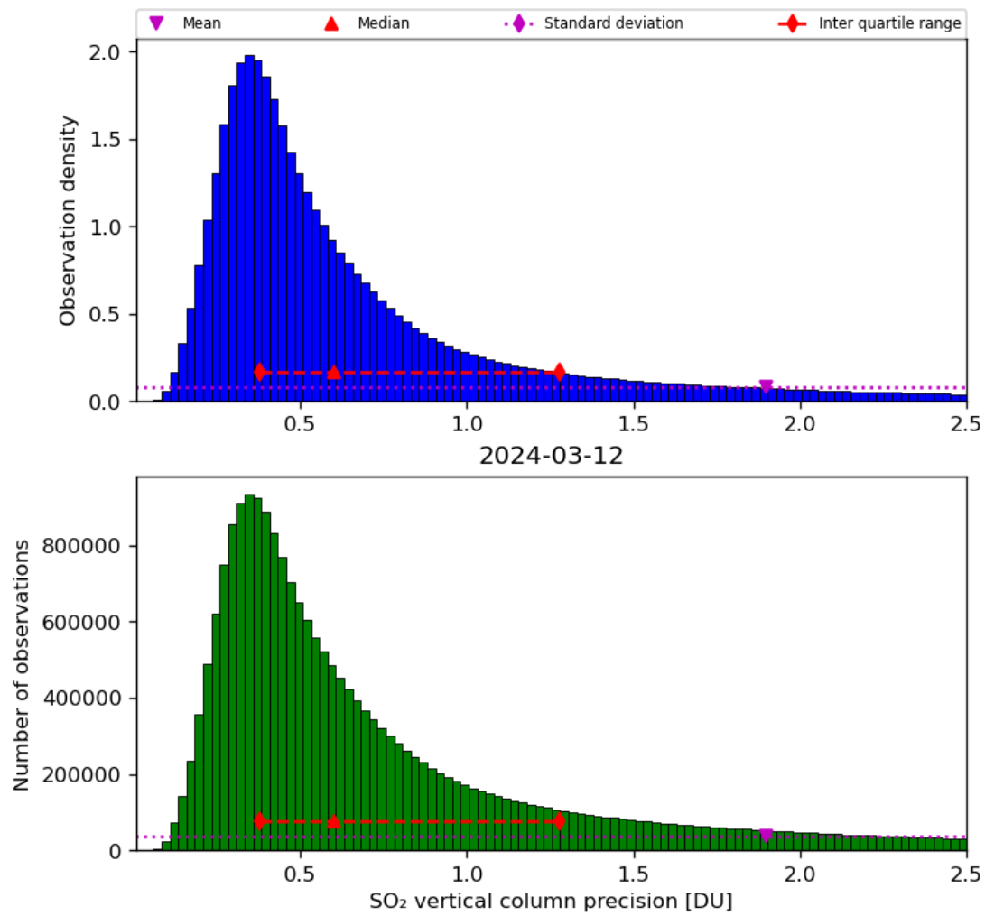
Figure 54: Histogram of “SO 2 vertical column precision” for 2024-03-11 to 2024-03-13
