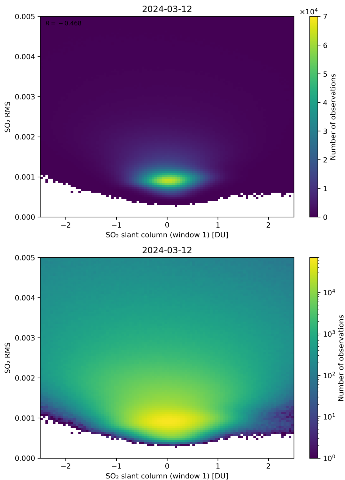
Figure 217: Scatter density plot of “SO 2 slant column (window 1)” against “SO 2 RMS” for 2024-03-11 to 2024-03-13.
