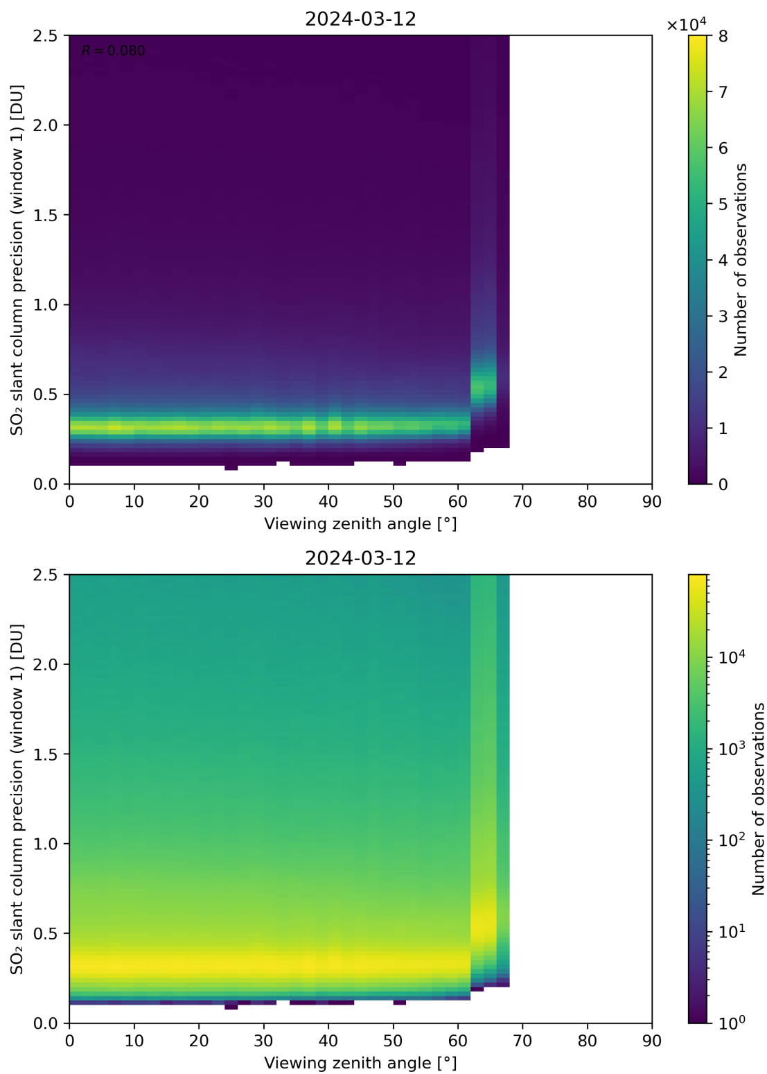
Figure 321: Scatter density plot of “Viewing zenith angle” against “SO 2 slant column precision (window 1)” for 2024-03-11 to 2024-03-13.
