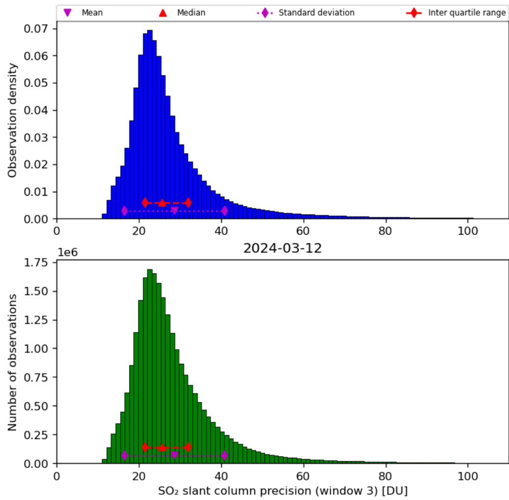
Figure 65: Histogram of “SO 2 slant column precision (window 3)” for 2024-03-11 to 2024-03-13
