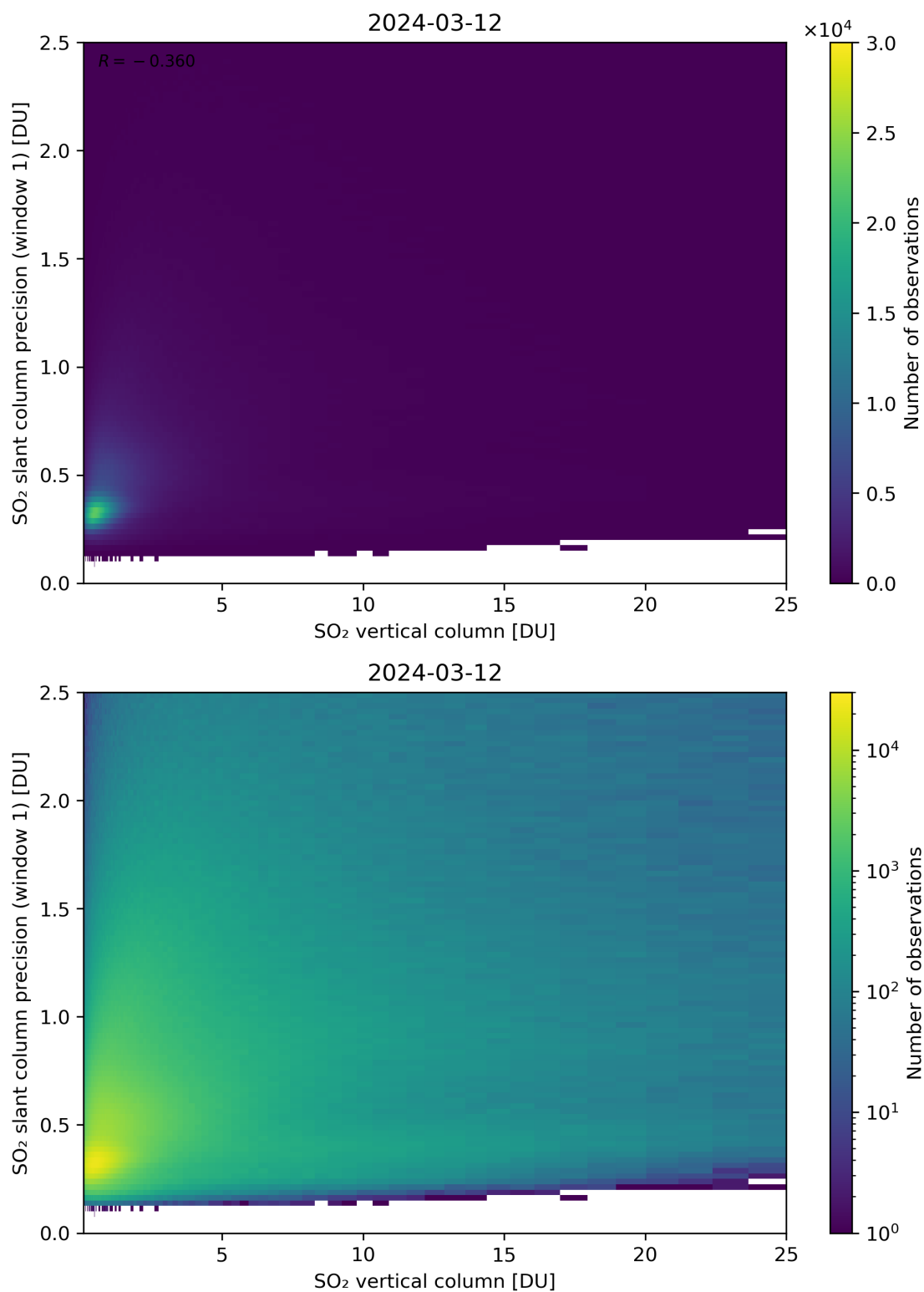
Figure 301: Scatter density plot of “SO 2 vertical column” against “SO 2 slant column precision (window 1)” for 2024-03-11 to 2024-03-13.
