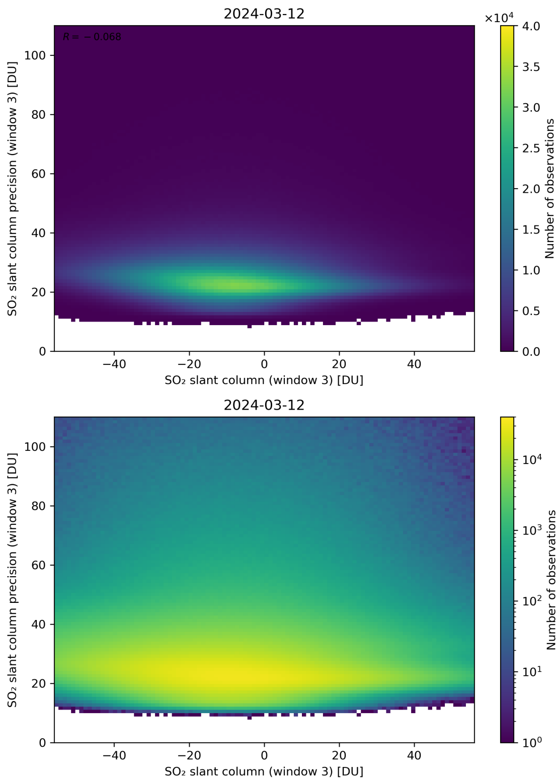
Figure 267: Scatter density plot of “SO 2 slant column (window 3)” against “SO 2 slant column precision (window 3)” for 2024-03-11 to 2024-03-13.
