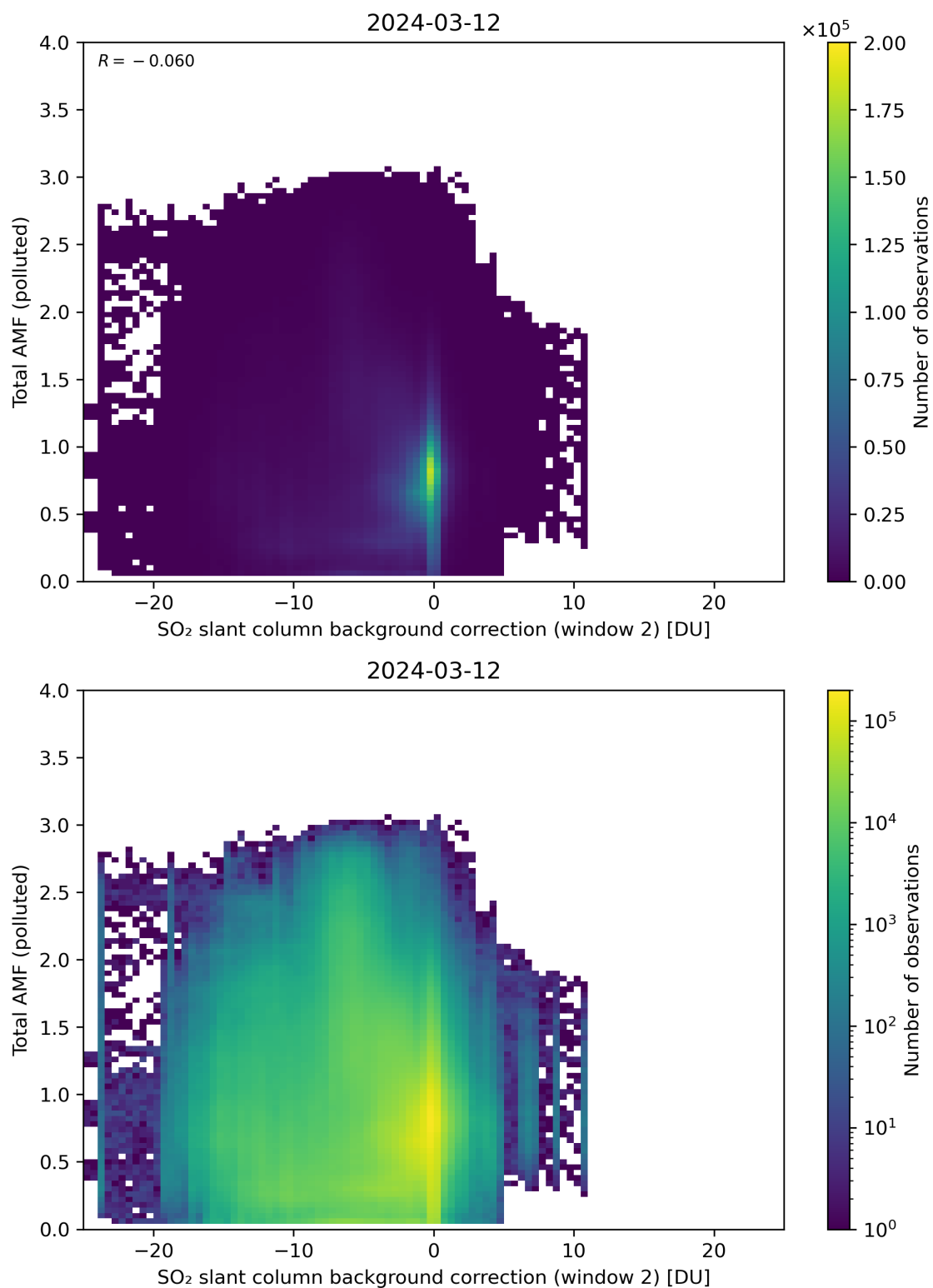
Figure 119: Scatter density plot of “SO 2 slant column background correction (window 2)” against “Total AMF (polluted)” for 2024-03-11 to 2024-03-13.
