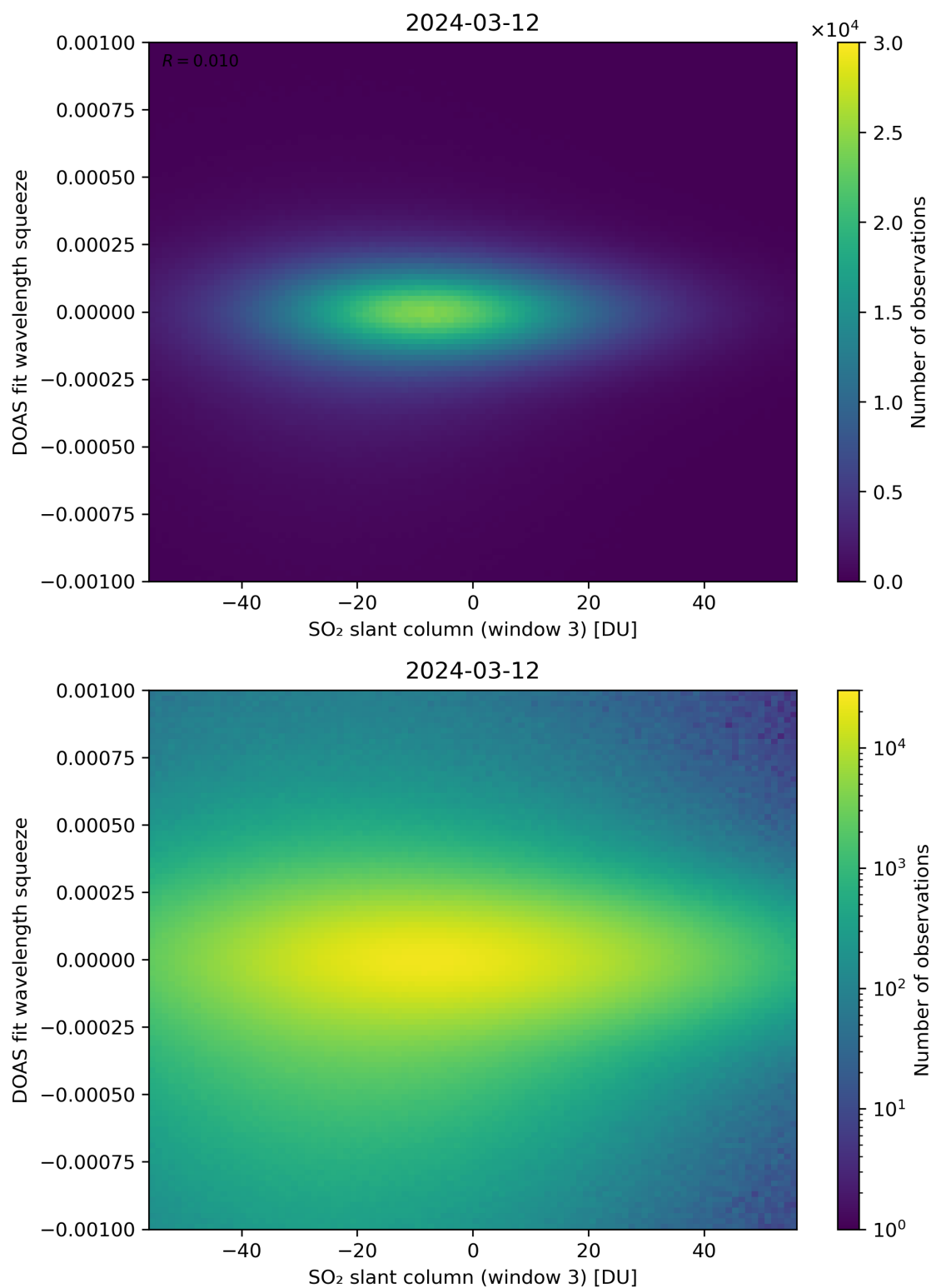
Figure 255: Scatter density plot of “SO 2 slant column (window 3)” against “DOAS fit wavelength squeeze” for 2024-03-11 to 2024-03-13.
