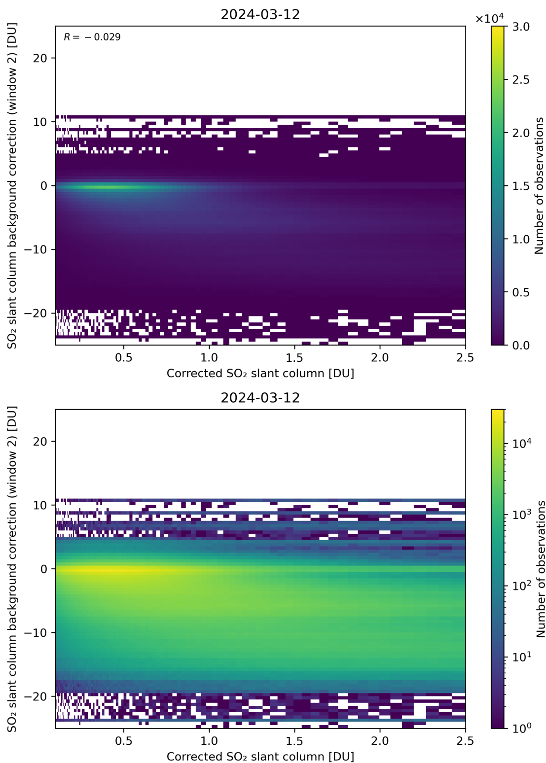
Figure 179: Scatter density plot of “Corrected SO 2 slant column” against “SO 2 slant column background correction (window 2)” for 2024-03-11 to 2024-03-13.
