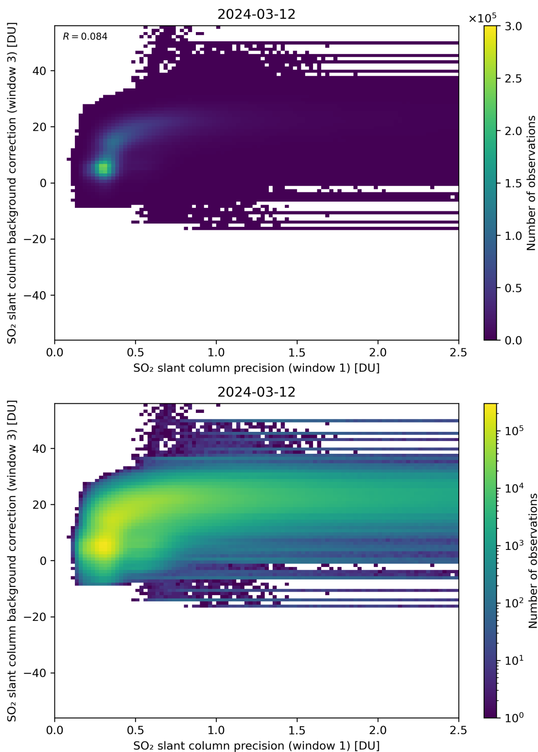
Figure 220: Scatter density plot of “SO 2 slant column precision (window 1)” against “SO 2 slant column background correction (window 3)” for 2024-03-11 to 2024-03-13.
