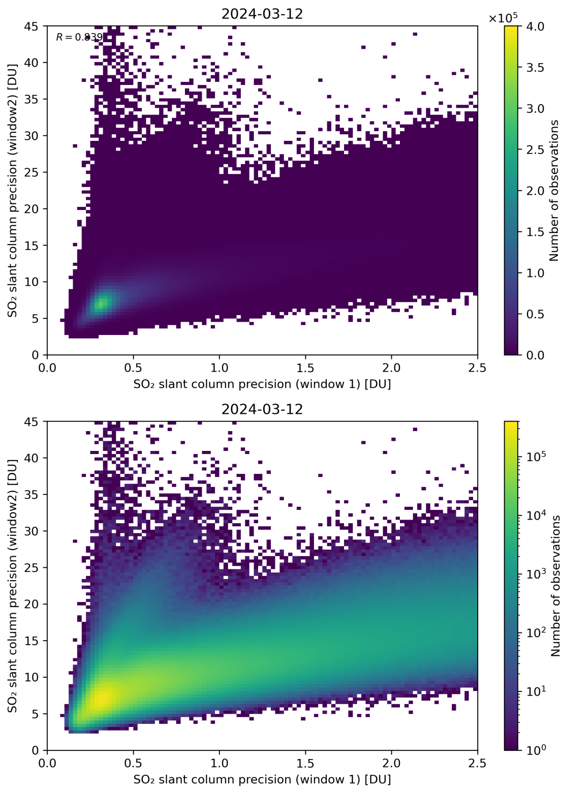
Figure 227: Scatter density plot of “SO 2 slant column precision (window 1)” against “SO 2 slant column precision (window2)” for 2024-03-11 to 2024-03-13.
