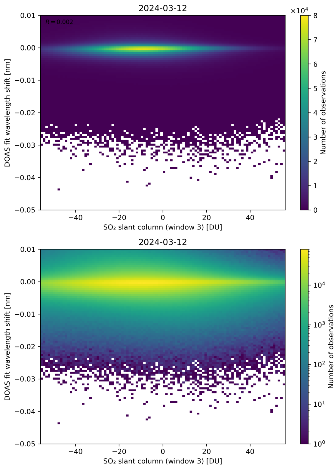
Figure 254: Scatter density plot of “SO 2 slant column (window 3)” against “DOAS fit wavelength shift” for 2024-03-11 to 2024-03-13.
