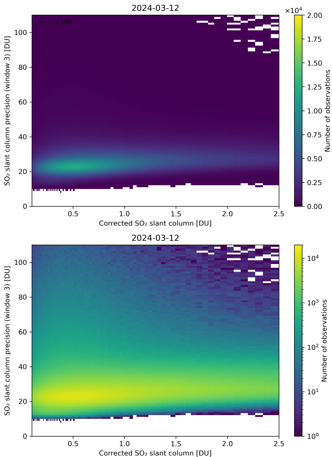
Figure 191: Scatter density plot of “Corrected SO 2 slant column” against “SO 2 slant column precision (window 3)” for 2024-03-11 to 2024-03-13.
