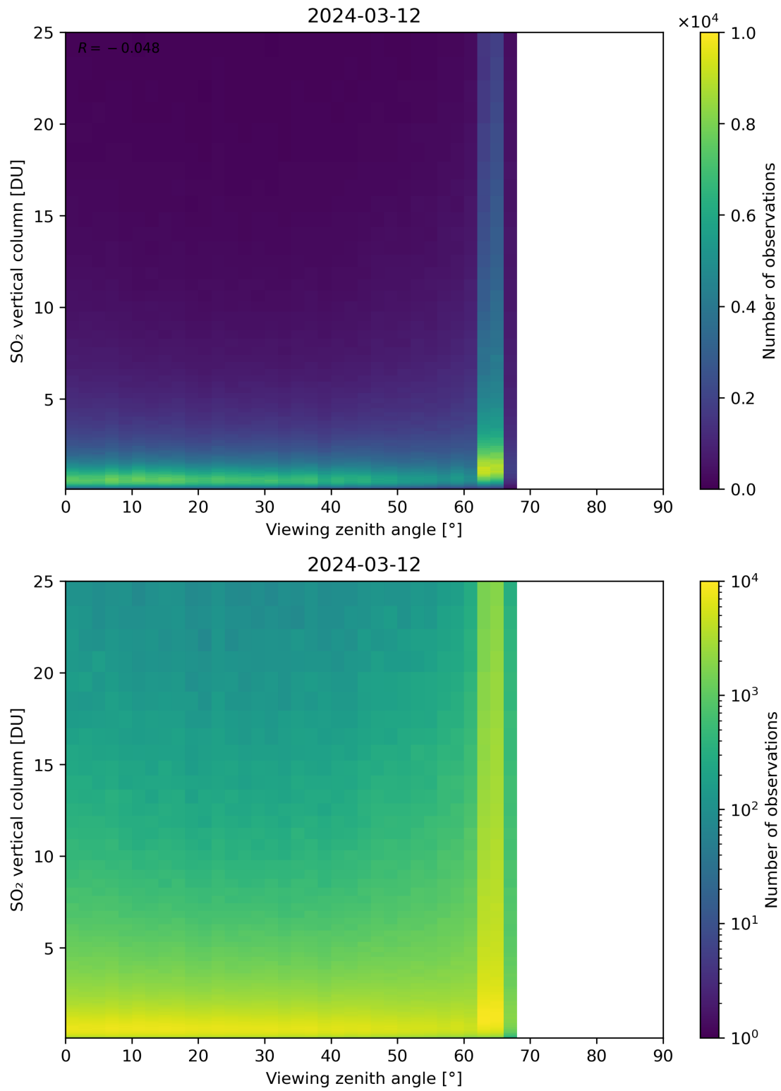
Figure 327: Scatter density plot of “Viewing zenith angle” against “SO 2 vertical column” for 2024-03-11 to 2024-03-13.
