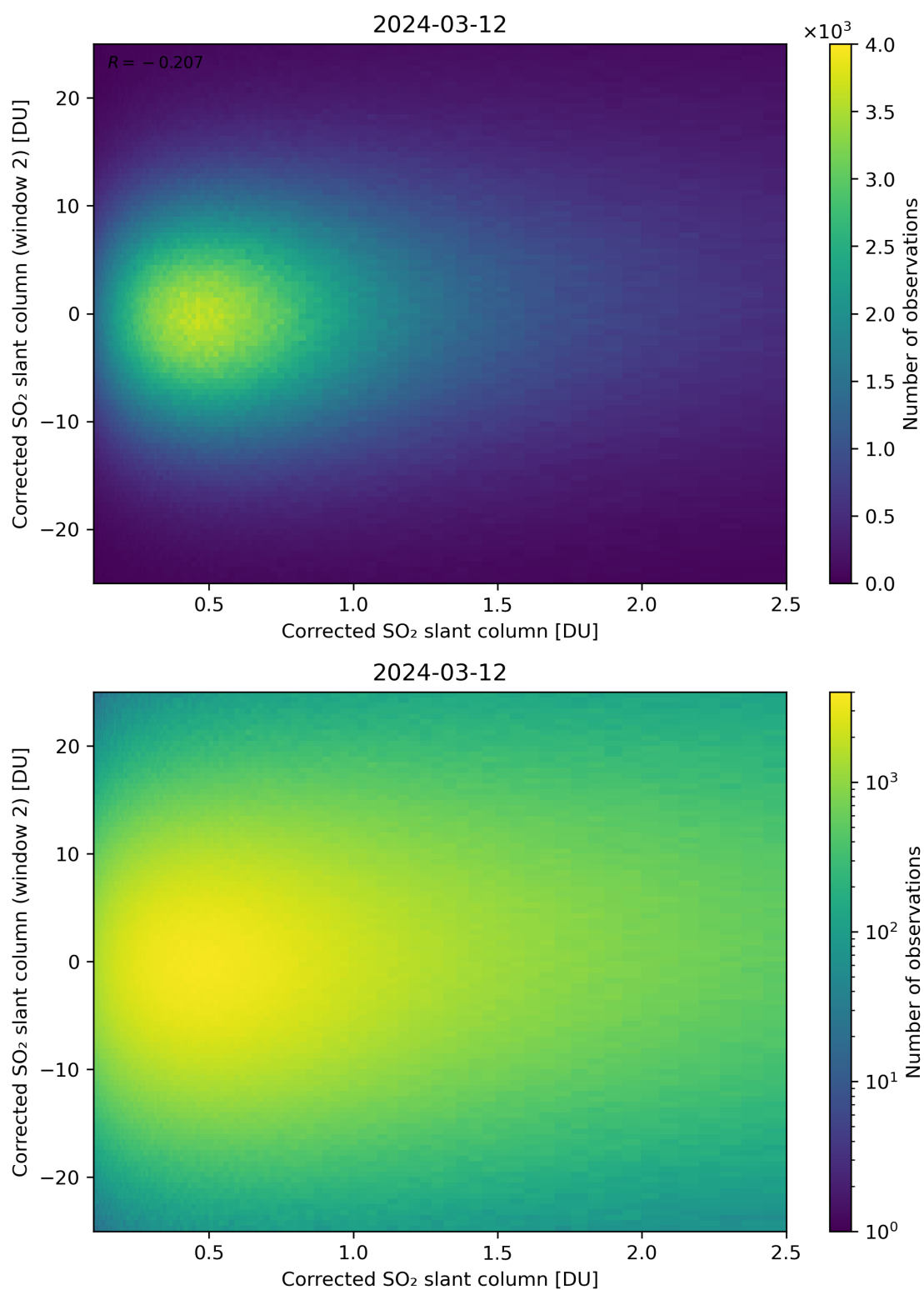
Figure 185: Scatter density plot of “Corrected SO 2 slant column” against “Corrected SO 2 slant column (window 2)” for 2024-03-11 to 2024-03-13.
