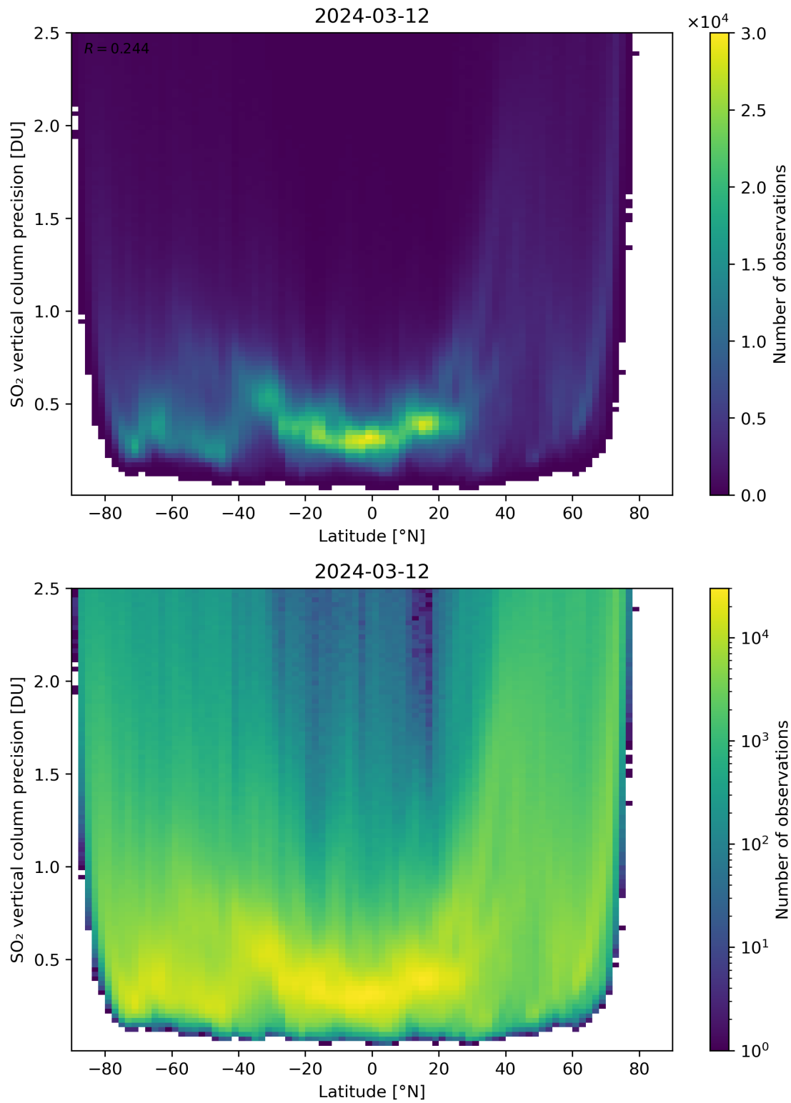
Figure 157: Scatter density plot of “Latitude” against “SO 2 vertical column precision” for 2024-03-11 to 2024-03-13.
