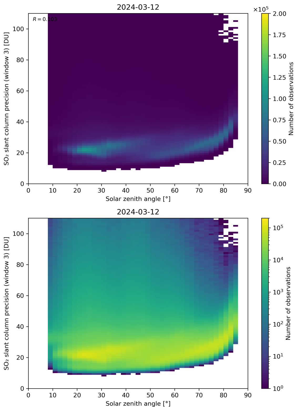
Figure 173: Scatter density plot of “Solar zenith angle” against “SO 2 slant column precision (window 3)” for 2024-03-11 to 2024-03-13.
