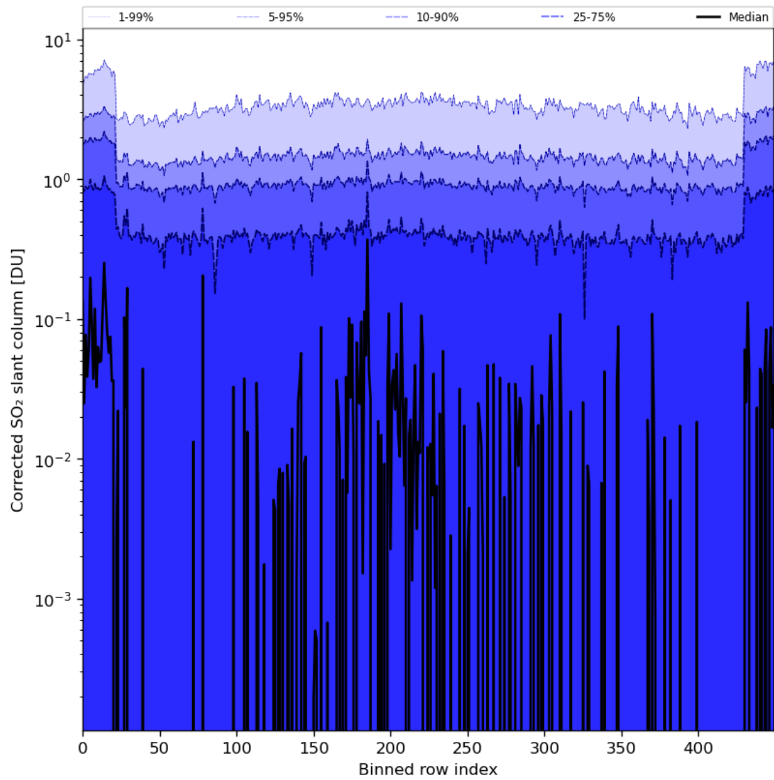
Figure 78: Along track statistics of “Corrected SO 2 slant column” for 2024-03-11 to 2024-03-13
