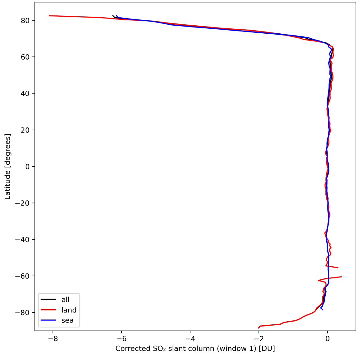
Figure 35: Zonal average of “Corrected SO 2 slant column (window 1)” for 2024-03-11 to 2024-03-13.
