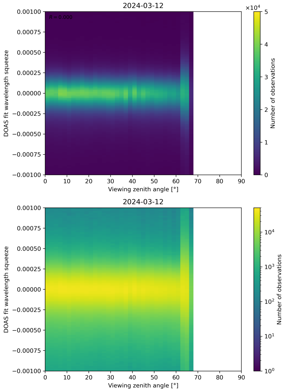
Figure 312: Scatter density plot of “Viewing zenith angle” against “DOAS fit wavelength squeeze” for 2024-03-11 to 2024-03-13.
