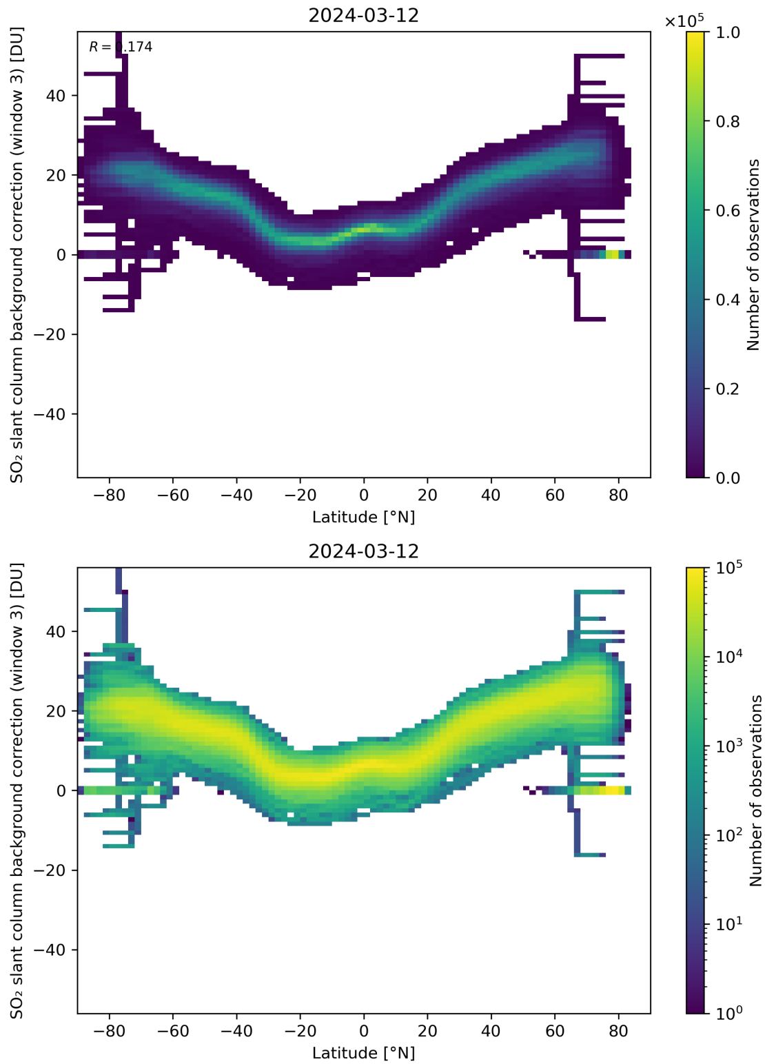
Figure 141: Scatter density plot of “Latitude” against “SO 2 slant column background correction (window 3)” for 2024-03-11 to 2024-03-13.
