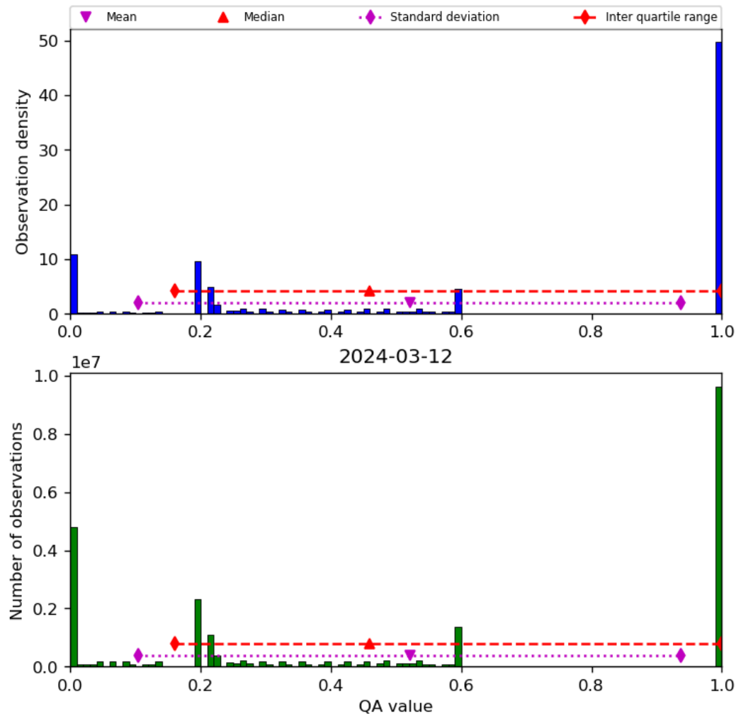
Figure 52: Histogram of “QA value” for 2024-03-11 to 2024-03-13
