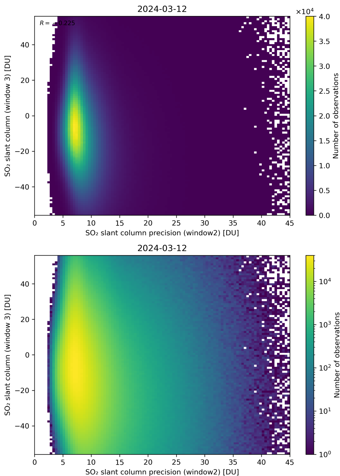
Figure 249: Scatter density plot of “SO 2 slant column precision (window2)” against “SO 2 slant column (window 3)” for 2024-03-11 to 2024-03-13.
