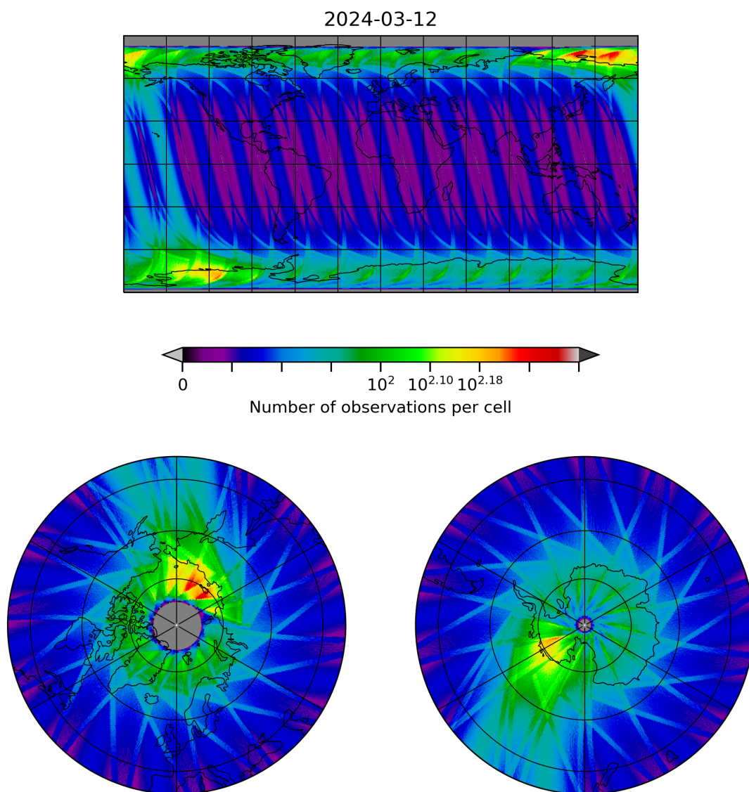
Figure 28: Map of the number of observations for 2024-03-11 to 2024-03-13
