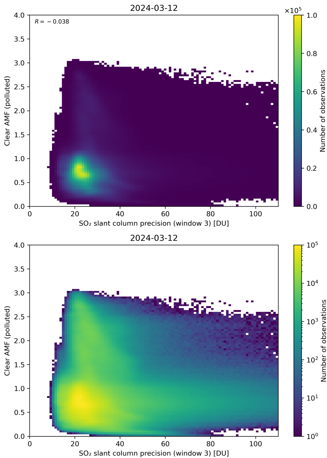
Figure 261: Scatter density plot of “SO 2 slant column precision (window 3)” against “Clear AMF (polluted)” for 2024-03-11 to 2024-03-13.
