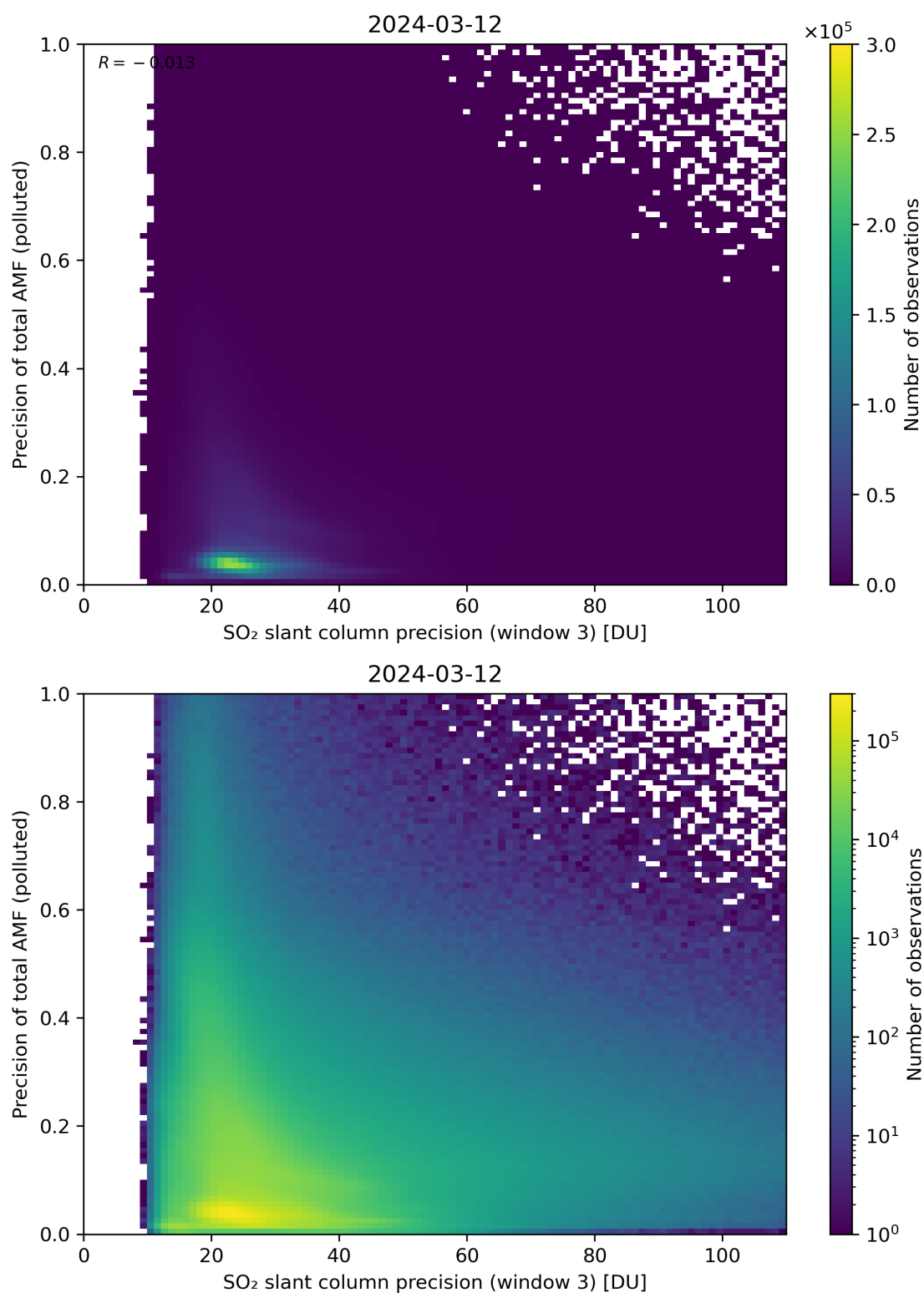
Figure 264: Scatter density plot of “SO 2 slant column precision (window 3)” against “Precision of total AMF (polluted)” for 2024-03-11 to 2024-03-13.
