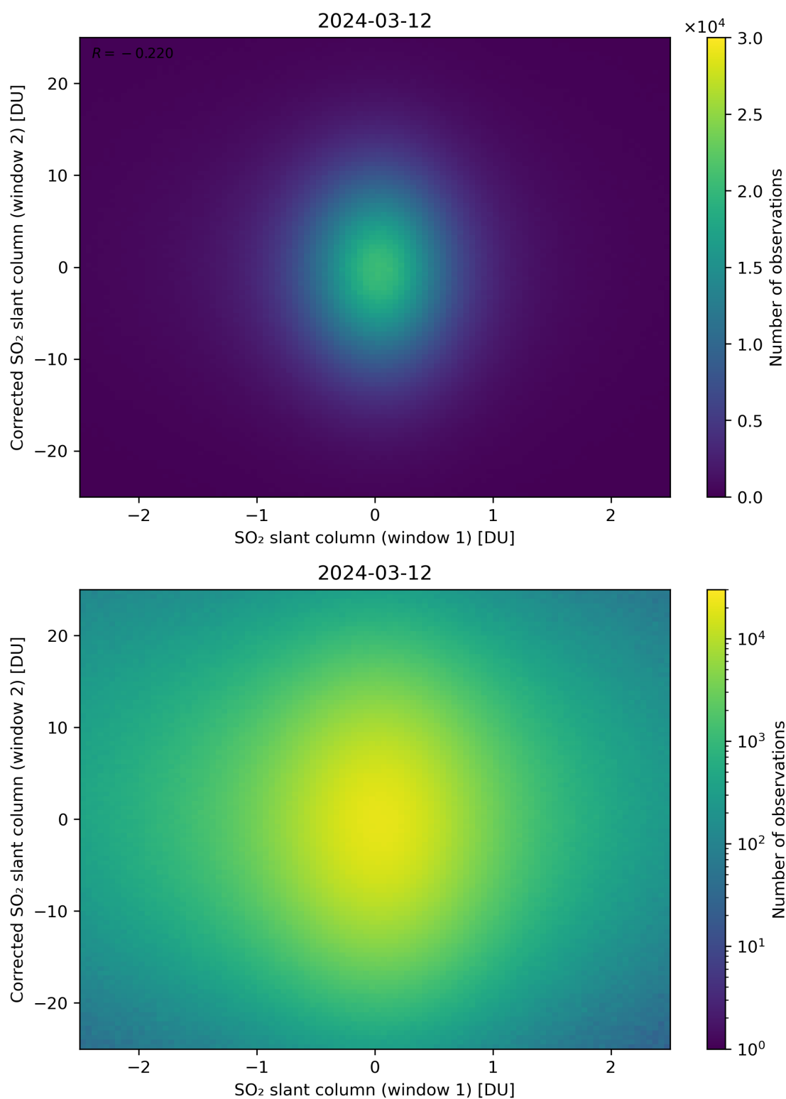
Figure 233: Scatter density plot of “SO 2 slant column (window 1)” against “Corrected SO 2 slant column (window 2)” for 2024-03-11 to 2024-03-13.
