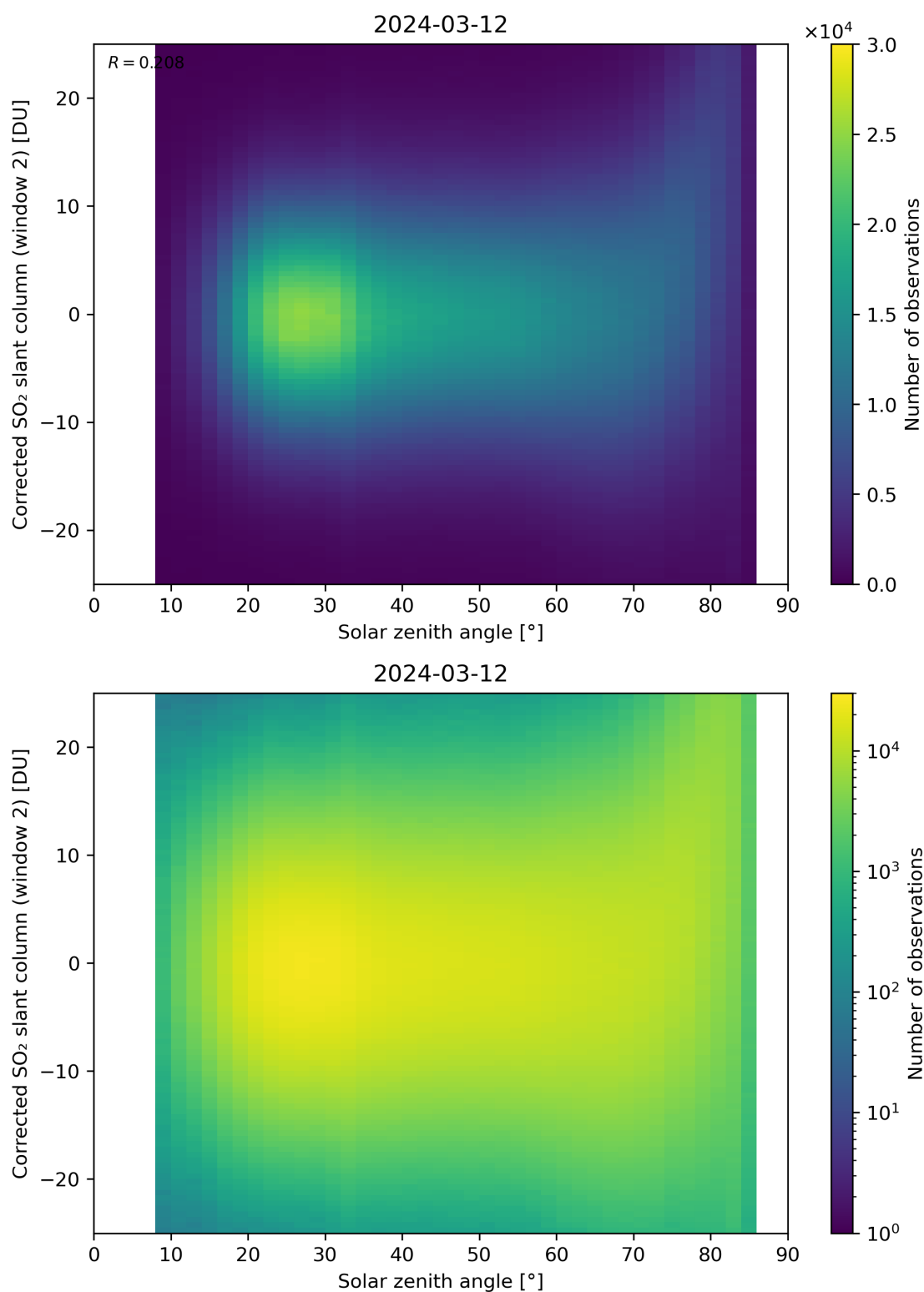
Figure 167: Scatter density plot of “Solar zenith angle” against “Corrected SO 2 slant column (window 2)” for 2024-03-11 to 2024-03-13.
