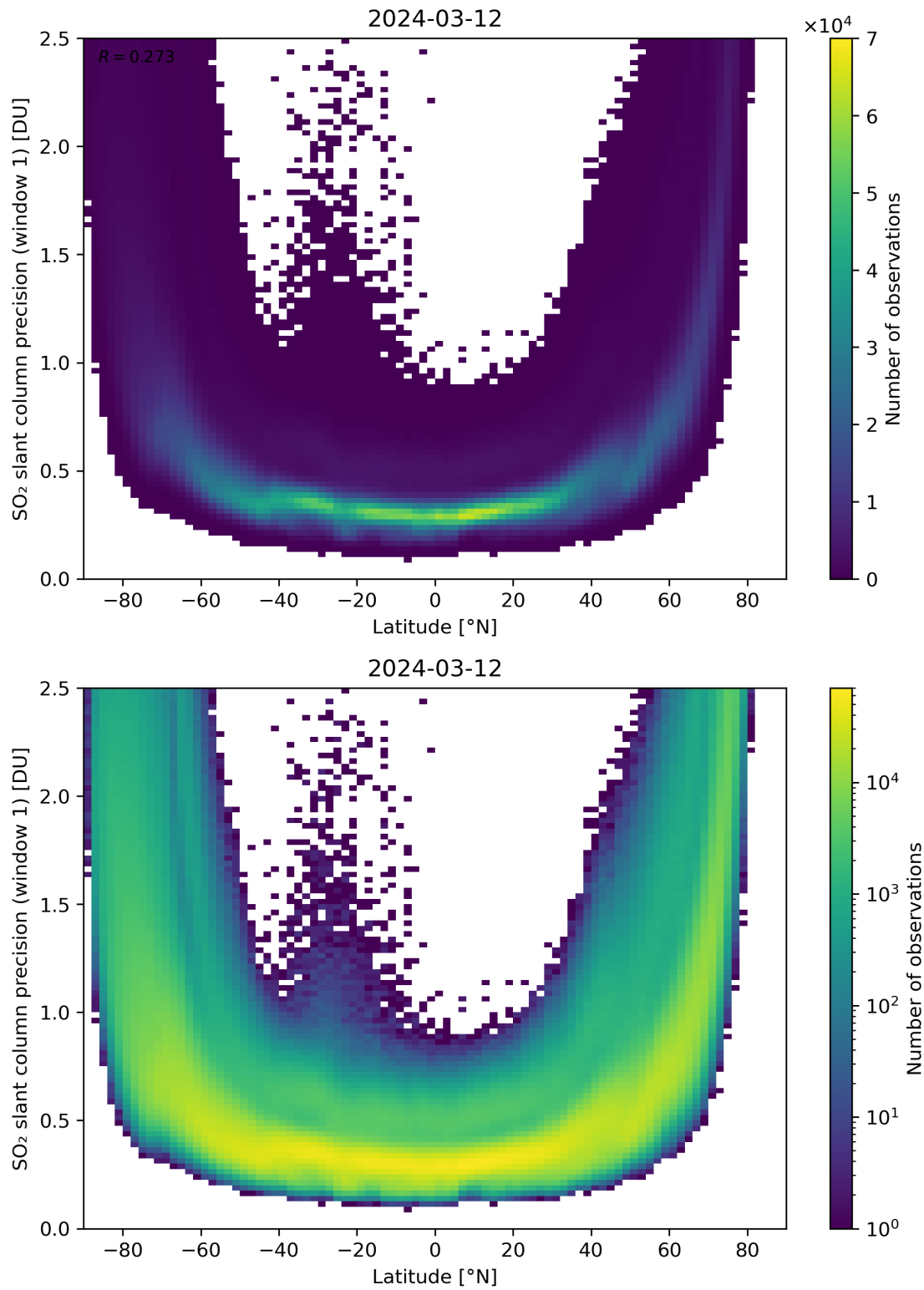
Figure 150: Scatter density plot of “Latitude” against “SO 2 slant column precision (window 1)” for 2024-03-11 to 2024-03-13.
