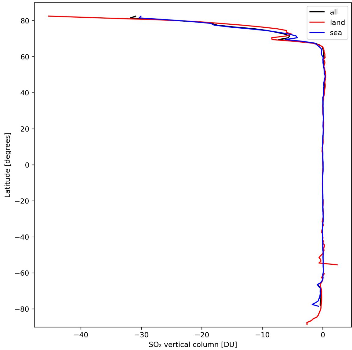
Figure 30: Zonal average of “SO 2 vertical column” for 2024-03-11 to 2024-03-13.
