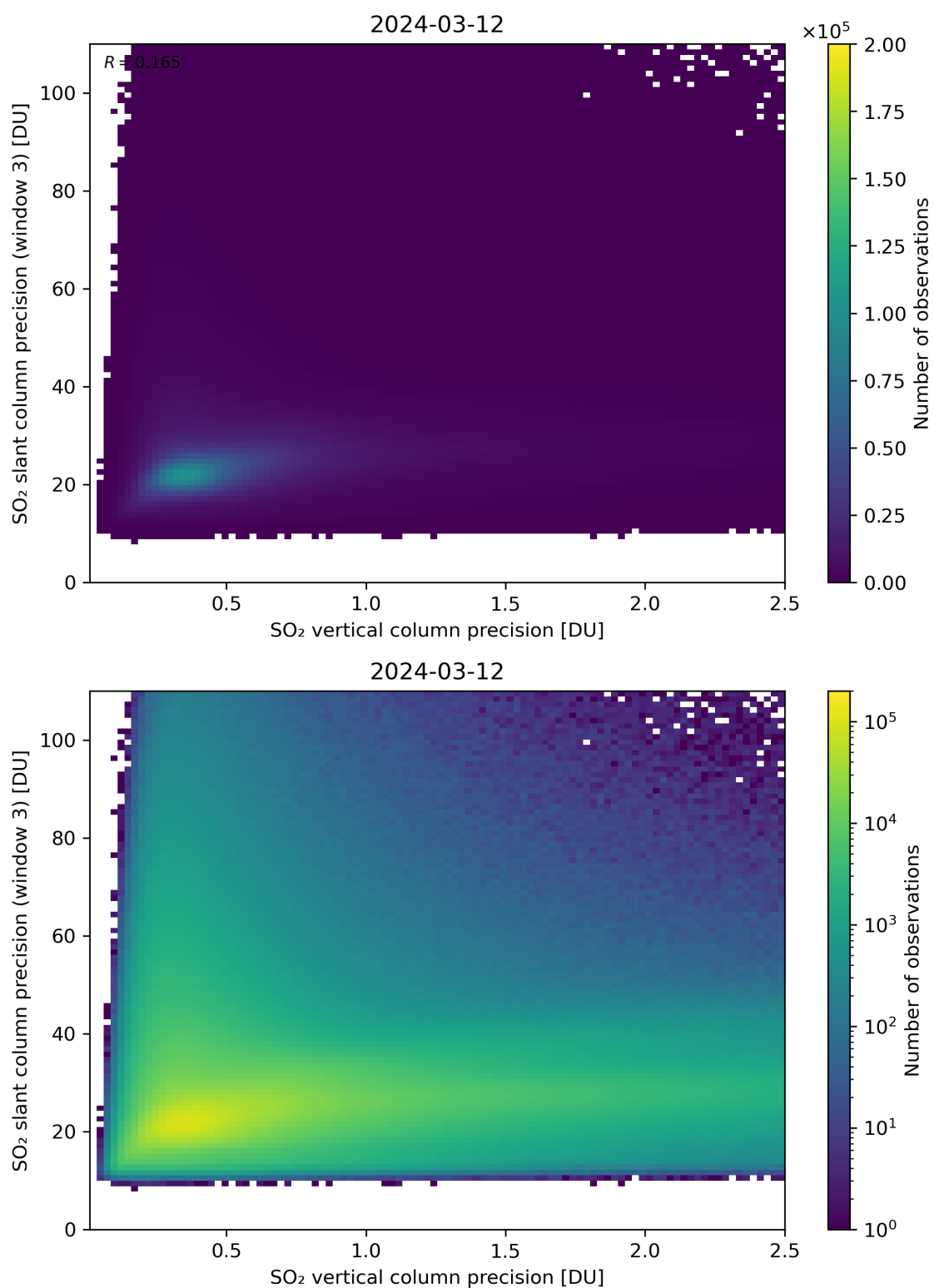
Figure 293: Scatter density plot of “SO 2 vertical column precision” against “SO 2 slant column precision (window 3)” for 2024-03-11 to 2024-03-13.
