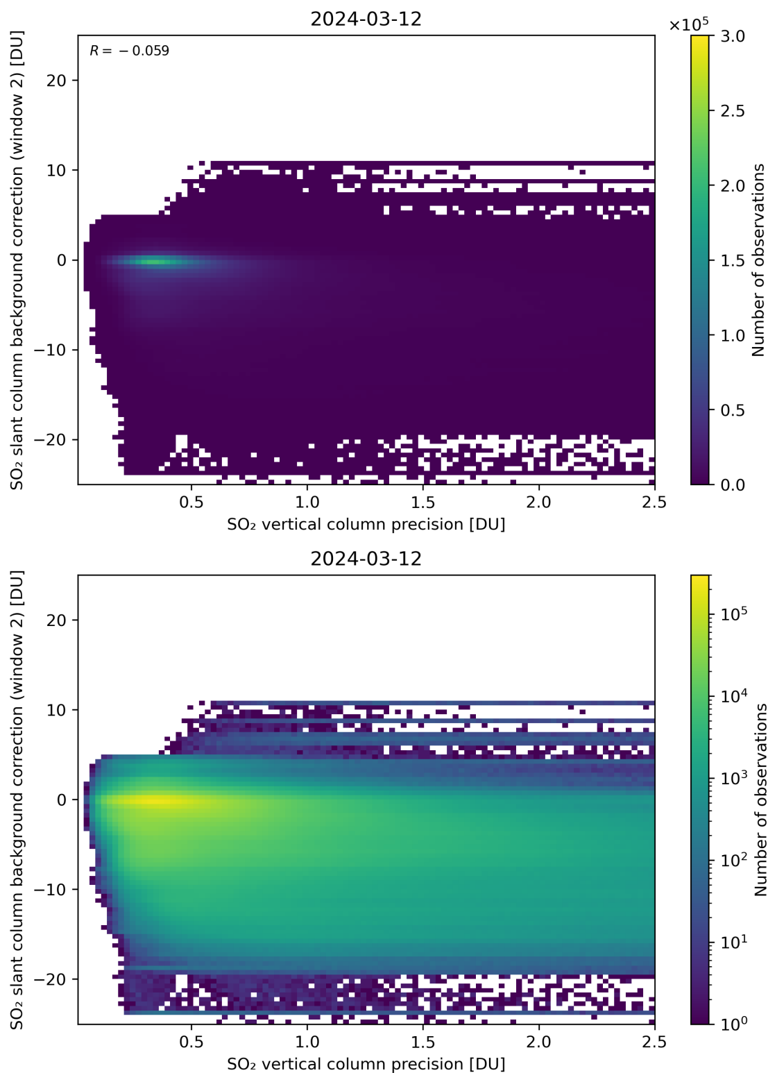
Figure 280: Scatter density plot of “SO 2 vertical column precision” against “SO 2 slant column background correction (window 2)” for 2024-03-11 to 2024-03-13.
