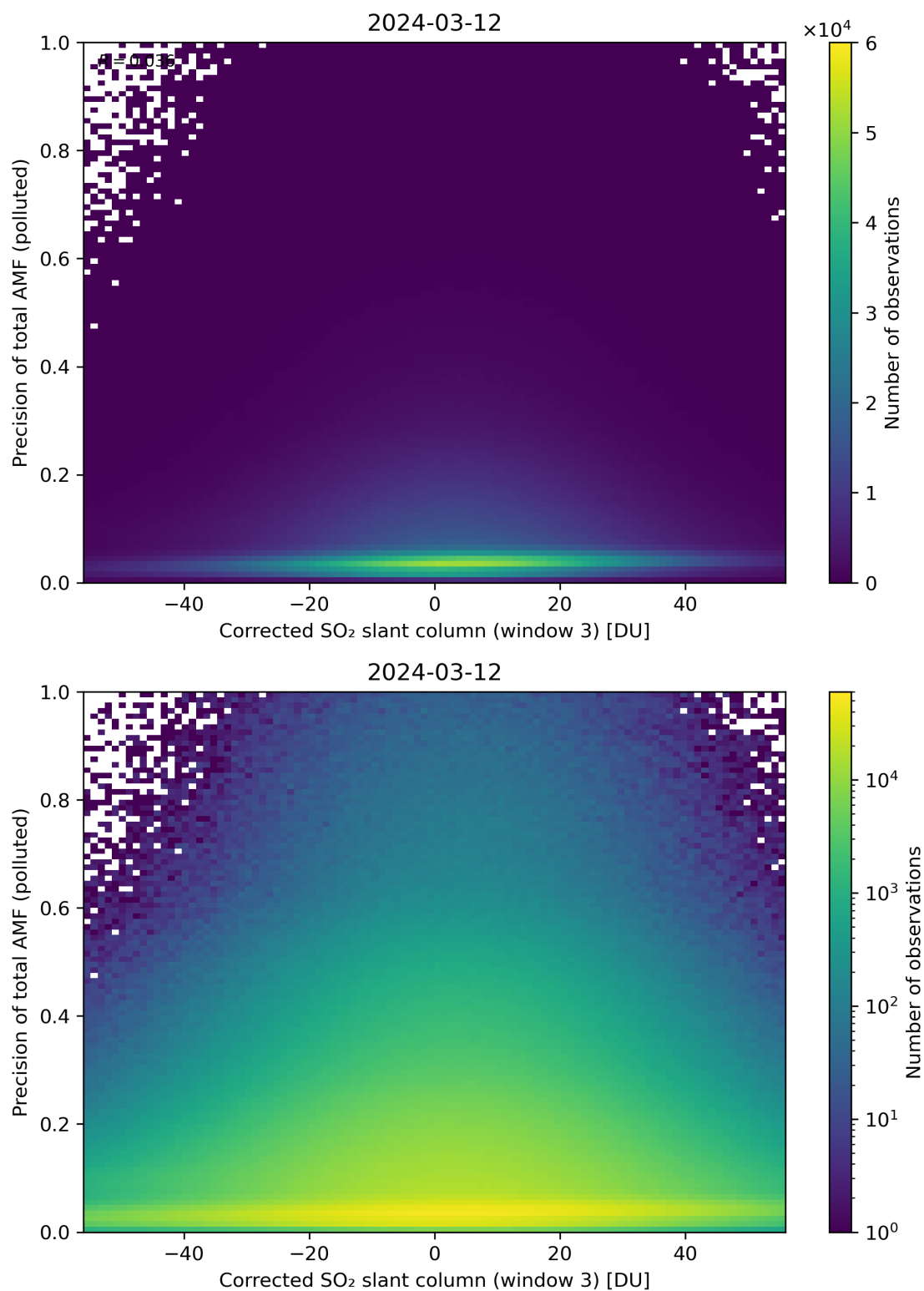
Figure 211: Scatter density plot of “Corrected SO 2 slant column (window 3)” against “Precision of total AMF (polluted)” for 2024-03-11 to 2024-03-13.
