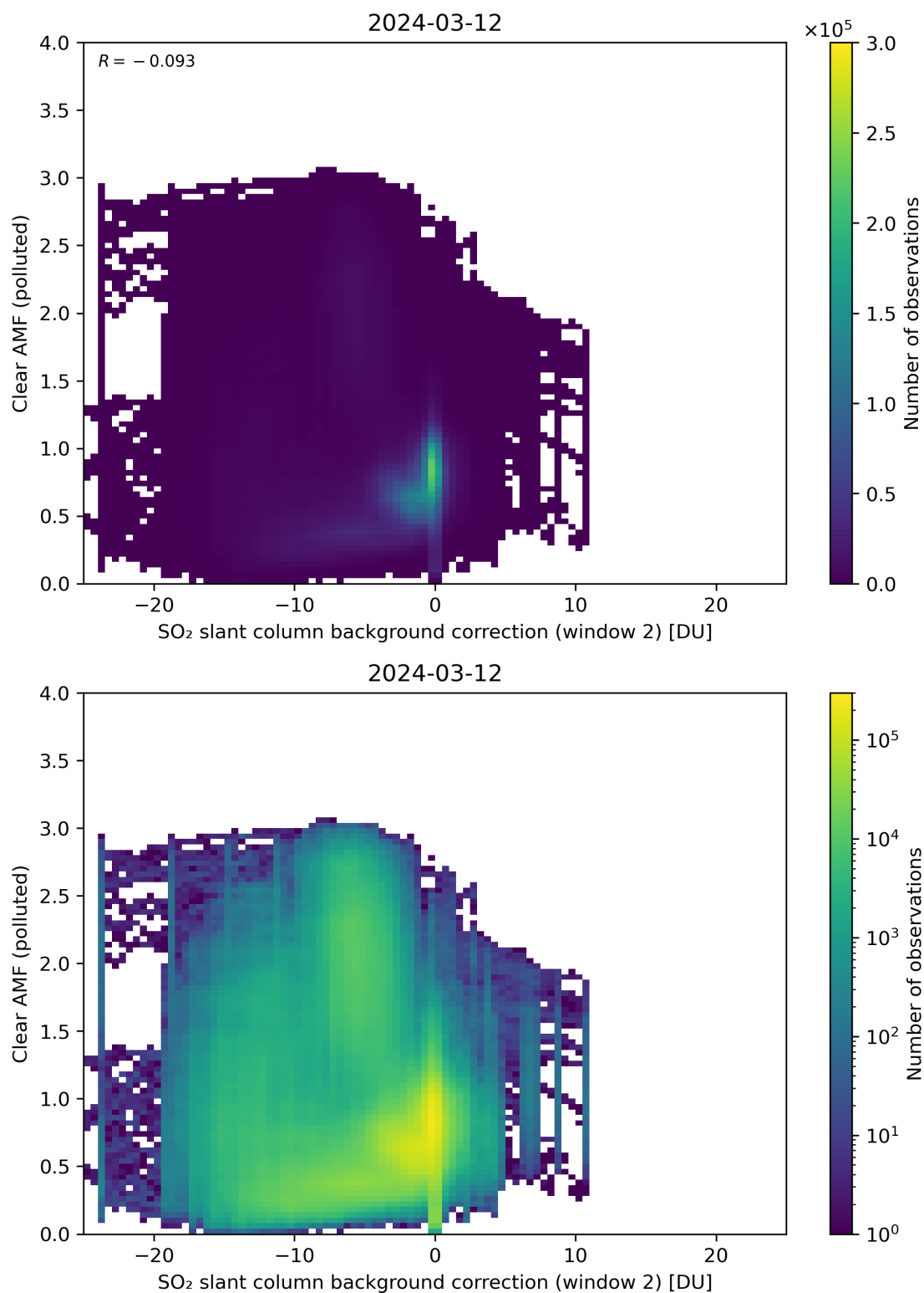
Figure 115: Scatter density plot of “SO 2 slant column background correction (window 2)” against “Clear AMF (polluted)” for 2024-03-11 to 2024-03-13.
