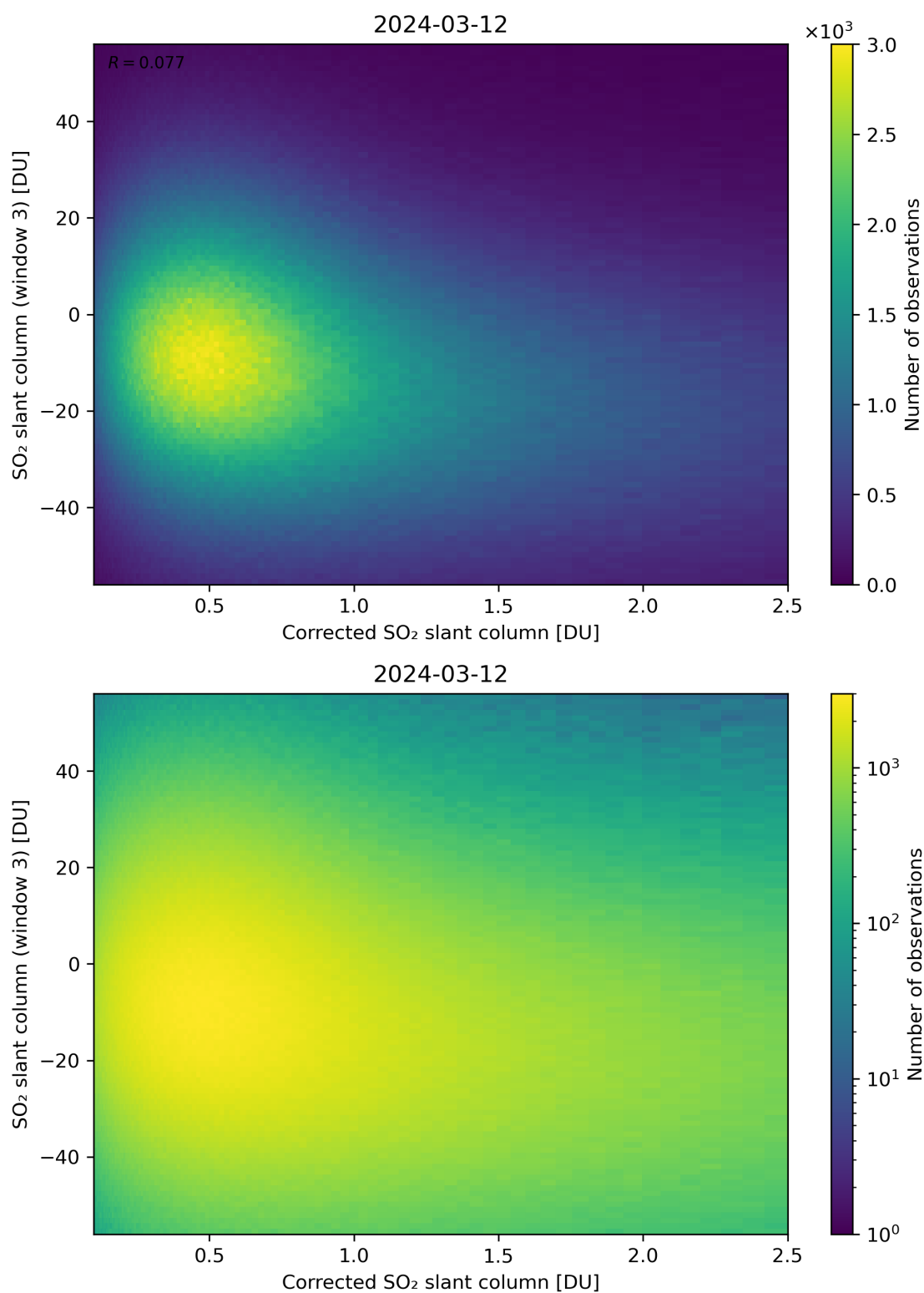
Figure 190: Scatter density plot of “Corrected SO 2 slant column” against “SO 2 slant column (window 3)” for 2024-03-11 to 2024-03-13.
