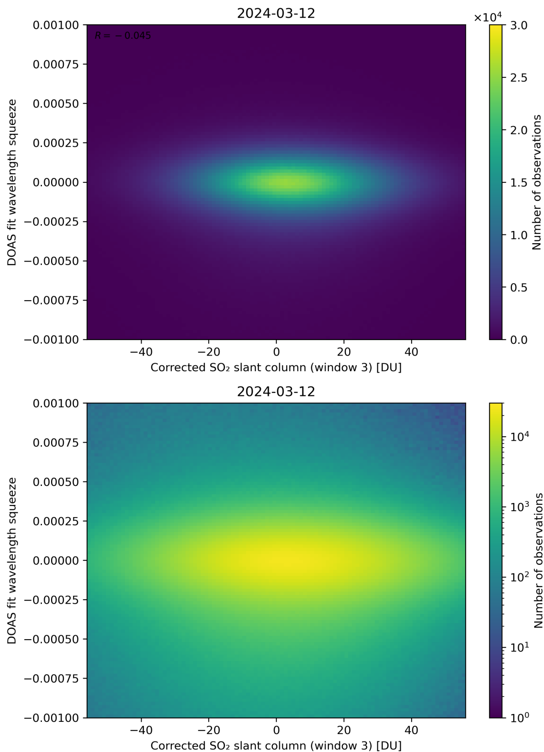
Figure 207: Scatter density plot of “Corrected SO 2 slant column (window 3)” against “DOAS fit wavelength squeeze” for 2024-03-11 to 2024-03-13.
