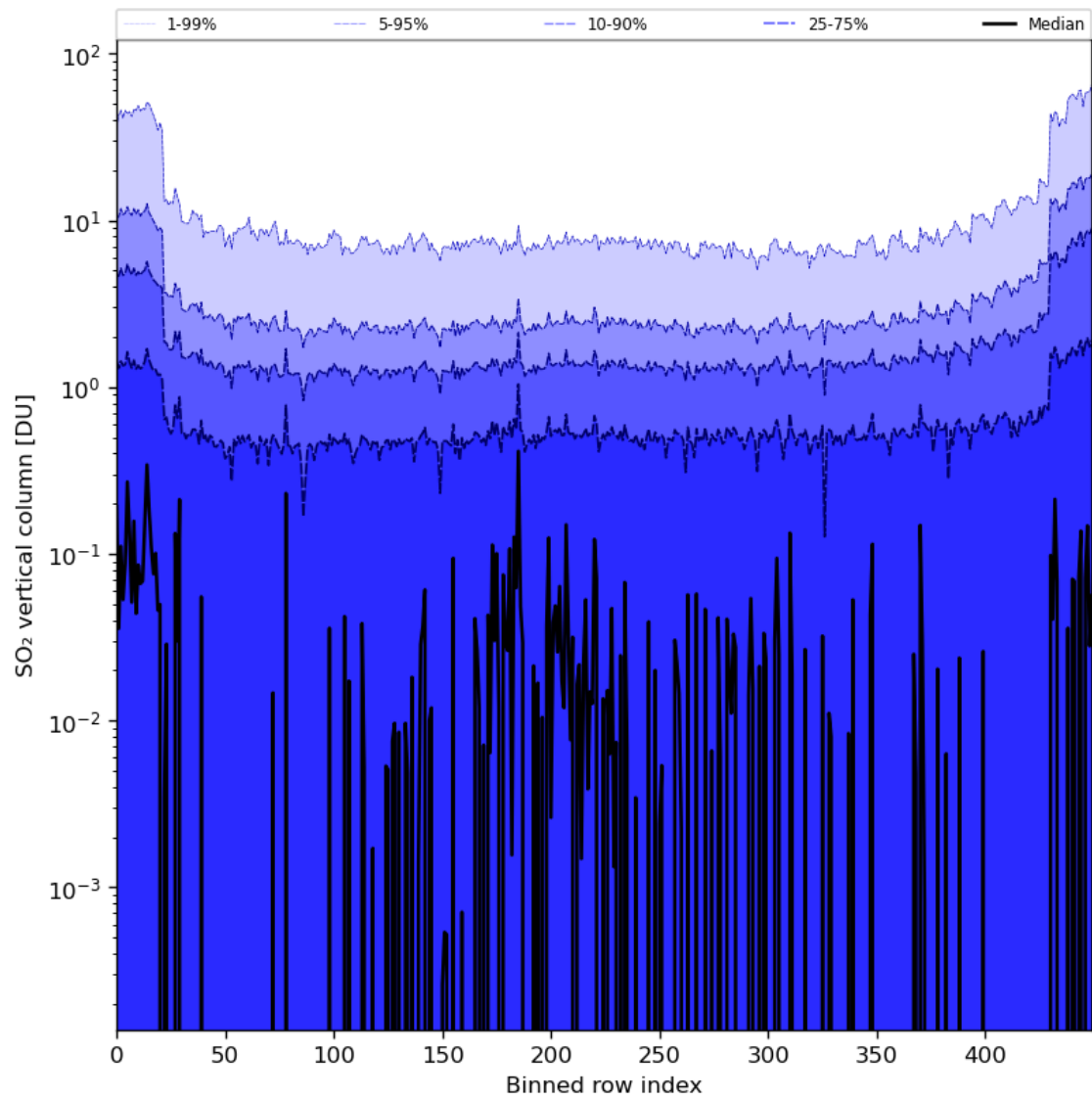
Figure 76: Along track statistics of “SO 2 vertical column” for 2024-03-11 to 2024-03-13
