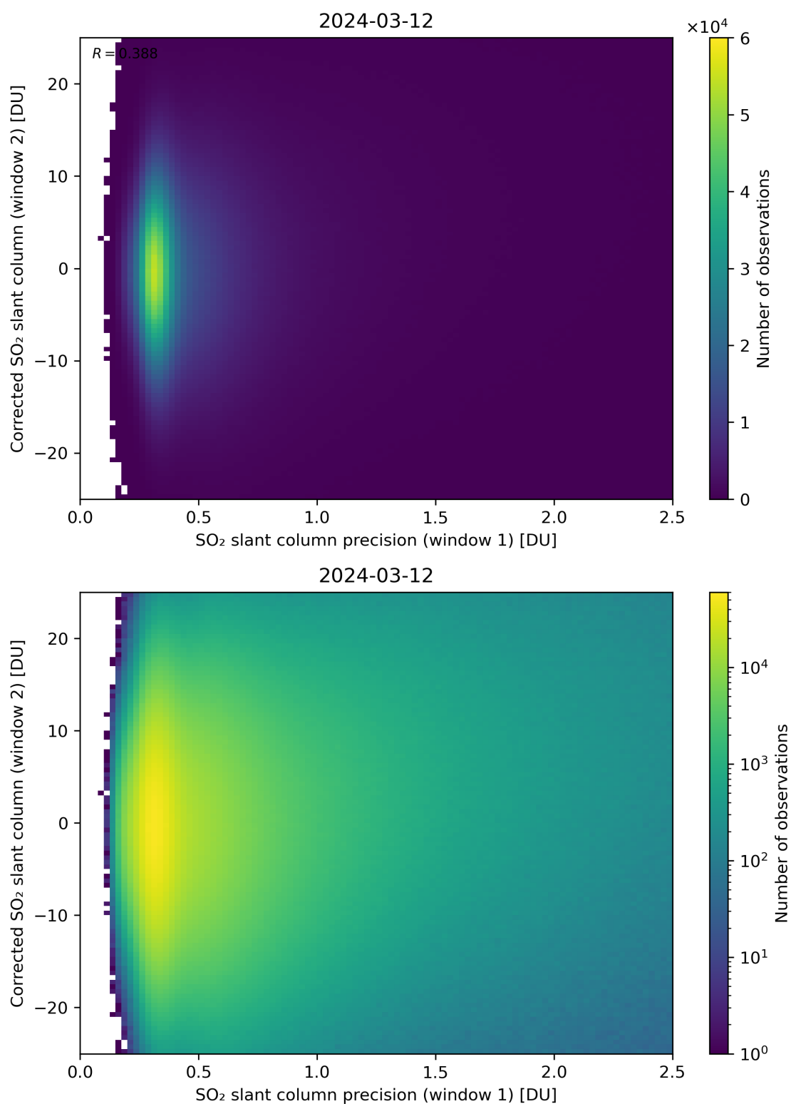
Figure 225: Scatter density plot of “SO 2 slant column precision (window 1)” against “Corrected SO 2 slant column (window 2)” for 2024-03-11 to 2024-03-13.
