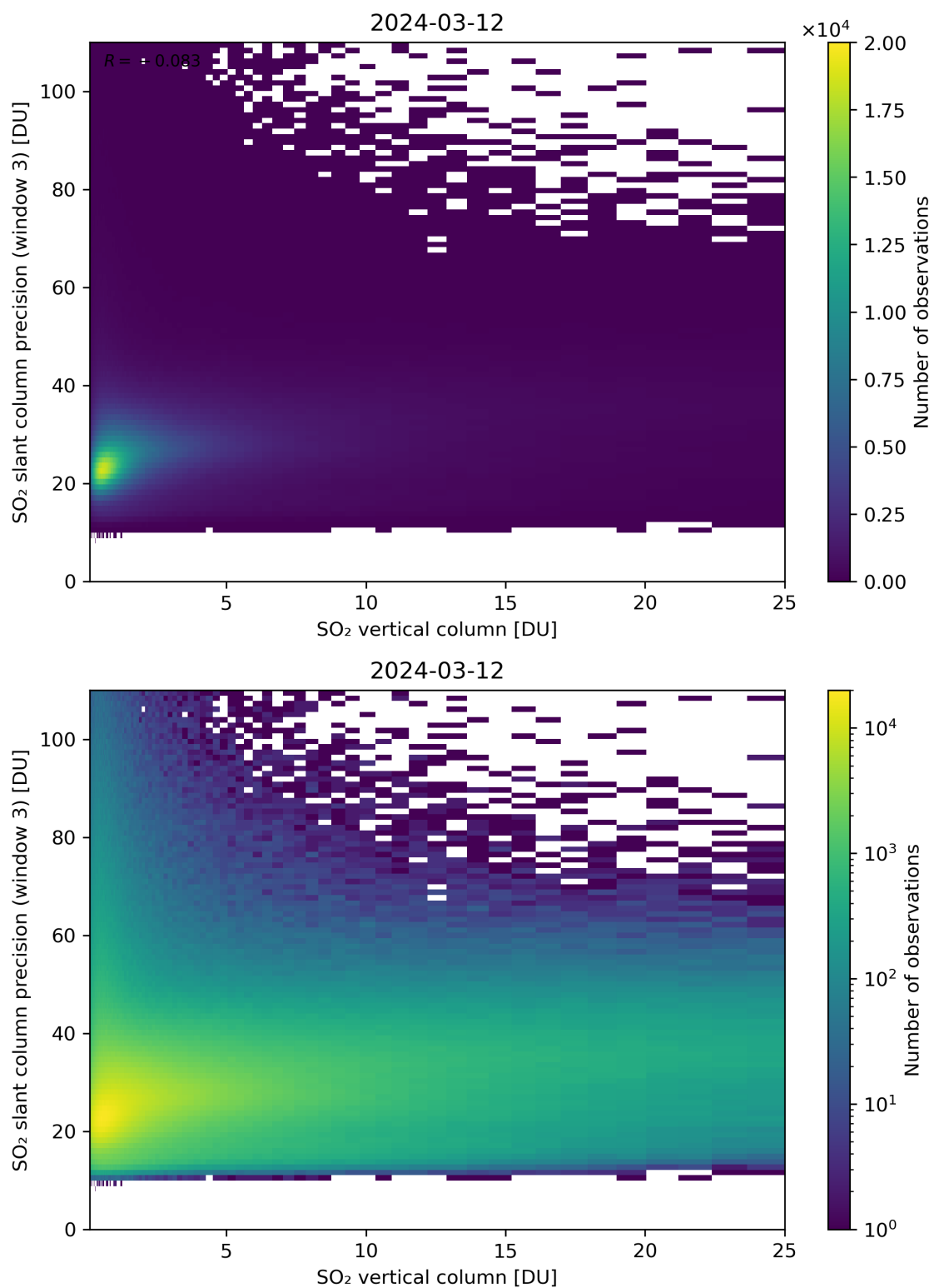
Figure 304: Scatter density plot of “SO 2 vertical column” against “SO 2 slant column precision (window 3)” for 2024-03-11 to 2024-03-13.
