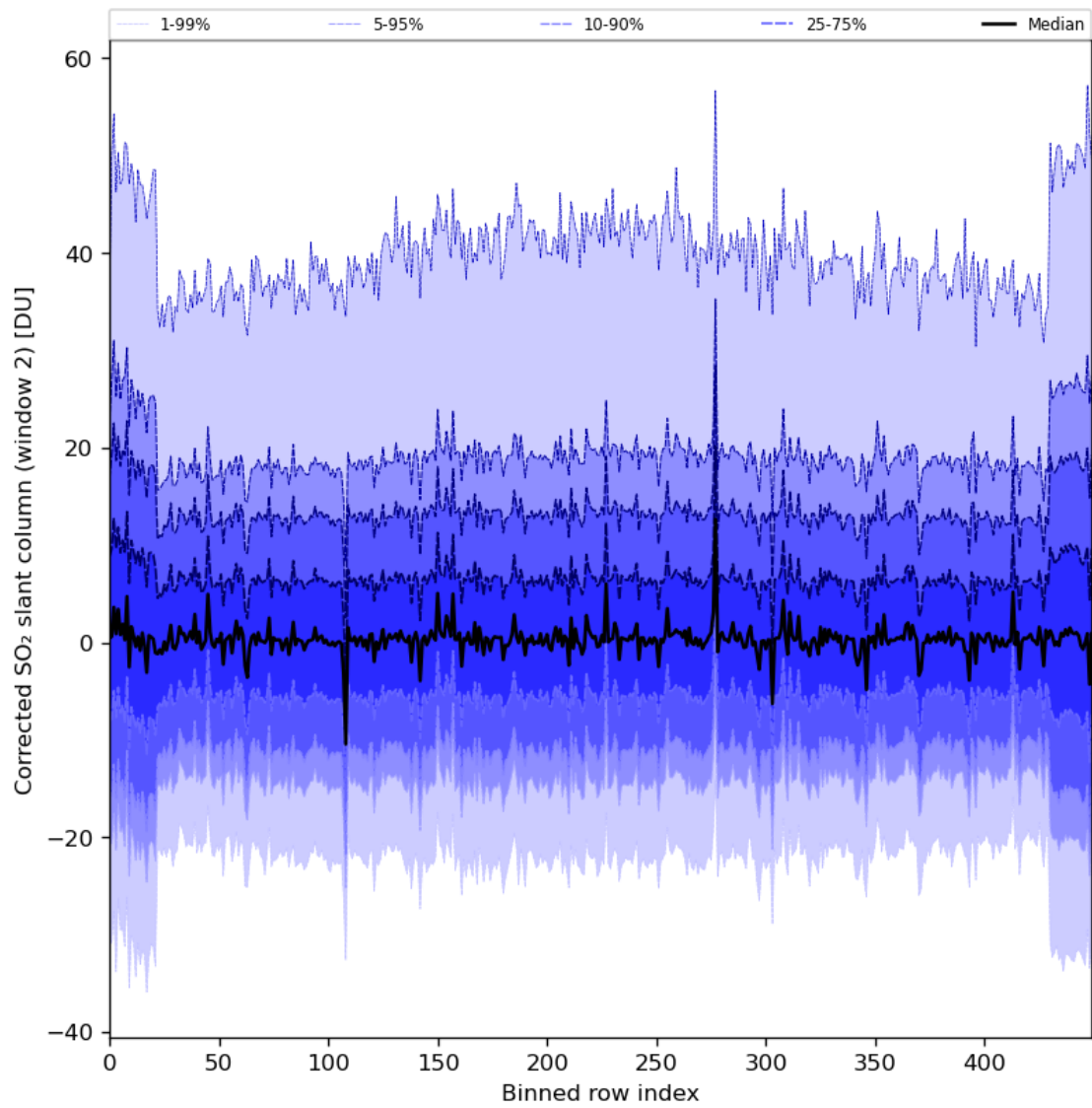
Figure 85: Along track statistics of “Corrected SO 2 slant column (window 2)” for 2024-03-11 to 2024-03-13
