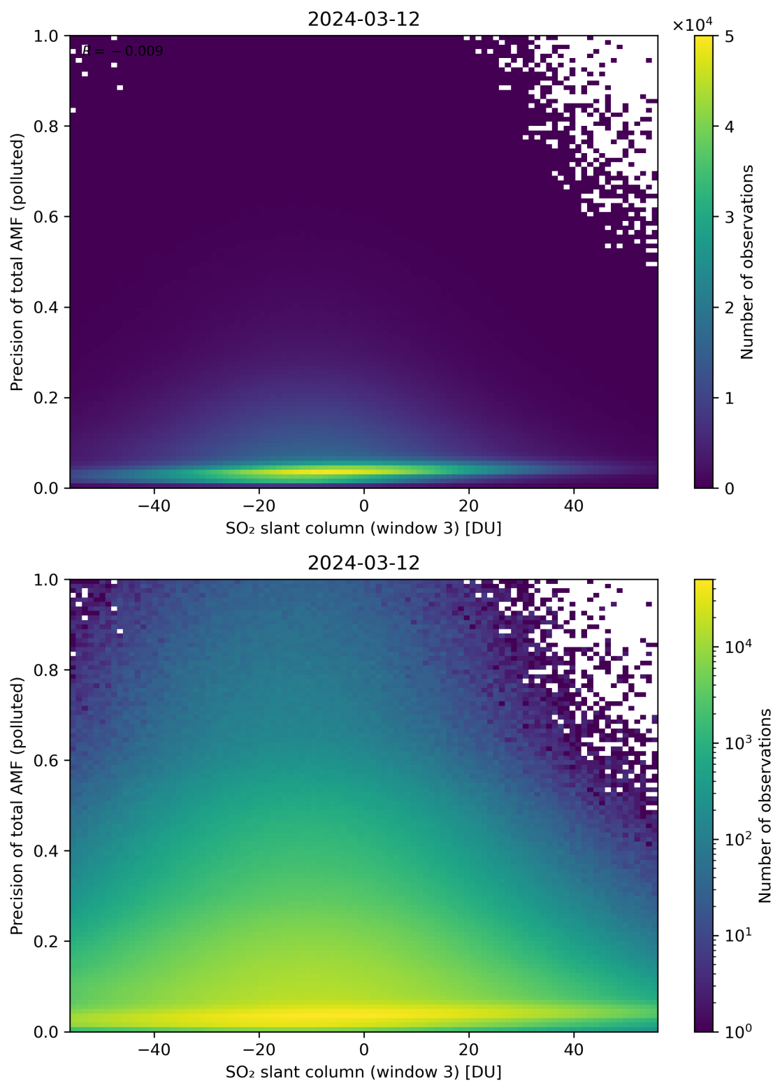
Figure 269: Scatter density plot of “SO 2 slant column (window 3)” against “Precision of total AMF (polluted)” for 2024-03-11 to 2024-03-13.
