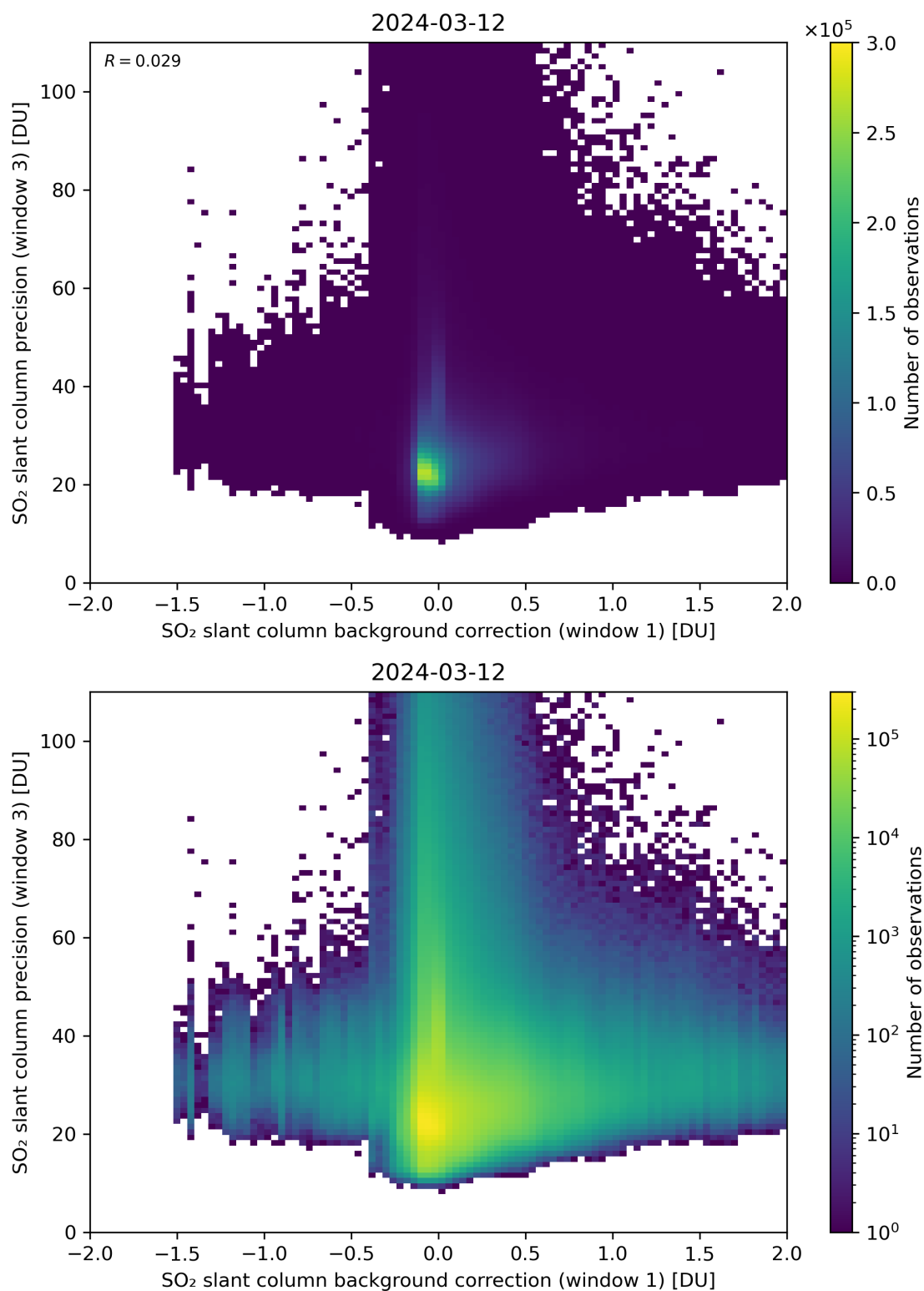
Figure 108: Scatter density plot of “SO 2 slant column background correction (window 1)” against “SO 2 slant column precision (window 3)” for 2024-03-11 to 2024-03-13.
