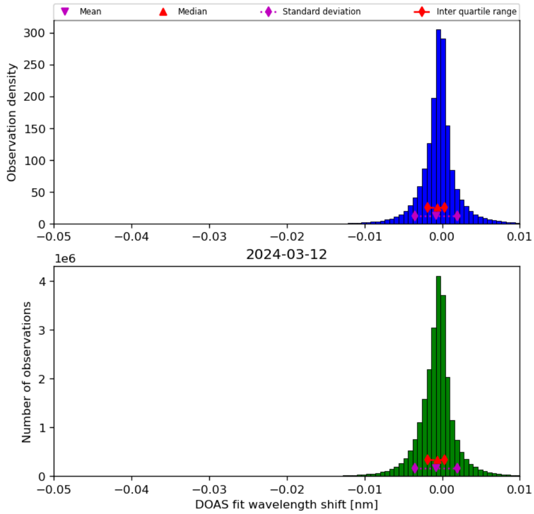
Figure 68: Histogram of “DOAS fit wavelength shift” for 2024-03-11 to 2024-03-13
