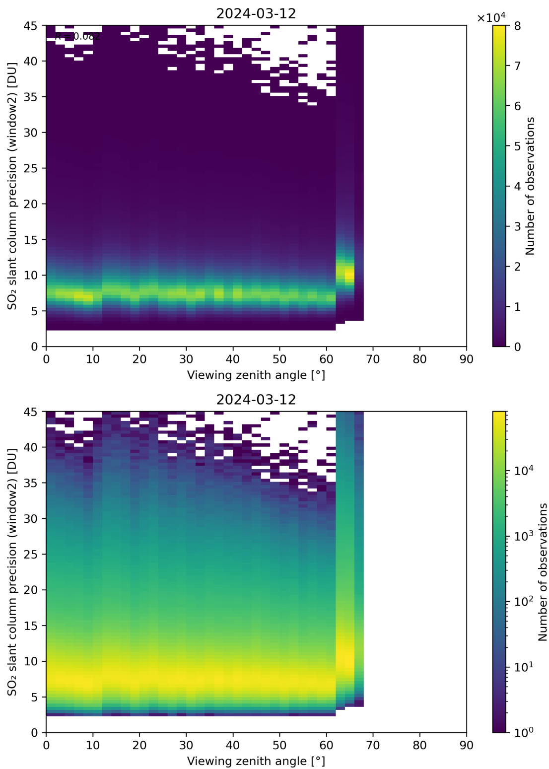
Figure 322: Scatter density plot of “Viewing zenith angle” against “SO 2 slant column precision (window2)” for 2024-03-11 to 2024-03-13.
