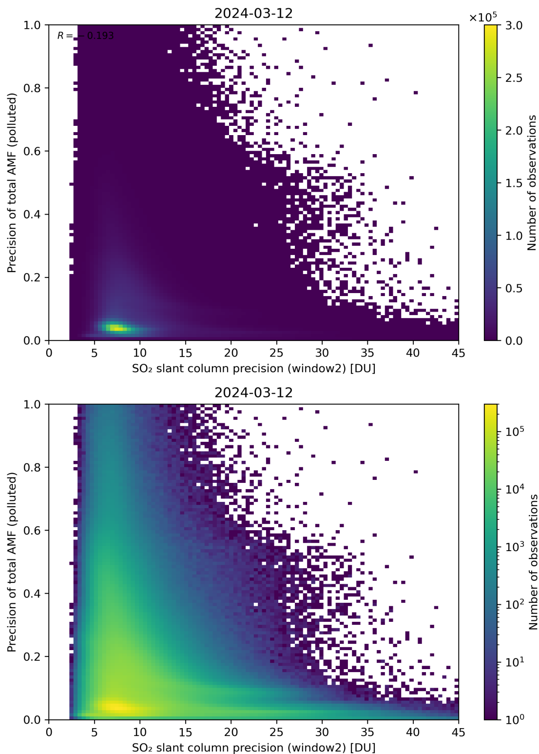
Figure 252: Scatter density plot of “SO 2 slant column precision (window2)” against “Precision of total AMF (polluted)” for 2024-03-11 to 2024-03-13.
