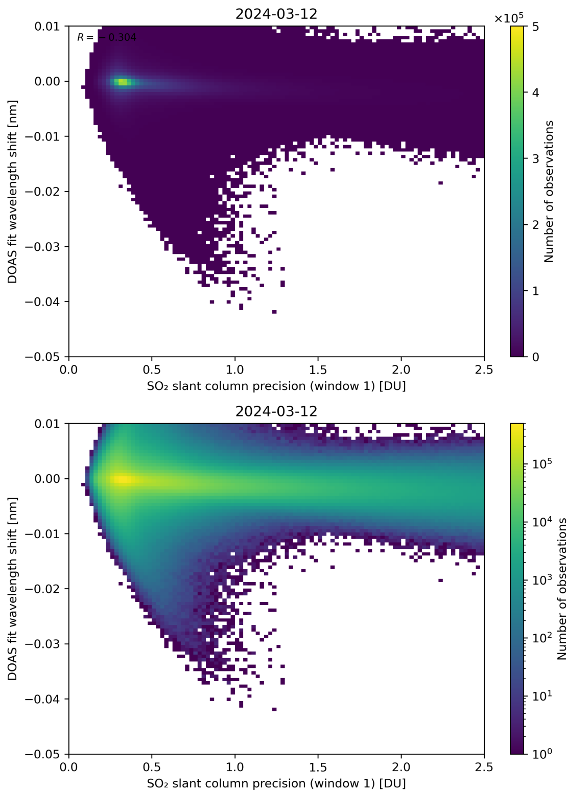
Figure 221: Scatter density plot of “SO 2 slant column precision (window 1)” against “DOAS fit wavelength shift” for 2024-03-11 to 2024-03-13.
