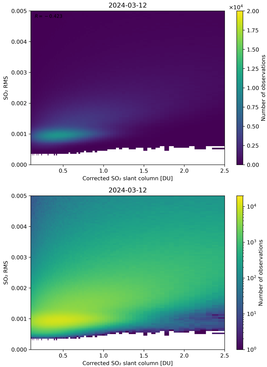
Figure 183: Scatter density plot of “Corrected SO 2 slant column” against “SO 2 RMS” for 2024-03-11 to 2024-03-13.
