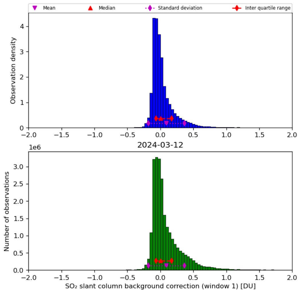
Figure 59: Histogram of “SO 2 slant column background correction (window 1)” for 2024-03-11 to 2024-03-13
