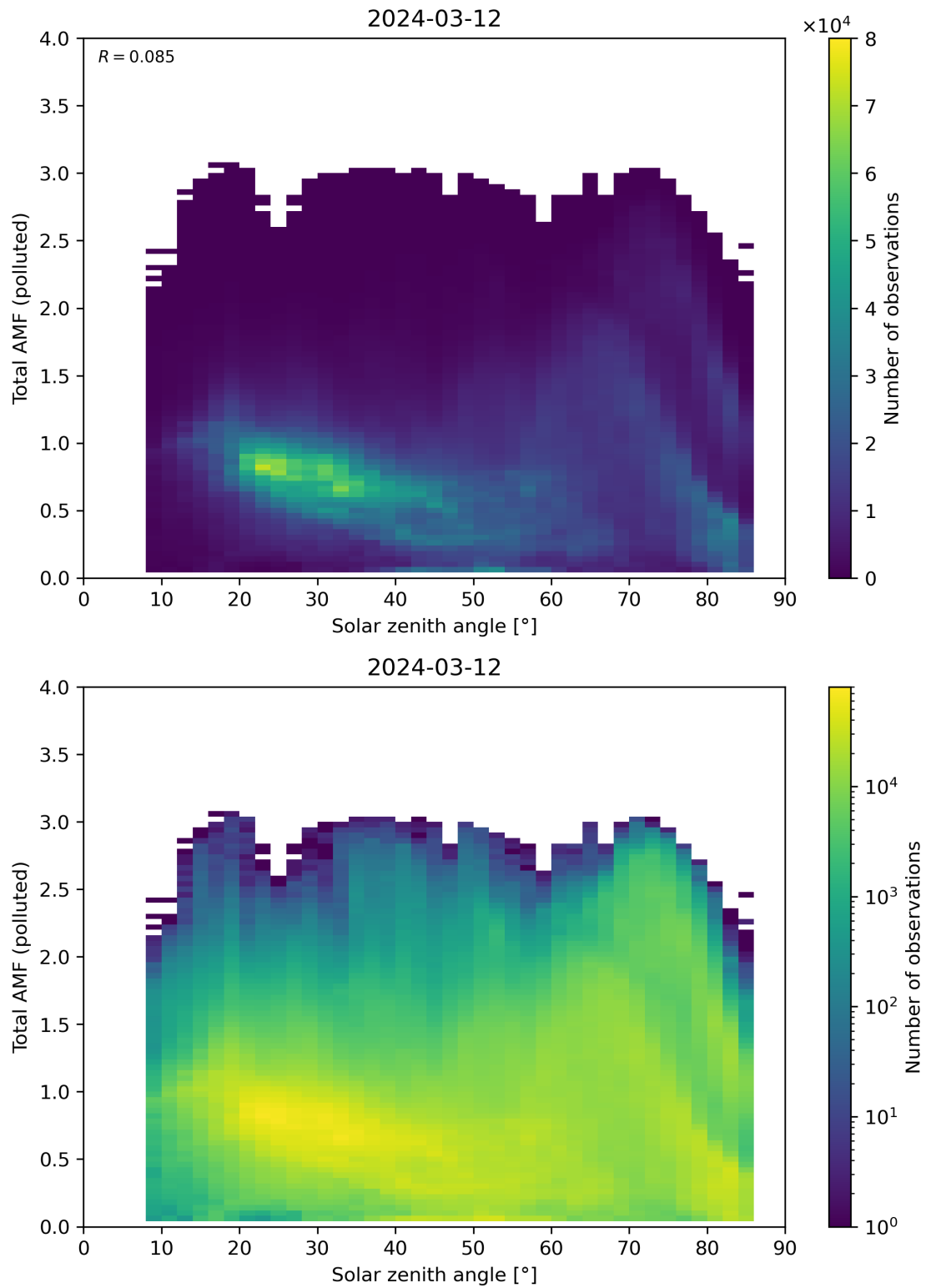
Figure 174: Scatter density plot of “Solar zenith angle” against “Total AMF (polluted)” for 2024-03-11 to 2024-03-13.
