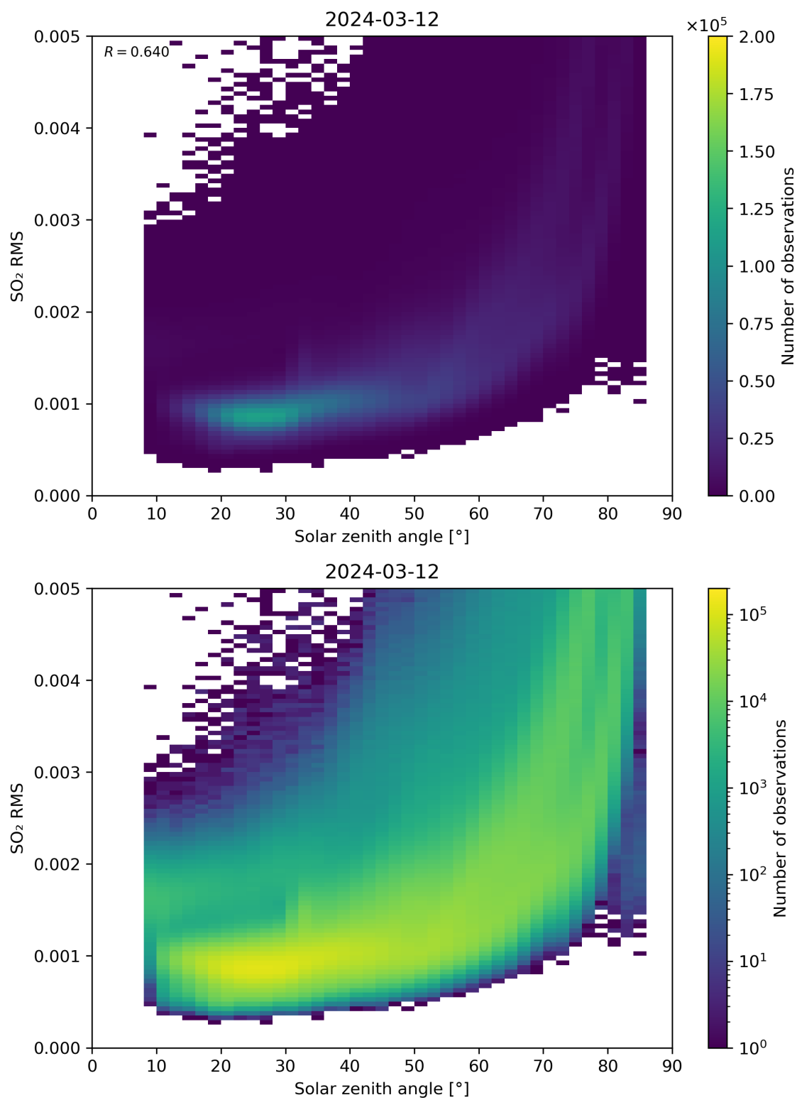
Figure 163: Scatter density plot of “Solar zenith angle” against “SO 2 RMS” for 2024-03-11 to 2024-03-13.
