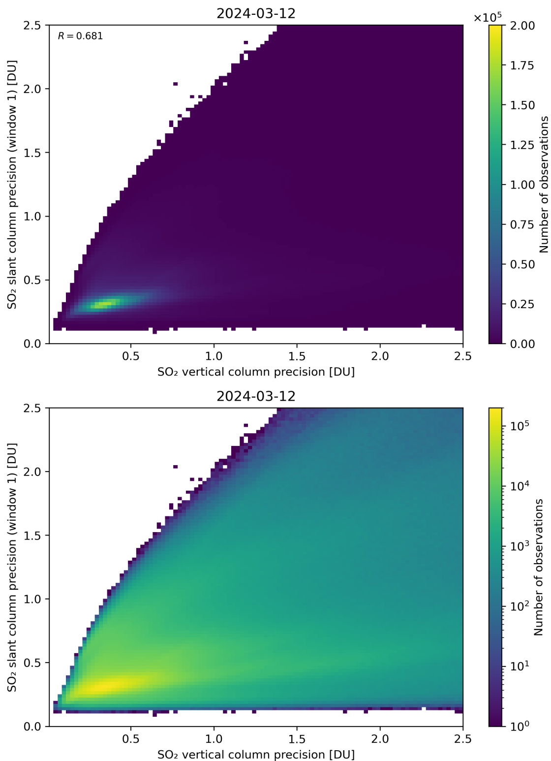
Figure 290: Scatter density plot of “SO 2 vertical column precision” against “SO 2 slant column precision (window 1)” for 2024-03-11 to 2024-03-13.
