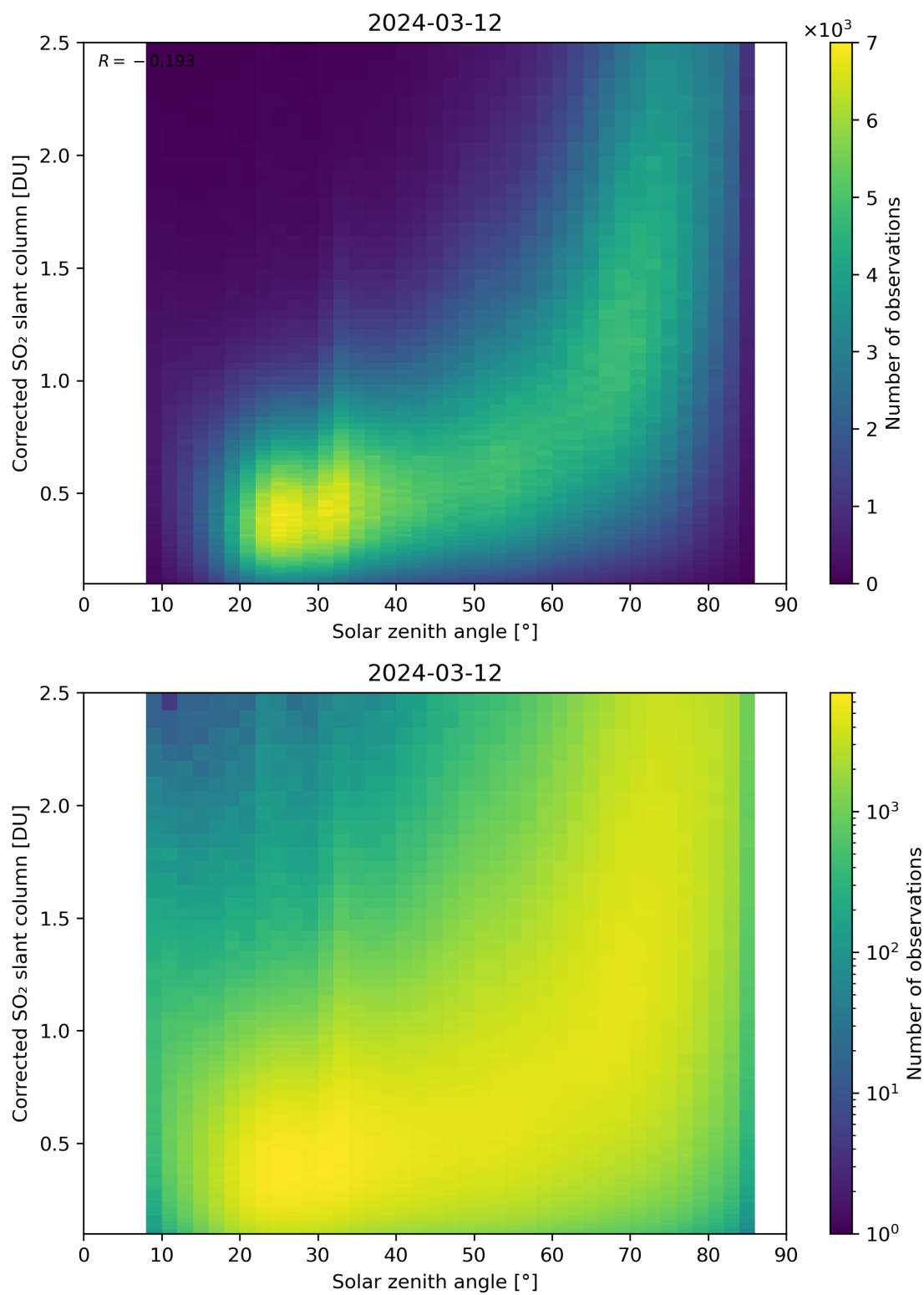
Figure 166: Scatter density plot of “Solar zenith angle” against “Corrected SO 2 slant column” for 2024-03-11 to 2024-03-13.
