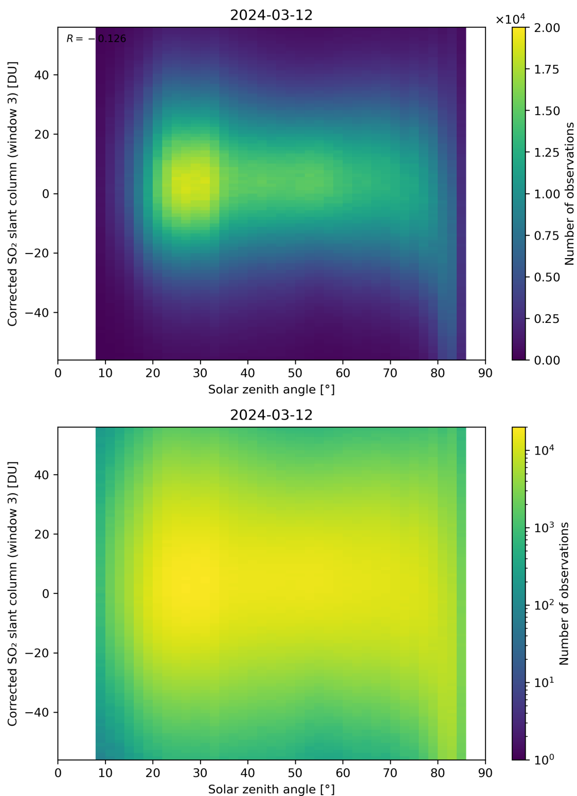
Figure 168: Scatter density plot of “Solar zenith angle” against “Corrected SO 2 slant column (window 3)” for 2024-03-11 to 2024-03-13.
