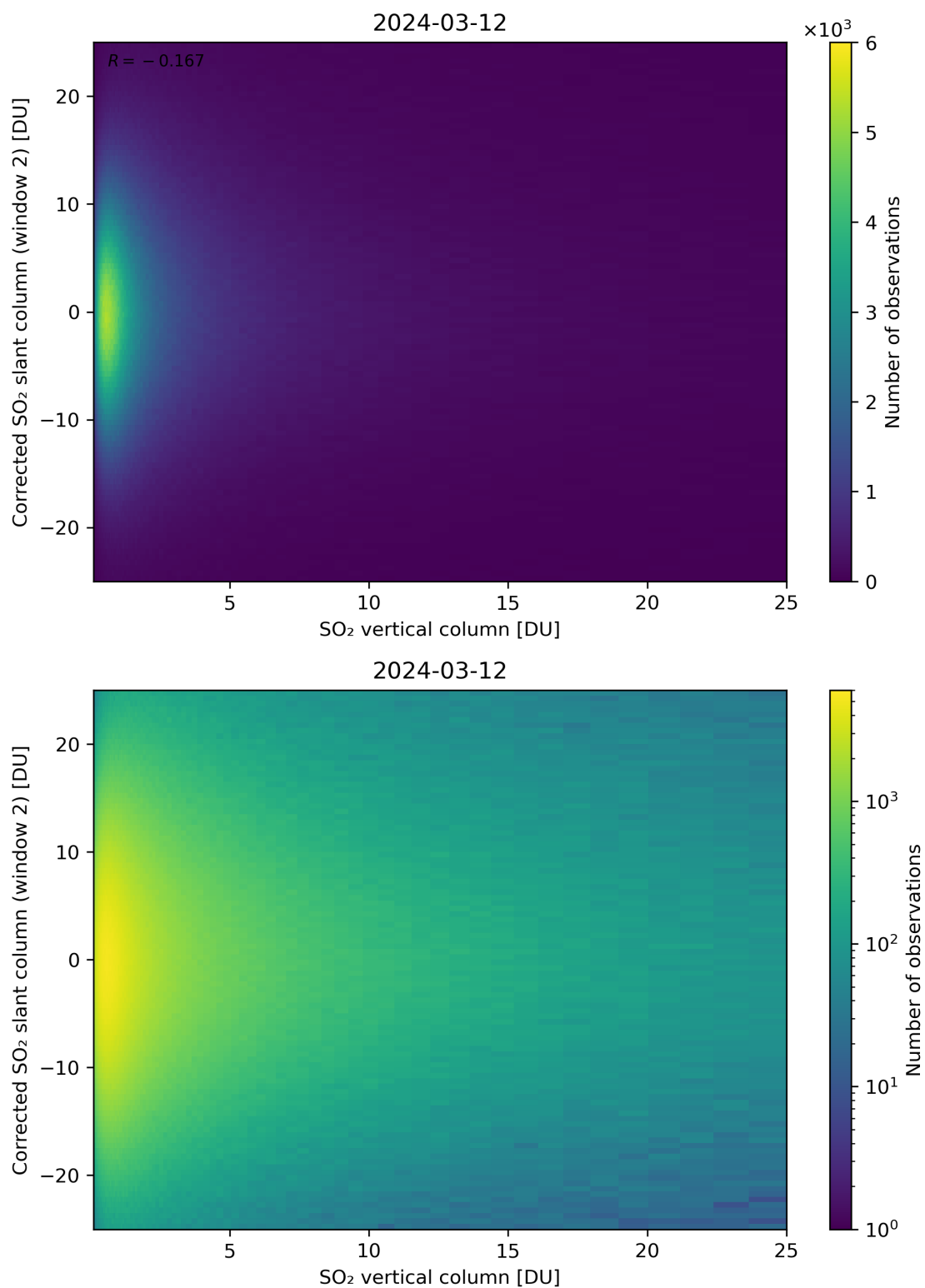
Figure 298: Scatter density plot of “SO 2 vertical column” against “Corrected SO 2 slant column (window 2)” for 2024-03-11 to 2024-03-13.
