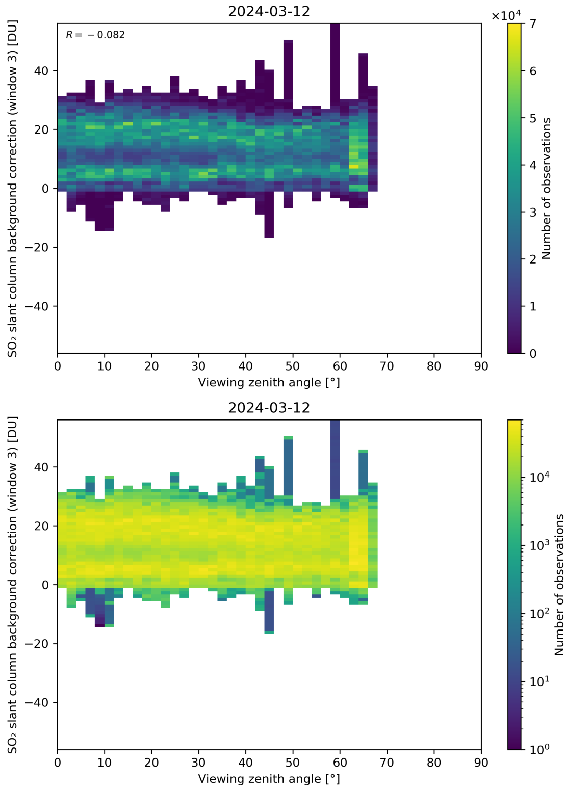
Figure 310: Scatter density plot of “Viewing zenith angle” against “SO 2 slant column background correction (window 3)” for 2024-03-11 to 2024-03-13.
