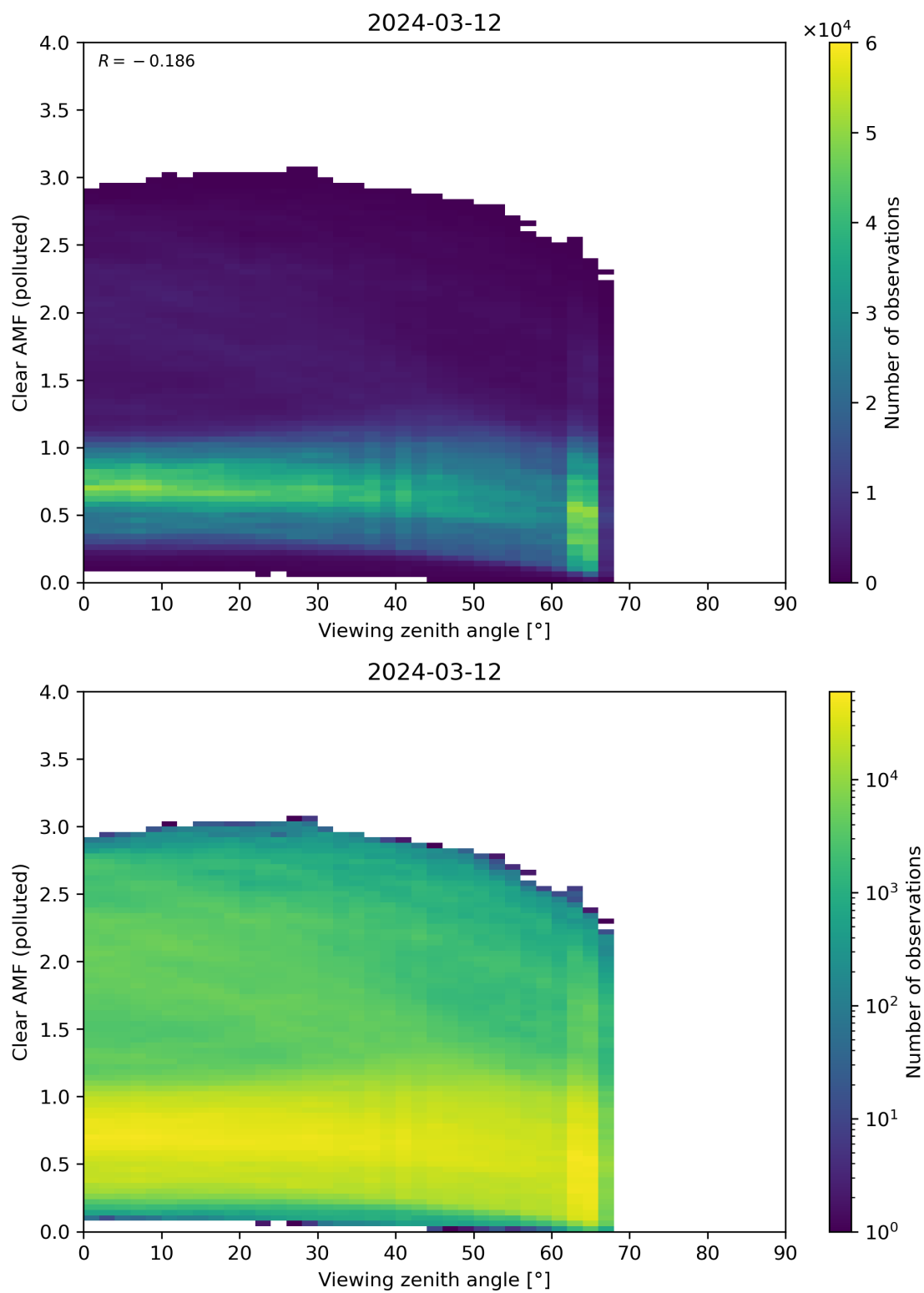
Figure 316: Scatter density plot of “Viewing zenith angle” against “Clear AMF (polluted)” for 2024-03-11 to 2024-03-13.
