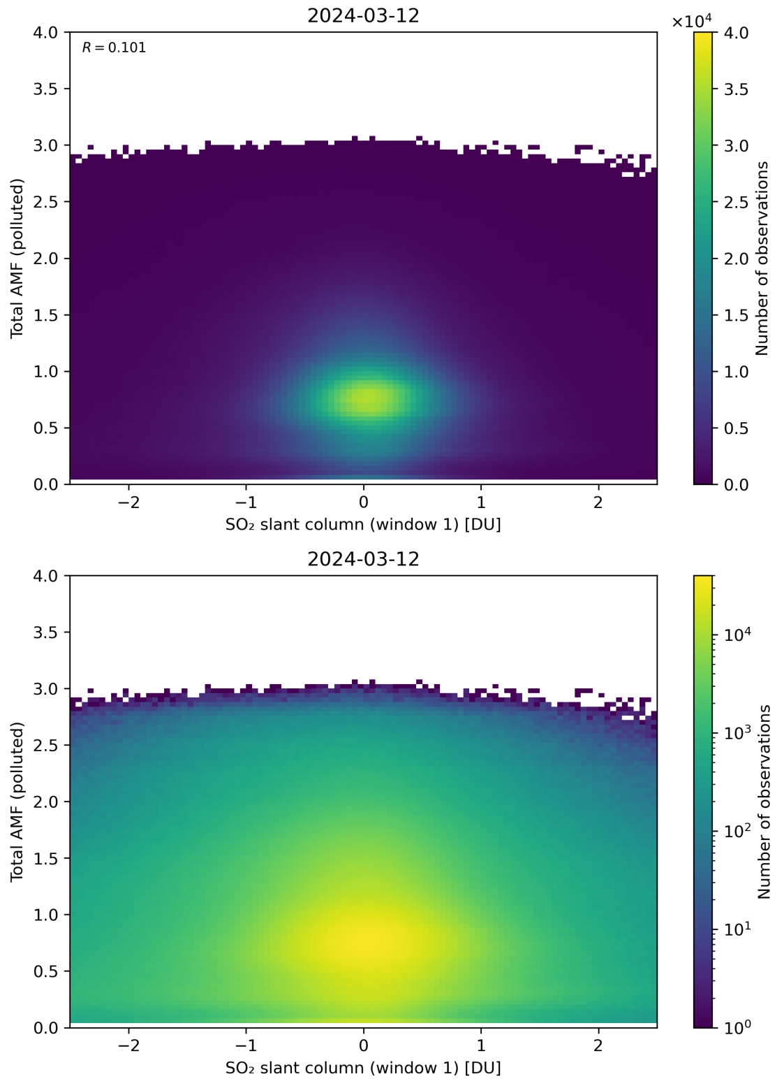
Figure 239: Scatter density plot of “SO 2 slant column (window 1)” against “Total AMF (polluted)” for 2024-03-11 to 2024-03-13.
