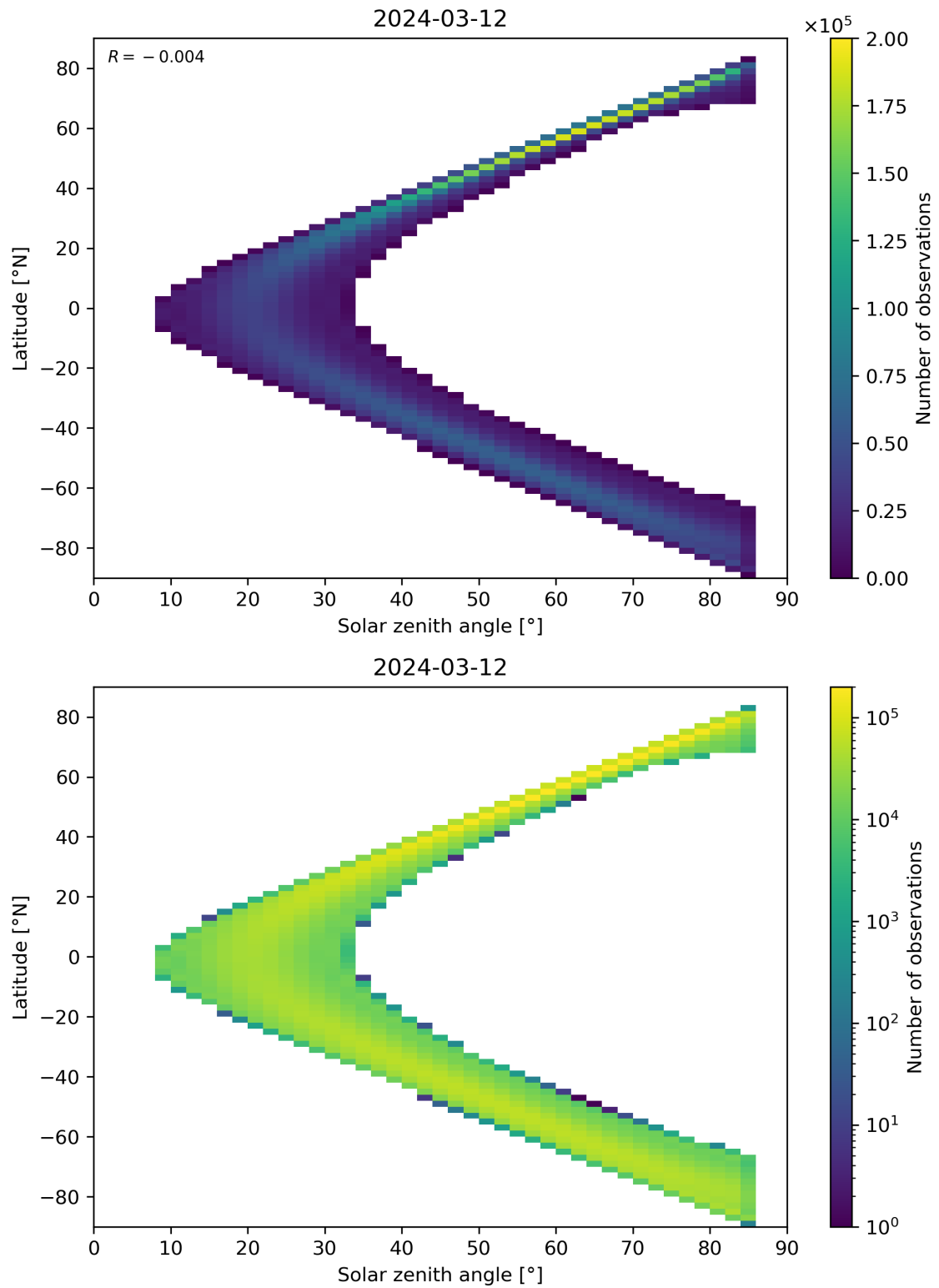
Figure 164: Scatter density plot of “Solar zenith angle” against “Latitude” for 2024-03-11 to 2024-03-13.
