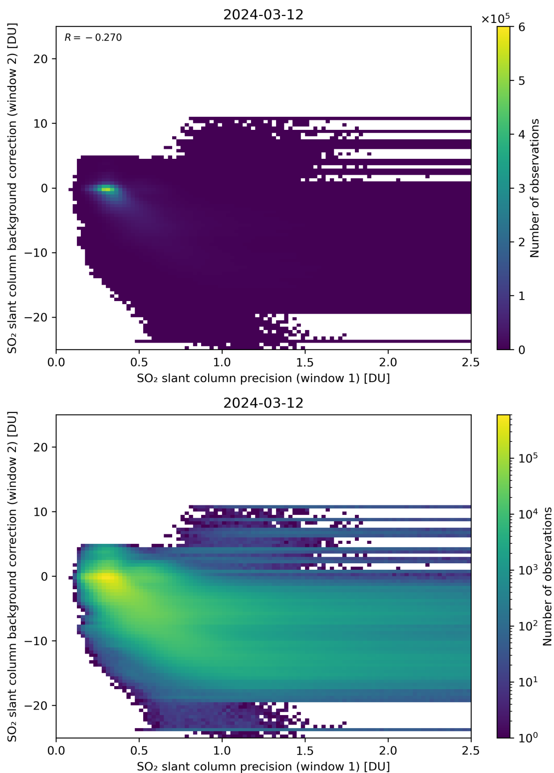
Figure 219: Scatter density plot of “SO 2 slant column precision (window 1)” against “SO 2 slant column background correction (window 2)” for 2024-03-11 to 2024-03-13.
