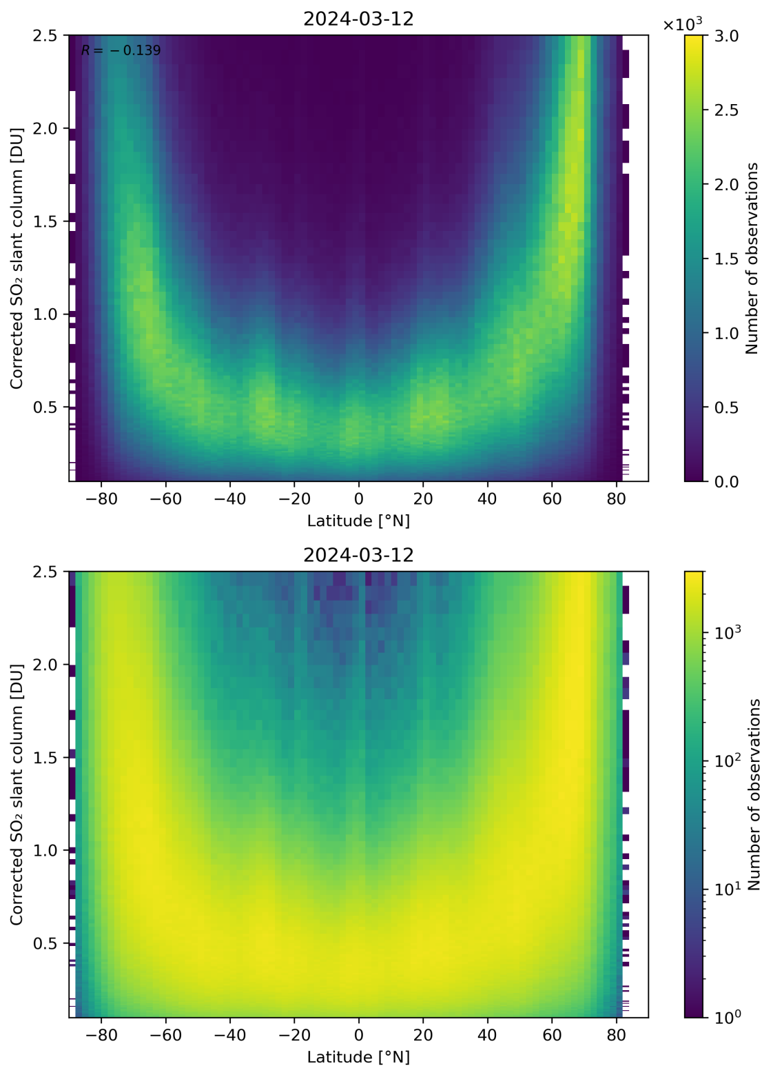
Figure 146: Scatter density plot of “Latitude” against “Corrected SO 2 slant column” for 2024-03-11 to 2024-03-13.
