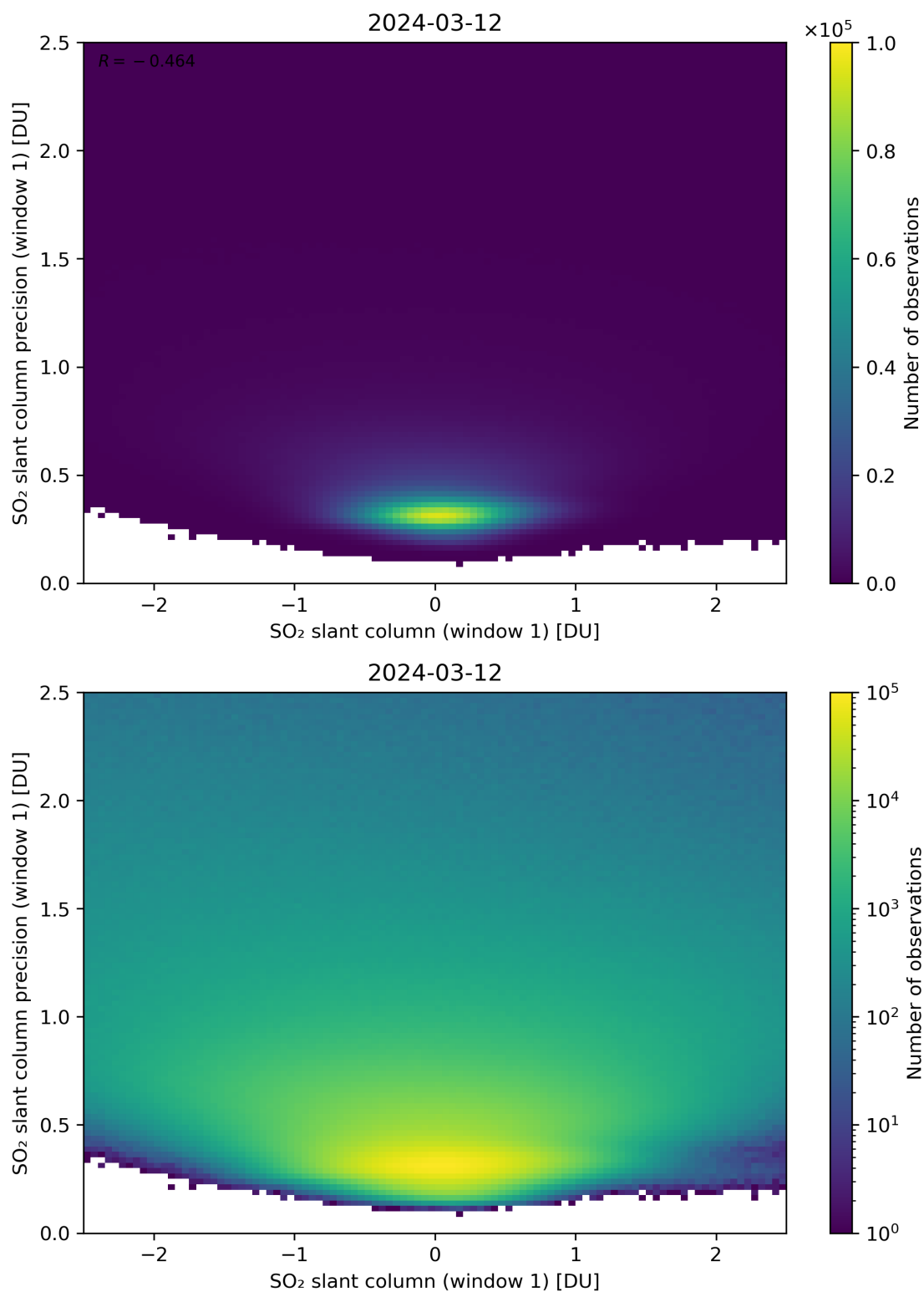
Figure 235: Scatter density plot of “SO 2 slant column (window 1)” against “SO 2 slant column precision (window 1)” for 2024-03-11 to 2024-03-13.
