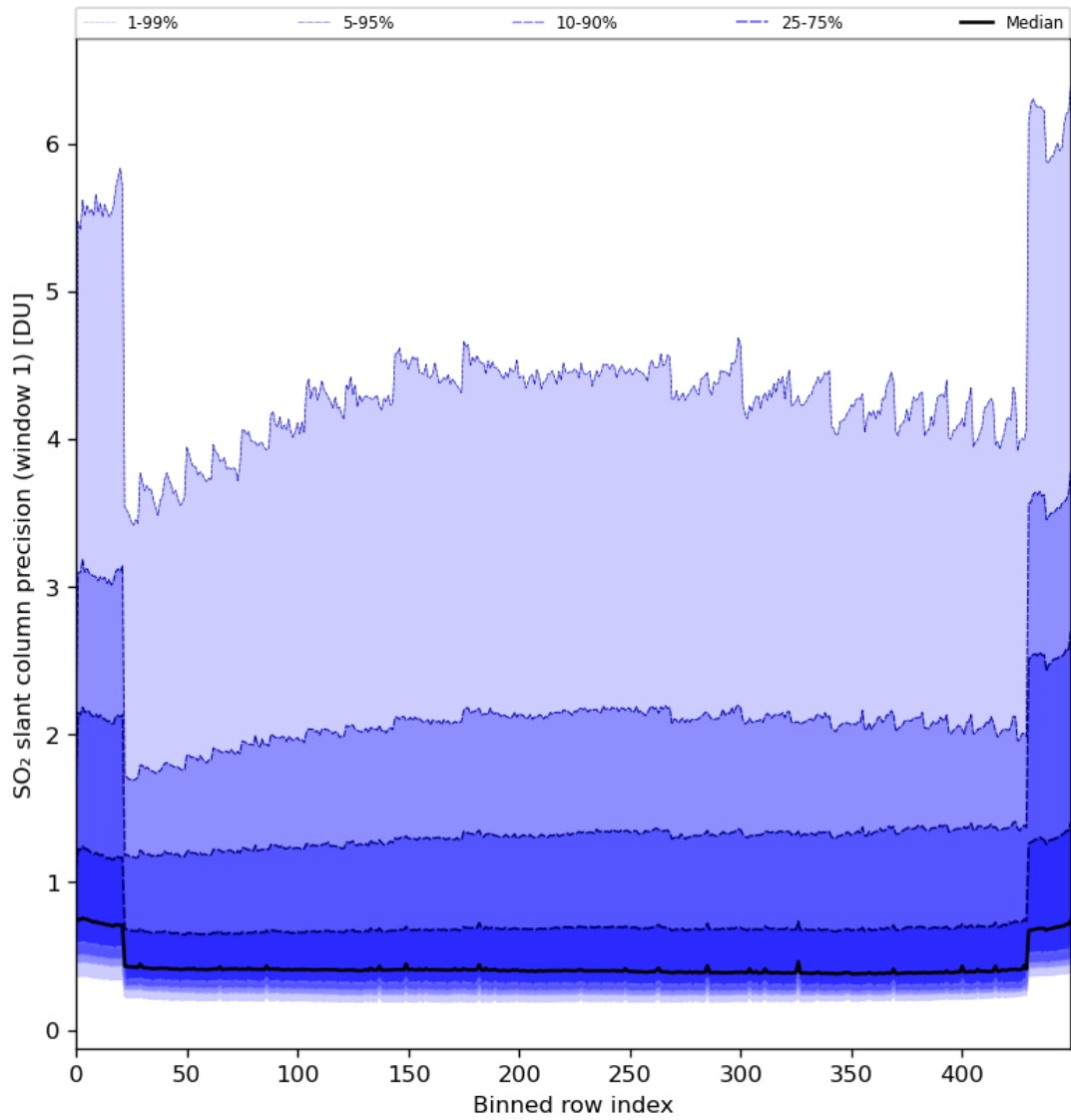
Figure 80: Along track statistics of “SO 2 slant column precision (window 1)” for 2024-03-11 to 2024-03-13
