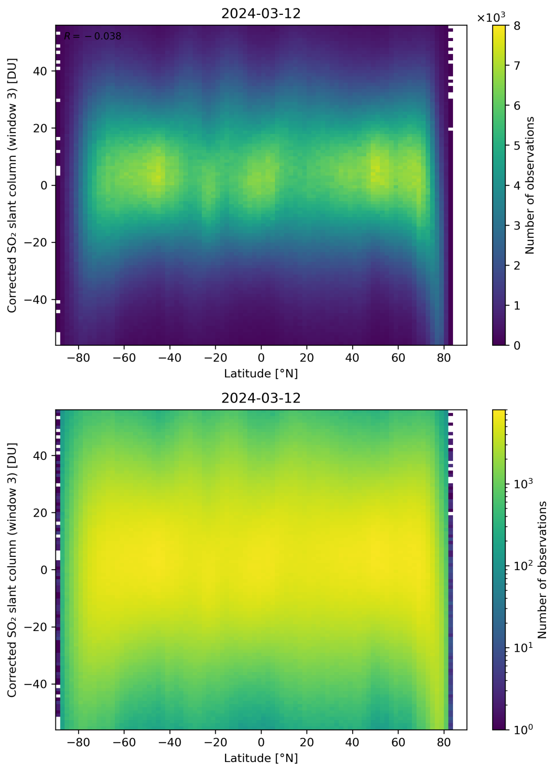
Figure 148: Scatter density plot of “Latitude” against “Corrected SO 2 slant column (window 3)” for 2024-03-11 to 2024-03-13.
