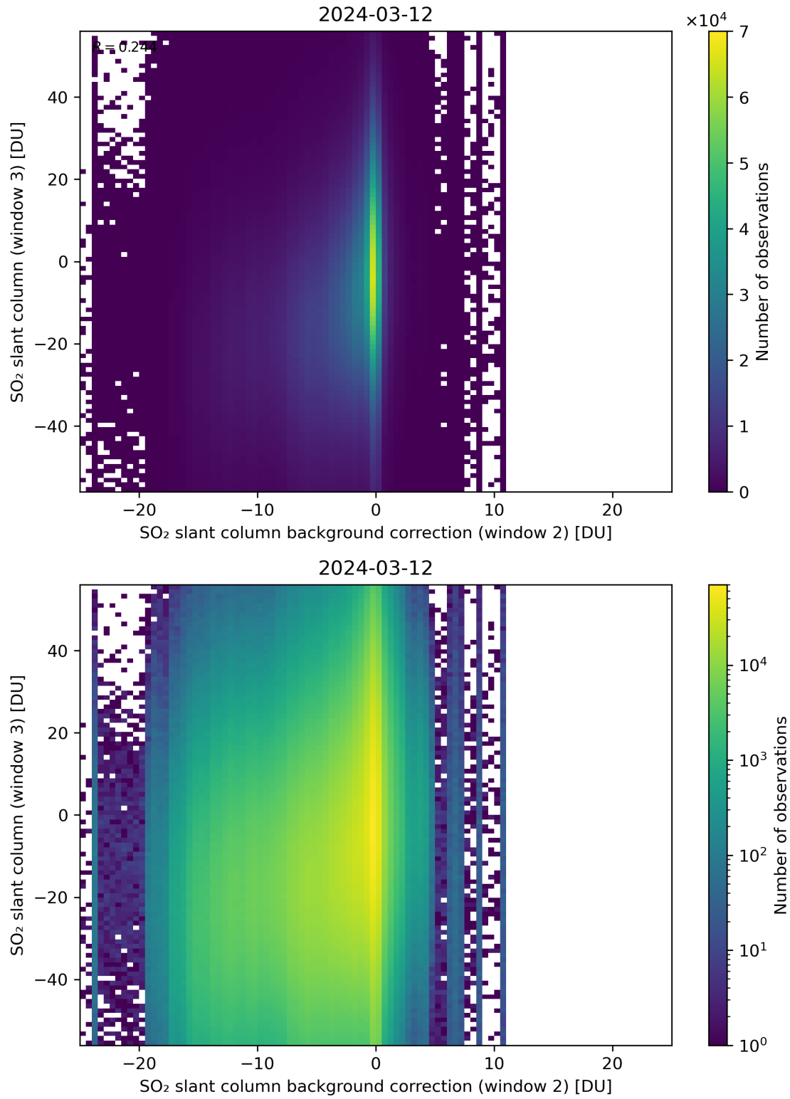
Figure 117: Scatter density plot of “SO 2 slant column background correction (window 2)” against “SO 2 slant column (window 3)” for 2024-03-11 to 2024-03-13.
