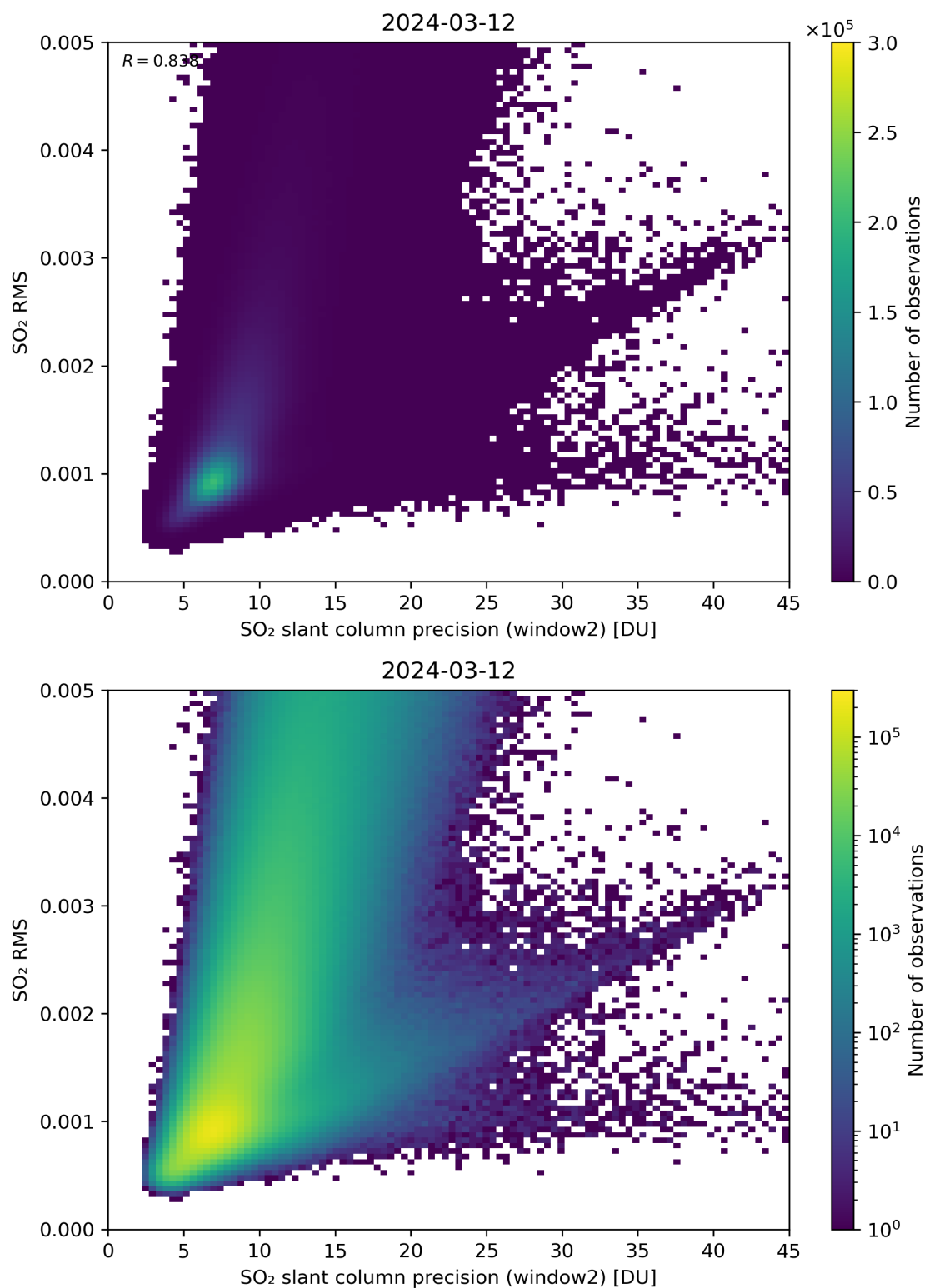
Figure 245: Scatter density plot of “SO 2 slant column precision (window2)” against “SO 2 RMS” for 2024-03-11 to 2024-03-13.
