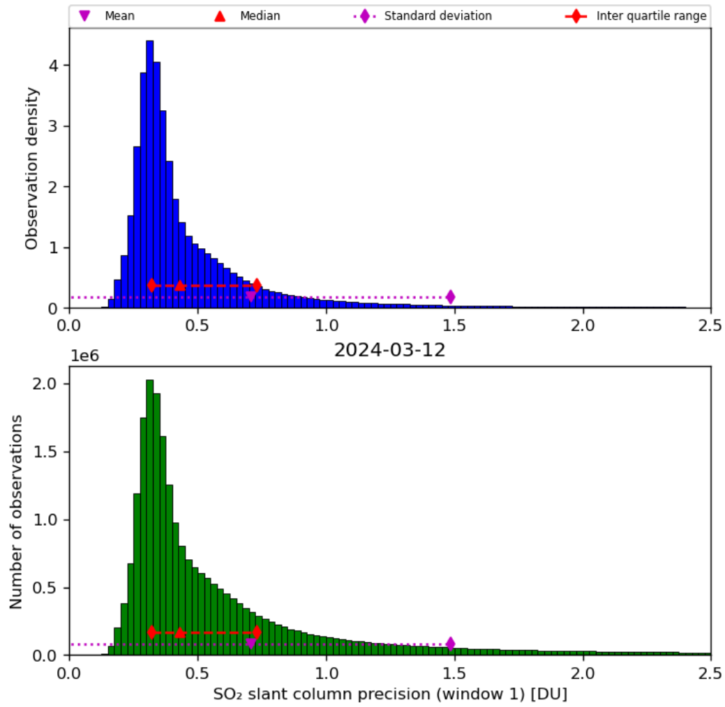
Figure 57: Histogram of “SO 2 slant column precision (window 1)” for 2024-03-11 to 2024-03-13
