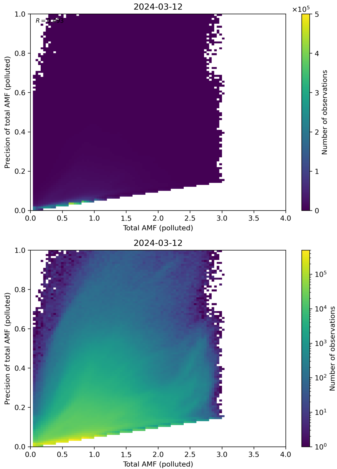
Figure 272: Scatter density plot of “Total AMF (polluted)” against “Precision of total AMF (polluted)” for 2024-03-11 to 2024-03-13.
