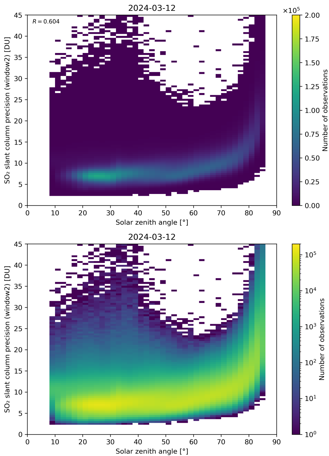
Figure 171: Scatter density plot of “Solar zenith angle” against “SO 2 slant column precision (window2)” for 2024-03-11 to 2024-03-13.
