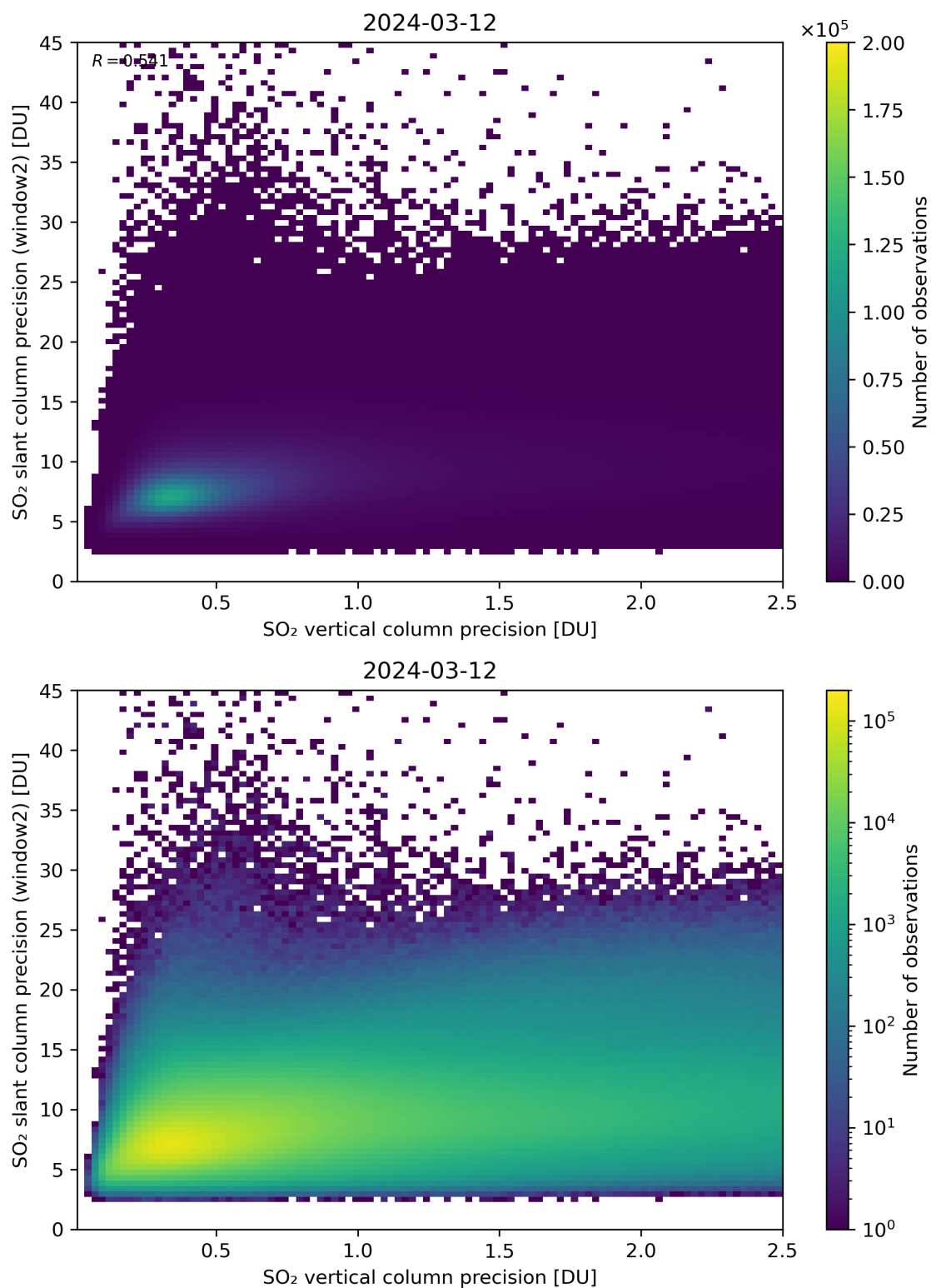
Figure 291: Scatter density plot of “SO 2 vertical column precision” against “SO 2 slant column precision (window2)” for 2024-03-11 to 2024-03-13.
