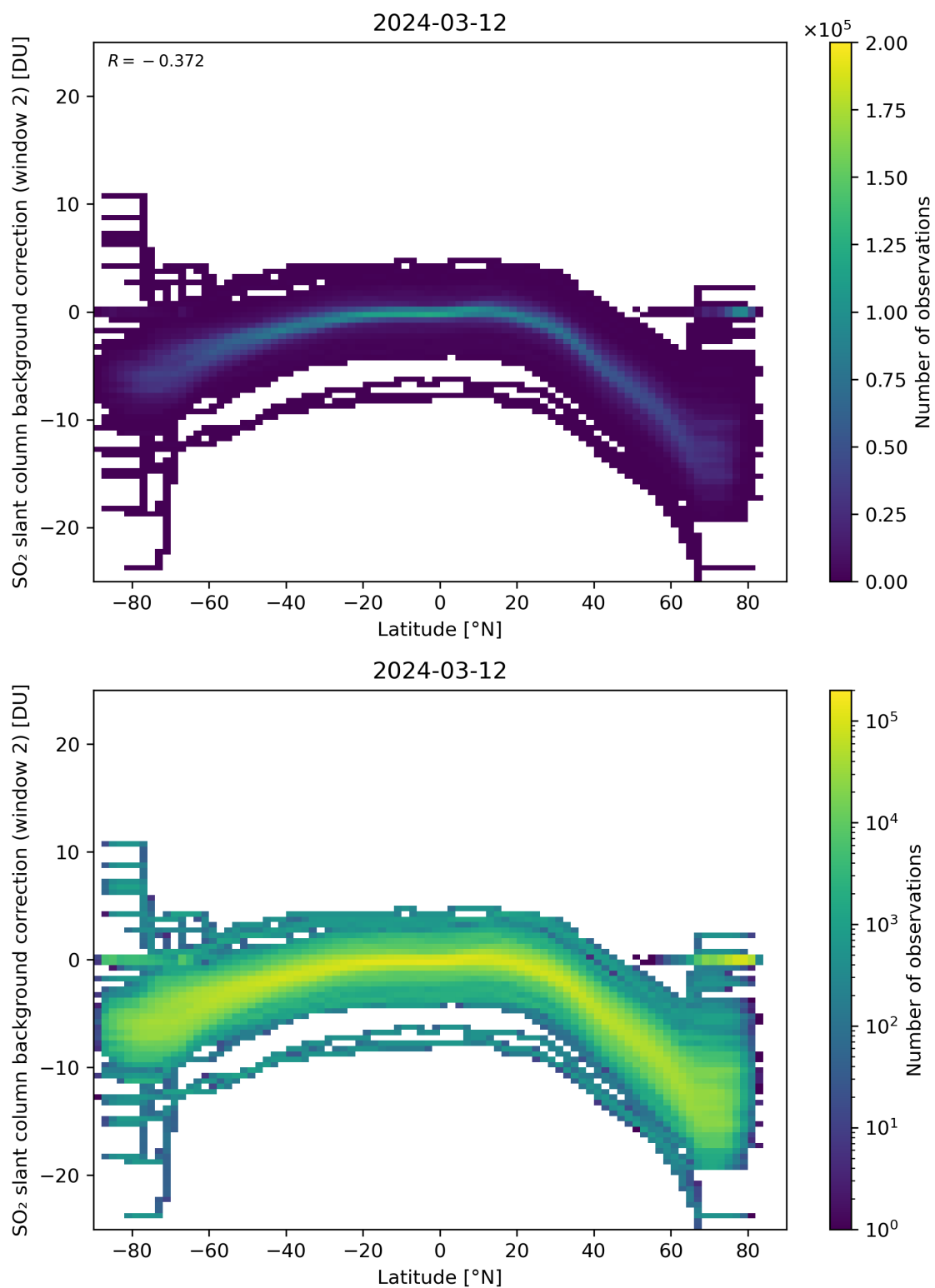
Figure 140: Scatter density plot of “Latitude” against “SO 2 slant column background correction (window 2)” for 2024-03-11 to 2024-03-13.
