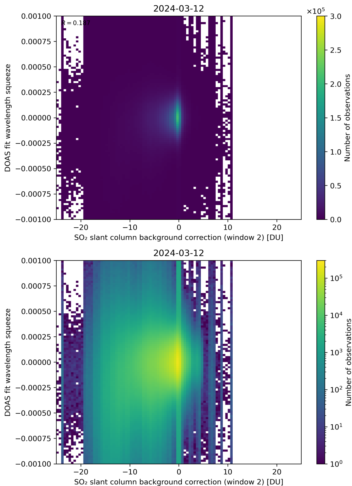
Figure 113: Scatter density plot of “SO 2 slant column background correction (window 2)” against “DOAS fit wavelength squeeze” for 2024-03-11 to 2024-03-13.
