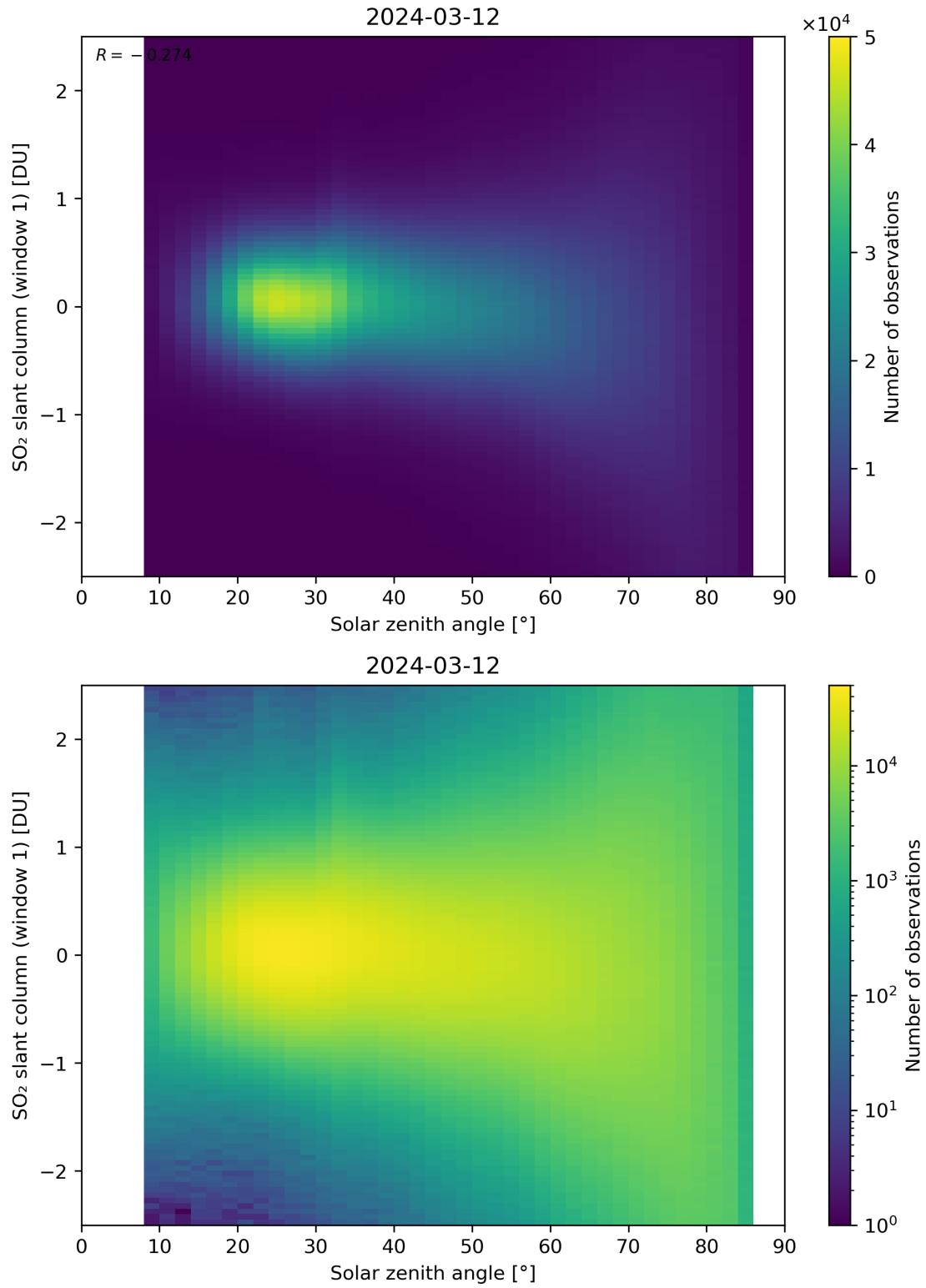
Figure 169: Scatter density plot of “Solar zenith angle” against “SO 2 slant column (window 1)” for 2024-03-11 to 2024-03-13.
