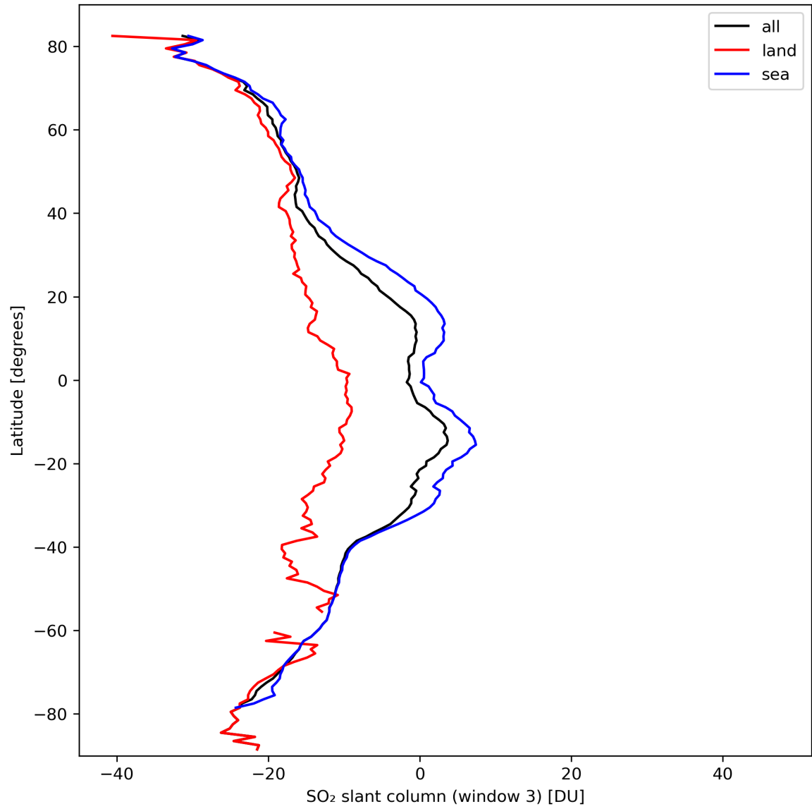
Figure 41: Zonal average of “SO 2 slant column (window 3)” for 2024-03-11 to 2024-03-13.
