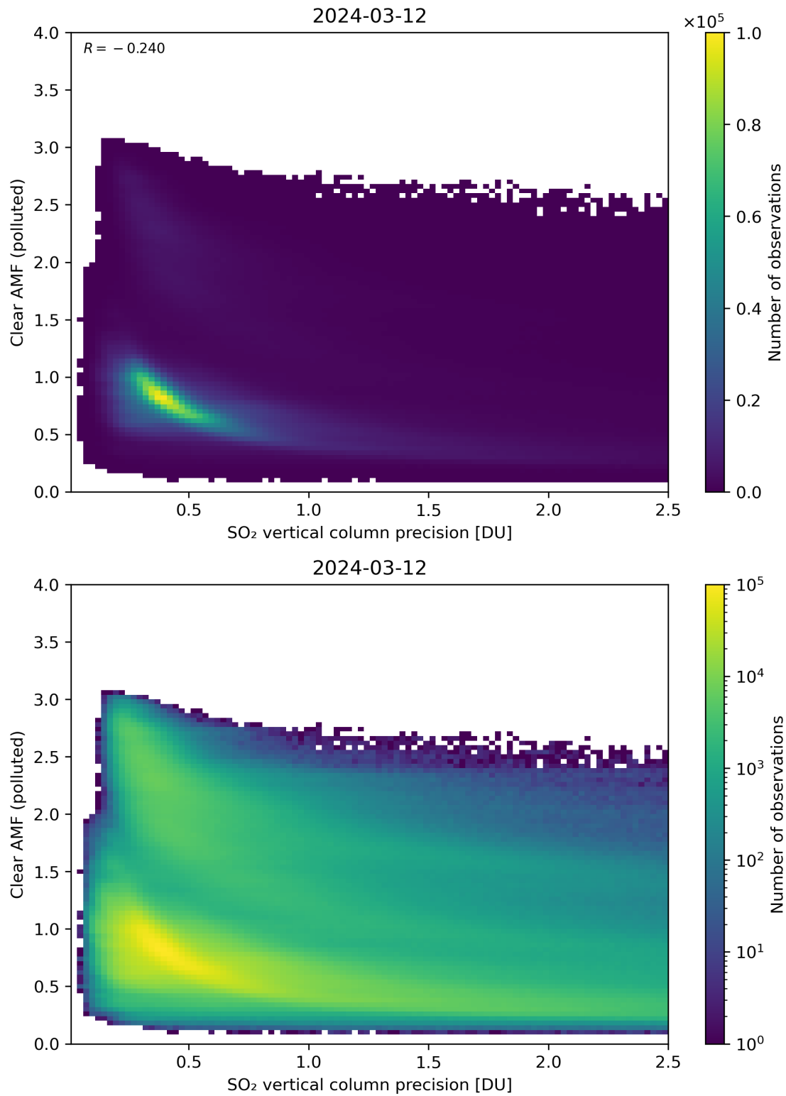
Figure 285: Scatter density plot of “SO 2 vertical column precision” against “Clear AMF (polluted)” for 2024-03-11 to 2024-03-13.
