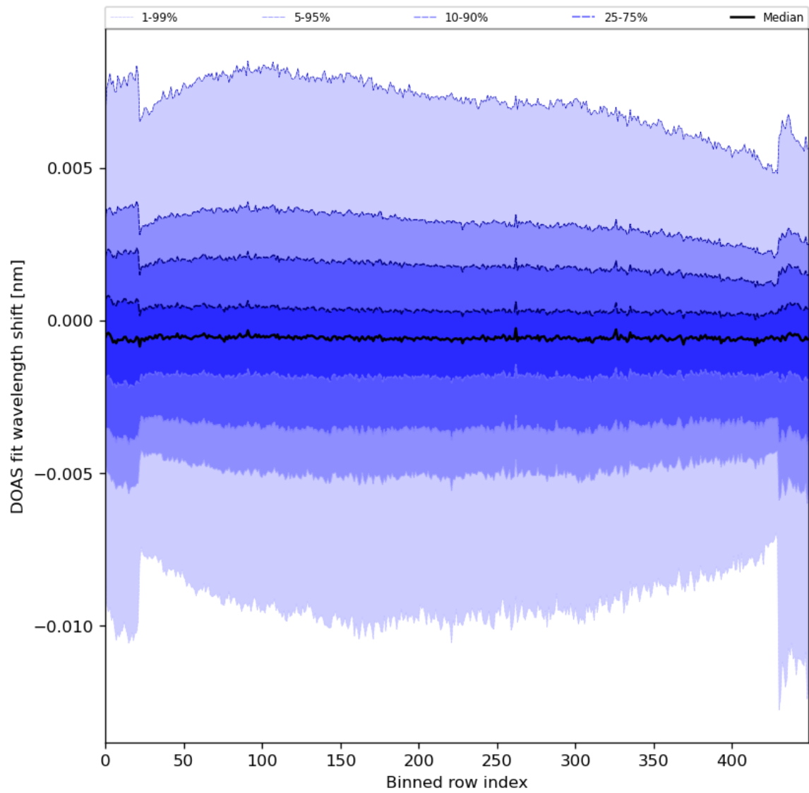
Figure 91: Along track statistics of “DOAS fit wavelength shift” for 2024-03-11 to 2024-03-13
