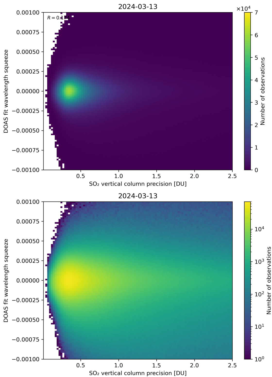
Figure 283: Scatter density plot of “SO 2 vertical column precision” against “DOAS fit wavelength squeeze” for 2024-03-12 to 2024-03-14.
