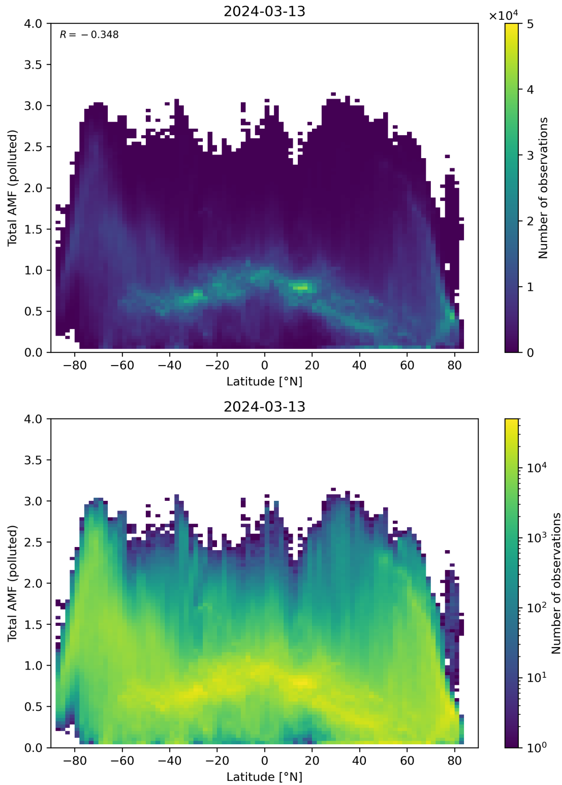
Figure 154: Scatter density plot of “Latitude” against “Total AMF (polluted)” for 2024-03-12 to 2024-03-14.
