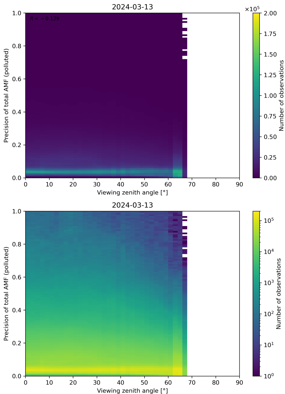
Figure 326: Scatter density plot of “Viewing zenith angle” against “Precision of total AMF (polluted)” for 2024-03-12 to 2024-03-14.
