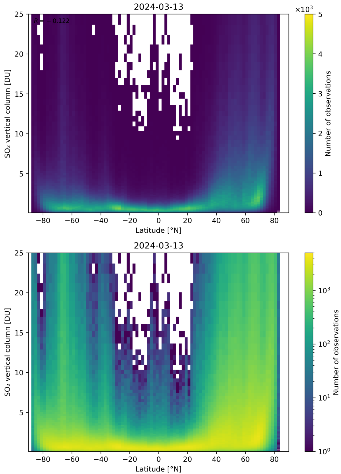
Figure 156: Scatter density plot of “Latitude” against “SO 2 vertical column” for 2024-03-12 to 2024-03-14.
