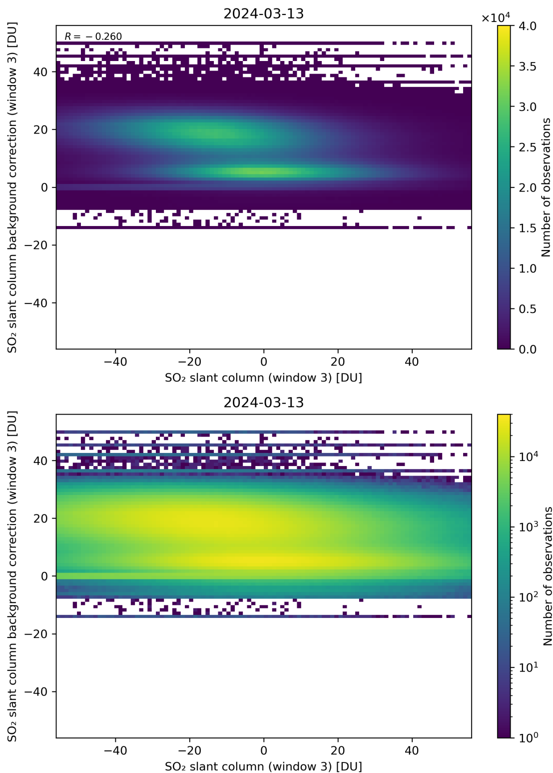
Figure 253: Scatter density plot of “SO 2 slant column (window 3)” against “SO 2 slant column background correction (window 3)” for 2024-03-12 to 2024-03-14.
