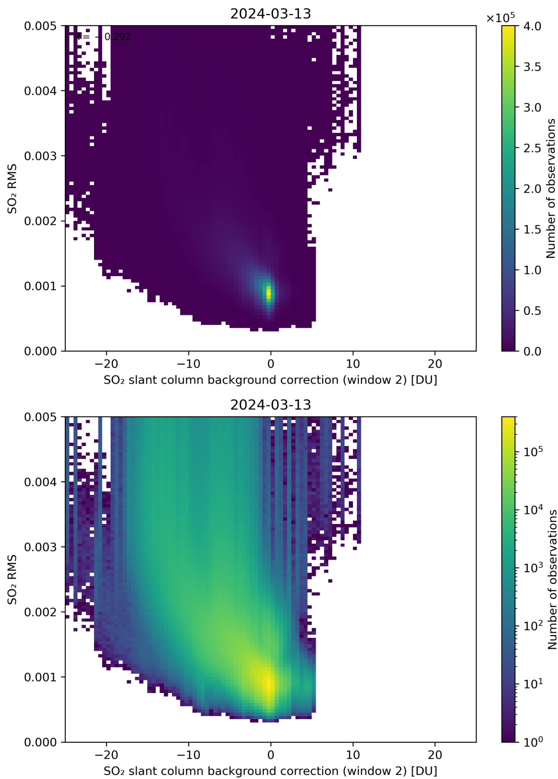
Figure 114: Scatter density plot of “SO 2 slant column background correction (window 2)” against “SO 2 RMS” for 2024-03-12 to 2024-03-14.
