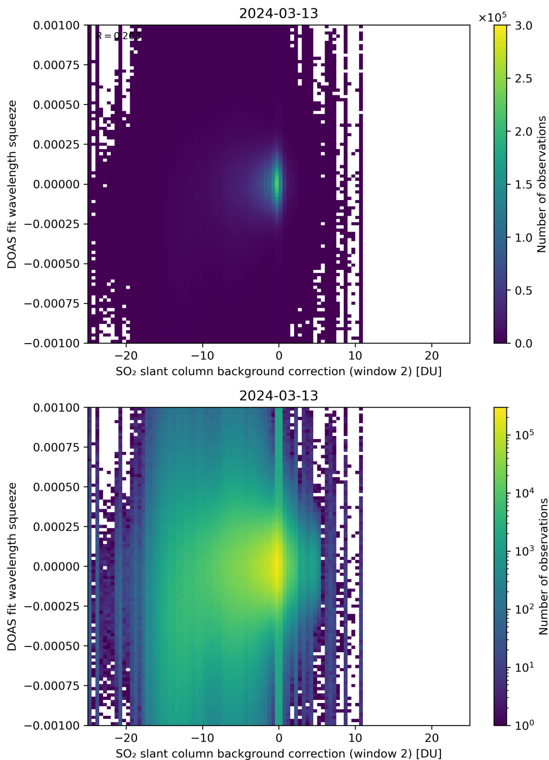
Figure 113: Scatter density plot of “SO 2 slant column background correction (window 2)” against “DOAS fit wavelength squeeze” for 2024-03-12 to 2024-03-14.
