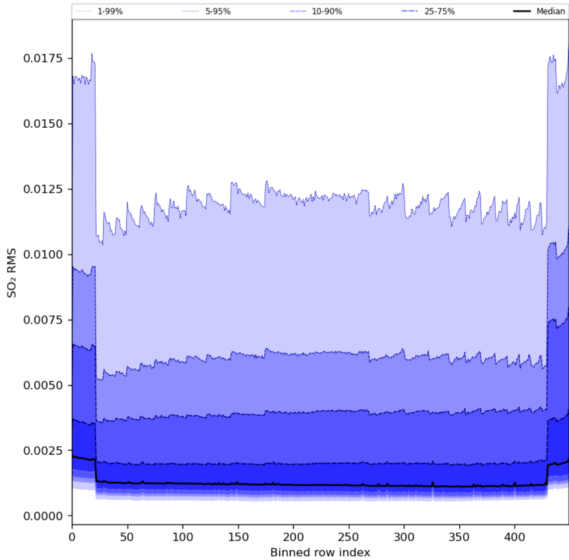
Figure 93: Along track statistics of “SO 2 RMS” for 2024-03-12 to 2024-03-14
