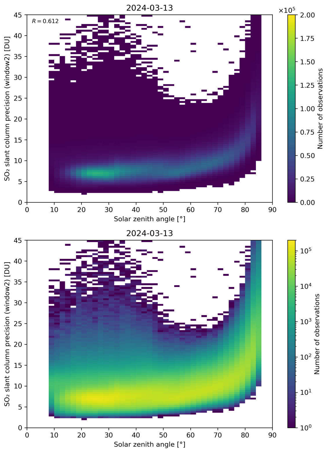
Figure 171: Scatter density plot of “Solar zenith angle” against “SO 2 slant column precision (window2)” for 2024-03-12 to 2024-03-14.
