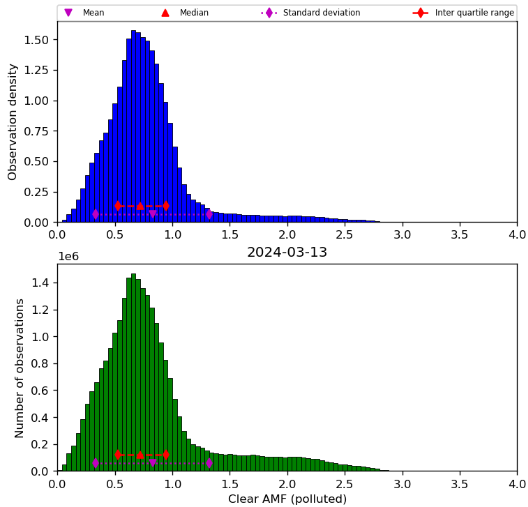
Figure 73: Histogram of “Clear AMF (polluted)” for 2024-03-12 to 2024-03-14
