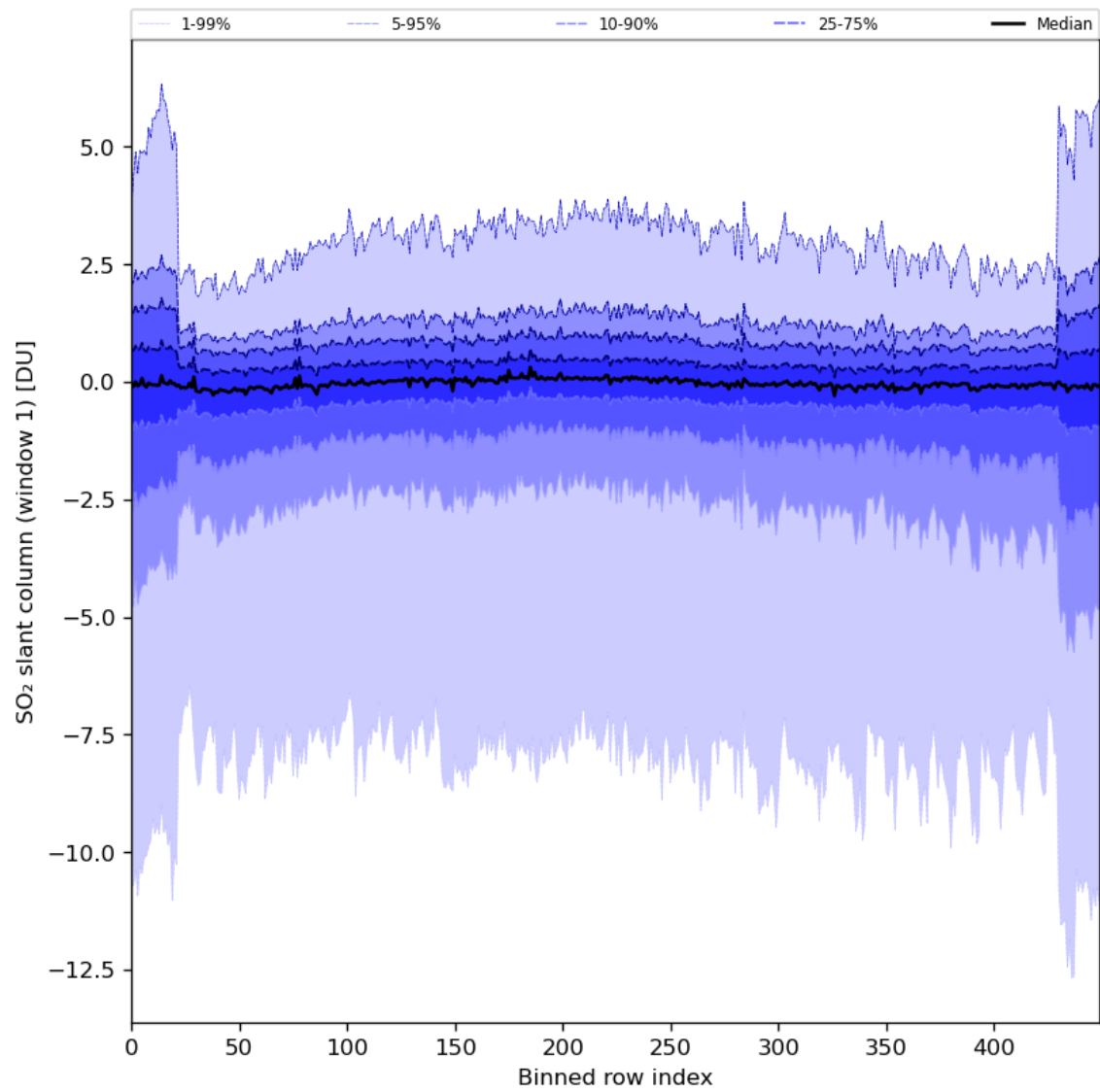
Figure 79: Along track statistics of “SO 2 slant column (window 1)” for 2024-03-12 to 2024-03-14
