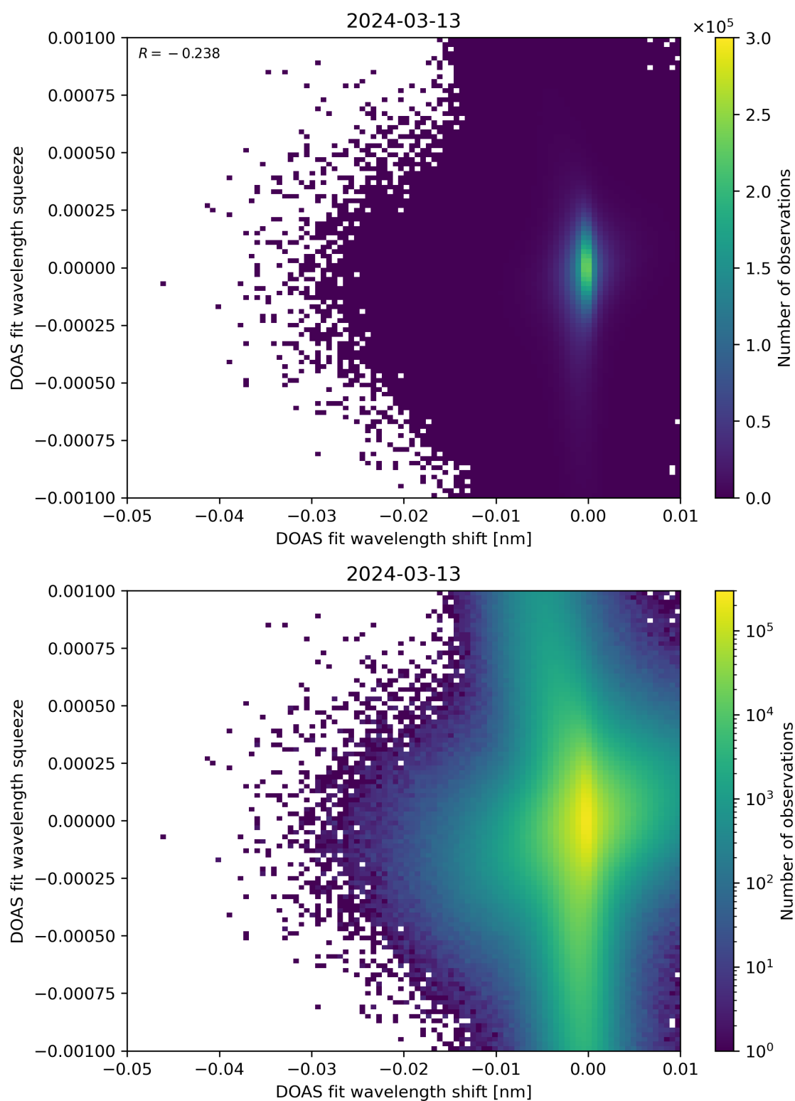
Figure 127: Scatter density plot of “DOAS fit wavelength shift” against “DOAS fit wavelength squeeze” for 2024-03-12 to 2024-03-14.
