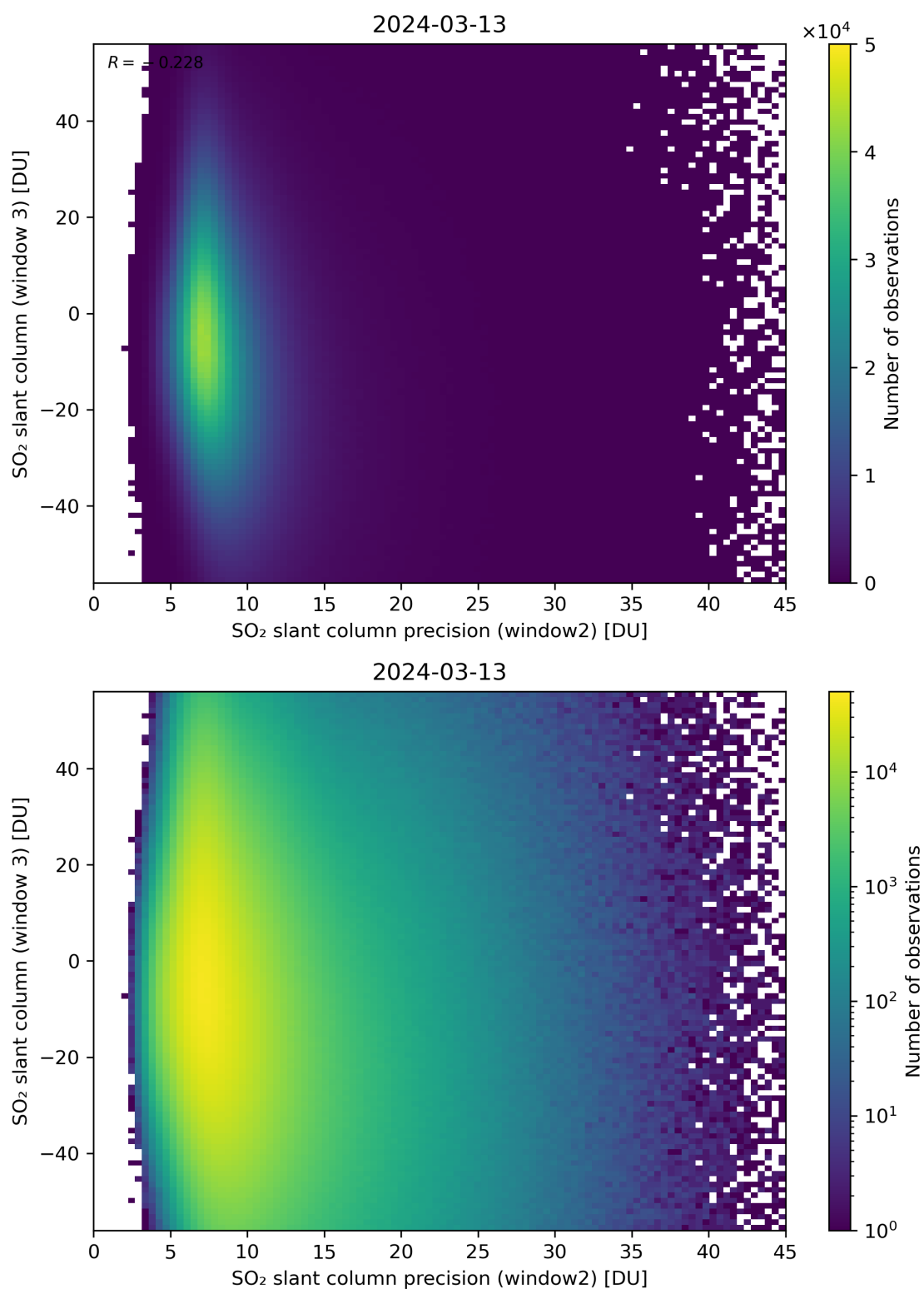
Figure 249: Scatter density plot of “SO 2 slant column precision (window2)” against “SO 2 slant column (window 3)” for 2024-03-12 to 2024-03-14.
