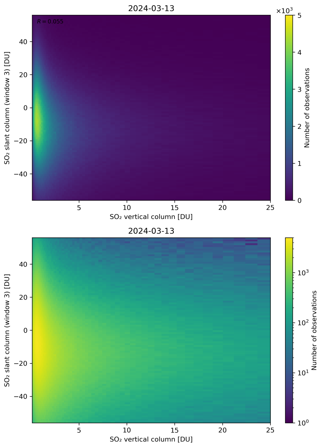
Figure 303: Scatter density plot of “SO 2 vertical column” against “SO 2 slant column (window 3)” for 2024-03-12 to 2024-03-14.
