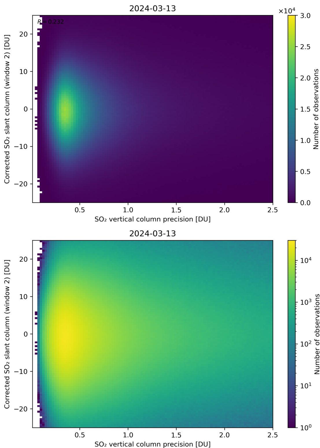
Figure 287: Scatter density plot of “SO 2 vertical column precision” against “Corrected SO 2 slant column (window 2)” for 2024-03-12 to 2024-03-14.
