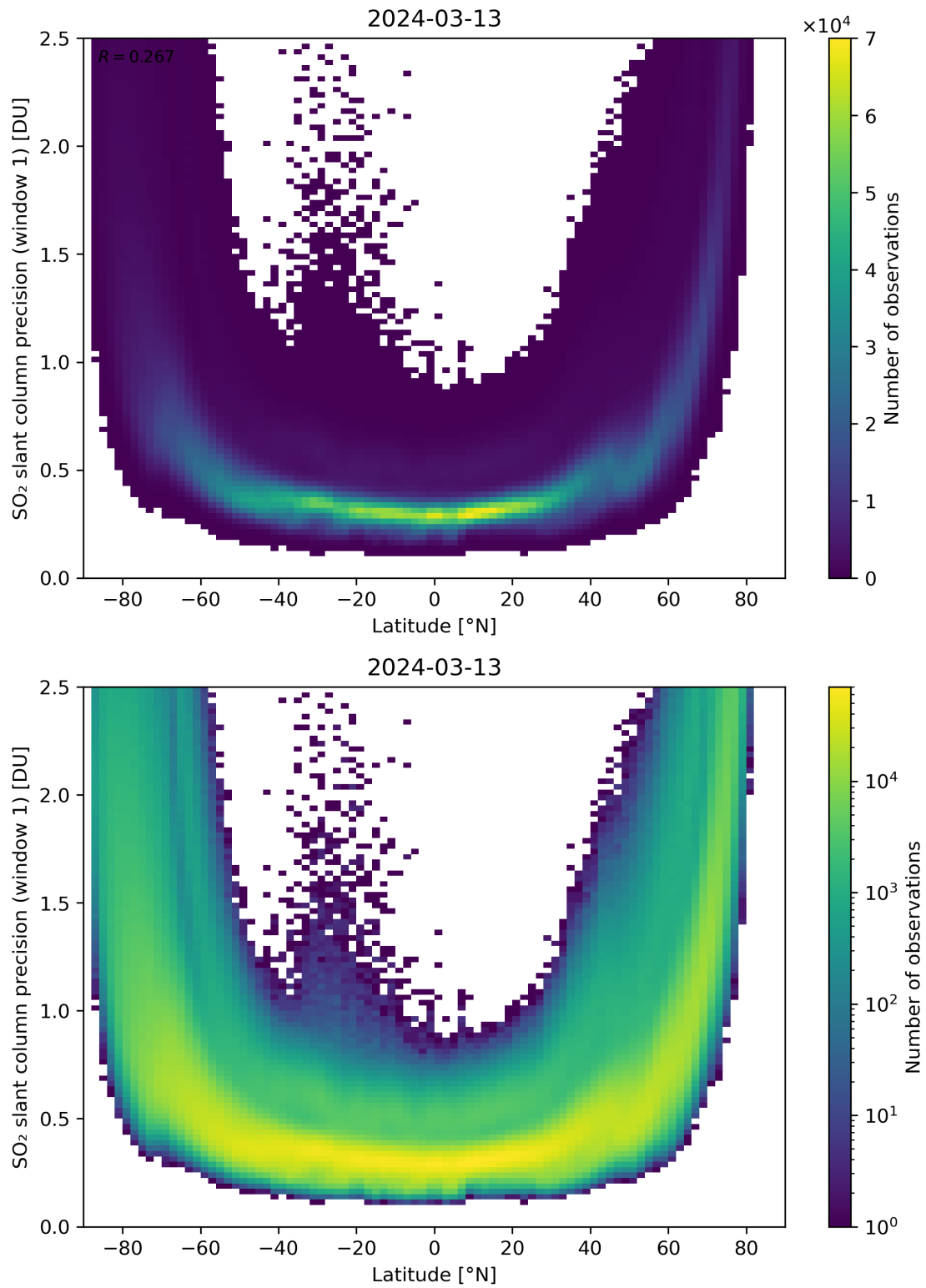
Figure 150: Scatter density plot of “Latitude” against “SO 2 slant column precision (window 1)” for 2024-03-12 to 2024-03-14.
