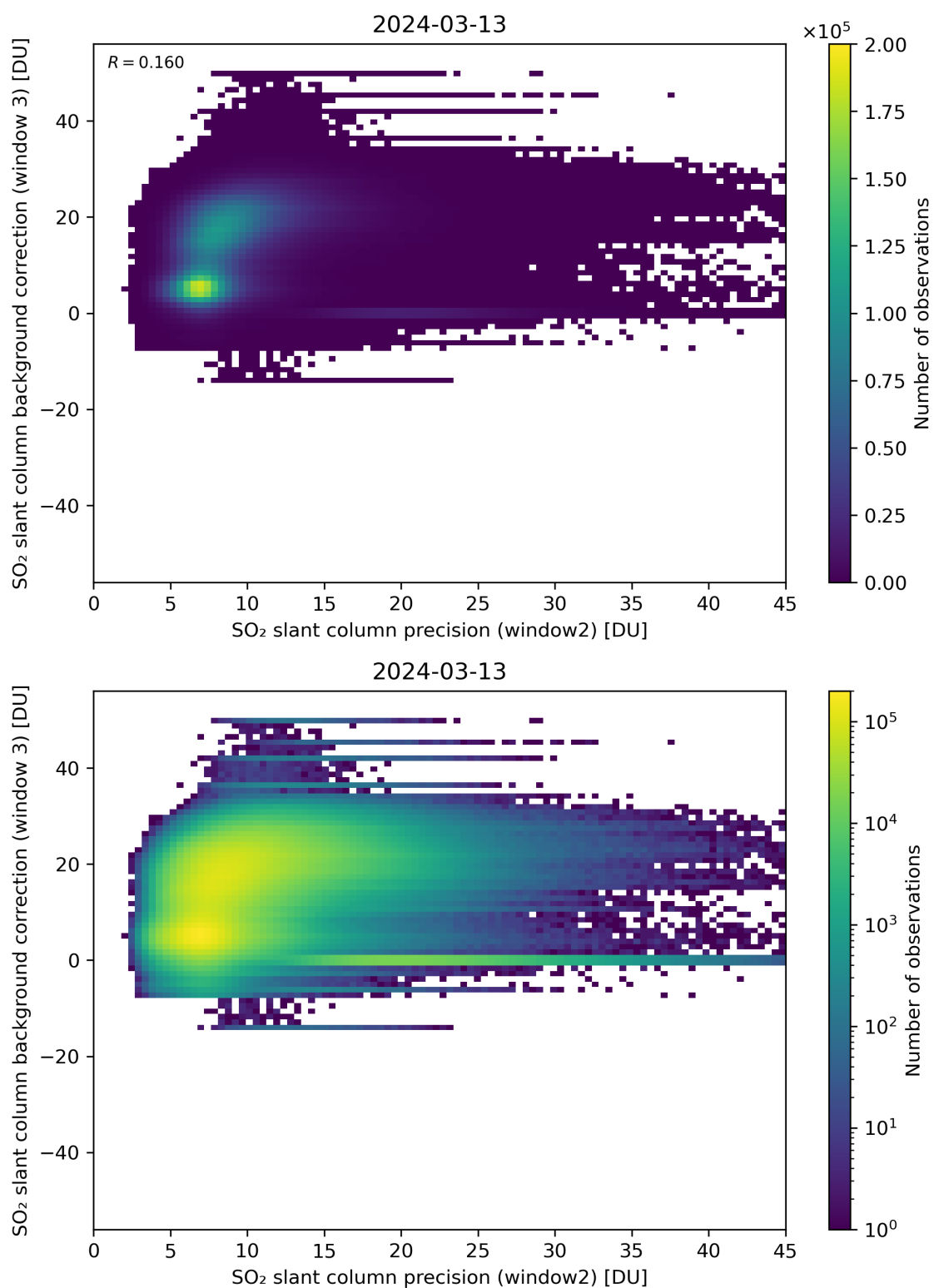
Figure 242: Scatter density plot of “SO 2 slant column precision (window2)” against “SO 2 slant column background correction (window 3)” for 2024-03-12 to 2024-03-14.
