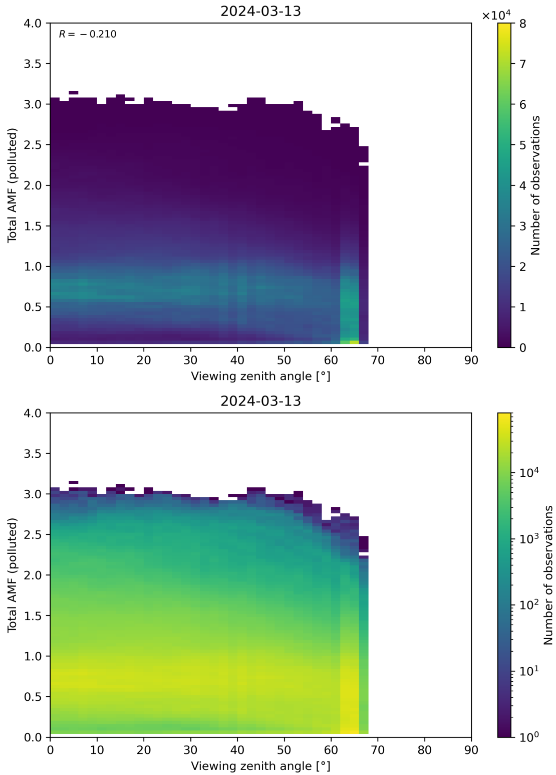
Figure 325: Scatter density plot of “Viewing zenith angle” against “Total AMF (polluted)” for 2024-03-12 to 2024-03-14.
