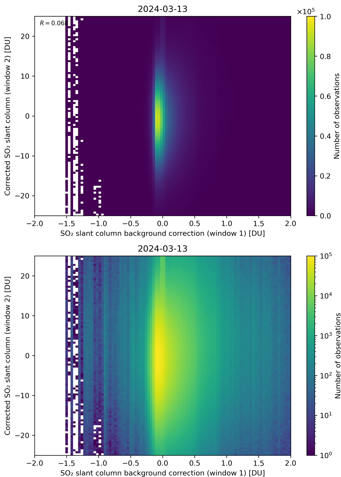
Figure 104: Scatter density plot of “SO 2 slant column background correction (window 1)” against “Corrected SO 2 slant column (window 2)” for 2024-03-12 to 2024-03-14.
