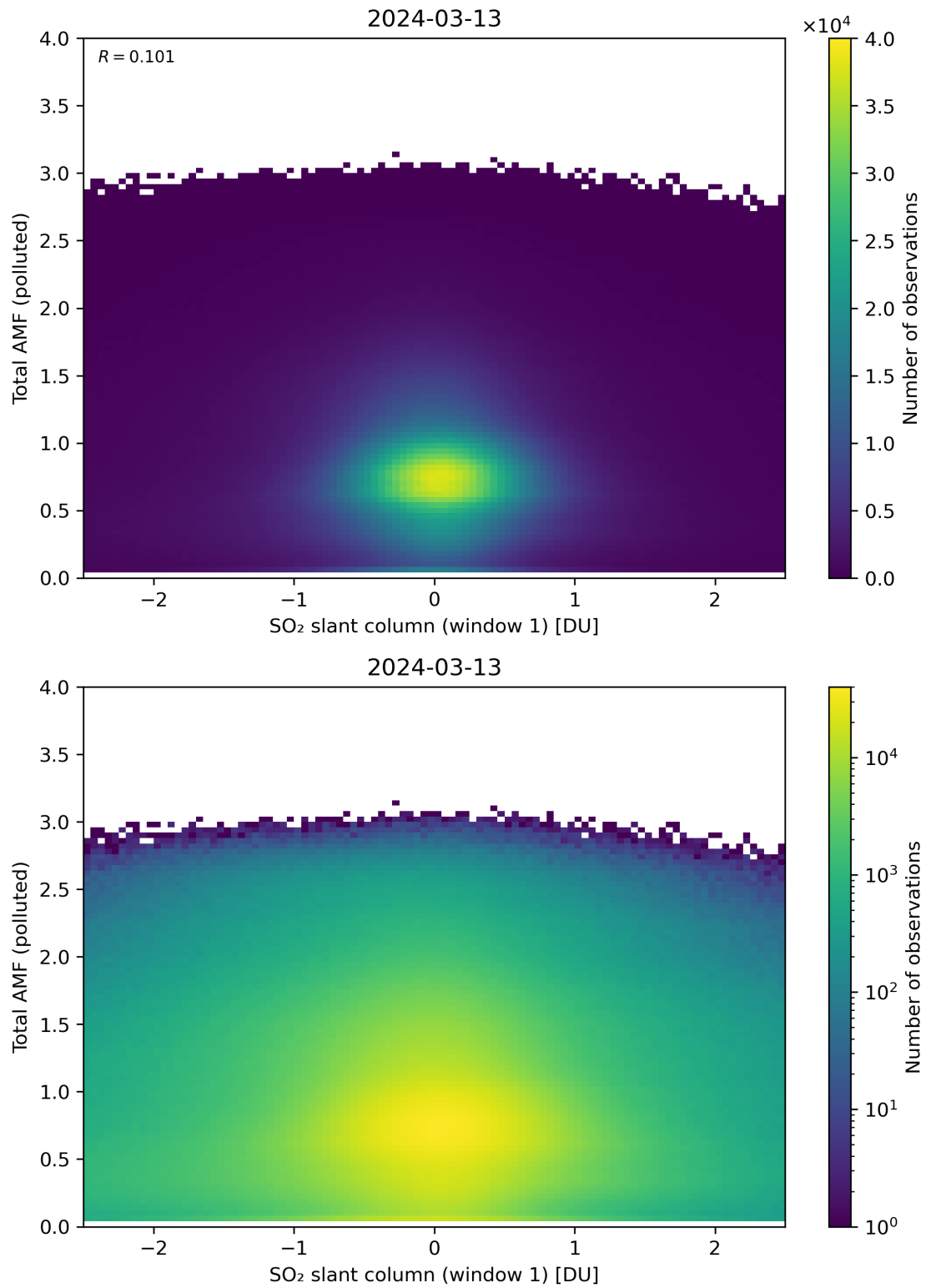
Figure 239: Scatter density plot of “SO 2 slant column (window 1)” against “Total AMF (polluted)” for 2024-03-12 to 2024-03-14.
