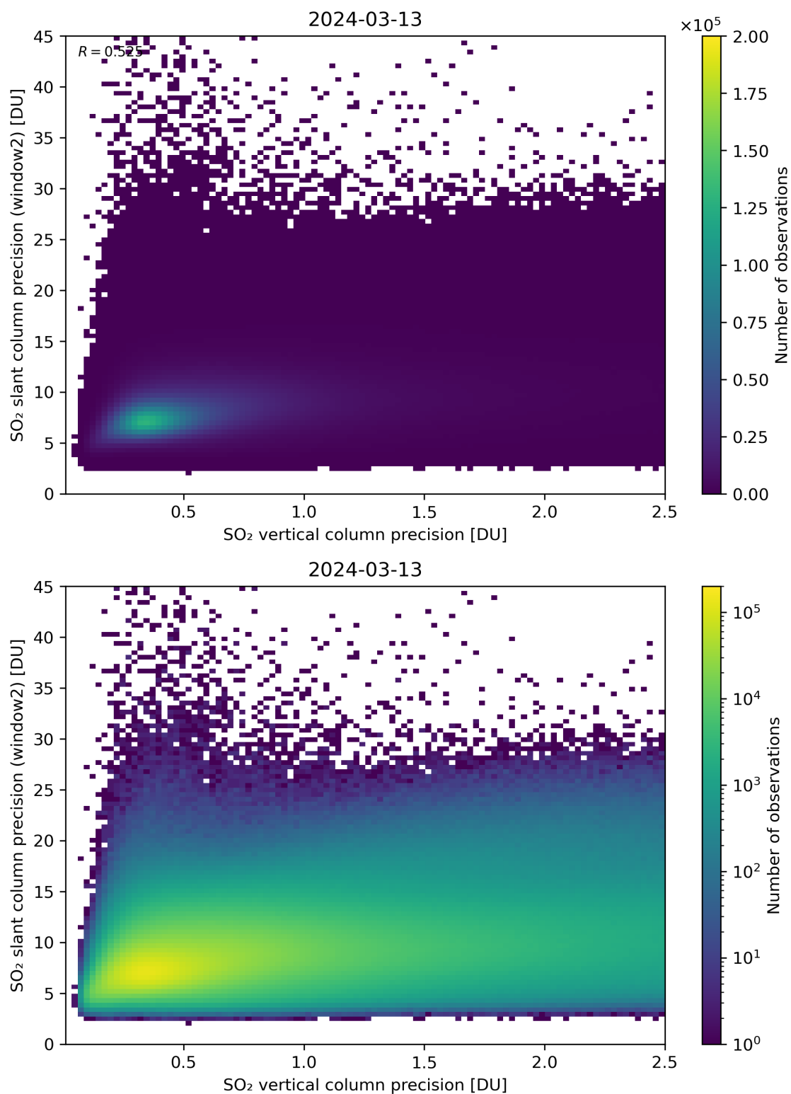
Figure 291: Scatter density plot of “SO 2 vertical column precision” against “SO 2 slant column precision (window2)” for 2024-03-12 to 2024-03-14.
