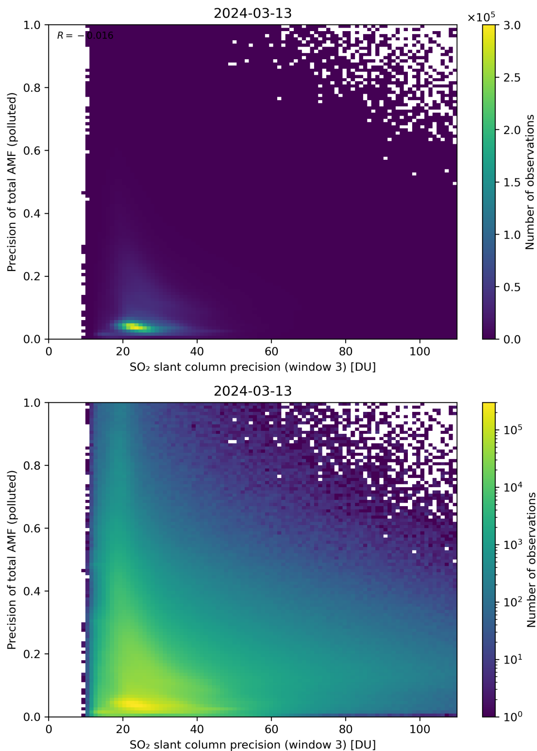
Figure 264: Scatter density plot of “SO 2 slant column precision (window 3)” against “Precision of total AMF (polluted)” for 2024-03-12 to 2024-03-14.
