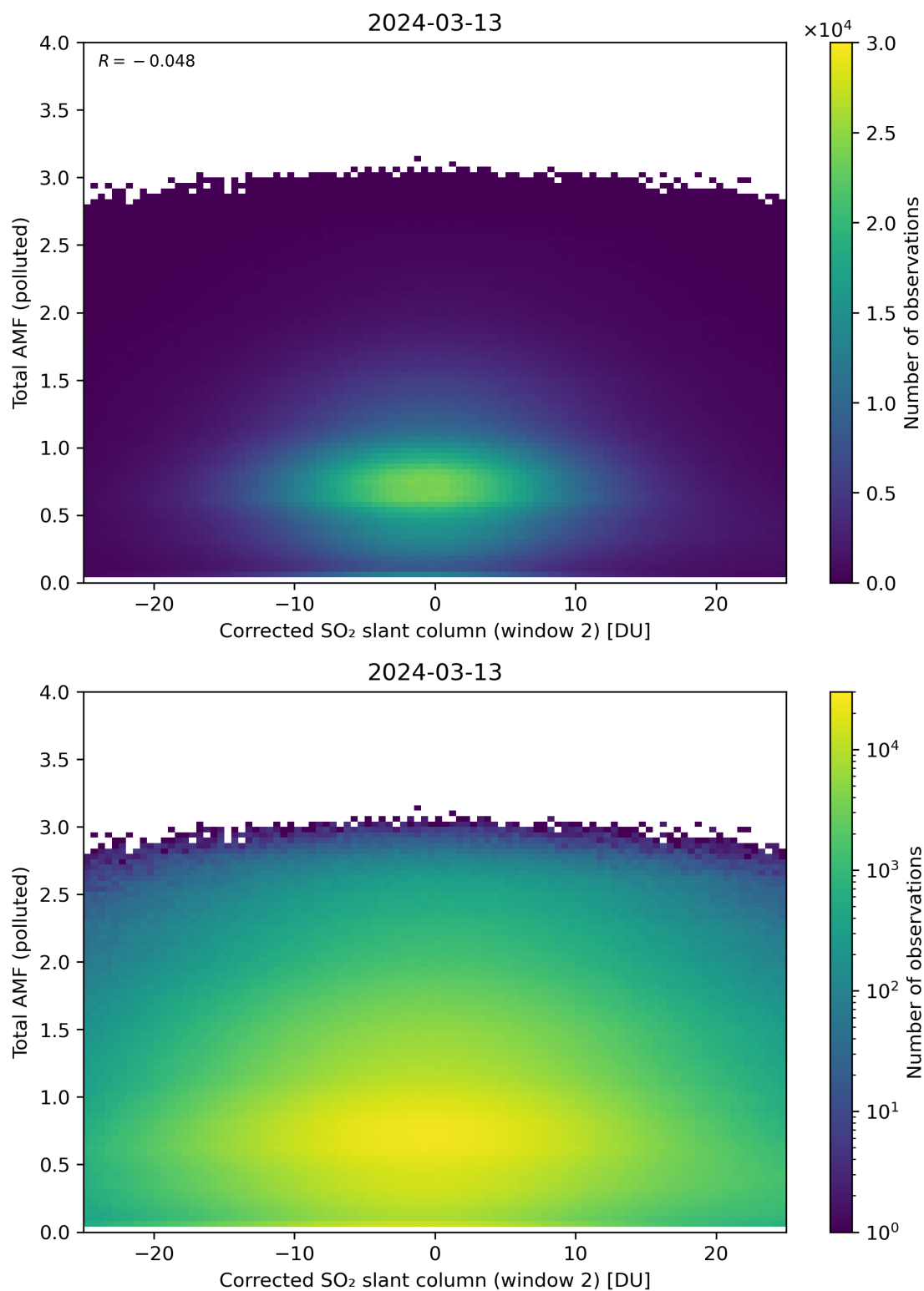
Figure 203: Scatter density plot of “Corrected SO 2 slant column (window 2)” against “Total AMF (polluted)” for 2024-03-12 to 2024-03-14.
