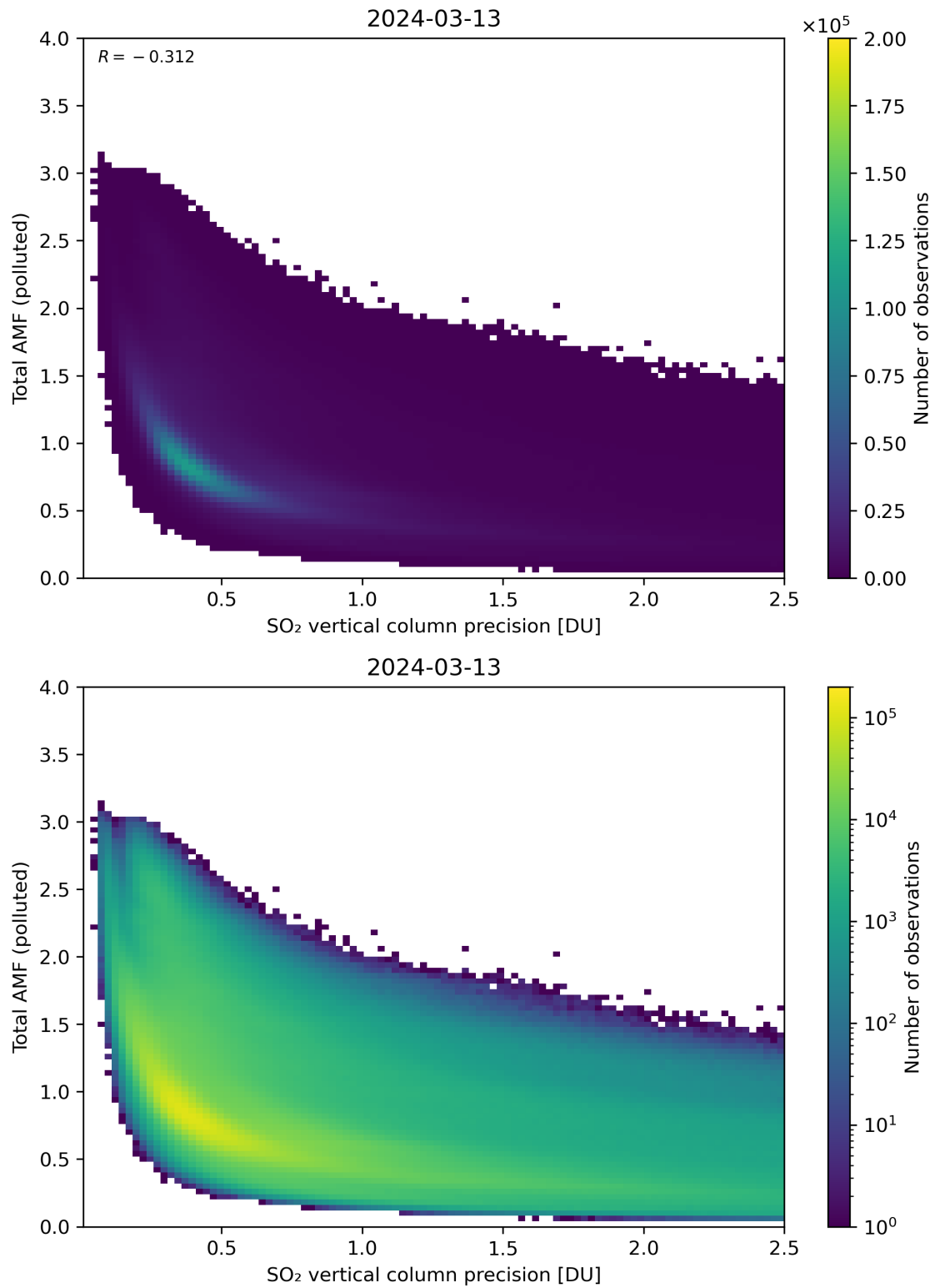
Figure 294: Scatter density plot of “SO 2 vertical column precision” against “Total AMF (polluted)” for 2024-03-12 to 2024-03-14.
