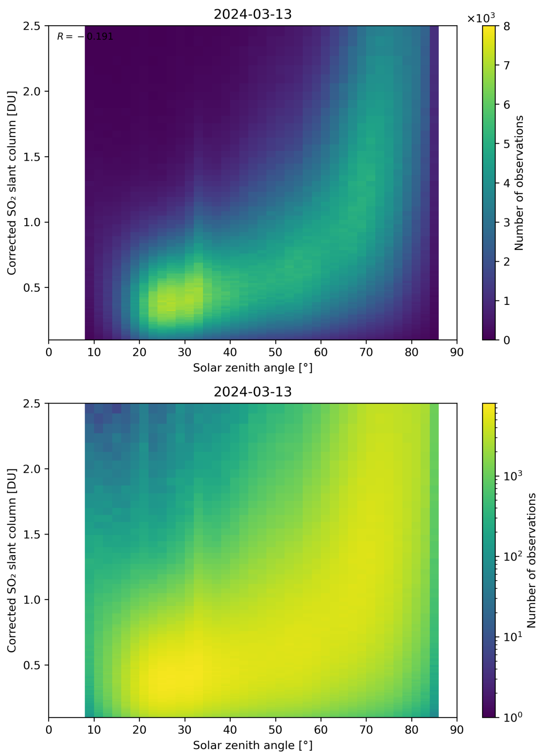
Figure 166: Scatter density plot of “Solar zenith angle” against “Corrected SO 2 slant column” for 2024-03-12 to 2024-03-14.
