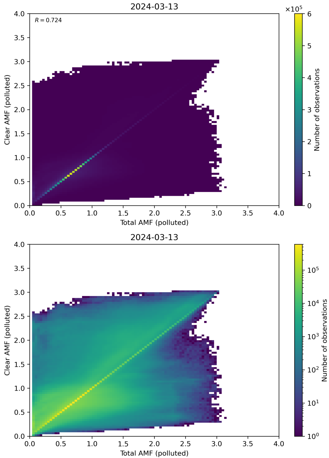
Figure 271: Scatter density plot of “Total AMF (polluted)” against “Clear AMF (polluted)” for 2024-03-12 to 2024-03-14.
