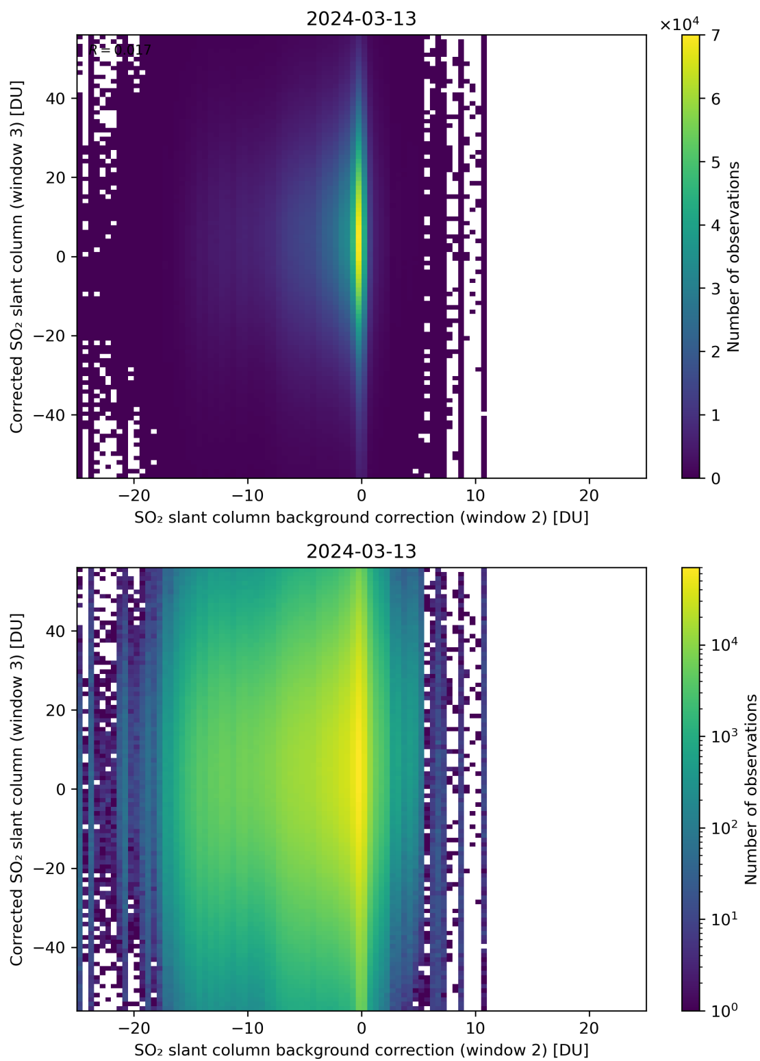
Figure 116: Scatter density plot of “SO 2 slant column background correction (window 2)” against “Corrected SO 2 slant column (window 3)” for 2024-03-12 to 2024-03-14.
