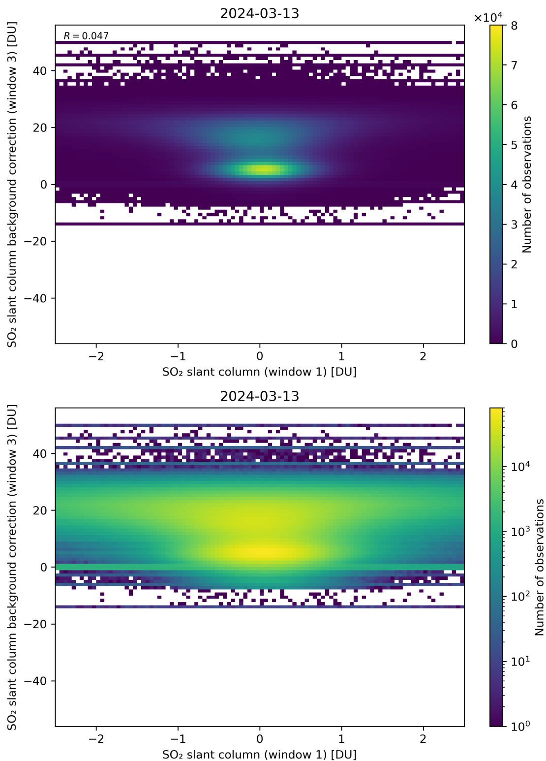
Figure 214: Scatter density plot of “SO 2 slant column (window 1)” against “SO 2 slant column background correction (window 3)” for 2024-03-12 to 2024-03-14.
