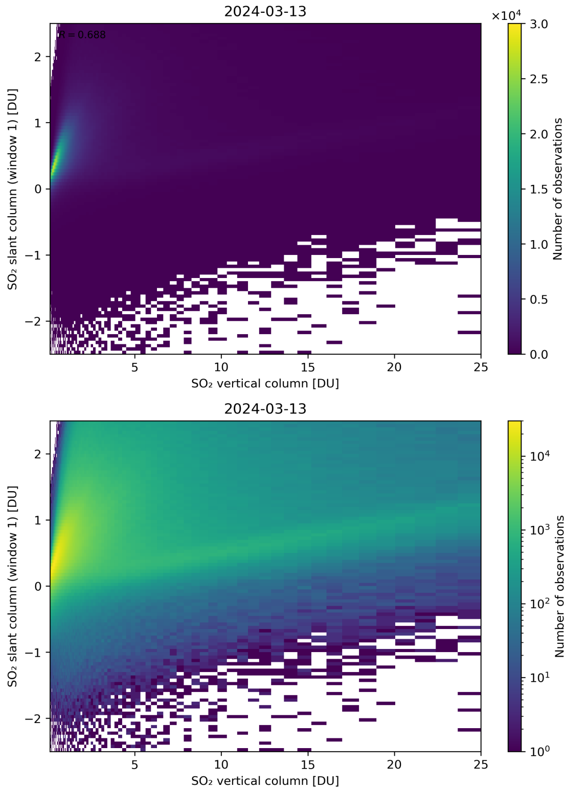
Figure 300: Scatter density plot of “SO 2 vertical column” against “SO 2 slant column (window 1)” for 2024-03-12 to 2024-03-14.
