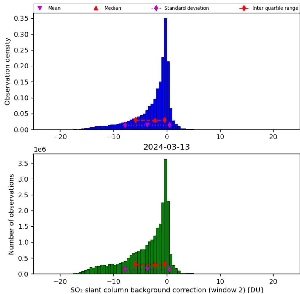
Figure 63: Histogram of “SO 2 slant column background correction (window 2)” for 2024-03-12 to 2024-03-14
