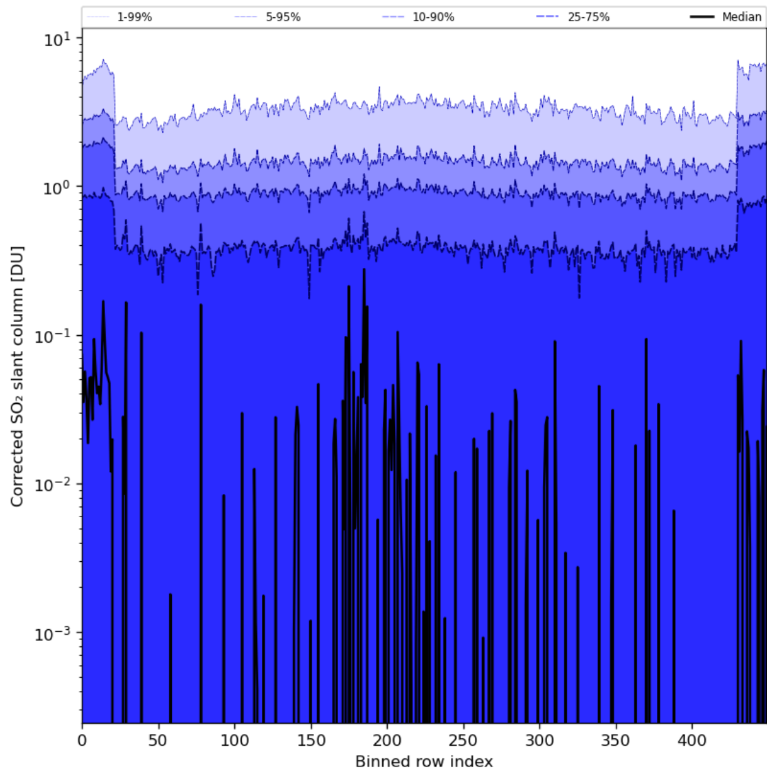
Figure 78: Along track statistics of “Corrected SO 2 slant column” for 2024-03-12 to 2024-03-14
