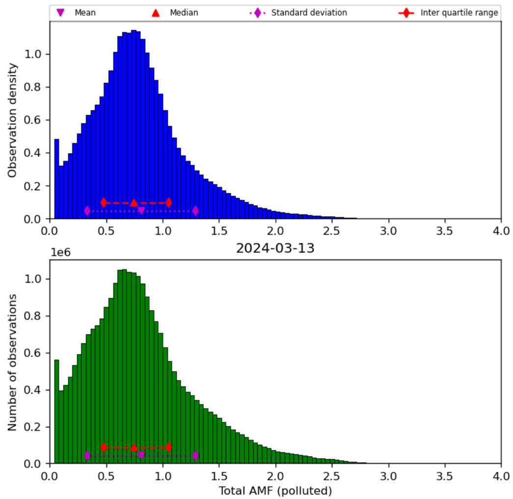
Figure 71: Histogram of “Total AMF (polluted)” for 2024-03-12 to 2024-03-14
