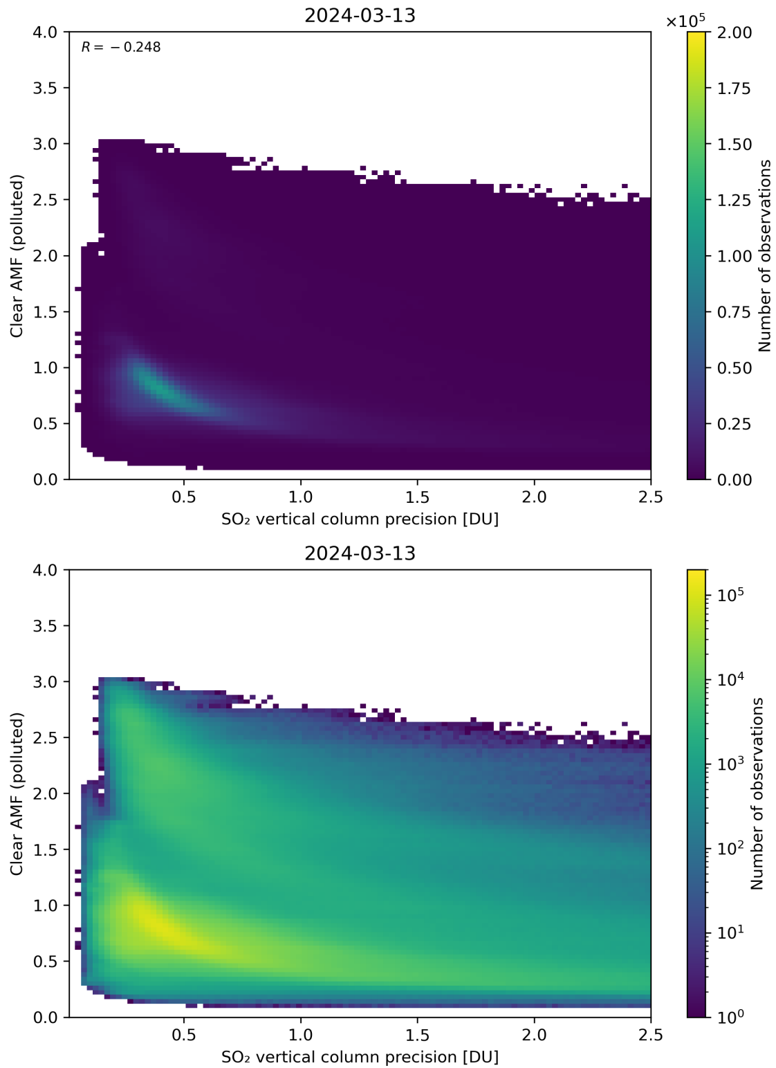
Figure 285: Scatter density plot of “SO 2 vertical column precision” against “Clear AMF (polluted)” for 2024-03-12 to 2024-03-14.
