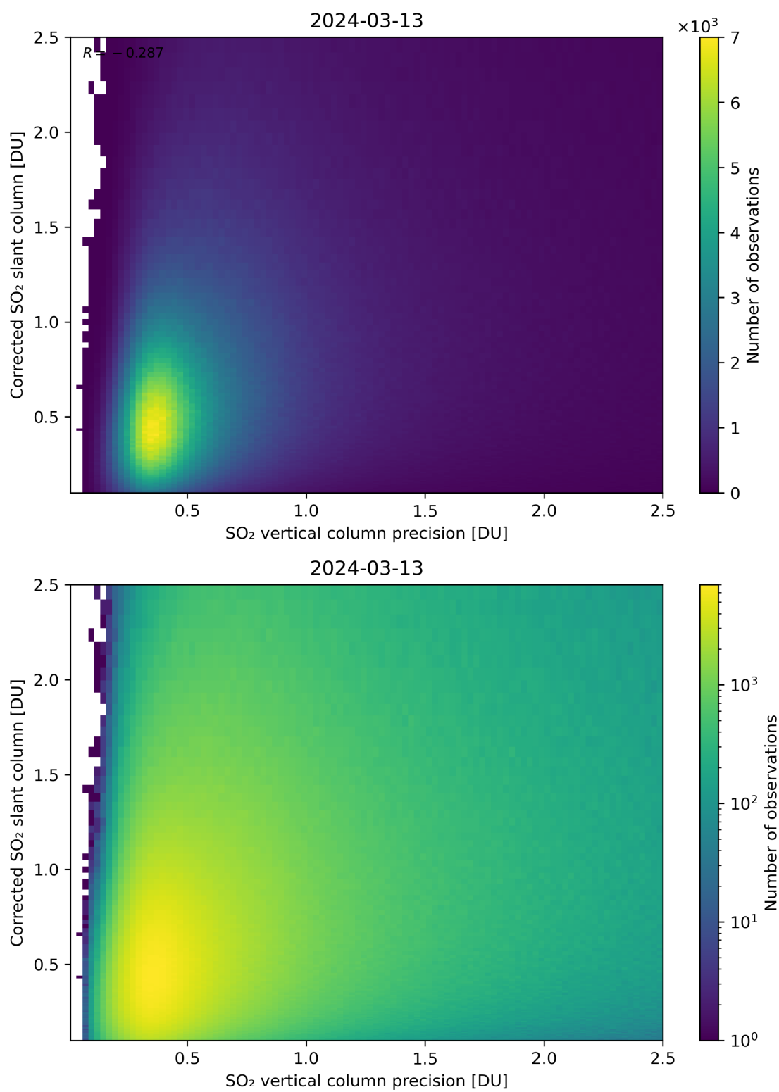
Figure 286: Scatter density plot of “SO 2 vertical column precision” against “Corrected SO 2 slant column” for 2024-03-12 to 2024-03-14.
