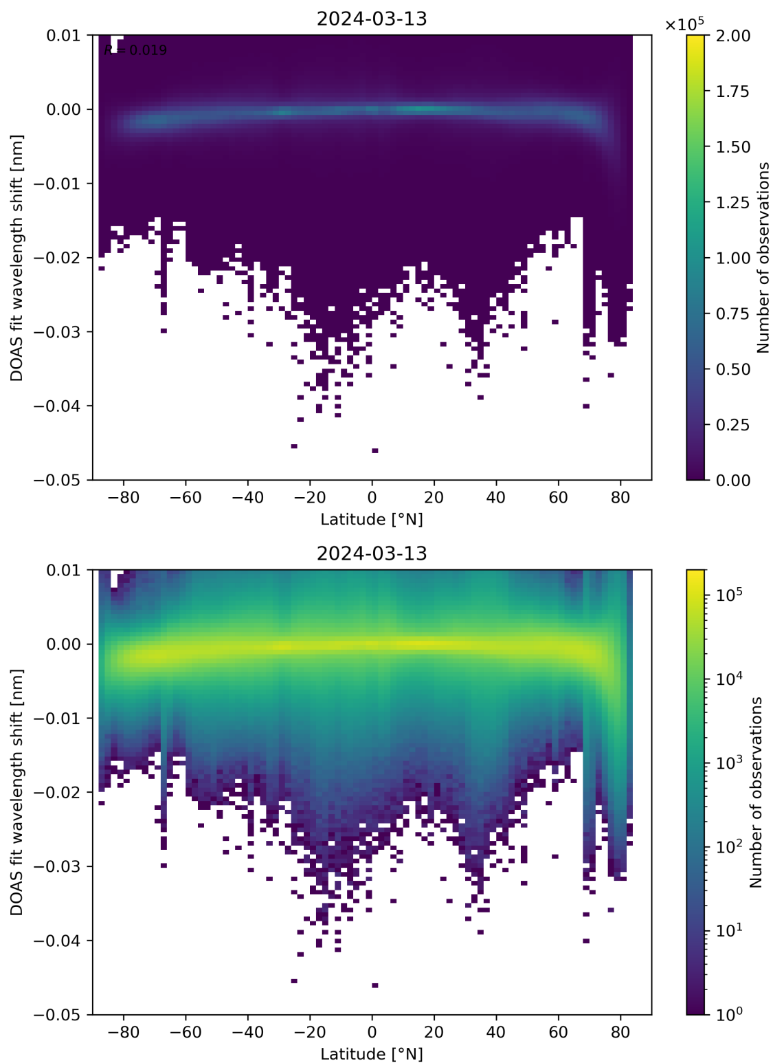
Figure 142: Scatter density plot of “Latitude” against “DOAS fit wavelength shift” for 2024-03-12 to 2024-03-14.
