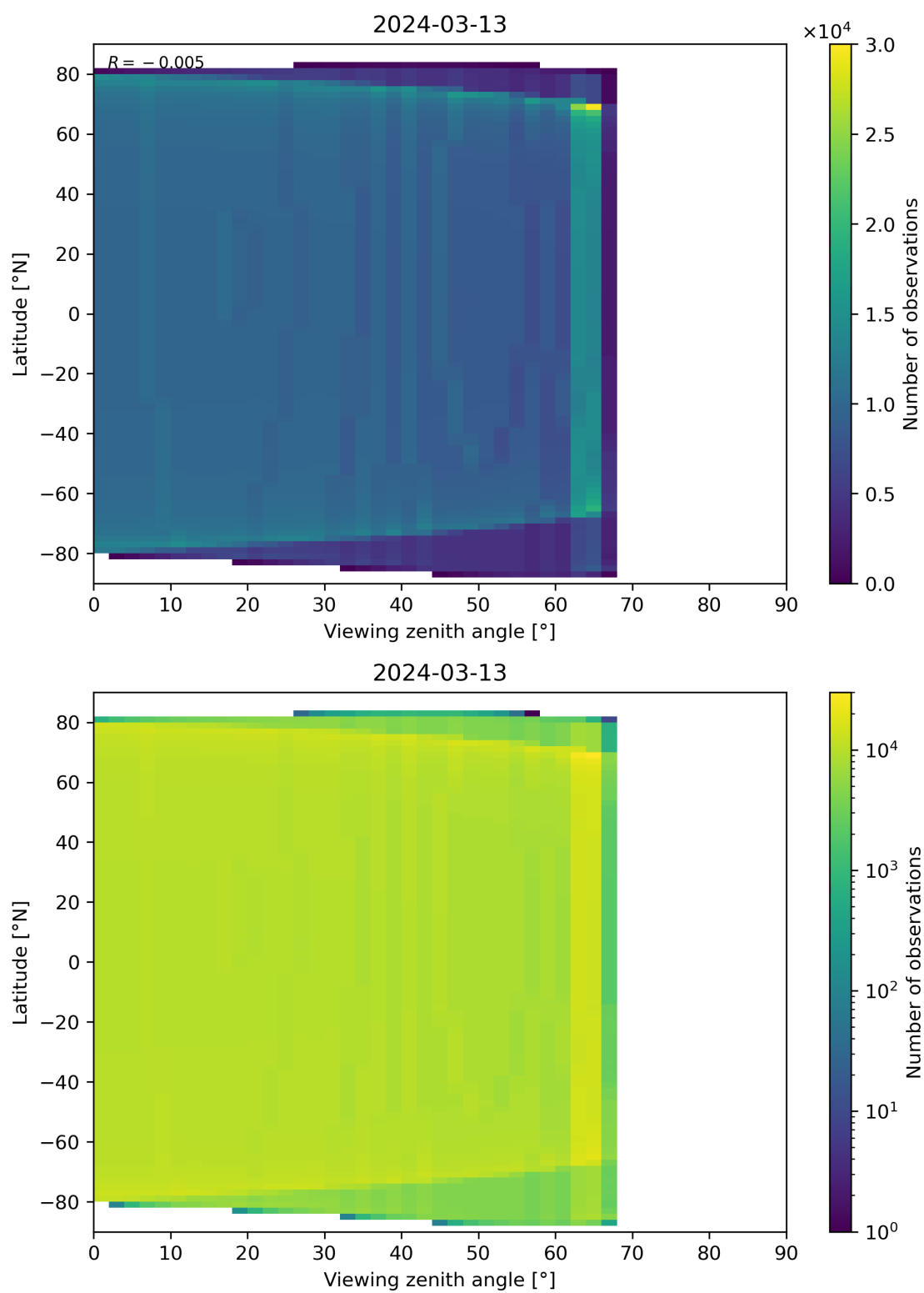
Figure 314: Scatter density plot of “Viewing zenith angle” against “Latitude” for 2024-03-12 to 2024-03-14.
