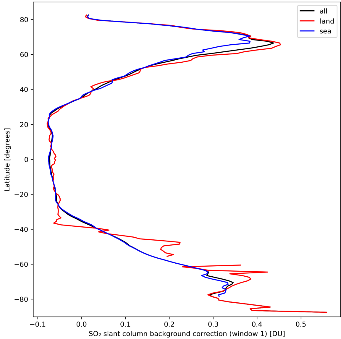
Figure 36: Zonal average of “SO 2 slant column background correction (window 1)” for 2024-03-12 to 2024-03-14.
