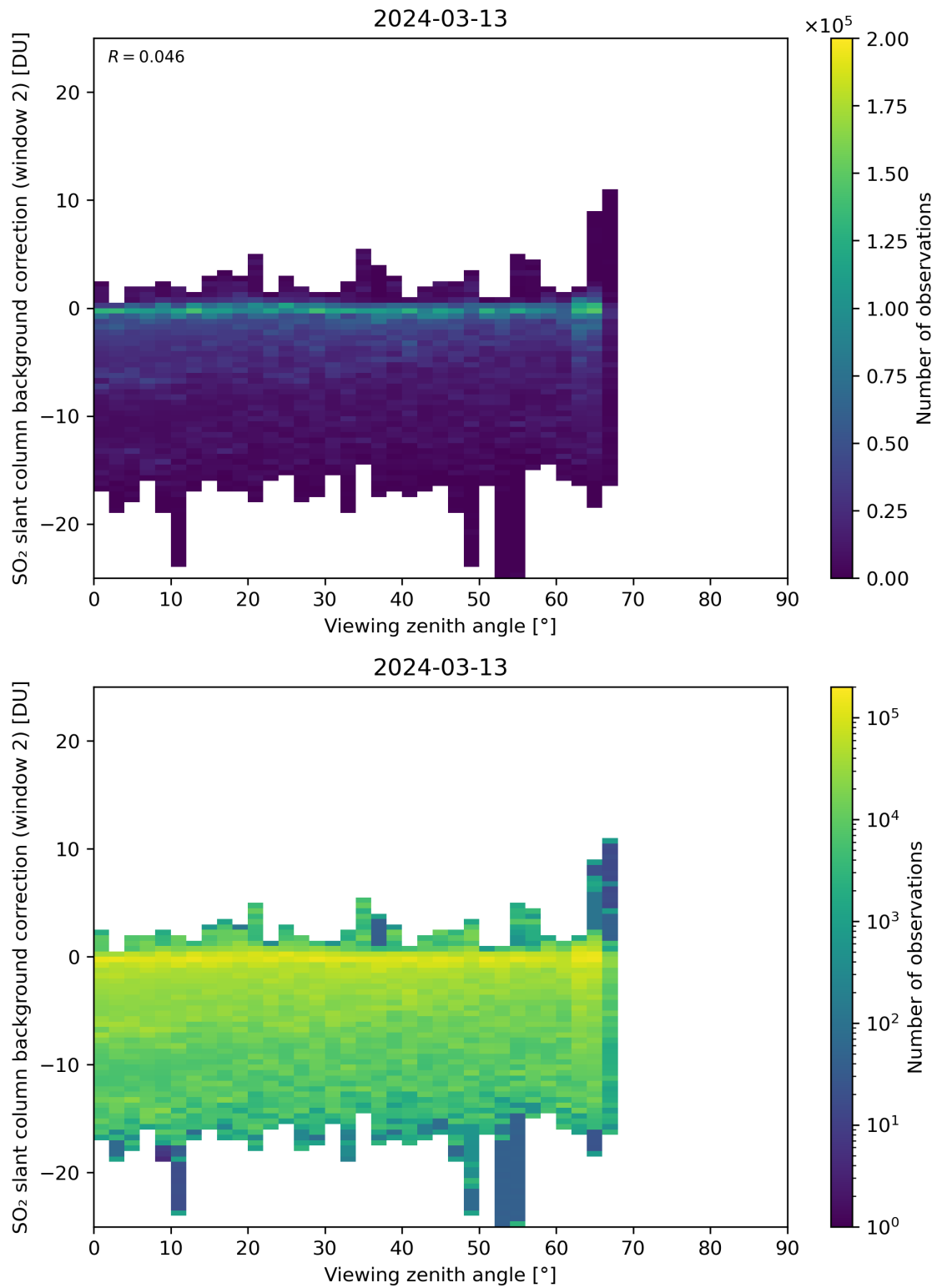
Figure 309: Scatter density plot of “Viewing zenith angle” against “SO 2 slant column background correction (window 2)” for 2024-03-12 to 2024-03-14.
