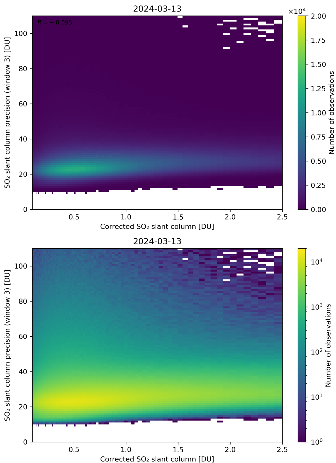
Figure 191: Scatter density plot of “Corrected SO 2 slant column” against “SO 2 slant column precision (window 3)” for 2024-03-12 to 2024-03-14.
