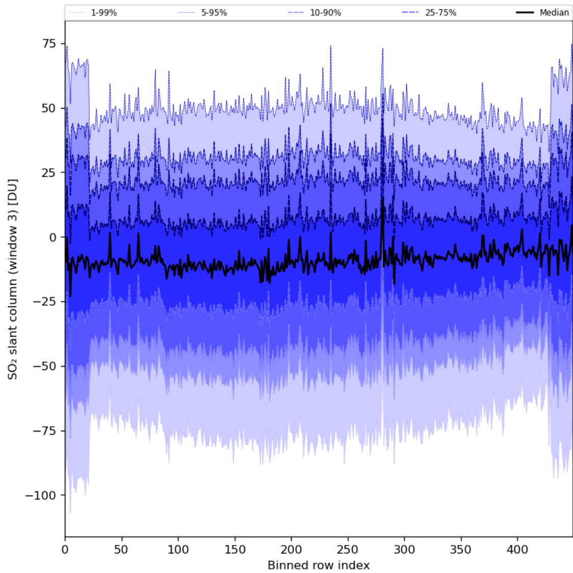
Figure 87: Along track statistics of “SO 2 slant column (window 3)” for 2024-03-12 to 2024-03-14
