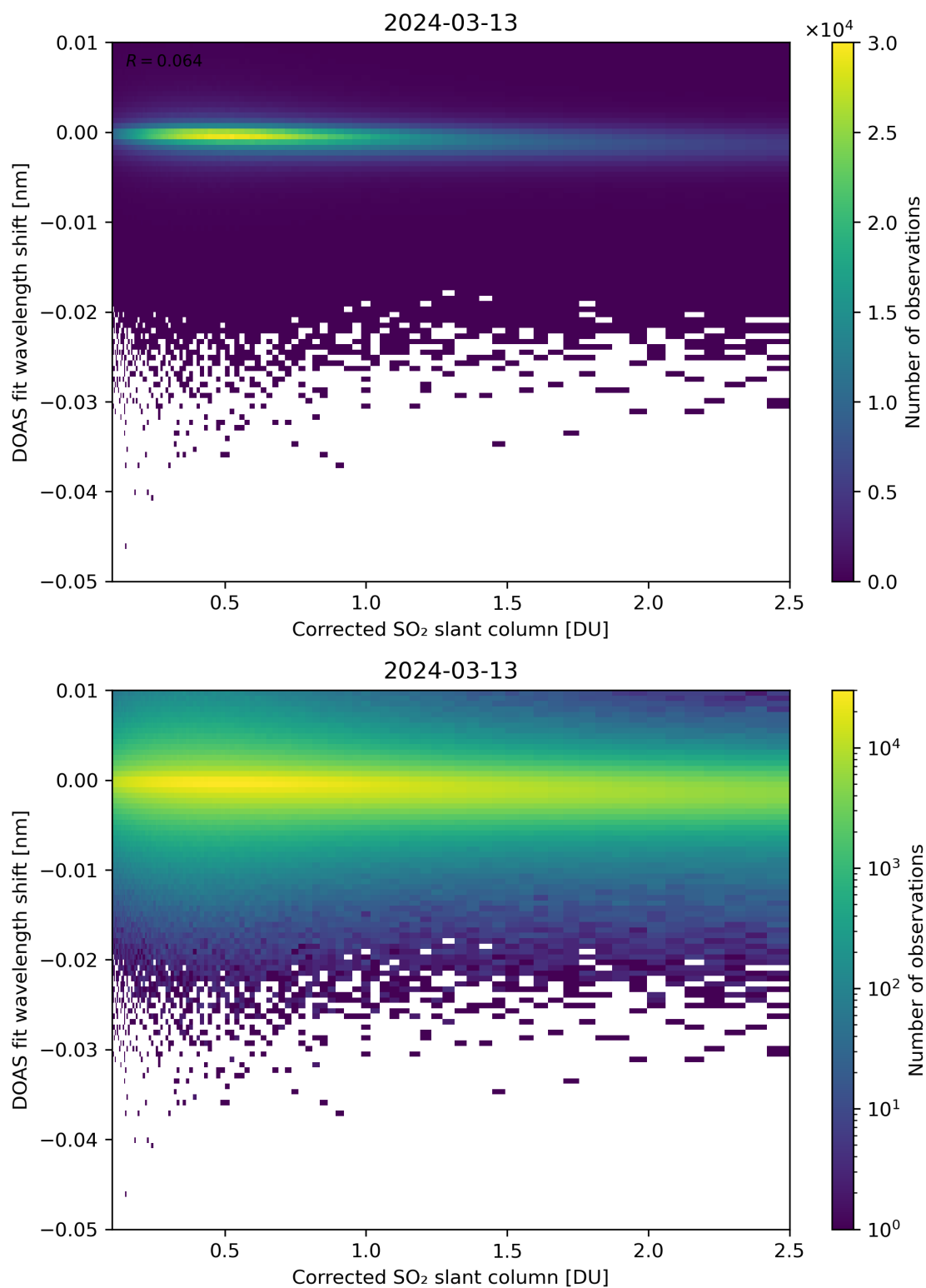
Figure 181: Scatter density plot of “Corrected SO 2 slant column” against “DOAS fit wavelength shift” for 2024-03-12 to 2024-03-14.
