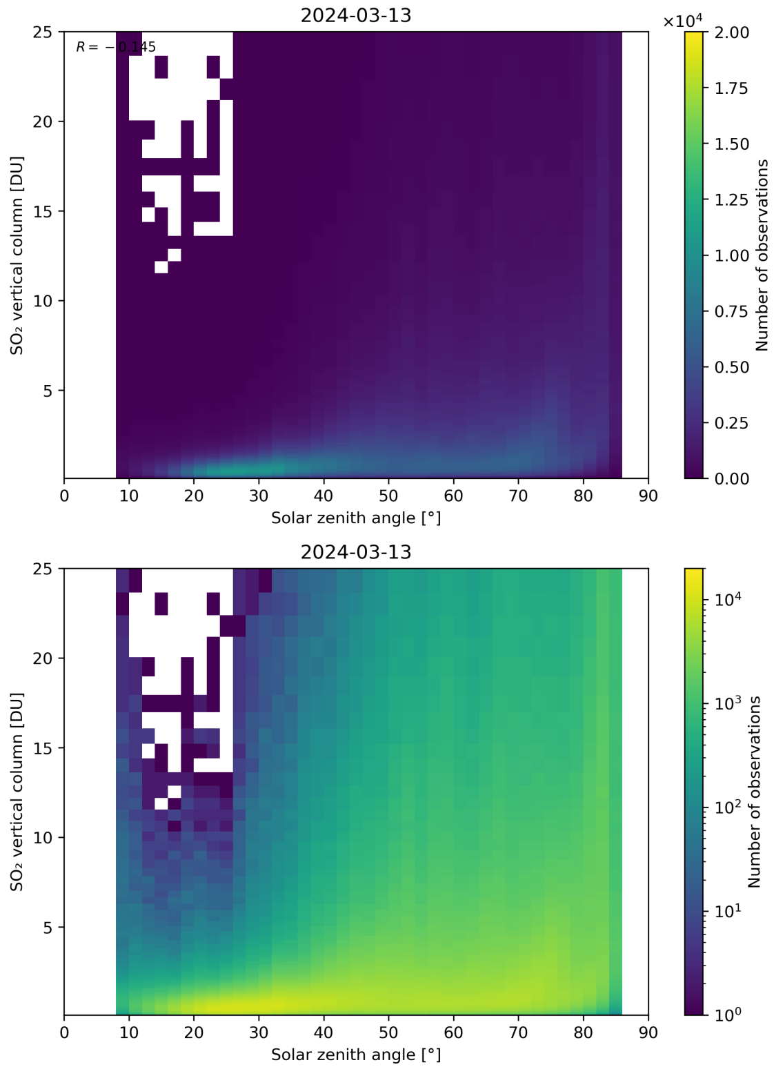
Figure 176: Scatter density plot of “Solar zenith angle” against “SO 2 vertical column” for 2024-03-12 to 2024-03-14.
