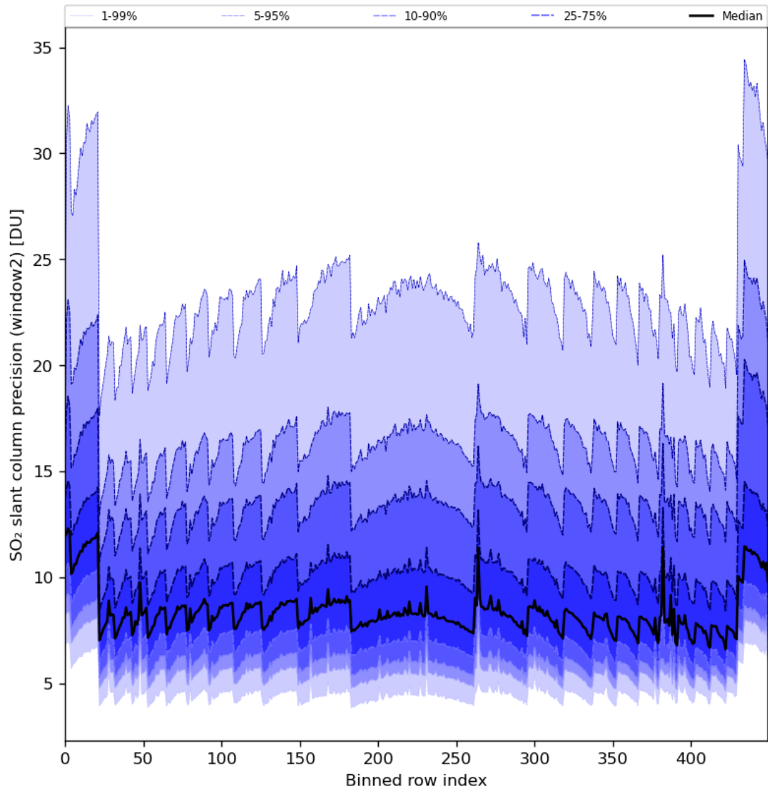
Figure 84: Along track statistics of “SO 2 slant column precision (window2)” for 2024-03-12 to 2024-03-14
