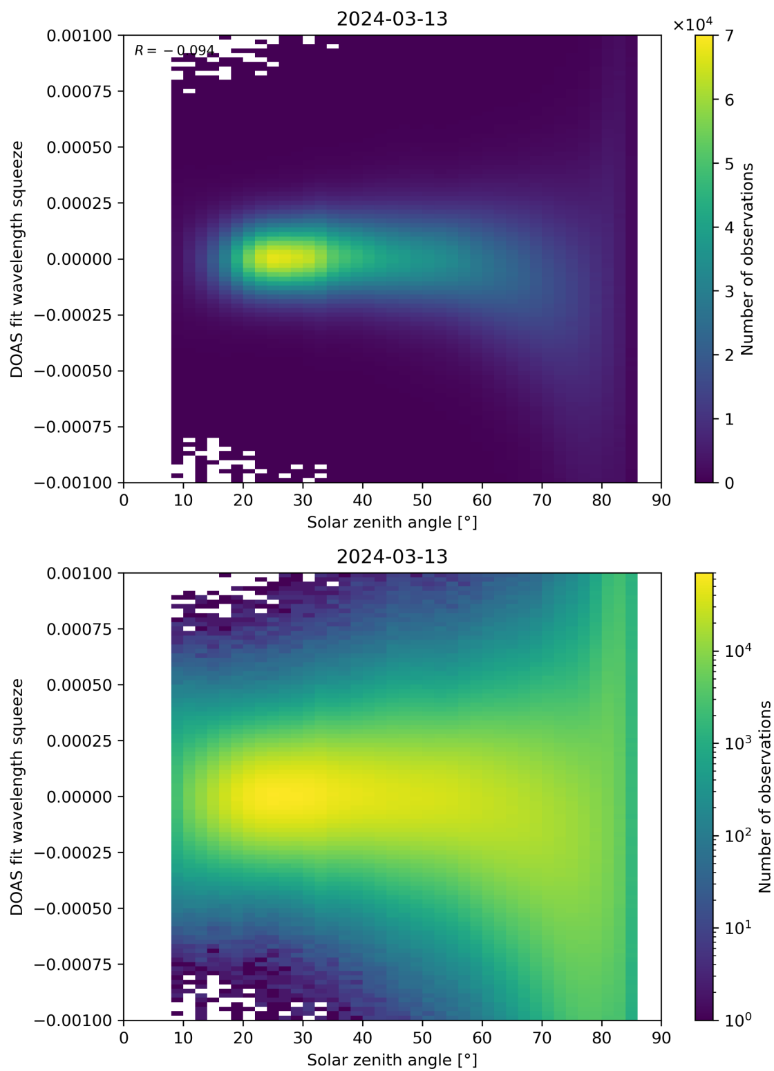
Figure 162: Scatter density plot of “Solar zenith angle” against “DOAS fit wavelength squeeze” for 2024-03-12 to 2024-03-14.
