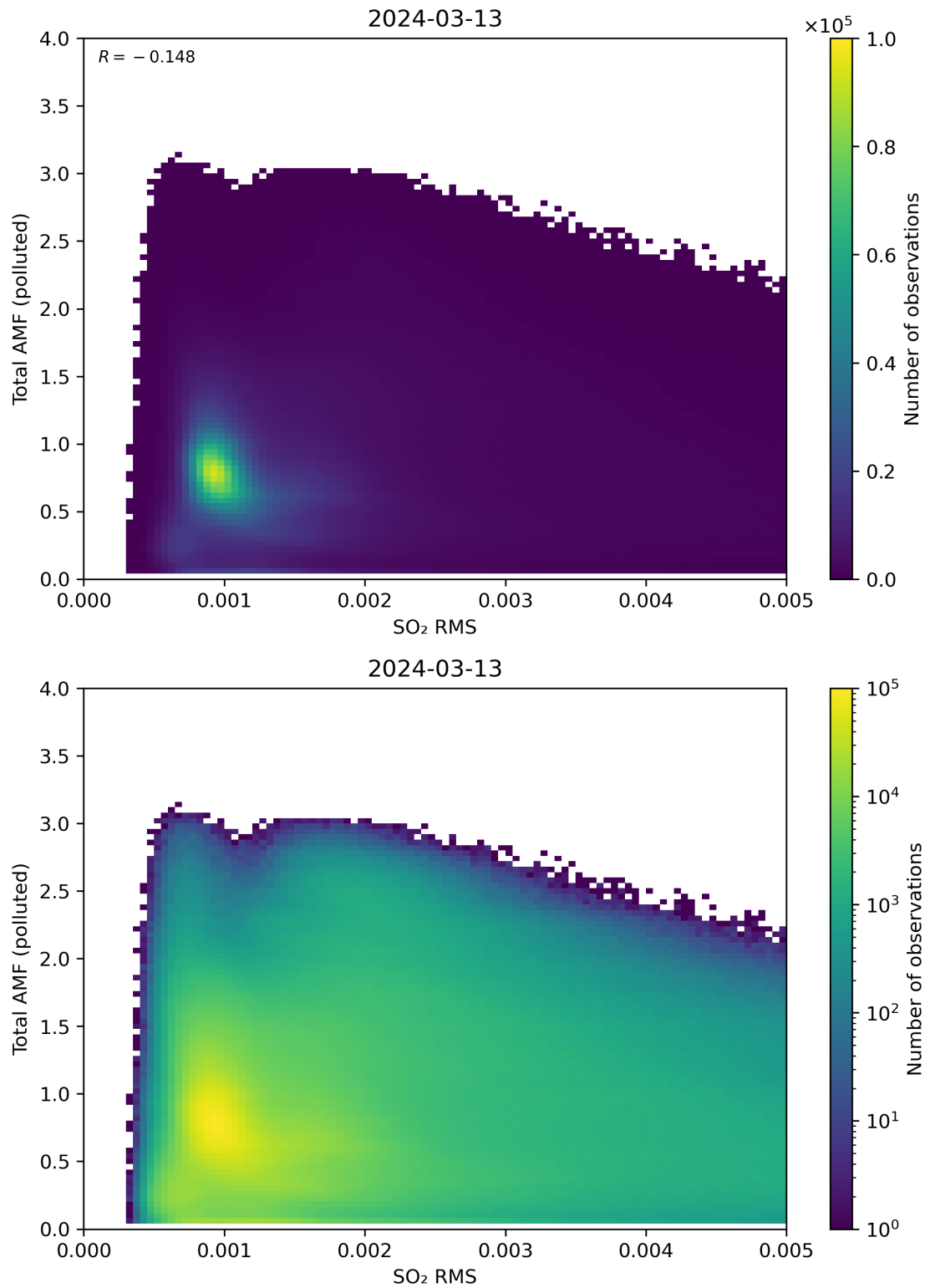
Figure 137: Scatter density plot of “SO 2 RMS” against “Total AMF (polluted)” for 2024-03-12 to 2024-03-14.
