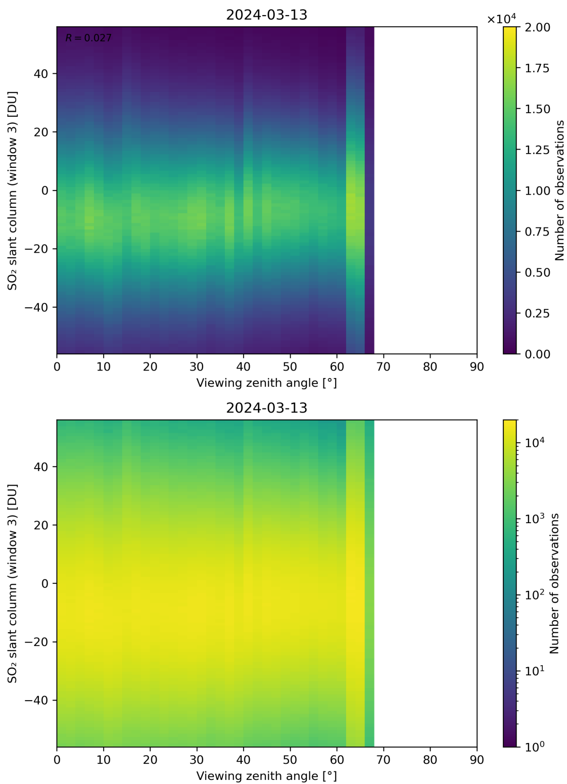
Figure 323: Scatter density plot of “Viewing zenith angle” against “SO 2 slant column (window 3)” for 2024-03-12 to 2024-03-14.
