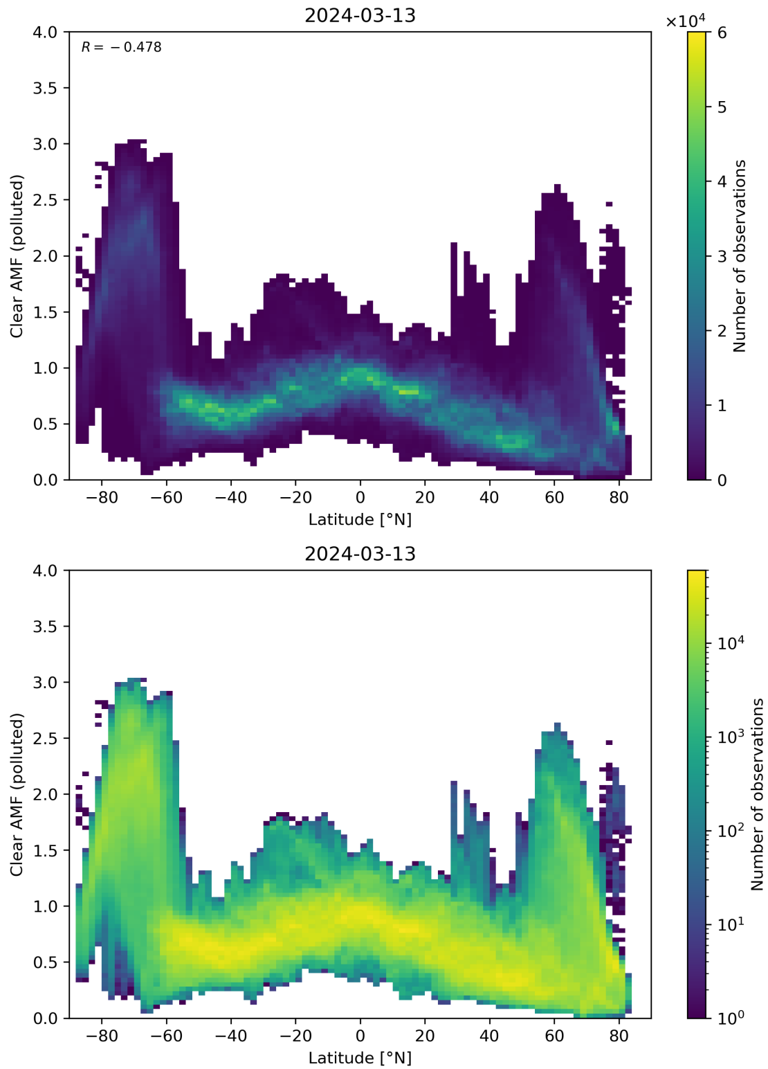
Figure 145: Scatter density plot of “Latitude” against “Clear AMF (polluted)” for 2024-03-12 to 2024-03-14.
