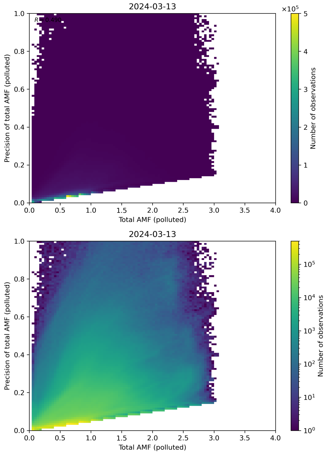
Figure 272: Scatter density plot of “Total AMF (polluted)” against “Precision of total AMF (polluted)” for 2024-03-12 to 2024-03-14.
