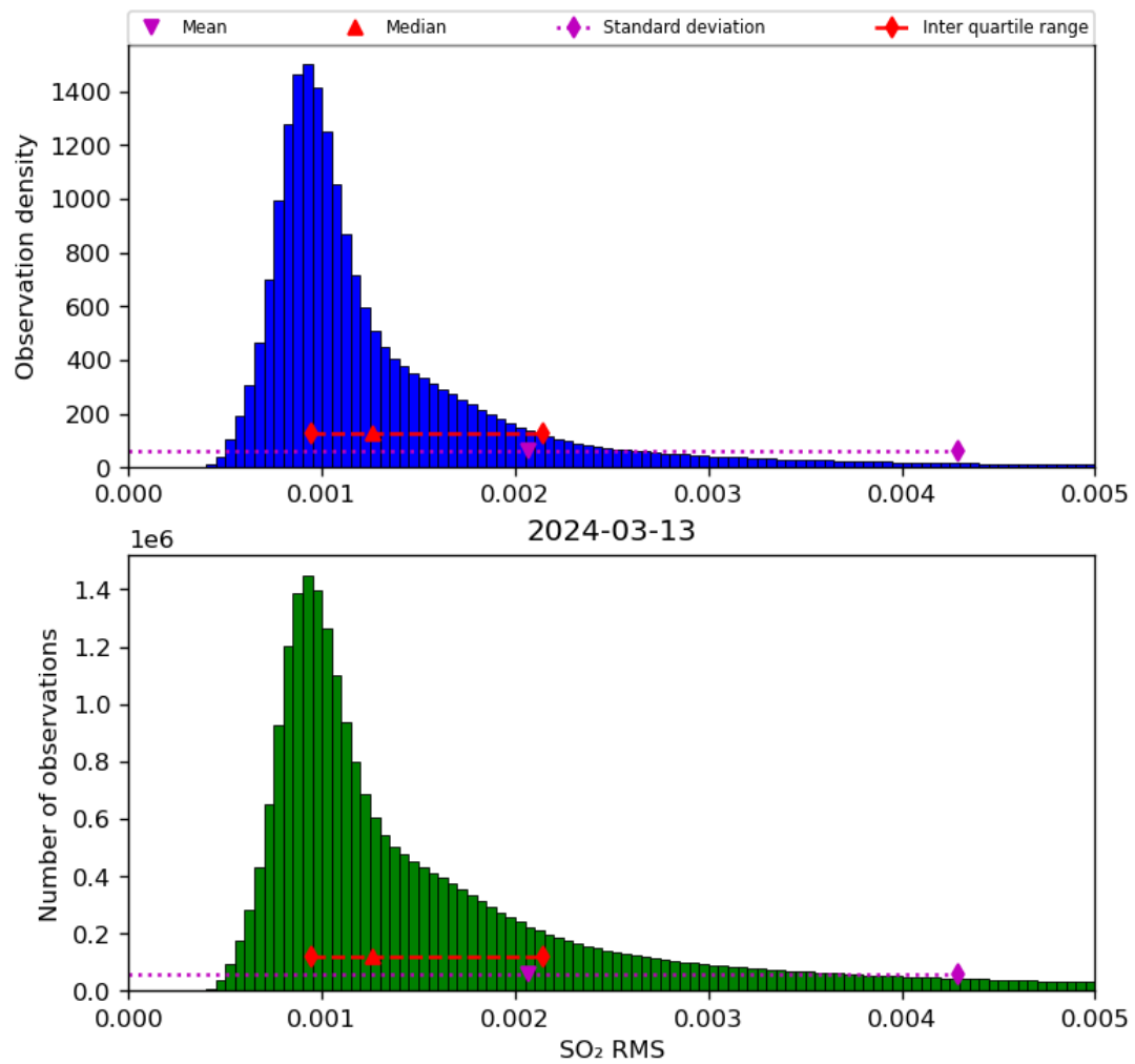
Figure 70: Histogram of “SO 2 RMS” for 2024-03-12 to 2024-03-14
