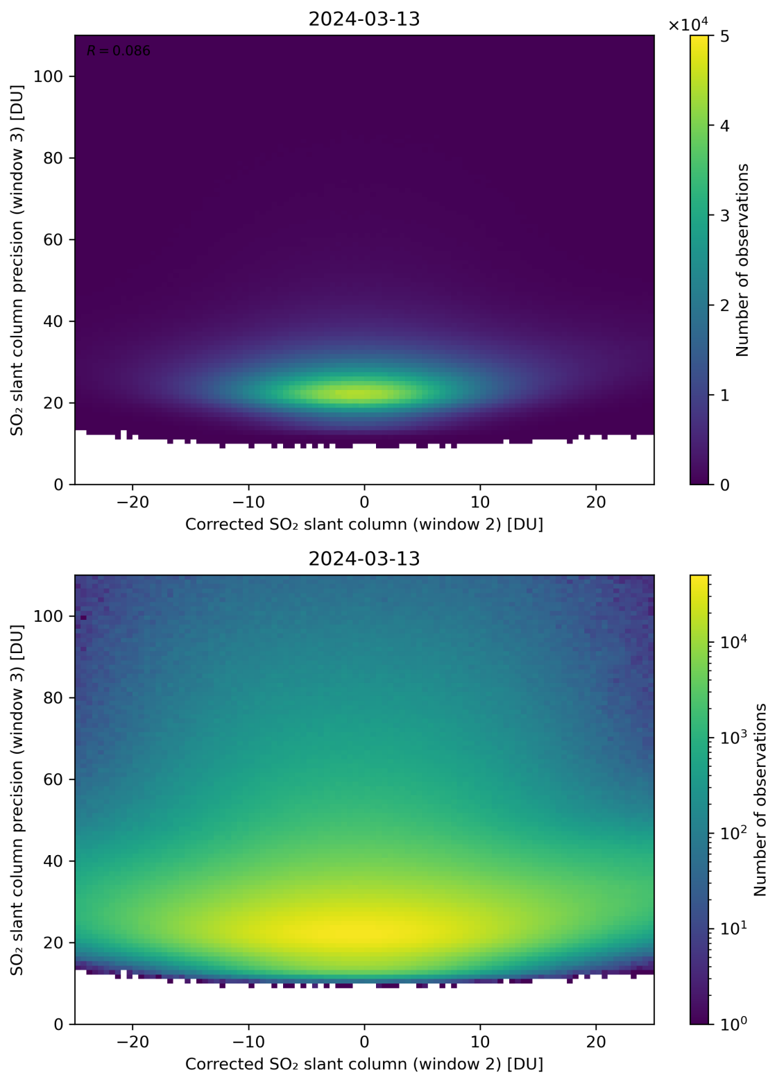
Figure 202: Scatter density plot of “Corrected SO 2 slant column (window 2)” against “SO 2 slant column precision (window 3)” for 2024-03-12 to 2024-03-14.
