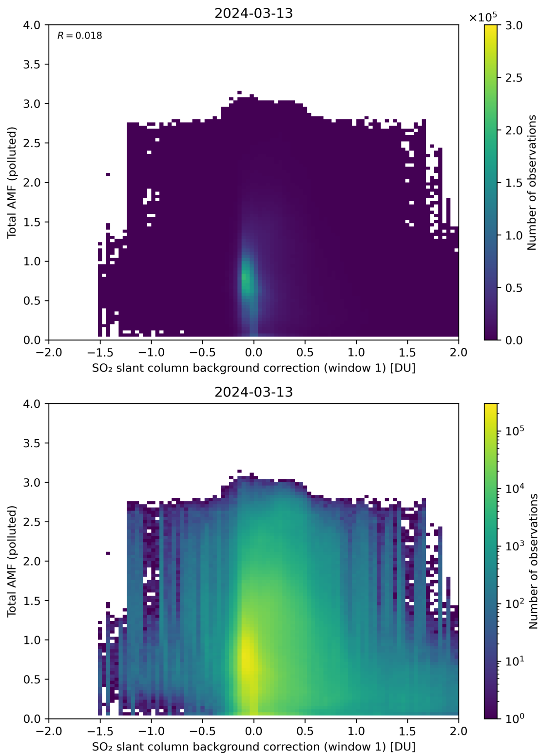
Figure 109: Scatter density plot of “SO 2 slant column background correction (window 1)” against “Total AMF (polluted)” for 2024-03-12 to 2024-03-14.
