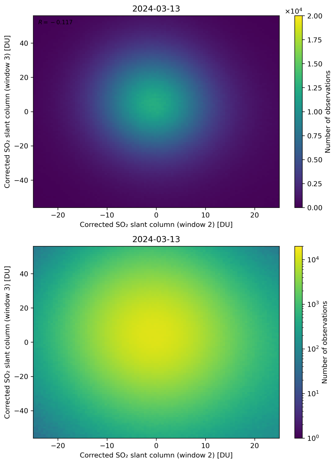
Figure 200: Scatter density plot of “Corrected SO 2 slant column (window 2)” against “Corrected SO 2 slant column (window 3)” for 2024-03-12 to 2024-03-14.
