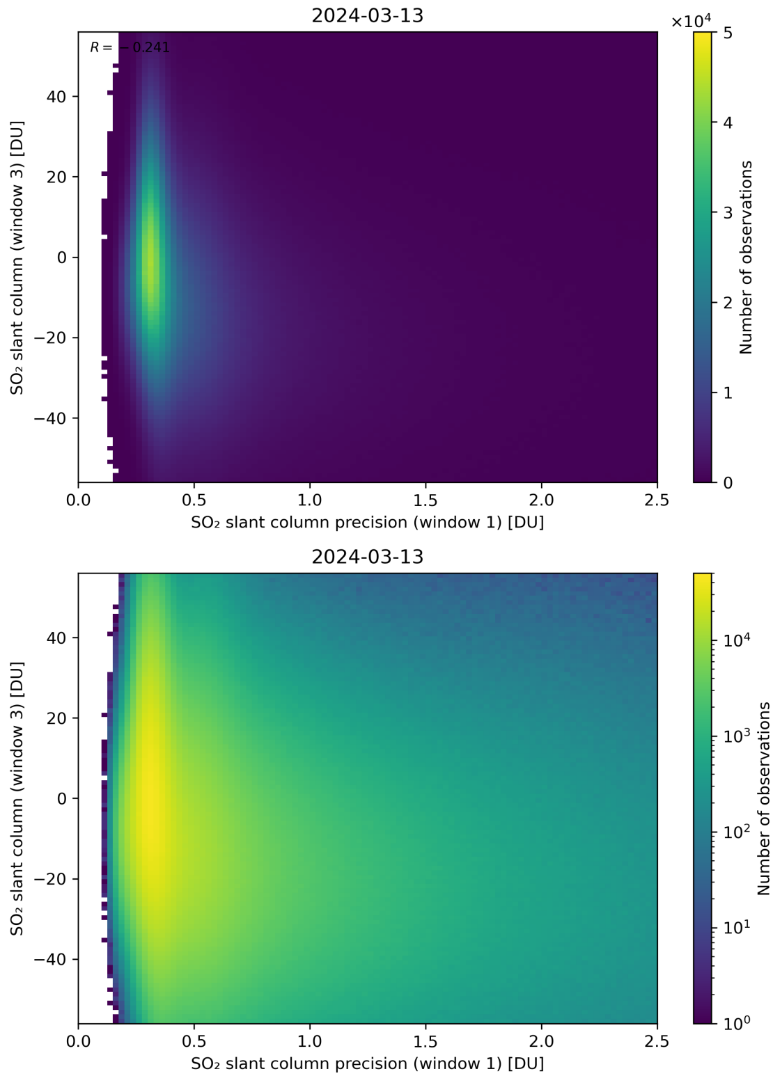
Figure 228: Scatter density plot of “SO 2 slant column precision (window 1)” against “SO 2 slant column (window 3)” for 2024-03-12 to 2024-03-14.
