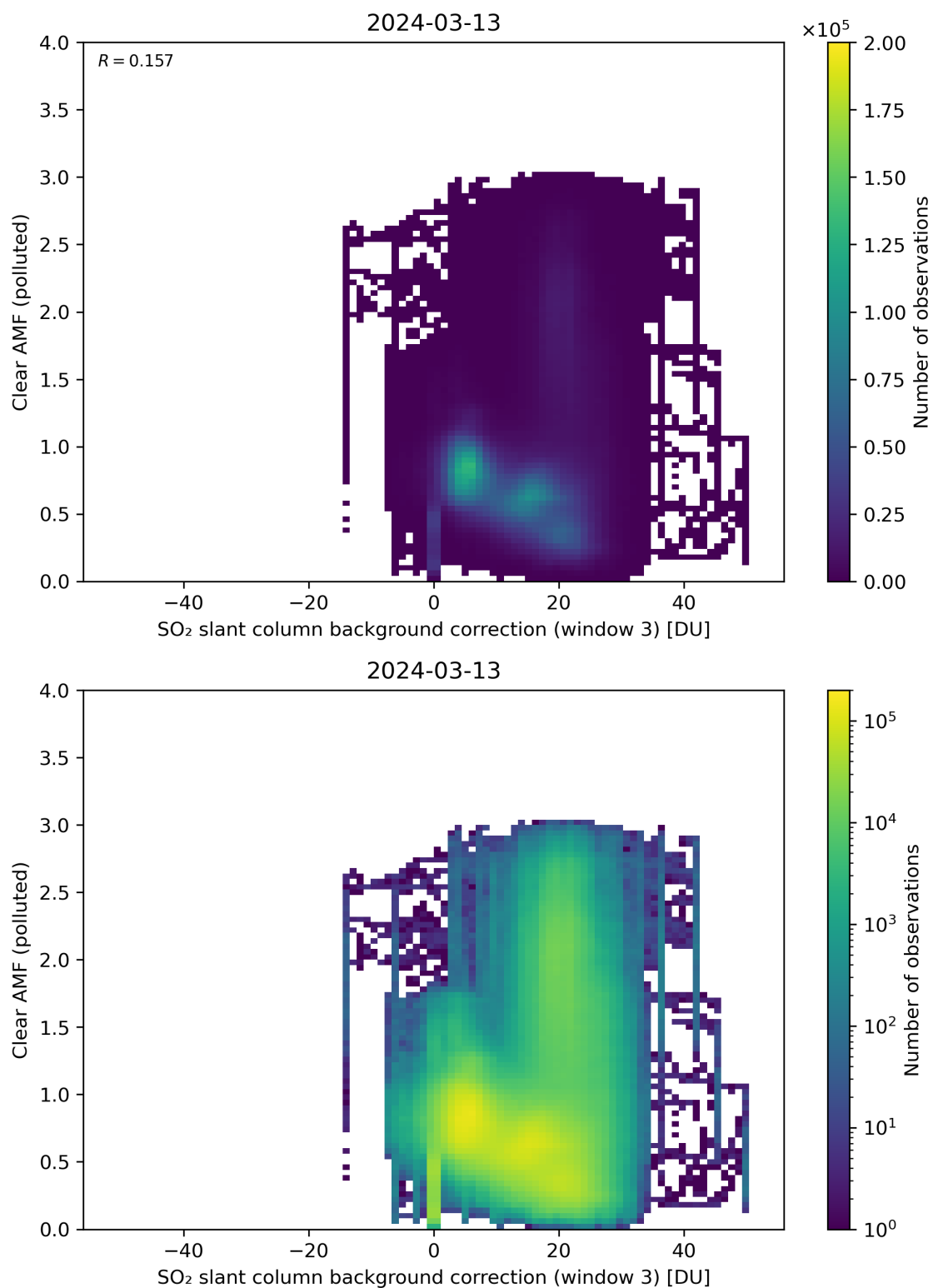
Figure 124: Scatter density plot of “SO 2 slant column background correction (window 3)” against “Clear AMF (polluted)” for 2024-03-12 to 2024-03-14.
