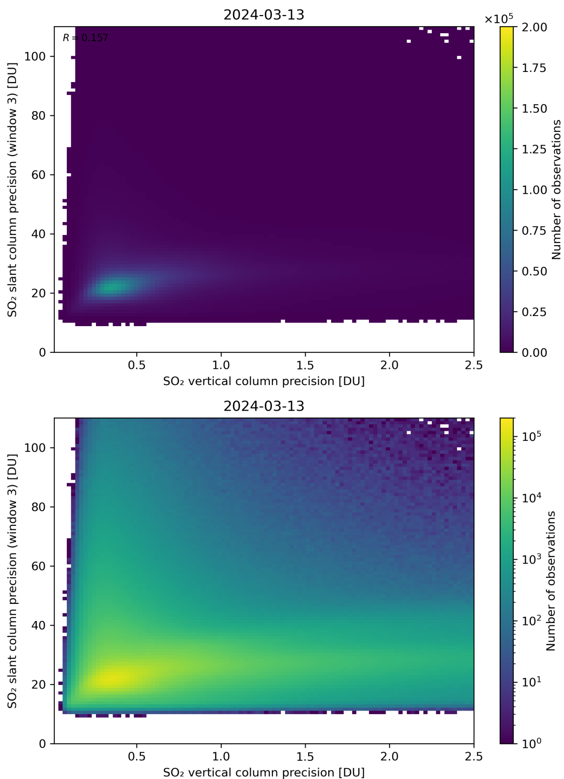
Figure 293: Scatter density plot of “SO 2 vertical column precision” against “SO 2 slant column precision (window 3)” for 2024-03-12 to 2024-03-14.
