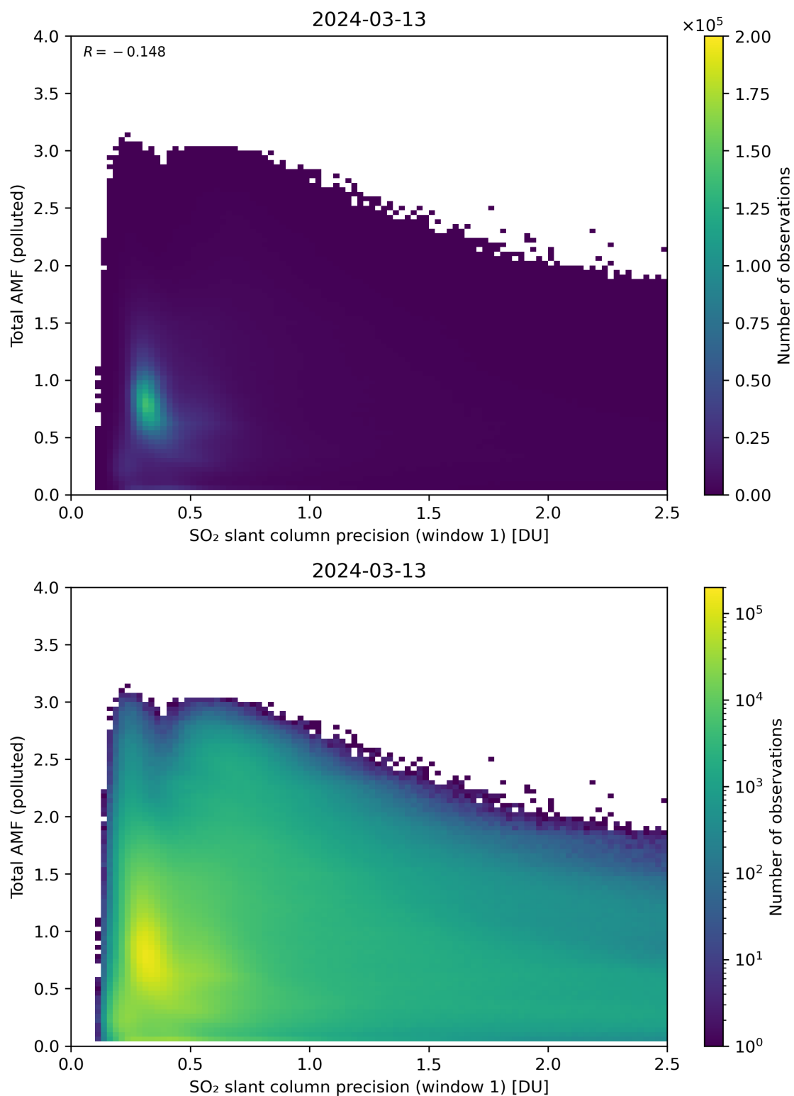
Figure 230: Scatter density plot of “SO 2 slant column precision (window 1)” against “Total AMF (polluted)” for 2024-03-12 to 2024-03-14.
