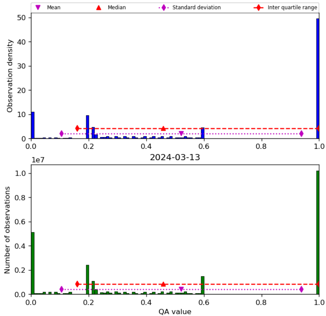
Figure 52: Histogram of “QA value” for 2024-03-12 to 2024-03-14
