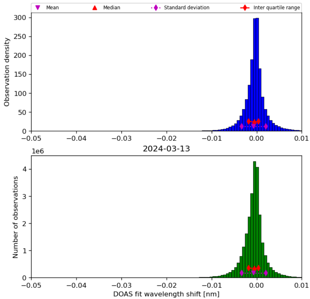
Figure 68: Histogram of “DOAS fit wavelength shift” for 2024-03-12 to 2024-03-14
