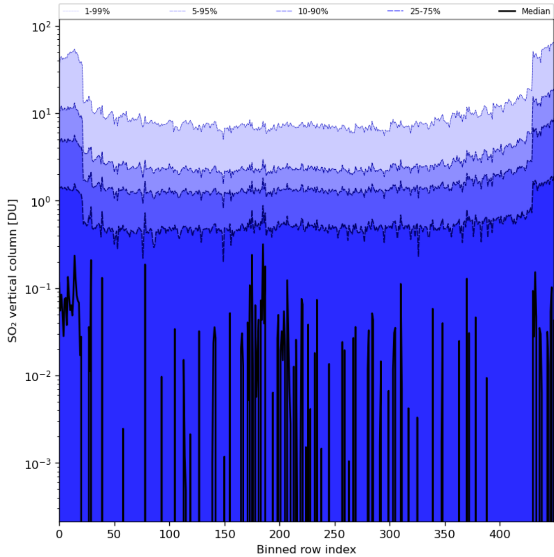
Figure 76: Along track statistics of “SO 2 vertical column” for 2024-03-12 to 2024-03-14
