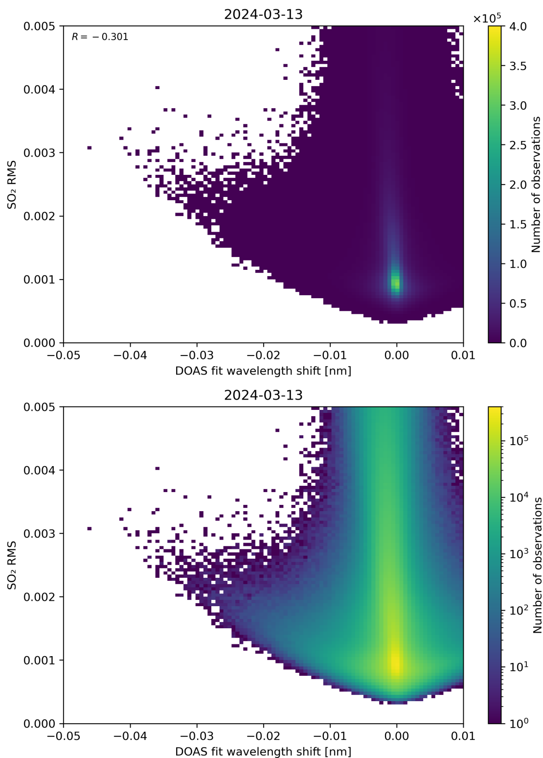
Figure 128: Scatter density plot of “DOAS fit wavelength shift” against “SO 2 RMS” for 2024-03-12 to 2024-03-14.
