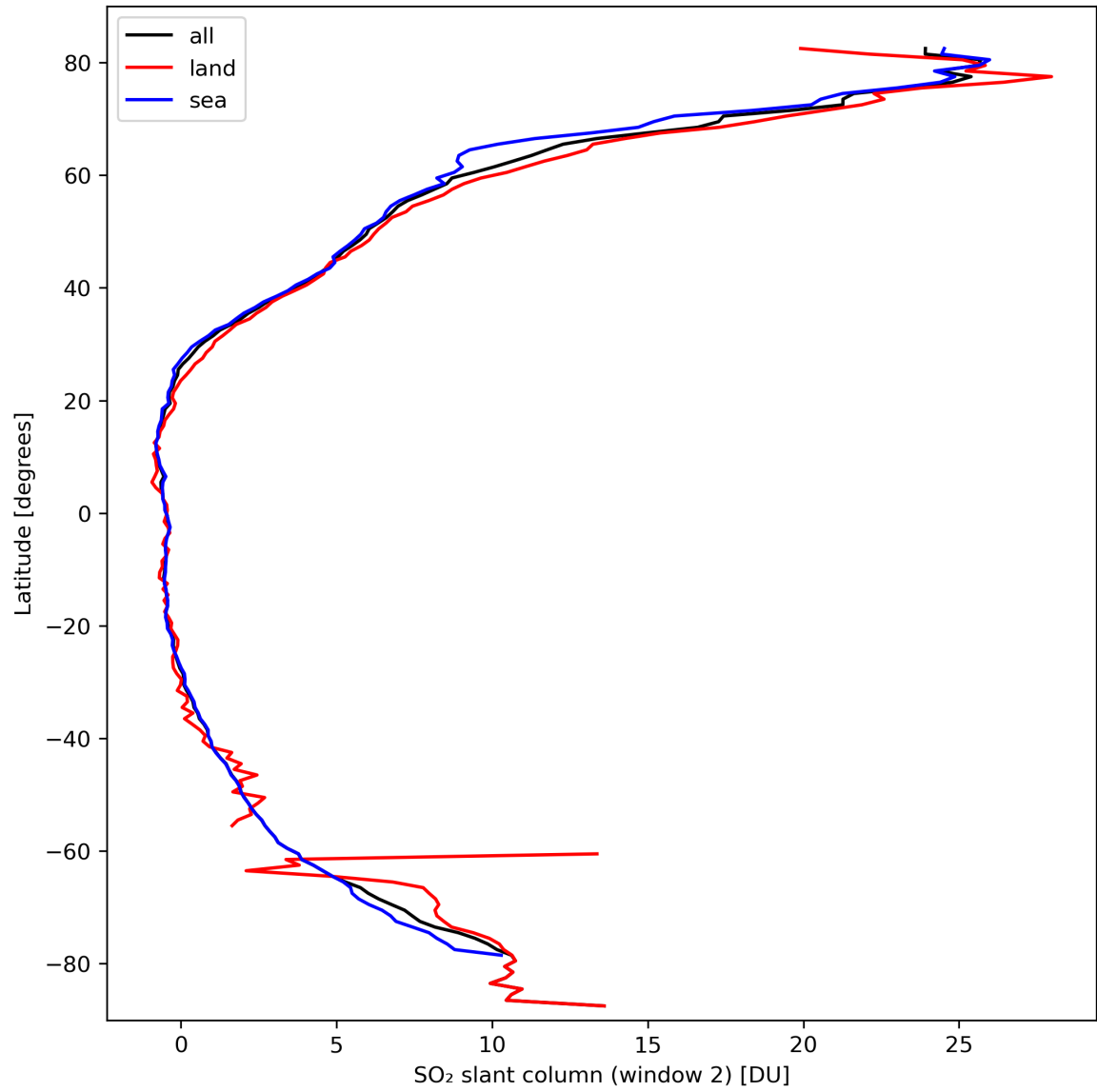
Figure 37: Zonal average of “SO 2 slant column (window 2)” for 2024-03-12 to 2024-03-14.
