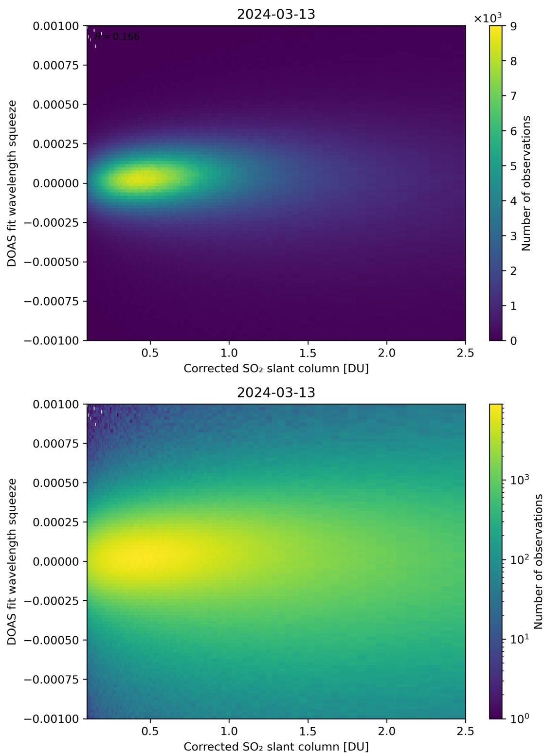
Figure 182: Scatter density plot of “Corrected SO 2 slant column” against “DOAS fit wavelength squeeze” for 2024-03-12 to 2024-03-14.
