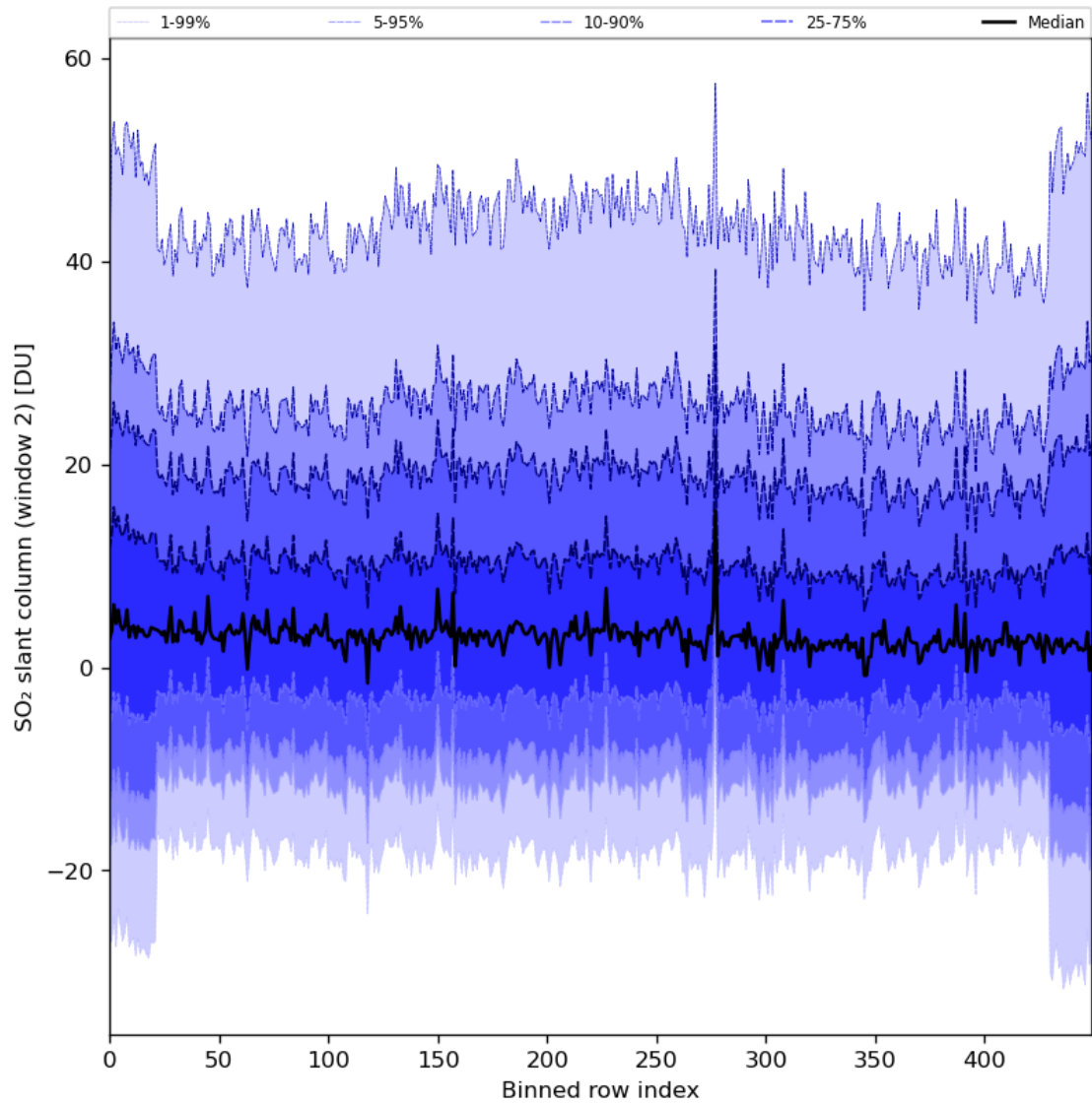
Figure 83: Along track statistics of “SO 2 slant column (window 2)” for 2024-03-12 to 2024-03-14
