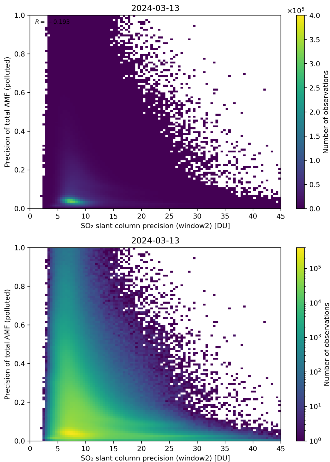
Figure 252: Scatter density plot of “SO 2 slant column precision (window2)” against “Precision of total AMF (polluted)” for 2024-03-12 to 2024-03-14.
