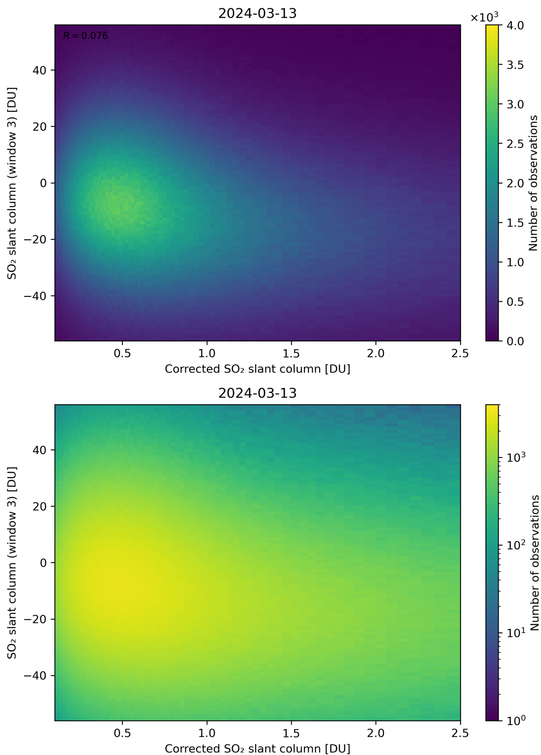
Figure 190: Scatter density plot of “Corrected SO 2 slant column” against “SO 2 slant column (window 3)” for 2024-03-12 to 2024-03-14.
