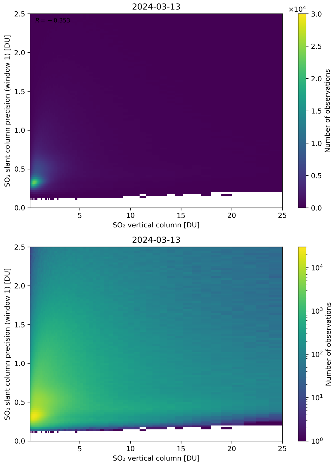
Figure 301: Scatter density plot of “SO 2 vertical column” against “SO 2 slant column precision (window 1)” for 2024-03-12 to 2024-03-14.
