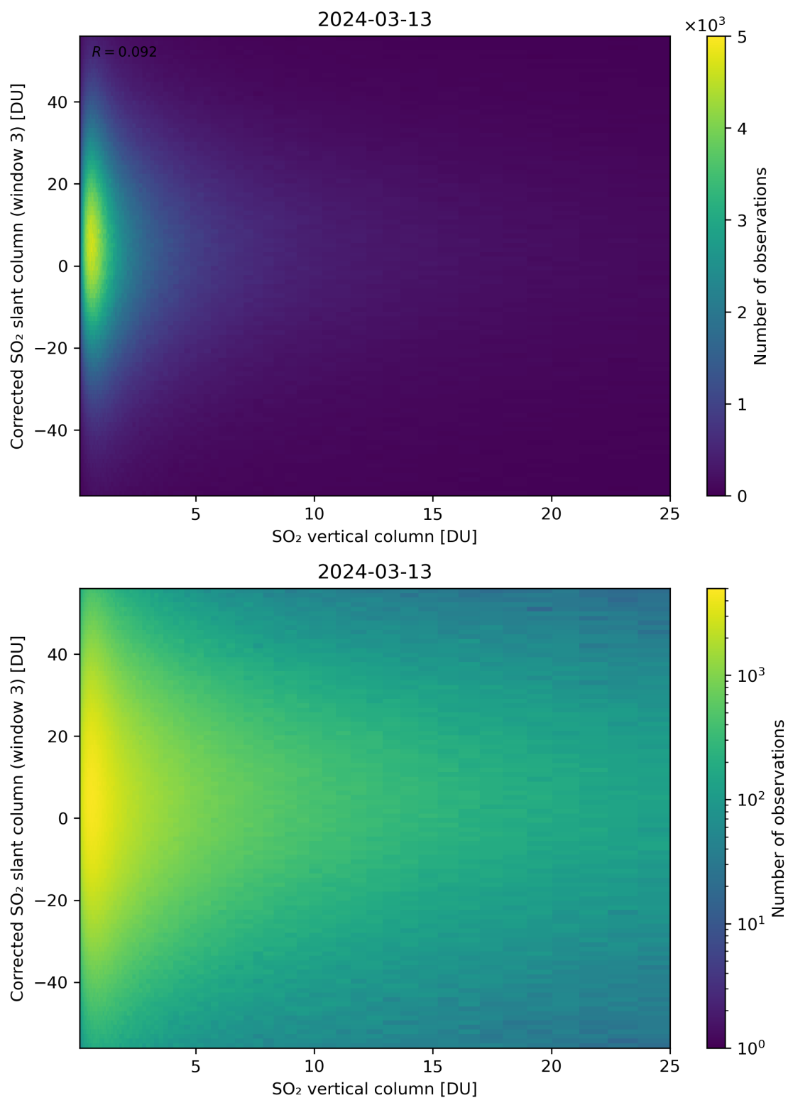
Figure 299: Scatter density plot of “SO 2 vertical column” against “Corrected SO 2 slant column (window 3)” for 2024-03-12 to 2024-03-14.
