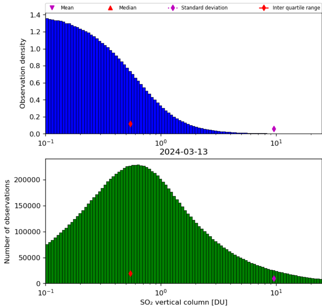
Figure 53: Histogram of “SO 2 vertical column” for 2024-03-12 to 2024-03-14
