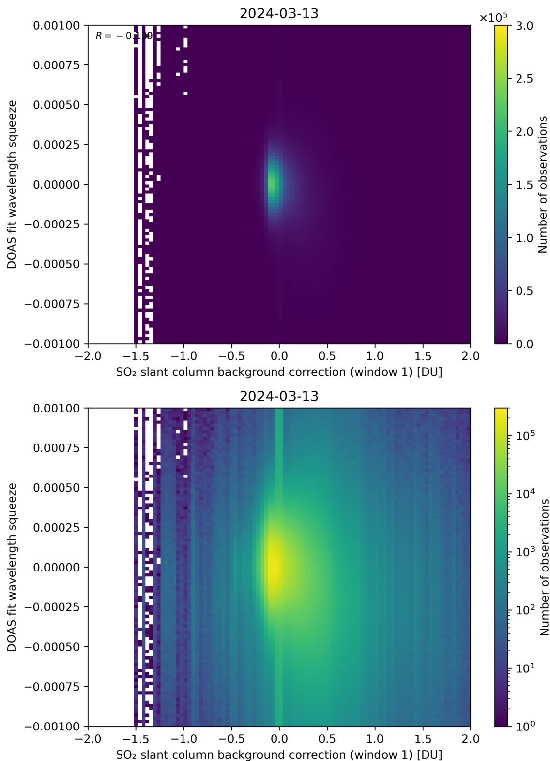
Figure 101: Scatter density plot of “SO 2 slant column background correction (window 1)” against “DOAS fit wavelength squeeze” for 2024-03-12 to 2024-03-14.
