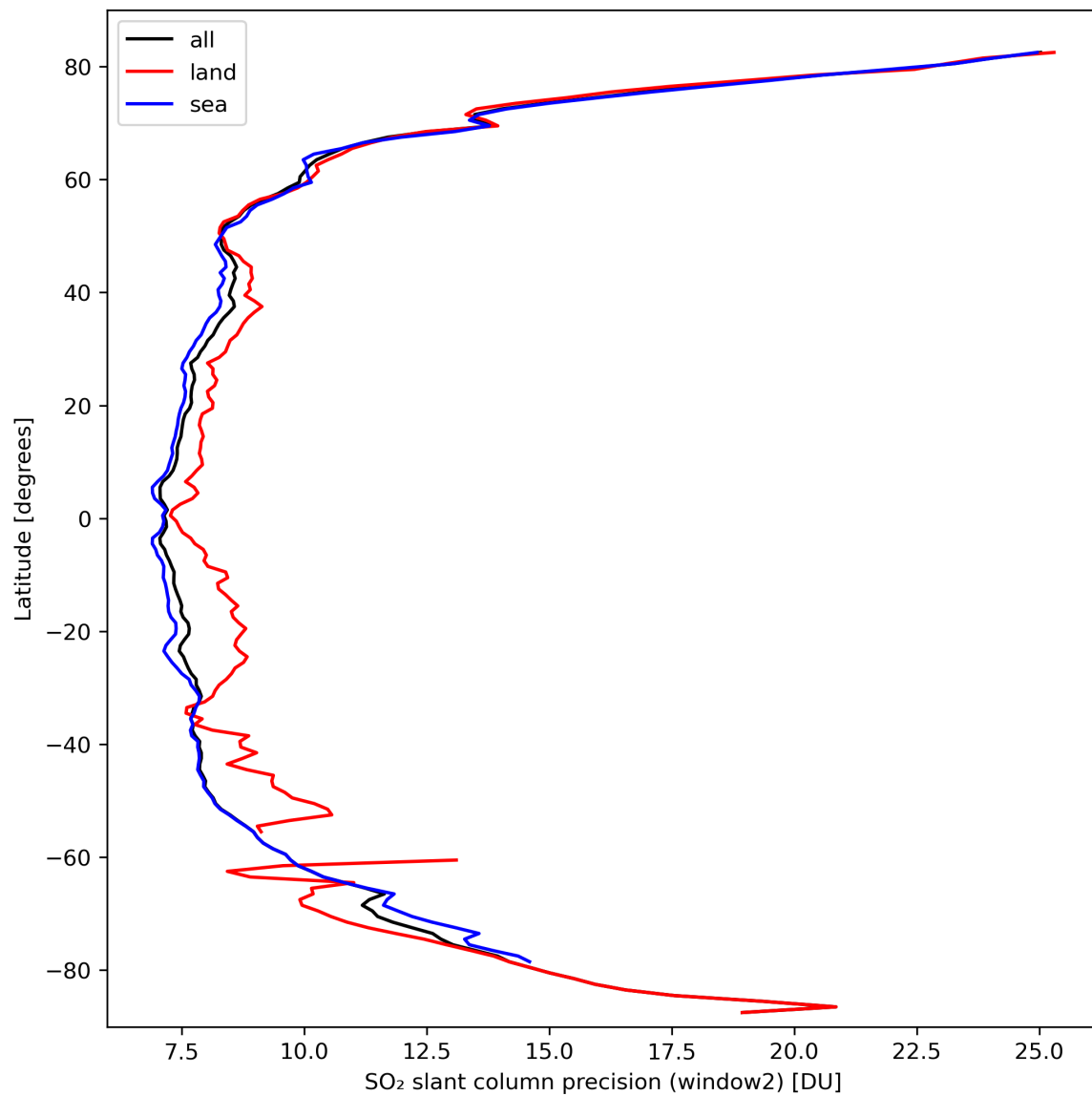
Figure 38: Zonal average of “SO 2 slant column precision (window2)” for 2024-03-12 to 2024-03-14.
