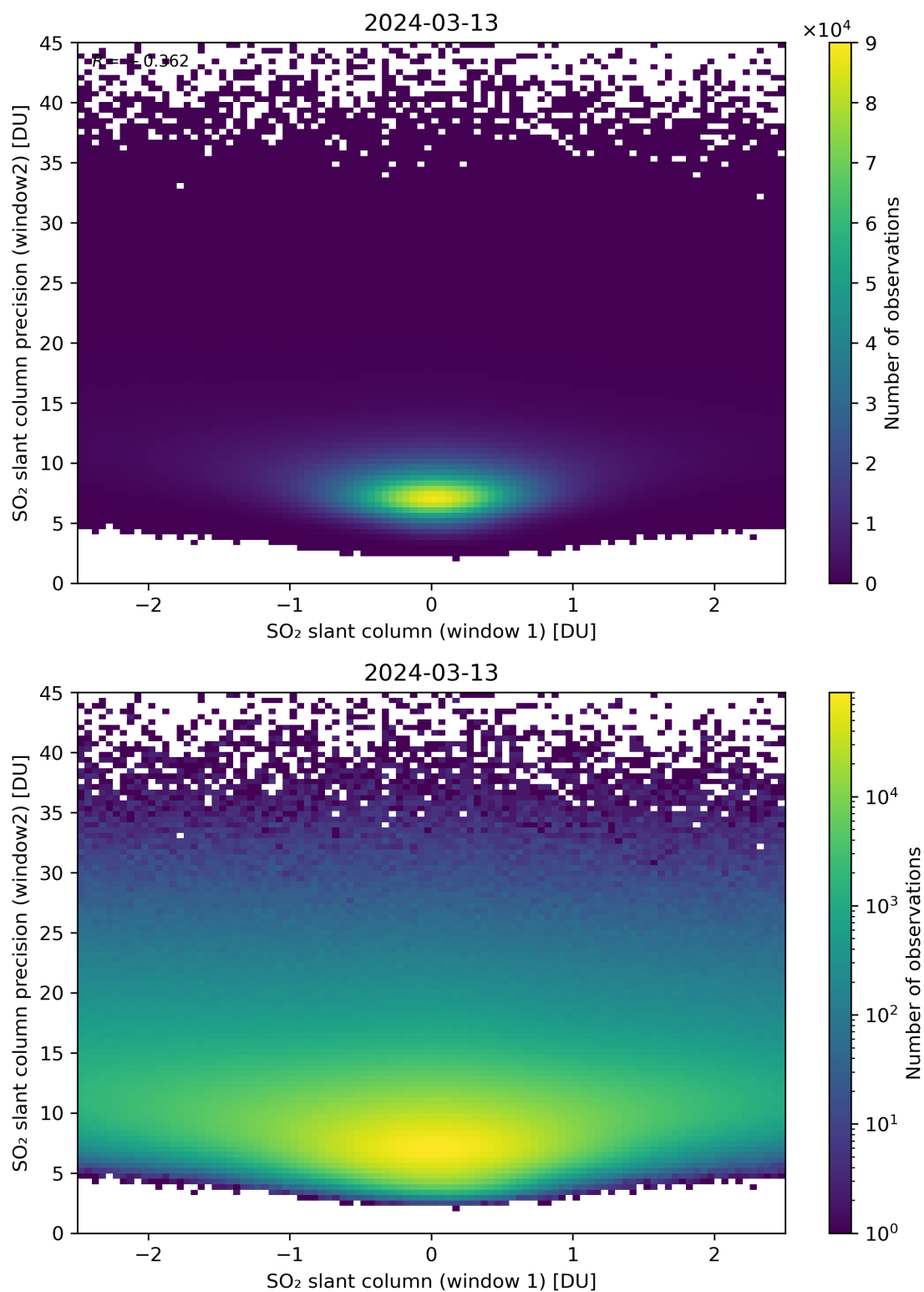
Figure 236: Scatter density plot of “SO 2 slant column (window 1)” against “SO 2 slant column precision (window2)” for 2024-03-12 to 2024-03-14.
