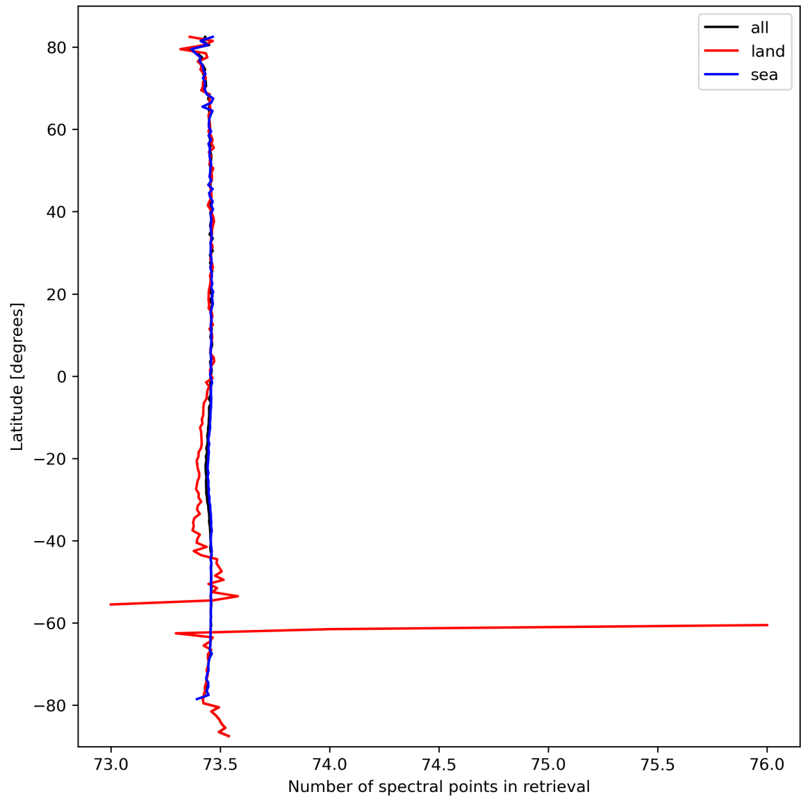
Figure 51: Zonal average of “Number of spectral points in retrieval” for 2024-03-12 to 2024-03-14.
