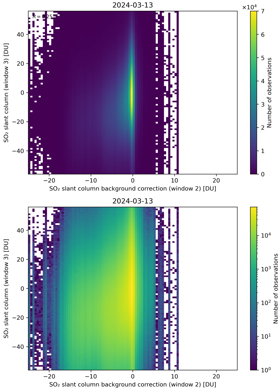
Figure 117: Scatter density plot of “SO 2 slant column background correction (window 2)” against “SO 2 slant column (window 3)” for 2024-03-12 to 2024-03-14.
