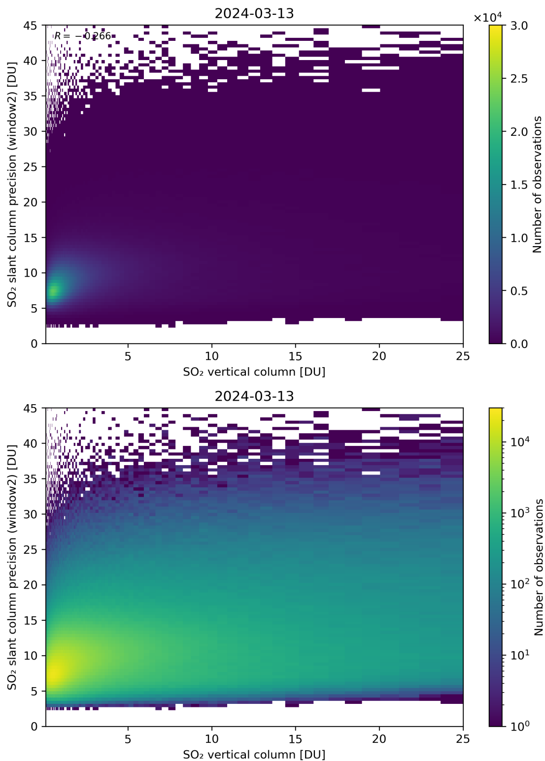
Figure 302: Scatter density plot of “SO 2 vertical column” against “SO 2 slant column precision (window2)” for 2024-03-12 to 2024-03-14.
