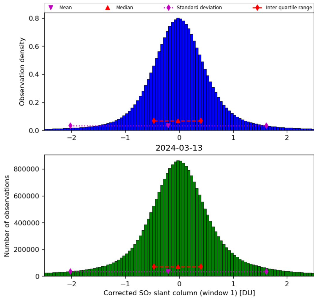
Figure 58: Histogram of “Corrected SO 2 slant column (window 1)” for 2024-03-12 to 2024-03-14
