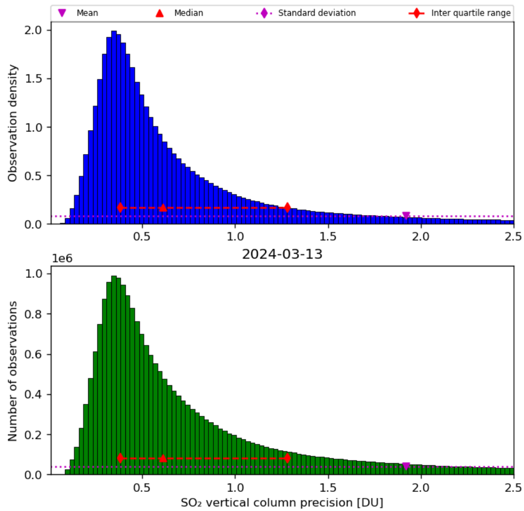
Figure 54: Histogram of “SO 2 vertical column precision” for 2024-03-12 to 2024-03-14
