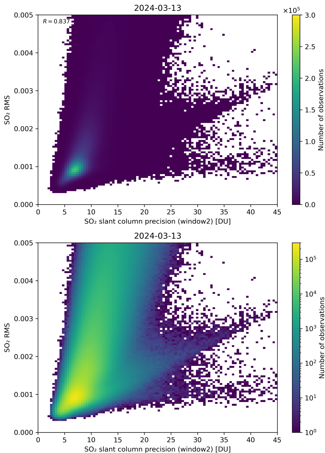
Figure 245: Scatter density plot of “SO 2 slant column precision (window2)” against “SO 2 RMS” for 2024-03-12 to 2024-03-14.
