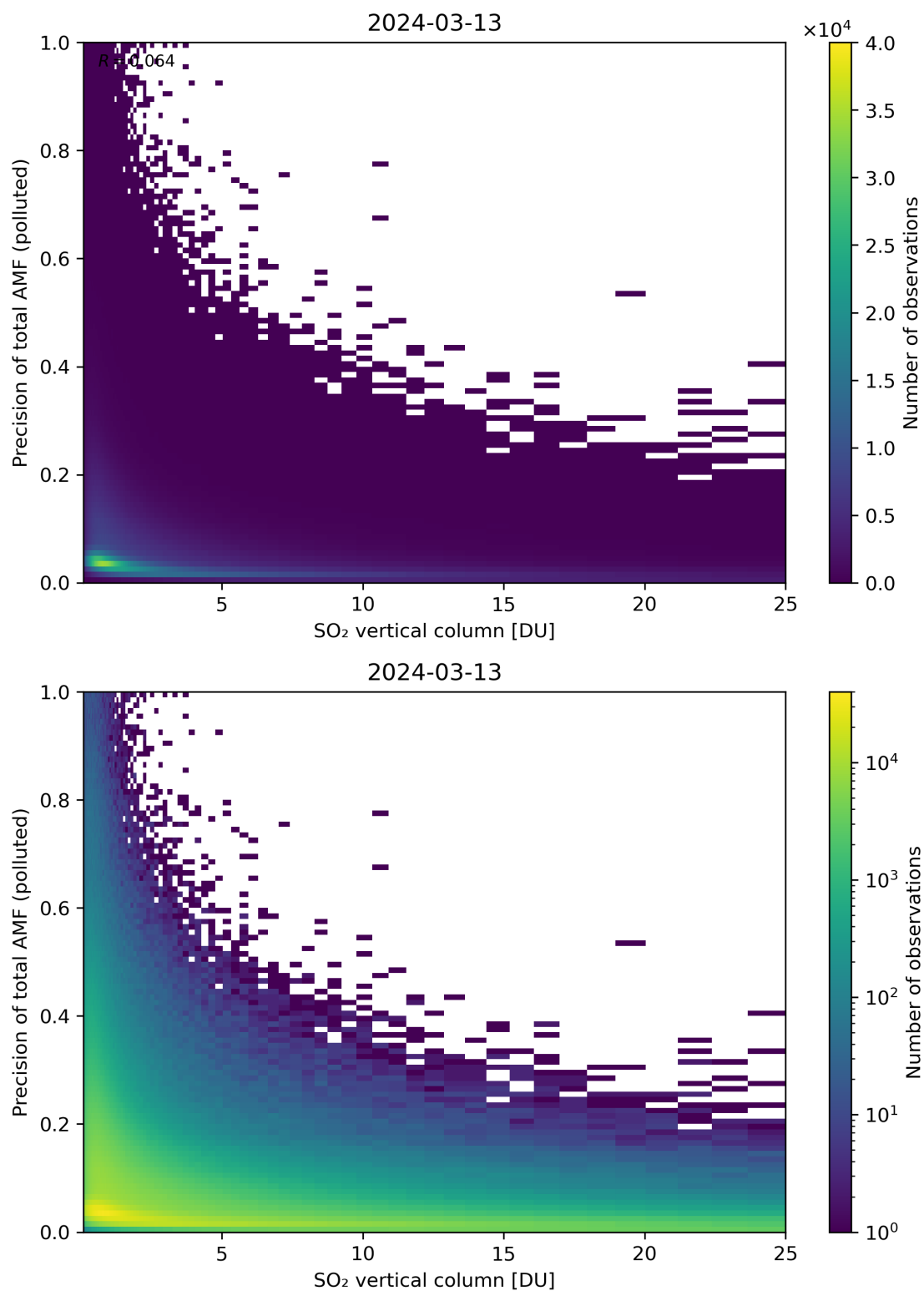
Figure 306: Scatter density plot of “SO 2 vertical column” against “Precision of total AMF (polluted)” for 2024-03-12 to 2024-03-14.
