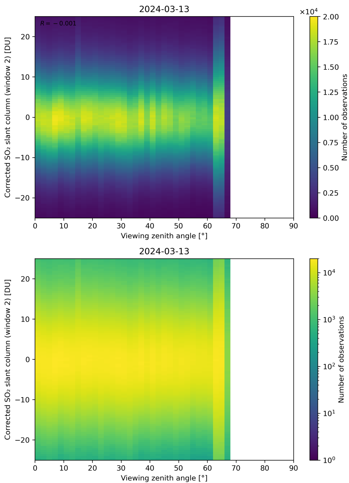
Figure 318: Scatter density plot of “Viewing zenith angle” against “Corrected SO 2 slant column (window 2)” for 2024-03-12 to 2024-03-14.
