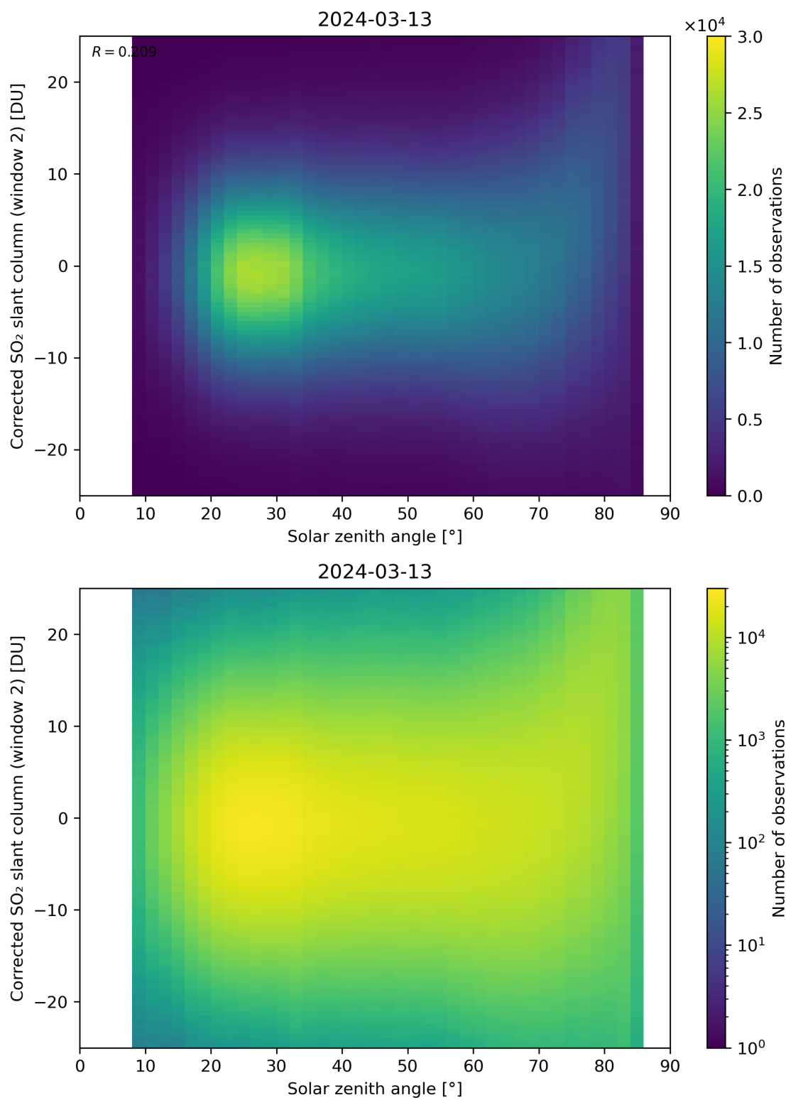
Figure 167: Scatter density plot of “Solar zenith angle” against “Corrected SO 2 slant column (window 2)” for 2024-03-12 to 2024-03-14.
