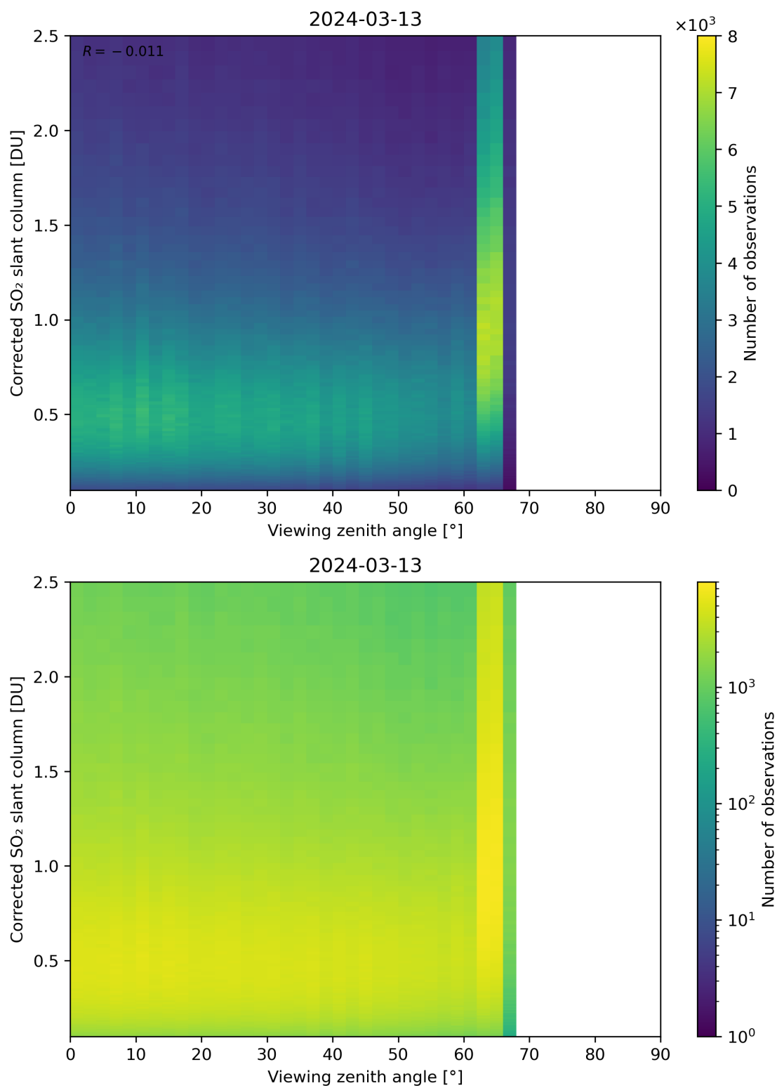
Figure 317: Scatter density plot of “Viewing zenith angle” against “Corrected SO 2 slant column” for 2024-03-12 to 2024-03-14.
