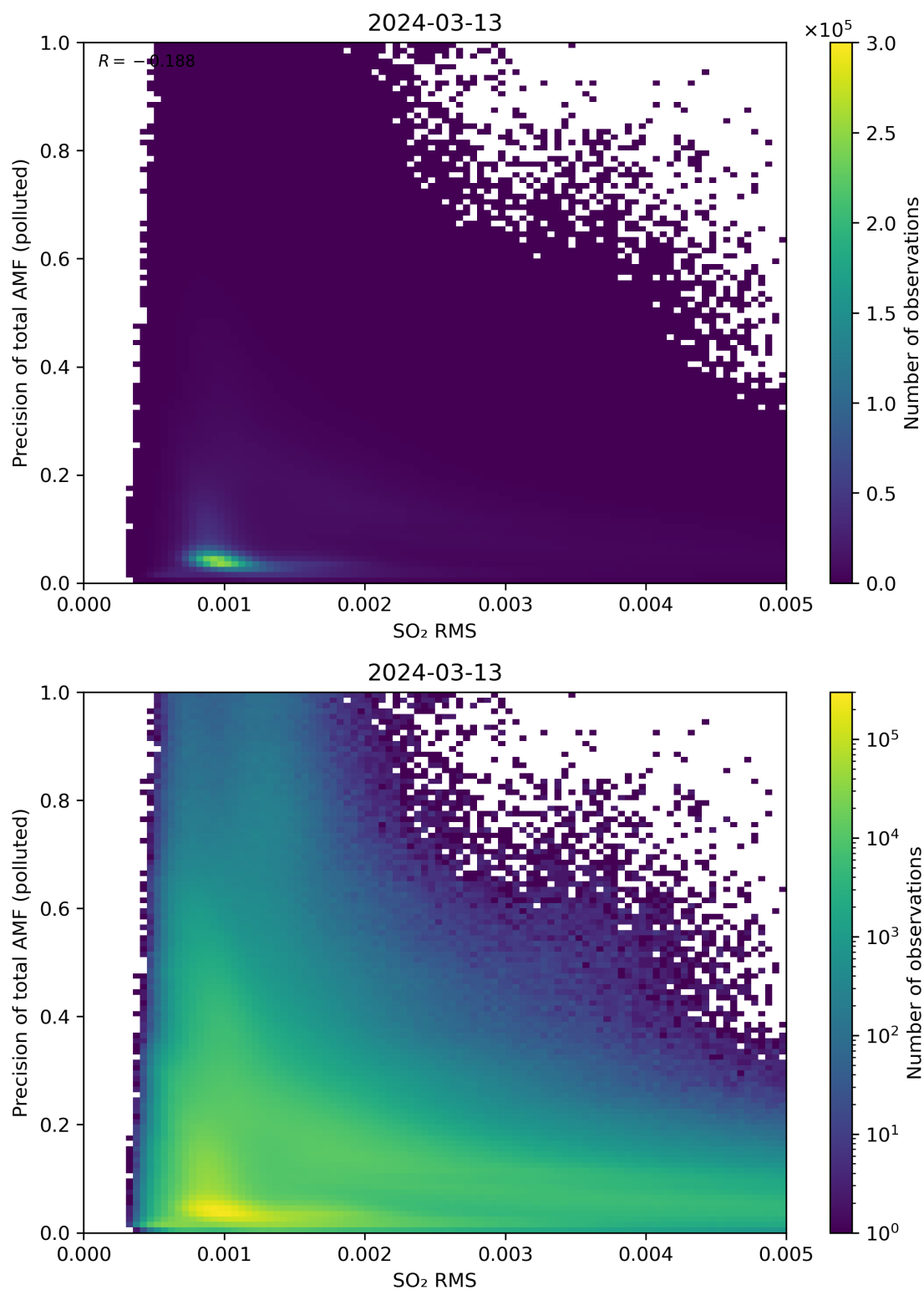
Figure 138: Scatter density plot of “SO 2 RMS” against “Precision of total AMF (polluted)” for 2024-03-12 to 2024-03-14.
