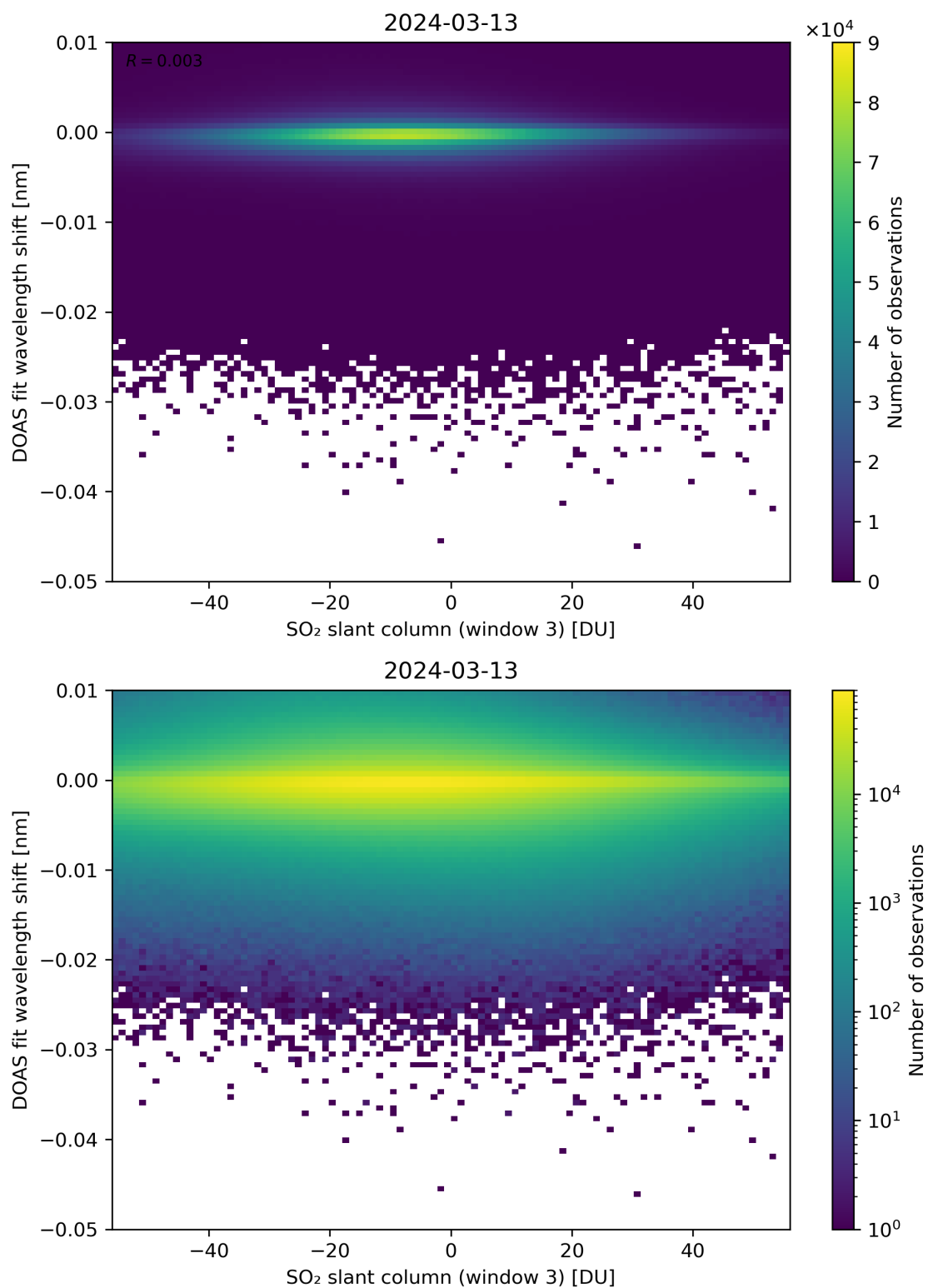
Figure 254: Scatter density plot of “SO 2 slant column (window 3)” against “DOAS fit wavelength shift” for 2024-03-12 to 2024-03-14.
