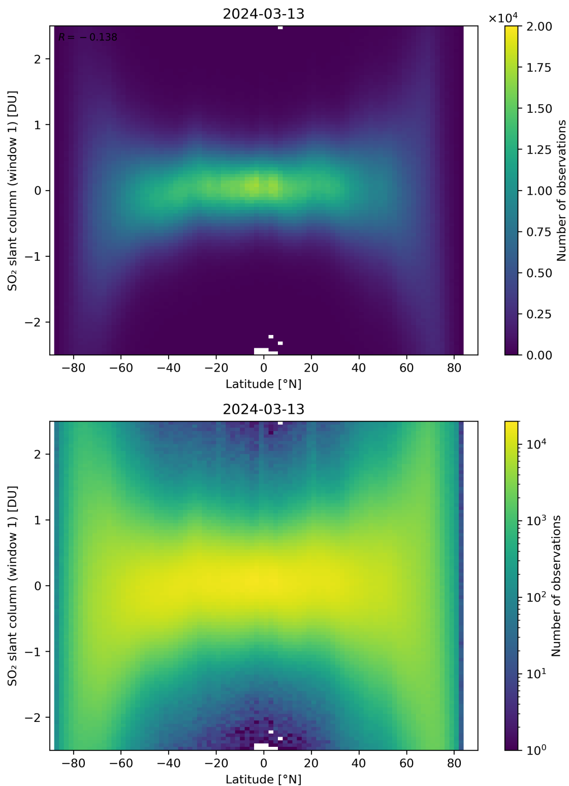
Figure 149: Scatter density plot of “Latitude” against “SO 2 slant column (window 1)” for 2024-03-12 to 2024-03-14.
