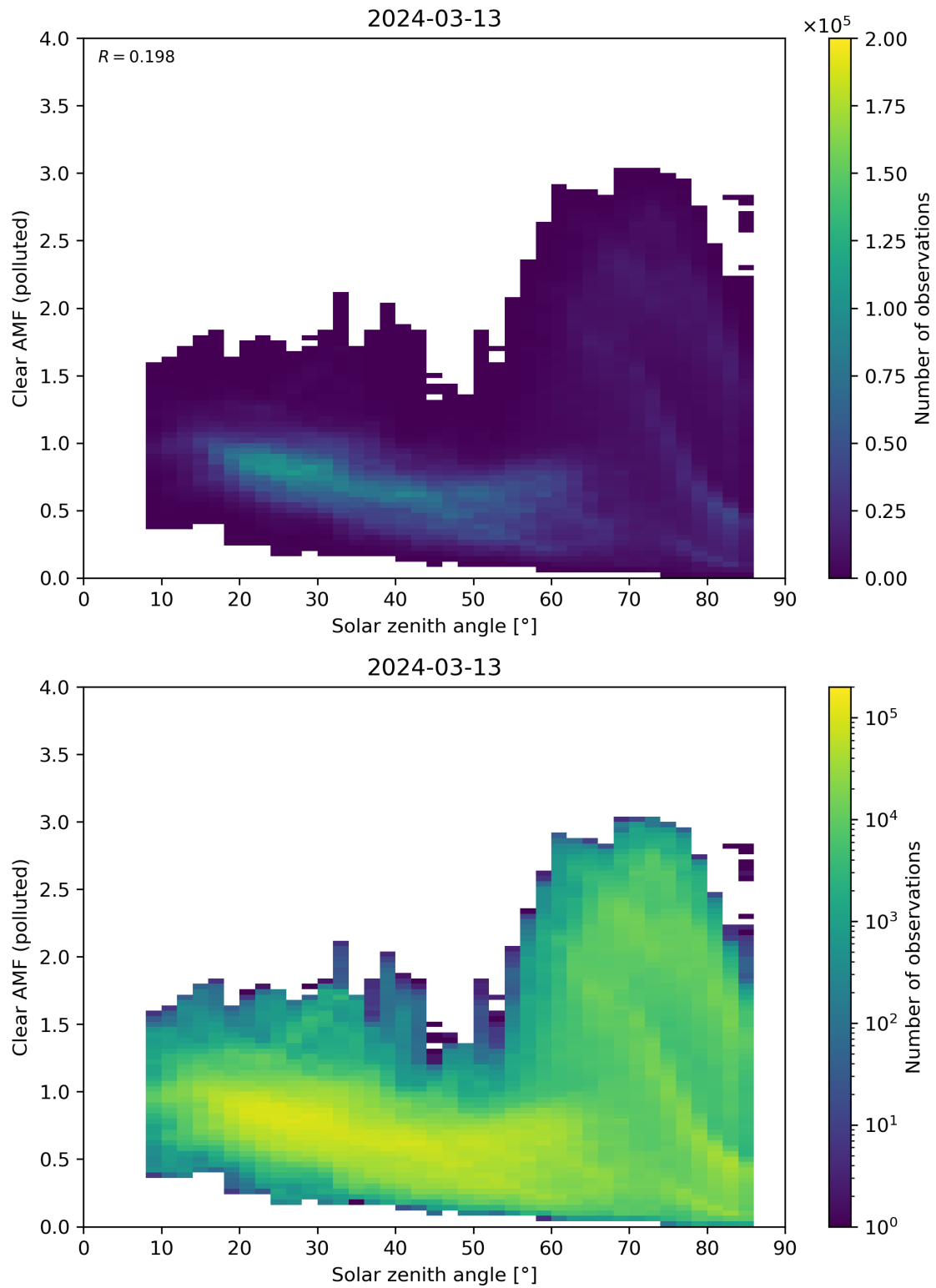
Figure 165: Scatter density plot of “Solar zenith angle” against “Clear AMF (polluted)” for 2024-03-12 to 2024-03-14.
