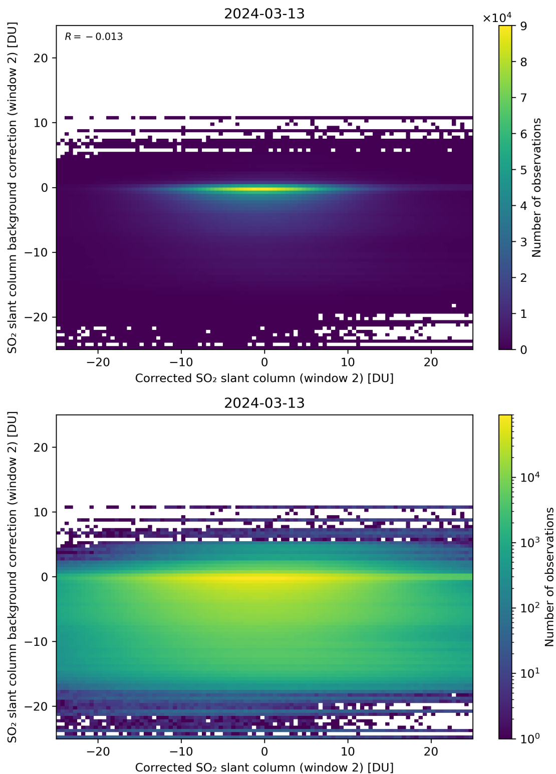
Figure 194: Scatter density plot of “Corrected SO 2 slant column (window 2)” against “SO 2 slant column background correction (window 2)” for 2024-03-12 to 2024-03-14.
