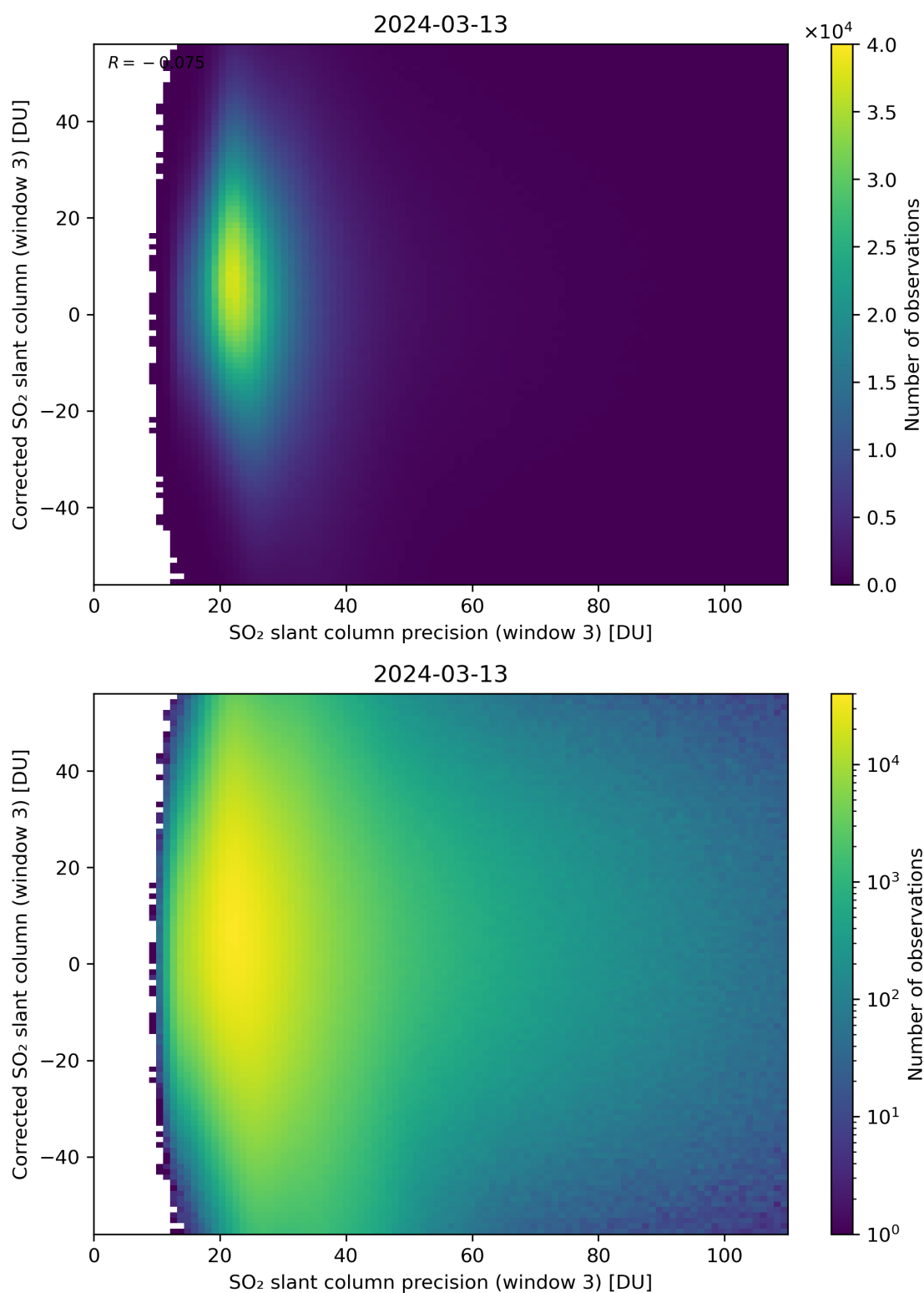
Figure 262: Scatter density plot of “SO 2 slant column precision (window 3)” against “Corrected SO 2 slant column (window 3)” for 2024-03-12 to 2024-03-14.
