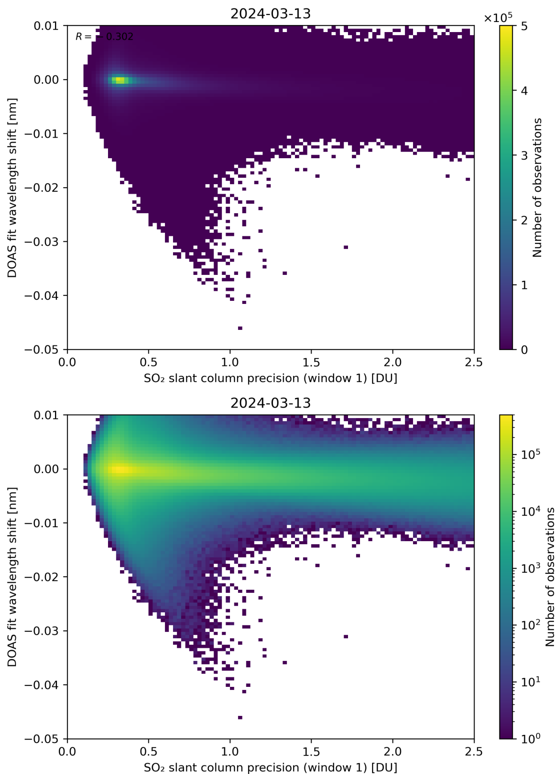
Figure 221: Scatter density plot of “SO 2 slant column precision (window 1)” against “DOAS fit wavelength shift” for 2024-03-12 to 2024-03-14.
