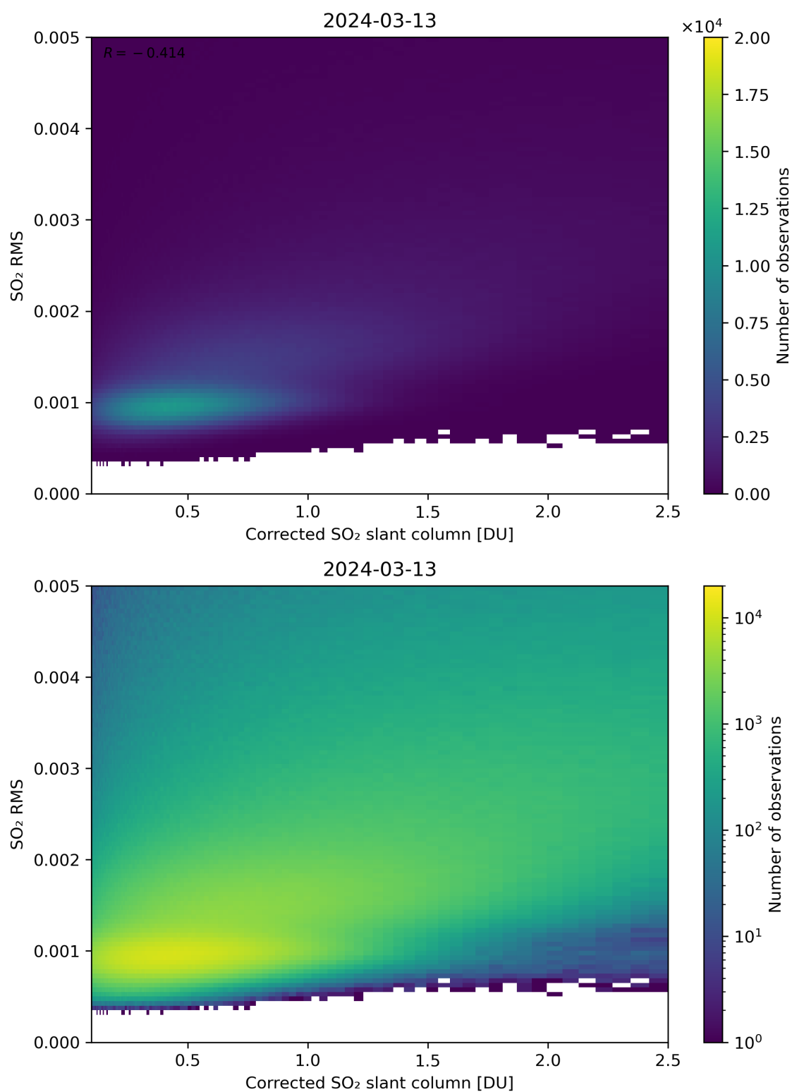
Figure 183: Scatter density plot of “Corrected SO 2 slant column” against “SO 2 RMS” for 2024-03-12 to 2024-03-14.
