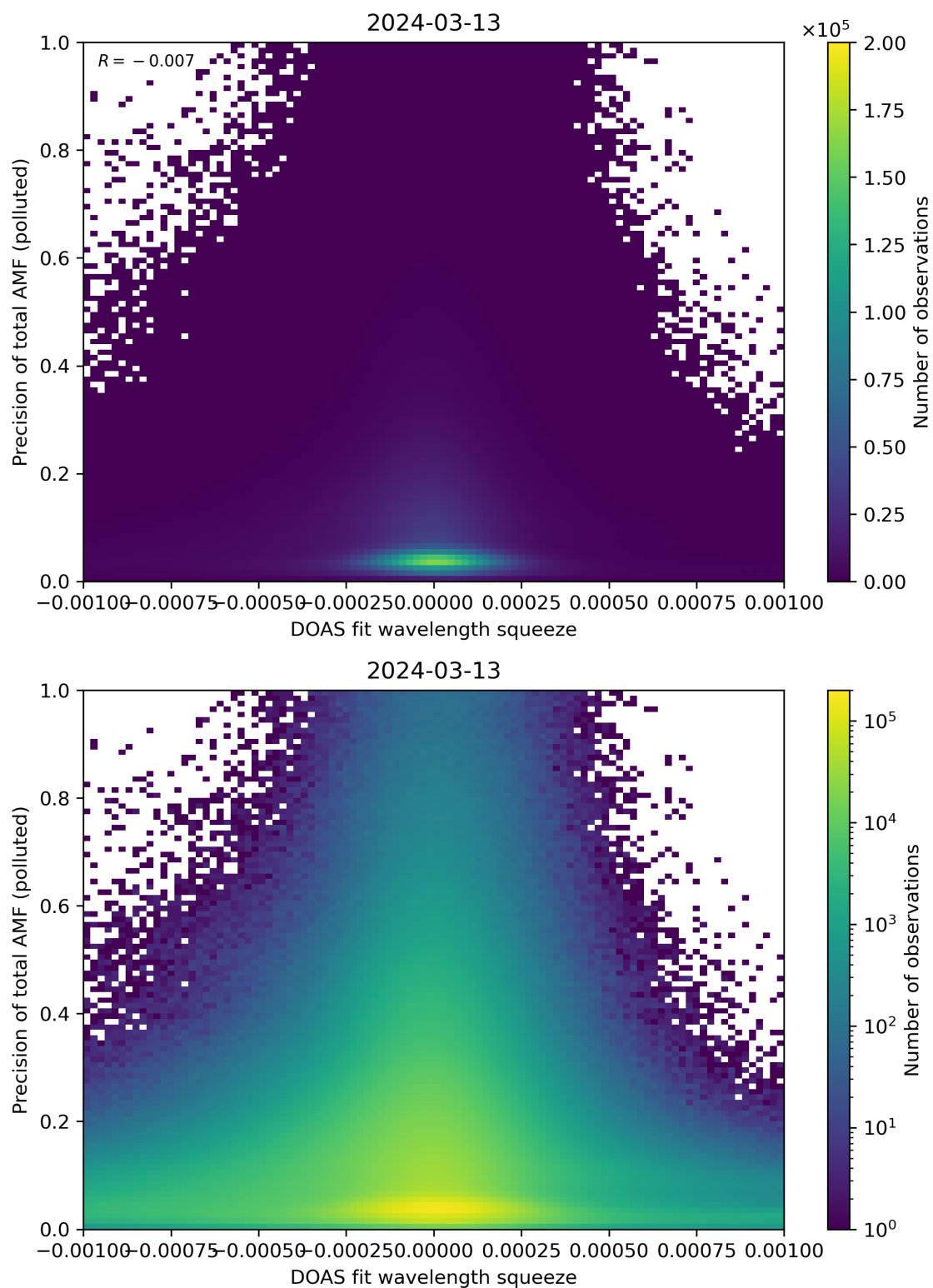
Figure 135: Scatter density plot of “DOAS fit wavelength squeeze” against “Precision of total AMF (polluted)” for 2024-03-12 to 2024-03-14.
