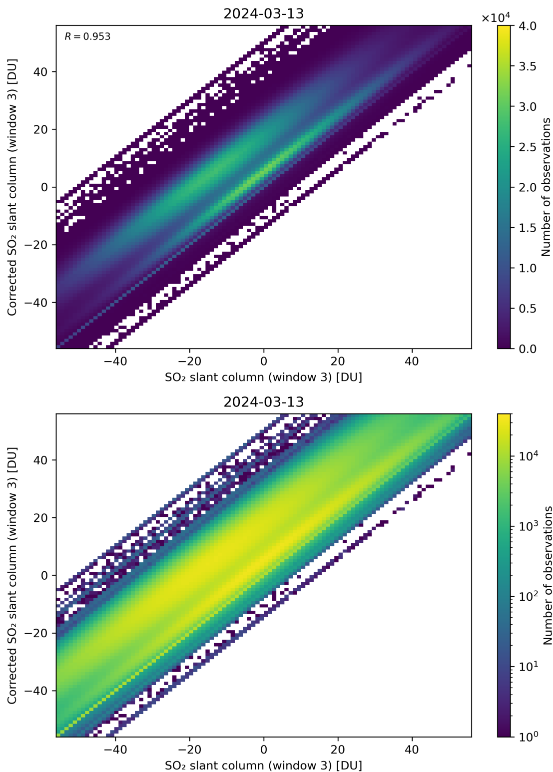
Figure 266: Scatter density plot of “SO 2 slant column (window 3)” against “Corrected SO 2 slant column (window 3)” for 2024-03-12 to 2024-03-14.
