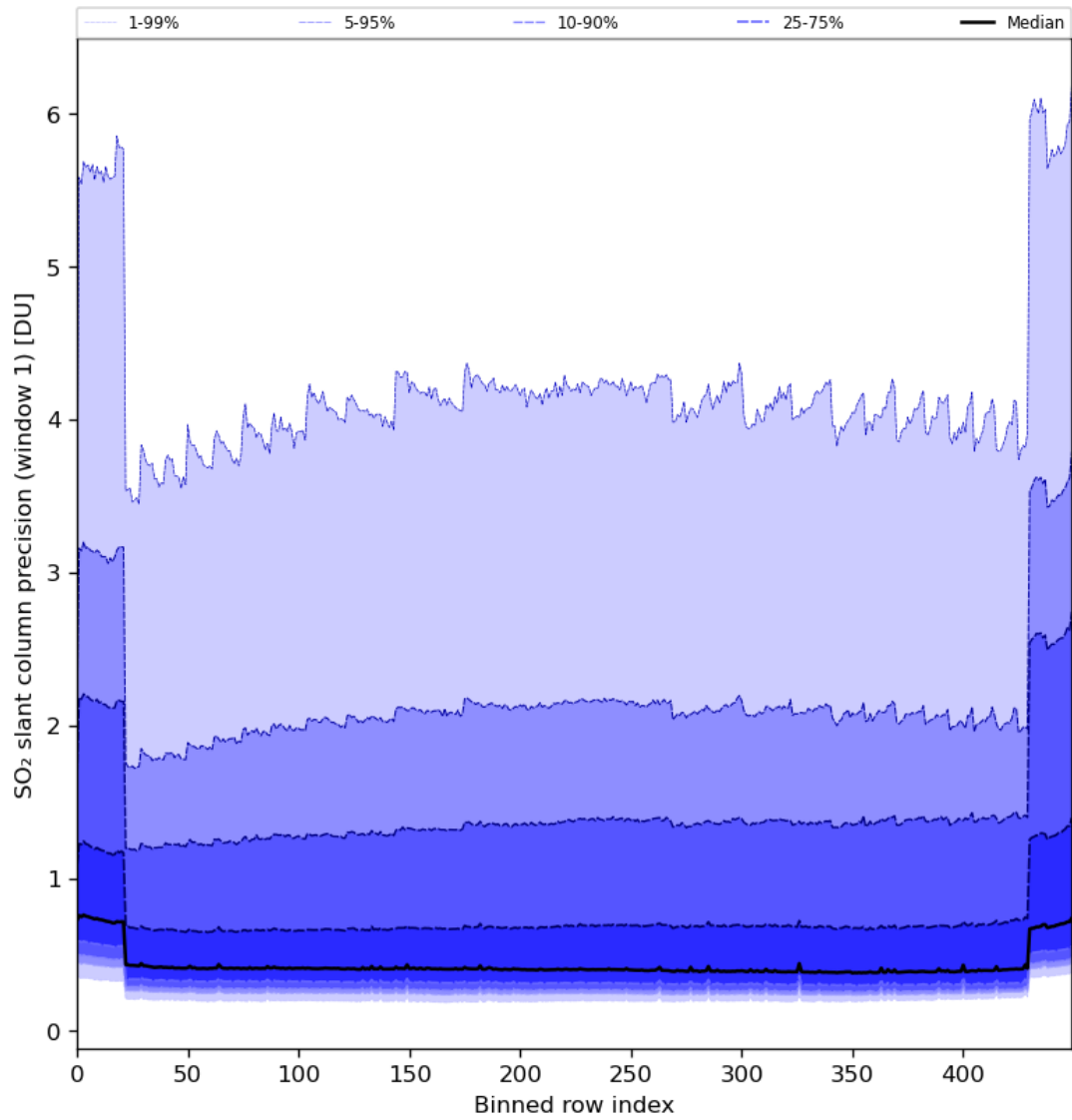
Figure 80: Along track statistics of “SO 2 slant column precision (window 1)” for 2024-03-12 to 2024-03-14
