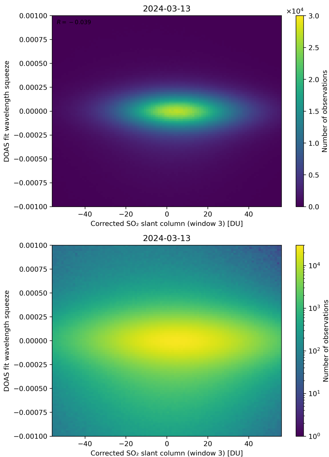
Figure 207: Scatter density plot of “Corrected SO 2 slant column (window 3)” against “DOAS fit wavelength squeeze” for 2024-03-12 to 2024-03-14.
