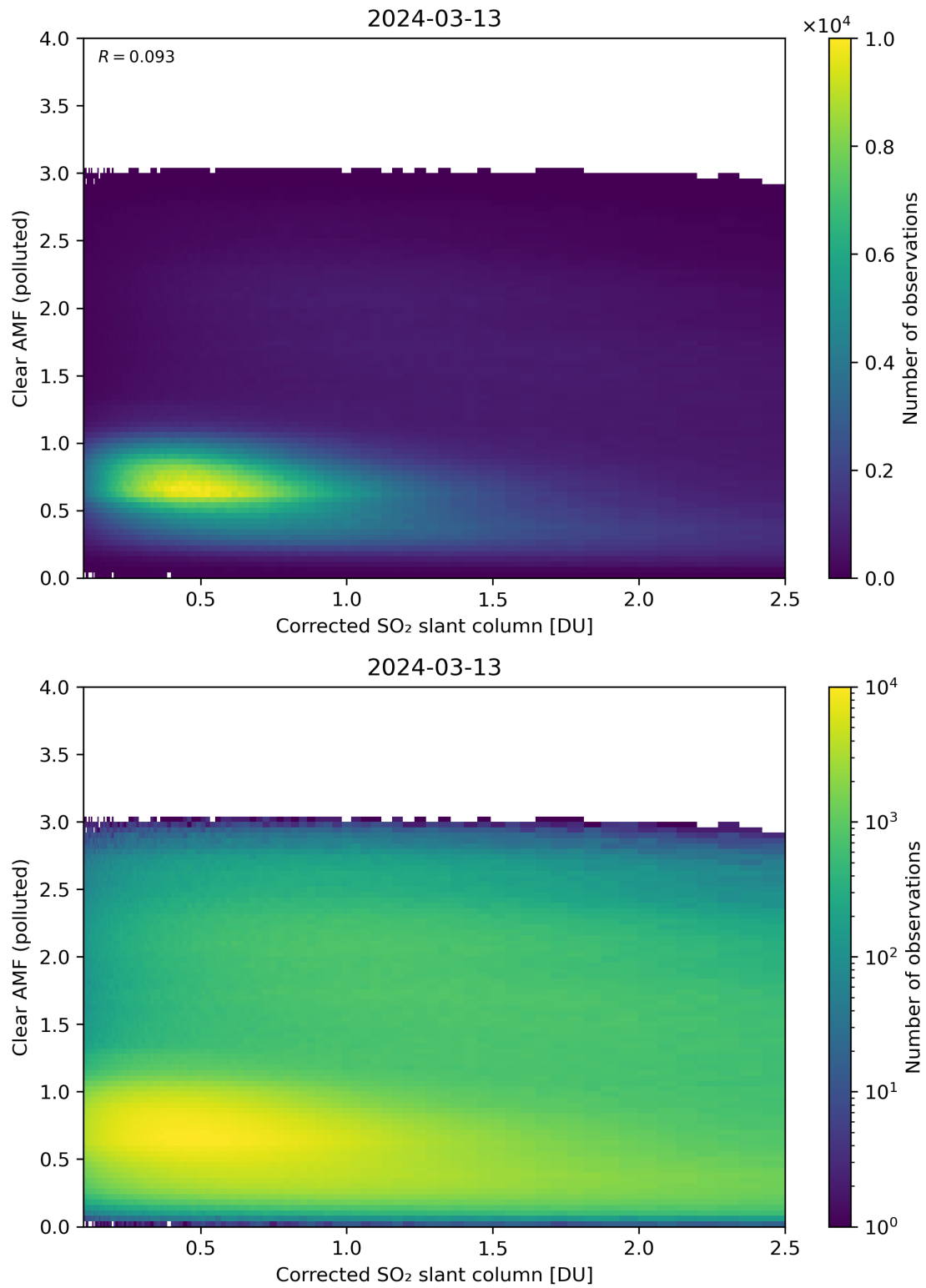
Figure 184: Scatter density plot of “Corrected SO 2 slant column” against “Clear AMF (polluted)” for 2024-03-12 to 2024-03-14.
