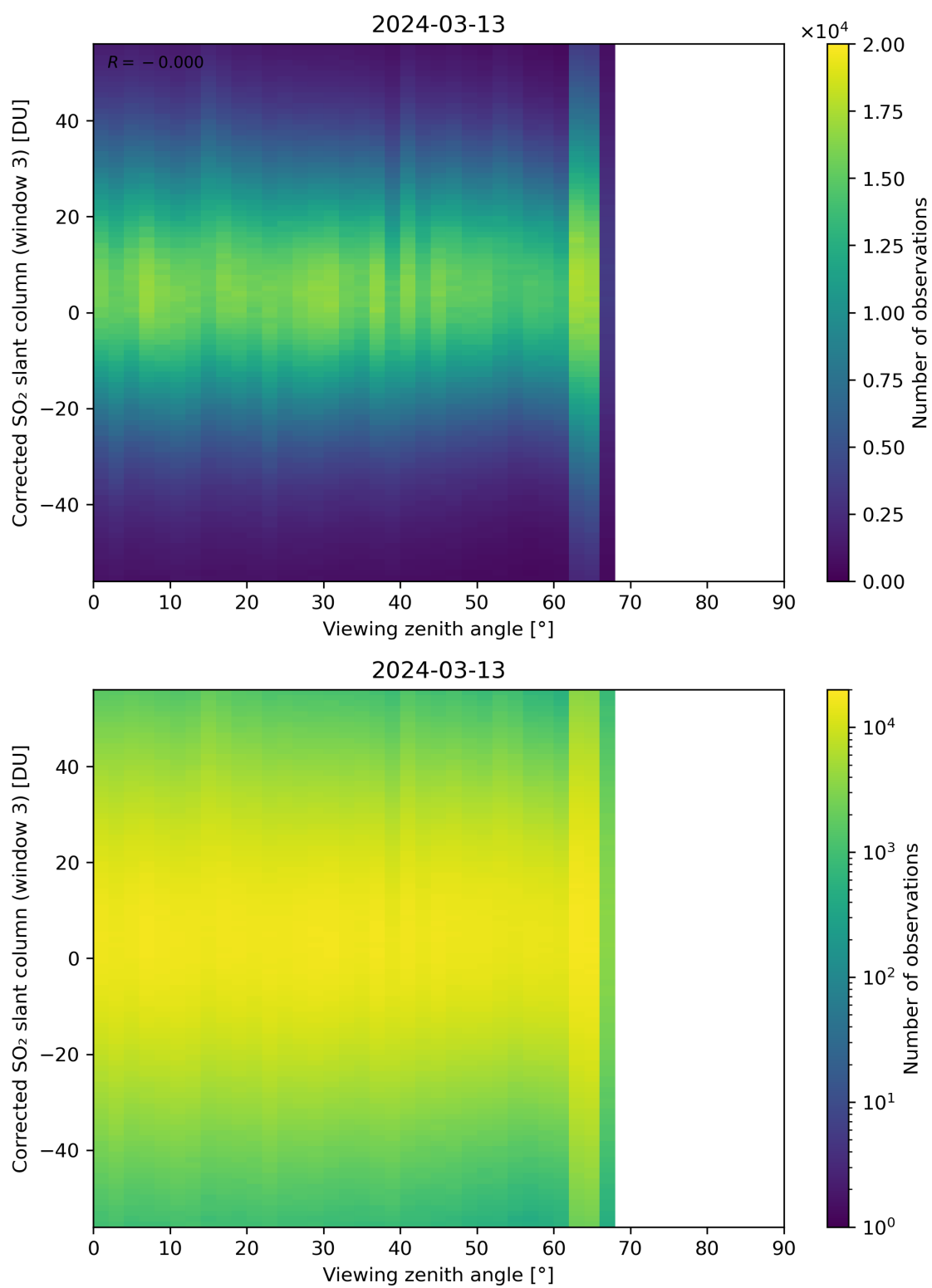
Figure 319: Scatter density plot of “Viewing zenith angle” against “Corrected SO 2 slant column (window 3)” for 2024-03-12 to 2024-03-14.
