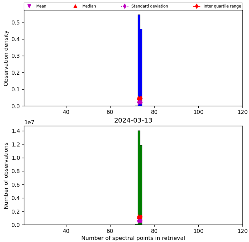
Figure 74: Histogram of “Number of spectral points in retrieval” for 2024-03-12 to 2024-03-14
