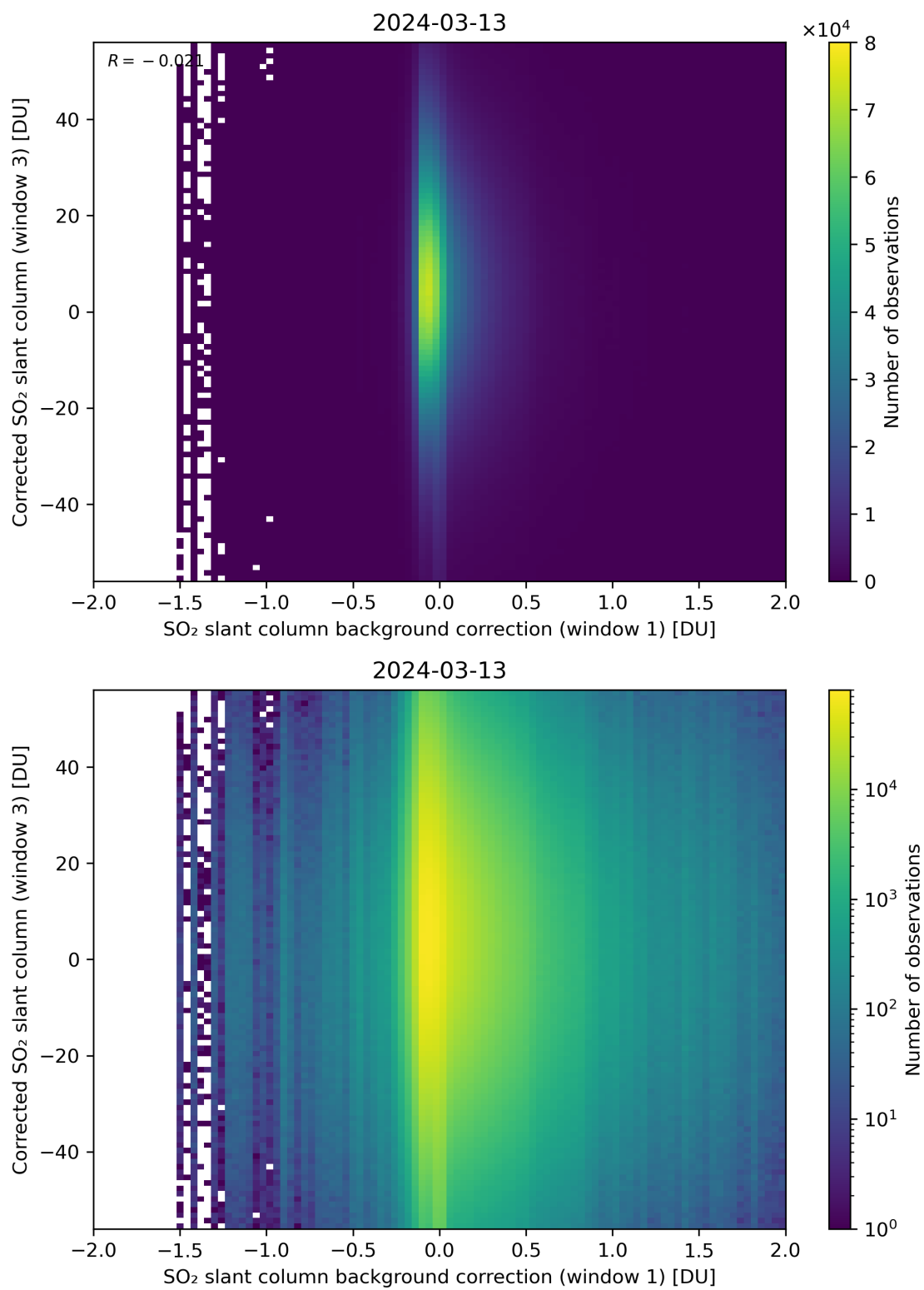
Figure 105: Scatter density plot of “SO 2 slant column background correction (window 1)” against “Corrected SO 2 slant column (window 3)” for 2024-03-12 to 2024-03-14.
