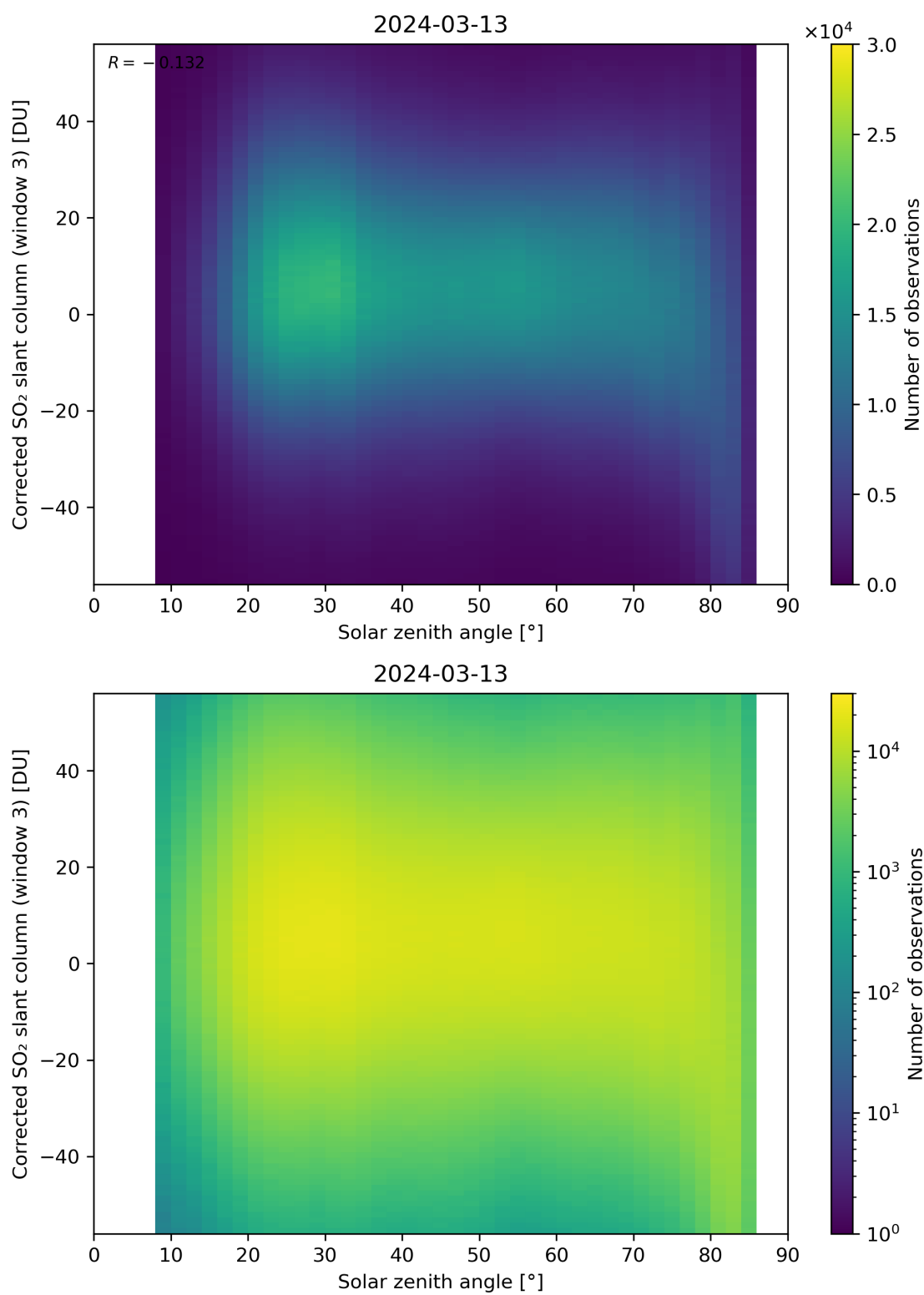
Figure 168: Scatter density plot of “Solar zenith angle” against “Corrected SO 2 slant column (window 3)” for 2024-03-12 to 2024-03-14.
