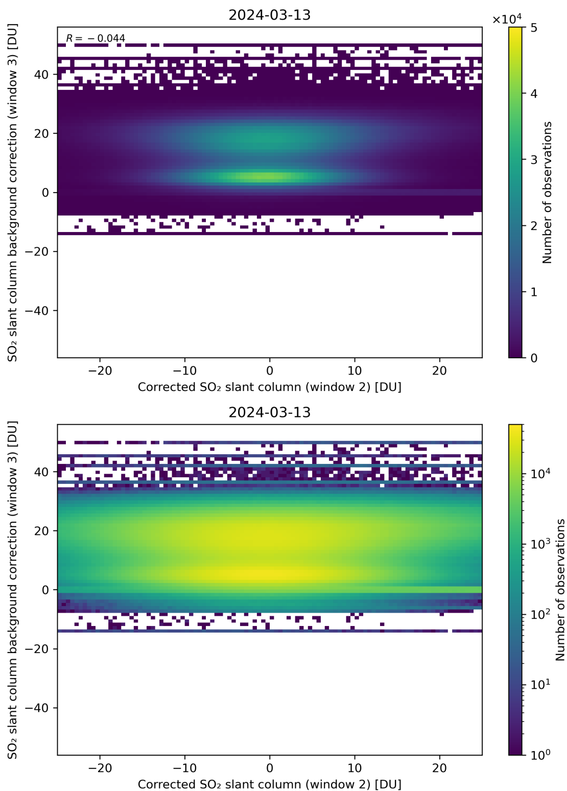
Figure 195: Scatter density plot of “Corrected SO 2 slant column (window 2)” against “SO 2 slant column background correction (window 3)” for 2024-03-12 to 2024-03-14.
