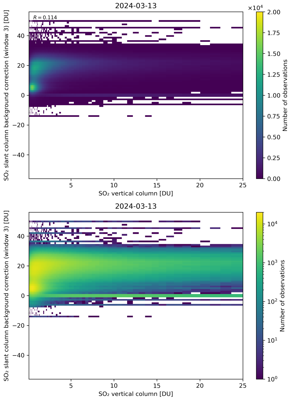
Figure 275: Scatter density plot of “SO 2 vertical column” against “SO 2 slant column background correction (window 3)” for 2024-03-12 to 2024-03-14.
