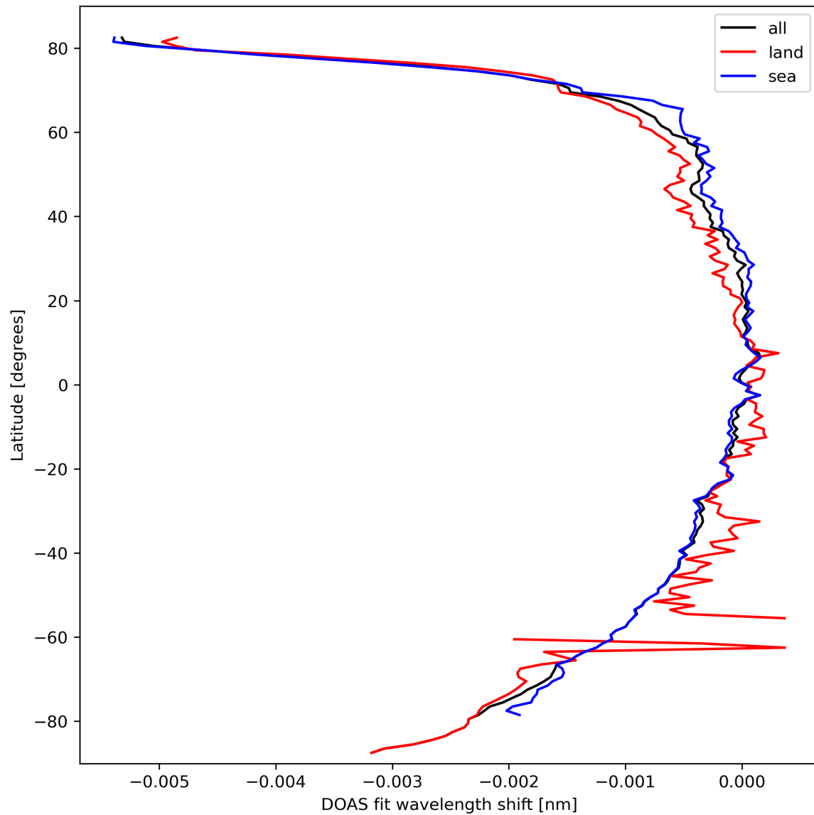
Figure 45: Zonal average of “DOAS fit wavelength shift” for 2024-03-12 to 2024-03-14.
