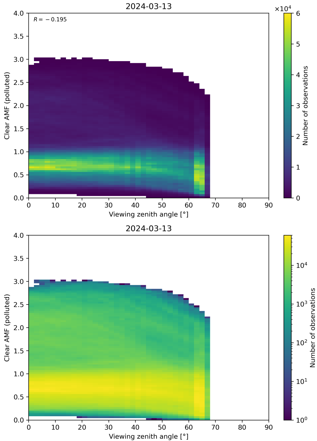
Figure 316: Scatter density plot of “Viewing zenith angle” against “Clear AMF (polluted)” for 2024-03-12 to 2024-03-14.
