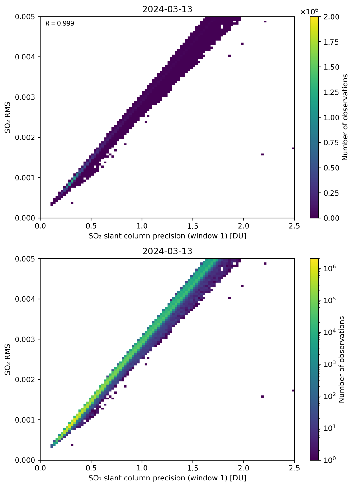
Figure 223: Scatter density plot of “SO 2 slant column precision (window 1)” against “SO 2 RMS” for 2024-03-12 to 2024-03-14.
