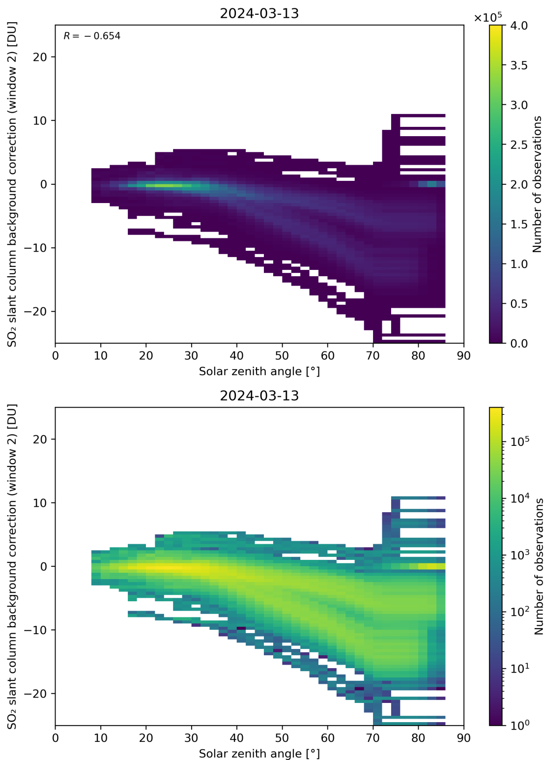
Figure 159: Scatter density plot of “Solar zenith angle” against “SO 2 slant column background correction (window 2)” for 2024-03-12 to 2024-03-14.
