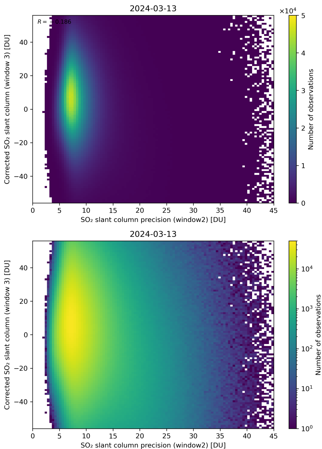
Figure 248: Scatter density plot of “SO 2 slant column precision (window2)” against “Corrected SO 2 slant column (window 3)” for 2024-03-12 to 2024-03-14.
