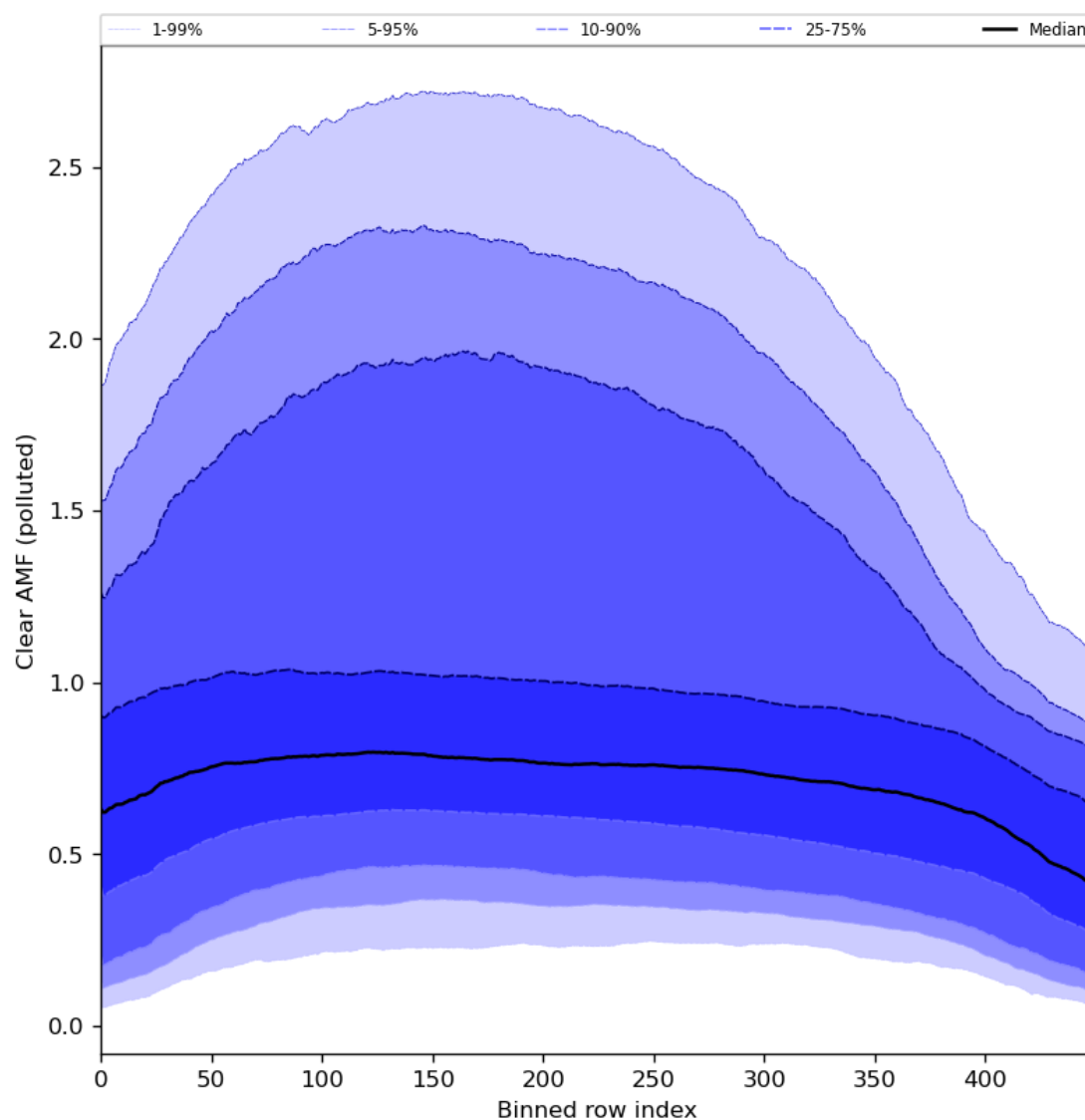
Figure 96: Along track statistics of “Clear AMF (polluted)” for 2024-03-12 to 2024-03-14
