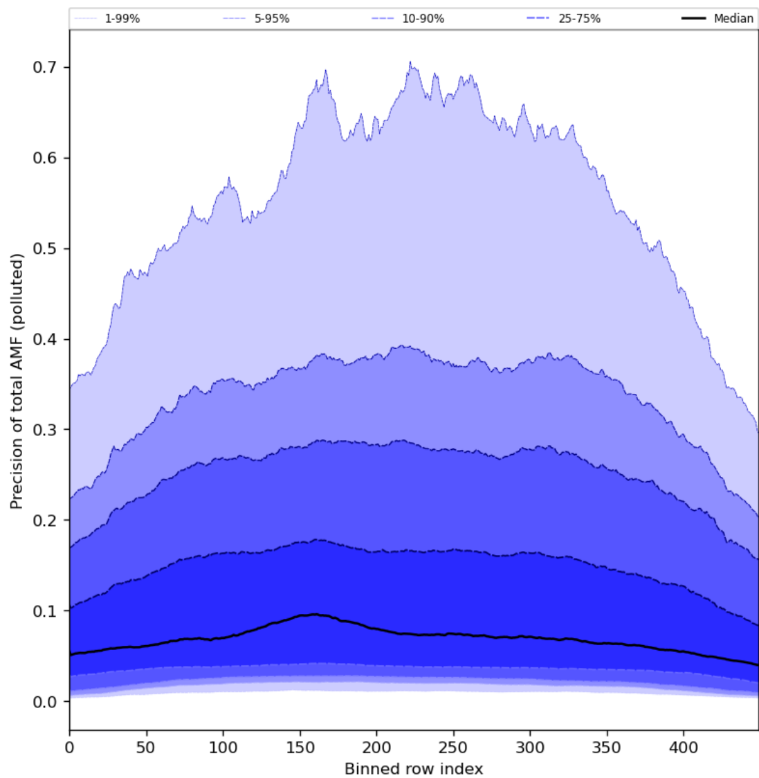
Figure 95: Along track statistics of “Precision of total AMF (polluted)” for 2024-03-12 to 2024-03-14
