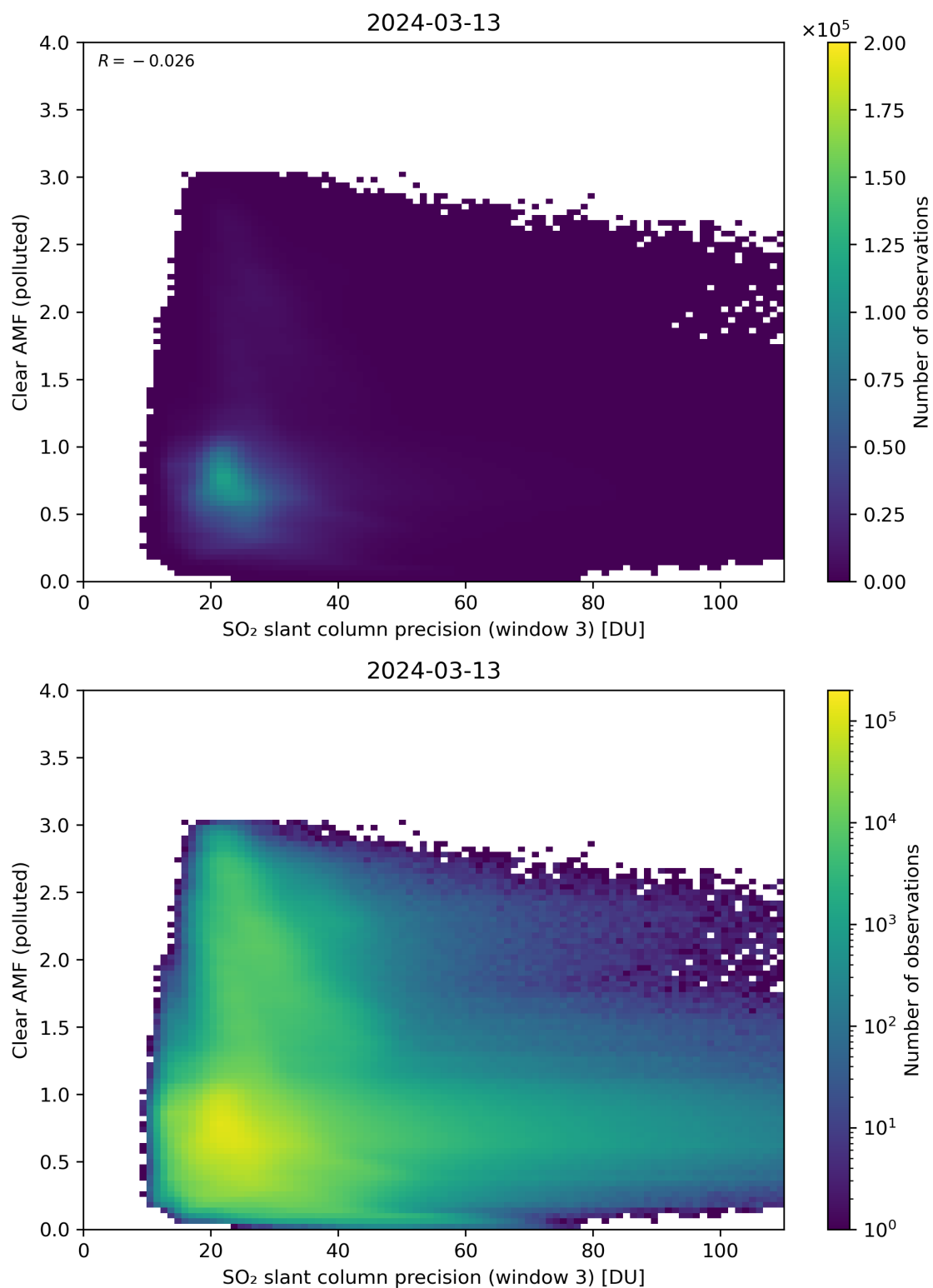
Figure 261: Scatter density plot of “SO 2 slant column precision (window 3)” against “Clear AMF (polluted)” for 2024-03-12 to 2024-03-14.
