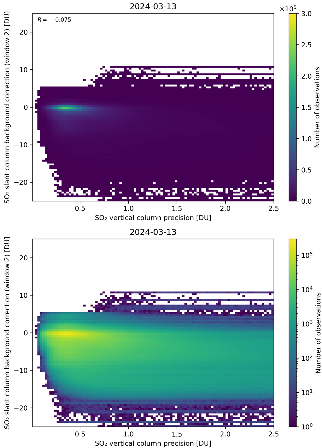
Figure 280: Scatter density plot of “SO 2 vertical column precision” against “SO 2 slant column background correction (window 2)” for 2024-03-12 to 2024-03-14.
