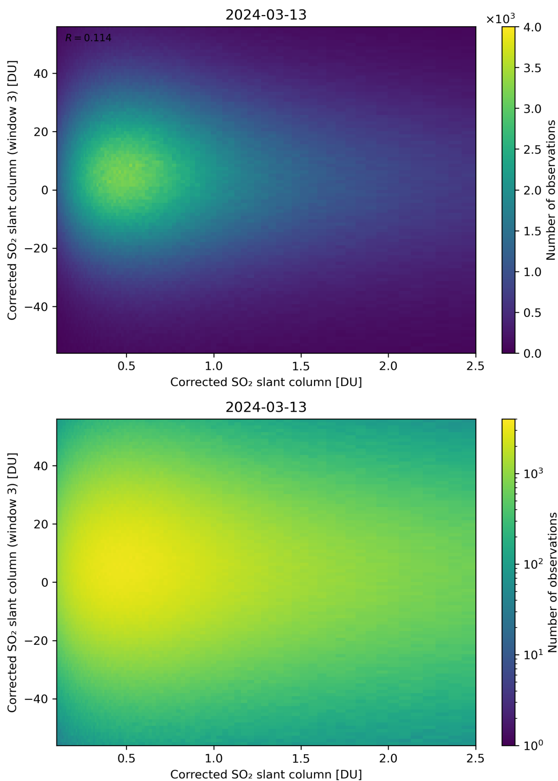
Figure 186: Scatter density plot of “Corrected SO 2 slant column” against “Corrected SO 2 slant column (window 3)” for 2024-03-12 to 2024-03-14.
