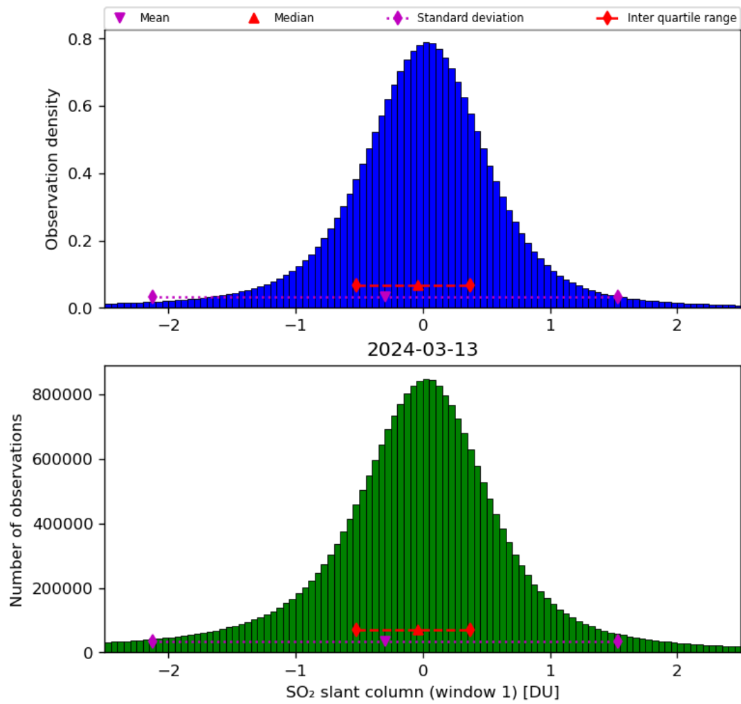
Figure 56: Histogram of “SO 2 slant column (window 1)” for 2024-03-12 to 2024-03-14
