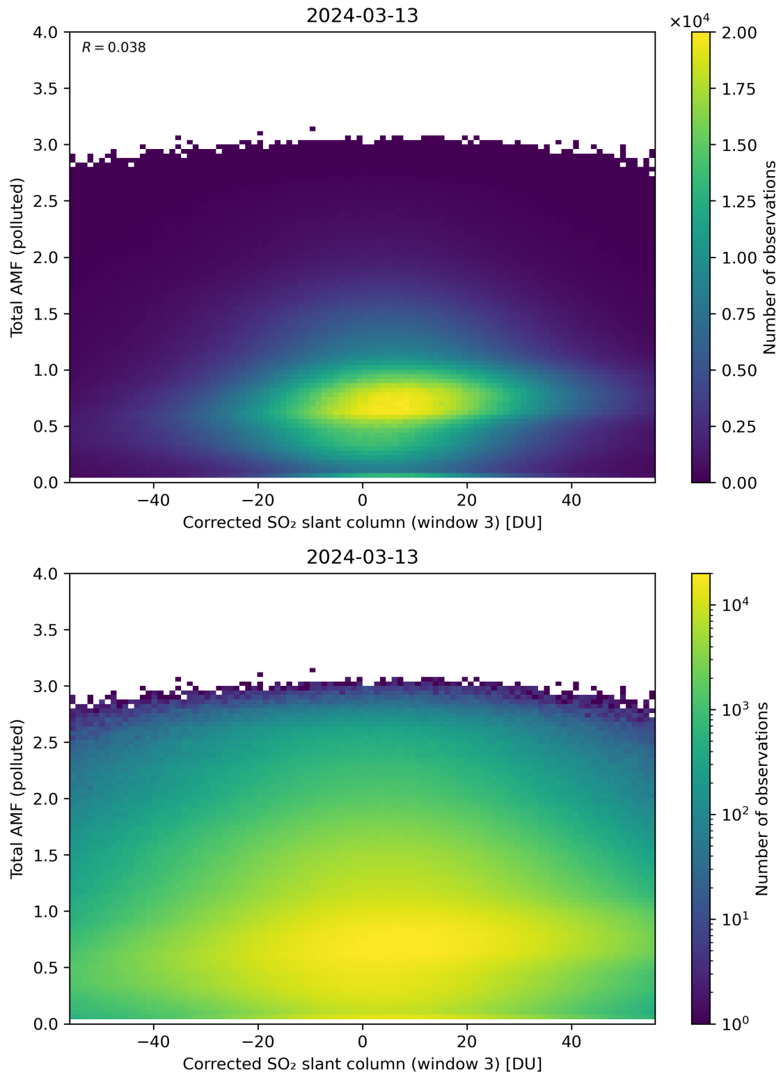
Figure 210: Scatter density plot of “Corrected SO 2 slant column (window 3)” against “Total AMF (polluted)” for 2024-03-12 to 2024-03-14.
