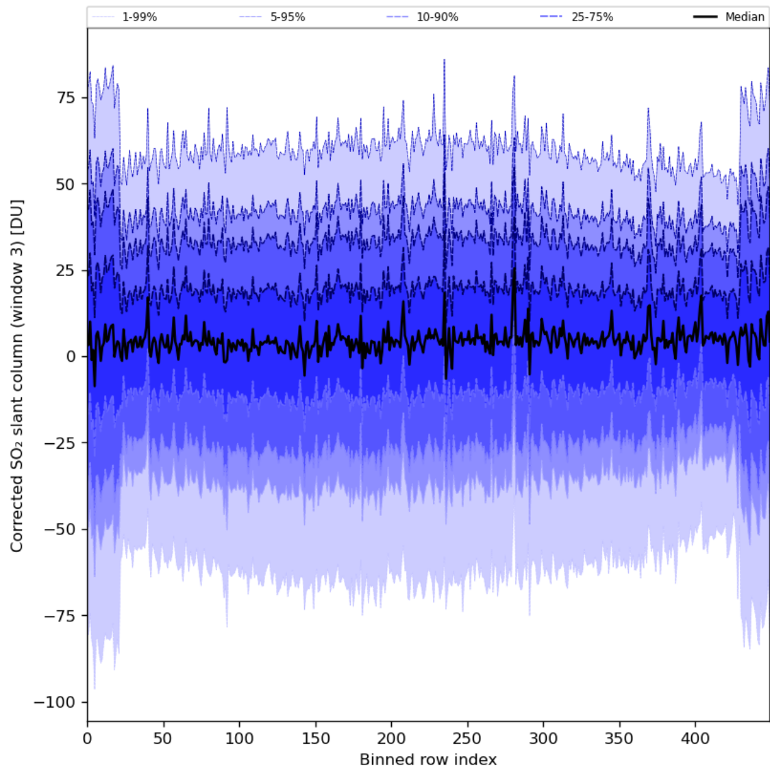
Figure 89: Along track statistics of “Corrected SO 2 slant column (window 3)” for 2024-03-12 to 2024-03-14
