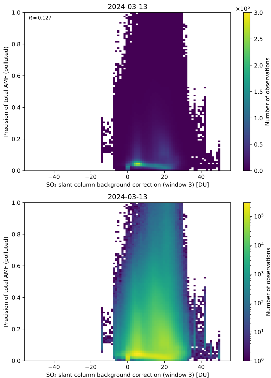
Figure 126: Scatter density plot of “SO 2 slant column background correction (window 3)” against “Precision of total AMF (polluted)” for 2024-03-12 to 2024-03-14.
