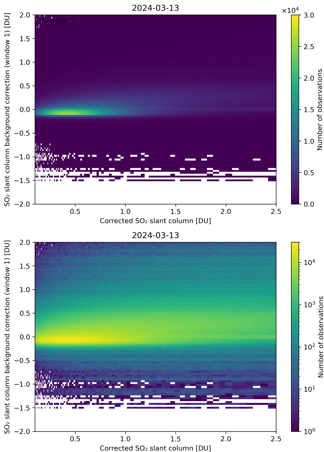
Figure 178: Scatter density plot of “Corrected SO 2 slant column” against “SO 2 slant column background correction (window 1)” for 2024-03-12 to 2024-03-14.
