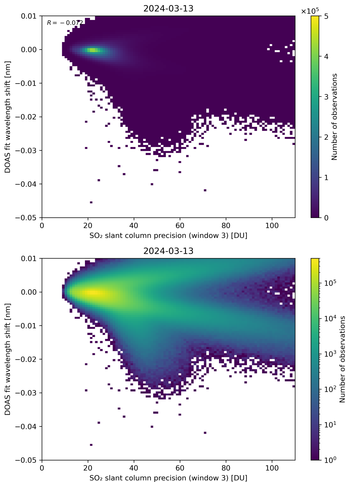
Figure 258: Scatter density plot of “SO 2 slant column precision (window 3)” against “DOAS fit wavelength shift” for 2024-03-12 to 2024-03-14.
