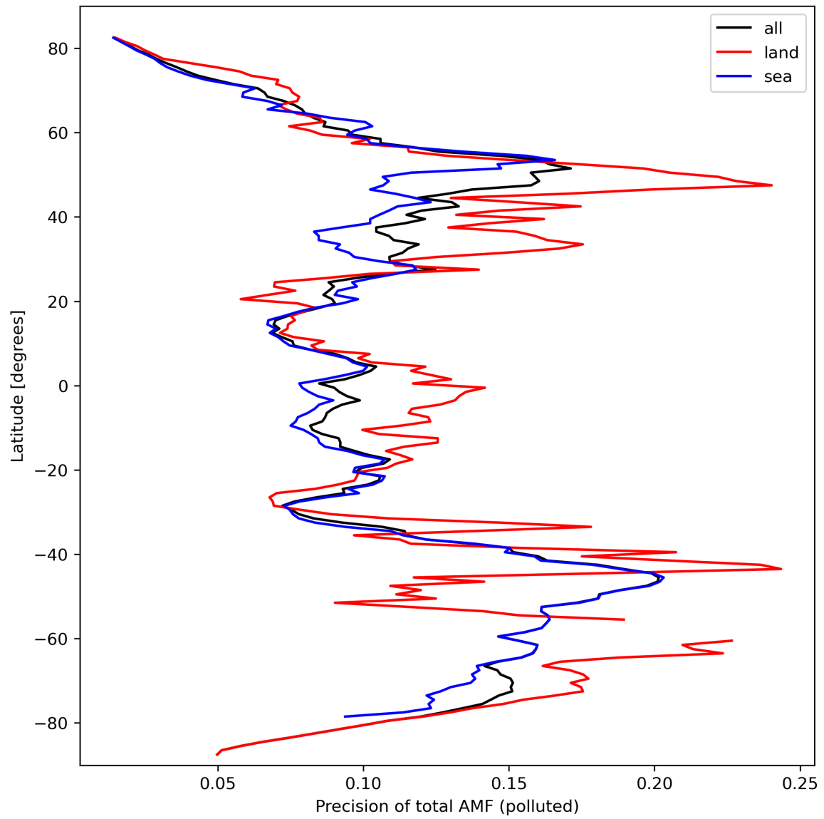
Figure 49: Zonal average of “Precision of total AMF (polluted)” for 2024-03-12 to 2024-03-14.
