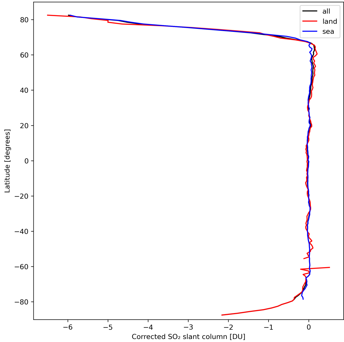
Figure 32: Zonal average of “Corrected SO 2 slant column” for 2024-03-12 to 2024-03-14.
