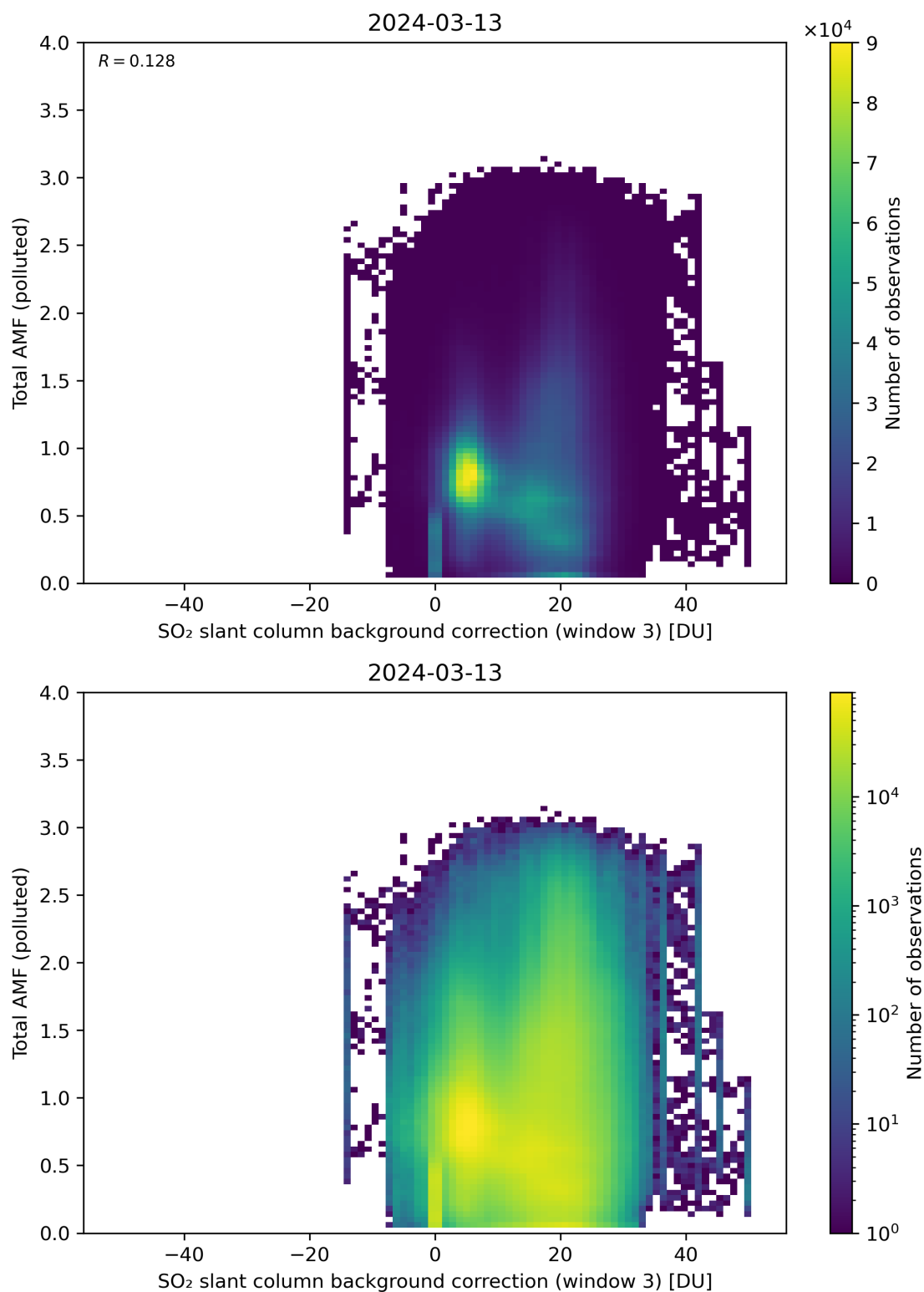
Figure 125: Scatter density plot of “SO 2 slant column background correction (window 3)” against “Total AMF (polluted)” for 2024-03-12 to 2024-03-14.
