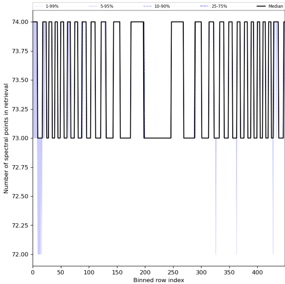
Figure 97: Along track statistics of “Number of spectral points in retrieval” for 2024-03-12 to 2024-03-14
