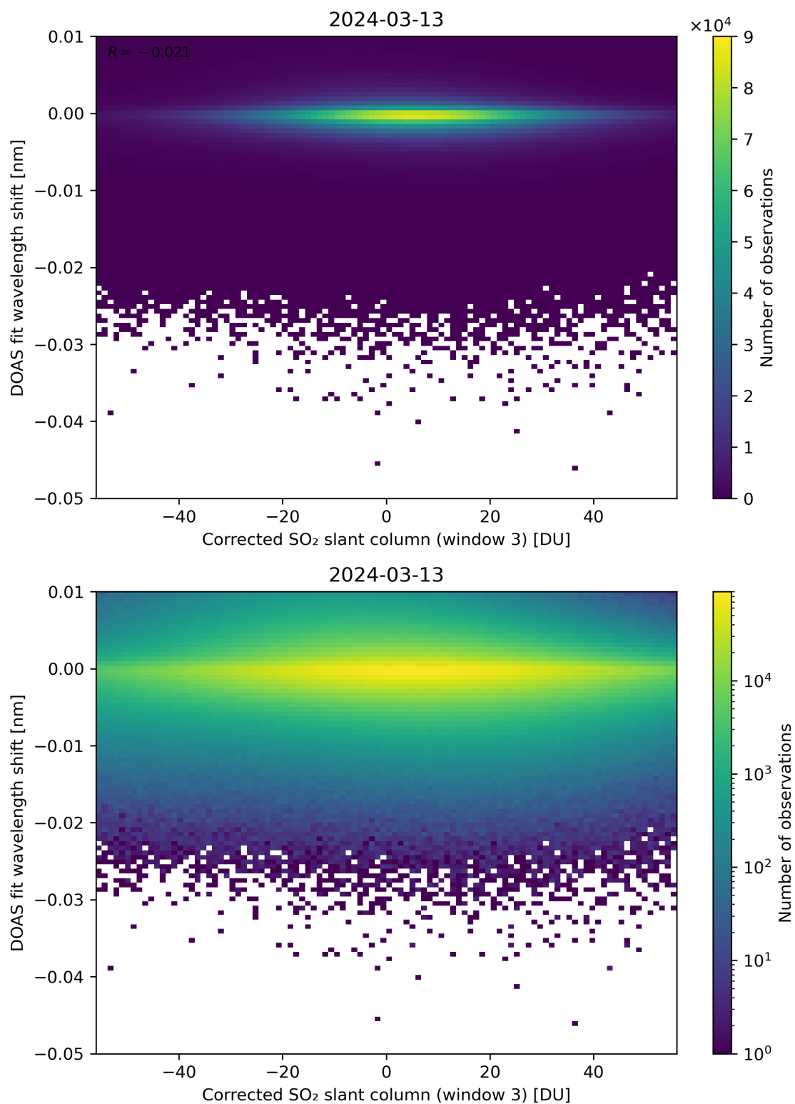
Figure 206: Scatter density plot of “Corrected SO 2 slant column (window 3)” against “DOAS fit wavelength shift” for 2024-03-12 to 2024-03-14.
