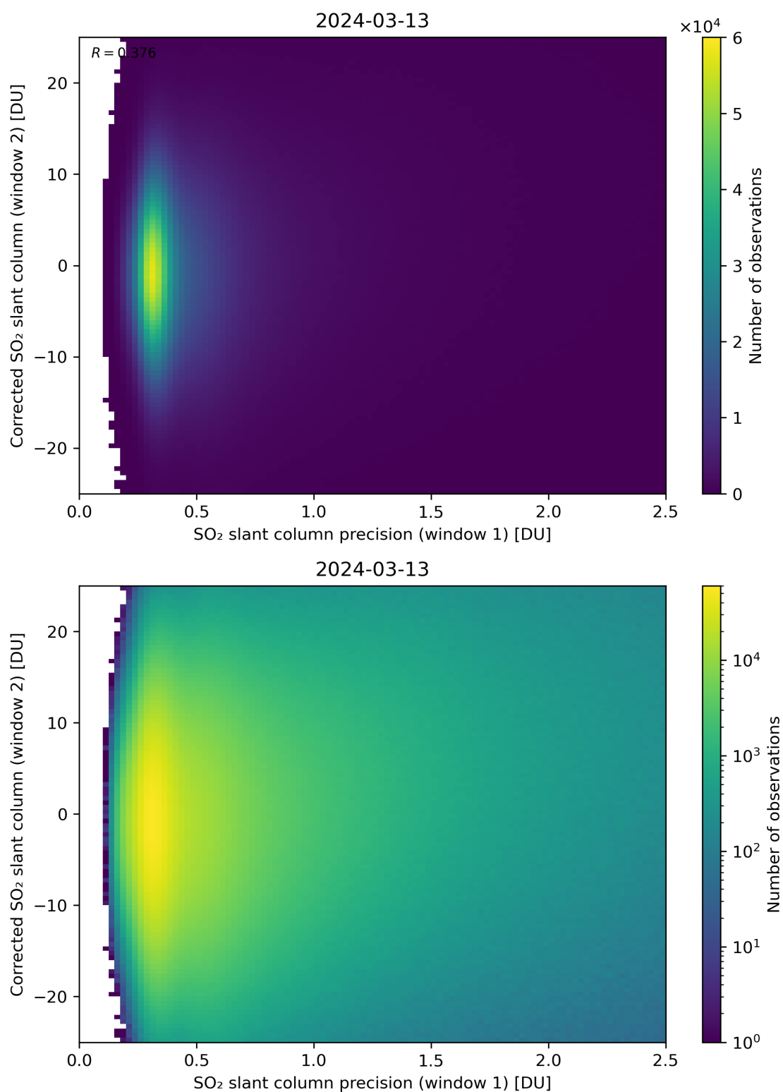
Figure 225: Scatter density plot of “SO 2 slant column precision (window 1)” against “Corrected SO 2 slant column (window 2)” for 2024-03-12 to 2024-03-14.
