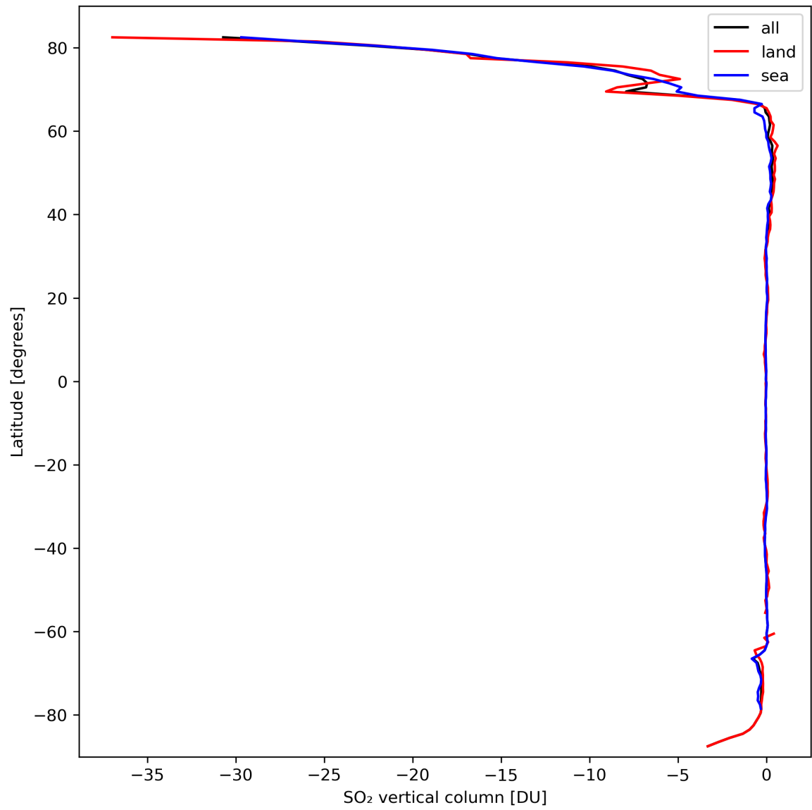
Figure 30: Zonal average of “SO 2 vertical column” for 2024-03-12 to 2024-03-14.
