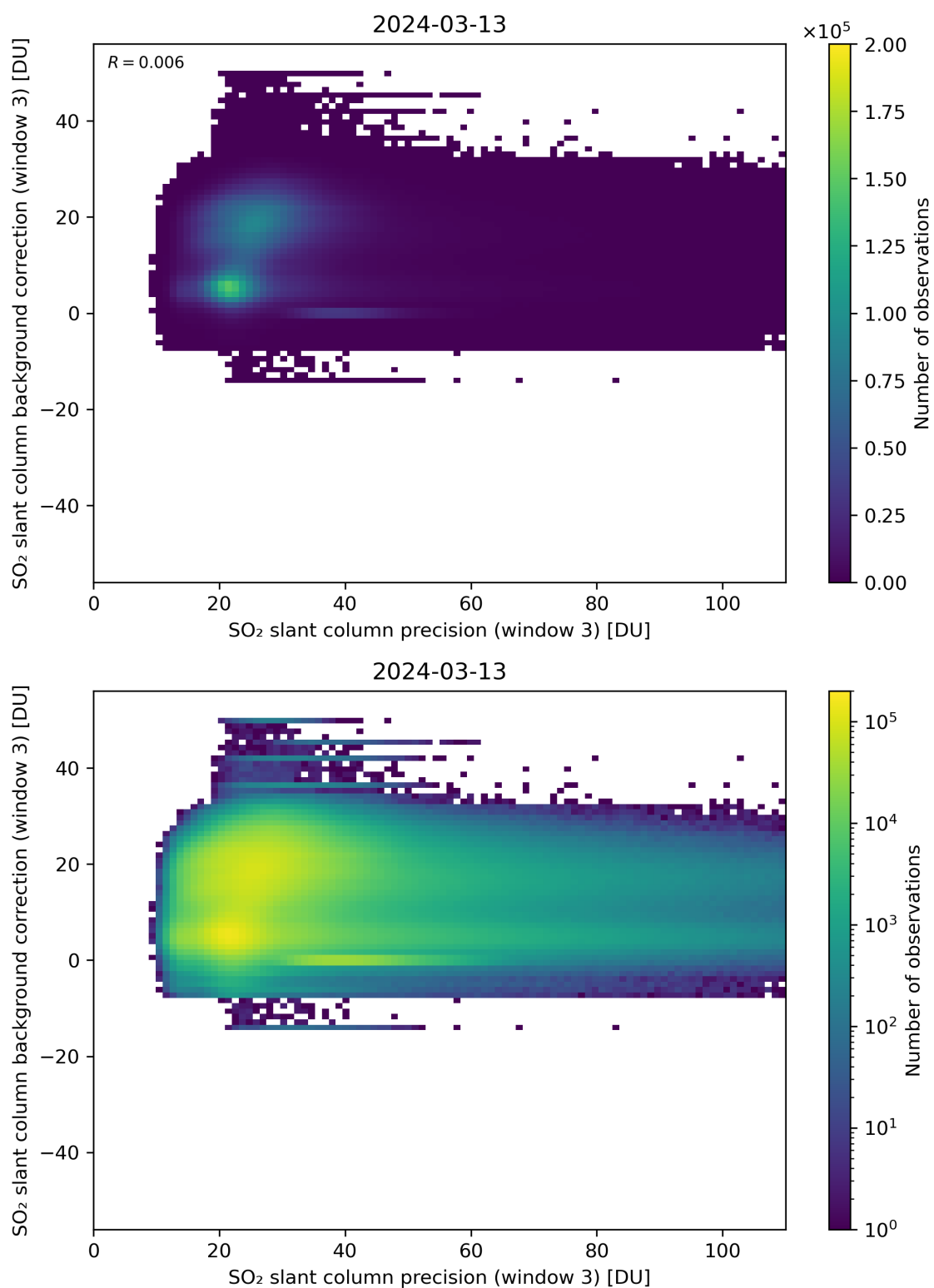
Figure 257: Scatter density plot of “SO 2 slant column precision (window 3)” against “SO 2 slant column background correction (window 3)” for 2024-03-12 to 2024-03-14.
