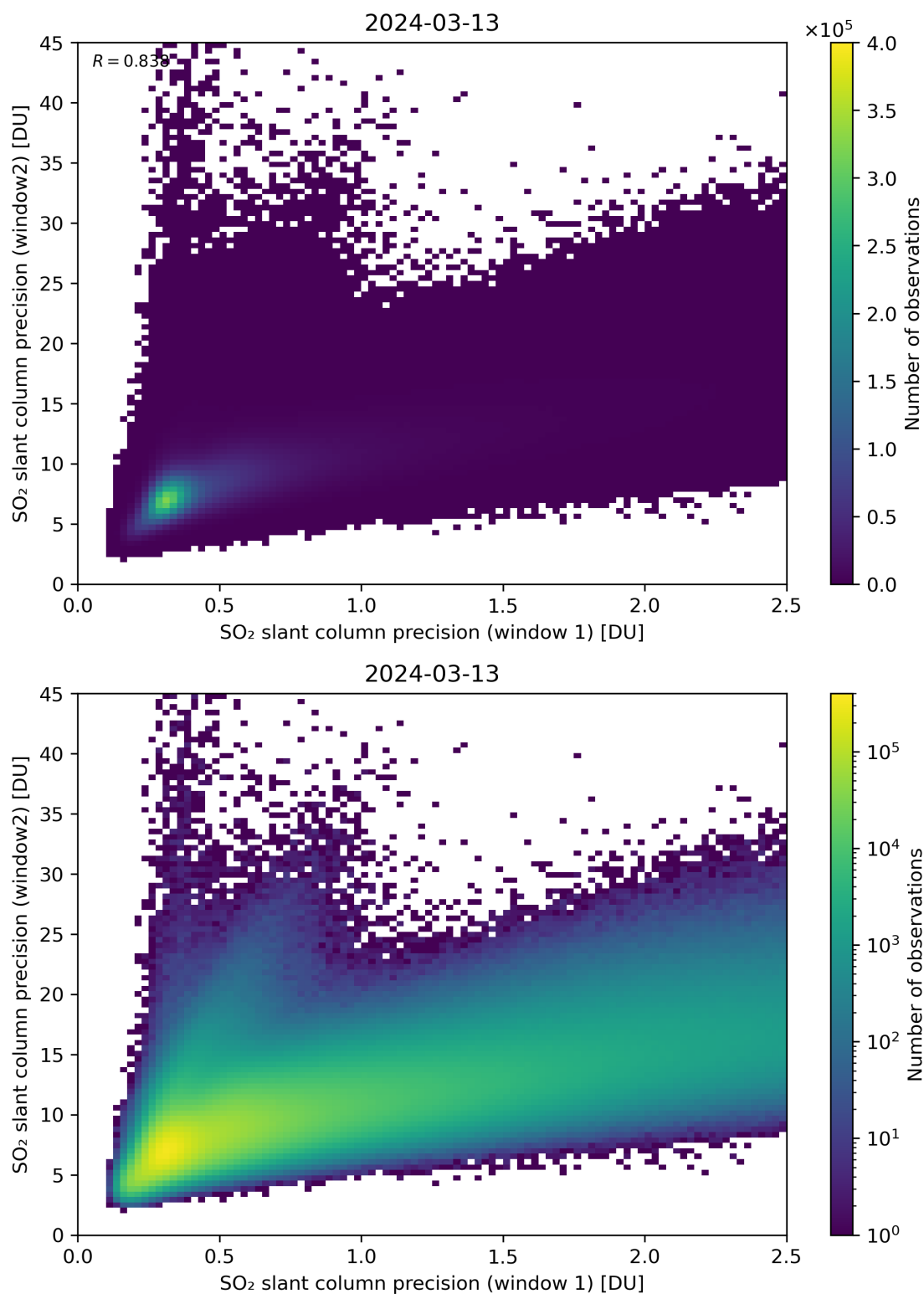
Figure 227: Scatter density plot of “SO 2 slant column precision (window 1)” against “SO 2 slant column precision (window2)” for 2024-03-12 to 2024-03-14.
