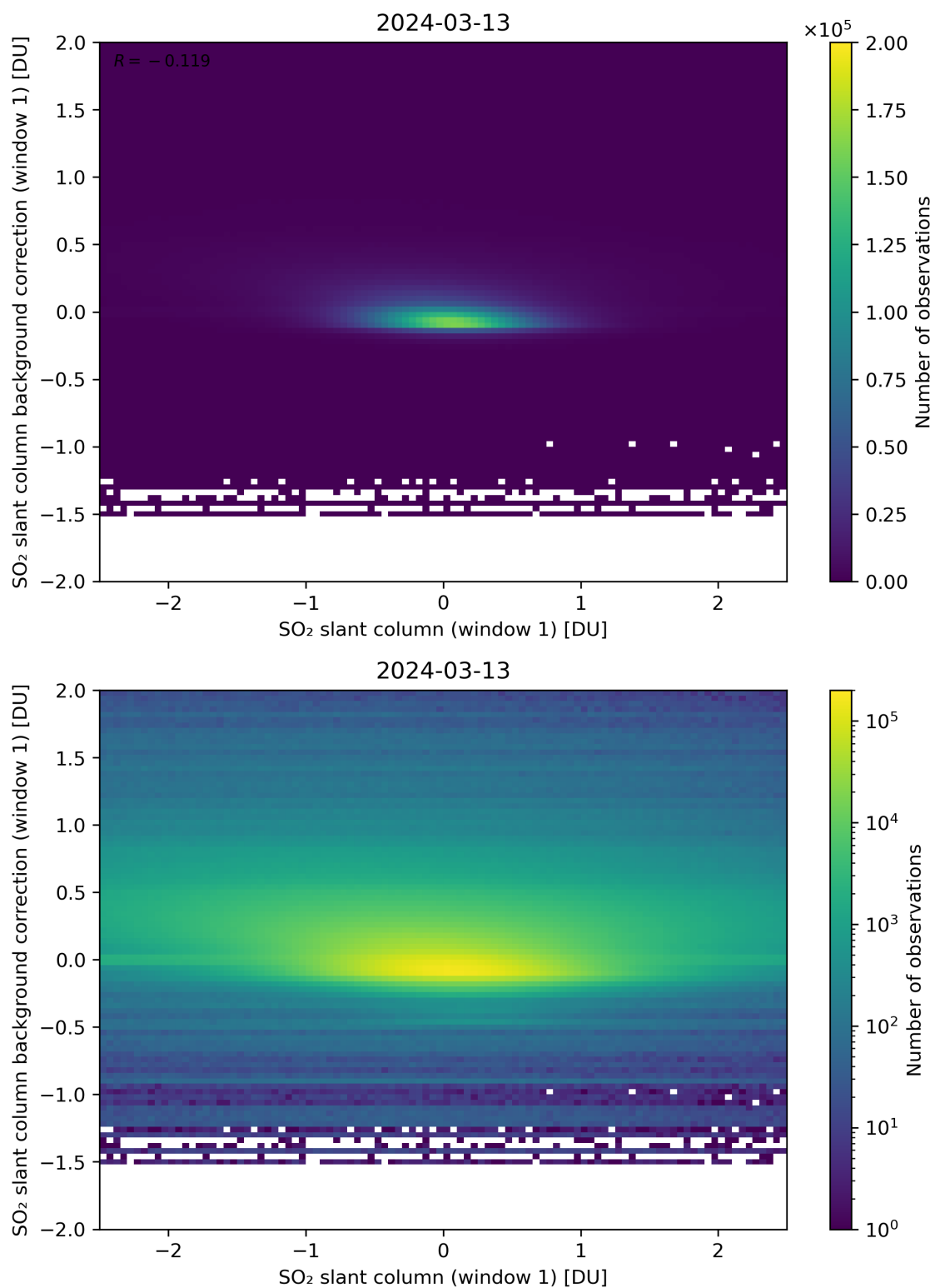
Figure 212: Scatter density plot of “SO 2 slant column (window 1)” against “SO 2 slant column background correction (window 1)” for 2024-03-12 to 2024-03-14.
