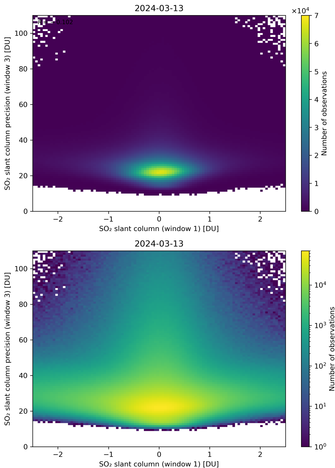
Figure 238: Scatter density plot of “SO 2 slant column (window 1)” against “SO 2 slant column precision (window 3)” for 2024-03-12 to 2024-03-14.
