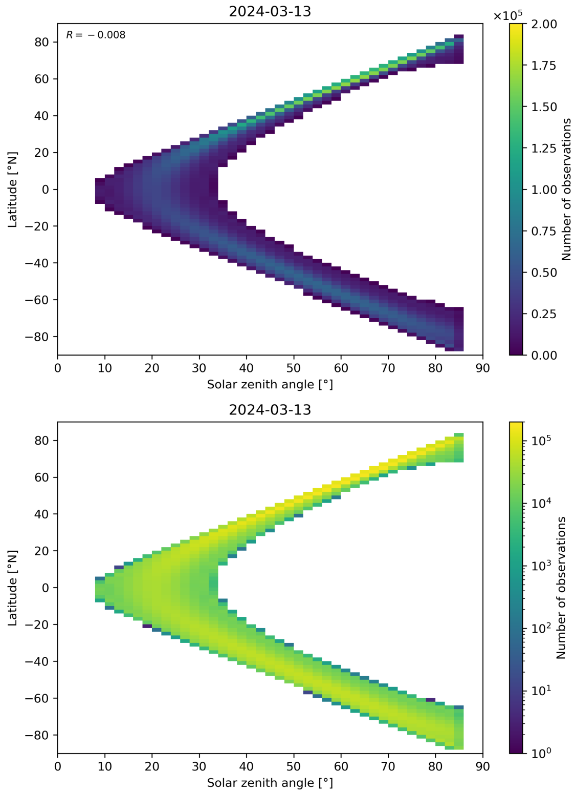
Figure 164: Scatter density plot of “Solar zenith angle” against “Latitude” for 2024-03-12 to 2024-03-14.
