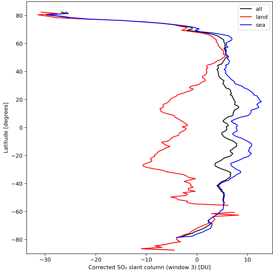
Figure 43: Zonal average of “Corrected SO 2 slant column (window 3)” for 2024-03-12 to 2024-03-14.
