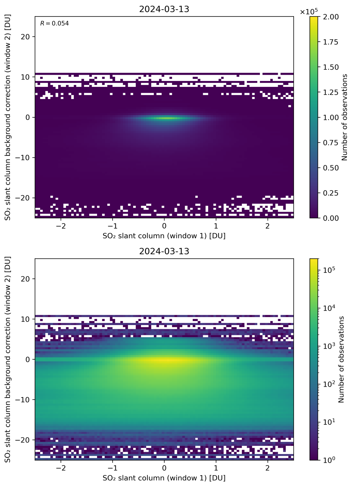
Figure 213: Scatter density plot of “SO 2 slant column (window 1)” against “SO 2 slant column background correction (window 2)” for 2024-03-12 to 2024-03-14.
