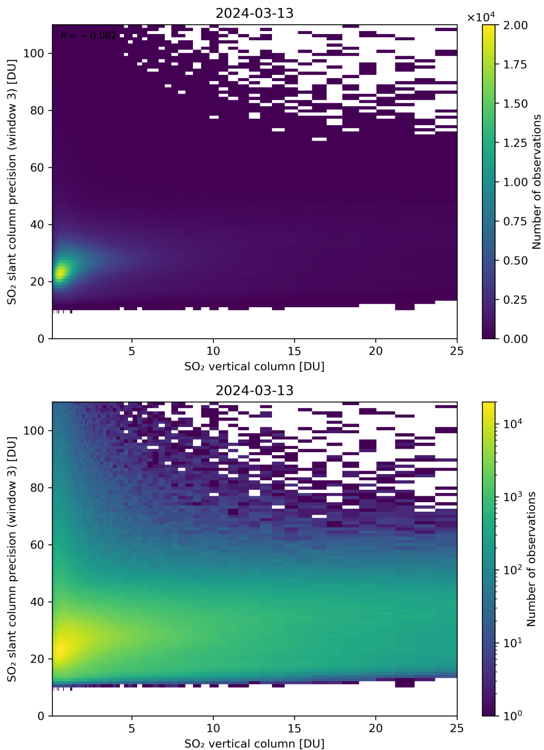
Figure 304: Scatter density plot of “SO 2 vertical column” against “SO 2 slant column precision (window 3)” for 2024-03-12 to 2024-03-14.
