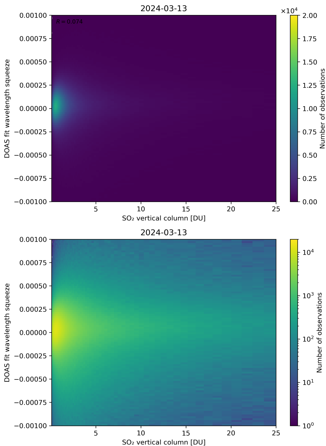
Figure 277: Scatter density plot of “SO 2 vertical column” against “DOAS fit wavelength squeeze” for 2024-03-12 to 2024-03-14.
