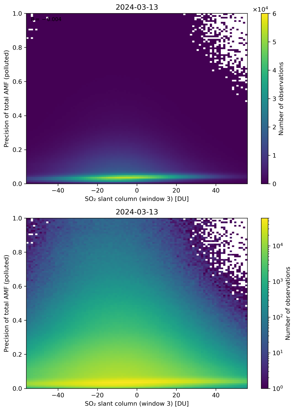
Figure 269: Scatter density plot of “SO 2 slant column (window 3)” against “Precision of total AMF (polluted)” for 2024-03-12 to 2024-03-14.
