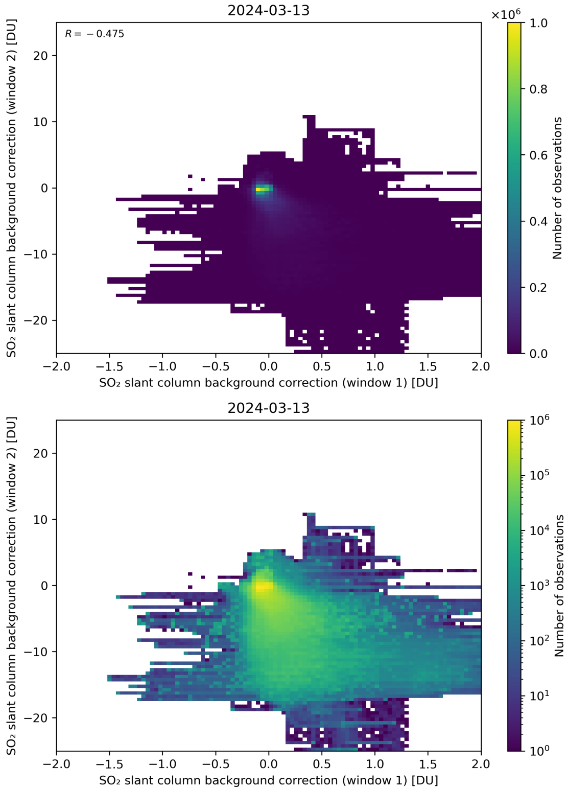
Figure 98: Scatter density plot of “SO 2 slant column background correction (window 1)” against “SO 2 slant column background correction (window 2)” for 2024-03-12 to 2024-03-14.
