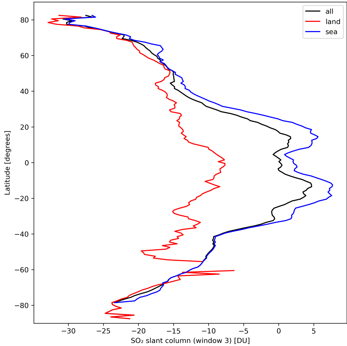
Figure 41: Zonal average of “SO 2 slant column (window 3)” for 2024-03-12 to 2024-03-14.
