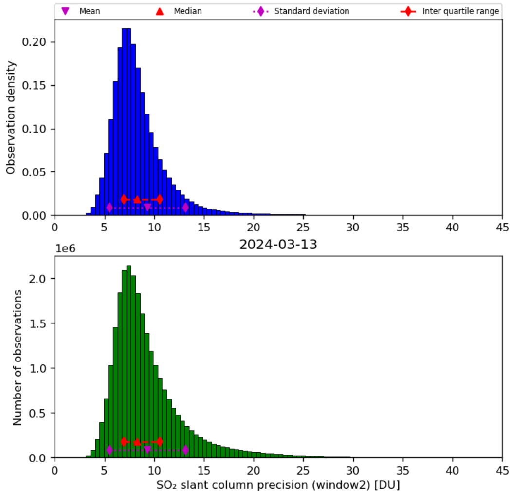
Figure 61: Histogram of “SO 2 slant column precision (window2)” for 2024-03-12 to 2024-03-14
