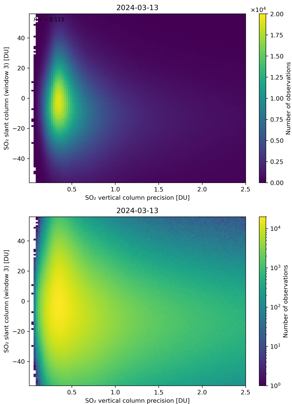
Figure 292: Scatter density plot of “SO 2 vertical column precision” against “SO 2 slant column (window 3)” for 2024-03-12 to 2024-03-14.
