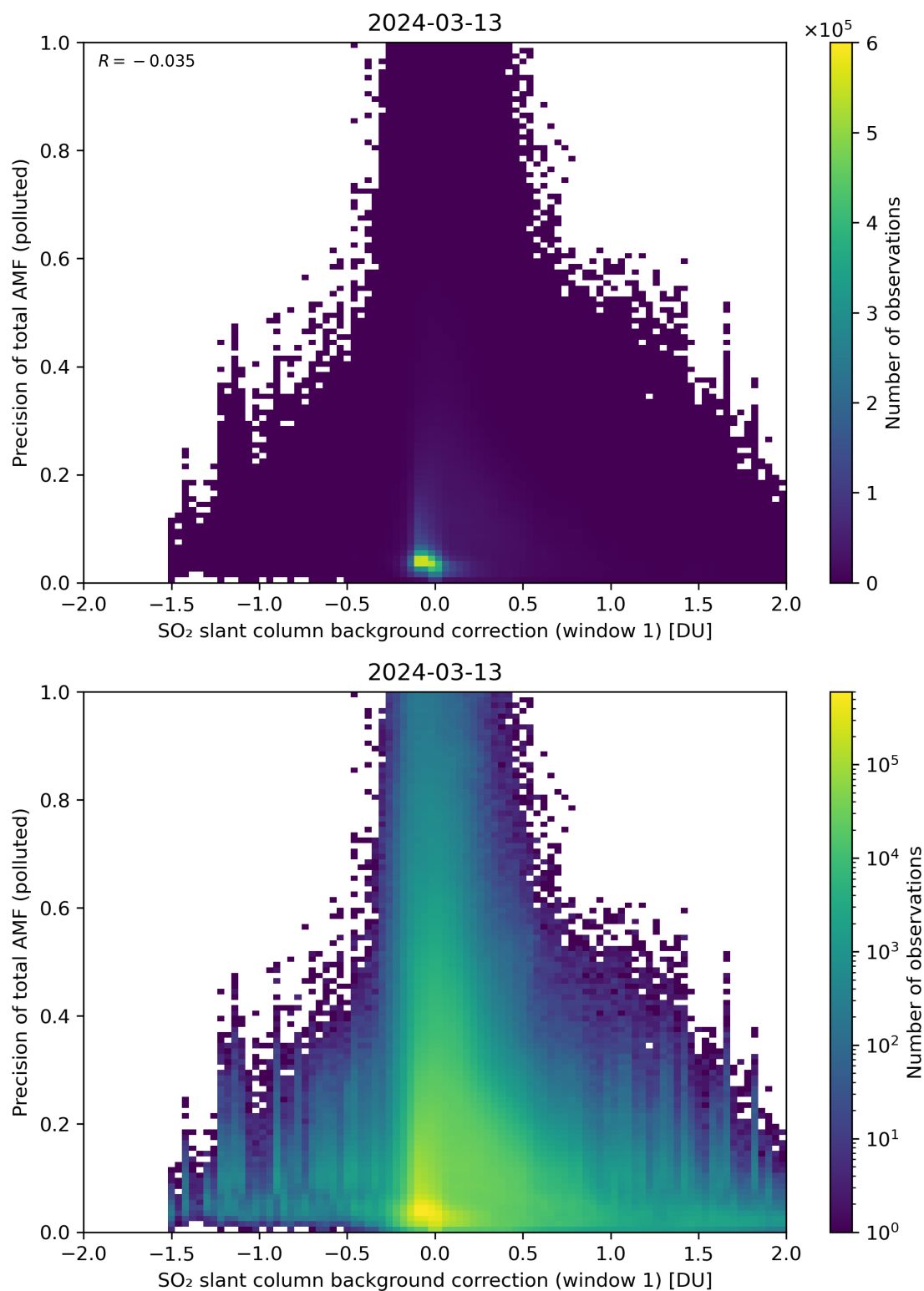
Figure 110: Scatter density plot of “SO 2 slant column background correction (window 1)” against “Precision of total AMF (polluted)” for 2024-03-12 to 2024-03-14.
