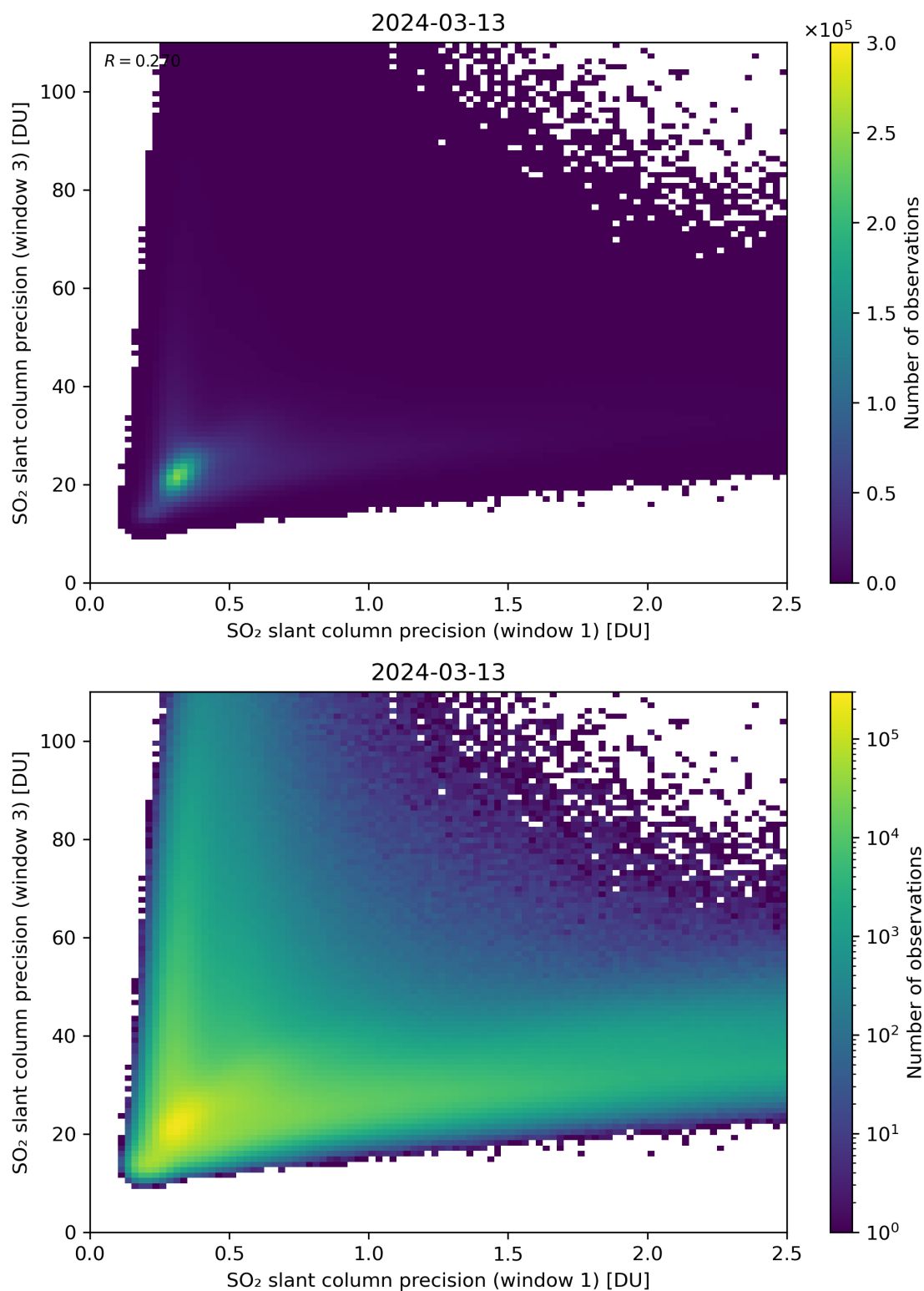
Figure 229: Scatter density plot of “SO 2 slant column precision (window 1)” against “SO 2 slant column precision (window 3)” for 2024-03-12 to 2024-03-14.
