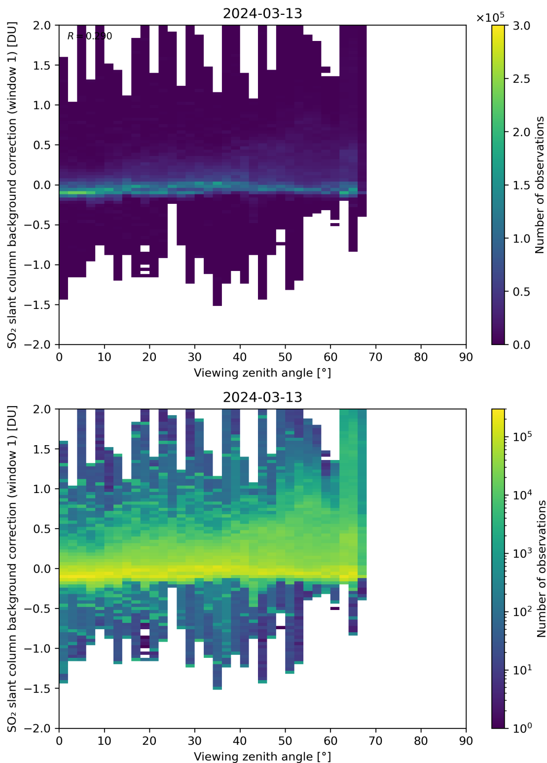
Figure 308: Scatter density plot of “Viewing zenith angle” against “SO 2 slant column background correction (window 1)” for 2024-03-12 to 2024-03-14.
