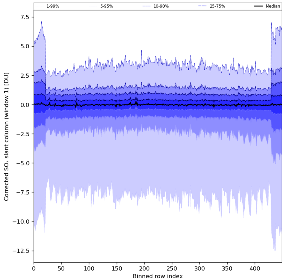
Figure 81: Along track statistics of “Corrected SO 2 slant column (window 1)” for 2024-03-12 to 2024-03-14
