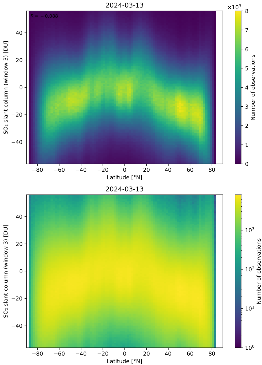
Figure 152: Scatter density plot of “Latitude” against “SO 2 slant column (window 3)” for 2024-03-12 to 2024-03-14.
