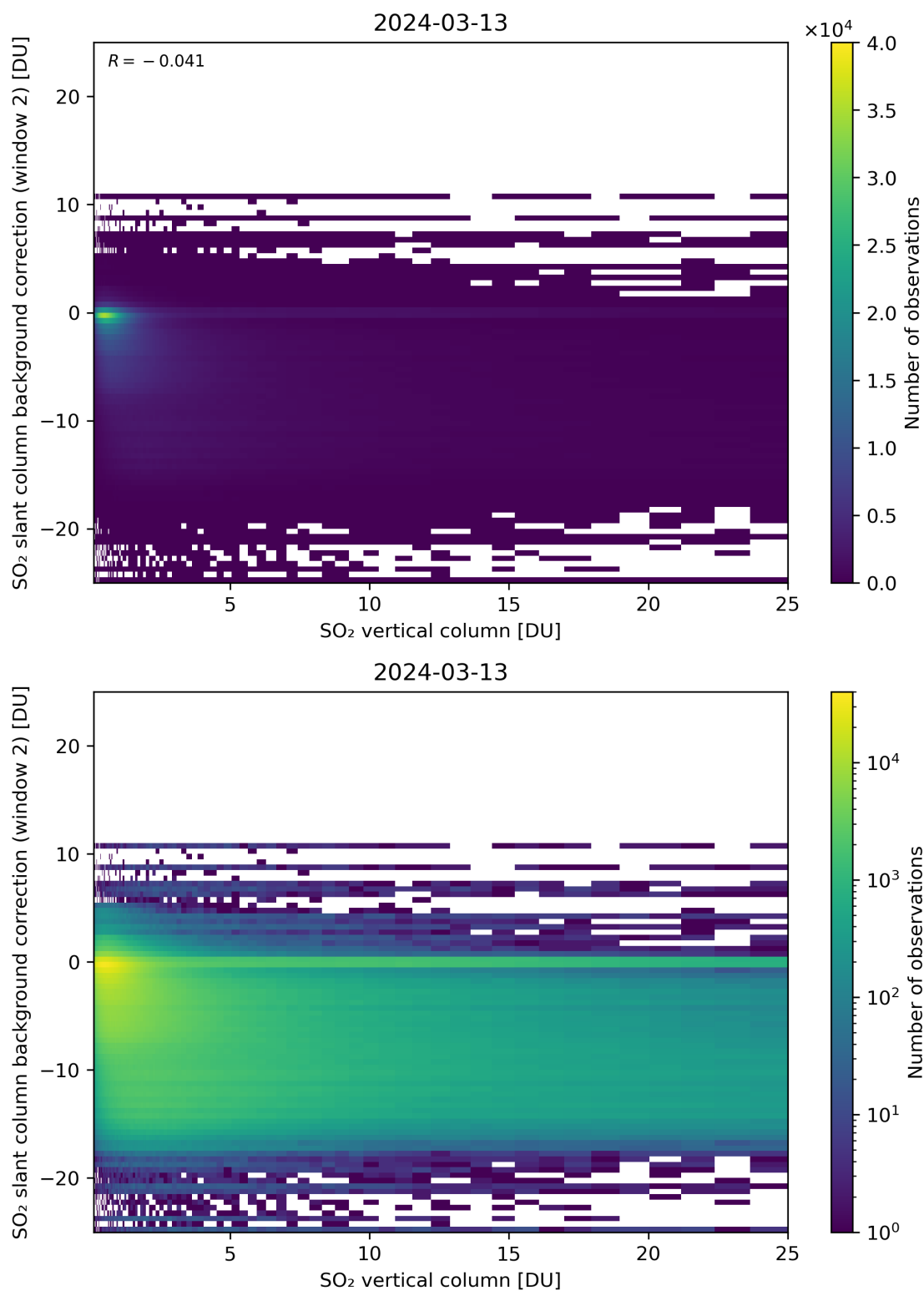
Figure 274: Scatter density plot of “SO 2 vertical column” against “SO 2 slant column background correction (window 2)” for 2024-03-12 to 2024-03-14.
