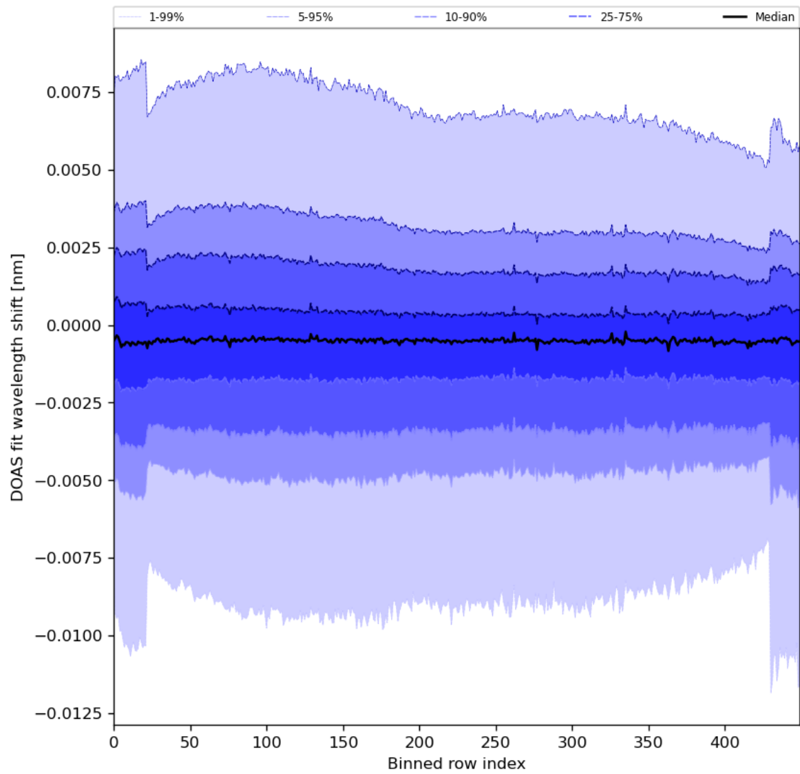
Figure 91: Along track statistics of “DOAS fit wavelength shift” for 2024-03-12 to 2024-03-14
