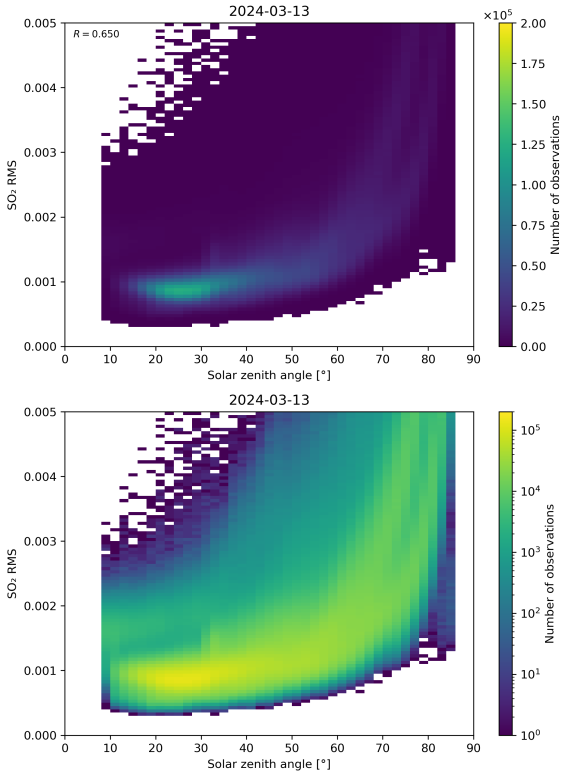
Figure 163: Scatter density plot of “Solar zenith angle” against “SO 2 RMS” for 2024-03-12 to 2024-03-14.
