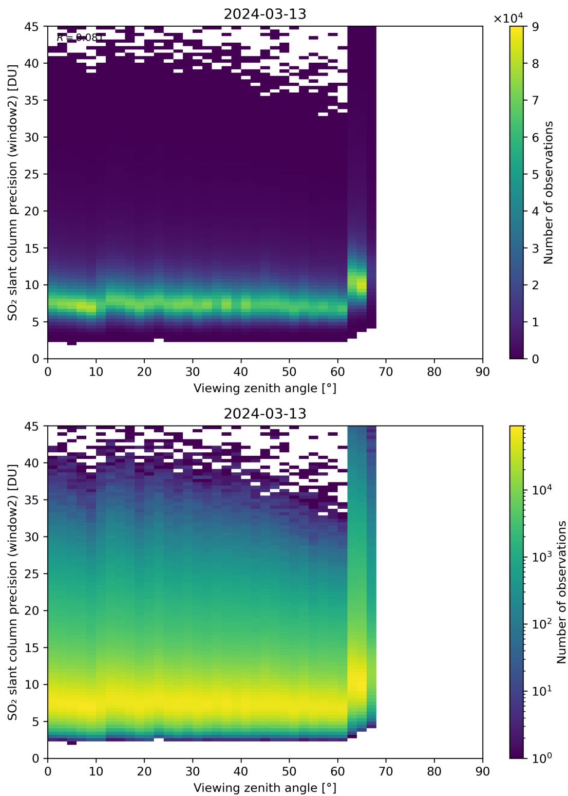
Figure 322: Scatter density plot of “Viewing zenith angle” against “SO 2 slant column precision (window2)” for 2024-03-12 to 2024-03-14.
