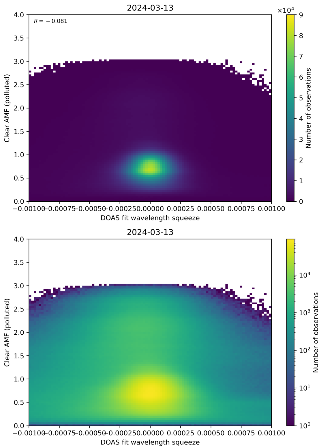
Figure 133: Scatter density plot of “DOAS fit wavelength squeeze” against “Clear AMF (polluted)” for 2024-03-12 to 2024-03-14.
