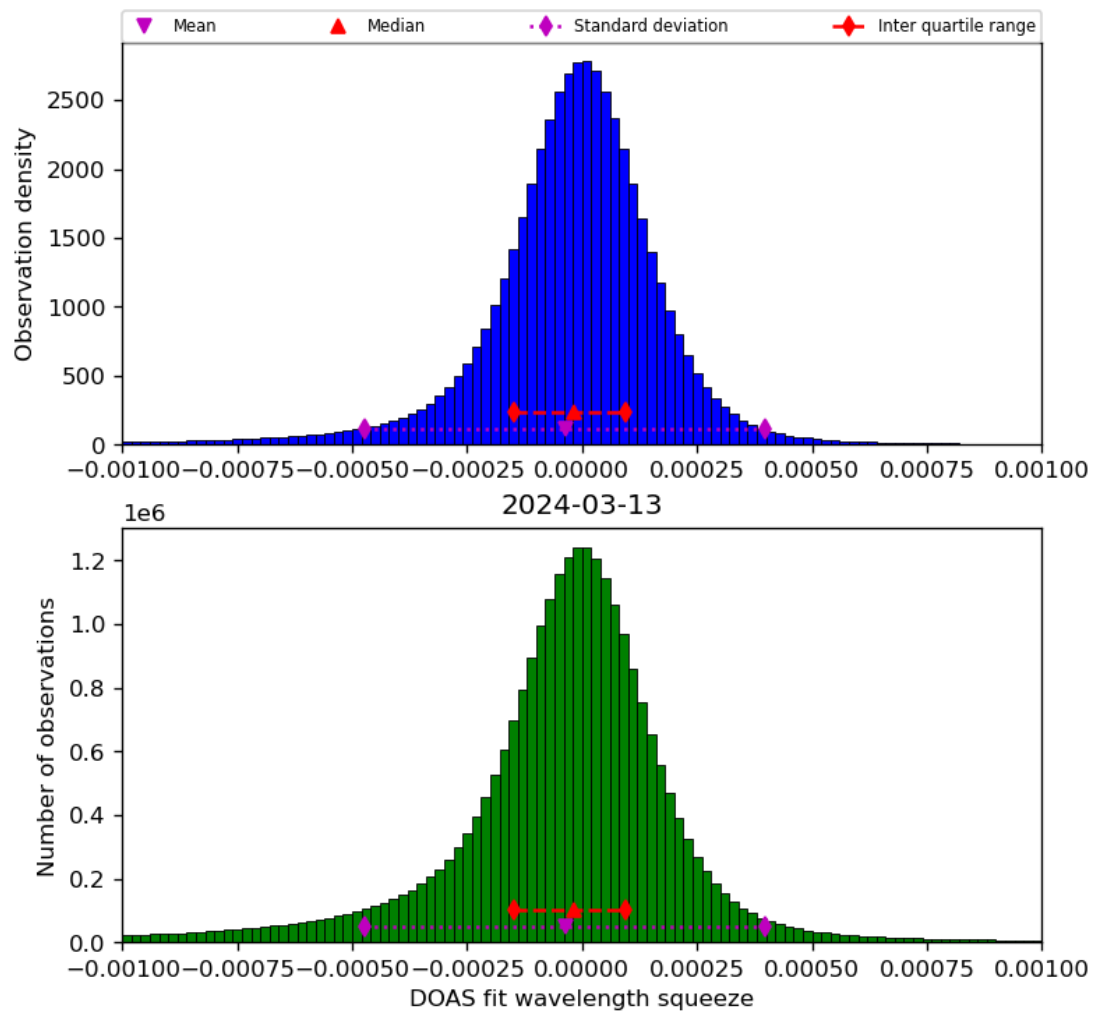
Figure 69: Histogram of “DOAS fit wavelength squeeze” for 2024-03-12 to 2024-03-14
