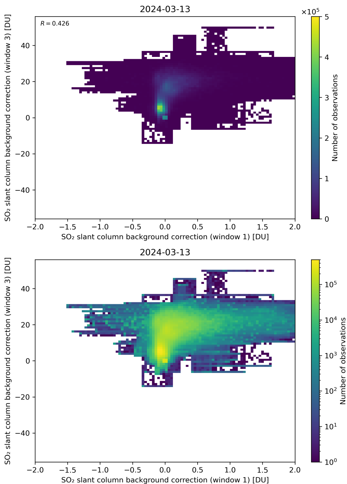
Figure 99: Scatter density plot of “SO 2 slant column background correction (window 1)” against “SO 2 slant column background correction (window 3)” for 2024-03-12 to 2024-03-14.
