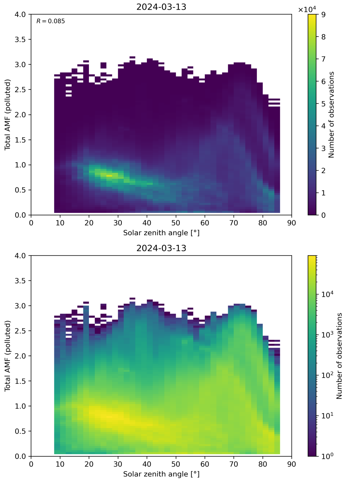
Figure 174: Scatter density plot of “Solar zenith angle” against “Total AMF (polluted)” for 2024-03-12 to 2024-03-14.
