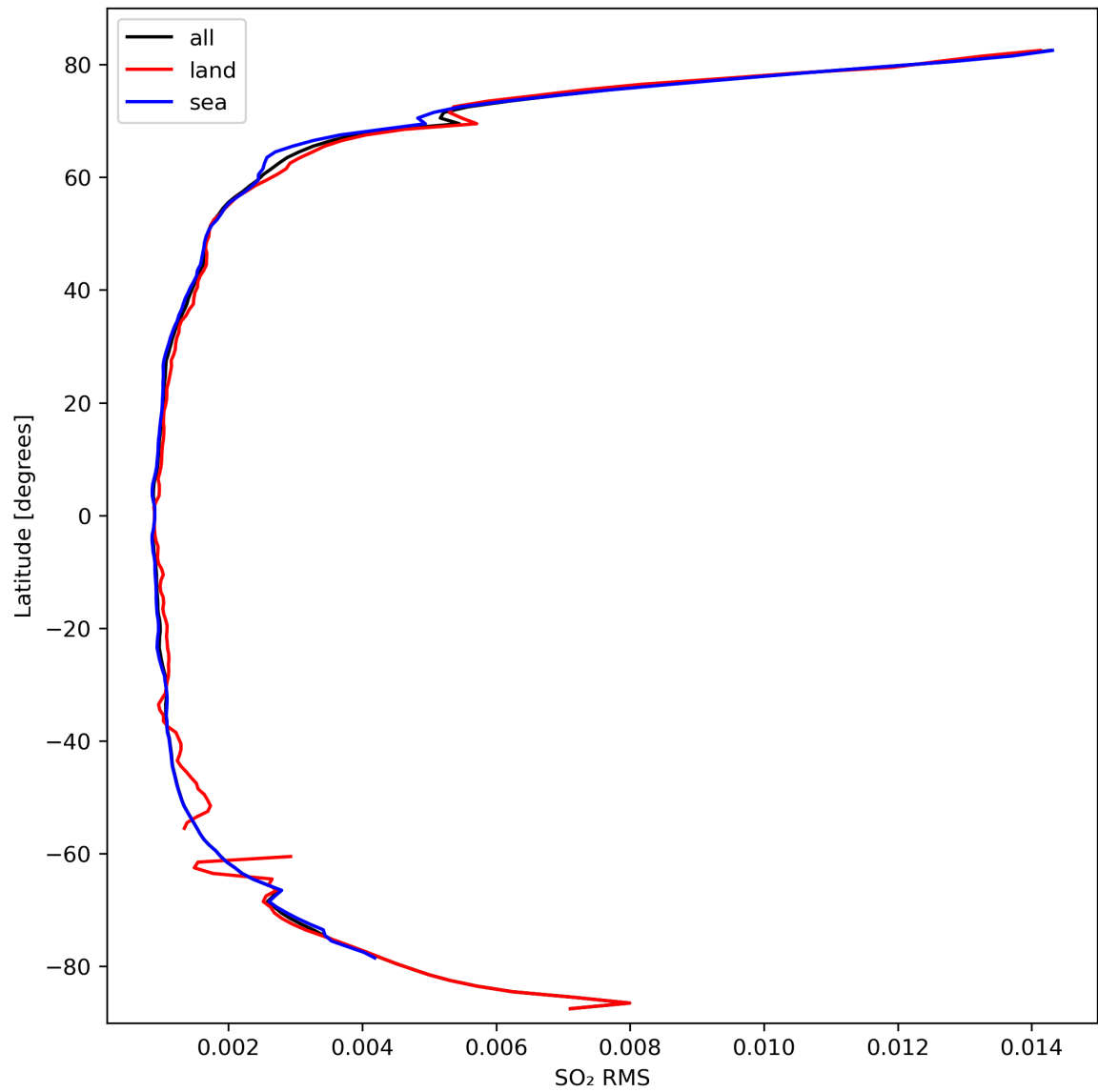
Figure 47: Zonal average of “SO 2 RMS” for 2024-03-12 to 2024-03-14.
