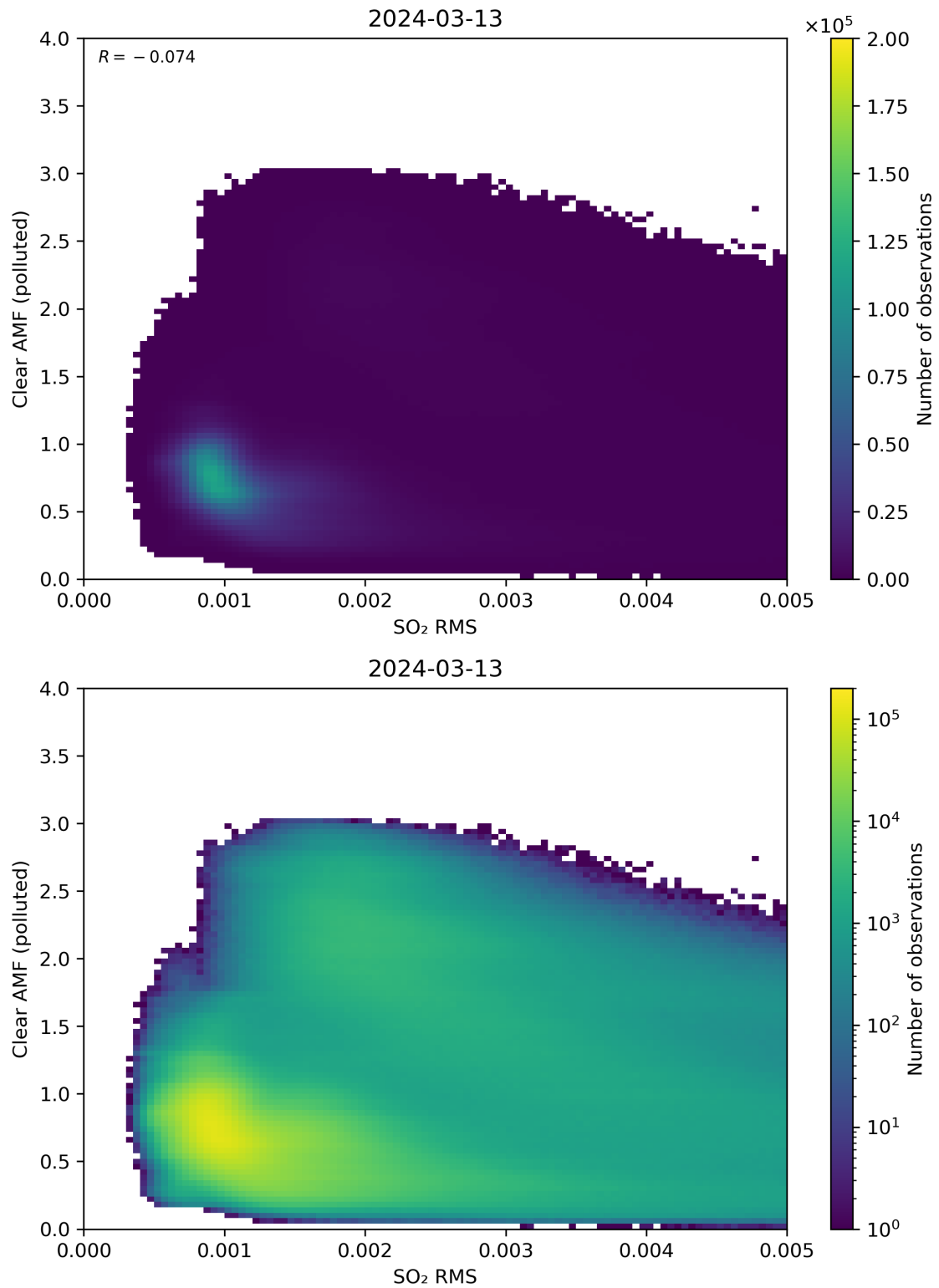
Figure 136: Scatter density plot of “SO 2 RMS” against “Clear AMF (polluted)” for 2024-03-12 to 2024-03-14.
