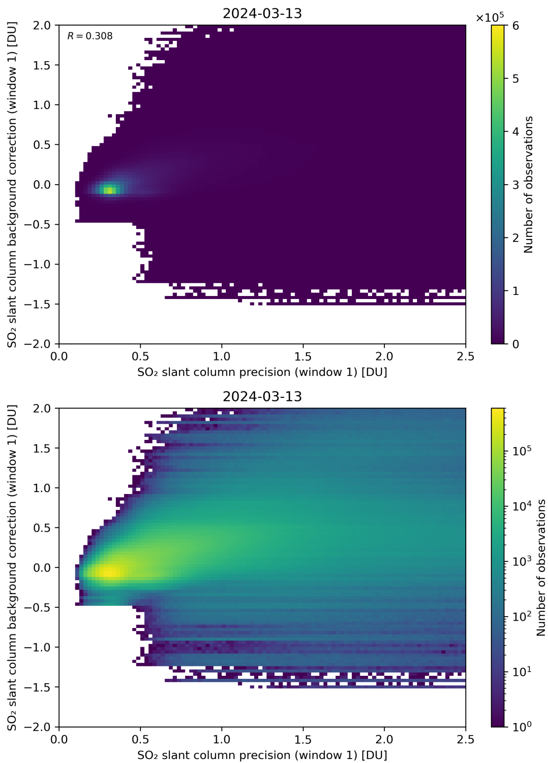
Figure 218: Scatter density plot of “SO 2 slant column precision (window 1)” against “SO 2 slant column background correction (window 1)” for 2024-03-12 to 2024-03-14.
