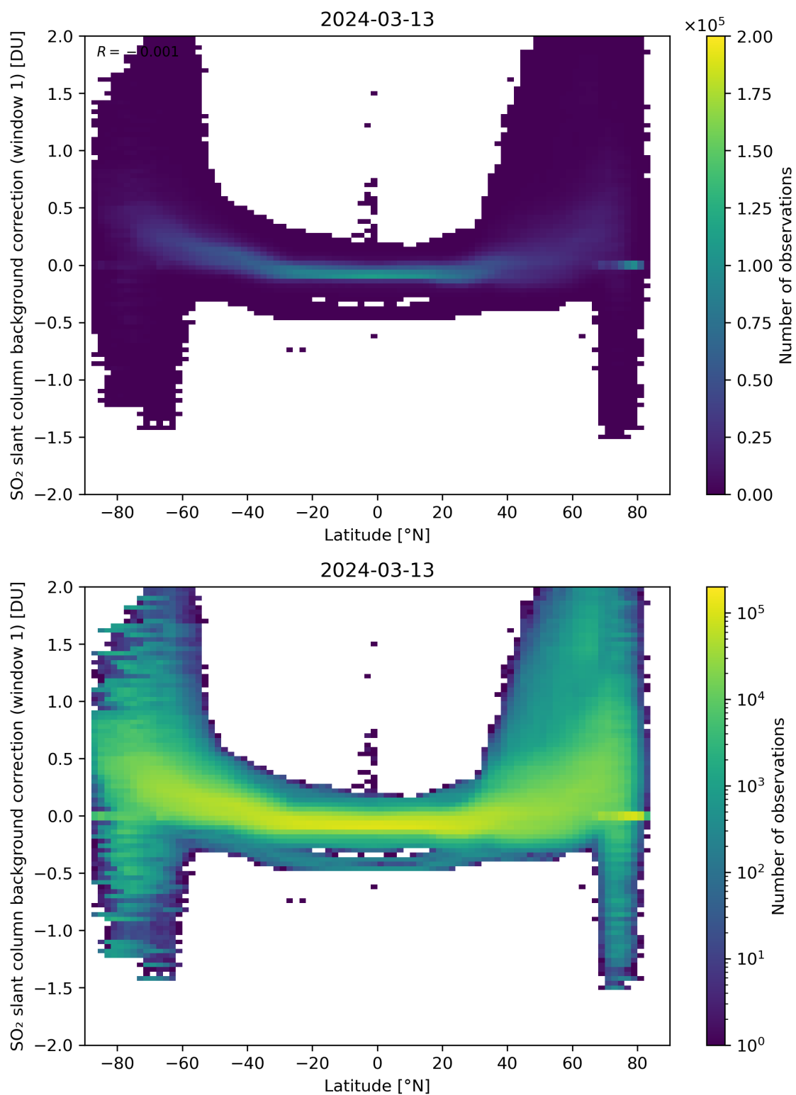
Figure 139: Scatter density plot of “Latitude” against “SO 2 slant column background correction (window 1)” for 2024-03-12 to 2024-03-14.
