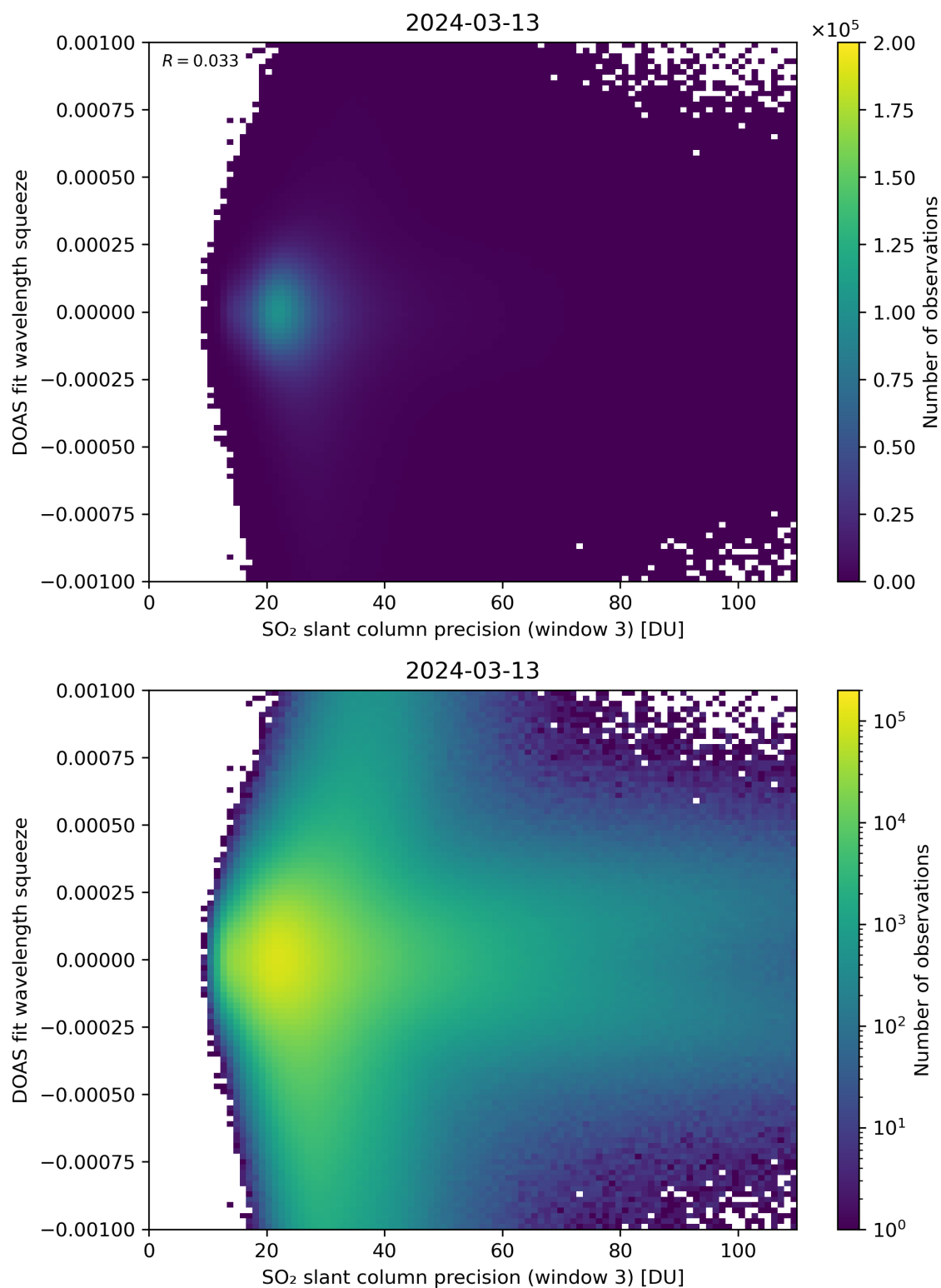
Figure 259: Scatter density plot of “SO 2 slant column precision (window 3)” against “DOAS fit wavelength squeeze” for 2024-03-12 to 2024-03-14.
