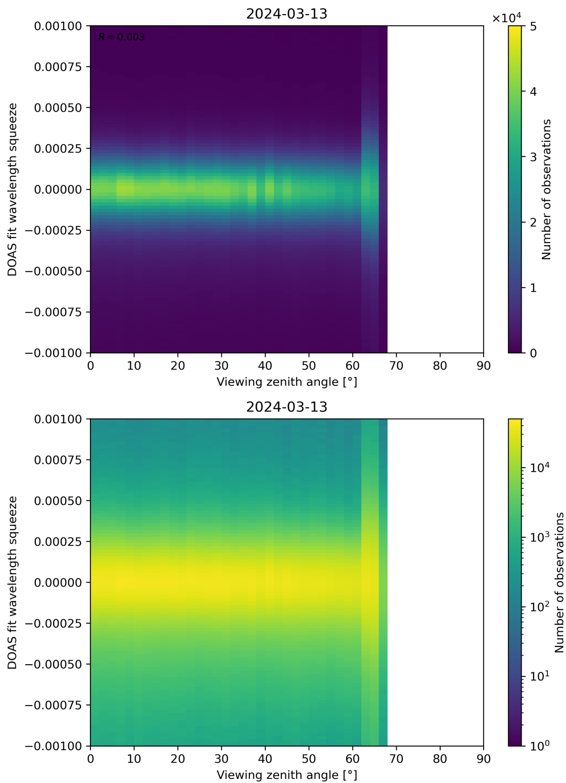
Figure 312: Scatter density plot of “Viewing zenith angle” against “DOAS fit wavelength squeeze” for 2024-03-12 to 2024-03-14.
