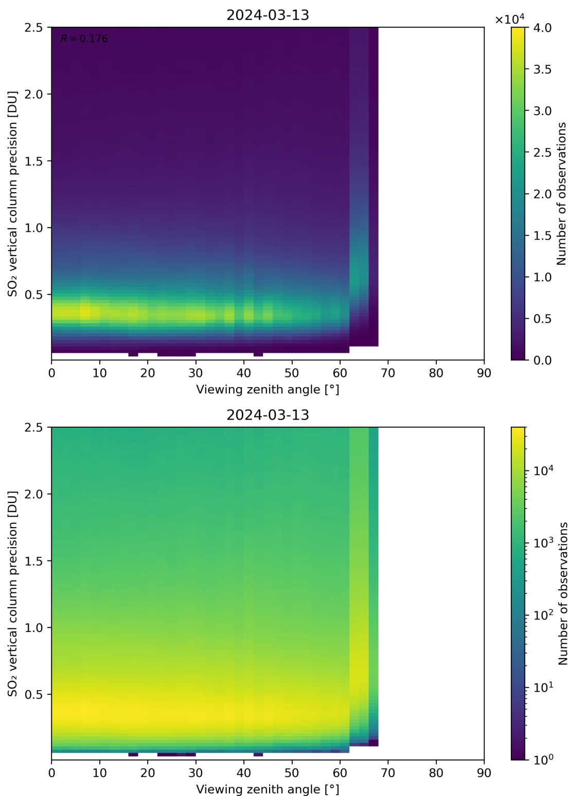
Figure 328: Scatter density plot of “Viewing zenith angle” against “SO 2 vertical column precision” for 2024-03-12 to 2024-03-14.
