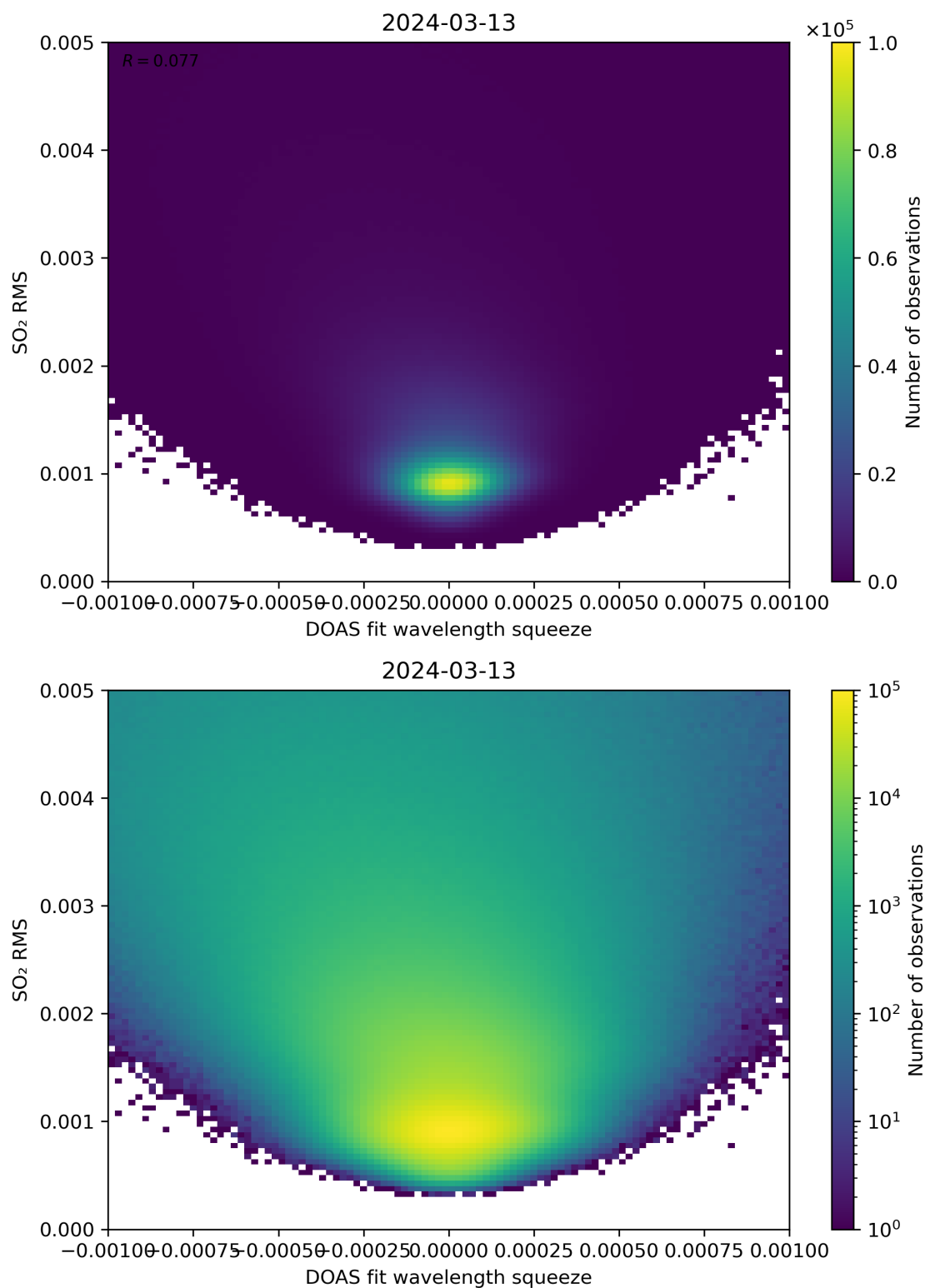
Figure 132: Scatter density plot of “DOAS fit wavelength squeeze” against “SO 2 RMS” for 2024-03-12 to 2024-03-14.
