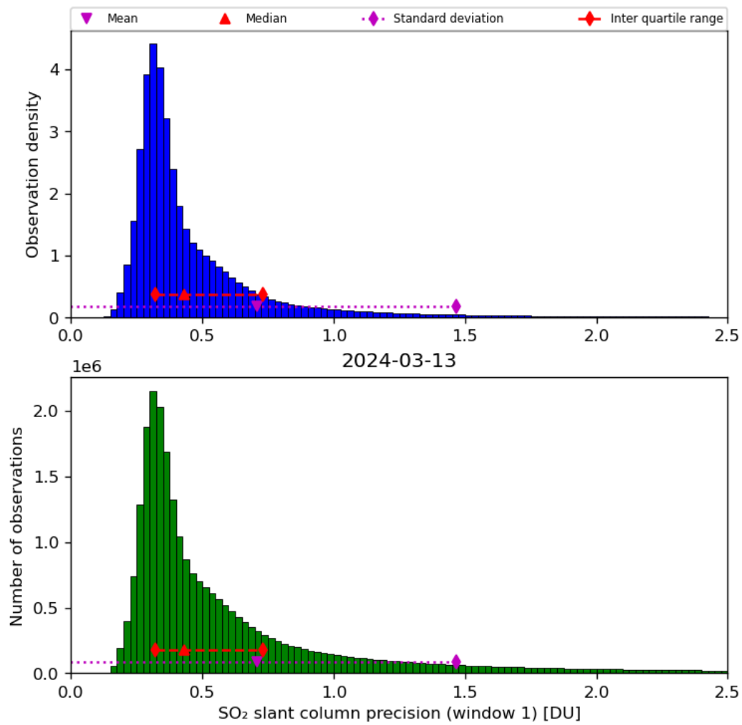
Figure 57: Histogram of “SO 2 slant column precision (window 1)” for 2024-03-12 to 2024-03-14
