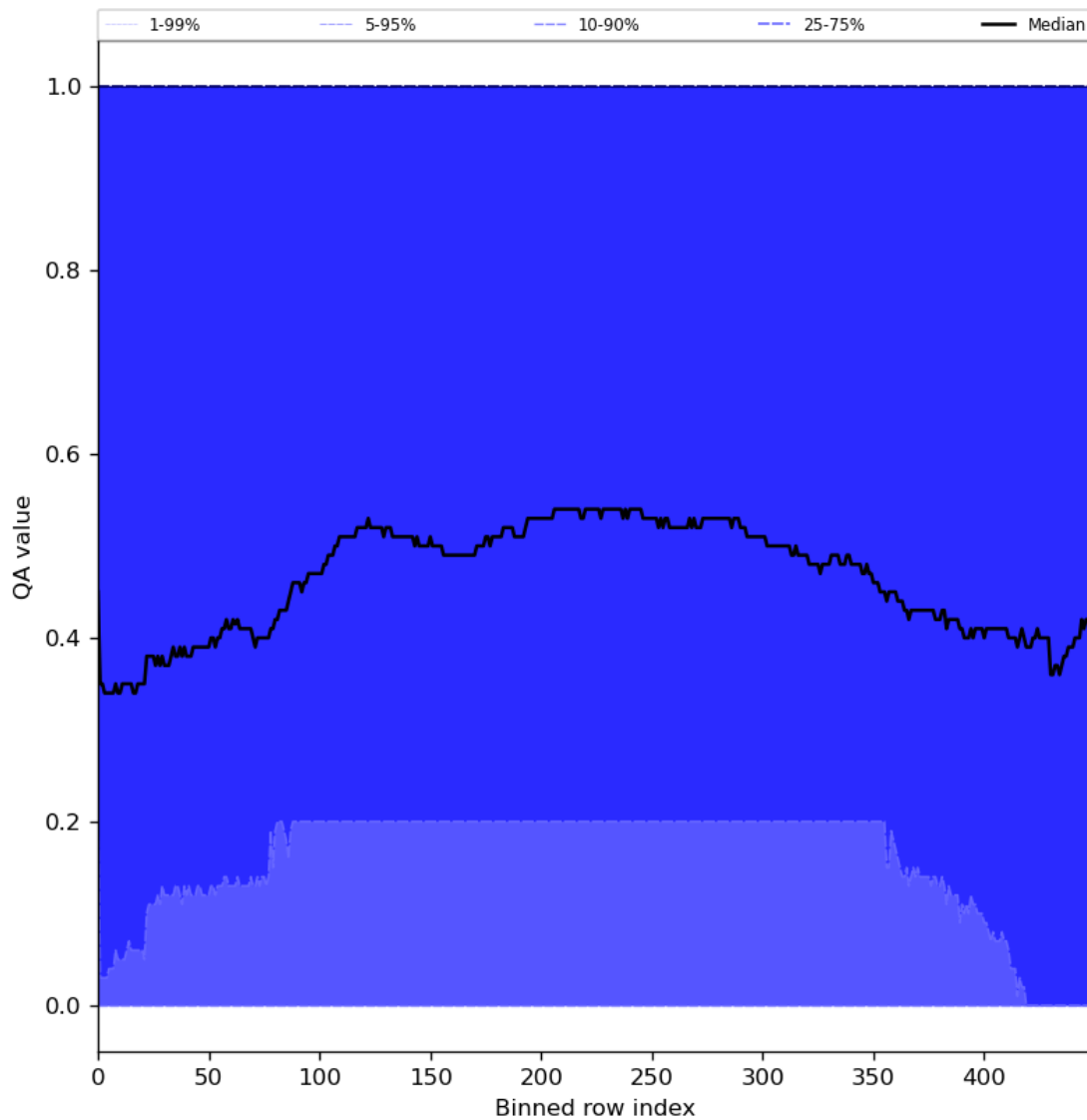
Figure 75: Along track statistics of “QA value” for 2024-03-12 to 2024-03-14
