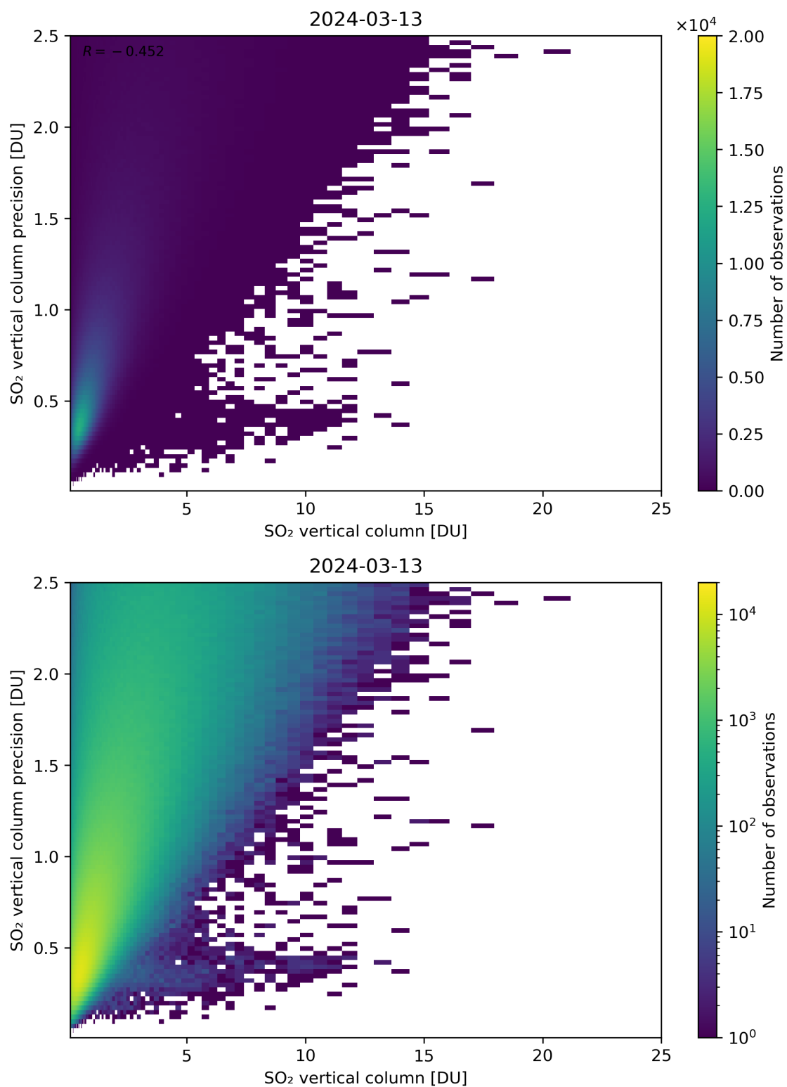
Figure 307: Scatter density plot of “SO 2 vertical column” against “SO 2 vertical column precision” for 2024-03-12 to 2024-03-14.
