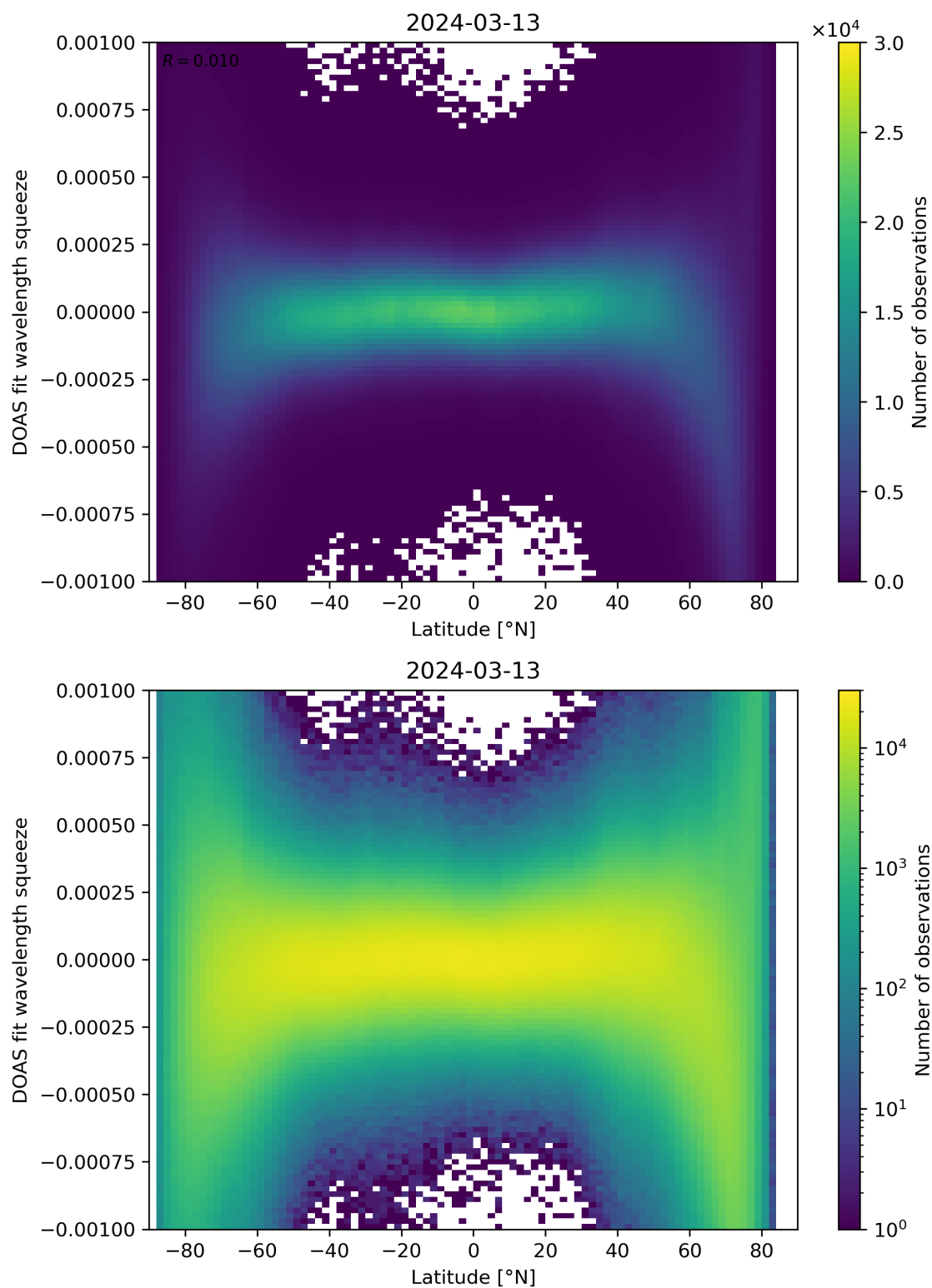
Figure 143: Scatter density plot of “Latitude” against “DOAS fit wavelength squeeze” for 2024-03-12 to 2024-03-14.
