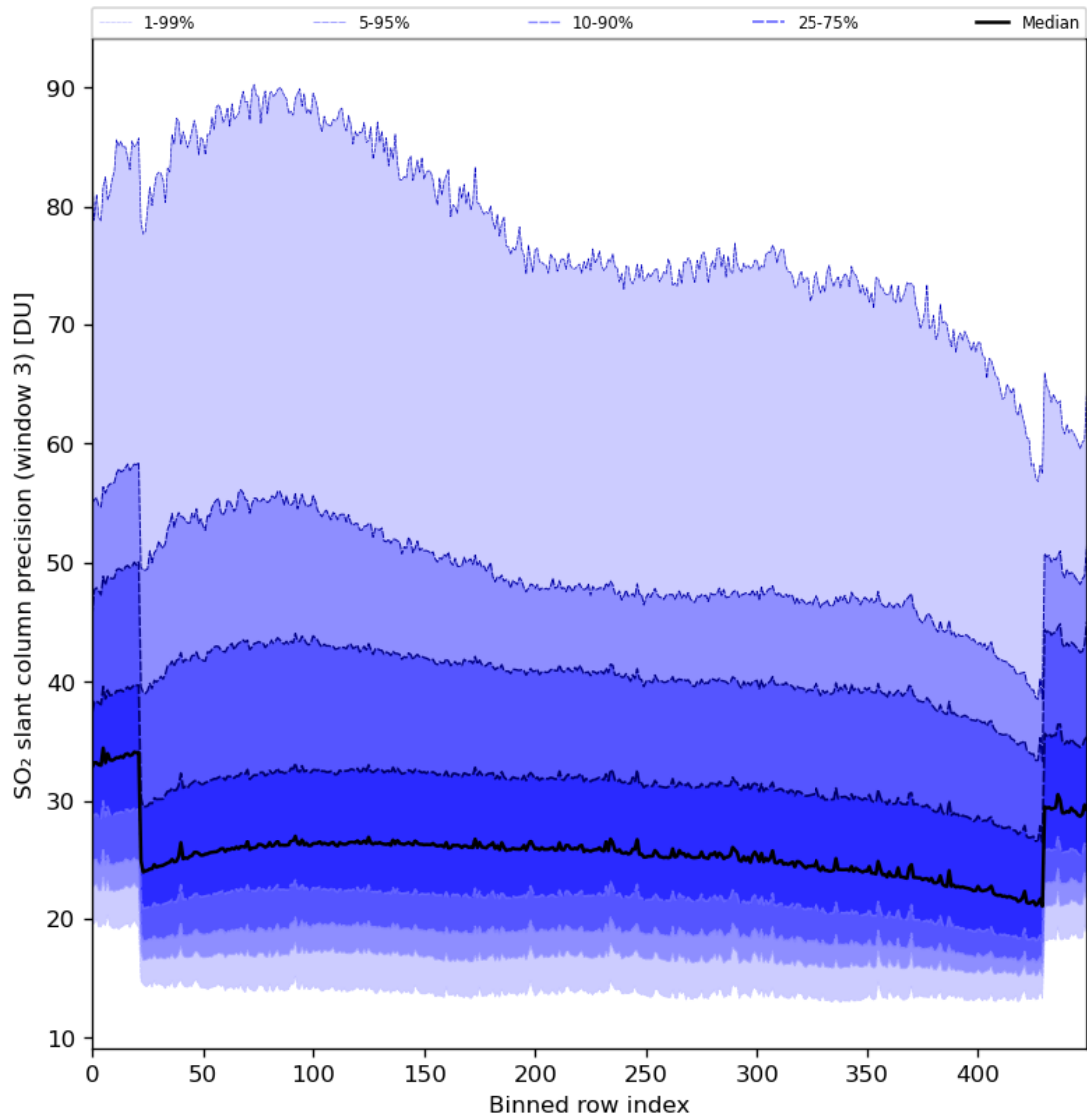
Figure 88: Along track statistics of “SO 2 slant column precision (window 3)” for 2024-03-12 to 2024-03-14
