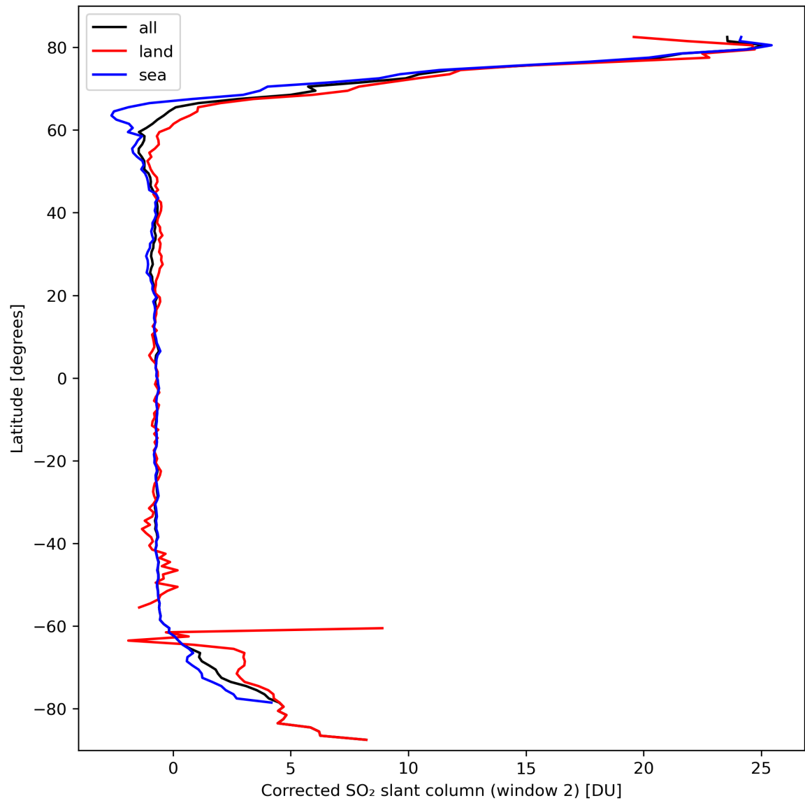
Figure 39: Zonal average of “Corrected SO 2 slant column (window 2)” for 2024-03-12 to 2024-03-14.
