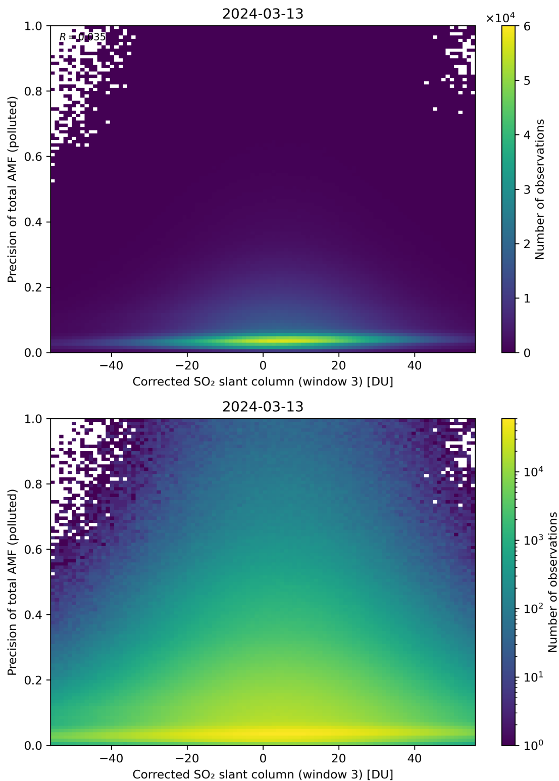
Figure 211: Scatter density plot of “Corrected SO 2 slant column (window 3)” against “Precision of total AMF (polluted)” for 2024-03-12 to 2024-03-14.
