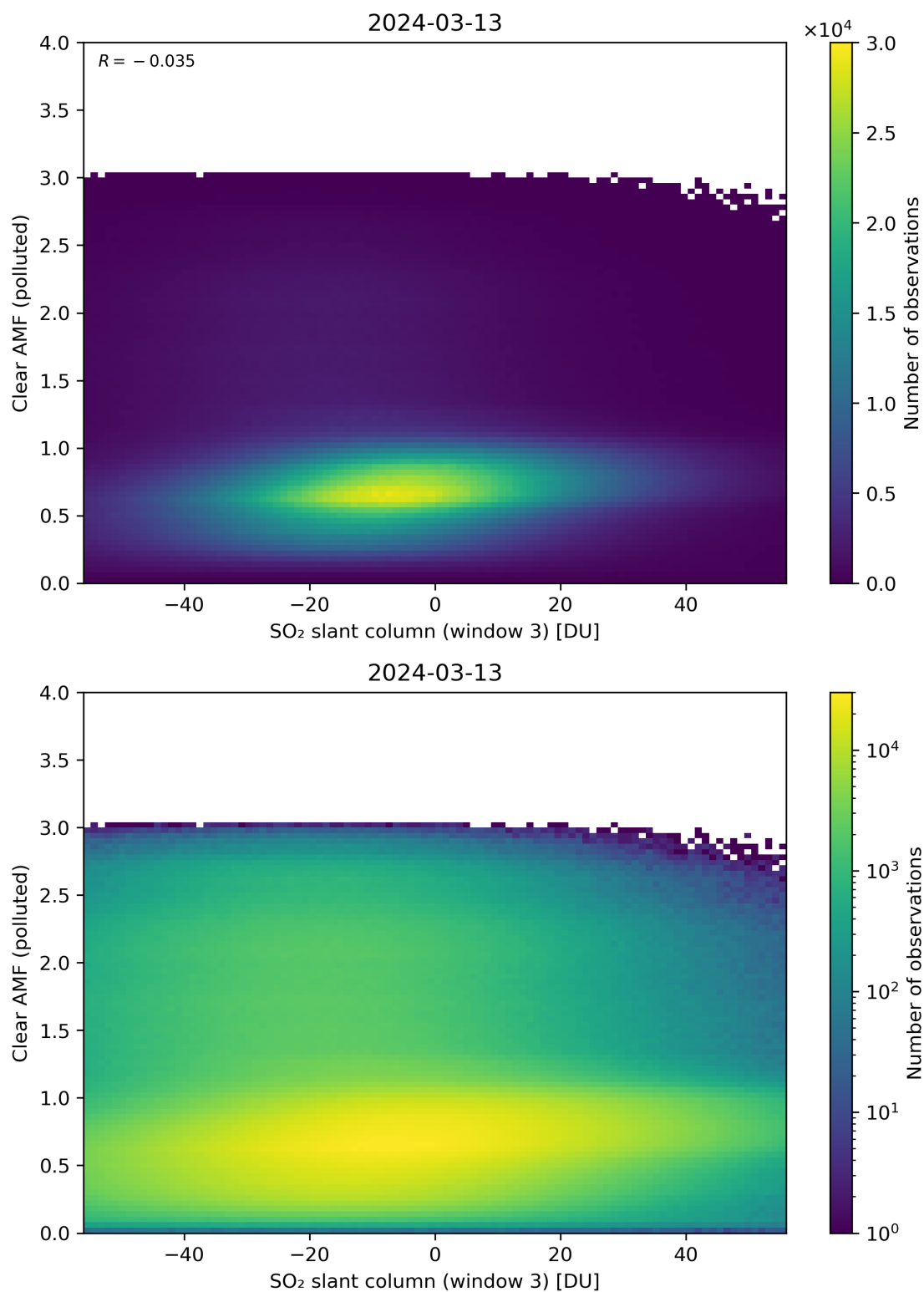
Figure 265: Scatter density plot of “SO 2 slant column (window 3)” against “Clear AMF (polluted)” for 2024-03-12 to 2024-03-14.
