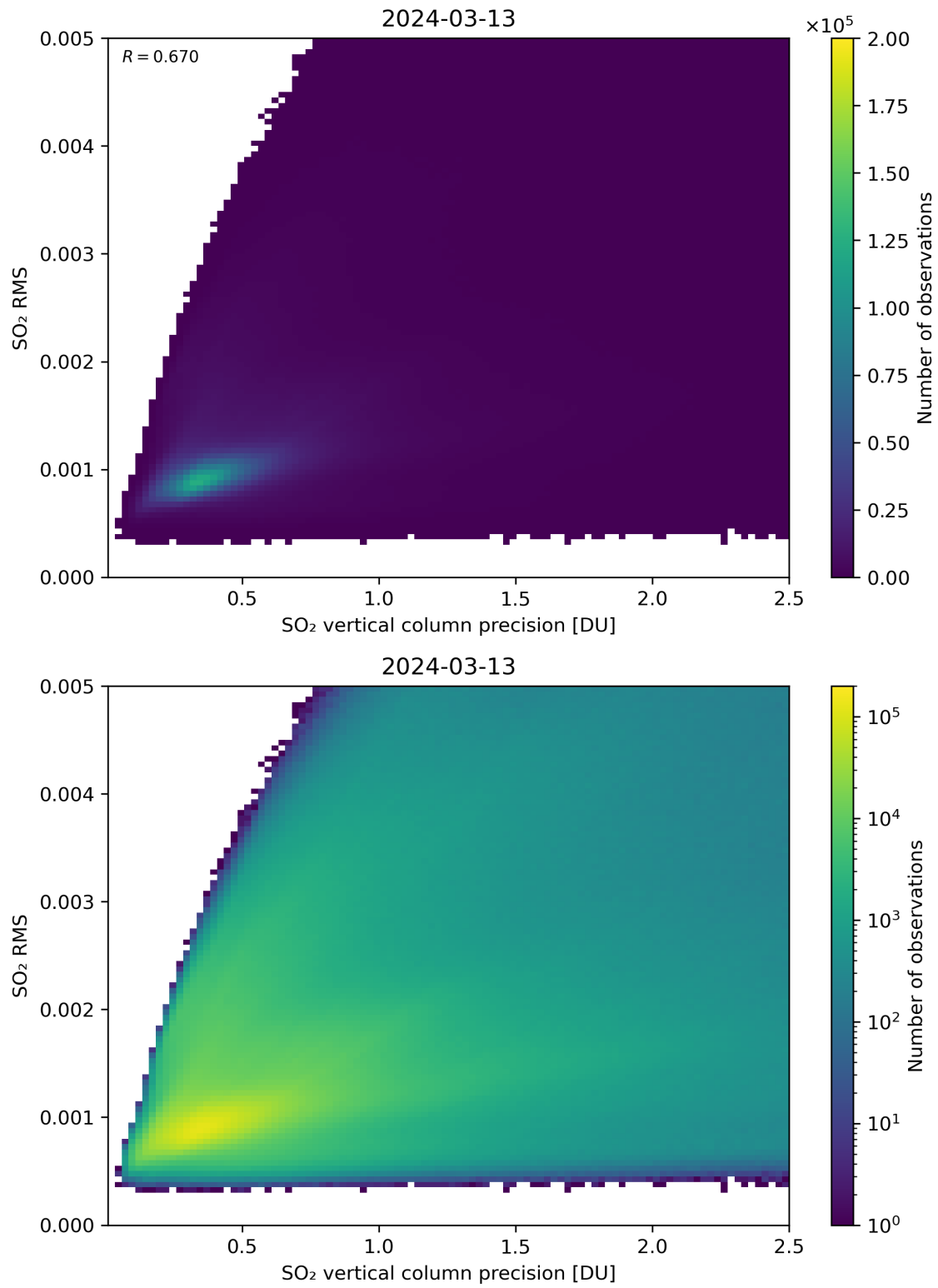
Figure 284: Scatter density plot of “SO 2 vertical column precision” against “SO 2 RMS” for 2024-03-12 to 2024-03-14.
