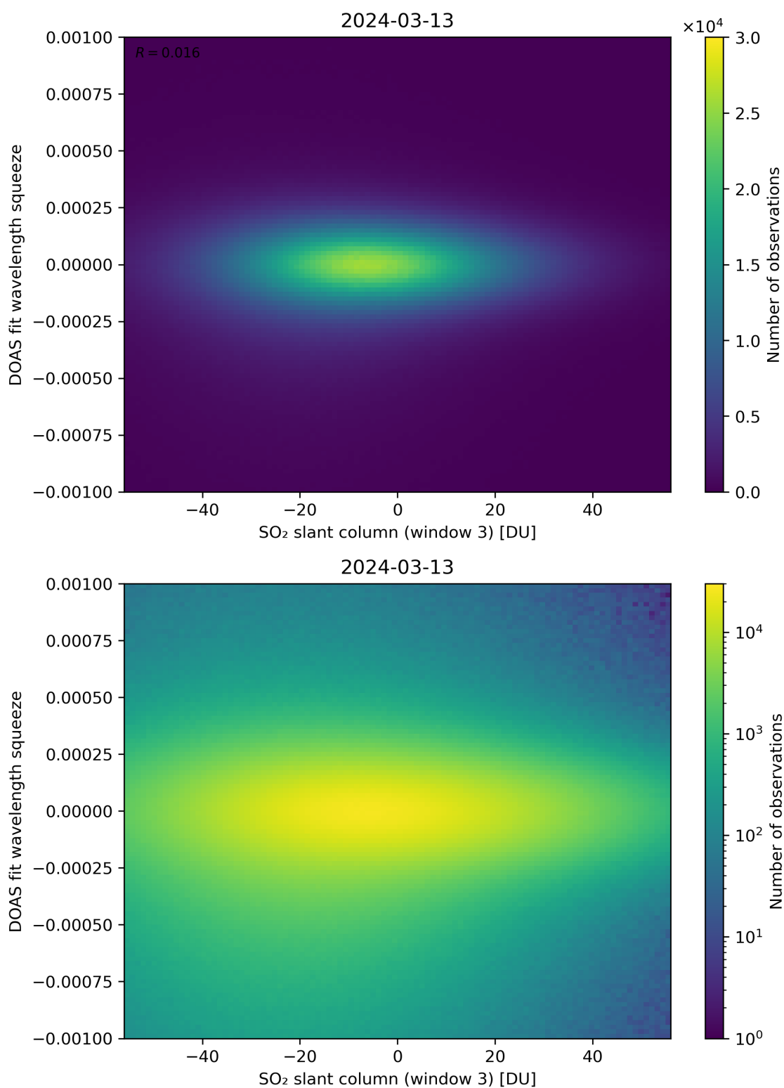
Figure 255: Scatter density plot of “SO 2 slant column (window 3)” against “DOAS fit wavelength squeeze” for 2024-03-12 to 2024-03-14.
