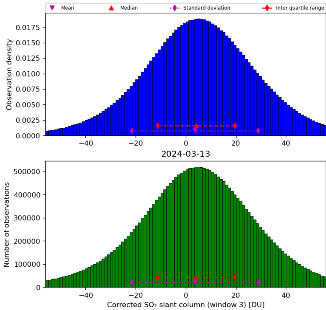
Figure 66: Histogram of “Corrected SO 2 slant column (window 3)” for 2024-03-12 to 2024-03-14
