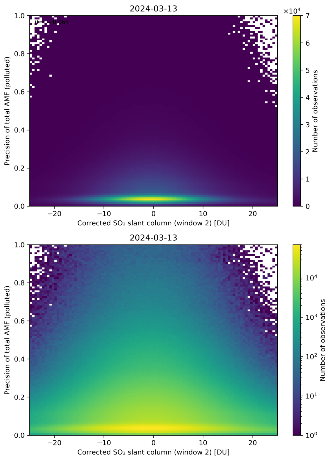
Figure 204: Scatter density plot of “Corrected SO 2 slant column (window 2)” against “Precision of total AMF (polluted)” for 2024-03-12 to 2024-03-14.
