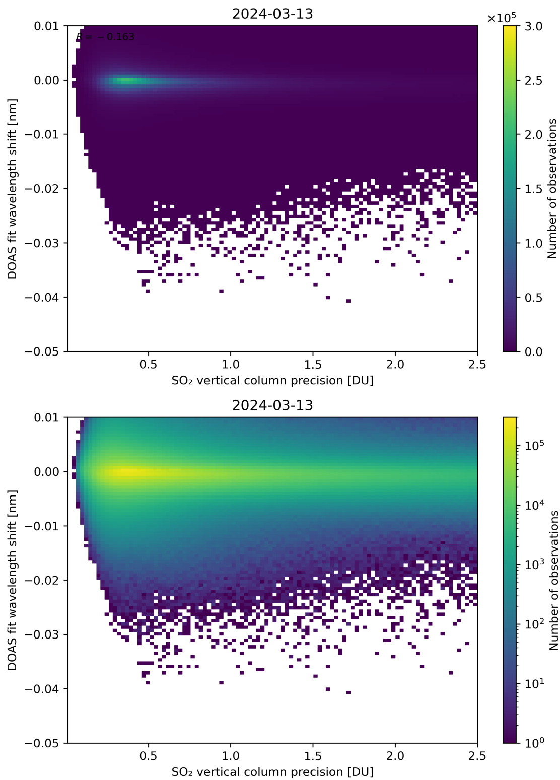
Figure 282: Scatter density plot of “SO 2 vertical column precision” against “DOAS fit wavelength shift” for 2024-03-12 to 2024-03-14.
