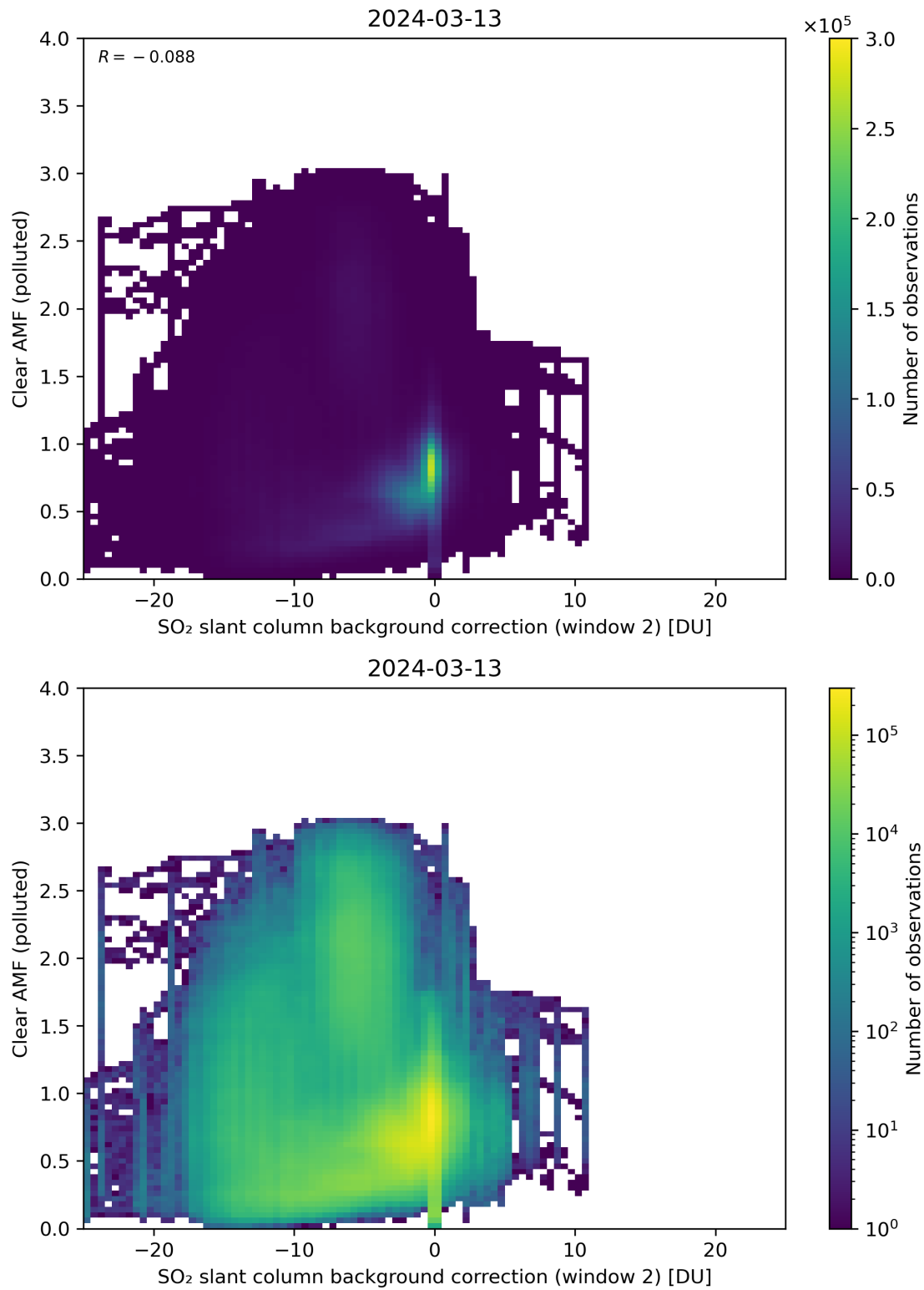
Figure 115: Scatter density plot of “SO 2 slant column background correction (window 2)” against “Clear AMF (polluted)” for 2024-03-12 to 2024-03-14.
