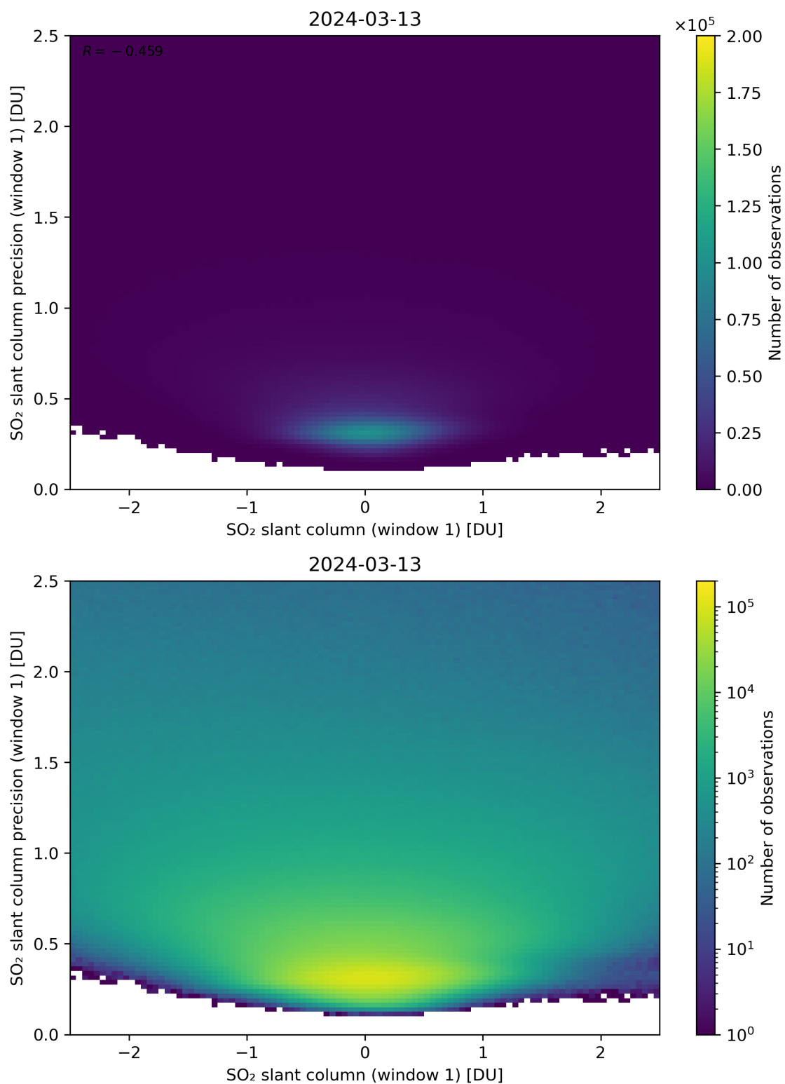
Figure 235: Scatter density plot of “SO 2 slant column (window 1)” against “SO 2 slant column precision (window 1)” for 2024-03-12 to 2024-03-14.
