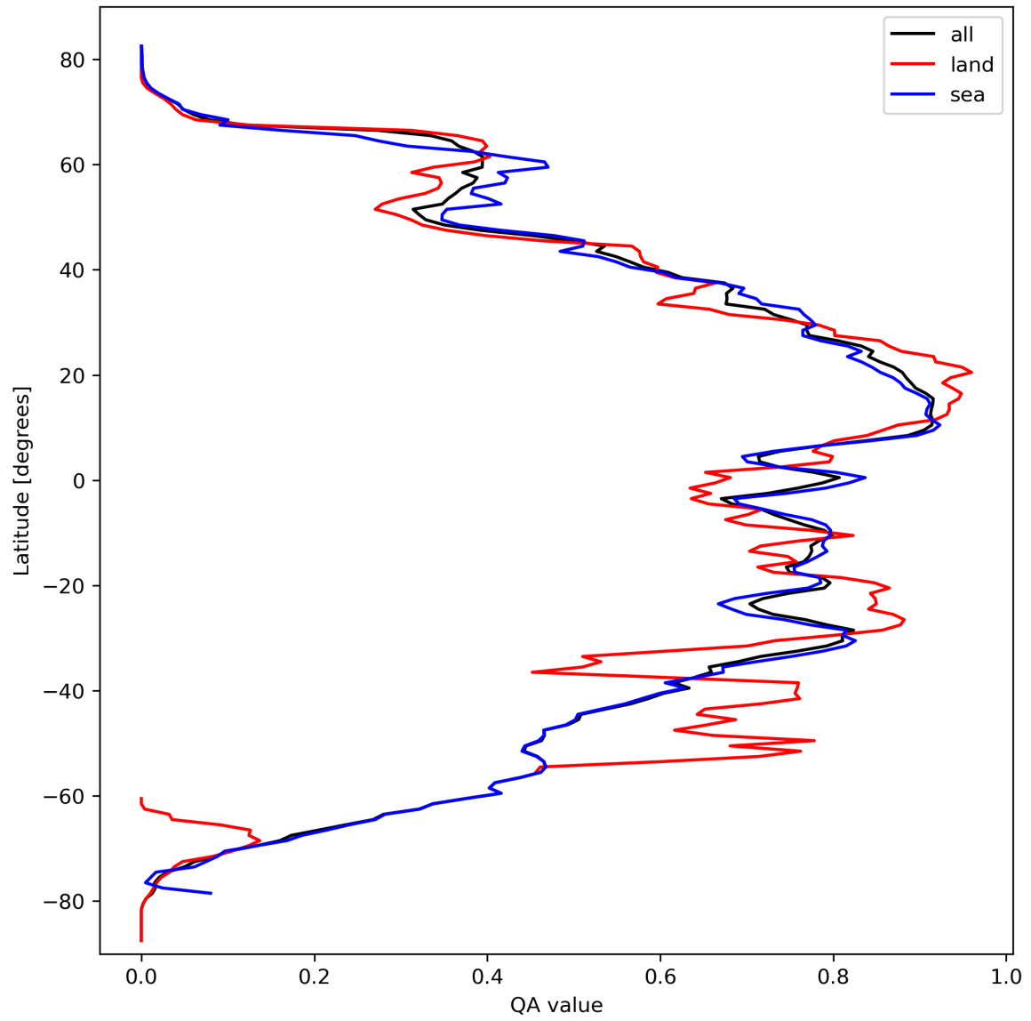
Figure 29: Zonal average of “QA value” for 2024-03-12 to 2024-03-14.
