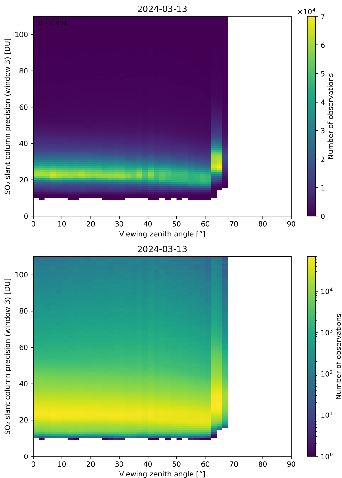
Figure 324: Scatter density plot of “Viewing zenith angle” against “SO 2 slant column precision (window 3)” for 2024-03-12 to 2024-03-14.
