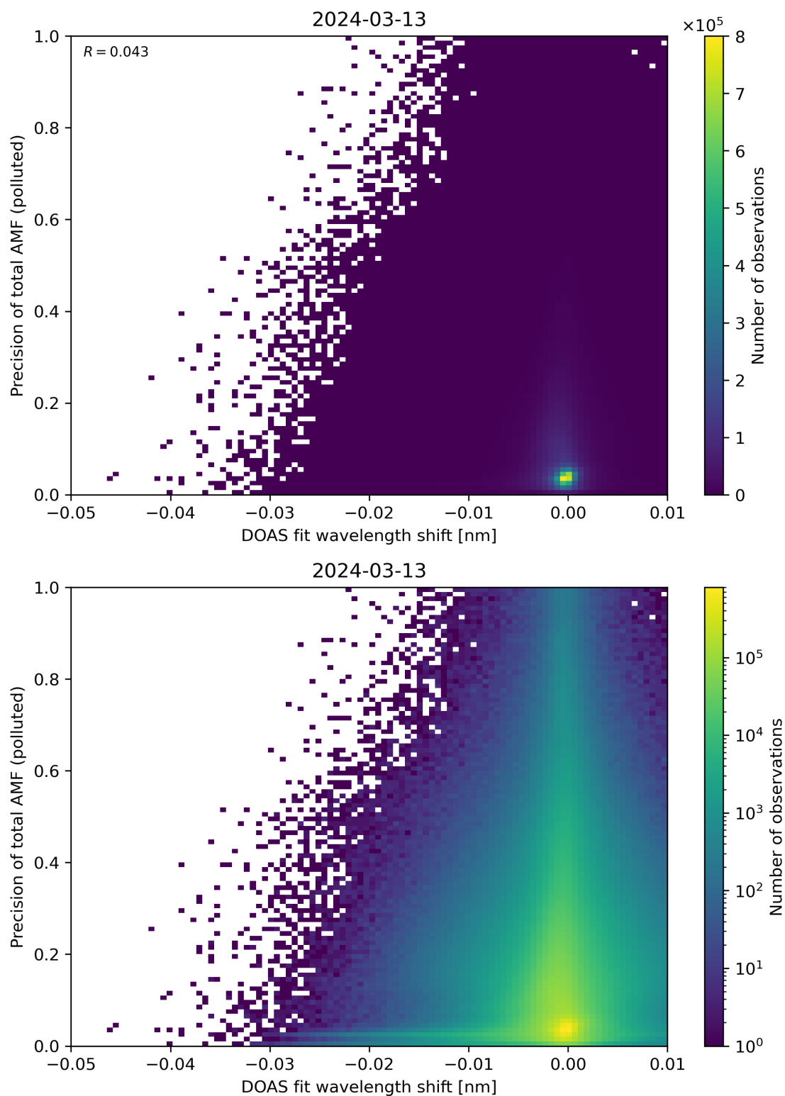
Figure 131: Scatter density plot of “DOAS fit wavelength shift” against “Precision of total AMF (polluted)” for 2024-03-12 to 2024-03-14.
