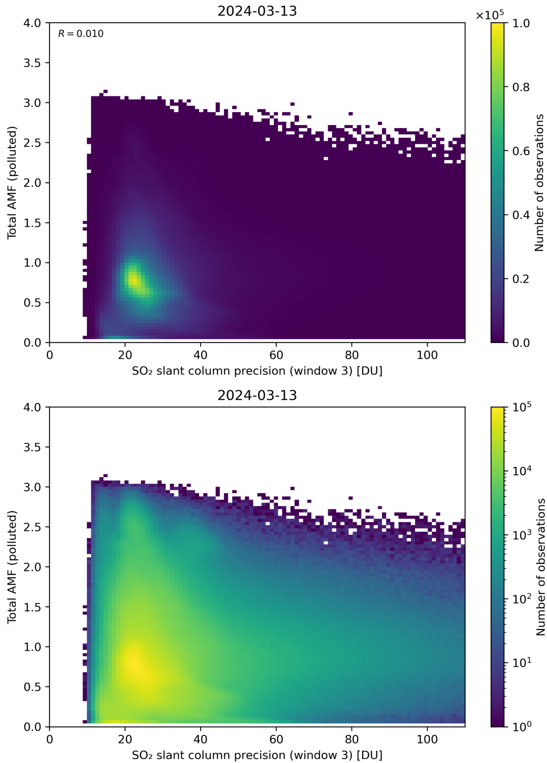
Figure 263: Scatter density plot of “SO 2 slant column precision (window 3)” against “Total AMF (polluted)” for 2024-03-12 to 2024-03-14.
