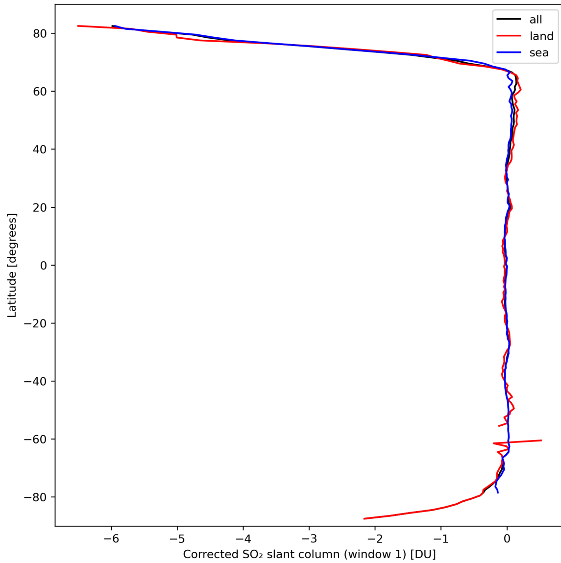
Figure 35: Zonal average of “Corrected SO 2 slant column (window 1)” for 2024-03-12 to 2024-03-14.
