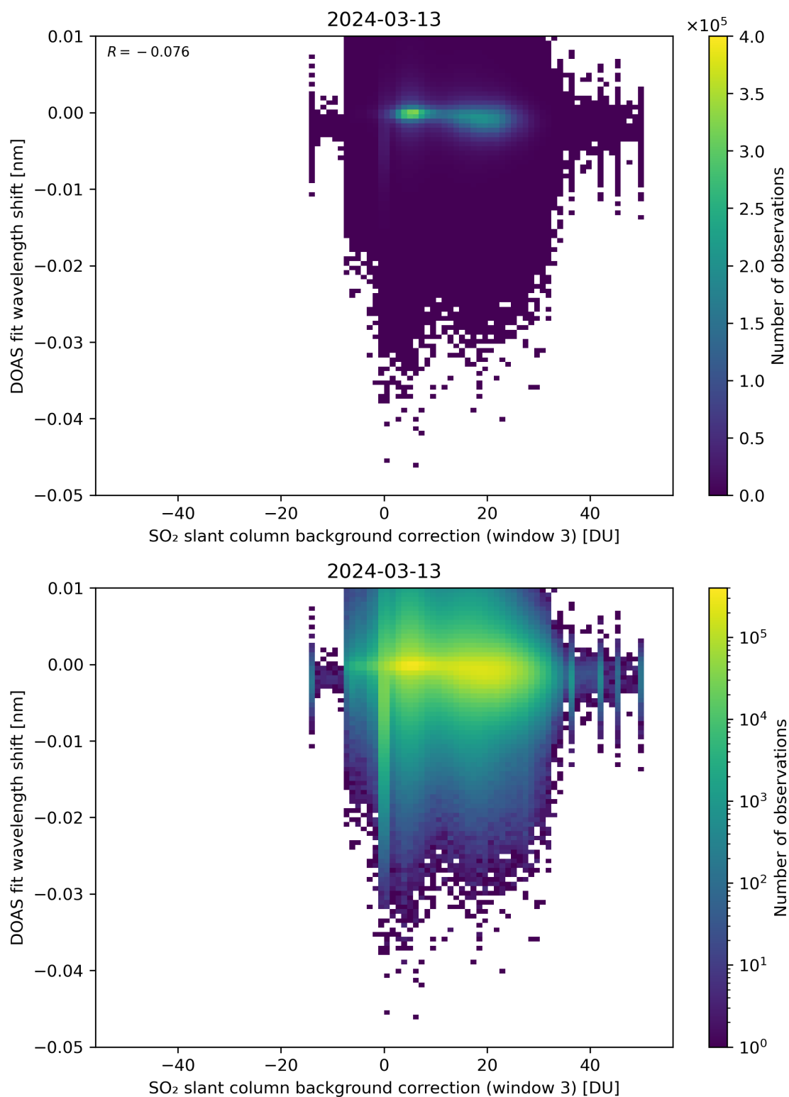
Figure 121: Scatter density plot of “SO 2 slant column background correction (window 3)” against “DOAS fit wavelength shift” for 2024-03-12 to 2024-03-14.
