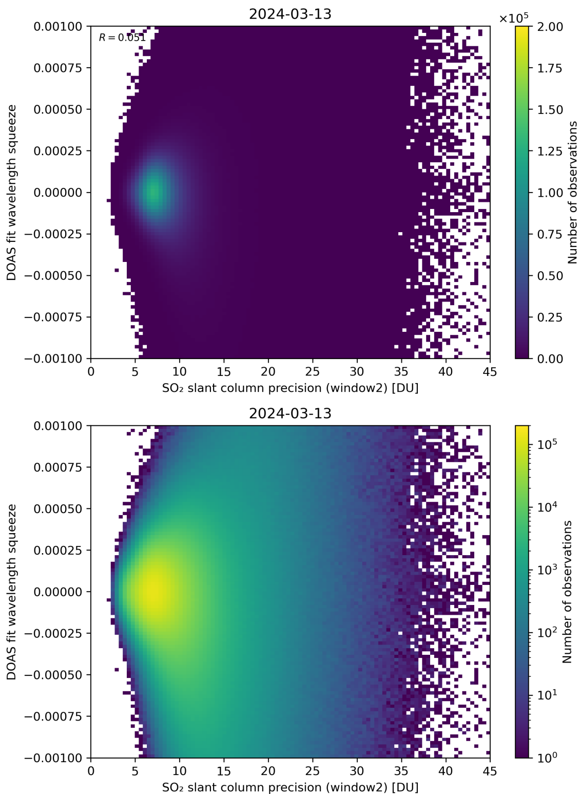
Figure 244: Scatter density plot of “SO 2 slant column precision (window2)” against “DOAS fit wavelength squeeze” for 2024-03-12 to 2024-03-14.
