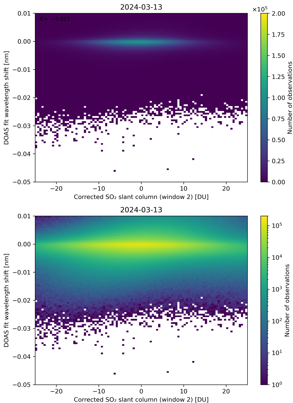
Figure 196: Scatter density plot of “Corrected SO 2 slant column (window 2)” against “DOAS fit wavelength shift” for 2024-03-12 to 2024-03-14.
