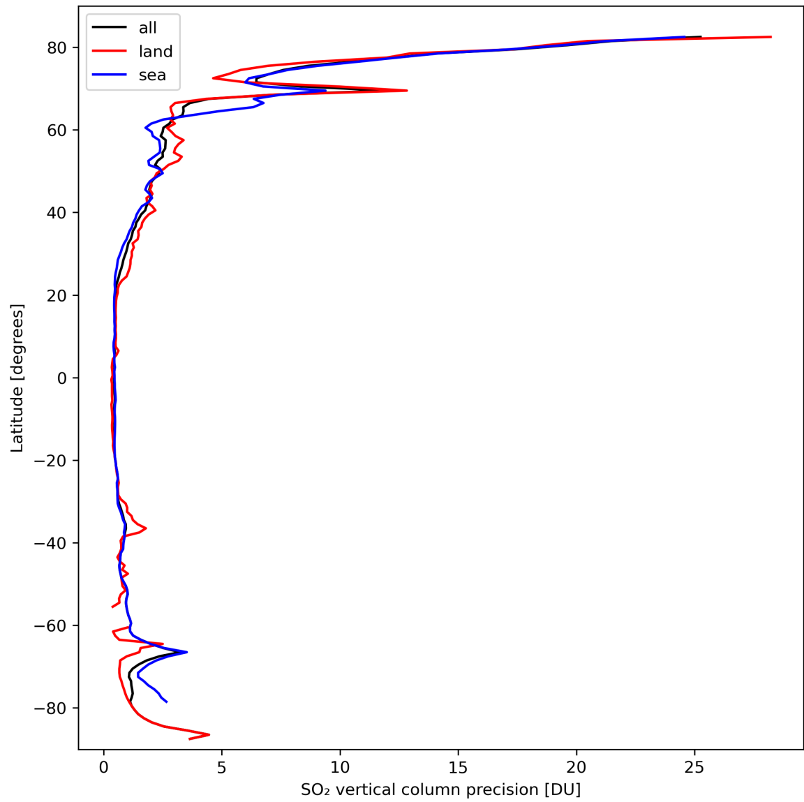
Figure 31: Zonal average of “SO 2 vertical column precision” for 2024-03-12 to 2024-03-14.
