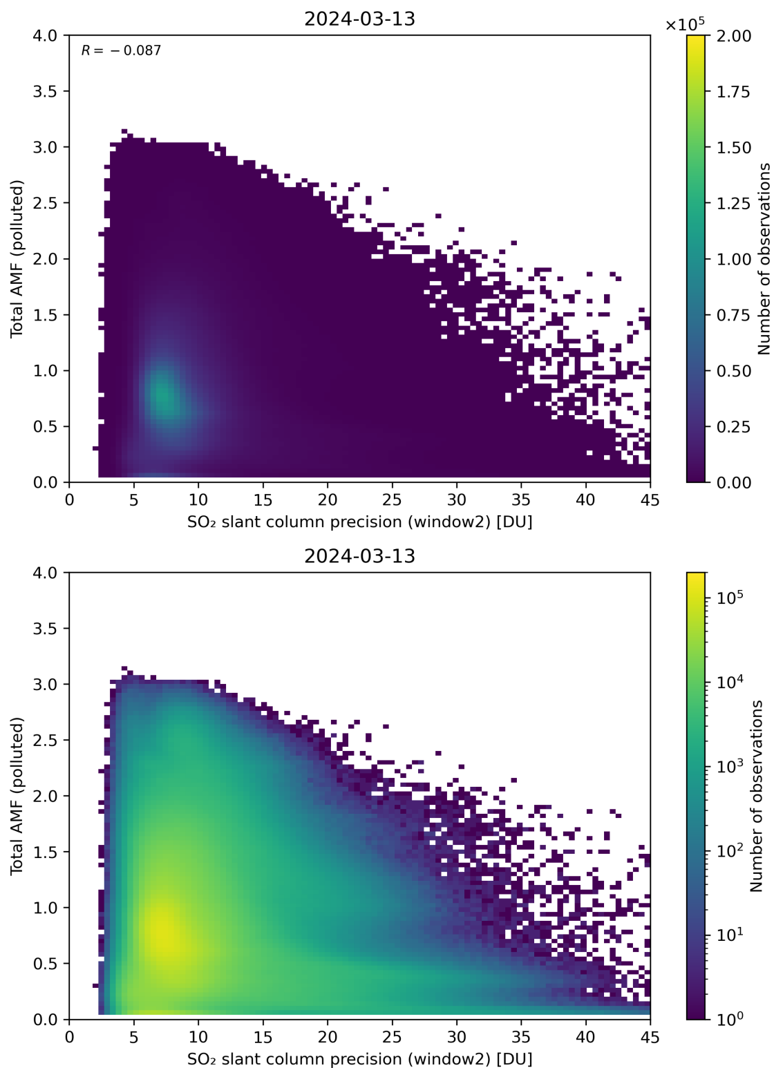
Figure 251: Scatter density plot of “SO 2 slant column precision (window2)” against “Total AMF (polluted)” for 2024-03-12 to 2024-03-14.
