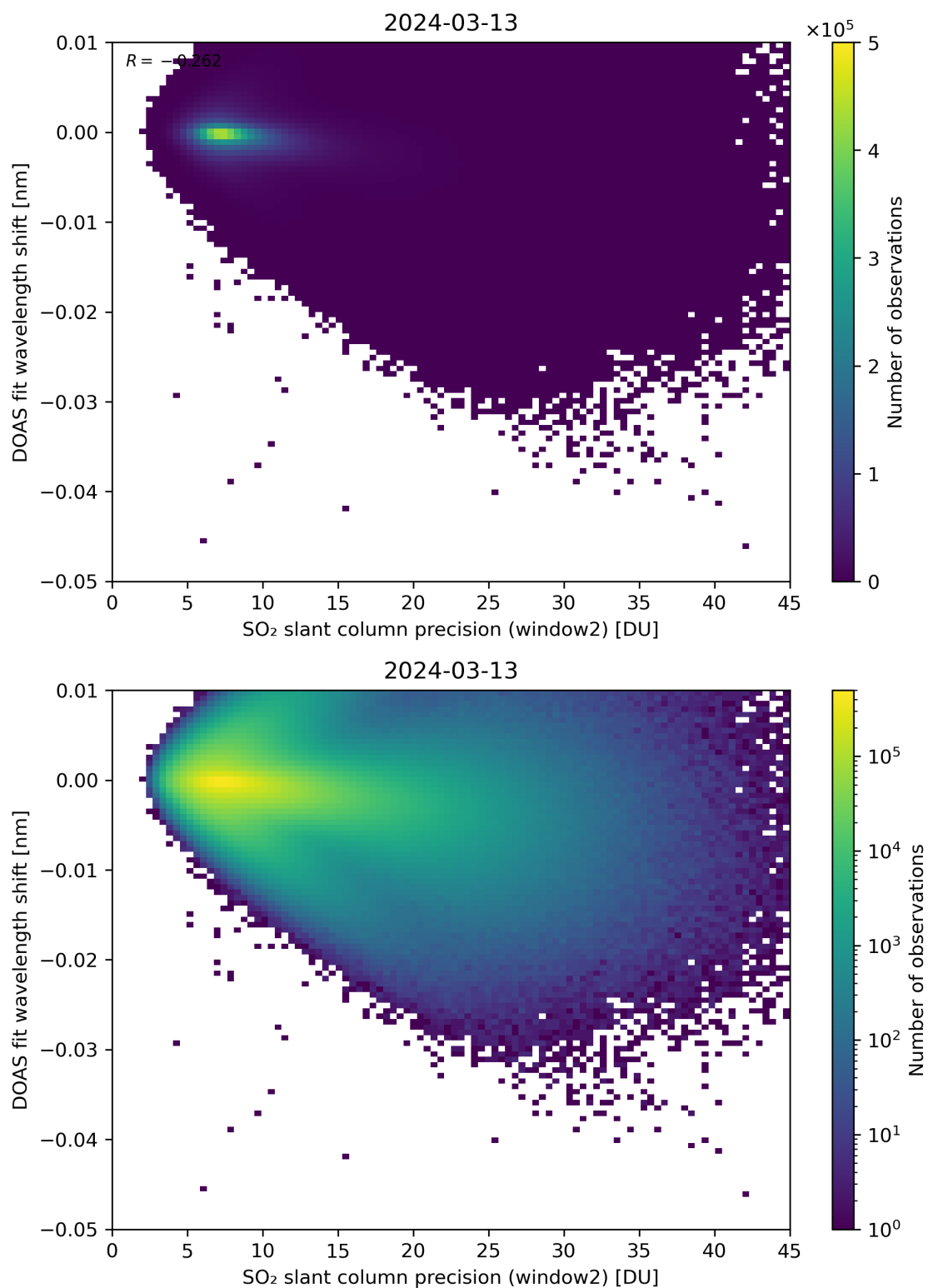
Figure 243: Scatter density plot of “SO 2 slant column precision (window2)” against “DOAS fit wavelength shift” for 2024-03-12 to 2024-03-14.
