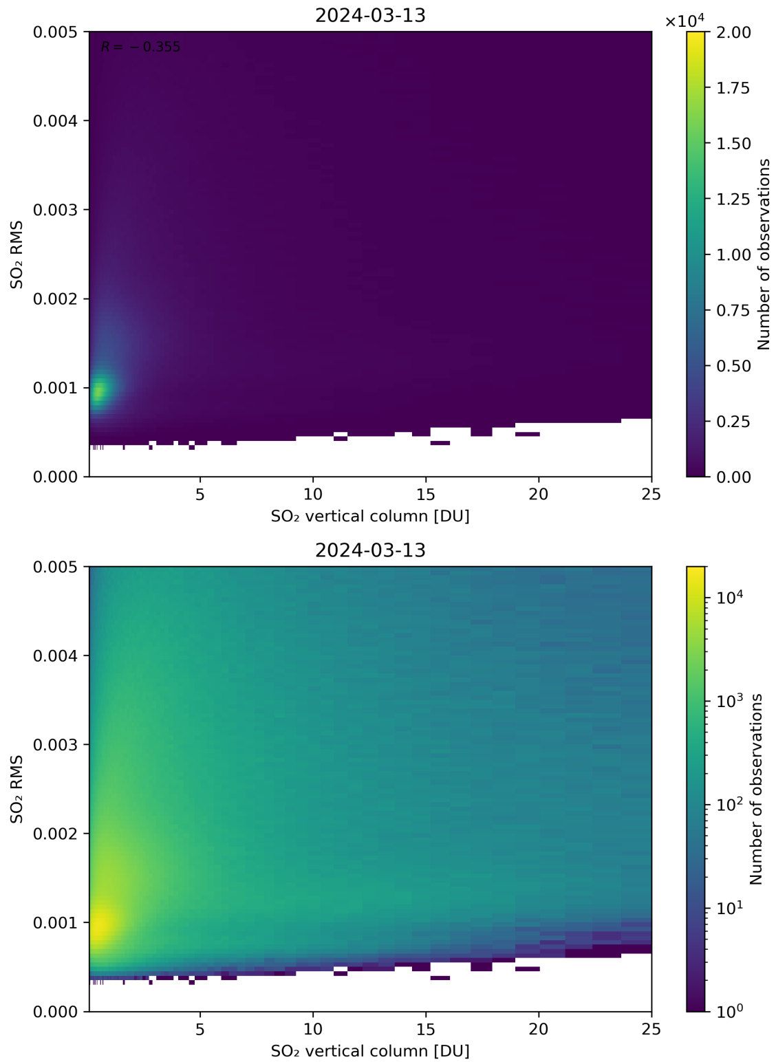
Figure 278: Scatter density plot of “SO 2 vertical column” against “SO 2 RMS” for 2024-03-12 to 2024-03-14.
