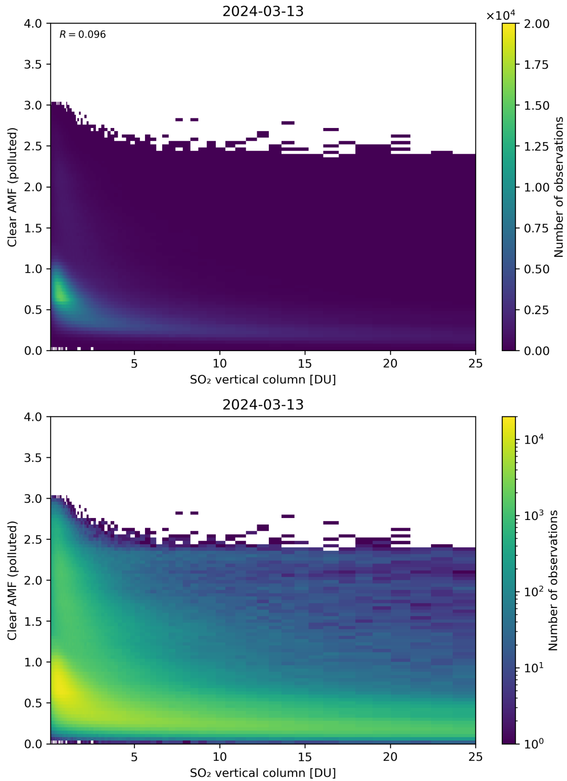
Figure 296: Scatter density plot of “SO 2 vertical column” against “Clear AMF (polluted)” for 2024-03-12 to 2024-03-14.
