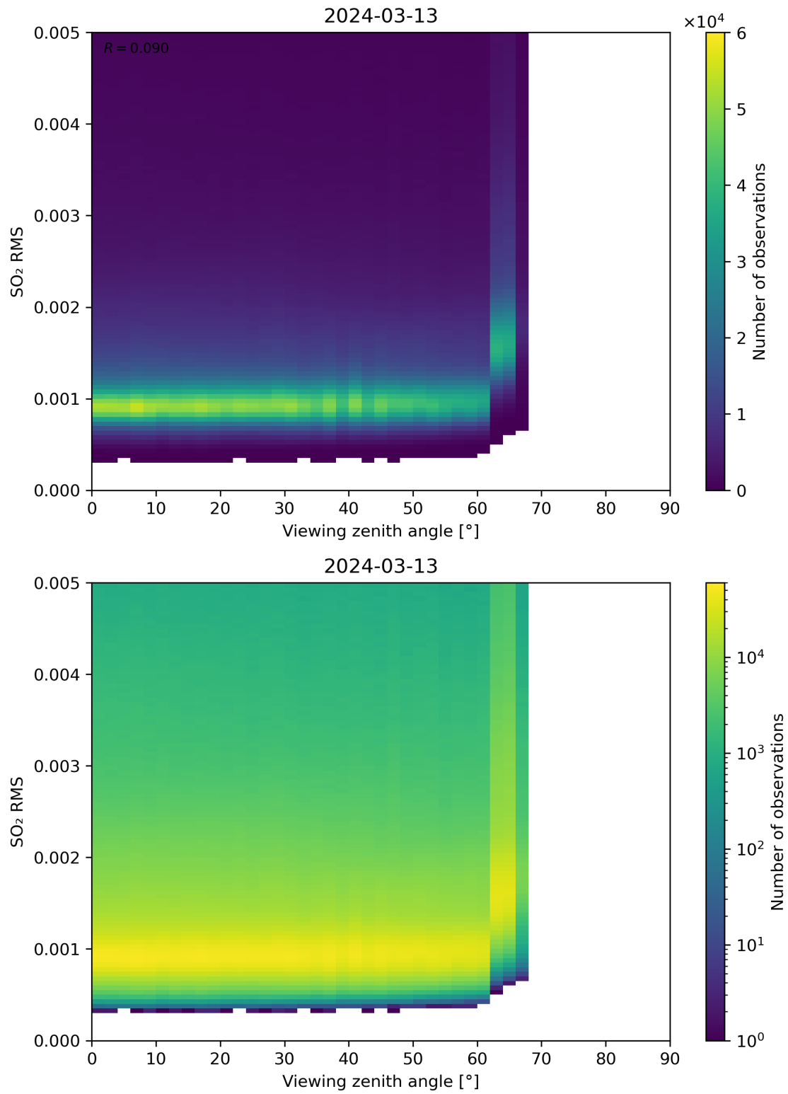
Figure 313: Scatter density plot of “Viewing zenith angle” against “SO 2 RMS” for 2024-03-12 to 2024-03-14.
