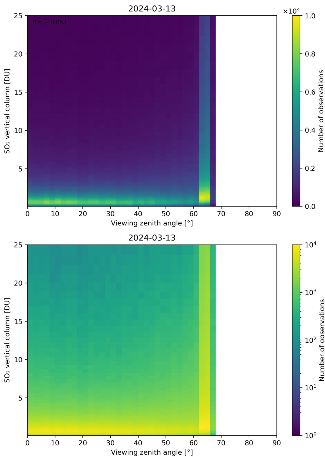
Figure 327: Scatter density plot of “Viewing zenith angle” against “SO 2 vertical column” for 2024-03-12 to 2024-03-14.
