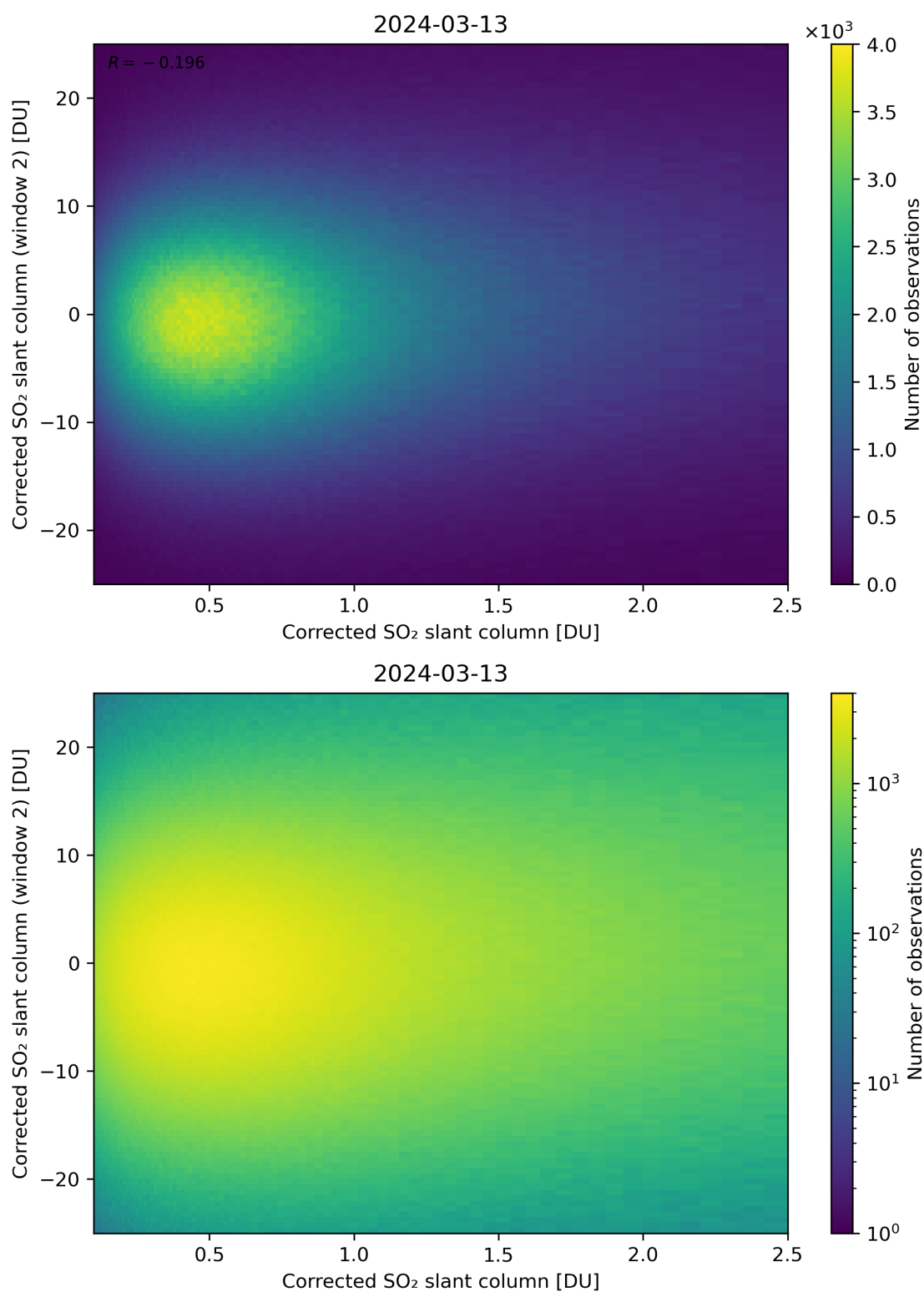
Figure 185: Scatter density plot of “Corrected SO 2 slant column” against “Corrected SO 2 slant column (window 2)” for 2024-03-12 to 2024-03-14.
