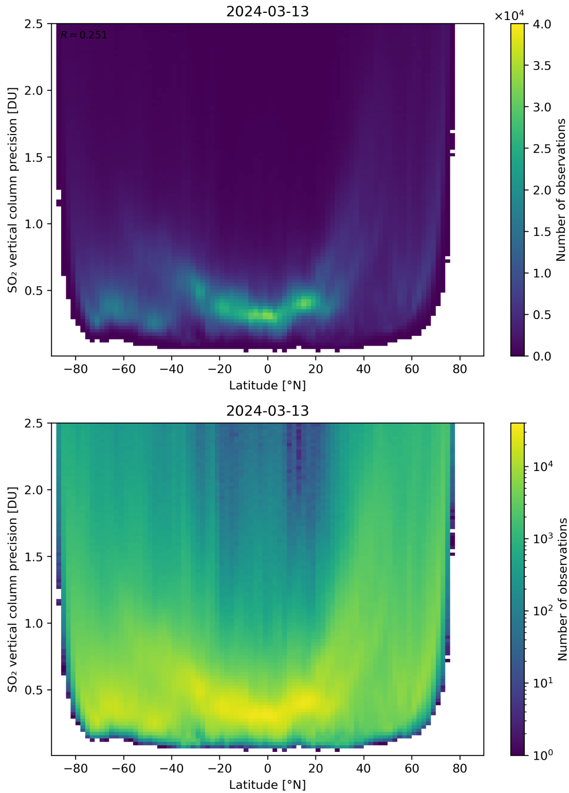
Figure 157: Scatter density plot of “Latitude” against “SO 2 vertical column precision” for 2024-03-12 to 2024-03-14.
