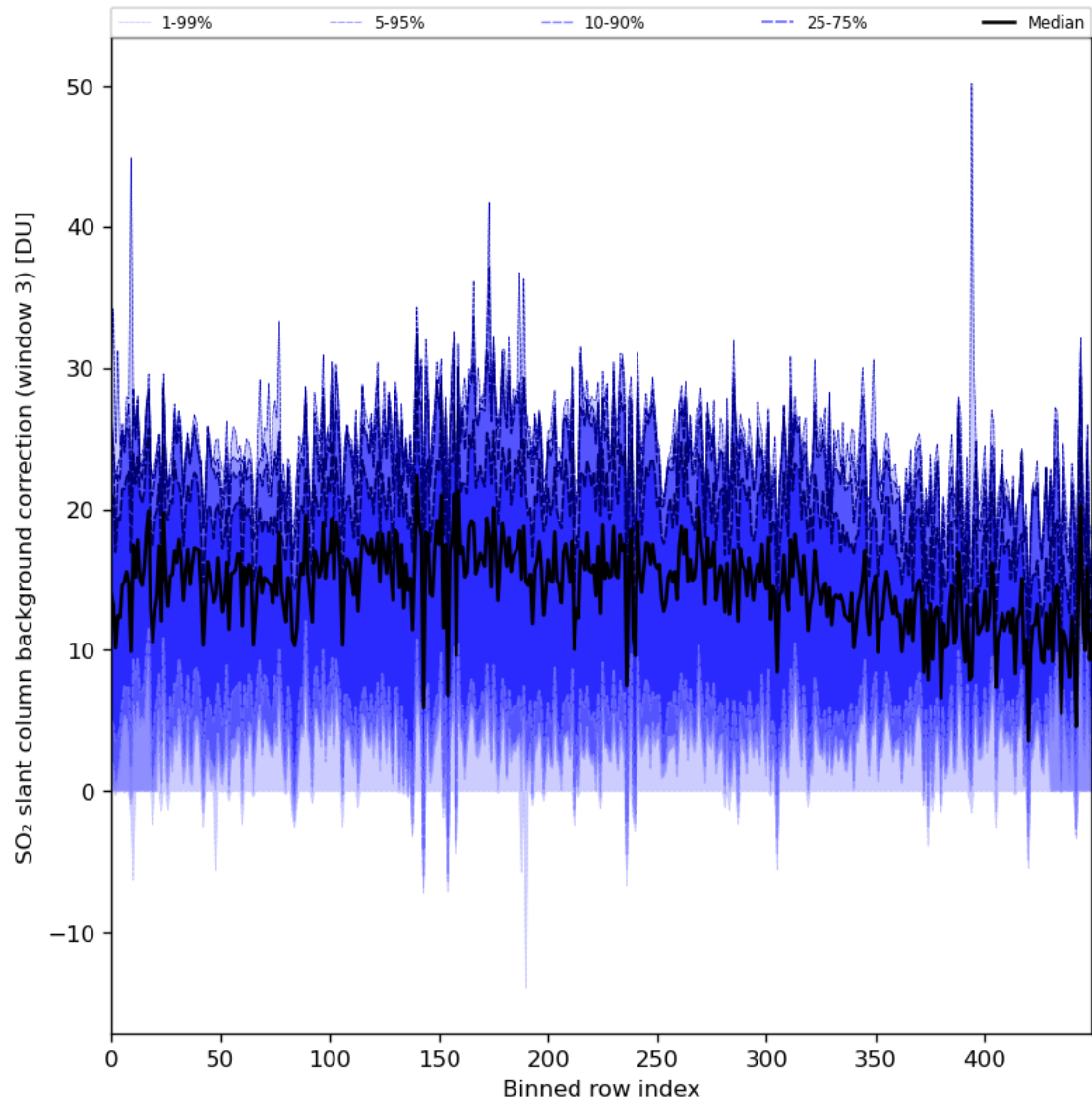
Figure 90: Along track statistics of “SO 2 slant column background correction (window 3)” for 2024-03-12 to 2024-03-14
