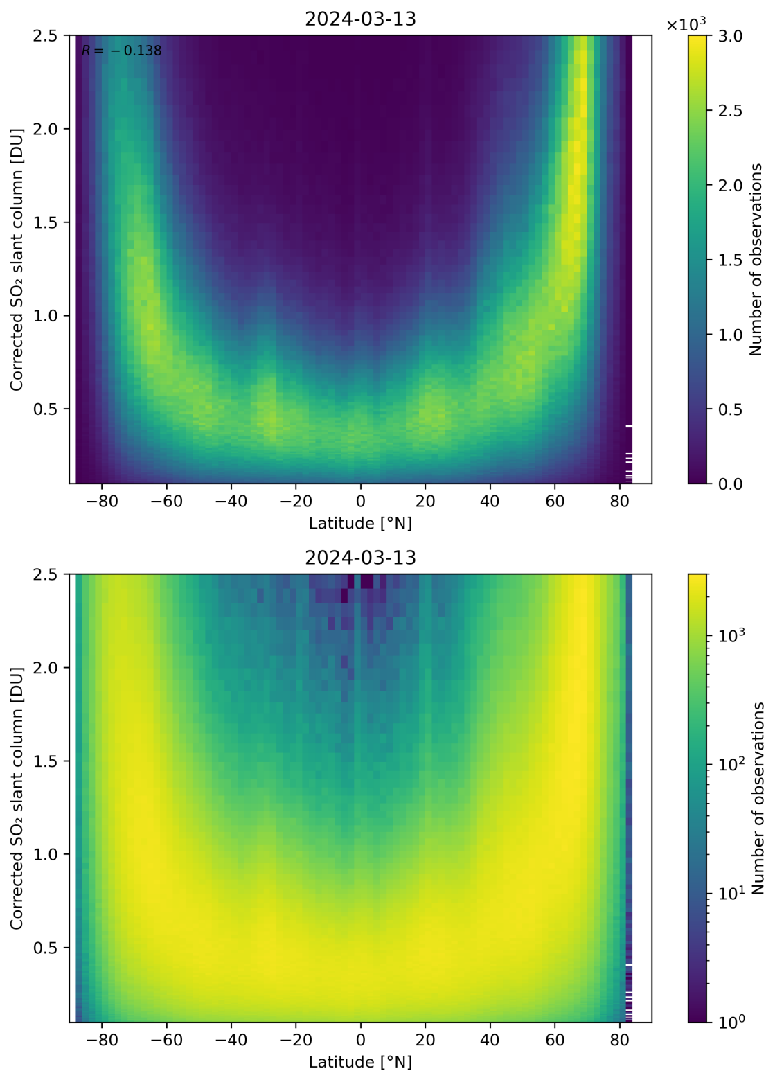
Figure 146: Scatter density plot of “Latitude” against “Corrected SO 2 slant column” for 2024-03-12 to 2024-03-14.
