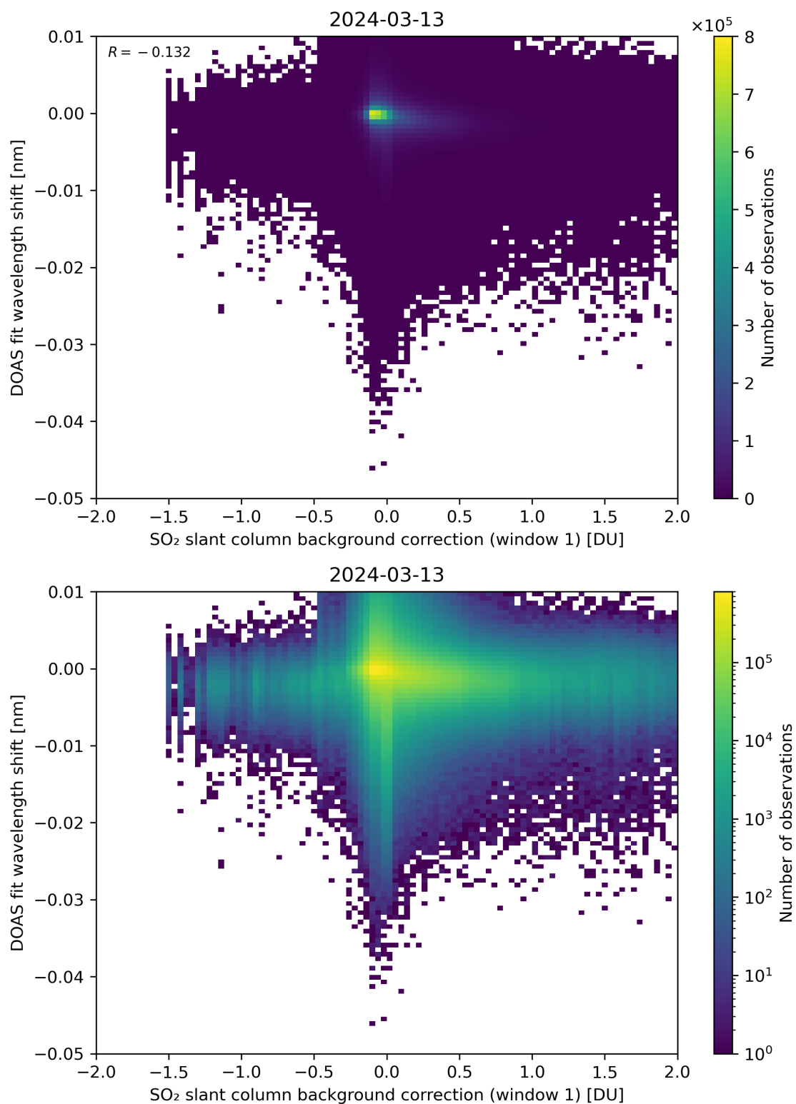
Figure 100: Scatter density plot of “SO 2 slant column background correction (window 1)” against “DOAS fit wavelength shift” for 2024-03-12 to 2024-03-14.
