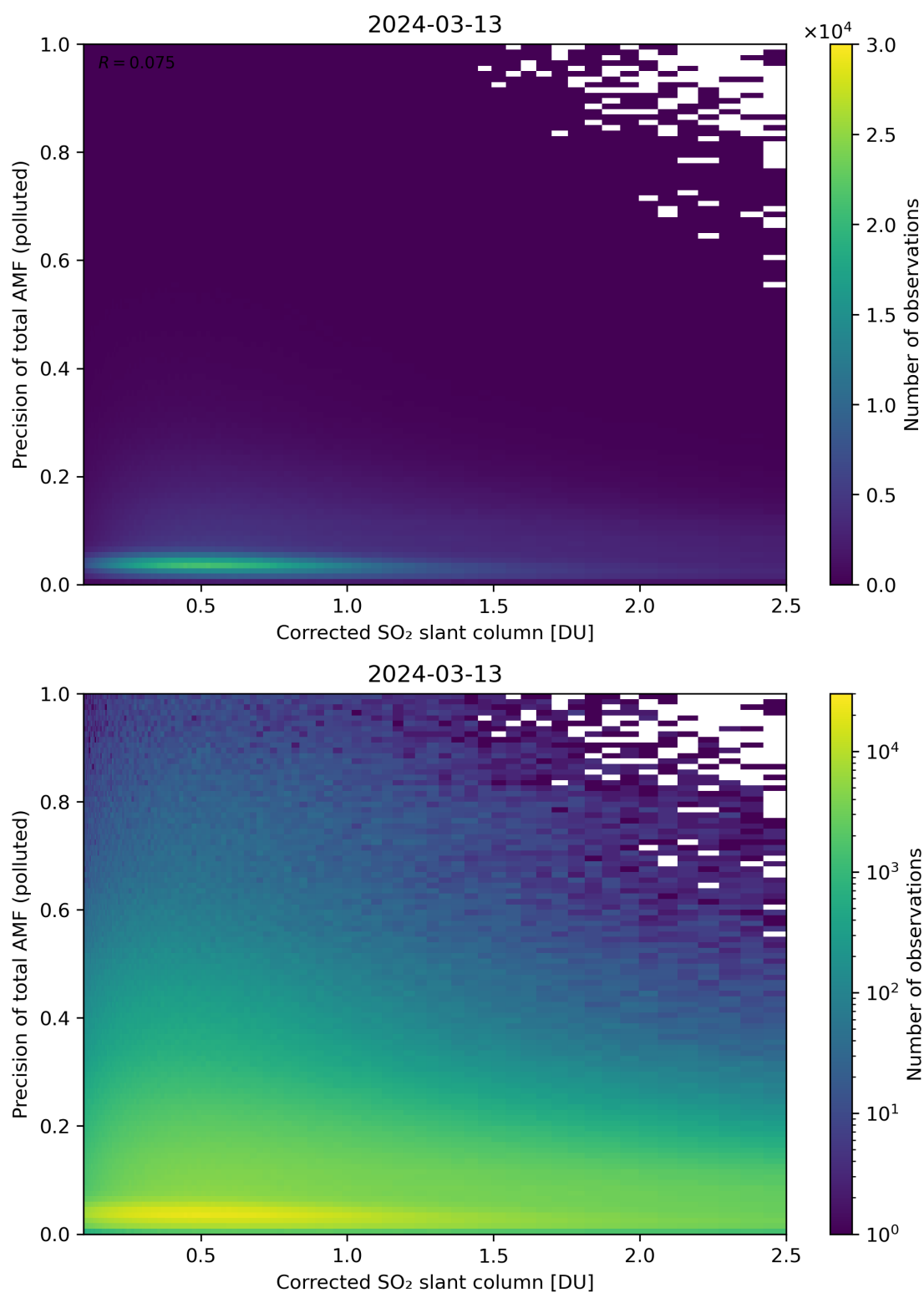
Figure 193: Scatter density plot of “Corrected SO 2 slant column” against “Precision of total AMF (polluted)” for 2024-03-12 to 2024-03-14.
