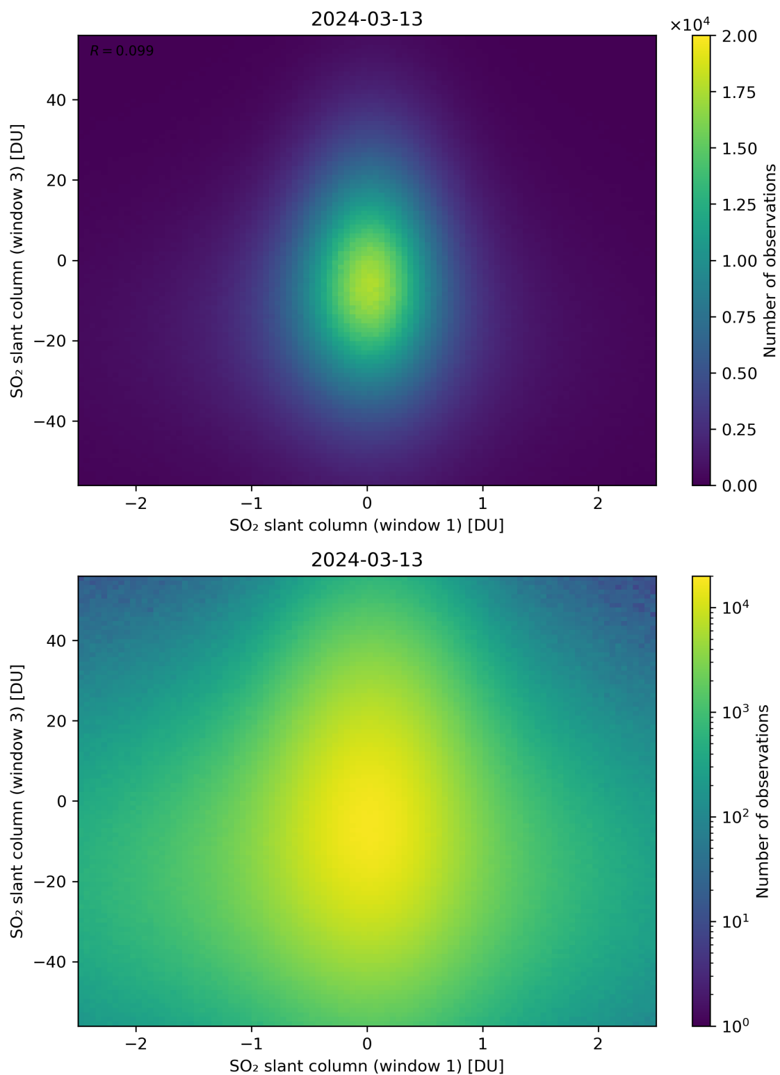
Figure 237: Scatter density plot of “SO 2 slant column (window 1)” against “SO 2 slant column (window 3)” for 2024-03-12 to 2024-03-14.
