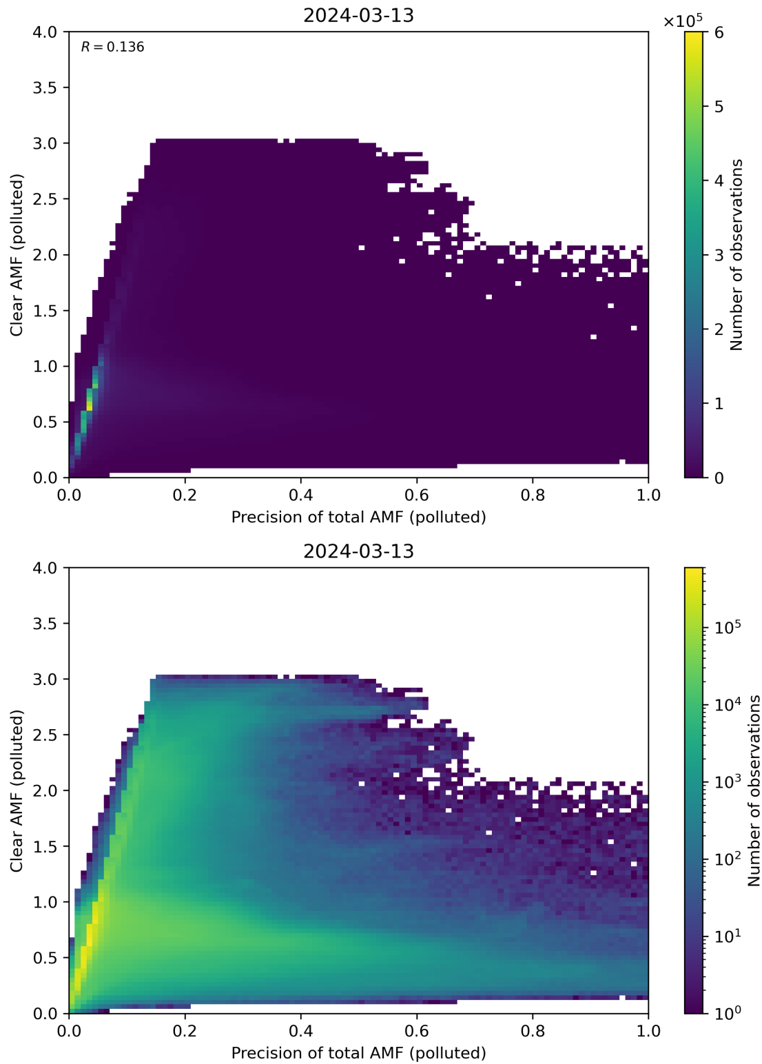
Figure 270: Scatter density plot of “Precision of total AMF (polluted)” against “Clear AMF (polluted)” for 2024-03-12 to 2024-03-14.
