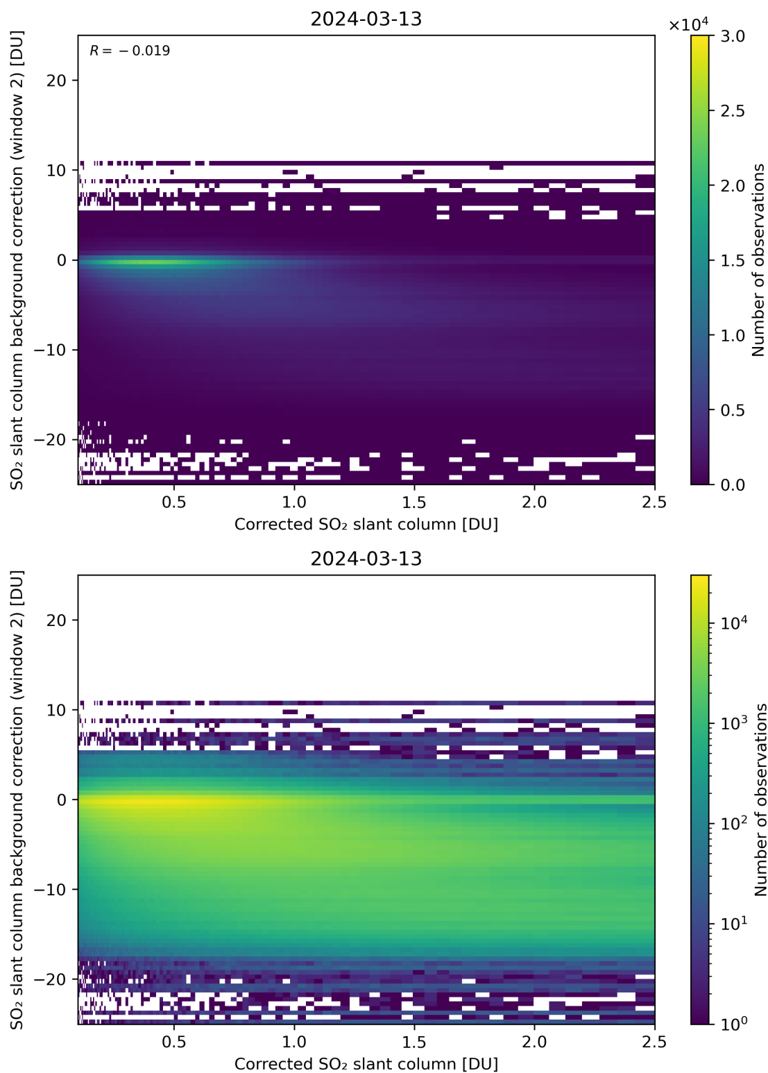
Figure 179: Scatter density plot of “Corrected SO 2 slant column” against “SO 2 slant column background correction (window 2)” for 2024-03-12 to 2024-03-14.
