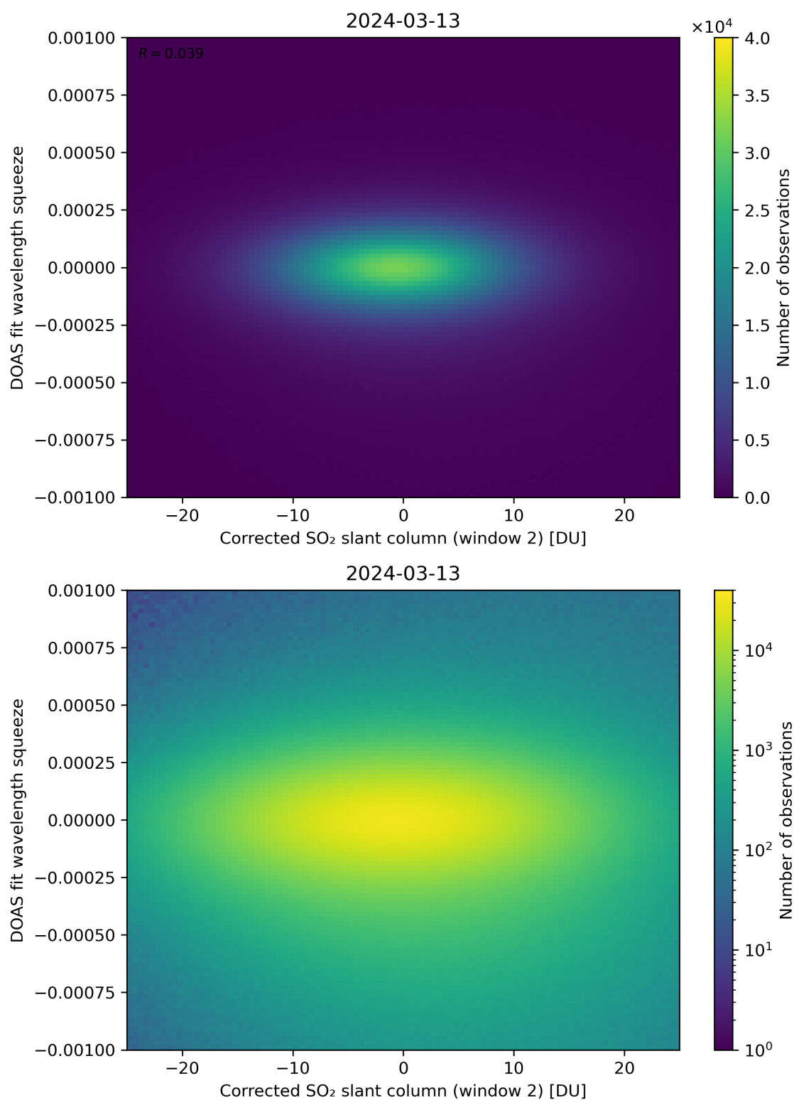
Figure 197: Scatter density plot of “Corrected SO 2 slant column (window 2)” against “DOAS fit wavelength squeeze” for 2024-03-12 to 2024-03-14.
