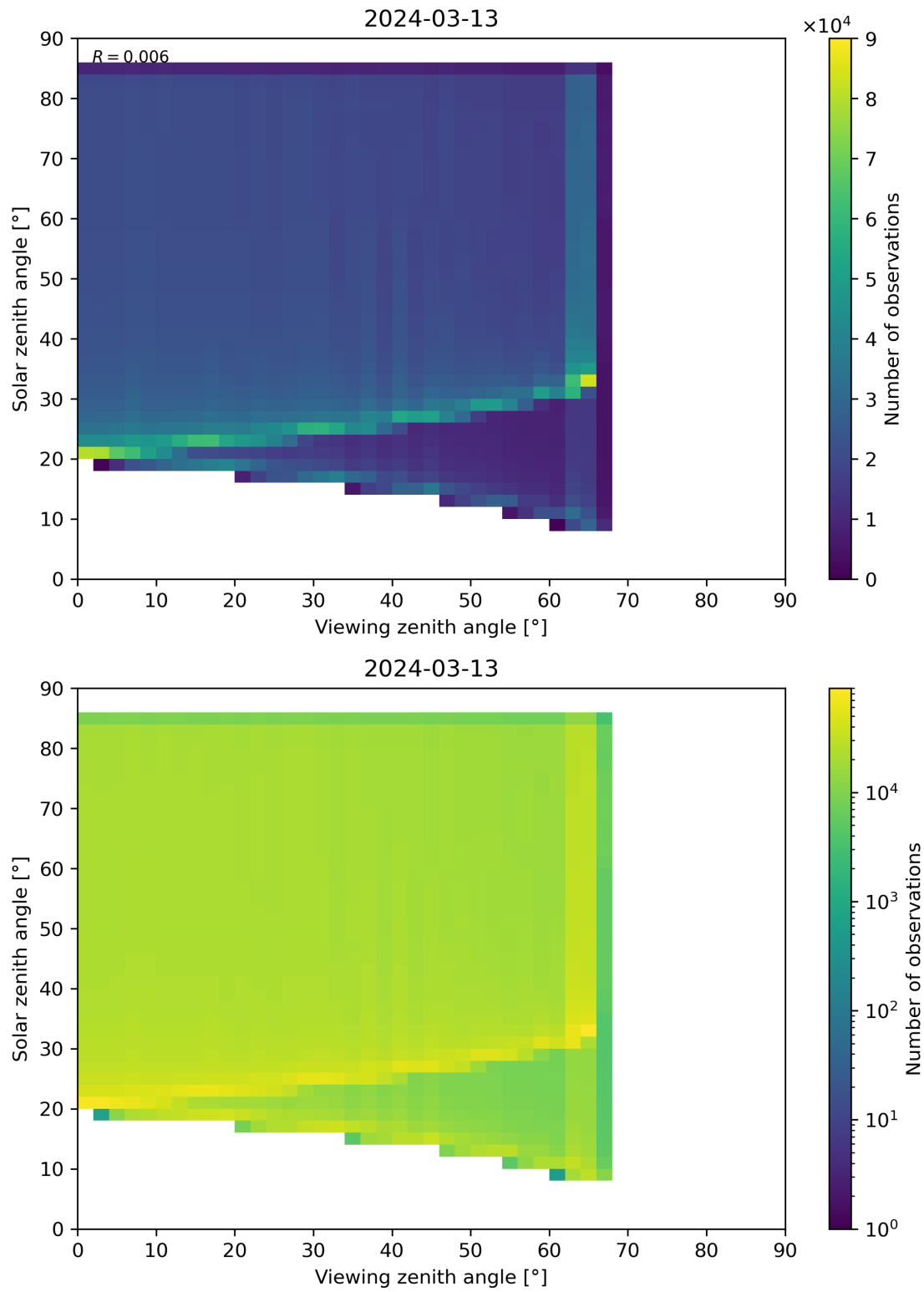
Figure 315: Scatter density plot of “Viewing zenith angle” against “Solar zenith angle” for 2024-03-12 to 2024-03-14.
