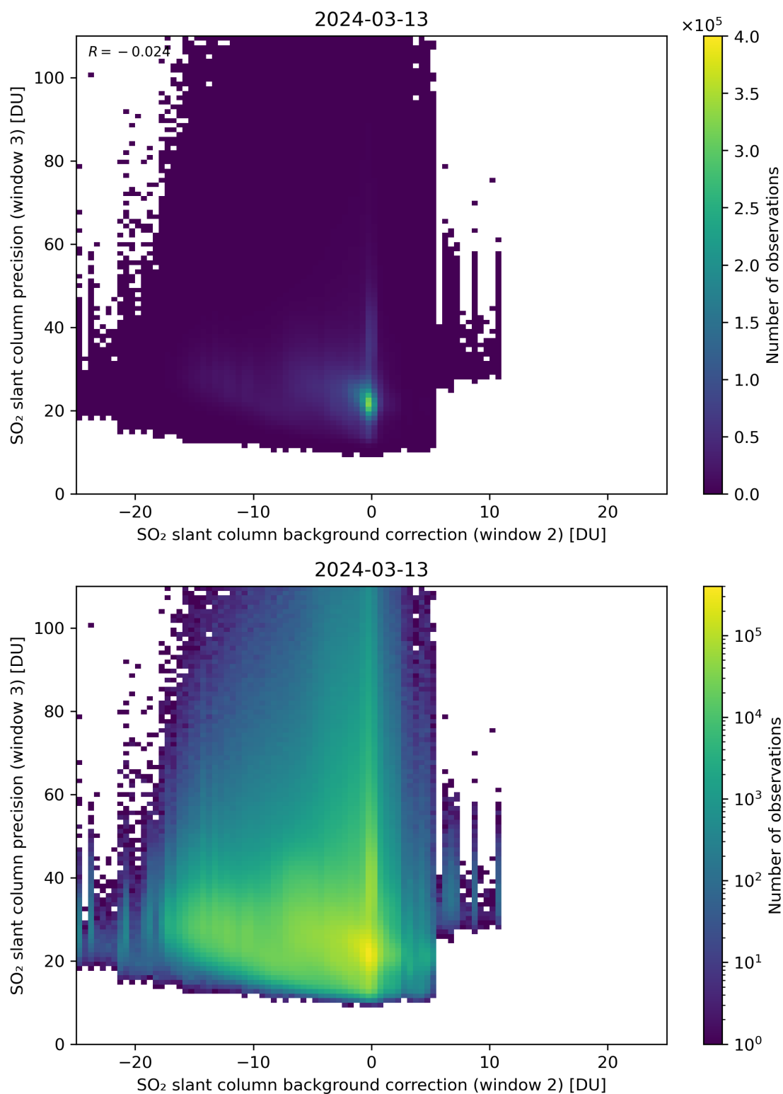
Figure 118: Scatter density plot of “SO 2 slant column background correction (window 2)” against “SO 2 slant column precision (window 3)” for 2024-03-12 to 2024-03-14.
