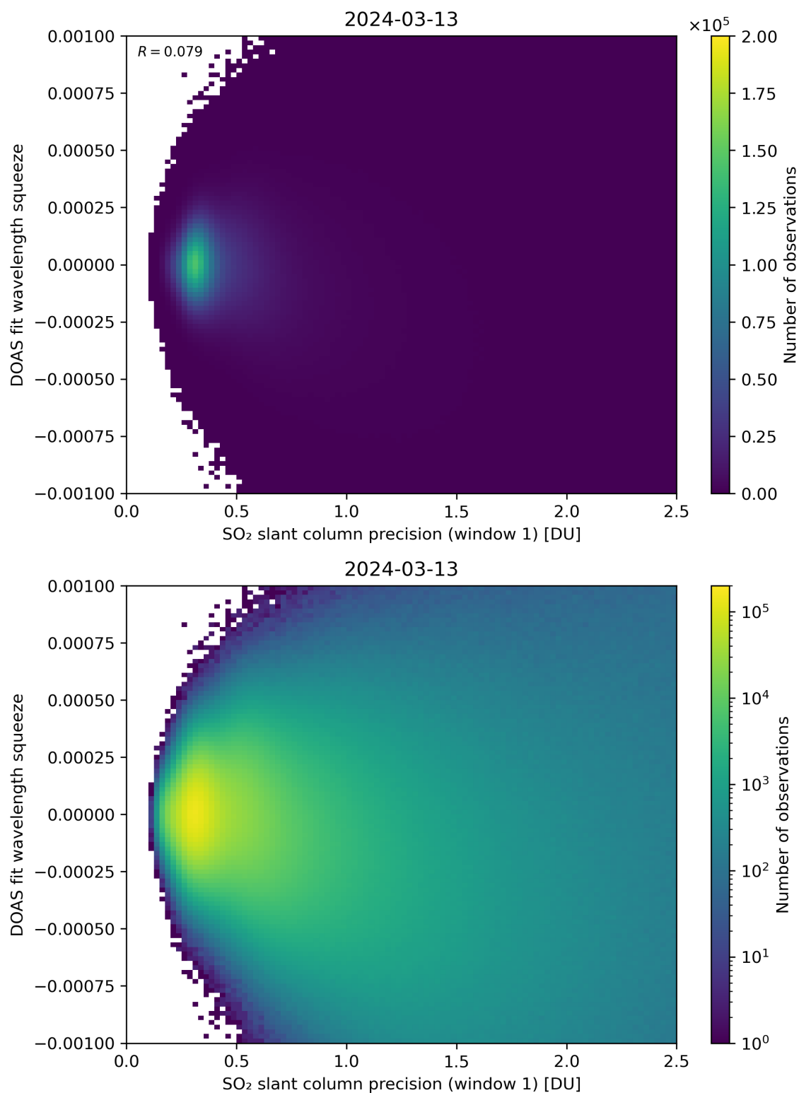
Figure 222: Scatter density plot of “SO 2 slant column precision (window 1)” against “DOAS fit wavelength squeeze” for 2024-03-12 to 2024-03-14.
