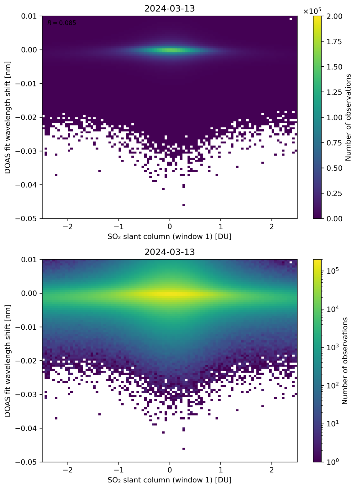
Figure 215: Scatter density plot of “SO 2 slant column (window 1)” against “DOAS fit wavelength shift” for 2024-03-12 to 2024-03-14.
