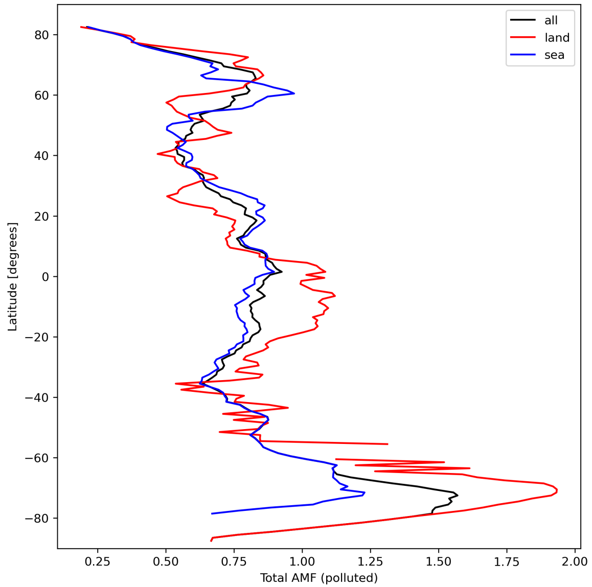
Figure 48: Zonal average of “Total AMF (polluted)” for 2024-03-12 to 2024-03-14.
