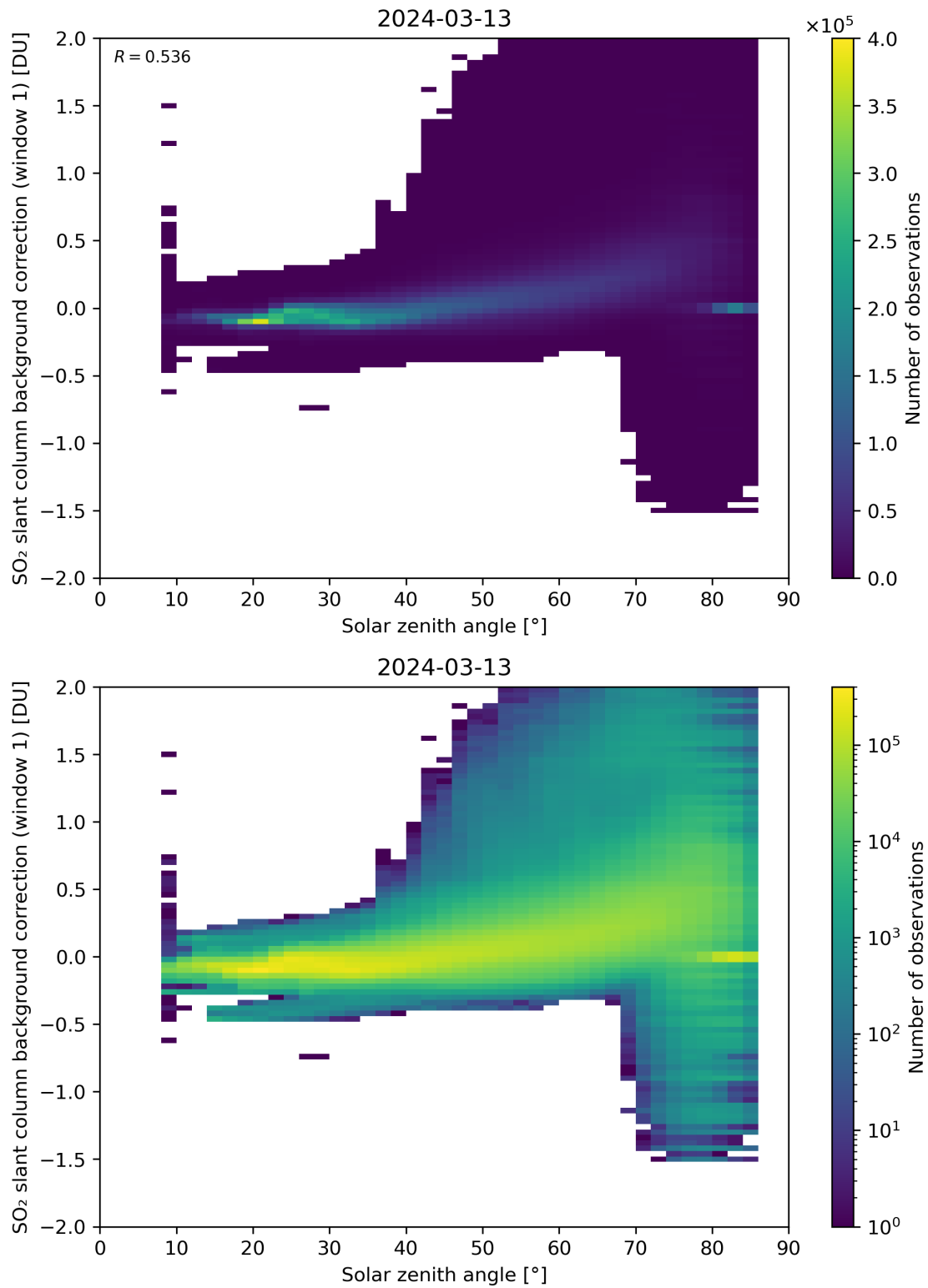
Figure 158: Scatter density plot of “Solar zenith angle” against “SO 2 slant column background correction (window 1)” for 2024-03-12 to 2024-03-14.
