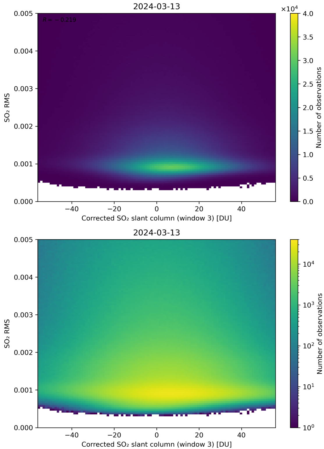
Figure 208: Scatter density plot of “Corrected SO 2 slant column (window 3)” against “SO 2 RMS” for 2024-03-12 to 2024-03-14.
