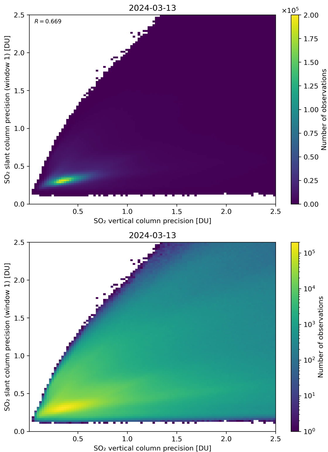
Figure 290: Scatter density plot of “SO 2 vertical column precision” against “SO 2 slant column precision (window 1)” for 2024-03-12 to 2024-03-14.
