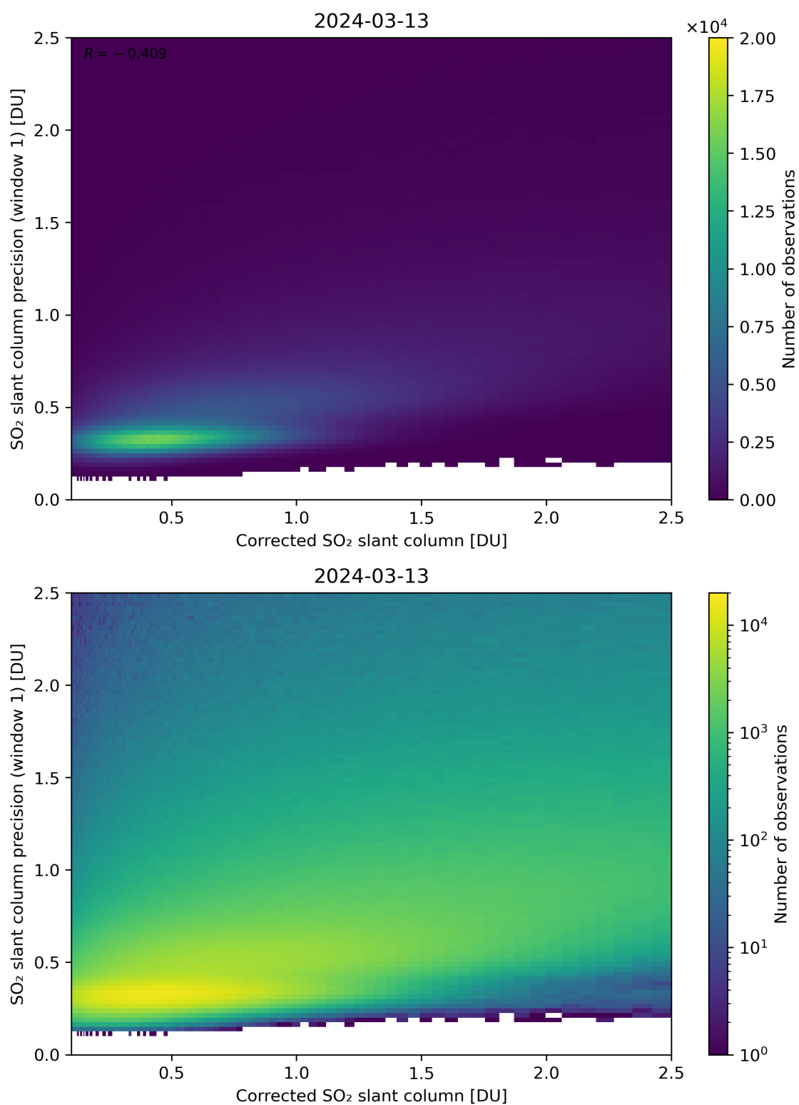
Figure 188: Scatter density plot of “Corrected SO 2 slant column” against “SO 2 slant column precision (window 1)” for 2024-03-12 to 2024-03-14.
