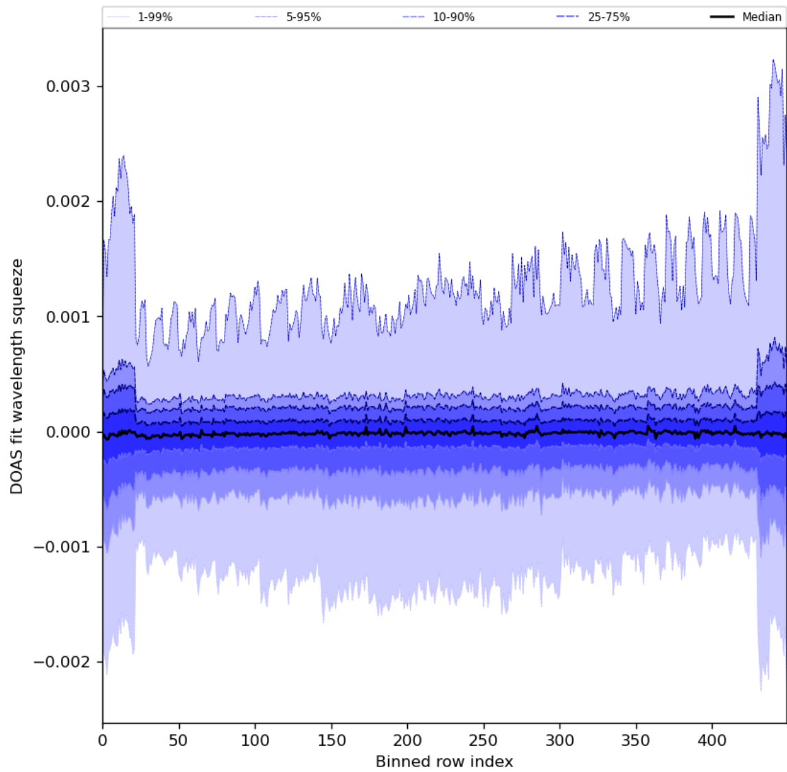
Figure 92: Along track statistics of “DOAS fit wavelength squeeze” for 2024-03-12 to 2024-03-14
