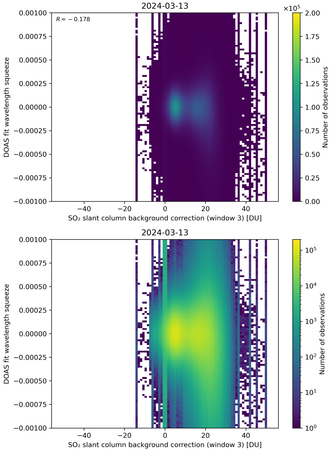
Figure 122: Scatter density plot of “SO 2 slant column background correction (window 3)” against “DOAS fit wavelength squeeze” for 2024-03-12 to 2024-03-14.
