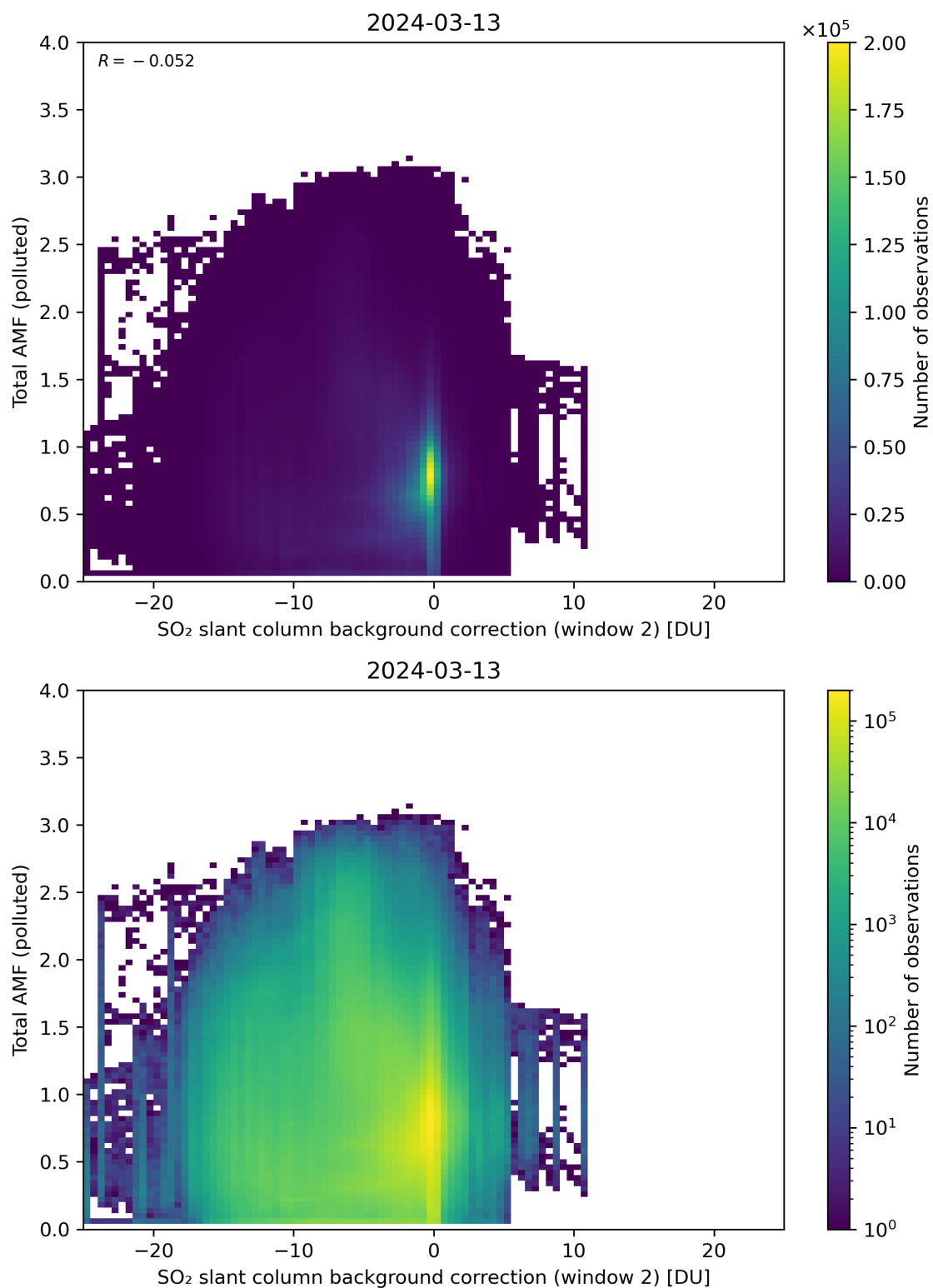
Figure 119: Scatter density plot of “SO 2 slant column background correction (window 2)” against “Total AMF (polluted)” for 2024-03-12 to 2024-03-14.
