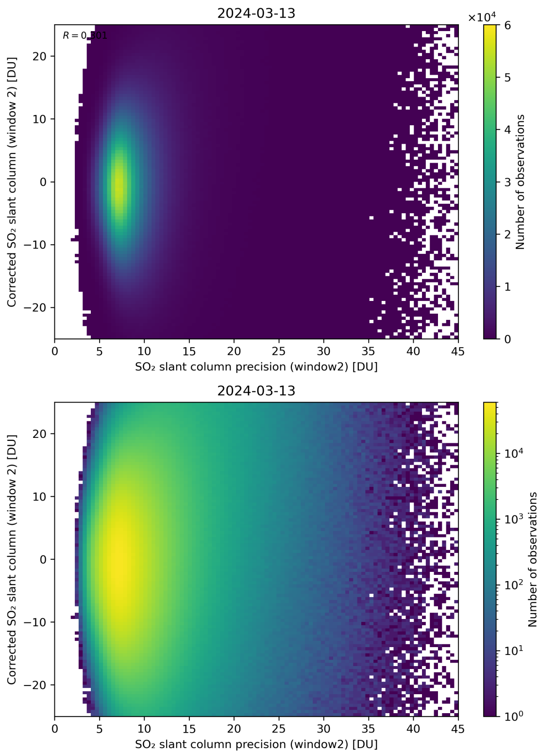
Figure 247: Scatter density plot of “SO 2 slant column precision (window2)” against “Corrected SO 2 slant column (window 2)” for 2024-03-12 to 2024-03-14.
