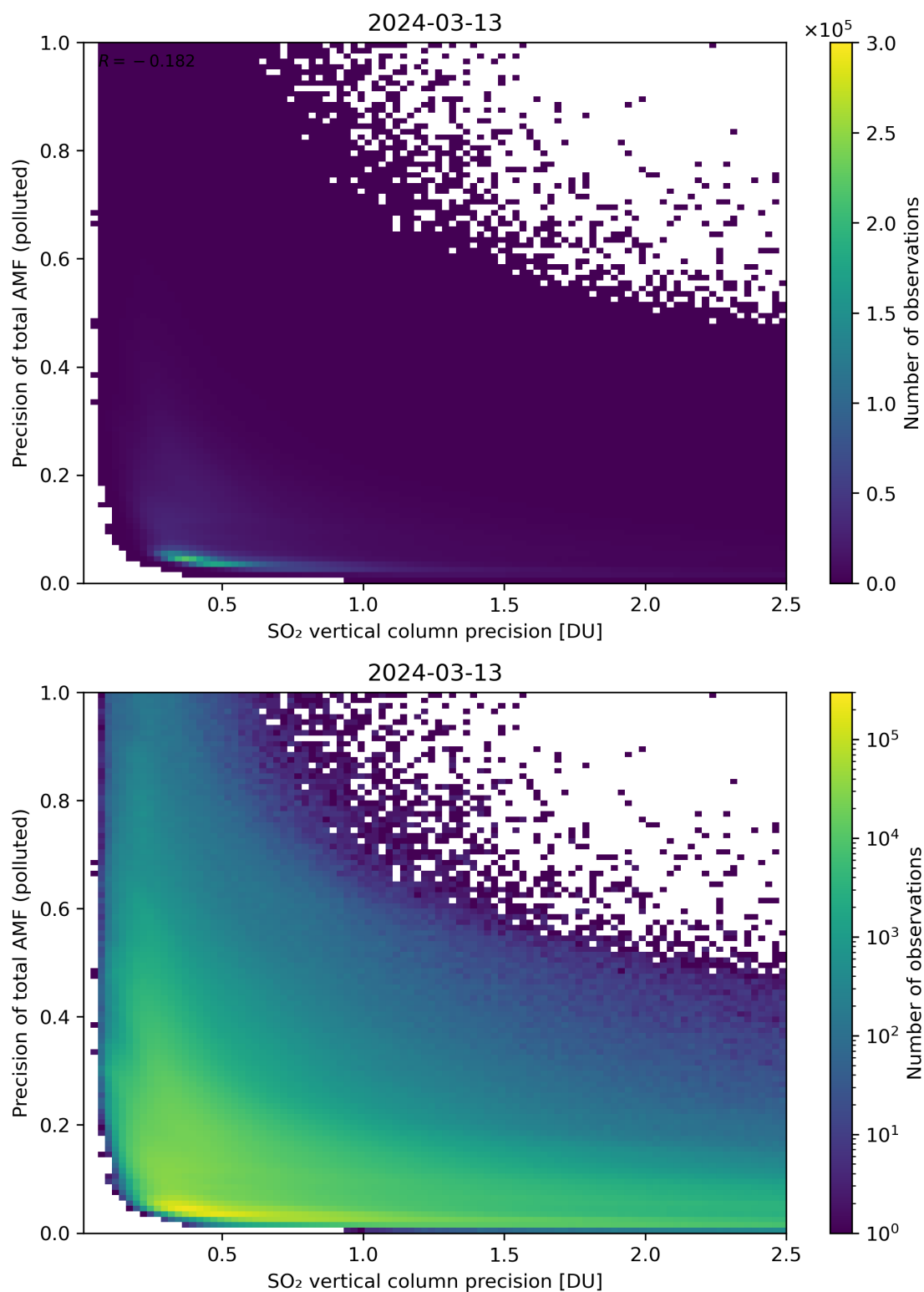
Figure 295: Scatter density plot of “SO 2 vertical column precision” against “Precision of total AMF (polluted)” for 2024-03-12 to 2024-03-14.
