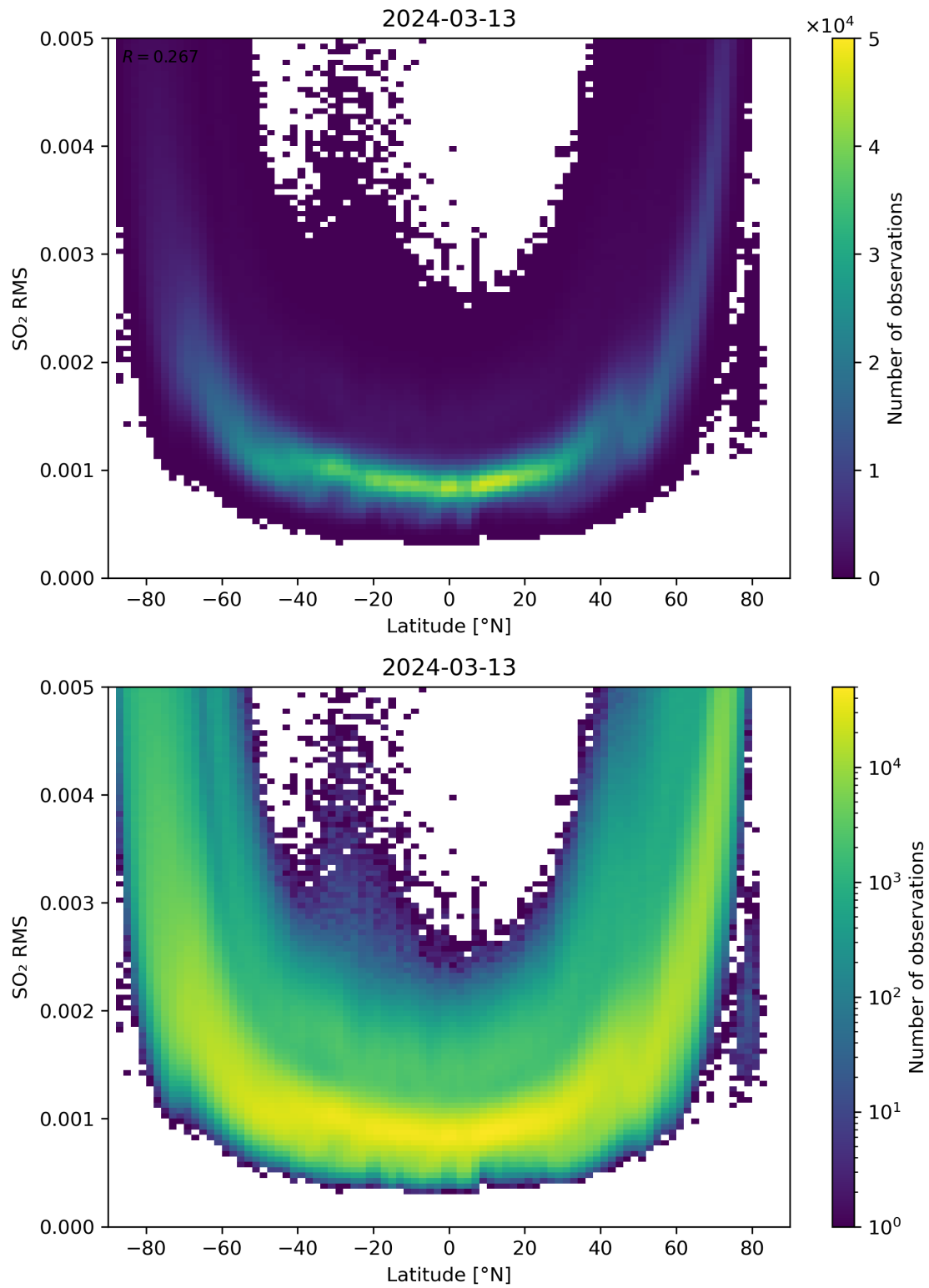
Figure 144: Scatter density plot of “Latitude” against “SO 2 RMS” for 2024-03-12 to 2024-03-14.
