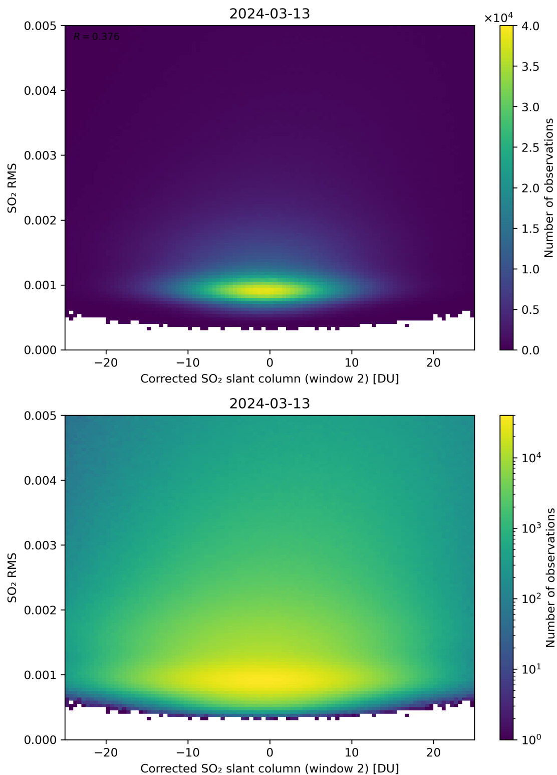
Figure 198: Scatter density plot of “Corrected SO 2 slant column (window 2)” against “SO 2 RMS” for 2024-03-12 to 2024-03-14.
