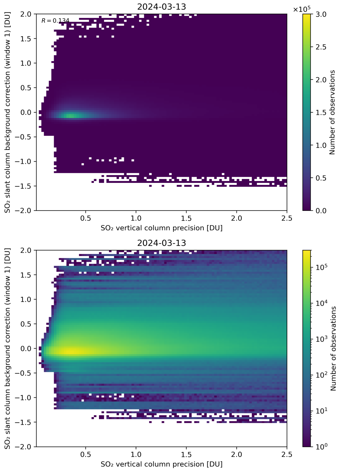
Figure 279: Scatter density plot of “SO 2 vertical column precision” against “SO 2 slant column background correction (window 1)” for 2024-03-12 to 2024-03-14.
