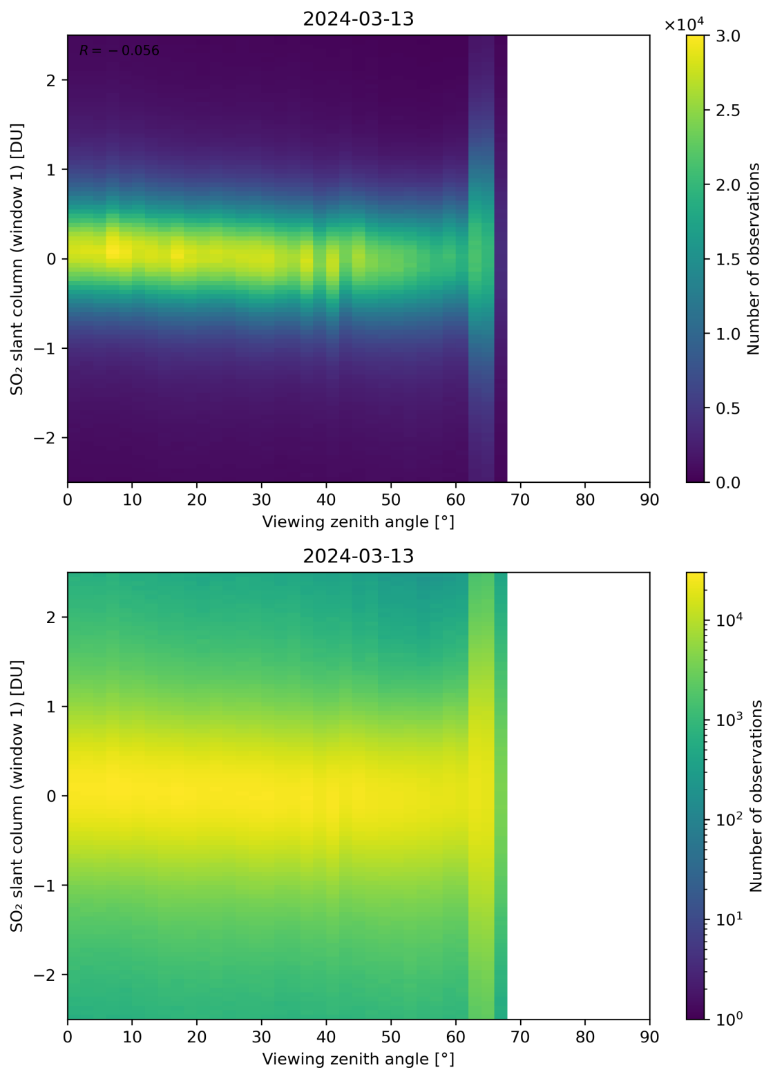
Figure 320: Scatter density plot of “Viewing zenith angle” against “SO 2 slant column (window 1)” for 2024-03-12 to 2024-03-14.
