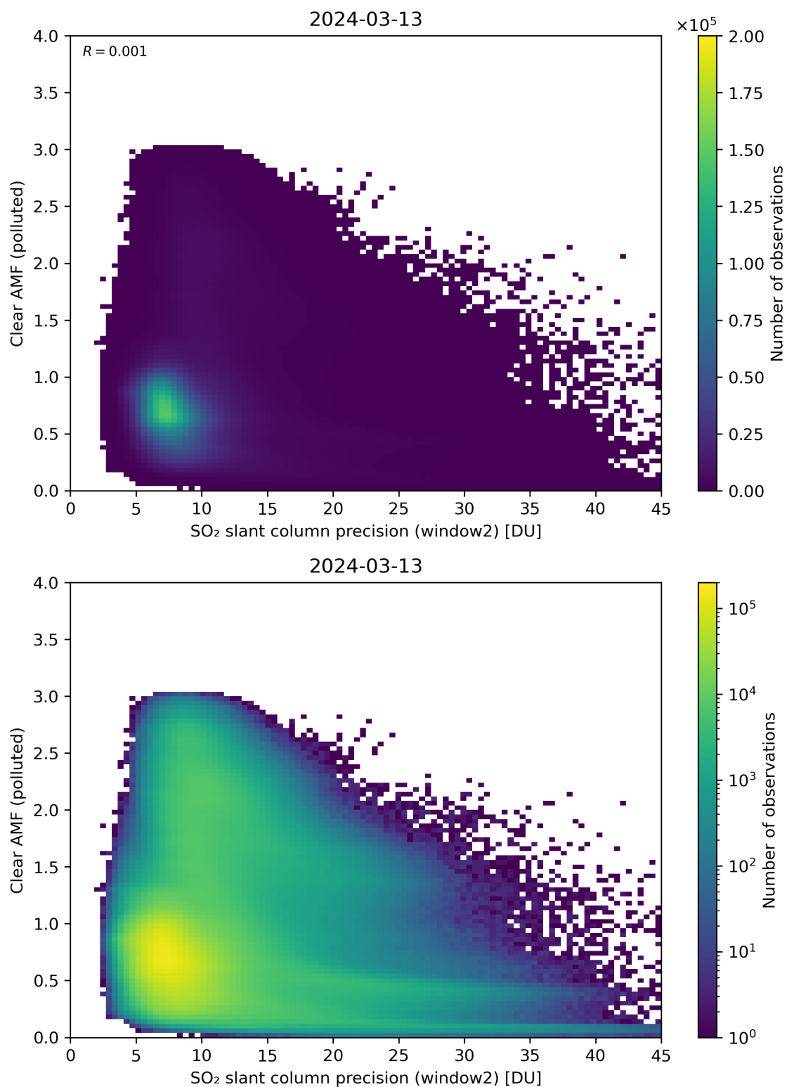
Figure 246: Scatter density plot of “SO 2 slant column precision (window2)” against “Clear AMF (polluted)” for 2024-03-12 to 2024-03-14.
