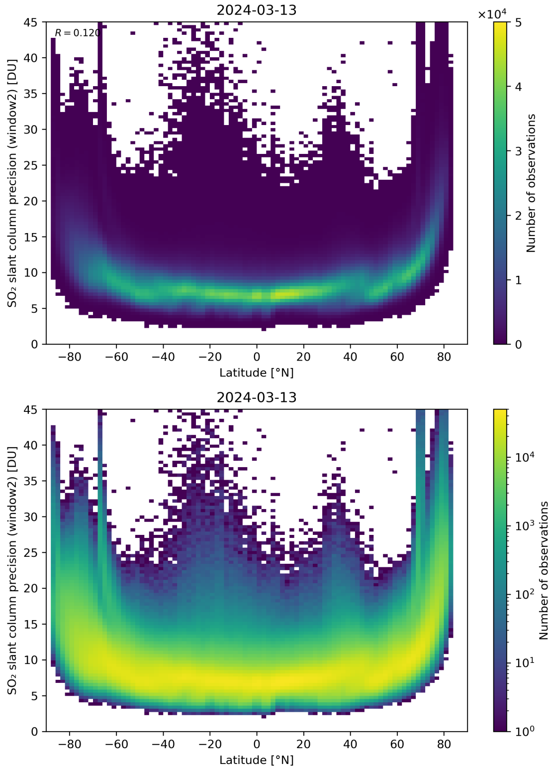
Figure 151: Scatter density plot of “Latitude” against “SO 2 slant column precision (window2)” for 2024-03-12 to 2024-03-14.
