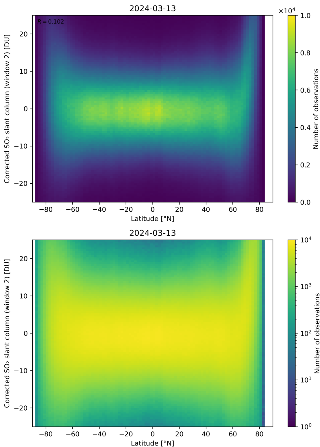
Figure 147: Scatter density plot of “Latitude” against “Corrected SO 2 slant column (window 2)” for 2024-03-12 to 2024-03-14.
