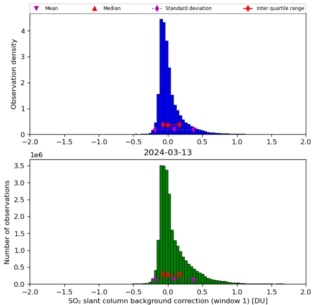
Figure 59: Histogram of “SO 2 slant column background correction (window 1)” for 2024-03-12 to 2024-03-14
