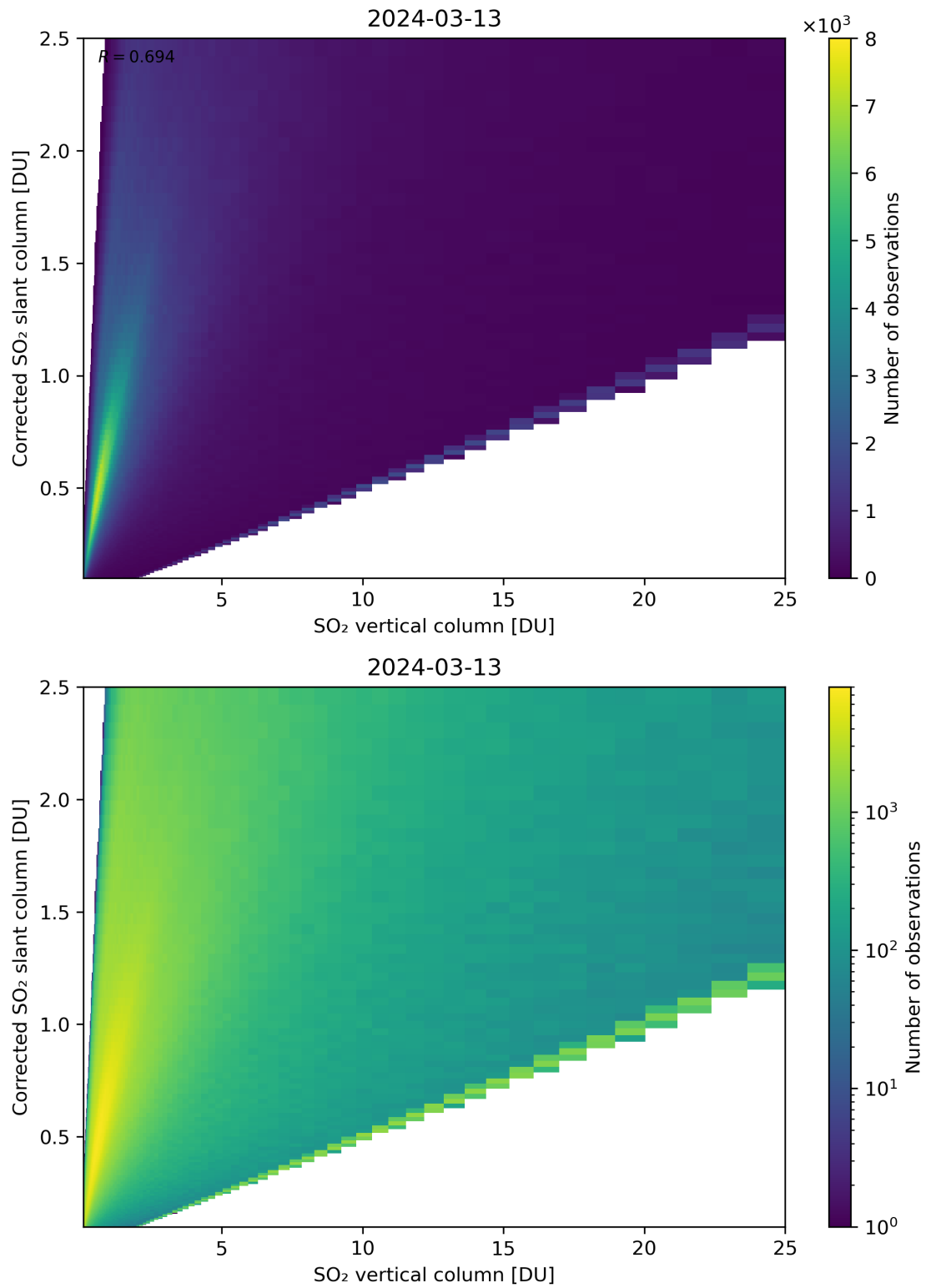
Figure 297: Scatter density plot of “SO 2 vertical column” against “Corrected SO 2 slant column” for 2024-03-12 to 2024-03-14.
