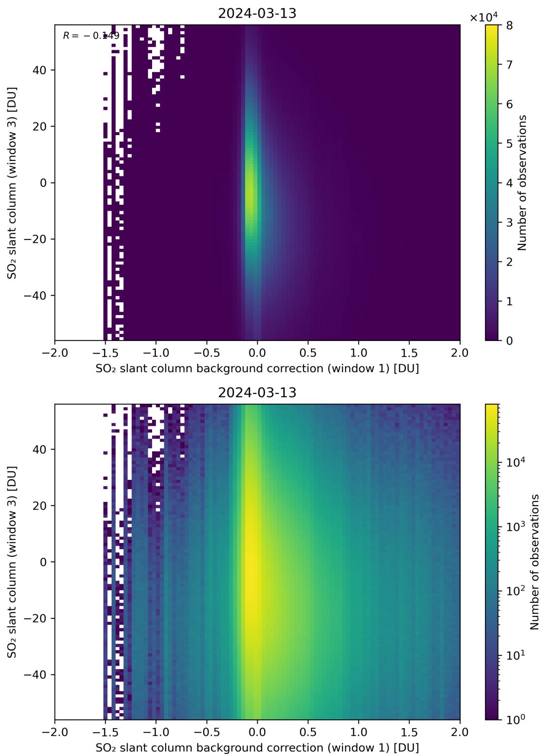
Figure 107: Scatter density plot of “SO 2 slant column background correction (window 1)” against “SO 2 slant column (window 3)” for 2024-03-12 to 2024-03-14.
