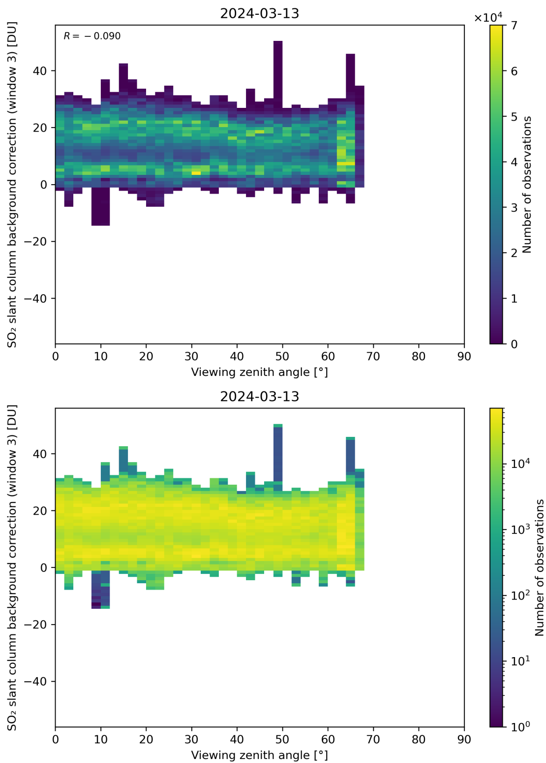
Figure 310: Scatter density plot of “Viewing zenith angle” against “SO 2 slant column background correction (window 3)” for 2024-03-12 to 2024-03-14.
