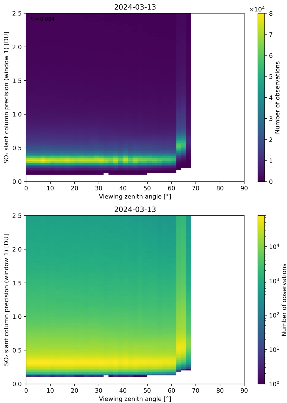
Figure 321: Scatter density plot of “Viewing zenith angle” against “SO 2 slant column precision (window 1)” for 2024-03-12 to 2024-03-14.
