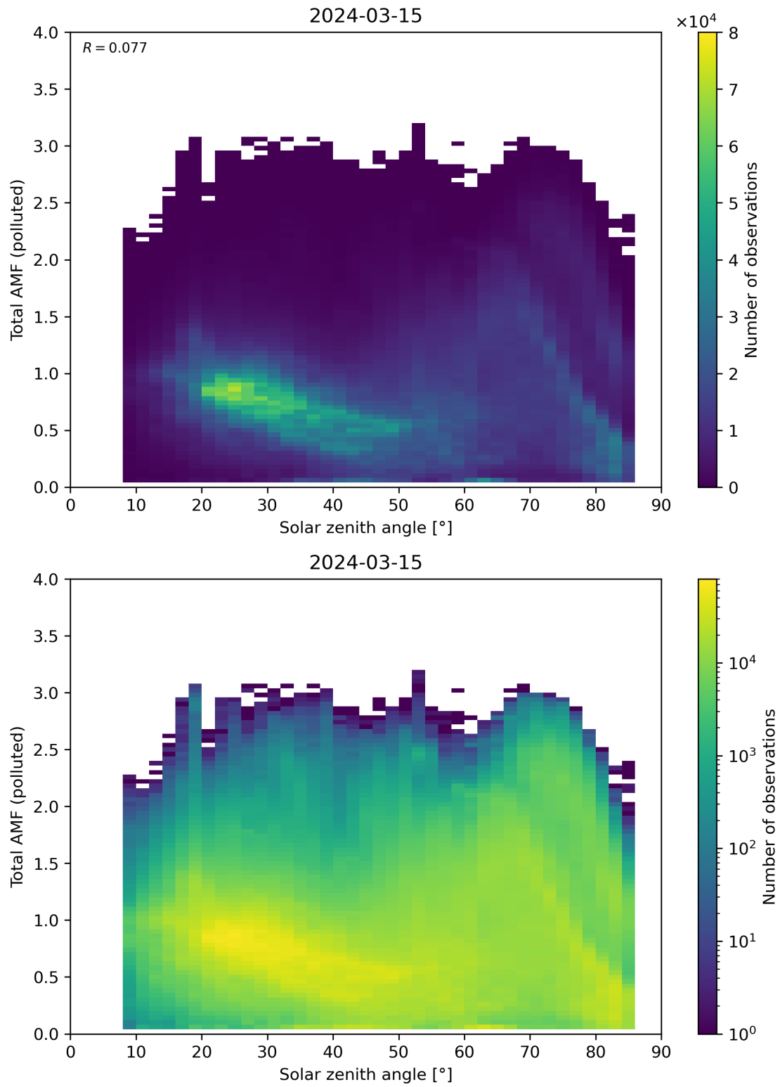
Figure 174: Scatter density plot of “Solar zenith angle” against “Total AMF (polluted)” for 2024-03-14 to 2024-03-16.
