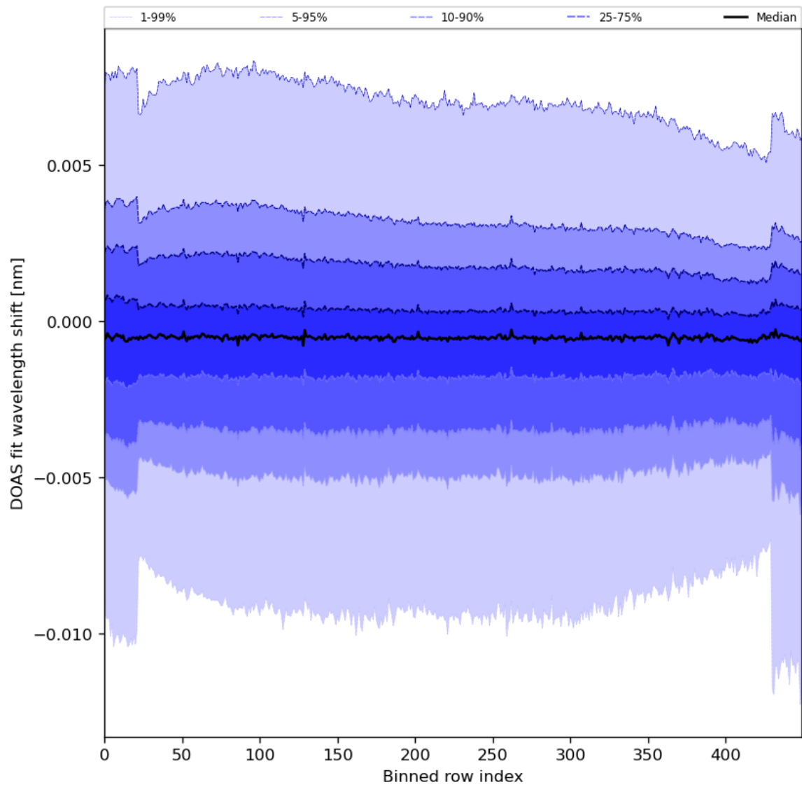
Figure 91: Along track statistics of “DOAS fit wavelength shift” for 2024-03-14 to 2024-03-16
