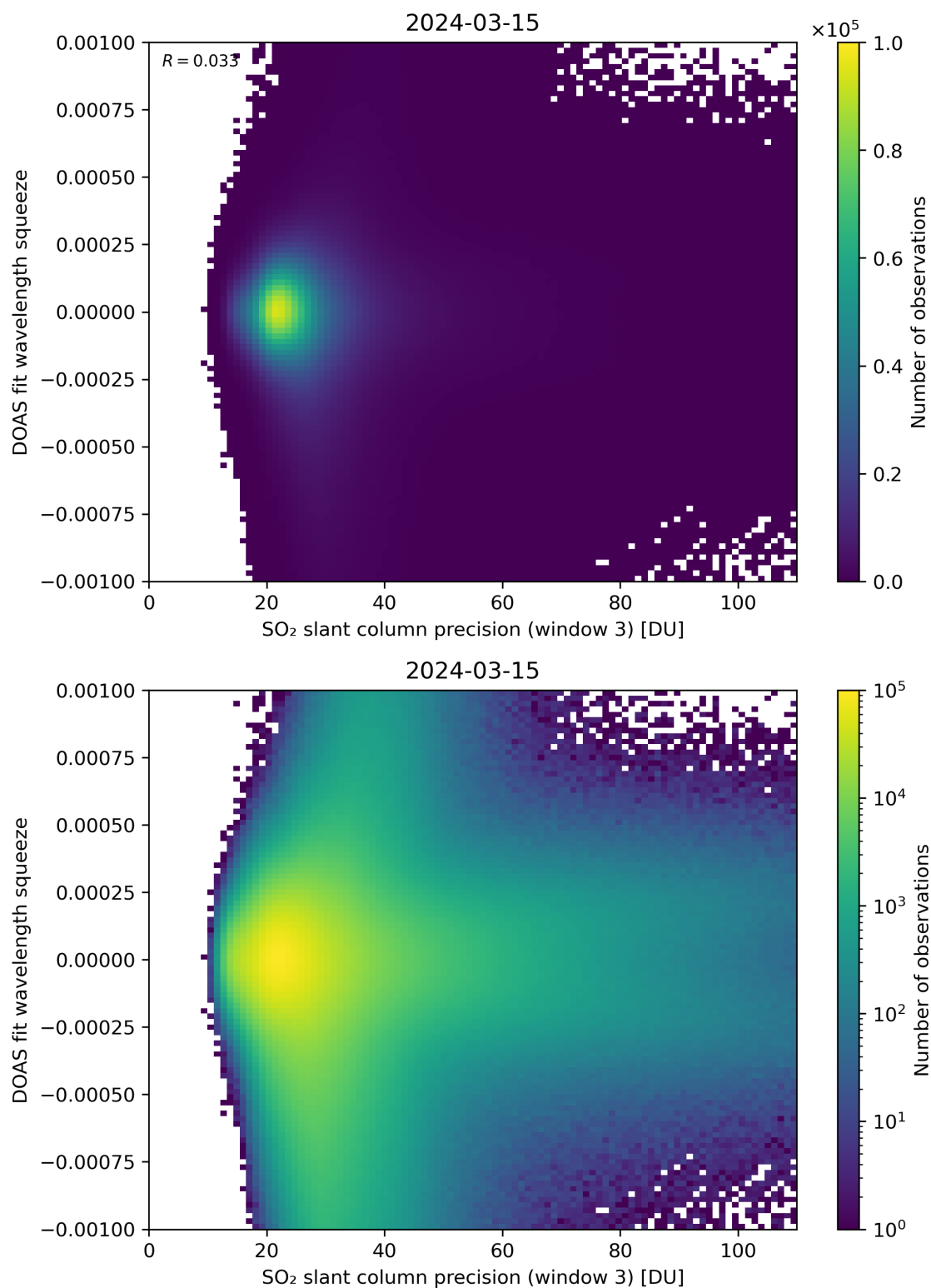
Figure 259: Scatter density plot of “SO 2 slant column precision (window 3)” against “DOAS fit wavelength squeeze” for 2024-03-14 to 2024-03-16.
