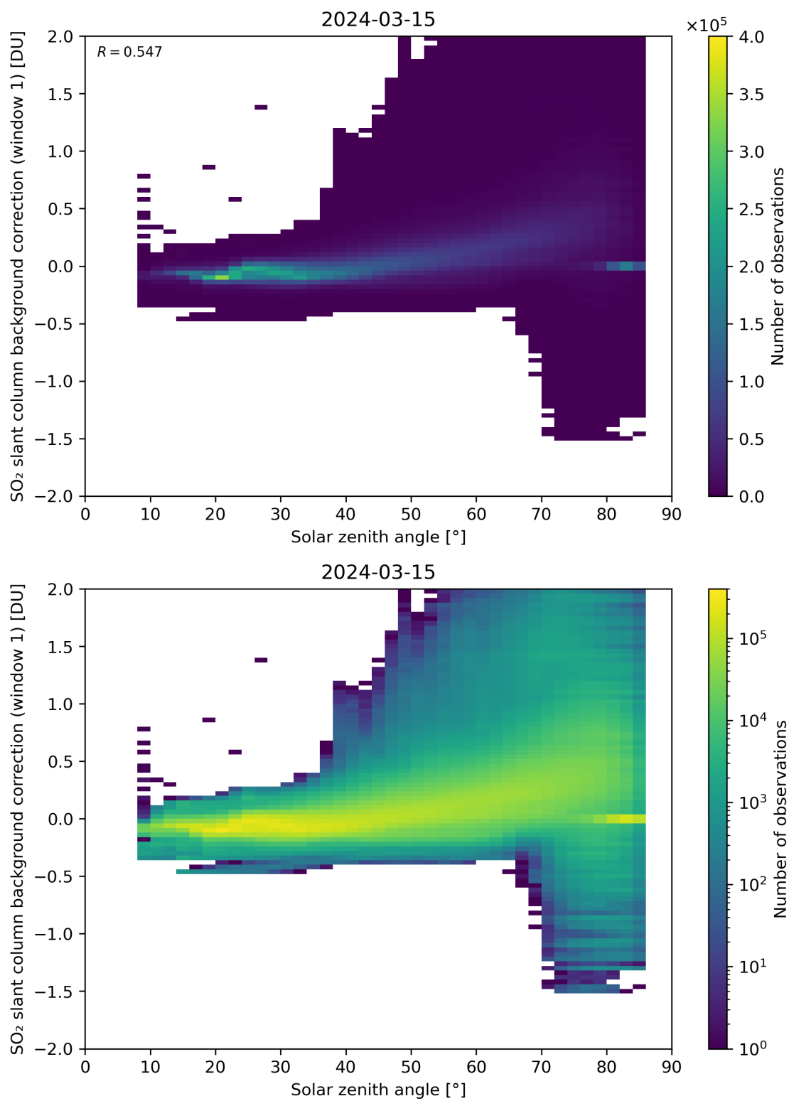
Figure 158: Scatter density plot of “Solar zenith angle” against “SO 2 slant column background correction (window 1)” for 2024-03-14 to 2024-03-16.
