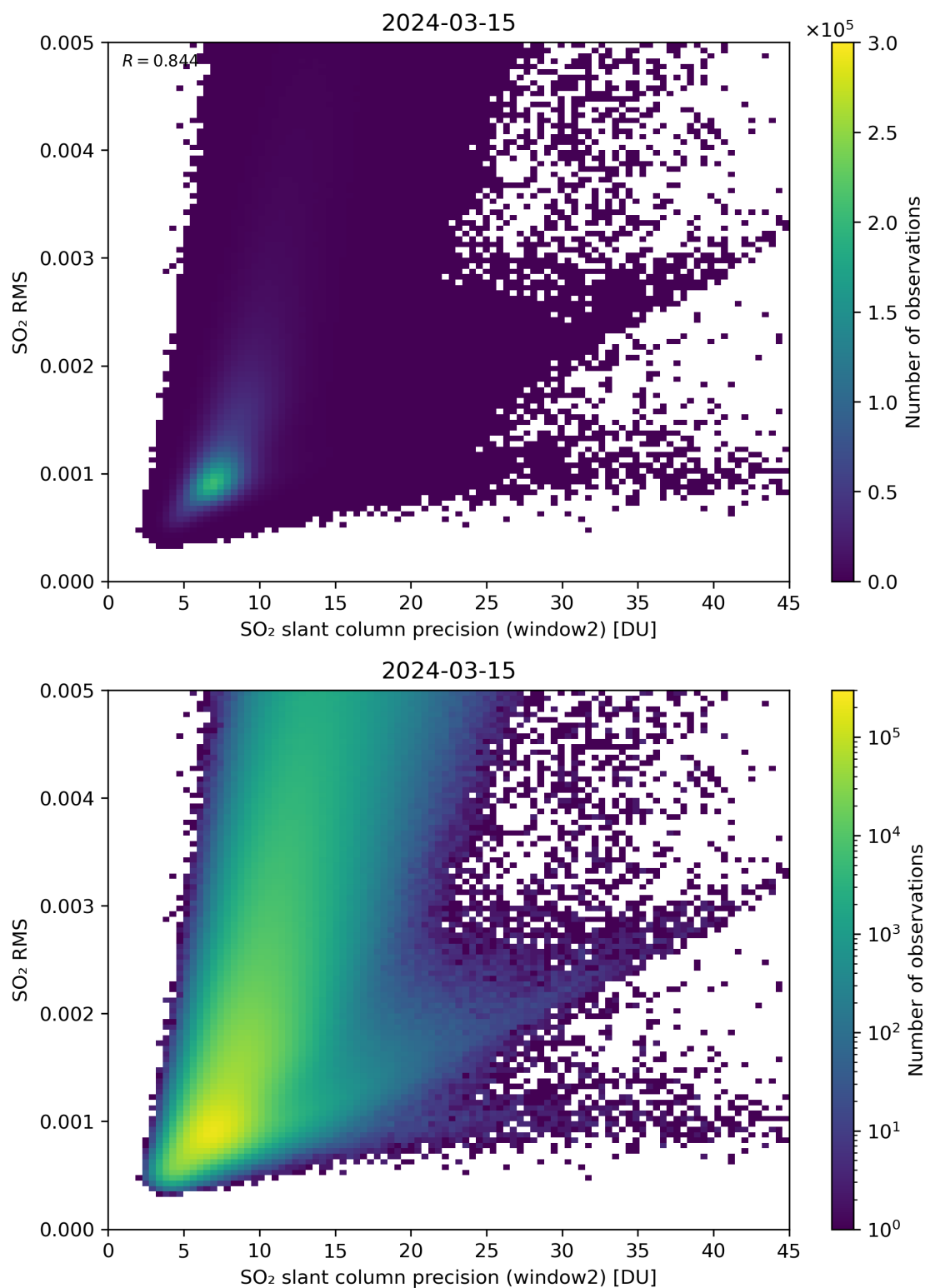
Figure 245: Scatter density plot of “SO 2 slant column precision (window2)” against “SO 2 RMS” for 2024-03-14 to 2024-03-16.
