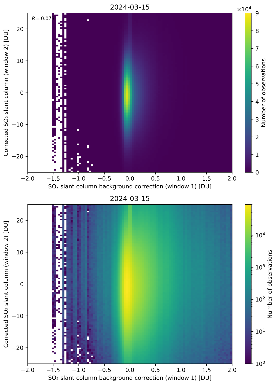
Figure 104: Scatter density plot of “SO 2 slant column background correction (window 1)” against “Corrected SO 2 slant column (window 2)” for 2024-03-14 to 2024-03-16.
