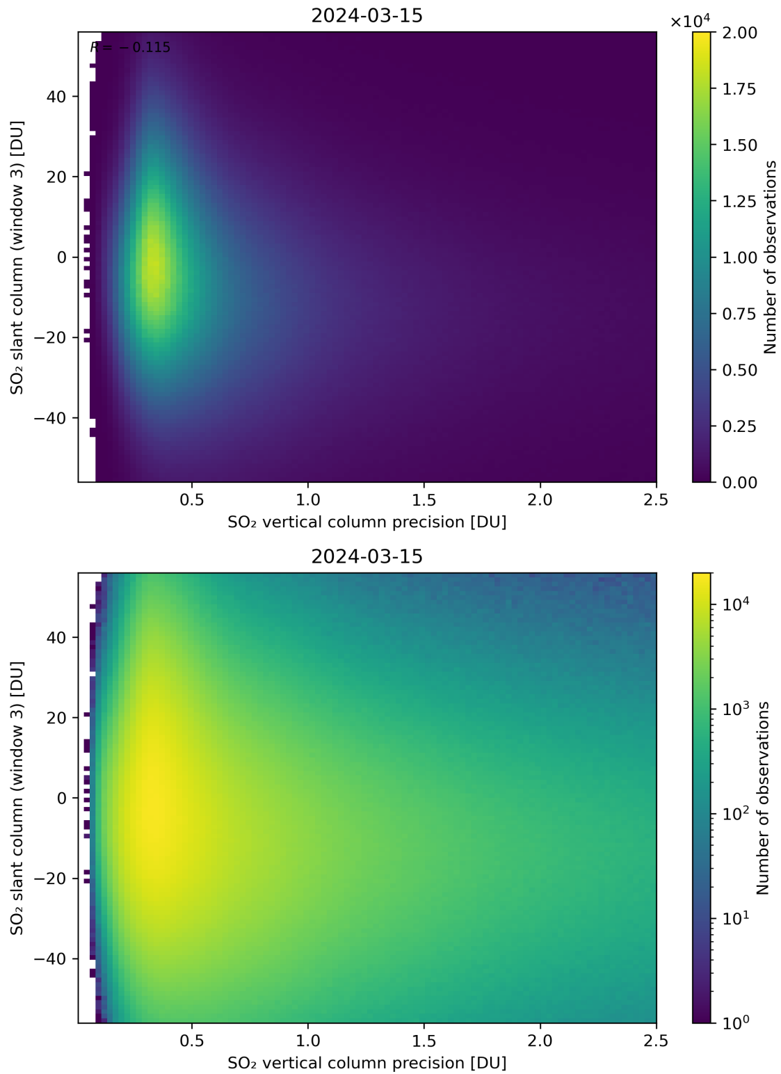
Figure 292: Scatter density plot of “SO 2 vertical column precision” against “SO 2 slant column (window 3)” for 2024-03-14 to 2024-03-16.
