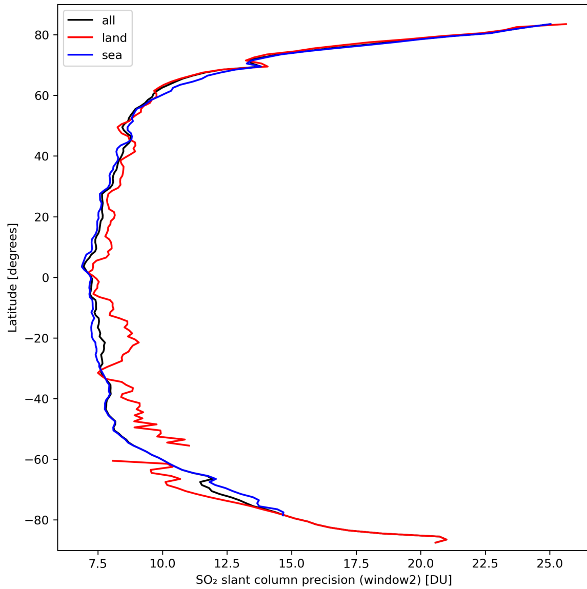
Figure 38: Zonal average of “SO 2 slant column precision (window2)” for 2024-03-14 to 2024-03-16.
