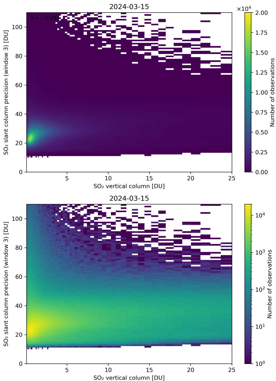
Figure 304: Scatter density plot of “SO 2 vertical column” against “SO 2 slant column precision (window 3)” for 2024-03-14 to 2024-03-16.
