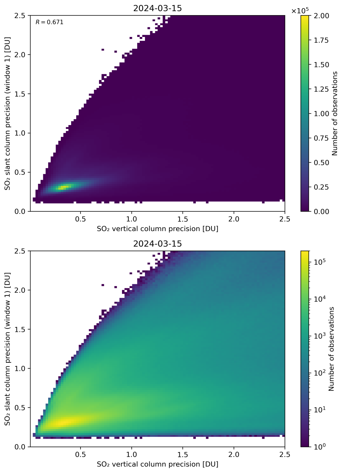
Figure 290: Scatter density plot of “SO 2 vertical column precision” against “SO 2 slant column precision (window 1)” for 2024-03-14 to 2024-03-16.
