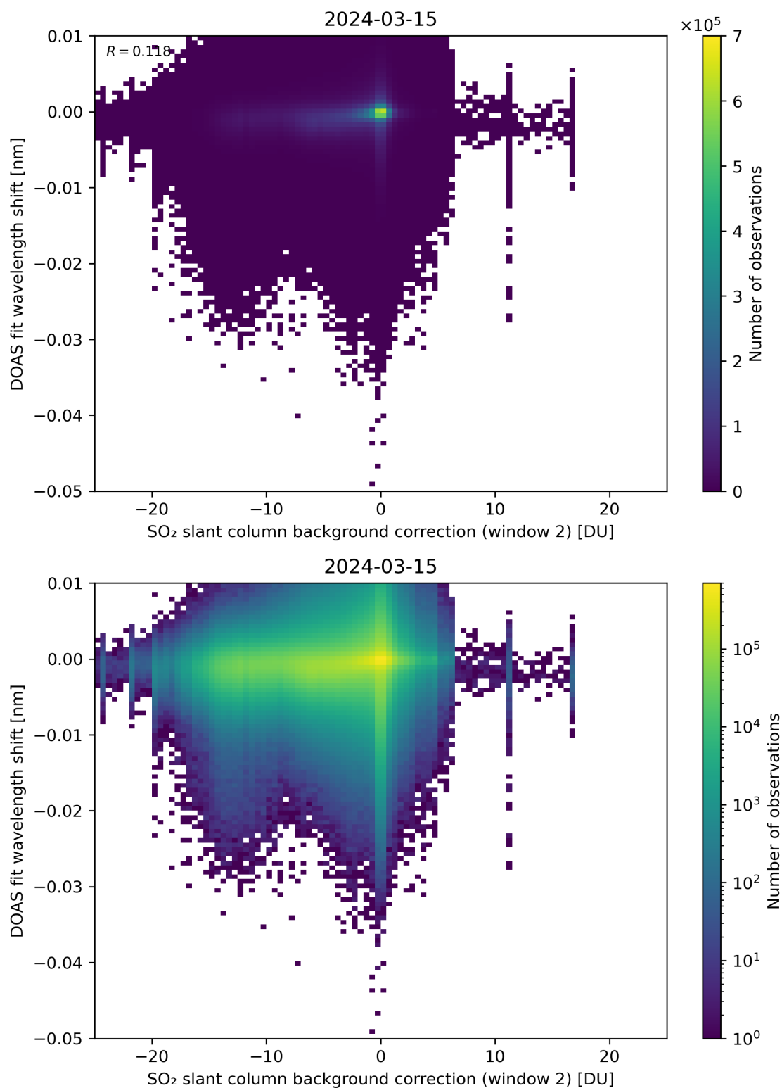
Figure 112: Scatter density plot of “SO 2 slant column background correction (window 2)” against “DOAS fit wavelength shift” for 2024-03-14 to 2024-03-16.
