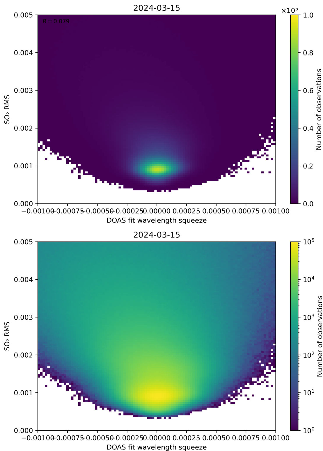
Figure 132: Scatter density plot of “DOAS fit wavelength squeeze” against “SO 2 RMS” for 2024-03-14 to 2024-03-16.
