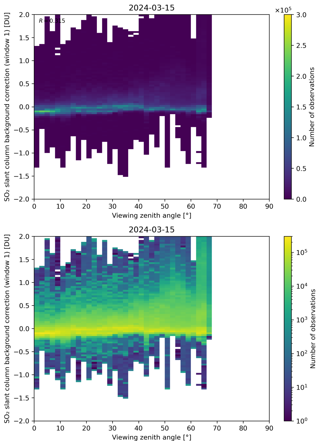
Figure 308: Scatter density plot of “Viewing zenith angle” against “SO 2 slant column background correction (window 1)” for 2024-03-14 to 2024-03-16.
