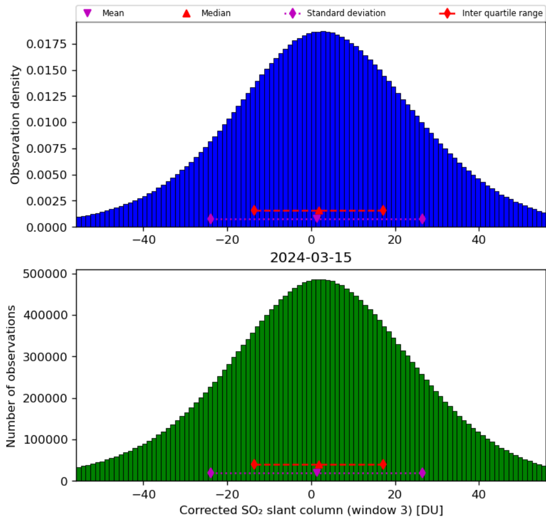
Figure 66: Histogram of "Corrected SO 2 slant column (window 3)" for 2024-03-14 to 2024-03-16
