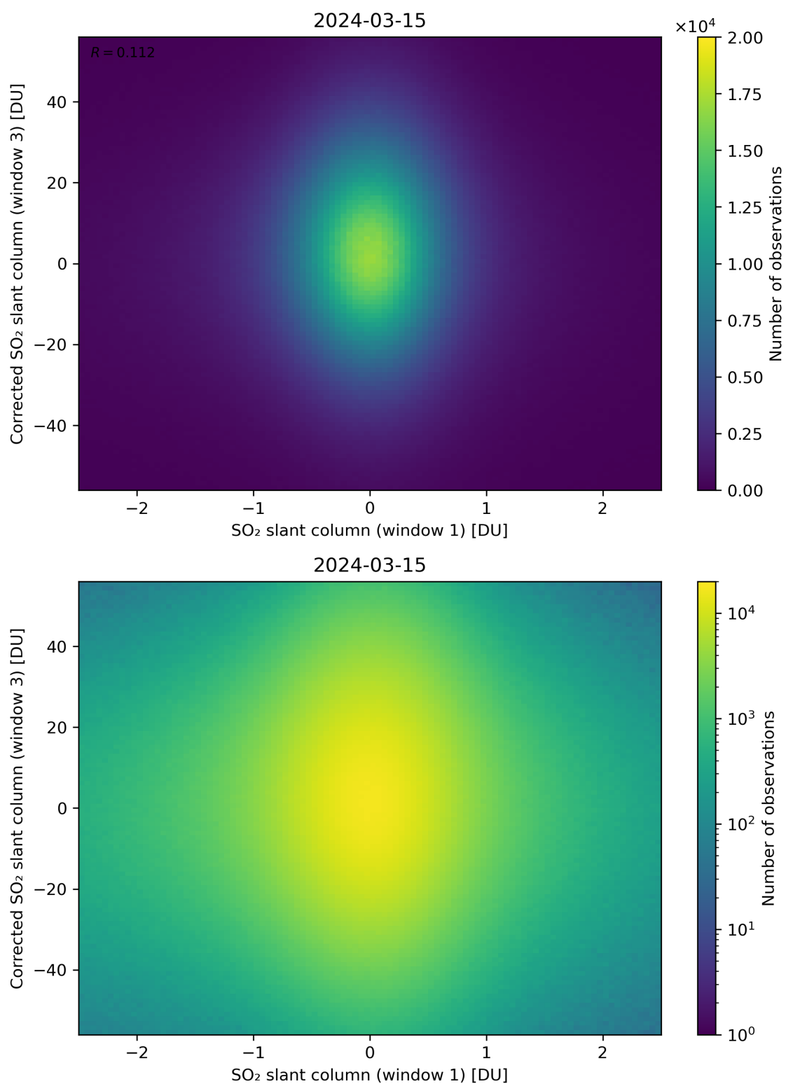
Figure 234: Scatter density plot of “SO 2 slant column (window 1)” against “Corrected SO 2 slant column (window 3)” for 2024-03-14 to 2024-03-16.
