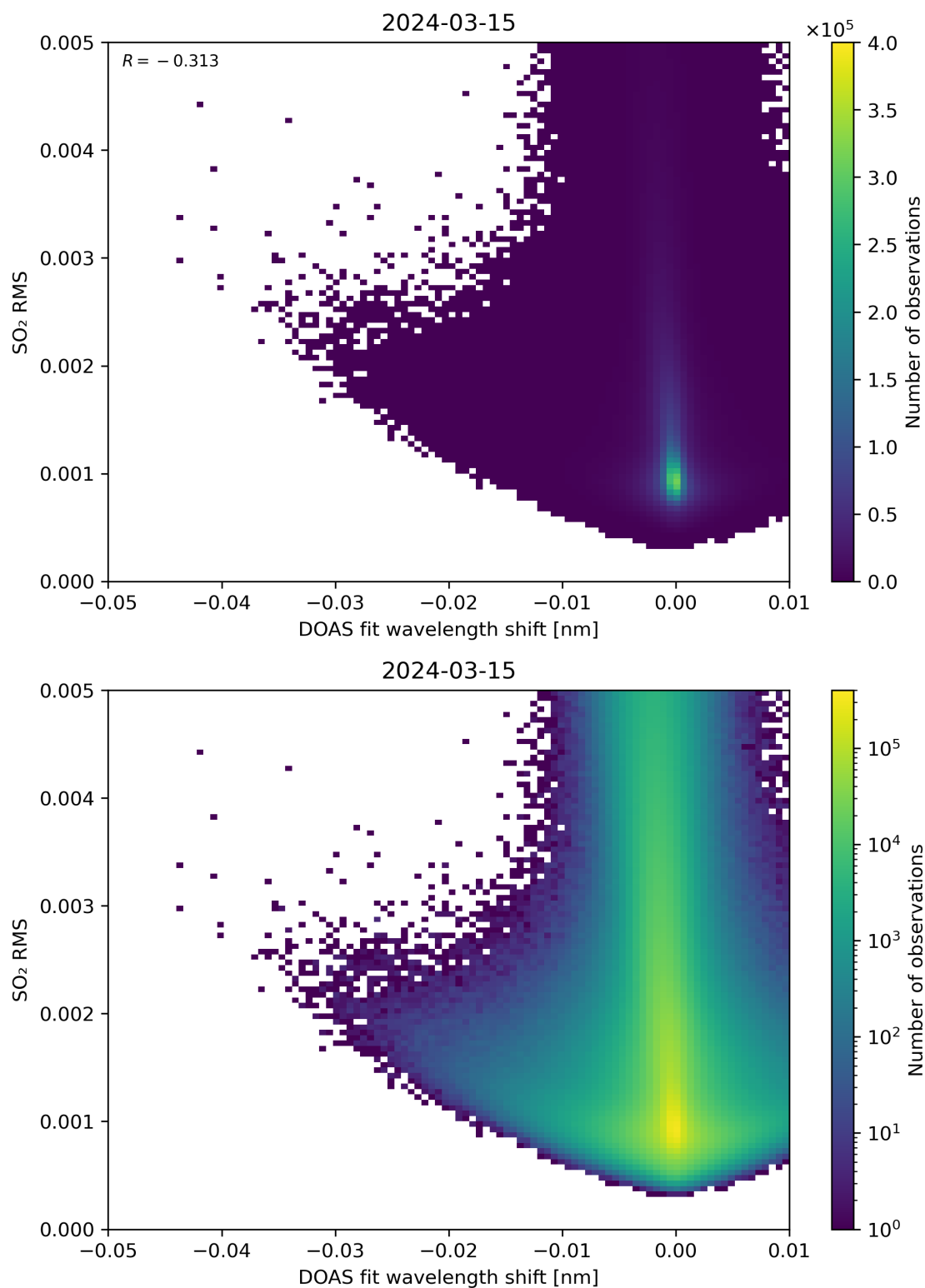
Figure 128: Scatter density plot of “DOAS fit wavelength shift” against “SO 2 RMS” for 2024-03-14 to 2024-03-16.
