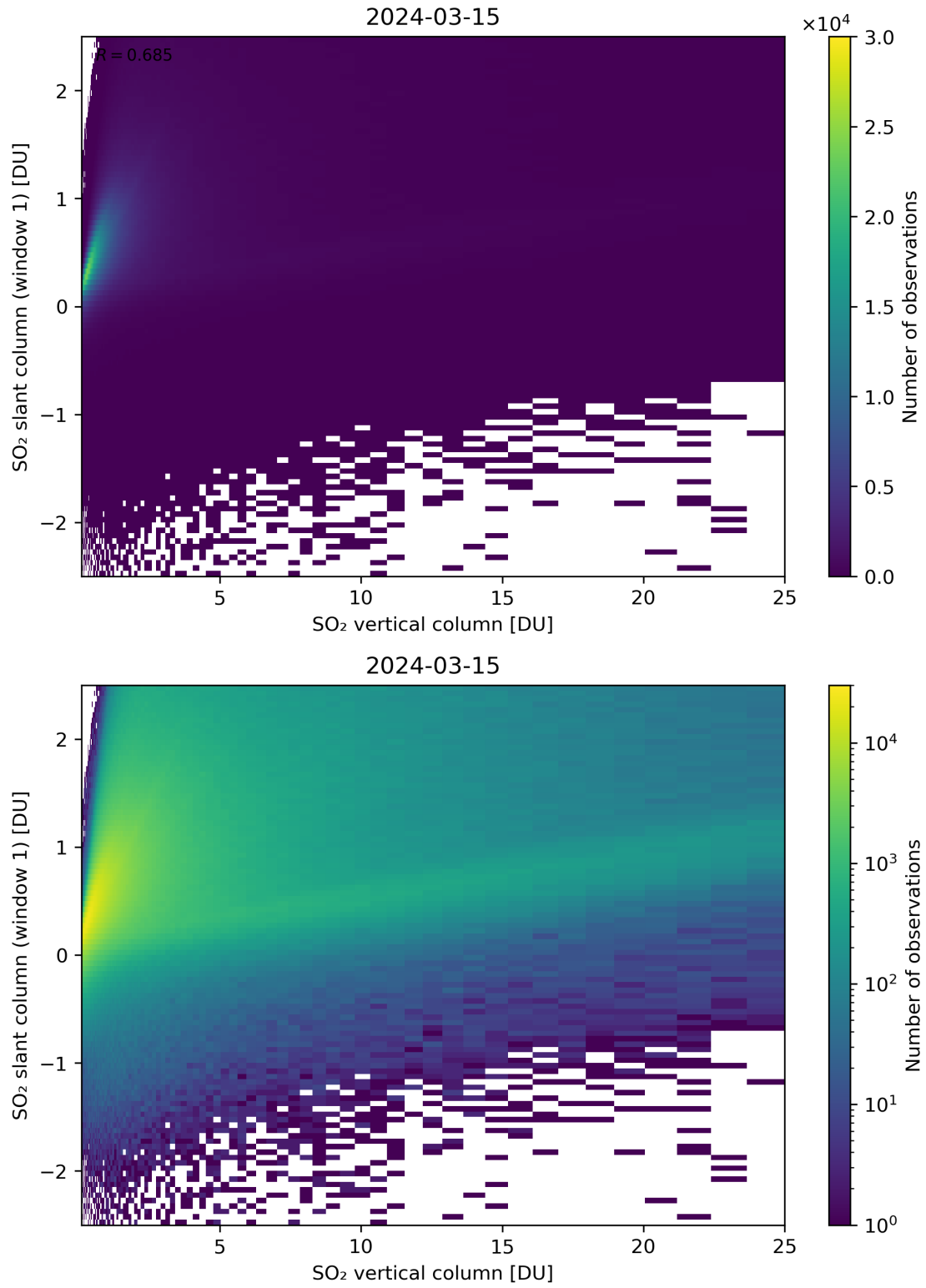
Figure 300: Scatter density plot of “SO 2 vertical column” against “SO 2 slant column (window 1)” for 2024-03-14 to 2024-03-16.
