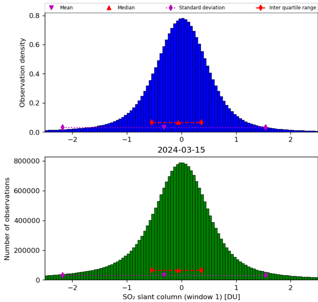
Figure 56: Histogram of “SO 2 slant column (window 1)” for 2024-03-14 to 2024-03-16
