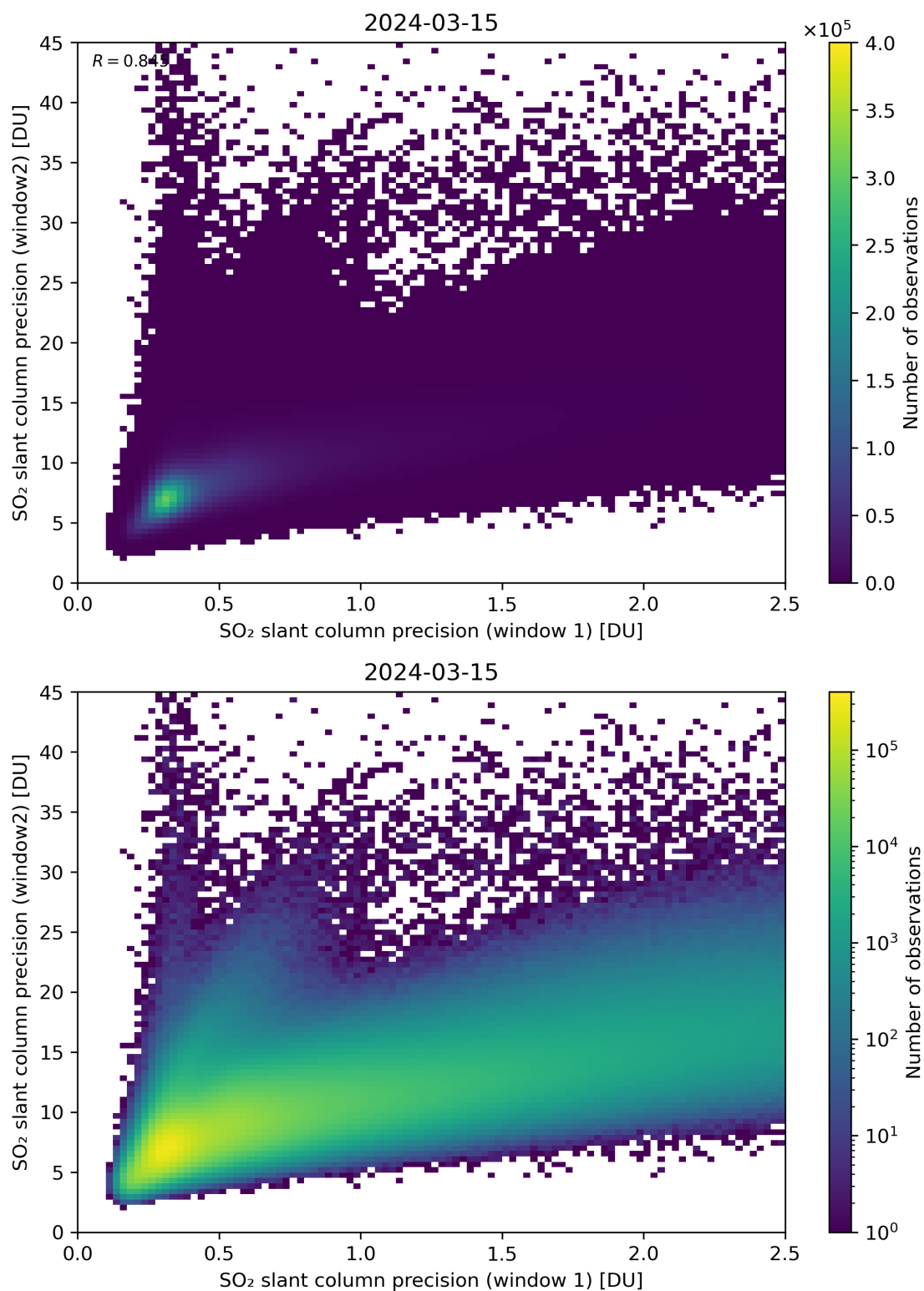
Figure 227: Scatter density plot of “SO 2 slant column precision (window 1)” against “SO 2 slant column precision (window2)” for 2024-03-14 to 2024-03-16.
