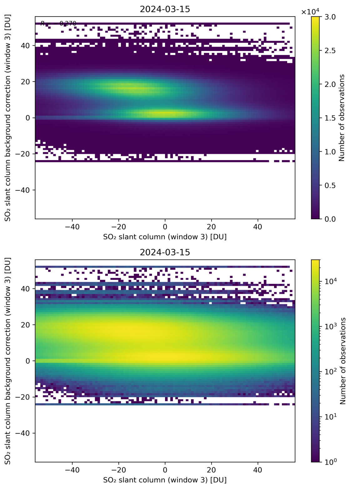
Figure 253: Scatter density plot of “SO 2 slant column (window 3)” against “SO 2 slant column background correction (window 3)” for 2024-03-14 to 2024-03-16.
