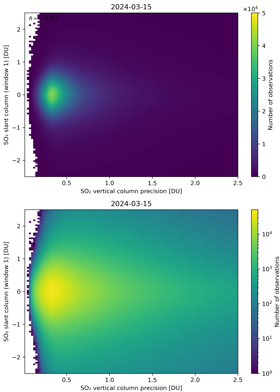
Figure 289: Scatter density plot of “SO 2 vertical column precision” against “SO 2 slant column (window 1)” for 2024-03-14 to 2024-03-16.
