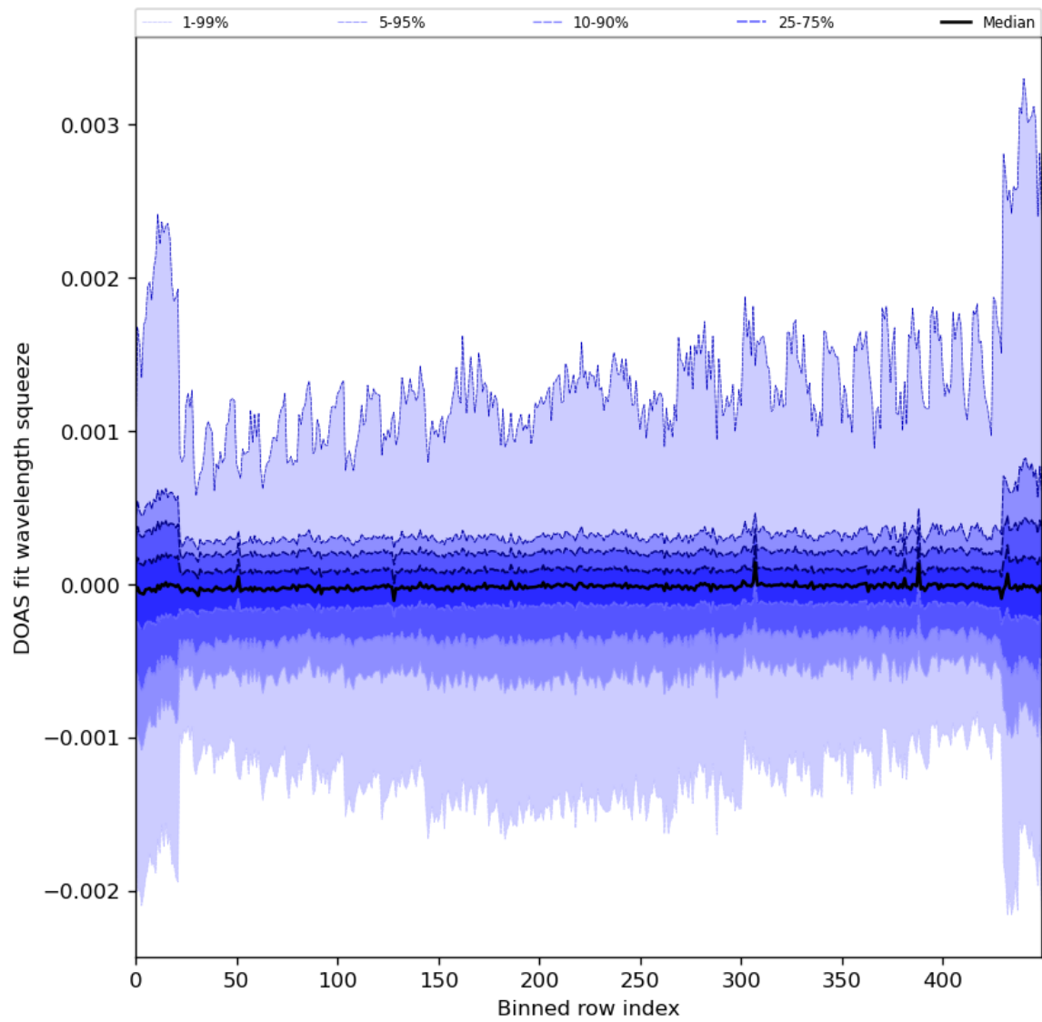
Figure 92: Along track statistics of “DOAS fit wavelength squeeze” for 2024-03-14 to 2024-03-16
