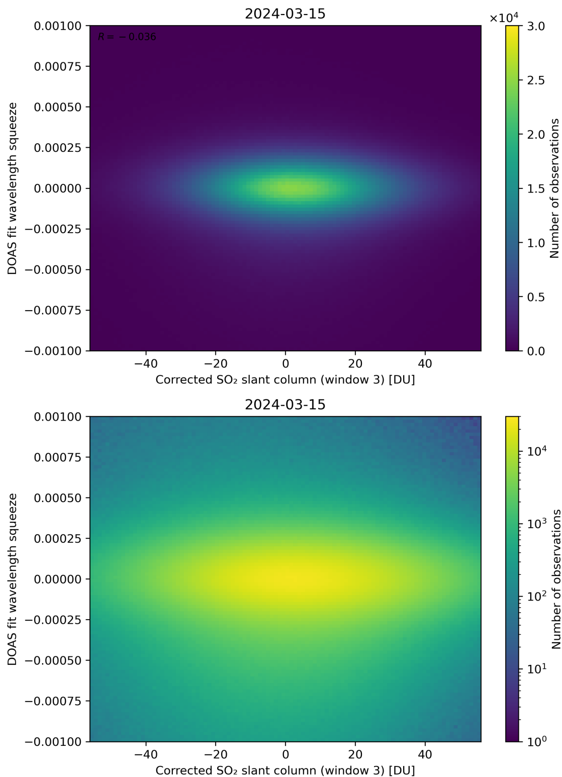
Figure 207: Scatter density plot of “Corrected SO 2 slant column (window 3)” against “DOAS fit wavelength squeeze” for 2024-03-14 to 2024-03-16.
