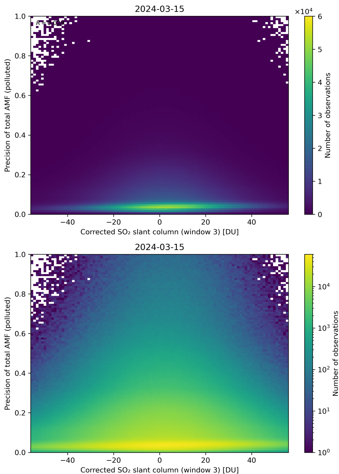
Figure 211: Scatter density plot of “Corrected SO 2 slant column (window 3)” against “Precision of total AMF (polluted)” for 2024-03-14 to 2024-03-16.
