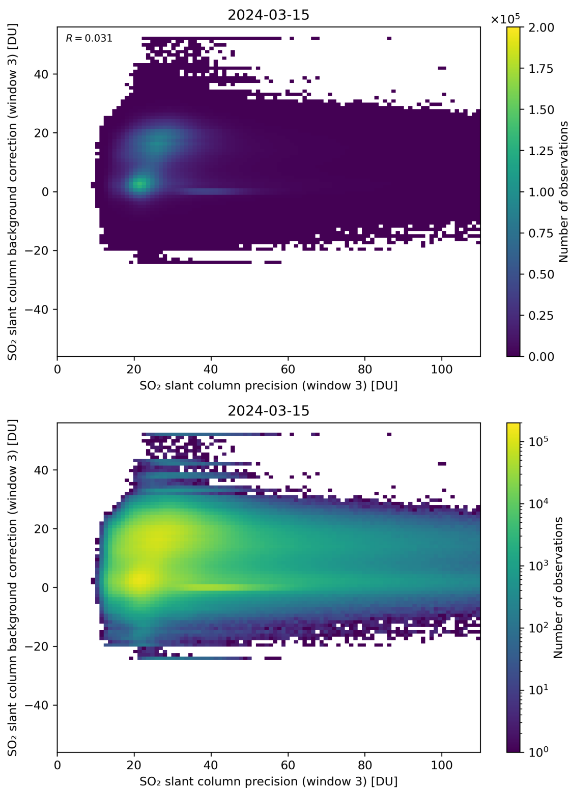
Figure 257: Scatter density plot of “SO 2 slant column precision (window 3)” against “SO 2 slant column background correction (window 3)” for 2024-03-14 to 2024-03-16.
