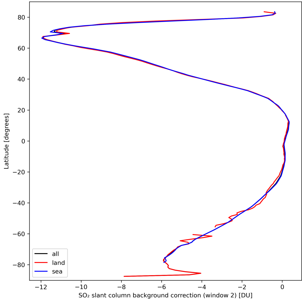
Figure 40: Zonal average of “SO 2 slant column background correction (window 2)” for 2024-03-14 to 2024-03-16.
