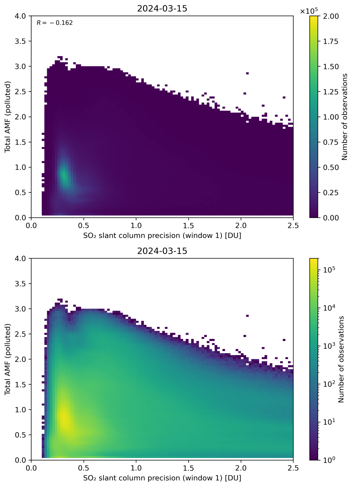
Figure 230: Scatter density plot of “SO 2 slant column precision (window 1)” against “Total AMF (polluted)” for 2024-03-14 to 2024-03-16.
