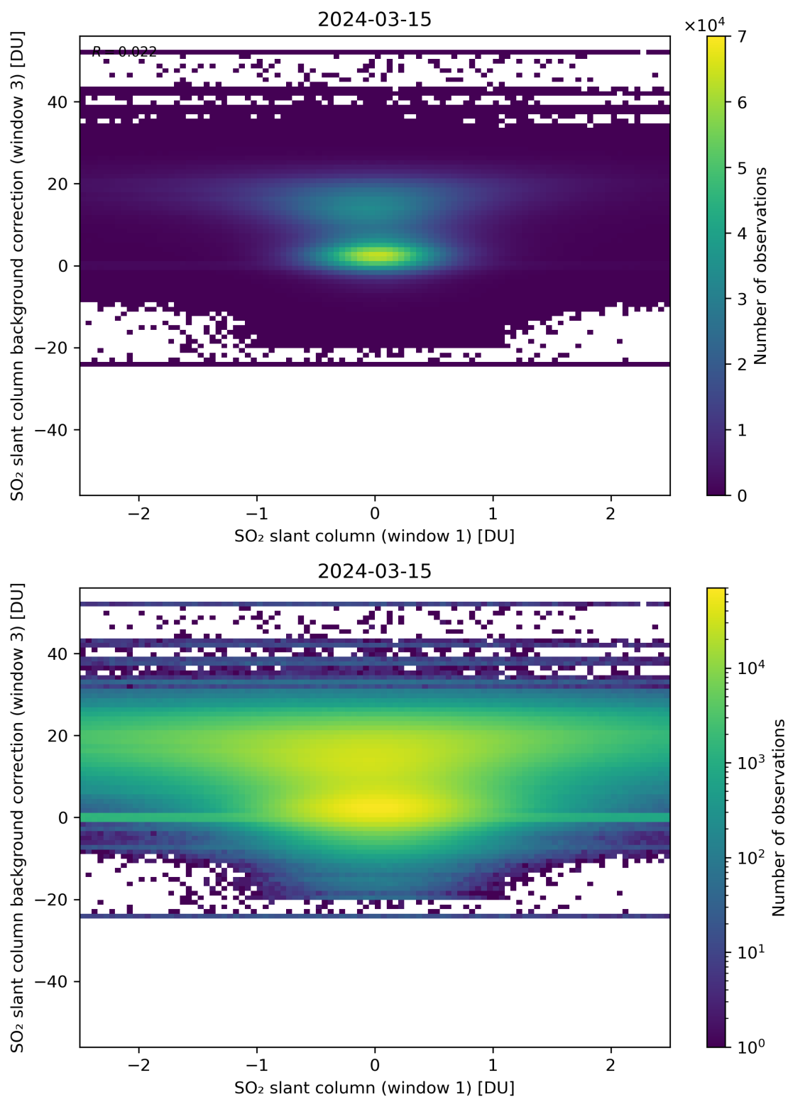
Figure 214: Scatter density plot of “SO 2 slant column (window 1)” against “SO 2 slant column background correction (window 3)” for 2024-03-14 to 2024-03-16.
