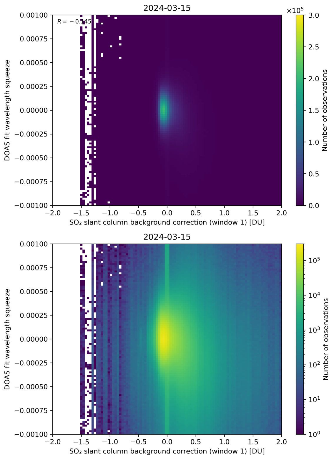
Figure 101: Scatter density plot of “SO 2 slant column background correction (window 1)” against “DOAS fit wavelength squeeze” for 2024-03-14 to 2024-03-16.
