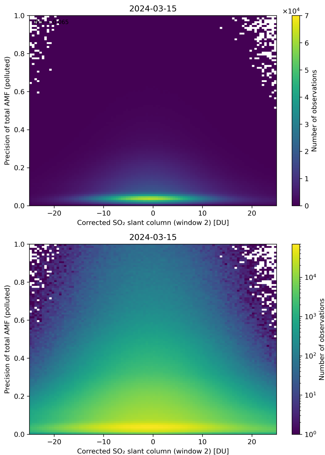
Figure 204: Scatter density plot of “Corrected SO 2 slant column (window 2)” against “Precision of total AMF (polluted)” for 2024-03-14 to 2024-03-16.
