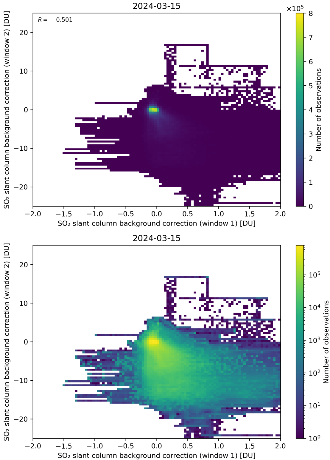
Figure 98: Scatter density plot of “SO 2 slant column background correction (window 1)” against “SO 2 slant column background correction (window 2)” for 2024-03-14 to 2024-03-16.
