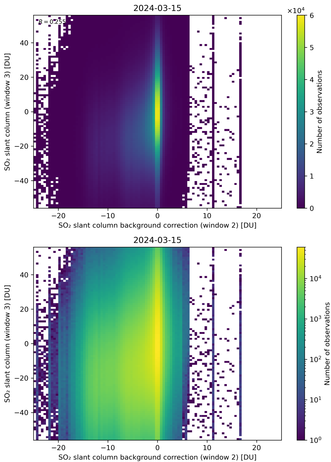
Figure 117: Scatter density plot of “SO 2 slant column background correction (window 2)” against “SO 2 slant column (window 3)” for 2024-03-14 to 2024-03-16.
