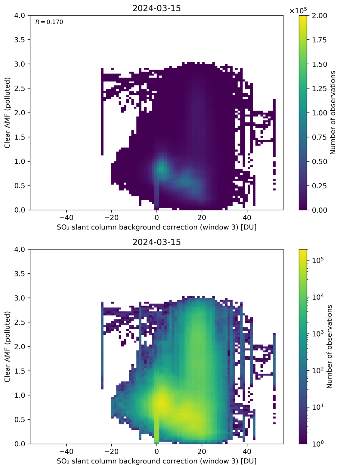
Figure 124: Scatter density plot of “SO 2 slant column background correction (window 3)” against “Clear AMF (polluted)” for 2024-03-14 to 2024-03-16.
