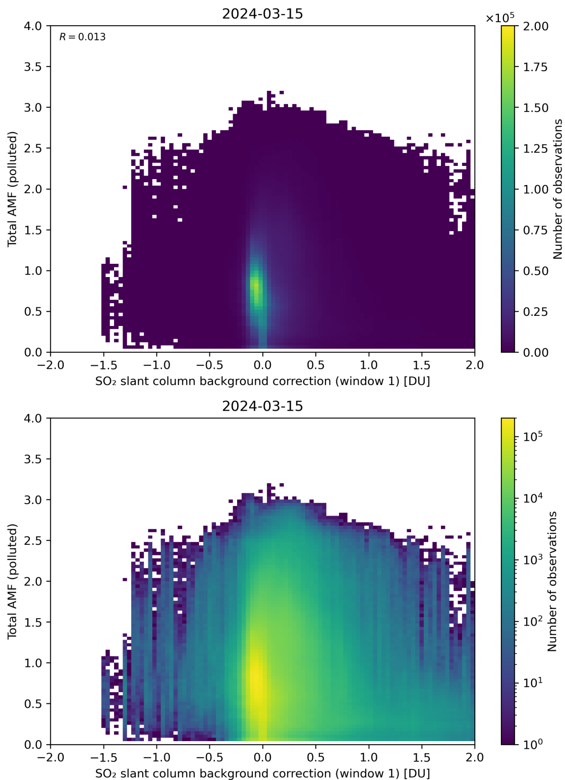
Figure 109: Scatter density plot of “SO 2 slant column background correction (window 1)” against “Total AMF (polluted)” for 2024-03-14 to 2024-03-16.
