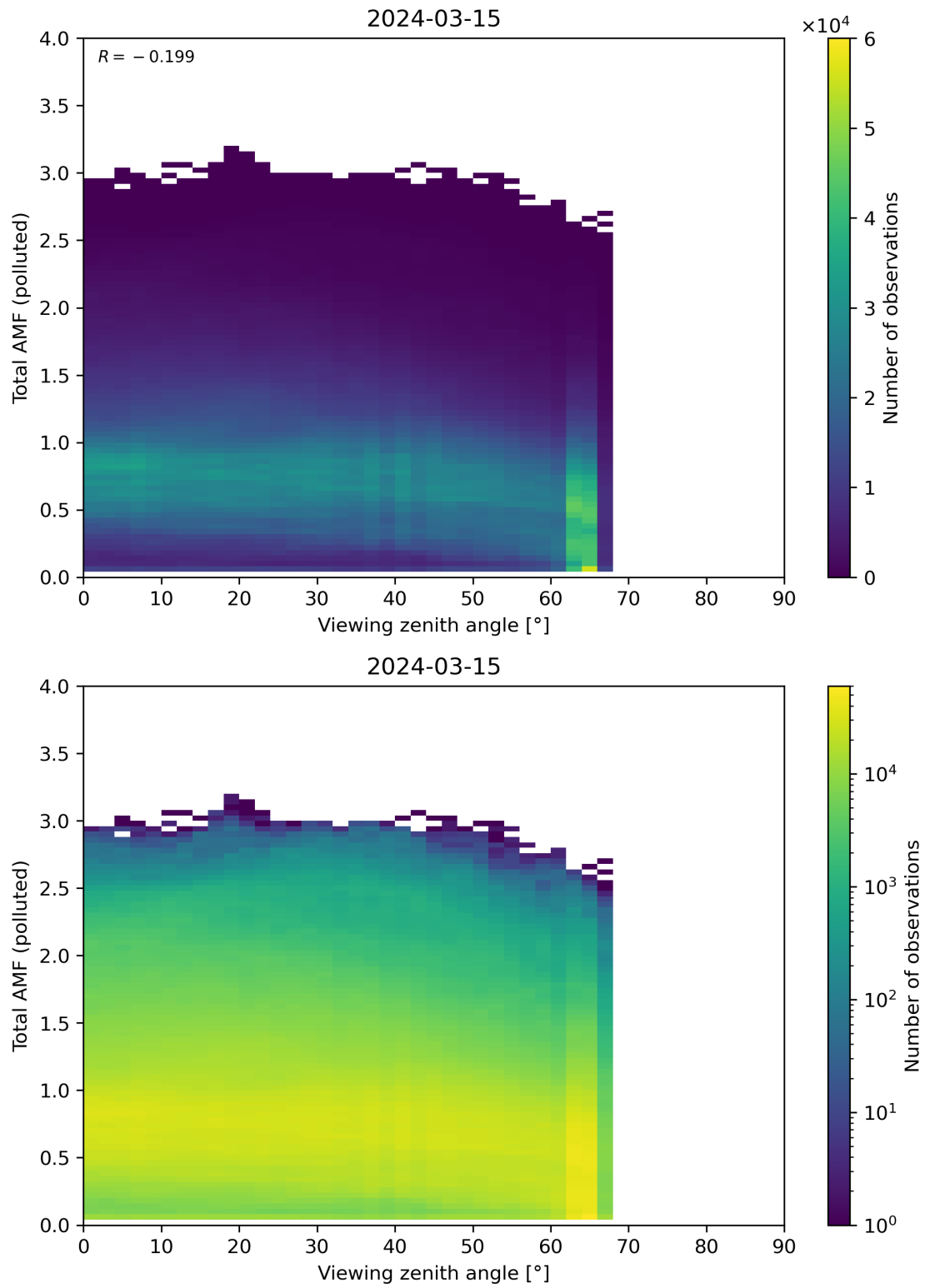
Figure 325: Scatter density plot of “Viewing zenith angle” against “Total AMF (polluted)” for 2024-03-14 to 2024-03-16.
