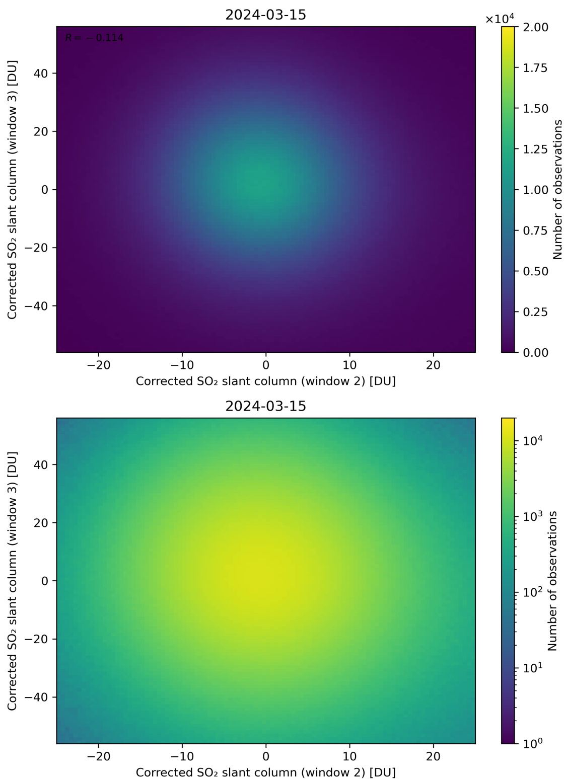
Figure 200: Scatter density plot of “Corrected SO 2 slant column (window 2)” against “Corrected SO 2 slant column (window 3)” for 2024-03-14 to 2024-03-16.
