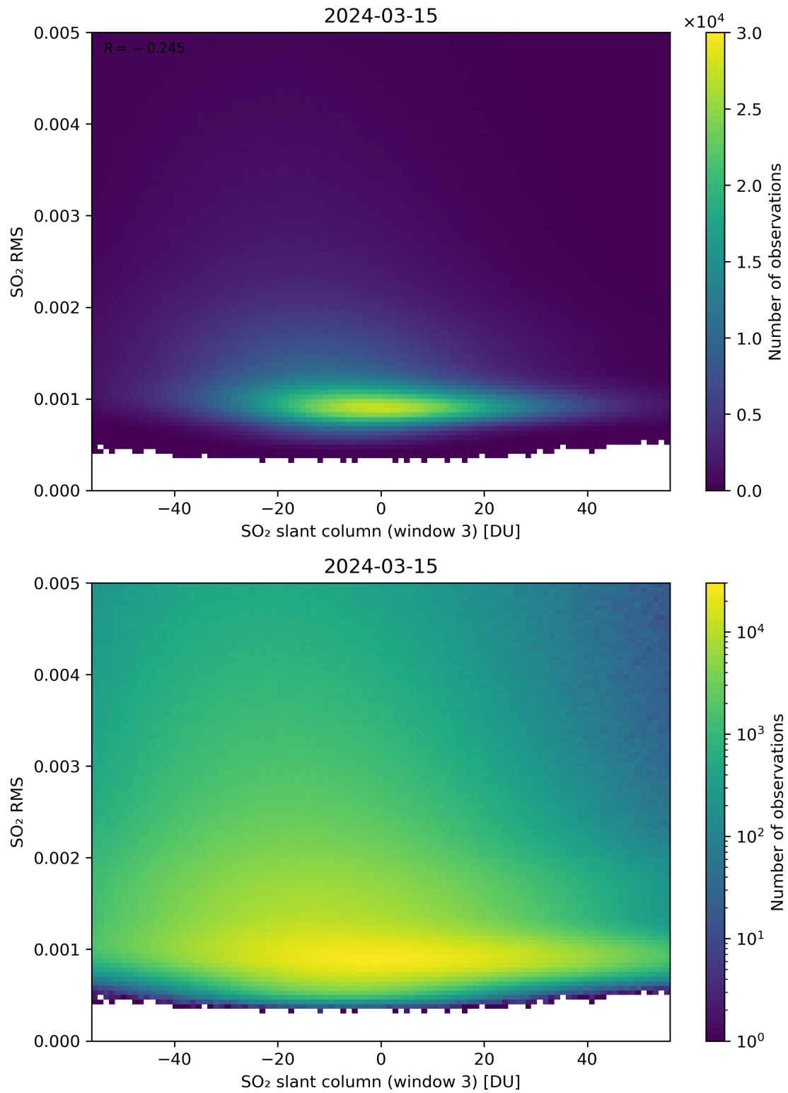
Figure 256: Scatter density plot of “SO 2 slant column (window 3)” against “SO 2 RMS” for 2024-03-14 to 2024-03-16.
