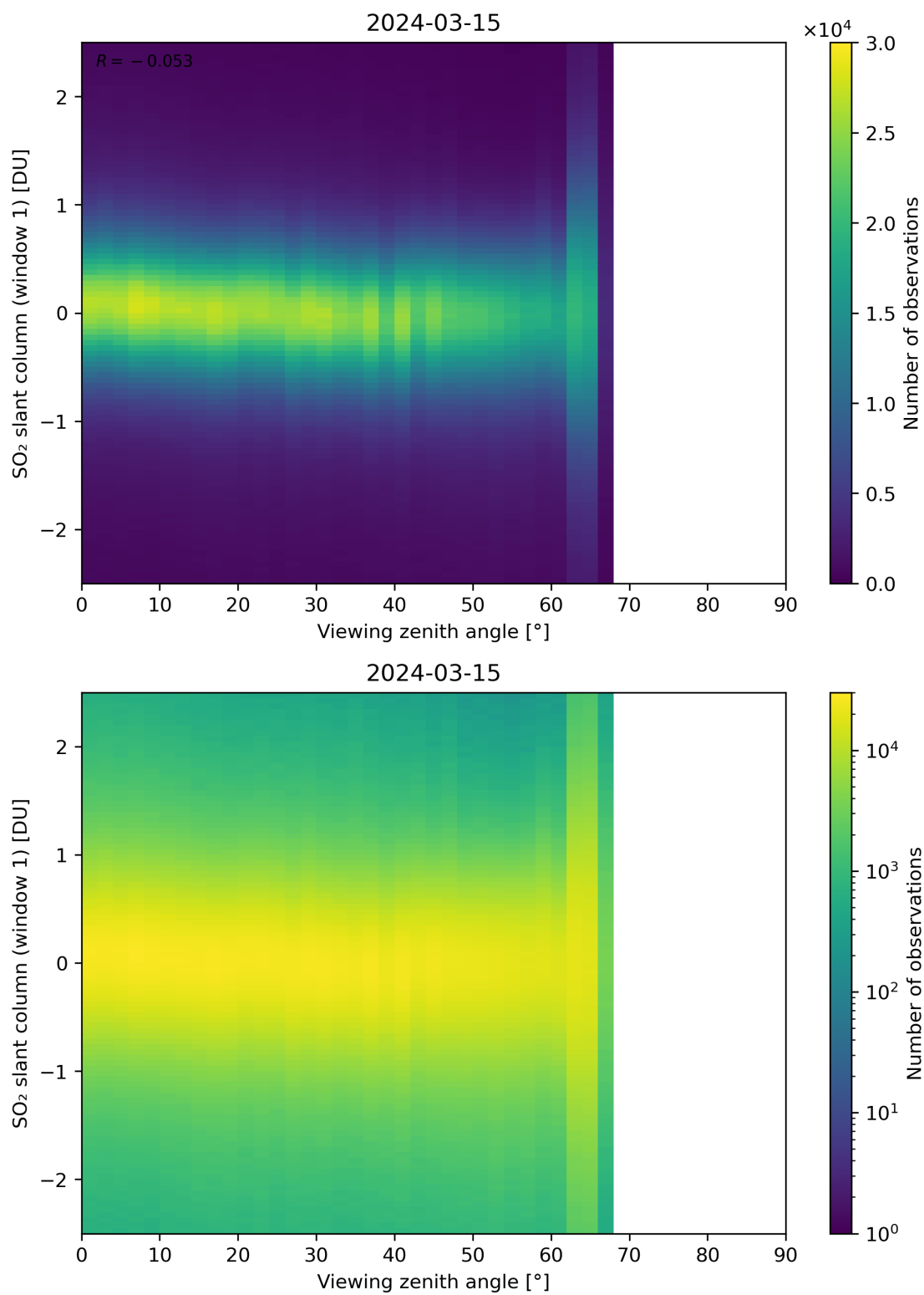
Figure 320: Scatter density plot of “Viewing zenith angle” against “SO 2 slant column (window 1)” for 2024-03-14 to 2024-03-16.
