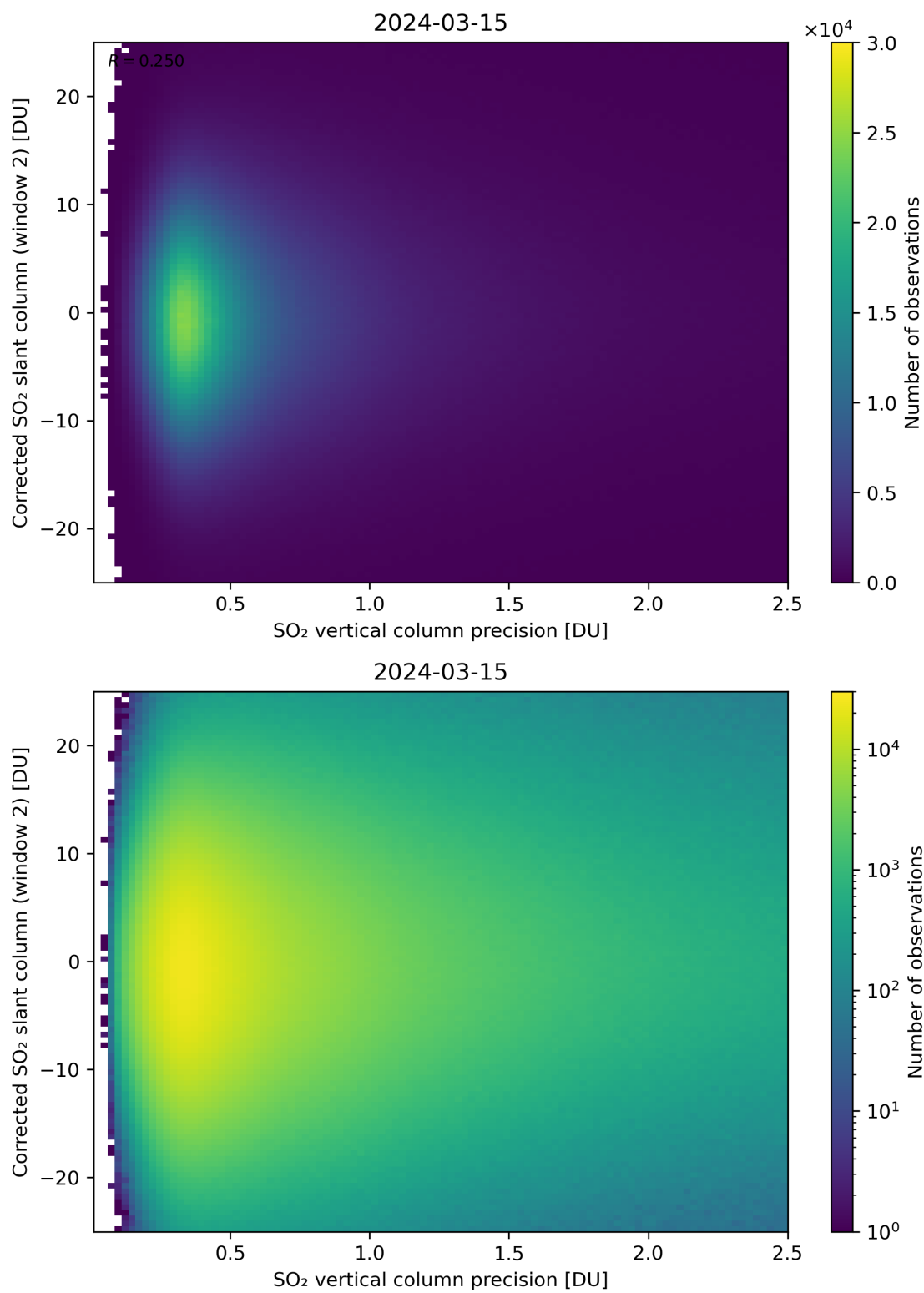
Figure 287: Scatter density plot of “SO 2 vertical column precision” against “Corrected SO 2 slant column (window 2)” for 2024-03-14 to 2024-03-16.
