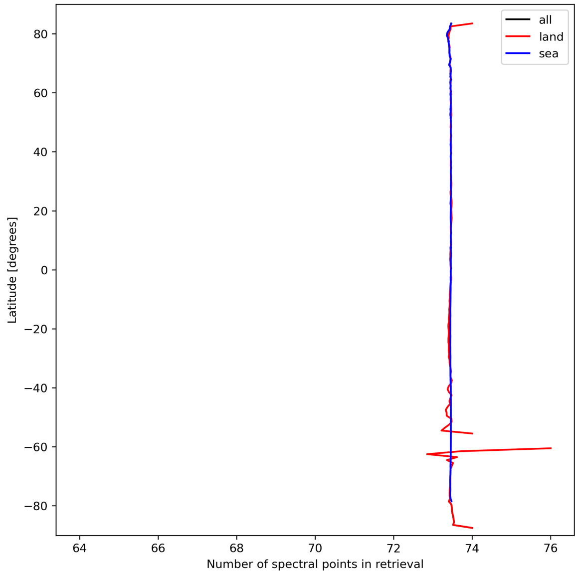
Figure 51: Zonal average of “Number of spectral points in retrieval” for 2024-03-14 to 2024-03-16.
