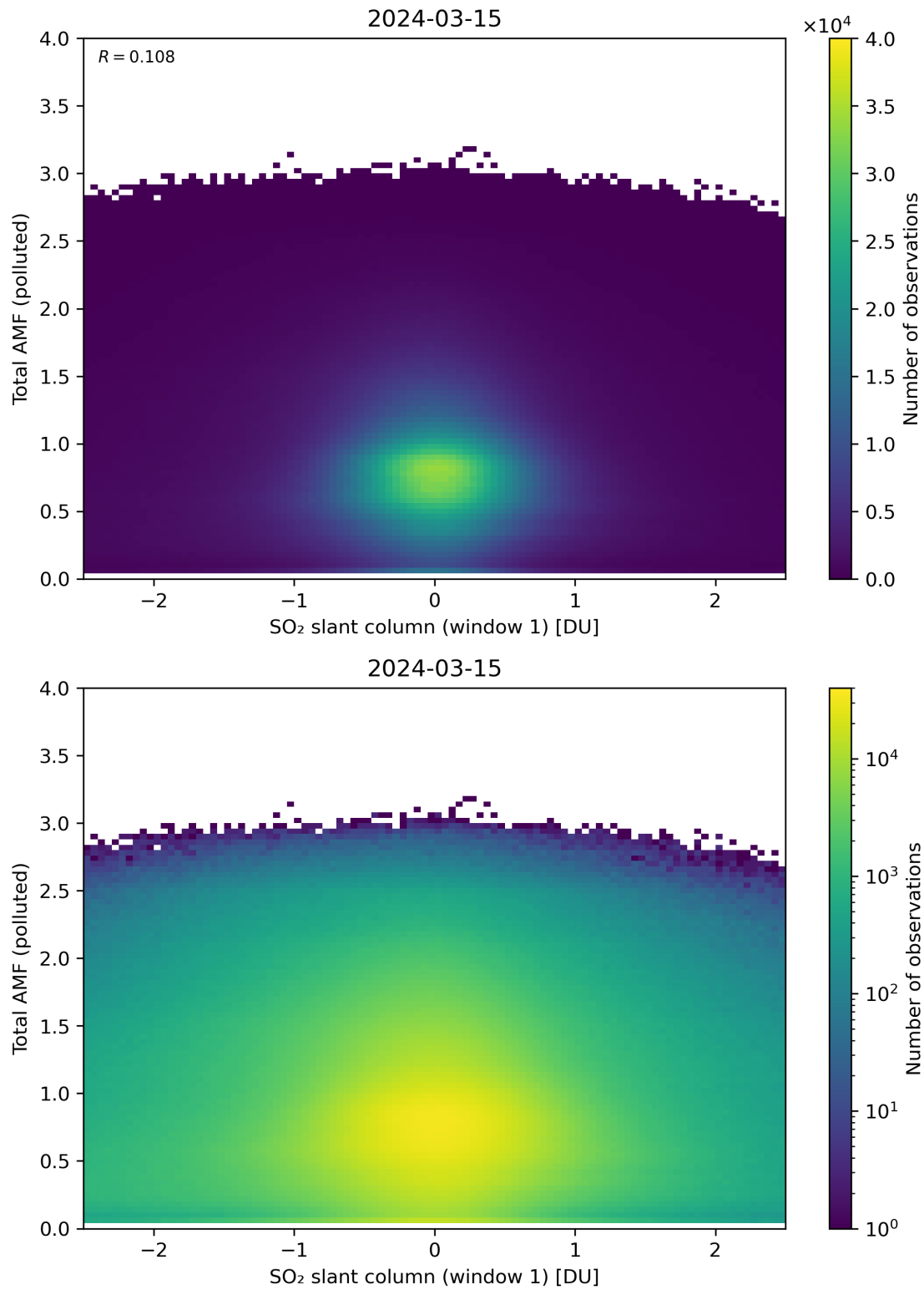
Figure 239: Scatter density plot of “SO 2 slant column (window 1)” against “Total AMF (polluted)” for 2024-03-14 to 2024-03-16.
