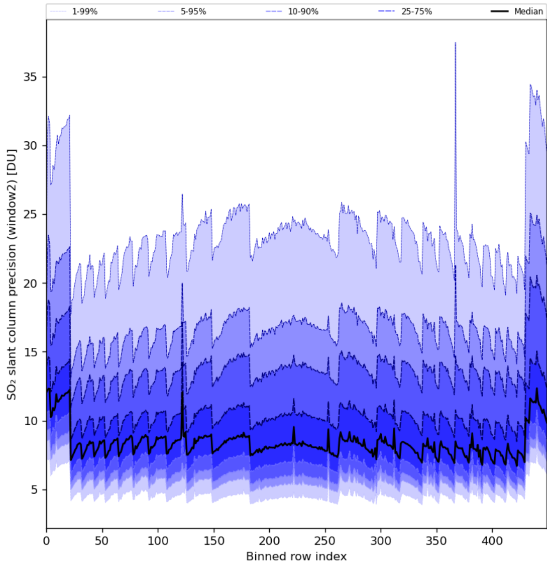
Figure 84: Along track statistics of “SO 2 slant column precision (window2)” for 2024-03-14 to 2024-03-16
