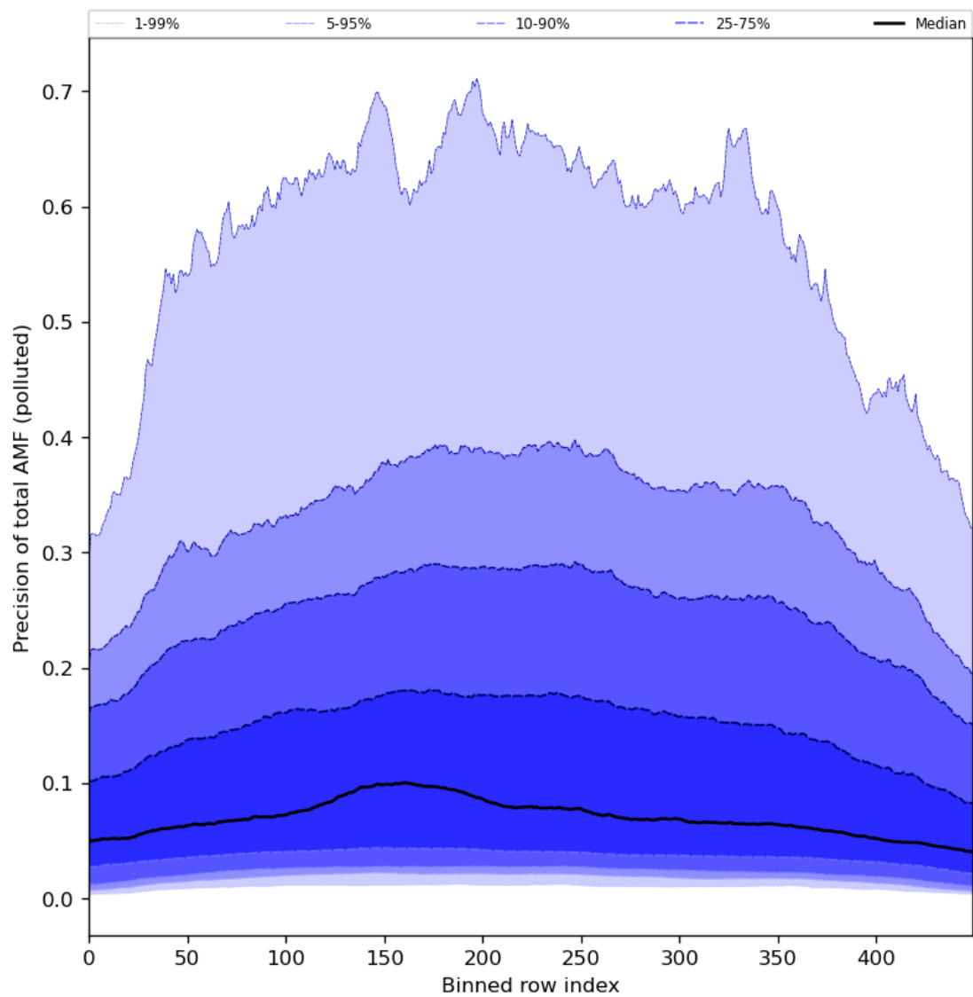
Figure 95: Along track statistics of “Precision of total AMF (polluted)” for 2024-03-14 to 2024-03-16
