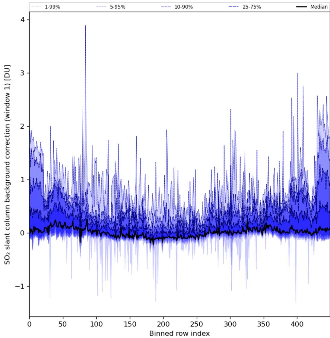
Figure 82: Along track statistics of “SO 2 slant column background correction (window 1)” for 2024-03-14 to 2024-03-16
