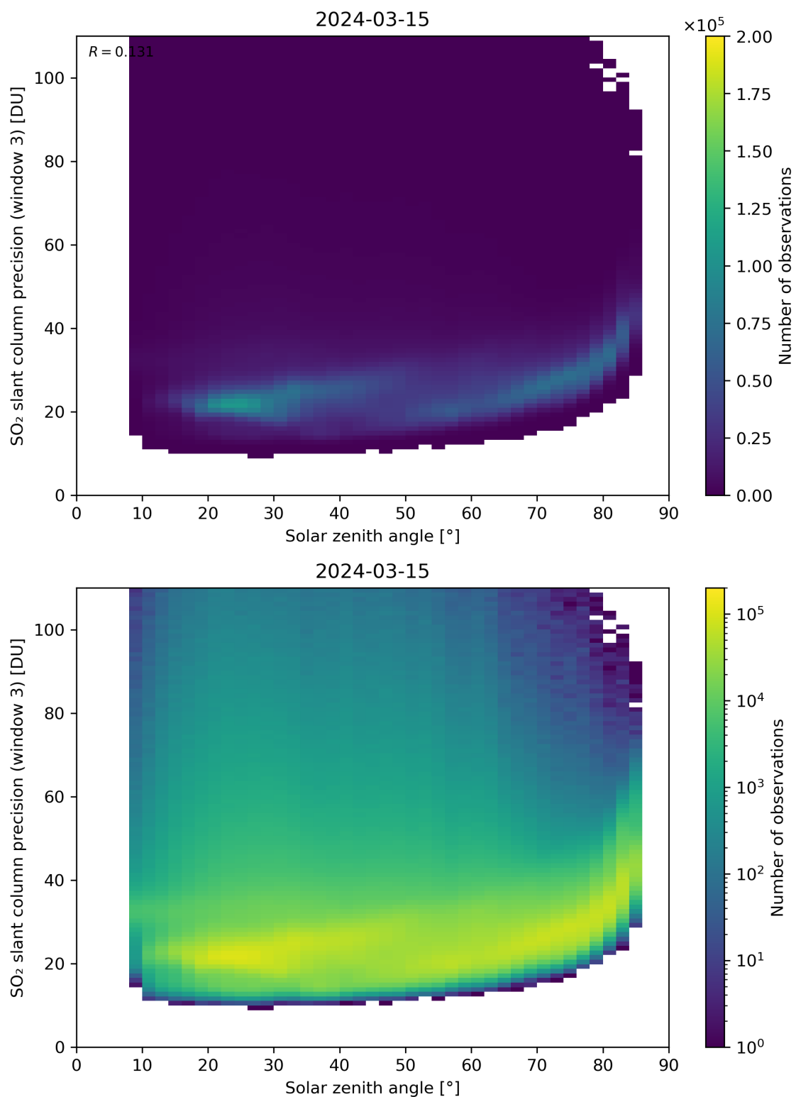
Figure 173: Scatter density plot of “Solar zenith angle” against “SO 2 slant column precision (window 3)” for 2024-03-14 to 2024-03-16.
