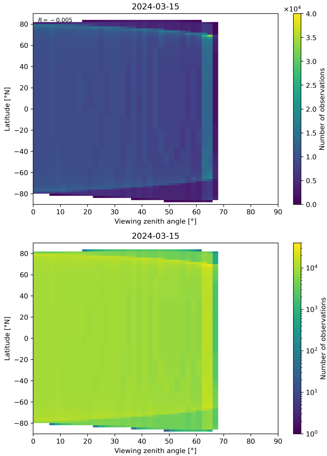
Figure 314: Scatter density plot of “Viewing zenith angle” against “Latitude” for 2024-03-14 to 2024-03-16.
