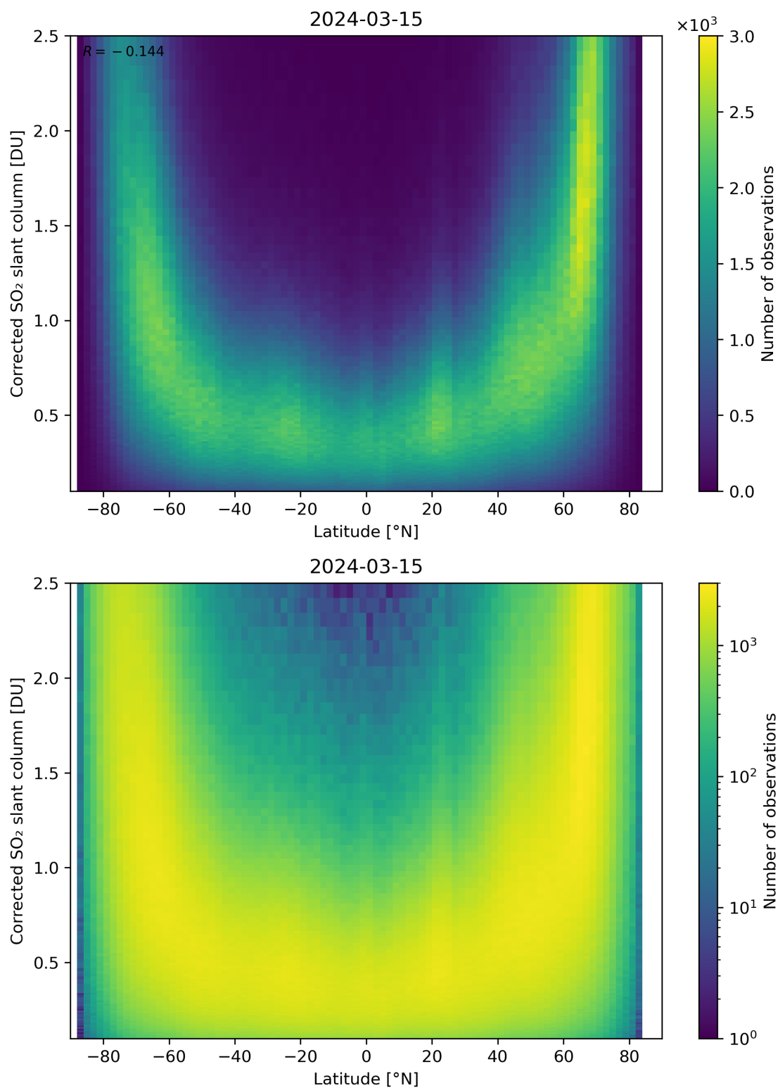
Figure 146: Scatter density plot of “Latitude” against “Corrected SO 2 slant column” for 2024-03-14 to 2024-03-16.
