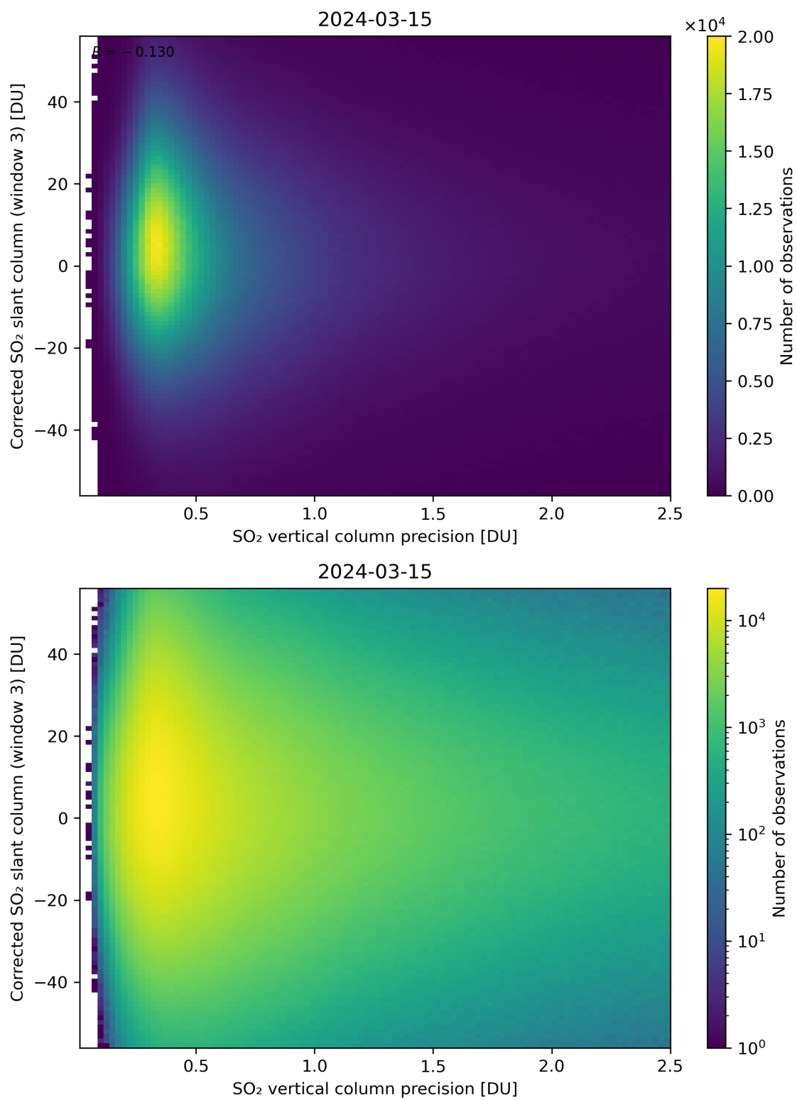
Figure 288: Scatter density plot of “SO 2 vertical column precision” against “Corrected SO 2 slant column (window 3)” for 2024-03-14 to 2024-03-16.
