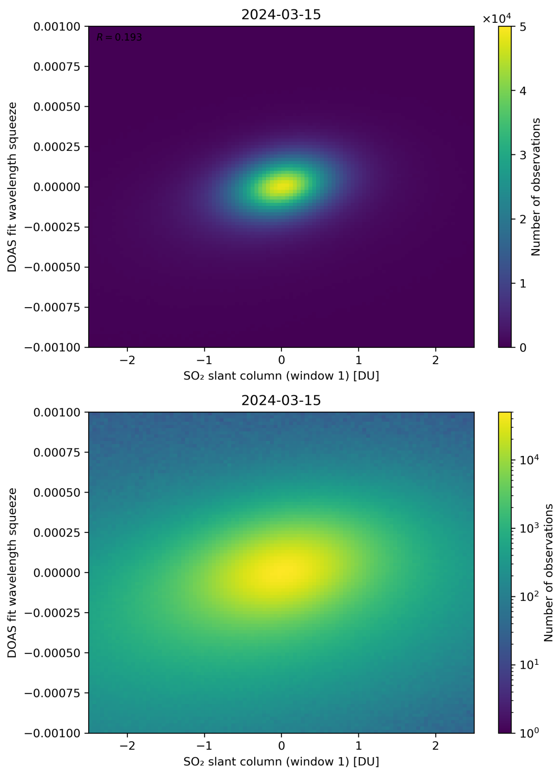
Figure 216: Scatter density plot of “SO 2 slant column (window 1)” against “DOAS fit wavelength squeeze” for 2024-03-14 to 2024-03-16.
