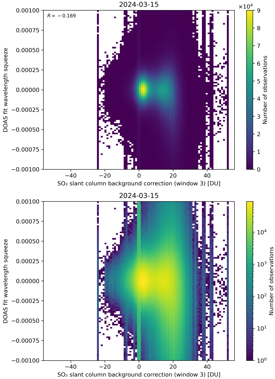
Figure 122: Scatter density plot of “SO 2 slant column background correction (window 3)” against “DOAS fit wavelength squeeze” for 2024-03-14 to 2024-03-16.
