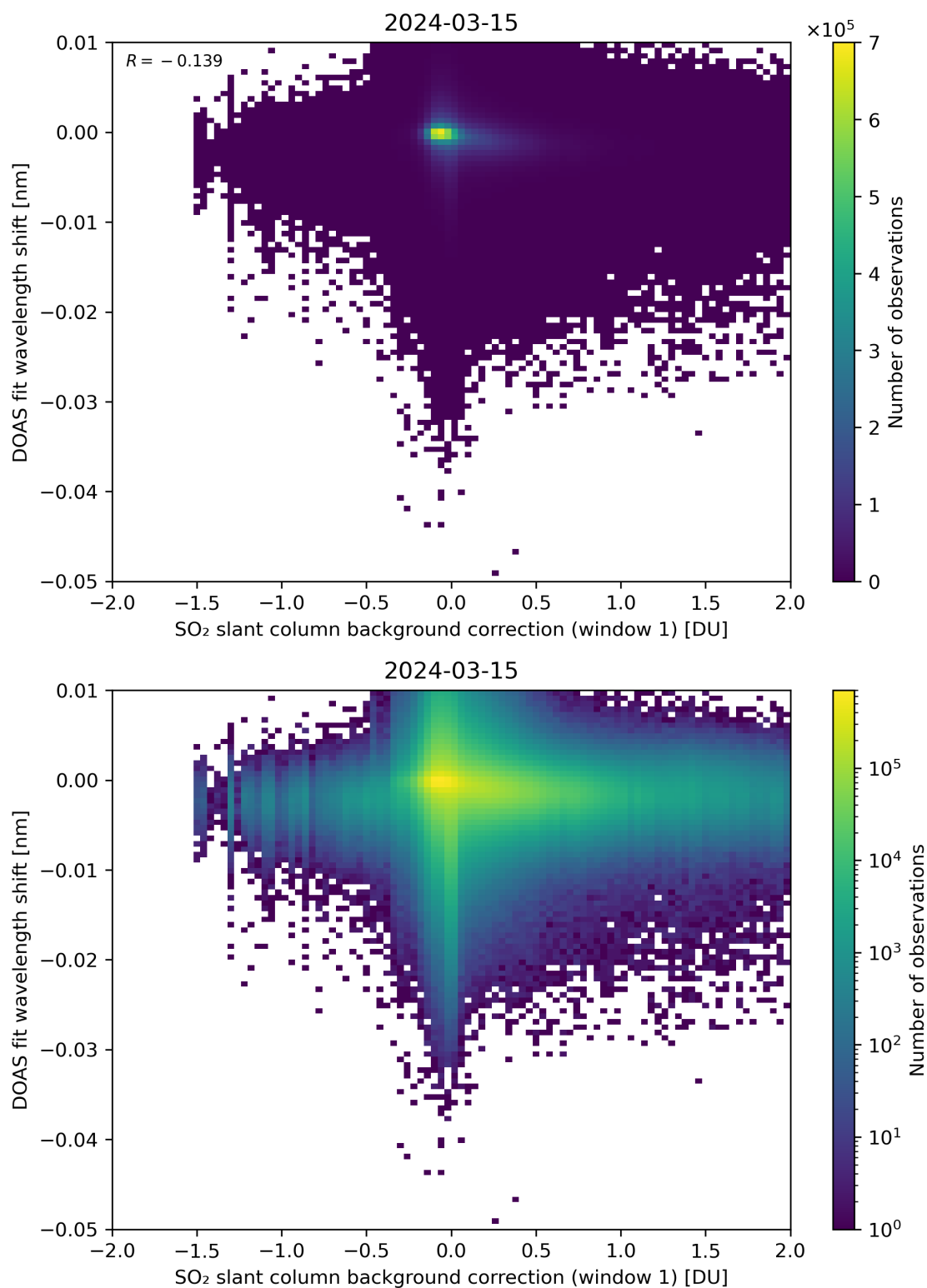
Figure 100: Scatter density plot of “SO 2 slant column background correction (window 1)” against “DOAS fit wavelength shift” for 2024-03-14 to 2024-03-16.
