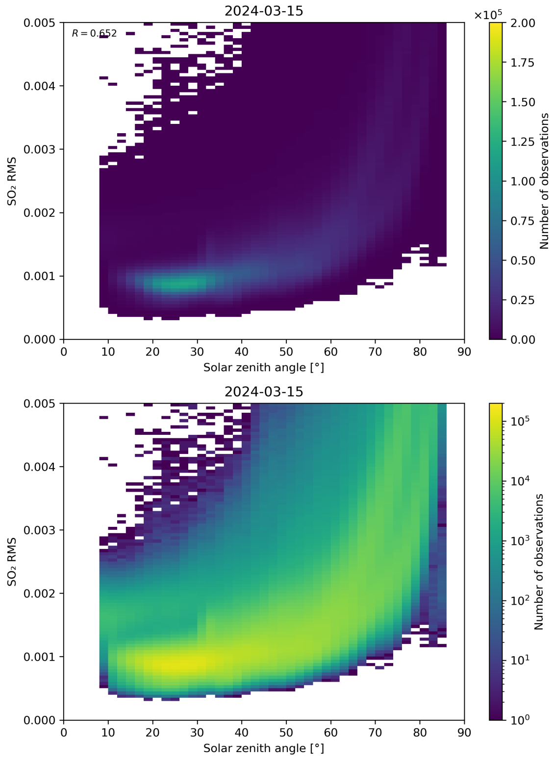
Figure 163: Scatter density plot of “Solar zenith angle” against “SO 2 RMS” for 2024-03-14 to 2024-03-16.
