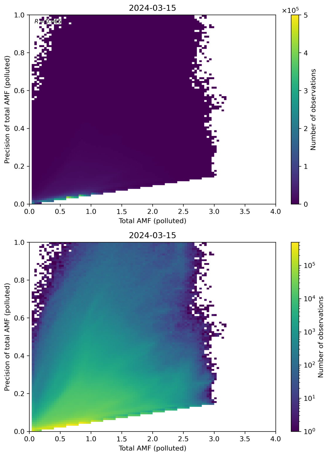
Figure 272: Scatter density plot of “Total AMF (polluted)” against “Precision of total AMF (polluted)” for 2024-03-14 to 2024-03-16.
