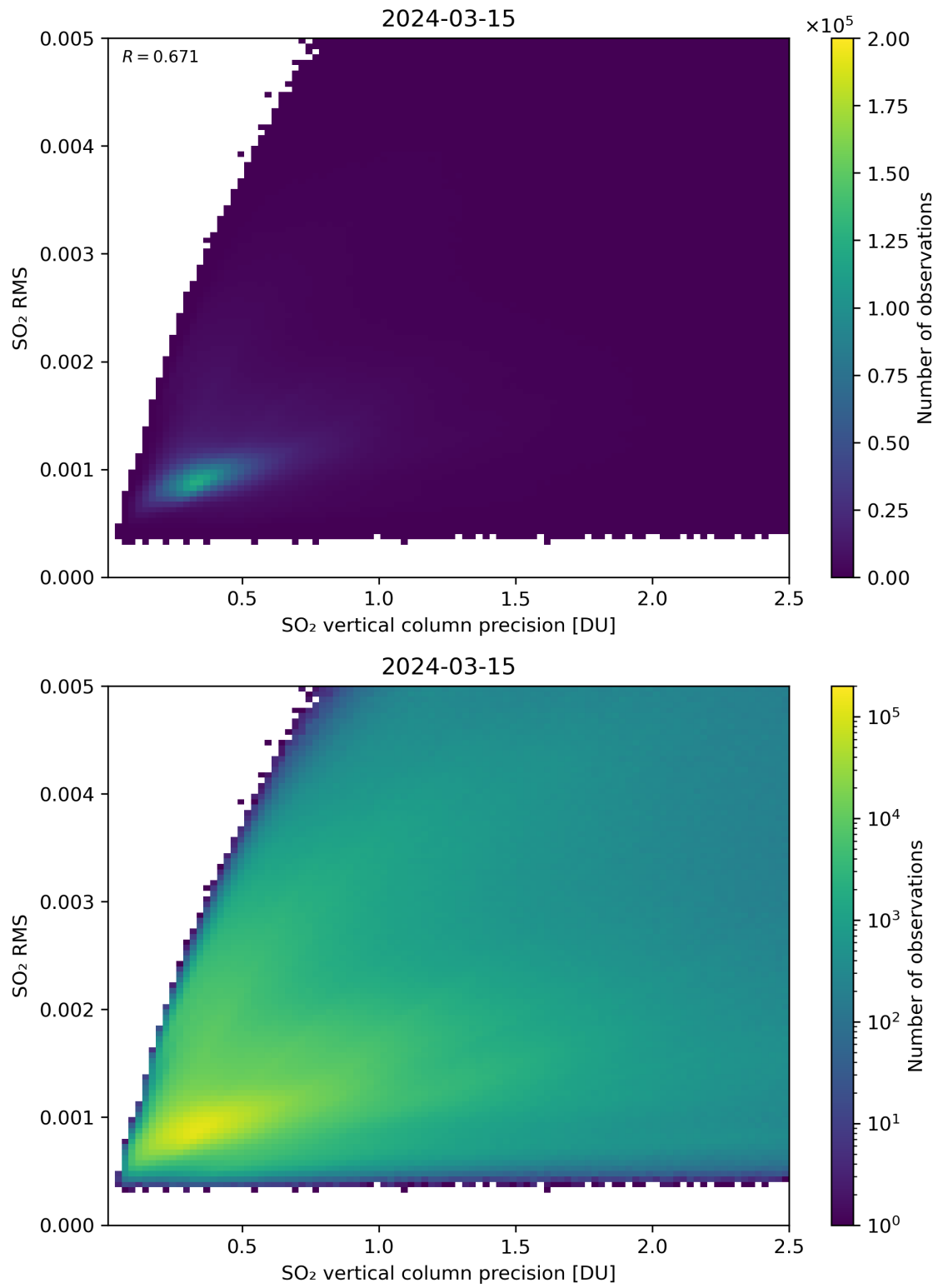
Figure 284: Scatter density plot of “SO 2 vertical column precision” against “SO 2 RMS” for 2024-03-14 to 2024-03-16.
