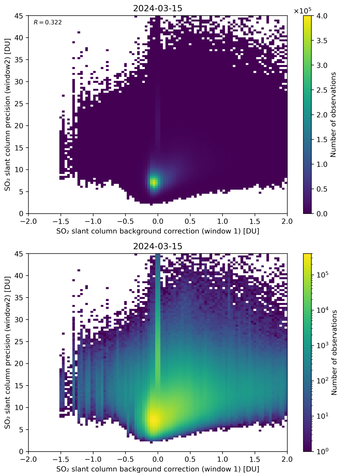
Figure 106: Scatter density plot of “SO 2 slant column background correction (window 1)” against “SO 2 slant column precision (window2)” for 2024-03-14 to 2024-03-16.
