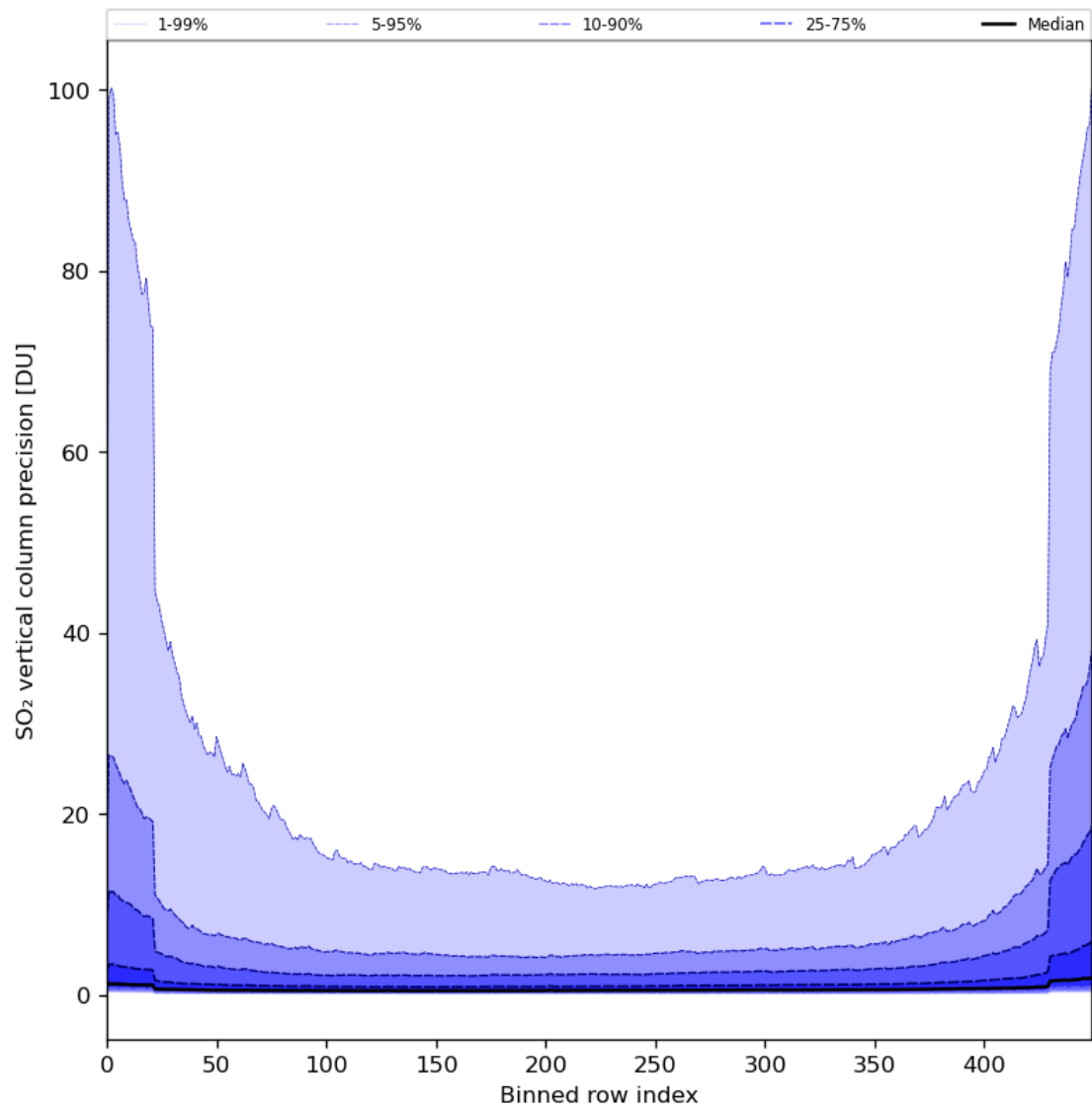
Figure 77: Along track statistics of “SO 2 vertical column precision” for 2024-03-14 to 2024-03-16
