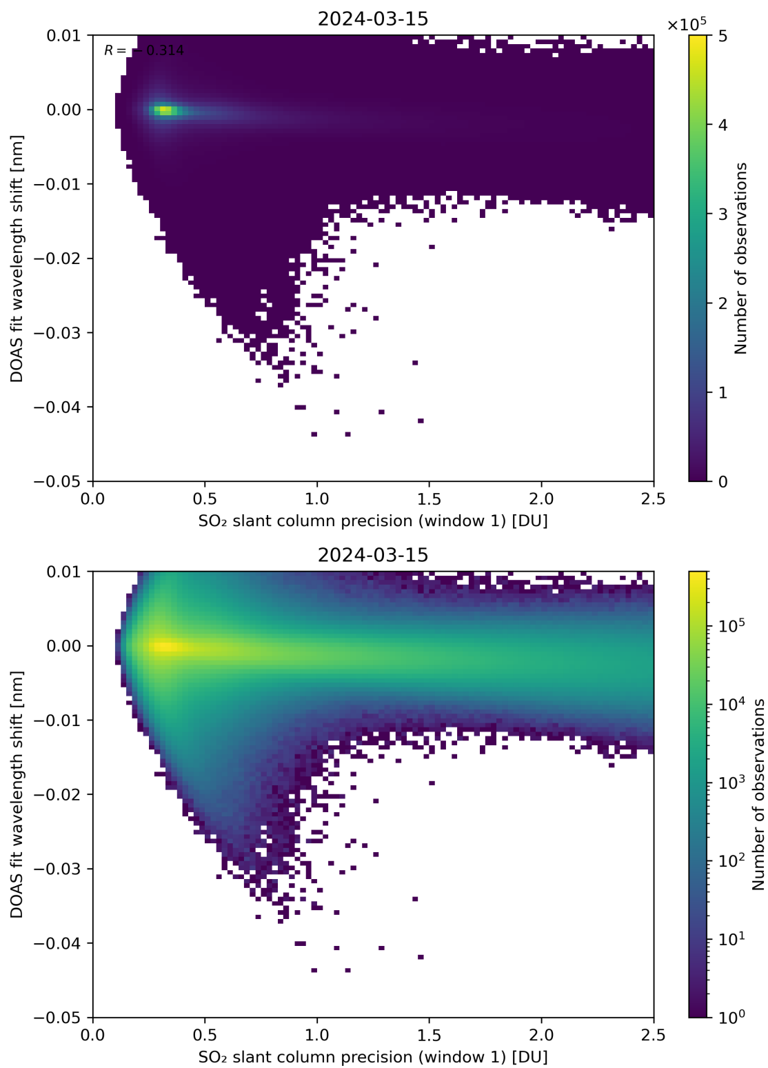
Figure 221: Scatter density plot of “SO 2 slant column precision (window 1)” against “DOAS fit wavelength shift” for 2024-03-14 to 2024-03-16.
