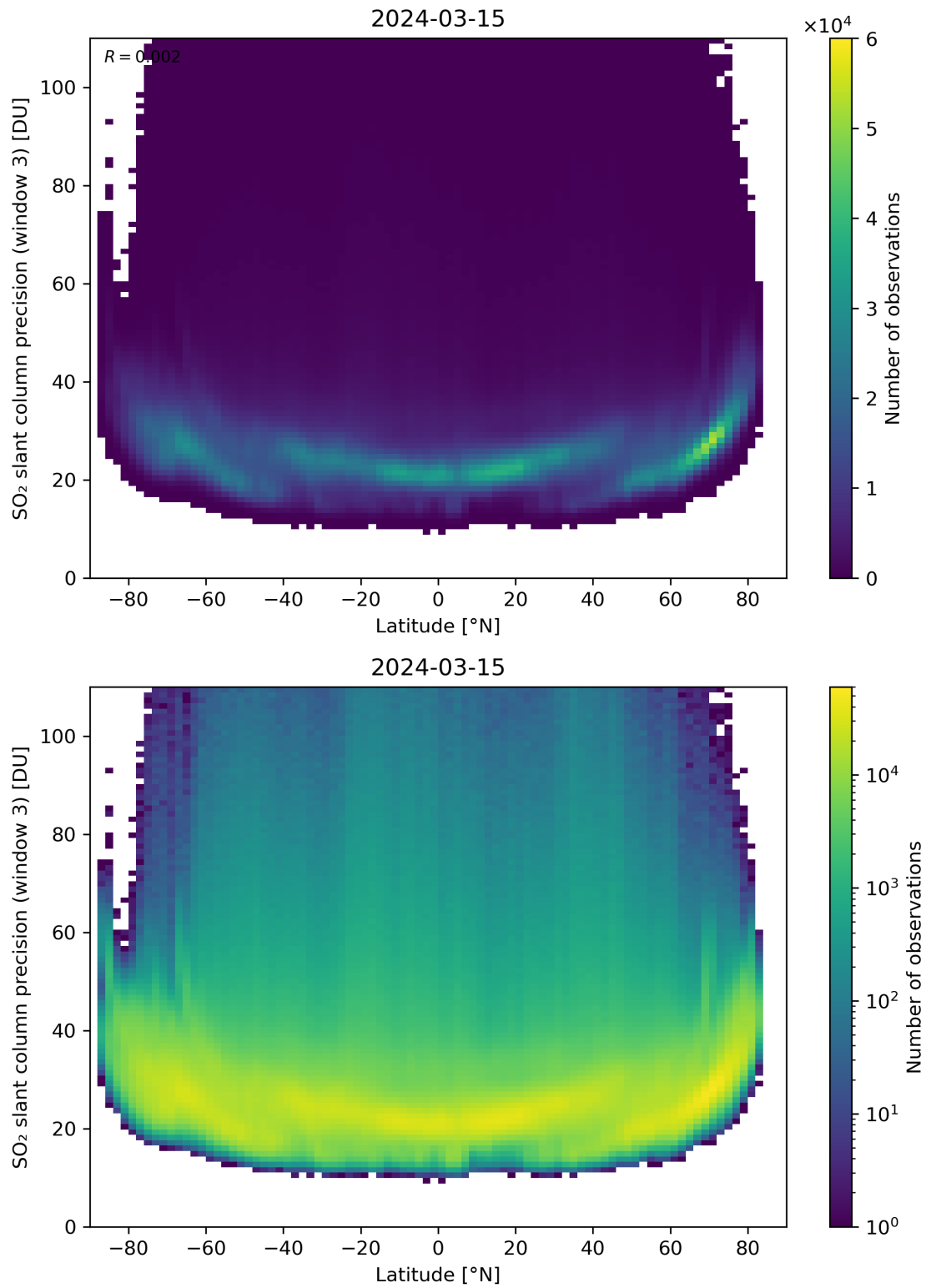
Figure 153: Scatter density plot of “Latitude” against “SO 2 slant column precision (window 3)” for 2024-03-14 to 2024-03-16.
