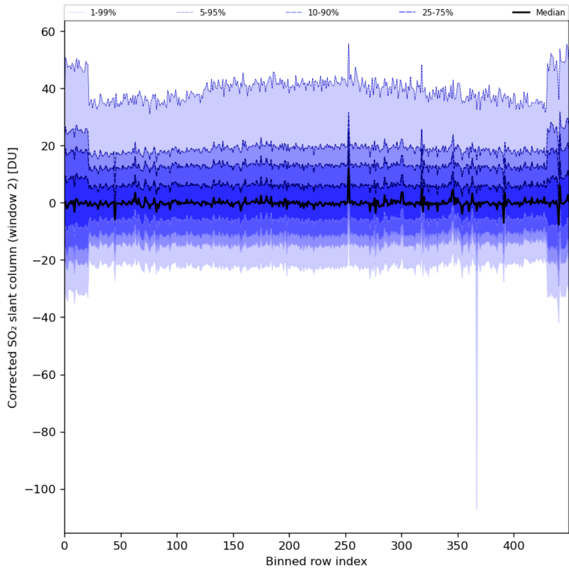
Figure 85: Along track statistics of “Corrected SO 2 slant column (window 2)” for 2024-03-14 to 2024-03-16
