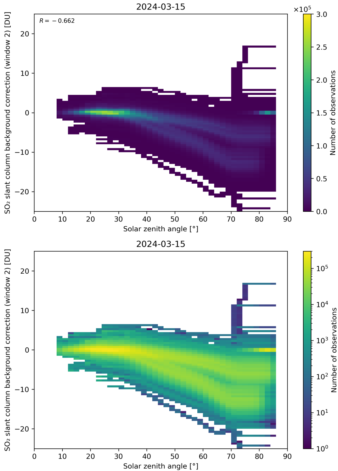
Figure 159: Scatter density plot of “Solar zenith angle” against “SO 2 slant column background correction (window 2)” for 2024-03-14 to 2024-03-16.
