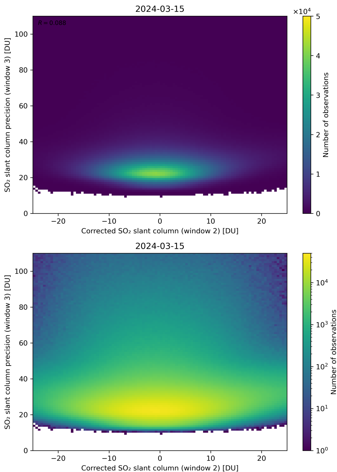
Figure 202: Scatter density plot of “Corrected SO 2 slant column (window 2)” against “SO 2 slant column precision (window 3)” for 2024-03-14 to 2024-03-16.
