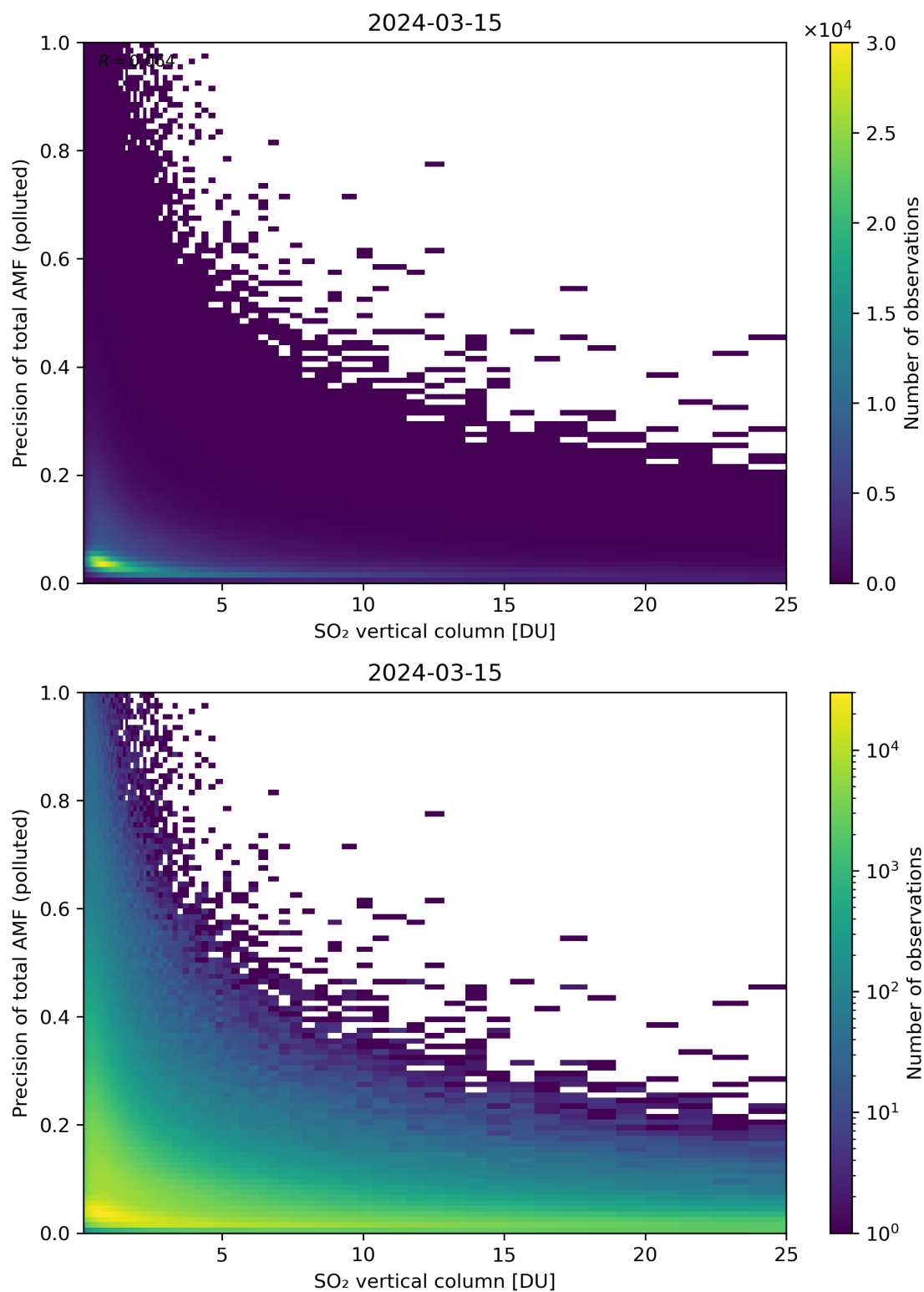
Figure 306: Scatter density plot of “SO 2 vertical column” against “Precision of total AMF (polluted)” for 2024-03-14 to 2024-03-16.
