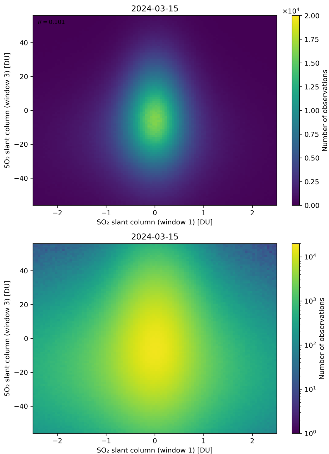
Figure 237: Scatter density plot of “SO 2 slant column (window 1)” against “SO 2 slant column (window 3)” for 2024-03-14 to 2024-03-16.
