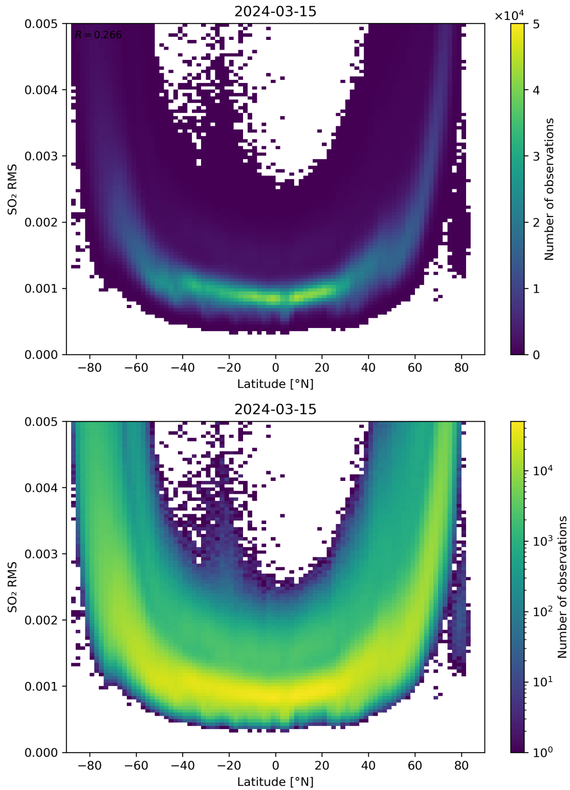
Figure 144: Scatter density plot of “Latitude” against “SO 2 RMS” for 2024-03-14 to 2024-03-16.
