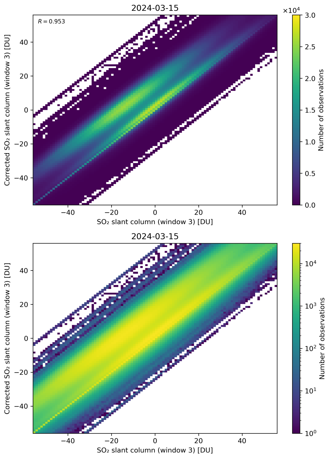
Figure 266: Scatter density plot of “SO 2 slant column (window 3)” against “Corrected SO 2 slant column (window 3)” for 2024-03-14 to 2024-03-16.
