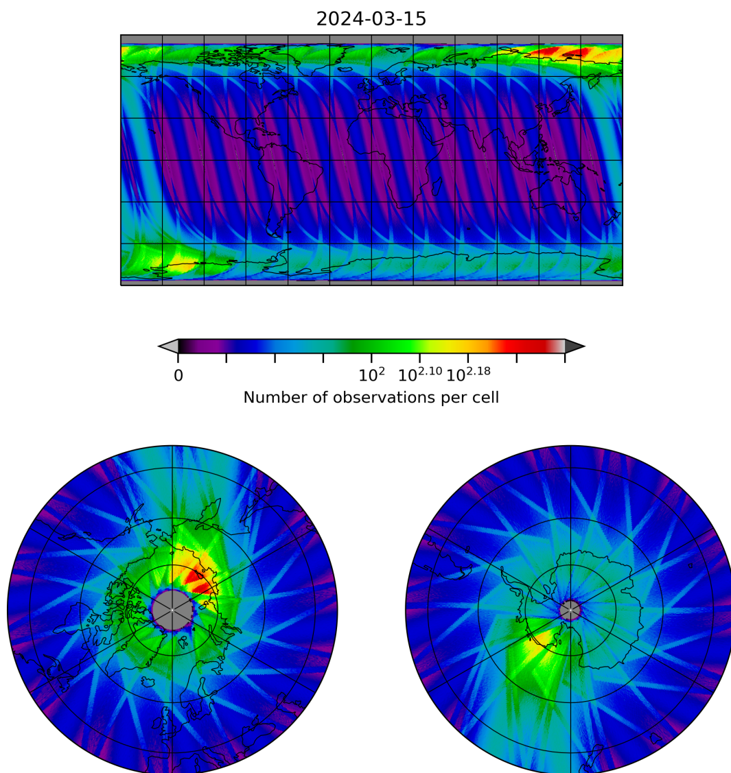
Figure 28: Map of the number of observations for 2024-03-14 to 2024-03-16
