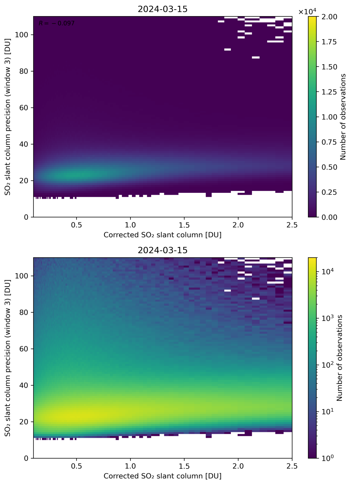
Figure 191: Scatter density plot of “Corrected SO 2 slant column” against “SO 2 slant column precision (window 3)” for 2024-03-14 to 2024-03-16.
