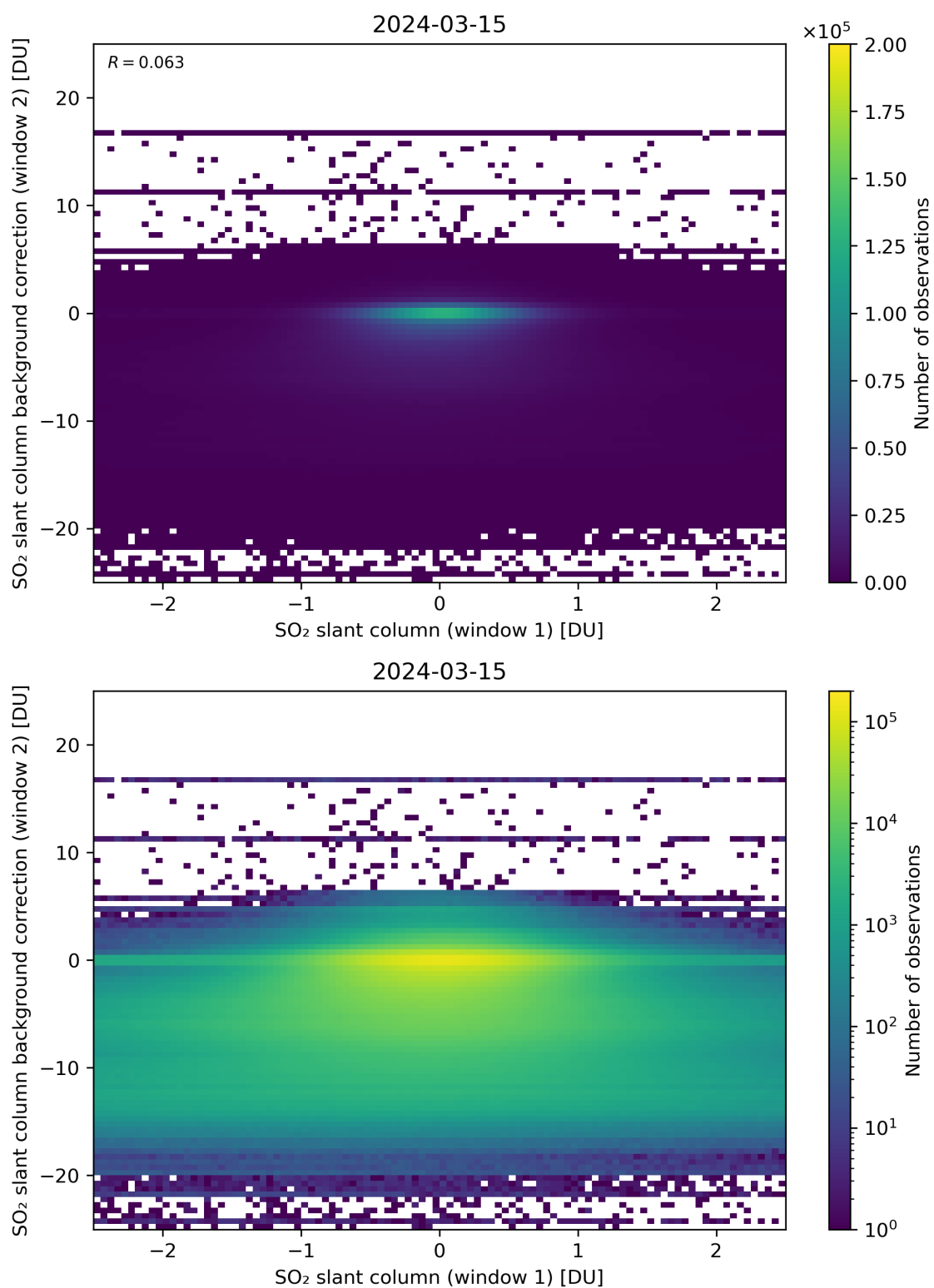
Figure 213: Scatter density plot of “SO 2 slant column (window 1)” against “SO 2 slant column background correction (window 2)” for 2024-03-14 to 2024-03-16.
