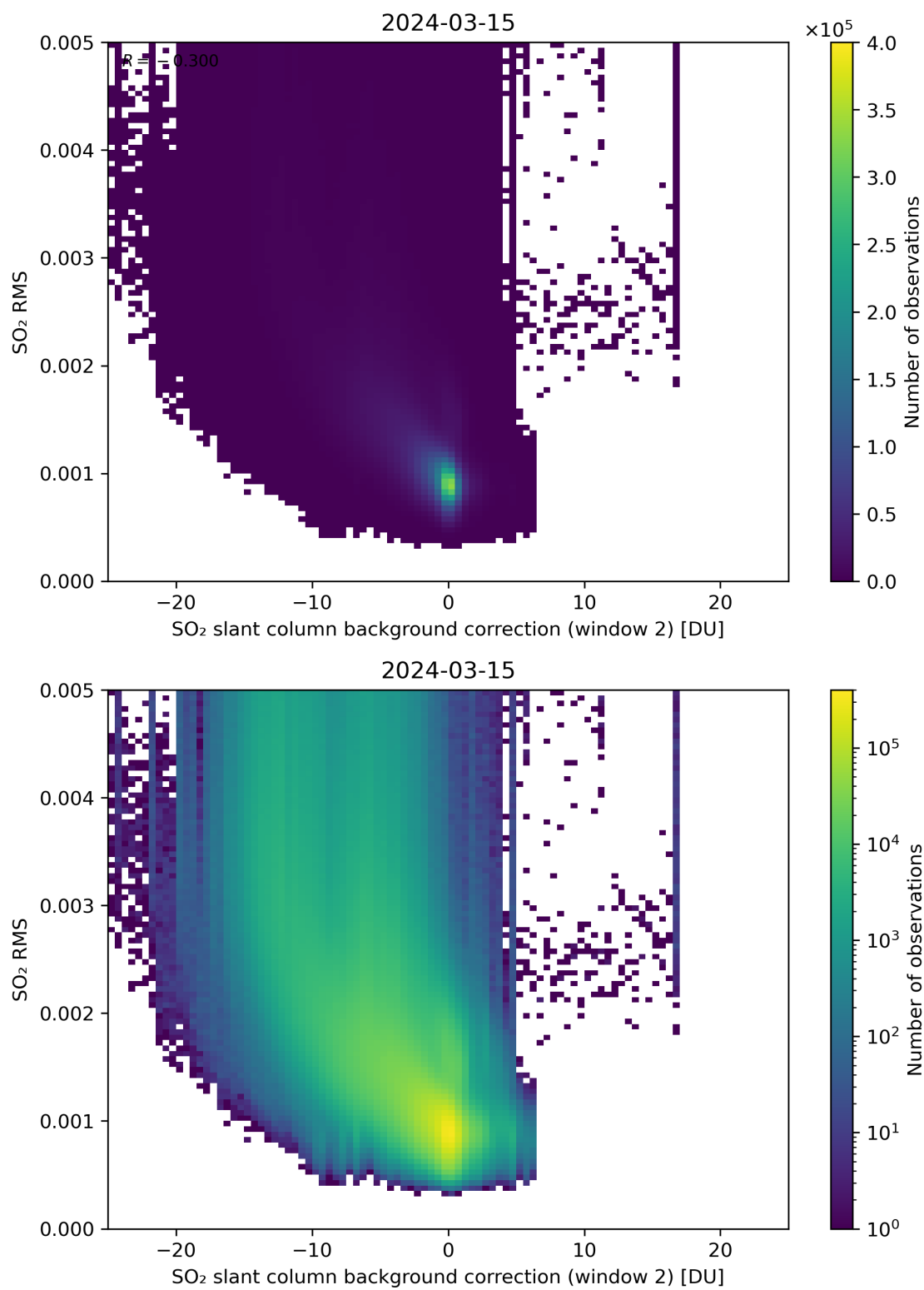
Figure 114: Scatter density plot of “SO 2 slant column background correction (window 2)” against “SO 2 RMS” for 2024-03-14 to 2024-03-16.
