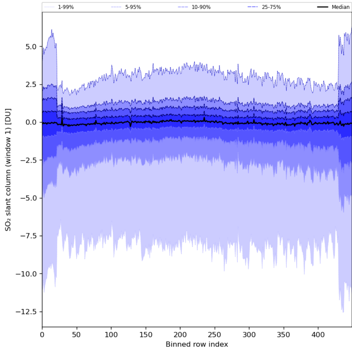
Figure 79: Along track statistics of “SO 2 slant column (window 1)” for 2024-03-14 to 2024-03-16
