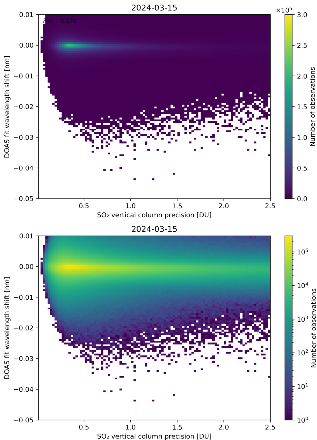
Figure 282: Scatter density plot of “SO 2 vertical column precision” against “DOAS fit wavelength shift” for 2024-03-14 to 2024-03-16.
