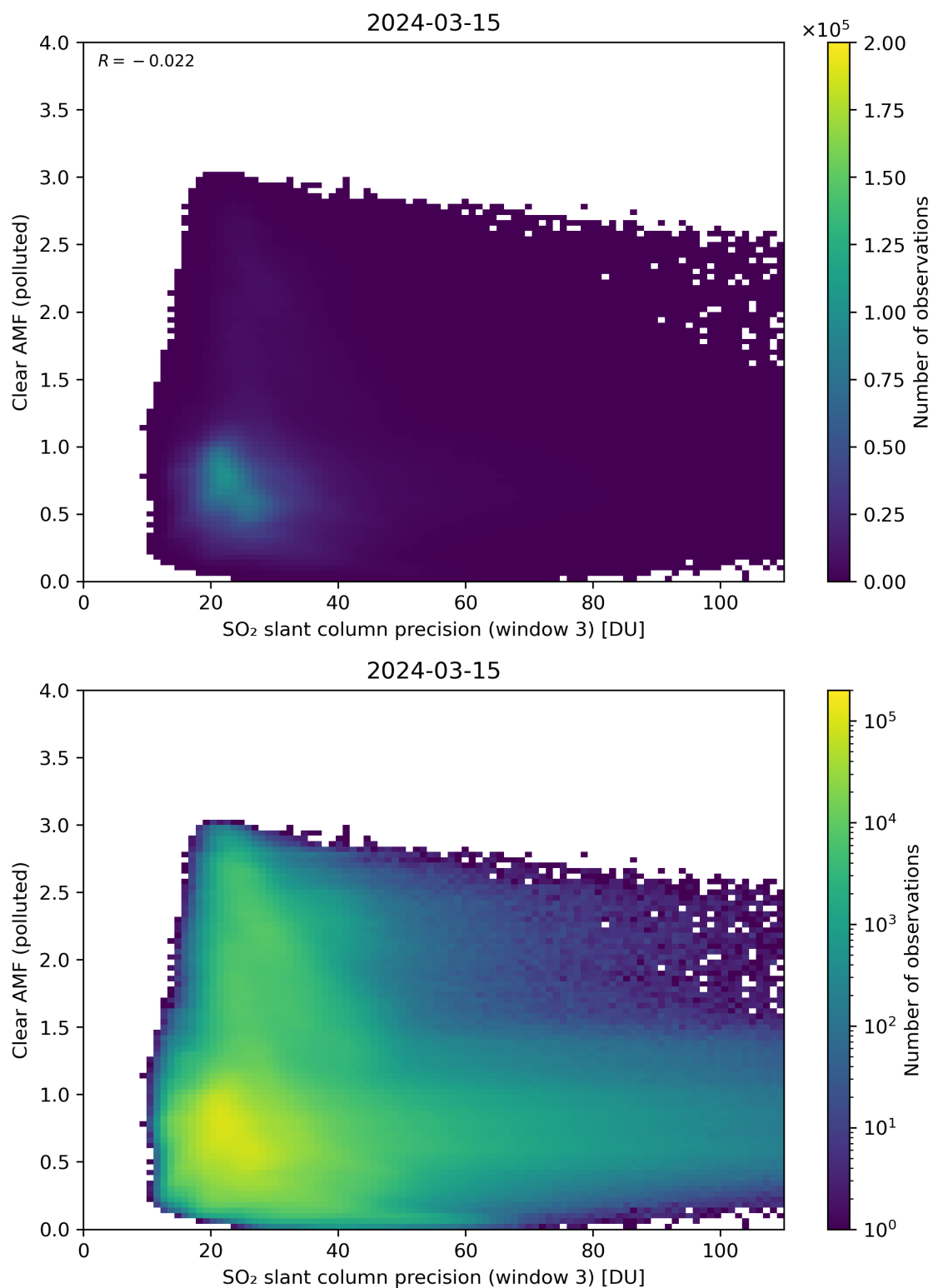
Figure 261: Scatter density plot of “SO 2 slant column precision (window 3)” against “Clear AMF (polluted)” for 2024-03-14 to 2024-03-16.
