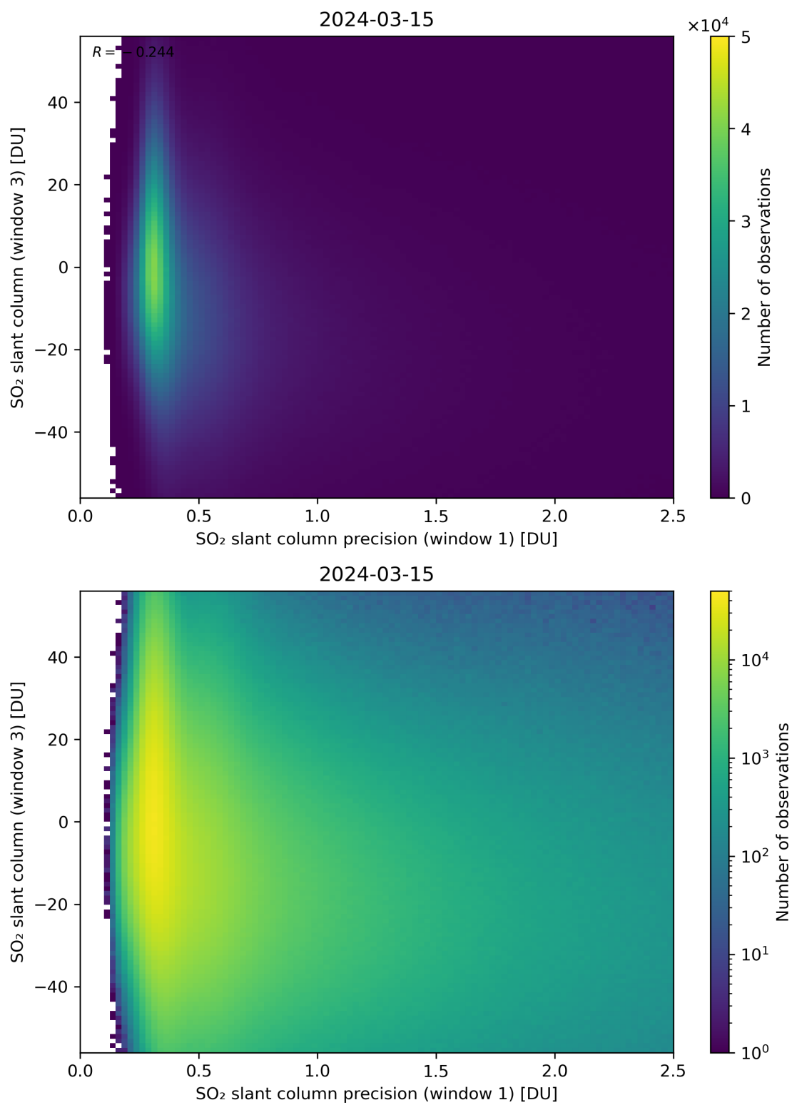
Figure 228: Scatter density plot of “SO 2 slant column precision (window 1)” against “SO 2 slant column (window 3)” for 2024-03-14 to 2024-03-16.
