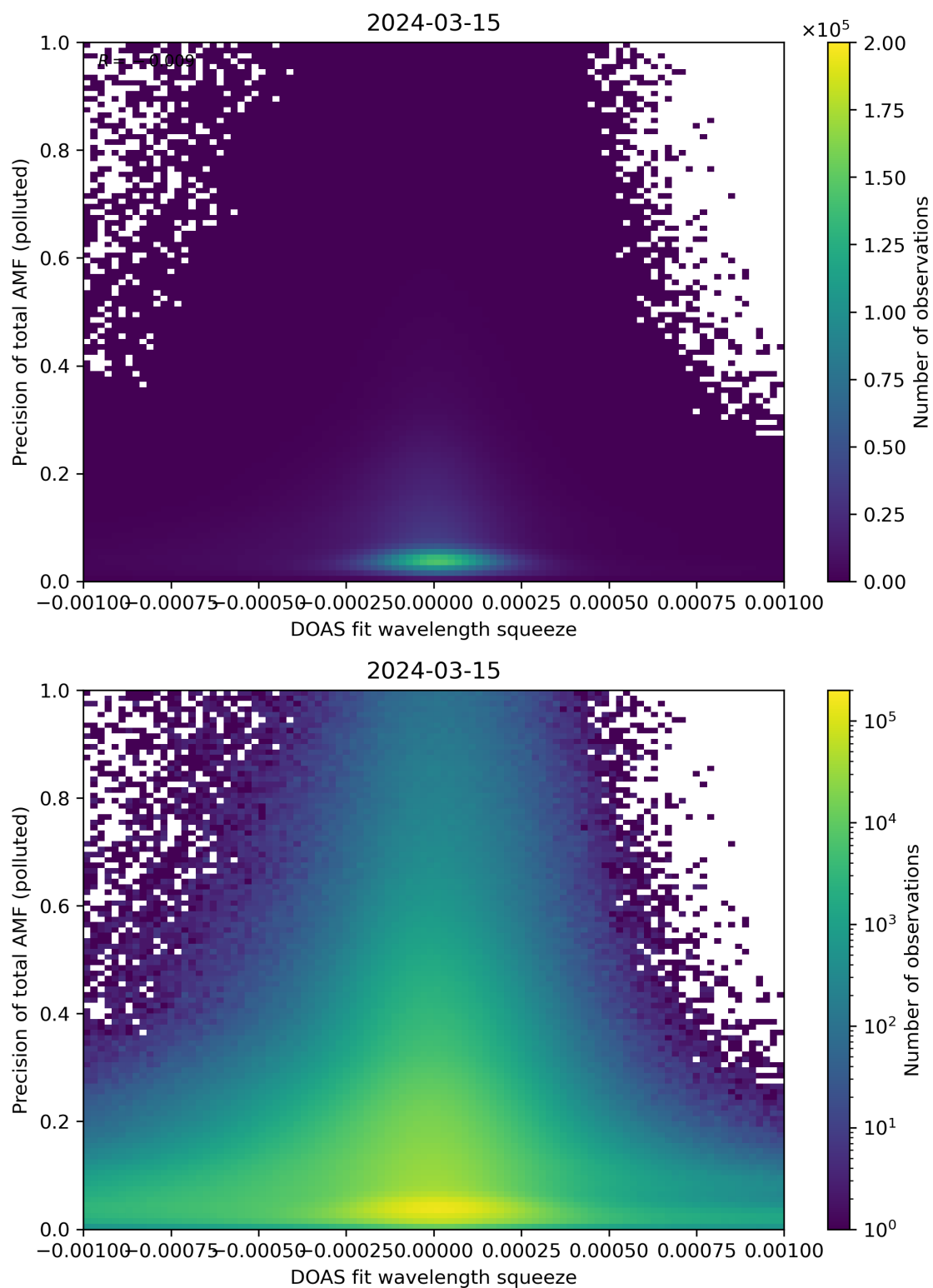
Figure 135: Scatter density plot of “DOAS fit wavelength squeeze” against “Precision of total AMF (polluted)” for 2024-03-14 to 2024-03-16.
