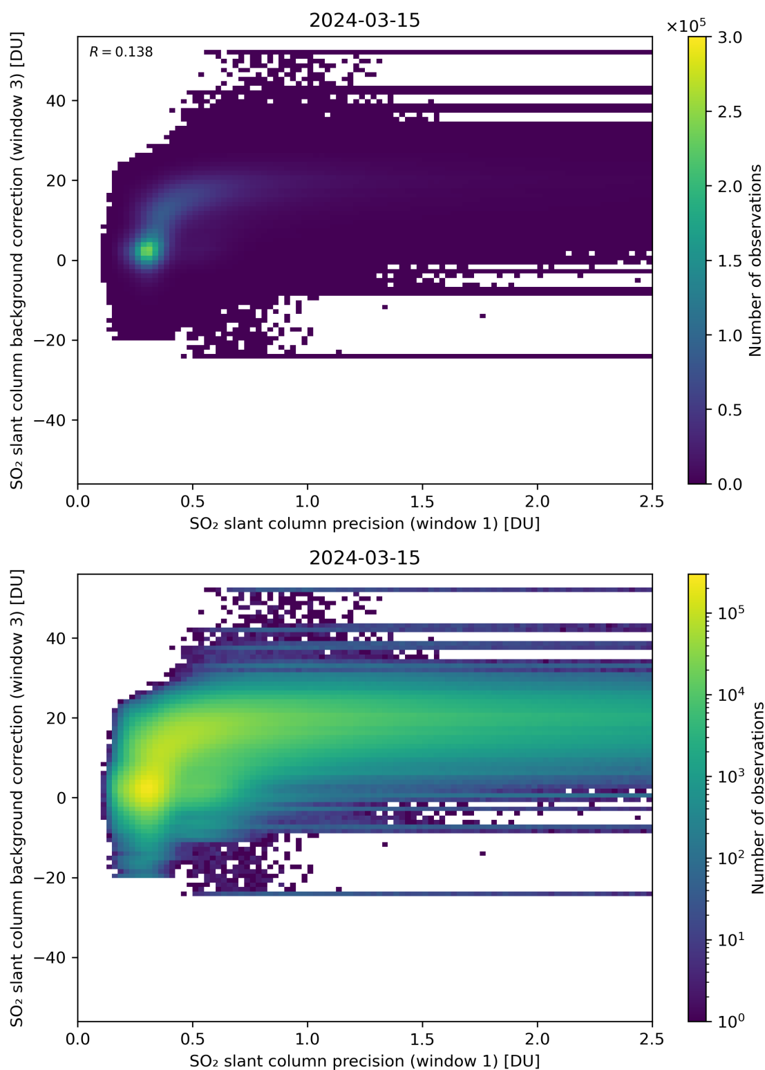
Figure 220: Scatter density plot of “SO 2 slant column precision (window 1)” against “SO 2 slant column background correction (window 3)” for 2024-03-14 to 2024-03-16.
