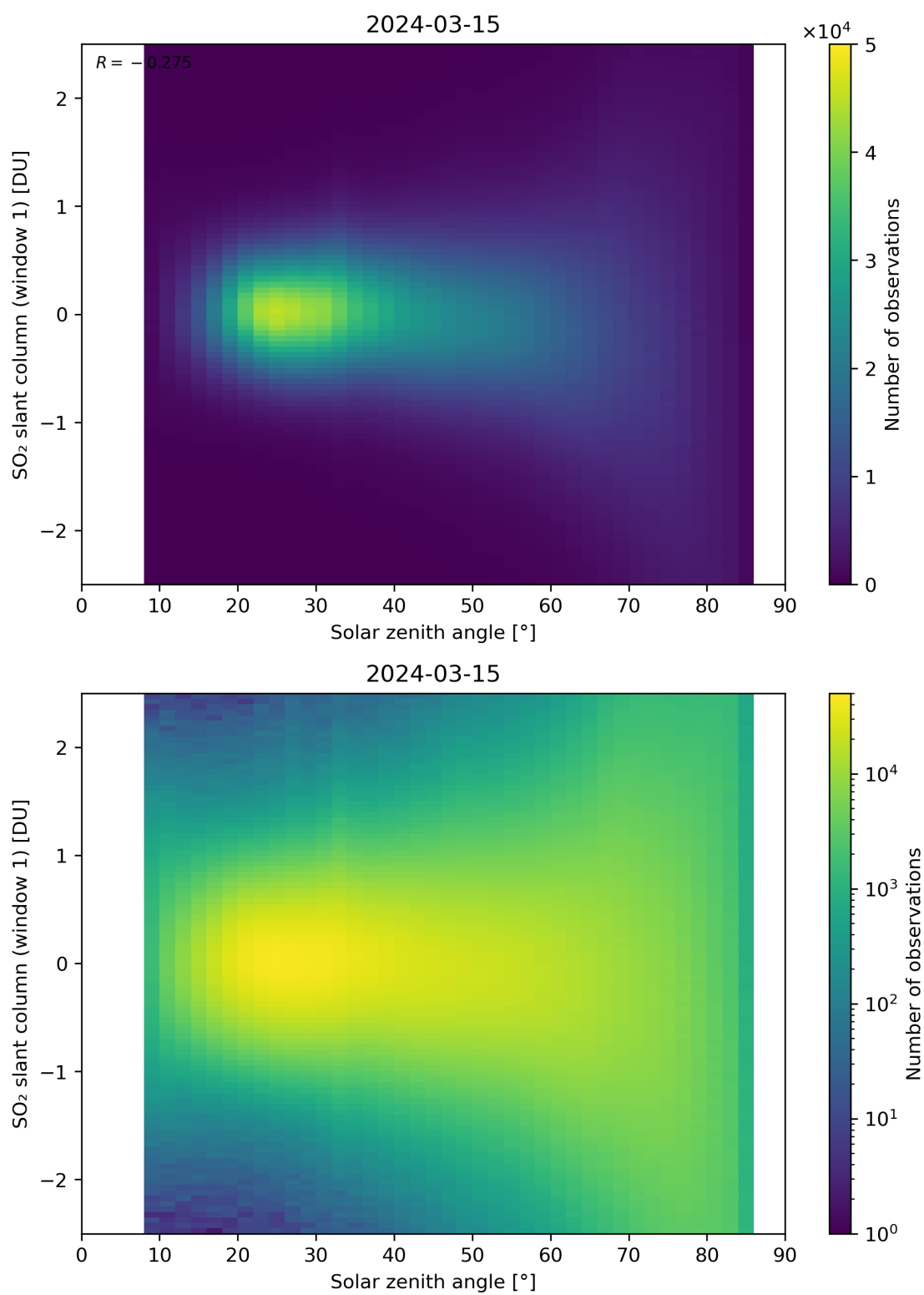
Figure 169: Scatter density plot of “Solar zenith angle” against “SO 2 slant column (window 1)” for 2024-03-14 to 2024-03-16.
