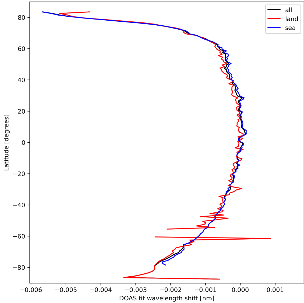
Figure 45: Zonal average of “DOAS fit wavelength shift” for 2024-03-14 to 2024-03-16.
