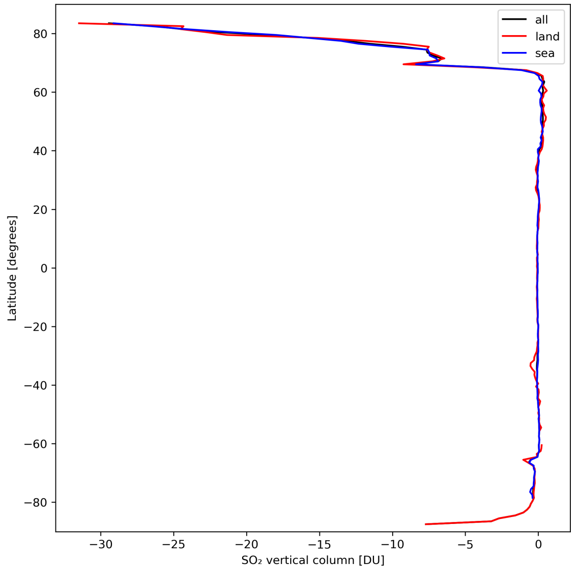
Figure 30: Zonal average of “SO 2 vertical column” for 2024-03-14 to 2024-03-16.
