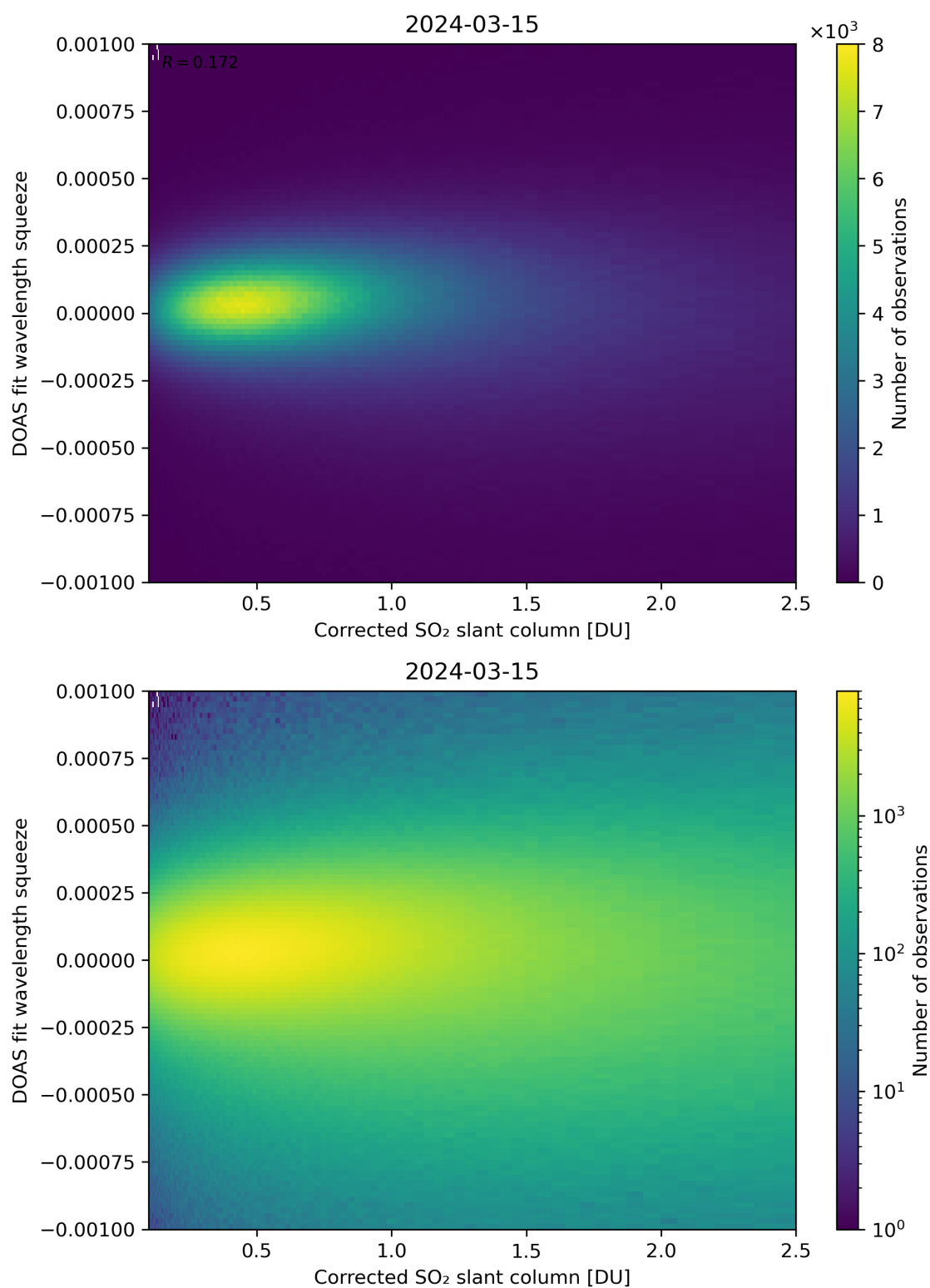
Figure 182: Scatter density plot of “Corrected SO 2 slant column” against “DOAS fit wavelength squeeze” for 2024-03-14 to 2024-03-16.
