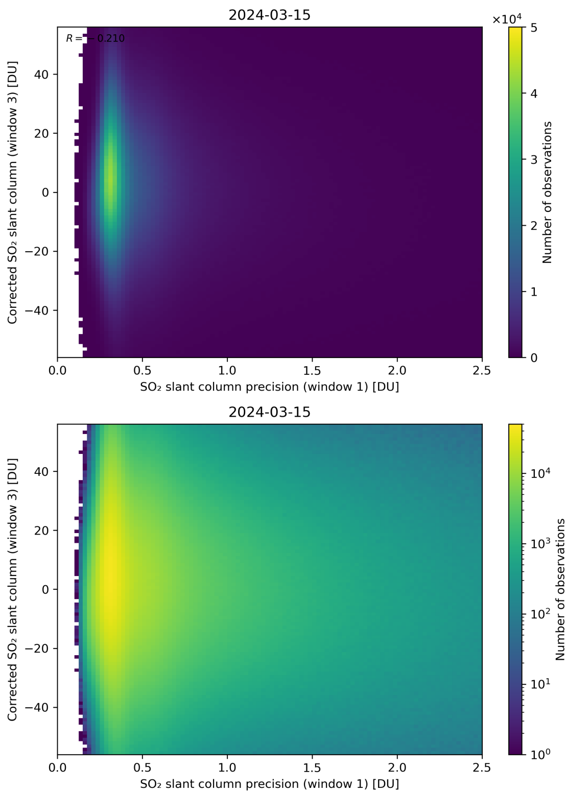
Figure 226: Scatter density plot of “SO 2 slant column precision (window 1)” against “Corrected SO 2 slant column (window 3)” for 2024-03-14 to 2024-03-16.
