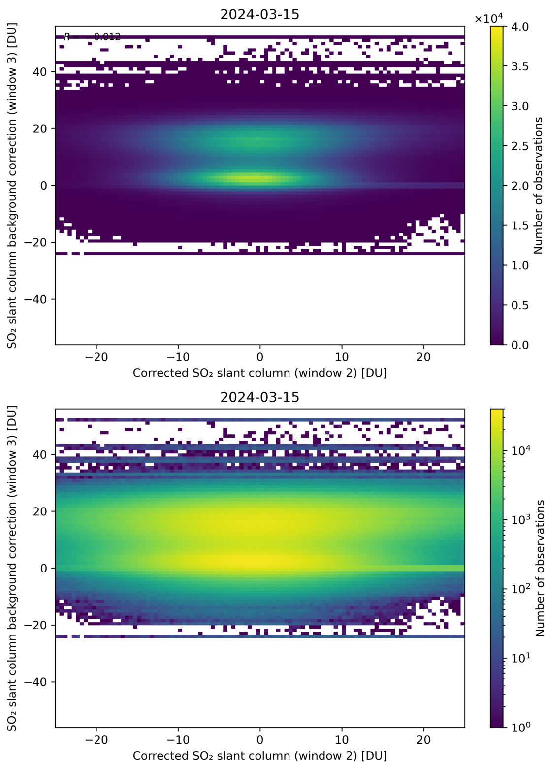
Figure 195: Scatter density plot of “Corrected SO 2 slant column (window 2)” against “SO 2 slant column background correction (window 3)” for 2024-03-14 to 2024-03-16.
