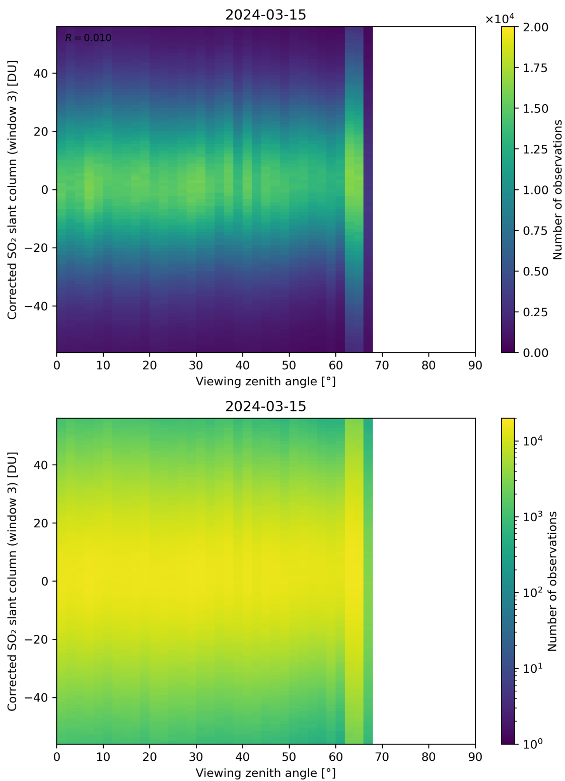
Figure 319: Scatter density plot of “Viewing zenith angle” against “Corrected SO 2 slant column (window 3)” for 2024-03-14 to 2024-03-16.
