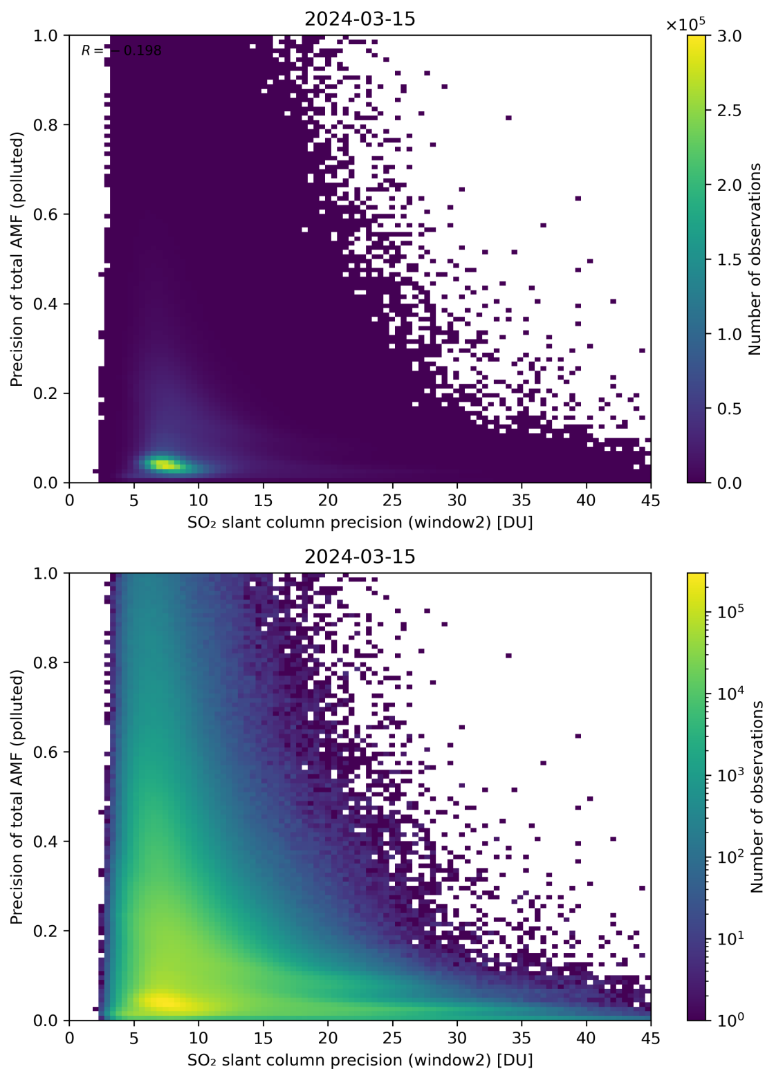
Figure 252: Scatter density plot of “SO 2 slant column precision (window2)” against “Precision of total AMF (polluted)” for 2024-03-14 to 2024-03-16.
