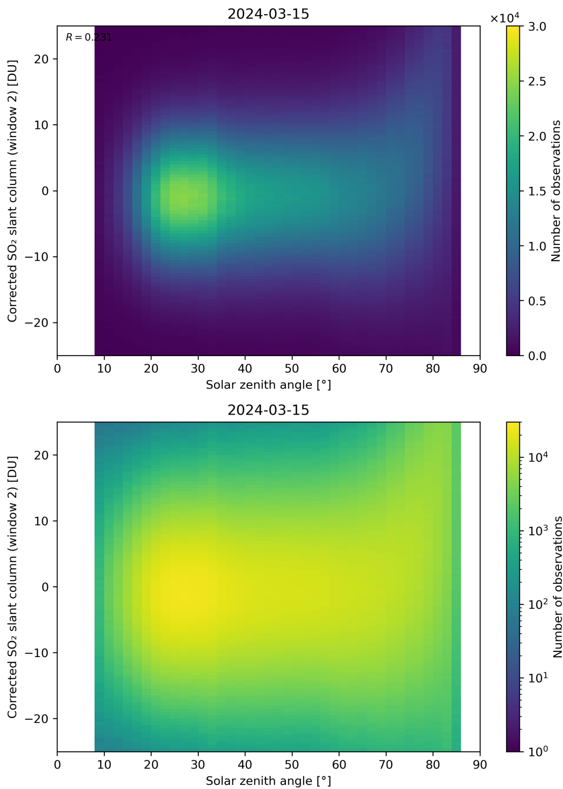
Figure 167: Scatter density plot of “Solar zenith angle” against “Corrected SO 2 slant column (window 2)” for 2024-03-14 to 2024-03-16.
