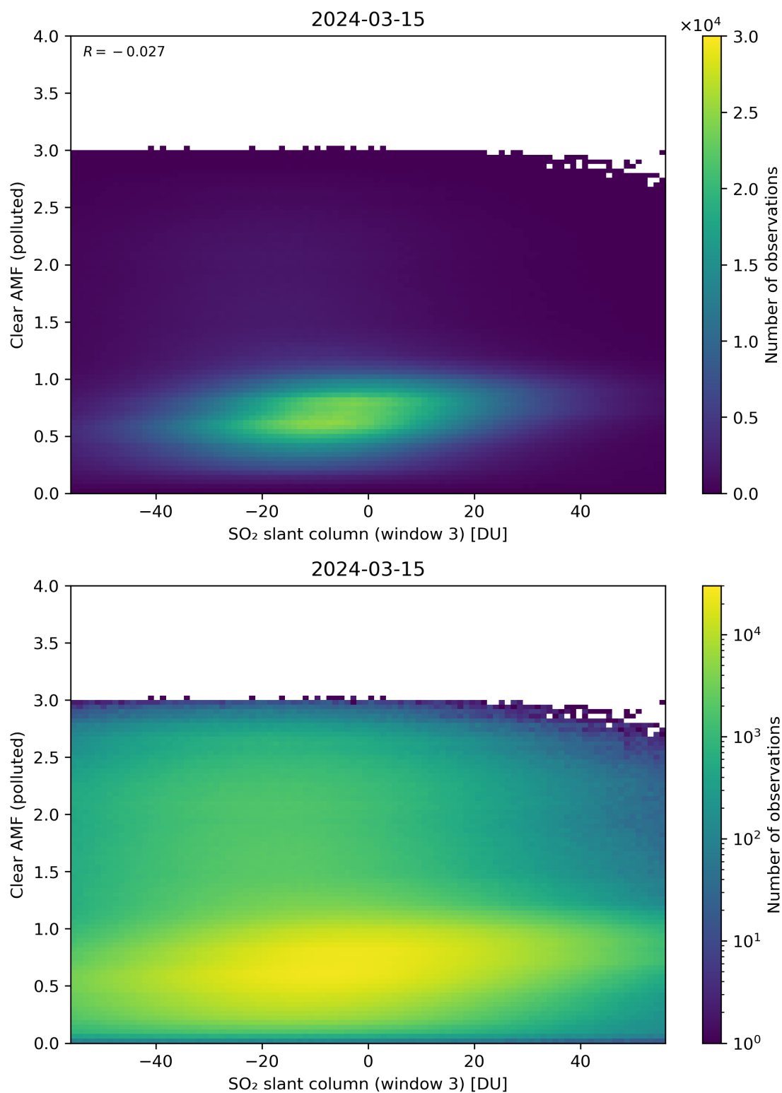
Figure 265: Scatter density plot of “SO 2 slant column (window 3)” against “Clear AMF (polluted)” for 2024-03-14 to 2024-03-16.
