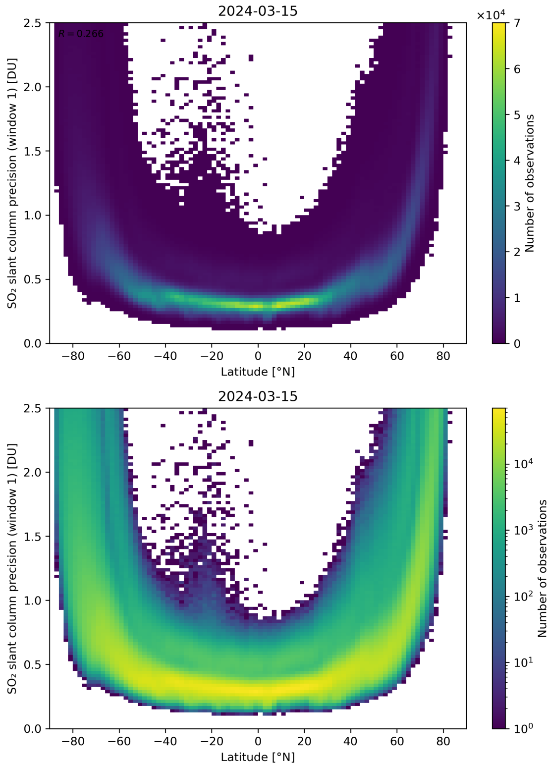
Figure 150: Scatter density plot of “Latitude” against “SO 2 slant column precision (window 1)” for 2024-03-14 to 2024-03-16.
