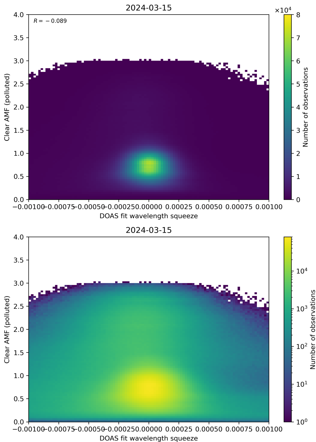
Figure 133: Scatter density plot of “DOAS fit wavelength squeeze” against “Clear AMF (polluted)” for 2024-03-14 to 2024-03-16.
