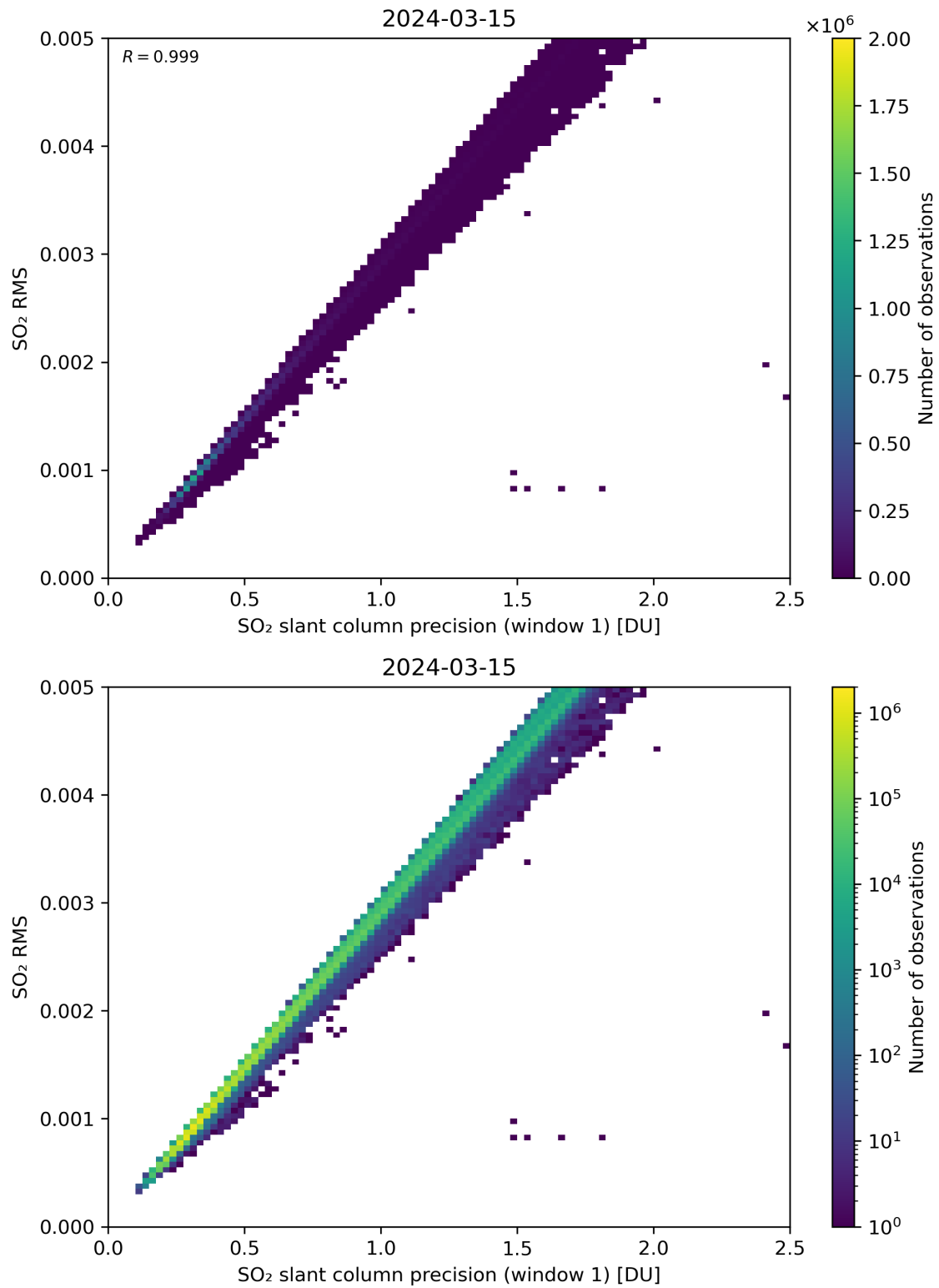
Figure 223: Scatter density plot of “SO 2 slant column precision (window 1)” against “SO 2 RMS” for 2024-03-14 to 2024-03-16.
