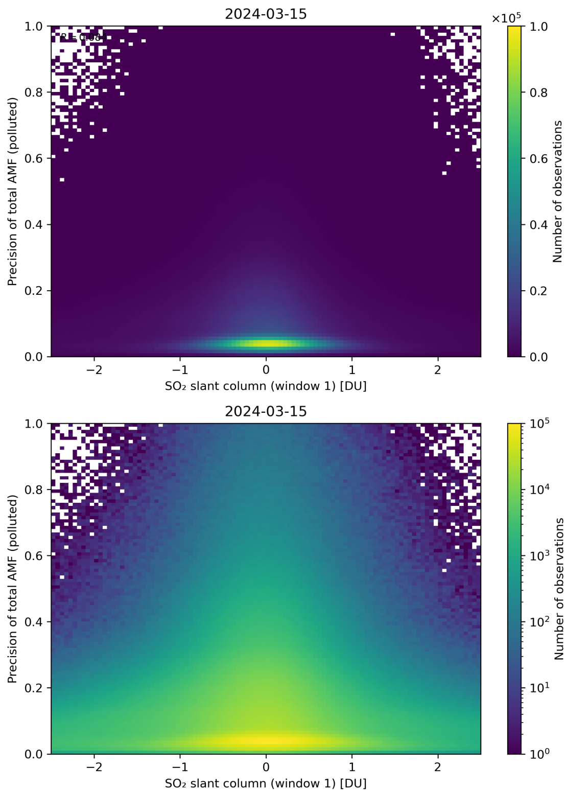
Figure 240: Scatter density plot of “SO 2 slant column (window 1)” against “Precision of total AMF (polluted)” for 2024-03-14 to 2024-03-16.
