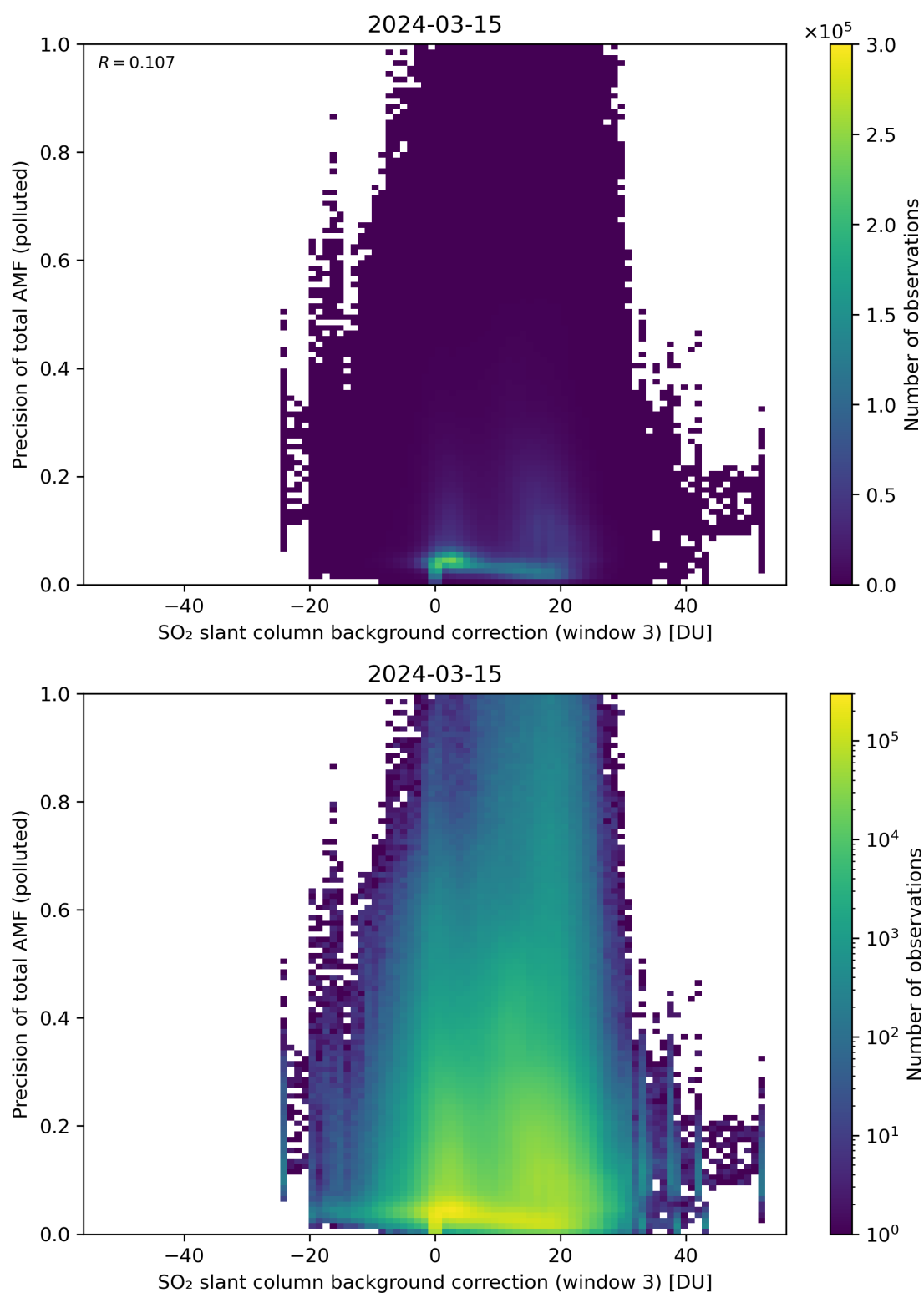
Figure 126: Scatter density plot of “SO 2 slant column background correction (window 3)” against “Precision of total AMF (polluted)” for 2024-03-14 to 2024-03-16.
