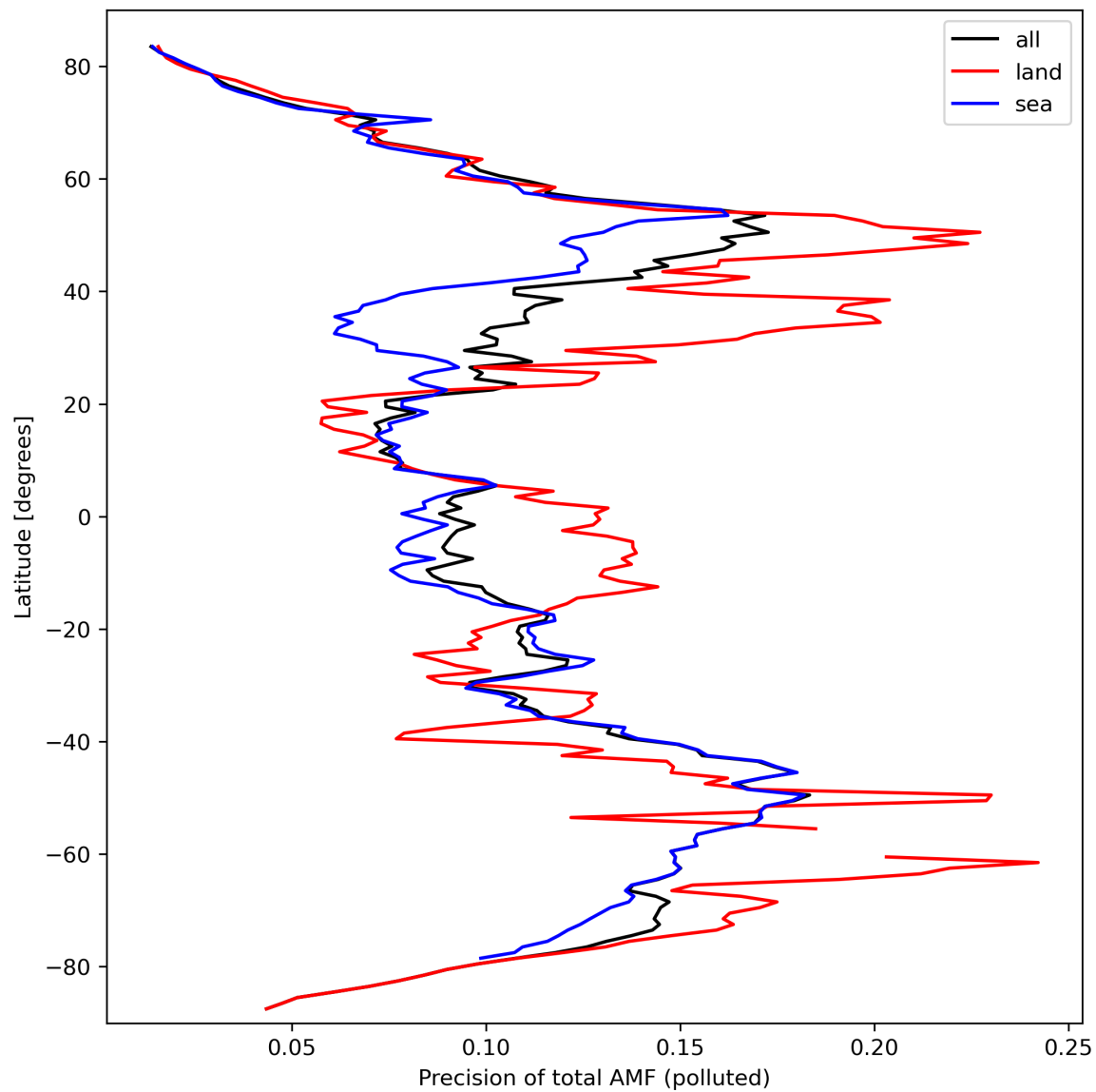
Figure 49: Zonal average of “Precision of total AMF (polluted)” for 2024-03-14 to 2024-03-16.
