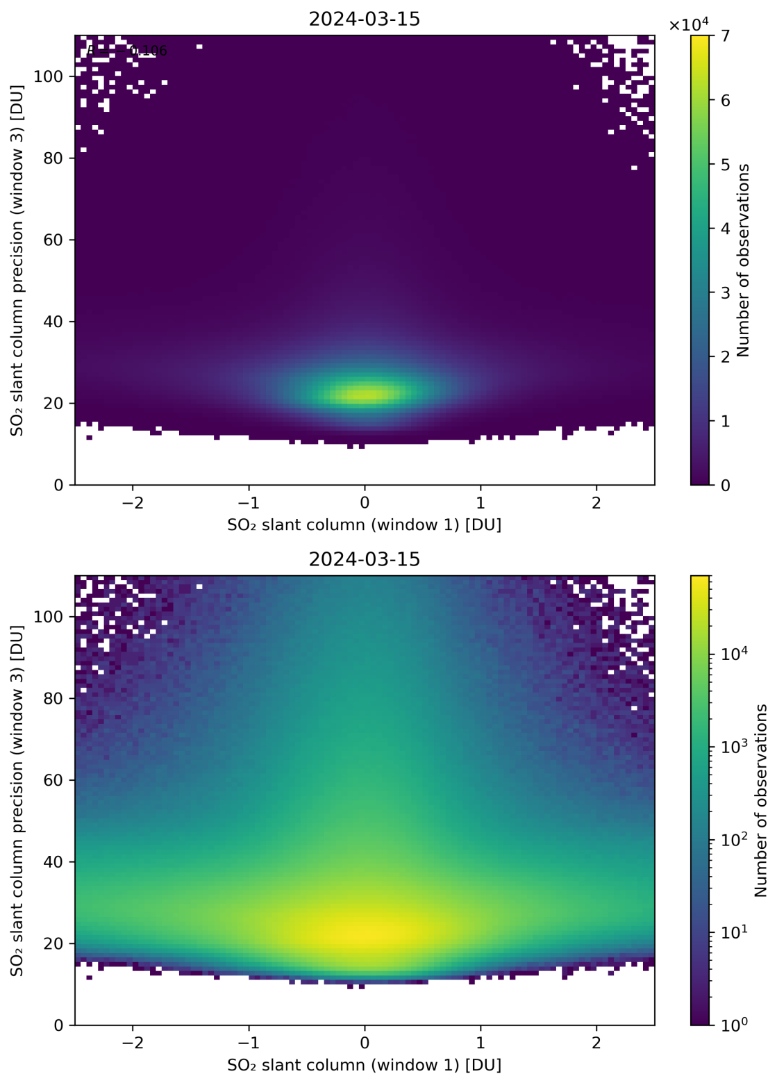
Figure 238: Scatter density plot of “SO 2 slant column (window 1)” against “SO 2 slant column precision (window 3)” for 2024-03-14 to 2024-03-16.
