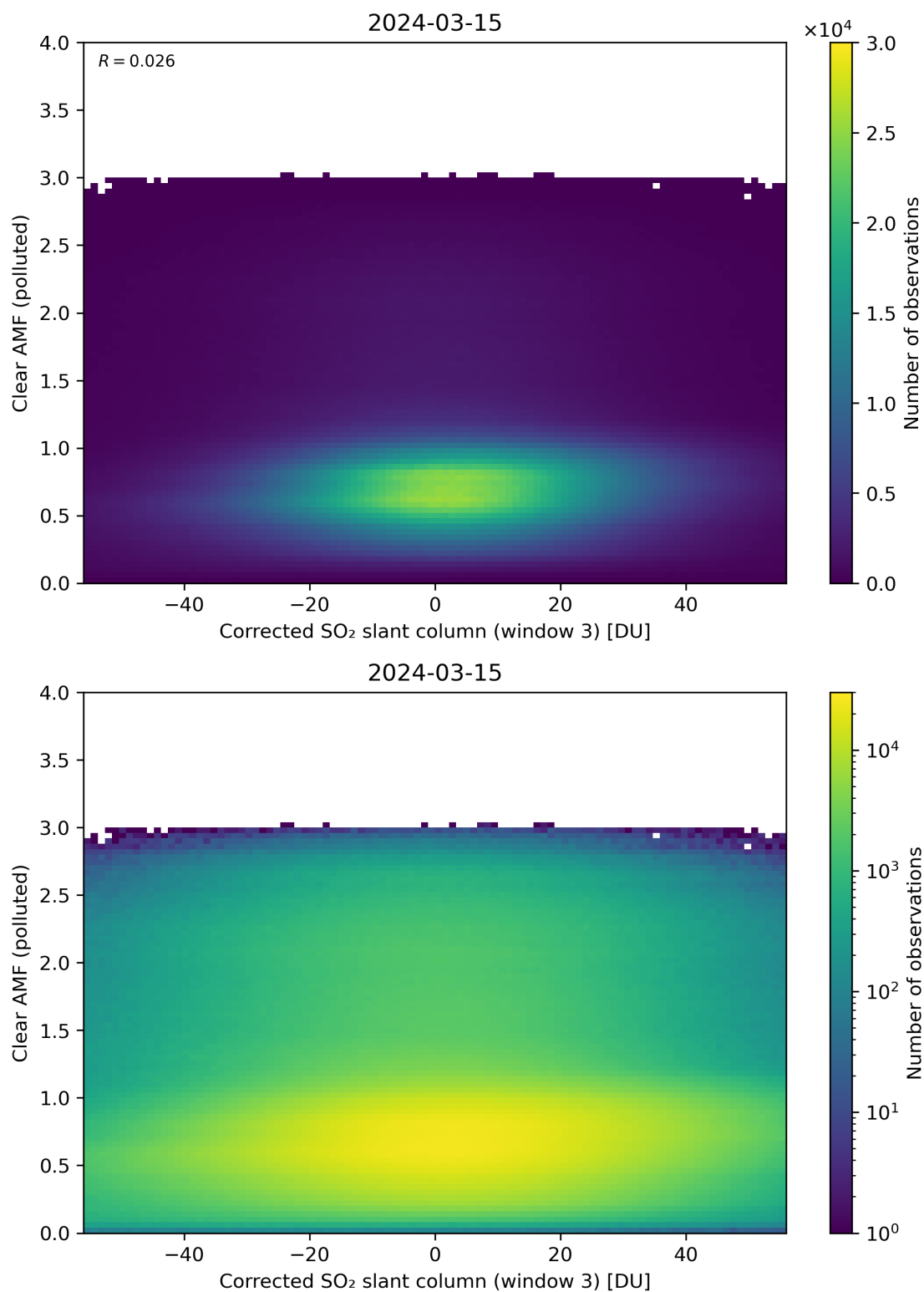
Figure 209: Scatter density plot of “Corrected SO 2 slant column (window 3)” against “Clear AMF (polluted)” for 2024-03-14 to 2024-03-16.
