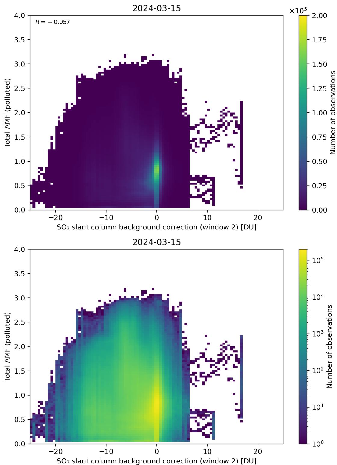
Figure 119: Scatter density plot of “SO 2 slant column background correction (window 2)” against “Total AMF (polluted)” for 2024-03-14 to 2024-03-16.
