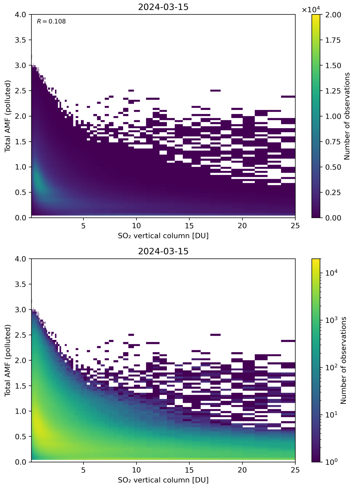
Figure 305: Scatter density plot of “SO 2 vertical column” against “Total AMF (polluted)” for 2024-03-14 to 2024-03-16.
