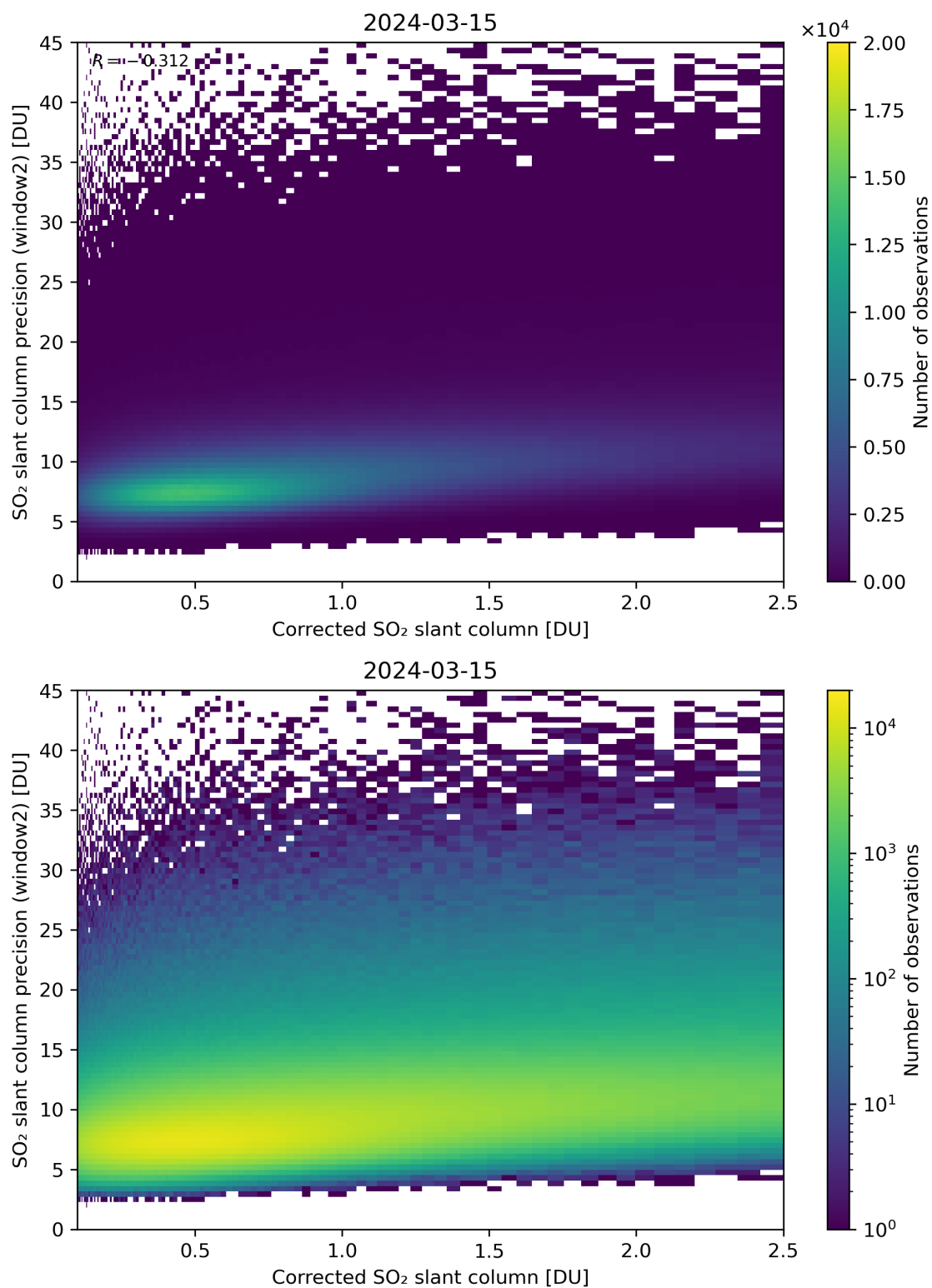
Figure 189: Scatter density plot of “Corrected SO 2 slant column” against “SO 2 slant column precision (window2)” for 2024-03-14 to 2024-03-16.
