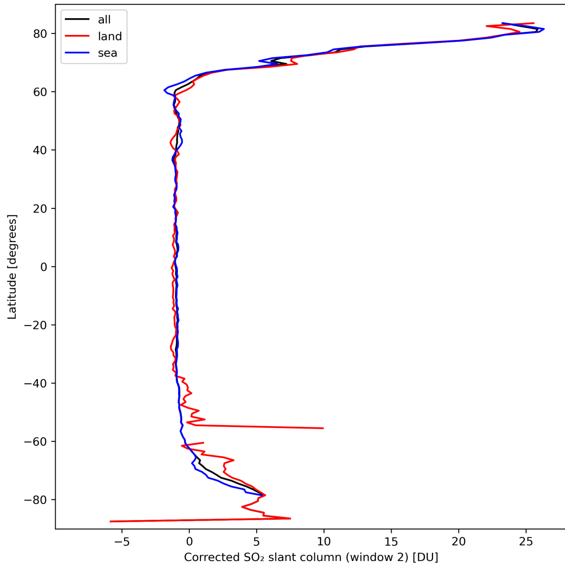
Figure 39: Zonal average of “Corrected SO 2 slant column (window 2)” for 2024-03-14 to 2024-03-16.
