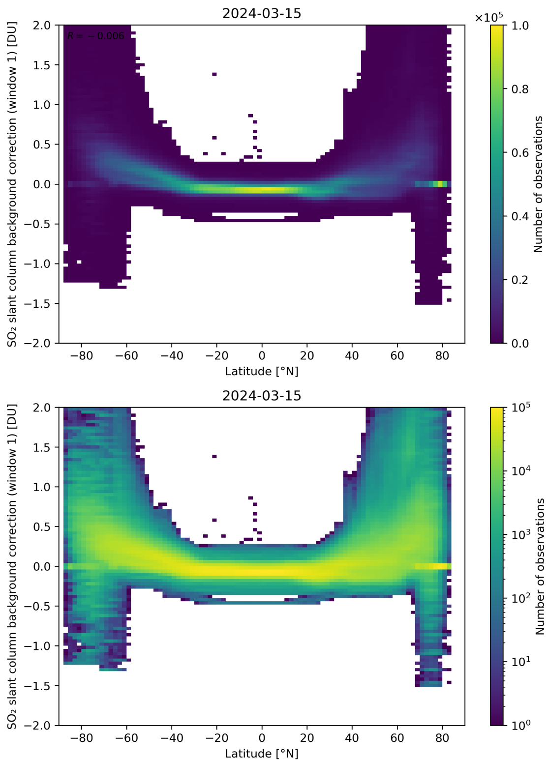
Figure 139: Scatter density plot of “Latitude” against “SO 2 slant column background correction (window 1)” for 2024-03-14 to 2024-03-16.
