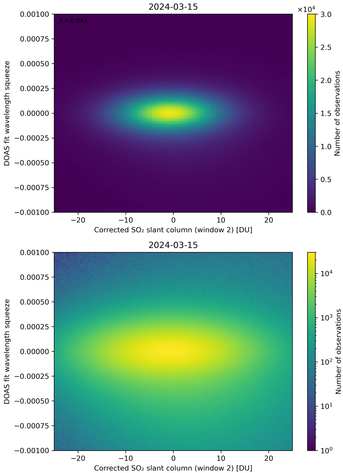
Figure 197: Scatter density plot of “Corrected SO 2 slant column (window 2)” against “DOAS fit wavelength squeeze” for 2024-03-14 to 2024-03-16.
