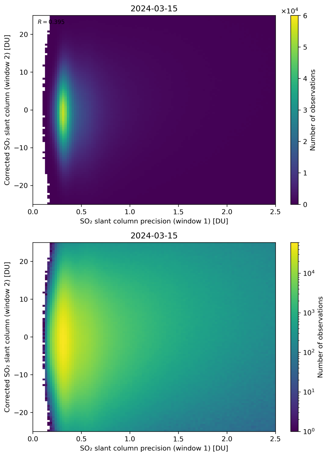
Figure 225: Scatter density plot of “SO 2 slant column precision (window 1)” against “Corrected SO 2 slant column (window 2)” for 2024-03-14 to 2024-03-16.
