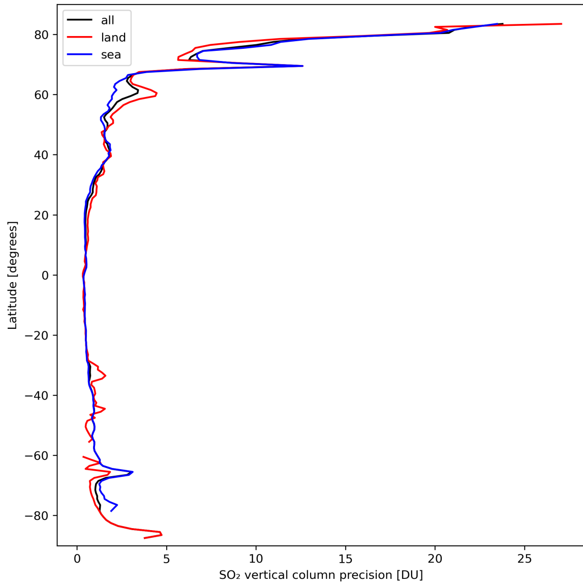
Figure 31: Zonal average of “SO 2 vertical column precision” for 2024-03-14 to 2024-03-16.
