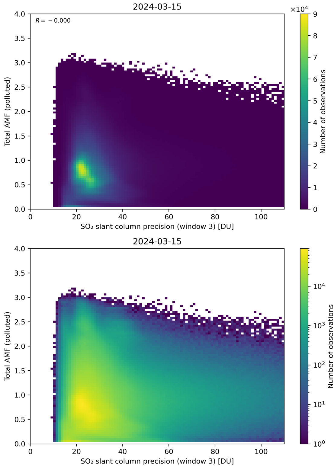
Figure 263: Scatter density plot of “SO 2 slant column precision (window 3)” against “Total AMF (polluted)” for 2024-03-14 to 2024-03-16.
