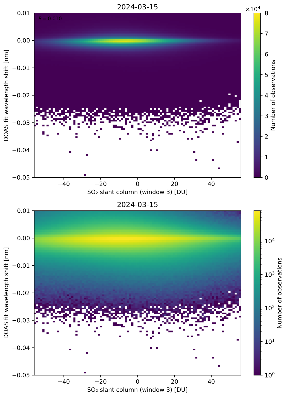
Figure 254: Scatter density plot of “SO 2 slant column (window 3)” against “DOAS fit wavelength shift” for 2024-03-14 to 2024-03-16.
