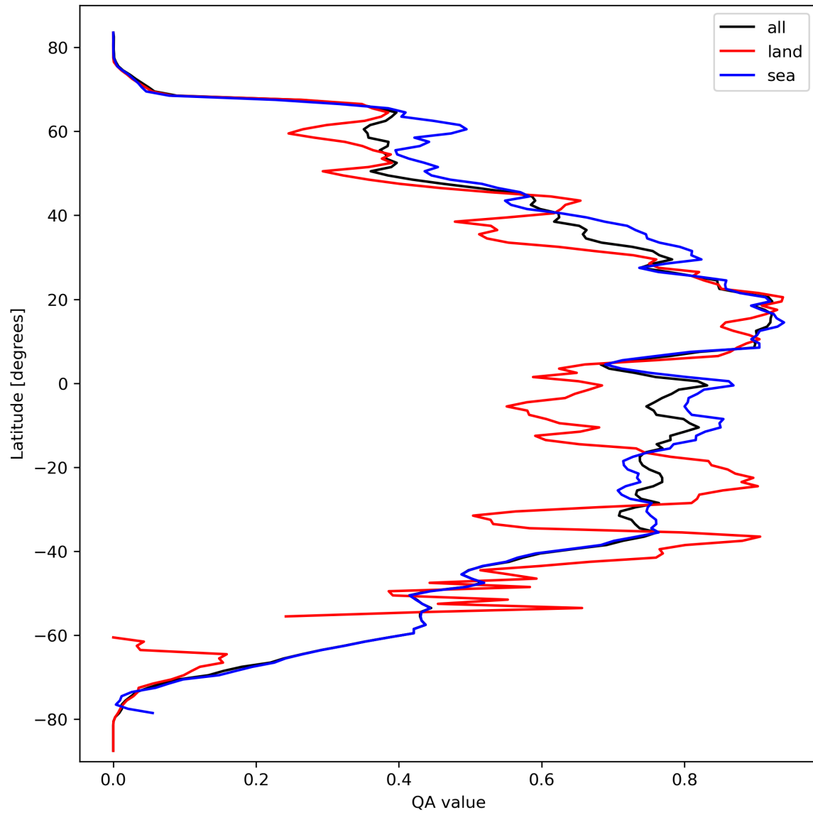
Figure 29: Zonal average of “QA value” for 2024-03-14 to 2024-03-16.
