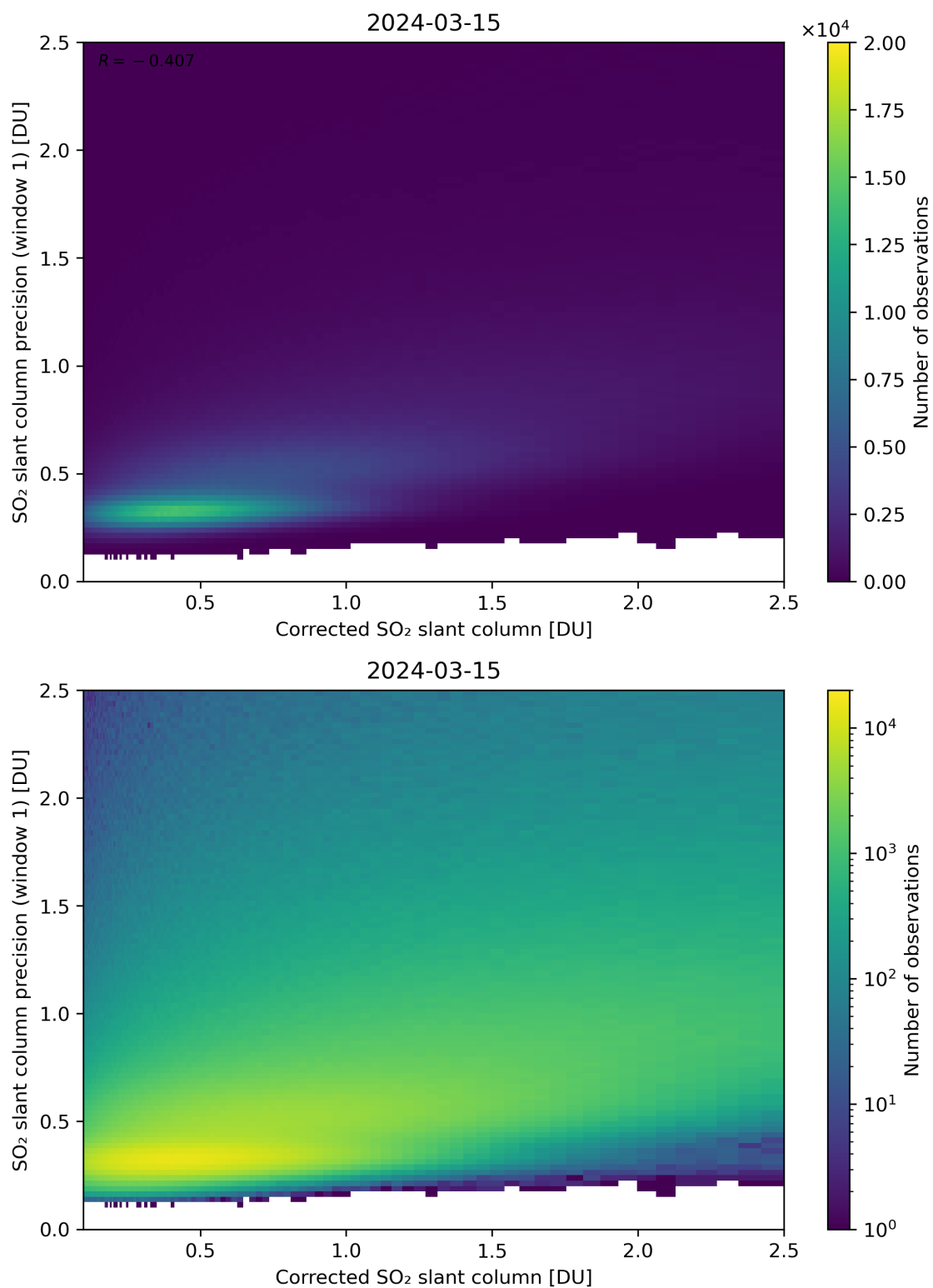
Figure 188: Scatter density plot of “Corrected SO 2 slant column” against “SO 2 slant column precision (window 1)” for 2024-03-14 to 2024-03-16.
