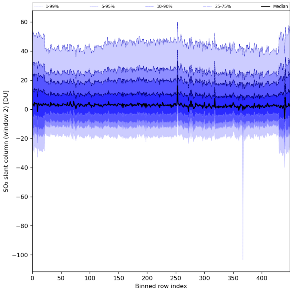
Figure 83: Along track statistics of “SO 2 slant column (window 2)” for 2024-03-14 to 2024-03-16
