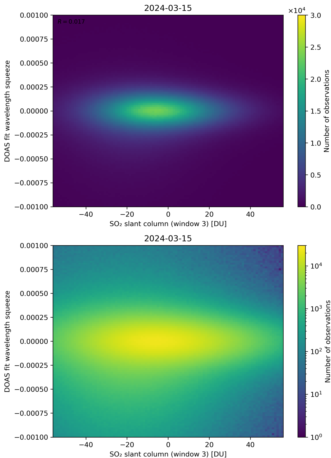
Figure 255: Scatter density plot of “SO 2 slant column (window 3)” against “DOAS fit wavelength squeeze” for 2024-03-14 to 2024-03-16.
