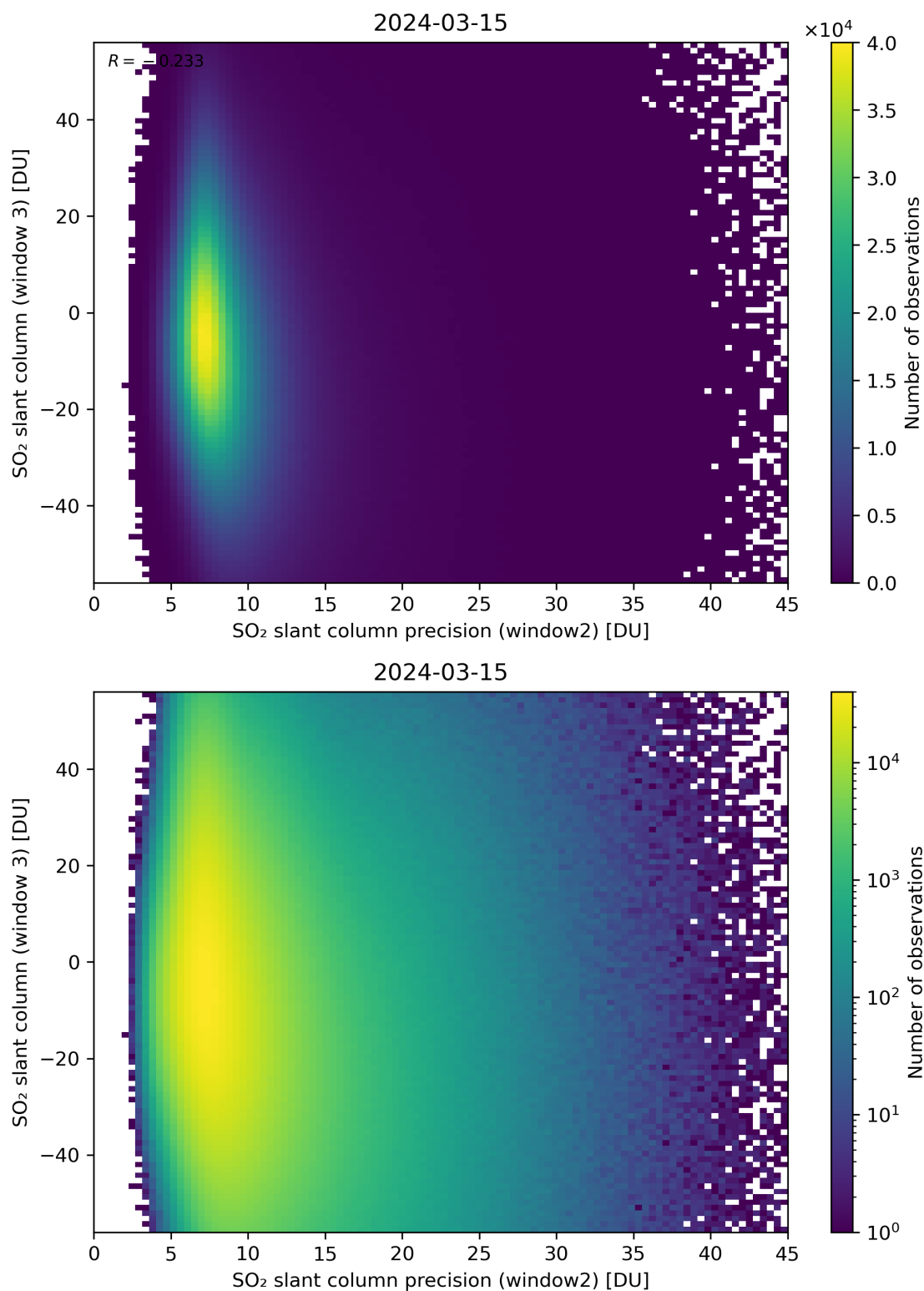
Figure 249: Scatter density plot of “SO 2 slant column precision (window2)” against “SO 2 slant column (window 3)” for 2024-03-14 to 2024-03-16.
