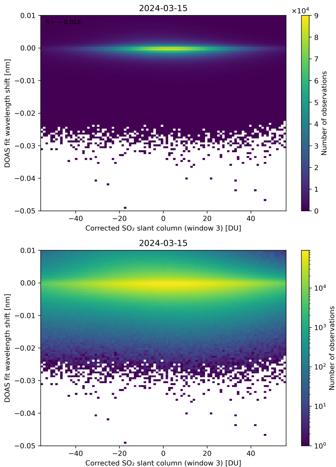
Figure 206: Scatter density plot of “Corrected SO 2 slant column (window 3)” against “DOAS fit wavelength shift” for 2024-03-14 to 2024-03-16.
