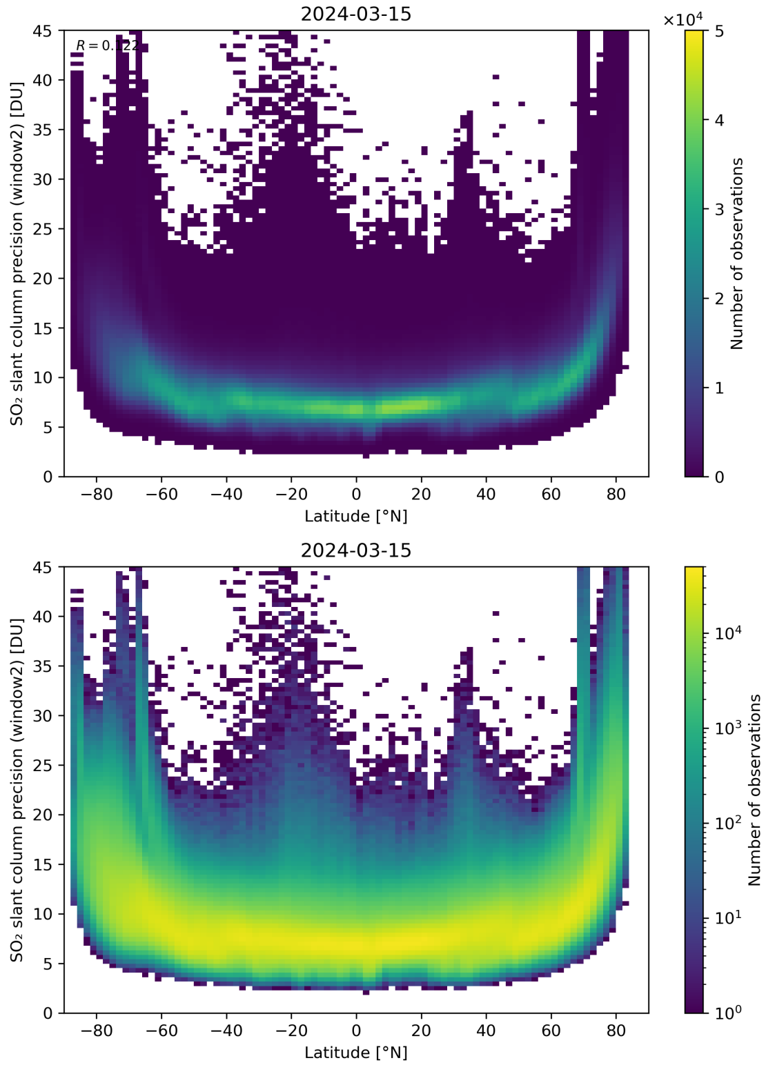
Figure 151: Scatter density plot of “Latitude” against “SO 2 slant column precision (window2)” for 2024-03-14 to 2024-03-16.
