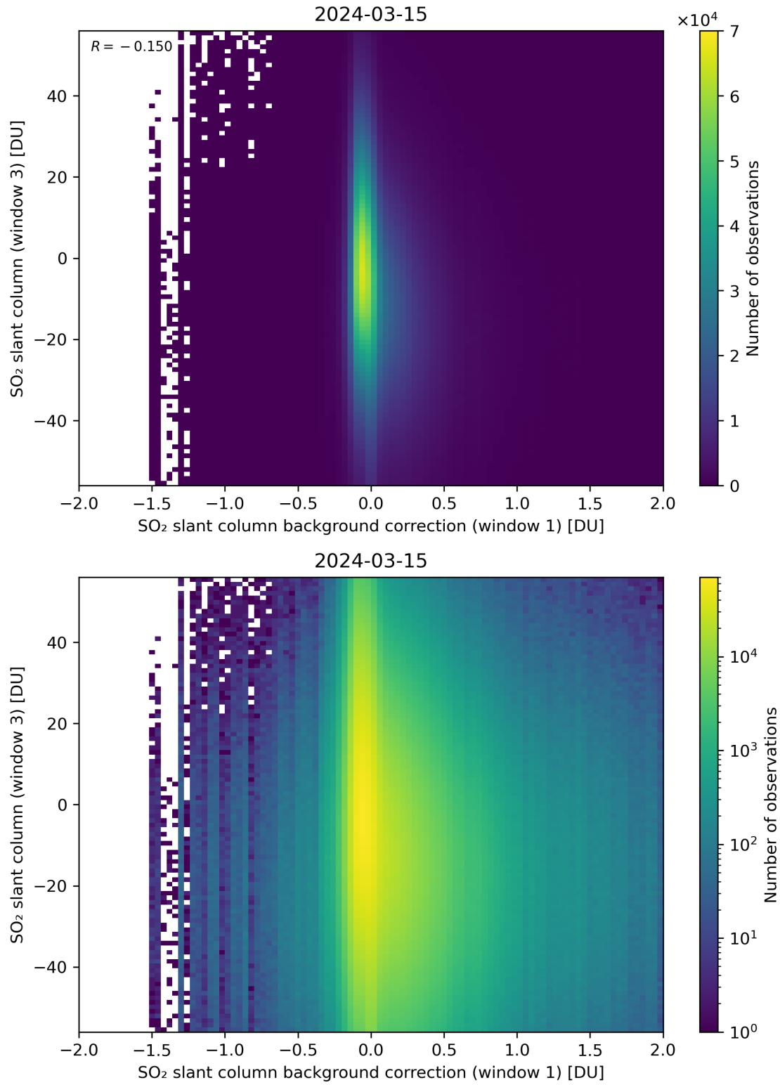
Figure 107: Scatter density plot of “SO 2 slant column background correction (window 1)” against “SO 2 slant column (window 3)” for 2024-03-14 to 2024-03-16.
