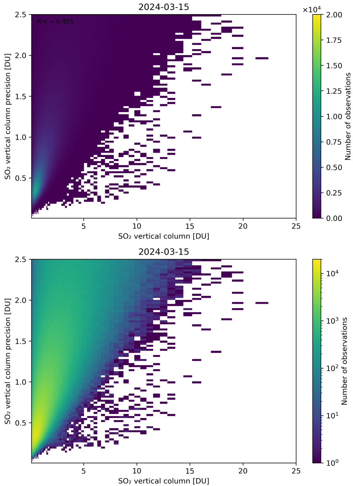
Figure 307: Scatter density plot of “SO 2 vertical column” against “SO 2 vertical column precision” for 2024-03-14 to 2024-03-16.
