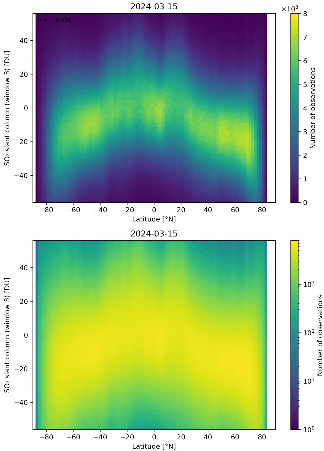
Figure 152: Scatter density plot of “Latitude” against “SO 2 slant column (window 3)” for 2024-03-14 to 2024-03-16.
