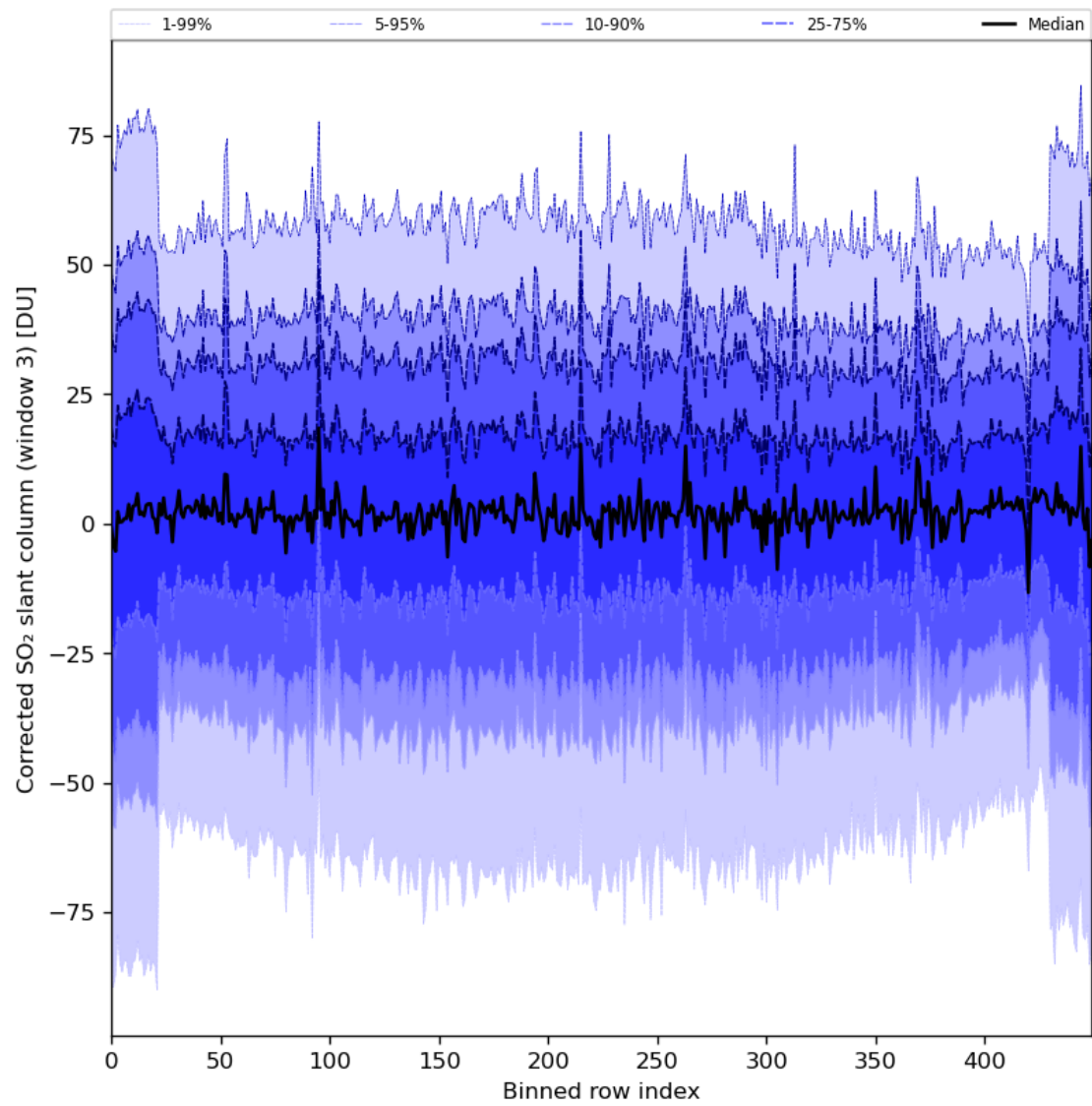
Figure 89: Along track statistics of “Corrected SO 2 slant column (window 3)” for 2024-03-14 to 2024-03-16
