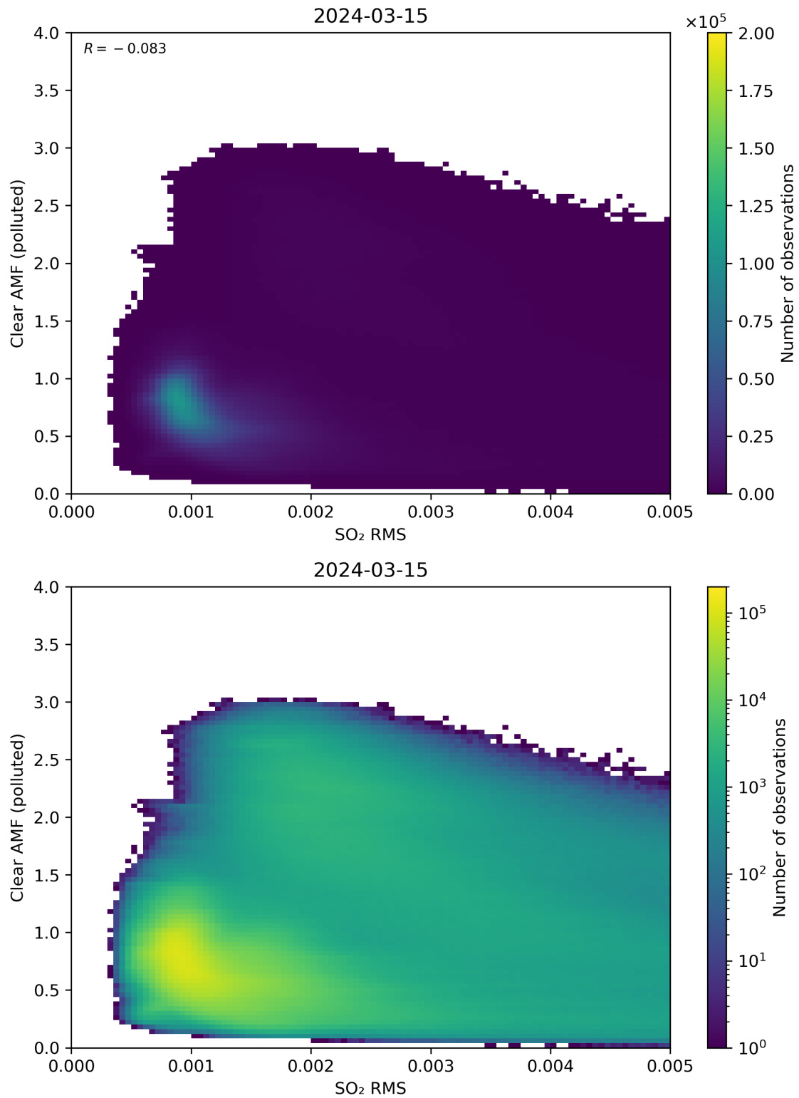
Figure 136: Scatter density plot of “SO 2 RMS” against “Clear AMF (polluted)” for 2024-03-14 to 2024-03-16.
