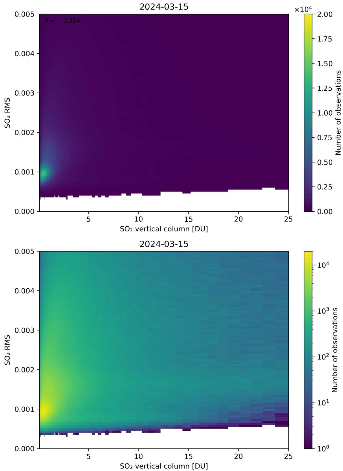
Figure 278: Scatter density plot of “SO 2 vertical column” against “SO 2 RMS” for 2024-03-14 to 2024-03-16.
