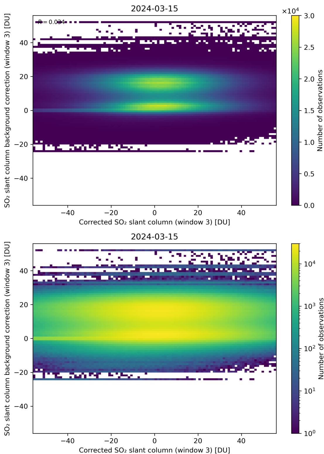
Figure 205: Scatter density plot of “Corrected SO 2 slant column (window 3)” against “SO 2 slant column background correction (window 3)” for 2024-03-14 to 2024-03-16.
