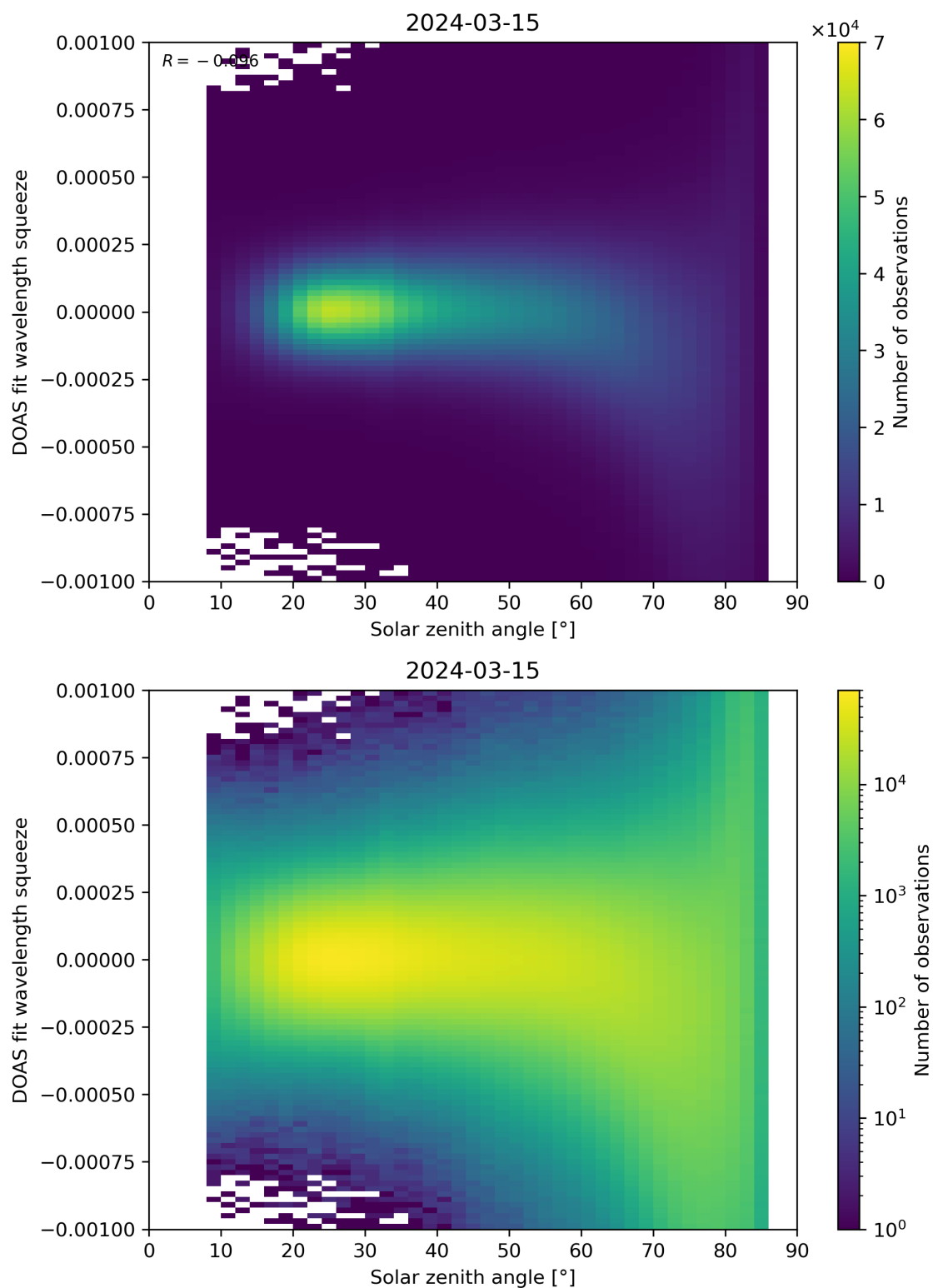
Figure 162: Scatter density plot of “Solar zenith angle” against “DOAS fit wavelength squeeze” for 2024-03-14 to 2024-03-16.
