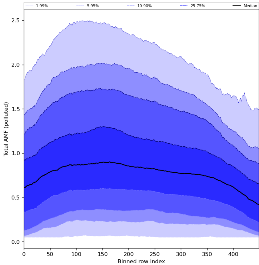
Figure 94: Along track statistics of “Total AMF (polluted)” for 2024-03-14 to 2024-03-16
