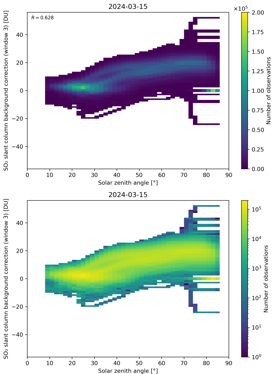
Figure 160: Scatter density plot of “Solar zenith angle” against “SO 2 slant column background correction (window 3)” for 2024-03-14 to 2024-03-16.
