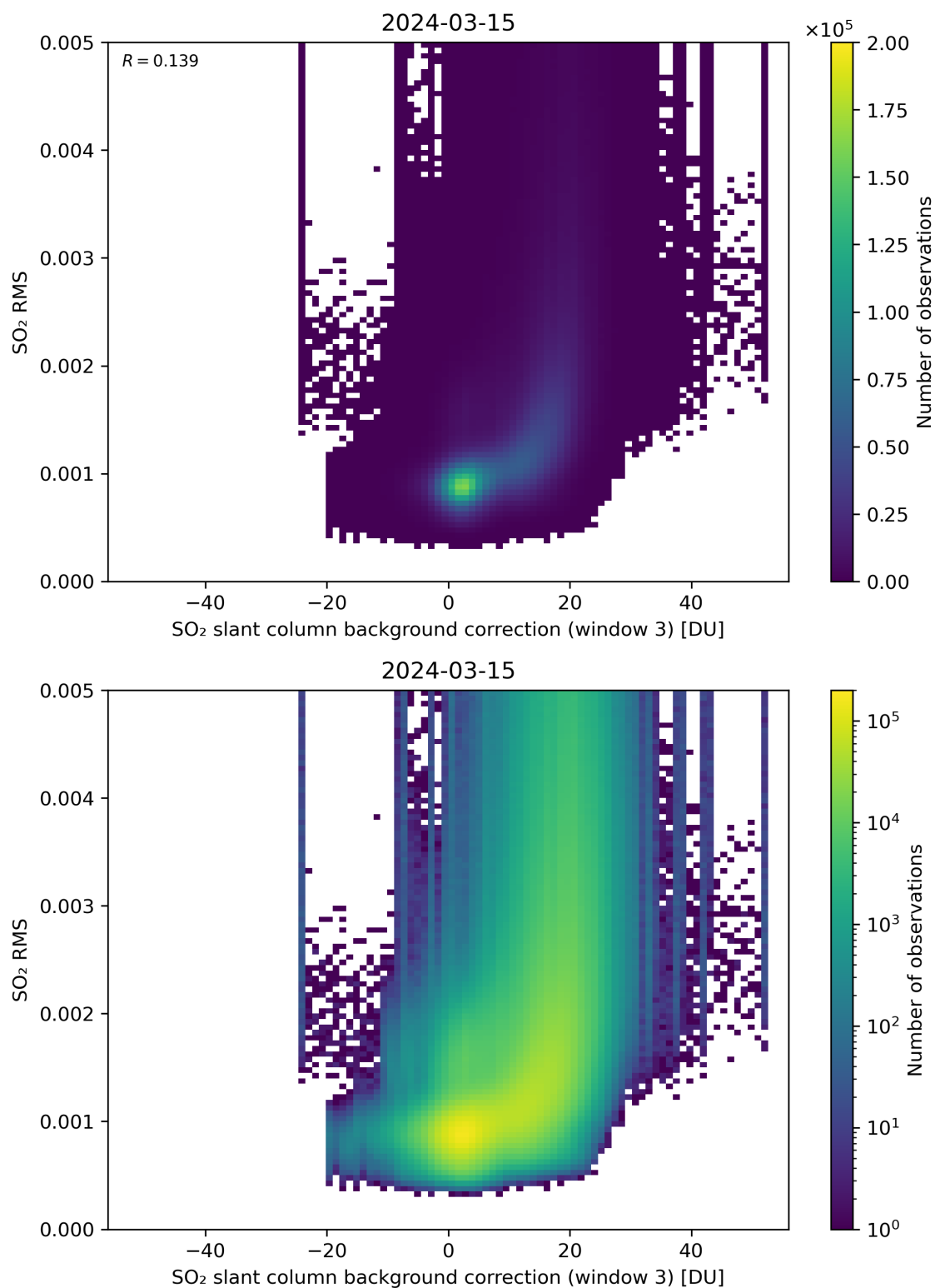
Figure 123: Scatter density plot of “SO 2 slant column background correction (window 3)” against “SO 2 RMS” for 2024-03-14 to 2024-03-16.
