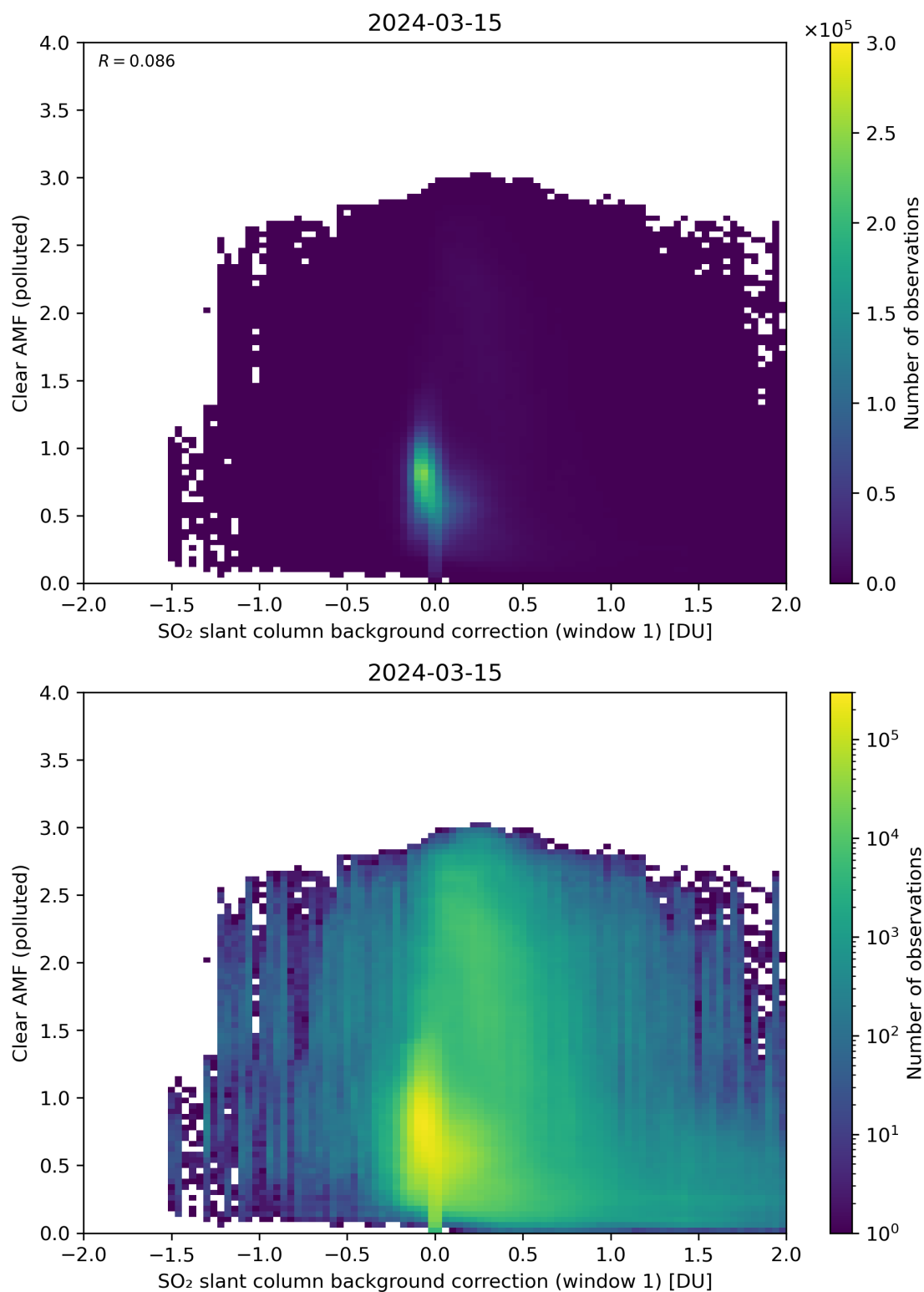
Figure 103: Scatter density plot of “SO 2 slant column background correction (window 1)” against “Clear AMF (polluted)” for 2024-03-14 to 2024-03-16.
