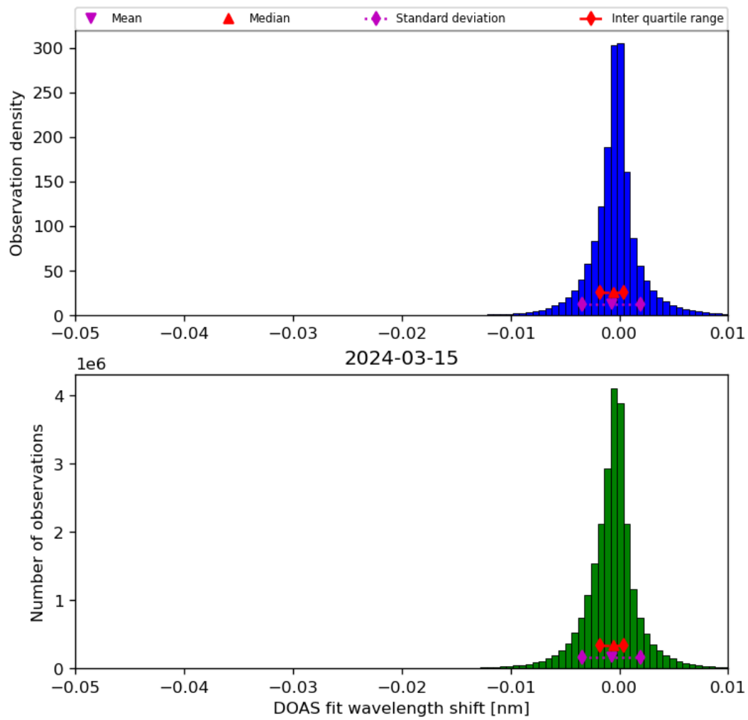
Figure 68: Histogram of “DOAS fit wavelength shift” for 2024-03-14 to 2024-03-16
