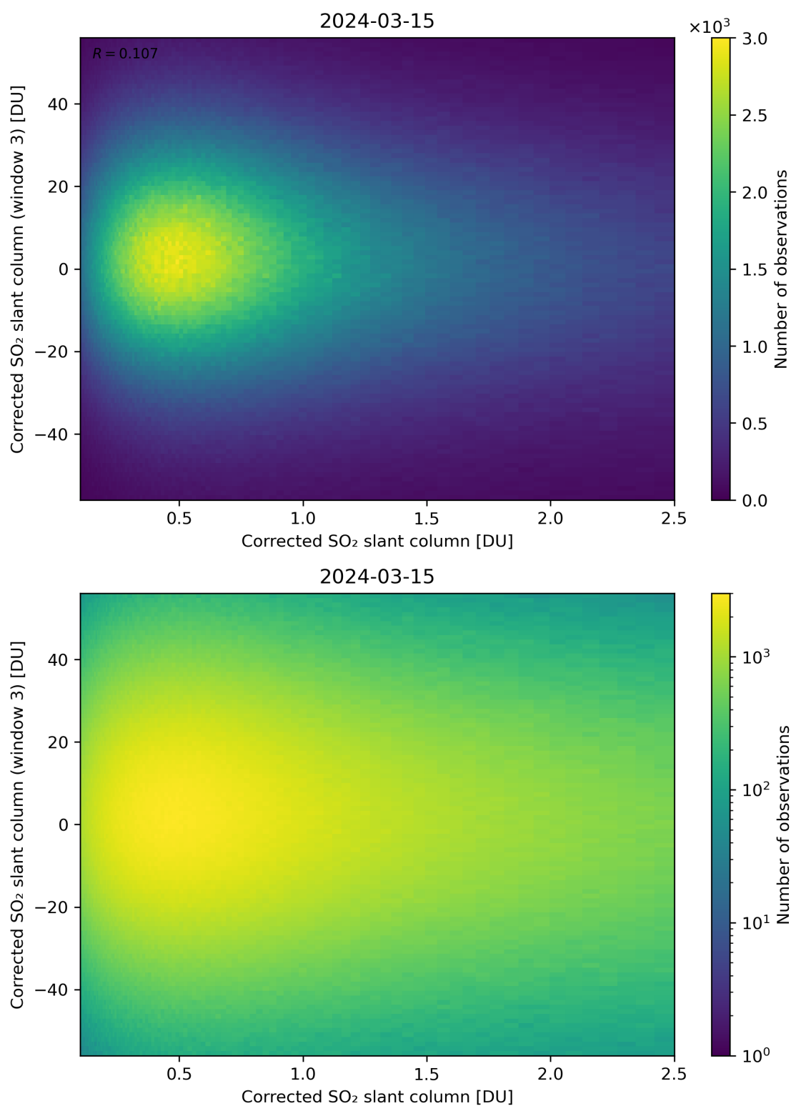
Figure 186: Scatter density plot of “Corrected SO 2 slant column” against “Corrected SO 2 slant column (window 3)” for 2024-03-14 to 2024-03-16.
