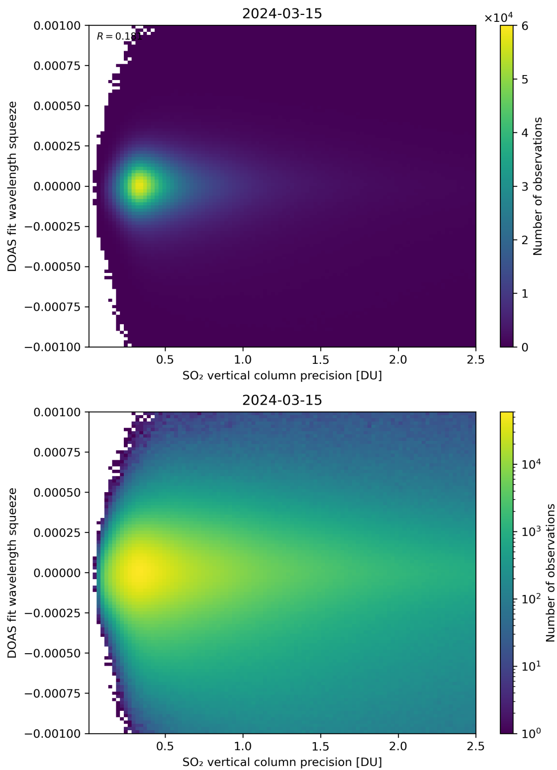
Figure 283: Scatter density plot of “SO 2 vertical column precision” against “DOAS fit wavelength squeeze” for 2024-03-14 to 2024-03-16.
