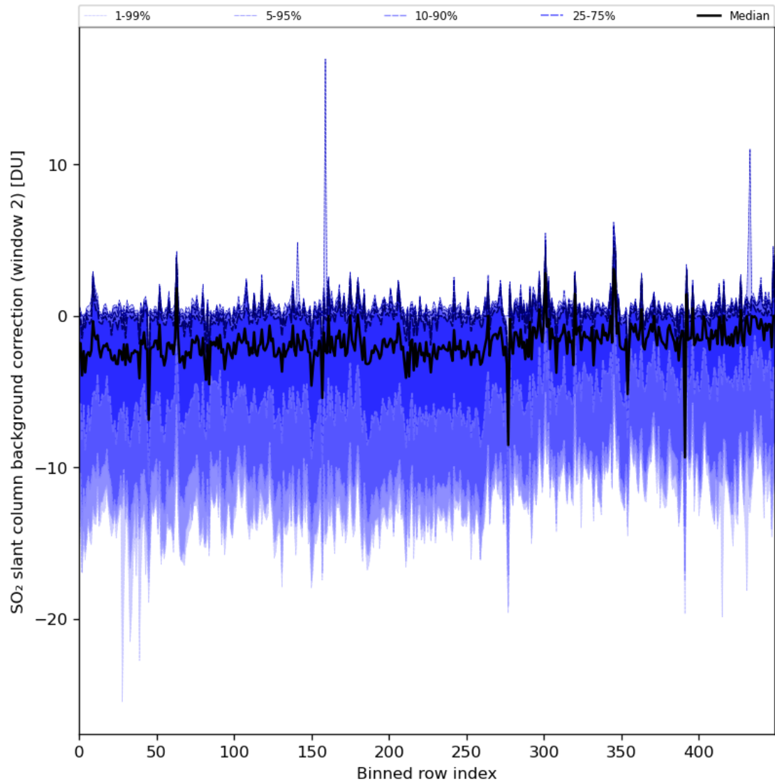
Figure 86: Along track statistics of “SO 2 slant column background correction (window 2)” for 2024-03-14 to 2024-03-16
