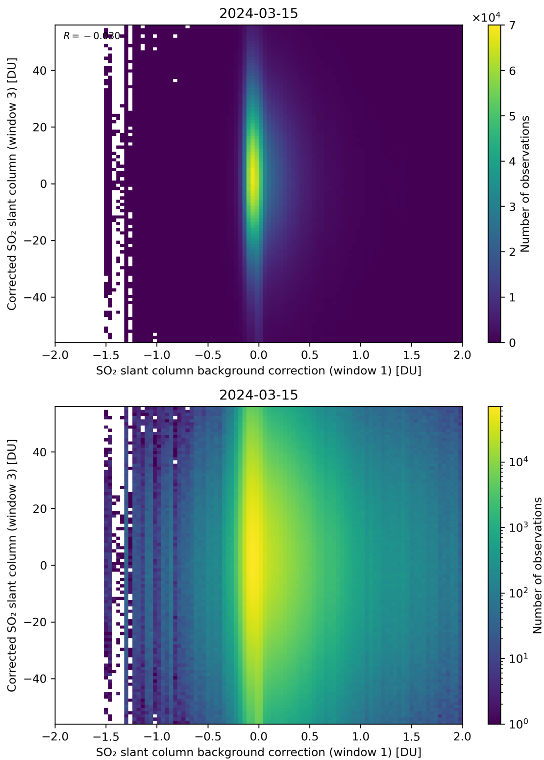
Figure 105: Scatter density plot of “SO 2 slant column background correction (window 1)” against “Corrected SO 2 slant column (window 3)” for 2024-03-14 to 2024-03-16.
