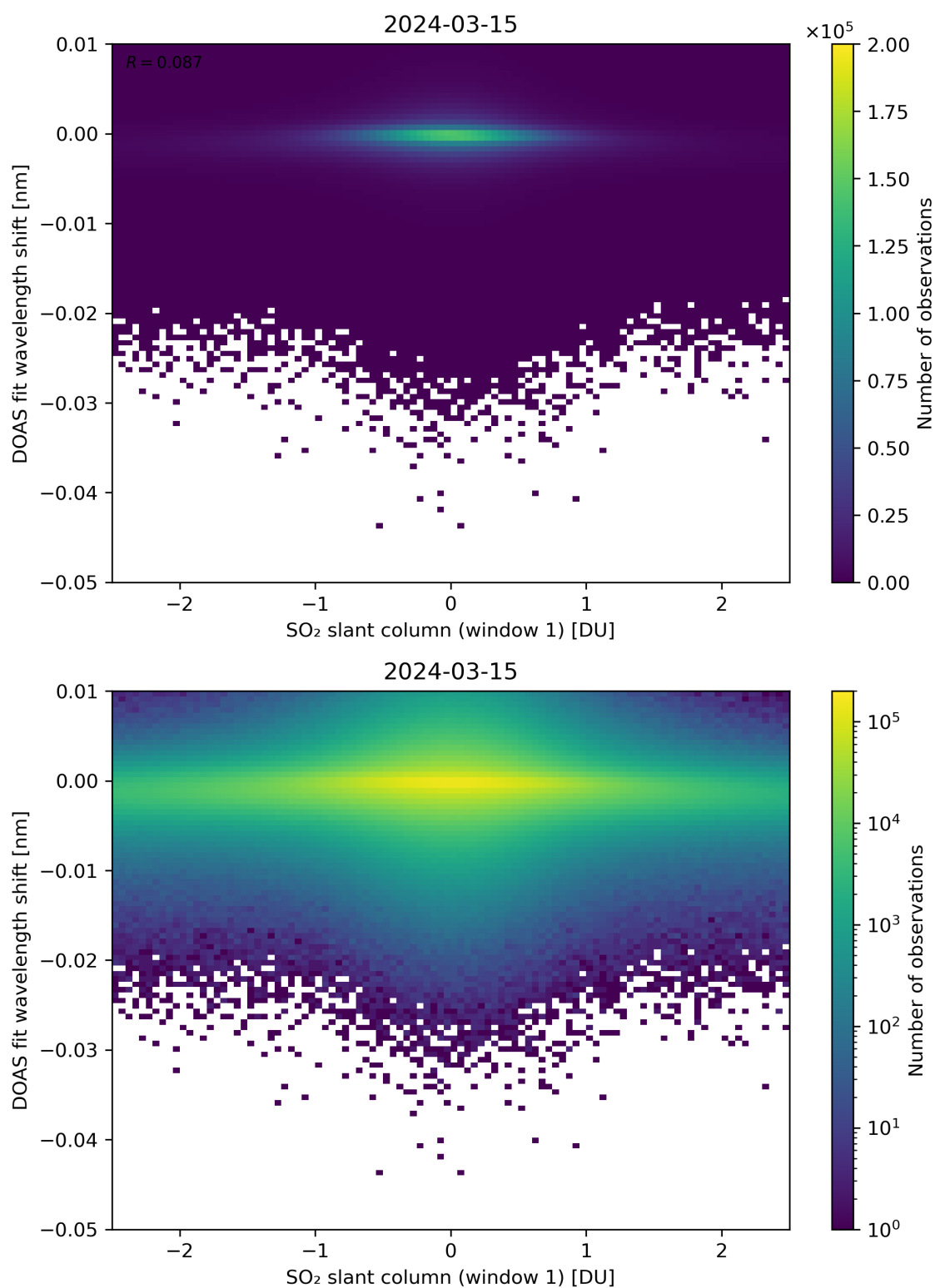
Figure 215: Scatter density plot of “SO 2 slant column (window 1)” against “DOAS fit wavelength shift” for 2024-03-14 to 2024-03-16.
