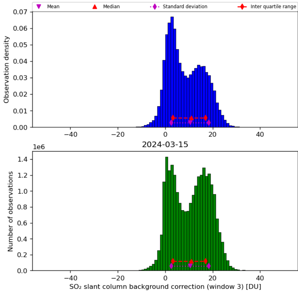
Figure 67: Histogram of “SO 2 slant column background correction (window 3)” for 2024-03-14 to 2024-03-16
