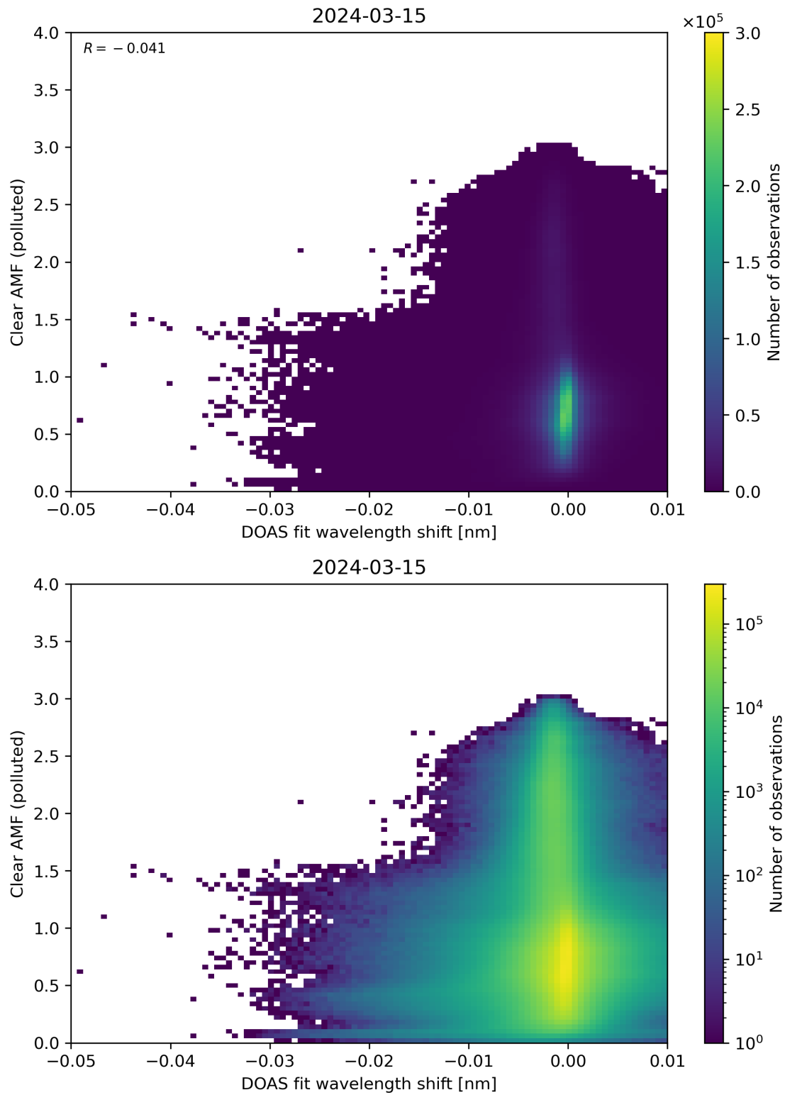
Figure 129: Scatter density plot of “DOAS fit wavelength shift” against “Clear AMF (polluted)” for 2024-03-14 to 2024-03-16.
