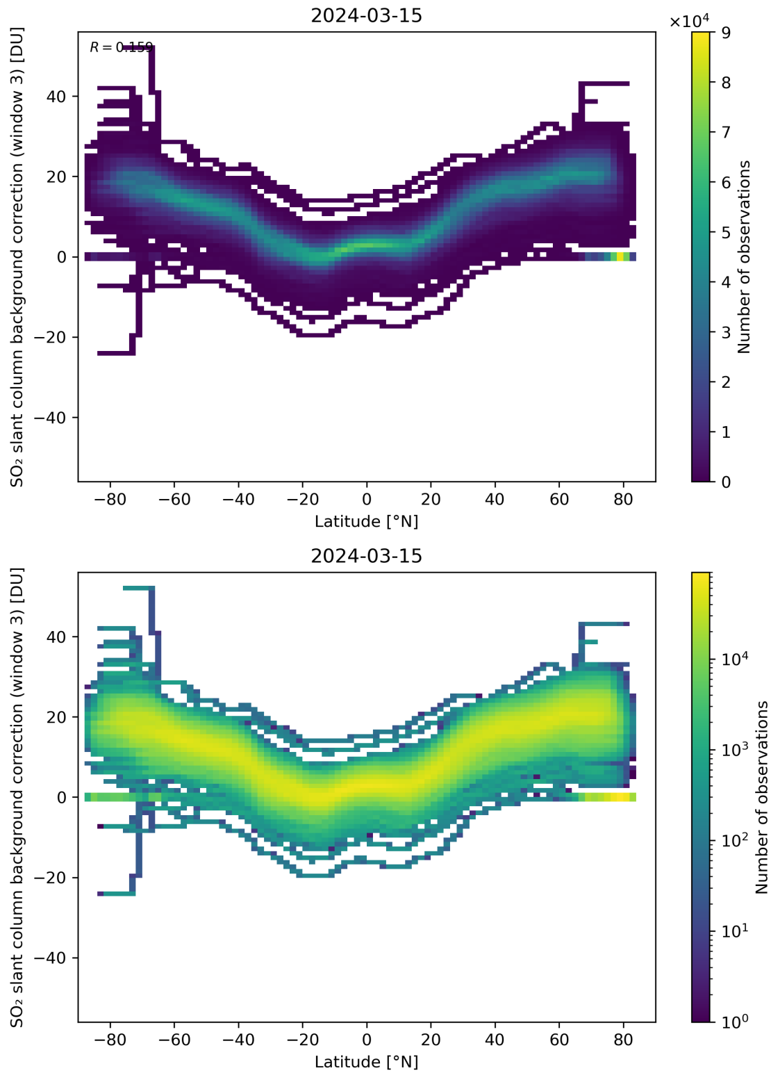
Figure 141: Scatter density plot of “Latitude” against “SO 2 slant column background correction (window 3)” for 2024-03-14 to 2024-03-16.
