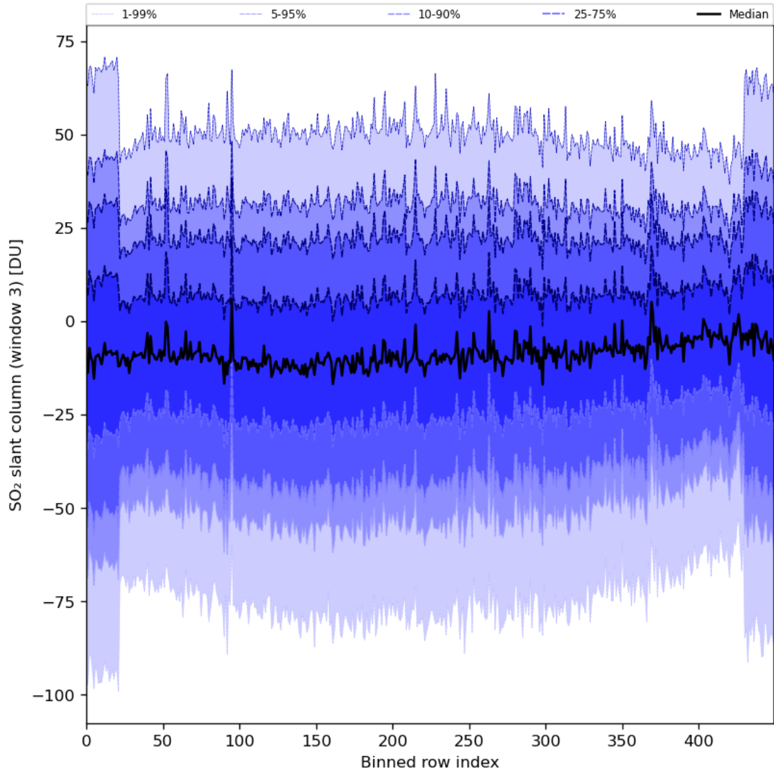
Figure 87: Along track statistics of “SO 2 slant column (window 3)” for 2024-03-14 to 2024-03-16
