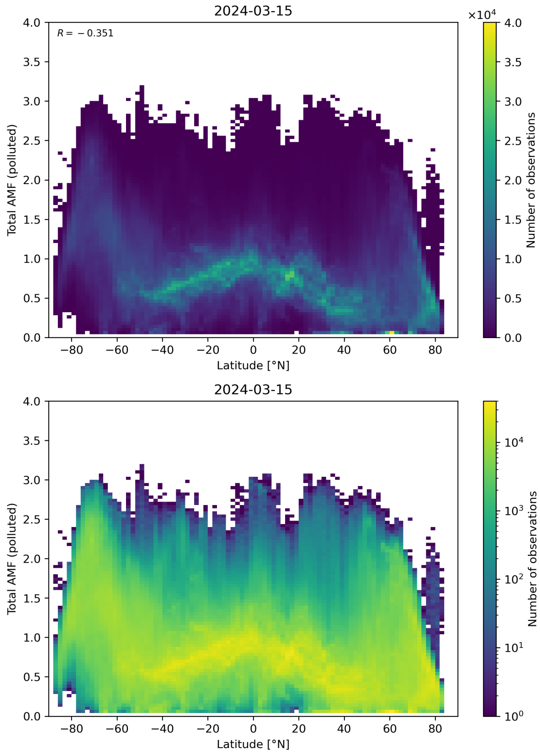
Figure 154: Scatter density plot of “Latitude” against “Total AMF (polluted)” for 2024-03-14 to 2024-03-16.
