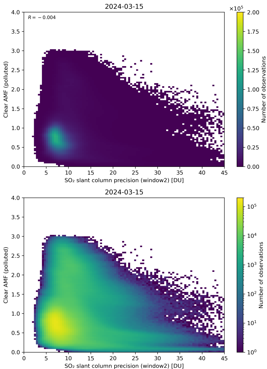
Figure 246: Scatter density plot of “SO 2 slant column precision (window2)” against “Clear AMF (polluted)” for 2024-03-14 to 2024-03-16.
