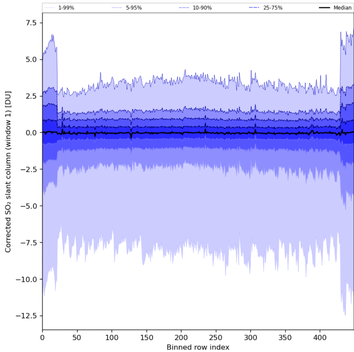
Figure 81: Along track statistics of “Corrected SO 2 slant column (window 1)” for 2024-03-14 to 2024-03-16
