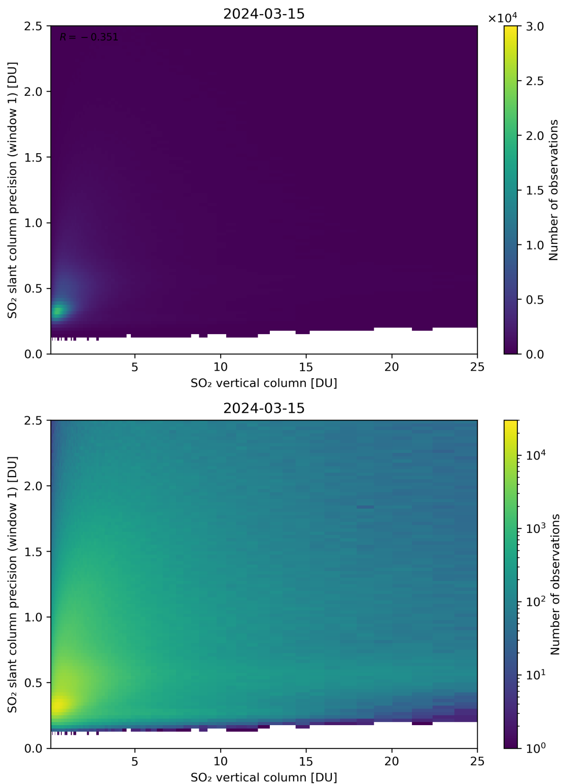
Figure 301: Scatter density plot of “SO 2 vertical column” against “SO 2 slant column precision (window 1)” for 2024-03-14 to 2024-03-16.
