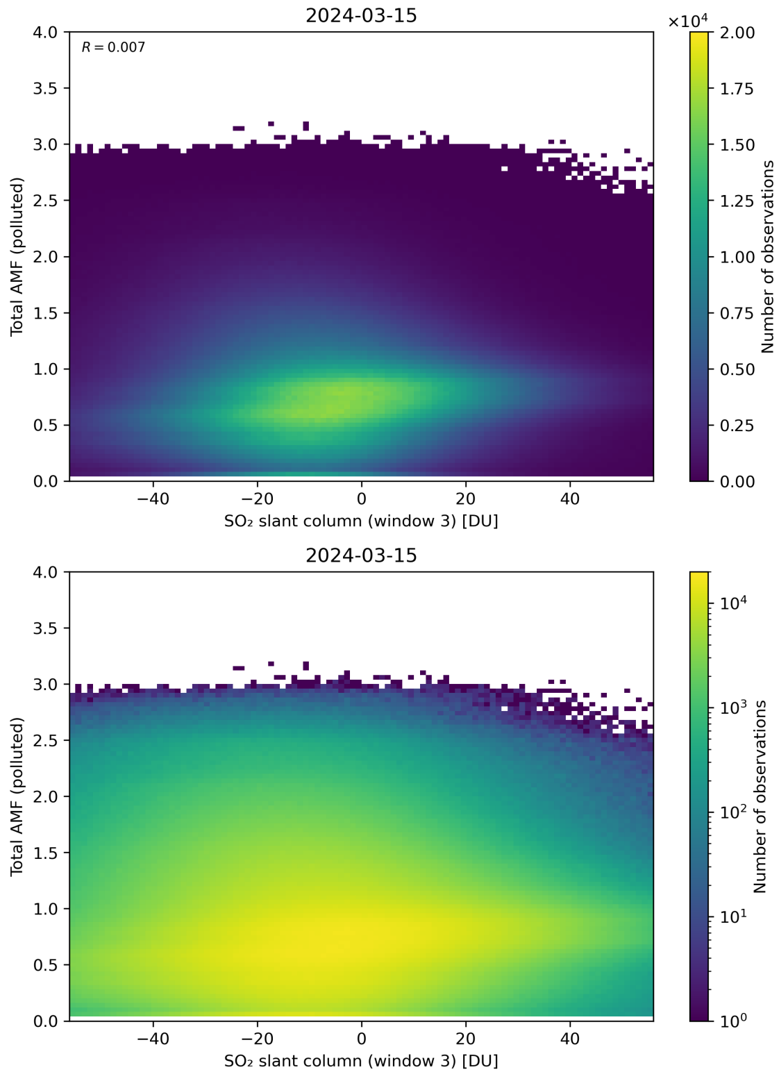
Figure 268: Scatter density plot of “SO 2 slant column (window 3)” against “Total AMF (polluted)” for 2024-03-14 to 2024-03-16.
