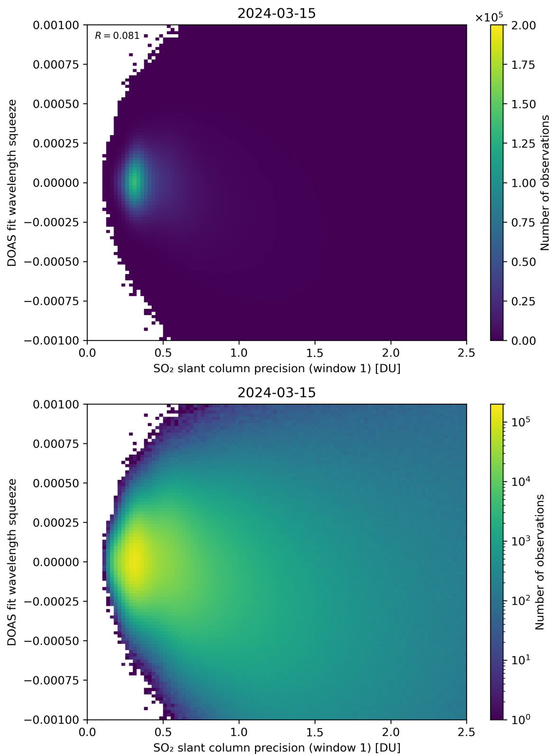
Figure 222: Scatter density plot of “SO 2 slant column precision (window 1)” against “DOAS fit wavelength squeeze” for 2024-03-14 to 2024-03-16.
