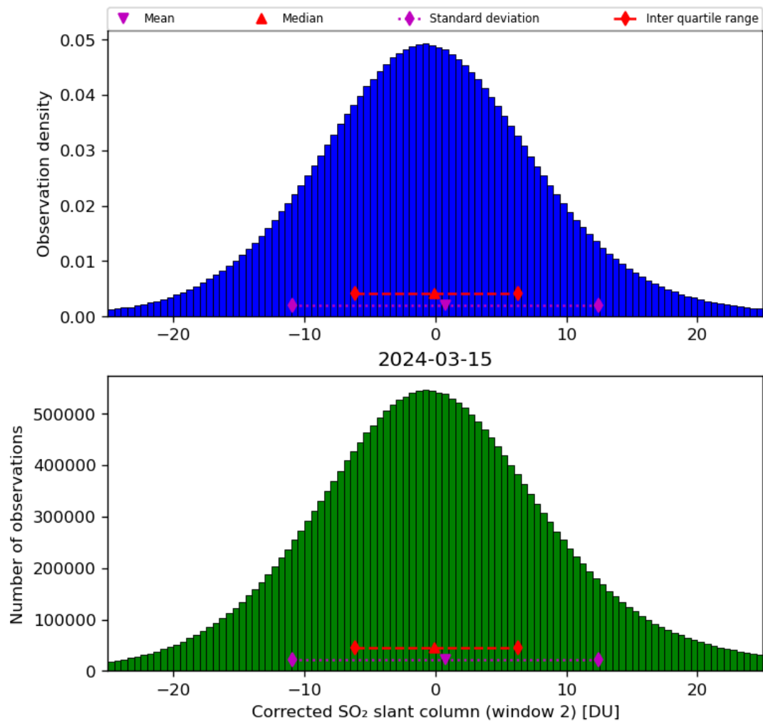
Figure 62: Histogram of “Corrected SO 2 slant column (window 2)” for 2024-03-14 to 2024-03-16
