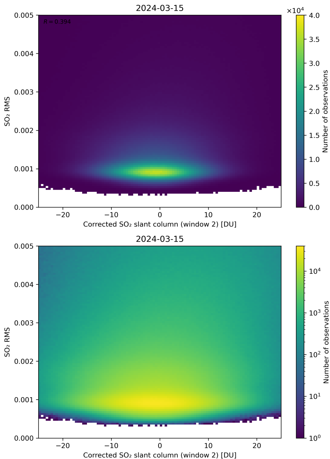
Figure 198: Scatter density plot of “Corrected SO 2 slant column (window 2)” against “SO 2 RMS” for 2024-03-14 to 2024-03-16.
