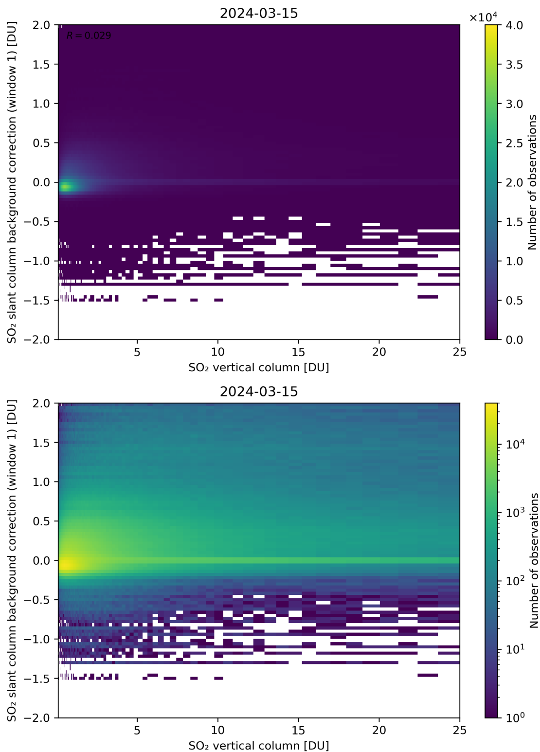
Figure 273: Scatter density plot of “SO 2 vertical column” against “SO 2 slant column background correction (window 1)” for 2024-03-14 to 2024-03-16.
