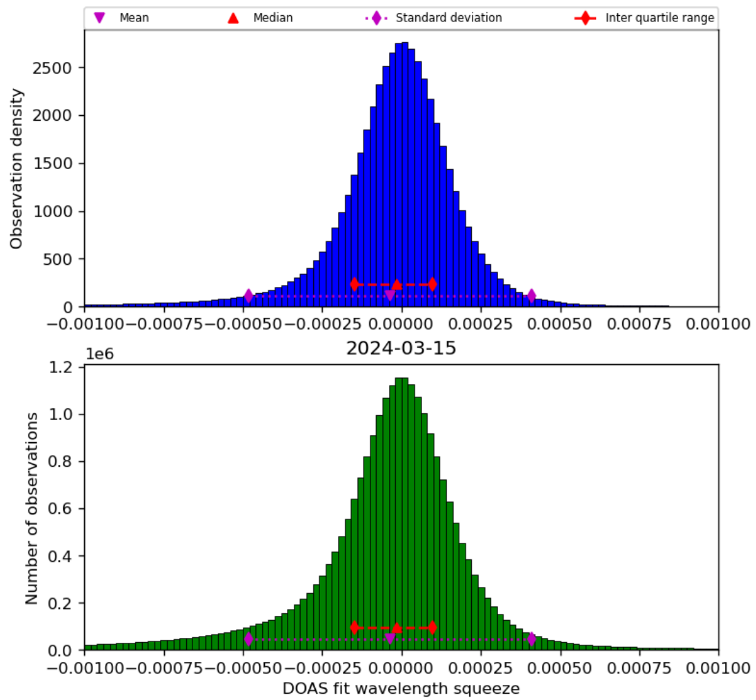
Figure 69: Histogram of “DOAS fit wavelength squeeze” for 2024-03-14 to 2024-03-16
