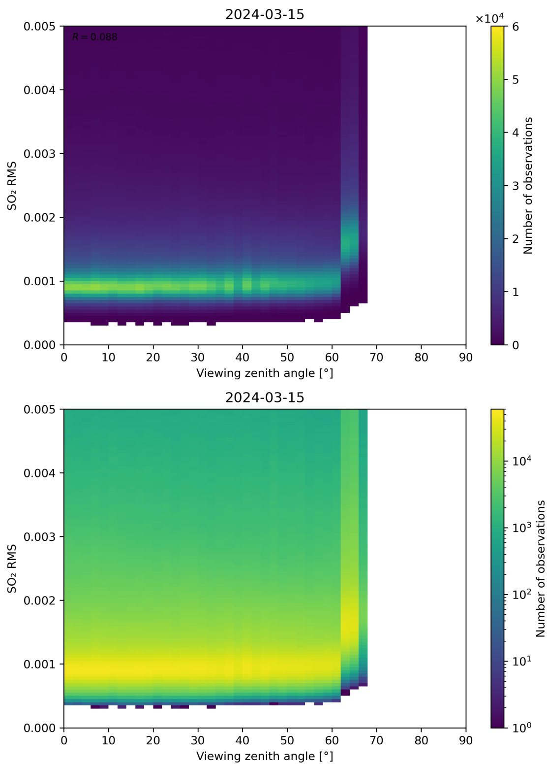
Figure 313: Scatter density plot of “Viewing zenith angle” against “SO 2 RMS” for 2024-03-14 to 2024-03-16.
