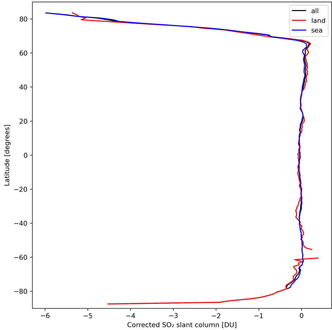
Figure 32: Zonal average of “Corrected SO 2 slant column” for 2024-03-14 to 2024-03-16.
