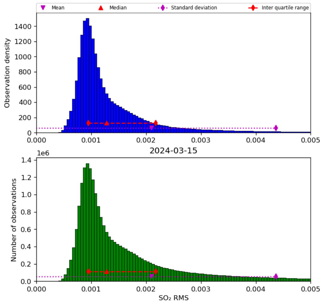
Figure 70: Histogram of “SO 2 RMS” for 2024-03-14 to 2024-03-16
