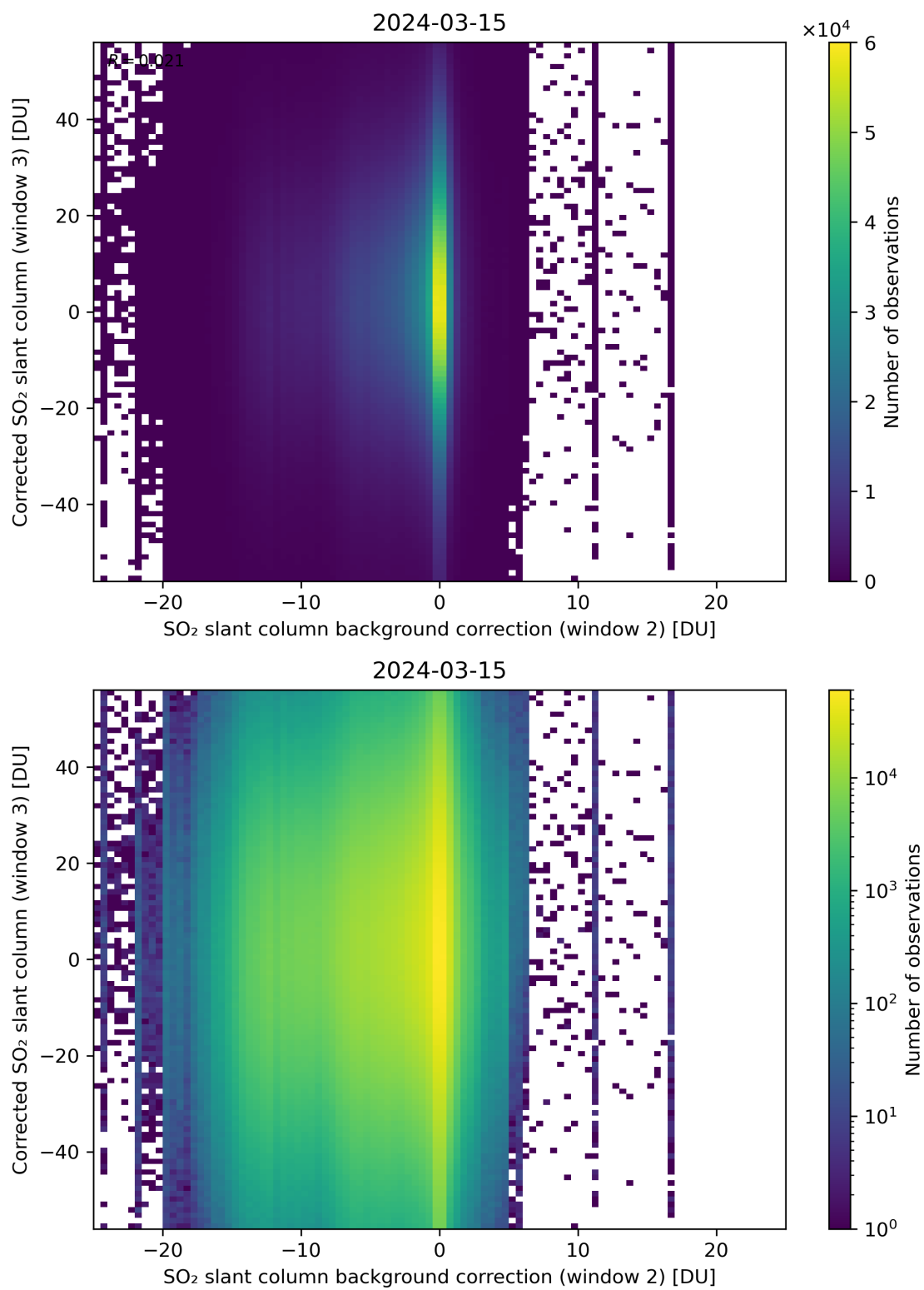
Figure 116: Scatter density plot of “SO 2 slant column background correction (window 2)” against “Corrected SO 2 slant column (window 3)” for 2024-03-14 to 2024-03-16.
