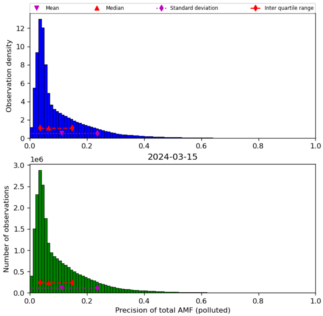
Figure 72: Histogram of “Precision of total AMF (polluted)” for 2024-03-14 to 2024-03-16
