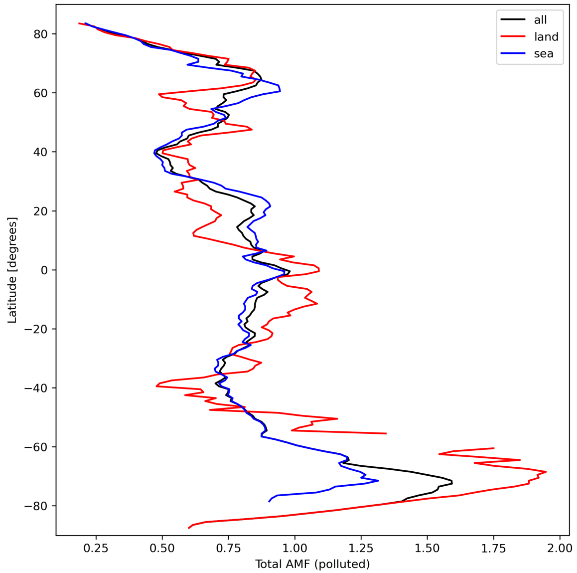
Figure 48: Zonal average of “Total AMF (polluted)” for 2024-03-14 to 2024-03-16.
