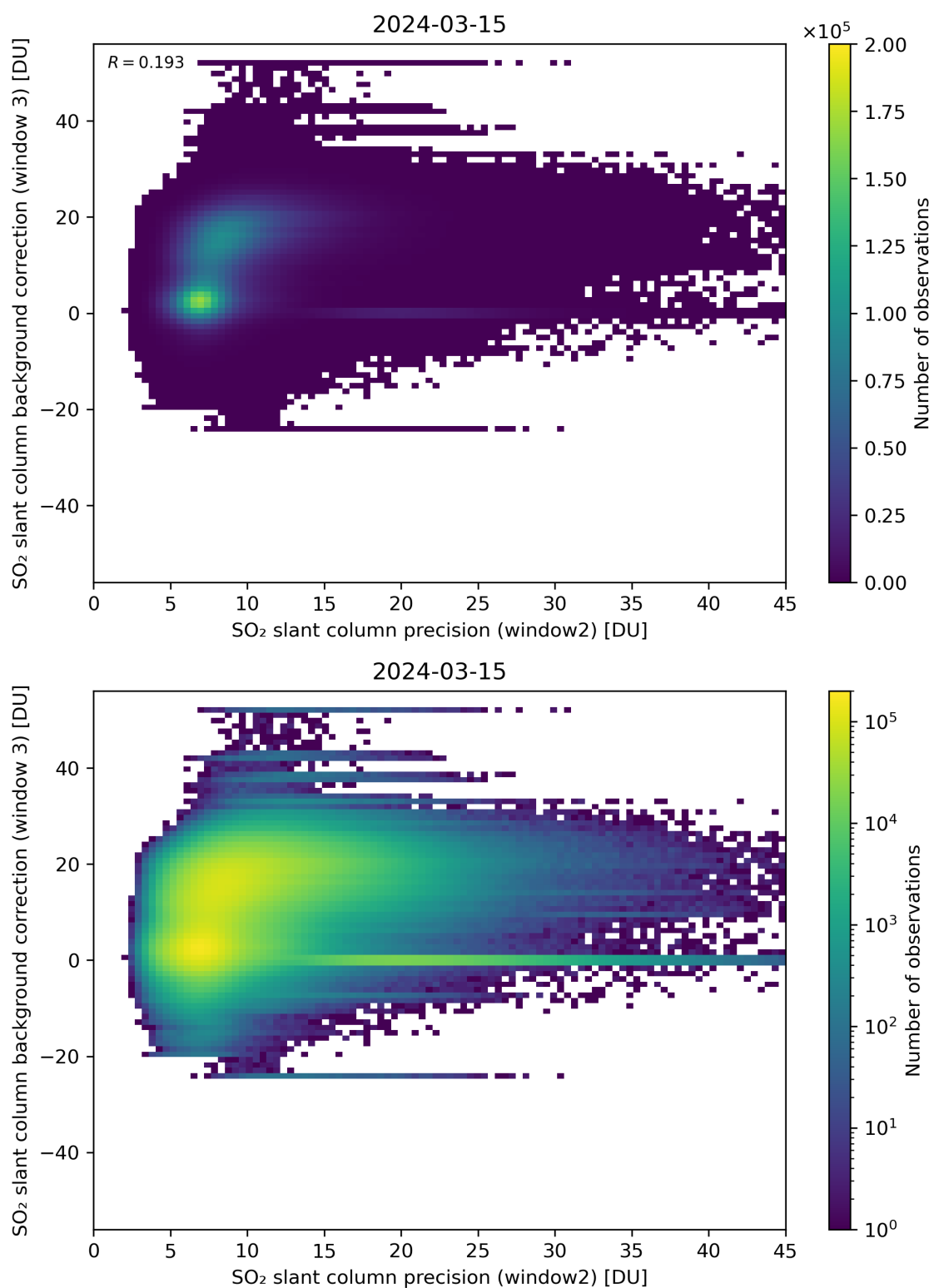
Figure 242: Scatter density plot of “SO 2 slant column precision (window2)” against “SO 2 slant column background correction (window 3)” for 2024-03-14 to 2024-03-16.
