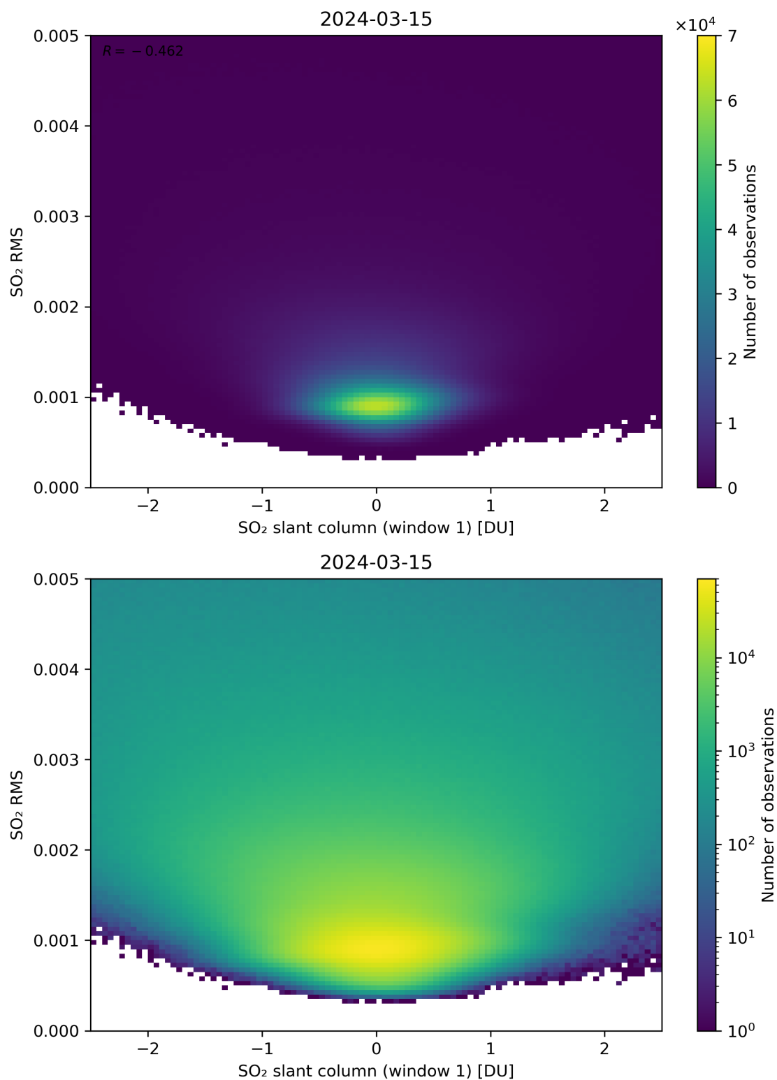
Figure 217: Scatter density plot of “SO 2 slant column (window 1)” against “SO 2 RMS” for 2024-03-14 to 2024-03-16.
