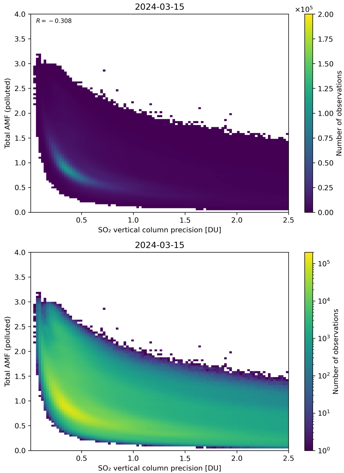
Figure 294: Scatter density plot of “SO 2 vertical column precision” against “Total AMF (polluted)” for 2024-03-14 to 2024-03-16.
