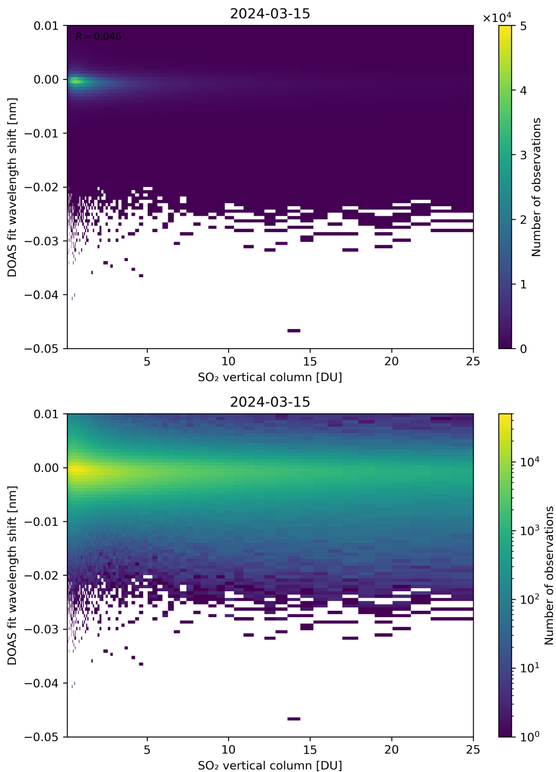
Figure 276: Scatter density plot of “SO 2 vertical column” against “DOAS fit wavelength shift” for 2024-03-14 to 2024-03-16.
