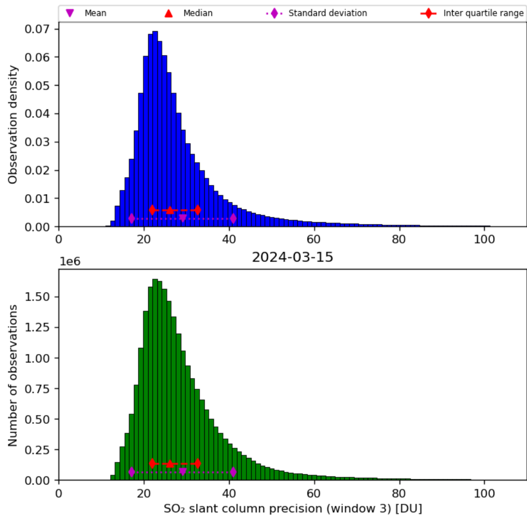
Figure 65: Histogram of “SO 2 slant column precision (window 3)” for 2024-03-14 to 2024-03-16
