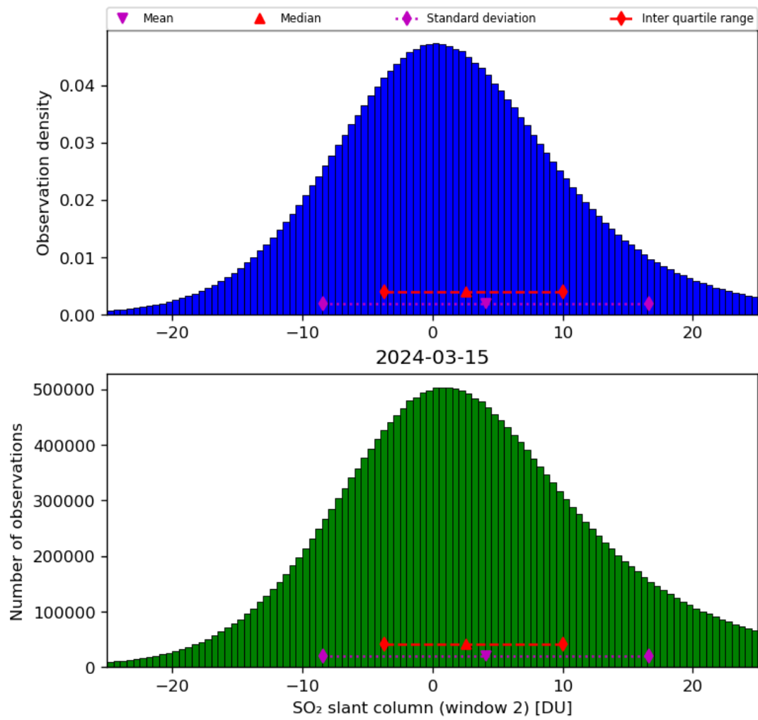
Figure 60: Histogram of “SO 2 slant column (window 2)” for 2024-03-14 to 2024-03-16
