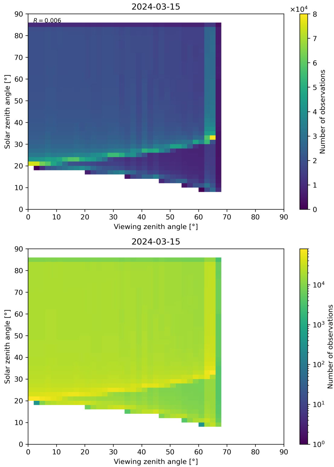
Figure 315: Scatter density plot of “Viewing zenith angle” against “Solar zenith angle” for 2024-03-14 to 2024-03-16.
