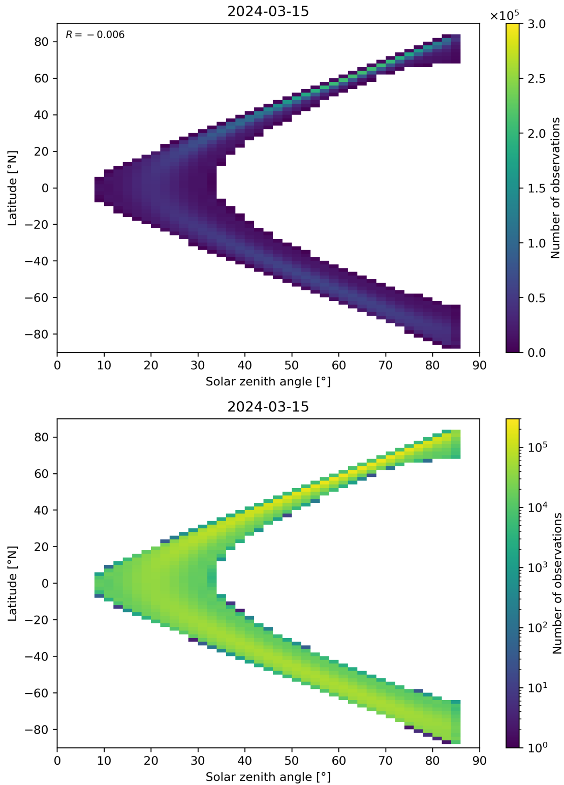
Figure 164: Scatter density plot of “Solar zenith angle” against “Latitude” for 2024-03-14 to 2024-03-16.
