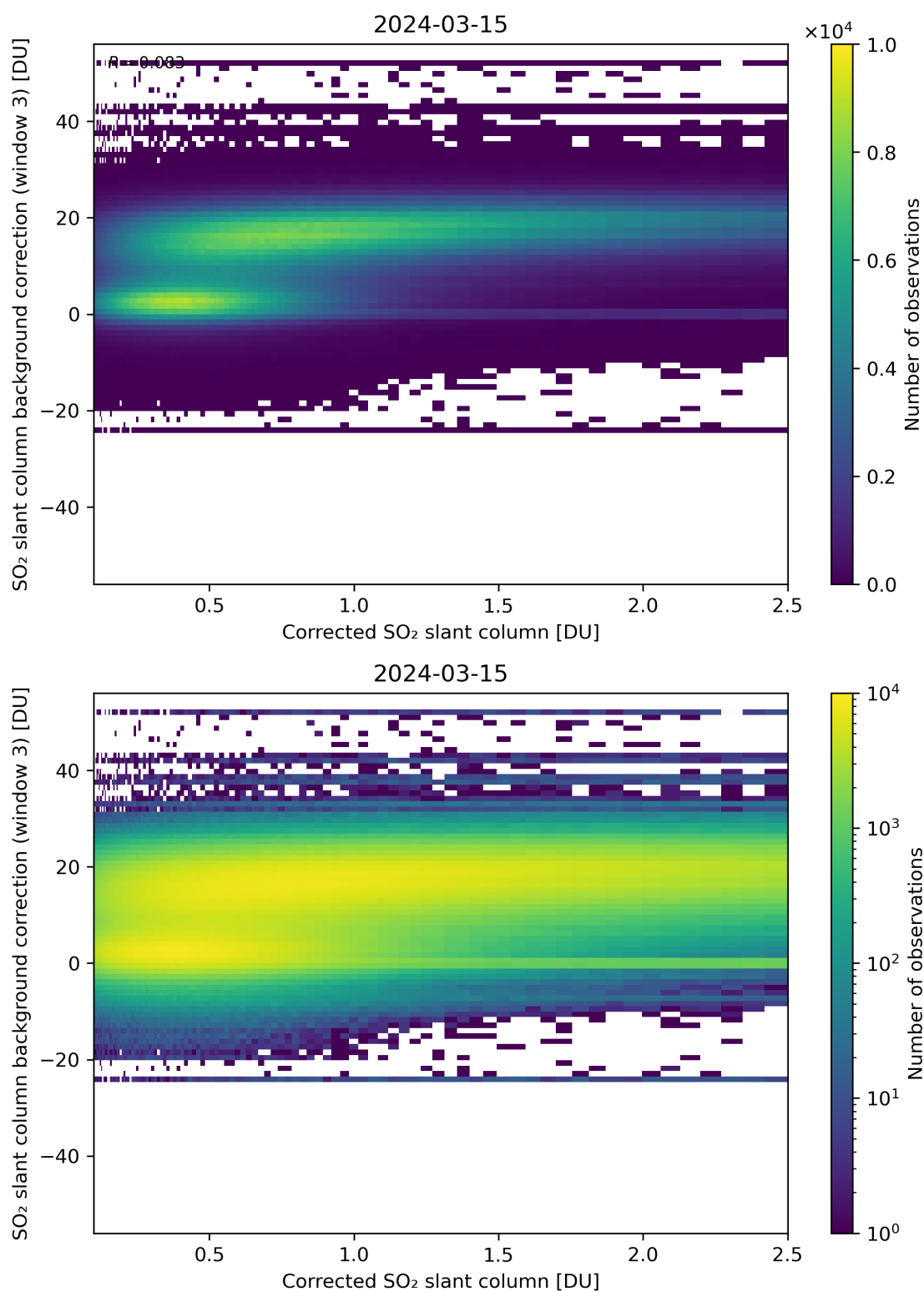
Figure 180: Scatter density plot of “Corrected SO 2 slant column” against “SO 2 slant column background correction (window 3)” for 2024-03-14 to 2024-03-16.
