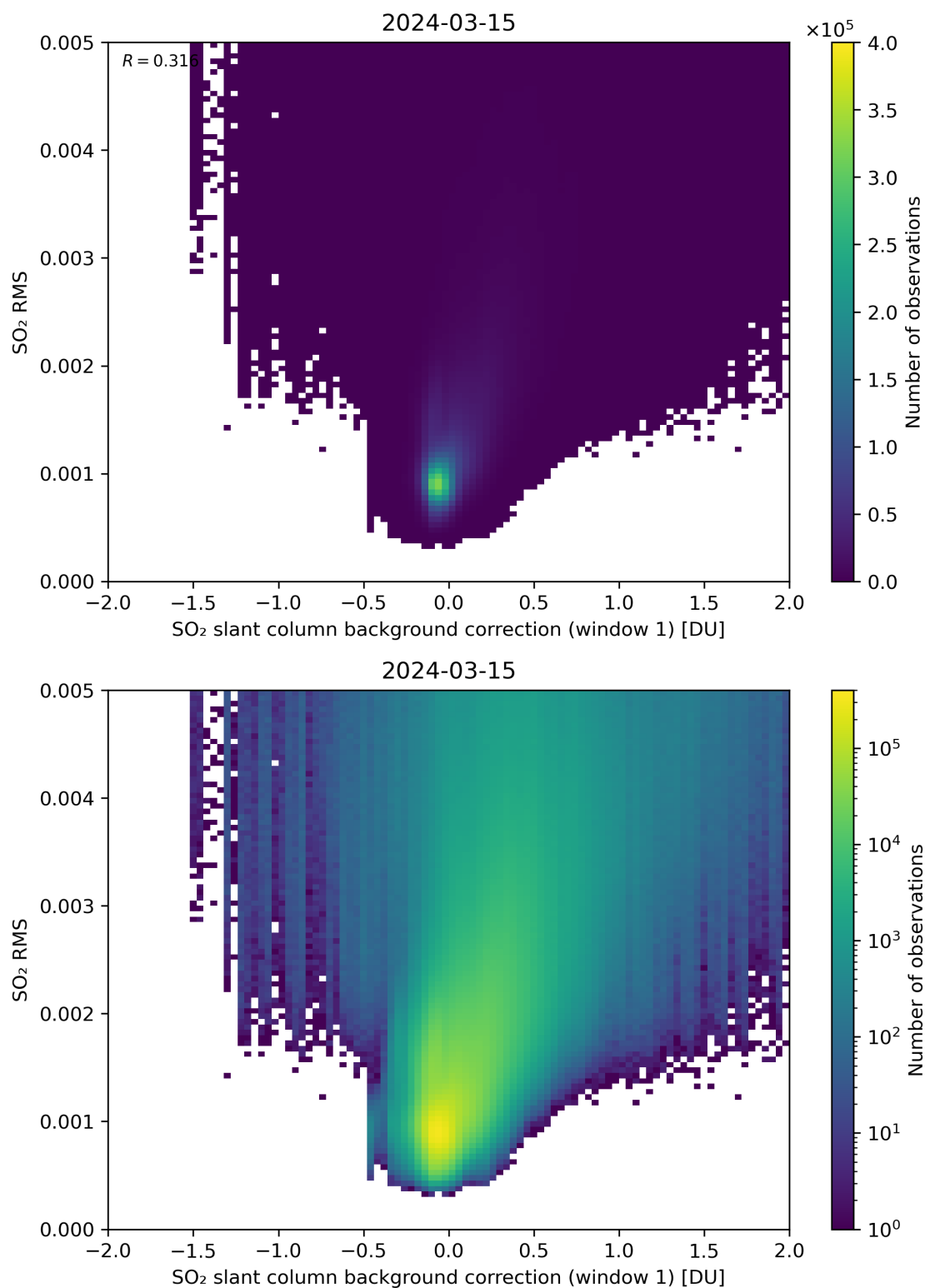
Figure 102: Scatter density plot of “SO 2 slant column background correction (window 1)” against “SO 2 RMS” for 2024-03-14 to 2024-03-16.
