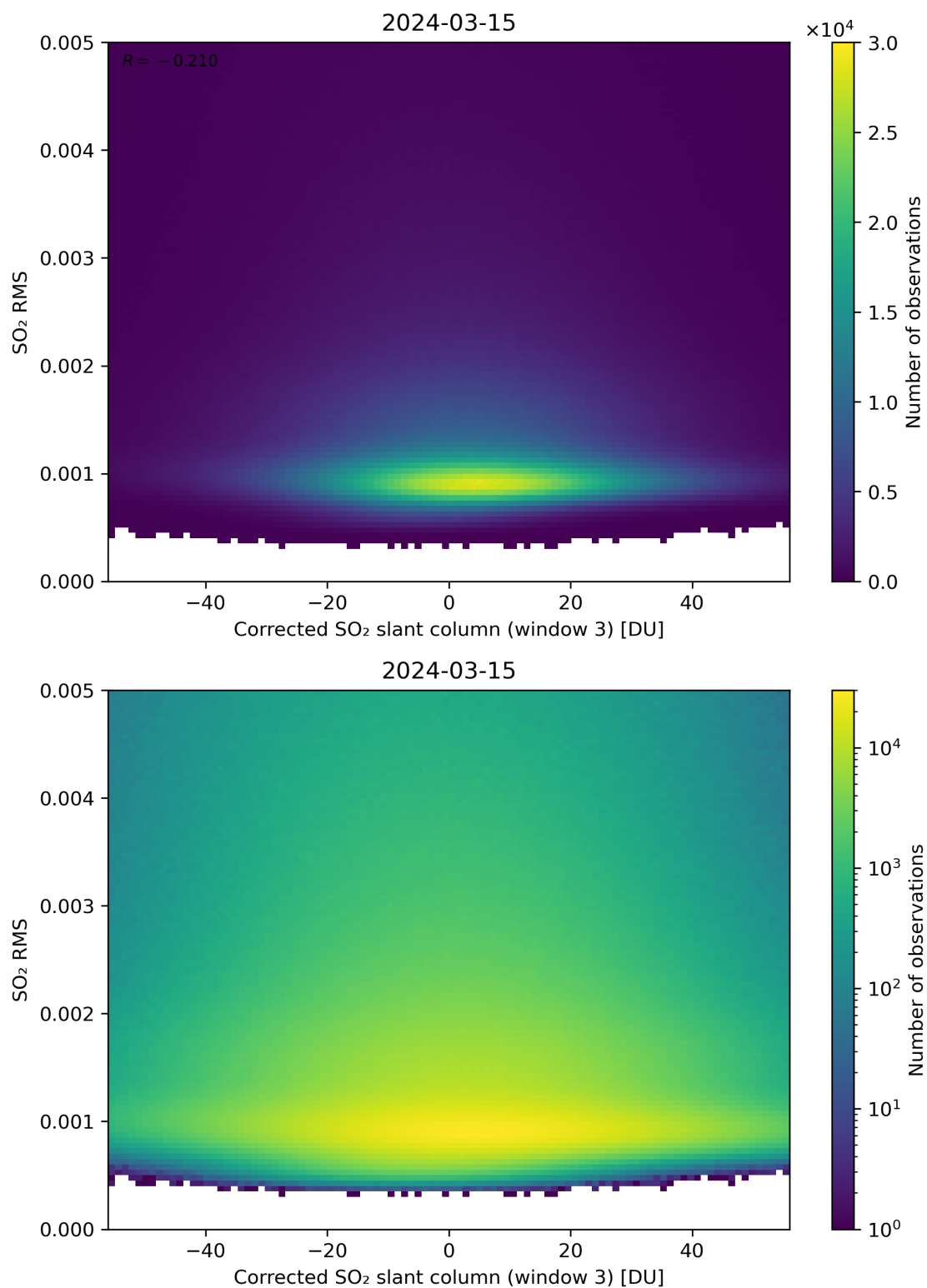
Figure 208: Scatter density plot of “Corrected SO 2 slant column (window 3)” against “SO 2 RMS” for 2024-03-14 to 2024-03-16.
