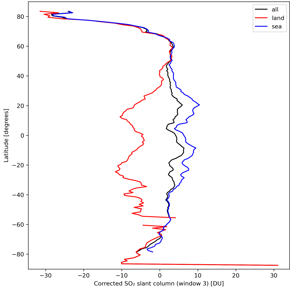
Figure 43: Zonal average of “Corrected SO 2 slant column (window 3)” for 2024-03-14 to 2024-03-16.
