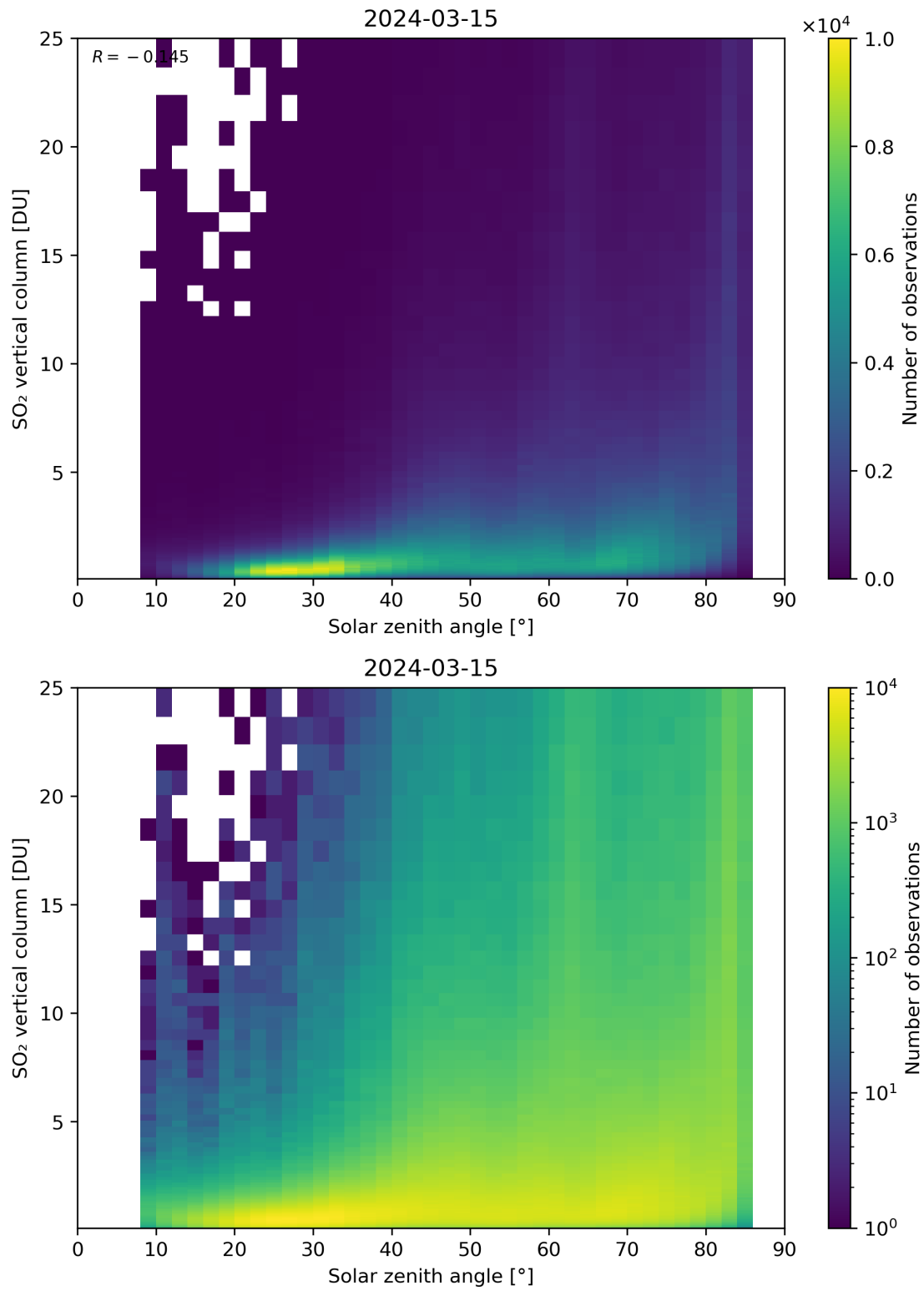
Figure 176: Scatter density plot of “Solar zenith angle” against “SO 2 vertical column” for 2024-03-14 to 2024-03-16.
