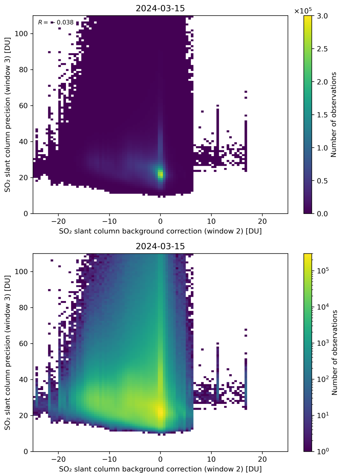
Figure 118: Scatter density plot of “SO 2 slant column background correction (window 2)” against “SO 2 slant column precision (window 3)” for 2024-03-14 to 2024-03-16.
