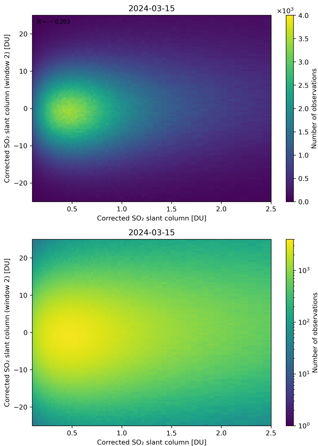
Figure 185: Scatter density plot of “Corrected SO 2 slant column” against “Corrected SO 2 slant column (window 2)” for 2024-03-14 to 2024-03-16.
