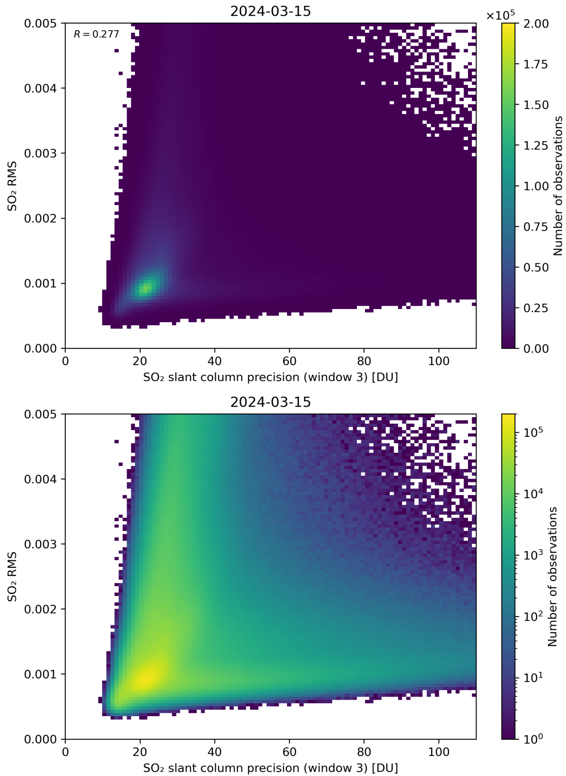
Figure 260: Scatter density plot of “SO 2 slant column precision (window 3)” against “SO 2 RMS” for 2024-03-14 to 2024-03-16.
