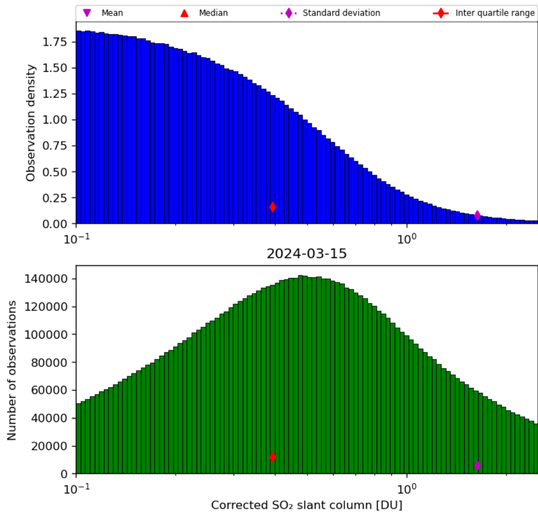
Figure 55: Histogram of “Corrected SO 2 slant column” for 2024-03-14 to 2024-03-16
