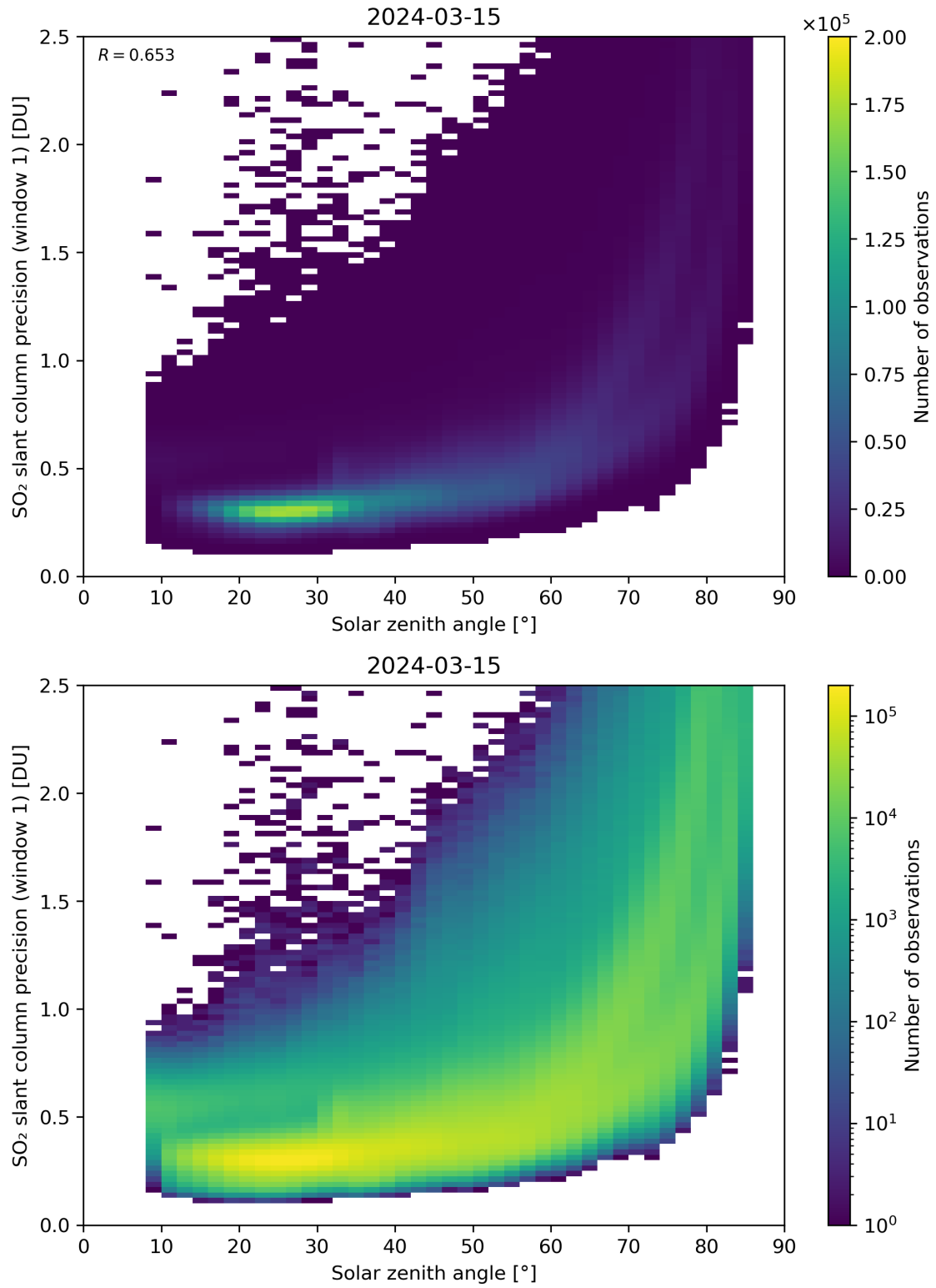
Figure 170: Scatter density plot of “Solar zenith angle” against “SO 2 slant column precision (window 1)” for 2024-03-14 to 2024-03-16.
