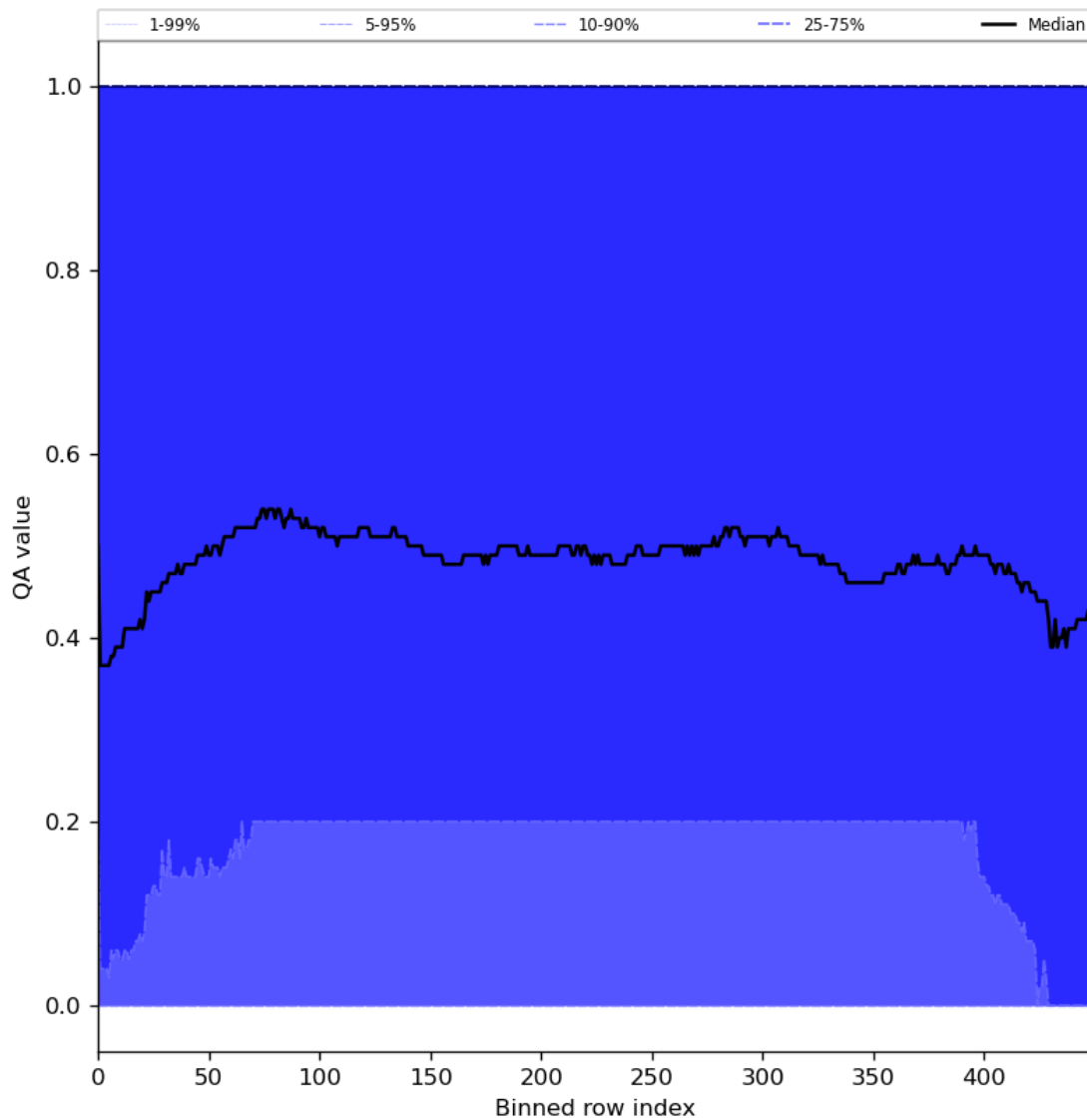
Figure 75: Along track statistics of “QA value” for 2024-03-14 to 2024-03-16
