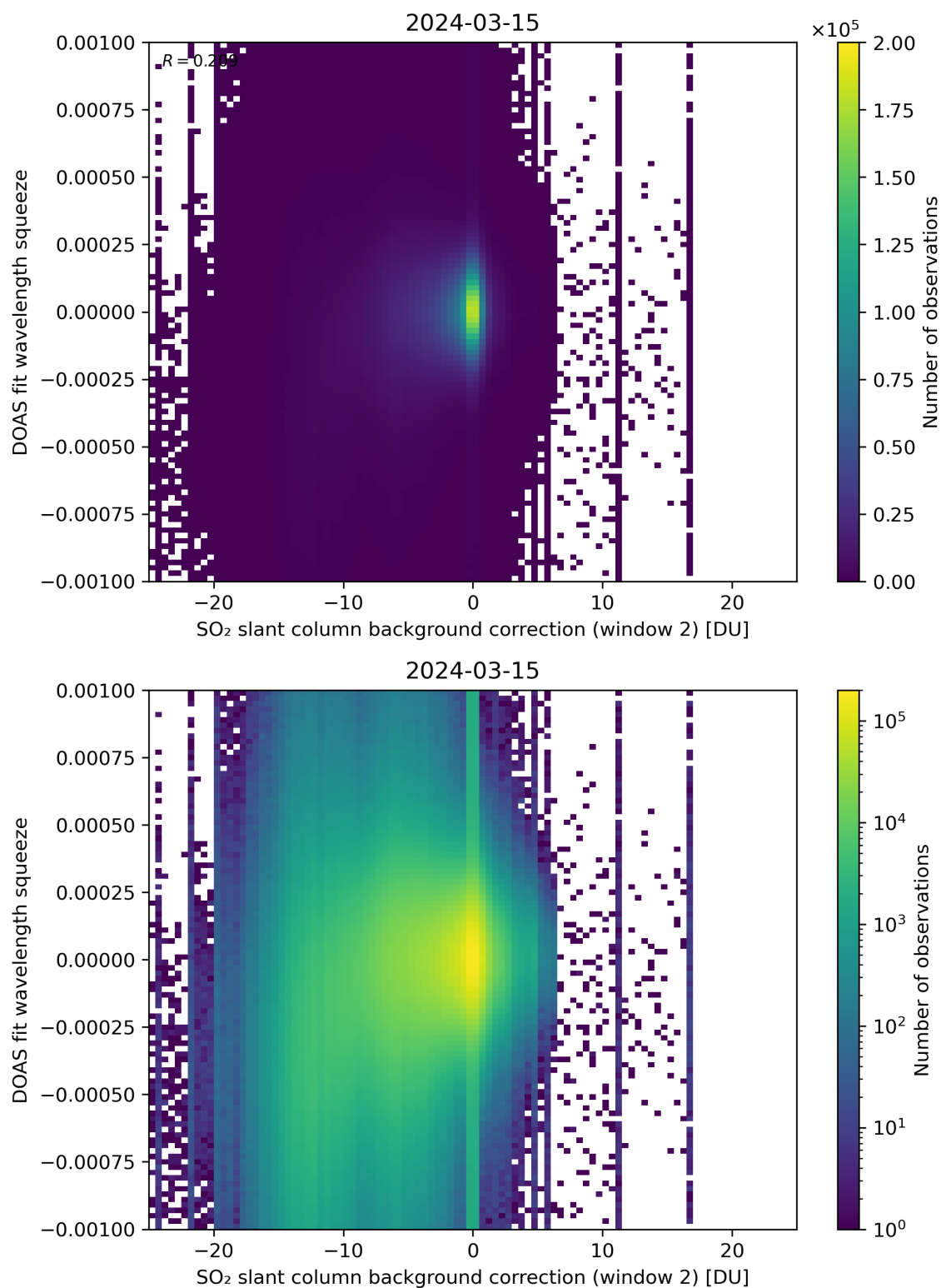
Figure 113: Scatter density plot of “SO 2 slant column background correction (window 2)” against “DOAS fit wavelength squeeze” for 2024-03-14 to 2024-03-16.
