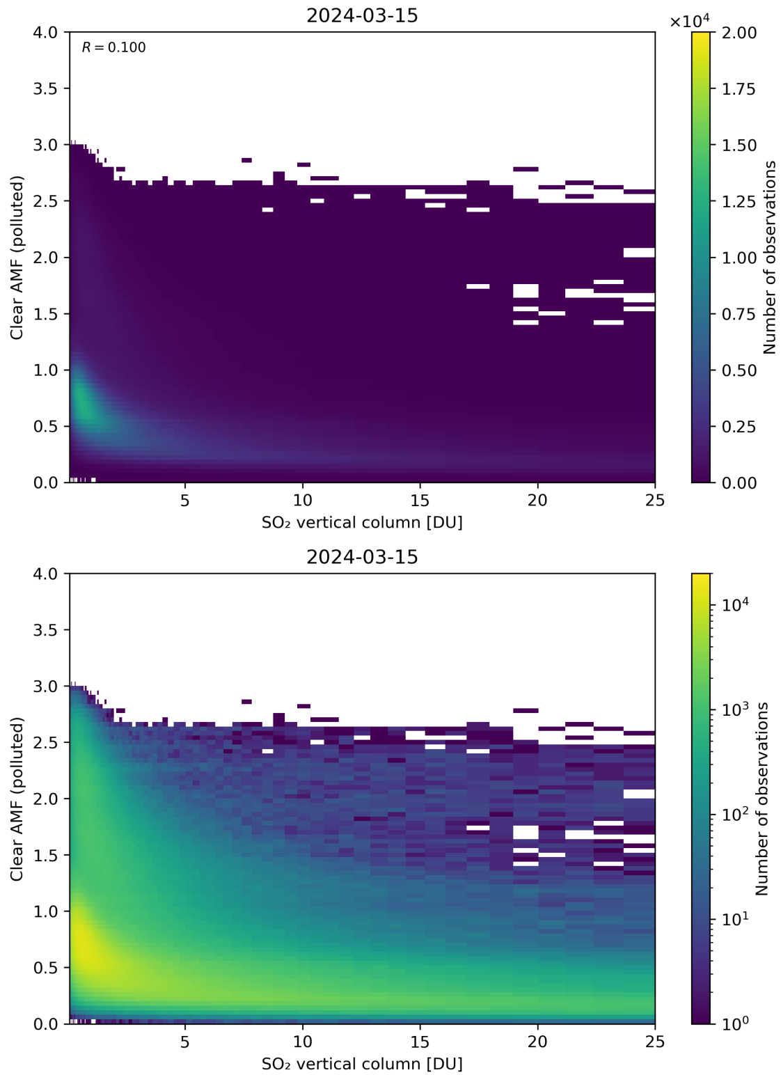
Figure 296: Scatter density plot of “SO 2 vertical column” against “Clear AMF (polluted)” for 2024-03-14 to 2024-03-16.
