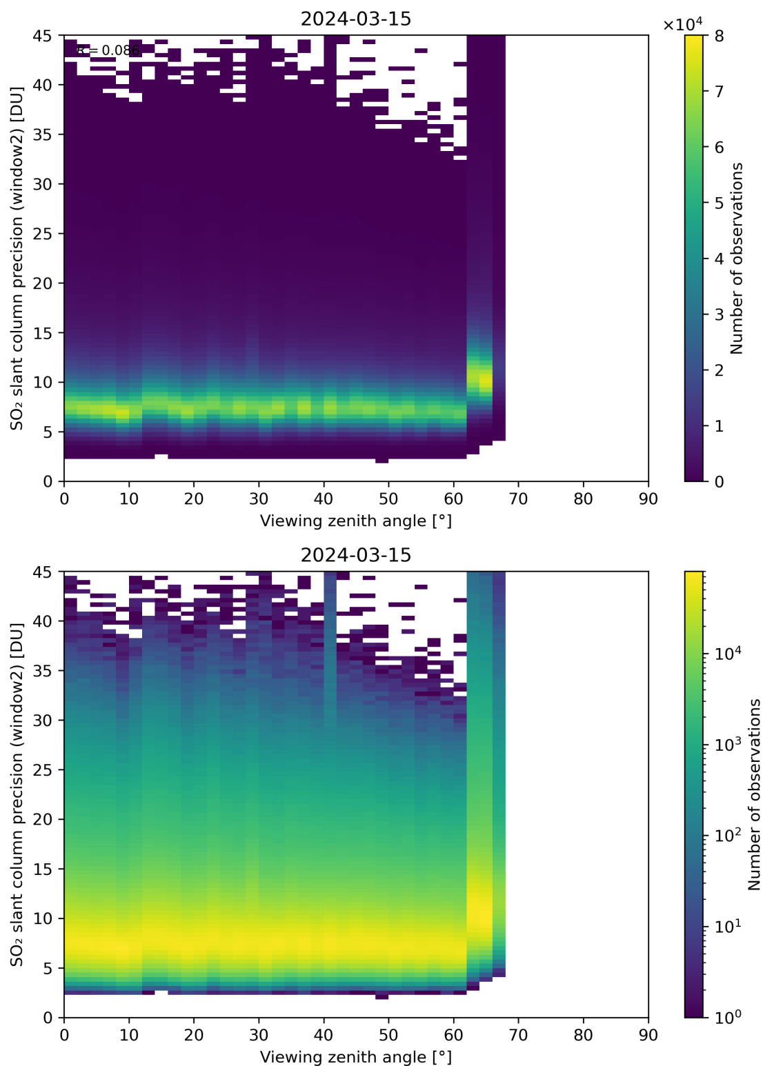
Figure 322: Scatter density plot of “Viewing zenith angle” against “SO 2 slant column precision (window2)” for 2024-03-14 to 2024-03-16.
