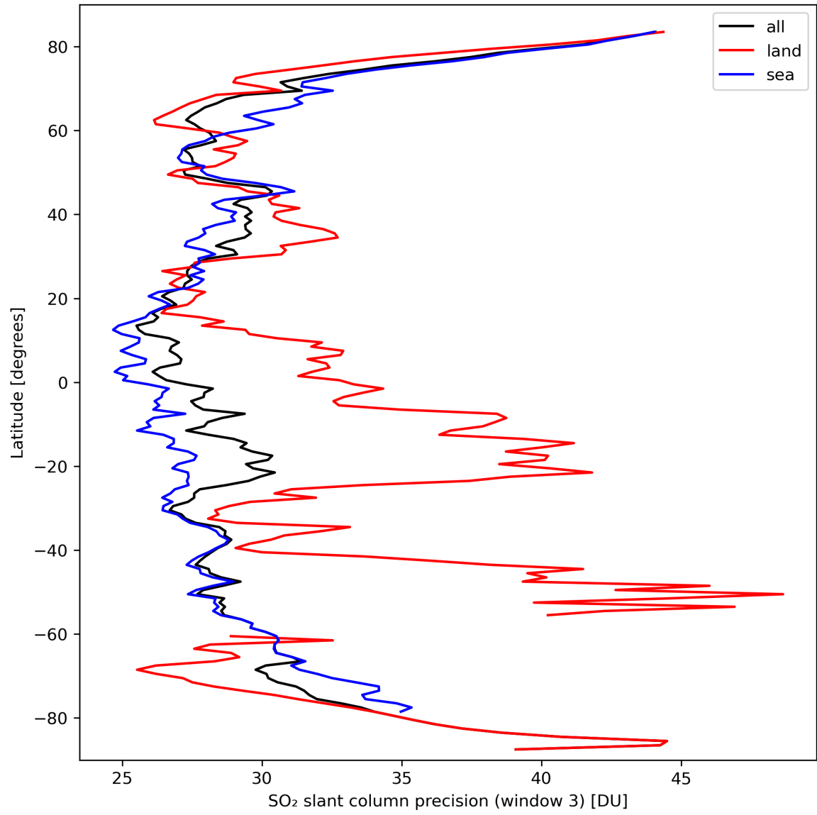
Figure 42: Zonal average of “SO 2 slant column precision (window 3)” for 2024-03-14 to 2024-03-16.
