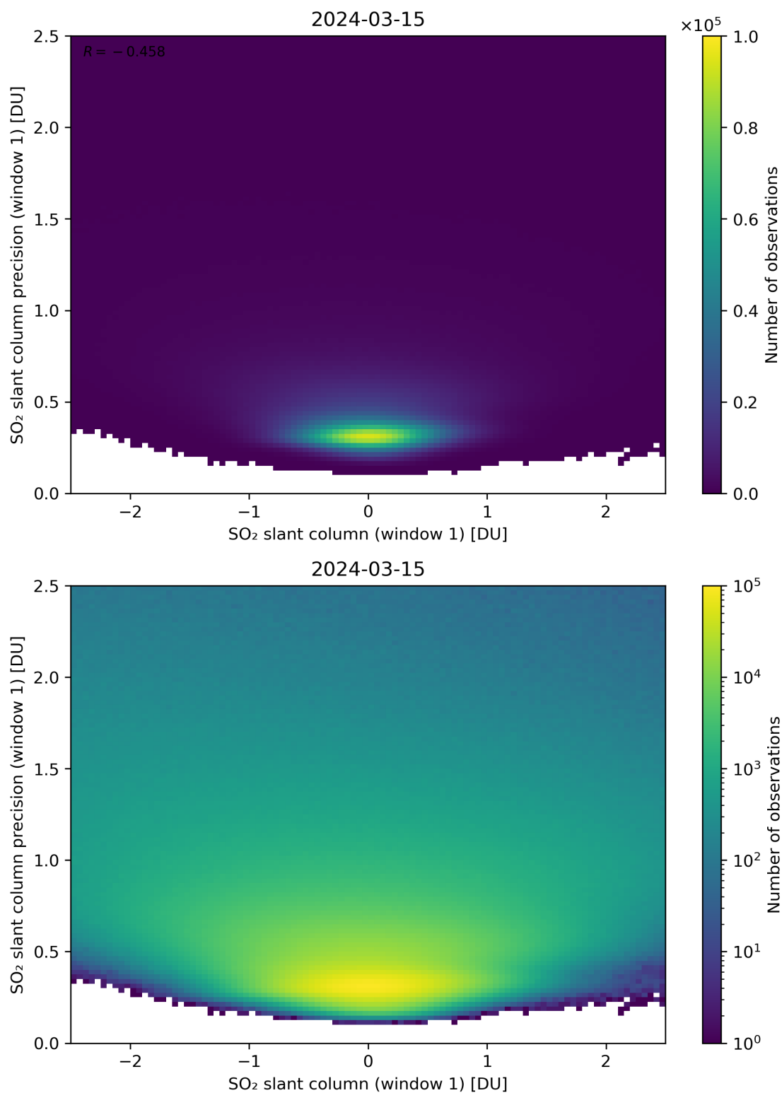
Figure 235: Scatter density plot of “SO 2 slant column (window 1)” against “SO 2 slant column precision (window 1)” for 2024-03-14 to 2024-03-16.
