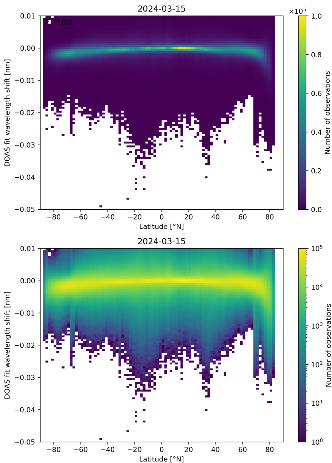
Figure 142: Scatter density plot of “Latitude” against “DOAS fit wavelength shift” for 2024-03-14 to 2024-03-16.
