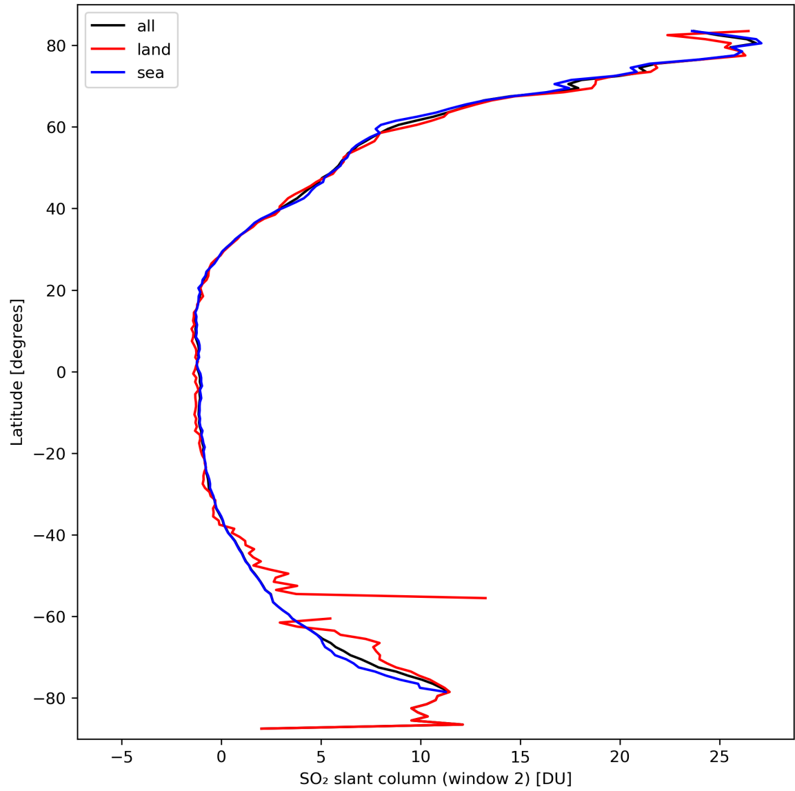
Figure 37: Zonal average of “SO 2 slant column (window 2)” for 2024-03-14 to 2024-03-16.
