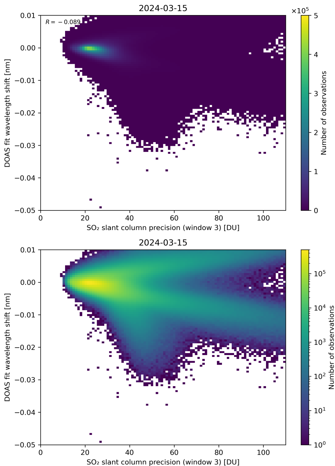
Figure 258: Scatter density plot of “SO 2 slant column precision (window 3)” against “DOAS fit wavelength shift” for 2024-03-14 to 2024-03-16.
