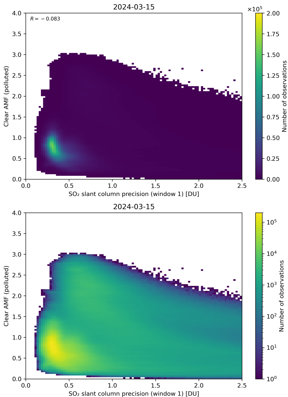
Figure 224: Scatter density plot of “SO 2 slant column precision (window 1)” against “Clear AMF (polluted)” for 2024-03-14 to 2024-03-16.
