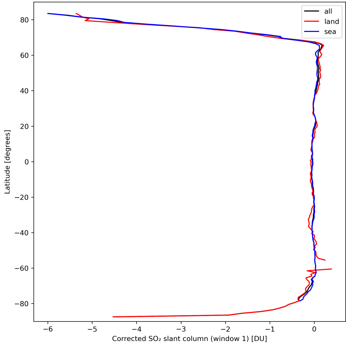
Figure 35: Zonal average of “Corrected SO 2 slant column (window 1)” for 2024-03-14 to 2024-03-16.
