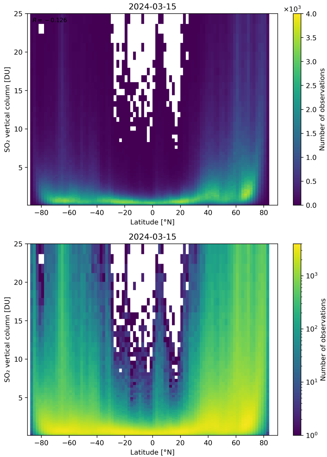
Figure 156: Scatter density plot of “Latitude” against “SO 2 vertical column” for 2024-03-14 to 2024-03-16.
