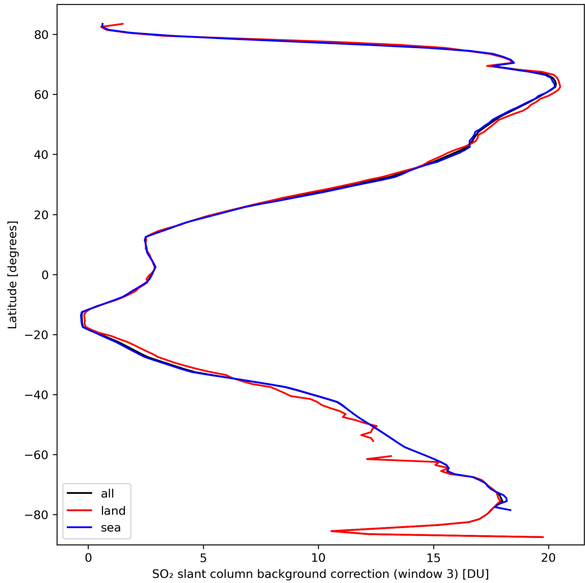
Figure 44: Zonal average of “SO 2 slant column background correction (window 3)” for 2024-03-14 to 2024-03-16.
