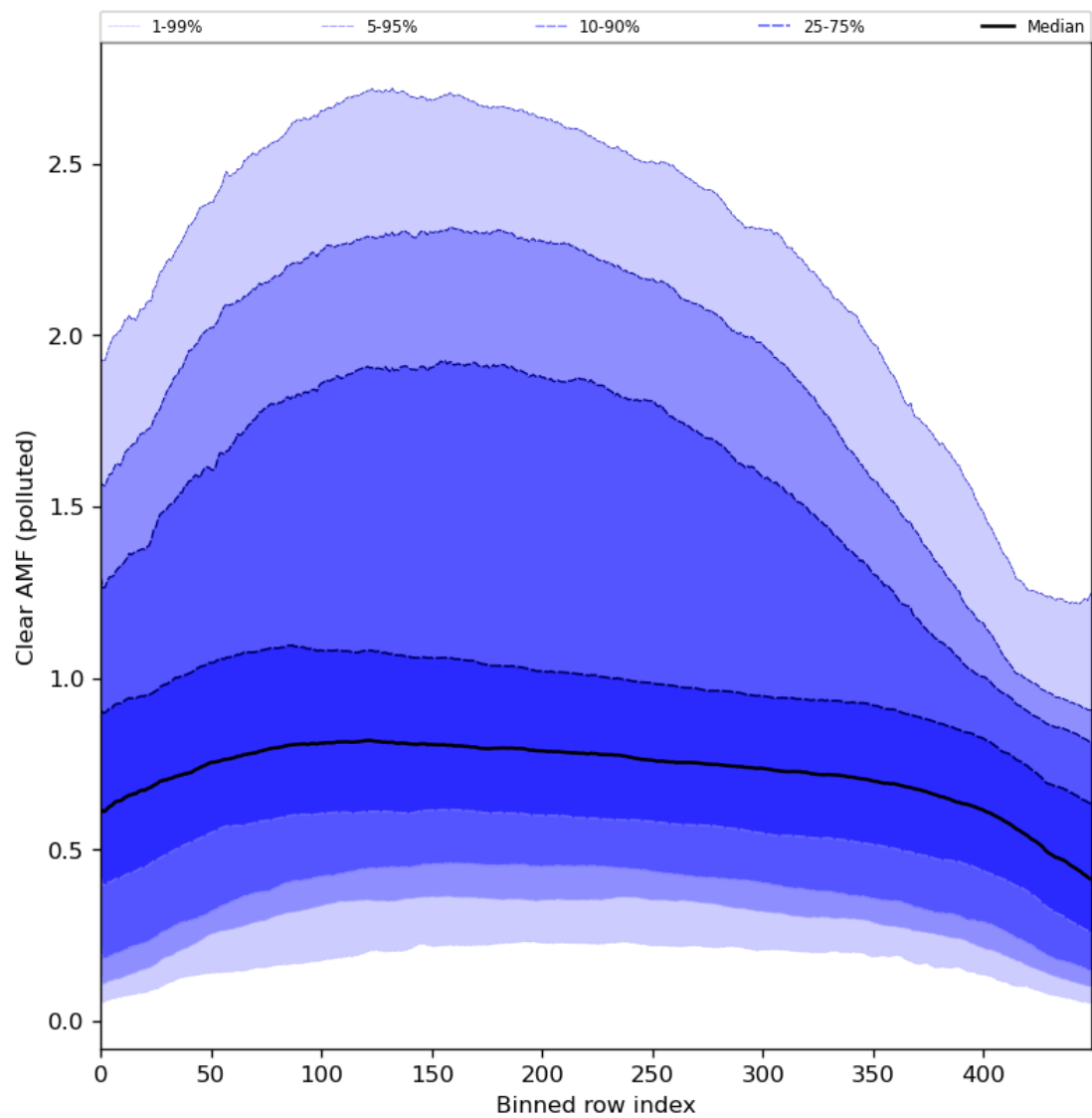
Figure 96: Along track statistics of “Clear AMF (polluted)” for 2024-03-14 to 2024-03-16
