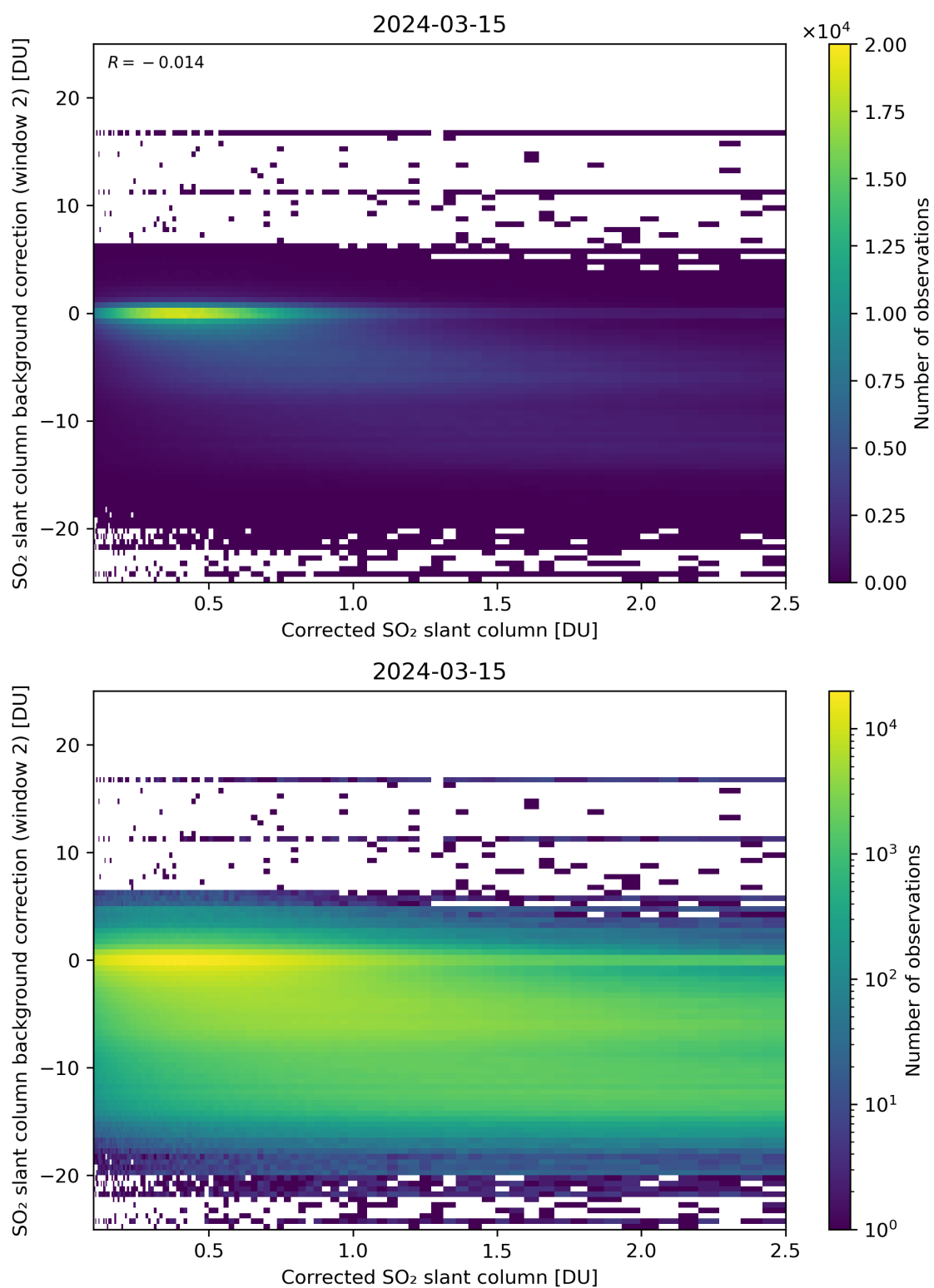
Figure 179: Scatter density plot of “Corrected SO 2 slant column” against “SO 2 slant column background correction (window 2)” for 2024-03-14 to 2024-03-16.
