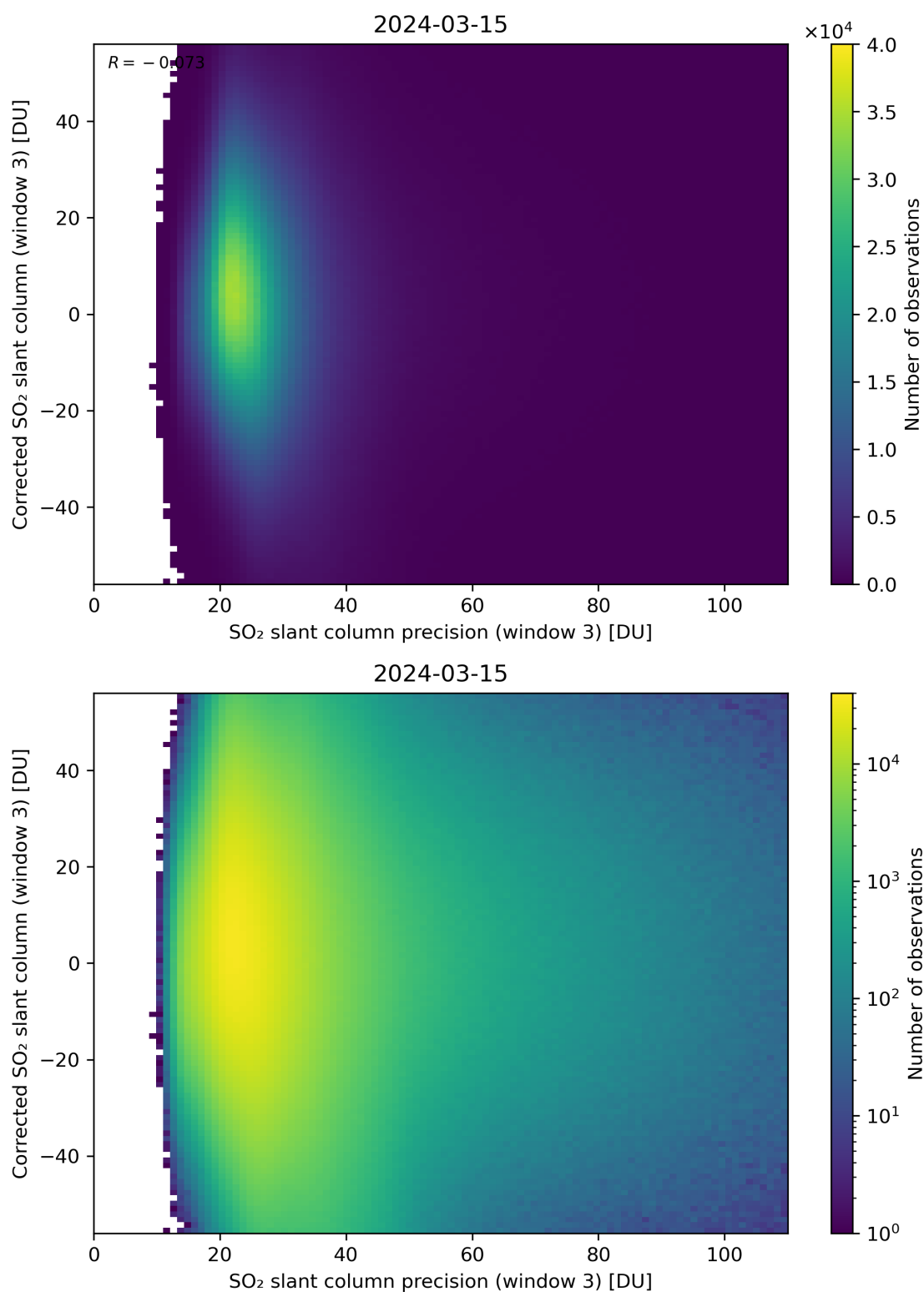
Figure 262: Scatter density plot of “SO 2 slant column precision (window 3)” against “Corrected SO 2 slant column (window 3)” for 2024-03-14 to 2024-03-16.
