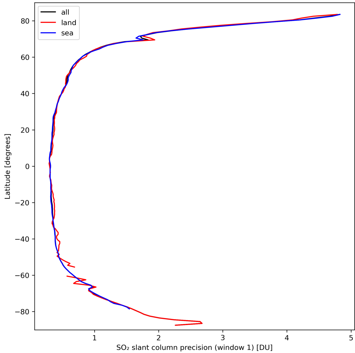
Figure 34: Zonal average of “SO 2 slant column precision (window 1)” for 2024-03-14 to 2024-03-16.
