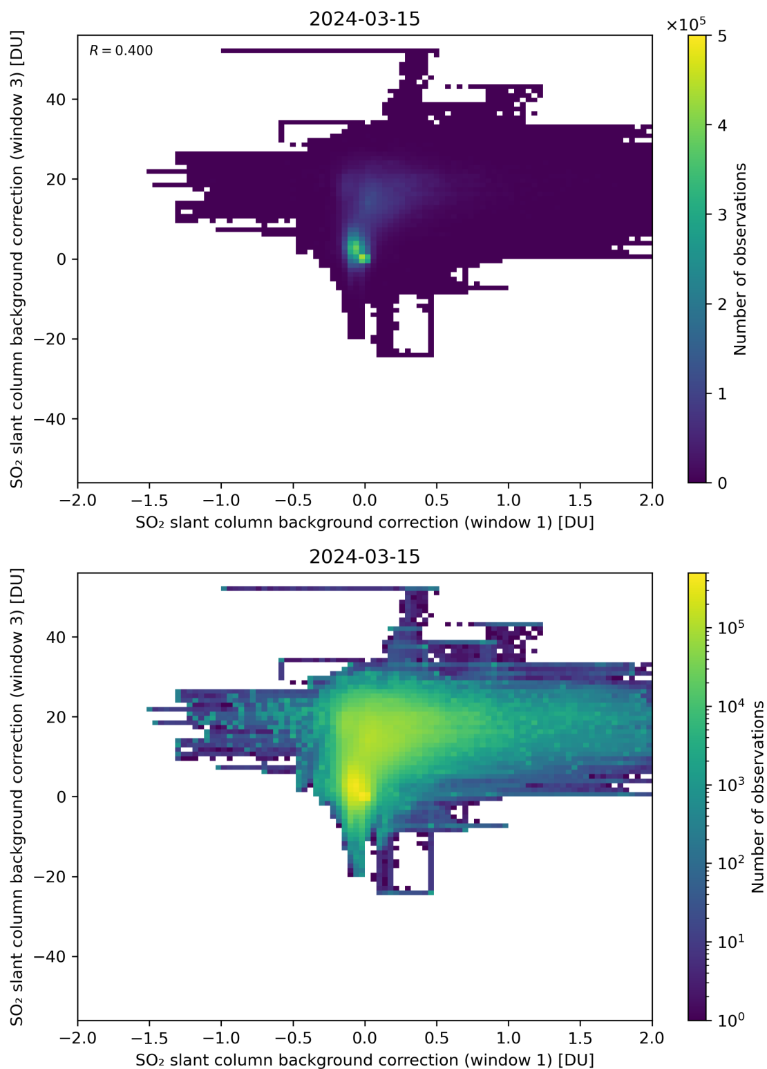
Figure 99: Scatter density plot of “SO 2 slant column background correction (window 1)” against “SO 2 slant column background correction (window 3)” for 2024-03-14 to 2024-03-16.
