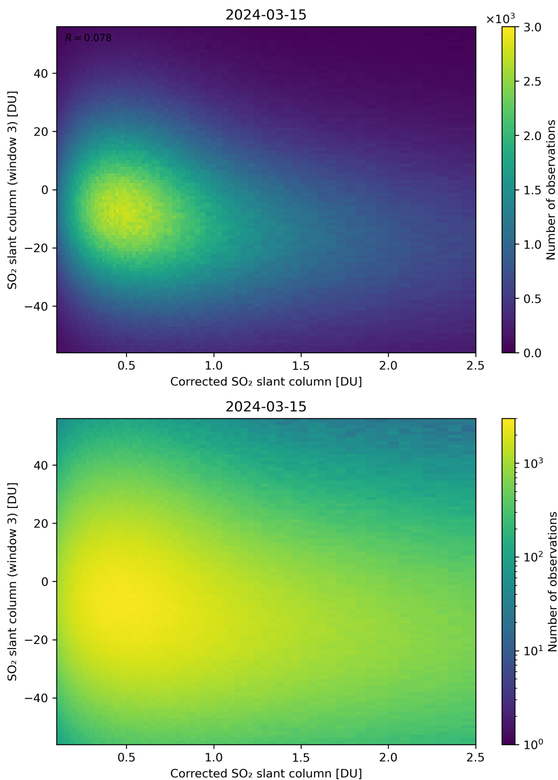
Figure 190: Scatter density plot of “Corrected SO 2 slant column” against “SO 2 slant column (window 3)” for 2024-03-14 to 2024-03-16.
