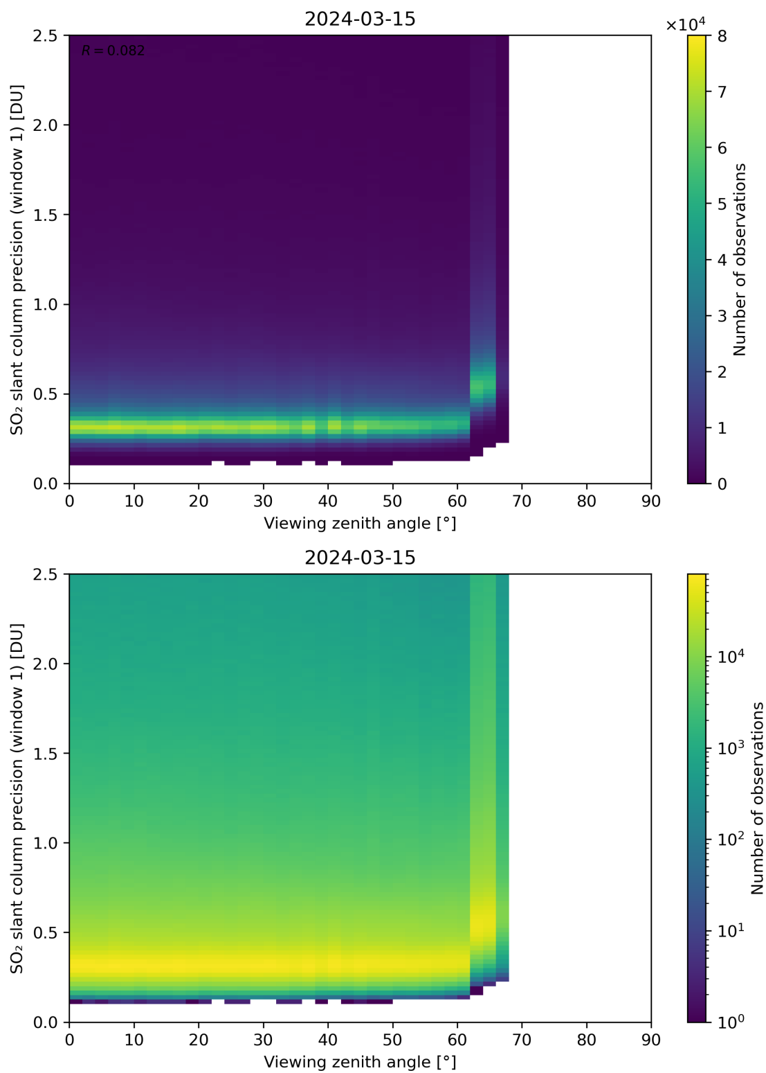
Figure 321: Scatter density plot of “Viewing zenith angle” against “SO 2 slant column precision (window 1)” for 2024-03-14 to 2024-03-16.
