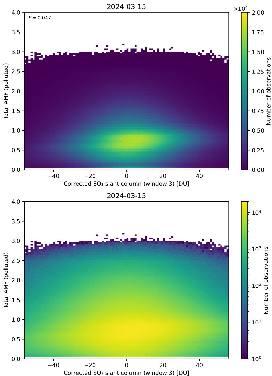
Figure 210: Scatter density plot of “Corrected SO 2 slant column (window 3)” against “Total AMF (polluted)” for 2024-03-14 to 2024-03-16.
