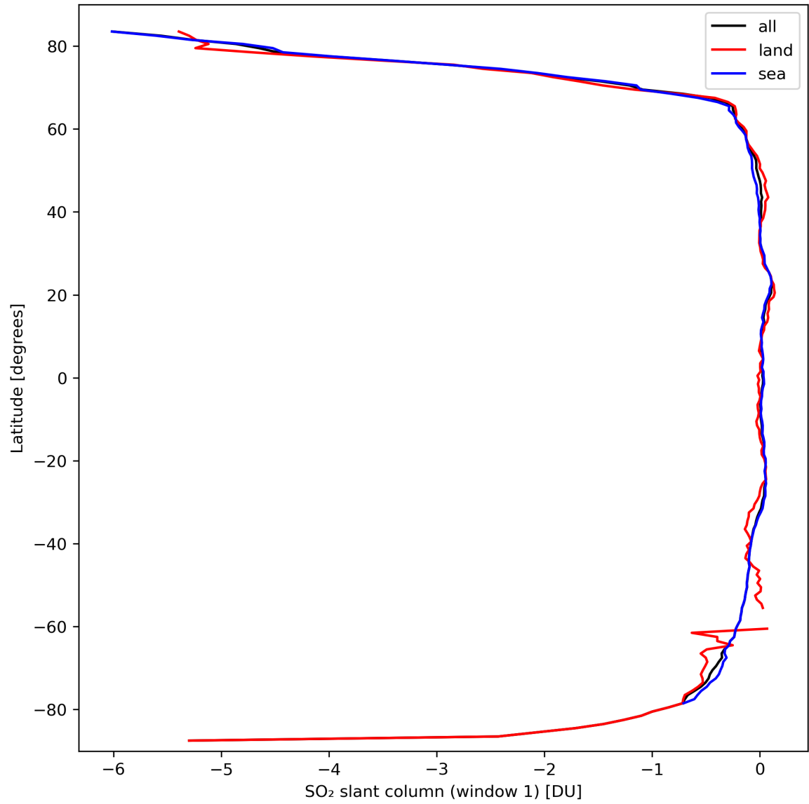
Figure 33: Zonal average of “SO 2 slant column (window 1)” for 2024-03-14 to 2024-03-16.
