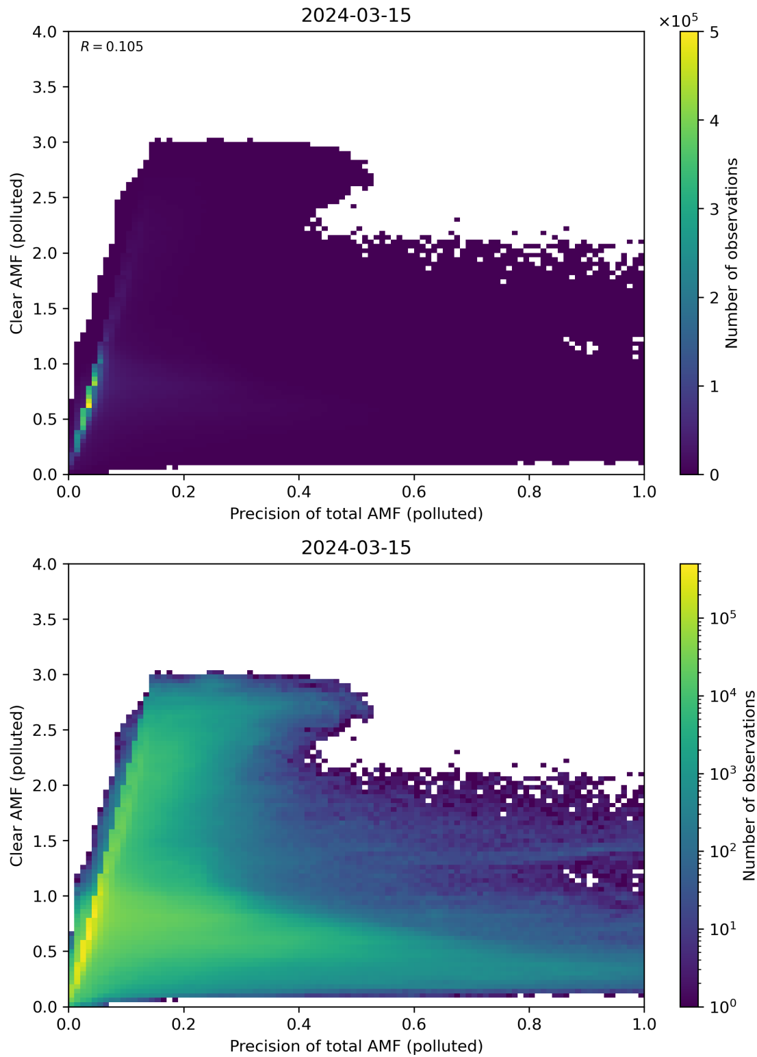
Figure 270: Scatter density plot of “Precision of total AMF (polluted)” against “Clear AMF (polluted)” for 2024-03-14 to 2024-03-16.
