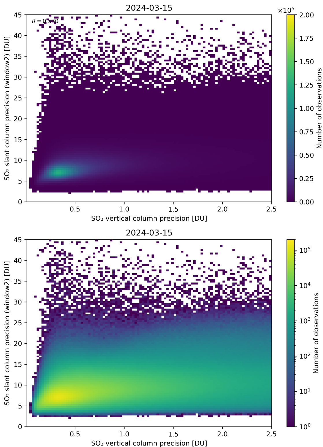
Figure 291: Scatter density plot of “SO 2 vertical column precision” against “SO 2 slant column precision (window2)” for 2024-03-14 to 2024-03-16.
