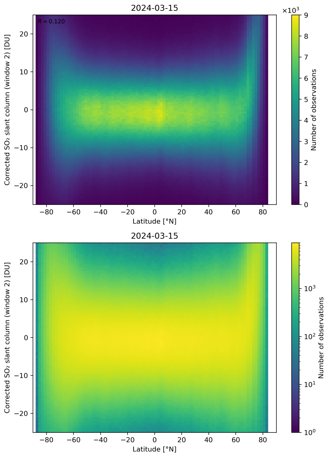
Figure 147: Scatter density plot of “Latitude” against “Corrected SO 2 slant column (window 2)” for 2024-03-14 to 2024-03-16.
