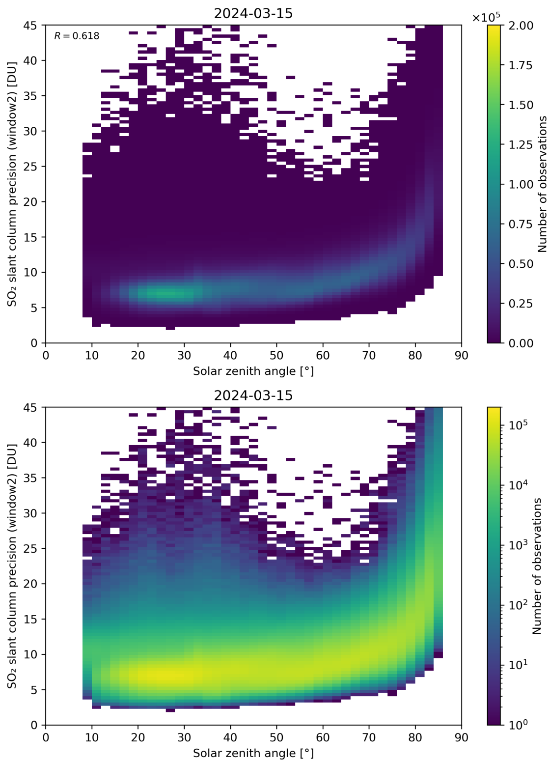
Figure 171: Scatter density plot of “Solar zenith angle” against “SO 2 slant column precision (window2)” for 2024-03-14 to 2024-03-16.
