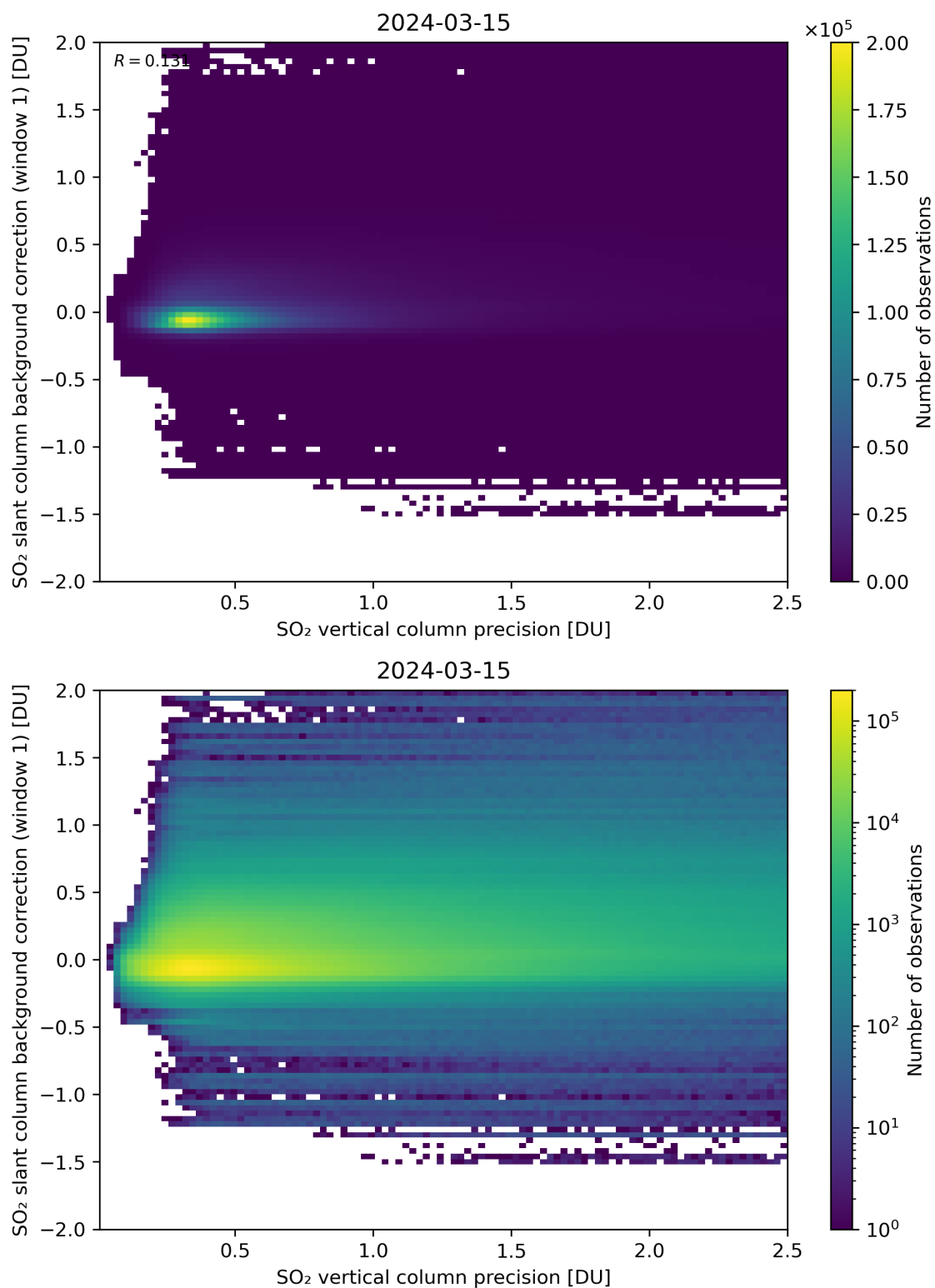
Figure 279: Scatter density plot of “SO 2 vertical column precision” against “SO 2 slant column background correction (window 1)” for 2024-03-14 to 2024-03-16.
