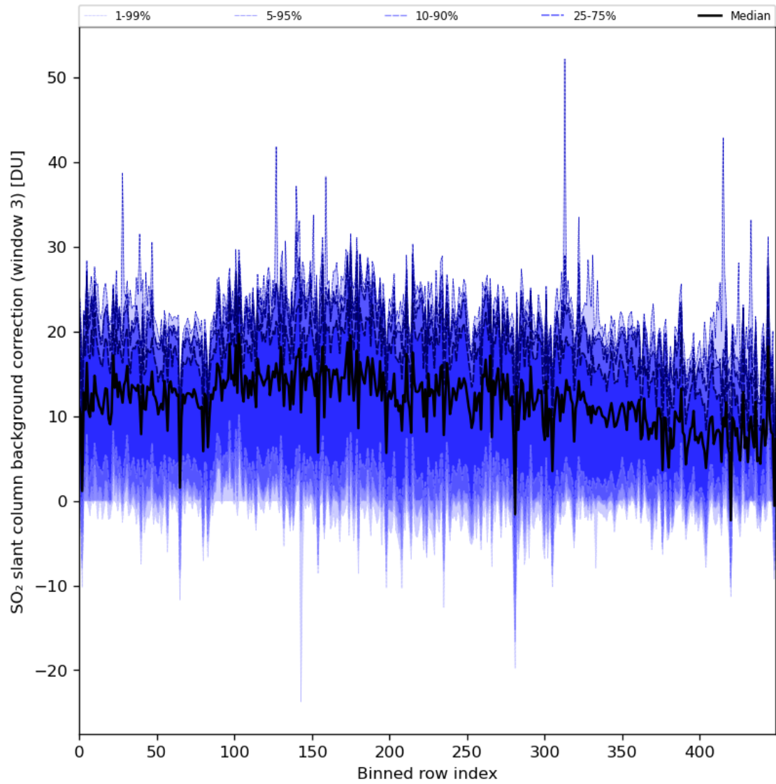
Figure 90: Along track statistics of “SO 2 slant column background correction (window 3)” for 2024-03-14 to 2024-03-16
