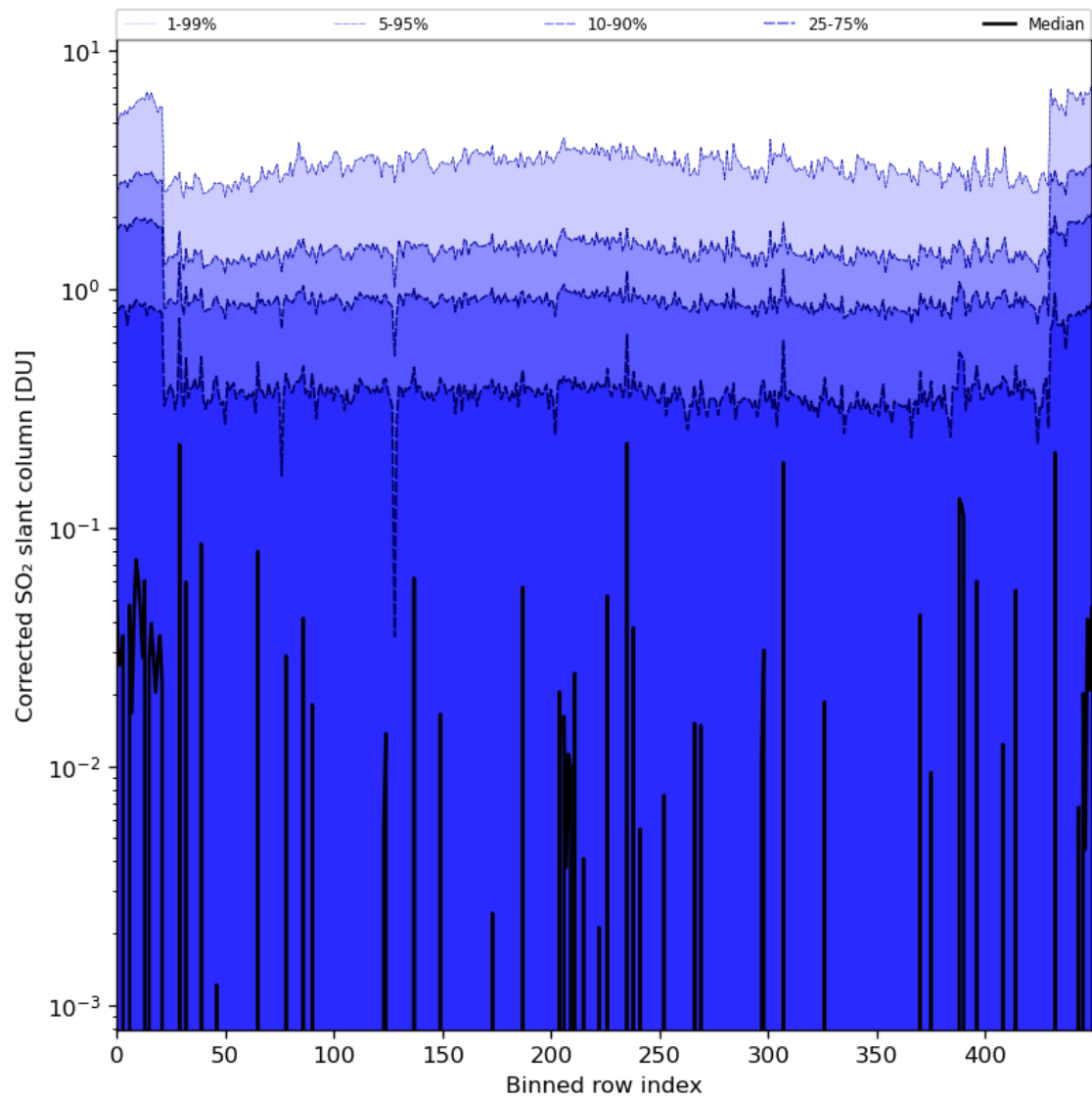
Figure 78: Along track statistics of “Corrected SO 2 slant column” for 2024-03-14 to 2024-03-16
