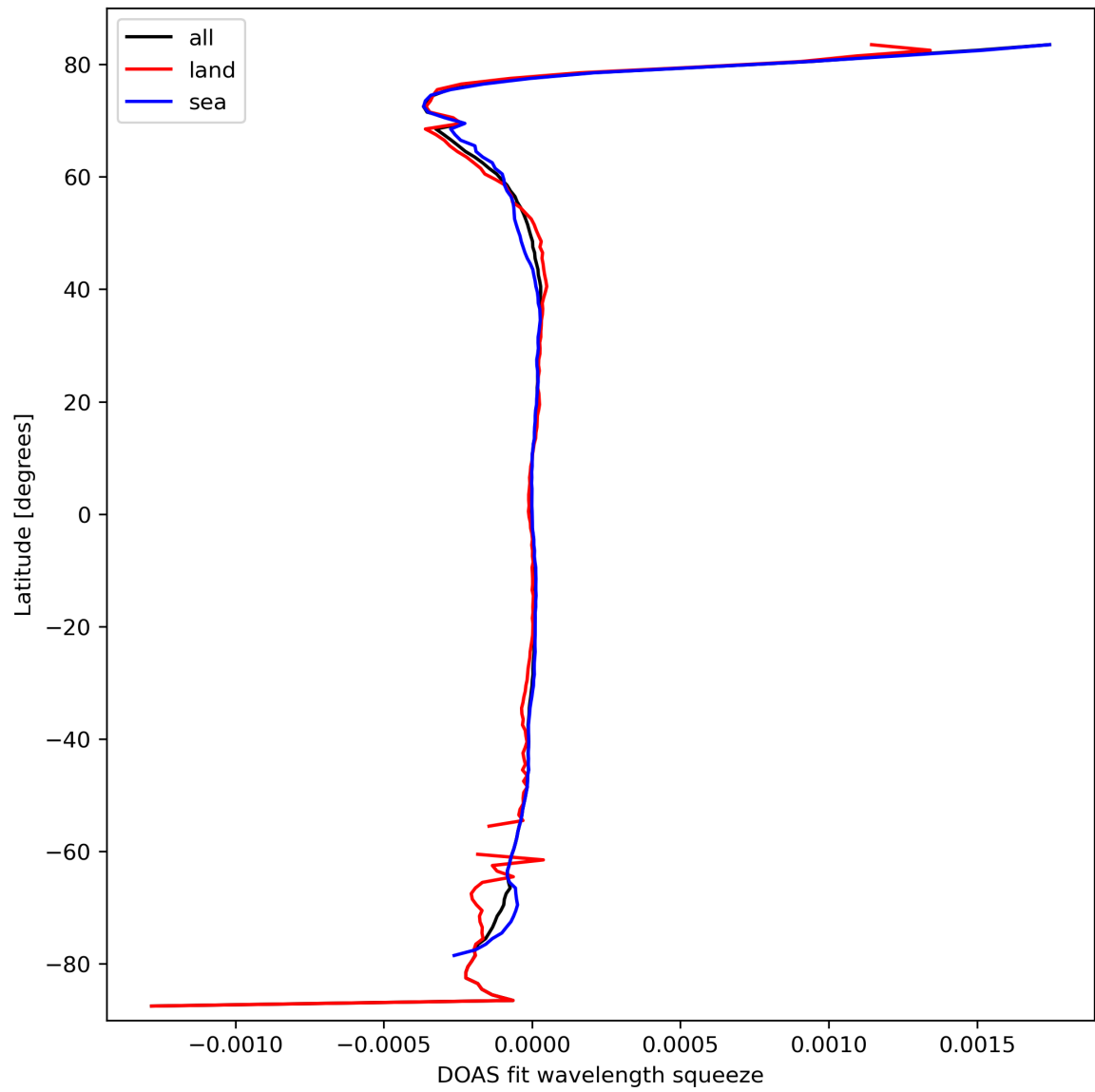
Figure 46: Zonal average of “DOAS fit wavelength squeeze” for 2024-03-14 to 2024-03-16.
