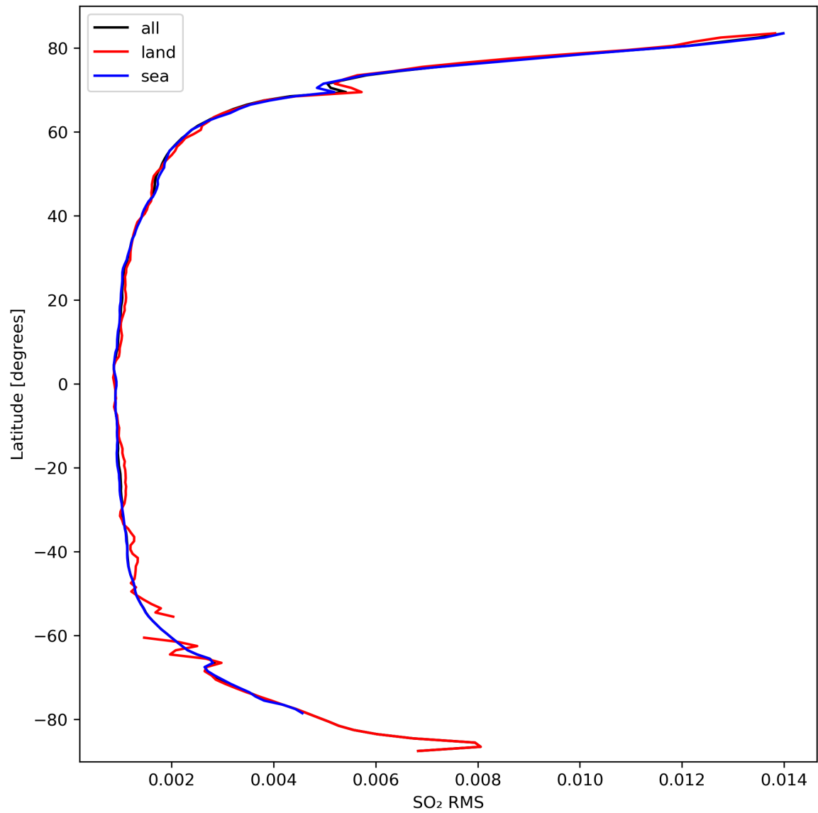
Figure 47: Zonal average of “SO 2 RMS” for 2024-03-14 to 2024-03-16.
