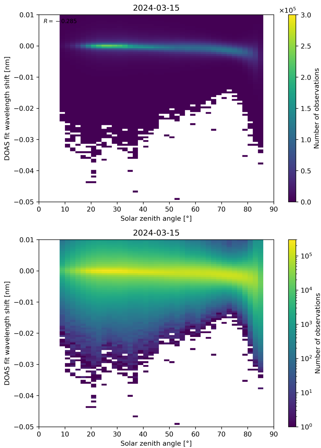
Figure 161: Scatter density plot of “Solar zenith angle” against “DOAS fit wavelength shift” for 2024-03-14 to 2024-03-16.
