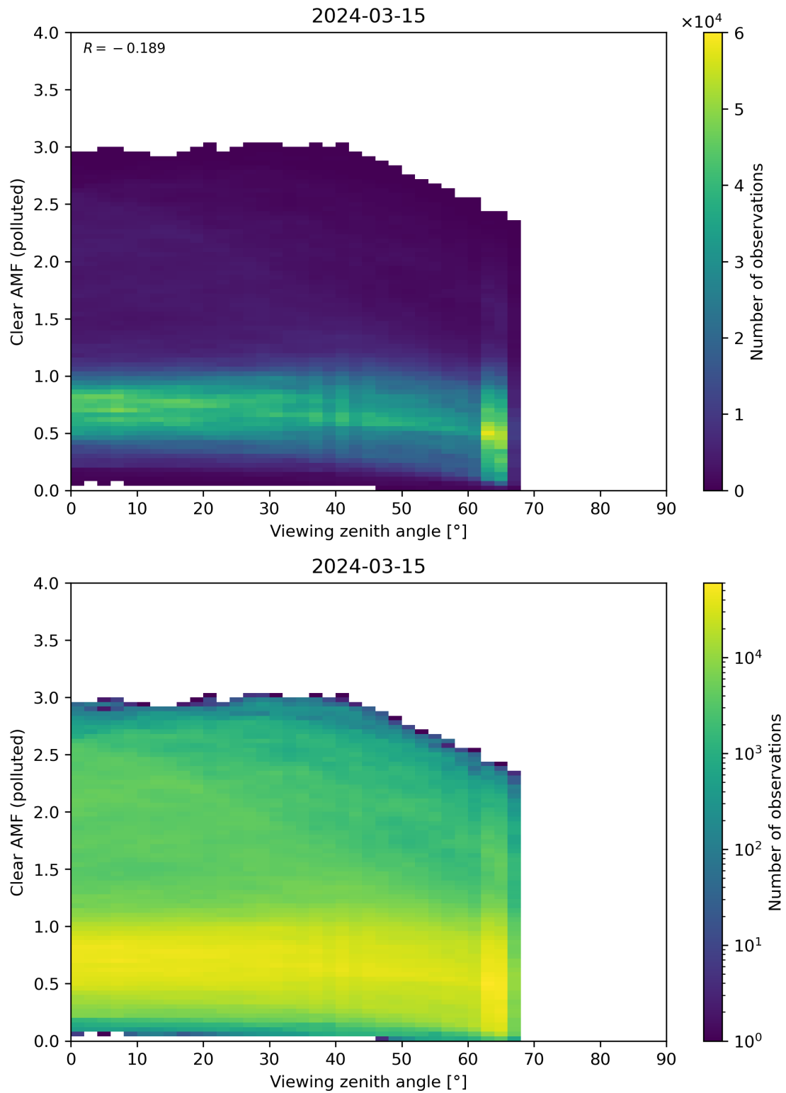
Figure 316: Scatter density plot of “Viewing zenith angle” against “Clear AMF (polluted)” for 2024-03-14 to 2024-03-16.
