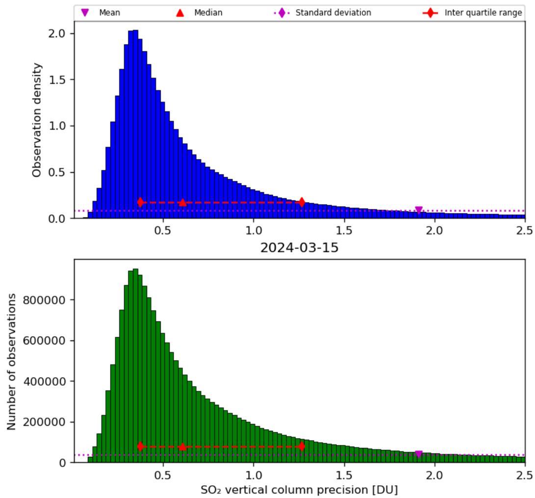
Figure 54: Histogram of “SO 2 vertical column precision” for 2024-03-14 to 2024-03-16
