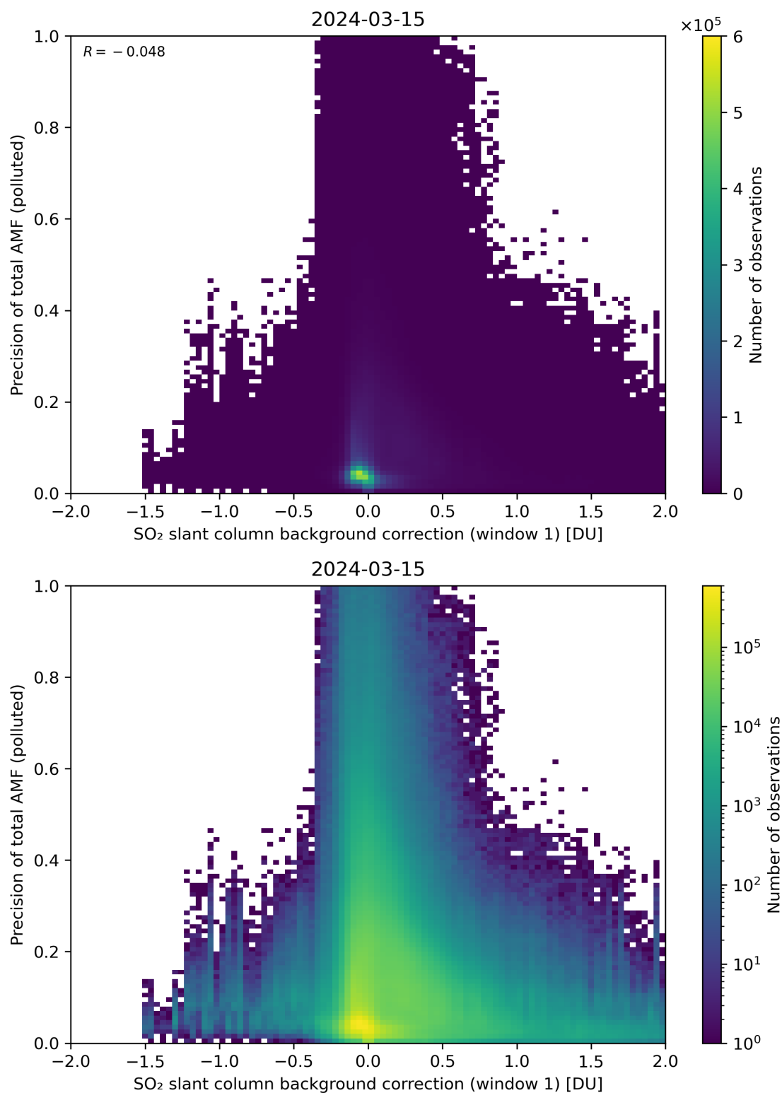
Figure 110: Scatter density plot of “SO 2 slant column background correction (window 1)” against “Precision of total AMF (polluted)” for 2024-03-14 to 2024-03-16.
