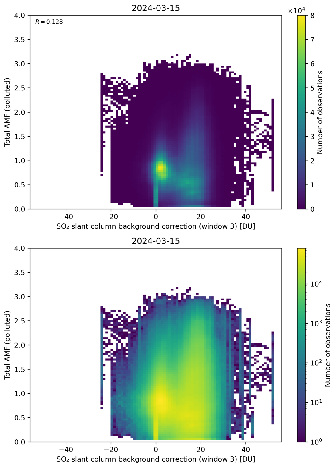
Figure 125: Scatter density plot of “SO 2 slant column background correction (window 3)” against “Total AMF (polluted)” for 2024-03-14 to 2024-03-16.
