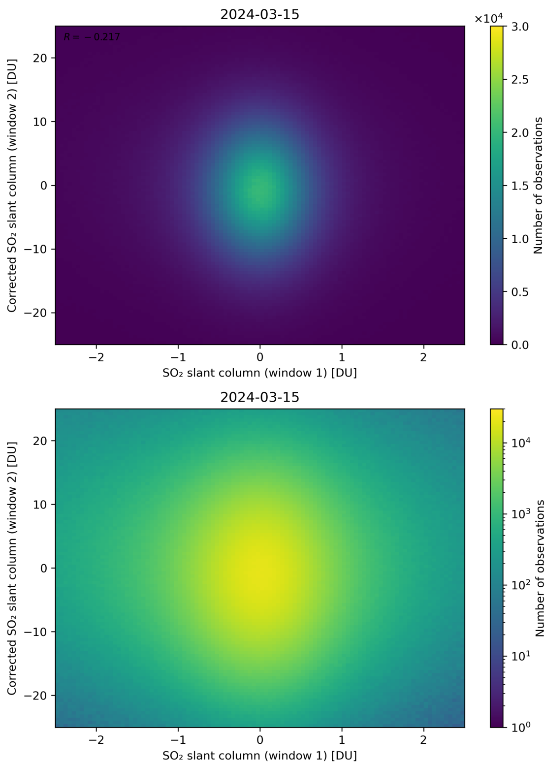
Figure 233: Scatter density plot of “SO 2 slant column (window 1)” against “Corrected SO 2 slant column (window 2)” for 2024-03-14 to 2024-03-16.
