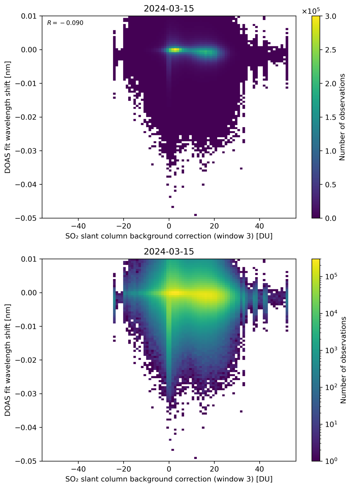
Figure 121: Scatter density plot of “SO 2 slant column background correction (window 3)” against “DOAS fit wavelength shift” for 2024-03-14 to 2024-03-16.
