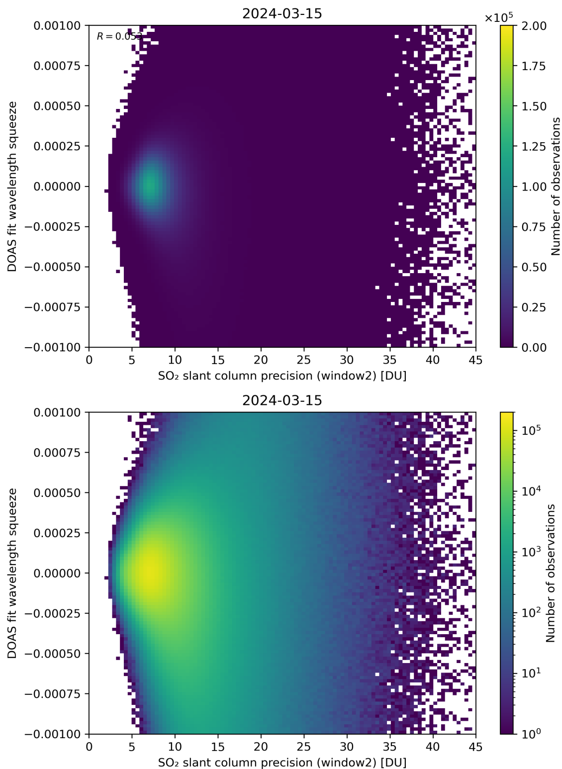
Figure 244: Scatter density plot of “SO 2 slant column precision (window2)” against “DOAS fit wavelength squeeze” for 2024-03-14 to 2024-03-16.
