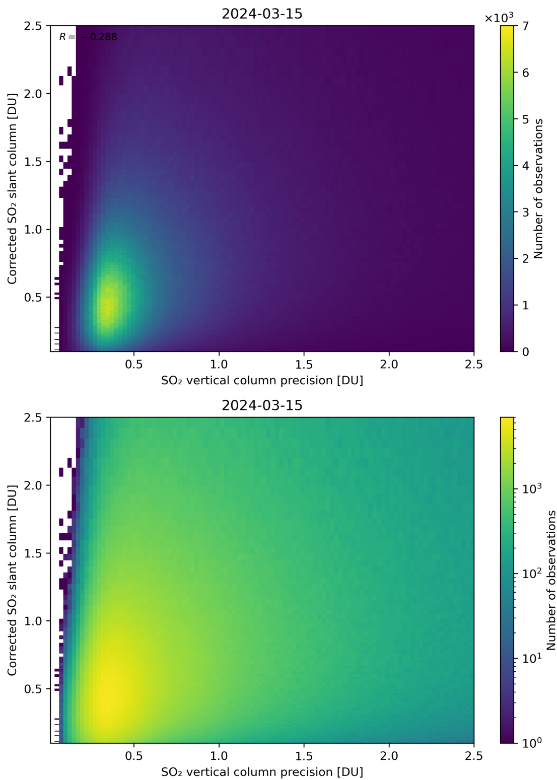
Figure 286: Scatter density plot of “SO 2 vertical column precision” against “Corrected SO 2 slant column” for 2024-03-14 to 2024-03-16.
