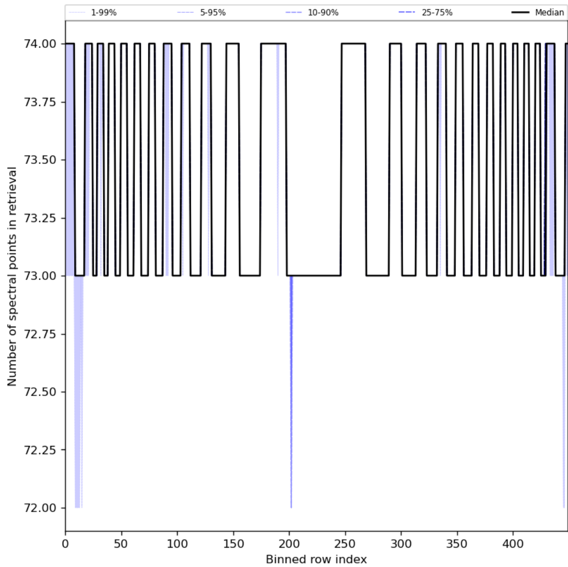
Figure 97: Along track statistics of “Number of spectral points in retrieval” for 2024-03-14 to 2024-03-16
