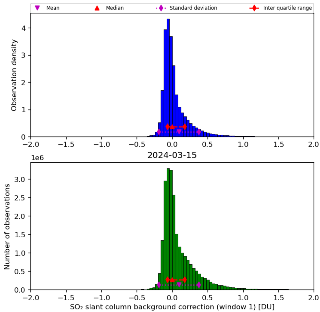
Figure 59: Histogram of “SO 2 slant column background correction (window 1)” for 2024-03-14 to 2024-03-16
