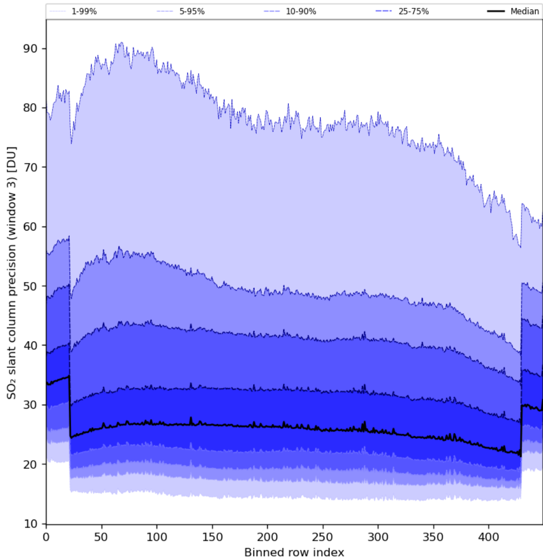
Figure 88: Along track statistics of “SO 2 slant column precision (window 3)” for 2024-03-14 to 2024-03-16
