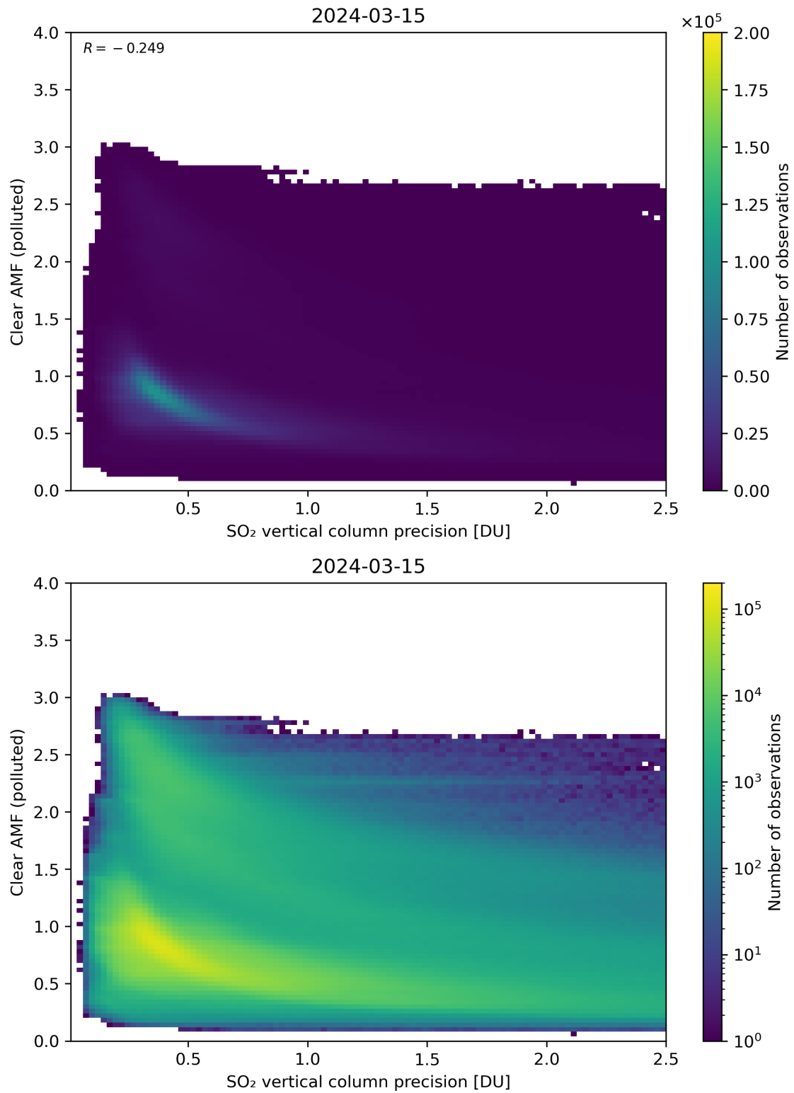
Figure 285: Scatter density plot of “SO 2 vertical column precision” against “Clear AMF (polluted)” for 2024-03-14 to 2024-03-16.
