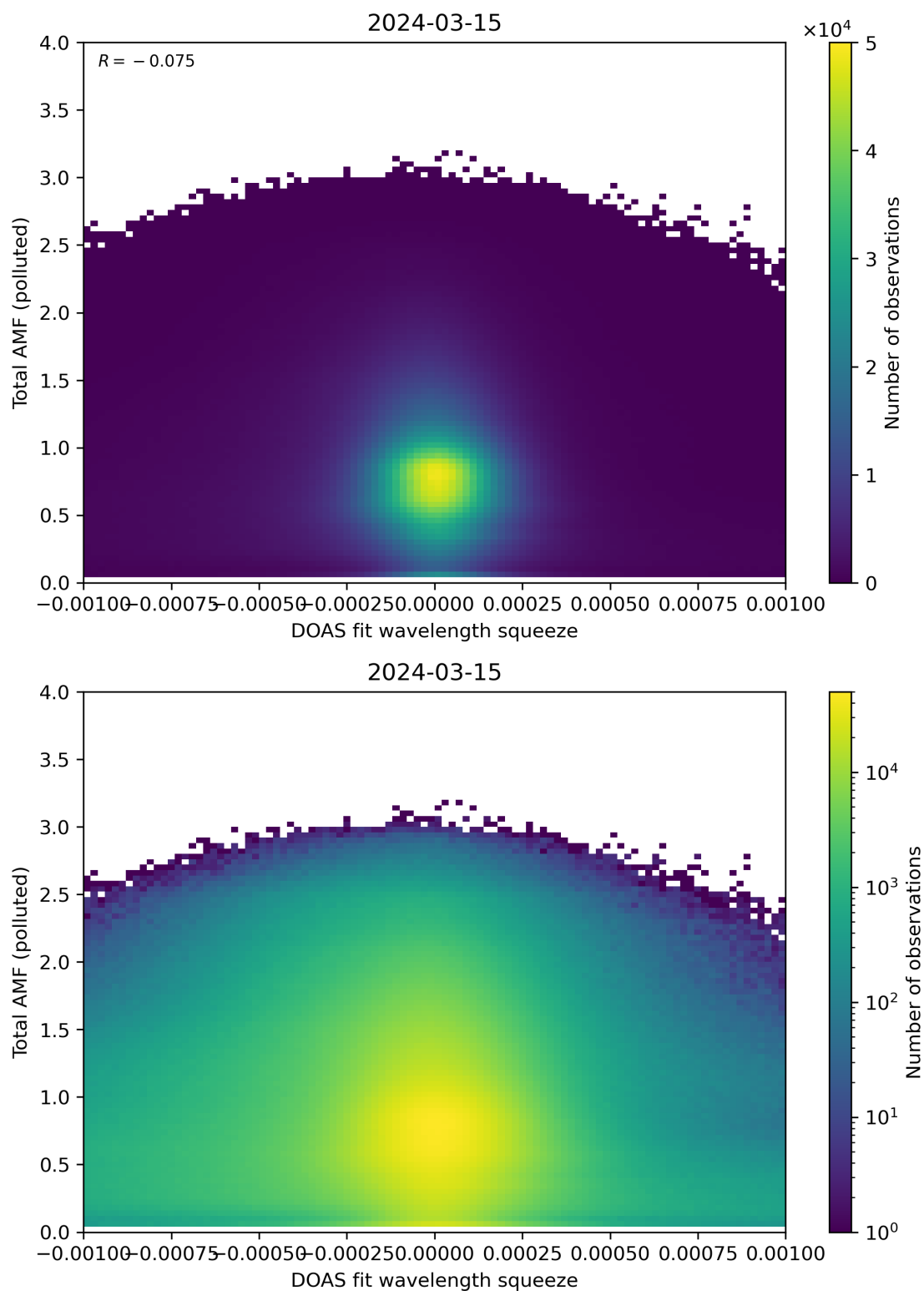
Figure 134: Scatter density plot of “DOAS fit wavelength squeeze” against “Total AMF (polluted)” for 2024-03-14 to 2024-03-16.
