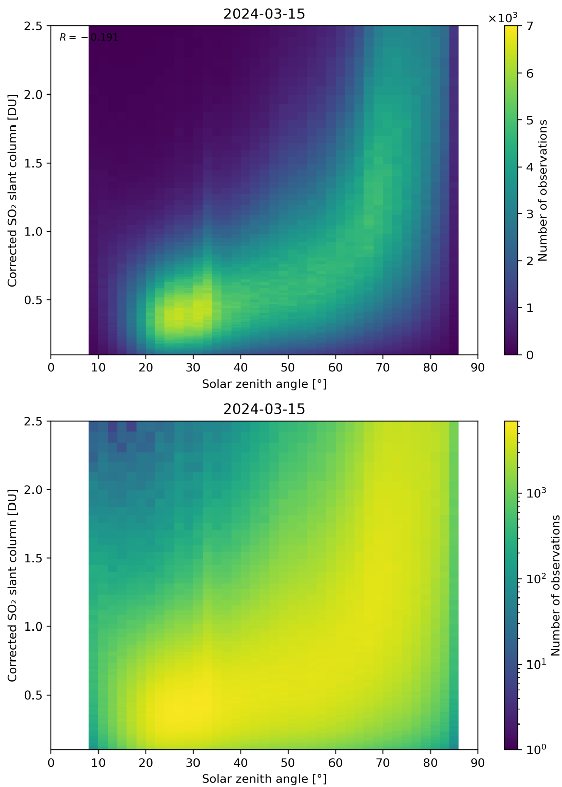
Figure 166: Scatter density plot of “Solar zenith angle” against “Corrected SO 2 slant column” for 2024-03-14 to 2024-03-16.
