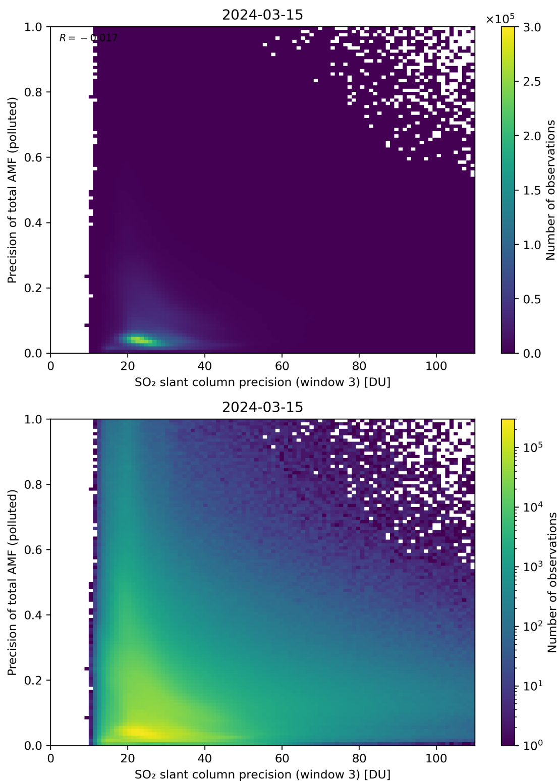
Figure 264: Scatter density plot of “SO 2 slant column precision (window 3)” against “Precision of total AMF (polluted)” for 2024-03-14 to 2024-03-16.
