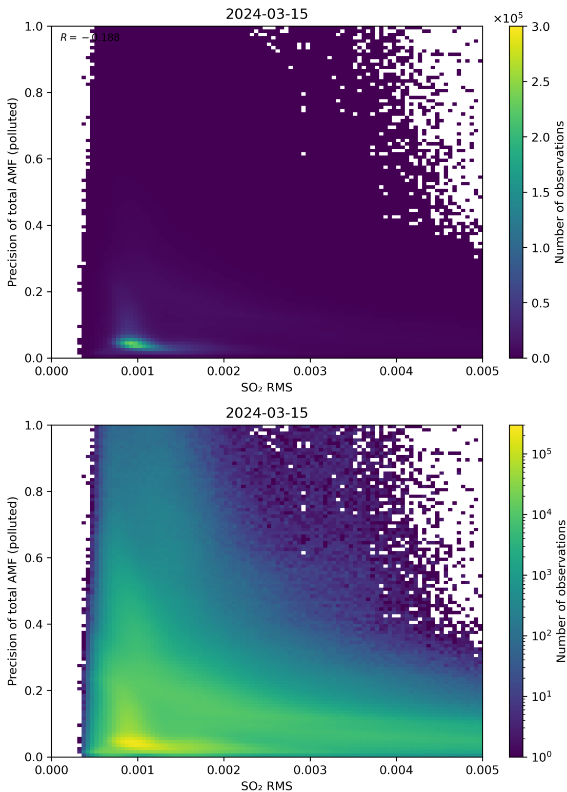
Figure 138: Scatter density plot of “SO 2 RMS” against “Precision of total AMF (polluted)” for 2024-03-14 to 2024-03-16.
