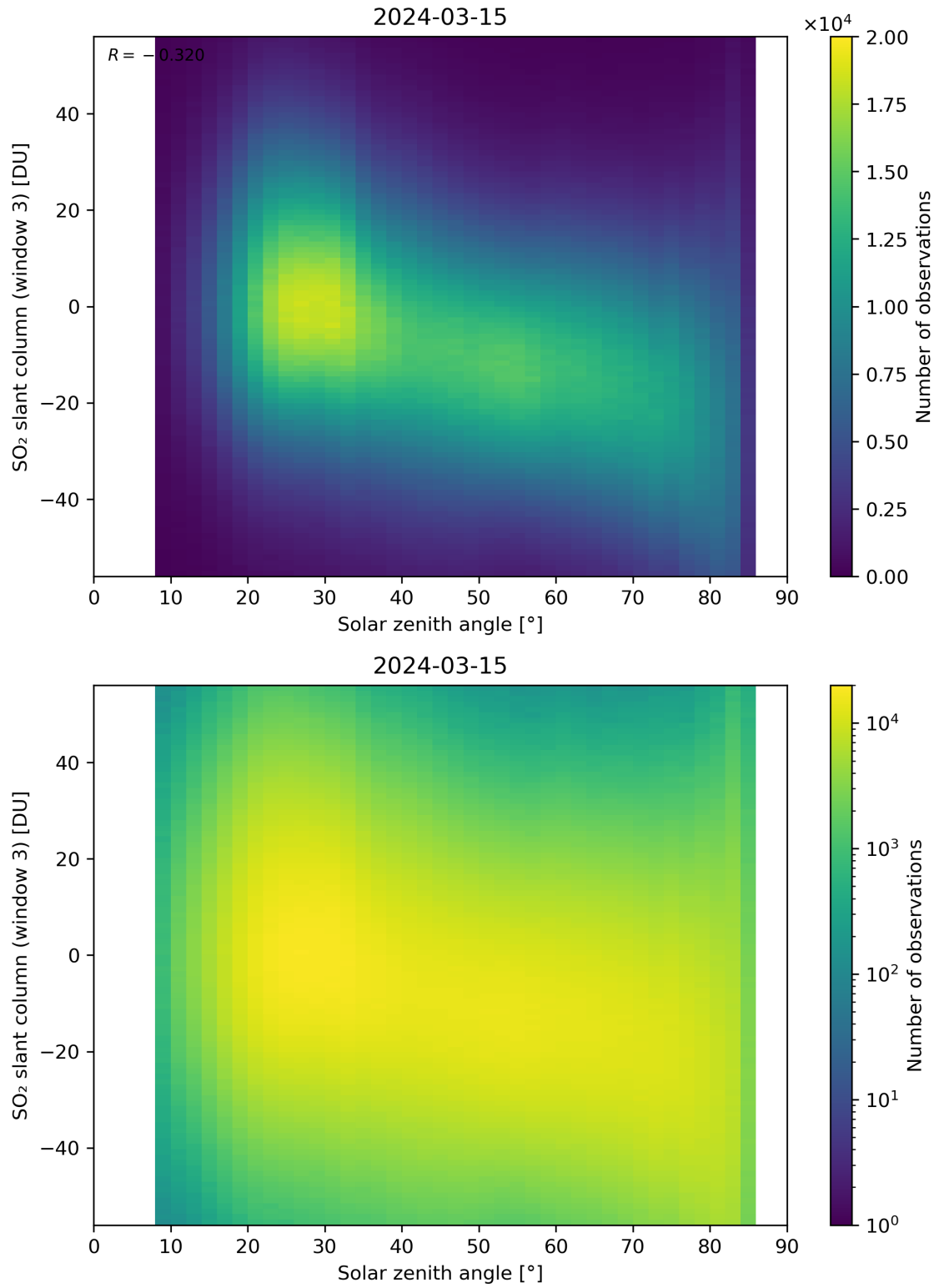
Figure 172: Scatter density plot of “Solar zenith angle” against “SO 2 slant column (window 3)” for 2024-03-14 to 2024-03-16.
