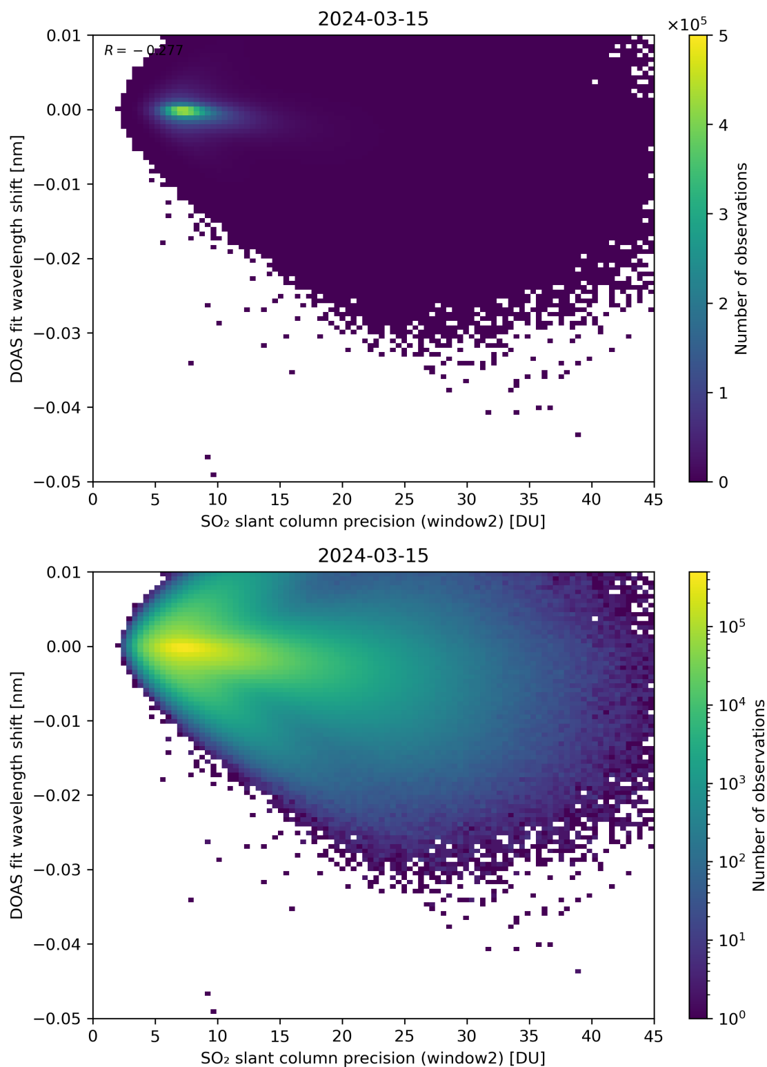
Figure 243: Scatter density plot of “SO 2 slant column precision (window2)” against “DOAS fit wavelength shift” for 2024-03-14 to 2024-03-16.
