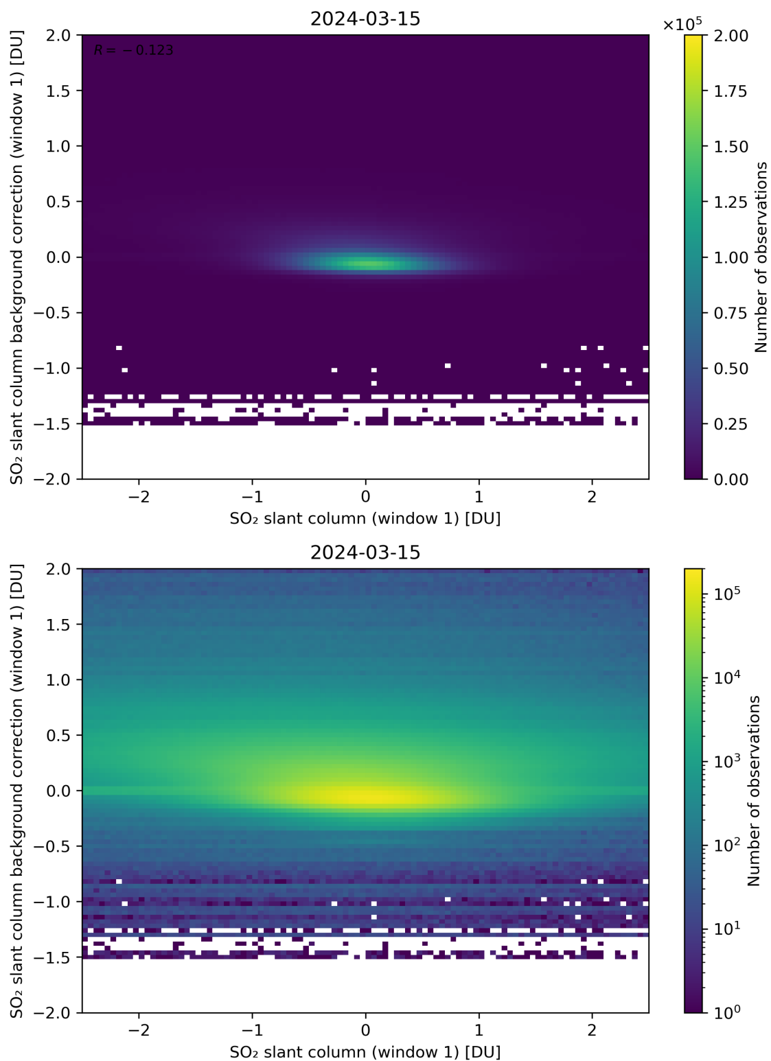
Figure 212: Scatter density plot of “SO 2 slant column (window 1)” against “SO 2 slant column background correction (window 1)” for 2024-03-14 to 2024-03-16.
