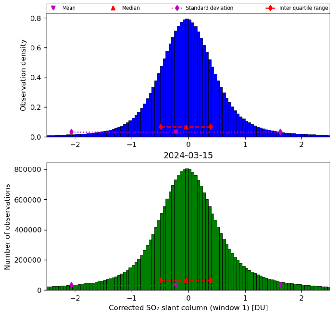
Figure 58: Histogram of “Corrected SO 2 slant column (window 1)” for 2024-03-14 to 2024-03-16
