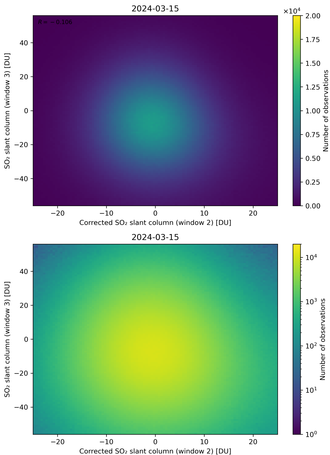
Figure 201: Scatter density plot of “Corrected SO 2 slant column (window 2)” against “SO 2 slant column (window 3)” for 2024-03-14 to 2024-03-16.
