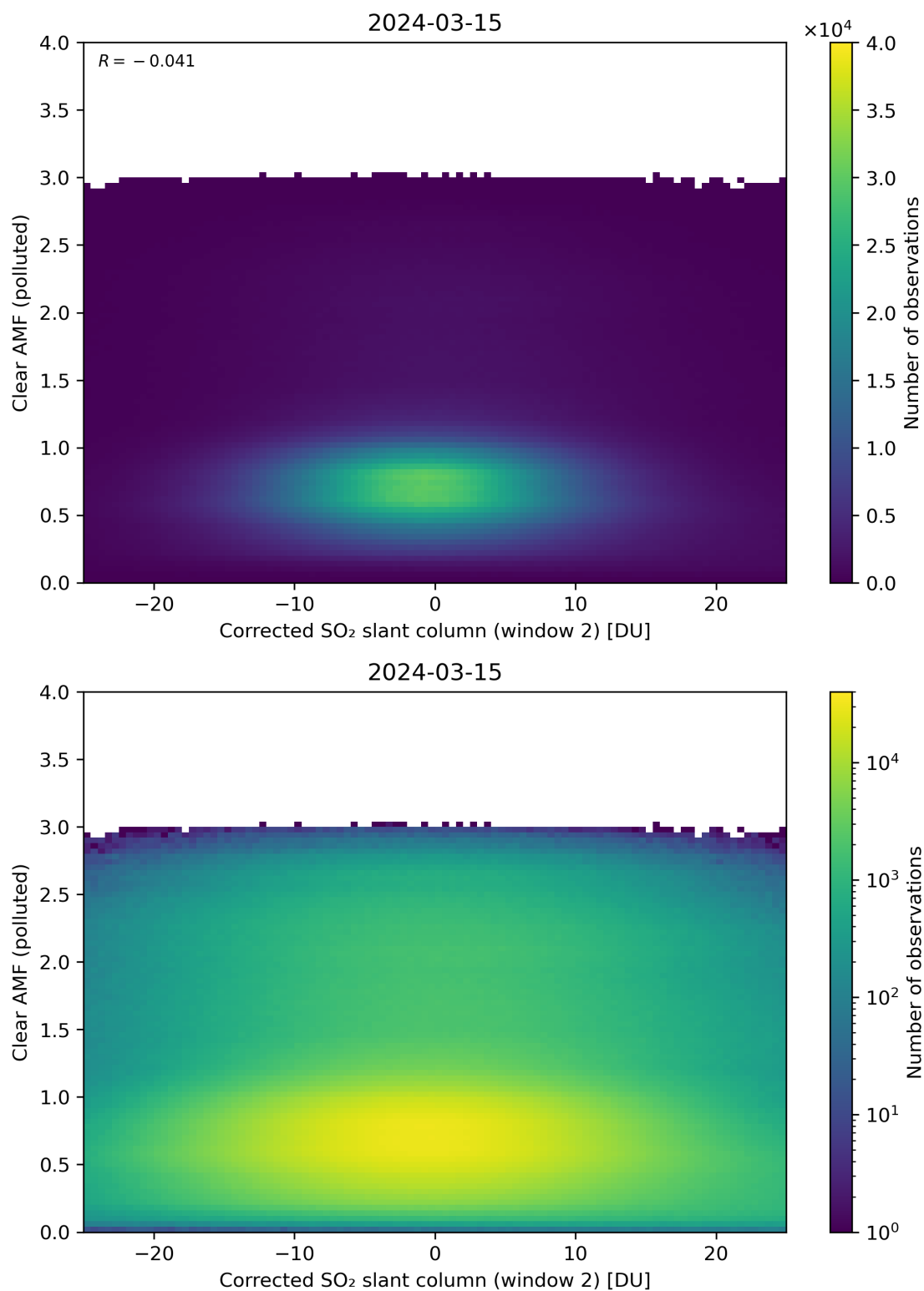
Figure 199: Scatter density plot of “Corrected SO 2 slant column (window 2)” against “Clear AMF (polluted)” for 2024-03-14 to 2024-03-16.
