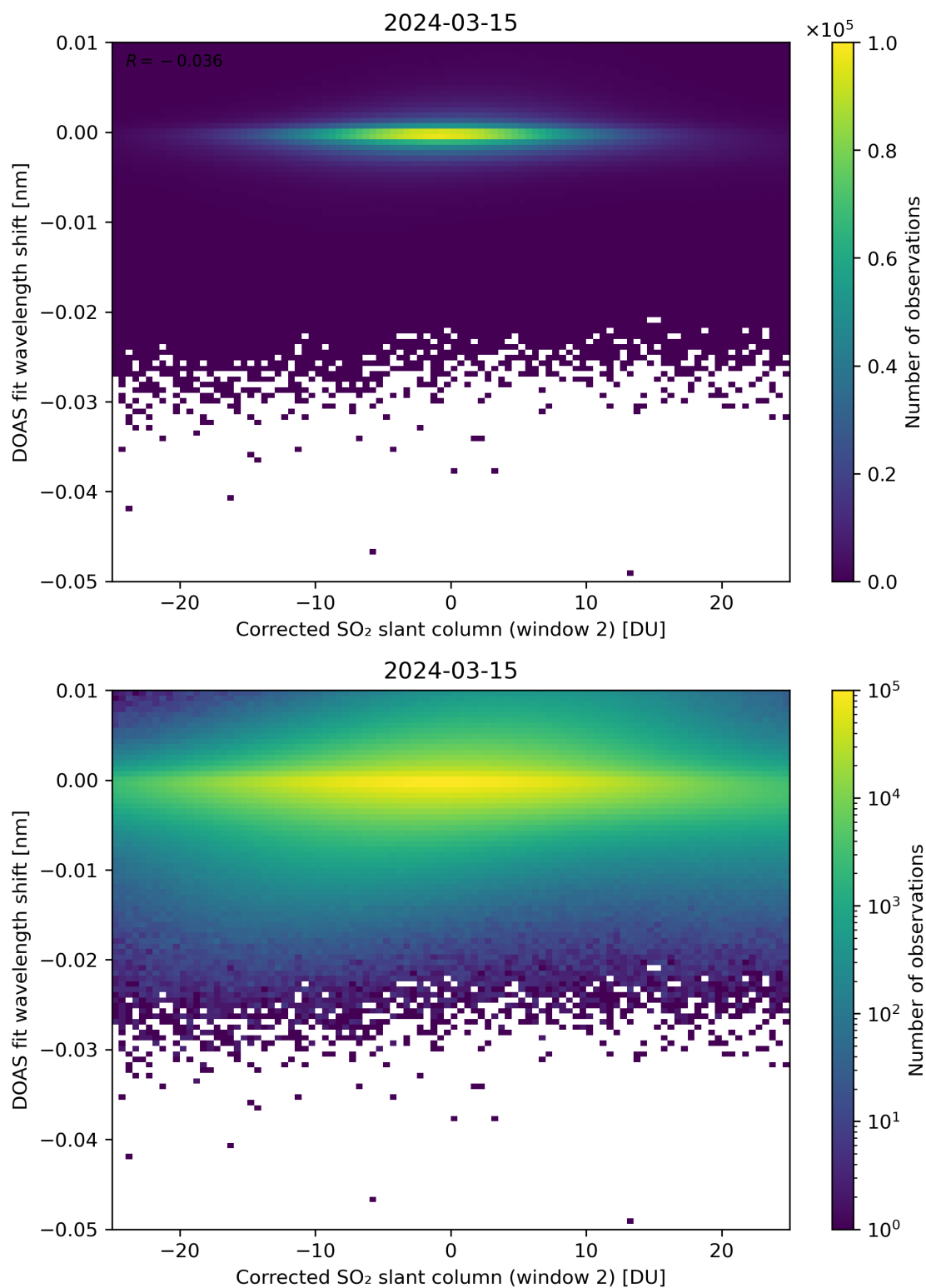
Figure 196: Scatter density plot of “Corrected SO 2 slant column (window 2)” against “DOAS fit wavelength shift” for 2024-03-14 to 2024-03-16.
