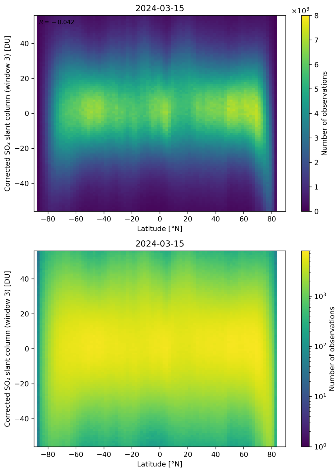
Figure 148: Scatter density plot of “Latitude” against “Corrected SO 2 slant column (window 3)” for 2024-03-14 to 2024-03-16.
