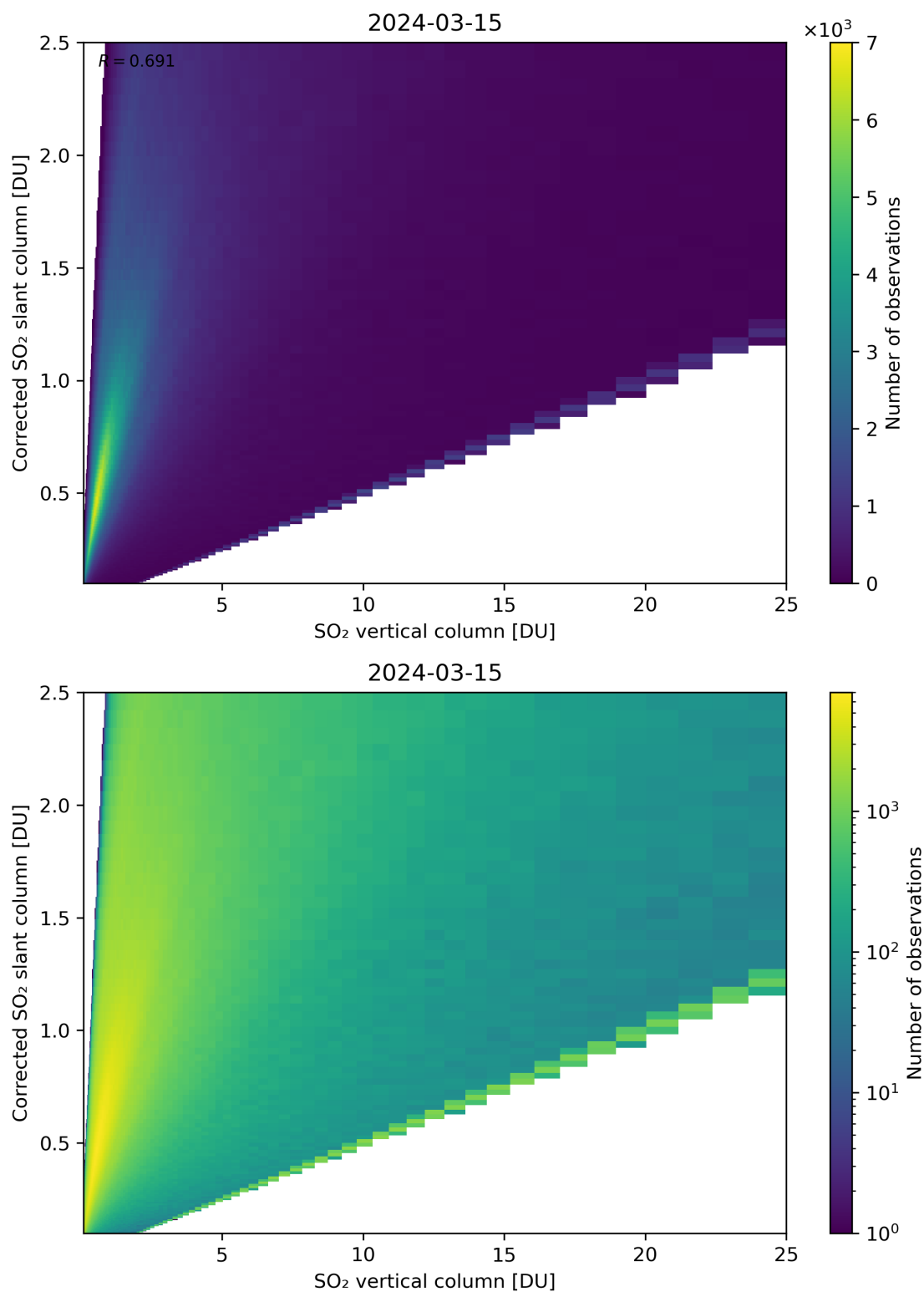
Figure 297: Scatter density plot of “SO 2 vertical column” against “Corrected SO 2 slant column” for 2024-03-14 to 2024-03-16.
