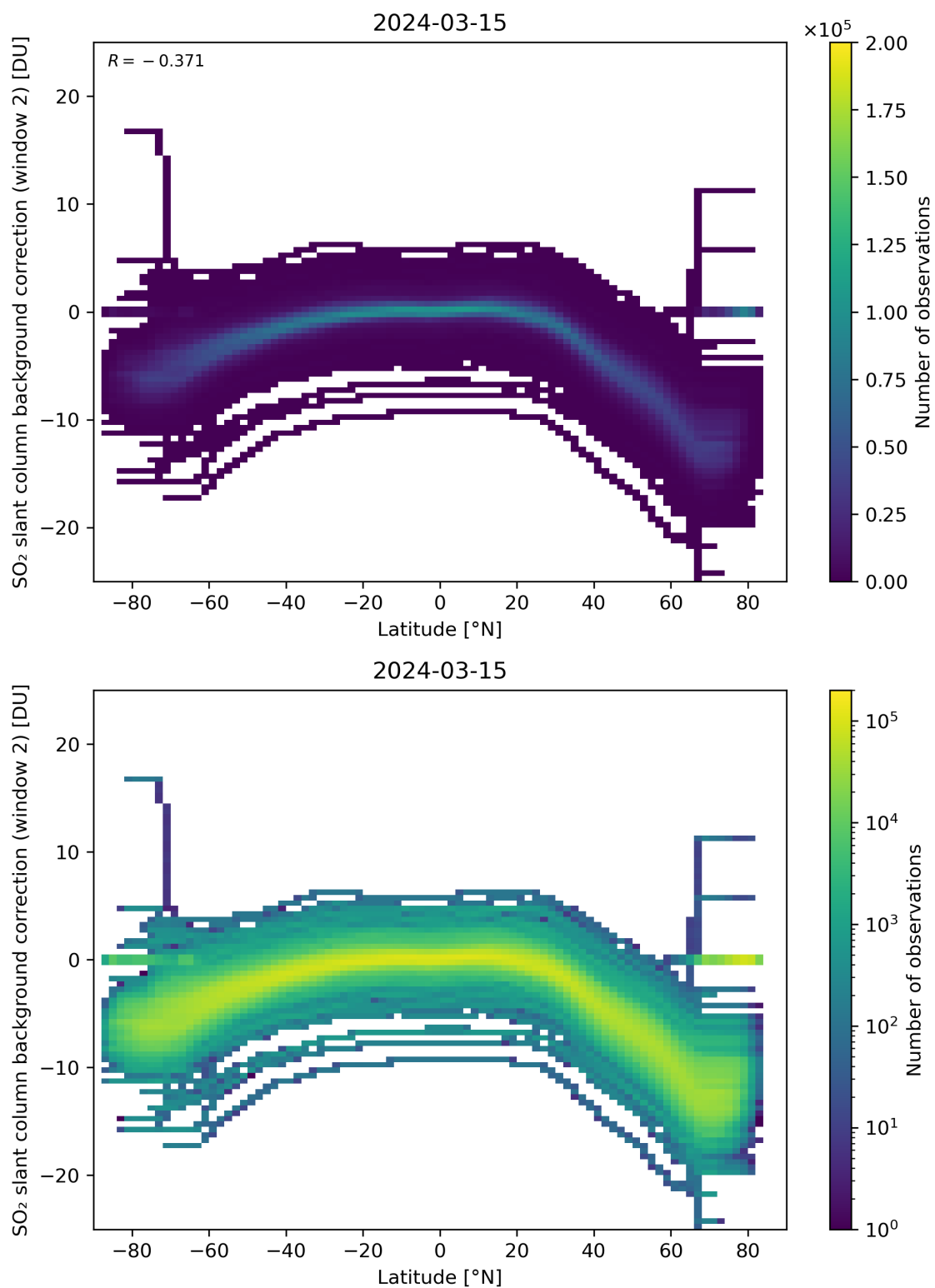
Figure 140: Scatter density plot of “Latitude” against “SO 2 slant column background correction (window 2)” for 2024-03-14 to 2024-03-16.
