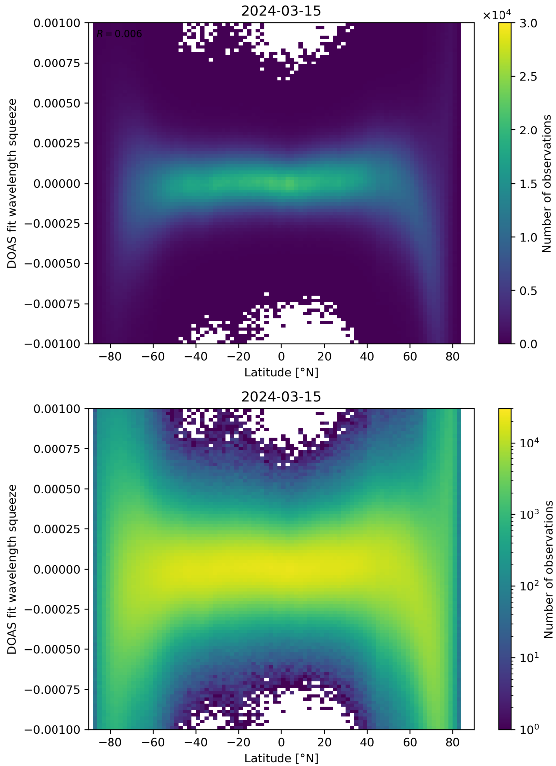
Figure 143: Scatter density plot of “Latitude” against “DOAS fit wavelength squeeze” for 2024-03-14 to 2024-03-16.
