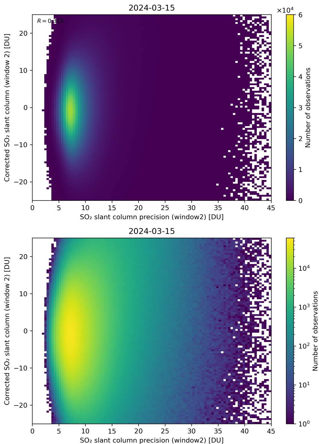
Figure 247: Scatter density plot of “SO 2 slant column precision (window2)” against “Corrected SO 2 slant column (window 2)” for 2024-03-14 to 2024-03-16.
