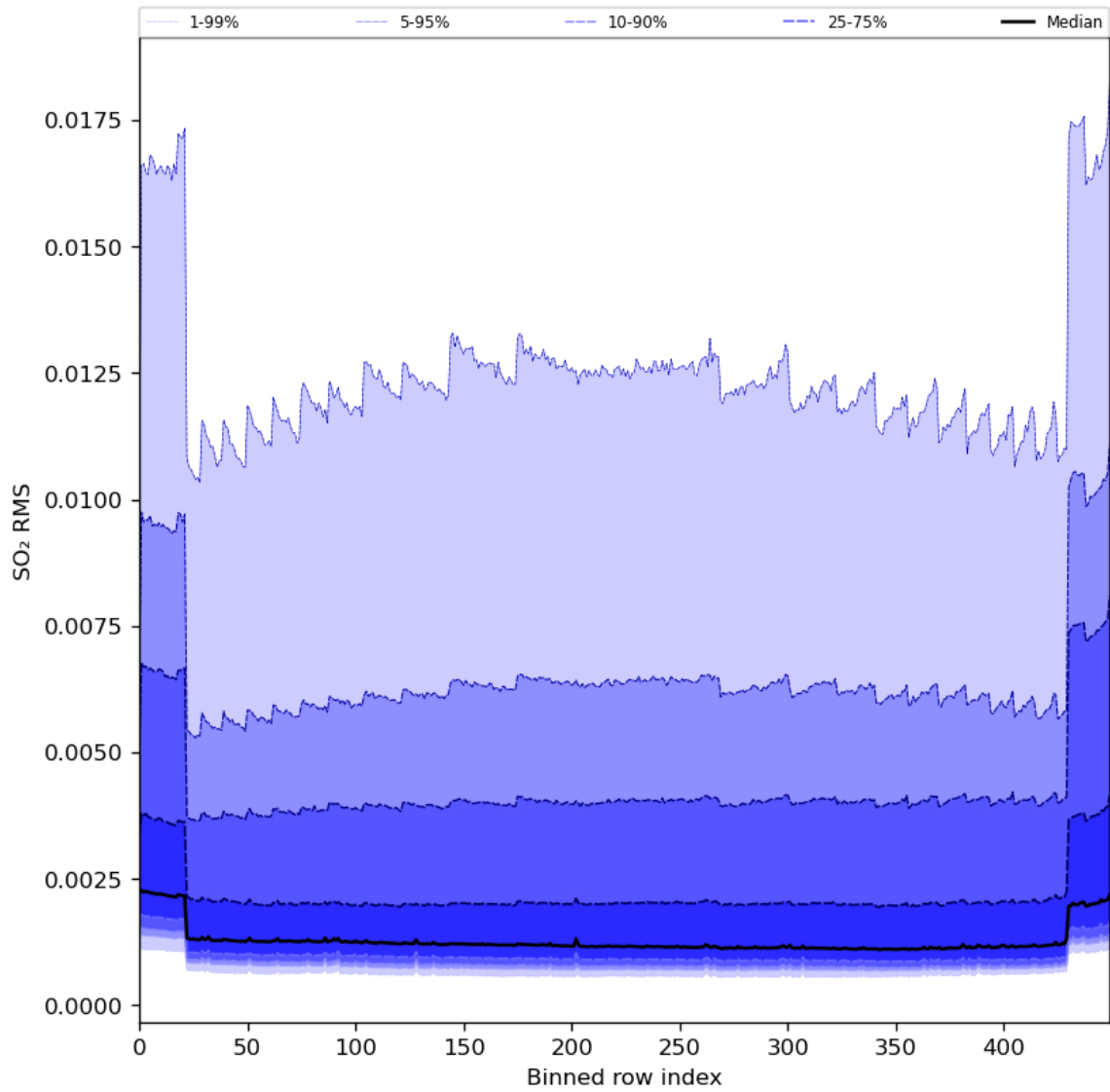
Figure 93: Along track statistics of “SO 2 RMS” for 2024-03-14 to 2024-03-16
