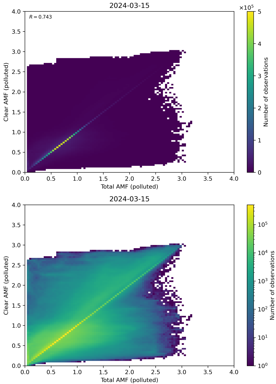
Figure 271: Scatter density plot of “Total AMF (polluted)” against “Clear AMF (polluted)” for 2024-03-14 to 2024-03-16.
