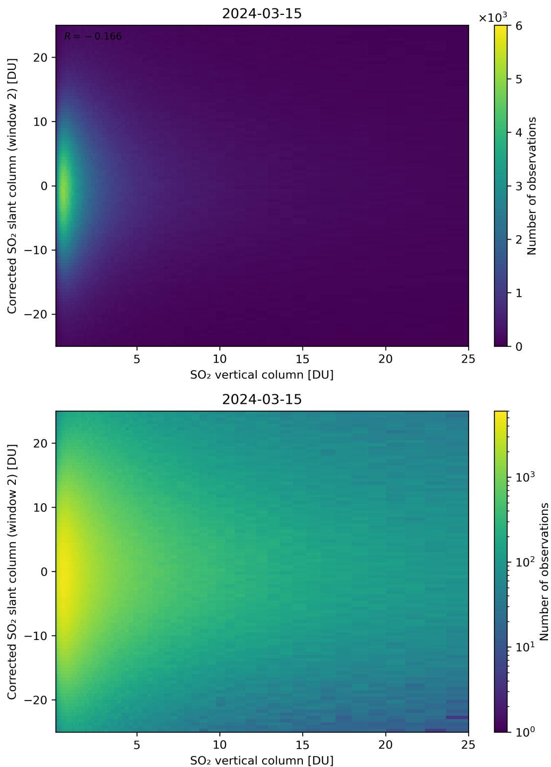
Figure 298: Scatter density plot of “SO 2 vertical column” against “Corrected SO 2 slant column (window 2)” for 2024-03-14 to 2024-03-16.
