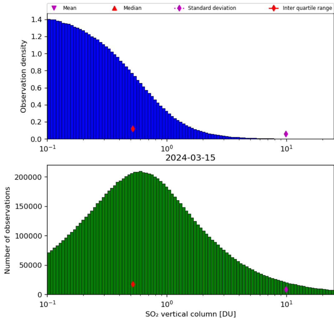
Figure 53: Histogram of “SO 2 vertical column” for 2024-03-14 to 2024-03-16
