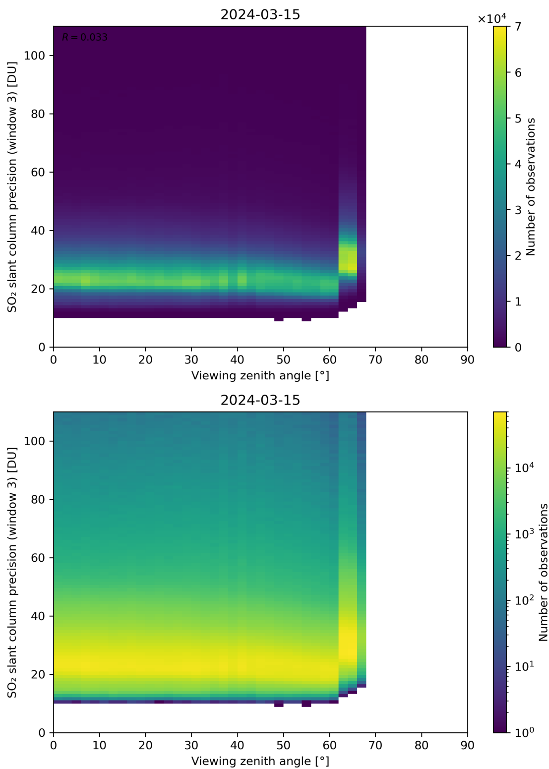
Figure 324: Scatter density plot of “Viewing zenith angle” against “SO 2 slant column precision (window 3)” for 2024-03-14 to 2024-03-16.
