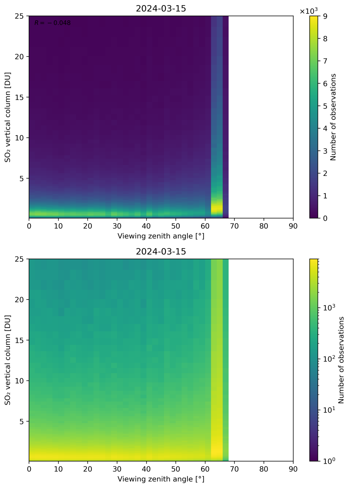
Figure 327: Scatter density plot of “Viewing zenith angle” against “SO 2 vertical column” for 2024-03-14 to 2024-03-16.
