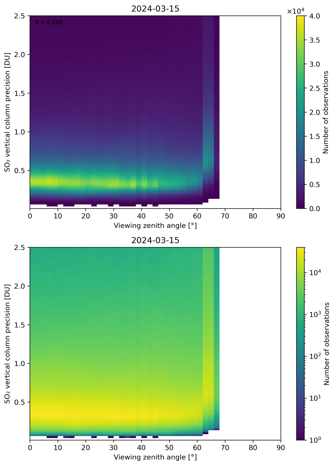
Figure 328: Scatter density plot of “Viewing zenith angle” against “SO 2 vertical column precision” for 2024-03-14 to 2024-03-16.
