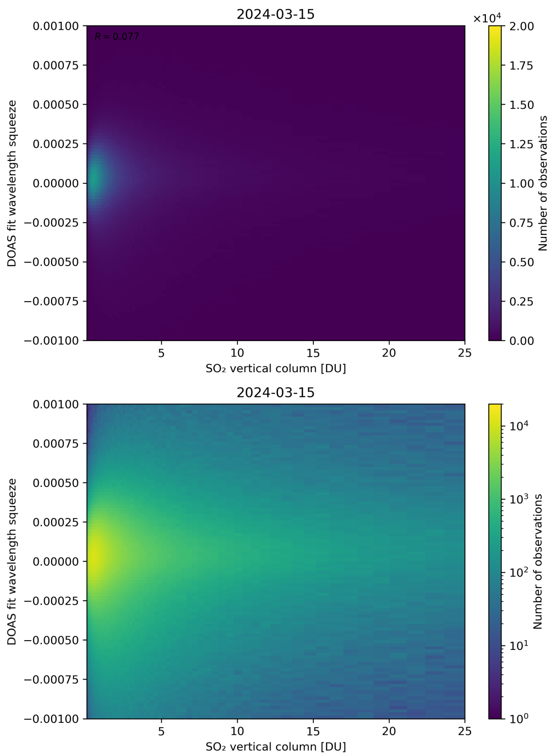
Figure 277: Scatter density plot of “SO 2 vertical column” against “DOAS fit wavelength squeeze” for 2024-03-14 to 2024-03-16.
