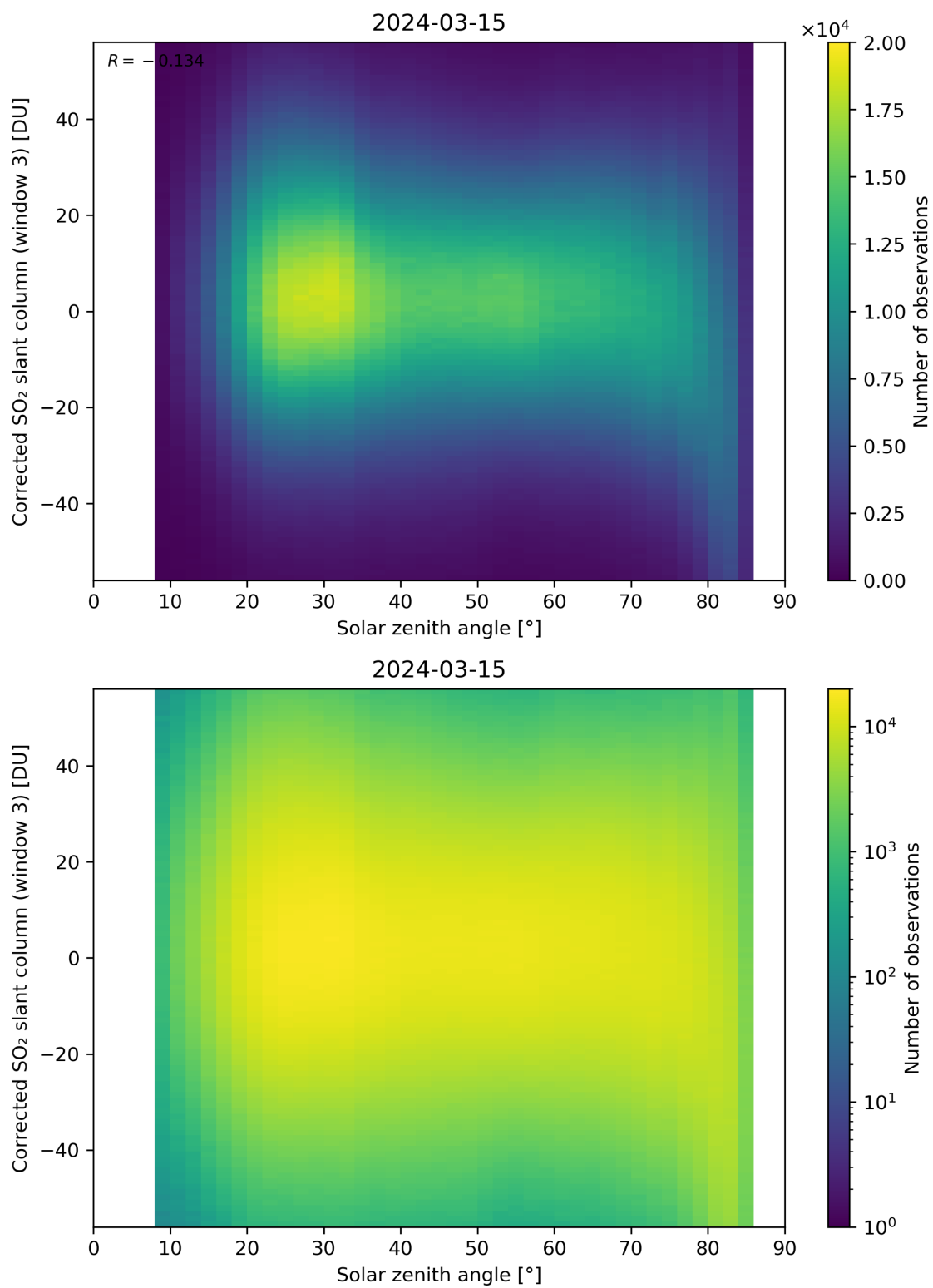
Figure 168: Scatter density plot of “Solar zenith angle” against “Corrected SO 2 slant column (window 3)” for 2024-03-14 to 2024-03-16.
