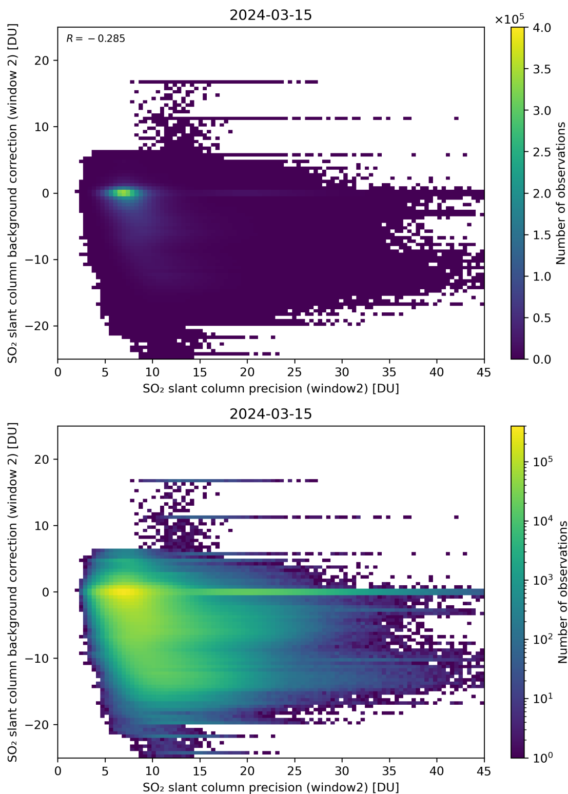
Figure 241: Scatter density plot of “SO 2 slant column precision (window2)” against “SO 2 slant column background correction (window 2)” for 2024-03-14 to 2024-03-16.
