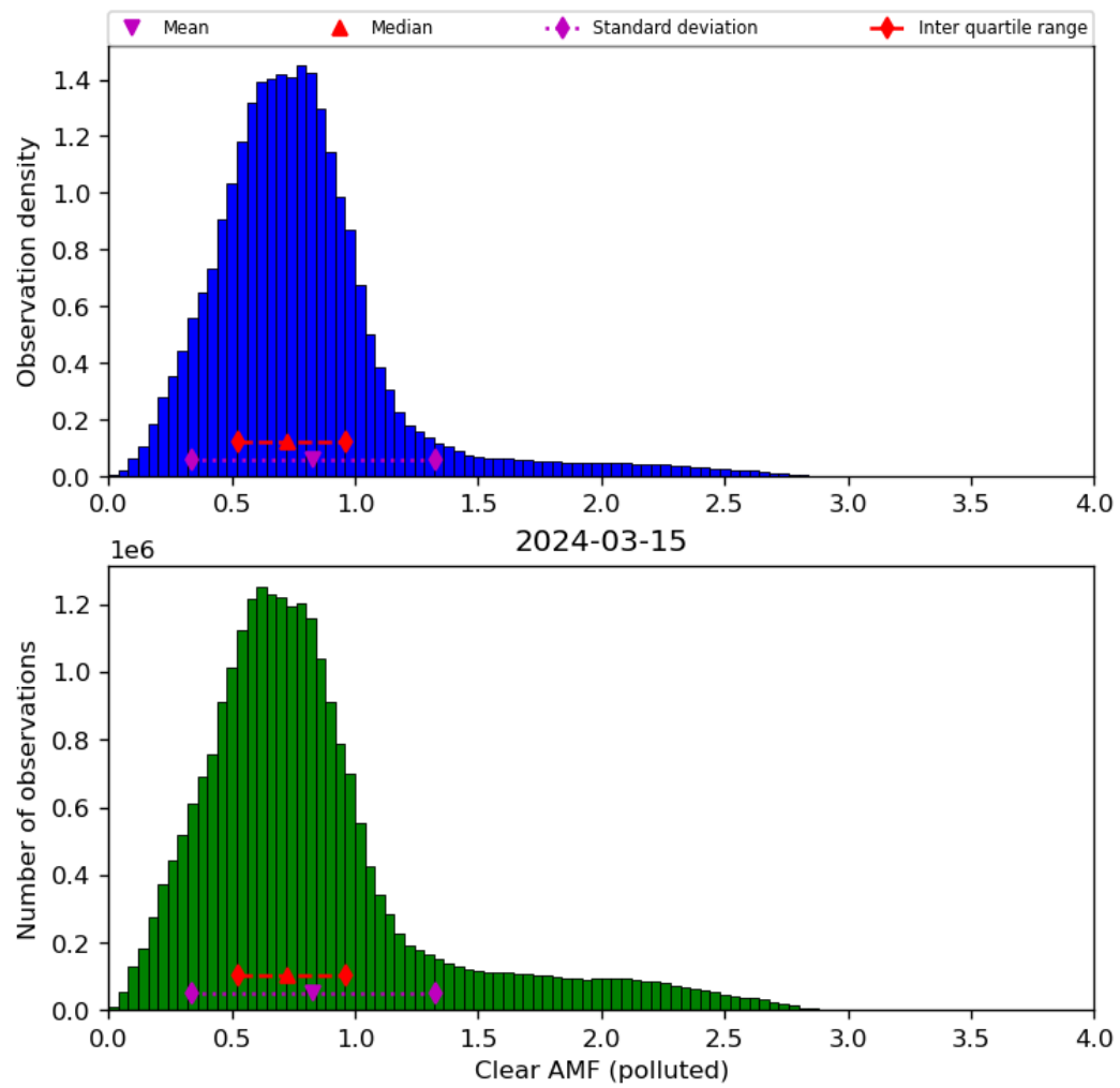
Figure 73: Histogram of “Clear AMF (polluted)” for 2024-03-14 to 2024-03-16
