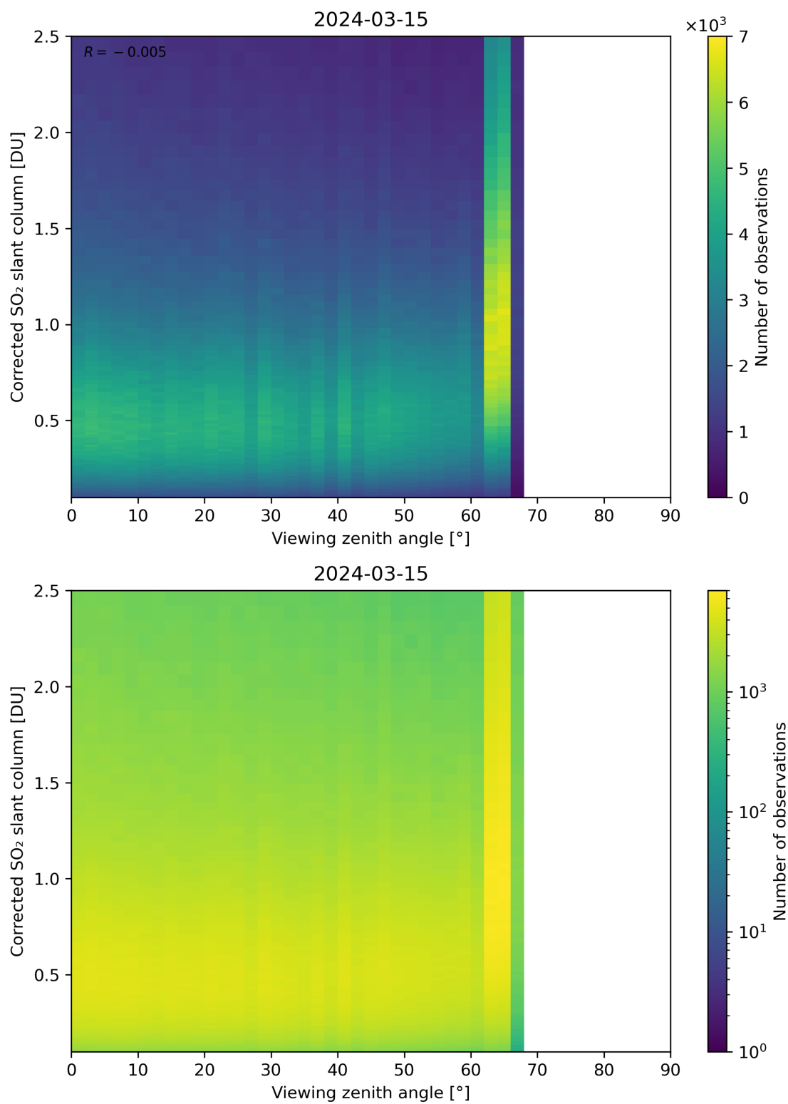
Figure 317: Scatter density plot of “Viewing zenith angle” against “Corrected SO 2 slant column” for 2024-03-14 to 2024-03-16.
