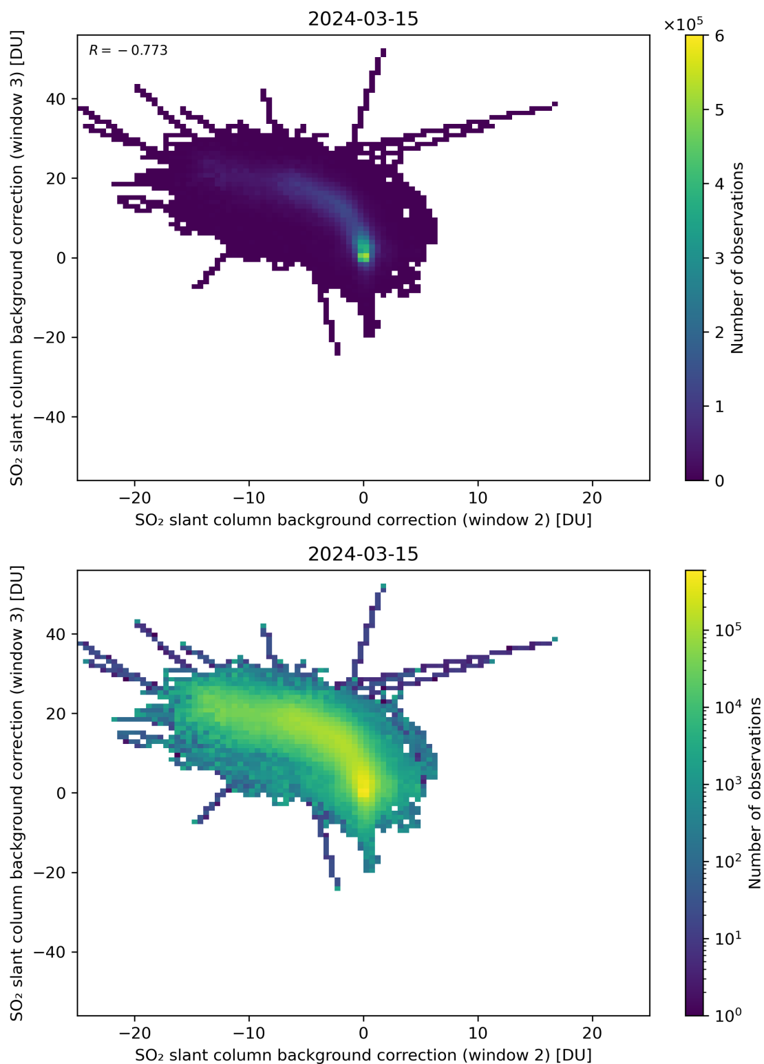
Figure 111: Scatter density plot of “SO 2 slant column background correction (window 2)” against “SO 2 slant column background correction (window 3)” for 2024-03-14 to 2024-03-16.
