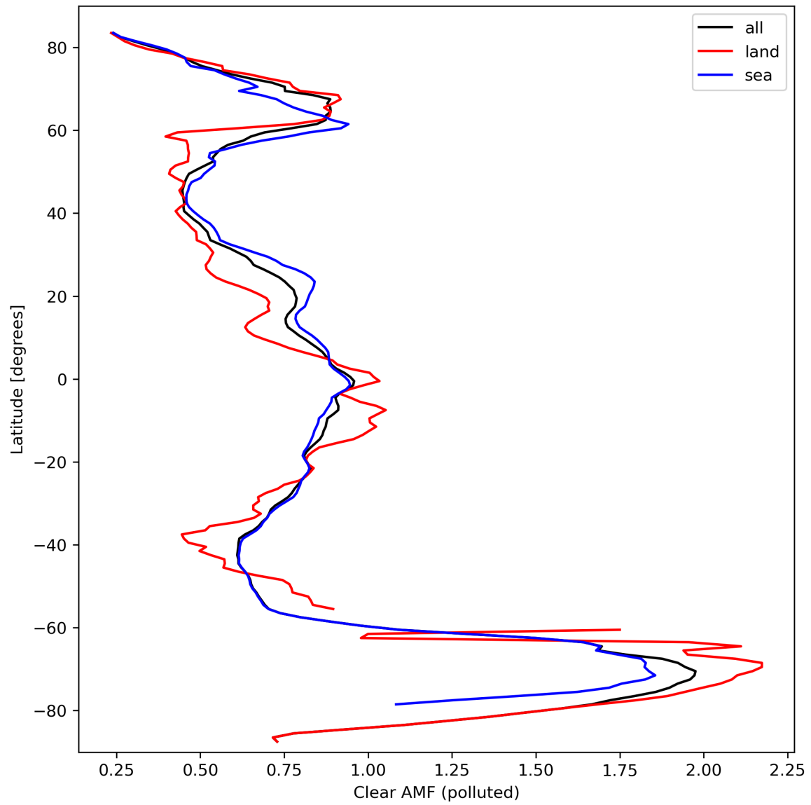
Figure 50: Zonal average of “Clear AMF (polluted)” for 2024-03-14 to 2024-03-16.
