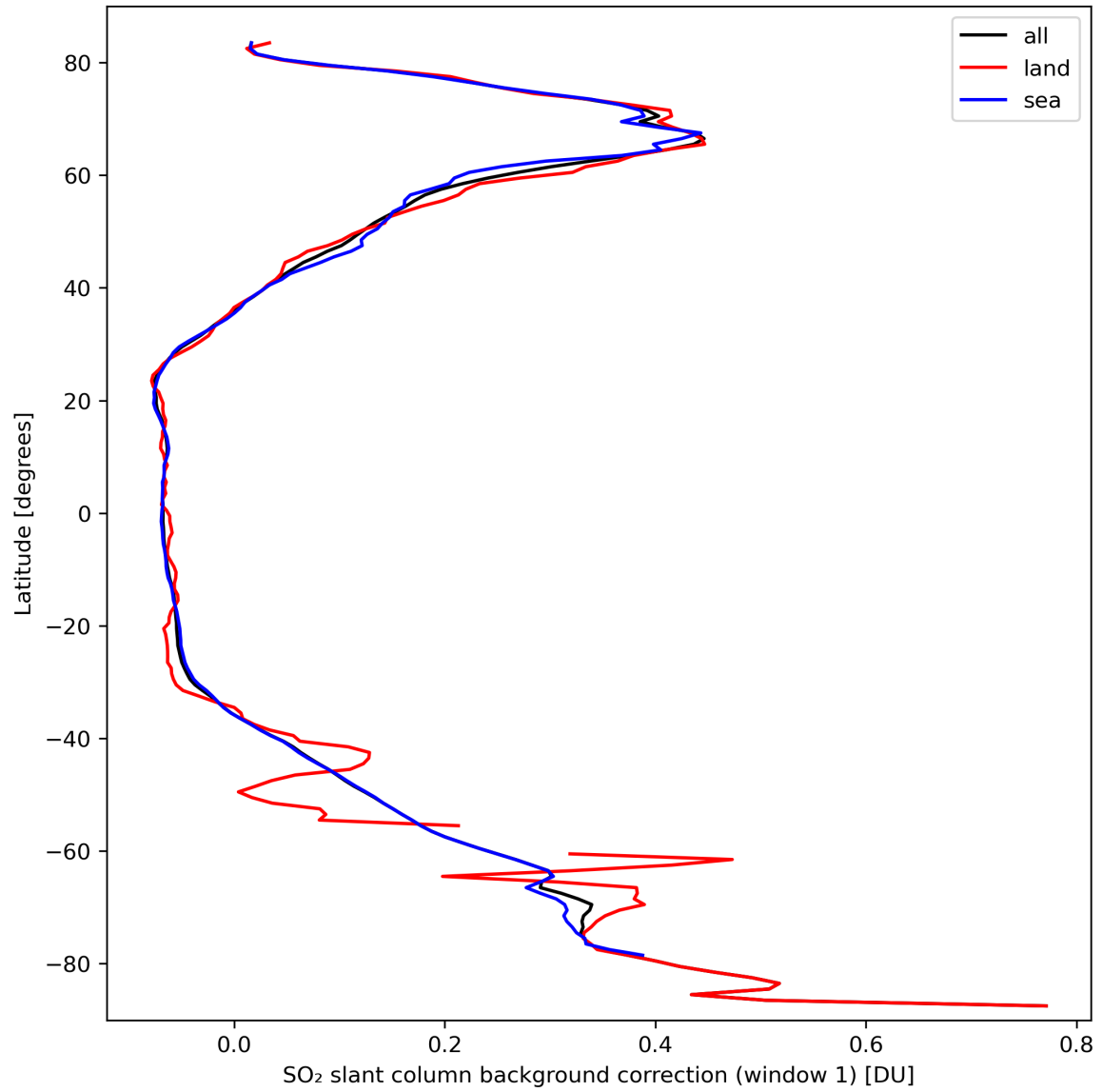
Figure 36: Zonal average of “SO 2 slant column background correction (window 1)” for 2024-03-14 to 2024-03-16.
