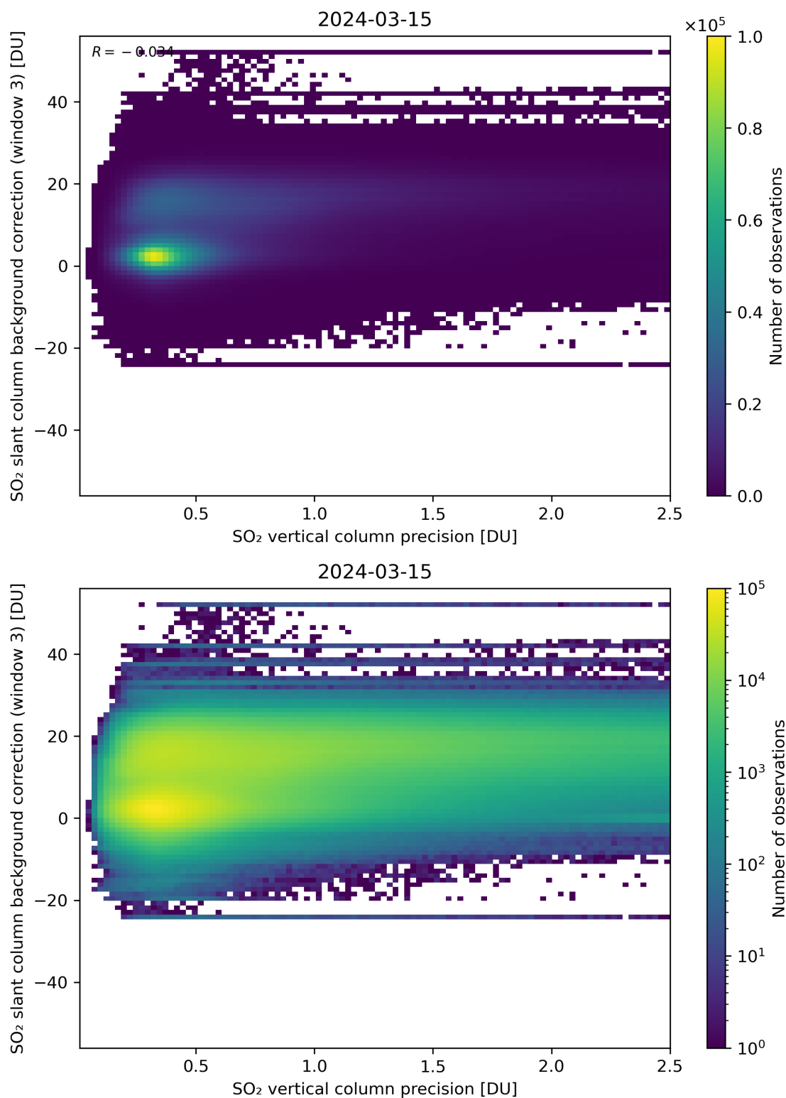
Figure 281: Scatter density plot of “SO 2 vertical column precision” against “SO 2 slant column background correction (window 3)” for 2024-03-14 to 2024-03-16.
