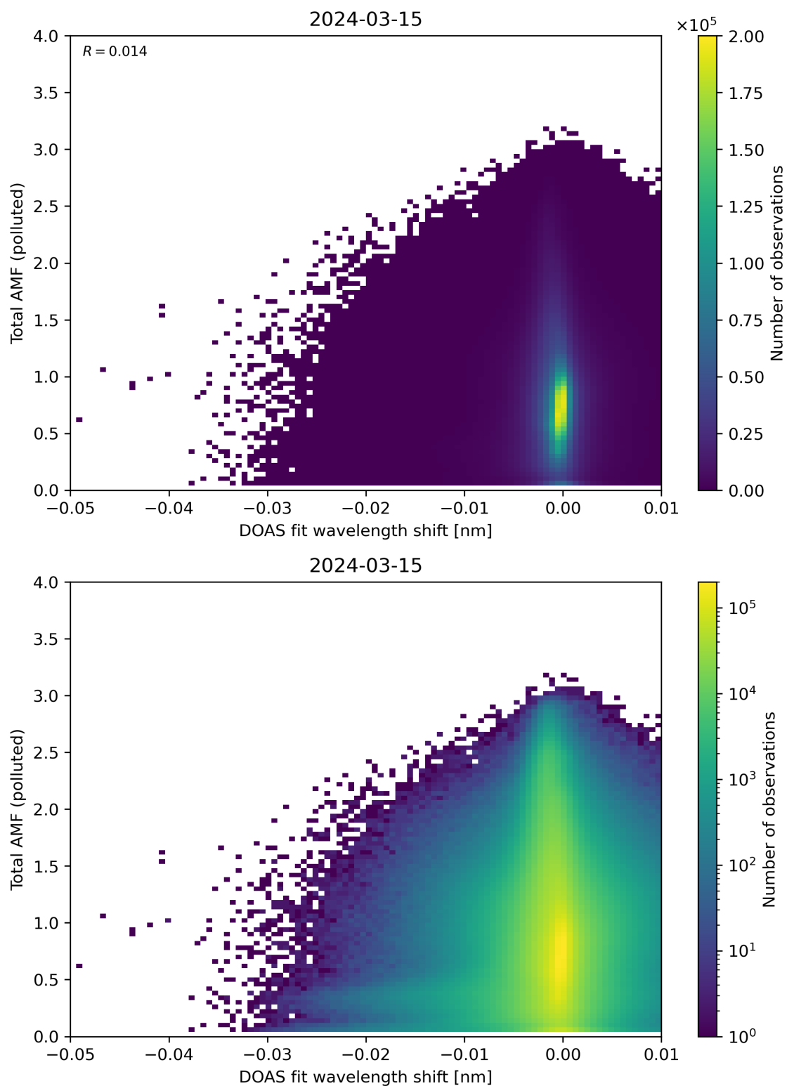
Figure 130: Scatter density plot of “DOAS fit wavelength shift” against “Total AMF (polluted)” for 2024-03-14 to 2024-03-16.
