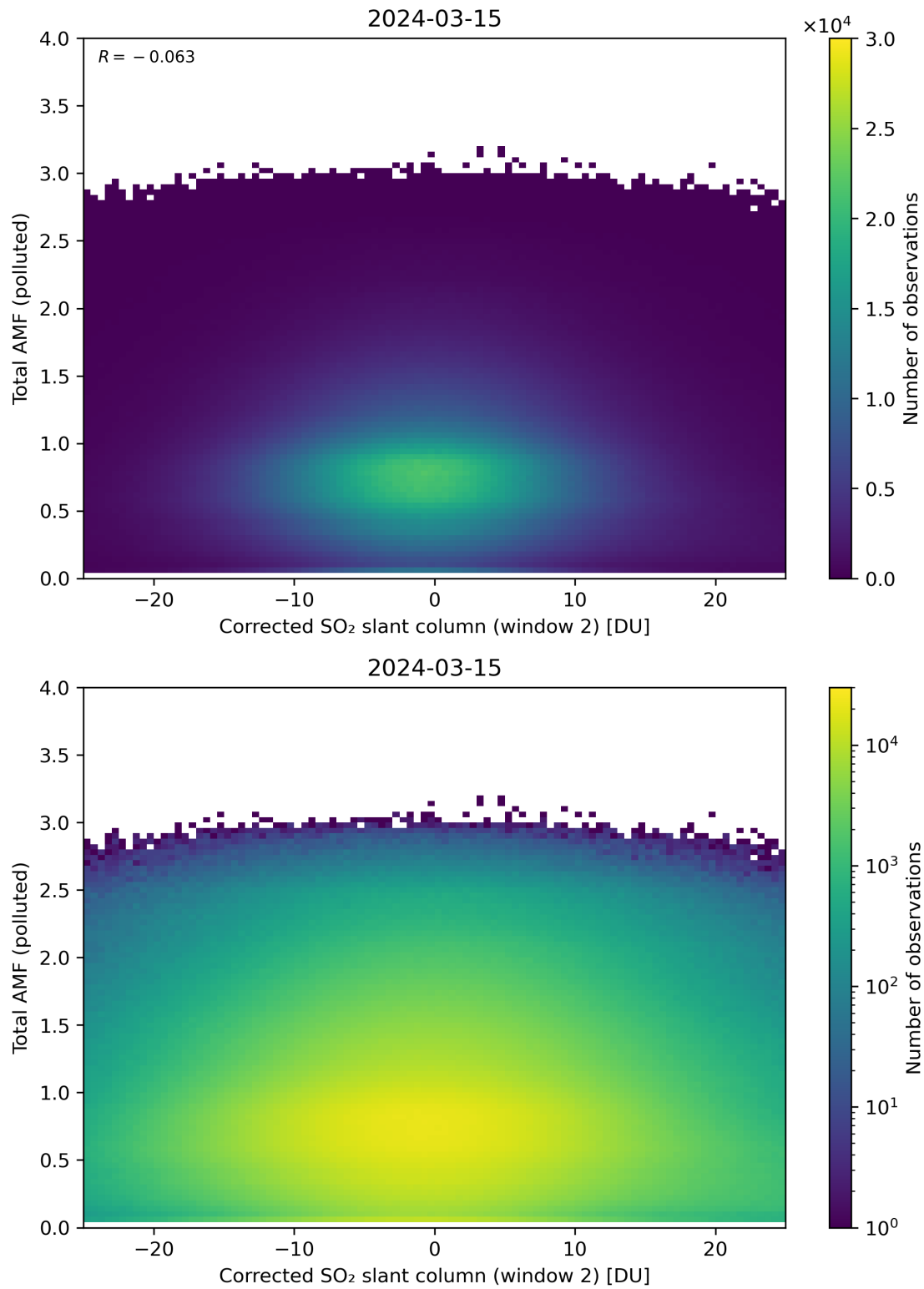
Figure 203: Scatter density plot of “Corrected SO 2 slant column (window 2)” against “Total AMF (polluted)” for 2024-03-14 to 2024-03-16.
