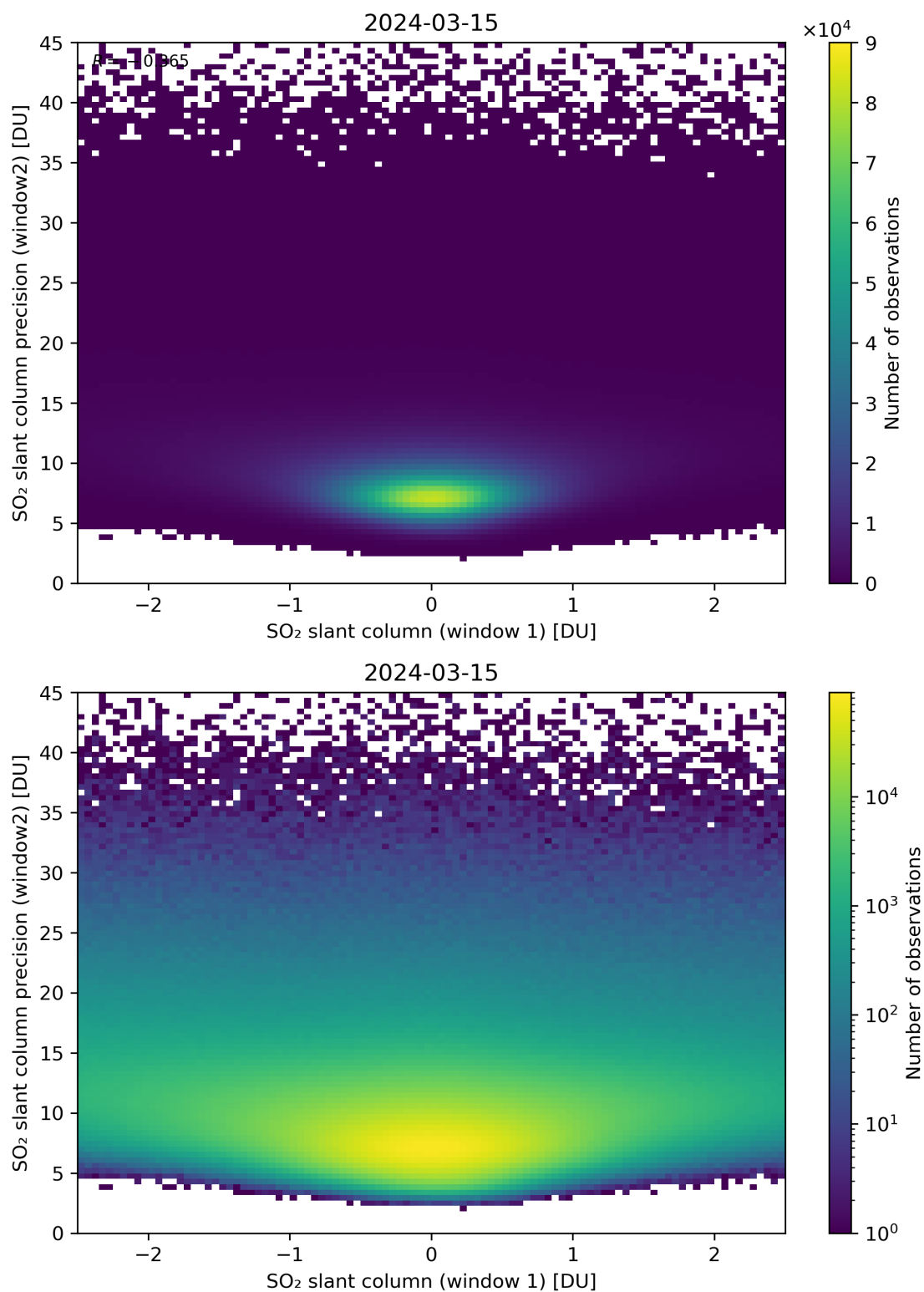
Figure 236: Scatter density plot of “SO 2 slant column (window 1)” against “SO 2 slant column precision (window2)” for 2024-03-14 to 2024-03-16.
