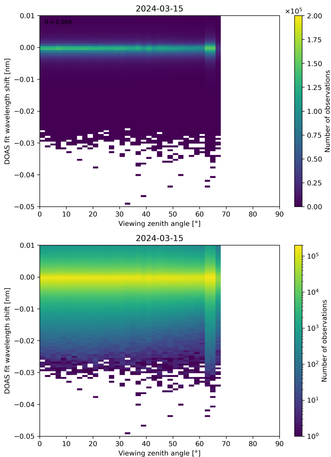
Figure 311: Scatter density plot of “Viewing zenith angle” against “DOAS fit wavelength shift” for 2024-03-14 to 2024-03-16.
