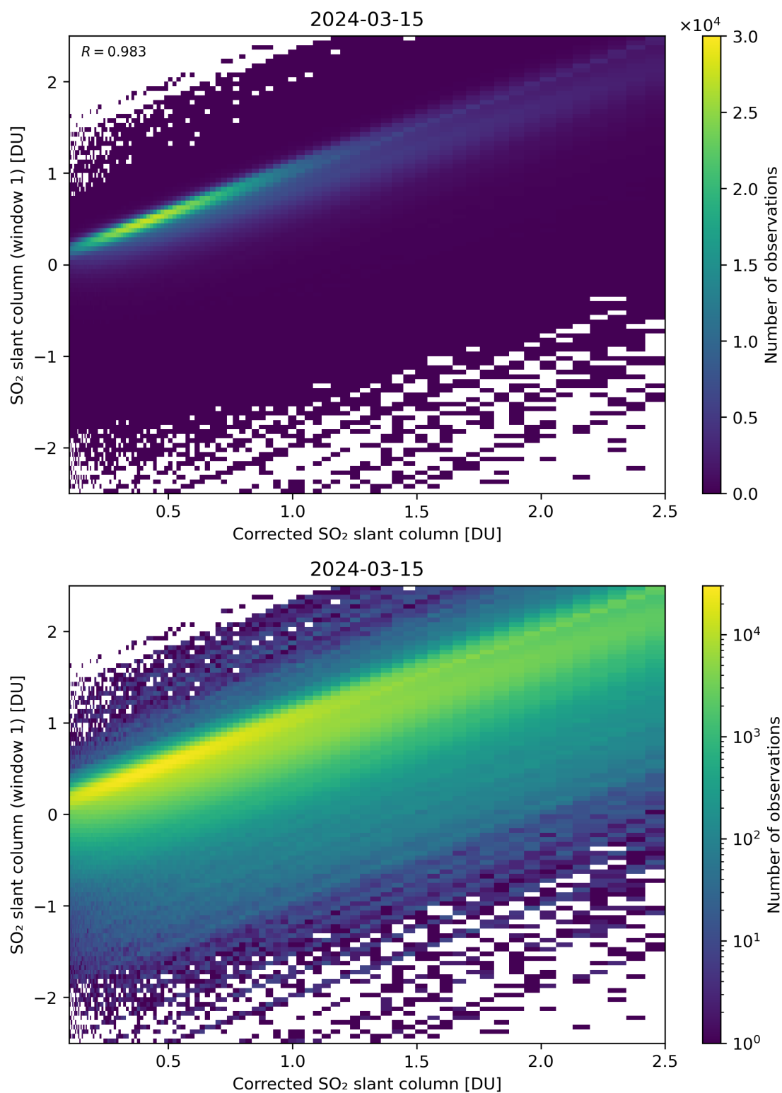
Figure 187: Scatter density plot of “Corrected SO 2 slant column” against “SO 2 slant column (window 1)” for 2024-03-14 to 2024-03-16.
