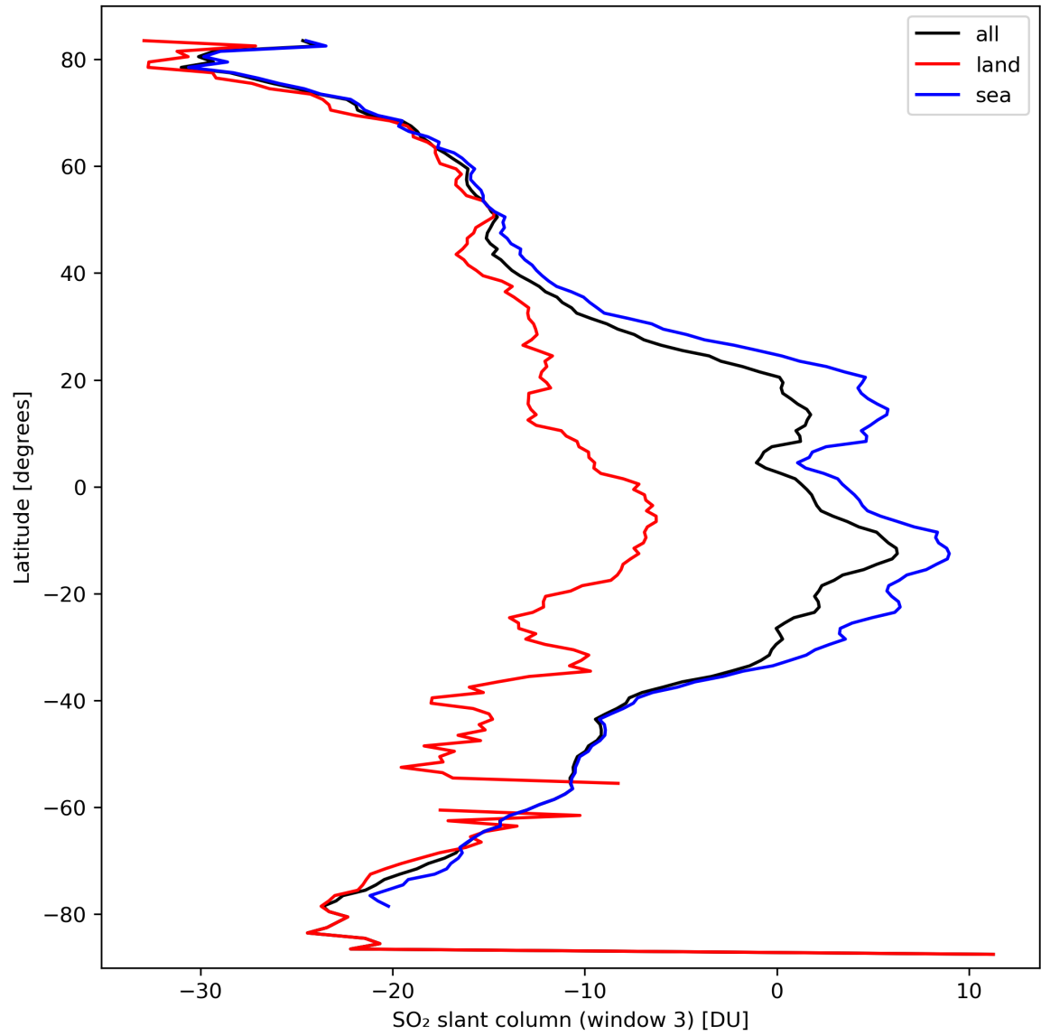
Figure 41: Zonal average of “SO 2 slant column (window 3)” for 2024-03-14 to 2024-03-16.
