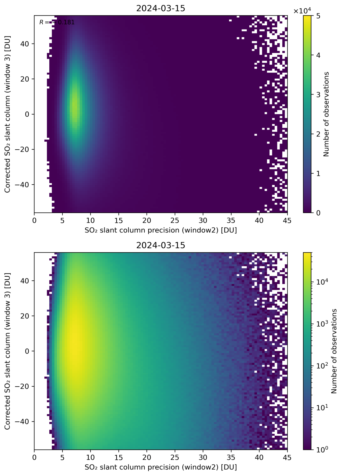
Figure 248: Scatter density plot of “SO 2 slant column precision (window2)” against “Corrected SO 2 slant column (window 3)” for 2024-03-14 to 2024-03-16.
