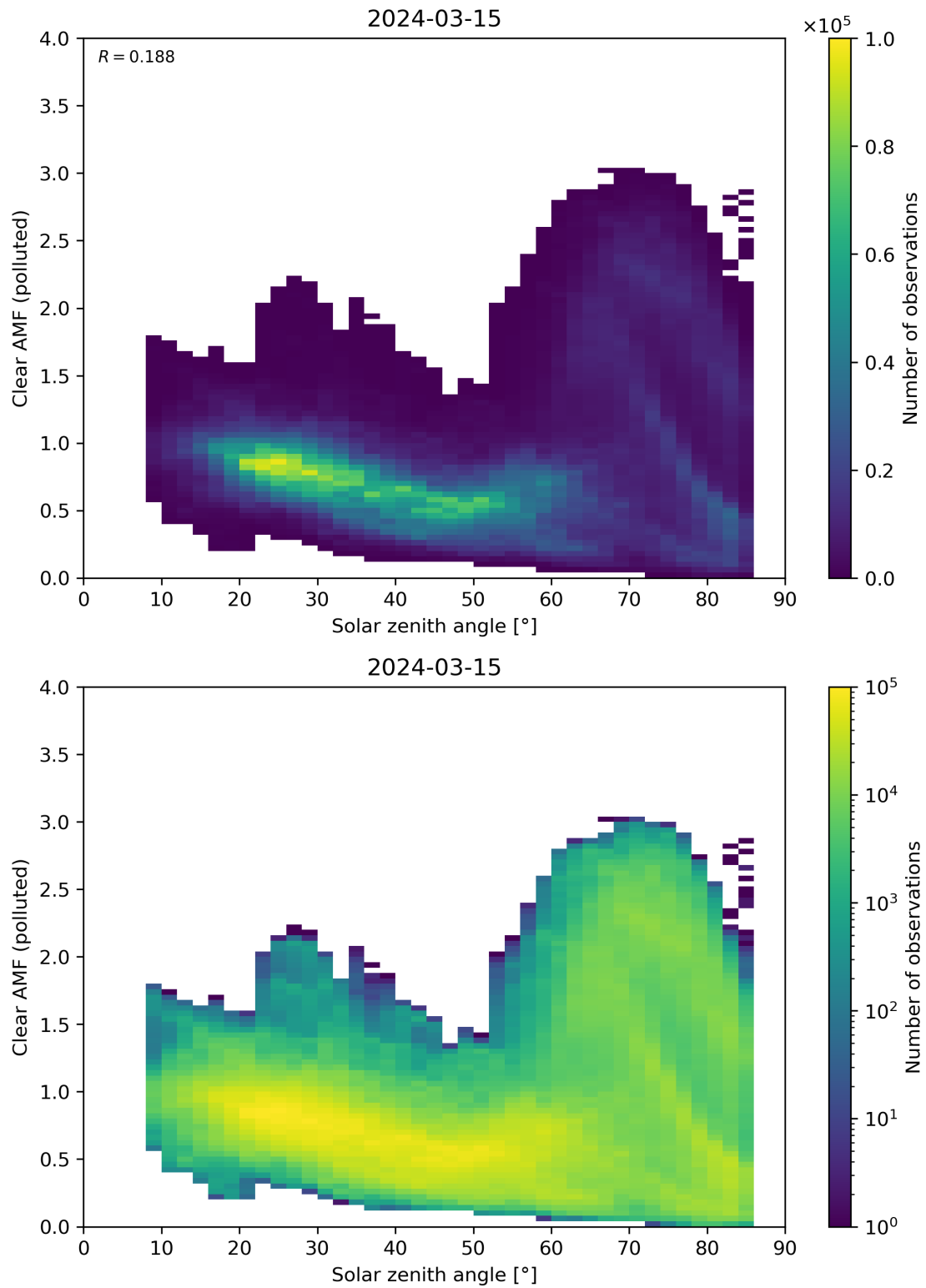
Figure 165: Scatter density plot of “Solar zenith angle” against “Clear AMF (polluted)” for 2024-03-14 to 2024-03-16.
