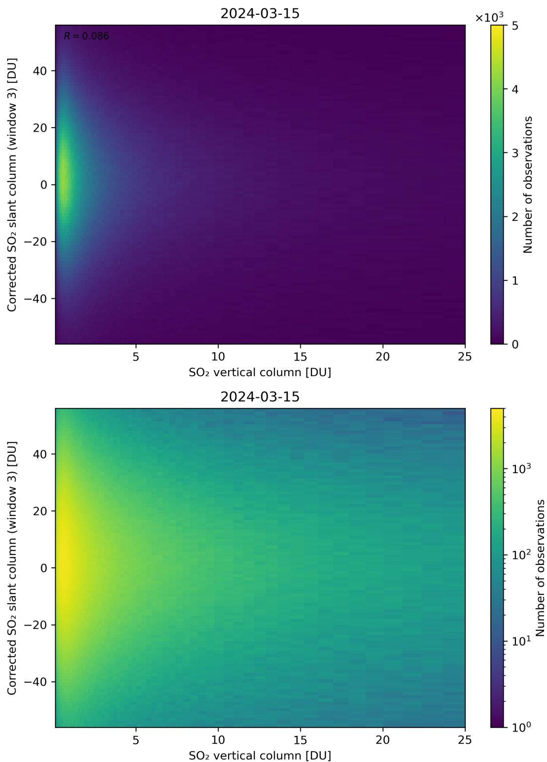
Figure 299: Scatter density plot of “SO 2 vertical column” against “Corrected SO 2 slant column (window 3)” for 2024-03-14 to 2024-03-16.
