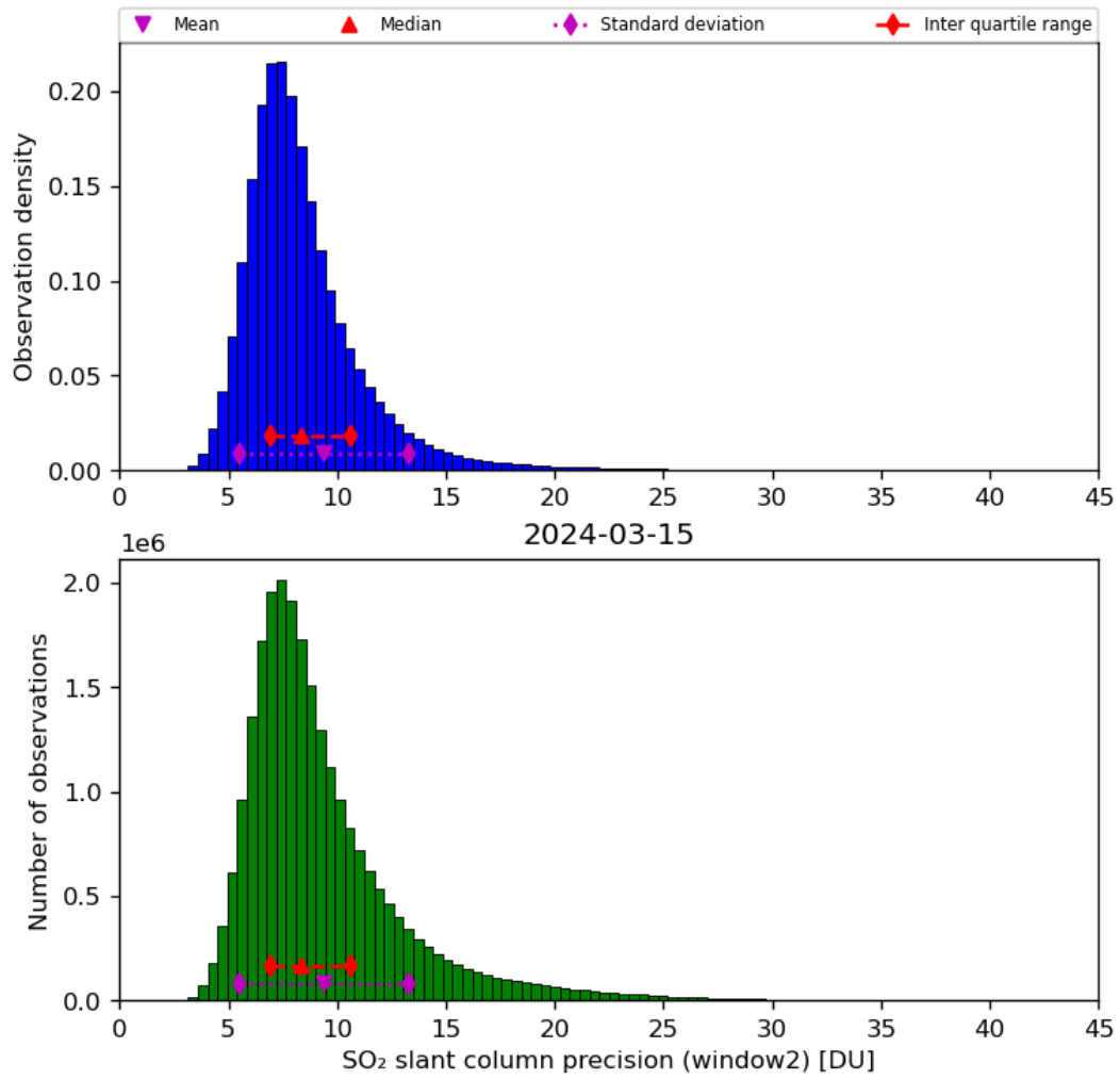
Figure 61: Histogram of “SO 2 slant column precision (window2)” for 2024-03-14 to 2024-03-16
