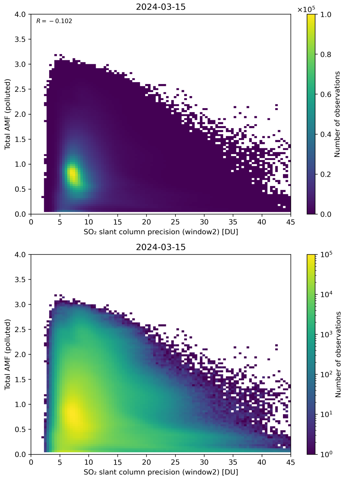
Figure 251: Scatter density plot of “SO 2 slant column precision (window2)” against “Total AMF (polluted)” for 2024-03-14 to 2024-03-16.
