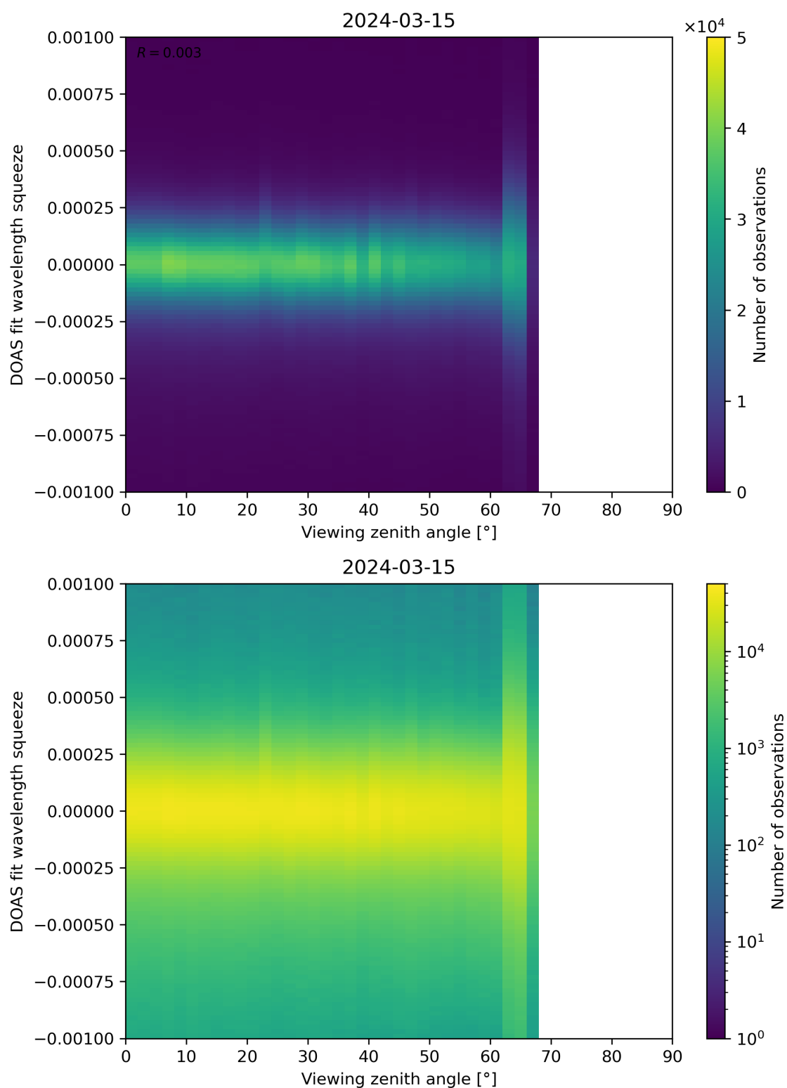
Figure 312: Scatter density plot of “Viewing zenith angle” against “DOAS fit wavelength squeeze” for 2024-03-14 to 2024-03-16.
