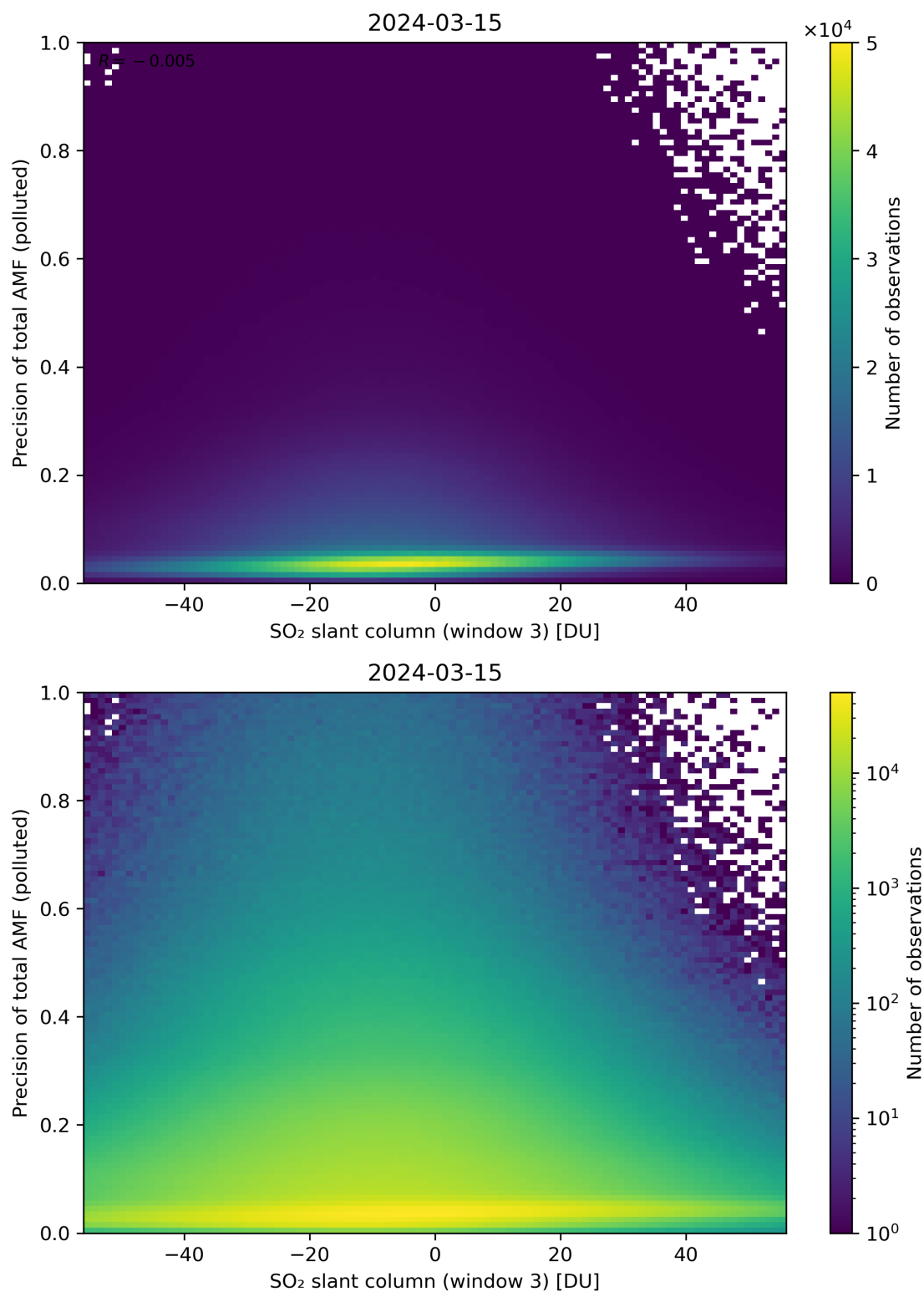
Figure 269: Scatter density plot of “SO 2 slant column (window 3)” against “Precision of total AMF (polluted)” for 2024-03-14 to 2024-03-16.
