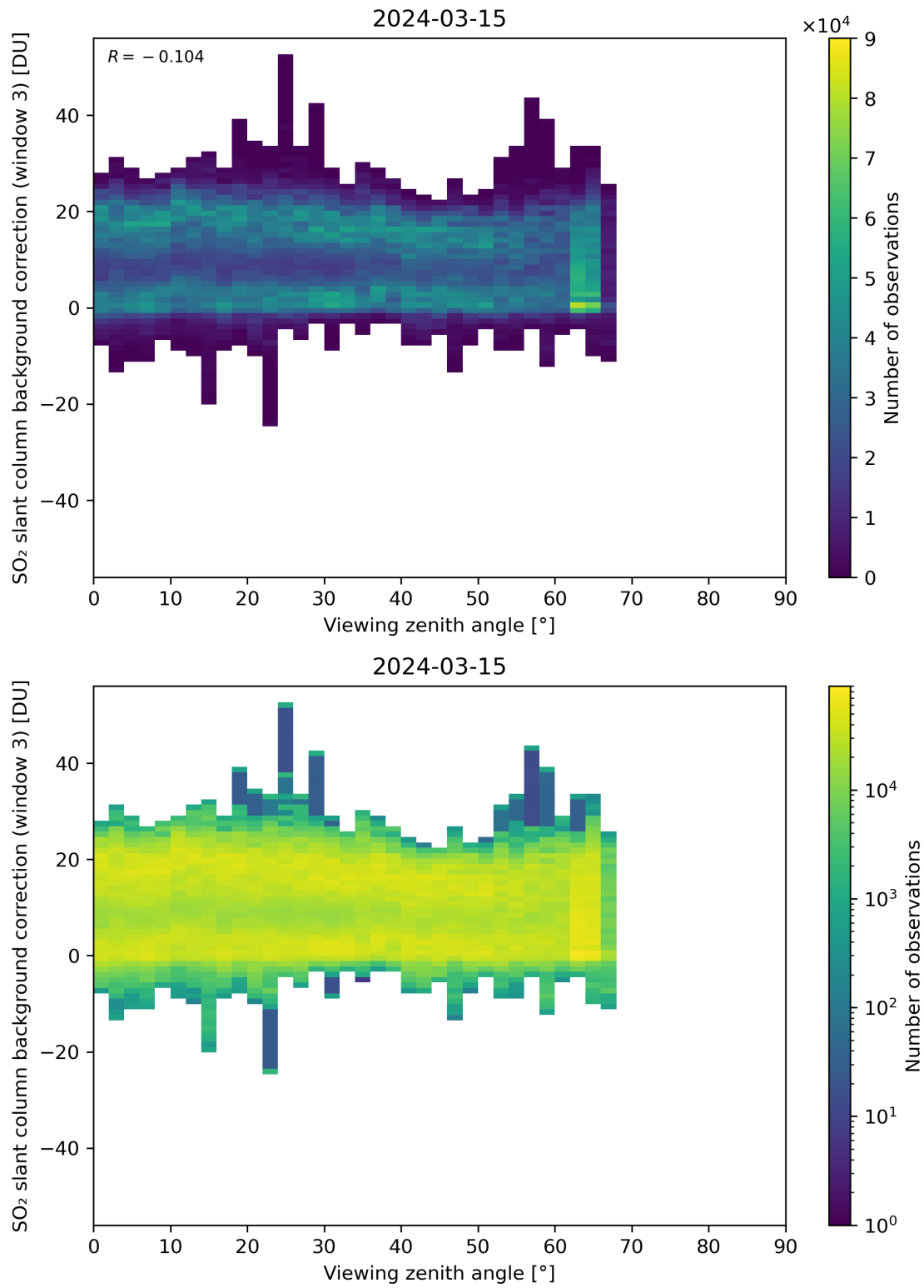
Figure 310: Scatter density plot of “Viewing zenith angle” against “SO 2 slant column background correction (window 3)” for 2024-03-14 to 2024-03-16.
