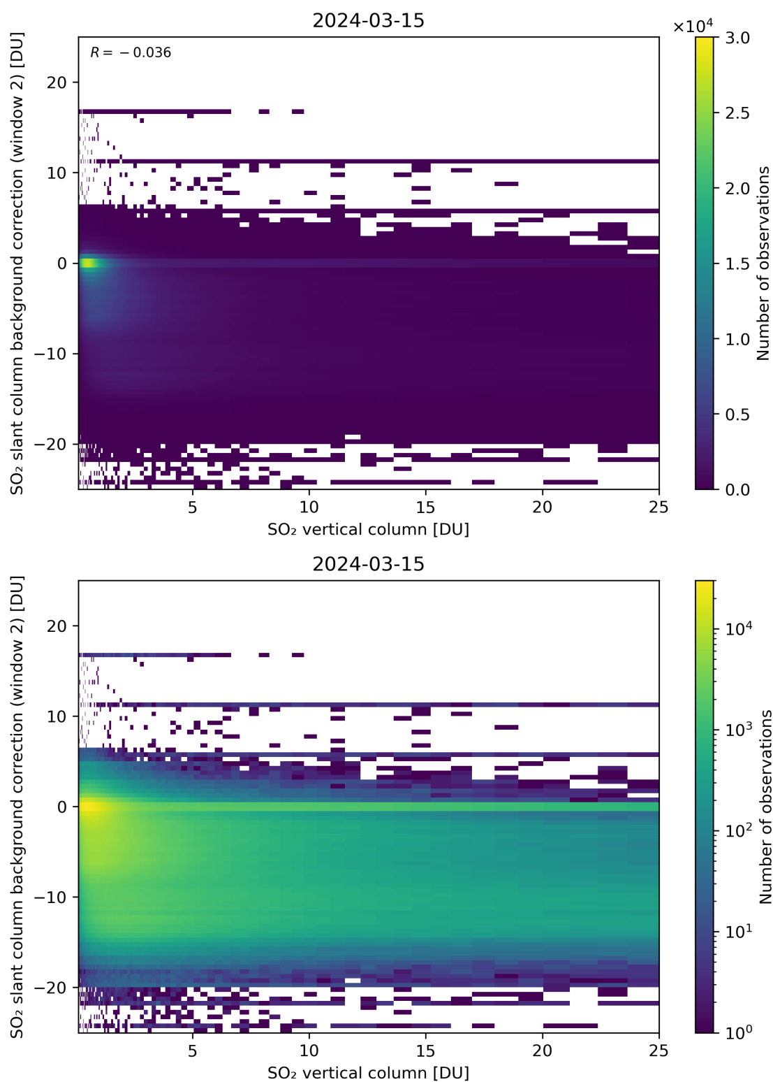
Figure 274: Scatter density plot of “SO 2 vertical column” against “SO 2 slant column background correction (window 2)” for 2024-03-14 to 2024-03-16.
