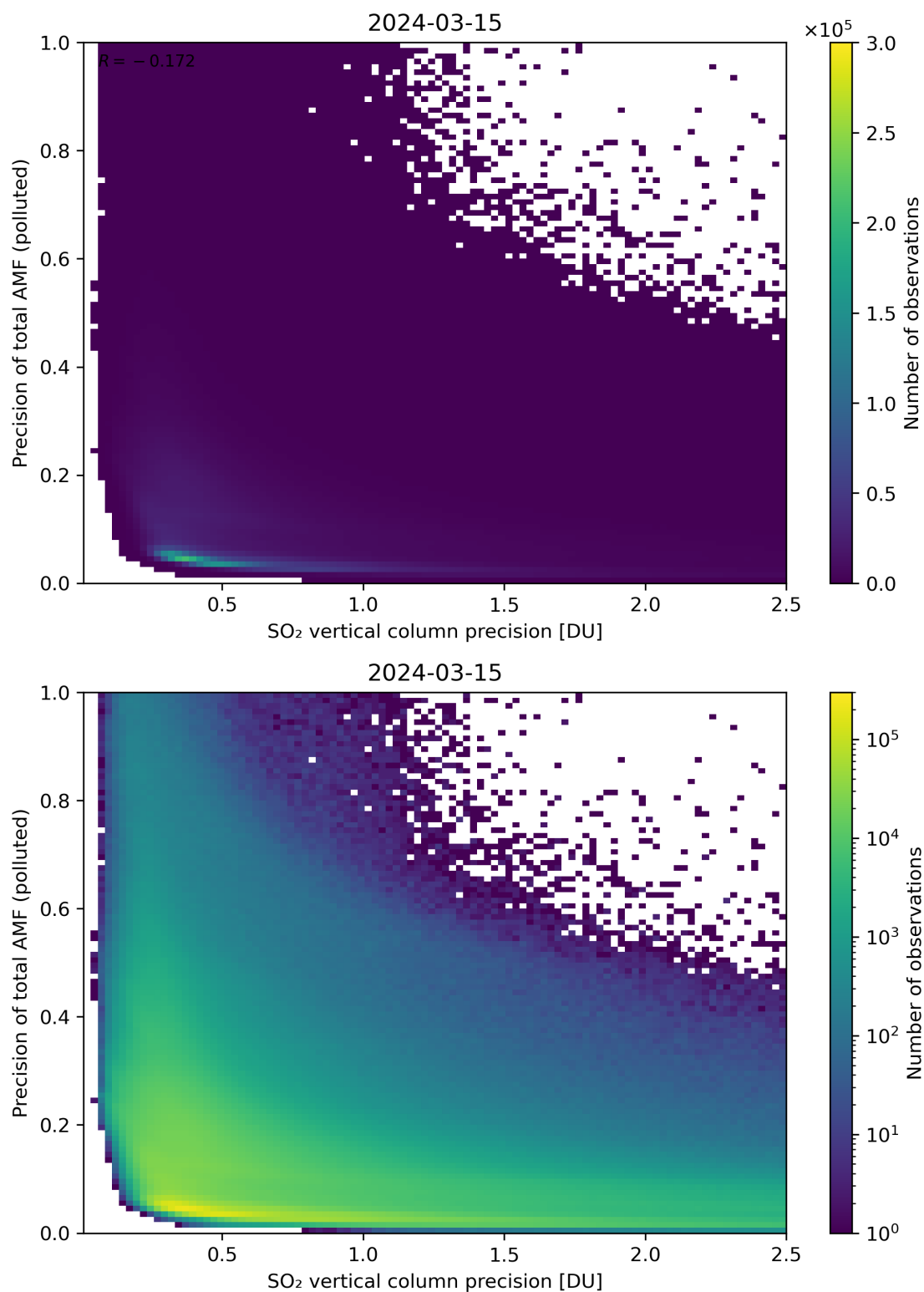
Figure 295: Scatter density plot of “SO 2 vertical column precision” against “Precision of total AMF (polluted)” for 2024-03-14 to 2024-03-16.
