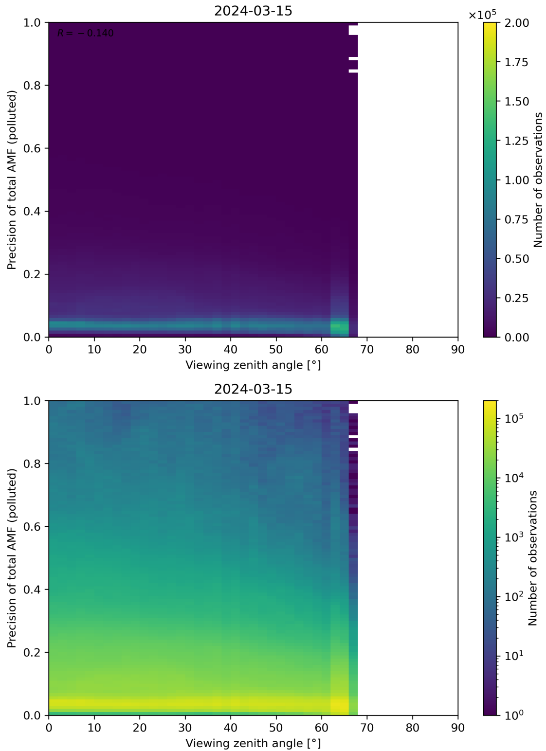
Figure 326: Scatter density plot of “Viewing zenith angle” against “Precision of total AMF (polluted)” for 2024-03-14 to 2024-03-16.
