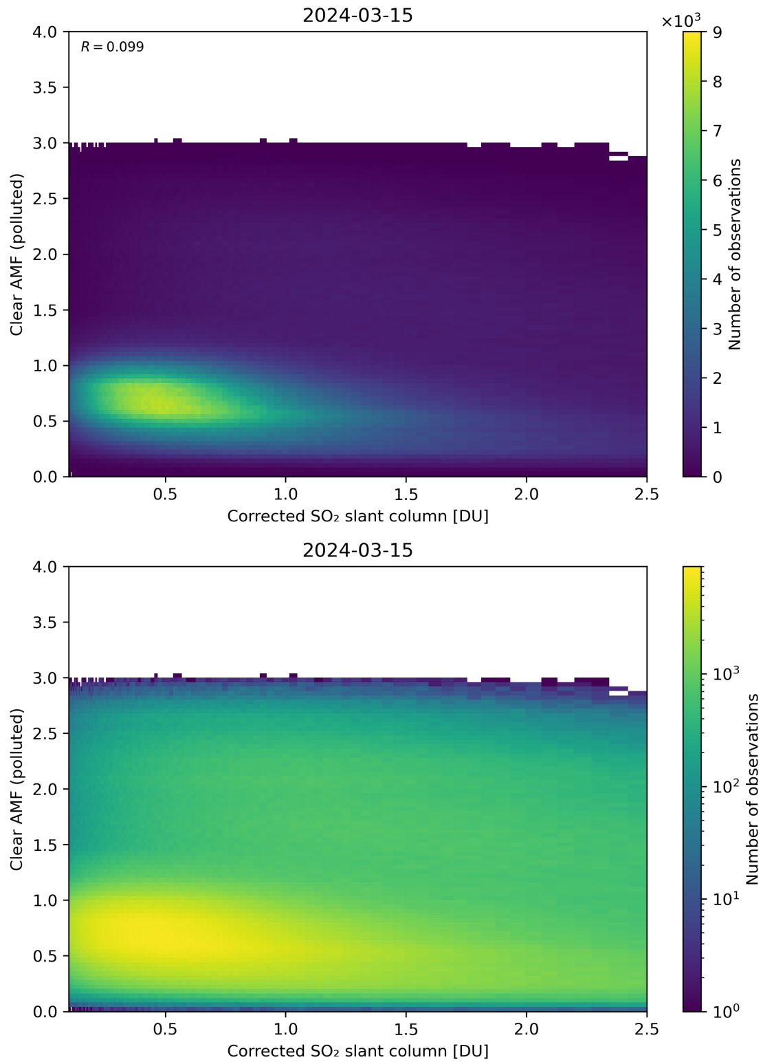
Figure 184: Scatter density plot of “Corrected SO 2 slant column” against “Clear AMF (polluted)” for 2024-03-14 to 2024-03-16.
