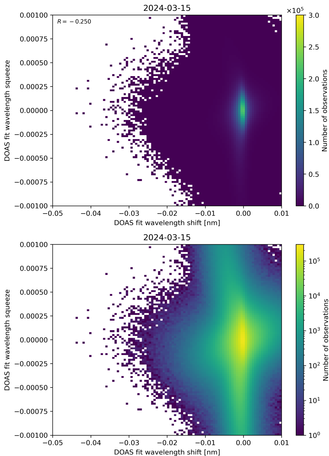
Figure 127: Scatter density plot of “DOAS fit wavelength shift” against “DOAS fit wavelength squeeze” for 2024-03-14 to 2024-03-16.
