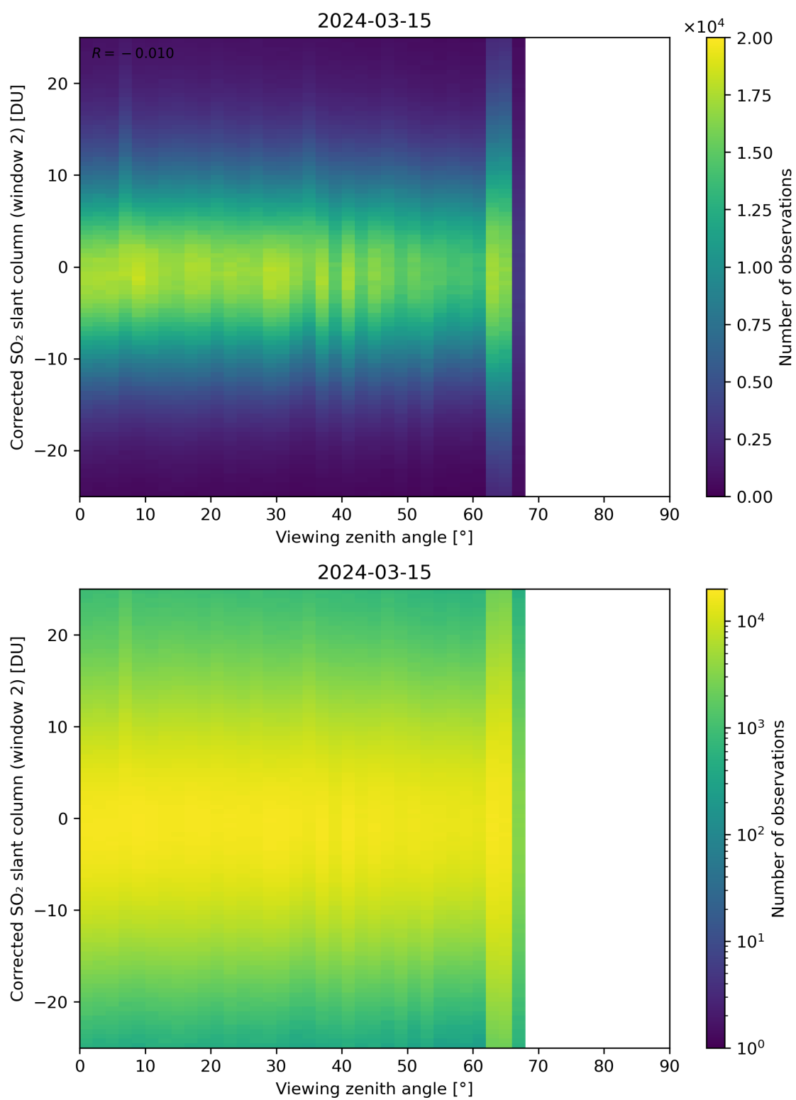
Figure 318: Scatter density plot of “Viewing zenith angle” against “Corrected SO 2 slant column (window 2)” for 2024-03-14 to 2024-03-16.
