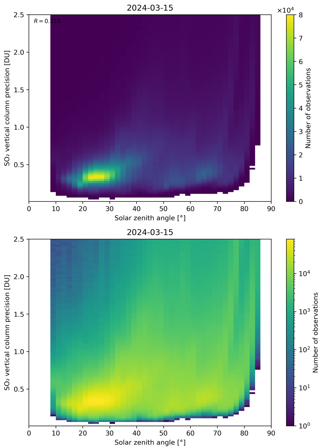
Figure 177: Scatter density plot of “Solar zenith angle” against “SO 2 vertical column precision” for 2024-03-14 to 2024-03-16.
