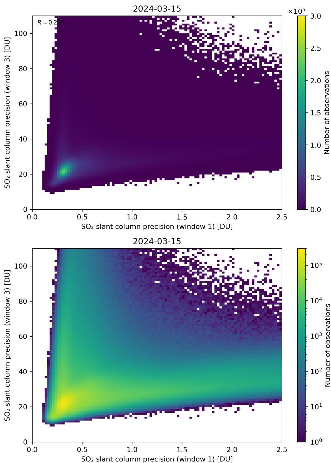
Figure 229: Scatter density plot of “SO 2 slant column precision (window 1)” against “SO 2 slant column precision (window 3)” for 2024-03-14 to 2024-03-16.
