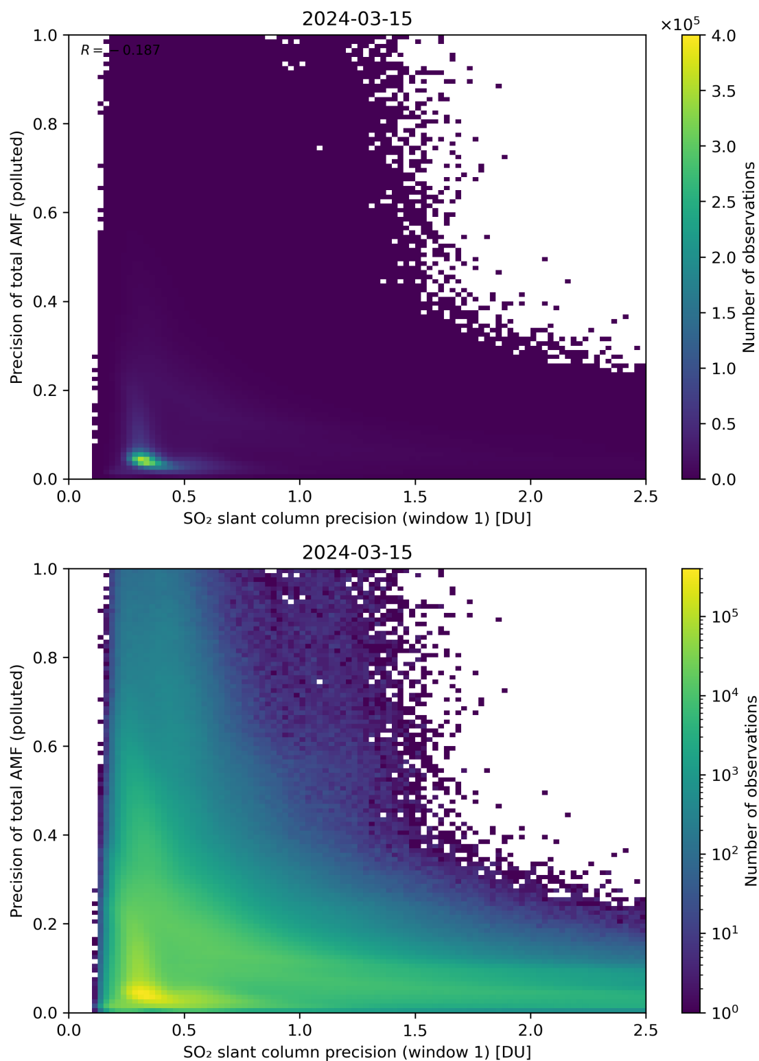
Figure 231: Scatter density plot of “SO 2 slant column precision (window 1)” against “Precision of total AMF (polluted)” for 2024-03-14 to 2024-03-16.
