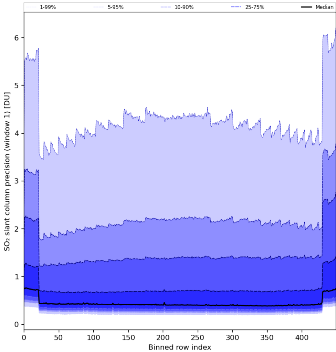
Figure 80: Along track statistics of “SO 2 slant column precision (window 1)” for 2024-03-14 to 2024-03-16
