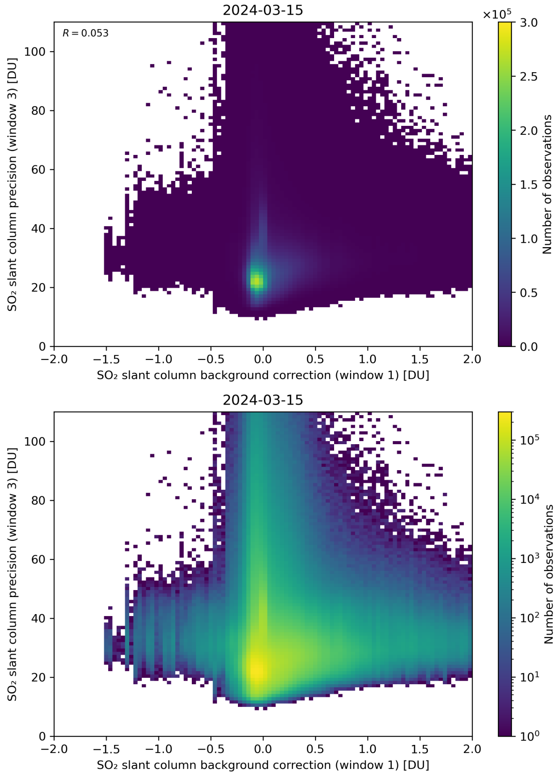
Figure 108: Scatter density plot of “SO 2 slant column background correction (window 1)” against “SO 2 slant column precision (window 3)” for 2024-03-14 to 2024-03-16.
