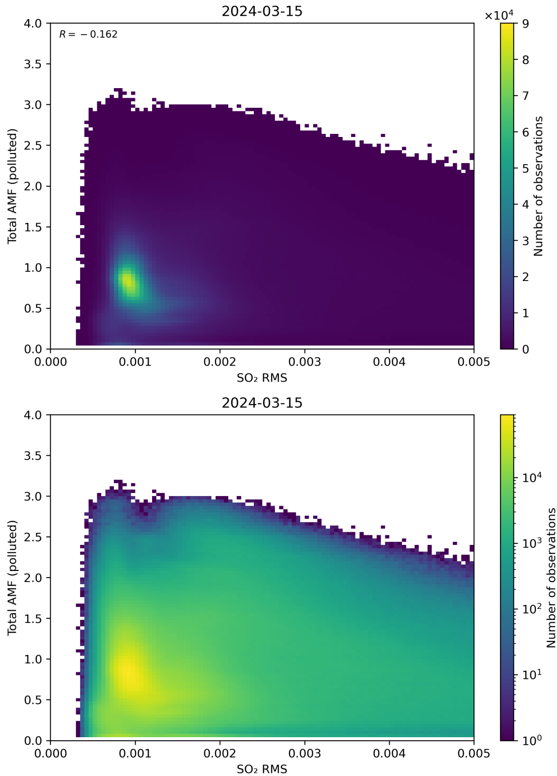
Figure 137: Scatter density plot of “SO 2 RMS” against “Total AMF (polluted)” for 2024-03-14 to 2024-03-16.
