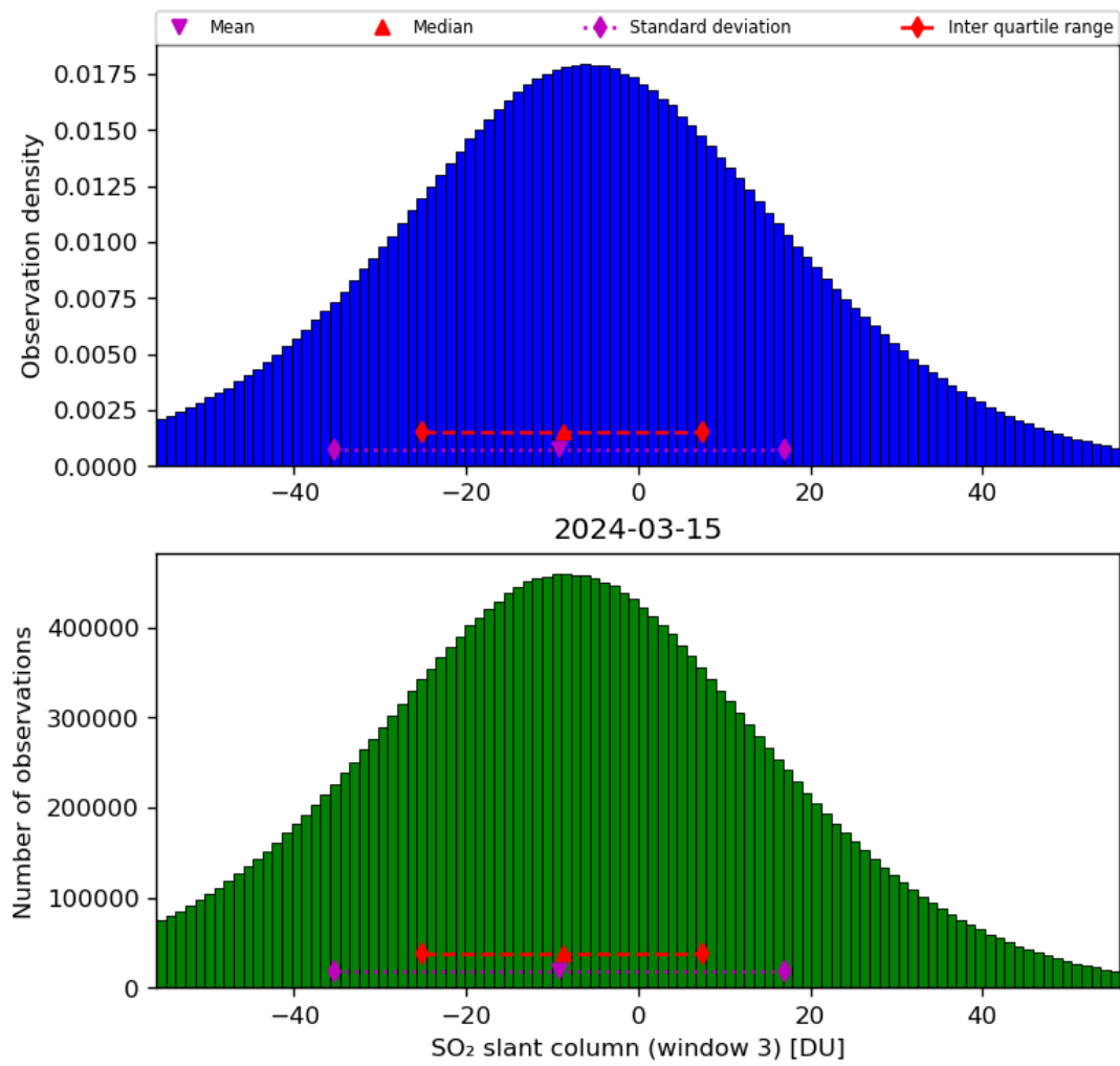
Figure 64: Histogram of “SO 2 slant column (window 3)” for 2024-03-14 to 2024-03-16
