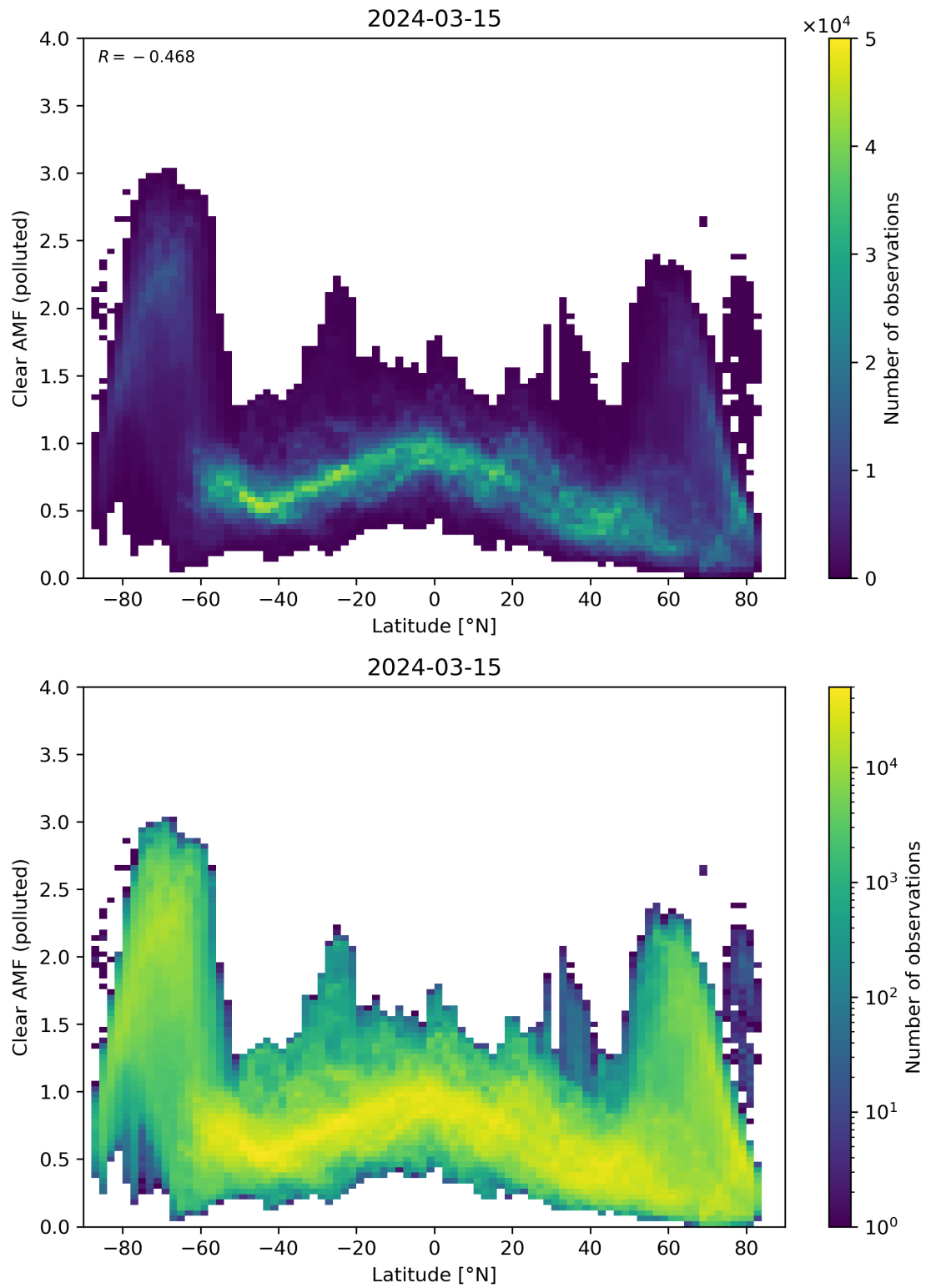
Figure 145: Scatter density plot of “Latitude” against “Clear AMF (polluted)” for 2024-03-14 to 2024-03-16.
