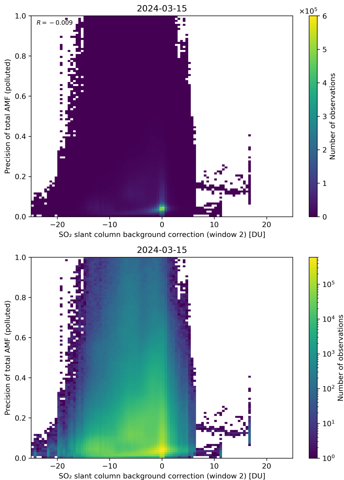
Figure 120: Scatter density plot of “SO 2 slant column background correction (window 2)” against “Precision of total AMF (polluted)” for 2024-03-14 to 2024-03-16.
