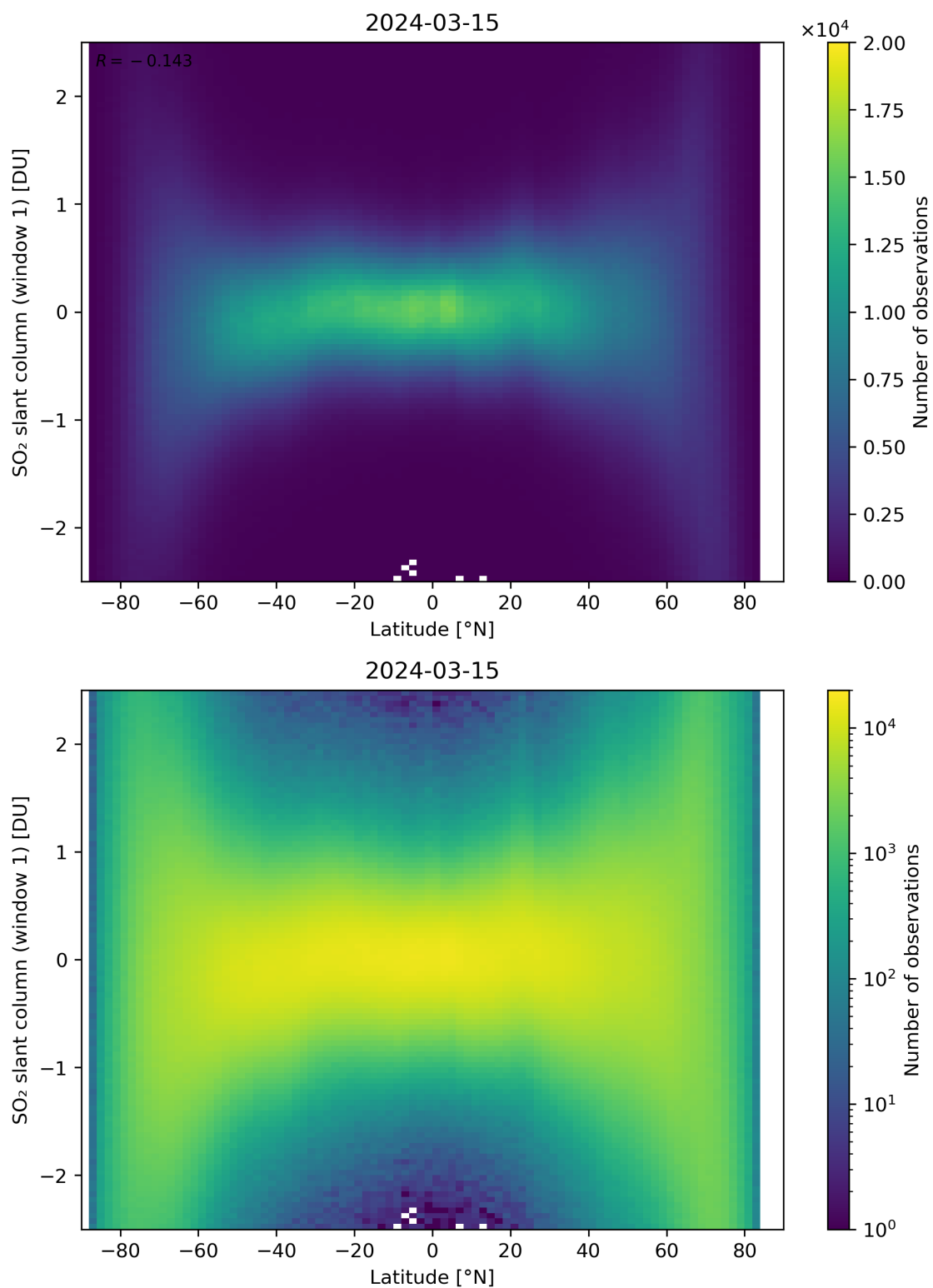
Figure 149: Scatter density plot of “Latitude” against “SO 2 slant column (window 1)” for 2024-03-14 to 2024-03-16.
