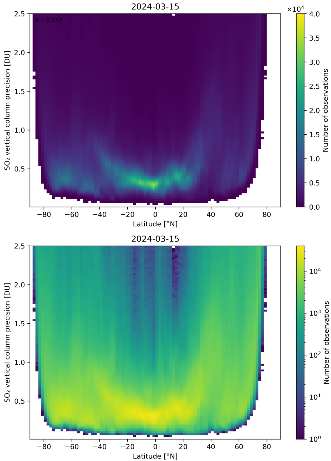
Figure 157: Scatter density plot of “Latitude” against “SO 2 vertical column precision” for 2024-03-14 to 2024-03-16.
