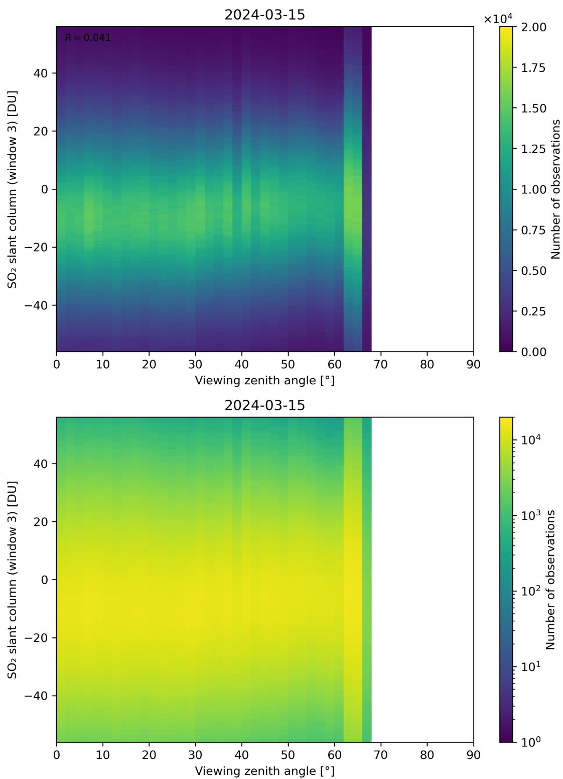
Figure 323: Scatter density plot of “Viewing zenith angle” against “SO 2 slant column (window 3)” for 2024-03-14 to 2024-03-16.
