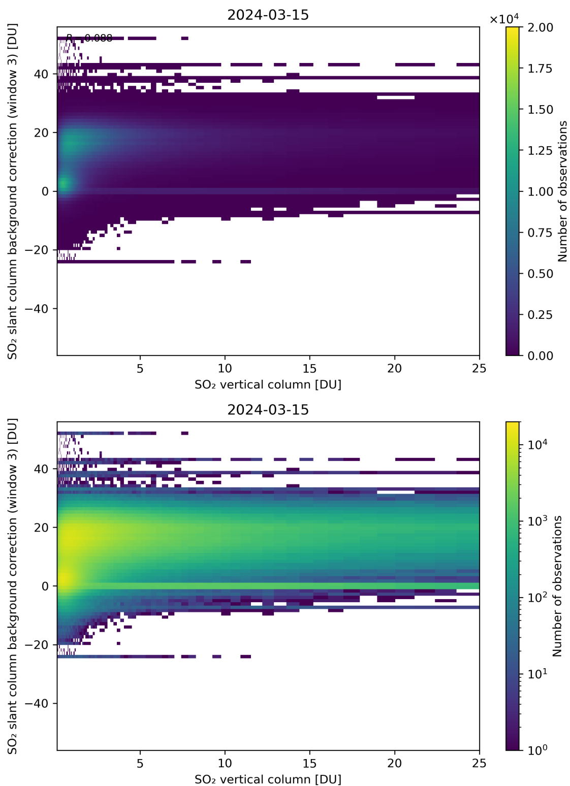
Figure 275: Scatter density plot of “SO 2 vertical column” against “SO 2 slant column background correction (window 3)” for 2024-03-14 to 2024-03-16.
