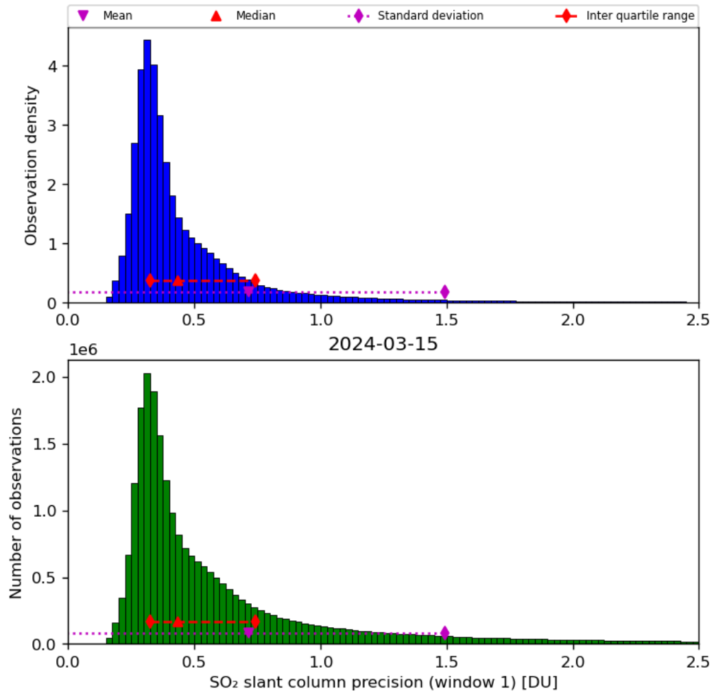
Figure 57: Histogram of “SO 2 slant column precision (window 1)” for 2024-03-14 to 2024-03-16
