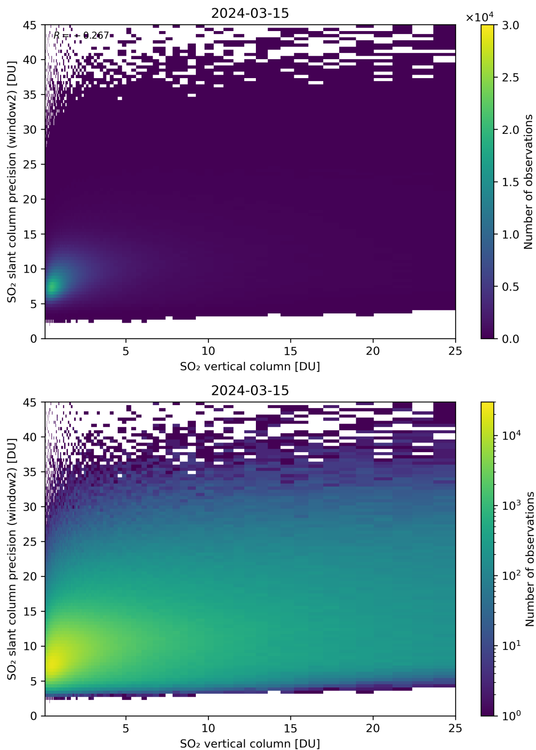
Figure 302: Scatter density plot of “SO 2 vertical column” against “SO 2 slant column precision (window2)” for 2024-03-14 to 2024-03-16.
