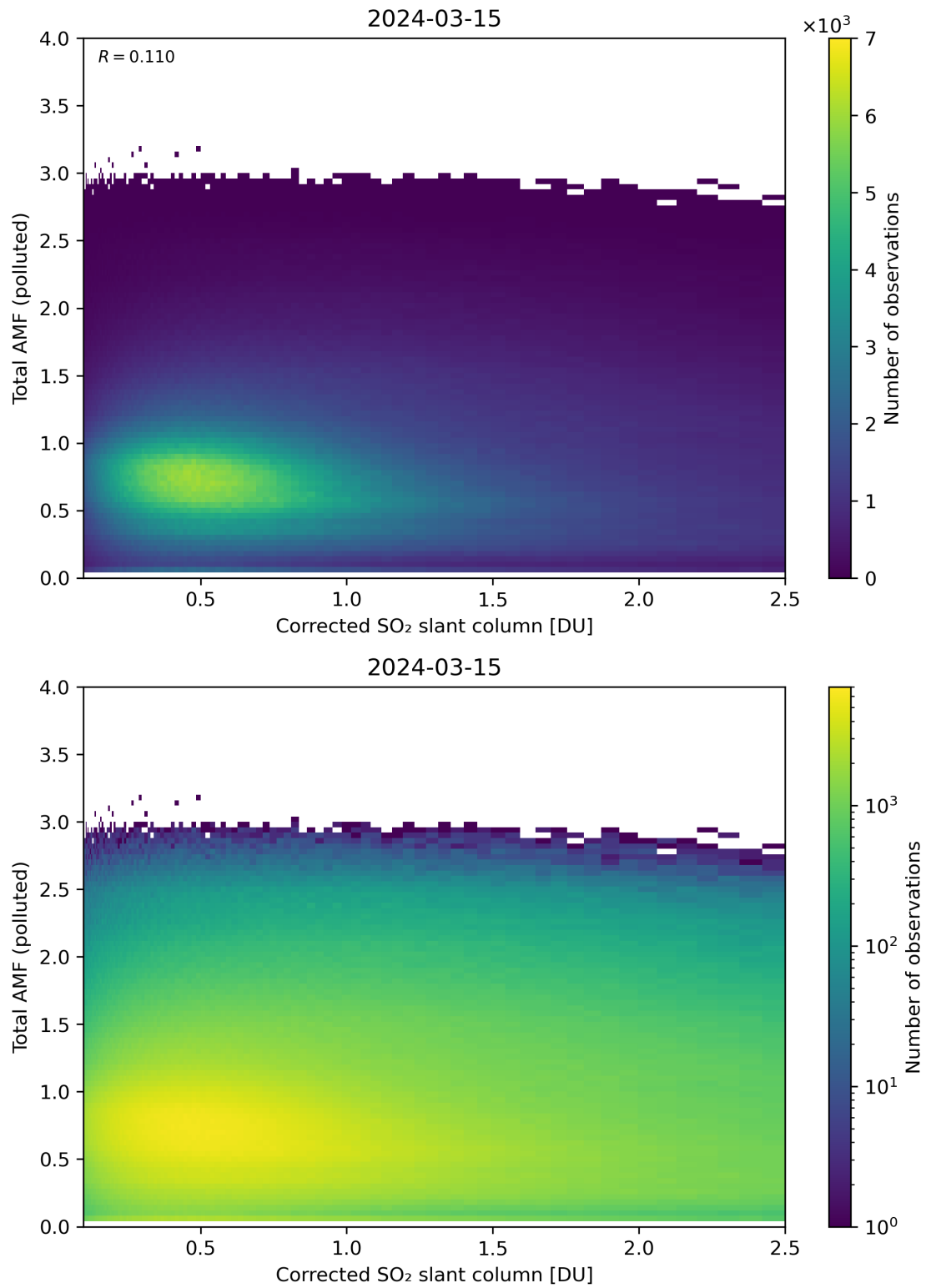
Figure 192: Scatter density plot of “Corrected SO 2 slant column” against “Total AMF (polluted)” for 2024-03-14 to 2024-03-16.
