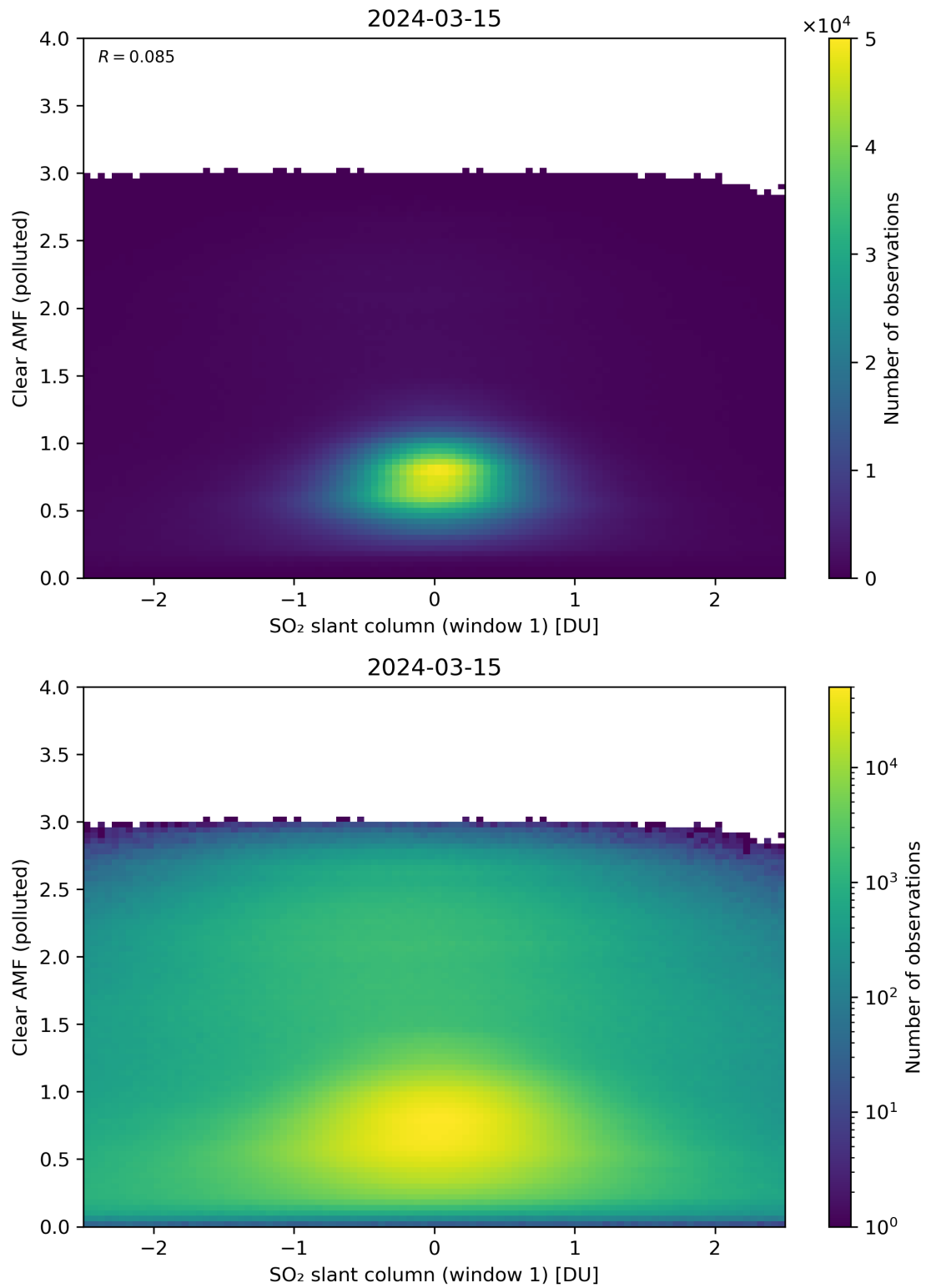
Figure 232: Scatter density plot of “SO 2 slant column (window 1)” against “Clear AMF (polluted)” for 2024-03-14 to 2024-03-16.
