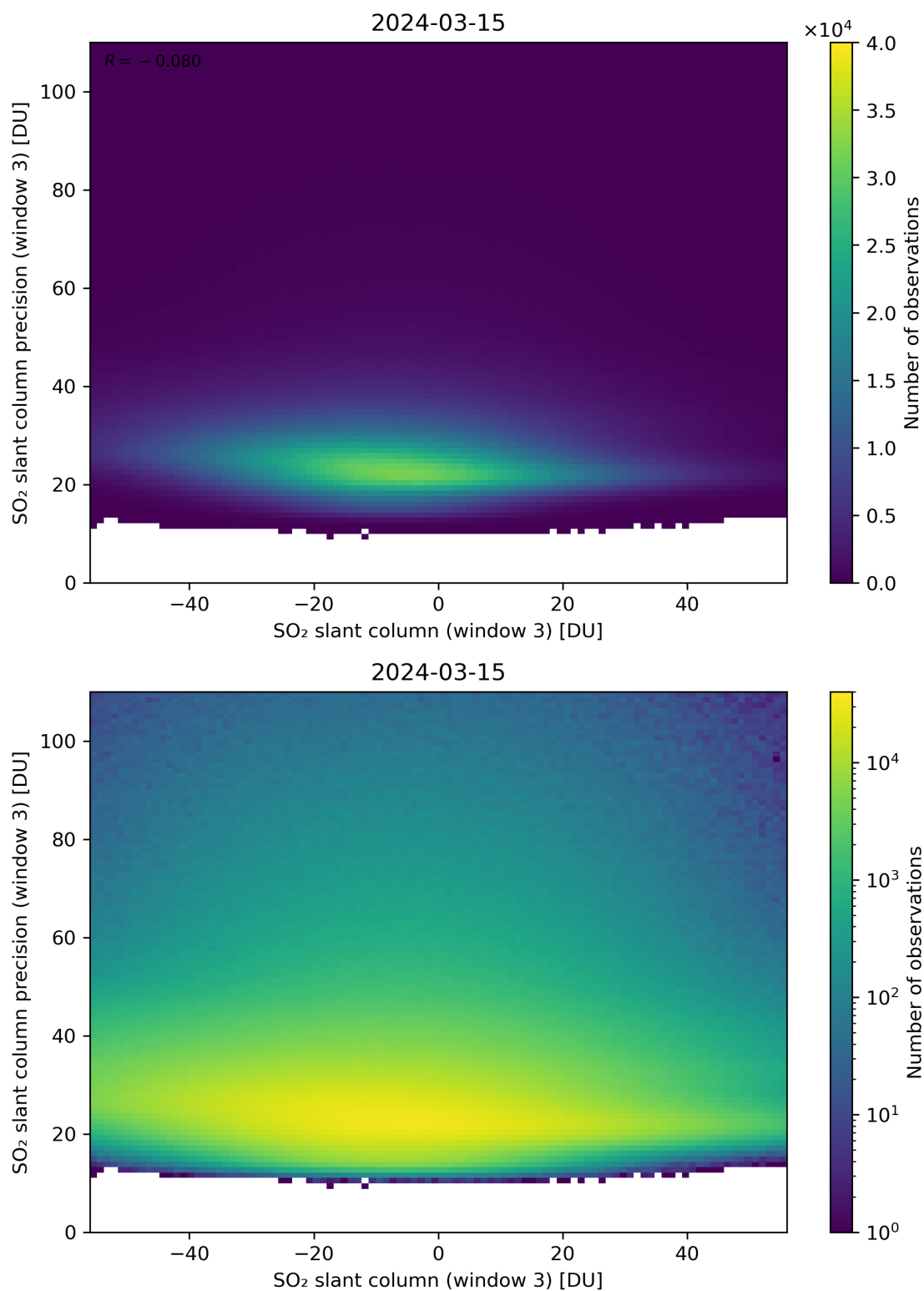
Figure 267: Scatter density plot of “SO 2 slant column (window 3)” against “SO 2 slant column precision (window 3)” for 2024-03-14 to 2024-03-16.
