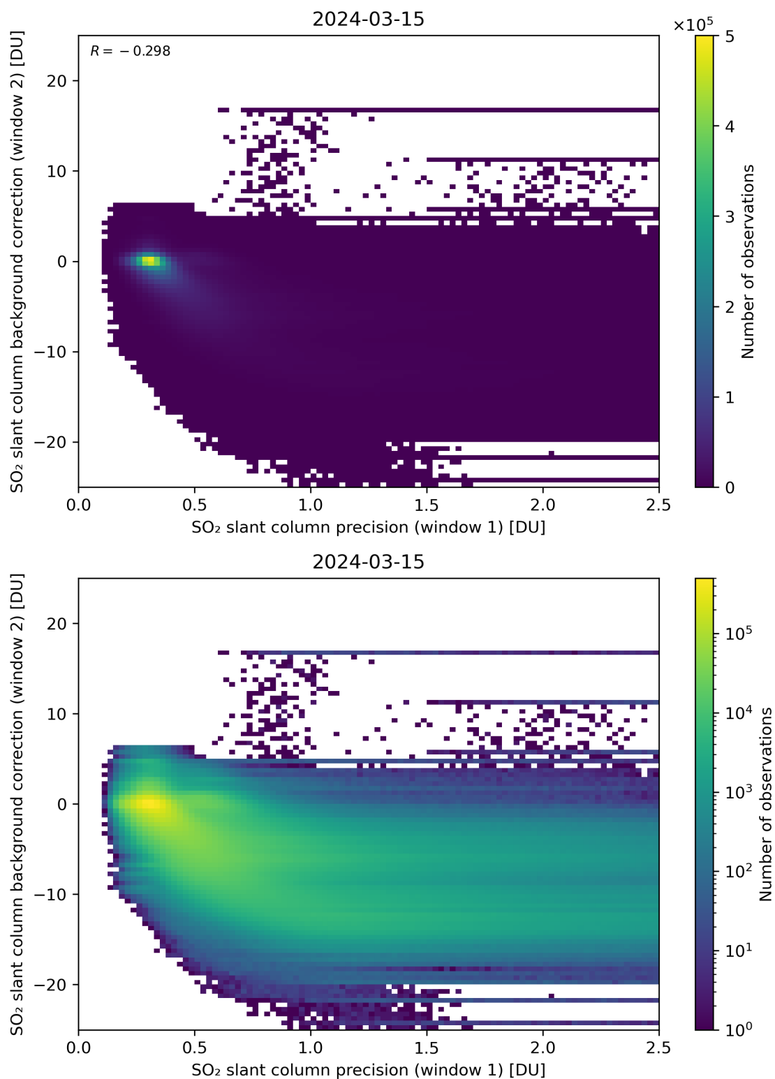
Figure 219: Scatter density plot of “SO 2 slant column precision (window 1)” against “SO 2 slant column background correction (window 2)” for 2024-03-14 to 2024-03-16.
