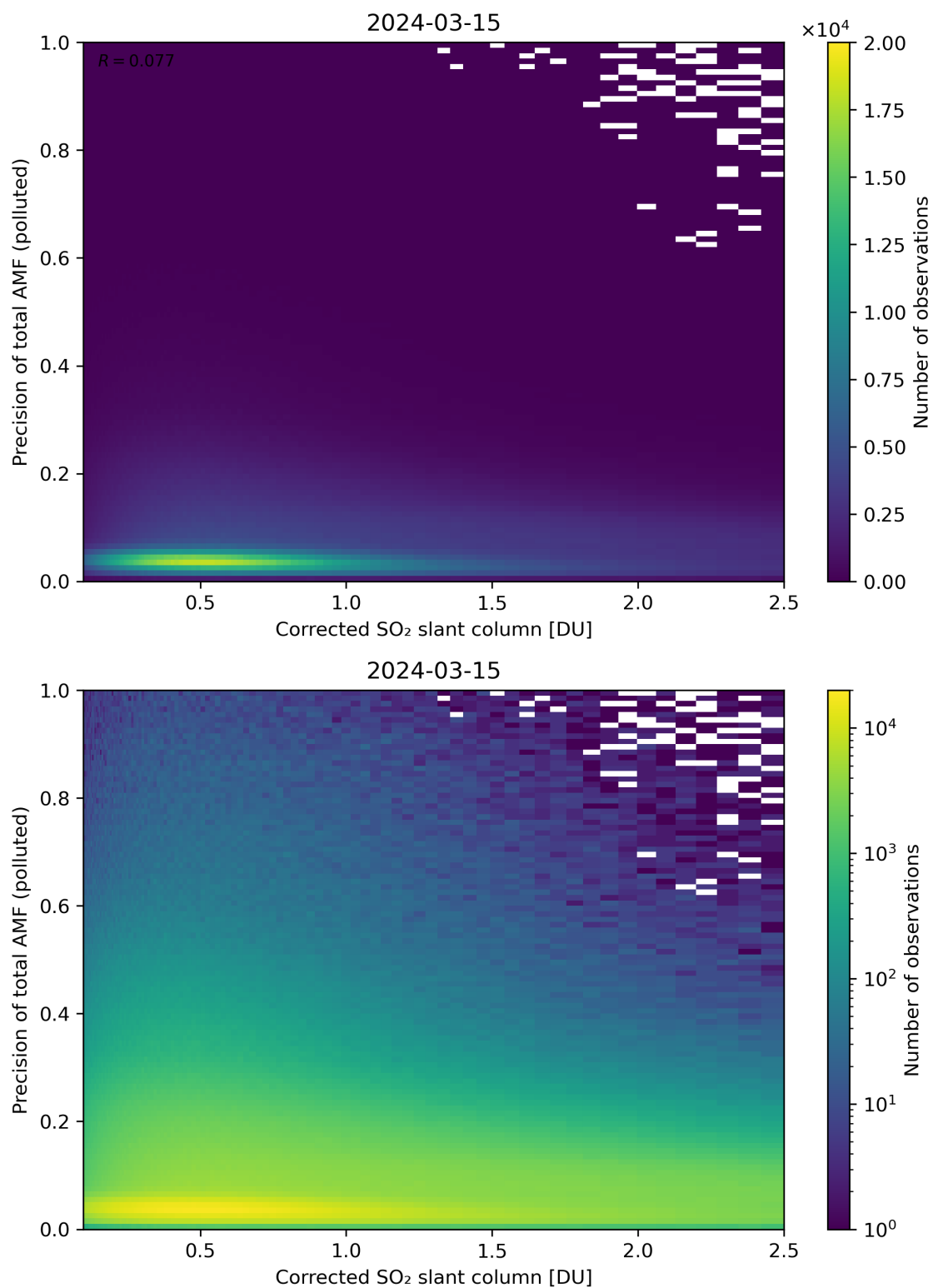
Figure 193: Scatter density plot of “Corrected SO 2 slant column” against “Precision of total AMF (polluted)” for 2024-03-14 to 2024-03-16.
