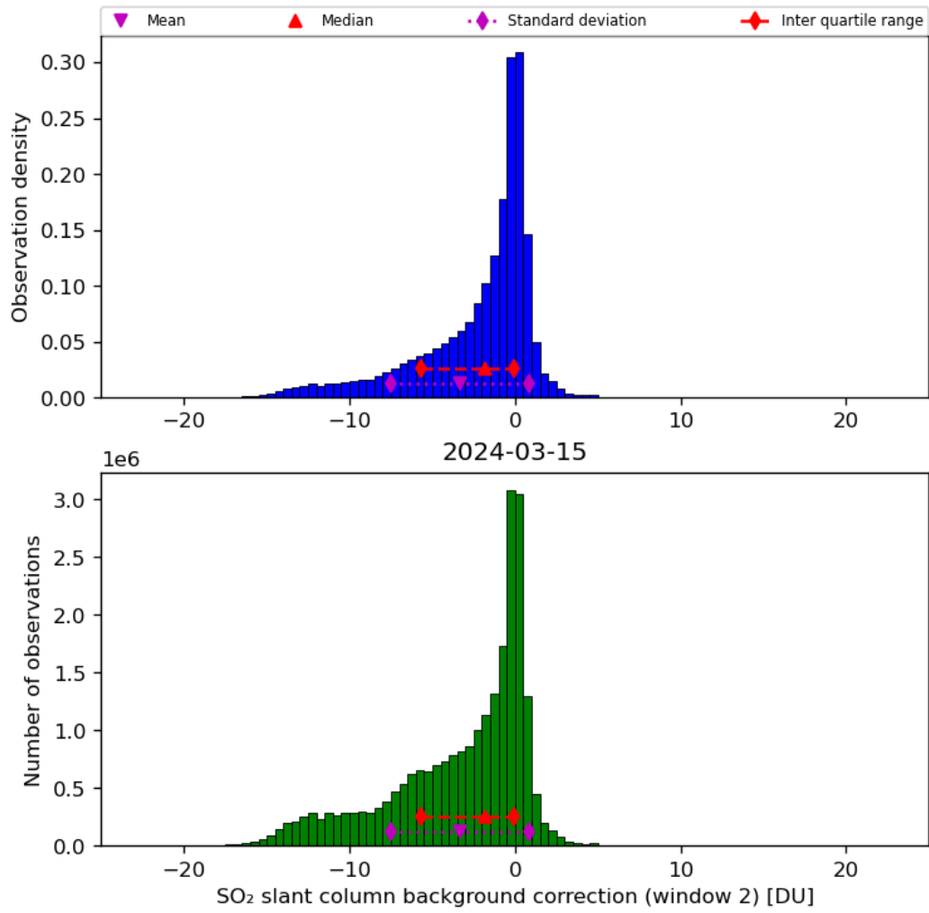
Figure 63: Histogram of “SO 2 slant column background correction (window 2)” for 2024-03-14 to 2024-03-16
