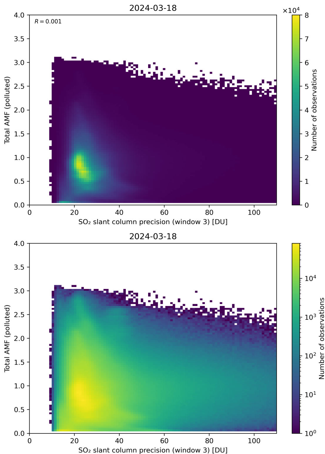
Figure 263: Scatter density plot of “SO 2 slant column precision (window 3)” against “Total AMF (polluted)” for 2024-03-17 to 2024-03-19.
