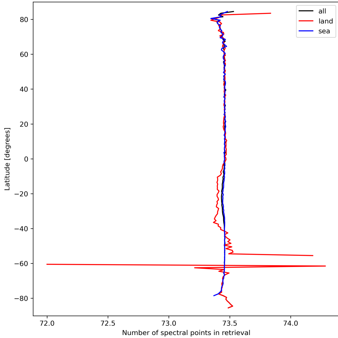
Figure 51: Zonal average of “Number of spectral points in retrieval” for 2024-03-17 to 2024-03-19.
