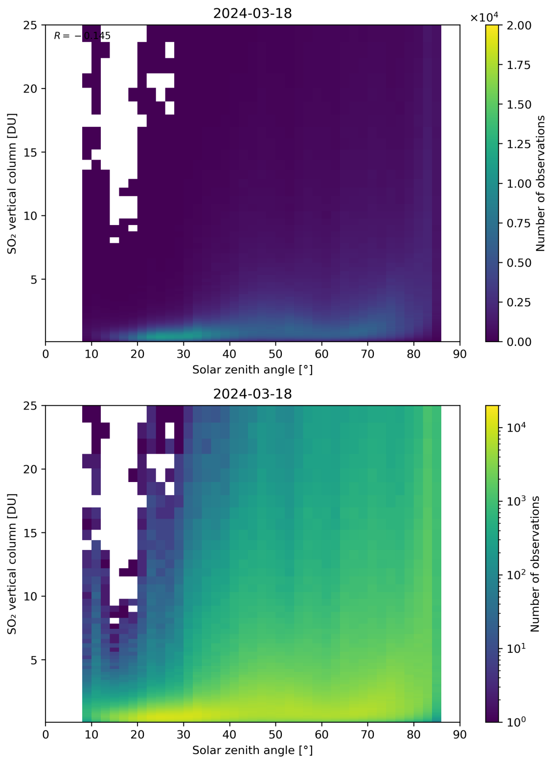
Figure 176: Scatter density plot of “Solar zenith angle” against “SO 2 vertical column” for 2024-03-17 to 2024-03-19.
