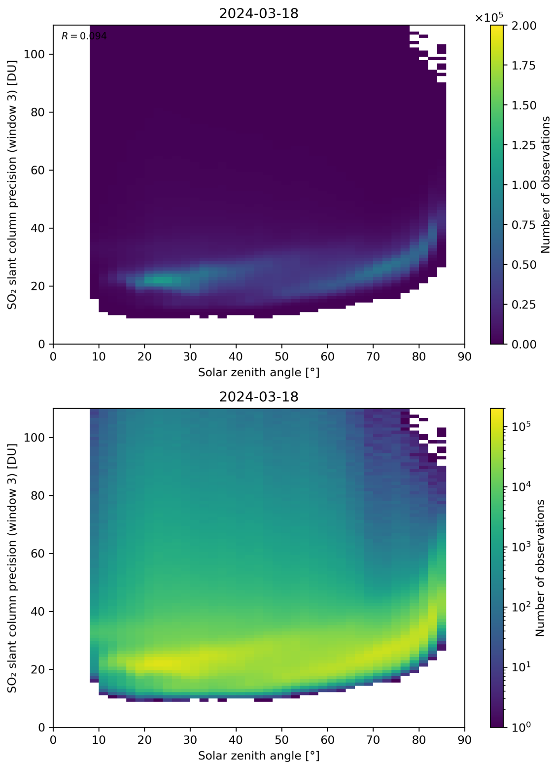
Figure 173: Scatter density plot of “Solar zenith angle” against “SO 2 slant column precision (window 3)” for 2024-03-17 to 2024-03-19.
