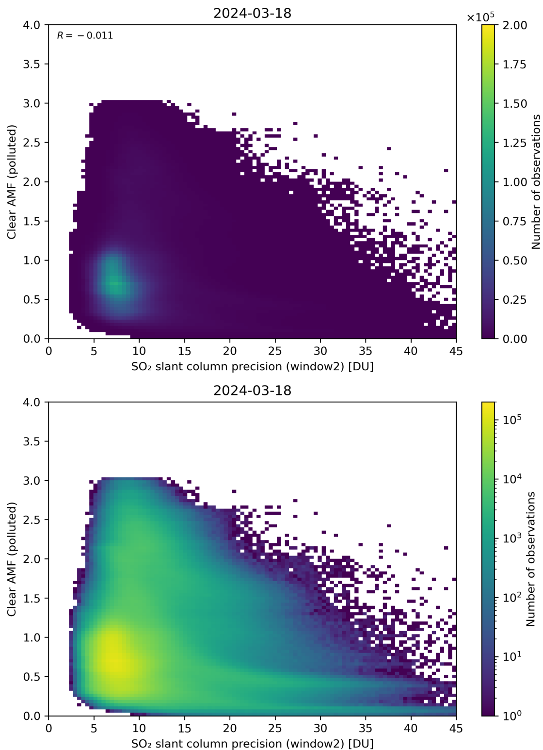
Figure 246: Scatter density plot of “SO 2 slant column precision (window2)” against “Clear AMF (polluted)” for 2024-03-17 to 2024-03-19.
