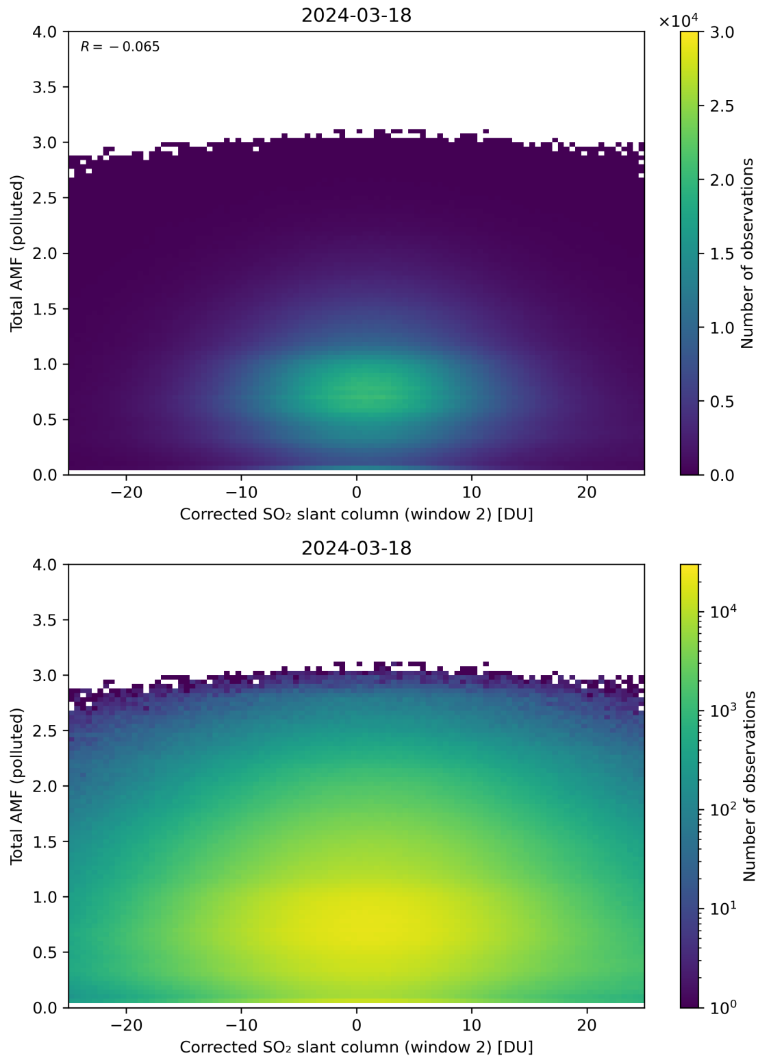
Figure 203: Scatter density plot of “Corrected SO 2 slant column (window 2)” against “Total AMF (polluted)” for 2024-03-17 to 2024-03-19.
