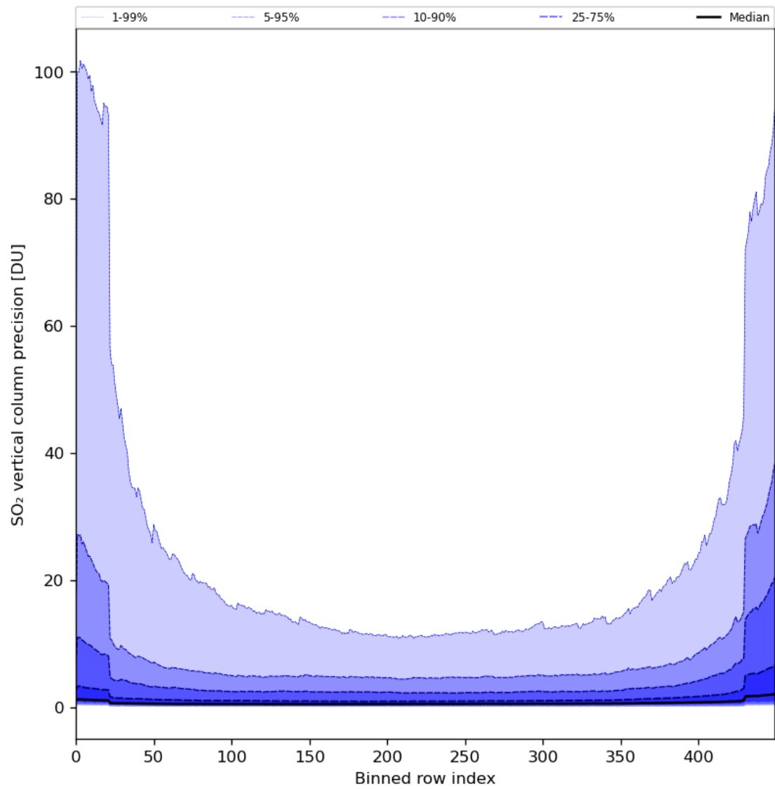
Figure 77: Along track statistics of “SO 2 vertical column precision” for 2024-03-17 to 2024-03-19
