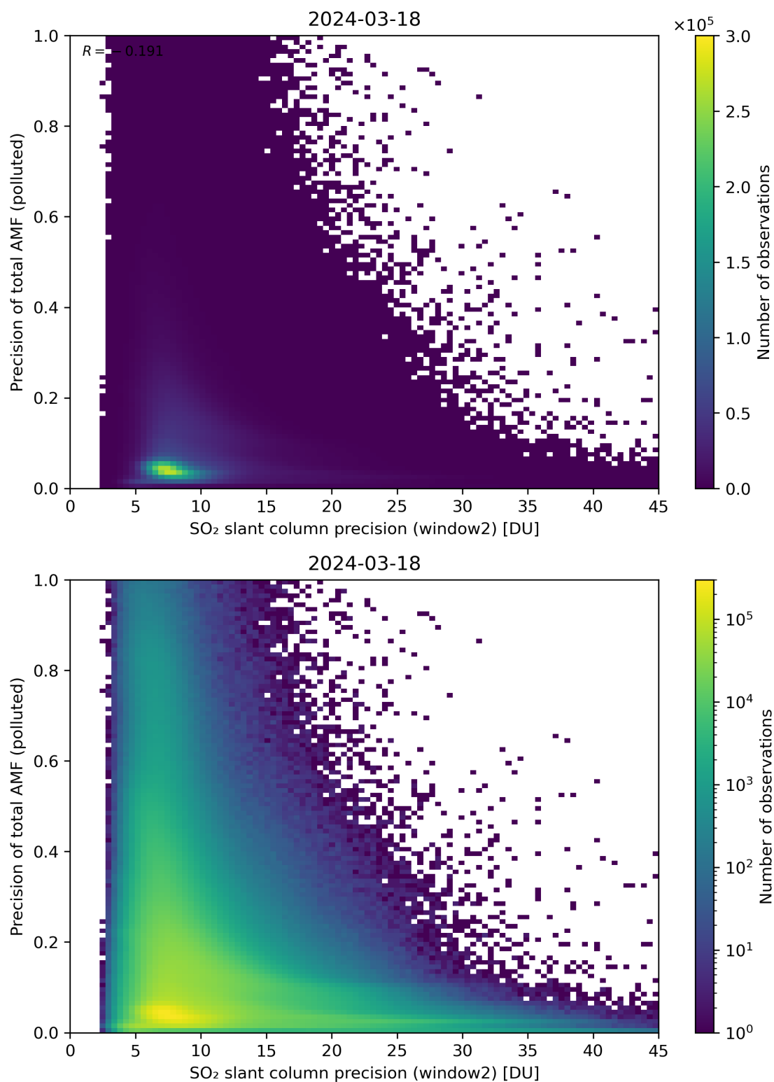
Figure 252: Scatter density plot of “SO 2 slant column precision (window2)” against “Precision of total AMF (polluted)” for 2024-03-17 to 2024-03-19.
