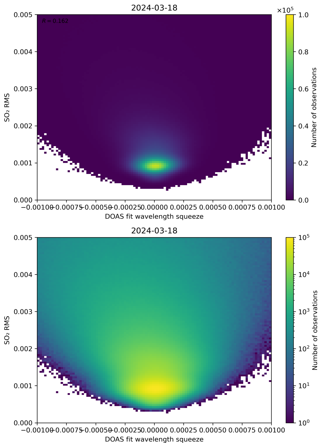
Figure 132: Scatter density plot of “DOAS fit wavelength squeeze” against “SO 2 RMS” for 2024-03-17 to 2024-03-19.
