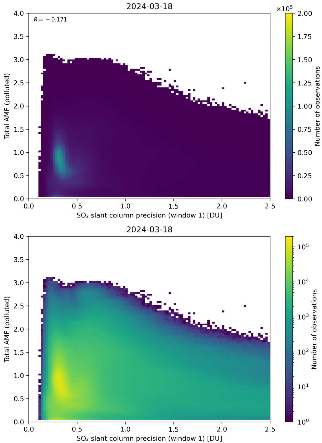
Figure 230: Scatter density plot of “SO 2 slant column precision (window 1)” against “Total AMF (polluted)” for 2024-03-17 to 2024-03-19.
