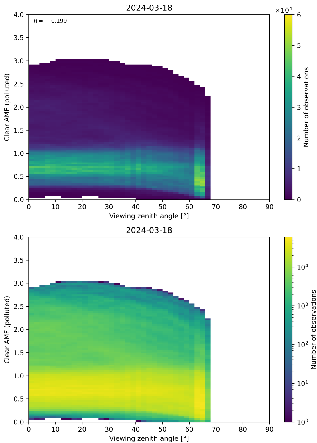
Figure 316: Scatter density plot of “Viewing zenith angle” against “Clear AMF (polluted)” for 2024-03-17 to 2024-03-19.
