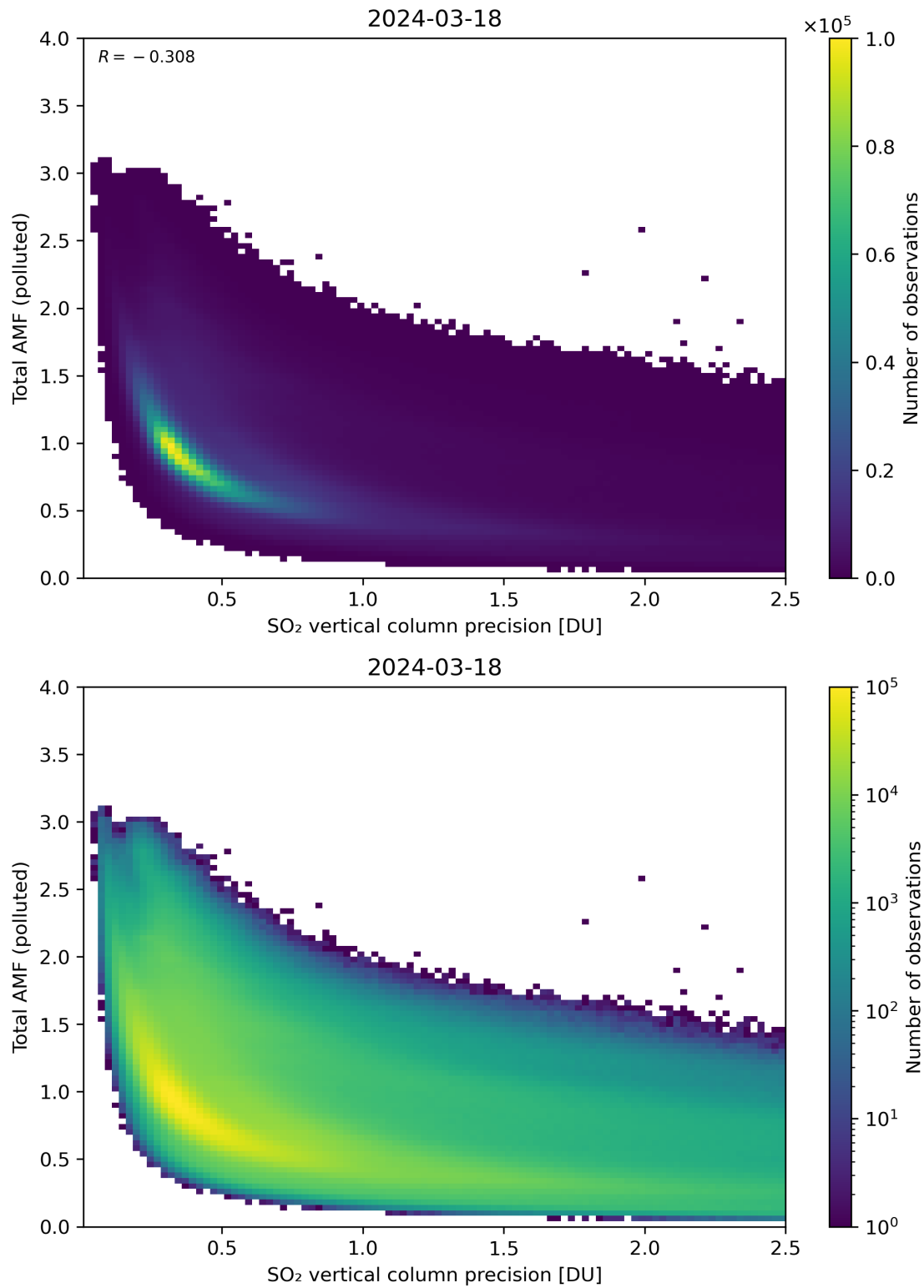
Figure 294: Scatter density plot of “SO 2 vertical column precision” against “Total AMF (polluted)” for 2024-03-17 to 2024-03-19.
