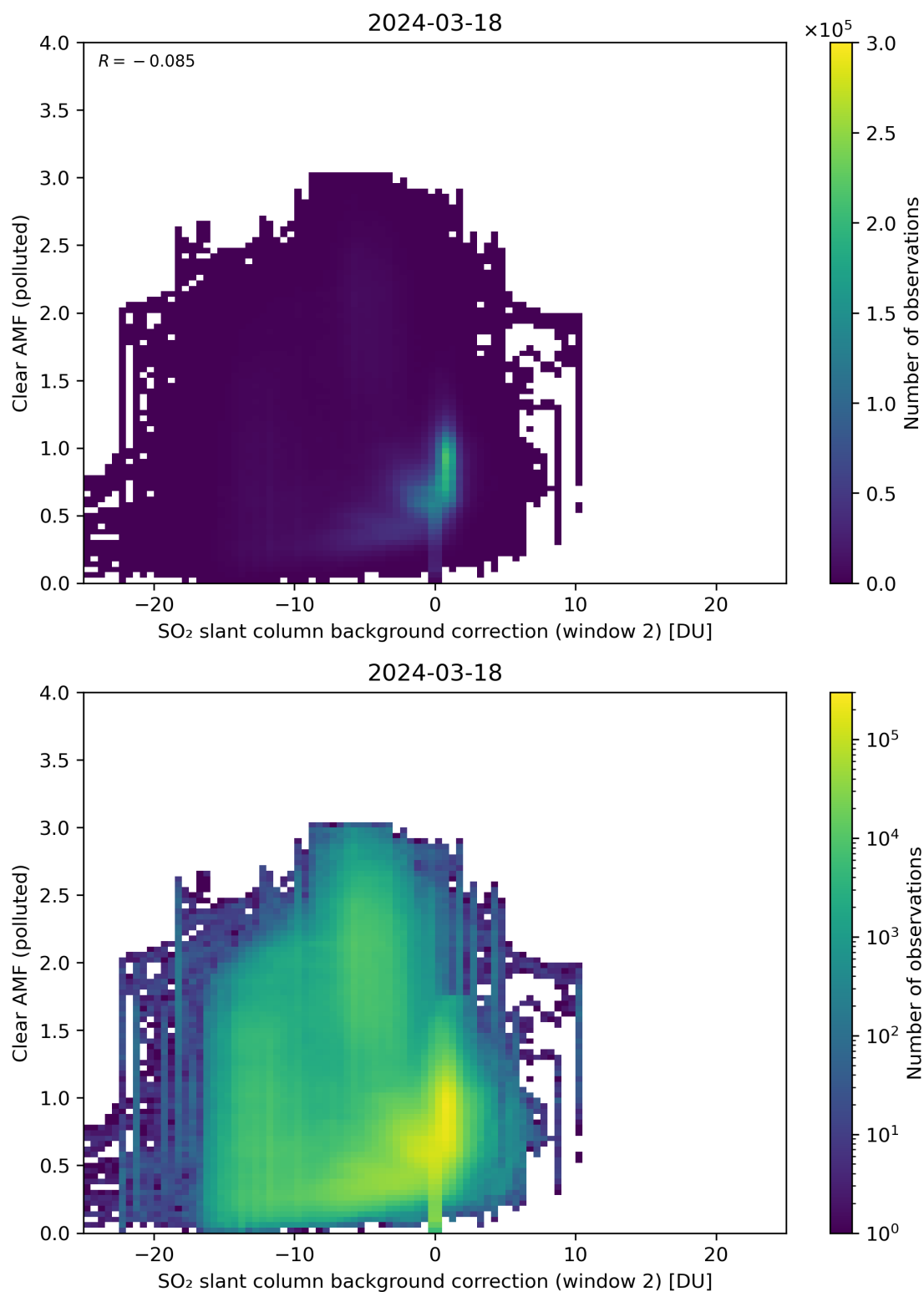
Figure 115: Scatter density plot of “SO 2 slant column background correction (window 2)” against “Clear AMF (polluted)” for 2024-03-17 to 2024-03-19.
