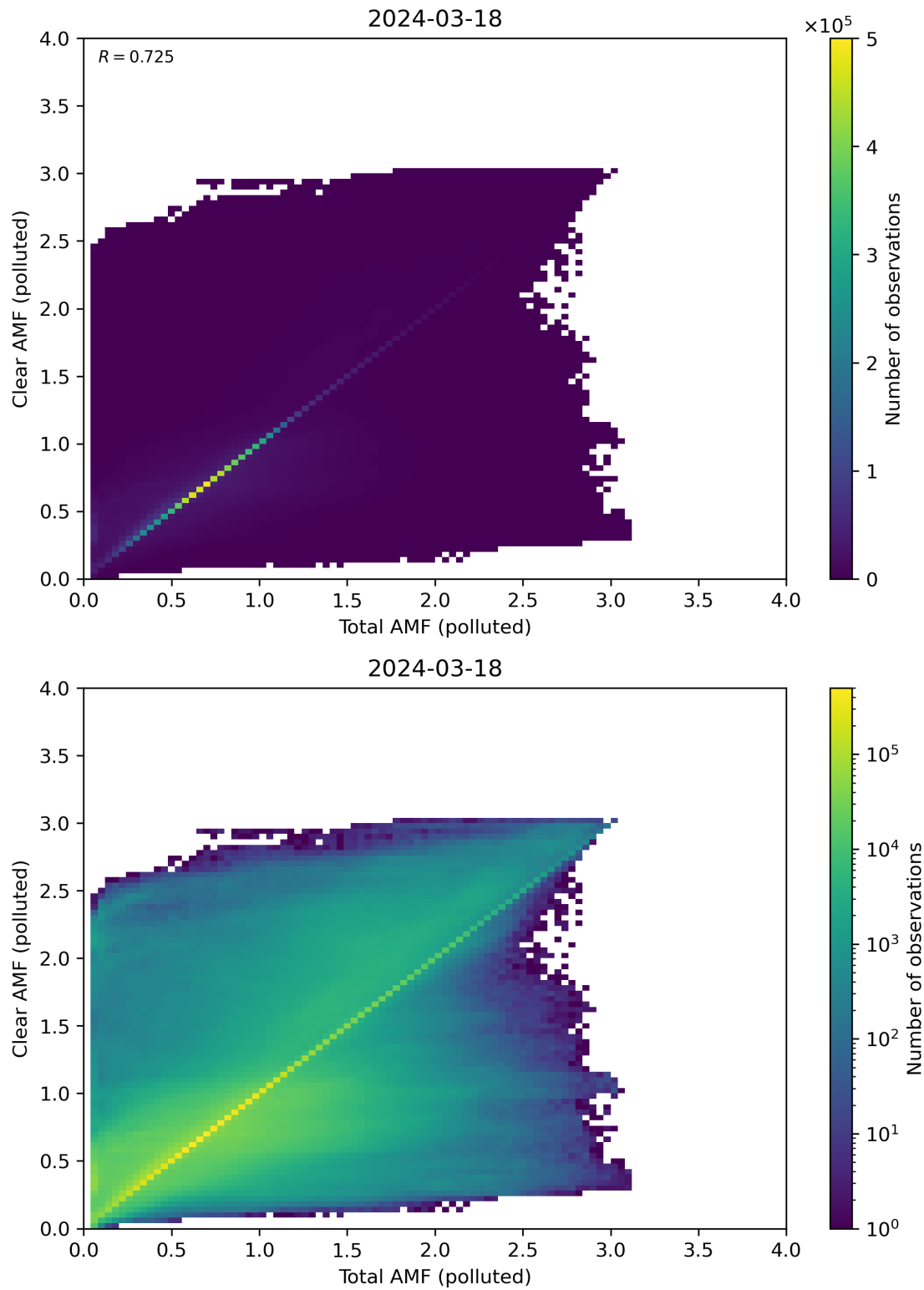
Figure 271: Scatter density plot of “Total AMF (polluted)” against “Clear AMF (polluted)” for 2024-03-17 to 2024-03-19.
