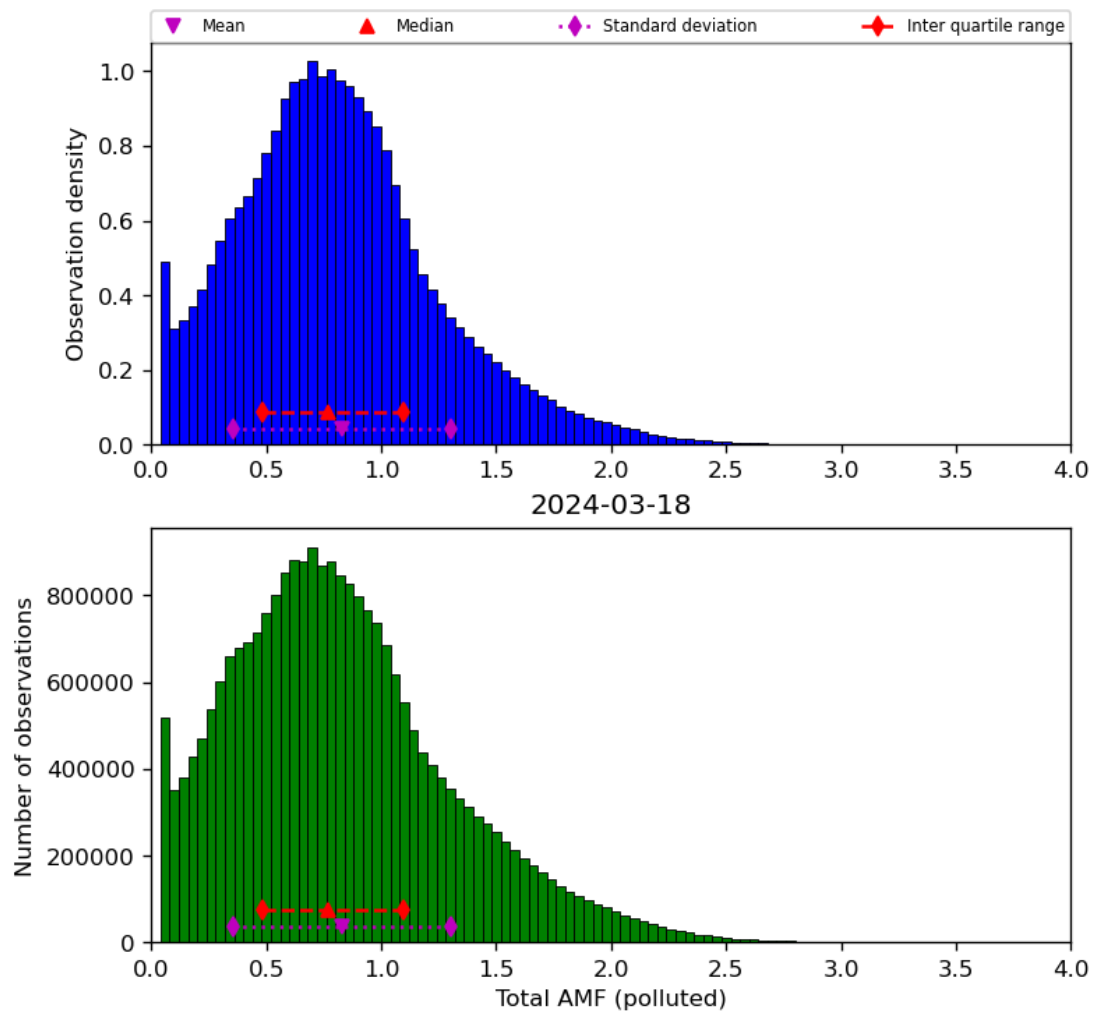
Figure 71: Histogram of “Total AMF (polluted)” for 2024-03-17 to 2024-03-19
