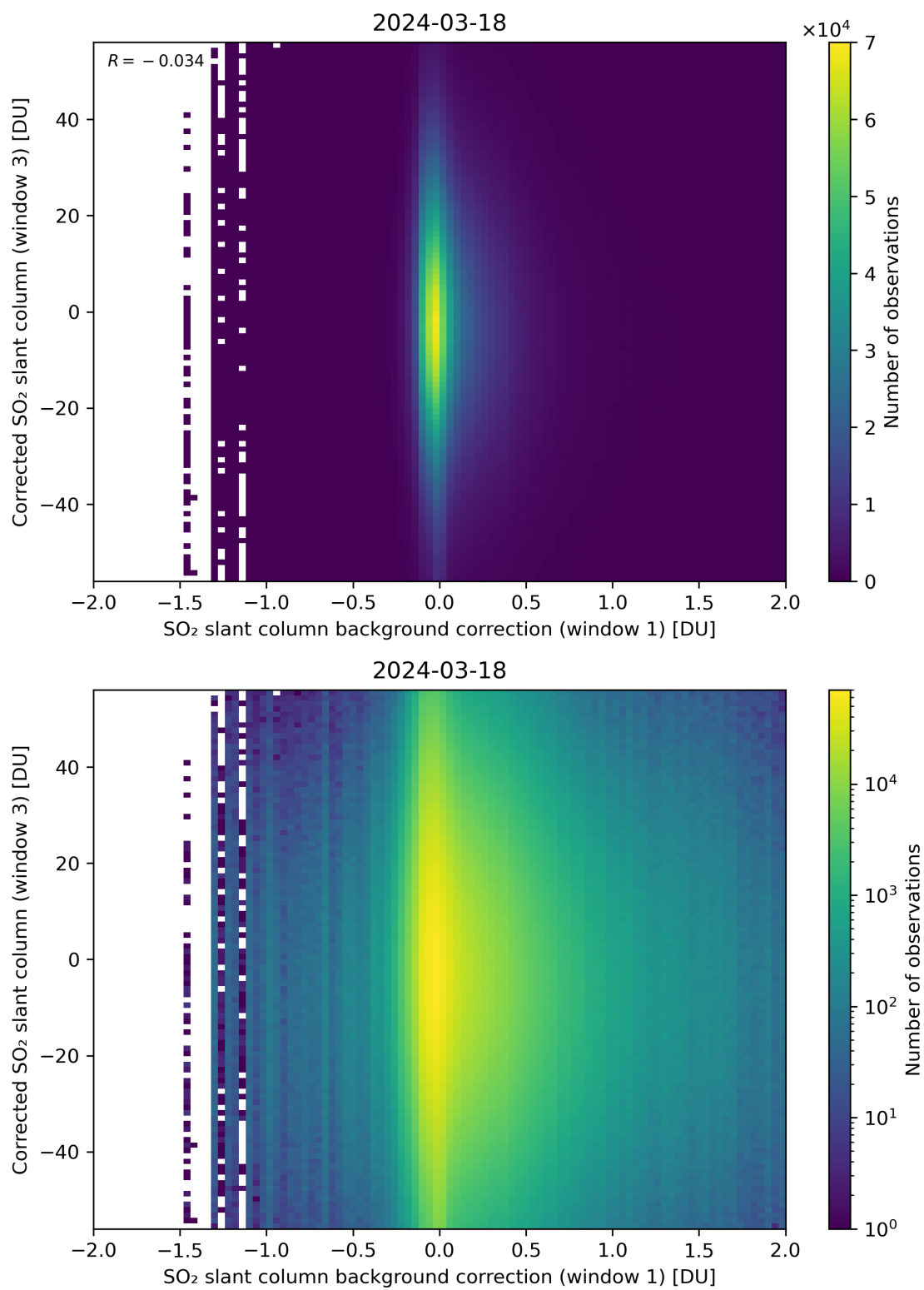
Figure 105: Scatter density plot of “SO 2 slant column background correction (window 1)” against “Corrected SO 2 slant column (window 3)” for 2024-03-17 to 2024-03-19.
