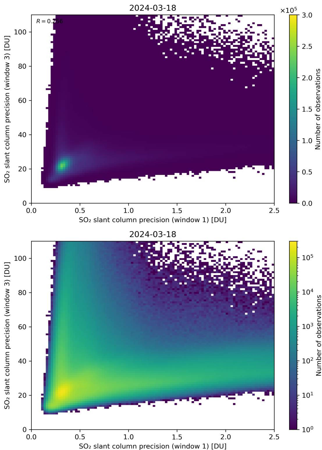
Figure 229: Scatter density plot of “SO 2 slant column precision (window 1)” against “SO 2 slant column precision (window 3)” for 2024-03-17 to 2024-03-19.
