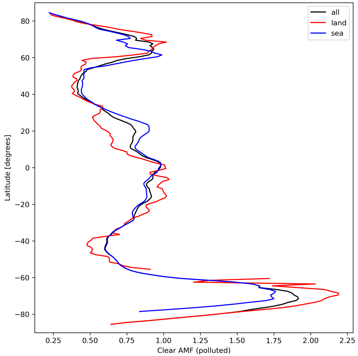
Figure 50: Zonal average of “Clear AMF (polluted)” for 2024-03-17 to 2024-03-19.
