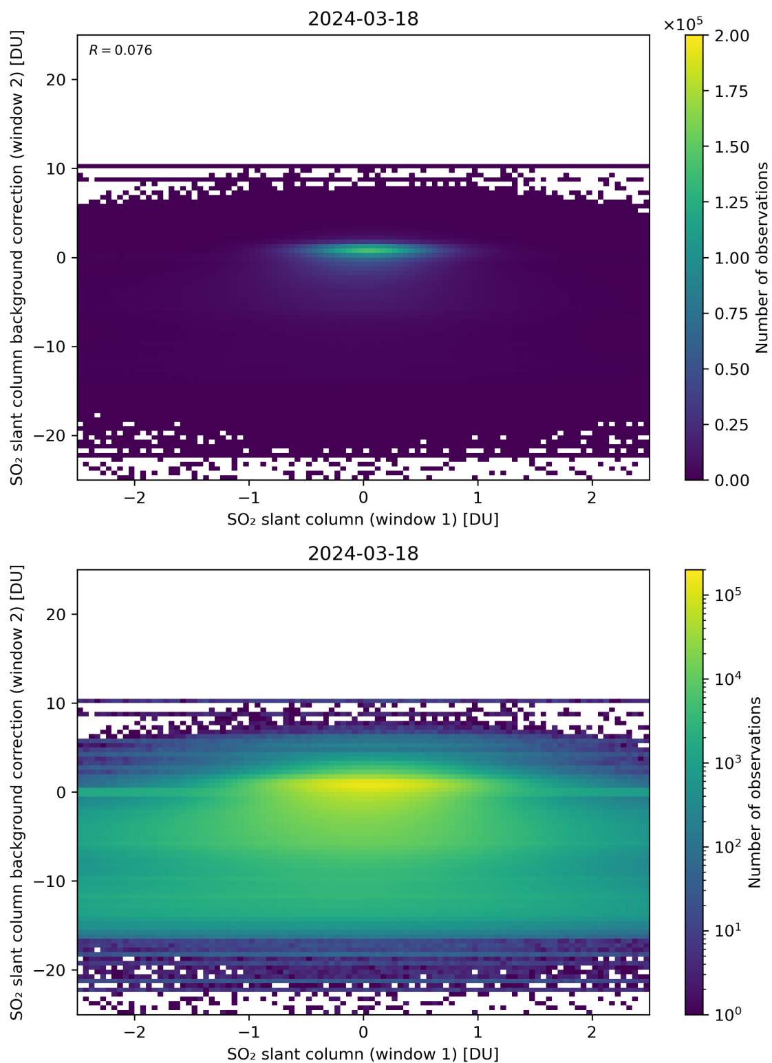
Figure 213: Scatter density plot of “SO 2 slant column (window 1)” against “SO 2 slant column background correction (window 2)” for 2024-03-17 to 2024-03-19.
