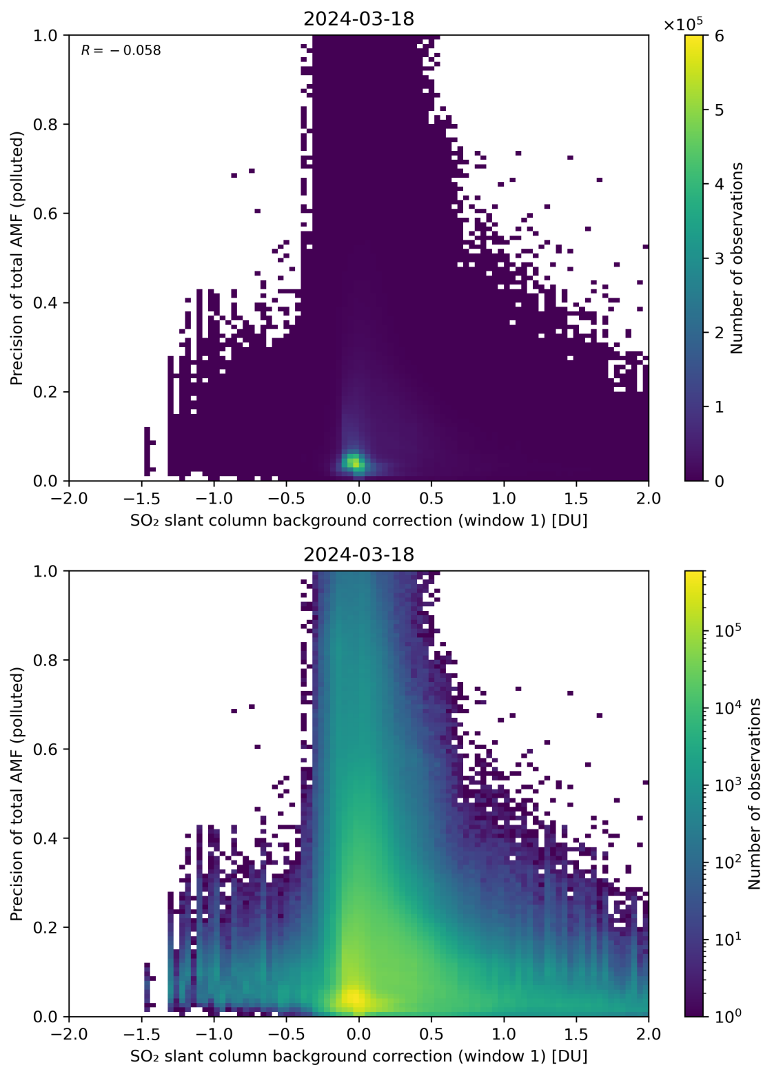
Figure 110: Scatter density plot of “SO 2 slant column background correction (window 1)” against “Precision of total AMF (polluted)” for 2024-03-17 to 2024-03-19.
