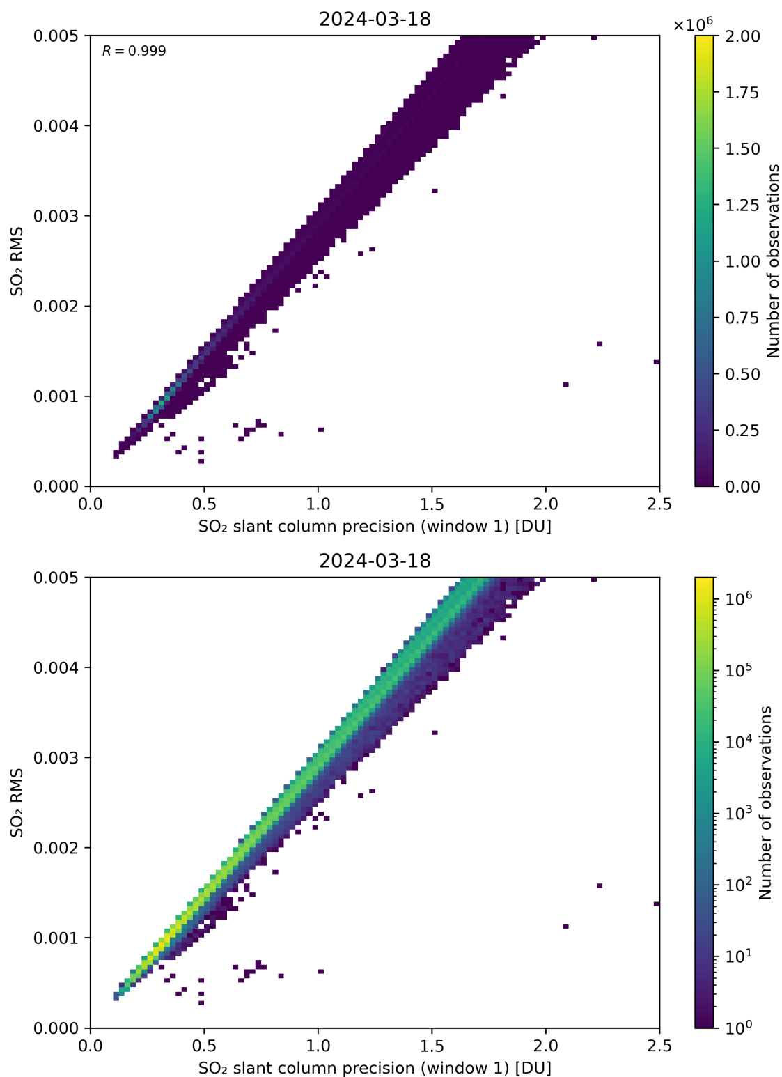
Figure 223: Scatter density plot of “SO 2 slant column precision (window 1)” against “SO 2 RMS” for 2024-03-17 to 2024-03-19.
