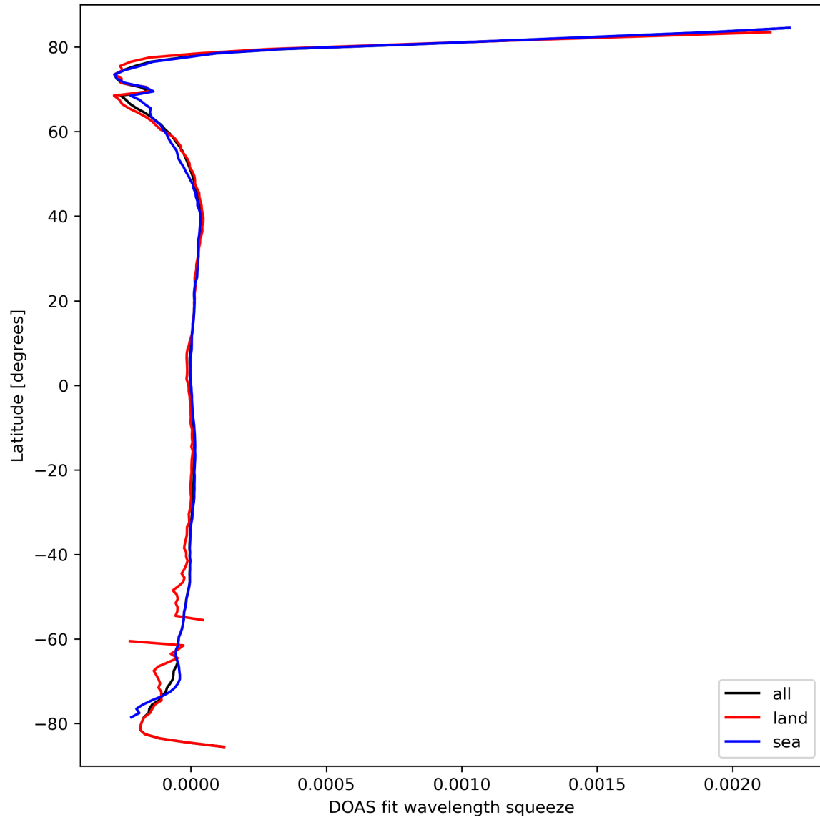
Figure 46: Zonal average of “DOAS fit wavelength squeeze” for 2024-03-17 to 2024-03-19.
