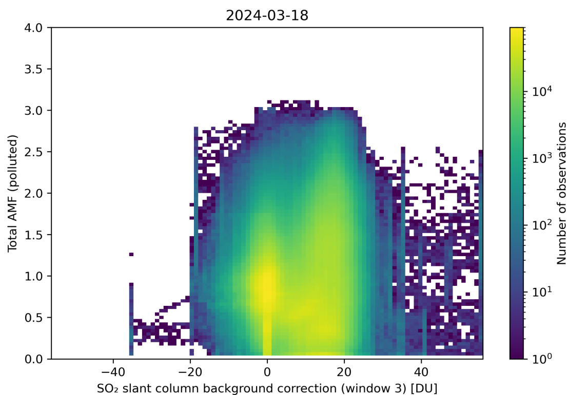
Figure 125: Scatter density plot of “SO 2 slant column background correction (window 3)” against “Total AMF (polluted)” for 2024-03-17 to 2024-03-19.
