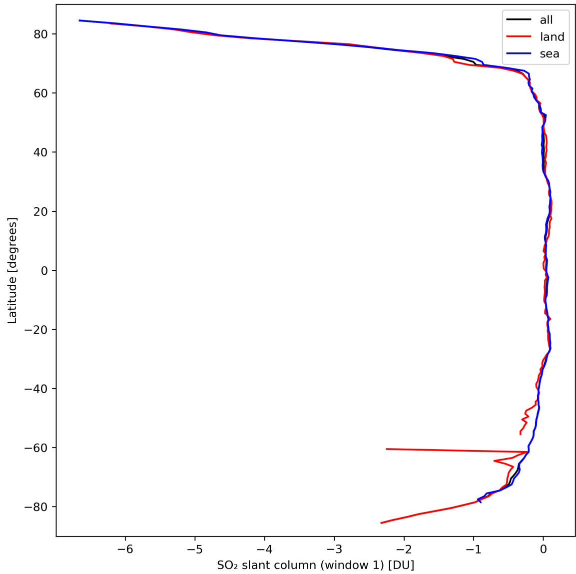
Figure 33: Zonal average of “SO 2 slant column (window 1)” for 2024-03-17 to 2024-03-19.
