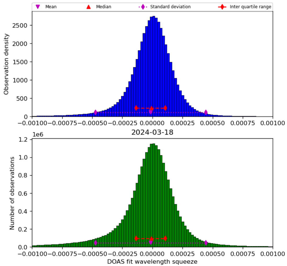
Figure 69: Histogram of “DOAS fit wavelength squeeze” for 2024-03-17 to 2024-03-19
