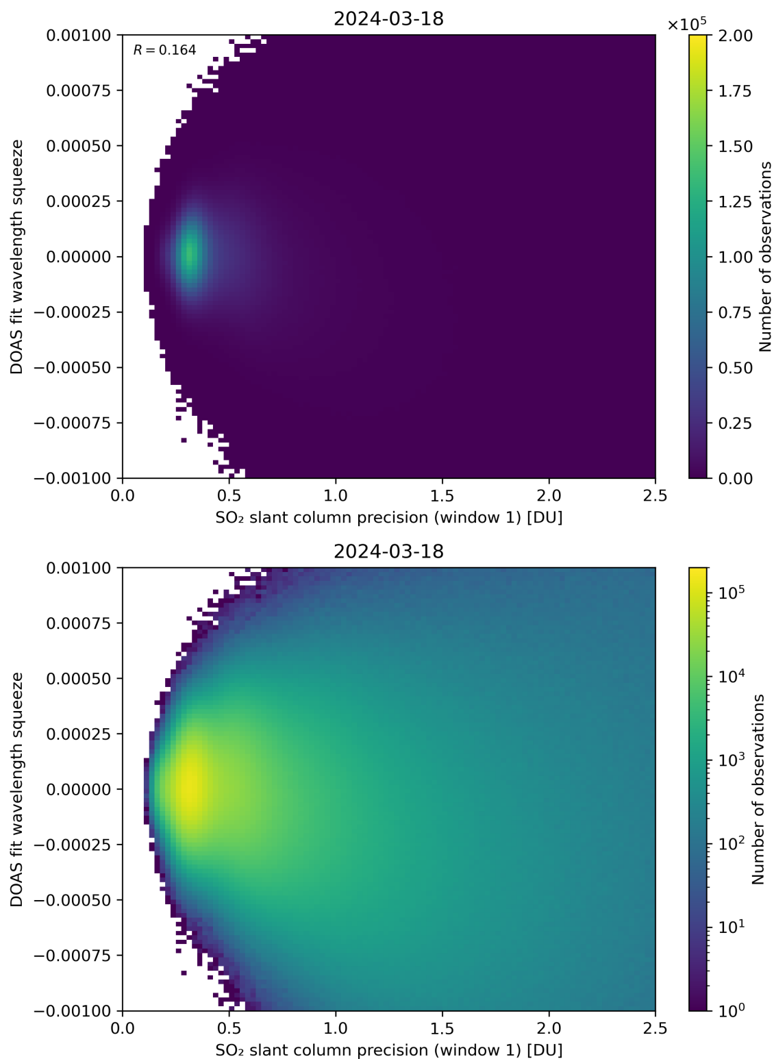
Figure 222: Scatter density plot of “SO 2 slant column precision (window 1)” against “DOAS fit wavelength squeeze” for 2024-03-17 to 2024-03-19.
