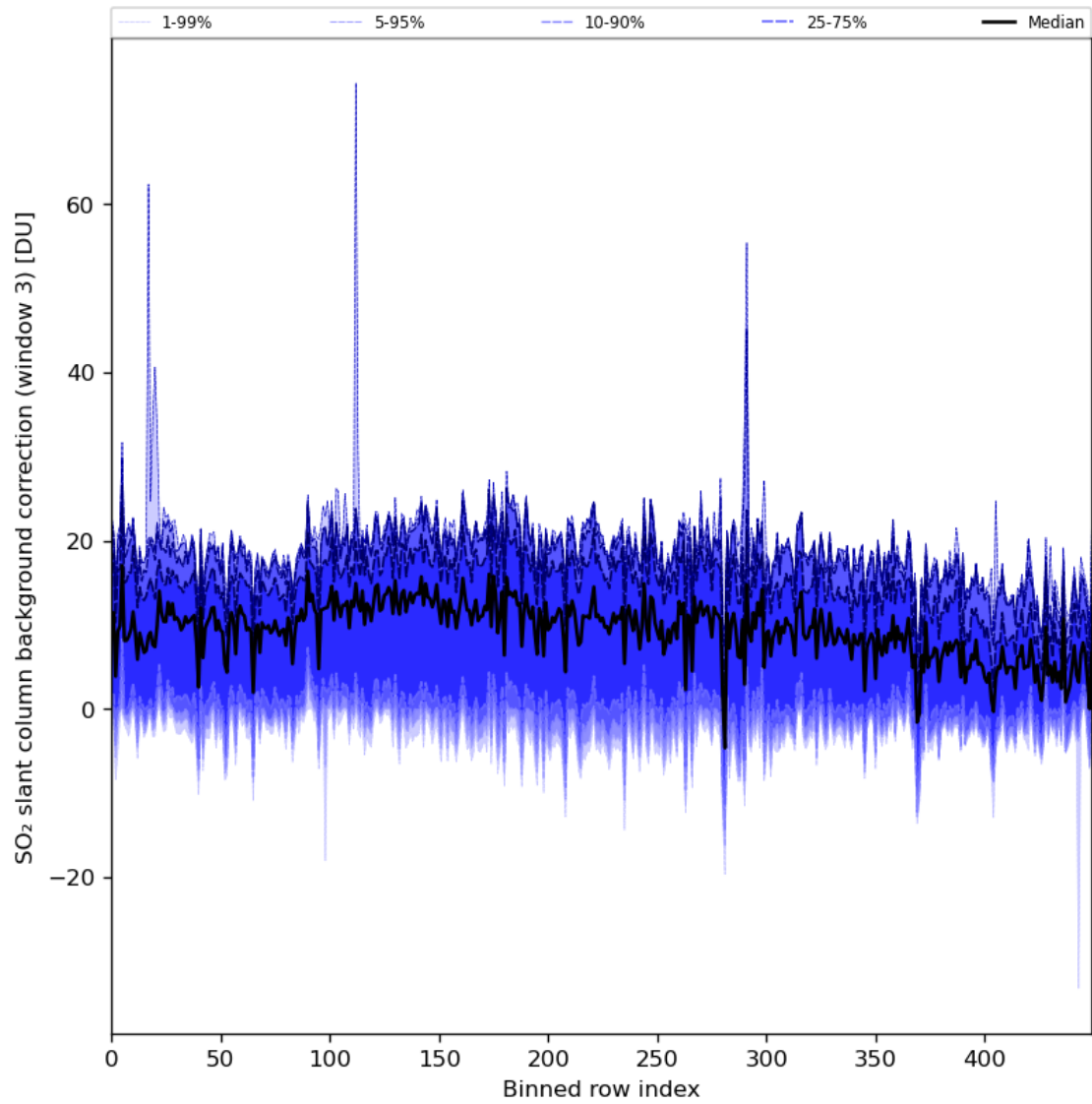
Figure 90: Along track statistics of “SO 2 slant column background correction (window 3)” for 2024-03-17 to 2024-03-19
