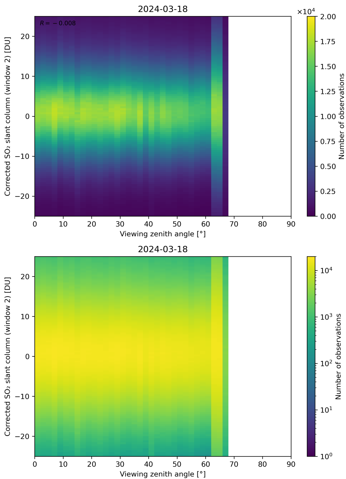
Figure 318: Scatter density plot of “Viewing zenith angle” against “Corrected SO 2 slant column (window 2)” for 2024-03-17 to 2024-03-19.
