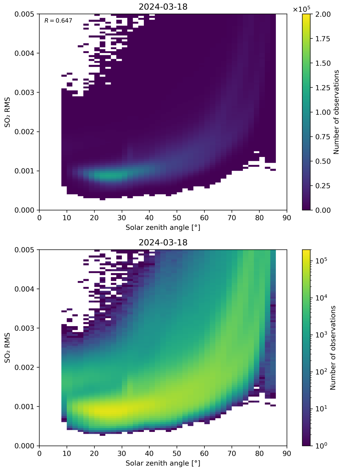
Figure 163: Scatter density plot of “Solar zenith angle” against “SO 2 RMS” for 2024-03-17 to 2024-03-19.
