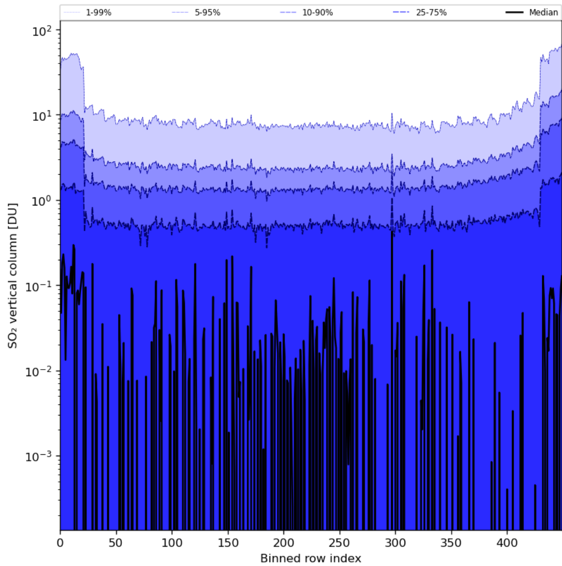
Figure 76: Along track statistics of “SO 2 vertical column” for 2024-03-17 to 2024-03-19
