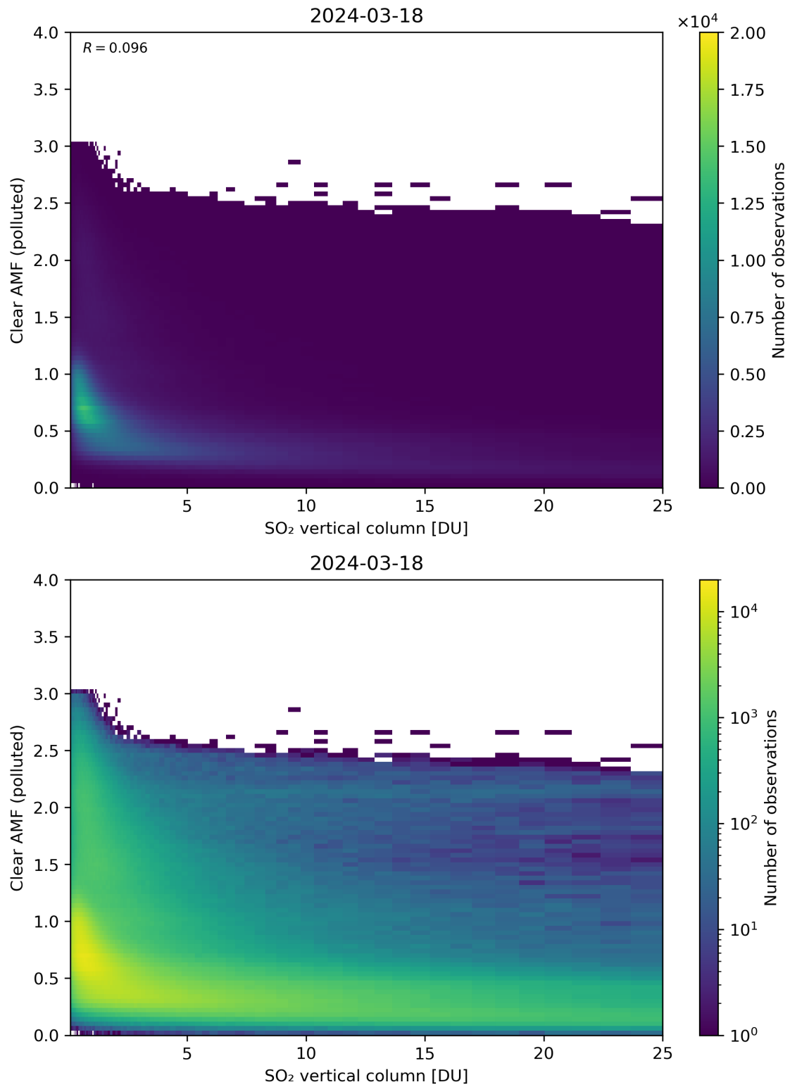
Figure 296: Scatter density plot of “SO 2 vertical column” against “Clear AMF (polluted)” for 2024-03-17 to 2024-03-19.
