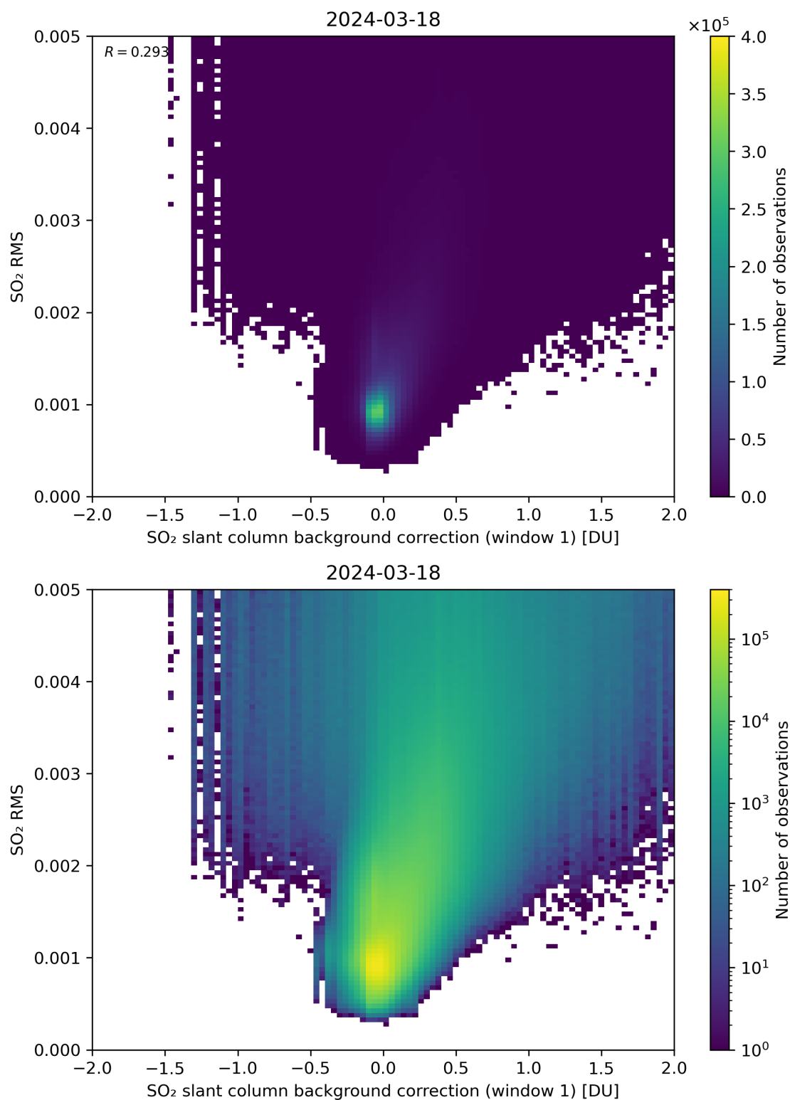
Figure 102: Scatter density plot of “SO 2 slant column background correction (window 1)” against “SO 2 RMS” for 2024-03-17 to 2024-03-19.
