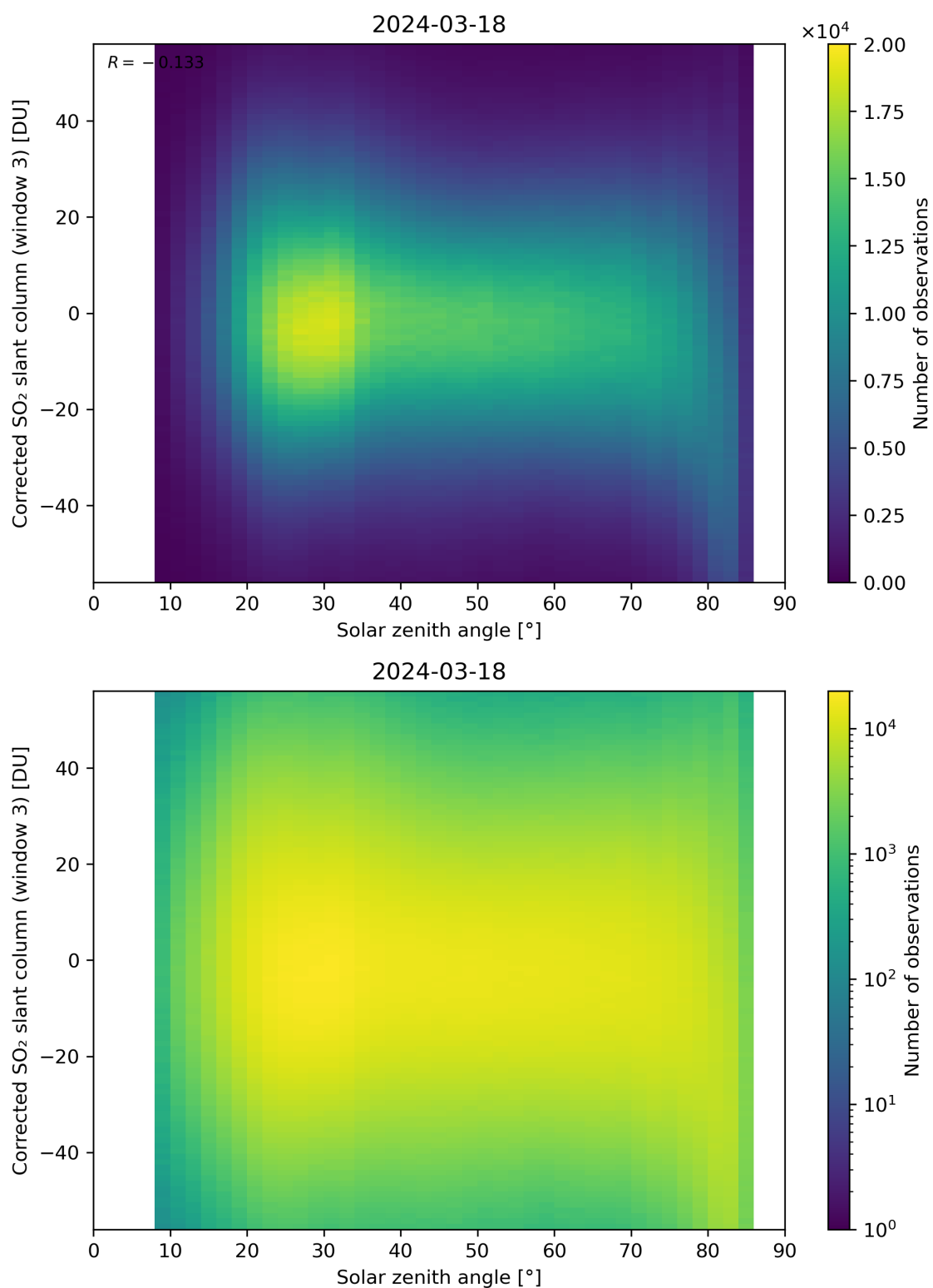
Figure 168: Scatter density plot of “Solar zenith angle” against “Corrected SO 2 slant column (window 3)” for 2024-03-17 to 2024-03-19.
