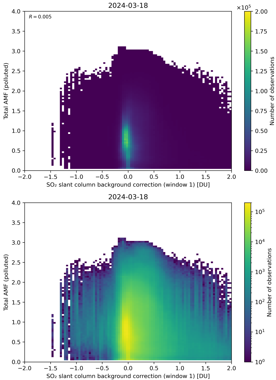
Figure 109: Scatter density plot of “SO 2 slant column background correction (window 1)” against “Total AMF (polluted)” for 2024-03-17 to 2024-03-19.
