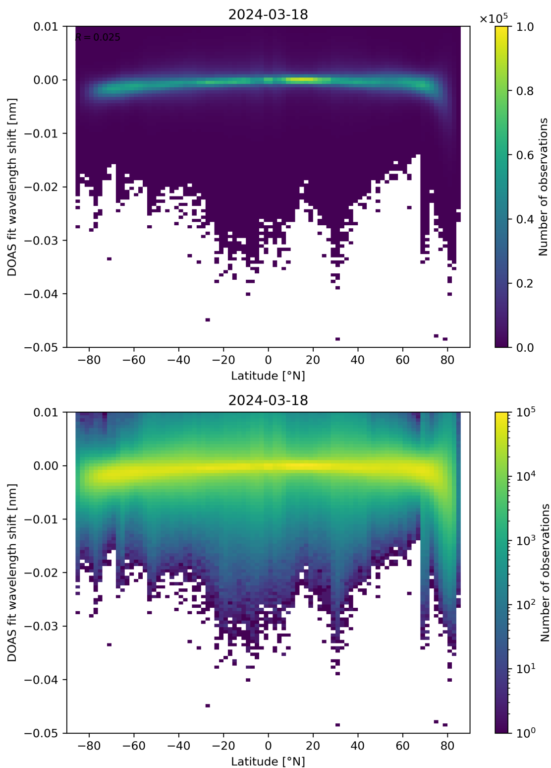
Figure 142: Scatter density plot of “Latitude” against “DOAS fit wavelength shift” for 2024-03-17 to 2024-03-19.
