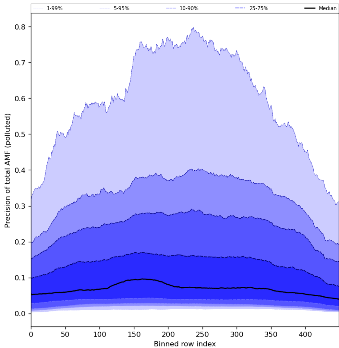
Figure 95: Along track statistics of “Precision of total AMF (polluted)” for 2024-03-17 to 2024-03-19
