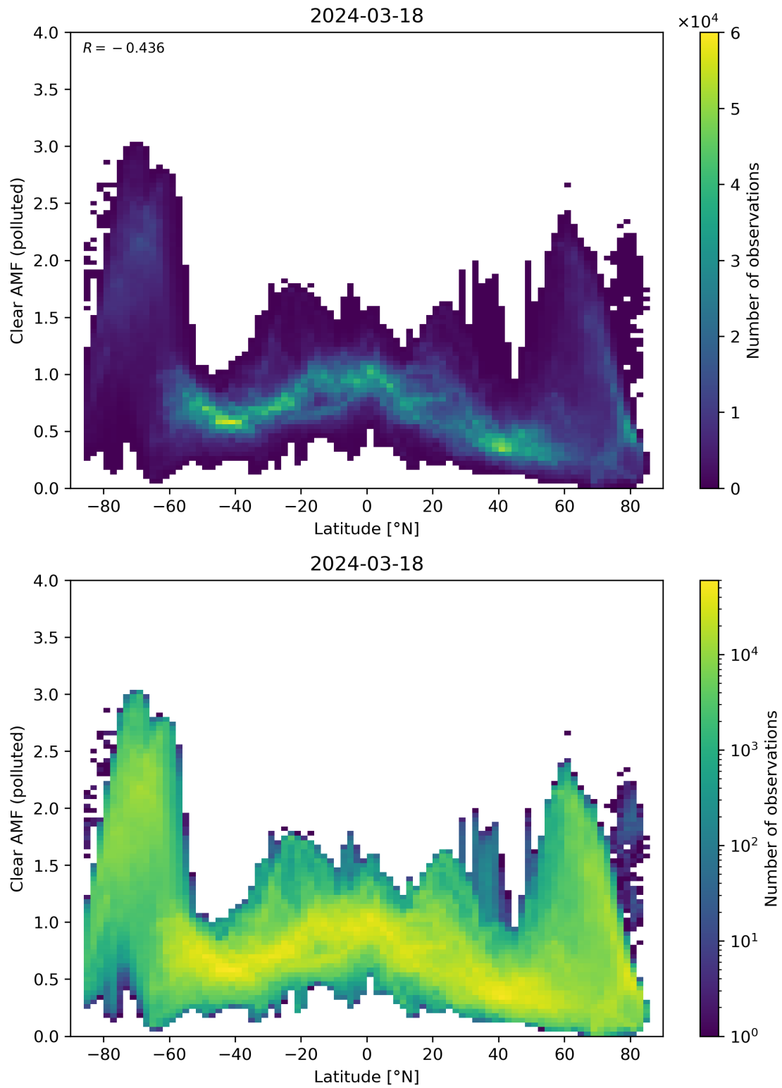
Figure 145: Scatter density plot of “Latitude” against “Clear AMF (polluted)” for 2024-03-17 to 2024-03-19.
