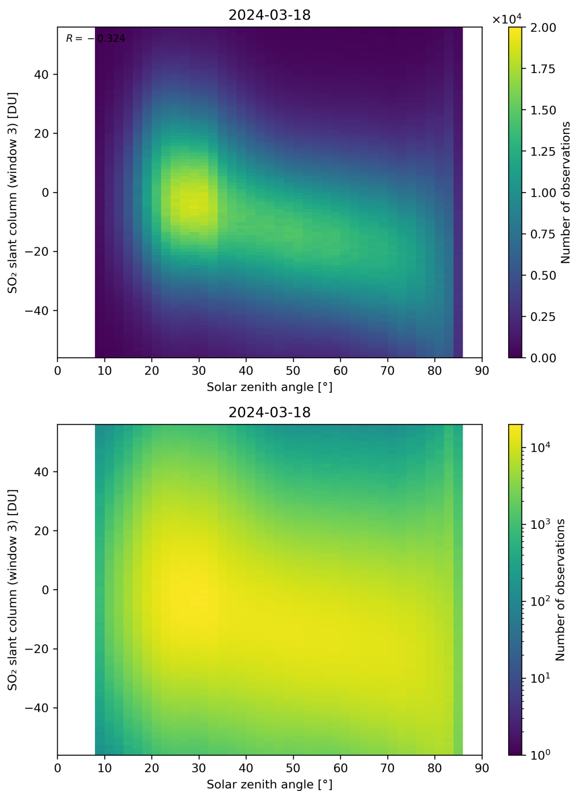
Figure 172: Scatter density plot of “Solar zenith angle” against “SO 2 slant column (window 3)” for 2024-03-17 to 2024-03-19.
