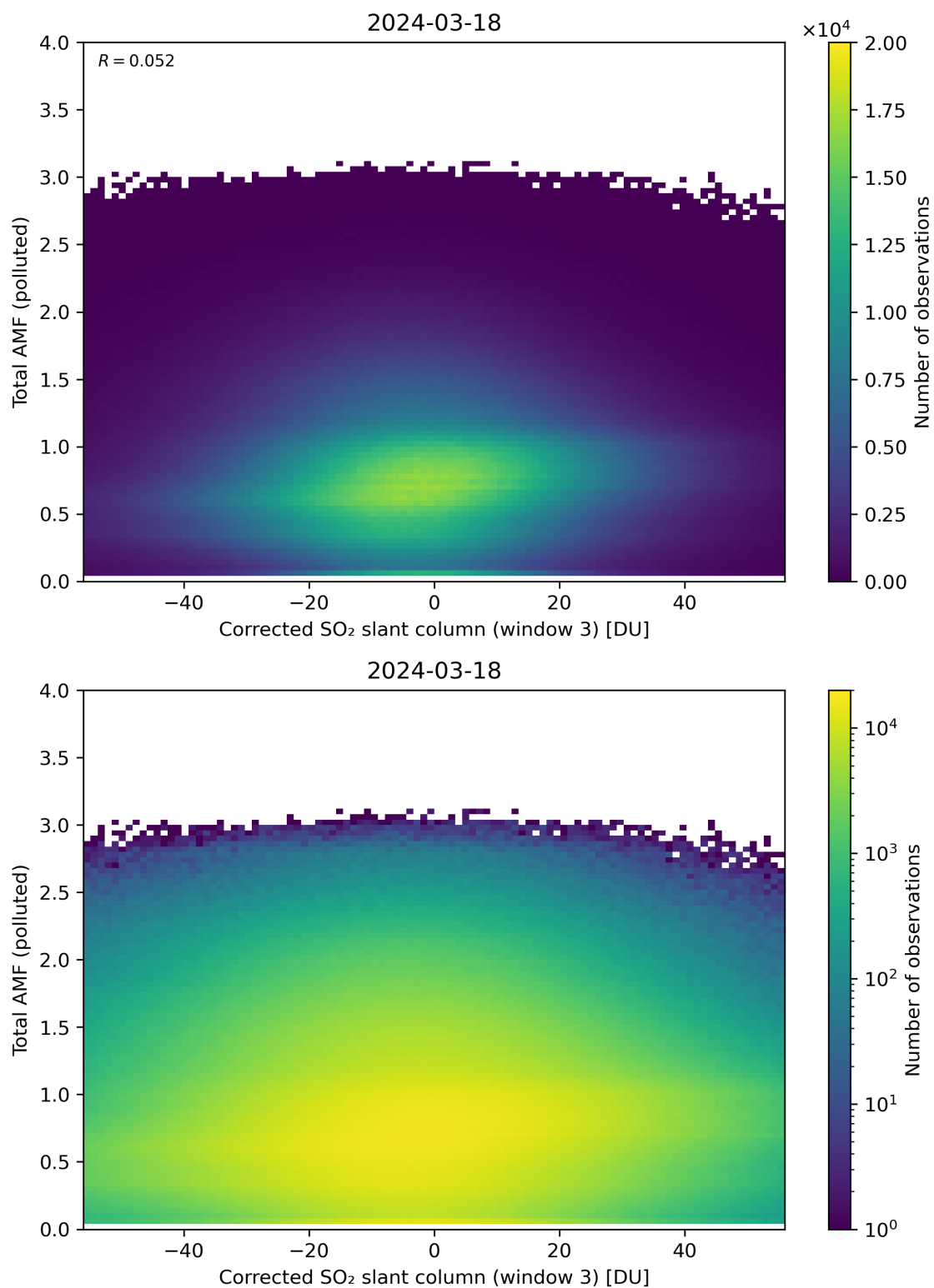
Figure 210: Scatter density plot of “Corrected SO 2 slant column (window 3)” against “Total AMF (polluted)” for 2024-03-17 to 2024-03-19.
