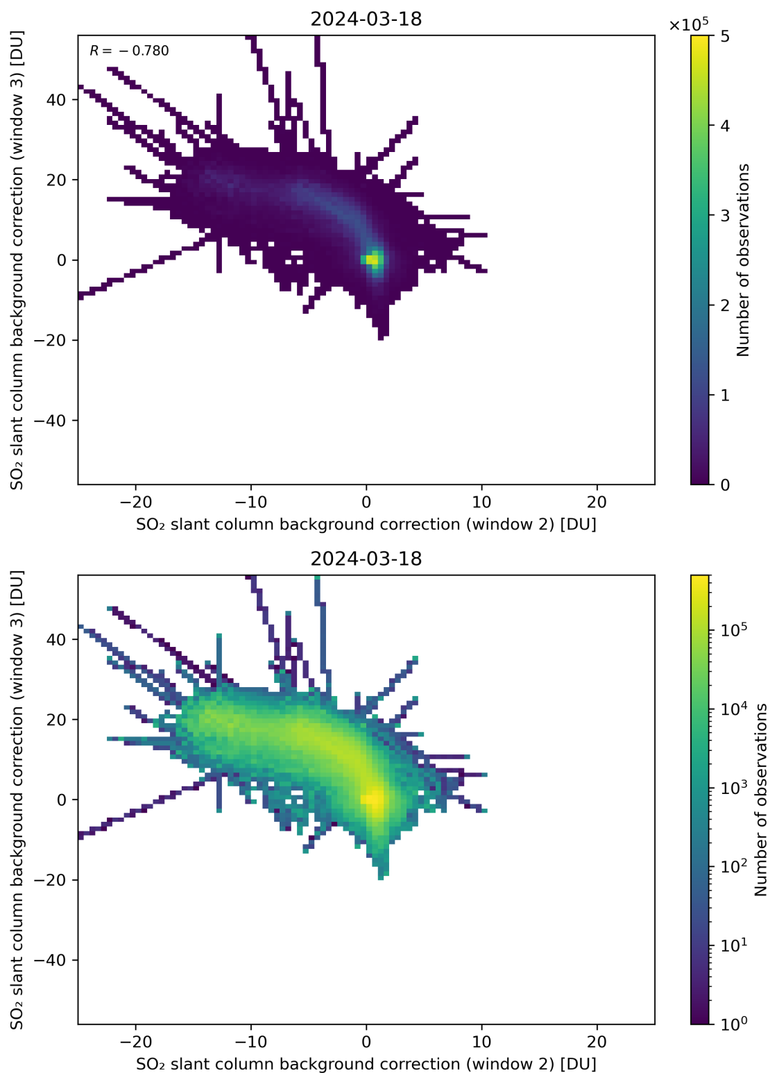
Figure 111: Scatter density plot of “SO 2 slant column background correction (window 2)” against “SO 2 slant column background correction (window 3)” for 2024-03-17 to 2024-03-19.
