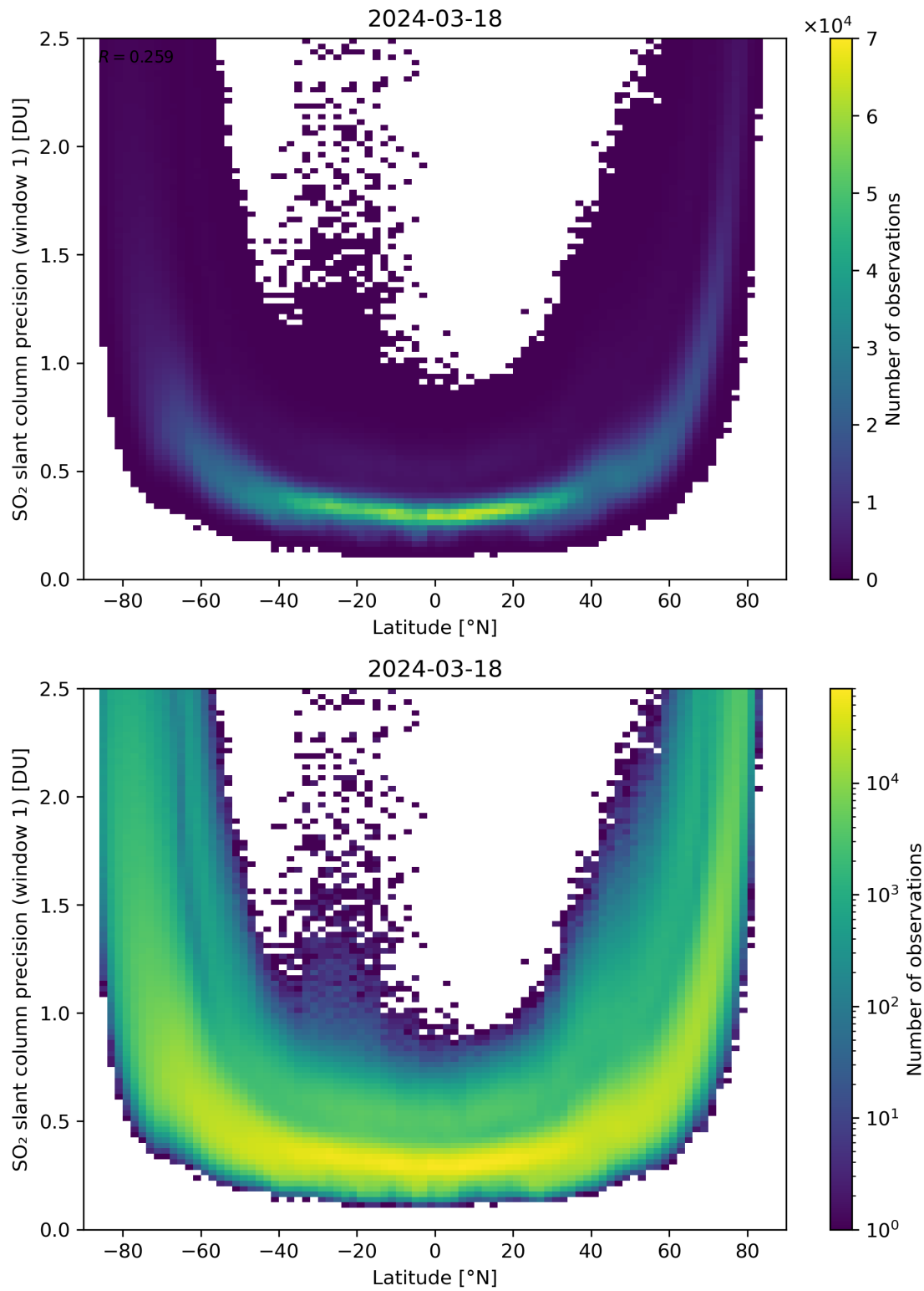
Figure 150: Scatter density plot of “Latitude” against “SO 2 slant column precision (window 1)” for 2024-03-17 to 2024-03-19.
