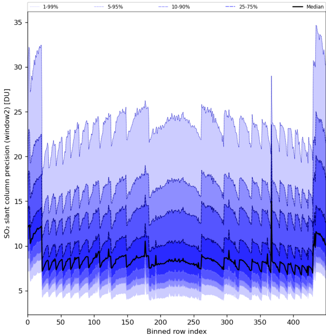
Figure 84: Along track statistics of “SO 2 slant column precision (window2)” for 2024-03-17 to 2024-03-19
