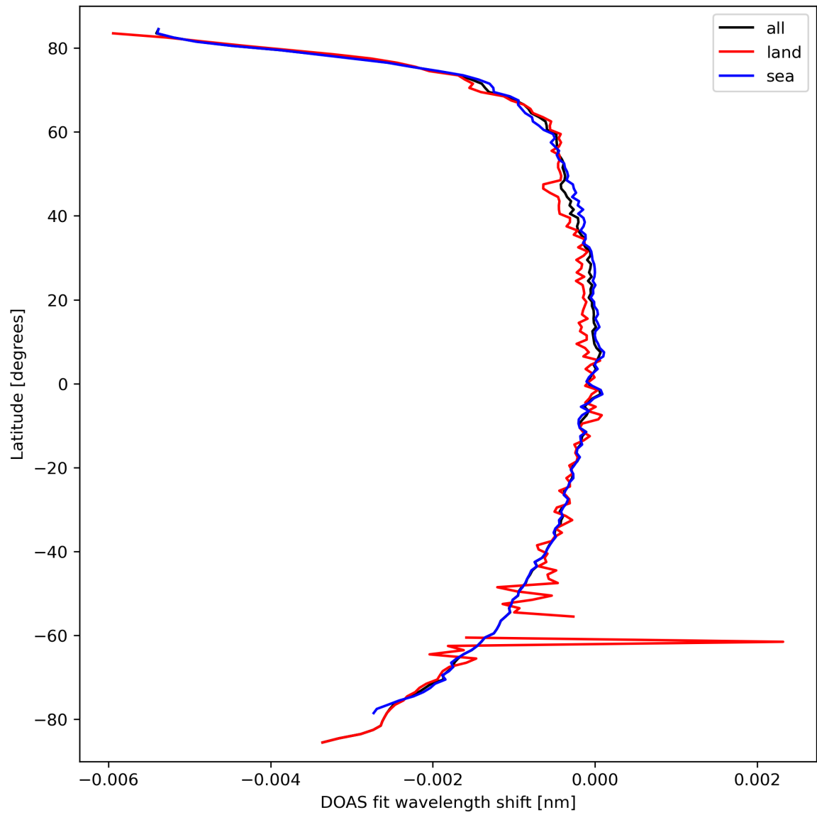
Figure 45: Zonal average of “DOAS fit wavelength shift” for 2024-03-17 to 2024-03-19.
