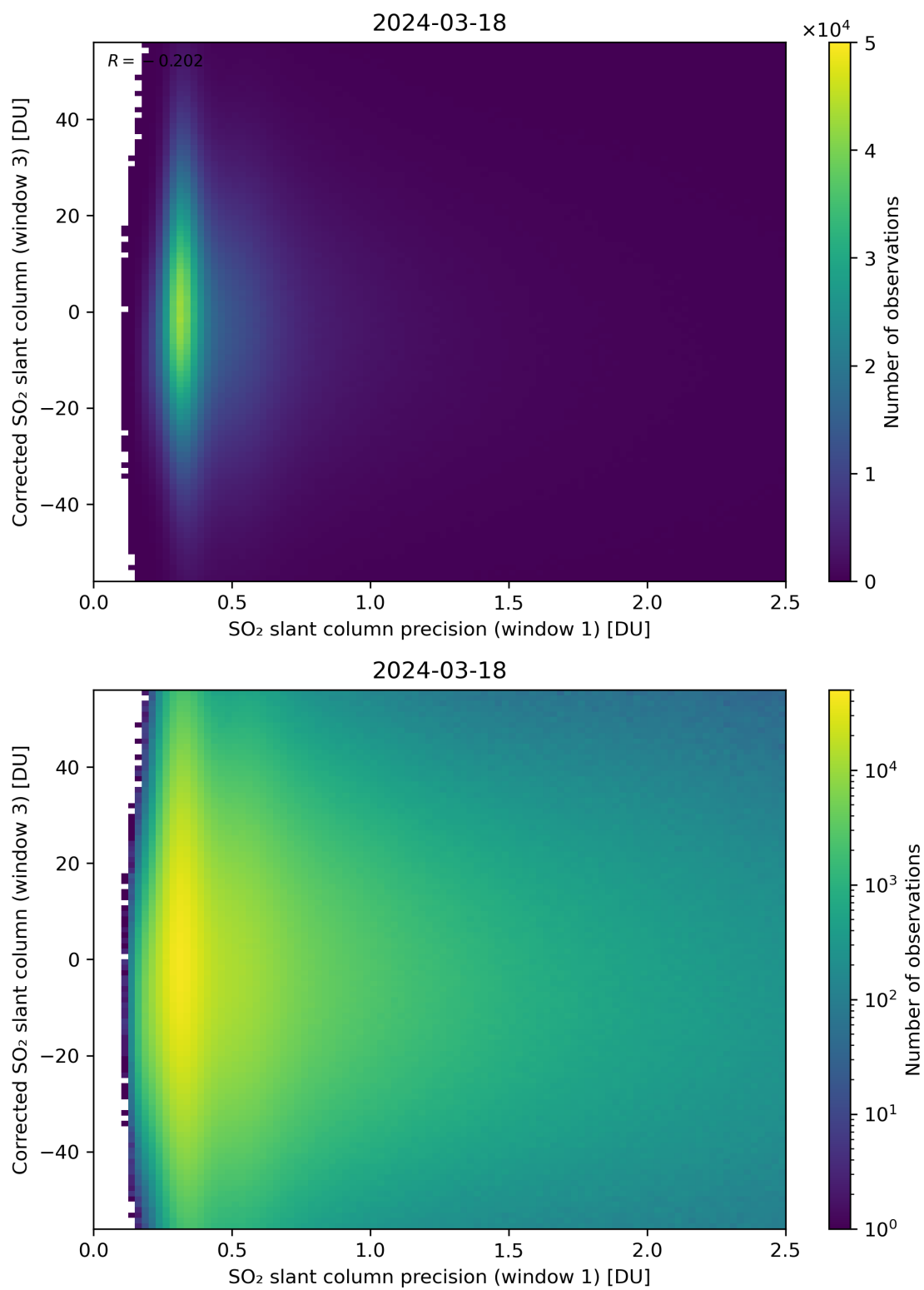
Figure 226: Scatter density plot of “SO 2 slant column precision (window 1)” against “Corrected SO 2 slant column (window 3)” for 2024-03-17 to 2024-03-19.
