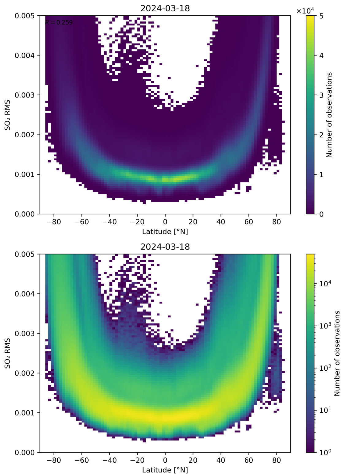
Figure 144: Scatter density plot of “Latitude” against “SO 2 RMS” for 2024-03-17 to 2024-03-19.
