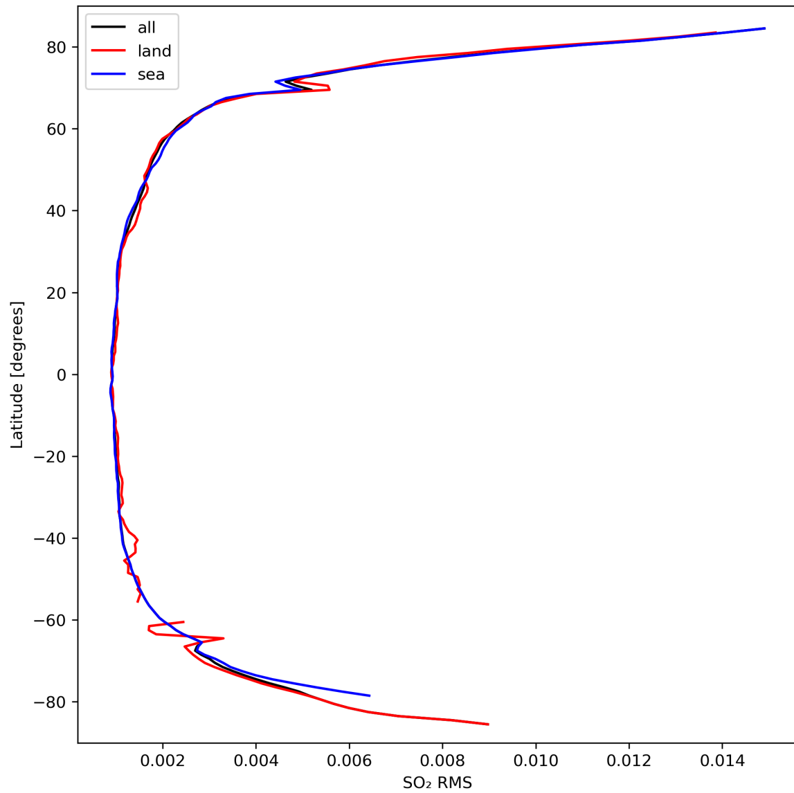
Figure 47: Zonal average of “SO 2 RMS” for 2024-03-17 to 2024-03-19.
