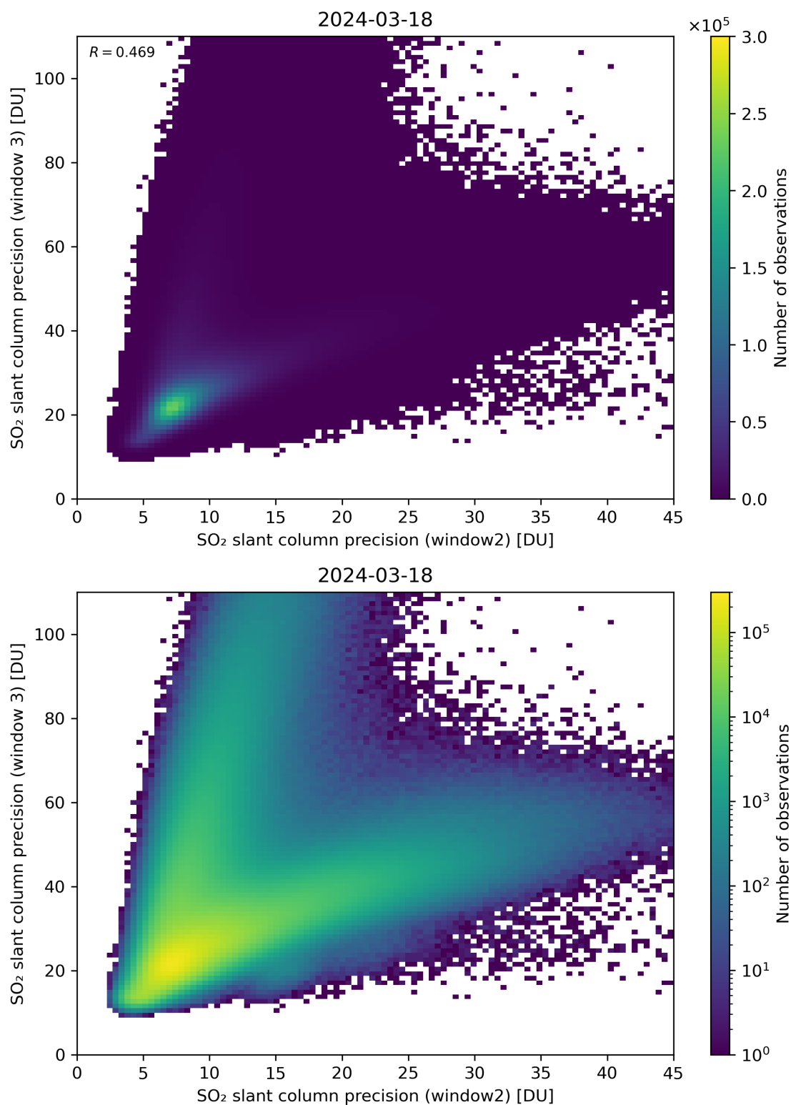
Figure 250: Scatter density plot of “SO 2 slant column precision (window2)” against “SO 2 slant column precision (window 3)” for 2024-03-17 to 2024-03-19.
