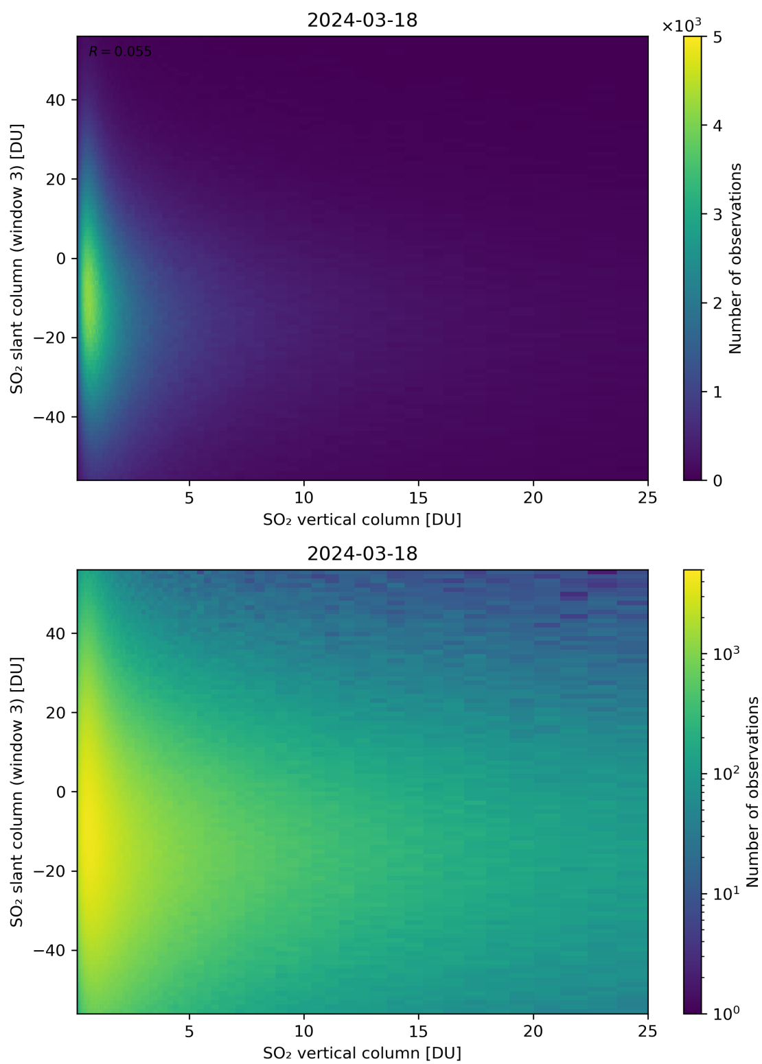
Figure 303: Scatter density plot of “SO 2 vertical column” against “SO 2 slant column (window 3)” for 2024-03-17 to 2024-03-19.
