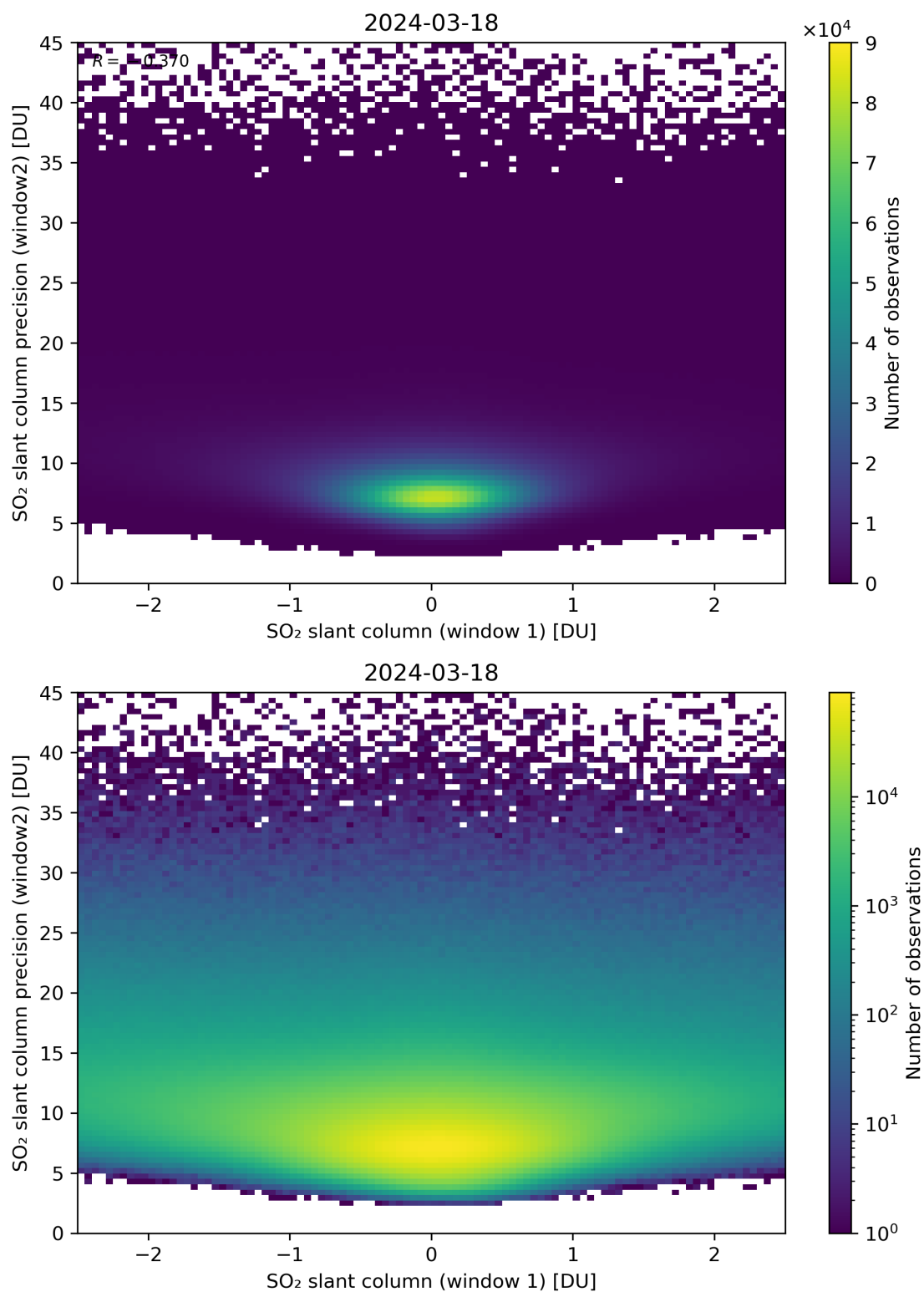
Figure 236: Scatter density plot of “SO 2 slant column (window 1)” against “SO 2 slant column precision (window2)” for 2024-03-17 to 2024-03-19.
