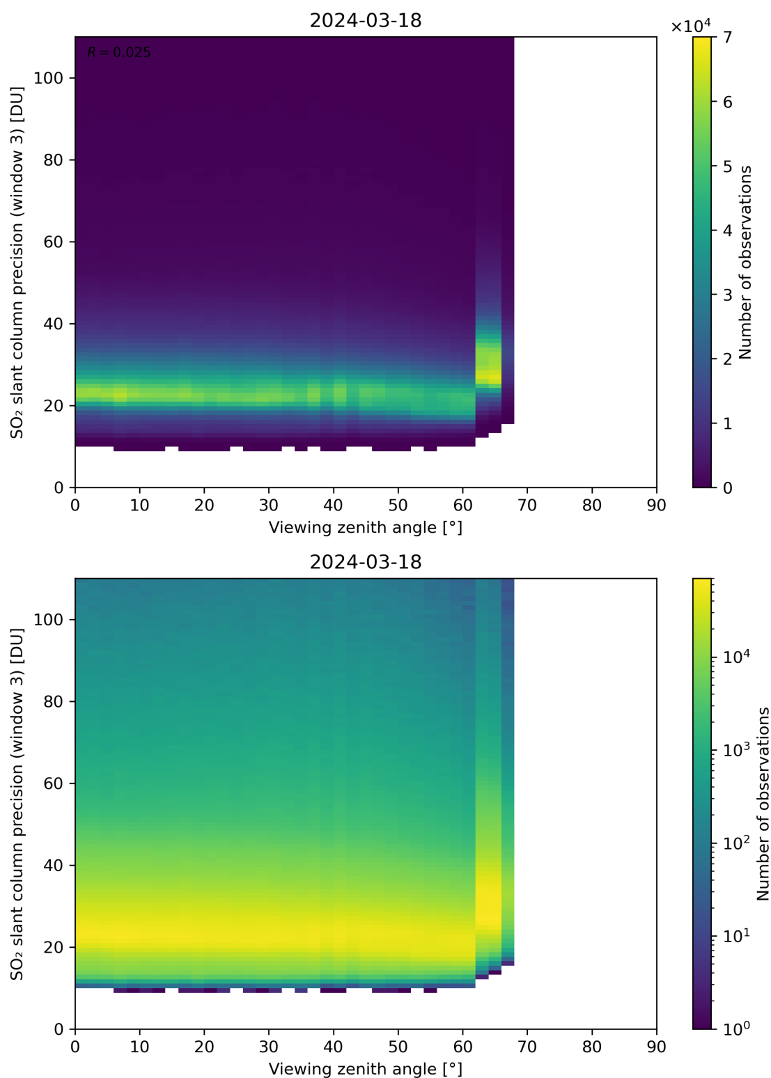
Figure 324: Scatter density plot of “Viewing zenith angle” against “SO 2 slant column precision (window 3)” for 2024-03-17 to 2024-03-19.
