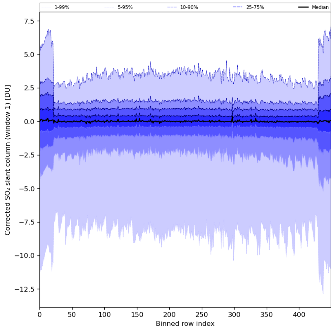
Figure 81: Along track statistics of “Corrected SO 2 slant column (window 1)” for 2024-03-17 to 2024-03-19
