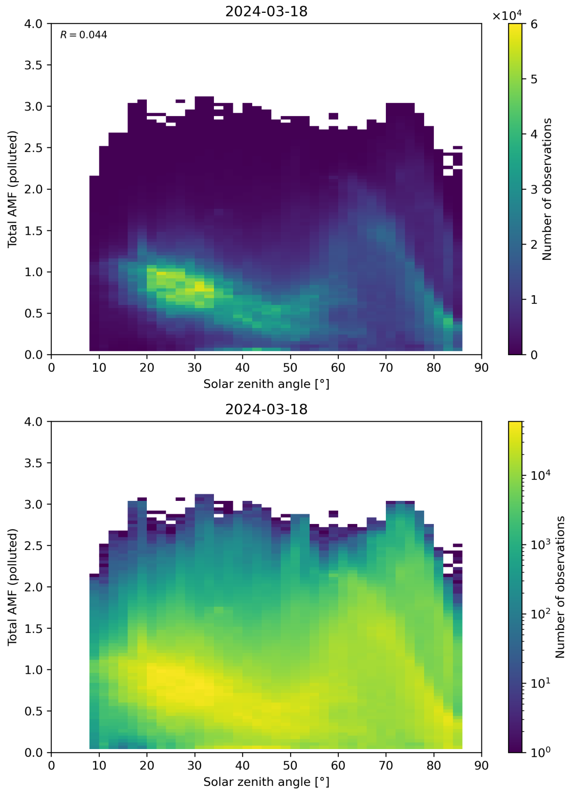
Figure 174: Scatter density plot of “Solar zenith angle” against “Total AMF (polluted)” for 2024-03-17 to 2024-03-19.
