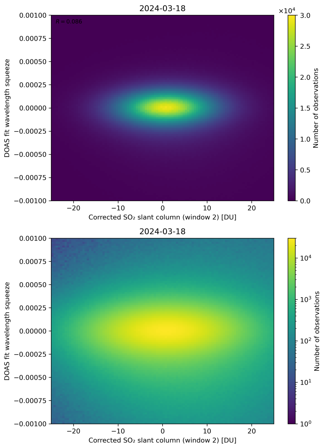
Figure 197: Scatter density plot of “Corrected SO 2 slant column (window 2)” against “DOAS fit wavelength squeeze” for 2024-03-17 to 2024-03-19.
