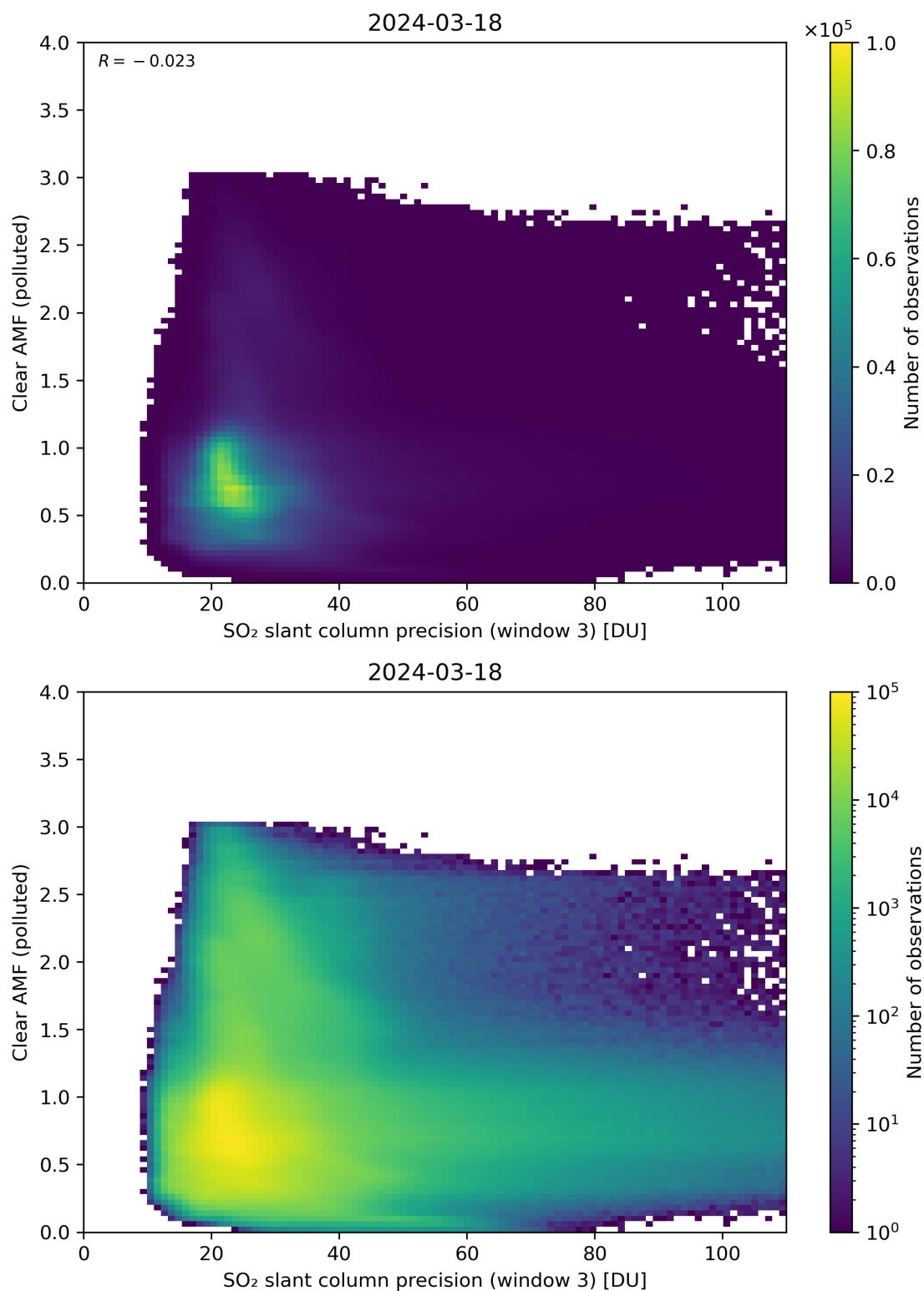
Figure 261: Scatter density plot of “SO 2 slant column precision (window 3)” against “Clear AMF (polluted)” for 2024-03-17 to 2024-03-19.
