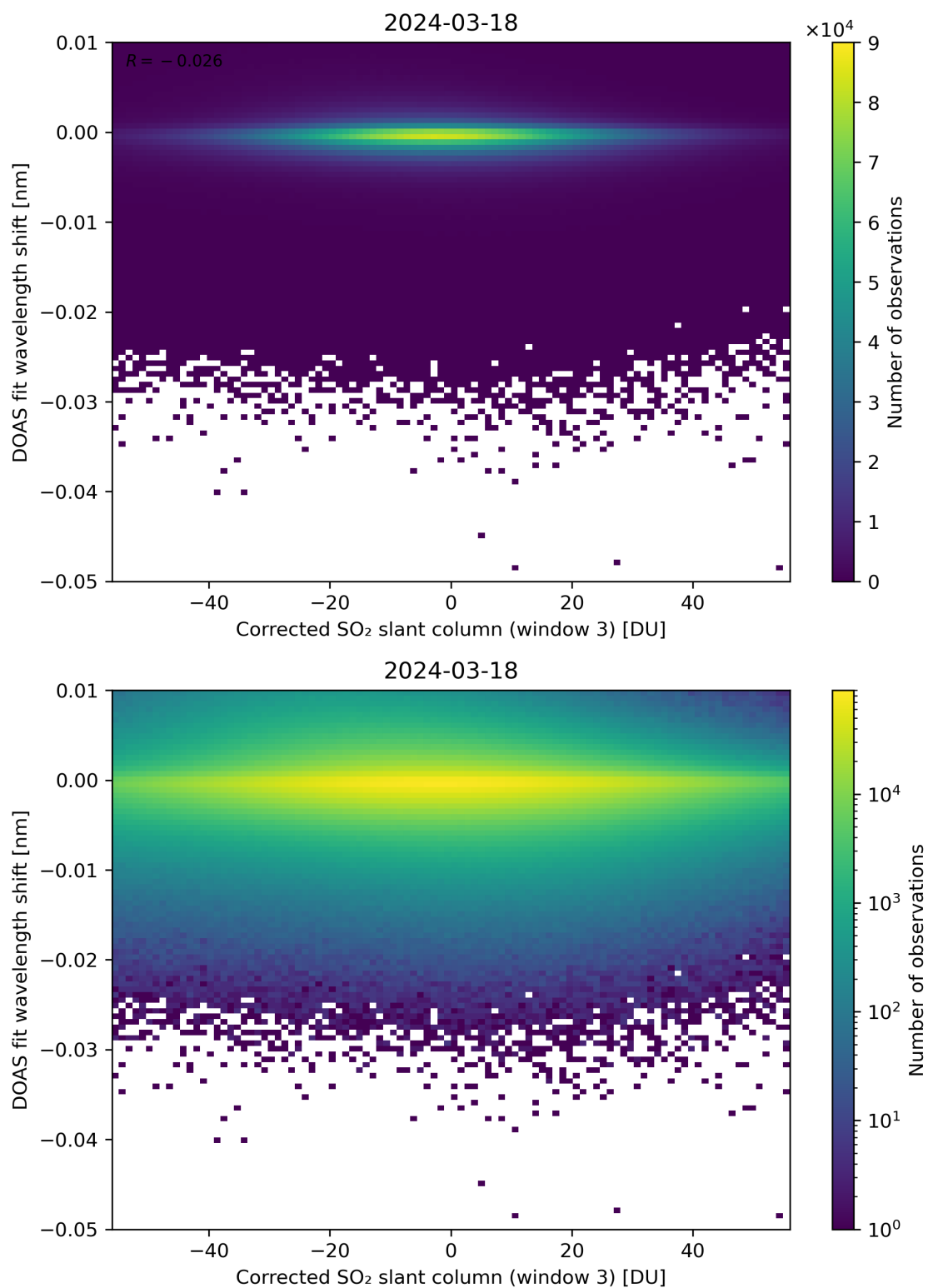
Figure 206: Scatter density plot of “Corrected SO 2 slant column (window 3)” against “DOAS fit wavelength shift” for 2024-03-17 to 2024-03-19.
