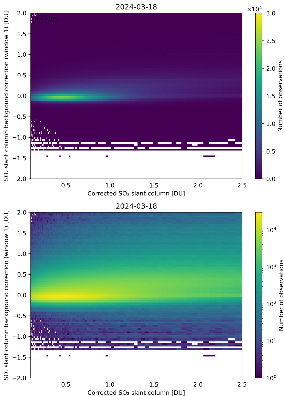
Figure 178: Scatter density plot of “Corrected SO 2 slant column” against “SO 2 slant column background correction (window 1)” for 2024-03-17 to 2024-03-19.
