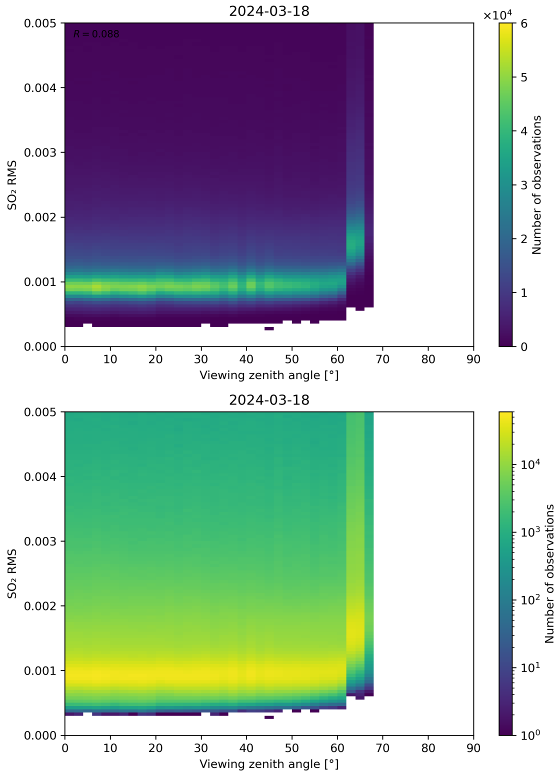
Figure 313: Scatter density plot of “Viewing zenith angle” against “SO 2 RMS” for 2024-03-17 to 2024-03-19.
