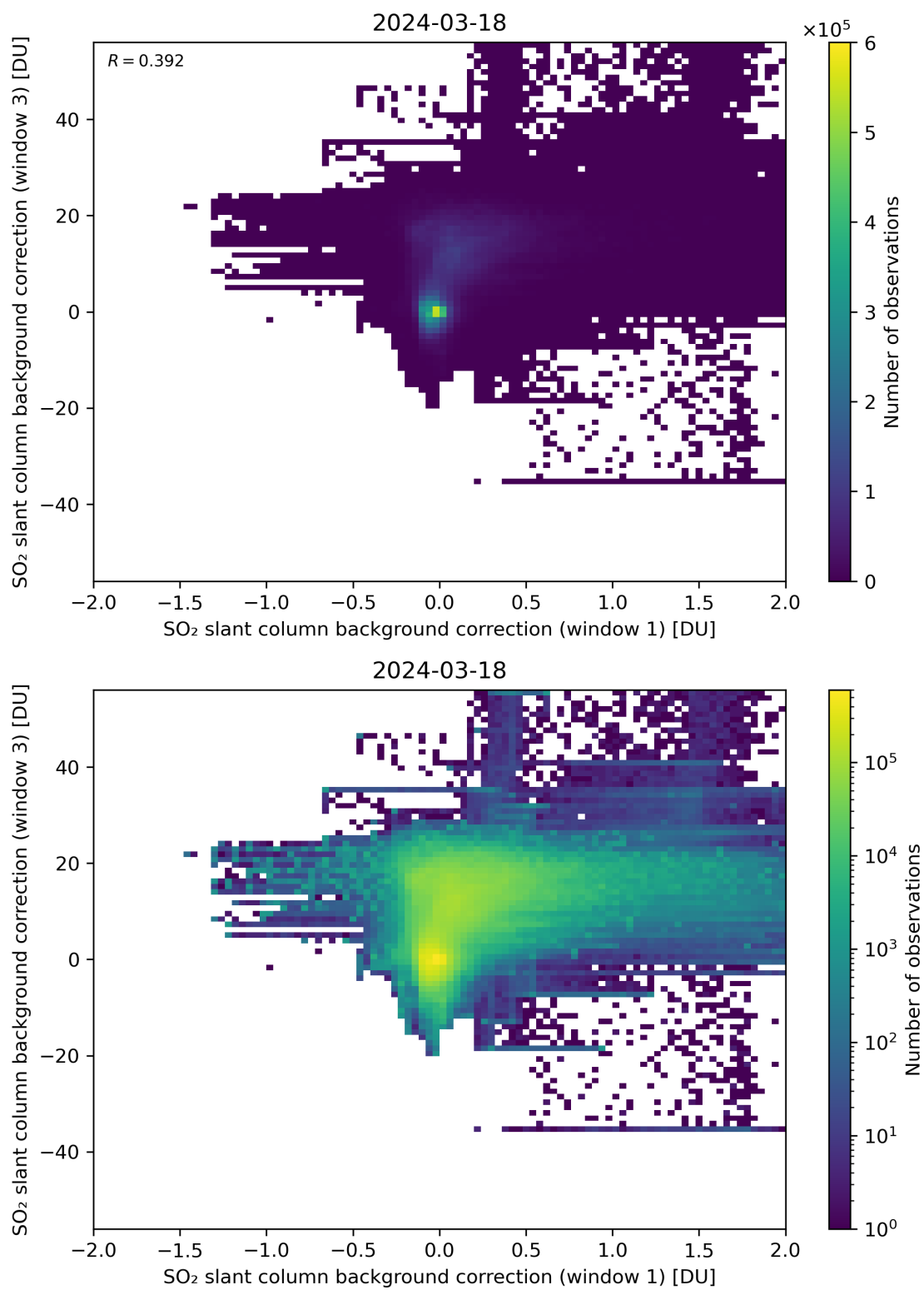
Figure 99: Scatter density plot of “SO 2 slant column background correction (window 1)” against “SO 2 slant column background correction (window 3)” for 2024-03-17 to 2024-03-19.
