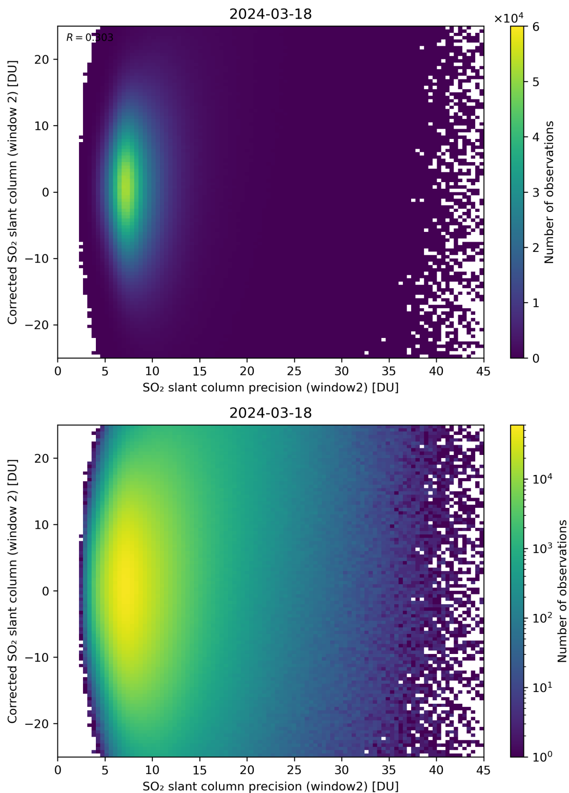
Figure 247: Scatter density plot of “SO 2 slant column precision (window2)” against “Corrected SO 2 slant column (window 2)” for 2024-03-17 to 2024-03-19.
