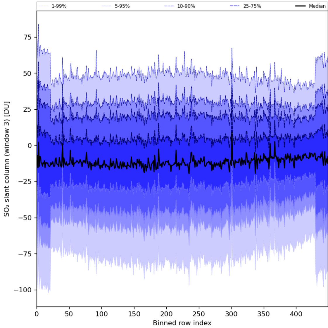
Figure 87: Along track statistics of “SO 2 slant column (window 3)” for 2024-03-17 to 2024-03-19
