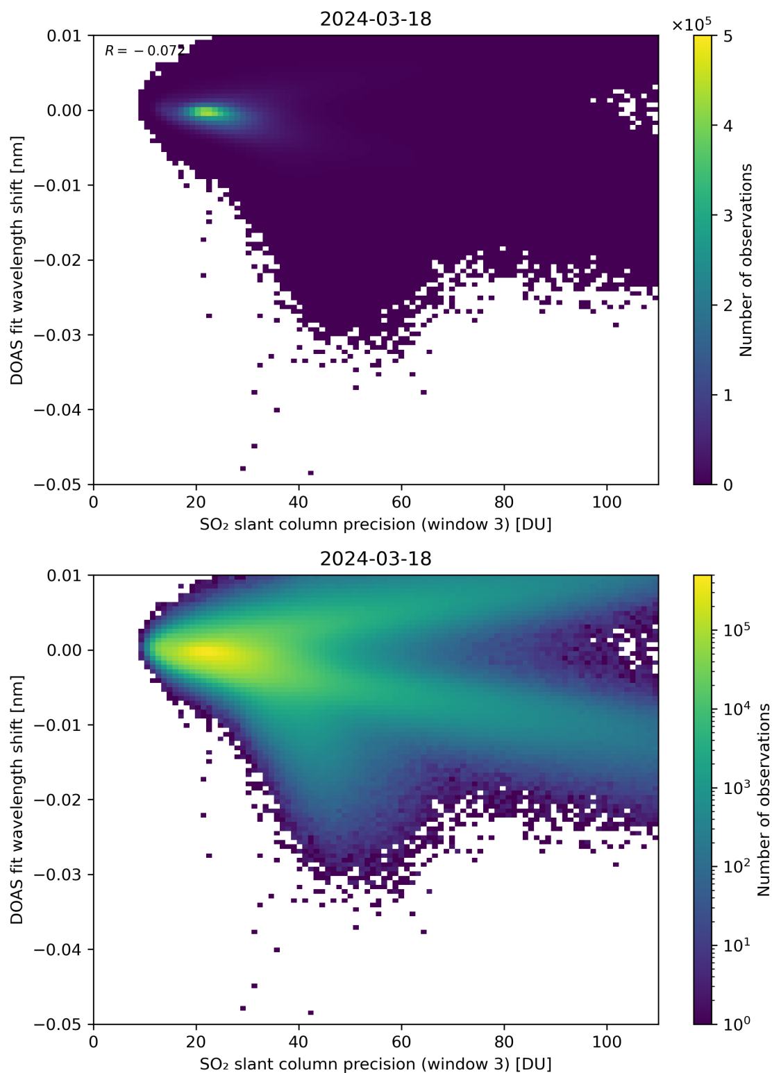
Figure 258: Scatter density plot of “SO 2 slant column precision (window 3)” against “DOAS fit wavelength shift” for 2024-03-17 to 2024-03-19.
