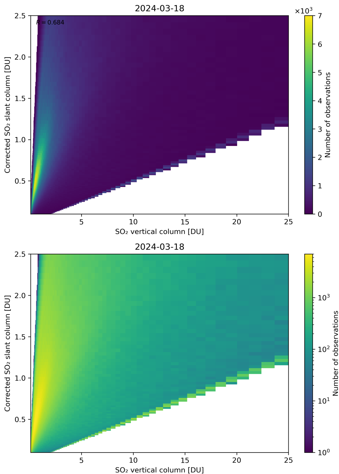
Figure 297: Scatter density plot of “SO 2 vertical column” against “Corrected SO 2 slant column” for 2024-03-17 to 2024-03-19.
