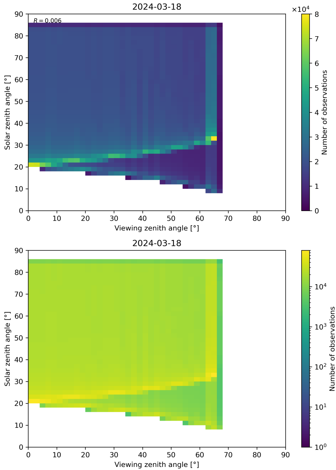
Figure 315: Scatter density plot of “Viewing zenith angle” against “Solar zenith angle” for 2024-03-17 to 2024-03-19.
