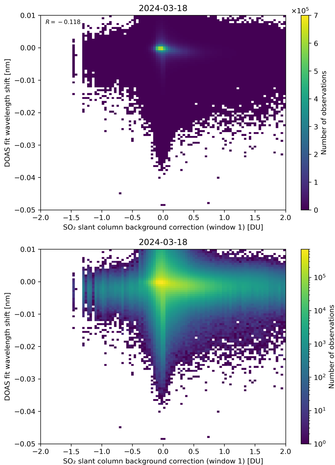
Figure 100: Scatter density plot of “SO 2 slant column background correction (window 1)” against “DOAS fit wavelength shift” for 2024-03-17 to 2024-03-19.
