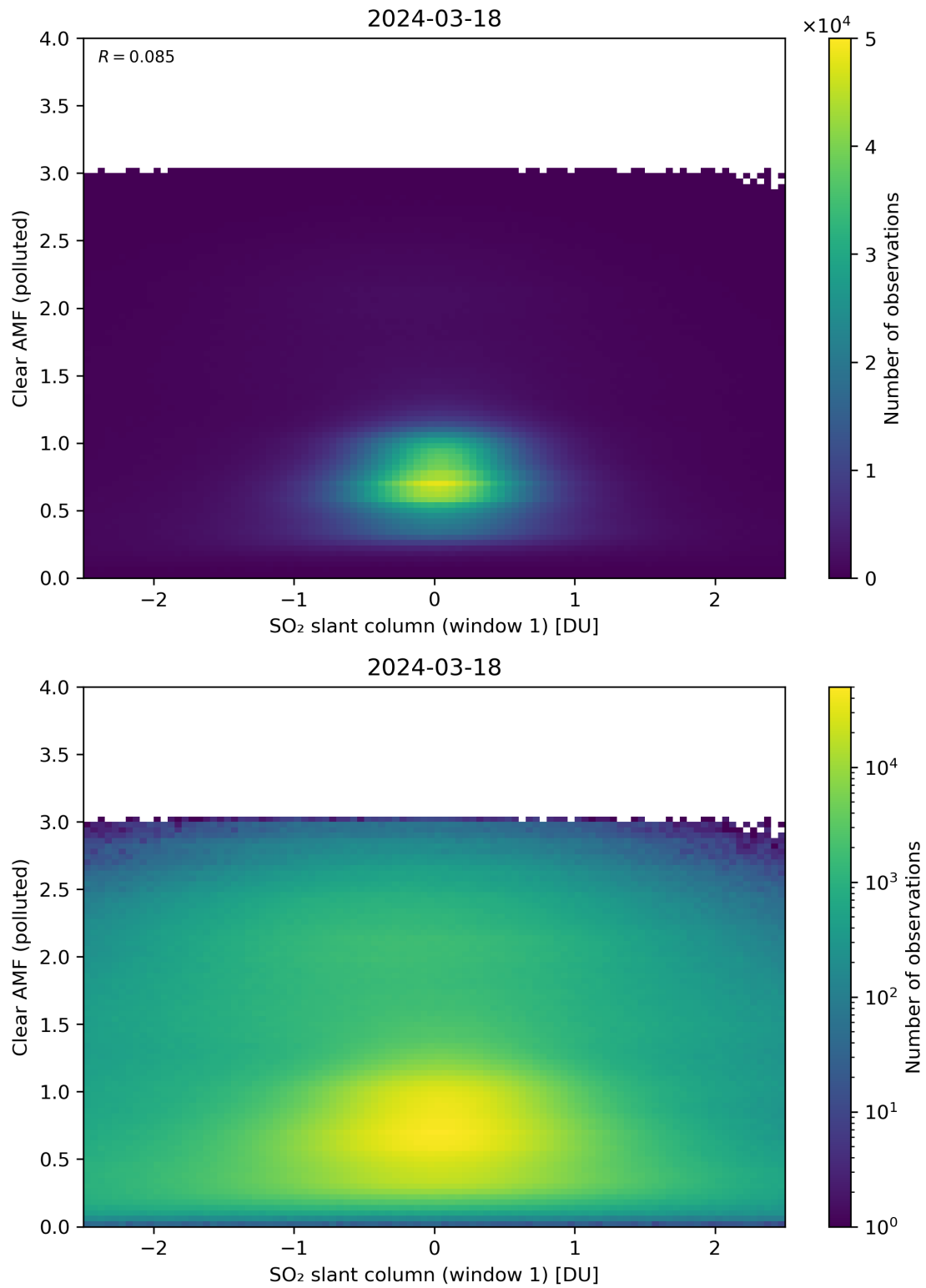
Figure 232: Scatter density plot of “SO 2 slant column (window 1)” against “Clear AMF (polluted)” for 2024-03-17 to 2024-03-19.
