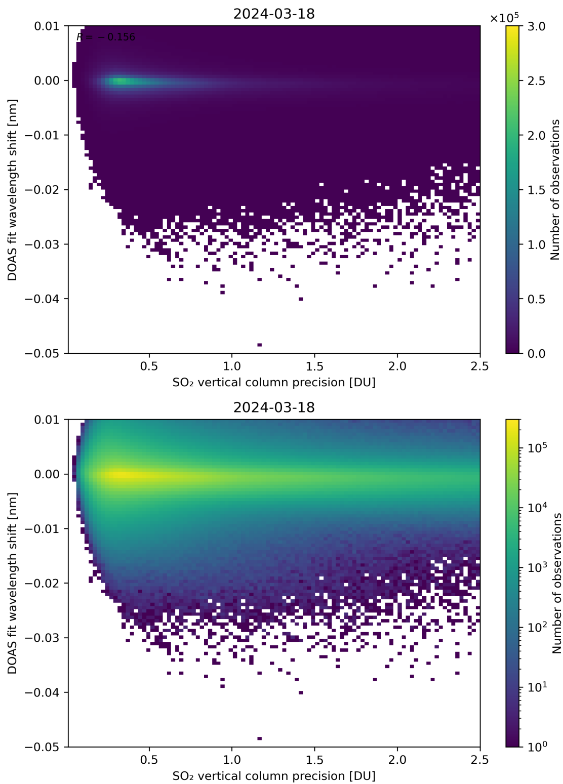
Figure 282: Scatter density plot of “SO 2 vertical column precision” against “DOAS fit wavelength shift” for 2024-03-17 to 2024-03-19.
