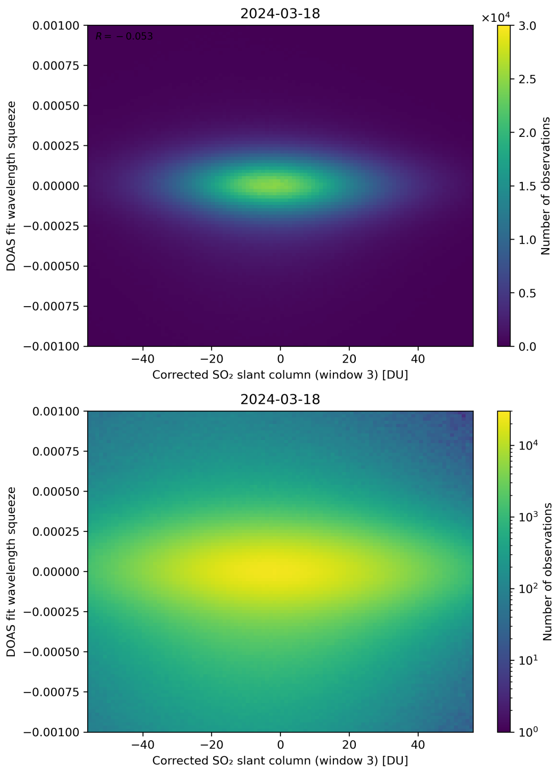
Figure 207: Scatter density plot of “Corrected SO 2 slant column (window 3)” against “DOAS fit wavelength squeeze” for 2024-03-17 to 2024-03-19.
