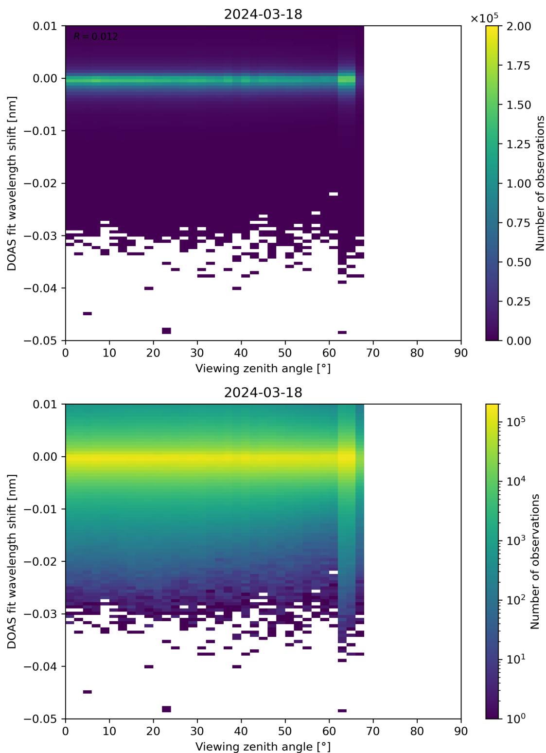
Figure 311: Scatter density plot of “Viewing zenith angle” against “DOAS fit wavelength shift” for 2024-03-17 to 2024-03-19.
