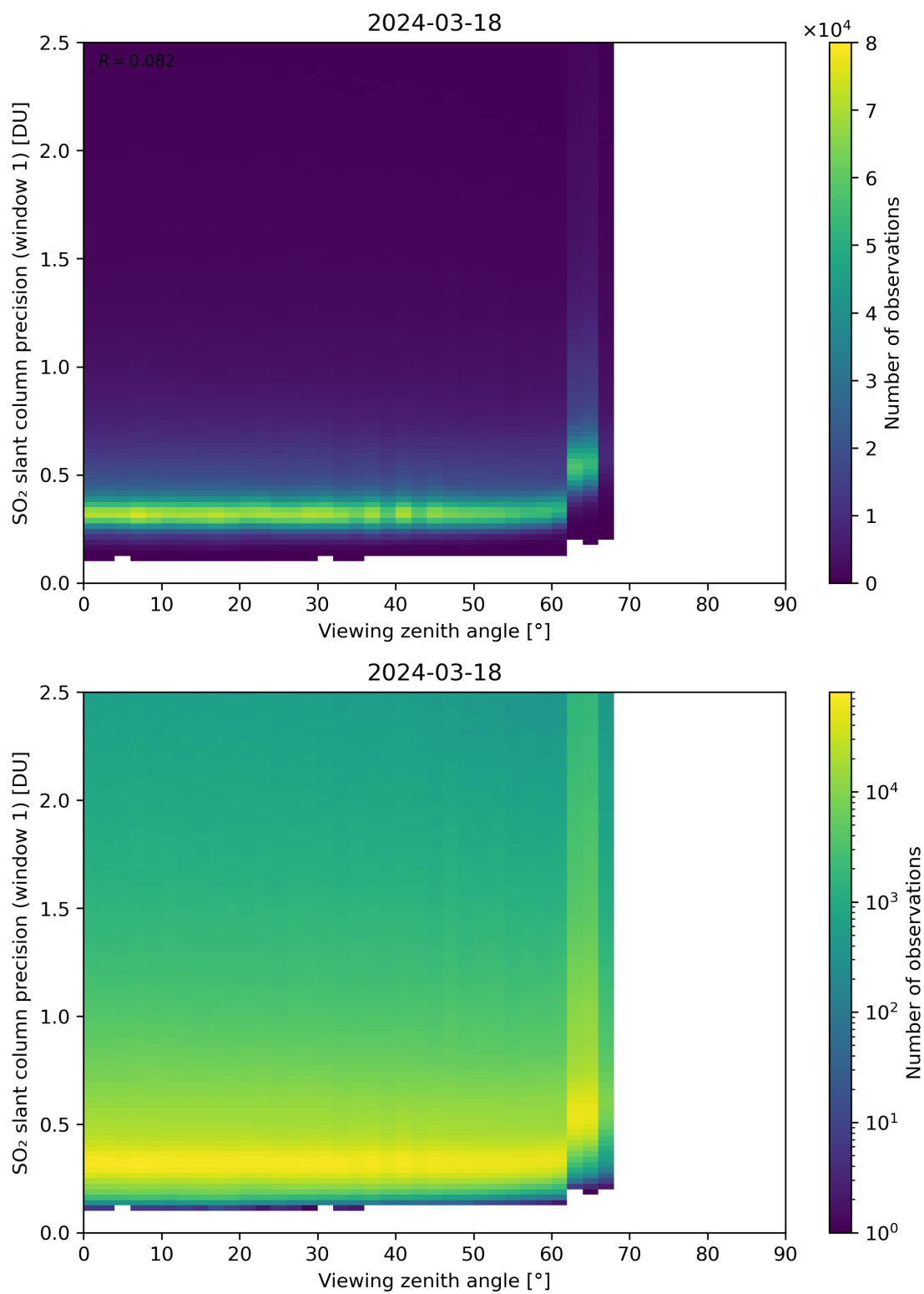
Figure 321: Scatter density plot of “Viewing zenith angle” against “SO 2 slant column precision (window 1)” for 2024-03-17 to 2024-03-19.
