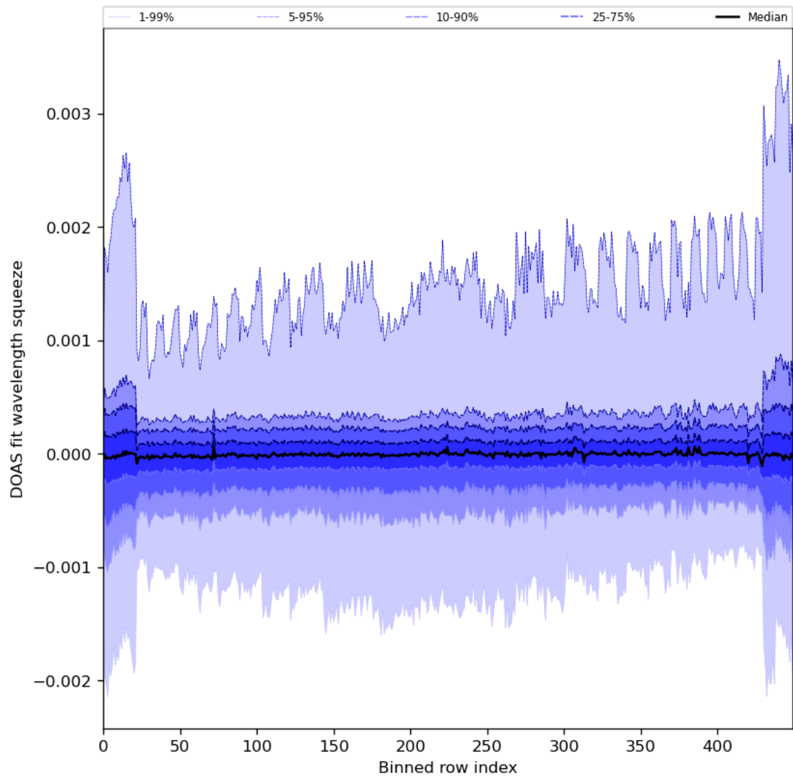
Figure 92: Along track statistics of “DOAS fit wavelength squeeze” for 2024-03-17 to 2024-03-19
