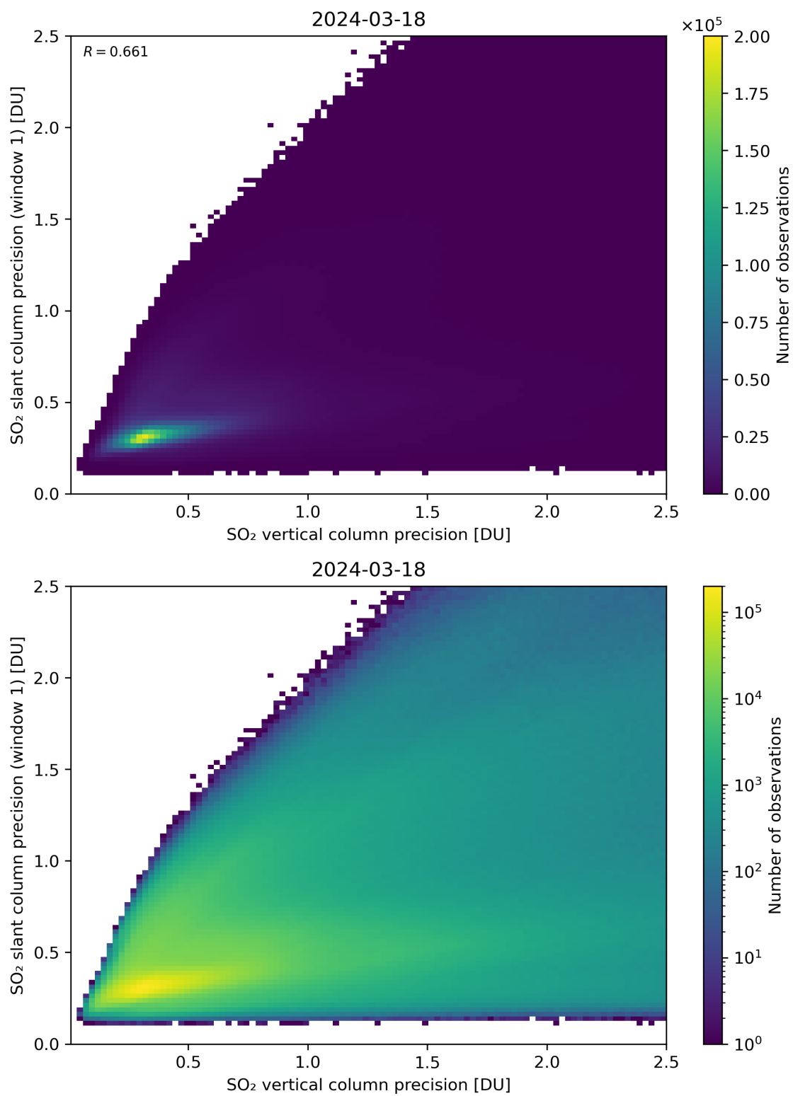
Figure 290: Scatter density plot of “SO 2 vertical column precision” against “SO 2 slant column precision (window 1)” for 2024-03-17 to 2024-03-19.
