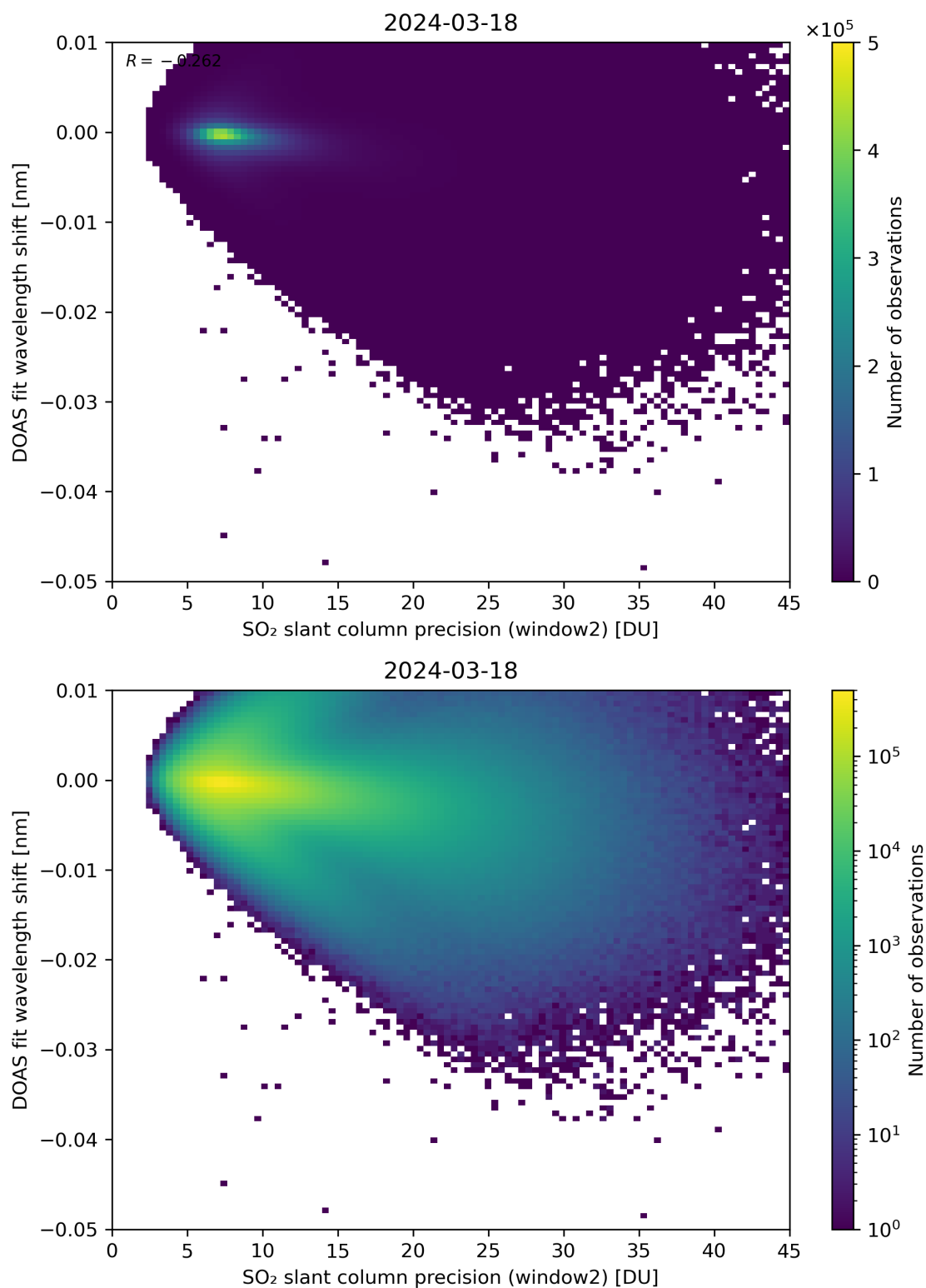
Figure 243: Scatter density plot of “SO 2 slant column precision (window2)” against “DOAS fit wavelength shift” for 2024-03-17 to 2024-03-19.
