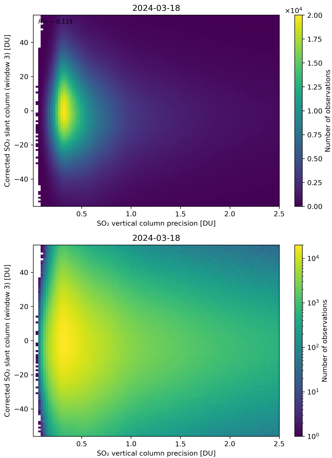
Figure 288: Scatter density plot of “SO 2 vertical column precision” against “Corrected SO 2 slant column (window 3)” for 2024-03-17 to 2024-03-19.
