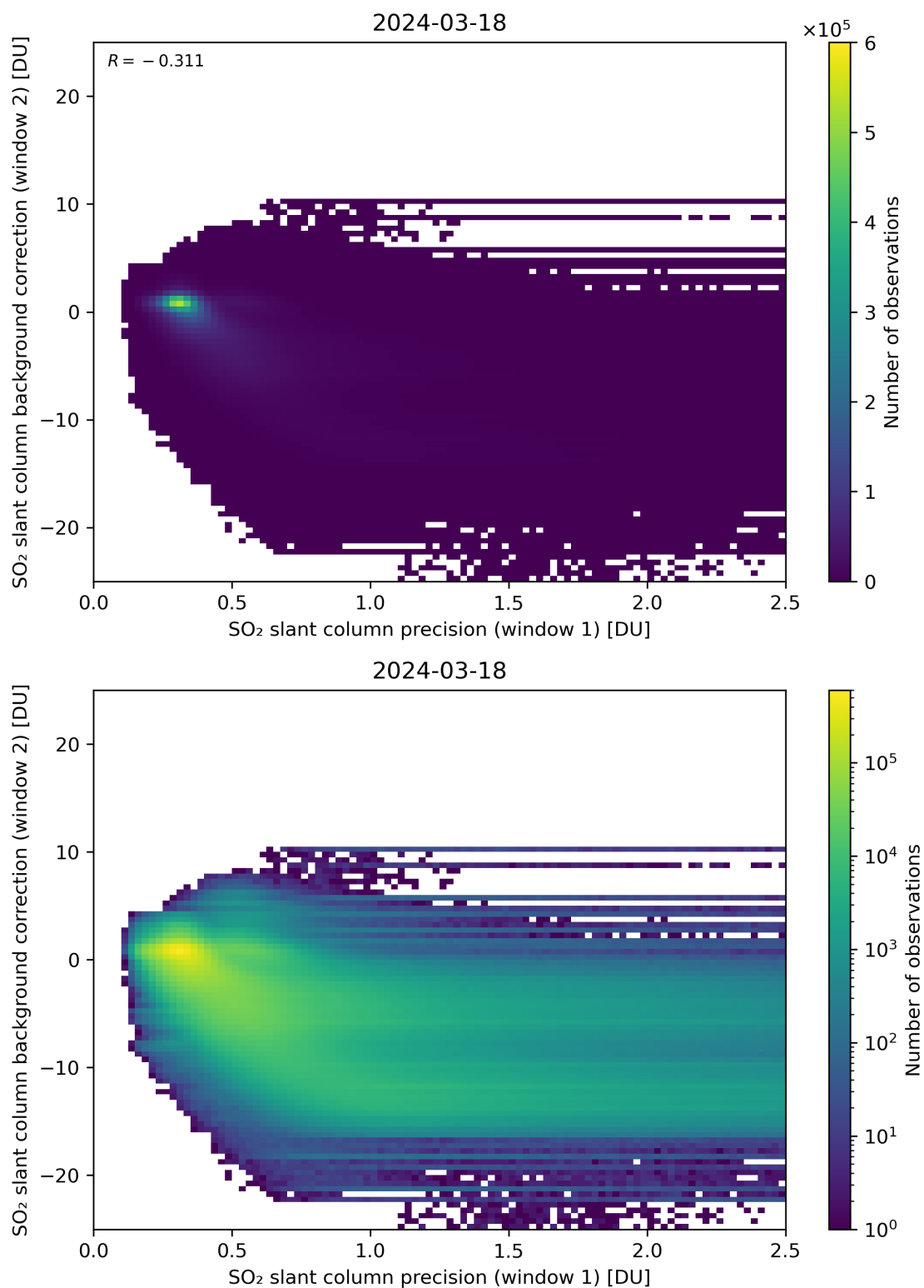
Figure 219: Scatter density plot of “SO 2 slant column precision (window 1)” against “SO 2 slant column background correction (window 2)” for 2024-03-17 to 2024-03-19.
