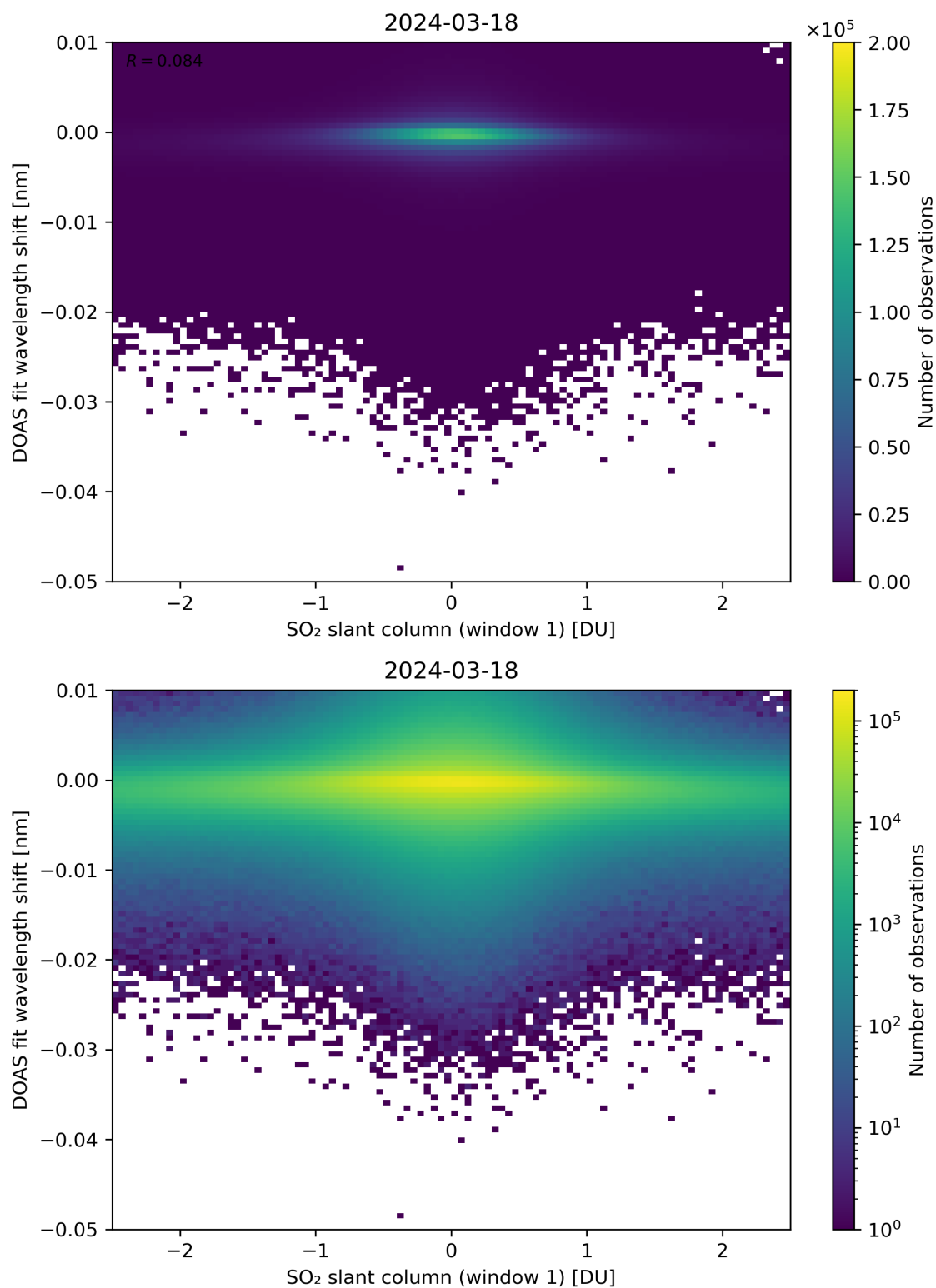
Figure 215: Scatter density plot of “SO 2 slant column (window 1)” against “DOAS fit wavelength shift” for 2024-03-17 to 2024-03-19.
