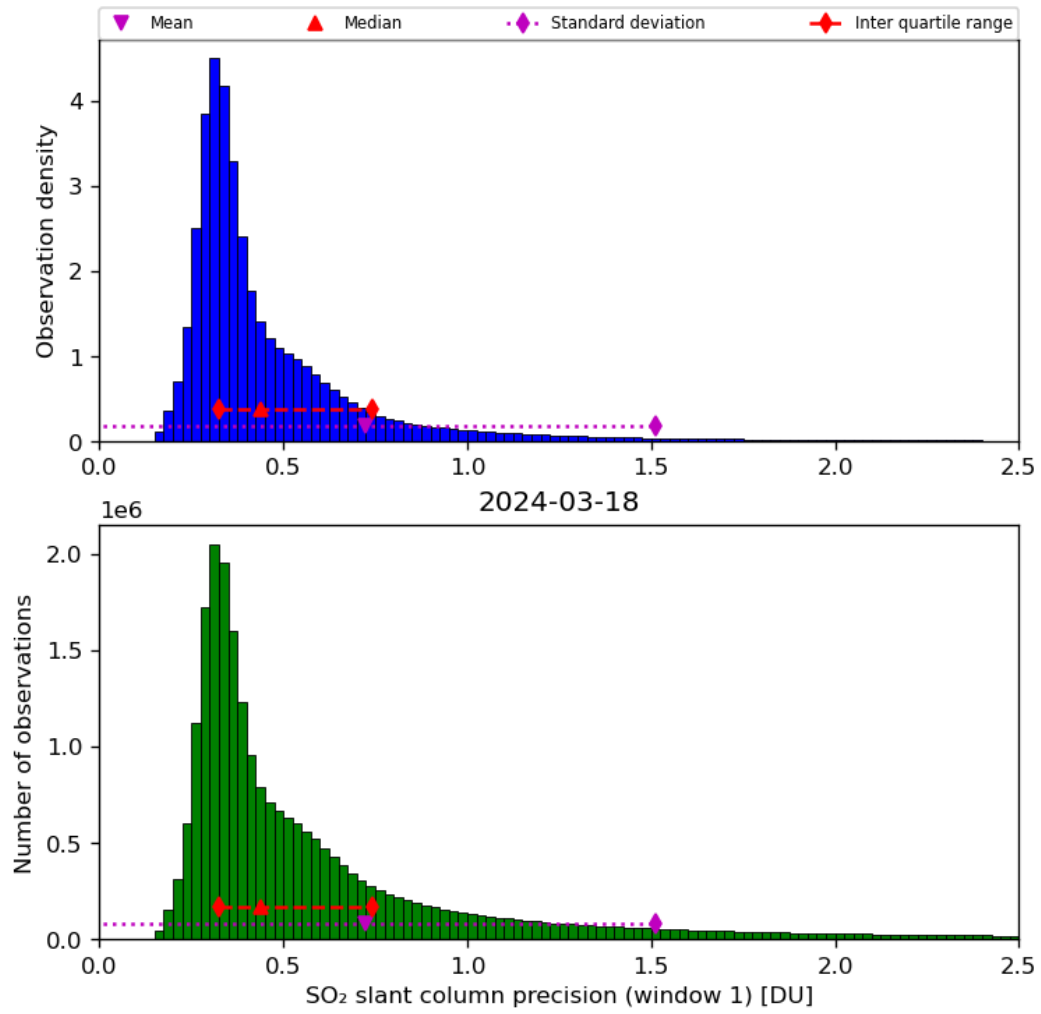
Figure 57: Histogram of “SO 2 slant column precision (window 1)” for 2024-03-17 to 2024-03-19
