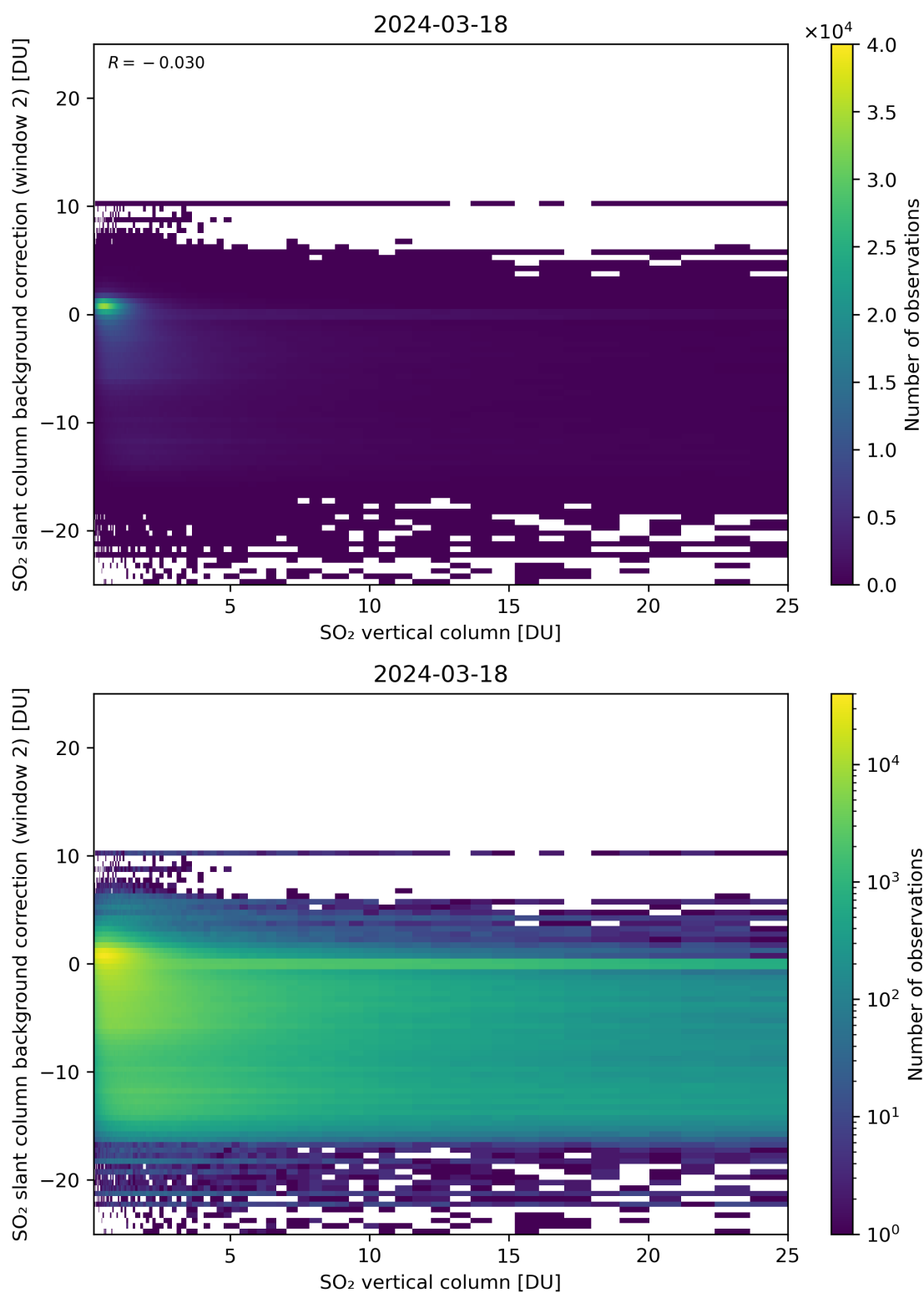
Figure 274: Scatter density plot of “SO 2 vertical column” against “SO 2 slant column background correction (window 2)” for 2024-03-17 to 2024-03-19.
