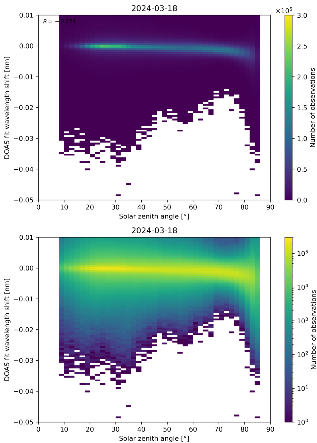
Figure 161: Scatter density plot of “Solar zenith angle” against “DOAS fit wavelength shift” for 2024-03-17 to 2024-03-19.
