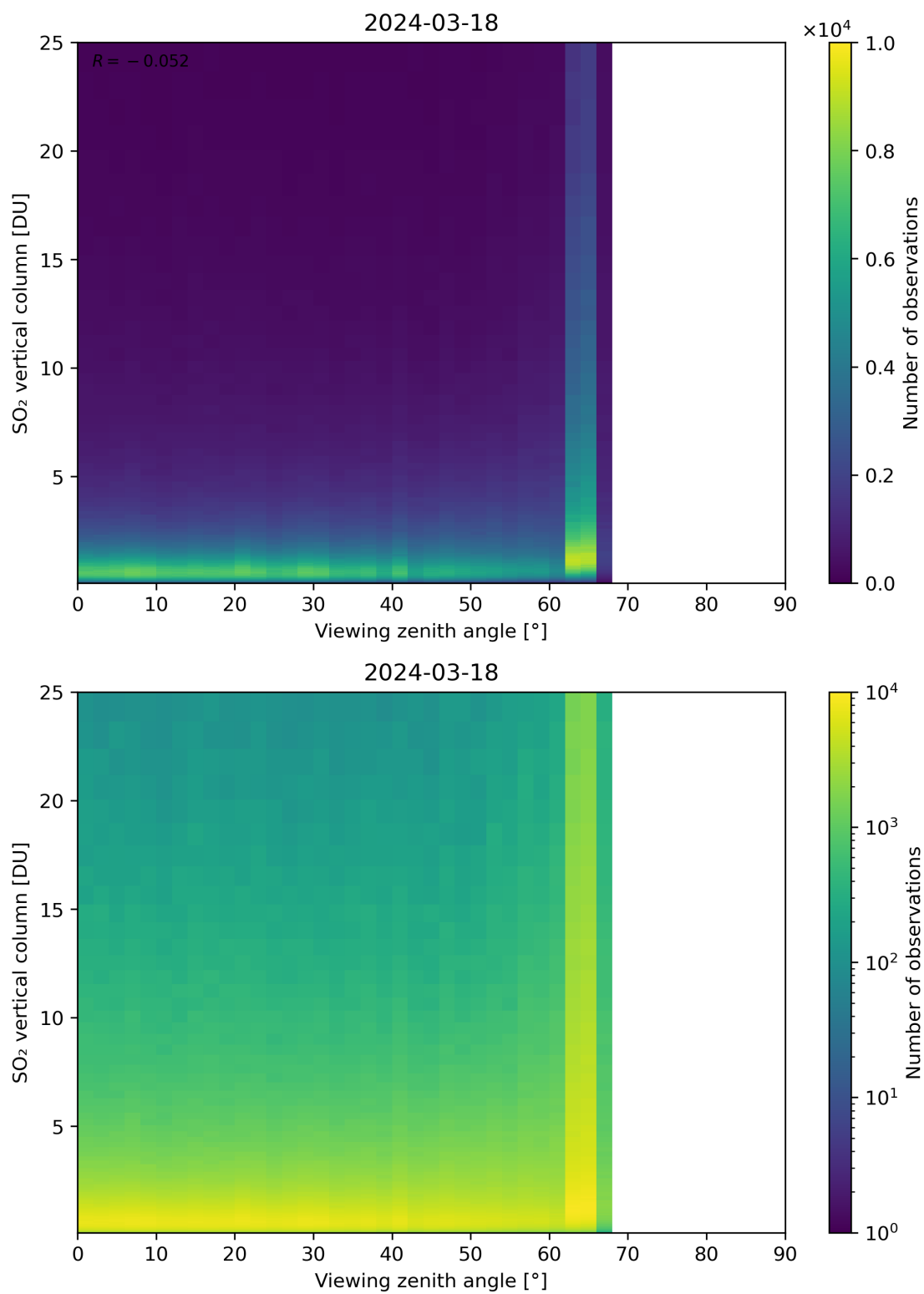
Figure 327: Scatter density plot of “Viewing zenith angle” against “SO 2 vertical column” for 2024-03-17 to 2024-03-19.
