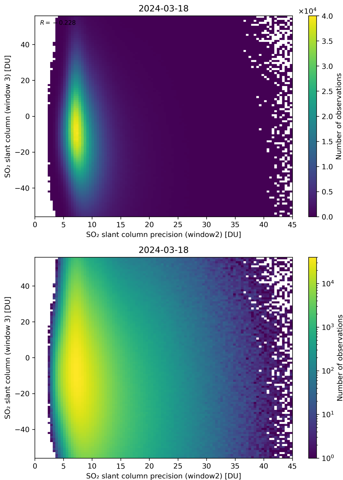
Figure 249: Scatter density plot of “SO 2 slant column precision (window2)” against “SO 2 slant column (window 3)” for 2024-03-17 to 2024-03-19.
