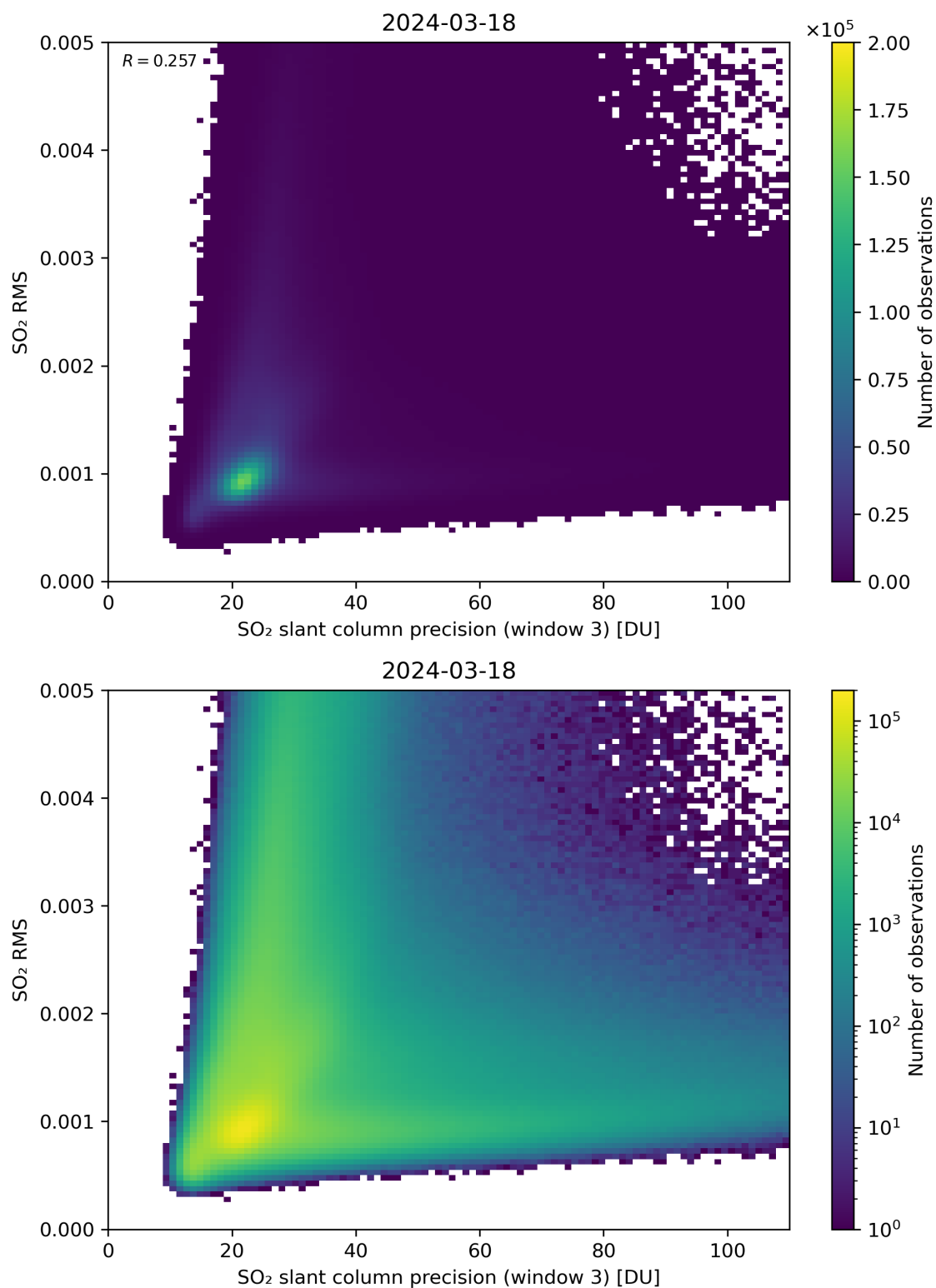
Figure 260: Scatter density plot of “SO 2 slant column precision (window 3)” against “SO 2 RMS” for 2024-03-17 to 2024-03-19.
