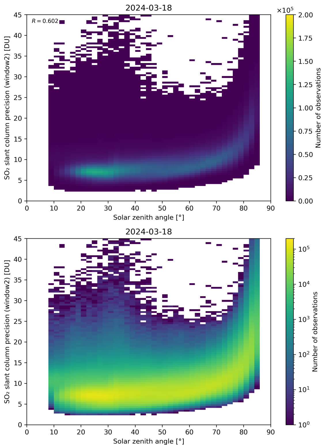
Figure 171: Scatter density plot of “Solar zenith angle” against “SO 2 slant column precision (window2)” for 2024-03-17 to 2024-03-19.
