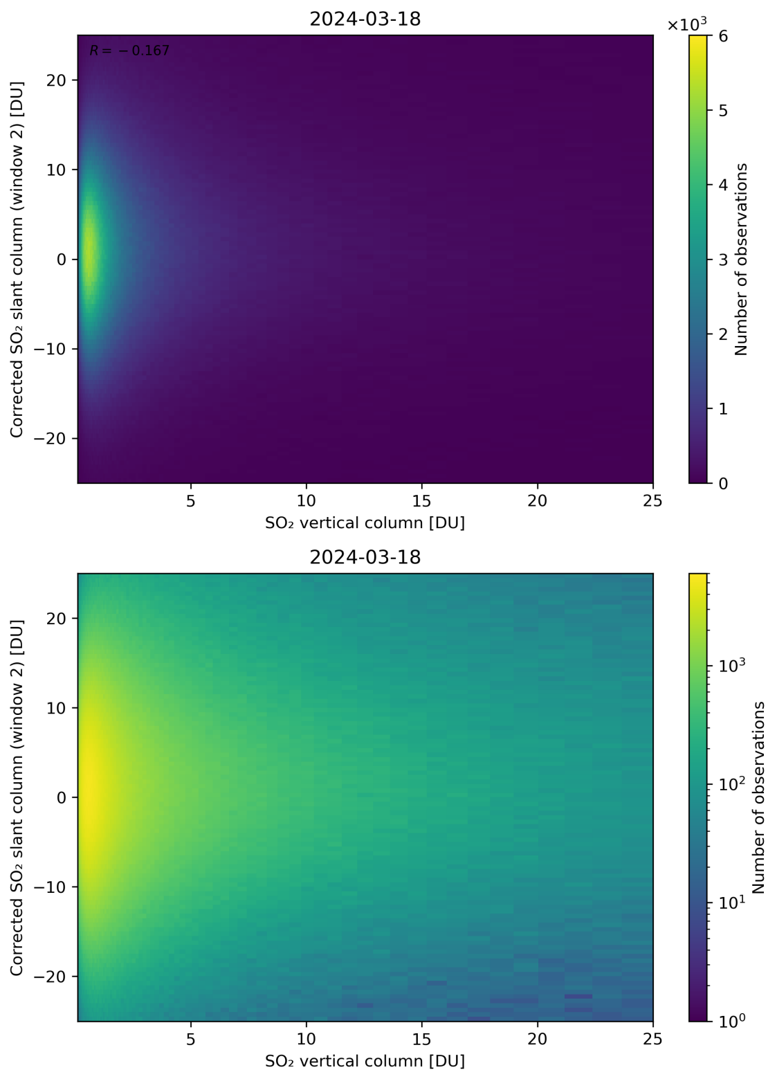
Figure 298: Scatter density plot of “SO 2 vertical column” against “Corrected SO 2 slant column (window 2)” for 2024-03-17 to 2024-03-19.
