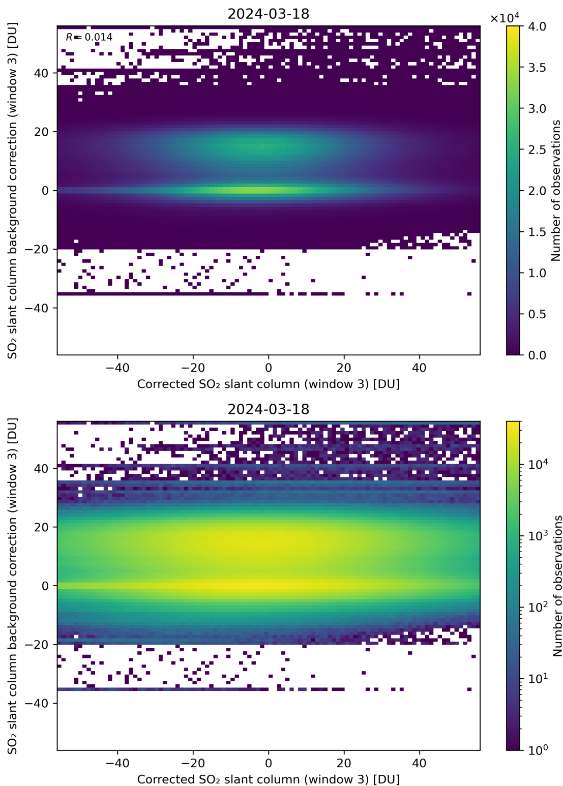
Figure 205: Scatter density plot of “Corrected SO 2 slant column (window 3)” against “SO 2 slant column background correction (window 3)” for 2024-03-17 to 2024-03-19.
