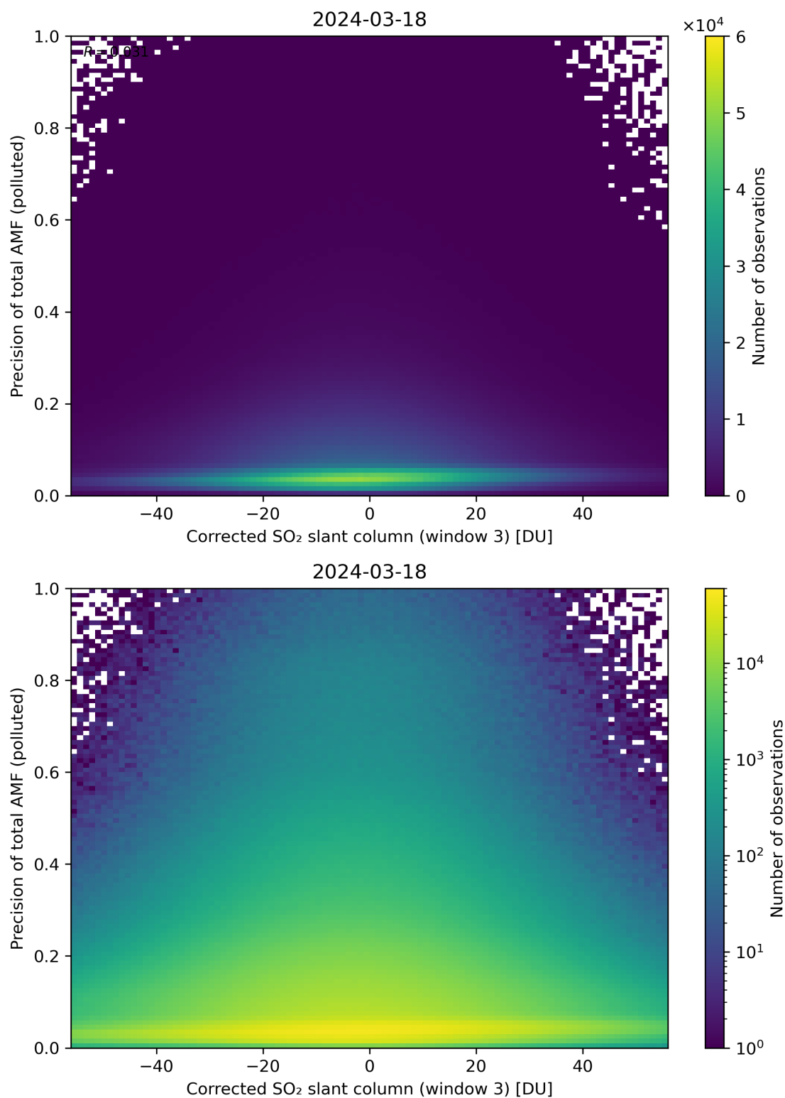
Figure 211: Scatter density plot of “Corrected SO 2 slant column (window 3)” against “Precision of total AMF (polluted)” for 2024-03-17 to 2024-03-19.
