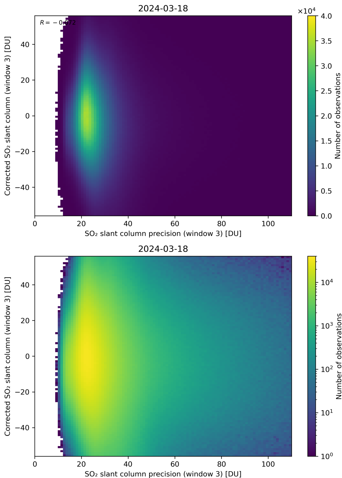
Figure 262: Scatter density plot of “SO 2 slant column precision (window 3)” against “Corrected SO 2 slant column (window 3)” for 2024-03-17 to 2024-03-19.
