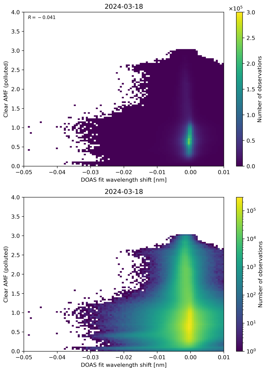
Figure 129: Scatter density plot of “DOAS fit wavelength shift” against “Clear AMF (polluted)” for 2024-03-17 to 2024-03-19.
