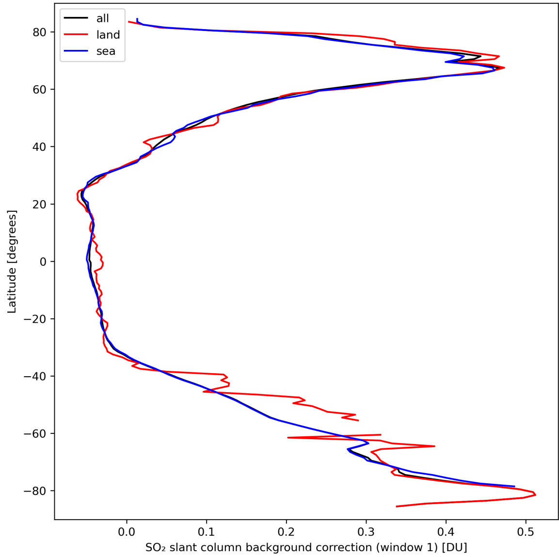
Figure 36: Zonal average of “SO 2 slant column background correction (window 1)” for 2024-03-17 to 2024-03-19.
