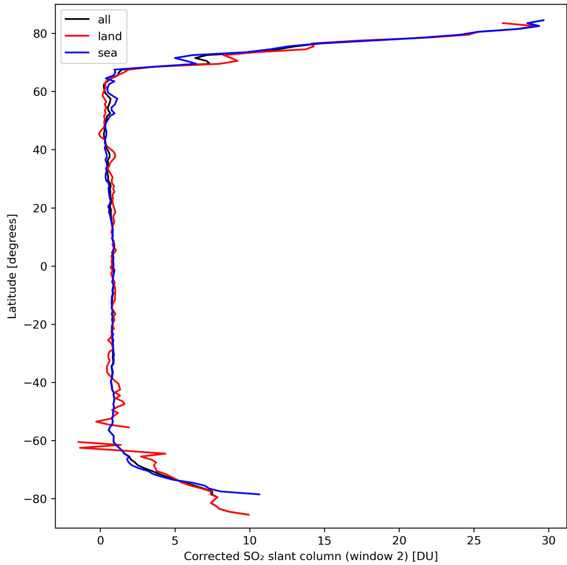
Figure 39: Zonal average of “Corrected SO 2 slant column (window 2)” for 2024-03-17 to 2024-03-19.
