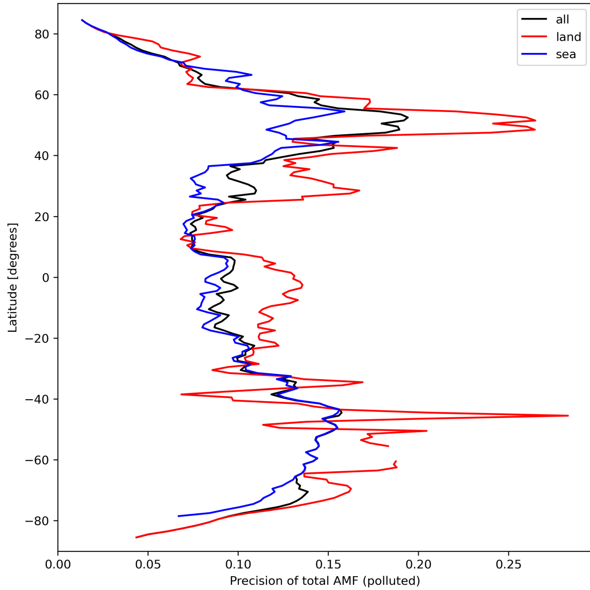
Figure 49: Zonal average of “Precision of total AMF (polluted)” for 2024-03-17 to 2024-03-19.
