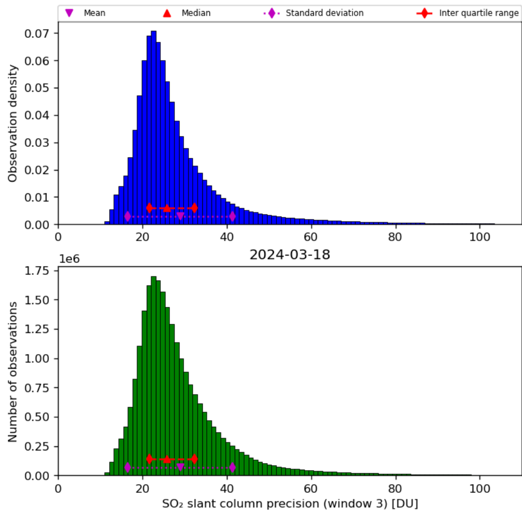
Figure 65: Histogram of “SO 2 slant column precision (window 3)” for 2024-03-17 to 2024-03-19
