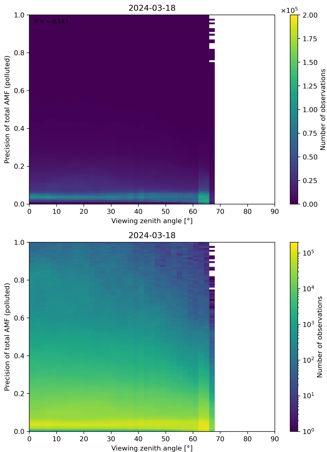
Figure 326: Scatter density plot of “Viewing zenith angle” against “Precision of total AMF (polluted)” for 2024-03-17 to 2024-03-19.
