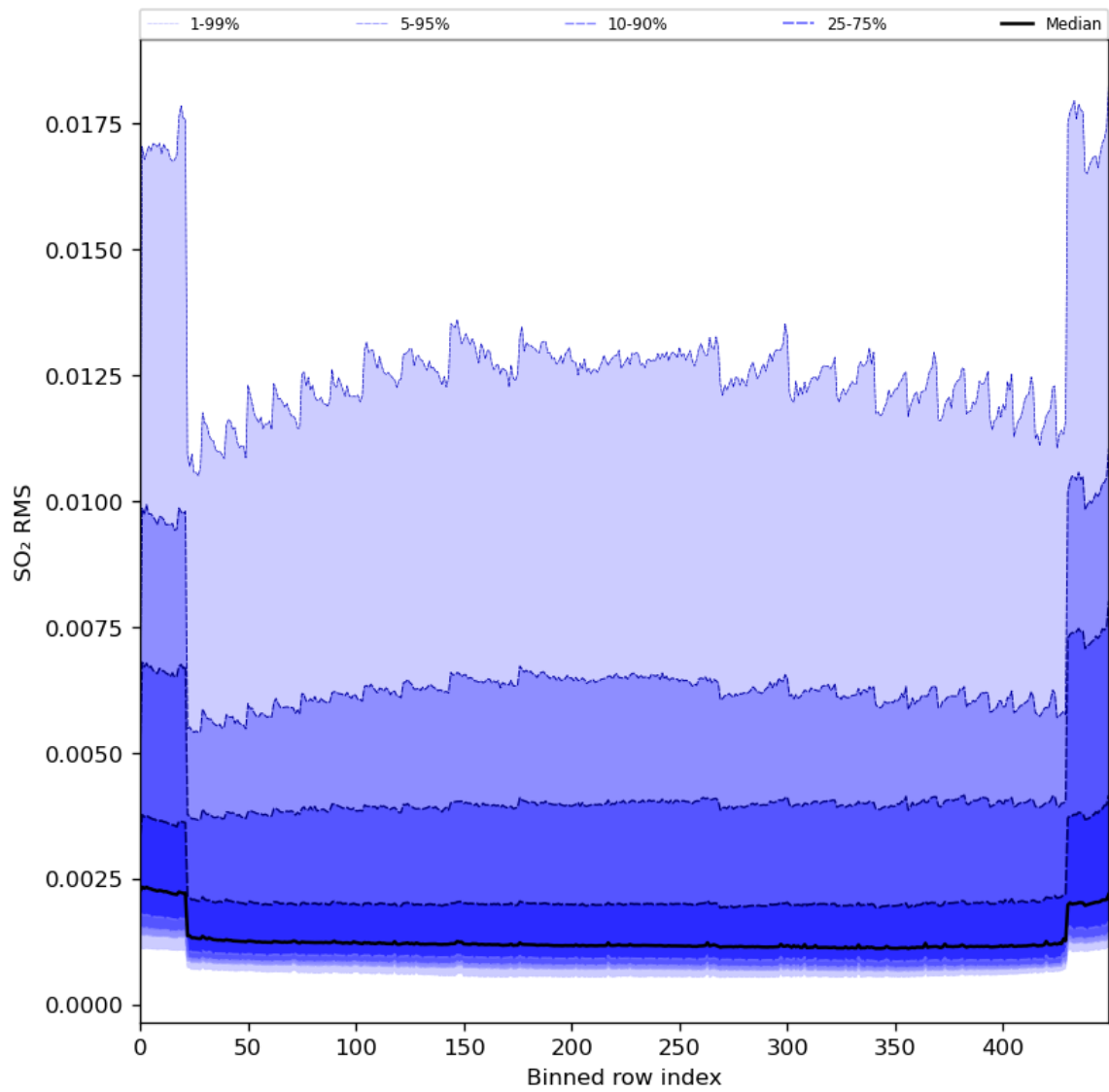
Figure 93: Along track statistics of “SO 2 RMS” for 2024-03-17 to 2024-03-19
