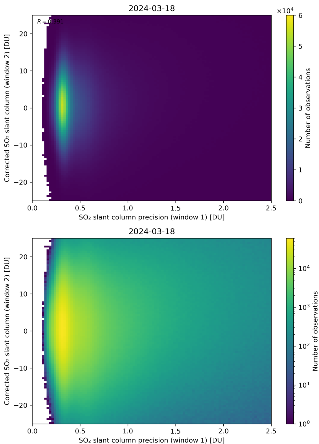
Figure 225: Scatter density plot of “SO 2 slant column precision (window 1)” against “Corrected SO 2 slant column (window 2)” for 2024-03-17 to 2024-03-19.
