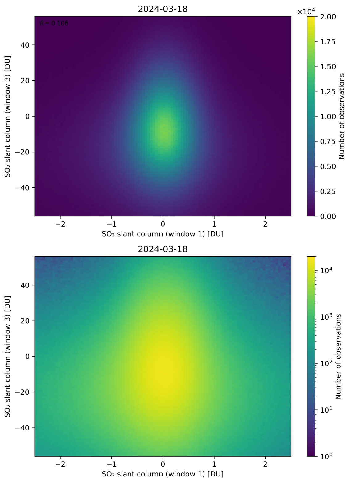
Figure 237: Scatter density plot of “SO 2 slant column (window 1)” against “SO 2 slant column (window 3)” for 2024-03-17 to 2024-03-19.
