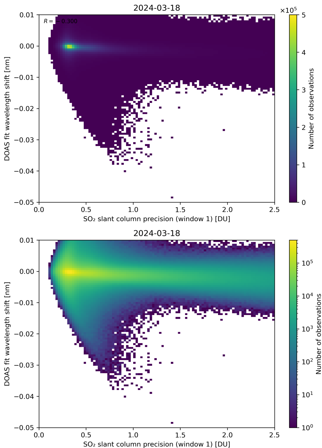
Figure 221: Scatter density plot of “SO 2 slant column precision (window 1)” against “DOAS fit wavelength shift” for 2024-03-17 to 2024-03-19.
