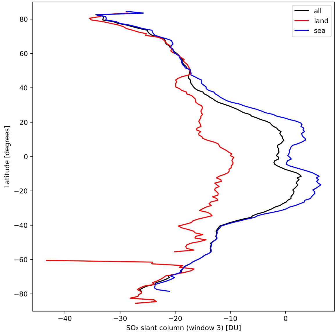
Figure 41: Zonal average of “SO 2 slant column (window 3)” for 2024-03-17 to 2024-03-19.
