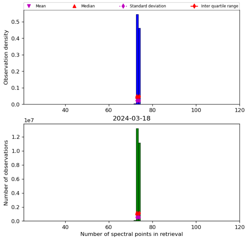
Figure 74: Histogram of “Number of spectral points in retrieval” for 2024-03-17 to 2024-03-19
