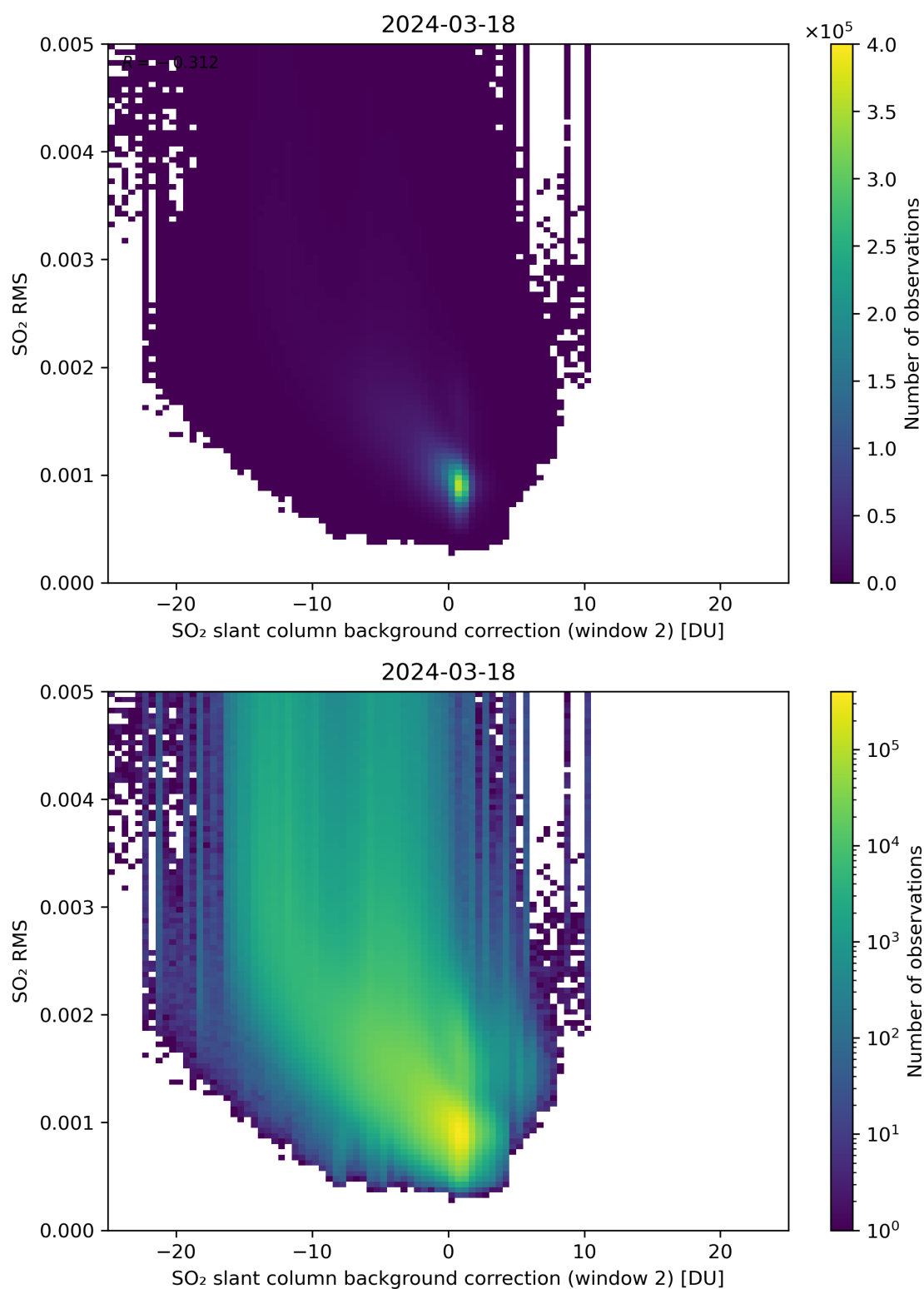
Figure 114: Scatter density plot of “SO 2 slant column background correction (window 2)” against “SO 2 RMS” for 2024-03-17 to 2024-03-19.
