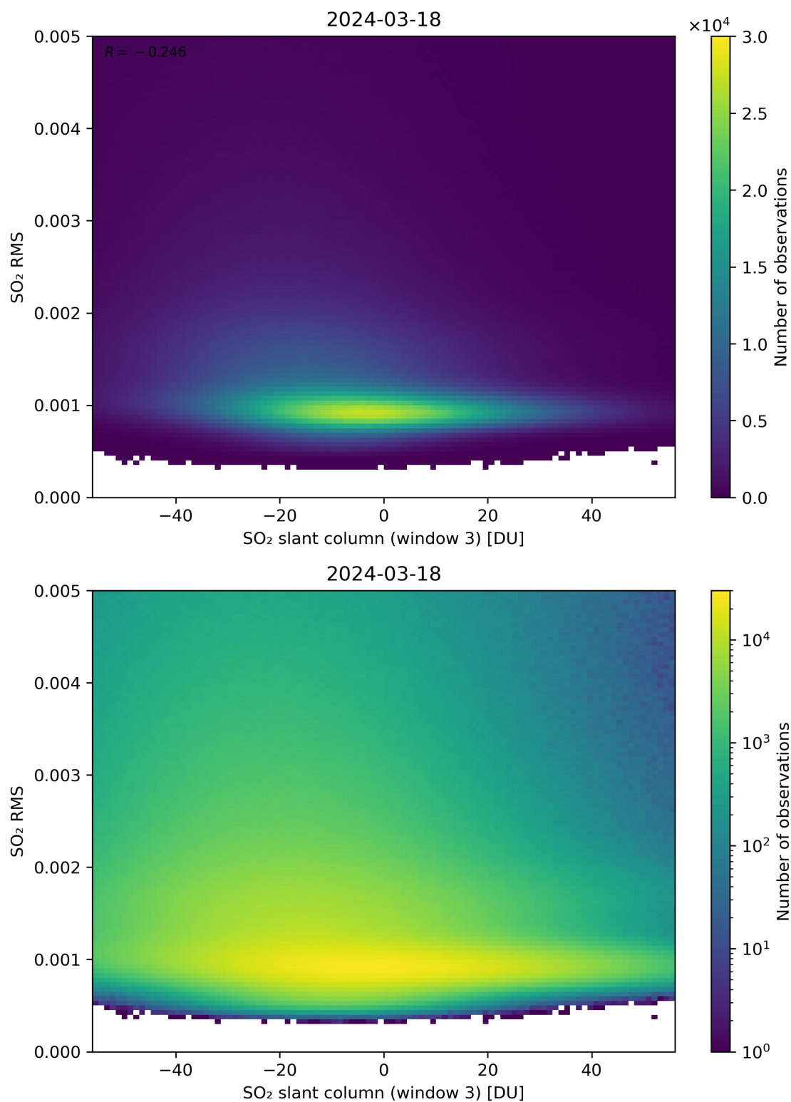
Figure 256: Scatter density plot of “SO 2 slant column (window 3)” against “SO 2 RMS” for 2024-03-17 to 2024-03-19.
