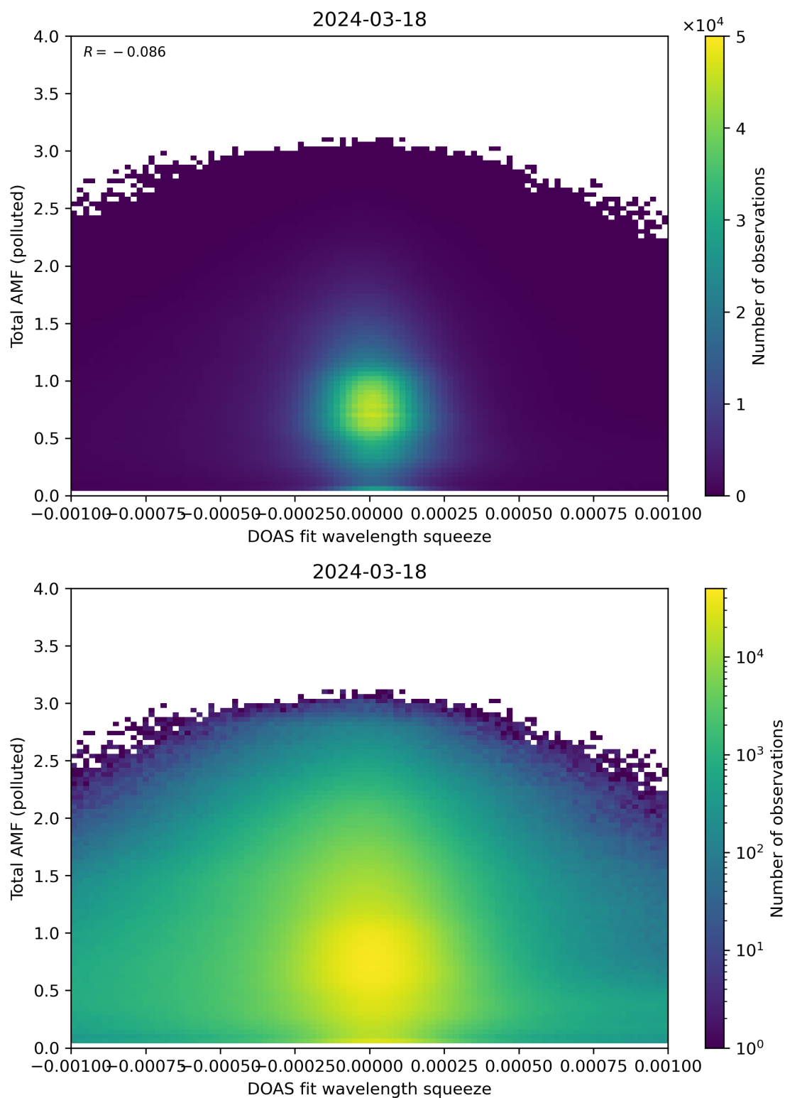
Figure 134: Scatter density plot of “DOAS fit wavelength squeeze” against “Total AMF (polluted)” for 2024-03-17 to 2024-03-19.
