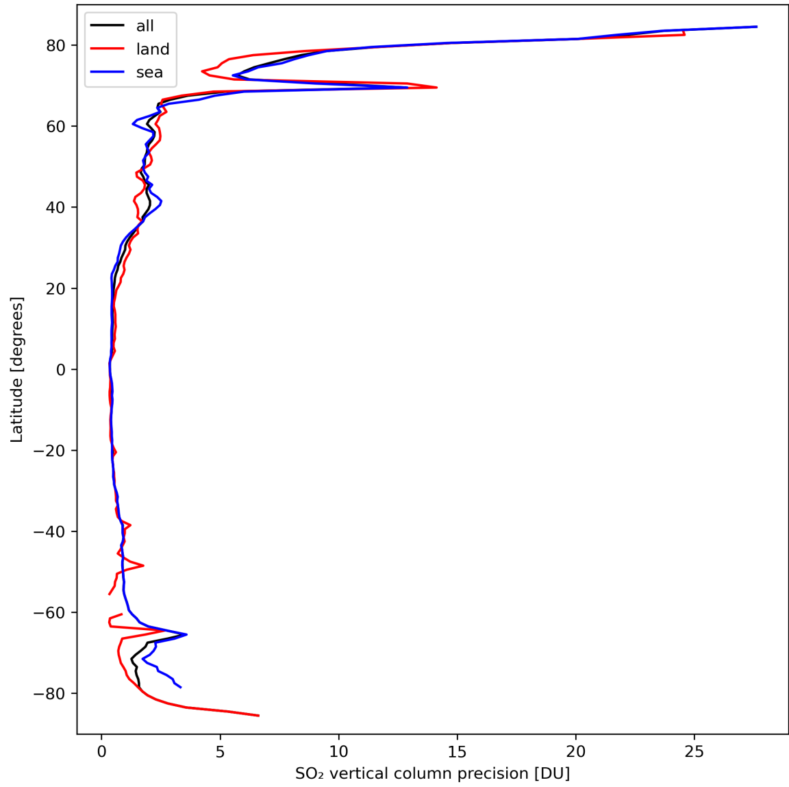
Figure 31: Zonal average of “SO 2 vertical column precision” for 2024-03-17 to 2024-03-19.
