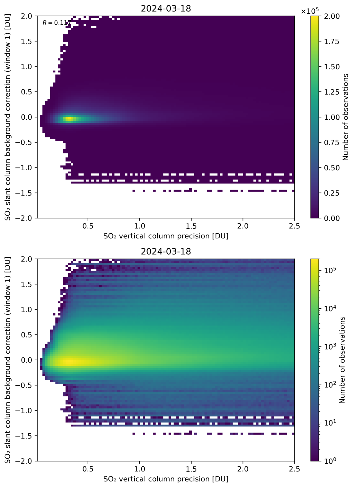
Figure 279: Scatter density plot of “SO 2 vertical column precision” against “SO 2 slant column background correction (window 1)” for 2024-03-17 to 2024-03-19.
