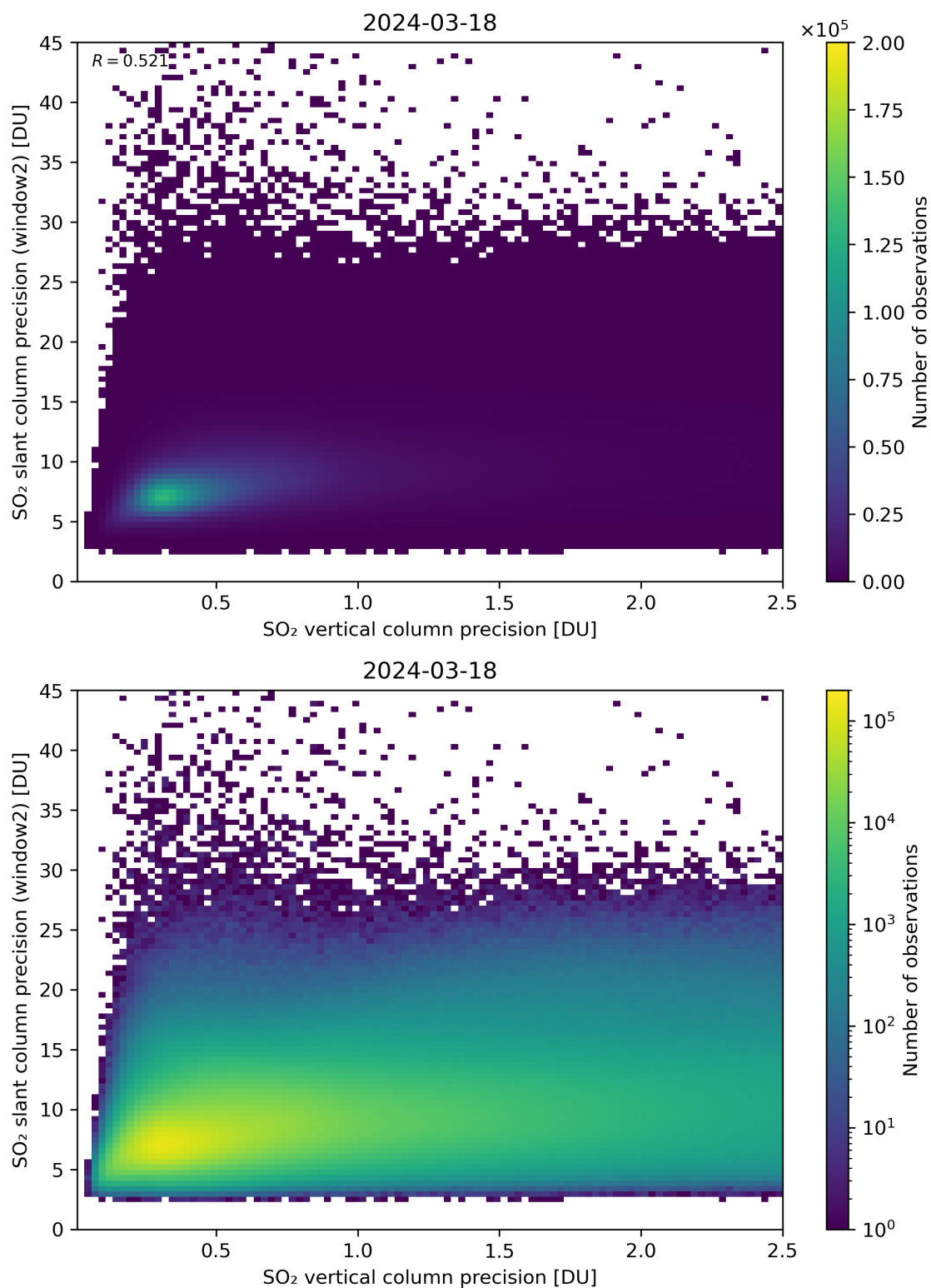
Figure 291: Scatter density plot of “SO 2 vertical column precision” against “SO 2 slant column precision (window2)” for 2024-03-17 to 2024-03-19.
