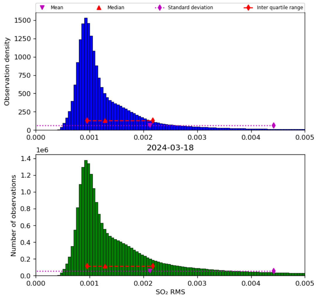
Figure 70: Histogram of “SO 2 RMS” for 2024-03-17 to 2024-03-19
