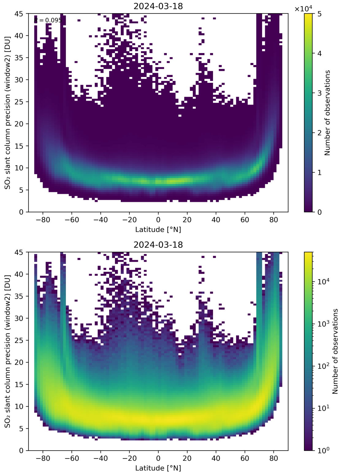
Figure 151: Scatter density plot of “Latitude” against “SO 2 slant column precision (window2)” for 2024-03-17 to 2024-03-19.
