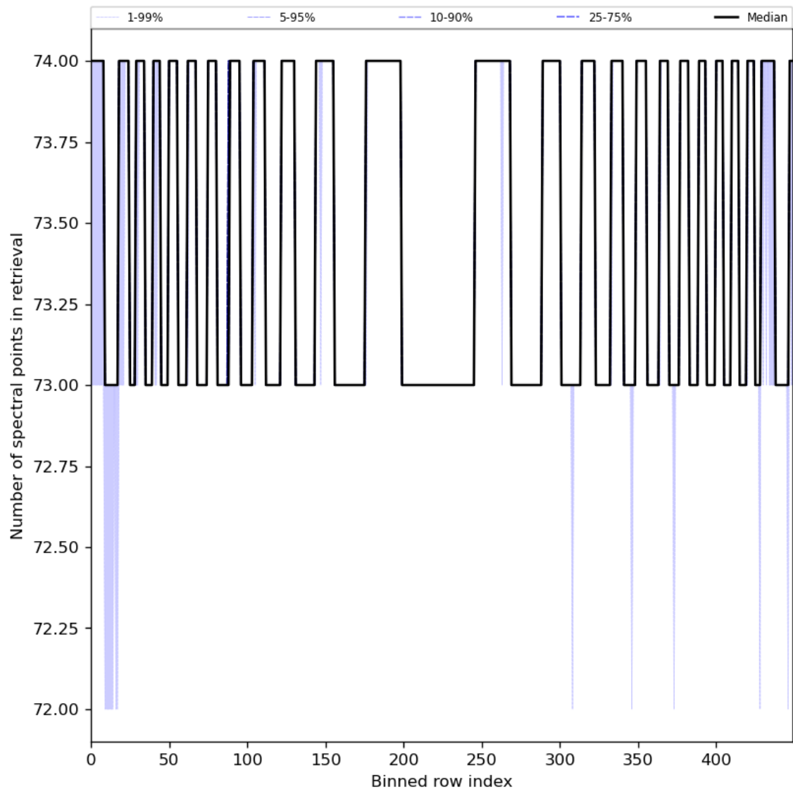
Figure 97: Along track statistics of “Number of spectral points in retrieval” for 2024-03-17 to 2024-03-19
