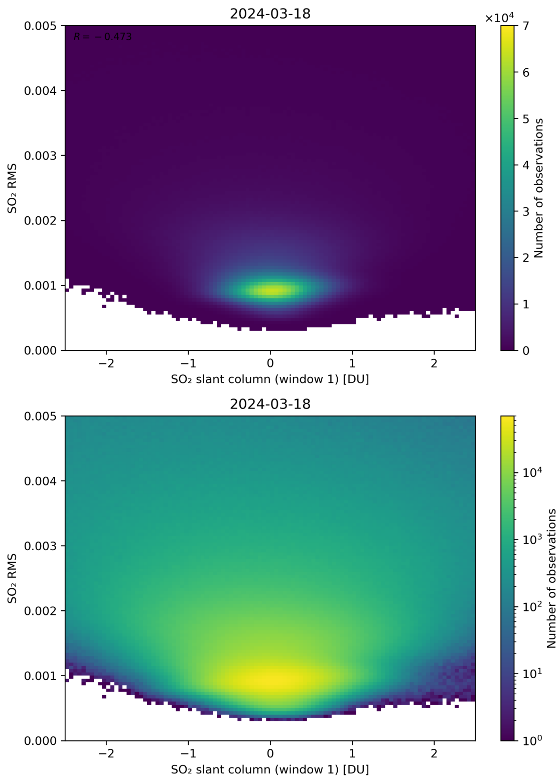
Figure 217: Scatter density plot of “SO 2 slant column (window 1)” against “SO 2 RMS” for 2024-03-17 to 2024-03-19.
