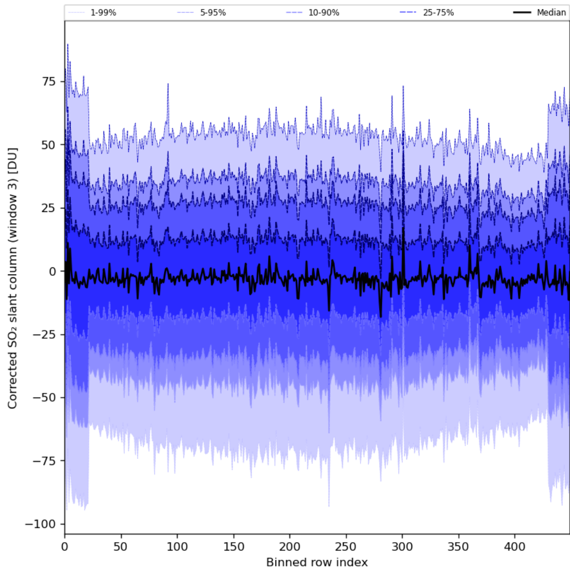
Figure 89: Along track statistics of “Corrected SO 2 slant column (window 3)” for 2024-03-17 to 2024-03-19
