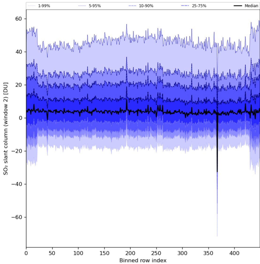
Figure 83: Along track statistics of “SO 2 slant column (window 2)” for 2024-03-17 to 2024-03-19
