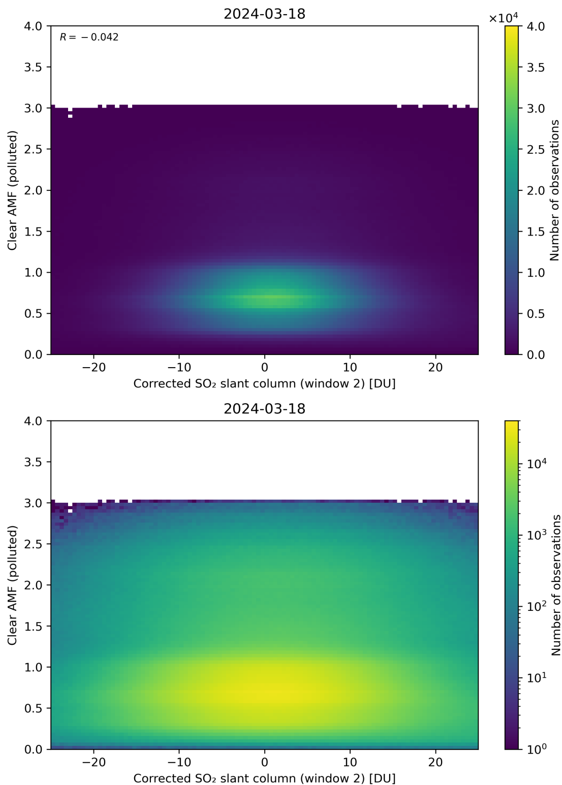
Figure 199: Scatter density plot of “Corrected SO 2 slant column (window 2)” against “Clear AMF (polluted)” for 2024-03-17 to 2024-03-19.
