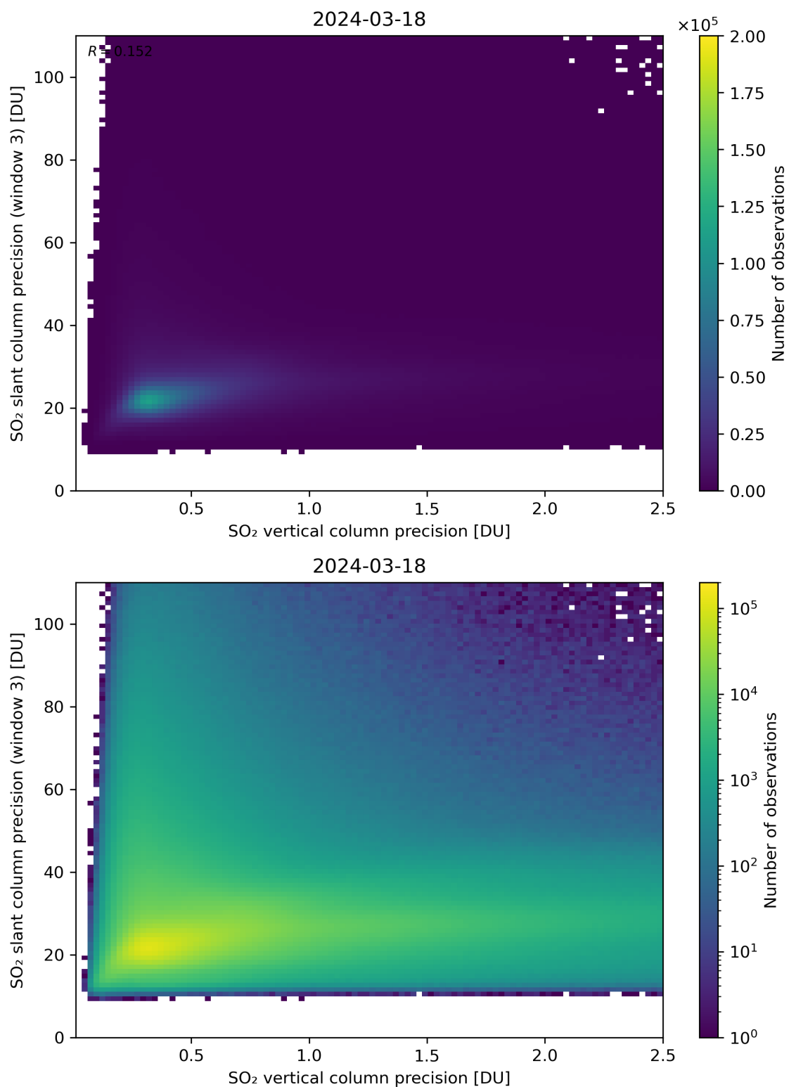
Figure 293: Scatter density plot of “SO 2 vertical column precision” against “SO 2 slant column precision (window 3)” for 2024-03-17 to 2024-03-19.
