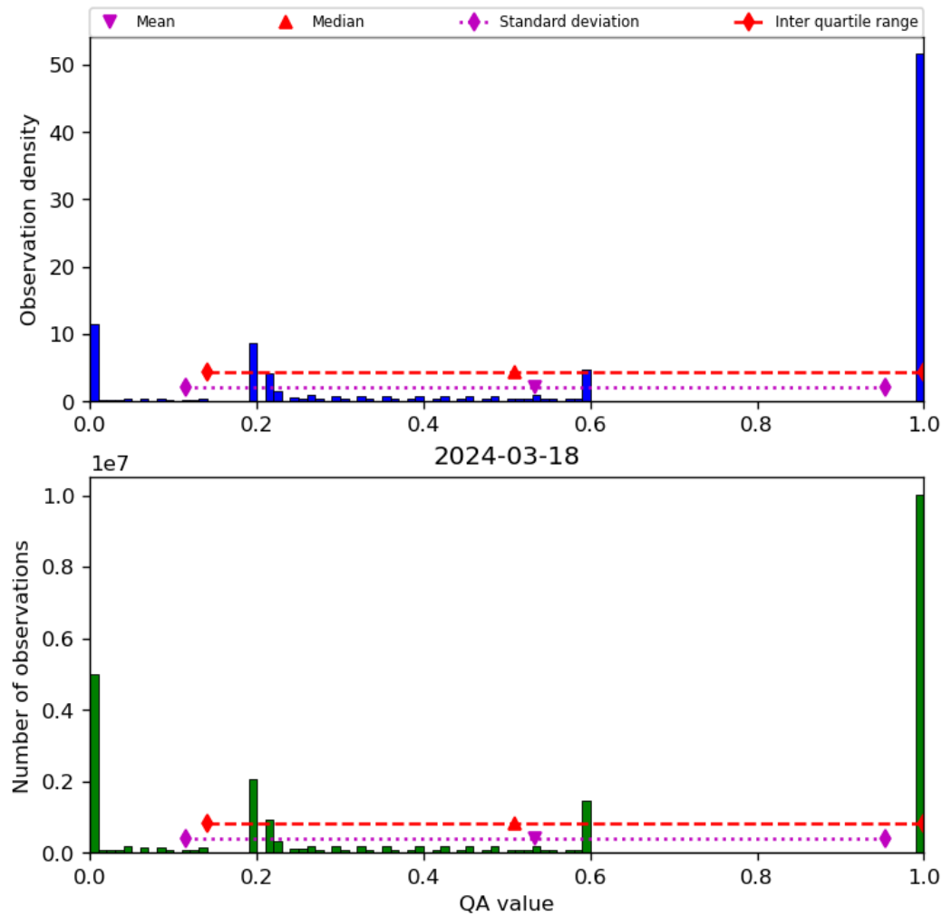
Figure 52: Histogram of “QA value” for 2024-03-17 to 2024-03-19
