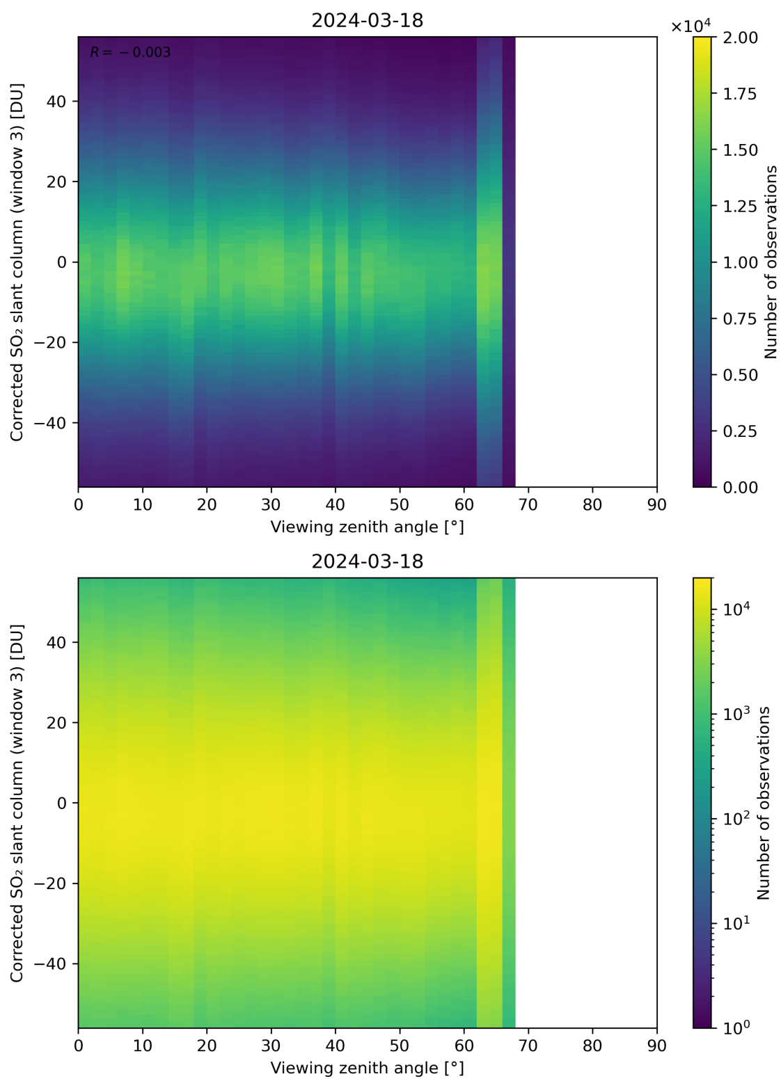
Figure 319: Scatter density plot of “Viewing zenith angle” against “Corrected SO 2 slant column (window 3)” for 2024-03-17 to 2024-03-19.
