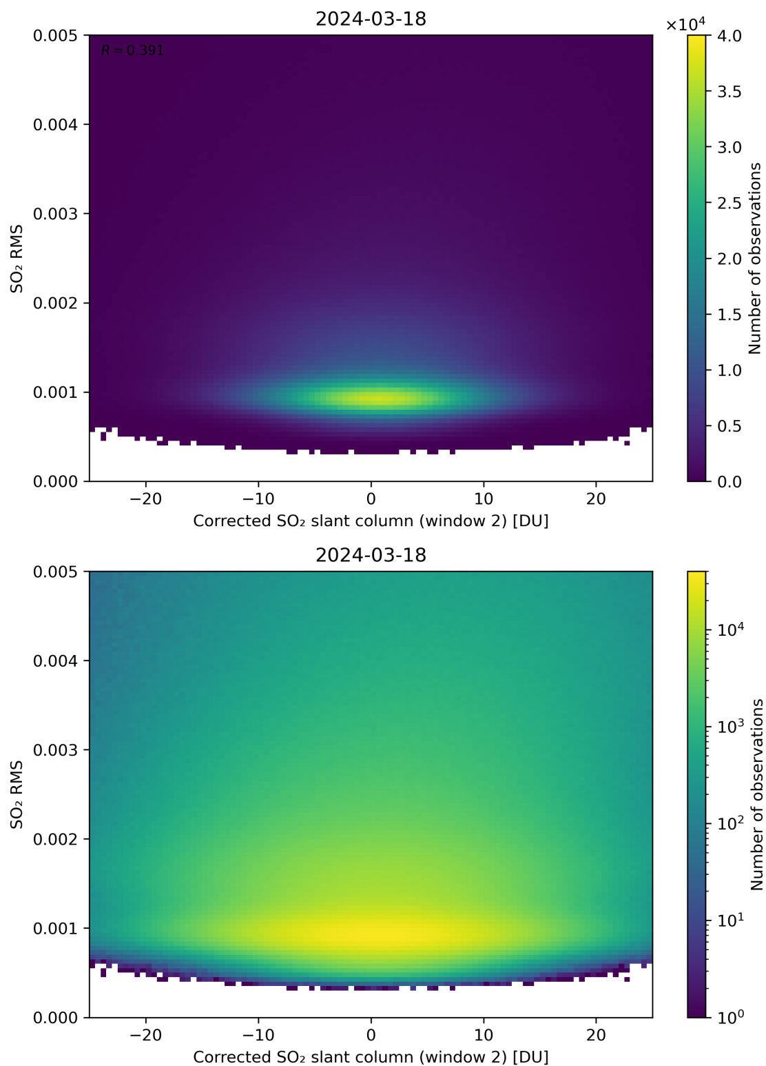
Figure 198: Scatter density plot of “Corrected SO 2 slant column (window 2)” against “SO 2 RMS” for 2024-03-17 to 2024-03-19.
