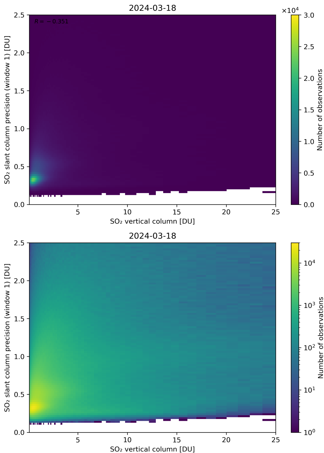
Figure 301: Scatter density plot of “SO 2 vertical column” against “SO 2 slant column precision (window 1)” for 2024-03-17 to 2024-03-19.
