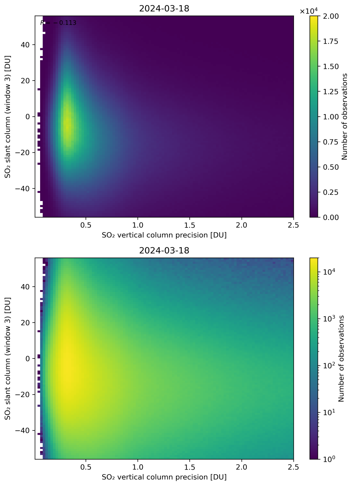
Figure 292: Scatter density plot of “SO 2 vertical column precision” against “SO 2 slant column (window 3)” for 2024-03-17 to 2024-03-19.
