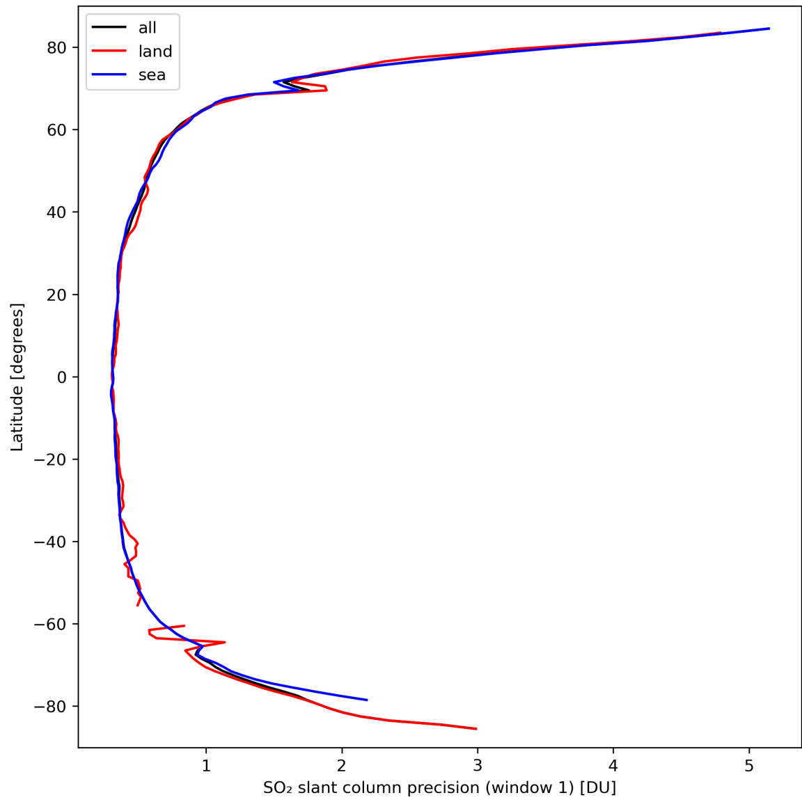
Figure 34: Zonal average of “SO 2 slant column precision (window 1)” for 2024-03-17 to 2024-03-19.
