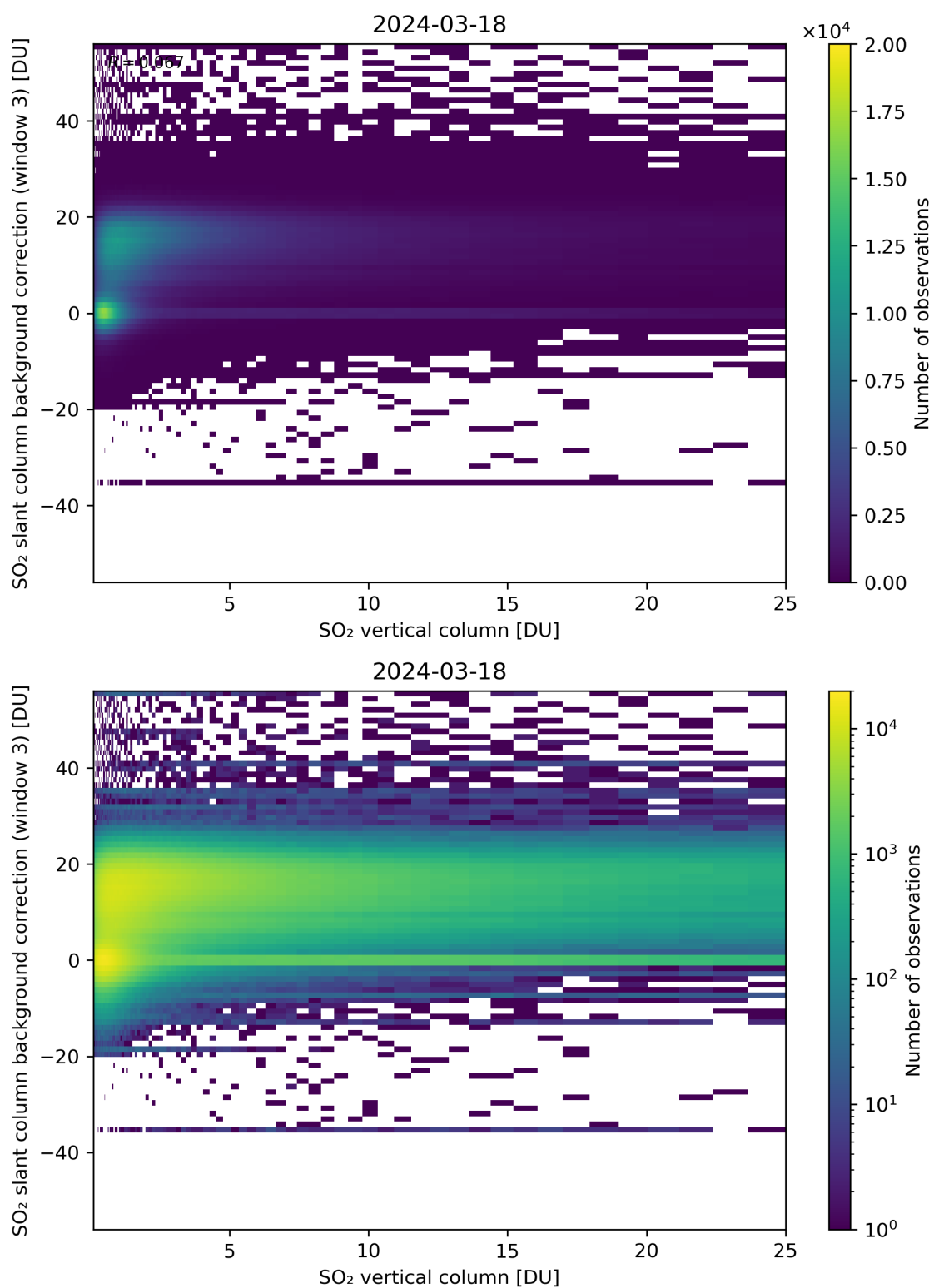
Figure 275: Scatter density plot of “SO 2 vertical column” against “SO 2 slant column background correction (window 3)” for 2024-03-17 to 2024-03-19.
