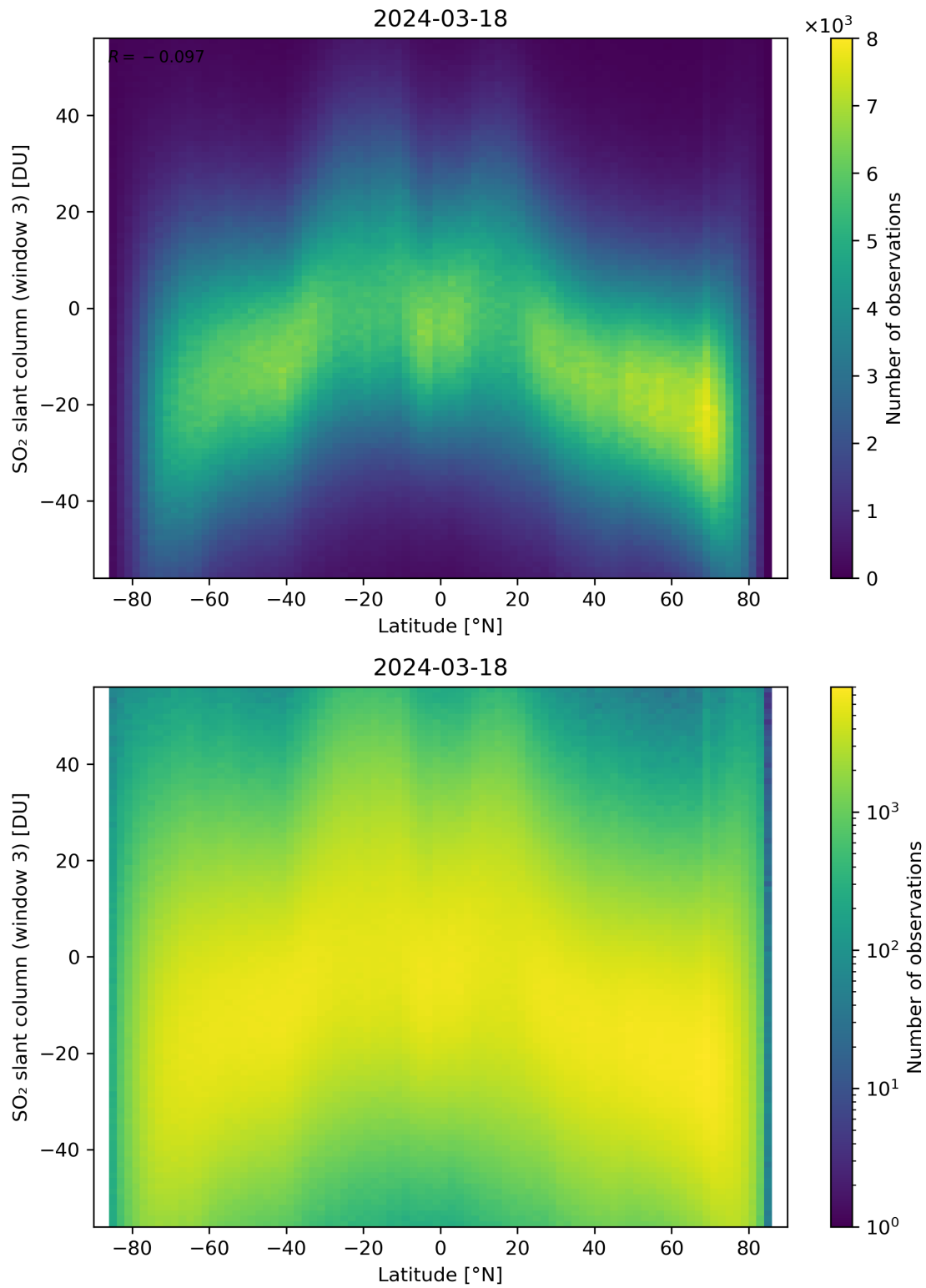
Figure 152: Scatter density plot of “Latitude” against “SO 2 slant column (window 3)” for 2024-03-17 to 2024-03-19.
