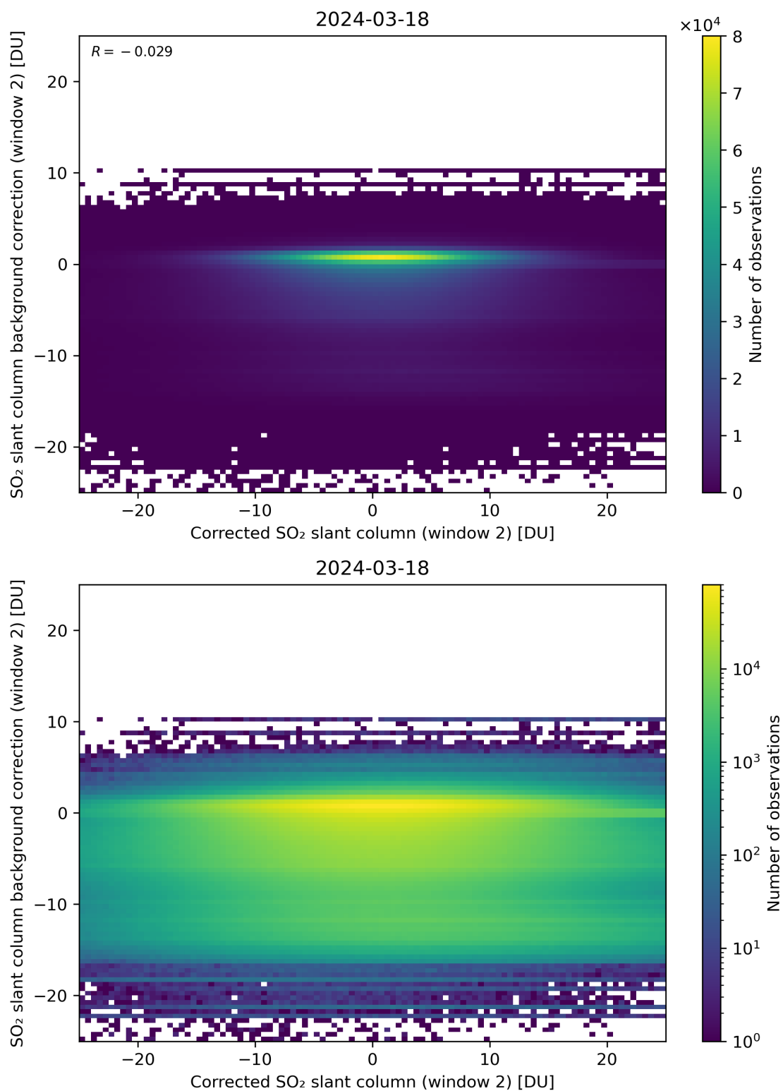
Figure 194: Scatter density plot of “Corrected SO 2 slant column (window 2)” against “SO 2 slant column background correction (window 2)” for 2024-03-17 to 2024-03-19.
