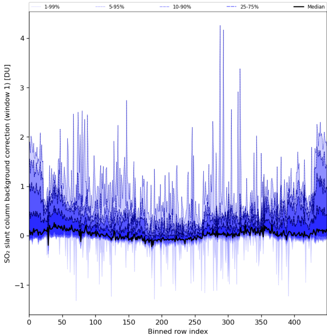
Figure 82: Along track statistics of “SO 2 slant column background correction (window 1)” for 2024-03-17 to 2024-03-19
