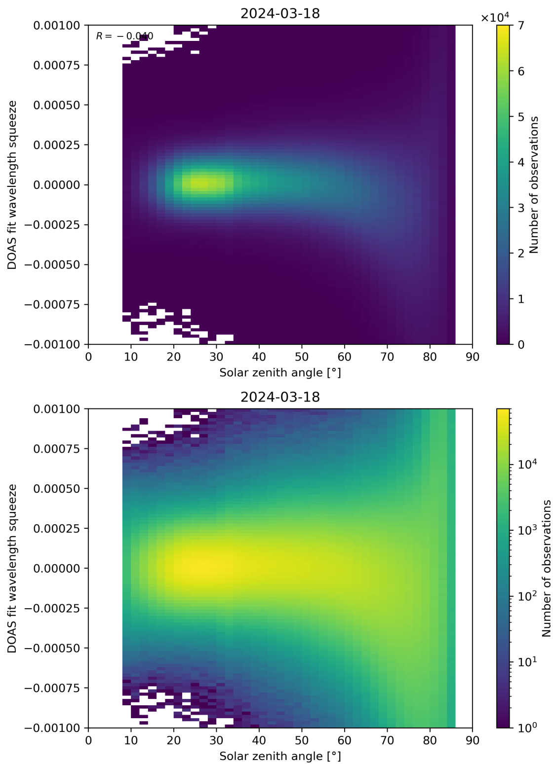
Figure 162: Scatter density plot of “Solar zenith angle” against “DOAS fit wavelength squeeze” for 2024-03-17 to 2024-03-19.
