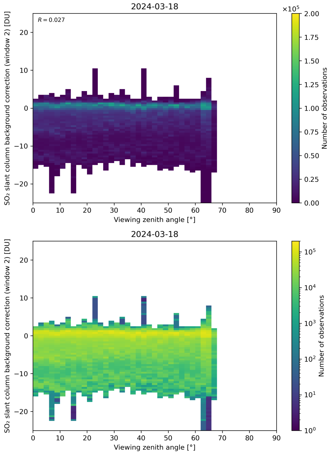
Figure 309: Scatter density plot of “Viewing zenith angle” against “SO 2 slant column background correction (window 2)” for 2024-03-17 to 2024-03-19.
