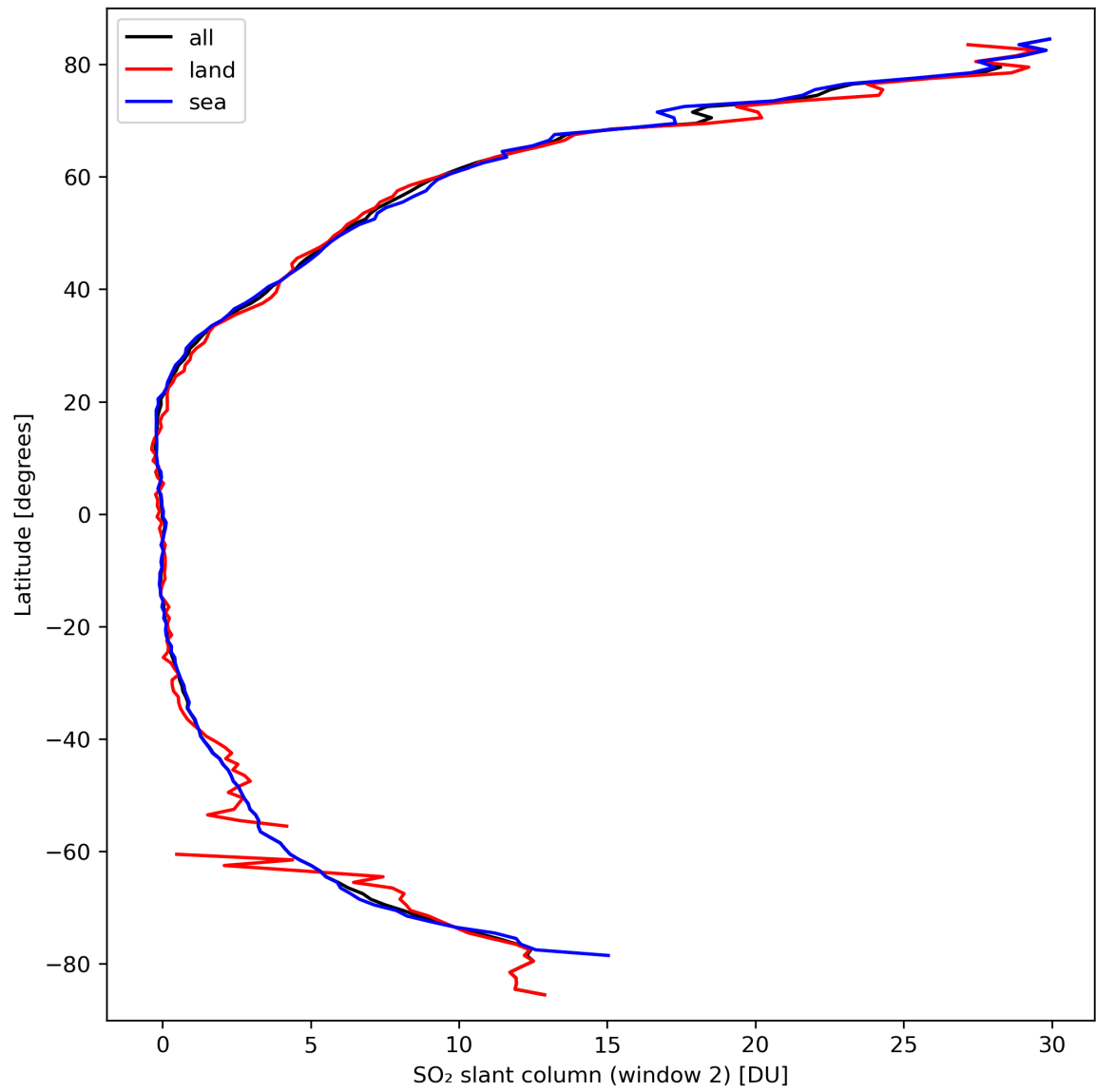
Figure 37: Zonal average of “SO 2 slant column (window 2)” for 2024-03-17 to 2024-03-19.
