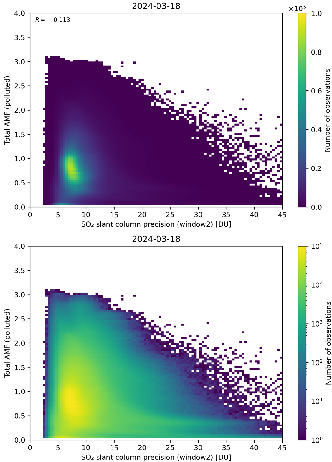
Figure 251: Scatter density plot of “SO 2 slant column precision (window2)” against “Total AMF (polluted)” for 2024-03-17 to 2024-03-19.
