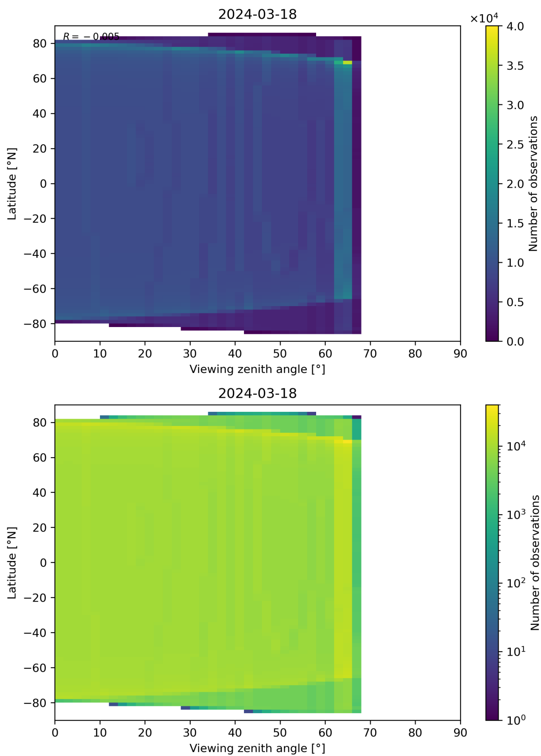
Figure 314: Scatter density plot of “Viewing zenith angle” against “Latitude” for 2024-03-17 to 2024-03-19.
