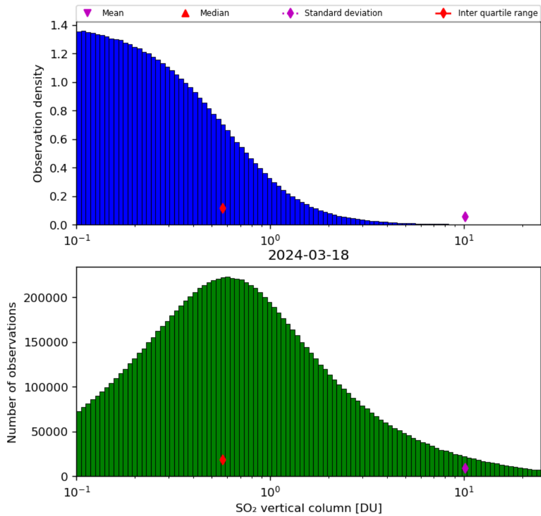
Figure 53: Histogram of “SO 2 vertical column” for 2024-03-17 to 2024-03-19
