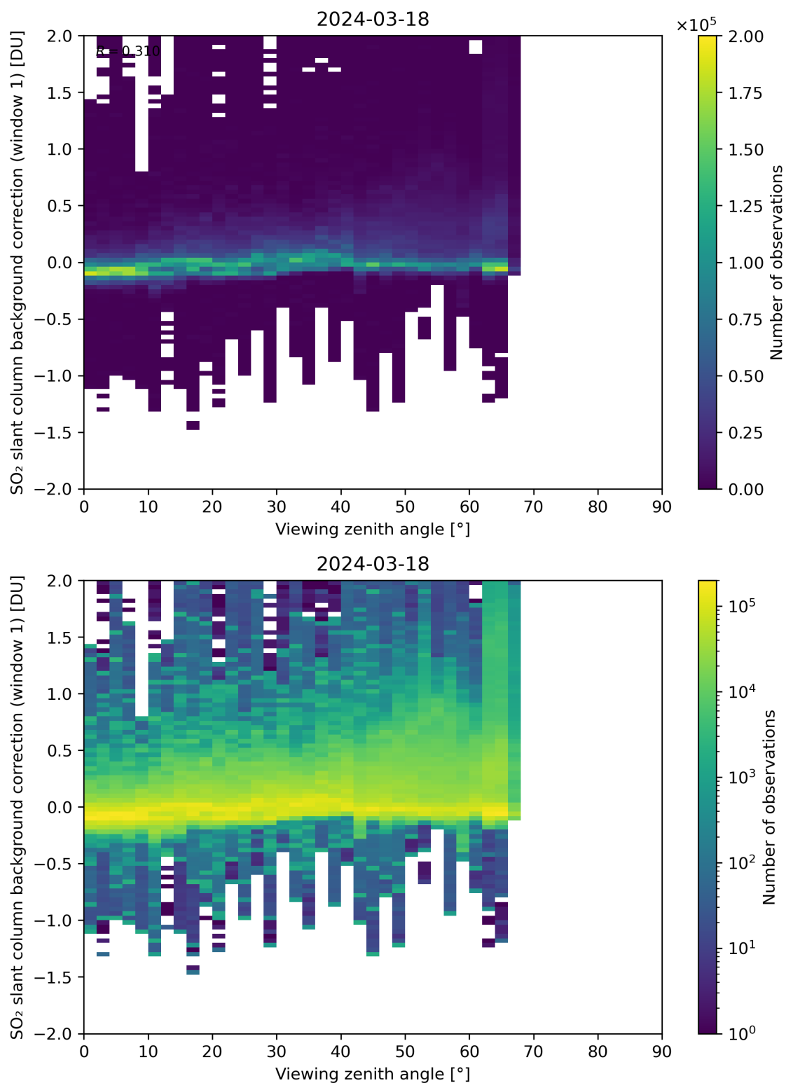
Figure 308: Scatter density plot of “Viewing zenith angle” against “SO 2 slant column background correction (window 1)” for 2024-03-17 to 2024-03-19.
