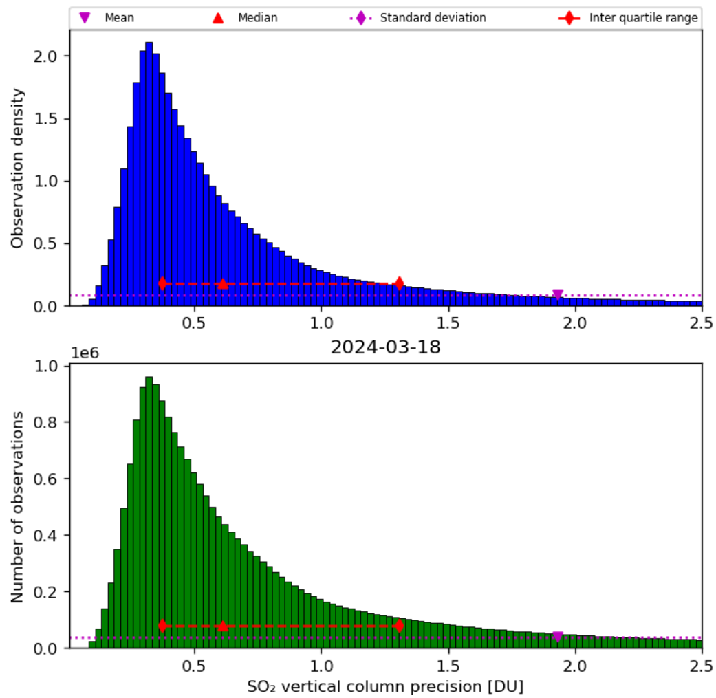
Figure 54: Histogram of “SO 2 vertical column precision” for 2024-03-17 to 2024-03-19
