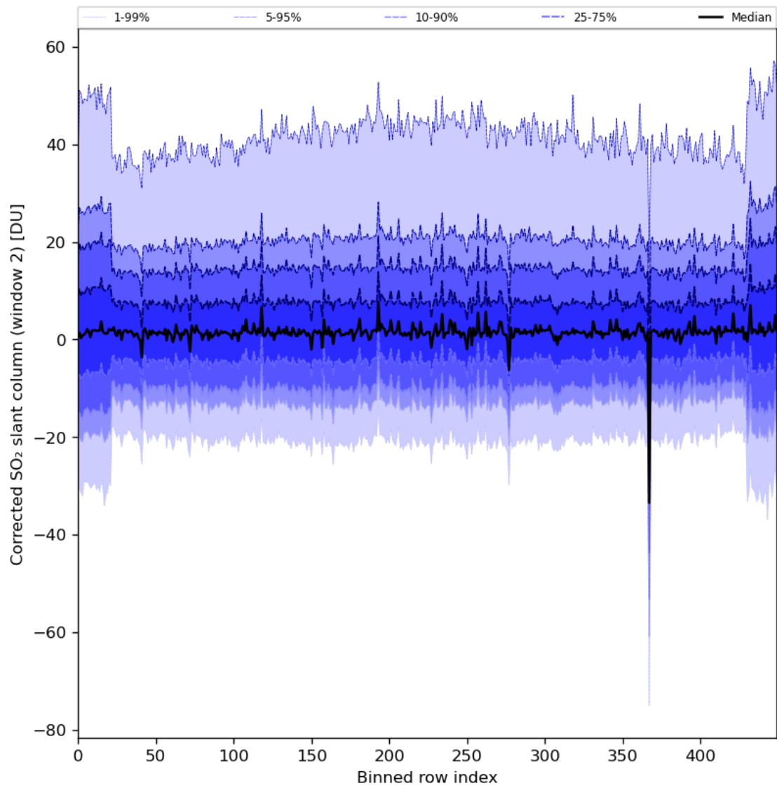
Figure 85: Along track statistics of “Corrected SO 2 slant column (window 2)” for 2024-03-17 to 2024-03-19
