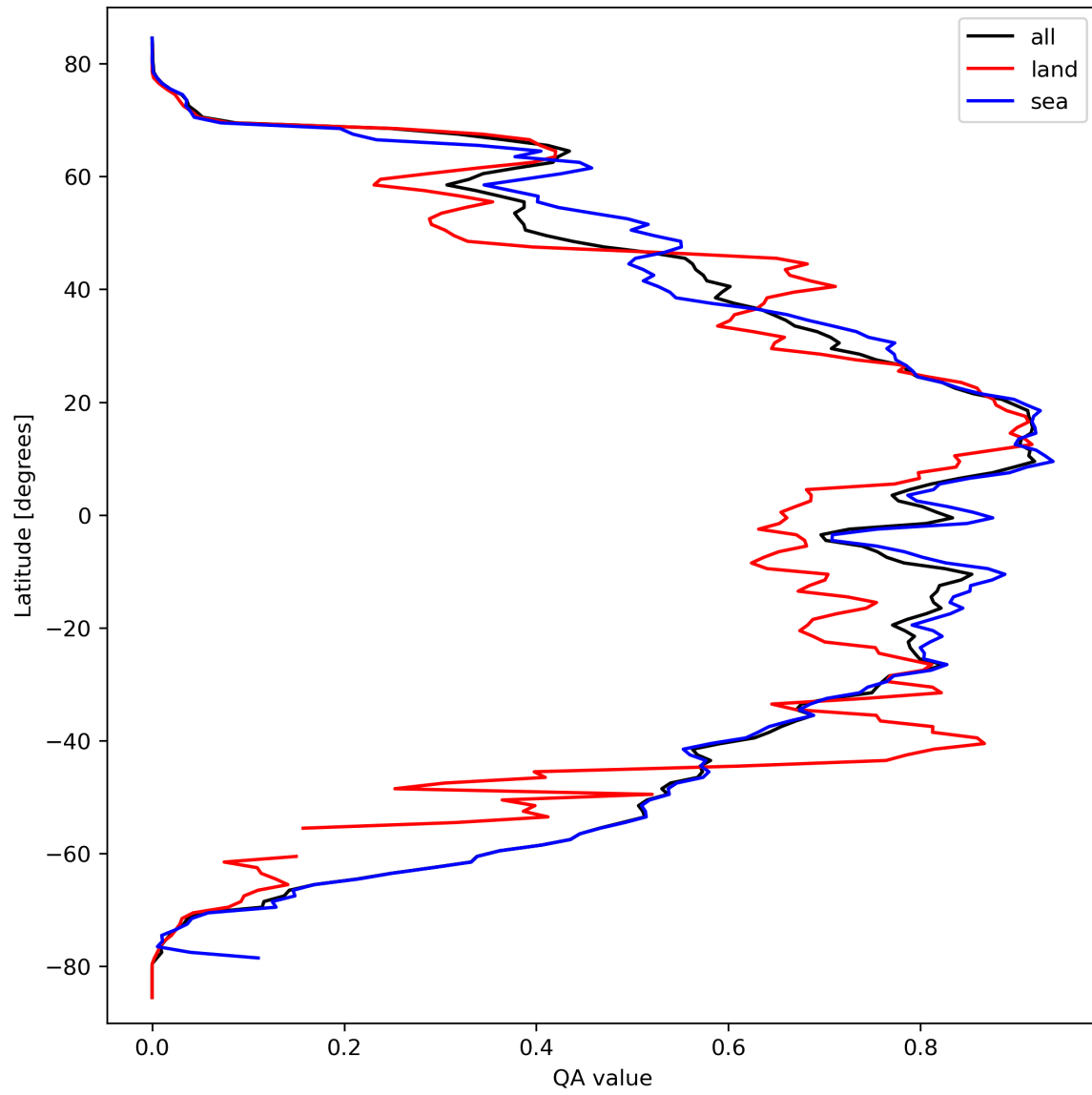
Figure 29: Zonal average of “QA value” for 2024-03-17 to 2024-03-19.
