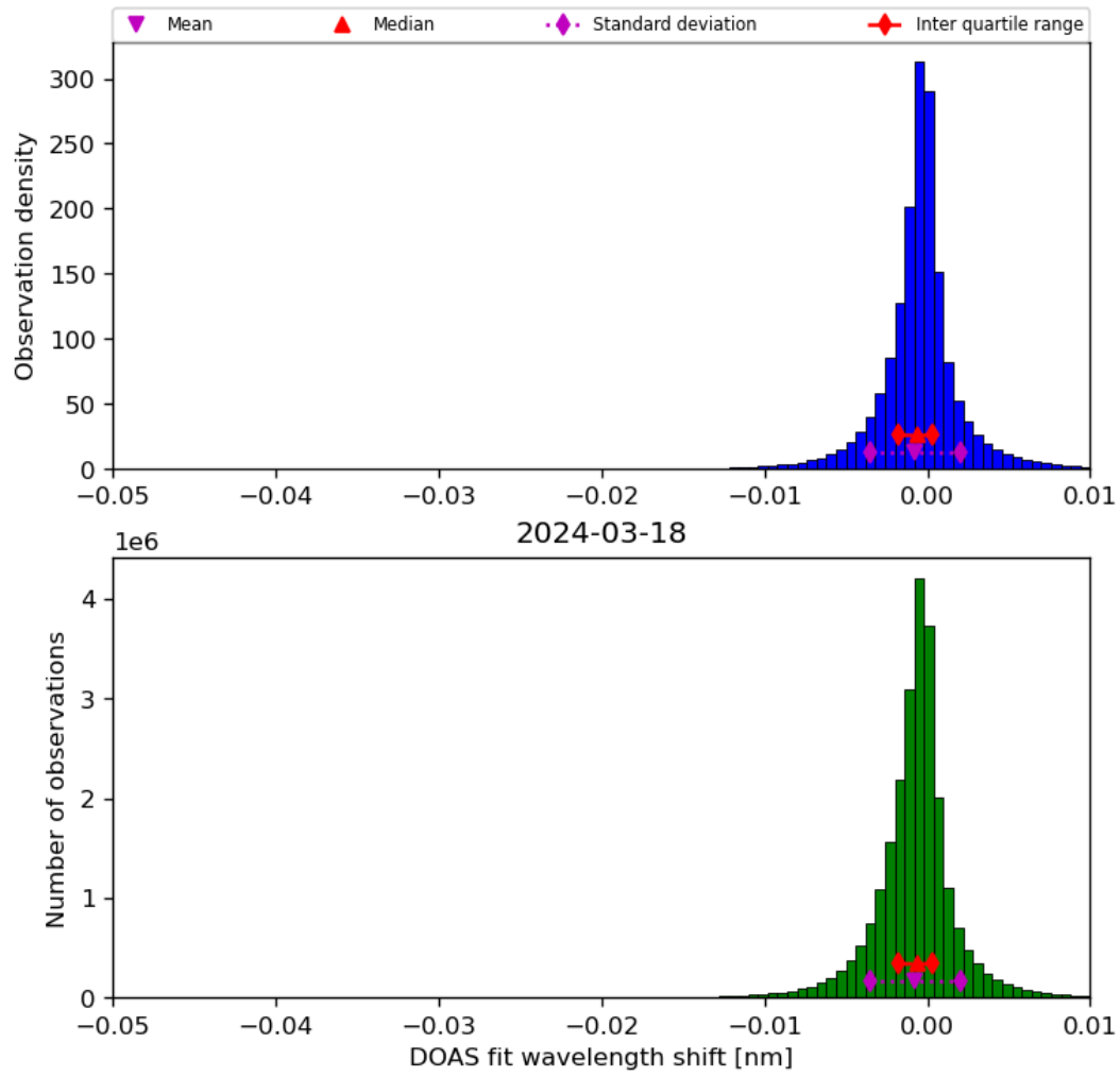
Figure 68: Histogram of “DOAS fit wavelength shift” for 2024-03-17 to 2024-03-19
