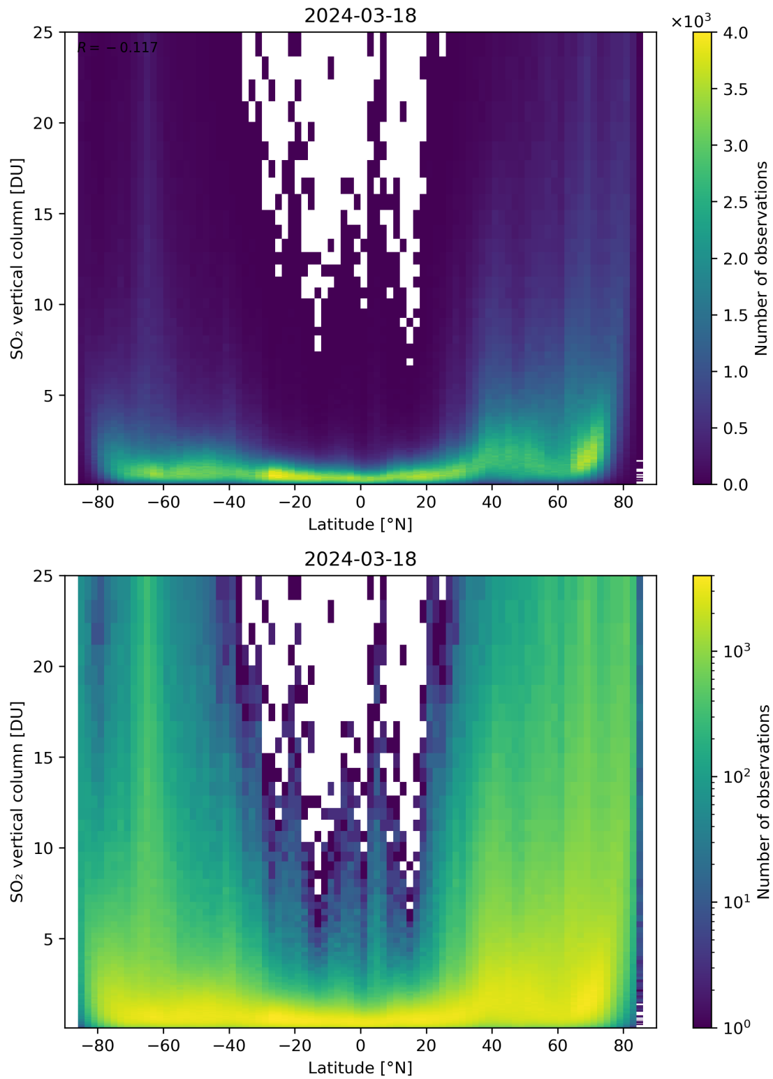
Figure 156: Scatter density plot of “Latitude” against “SO 2 vertical column” for 2024-03-17 to 2024-03-19.
