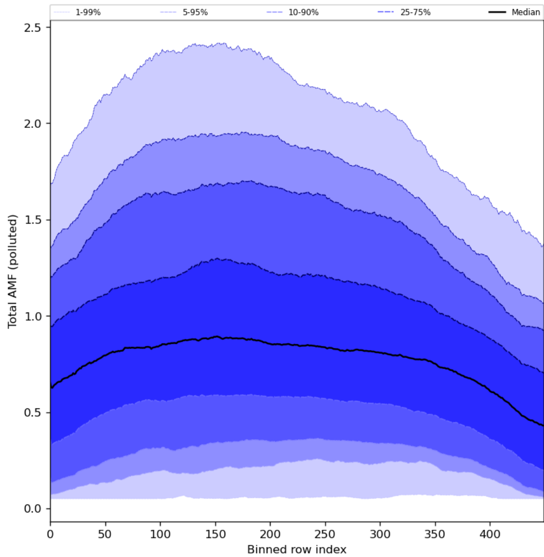
Figure 94: Along track statistics of “Total AMF (polluted)” for 2024-03-17 to 2024-03-19
