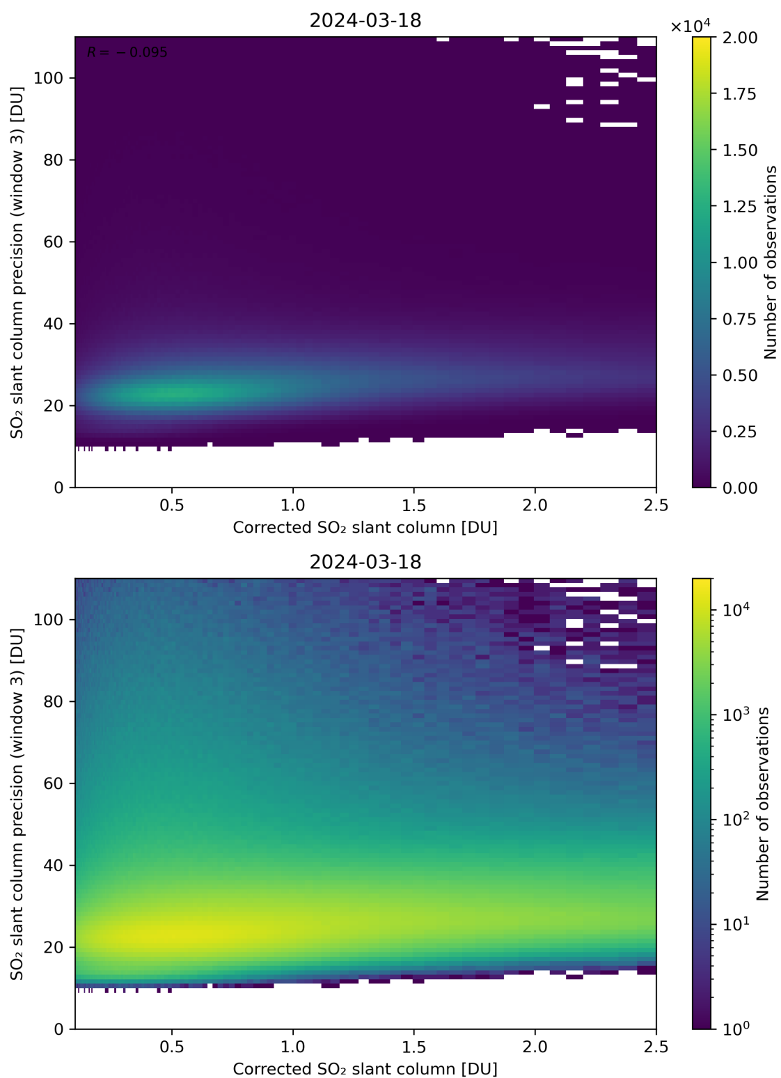
Figure 191: Scatter density plot of “Corrected SO 2 slant column” against “SO 2 slant column precision (window 3)” for 2024-03-17 to 2024-03-19.
