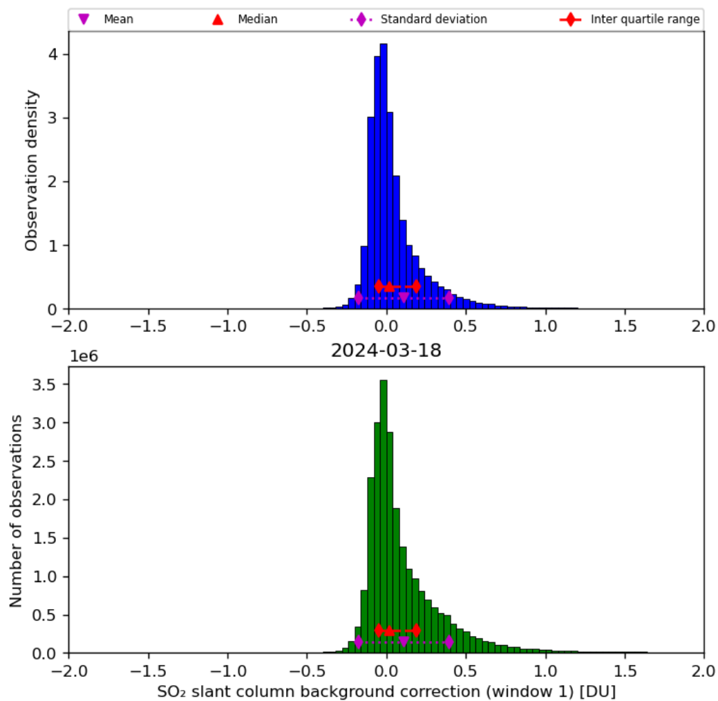
Figure 59: Histogram of “SO 2 slant column background correction (window 1)” for 2024-03-17 to 2024-03-19
