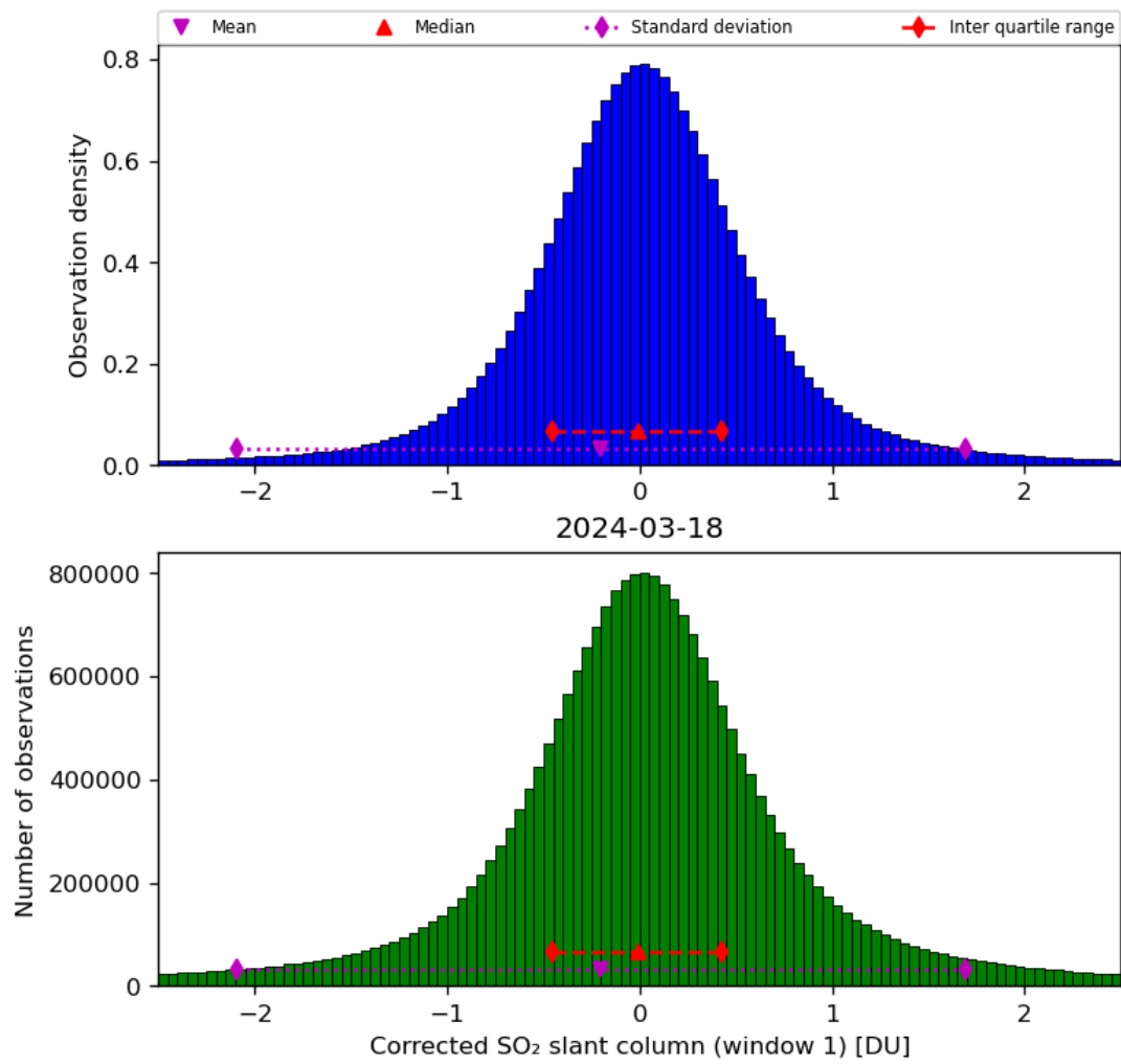
Figure 58: Histogram of “Corrected SO 2 slant column (window 1)” for 2024-03-17 to 2024-03-19
