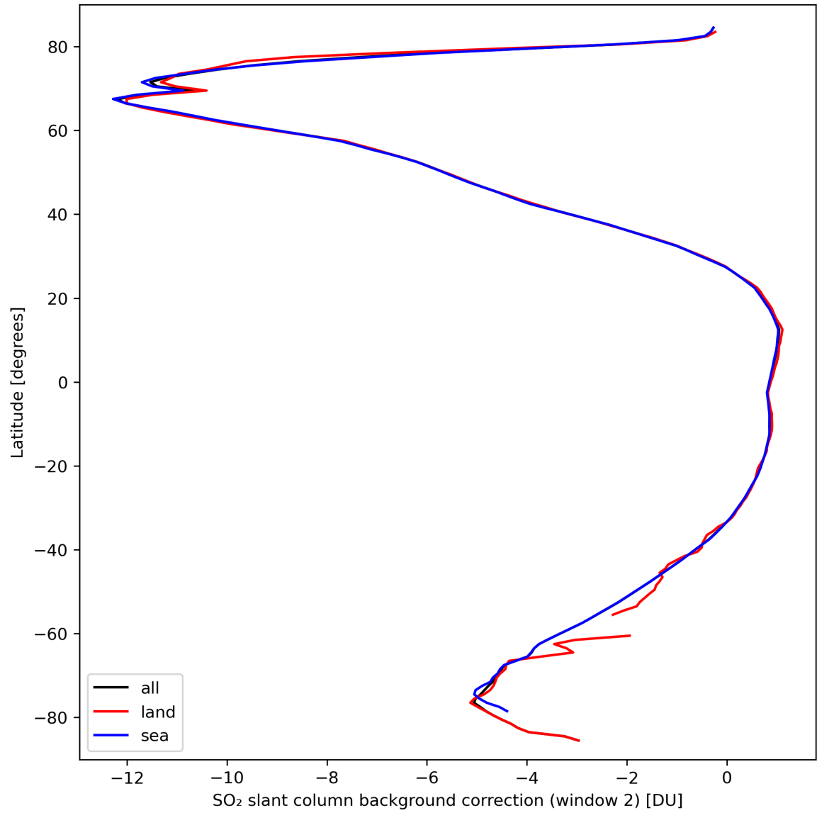
Figure 40: Zonal average of “SO 2 slant column background correction (window 2)” for 2024-03-17 to 2024-03-19.
