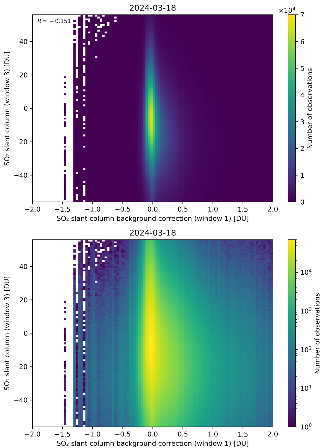
Figure 107: Scatter density plot of “SO 2 slant column background correction (window 1)” against “SO 2 slant column (window 3)” for 2024-03-17 to 2024-03-19.
