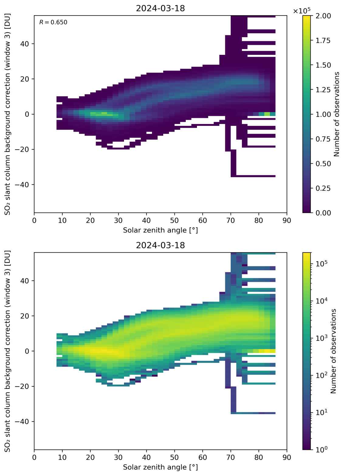
Figure 160: Scatter density plot of “Solar zenith angle” against “SO 2 slant column background correction (window 3)” for 2024-03-17 to 2024-03-19.
