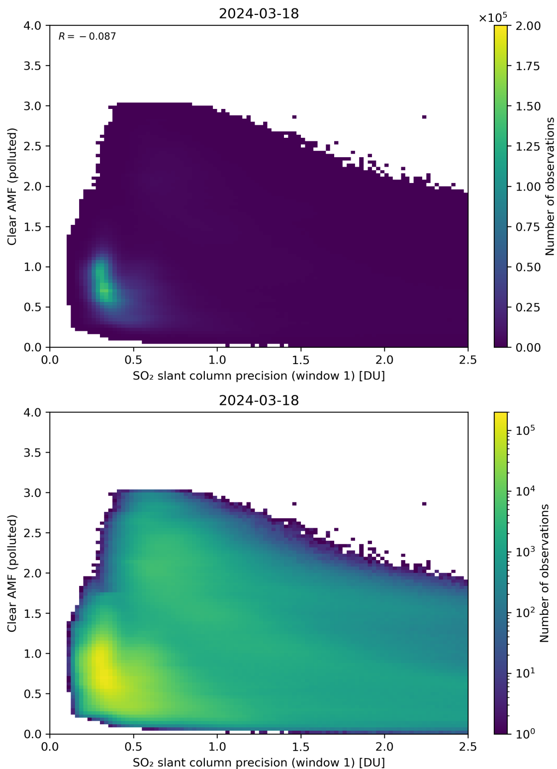
Figure 224: Scatter density plot of “SO 2 slant column precision (window 1)” against “Clear AMF (polluted)” for 2024-03-17 to 2024-03-19.
