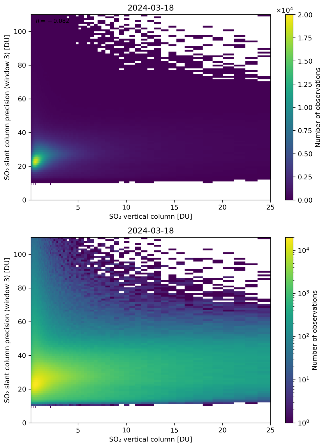
Figure 304: Scatter density plot of “SO 2 vertical column” against “SO 2 slant column precision (window 3)” for 2024-03-17 to 2024-03-19.
