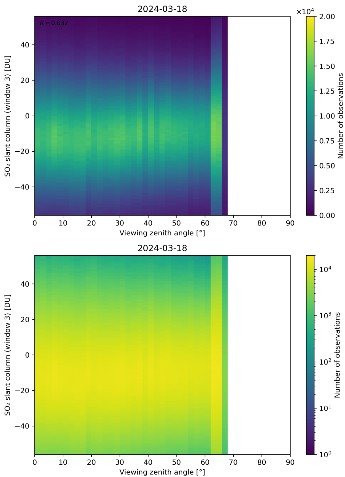
Figure 323: Scatter density plot of “Viewing zenith angle” against “SO 2 slant column (window 3)” for 2024-03-17 to 2024-03-19.
