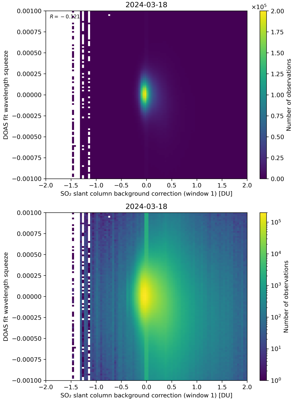
Figure 101: Scatter density plot of “SO 2 slant column background correction (window 1)” against “DOAS fit wavelength squeeze” for 2024-03-17 to 2024-03-19.
