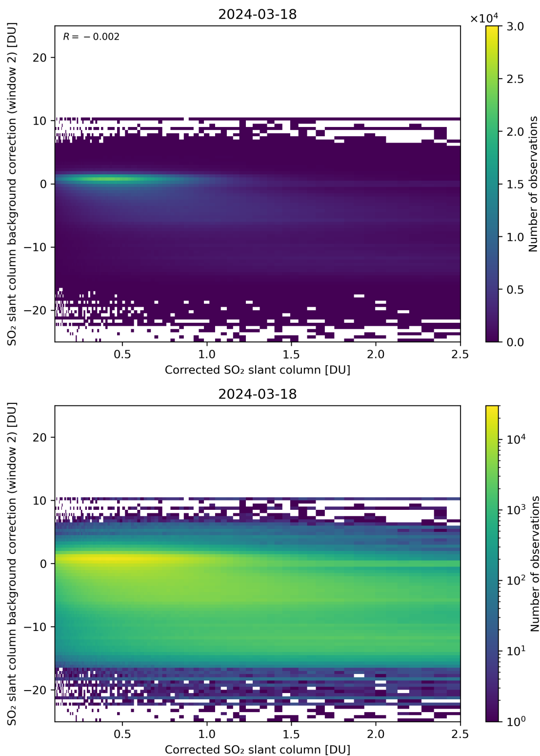
Figure 179: Scatter density plot of “Corrected SO 2 slant column” against “SO 2 slant column background correction (window 2)” for 2024-03-17 to 2024-03-19.
