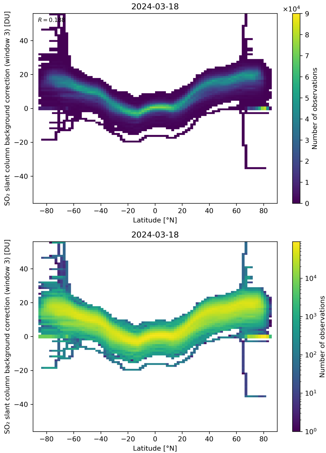
Figure 141: Scatter density plot of “Latitude” against “SO 2 slant column background correction (window 3)” for 2024-03-17 to 2024-03-19.
