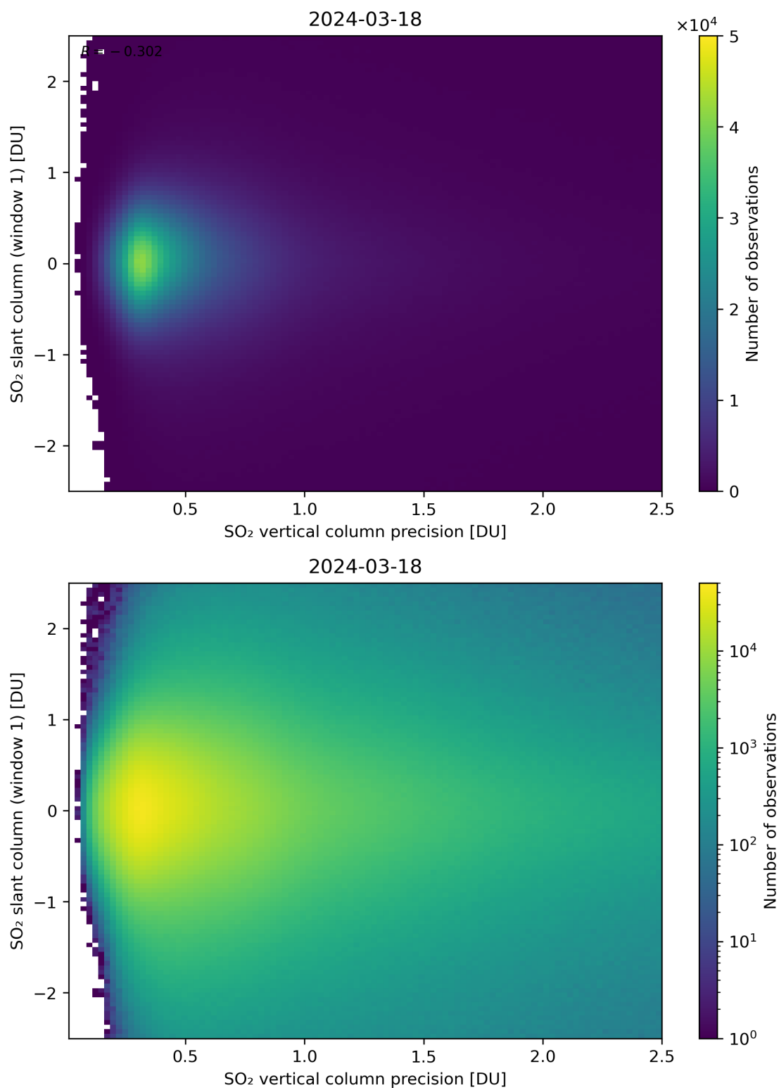
Figure 289: Scatter density plot of “SO 2 vertical column precision” against “SO 2 slant column (window 1)” for 2024-03-17 to 2024-03-19.
