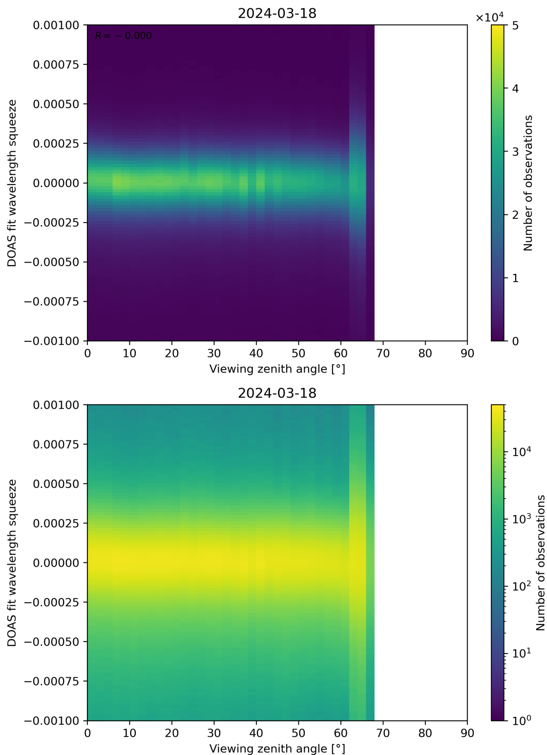
Figure 312: Scatter density plot of “Viewing zenith angle” against “DOAS fit wavelength squeeze” for 2024-03-17 to 2024-03-19.
