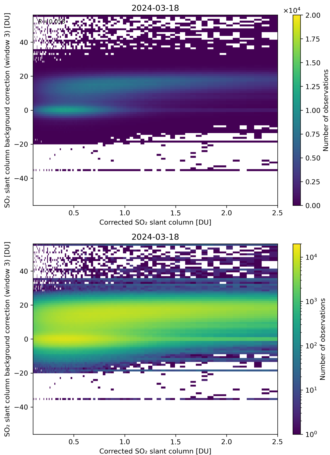
Figure 180: Scatter density plot of “Corrected SO 2 slant column” against “SO 2 slant column background correction (window 3)” for 2024-03-17 to 2024-03-19.
