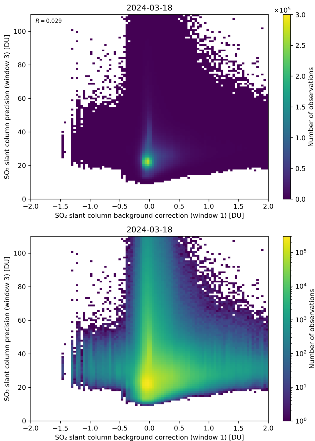
Figure 108: Scatter density plot of “SO 2 slant column background correction (window 1)” against “SO 2 slant column precision (window 3)” for 2024-03-17 to 2024-03-19.
