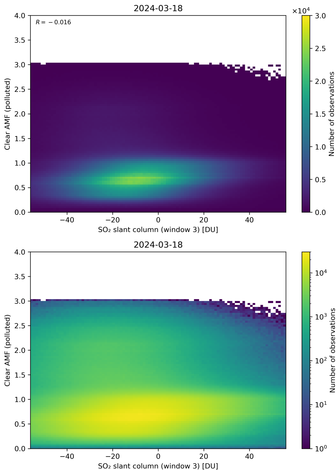
Figure 265: Scatter density plot of “SO 2 slant column (window 3)” against “Clear AMF (polluted)” for 2024-03-17 to 2024-03-19.
