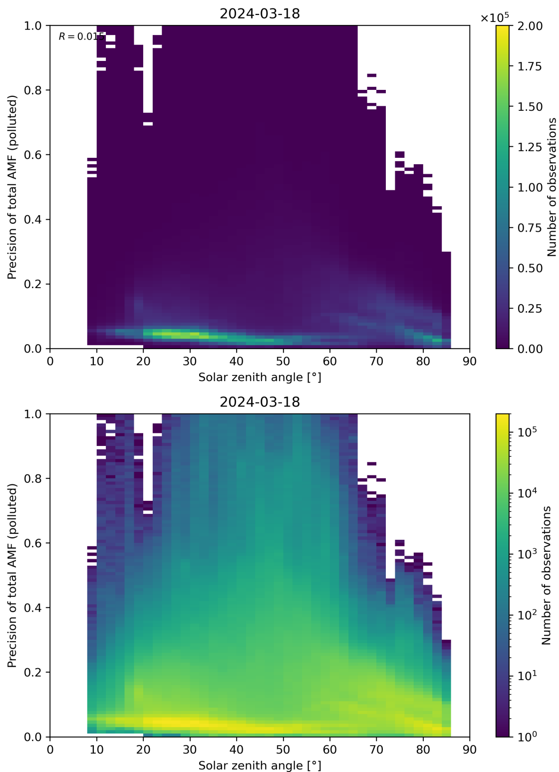
Figure 175: Scatter density plot of “Solar zenith angle” against “Precision of total AMF (polluted)” for 2024-03-17 to 2024-03-19.
