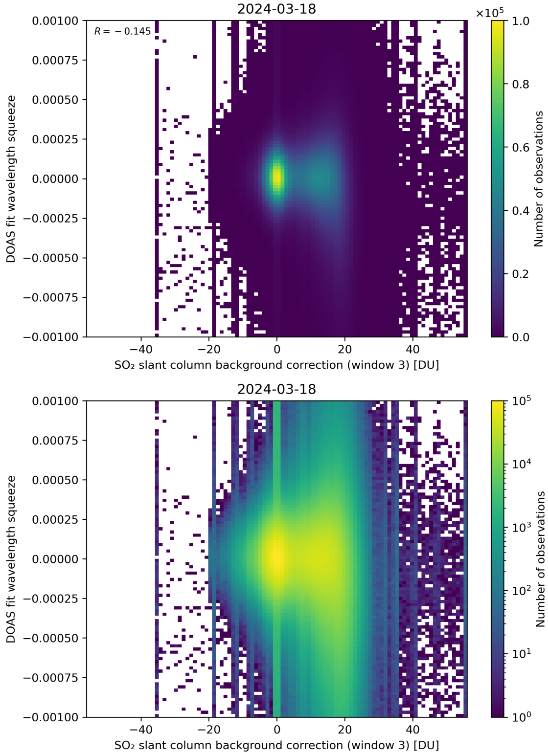
Figure 122: Scatter density plot of “SO 2 slant column background correction (window 3)” against “DOAS fit wavelength squeeze” for 2024-03-17 to 2024-03-19.
