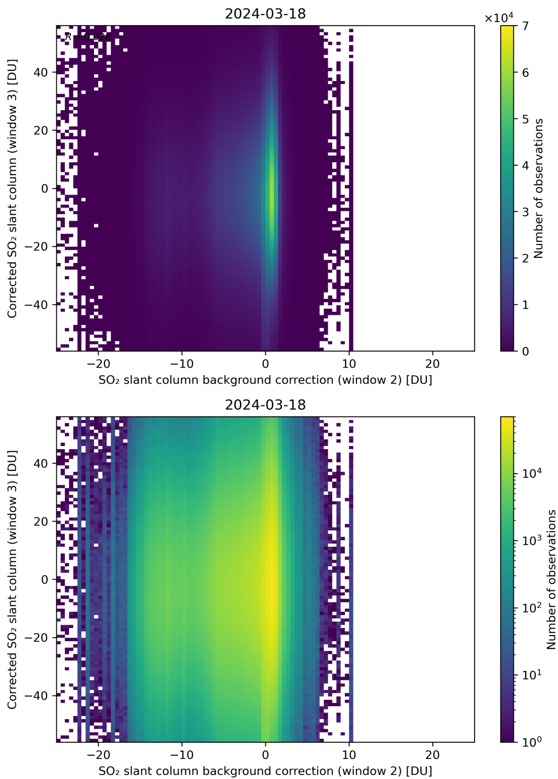
Figure 116: Scatter density plot of “SO 2 slant column background correction (window 2)” against “Corrected SO 2 slant column (window 3)” for 2024-03-17 to 2024-03-19.
