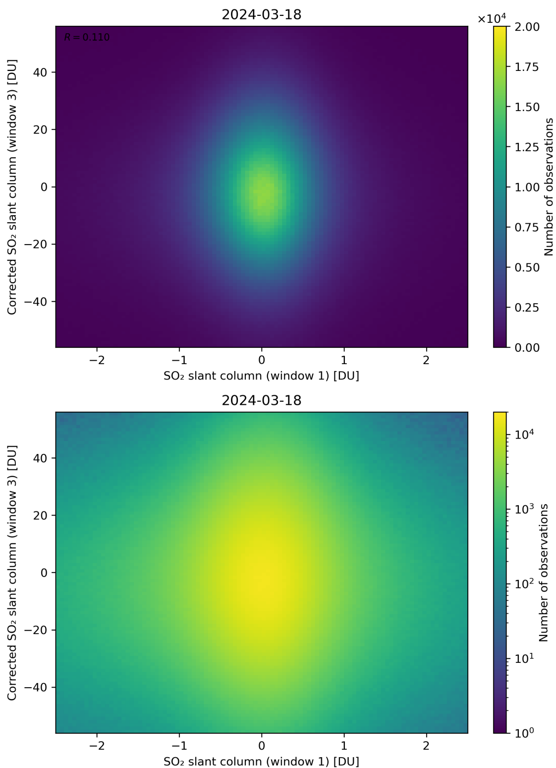
Figure 234: Scatter density plot of “SO 2 slant column (window 1)” against “Corrected SO 2 slant column (window 3)” for 2024-03-17 to 2024-03-19.
