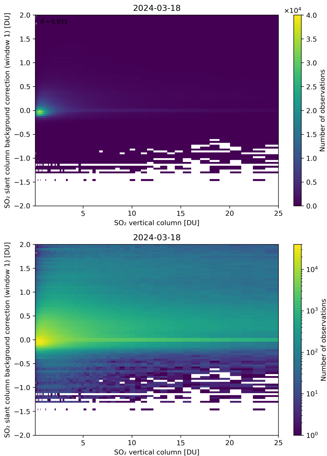
Figure 273: Scatter density plot of “SO 2 vertical column” against “SO 2 slant column background correction (window 1)” for 2024-03-17 to 2024-03-19.
