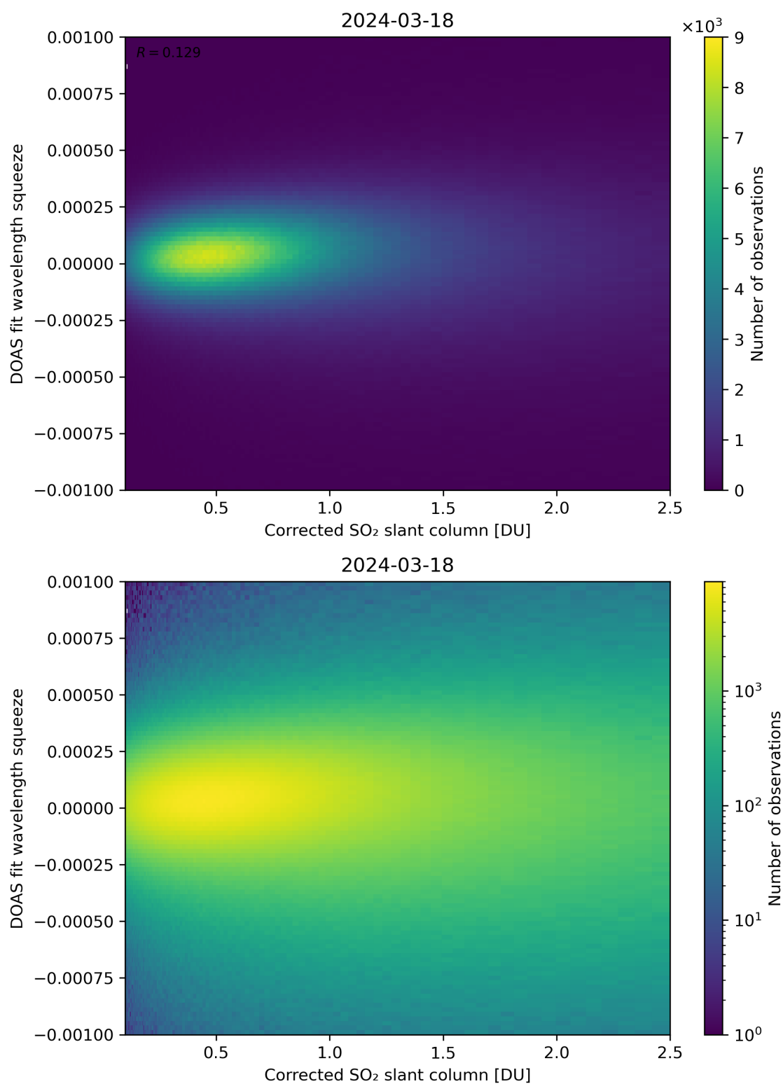
Figure 182: Scatter density plot of “Corrected SO 2 slant column” against “DOAS fit wavelength squeeze” for 2024-03-17 to 2024-03-19.
