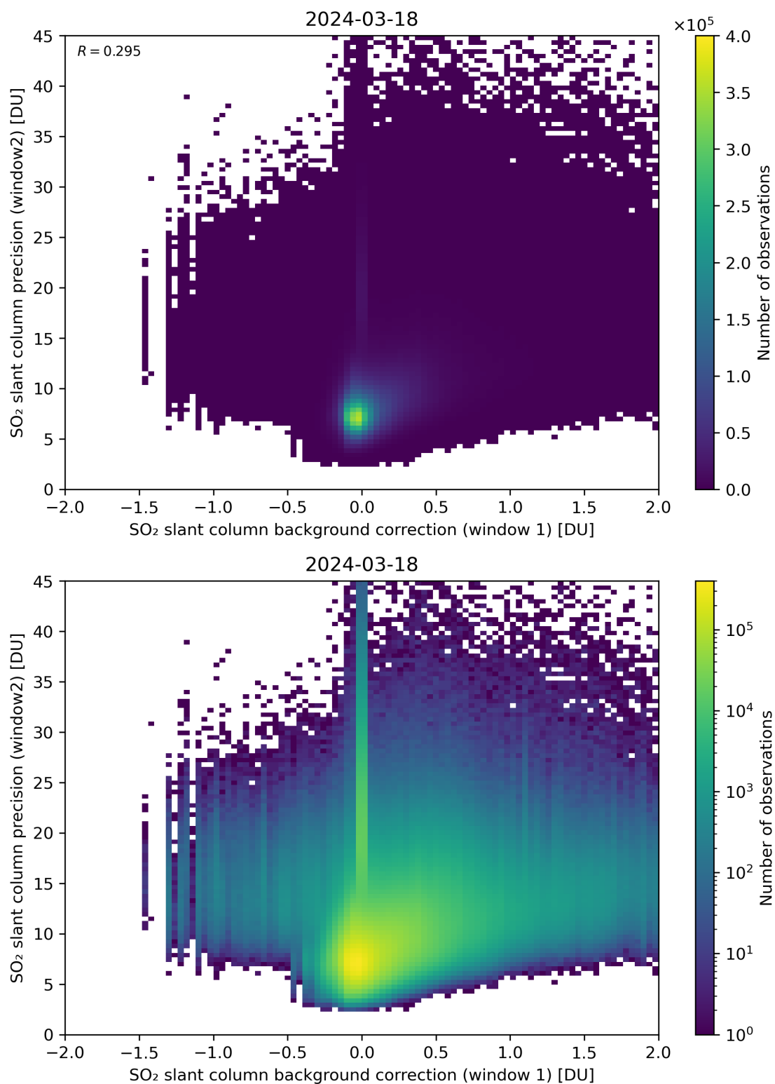
Figure 106: Scatter density plot of “SO 2 slant column background correction (window 1)” against “SO 2 slant column precision (window2)” for 2024-03-17 to 2024-03-19.
