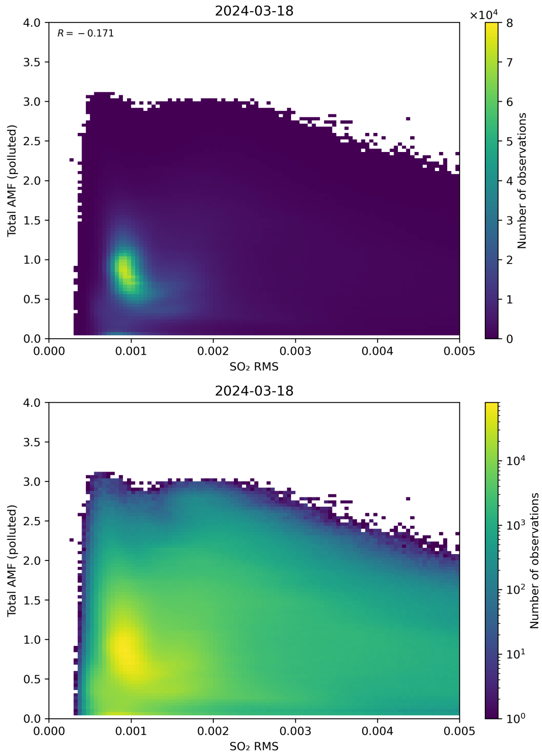
Figure 137: Scatter density plot of “SO 2 RMS” against “Total AMF (polluted)” for 2024-03-17 to 2024-03-19.
