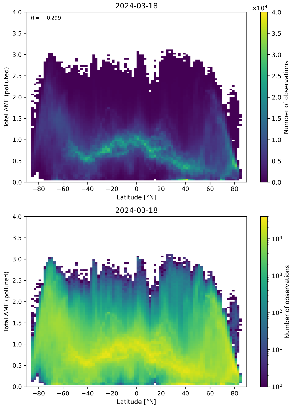
Figure 154: Scatter density plot of “Latitude” against “Total AMF (polluted)” for 2024-03-17 to 2024-03-19.
