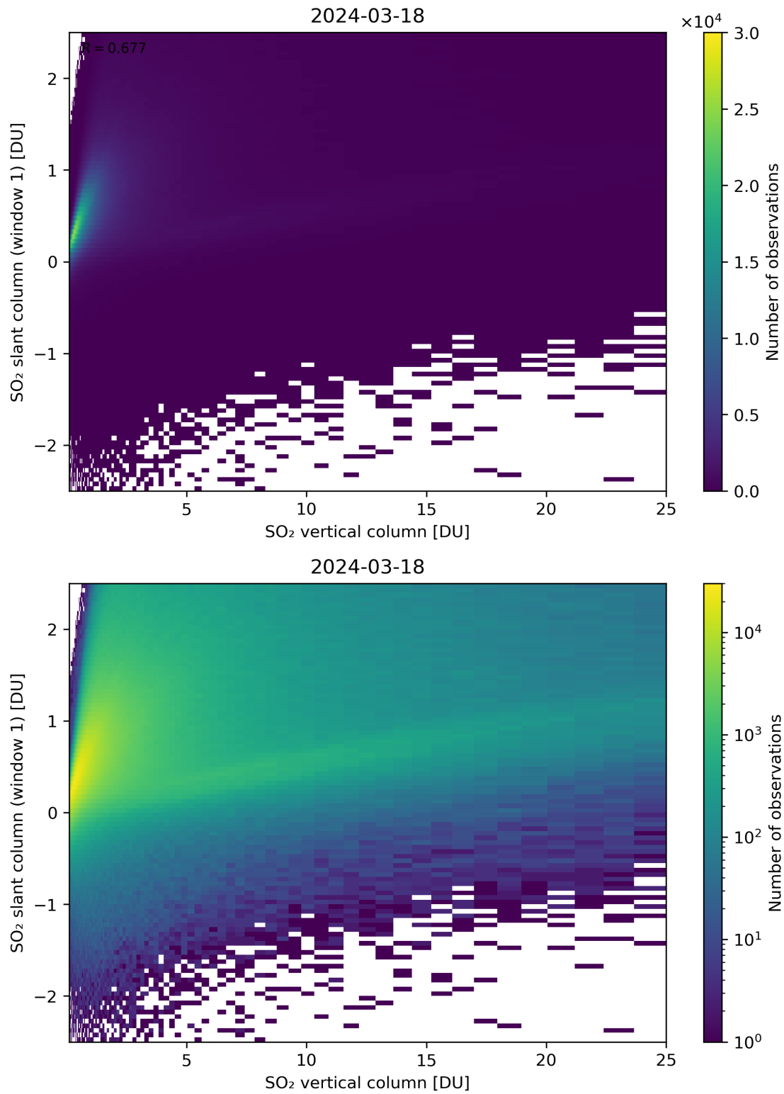
Figure 300: Scatter density plot of “SO 2 vertical column” against “SO 2 slant column (window 1)” for 2024-03-17 to 2024-03-19.
