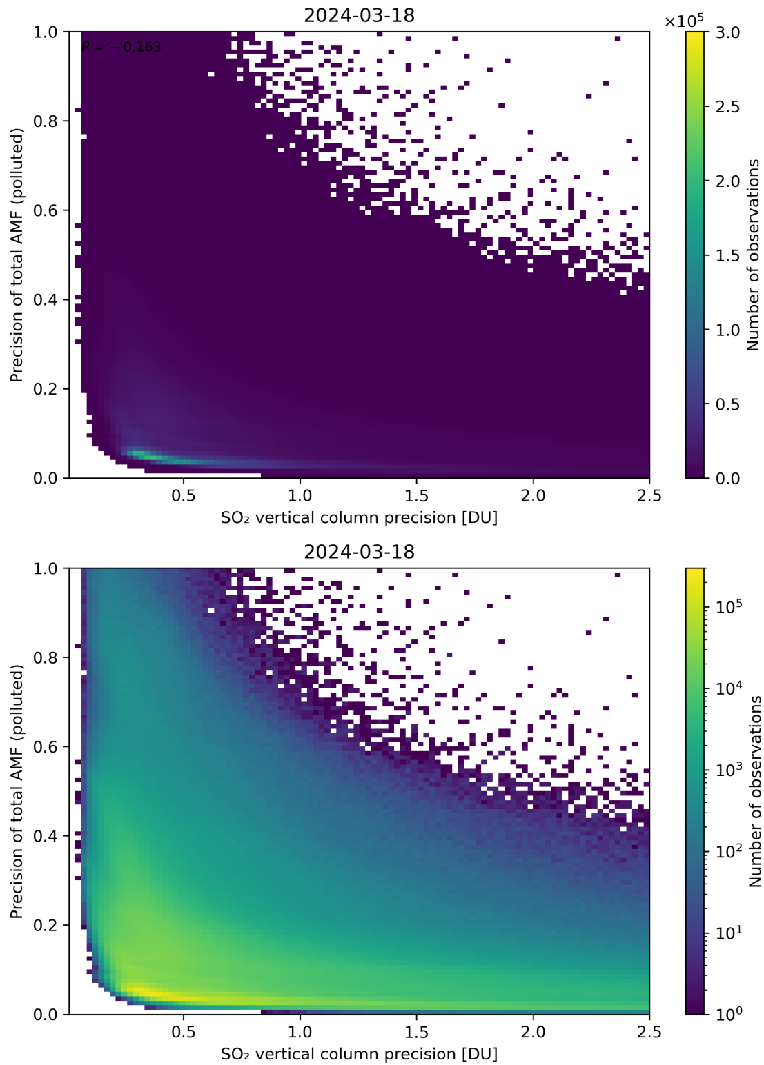
Figure 295: Scatter density plot of “SO 2 vertical column precision” against “Precision of total AMF (polluted)” for 2024-03-17 to 2024-03-19.
