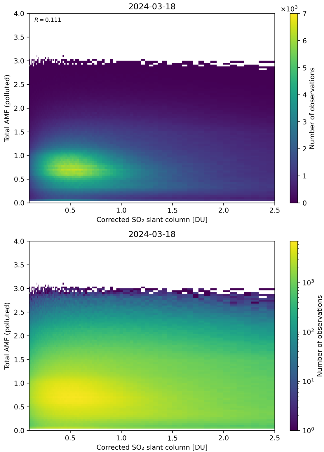
Figure 192: Scatter density plot of “Corrected SO 2 slant column” against “Total AMF (polluted)” for 2024-03-17 to 2024-03-19.
