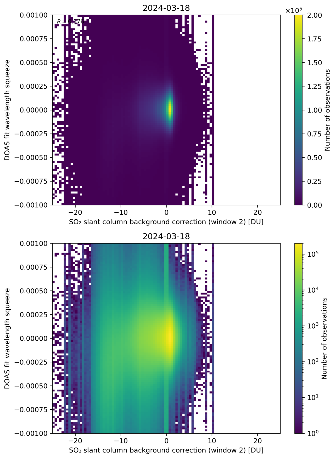
Figure 113: Scatter density plot of “SO 2 slant column background correction (window 2)” against “DOAS fit wavelength squeeze” for 2024-03-17 to 2024-03-19.
