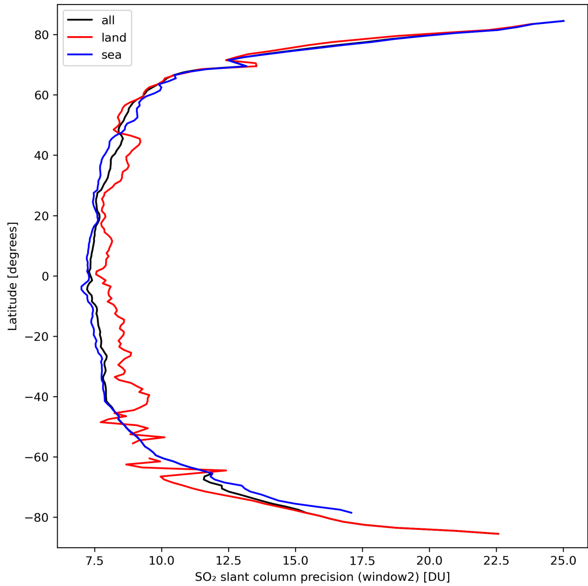
Figure 38: Zonal average of “SO 2 slant column precision (window2)” for 2024-03-17 to 2024-03-19.
