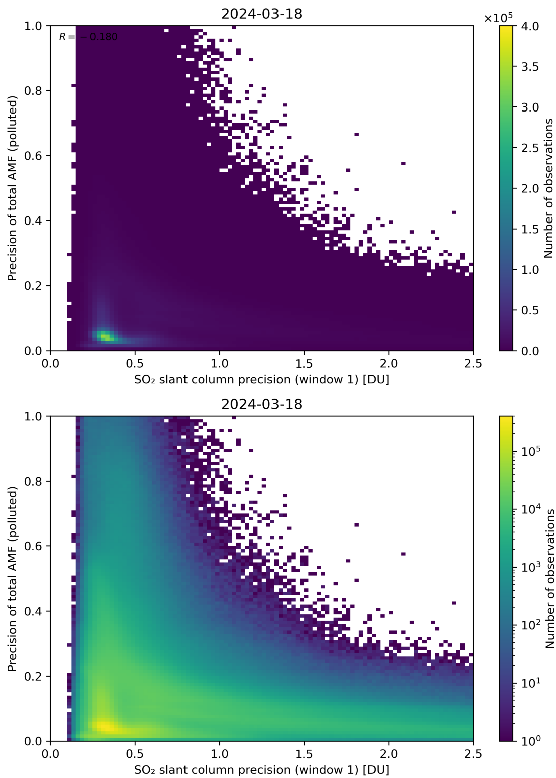
Figure 231: Scatter density plot of “SO 2 slant column precision (window 1)” against “Precision of total AMF (polluted)” for 2024-03-17 to 2024-03-19.
