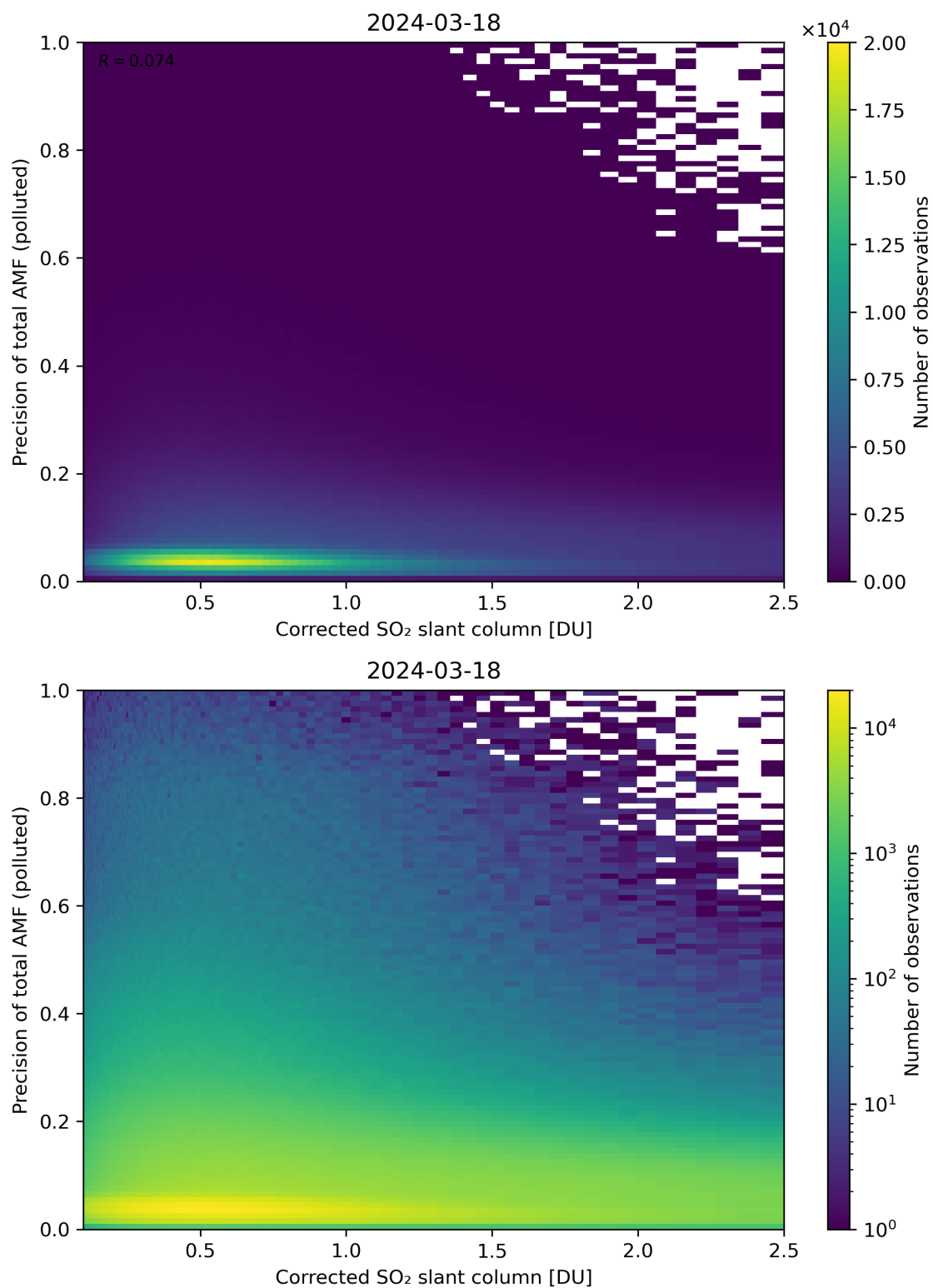
Figure 193: Scatter density plot of “Corrected SO 2 slant column” against “Precision of total AMF (polluted)” for 2024-03-17 to 2024-03-19.
