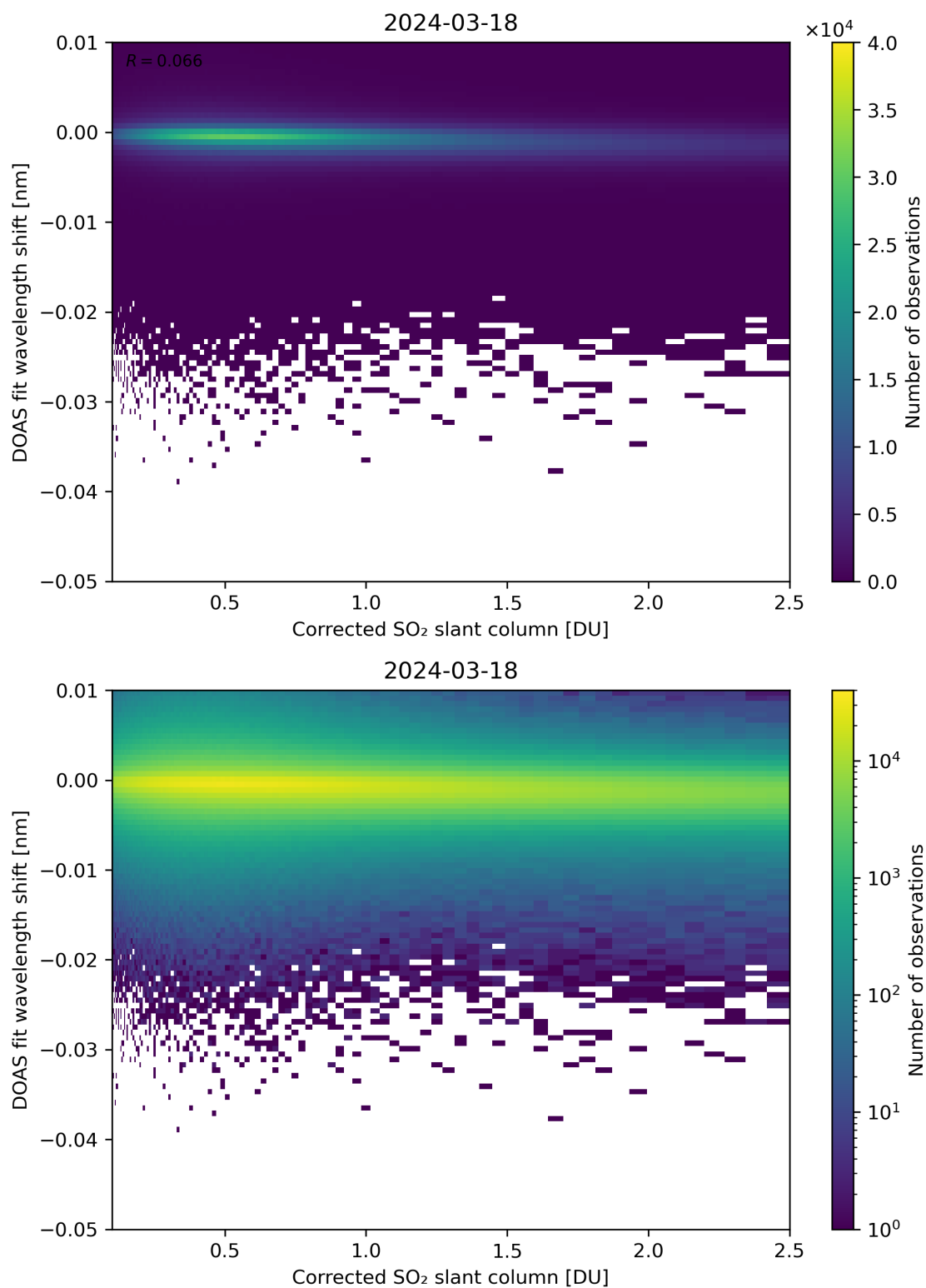
Figure 181: Scatter density plot of “Corrected SO 2 slant column” against “DOAS fit wavelength shift” for 2024-03-17 to 2024-03-19.
