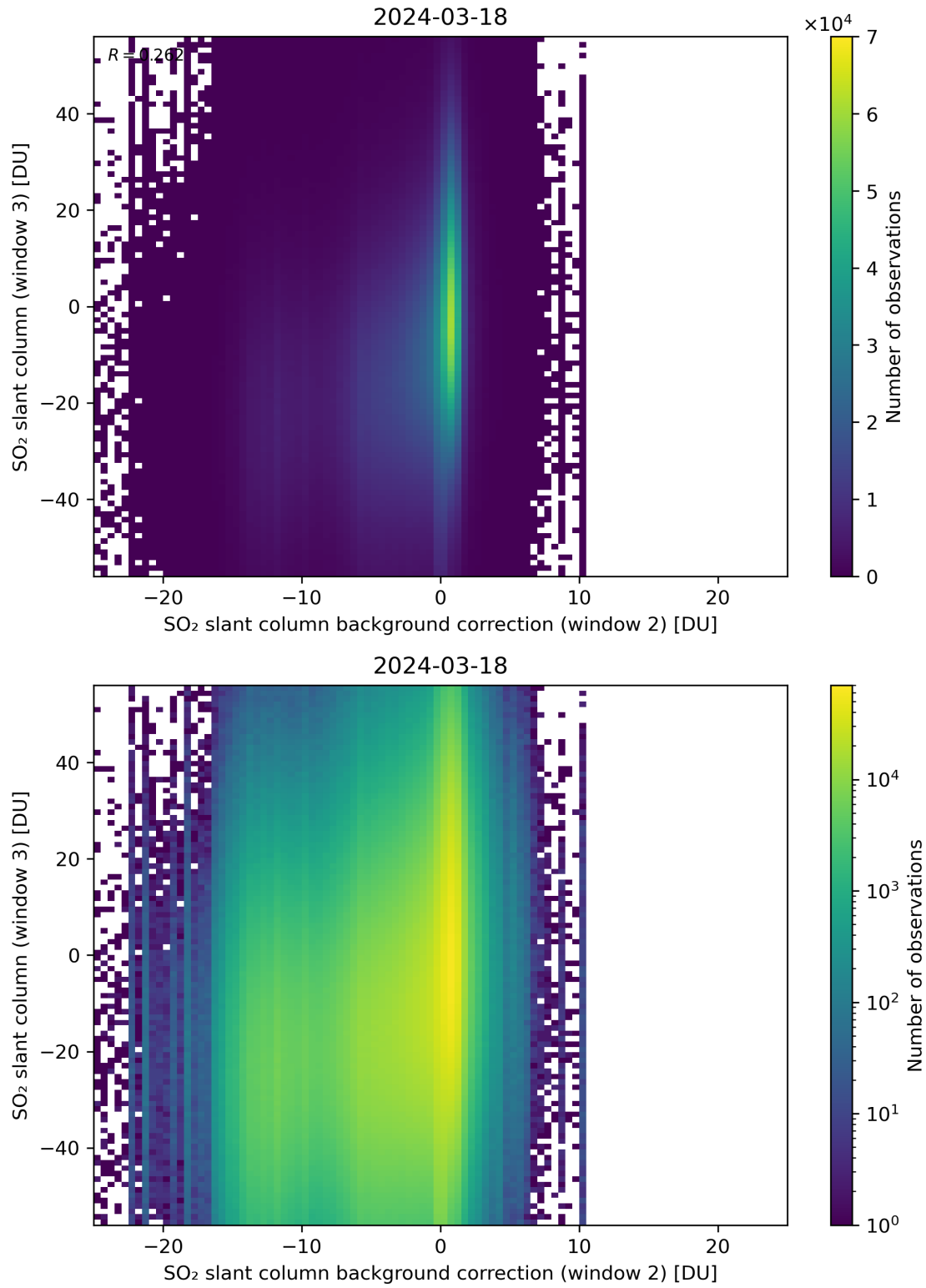
Figure 117: Scatter density plot of “SO 2 slant column background correction (window 2)” against “SO 2 slant column (window 3)” for 2024-03-17 to 2024-03-19.
