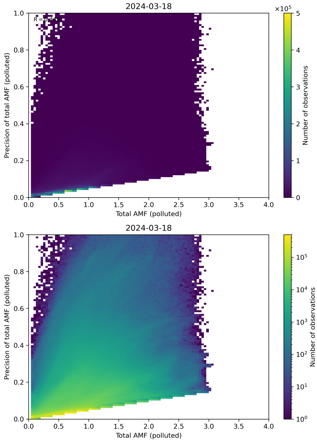
Figure 272: Scatter density plot of “Total AMF (polluted)” against “Precision of total AMF (polluted)” for 2024-03-17 to 2024-03-19.
