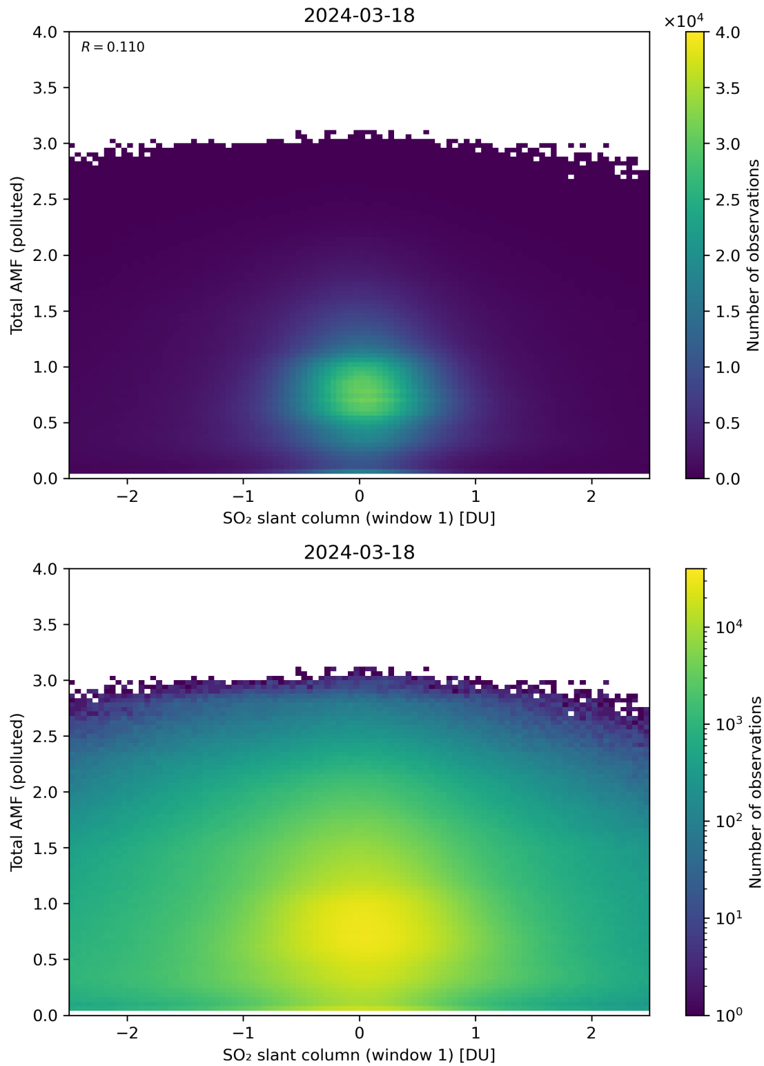
Figure 239: Scatter density plot of “SO 2 slant column (window 1)” against “Total AMF (polluted)” for 2024-03-17 to 2024-03-19.
