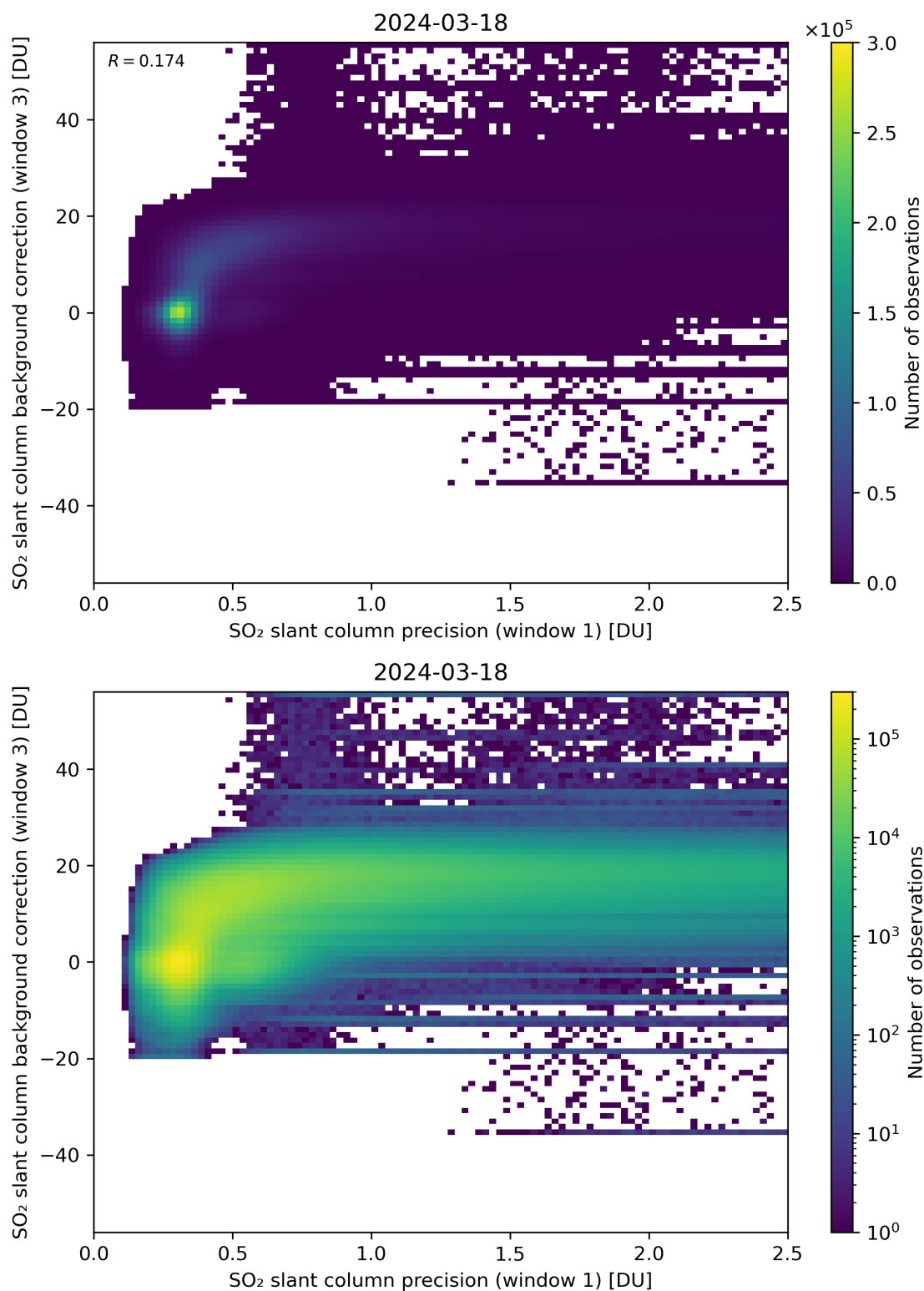
Figure 220: Scatter density plot of “SO 2 slant column precision (window 1)” against “SO 2 slant column background correction (window 3)” for 2024-03-17 to 2024-03-19.
