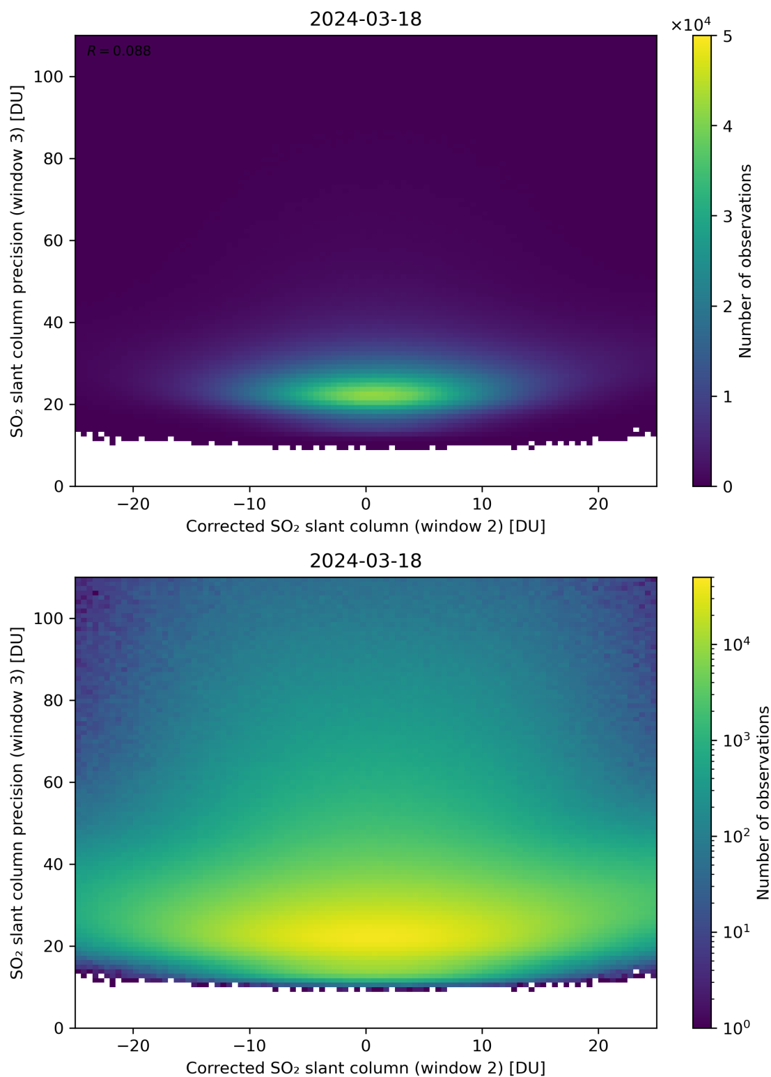
Figure 202: Scatter density plot of “Corrected SO 2 slant column (window 2)” against “SO 2 slant column precision (window 3)” for 2024-03-17 to 2024-03-19.
