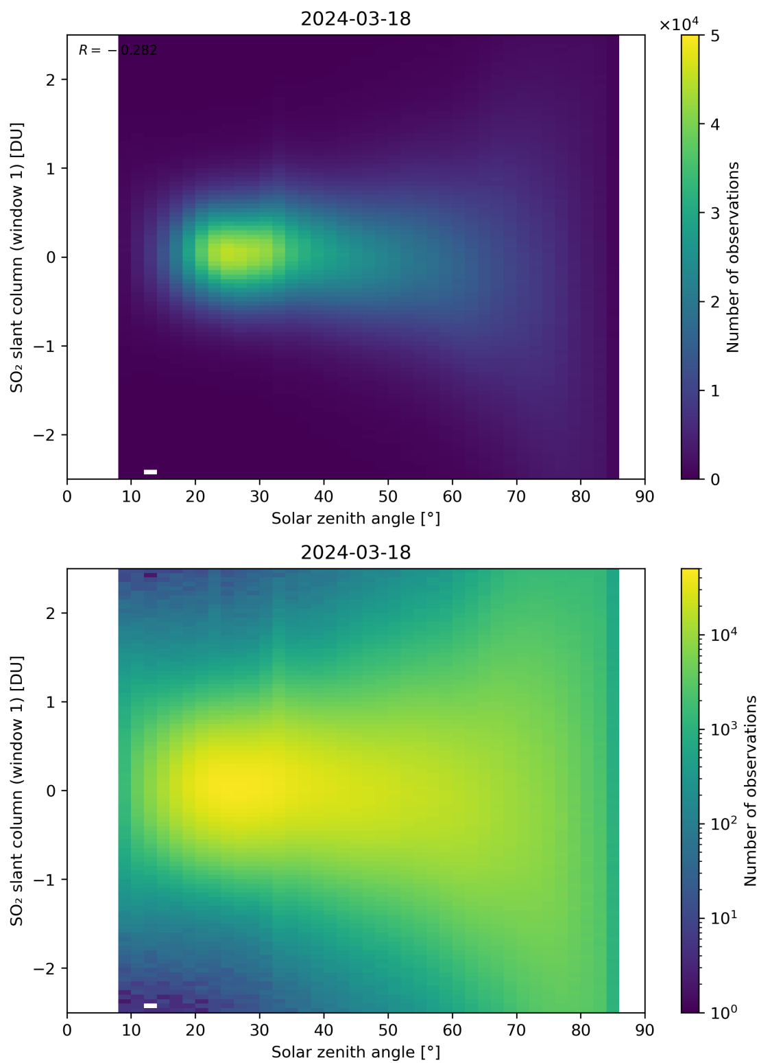
Figure 169: Scatter density plot of “Solar zenith angle” against “SO 2 slant column (window 1)” for 2024-03-17 to 2024-03-19.
