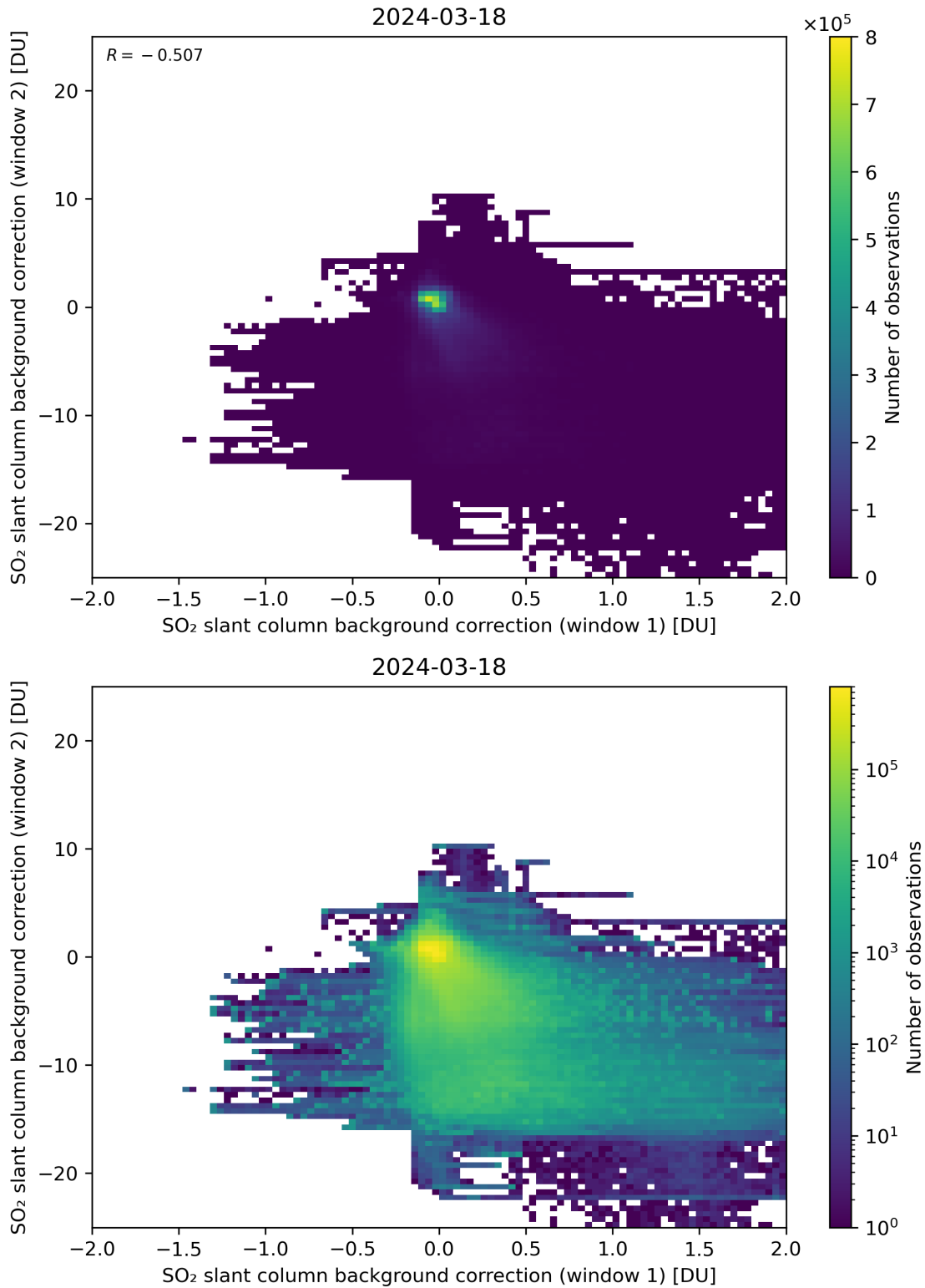
Figure 98: Scatter density plot of “SO 2 slant column background correction (window 1)” against “SO 2 slant column background correction (window 2)” for 2024-03-17 to 2024-03-19.
