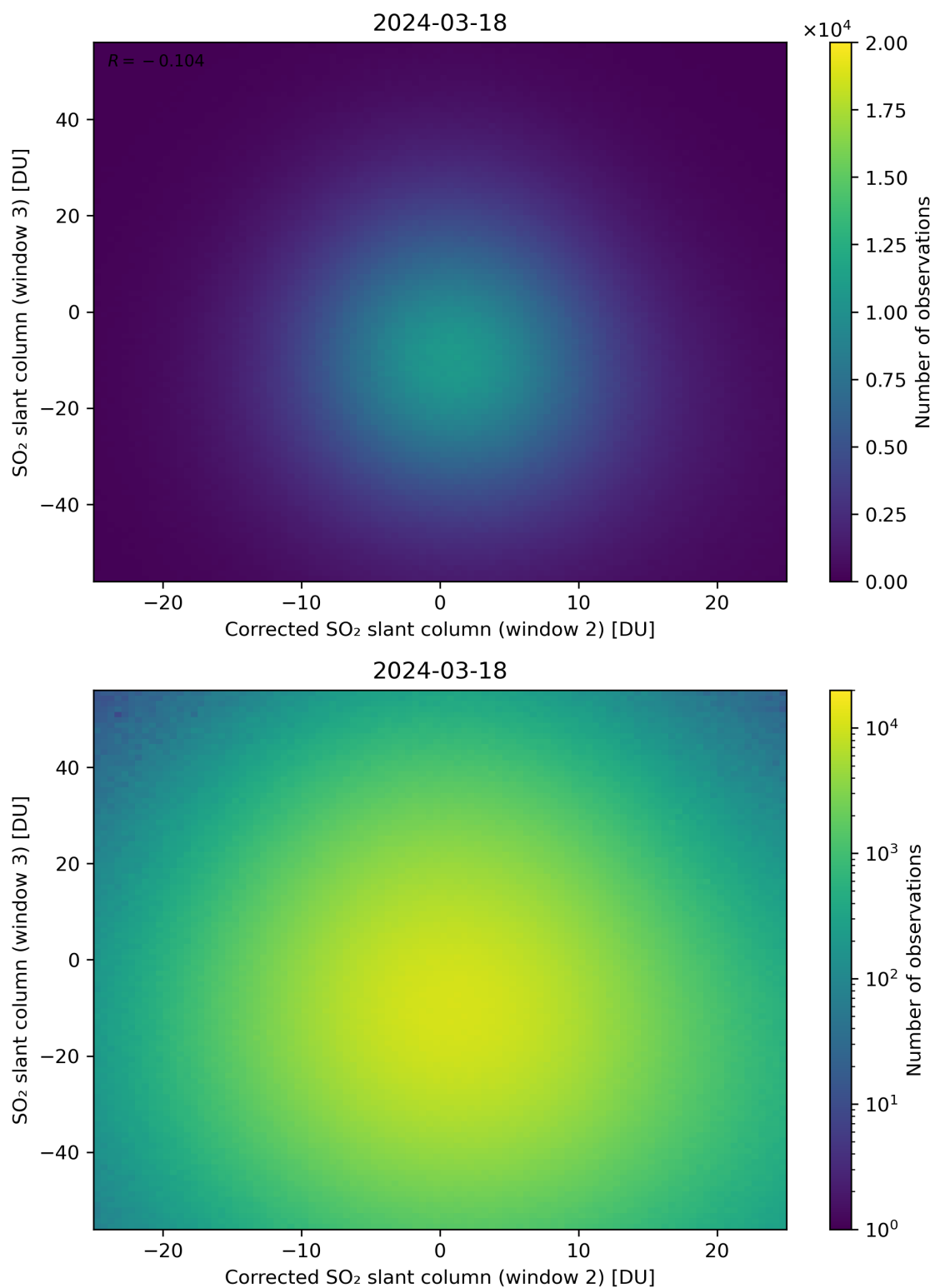
Figure 201: Scatter density plot of “Corrected SO 2 slant column (window 2)” against “SO 2 slant column (window 3)” for 2024-03-17 to 2024-03-19.
