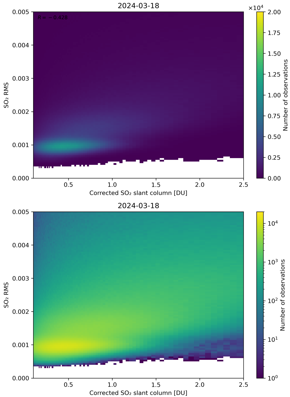
Figure 183: Scatter density plot of “Corrected SO 2 slant column” against “SO 2 RMS” for 2024-03-17 to 2024-03-19.
