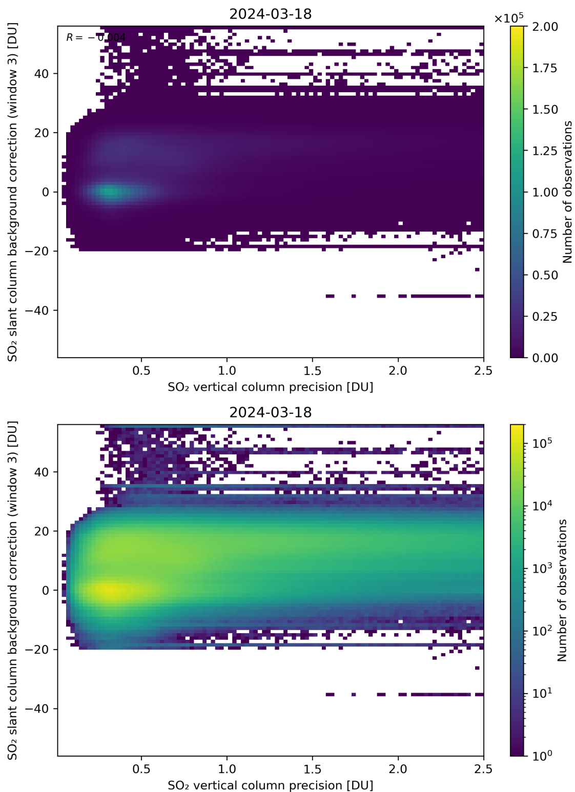
Figure 281: Scatter density plot of “SO 2 vertical column precision” against “SO 2 slant column background correction (window 3)” for 2024-03-17 to 2024-03-19.
