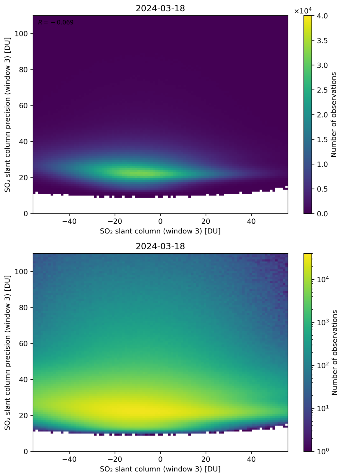
Figure 267: Scatter density plot of “SO 2 slant column (window 3)” against “SO 2 slant column precision (window 3)” for 2024-03-17 to 2024-03-19.
