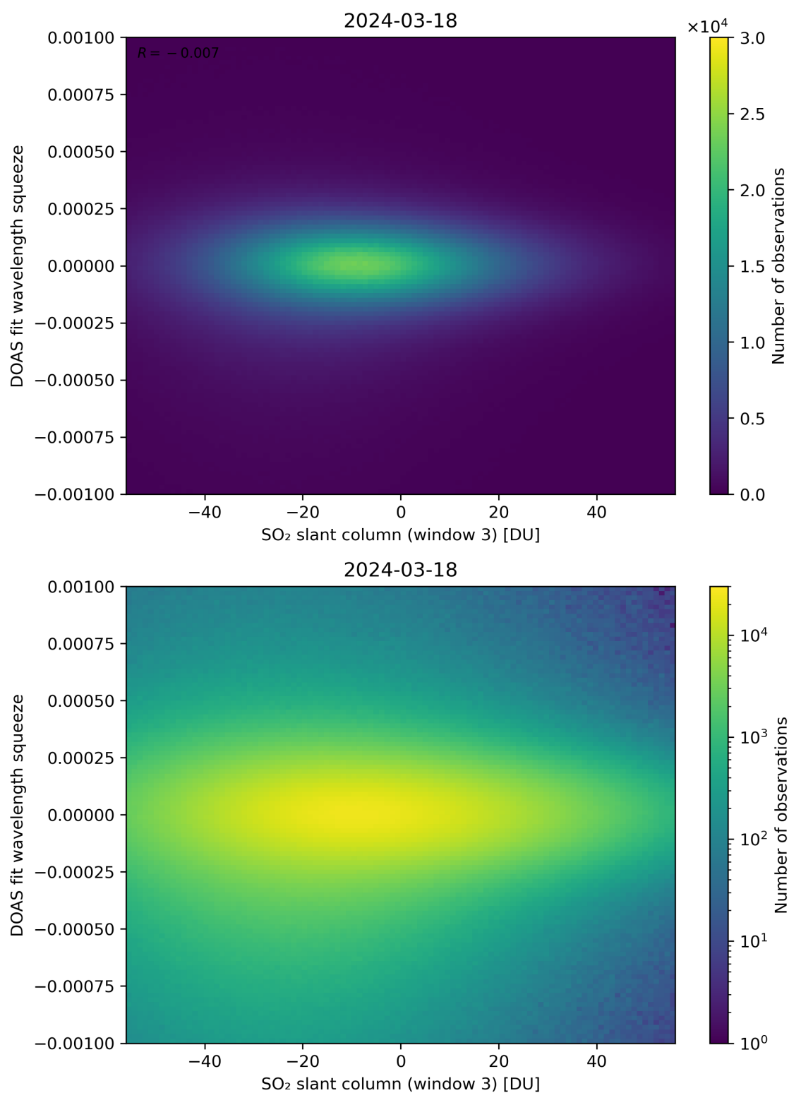
Figure 255: Scatter density plot of “SO 2 slant column (window 3)” against “DOAS fit wavelength squeeze” for 2024-03-17 to 2024-03-19.
