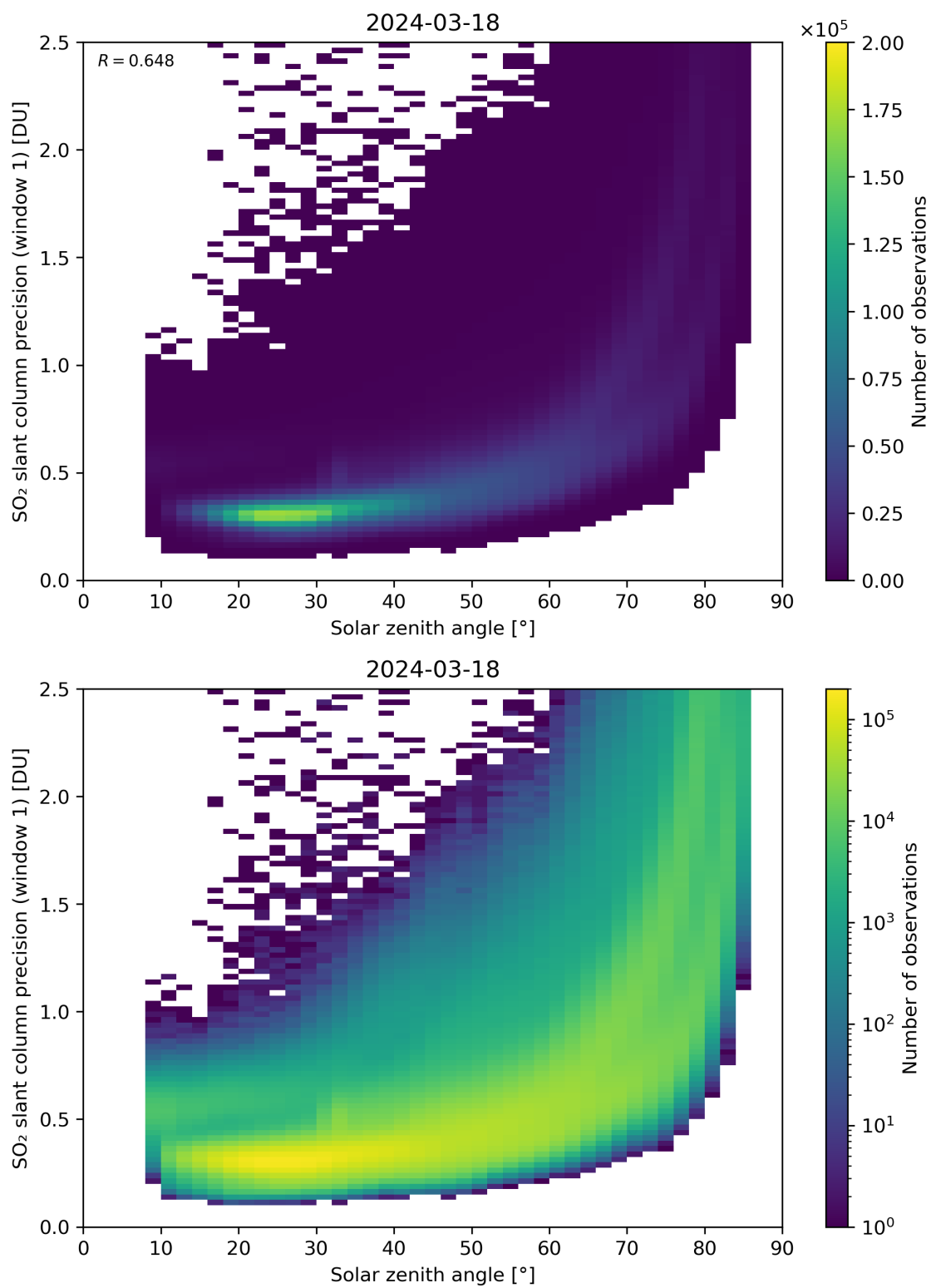
Figure 170: Scatter density plot of “Solar zenith angle” against “SO 2 slant column precision (window 1)” for 2024-03-17 to 2024-03-19.
