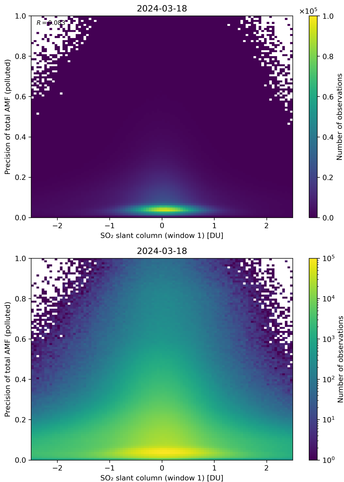
Figure 240: Scatter density plot of “SO 2 slant column (window 1)” against “Precision of total AMF (polluted)” for 2024-03-17 to 2024-03-19.
