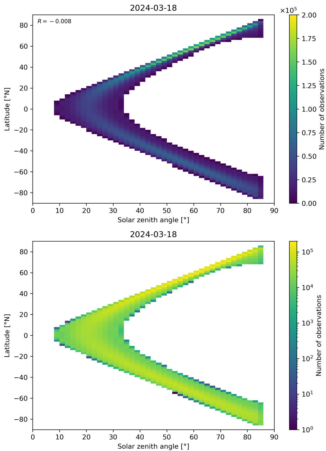
Figure 164: Scatter density plot of “Solar zenith angle” against “Latitude” for 2024-03-17 to 2024-03-19.
