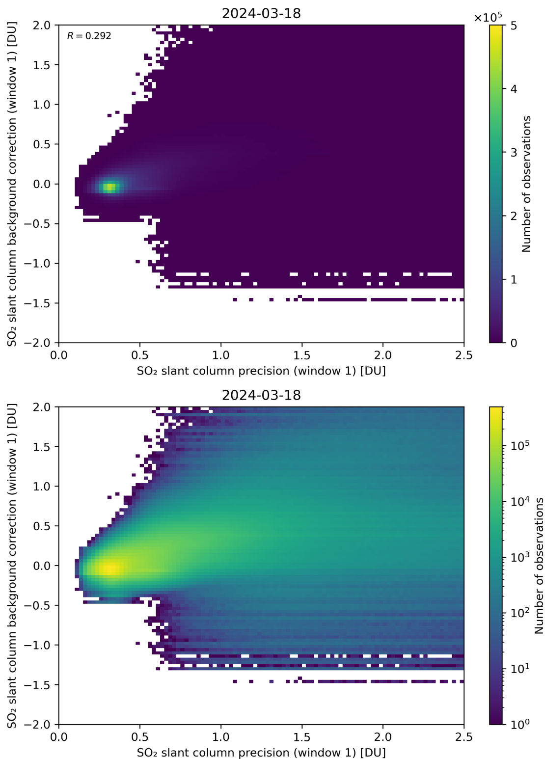
Figure 218: Scatter density plot of “SO 2 slant column precision (window 1)” against “SO 2 slant column background correction (window 1)” for 2024-03-17 to 2024-03-19.
