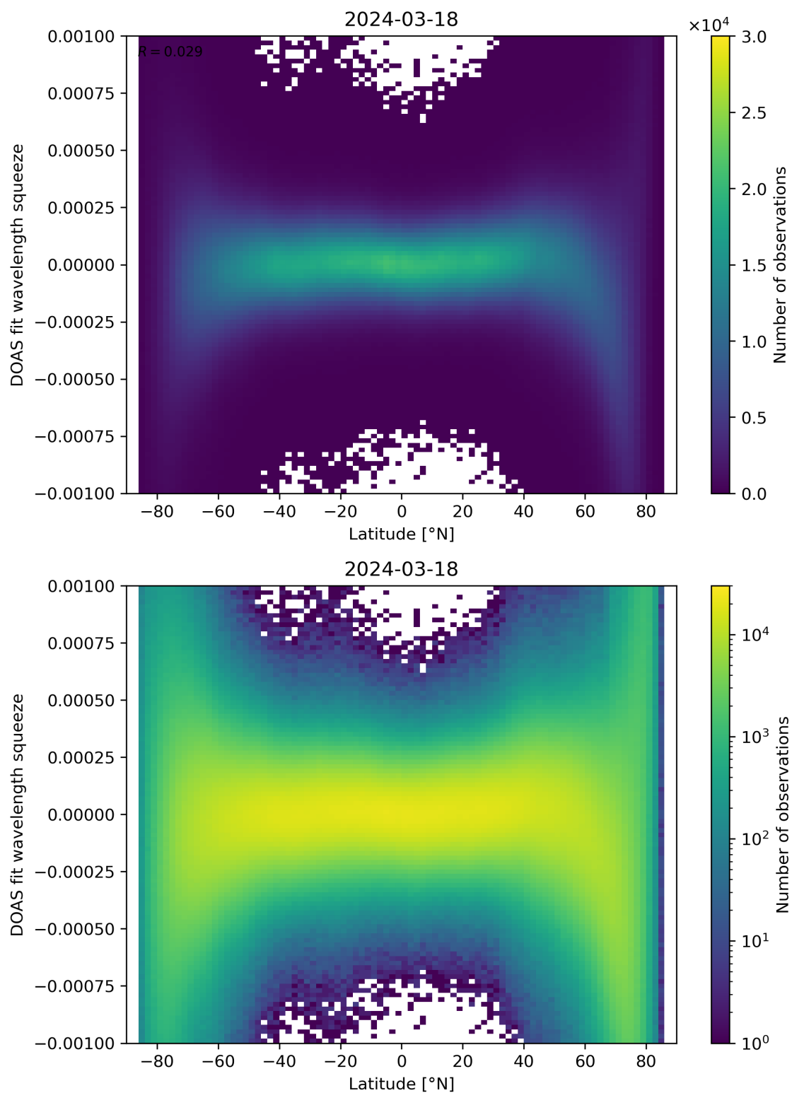
Figure 143: Scatter density plot of “Latitude” against “DOAS fit wavelength squeeze” for 2024-03-17 to 2024-03-19.
