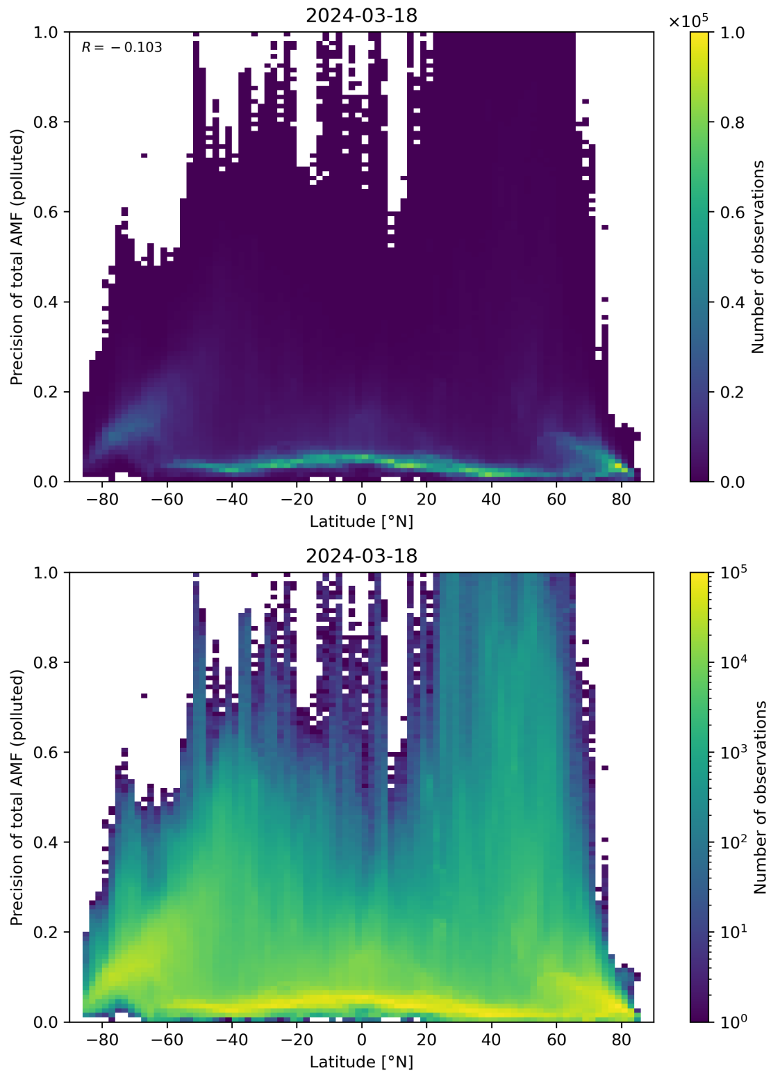
Figure 155: Scatter density plot of “Latitude” against “Precision of total AMF (polluted)” for 2024-03-17 to 2024-03-19.
