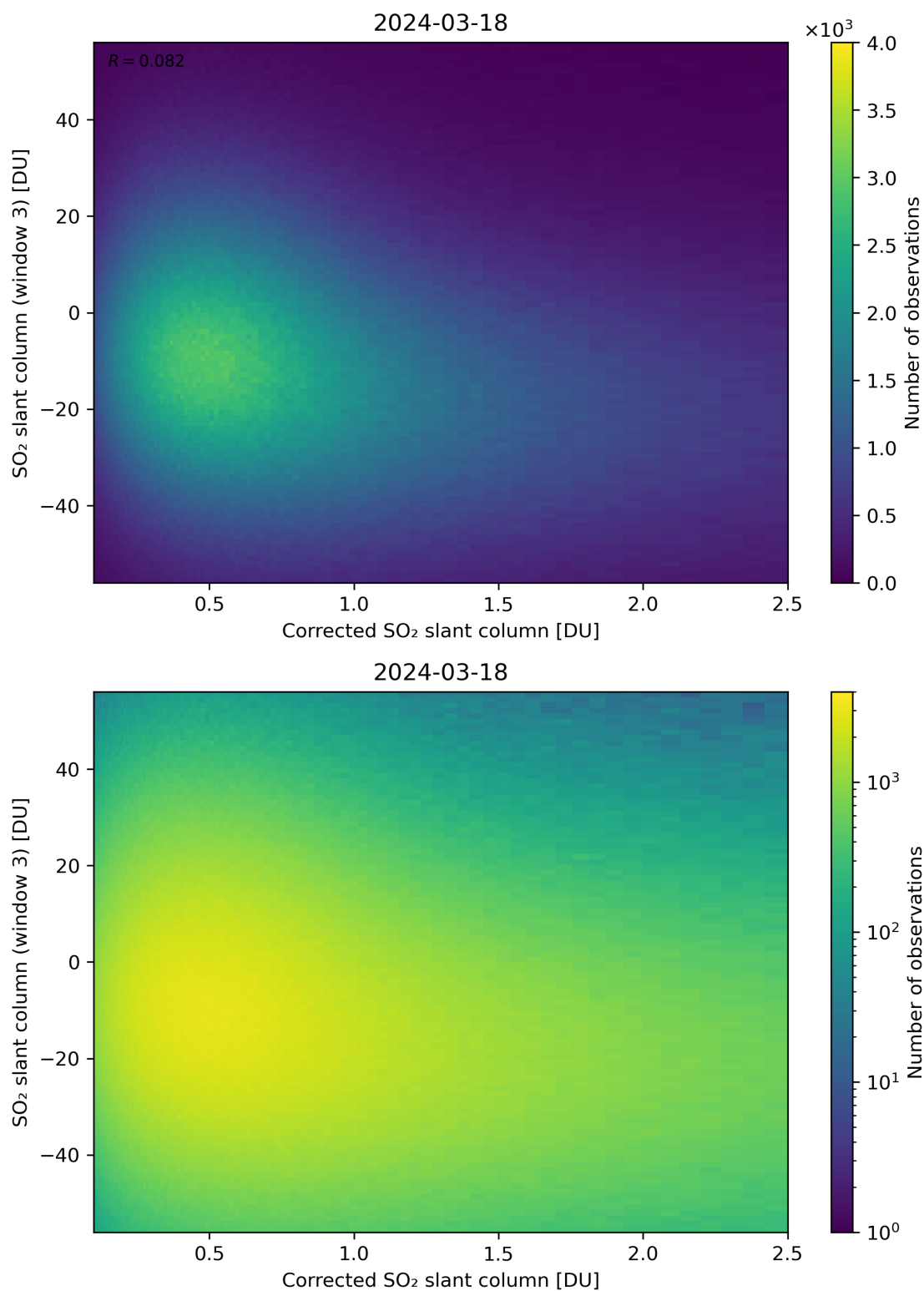
Figure 190: Scatter density plot of “Corrected SO 2 slant column” against “SO 2 slant column (window 3)” for 2024-03-17 to 2024-03-19.
