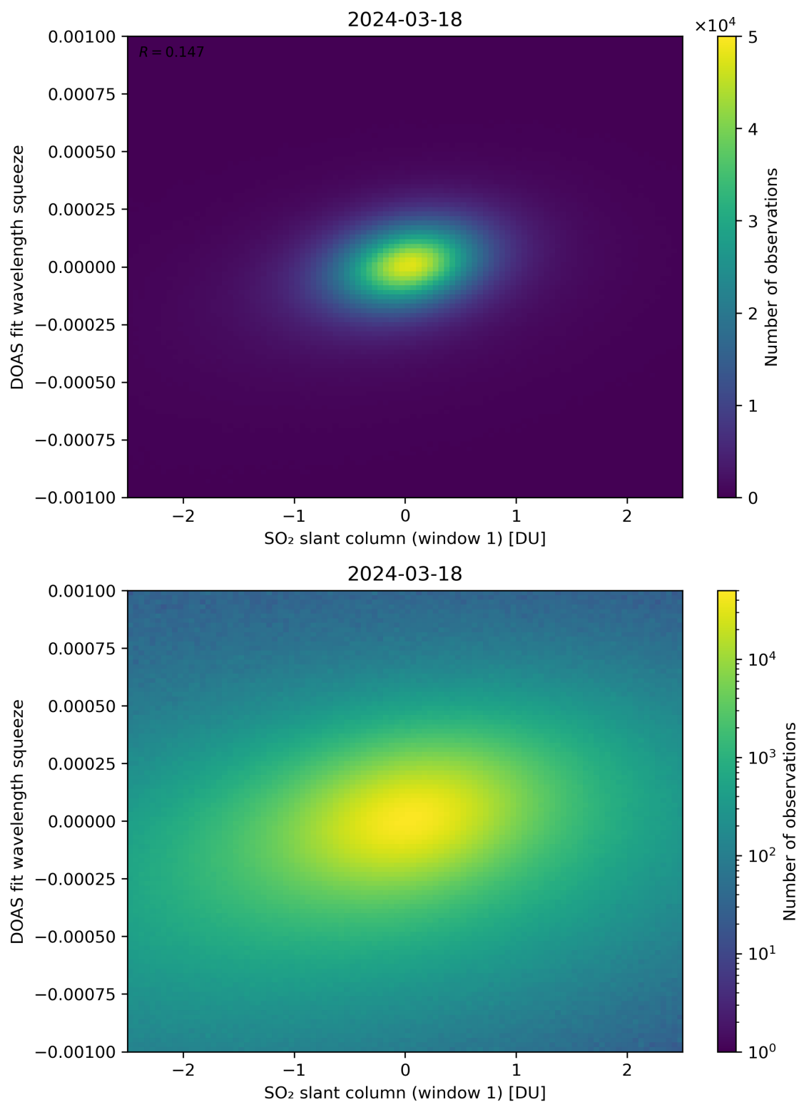
Figure 216: Scatter density plot of “SO 2 slant column (window 1)” against “DOAS fit wavelength squeeze” for 2024-03-17 to 2024-03-19.
