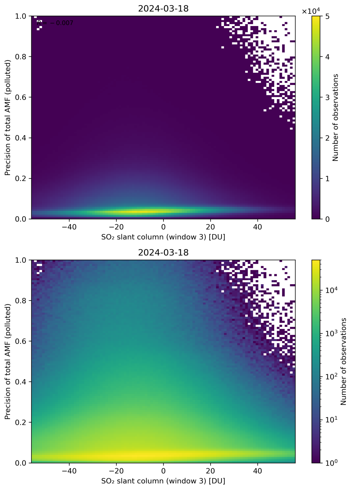
Figure 269: Scatter density plot of “SO 2 slant column (window 3)” against “Precision of total AMF (polluted)” for 2024-03-17 to 2024-03-19.
