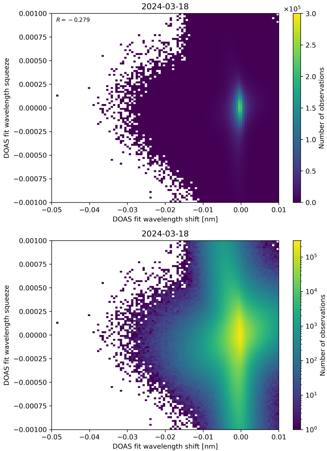
Figure 127: Scatter density plot of “DOAS fit wavelength shift” against “DOAS fit wavelength squeeze” for 2024-03-17 to 2024-03-19.
