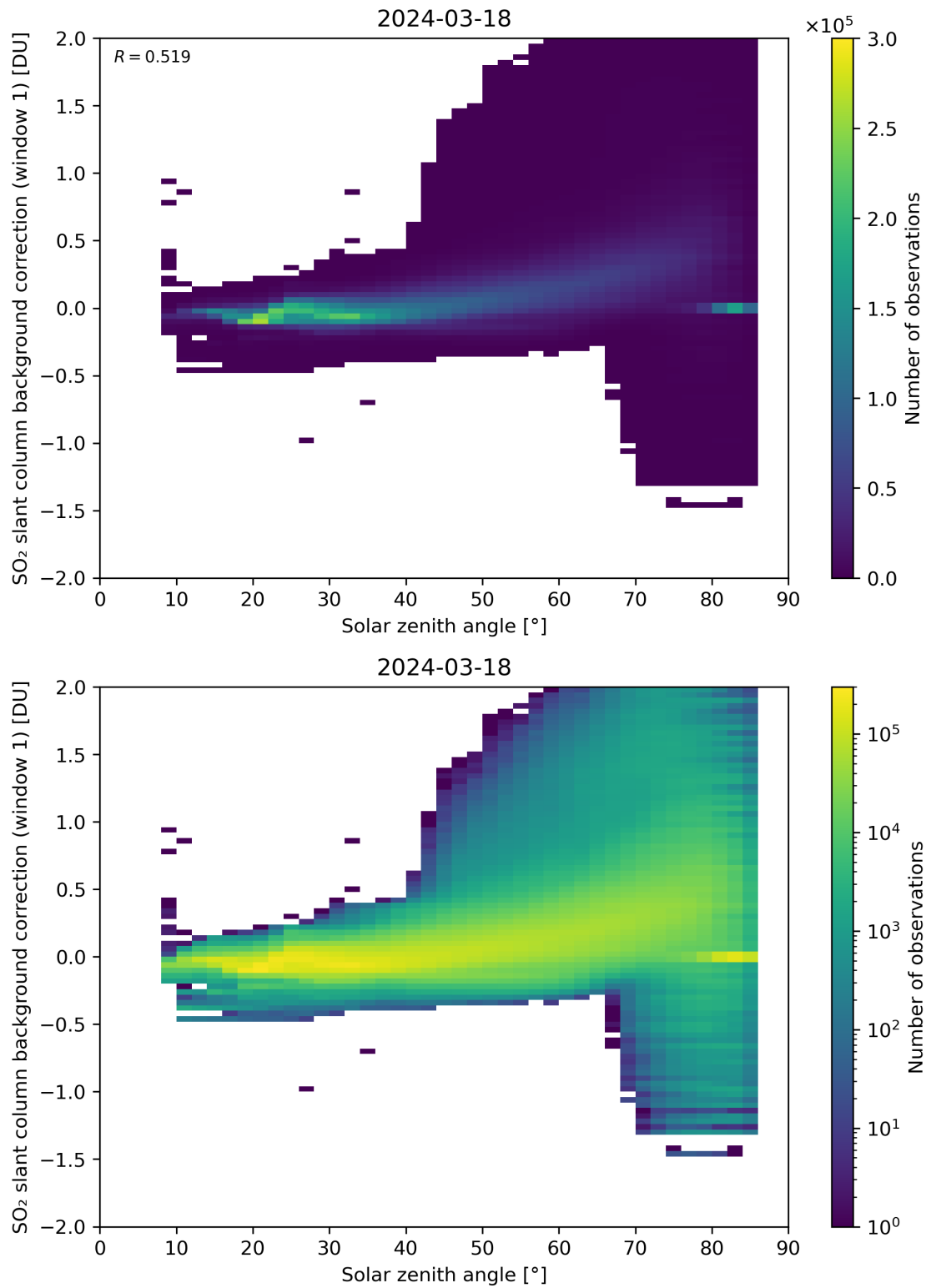
Figure 158: Scatter density plot of “Solar zenith angle” against “SO 2 slant column background correction (window 1)” for 2024-03-17 to 2024-03-19.
