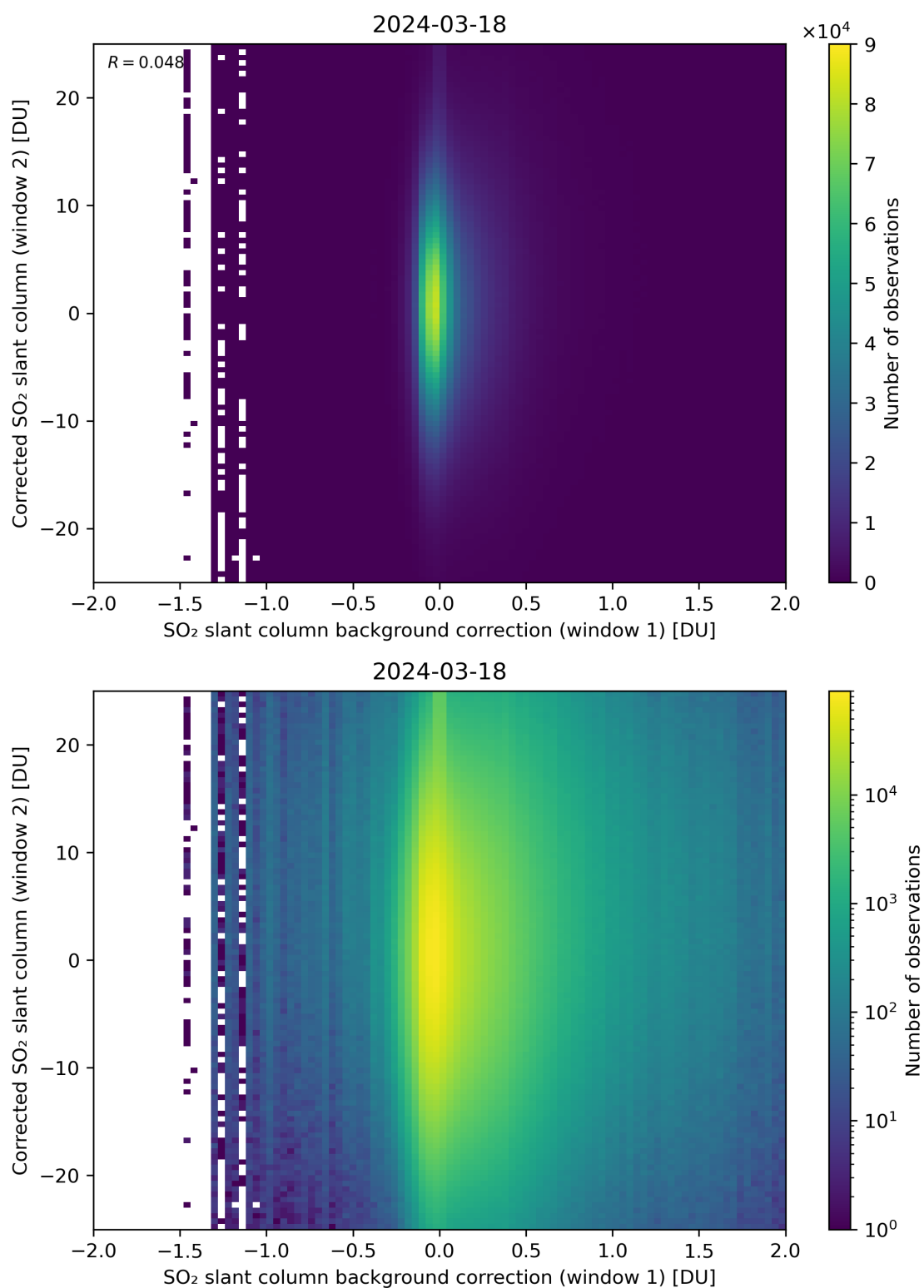
Figure 104: Scatter density plot of “SO 2 slant column background correction (window 1)” against “Corrected SO 2 slant column (window 2)” for 2024-03-17 to 2024-03-19.
