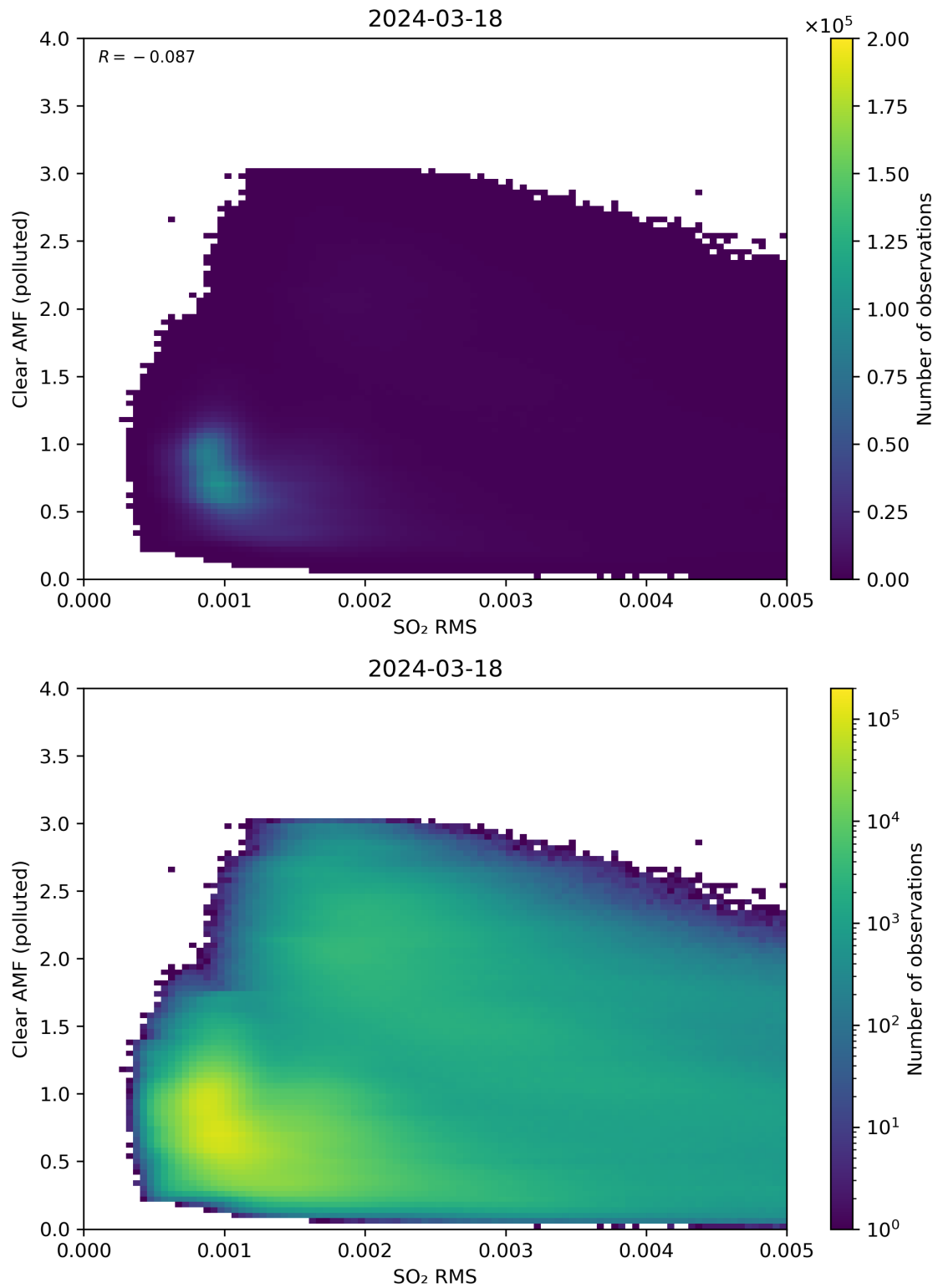
Figure 136: Scatter density plot of “SO 2 RMS” against “Clear AMF (polluted)” for 2024-03-17 to 2024-03-19.
