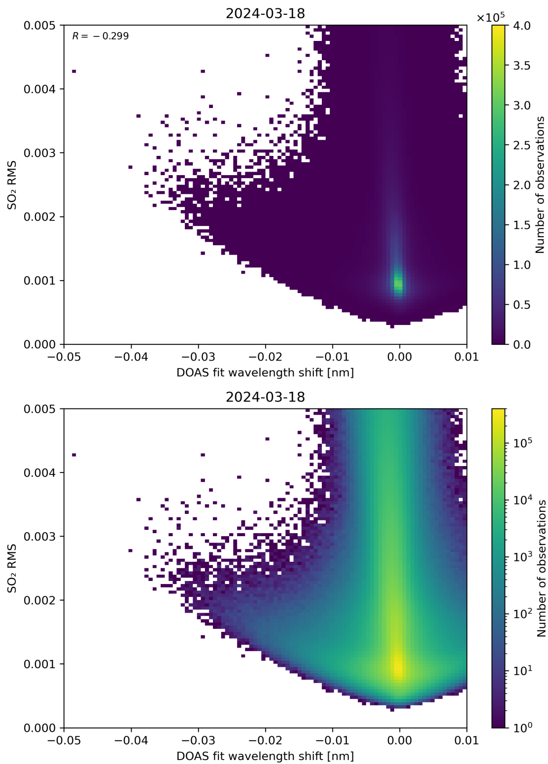
Figure 128: Scatter density plot of “DOAS fit wavelength shift” against “SO 2 RMS” for 2024-03-17 to 2024-03-19.
