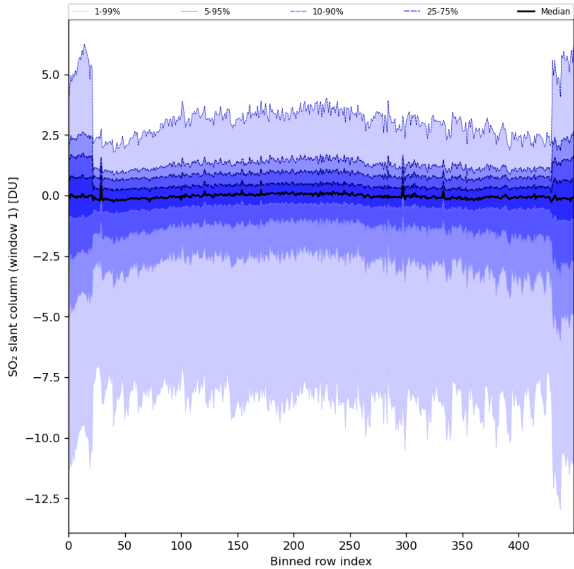
Figure 79: Along track statistics of "SO 2 slant column (window 1)" for 2024-03-17 to 2024-03-19
