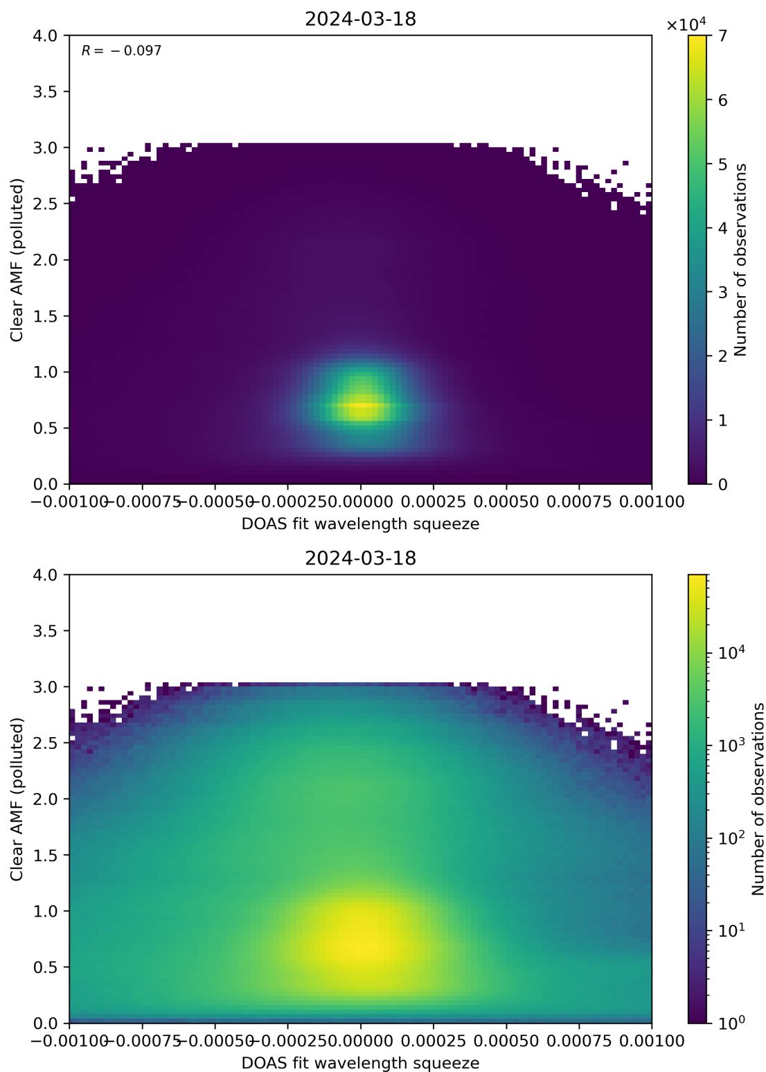
Figure 133: Scatter density plot of “DOAS fit wavelength squeeze” against “Clear AMF (polluted)” for 2024-03-17 to 2024-03-19.
