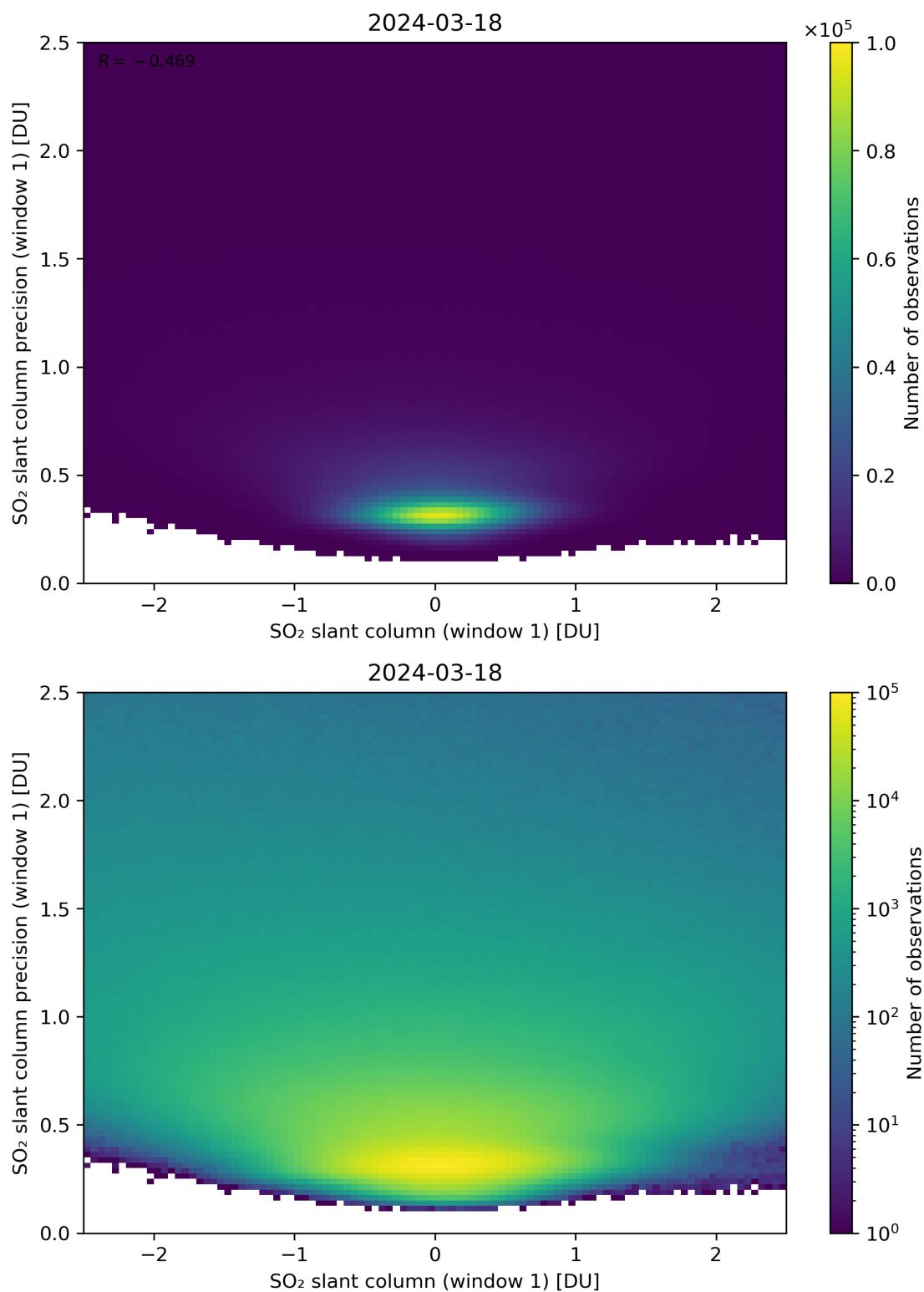
Figure 235: Scatter density plot of “SO 2 slant column (window 1)” against “SO 2 slant column precision (window 1)” for 2024-03-17 to 2024-03-19.
