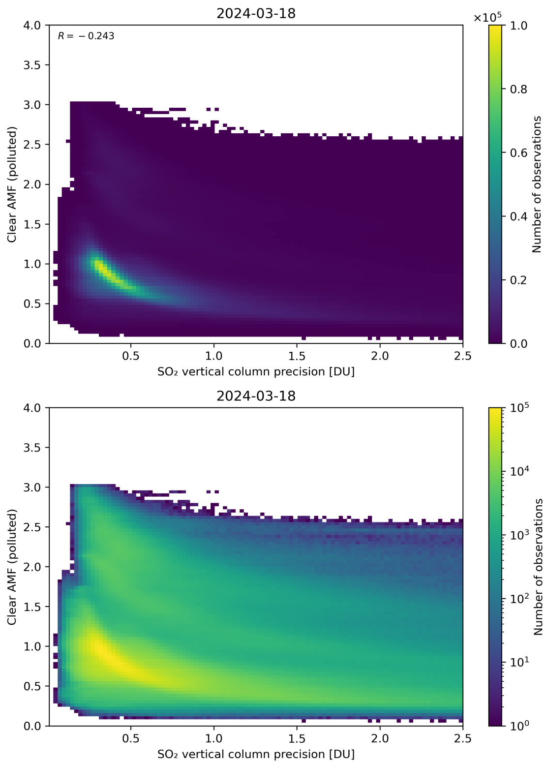
Figure 285: Scatter density plot of “SO 2 vertical column precision” against “Clear AMF (polluted)” for 2024-03-17 to 2024-03-19.
