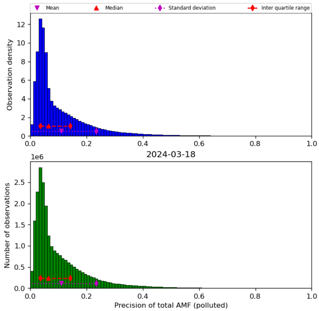
Figure 72: Histogram of “Precision of total AMF (polluted)” for 2024-03-17 to 2024-03-19
