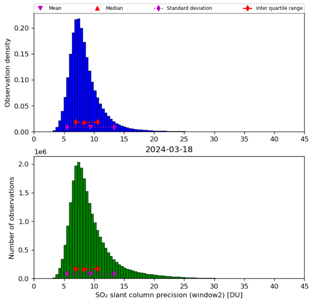
Figure 61: Histogram of “SO 2 slant column precision (window2)” for 2024-03-17 to 2024-03-19
