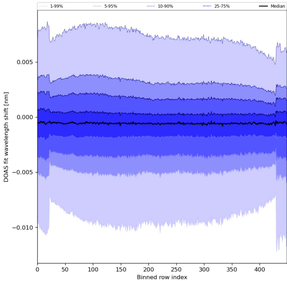
Figure 91: Along track statistics of “DOAS fit wavelength shift” for 2024-03-17 to 2024-03-19
