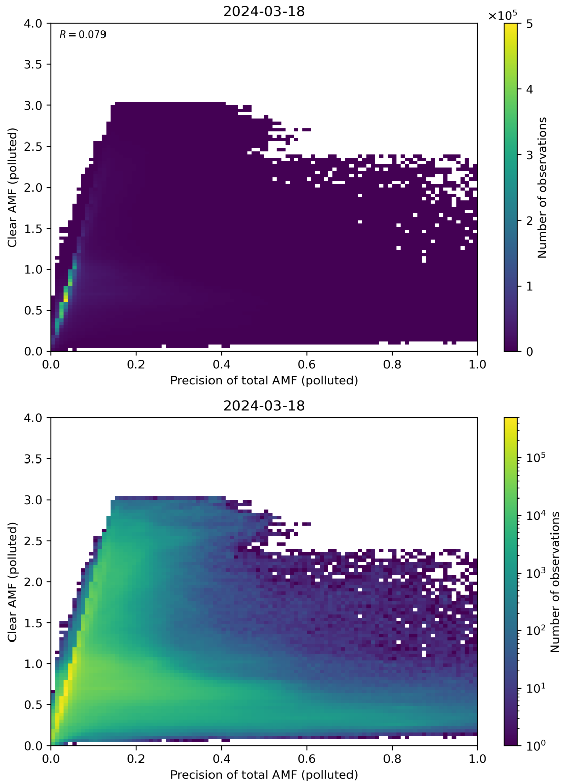
Figure 270: Scatter density plot of “Precision of total AMF (polluted)” against “Clear AMF (polluted)” for 2024-03-17 to 2024-03-19.
