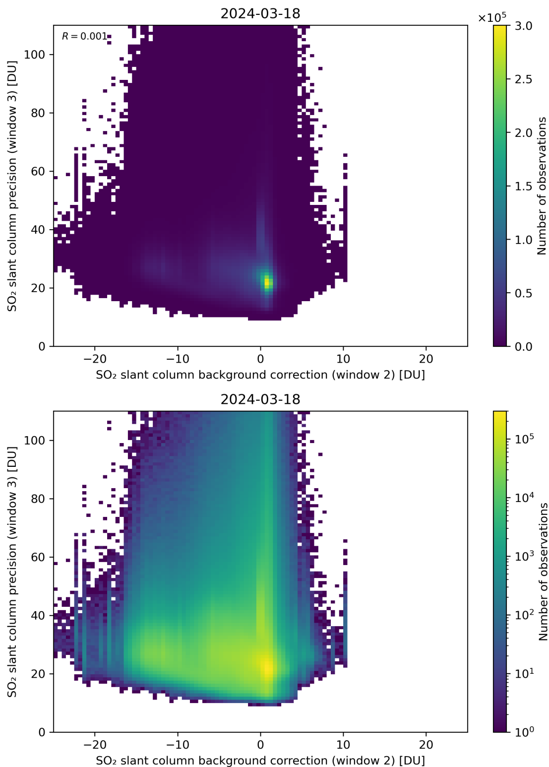
Figure 118: Scatter density plot of “SO 2 slant column background correction (window 2)” against “SO 2 slant column precision (window 3)” for 2024-03-17 to 2024-03-19.
