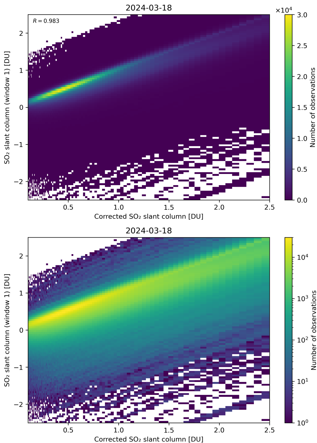
Figure 187: Scatter density plot of “Corrected SO 2 slant column” against “SO 2 slant column (window 1)” for 2024-03-17 to 2024-03-19.
