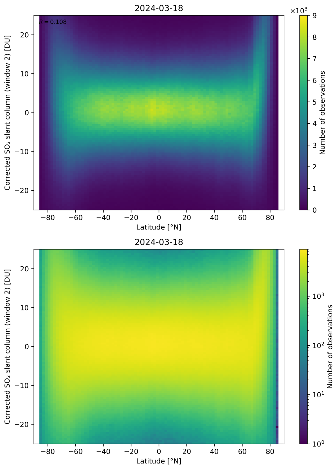
Figure 147: Scatter density plot of “Latitude” against “Corrected SO 2 slant column (window 2)” for 2024-03-17 to 2024-03-19.
