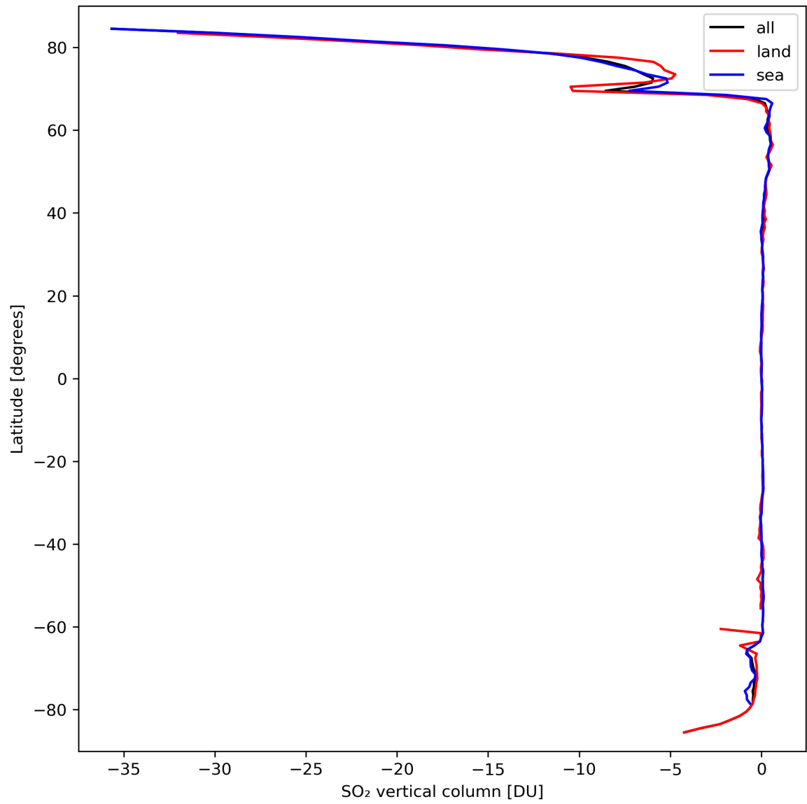
Figure 30: Zonal average of “SO 2 vertical column” for 2024-03-17 to 2024-03-19.
