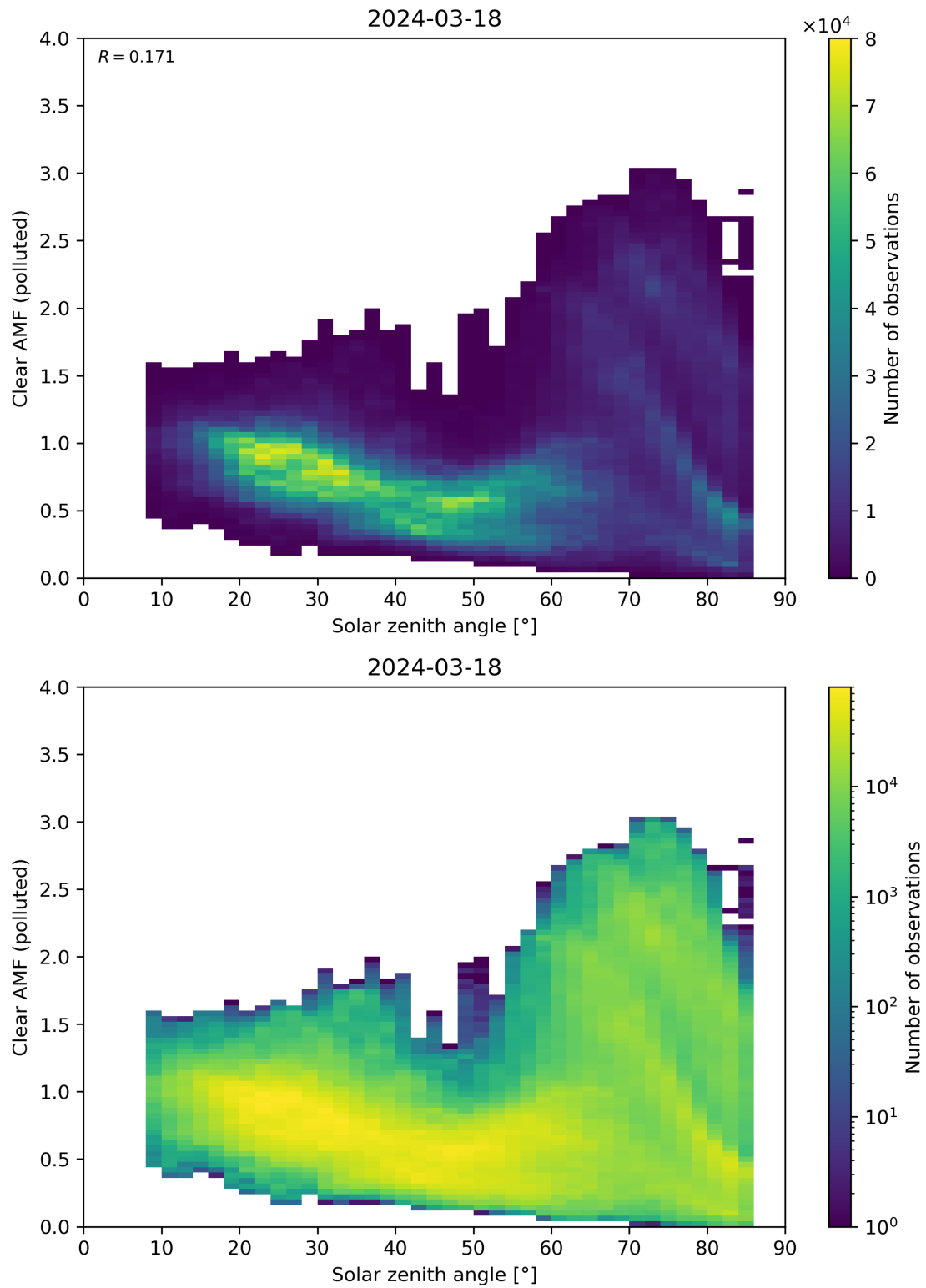
Figure 165: Scatter density plot of “Solar zenith angle” against “Clear AMF (polluted)” for 2024-03-17 to 2024-03-19.
