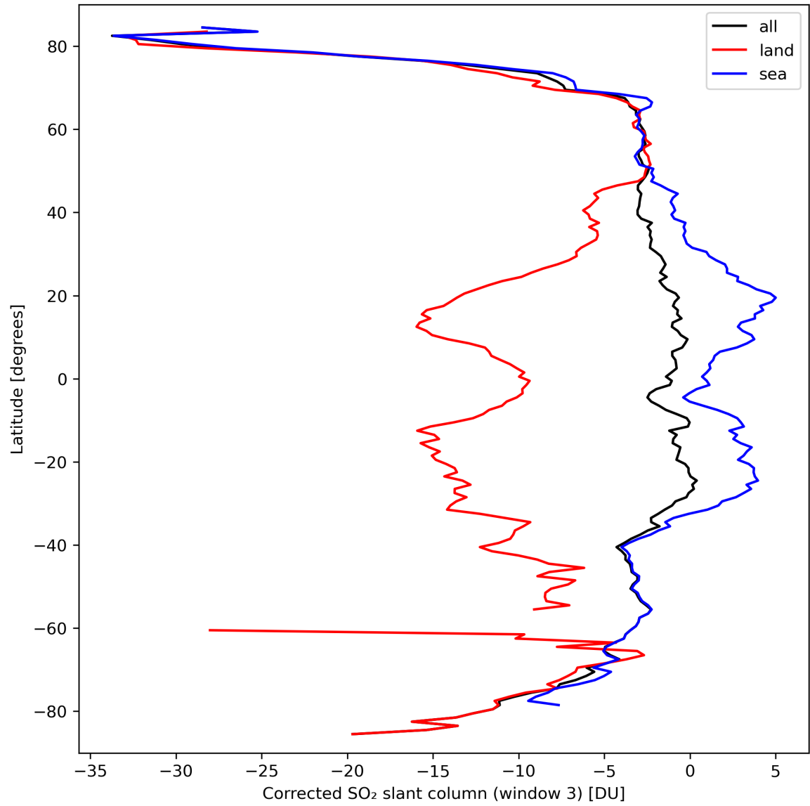
Figure 43: Zonal average of “Corrected SO 2 slant column (window 3)” for 2024-03-17 to 2024-03-19.
