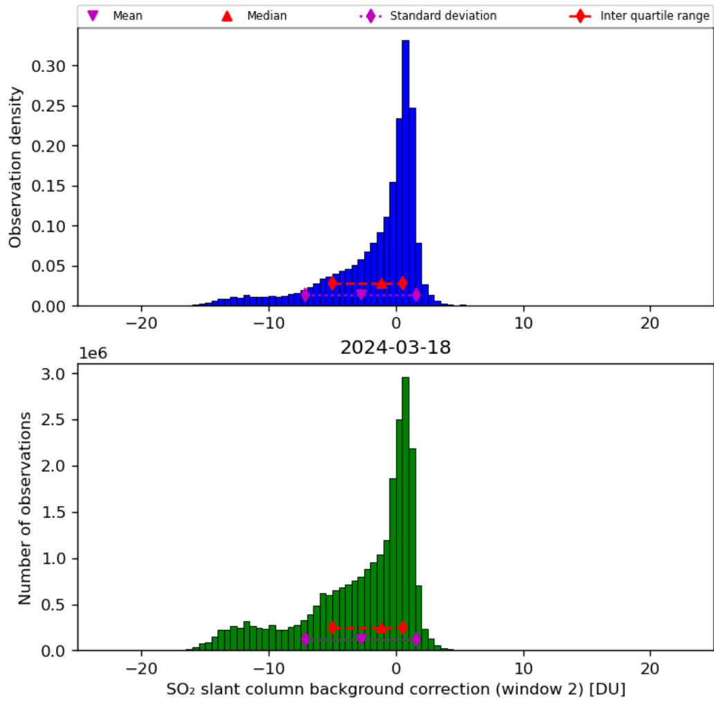
Figure 63: Histogram of “SO 2 slant column background correction (window 2)” for 2024-03-17 to 2024-03-19
