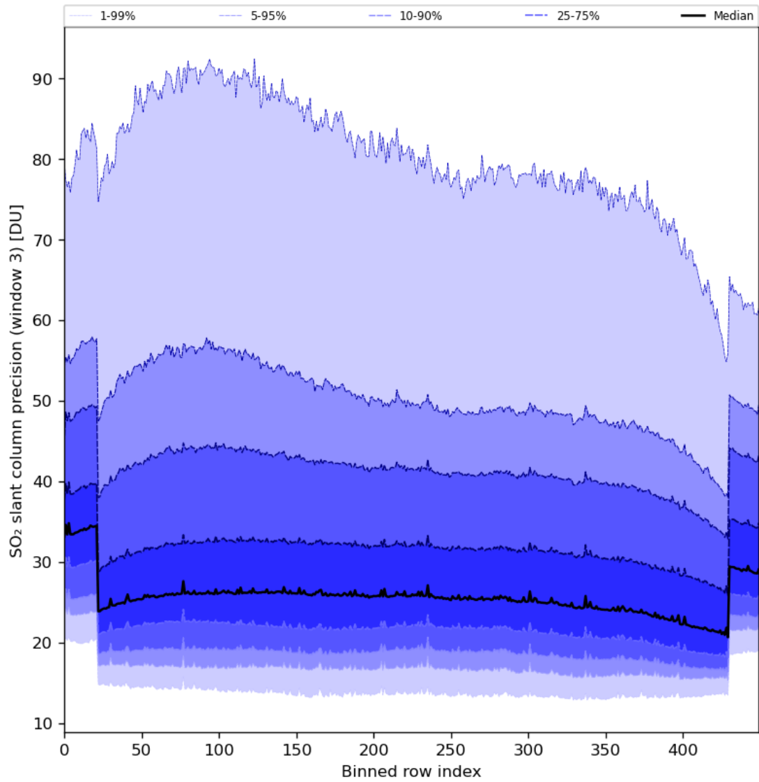
Figure 88: Along track statistics of “SO 2 slant column precision (window 3)” for 2024-03-17 to 2024-03-19
