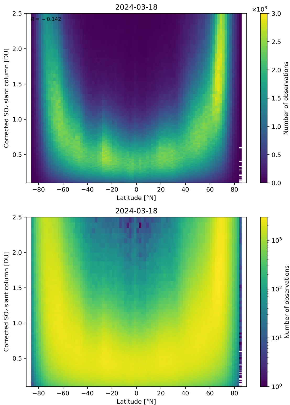
Figure 146: Scatter density plot of “Latitude” against “Corrected SO 2 slant column” for 2024-03-17 to 2024-03-19.
