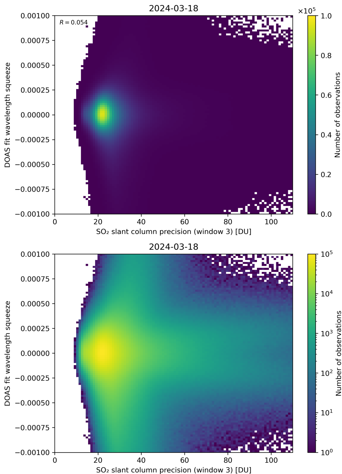
Figure 259: Scatter density plot of “SO 2 slant column precision (window 3)” against “DOAS fit wavelength squeeze” for 2024-03-17 to 2024-03-19.
