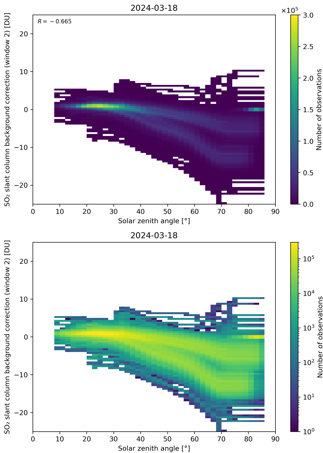
Figure 159: Scatter density plot of “Solar zenith angle” against “SO 2 slant column background correction (window 2)” for 2024-03-17 to 2024-03-19.
