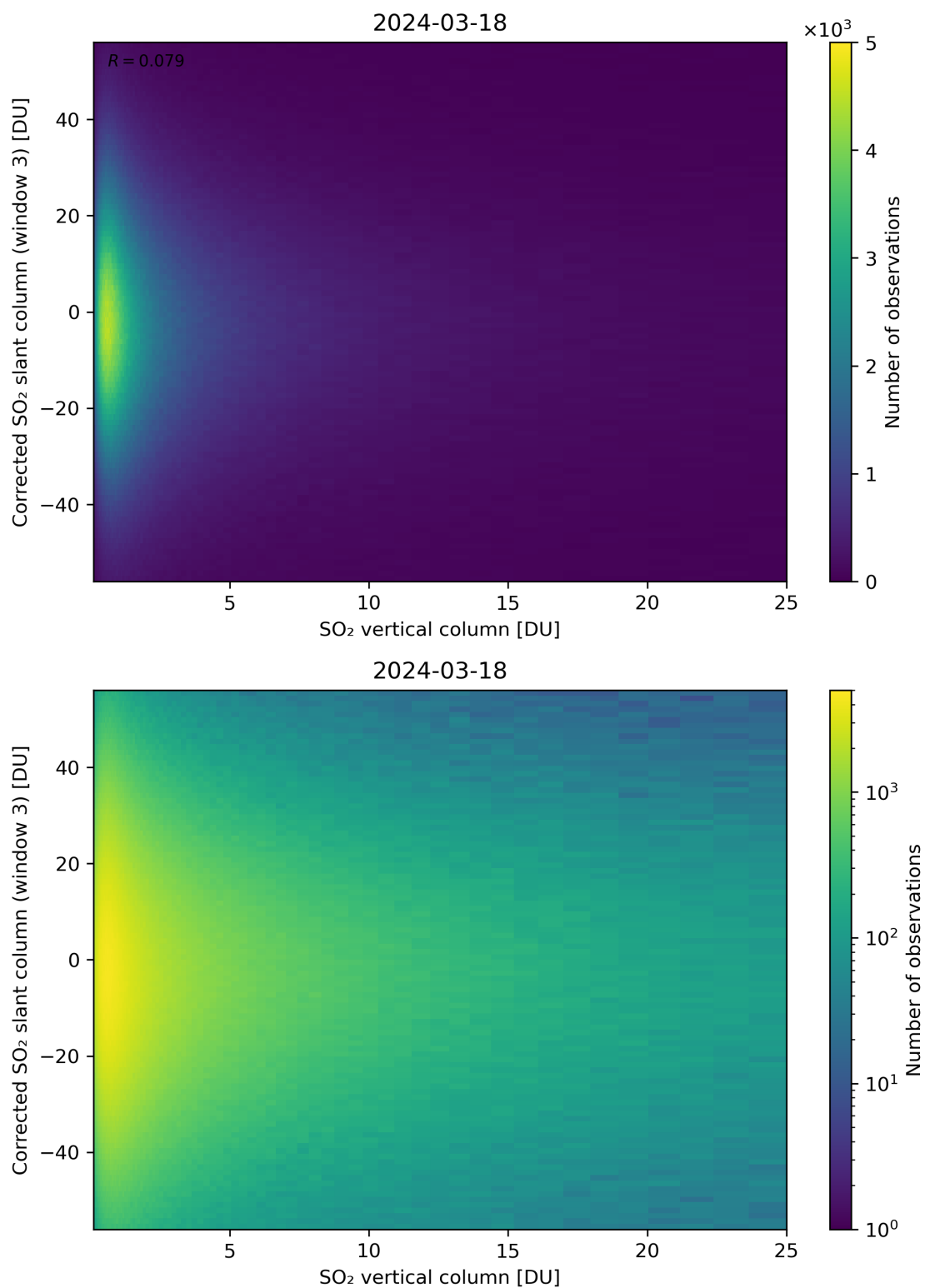
Figure 299: Scatter density plot of “SO 2 vertical column” against “Corrected SO 2 slant column (window 3)” for 2024-03-17 to 2024-03-19.
