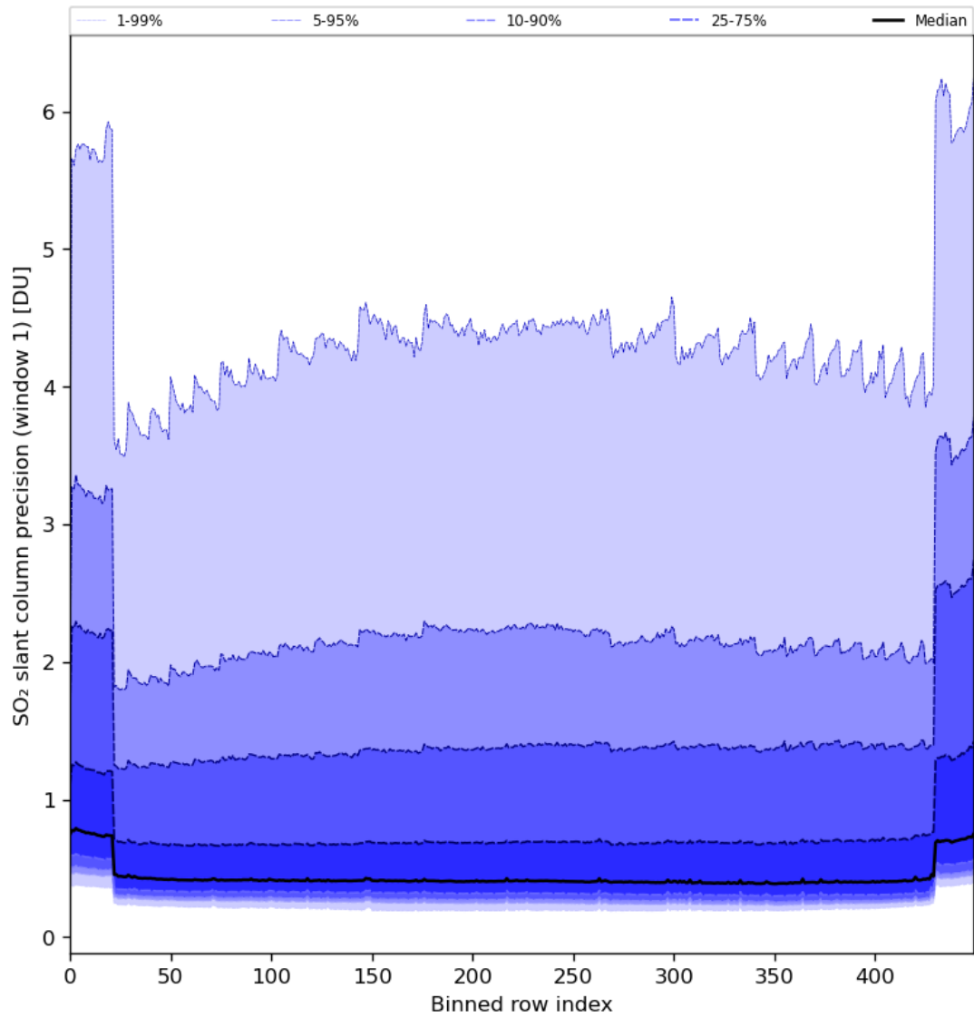
Figure 80: Along track statistics of “SO 2 slant column precision (window 1)” for 2024-03-17 to 2024-03-19
