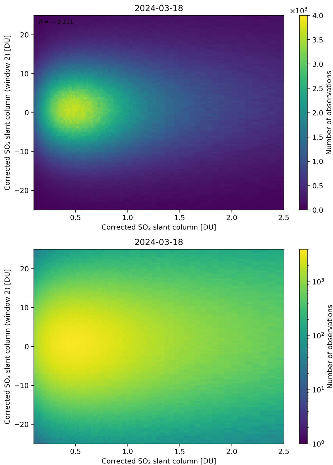
Figure 185: Scatter density plot of “Corrected SO 2 slant column” against “Corrected SO 2 slant column (window 2)” for 2024-03-17 to 2024-03-19.
