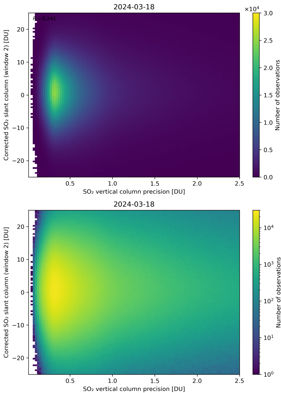
Figure 287: Scatter density plot of “SO 2 vertical column precision” against “Corrected SO 2 slant column (window 2)” for 2024-03-17 to 2024-03-19.
