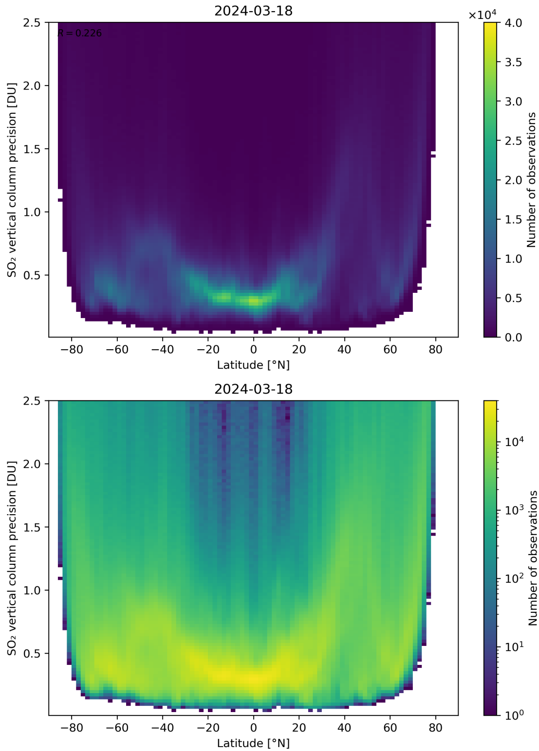
Figure 157: Scatter density plot of “Latitude” against “SO 2 vertical column precision” for 2024-03-17 to 2024-03-19.
