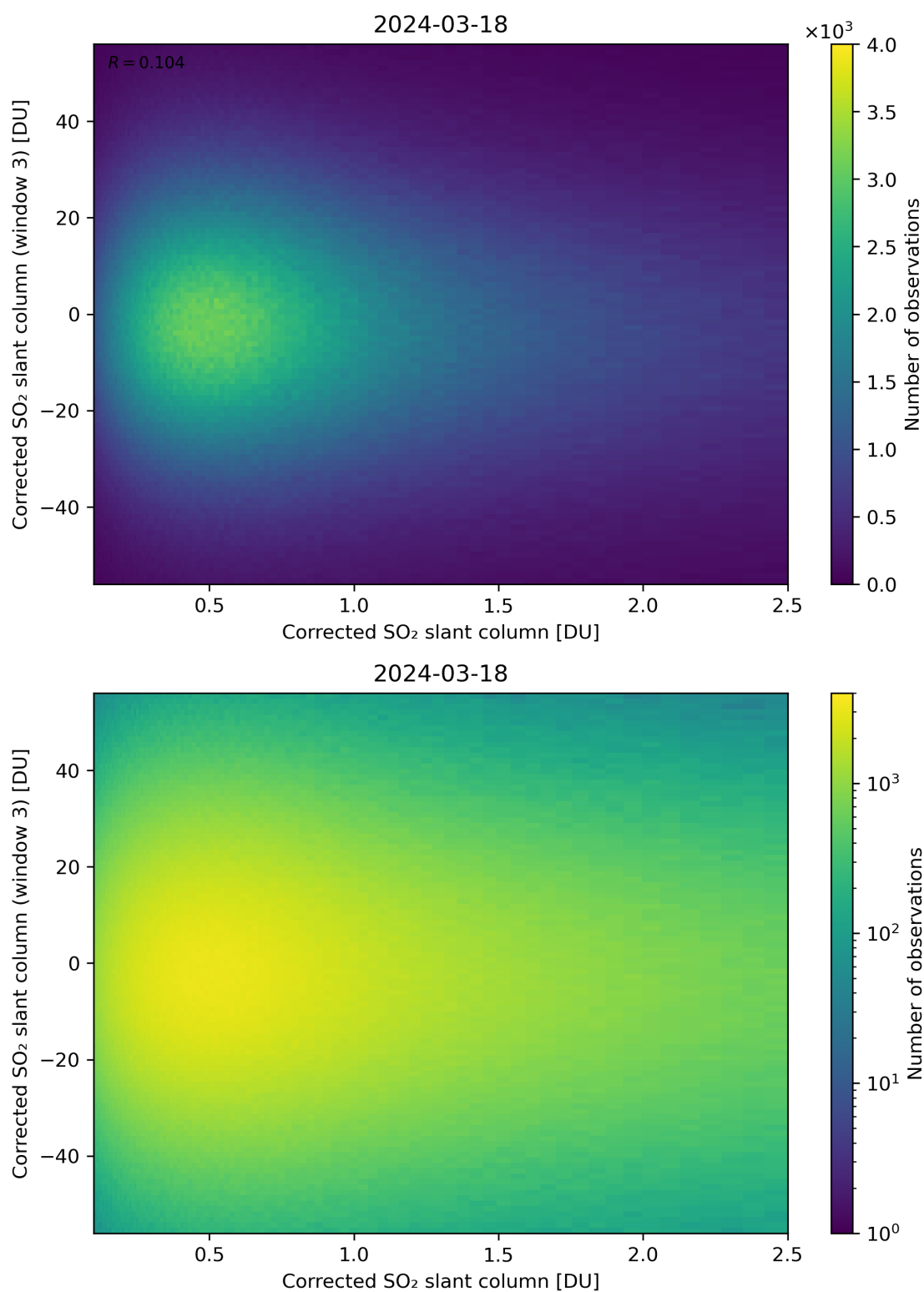
Figure 186: Scatter density plot of “Corrected SO 2 slant column” against “Corrected SO 2 slant column (window 3)” for 2024-03-17 to 2024-03-19.
