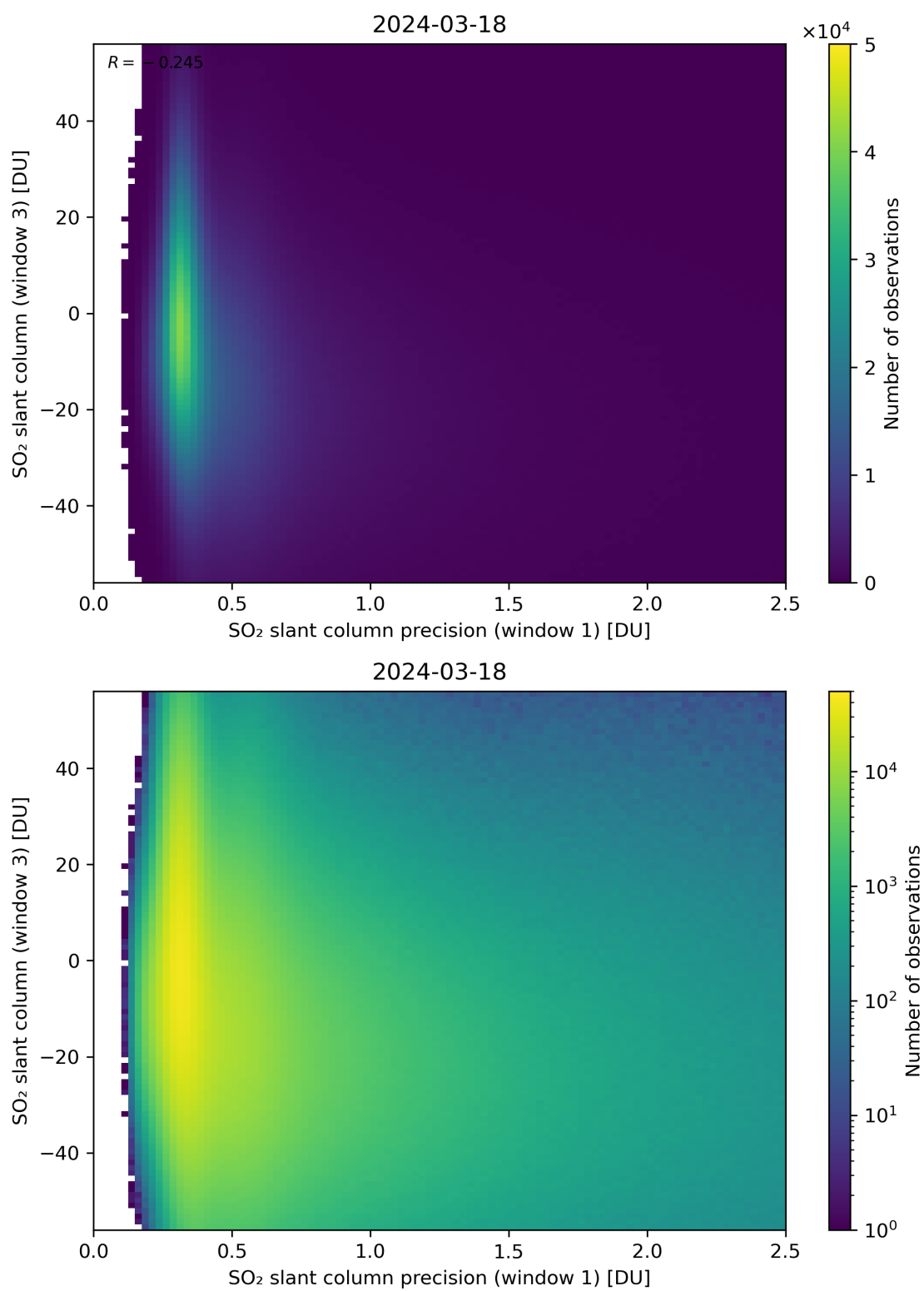
Figure 228: Scatter density plot of “SO 2 slant column precision (window 1)” against “SO 2 slant column (window 3)” for 2024-03-17 to 2024-03-19.
