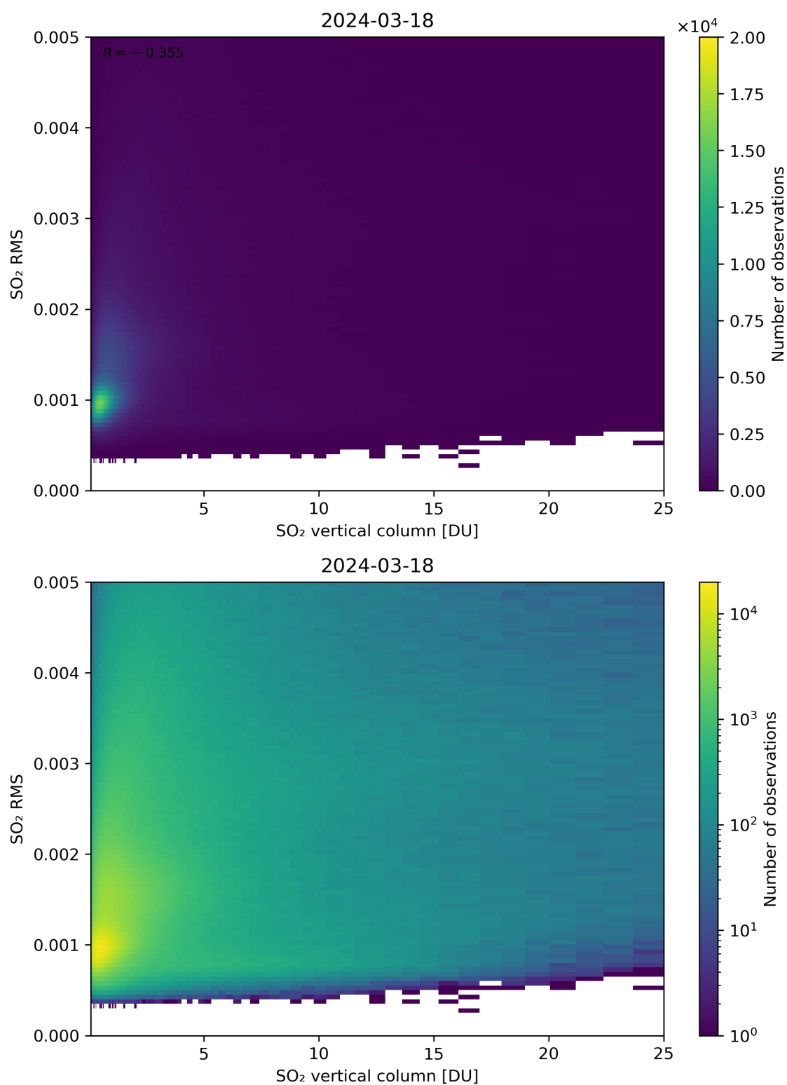
Figure 278: Scatter density plot of “SO 2 vertical column” against “SO 2 RMS” for 2024-03-17 to 2024-03-19.
