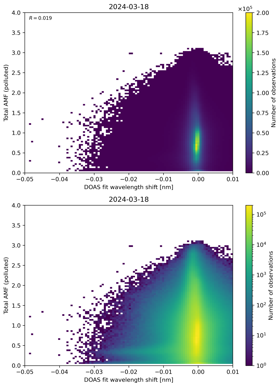
Figure 130: Scatter density plot of “DOAS fit wavelength shift” against “Total AMF (polluted)” for 2024-03-17 to 2024-03-19.
