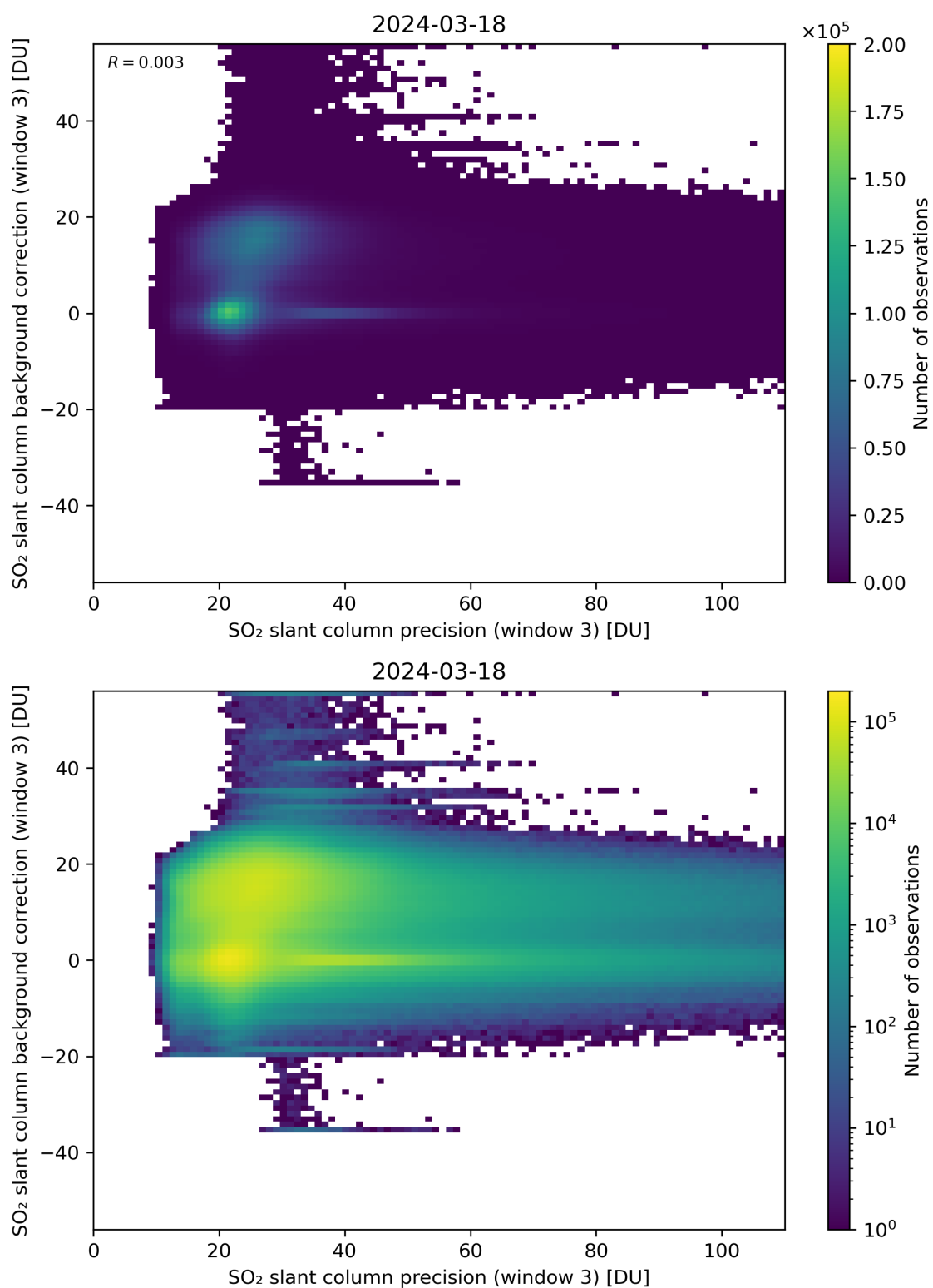
Figure 257: Scatter density plot of “SO 2 slant column precision (window 3)” against “SO 2 slant column background correction (window 3)” for 2024-03-17 to 2024-03-19.
