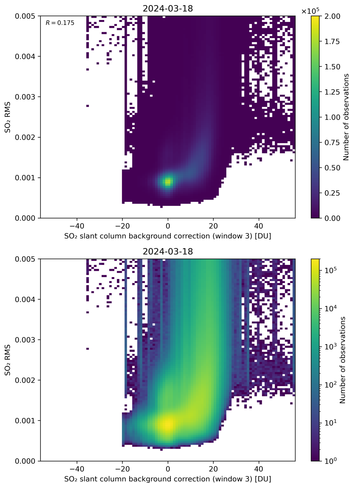
Figure 123: Scatter density plot of “SO 2 slant column background correction (window 3)” against “SO 2 RMS” for 2024-03-17 to 2024-03-19.
