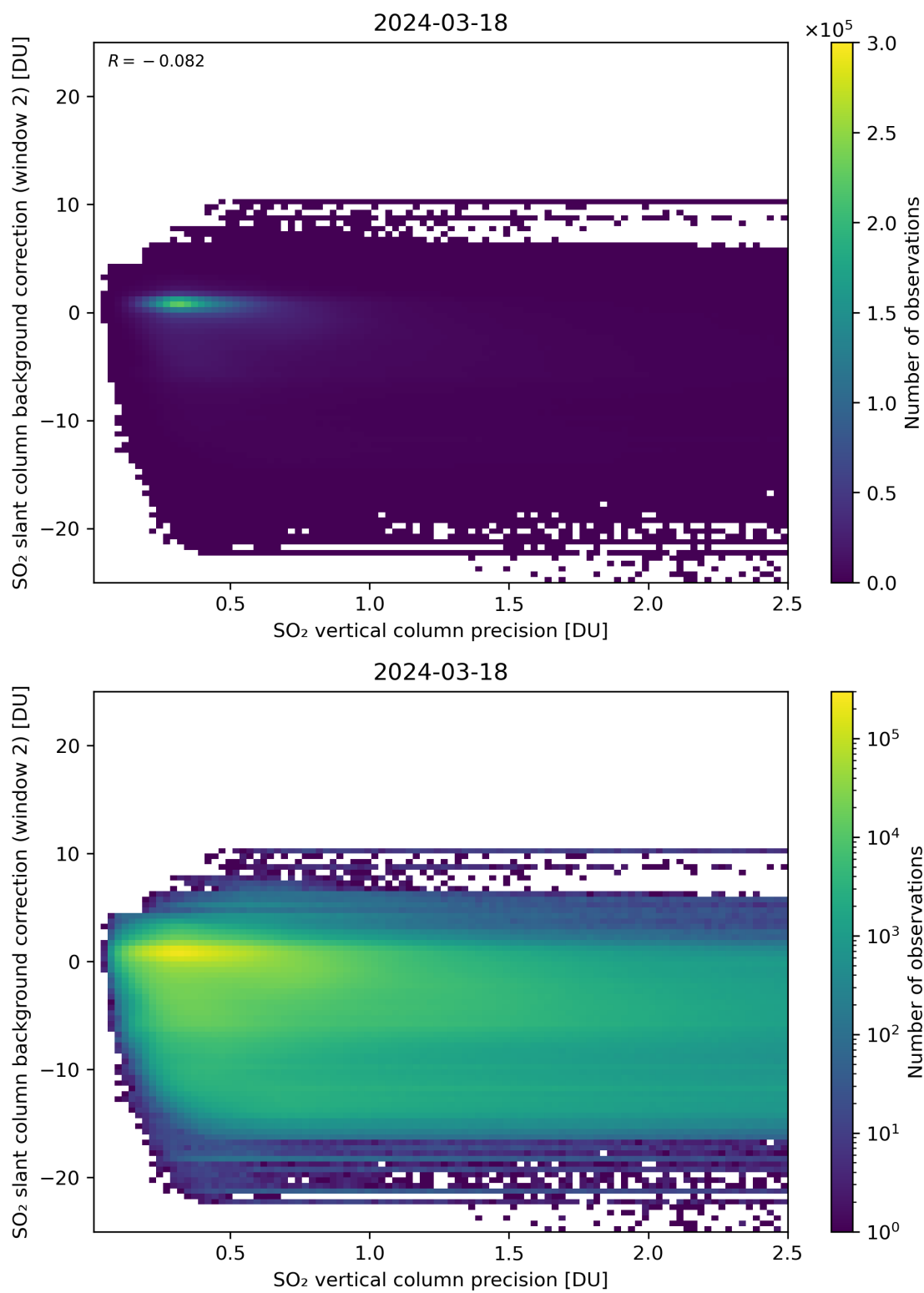
Figure 280: Scatter density plot of “SO 2 vertical column precision” against “SO 2 slant column background correction (window 2)” for 2024-03-17 to 2024-03-19.
