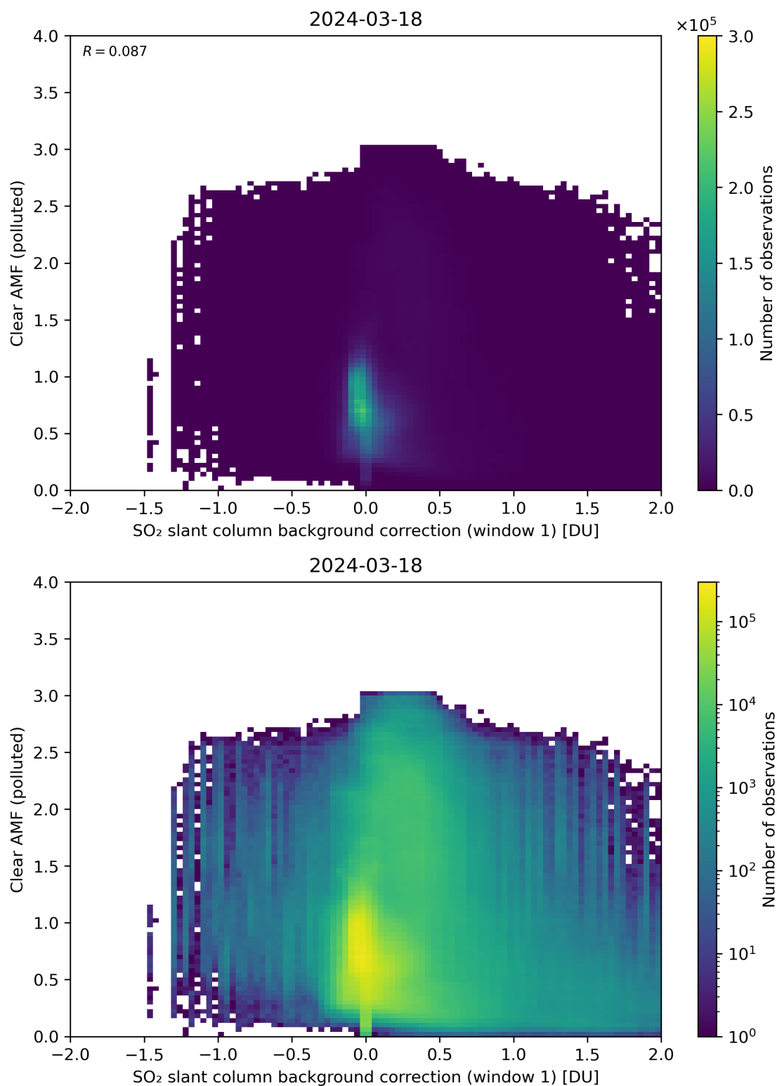
Figure 103: Scatter density plot of “SO 2 slant column background correction (window 1)” against “Clear AMF (polluted)” for 2024-03-17 to 2024-03-19.
