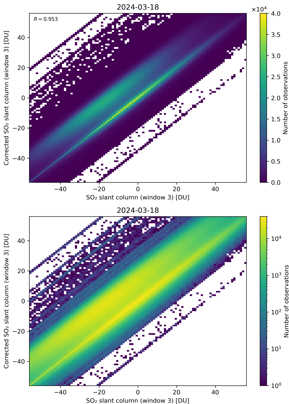
Figure 266: Scatter density plot of “SO 2 slant column (window 3)” against “Corrected SO 2 slant column (window 3)” for 2024-03-17 to 2024-03-19.
