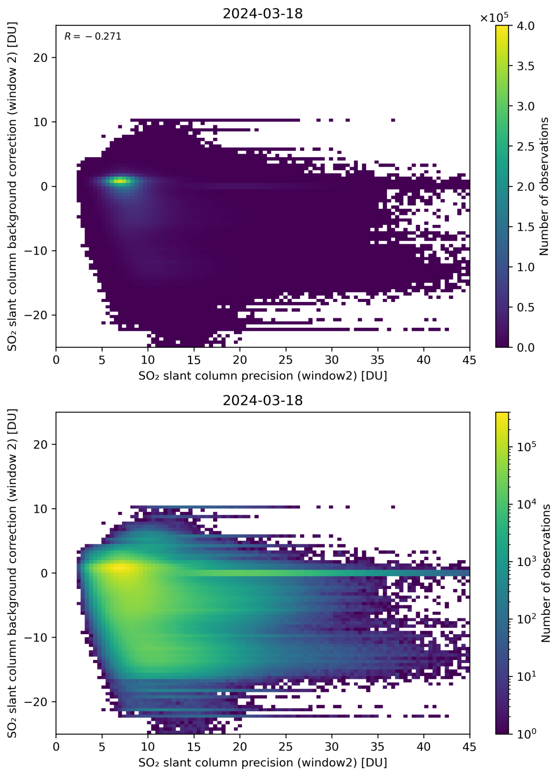
Figure 241: Scatter density plot of “SO 2 slant column precision (window2)” against “SO 2 slant column background correction (window 2)” for 2024-03-17 to 2024-03-19.
