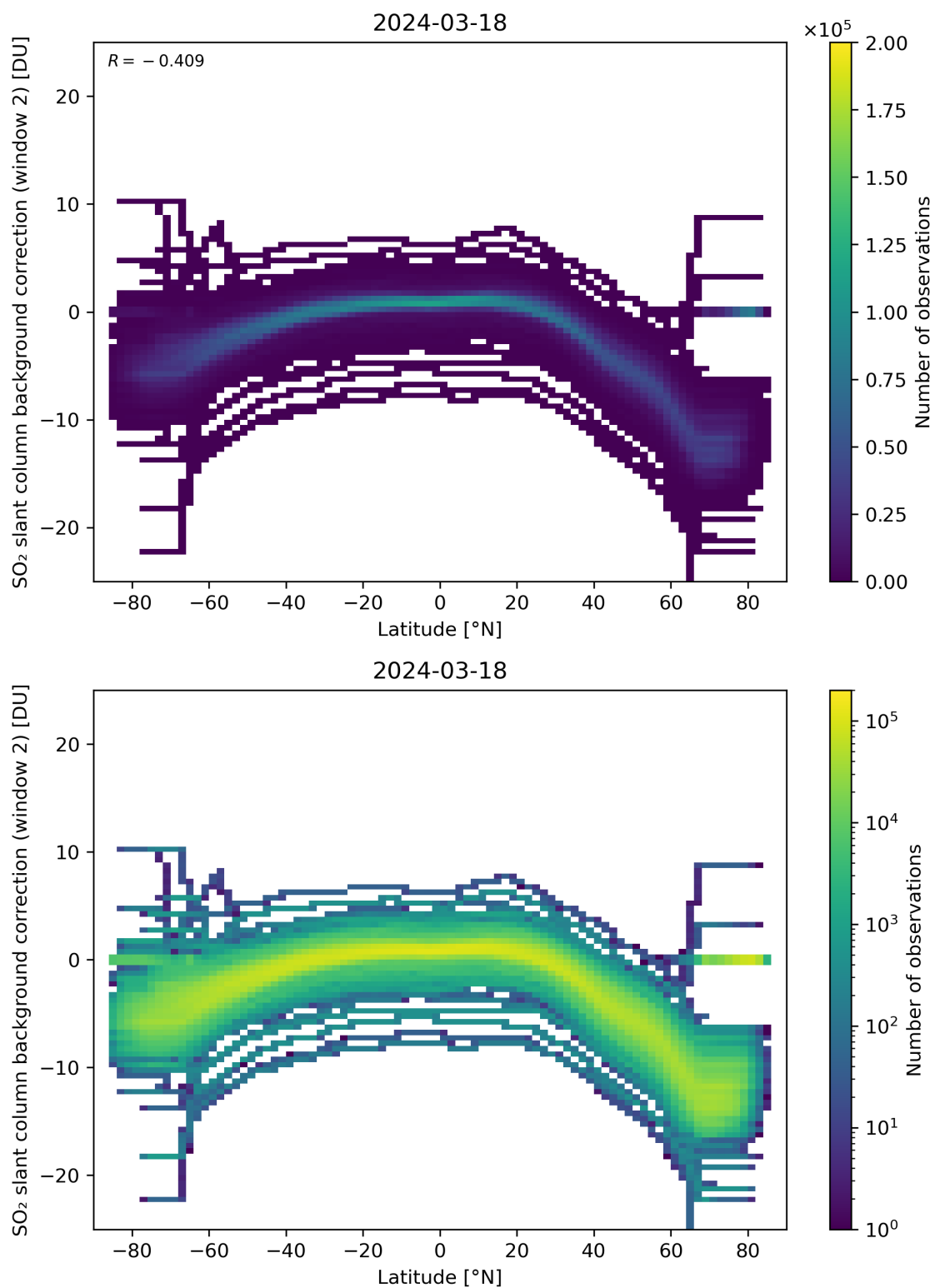
Figure 140: Scatter density plot of “Latitude” against “SO 2 slant column background correction (window 2)” for 2024-03-17 to 2024-03-19.
