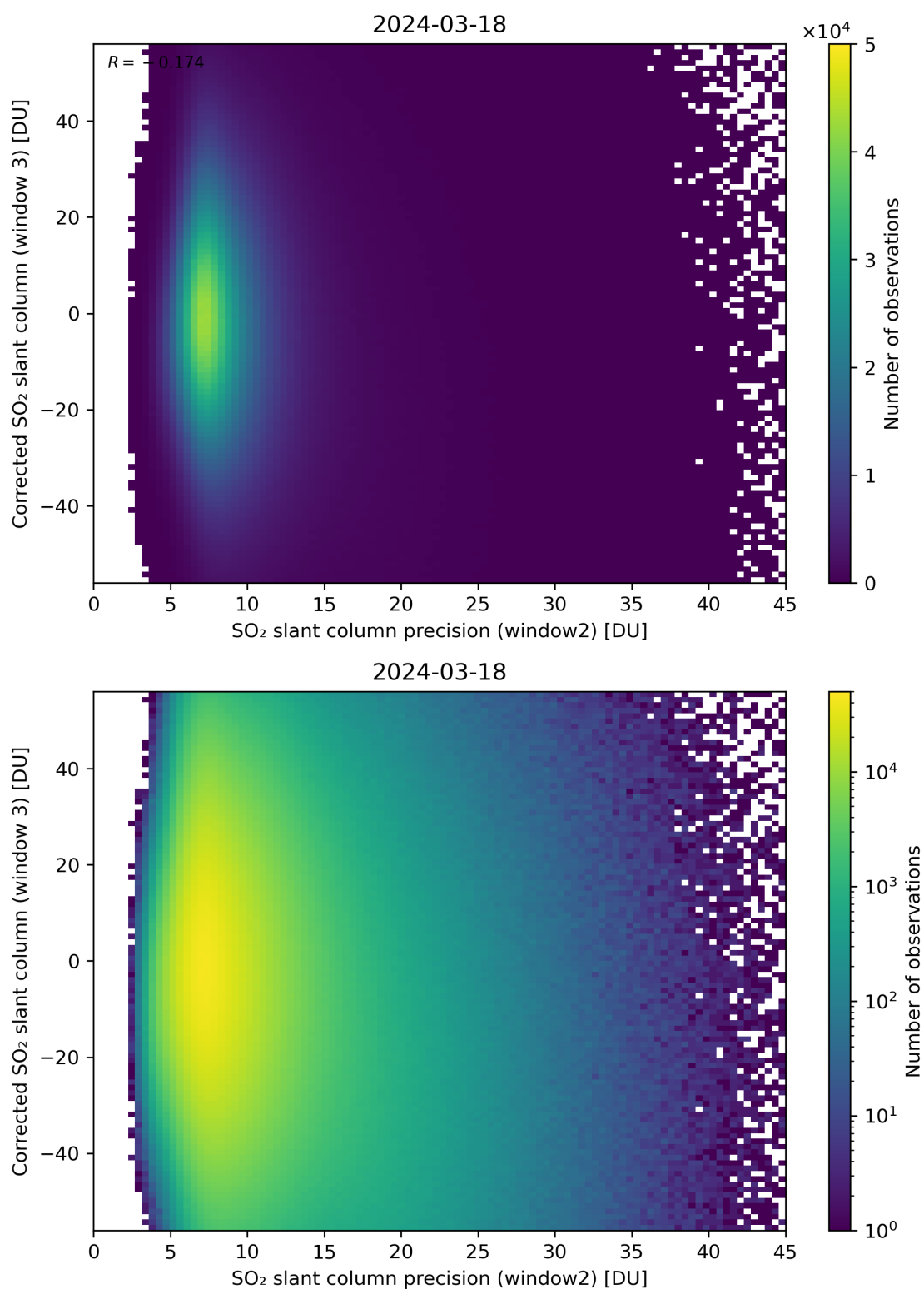
Figure 248: Scatter density plot of “SO 2 slant column precision (window2)” against “Corrected SO 2 slant column (window 3)” for 2024-03-17 to 2024-03-19.
