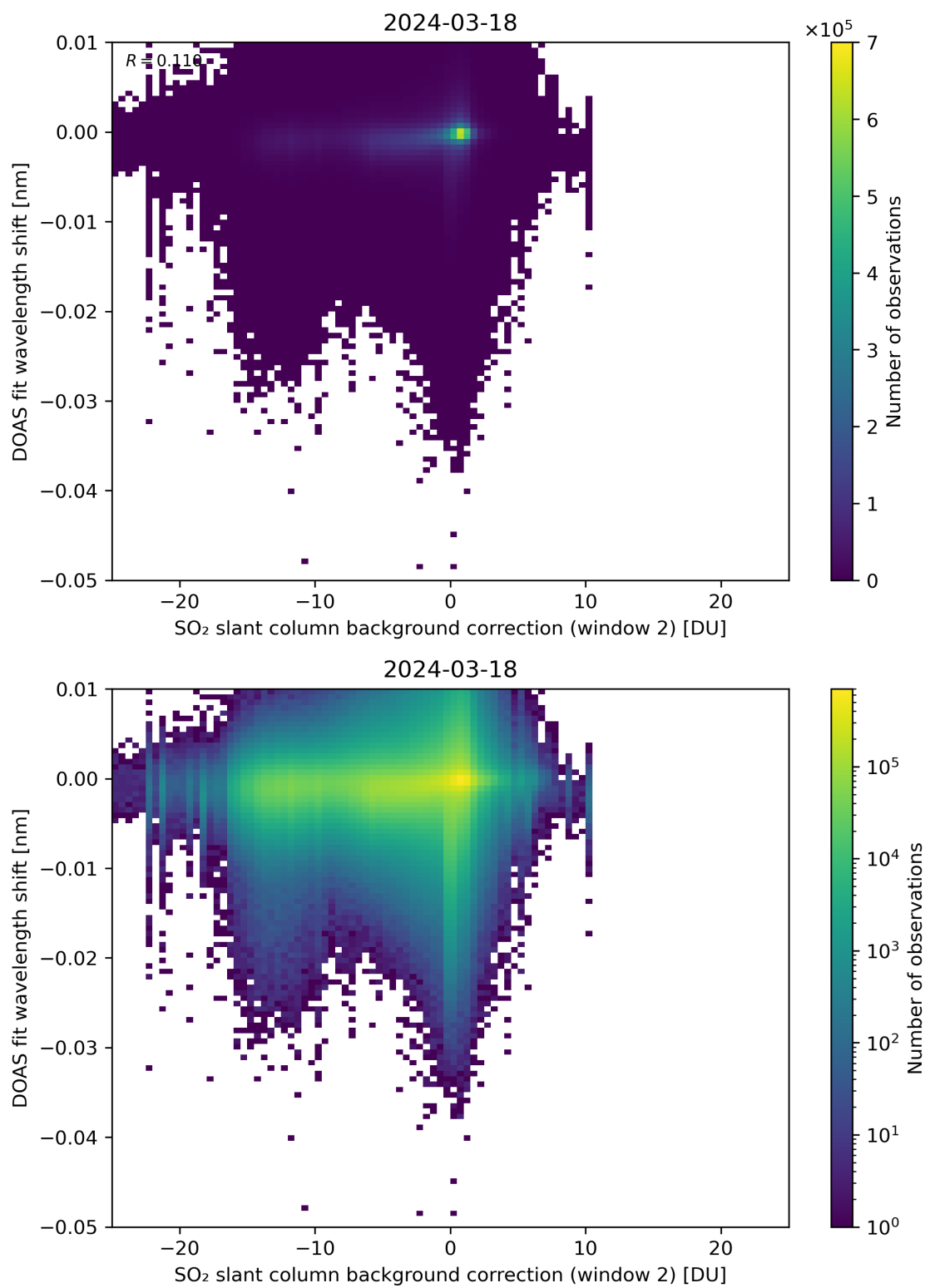
Figure 112: Scatter density plot of “SO 2 slant column background correction (window 2)” against “DOAS fit wavelength shift” for 2024-03-17 to 2024-03-19.
