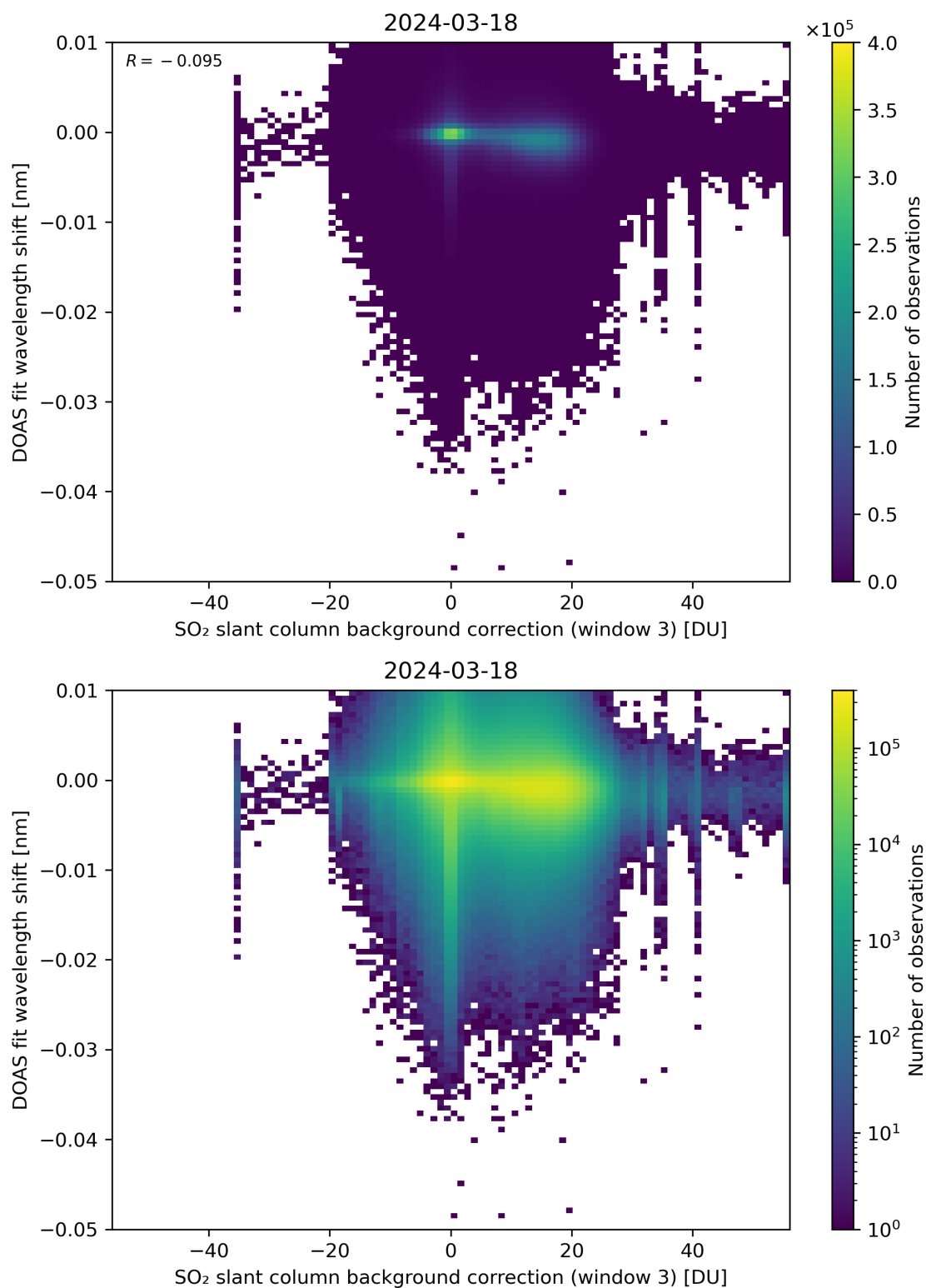
Figure 121: Scatter density plot of “SO 2 slant column background correction (window 3)” against “DOAS fit wavelength shift” for 2024-03-17 to 2024-03-19.
