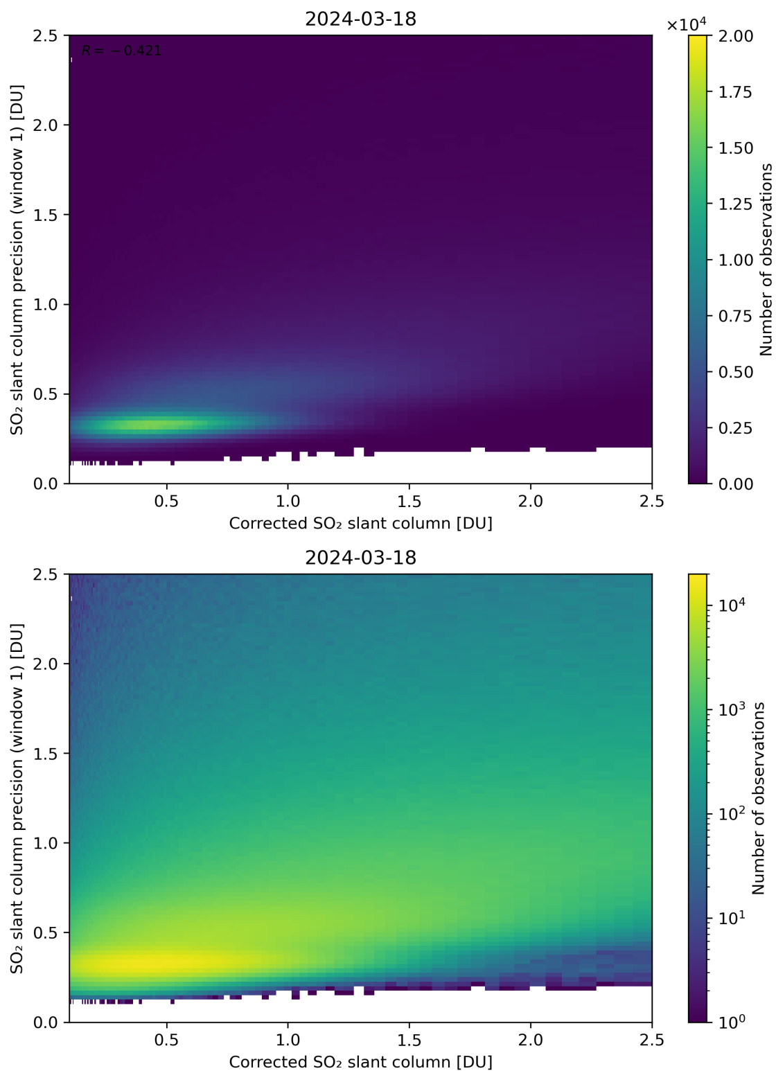
Figure 188: Scatter density plot of “Corrected SO 2 slant column” against “SO 2 slant column precision (window 1)” for 2024-03-17 to 2024-03-19.
