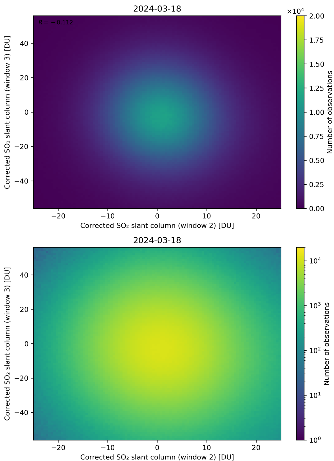
Figure 200: Scatter density plot of “Corrected SO 2 slant column (window 2)” against “Corrected SO 2 slant column (window 3)” for 2024-03-17 to 2024-03-19.
