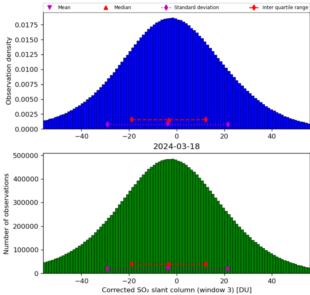
Figure 66: Histogram of "Corrected SO 2 slant column (window 3)" for 2024-03-17 to 2024-03-19
