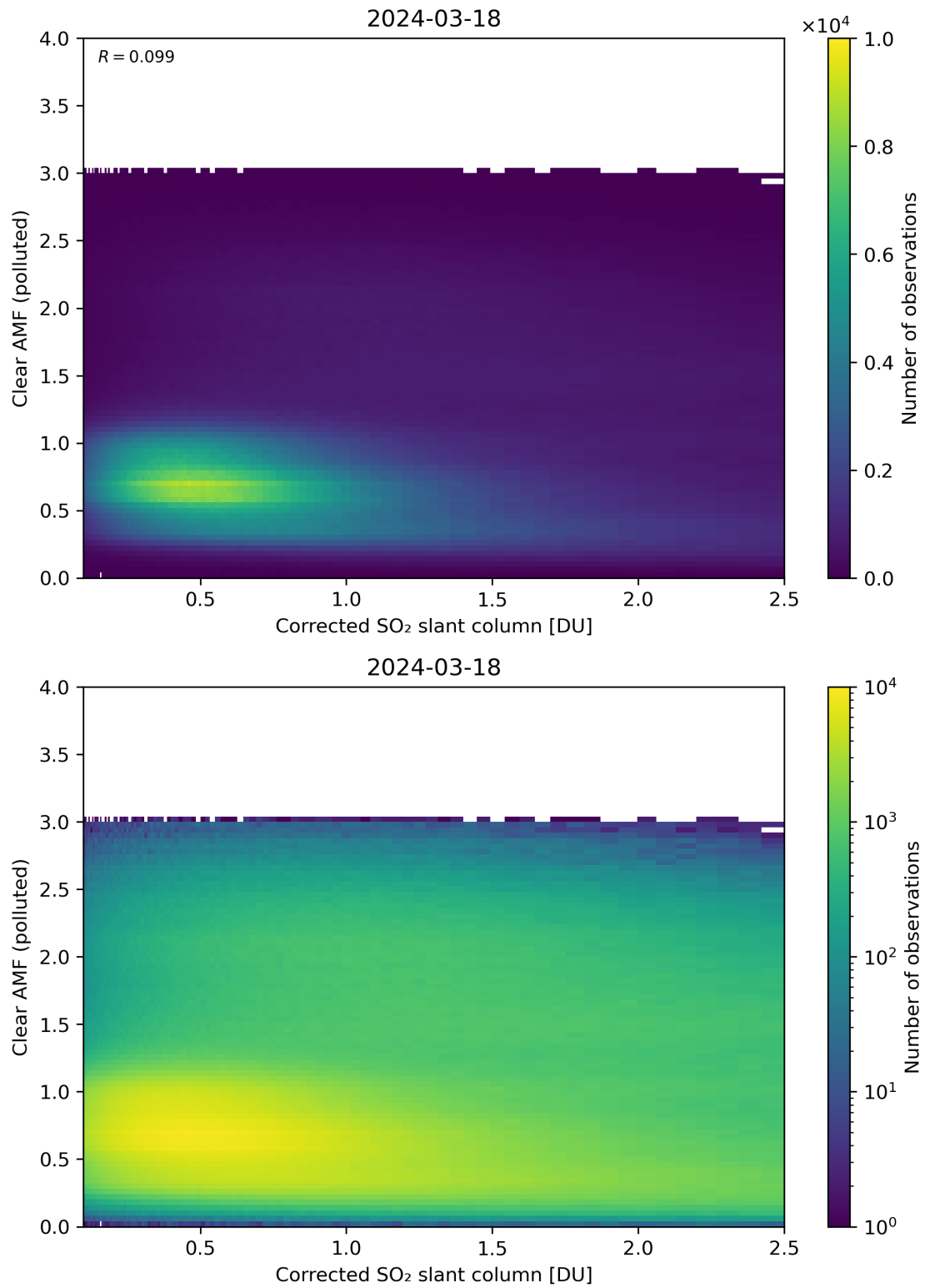
Figure 184: Scatter density plot of “Corrected SO 2 slant column” against “Clear AMF (polluted)” for 2024-03-17 to 2024-03-19.
