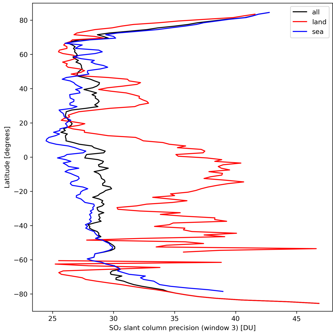
Figure 42: Zonal average of “SO 2 slant column precision (window 3)” for 2024-03-17 to 2024-03-19.
