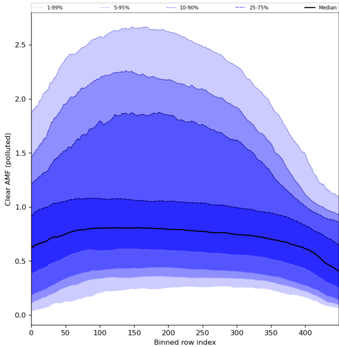
Figure 96: Along track statistics of “Clear AMF (polluted)” for 2024-03-17 to 2024-03-19
