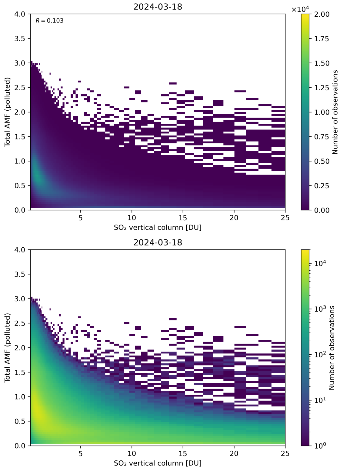
Figure 305: Scatter density plot of “SO 2 vertical column” against “Total AMF (polluted)” for 2024-03-17 to 2024-03-19.
