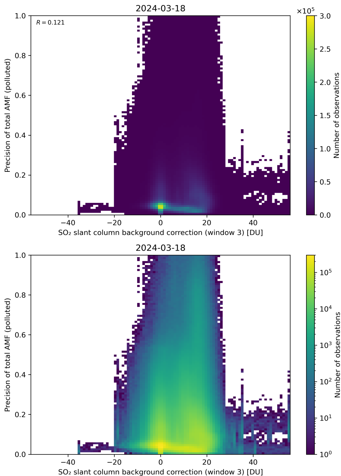
Figure 126: Scatter density plot of “SO 2 slant column background correction (window 3)” against “Precision of total AMF (polluted)” for 2024-03-17 to 2024-03-19.
