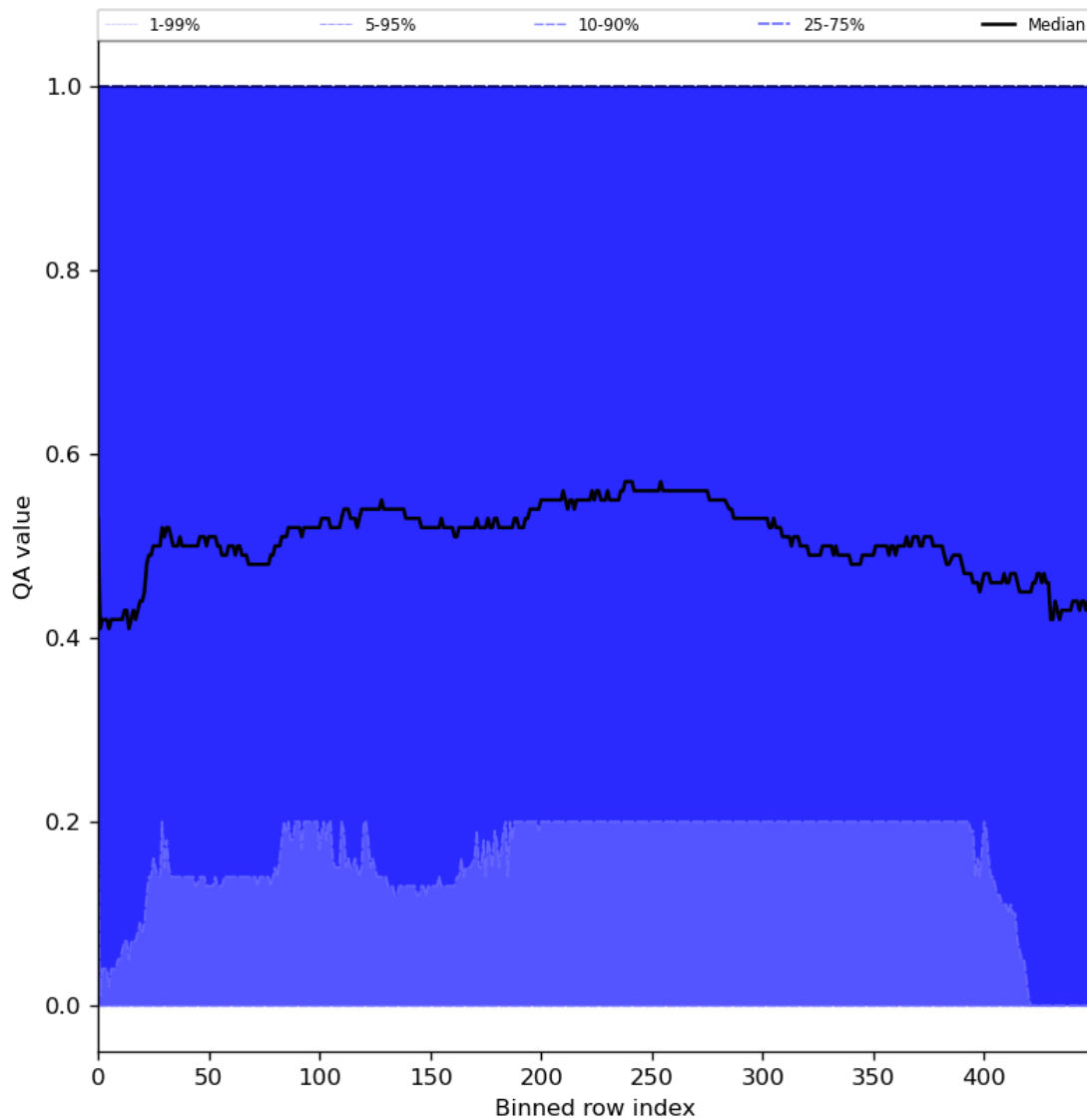
Figure 75: Along track statistics of “QA value” for 2024-03-17 to 2024-03-19
