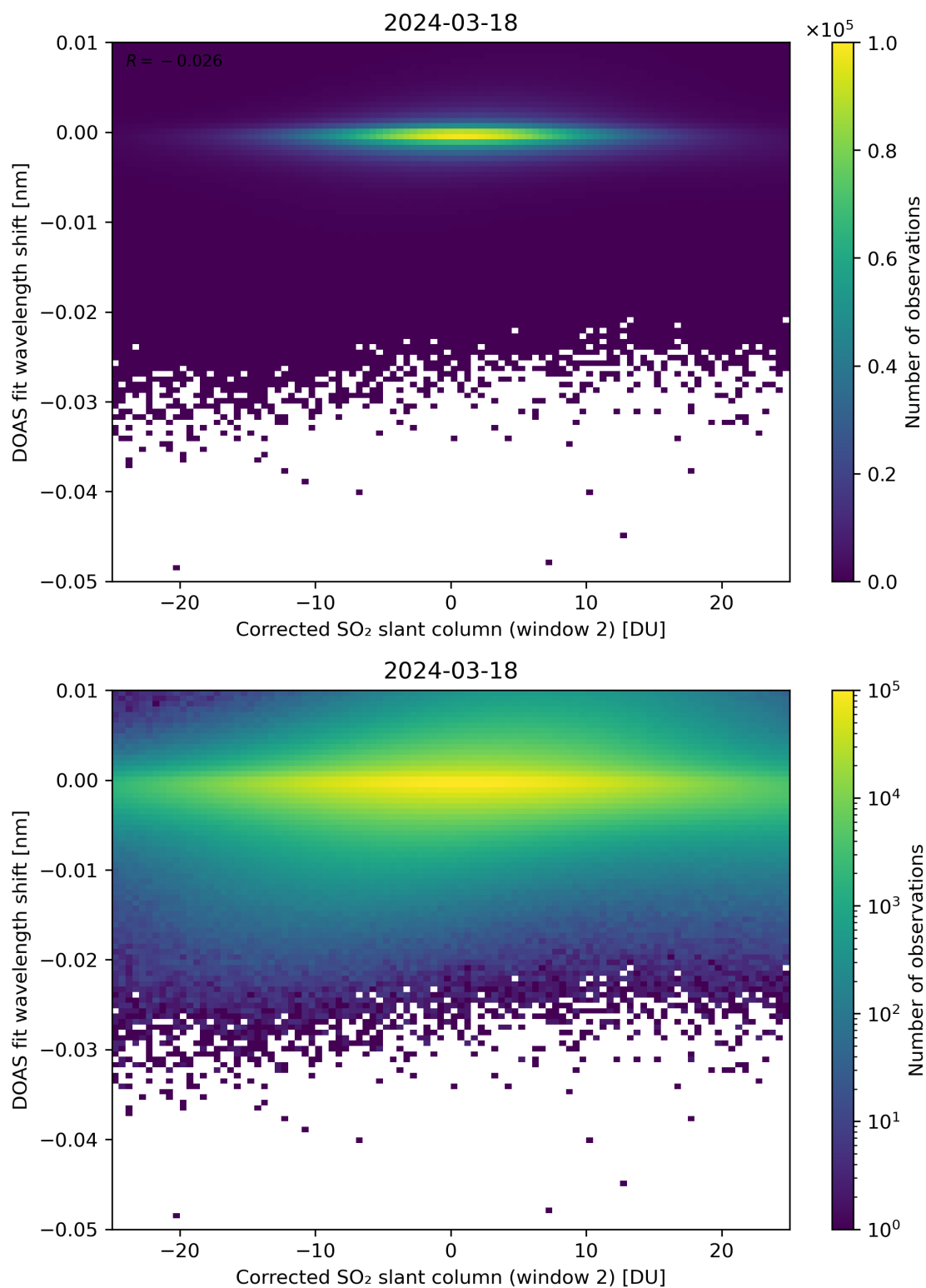
Figure 196: Scatter density plot of “Corrected SO 2 slant column (window 2)” against “DOAS fit wavelength shift” for 2024-03-17 to 2024-03-19.
