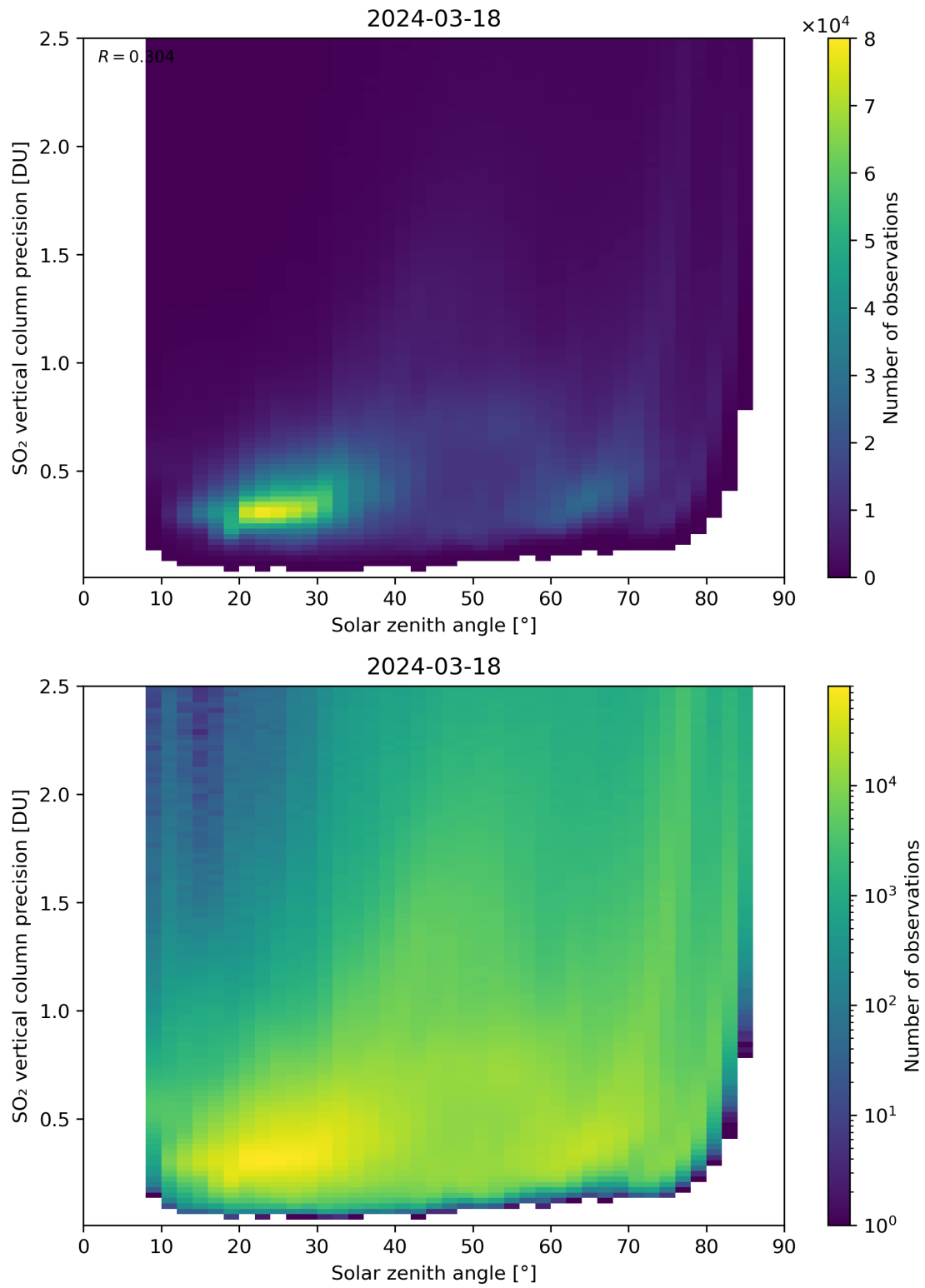
Figure 177: Scatter density plot of “Solar zenith angle” against “SO 2 vertical column precision” for 2024-03-17 to 2024-03-19.
