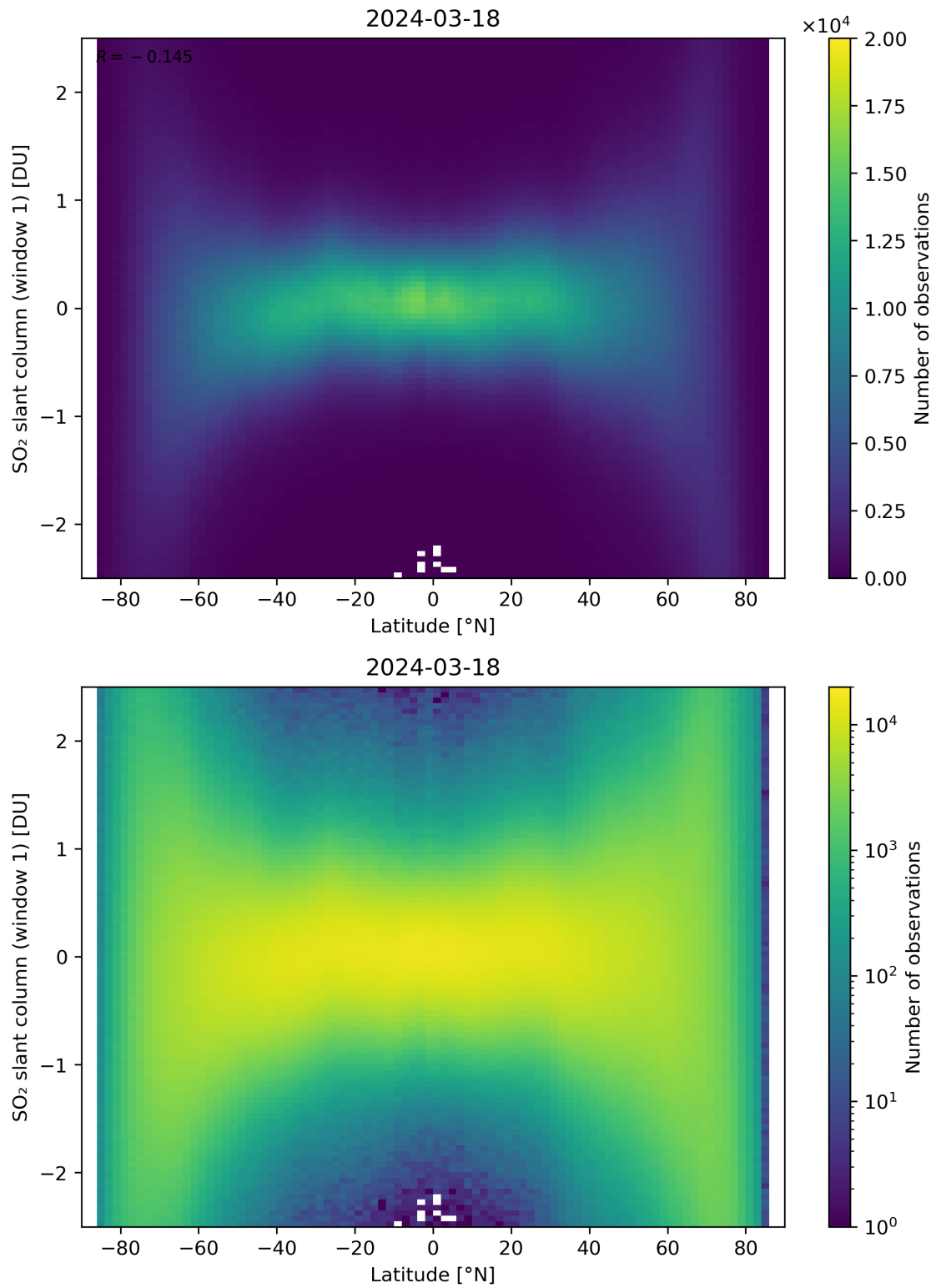
Figure 149: Scatter density plot of “Latitude” against “SO 2 slant column (window 1)” for 2024-03-17 to 2024-03-19.
