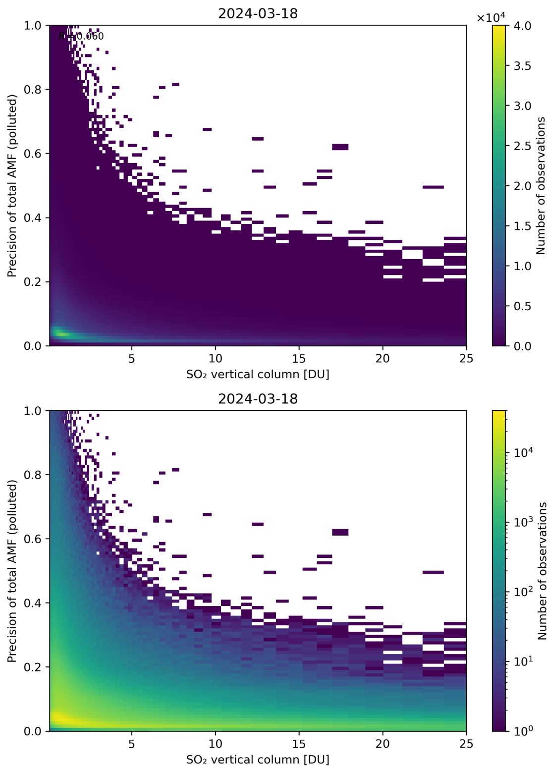
Figure 306: Scatter density plot of “SO 2 vertical column” against “Precision of total AMF (polluted)” for 2024-03-17 to 2024-03-19.
