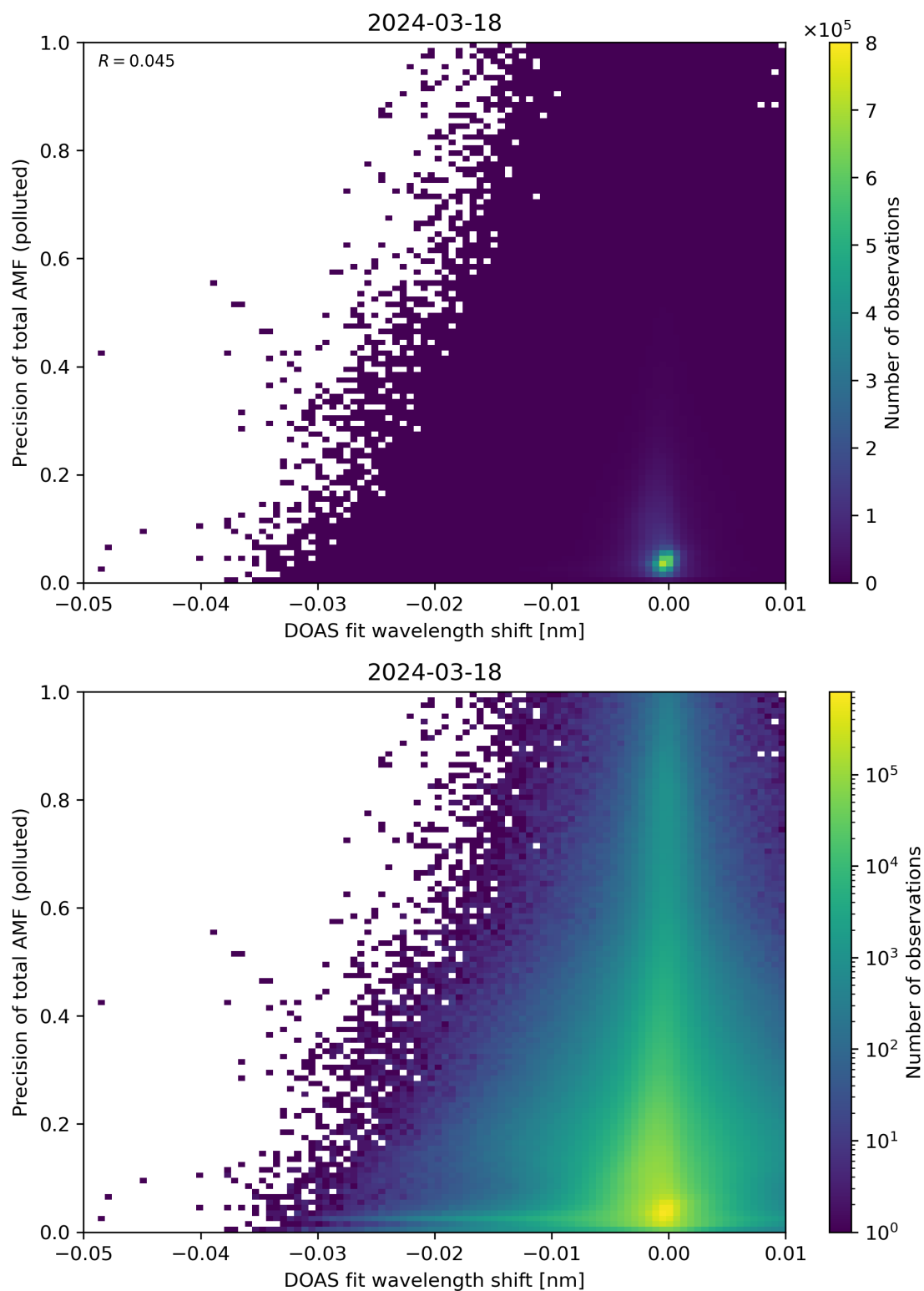
Figure 131: Scatter density plot of “DOAS fit wavelength shift” against “Precision of total AMF (polluted)” for 2024-03-17 to 2024-03-19.
