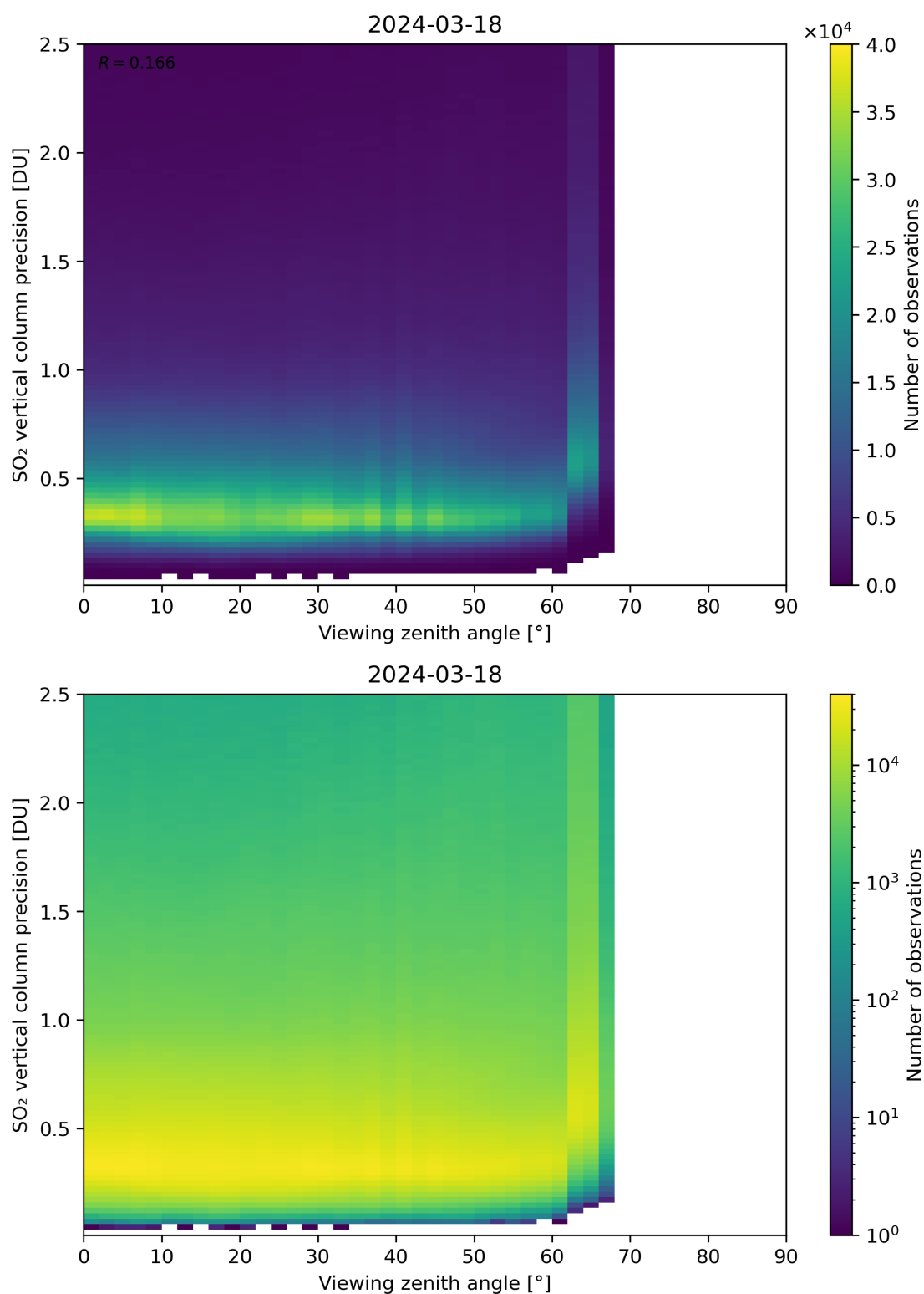
Figure 328: Scatter density plot of “Viewing zenith angle” against “SO 2 vertical column precision” for 2024-03-17 to 2024-03-19.
