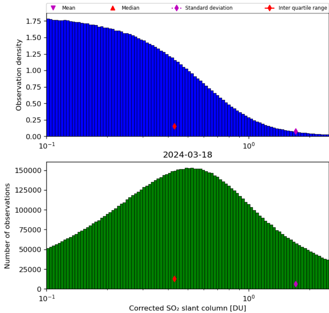
Figure 55: Histogram of “Corrected SO 2 slant column” for 2024-03-17 to 2024-03-19
