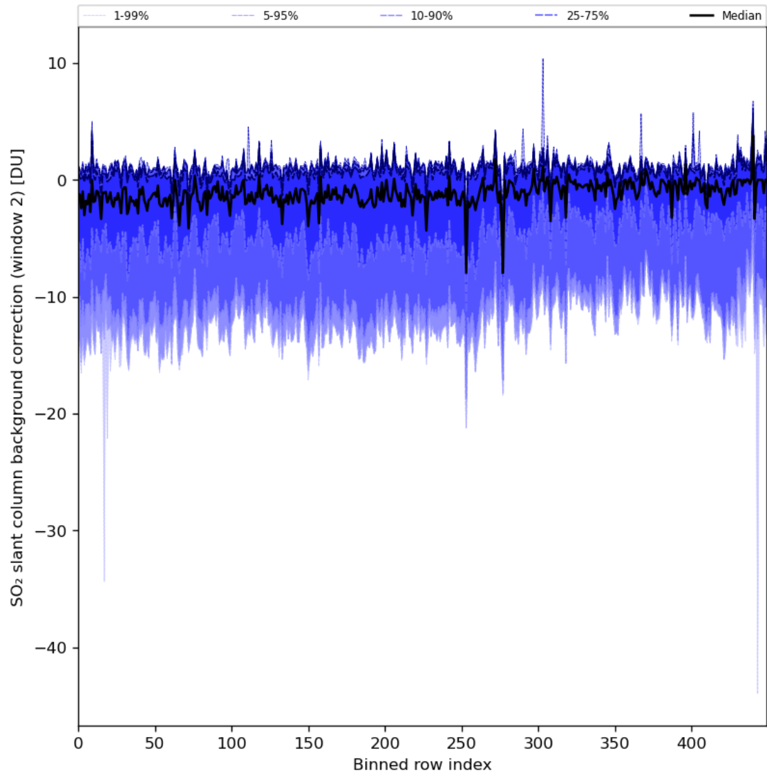
Figure 86: Along track statistics of “SO 2 slant column background correction (window 2)” for 2024-03-17 to 2024-03-19
