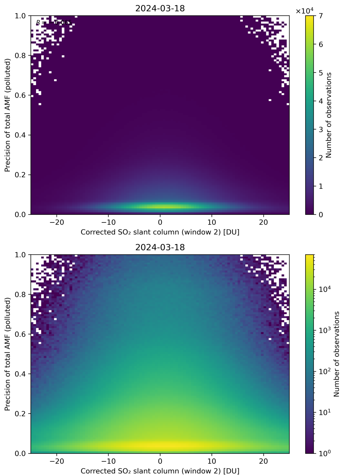
Figure 204: Scatter density plot of “Corrected SO 2 slant column (window 2)” against “Precision of total AMF (polluted)” for 2024-03-17 to 2024-03-19.
