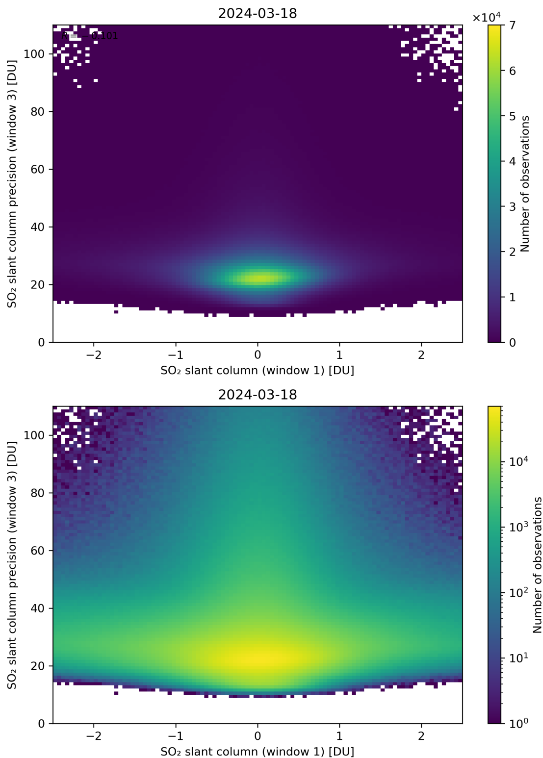
Figure 238: Scatter density plot of “SO 2 slant column (window 1)” against “SO 2 slant column precision (window 3)” for 2024-03-17 to 2024-03-19.
