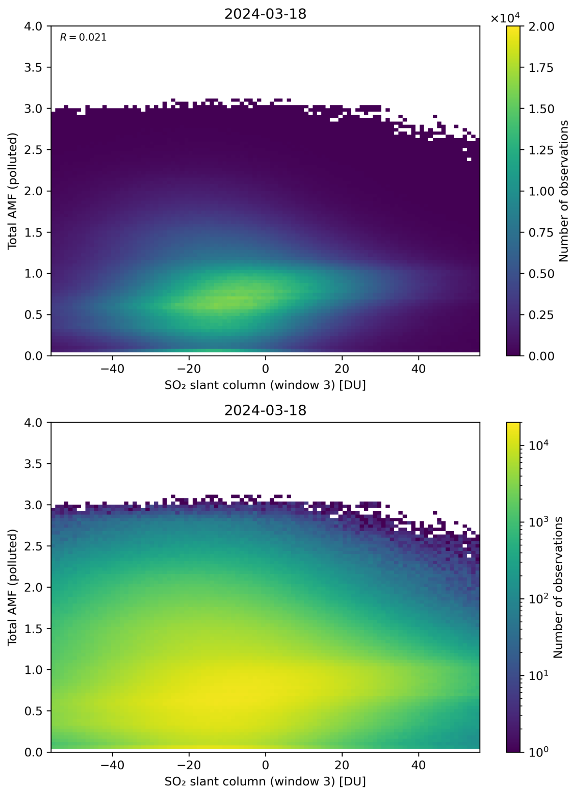
Figure 268: Scatter density plot of “SO 2 slant column (window 3)” against “Total AMF (polluted)” for 2024-03-17 to 2024-03-19.
