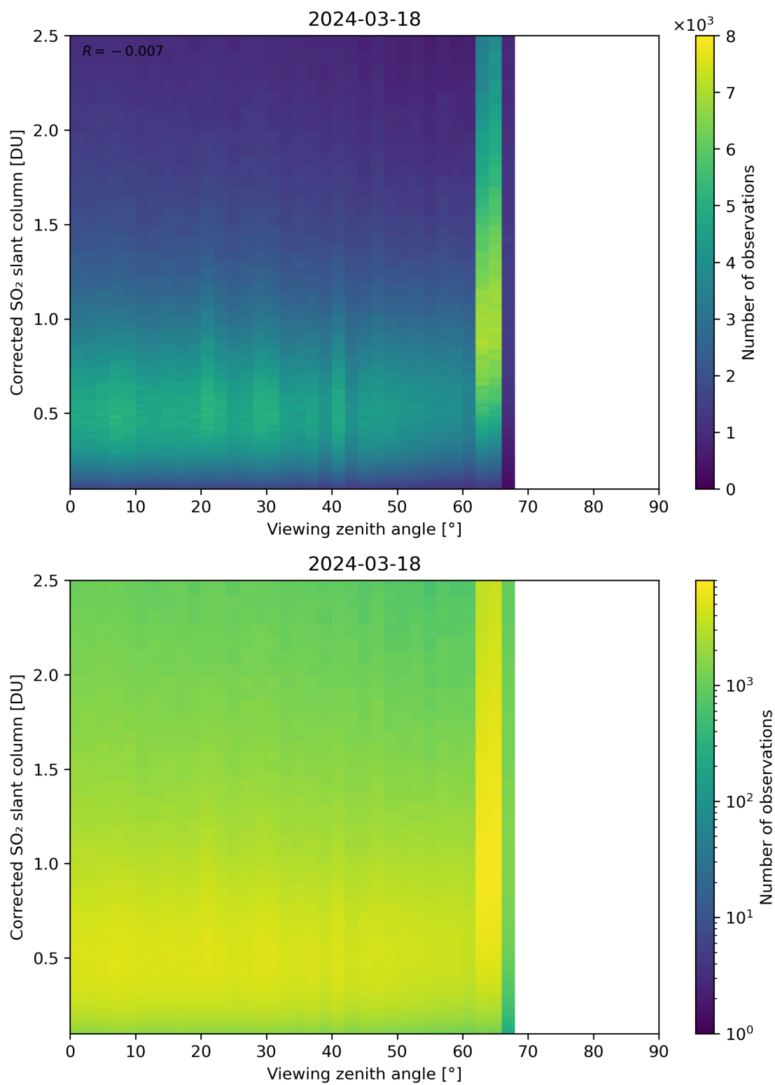
Figure 317: Scatter density plot of “Viewing zenith angle” against “Corrected SO 2 slant column” for 2024-03-17 to 2024-03-19.
