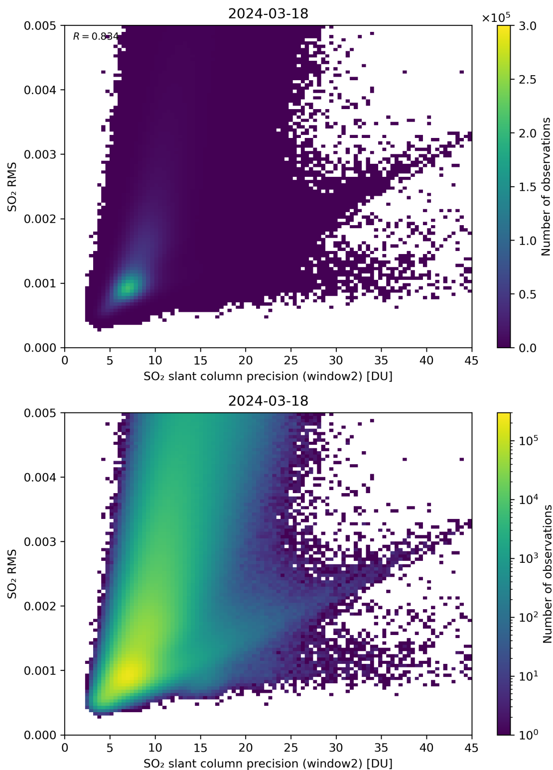
Figure 245: Scatter density plot of “SO 2 slant column precision (window2)” against “SO 2 RMS” for 2024-03-17 to 2024-03-19.
