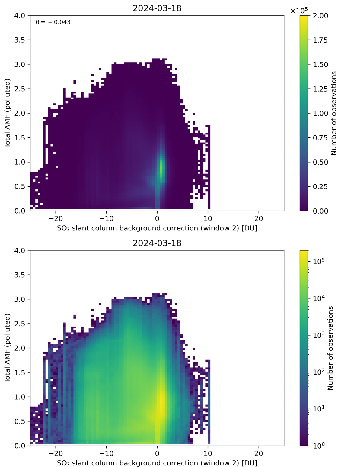
Figure 119: Scatter density plot of “SO 2 slant column background correction (window 2)” against “Total AMF (polluted)” for 2024-03-17 to 2024-03-19.
