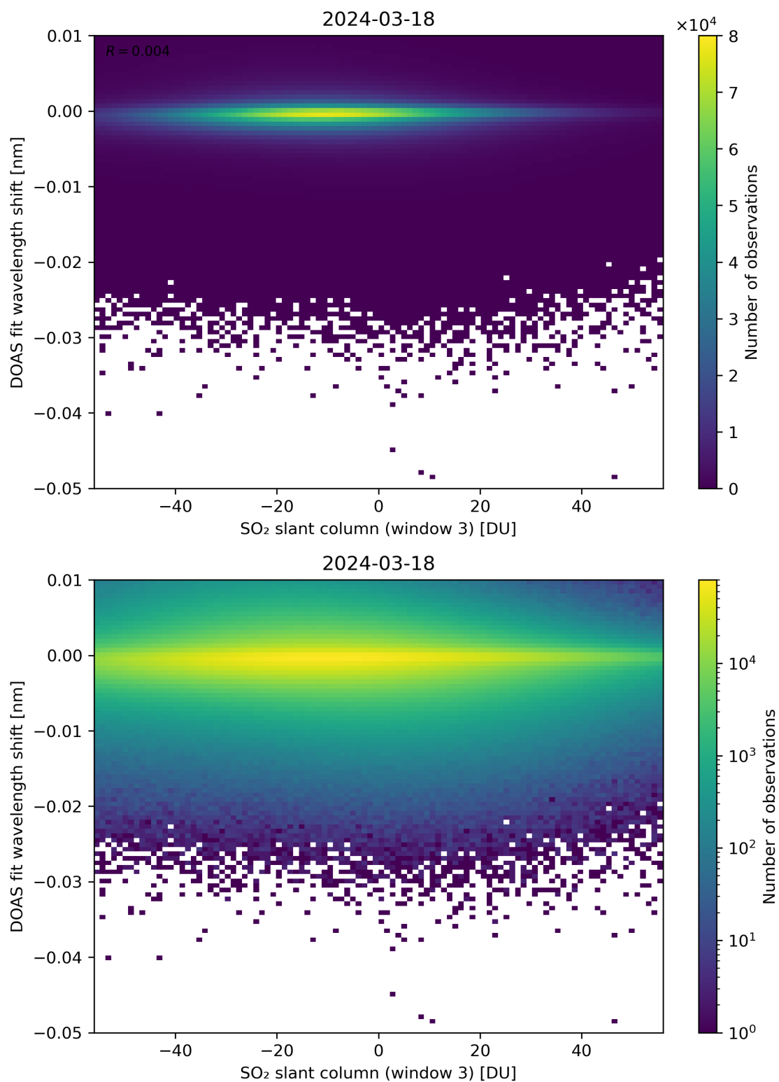
Figure 254: Scatter density plot of “SO 2 slant column (window 3)” against “DOAS fit wavelength shift” for 2024-03-17 to 2024-03-19.
