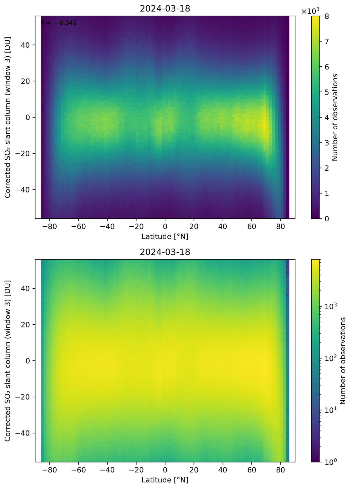
Figure 148: Scatter density plot of “Latitude” against “Corrected SO 2 slant column (window 3)” for 2024-03-17 to 2024-03-19.
