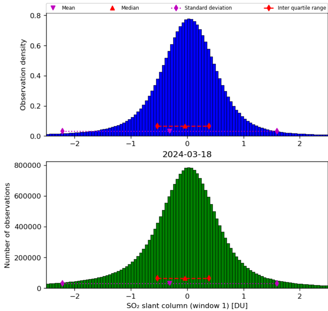
Figure 56: Histogram of “SO 2 slant column (window 1)” for 2024-03-17 to 2024-03-19
