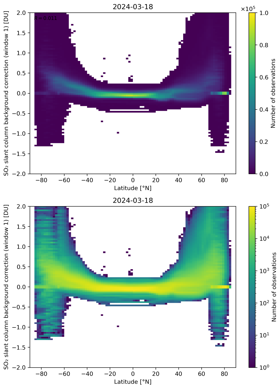
Figure 139: Scatter density plot of “Latitude” against “SO 2 slant column background correction (window 1)” for 2024-03-17 to 2024-03-19.
