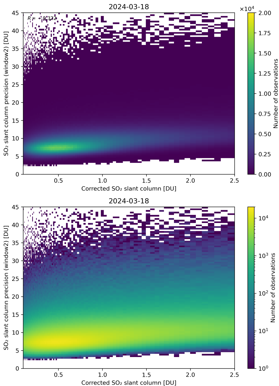
Figure 189: Scatter density plot of “Corrected SO 2 slant column” against “SO 2 slant column precision (window2)” for 2024-03-17 to 2024-03-19.
