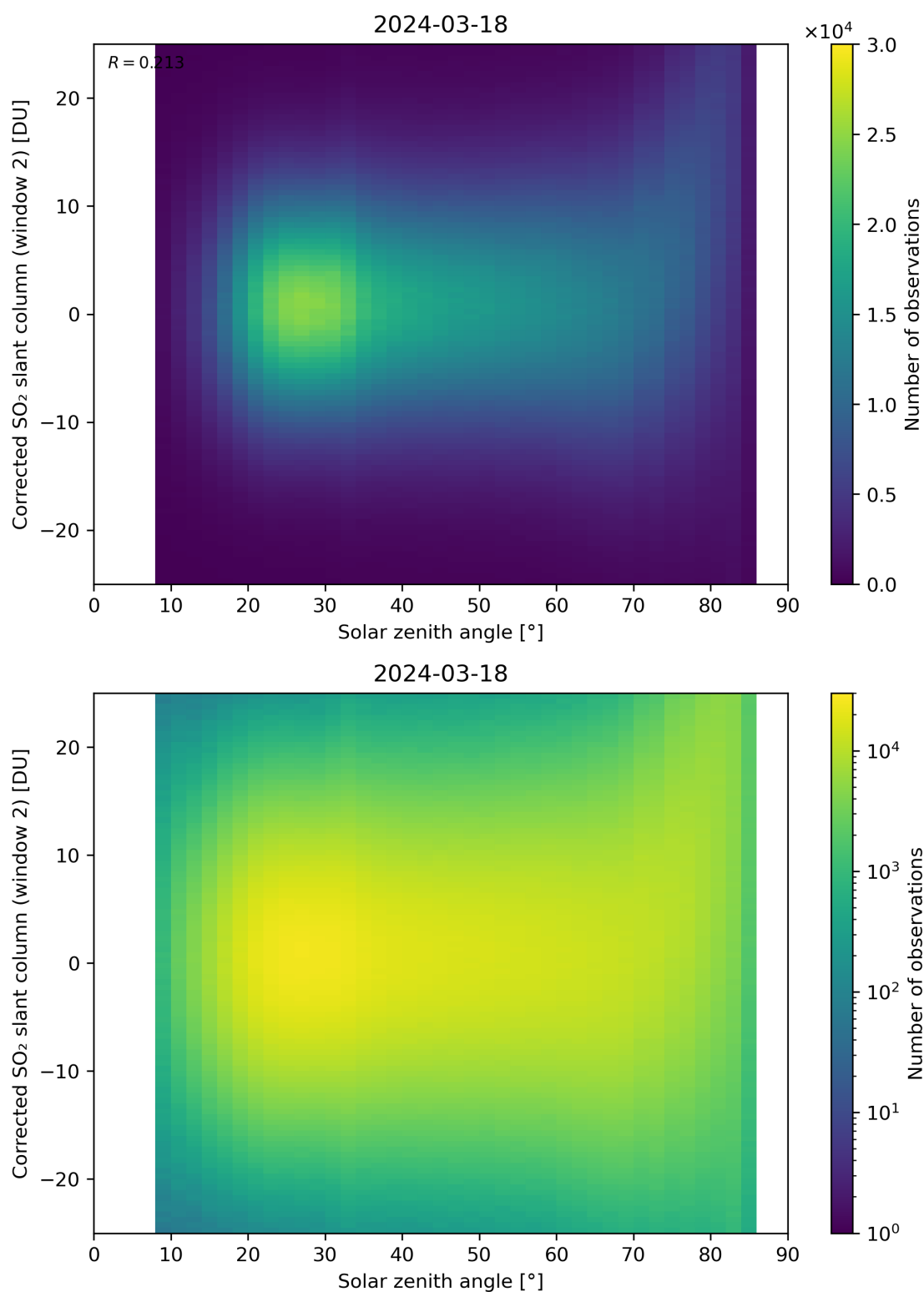
Figure 167: Scatter density plot of “Solar zenith angle” against “Corrected SO 2 slant column (window 2)” for 2024-03-17 to 2024-03-19.
