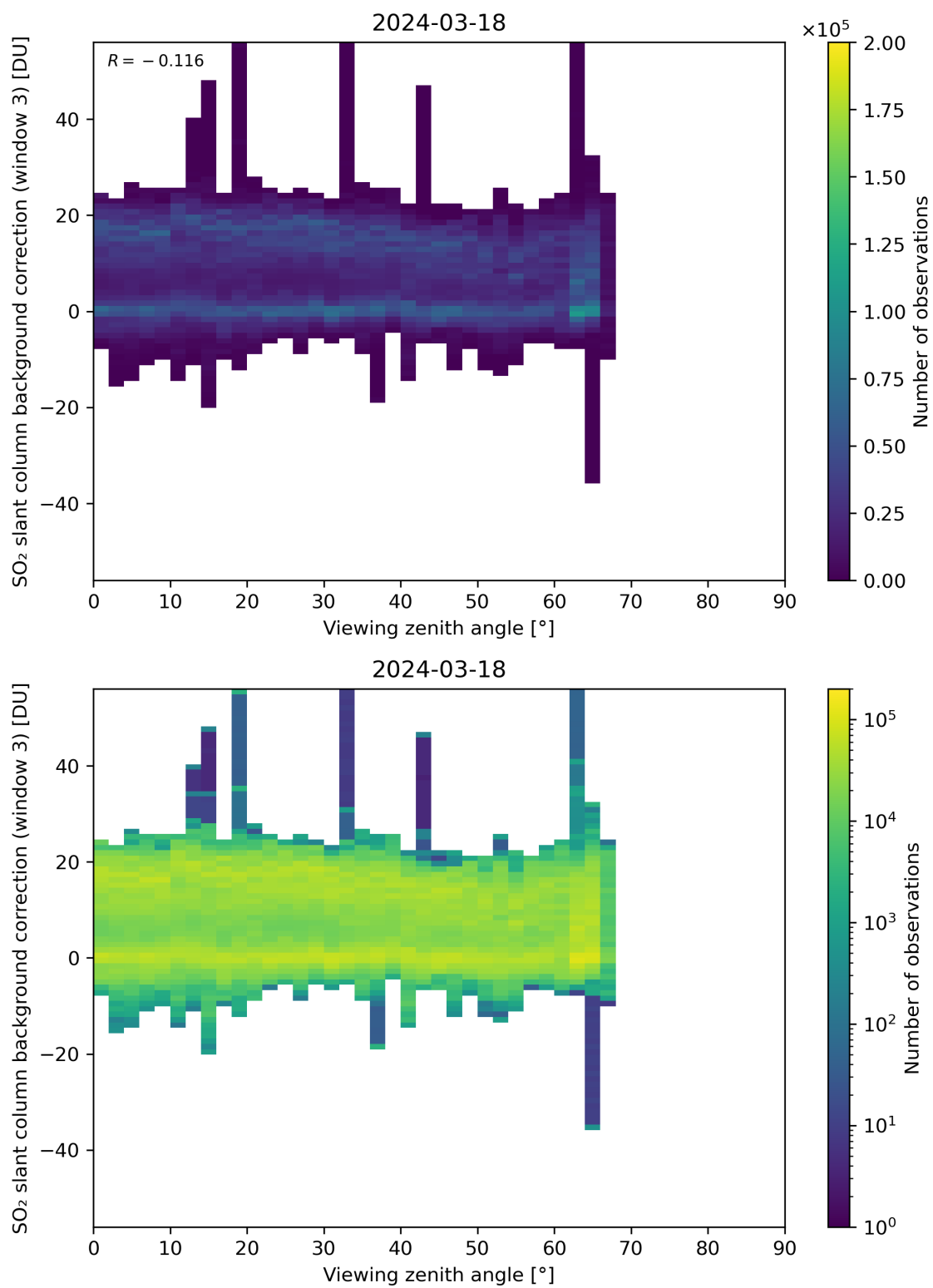
Figure 310: Scatter density plot of “Viewing zenith angle” against “SO 2 slant column background correction (window 3)” for 2024-03-17 to 2024-03-19.
