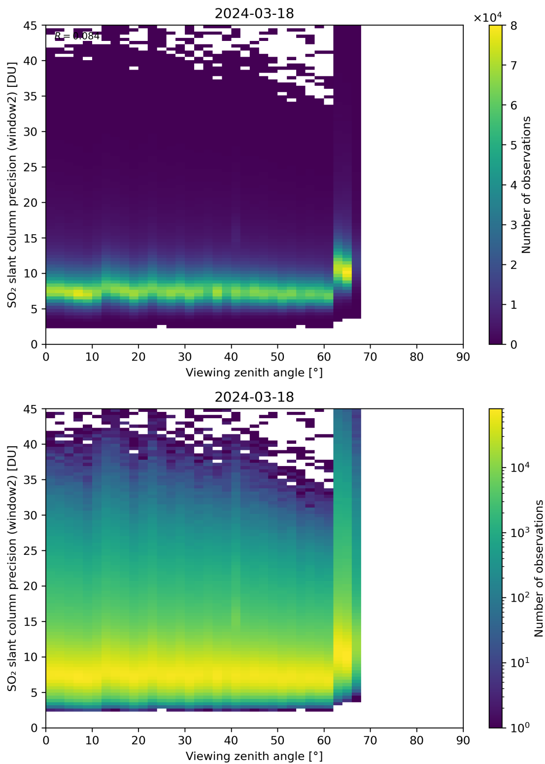
Figure 322: Scatter density plot of “Viewing zenith angle” against “SO 2 slant column precision (window2)” for 2024-03-17 to 2024-03-19.
