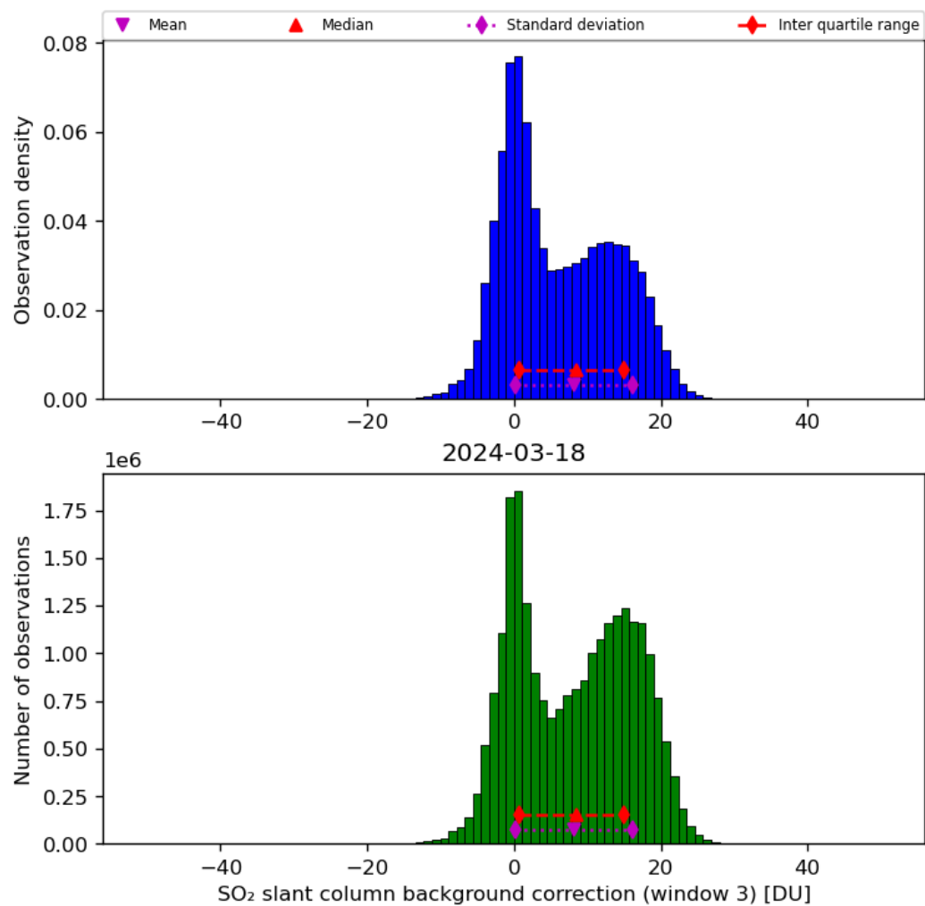
Figure 67: Histogram of “SO 2 slant column background correction (window 3)” for 2024-03-17 to 2024-03-19
