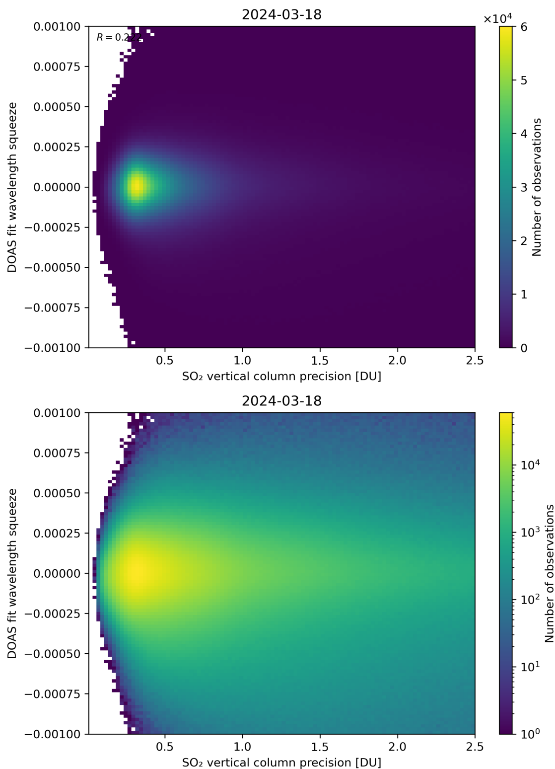
Figure 283: Scatter density plot of “SO 2 vertical column precision” against “DOAS fit wavelength squeeze” for 2024-03-17 to 2024-03-19.
