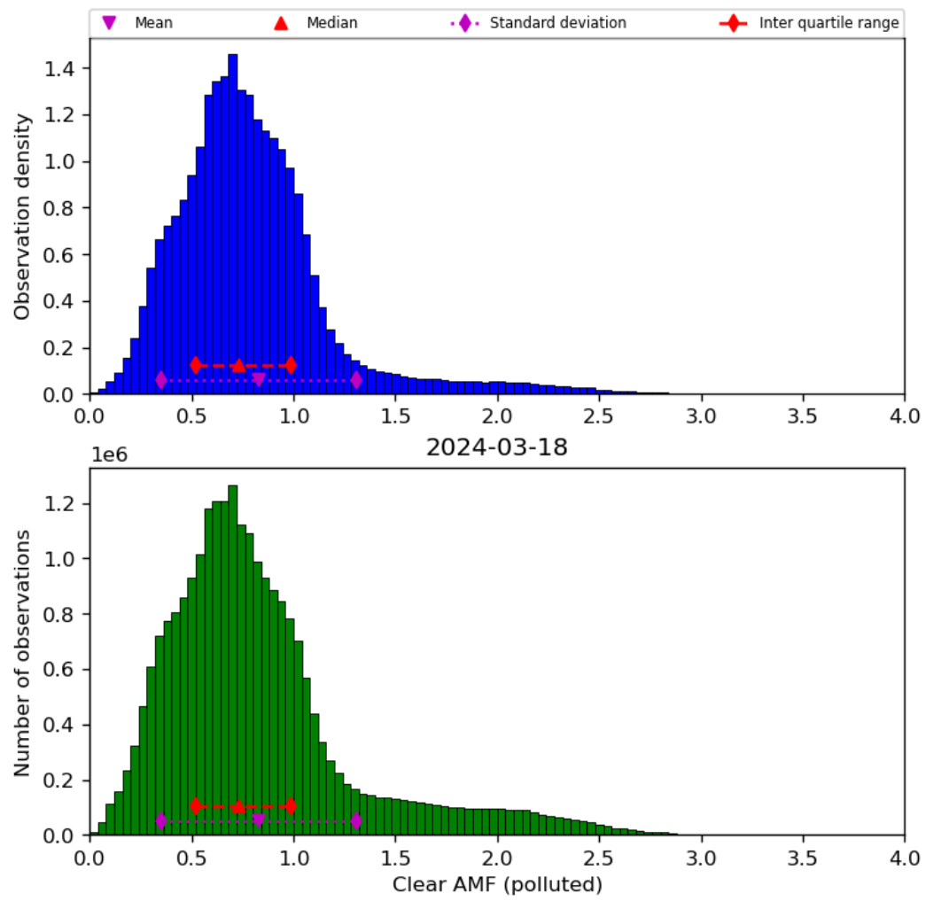
Figure 73: Histogram of “Clear AMF (polluted)” for 2024-03-17 to 2024-03-19
