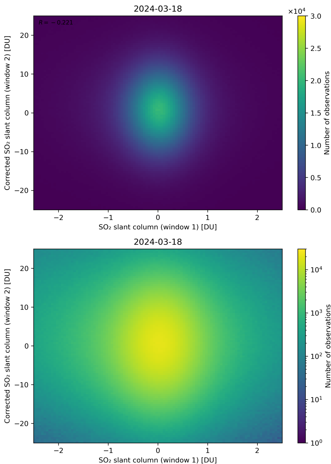
Figure 233: Scatter density plot of “SO 2 slant column (window 1)” against “Corrected SO 2 slant column (window 2)” for 2024-03-17 to 2024-03-19.
