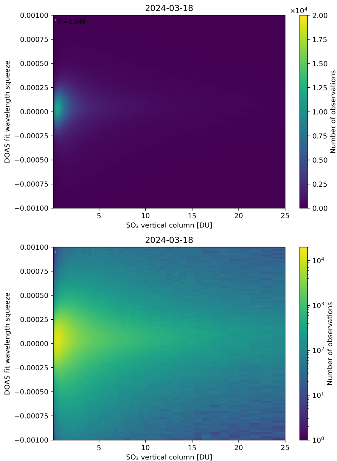
Figure 277: Scatter density plot of “SO 2 vertical column” against “DOAS fit wavelength squeeze” for 2024-03-17 to 2024-03-19.
