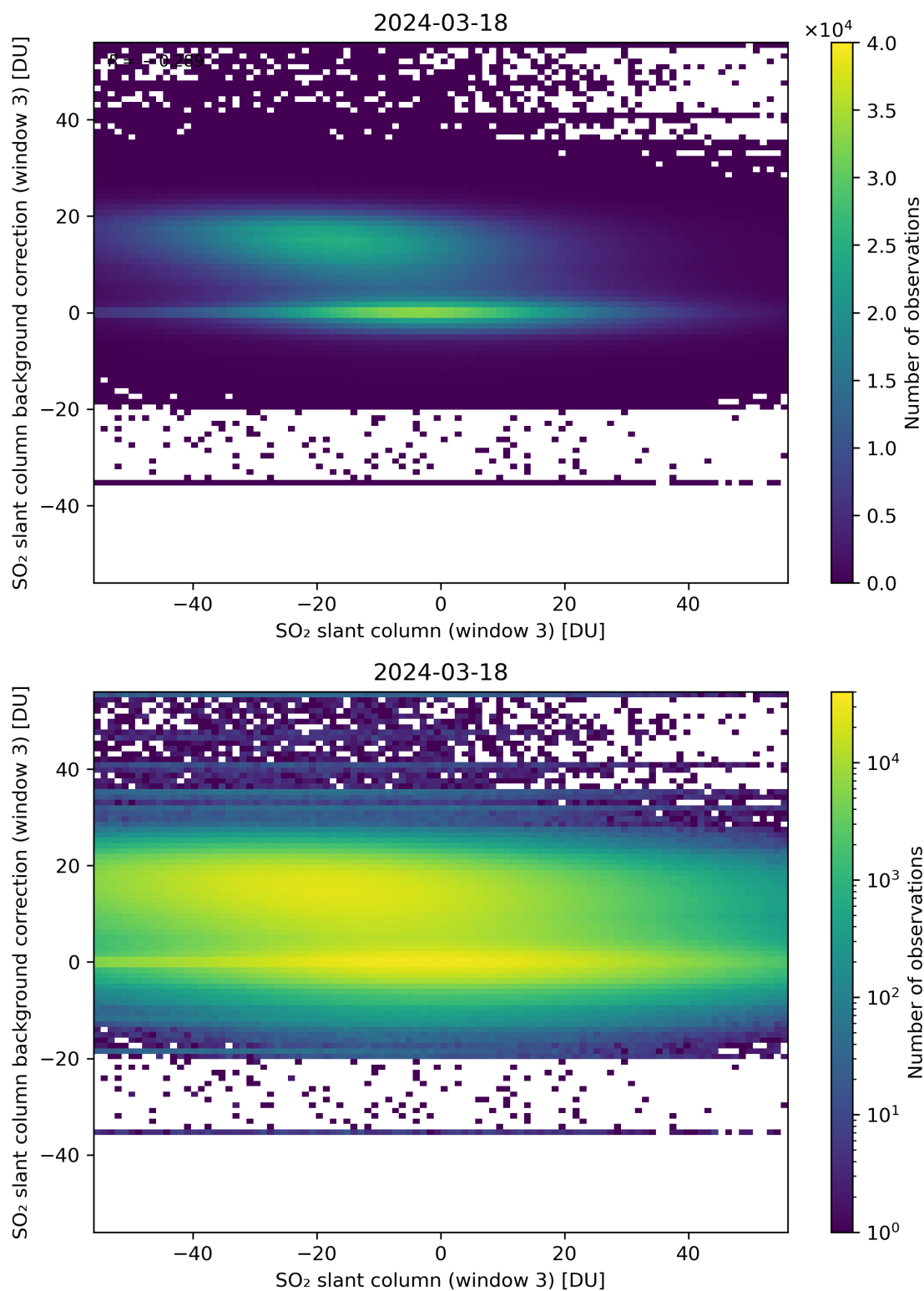
Figure 253: Scatter density plot of “SO 2 slant column (window 3)” against “SO 2 slant column background correction (window 3)” for 2024-03-17 to 2024-03-19.
