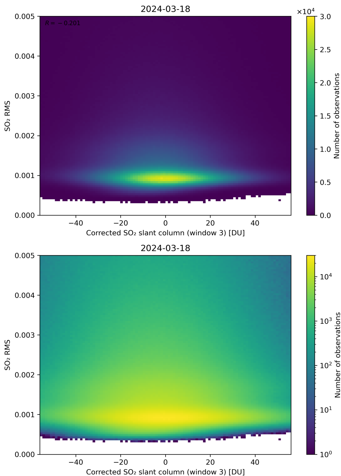
Figure 208: Scatter density plot of “Corrected SO 2 slant column (window 3)” against “SO 2 RMS” for 2024-03-17 to 2024-03-19.
