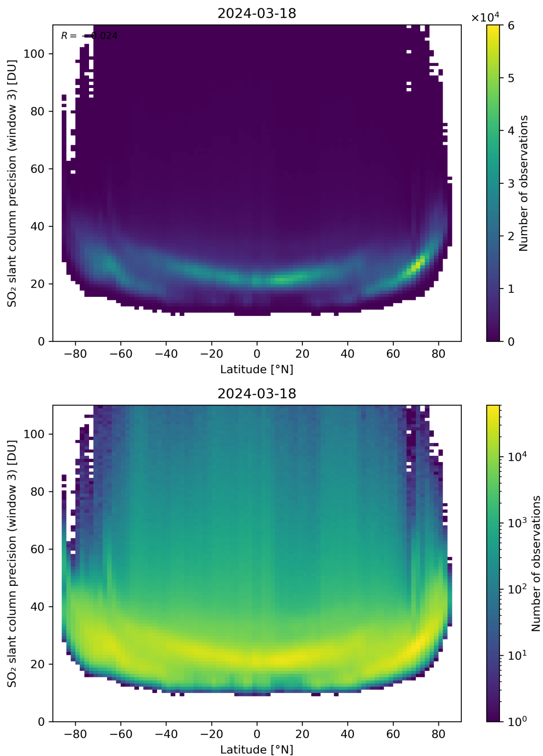
Figure 153: Scatter density plot of “Latitude” against “SO 2 slant column precision (window 3)” for 2024-03-17 to 2024-03-19.
