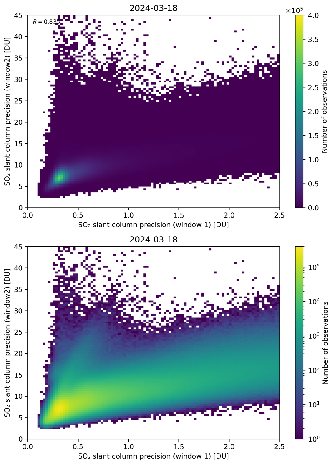
Figure 227: Scatter density plot of “SO 2 slant column precision (window 1)” against “SO 2 slant column precision (window2)” for 2024-03-17 to 2024-03-19.
