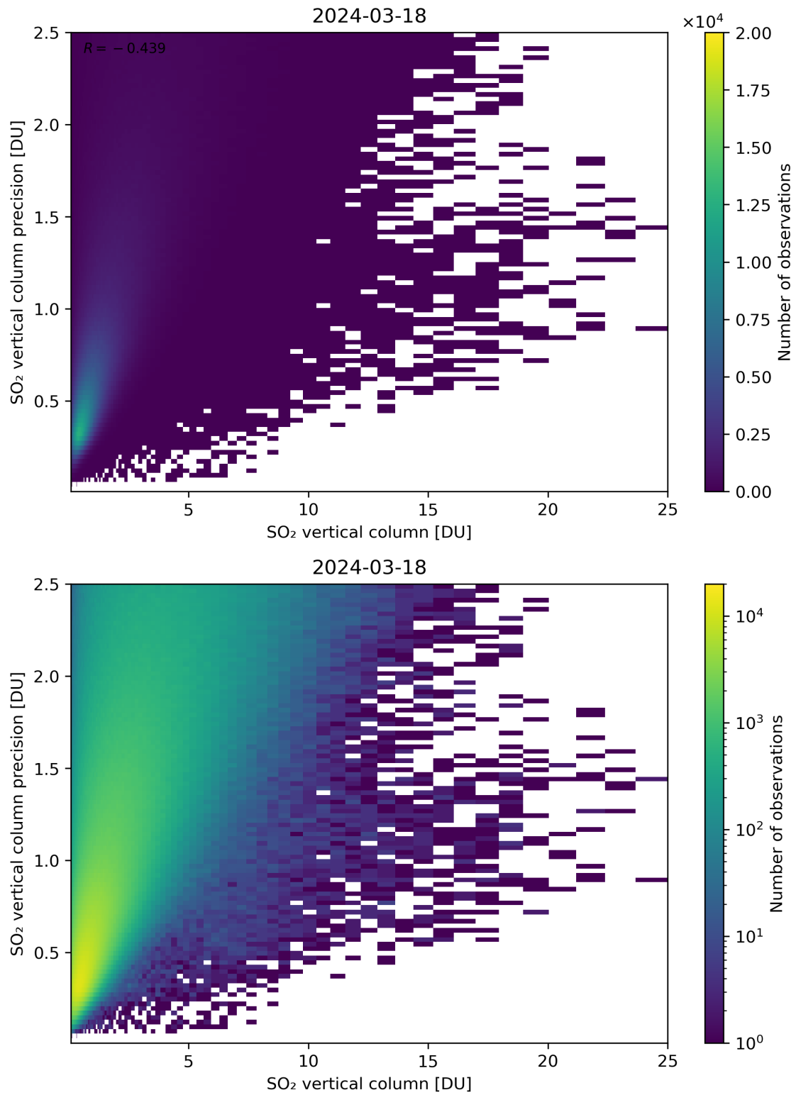
Figure 307: Scatter density plot of “SO 2 vertical column” against “SO 2 vertical column precision” for 2024-03-17 to 2024-03-19.
