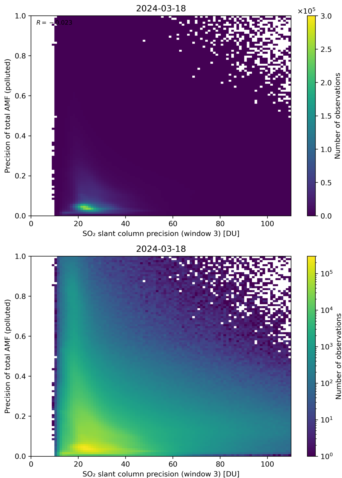
Figure 264: Scatter density plot of “SO 2 slant column precision (window 3)” against “Precision of total AMF (polluted)” for 2024-03-17 to 2024-03-19.
