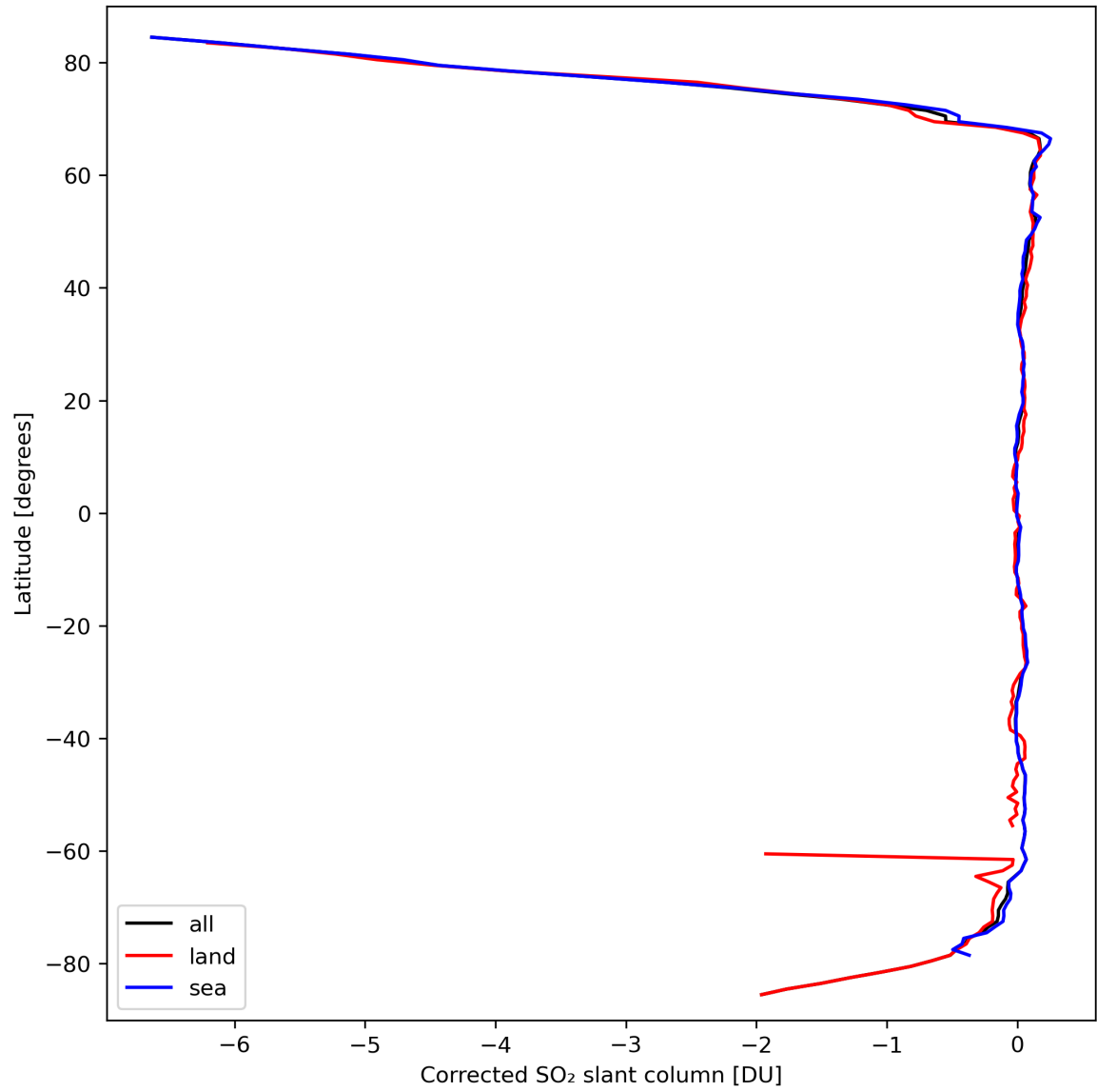
Figure 32: Zonal average of “Corrected SO 2 slant column” for 2024-03-17 to 2024-03-19.
