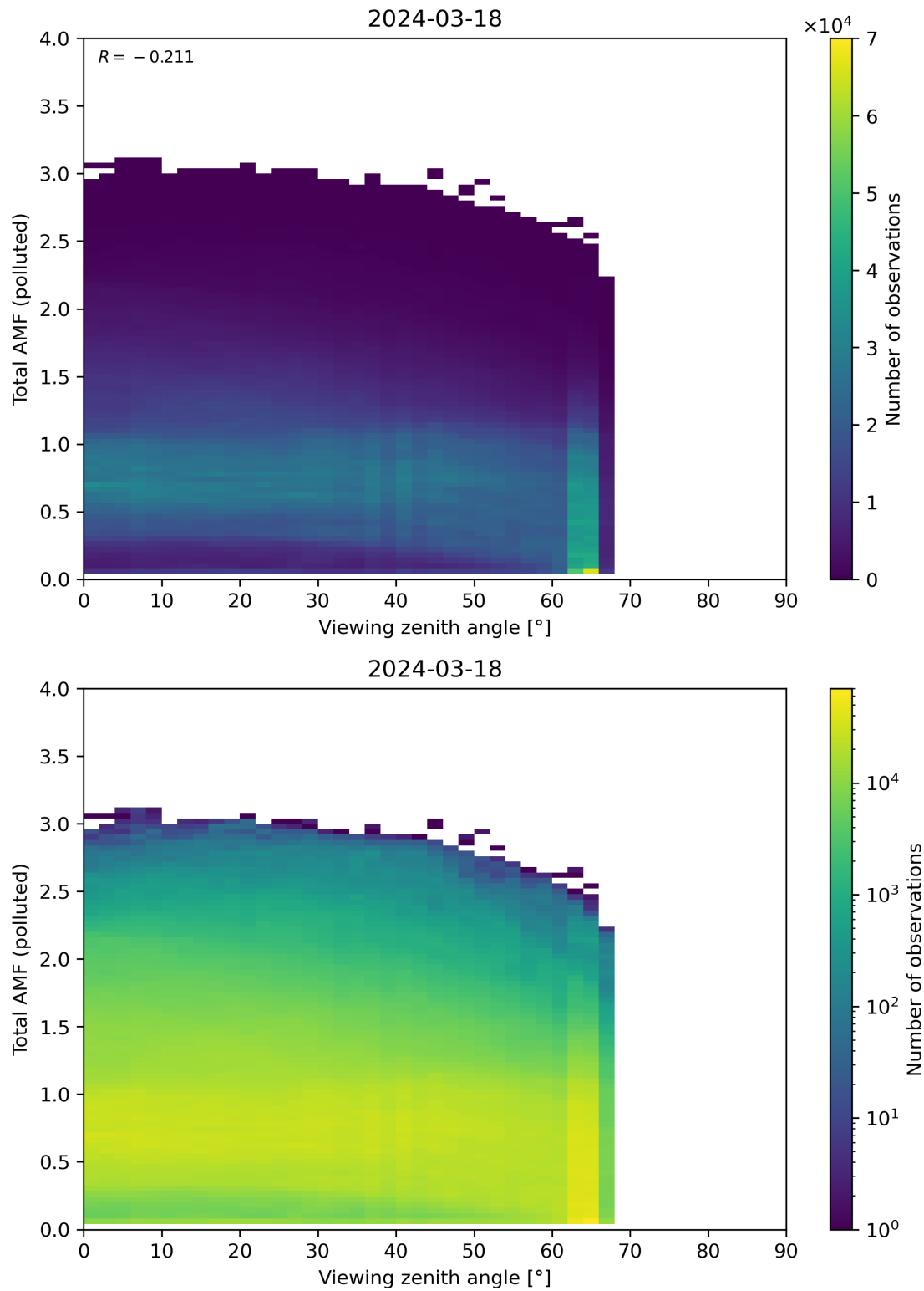
Figure 325: Scatter density plot of “Viewing zenith angle” against “Total AMF (polluted)” for 2024-03-17 to 2024-03-19.
