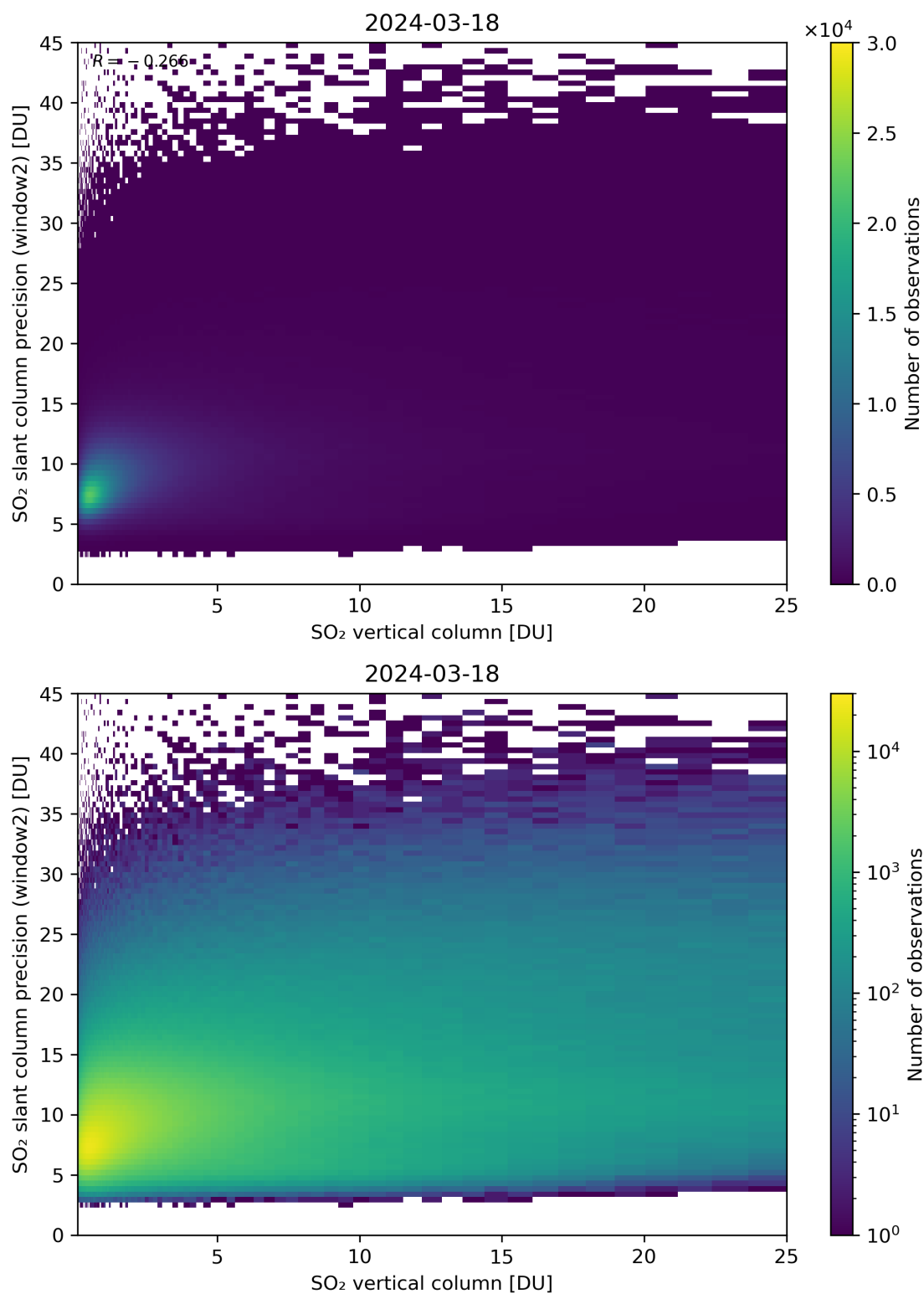
Figure 302: Scatter density plot of “SO 2 vertical column” against “SO 2 slant column precision (window2)” for 2024-03-17 to 2024-03-19.
