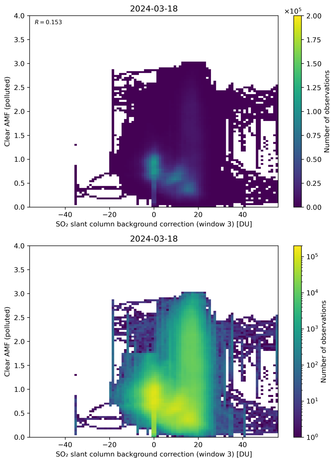
Figure 124: Scatter density plot of “SO 2 slant column background correction (window 3)” against “Clear AMF (polluted)” for 2024-03-17 to 2024-03-19.
