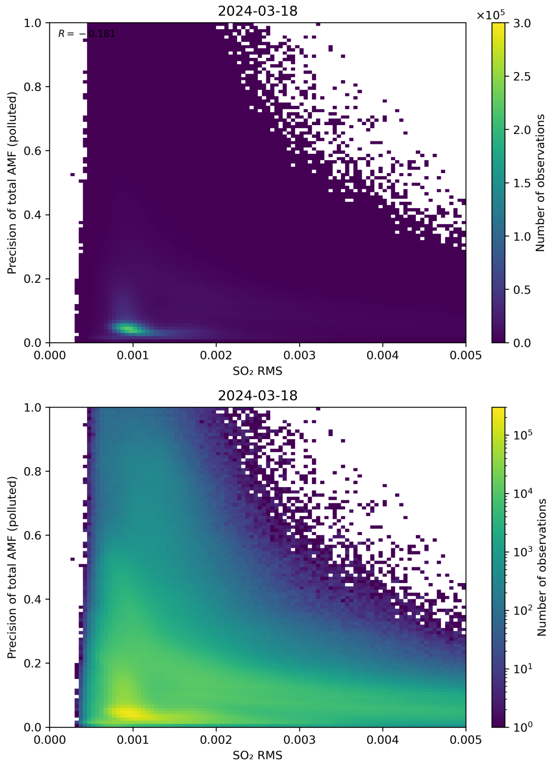
Figure 138: Scatter density plot of “SO 2 RMS” against “Precision of total AMF (polluted)” for 2024-03-17 to 2024-03-19.
