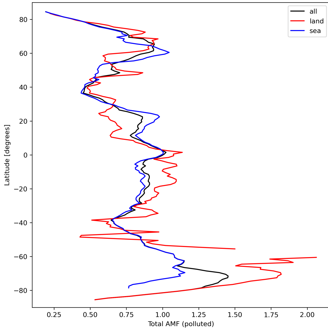
Figure 48: Zonal average of “Total AMF (polluted)” for 2024-03-17 to 2024-03-19.
