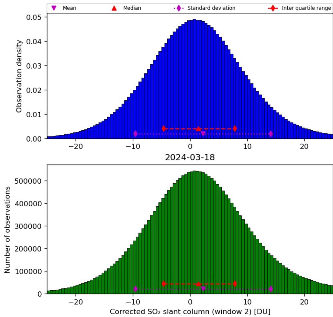
Figure 62: Histogram of “Corrected SO 2 slant column (window 2)” for 2024-03-17 to 2024-03-19
