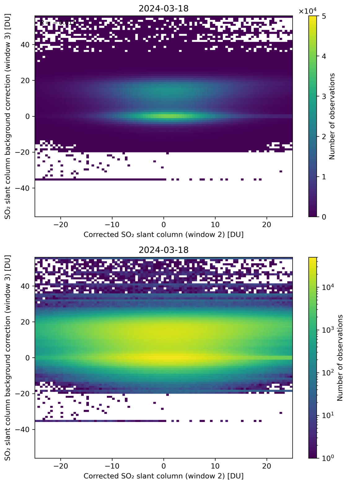
Figure 195: Scatter density plot of “Corrected SO 2 slant column (window 2)” against “SO 2 slant column background correction (window 3)” for 2024-03-17 to 2024-03-19.
