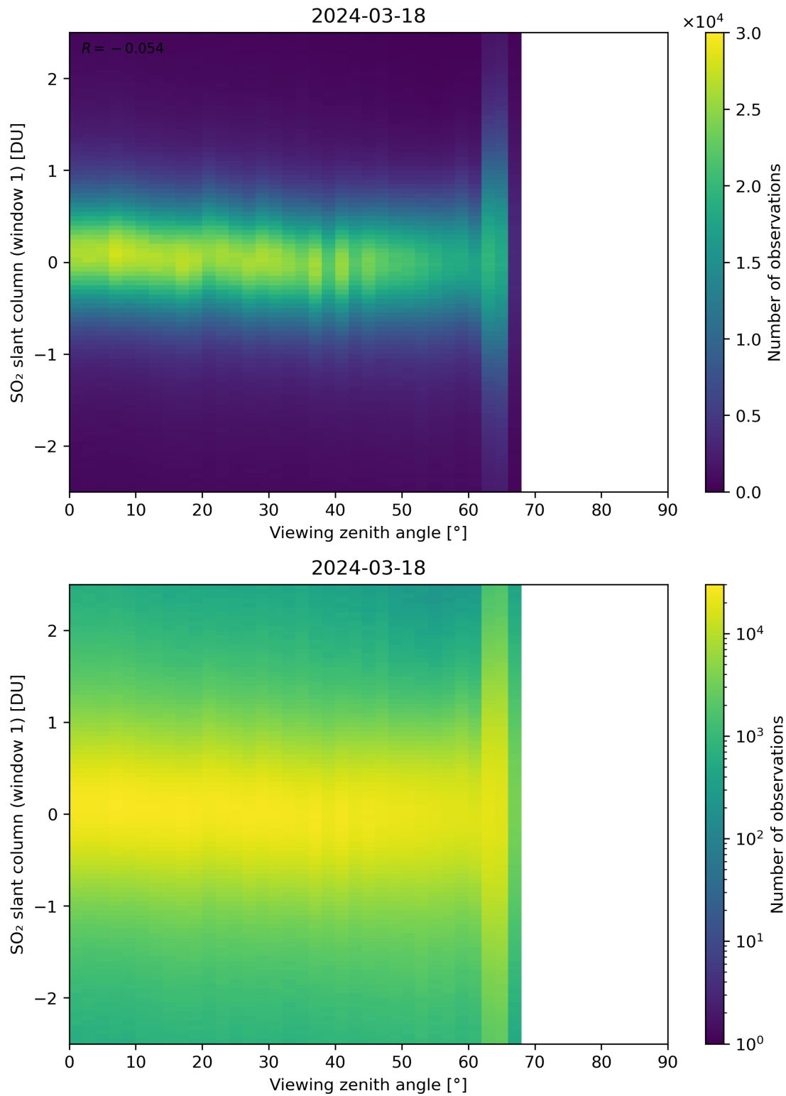
Figure 320: Scatter density plot of “Viewing zenith angle” against “SO 2 slant column (window 1)” for 2024-03-17 to 2024-03-19.
