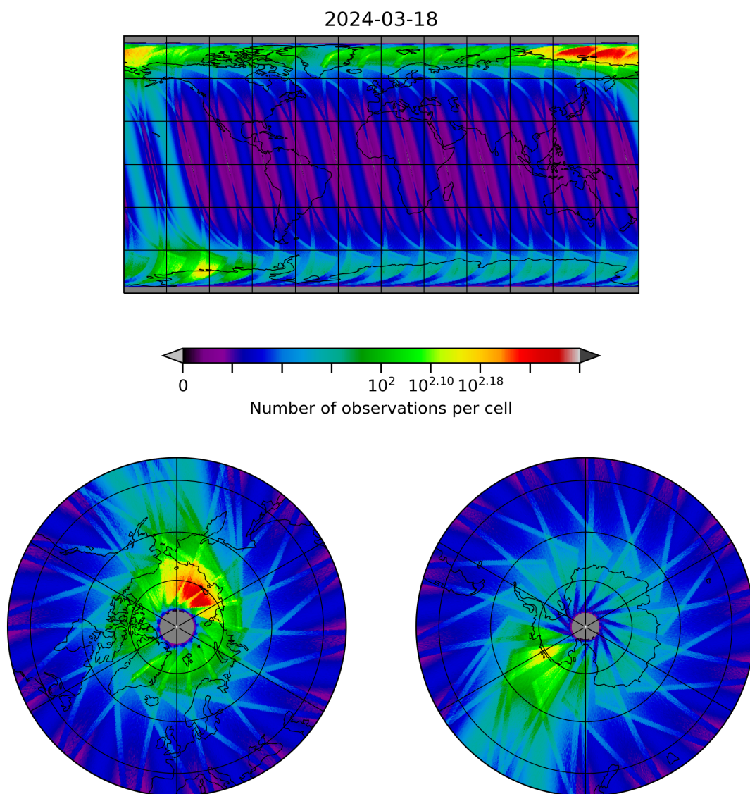
Figure 28: Map of the number of observations for 2024-03-17 to 2024-03-19
