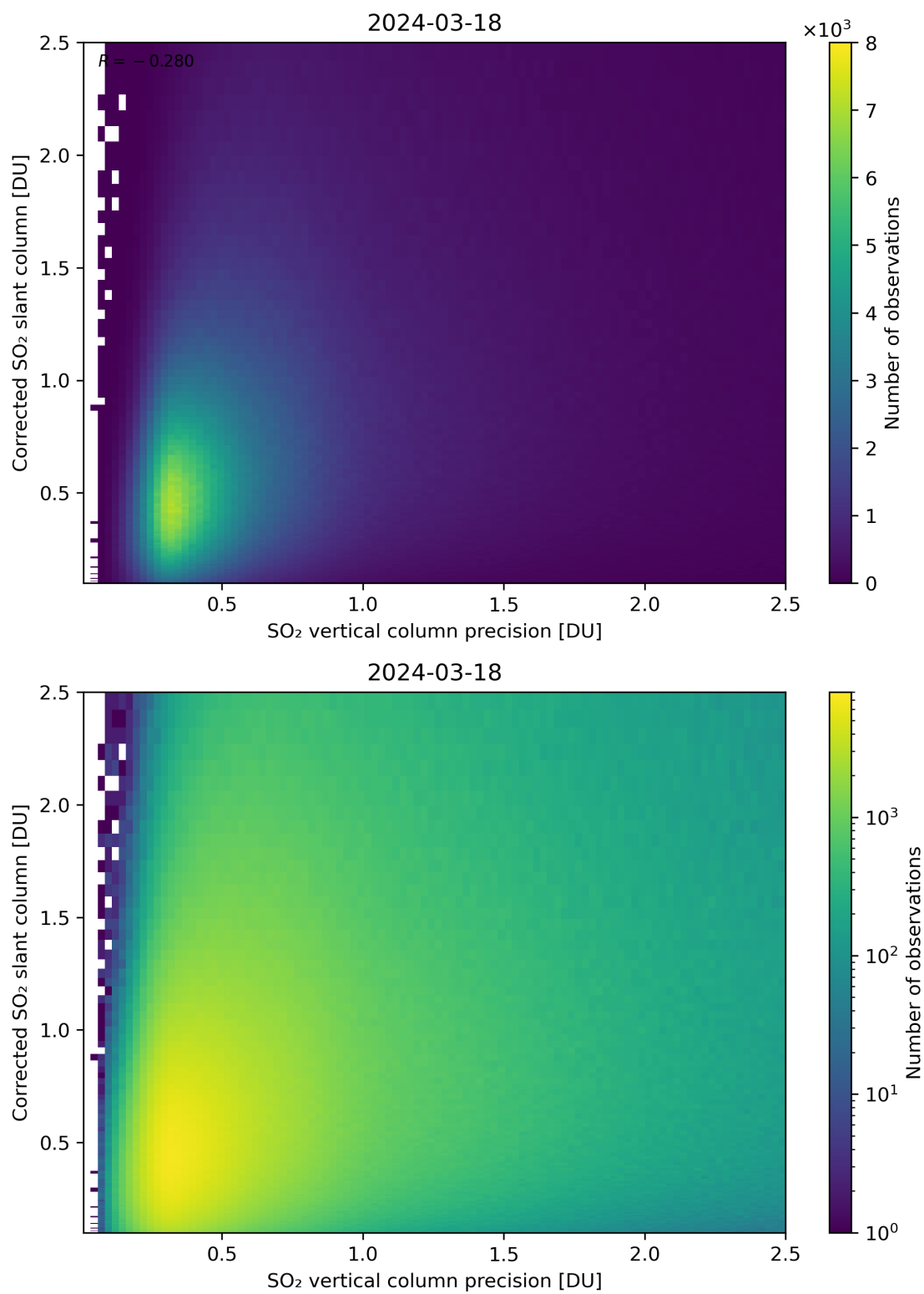
Figure 286: Scatter density plot of “SO 2 vertical column precision” against “Corrected SO 2 slant column” for 2024-03-17 to 2024-03-19.
