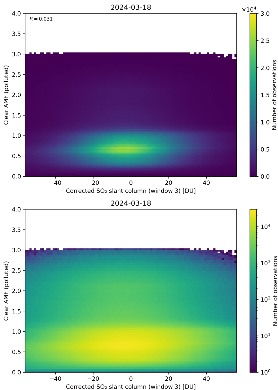
Figure 209: Scatter density plot of “Corrected SO 2 slant column (window 3)” against “Clear AMF (polluted)” for 2024-03-17 to 2024-03-19.
