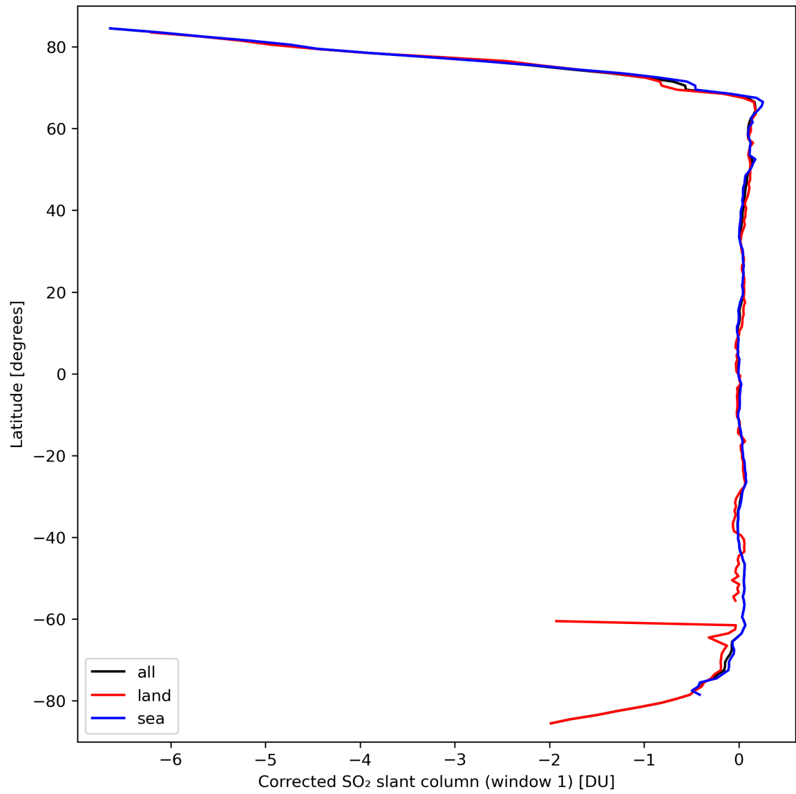
Figure 35: Zonal average of “Corrected SO 2 slant column (window 1)” for 2024-03-17 to 2024-03-19.
