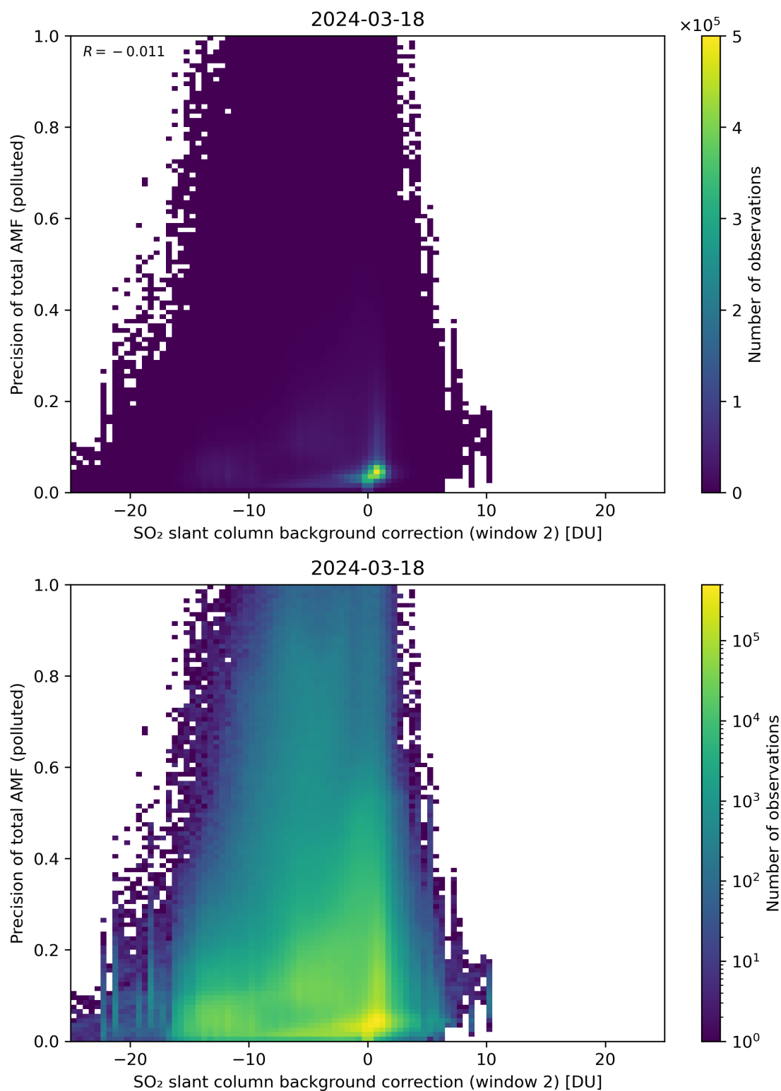
Figure 120: Scatter density plot of “SO 2 slant column background correction (window 2)” against “Precision of total AMF (polluted)” for 2024-03-17 to 2024-03-19.
