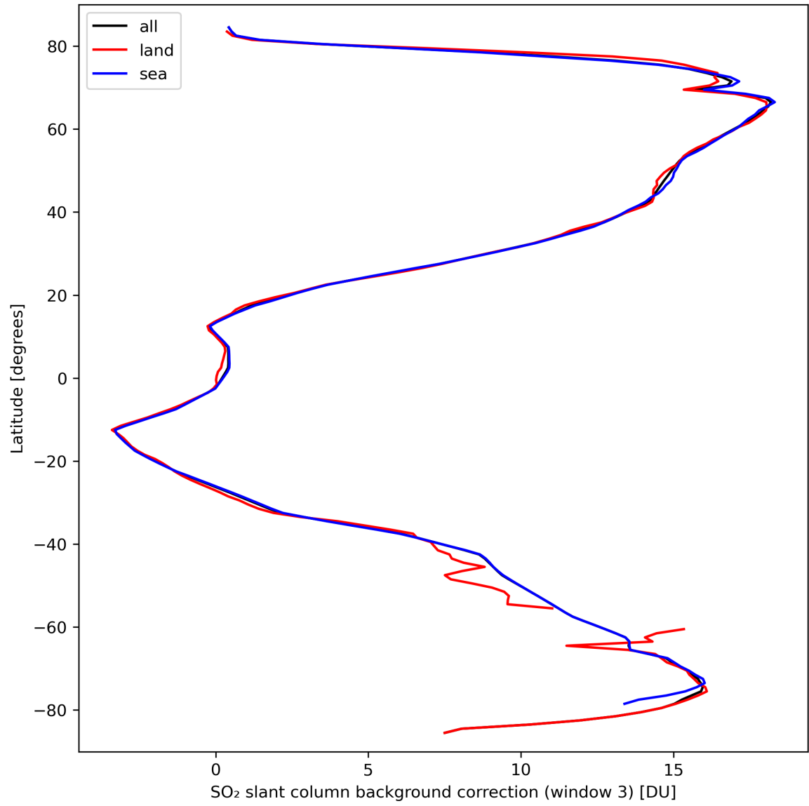
Figure 44: Zonal average of "SO 2 slant column background correction (window 3)" for 2024-03-17 to 2024-03-19.
