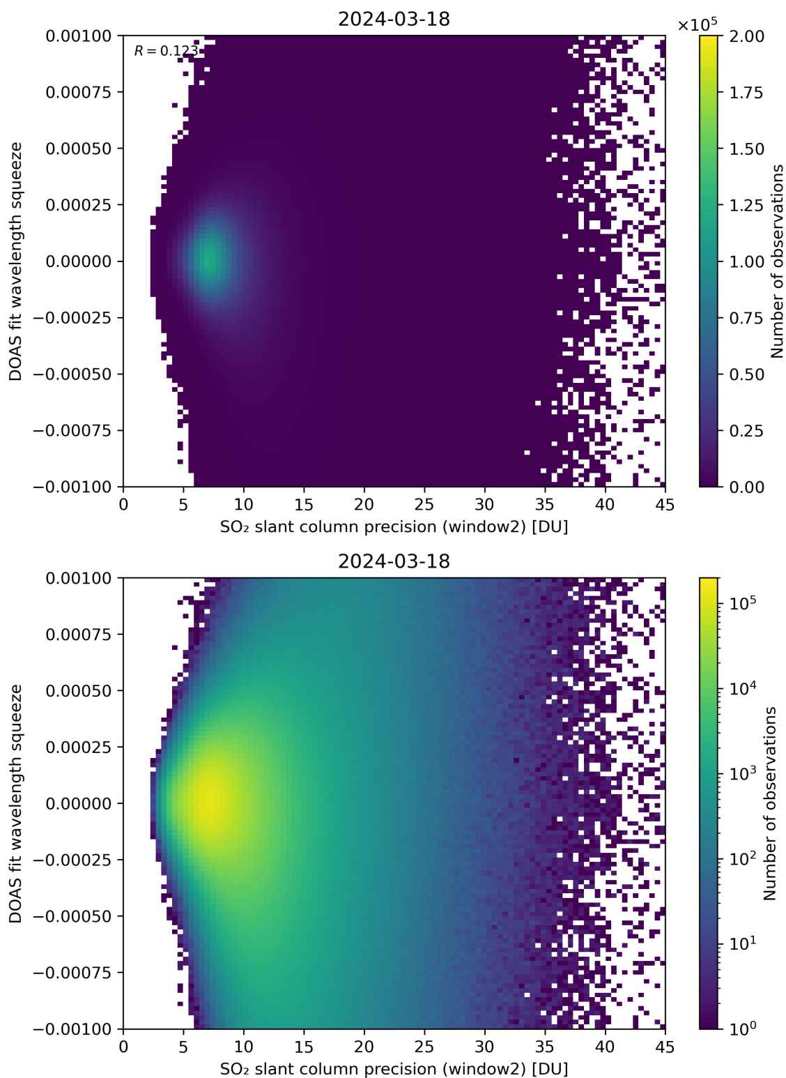
Figure 244: Scatter density plot of “SO 2 slant column precision (window2)” against “DOAS fit wavelength squeeze” for 2024-03-17 to 2024-03-19.
