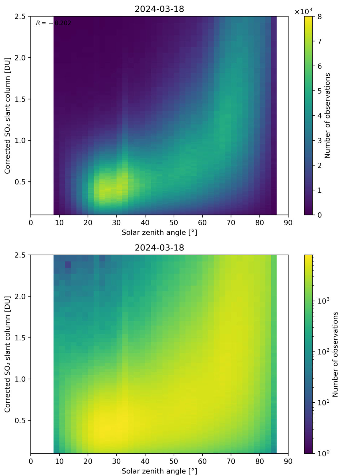
Figure 166: Scatter density plot of “Solar zenith angle” against “Corrected SO 2 slant column” for 2024-03-17 to 2024-03-19.
