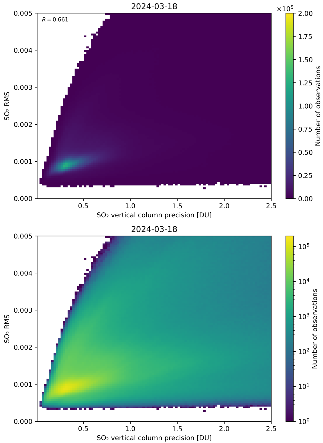
Figure 284: Scatter density plot of “SO 2 vertical column precision” against “SO 2 RMS” for 2024-03-17 to 2024-03-19.
