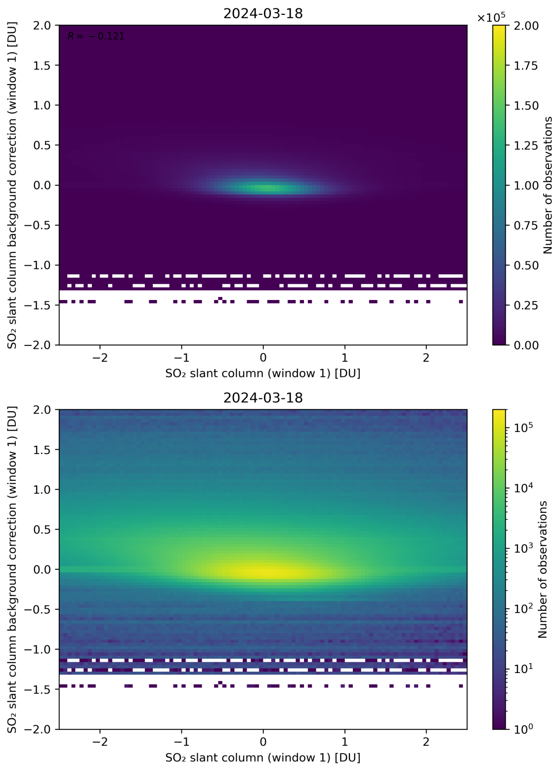
Figure 212: Scatter density plot of “SO 2 slant column (window 1)” against “SO 2 slant column background correction (window 1)” for 2024-03-17 to 2024-03-19.
