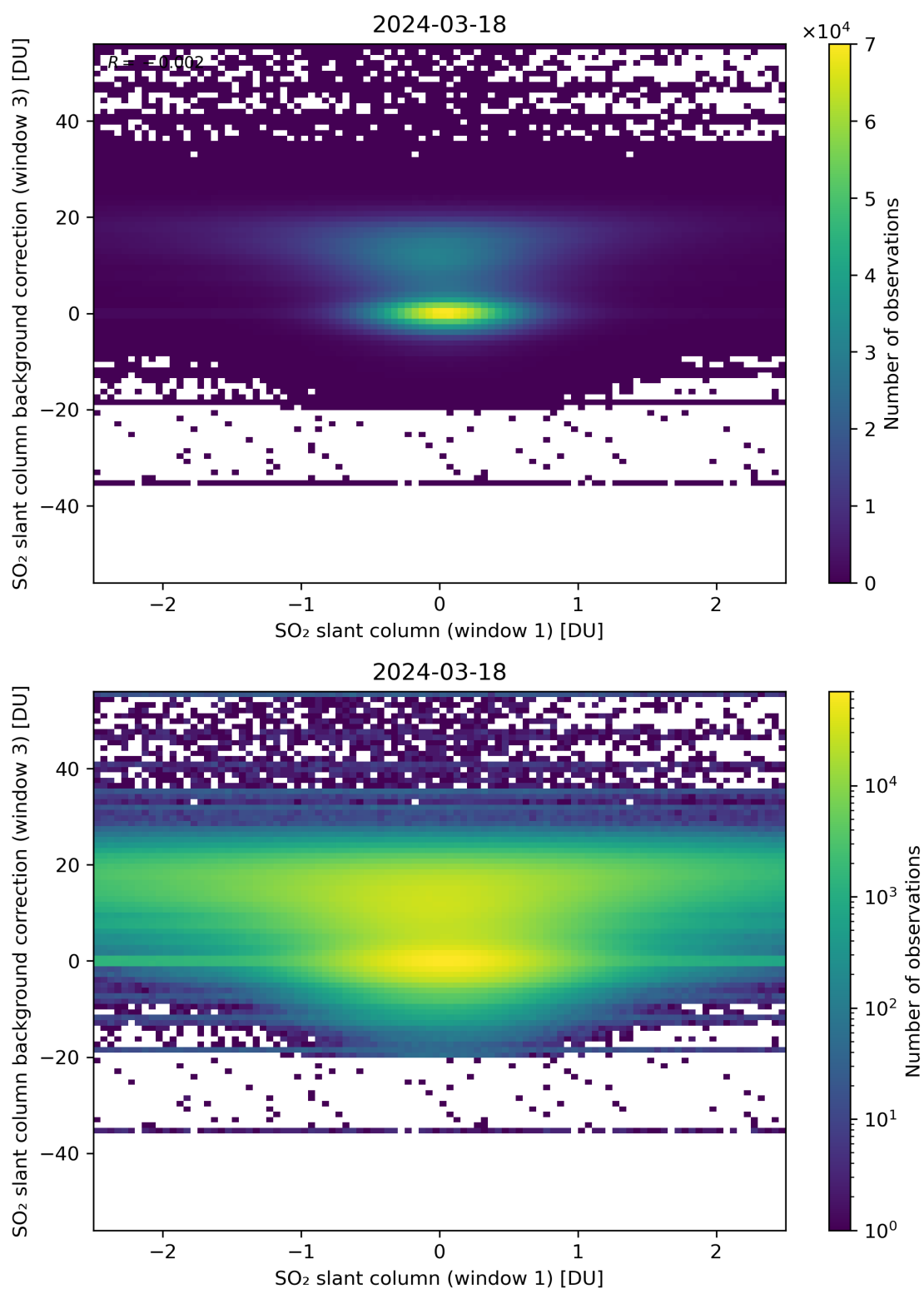
Figure 214: Scatter density plot of “SO 2 slant column (window 1)” against “SO 2 slant column background correction (window 3)” for 2024-03-17 to 2024-03-19.
