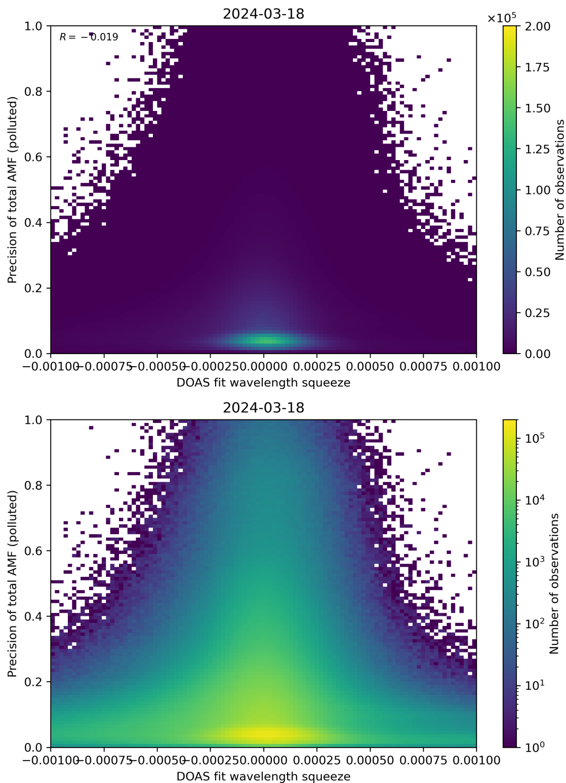
Figure 135: Scatter density plot of “DOAS fit wavelength squeeze” against “Precision of total AMF (polluted)” for 2024-03-17 to 2024-03-19.
