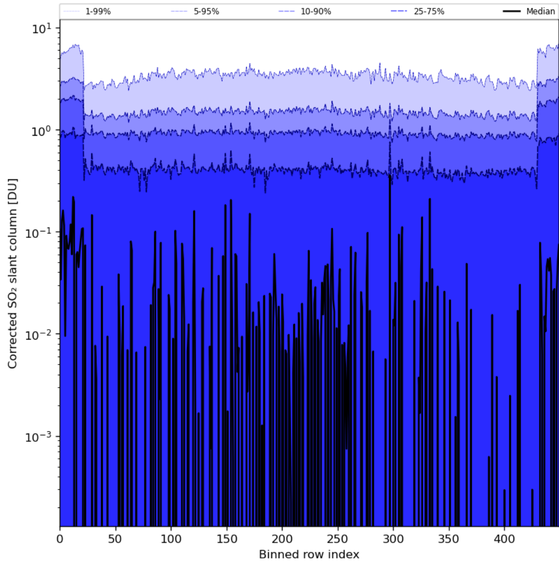
Figure 78: Along track statistics of “Corrected SO 2 slant column” for 2024-03-17 to 2024-03-19
