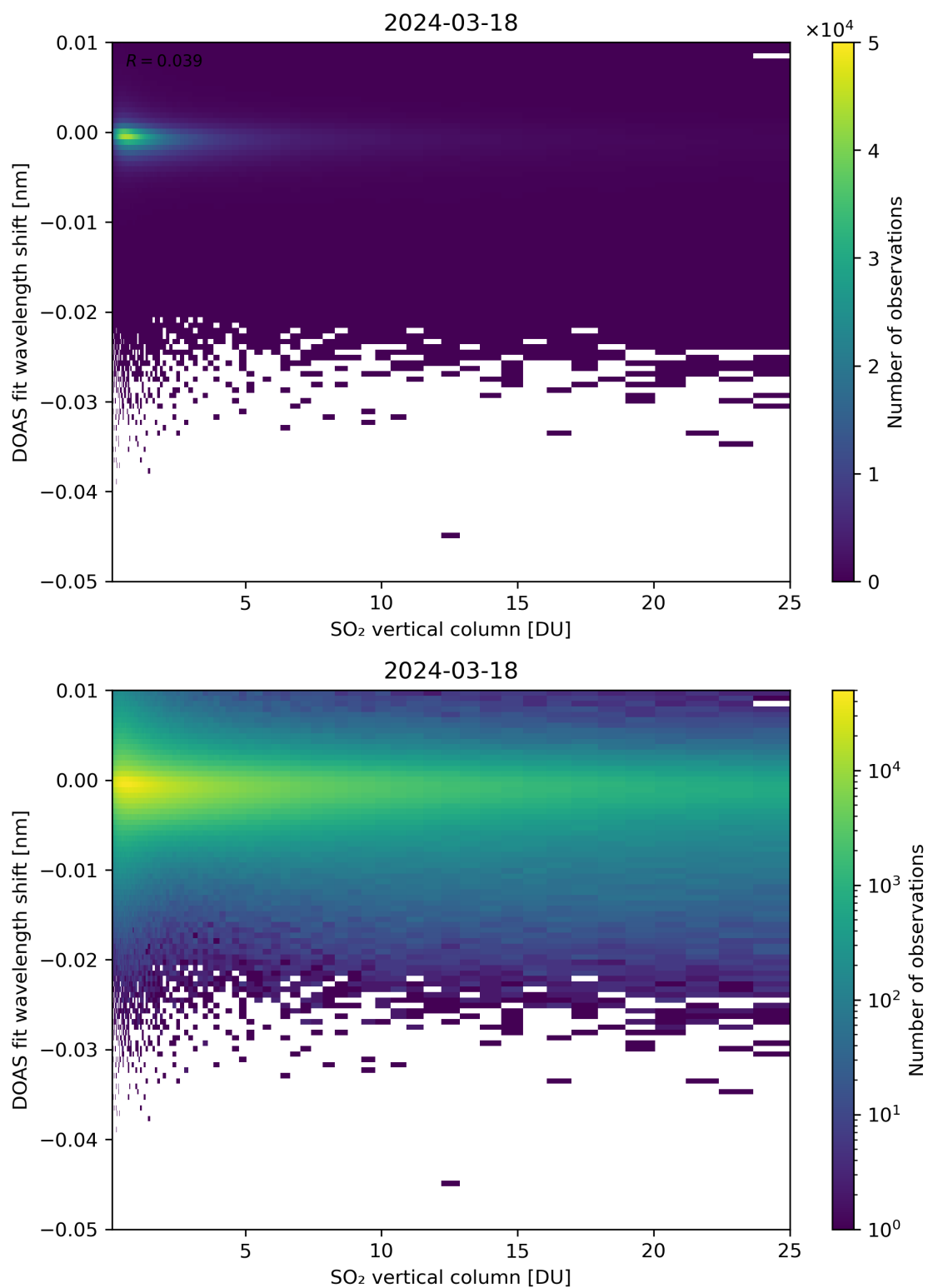
Figure 276: Scatter density plot of “SO 2 vertical column” against “DOAS fit wavelength shift” for 2024-03-17 to 2024-03-19.
