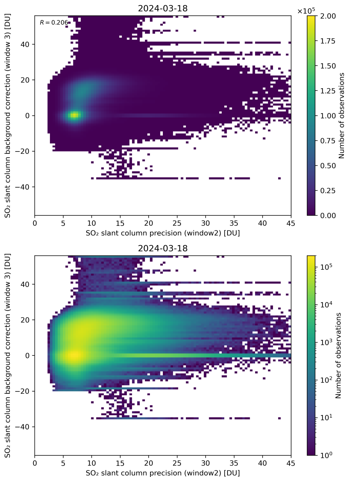
Figure 242: Scatter density plot of “SO 2 slant column precision (window2)” against “SO 2 slant column background correction (window 3)” for 2024-03-17 to 2024-03-19.
