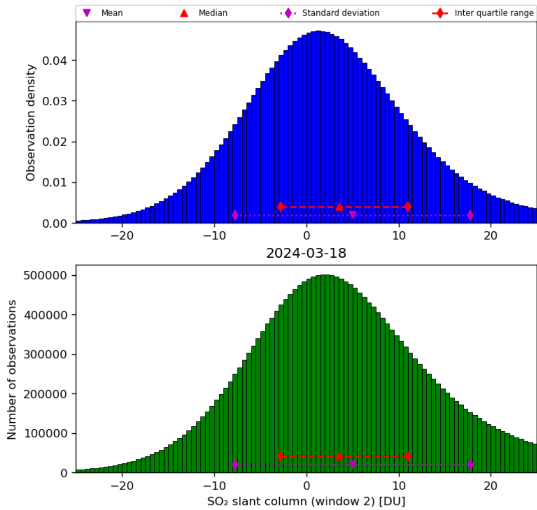
Figure 60: Histogram of “SO 2 slant column (window 2)” for 2024-03-17 to 2024-03-19
