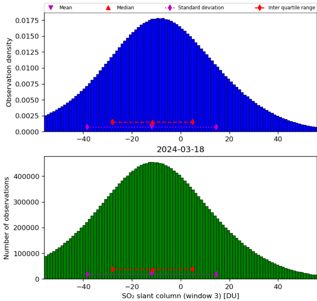
Figure 64: Histogram of “SO 2 slant column (window 3)” for 2024-03-17 to 2024-03-19
