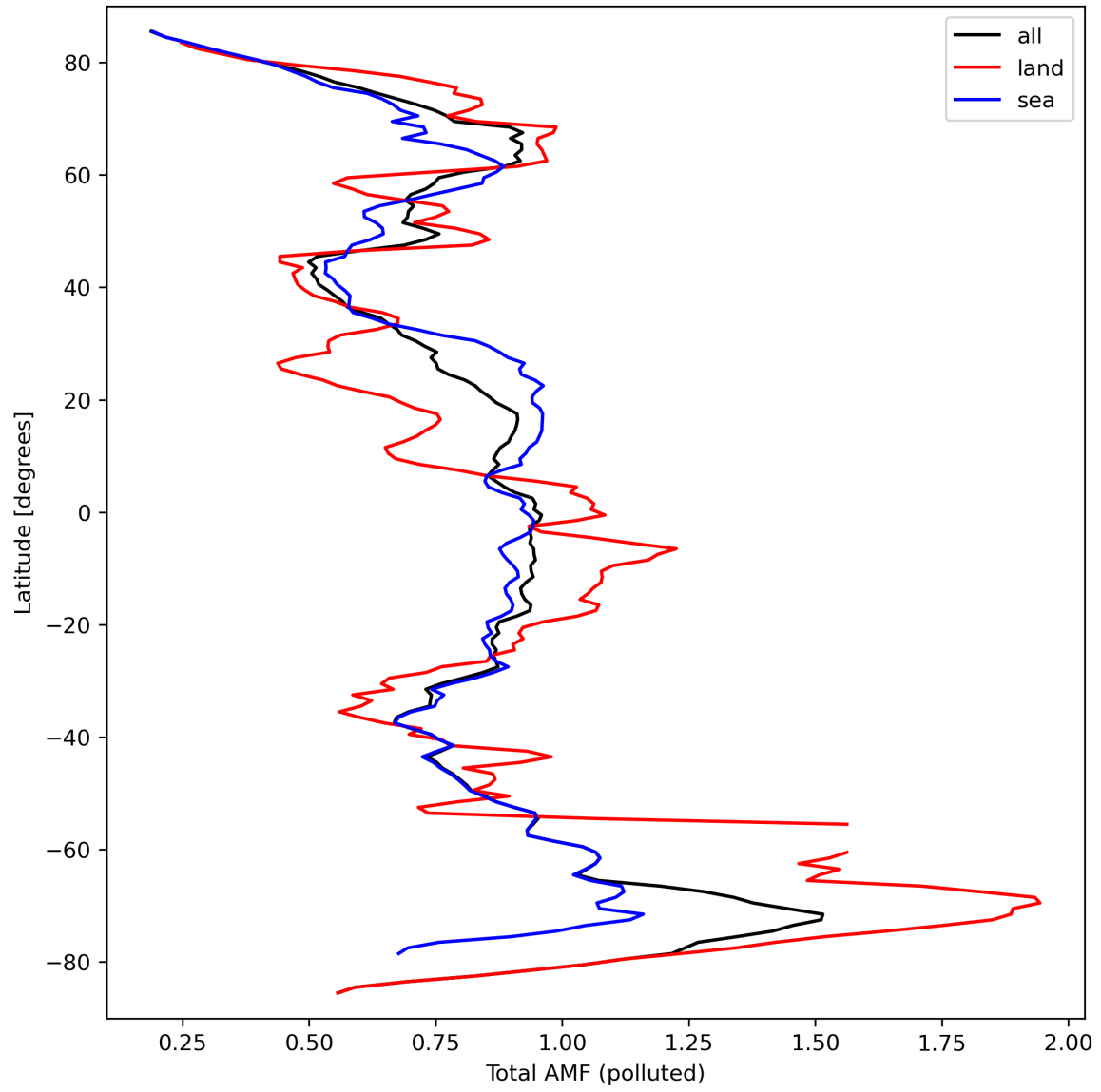
Figure 48: Zonal average of “Total AMF (polluted)” for 2024-03-20 to 2024-03-21.
