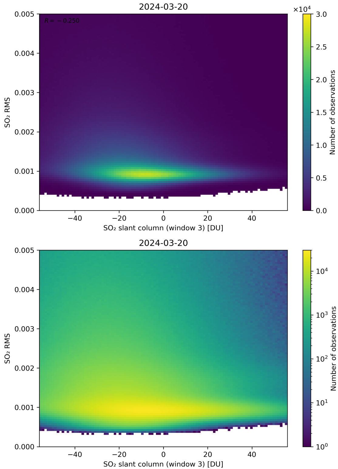
Figure 256: Scatter density plot of “SO 2 slant column (window 3)” against “SO 2 RMS” for 2024-03-20 to 2024-03-21.
