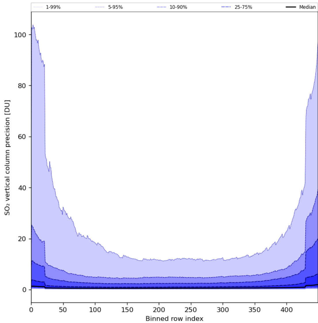
Figure 77: Along track statistics of “SO 2 vertical column precision” for 2024-03-20 to 2024-03-21
