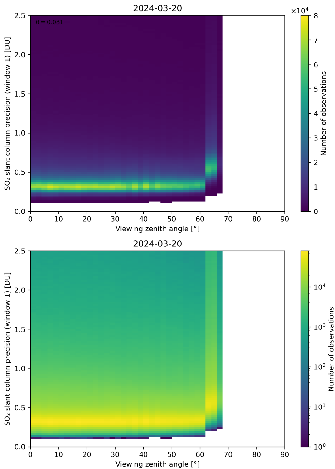
Figure 321: Scatter density plot of “Viewing zenith angle” against “SO 2 slant column precision (window 1)” for 2024-03-20 to 2024-03-21.
