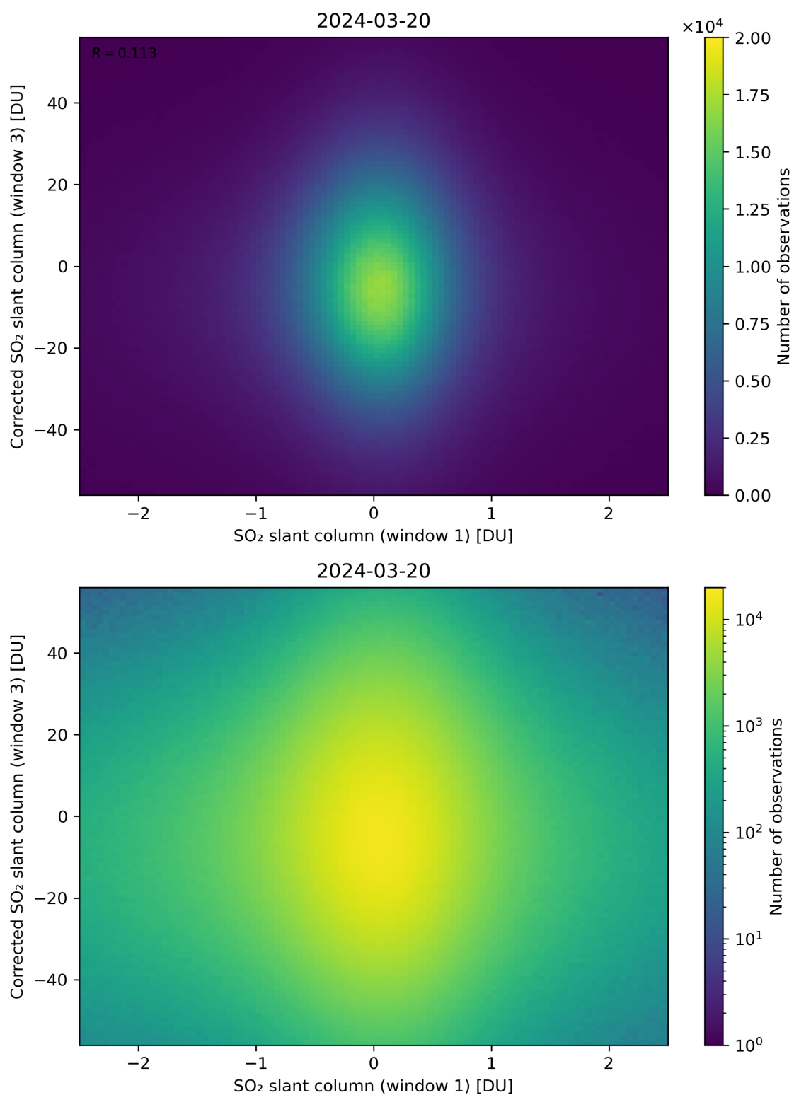
Figure 234: Scatter density plot of “SO 2 slant column (window 1)” against “Corrected SO 2 slant column (window 3)” for 2024-03-20 to 2024-03-21.
