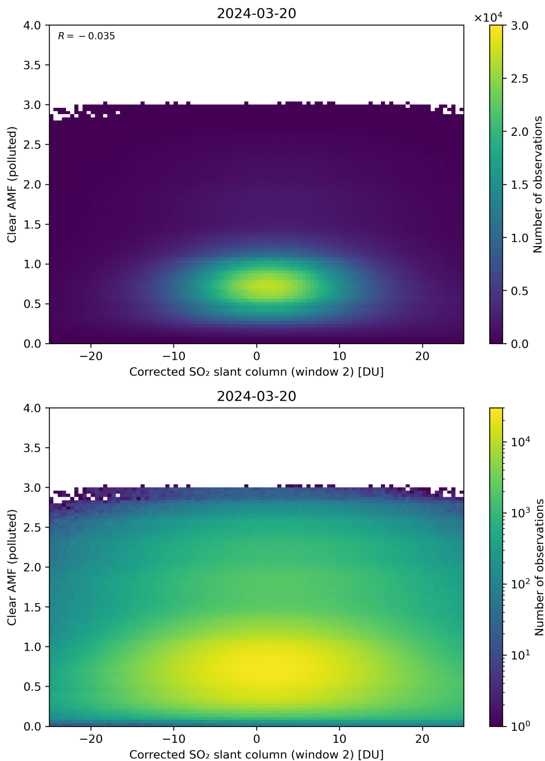
Figure 199: Scatter density plot of “Corrected SO 2 slant column (window 2)” against “Clear AMF (polluted)” for 2024-03-20 to 2024-03-21.
