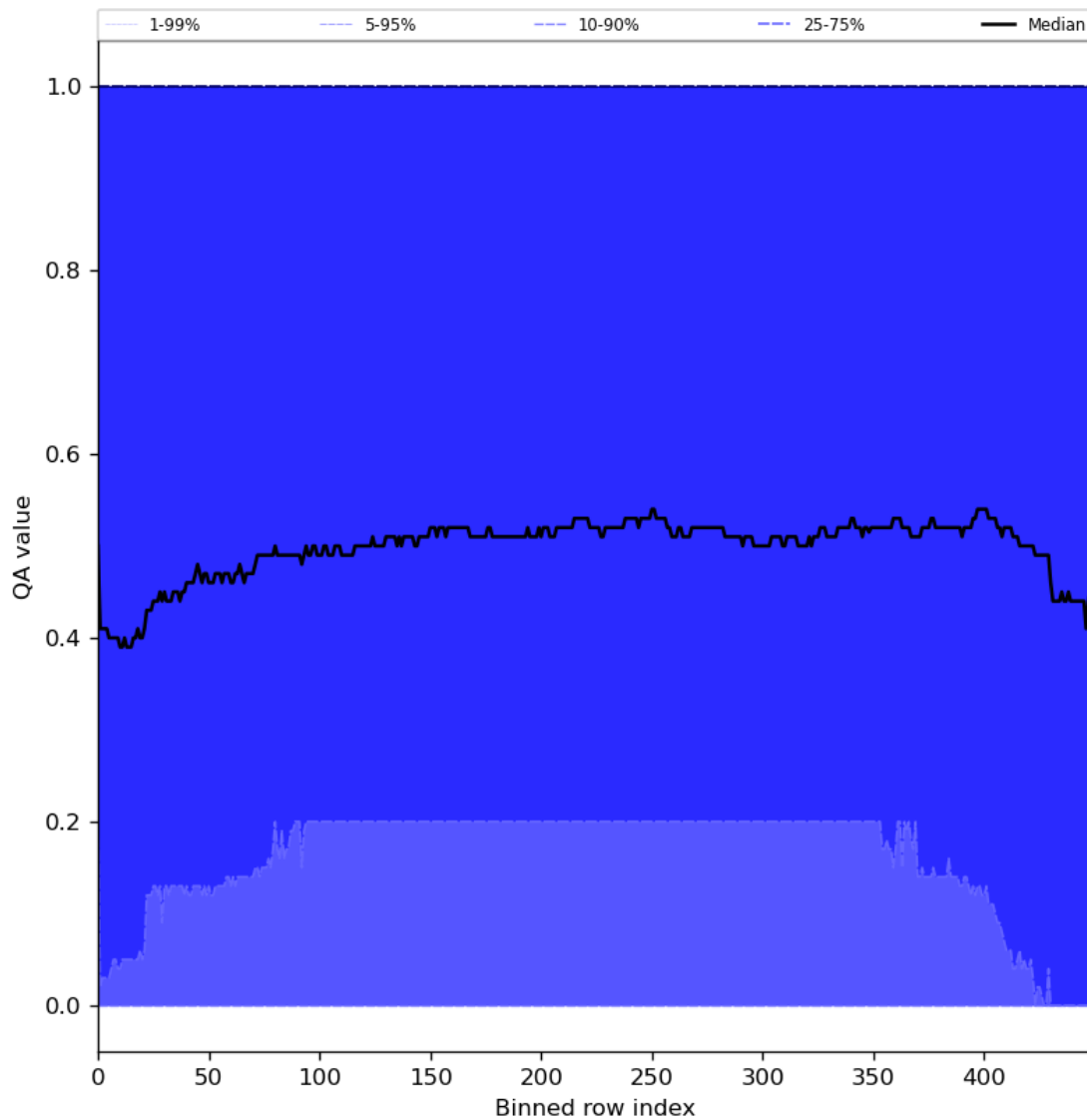
Figure 75: Along track statistics of “QA value” for 2024-03-20 to 2024-03-21
