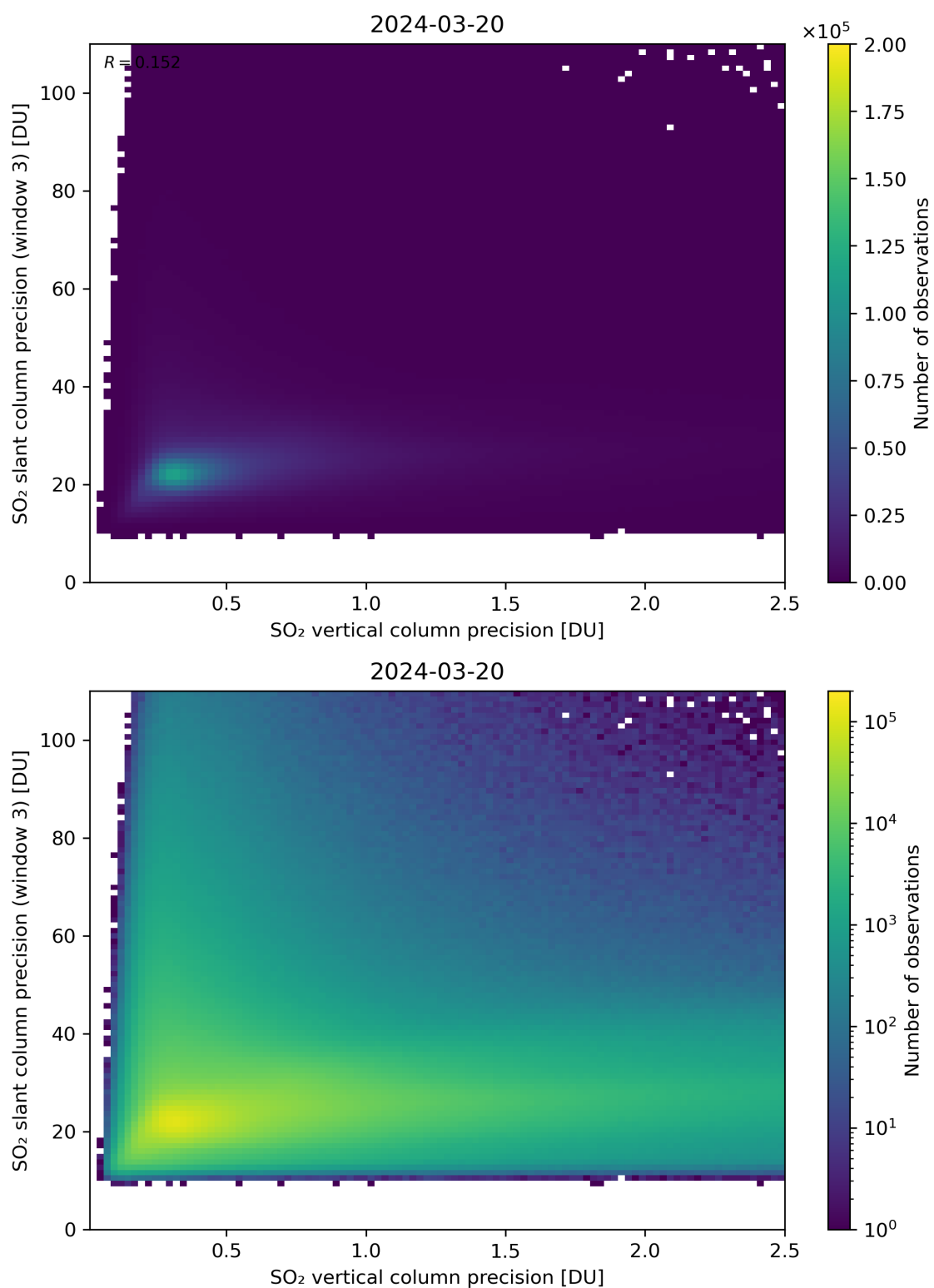
Figure 293: Scatter density plot of “SO 2 vertical column precision” against “SO 2 slant column precision (window 3)” for 2024-03-20 to 2024-03-21.
