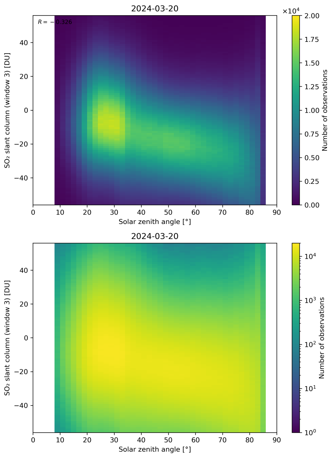
Figure 172: Scatter density plot of “Solar zenith angle” against “SO 2 slant column (window 3)” for 2024-03-20 to 2024-03-21.
