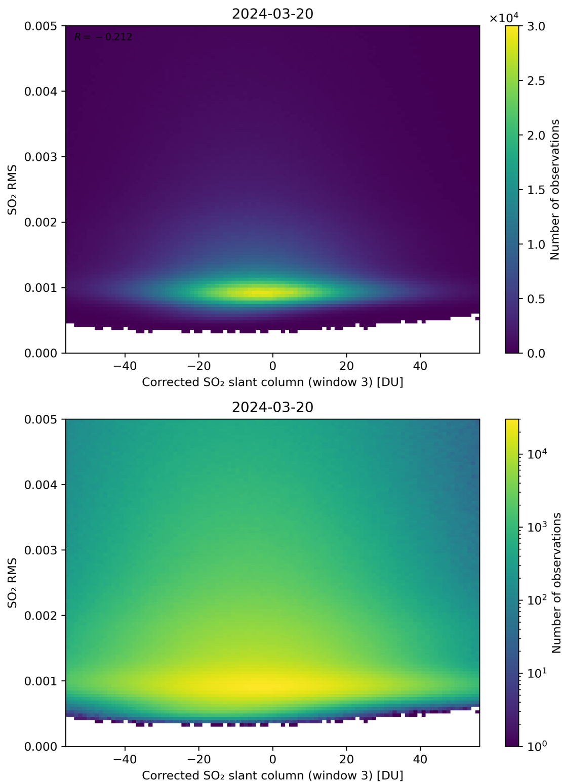
Figure 208: Scatter density plot of “Corrected SO 2 slant column (window 3)” against “SO 2 RMS” for 2024-03-20 to 2024-03-21.
