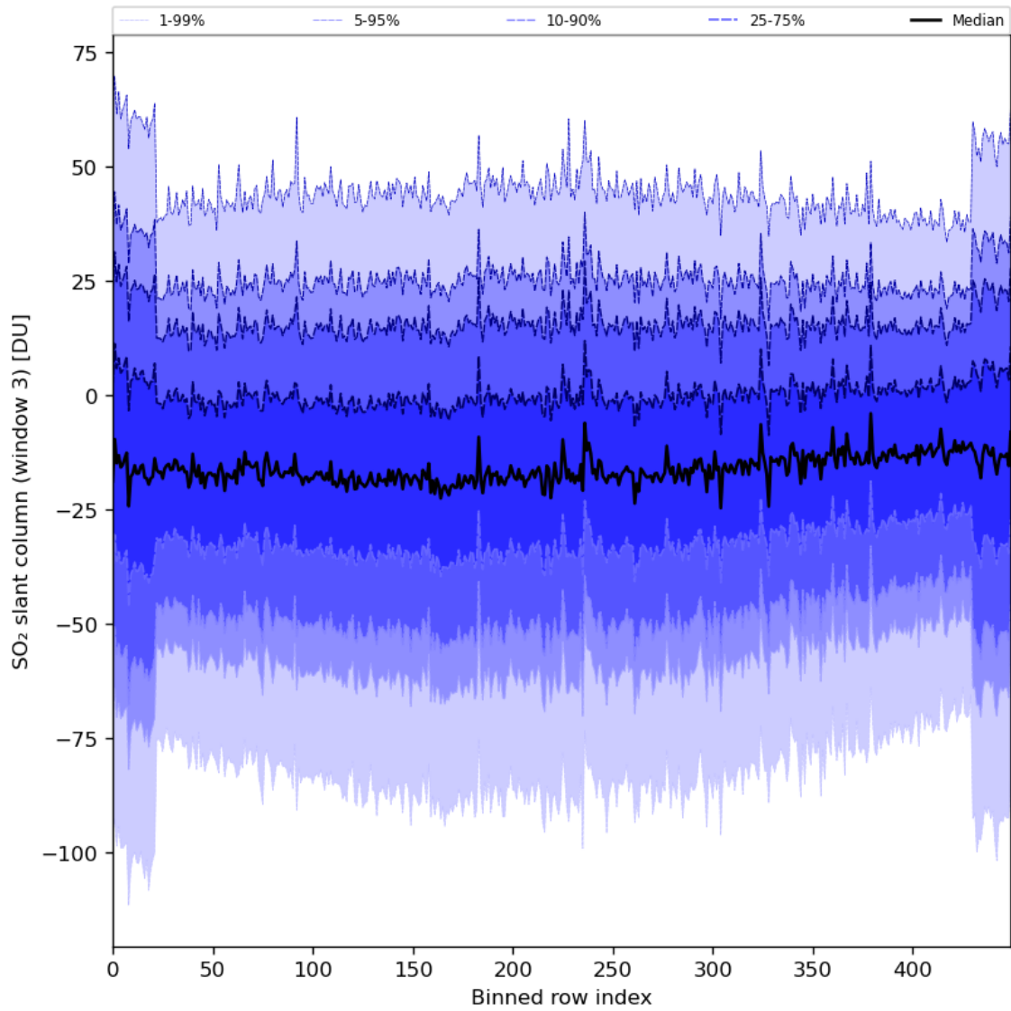
Figure 87: Along track statistics of “SO 2 slant column (window 3)” for 2024-03-20 to 2024-03-21
