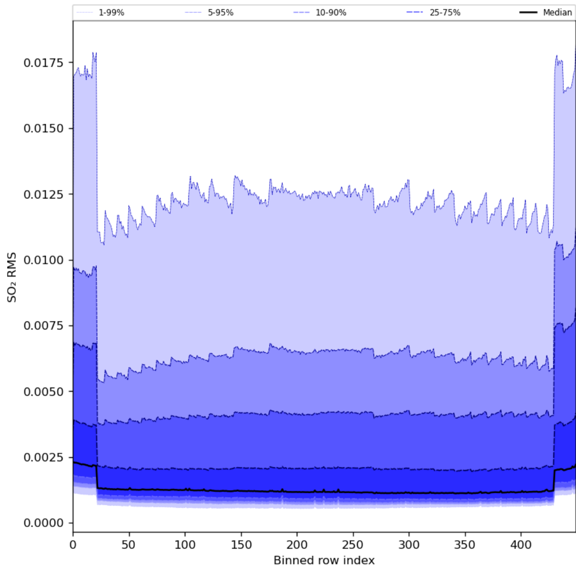
Figure 93: Along track statistics of “SO 2 RMS” for 2024-03-20 to 2024-03-21
