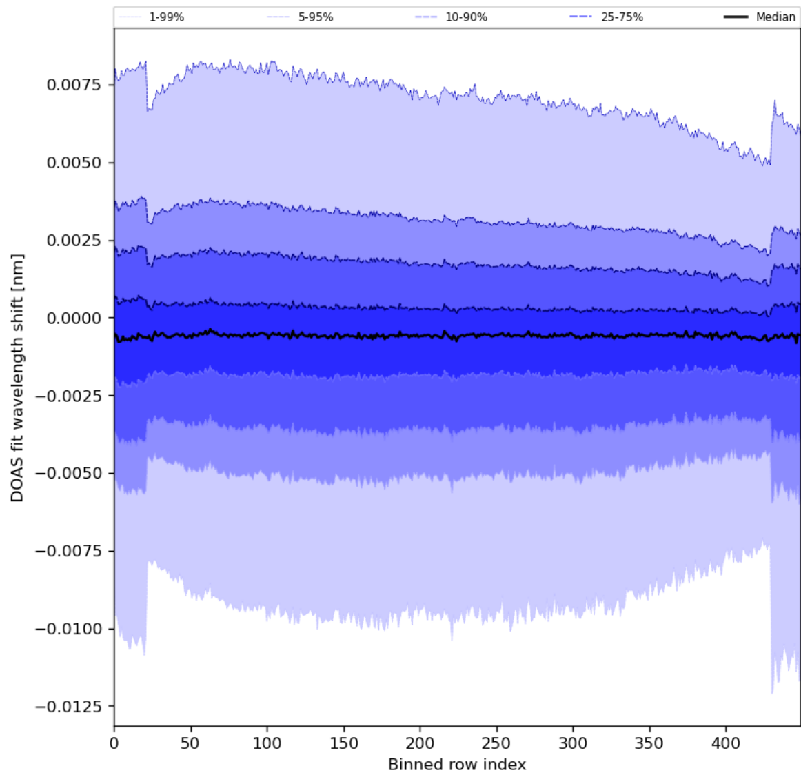
Figure 91: Along track statistics of “DOAS fit wavelength shift” for 2024-03-20 to 2024-03-21
