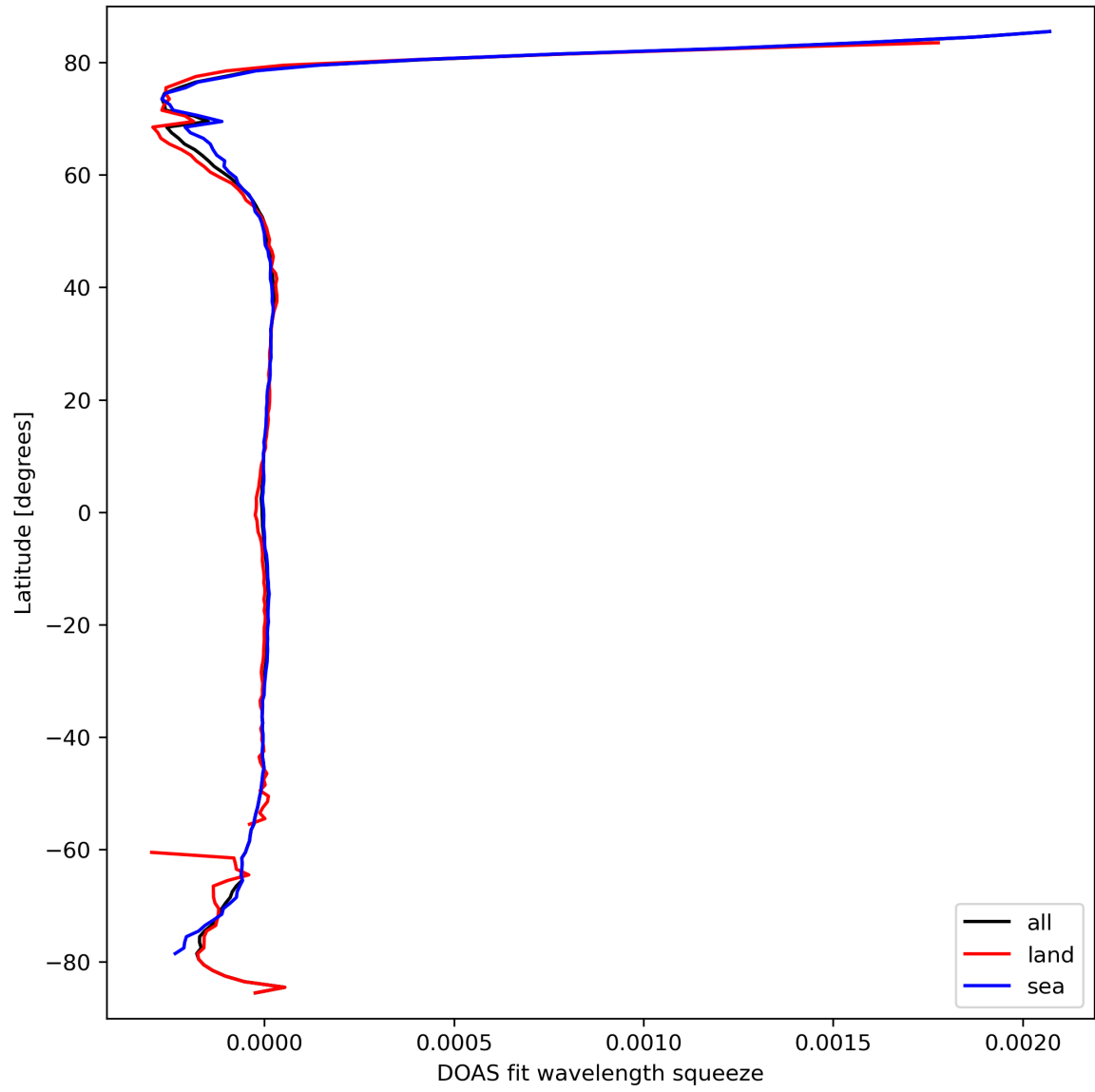
Figure 46: Zonal average of “DOAS fit wavelength squeeze” for 2024-03-20 to 2024-03-21.
