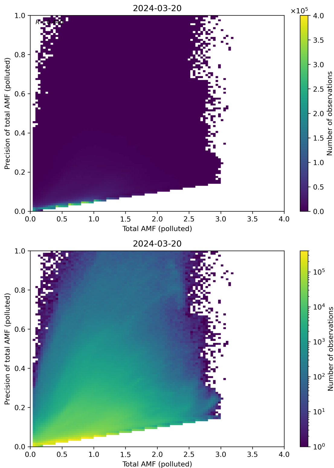
Figure 272: Scatter density plot of “Total AMF (polluted)” against “Precision of total AMF (polluted)” for 2024-03-20 to 2024-03-21.
