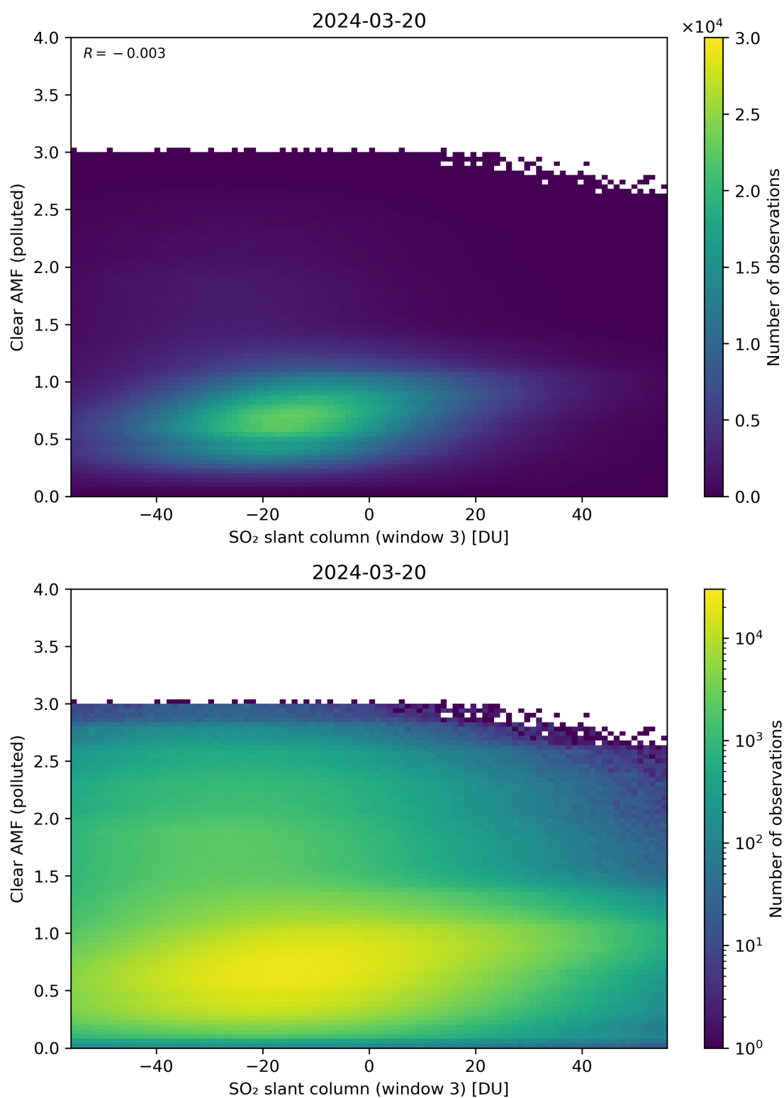
Figure 265: Scatter density plot of “SO 2 slant column (window 3)” against “Clear AMF (polluted)” for 2024-03-20 to 2024-03-21.
