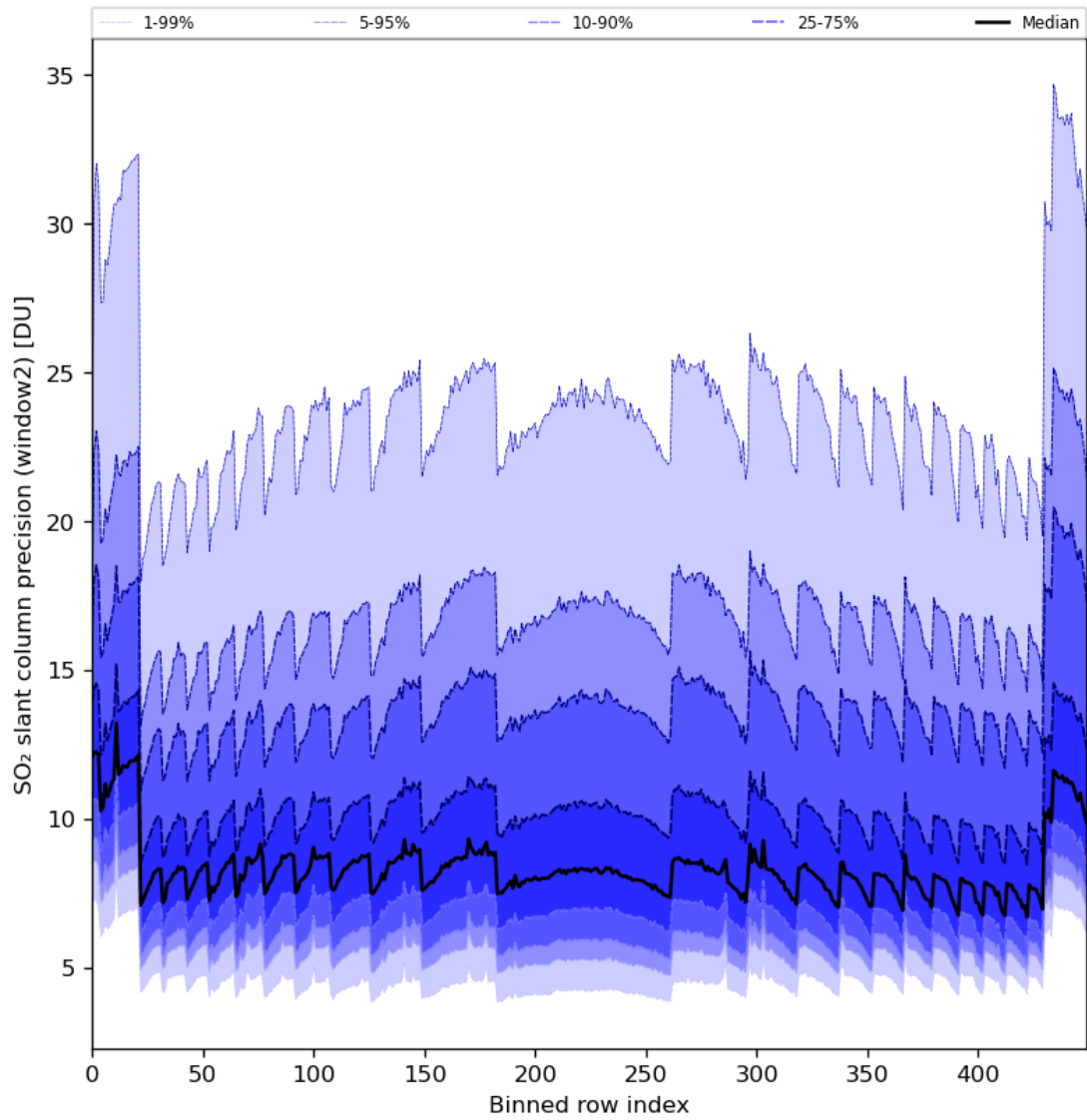
Figure 84: Along track statistics of “SO 2 slant column precision (window2)” for 2024-03-20 to 2024-03-21
