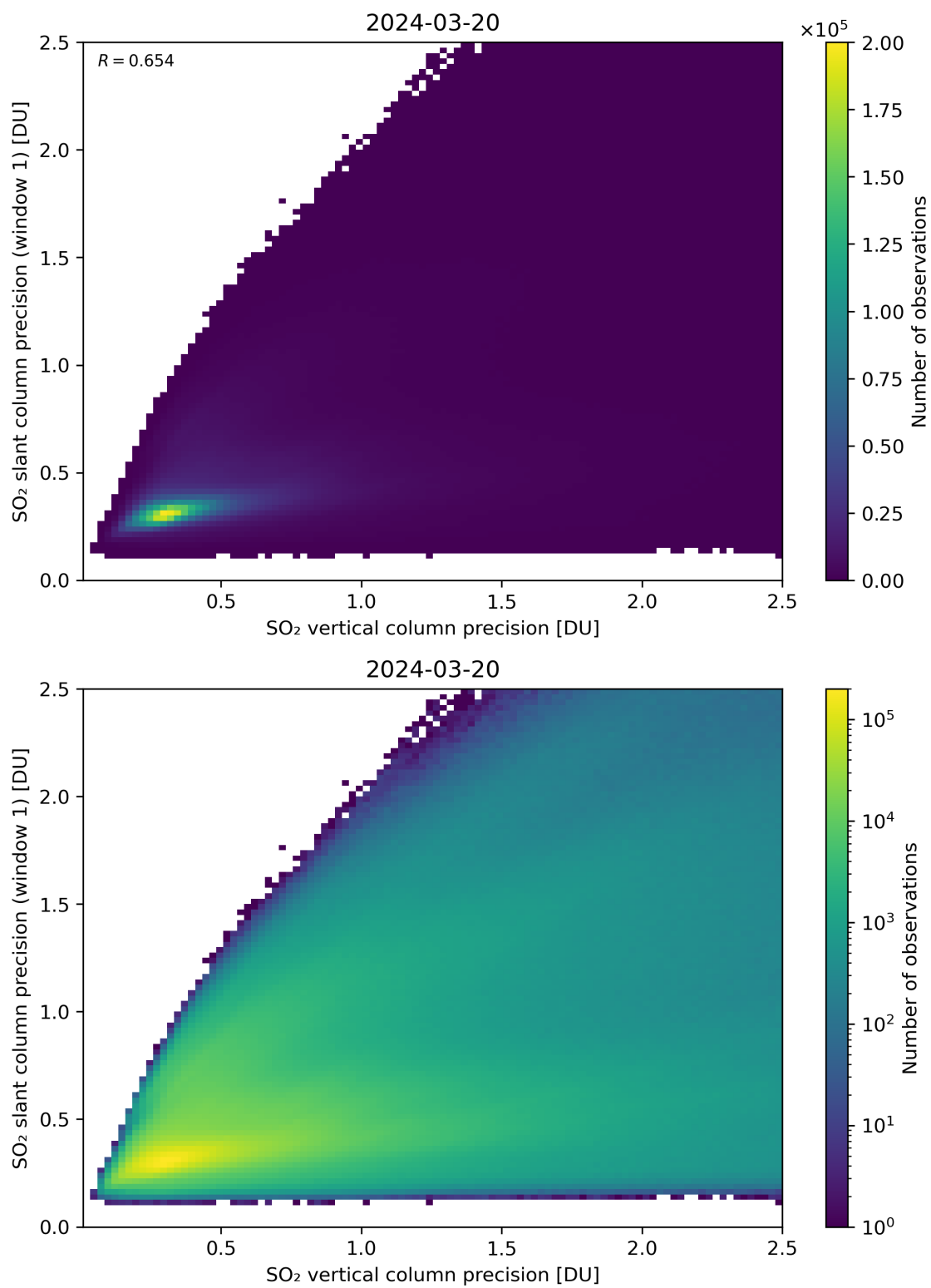
Figure 290: Scatter density plot of “SO 2 vertical column precision” against “SO 2 slant column precision (window 1)” for 2024-03-20 to 2024-03-21.
