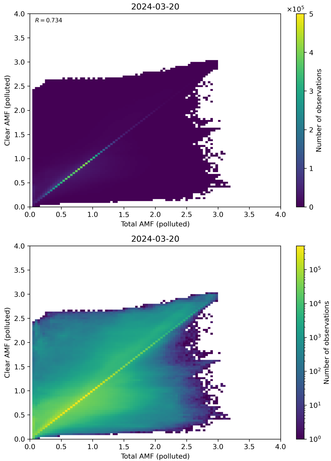
Figure 271: Scatter density plot of “Total AMF (polluted)” against “Clear AMF (polluted)” for 2024-03-20 to 2024-03-21.
