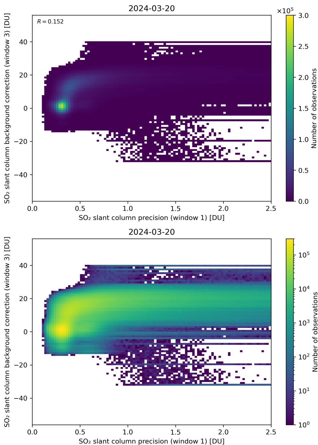
Figure 220: Scatter density plot of “SO 2 slant column precision (window 1)” against “SO 2 slant column background correction (window 3)” for 2024-03-20 to 2024-03-21.
