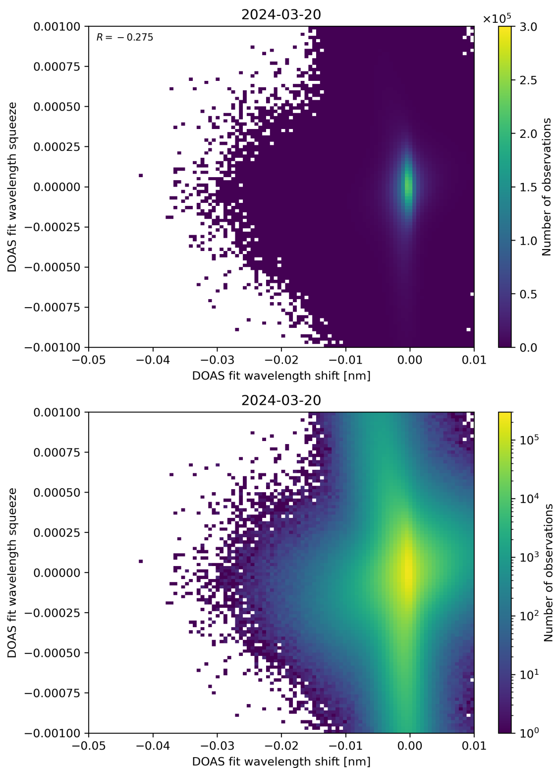
Figure 127: Scatter density plot of “DOAS fit wavelength shift” against “DOAS fit wavelength squeeze” for 2024-03-20 to 2024-03-21.
