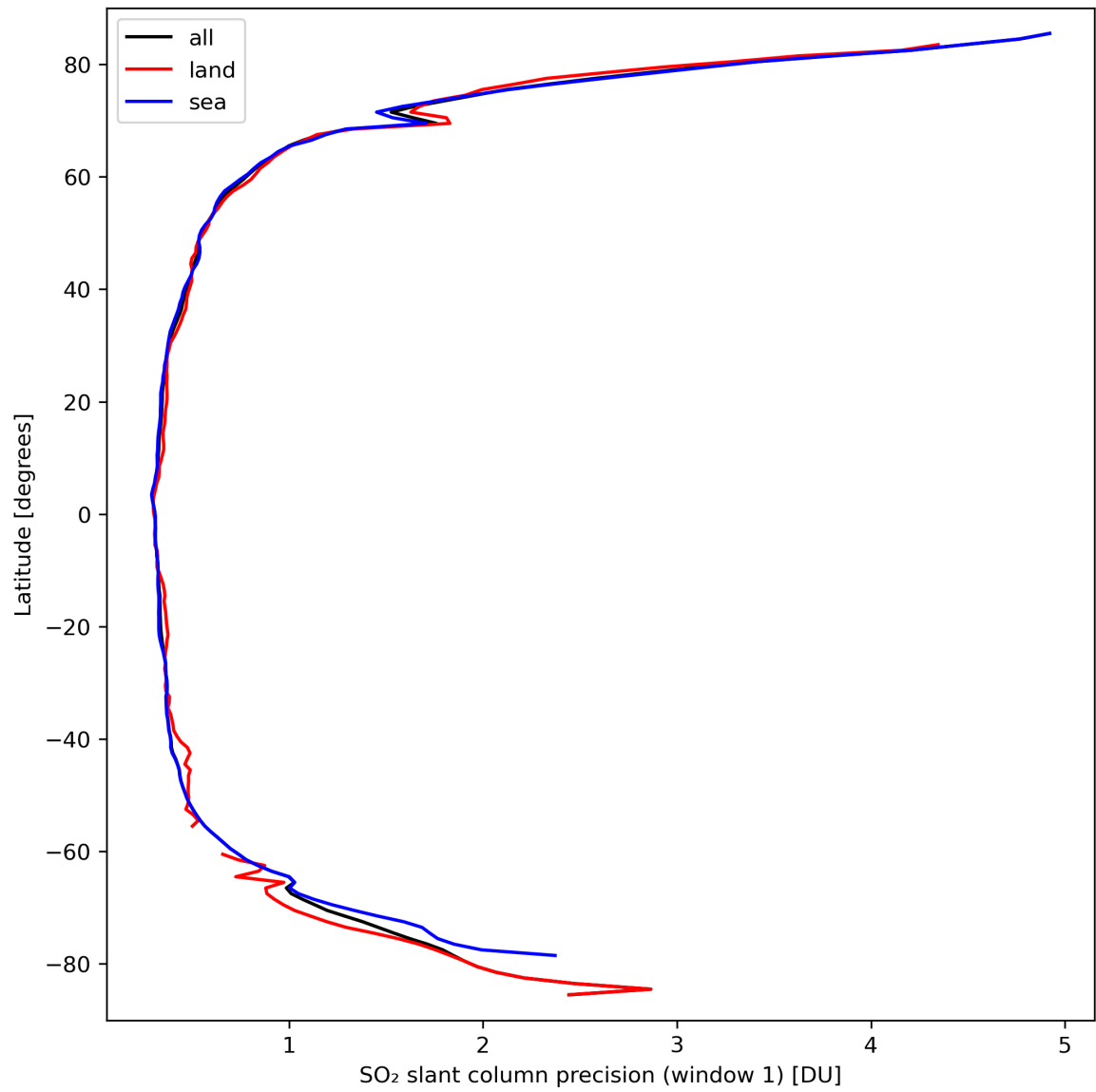
Figure 34: Zonal average of “SO 2 slant column precision (window 1)” for 2024-03-20 to 2024-03-21.
