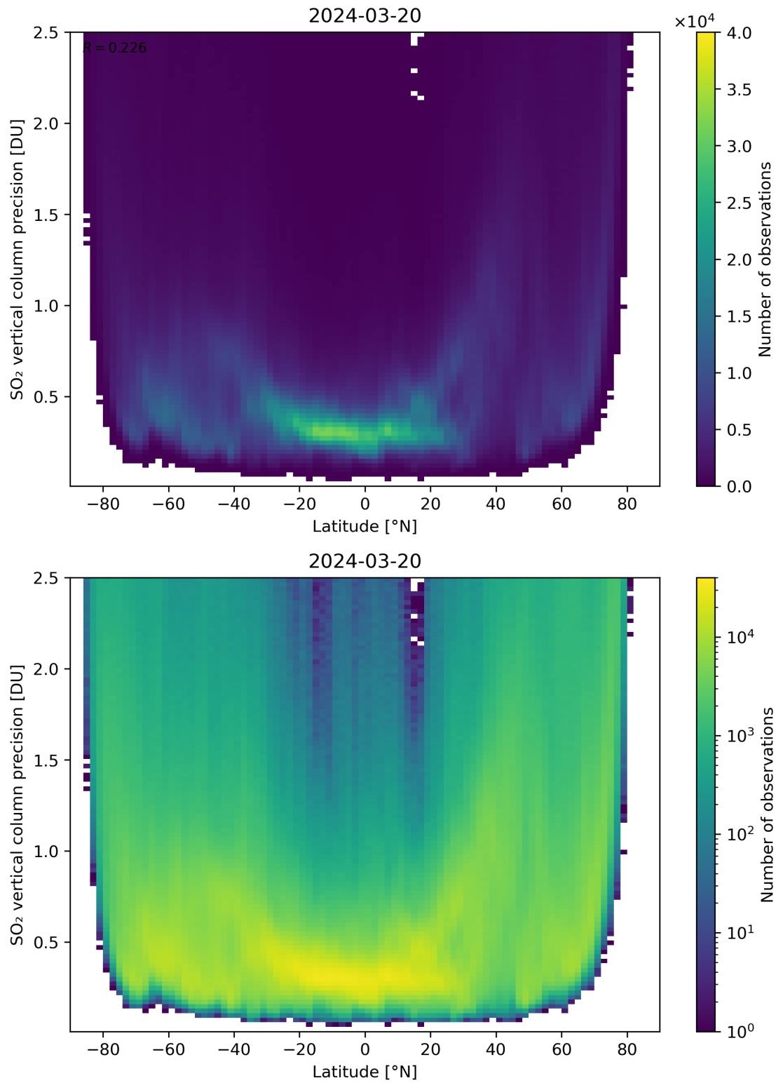
Figure 157: Scatter density plot of “Latitude” against “SO 2 vertical column precision” for 2024-03-20 to 2024-03-21.
