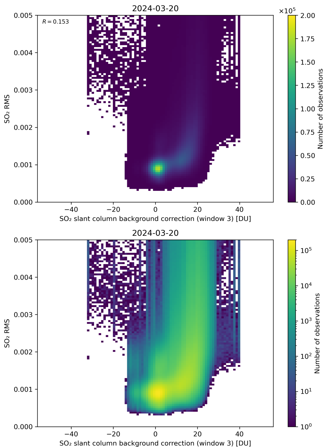
Figure 123: Scatter density plot of “SO 2 slant column background correction (window 3)” against “SO 2 RMS” for 2024-03-20 to 2024-03-21.
