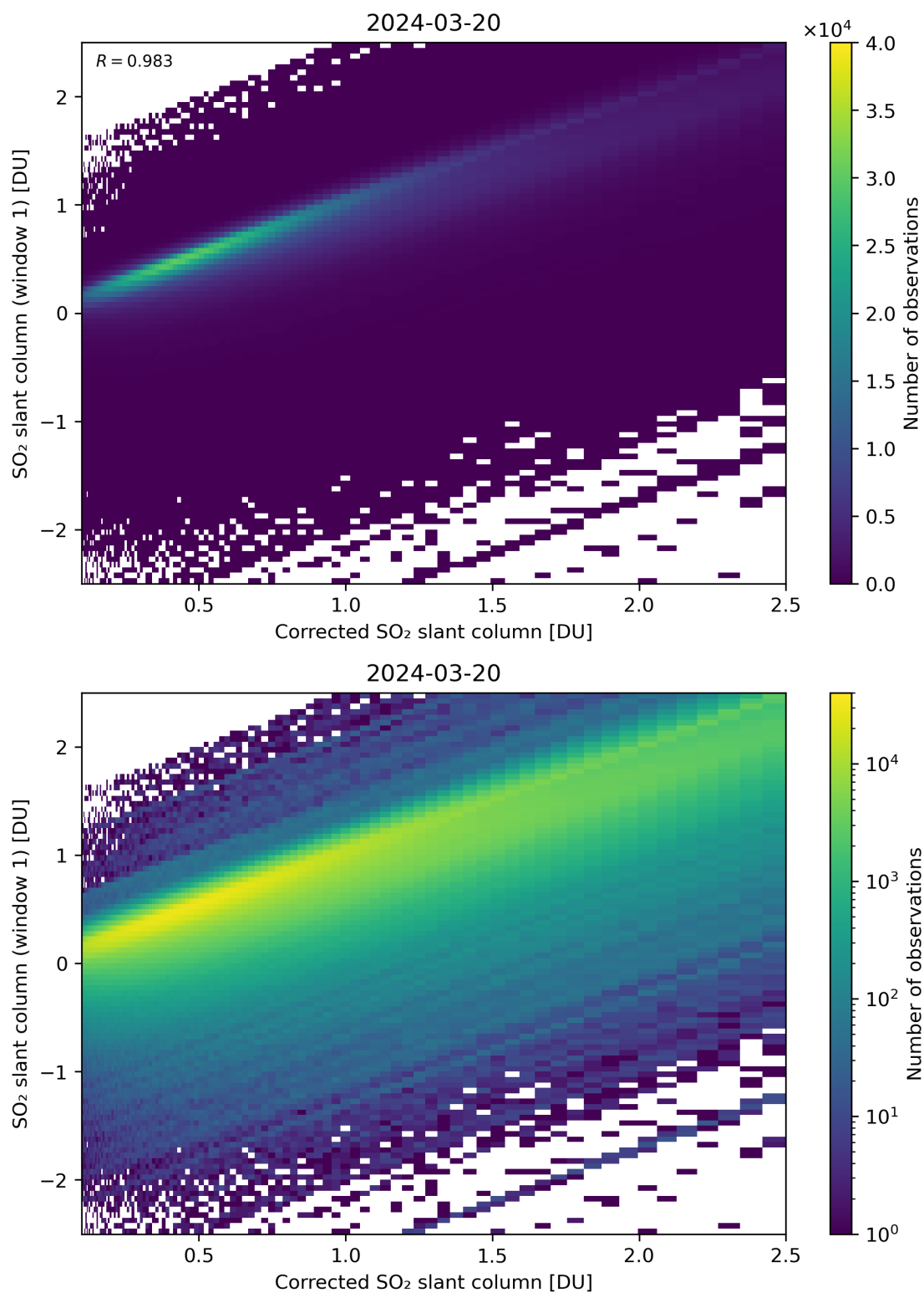
Figure 187: Scatter density plot of “Corrected SO 2 slant column” against “SO 2 slant column (window 1)” for 2024-03-20 to 2024-03-21.
