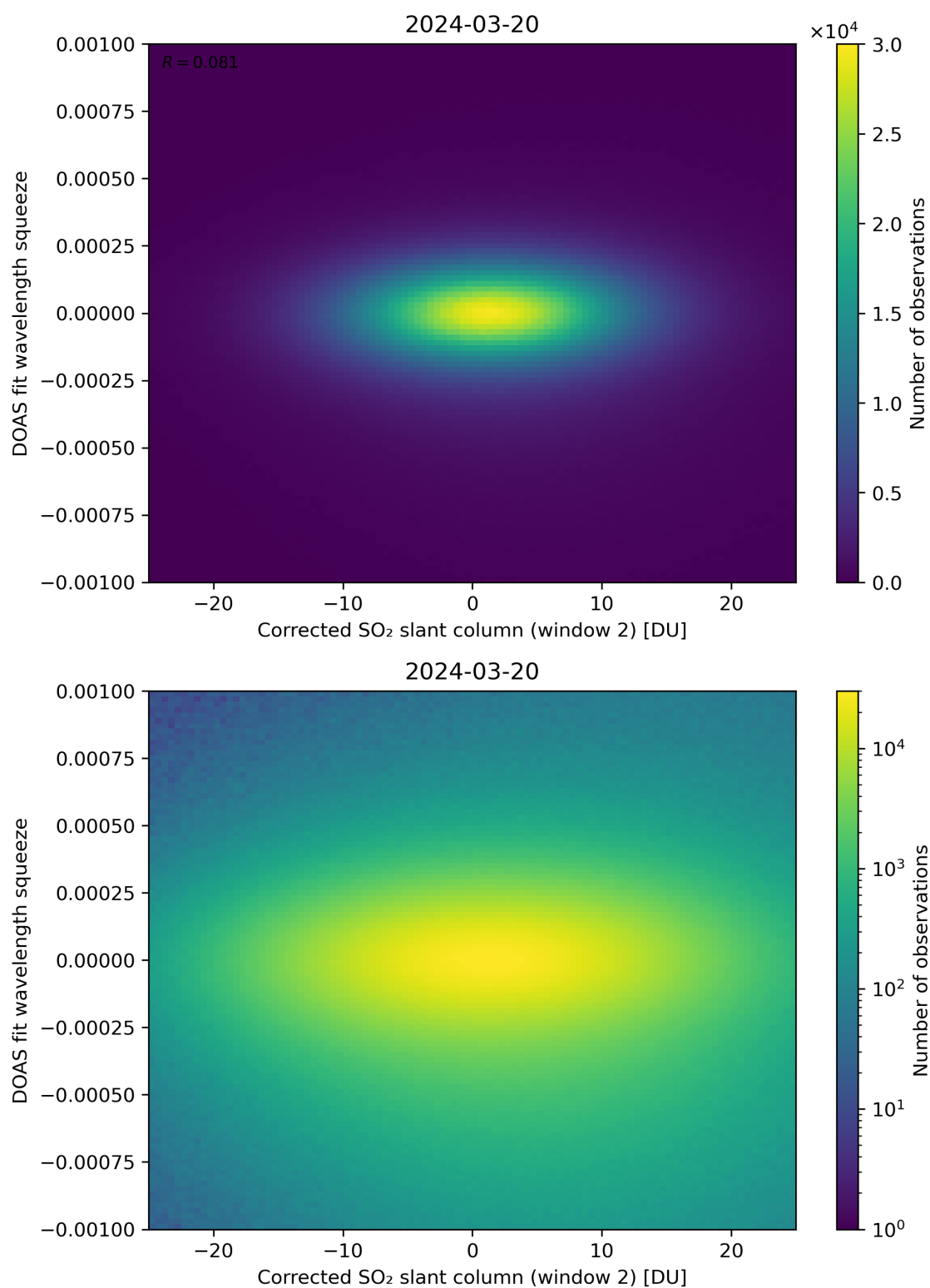
Figure 197: Scatter density plot of “Corrected SO 2 slant column (window 2)” against “DOAS fit wavelength squeeze” for 2024-03-20 to 2024-03-21.
