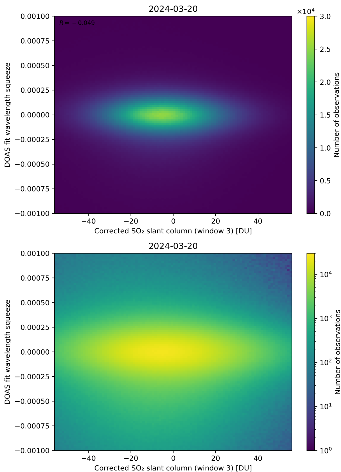
Figure 207: Scatter density plot of “Corrected SO 2 slant column (window 3)” against “DOAS fit wavelength squeeze” for 2024-03-20 to 2024-03-21.
