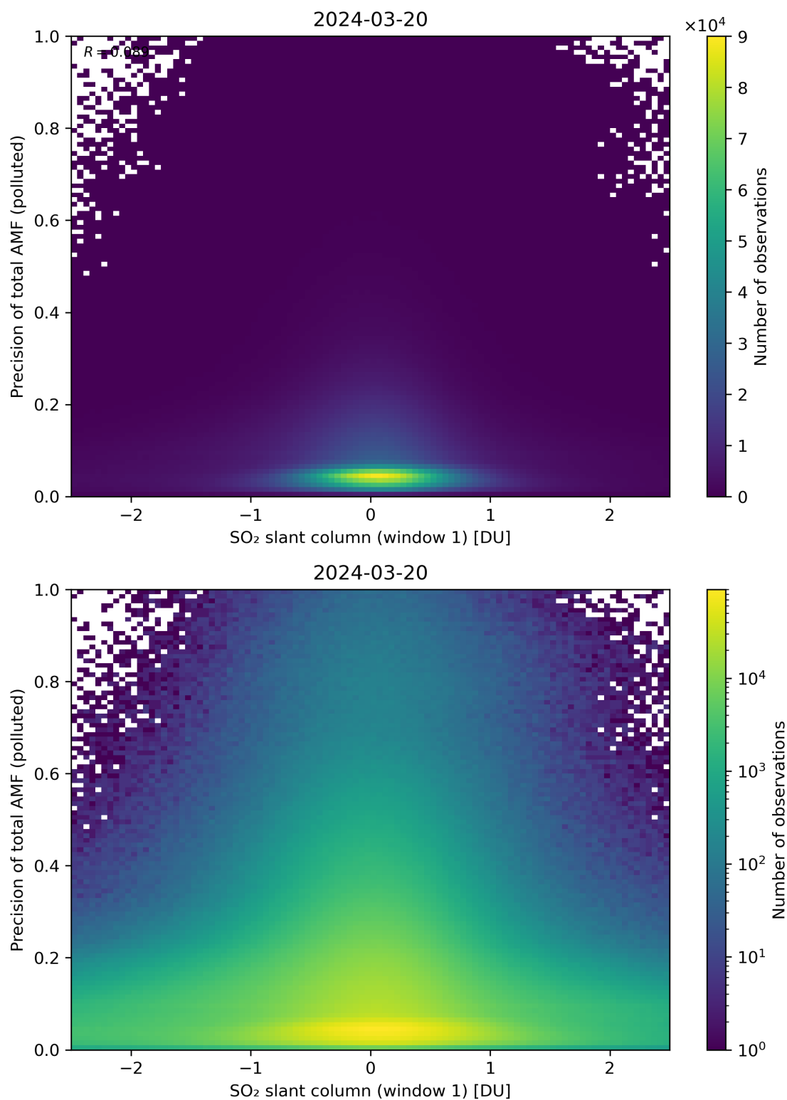
Figure 240: Scatter density plot of “SO 2 slant column (window 1)” against “Precision of total AMF (polluted)” for 2024-03-20 to 2024-03-21.
