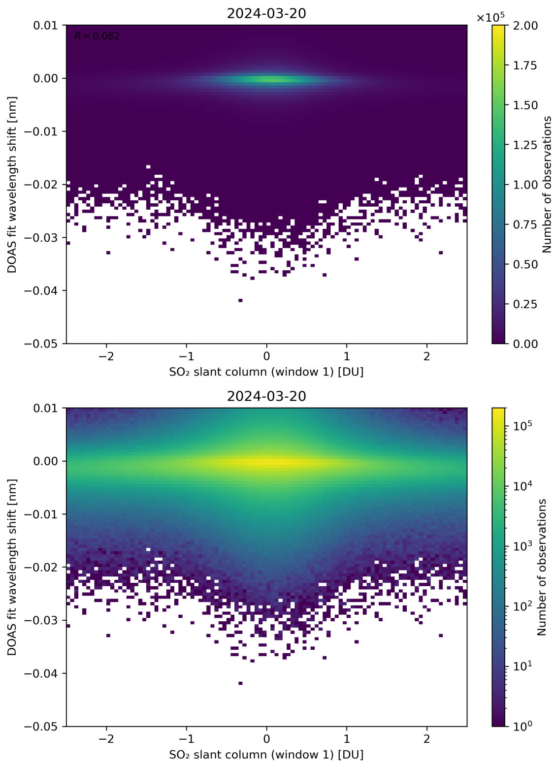
Figure 215: Scatter density plot of “SO 2 slant column (window 1)” against “DOAS fit wavelength shift” for 2024-03-20 to 2024-03-21.
