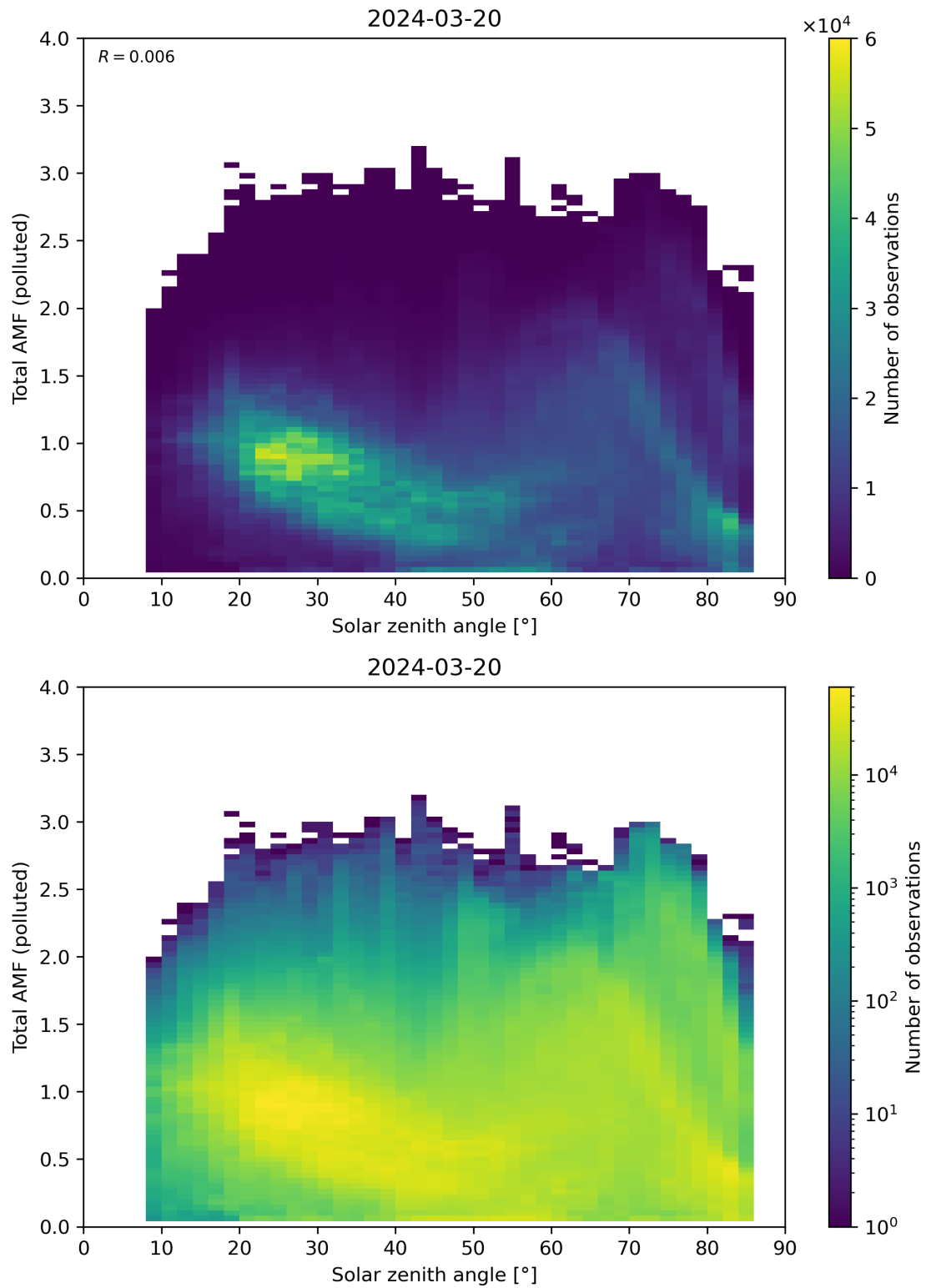
Figure 174: Scatter density plot of “Solar zenith angle” against “Total AMF (polluted)” for 2024-03-20 to 2024-03-21.
