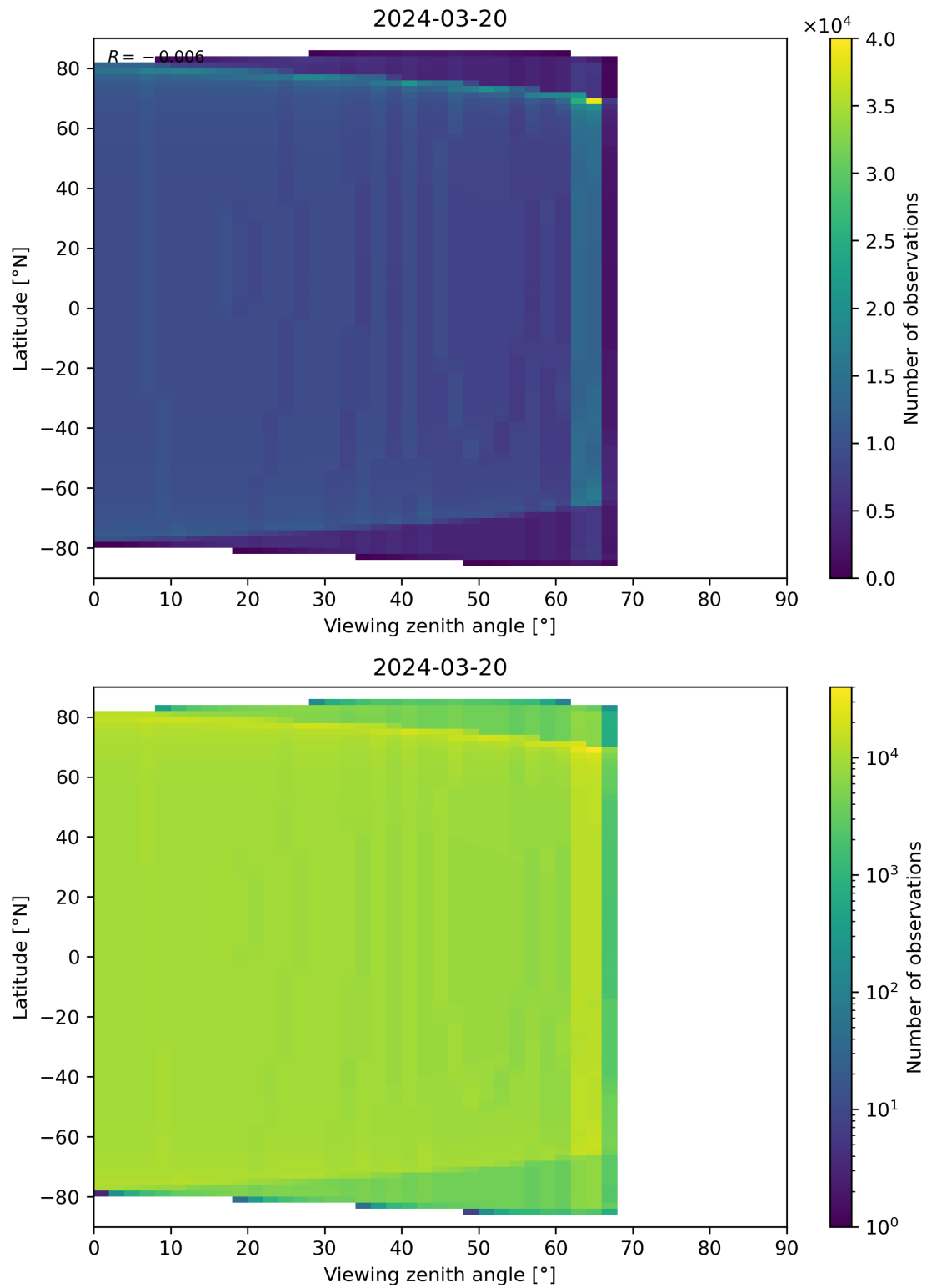
Figure 314: Scatter density plot of “Viewing zenith angle” against “Latitude” for 2024-03-20 to 2024-03-21.
