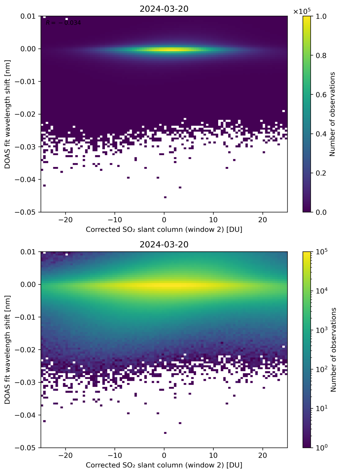
Figure 196: Scatter density plot of “Corrected SO 2 slant column (window 2)” against “DOAS fit wavelength shift” for 2024-03-20 to 2024-03-21.
