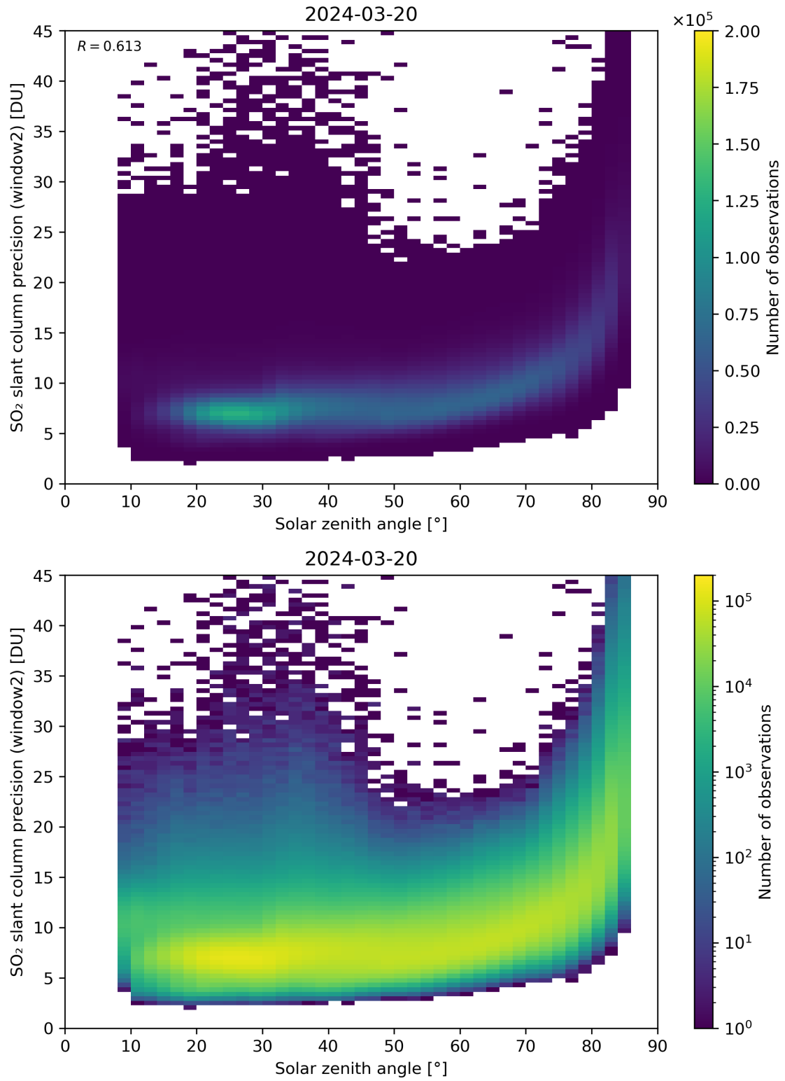
Figure 171: Scatter density plot of “Solar zenith angle” against “SO 2 slant column precision (window2)” for 2024-03-20 to 2024-03-21.
