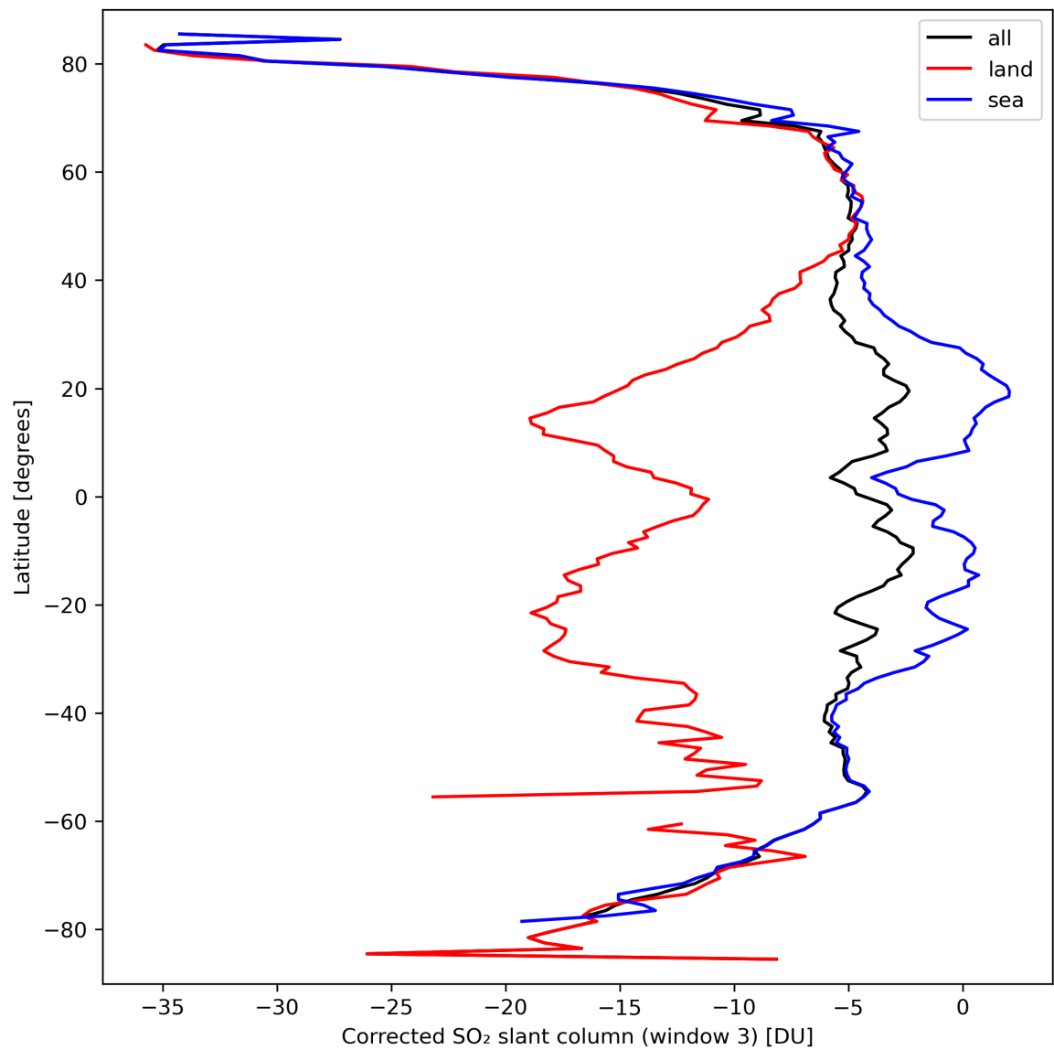
Figure 43: Zonal average of “Corrected SO 2 slant column (window 3)” for 2024-03-20 to 2024-03-21.
