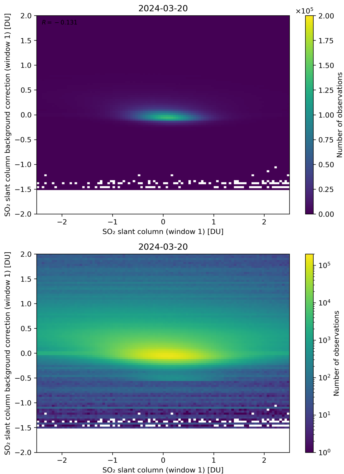
Figure 212: Scatter density plot of “SO 2 slant column (window 1)” against “SO 2 slant column background correction (window 1)” for 2024-03-20 to 2024-03-21.
