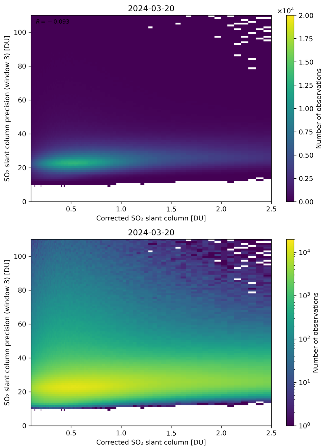
Figure 191: Scatter density plot of “Corrected SO 2 slant column” against “SO 2 slant column precision (window 3)” for 2024-03-20 to 2024-03-21.
