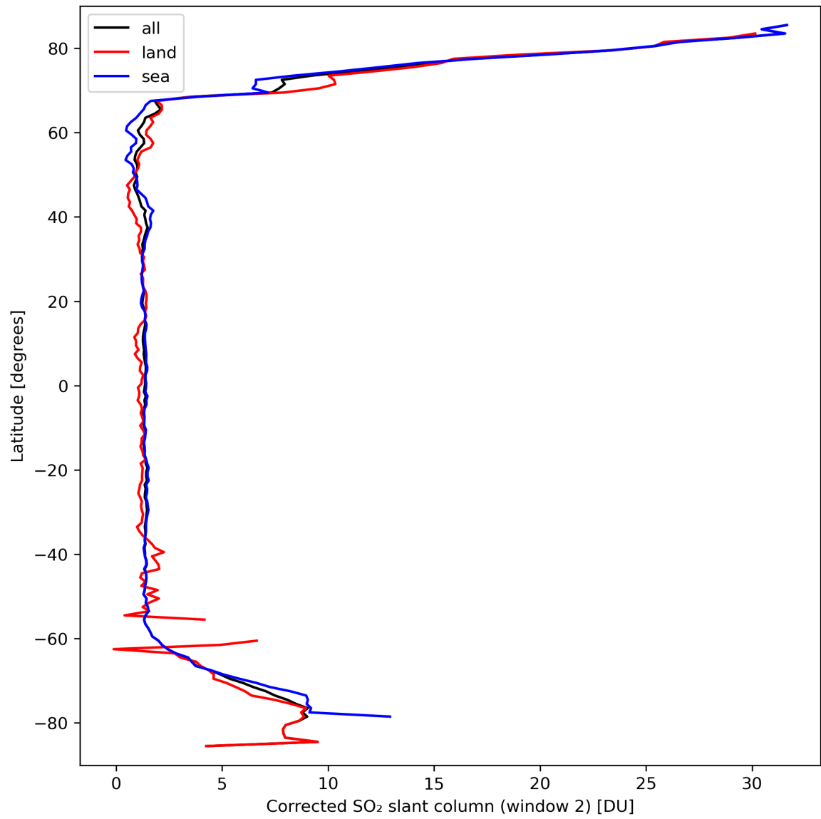
Figure 39: Zonal average of “Corrected SO 2 slant column (window 2)” for 2024-03-20 to 2024-03-21.
