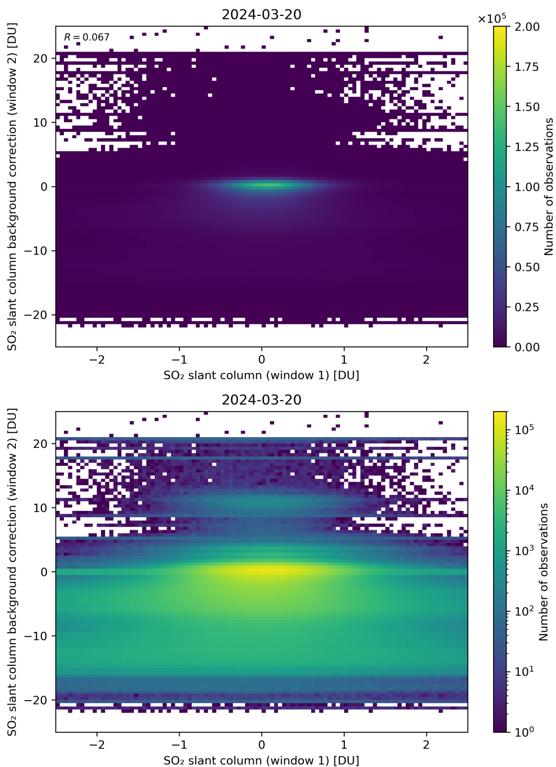
Figure 213: Scatter density plot of “SO 2 slant column (window 1)” against “SO 2 slant column background correction (window 2)” for 2024-03-20 to 2024-03-21.
