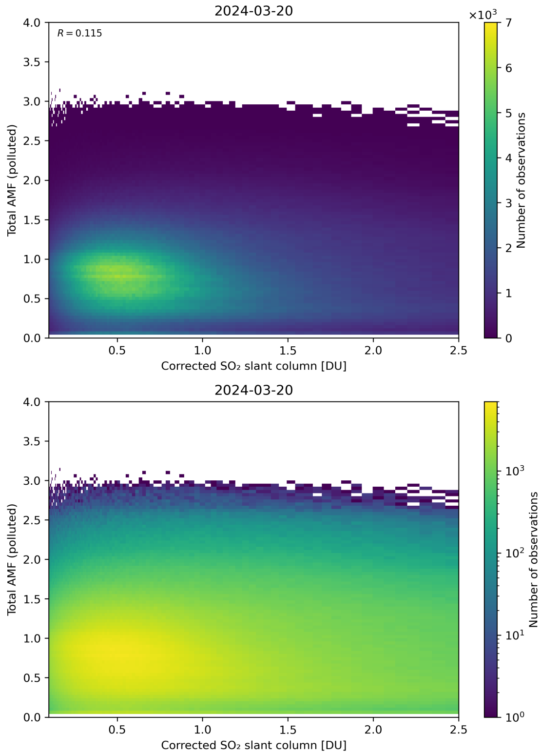
Figure 192: Scatter density plot of “Corrected SO 2 slant column” against “Total AMF (polluted)” for 2024-03-20 to 2024-03-21.
