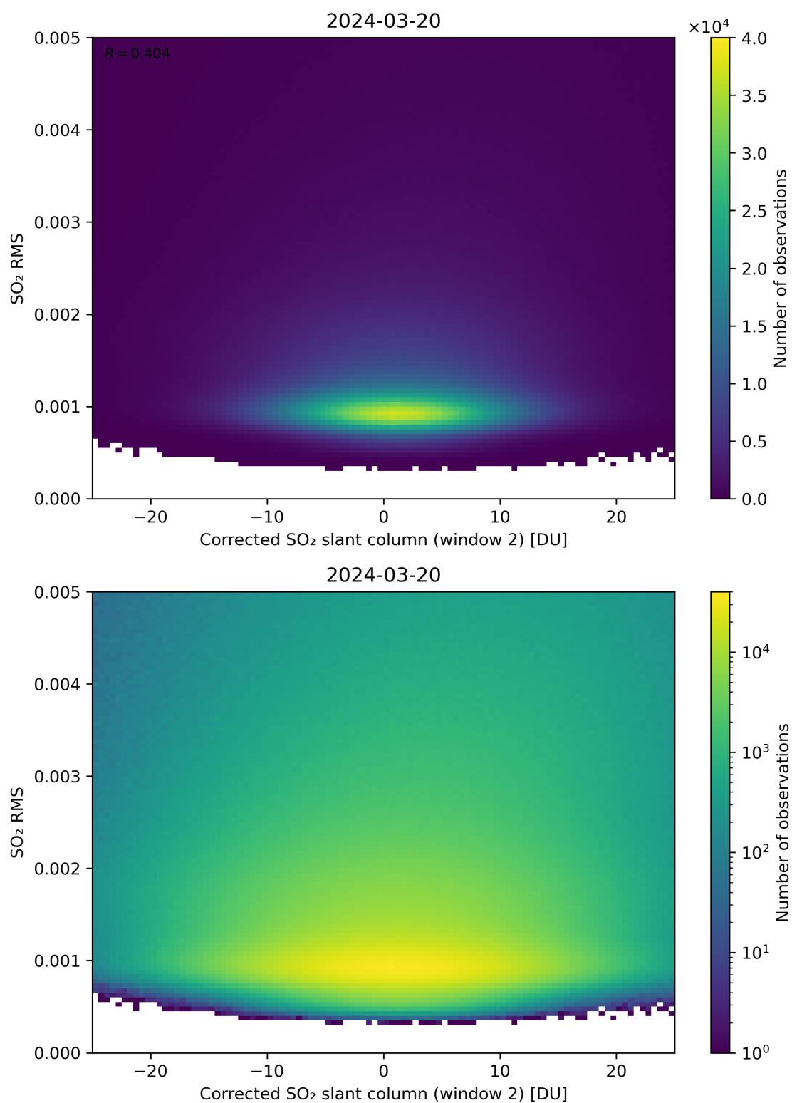
Figure 198: Scatter density plot of “Corrected SO 2 slant column (window 2)” against “SO 2 RMS” for 2024-03-20 to 2024-03-21.
