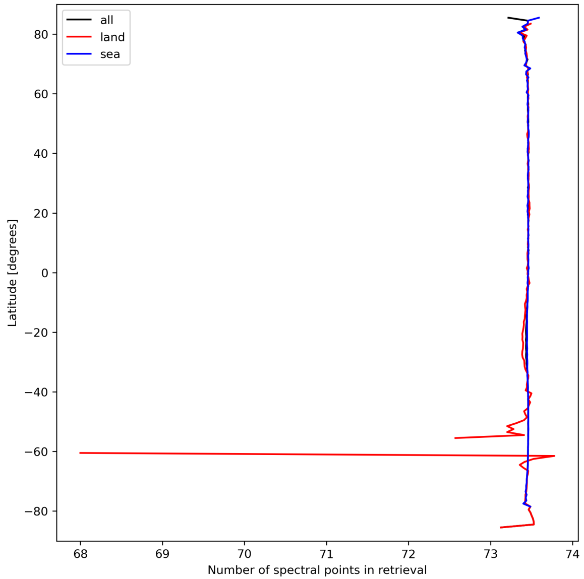
Figure 51: Zonal average of “Number of spectral points in retrieval” for 2024-03-20 to 2024-03-21.
