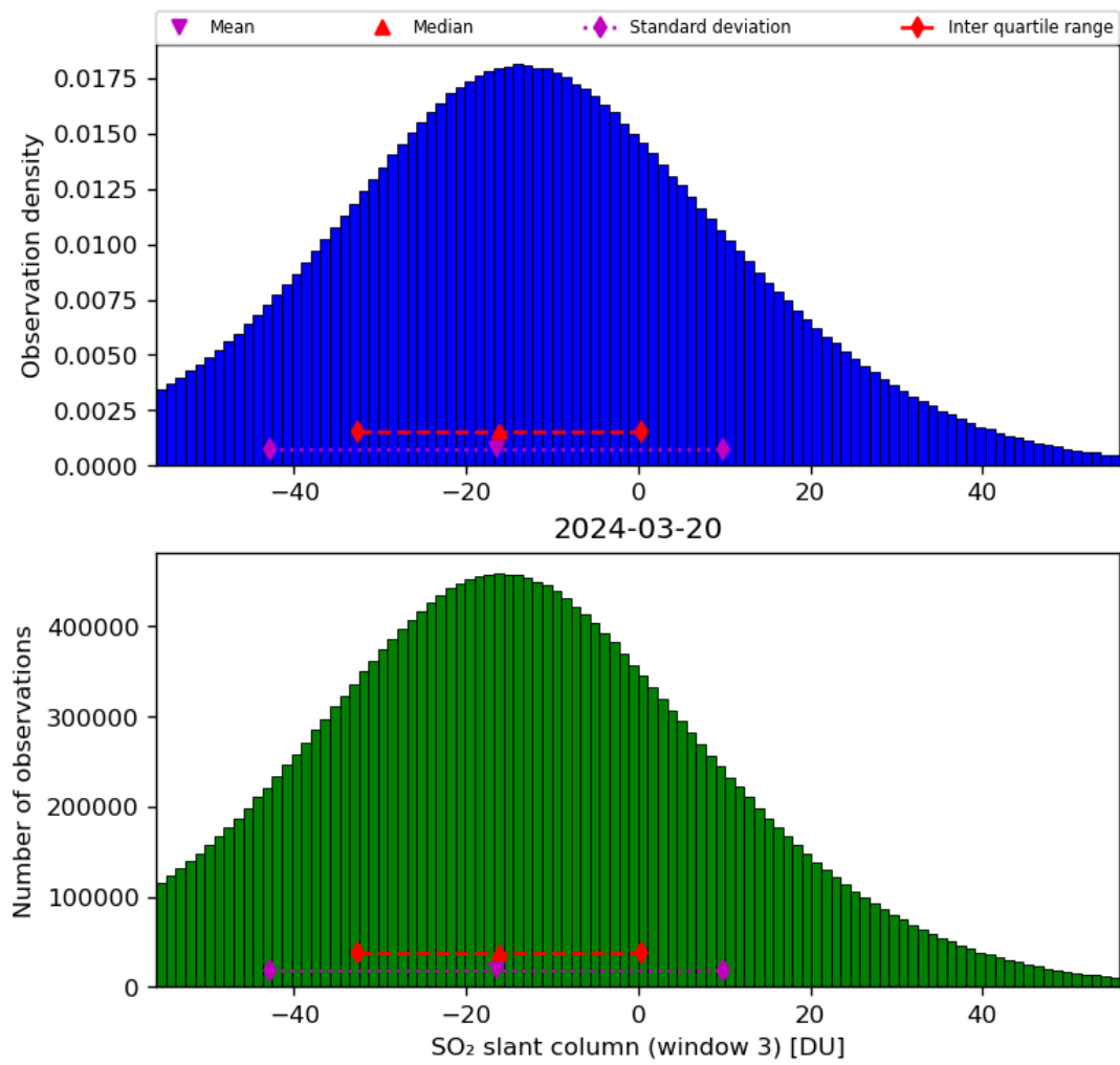
Figure 64: Histogram of “SO 2 slant column (window 3)” for 2024-03-20 to 2024-03-21
