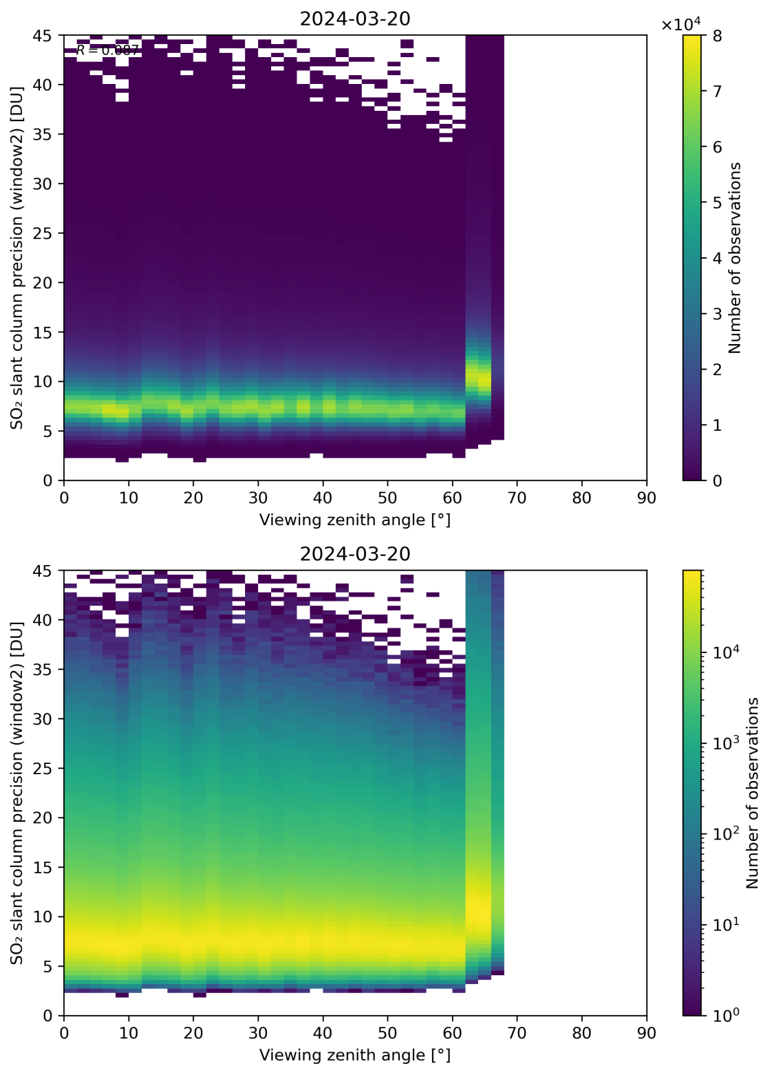
Figure 322: Scatter density plot of “Viewing zenith angle” against “SO 2 slant column precision (window2)” for 2024-03-20 to 2024-03-21.
