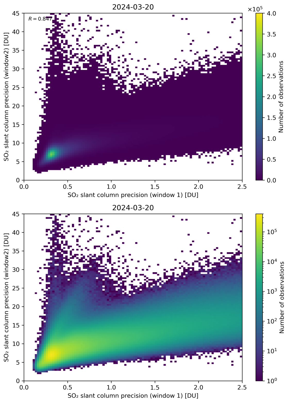
Figure 227: Scatter density plot of “SO 2 slant column precision (window 1)” against “SO 2 slant column precision (window2)” for 2024-03-20 to 2024-03-21.
