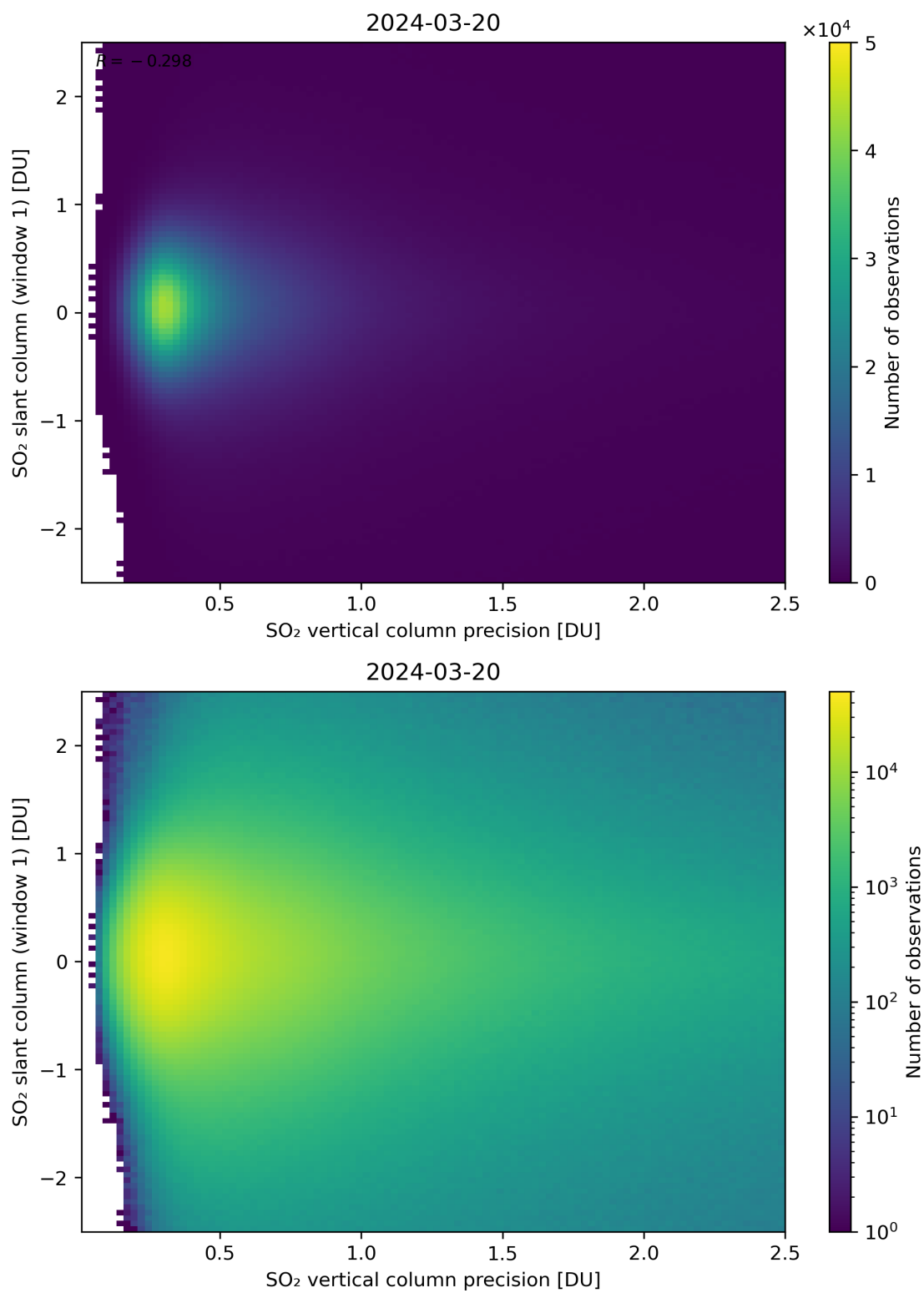
Figure 289: Scatter density plot of “SO 2 vertical column precision” against “SO 2 slant column (window 1)” for 2024-03-20 to 2024-03-21.
