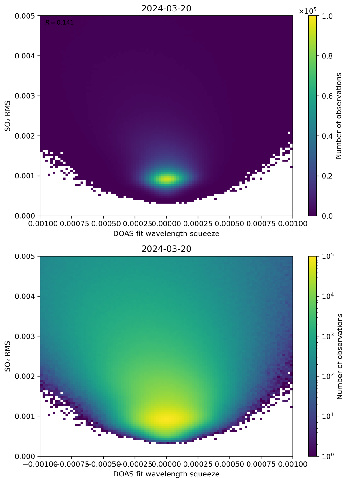
Figure 132: Scatter density plot of “DOAS fit wavelength squeeze” against “SO 2 RMS” for 2024-03-20 to 2024-03-21.
