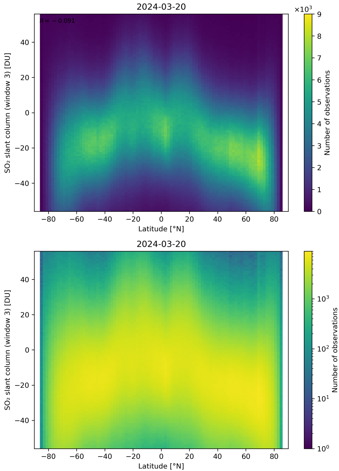
Figure 152: Scatter density plot of “Latitude” against “SO 2 slant column (window 3)” for 2024-03-20 to 2024-03-21.
