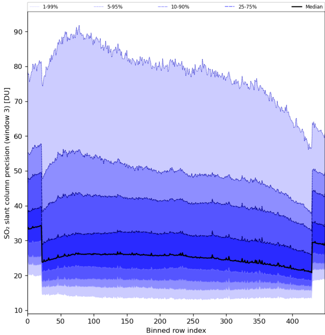
Figure 88: Along track statistics of “SO 2 slant column precision (window 3)” for 2024-03-20 to 2024-03-21
