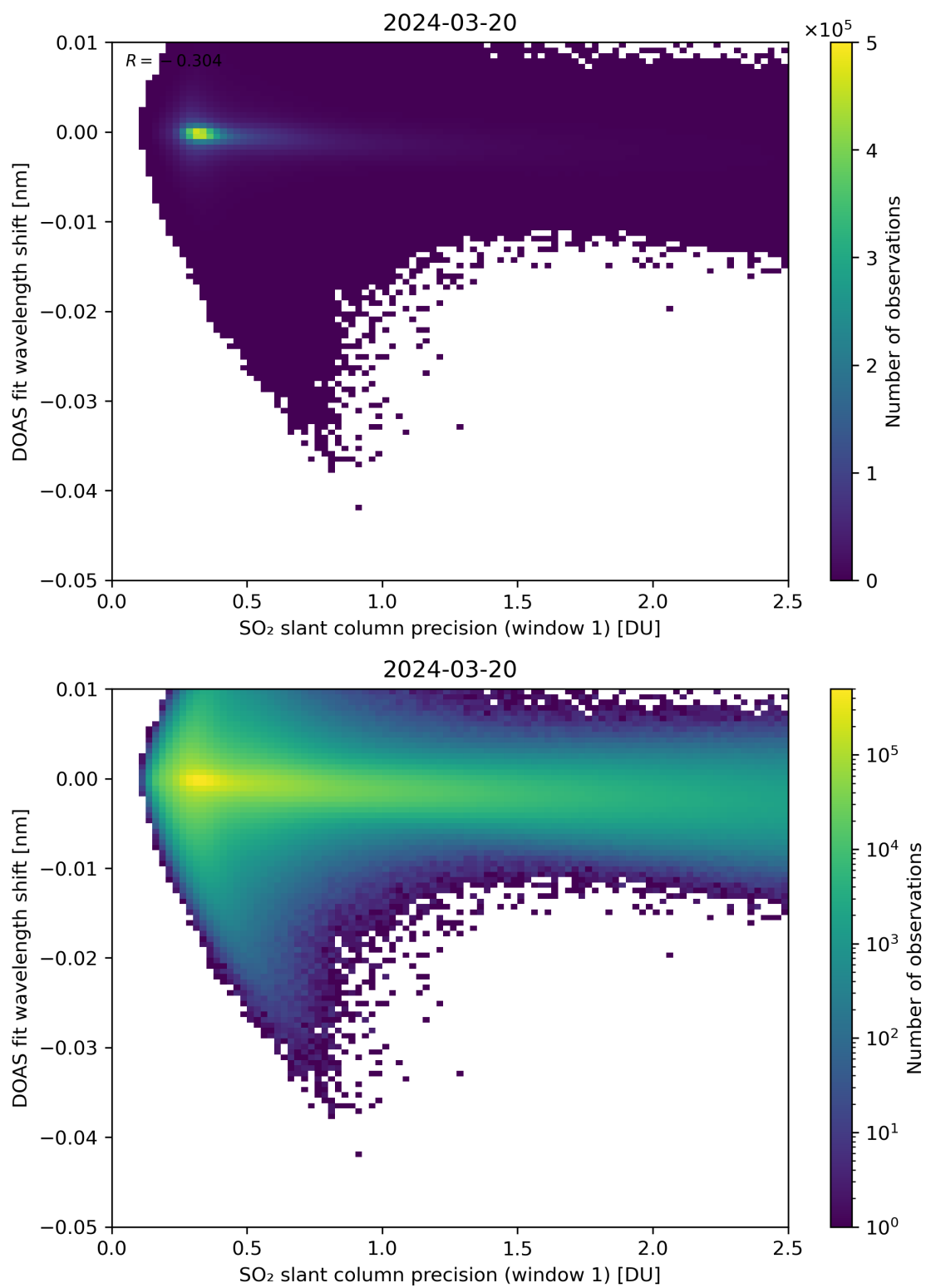
Figure 221: Scatter density plot of “SO 2 slant column precision (window 1)” against “DOAS fit wavelength shift” for 2024-03-20 to 2024-03-21.
