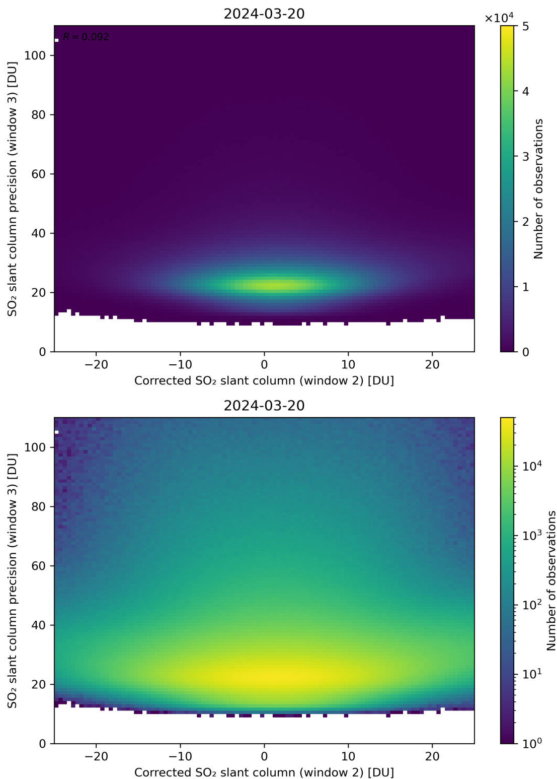
Figure 202: Scatter density plot of “Corrected SO 2 slant column (window 2)” against “SO 2 slant column precision (window 3)” for 2024-03-20 to 2024-03-21.
