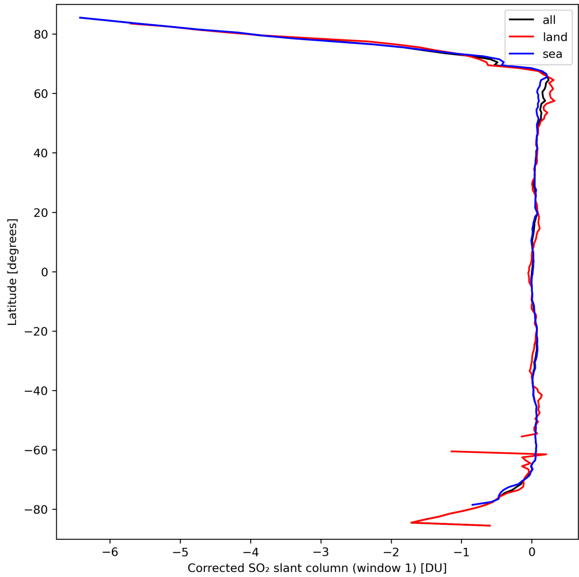
Figure 35: Zonal average of “Corrected SO 2 slant column (window 1)” for 2024-03-20 to 2024-03-21.
