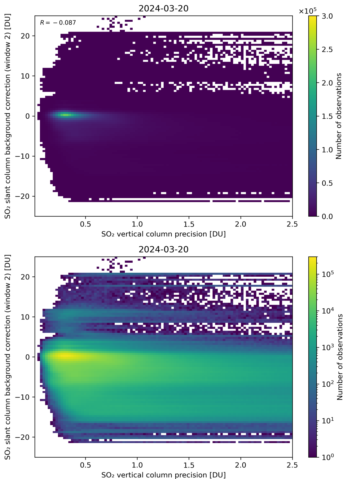
Figure 280: Scatter density plot of “SO 2 vertical column precision” against “SO 2 slant column background correction (window 2)” for 2024-03-20 to 2024-03-21.
