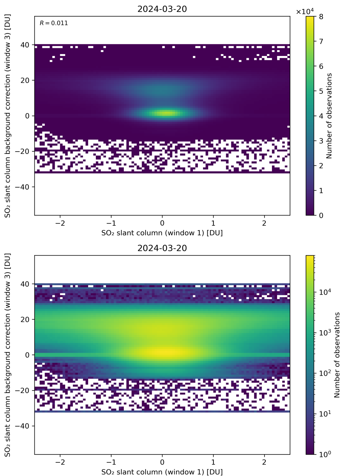
Figure 214: Scatter density plot of “SO 2 slant column (window 1)” against “SO 2 slant column background correction (window 3)” for 2024-03-20 to 2024-03-21.
