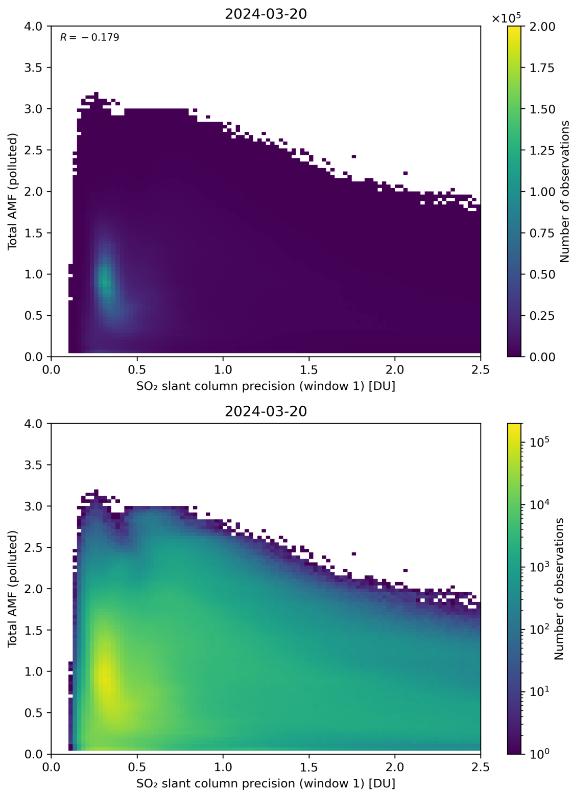
Figure 230: Scatter density plot of “SO 2 slant column precision (window 1)” against “Total AMF (polluted)” for 2024-03-20 to 2024-03-21.
