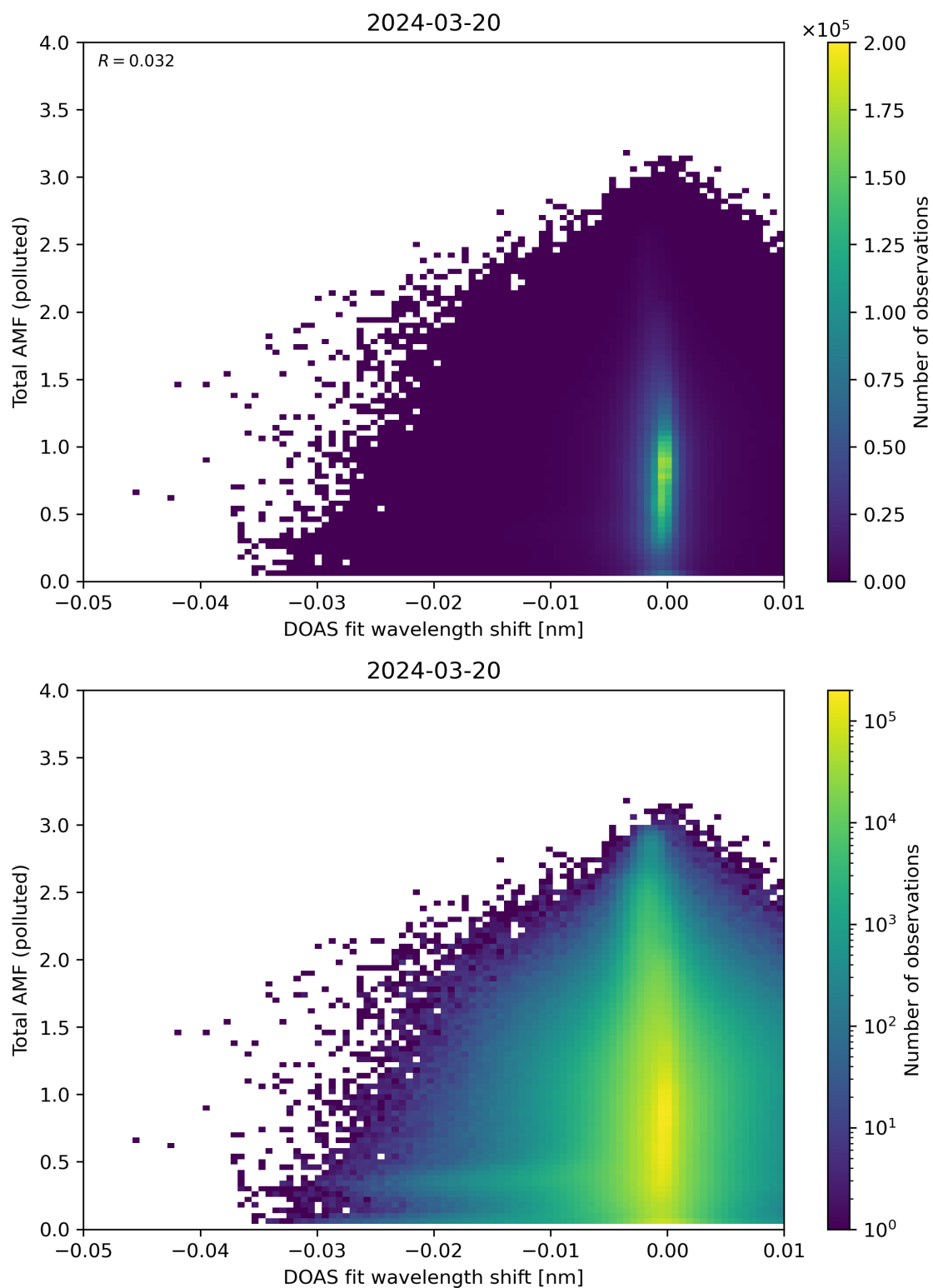
Figure 130: Scatter density plot of “DOAS fit wavelength shift” against “Total AMF (polluted)” for 2024-03-20 to 2024-03-21.
