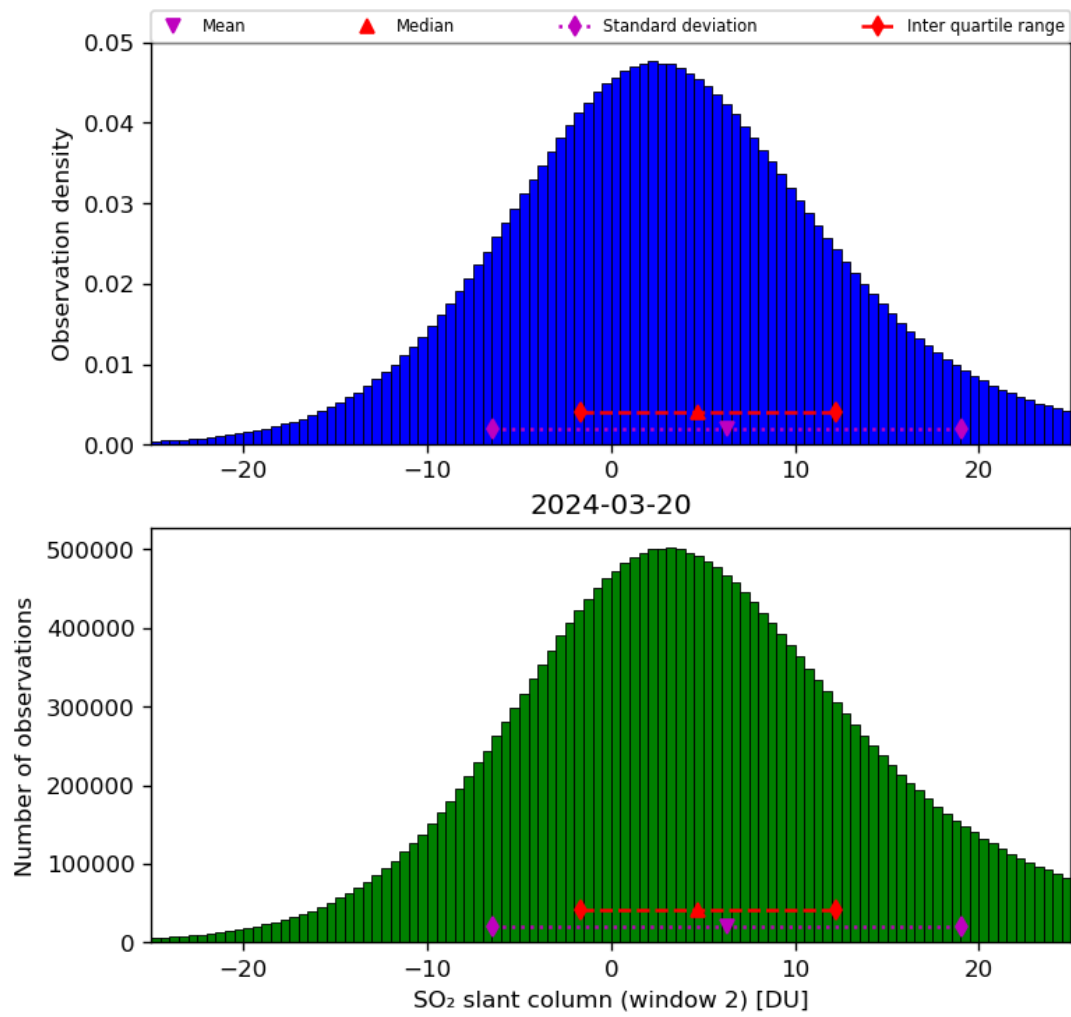
Figure 60: Histogram of “SO 2 slant column (window 2)” for 2024-03-20 to 2024-03-21
