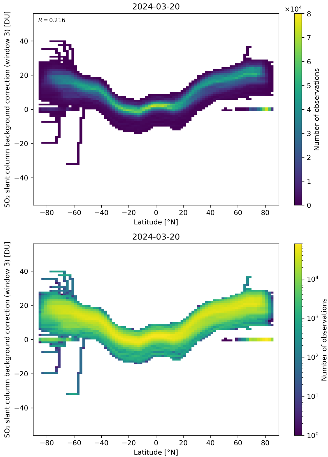
Figure 141: Scatter density plot of “Latitude” against “SO 2 slant column background correction (window 3)” for 2024-03-20 to 2024-03-21.
