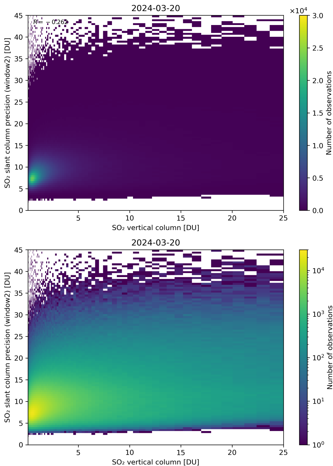
Figure 302: Scatter density plot of “SO 2 vertical column” against “SO 2 slant column precision (window2)” for 2024-03-20 to 2024-03-21.
