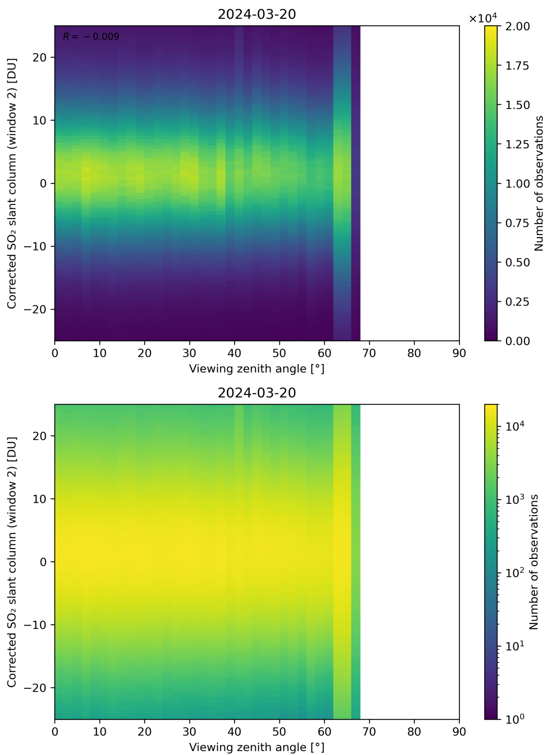
Figure 318: Scatter density plot of “Viewing zenith angle” against “Corrected SO 2 slant column (window 2)” for 2024-03-20 to 2024-03-21.
