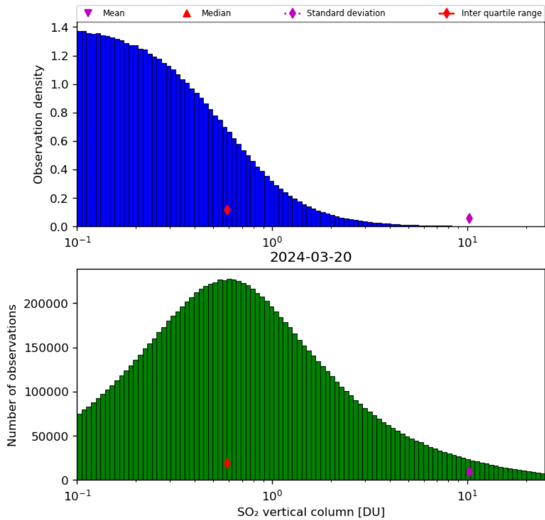
Figure 53: Histogram of “SO 2 vertical column” for 2024-03-20 to 2024-03-21
