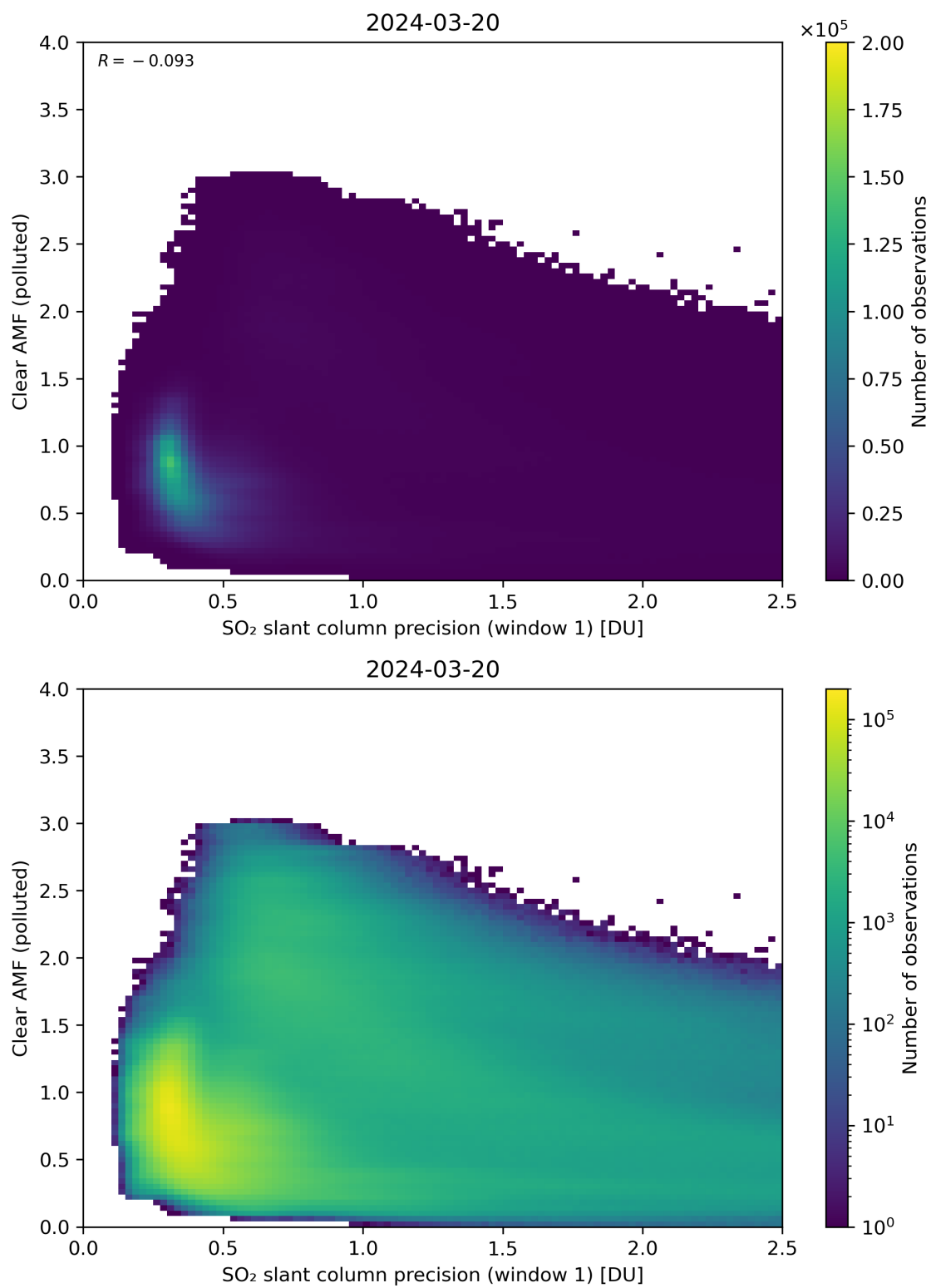
Figure 224: Scatter density plot of “SO 2 slant column precision (window 1)” against “Clear AMF (polluted)” for 2024-03-20 to 2024-03-21.
