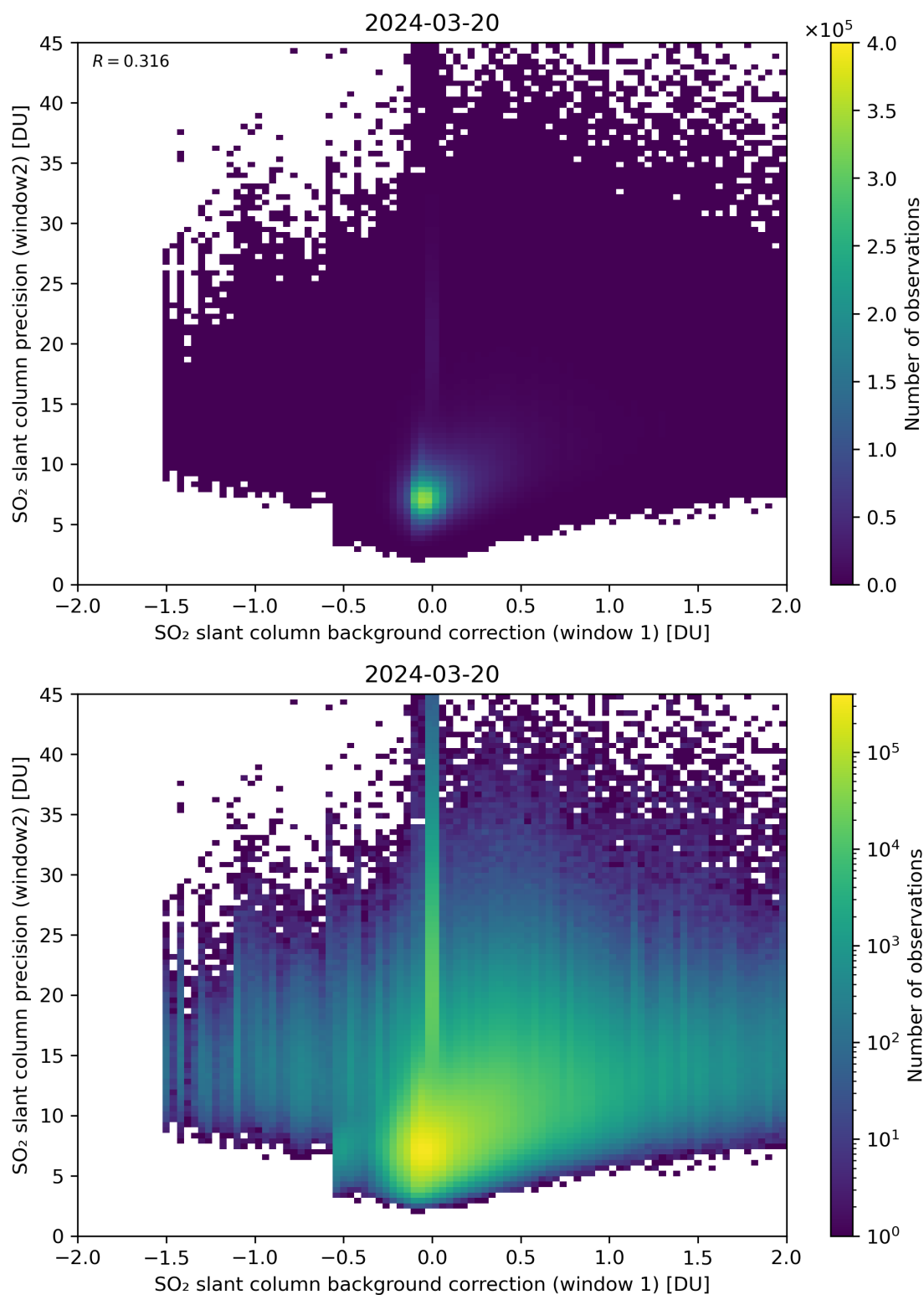
Figure 106: Scatter density plot of “SO 2 slant column background correction (window 1)” against “SO 2 slant column precision (window2)” for 2024-03-20 to 2024-03-21.
