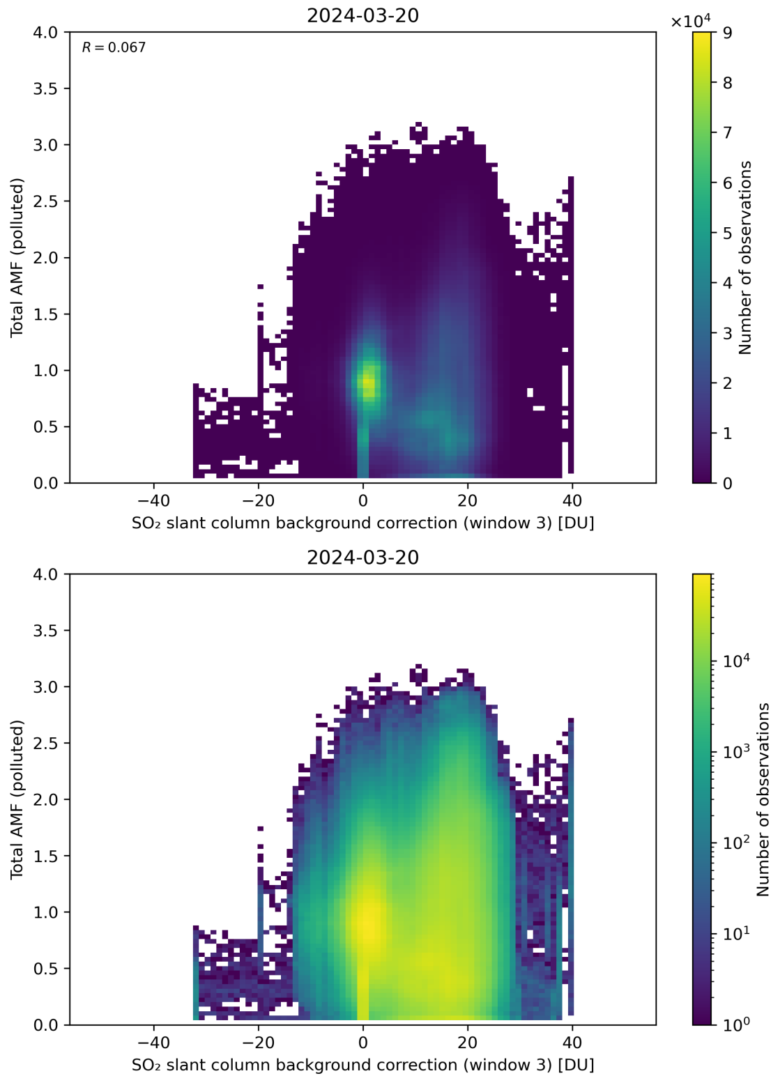
Figure 125: Scatter density plot of “SO 2 slant column background correction (window 3)” against “Total AMF (polluted)” for 2024-03-20 to 2024-03-21.
