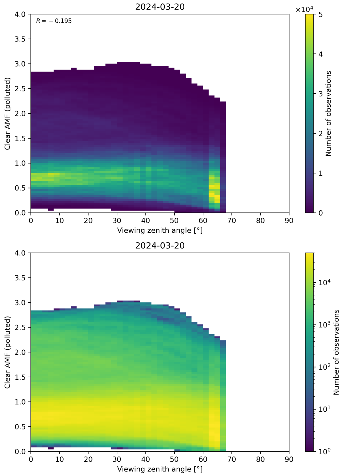
Figure 316: Scatter density plot of “Viewing zenith angle” against “Clear AMF (polluted)” for 2024-03-20 to 2024-03-21.
