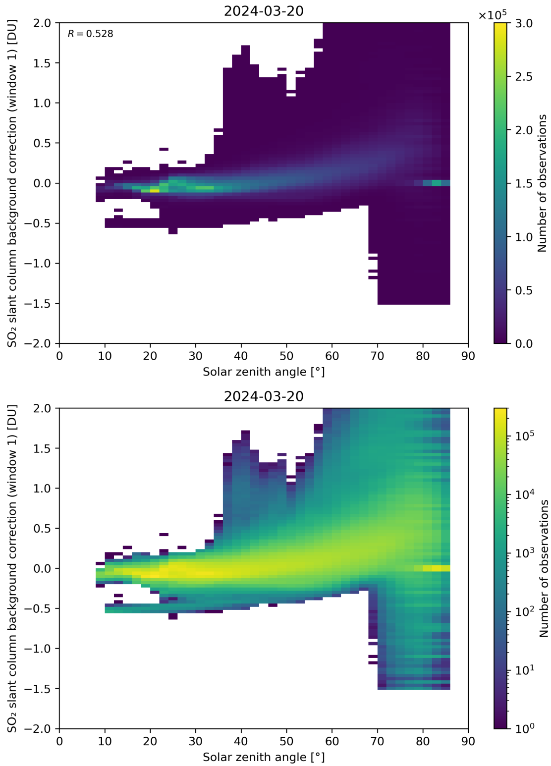
Figure 158: Scatter density plot of “Solar zenith angle” against “SO 2 slant column background correction (window 1)” for 2024-03-20 to 2024-03-21.
