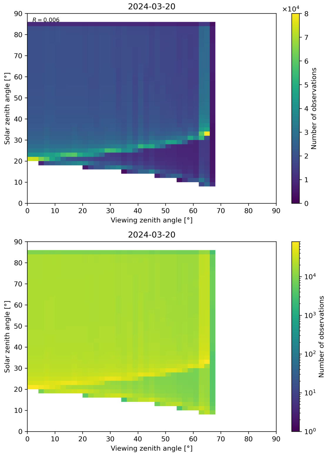
Figure 315: Scatter density plot of “Viewing zenith angle” against “Solar zenith angle” for 2024-03-20 to 2024-03-21.
