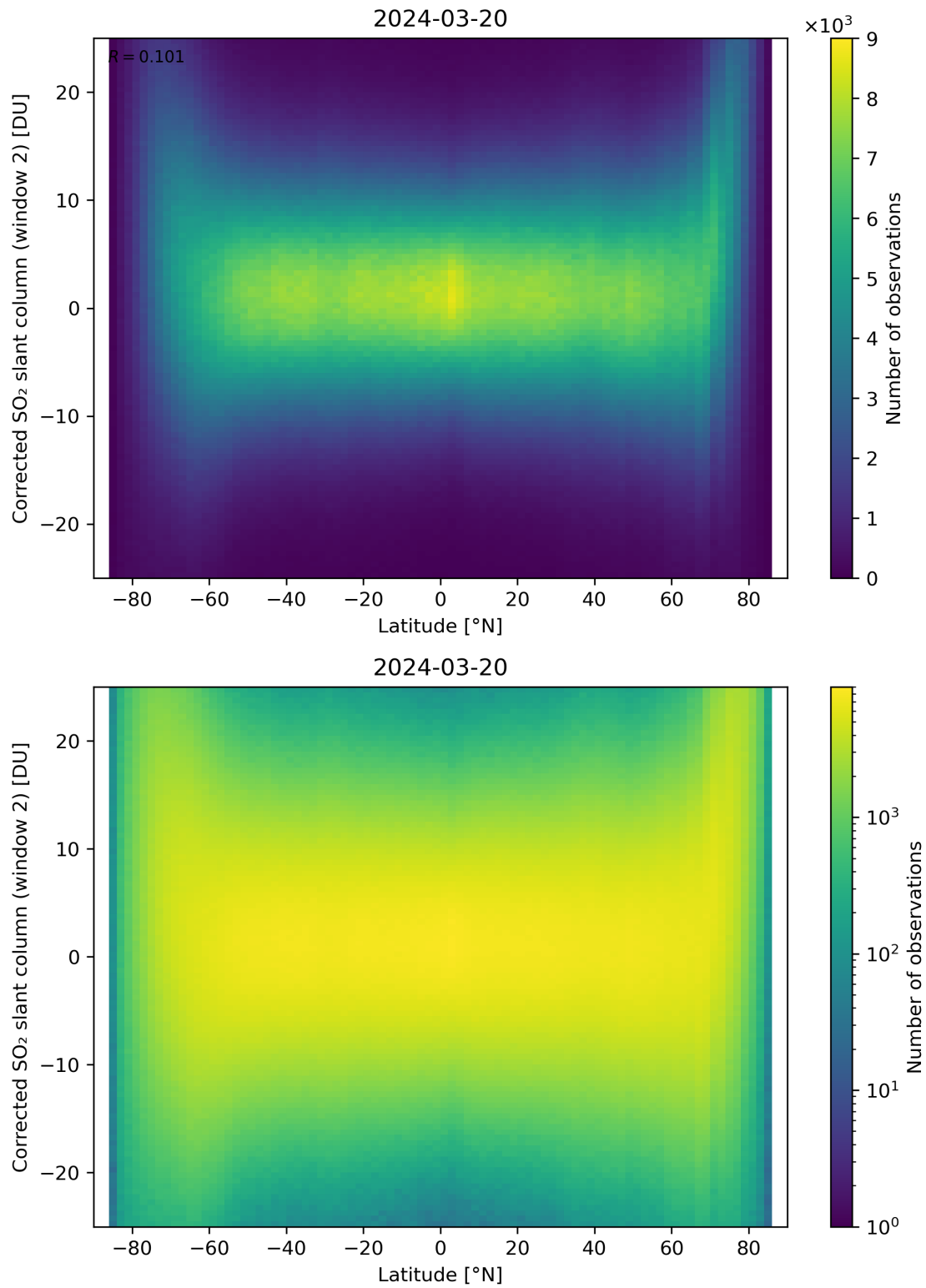
Figure 147: Scatter density plot of “Latitude” against “Corrected SO 2 slant column (window 2)” for 2024-03-20 to 2024-03-21.
