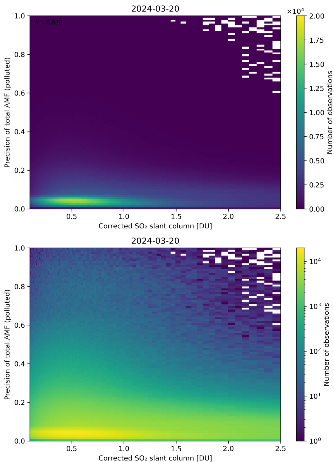
Figure 193: Scatter density plot of “Corrected SO 2 slant column” against “Precision of total AMF (polluted)” for 2024-03-20 to 2024-03-21.
