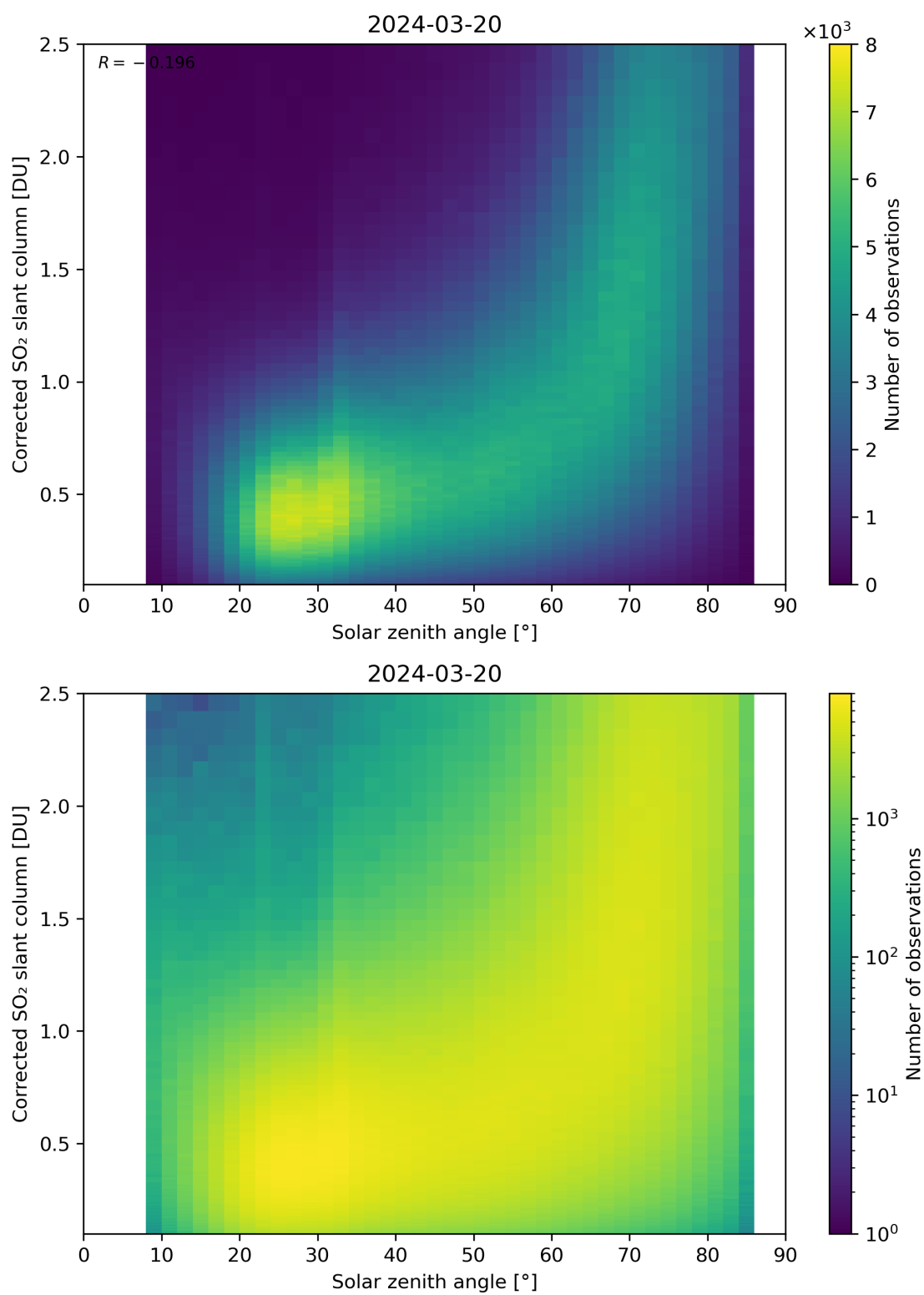
Figure 166: Scatter density plot of “Solar zenith angle” against “Corrected SO 2 slant column” for 2024-03-20 to 2024-03-21.
