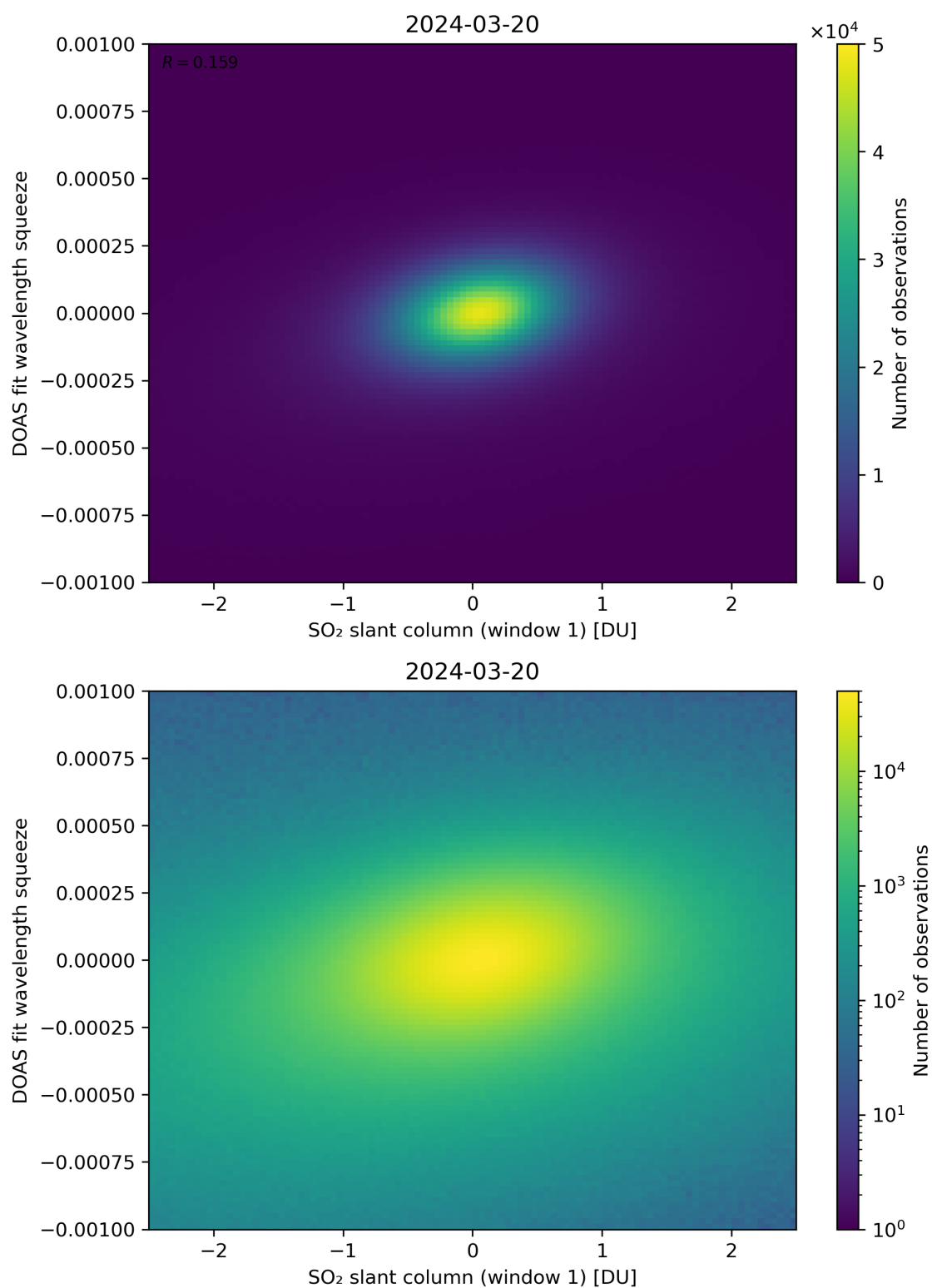
Figure 216: Scatter density plot of “SO 2 slant column (window 1)” against “DOAS fit wavelength squeeze” for 2024-03-20 to 2024-03-21.
