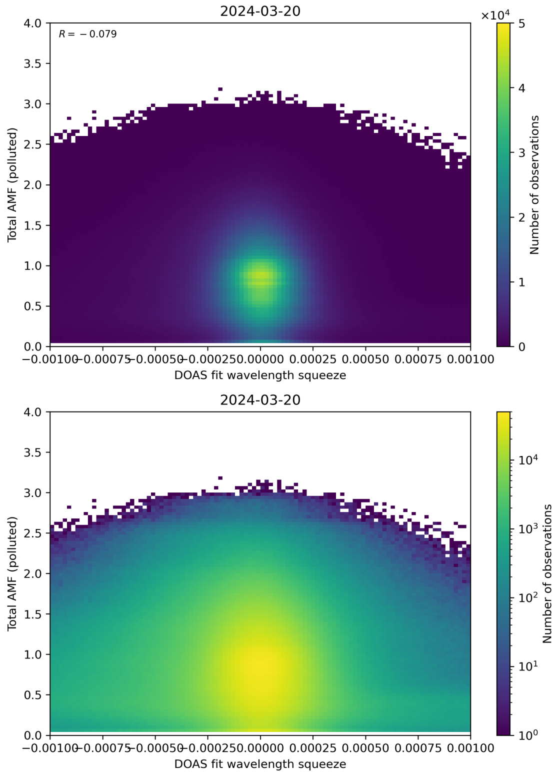
Figure 134: Scatter density plot of “DOAS fit wavelength squeeze” against “Total AMF (polluted)” for 2024-03-20 to 2024-03-21.
