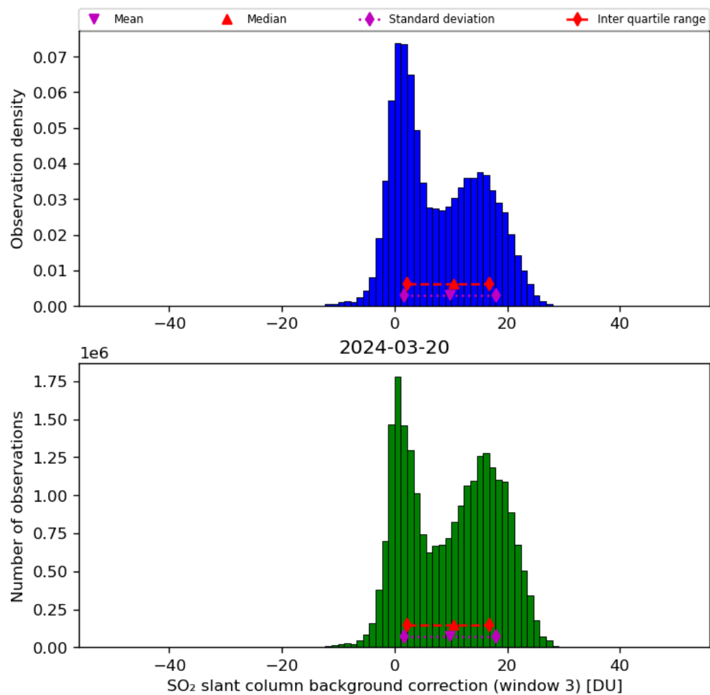
Figure 67: Histogram of “SO 2 slant column background correction (window 3)” for 2024-03-20 to 2024-03-21
