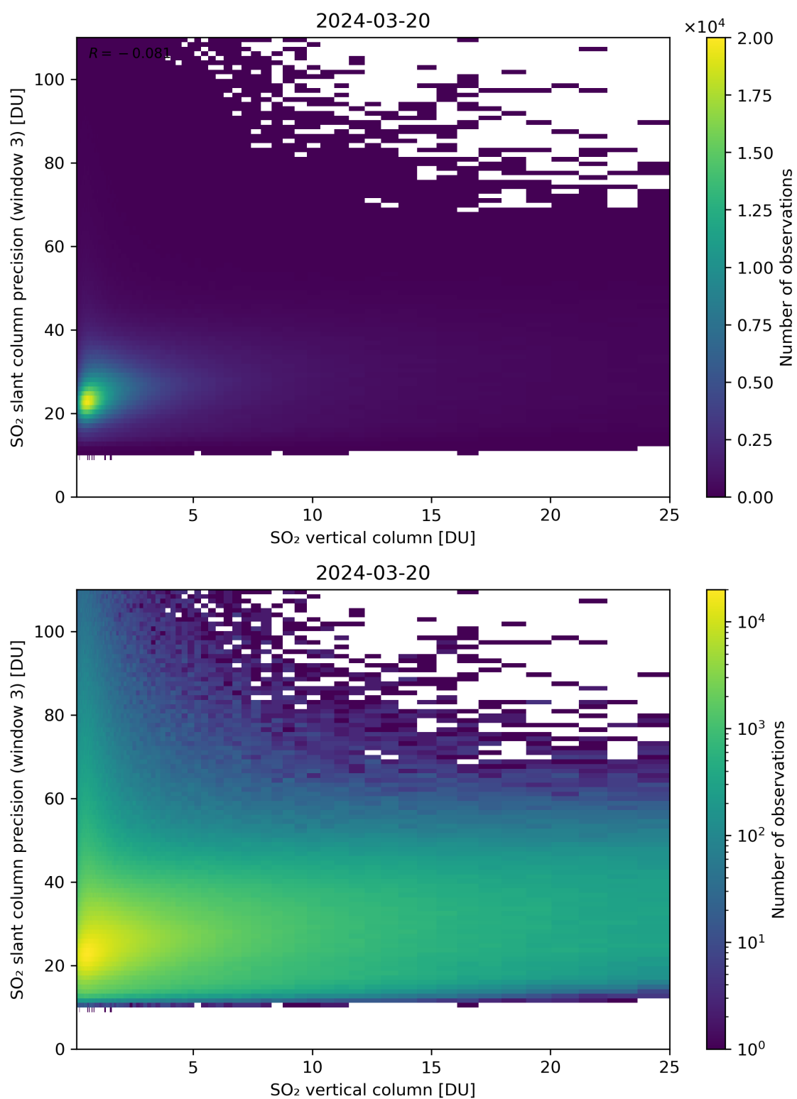
Figure 304: Scatter density plot of “SO 2 vertical column” against “SO 2 slant column precision (window 3)” for 2024-03-20 to 2024-03-21.
