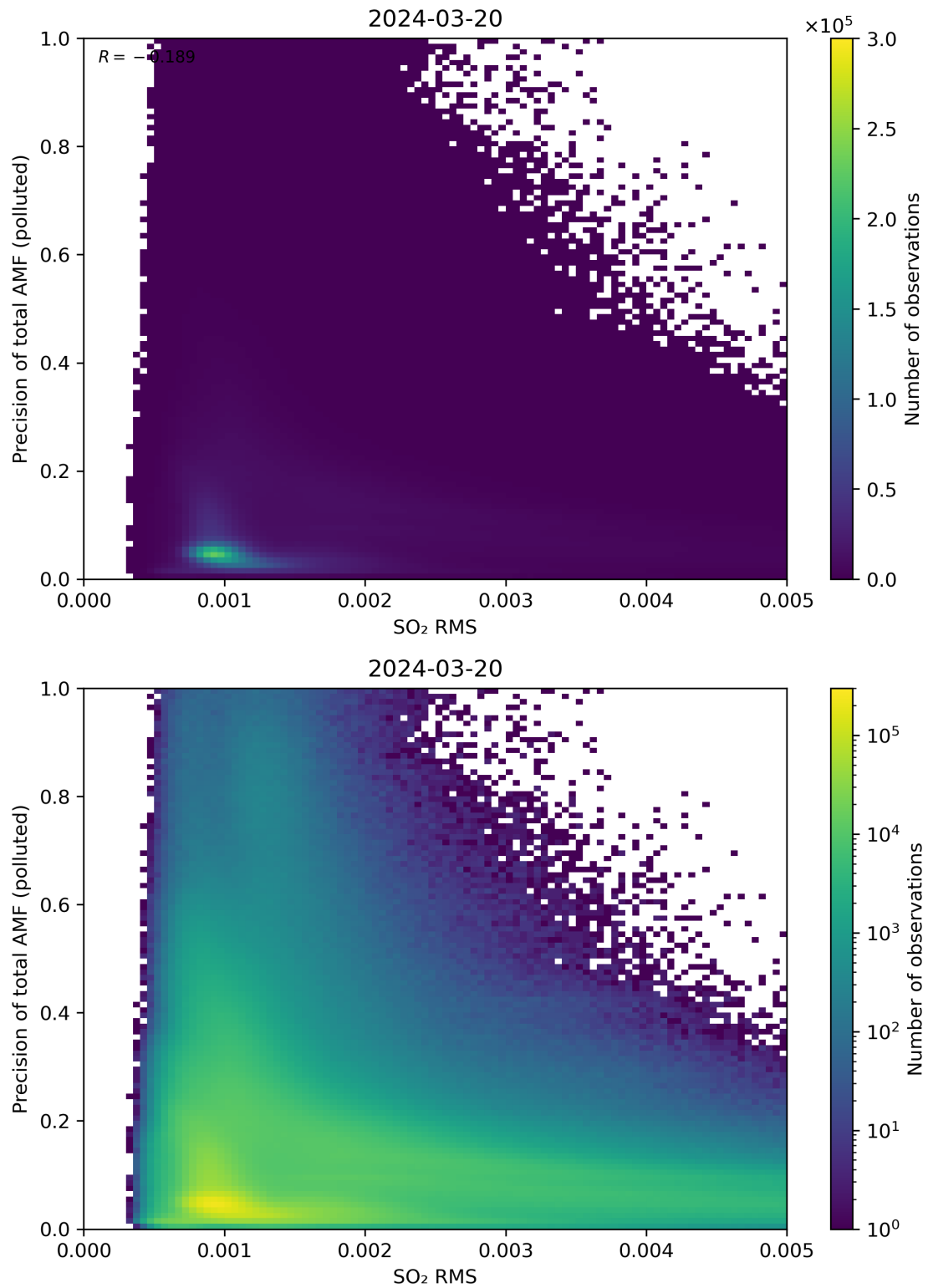
Figure 138: Scatter density plot of “SO 2 RMS” against “Precision of total AMF (polluted)” for 2024-03-20 to 2024-03-21.
