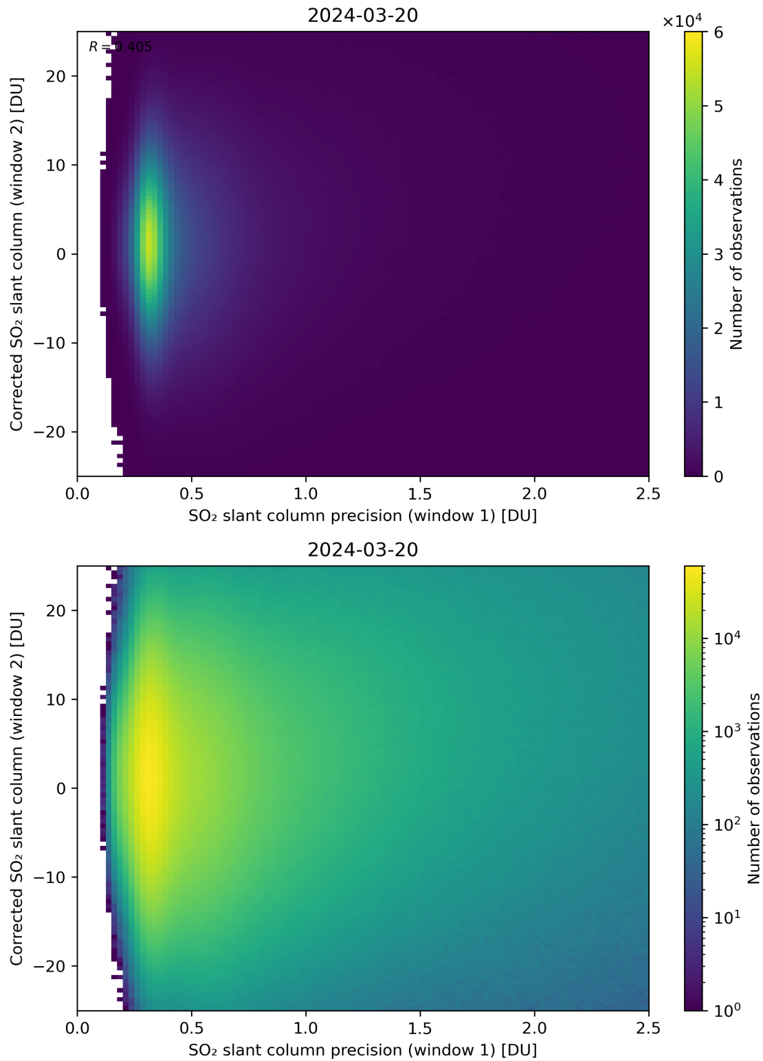
Figure 225: Scatter density plot of “SO 2 slant column precision (window 1)” against “Corrected SO 2 slant column (window 2)” for 2024-03-20 to 2024-03-21.
