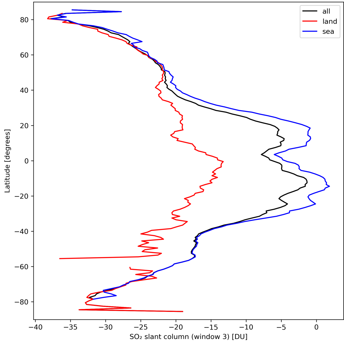
Figure 41: Zonal average of “SO 2 slant column (window 3)” for 2024-03-20 to 2024-03-21.
