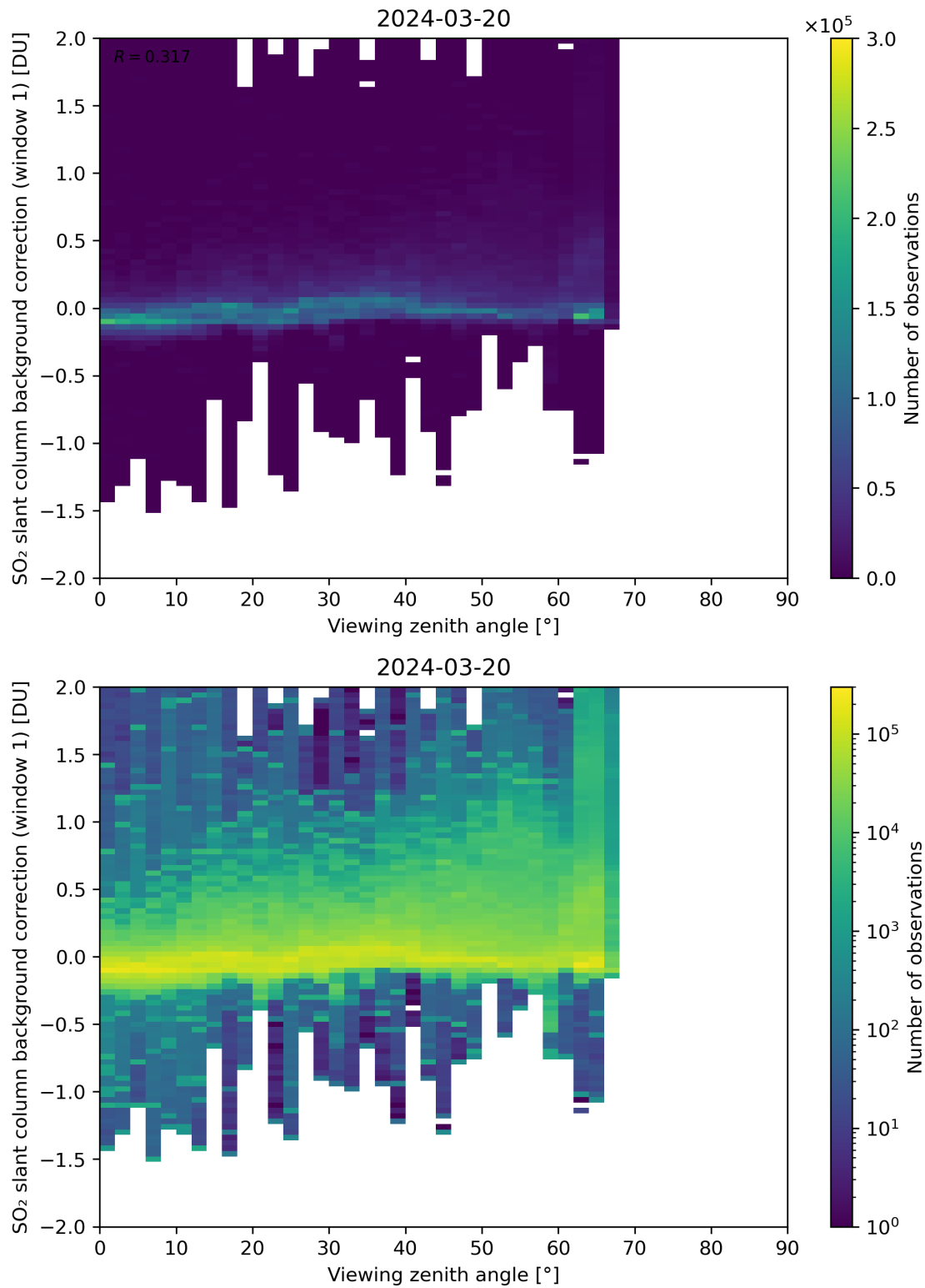
Figure 308: Scatter density plot of “Viewing zenith angle” against “SO 2 slant column background correction (window 1)” for 2024-03-20 to 2024-03-21.
