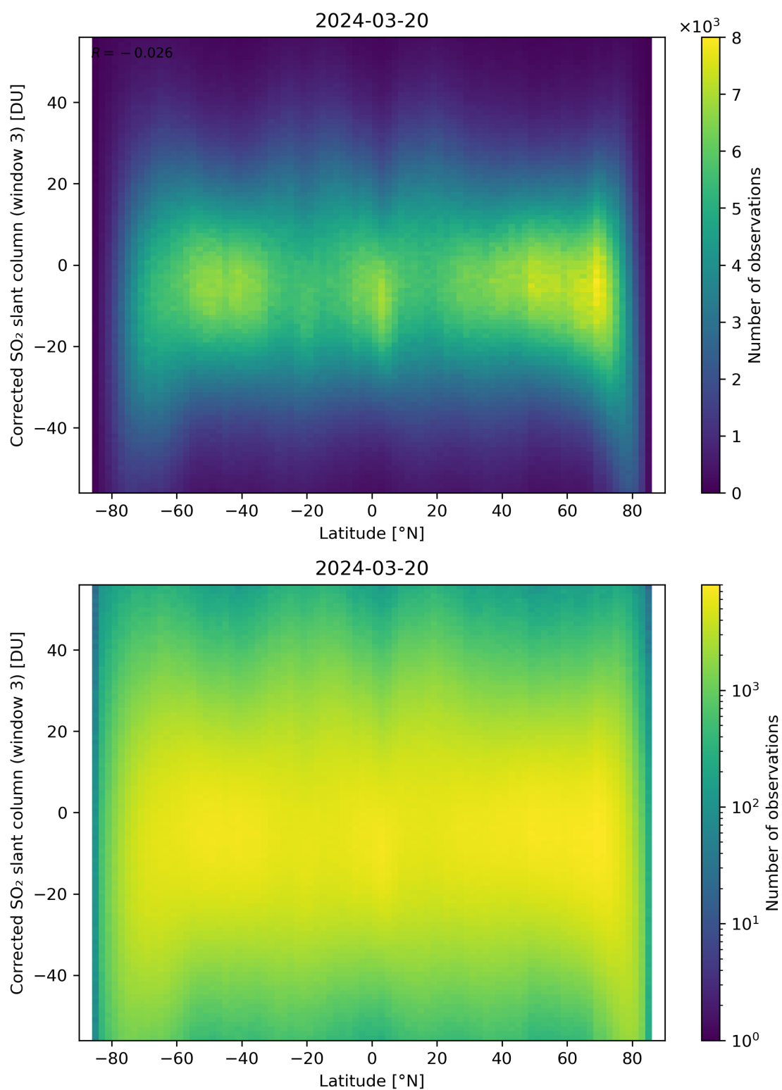
Figure 148: Scatter density plot of “Latitude” against “Corrected SO 2 slant column (window 3)” for 2024-03-20 to 2024-03-21.
