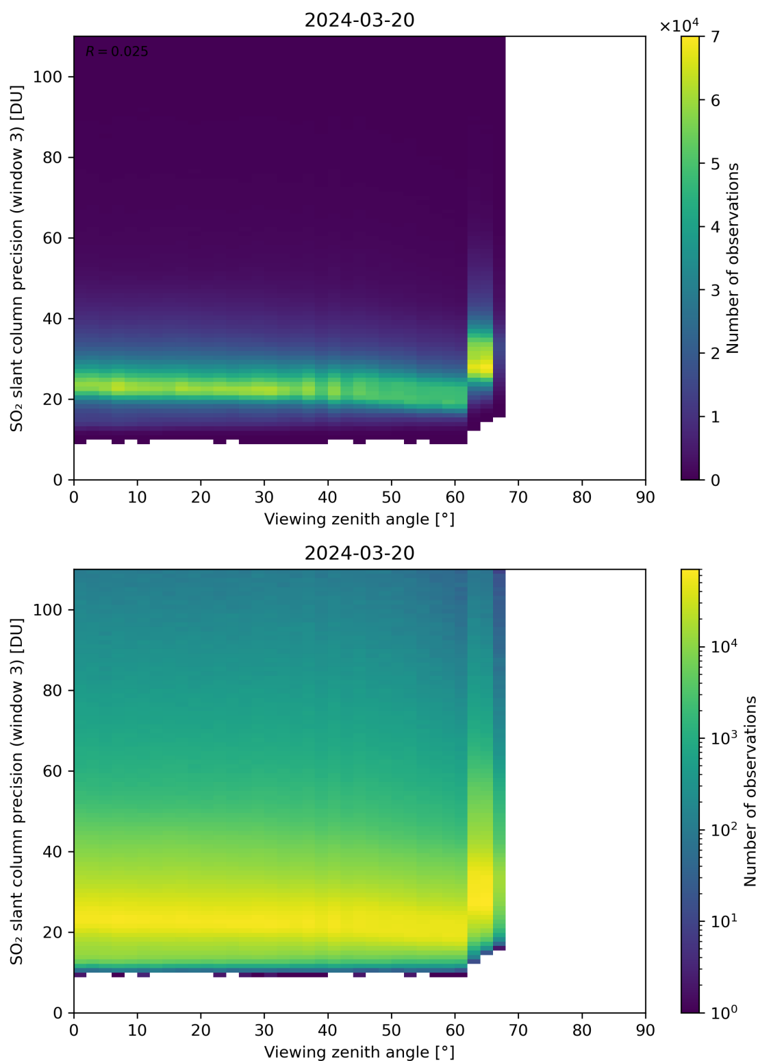
Figure 324: Scatter density plot of “Viewing zenith angle” against “SO 2 slant column precision (window 3)” for 2024-03-20 to 2024-03-21.
