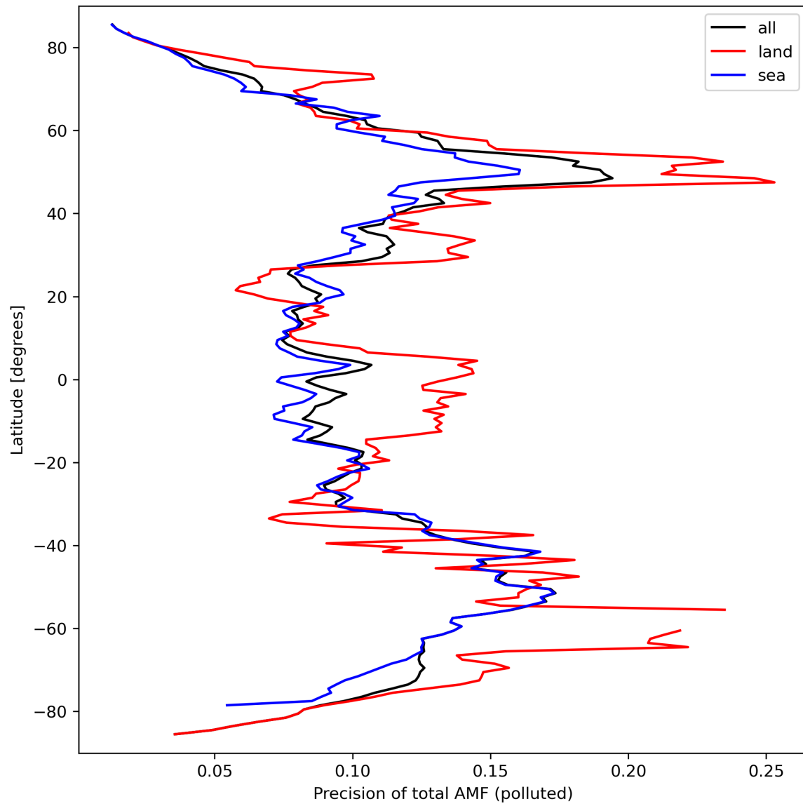
Figure 49: Zonal average of “Precision of total AMF (polluted)” for 2024-03-20 to 2024-03-21.
