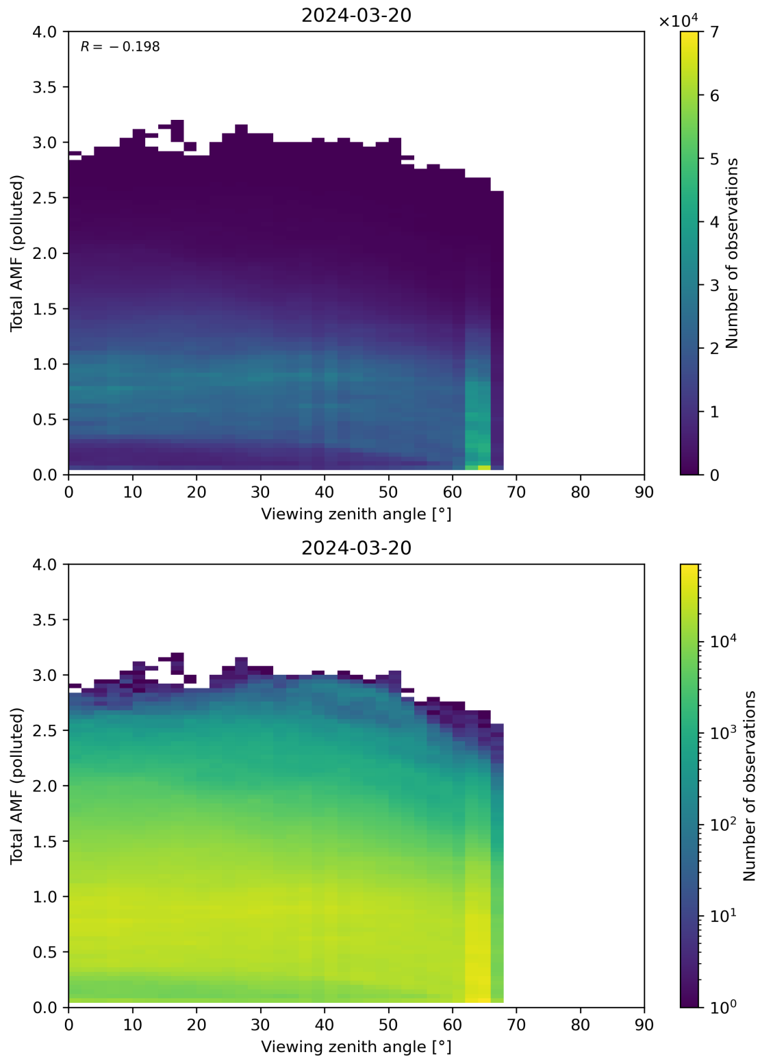
Figure 325: Scatter density plot of “Viewing zenith angle” against “Total AMF (polluted)” for 2024-03-20 to 2024-03-21.
