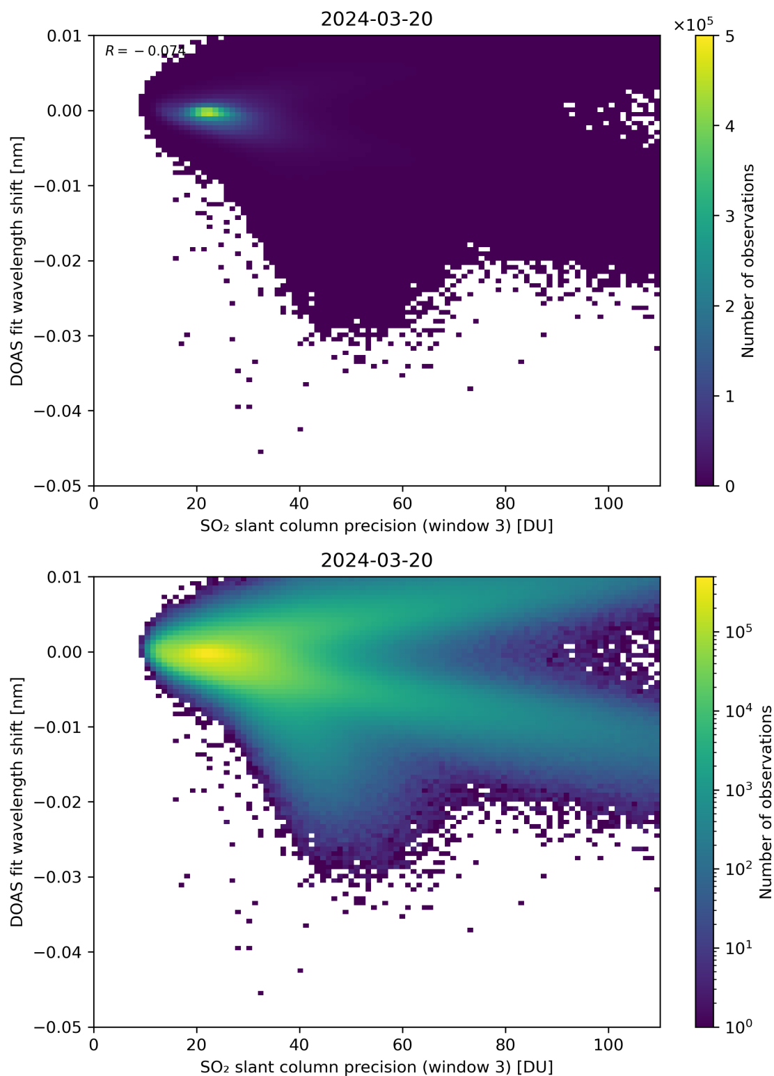
Figure 258: Scatter density plot of “SO 2 slant column precision (window 3)” against “DOAS fit wavelength shift” for 2024-03-20 to 2024-03-21.
