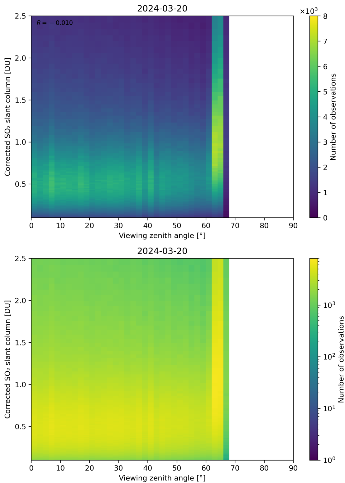
Figure 317: Scatter density plot of “Viewing zenith angle” against “Corrected SO 2 slant column” for 2024-03-20 to 2024-03-21.
