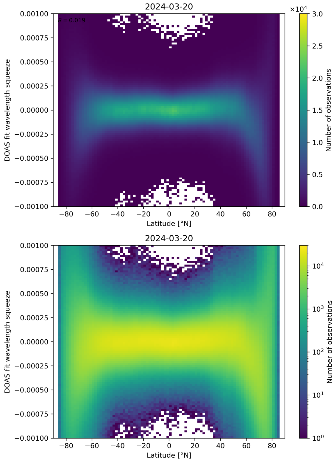
Figure 143: Scatter density plot of “Latitude” against “DOAS fit wavelength squeeze” for 2024-03-20 to 2024-03-21.
