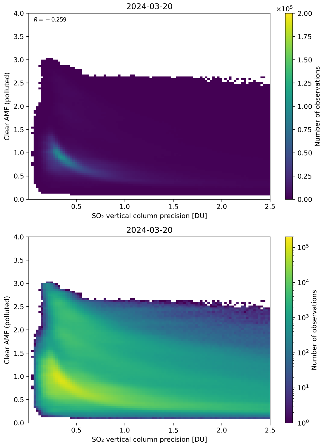
Figure 285: Scatter density plot of “SO 2 vertical column precision” against “Clear AMF (polluted)” for 2024-03-20 to 2024-03-21.
