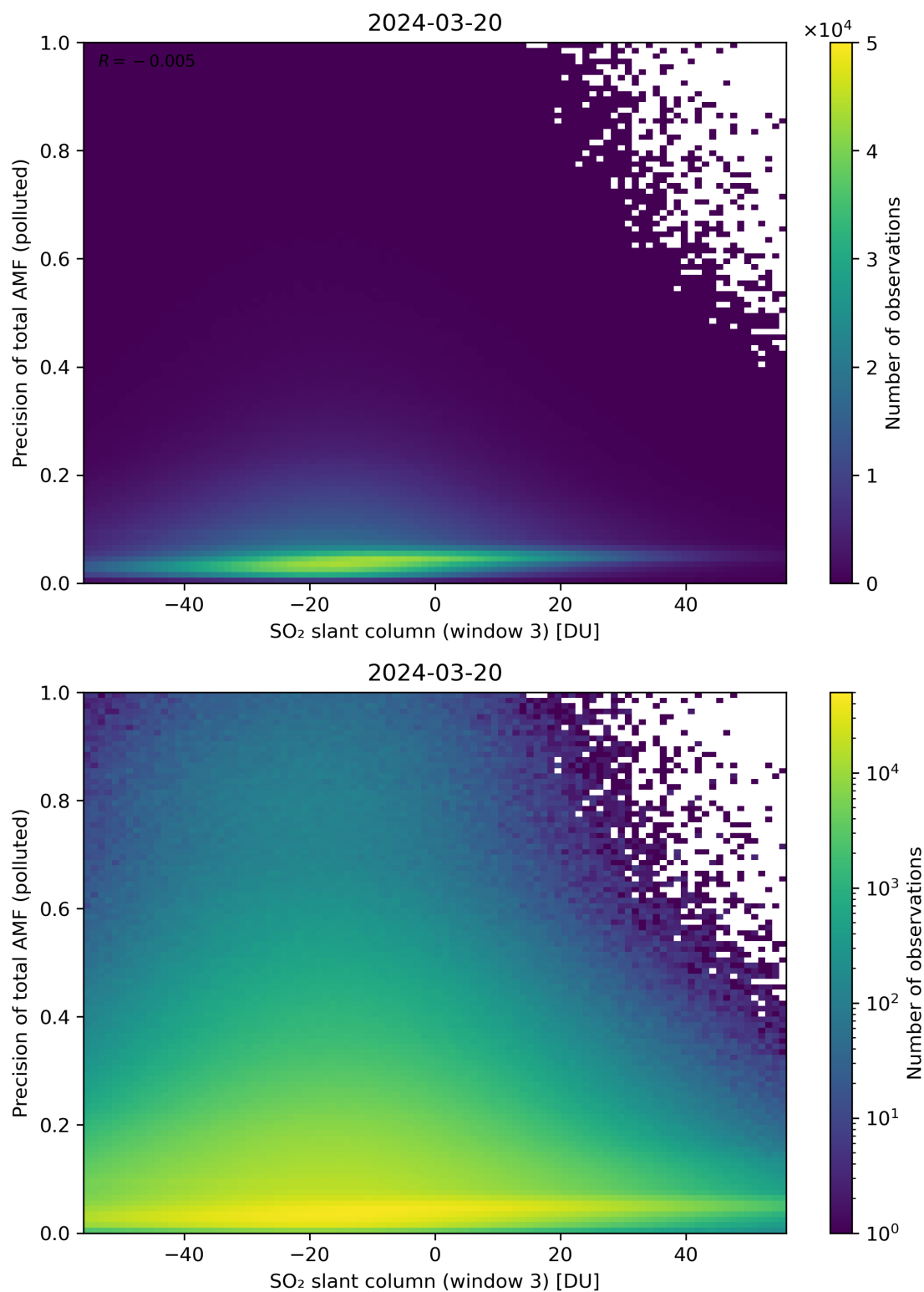
Figure 269: Scatter density plot of “SO 2 slant column (window 3)” against “Precision of total AMF (polluted)” for 2024-03-20 to 2024-03-21.
