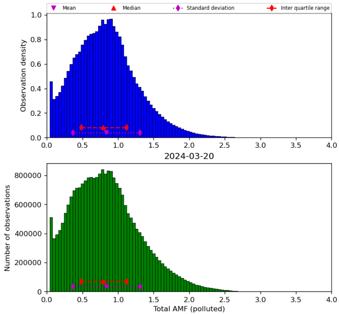
Figure 71: Histogram of “Total AMF (polluted)” for 2024-03-20 to 2024-03-21
