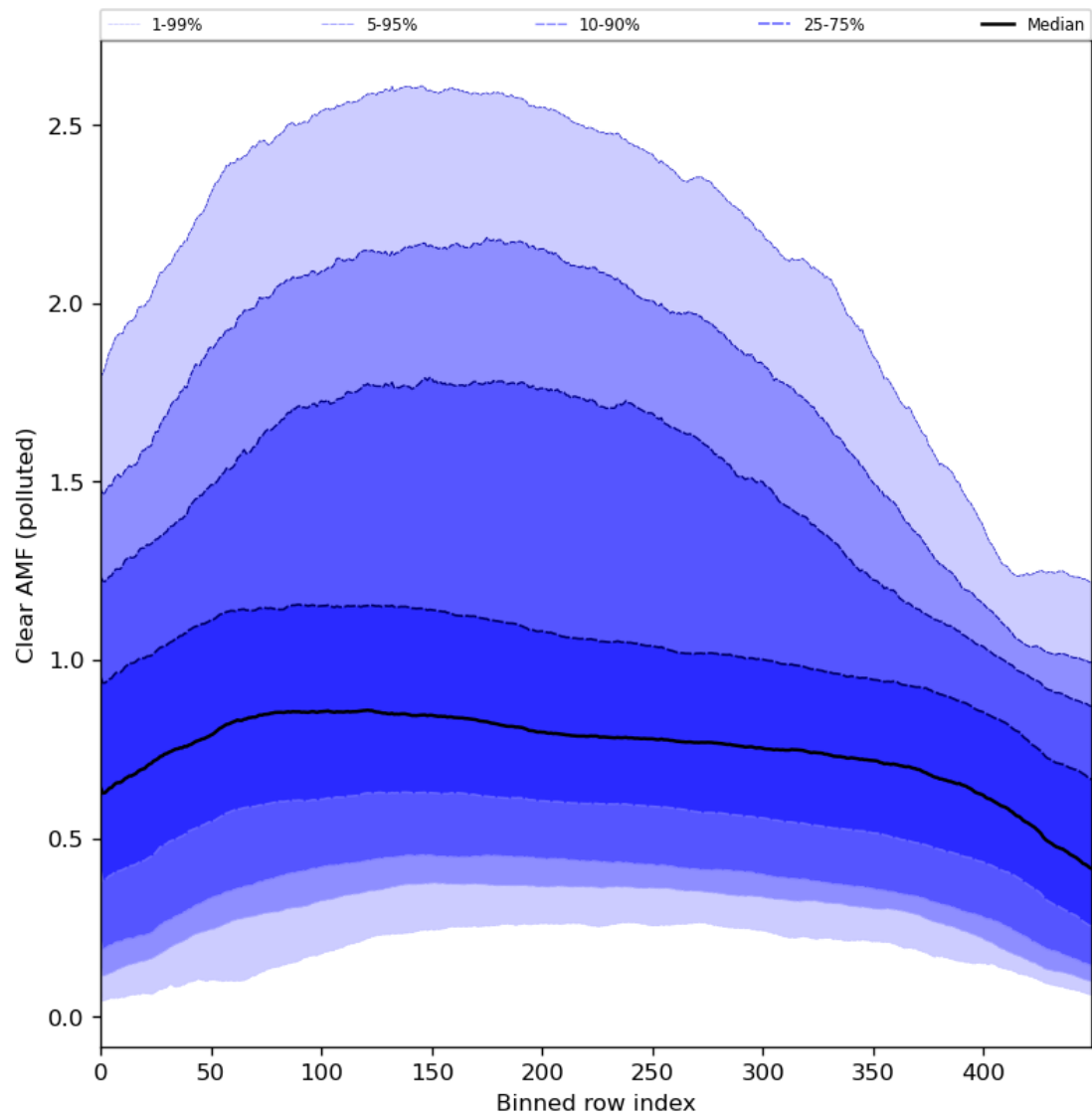
Figure 96: Along track statistics of “Clear AMF (polluted)” for 2024-03-20 to 2024-03-21
