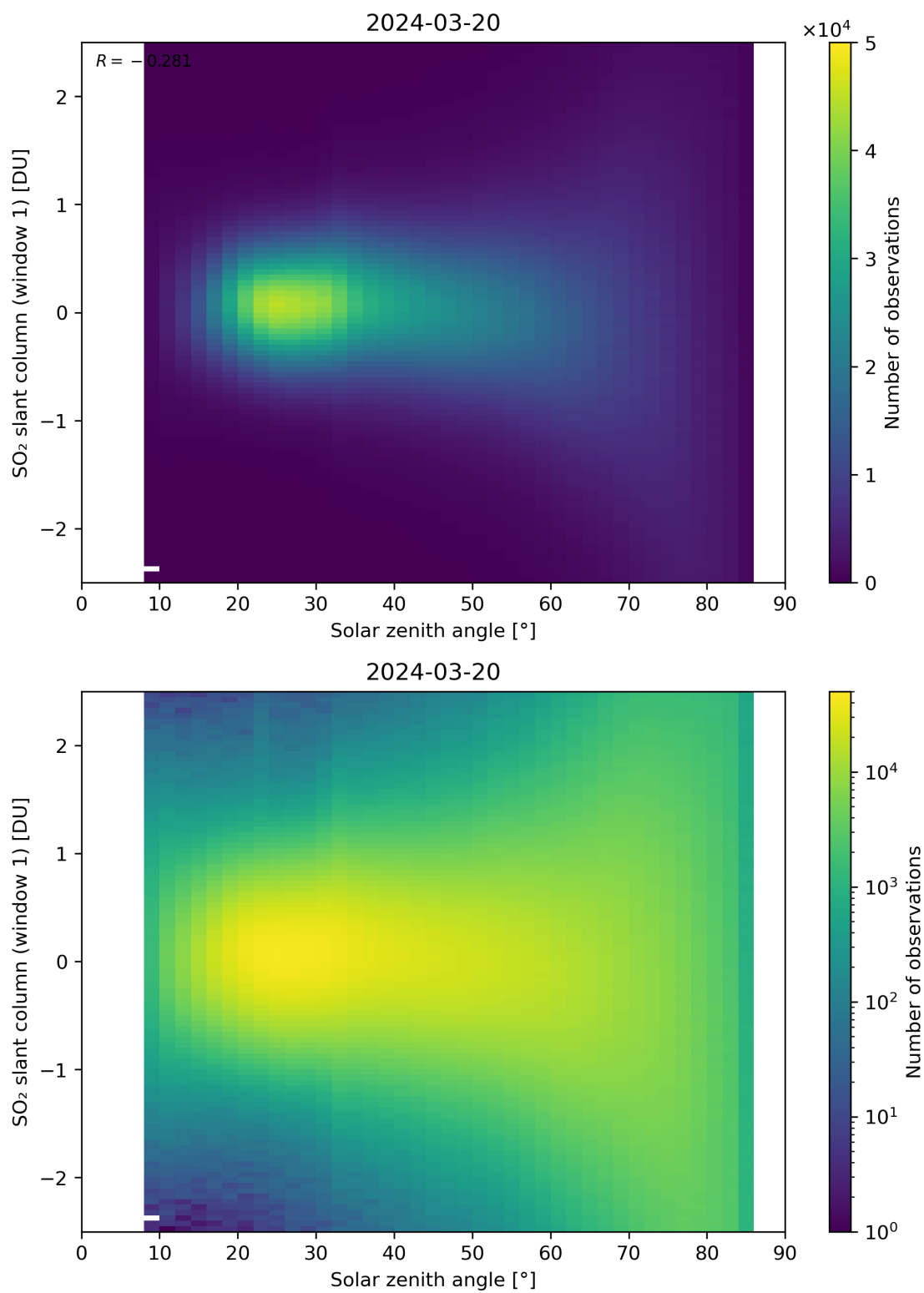
Figure 169: Scatter density plot of “Solar zenith angle” against “SO 2 slant column (window 1)” for 2024-03-20 to 2024-03-21.
