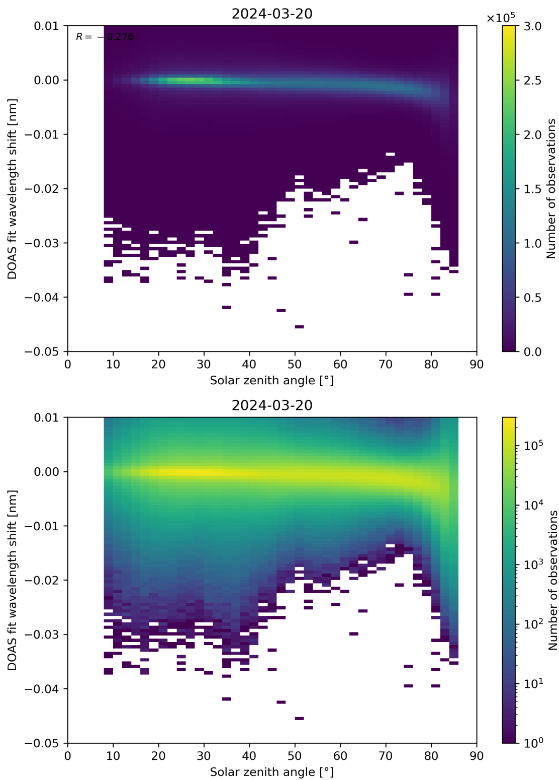
Figure 161: Scatter density plot of “Solar zenith angle” against “DOAS fit wavelength shift” for 2024-03-20 to 2024-03-21.
