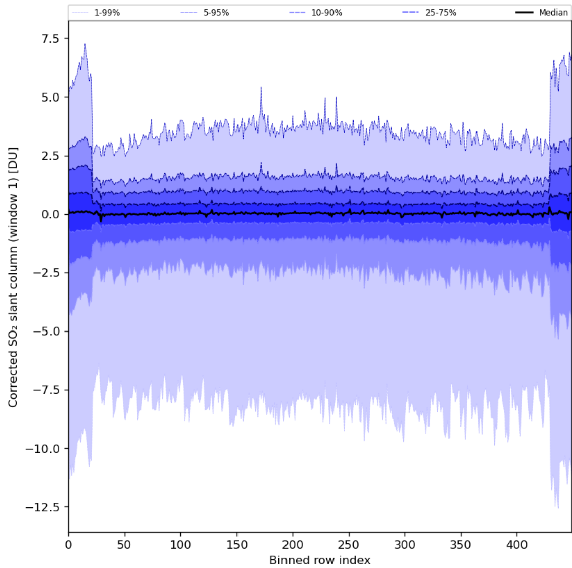
Figure 81: Along track statistics of “Corrected SO 2 slant column (window 1)” for 2024-03-20 to 2024-03-21
