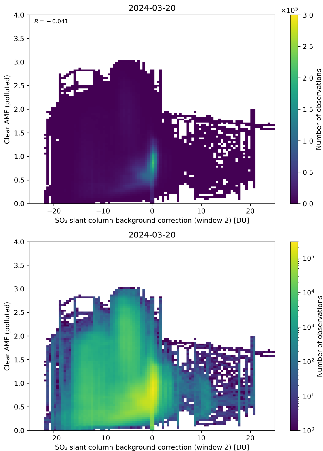
Figure 115: Scatter density plot of “SO 2 slant column background correction (window 2)” against “Clear AMF (polluted)” for 2024-03-20 to 2024-03-21.
