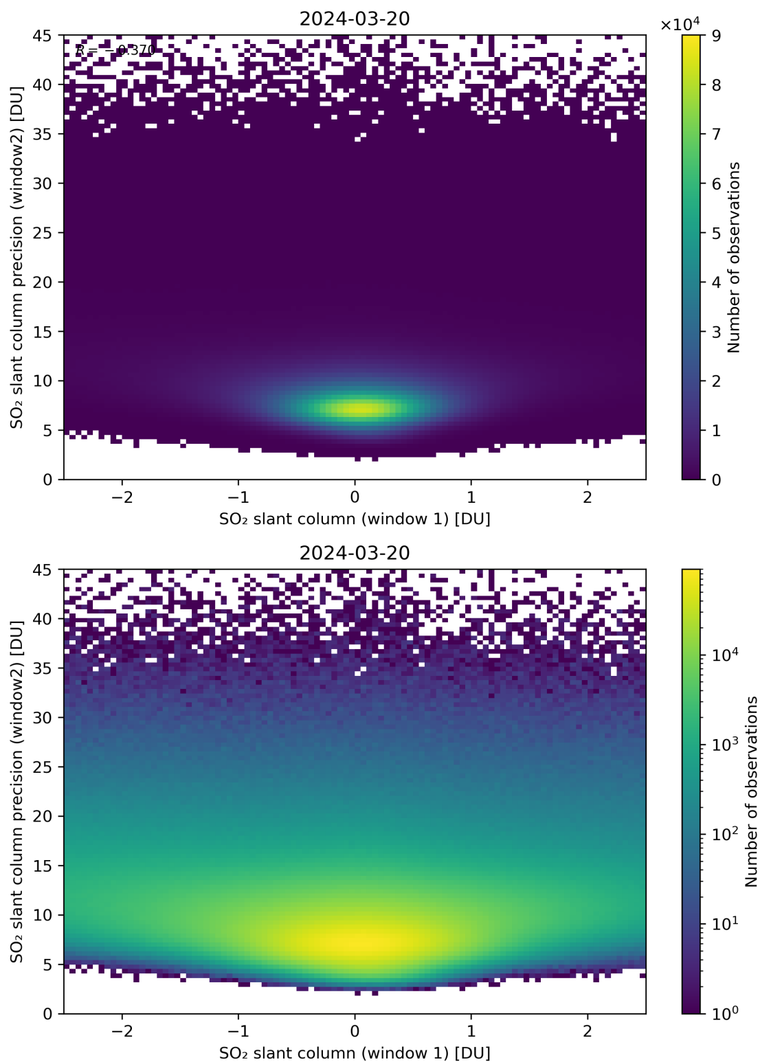
Figure 236: Scatter density plot of “SO 2 slant column (window 1)” against “SO 2 slant column precision (window2)” for 2024-03-20 to 2024-03-21.
