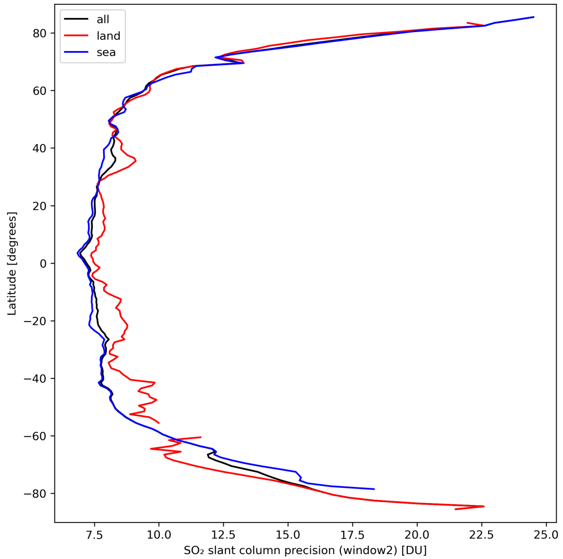
Figure 38: Zonal average of “SO 2 slant column precision (window2)” for 2024-03-20 to 2024-03-21.
