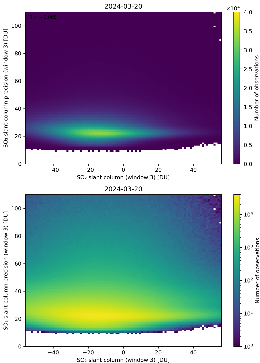
Figure 267: Scatter density plot of “SO 2 slant column (window 3)” against “SO 2 slant column precision (window 3)” for 2024-03-20 to 2024-03-21.
