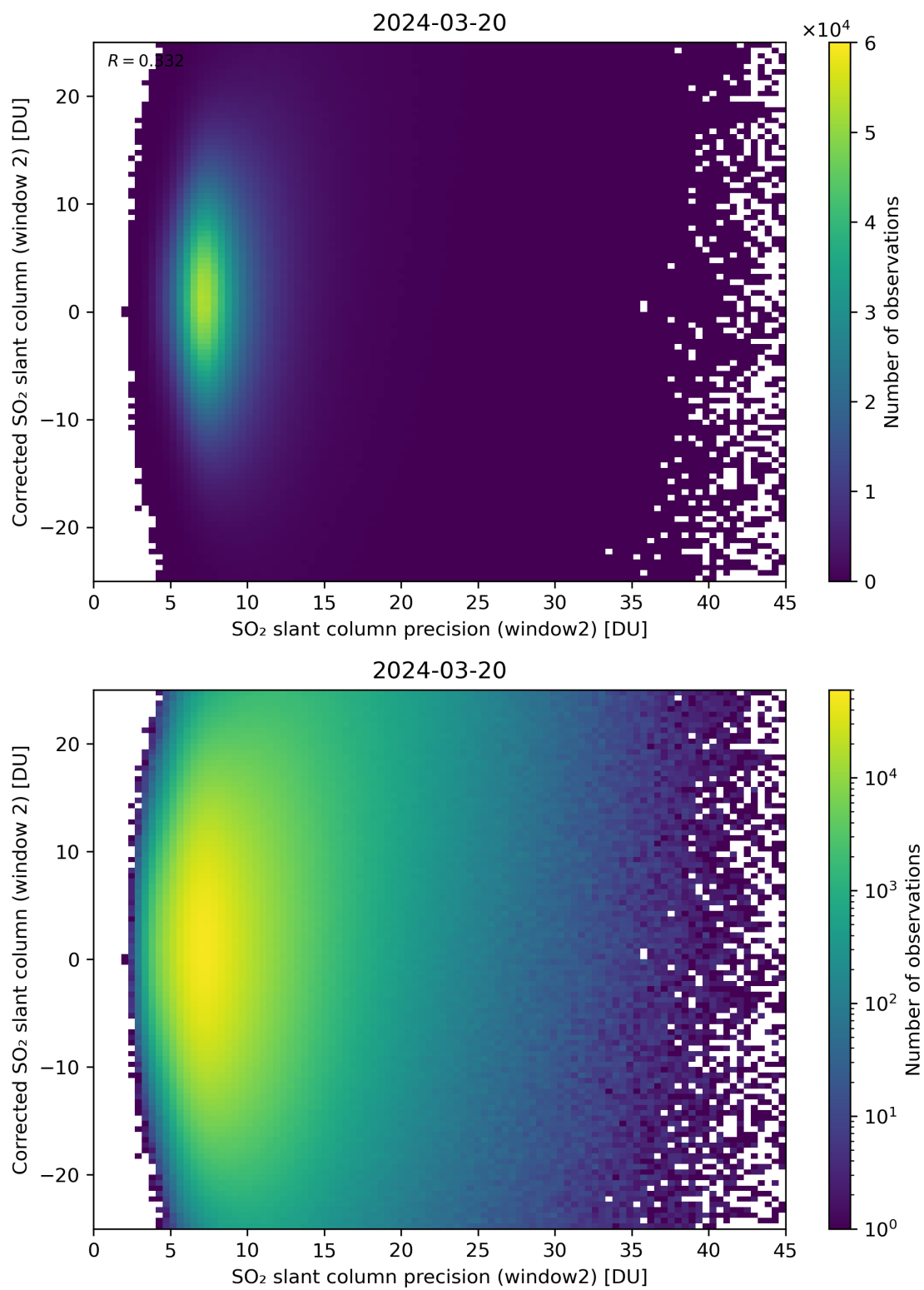
Figure 247: Scatter density plot of “SO 2 slant column precision (window2)” against “Corrected SO 2 slant column (window 2)” for 2024-03-20 to 2024-03-21.
