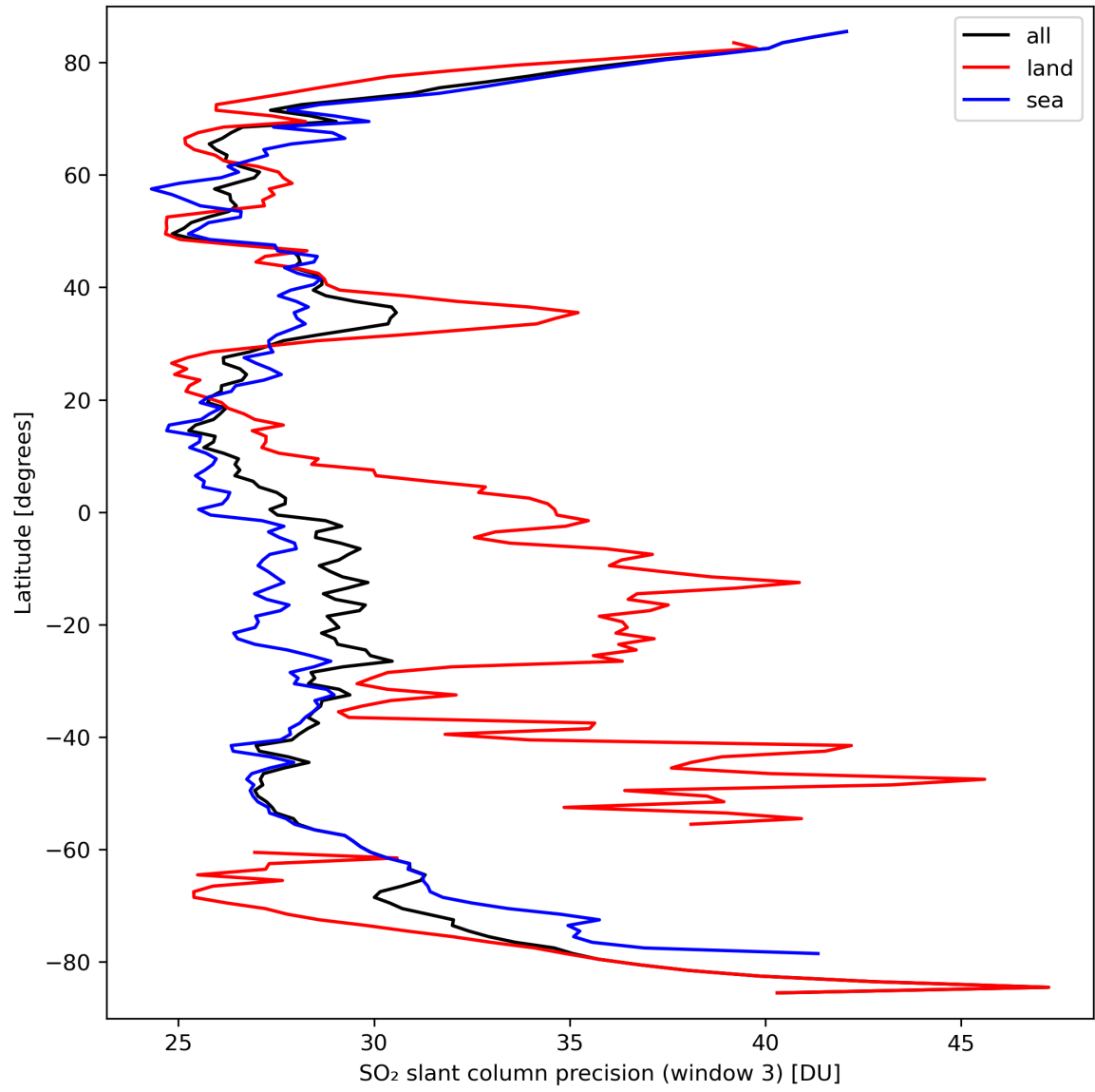
Figure 42: Zonal average of “SO 2 slant column precision (window 3)” for 2024-03-20 to 2024-03-21.
