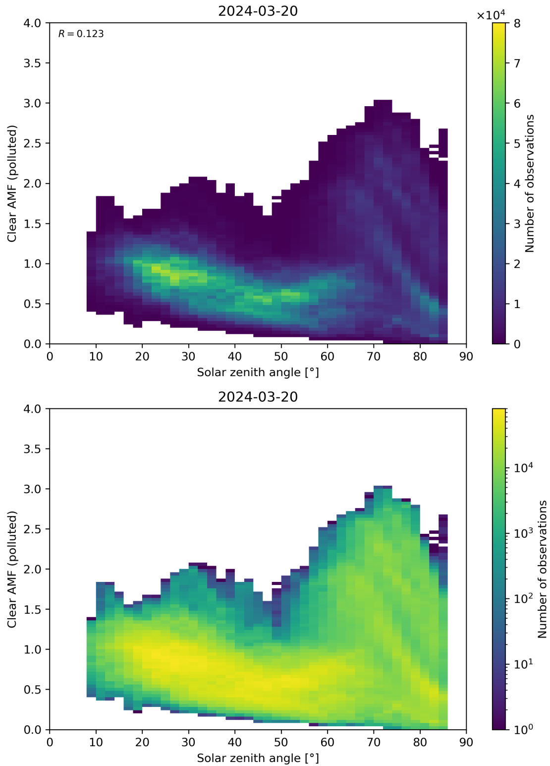
Figure 165: Scatter density plot of “Solar zenith angle” against “Clear AMF (polluted)” for 2024-03-20 to 2024-03-21.
