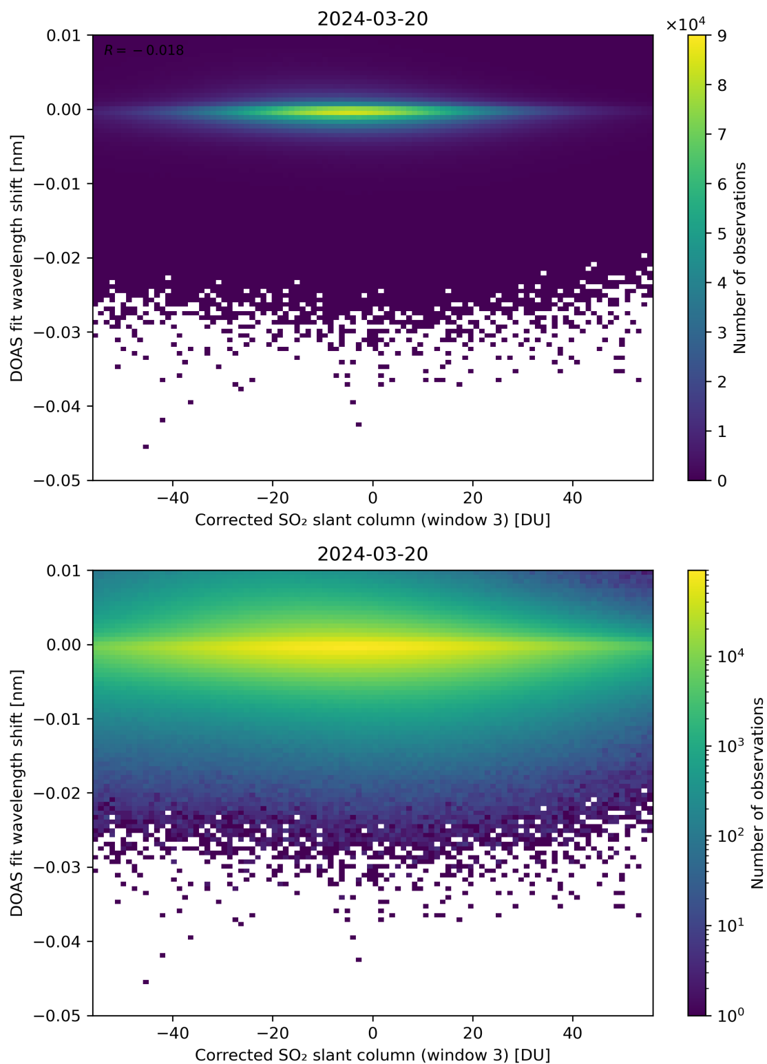
Figure 206: Scatter density plot of “Corrected SO 2 slant column (window 3)” against “DOAS fit wavelength shift” for 2024-03-20 to 2024-03-21.
