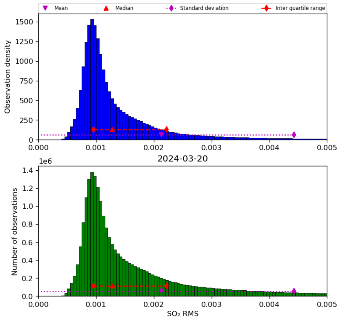
Figure 70: Histogram of “SO 2 RMS” for 2024-03-20 to 2024-03-21
