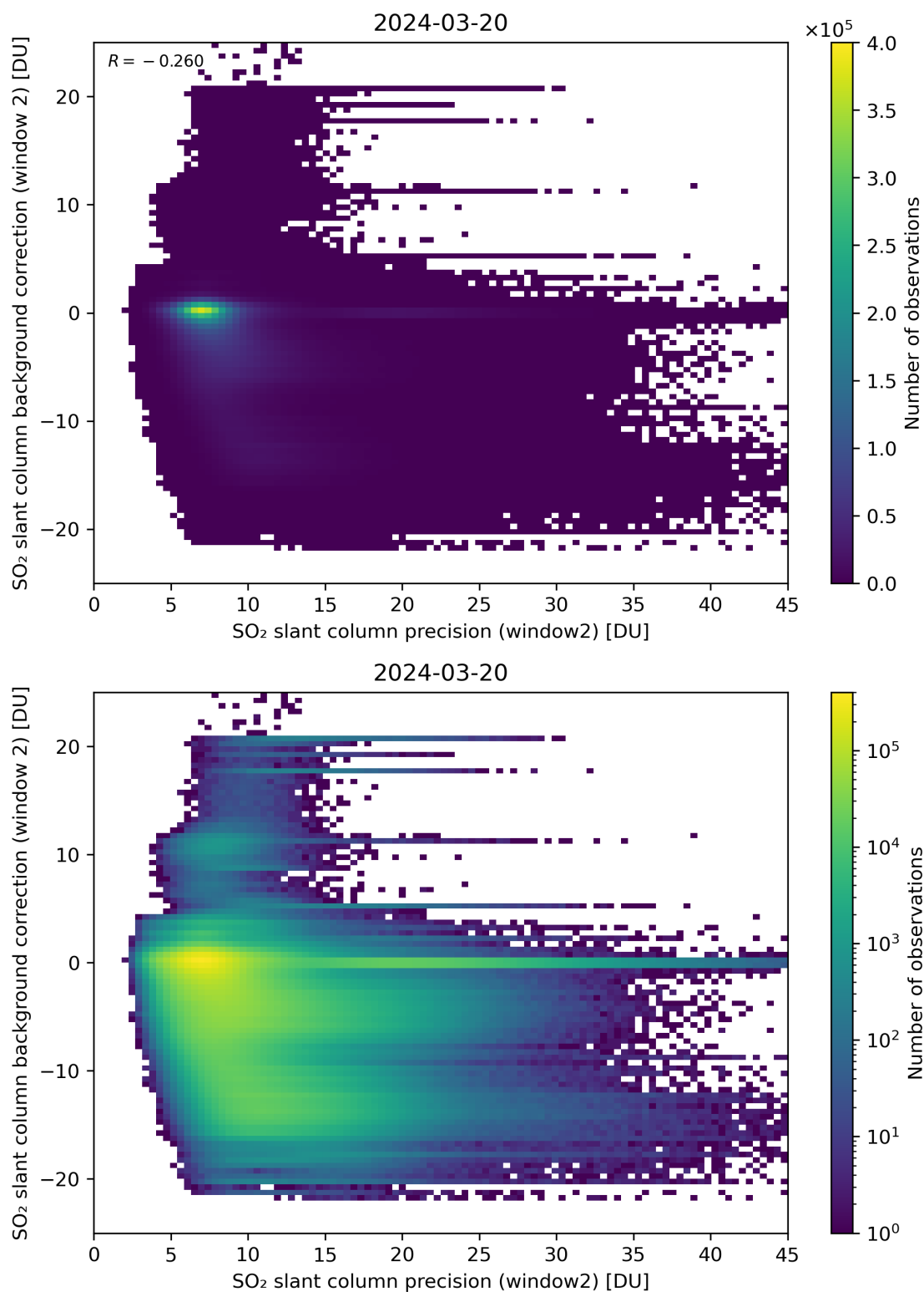
Figure 241: Scatter density plot of “SO 2 slant column precision (window2)” against “SO 2 slant column background correction (window 2)” for 2024-03-20 to 2024-03-21.
