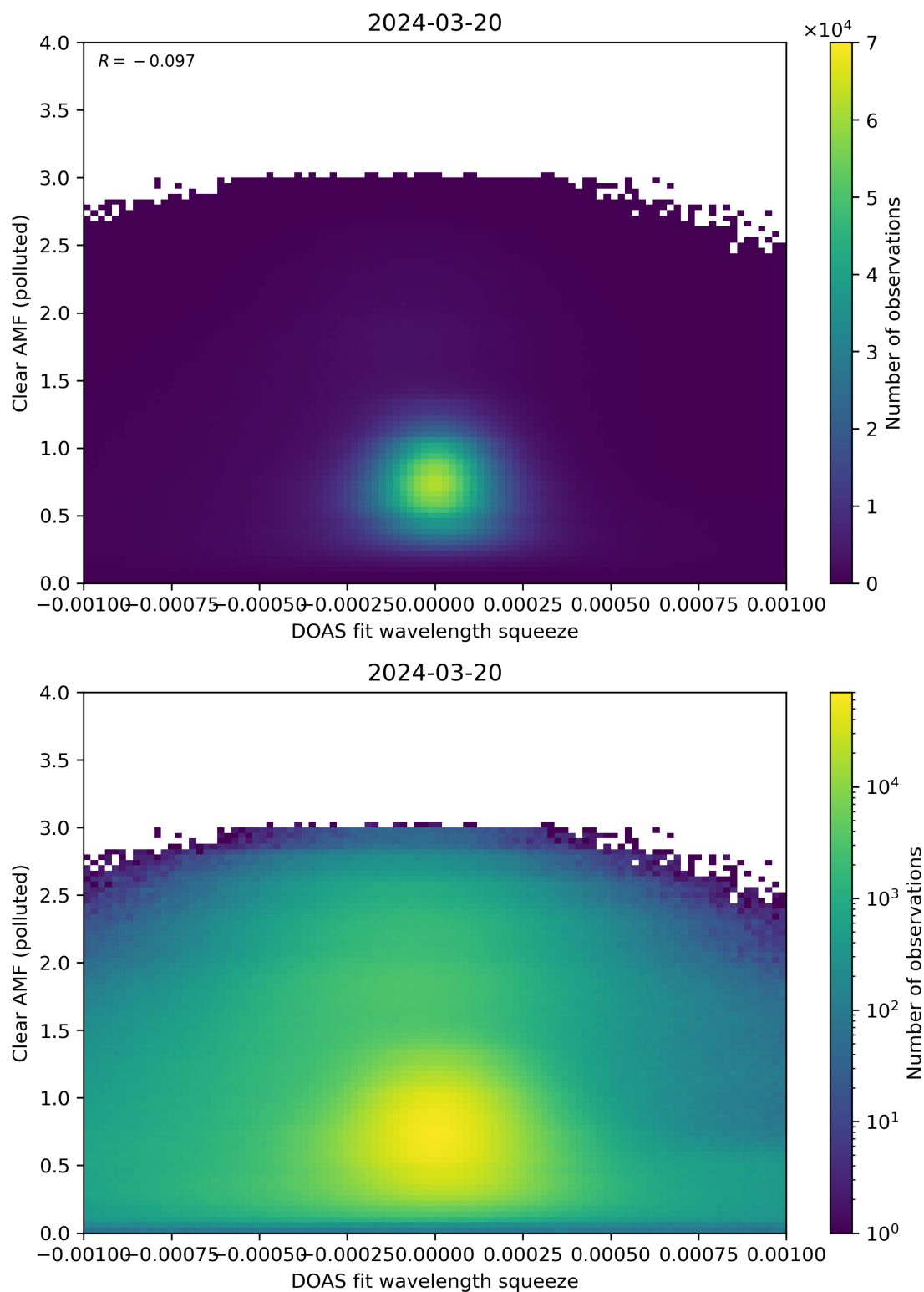
Figure 133: Scatter density plot of “DOAS fit wavelength squeeze” against “Clear AMF (polluted)” for 2024-03-20 to 2024-03-21.
