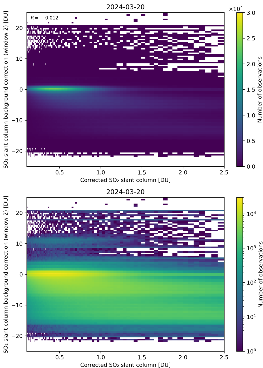
Figure 179: Scatter density plot of “Corrected SO 2 slant column” against “SO 2 slant column background correction (window 2)” for 2024-03-20 to 2024-03-21.
