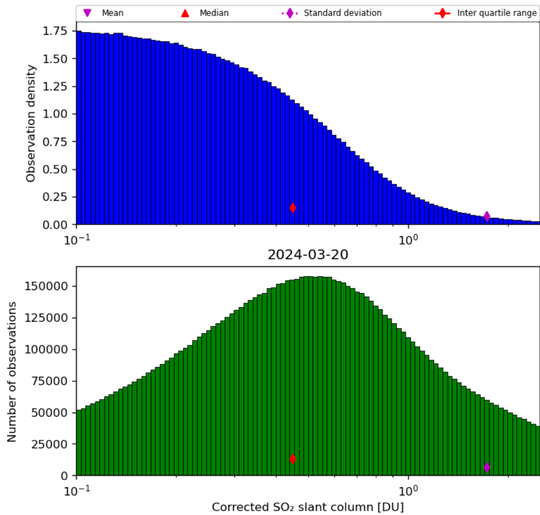
Figure 55: Histogram of “Corrected SO 2 slant column” for 2024-03-20 to 2024-03-21
