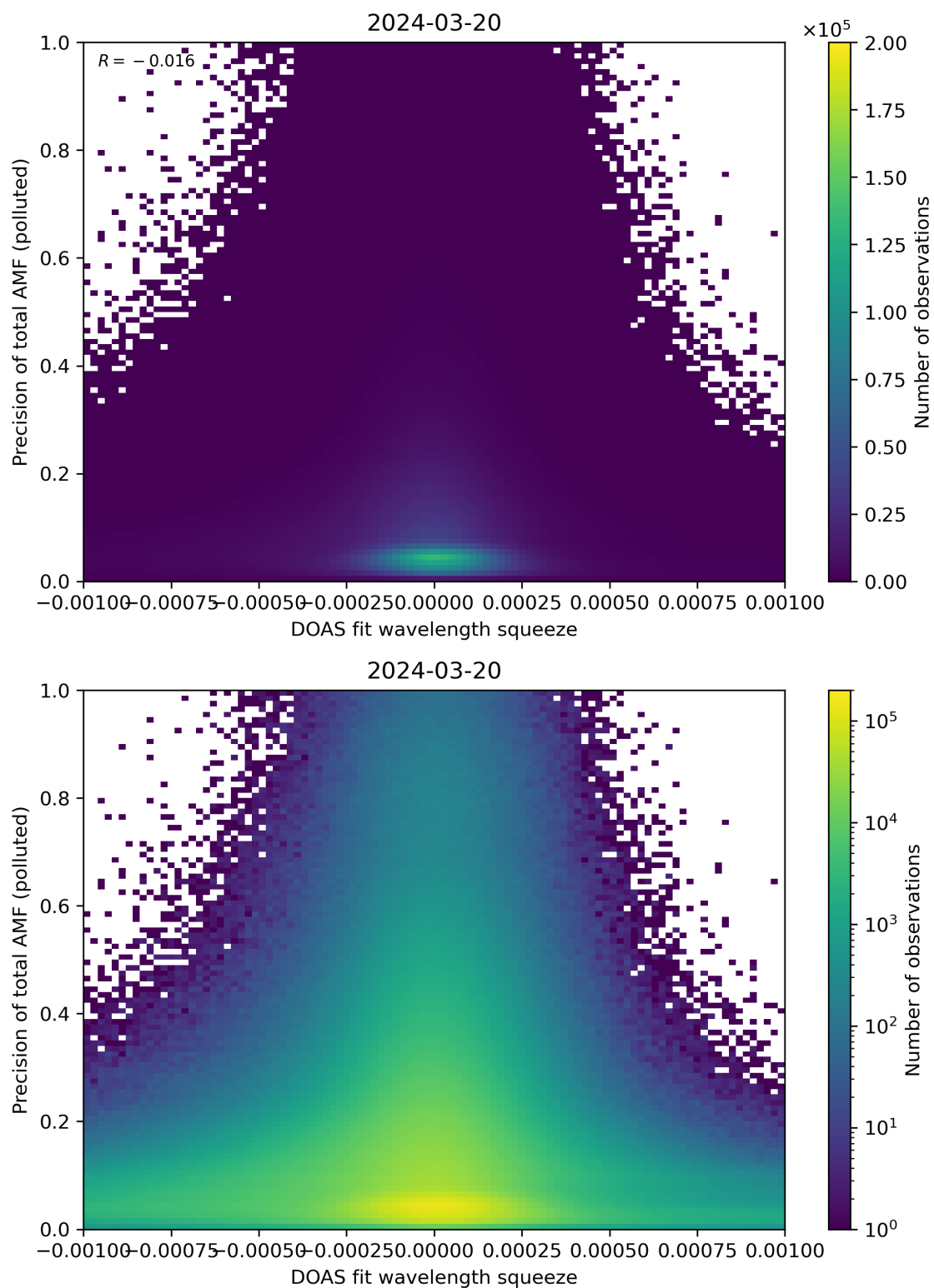
Figure 135: Scatter density plot of “DOAS fit wavelength squeeze” against “Precision of total AMF (polluted)” for 2024-03-20 to 2024-03-21.
