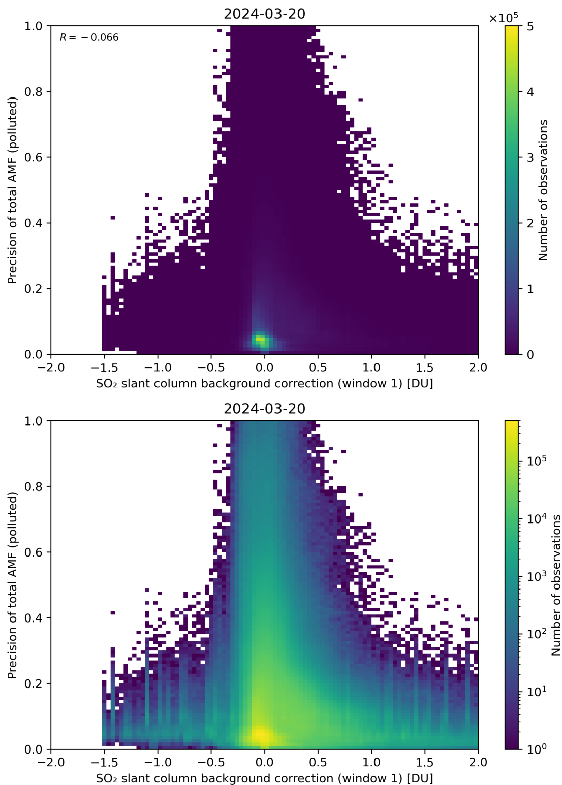
Figure 110: Scatter density plot of “SO 2 slant column background correction (window 1)” against “Precision of total AMF (polluted)” for 2024-03-20 to 2024-03-21.
