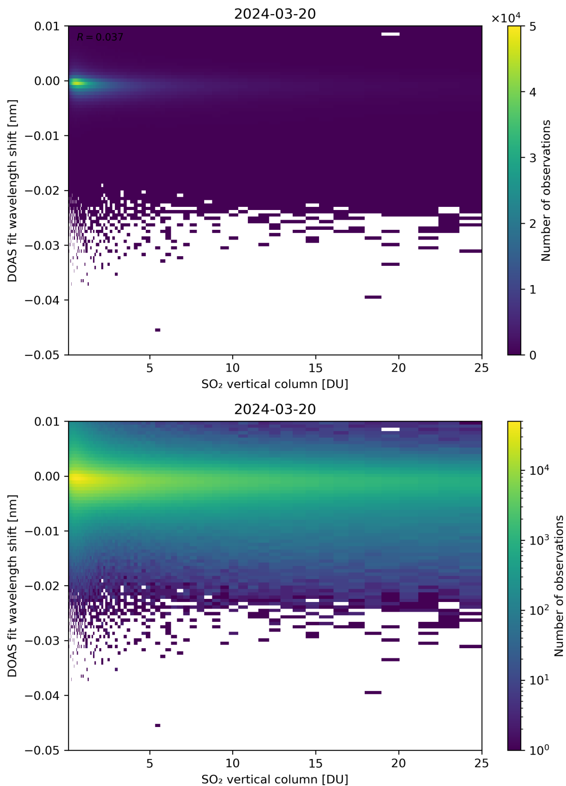
Figure 276: Scatter density plot of “SO 2 vertical column” against “DOAS fit wavelength shift” for 2024-03-20 to 2024-03-21.
