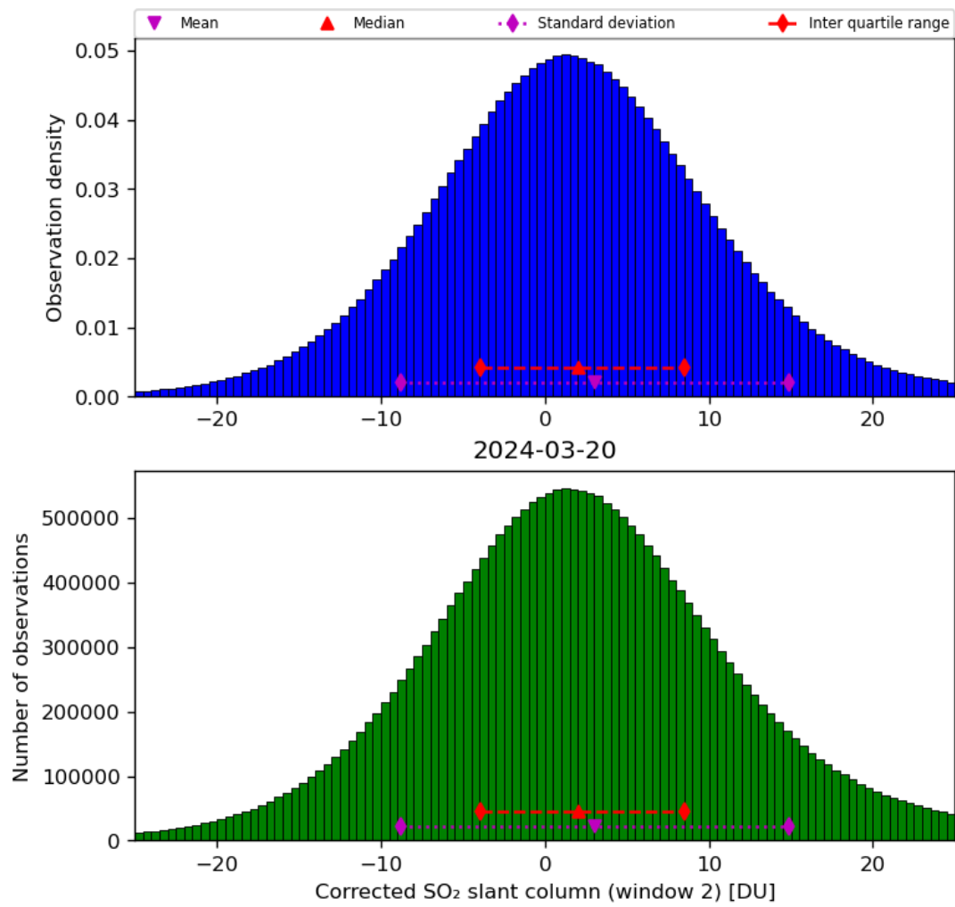
Figure 62: Histogram of “Corrected SO 2 slant column (window 2)” for 2024-03-20 to 2024-03-21
