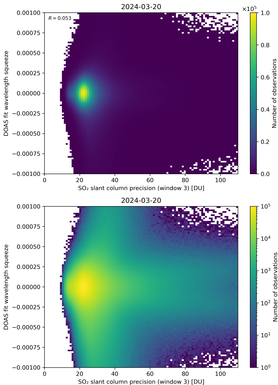
Figure 259: Scatter density plot of “SO 2 slant column precision (window 3)” against “DOAS fit wavelength squeeze” for 2024-03-20 to 2024-03-21.
