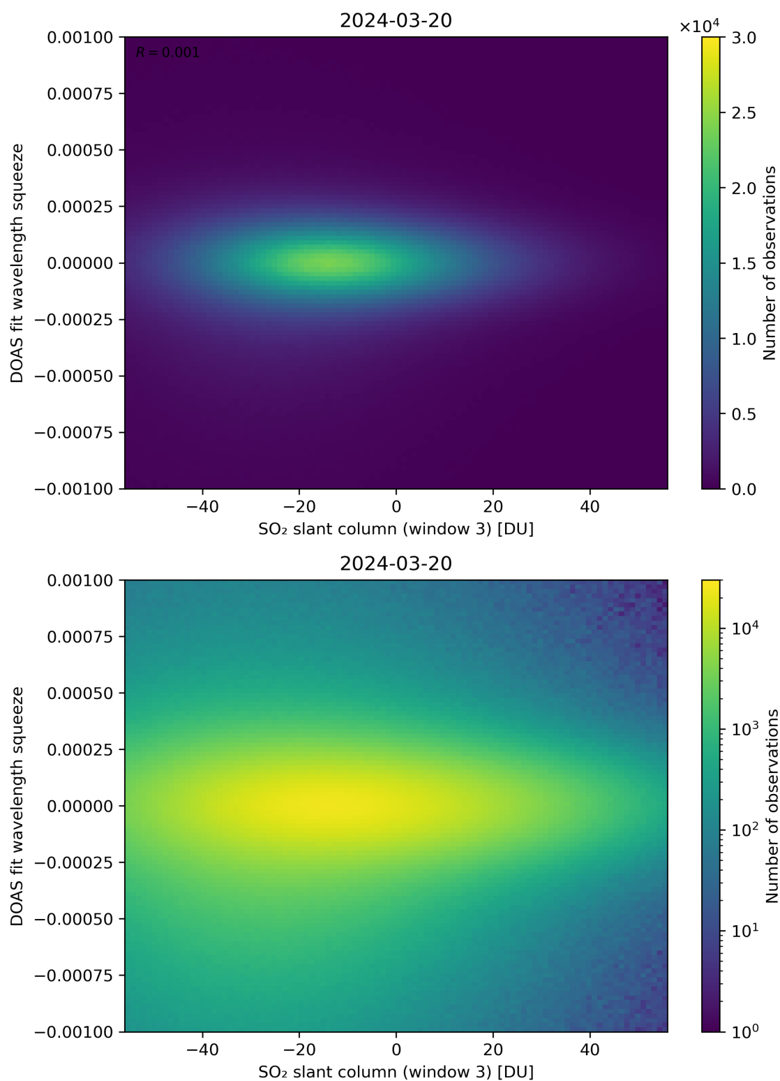
Figure 255: Scatter density plot of “SO 2 slant column (window 3)” against “DOAS fit wavelength squeeze” for 2024-03-20 to 2024-03-21.
