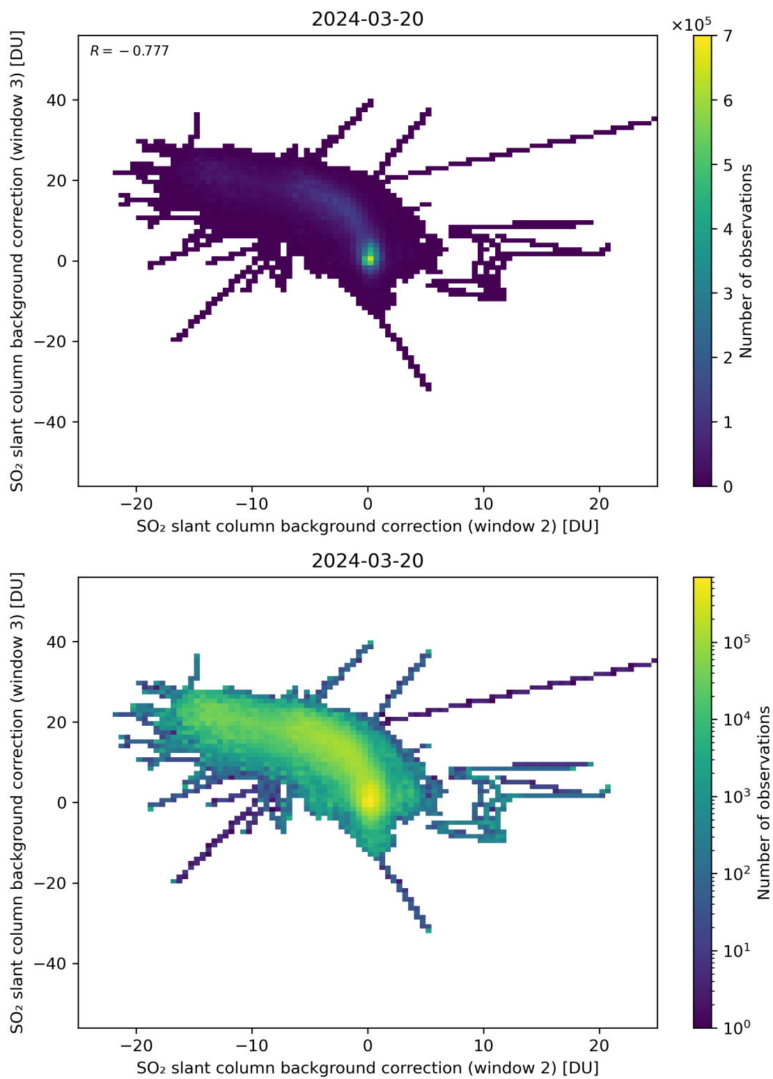
Figure 111: Scatter density plot of “SO 2 slant column background correction (window 2)” against “SO 2 slant column background correction (window 3)” for 2024-03-20 to 2024-03-21.
