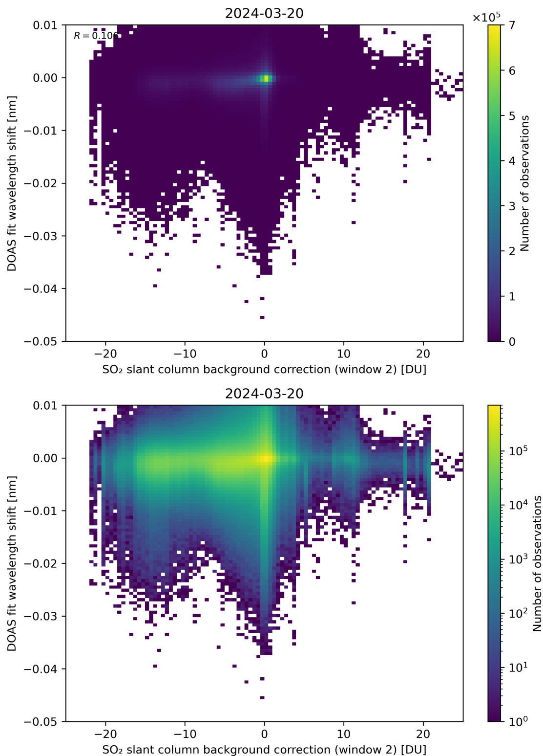
Figure 112: Scatter density plot of “SO 2 slant column background correction (window 2)” against “DOAS fit wavelength shift” for 2024-03-20 to 2024-03-21.
