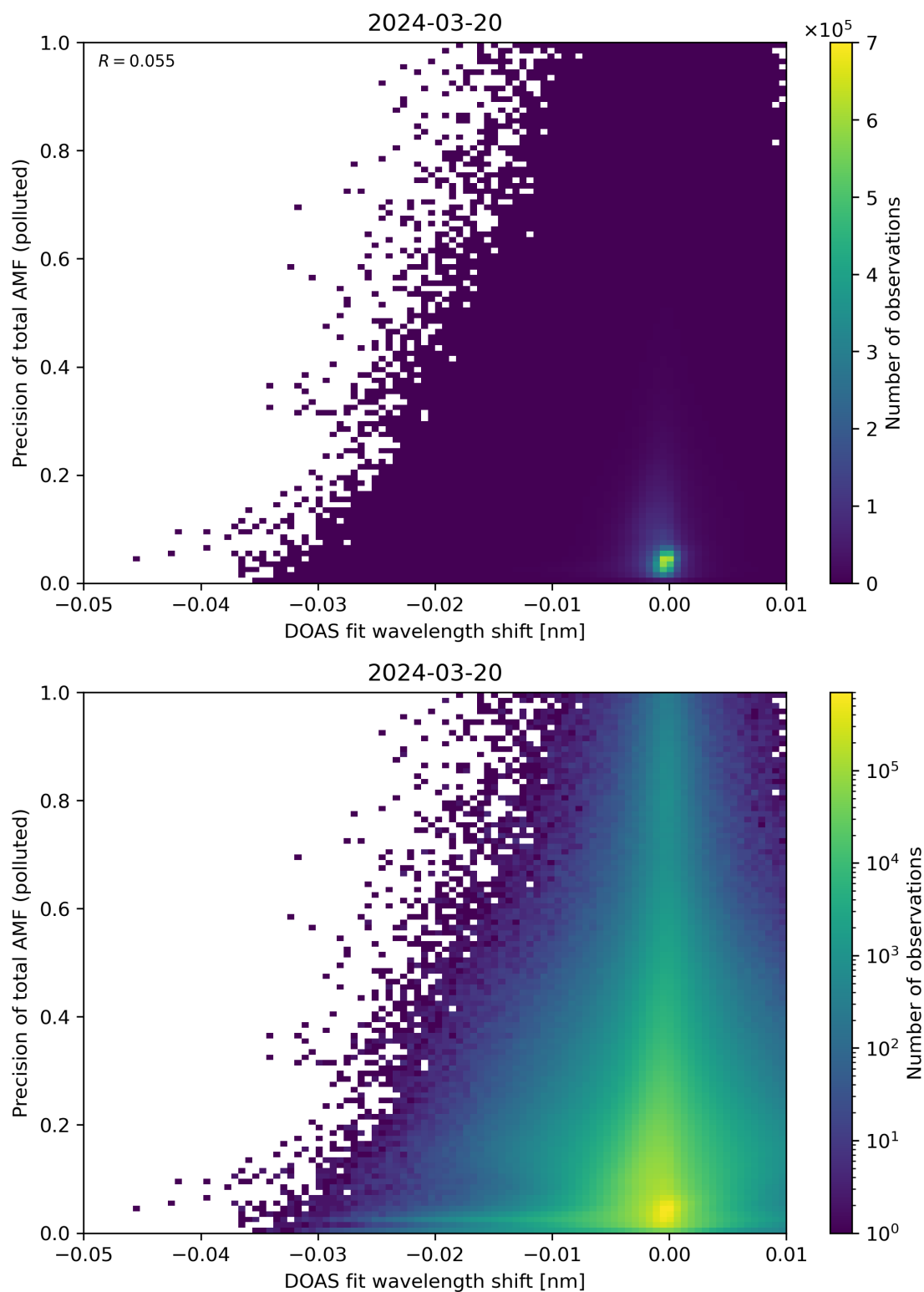
Figure 131: Scatter density plot of “DOAS fit wavelength shift” against “Precision of total AMF (polluted)” for 2024-03-20 to 2024-03-21.
