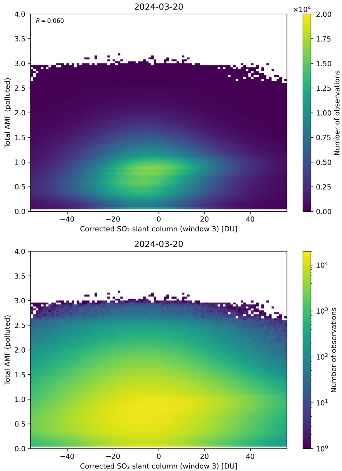
Figure 210: Scatter density plot of “Corrected SO 2 slant column (window 3)” against “Total AMF (polluted)” for 2024-03-20 to 2024-03-21.
