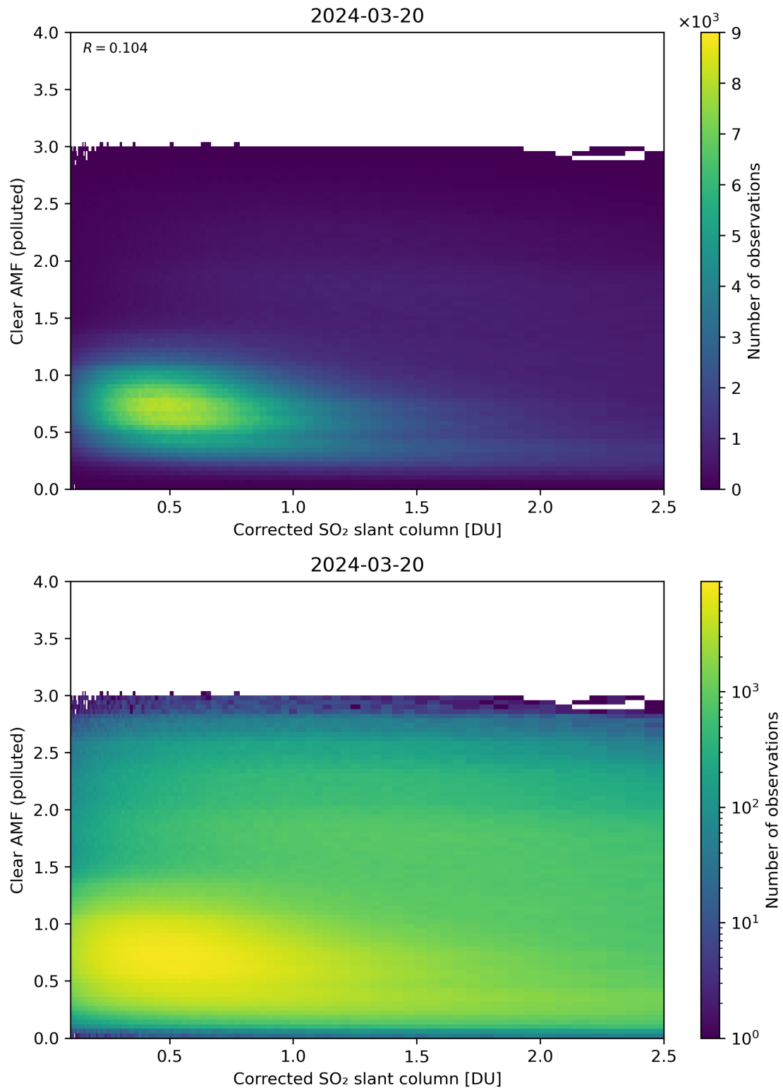
Figure 184: Scatter density plot of “Corrected SO 2 slant column” against “Clear AMF (polluted)” for 2024-03-20 to 2024-03-21.
