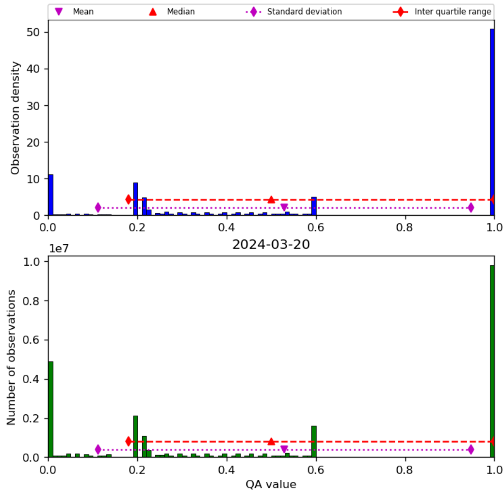
Figure 52: Histogram of “QA value” for 2024-03-20 to 2024-03-21
