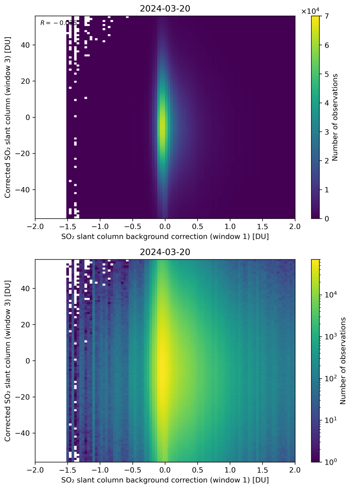
Figure 105: Scatter density plot of “SO 2 slant column background correction (window 1)” against “Corrected SO 2 slant column (window 3)” for 2024-03-20 to 2024-03-21.
