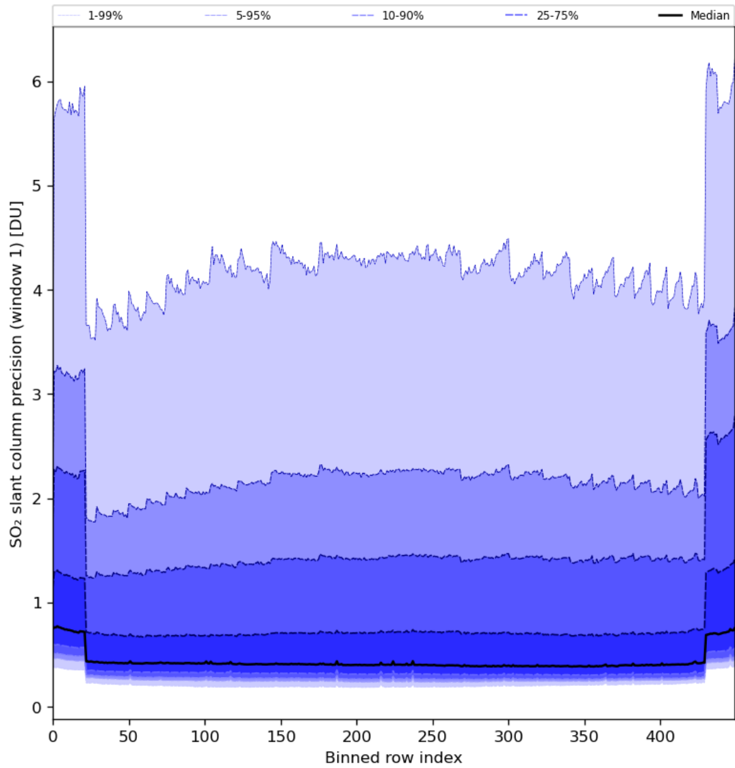
Figure 80: Along track statistics of “SO 2 slant column precision (window 1)” for 2024-03-20 to 2024-03-21
