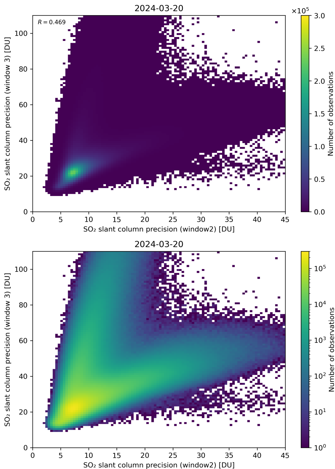
Figure 250: Scatter density plot of “SO 2 slant column precision (window2)” against “SO 2 slant column precision (window 3)” for 2024-03-20 to 2024-03-21.
