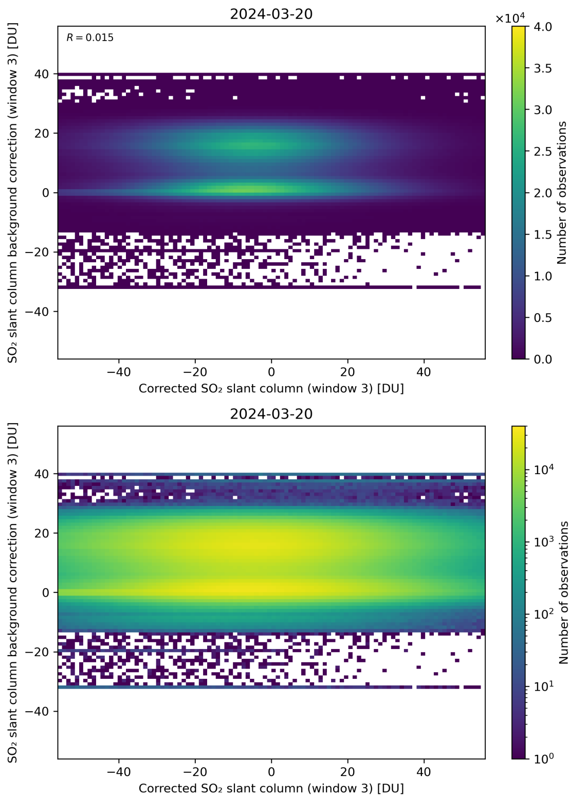
Figure 205: Scatter density plot of “Corrected SO 2 slant column (window 3)” against “SO 2 slant column background correction (window 3)” for 2024-03-20 to 2024-03-21.
