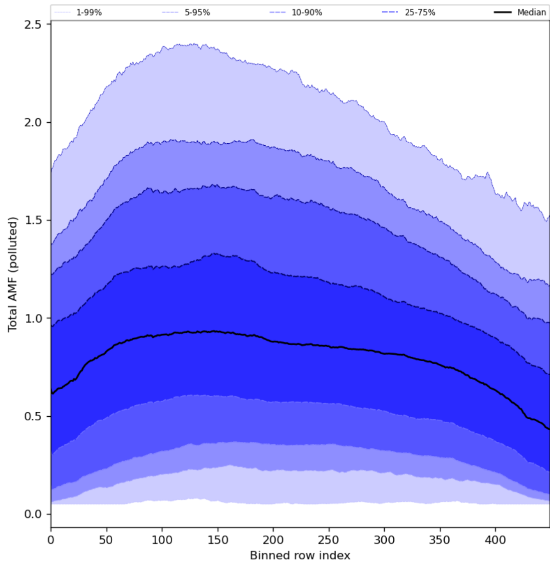
Figure 94: Along track statistics of “Total AMF (polluted)” for 2024-03-20 to 2024-03-21
