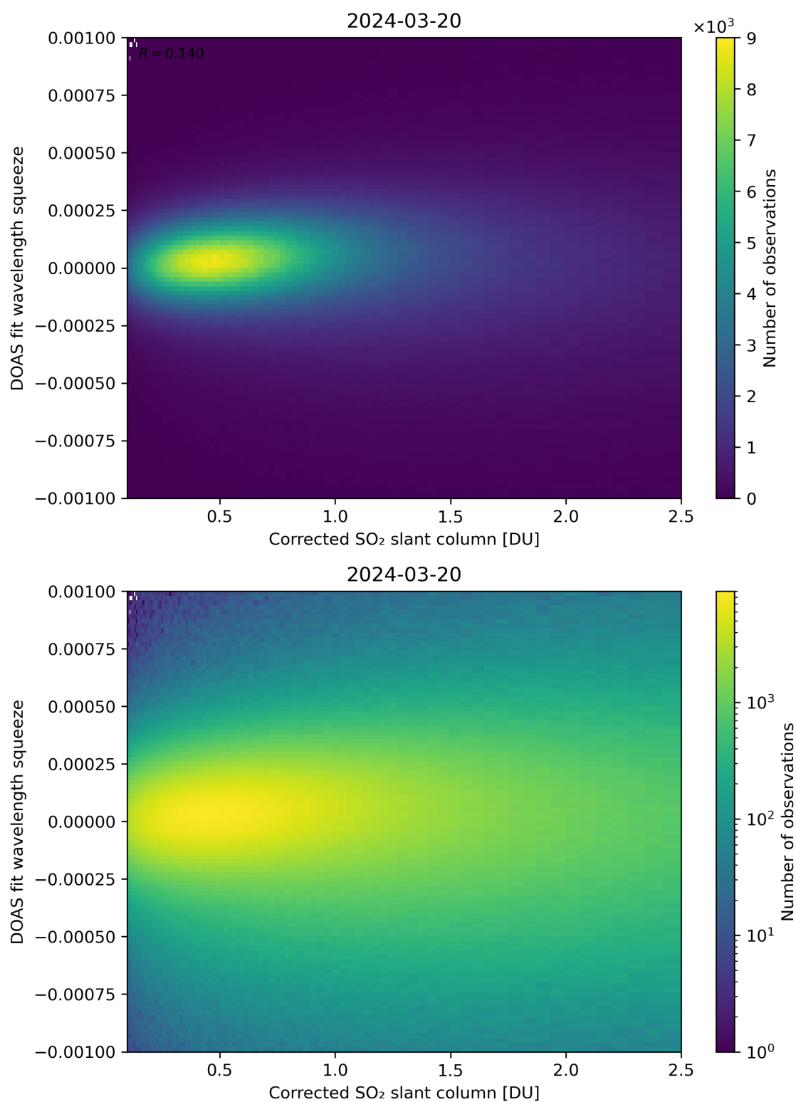
Figure 182: Scatter density plot of “Corrected SO 2 slant column” against “DOAS fit wavelength squeeze” for 2024-03-20 to 2024-03-21.
