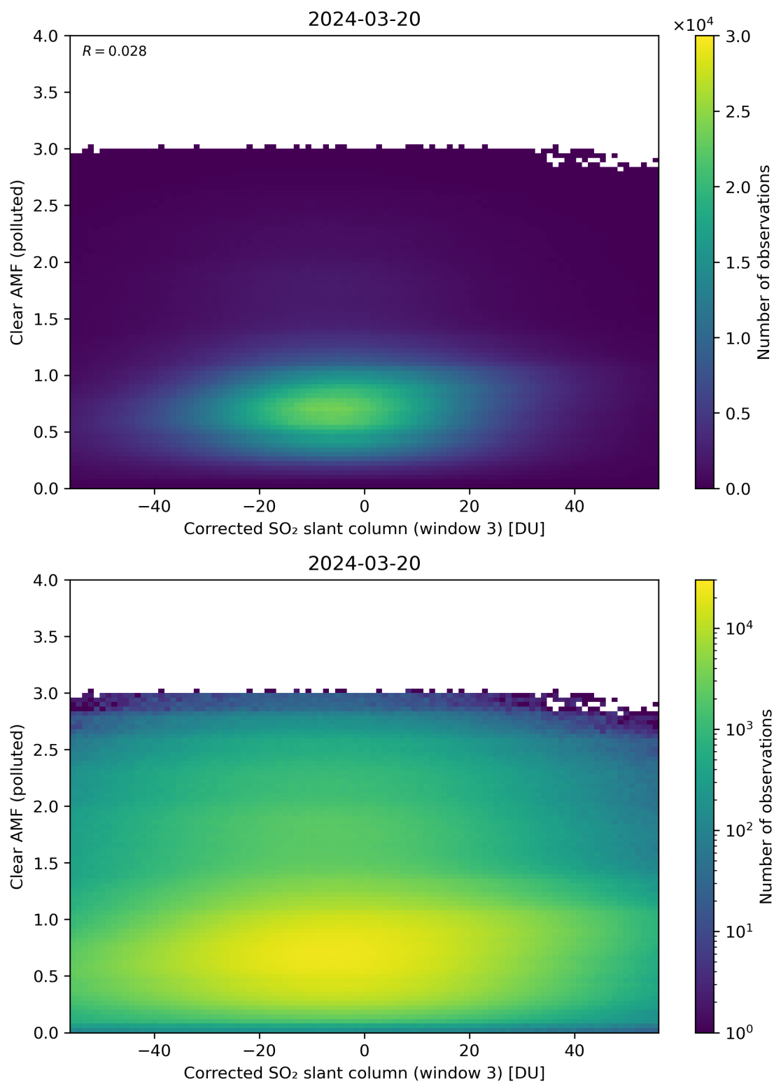
Figure 209: Scatter density plot of “Corrected SO 2 slant column (window 3)” against “Clear AMF (polluted)” for 2024-03-20 to 2024-03-21.
