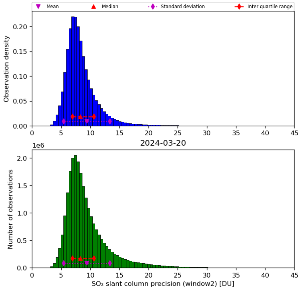
Figure 61: Histogram of “SO 2 slant column precision (window2)” for 2024-03-20 to 2024-03-21
