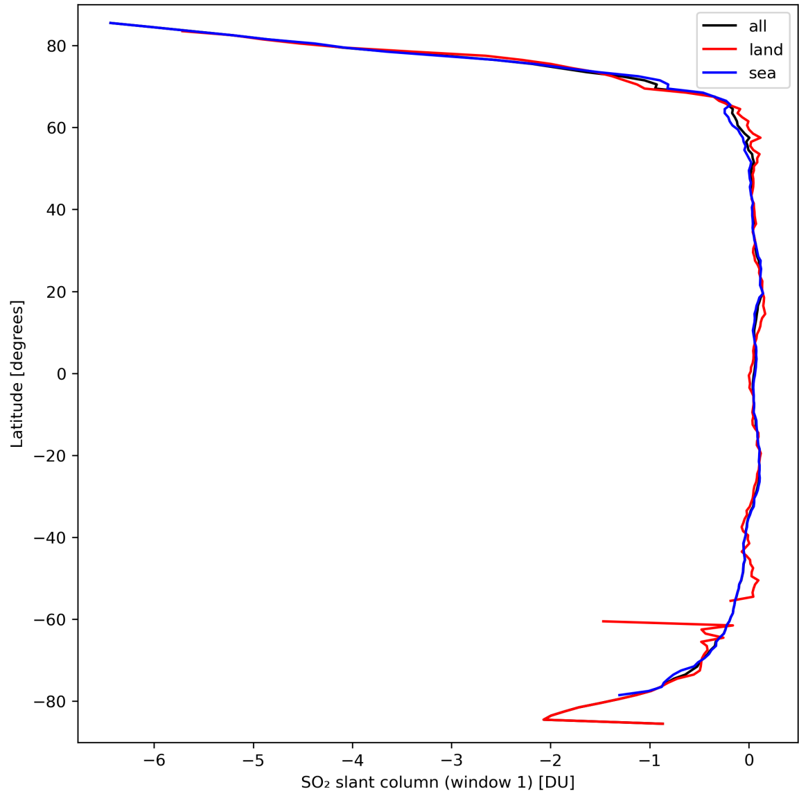
Figure 33: Zonal average of “SO 2 slant column (window 1)” for 2024-03-20 to 2024-03-21.
