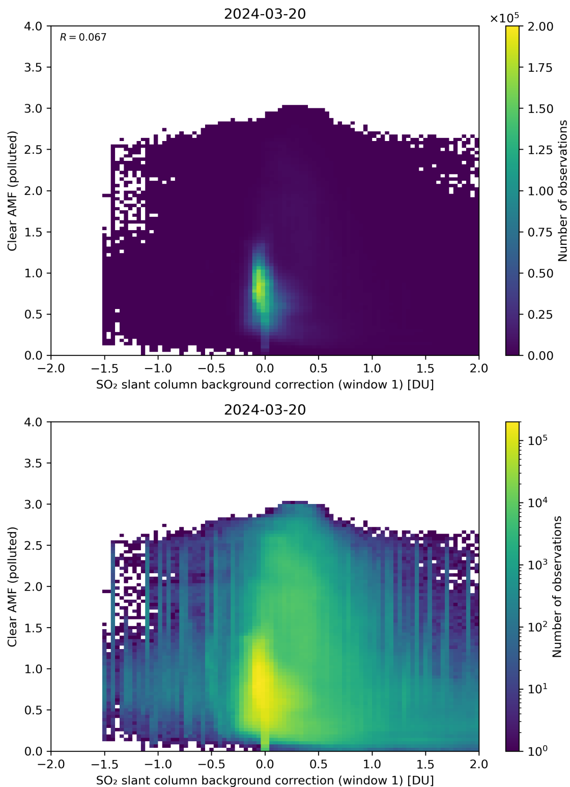
Figure 103: Scatter density plot of “SO 2 slant column background correction (window 1)” against “Clear AMF (polluted)” for 2024-03-20 to 2024-03-21.
