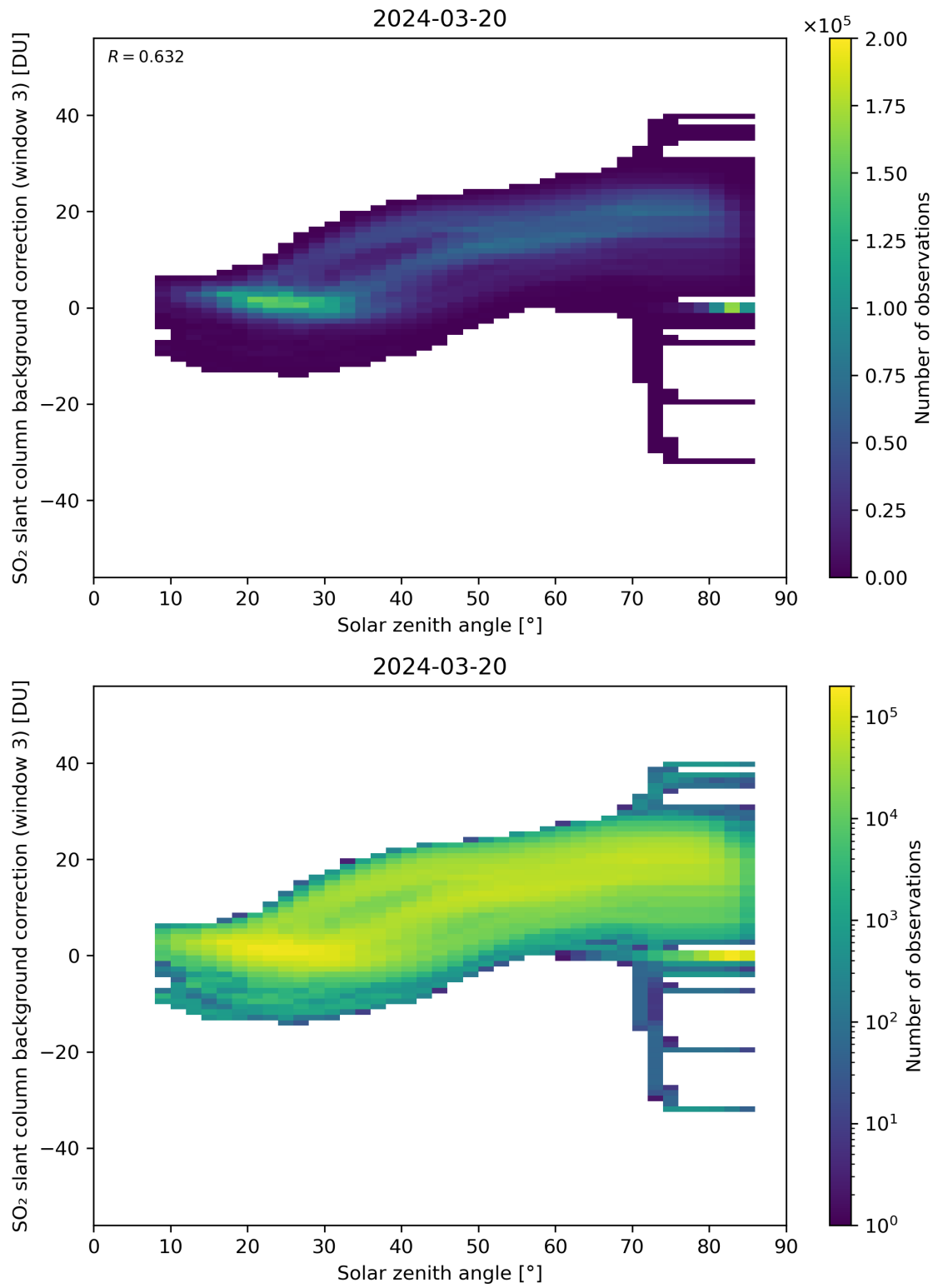
Figure 160: Scatter density plot of “Solar zenith angle” against “SO 2 slant column background correction (window 3)” for 2024-03-20 to 2024-03-21.
