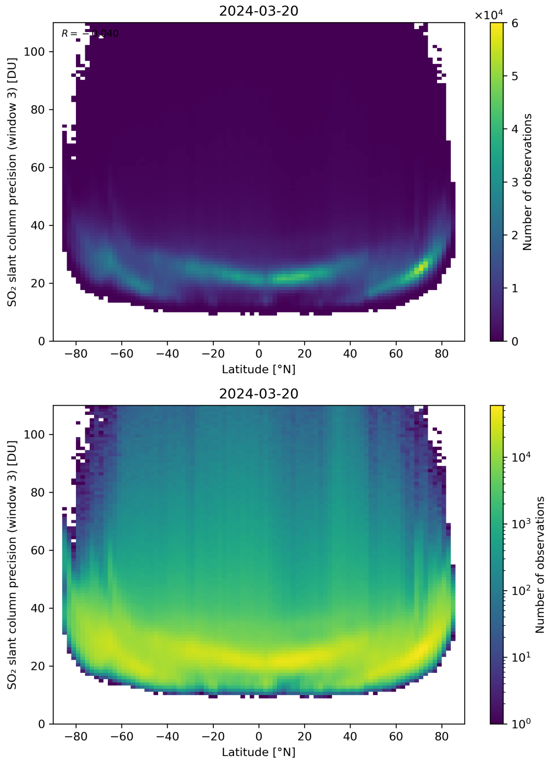
Figure 153: Scatter density plot of “Latitude” against “SO 2 slant column precision (window 3)” for 2024-03-20 to 2024-03-21.
