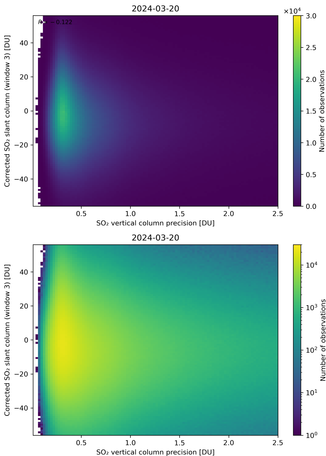
Figure 288: Scatter density plot of “SO 2 vertical column precision” against “Corrected SO 2 slant column (window 3)” for 2024-03-20 to 2024-03-21.
