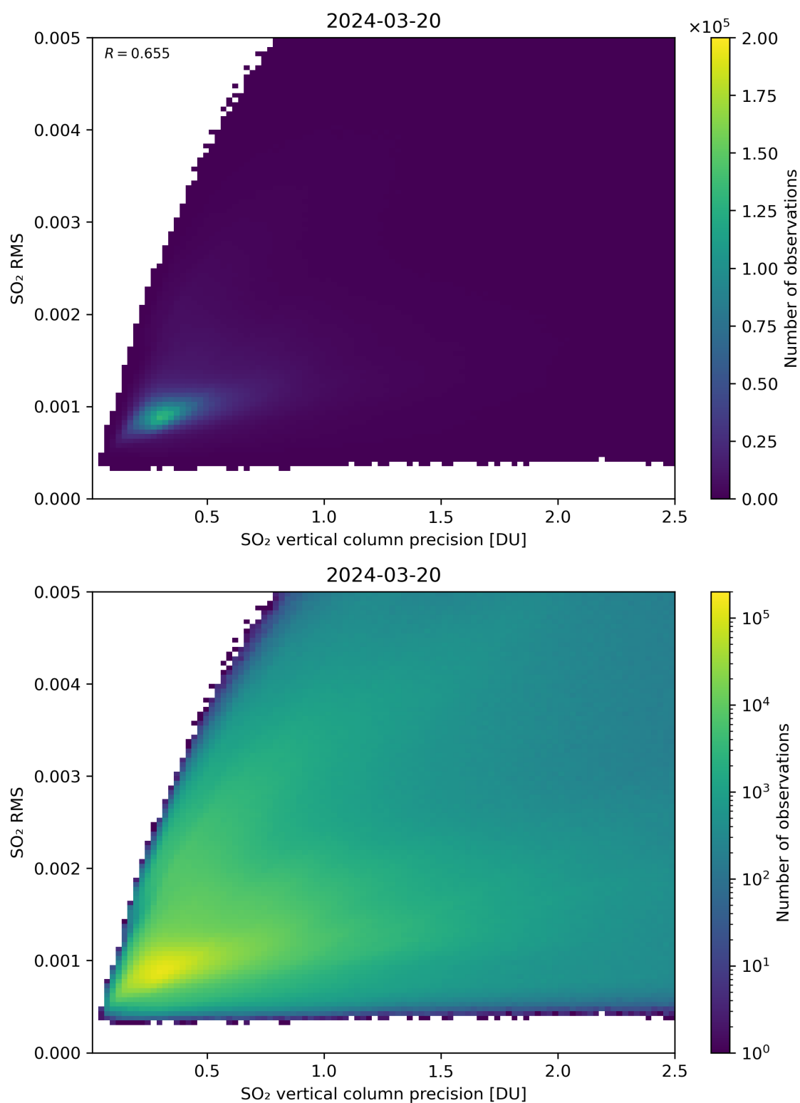
Figure 284: Scatter density plot of “SO 2 vertical column precision” against “SO 2 RMS” for 2024-03-20 to 2024-03-21.
