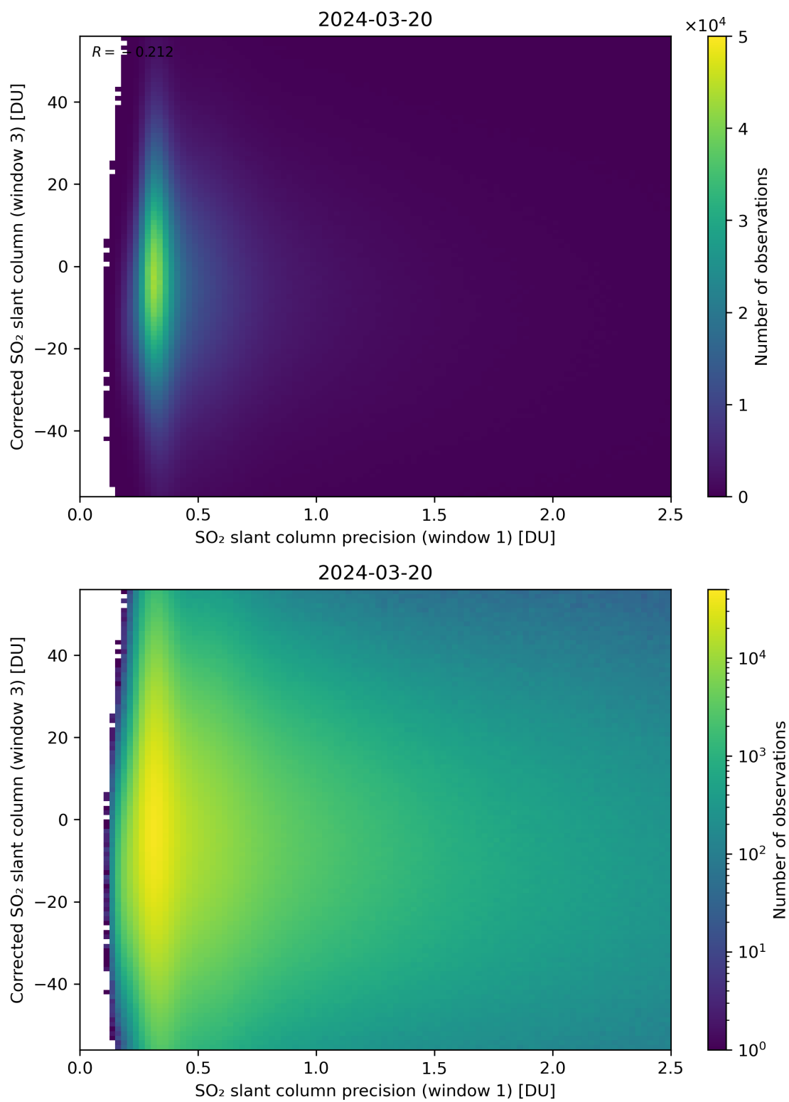
Figure 226: Scatter density plot of “SO 2 slant column precision (window 1)” against “Corrected SO 2 slant column (window 3)” for 2024-03-20 to 2024-03-21.
