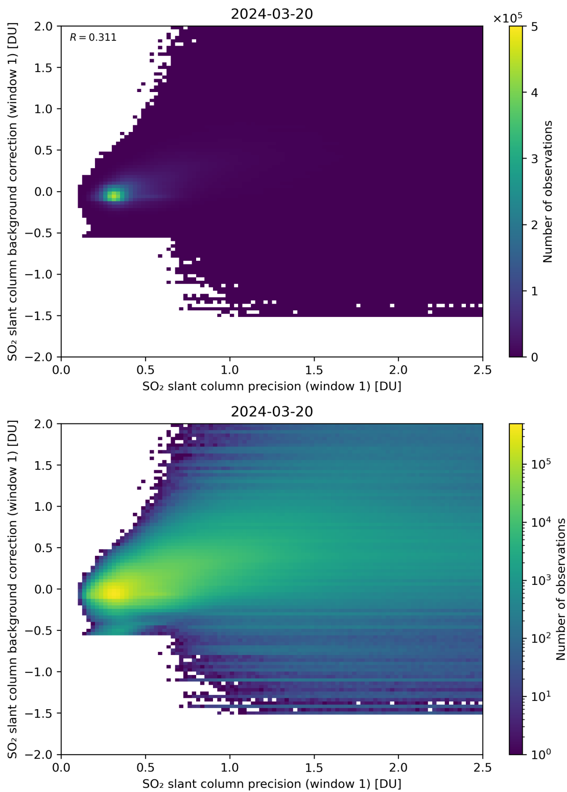
Figure 218: Scatter density plot of “SO 2 slant column precision (window 1)” against “SO 2 slant column background correction (window 1)” for 2024-03-20 to 2024-03-21.
