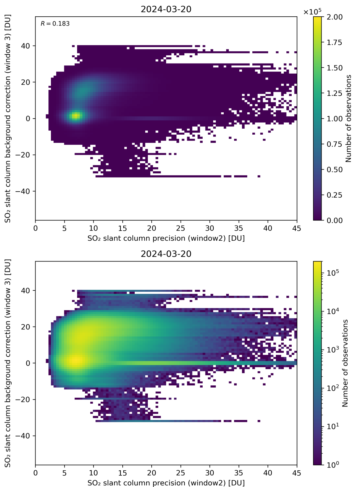
Figure 242: Scatter density plot of “SO 2 slant column precision (window2)” against “SO 2 slant column background correction (window 3)” for 2024-03-20 to 2024-03-21.
