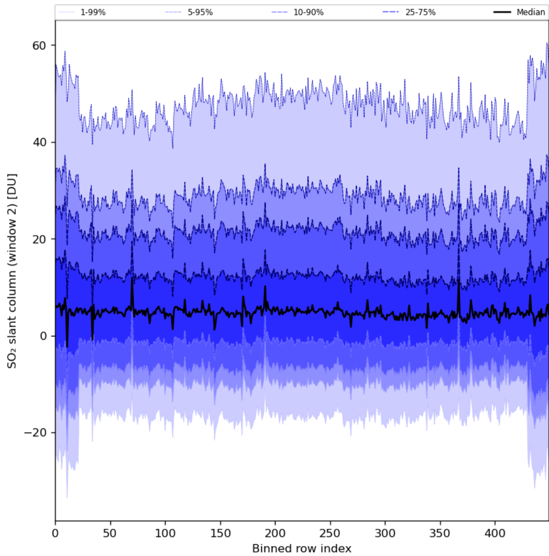
Figure 83: Along track statistics of “SO 2 slant column (window 2)” for 2024-03-20 to 2024-03-21
