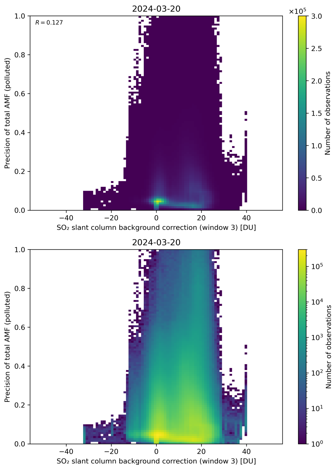
Figure 126: Scatter density plot of “SO 2 slant column background correction (window 3)” against “Precision of total AMF (polluted)” for 2024-03-20 to 2024-03-21.
