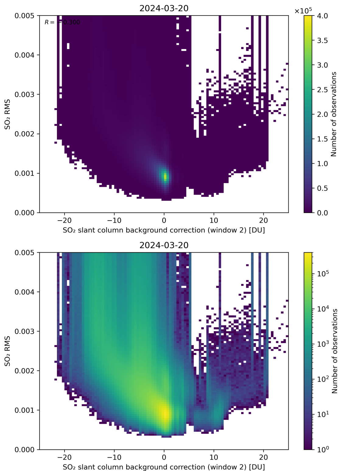
Figure 114: Scatter density plot of “SO 2 slant column background correction (window 2)” against “SO 2 RMS” for 2024-03-20 to 2024-03-21.
