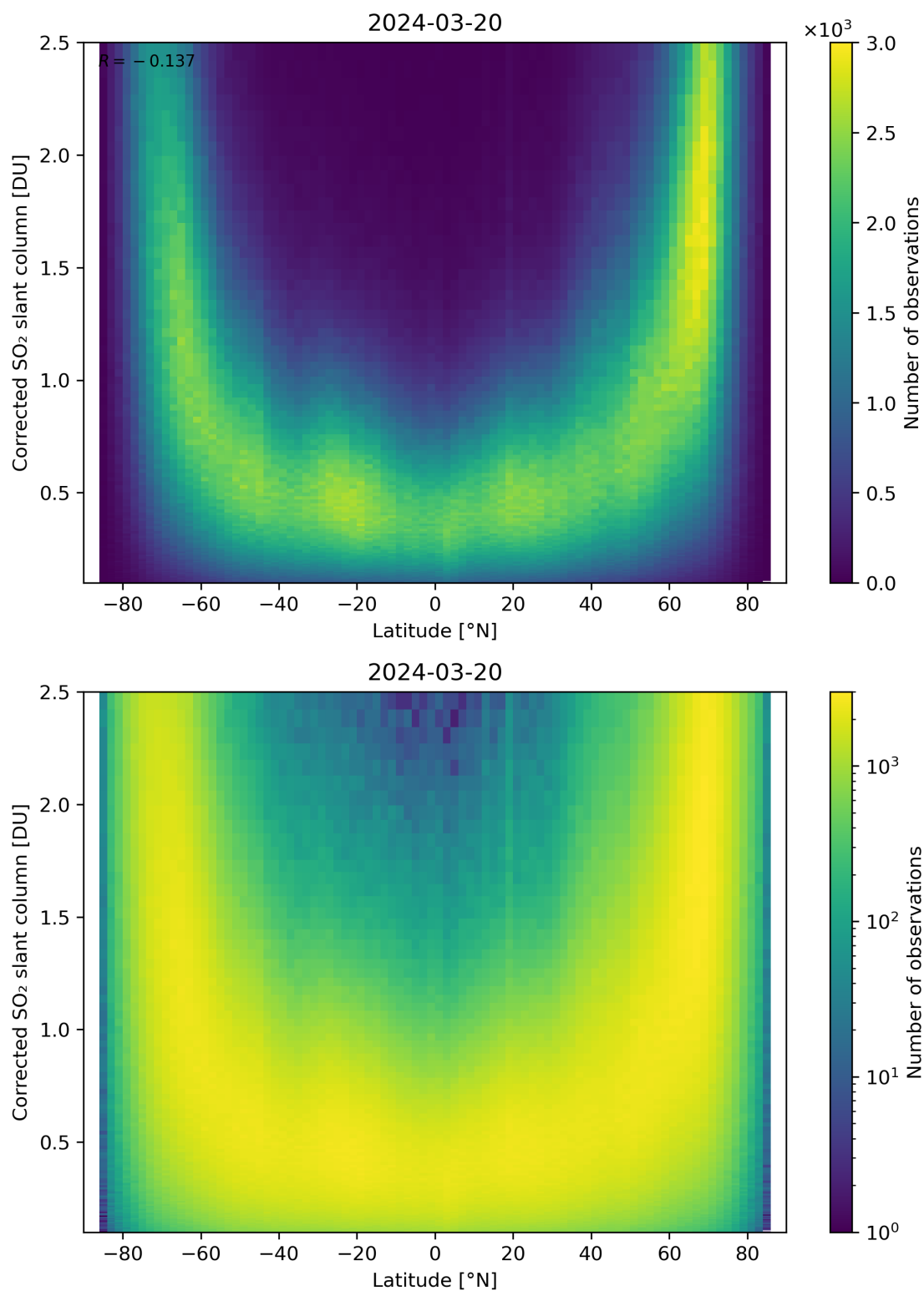
Figure 146: Scatter density plot of “Latitude” against “Corrected SO 2 slant column” for 2024-03-20 to 2024-03-21.
