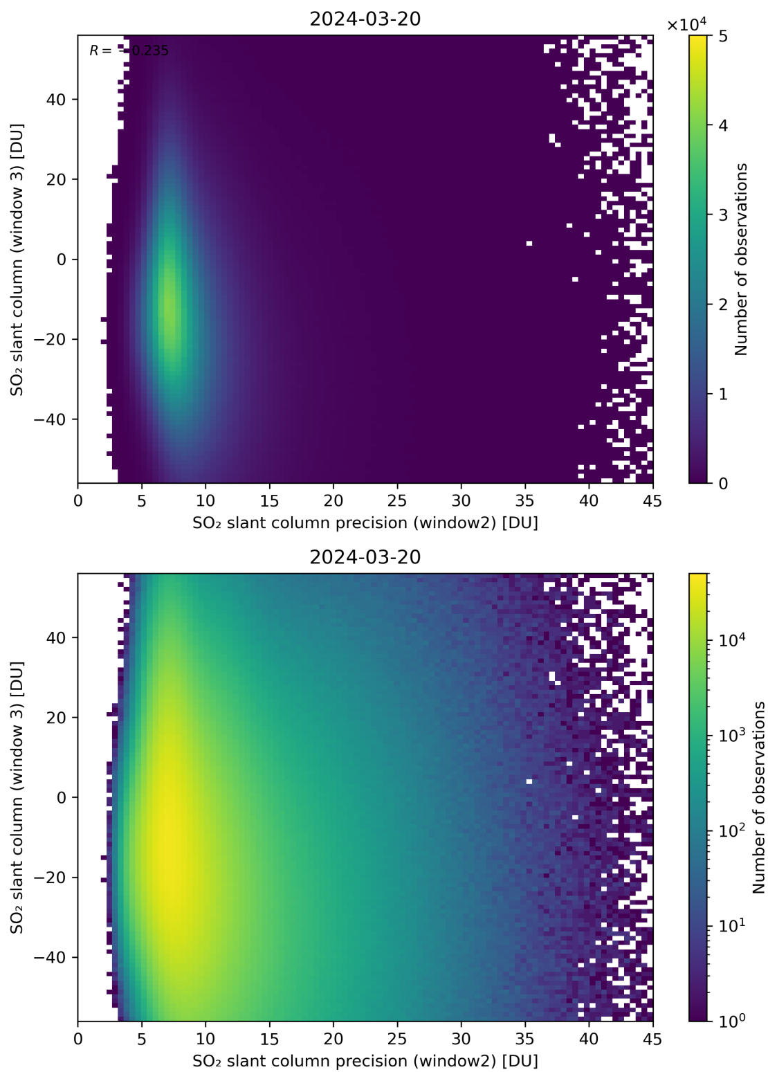
Figure 249: Scatter density plot of “SO 2 slant column precision (window2)” against “SO 2 slant column (window 3)” for 2024-03-20 to 2024-03-21.
