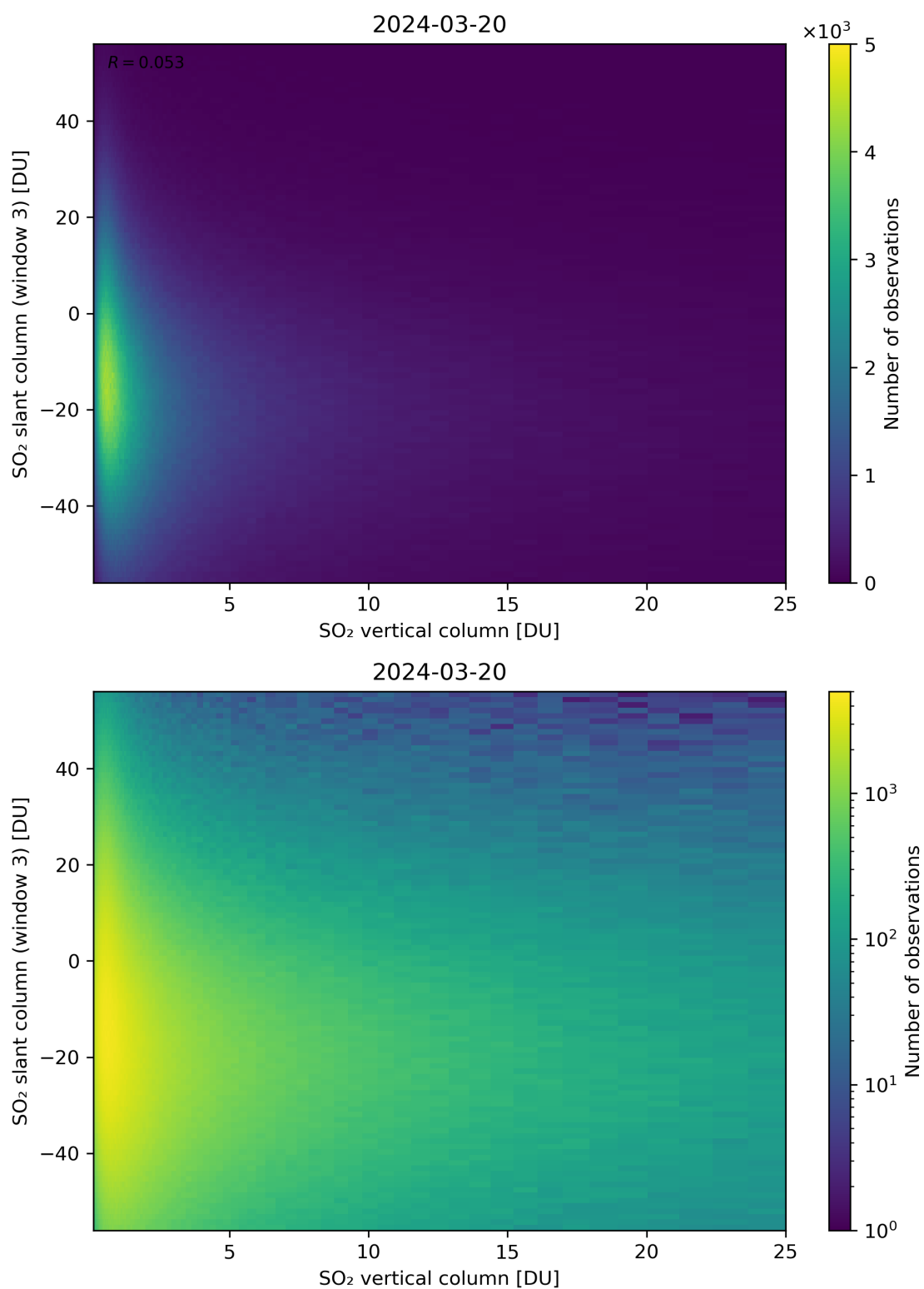
Figure 303: Scatter density plot of “SO 2 vertical column” against “SO 2 slant column (window 3)” for 2024-03-20 to 2024-03-21.
