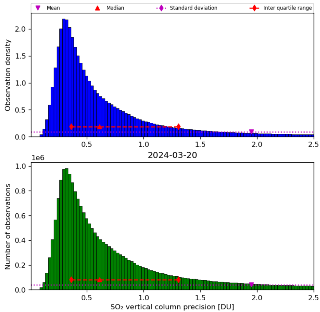
Figure 54: Histogram of “SO 2 vertical column precision” for 2024-03-20 to 2024-03-21
