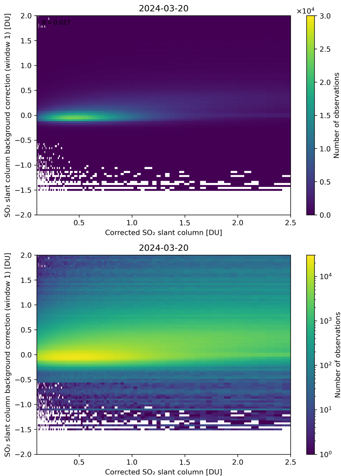
Figure 178: Scatter density plot of “Corrected SO 2 slant column” against “SO 2 slant column background correction (window 1)” for 2024-03-20 to 2024-03-21.
