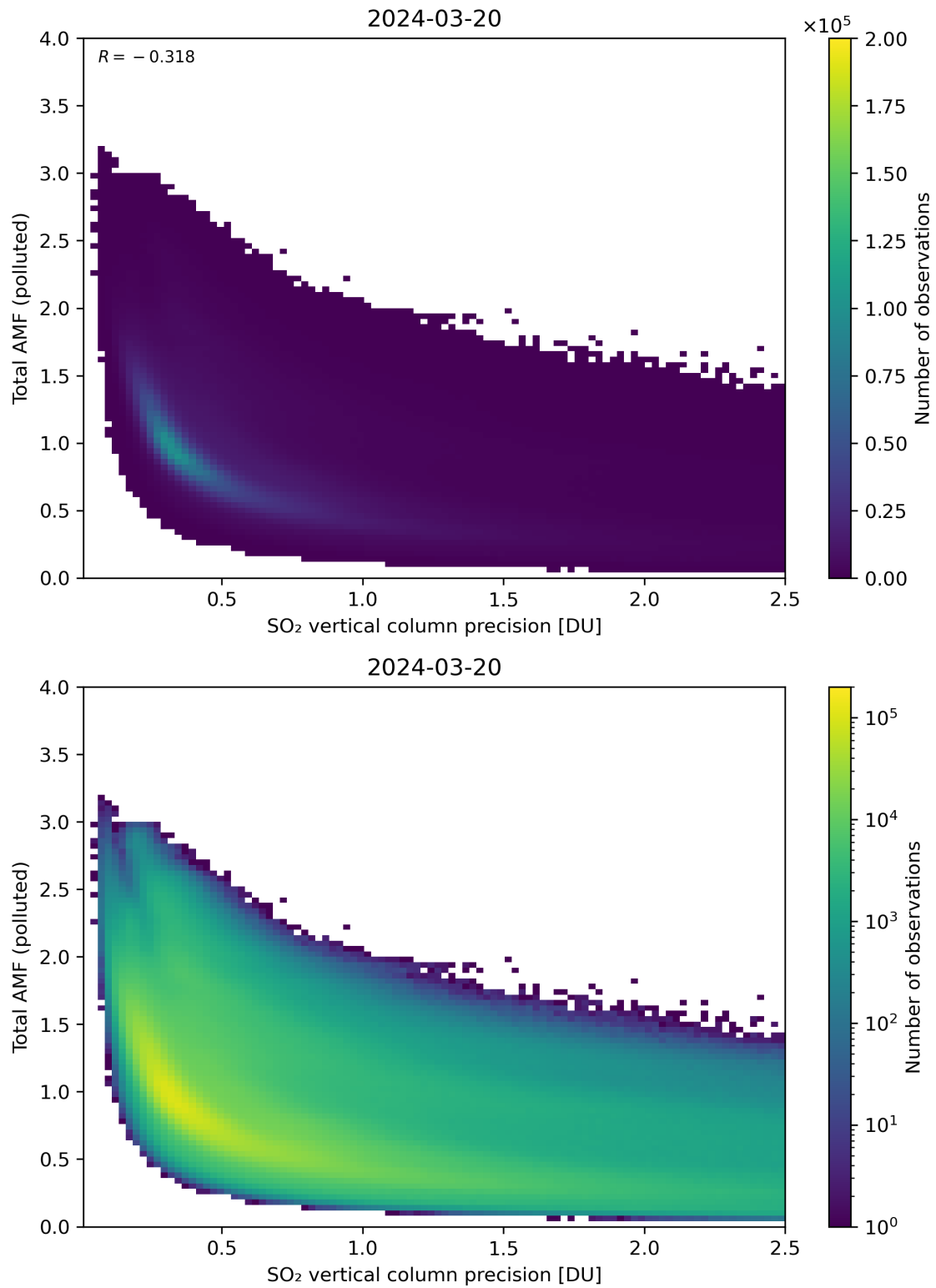
Figure 294: Scatter density plot of “SO 2 vertical column precision” against “Total AMF (polluted)” for 2024-03-20 to 2024-03-21.
