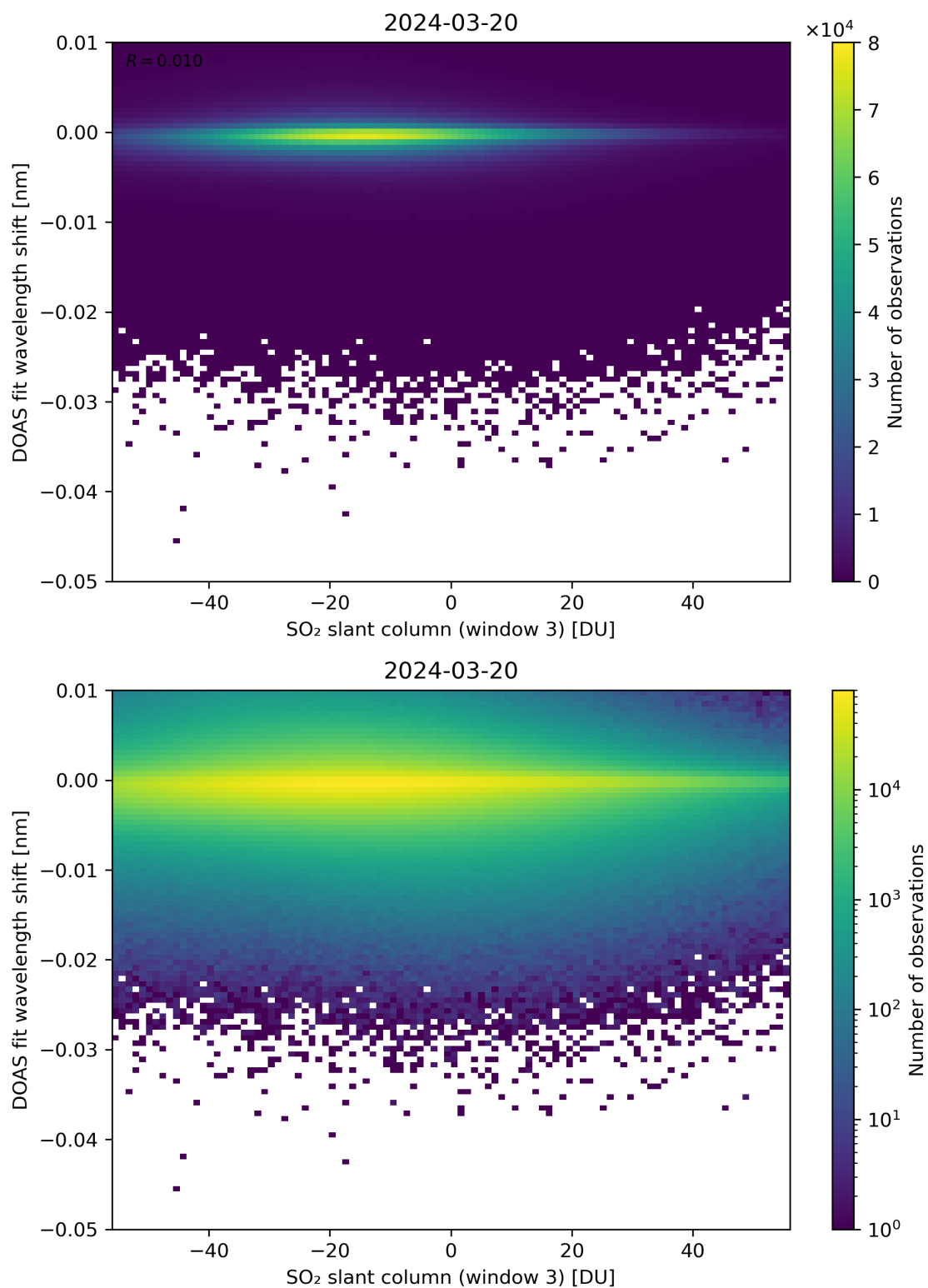
Figure 254: Scatter density plot of “SO 2 slant column (window 3)” against “DOAS fit wavelength shift” for 2024-03-20 to 2024-03-21.
