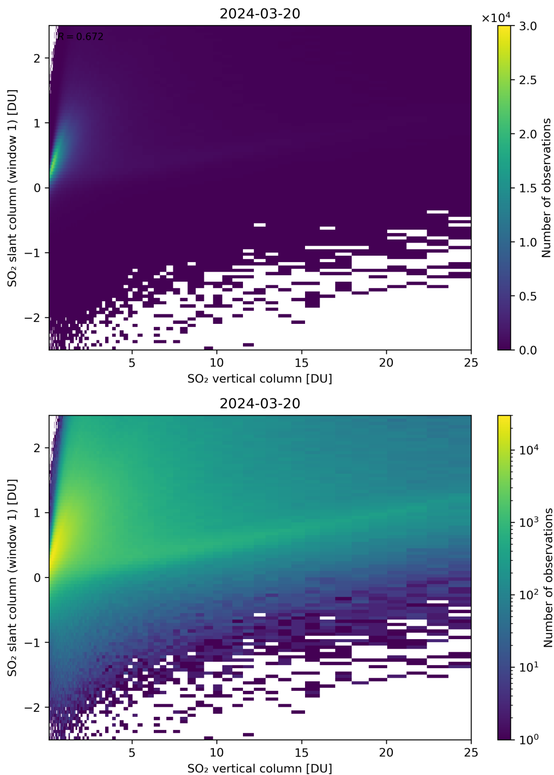
Figure 300: Scatter density plot of “SO 2 vertical column” against “SO 2 slant column (window 1)” for 2024-03-20 to 2024-03-21.
