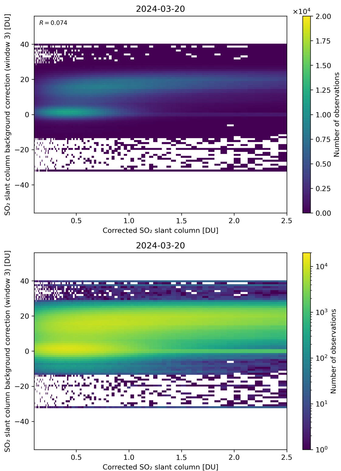
Figure 180: Scatter density plot of “Corrected SO 2 slant column” against “SO 2 slant column background correction (window 3)” for 2024-03-20 to 2024-03-21.
