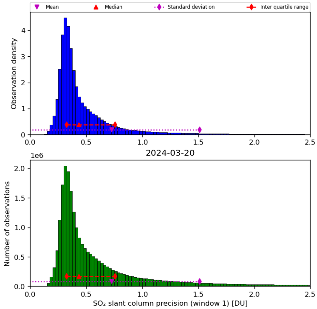
Figure 57: Histogram of “SO 2 slant column precision (window 1)” for 2024-03-20 to 2024-03-21
