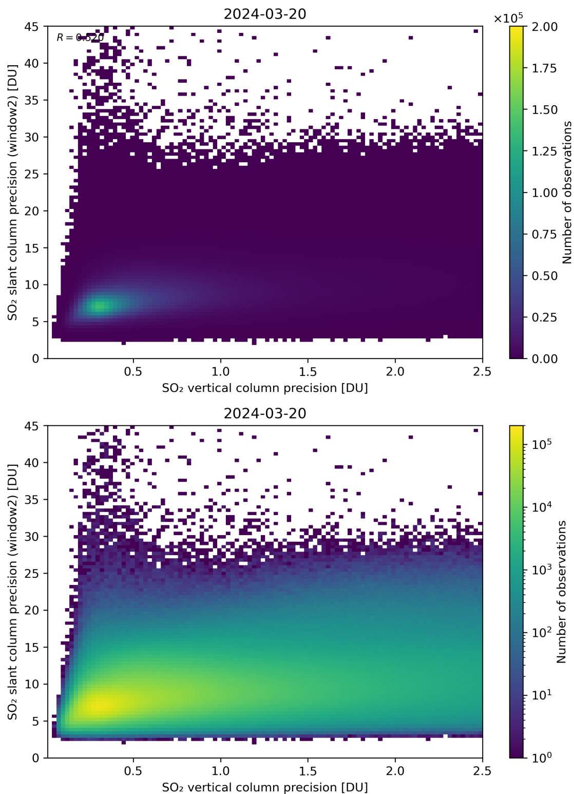
Figure 291: Scatter density plot of “SO 2 vertical column precision” against “SO 2 slant column precision (window2)” for 2024-03-20 to 2024-03-21.
