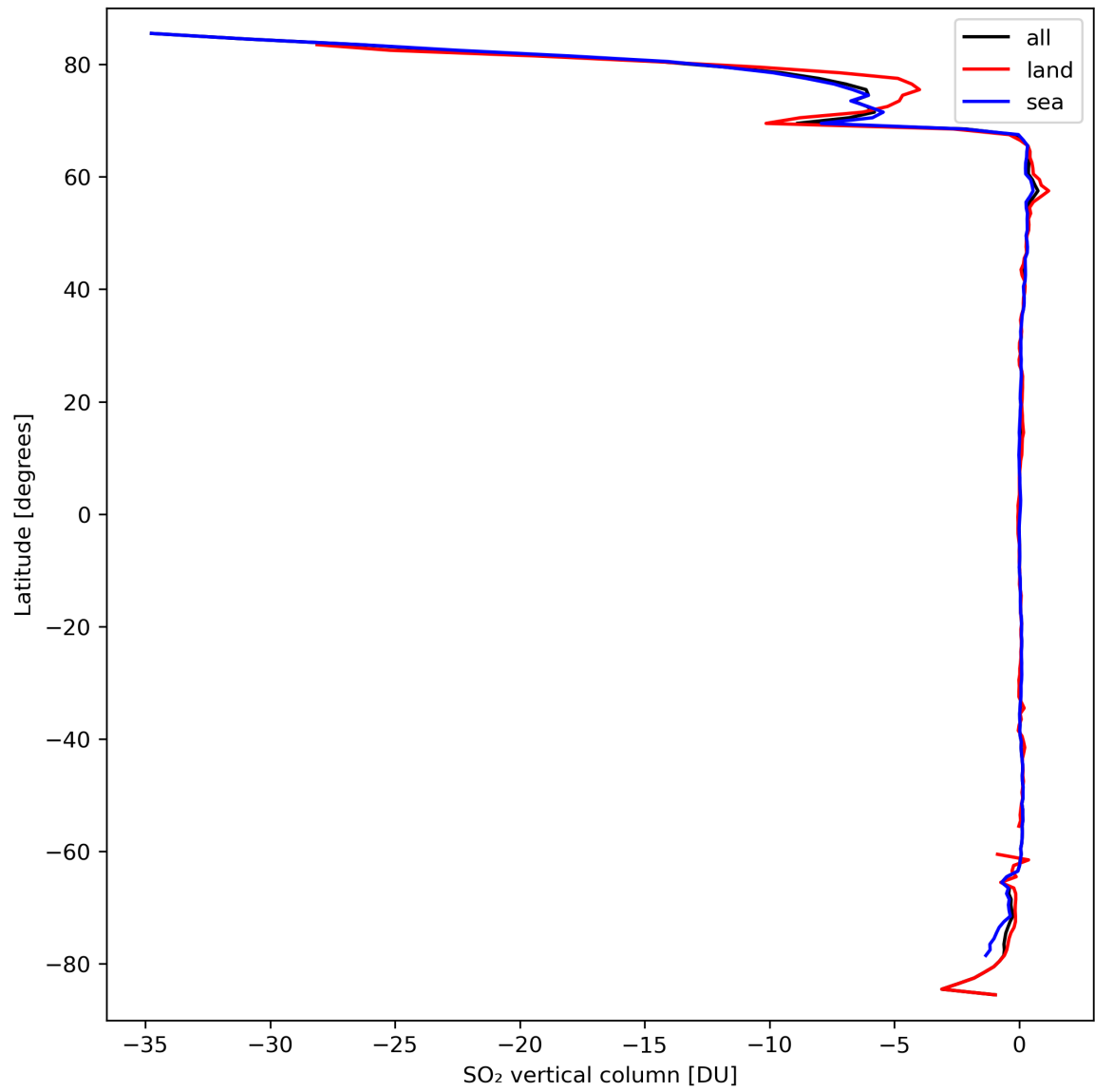
Figure 30: Zonal average of “SO 2 vertical column” for 2024-03-20 to 2024-03-21.
