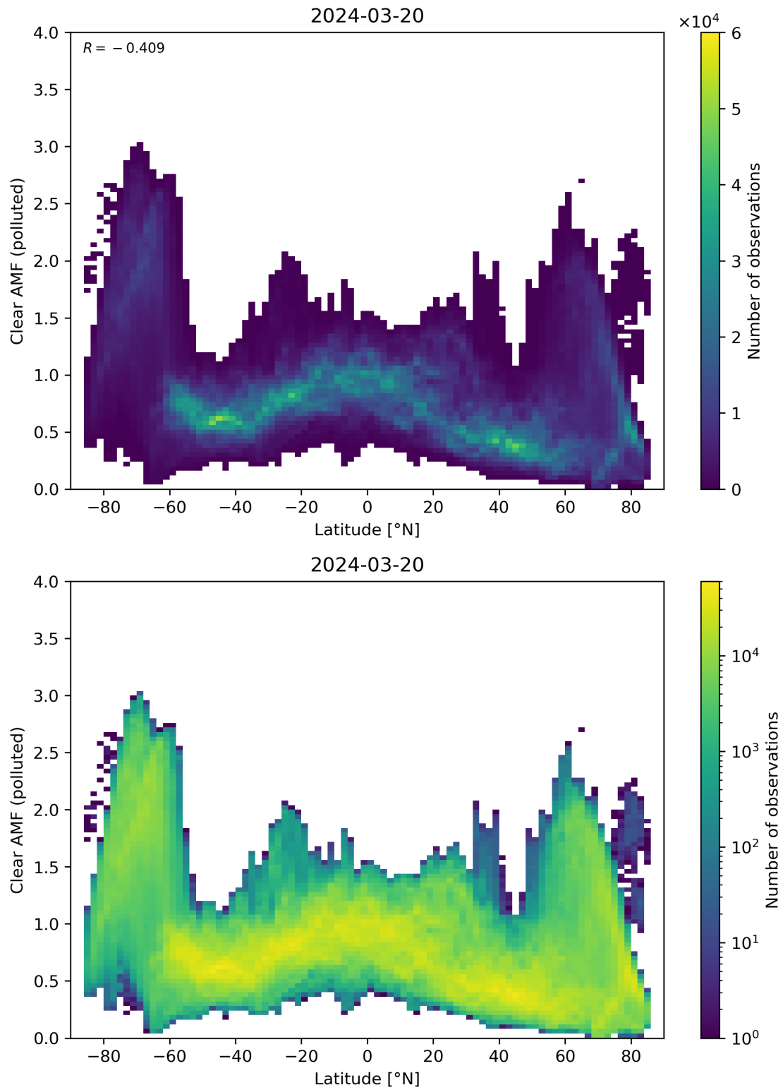
Figure 145: Scatter density plot of “Latitude” against “Clear AMF (polluted)” for 2024-03-20 to 2024-03-21.
