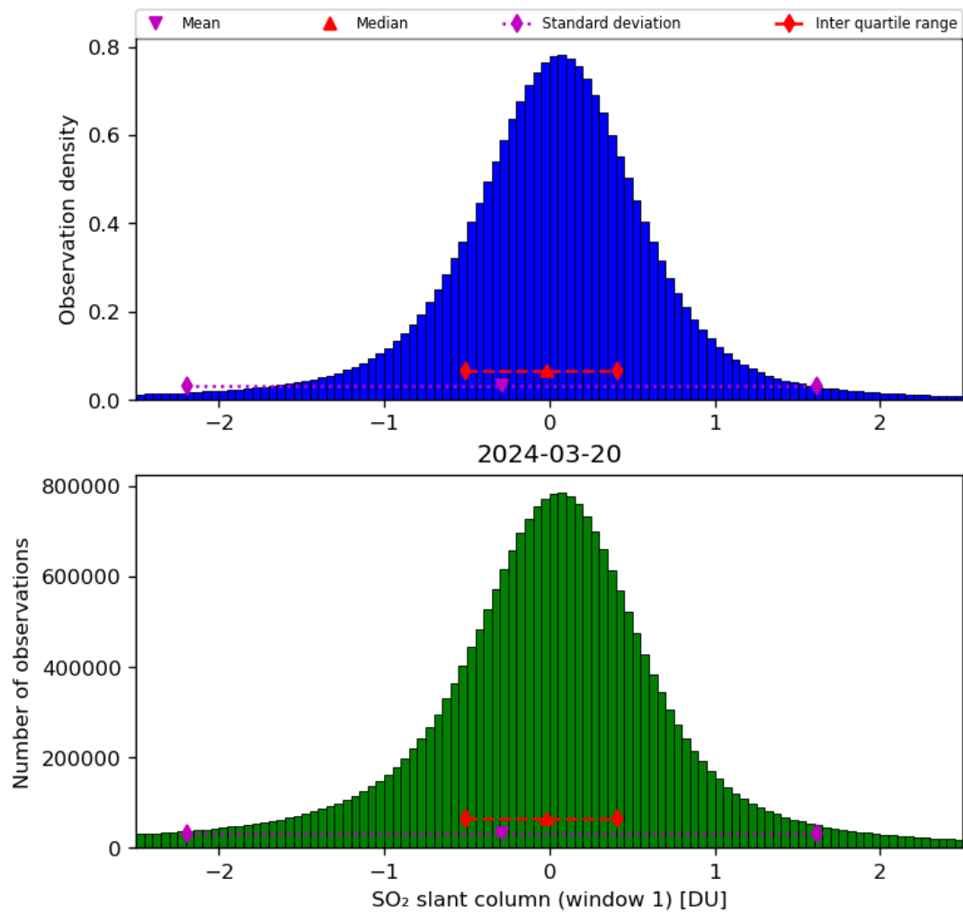
Figure 56: Histogram of “SO 2 slant column (window 1)” for 2024-03-20 to 2024-03-21
