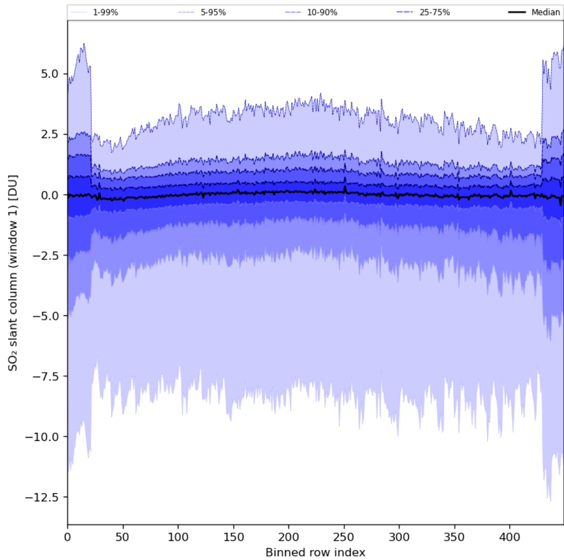
Figure 79: Along track statistics of “SO 2 slant column (window 1)” for 2024-03-20 to 2024-03-21
