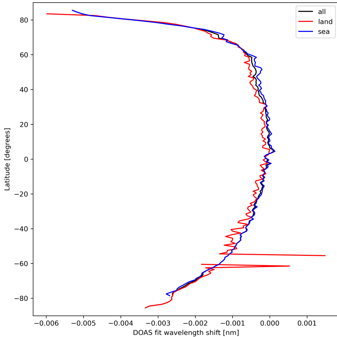
Figure 45: Zonal average of “DOAS fit wavelength shift” for 2024-03-20 to 2024-03-21.
