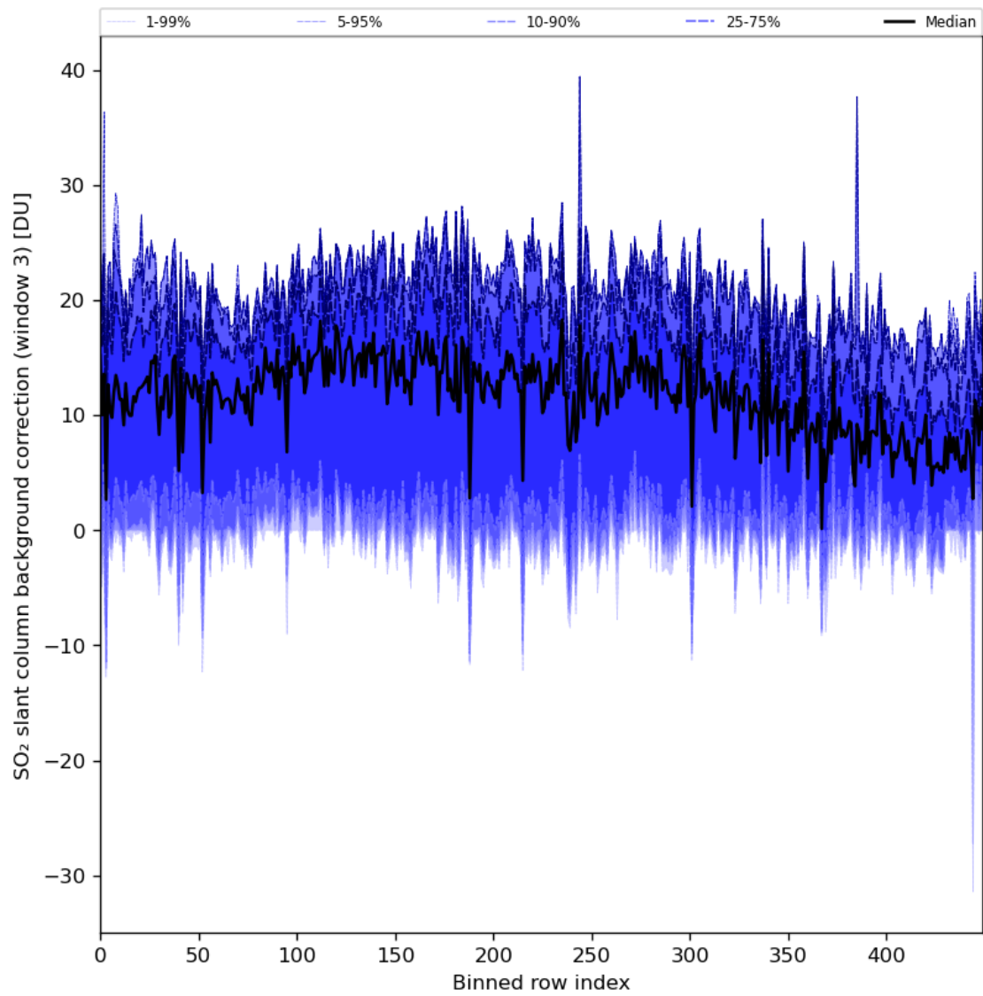
Figure 90: Along track statistics of “SO 2 slant column background correction (window 3)” for 2024-03-20 to 2024-03-21
