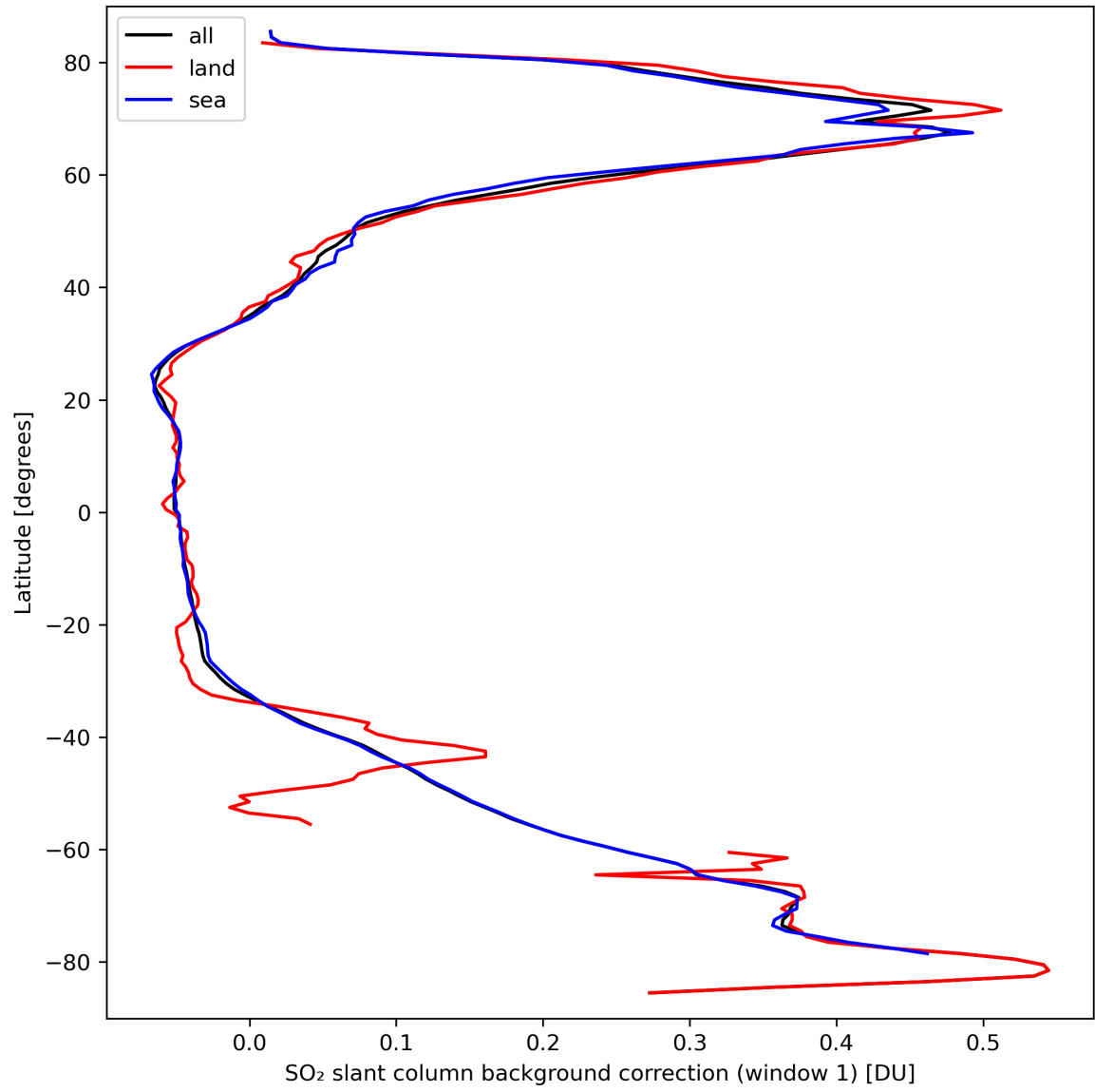
Figure 36: Zonal average of “SO 2 slant column background correction (window 1)” for 2024-03-20 to 2024-03-21.
