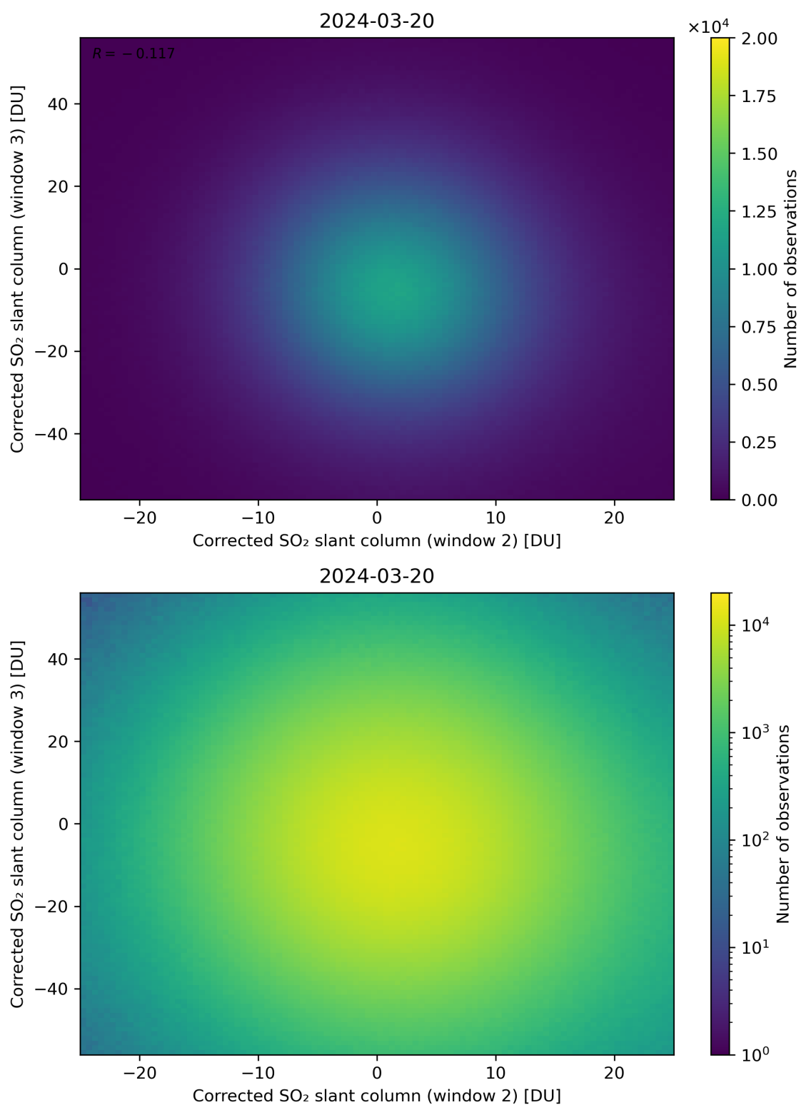
Figure 200: Scatter density plot of “Corrected SO 2 slant column (window 2)” against “Corrected SO 2 slant column (window 3)” for 2024-03-20 to 2024-03-21.
