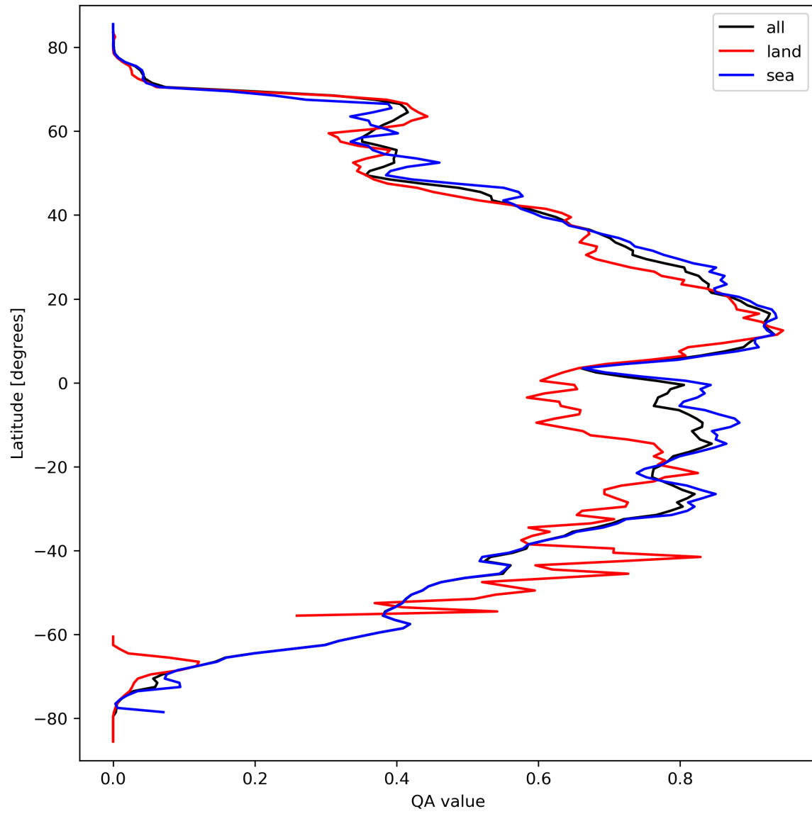
Figure 29: Zonal average of “QA value” for 2024-03-20 to 2024-03-21.
