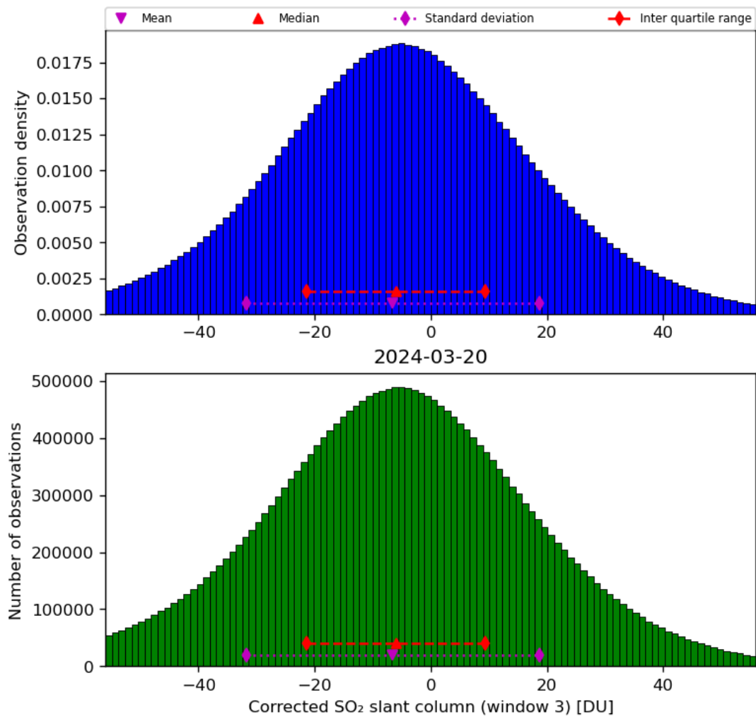
Figure 66: Histogram of “Corrected SO 2 slant column (window 3)” for 2024-03-20 to 2024-03-21
