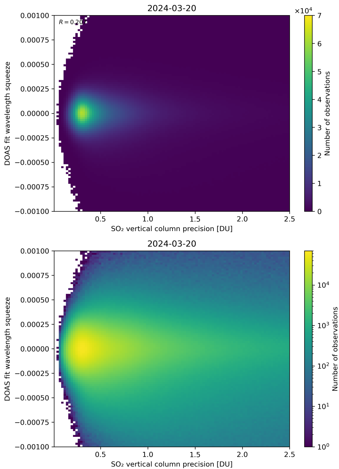
Figure 283: Scatter density plot of “SO 2 vertical column precision” against “DOAS fit wavelength squeeze” for 2024-03-20 to 2024-03-21.
