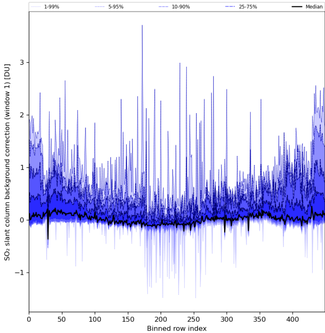
Figure 82: Along track statistics of “SO 2 slant column background correction (window 1)” for 2024-03-20 to 2024-03-21
