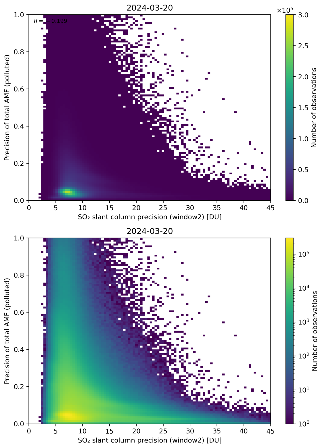
Figure 252: Scatter density plot of “SO 2 slant column precision (window2)” against “Precision of total AMF (polluted)” for 2024-03-20 to 2024-03-21.
