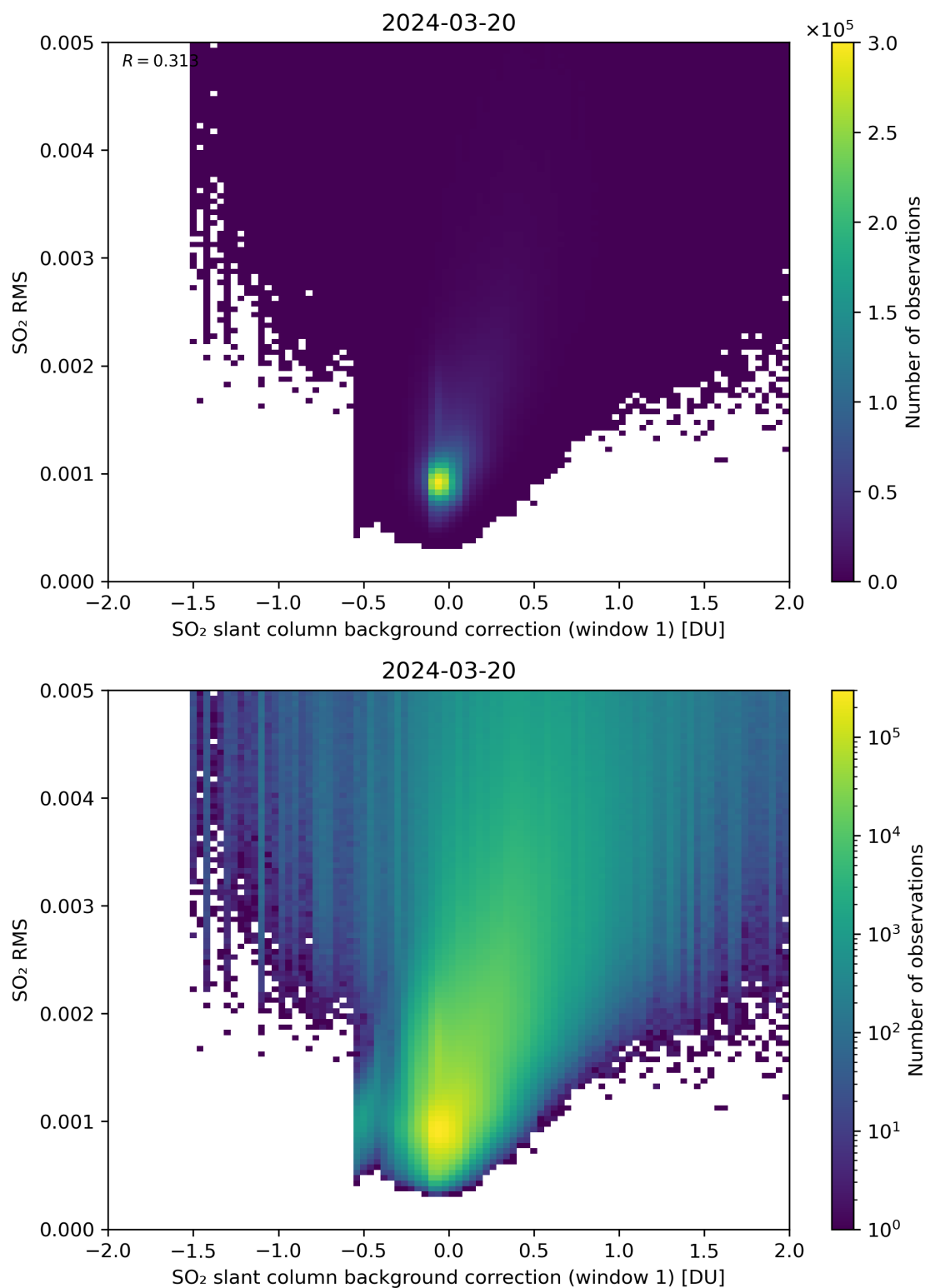
Figure 102: Scatter density plot of “SO 2 slant column background correction (window 1)” against “SO 2 RMS” for 2024-03-20 to 2024-03-21.
