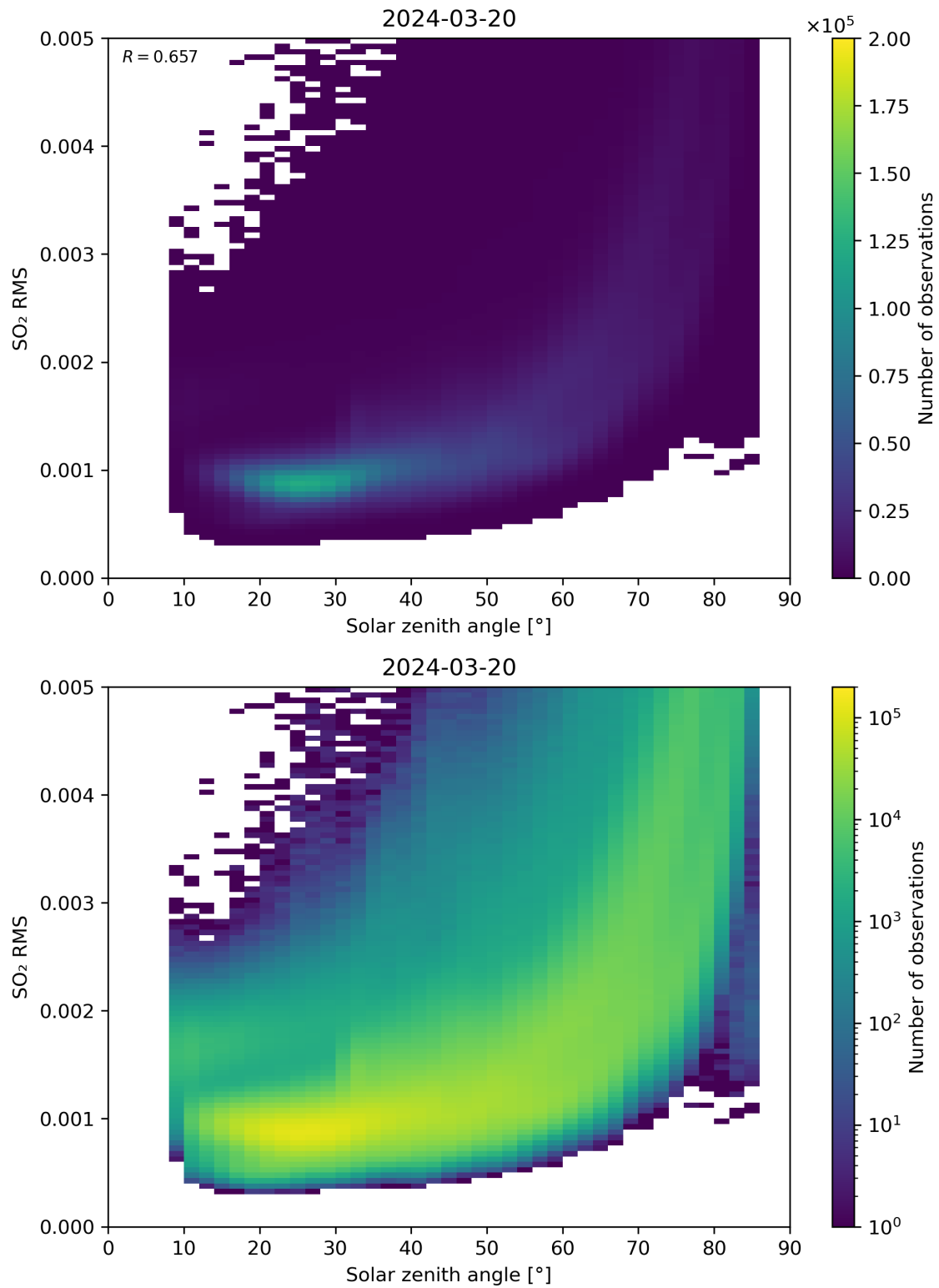
Figure 163: Scatter density plot of “Solar zenith angle” against “SO 2 RMS” for 2024-03-20 to 2024-03-21.
