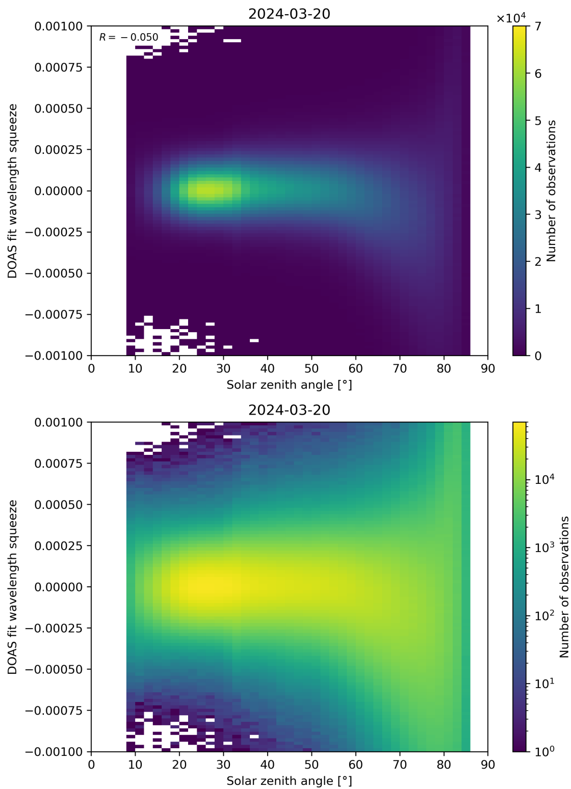
Figure 162: Scatter density plot of “Solar zenith angle” against “DOAS fit wavelength squeeze” for 2024-03-20 to 2024-03-21.
