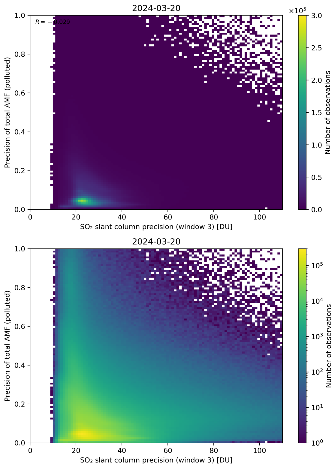
Figure 264: Scatter density plot of “SO 2 slant column precision (window 3)” against “Precision of total AMF (polluted)” for 2024-03-20 to 2024-03-21.
