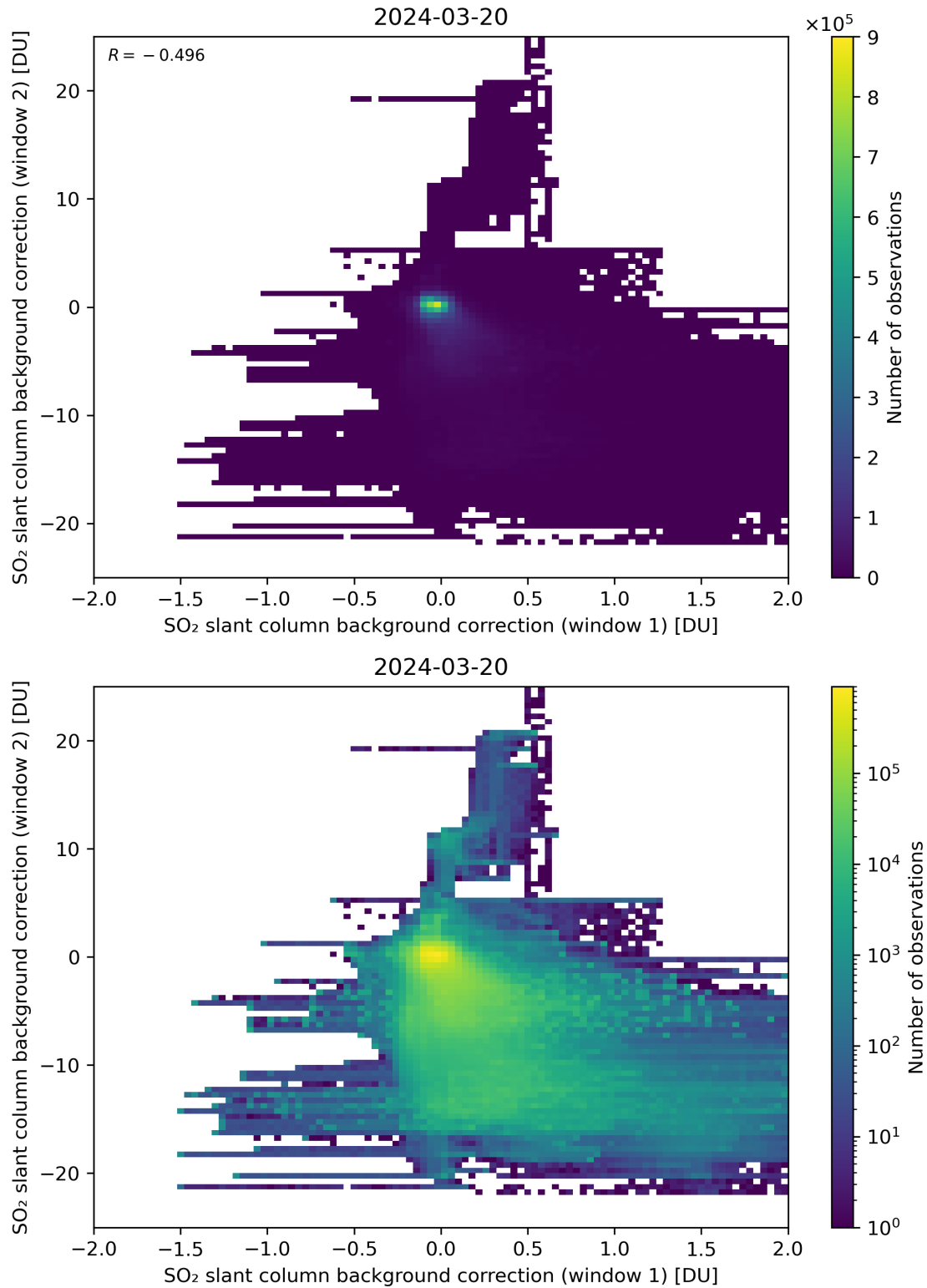
Figure 98: Scatter density plot of “SO 2 slant column background correction (window 1)” against “SO 2 slant column background correction (window 2)” for 2024-03-20 to 2024-03-21.
