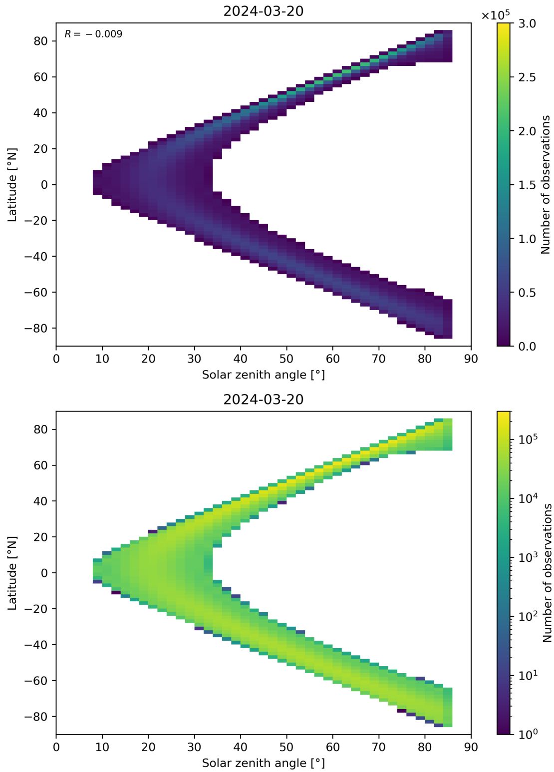
Figure 164: Scatter density plot of “Solar zenith angle” against “Latitude” for 2024-03-20 to 2024-03-21.
