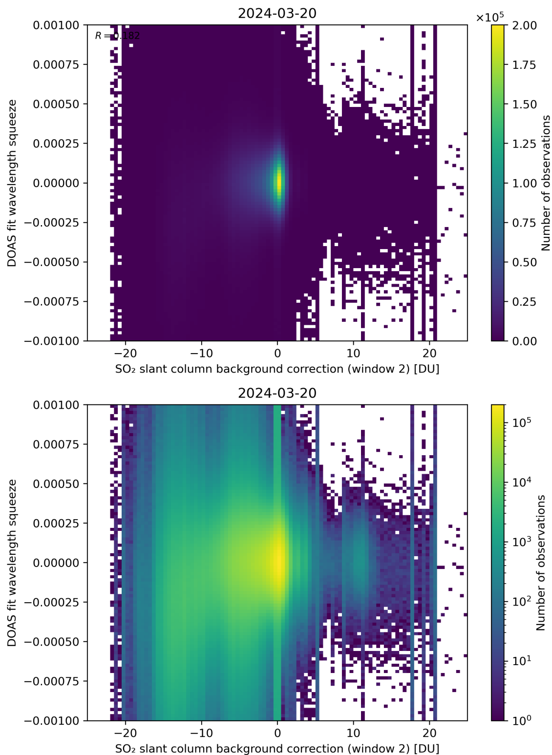
Figure 113: Scatter density plot of “SO 2 slant column background correction (window 2)” against “DOAS fit wavelength squeeze” for 2024-03-20 to 2024-03-21.
