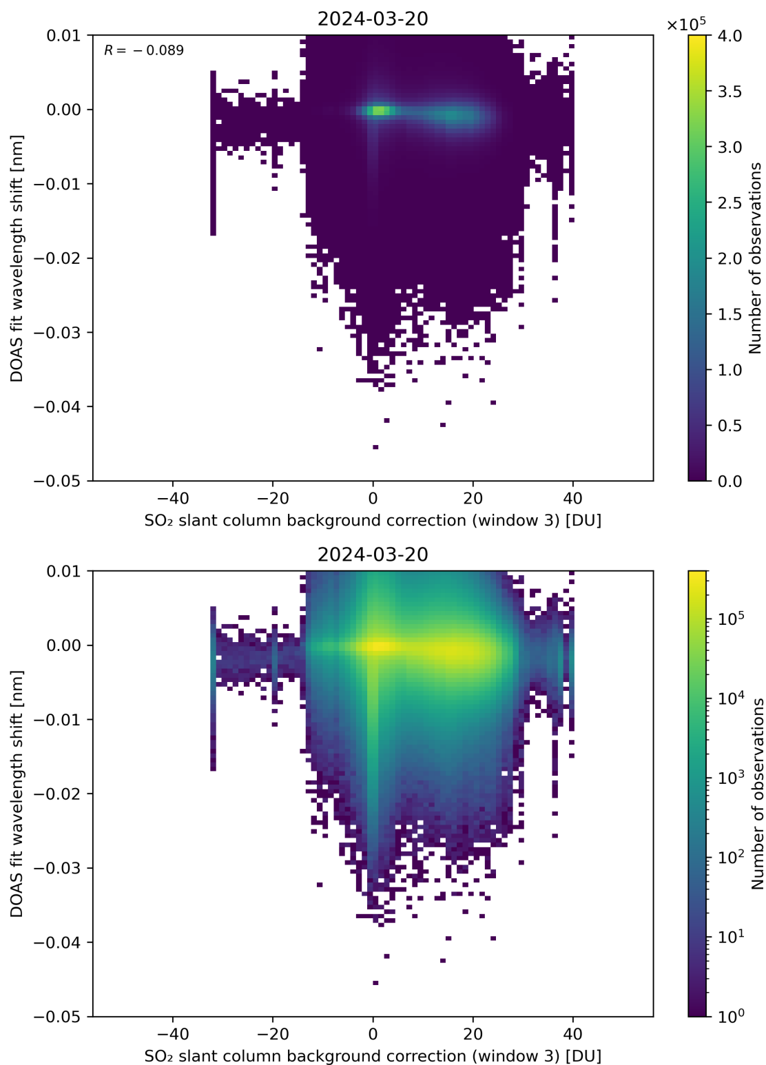
Figure 121: Scatter density plot of “SO 2 slant column background correction (window 3)” against “DOAS fit wavelength shift” for 2024-03-20 to 2024-03-21.
