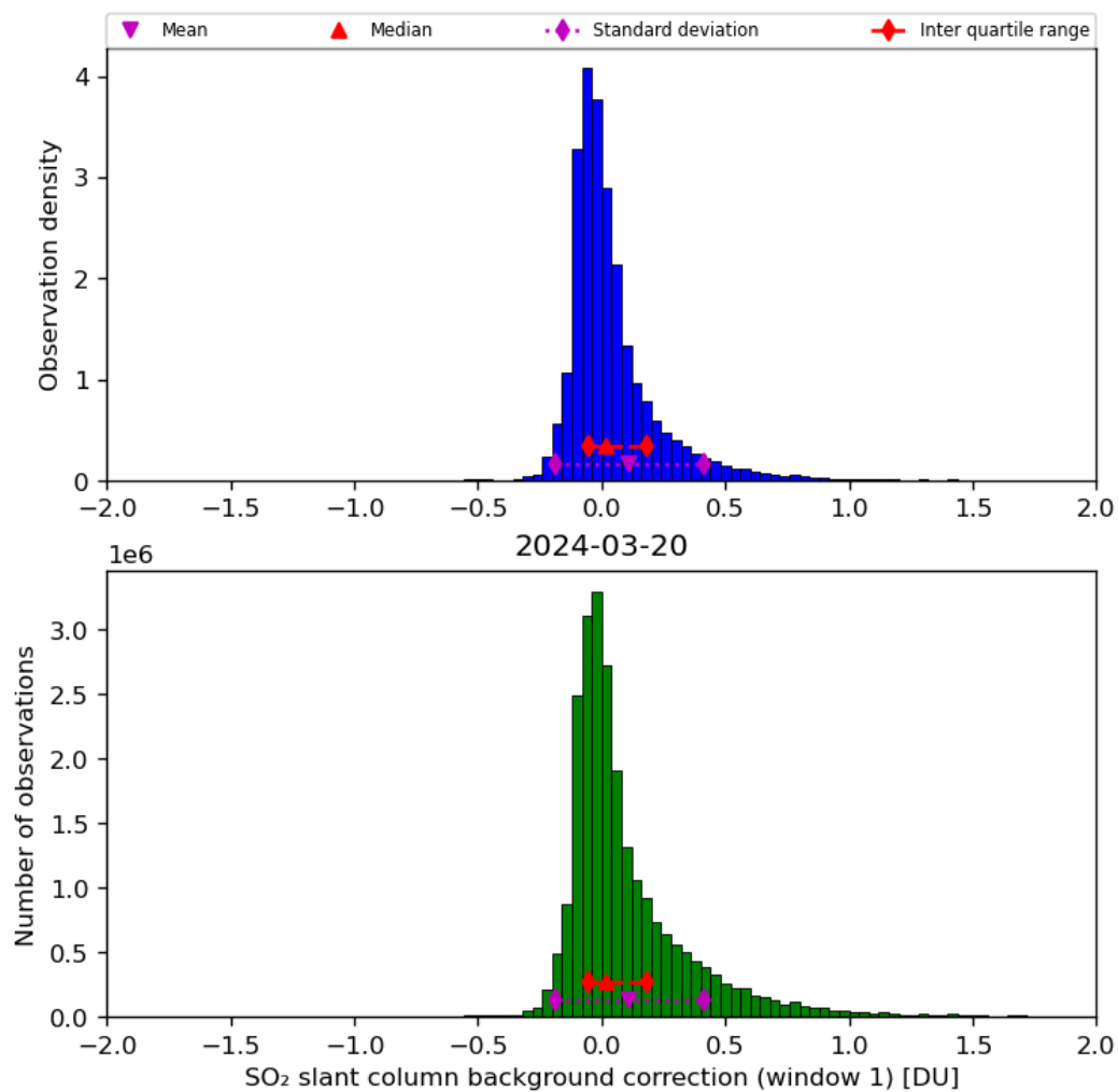
Figure 59: Histogram of “SO 2 slant column background correction (window 1)” for 2024-03-20 to 2024-03-21
