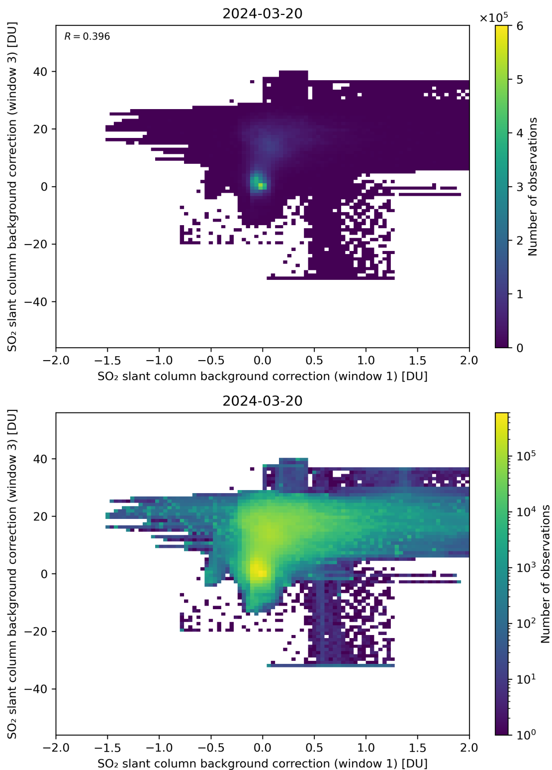
Figure 99: Scatter density plot of “SO 2 slant column background correction (window 1)” against “SO 2 slant column background correction (window 3)” for 2024-03-20 to 2024-03-21.
