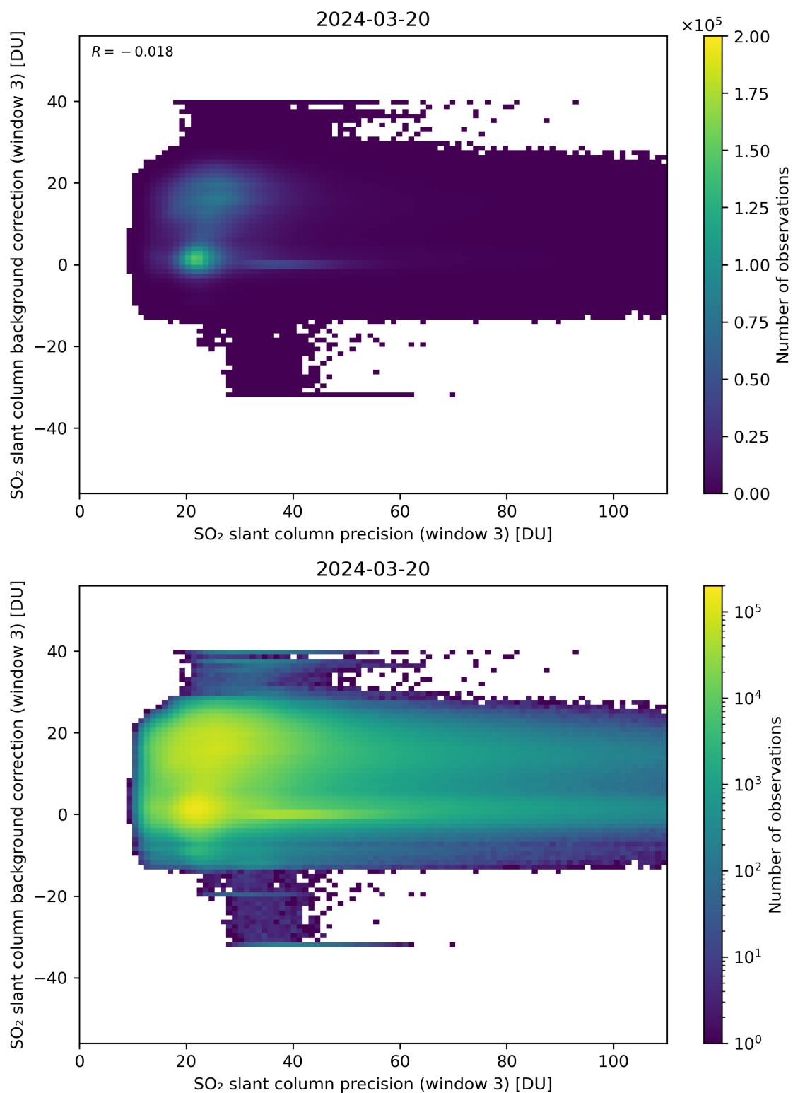
Figure 257: Scatter density plot of “SO 2 slant column precision (window 3)” against “SO 2 slant column background correction (window 3)” for 2024-03-20 to 2024-03-21.
