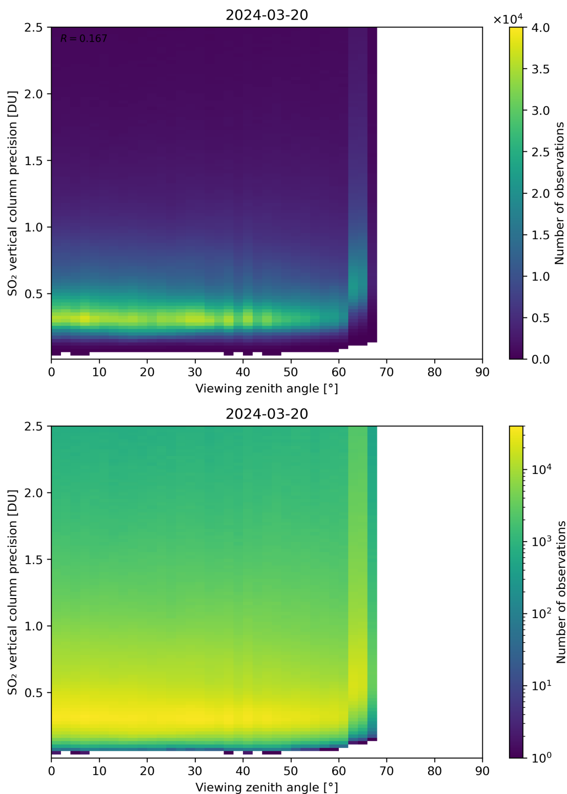
Figure 328: Scatter density plot of “Viewing zenith angle” against “SO 2 vertical column precision” for 2024-03-20 to 2024-03-21.
