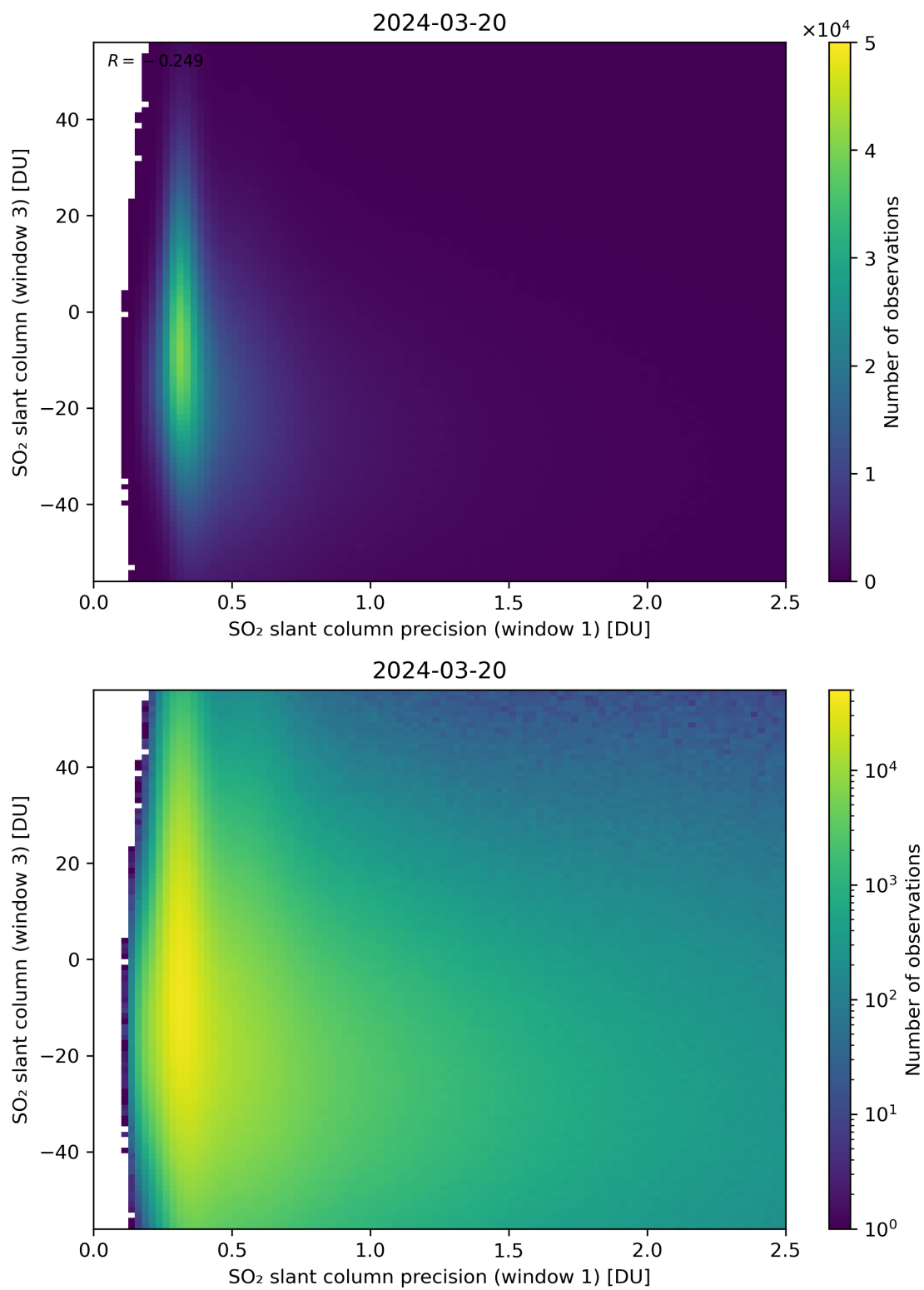
Figure 228: Scatter density plot of “SO 2 slant column precision (window 1)” against “SO 2 slant column (window 3)” for 2024-03-20 to 2024-03-21.
