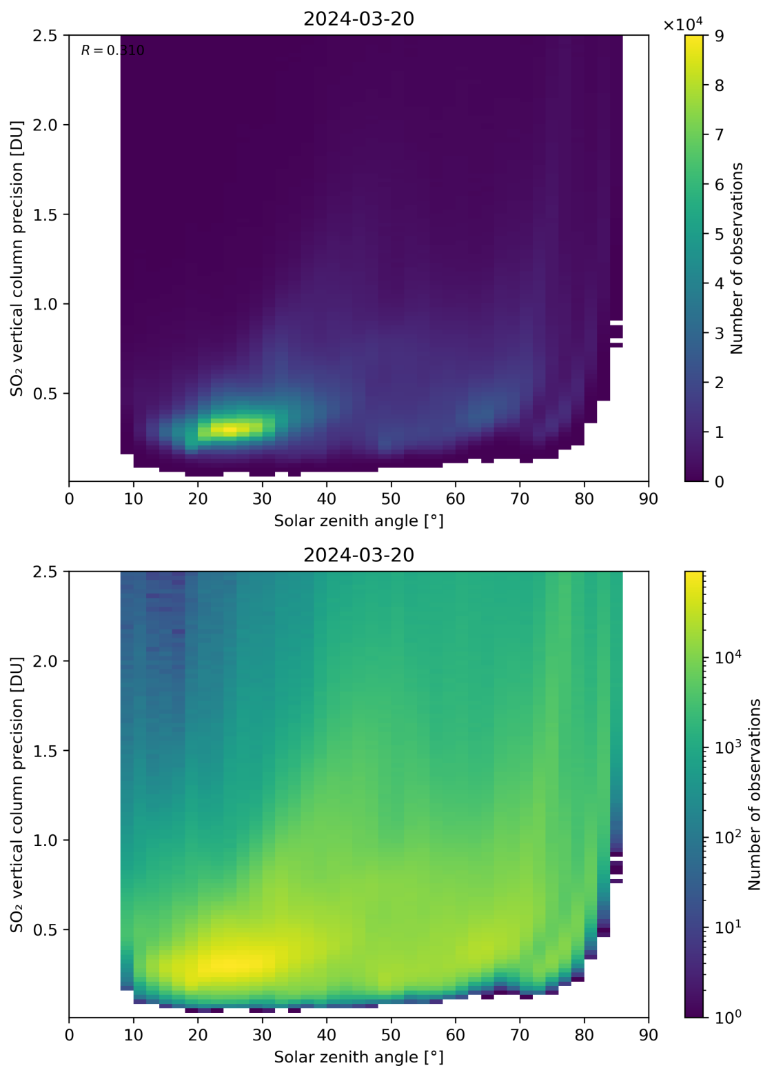
Figure 177: Scatter density plot of “Solar zenith angle” against “SO 2 vertical column precision” for 2024-03-20 to 2024-03-21.
