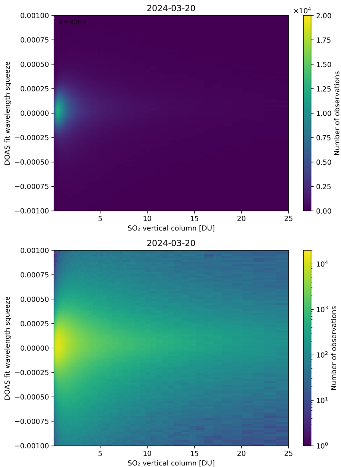
Figure 277: Scatter density plot of “SO 2 vertical column” against “DOAS fit wavelength squeeze” for 2024-03-20 to 2024-03-21.
