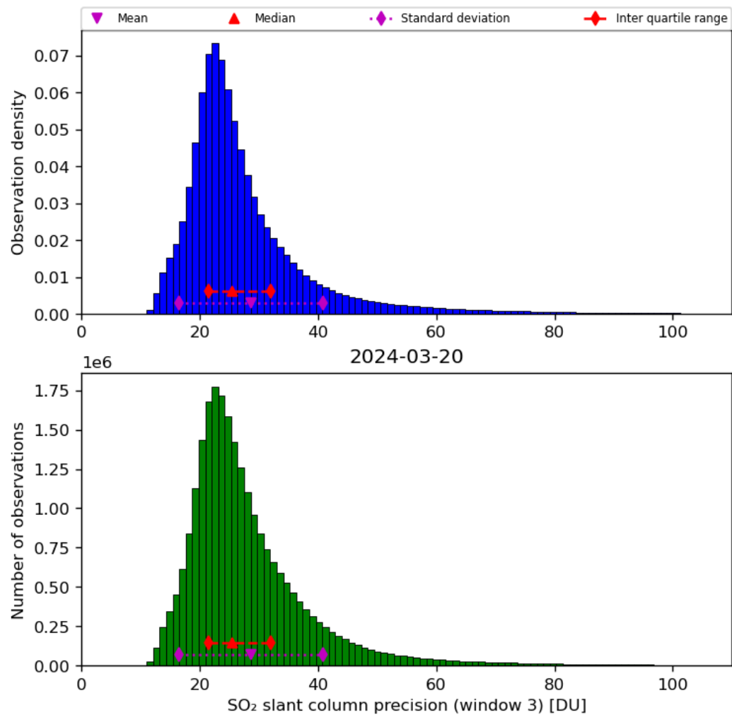
Figure 65: Histogram of “SO 2 slant column precision (window 3)” for 2024-03-20 to 2024-03-21
