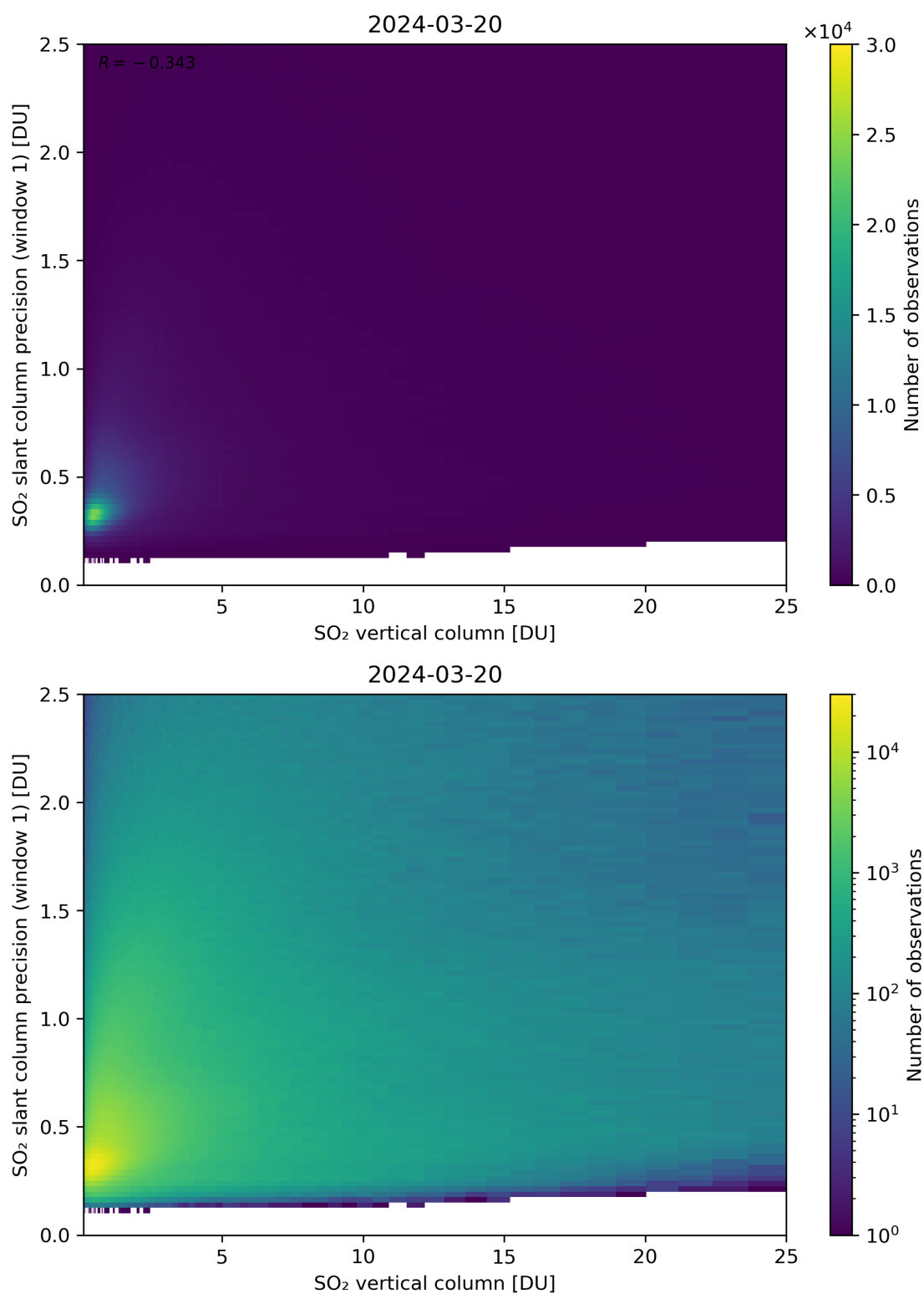
Figure 301: Scatter density plot of “SO 2 vertical column” against “SO 2 slant column precision (window 1)” for 2024-03-20 to 2024-03-21.
