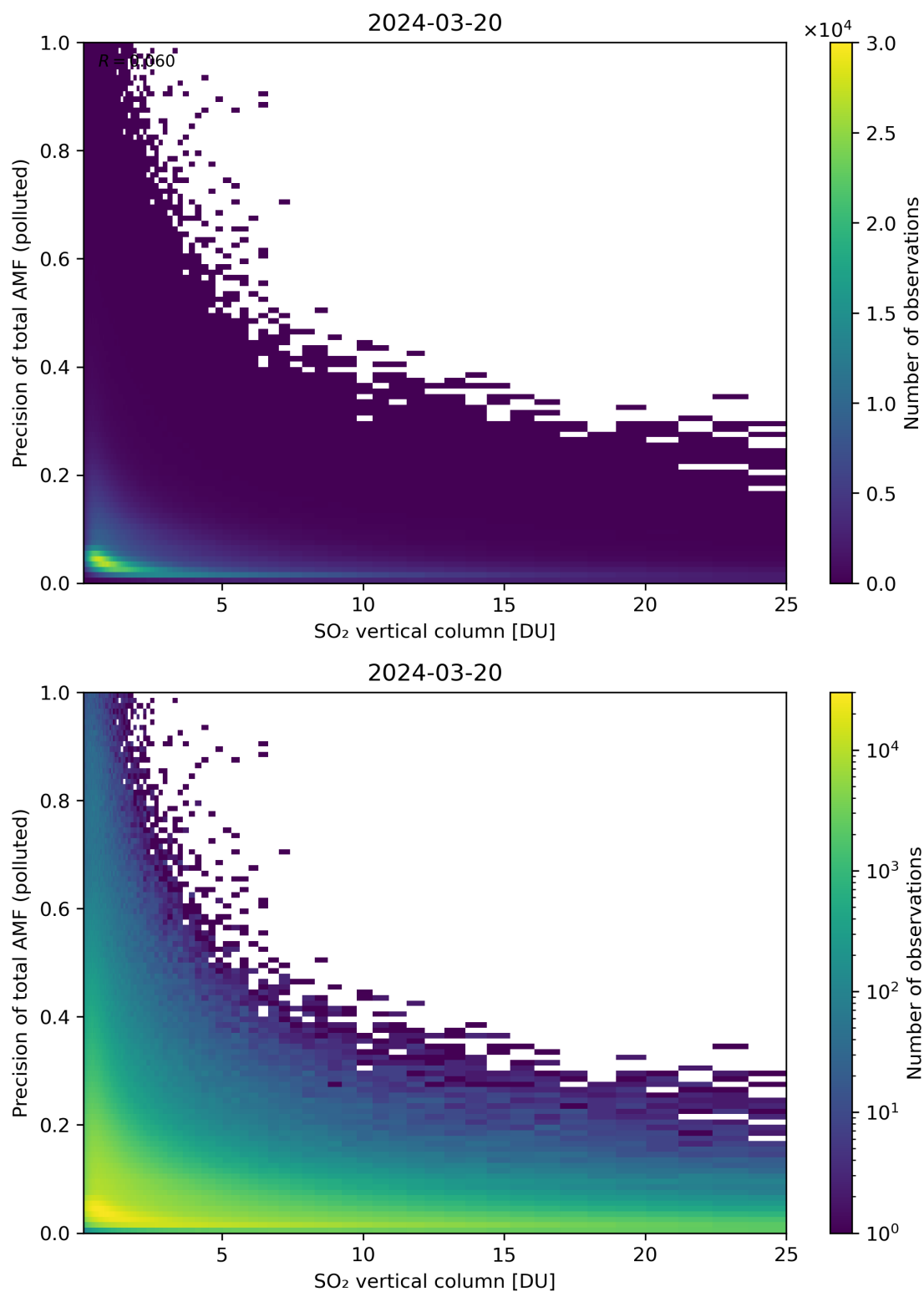
Figure 306: Scatter density plot of “SO 2 vertical column” against “Precision of total AMF (polluted)” for 2024-03-20 to 2024-03-21.
