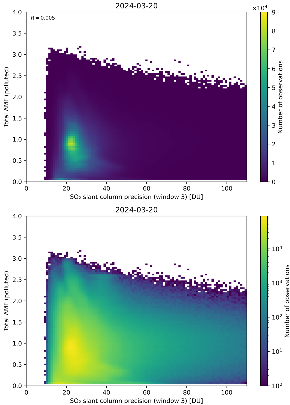
Figure 263: Scatter density plot of “SO 2 slant column precision (window 3)” against “Total AMF (polluted)” for 2024-03-20 to 2024-03-21.
