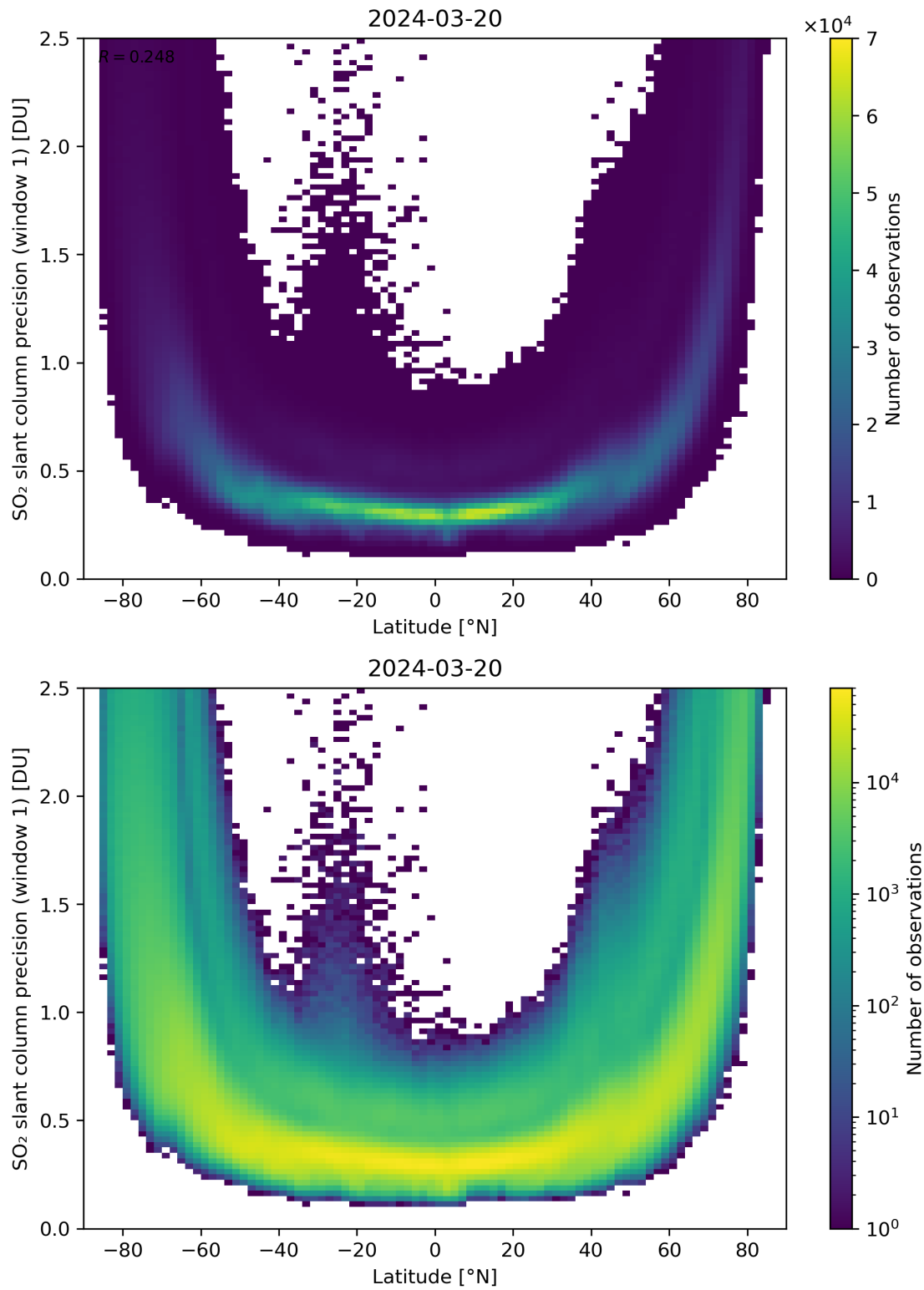
Figure 150: Scatter density plot of “Latitude” against “SO 2 slant column precision (window 1)” for 2024-03-20 to 2024-03-21.
