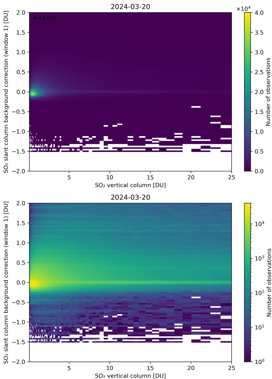
Figure 273: Scatter density plot of “SO 2 vertical column” against “SO 2 slant column background correction (window 1)” for 2024-03-20 to 2024-03-21.
