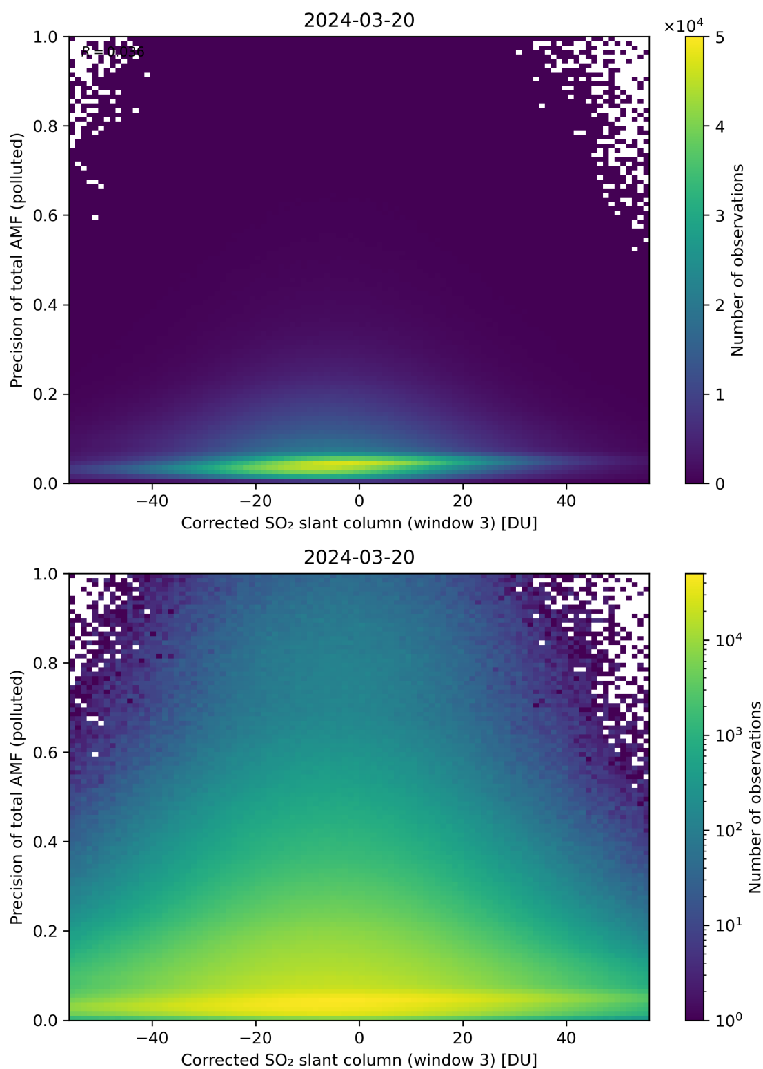
Figure 211: Scatter density plot of “Corrected SO 2 slant column (window 3)” against “Precision of total AMF (polluted)” for 2024-03-20 to 2024-03-21.
