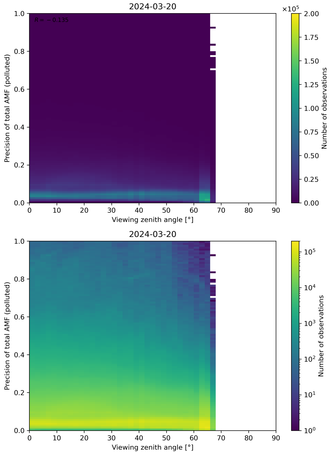
Figure 326: Scatter density plot of “Viewing zenith angle” against “Precision of total AMF (polluted)” for 2024-03-20 to 2024-03-21.
