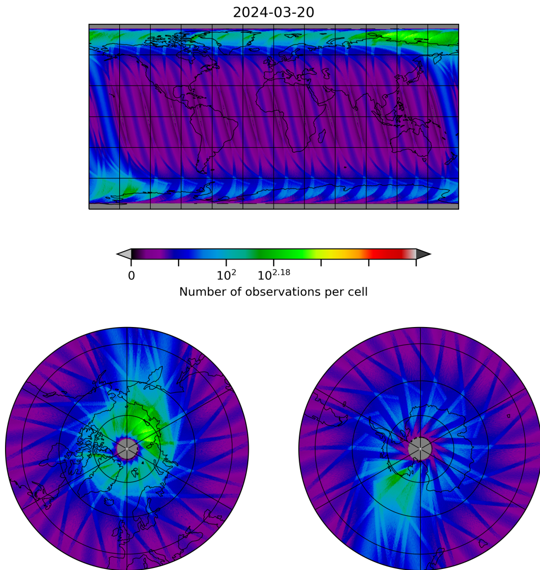
Figure 28: Map of the number of observations for 2024-03-20 to 2024-03-21
