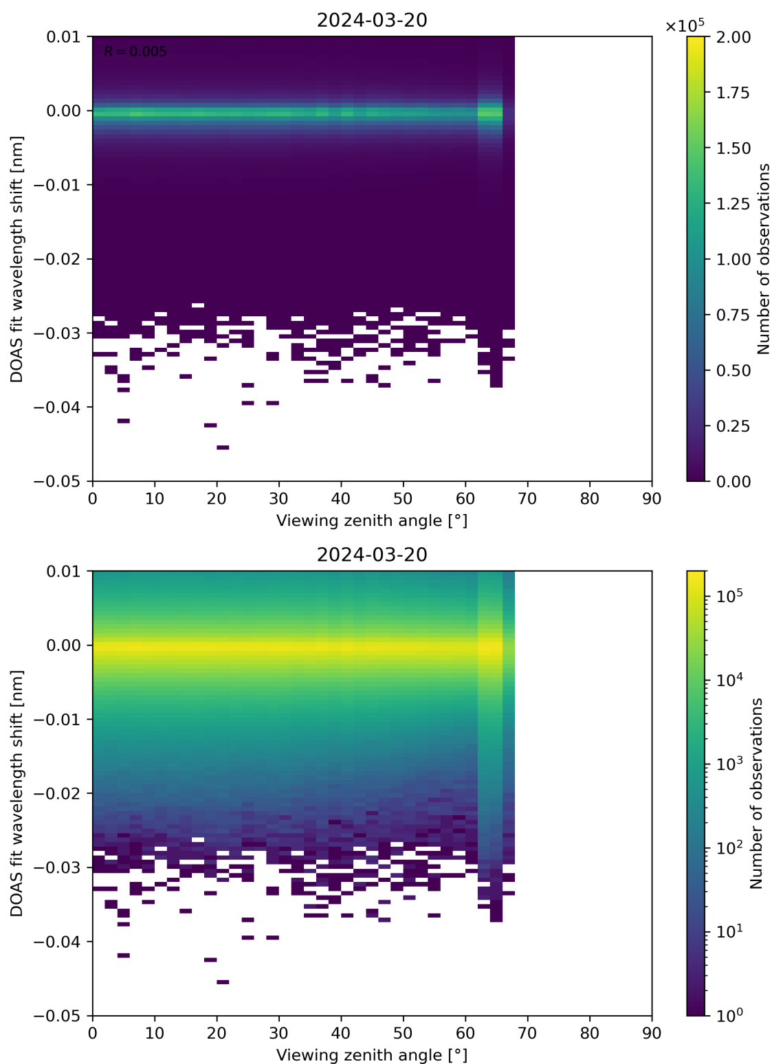
Figure 311: Scatter density plot of “Viewing zenith angle” against “DOAS fit wavelength shift” for 2024-03-20 to 2024-03-21.
