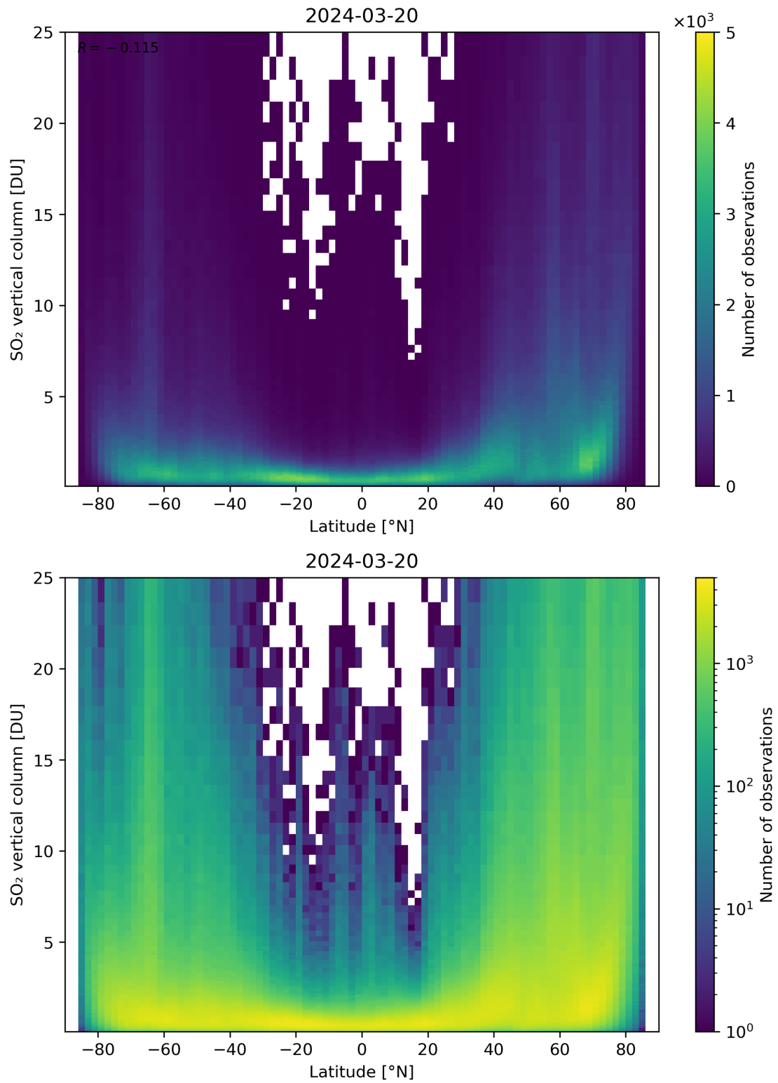
Figure 156: Scatter density plot of “Latitude” against “SO 2 vertical column” for 2024-03-20 to 2024-03-21.
