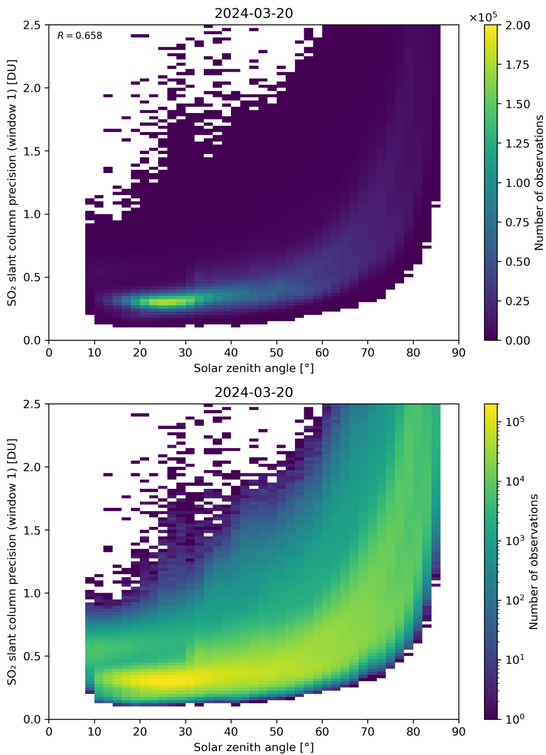
Figure 170: Scatter density plot of “Solar zenith angle” against “SO 2 slant column precision (window 1)” for 2024-03-20 to 2024-03-21.
