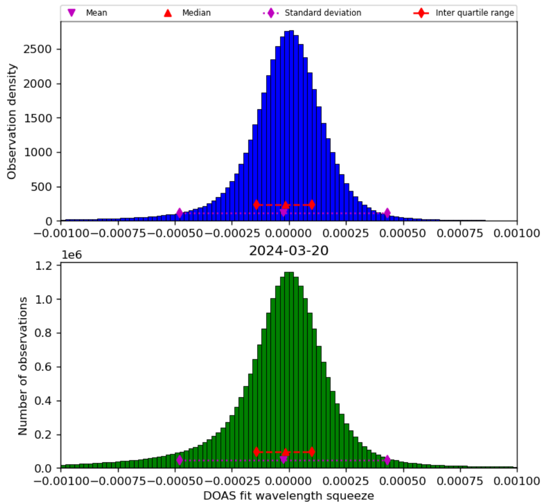
Figure 69: Histogram of “DOAS fit wavelength squeeze” for 2024-03-20 to 2024-03-21
