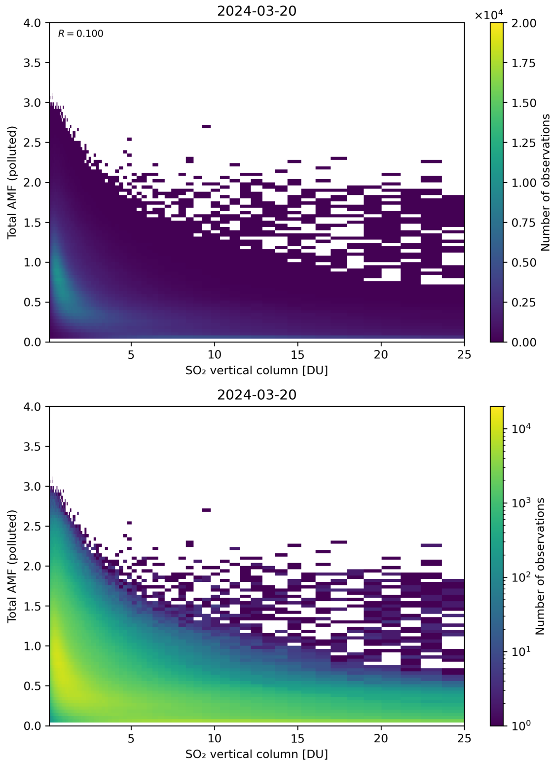
Figure 305: Scatter density plot of “SO 2 vertical column” against “Total AMF (polluted)” for 2024-03-20 to 2024-03-21.
