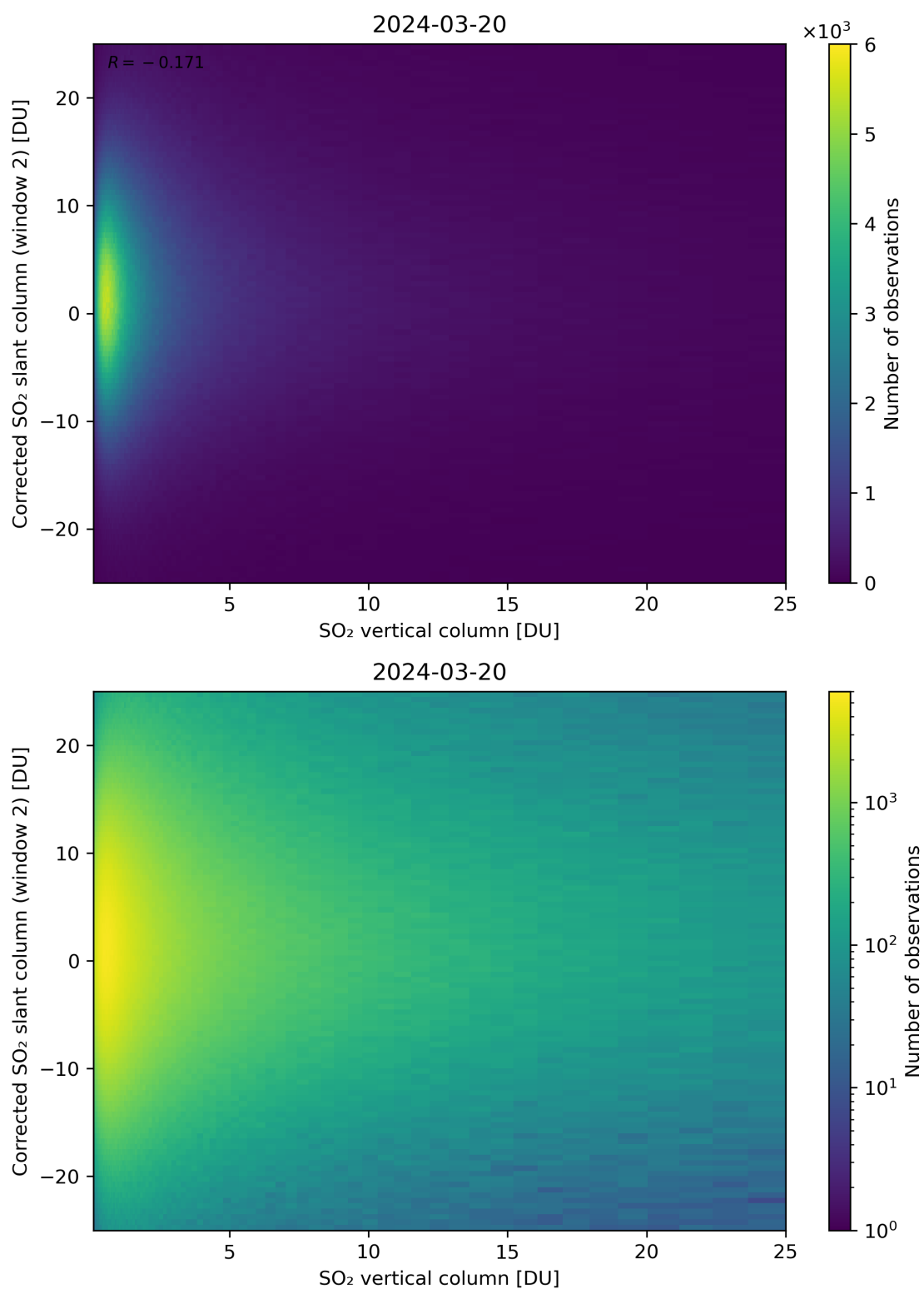
Figure 298: Scatter density plot of “SO 2 vertical column” against “Corrected SO 2 slant column (window 2)” for 2024-03-20 to 2024-03-21.
