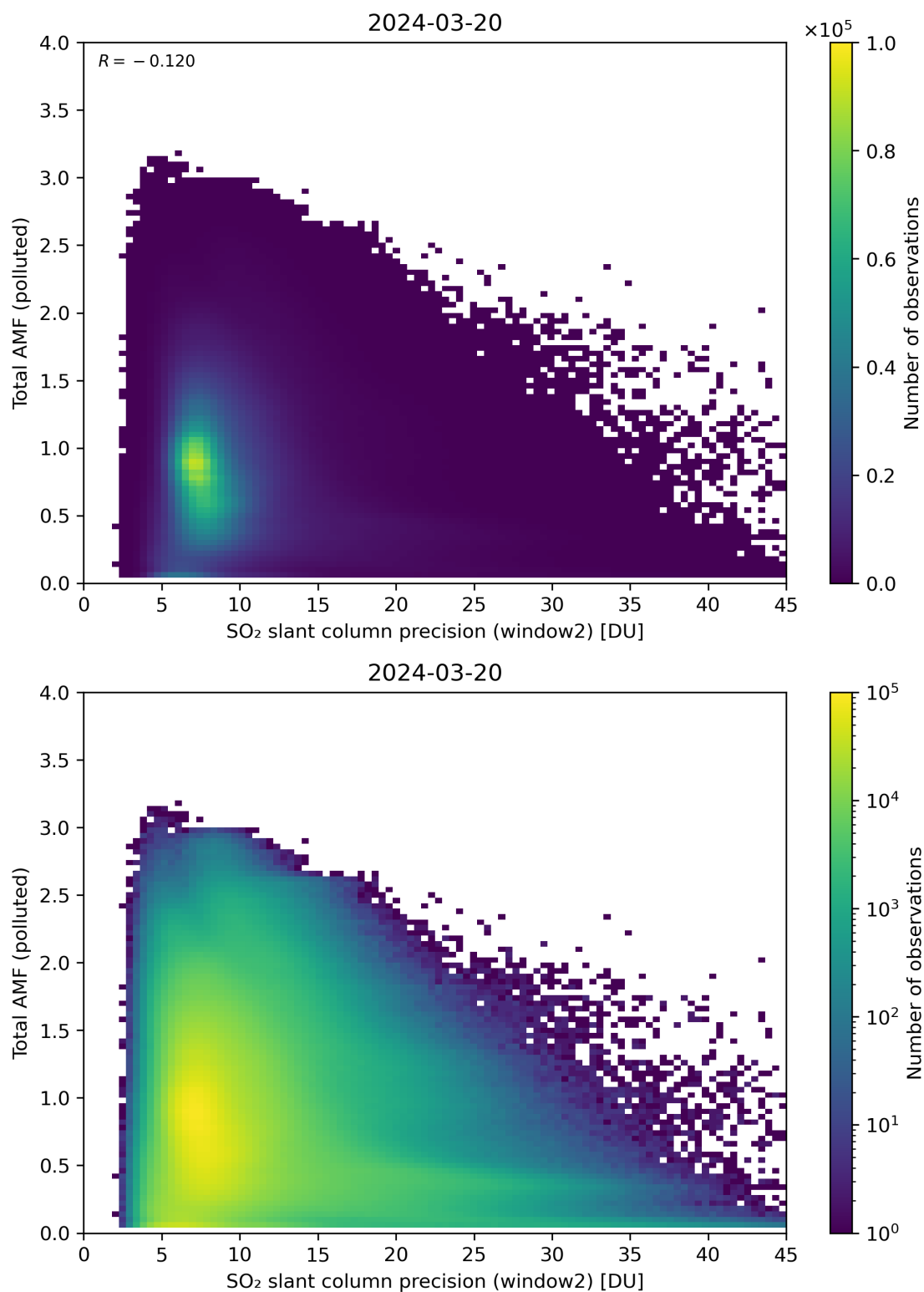
Figure 251: Scatter density plot of “SO 2 slant column precision (window2)” against “Total AMF (polluted)” for 2024-03-20 to 2024-03-21.
