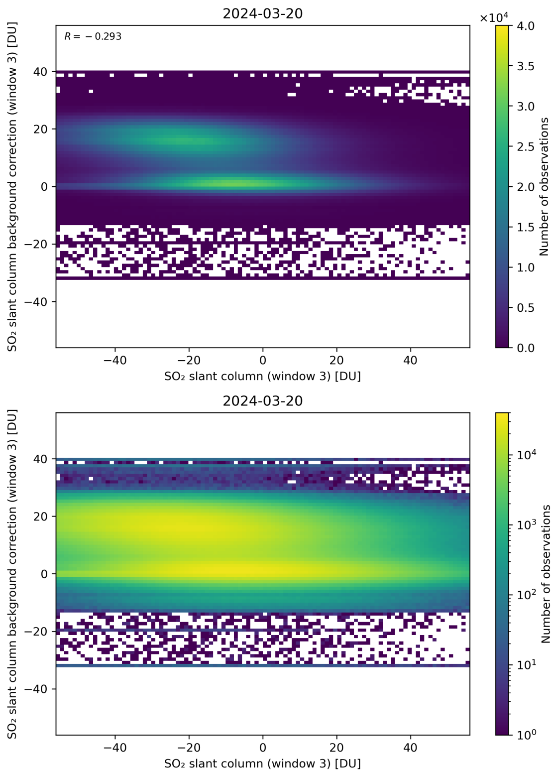
Figure 253: Scatter density plot of “SO 2 slant column (window 3)” against “SO 2 slant column background correction (window 3)” for 2024-03-20 to 2024-03-21.
