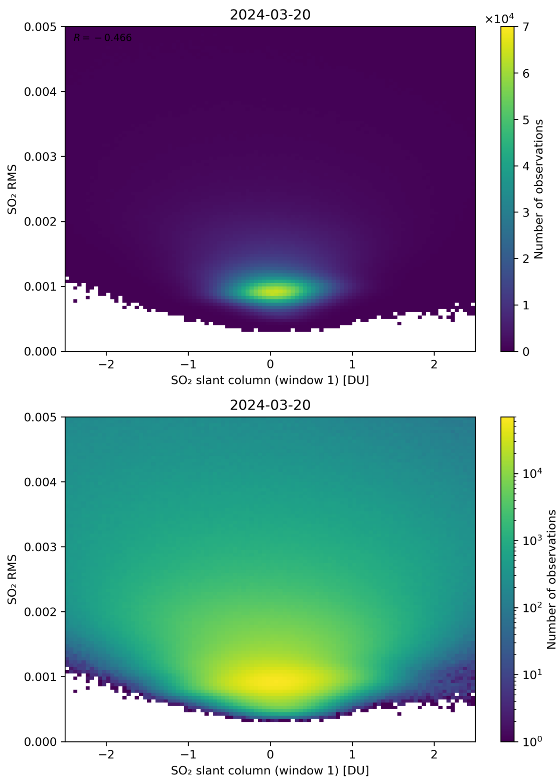
Figure 217: Scatter density plot of “SO 2 slant column (window 1)” against “SO 2 RMS” for 2024-03-20 to 2024-03-21.
