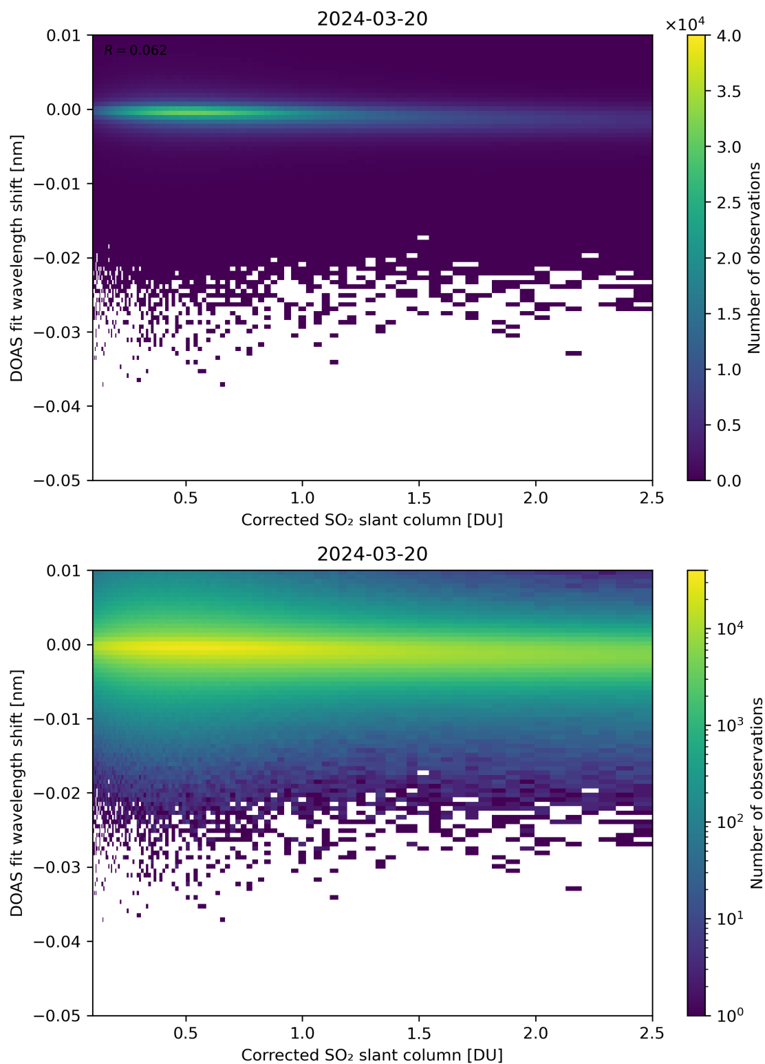
Figure 181: Scatter density plot of “Corrected SO 2 slant column” against “DOAS fit wavelength shift” for 2024-03-20 to 2024-03-21.
