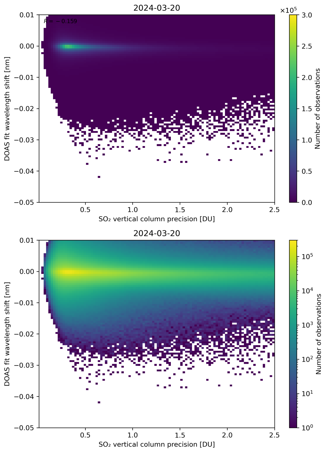
Figure 282: Scatter density plot of “SO 2 vertical column precision” against “DOAS fit wavelength shift” for 2024-03-20 to 2024-03-21.
