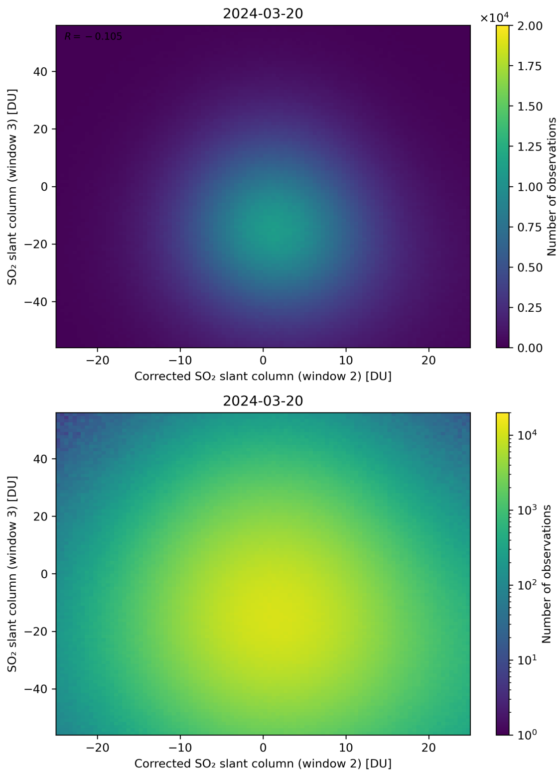
Figure 201: Scatter density plot of “Corrected SO 2 slant column (window 2)” against “SO 2 slant column (window 3)” for 2024-03-20 to 2024-03-21.
