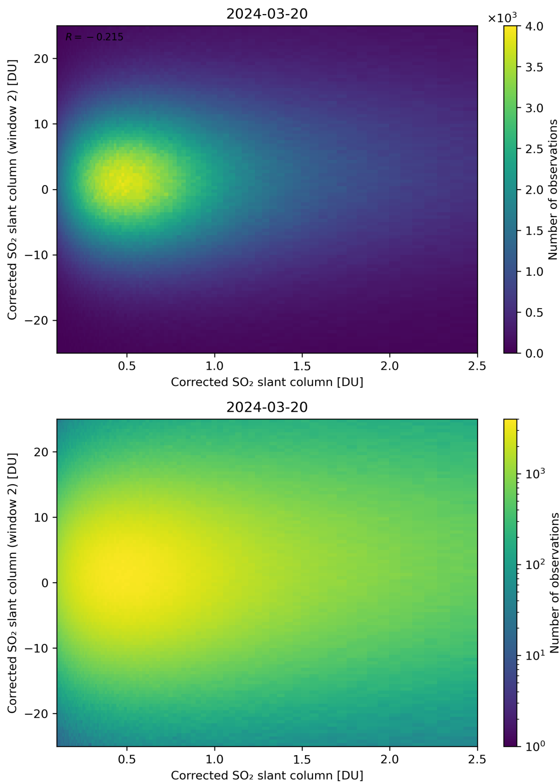
Figure 185: Scatter density plot of “Corrected SO 2 slant column” against “Corrected SO 2 slant column (window 2)” for 2024-03-20 to 2024-03-21.
