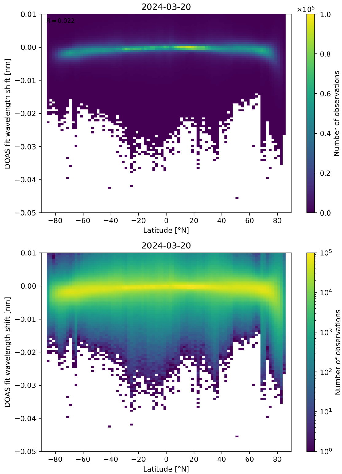
Figure 142: Scatter density plot of “Latitude” against “DOAS fit wavelength shift” for 2024-03-20 to 2024-03-21.
