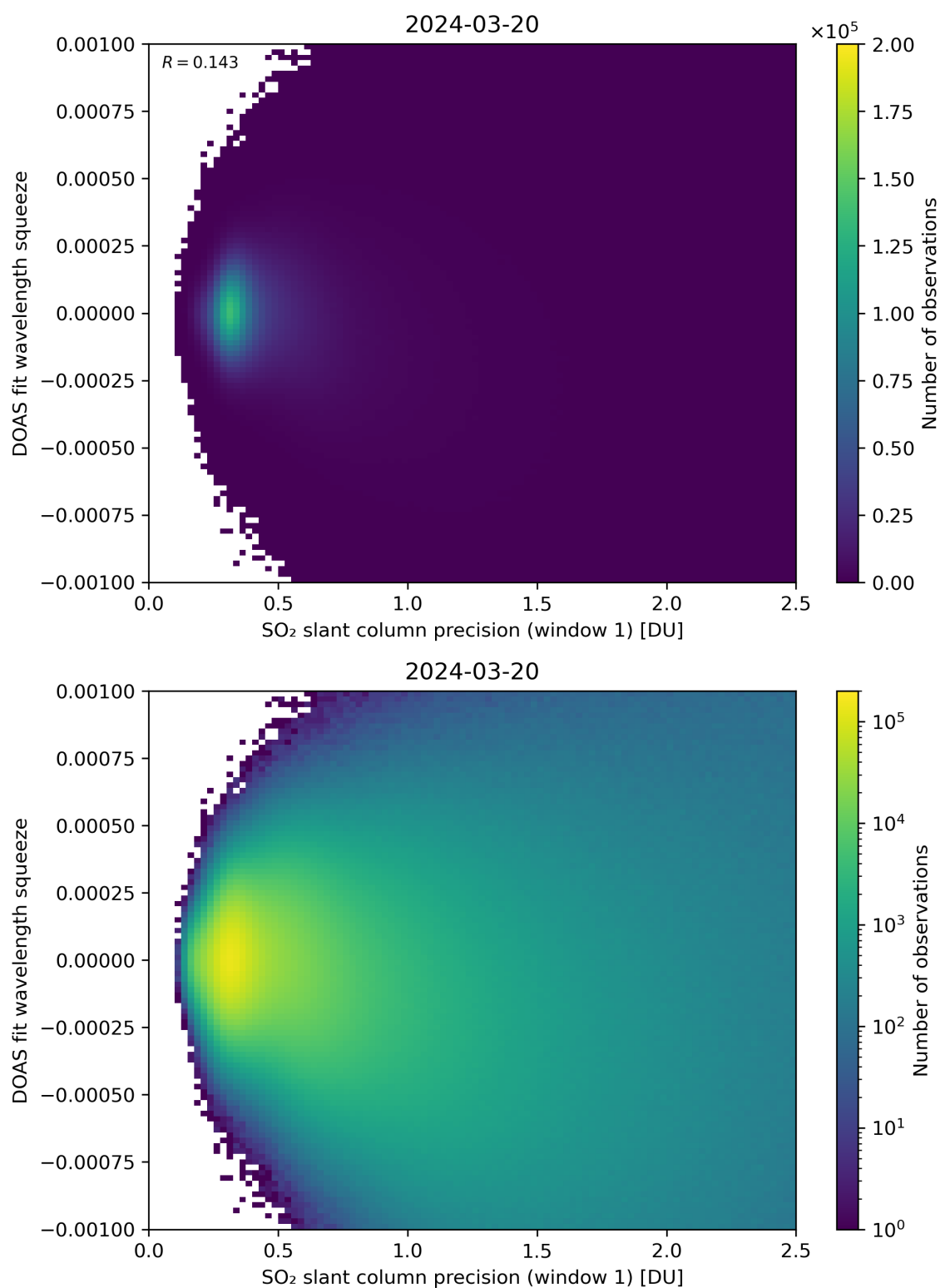
Figure 222: Scatter density plot of “SO 2 slant column precision (window 1)” against “DOAS fit wavelength squeeze” for 2024-03-20 to 2024-03-21.
