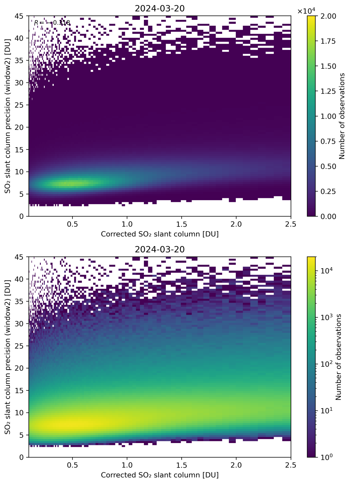
Figure 189: Scatter density plot of “Corrected SO 2 slant column” against “SO 2 slant column precision (window2)” for 2024-03-20 to 2024-03-21.
