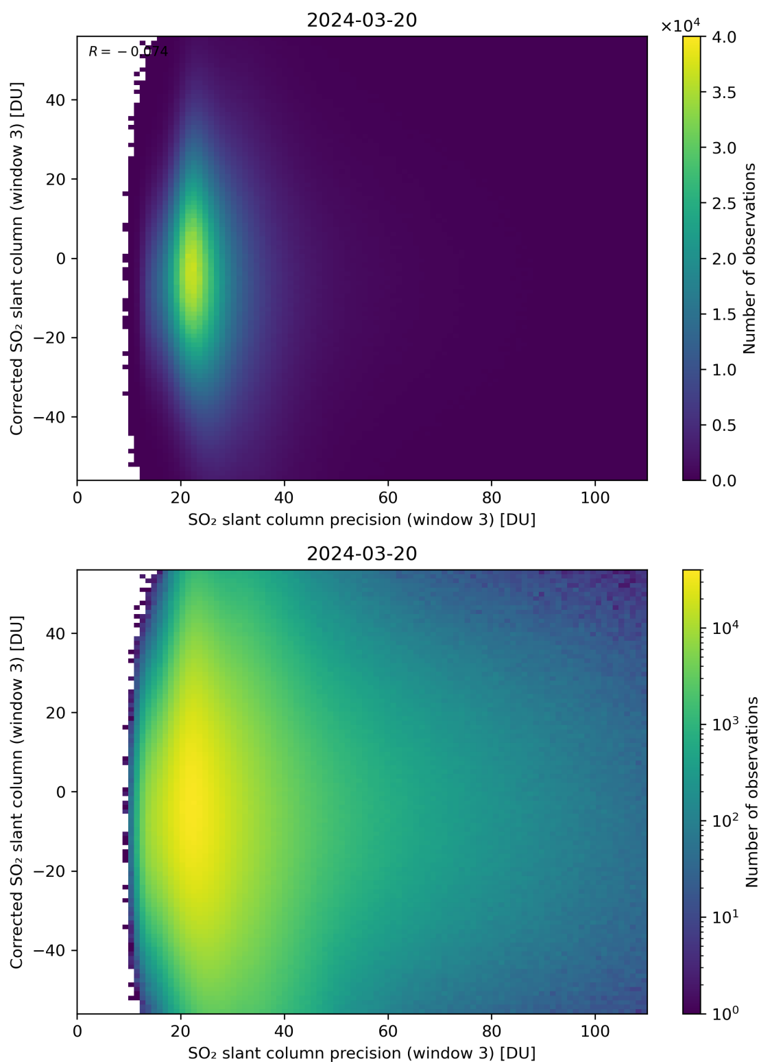
Figure 262: Scatter density plot of “SO 2 slant column precision (window 3)” against “Corrected SO 2 slant column (window 3)” for 2024-03-20 to 2024-03-21.
