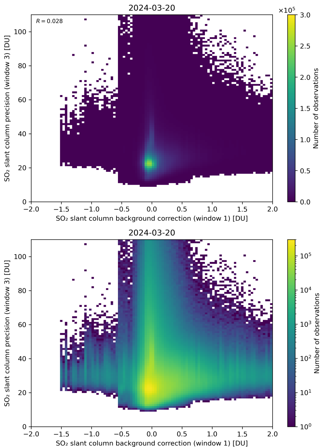
Figure 108: Scatter density plot of “SO 2 slant column background correction (window 1)” against “SO 2 slant column precision (window 3)” for 2024-03-20 to 2024-03-21.
