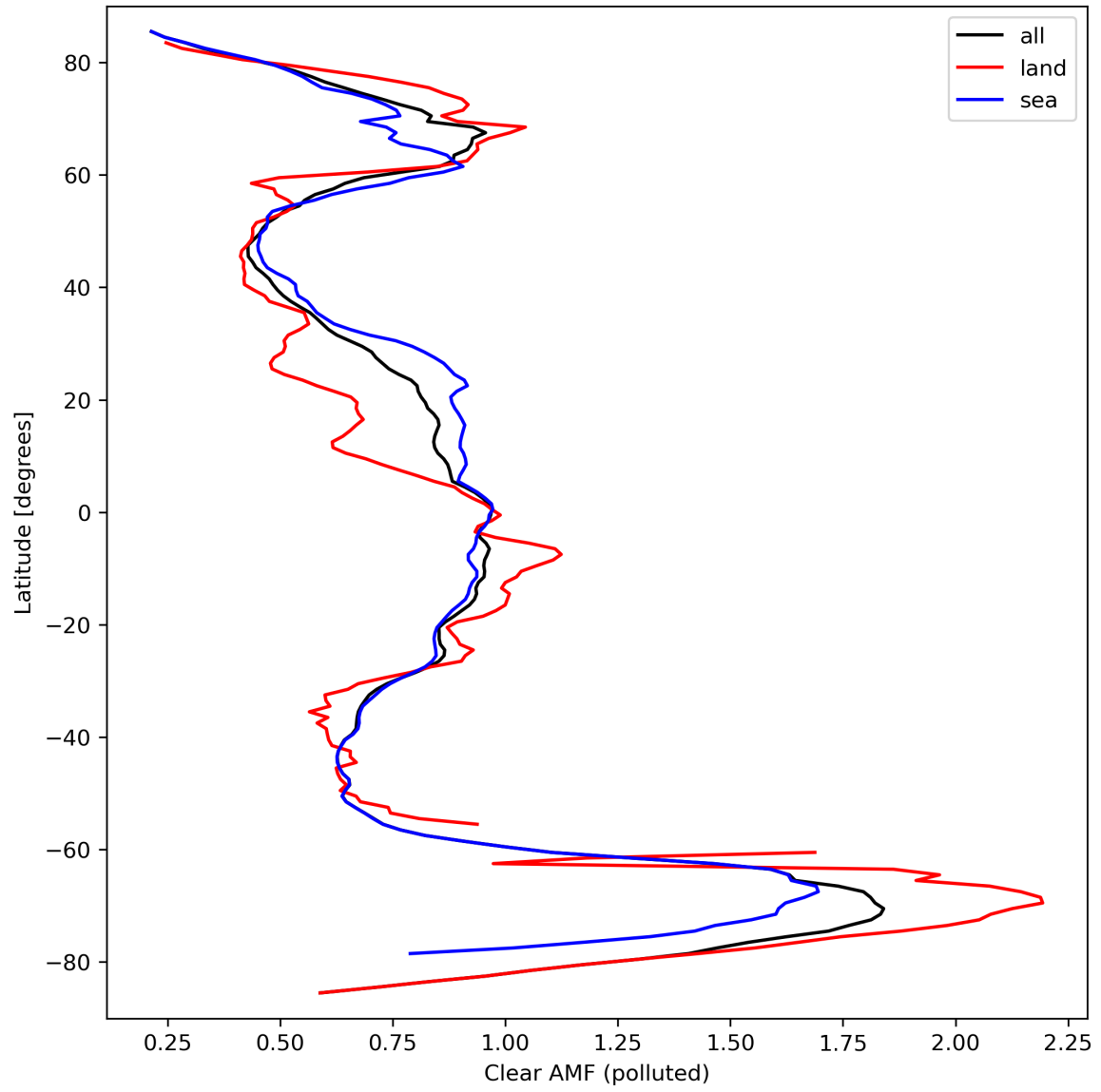
Figure 50: Zonal average of “Clear AMF (polluted)” for 2024-03-20 to 2024-03-21.
