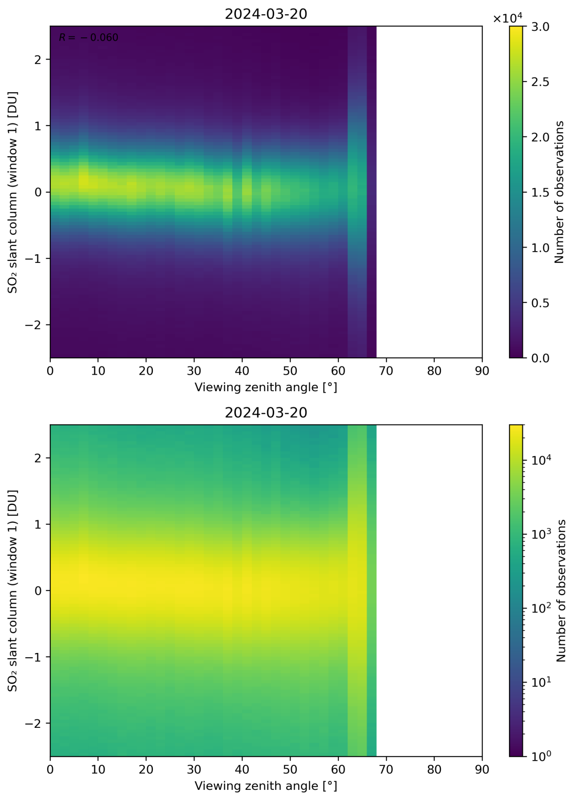
Figure 320: Scatter density plot of “Viewing zenith angle” against “SO 2 slant column (window 1)” for 2024-03-20 to 2024-03-21.
