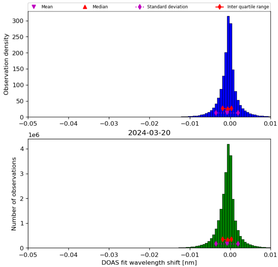
Figure 68: Histogram of “DOAS fit wavelength shift” for 2024-03-20 to 2024-03-21
