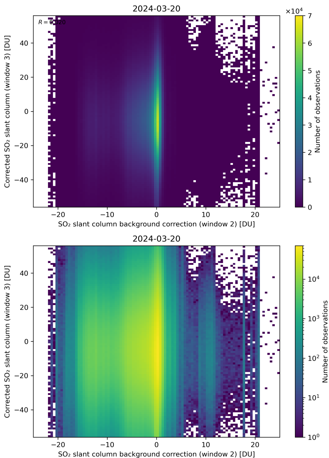
Figure 116: Scatter density plot of “SO 2 slant column background correction (window 2)” against “Corrected SO 2 slant column (window 3)” for 2024-03-20 to 2024-03-21.
