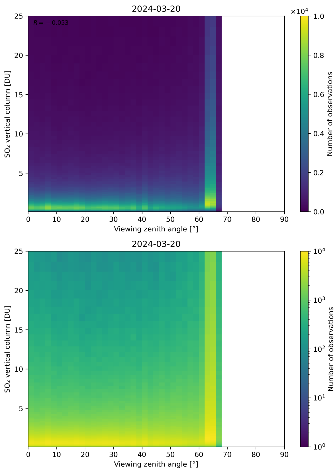
Figure 327: Scatter density plot of “Viewing zenith angle” against “SO 2 vertical column” for 2024-03-20 to 2024-03-21.
