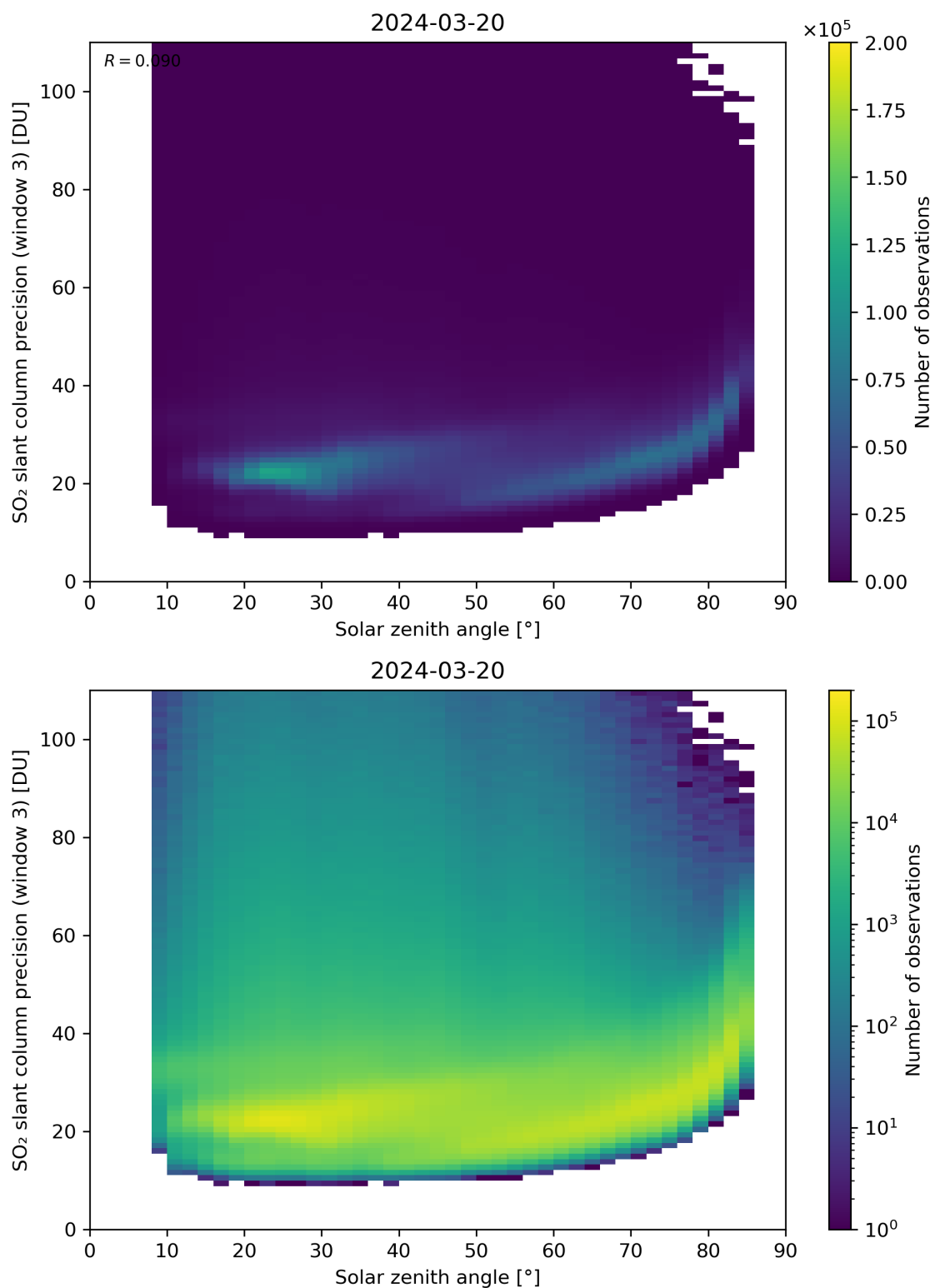
Figure 173: Scatter density plot of “Solar zenith angle” against “SO 2 slant column precision (window 3)” for 2024-03-20 to 2024-03-21.
