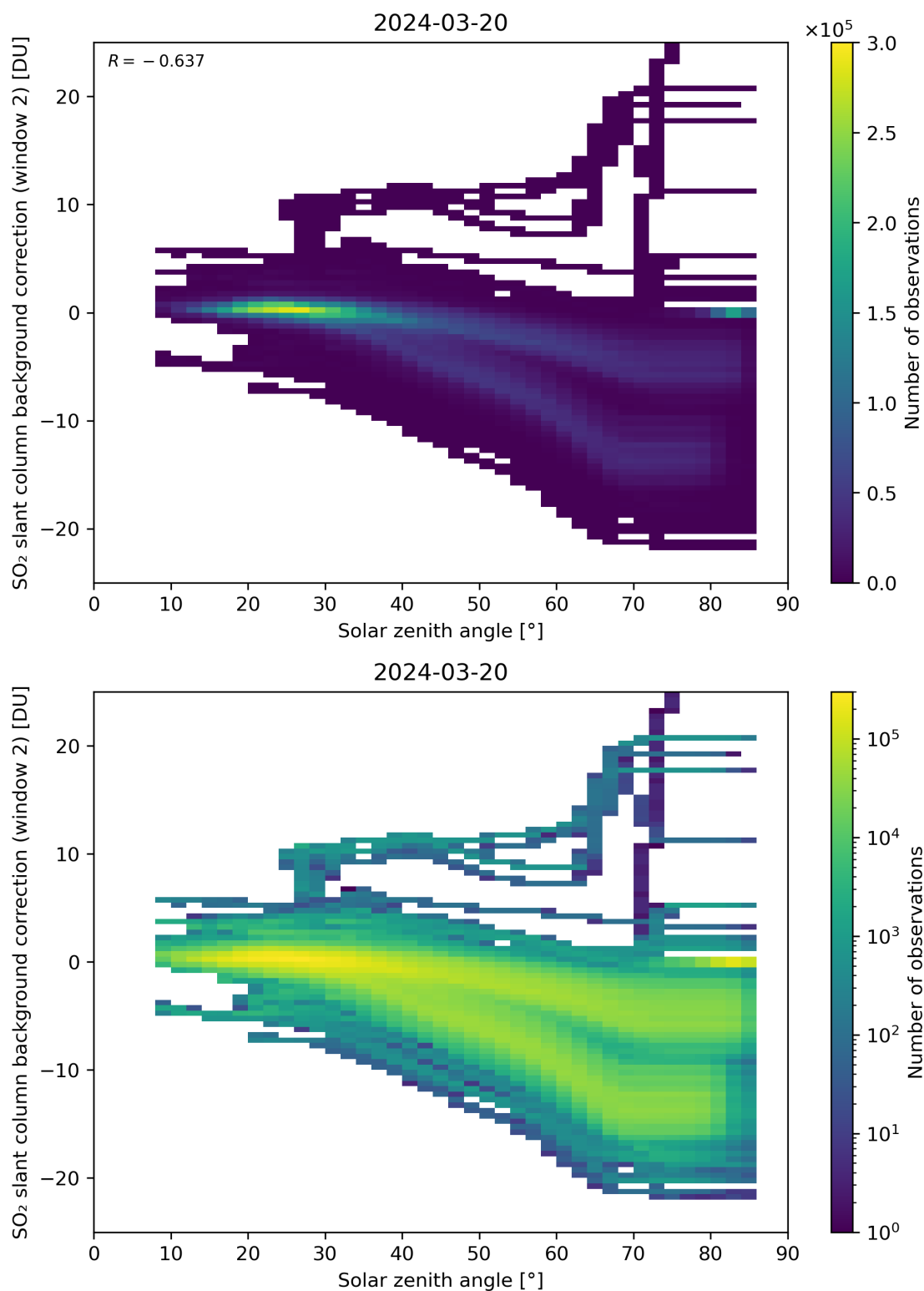
Figure 159: Scatter density plot of “Solar zenith angle” against “SO 2 slant column background correction (window 2)” for 2024-03-20 to 2024-03-21.
