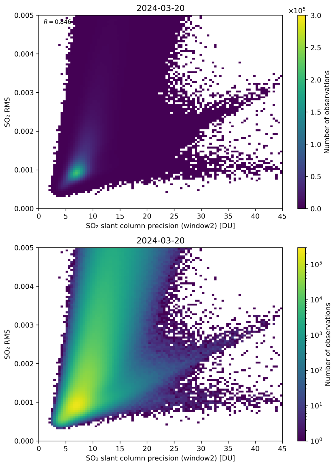
Figure 245: Scatter density plot of “SO 2 slant column precision (window2)” against “SO 2 RMS” for 2024-03-20 to 2024-03-21.
