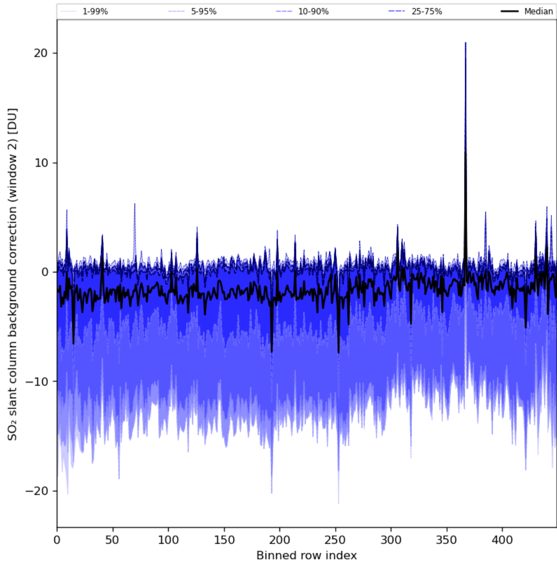
Figure 86: Along track statistics of “SO 2 slant column background correction (window 2)” for 2024-03-20 to 2024-03-21
