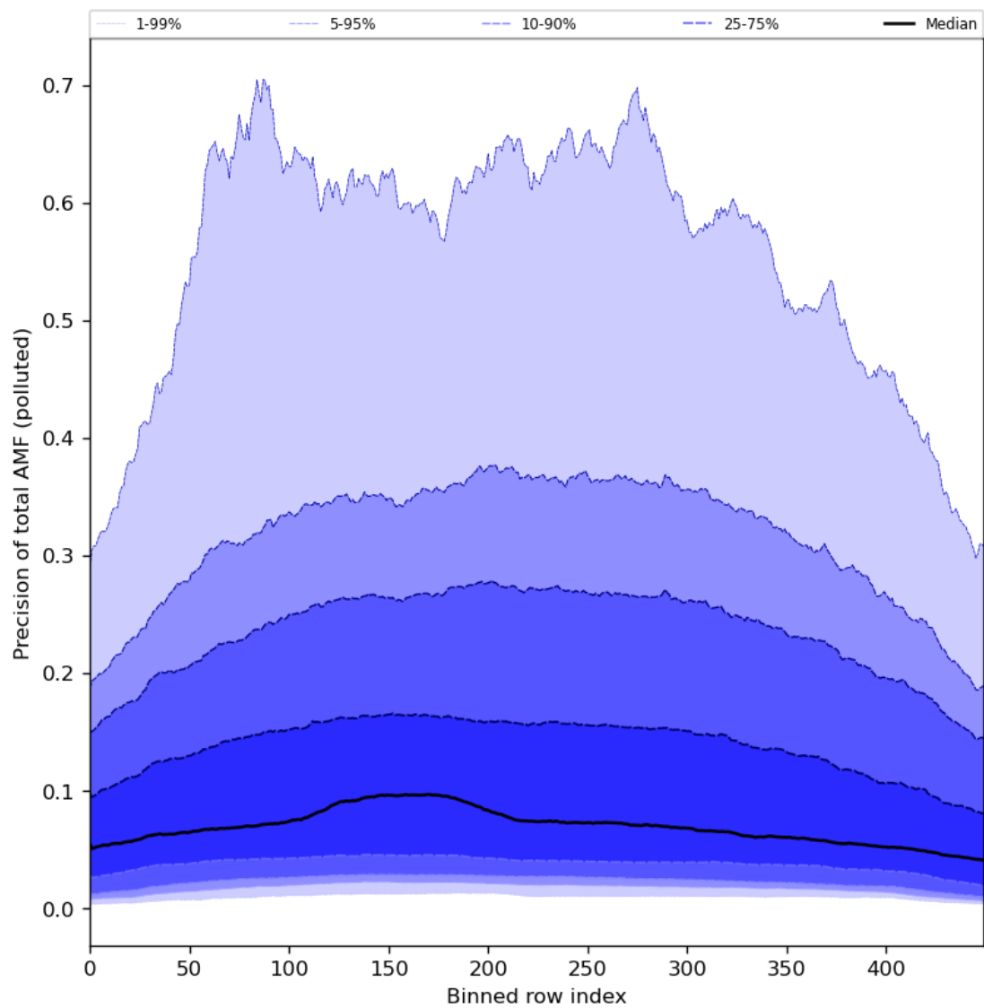
Figure 95: Along track statistics of “Precision of total AMF (polluted)” for 2024-03-20 to 2024-03-21
