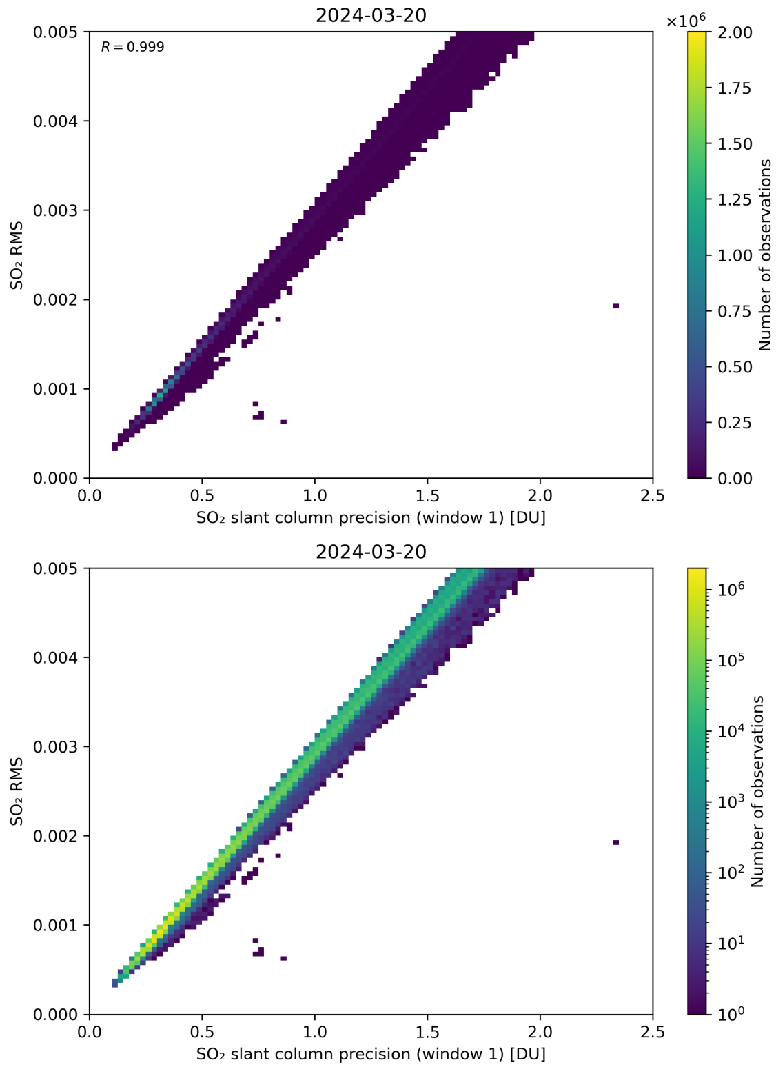
Figure 223: Scatter density plot of “SO 2 slant column precision (window 1)” against “SO 2 RMS” for 2024-03-20 to 2024-03-21.
