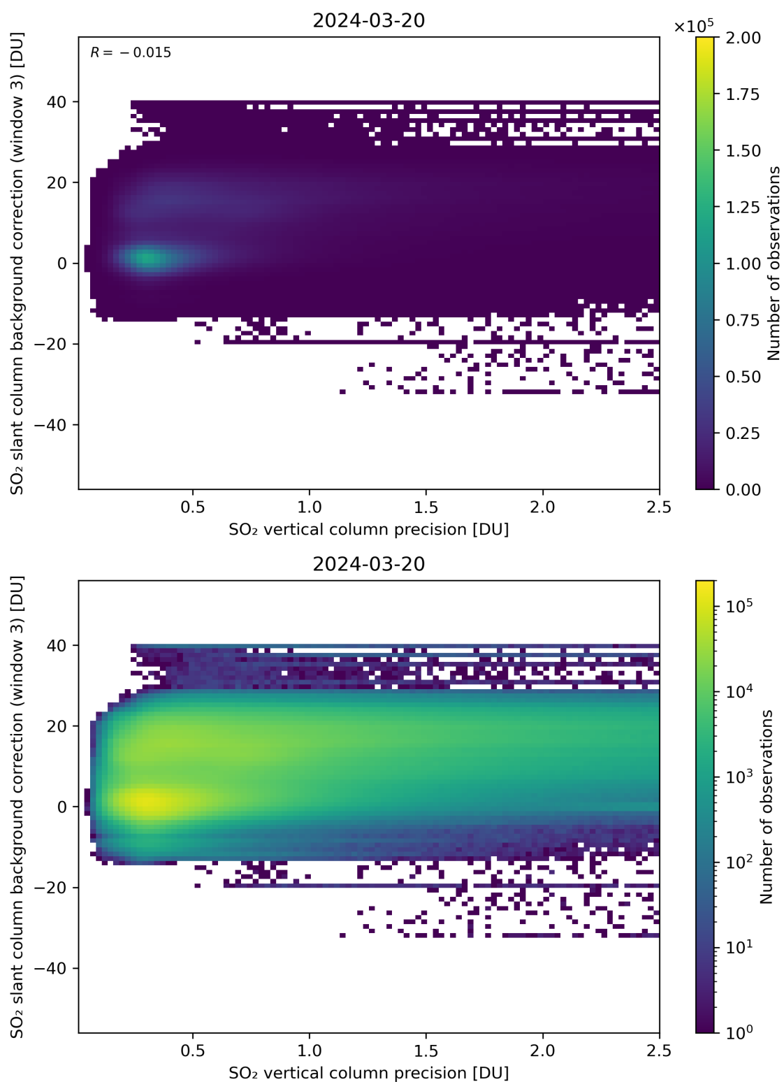
Figure 281: Scatter density plot of “SO 2 vertical column precision” against “SO 2 slant column background correction (window 3)” for 2024-03-20 to 2024-03-21.
