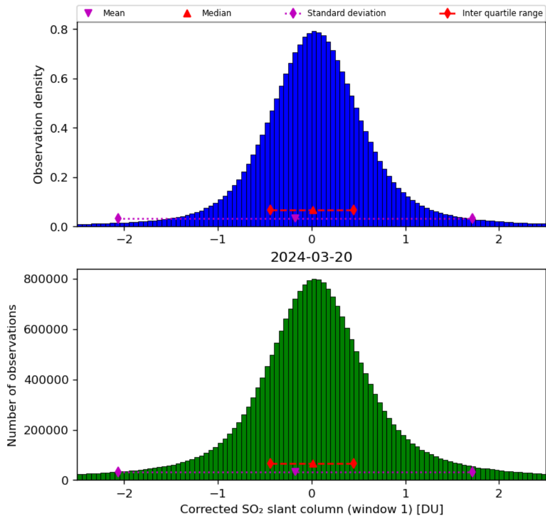
Figure 58: Histogram of “Corrected SO 2 slant column (window 1)” for 2024-03-20 to 2024-03-21
