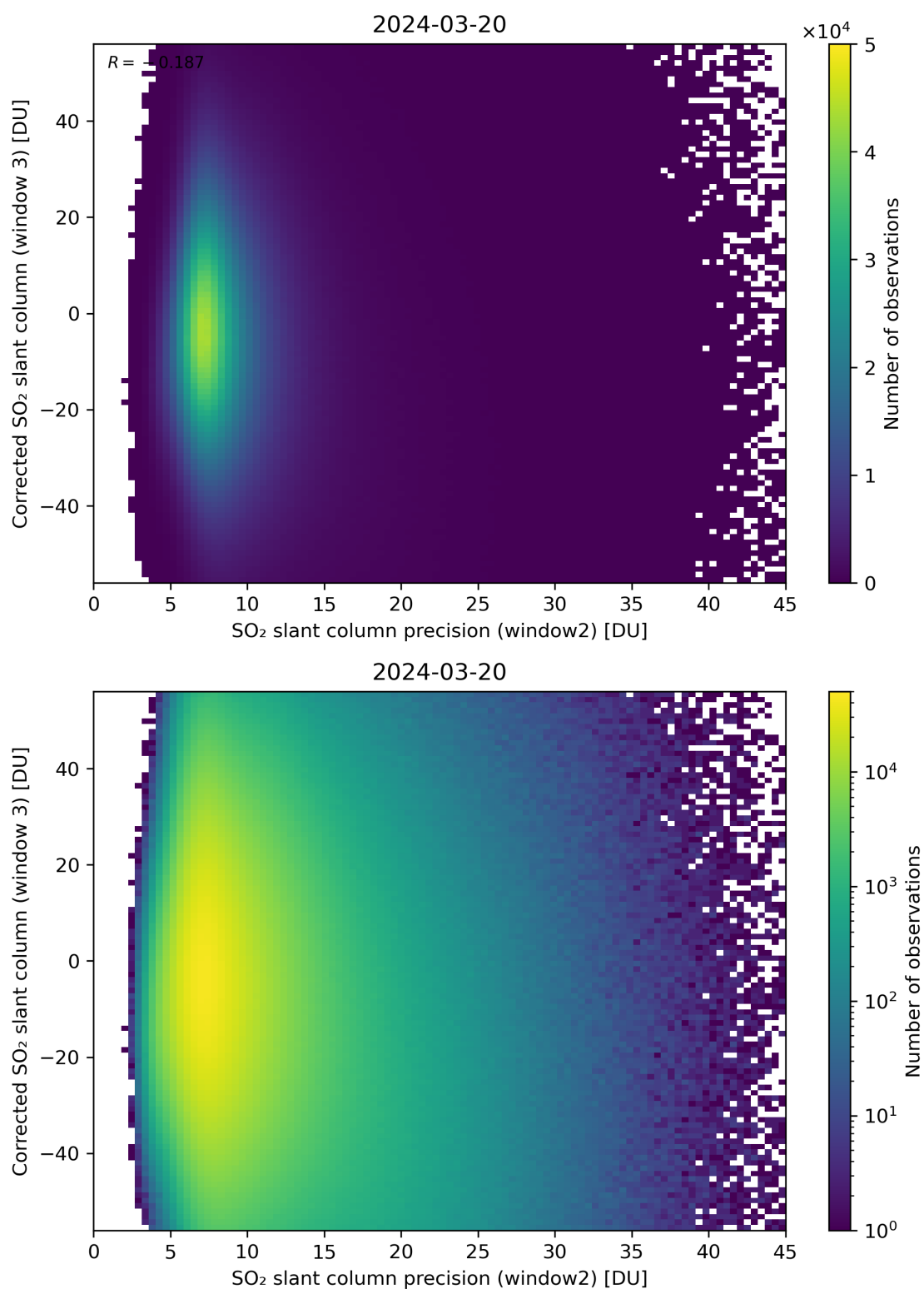
Figure 248: Scatter density plot of “SO 2 slant column precision (window2)” against “Corrected SO 2 slant column (window 3)” for 2024-03-20 to 2024-03-21.
