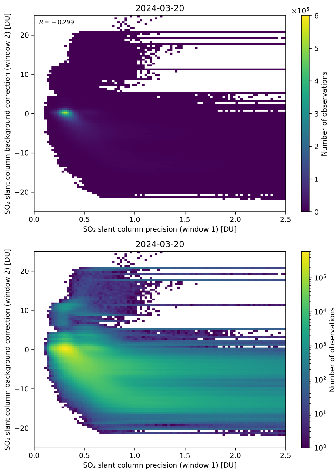
Figure 219: Scatter density plot of “SO 2 slant column precision (window 1)” against “SO 2 slant column background correction (window 2)” for 2024-03-20 to 2024-03-21.
