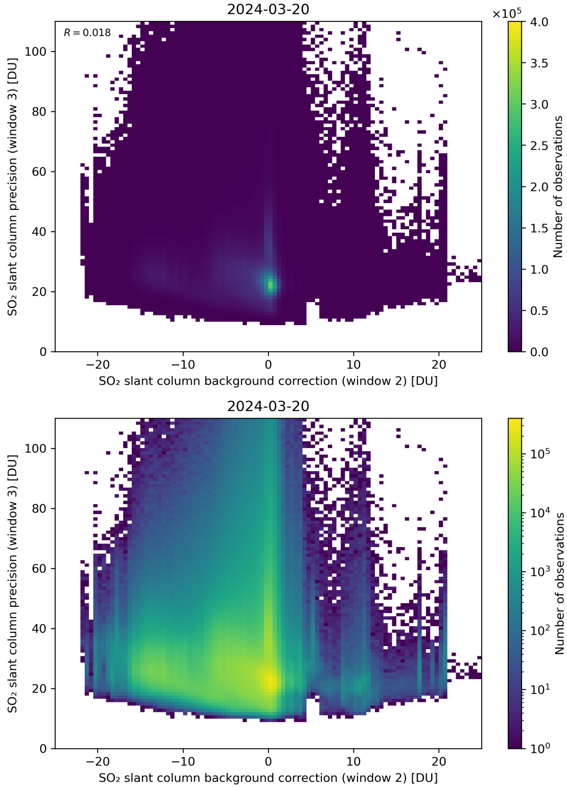
Figure 118: Scatter density plot of “SO 2 slant column background correction (window 2)” against “SO 2 slant column precision (window 3)” for 2024-03-20 to 2024-03-21.
