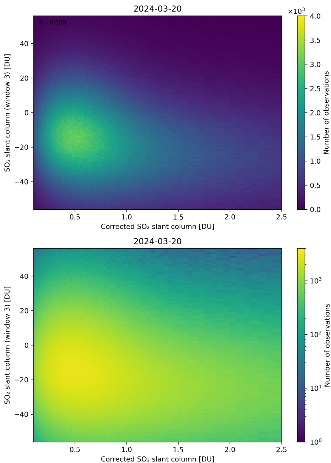
Figure 190: Scatter density plot of “Corrected SO 2 slant column” against “SO 2 slant column (window 3)” for 2024-03-20 to 2024-03-21.
