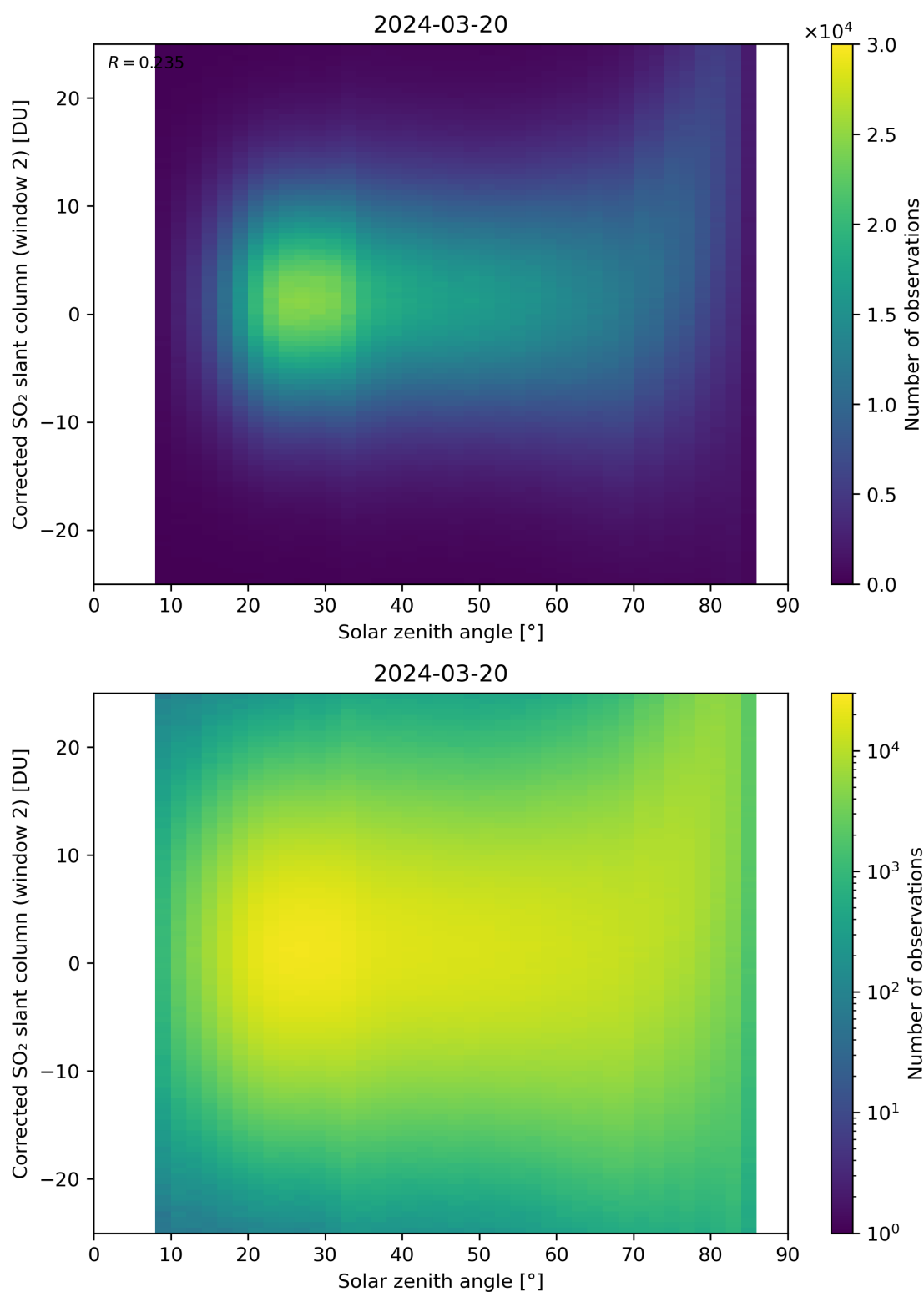
Figure 167: Scatter density plot of “Solar zenith angle” against “Corrected SO 2 slant column (window 2)” for 2024-03-20 to 2024-03-21.
