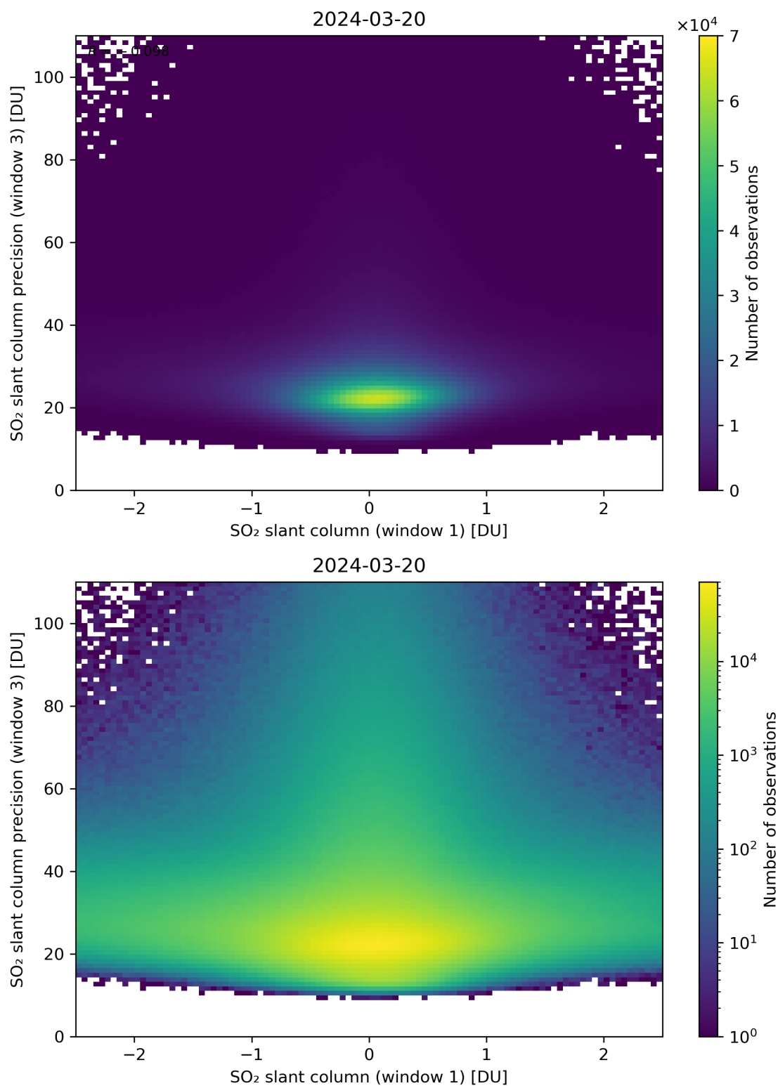
Figure 238: Scatter density plot of “SO 2 slant column (window 1)” against “SO 2 slant column precision (window 3)” for 2024-03-20 to 2024-03-21.
