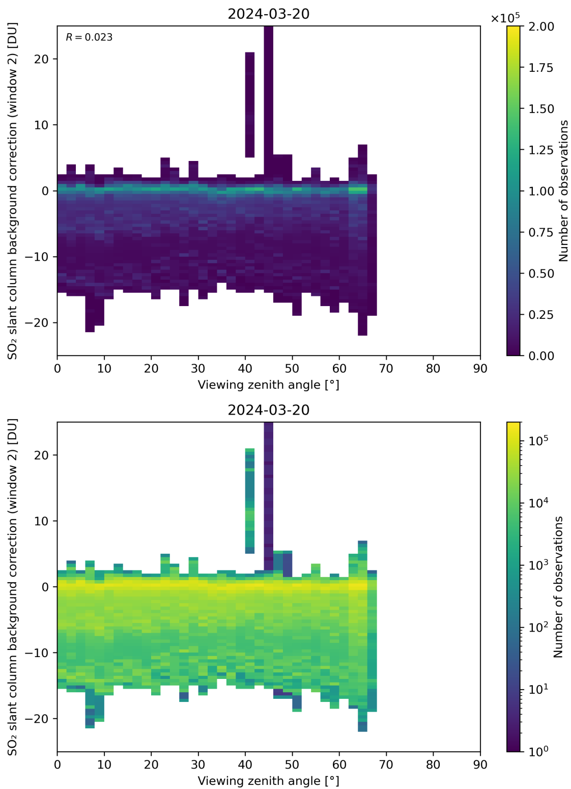
Figure 309: Scatter density plot of “Viewing zenith angle” against “SO 2 slant column background correction (window 2)” for 2024-03-20 to 2024-03-21.
