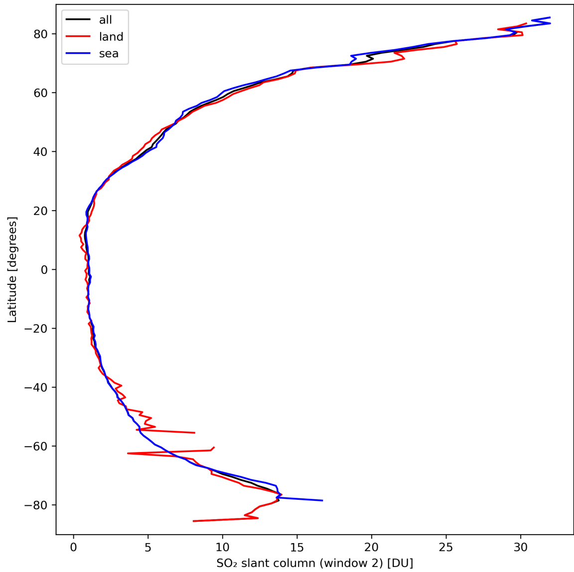
Figure 37: Zonal average of “SO 2 slant column (window 2)” for 2024-03-20 to 2024-03-21.
