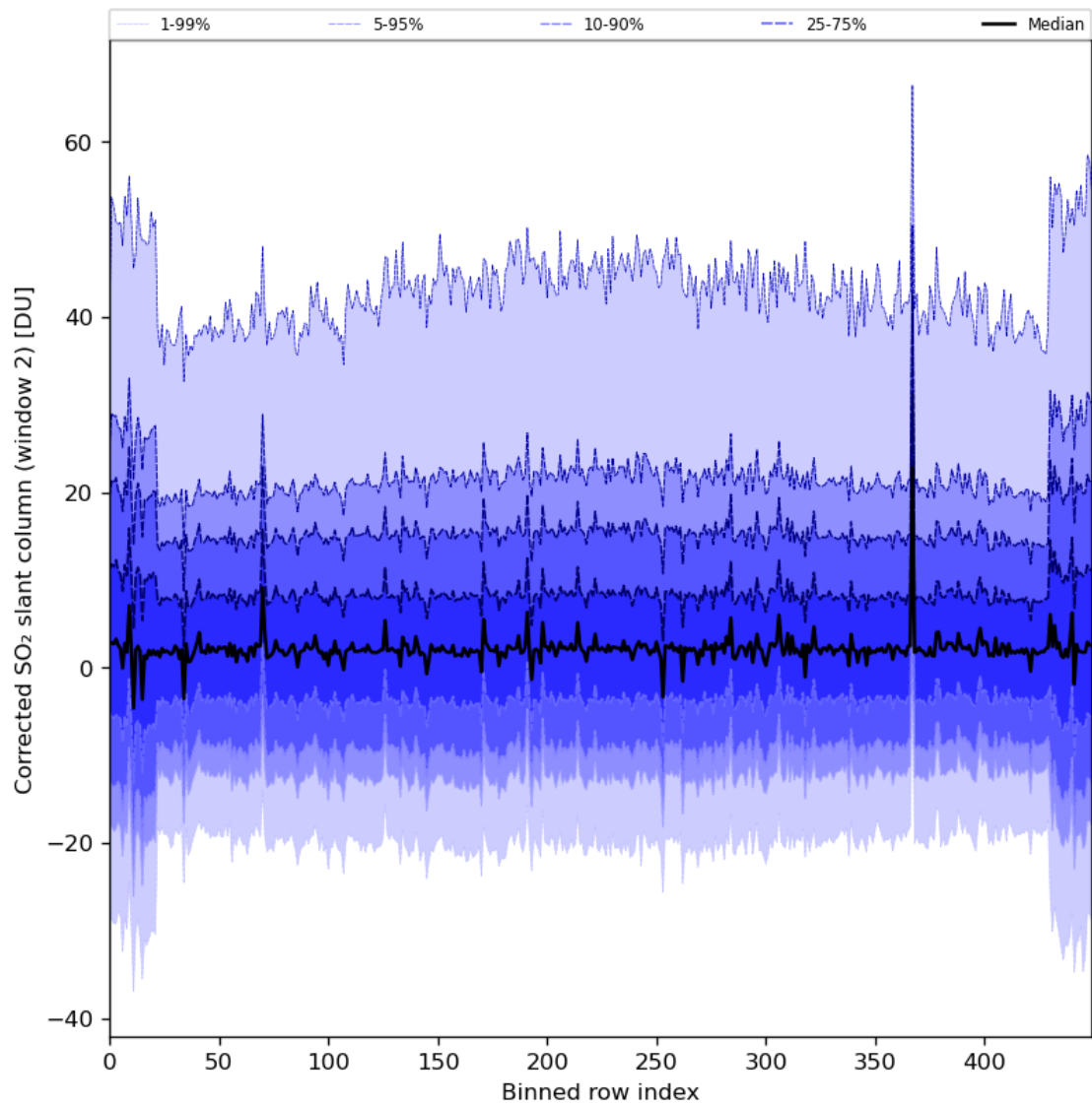
Figure 85: Along track statistics of “Corrected SO 2 slant column (window 2)” for 2024-03-20 to 2024-03-21
