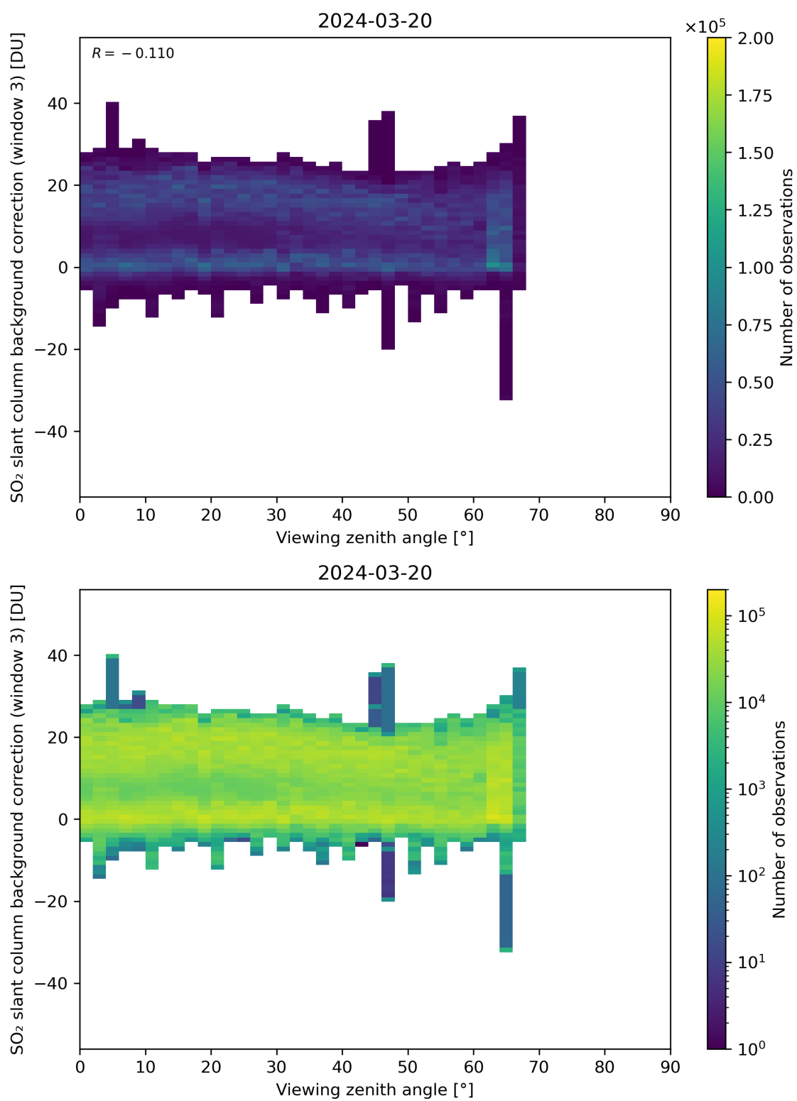
Figure 310: Scatter density plot of “Viewing zenith angle” against “SO 2 slant column background correction (window 3)” for 2024-03-20 to 2024-03-21.
