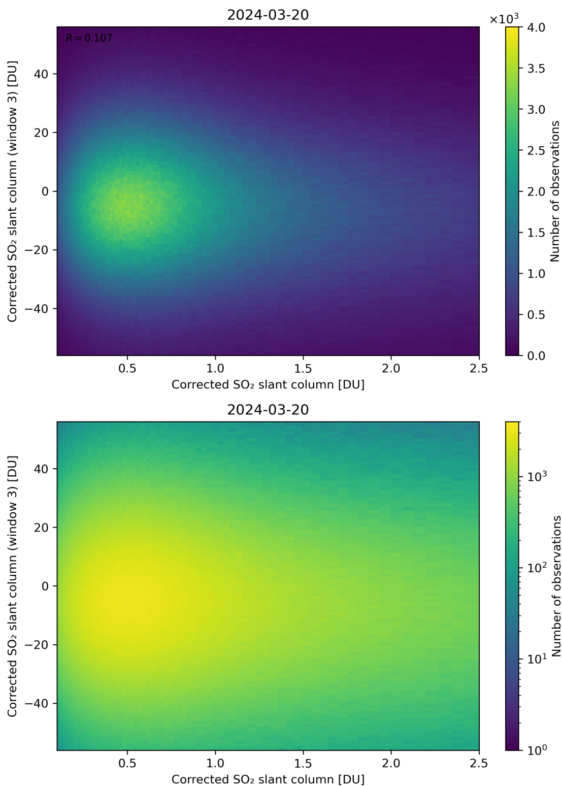
Figure 186: Scatter density plot of “Corrected SO 2 slant column” against “Corrected SO 2 slant column (window 3)” for 2024-03-20 to 2024-03-21.
