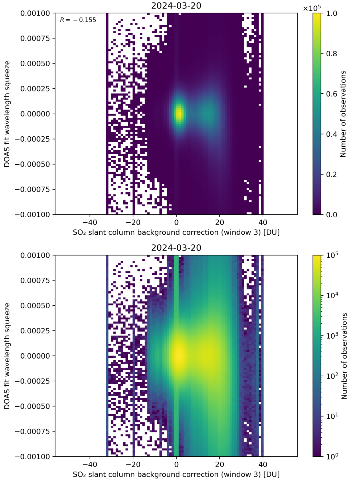
Figure 122: Scatter density plot of “SO 2 slant column background correction (window 3)” against “DOAS fit wavelength squeeze” for 2024-03-20 to 2024-03-21.
