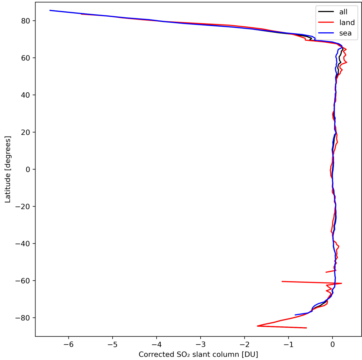
Figure 32: Zonal average of “Corrected SO 2 slant column” for 2024-03-20 to 2024-03-21.
