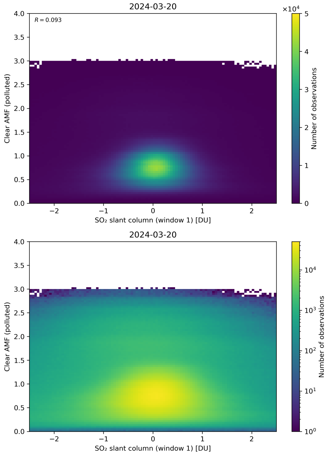
Figure 232: Scatter density plot of “SO 2 slant column (window 1)” against “Clear AMF (polluted)” for 2024-03-20 to 2024-03-21.
