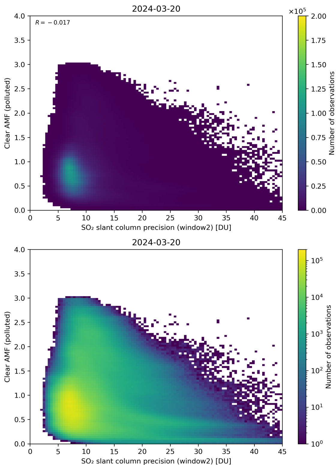
Figure 246: Scatter density plot of “SO 2 slant column precision (window2)” against “Clear AMF (polluted)” for 2024-03-20 to 2024-03-21.
