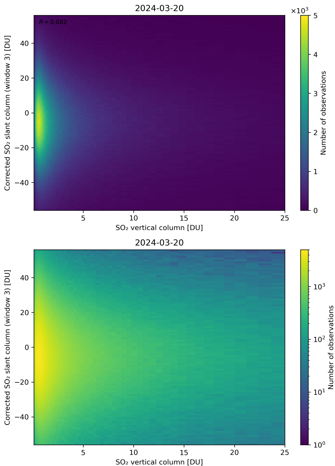
Figure 299: Scatter density plot of “SO 2 vertical column” against “Corrected SO 2 slant column (window 3)” for 2024-03-20 to 2024-03-21.
