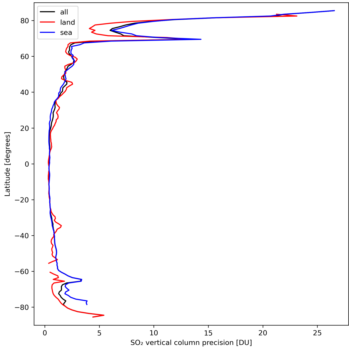
Figure 31: Zonal average of “SO 2 vertical column precision” for 2024-03-20 to 2024-03-21.
