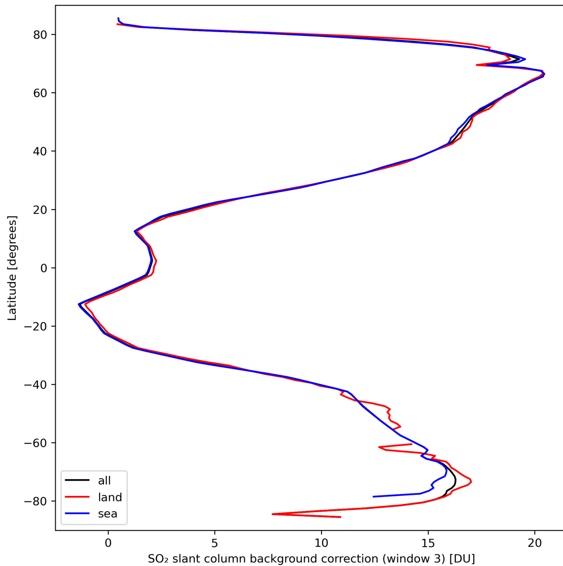
Figure 44: Zonal average of “SO 2 slant column background correction (window 3)” for 2024-03-20 to 2024-03-21.
