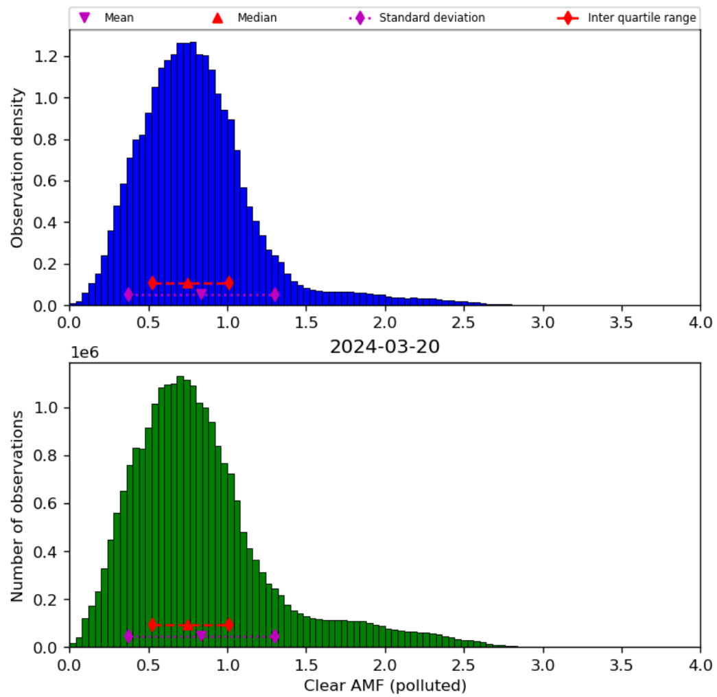
Figure 73: Histogram of “Clear AMF (polluted)” for 2024-03-20 to 2024-03-21
