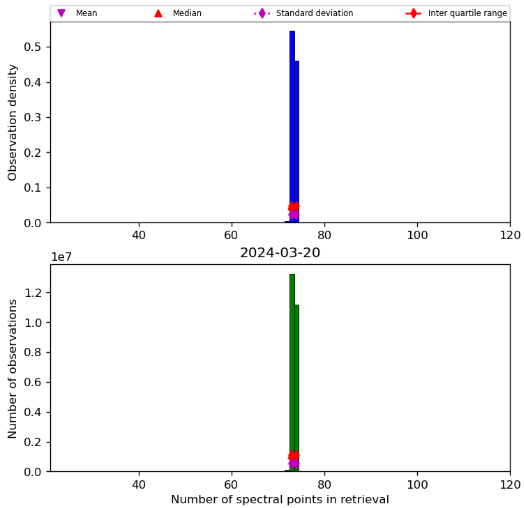
Figure 74: Histogram of “Number of spectral points in retrieval” for 2024-03-20 to 2024-03-21
