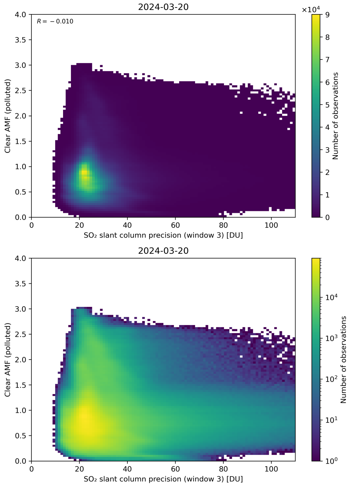
Figure 261: Scatter density plot of “SO 2 slant column precision (window 3)” against “Clear AMF (polluted)” for 2024-03-20 to 2024-03-21.
