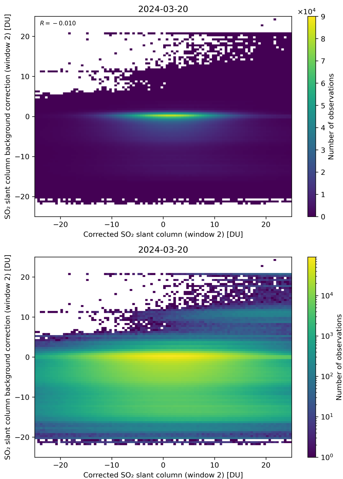
Figure 194: Scatter density plot of “Corrected SO 2 slant column (window 2)” against “SO 2 slant column background correction (window 2)” for 2024-03-20 to 2024-03-21.
