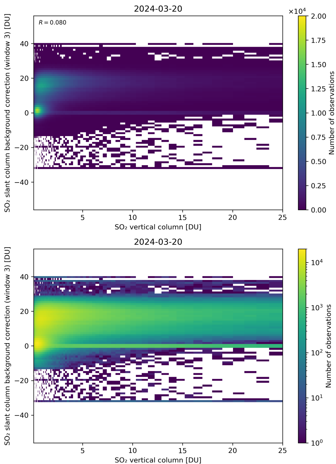
Figure 275: Scatter density plot of “SO 2 vertical column” against “SO 2 slant column background correction (window 3)” for 2024-03-20 to 2024-03-21.
