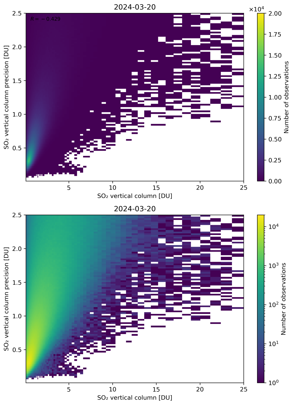
Figure 307: Scatter density plot of “SO 2 vertical column” against “SO 2 vertical column precision” for 2024-03-20 to 2024-03-21.
