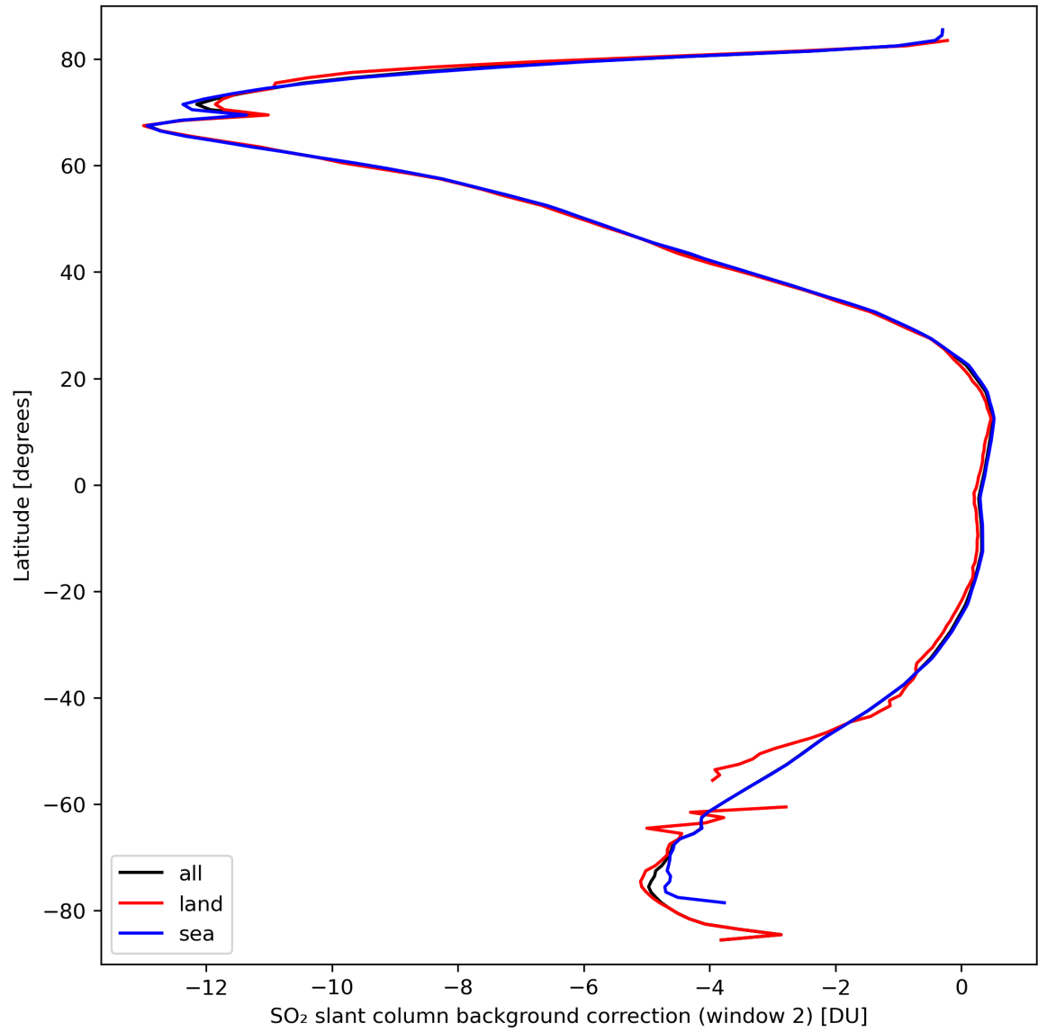
Figure 40: Zonal average of “SO 2 slant column background correction (window 2)” for 2024-03-20 to 2024-03-21.
