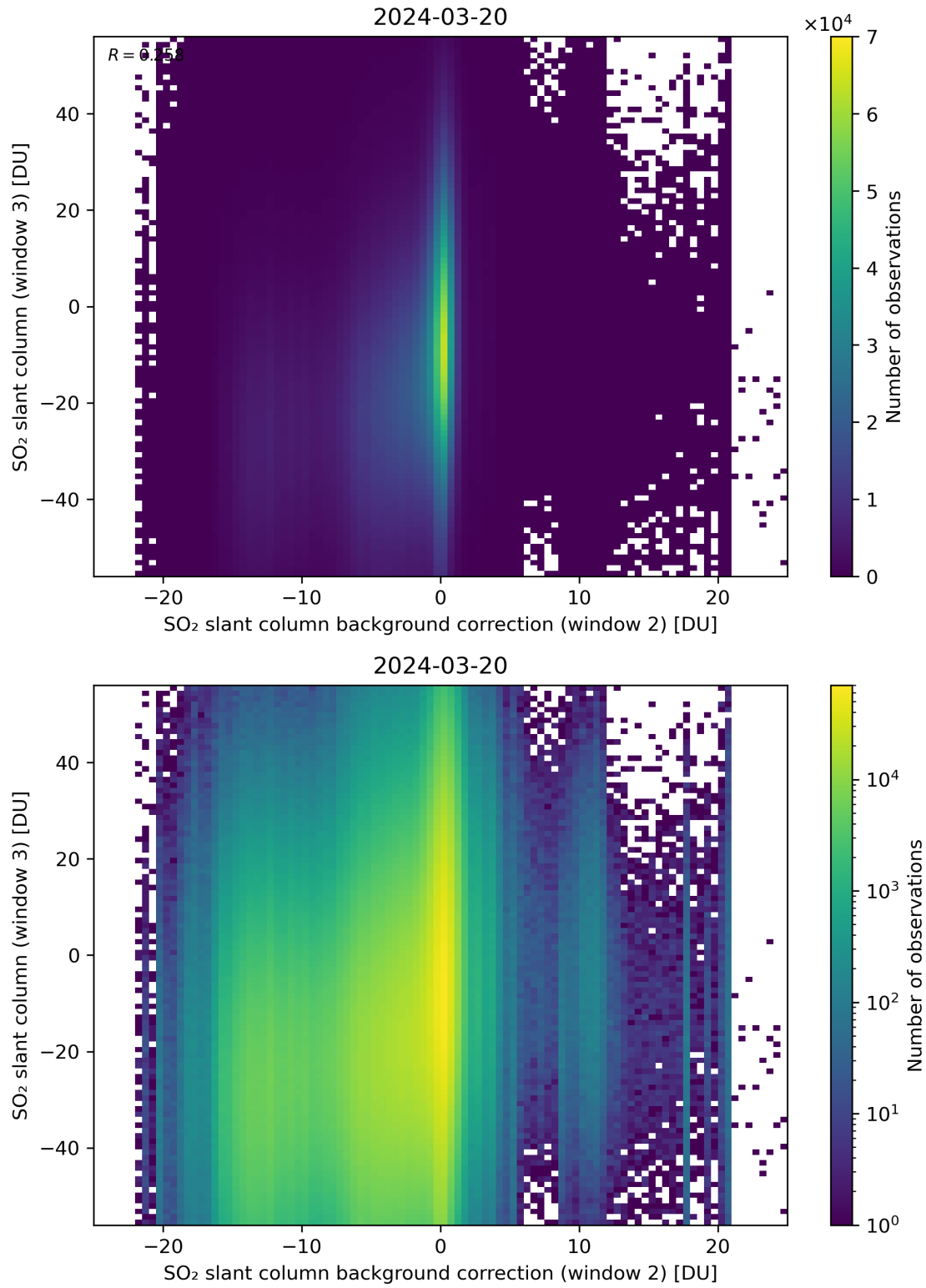
Figure 117: Scatter density plot of “SO 2 slant column background correction (window 2)” against “SO 2 slant column (window 3)” for 2024-03-20 to 2024-03-21.
