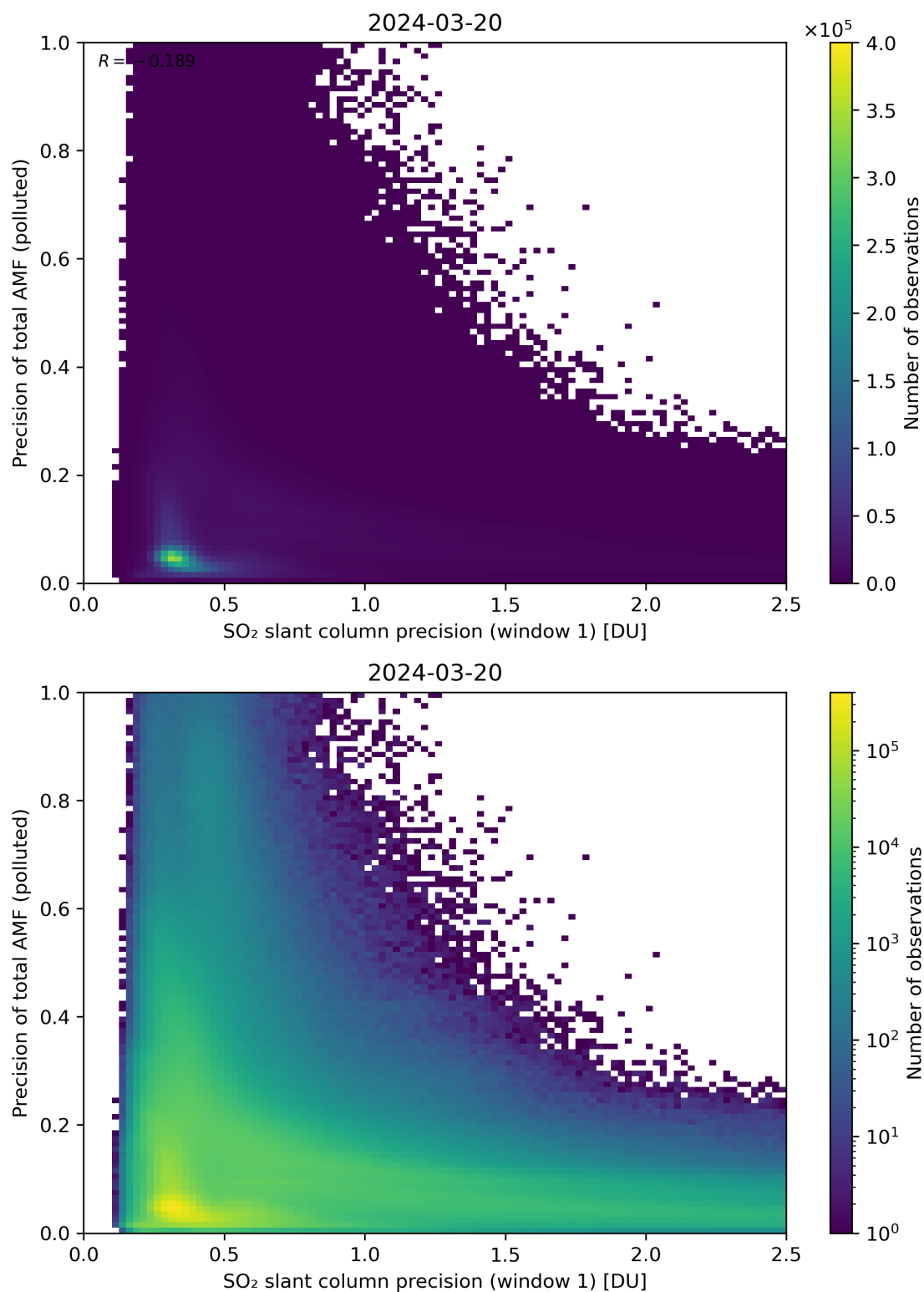
Figure 231: Scatter density plot of “SO 2 slant column precision (window 1)” against “Precision of total AMF (polluted)” for 2024-03-20 to 2024-03-21.
