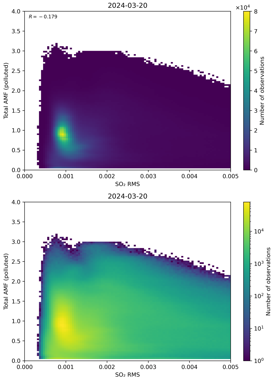
Figure 137: Scatter density plot of “SO 2 RMS” against “Total AMF (polluted)” for 2024-03-20 to 2024-03-21.
