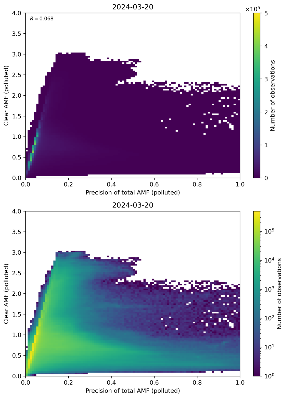
Figure 270: Scatter density plot of “Precision of total AMF (polluted)” against “Clear AMF (polluted)” for 2024-03-20 to 2024-03-21.
