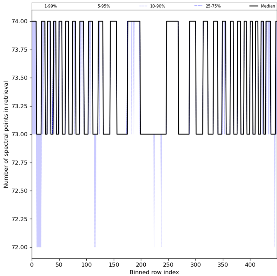
Figure 97: Along track statistics of “Number of spectral points in retrieval” for 2024-03-20 to 2024-03-21
