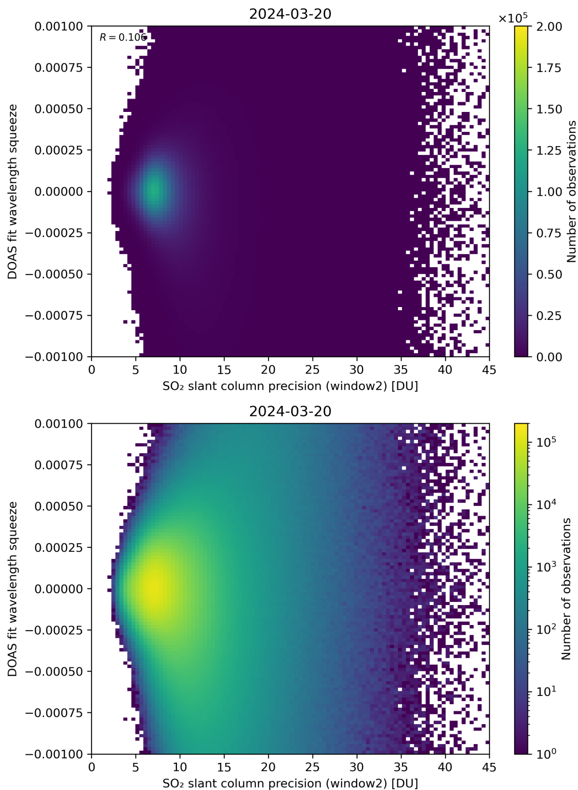
Figure 244: Scatter density plot of “SO 2 slant column precision (window2)” against “DOAS fit wavelength squeeze” for 2024-03-20 to 2024-03-21.
