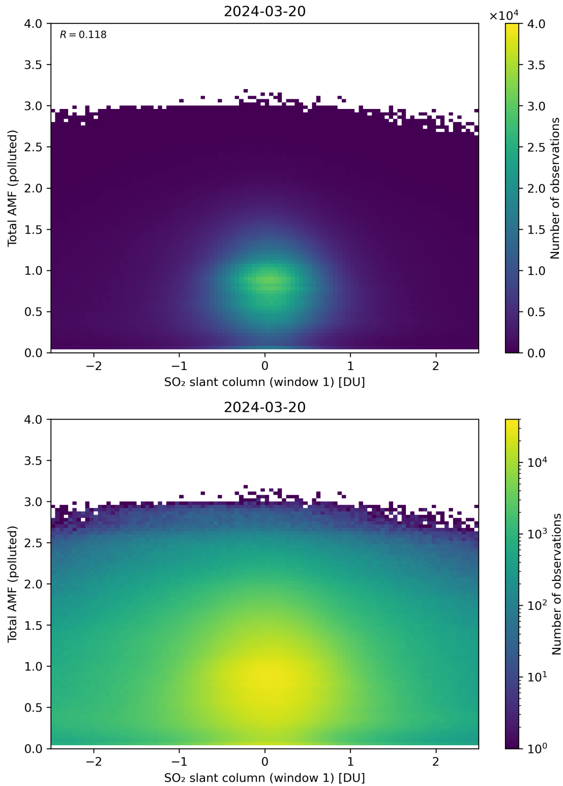
Figure 239: Scatter density plot of “SO 2 slant column (window 1)” against “Total AMF (polluted)” for 2024-03-20 to 2024-03-21.
