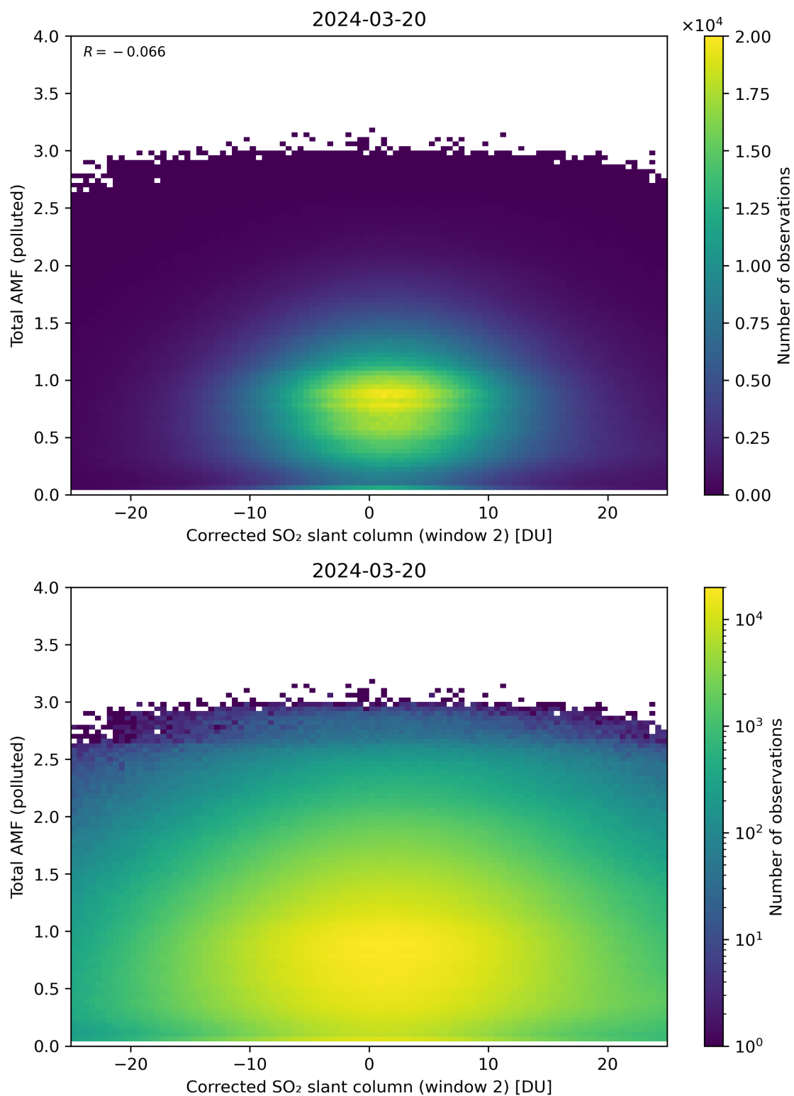
Figure 203: Scatter density plot of “Corrected SO 2 slant column (window 2)” against “Total AMF (polluted)” for 2024-03-20 to 2024-03-21.
