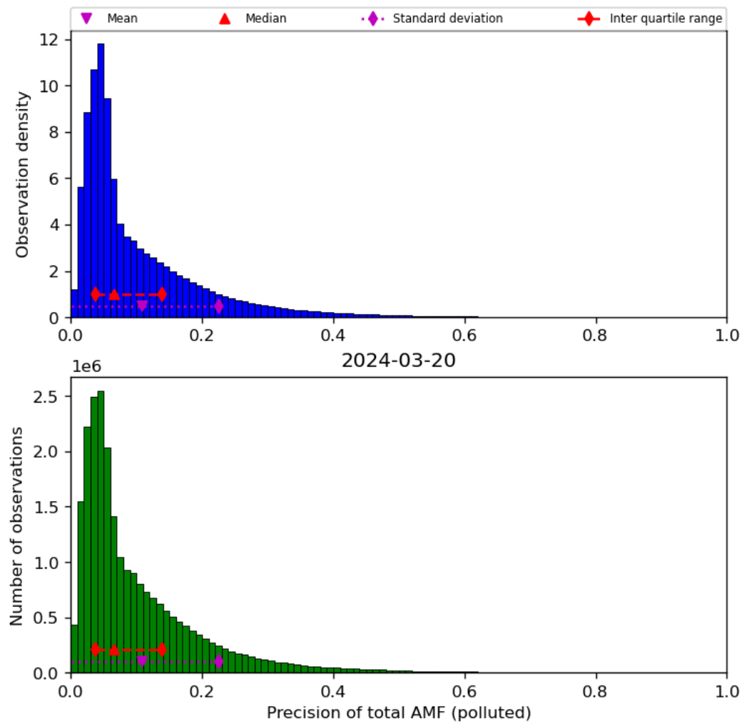
Figure 72: Histogram of “Precision of total AMF (polluted)” for 2024-03-20 to 2024-03-21
