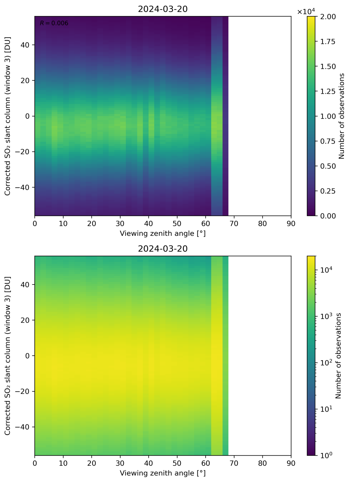
Figure 319: Scatter density plot of “Viewing zenith angle” against “Corrected SO 2 slant column (window 3)” for 2024-03-20 to 2024-03-21.
