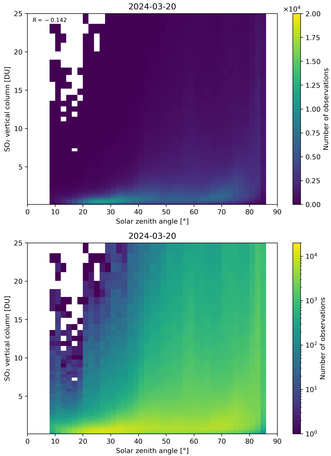
Figure 176: Scatter density plot of “Solar zenith angle” against “SO 2 vertical column” for 2024-03-20 to 2024-03-21.
