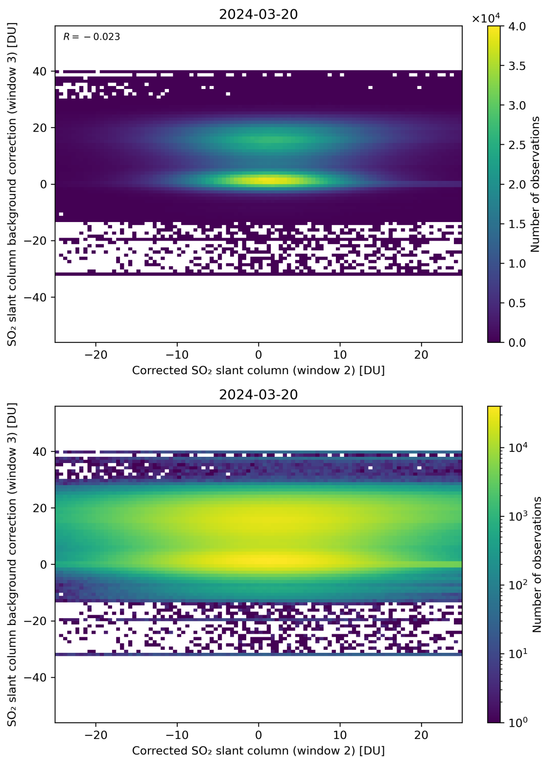
Figure 195: Scatter density plot of “Corrected SO 2 slant column (window 2)” against “SO 2 slant column background correction (window 3)” for 2024-03-20 to 2024-03-21.
