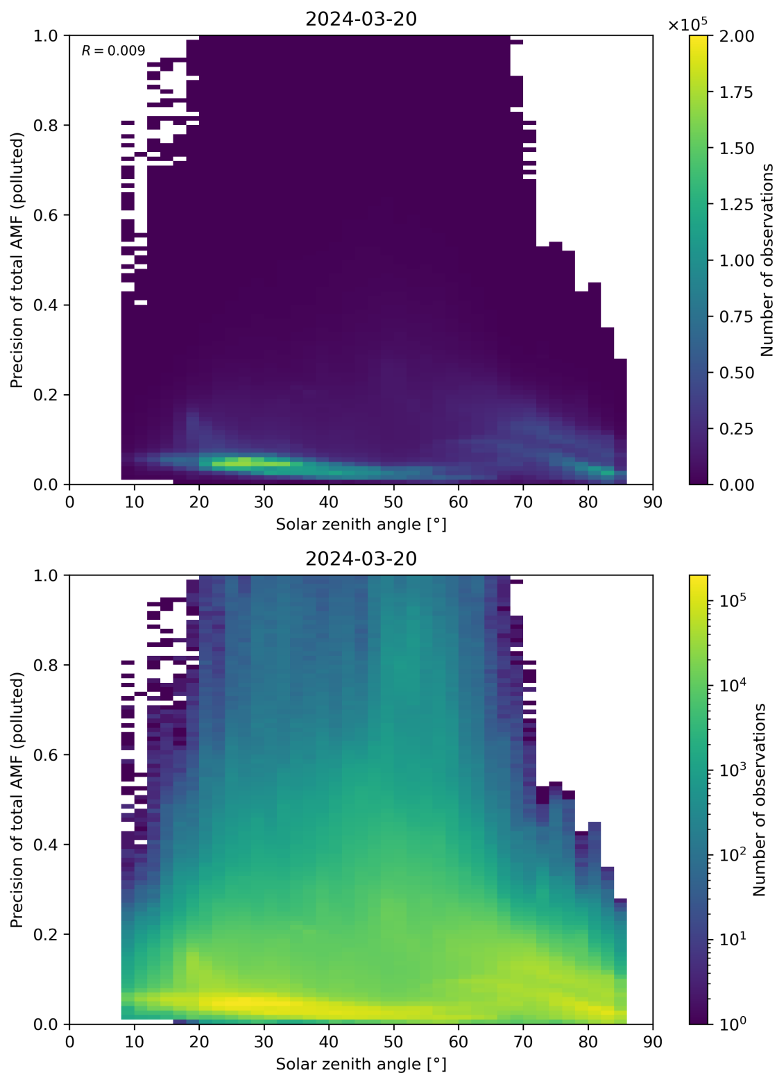
Figure 175: Scatter density plot of “Solar zenith angle” against “Precision of total AMF (polluted)” for 2024-03-20 to 2024-03-21.
