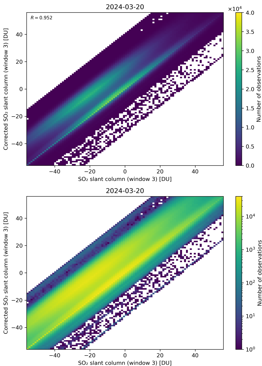
Figure 266: Scatter density plot of “SO 2 slant column (window 3)” against “Corrected SO 2 slant column (window 3)” for 2024-03-20 to 2024-03-21.
