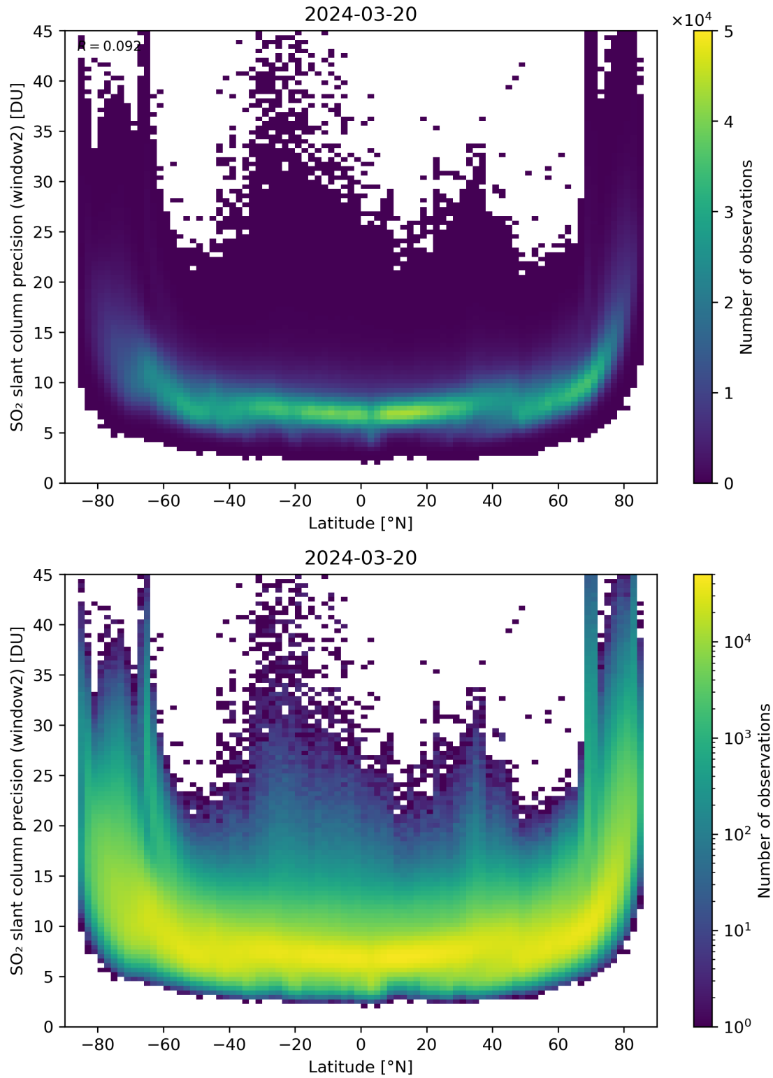
Figure 151: Scatter density plot of “Latitude” against “SO 2 slant column precision (window2)” for 2024-03-20 to 2024-03-21.
