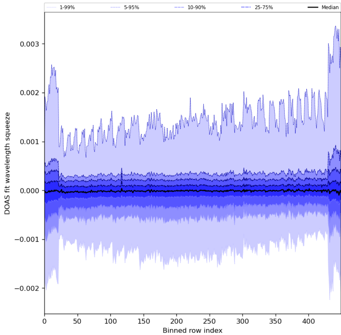
Figure 92: Along track statistics of “DOAS fit wavelength squeeze” for 2024-03-20 to 2024-03-21
