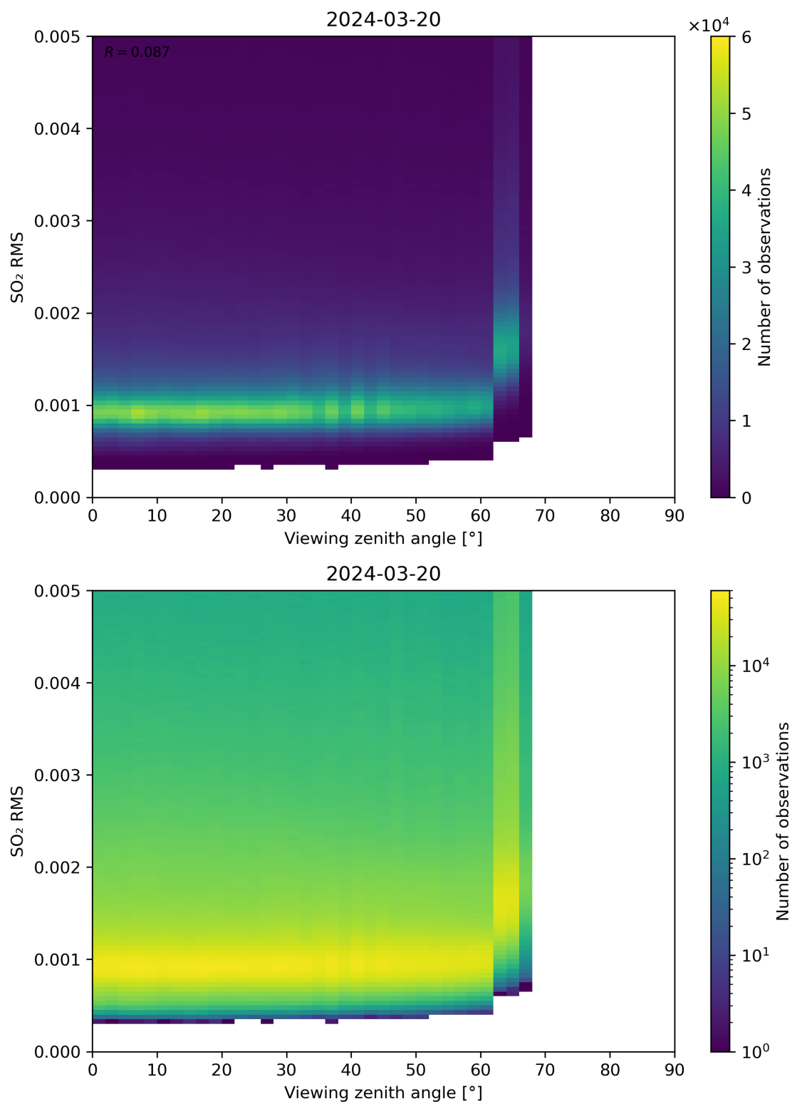
Figure 313: Scatter density plot of “Viewing zenith angle” against “SO 2 RMS” for 2024-03-20 to 2024-03-21.
