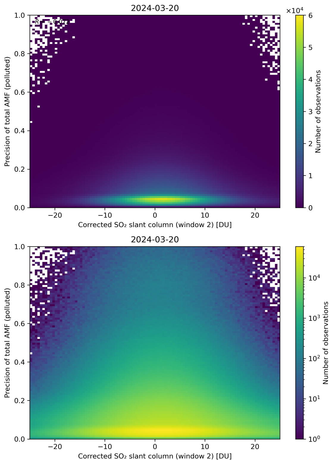
Figure 204: Scatter density plot of “Corrected SO 2 slant column (window 2)” against “Precision of total AMF (polluted)” for 2024-03-20 to 2024-03-21.
