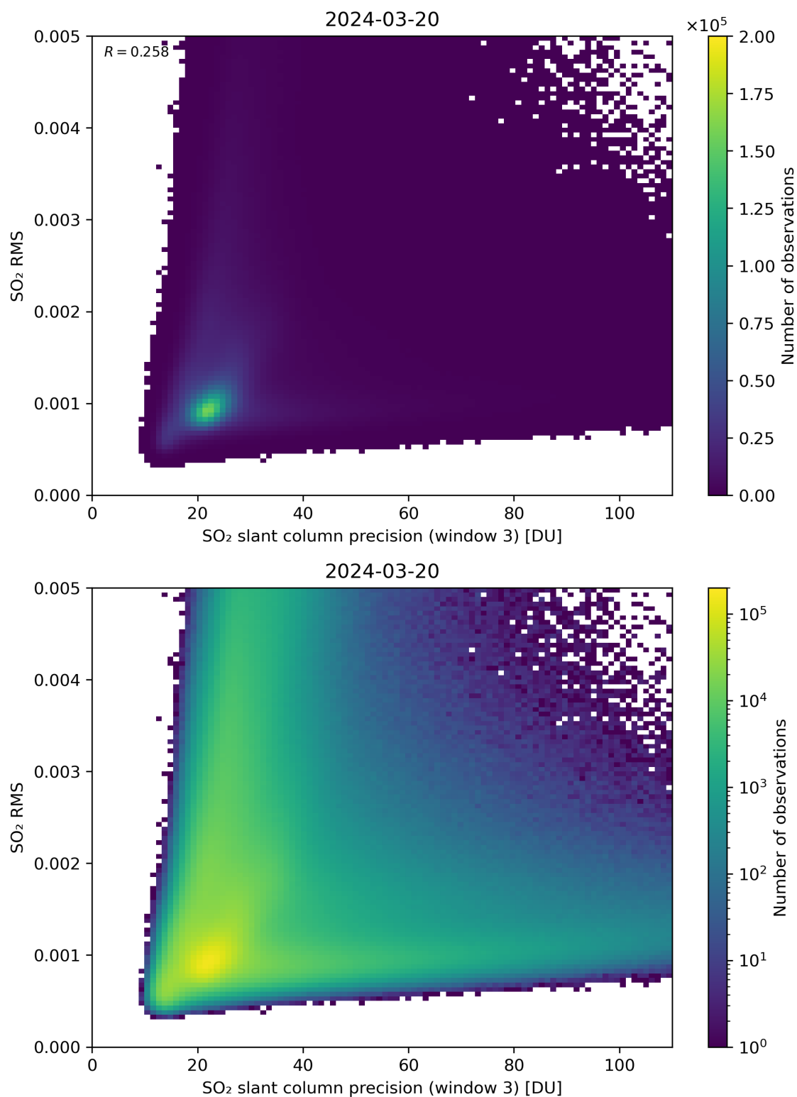
Figure 260: Scatter density plot of “SO 2 slant column precision (window 3)” against “SO 2 RMS” for 2024-03-20 to 2024-03-21.
