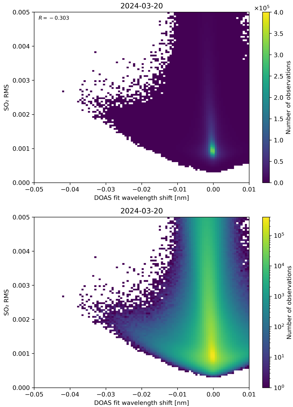
Figure 128: Scatter density plot of “DOAS fit wavelength shift” against “SO 2 RMS” for 2024-03-20 to 2024-03-21.
