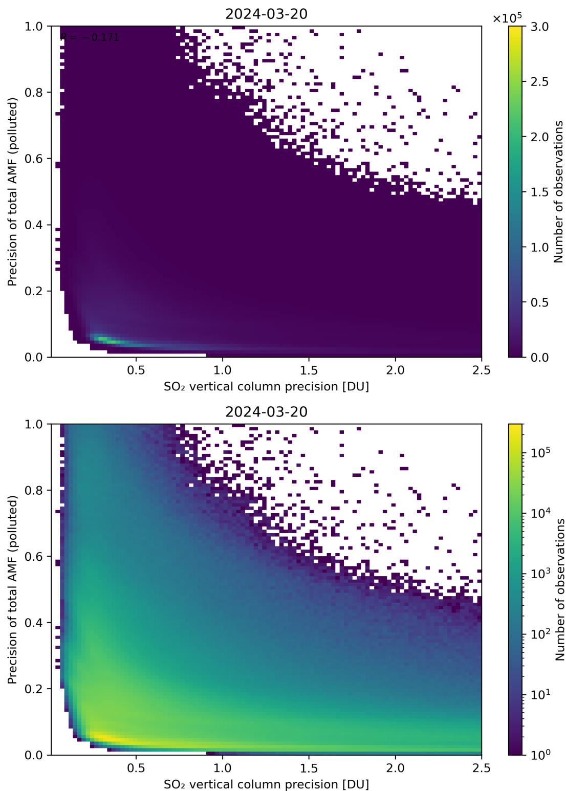
Figure 295: Scatter density plot of “SO 2 vertical column precision” against “Precision of total AMF (polluted)” for 2024-03-20 to 2024-03-21.
