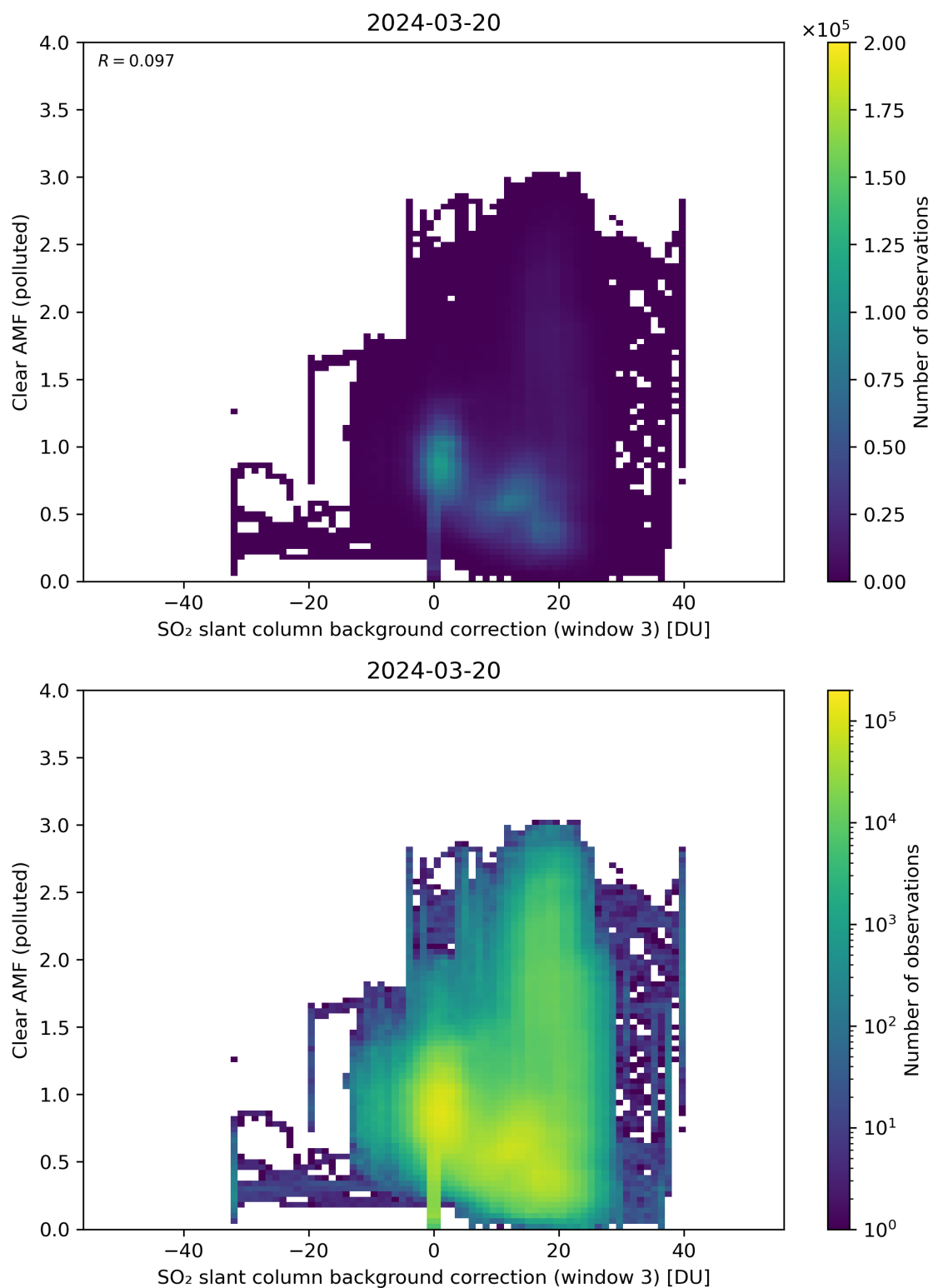
Figure 124: Scatter density plot of “SO 2 slant column background correction (window 3)” against “Clear AMF (polluted)” for 2024-03-20 to 2024-03-21.
