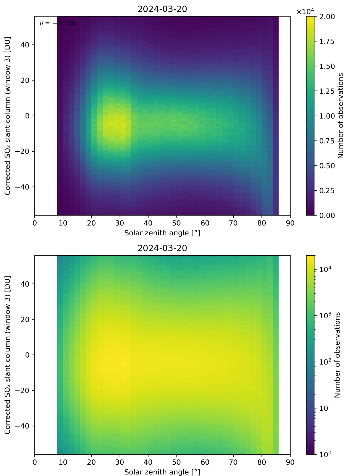
Figure 168: Scatter density plot of “Solar zenith angle” against “Corrected SO 2 slant column (window 3)” for 2024-03-20 to 2024-03-21.
