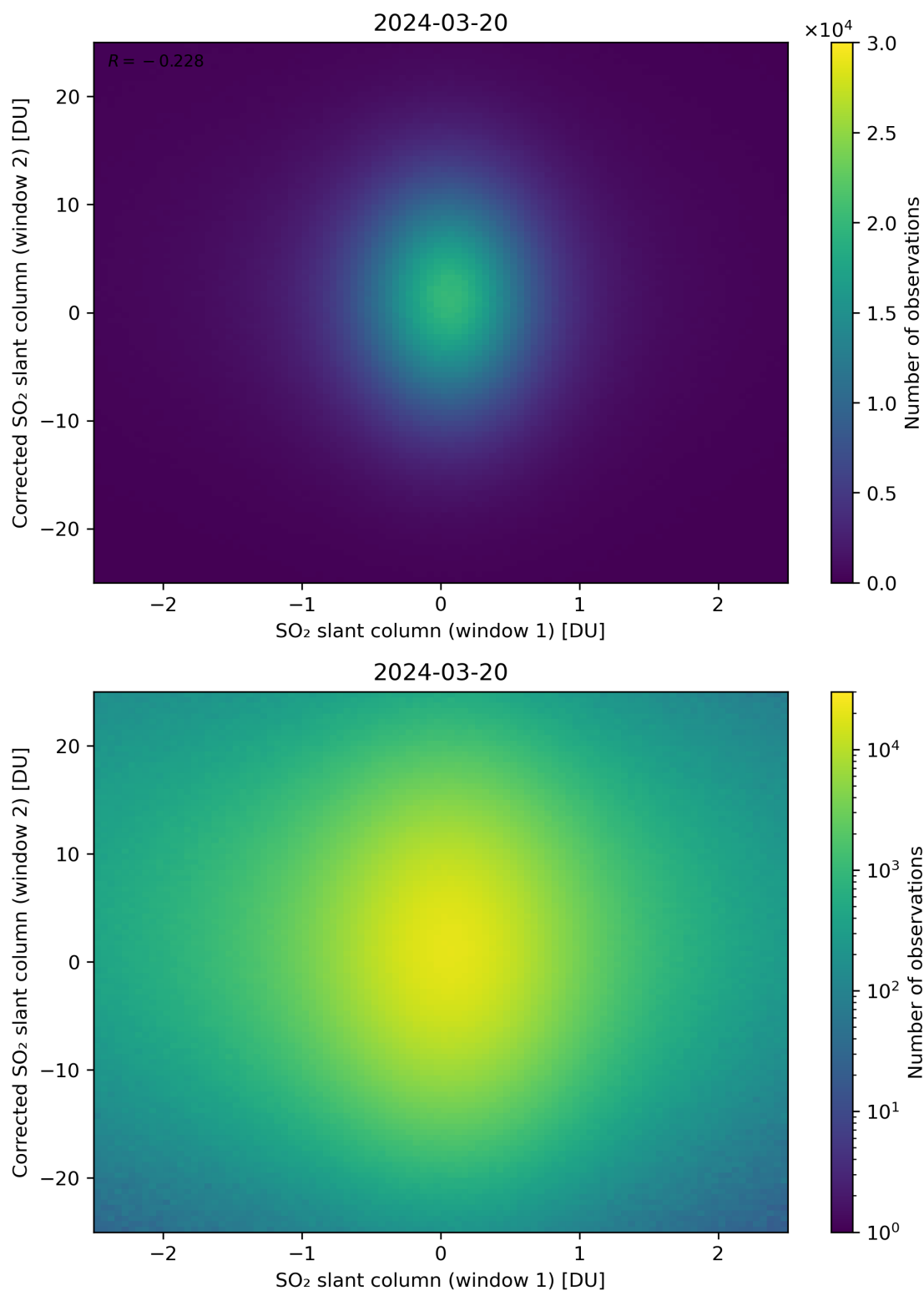
Figure 233: Scatter density plot of “SO 2 slant column (window 1)” against “Corrected SO 2 slant column (window 2)” for 2024-03-20 to 2024-03-21.
