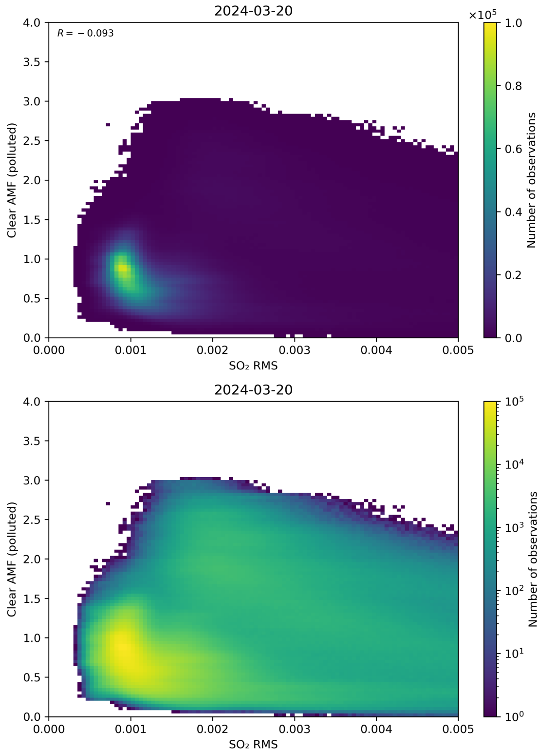
Figure 136: Scatter density plot of “SO 2 RMS” against “Clear AMF (polluted)” for 2024-03-20 to 2024-03-21.
