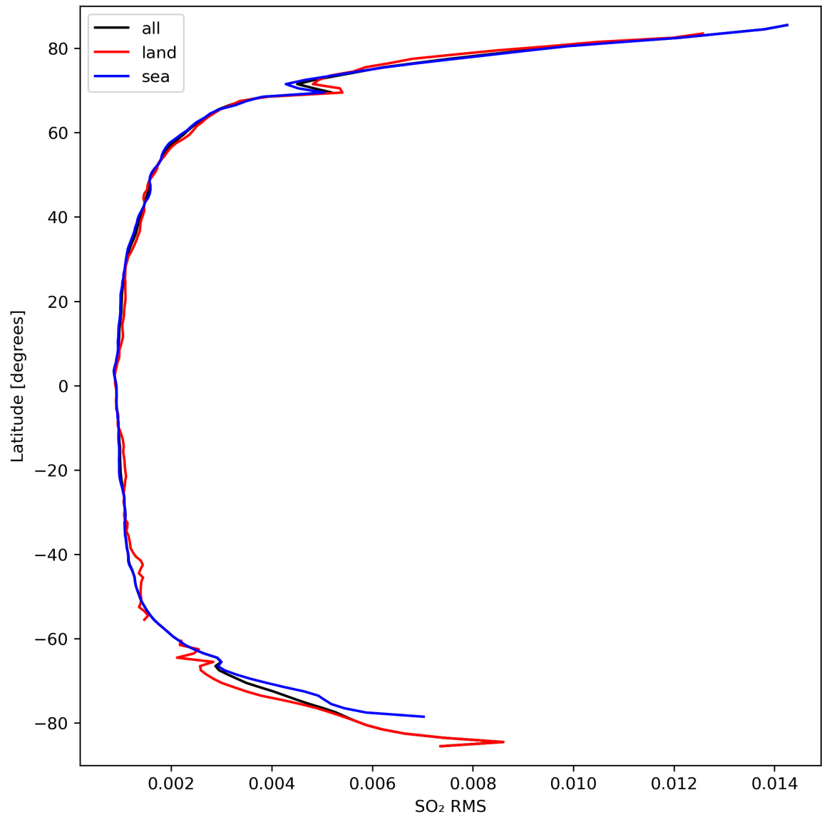
Figure 47: Zonal average of “SO 2 RMS” for 2024-03-20 to 2024-03-21.
