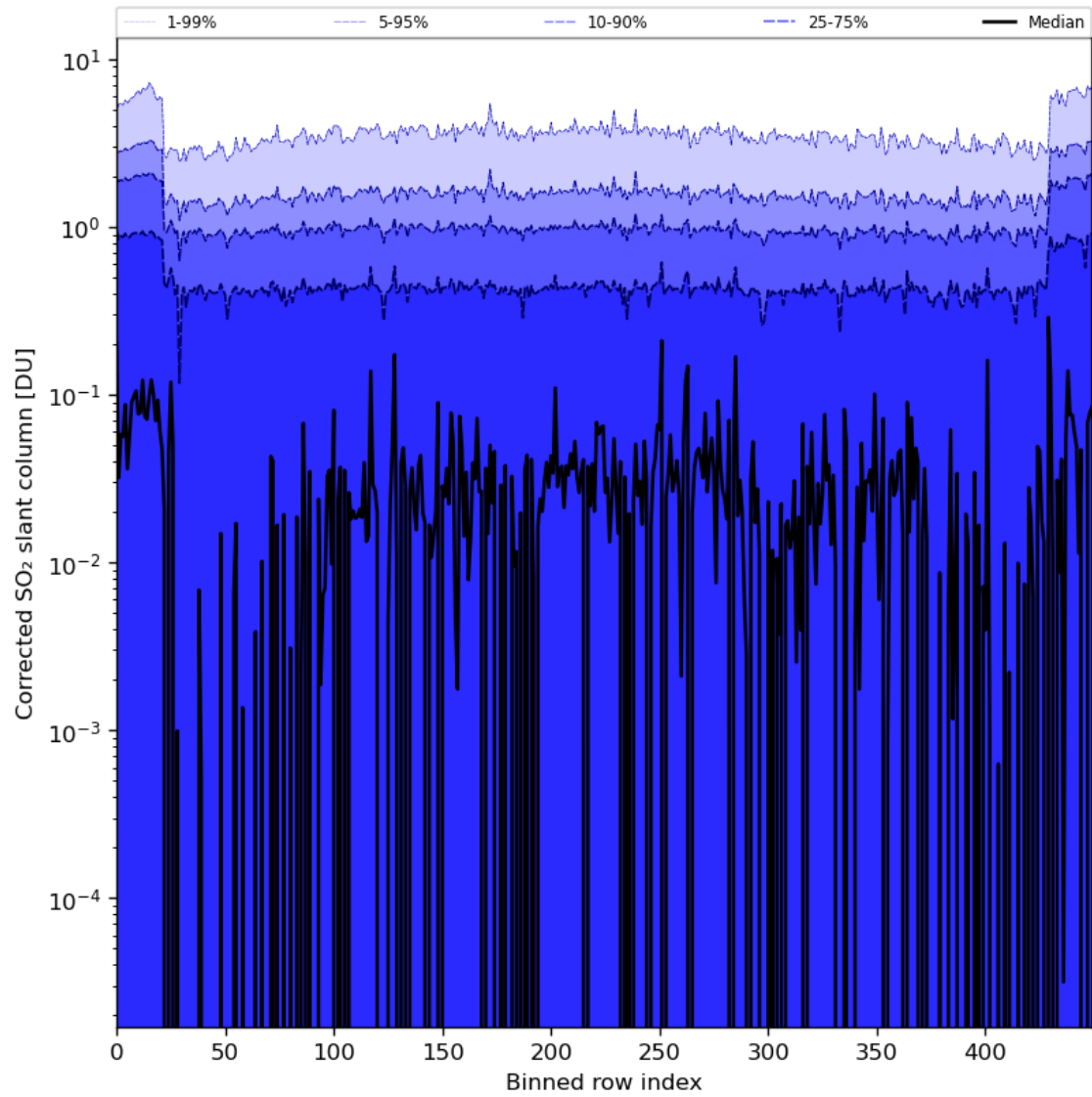
Figure 78: Along track statistics of “Corrected SO 2 slant column” for 2024-03-20 to 2024-03-21
