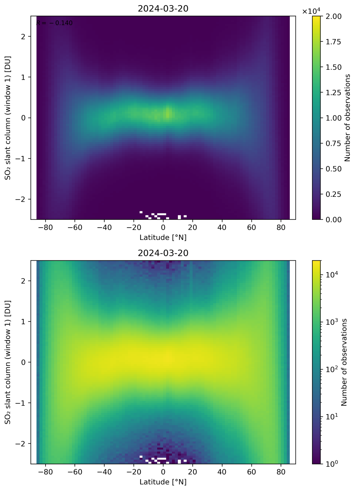
Figure 149: Scatter density plot of “Latitude” against “SO 2 slant column (window 1)” for 2024-03-20 to 2024-03-21.
