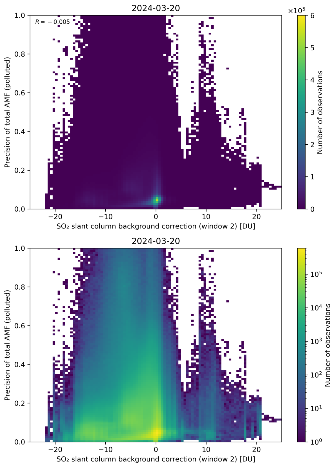
Figure 120: Scatter density plot of “SO 2 slant column background correction (window 2)” against “Precision of total AMF (polluted)” for 2024-03-20 to 2024-03-21.
