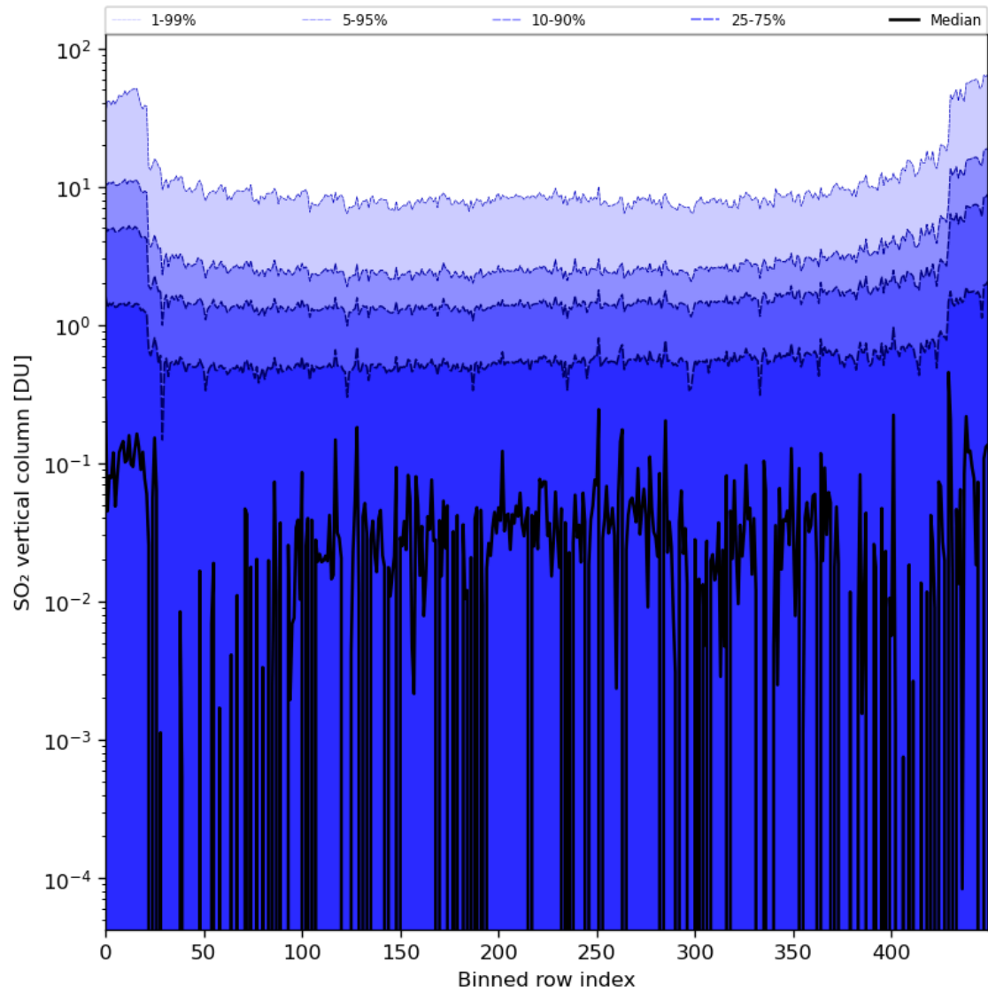
Figure 76: Along track statistics of “SO 2 vertical column” for 2024-03-20 to 2024-03-21
