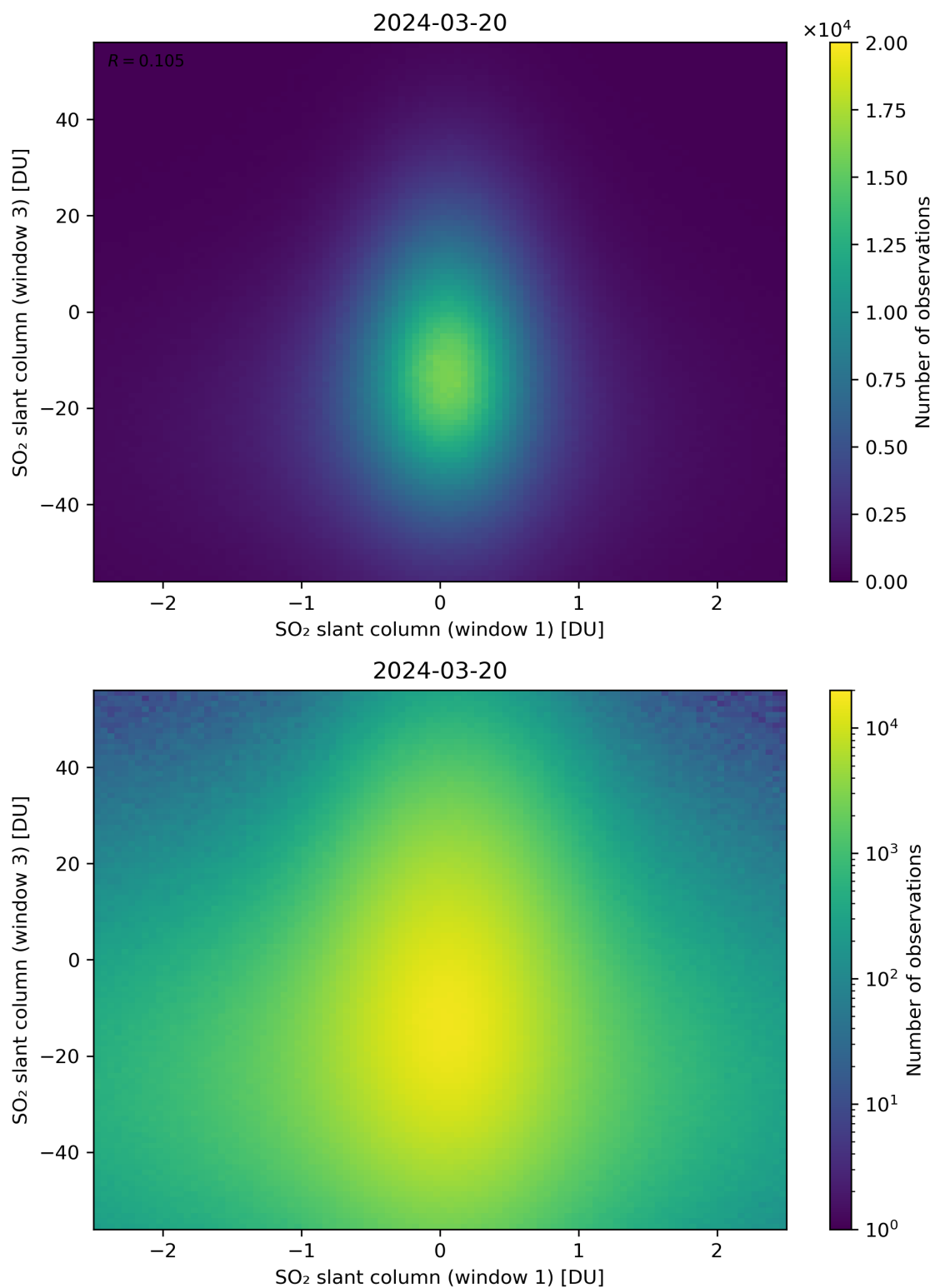
Figure 237: Scatter density plot of “SO 2 slant column (window 1)” against “SO 2 slant column (window 3)” for 2024-03-20 to 2024-03-21.
