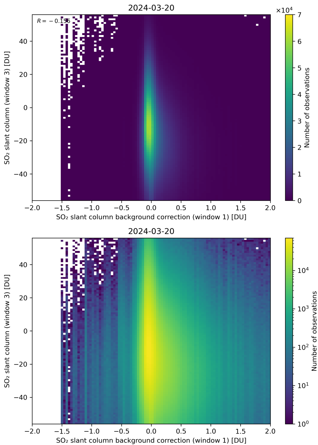
Figure 107: Scatter density plot of “SO 2 slant column background correction (window 1)” against “SO 2 slant column (window 3)” for 2024-03-20 to 2024-03-21.
