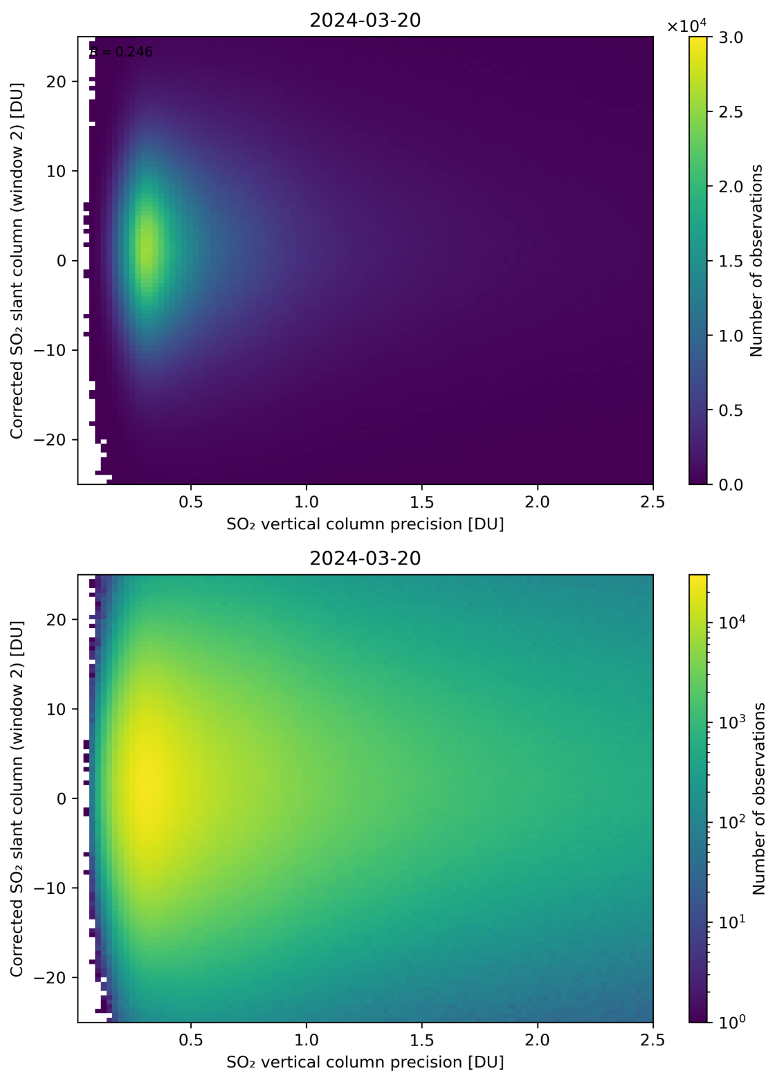
Figure 287: Scatter density plot of “SO 2 vertical column precision” against “Corrected SO 2 slant column (window 2)” for 2024-03-20 to 2024-03-21.
