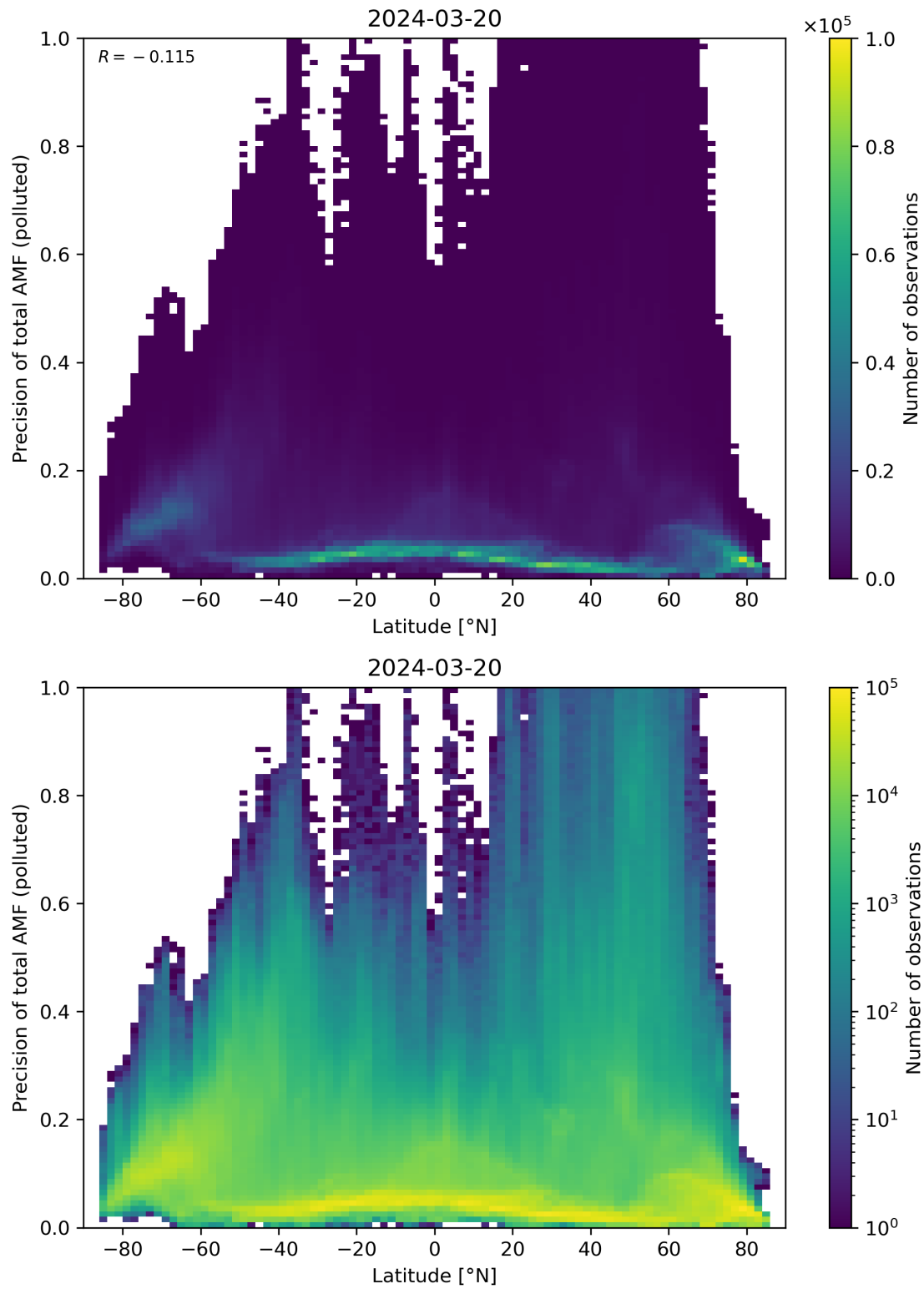
Figure 155: Scatter density plot of “Latitude” against “Precision of total AMF (polluted)” for 2024-03-20 to 2024-03-21.
