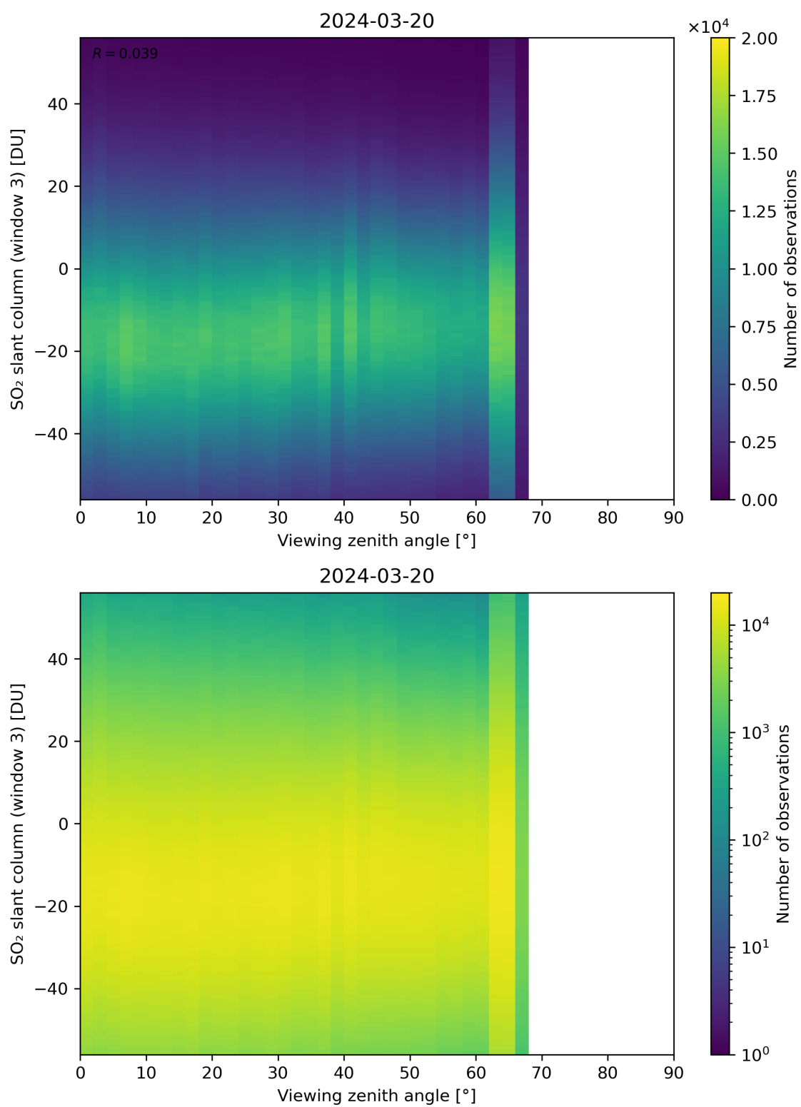
Figure 323: Scatter density plot of “Viewing zenith angle” against “SO 2 slant column (window 3)” for 2024-03-20 to 2024-03-21.
