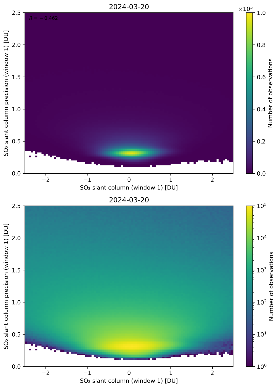
Figure 235: Scatter density plot of “SO 2 slant column (window 1)” against “SO 2 slant column precision (window 1)” for 2024-03-20 to 2024-03-21.
