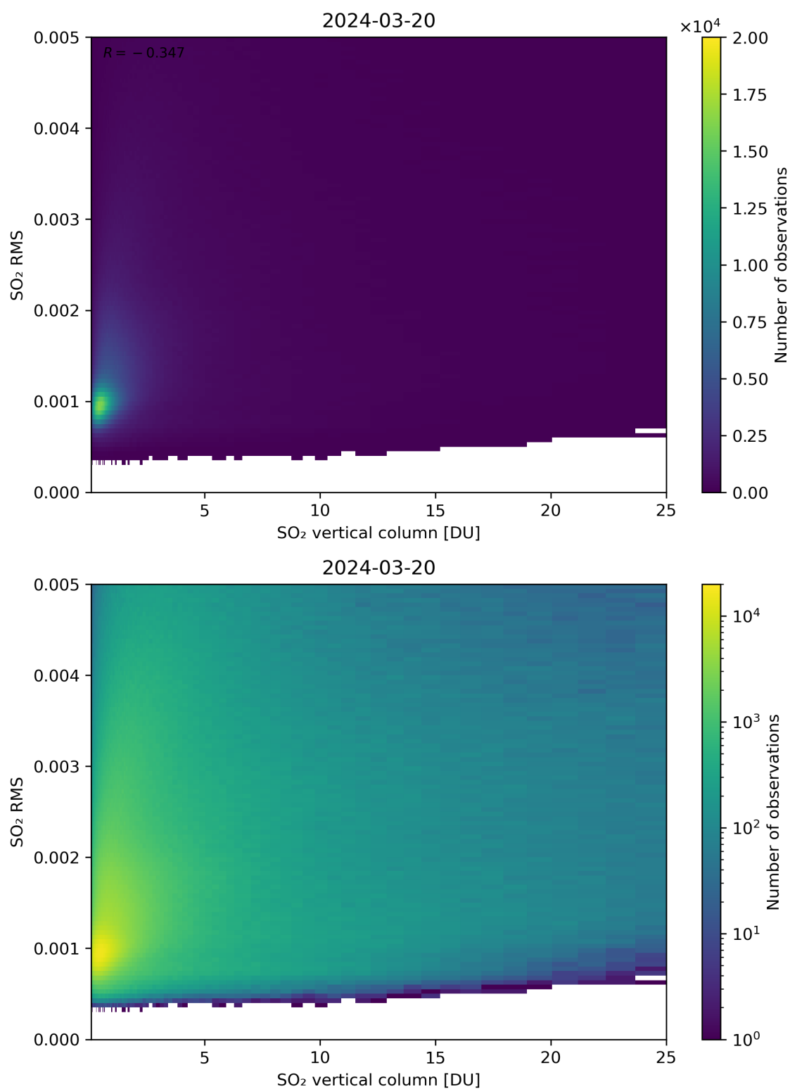
Figure 278: Scatter density plot of “SO 2 vertical column” against “SO 2 RMS” for 2024-03-20 to 2024-03-21.
