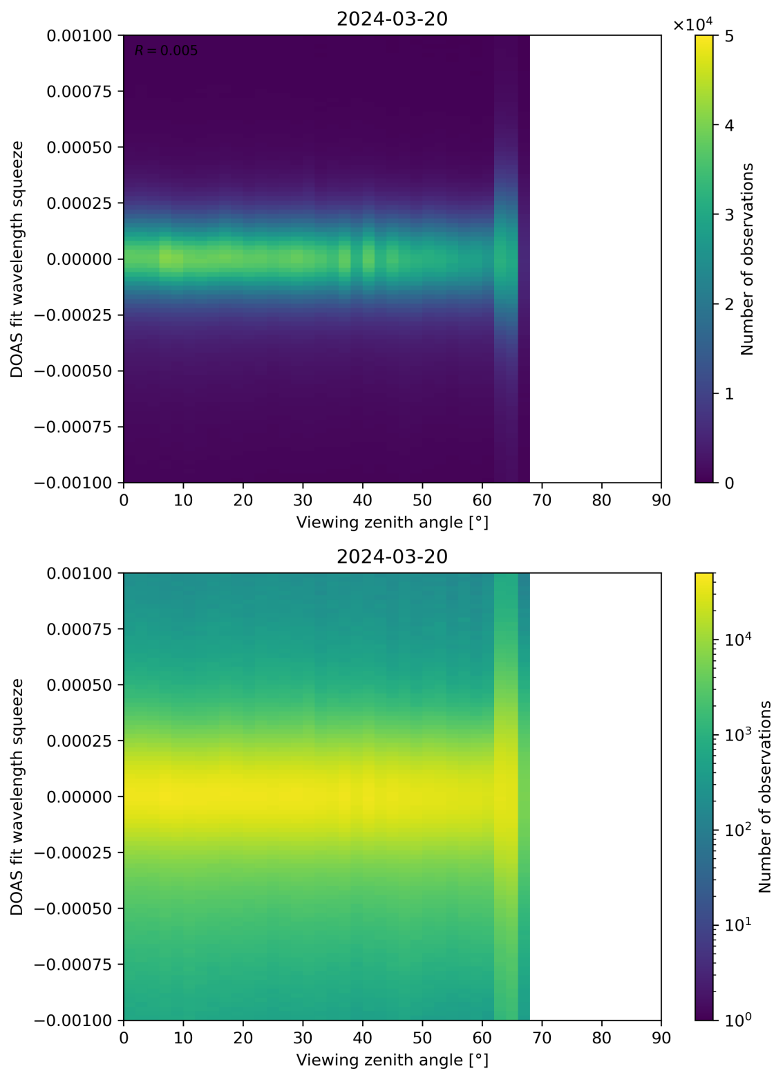
Figure 312: Scatter density plot of “Viewing zenith angle” against “DOAS fit wavelength squeeze” for 2024-03-20 to 2024-03-21.
