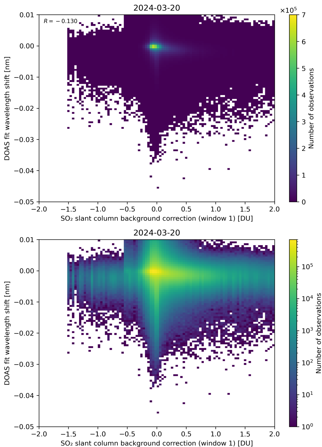
Figure 100: Scatter density plot of “SO 2 slant column background correction (window 1)” against “DOAS fit wavelength shift” for 2024-03-20 to 2024-03-21.
