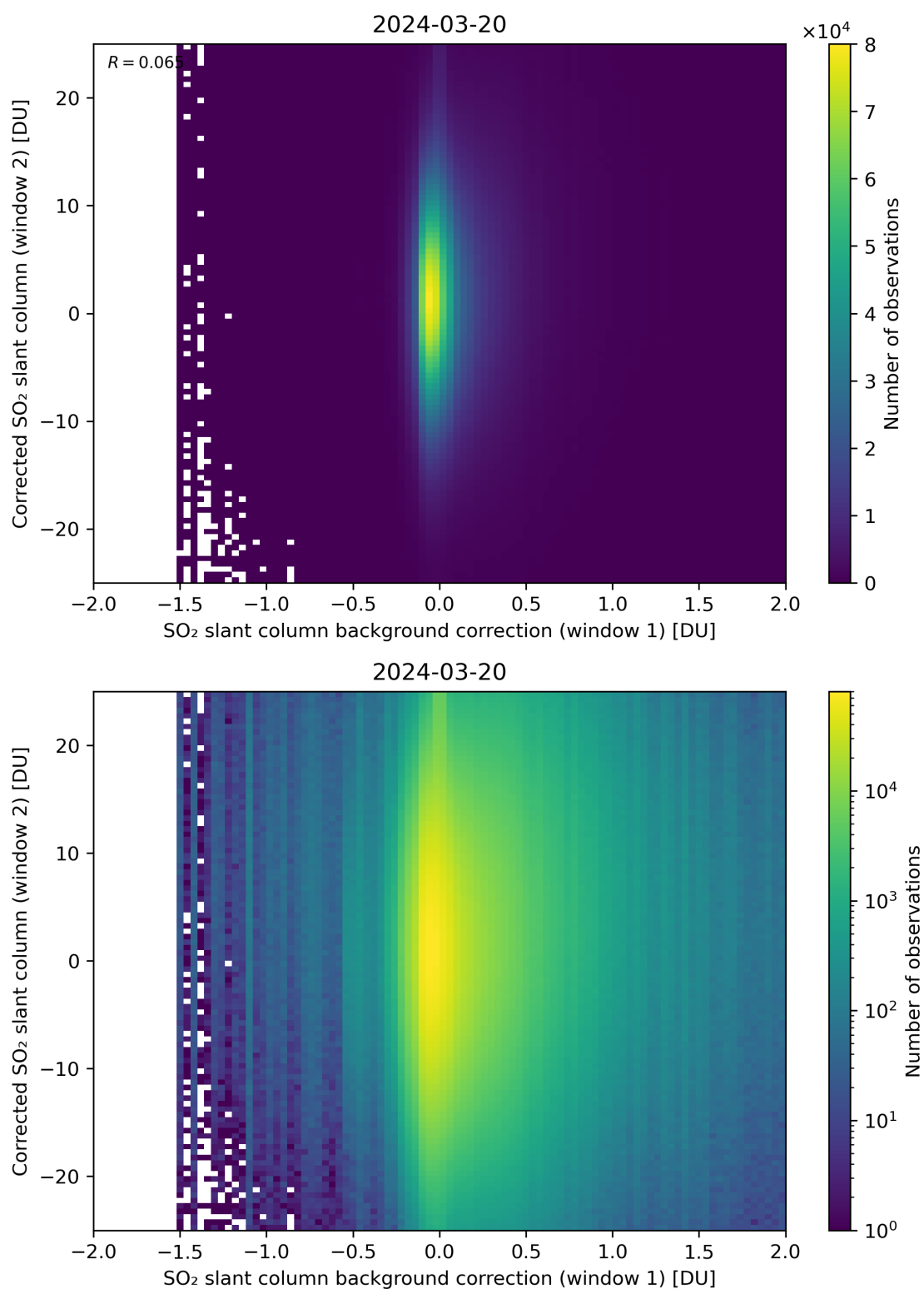
Figure 104: Scatter density plot of “SO 2 slant column background correction (window 1)” against “Corrected SO 2 slant column (window 2)” for 2024-03-20 to 2024-03-21.
