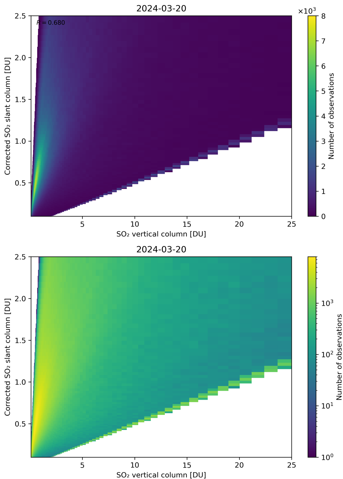
Figure 297: Scatter density plot of “SO 2 vertical column” against “Corrected SO 2 slant column” for 2024-03-20 to 2024-03-21.
