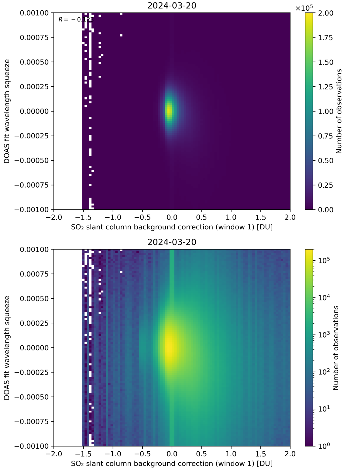
Figure 101: Scatter density plot of “SO 2 slant column background correction (window 1)” against “DOAS fit wavelength squeeze” for 2024-03-20 to 2024-03-21.
