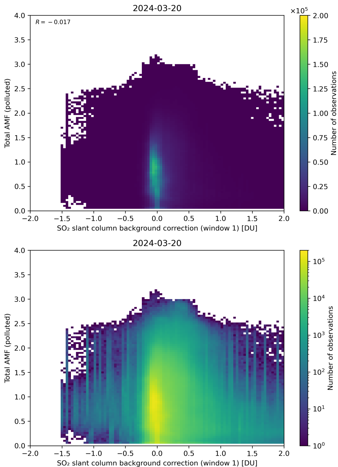
Figure 109: Scatter density plot of “SO 2 slant column background correction (window 1)” against “Total AMF (polluted)” for 2024-03-20 to 2024-03-21.
