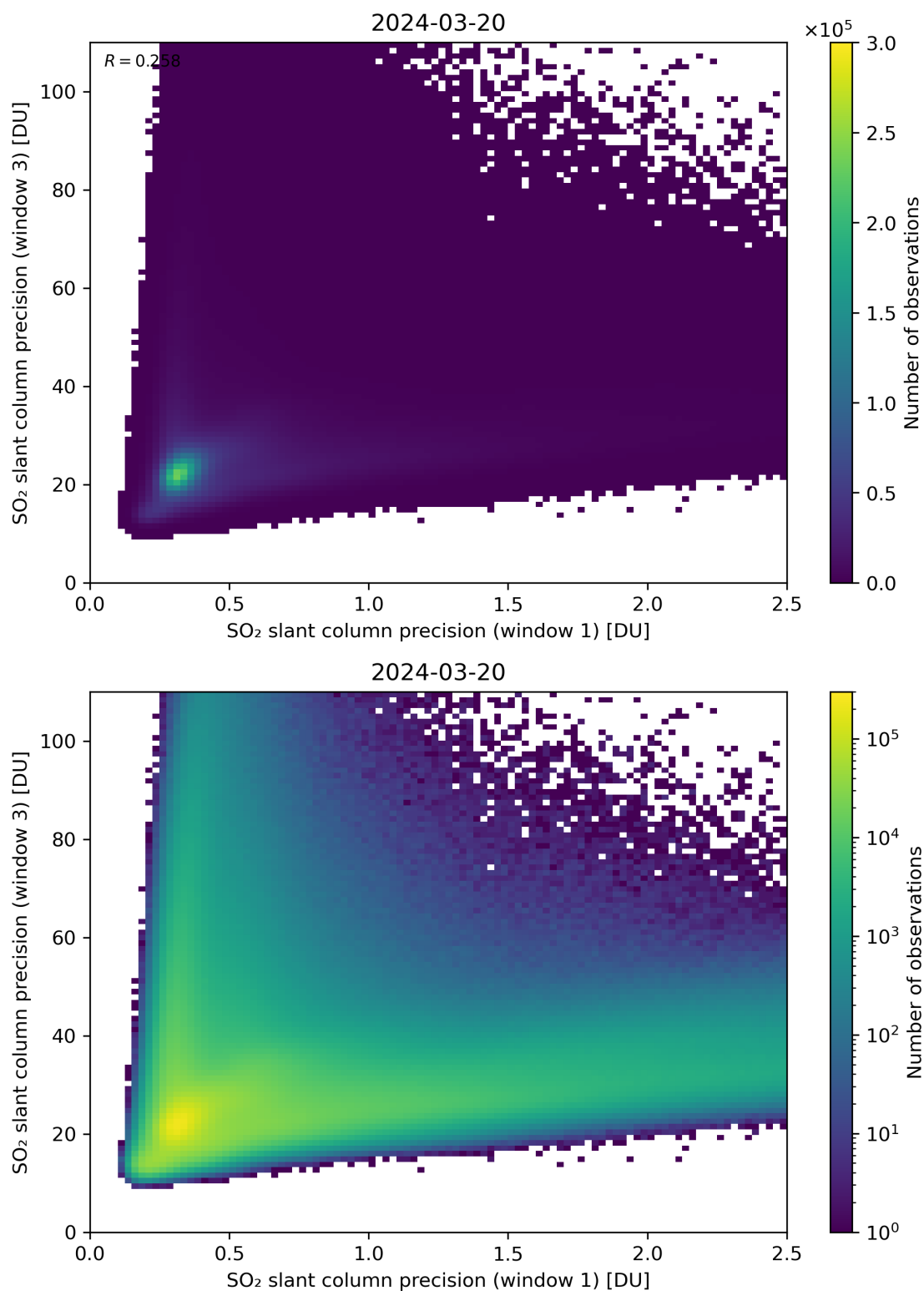
Figure 229: Scatter density plot of “SO 2 slant column precision (window 1)” against “SO 2 slant column precision (window 3)” for 2024-03-20 to 2024-03-21.
