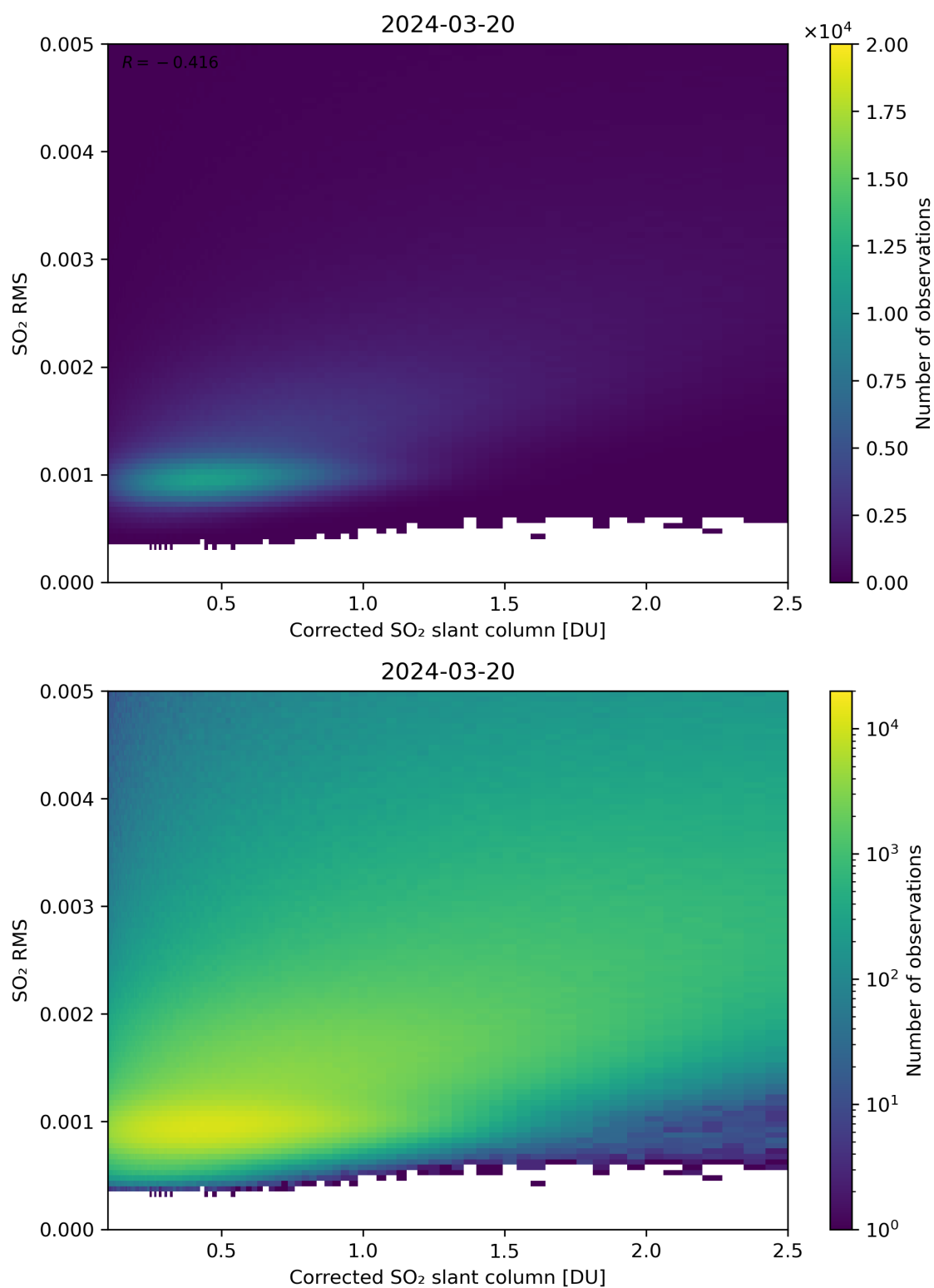
Figure 183: Scatter density plot of “Corrected SO 2 slant column” against “SO 2 RMS” for 2024-03-20 to 2024-03-21.
