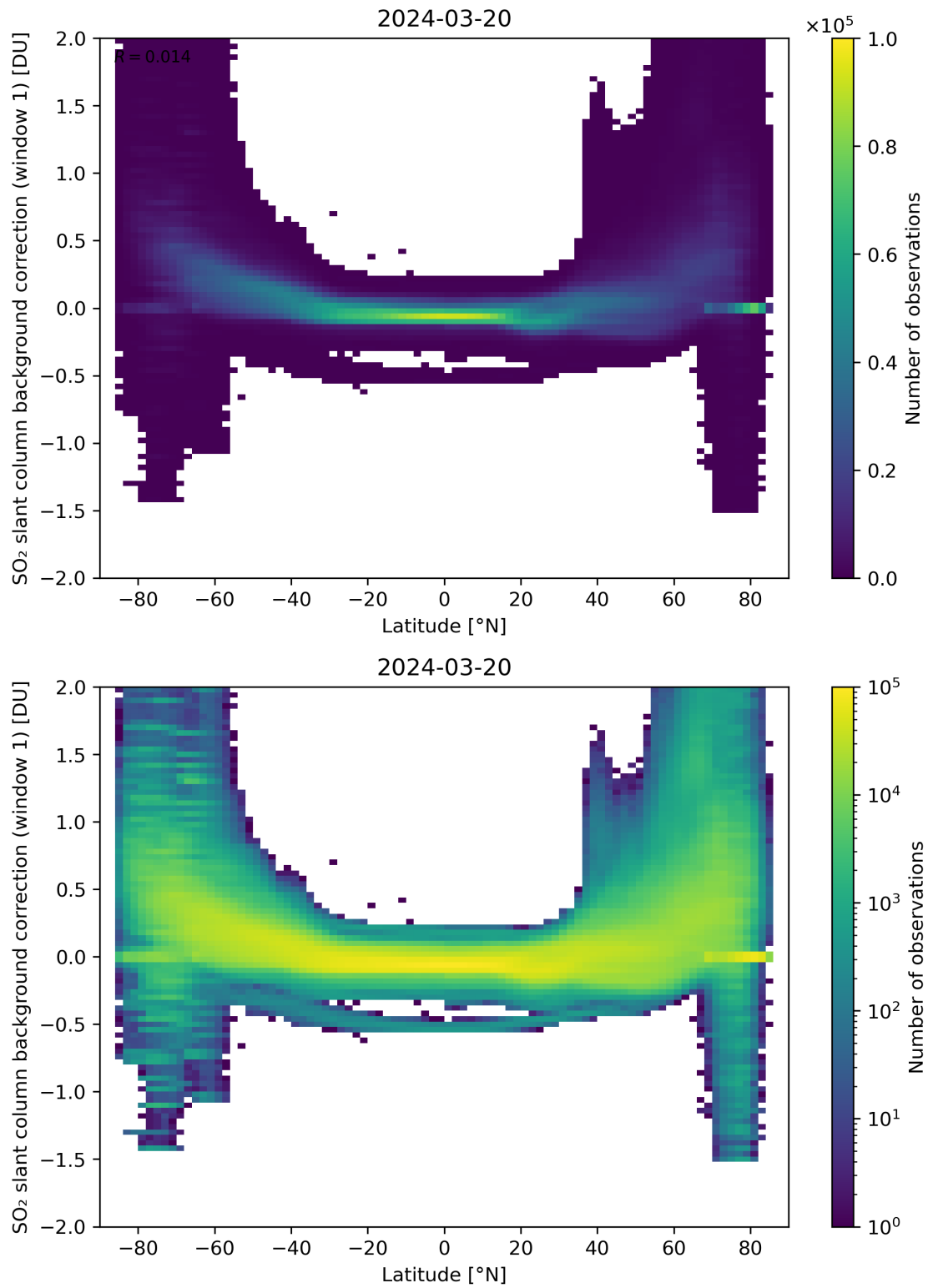
Figure 139: Scatter density plot of “Latitude” against “SO 2 slant column background correction (window 1)” for 2024-03-20 to 2024-03-21.
