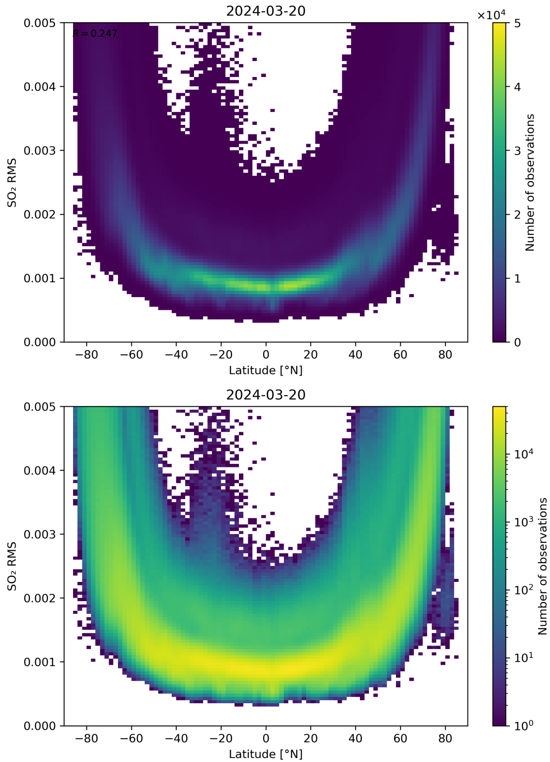
Figure 144: Scatter density plot of “Latitude” against “SO 2 RMS” for 2024-03-20 to 2024-03-21.
