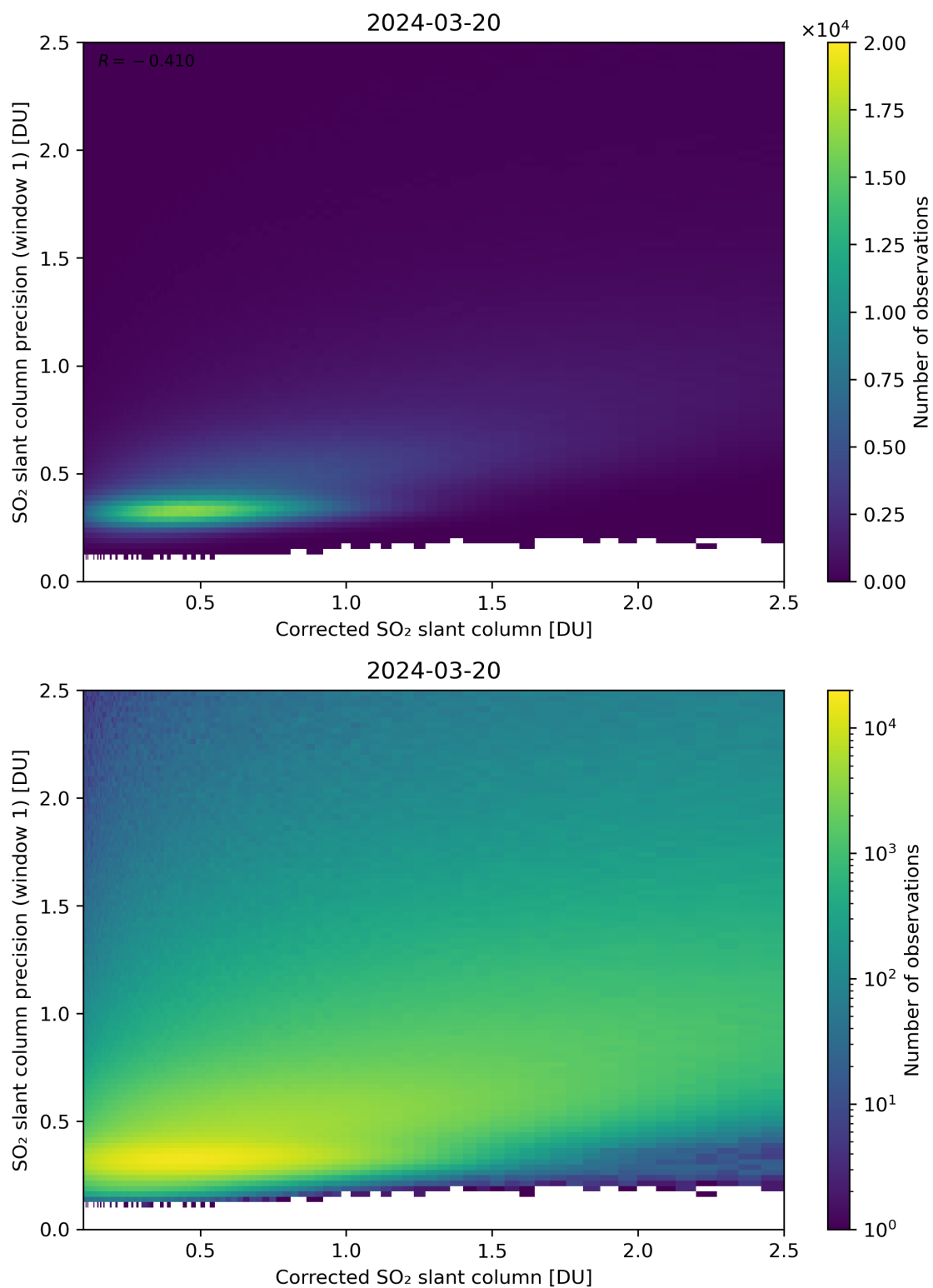
Figure 188: Scatter density plot of “Corrected SO 2 slant column” against “SO 2 slant column precision (window 1)” for 2024-03-20 to 2024-03-21.
