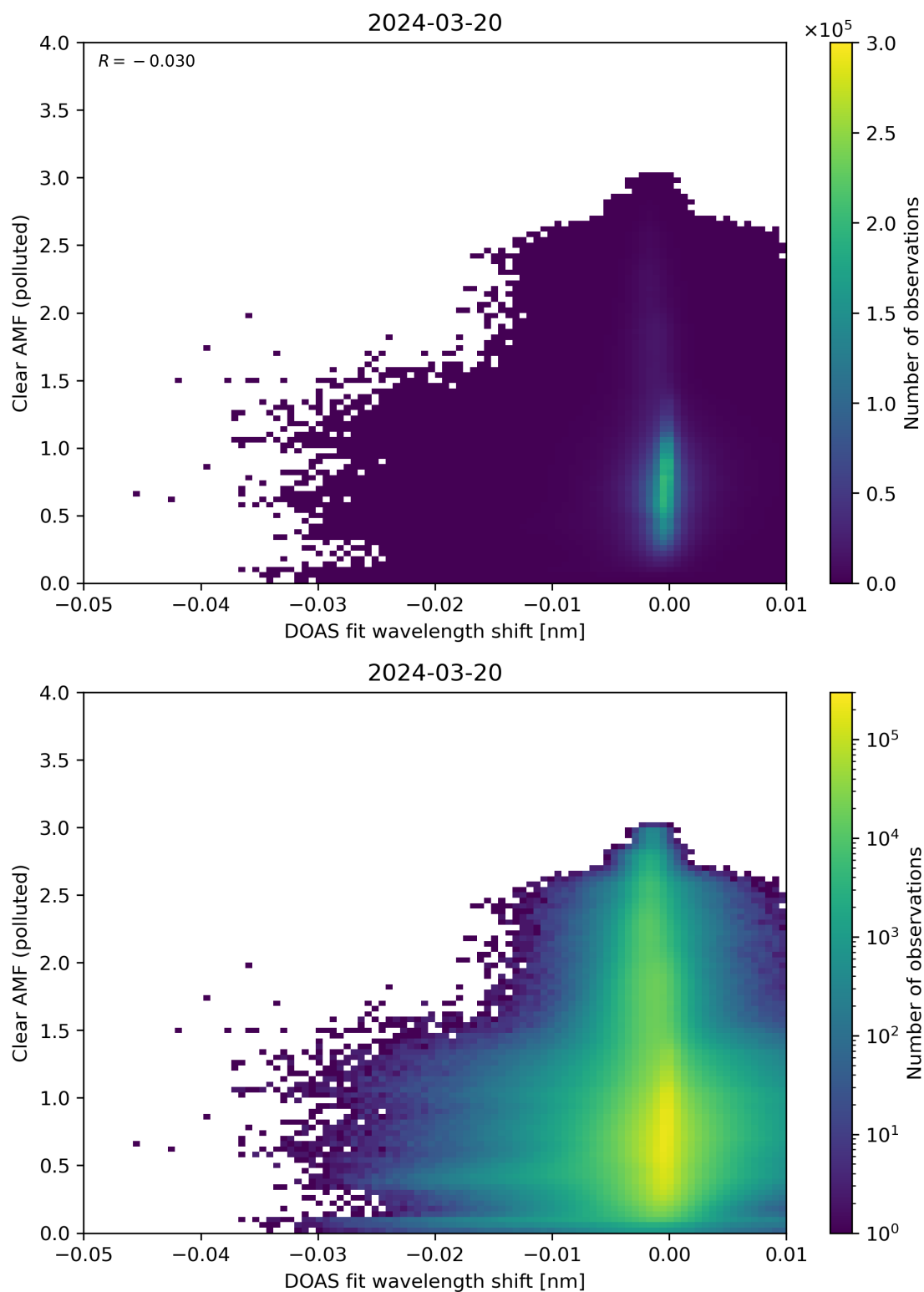
Figure 129: Scatter density plot of “DOAS fit wavelength shift” against “Clear AMF (polluted)” for 2024-03-20 to 2024-03-21.
