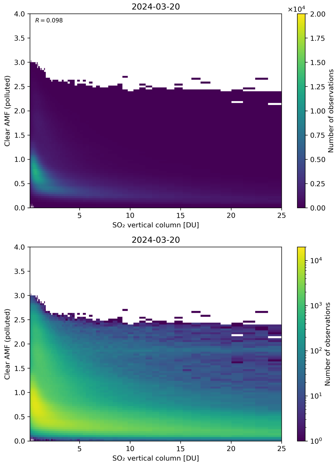
Figure 296: Scatter density plot of “SO 2 vertical column” against “Clear AMF (polluted)” for 2024-03-20 to 2024-03-21.
