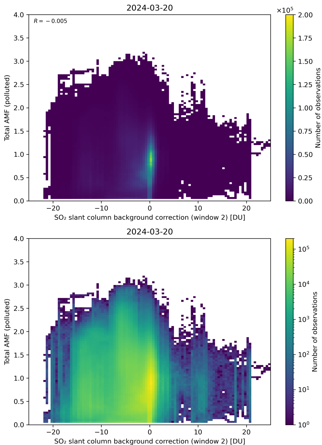
Figure 119: Scatter density plot of “SO 2 slant column background correction (window 2)” against “Total AMF (polluted)” for 2024-03-20 to 2024-03-21.
