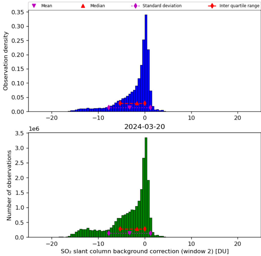
Figure 63: Histogram of “SO 2 slant column background correction (window 2)” for 2024-03-20 to 2024-03-21
