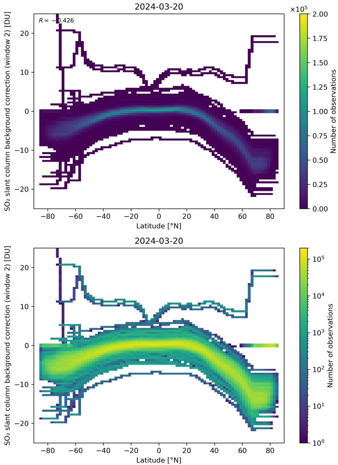
Figure 140: Scatter density plot of “Latitude” against “SO 2 slant column background correction (window 2)” for 2024-03-20 to 2024-03-21.
