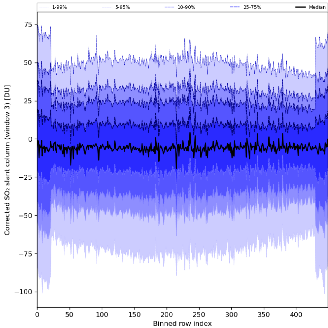
Figure 89: Along track statistics of “Corrected SO 2 slant column (window 3)” for 2024-03-20 to 2024-03-21
