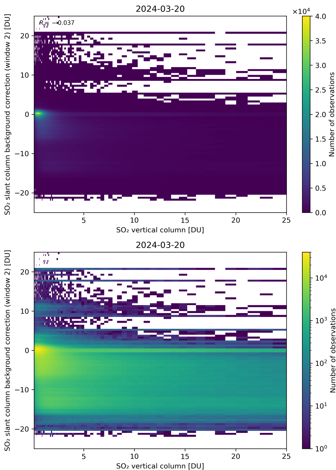
Figure 274: Scatter density plot of “SO 2 vertical column” against “SO 2 slant column background correction (window 2)” for 2024-03-20 to 2024-03-21.
