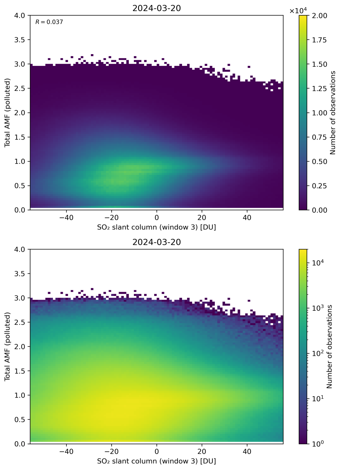
Figure 268: Scatter density plot of “SO 2 slant column (window 3)” against “Total AMF (polluted)” for 2024-03-20 to 2024-03-21.
