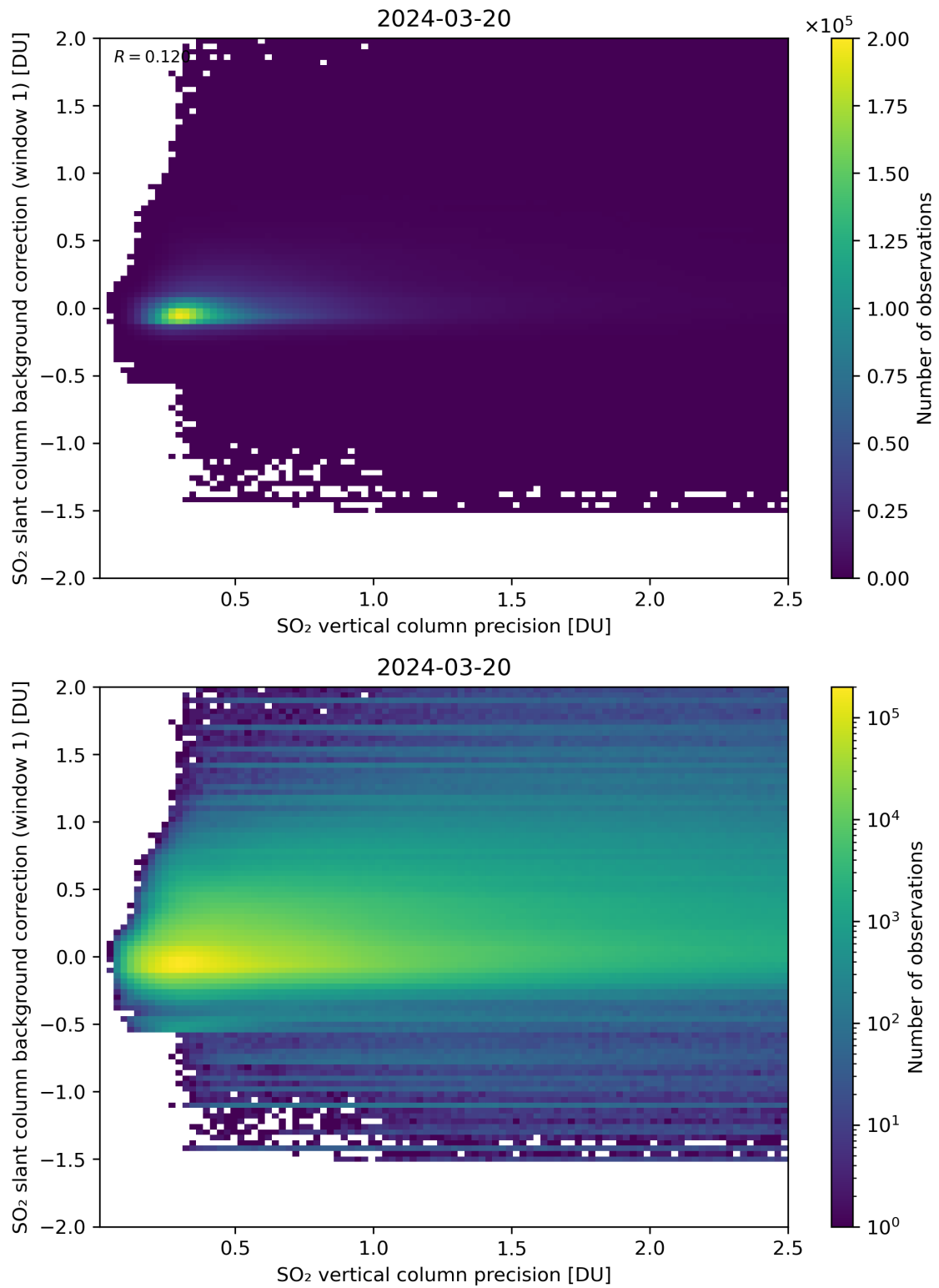
Figure 279: Scatter density plot of “SO 2 vertical column precision” against “SO 2 slant column background correction (window 1)” for 2024-03-20 to 2024-03-21.
