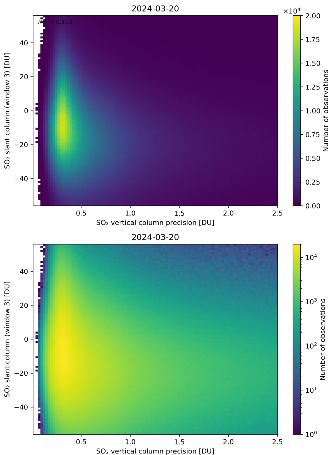
Figure 292: Scatter density plot of “SO 2 vertical column precision” against “SO 2 slant column (window 3)” for 2024-03-20 to 2024-03-21.
