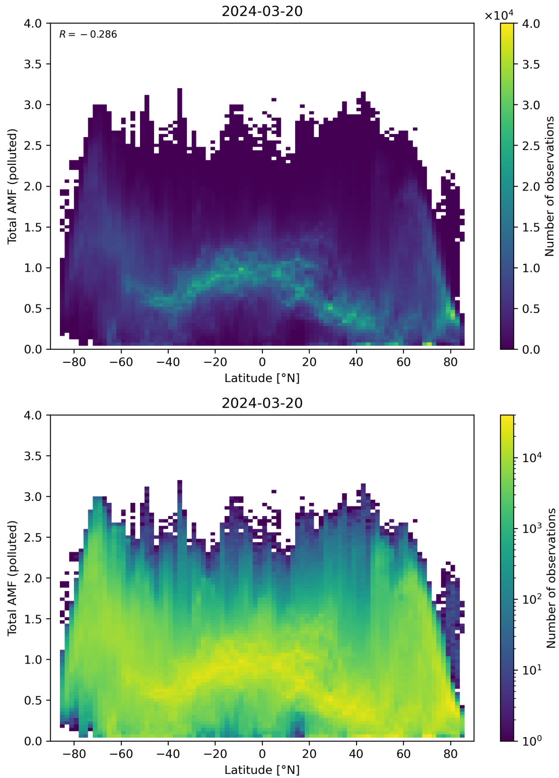
Figure 154: Scatter density plot of “Latitude” against “Total AMF (polluted)” for 2024-03-20 to 2024-03-21.
