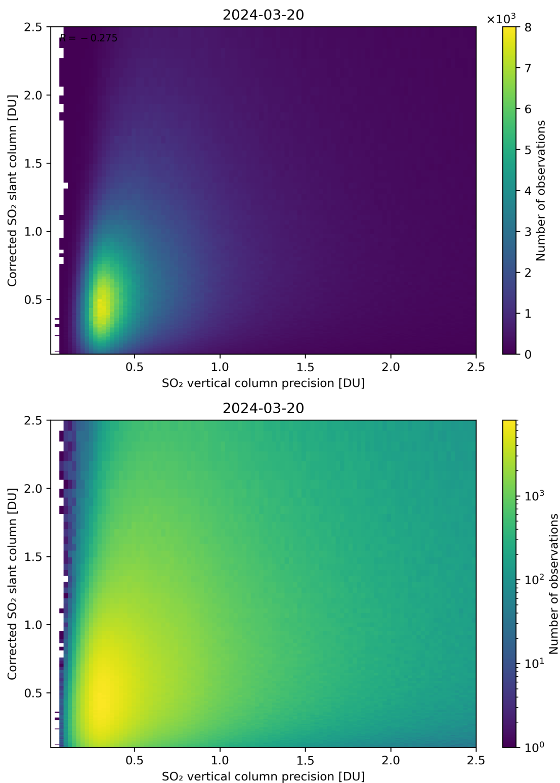
Figure 286: Scatter density plot of “SO 2 vertical column precision” against “Corrected SO 2 slant column” for 2024-03-20 to 2024-03-21.
