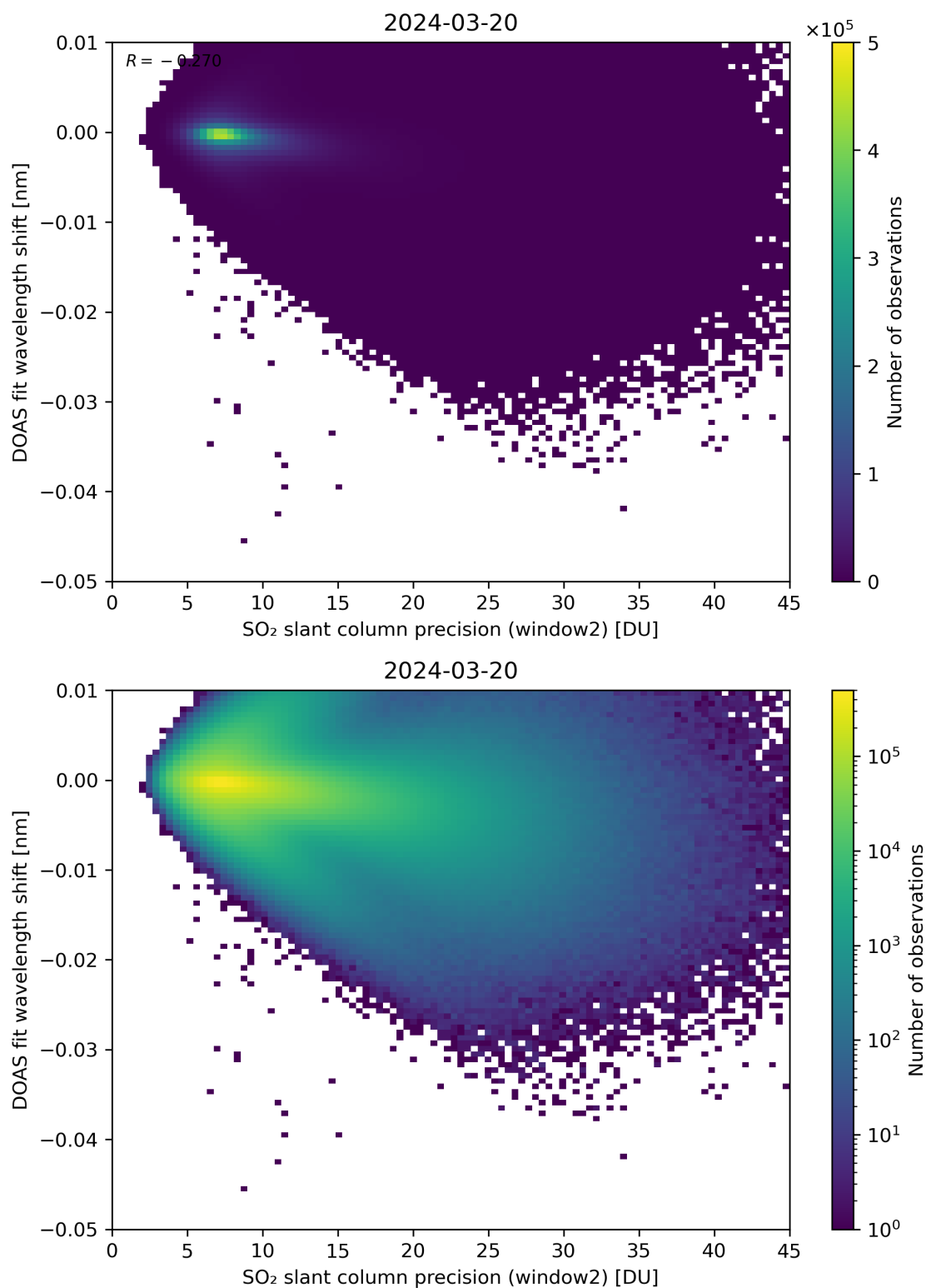
Figure 243: Scatter density plot of “SO 2 slant column precision (window2)” against “DOAS fit wavelength shift” for 2024-03-20 to 2024-03-21.
