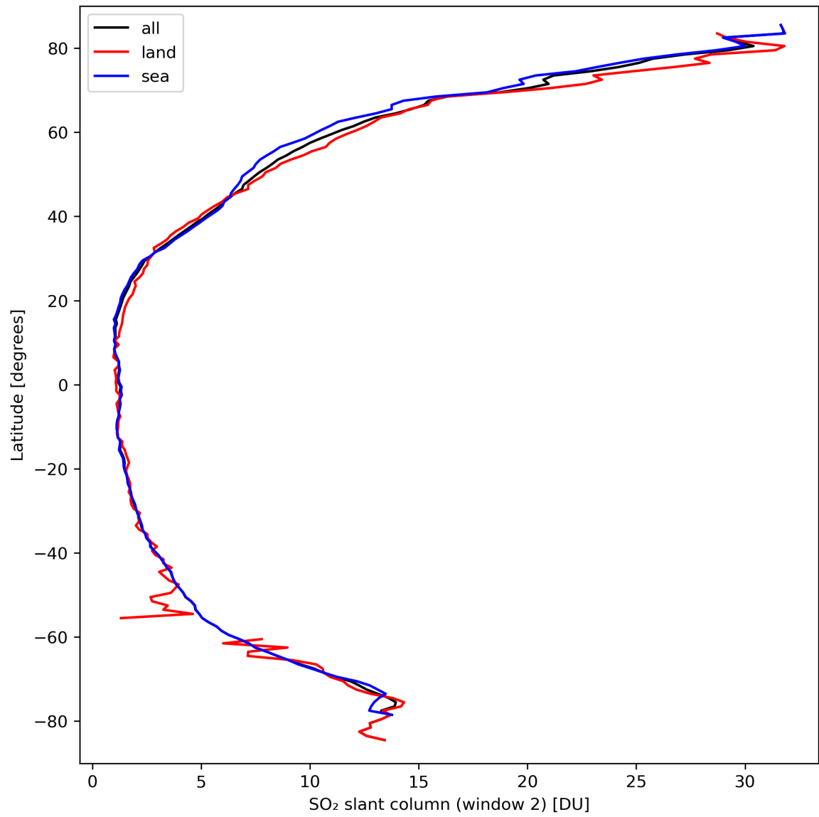
Figure 37: Zonal average of “SO 2 slant column (window 2)” for 2024-03-20 to 2024-03-22.
