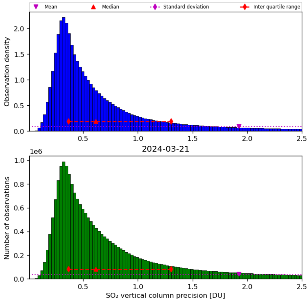
Figure 54: Histogram of “SO 2 vertical column precision” for 2024-03-20 to 2024-03-22
