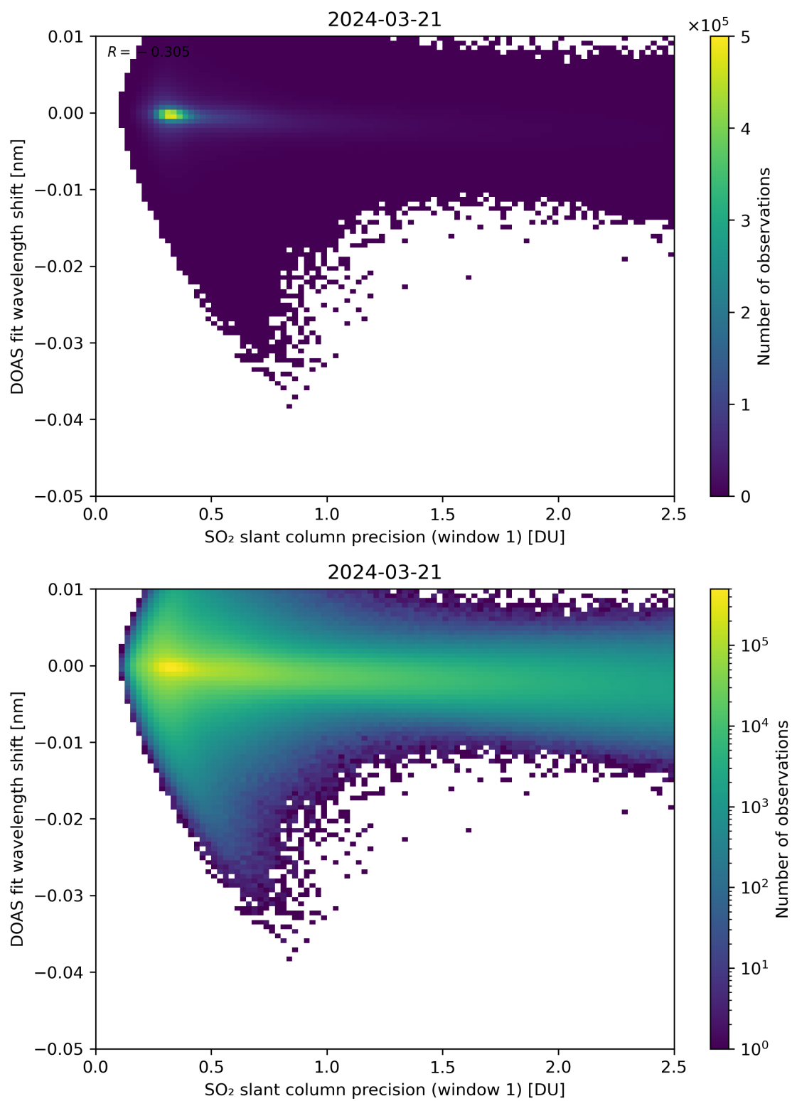
Figure 221: Scatter density plot of “SO 2 slant column precision (window 1)” against “DOAS fit wavelength shift” for 2024-03-20 to 2024-03-22.
