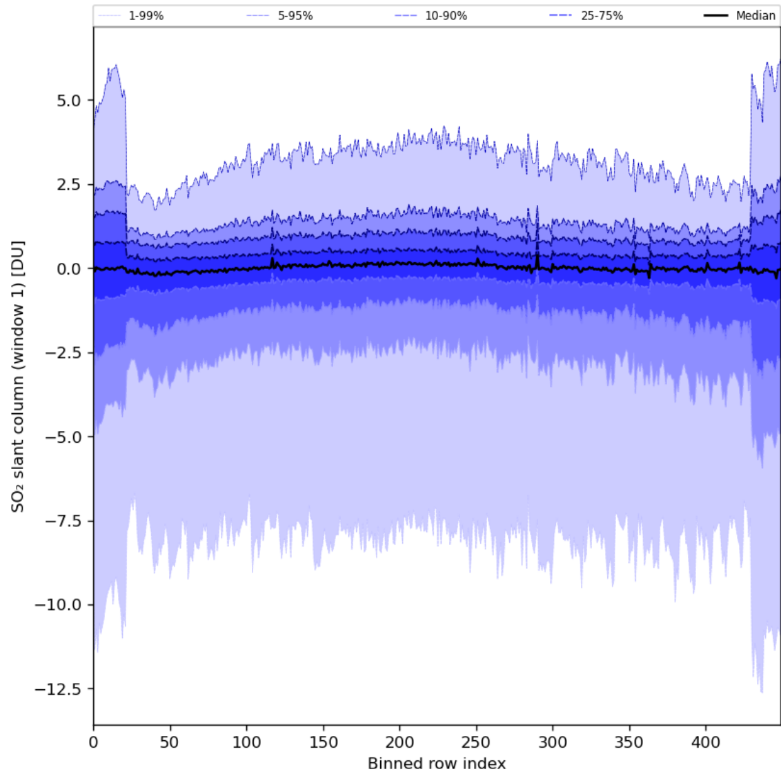
Figure 79: Along track statistics of “SO 2 slant column (window 1)” for 2024-03-20 to 2024-03-22
