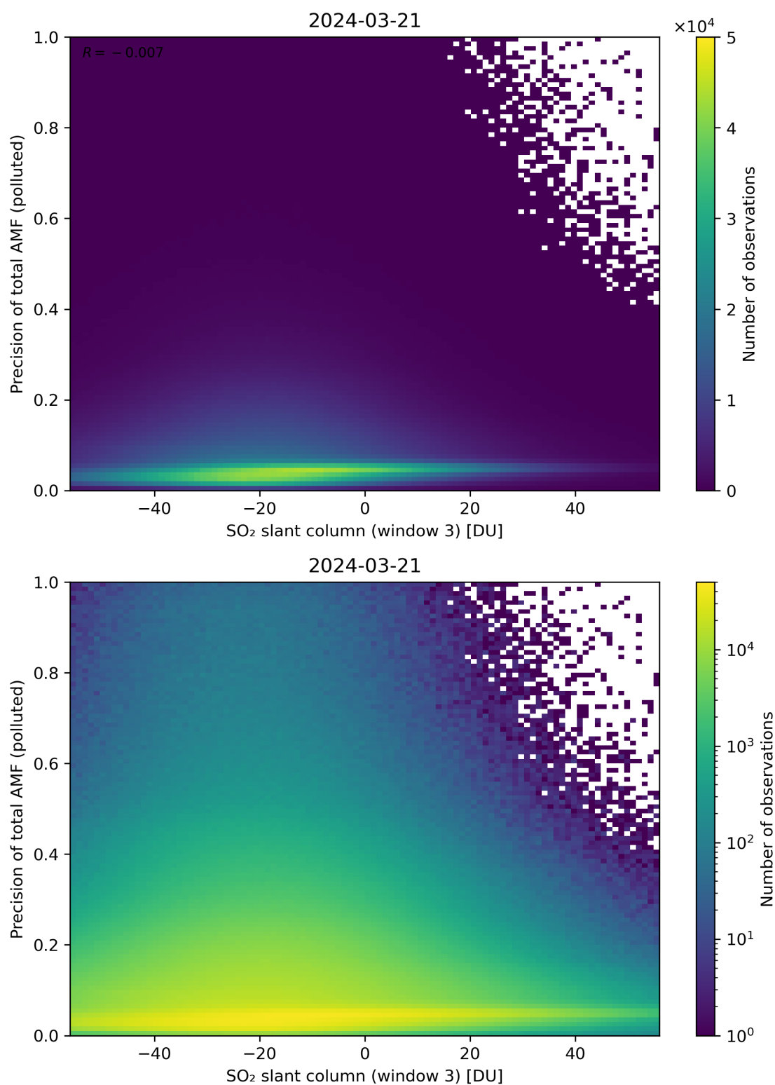
Figure 269: Scatter density plot of “SO 2 slant column (window 3)” against “Precision of total AMF (polluted)” for 2024-03-20 to 2024-03-22.
