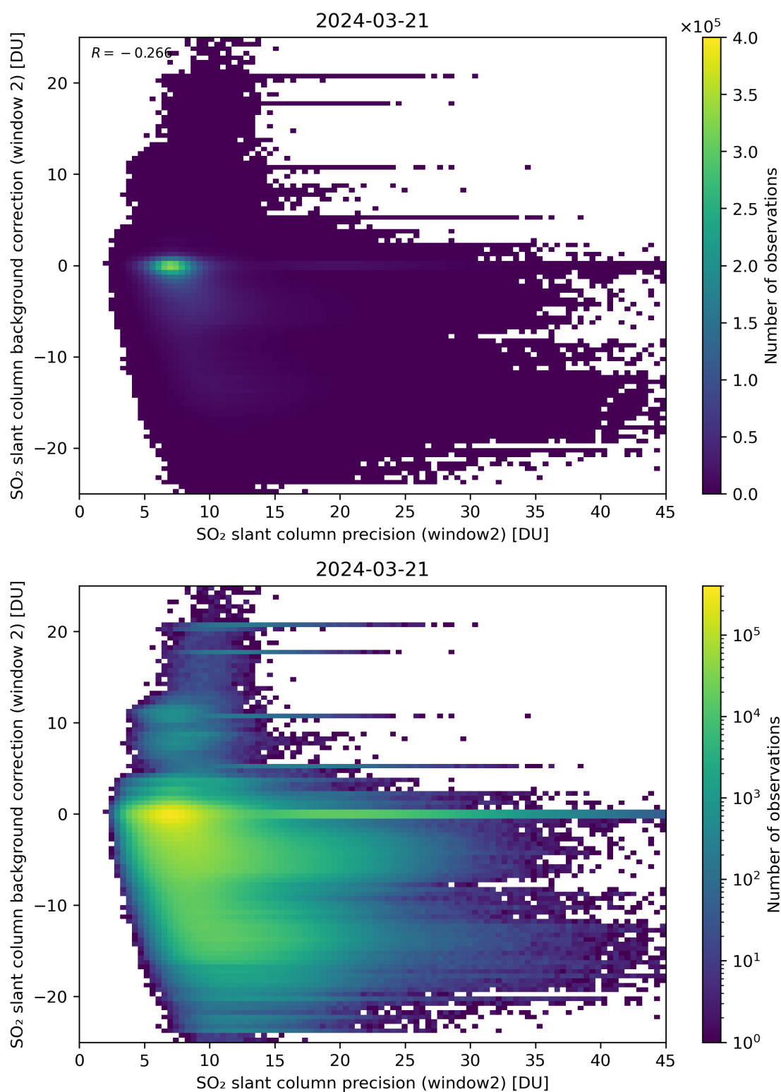
Figure 241: Scatter density plot of “SO 2 slant column precision (window2)” against “SO 2 slant column background correction (window 2)” for 2024-03-20 to 2024-03-22.
