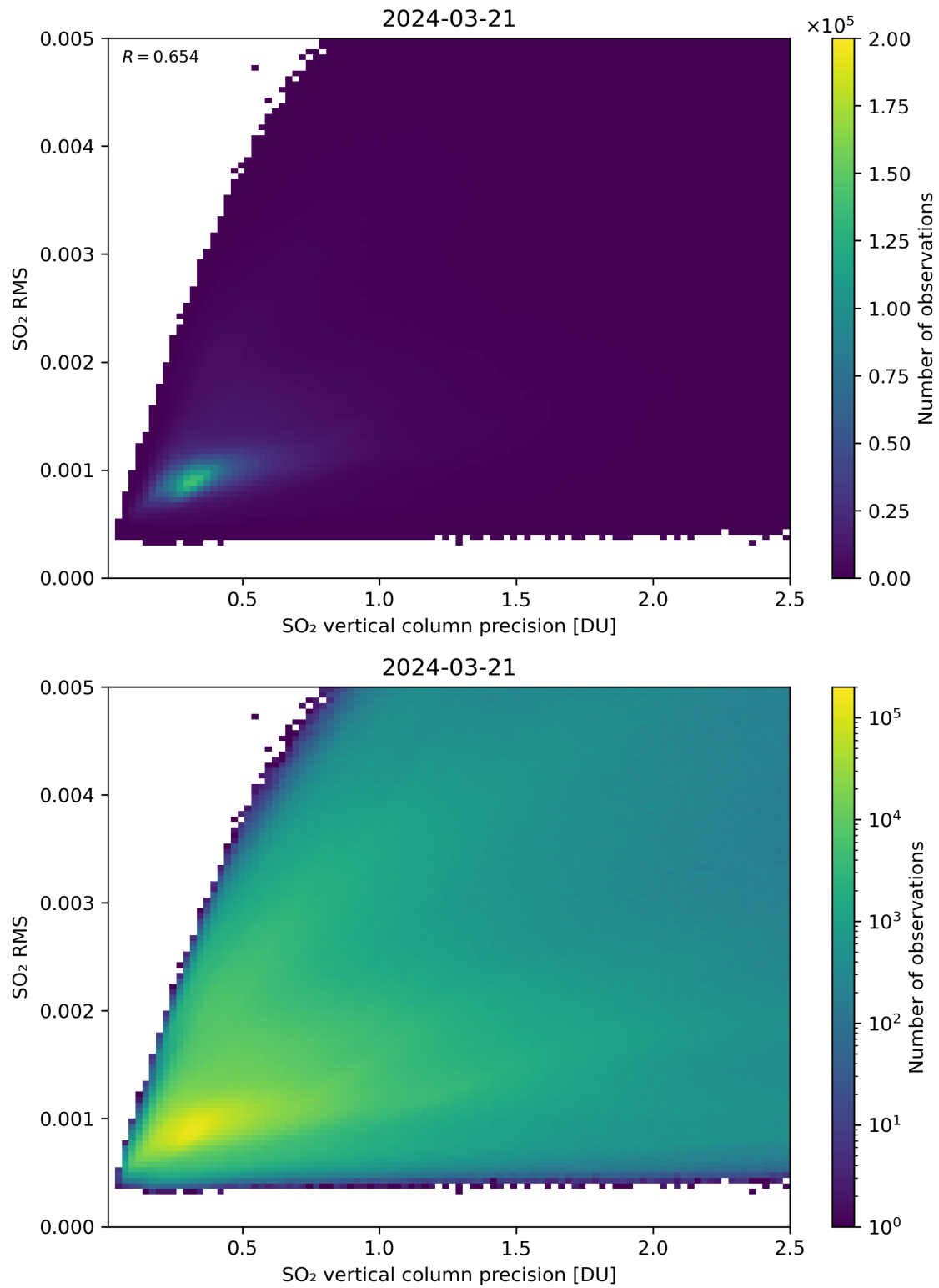
Figure 284: Scatter density plot of “SO 2 vertical column precision” against “SO 2 RMS” for 2024-03-20 to 2024-03-22.
