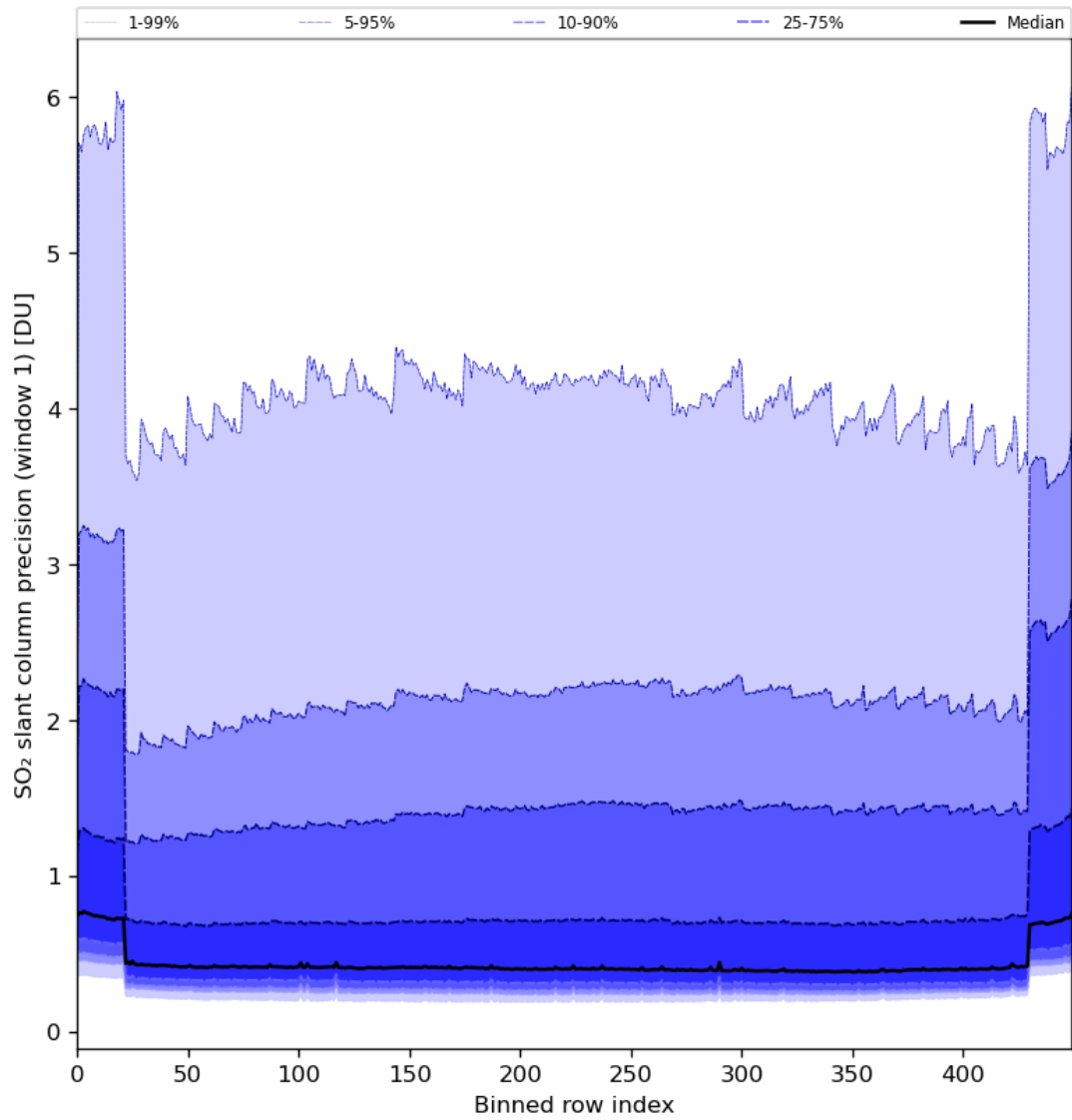
Figure 80: Along track statistics of “SO 2 slant column precision (window 1)” for 2024-03-20 to 2024-03-22
