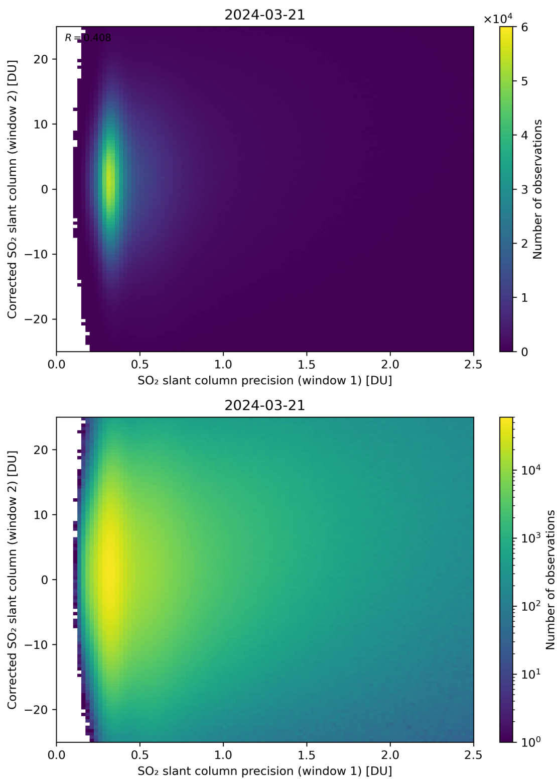
Figure 225: Scatter density plot of “SO 2 slant column precision (window 1)” against “Corrected SO 2 slant column (window 2)” for 2024-03-20 to 2024-03-22.
