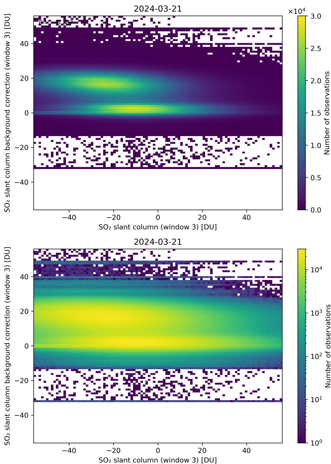
Figure 253: Scatter density plot of “SO 2 slant column (window 3)” against “SO 2 slant column background correction (window 3)” for 2024-03-20 to 2024-03-22.
