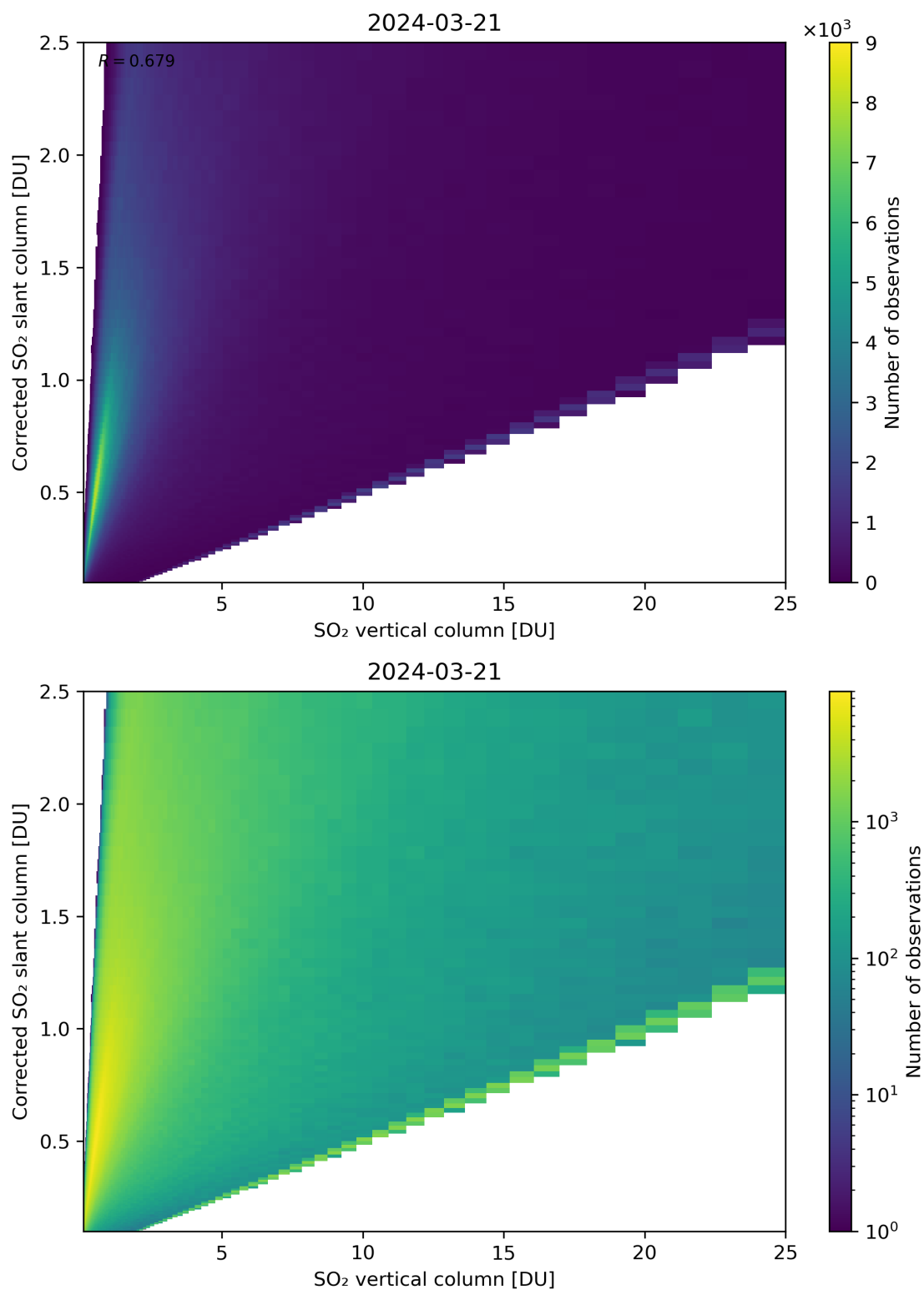
Figure 297: Scatter density plot of “SO 2 vertical column” against “Corrected SO 2 slant column” for 2024-03-20 to 2024-03-22.
