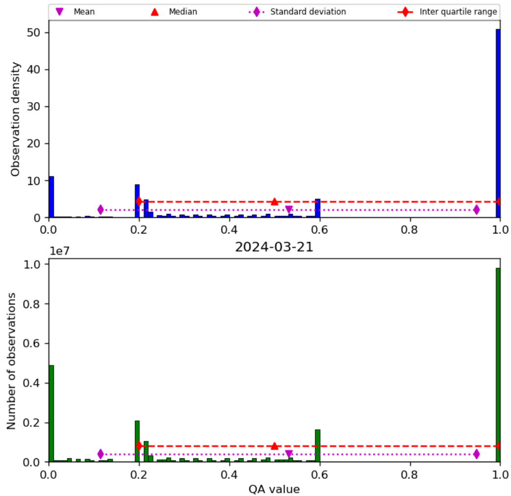
Figure 52: Histogram of “QA value” for 2024-03-20 to 2024-03-22
