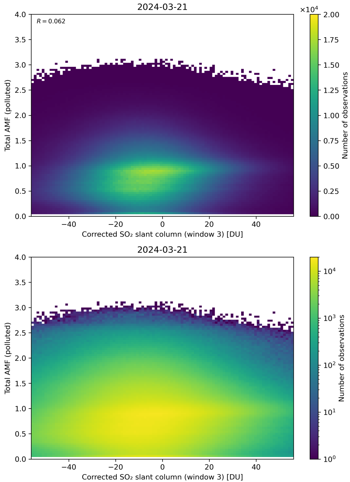
Figure 210: Scatter density plot of “Corrected SO 2 slant column (window 3)” against “Total AMF (polluted)” for 2024-03-20 to 2024-03-22.
