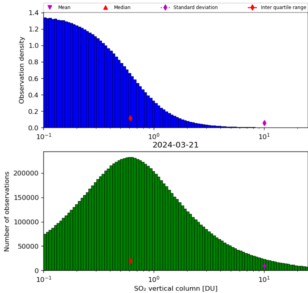
Figure 53: Histogram of “SO 2 vertical column” for 2024-03-20 to 2024-03-22
