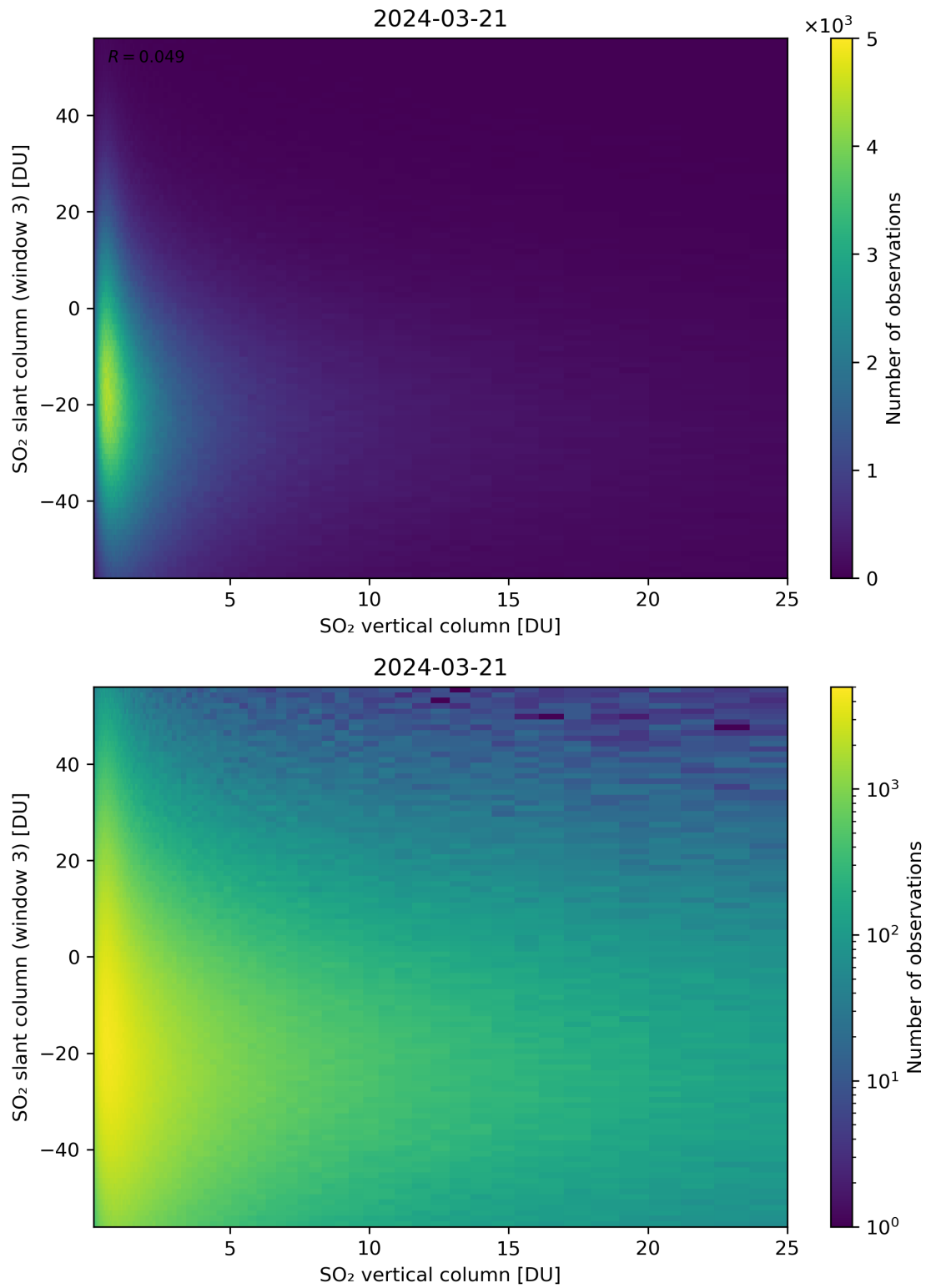
Figure 303: Scatter density plot of “SO 2 vertical column” against “SO 2 slant column (window 3)” for 2024-03-20 to 2024-03-22.
