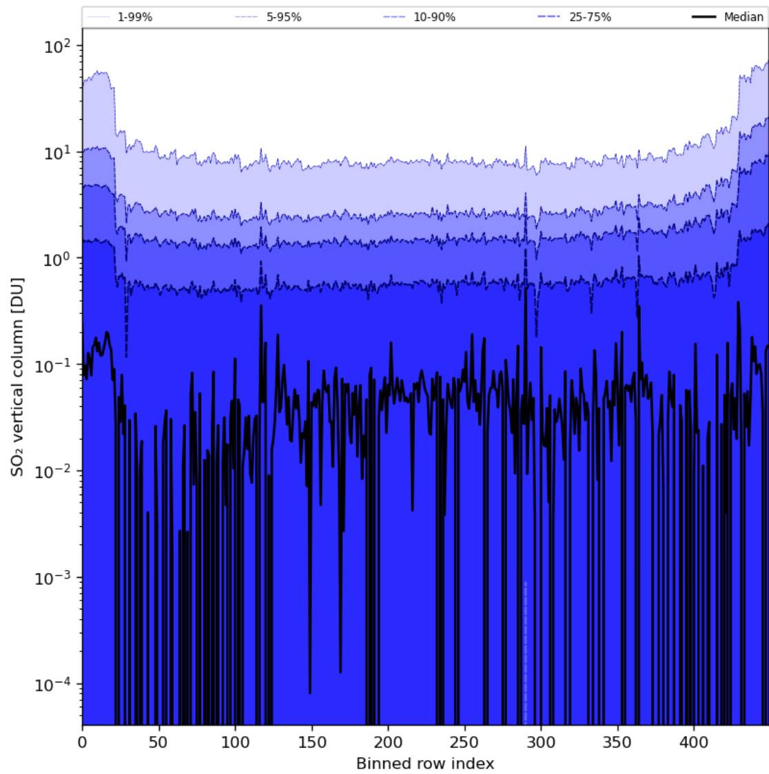
Figure 76: Along track statistics of “SO 2 vertical column” for 2024-03-20 to 2024-03-22
