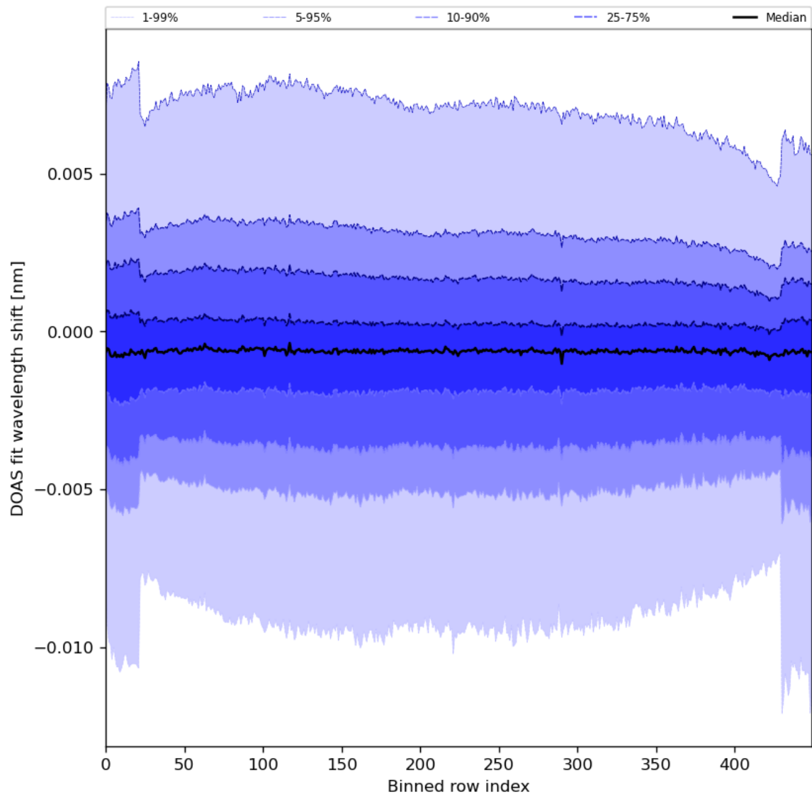
Figure 91: Along track statistics of “DOAS fit wavelength shift” for 2024-03-20 to 2024-03-22
