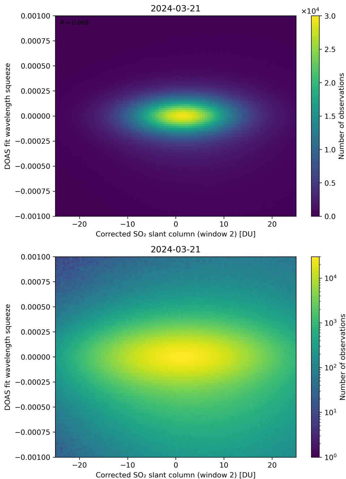
Figure 197: Scatter density plot of “Corrected SO 2 slant column (window 2)” against “DOAS fit wavelength squeeze” for 2024-03-20 to 2024-03-22.
