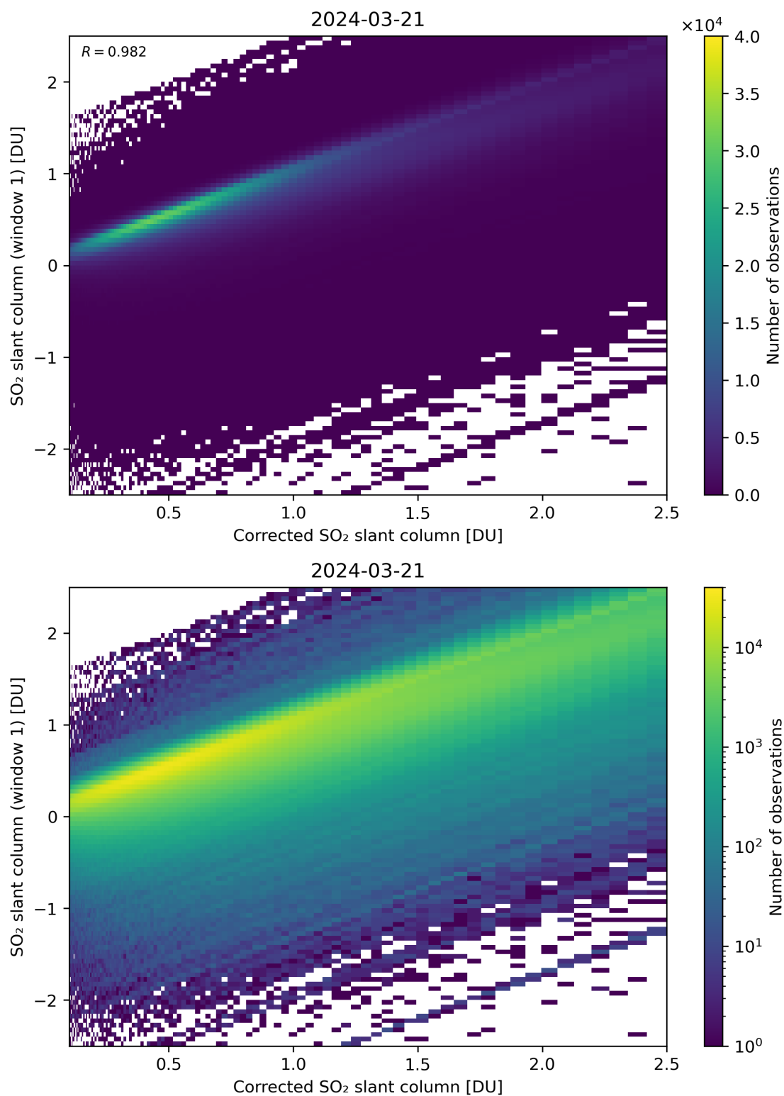
Figure 187: Scatter density plot of “Corrected SO 2 slant column” against “SO 2 slant column (window 1)” for 2024-03-20 to 2024-03-22.
