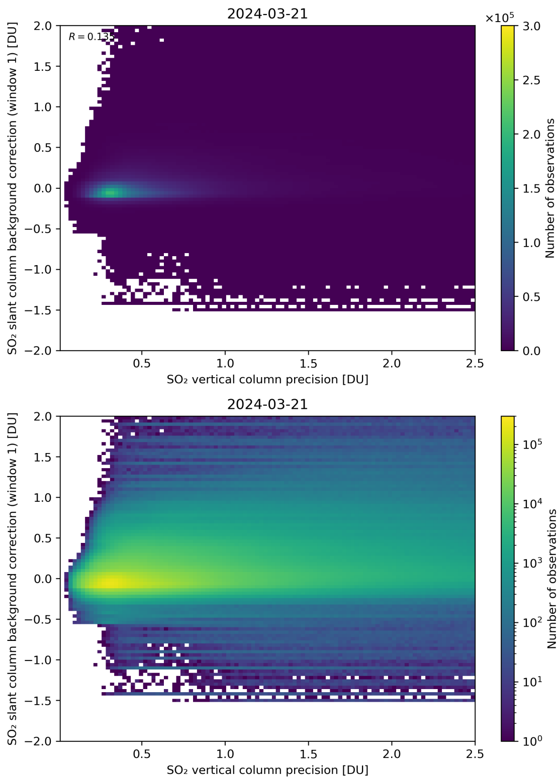
Figure 279: Scatter density plot of “SO 2 vertical column precision” against “SO 2 slant column background correction (window 1)” for 2024-03-20 to 2024-03-22.
