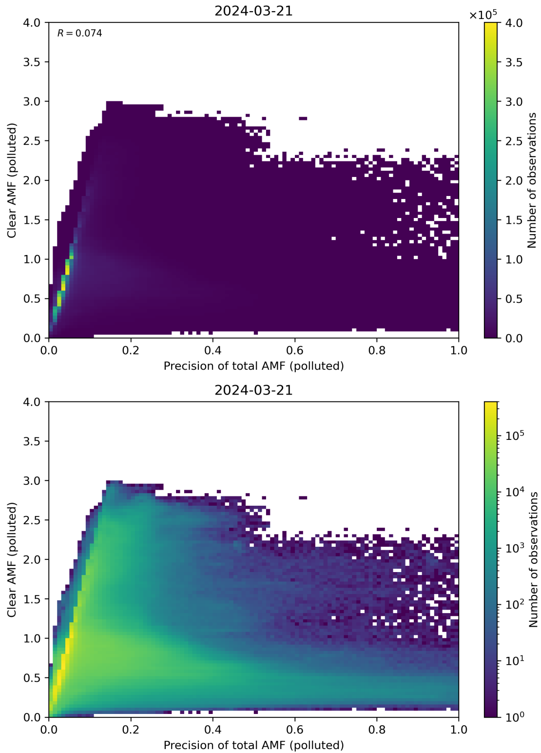
Figure 270: Scatter density plot of “Precision of total AMF (polluted)” against “Clear AMF (polluted)” for 2024-03-20 to 2024-03-22.
