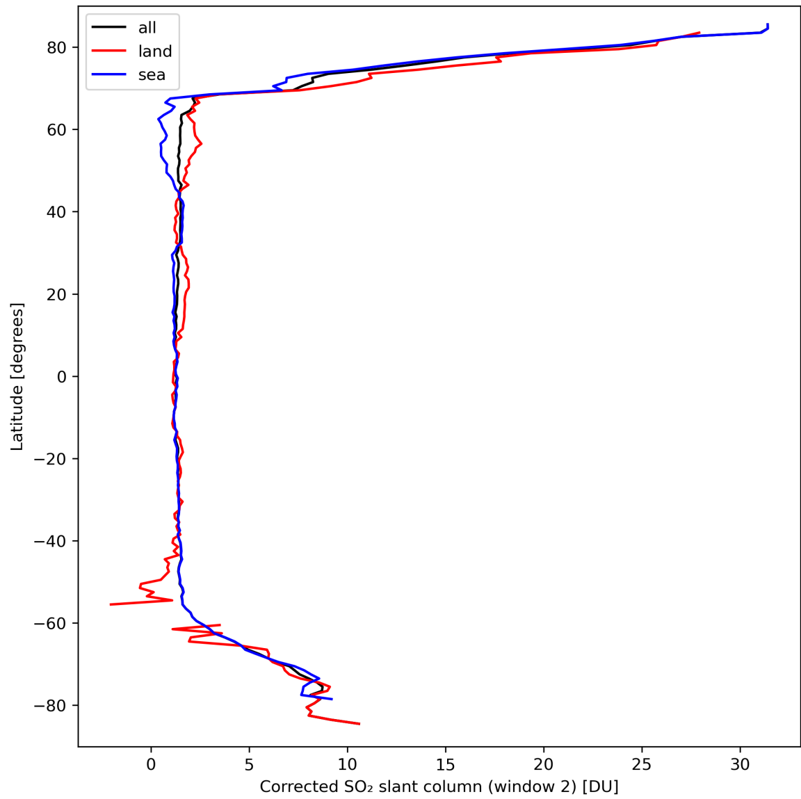
Figure 39: Zonal average of “Corrected SO 2 slant column (window 2)” for 2024-03-20 to 2024-03-22.
