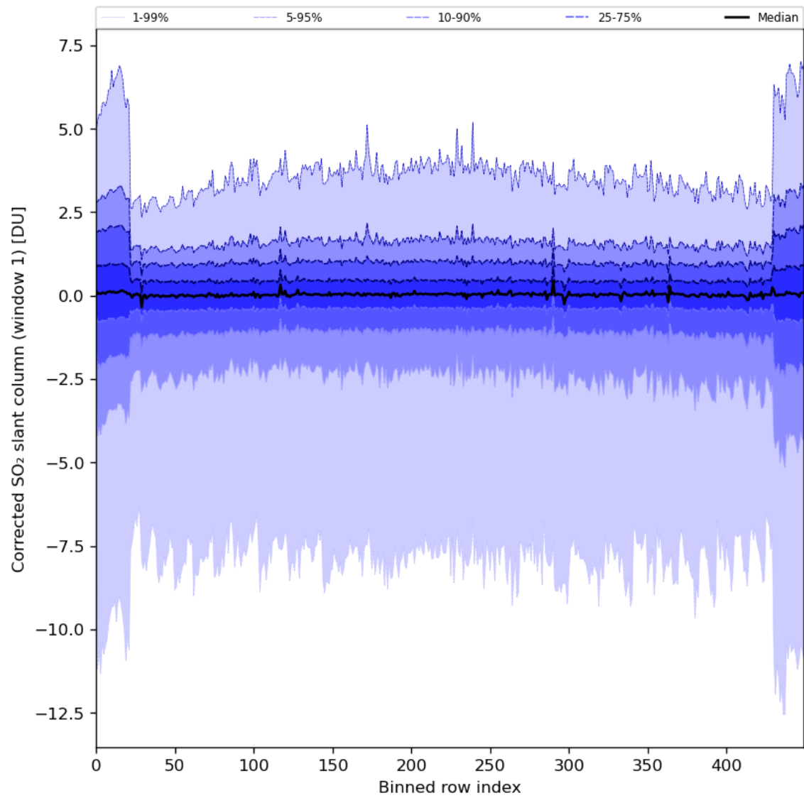
Figure 81: Along track statistics of “Corrected SO 2 slant column (window 1)” for 2024-03-20 to 2024-03-22
