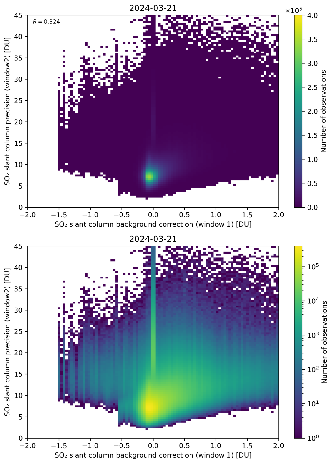
Figure 106: Scatter density plot of “SO 2 slant column background correction (window 1)” against “SO 2 slant column precision (window2)” for 2024-03-20 to 2024-03-22.
