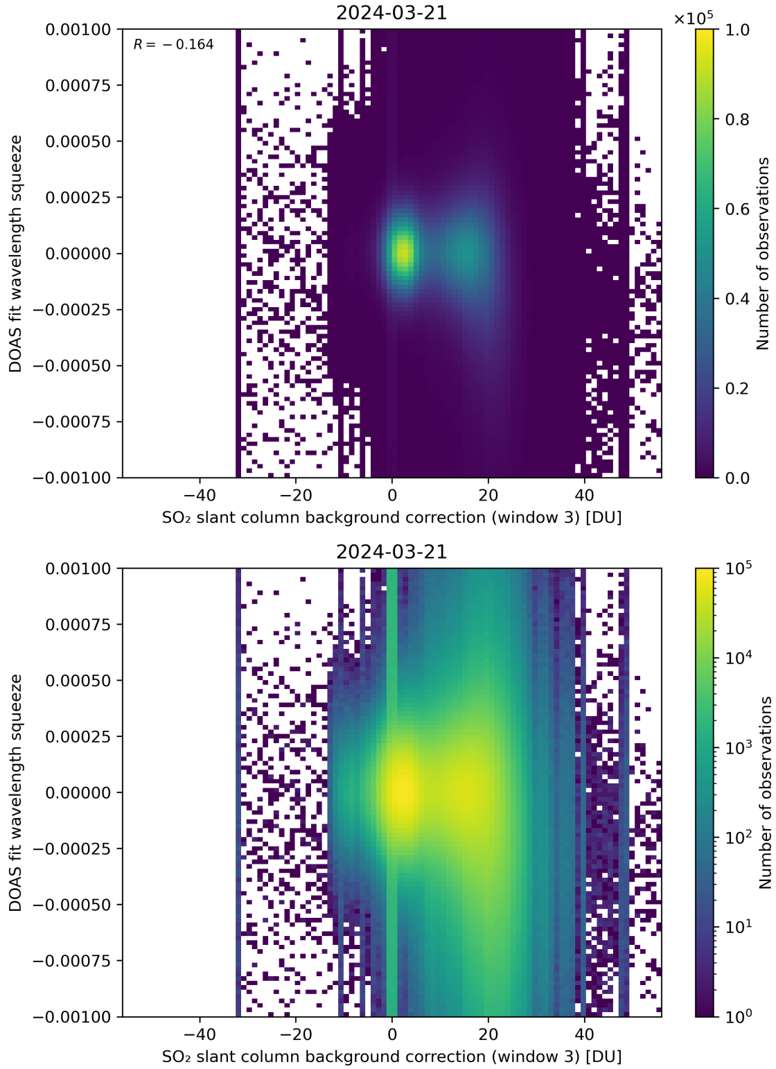
Figure 122: Scatter density plot of “SO 2 slant column background correction (window 3)” against “DOAS fit wavelength squeeze” for 2024-03-20 to 2024-03-22.
