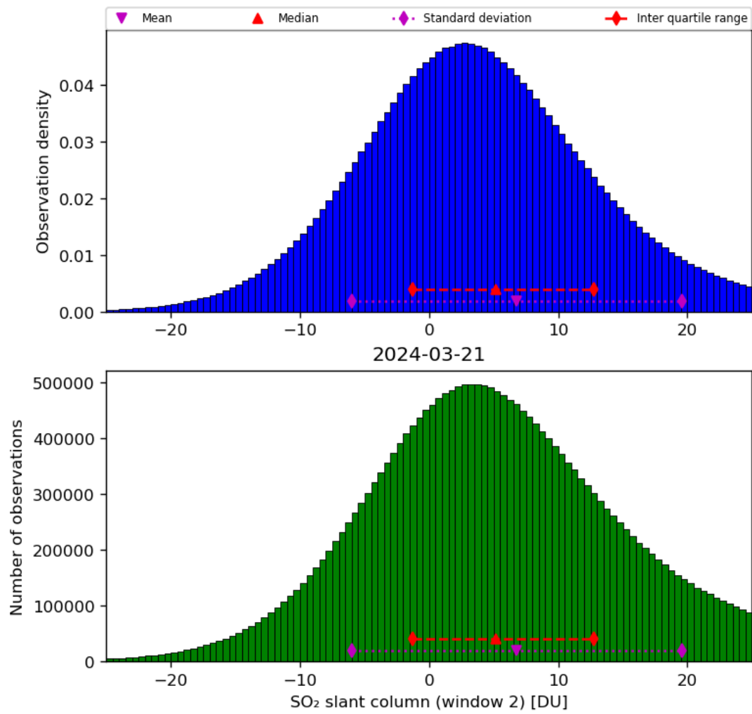
Figure 60: Histogram of “SO 2 slant column (window 2)” for 2024-03-20 to 2024-03-22
