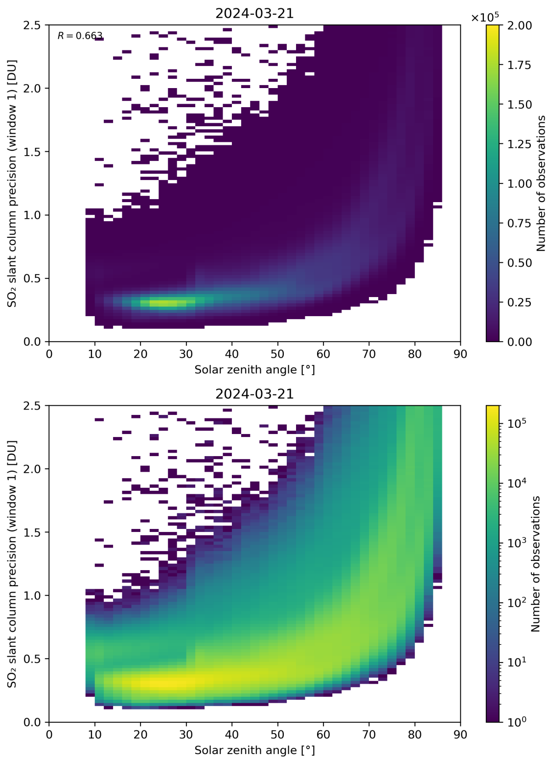
Figure 170: Scatter density plot of “Solar zenith angle” against “SO 2 slant column precision (window 1)” for 2024-03-20 to 2024-03-22.
