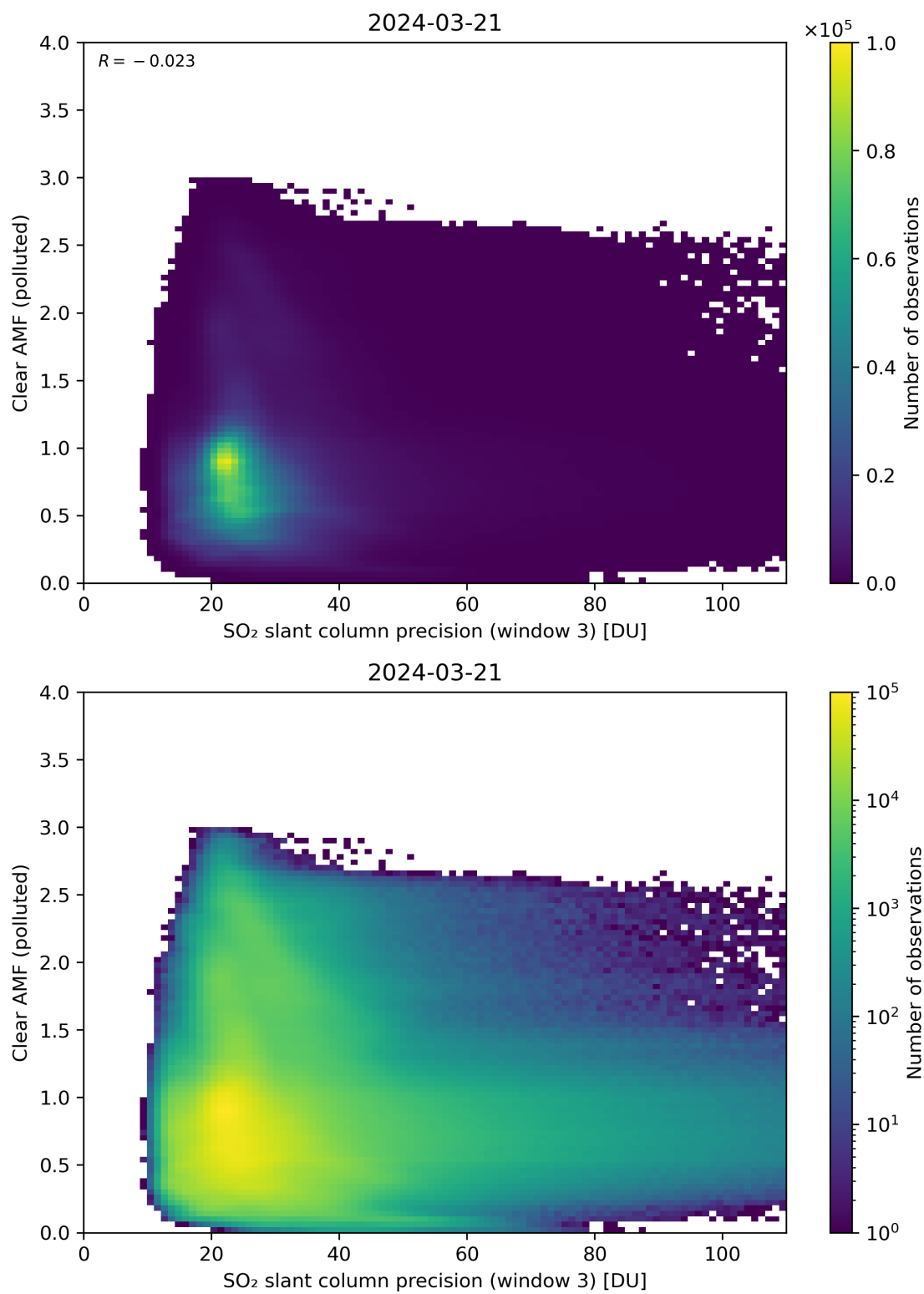
Figure 261: Scatter density plot of “SO 2 slant column precision (window 3)” against “Clear AMF (polluted)” for 2024-03-20 to 2024-03-22.
