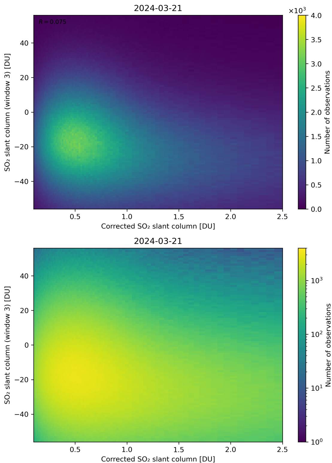
Figure 190: Scatter density plot of “Corrected SO 2 slant column” against “SO 2 slant column (window 3)” for 2024-03-20 to 2024-03-22.
