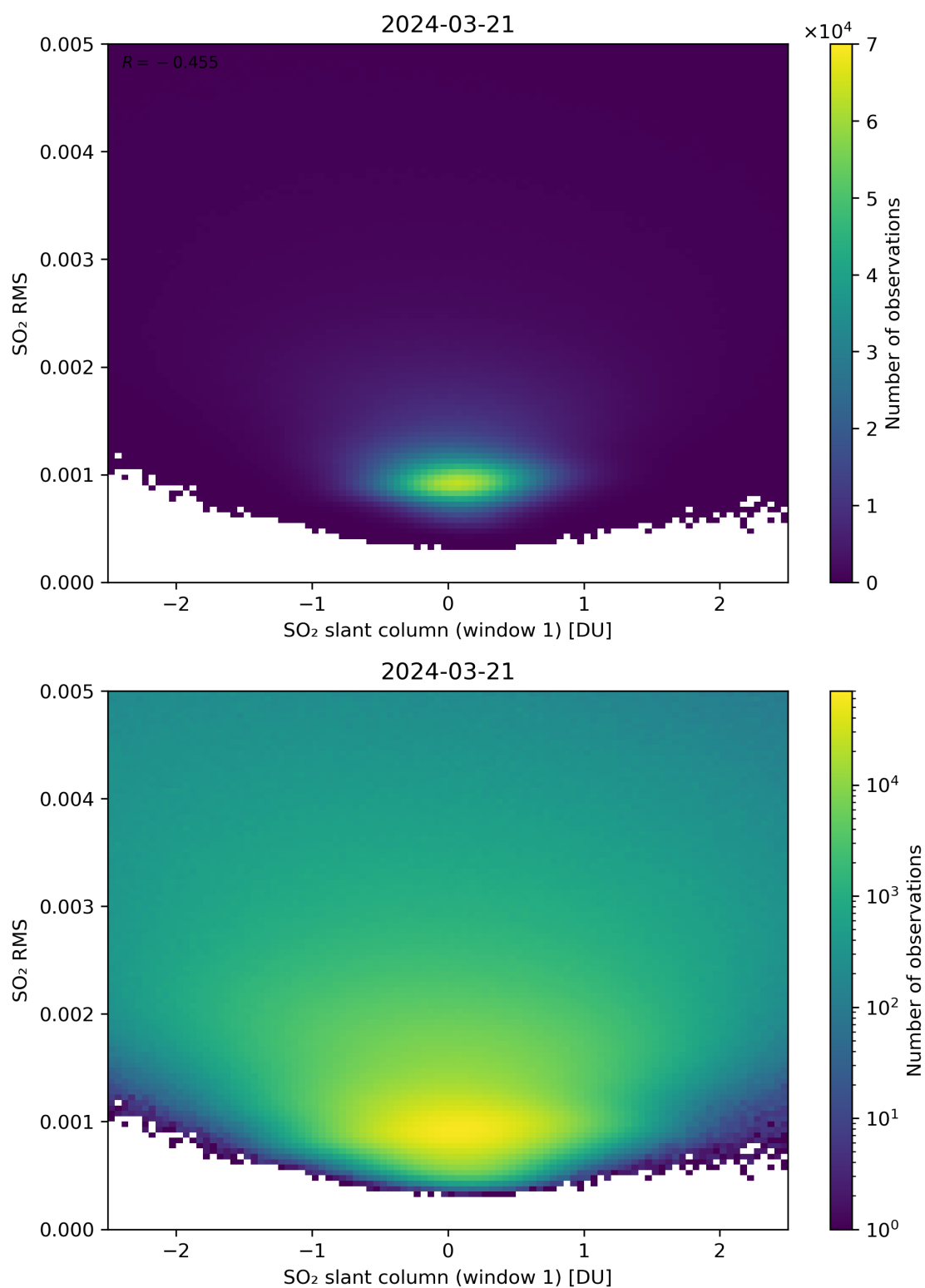
Figure 217: Scatter density plot of “SO 2 slant column (window 1)” against “SO 2 RMS” for 2024-03-20 to 2024-03-22.
