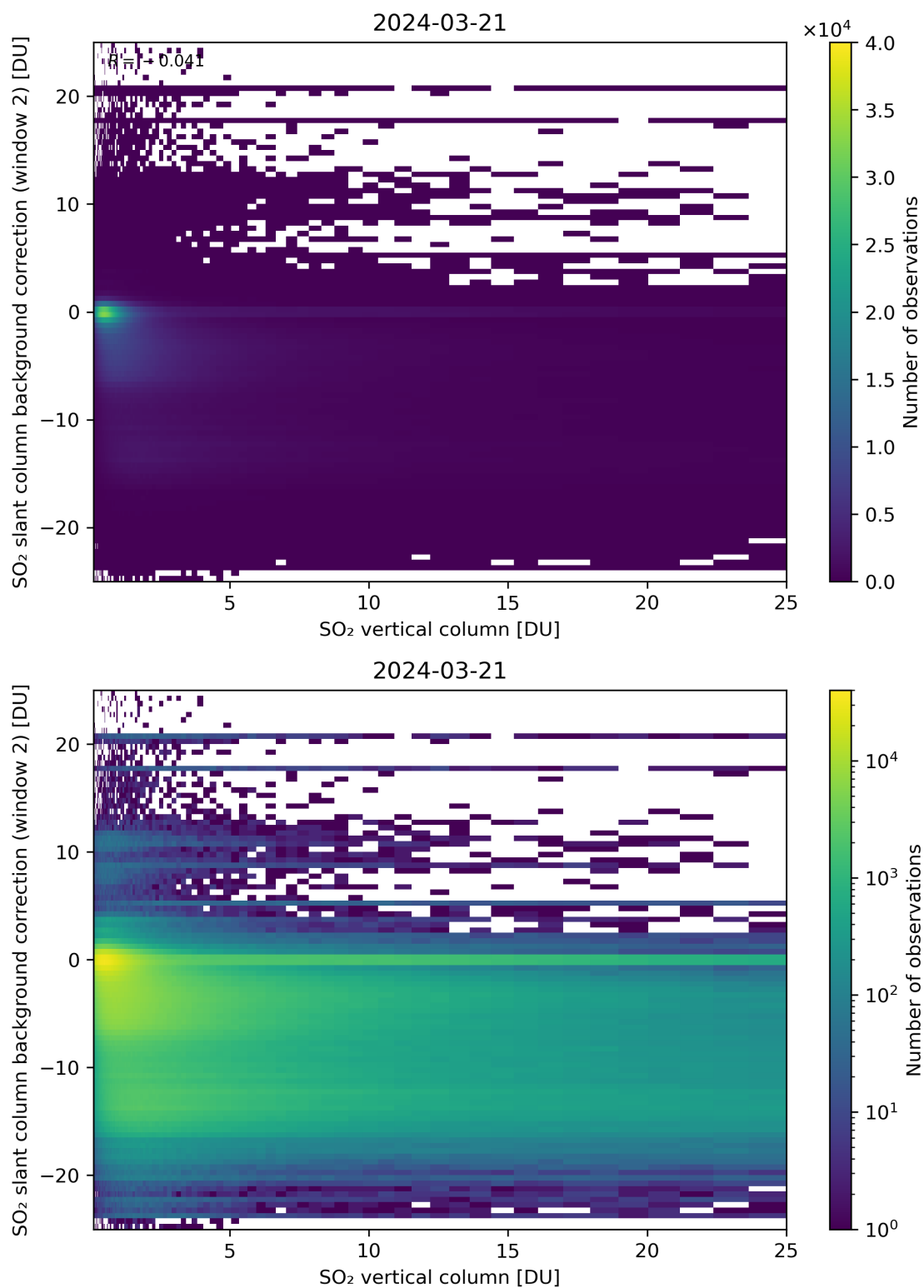
Figure 274: Scatter density plot of “SO 2 vertical column” against “SO 2 slant column background correction (window 2)” for 2024-03-20 to 2024-03-22.
