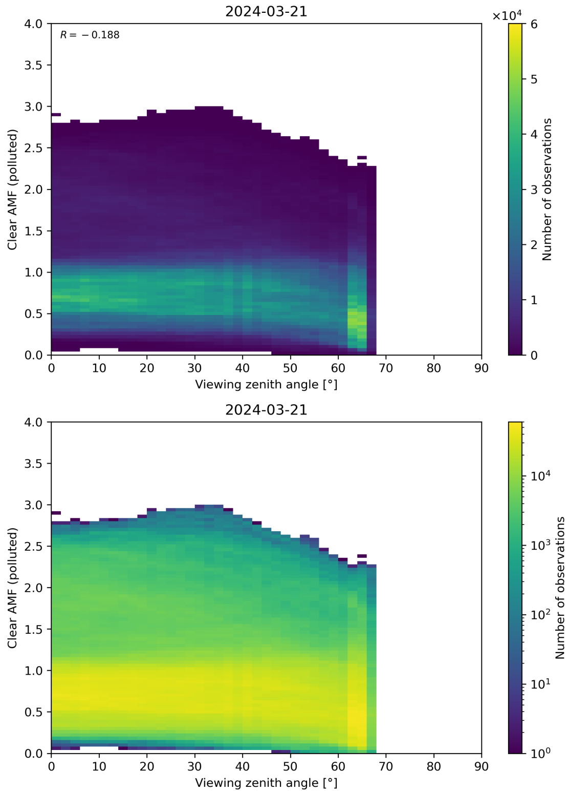
Figure 316: Scatter density plot of “Viewing zenith angle” against “Clear AMF (polluted)” for 2024-03-20 to 2024-03-22.
