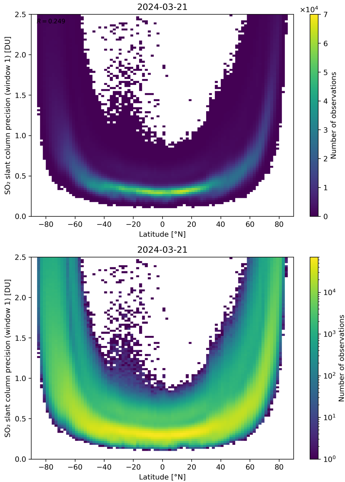
Figure 150: Scatter density plot of “Latitude” against “SO 2 slant column precision (window 1)” for 2024-03-20 to 2024-03-22.
