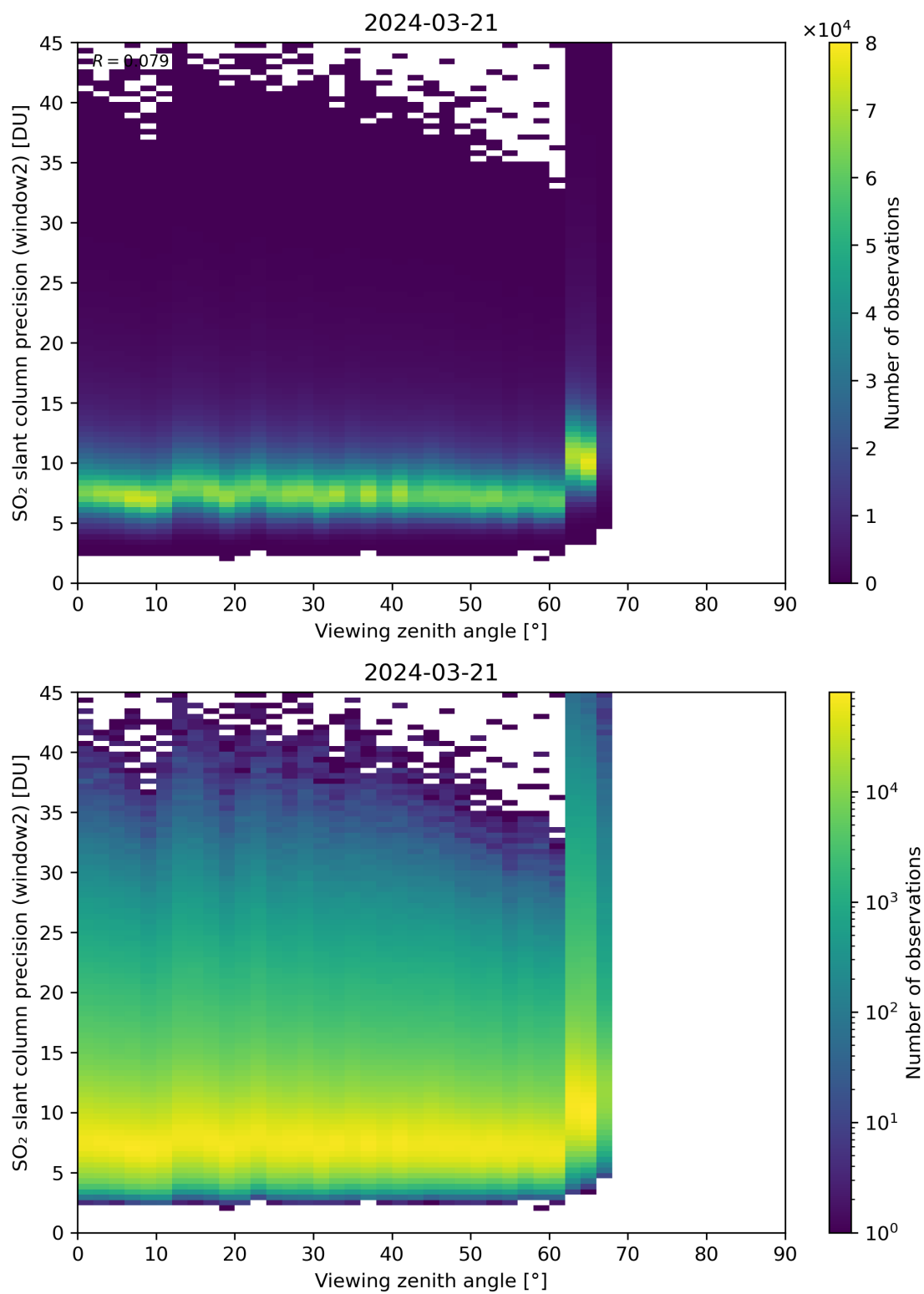
Figure 322: Scatter density plot of “Viewing zenith angle” against “SO 2 slant column precision (window2)” for 2024-03-20 to 2024-03-22.
