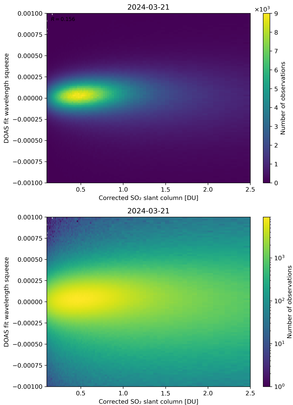
Figure 182: Scatter density plot of “Corrected SO 2 slant column” against “DOAS fit wavelength squeeze” for 2024-03-20 to 2024-03-22.
