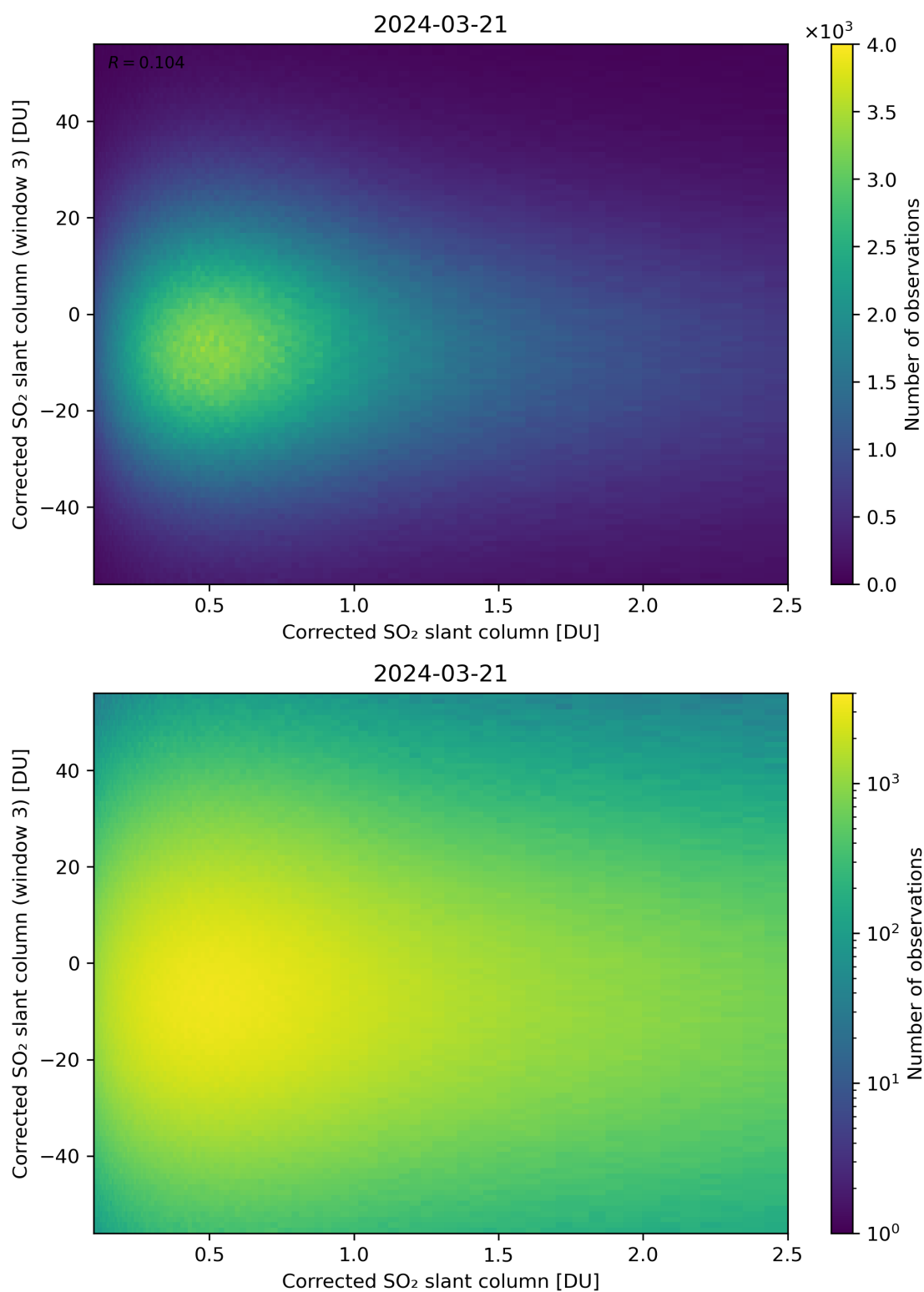
Figure 186: Scatter density plot of “Corrected SO 2 slant column” against “Corrected SO 2 slant column (window 3)” for 2024-03-20 to 2024-03-22.
