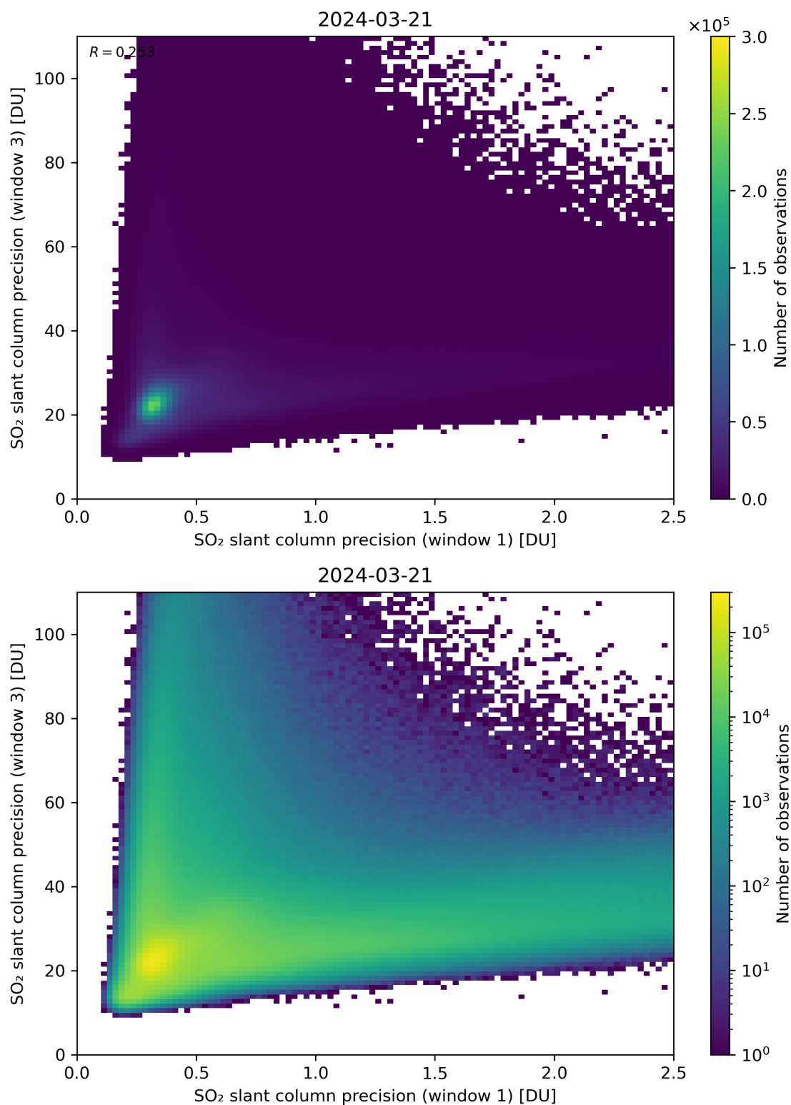
Figure 229: Scatter density plot of “SO 2 slant column precision (window 1)” against “SO 2 slant column precision (window 3)” for 2024-03-20 to 2024-03-22.
