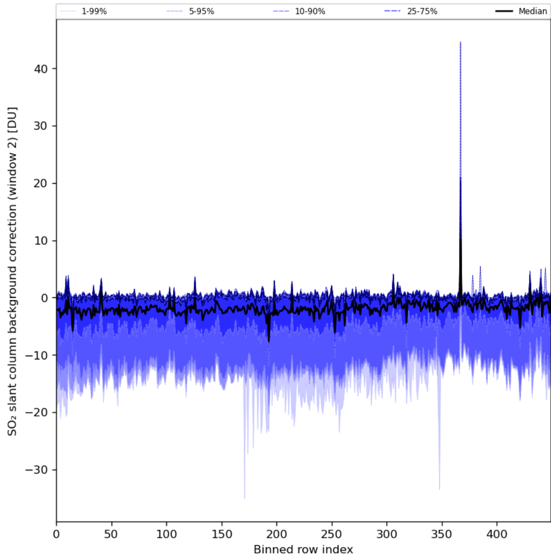
Figure 86: Along track statistics of “SO 2 slant column background correction (window 2)” for 2024-03-20 to 2024-03-22
