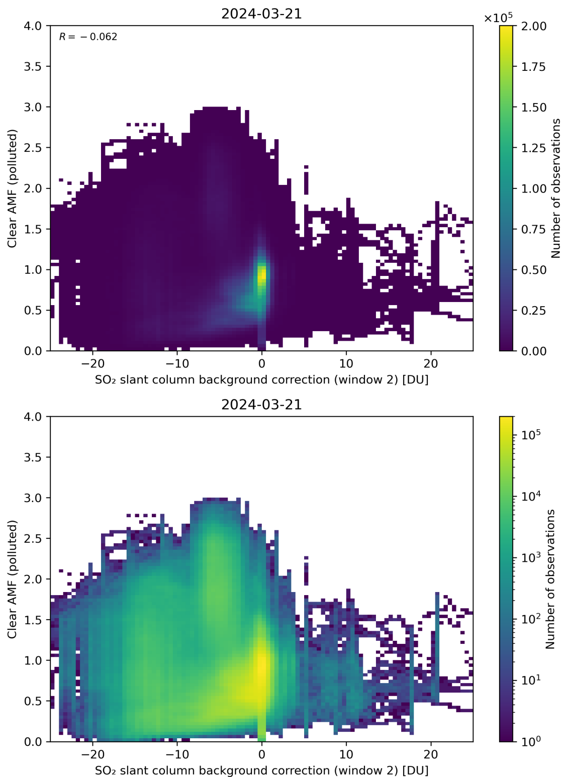
Figure 115: Scatter density plot of “SO 2 slant column background correction (window 2)” against “Clear AMF (polluted)” for 2024-03-20 to 2024-03-22.
