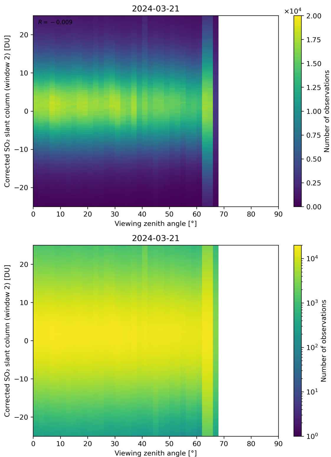
Figure 318: Scatter density plot of “Viewing zenith angle” against “Corrected SO 2 slant column (window 2)” for 2024-03-20 to 2024-03-22.
