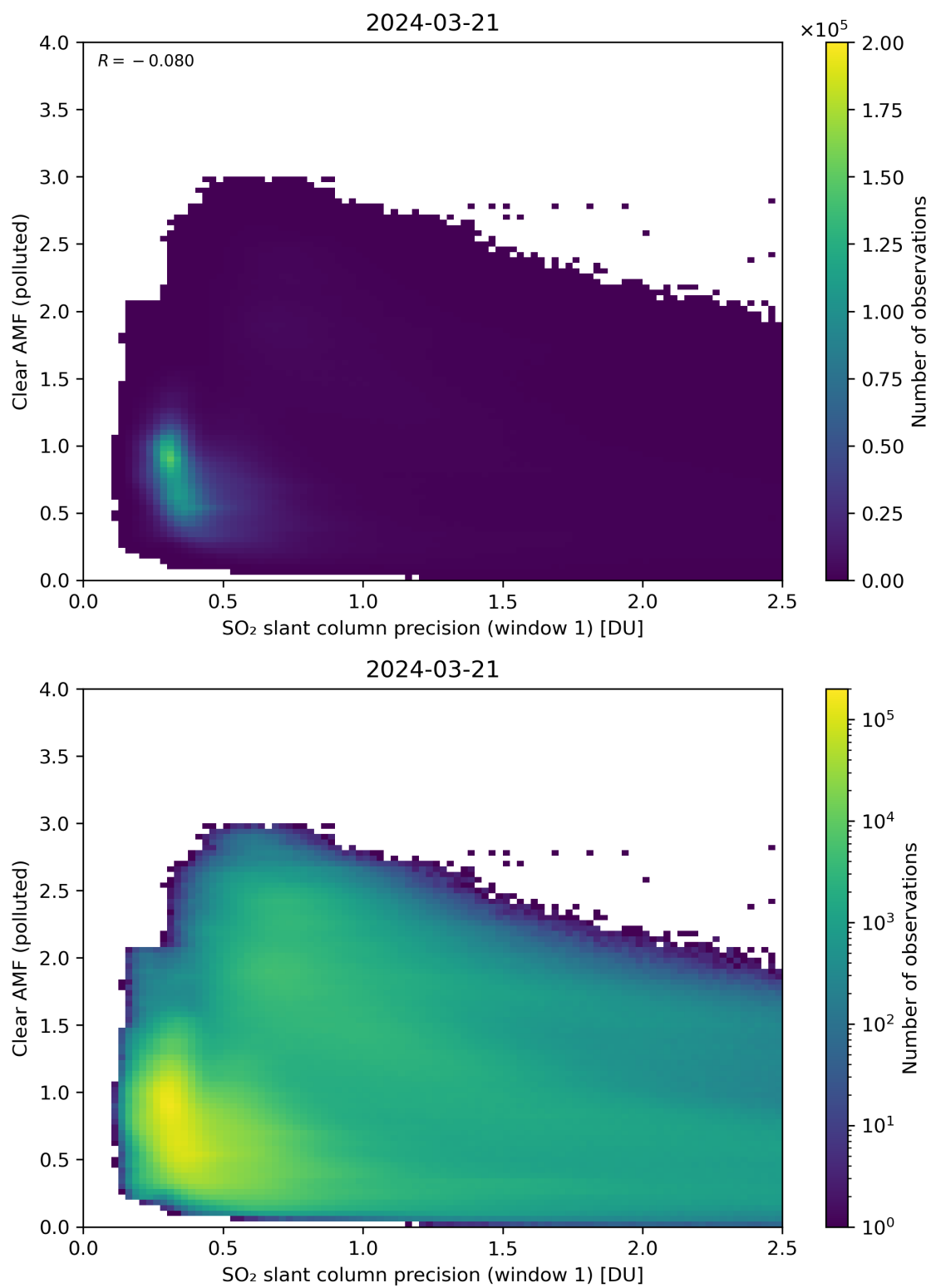
Figure 224: Scatter density plot of “SO 2 slant column precision (window 1)” against “Clear AMF (polluted)” for 2024-03-20 to 2024-03-22.
