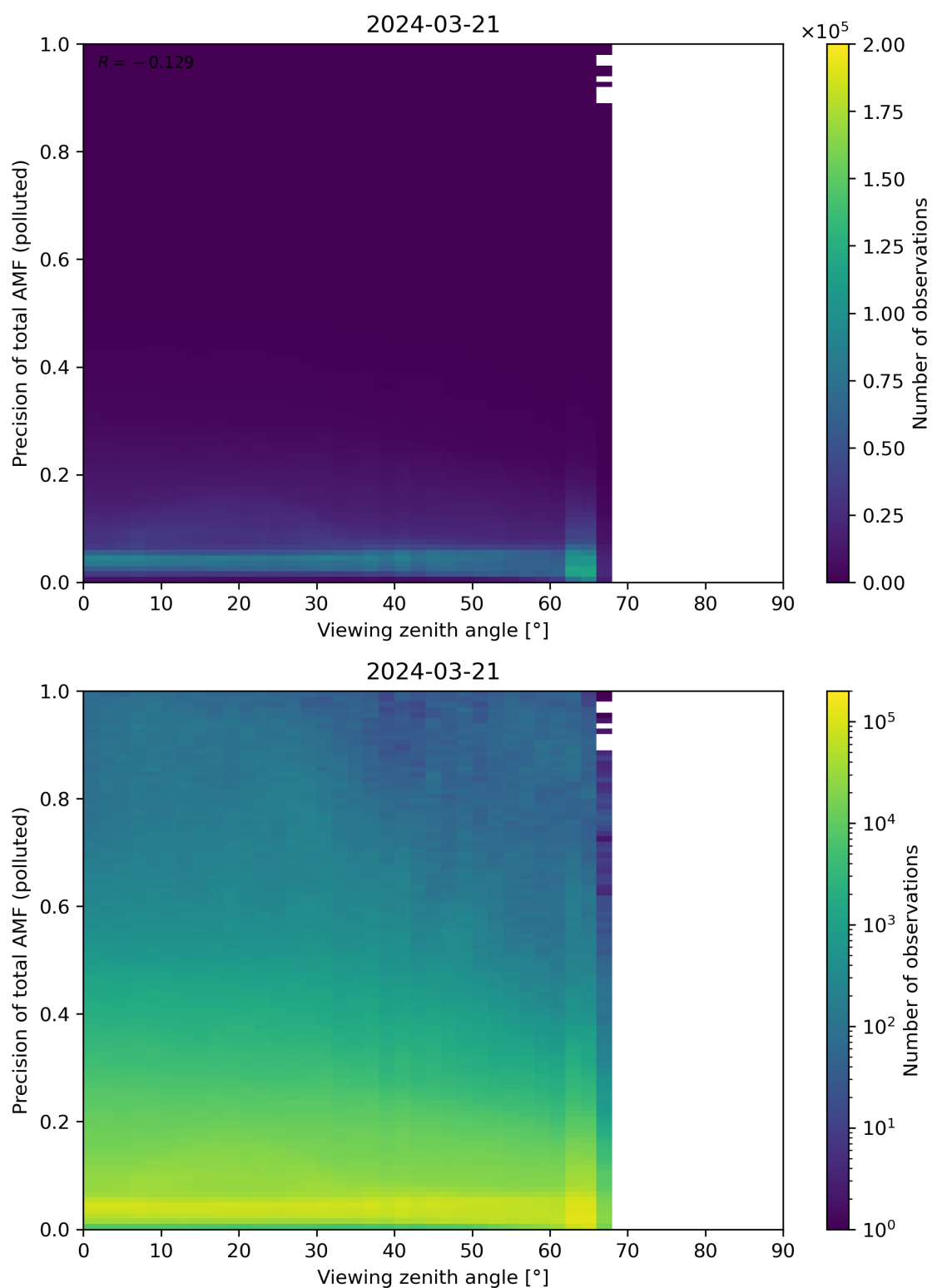
Figure 326: Scatter density plot of “Viewing zenith angle” against “Precision of total AMF (polluted)” for 2024-03-20 to 2024-03-22.
