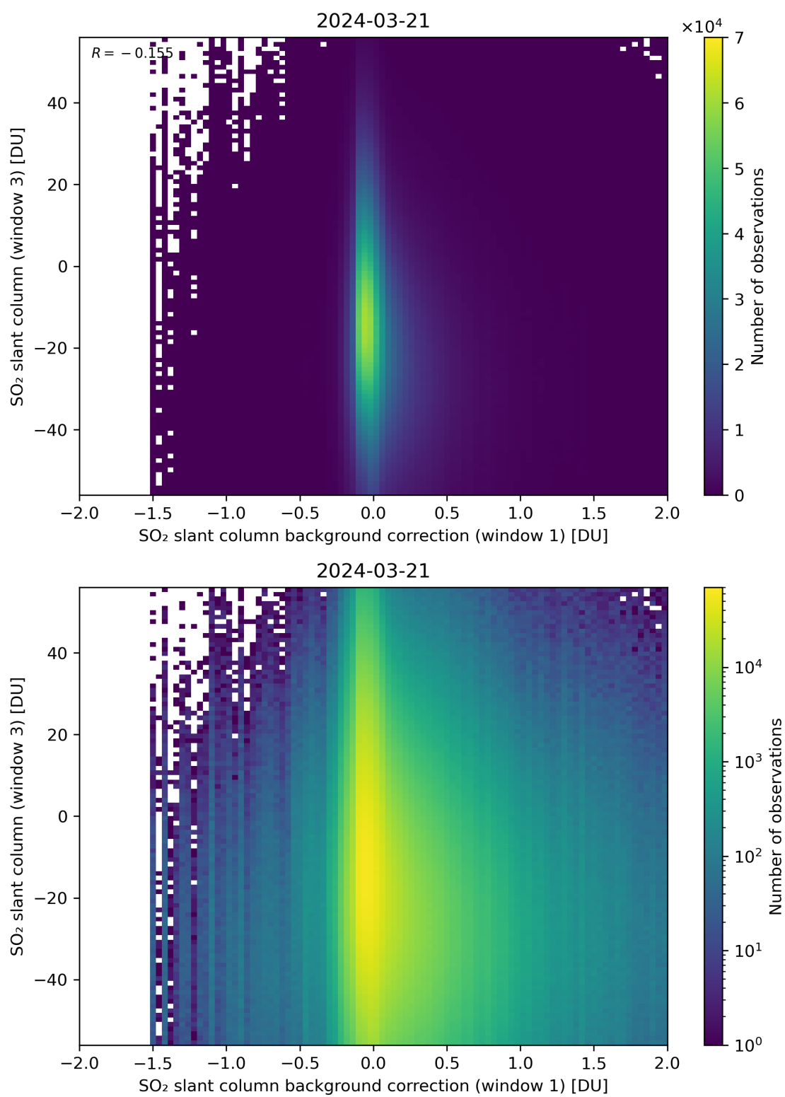
Figure 107: Scatter density plot of “SO 2 slant column background correction (window 1)” against “SO 2 slant column (window 3)” for 2024-03-20 to 2024-03-22.
