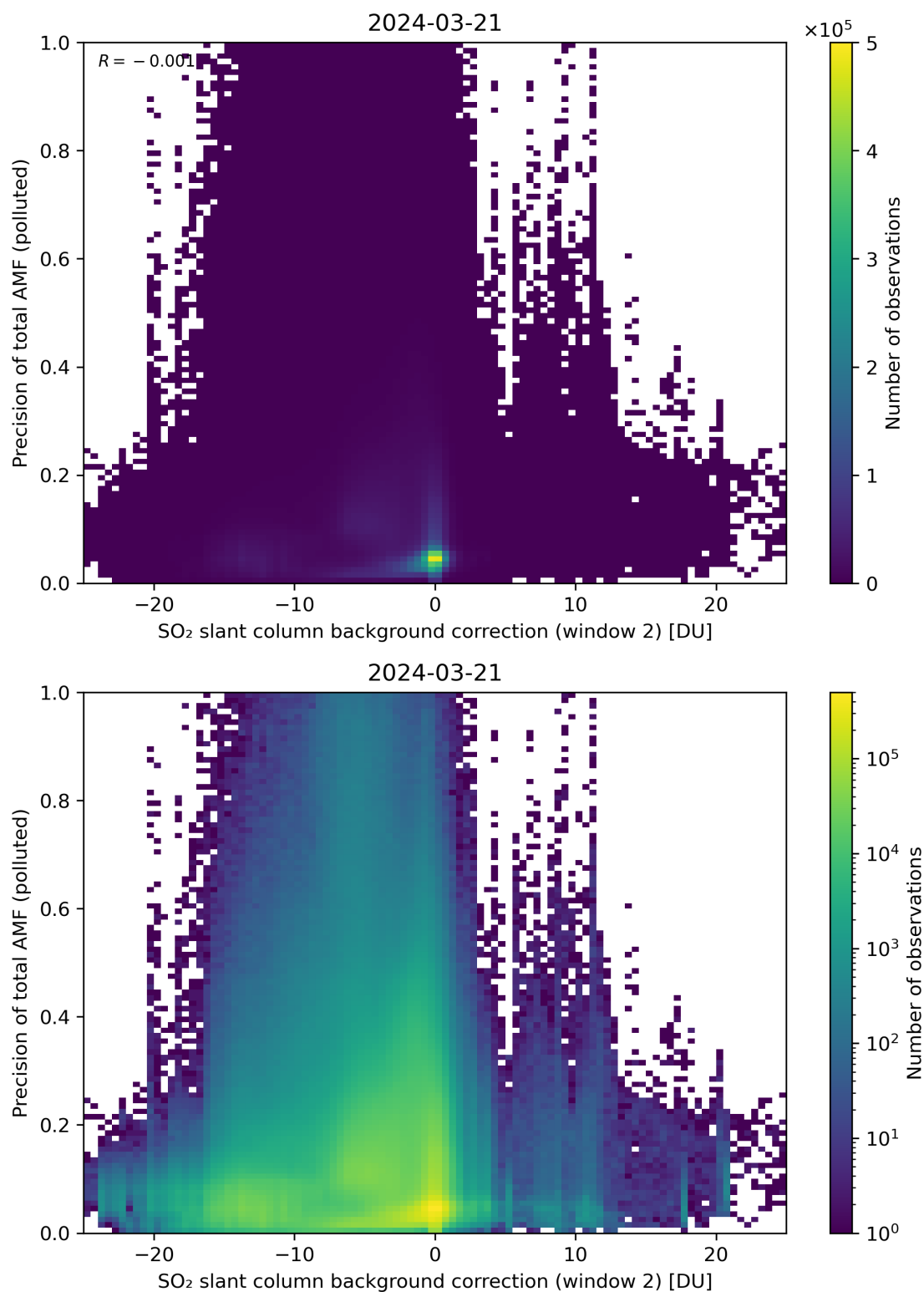
Figure 120: Scatter density plot of “SO 2 slant column background correction (window 2)” against “Precision of total AMF (polluted)” for 2024-03-20 to 2024-03-22.
