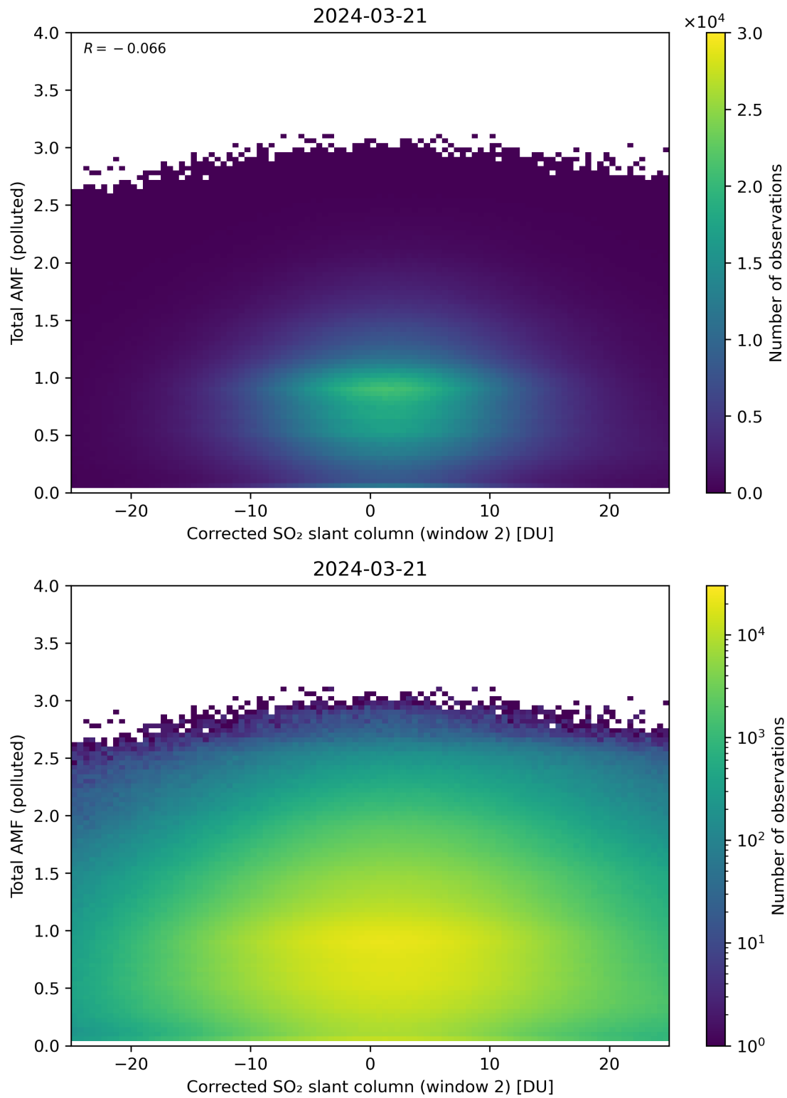
Figure 203: Scatter density plot of “Corrected SO 2 slant column (window 2)” against “Total AMF (polluted)” for 2024-03-20 to 2024-03-22.
