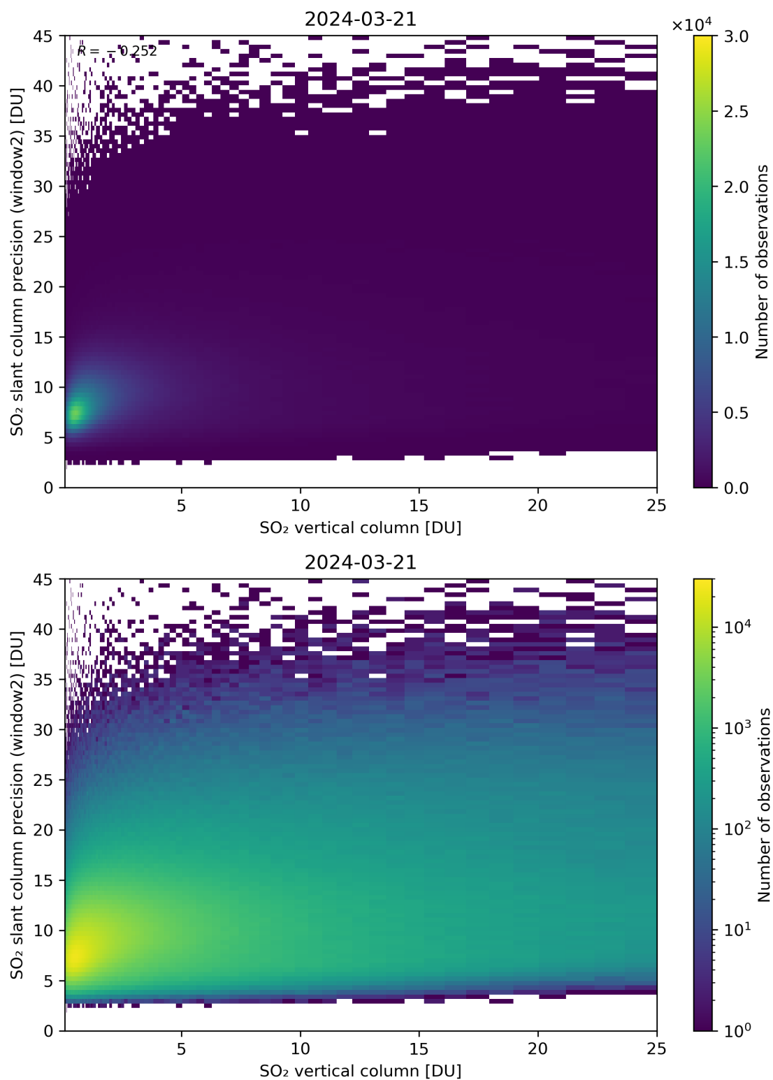
Figure 302: Scatter density plot of “SO 2 vertical column” against “SO 2 slant column precision (window2)” for 2024-03-20 to 2024-03-22.
