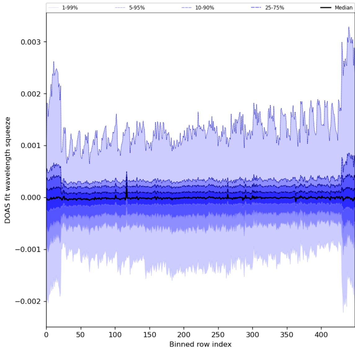
Figure 92: Along track statistics of “DOAS fit wavelength squeeze” for 2024-03-20 to 2024-03-22
