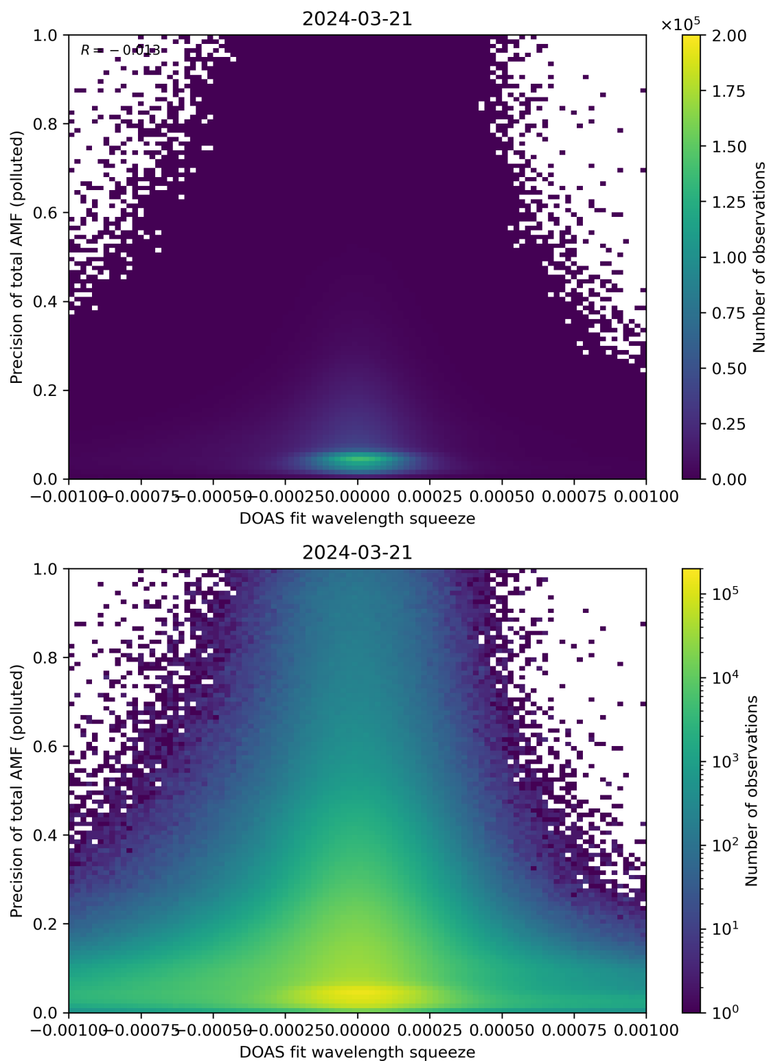
Figure 135: Scatter density plot of “DOAS fit wavelength squeeze” against “Precision of total AMF (polluted)” for 2024-03-20 to 2024-03-22.
