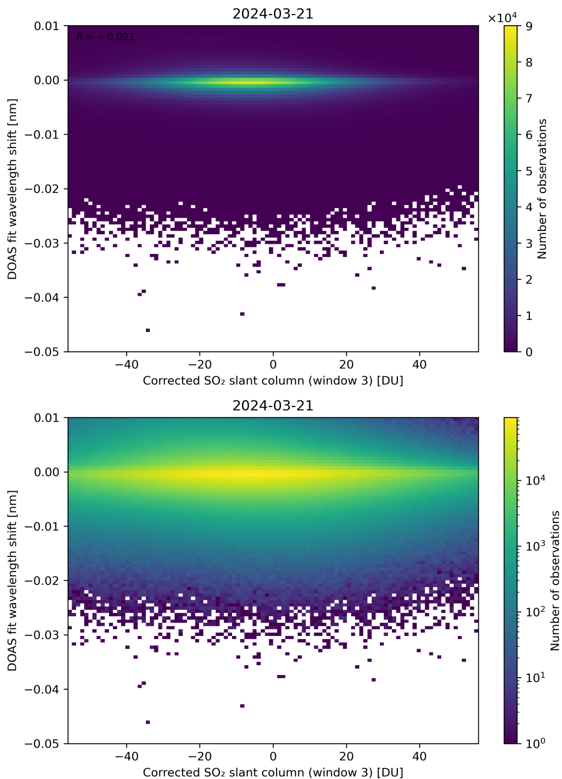
Figure 206: Scatter density plot of “Corrected SO 2 slant column (window 3)” against “DOAS fit wavelength shift” for 2024-03-20 to 2024-03-22.
