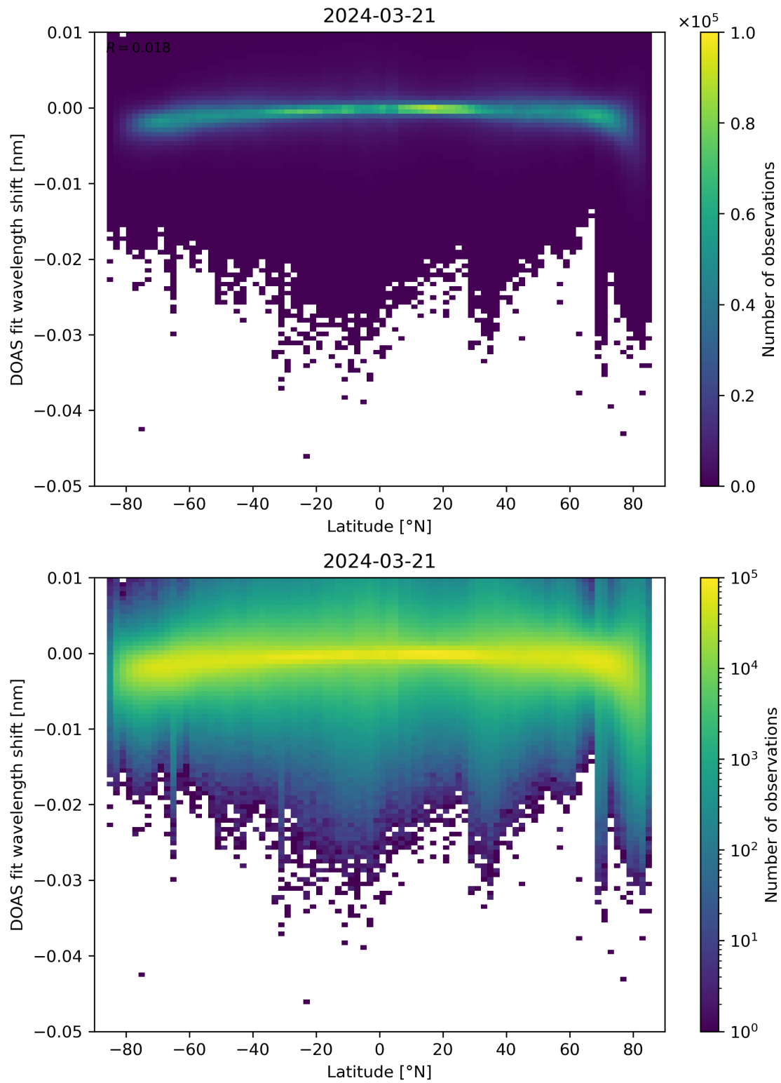
Figure 142: Scatter density plot of “Latitude” against “DOAS fit wavelength shift” for 2024-03-20 to 2024-03-22.
