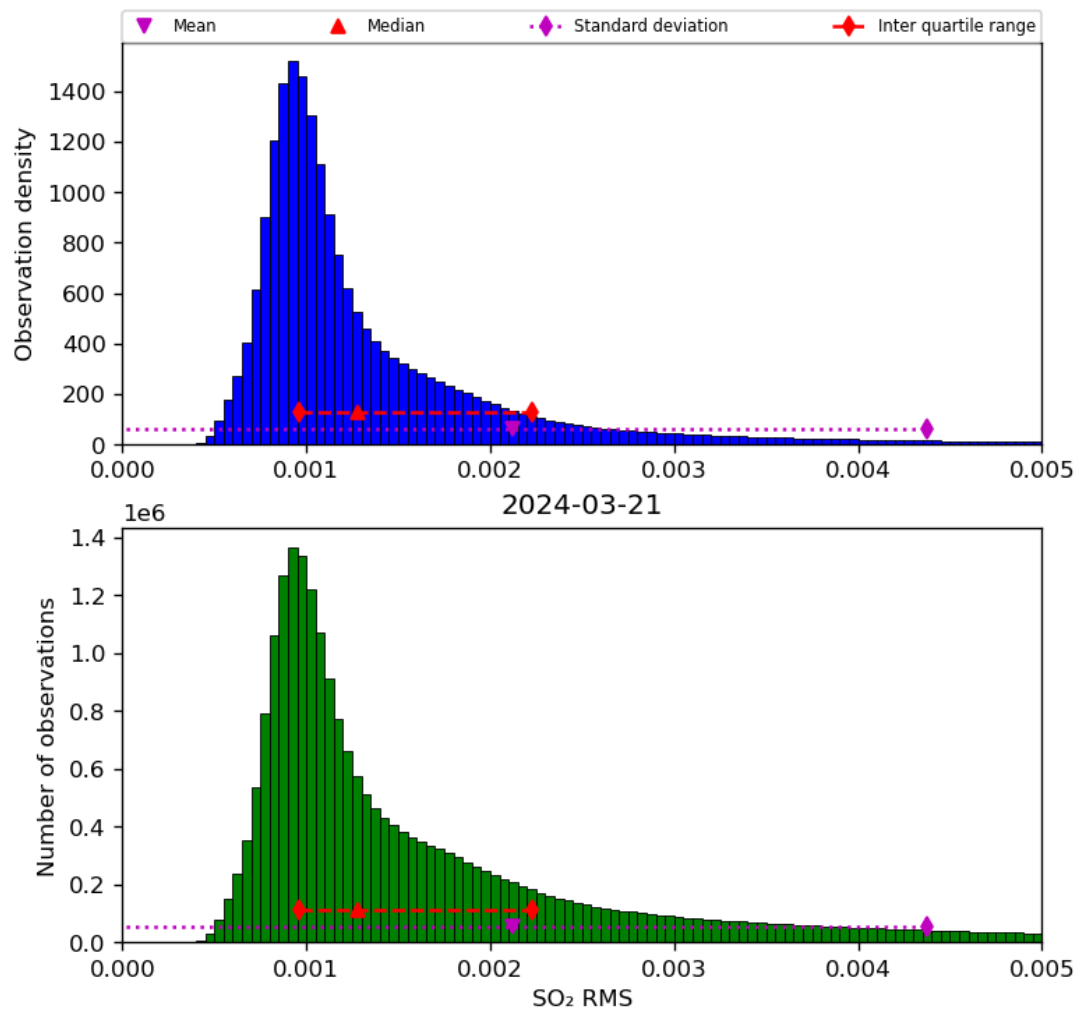
Figure 70: Histogram of “SO 2 RMS” for 2024-03-20 to 2024-03-22
