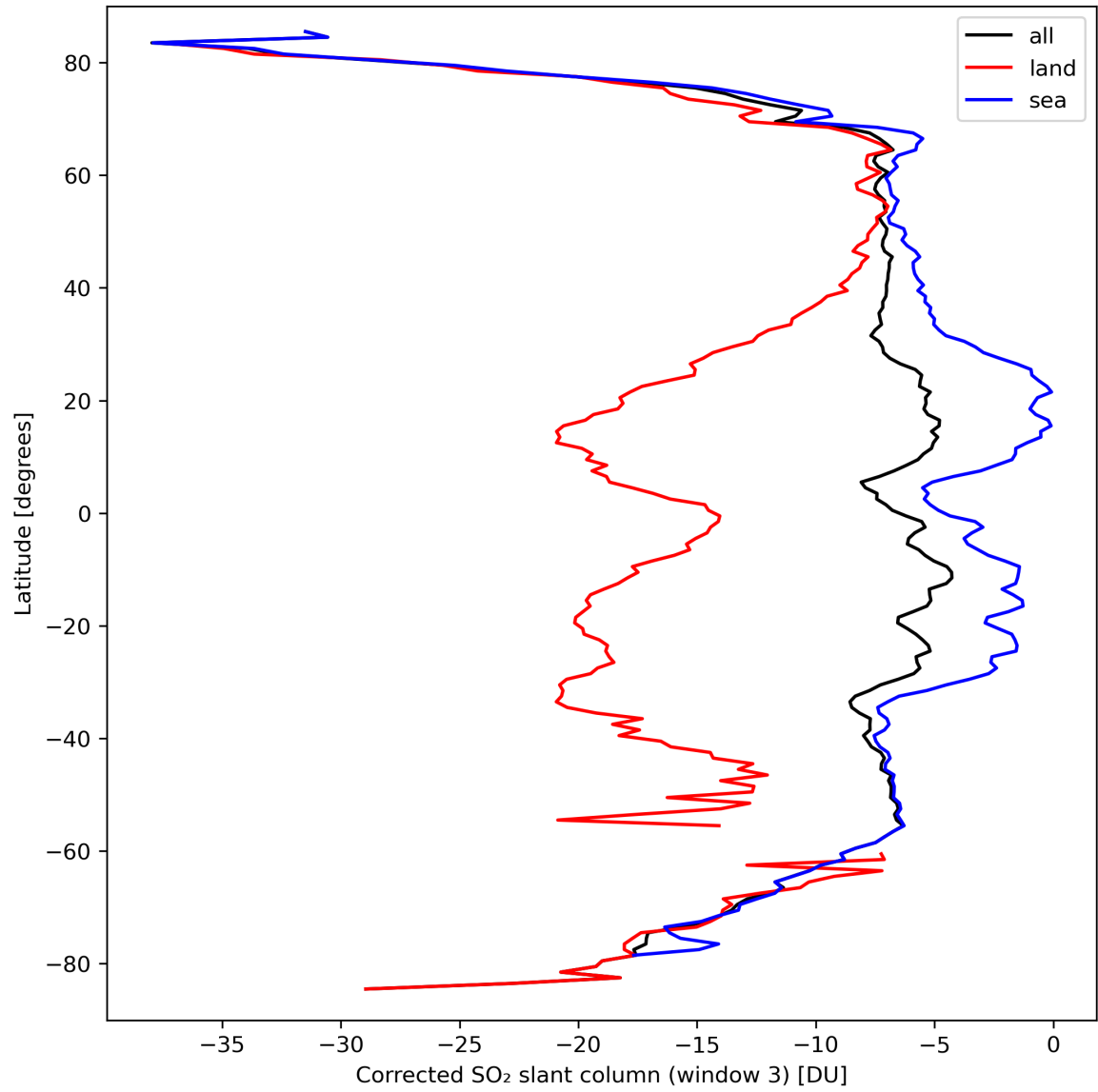
Figure 43: Zonal average of “Corrected SO 2 slant column (window 3)” for 2024-03-20 to 2024-03-22.
