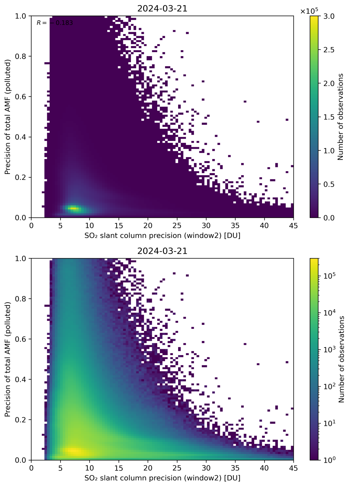
Figure 252: Scatter density plot of “SO 2 slant column precision (window2)” against “Precision of total AMF (polluted)” for 2024-03-20 to 2024-03-22.
