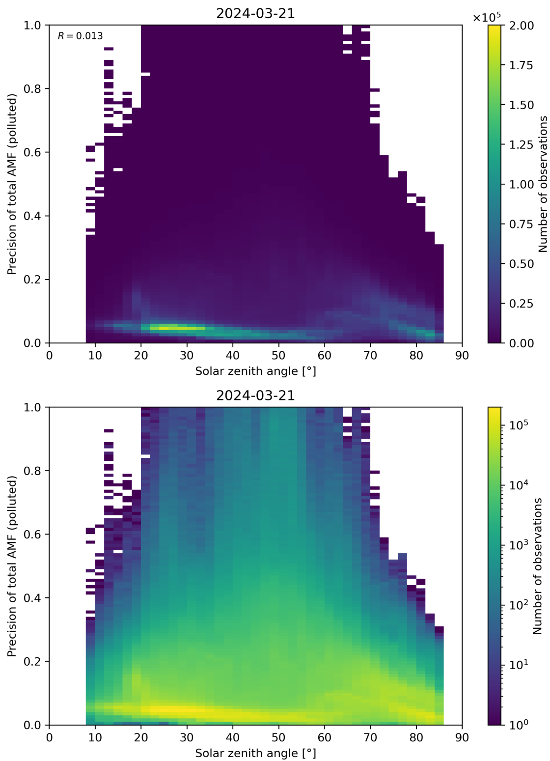
Figure 175: Scatter density plot of “Solar zenith angle” against “Precision of total AMF (polluted)” for 2024-03-20 to 2024-03-22.
