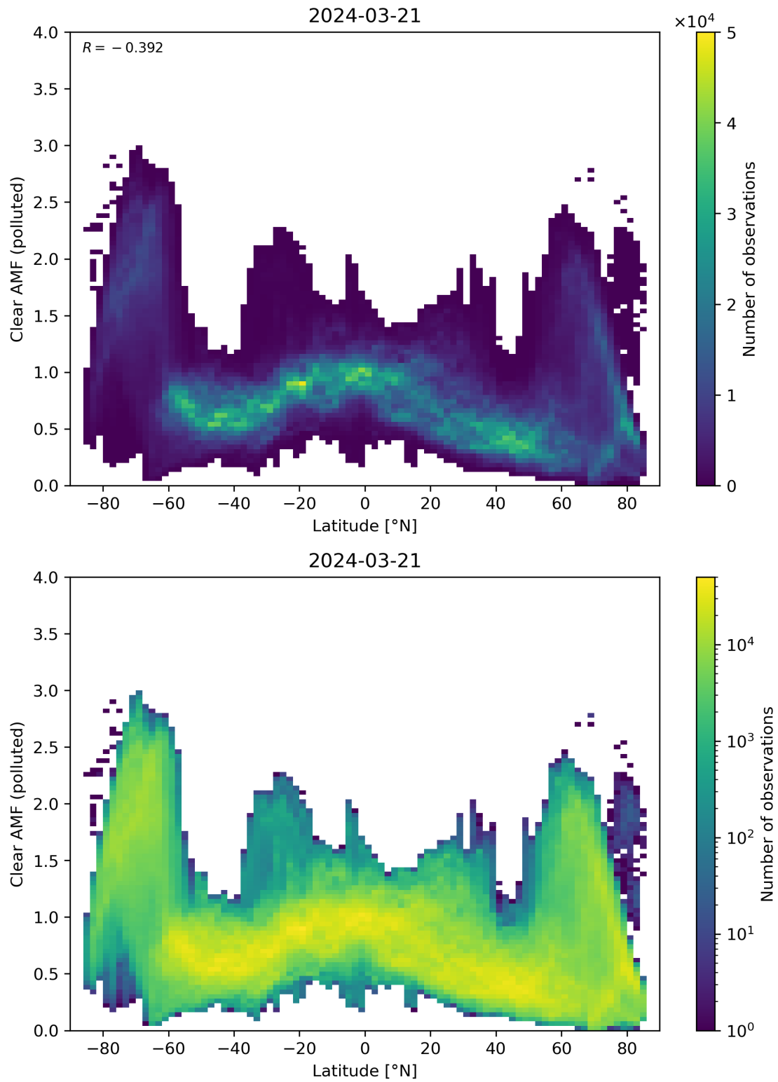
Figure 145: Scatter density plot of “Latitude” against “Clear AMF (polluted)” for 2024-03-20 to 2024-03-22.
