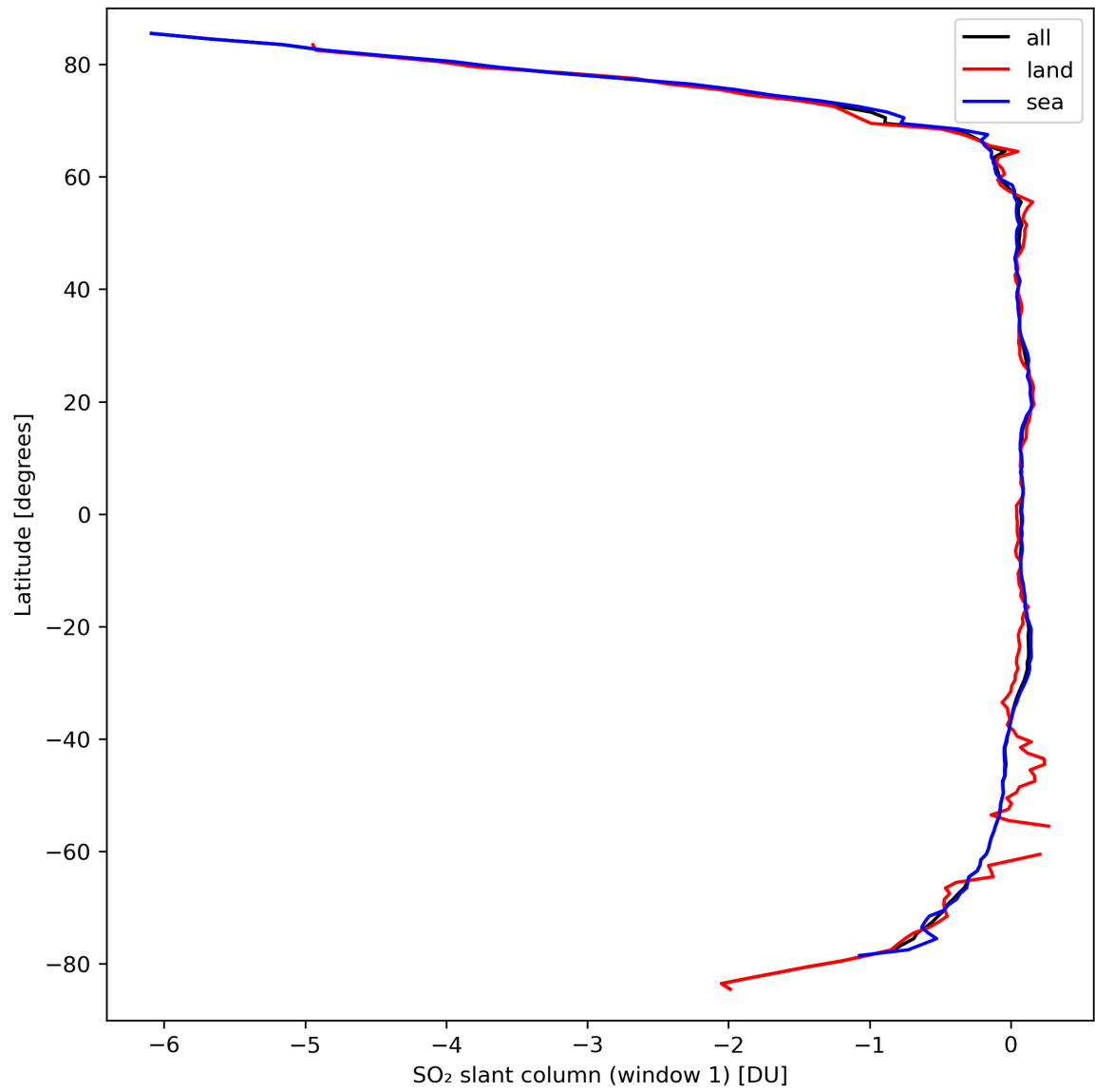
Figure 33: Zonal average of “SO 2 slant column (window 1)” for 2024-03-20 to 2024-03-22.
