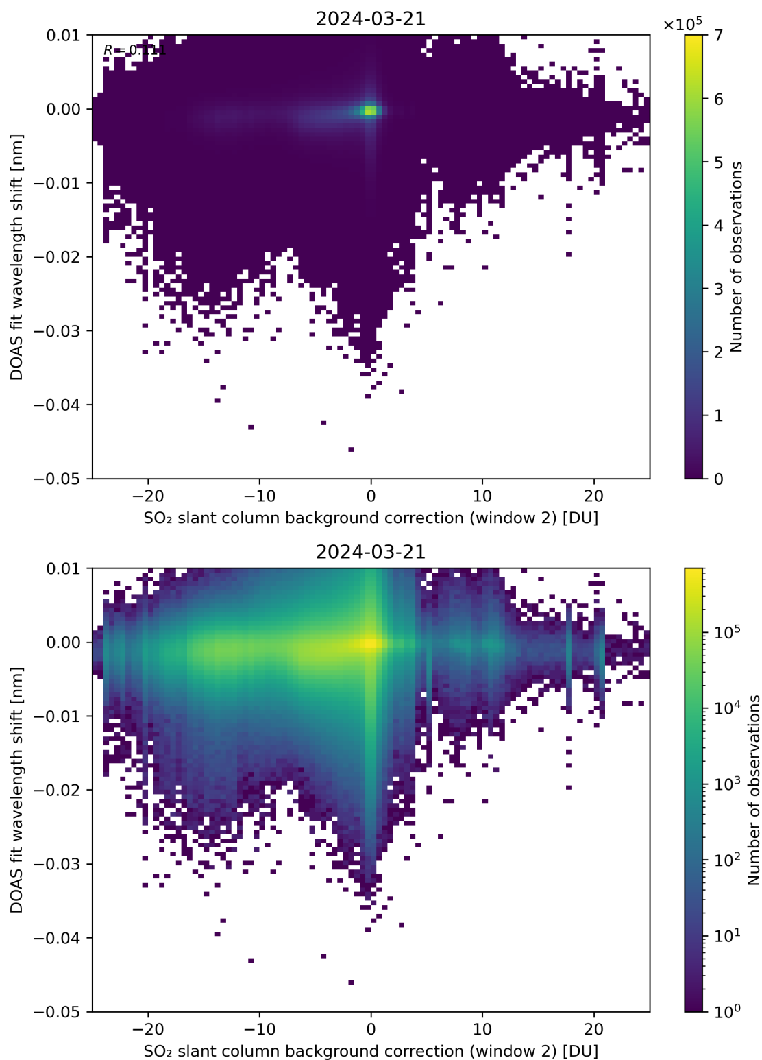
Figure 112: Scatter density plot of “SO 2 slant column background correction (window 2)” against “DOAS fit wavelength shift” for 2024-03-20 to 2024-03-22.
