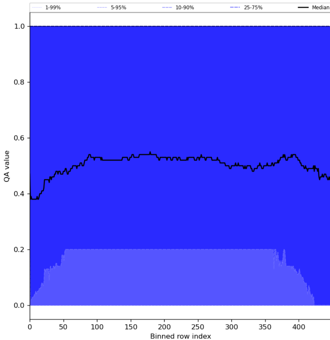
Figure 75: Along track statistics of “QA value” for 2024-03-20 to 2024-03-22
