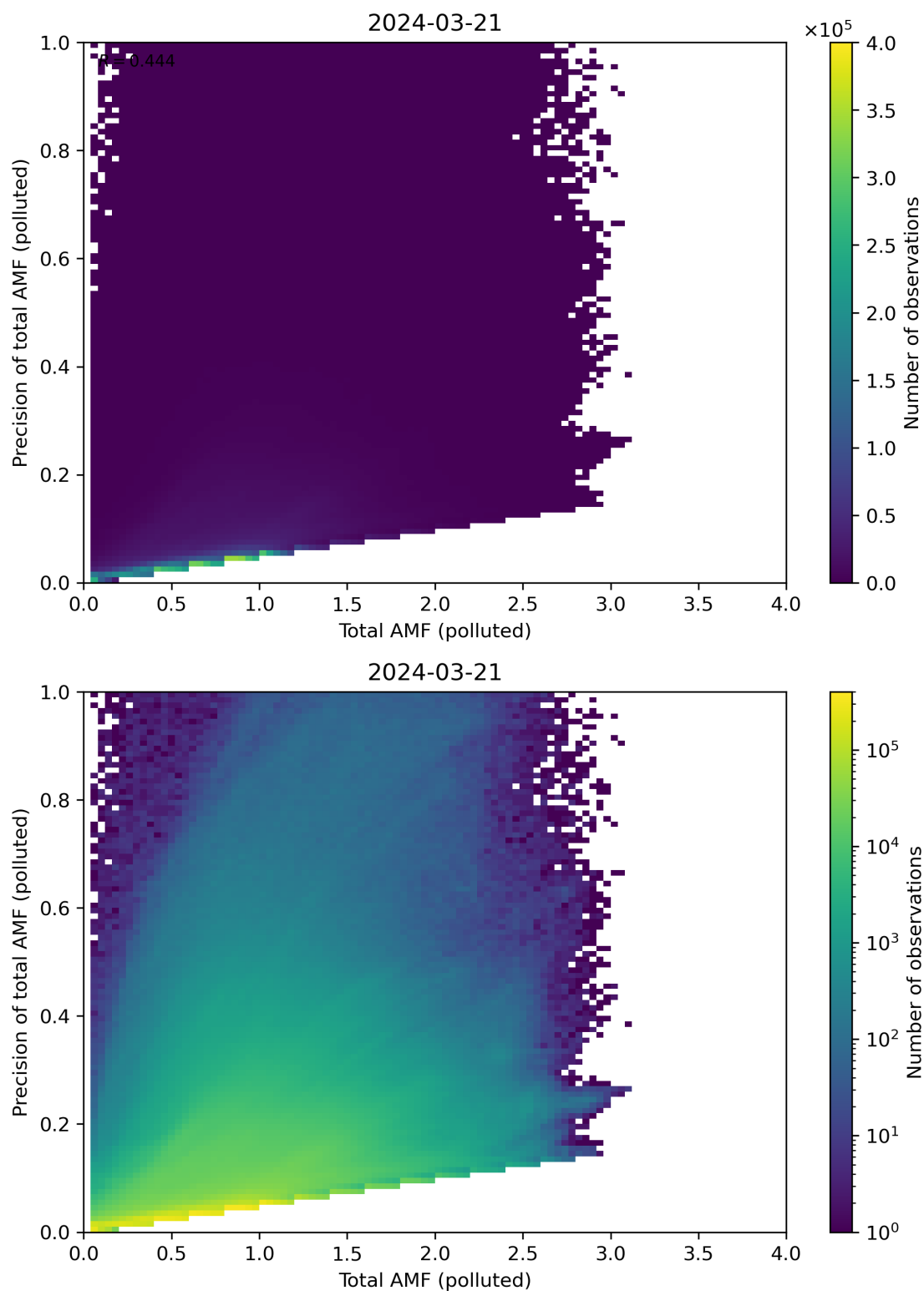
Figure 272: Scatter density plot of “Total AMF (polluted)” against “Precision of total AMF (polluted)” for 2024-03-20 to 2024-03-22.
