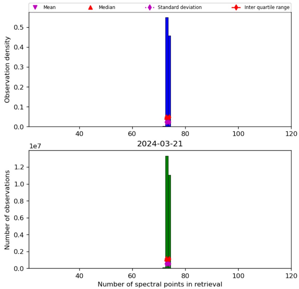
Figure 74: Histogram of “Number of spectral points in retrieval” for 2024-03-20 to 2024-03-22
