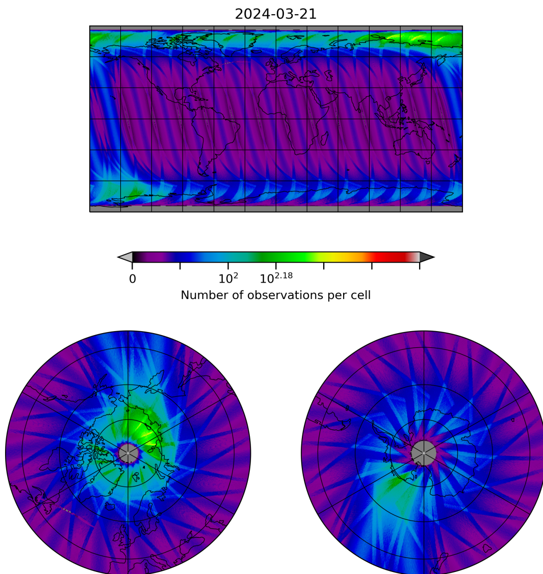
Figure 28: Map of the number of observations for 2024-03-20 to 2024-03-22
