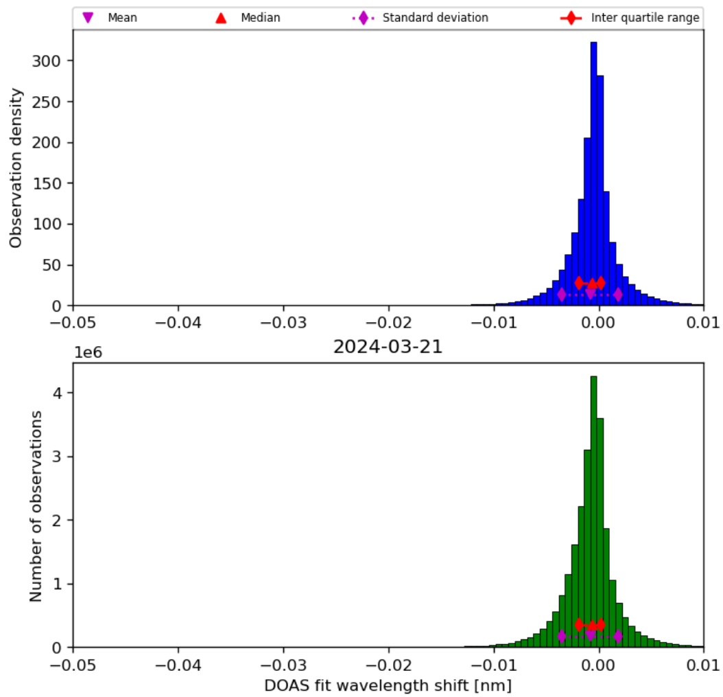
Figure 68: Histogram of “DOAS fit wavelength shift” for 2024-03-20 to 2024-03-22
