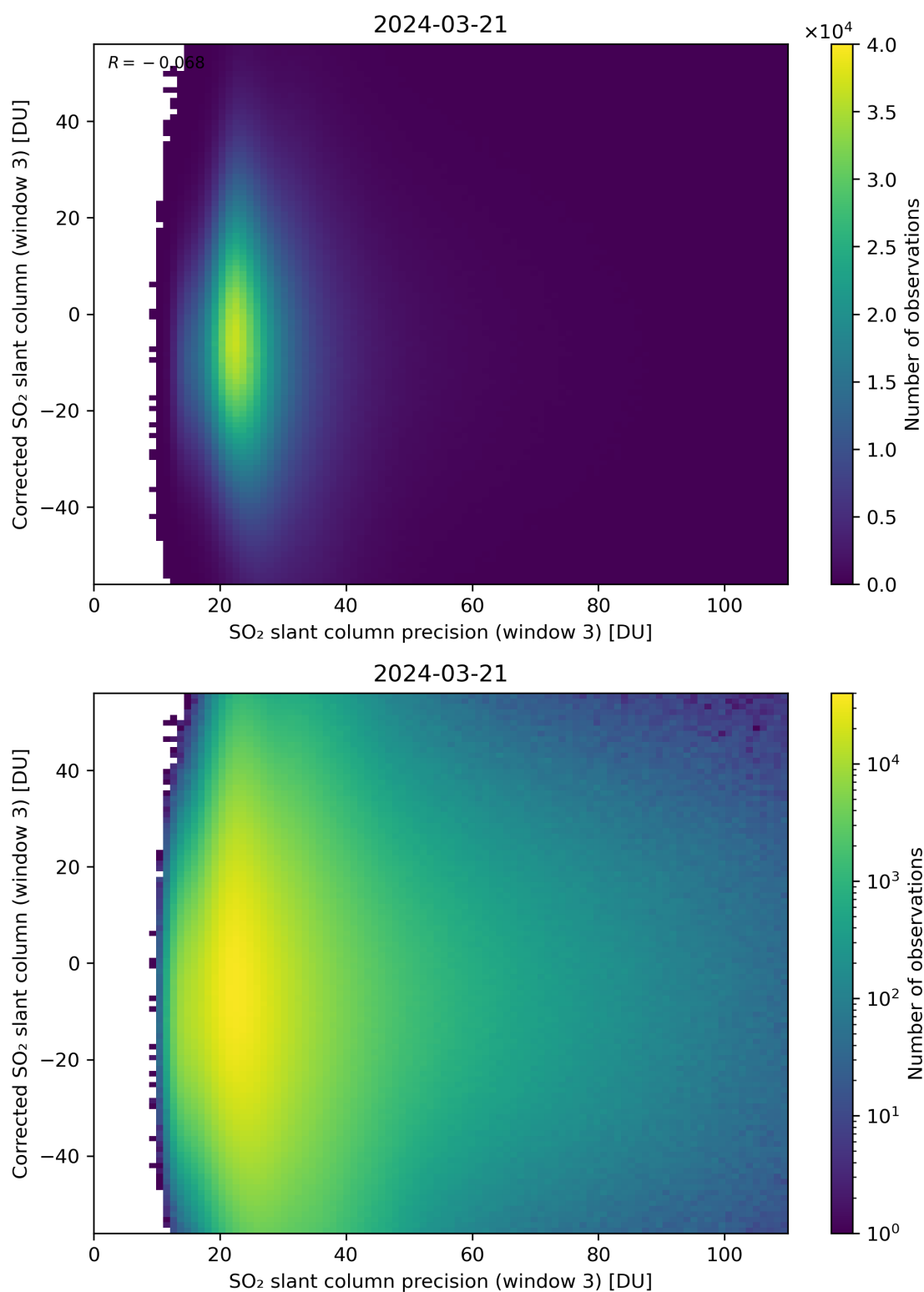
Figure 262: Scatter density plot of “SO 2 slant column precision (window 3)” against “Corrected SO 2 slant column (window 3)” for 2024-03-20 to 2024-03-22.
