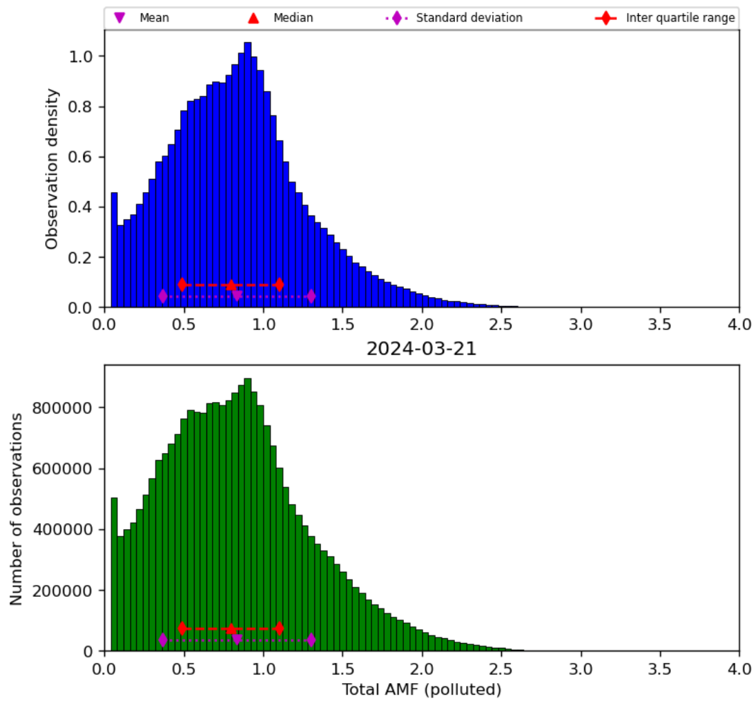
Figure 71: Histogram of “Total AMF (polluted)” for 2024-03-20 to 2024-03-22
