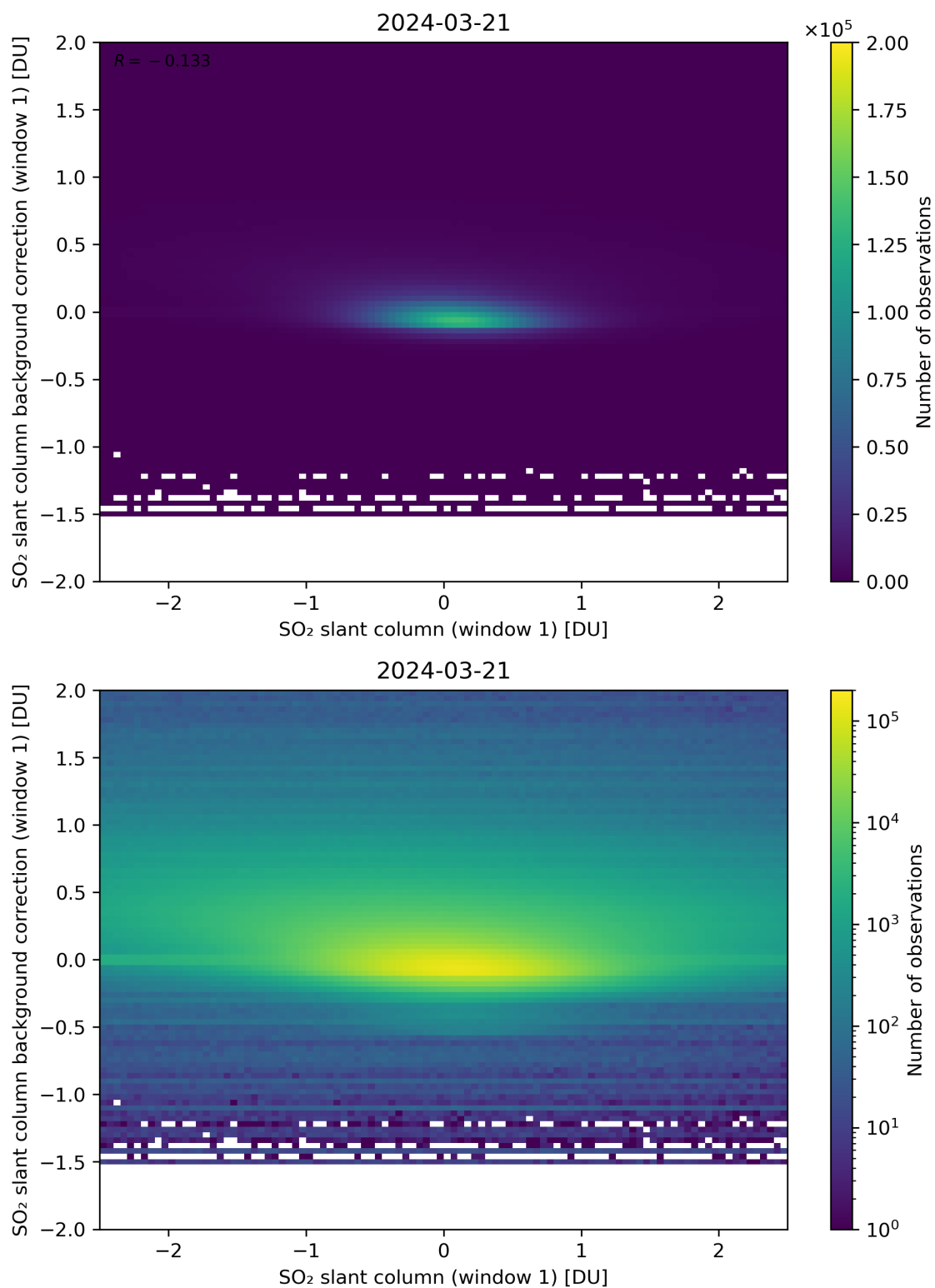
Figure 212: Scatter density plot of “SO 2 slant column (window 1)” against “SO 2 slant column background correction (window 1)” for 2024-03-20 to 2024-03-22.
