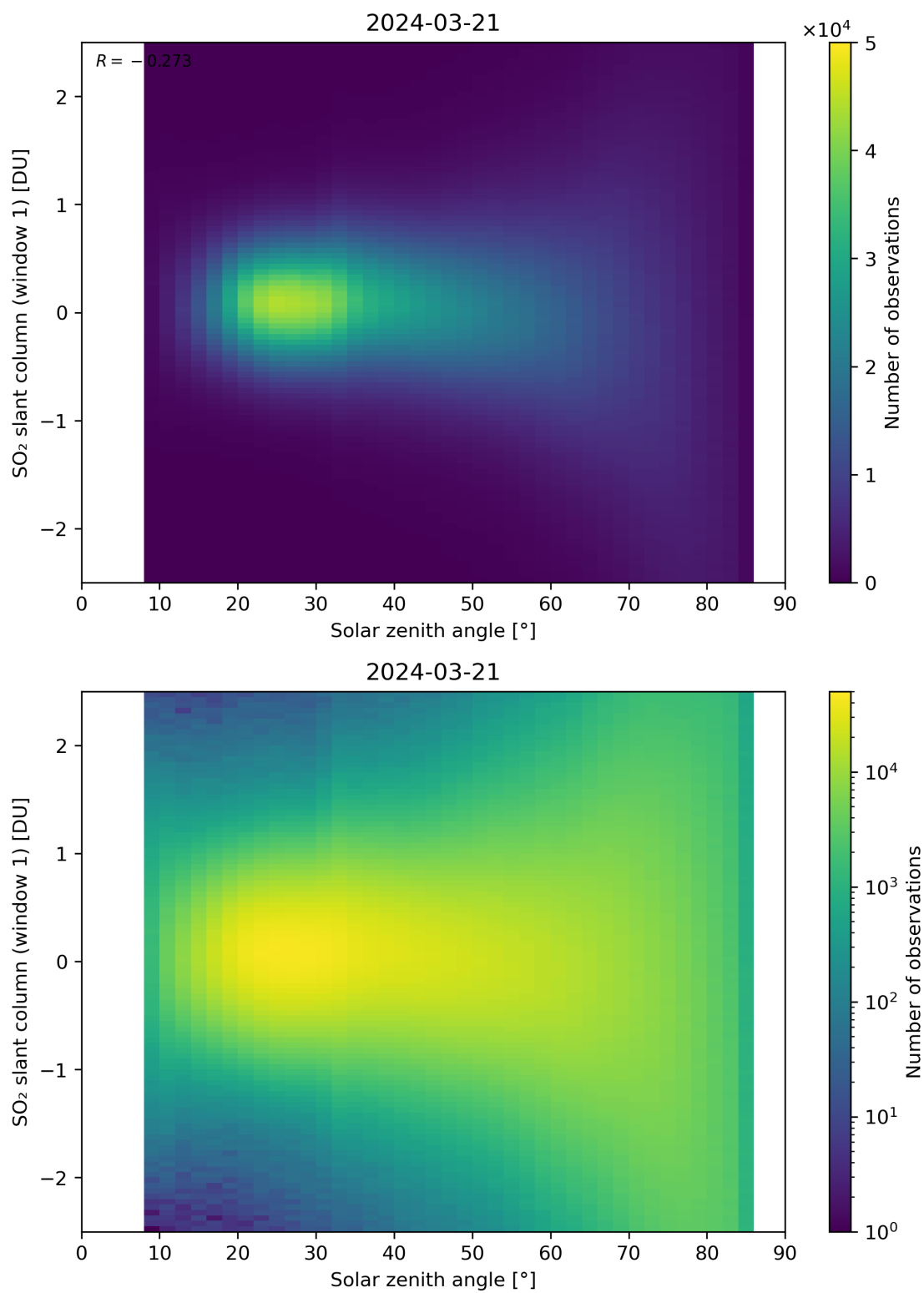
Figure 169: Scatter density plot of “Solar zenith angle” against “SO 2 slant column (window 1)” for 2024-03-20 to 2024-03-22.
