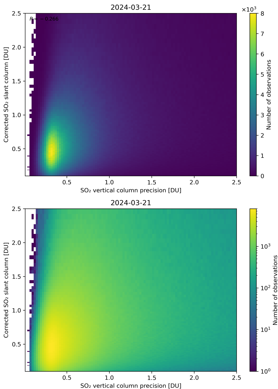
Figure 286: Scatter density plot of “SO 2 vertical column precision” against “Corrected SO 2 slant column” for 2024-03-20 to 2024-03-22.
