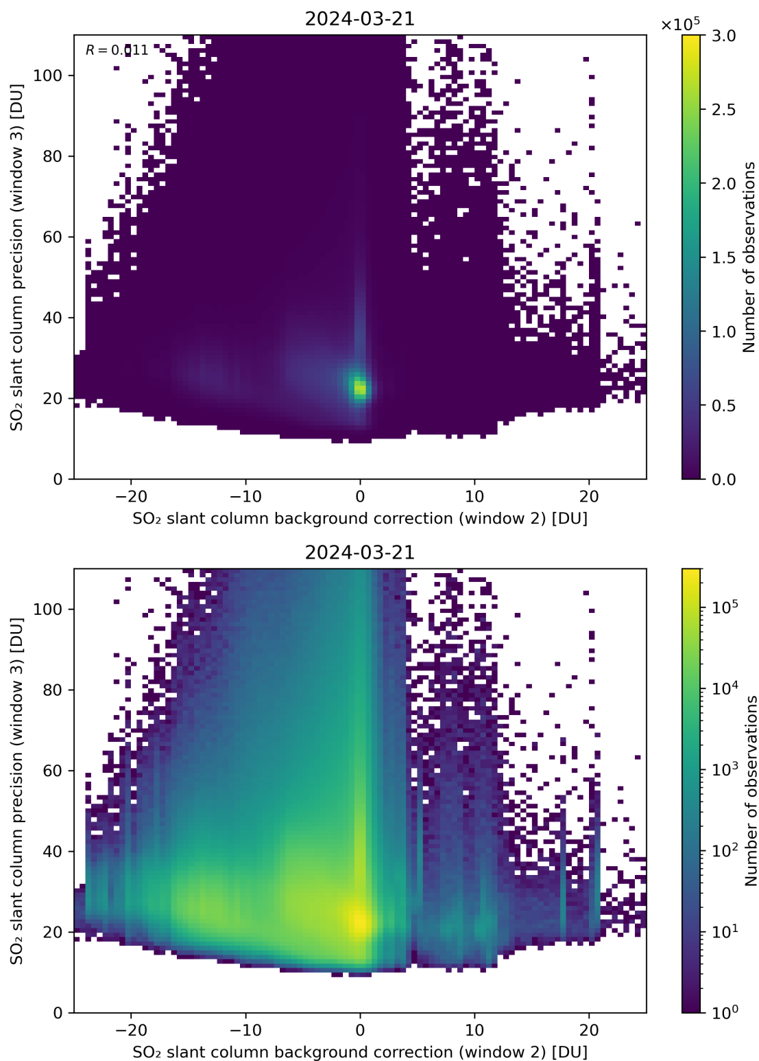
Figure 118: Scatter density plot of “SO 2 slant column background correction (window 2)” against “SO 2 slant column precision (window 3)” for 2024-03-20 to 2024-03-22.
