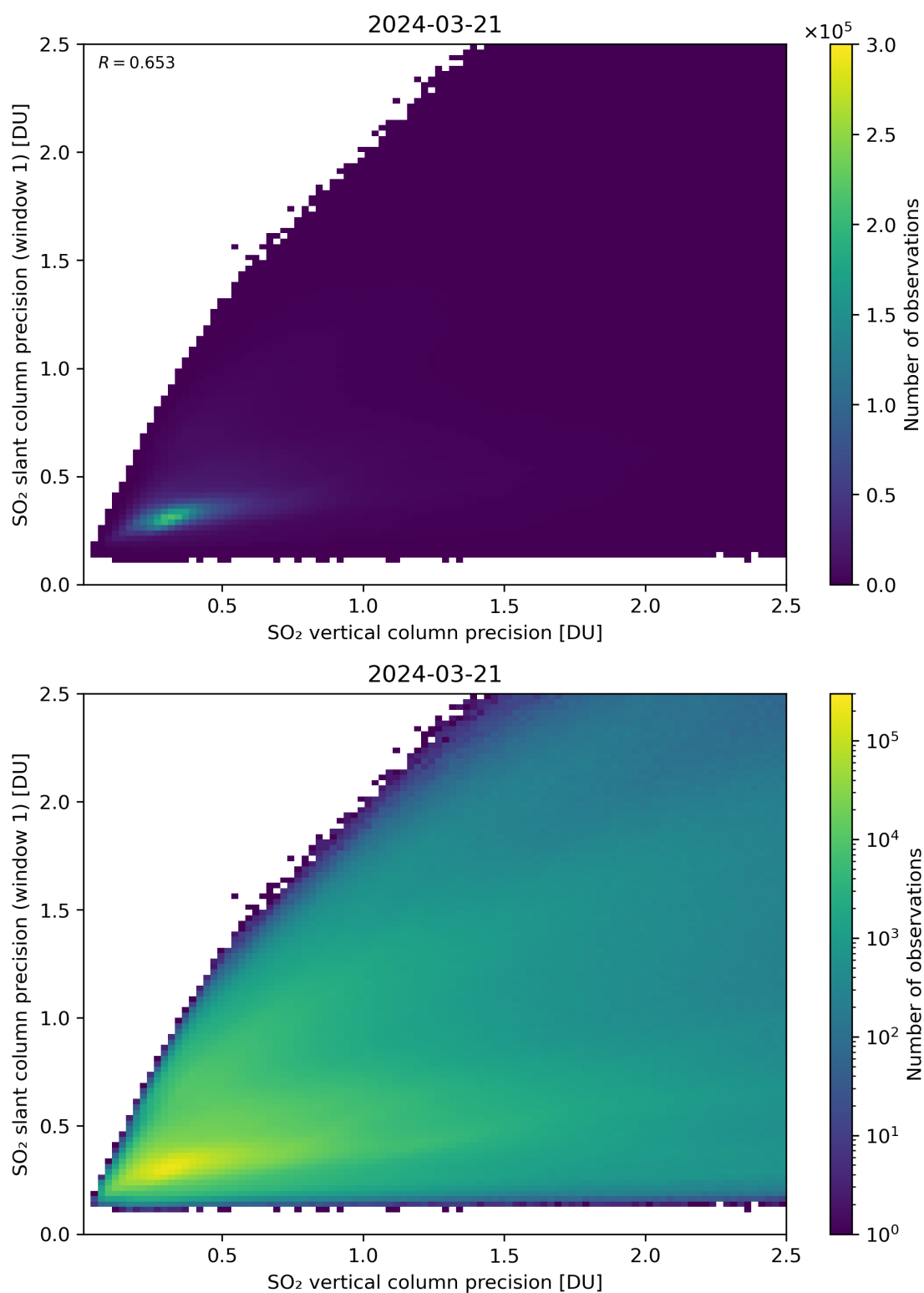
Figure 290: Scatter density plot of “SO 2 vertical column precision” against “SO 2 slant column precision (window 1)” for 2024-03-20 to 2024-03-22.
