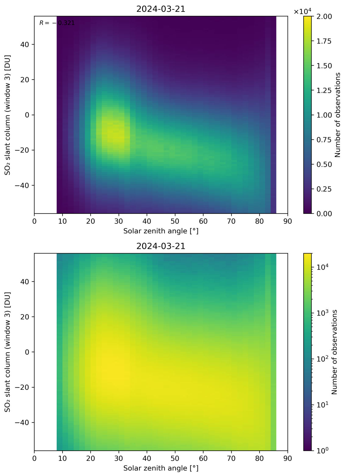
Figure 172: Scatter density plot of “Solar zenith angle” against “SO 2 slant column (window 3)” for 2024-03-20 to 2024-03-22.
