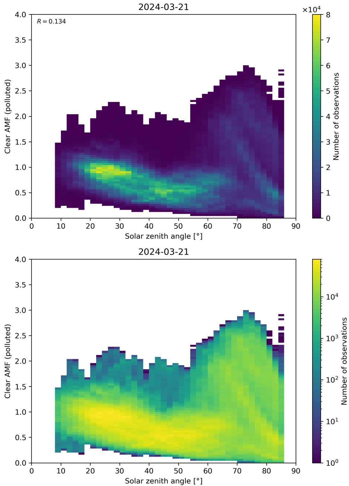
Figure 165: Scatter density plot of “Solar zenith angle” against “Clear AMF (polluted)” for 2024-03-20 to 2024-03-22.
