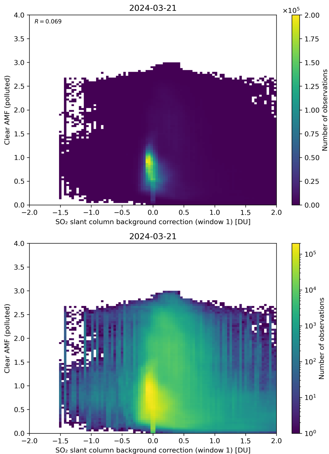
Figure 103: Scatter density plot of “SO 2 slant column background correction (window 1)” against “Clear AMF (polluted)” for 2024-03-20 to 2024-03-22.
