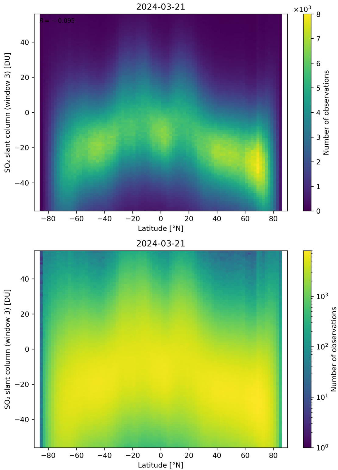
Figure 152: Scatter density plot of “Latitude” against “SO 2 slant column (window 3)” for 2024-03-20 to 2024-03-22.
