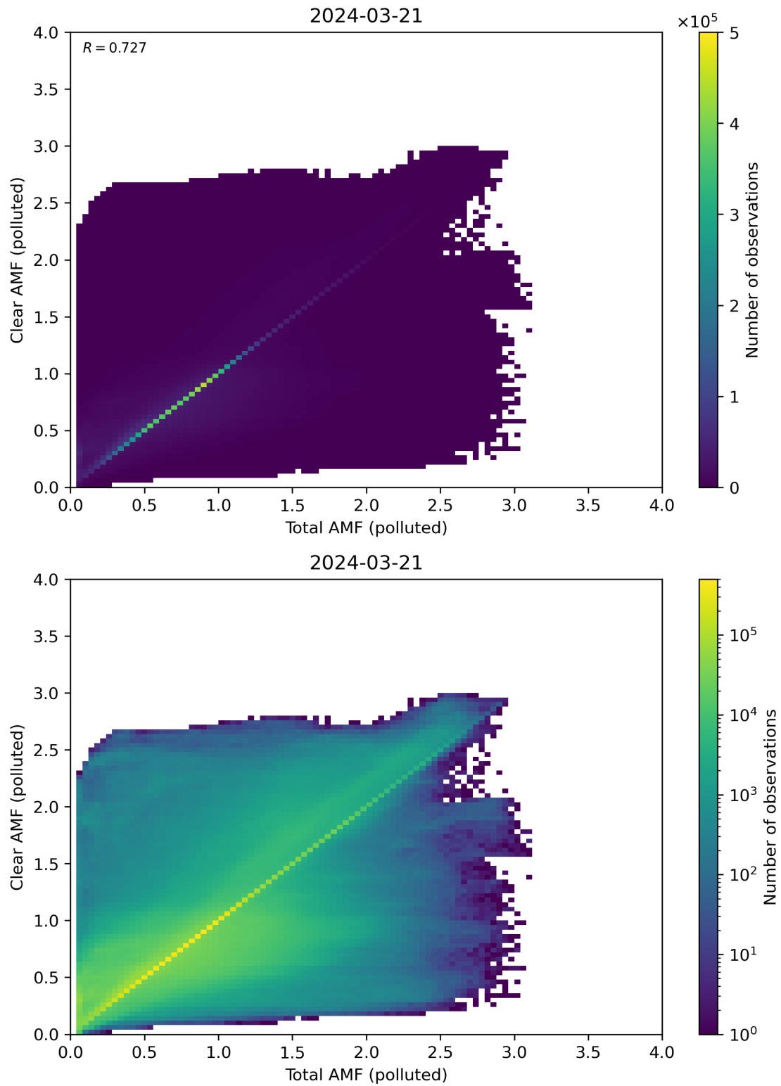
Figure 271: Scatter density plot of “Total AMF (polluted)” against “Clear AMF (polluted)” for 2024-03-20 to 2024-03-22.
