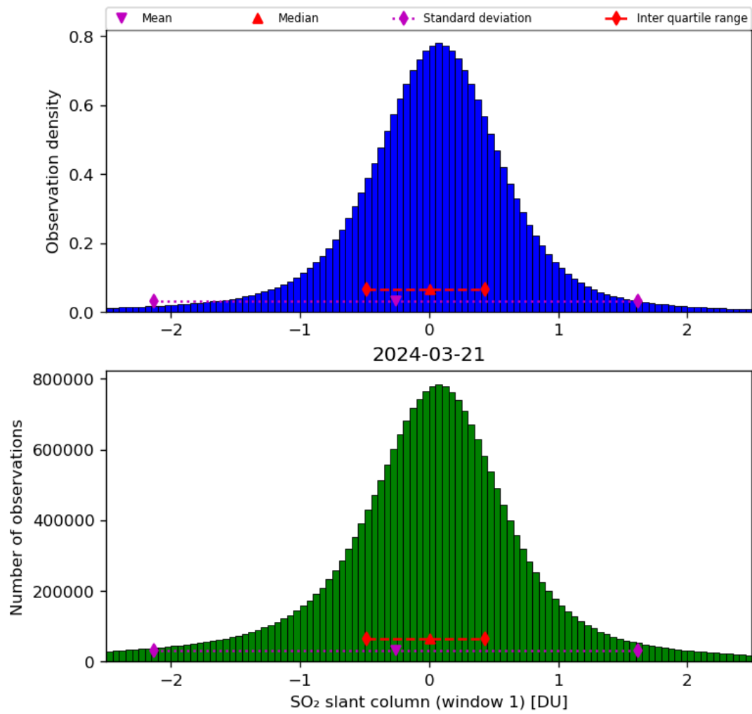
Figure 56: Histogram of “SO 2 slant column (window 1)” for 2024-03-20 to 2024-03-22
