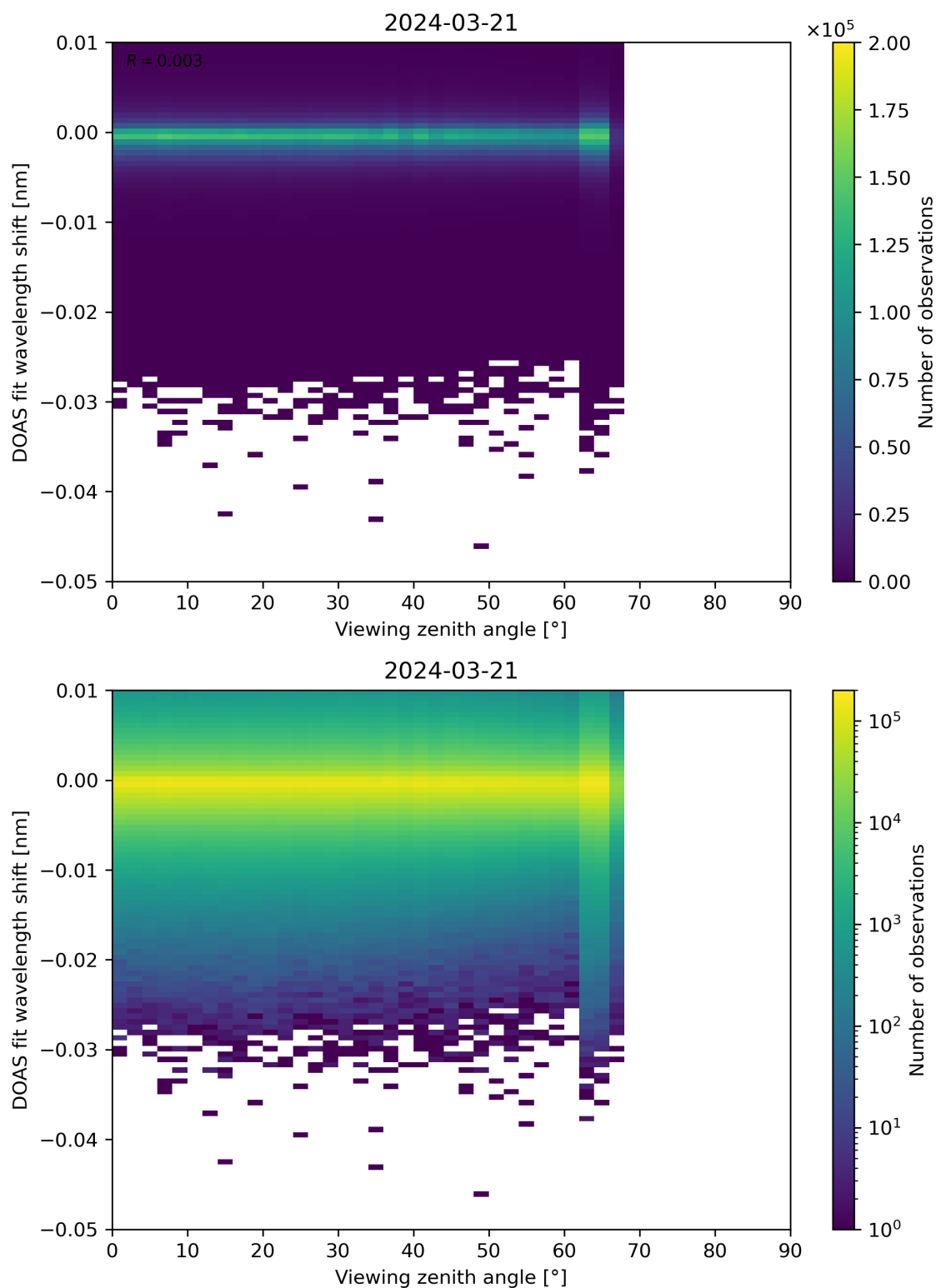
Figure 311: Scatter density plot of “Viewing zenith angle” against “DOAS fit wavelength shift” for 2024-03-20 to 2024-03-22.
