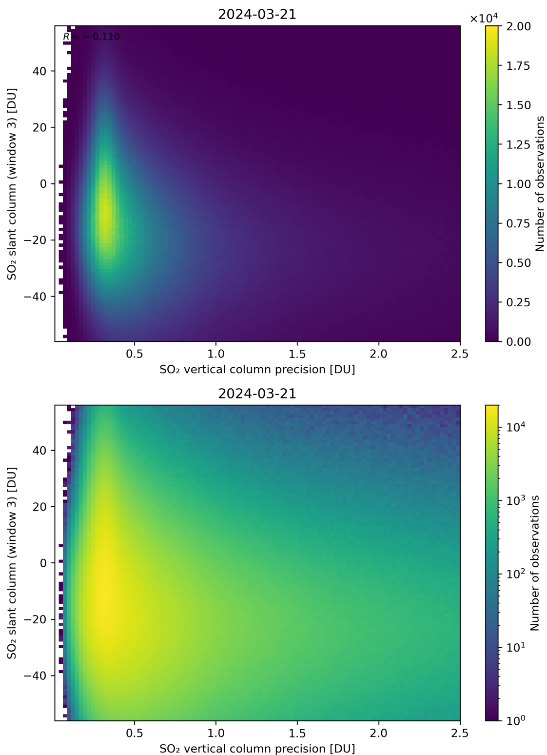
Figure 292: Scatter density plot of “SO 2 vertical column precision” against “SO 2 slant column (window 3)” for 2024-03-20 to 2024-03-22.
