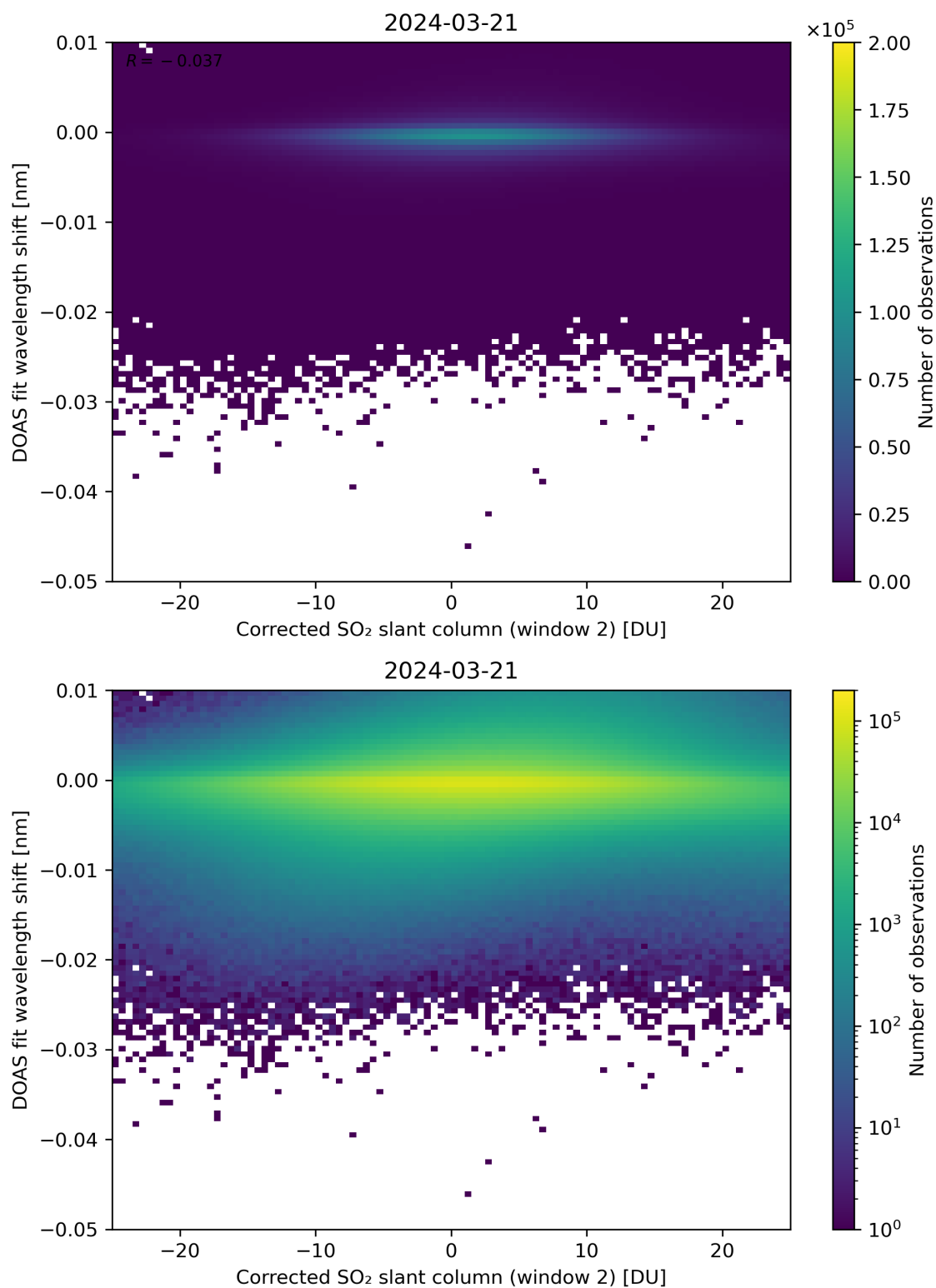
Figure 196: Scatter density plot of “Corrected SO 2 slant column (window 2)” against “DOAS fit wavelength shift” for 2024-03-20 to 2024-03-22.
