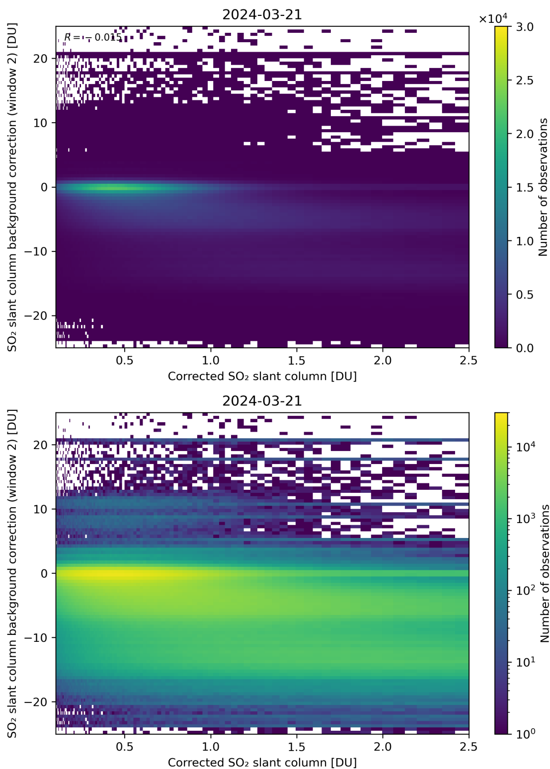
Figure 179: Scatter density plot of “Corrected SO 2 slant column” against “SO 2 slant column background correction (window 2)” for 2024-03-20 to 2024-03-22.
