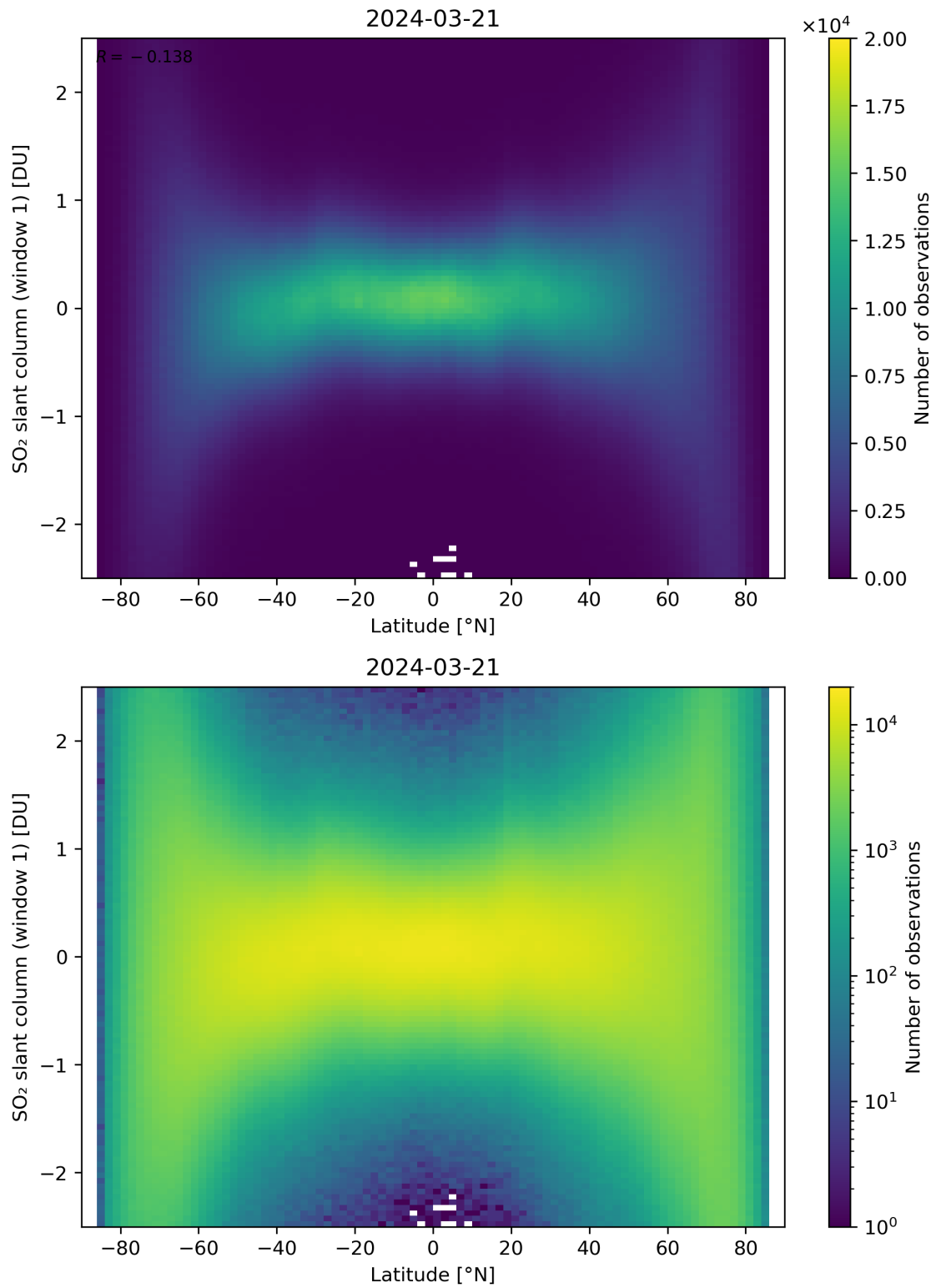
Figure 149: Scatter density plot of “Latitude” against “SO 2 slant column (window 1)” for 2024-03-20 to 2024-03-22.
