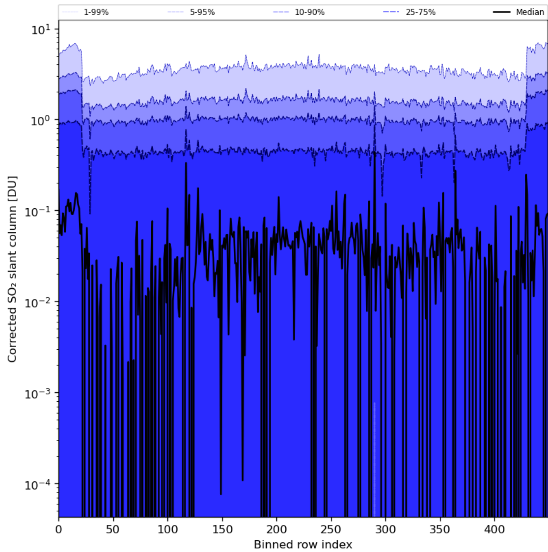
Figure 78: Along track statistics of “Corrected SO 2 slant column” for 2024-03-20 to 2024-03-22
