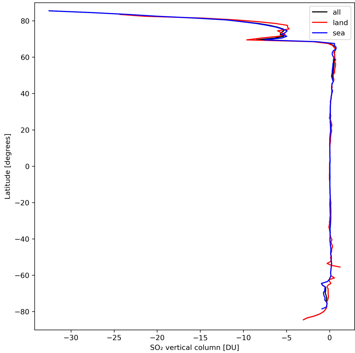
Figure 30: Zonal average of “SO 2 vertical column” for 2024-03-20 to 2024-03-22.
