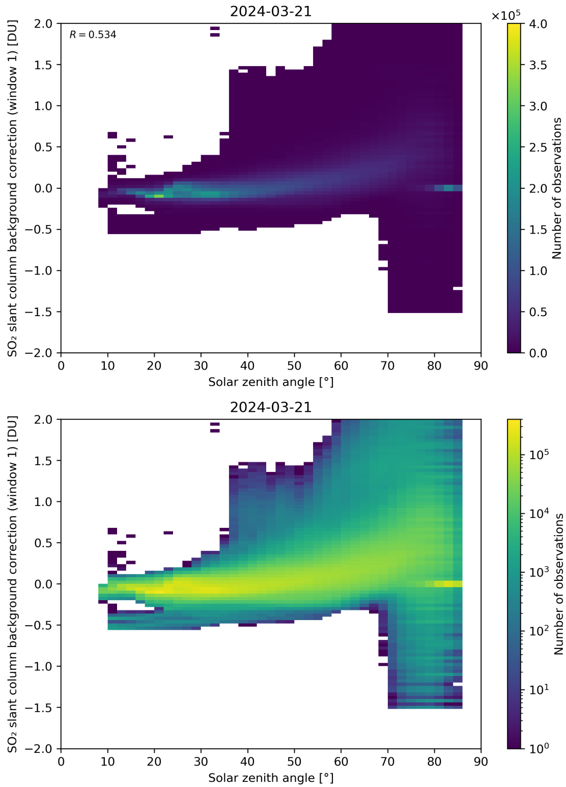
Figure 158: Scatter density plot of “Solar zenith angle” against “SO 2 slant column background correction (window 1)” for 2024-03-20 to 2024-03-22.
