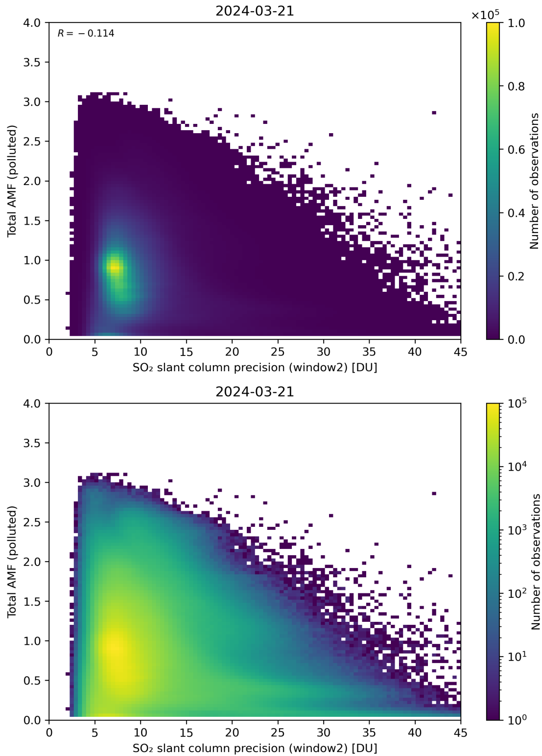
Figure 251: Scatter density plot of “SO 2 slant column precision (window2)” against “Total AMF (polluted)” for 2024-03-20 to 2024-03-22.
