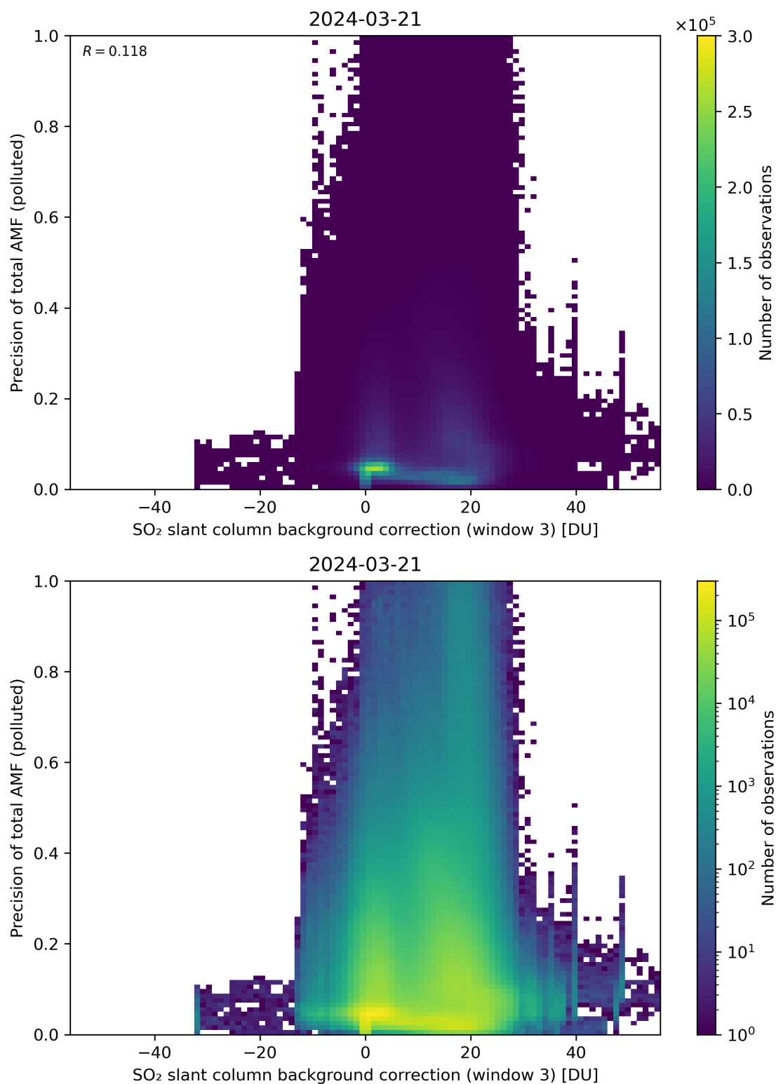
Figure 126: Scatter density plot of “SO 2 slant column background correction (window 3)” against “Precision of total AMF (polluted)” for 2024-03-20 to 2024-03-22.
