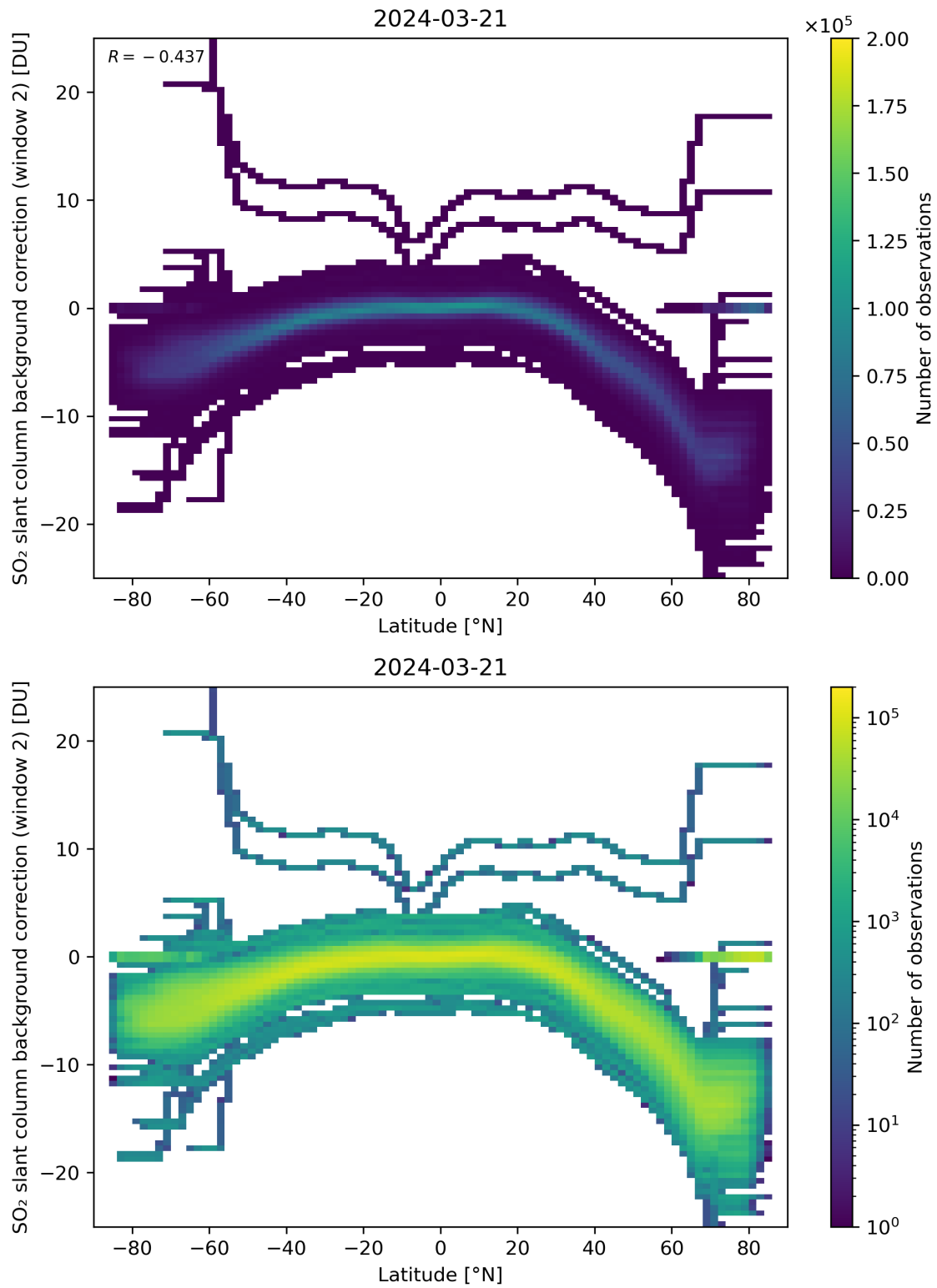
Figure 140: Scatter density plot of “Latitude” against “SO 2 slant column background correction (window 2)” for 2024-03-20 to 2024-03-22.
