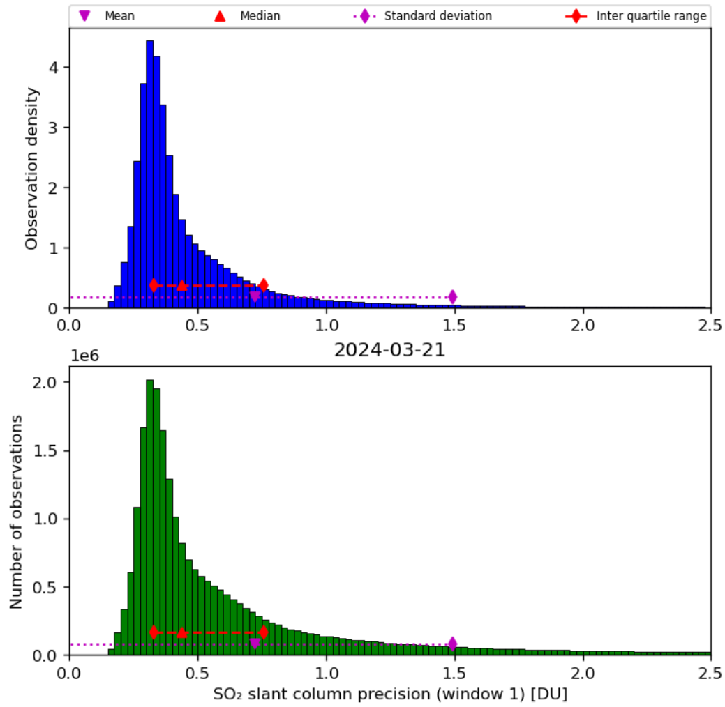
Figure 57: Histogram of “SO 2 slant column precision (window 1)” for 2024-03-20 to 2024-03-22
