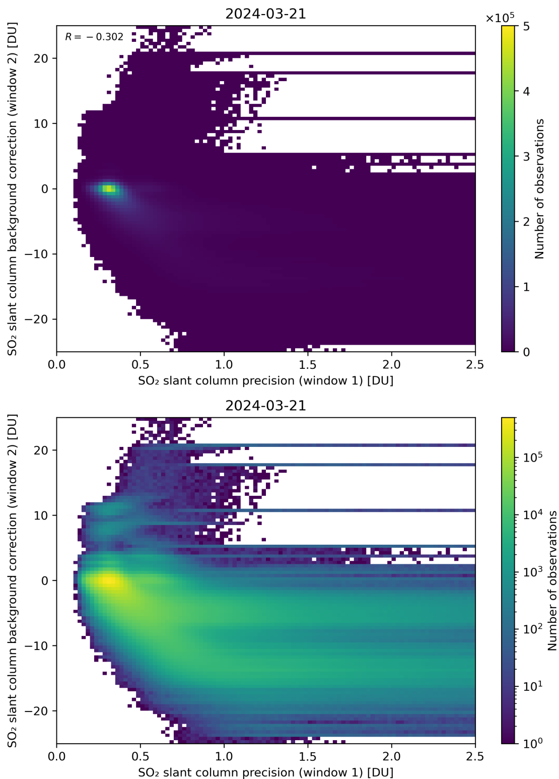
Figure 219: Scatter density plot of “SO 2 slant column precision (window 1)” against “SO 2 slant column background correction (window 2)” for 2024-03-20 to 2024-03-22.
