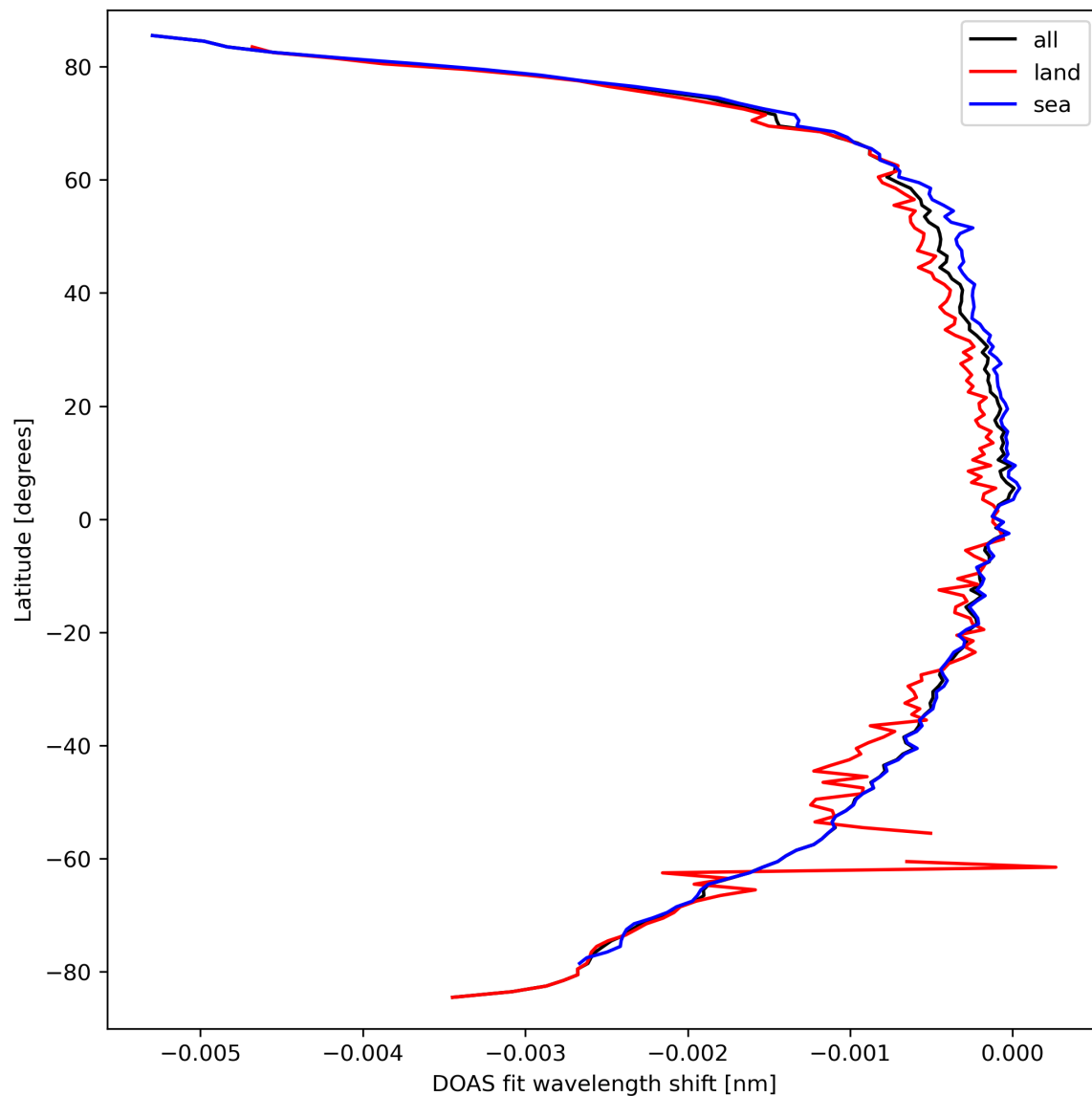
Figure 45: Zonal average of “DOAS fit wavelength shift” for 2024-03-20 to 2024-03-22.
