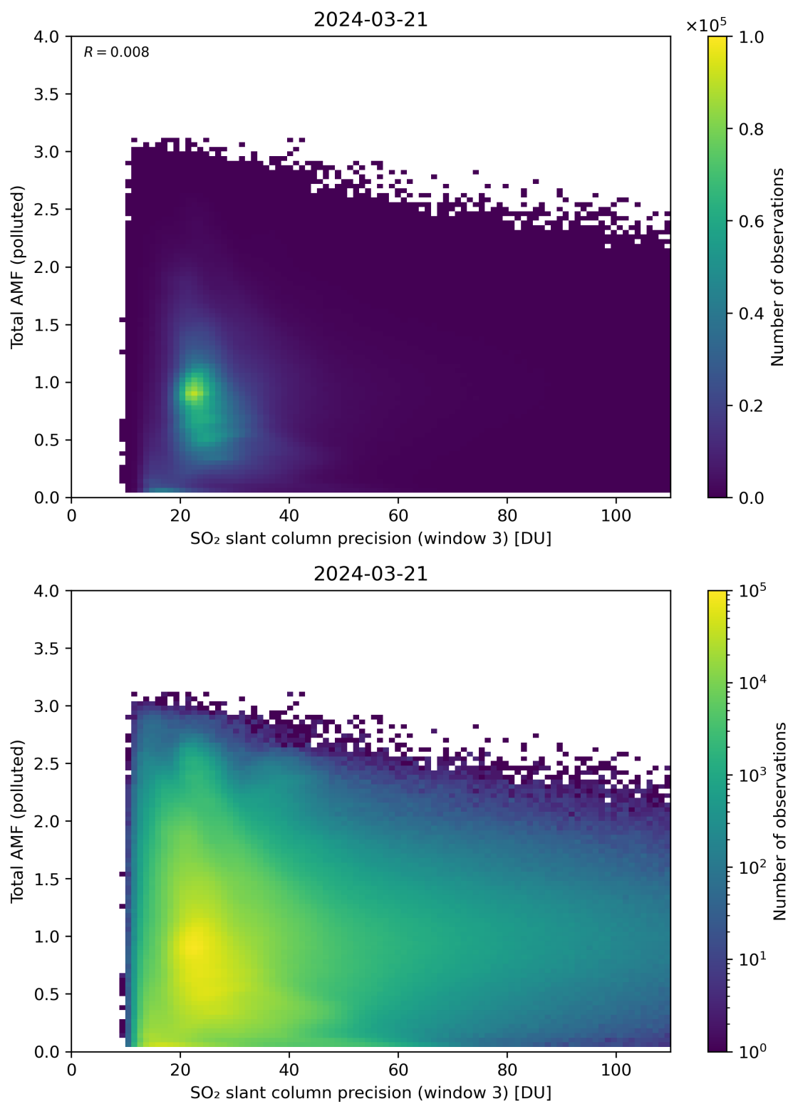
Figure 263: Scatter density plot of “SO 2 slant column precision (window 3)” against “Total AMF (polluted)” for 2024-03-20 to 2024-03-22.
