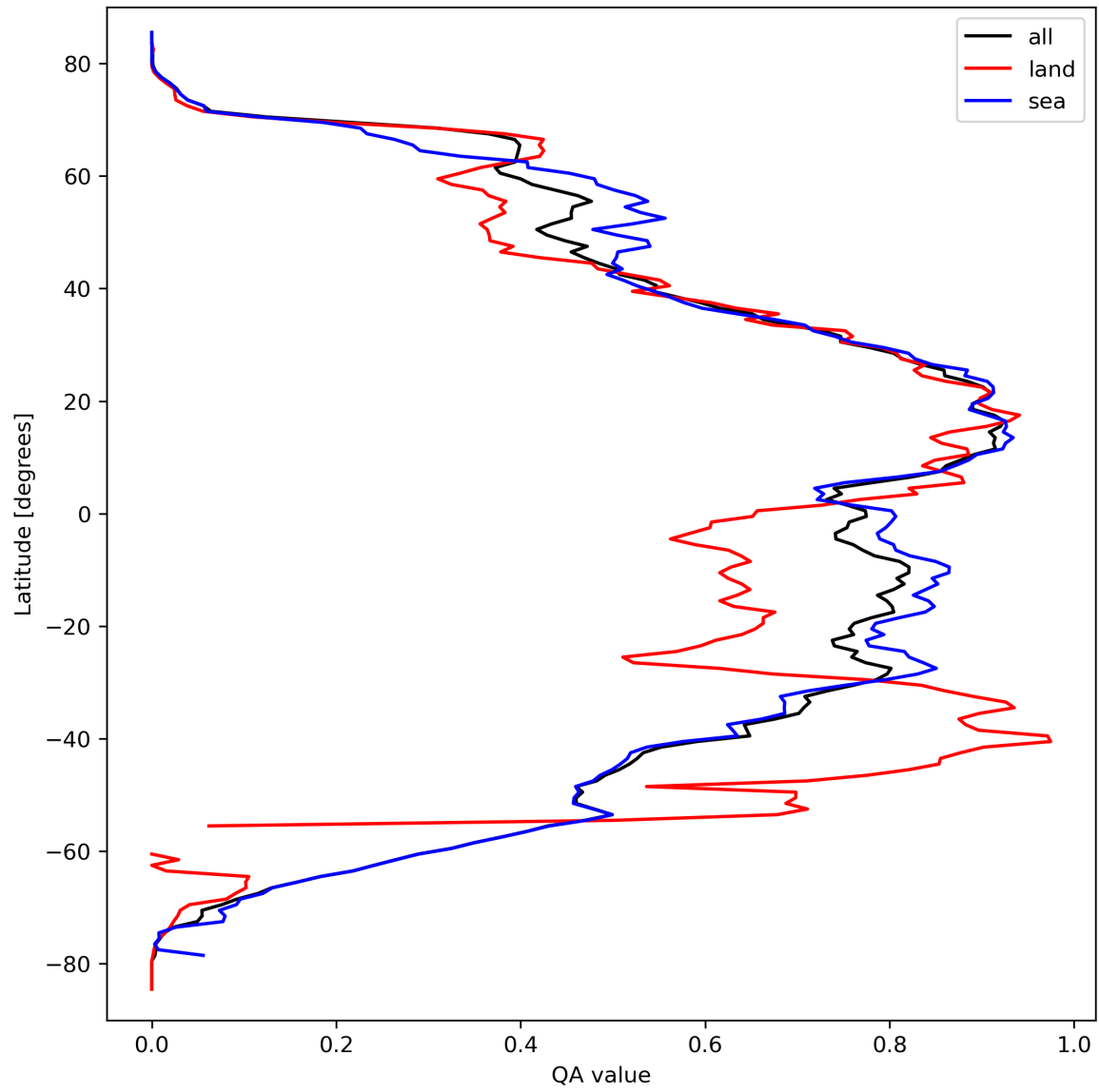
Figure 29: Zonal average of “QA value” for 2024-03-20 to 2024-03-22.
