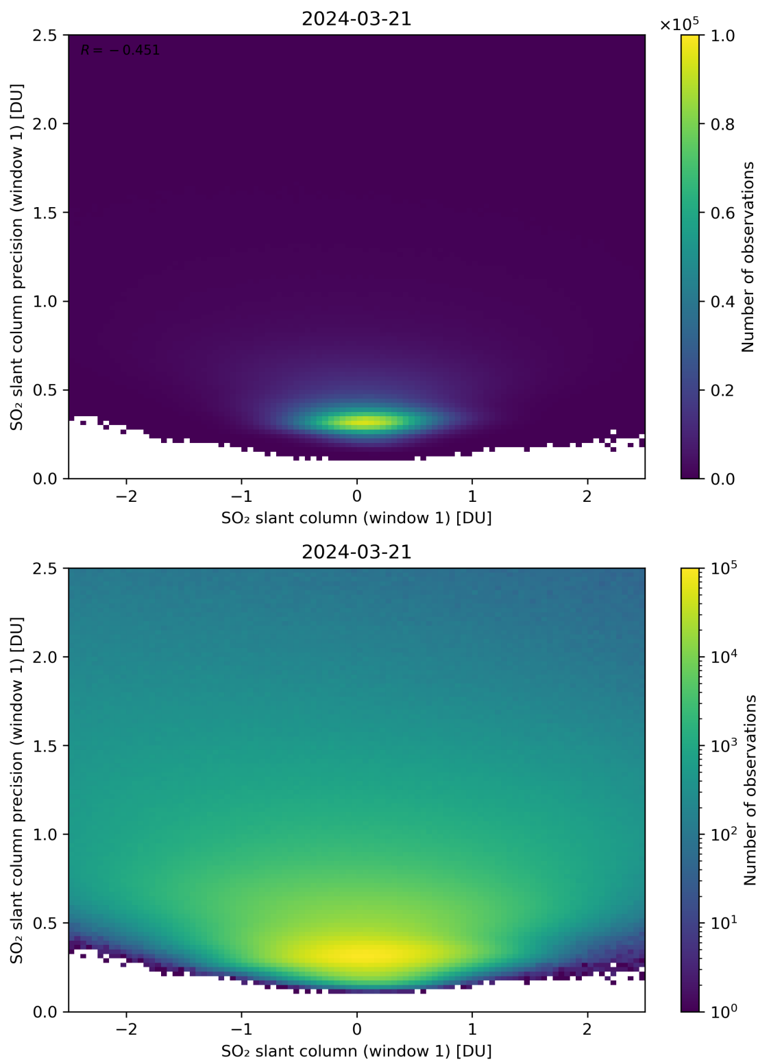
Figure 235: Scatter density plot of “SO 2 slant column (window 1)” against “SO 2 slant column precision (window 1)” for 2024-03-20 to 2024-03-22.
