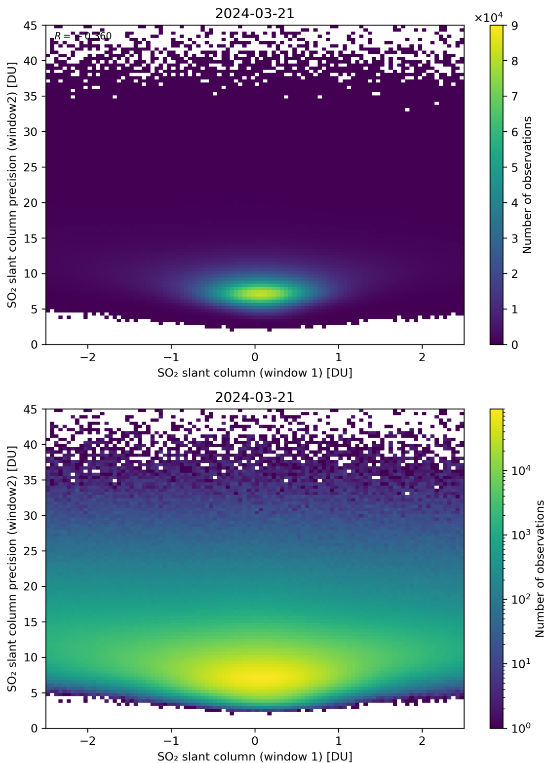
Figure 236: Scatter density plot of “SO 2 slant column (window 1)” against “SO 2 slant column precision (window2)” for 2024-03-20 to 2024-03-22.
