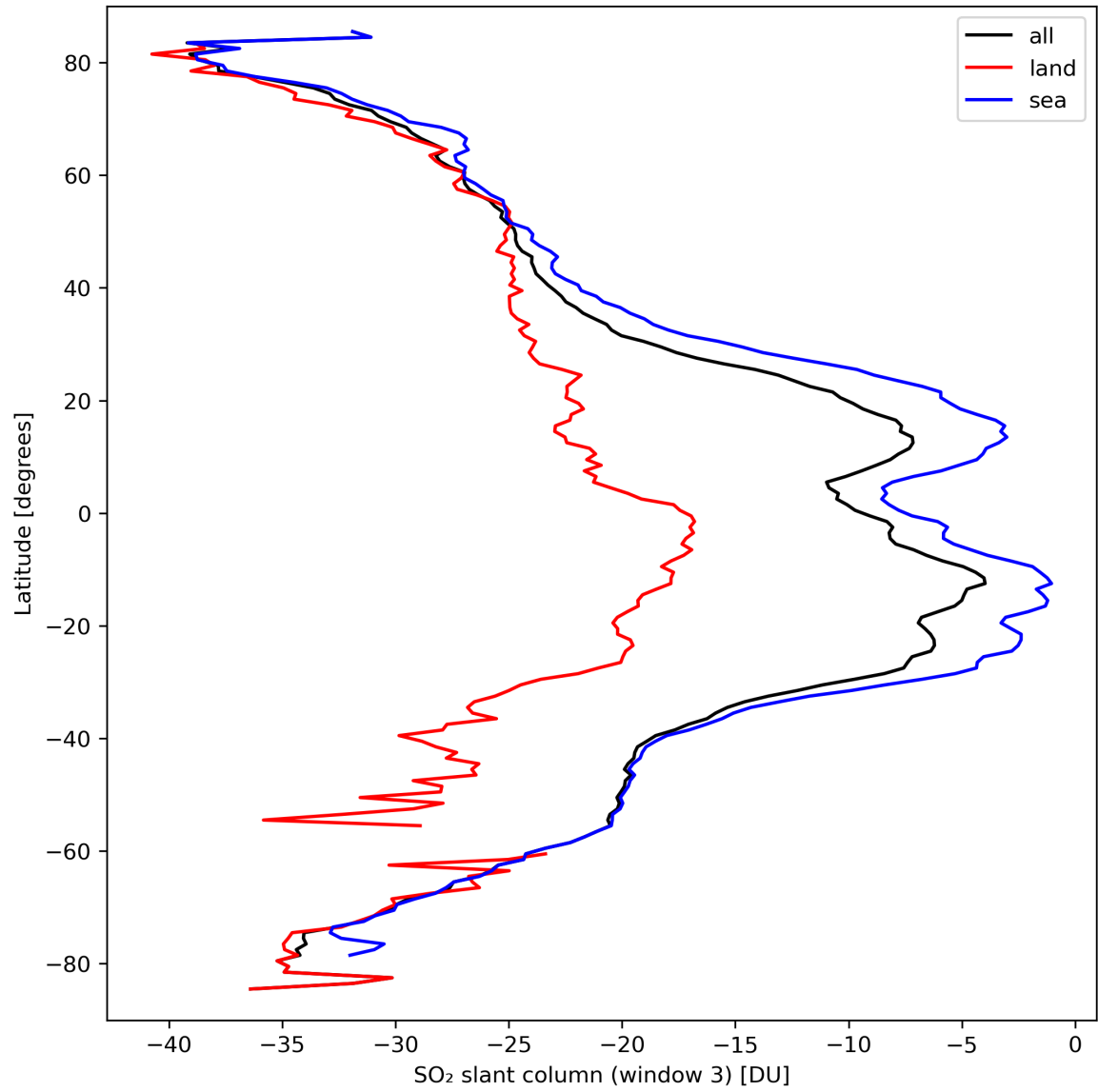
Figure 41: Zonal average of “SO 2 slant column (window 3)” for 2024-03-20 to 2024-03-22.
