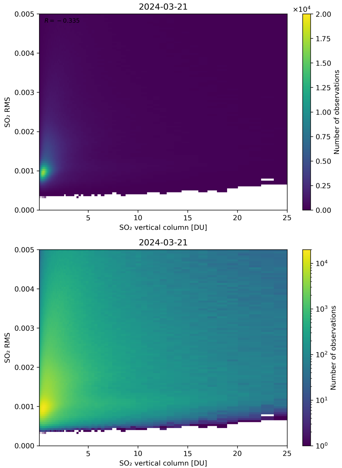
Figure 278: Scatter density plot of “SO 2 vertical column” against “SO 2 RMS” for 2024-03-20 to 2024-03-22.
