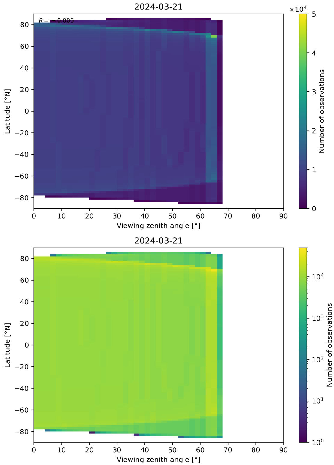
Figure 314: Scatter density plot of “Viewing zenith angle” against “Latitude” for 2024-03-20 to 2024-03-22.
