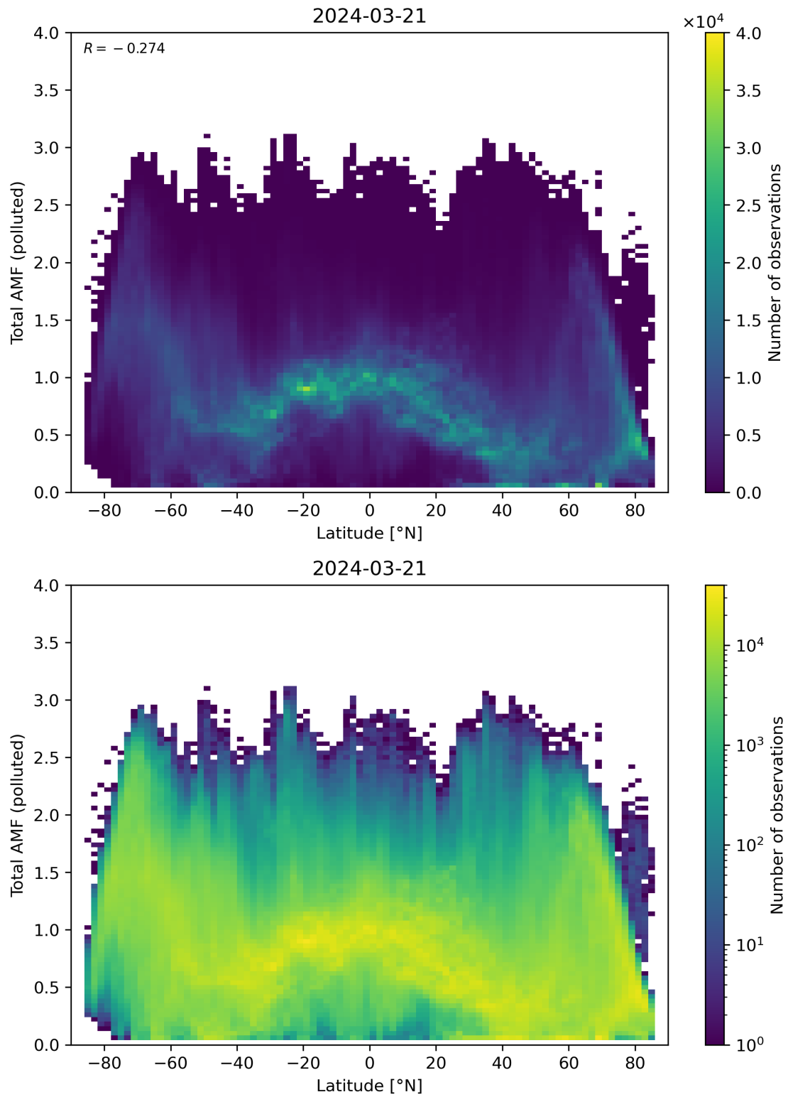
Figure 154: Scatter density plot of “Latitude” against “Total AMF (polluted)” for 2024-03-20 to 2024-03-22.
