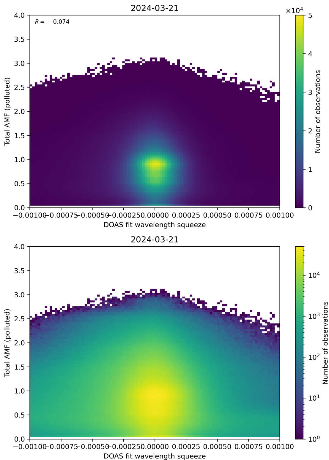
Figure 134: Scatter density plot of “DOAS fit wavelength squeeze” against “Total AMF (polluted)” for 2024-03-20 to 2024-03-22.
