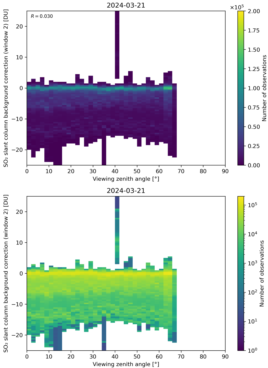
Figure 309: Scatter density plot of “Viewing zenith angle” against “SO 2 slant column background correction (window 2)” for 2024-03-20 to 2024-03-22.
