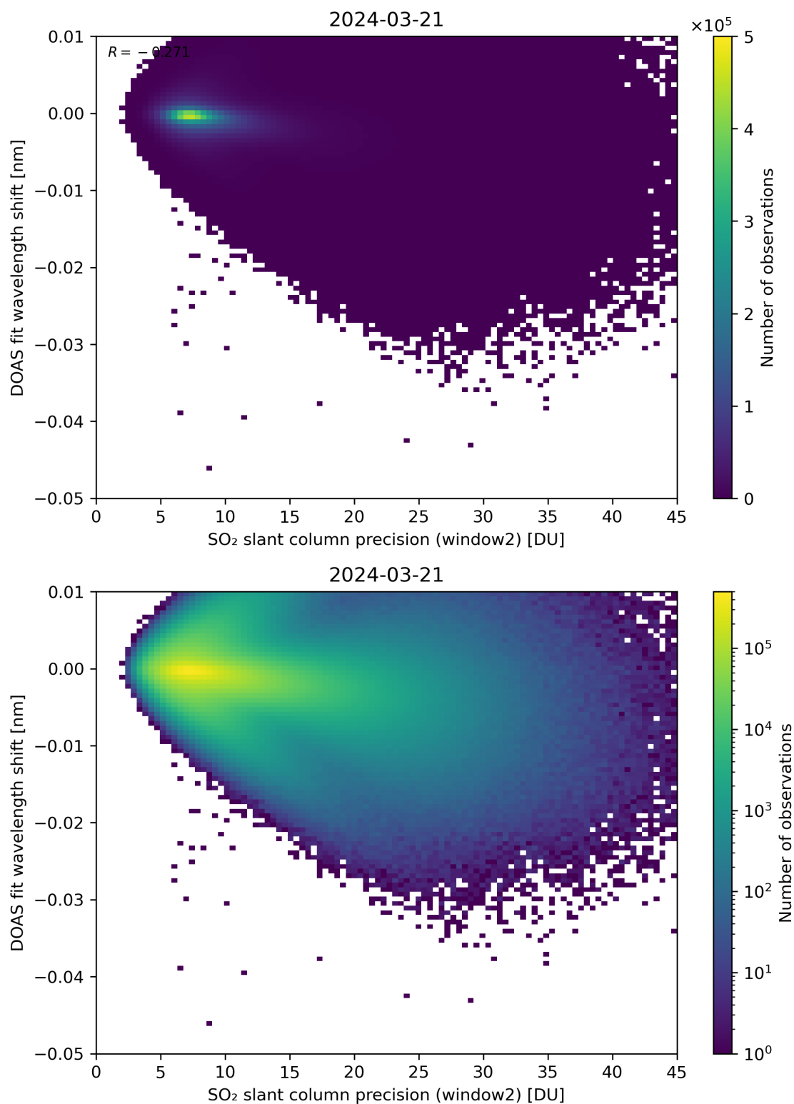
Figure 243: Scatter density plot of “SO 2 slant column precision (window2)” against “DOAS fit wavelength shift” for 2024-03-20 to 2024-03-22.
