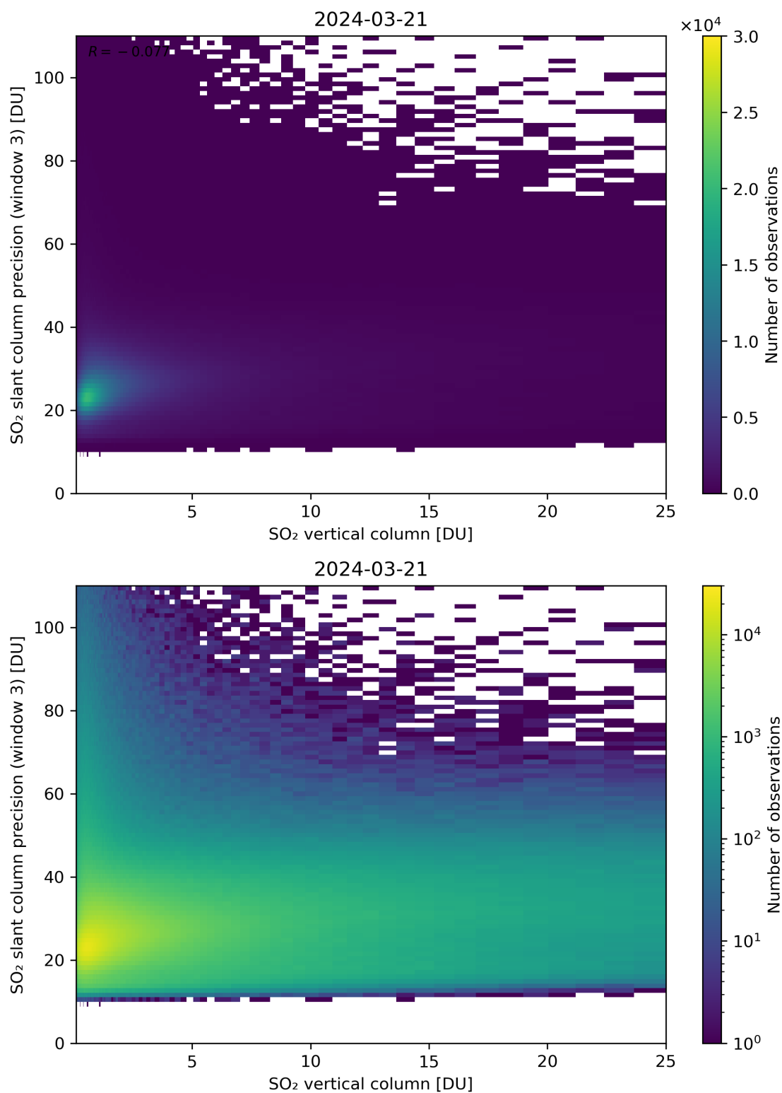
Figure 304: Scatter density plot of “SO 2 vertical column” against “SO 2 slant column precision (window 3)” for 2024-03-20 to 2024-03-22.
