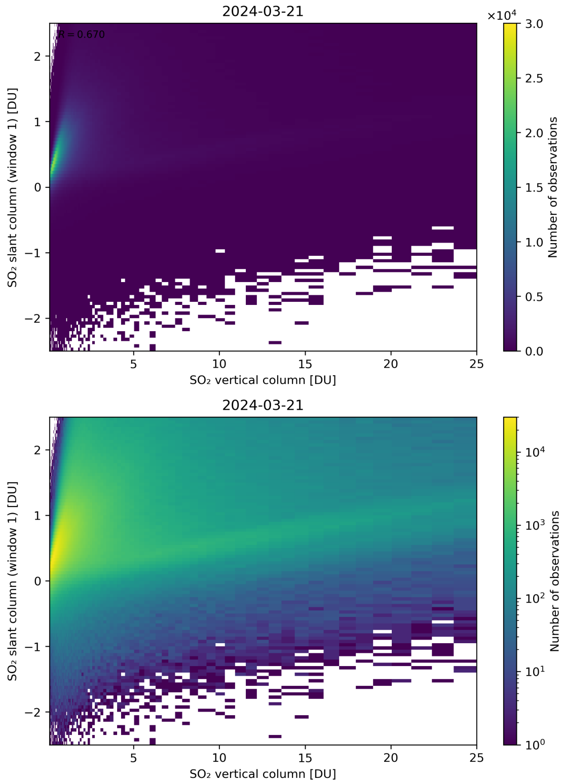
Figure 300: Scatter density plot of “SO 2 vertical column” against “SO 2 slant column (window 1)” for 2024-03-20 to 2024-03-22.
