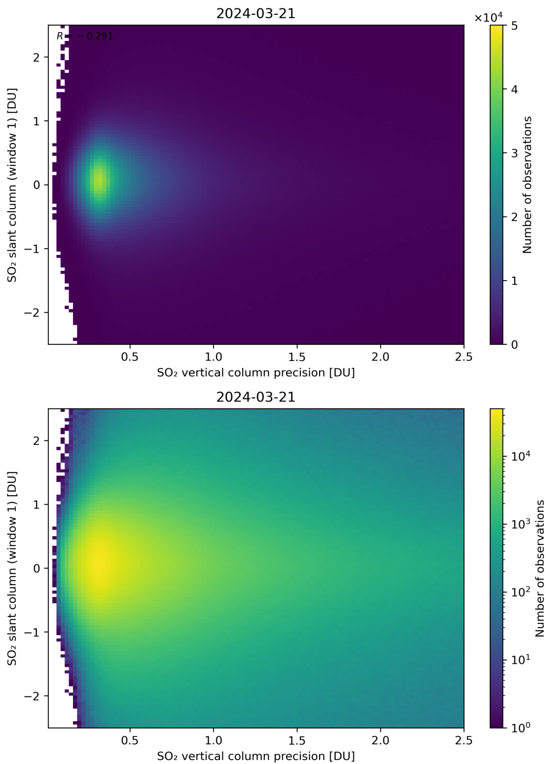
Figure 289: Scatter density plot of “SO 2 vertical column precision” against “SO 2 slant column (window 1)” for 2024-03-20 to 2024-03-22.
