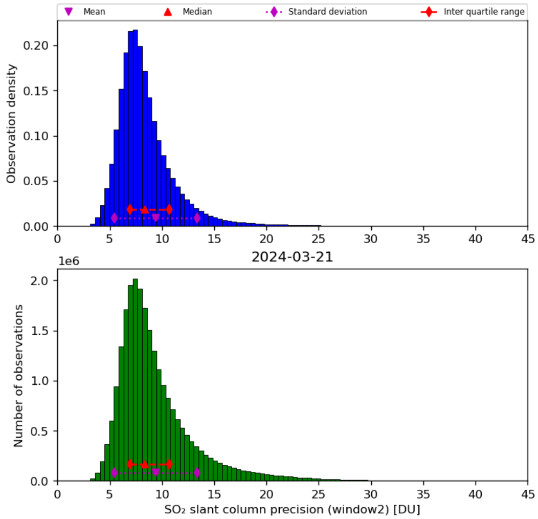
Figure 61: Histogram of “SO 2 slant column precision (window2)” for 2024-03-20 to 2024-03-22
