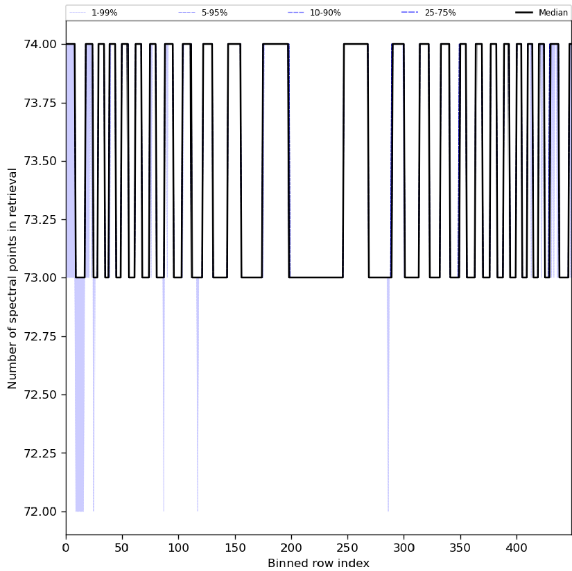
Figure 97: Along track statistics of “Number of spectral points in retrieval” for 2024-03-20 to 2024-03-22
