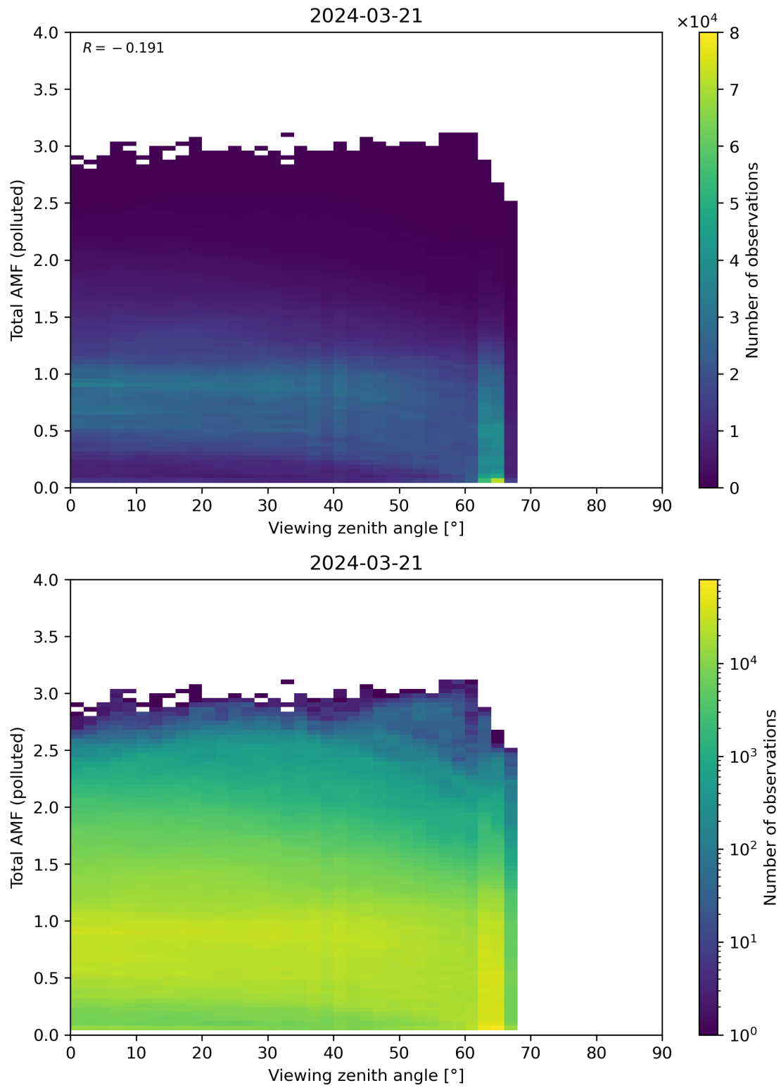
Figure 325: Scatter density plot of “Viewing zenith angle” against “Total AMF (polluted)” for 2024-03-20 to 2024-03-22.
