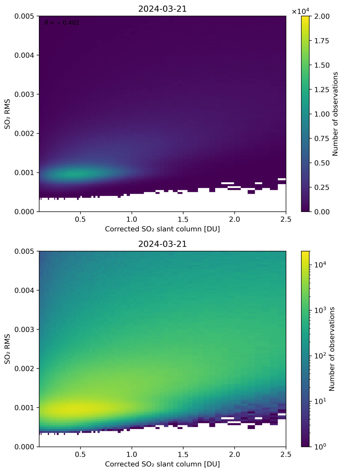
Figure 183: Scatter density plot of “Corrected SO 2 slant column” against “SO 2 RMS” for 2024-03-20 to 2024-03-22.
