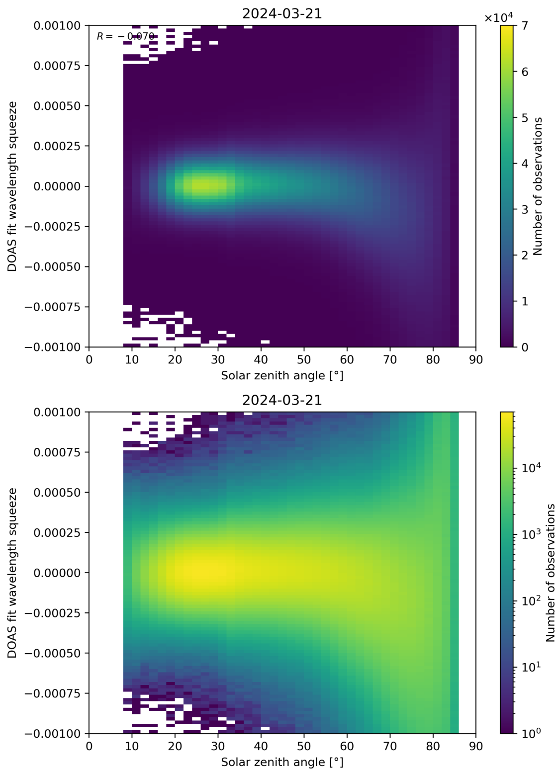
Figure 162: Scatter density plot of “Solar zenith angle” against “DOAS fit wavelength squeeze” for 2024-03-20 to 2024-03-22.
