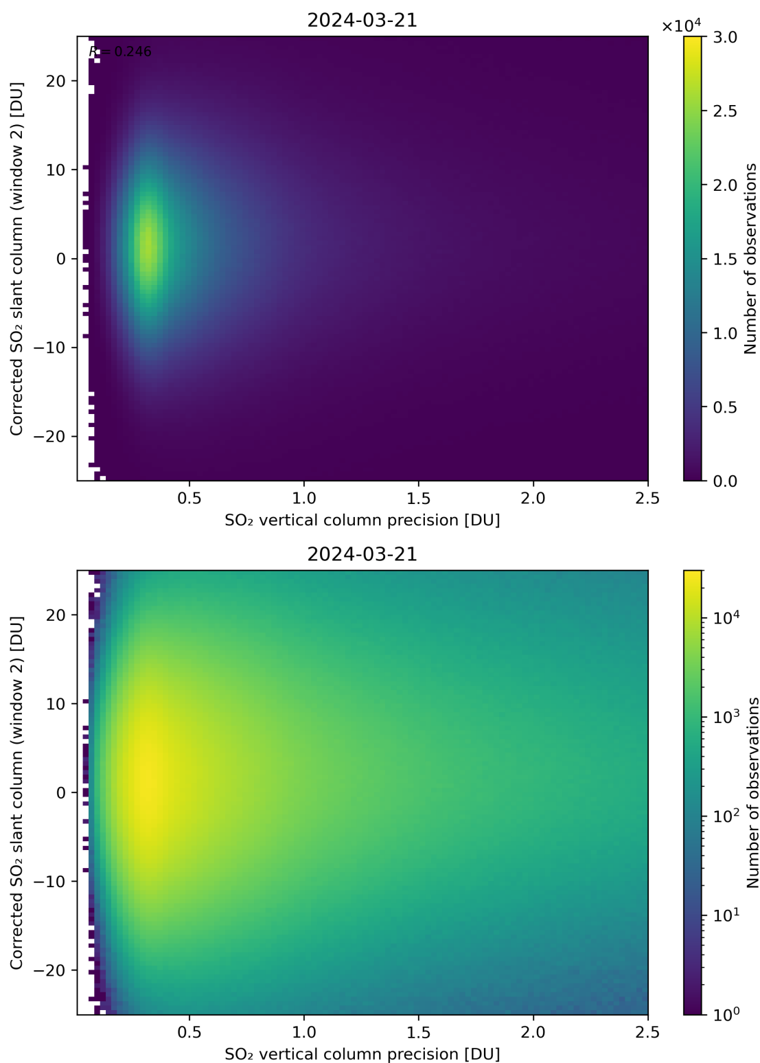
Figure 287: Scatter density plot of “SO 2 vertical column precision” against “Corrected SO 2 slant column (window 2)” for 2024-03-20 to 2024-03-22.
