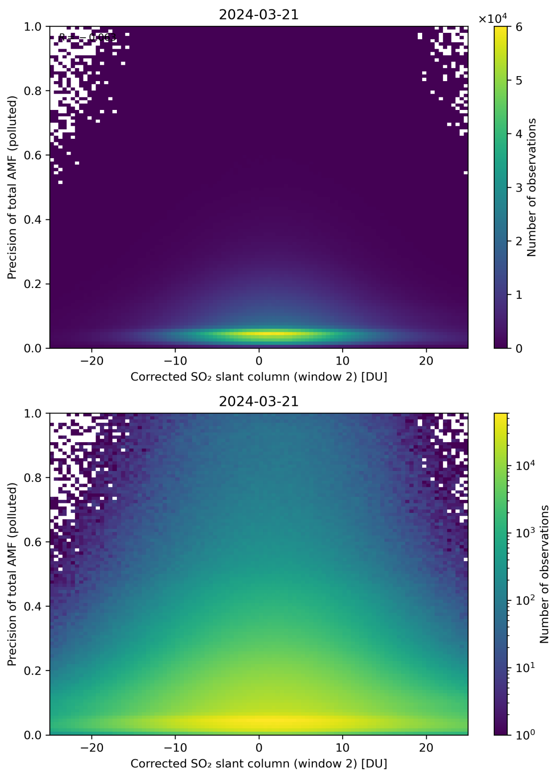
Figure 204: Scatter density plot of “Corrected SO 2 slant column (window 2)” against “Precision of total AMF (polluted)” for 2024-03-20 to 2024-03-22.
