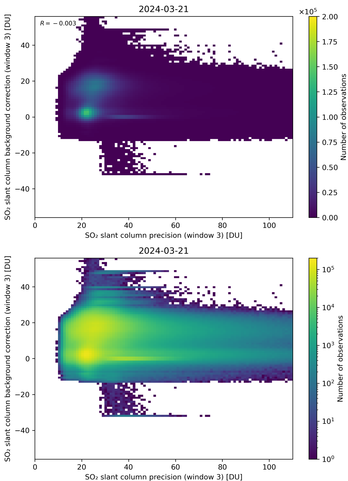
Figure 257: Scatter density plot of “SO 2 slant column precision (window 3)” against “SO 2 slant column background correction (window 3)” for 2024-03-20 to 2024-03-22.
