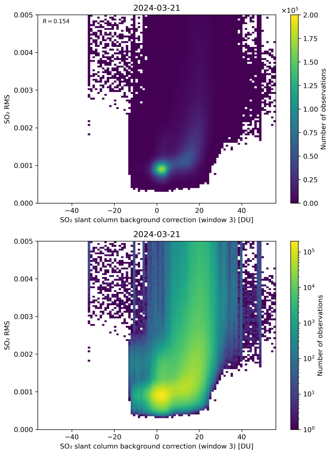
Figure 123: Scatter density plot of “SO 2 slant column background correction (window 3)” against “SO 2 RMS” for 2024-03-20 to 2024-03-22.
