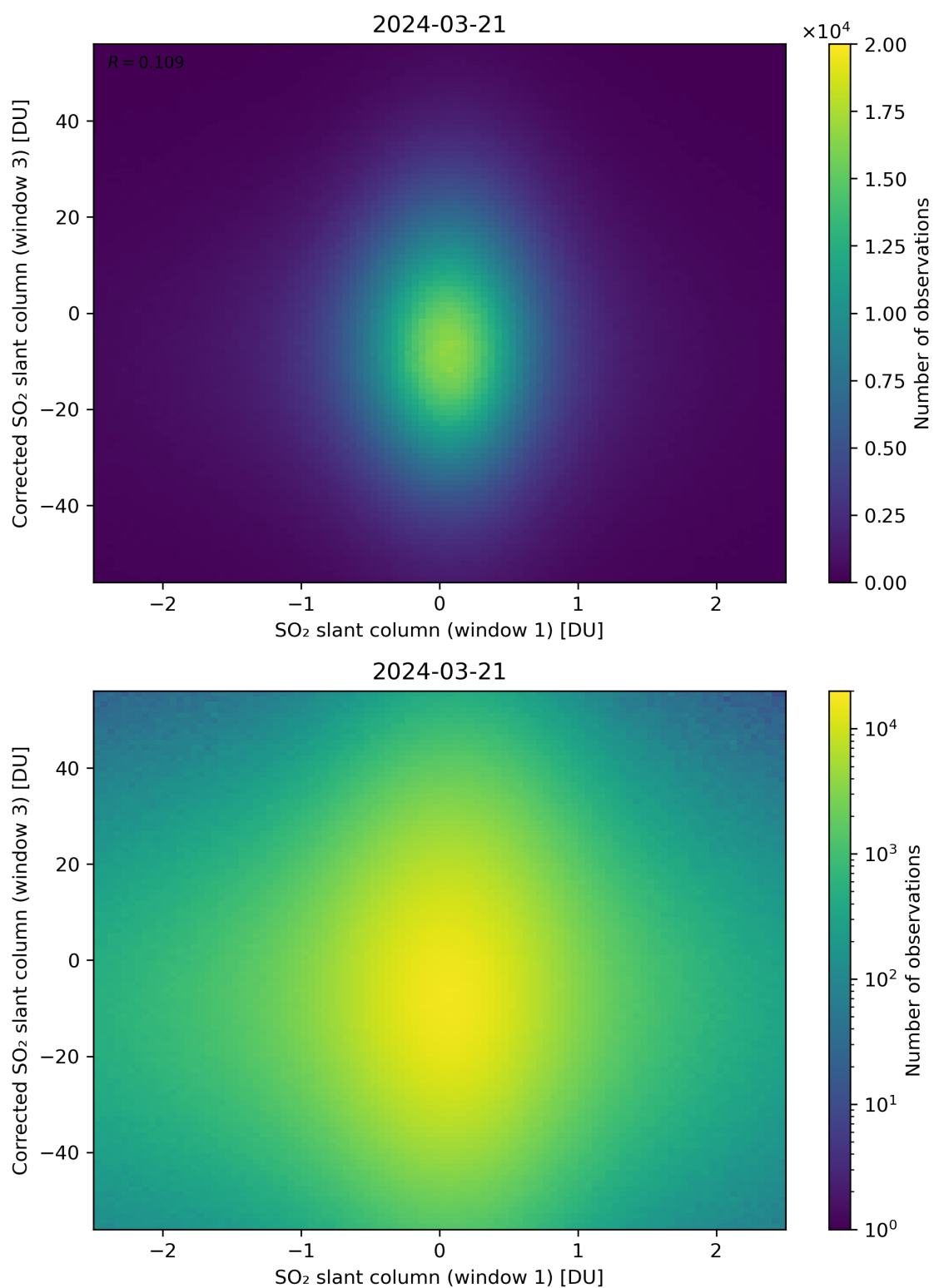
Figure 234: Scatter density plot of “SO 2 slant column (window 1)” against “Corrected SO 2 slant column (window 3)” for 2024-03-20 to 2024-03-22.
