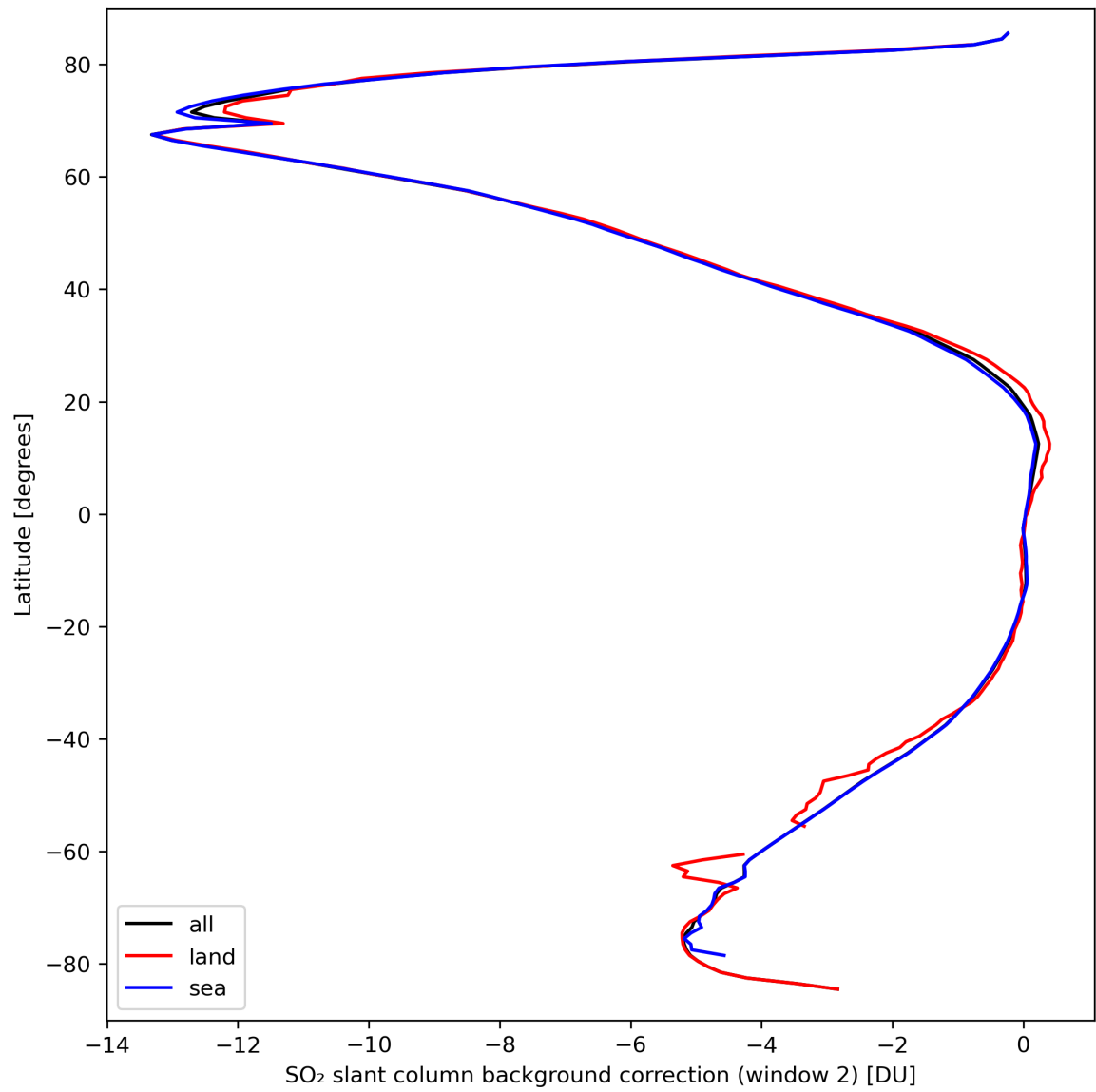
Figure 40: Zonal average of “SO 2 slant column background correction (window 2)” for 2024-03-20 to 2024-03-22.
