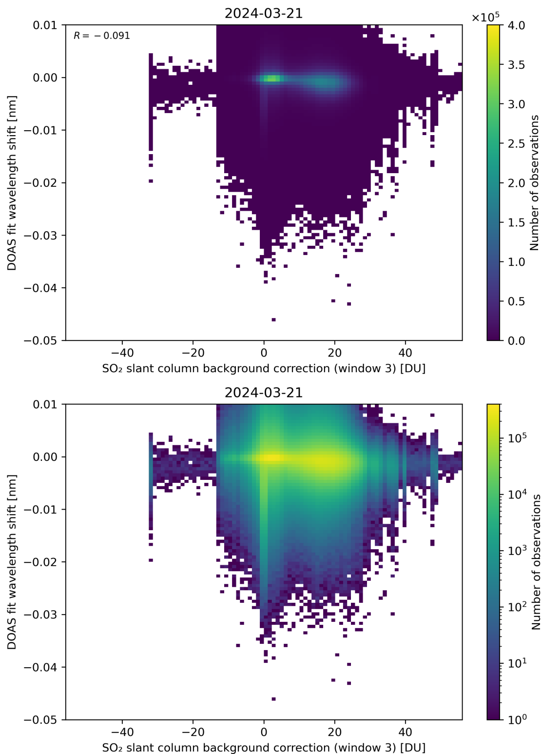
Figure 121: Scatter density plot of “SO 2 slant column background correction (window 3)” against “DOAS fit wavelength shift” for 2024-03-20 to 2024-03-22.
