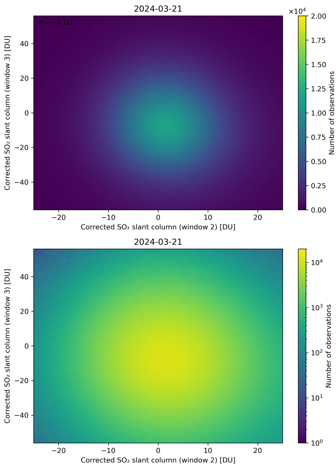
Figure 200: Scatter density plot of “Corrected SO 2 slant column (window 2)” against “Corrected SO 2 slant column (window 3)” for 2024-03-20 to 2024-03-22.
