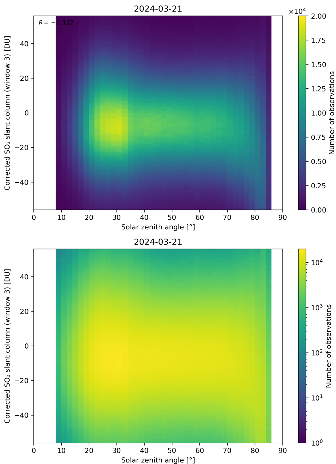
Figure 168: Scatter density plot of “Solar zenith angle” against “Corrected SO 2 slant column (window 3)” for 2024-03-20 to 2024-03-22.
