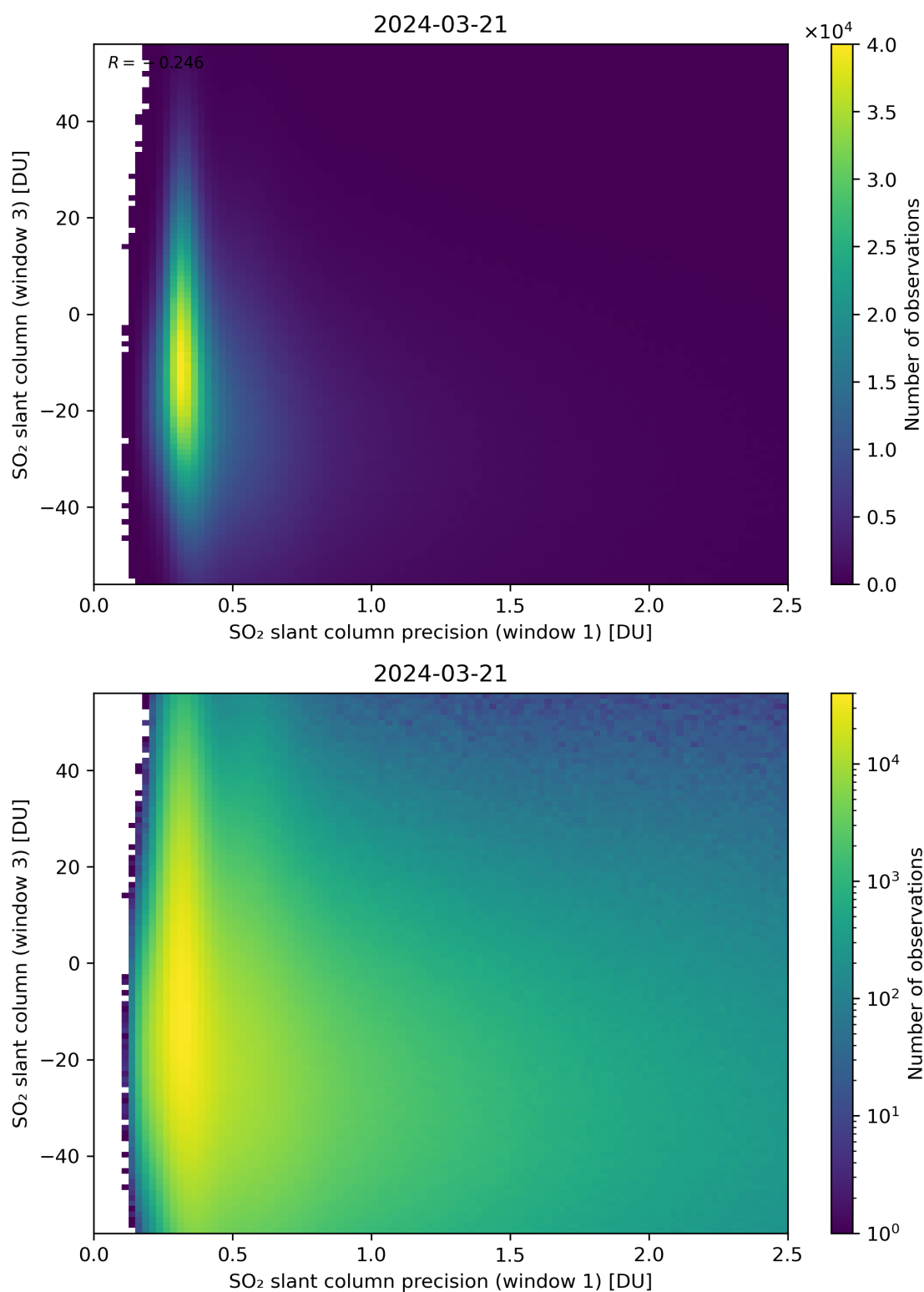
Figure 228: Scatter density plot of “SO 2 slant column precision (window 1)” against “SO 2 slant column (window 3)” for 2024-03-20 to 2024-03-22.
