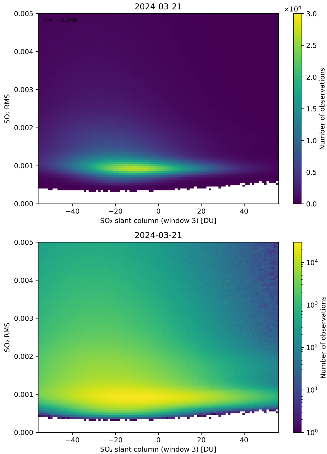
Figure 256: Scatter density plot of “SO 2 slant column (window 3)” against “SO 2 RMS” for 2024-03-20 to 2024-03-22.
