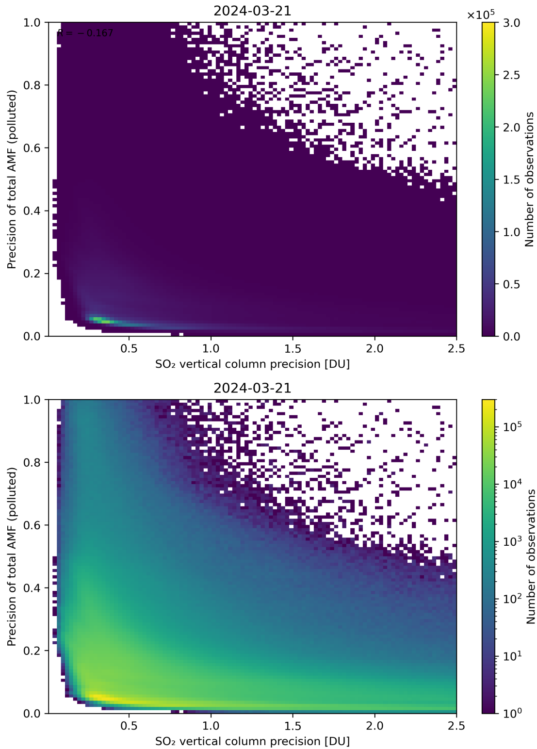
Figure 295: Scatter density plot of “SO 2 vertical column precision” against “Precision of total AMF (polluted)” for 2024-03-20 to 2024-03-22.
