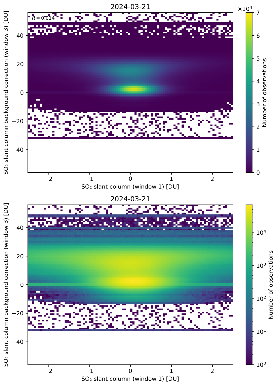
Figure 214: Scatter density plot of “SO 2 slant column (window 1)” against “SO 2 slant column background correction (window 3)” for 2024-03-20 to 2024-03-22.
