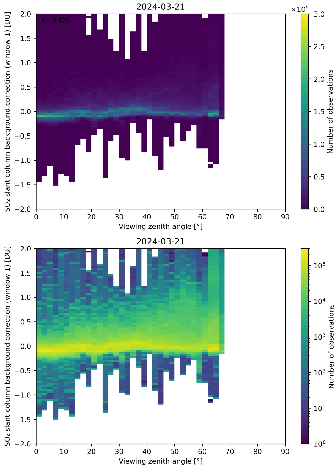
Figure 308: Scatter density plot of “Viewing zenith angle” against “SO 2 slant column background correction (window 1)” for 2024-03-20 to 2024-03-22.
