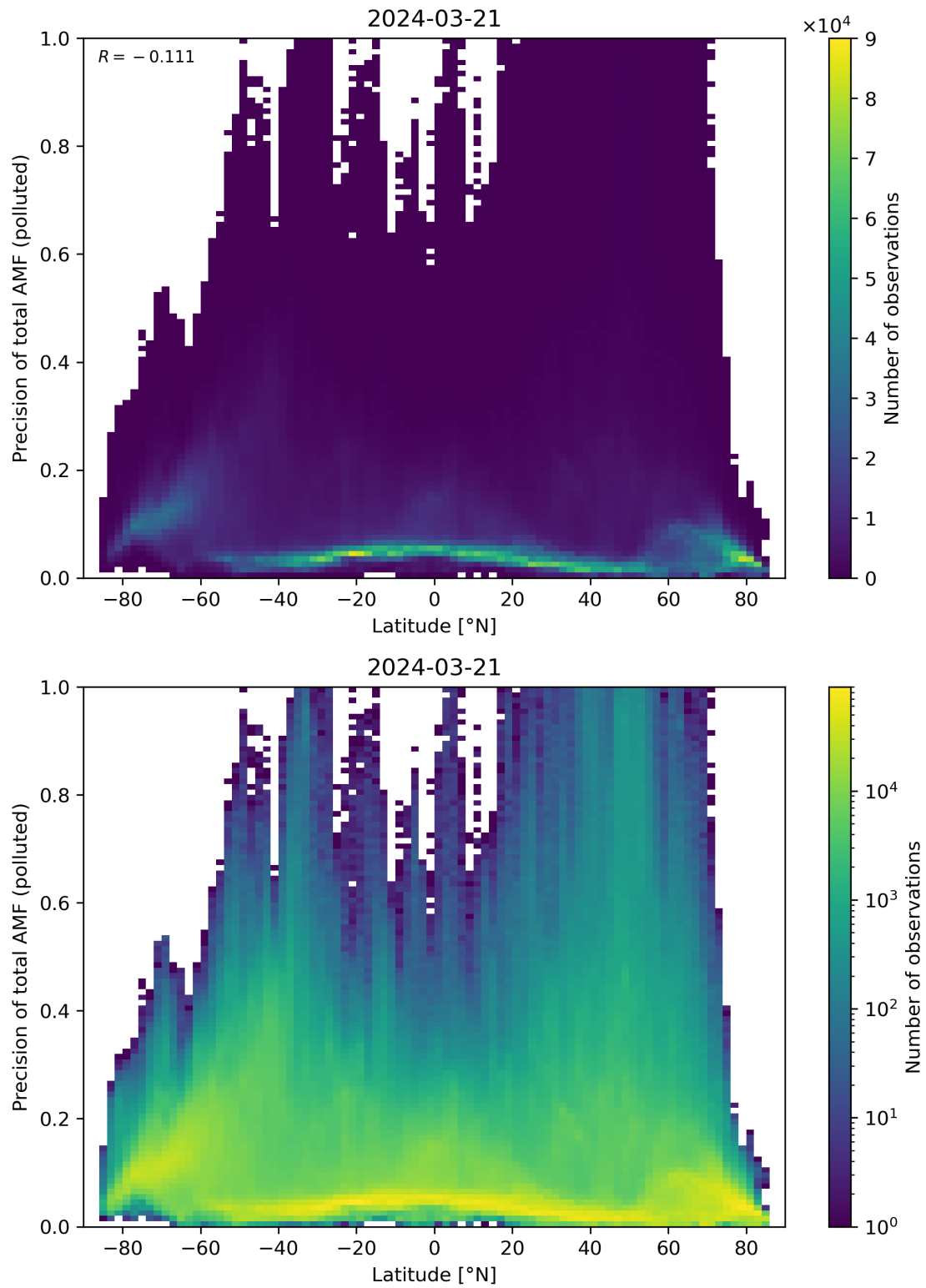
Figure 155: Scatter density plot of “Latitude” against “Precision of total AMF (polluted)” for 2024-03-20 to 2024-03-22.
