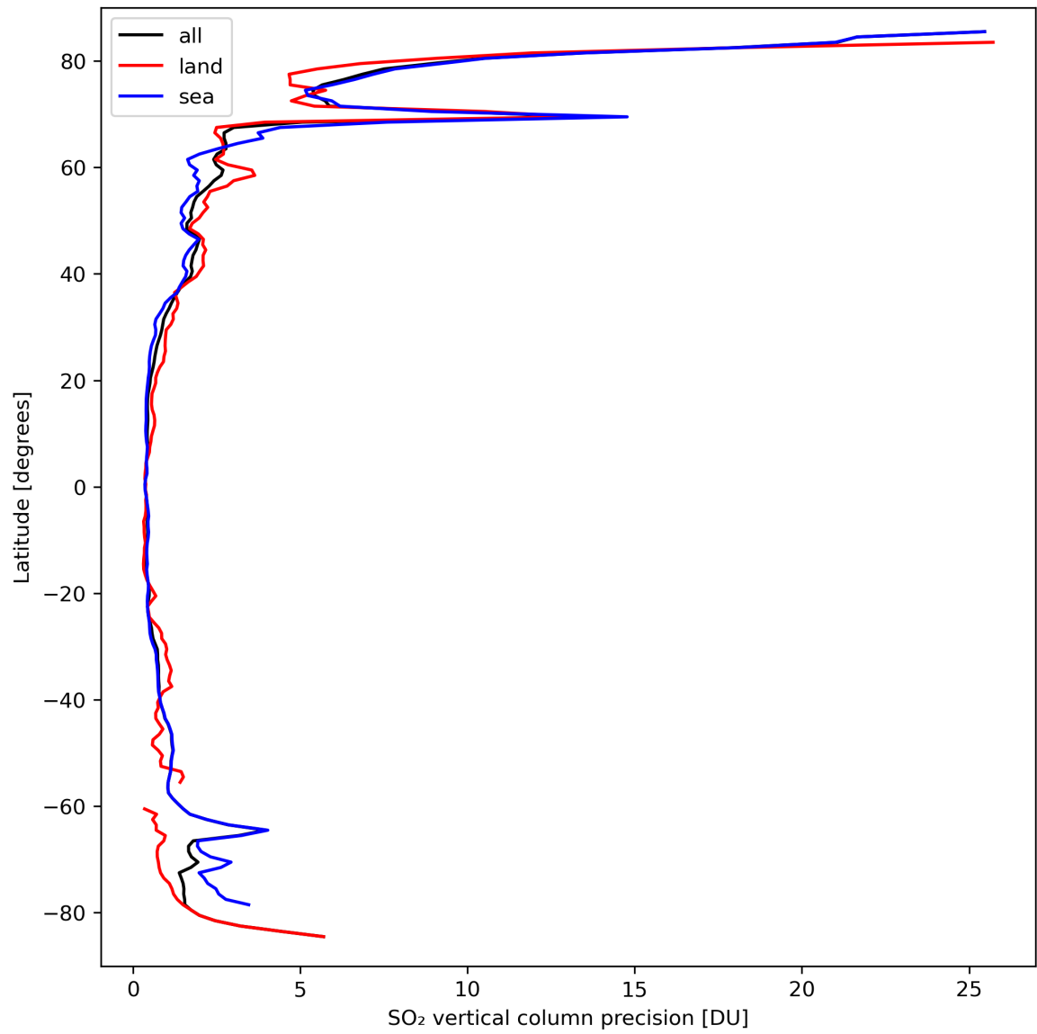
Figure 31: Zonal average of “SO 2 vertical column precision” for 2024-03-20 to 2024-03-22.
