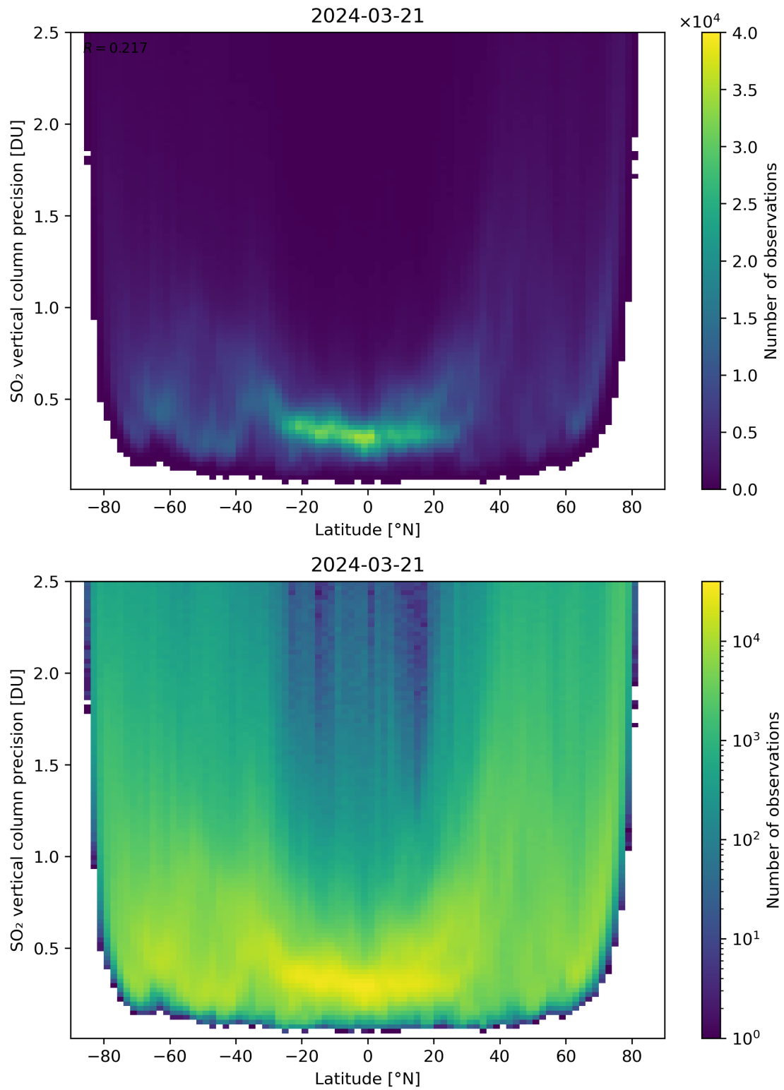
Figure 157: Scatter density plot of “Latitude” against “SO 2 vertical column precision” for 2024-03-20 to 2024-03-22.
