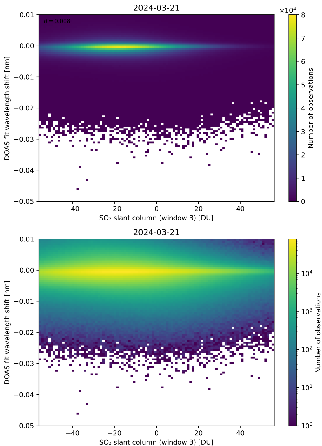
Figure 254: Scatter density plot of “SO 2 slant column (window 3)” against “DOAS fit wavelength shift” for 2024-03-20 to 2024-03-22.
