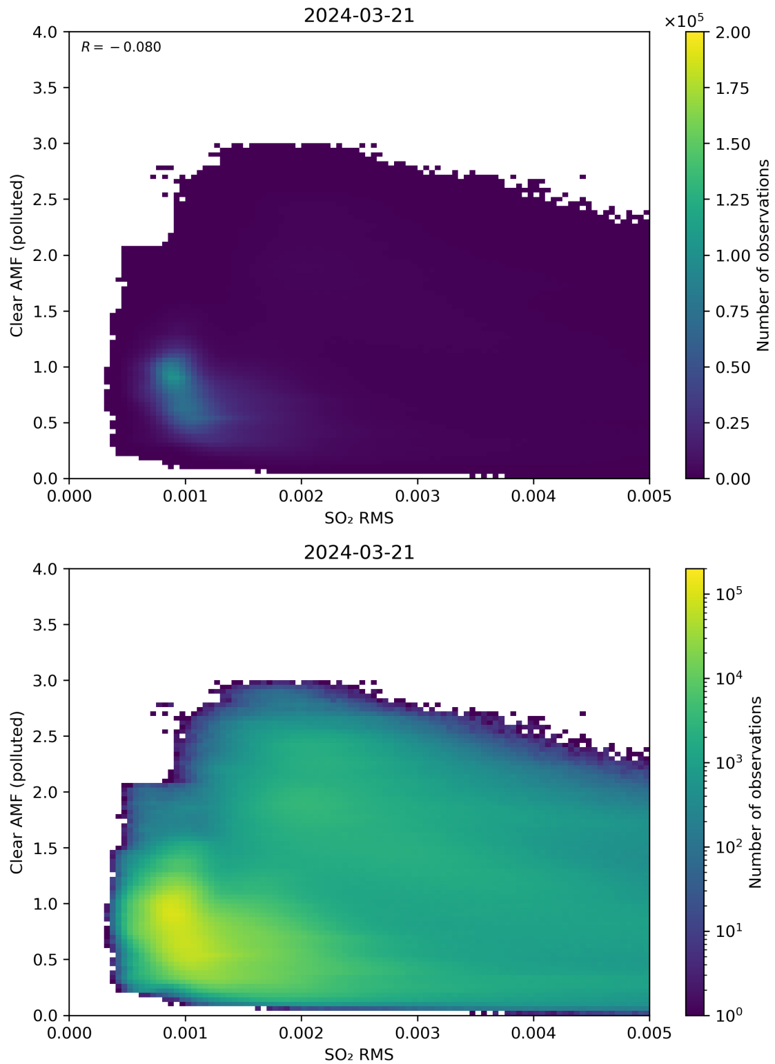
Figure 136: Scatter density plot of “SO 2 RMS” against “Clear AMF (polluted)” for 2024-03-20 to 2024-03-22.
