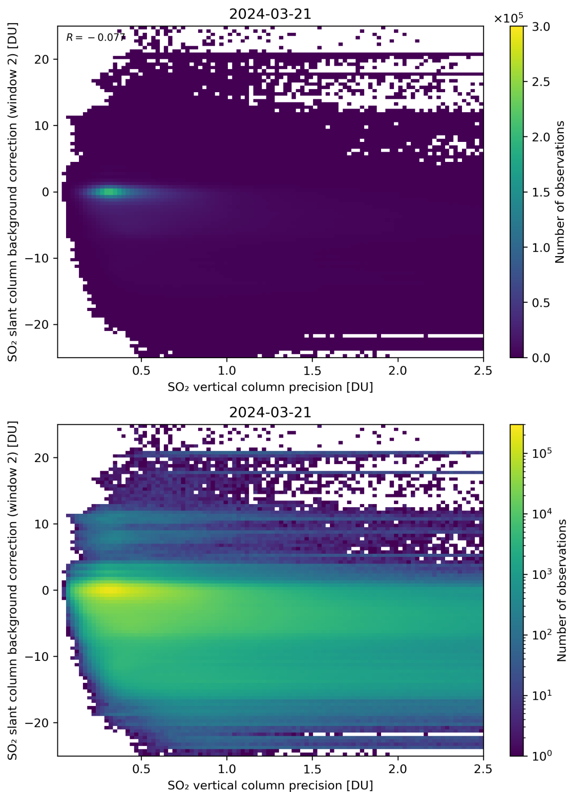
Figure 280: Scatter density plot of “SO 2 vertical column precision” against “SO 2 slant column background correction (window 2)” for 2024-03-20 to 2024-03-22.
