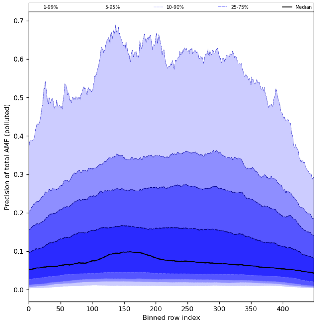
Figure 95: Along track statistics of “Precision of total AMF (polluted)” for 2024-03-20 to 2024-03-22
