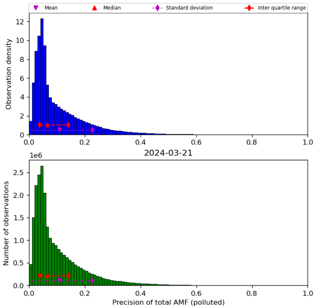
Figure 72: Histogram of “Precision of total AMF (polluted)” for 2024-03-20 to 2024-03-22
