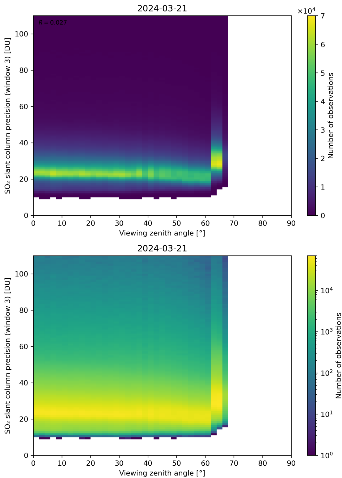
Figure 324: Scatter density plot of “Viewing zenith angle” against “SO 2 slant column precision (window 3)” for 2024-03-20 to 2024-03-22.
