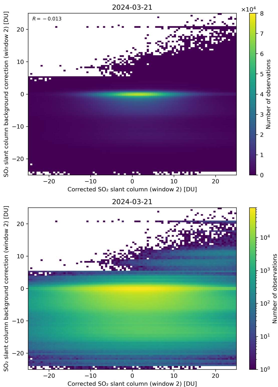
Figure 194: Scatter density plot of “Corrected SO 2 slant column (window 2)” against “SO 2 slant column background correction (window 2)” for 2024-03-20 to 2024-03-22.
