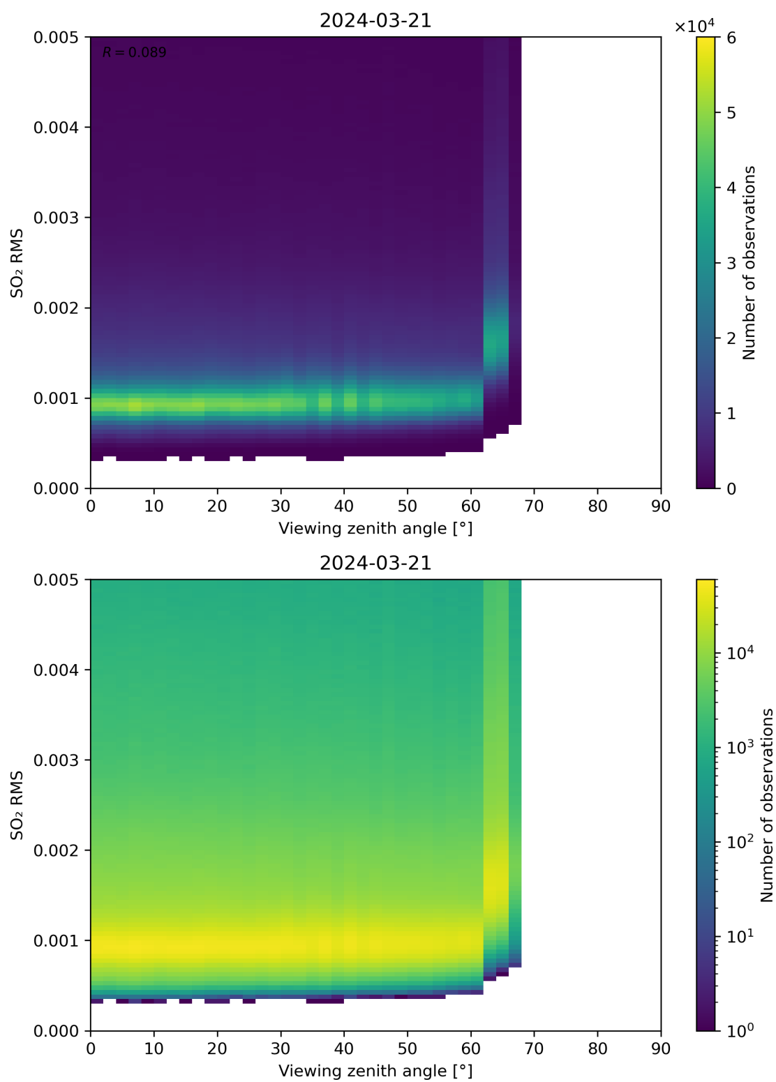
Figure 313: Scatter density plot of “Viewing zenith angle” against “SO 2 RMS” for 2024-03-20 to 2024-03-22.
