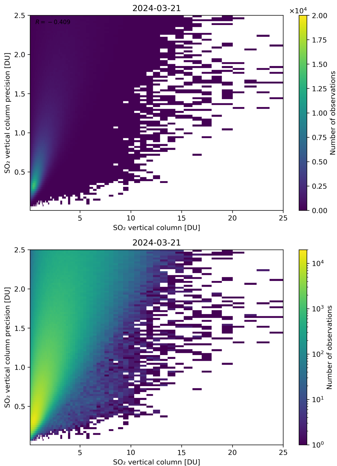
Figure 307: Scatter density plot of “SO 2 vertical column” against “SO 2 vertical column precision” for 2024-03-20 to 2024-03-22.
