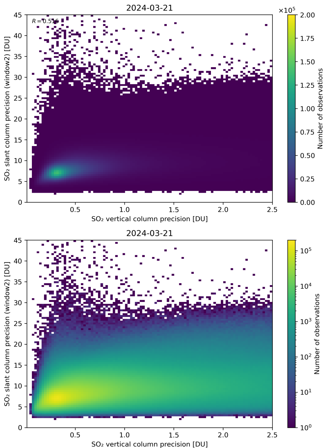
Figure 291: Scatter density plot of “SO 2 vertical column precision” against “SO 2 slant column precision (window2)” for 2024-03-20 to 2024-03-22.
