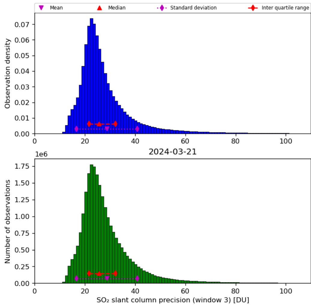
Figure 65: Histogram of “SO 2 slant column precision (window 3)” for 2024-03-20 to 2024-03-22
