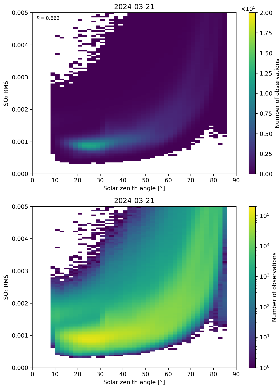
Figure 163: Scatter density plot of “Solar zenith angle” against “SO 2 RMS” for 2024-03-20 to 2024-03-22.
