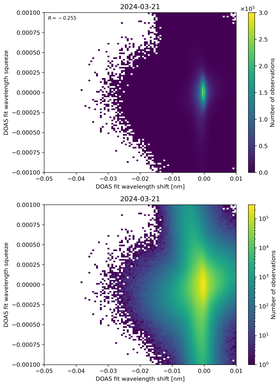
Figure 127: Scatter density plot of “DOAS fit wavelength shift” against “DOAS fit wavelength squeeze” for 2024-03-20 to 2024-03-22.
