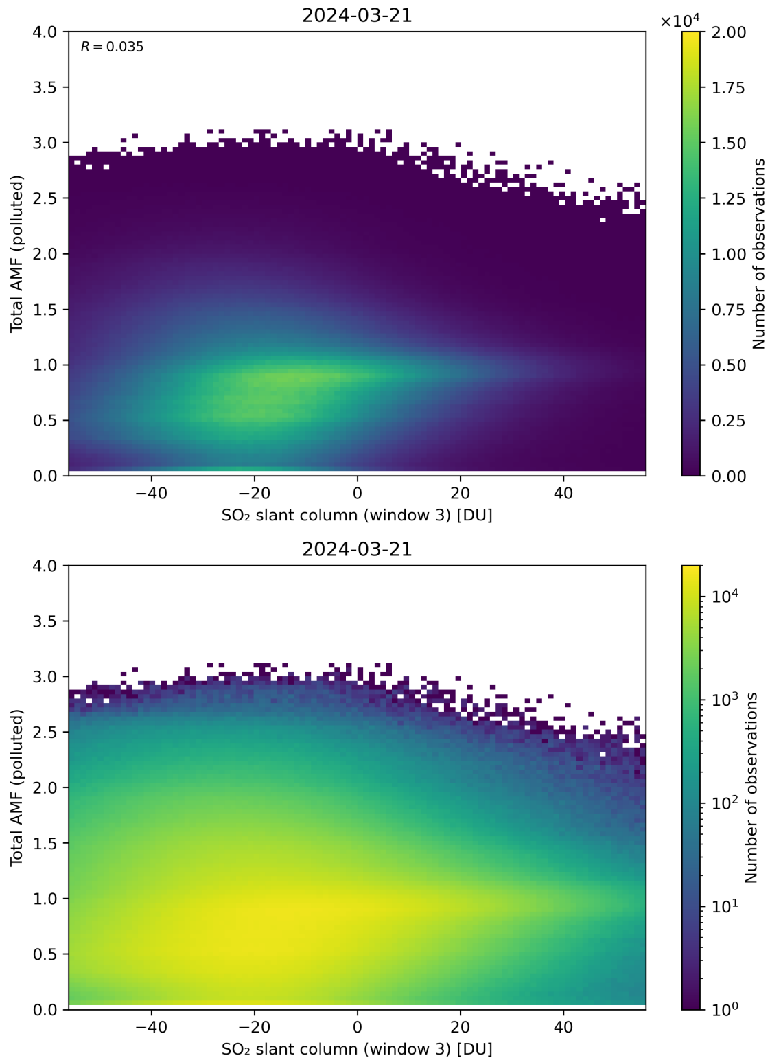
Figure 268: Scatter density plot of “SO 2 slant column (window 3)” against “Total AMF (polluted)” for 2024-03-20 to 2024-03-22.
