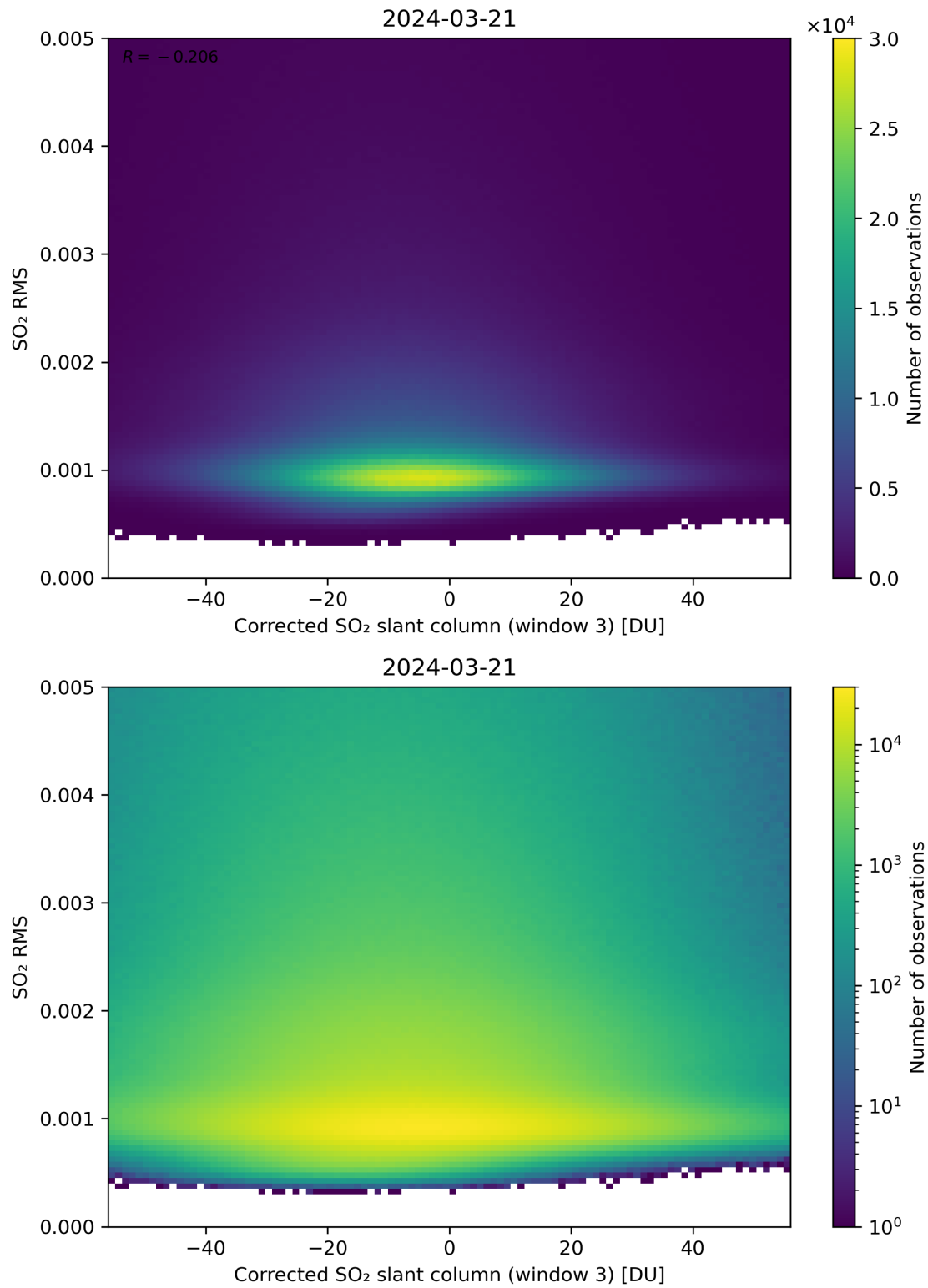
Figure 208: Scatter density plot of “Corrected SO 2 slant column (window 3)” against “SO 2 RMS” for 2024-03-20 to 2024-03-22.
