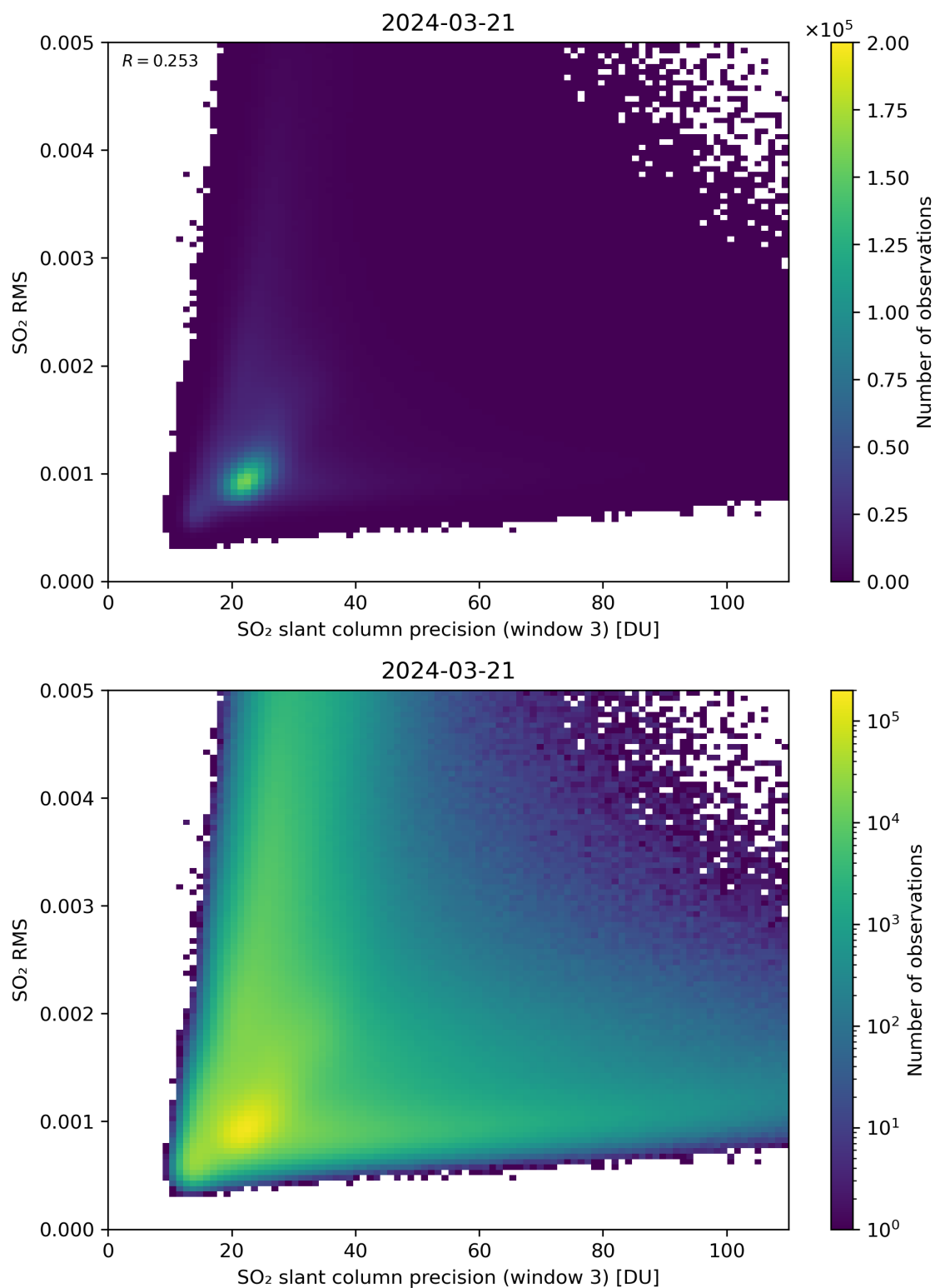
Figure 260: Scatter density plot of “SO 2 slant column precision (window 3)” against “SO 2 RMS” for 2024-03-20 to 2024-03-22.
