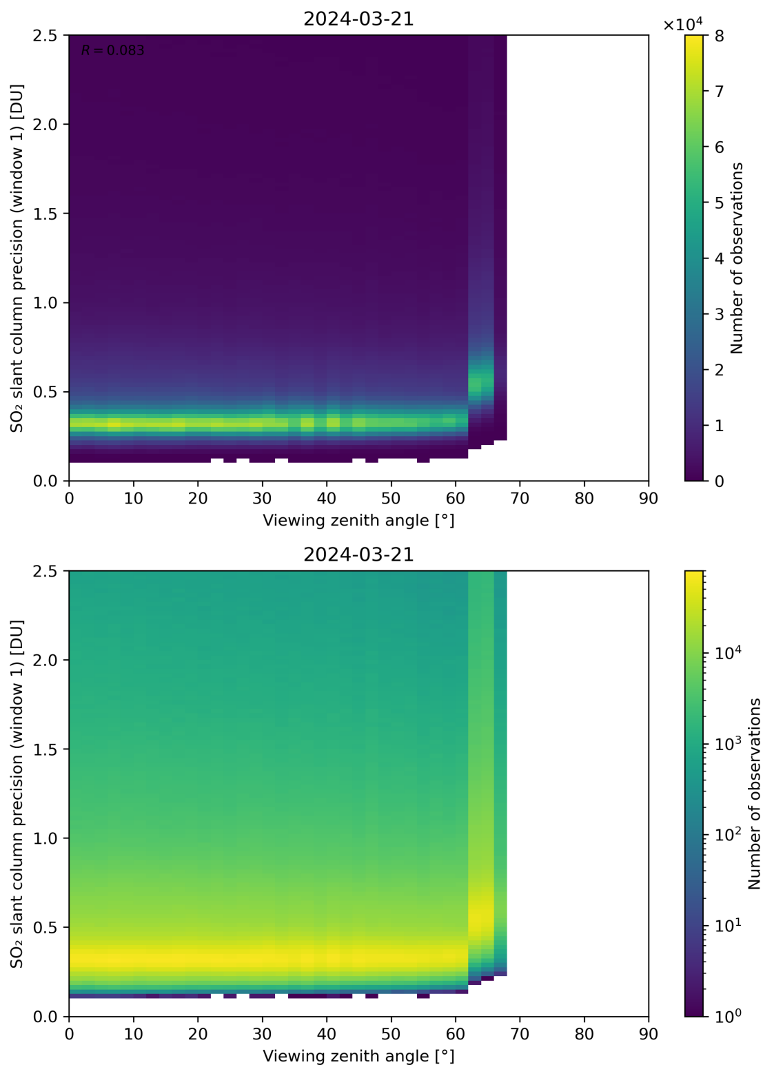
Figure 321: Scatter density plot of “Viewing zenith angle” against “SO 2 slant column precision (window 1)” for 2024-03-20 to 2024-03-22.
