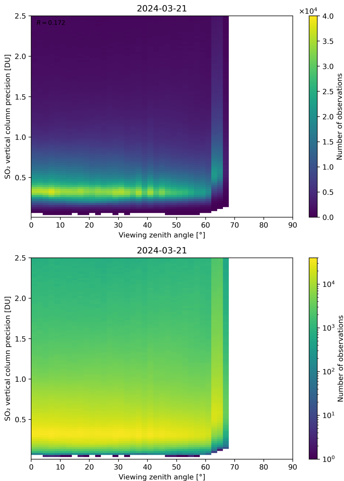
Figure 328: Scatter density plot of “Viewing zenith angle” against “SO 2 vertical column precision” for 2024-03-20 to 2024-03-22.
