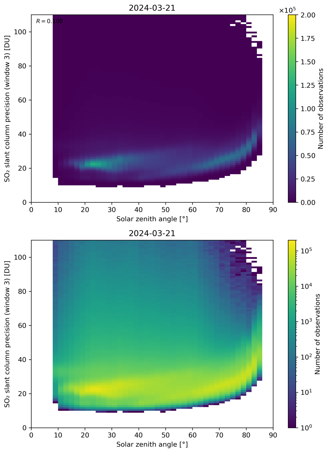
Figure 173: Scatter density plot of “Solar zenith angle” against “SO 2 slant column precision (window 3)” for 2024-03-20 to 2024-03-22.
