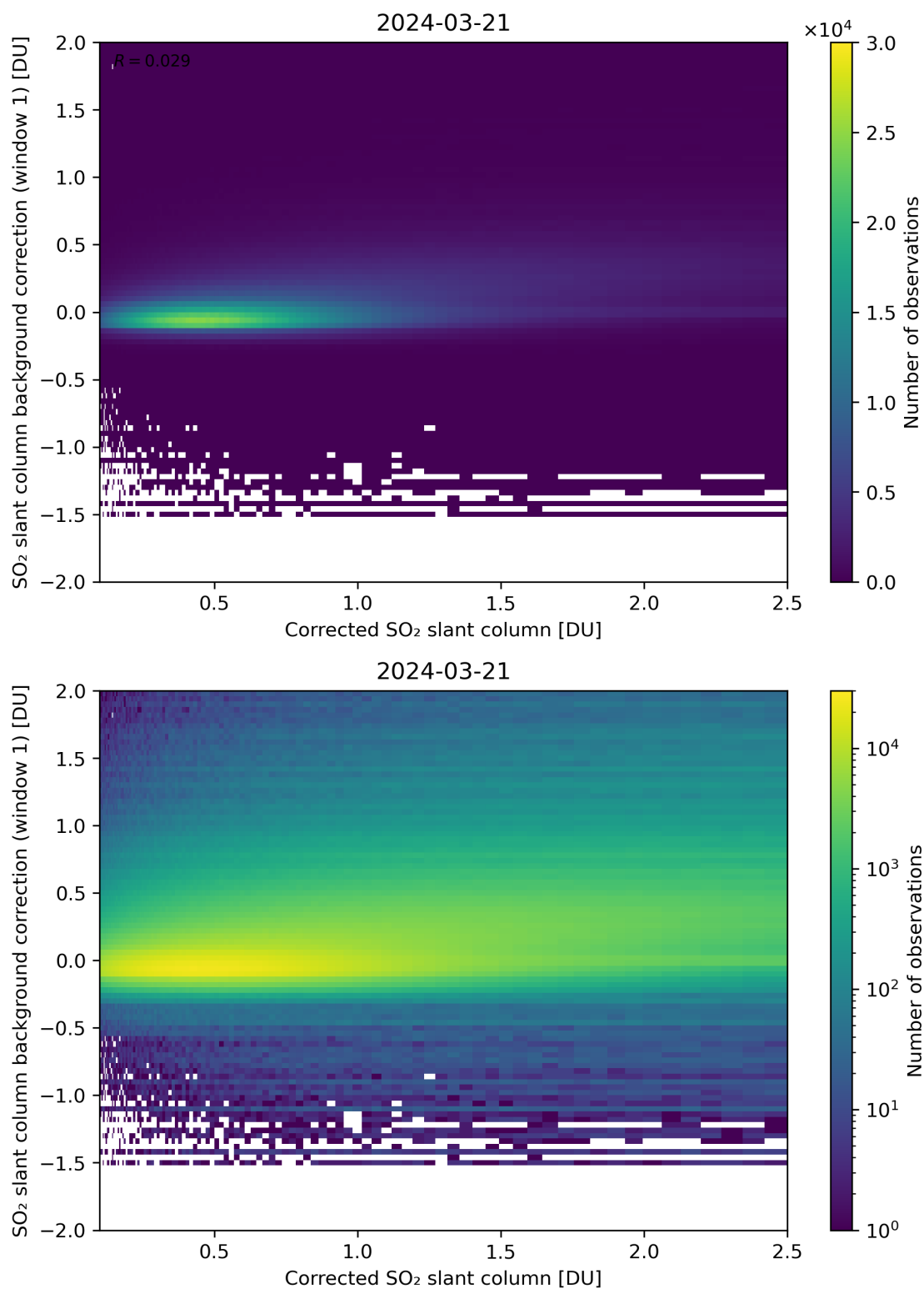
Figure 178: Scatter density plot of “Corrected SO 2 slant column” against “SO 2 slant column background correction (window 1)” for 2024-03-20 to 2024-03-22.
