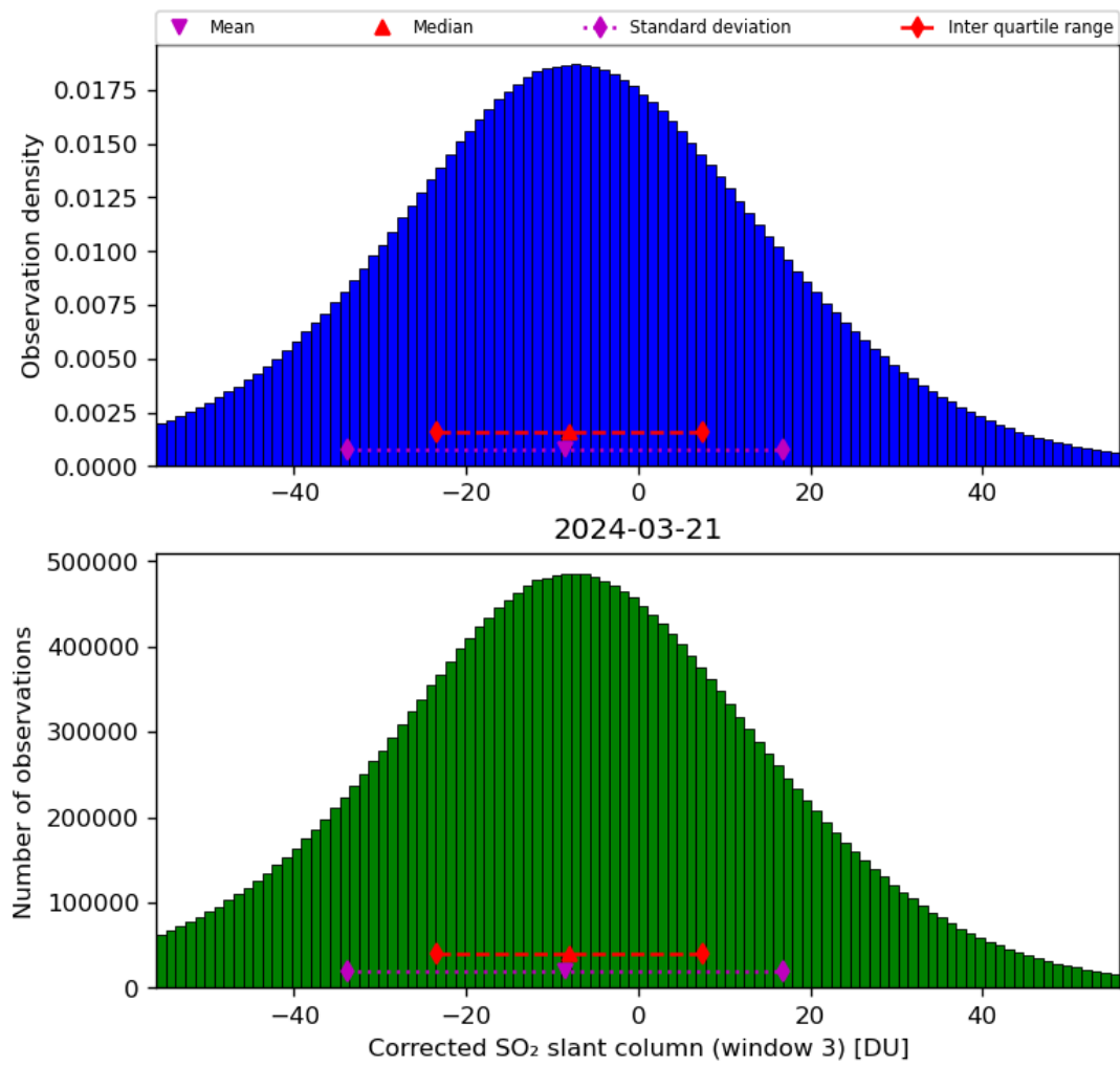
Figure 66: Histogram of "Corrected SO 2 slant column (window 3)" for 2024-03-20 to 2024-03-22
