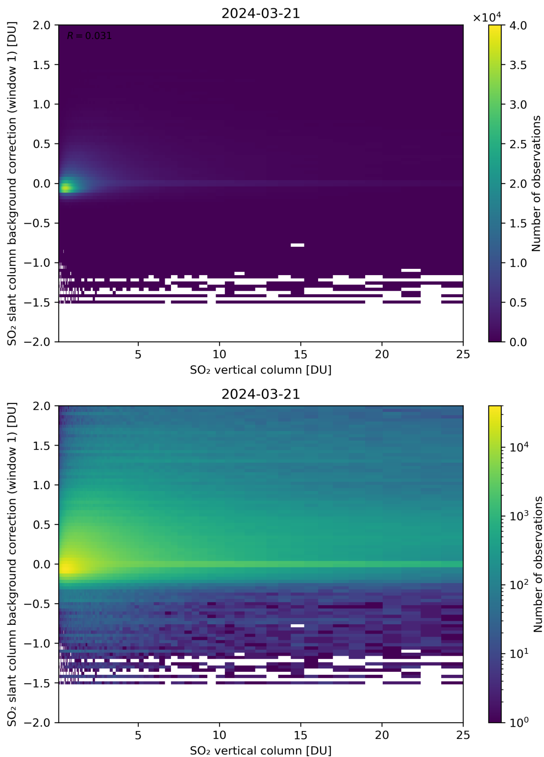
Figure 273: Scatter density plot of “SO 2 vertical column” against “SO 2 slant column background correction (window 1)” for 2024-03-20 to 2024-03-22.
