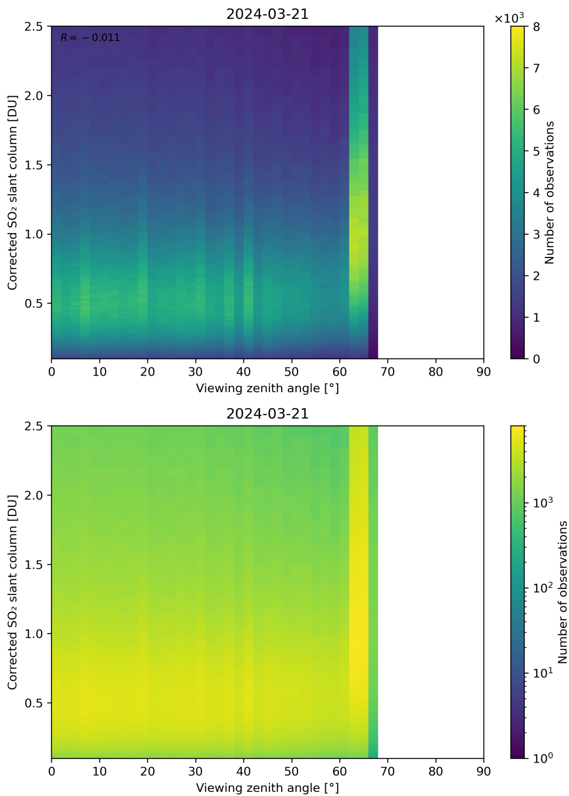
Figure 317: Scatter density plot of “Viewing zenith angle” against “Corrected SO 2 slant column” for 2024-03-20 to 2024-03-22.
