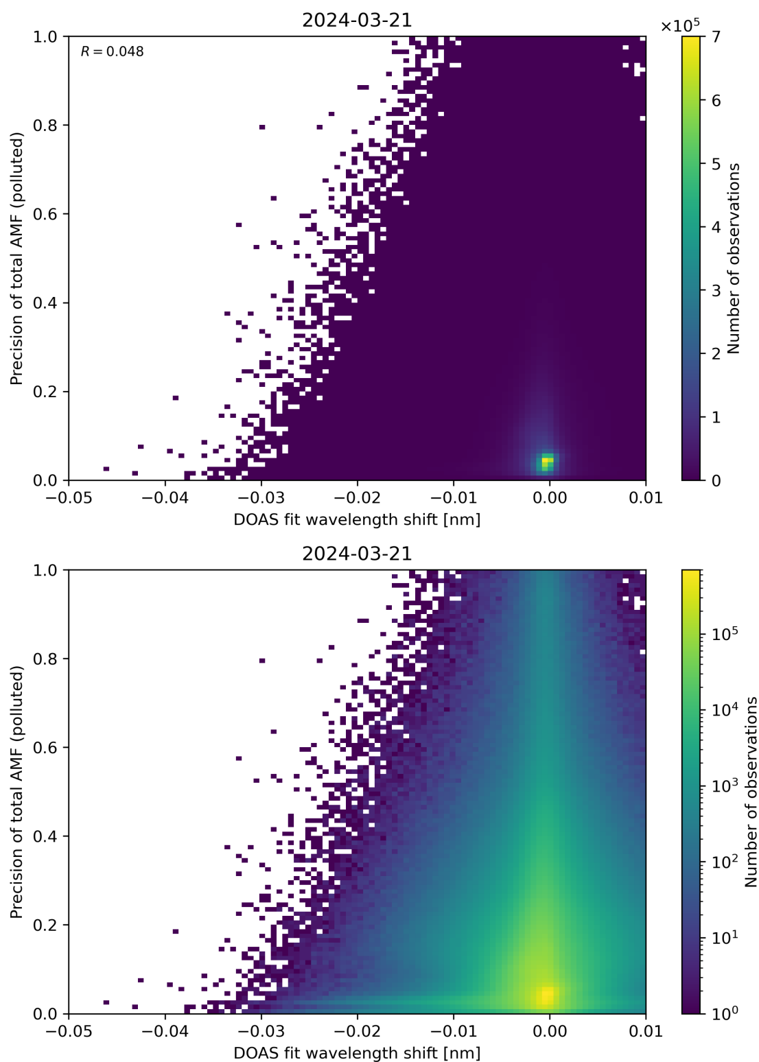
Figure 131: Scatter density plot of “DOAS fit wavelength shift” against “Precision of total AMF (polluted)” for 2024-03-20 to 2024-03-22.
