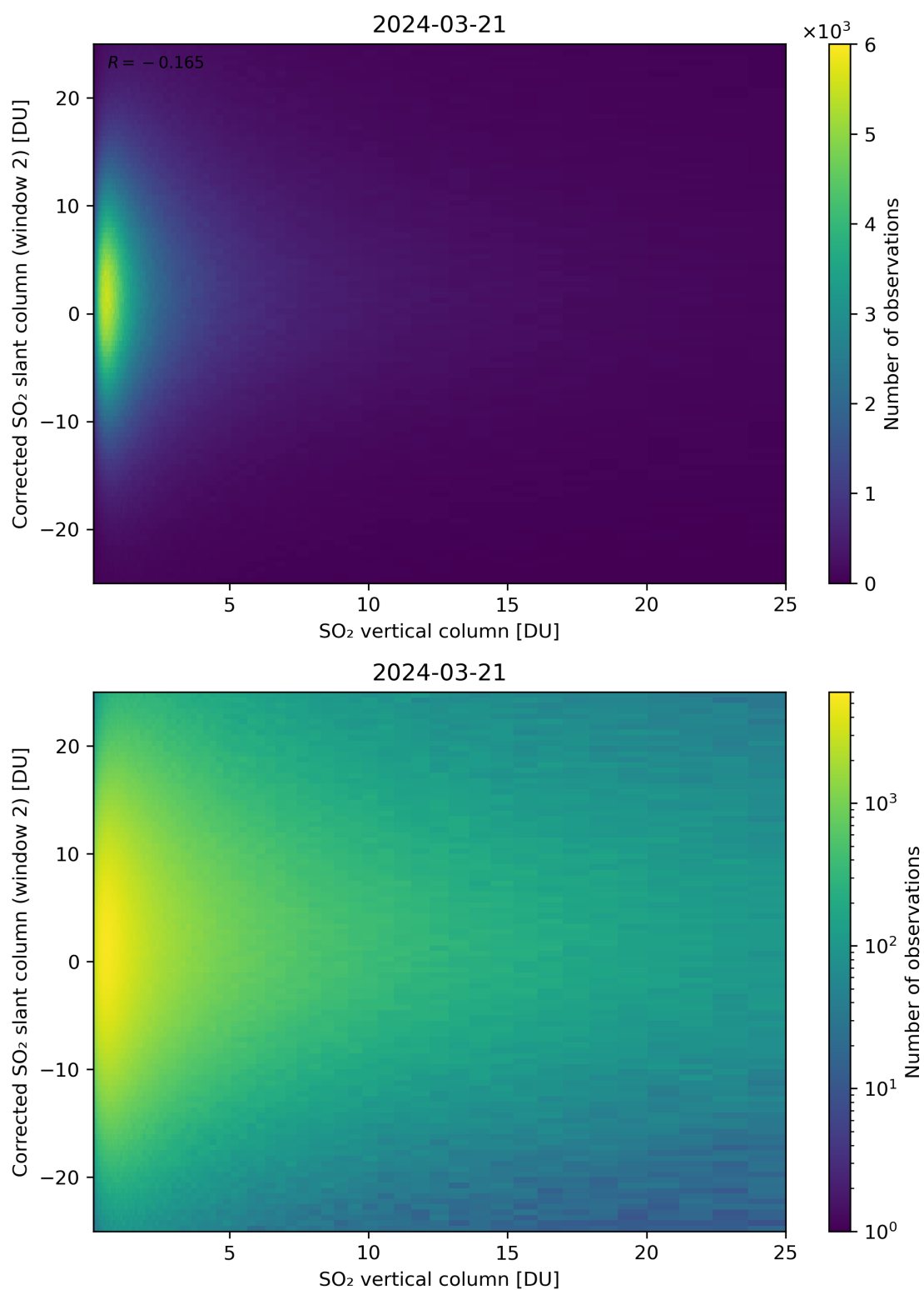
Figure 298: Scatter density plot of “SO 2 vertical column” against “Corrected SO 2 slant column (window 2)” for 2024-03-20 to 2024-03-22.
