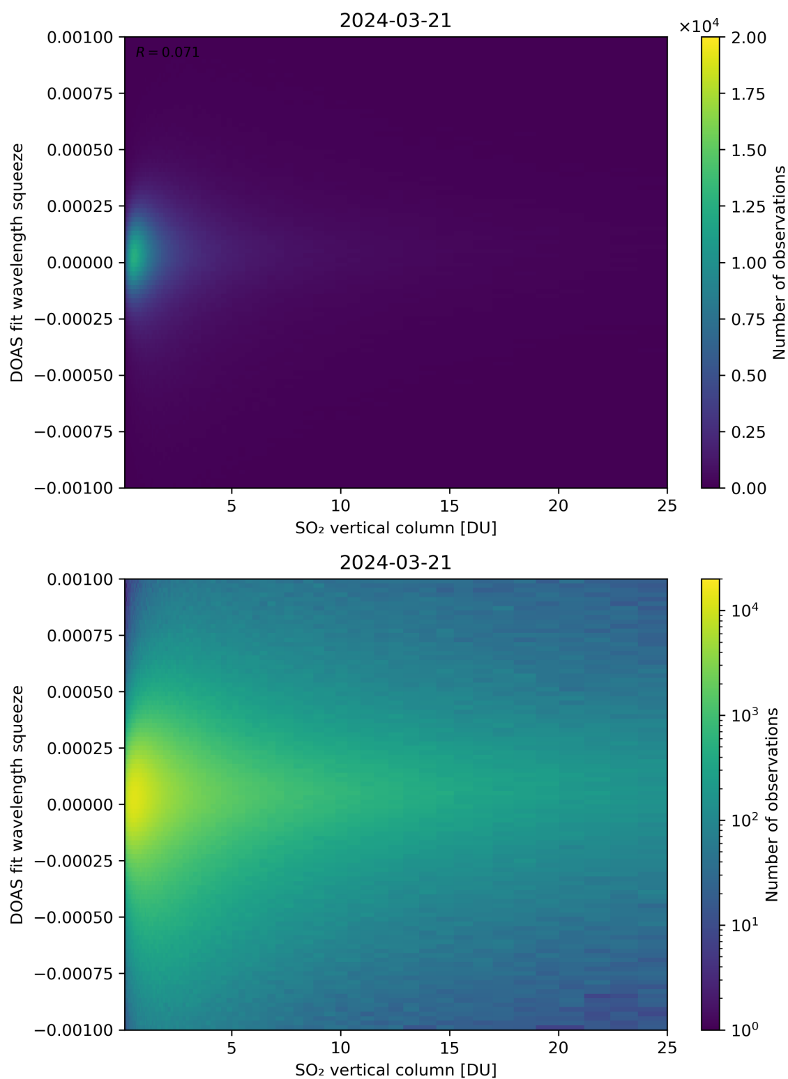
Figure 277: Scatter density plot of “SO 2 vertical column” against “DOAS fit wavelength squeeze” for 2024-03-20 to 2024-03-22.
