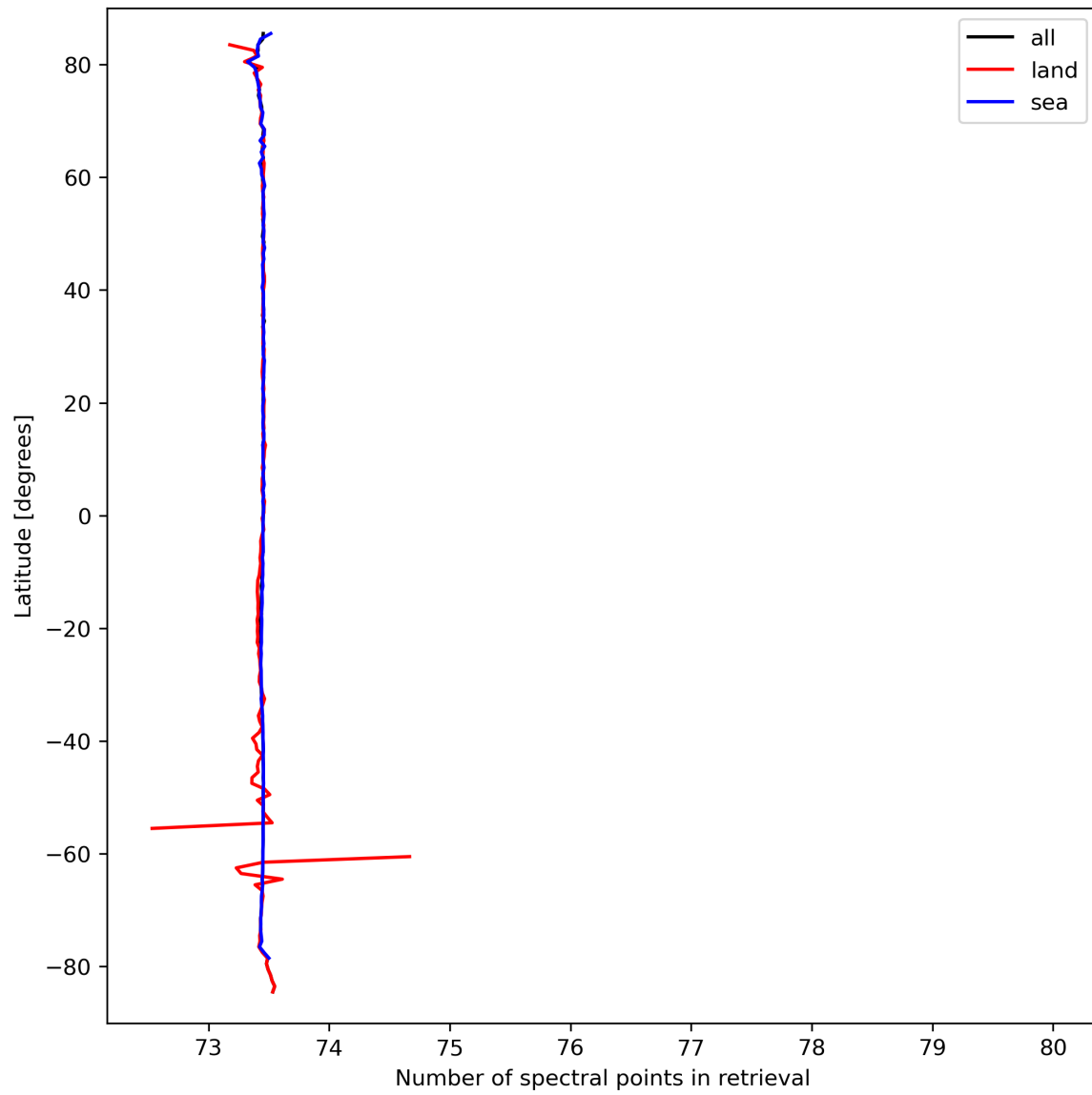
Figure 51: Zonal average of “Number of spectral points in retrieval” for 2024-03-20 to 2024-03-22.
