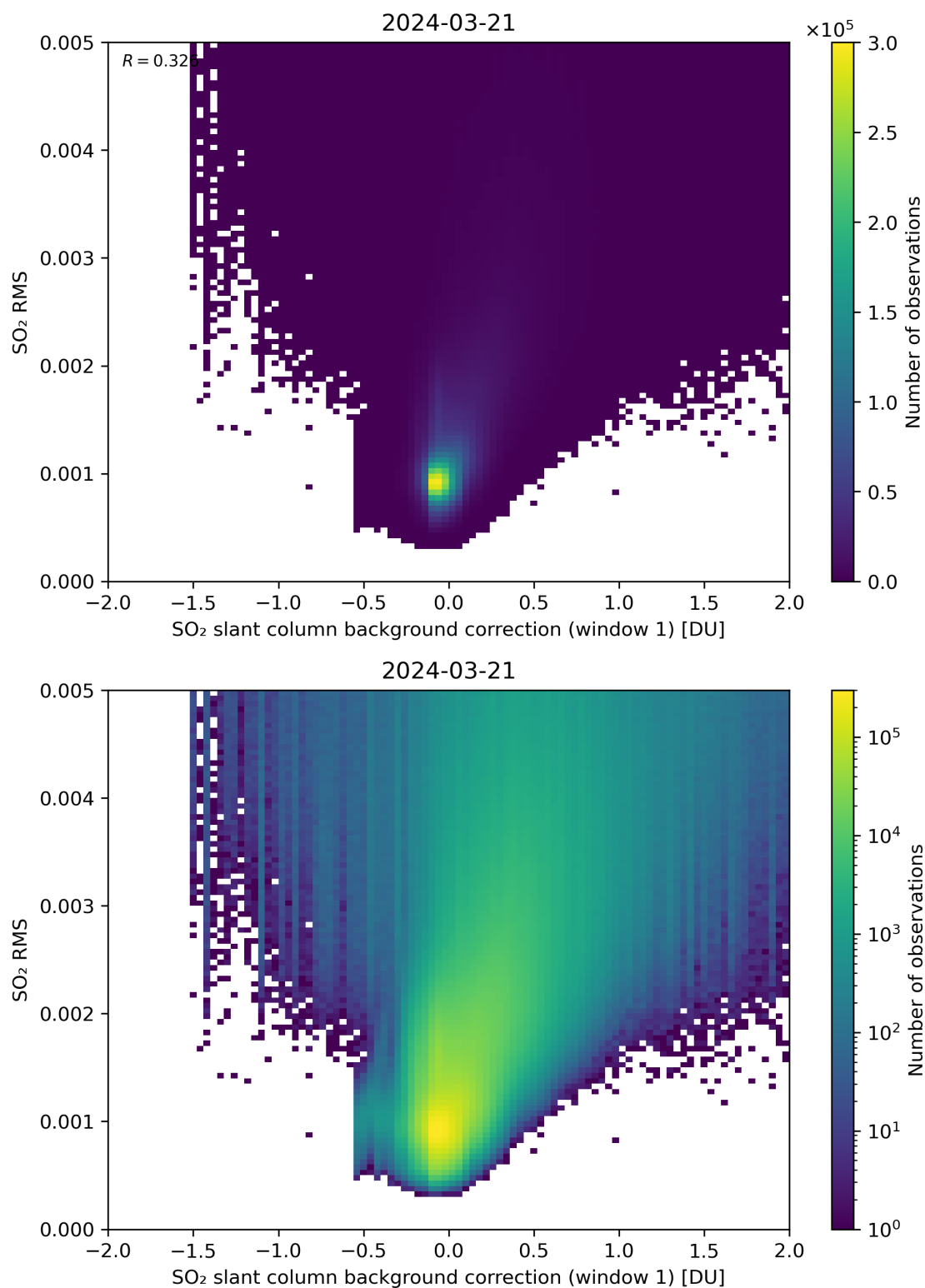
Figure 102: Scatter density plot of “SO 2 slant column background correction (window 1)” against “SO 2 RMS” for 2024-03-20 to 2024-03-22.
