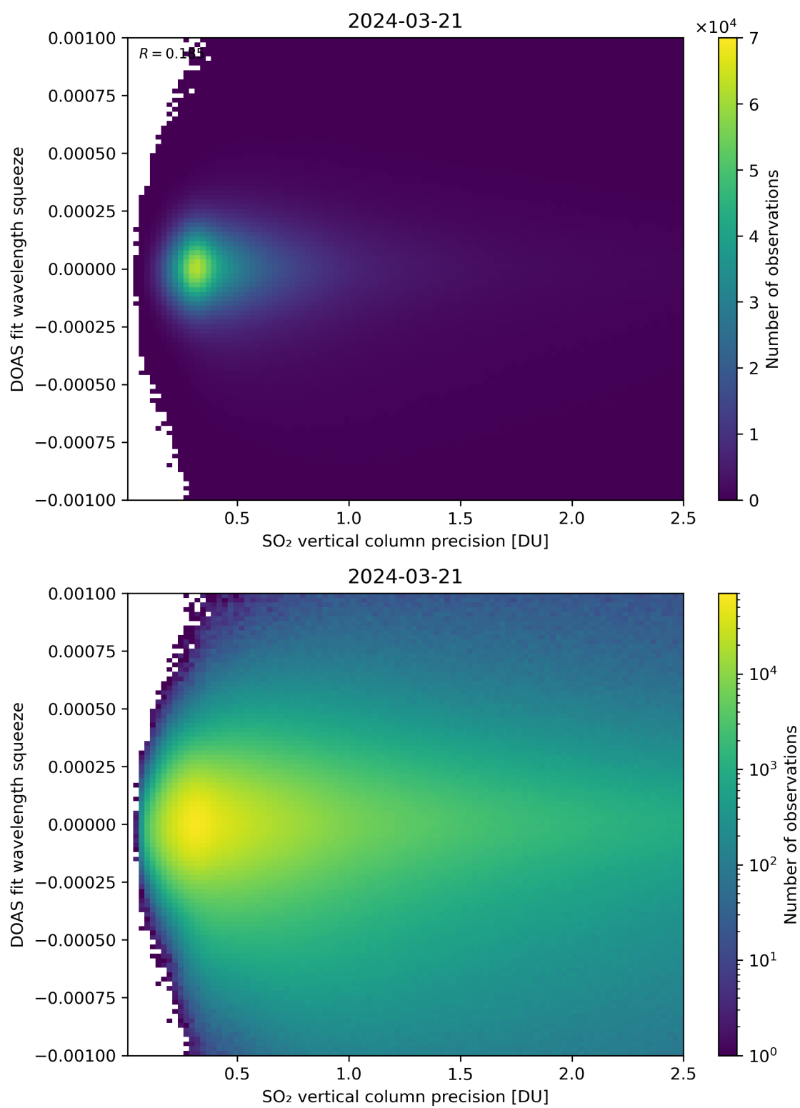
Figure 283: Scatter density plot of “SO 2 vertical column precision” against “DOAS fit wavelength squeeze” for 2024-03-20 to 2024-03-22.
