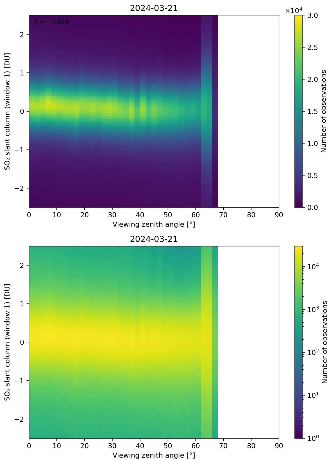
Figure 320: Scatter density plot of “Viewing zenith angle” against “SO 2 slant column (window 1)” for 2024-03-20 to 2024-03-22.
