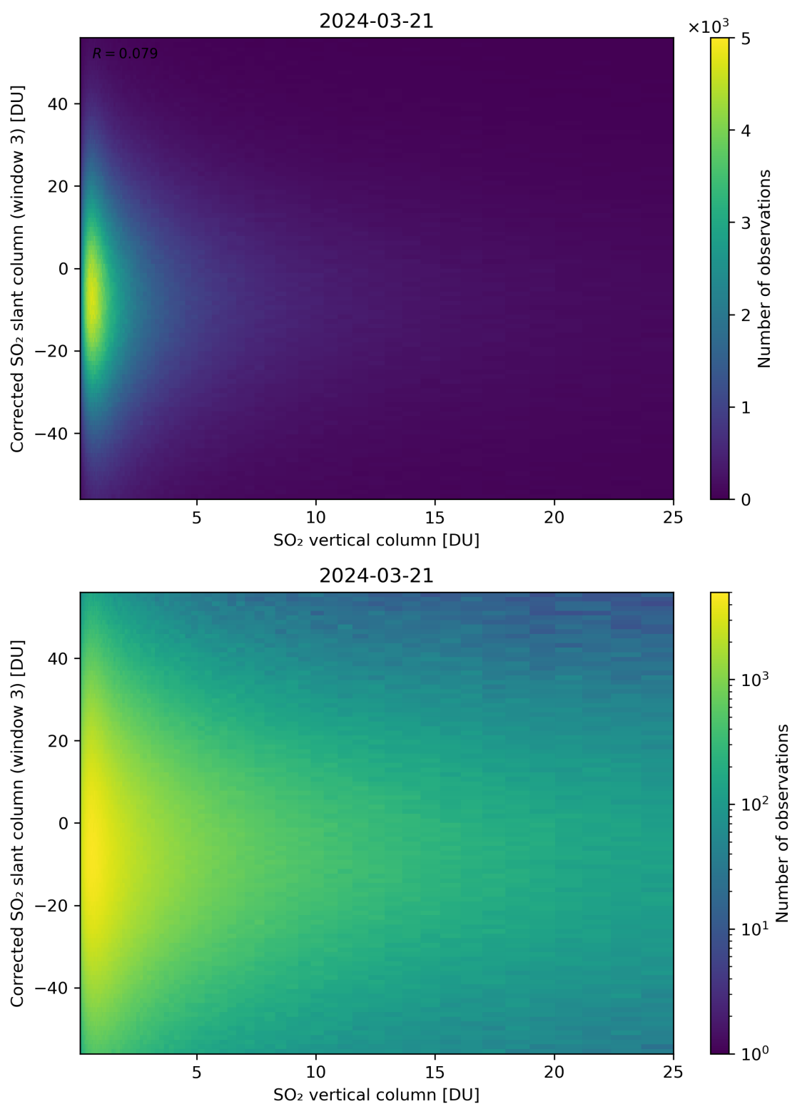
Figure 299: Scatter density plot of “SO 2 vertical column” against “Corrected SO 2 slant column (window 3)” for 2024-03-20 to 2024-03-22.
