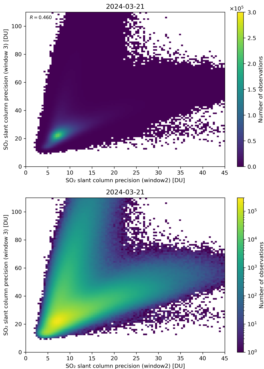
Figure 250: Scatter density plot of “SO 2 slant column precision (window2)” against “SO 2 slant column precision (window 3)” for 2024-03-20 to 2024-03-22.
