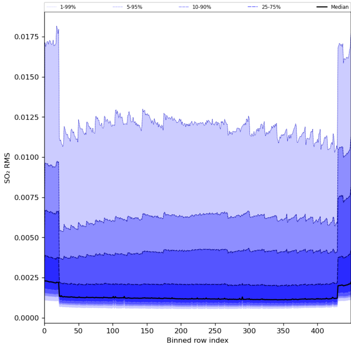
Figure 93: Along track statistics of "SO 2 RMS" for 2024-03-20 to 2024-03-22
