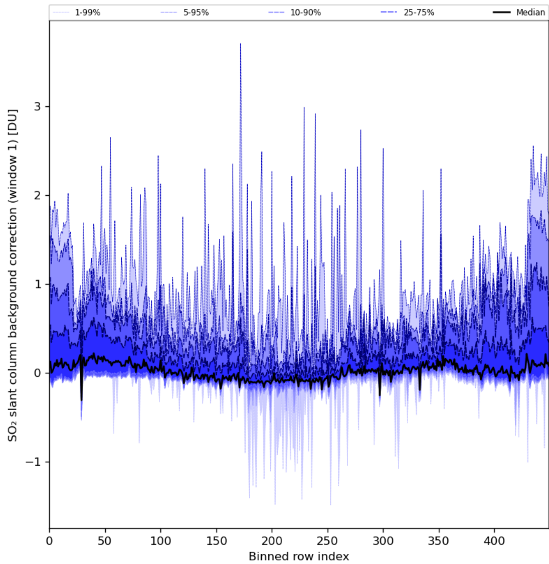
Figure 82: Along track statistics of “SO 2 slant column background correction (window 1)” for 2024-03-20 to 2024-03-22
