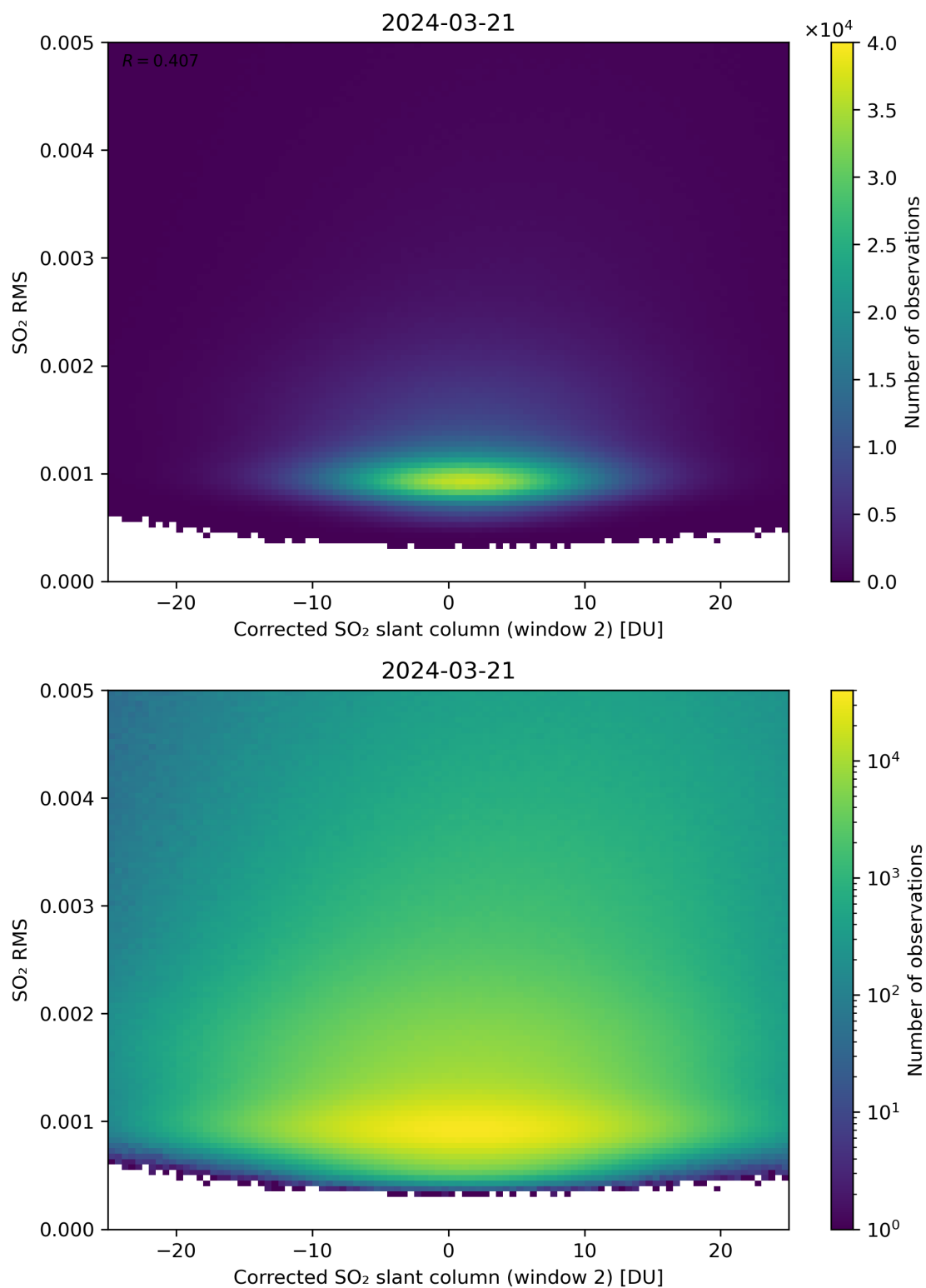
Figure 198: Scatter density plot of “Corrected SO 2 slant column (window 2)” against “SO 2 RMS” for 2024-03-20 to 2024-03-22.
