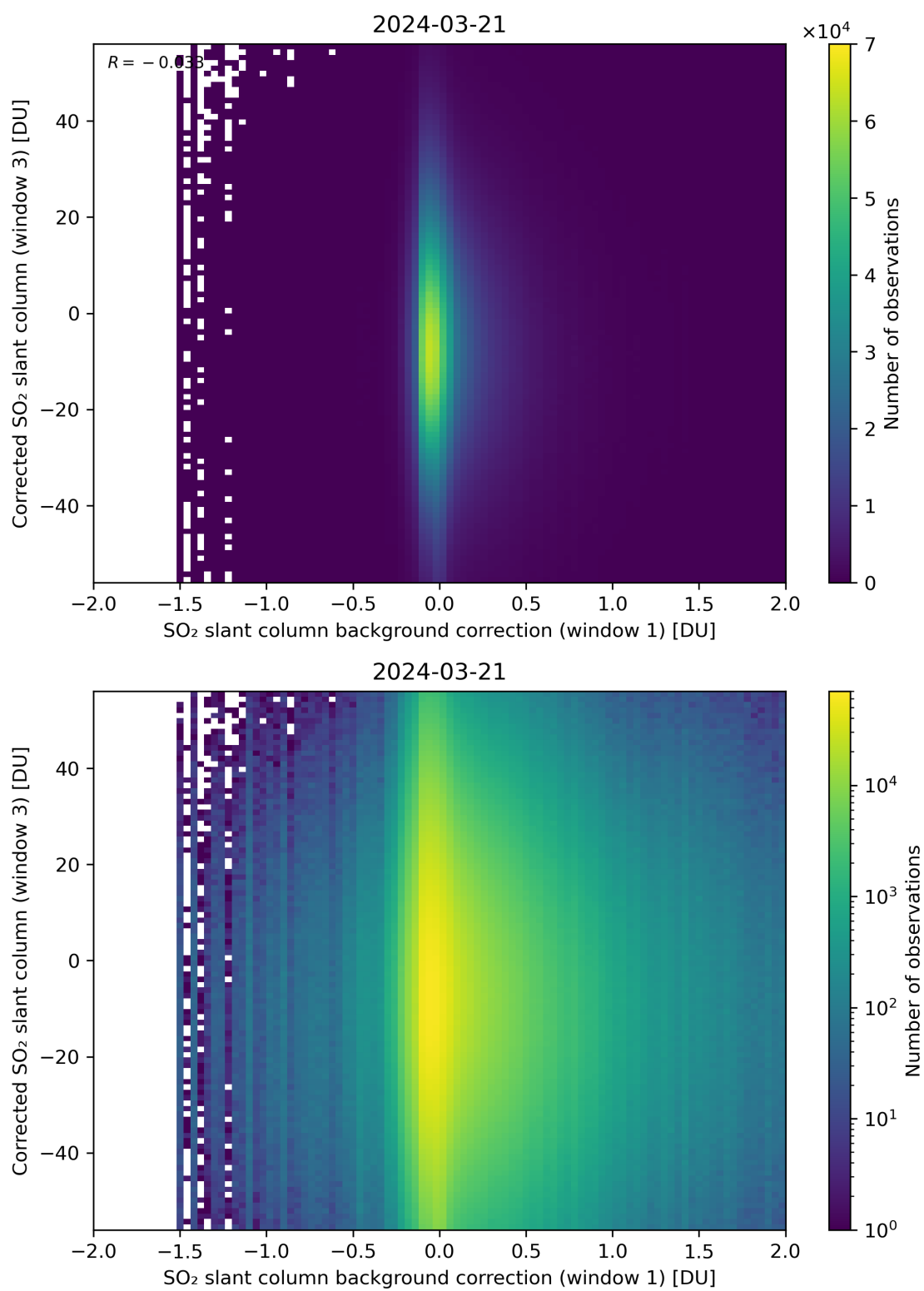
Figure 105: Scatter density plot of “SO 2 slant column background correction (window 1)” against “Corrected SO 2 slant column (window 3)” for 2024-03-20 to 2024-03-22.
