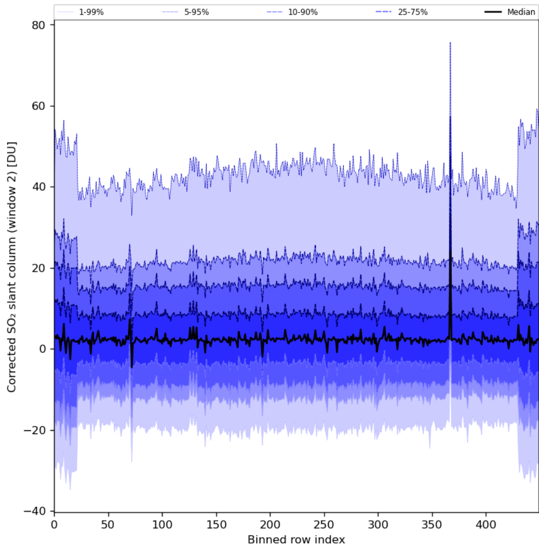
Figure 85: Along track statistics of “Corrected SO 2 slant column (window 2)” for 2024-03-20 to 2024-03-22
