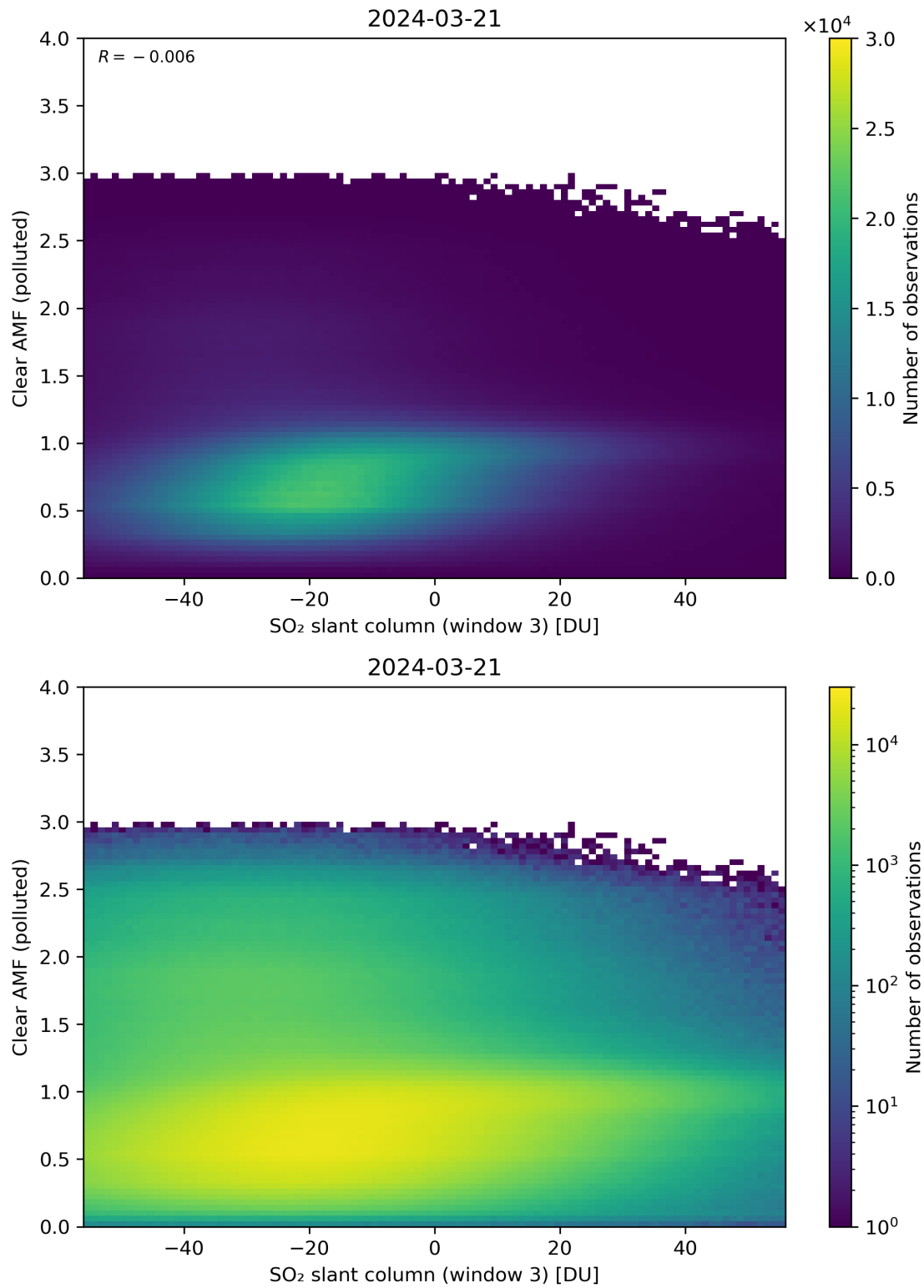
Figure 265: Scatter density plot of “SO 2 slant column (window 3)” against “Clear AMF (polluted)” for 2024-03-20 to 2024-03-22.
