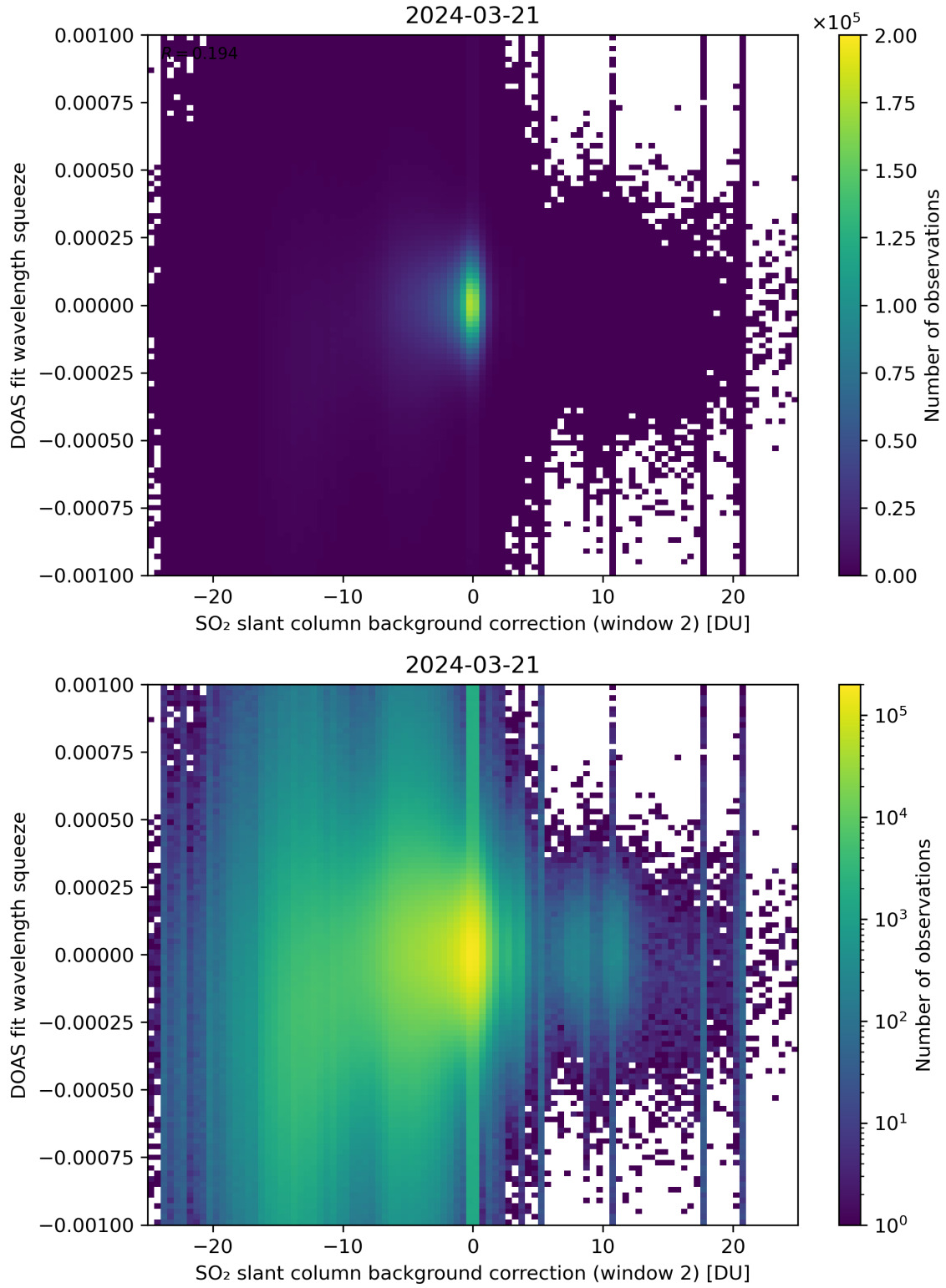
Figure 113: Scatter density plot of “SO 2 slant column background correction (window 2)” against “DOAS fit wavelength squeeze” for 2024-03-20 to 2024-03-22.
