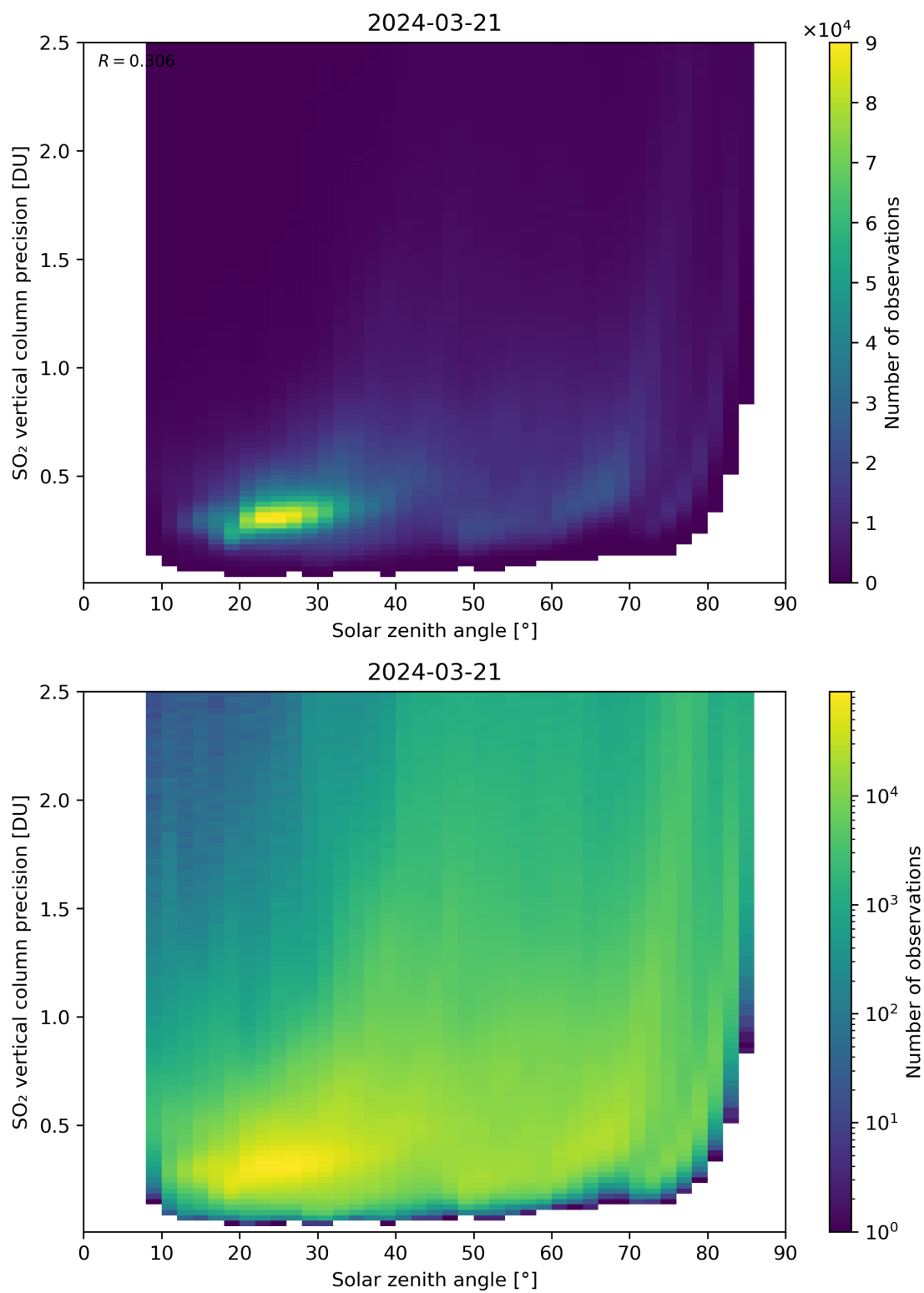
Figure 177: Scatter density plot of “Solar zenith angle” against “SO 2 vertical column precision” for 2024-03-20 to 2024-03-22.
