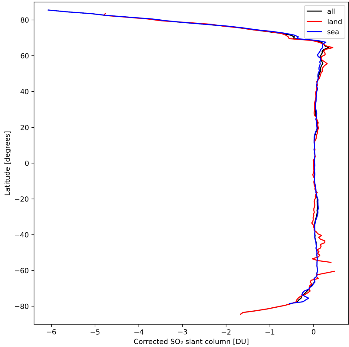
Figure 32: Zonal average of “Corrected SO 2 slant column” for 2024-03-20 to 2024-03-22.
