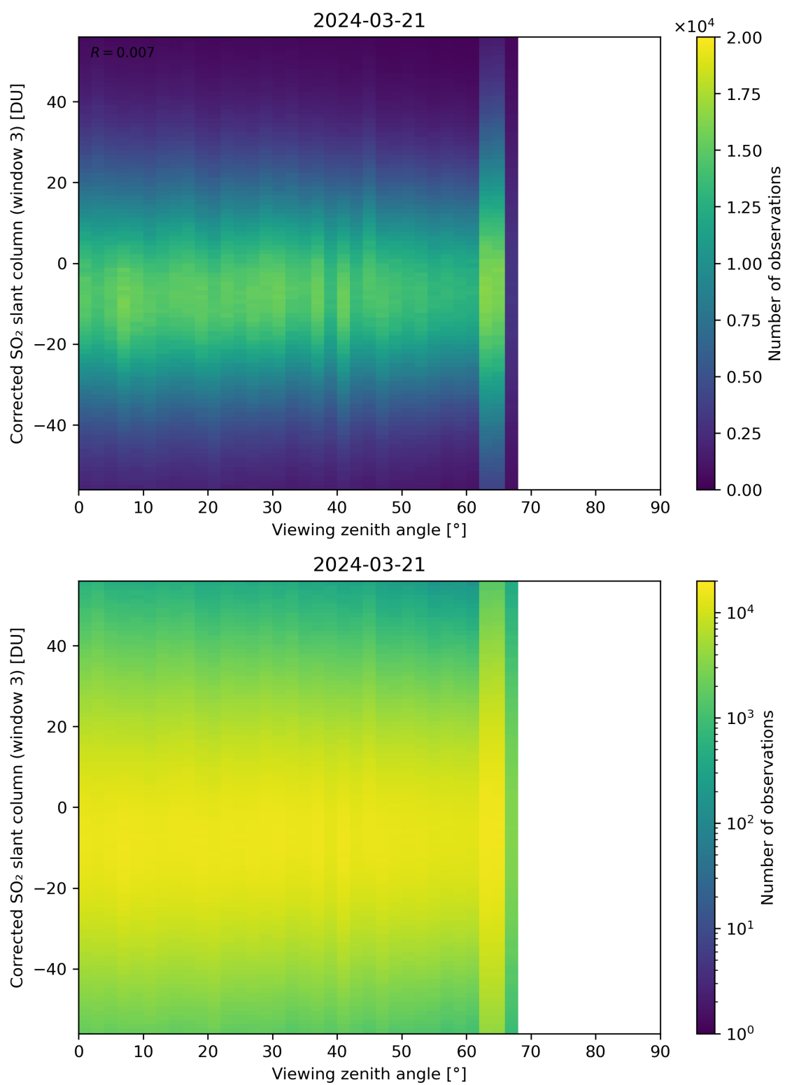
Figure 319: Scatter density plot of “Viewing zenith angle” against “Corrected SO 2 slant column (window 3)” for 2024-03-20 to 2024-03-22.
