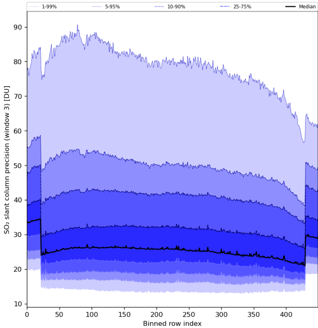
Figure 88: Along track statistics of “SO 2 slant column precision (window 3)” for 2024-03-20 to 2024-03-22
