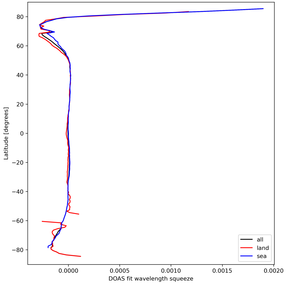
Figure 46: Zonal average of “DOAS fit wavelength squeeze” for 2024-03-20 to 2024-03-22.
