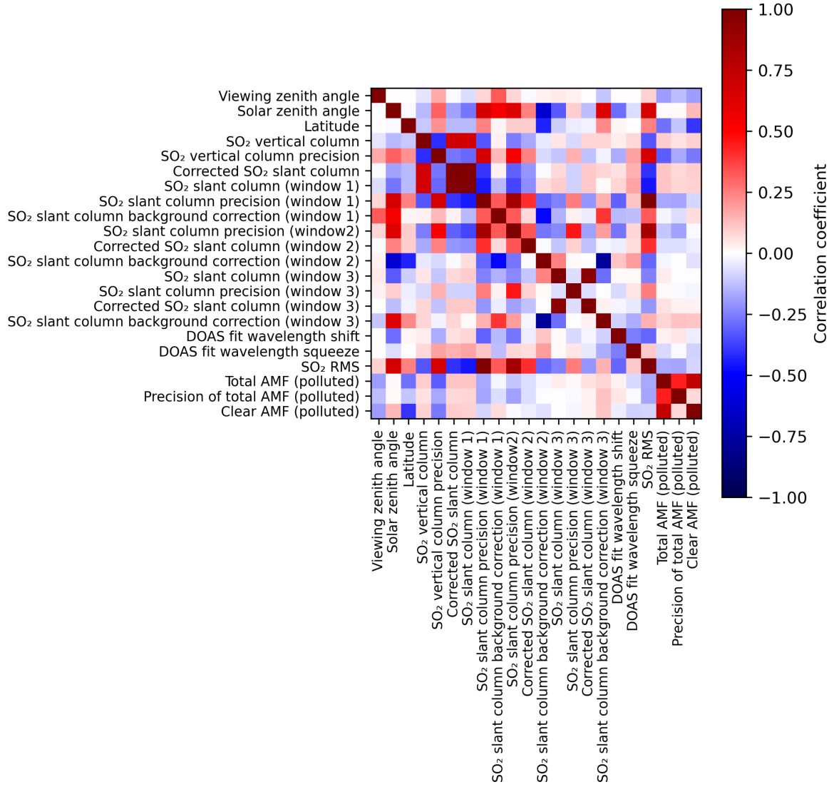
Figure 2: Map of correlation matrix for 2024-03-20 to 2024-03-22.
