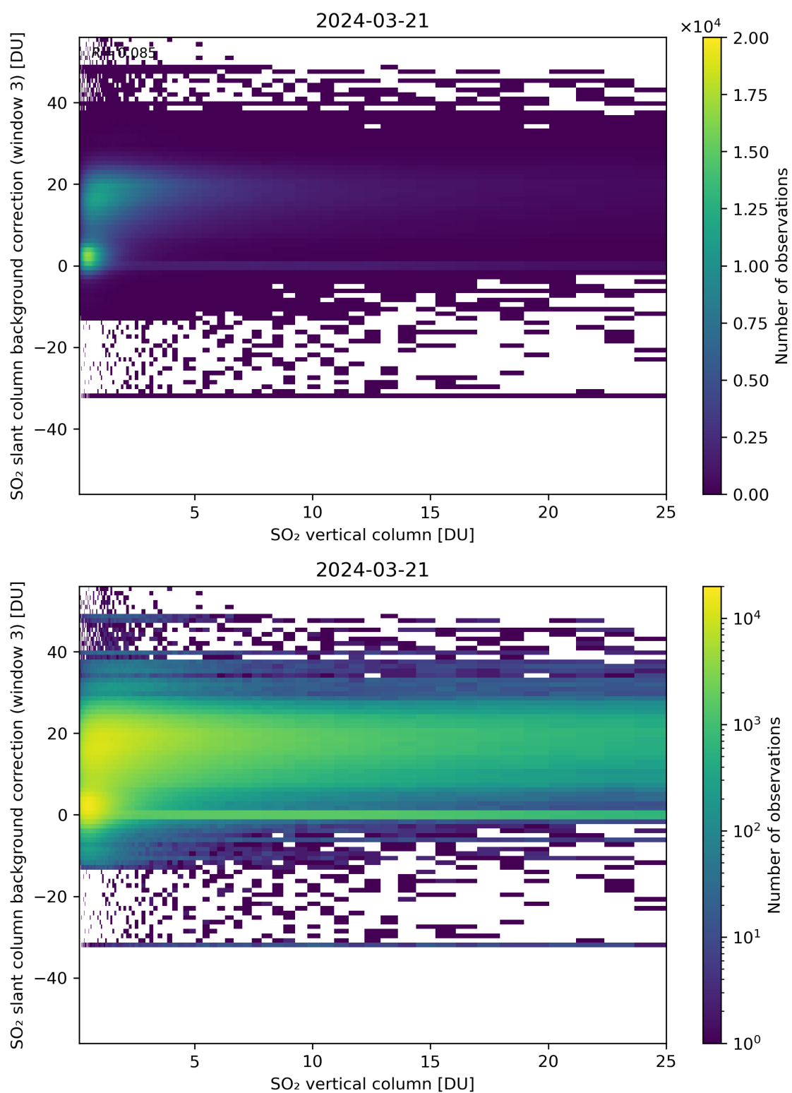
Figure 275: Scatter density plot of “SO 2 vertical column” against “SO 2 slant column background correction (window 3)” for 2024-03-20 to 2024-03-22.
