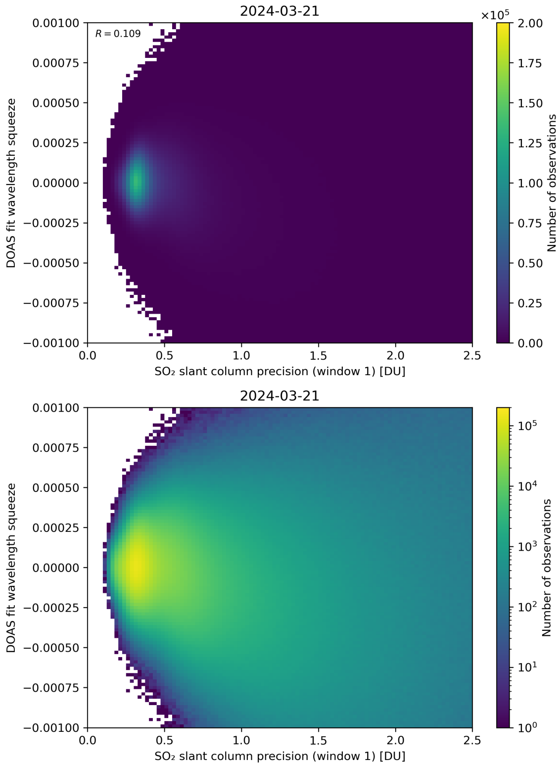
Figure 222: Scatter density plot of “SO 2 slant column precision (window 1)” against “DOAS fit wavelength squeeze” for 2024-03-20 to 2024-03-22.
