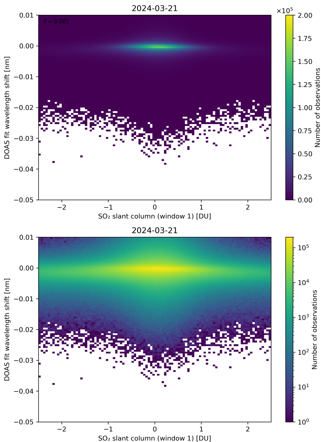
Figure 215: Scatter density plot of “SO 2 slant column (window 1)” against “DOAS fit wavelength shift” for 2024-03-20 to 2024-03-22.
