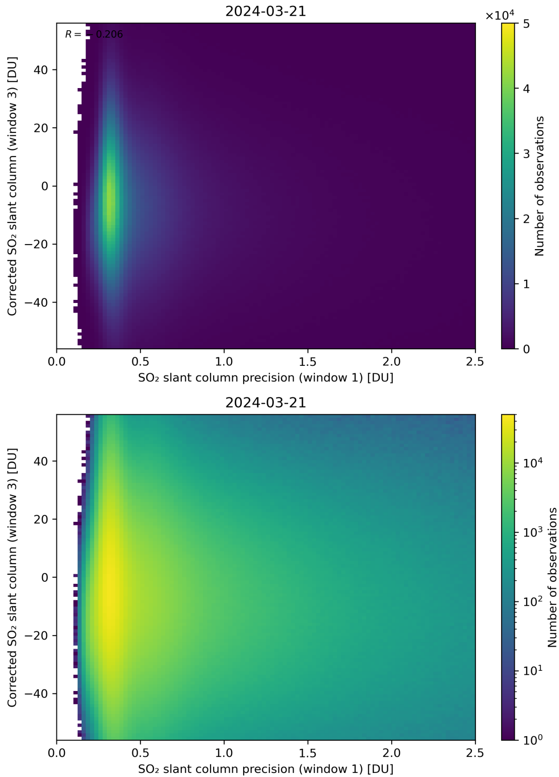
Figure 226: Scatter density plot of “SO 2 slant column precision (window 1)” against “Corrected SO 2 slant column (window 3)” for 2024-03-20 to 2024-03-22.
