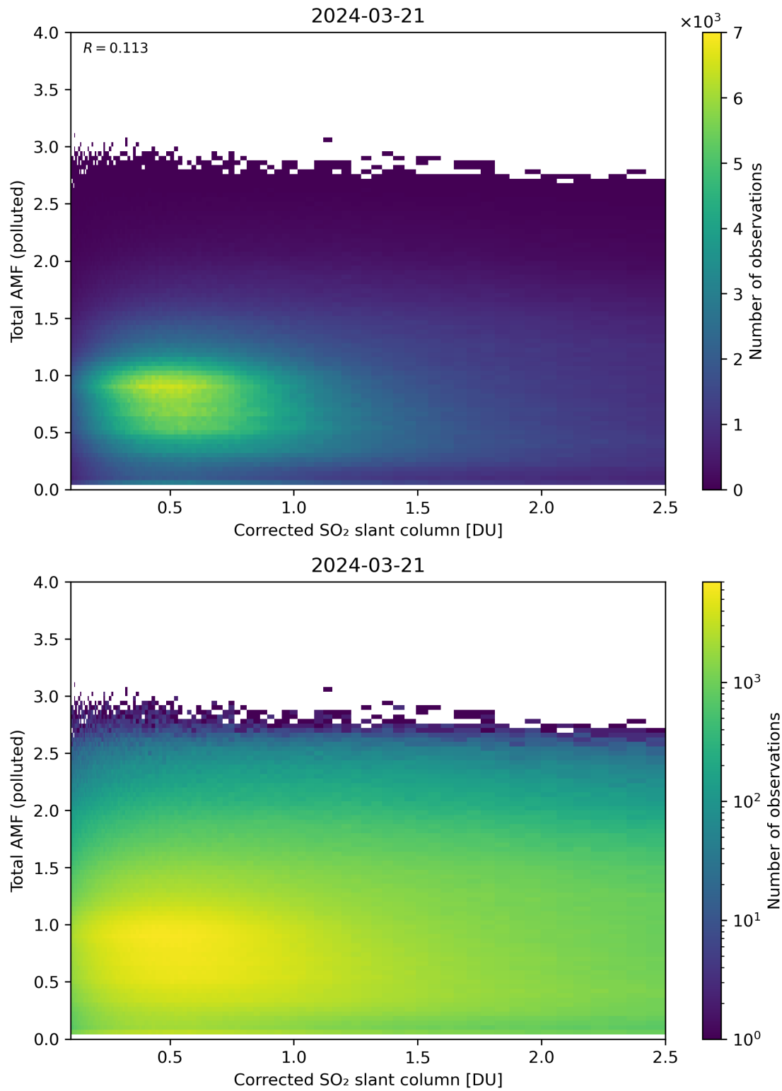
Figure 192: Scatter density plot of “Corrected SO 2 slant column” against “Total AMF (polluted)” for 2024-03-20 to 2024-03-22.
