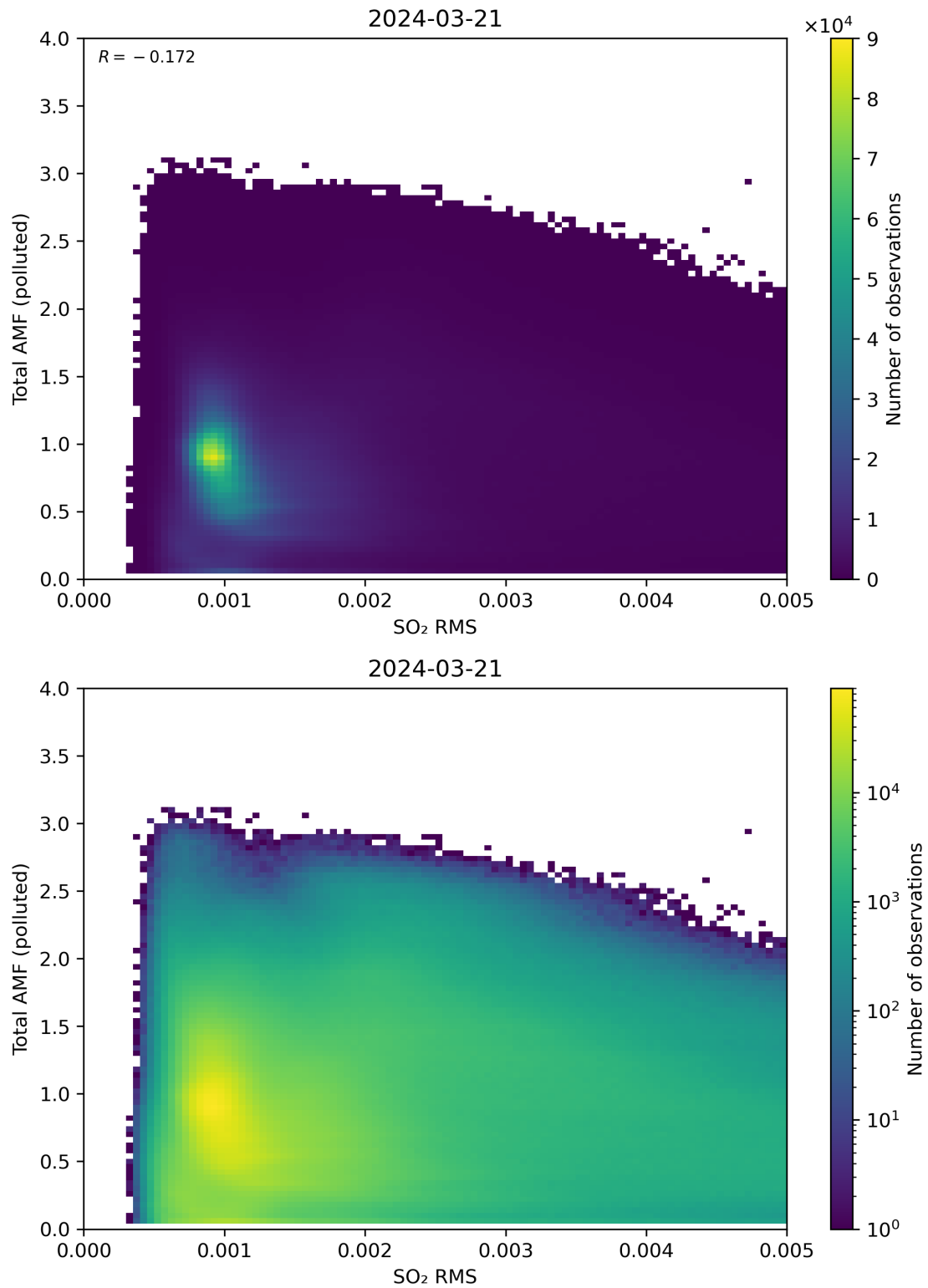
Figure 137: Scatter density plot of “SO 2 RMS” against “Total AMF (polluted)” for 2024-03-20 to 2024-03-22.
