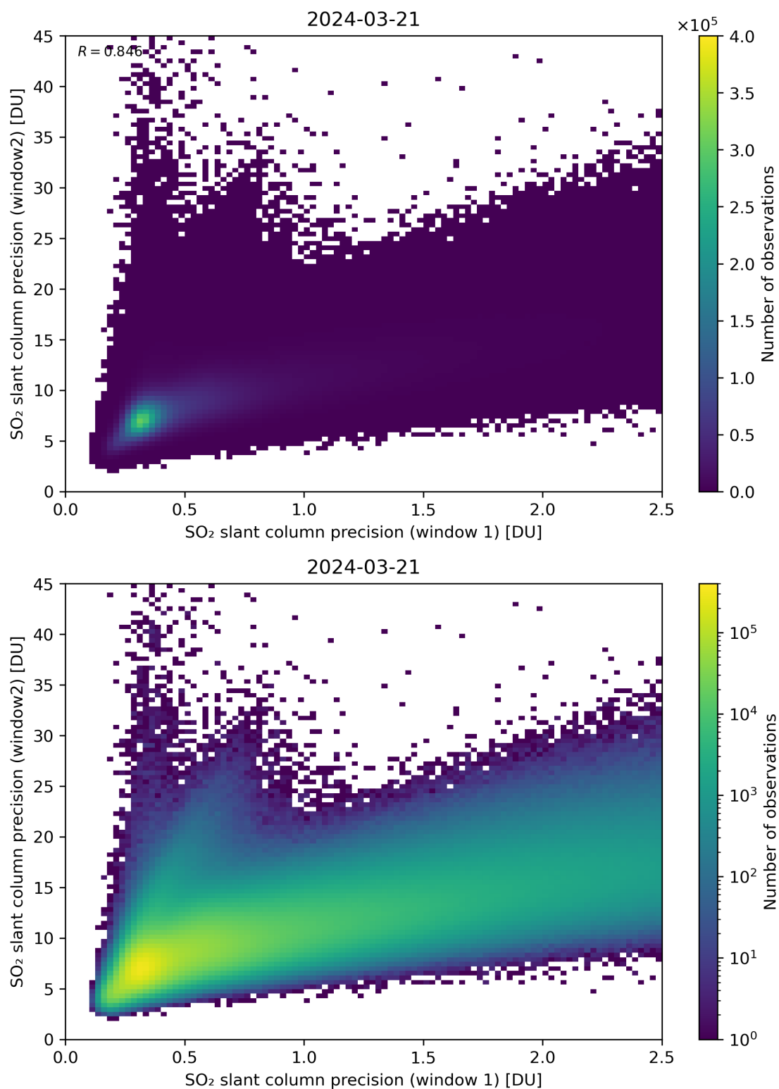
Figure 227: Scatter density plot of “SO 2 slant column precision (window 1)” against “SO 2 slant column precision (window2)” for 2024-03-20 to 2024-03-22.
