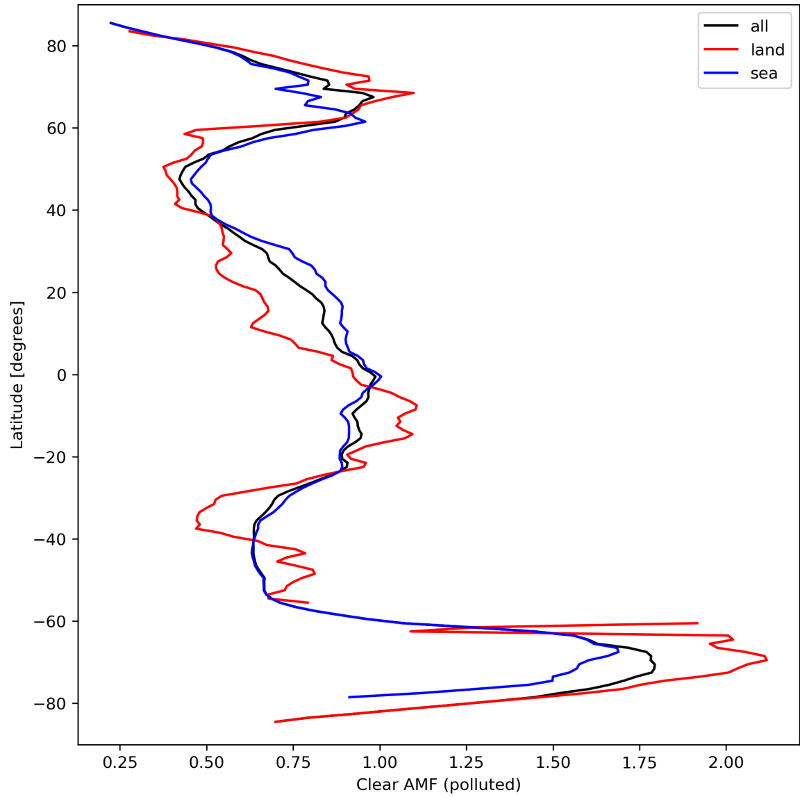
Figure 50: Zonal average of “Clear AMF (polluted)” for 2024-03-20 to 2024-03-22.
