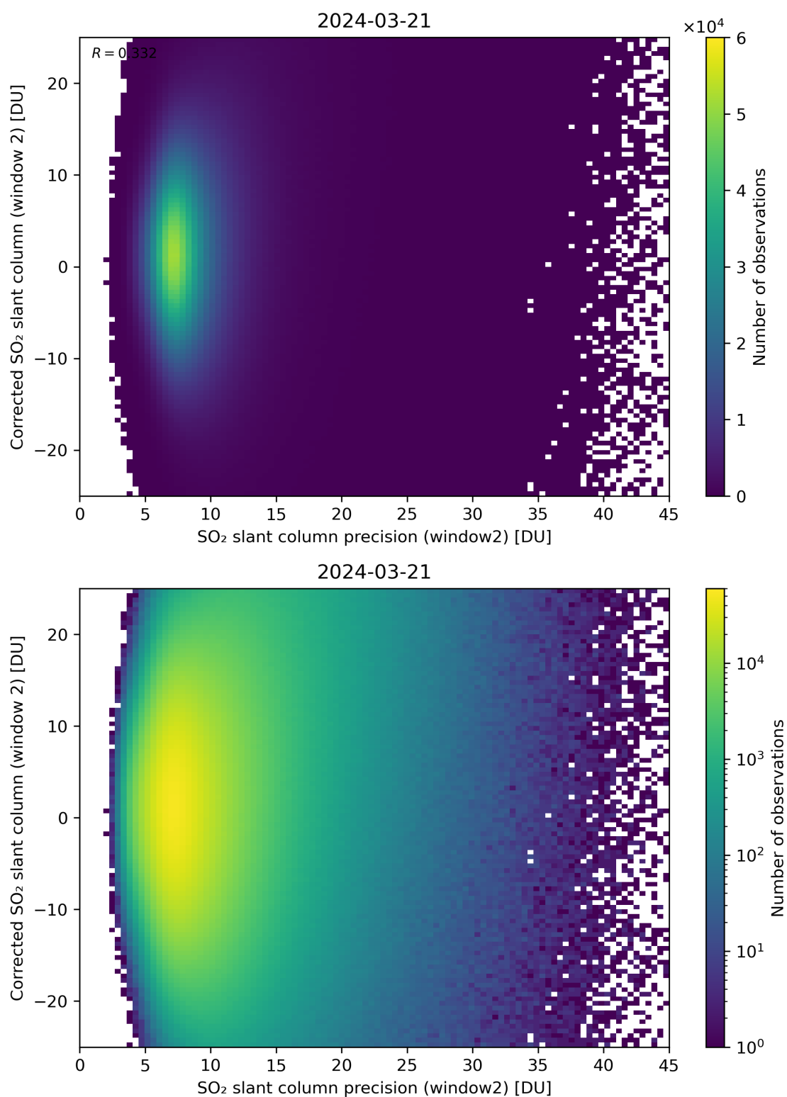
Figure 247: Scatter density plot of “SO 2 slant column precision (window2)” against “Corrected SO 2 slant column (window 2)” for 2024-03-20 to 2024-03-22.
