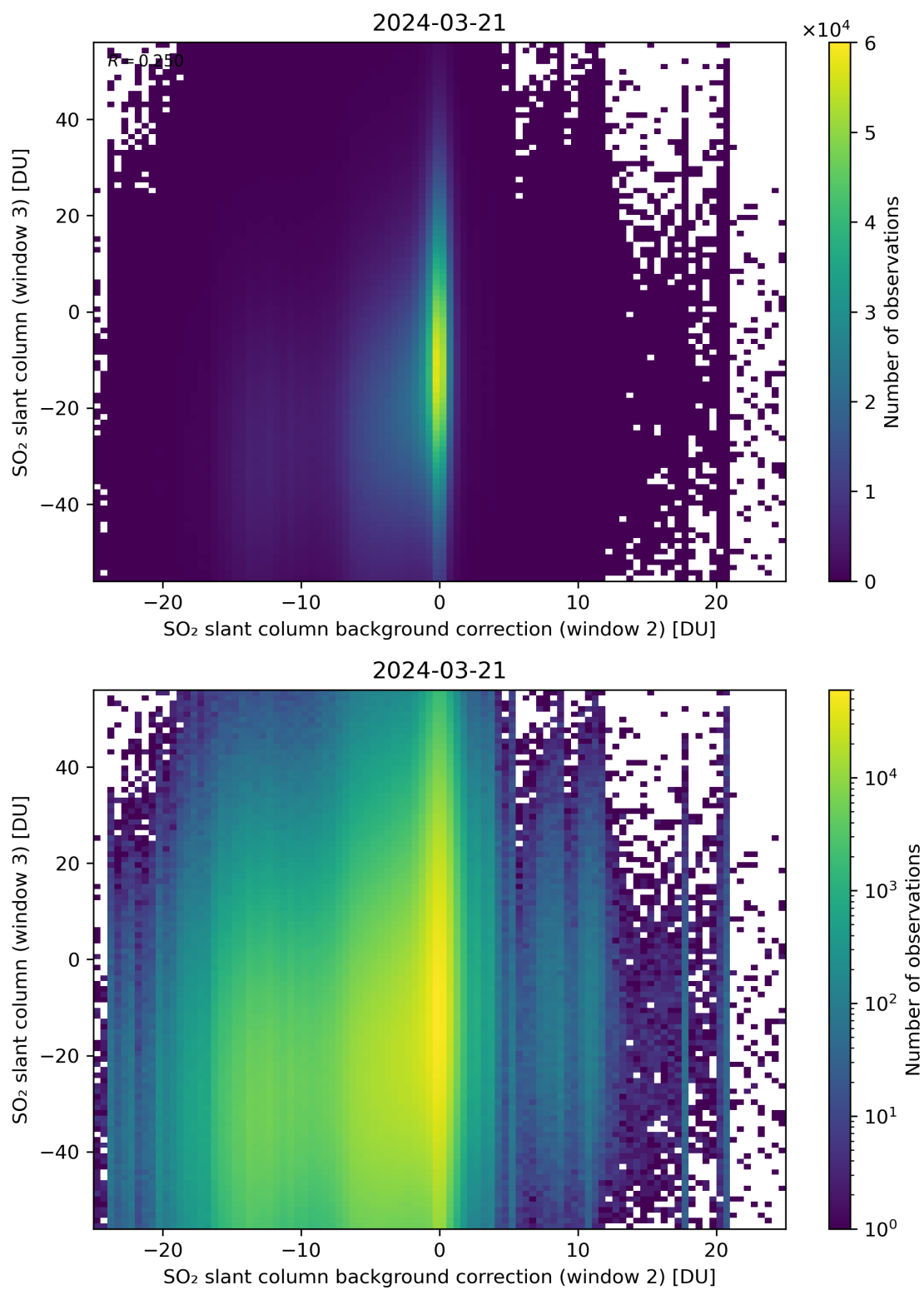
Figure 117: Scatter density plot of “SO 2 slant column background correction (window 2)” against “SO 2 slant column (window 3)” for 2024-03-20 to 2024-03-22.
