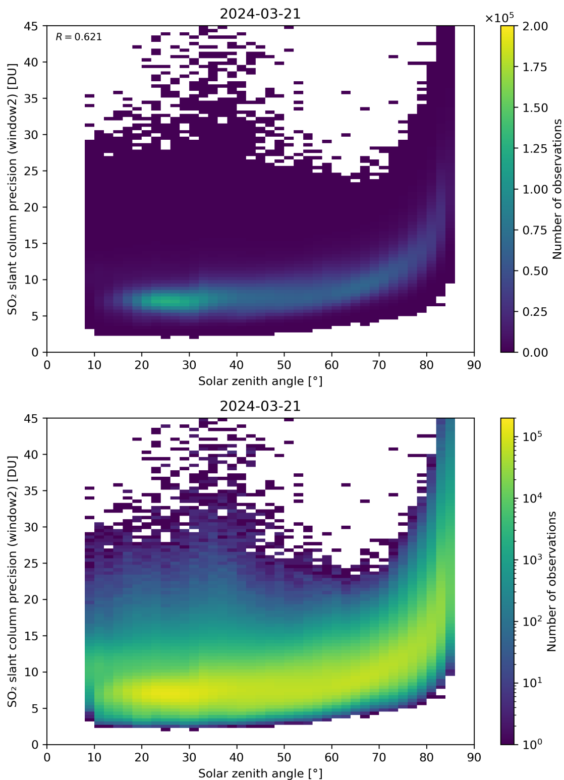
Figure 171: Scatter density plot of “Solar zenith angle” against “SO 2 slant column precision (window2)” for 2024-03-20 to 2024-03-22.
