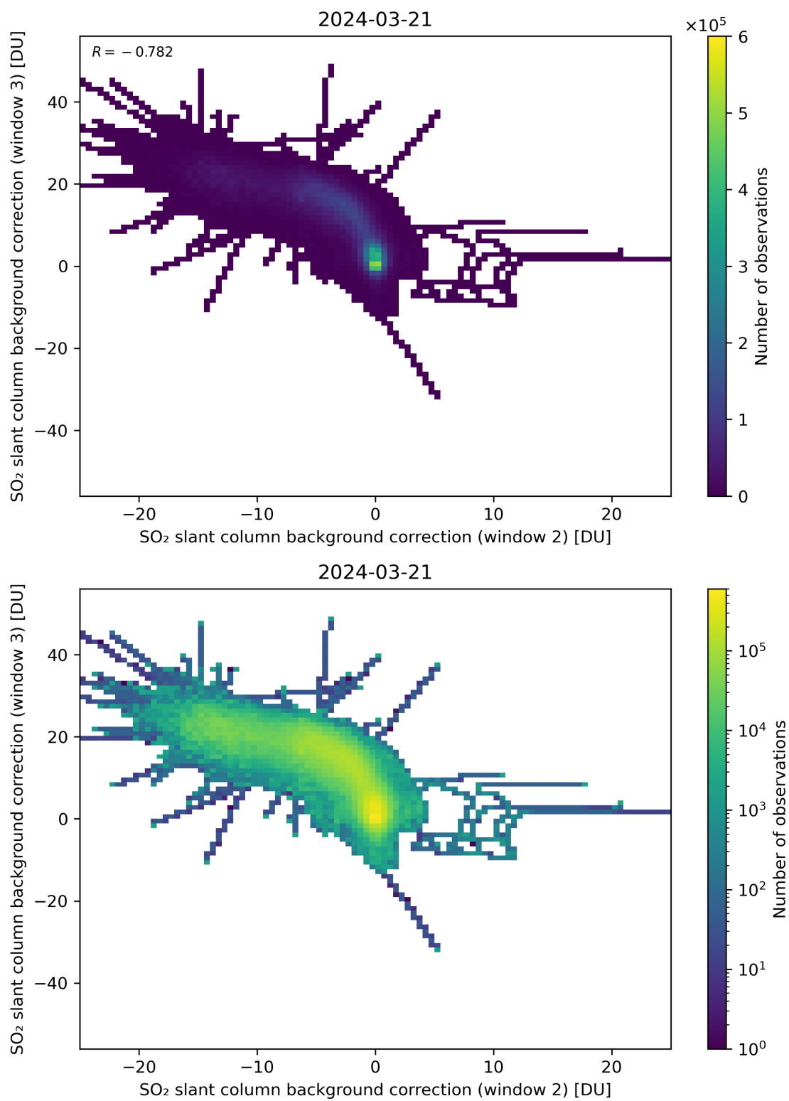
Figure 111: Scatter density plot of “SO 2 slant column background correction (window 2)” against “SO 2 slant column background correction (window 3)” for 2024-03-20 to 2024-03-22.
