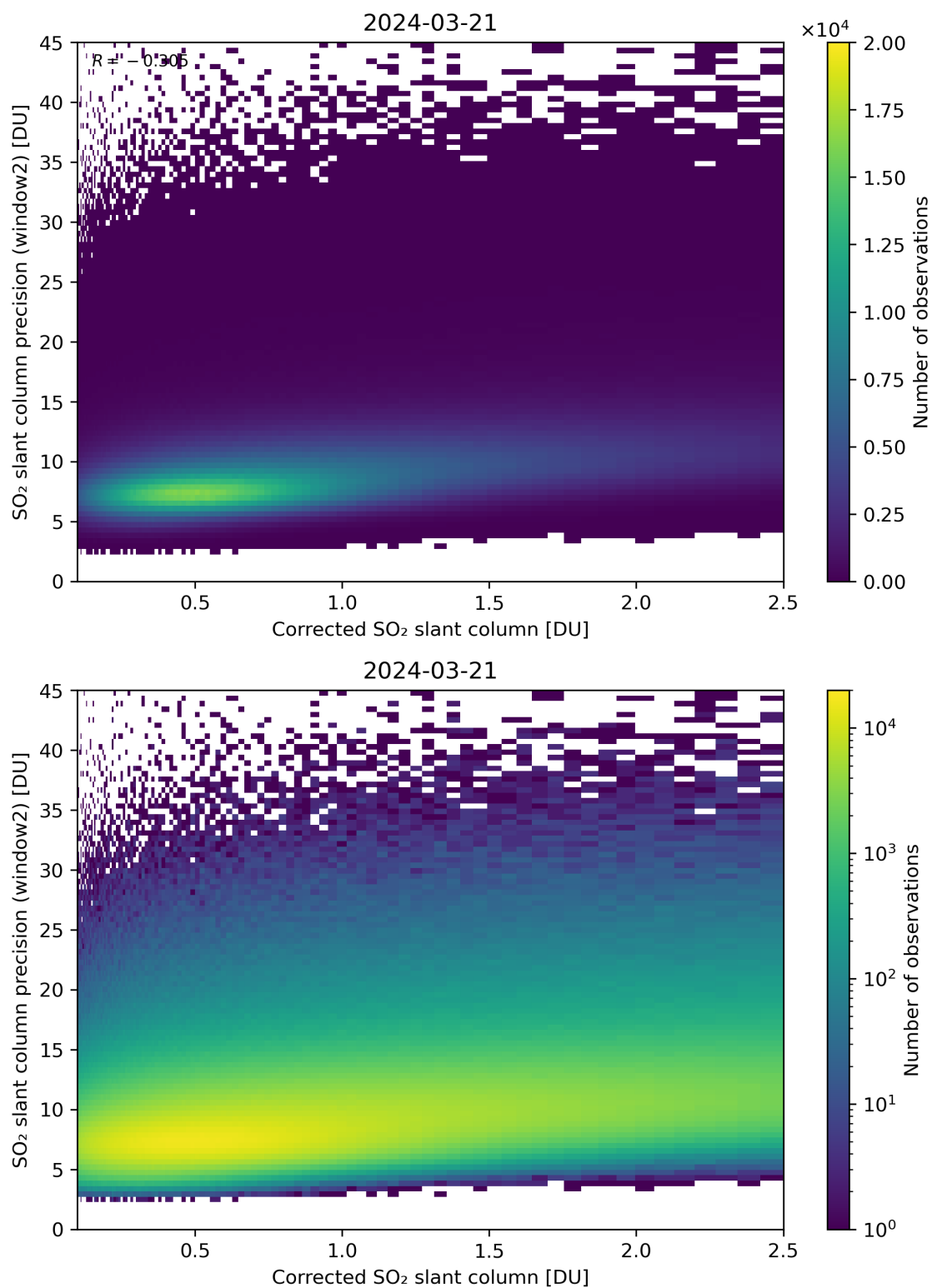
Figure 189: Scatter density plot of “Corrected SO 2 slant column” against “SO 2 slant column precision (window2)” for 2024-03-20 to 2024-03-22.
