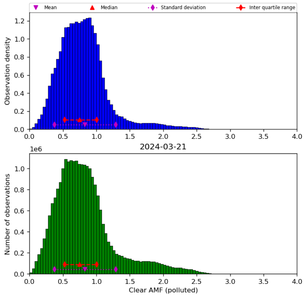
Figure 73: Histogram of “Clear AMF (polluted)” for 2024-03-20 to 2024-03-22
