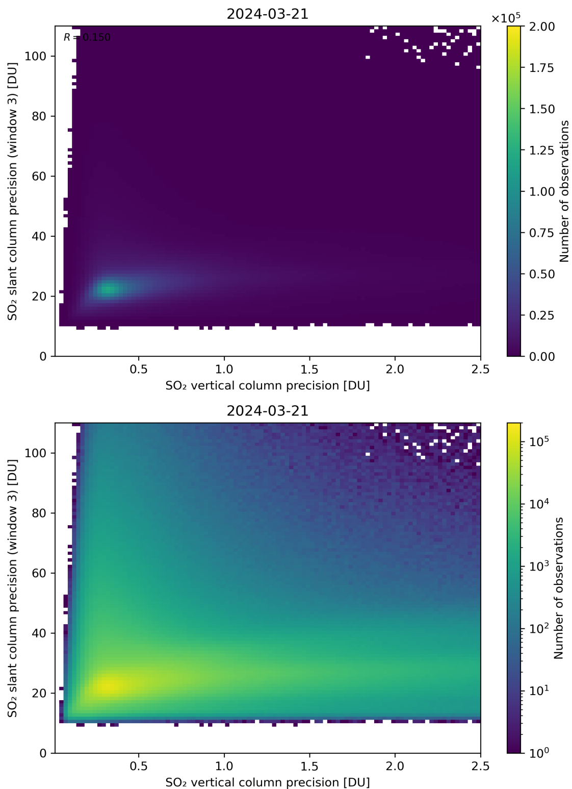
Figure 293: Scatter density plot of “SO 2 vertical column precision” against “SO 2 slant column precision (window 3)” for 2024-03-20 to 2024-03-22.
