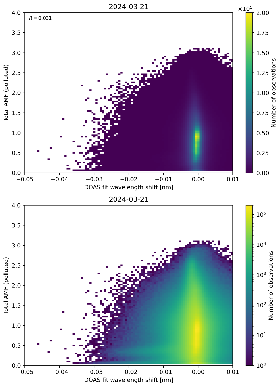
Figure 130: Scatter density plot of “DOAS fit wavelength shift” against “Total AMF (polluted)” for 2024-03-20 to 2024-03-22.
