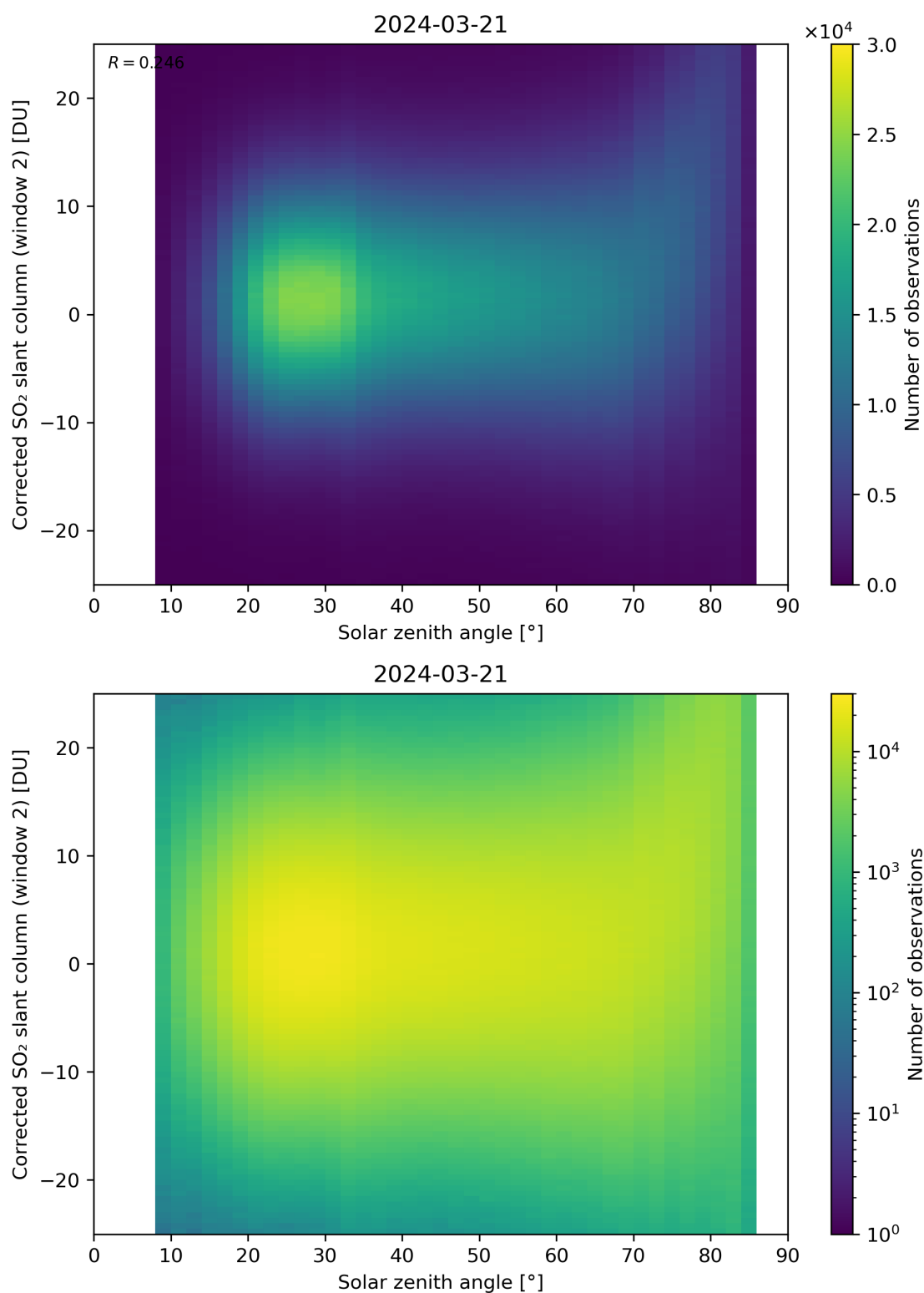
Figure 167: Scatter density plot of “Solar zenith angle” against “Corrected SO 2 slant column (window 2)” for 2024-03-20 to 2024-03-22.
