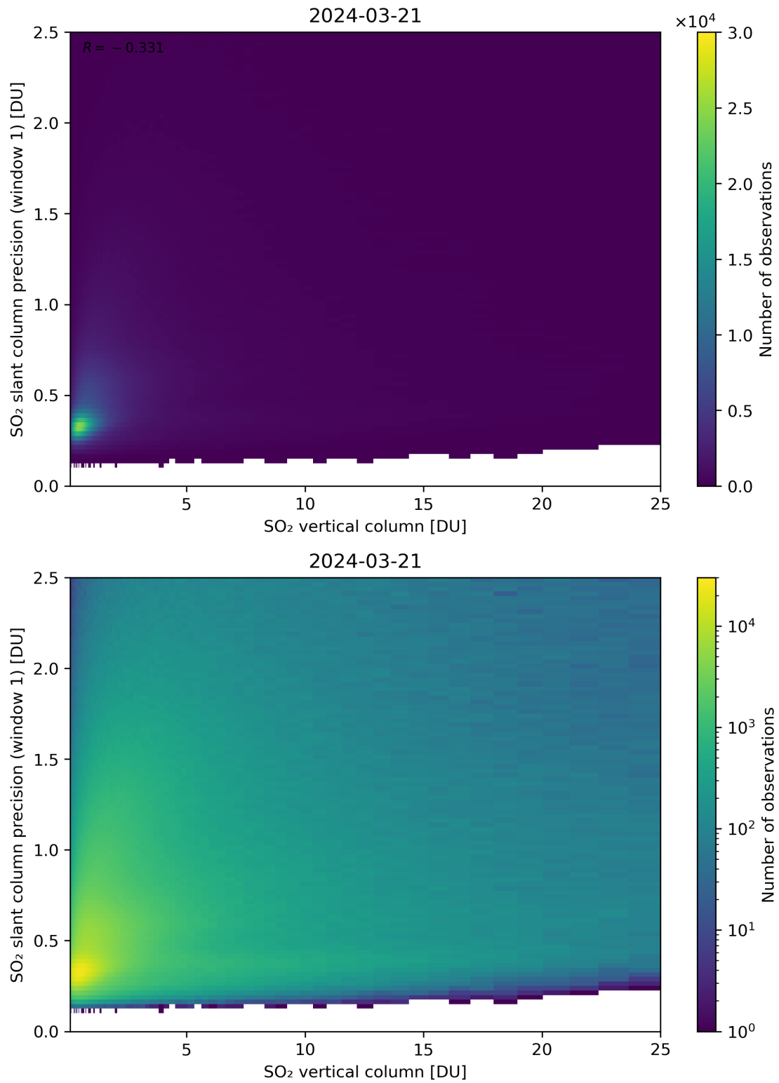
Figure 301: Scatter density plot of “SO 2 vertical column” against “SO 2 slant column precision (window 1)” for 2024-03-20 to 2024-03-22.
