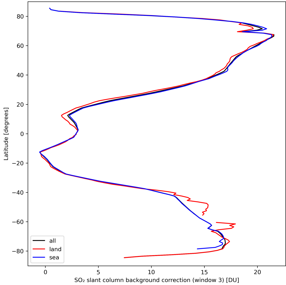
Figure 44: Zonal average of “SO 2 slant column background correction (window 3)” for 2024-03-20 to 2024-03-22.
