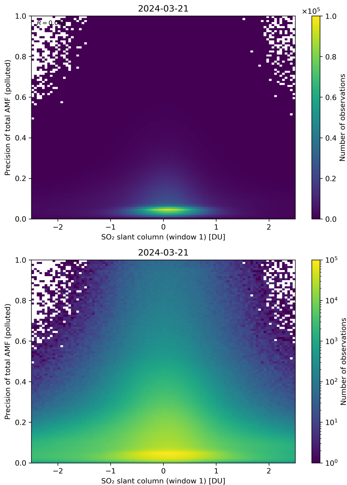
Figure 240: Scatter density plot of “SO 2 slant column (window 1)” against “Precision of total AMF (polluted)” for 2024-03-20 to 2024-03-22.
