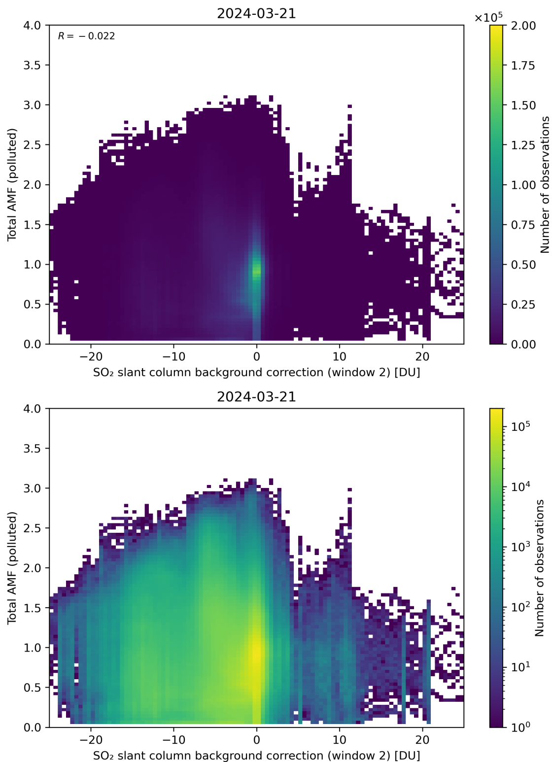
Figure 119: Scatter density plot of “SO 2 slant column background correction (window 2)” against “Total AMF (polluted)” for 2024-03-20 to 2024-03-22.
