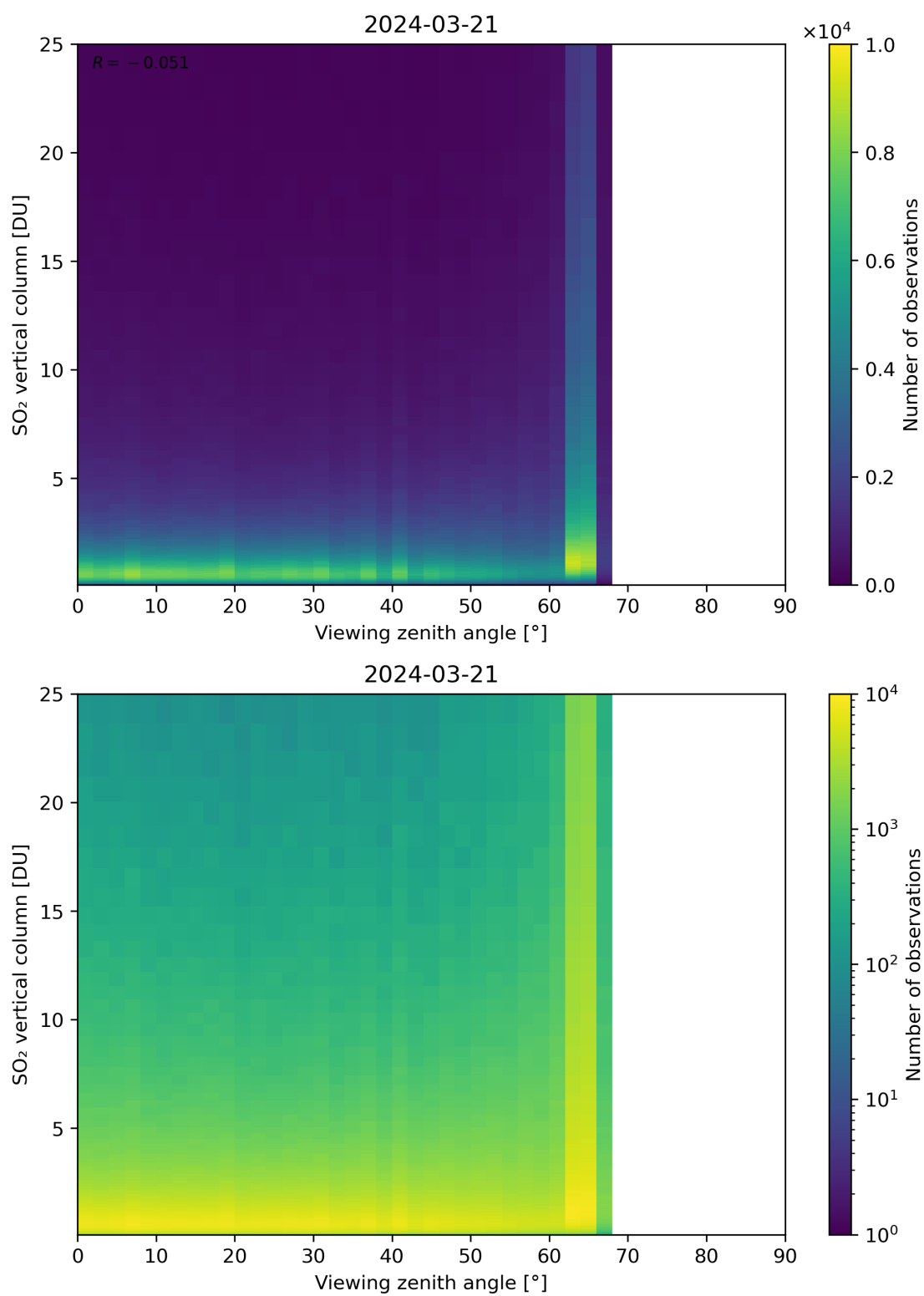
Figure 327: Scatter density plot of “Viewing zenith angle” against “SO 2 vertical column” for 2024-03-20 to 2024-03-22.
