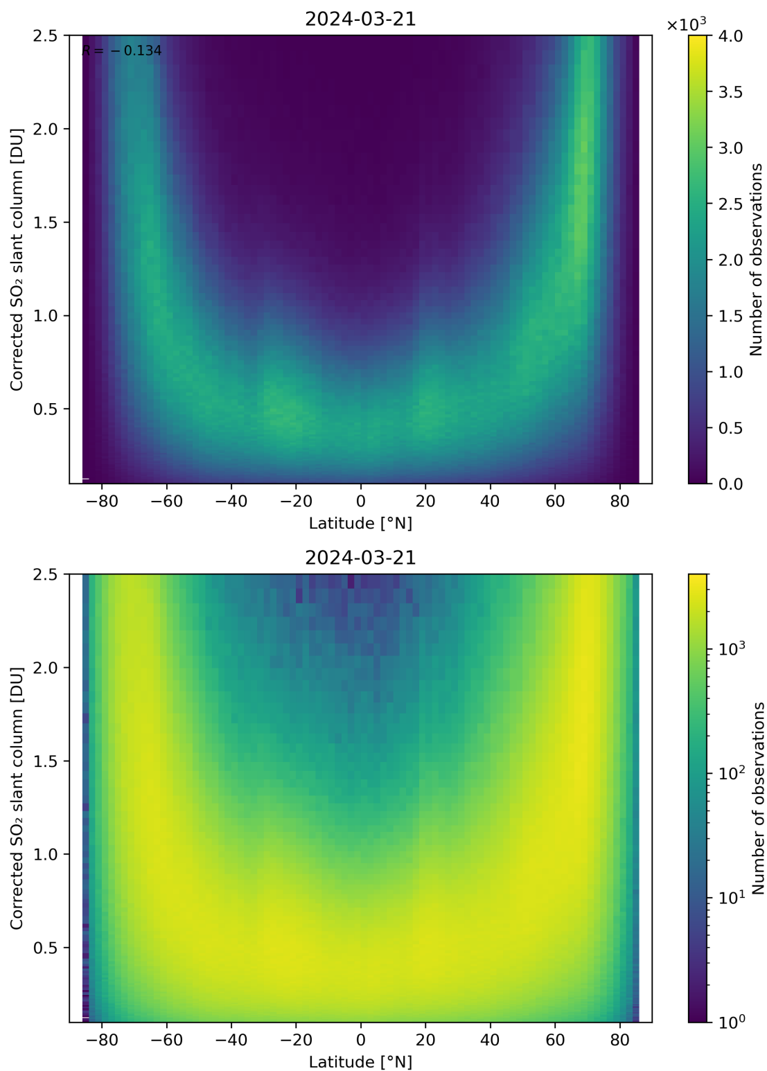
Figure 146: Scatter density plot of “Latitude” against “Corrected SO 2 slant column” for 2024-03-20 to 2024-03-22.
