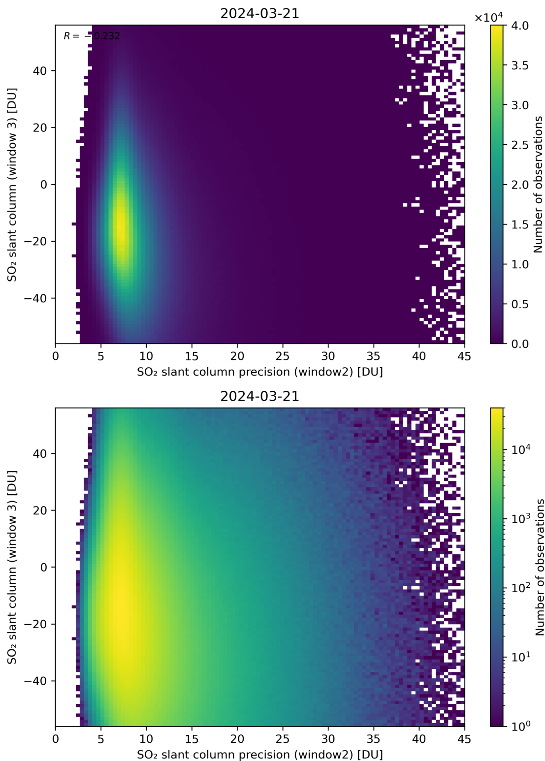
Figure 249: Scatter density plot of “SO 2 slant column precision (window2)” against “SO 2 slant column (window 3)” for 2024-03-20 to 2024-03-22.
