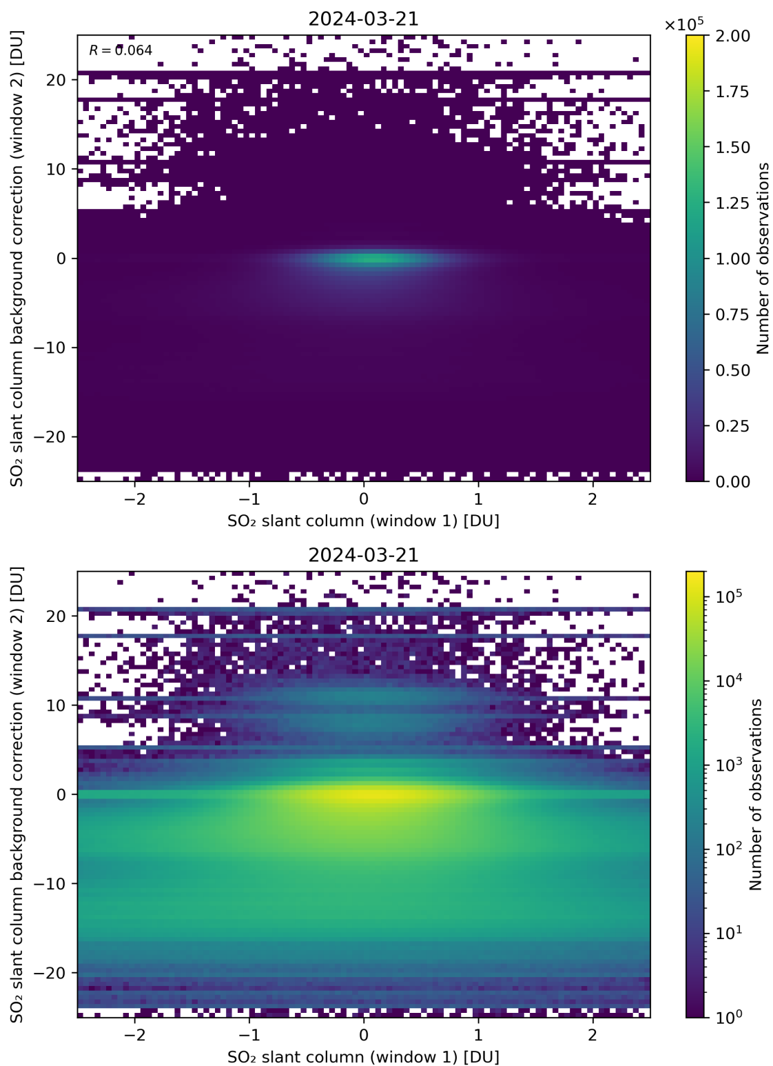
Figure 213: Scatter density plot of “SO 2 slant column (window 1)” against “SO 2 slant column background correction (window 2)” for 2024-03-20 to 2024-03-22.
