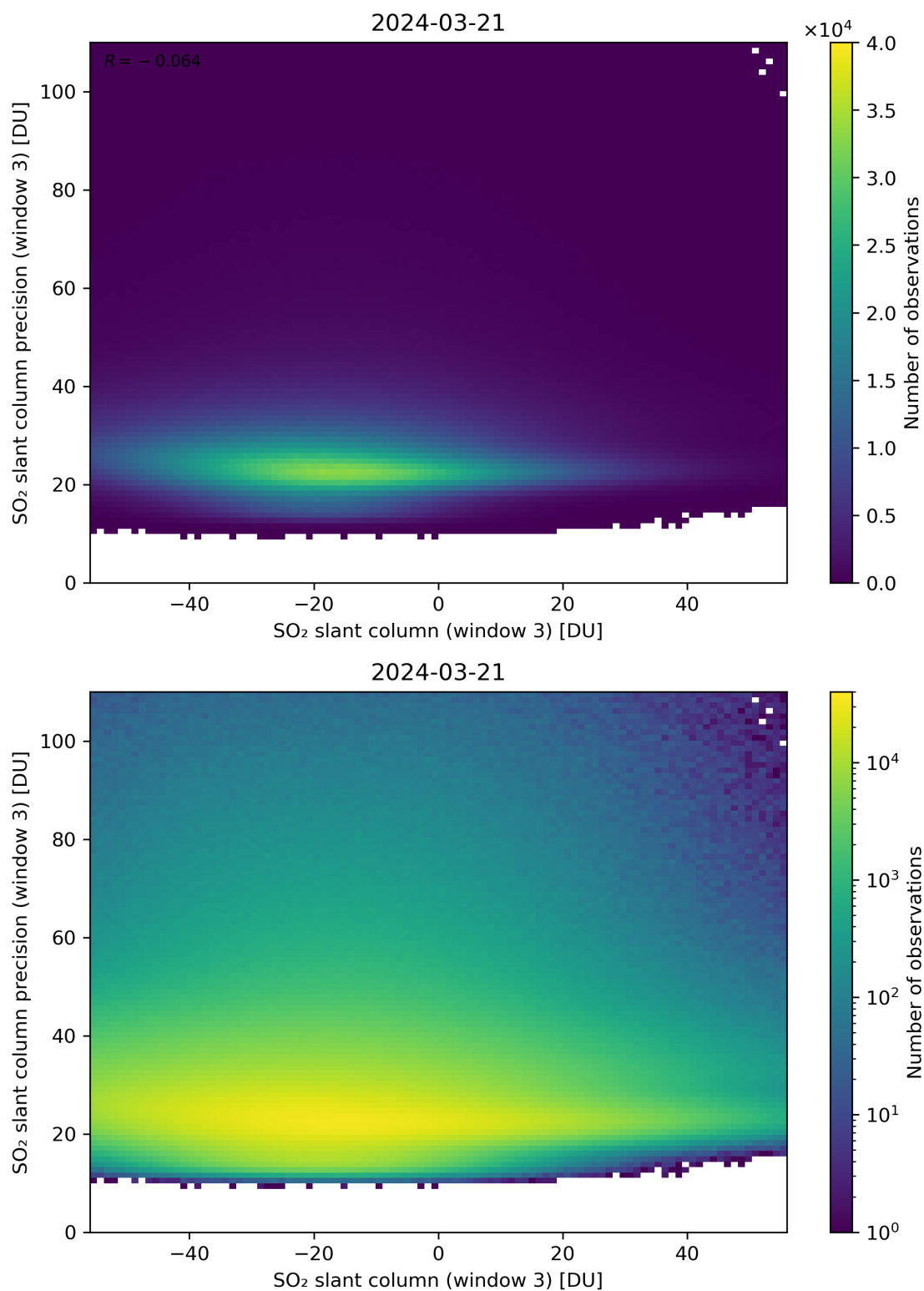
Figure 267: Scatter density plot of “SO 2 slant column (window 3)” against “SO 2 slant column precision (window 3)” for 2024-03-20 to 2024-03-22.
