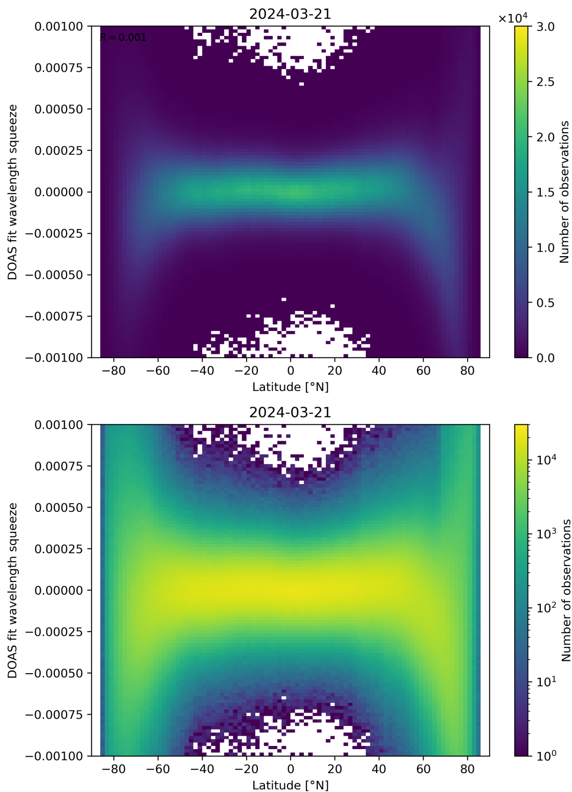
Figure 143: Scatter density plot of “Latitude” against “DOAS fit wavelength squeeze” for 2024-03-20 to 2024-03-22.
