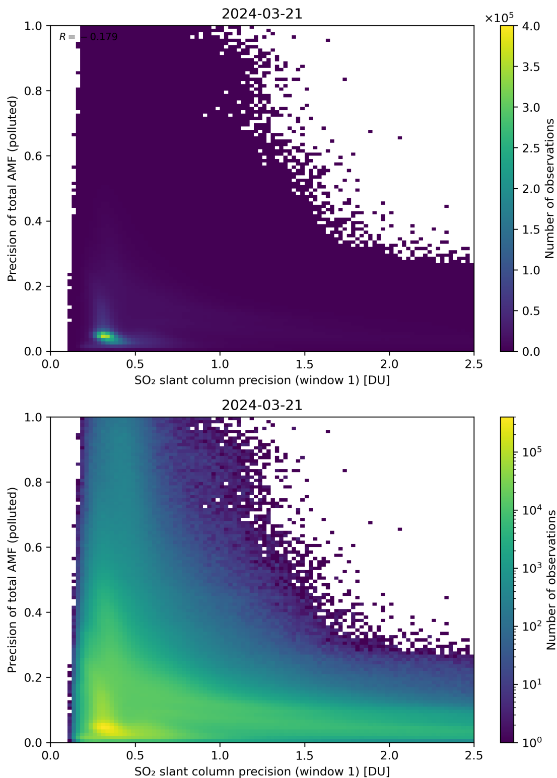
Figure 231: Scatter density plot of “SO 2 slant column precision (window 1)” against “Precision of total AMF (polluted)” for 2024-03-20 to 2024-03-22.
