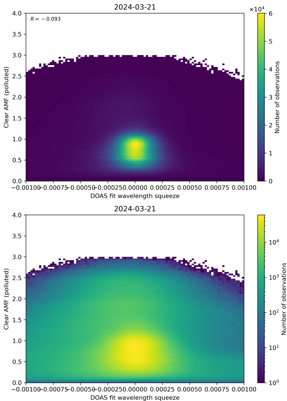
Figure 133: Scatter density plot of “DOAS fit wavelength squeeze” against “Clear AMF (polluted)” for 2024-03-20 to 2024-03-22.
