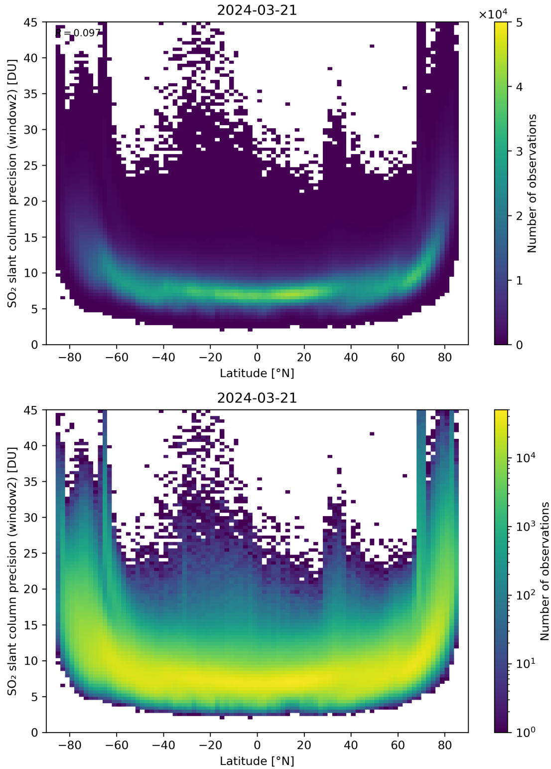
Figure 151: Scatter density plot of “Latitude” against “SO 2 slant column precision (window2)” for 2024-03-20 to 2024-03-22.
