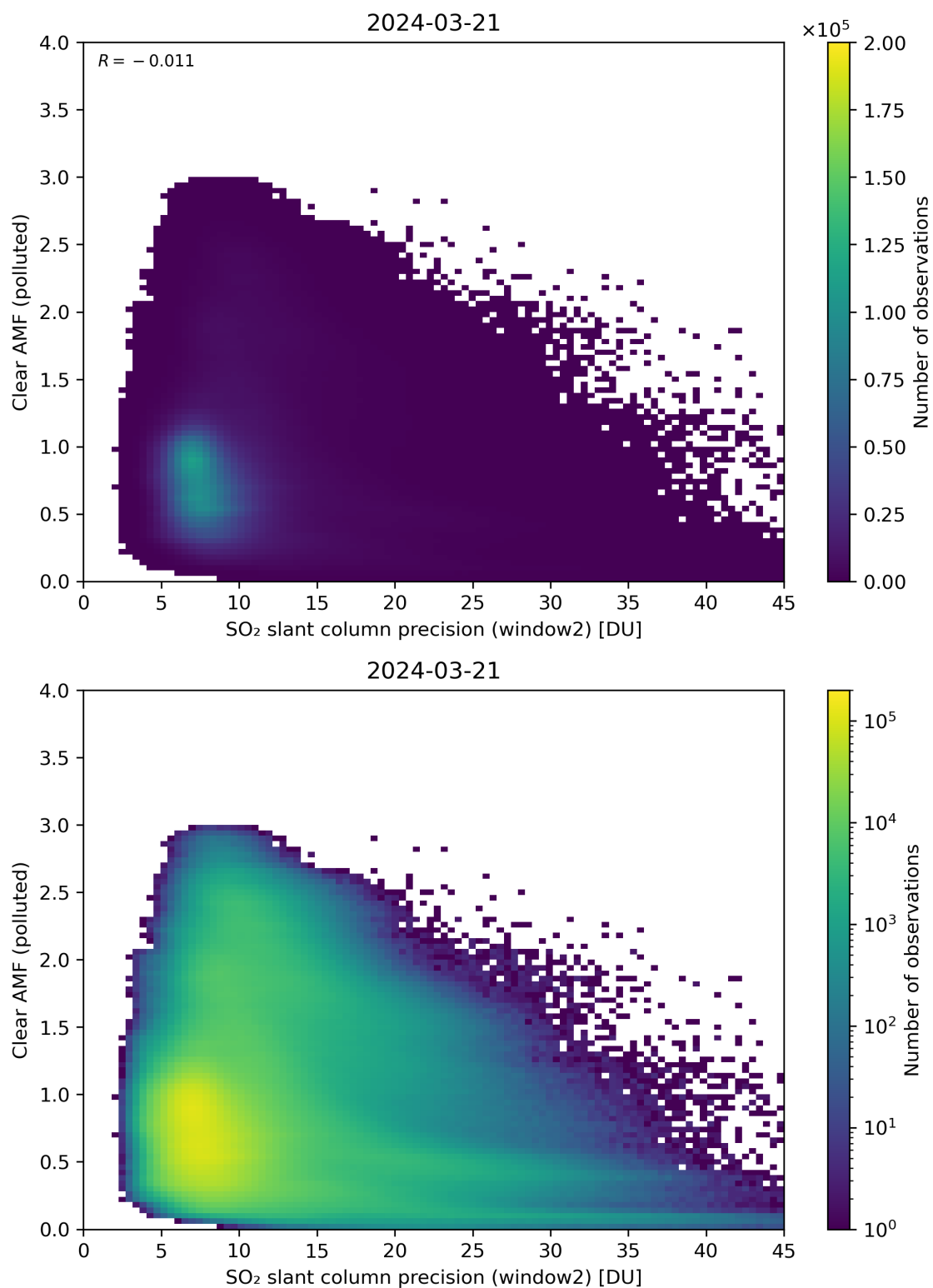
Figure 246: Scatter density plot of “SO 2 slant column precision (window2)” against “Clear AMF (polluted)” for 2024-03-20 to 2024-03-22.
