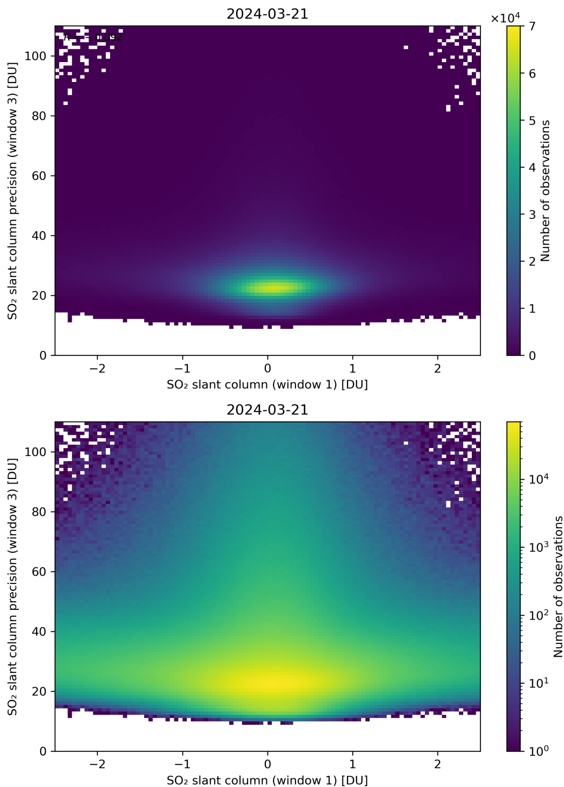
Figure 238: Scatter density plot of “SO 2 slant column (window 1)” against “SO 2 slant column precision (window 3)” for 2024-03-20 to 2024-03-22.
