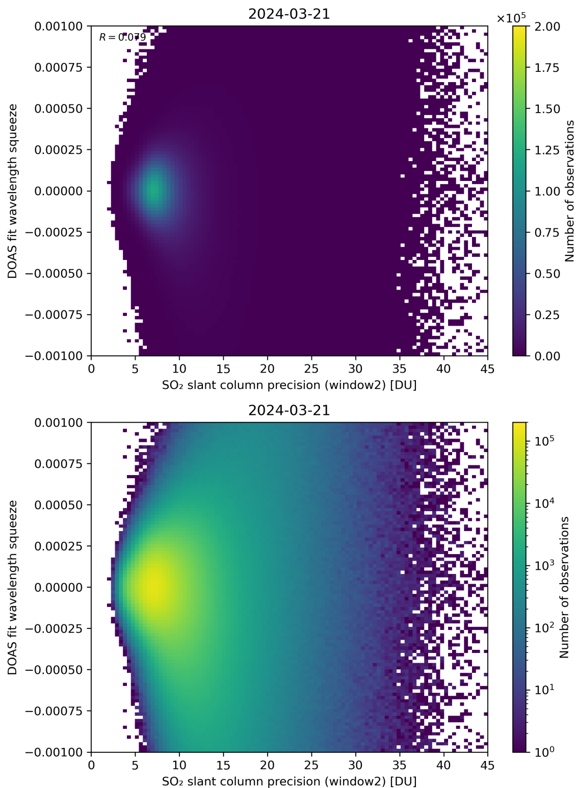
Figure 244: Scatter density plot of “SO 2 slant column precision (window2)” against “DOAS fit wavelength squeeze” for 2024-03-20 to 2024-03-22.
