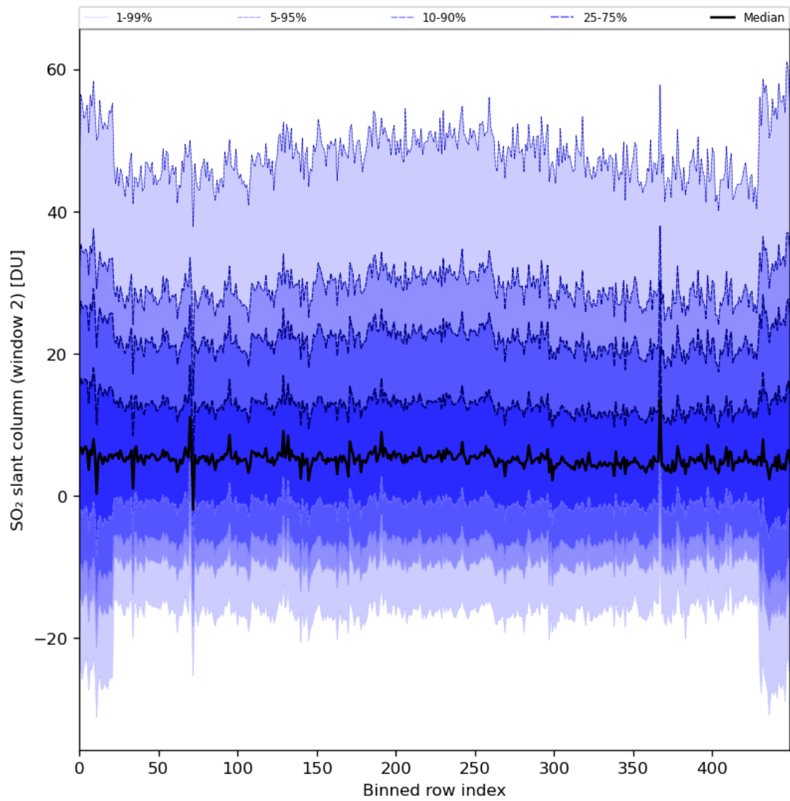
Figure 83: Along track statistics of “SO 2 slant column (window 2)” for 2024-03-20 to 2024-03-22
