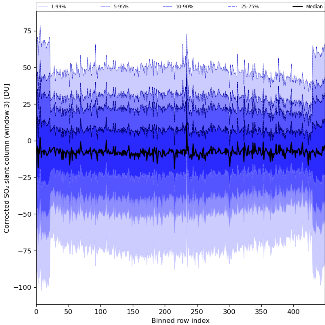
Figure 89: Along track statistics of “Corrected SO 2 slant column (window 3)” for 2024-03-20 to 2024-03-22
