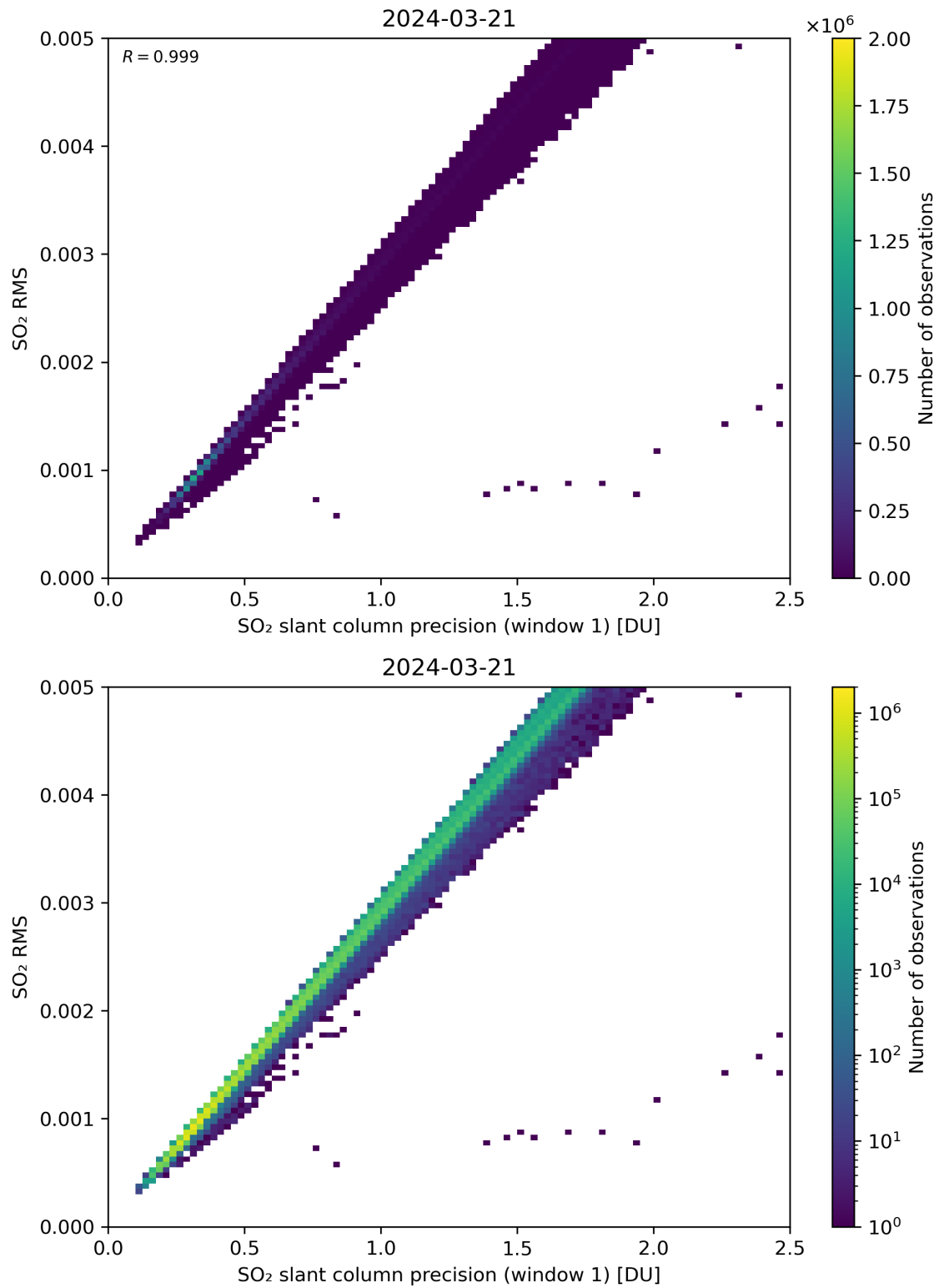
Figure 223: Scatter density plot of “SO 2 slant column precision (window 1)” against “SO 2 RMS” for 2024-03-20 to 2024-03-22.
