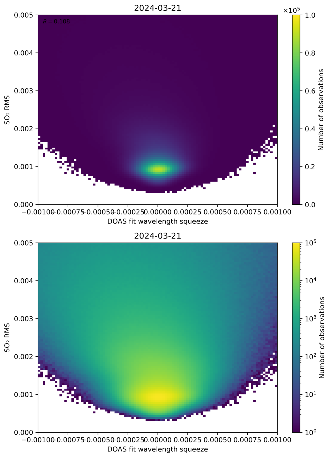
Figure 132: Scatter density plot of “DOAS fit wavelength squeeze” against “SO 2 RMS” for 2024-03-20 to 2024-03-22.
