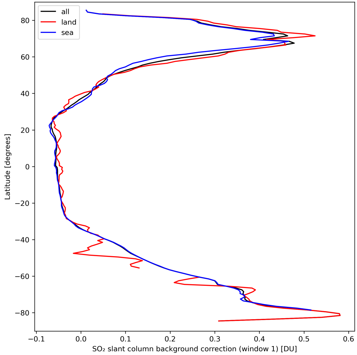
Figure 36: Zonal average of “SO 2 slant column background correction (window 1)” for 2024-03-20 to 2024-03-22.
