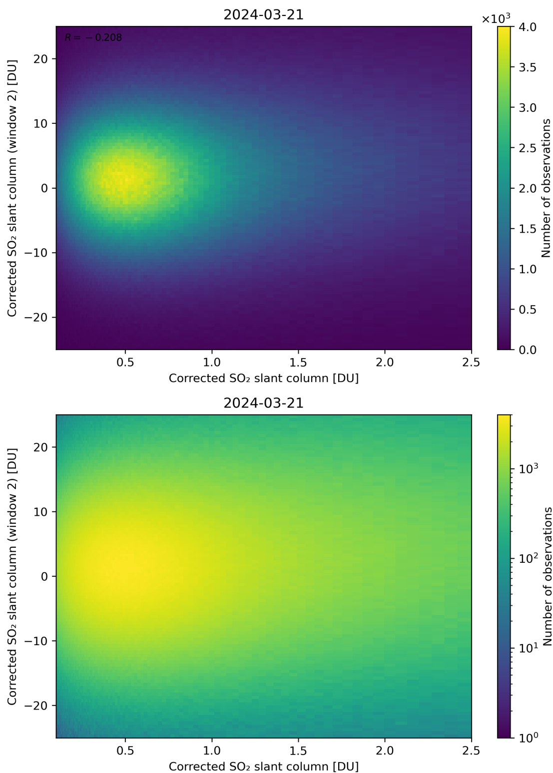
Figure 185: Scatter density plot of “Corrected SO 2 slant column” against “Corrected SO 2 slant column (window 2)” for 2024-03-20 to 2024-03-22.
