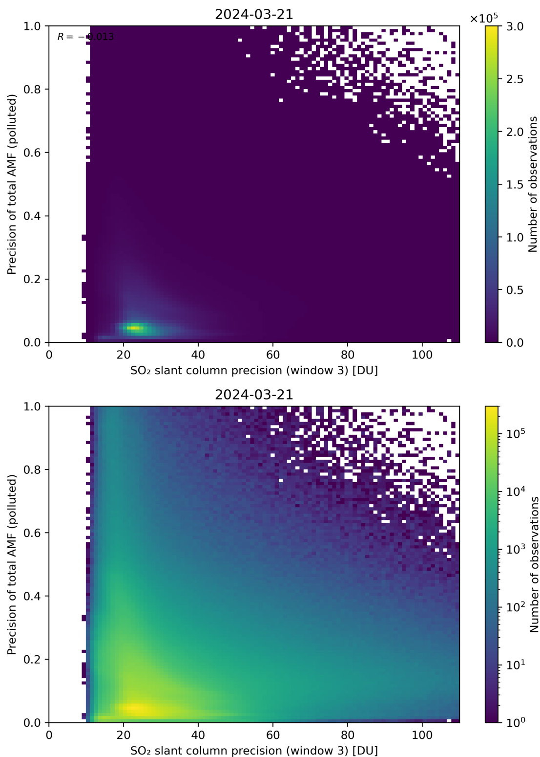
Figure 264: Scatter density plot of “SO 2 slant column precision (window 3)” against “Precision of total AMF (polluted)” for 2024-03-20 to 2024-03-22.
