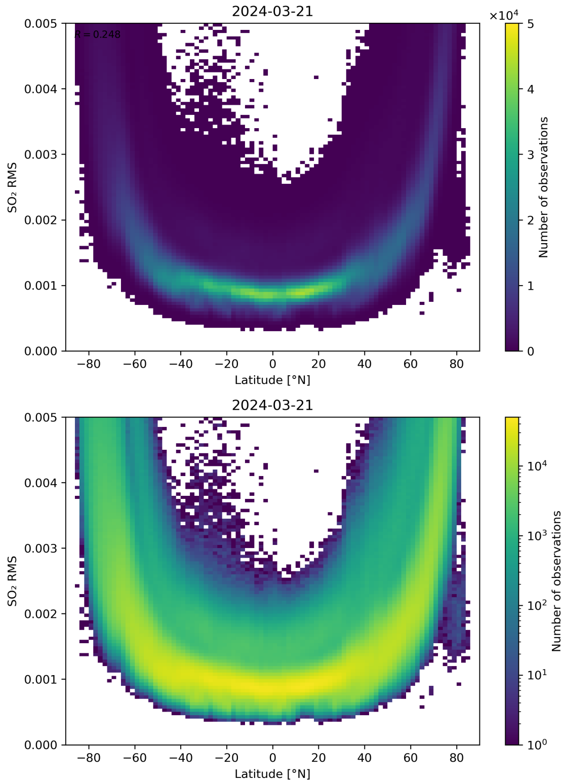
Figure 144: Scatter density plot of “Latitude” against “SO 2 RMS” for 2024-03-20 to 2024-03-22.
