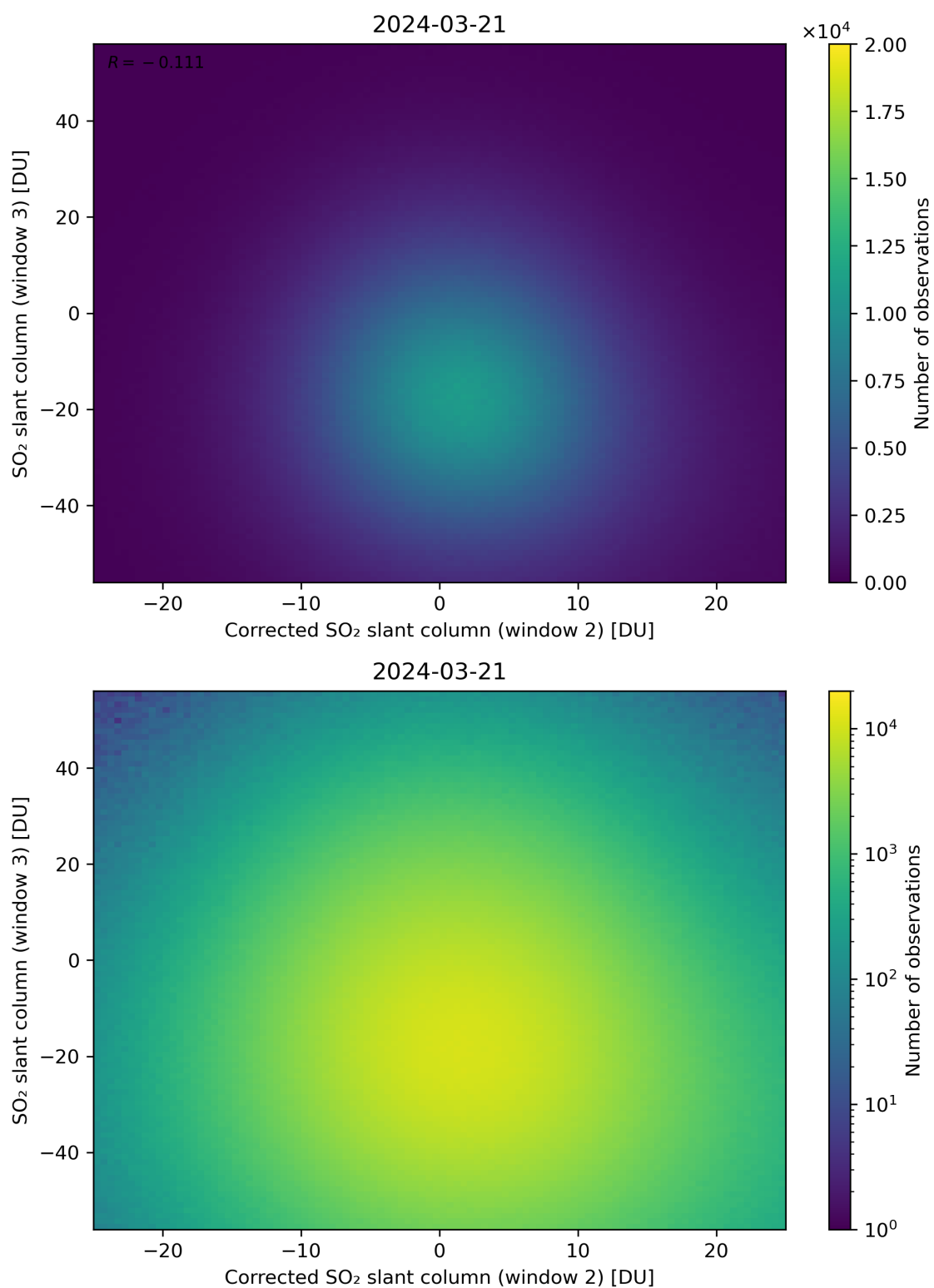
Figure 201: Scatter density plot of “Corrected SO 2 slant column (window 2)” against “SO 2 slant column (window 3)” for 2024-03-20 to 2024-03-22.
