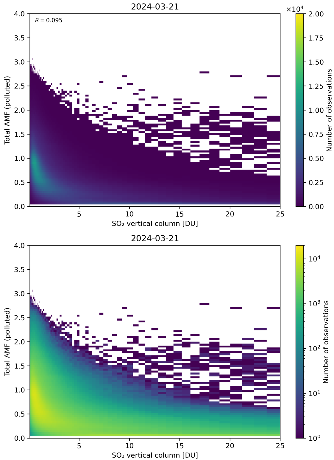
Figure 305: Scatter density plot of “SO 2 vertical column” against “Total AMF (polluted)” for 2024-03-20 to 2024-03-22.
