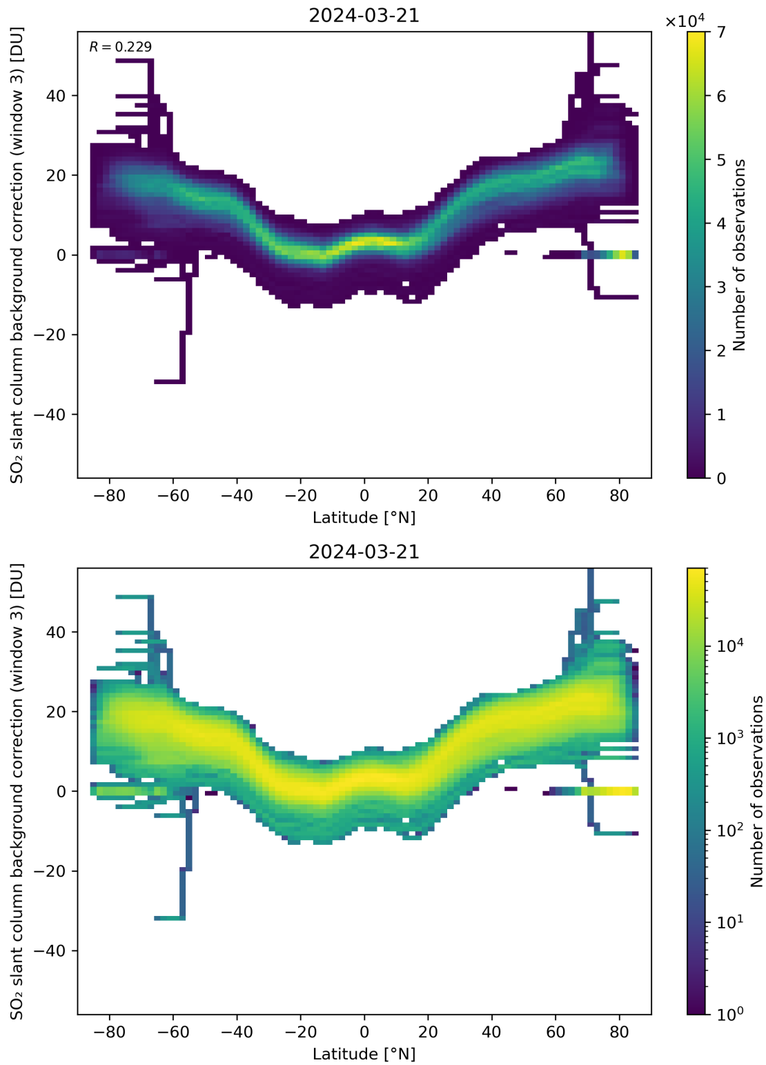
Figure 141: Scatter density plot of “Latitude” against “SO 2 slant column background correction (window 3)” for 2024-03-20 to 2024-03-22.
