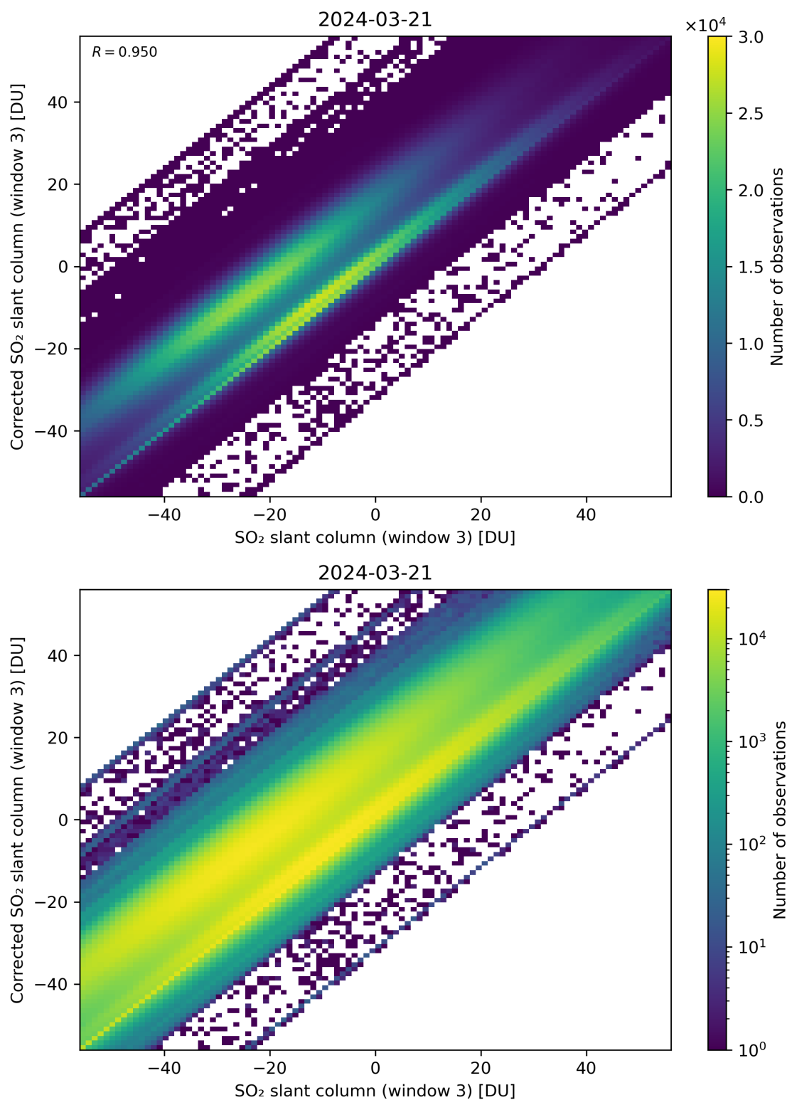
Figure 266: Scatter density plot of “SO 2 slant column (window 3)” against “Corrected SO 2 slant column (window 3)” for 2024-03-20 to 2024-03-22.
