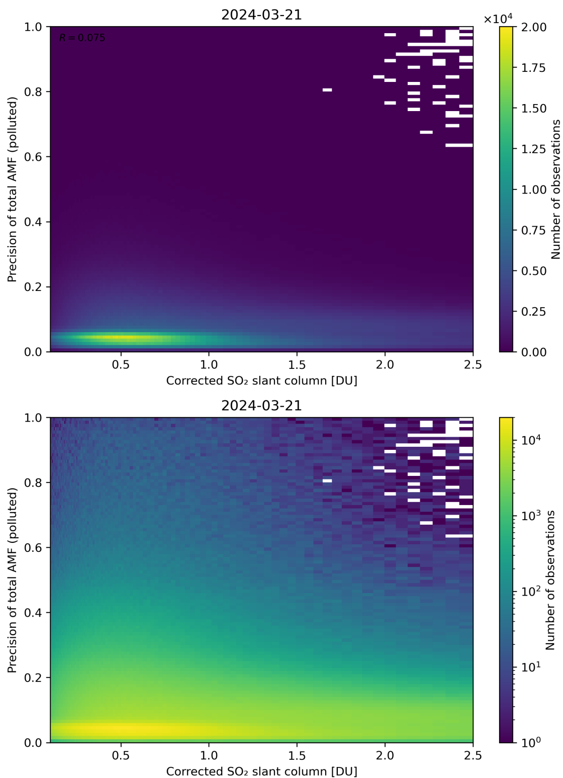
Figure 193: Scatter density plot of “Corrected SO 2 slant column” against “Precision of total AMF (polluted)” for 2024-03-20 to 2024-03-22.
