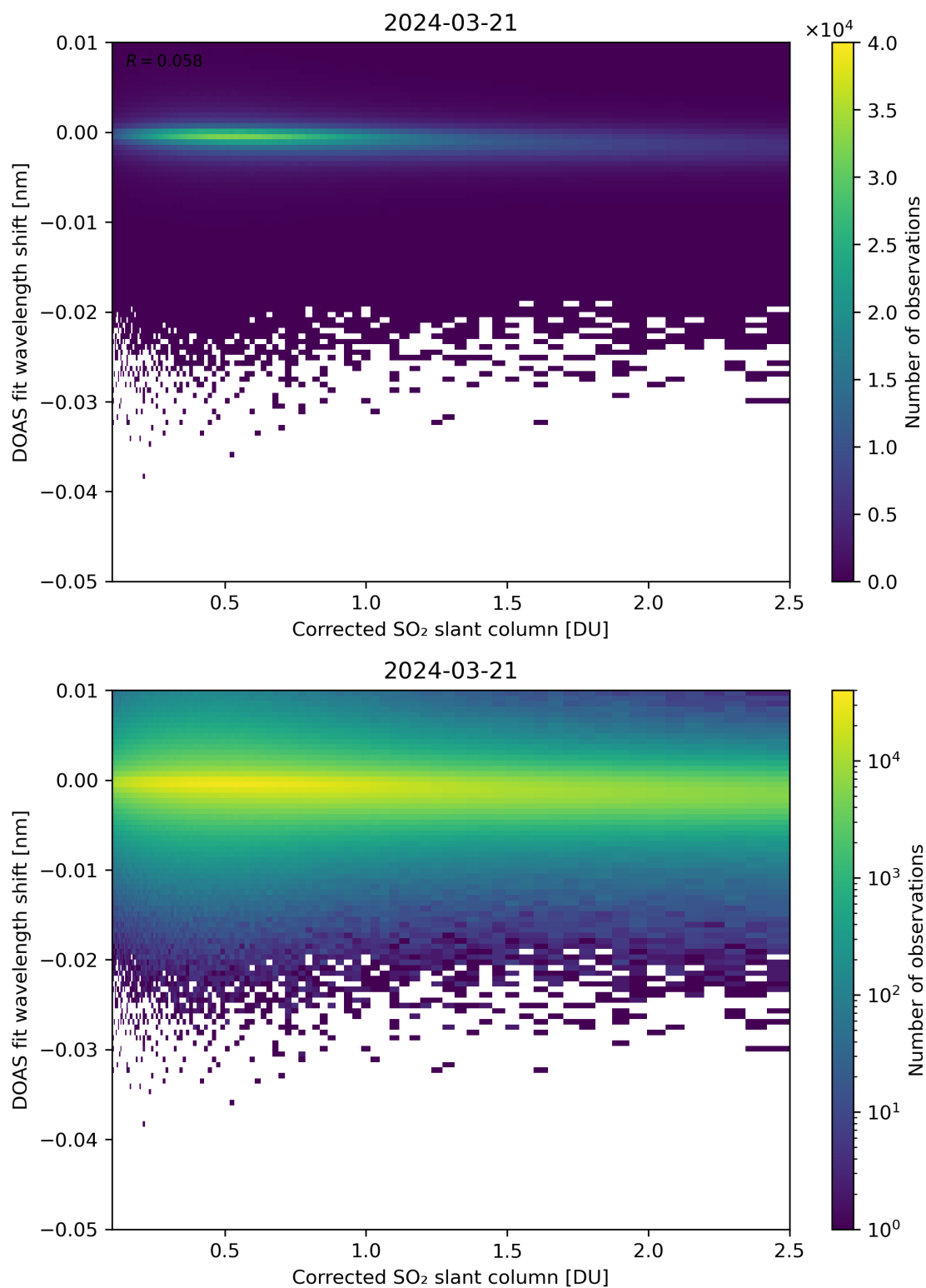
Figure 181: Scatter density plot of “Corrected SO 2 slant column” against “DOAS fit wavelength shift” for 2024-03-20 to 2024-03-22.
