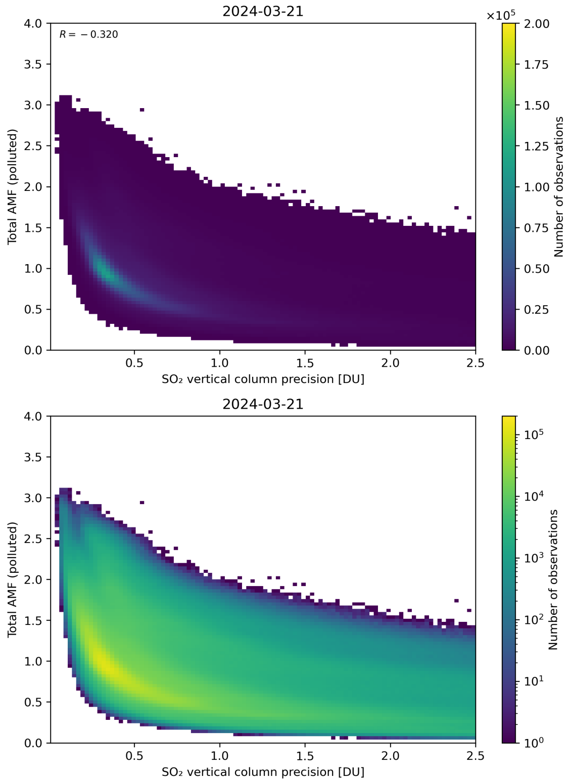
Figure 294: Scatter density plot of “SO 2 vertical column precision” against “Total AMF (polluted)” for 2024-03-20 to 2024-03-22.
