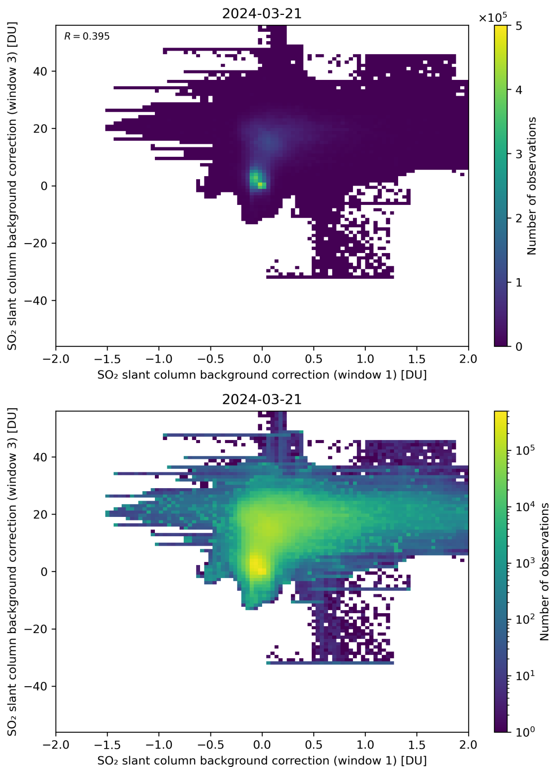
Figure 99: Scatter density plot of “SO 2 slant column background correction (window 1)” against “SO 2 slant column background correction (window 3)” for 2024-03-20 to 2024-03-22.
