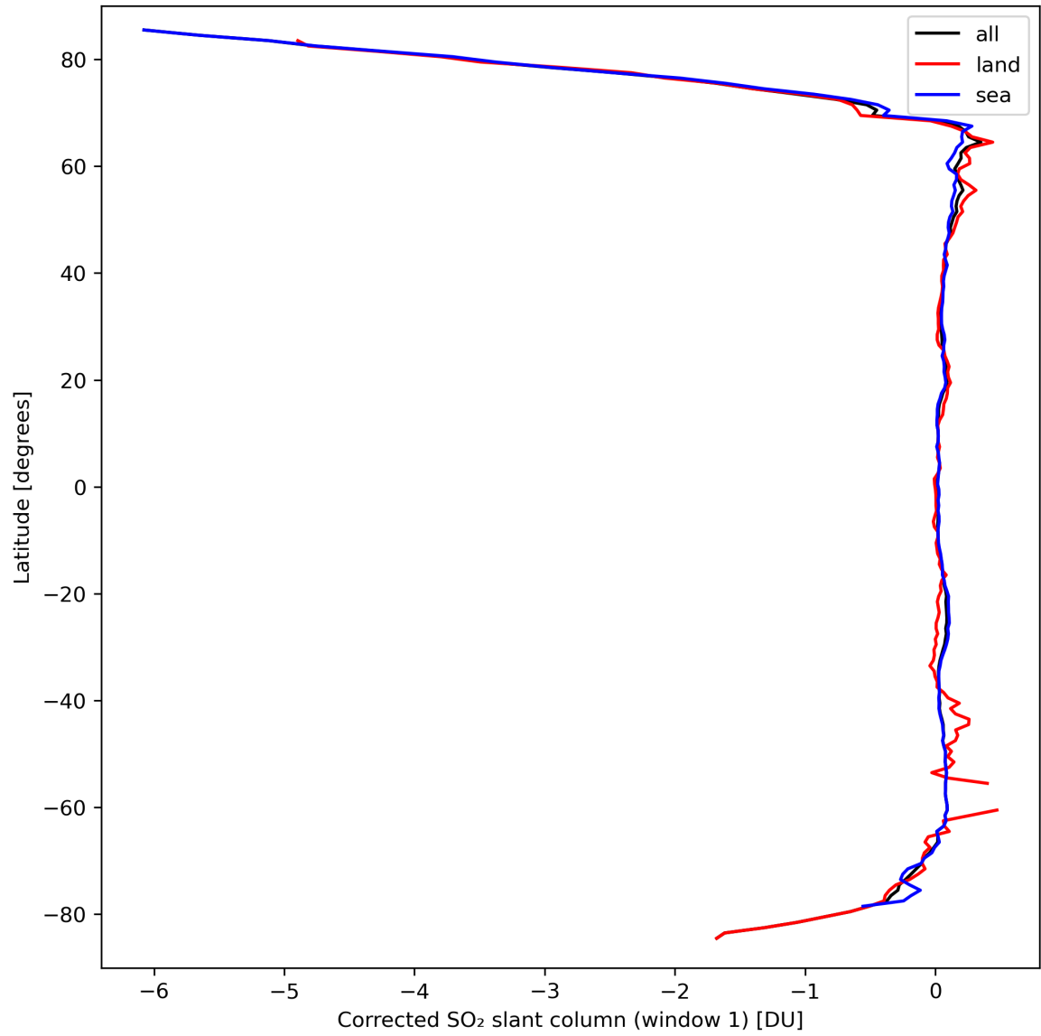
Figure 35: Zonal average of “Corrected SO 2 slant column (window 1)” for 2024-03-20 to 2024-03-22.
