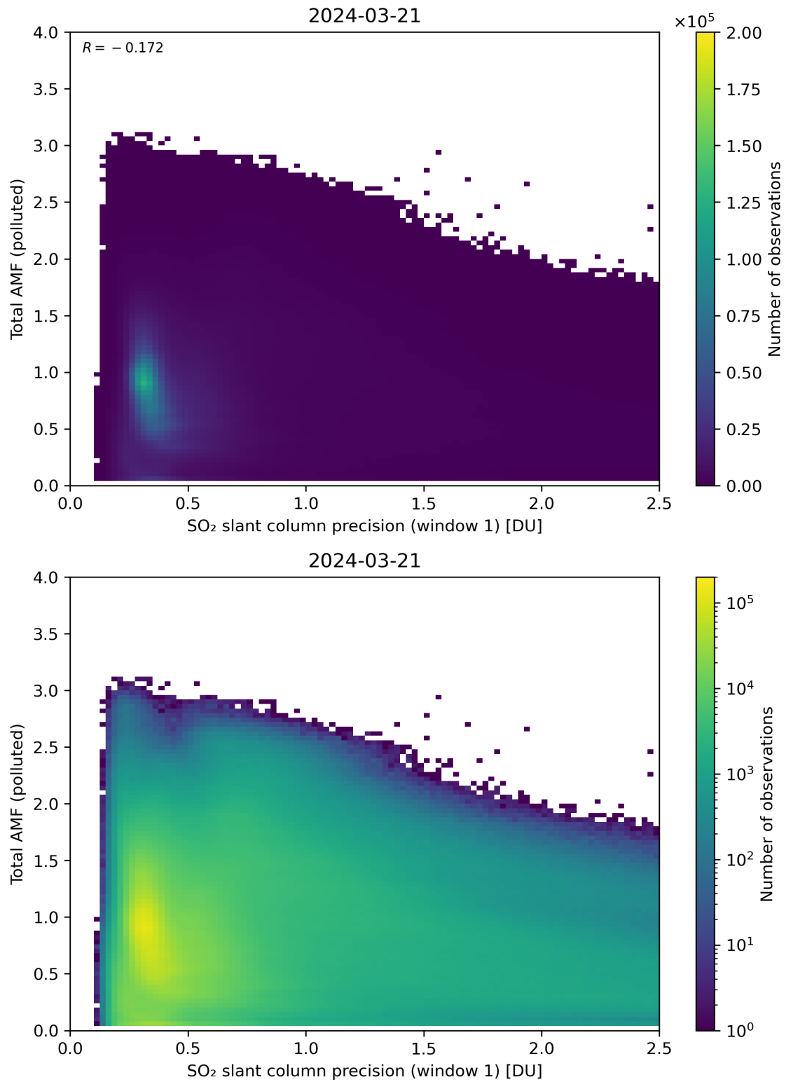
Figure 230: Scatter density plot of “SO 2 slant column precision (window 1)” against “Total AMF (polluted)” for 2024-03-20 to 2024-03-22.
