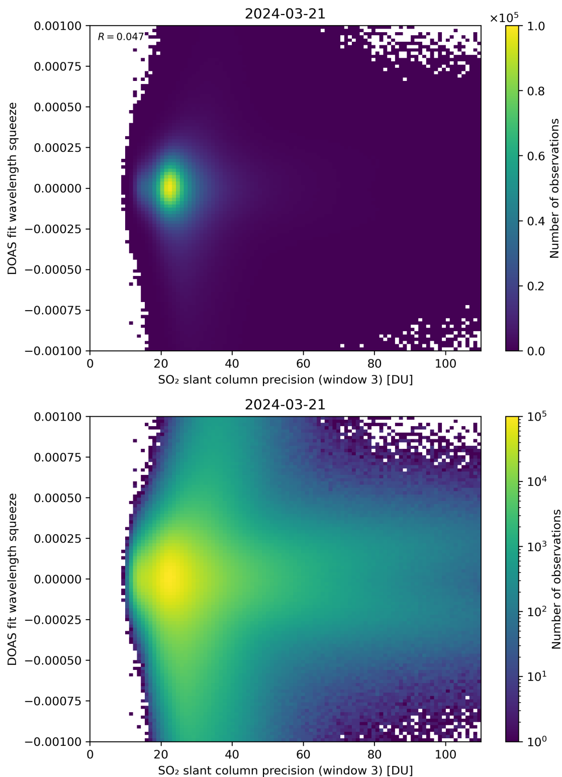
Figure 259: Scatter density plot of “SO 2 slant column precision (window 3)” against “DOAS fit wavelength squeeze” for 2024-03-20 to 2024-03-22.
