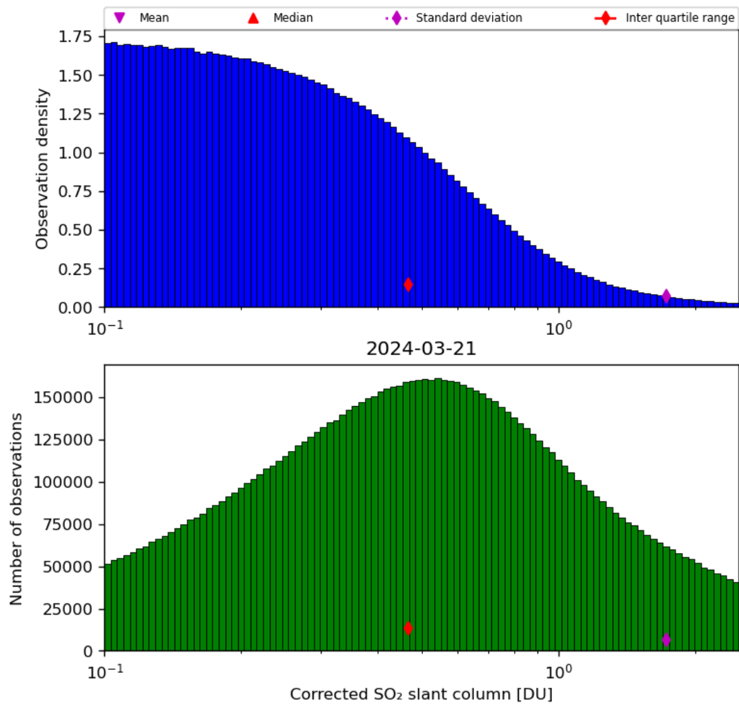
Figure 55: Histogram of “Corrected SO 2 slant column” for 2024-03-20 to 2024-03-22
