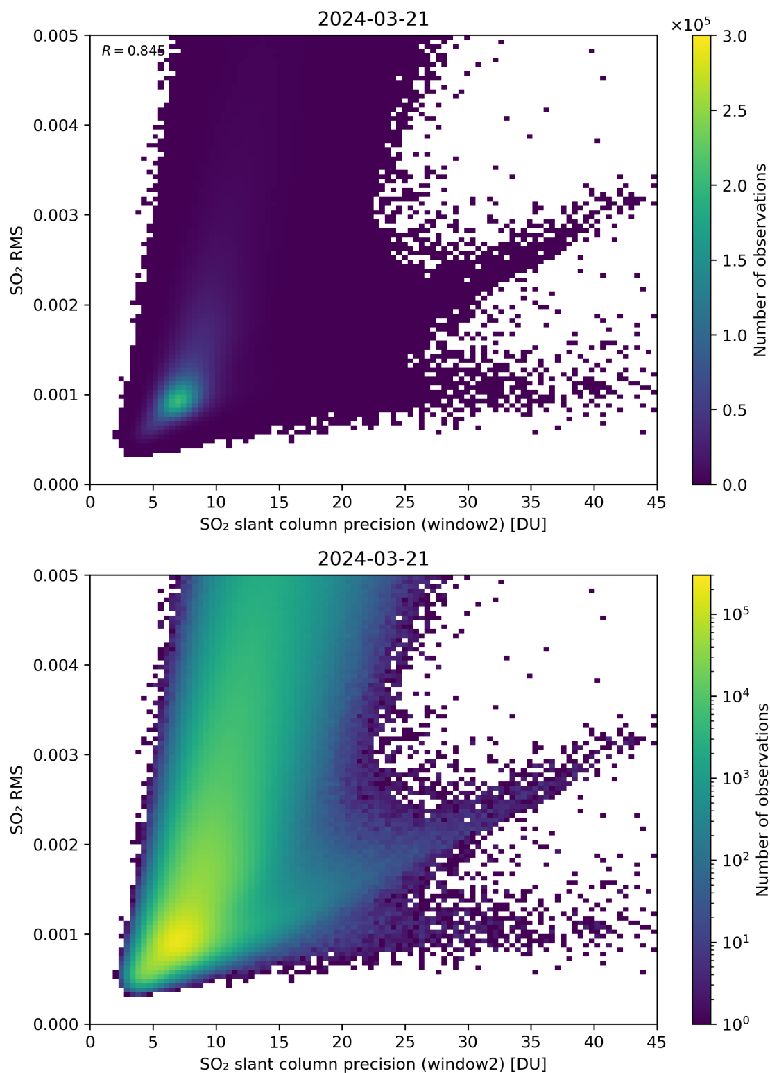
Figure 245: Scatter density plot of “SO 2 slant column precision (window2)” against “SO 2 RMS” for 2024-03-20 to 2024-03-22.
