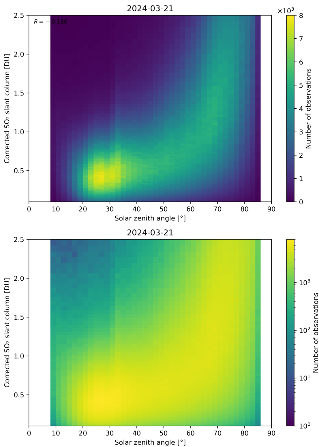
Figure 166: Scatter density plot of “Solar zenith angle” against “Corrected SO 2 slant column” for 2024-03-20 to 2024-03-22.
