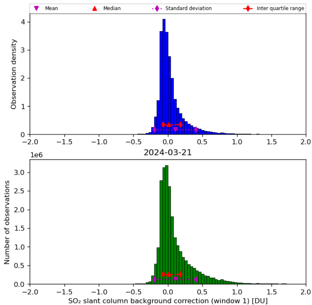
Figure 59: Histogram of “SO 2 slant column background correction (window 1)” for 2024-03-20 to 2024-03-22
