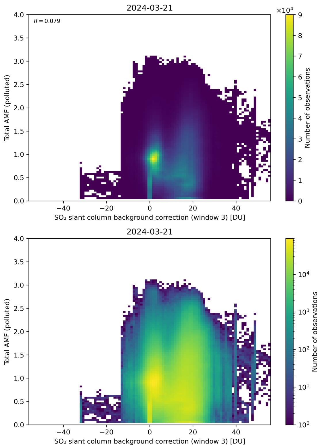
Figure 125: Scatter density plot of “SO 2 slant column background correction (window 3)” against “Total AMF (polluted)” for 2024-03-20 to 2024-03-22.
