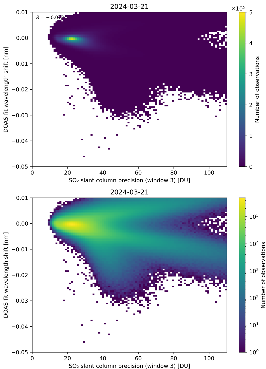
Figure 258: Scatter density plot of “SO 2 slant column precision (window 3)” against “DOAS fit wavelength shift” for 2024-03-20 to 2024-03-22.
