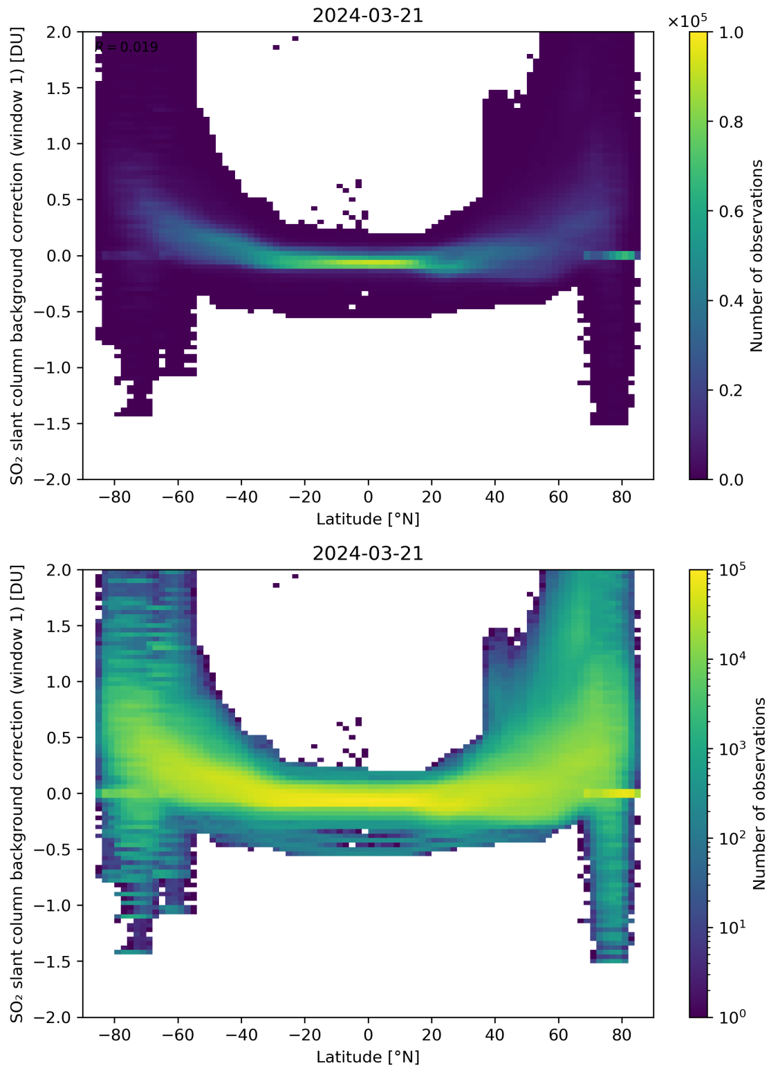
Figure 139: Scatter density plot of “Latitude” against “SO 2 slant column background correction (window 1)” for 2024-03-20 to 2024-03-22.
