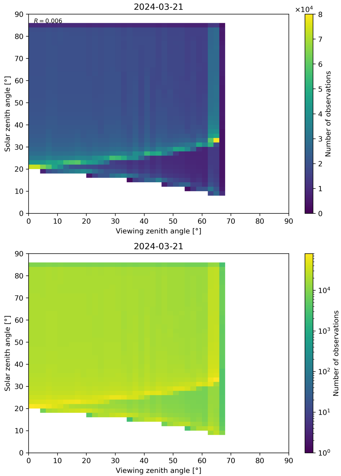
Figure 315: Scatter density plot of “Viewing zenith angle” against “Solar zenith angle” for 2024-03-20 to 2024-03-22.
