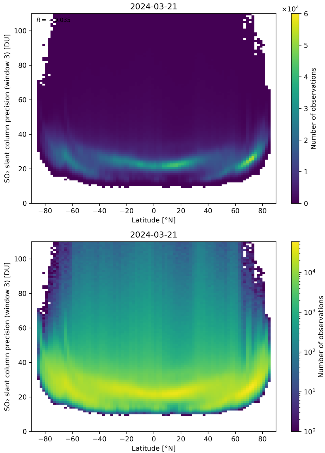
Figure 153: Scatter density plot of “Latitude” against “SO 2 slant column precision (window 3)” for 2024-03-20 to 2024-03-22.
