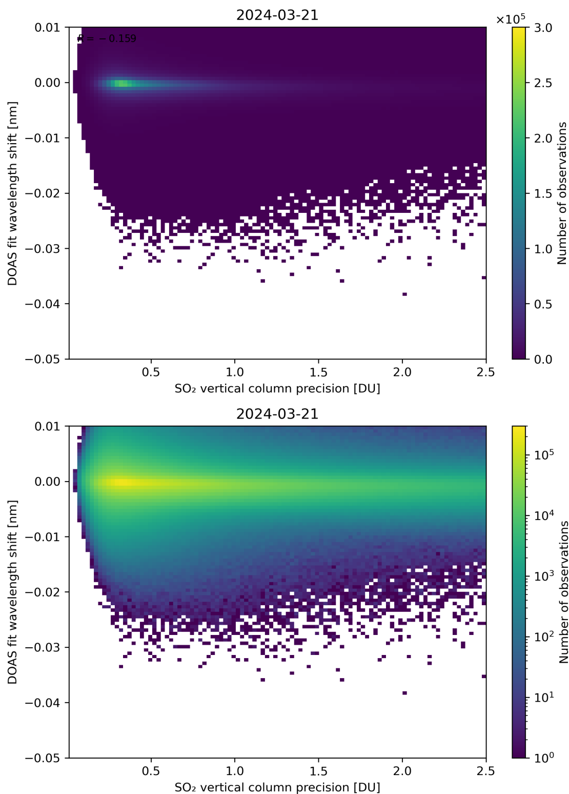
Figure 282: Scatter density plot of “SO 2 vertical column precision” against “DOAS fit wavelength shift” for 2024-03-20 to 2024-03-22.
