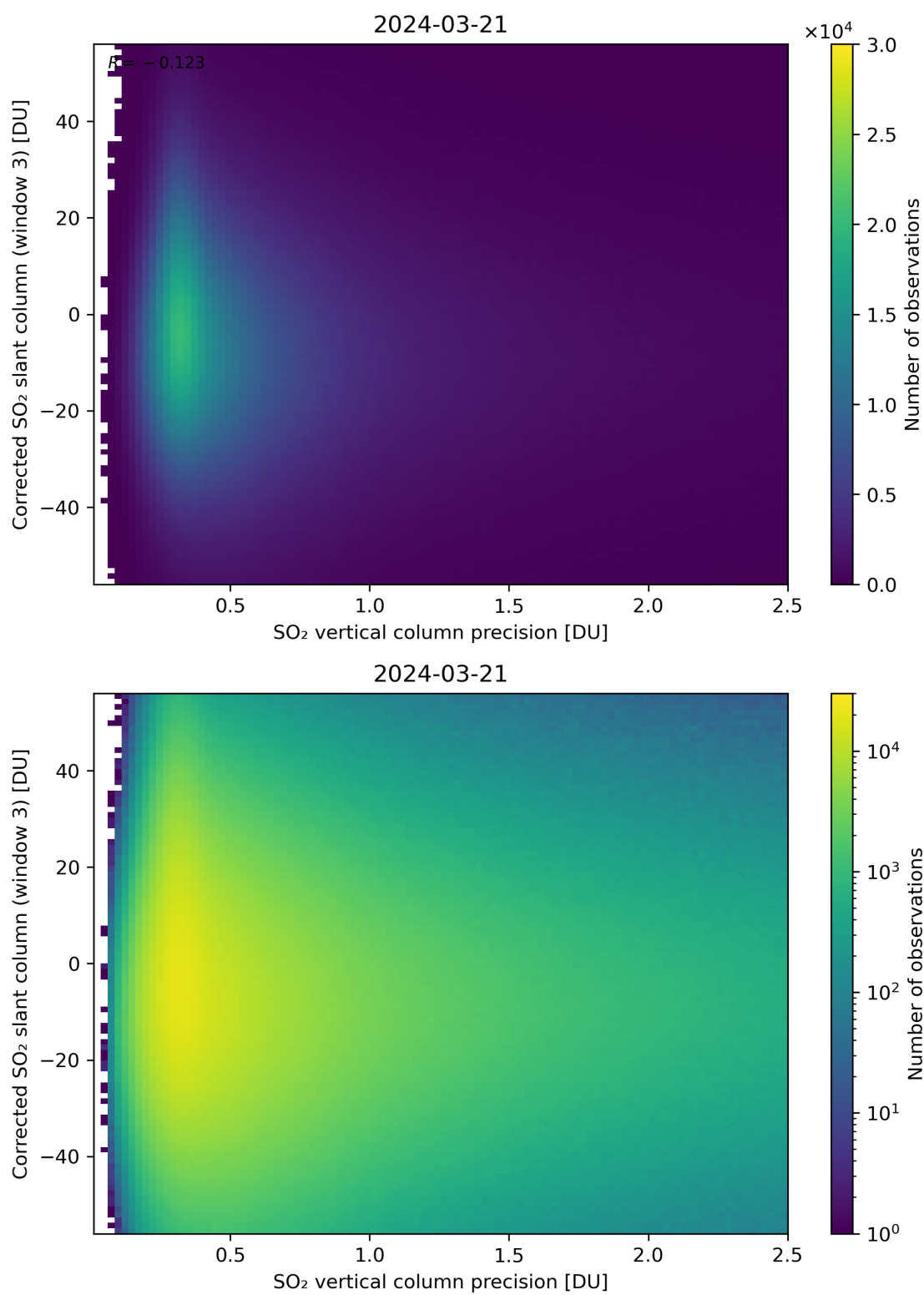
Figure 288: Scatter density plot of “SO 2 vertical column precision” against “Corrected SO 2 slant column (window 3)” for 2024-03-20 to 2024-03-22.
