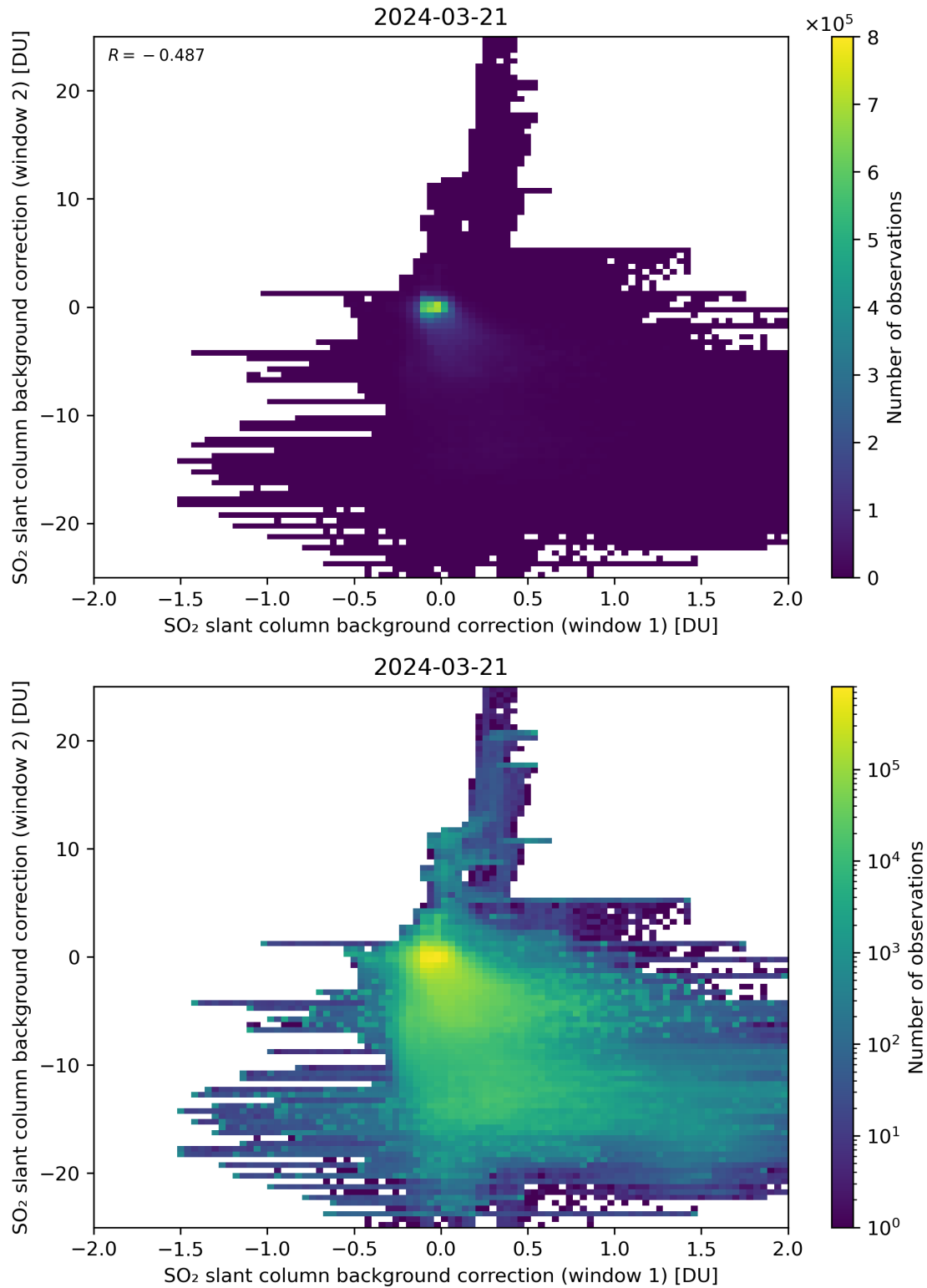
Figure 98: Scatter density plot of “SO 2 slant column background correction (window 1)” against “SO 2 slant column background correction (window 2)” for 2024-03-20 to 2024-03-22.
