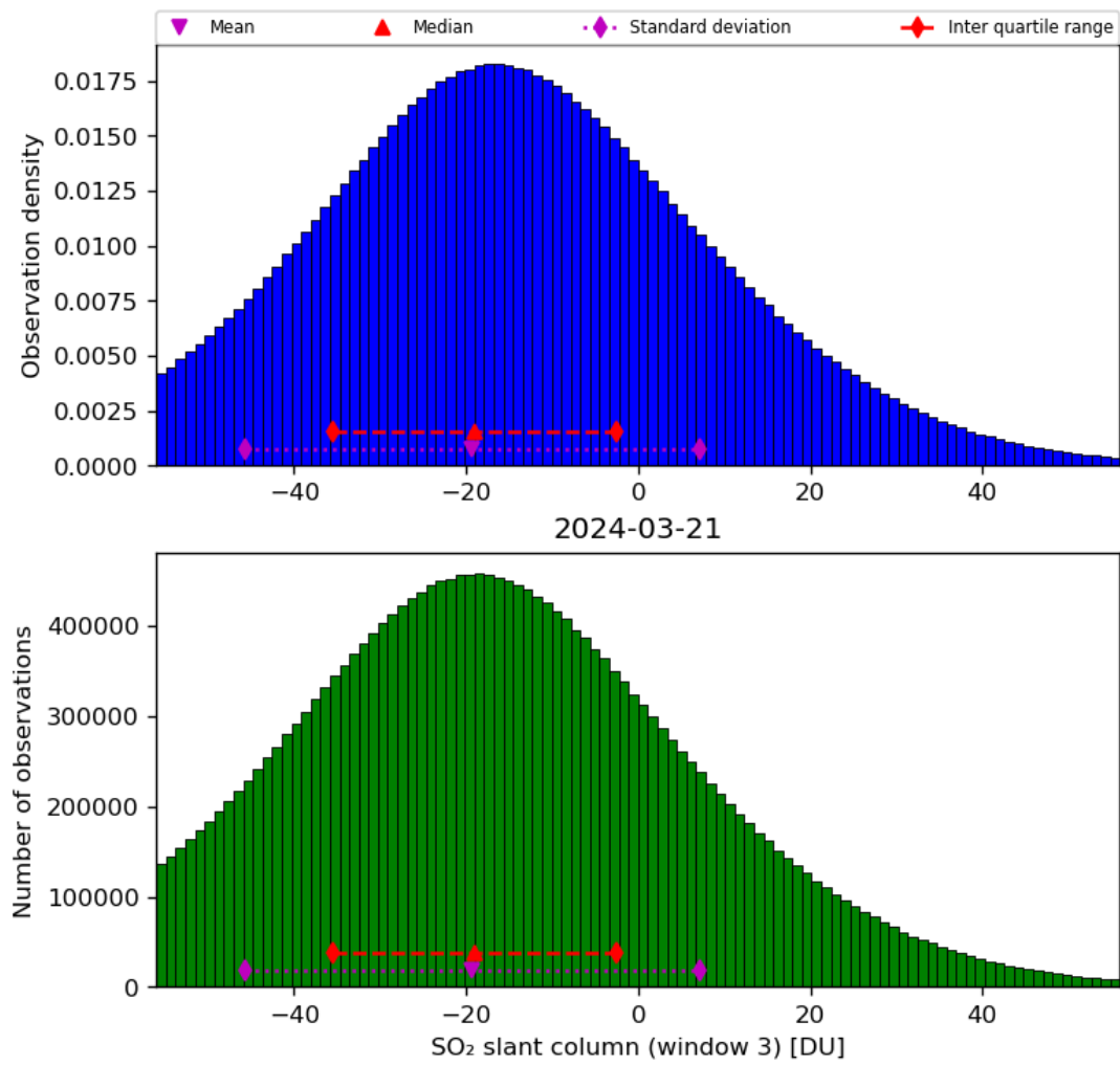
Figure 64: Histogram of “SO 2 slant column (window 3)” for 2024-03-20 to 2024-03-22
