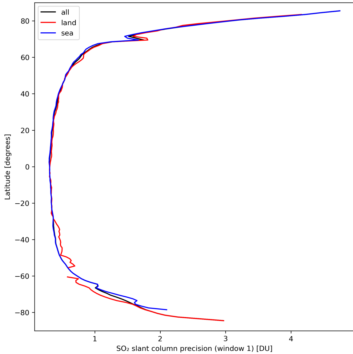
Figure 34: Zonal average of “SO 2 slant column precision (window 1)” for 2024-03-20 to 2024-03-22.
