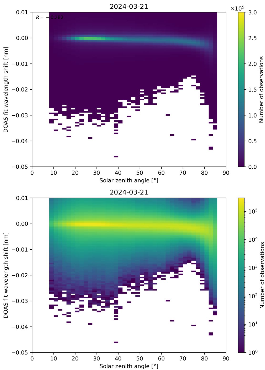
Figure 161: Scatter density plot of “Solar zenith angle” against “DOAS fit wavelength shift” for 2024-03-20 to 2024-03-22.
