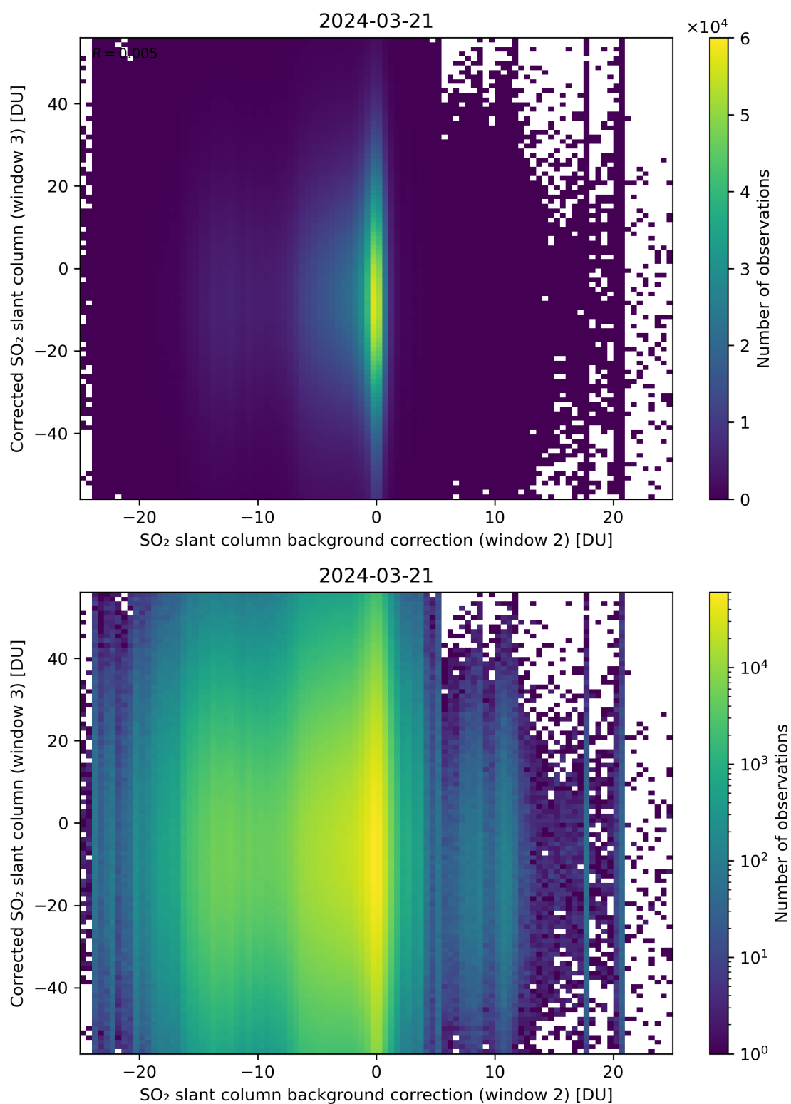
Figure 116: Scatter density plot of “SO 2 slant column background correction (window 2)” against “Corrected SO 2 slant column (window 3)” for 2024-03-20 to 2024-03-22.
