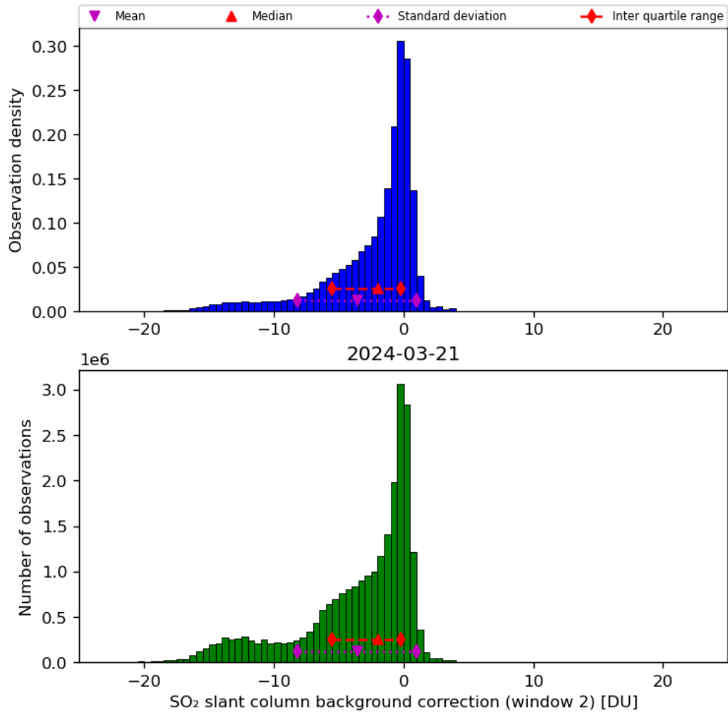
Figure 63: Histogram of “SO 2 slant column background correction (window 2)” for 2024-03-20 to 2024-03-22
