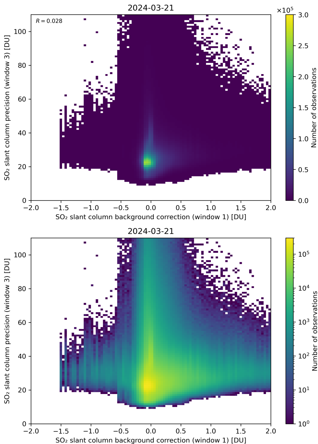
Figure 108: Scatter density plot of “SO 2 slant column background correction (window 1)” against “SO 2 slant column precision (window 3)” for 2024-03-20 to 2024-03-22.
