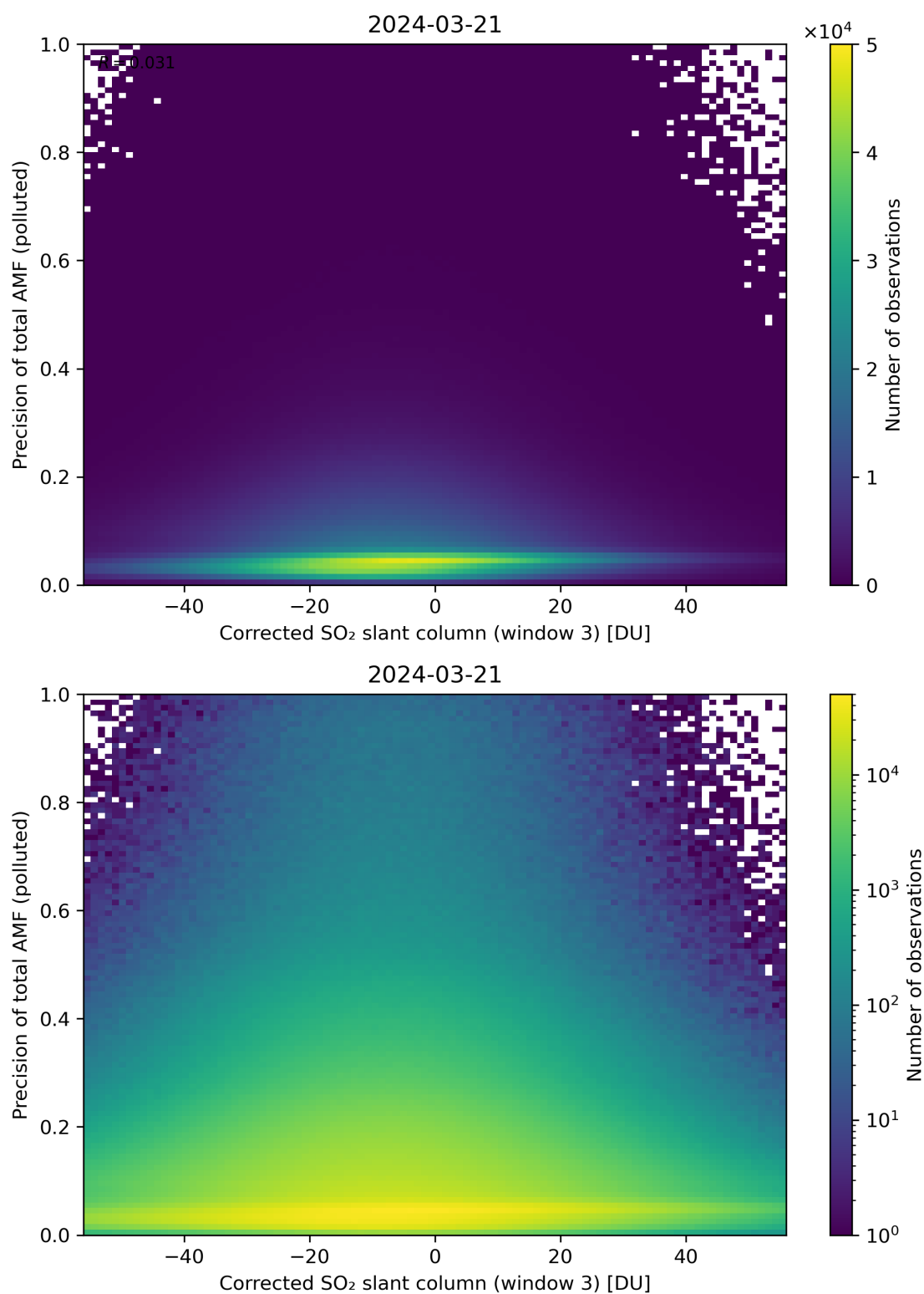
Figure 211: Scatter density plot of “Corrected SO 2 slant column (window 3)” against “Precision of total AMF (polluted)” for 2024-03-20 to 2024-03-22.
