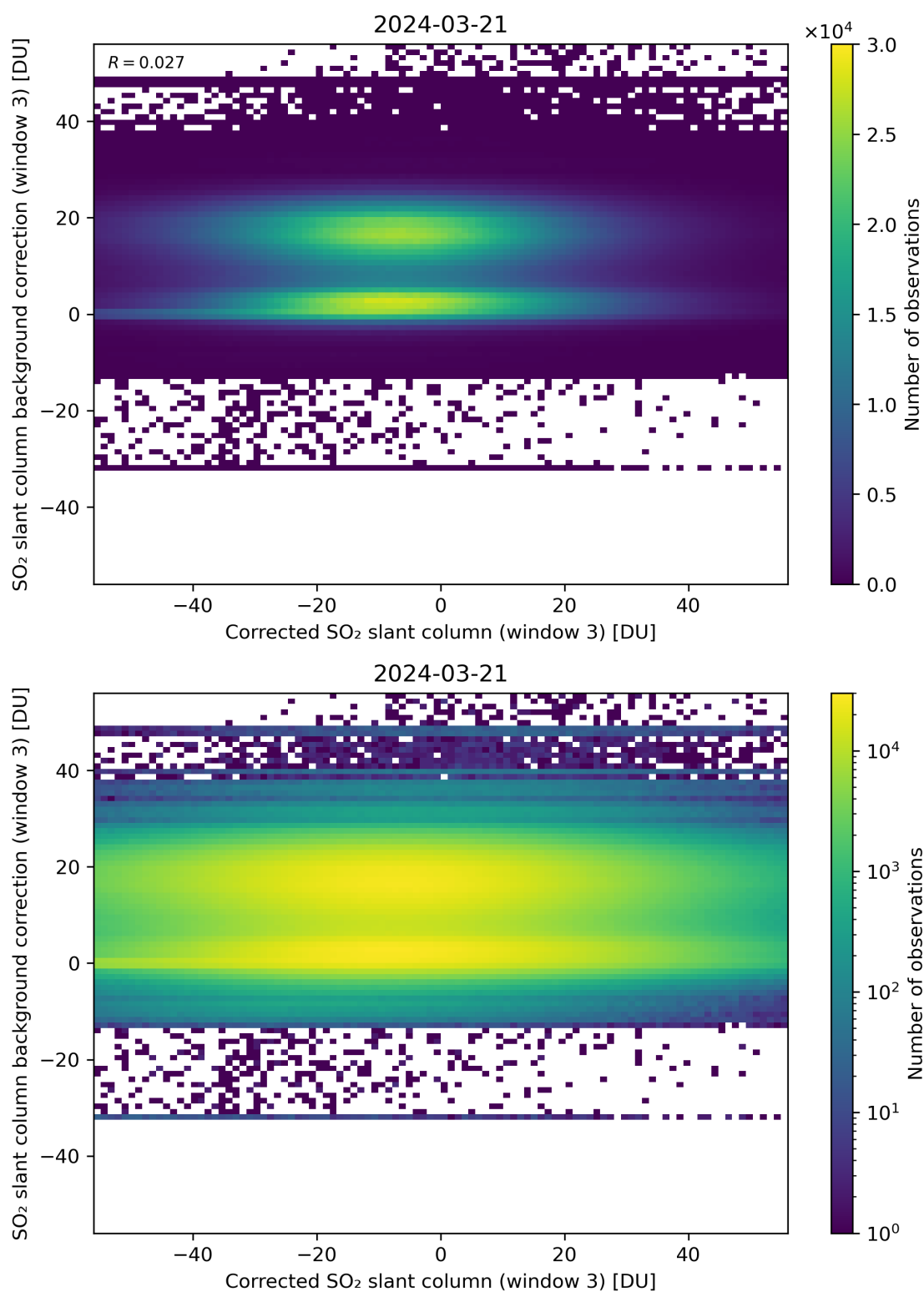
Figure 205: Scatter density plot of “Corrected SO 2 slant column (window 3)” against “SO 2 slant column background correction (window 3)” for 2024-03-20 to 2024-03-22.
