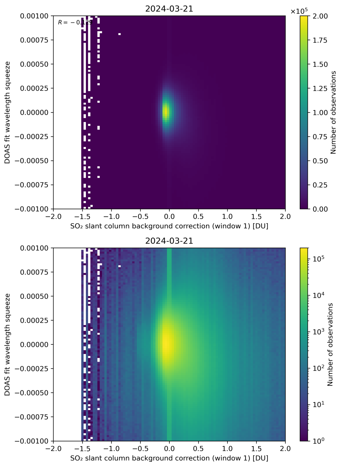
Figure 101: Scatter density plot of “SO 2 slant column background correction (window 1)” against “DOAS fit wavelength squeeze” for 2024-03-20 to 2024-03-22.
