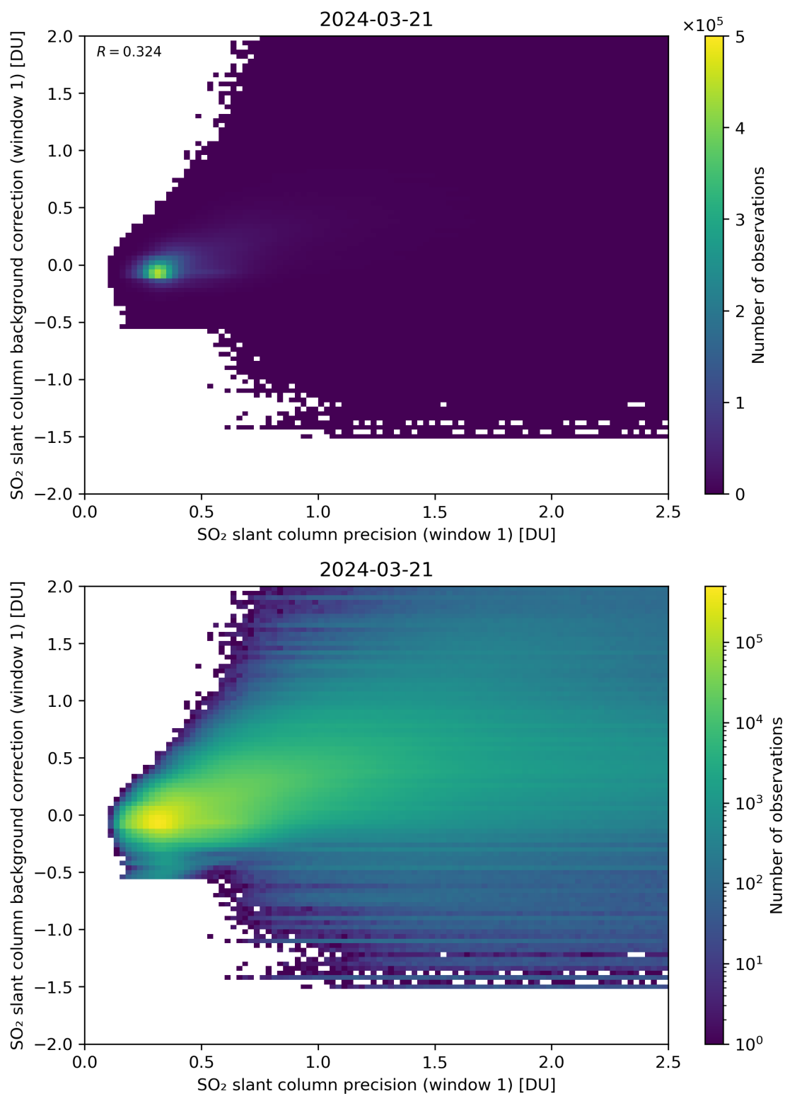
Figure 218: Scatter density plot of “SO 2 slant column precision (window 1)” against “SO 2 slant column background correction (window 1)” for 2024-03-20 to 2024-03-22.
