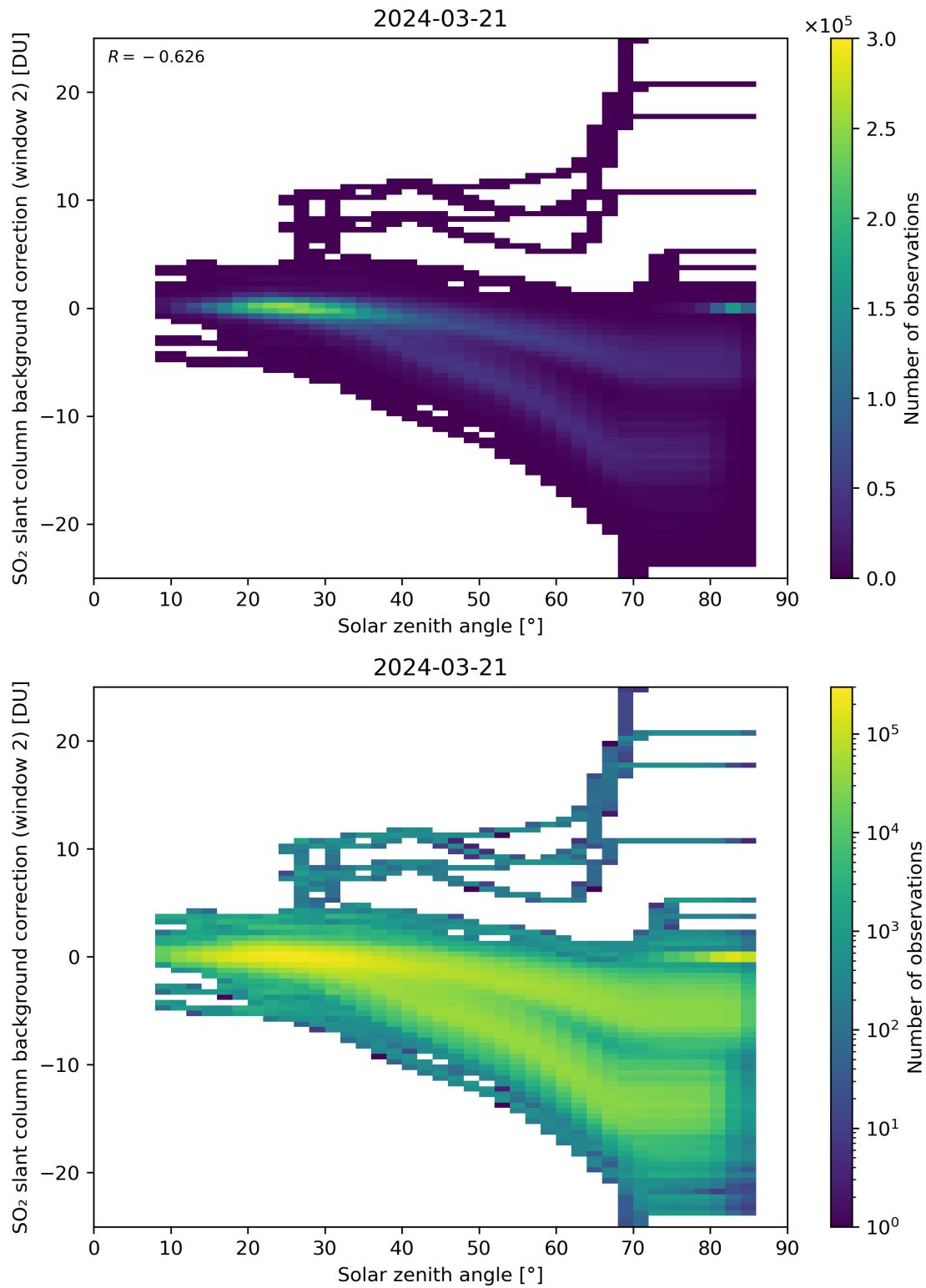
Figure 159: Scatter density plot of “Solar zenith angle” against “SO 2 slant column background correction (window 2)” for 2024-03-20 to 2024-03-22.
