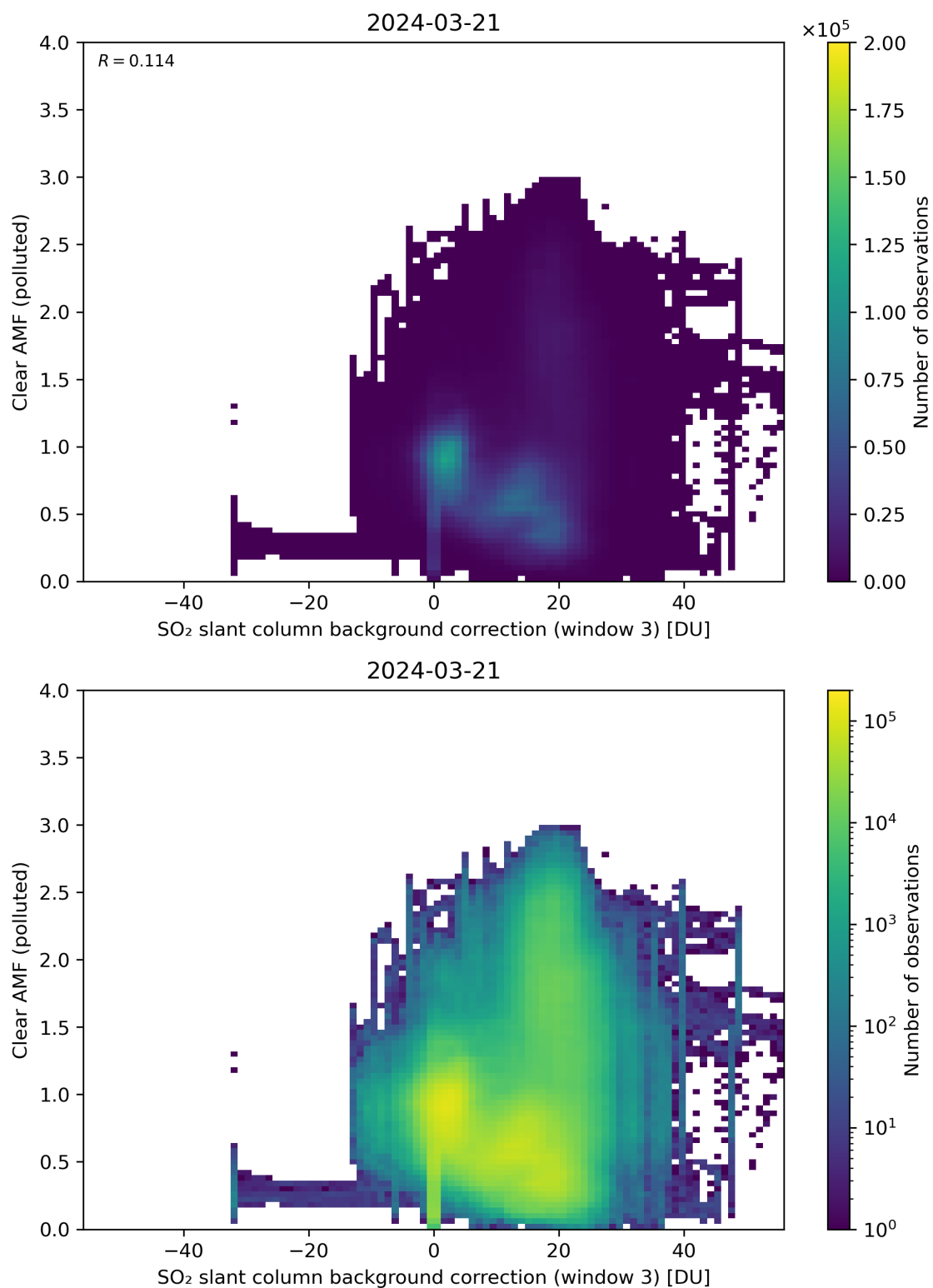
Figure 124: Scatter density plot of “SO 2 slant column background correction (window 3)” against “Clear AMF (polluted)” for 2024-03-20 to 2024-03-22.
