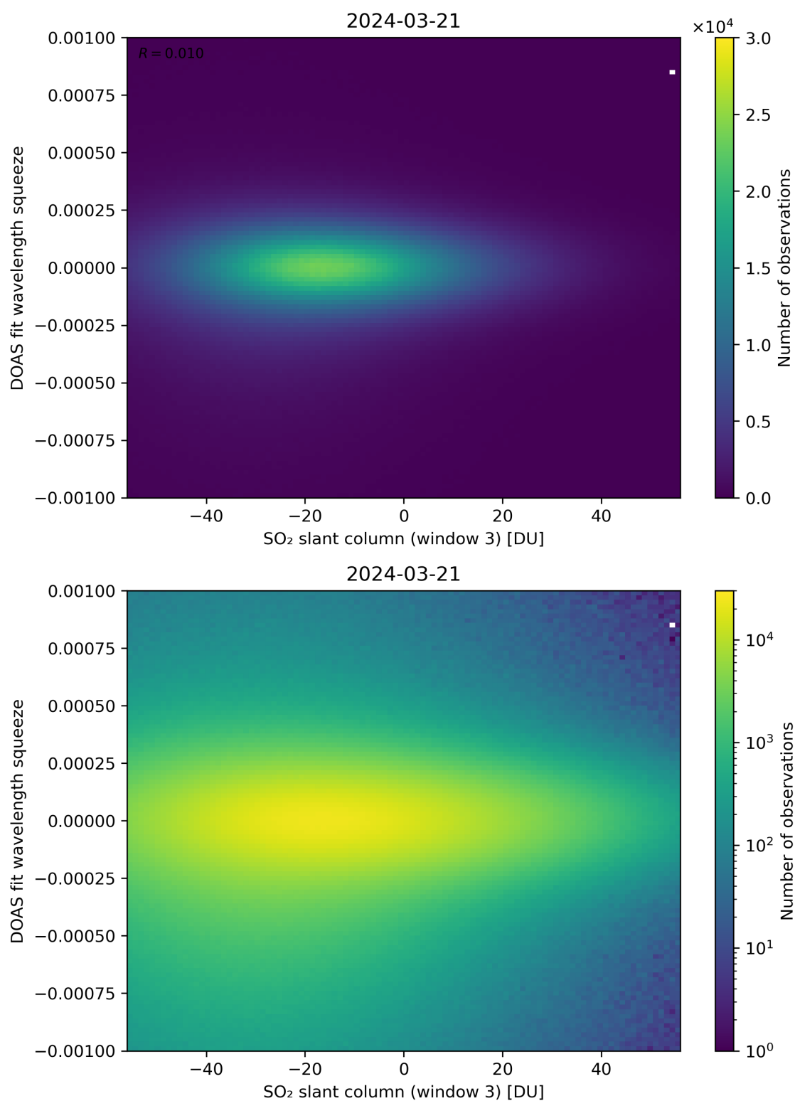
Figure 255: Scatter density plot of “SO 2 slant column (window 3)” against “DOAS fit wavelength squeeze” for 2024-03-20 to 2024-03-22.
