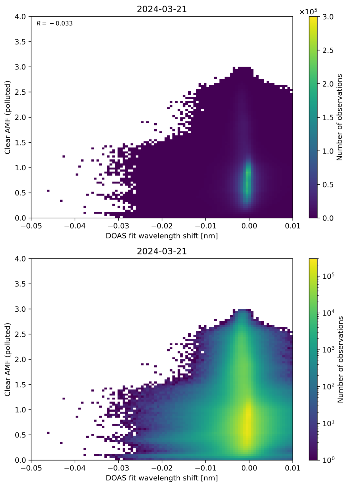
Figure 129: Scatter density plot of “DOAS fit wavelength shift” against “Clear AMF (polluted)” for 2024-03-20 to 2024-03-22.
