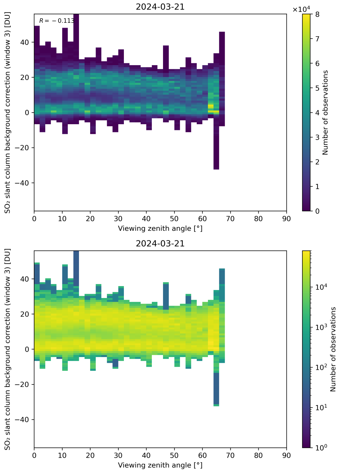
Figure 310: Scatter density plot of “Viewing zenith angle” against “SO 2 slant column background correction (window 3)” for 2024-03-20 to 2024-03-22.
