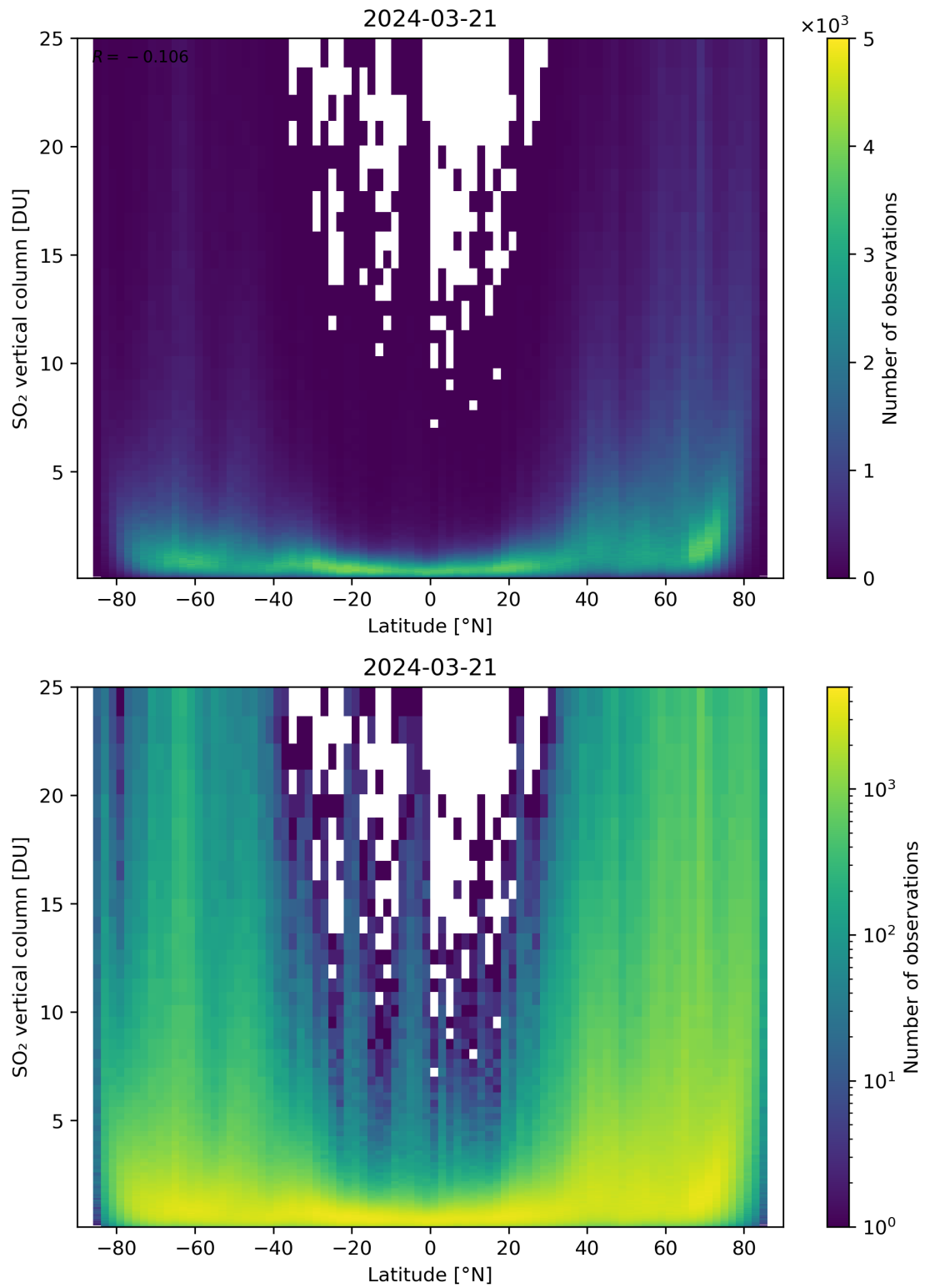
Figure 156: Scatter density plot of “Latitude” against “SO 2 vertical column” for 2024-03-20 to 2024-03-22.
