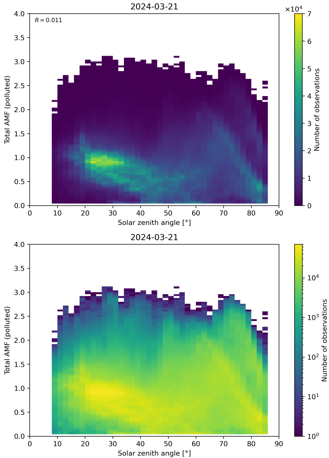
Figure 174: Scatter density plot of “Solar zenith angle” against “Total AMF (polluted)” for 2024-03-20 to 2024-03-22.
