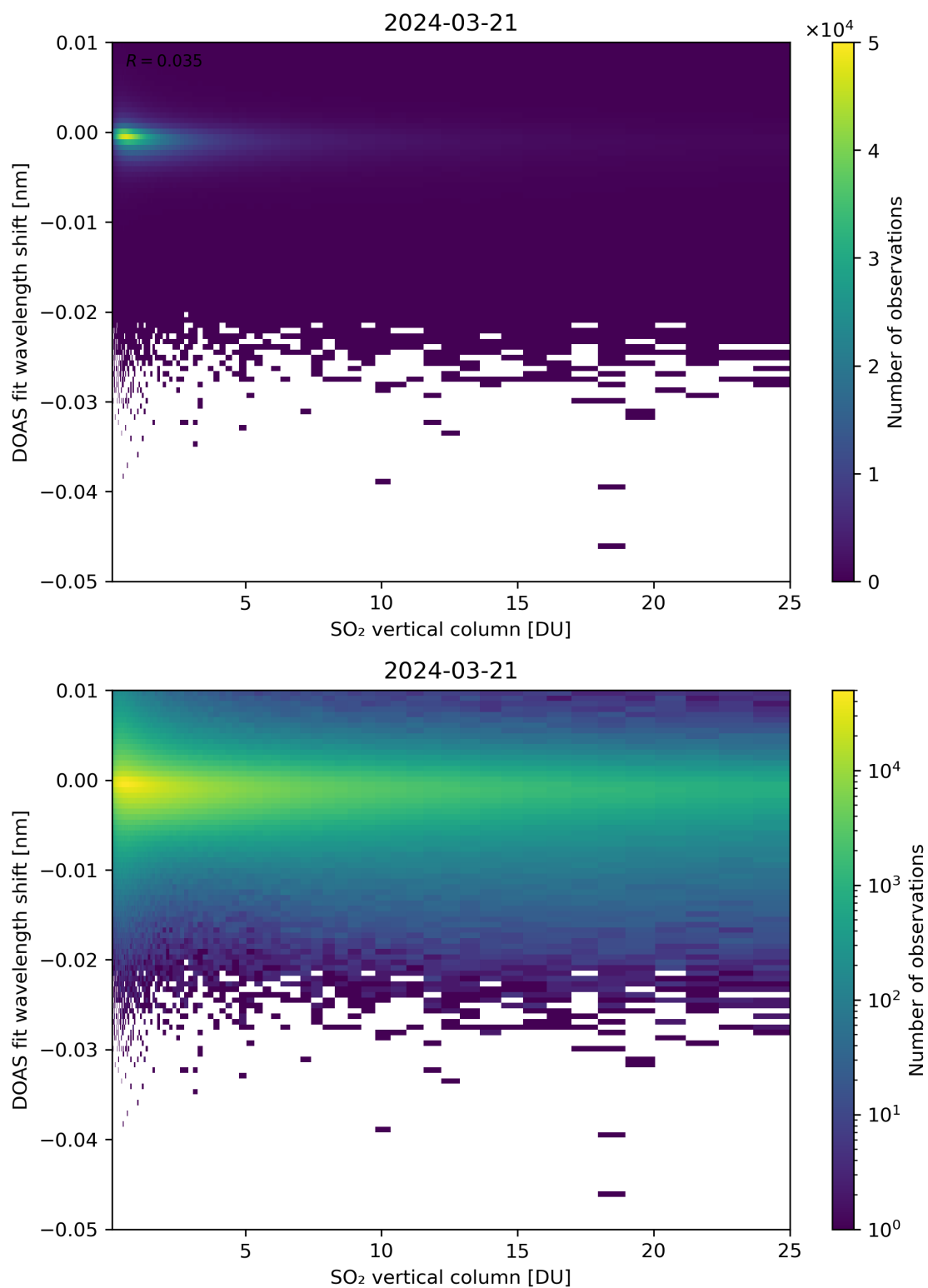
Figure 276: Scatter density plot of “SO 2 vertical column” against “DOAS fit wavelength shift” for 2024-03-20 to 2024-03-22.
