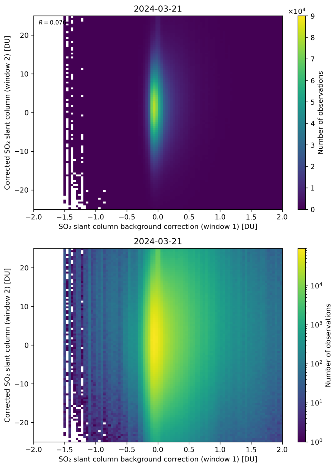
Figure 104: Scatter density plot of “SO 2 slant column background correction (window 1)” against “Corrected SO 2 slant column (window 2)” for 2024-03-20 to 2024-03-22.
