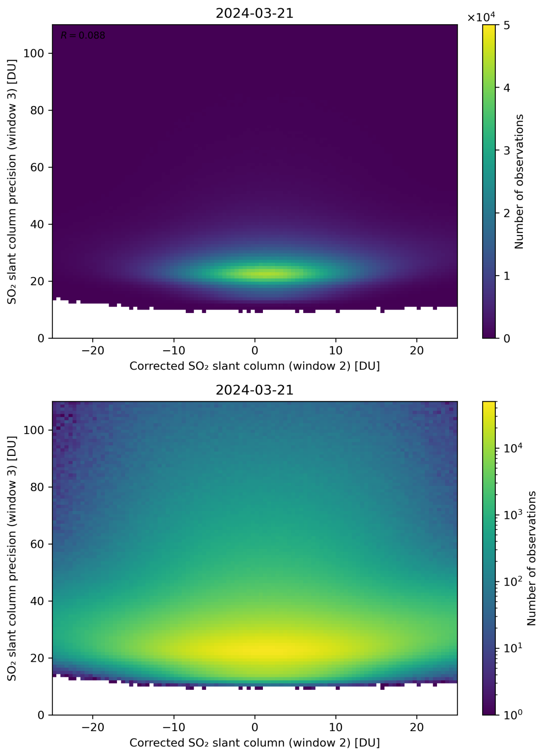
Figure 202: Scatter density plot of “Corrected SO 2 slant column (window 2)” against “SO 2 slant column precision (window 3)” for 2024-03-20 to 2024-03-22.
