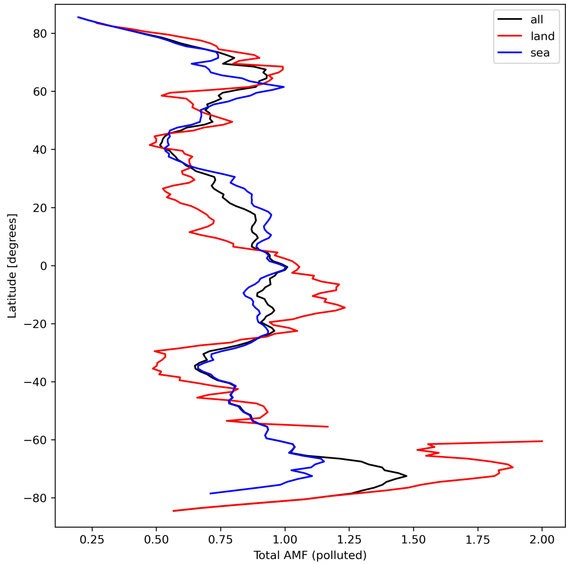
Figure 48: Zonal average of “Total AMF (polluted)” for 2024-03-20 to 2024-03-22.
