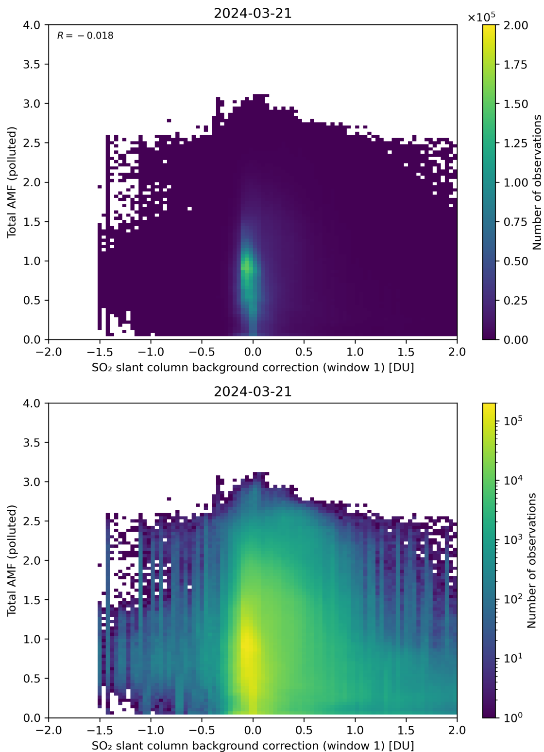
Figure 109: Scatter density plot of “SO 2 slant column background correction (window 1)” against “Total AMF (polluted)” for 2024-03-20 to 2024-03-22.
