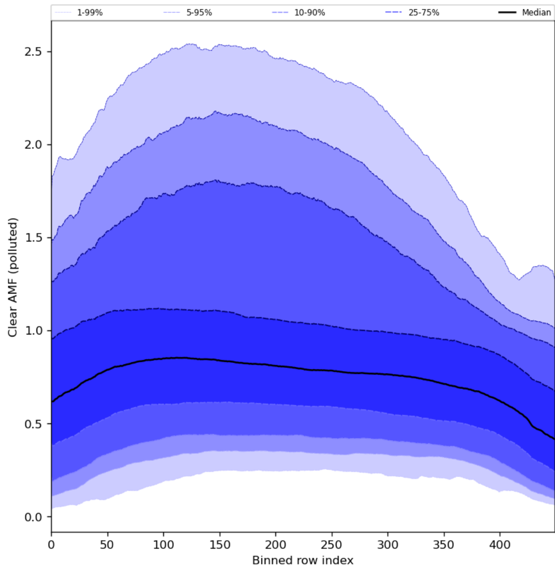
Figure 96: Along track statistics of “Clear AMF (polluted)” for 2024-03-20 to 2024-03-22
