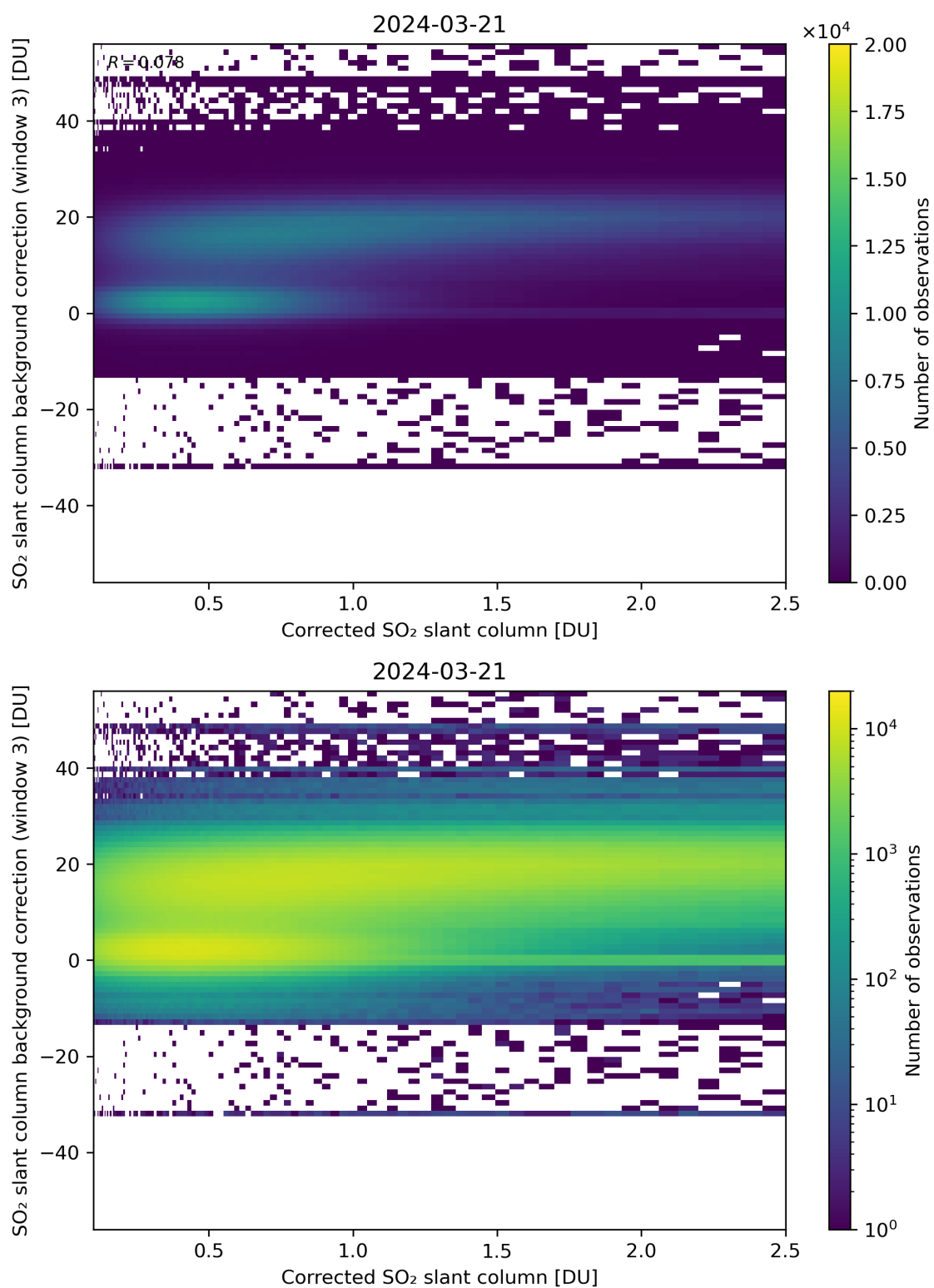
Figure 180: Scatter density plot of “Corrected SO 2 slant column” against “SO 2 slant column background correction (window 3)” for 2024-03-20 to 2024-03-22.
