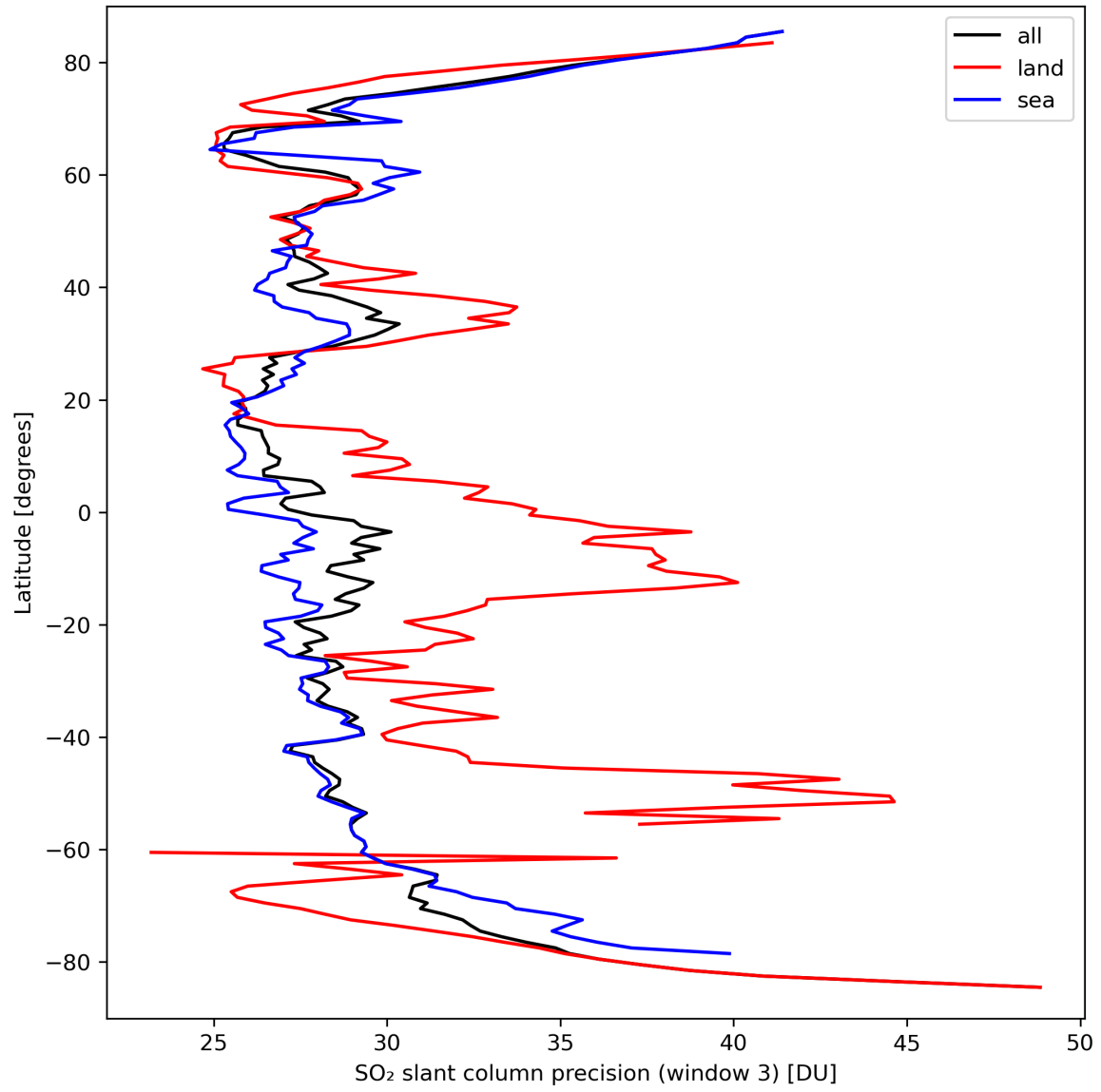
Figure 42: Zonal average of “SO 2 slant column precision (window 3)” for 2024-03-20 to 2024-03-22.
