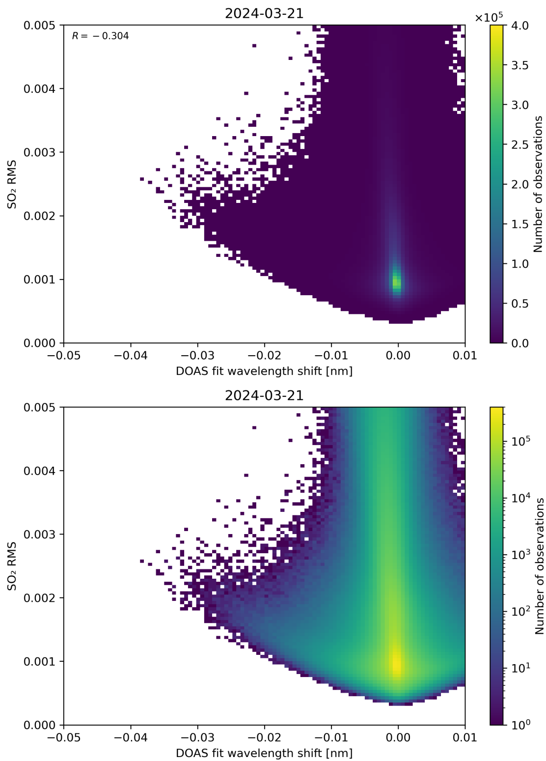
Figure 128: Scatter density plot of “DOAS fit wavelength shift” against “SO 2 RMS” for 2024-03-20 to 2024-03-22.
