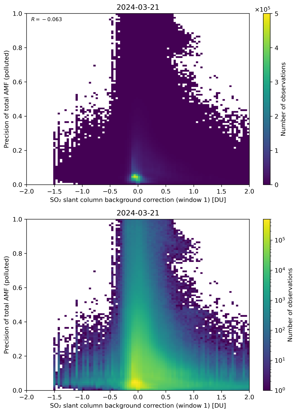
Figure 110: Scatter density plot of “SO 2 slant column background correction (window 1)” against “Precision of total AMF (polluted)” for 2024-03-20 to 2024-03-22.
