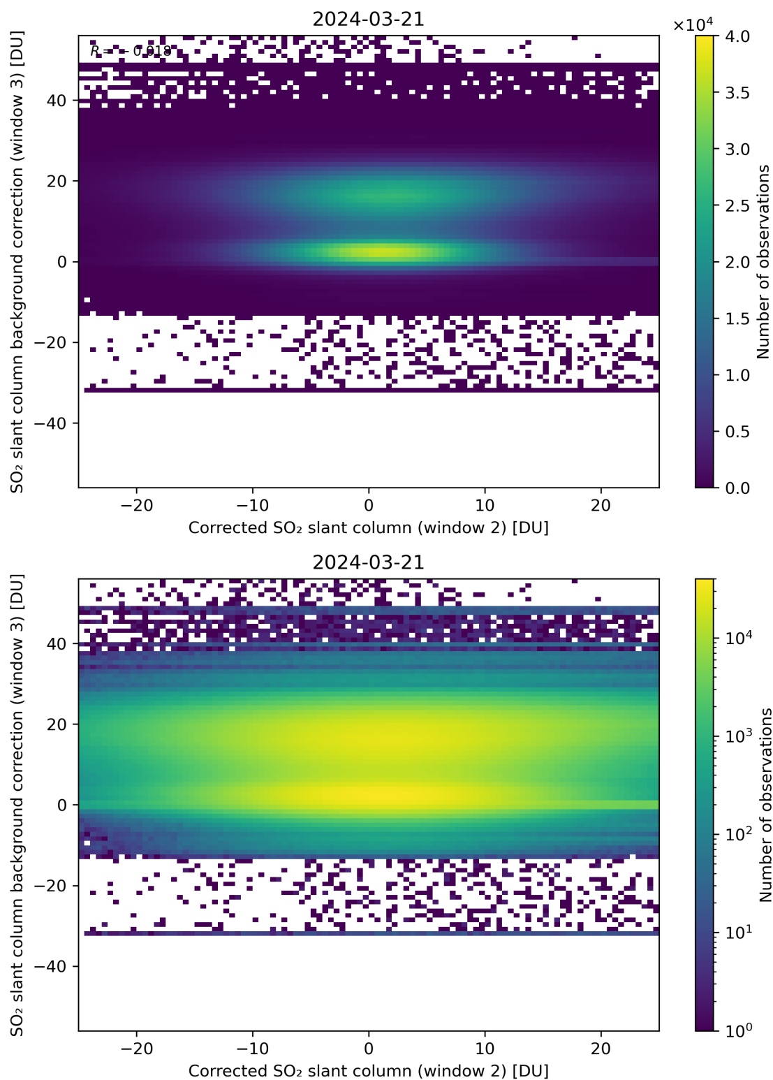
Figure 195: Scatter density plot of “Corrected SO 2 slant column (window 2)” against “SO 2 slant column background correction (window 3)” for 2024-03-20 to 2024-03-22.
