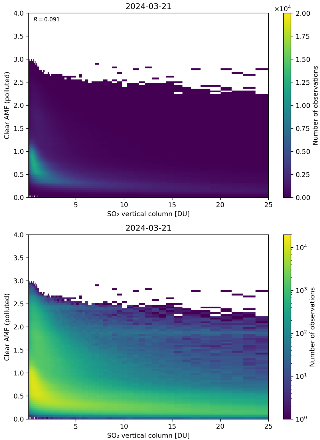
Figure 296: Scatter density plot of “SO 2 vertical column” against “Clear AMF (polluted)” for 2024-03-20 to 2024-03-22.
