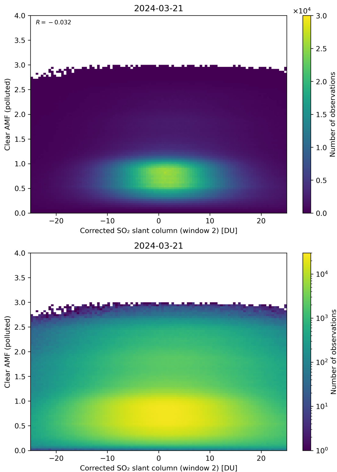
Figure 199: Scatter density plot of “Corrected SO 2 slant column (window 2)” against “Clear AMF (polluted)” for 2024-03-20 to 2024-03-22.
