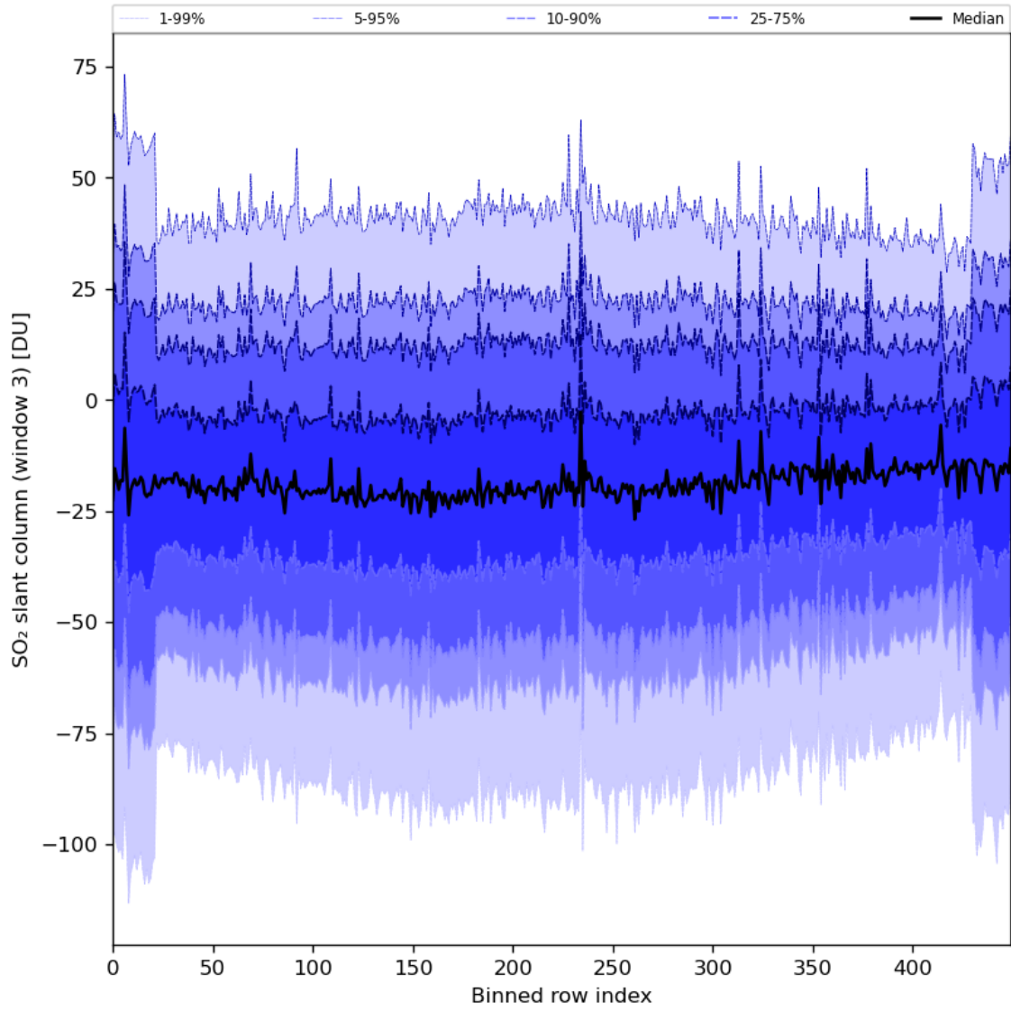
Figure 87: Along track statistics of “SO 2 slant column (window 3)” for 2024-03-20 to 2024-03-22
