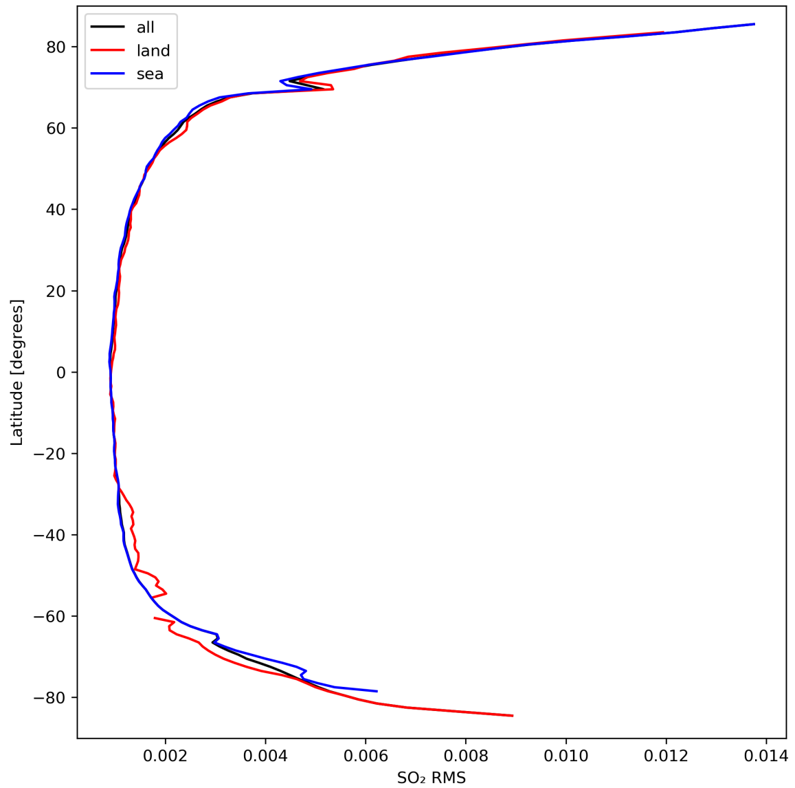
Figure 47: Zonal average of “SO 2 RMS” for 2024-03-20 to 2024-03-22.
