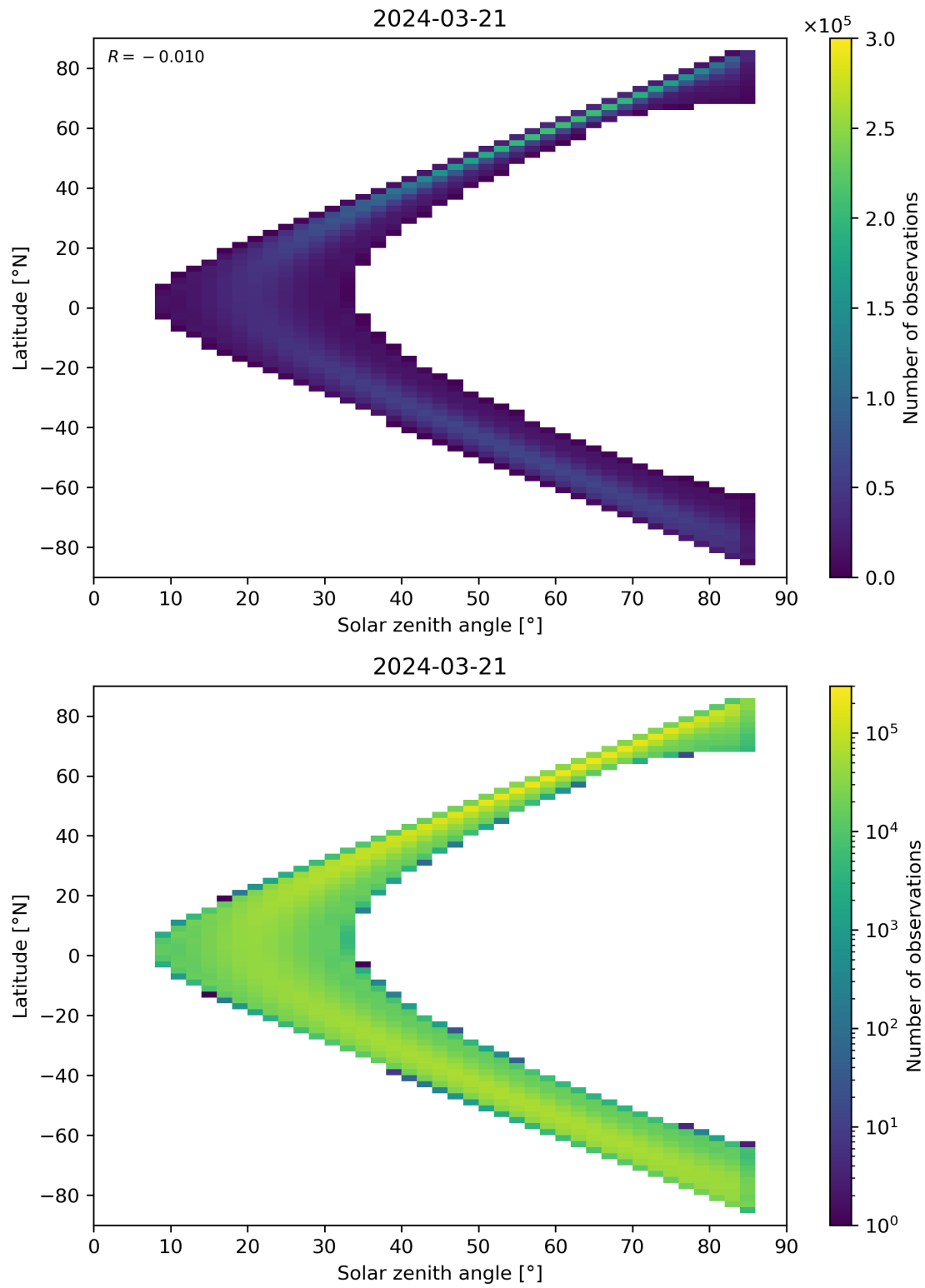
Figure 164: Scatter density plot of “Solar zenith angle” against “Latitude” for 2024-03-20 to 2024-03-22.
