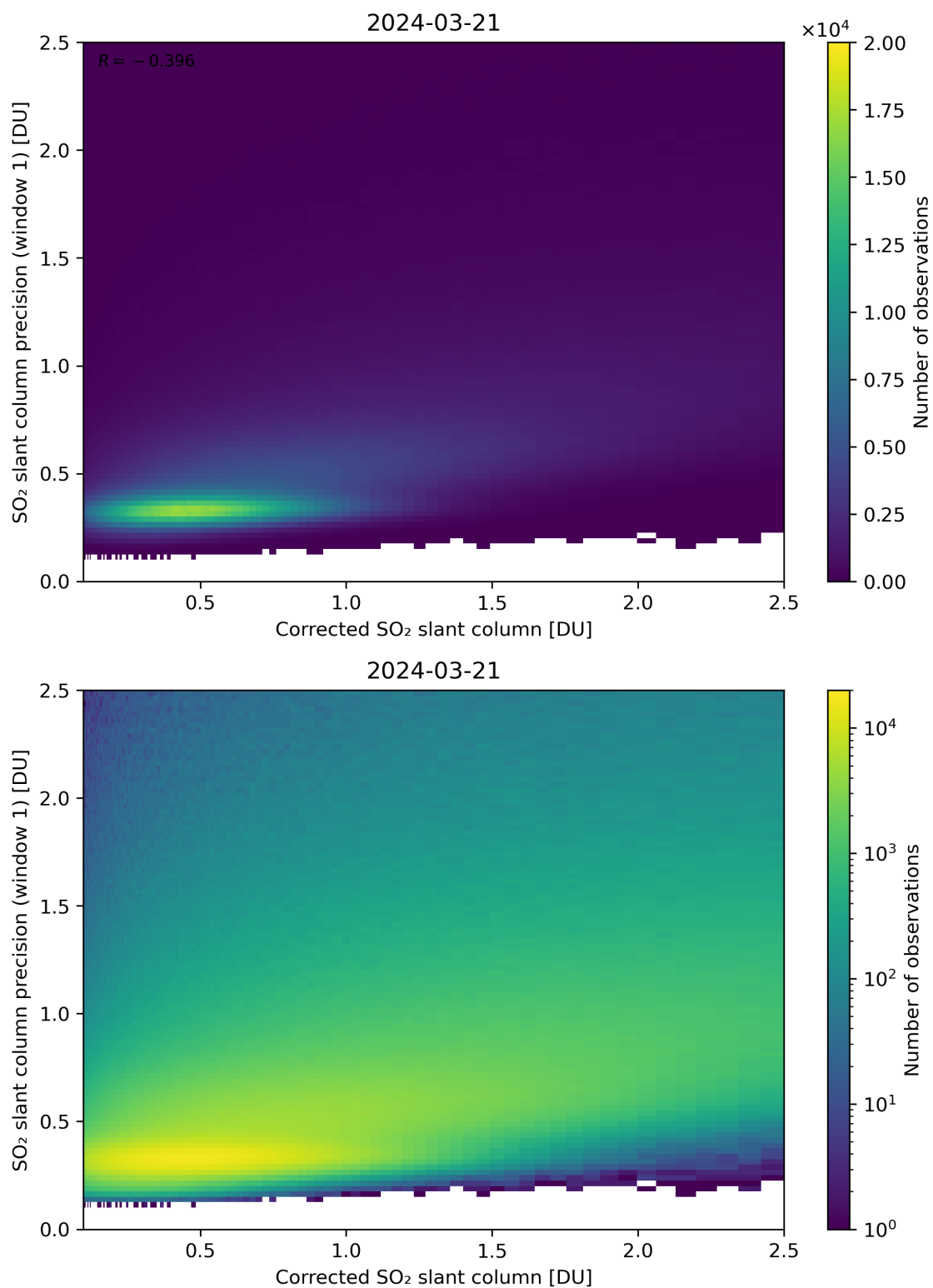
Figure 188: Scatter density plot of “Corrected SO 2 slant column” against “SO 2 slant column precision (window 1)” for 2024-03-20 to 2024-03-22.
