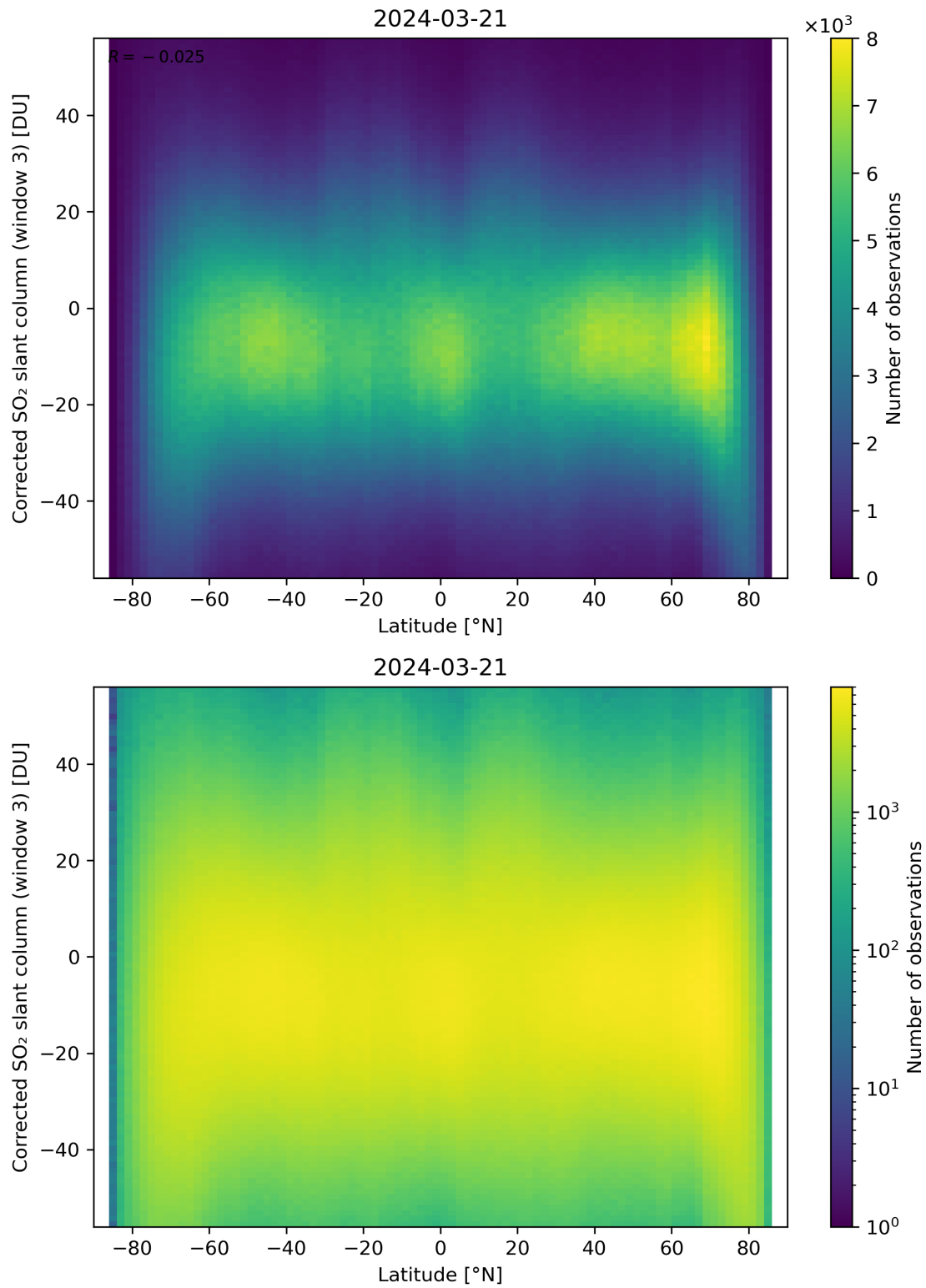
Figure 148: Scatter density plot of “Latitude” against “Corrected SO 2 slant column (window 3)” for 2024-03-20 to 2024-03-22.
