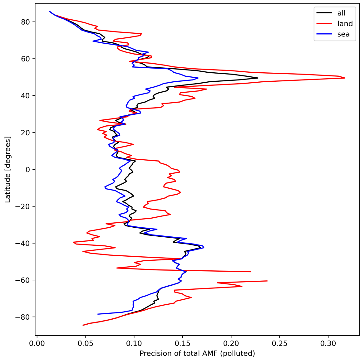
Figure 49: Zonal average of “Precision of total AMF (polluted)” for 2024-03-20 to 2024-03-22.
