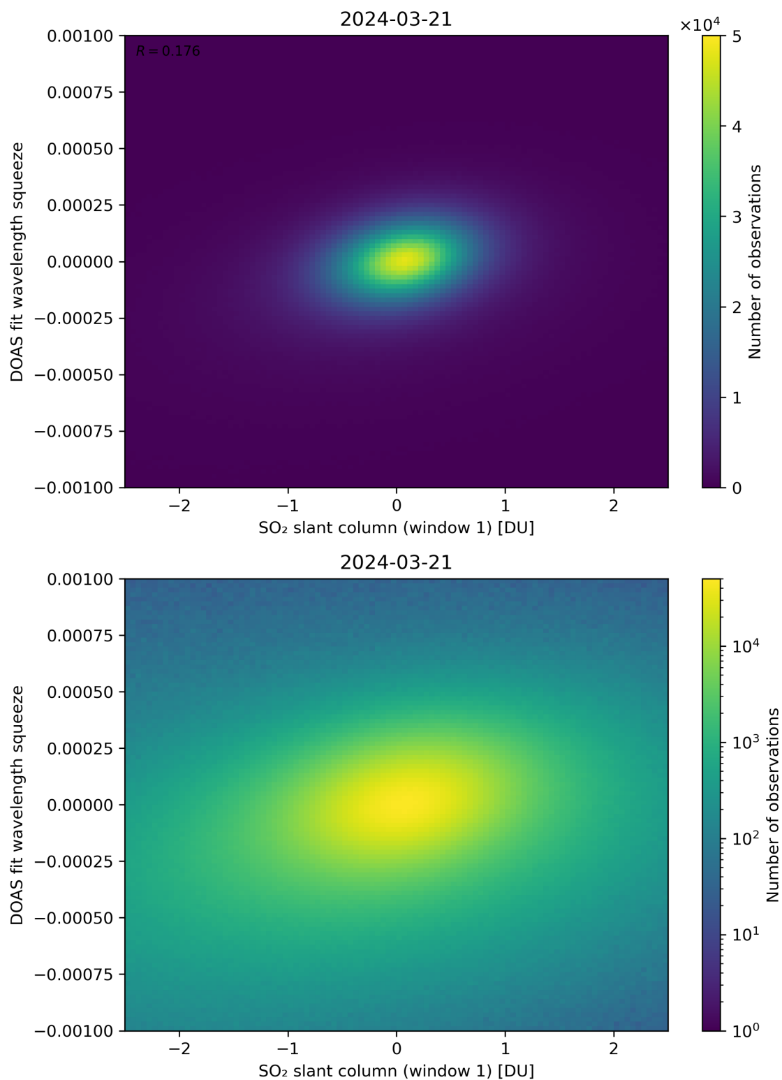
Figure 216: Scatter density plot of “SO 2 slant column (window 1)” against “DOAS fit wavelength squeeze” for 2024-03-20 to 2024-03-22.
