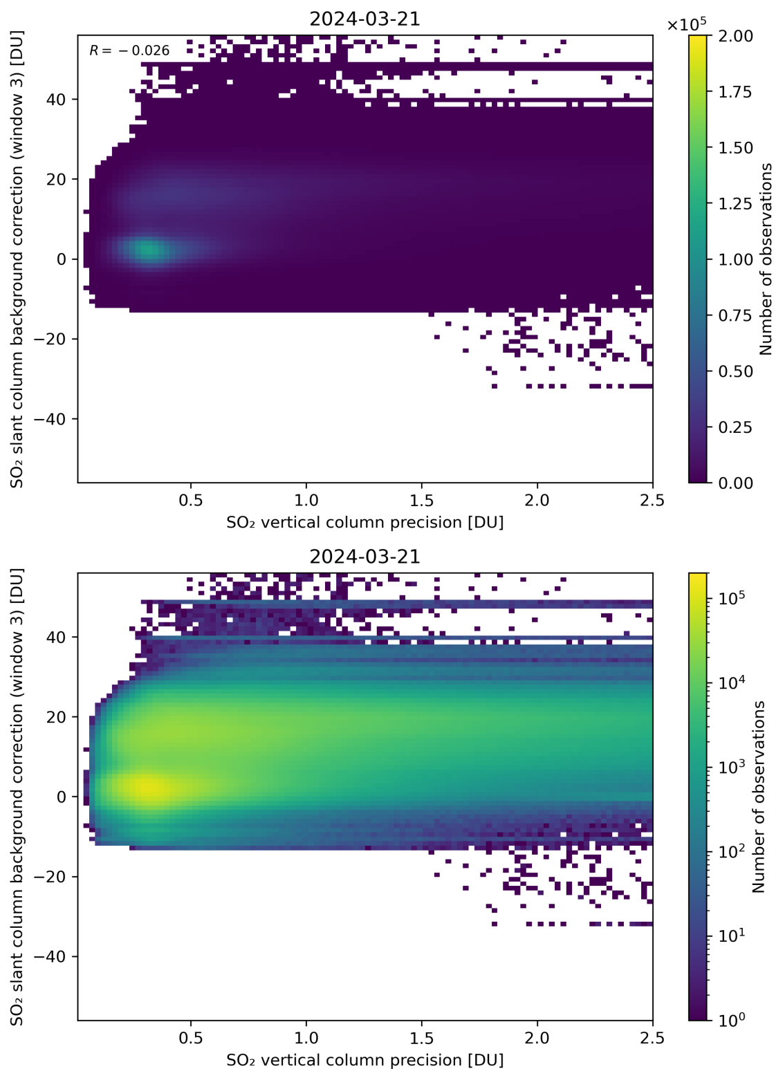
Figure 281: Scatter density plot of “SO 2 vertical column precision” against “SO 2 slant column background correction (window 3)” for 2024-03-20 to 2024-03-22.
