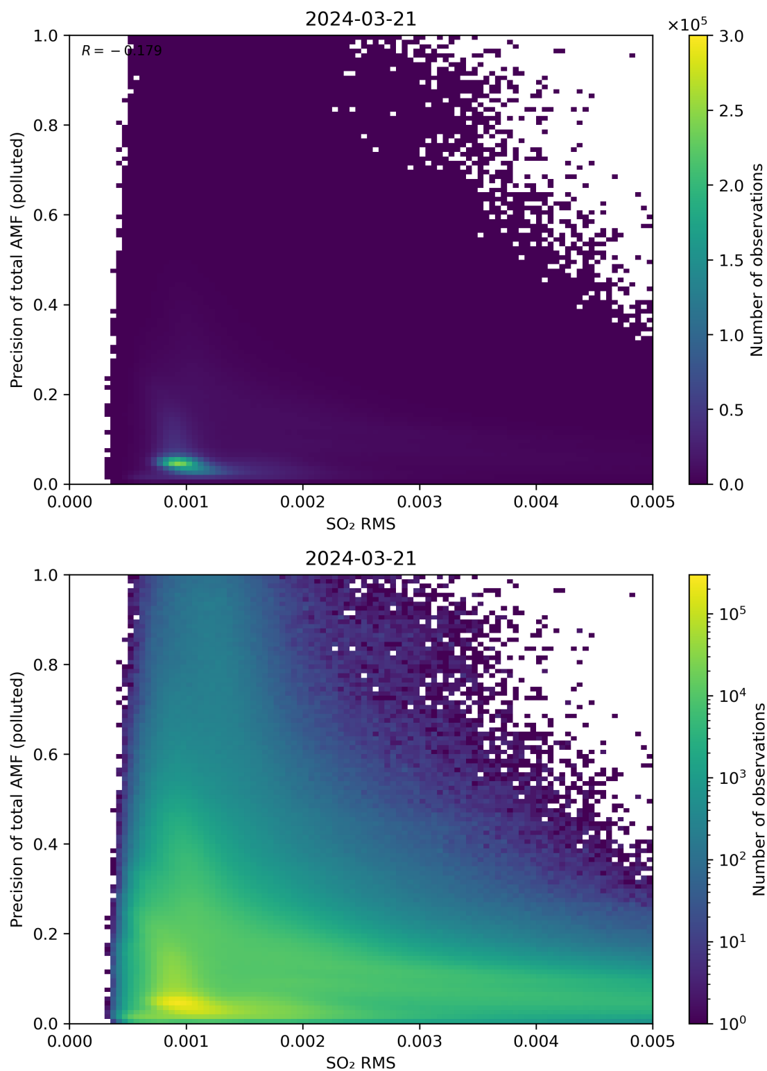
Figure 138: Scatter density plot of “SO 2 RMS” against “Precision of total AMF (polluted)” for 2024-03-20 to 2024-03-22.
