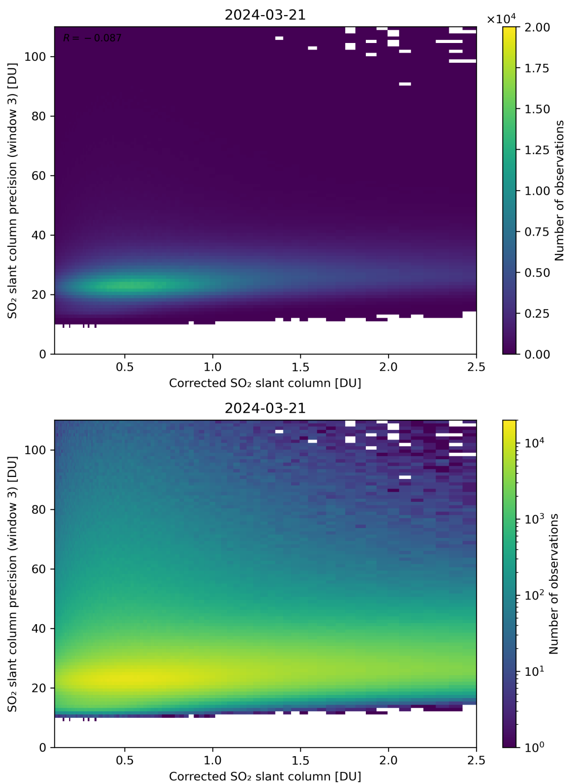
Figure 191: Scatter density plot of “Corrected SO 2 slant column” against “SO 2 slant column precision (window 3)” for 2024-03-20 to 2024-03-22.
