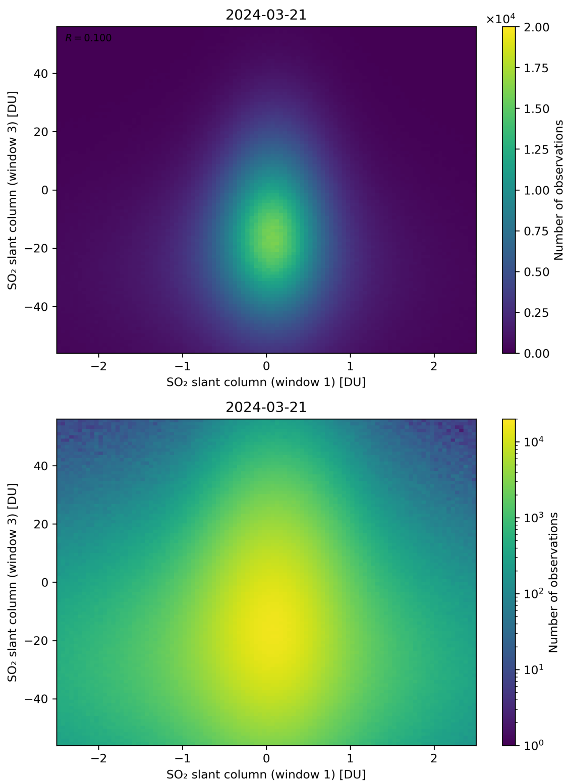
Figure 237: Scatter density plot of “SO 2 slant column (window 1)” against “SO 2 slant column (window 3)” for 2024-03-20 to 2024-03-22.
