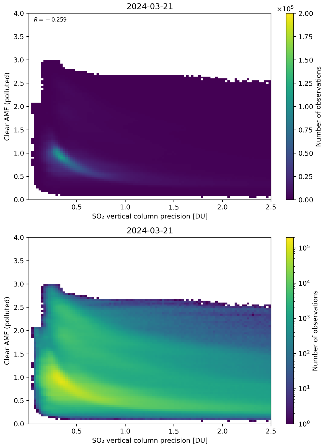
Figure 285: Scatter density plot of “SO 2 vertical column precision” against “Clear AMF (polluted)” for 2024-03-20 to 2024-03-22.
