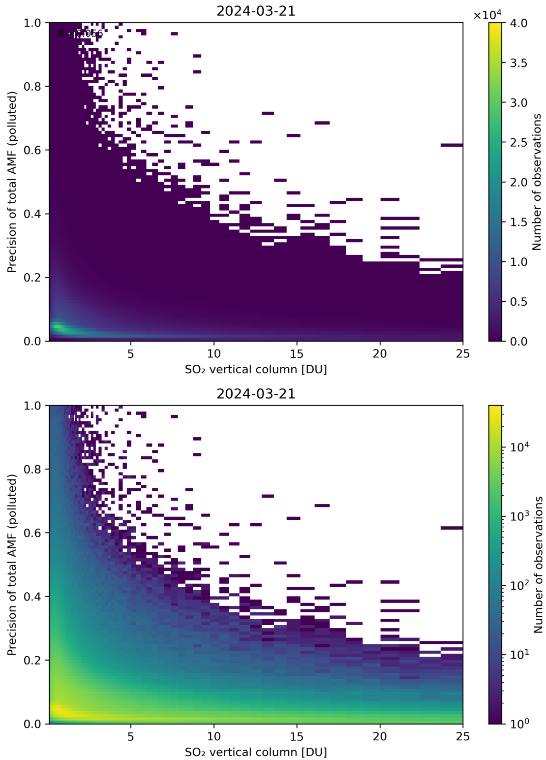
Figure 306: Scatter density plot of “SO 2 vertical column” against “Precision of total AMF (polluted)” for 2024-03-20 to 2024-03-22.
