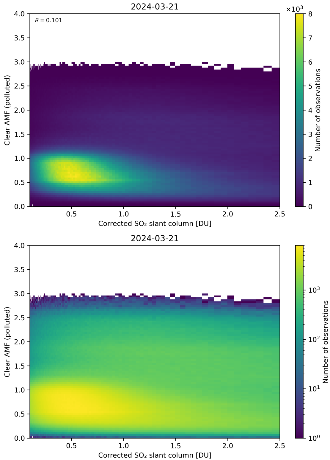
Figure 184: Scatter density plot of “Corrected SO 2 slant column” against “Clear AMF (polluted)” for 2024-03-20 to 2024-03-22.
