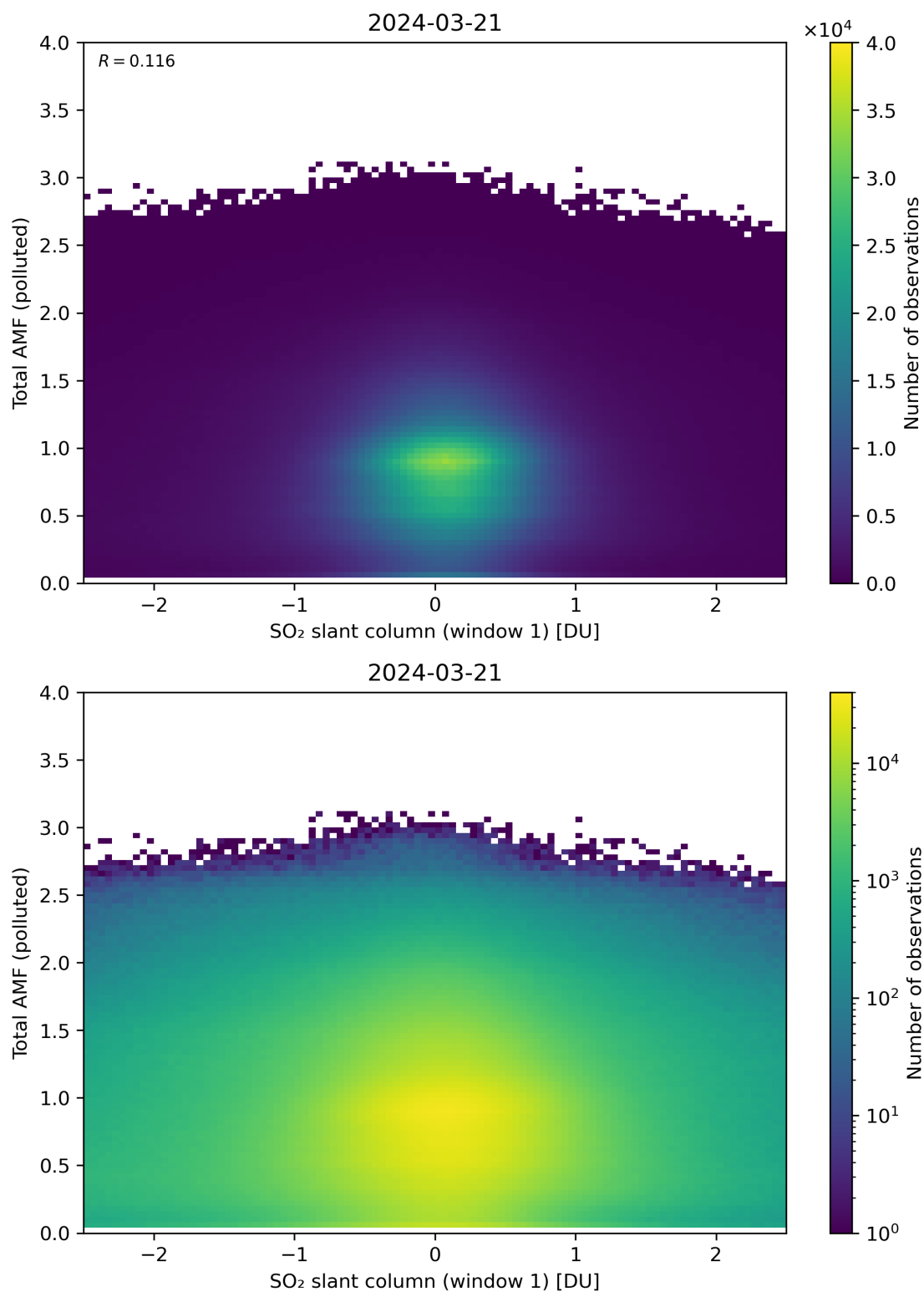
Figure 239: Scatter density plot of “SO 2 slant column (window 1)” against “Total AMF (polluted)” for 2024-03-20 to 2024-03-22.
