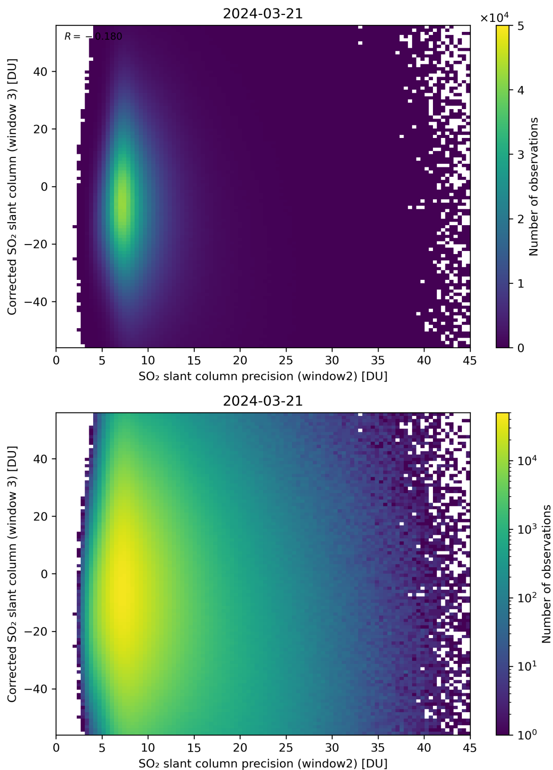
Figure 248: Scatter density plot of “SO 2 slant column precision (window2)” against “Corrected SO 2 slant column (window 3)” for 2024-03-20 to 2024-03-22.
