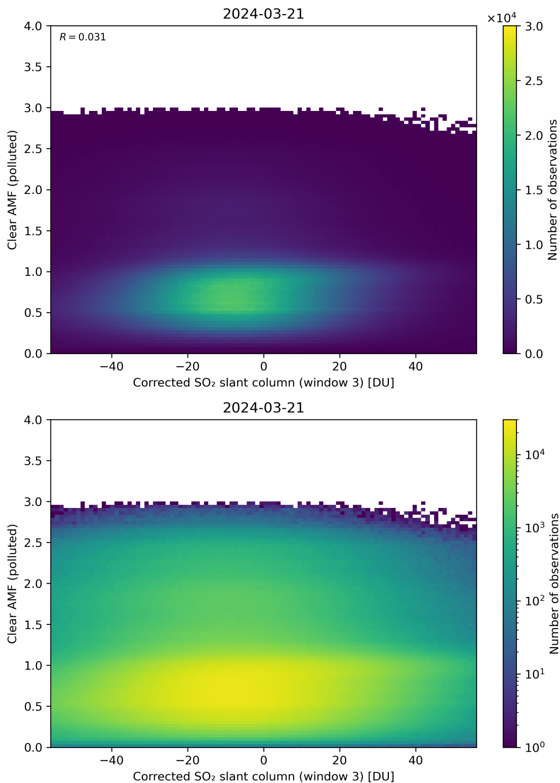
Figure 209: Scatter density plot of “Corrected SO 2 slant column (window 3)” against “Clear AMF (polluted)” for 2024-03-20 to 2024-03-22.
