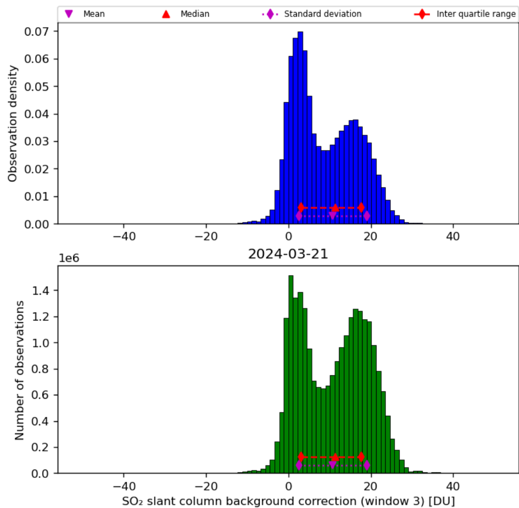
Figure 67: Histogram of “SO 2 slant column background correction (window 3)” for 2024-03-20 to 2024-03-22
