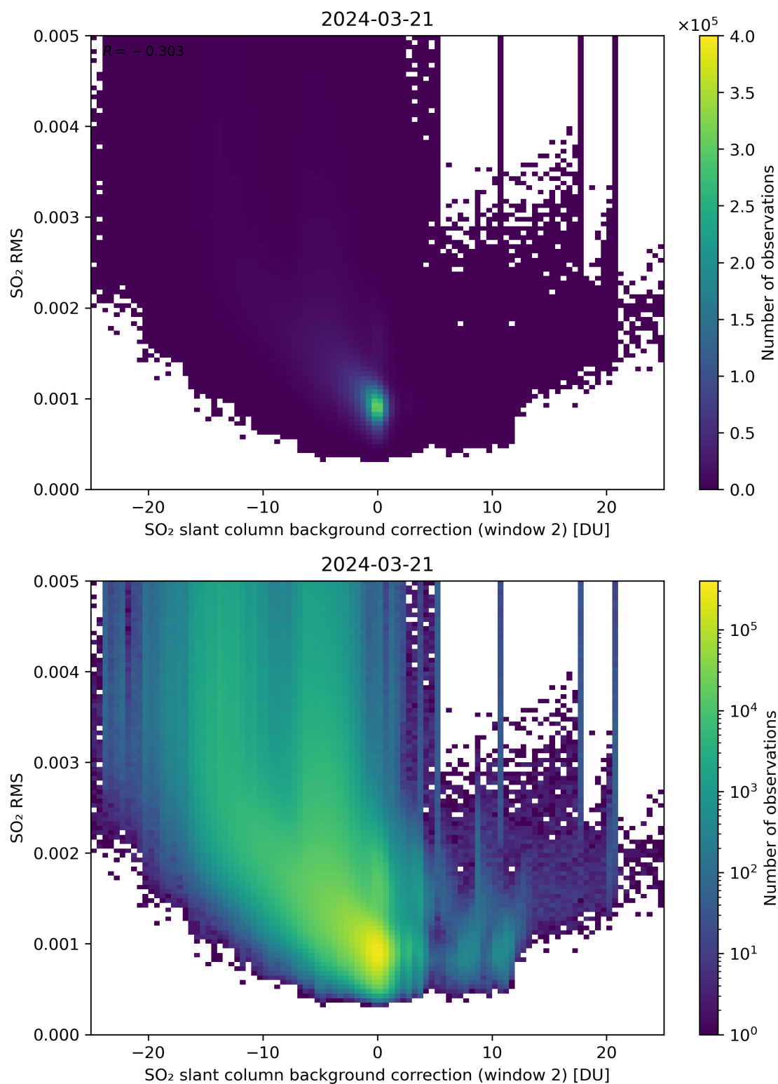
Figure 114: Scatter density plot of “SO 2 slant column background correction (window 2)” against “SO 2 RMS” for 2024-03-20 to 2024-03-22.
