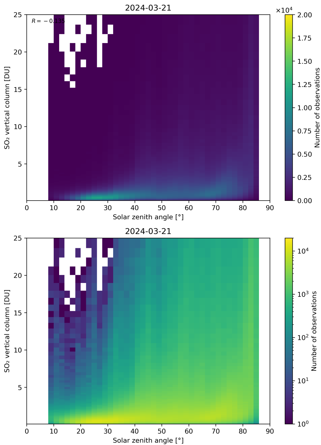
Figure 176: Scatter density plot of “Solar zenith angle” against “SO 2 vertical column” for 2024-03-20 to 2024-03-22.
