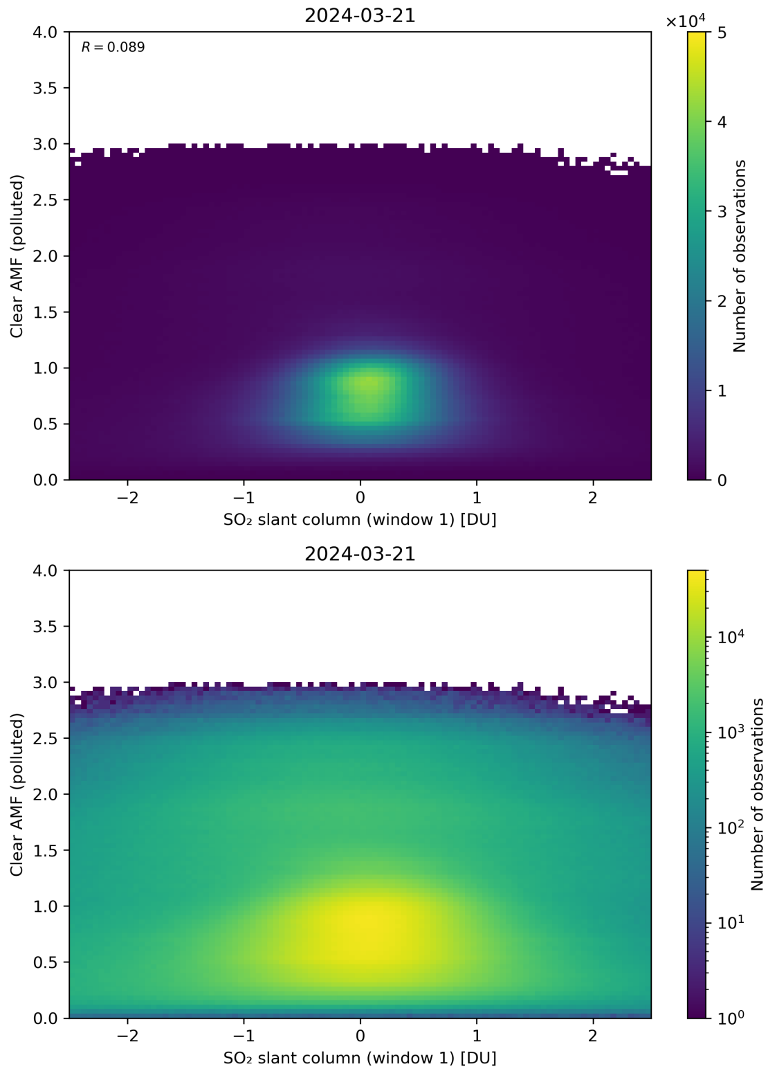
Figure 232: Scatter density plot of “SO 2 slant column (window 1)” against “Clear AMF (polluted)” for 2024-03-20 to 2024-03-22.
