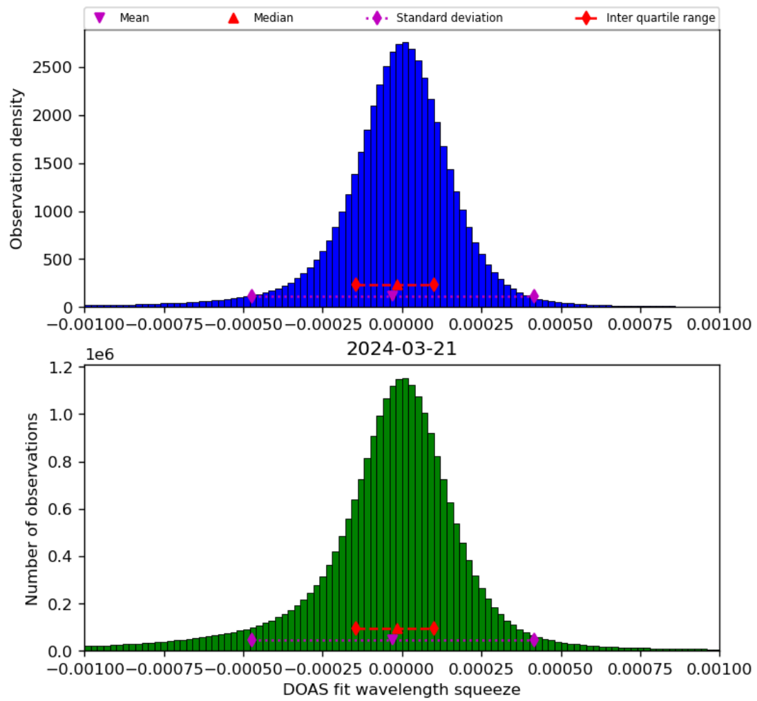
Figure 69: Histogram of “DOAS fit wavelength squeeze” for 2024-03-20 to 2024-03-22
