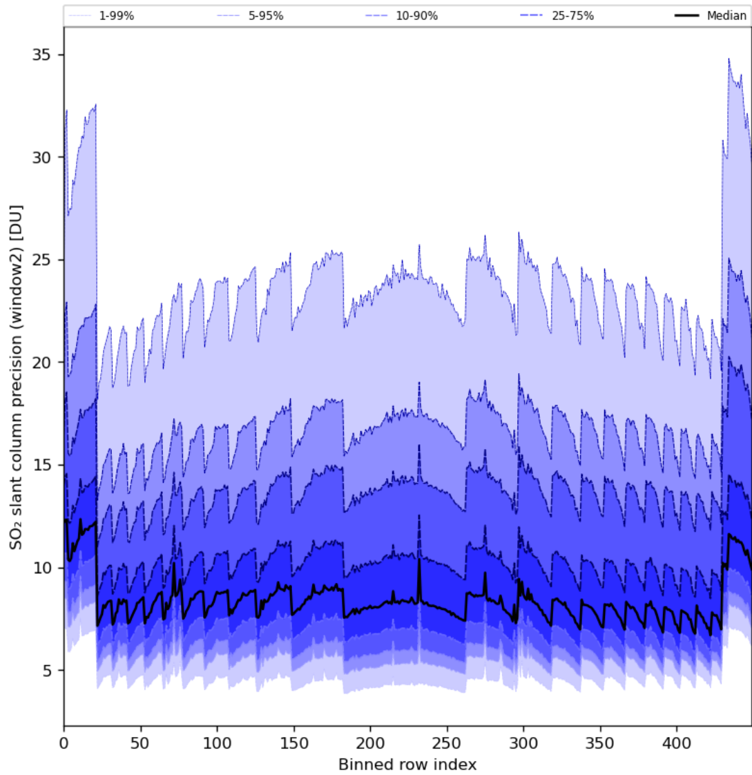
Figure 84: Along track statistics of “SO 2 slant column precision (window2)” for 2024-03-20 to 2024-03-22
