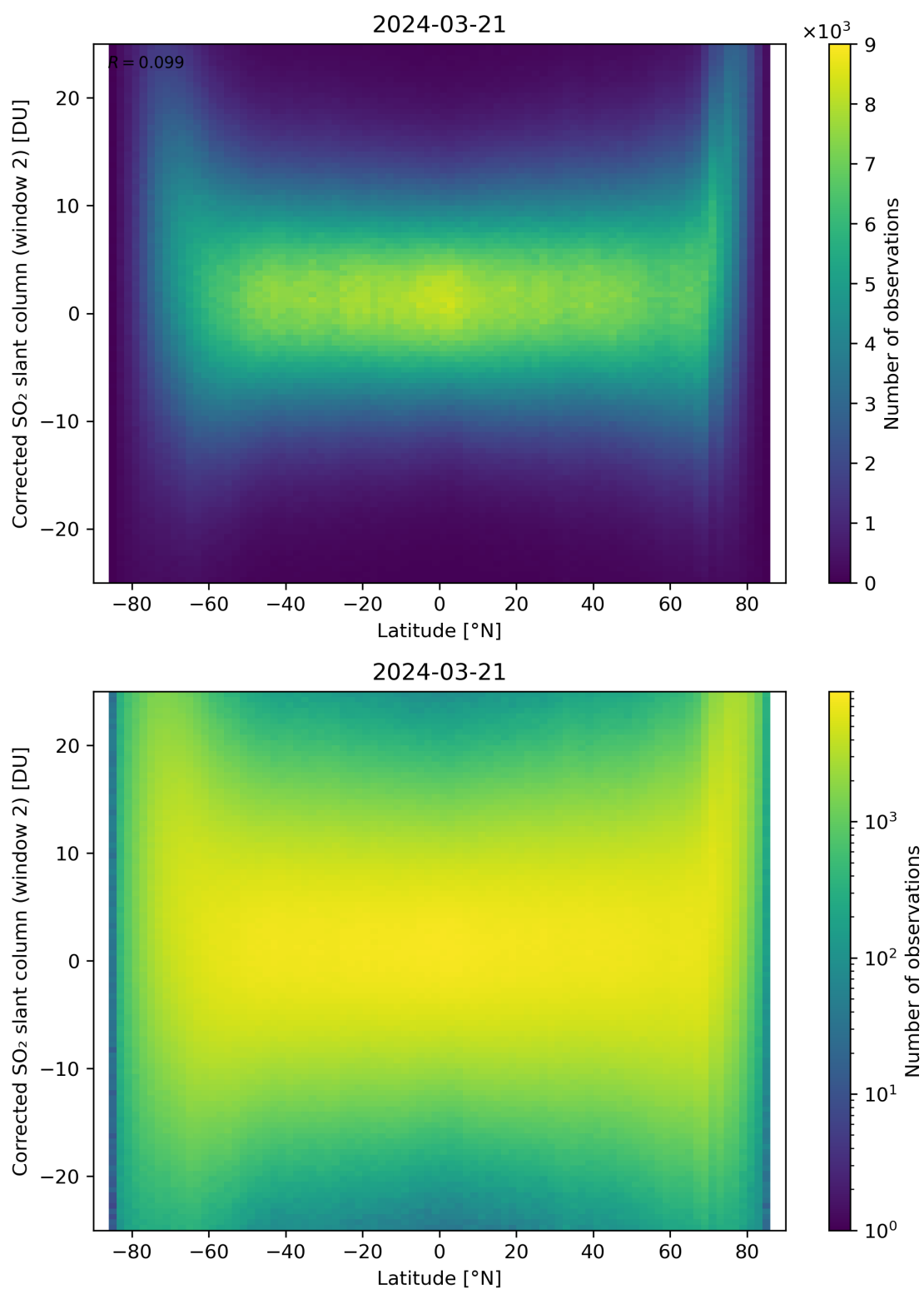
Figure 147: Scatter density plot of “Latitude” against “Corrected SO 2 slant column (window 2)” for 2024-03-20 to 2024-03-22.
