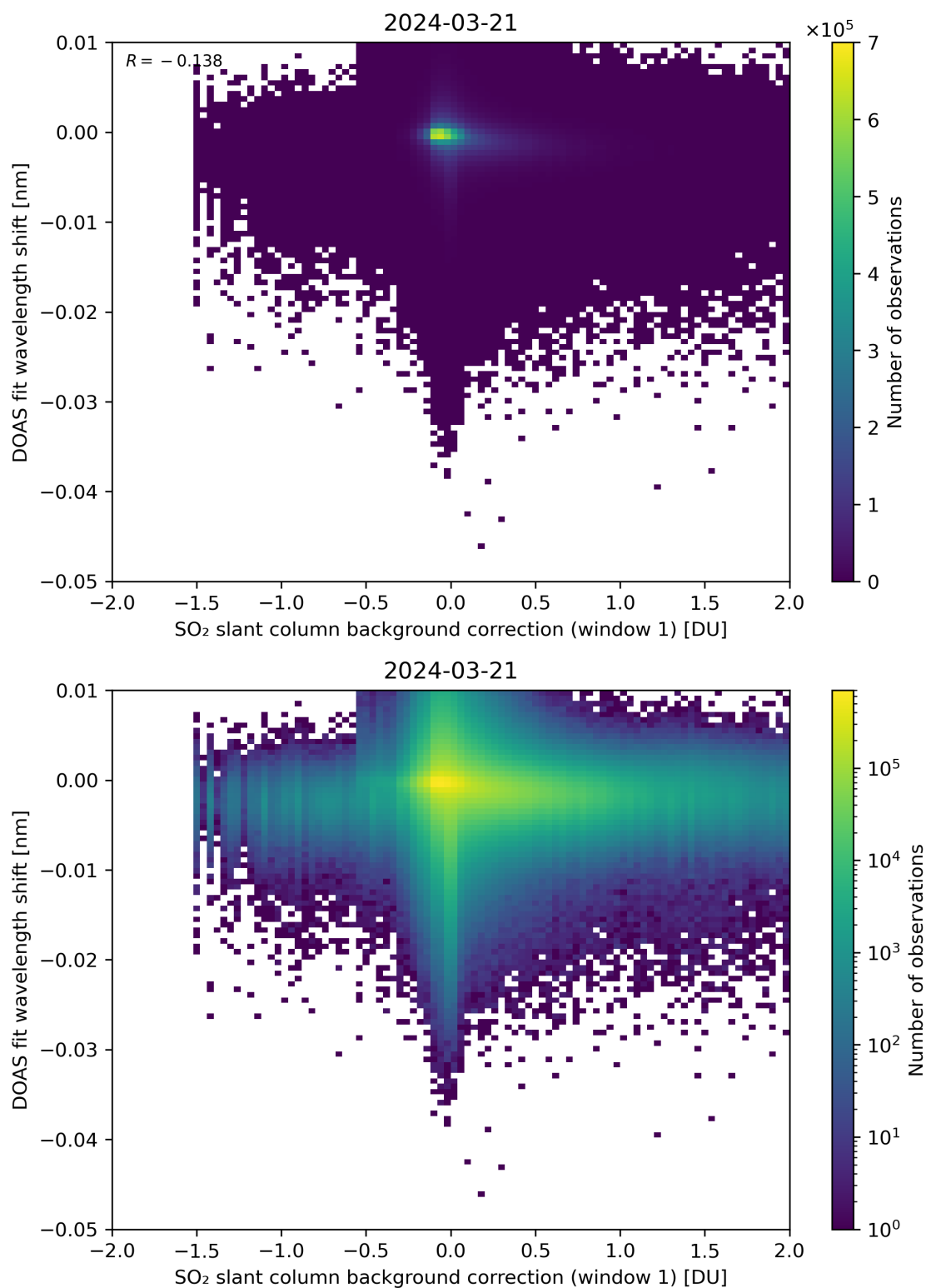
Figure 100: Scatter density plot of “SO 2 slant column background correction (window 1)” against “DOAS fit wavelength shift” for 2024-03-20 to 2024-03-22.
