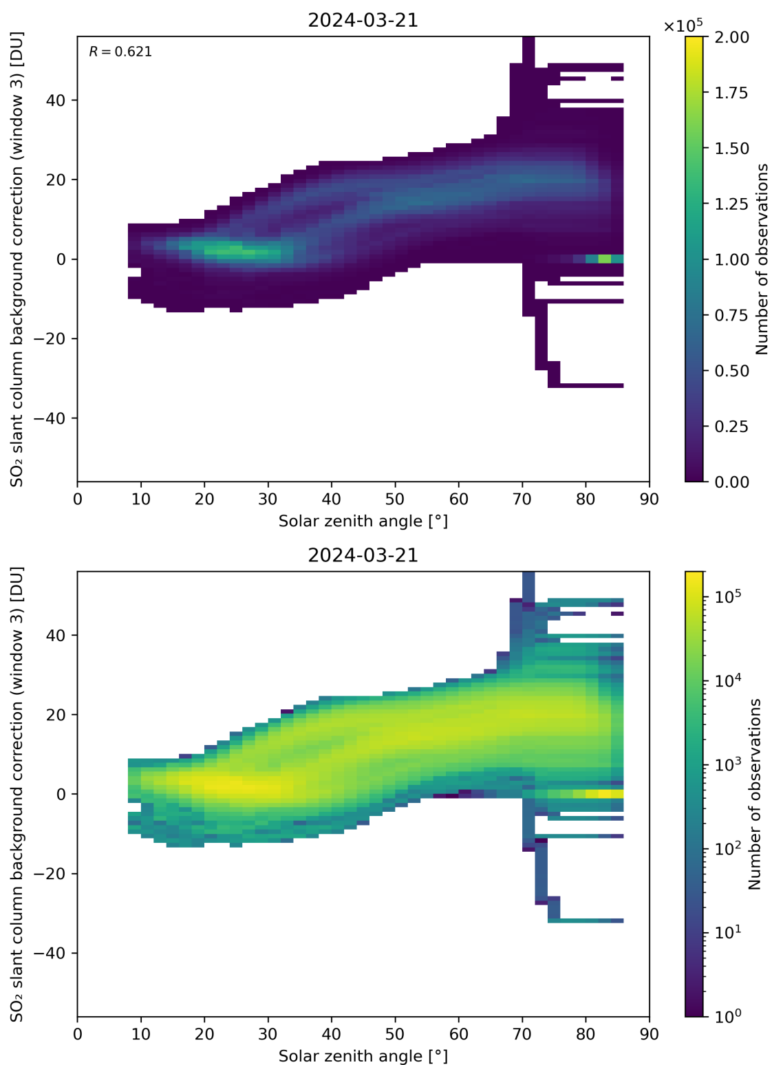
Figure 160: Scatter density plot of “Solar zenith angle” against “SO 2 slant column background correction (window 3)” for 2024-03-20 to 2024-03-22.
