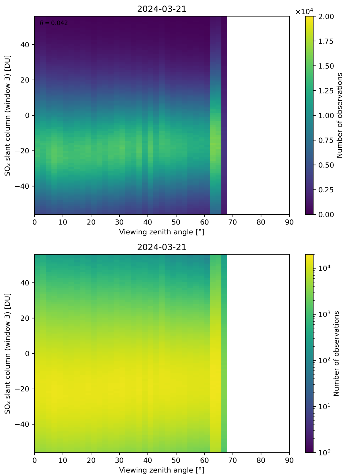
Figure 323: Scatter density plot of “Viewing zenith angle” against “SO 2 slant column (window 3)” for 2024-03-20 to 2024-03-22.
