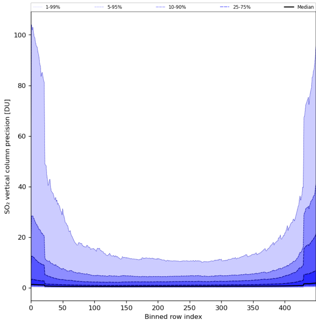
Figure 77: Along track statistics of “SO 2 vertical column precision” for 2024-03-20 to 2024-03-22
