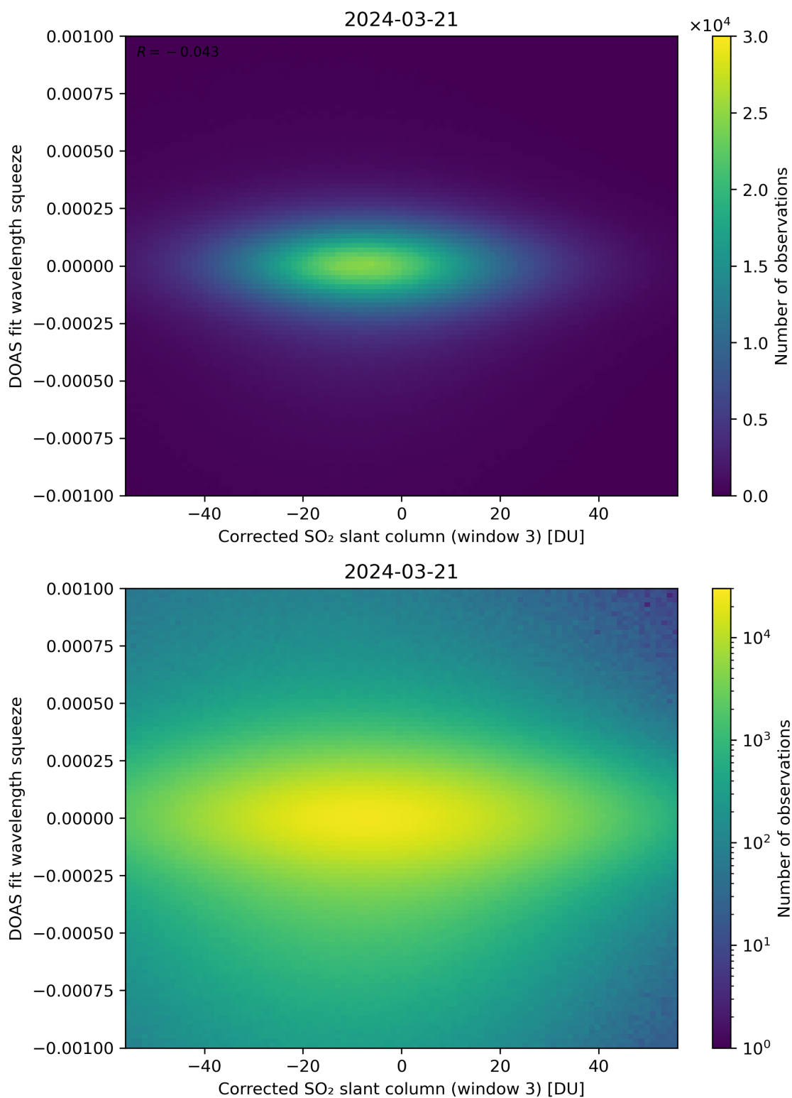
Figure 207: Scatter density plot of “Corrected SO 2 slant column (window 3)” against “DOAS fit wavelength squeeze” for 2024-03-20 to 2024-03-22.
