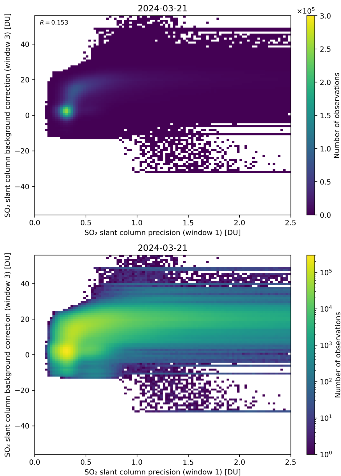
Figure 220: Scatter density plot of “SO 2 slant column precision (window 1)” against “SO 2 slant column background correction (window 3)” for 2024-03-20 to 2024-03-22.
