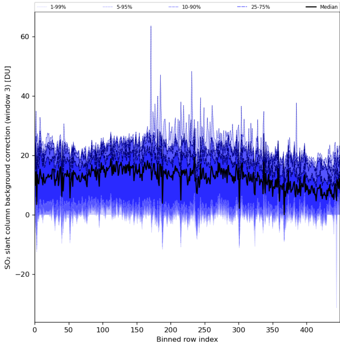
Figure 90: Along track statistics of “SO 2 slant column background correction (window 3)” for 2024-03-20 to 2024-03-22
