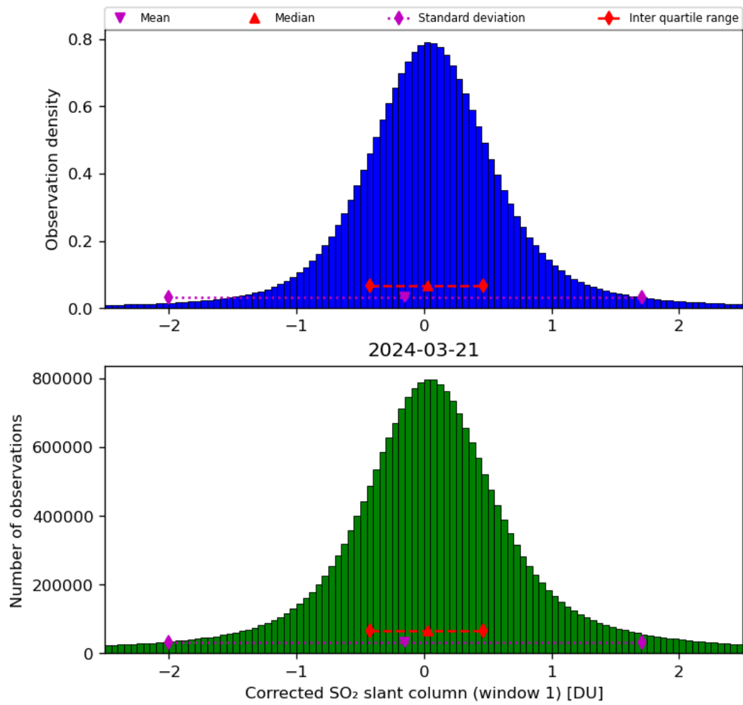
Figure 58: Histogram of “Corrected SO 2 slant column (window 1)” for 2024-03-20 to 2024-03-22
