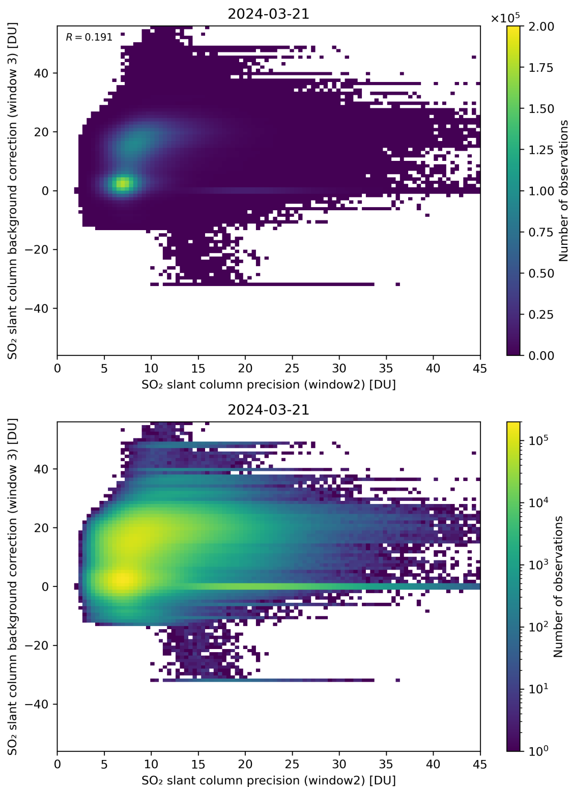
Figure 242: Scatter density plot of “SO 2 slant column precision (window2)” against “SO 2 slant column background correction (window 3)” for 2024-03-20 to 2024-03-22.
