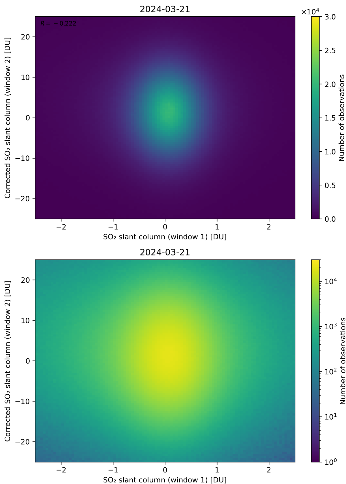
Figure 233: Scatter density plot of “SO 2 slant column (window 1)” against “Corrected SO 2 slant column (window 2)” for 2024-03-20 to 2024-03-22.
