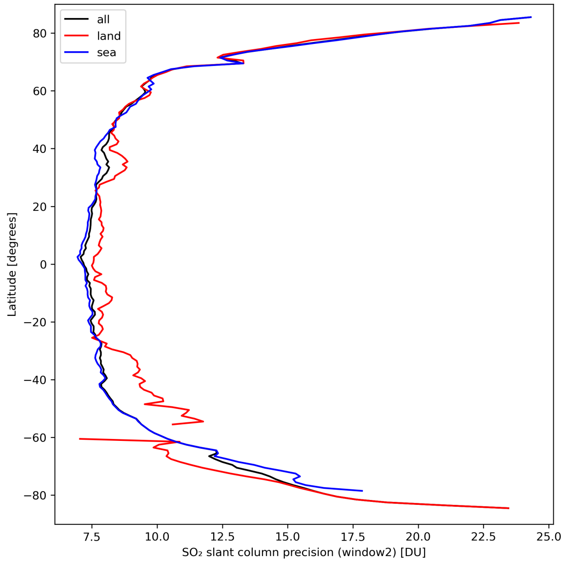
Figure 38: Zonal average of “SO 2 slant column precision (window2)” for 2024-03-20 to 2024-03-22.
