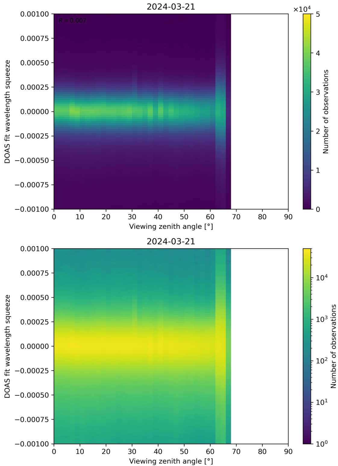
Figure 312: Scatter density plot of “Viewing zenith angle” against “DOAS fit wavelength squeeze” for 2024-03-20 to 2024-03-22.
