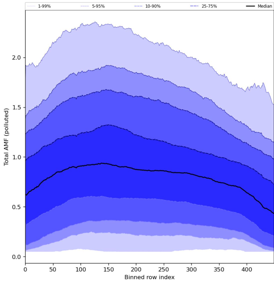
Figure 94: Along track statistics of “Total AMF (polluted)” for 2024-03-20 to 2024-03-22
