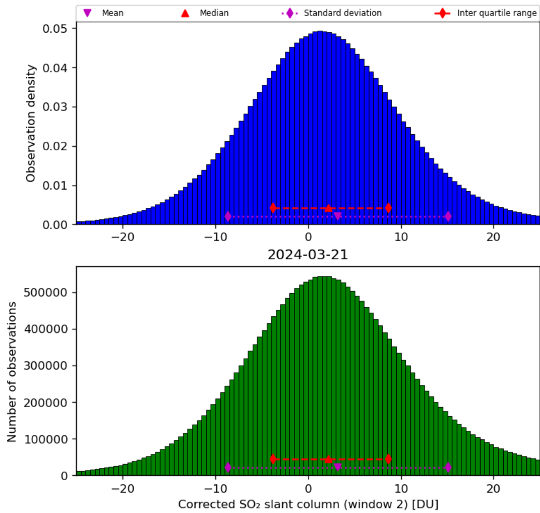
Figure 62: Histogram of “Corrected SO 2 slant column (window 2)” for 2024-03-20 to 2024-03-22
