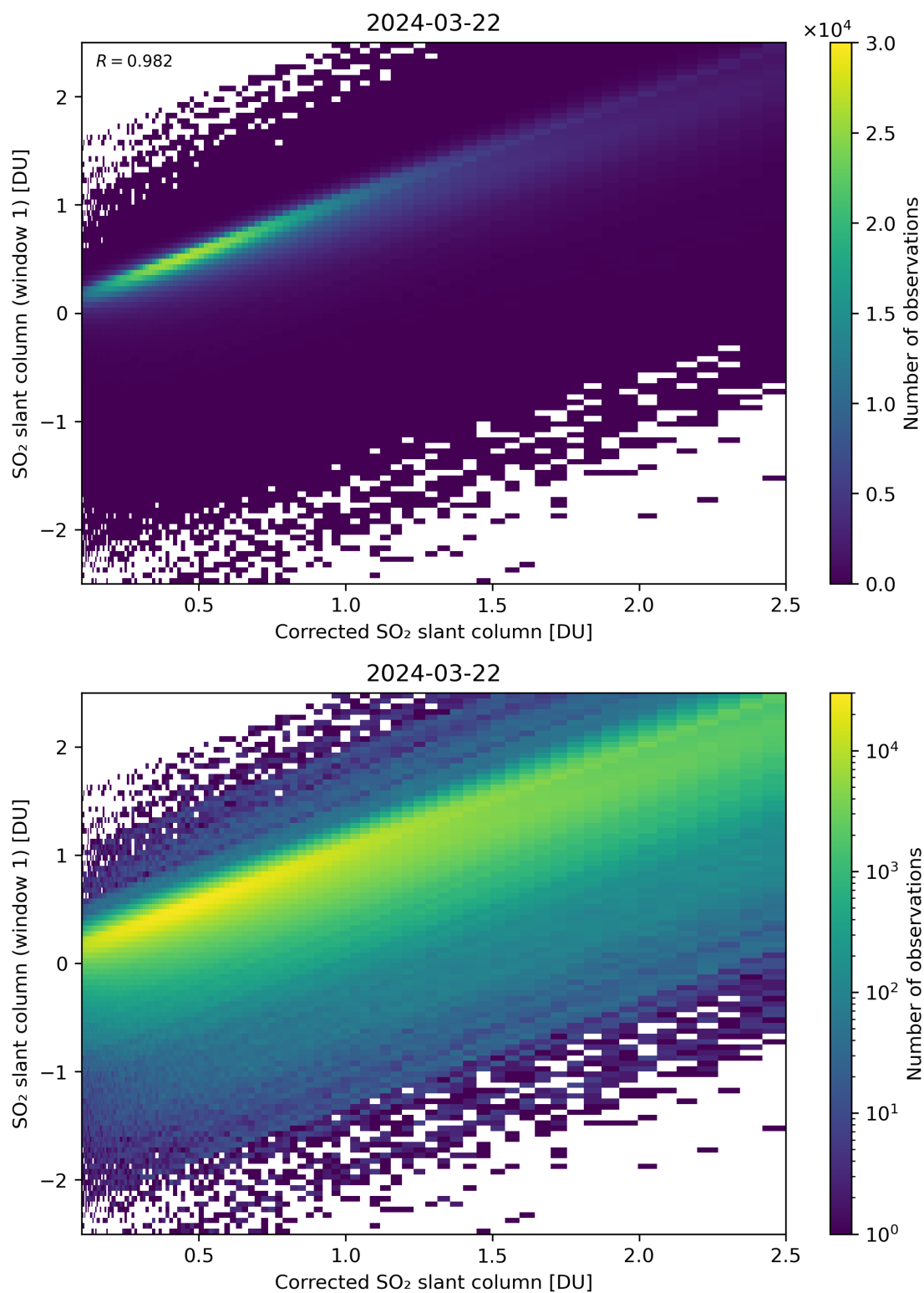
Figure 187: Scatter density plot of “Corrected SO 2 slant column” against “SO 2 slant column (window 1)” for 2024-03-21 to 2024-03-22.
