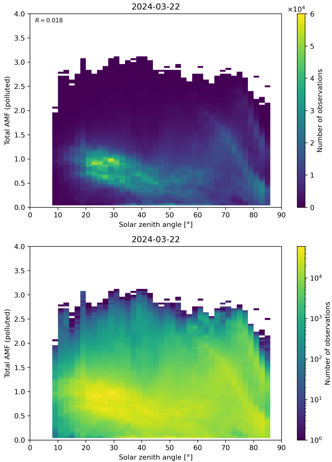
Figure 174: Scatter density plot of “Solar zenith angle” against “Total AMF (polluted)” for 2024-03-21 to 2024-03-22.
