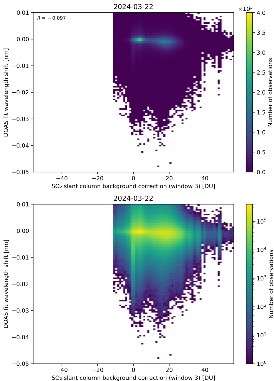
Figure 121: Scatter density plot of “SO 2 slant column background correction (window 3)” against “DOAS fit wavelength shift” for 2024-03-21 to 2024-03-22.
