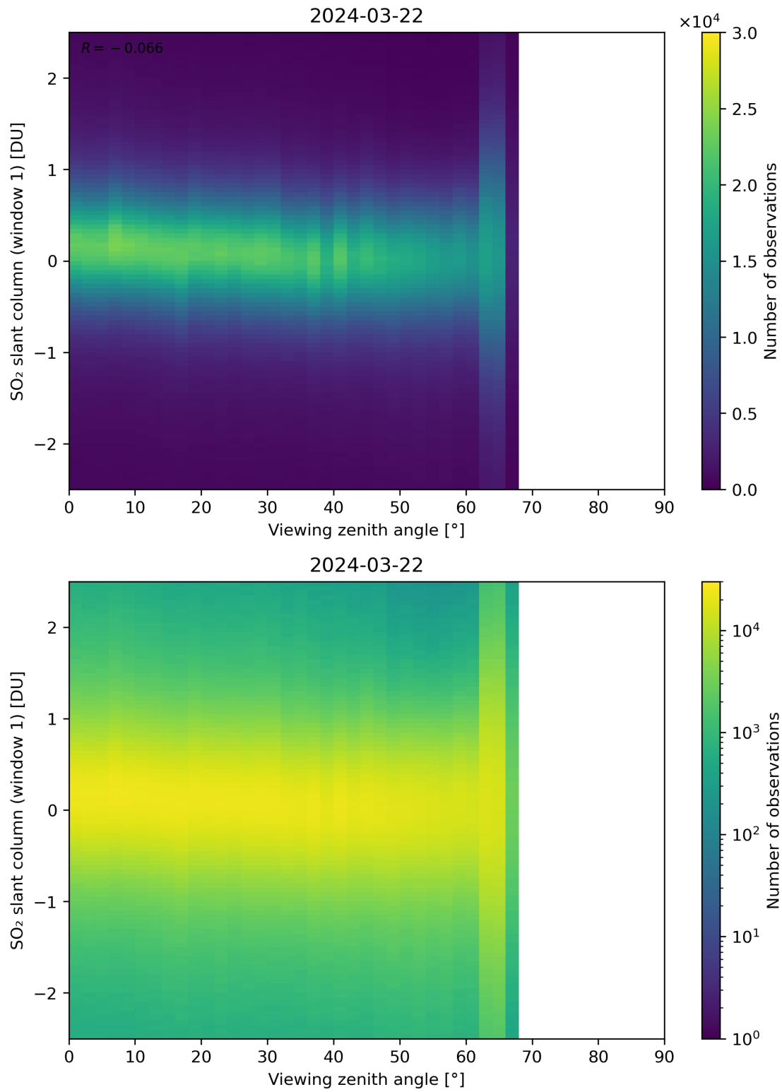
Figure 320: Scatter density plot of “Viewing zenith angle” against “SO 2 slant column (window 1)” for 2024-03-21 to 2024-03-22.
