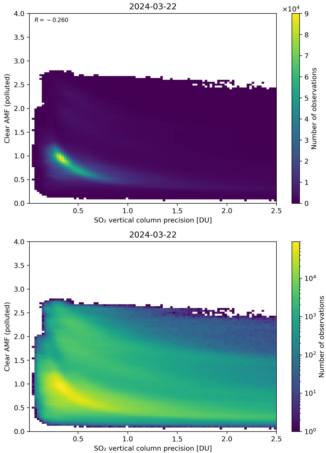
Figure 285: Scatter density plot of “SO 2 vertical column precision” against “Clear AMF (polluted)” for 2024-03-21 to 2024-03-22.
