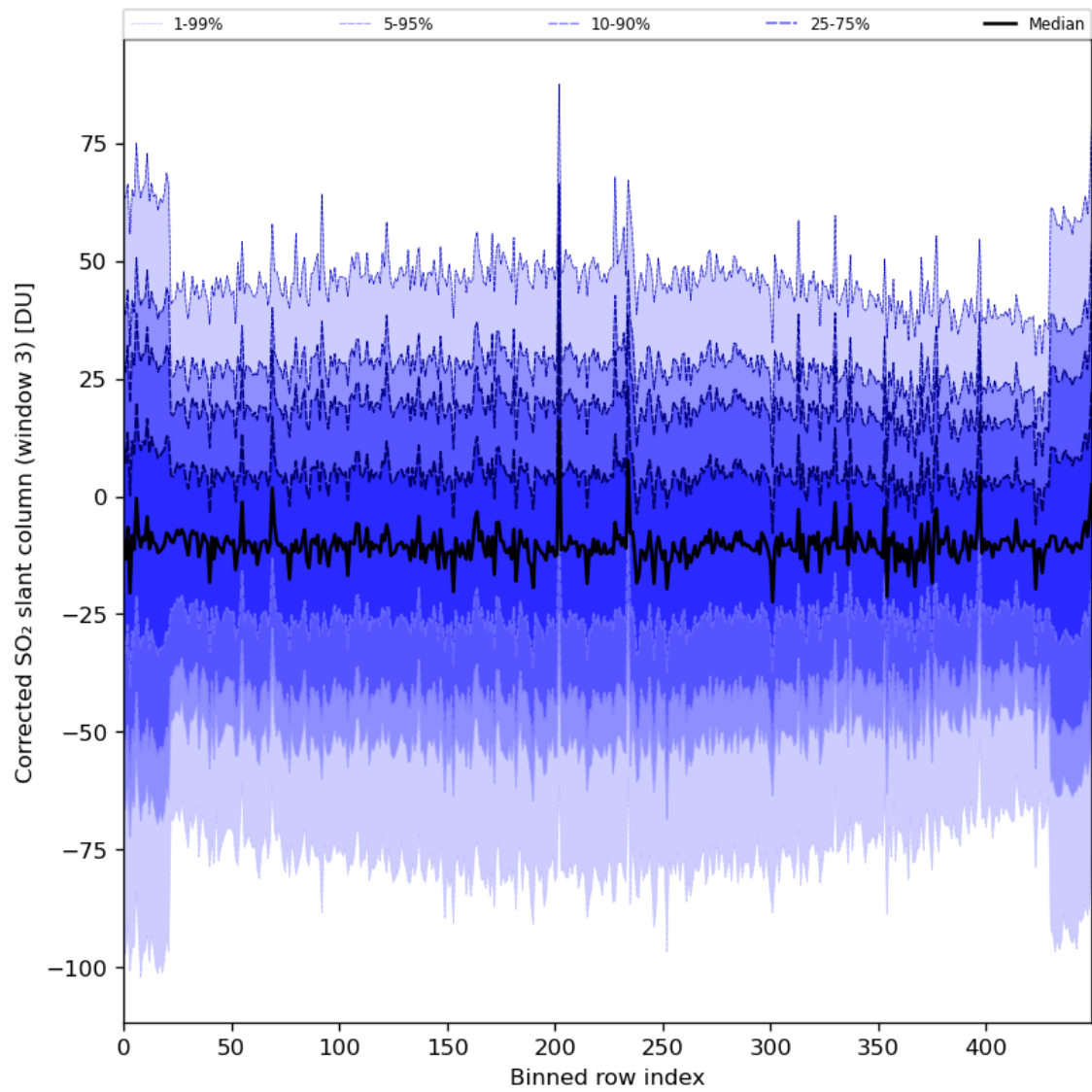
Figure 89: Along track statistics of “Corrected SO 2 slant column (window 3)” for 2024-03-21 to 2024-03-22
