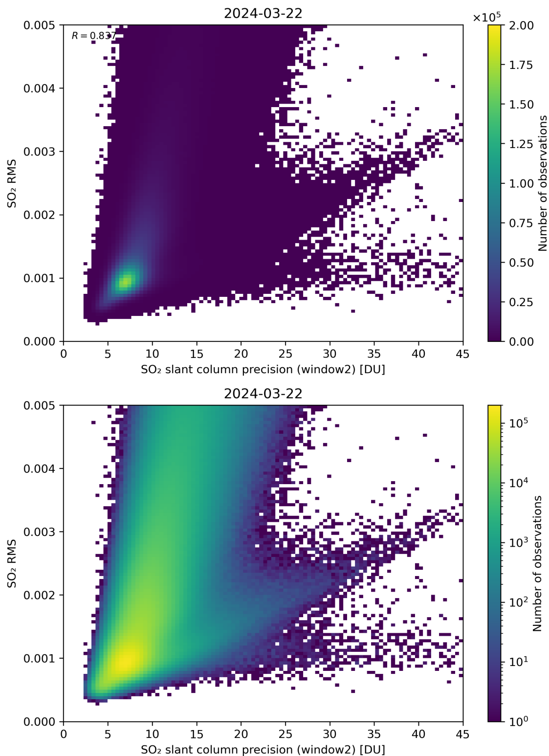
Figure 245: Scatter density plot of “SO 2 slant column precision (window2)” against “SO 2 RMS” for 2024-03-21 to 2024-03-22.
