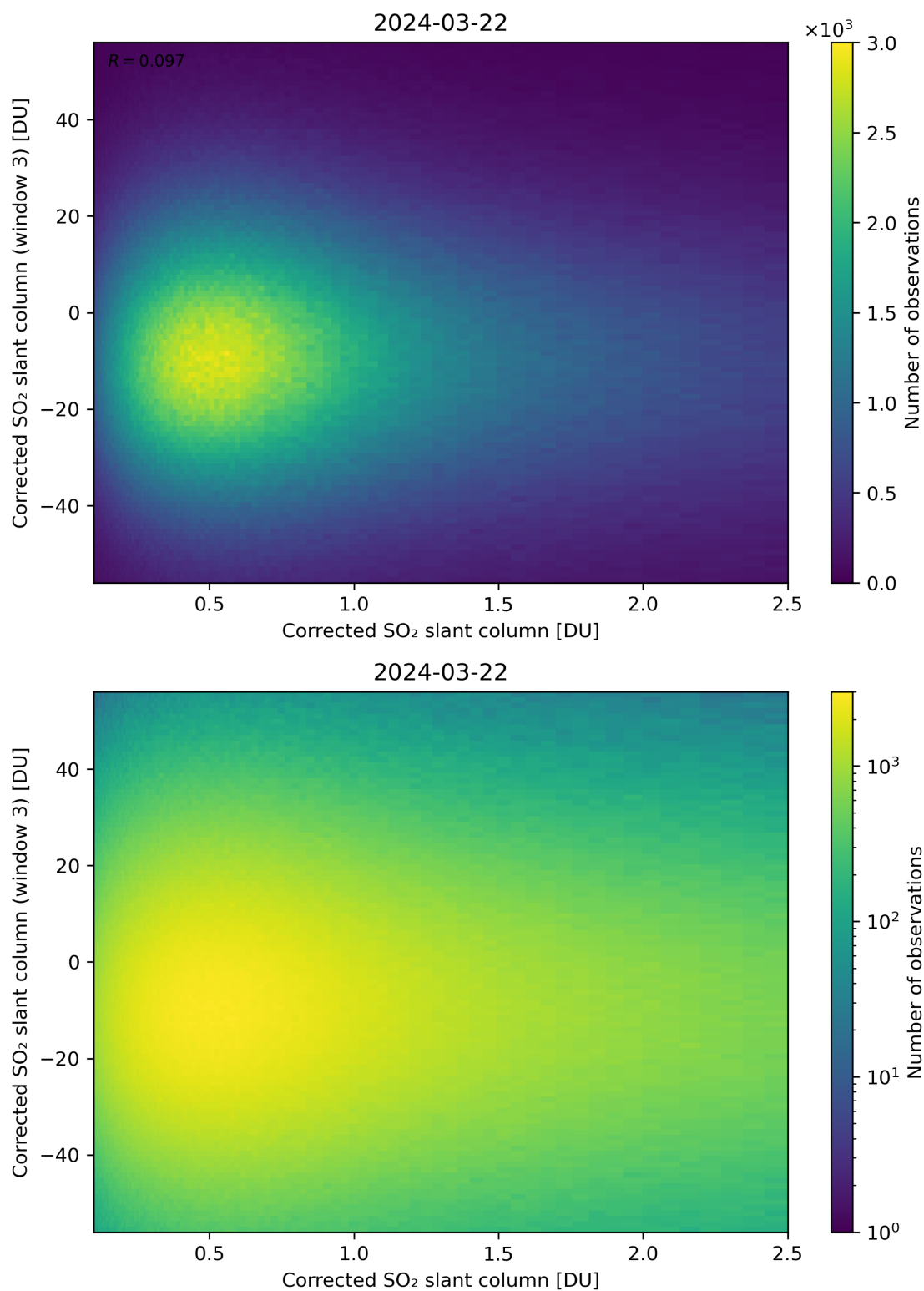
Figure 186: Scatter density plot of “Corrected SO 2 slant column” against “Corrected SO 2 slant column (window 3)” for 2024-03-21 to 2024-03-22.
