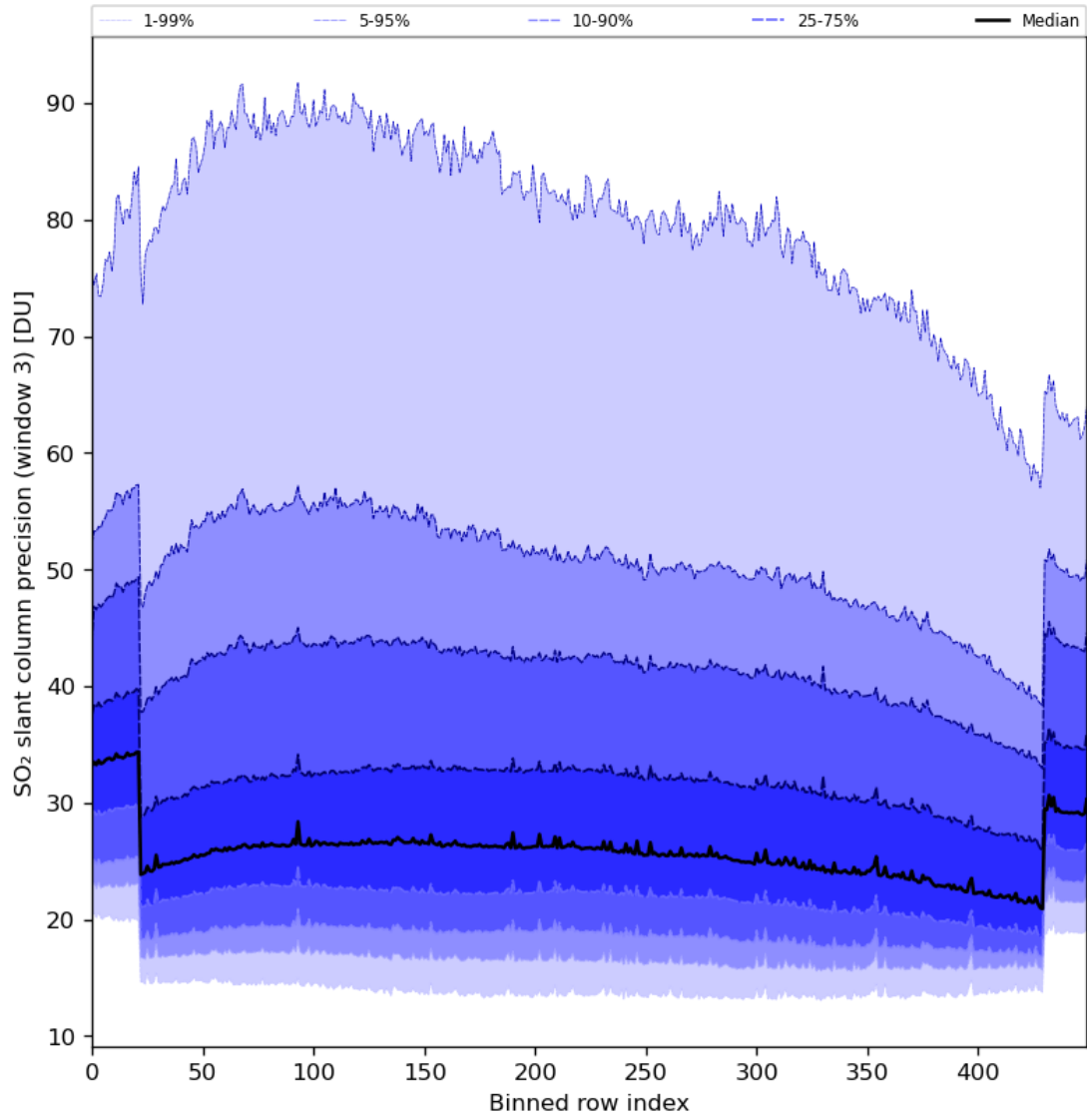
Figure 88: Along track statistics of “SO 2 slant column precision (window 3)” for 2024-03-21 to 2024-03-22
