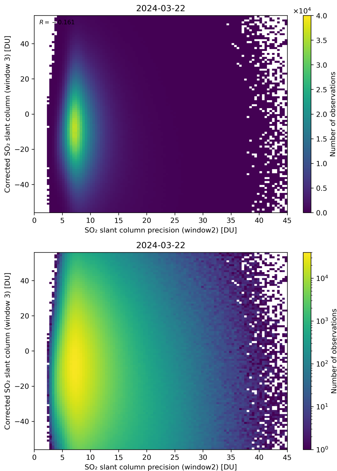
Figure 248: Scatter density plot of “SO 2 slant column precision (window2)” against “Corrected SO 2 slant column (window 3)” for 2024-03-21 to 2024-03-22.
