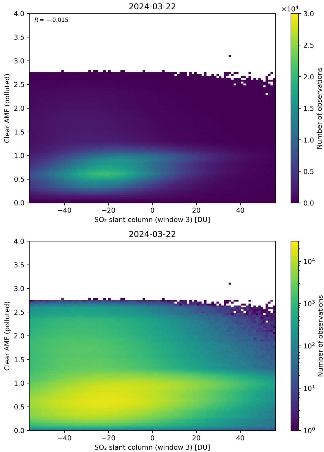
Figure 265: Scatter density plot of “SO 2 slant column (window 3)” against “Clear AMF (polluted)” for 2024-03-21 to 2024-03-22.
