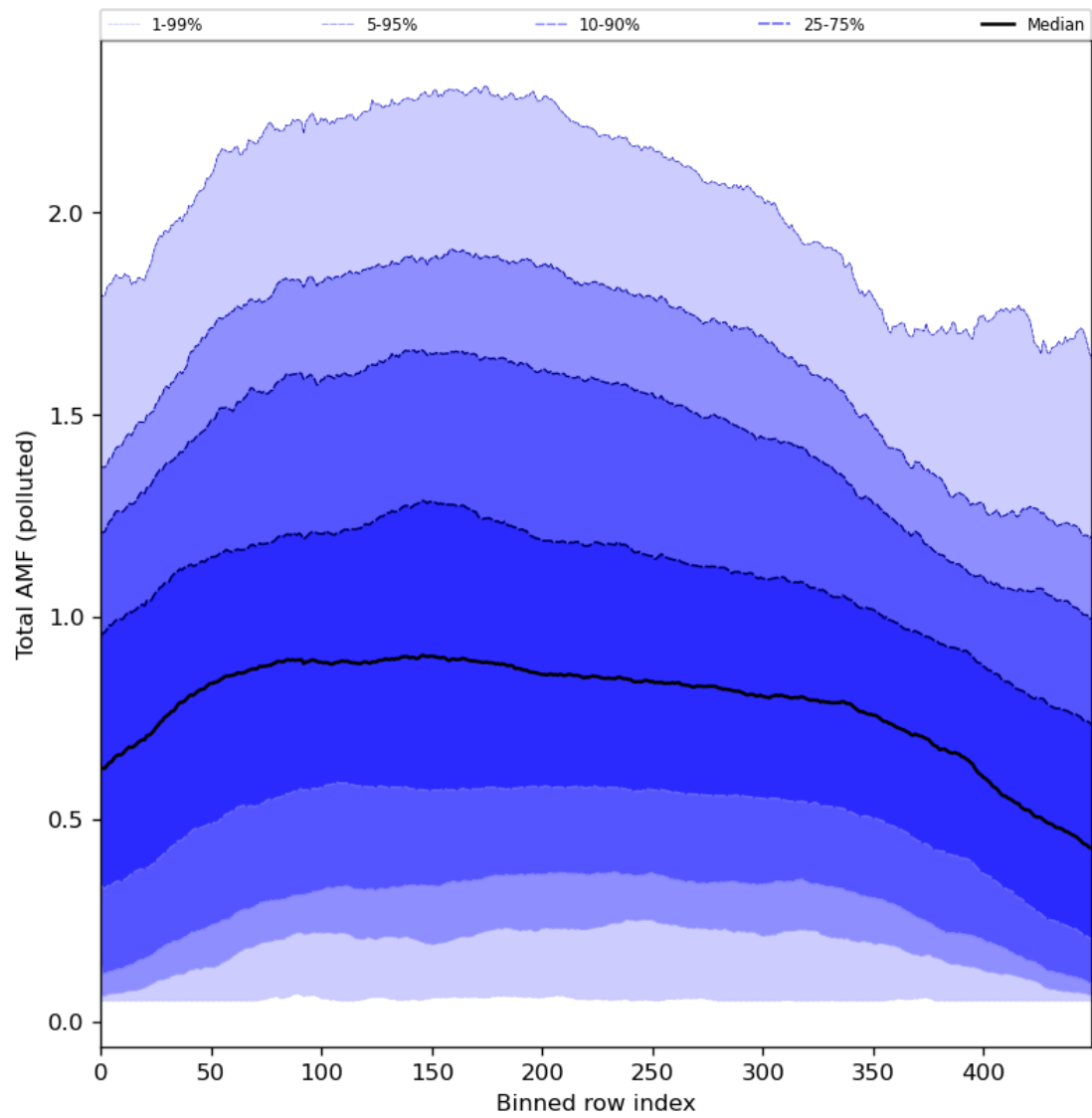
Figure 94: Along track statistics of “Total AMF (polluted)” for 2024-03-21 to 2024-03-22
