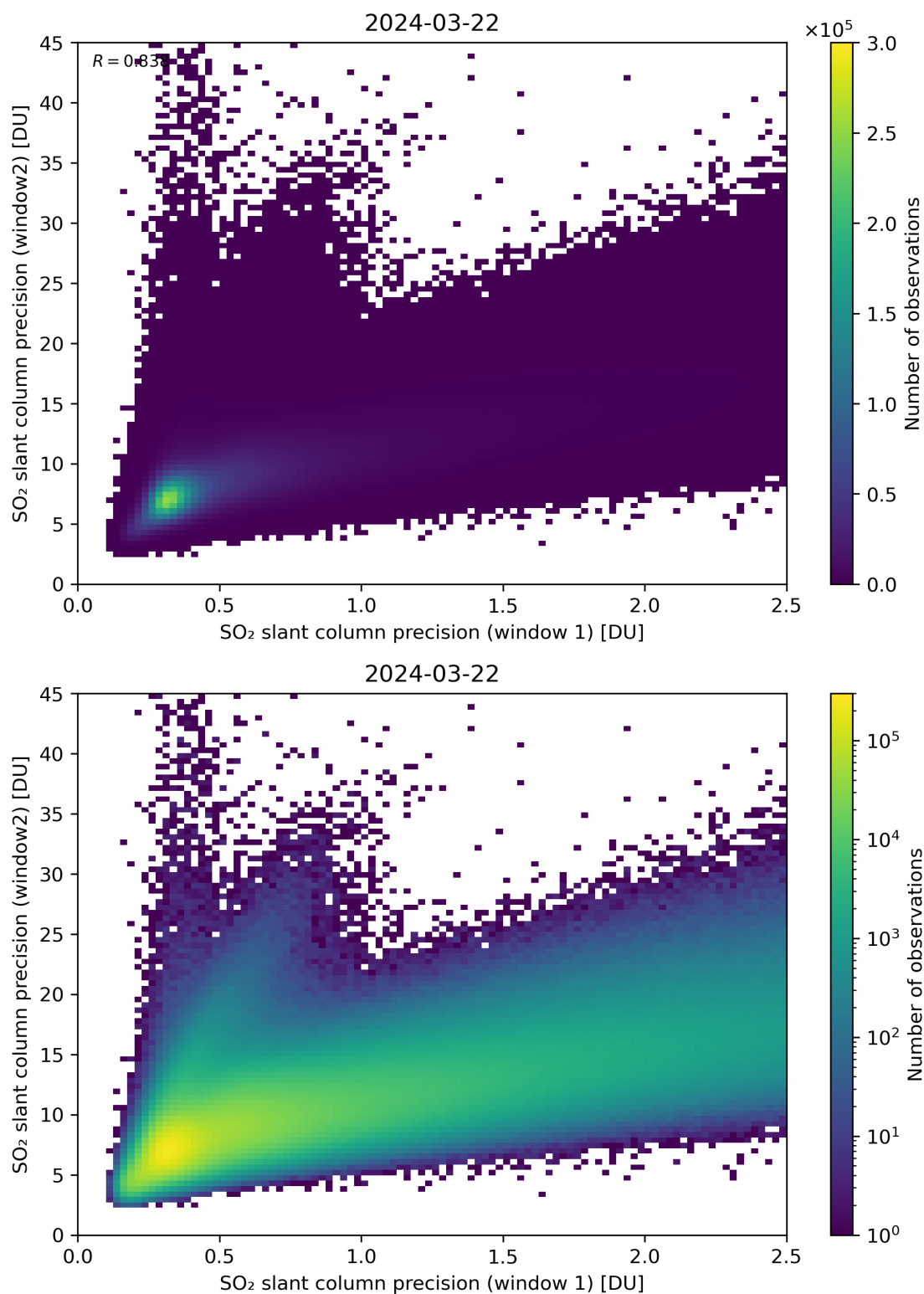
Figure 227: Scatter density plot of “SO 2 slant column precision (window 1)” against “SO 2 slant column precision (window2)” for 2024-03-21 to 2024-03-22.
