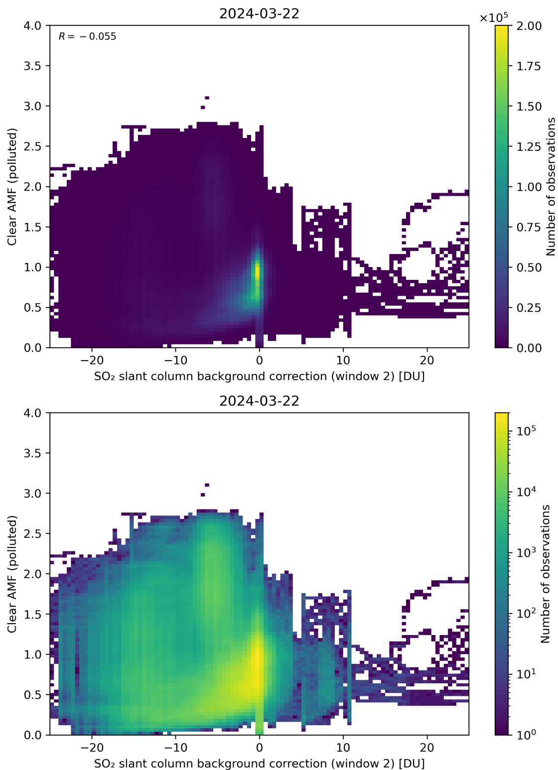
Figure 115: Scatter density plot of “SO 2 slant column background correction (window 2)” against “Clear AMF (polluted)” for 2024-03-21 to 2024-03-22.
