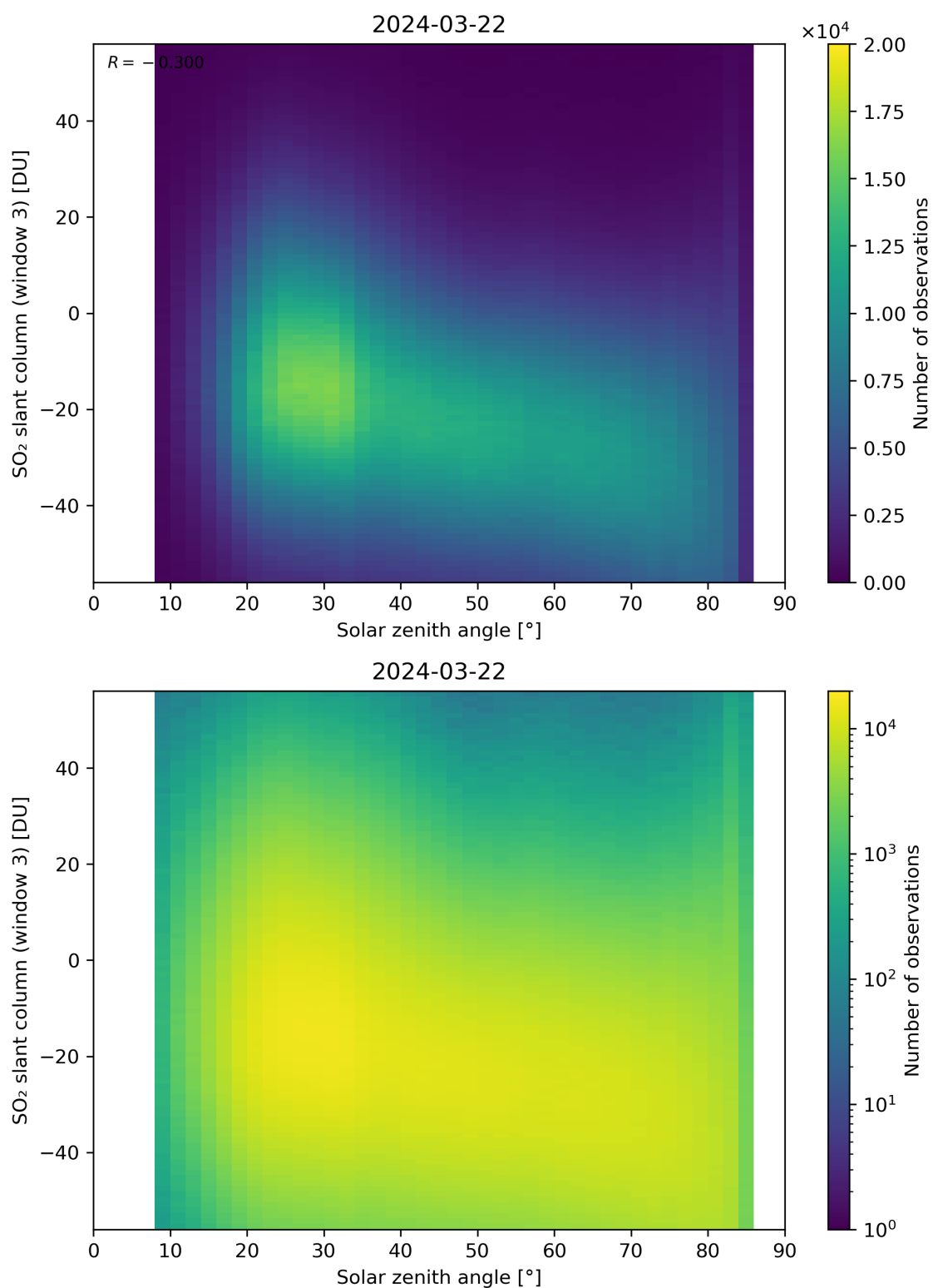
Figure 172: Scatter density plot of “Solar zenith angle” against “SO 2 slant column (window 3)” for 2024-03-21 to 2024-03-22.
