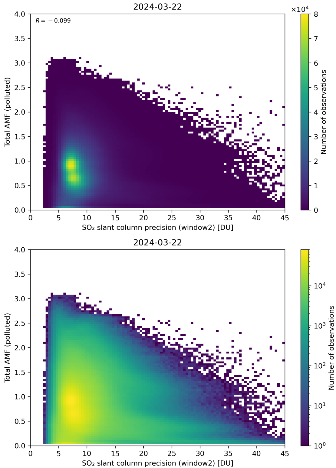
Figure 251: Scatter density plot of “SO 2 slant column precision (window2)” against “Total AMF (polluted)” for 2024-03-21 to 2024-03-22.
