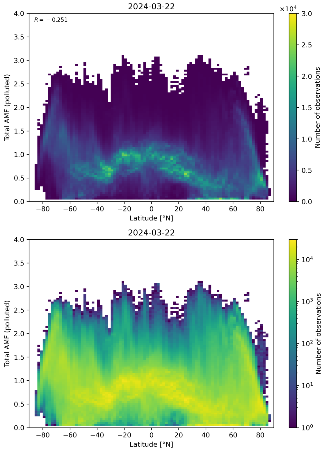
Figure 154: Scatter density plot of “Latitude” against “Total AMF (polluted)” for 2024-03-21 to 2024-03-22.
