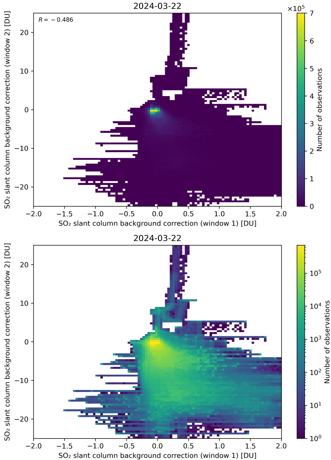
Figure 98: Scatter density plot of “SO 2 slant column background correction (window 1)” against “SO 2 slant column background correction (window 2)” for 2024-03-21 to 2024-03-22.
