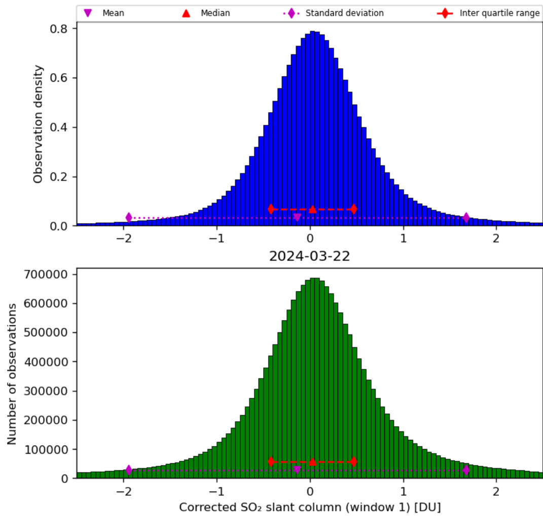
Figure 58: Histogram of “Corrected SO 2 slant column (window 1)” for 2024-03-21 to 2024-03-22
