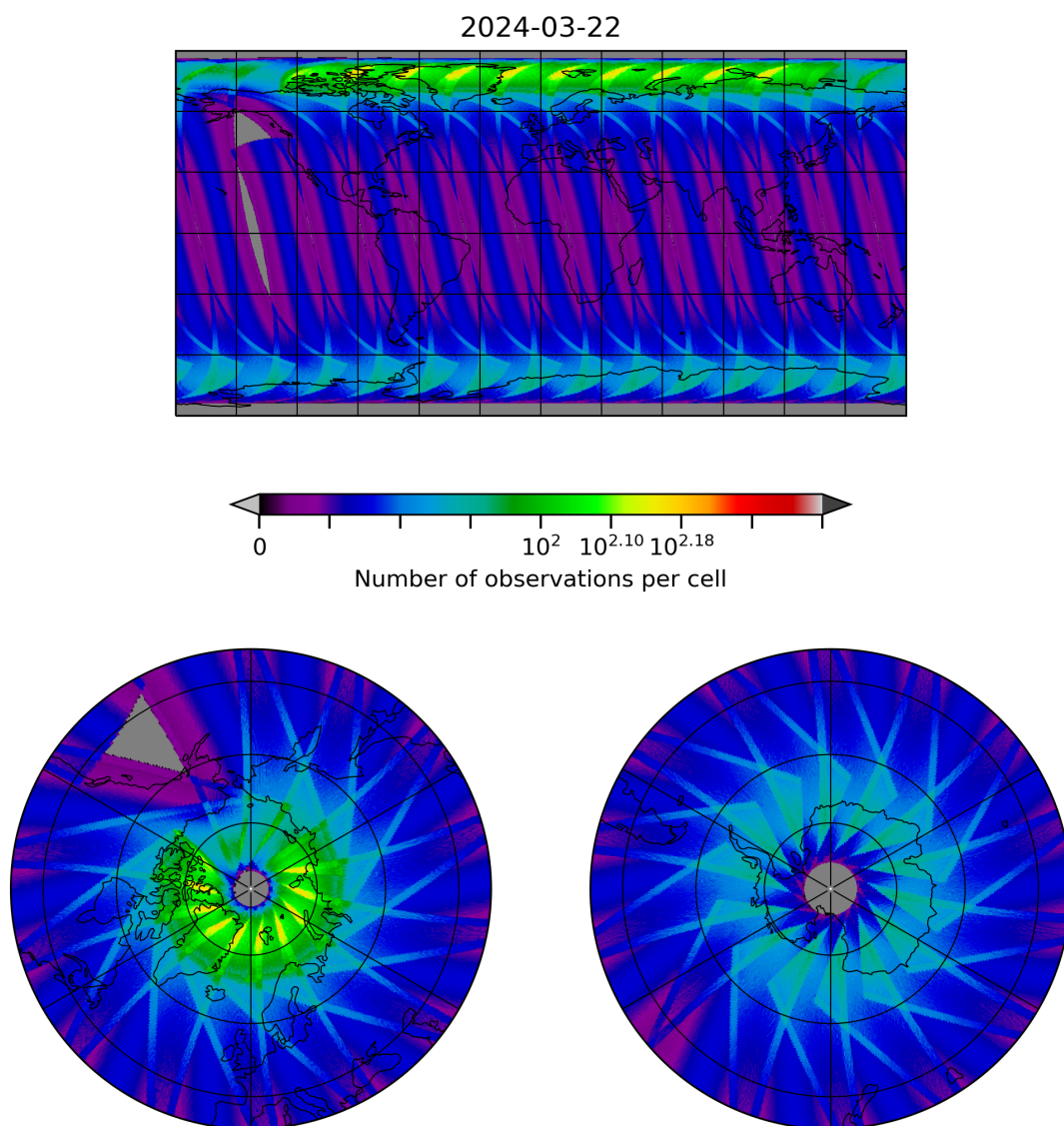
Figure 28: Map of the number of observations for 2024-03-21 to 2024-03-22
