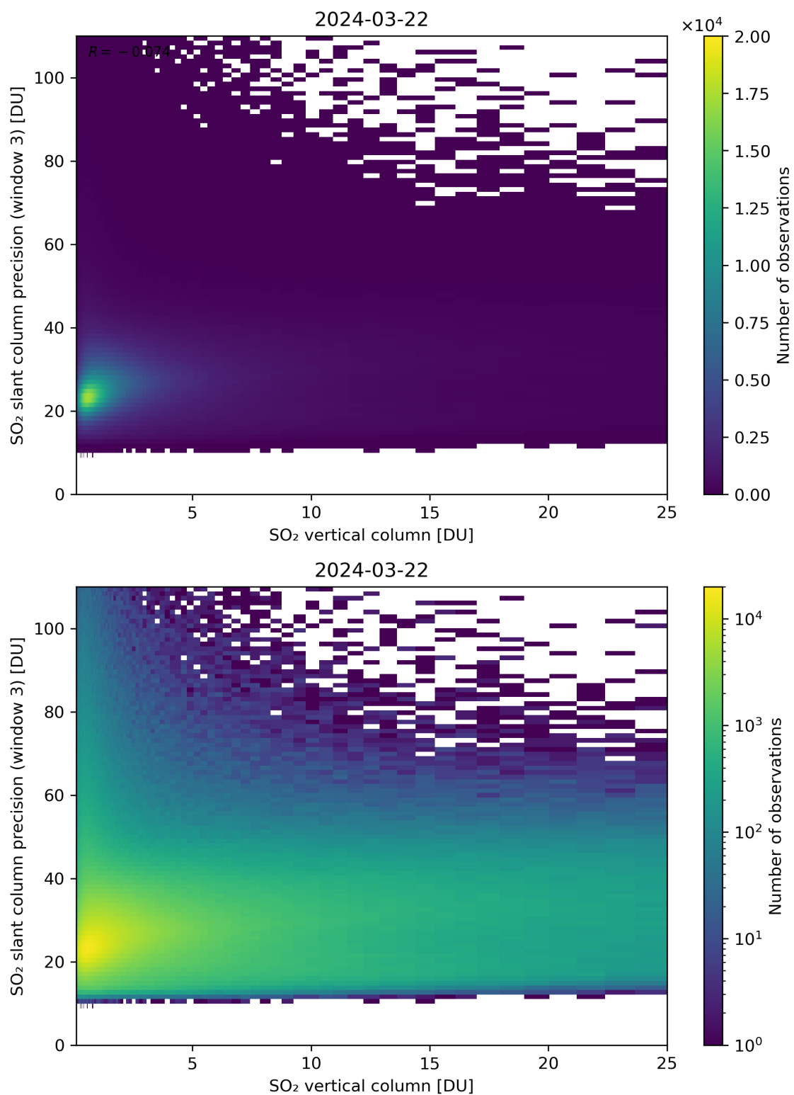
Figure 304: Scatter density plot of “SO 2 vertical column” against “SO 2 slant column precision (window 3)” for 2024-03-21 to 2024-03-22.
