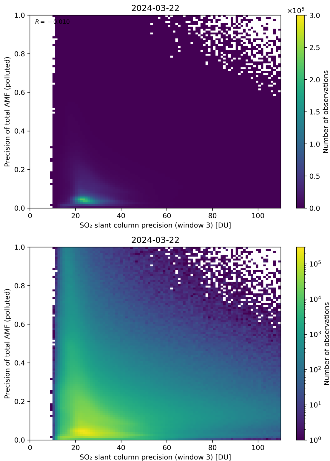
Figure 264: Scatter density plot of “SO 2 slant column precision (window 3)” against “Precision of total AMF (polluted)” for 2024-03-21 to 2024-03-22.
