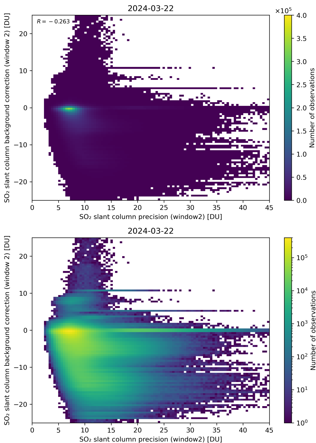
Figure 241: Scatter density plot of “SO 2 slant column precision (window2)” against “SO 2 slant column background correction (window 2)” for 2024-03-21 to 2024-03-22.
