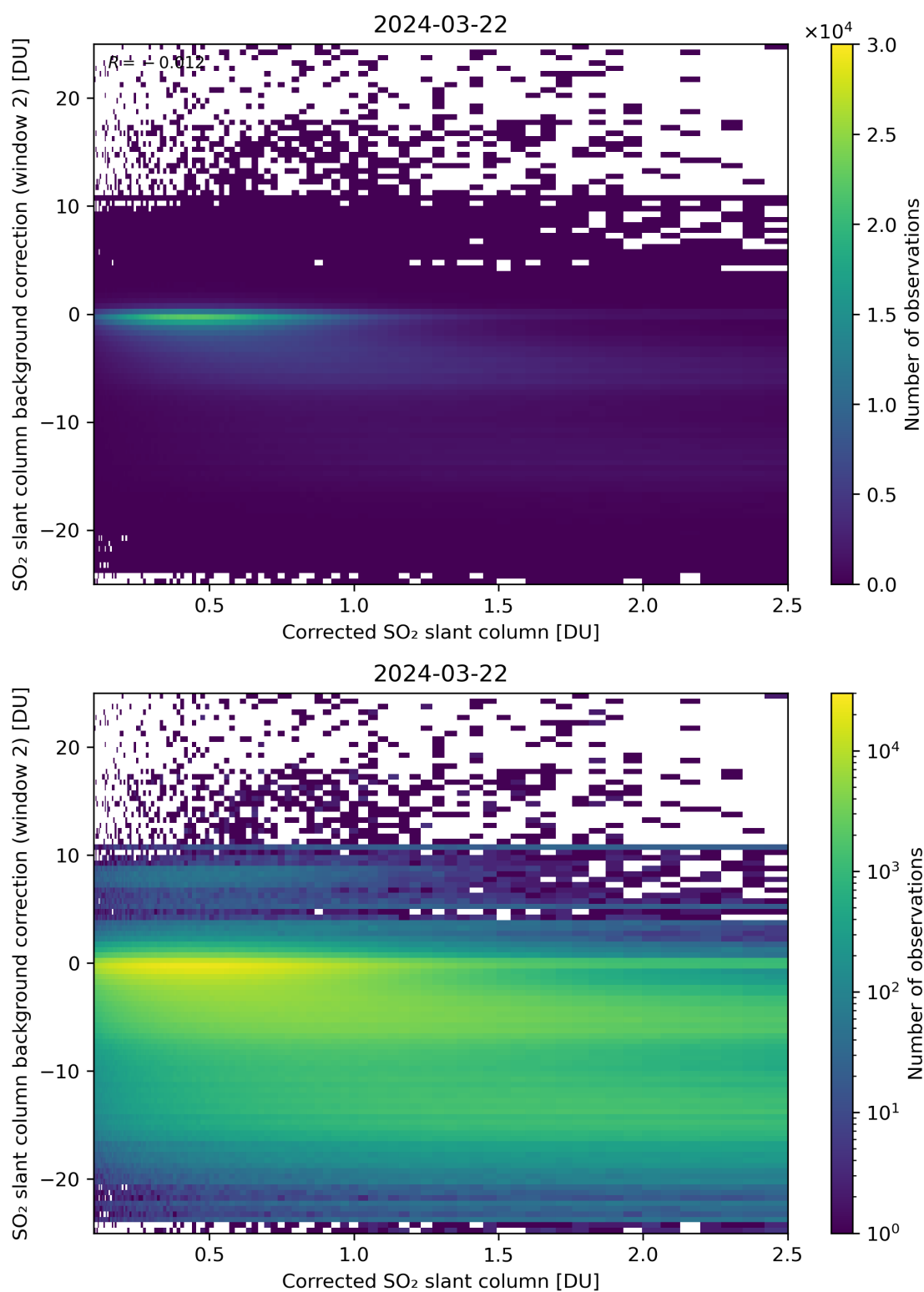
Figure 179: Scatter density plot of “Corrected SO 2 slant column” against “SO 2 slant column background correction (window 2)” for 2024-03-21 to 2024-03-22.
