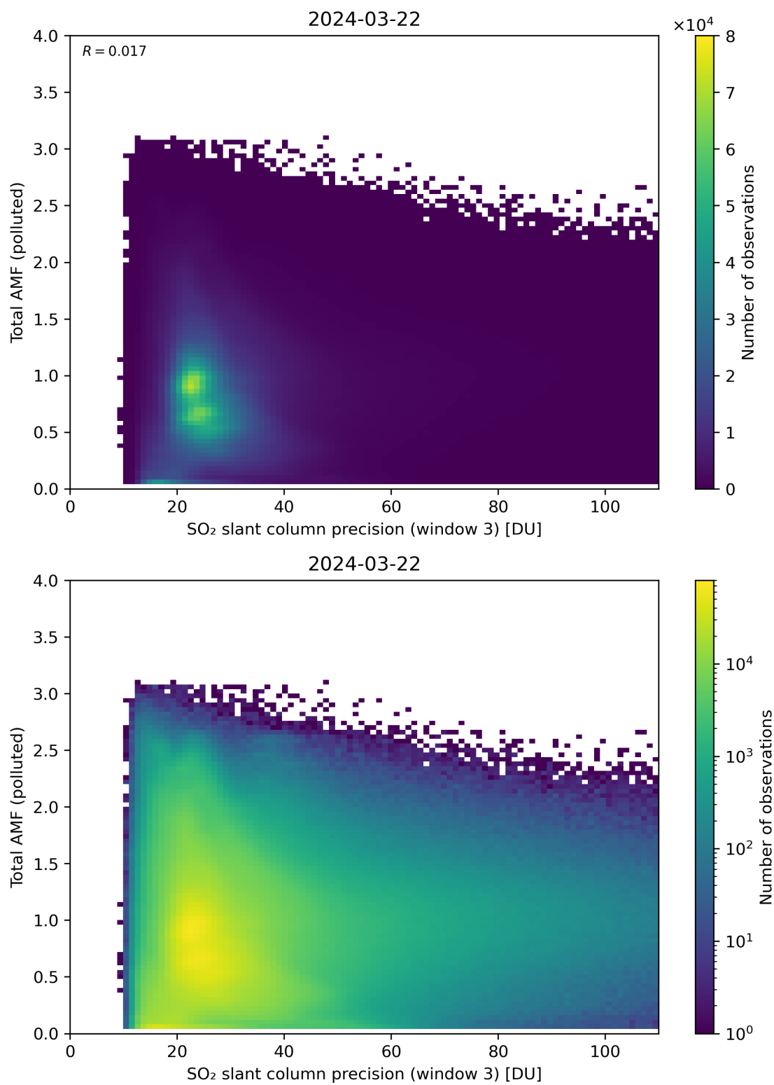
Figure 263: Scatter density plot of “SO 2 slant column precision (window 3)” against “Total AMF (polluted)” for 2024-03-21 to 2024-03-22.
