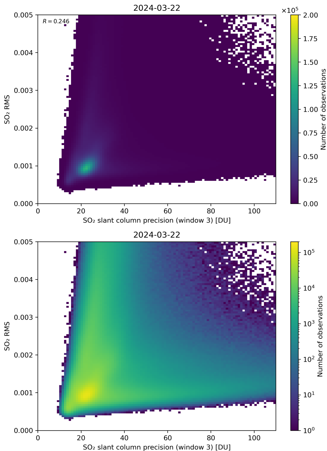
Figure 260: Scatter density plot of “SO 2 slant column precision (window 3)” against “SO 2 RMS” for 2024-03-21 to 2024-03-22.
