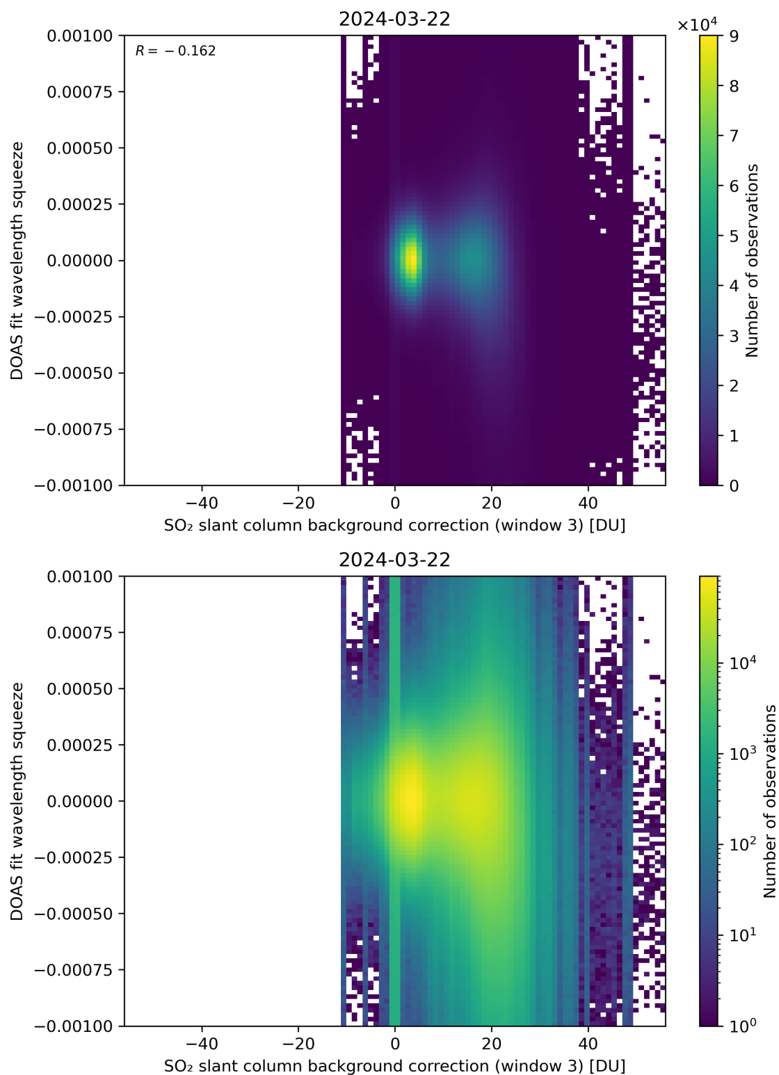
Figure 122: Scatter density plot of “SO 2 slant column background correction (window 3)” against “DOAS fit wavelength squeeze” for 2024-03-21 to 2024-03-22.
