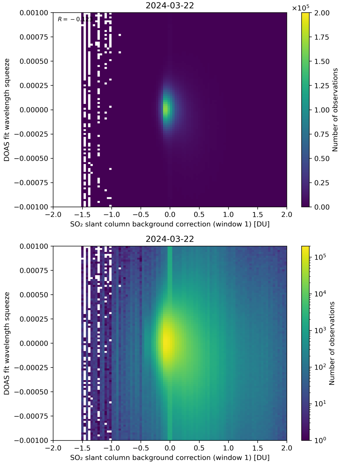
Figure 101: Scatter density plot of “SO 2 slant column background correction (window 1)” against “DOAS fit wavelength squeeze” for 2024-03-21 to 2024-03-22.
