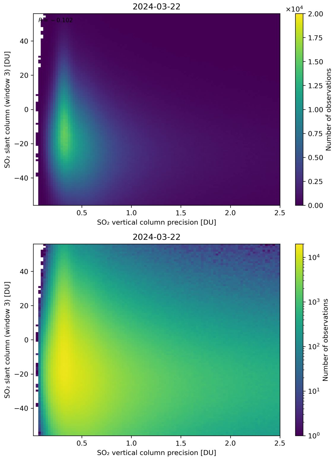
Figure 292: Scatter density plot of “SO 2 vertical column precision” against “SO 2 slant column (window 3)” for 2024-03-21 to 2024-03-22.
