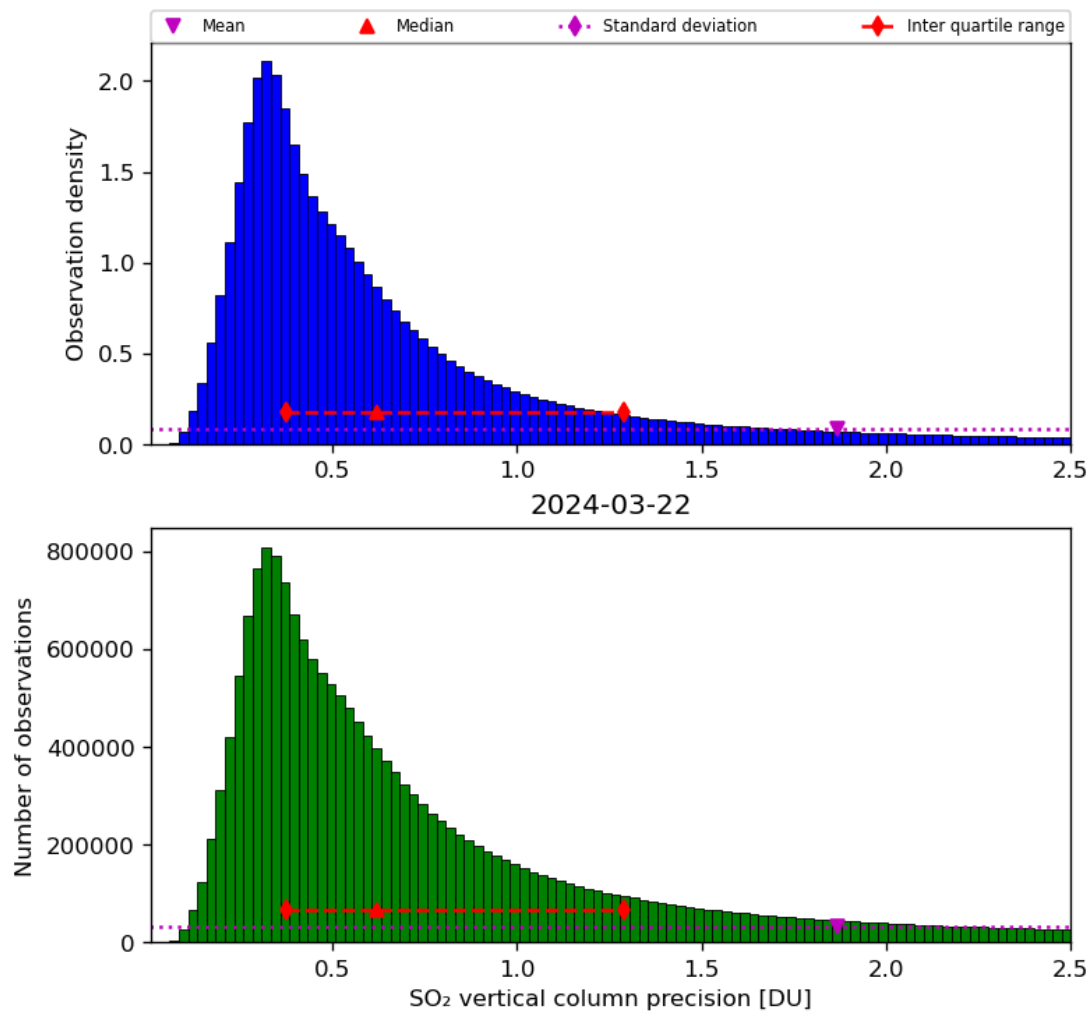
Figure 54: Histogram of “SO 2 vertical column precision” for 2024-03-21 to 2024-03-22
