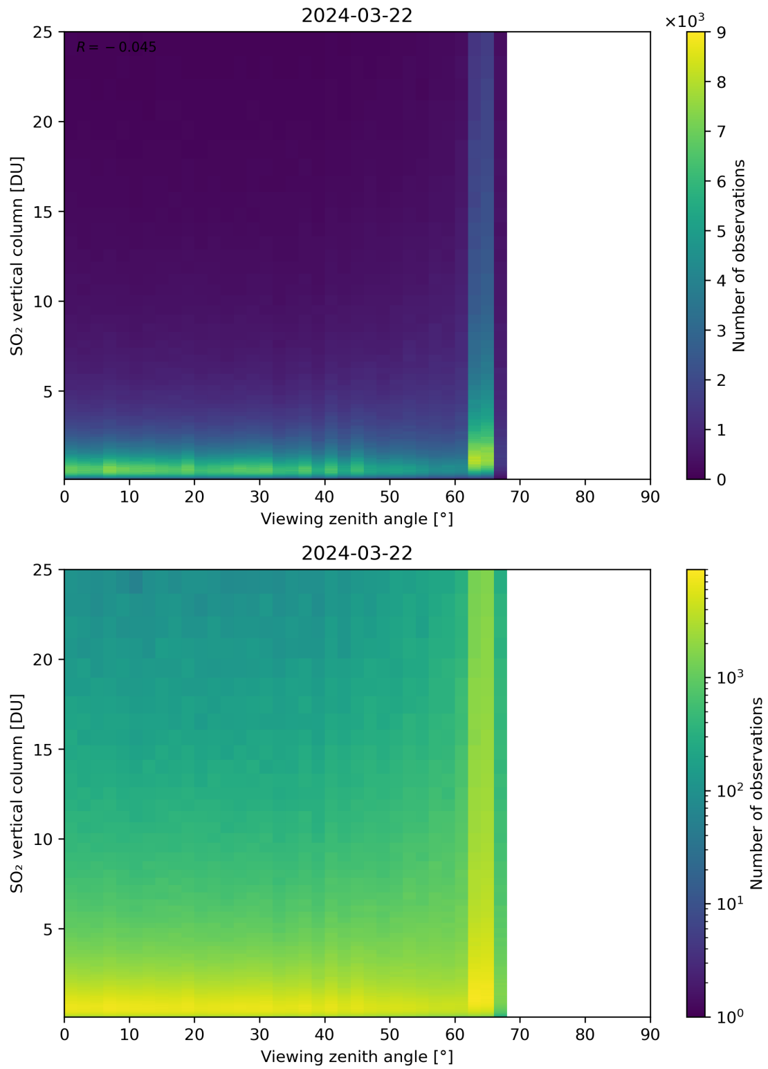
Figure 327: Scatter density plot of “Viewing zenith angle” against “SO 2 vertical column” for 2024-03-21 to 2024-03-22.
