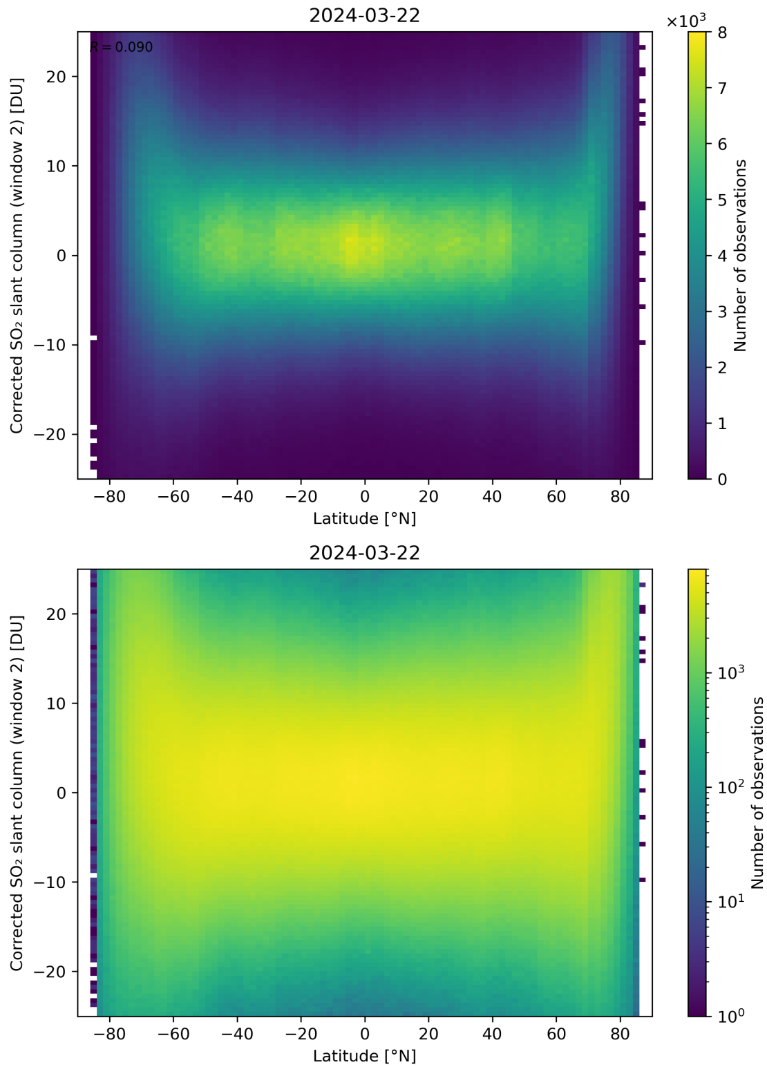
Figure 147: Scatter density plot of “Latitude” against “Corrected SO 2 slant column (window 2)” for 2024-03-21 to 2024-03-22.
