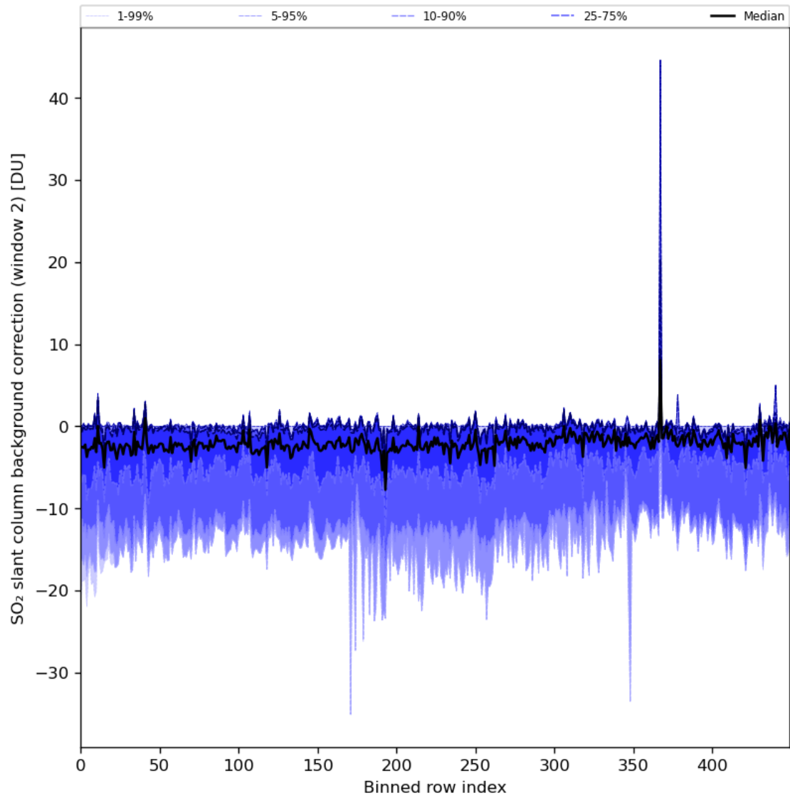
Figure 86: Along track statistics of “SO 2 slant column background correction (window 2)” for 2024-03-21 to 2024-03-22
