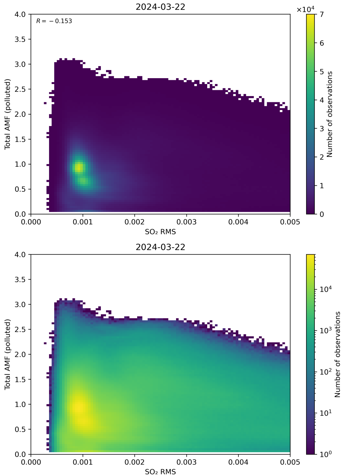
Figure 137: Scatter density plot of “SO 2 RMS” against “Total AMF (polluted)” for 2024-03-21 to 2024-03-22.
