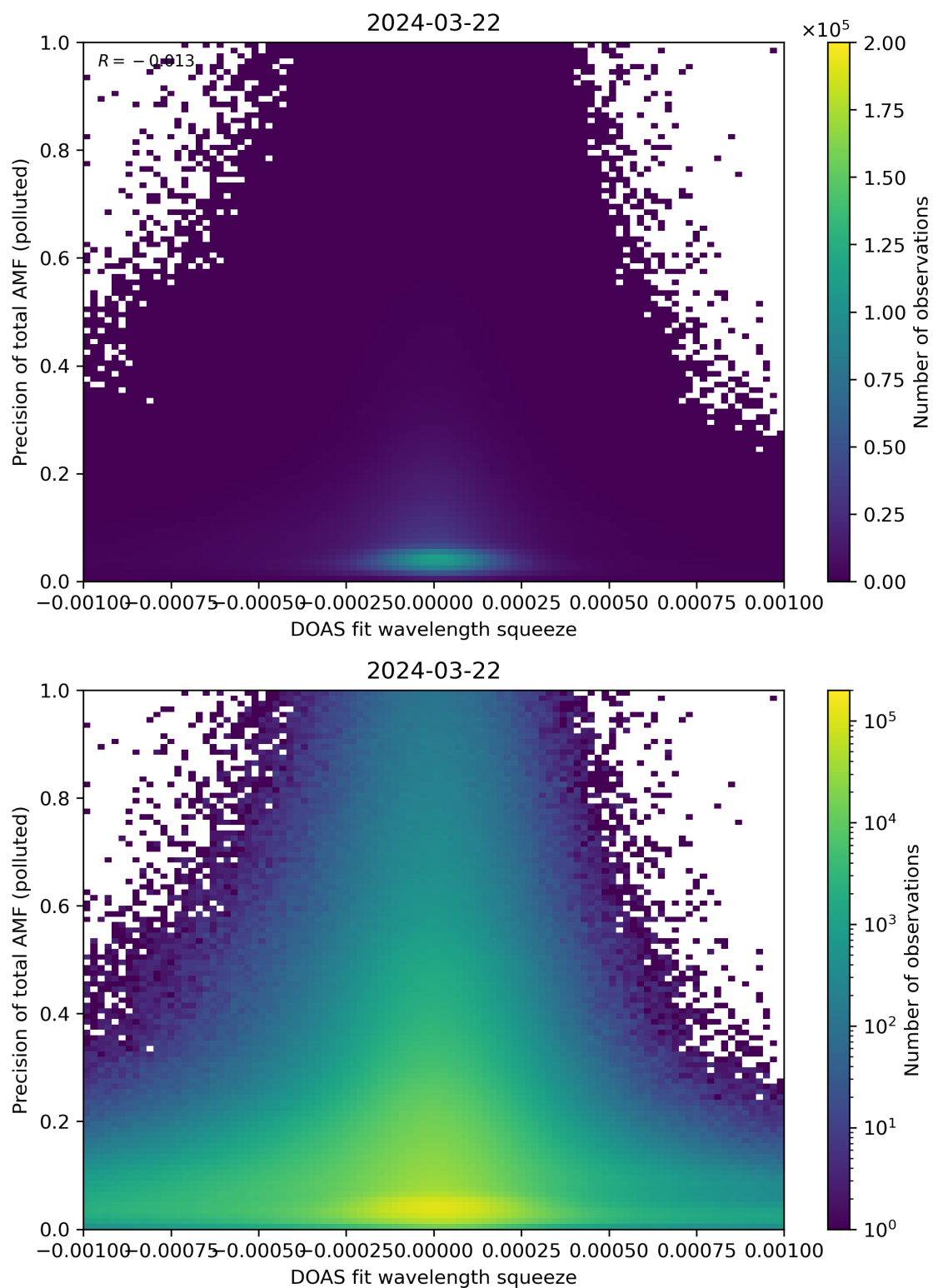
Figure 135: Scatter density plot of “DOAS fit wavelength squeeze” against “Precision of total AMF (polluted)” for 2024-03-21 to 2024-03-22.
