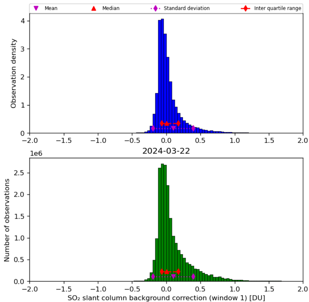
Figure 59: Histogram of “SO 2 slant column background correction (window 1)” for 2024-03-21 to 2024-03-22
