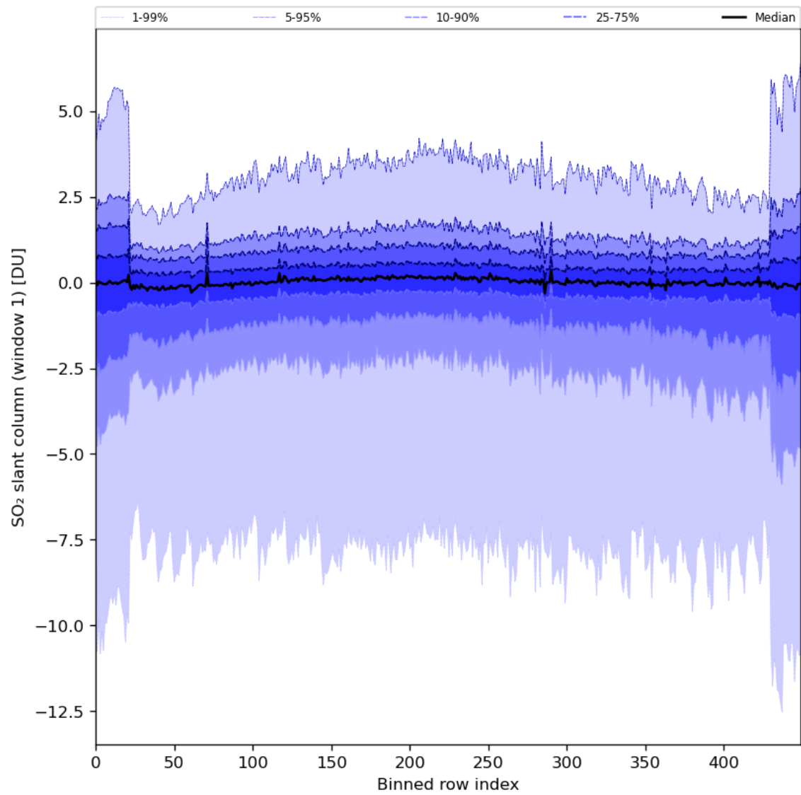
Figure 79: Along track statistics of “SO 2 slant column (window 1)” for 2024-03-21 to 2024-03-22
