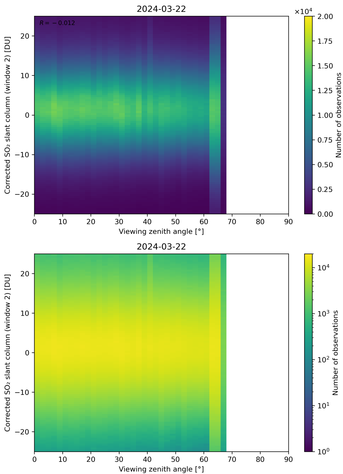
Figure 318: Scatter density plot of “Viewing zenith angle” against “Corrected SO 2 slant column (window 2)” for 2024-03-21 to 2024-03-22.
