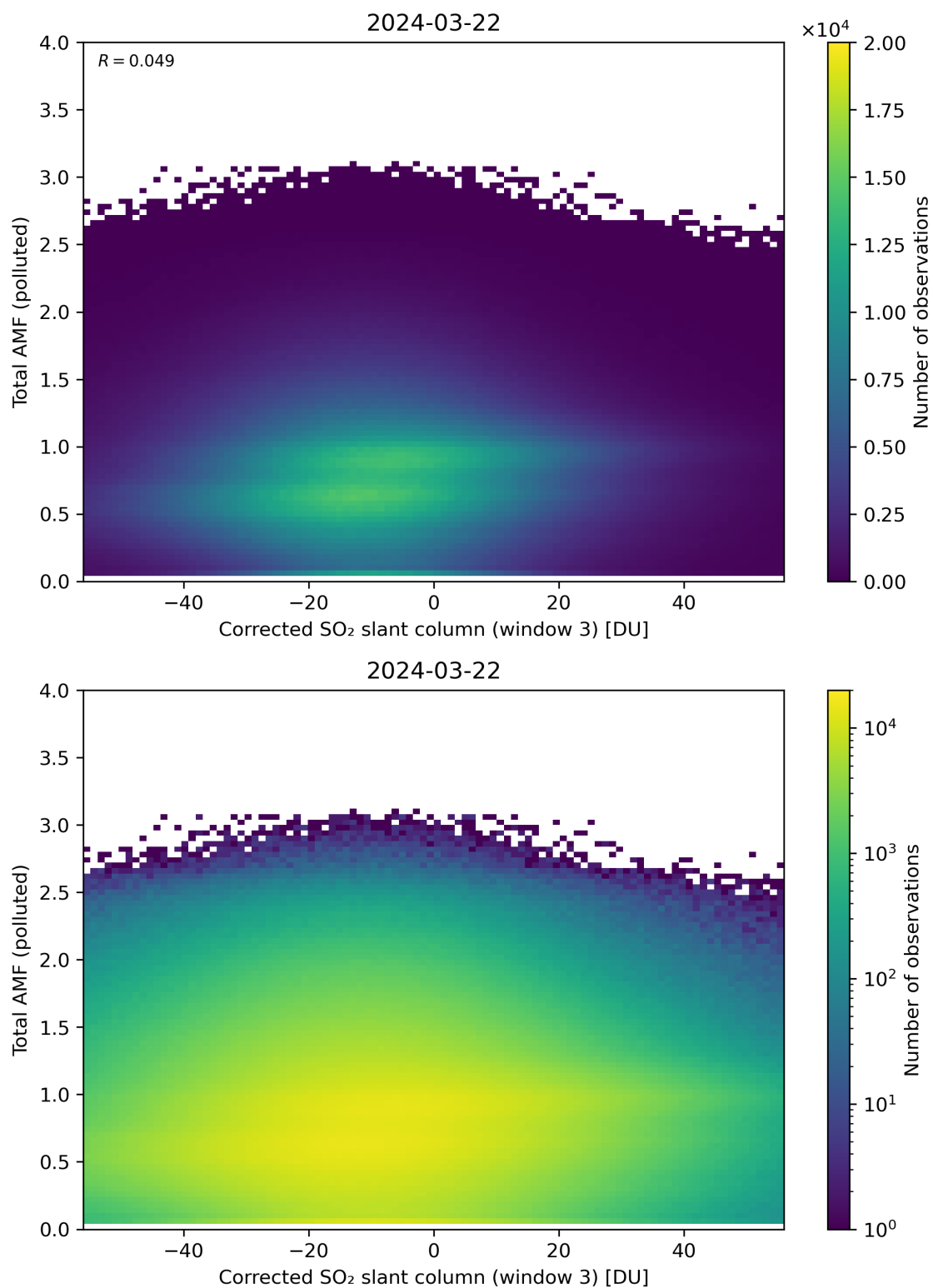
Figure 210: Scatter density plot of “Corrected SO 2 slant column (window 3)” against “Total AMF (polluted)” for 2024-03-21 to 2024-03-22.
