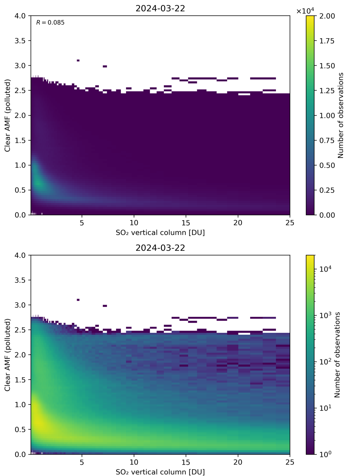
Figure 296: Scatter density plot of “SO 2 vertical column” against “Clear AMF (polluted)” for 2024-03-21 to 2024-03-22.
