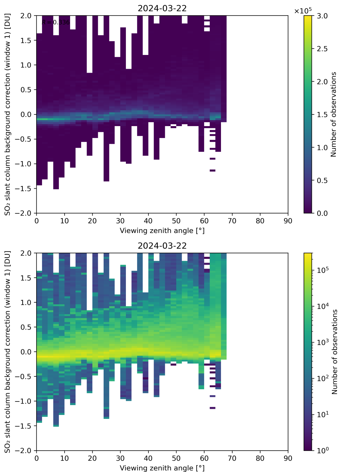
Figure 308: Scatter density plot of “Viewing zenith angle” against “SO 2 slant column background correction (window 1)” for 2024-03-21 to 2024-03-22.
