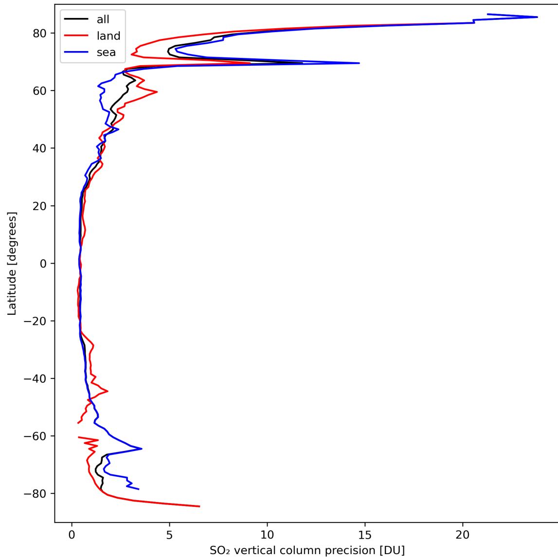
Figure 31: Zonal average of “SO 2 vertical column precision” for 2024-03-21 to 2024-03-22.
