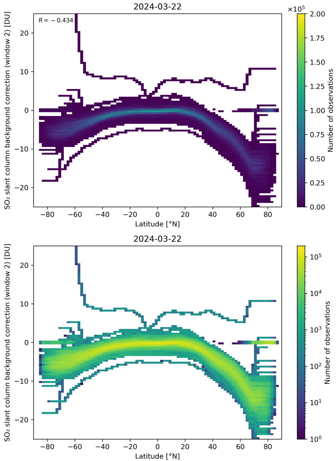
Figure 140: Scatter density plot of “Latitude” against “SO 2 slant column background correction (window 2)” for 2024-03-21 to 2024-03-22.
