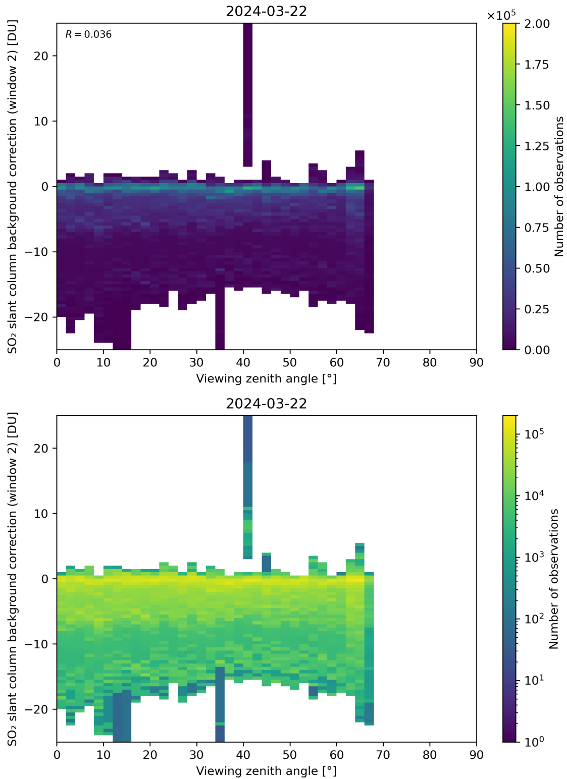
Figure 309: Scatter density plot of “Viewing zenith angle” against “SO 2 slant column background correction (window 2)” for 2024-03-21 to 2024-03-22.
