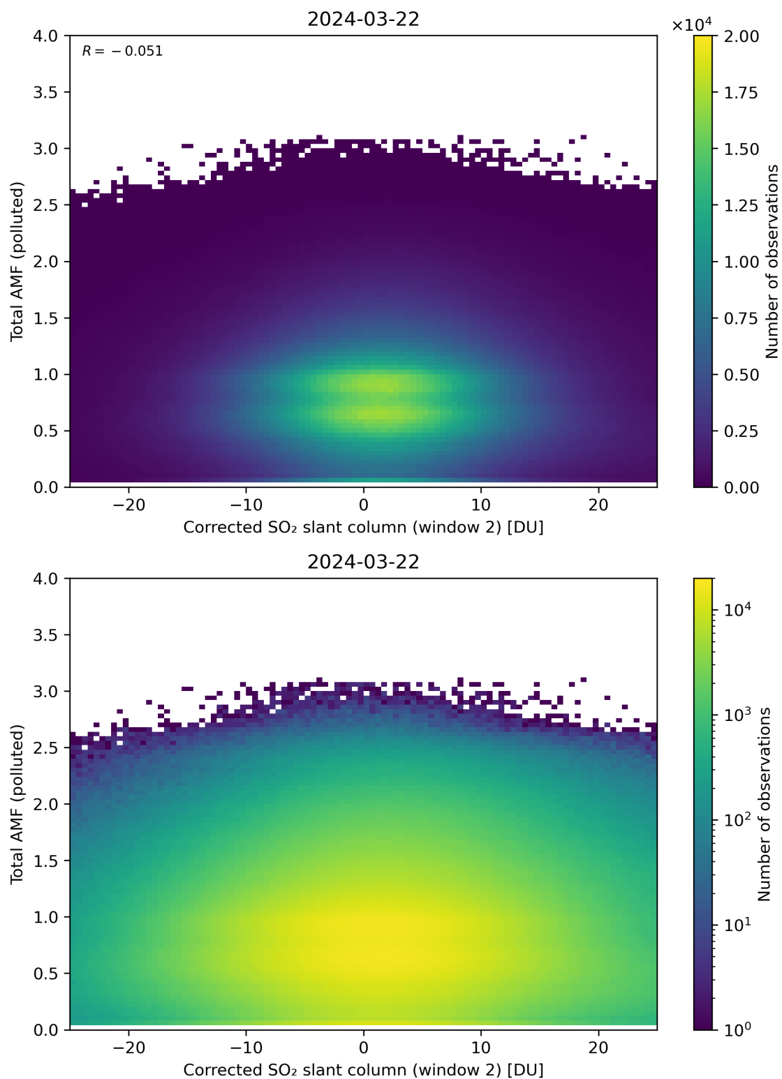
Figure 203: Scatter density plot of “Corrected SO 2 slant column (window 2)” against “Total AMF (polluted)” for 2024-03-21 to 2024-03-22.
