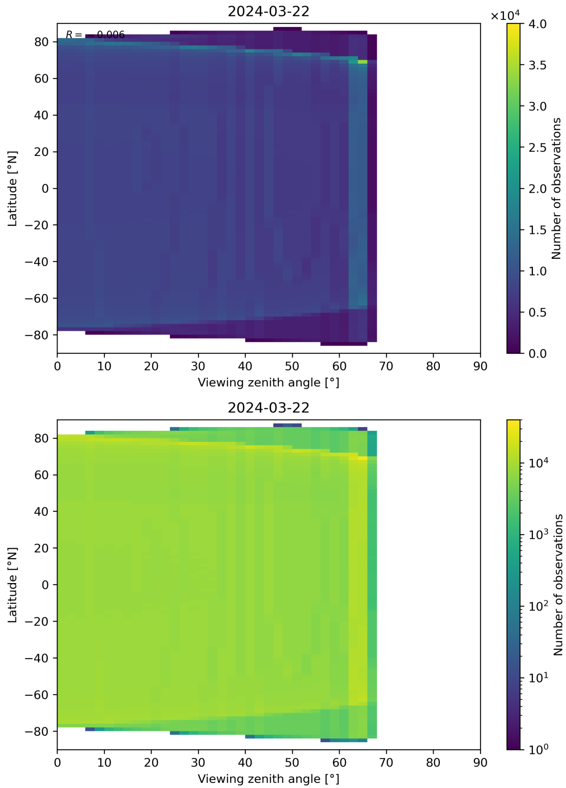
Figure 314: Scatter density plot of “Viewing zenith angle” against “Latitude” for 2024-03-21 to 2024-03-22.
