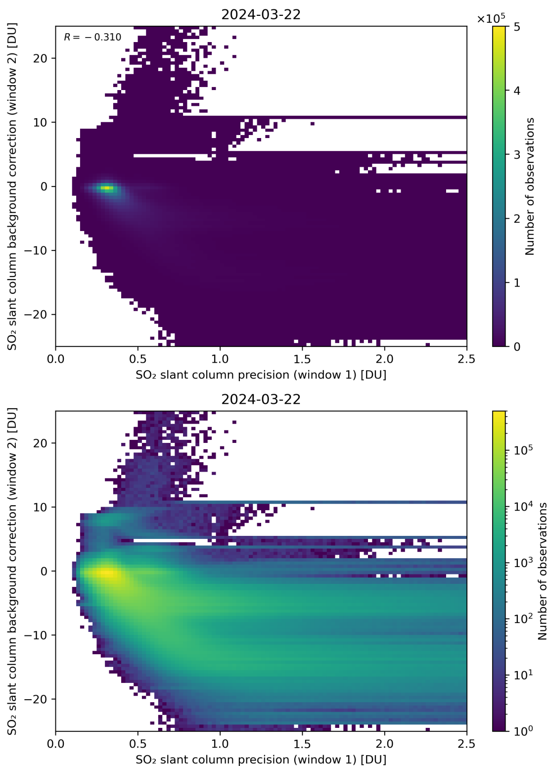
Figure 219: Scatter density plot of “SO 2 slant column precision (window 1)” against “SO 2 slant column background correction (window 2)” for 2024-03-21 to 2024-03-22.
