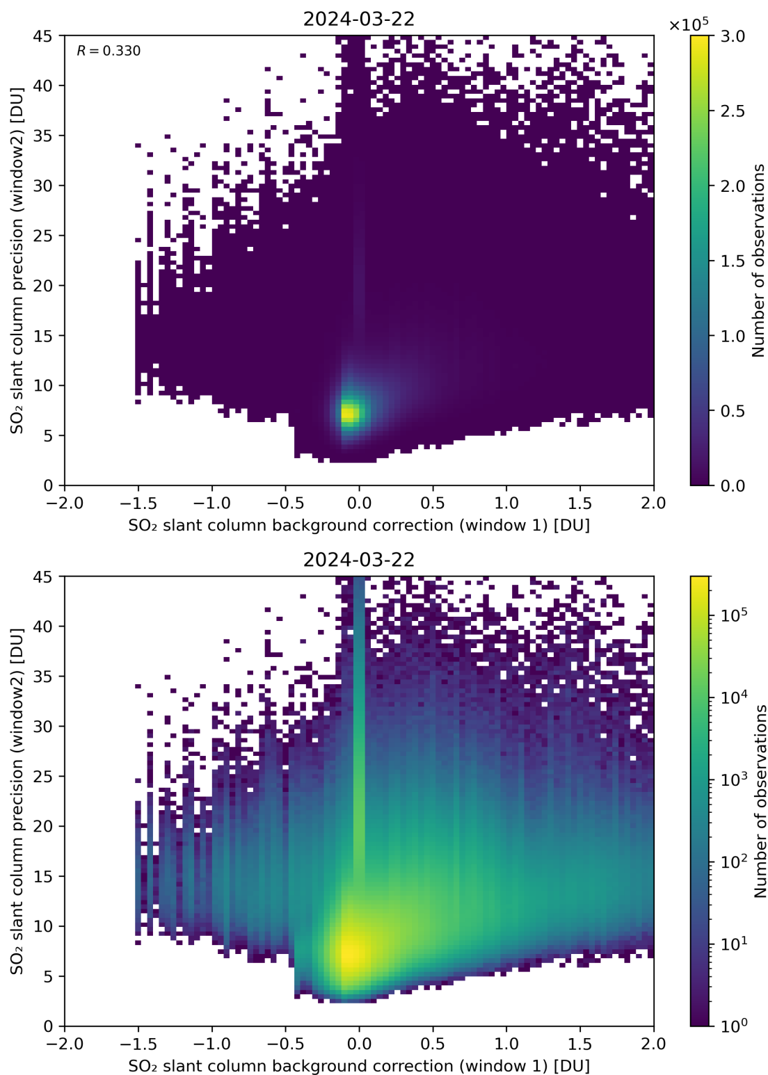
Figure 106: Scatter density plot of “SO 2 slant column background correction (window 1)” against “SO 2 slant column precision (window2)” for 2024-03-21 to 2024-03-22.
