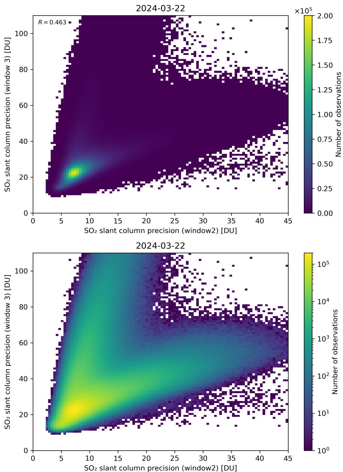
Figure 250: Scatter density plot of “SO 2 slant column precision (window2)” against “SO 2 slant column precision (window 3)” for 2024-03-21 to 2024-03-22.
