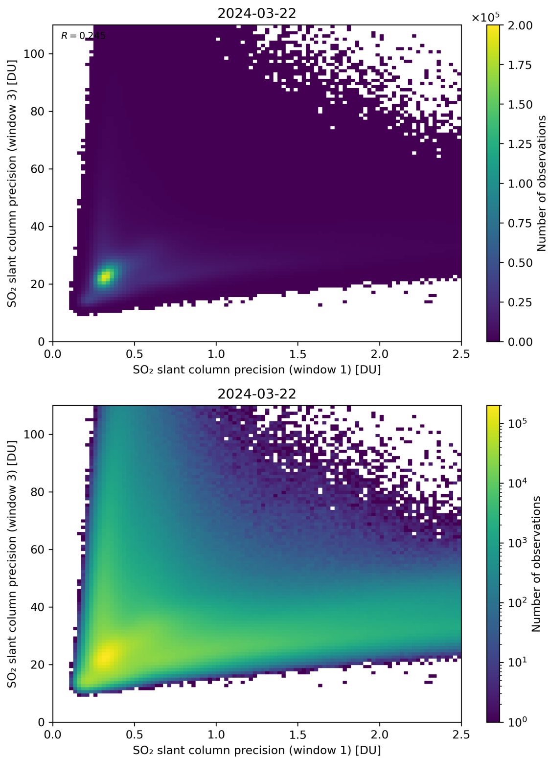
Figure 229: Scatter density plot of “SO 2 slant column precision (window 1)” against “SO 2 slant column precision (window 3)” for 2024-03-21 to 2024-03-22.
