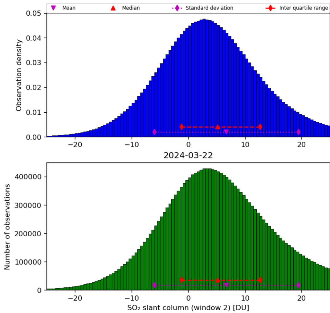
Figure 60: Histogram of “SO 2 slant column (window 2)” for 2024-03-21 to 2024-03-22
