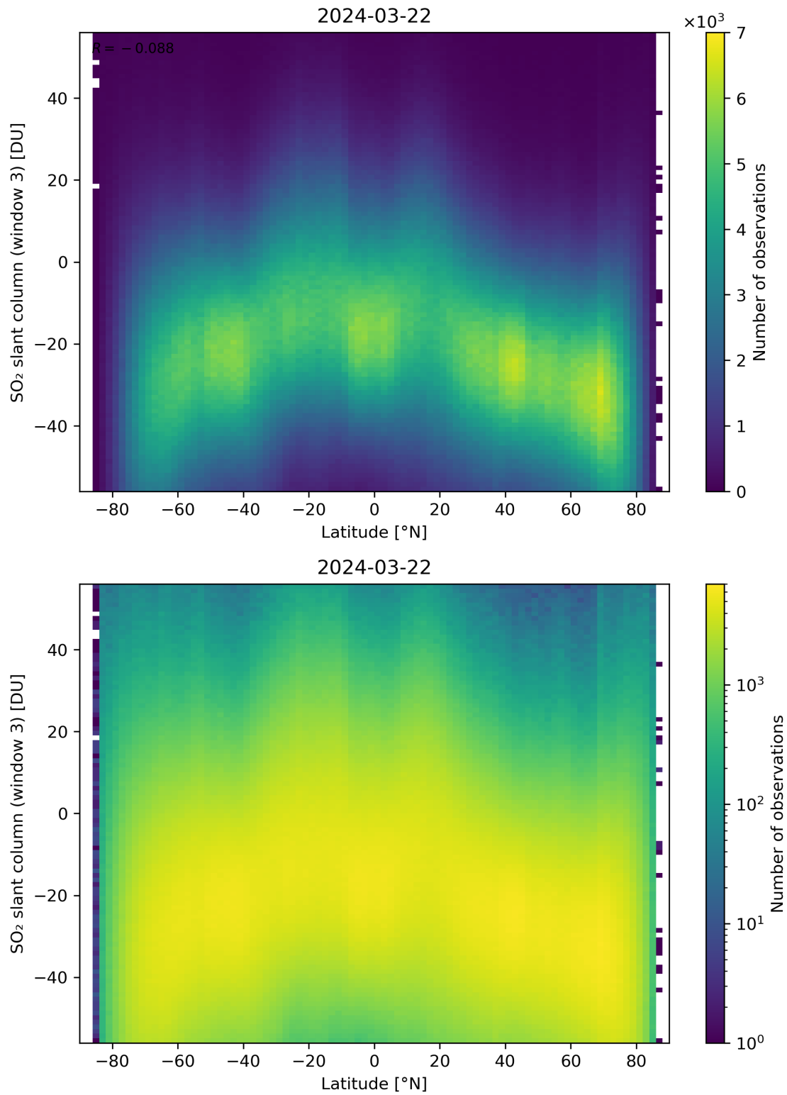
Figure 152: Scatter density plot of “Latitude” against “SO 2 slant column (window 3)” for 2024-03-21 to 2024-03-22.
