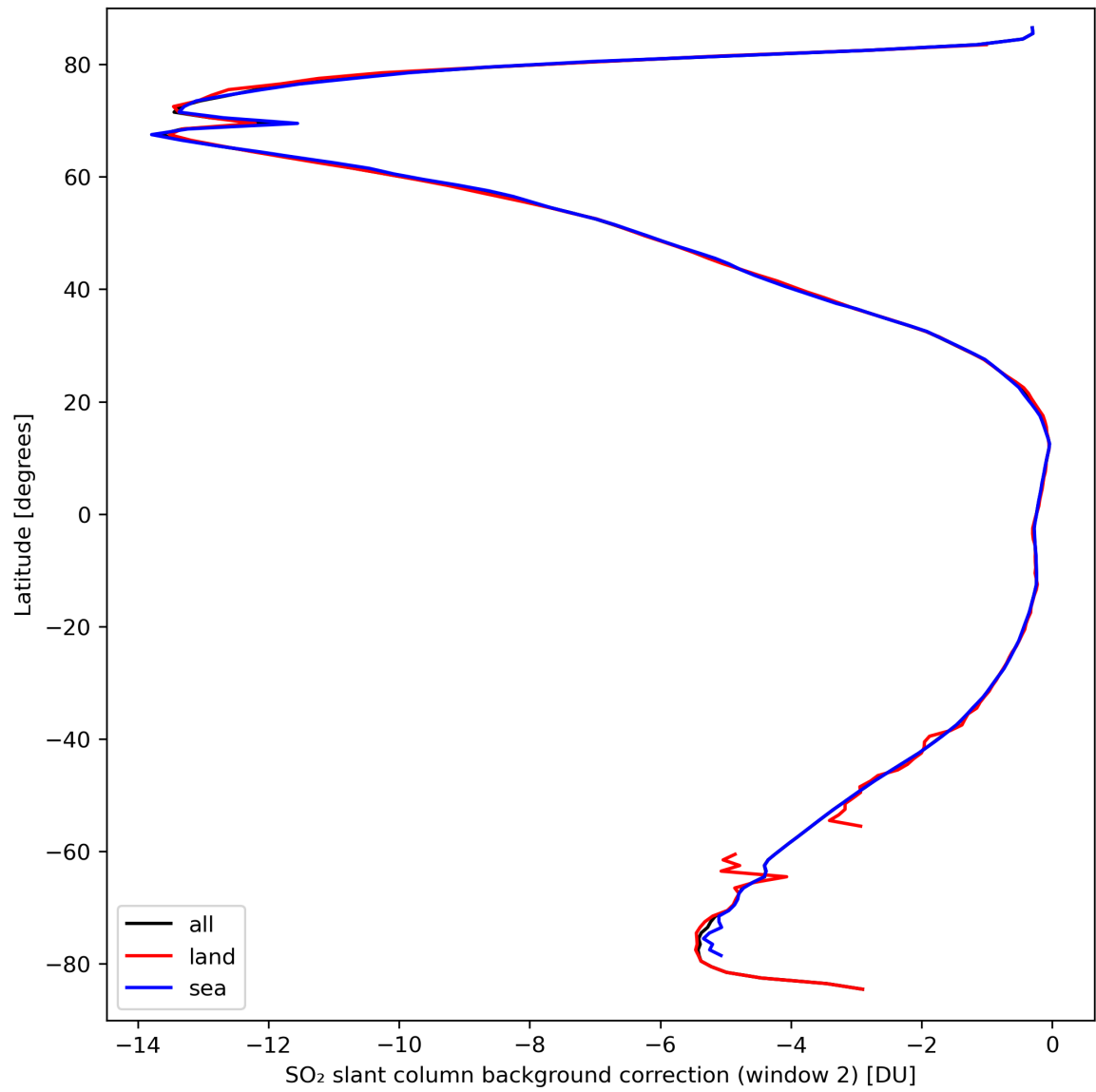
Figure 40: Zonal average of “SO 2 slant column background correction (window 2)” for 2024-03-21 to 2024-03-22.
