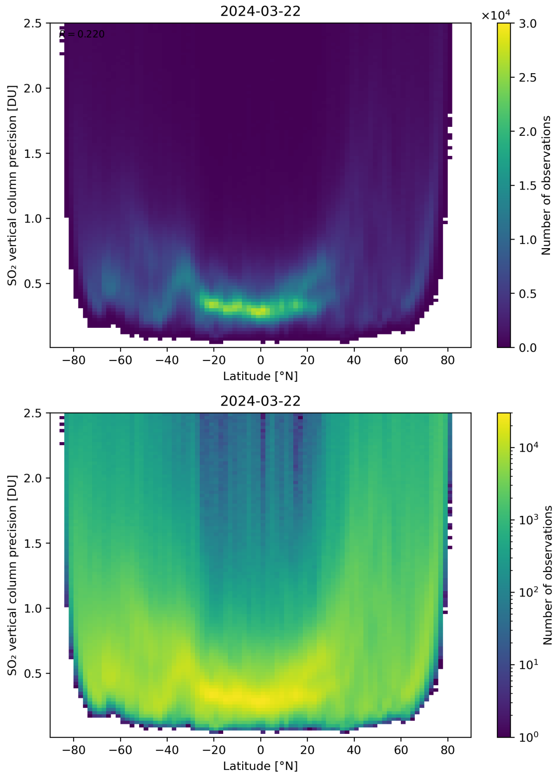
Figure 157: Scatter density plot of “Latitude” against “SO 2 vertical column precision” for 2024-03-21 to 2024-03-22.
