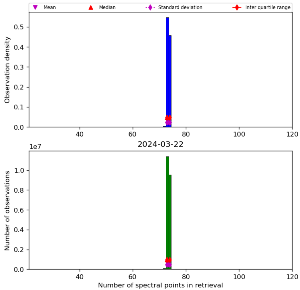
Figure 74: Histogram of “Number of spectral points in retrieval” for 2024-03-21 to 2024-03-22
