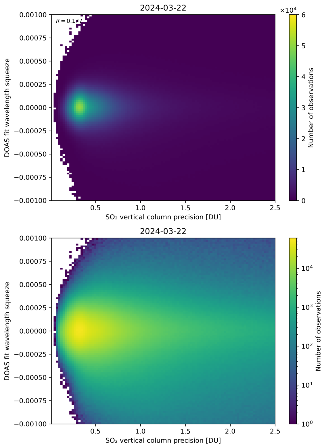
Figure 283: Scatter density plot of “SO 2 vertical column precision” against “DOAS fit wavelength squeeze” for 2024-03-21 to 2024-03-22.
