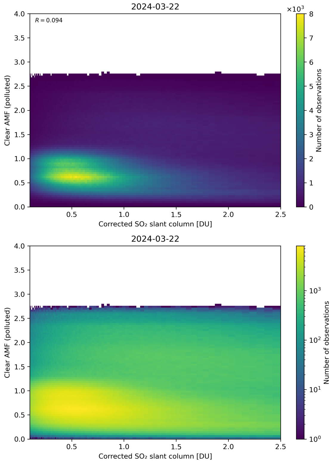
Figure 184: Scatter density plot of “Corrected SO 2 slant column” against “Clear AMF (polluted)” for 2024-03-21 to 2024-03-22.
