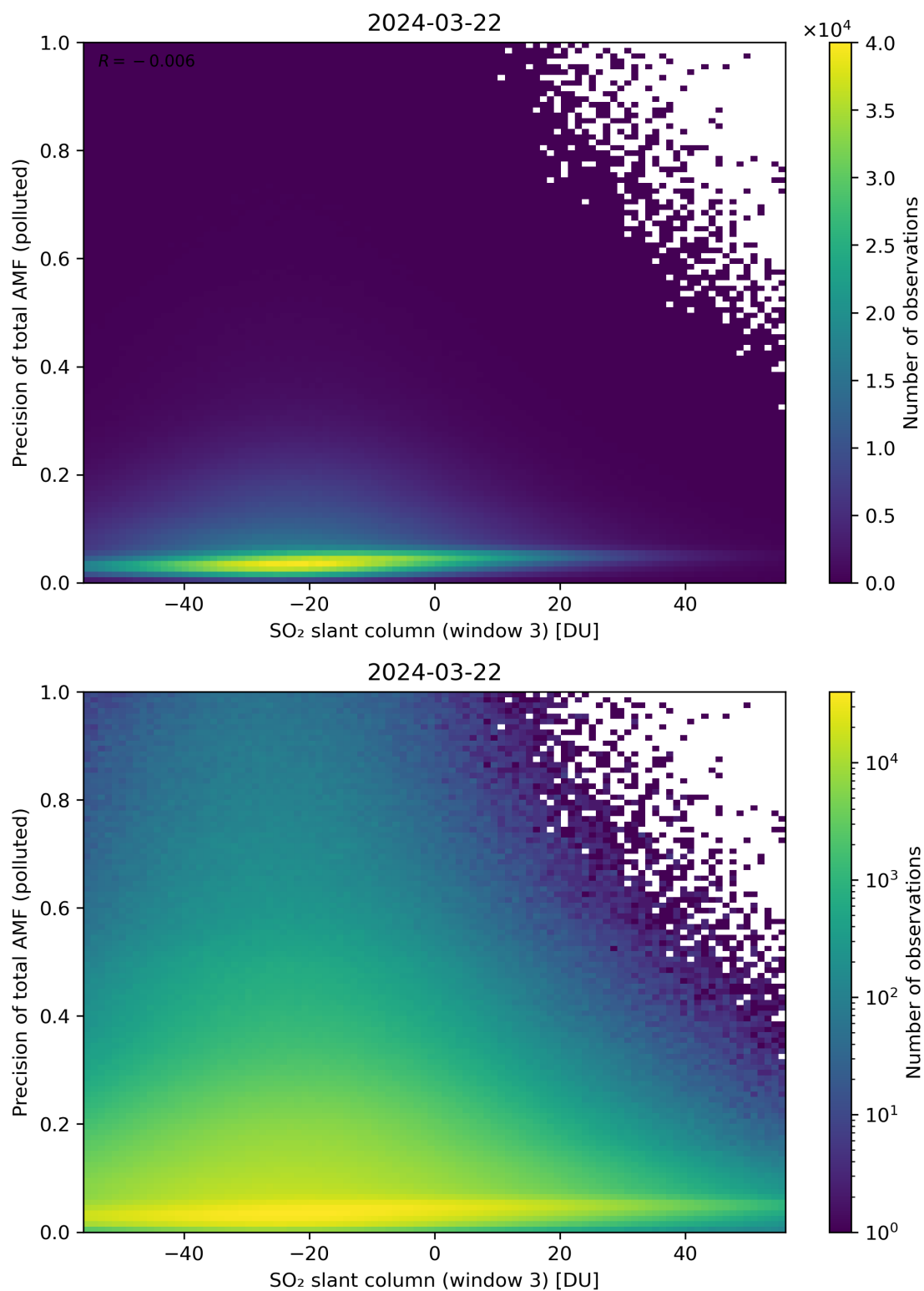
Figure 269: Scatter density plot of “SO 2 slant column (window 3)” against “Precision of total AMF (polluted)” for 2024-03-21 to 2024-03-22.
