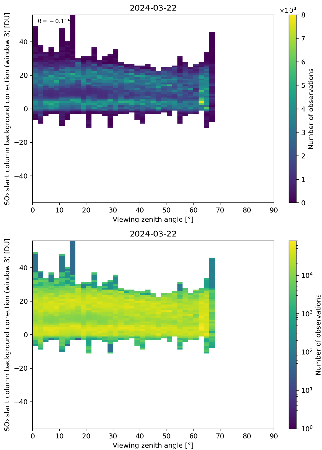
Figure 310: Scatter density plot of “Viewing zenith angle” against “SO 2 slant column background correction (window 3)” for 2024-03-21 to 2024-03-22.
