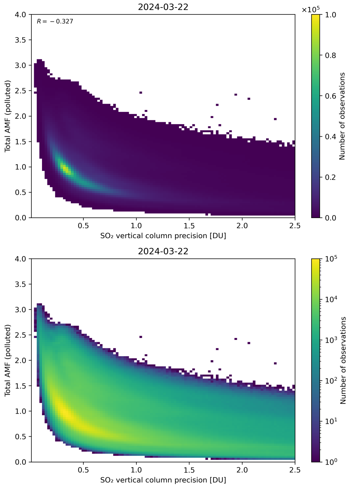
Figure 294: Scatter density plot of “SO 2 vertical column precision” against “Total AMF (polluted)” for 2024-03-21 to 2024-03-22.
