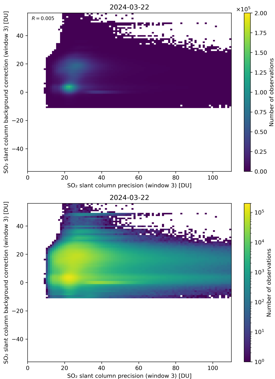
Figure 257: Scatter density plot of “SO 2 slant column precision (window 3)” against “SO 2 slant column background correction (window 3)” for 2024-03-21 to 2024-03-22.
