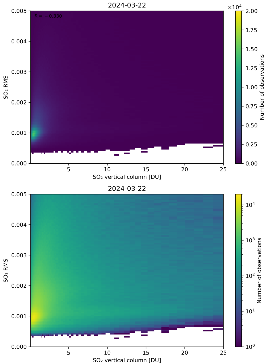
Figure 278: Scatter density plot of “SO 2 vertical column” against “SO 2 RMS” for 2024-03-21 to 2024-03-22.
