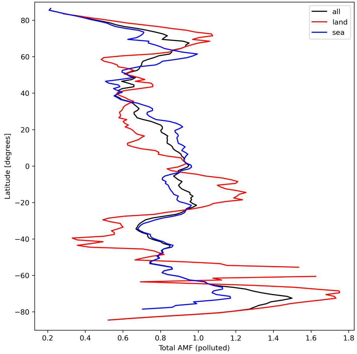
Figure 48: Zonal average of “Total AMF (polluted)” for 2024-03-21 to 2024-03-22.
