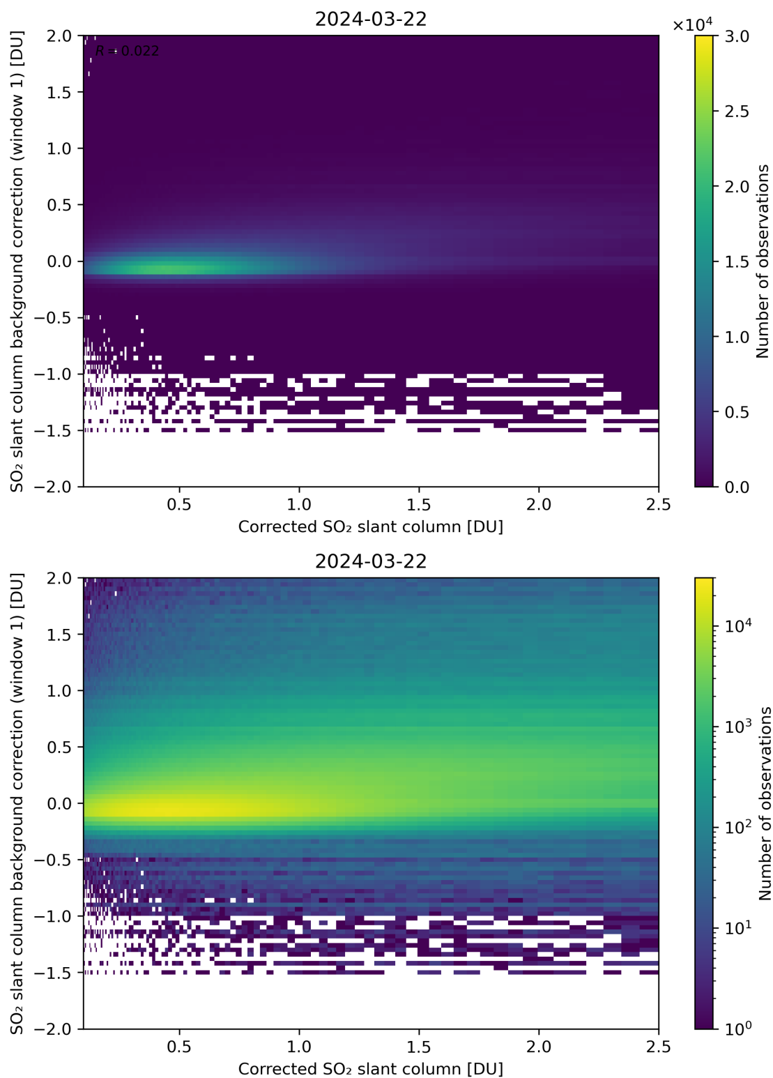
Figure 178: Scatter density plot of “Corrected SO 2 slant column” against “SO 2 slant column background correction (window 1)” for 2024-03-21 to 2024-03-22.
