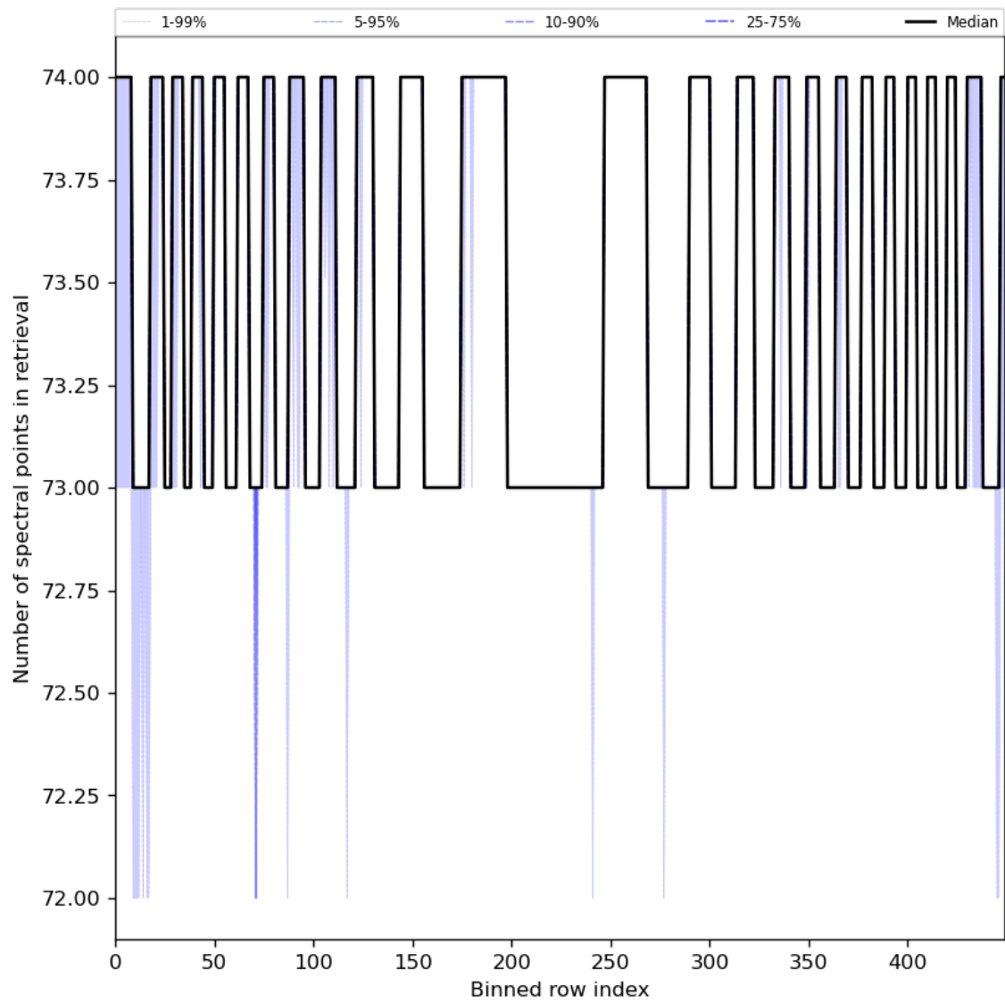
Figure 97: Along track statistics of “Number of spectral points in retrieval” for 2024-03-21 to 2024-03-22
