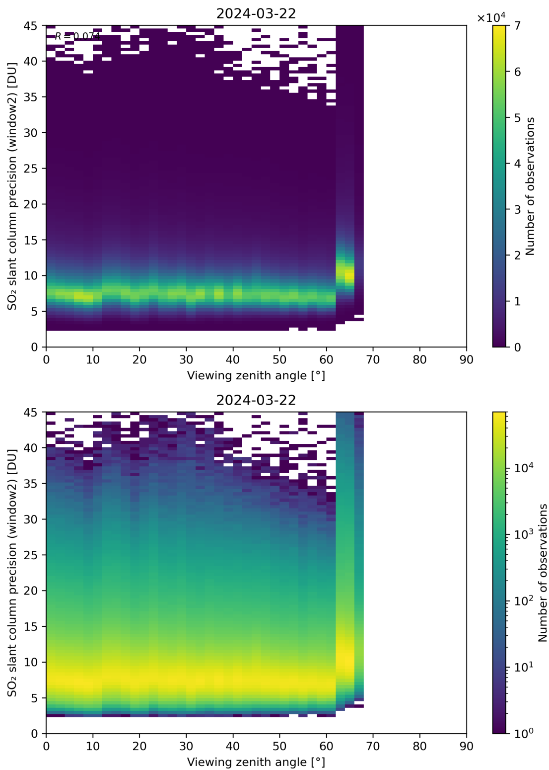
Figure 322: Scatter density plot of “Viewing zenith angle” against “SO 2 slant column precision (window2)” for 2024-03-21 to 2024-03-22.
