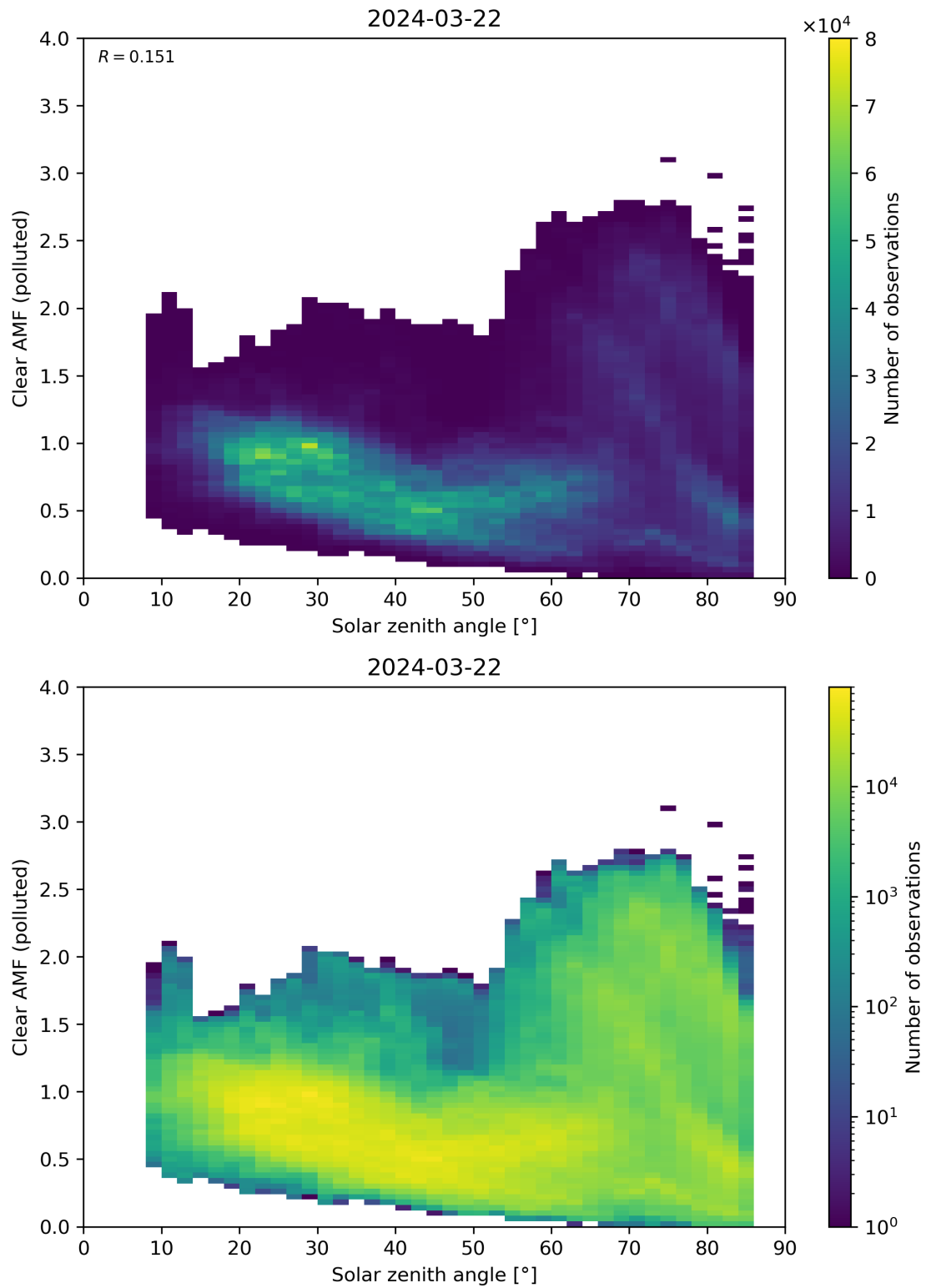
Figure 165: Scatter density plot of “Solar zenith angle” against “Clear AMF (polluted)” for 2024-03-21 to 2024-03-22.
