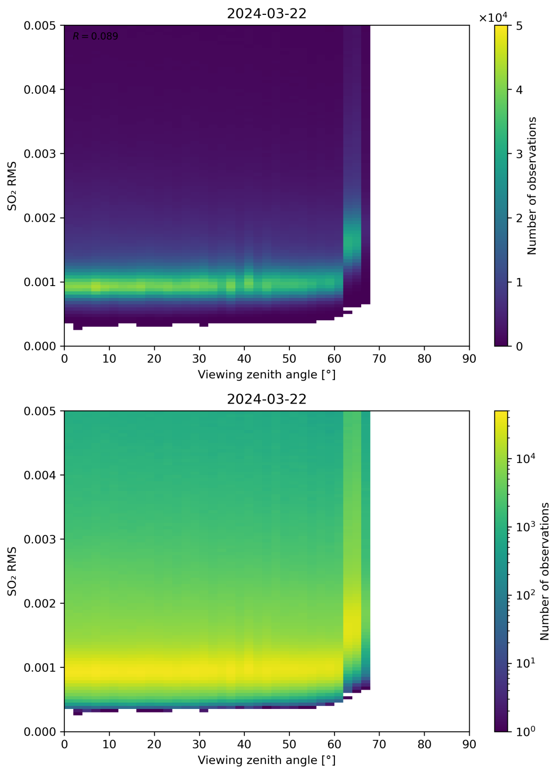
Figure 313: Scatter density plot of “Viewing zenith angle” against “SO 2 RMS” for 2024-03-21 to 2024-03-22.
