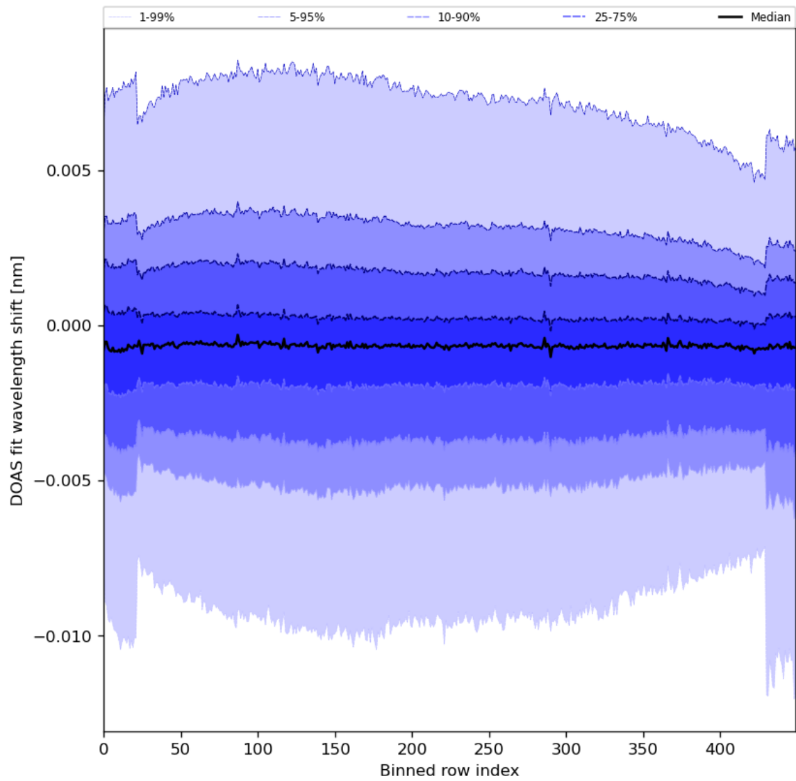
Figure 91: Along track statistics of “DOAS fit wavelength shift” for 2024-03-21 to 2024-03-22
