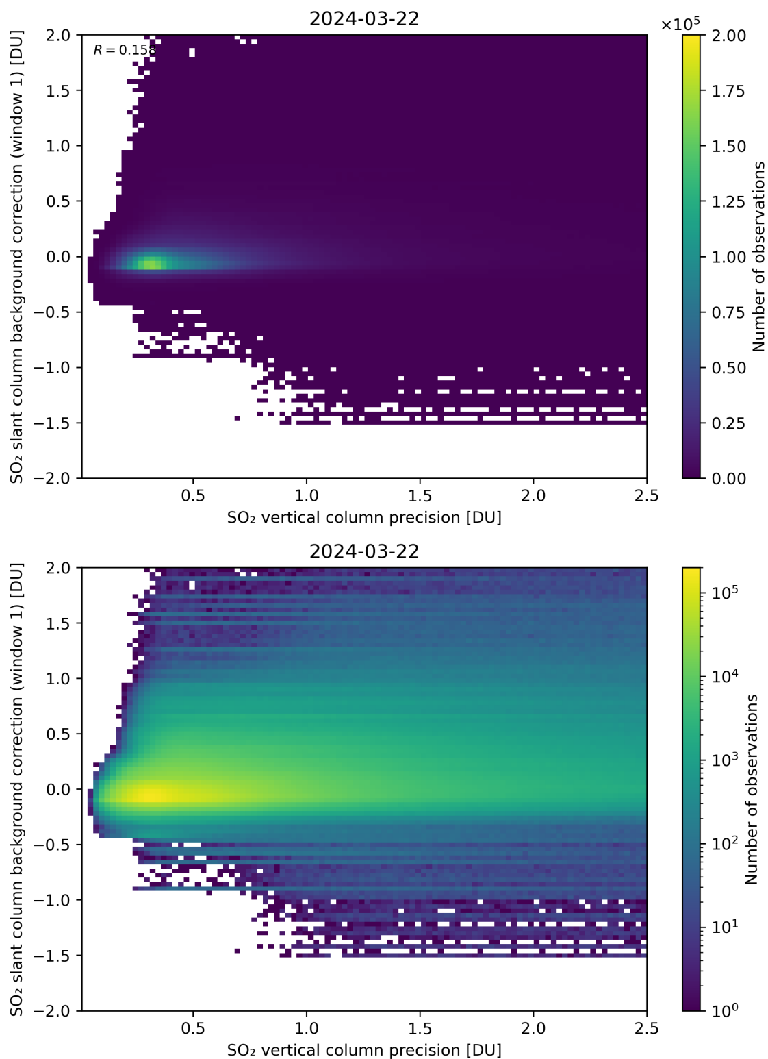
Figure 279: Scatter density plot of “SO 2 vertical column precision” against “SO 2 slant column background correction (window 1)” for 2024-03-21 to 2024-03-22.
