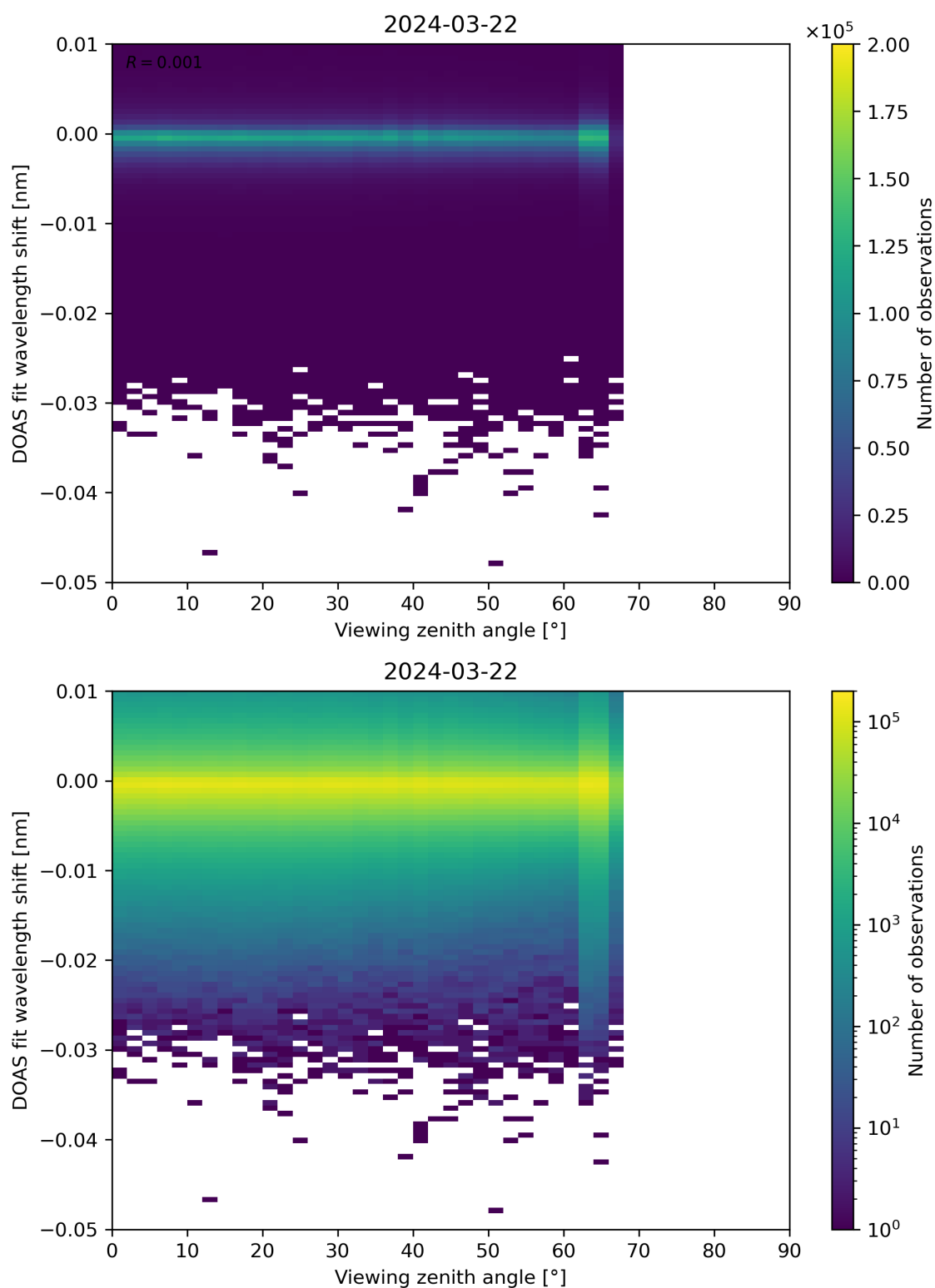
Figure 311: Scatter density plot of “Viewing zenith angle” against “DOAS fit wavelength shift” for 2024-03-21 to 2024-03-22.
