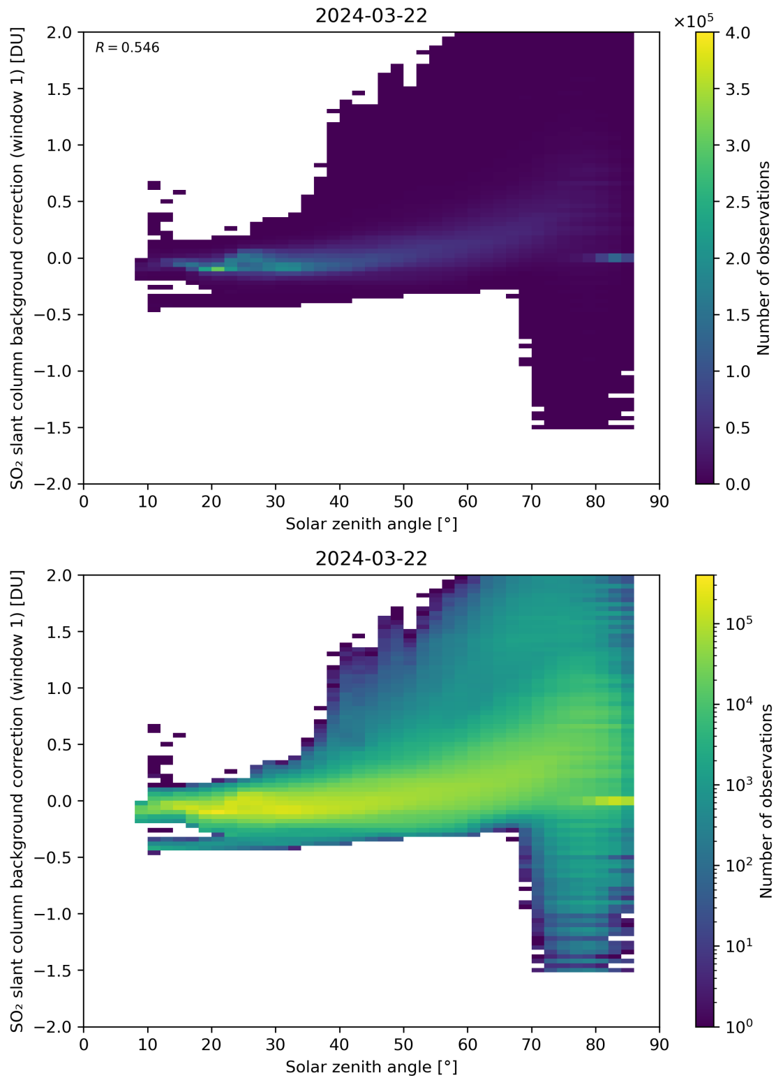
Figure 158: Scatter density plot of “Solar zenith angle” against “SO 2 slant column background correction (window 1)” for 2024-03-21 to 2024-03-22.
