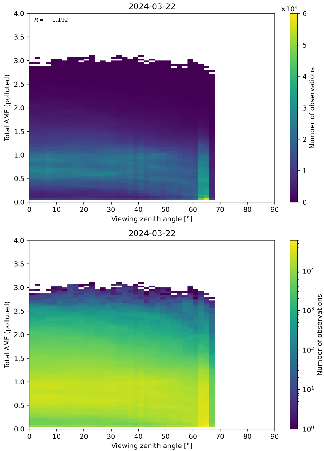
Figure 325: Scatter density plot of “Viewing zenith angle” against “Total AMF (polluted)” for 2024-03-21 to 2024-03-22.
