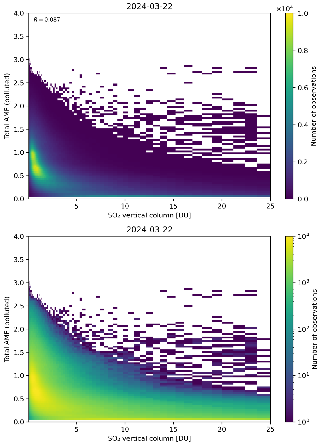
Figure 305: Scatter density plot of “SO 2 vertical column” against “Total AMF (polluted)” for 2024-03-21 to 2024-03-22.
