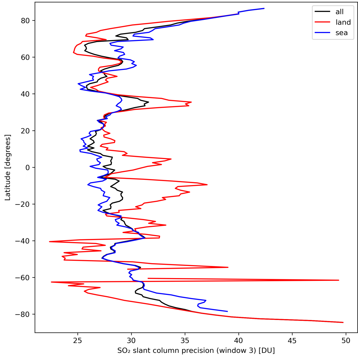
Figure 42: Zonal average of “SO 2 slant column precision (window 3)” for 2024-03-21 to 2024-03-22.
