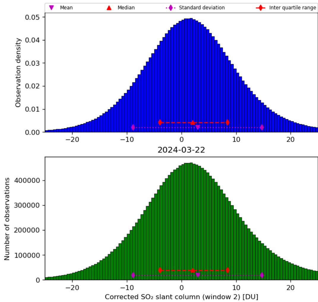
Figure 62: Histogram of “Corrected SO 2 slant column (window 2)” for 2024-03-21 to 2024-03-22
