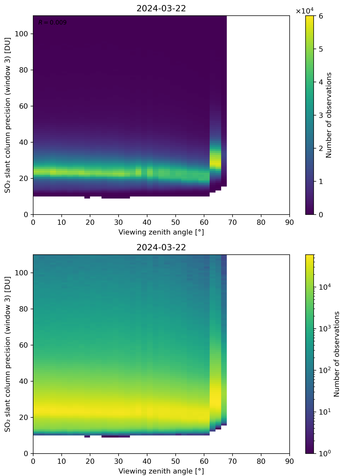
Figure 324: Scatter density plot of “Viewing zenith angle” against “SO 2 slant column precision (window 3)” for 2024-03-21 to 2024-03-22.
