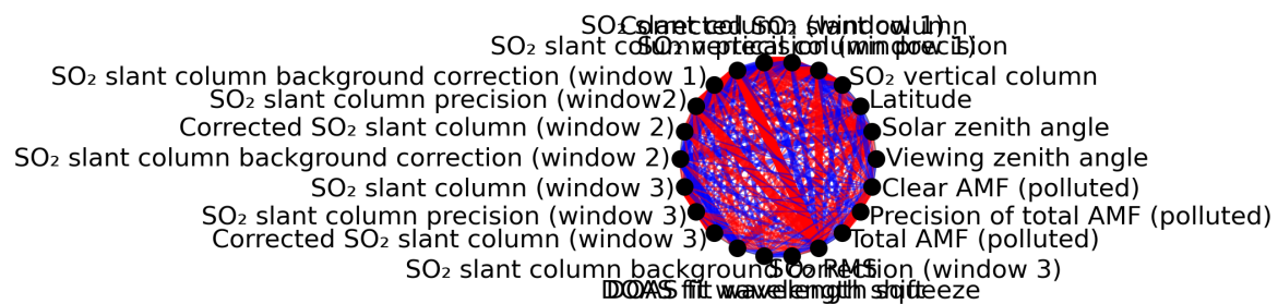
Figure 1: Map of correlation graph for 2024-03-21 to 2024-03-22.
