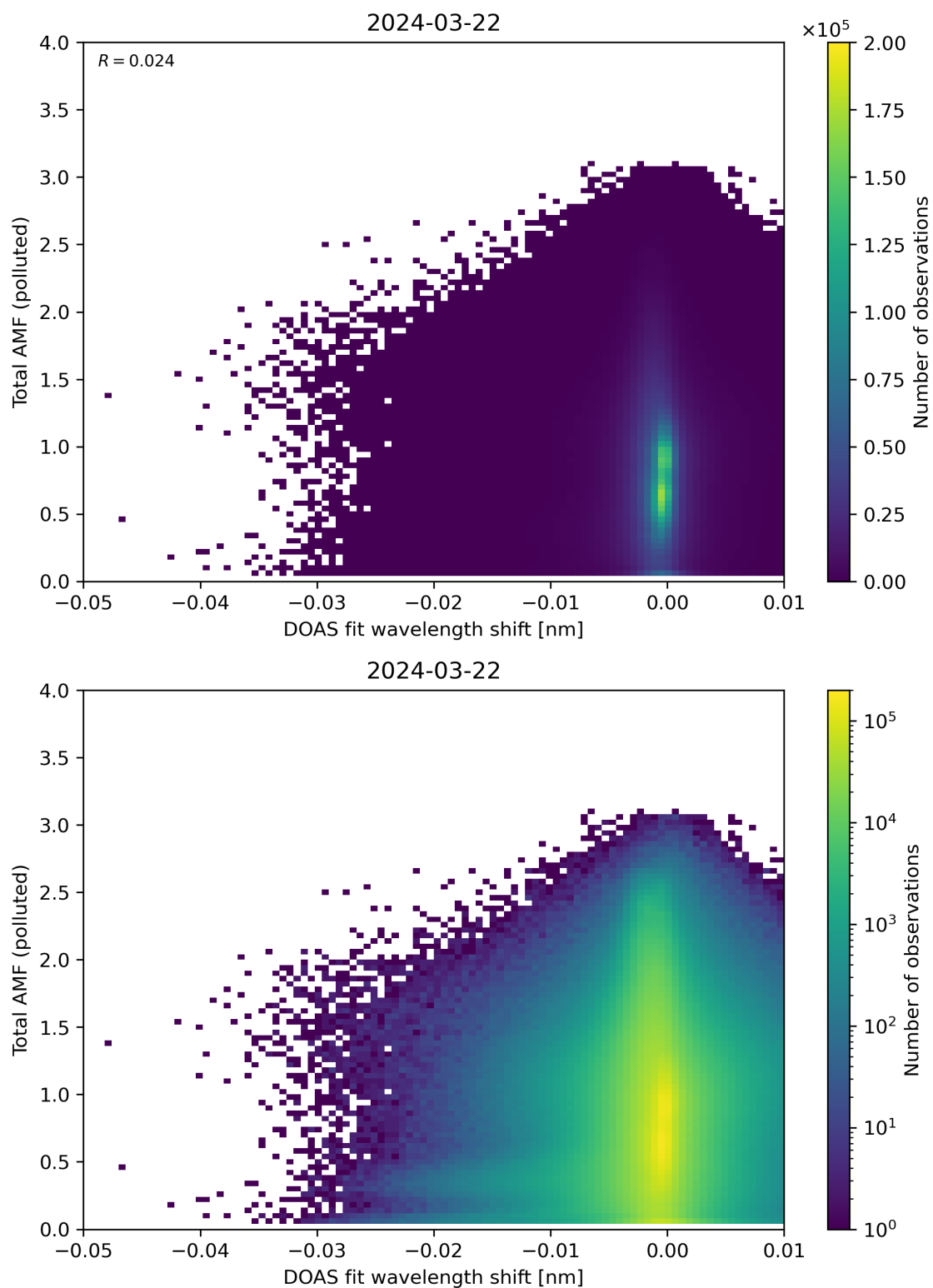
Figure 130: Scatter density plot of “DOAS fit wavelength shift” against “Total AMF (polluted)” for 2024-03-21 to 2024-03-22.
