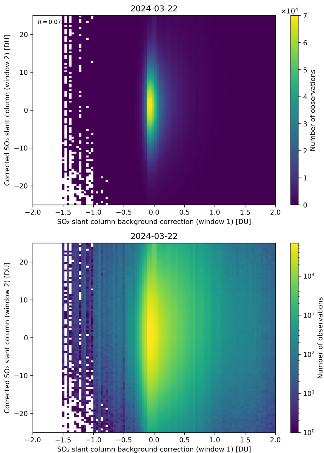
Figure 104: Scatter density plot of “SO 2 slant column background correction (window 1)” against “Corrected SO 2 slant column (window 2)” for 2024-03-21 to 2024-03-22.
