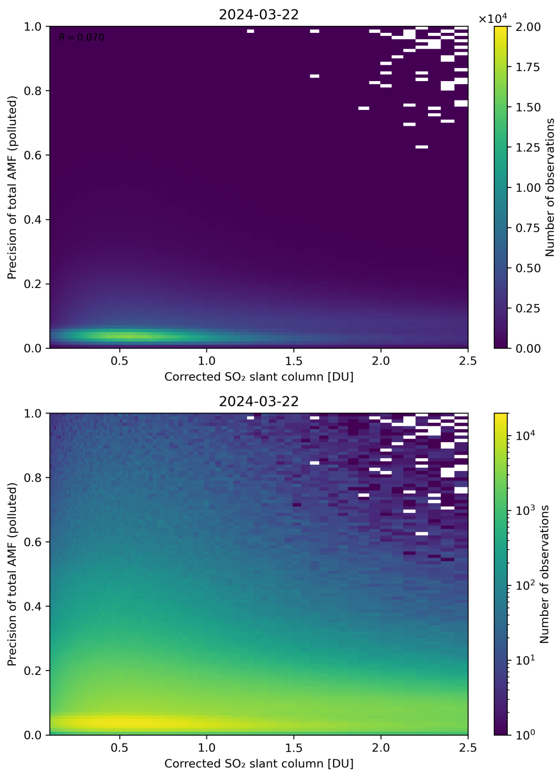
Figure 193: Scatter density plot of “Corrected SO 2 slant column” against “Precision of total AMF (polluted)” for 2024-03-21 to 2024-03-22.
