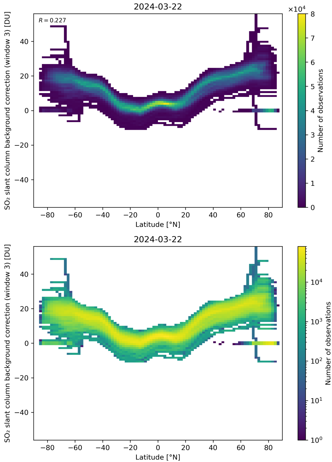
Figure 141: Scatter density plot of “Latitude” against “SO 2 slant column background correction (window 3)” for 2024-03-21 to 2024-03-22.
