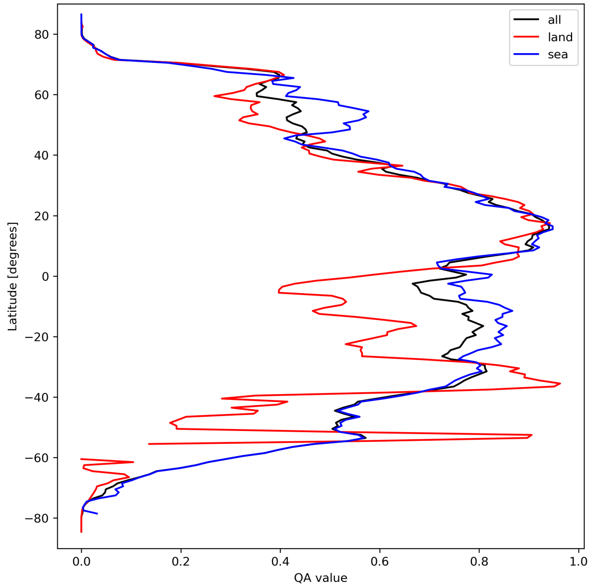
Figure 29: Zonal average of “QA value” for 2024-03-21 to 2024-03-22.
