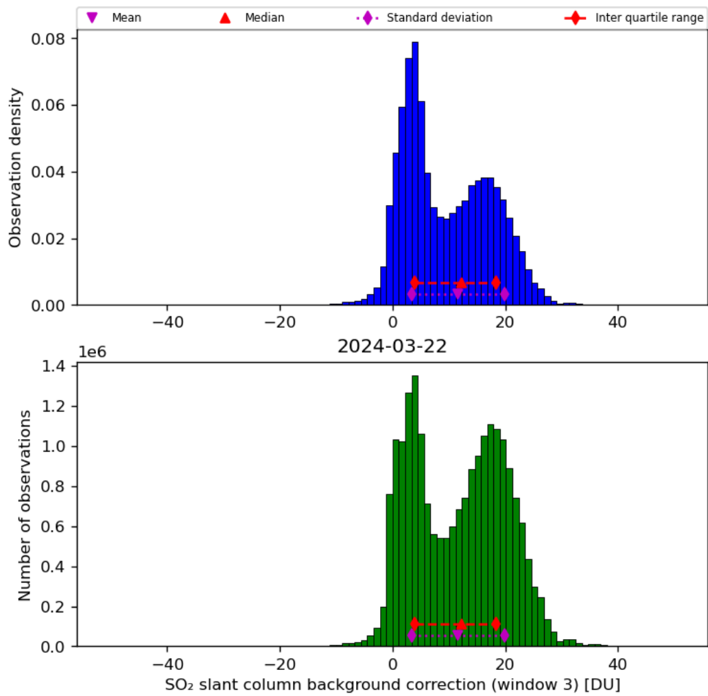
Figure 67: Histogram of “SO 2 slant column background correction (window 3)” for 2024-03-21 to 2024-03-22
