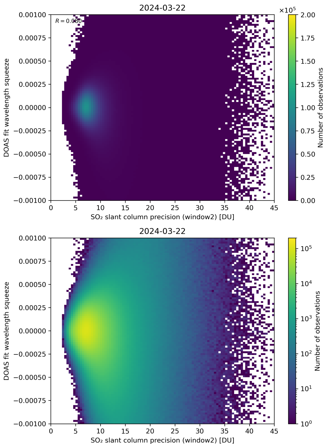
Figure 244: Scatter density plot of “SO 2 slant column precision (window2)” against “DOAS fit wavelength squeeze” for 2024-03-21 to 2024-03-22.
