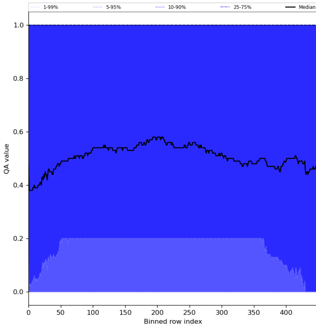
Figure 75: Along track statistics of “QA value” for 2024-03-21 to 2024-03-22
