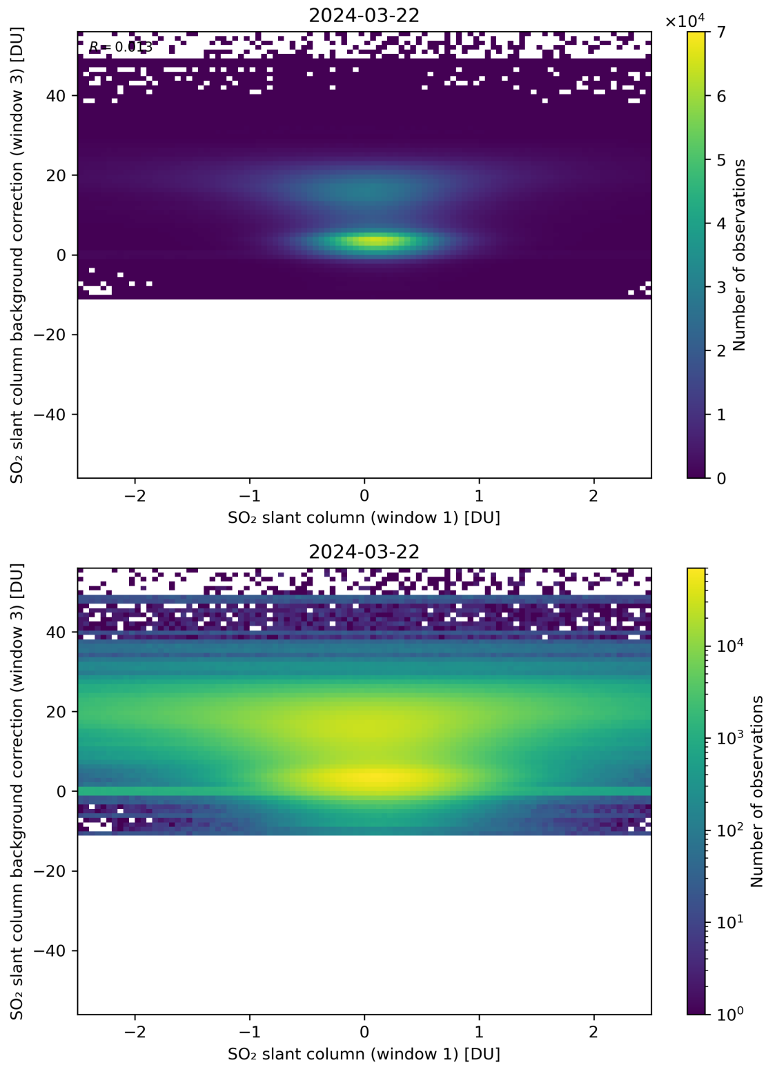
Figure 214: Scatter density plot of “SO 2 slant column (window 1)” against “SO 2 slant column background correction (window 3)” for 2024-03-21 to 2024-03-22.
