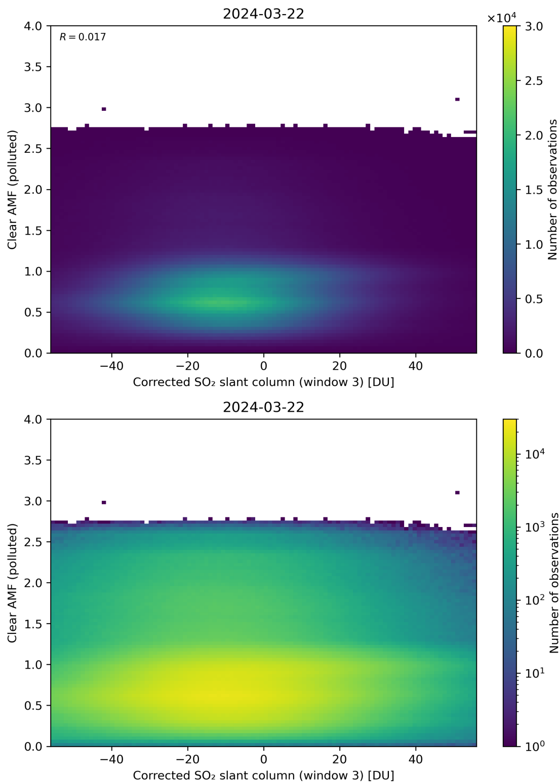
Figure 209: Scatter density plot of “Corrected SO 2 slant column (window 3)” against “Clear AMF (polluted)” for 2024-03-21 to 2024-03-22.
