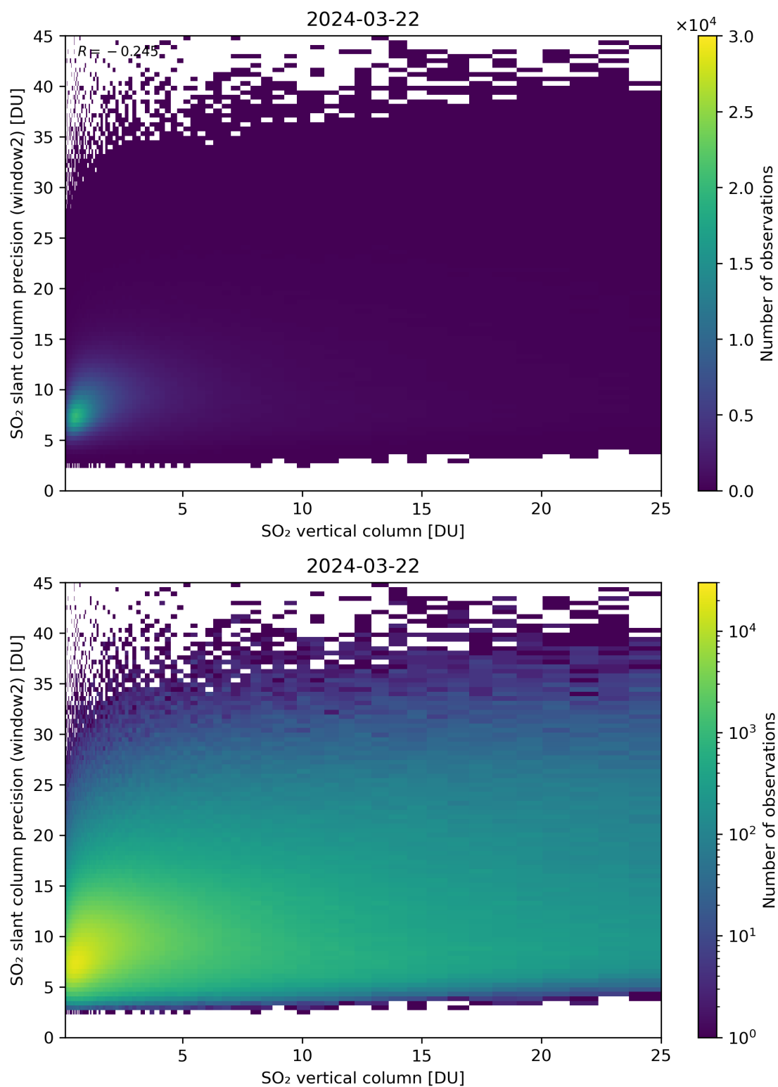
Figure 302: Scatter density plot of “SO 2 vertical column” against “SO 2 slant column precision (window2)” for 2024-03-21 to 2024-03-22.
