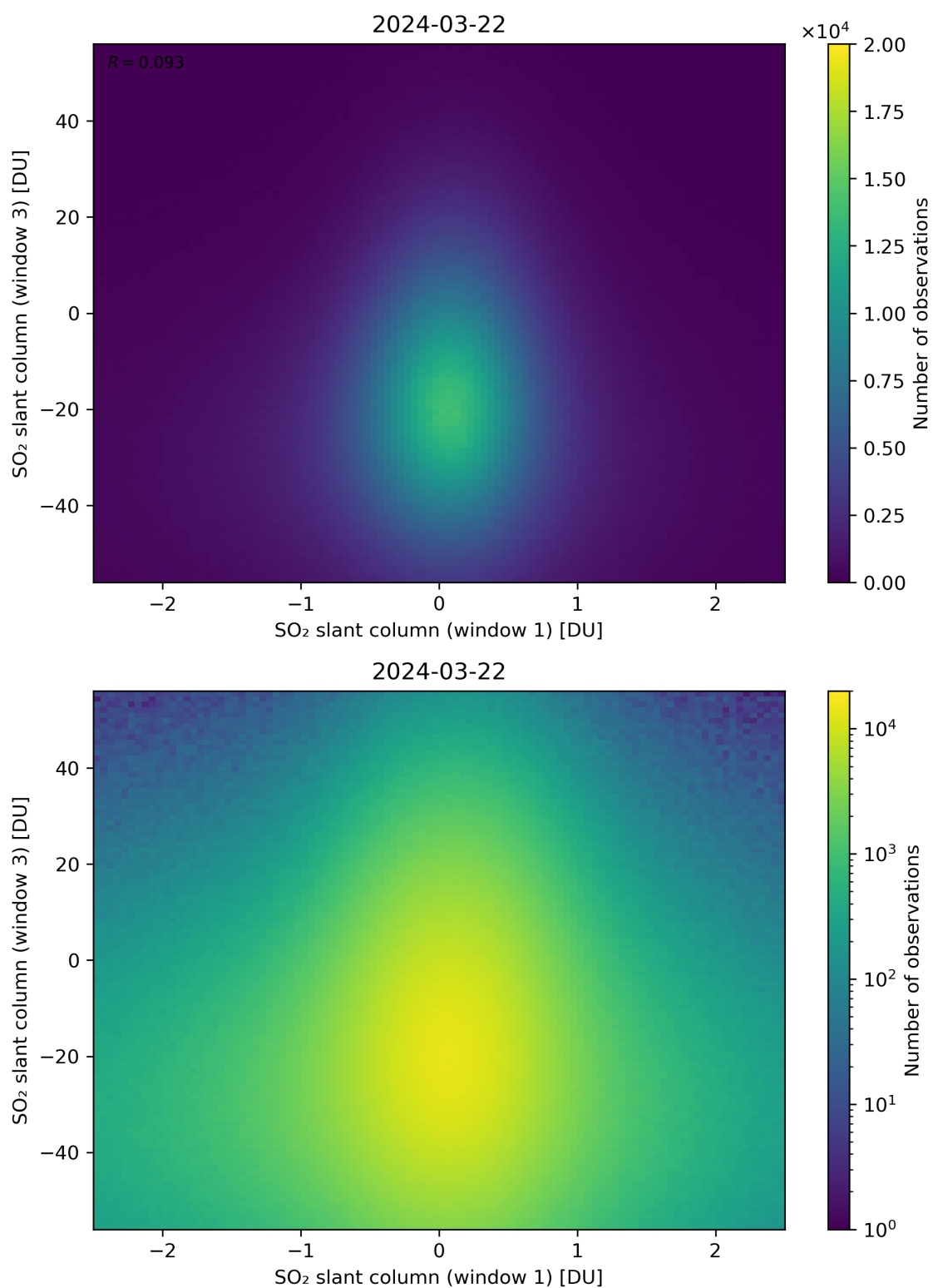
Figure 237: Scatter density plot of “SO 2 slant column (window 1)” against “SO 2 slant column (window 3)” for 2024-03-21 to 2024-03-22.
