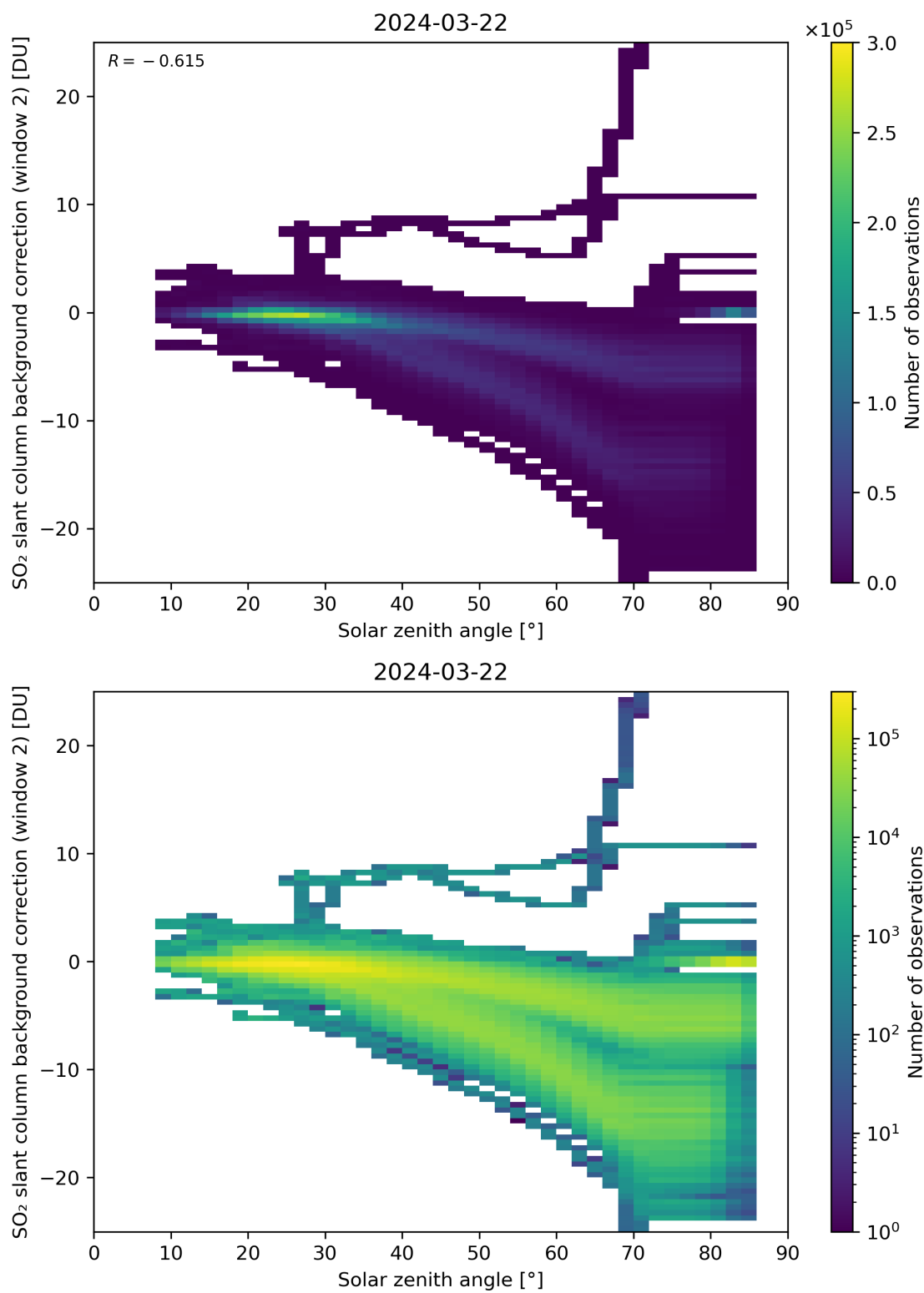
Figure 159: Scatter density plot of “Solar zenith angle” against “SO 2 slant column background correction (window 2)” for 2024-03-21 to 2024-03-22.
