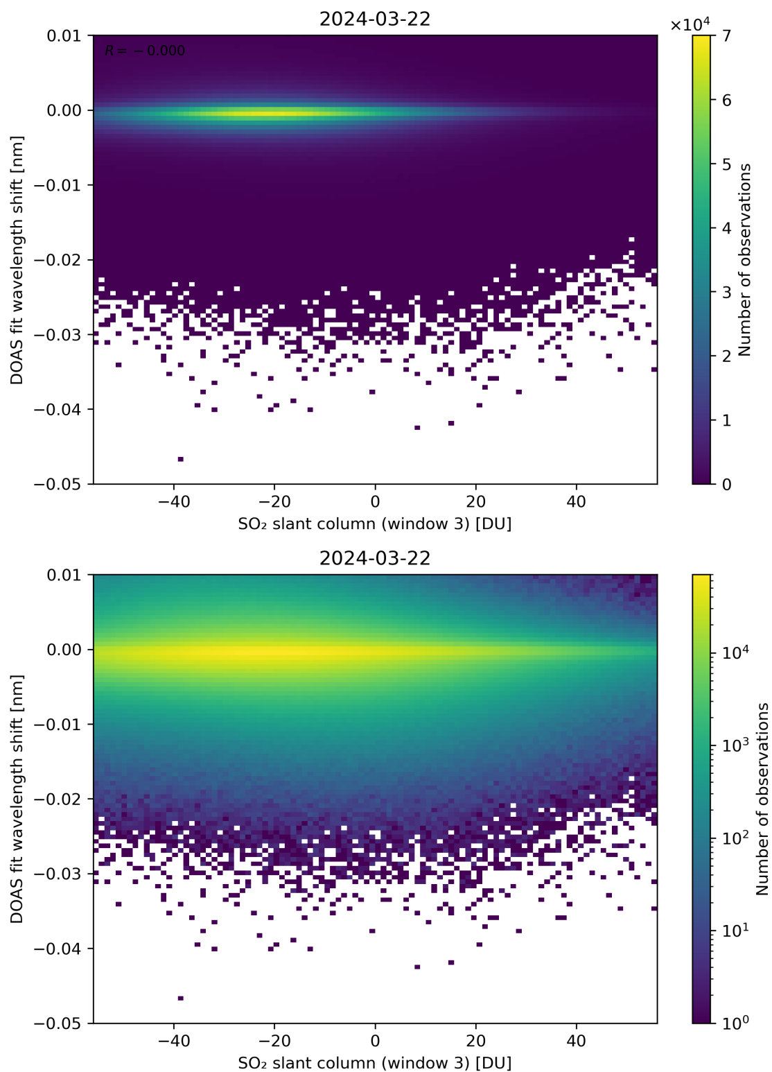
Figure 254: Scatter density plot of “SO 2 slant column (window 3)” against “DOAS fit wavelength shift” for 2024-03-21 to 2024-03-22.
