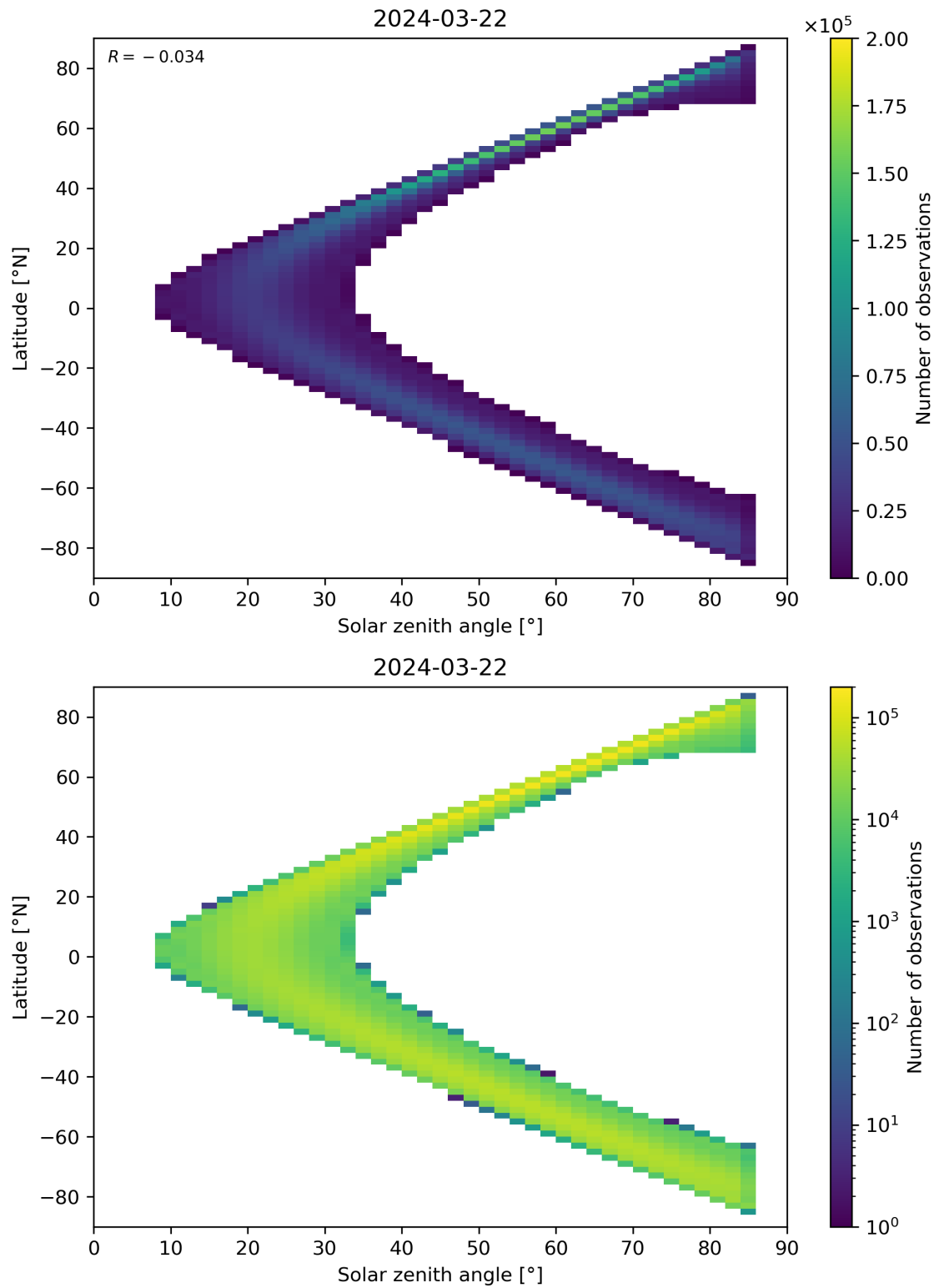
Figure 164: Scatter density plot of “Solar zenith angle” against “Latitude” for 2024-03-21 to 2024-03-22.
