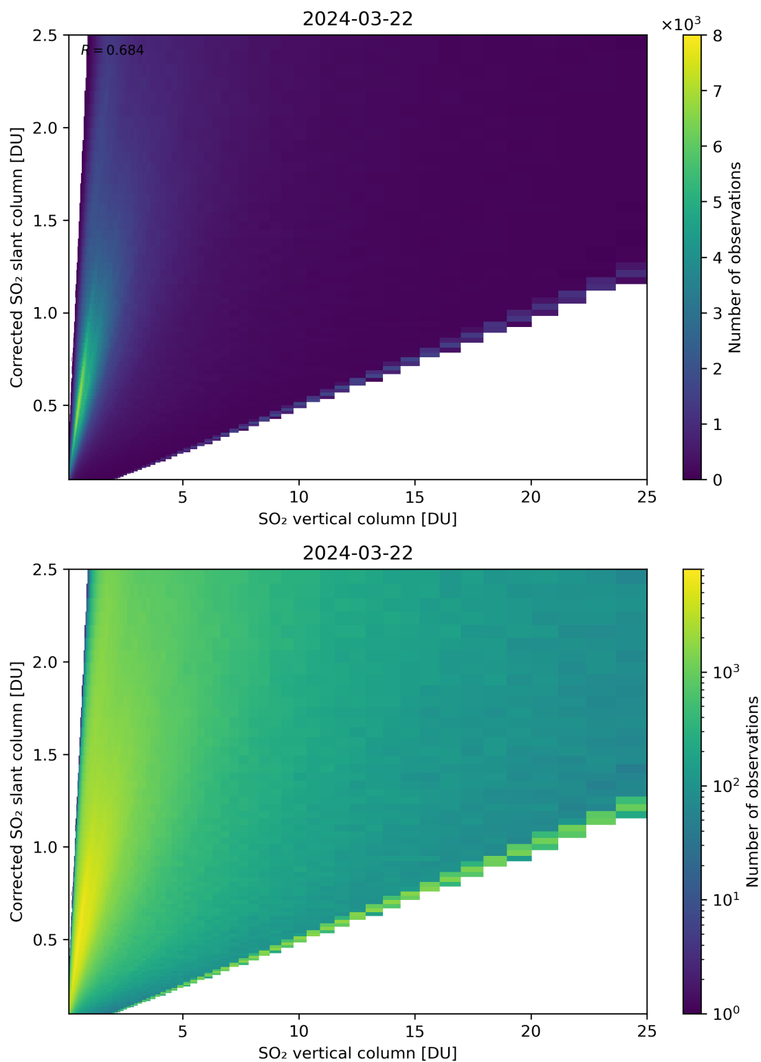
Figure 297: Scatter density plot of “SO 2 vertical column” against “Corrected SO 2 slant column” for 2024-03-21 to 2024-03-22.
