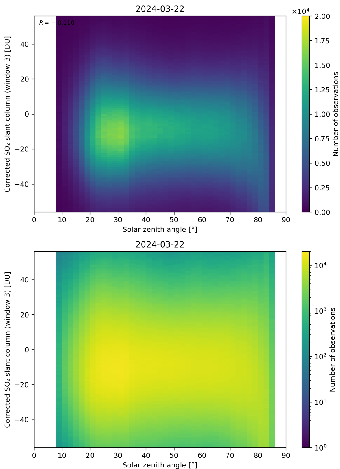
Figure 168: Scatter density plot of “Solar zenith angle” against “Corrected SO 2 slant column (window 3)” for 2024-03-21 to 2024-03-22.
