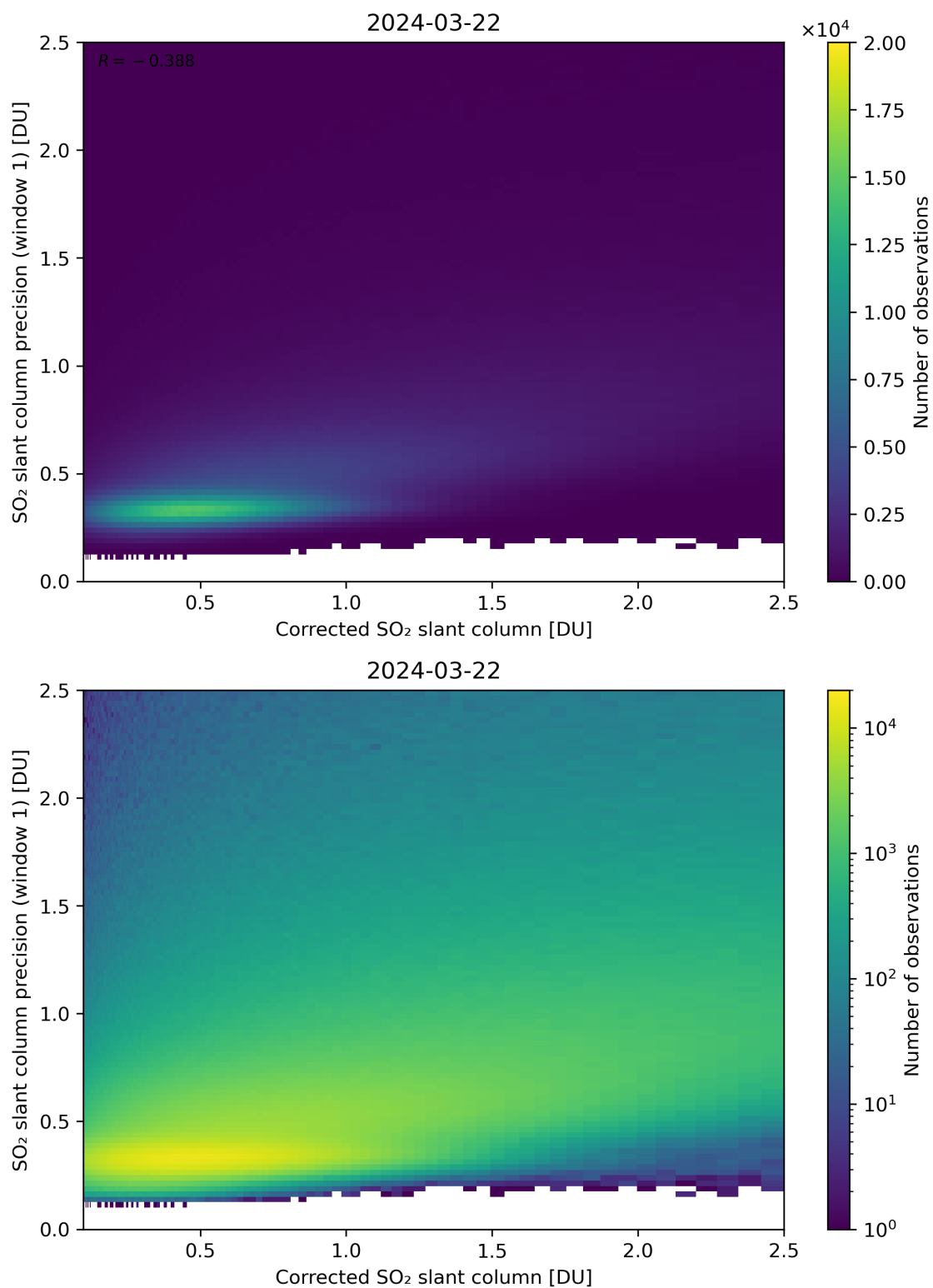
Figure 188: Scatter density plot of “Corrected SO 2 slant column” against “SO 2 slant column precision (window 1)” for 2024-03-21 to 2024-03-22.
