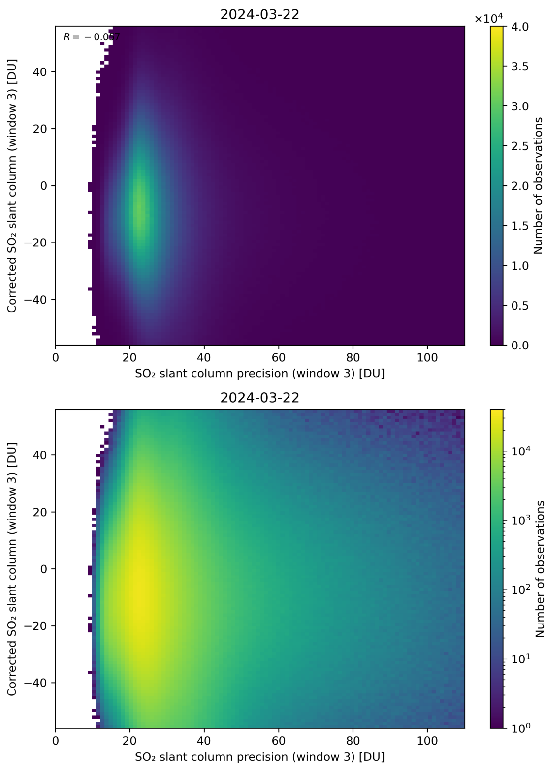
Figure 262: Scatter density plot of “SO 2 slant column precision (window 3)” against “Corrected SO 2 slant column (window 3)” for 2024-03-21 to 2024-03-22.
