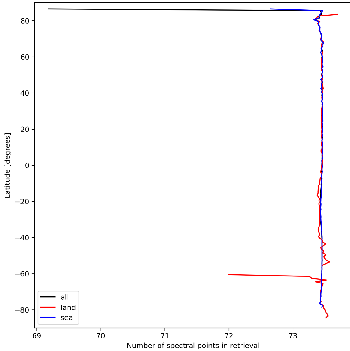
Figure 51: Zonal average of “Number of spectral points in retrieval” for 2024-03-21 to 2024-03-22.
