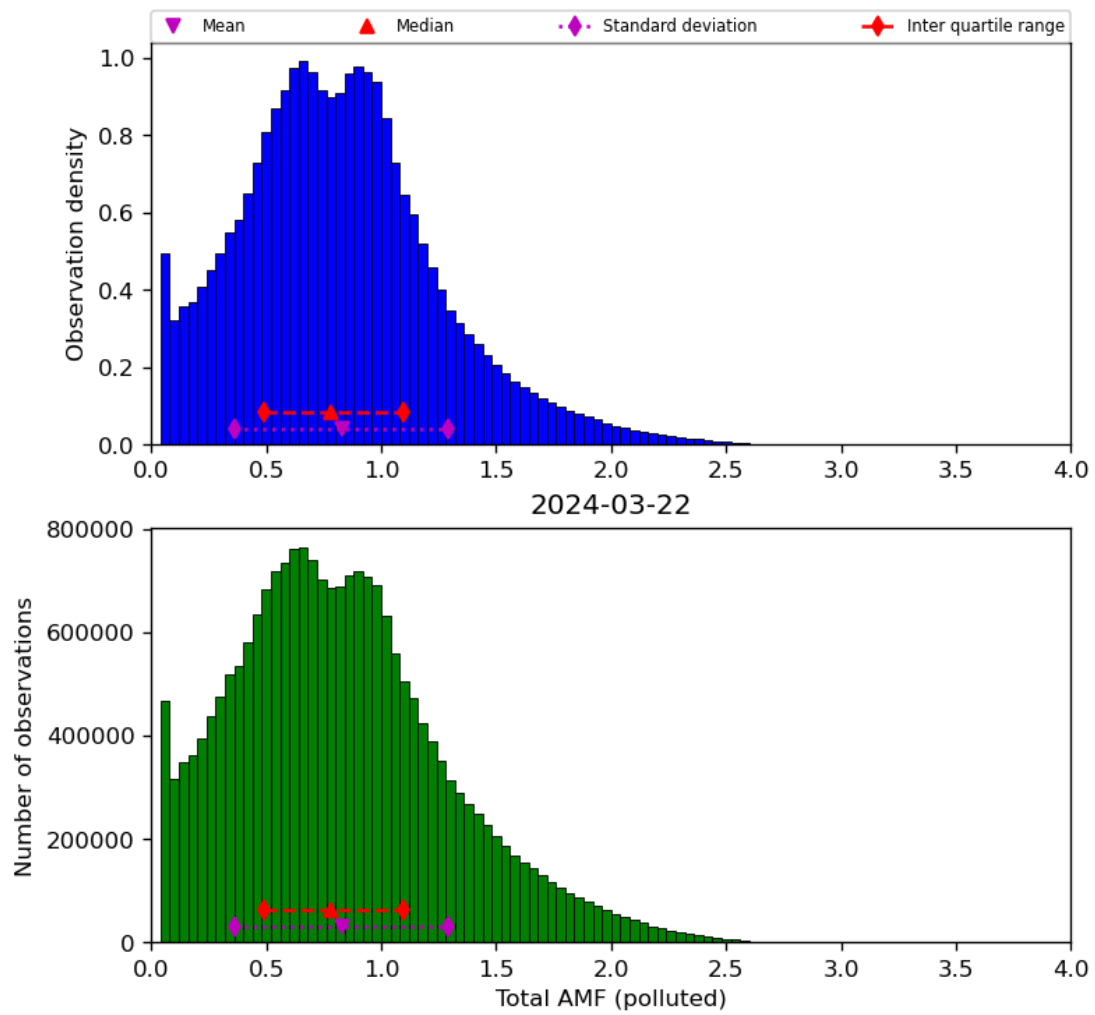
Figure 71: Histogram of “Total AMF (polluted)” for 2024-03-21 to 2024-03-22
