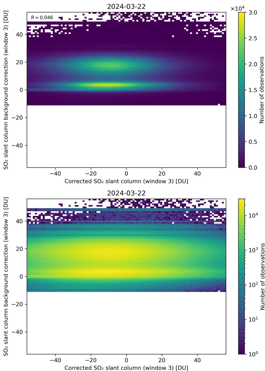
Figure 205: Scatter density plot of “Corrected SO 2 slant column (window 3)” against “SO 2 slant column background correction (window 3)” for 2024-03-21 to 2024-03-22.
