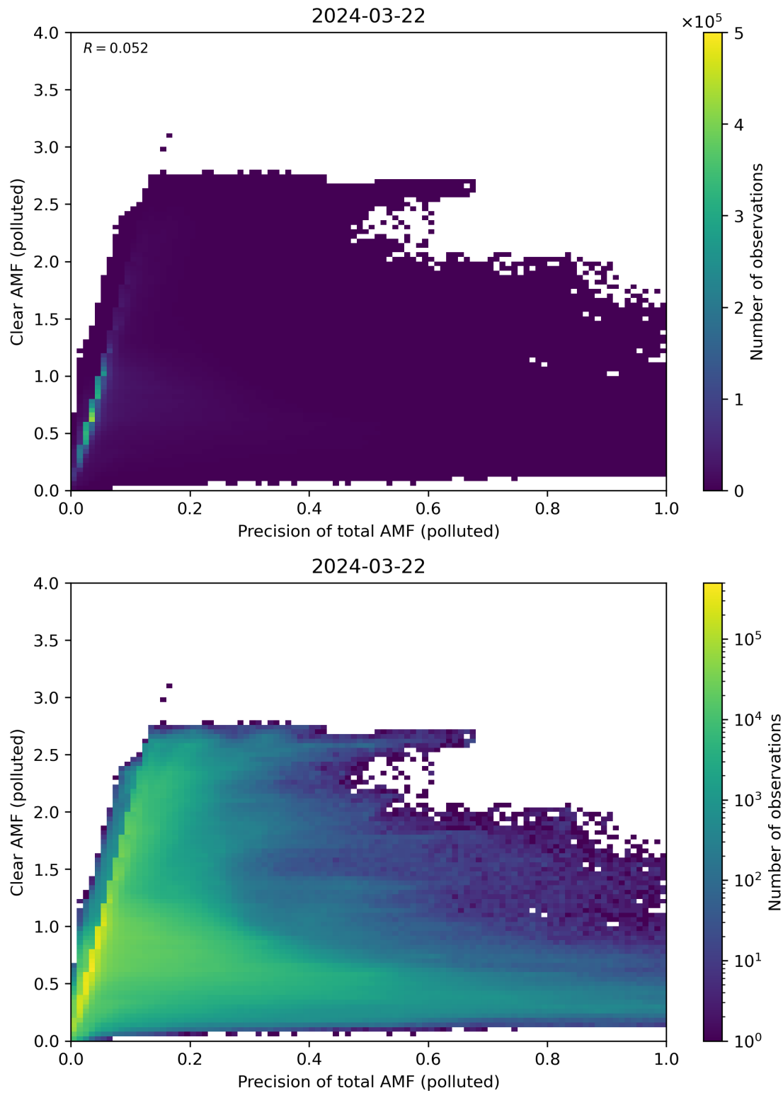
Figure 270: Scatter density plot of “Precision of total AMF (polluted)” against “Clear AMF (polluted)” for 2024-03-21 to 2024-03-22.
