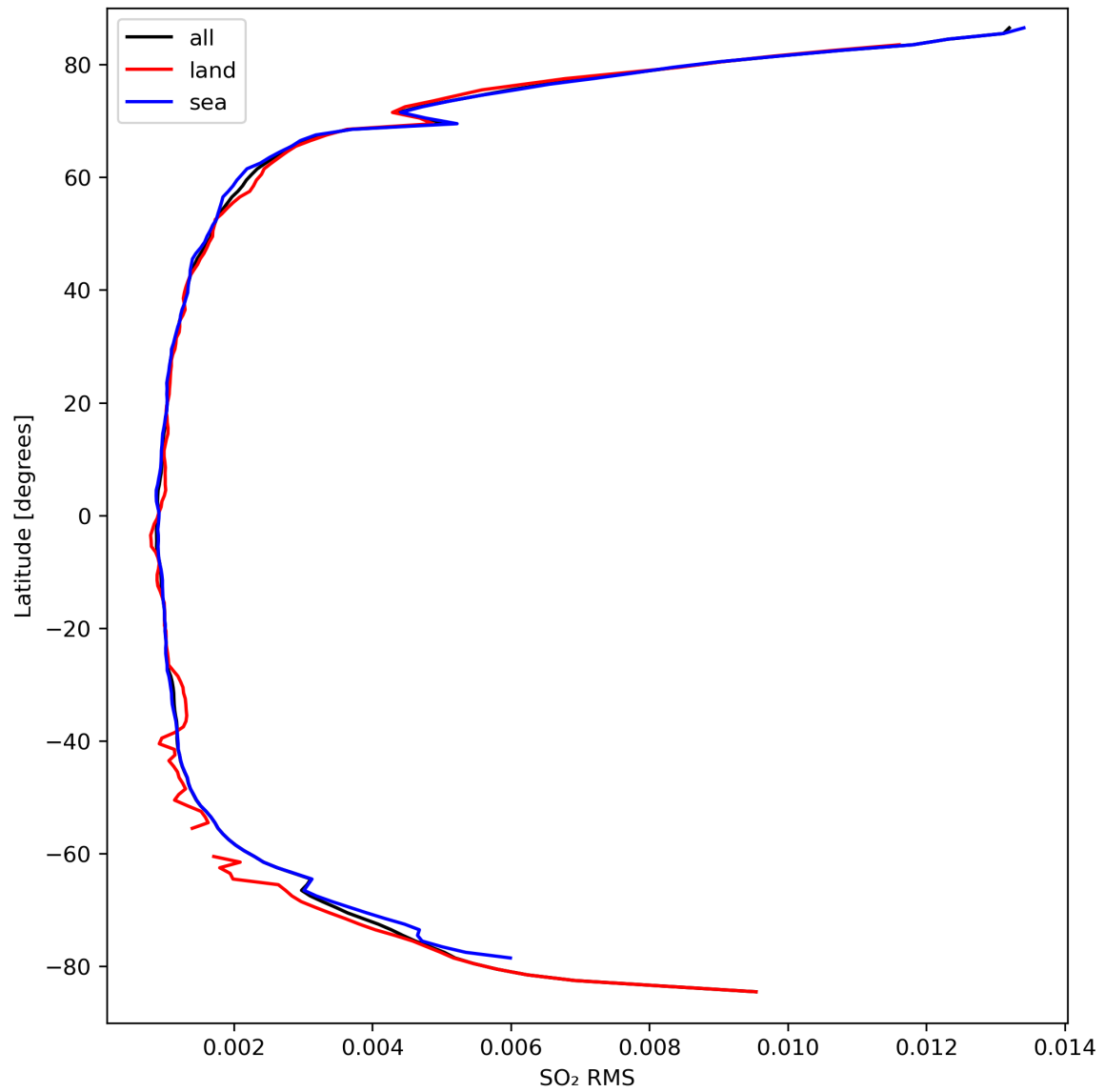
Figure 47: Zonal average of “SO 2 RMS” for 2024-03-21 to 2024-03-22.
