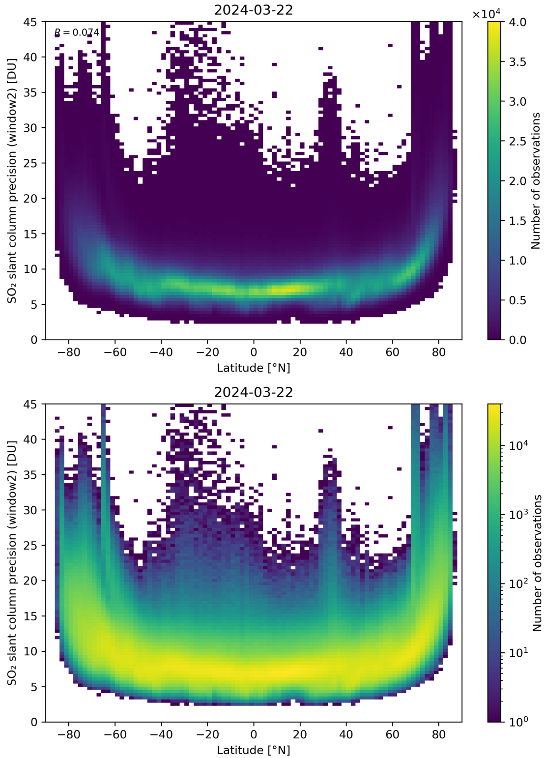
Figure 151: Scatter density plot of “Latitude” against “SO 2 slant column precision (window2)” for 2024-03-21 to 2024-03-22.
