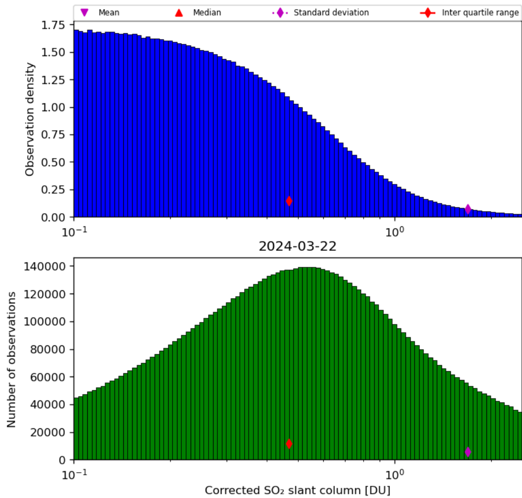
Figure 55: Histogram of “Corrected SO 2 slant column” for 2024-03-21 to 2024-03-22
