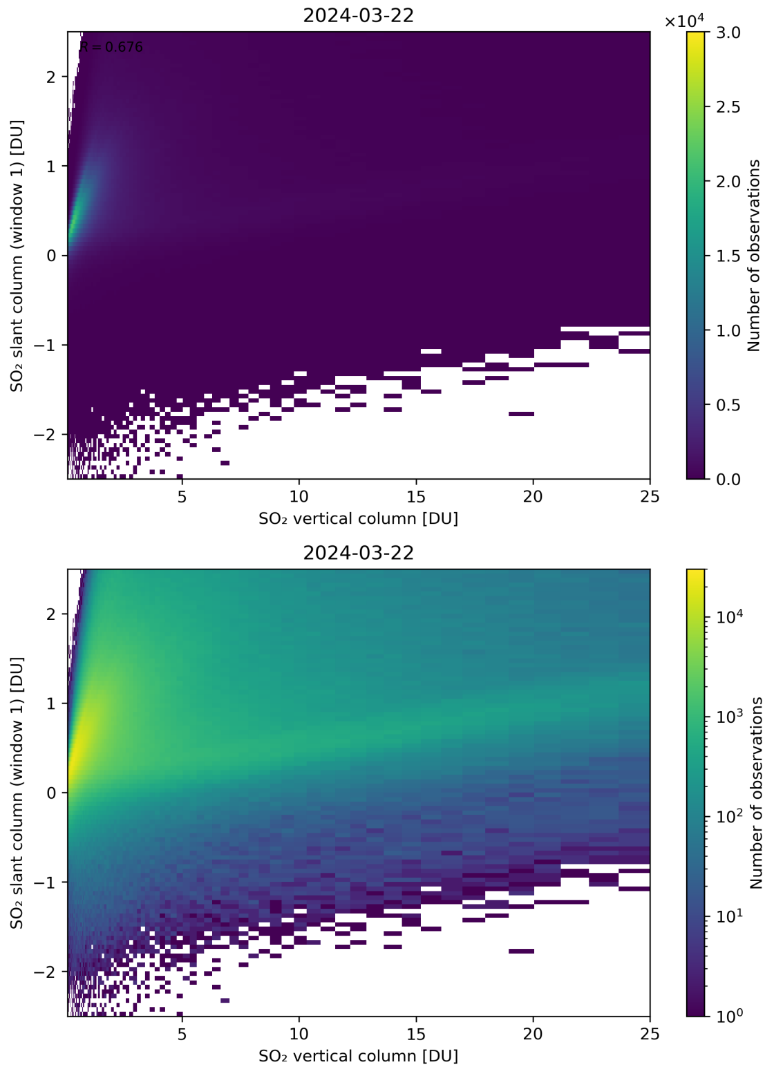
Figure 300: Scatter density plot of “SO 2 vertical column” against “SO 2 slant column (window 1)” for 2024-03-21 to 2024-03-22.
