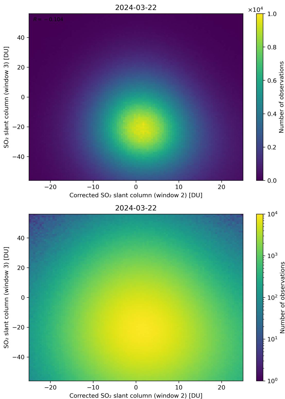
Figure 201: Scatter density plot of “Corrected SO 2 slant column (window 2)” against “SO 2 slant column (window 3)” for 2024-03-21 to 2024-03-22.
