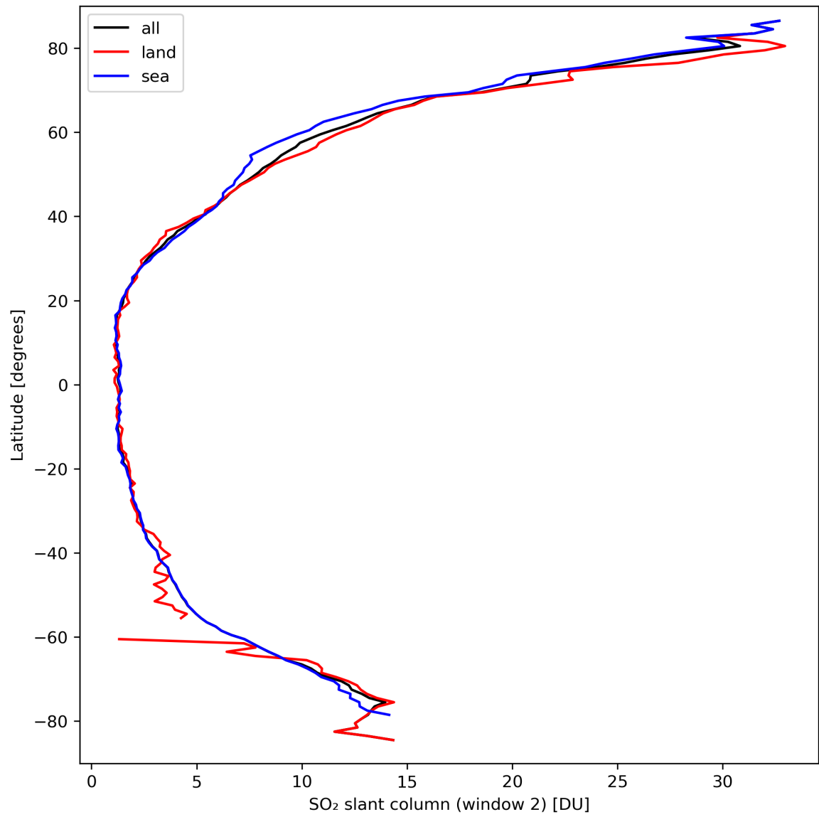
Figure 37: Zonal average of “SO 2 slant column (window 2)” for 2024-03-21 to 2024-03-22.
