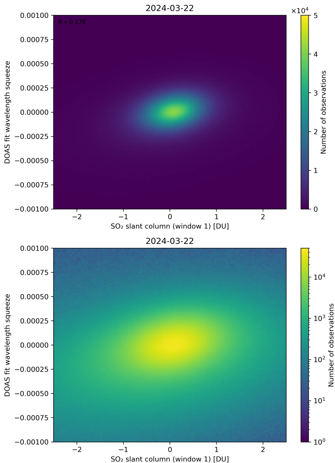
Figure 216: Scatter density plot of “SO 2 slant column (window 1)” against “DOAS fit wavelength squeeze” for 2024-03-21 to 2024-03-22.
