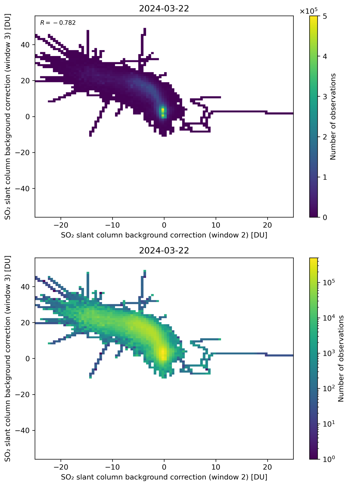
Figure 111: Scatter density plot of “SO 2 slant column background correction (window 2)” against “SO 2 slant column background correction (window 3)” for 2024-03-21 to 2024-03-22.
