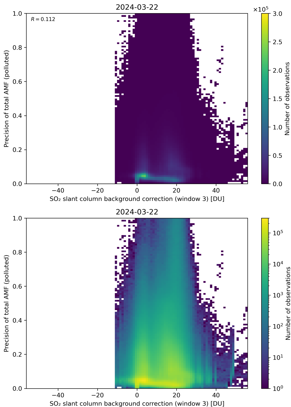
Figure 126: Scatter density plot of “SO 2 slant column background correction (window 3)” against “Precision of total AMF (polluted)” for 2024-03-21 to 2024-03-22.
