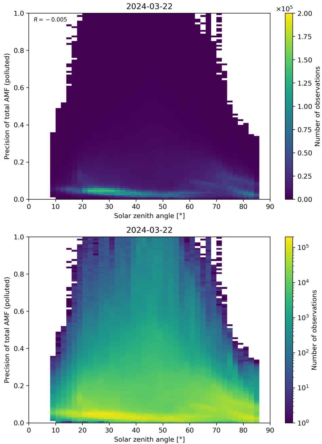
Figure 175: Scatter density plot of “Solar zenith angle” against “Precision of total AMF (polluted)” for 2024-03-21 to 2024-03-22.
