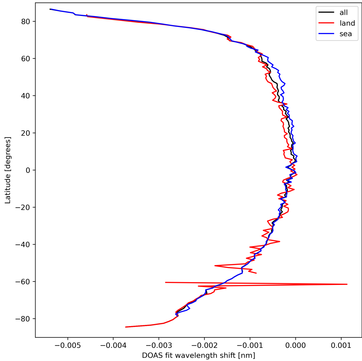
Figure 45: Zonal average of “DOAS fit wavelength shift” for 2024-03-21 to 2024-03-22.
