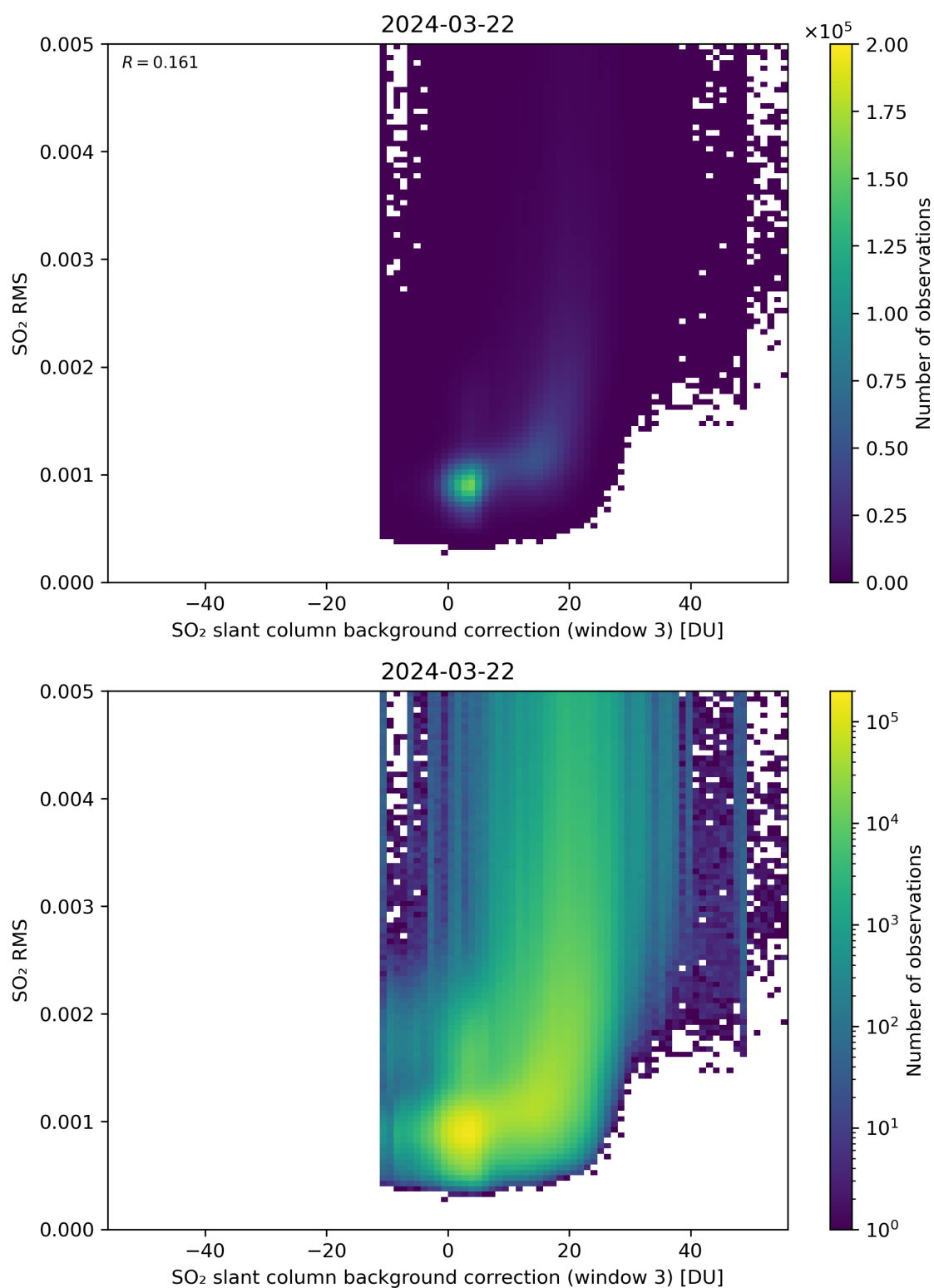
Figure 123: Scatter density plot of “SO 2 slant column background correction (window 3)” against “SO 2 RMS” for 2024-03-21 to 2024-03-22.
