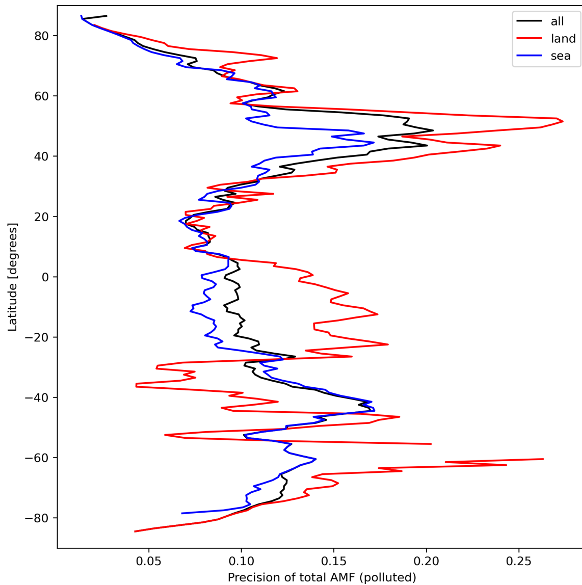
Figure 49: Zonal average of “Precision of total AMF (polluted)” for 2024-03-21 to 2024-03-22.
