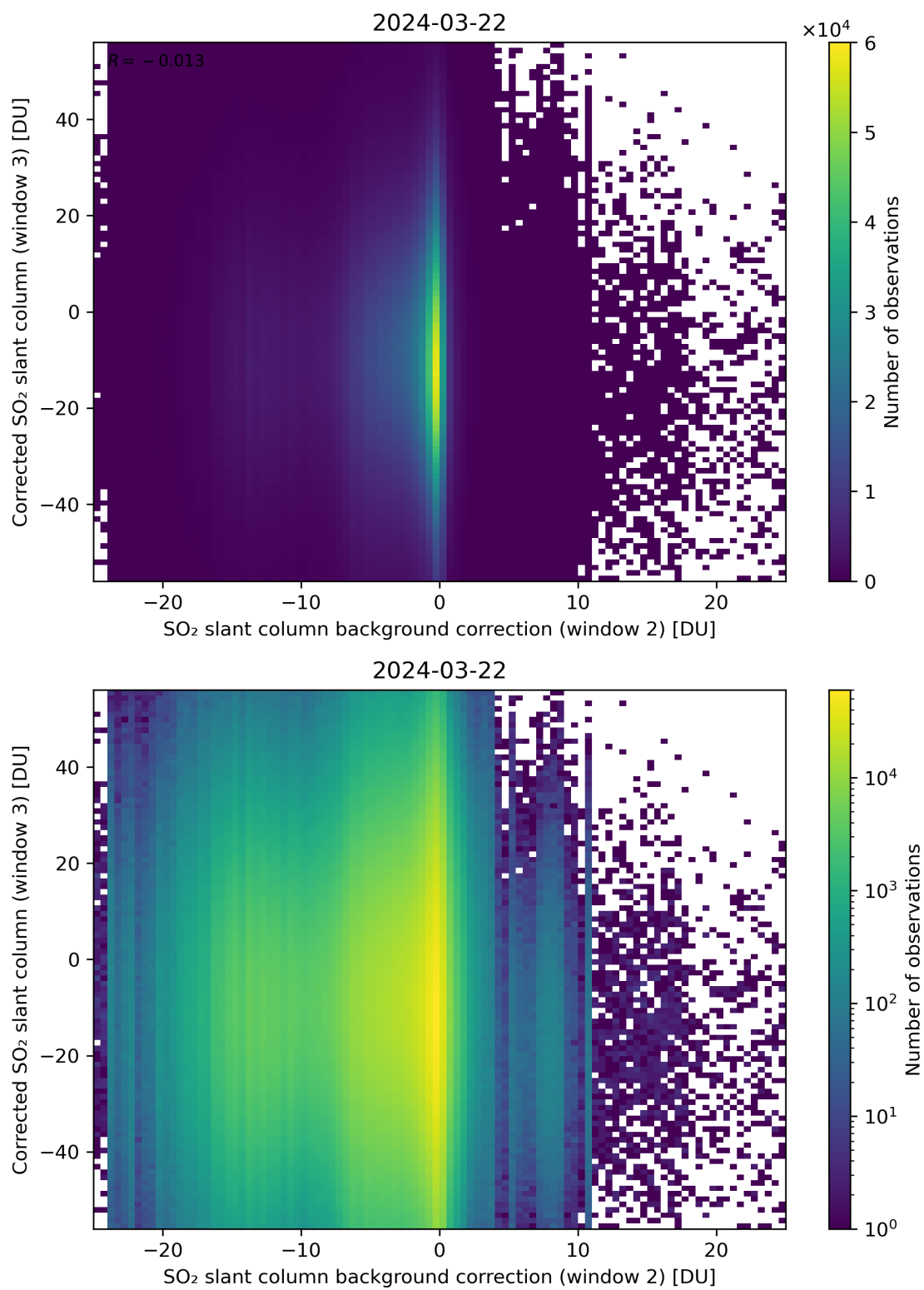
Figure 116: Scatter density plot of “SO 2 slant column background correction (window 2)” against “Corrected SO 2 slant column (window 3)” for 2024-03-21 to 2024-03-22.
