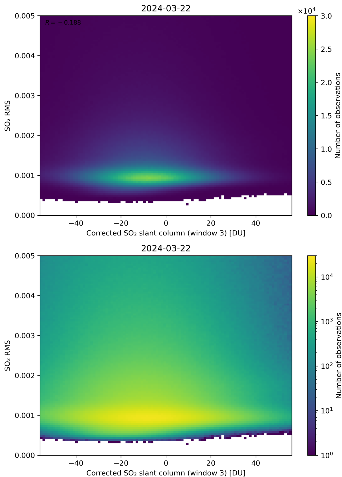
Figure 208: Scatter density plot of “Corrected SO 2 slant column (window 3)” against “SO 2 RMS” for 2024-03-21 to 2024-03-22.
