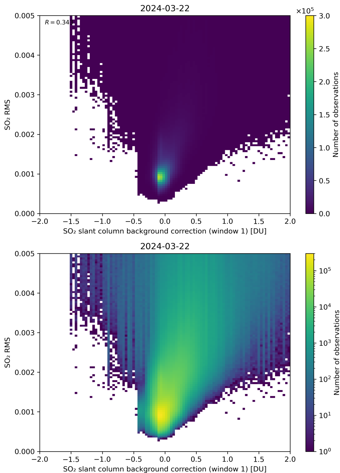
Figure 102: Scatter density plot of “SO 2 slant column background correction (window 1)” against “SO 2 RMS” for 2024-03-21 to 2024-03-22.
