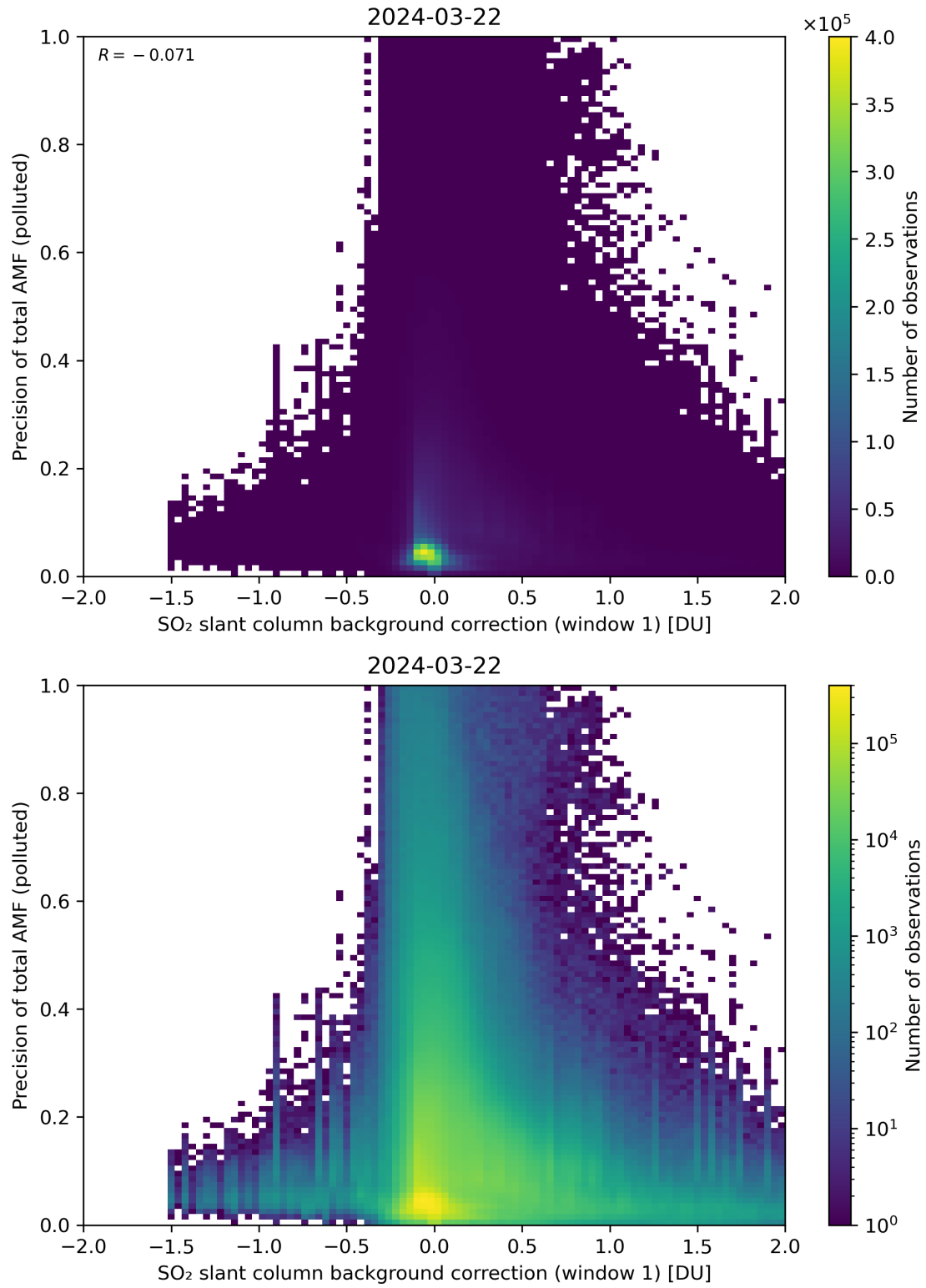
Figure 110: Scatter density plot of “SO 2 slant column background correction (window 1)” against “Precision of total AMF (polluted)” for 2024-03-21 to 2024-03-22.
