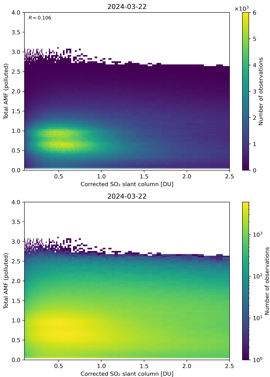
Figure 192: Scatter density plot of “Corrected SO 2 slant column” against “Total AMF (polluted)” for 2024-03-21 to 2024-03-22.
