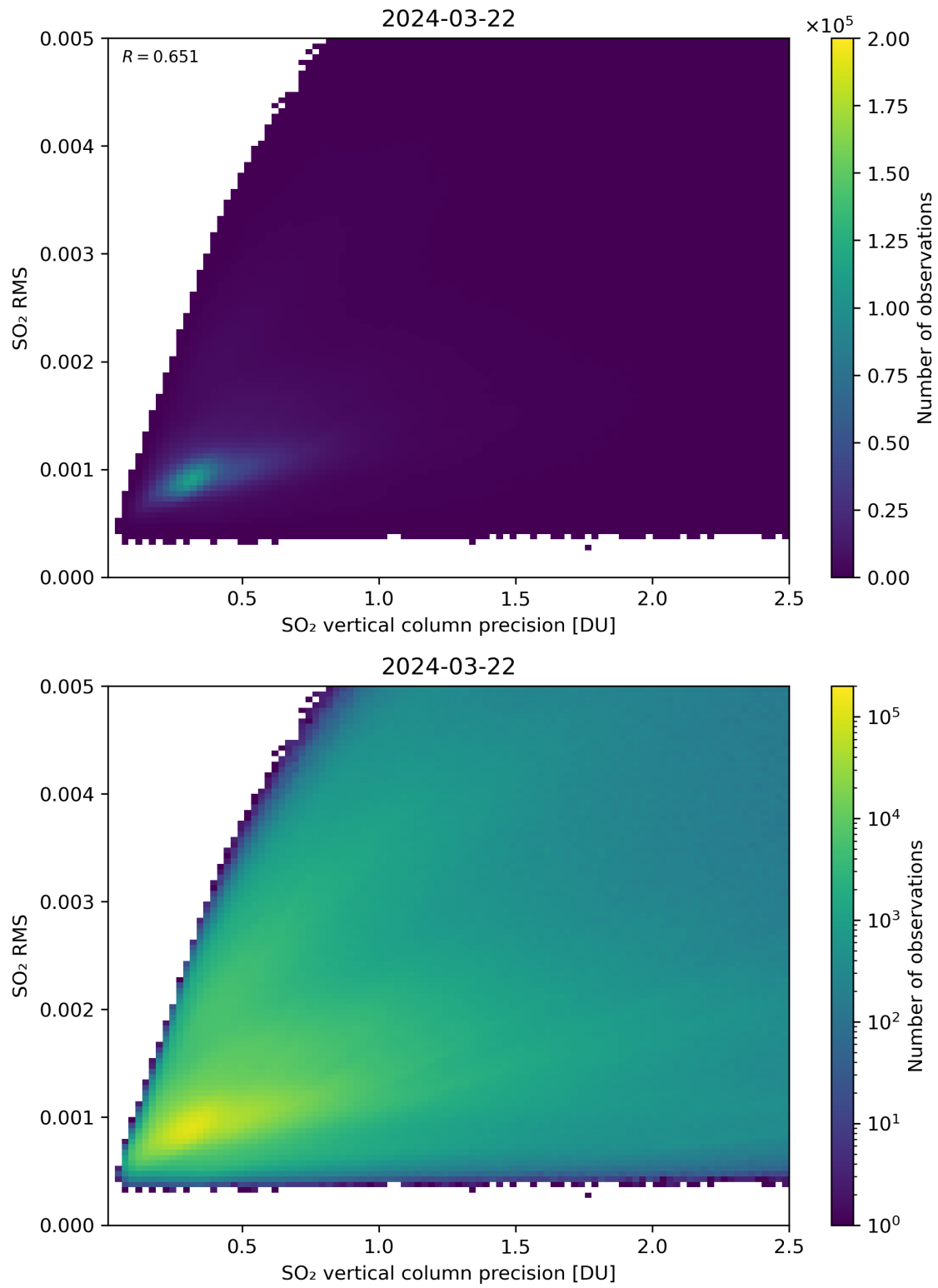
Figure 284: Scatter density plot of “SO 2 vertical column precision” against “SO 2 RMS” for 2024-03-21 to 2024-03-22.
