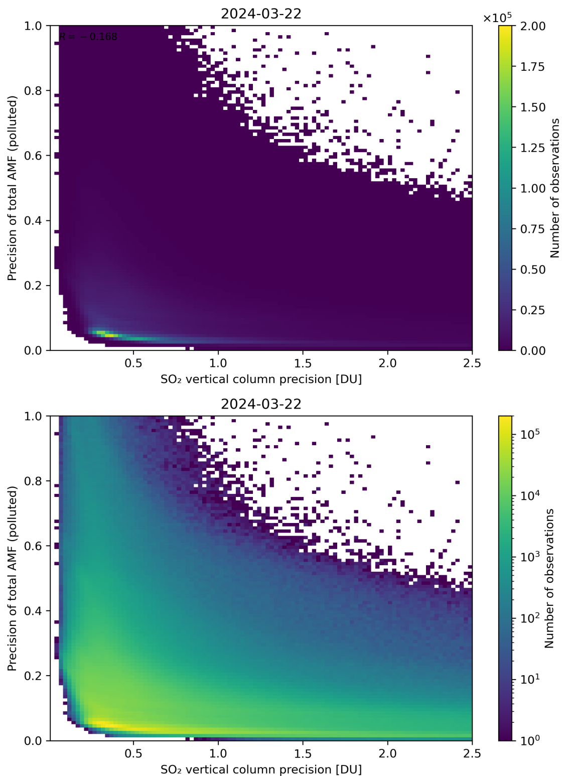
Figure 295: Scatter density plot of “SO 2 vertical column precision” against “Precision of total AMF (polluted)” for 2024-03-21 to 2024-03-22.
