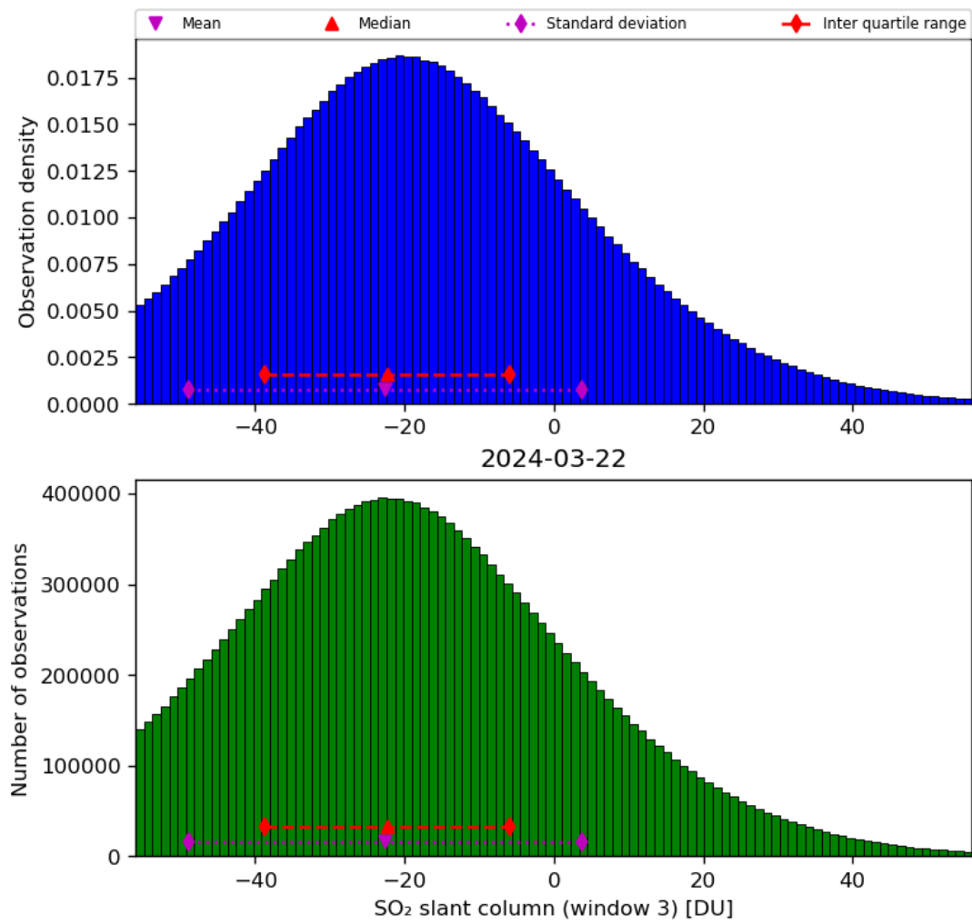
Figure 64: Histogram of “SO 2 slant column (window 3)” for 2024-03-21 to 2024-03-22
