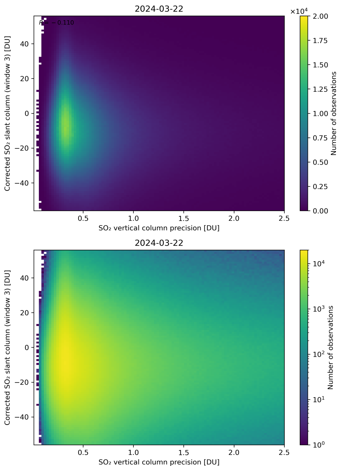
Figure 288: Scatter density plot of “SO 2 vertical column precision” against “Corrected SO 2 slant column (window 3)” for 2024-03-21 to 2024-03-22.
