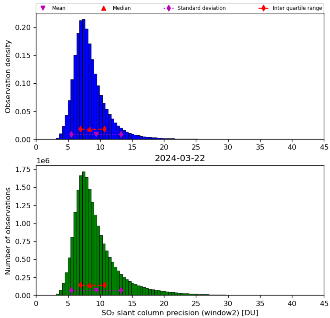
Figure 61: Histogram of “SO 2 slant column precision (window2)” for 2024-03-21 to 2024-03-22
