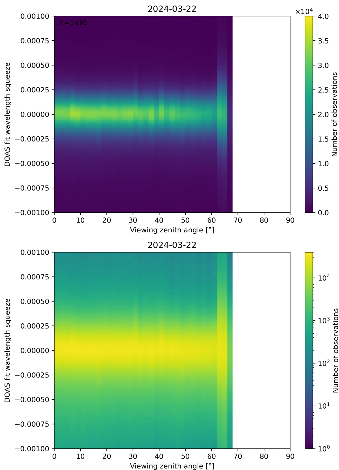
Figure 312: Scatter density plot of “Viewing zenith angle” against “DOAS fit wavelength squeeze” for 2024-03-21 to 2024-03-22.
