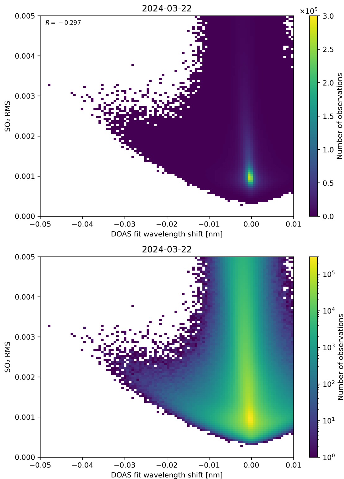
Figure 128: Scatter density plot of “DOAS fit wavelength shift” against “SO 2 RMS” for 2024-03-21 to 2024-03-22.
