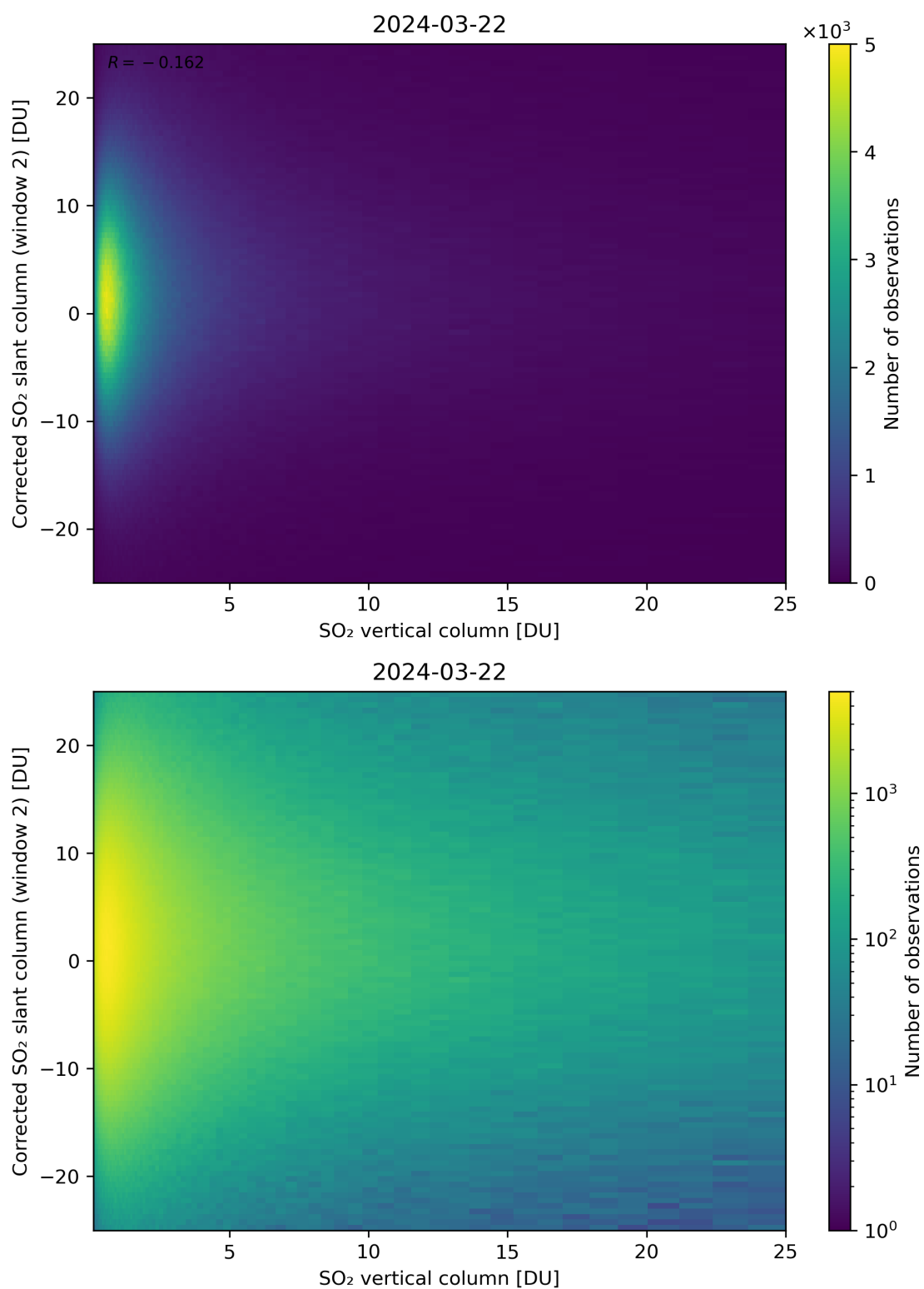
Figure 298: Scatter density plot of “SO 2 vertical column” against “Corrected SO 2 slant column (window 2)” for 2024-03-21 to 2024-03-22.
