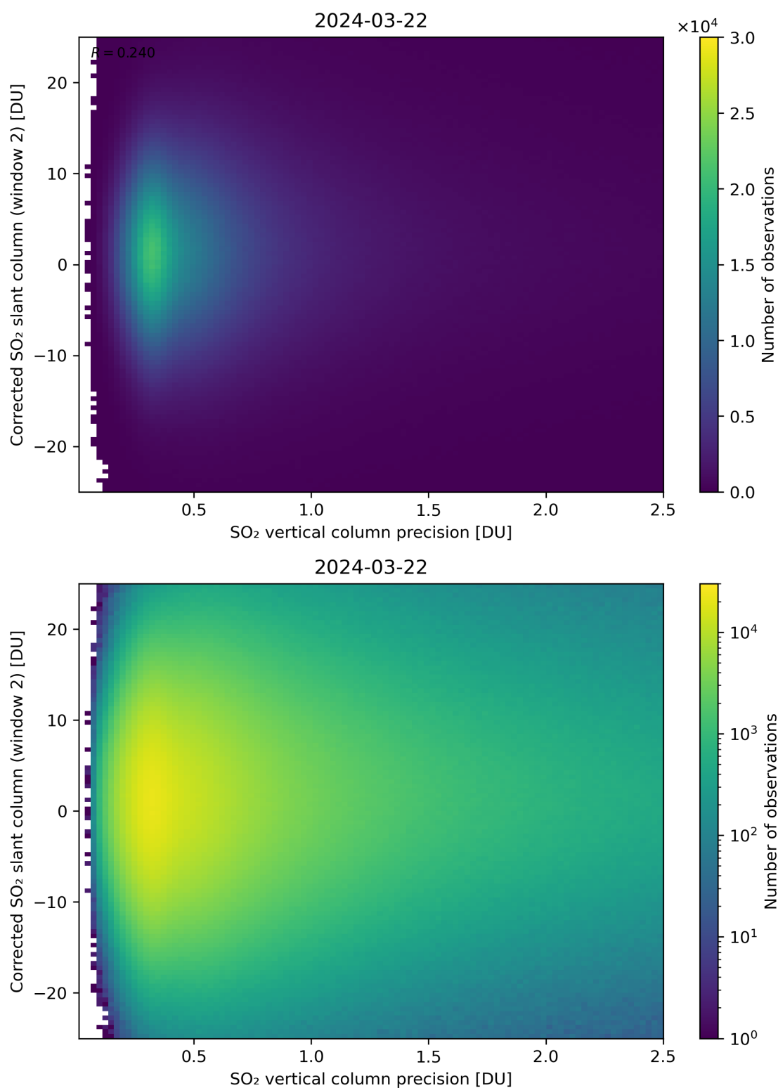
Figure 287: Scatter density plot of “SO 2 vertical column precision” against “Corrected SO 2 slant column (window 2)” for 2024-03-21 to 2024-03-22.
