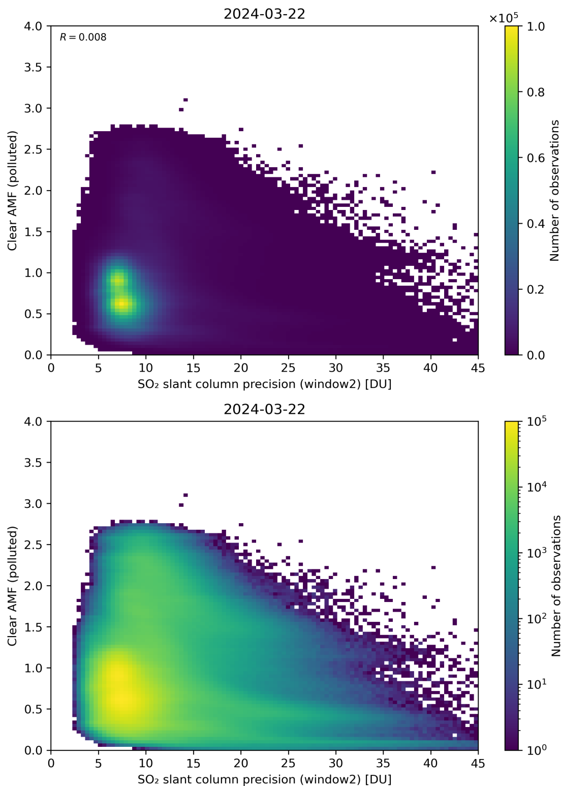
Figure 246: Scatter density plot of “SO 2 slant column precision (window2)” against “Clear AMF (polluted)” for 2024-03-21 to 2024-03-22.
