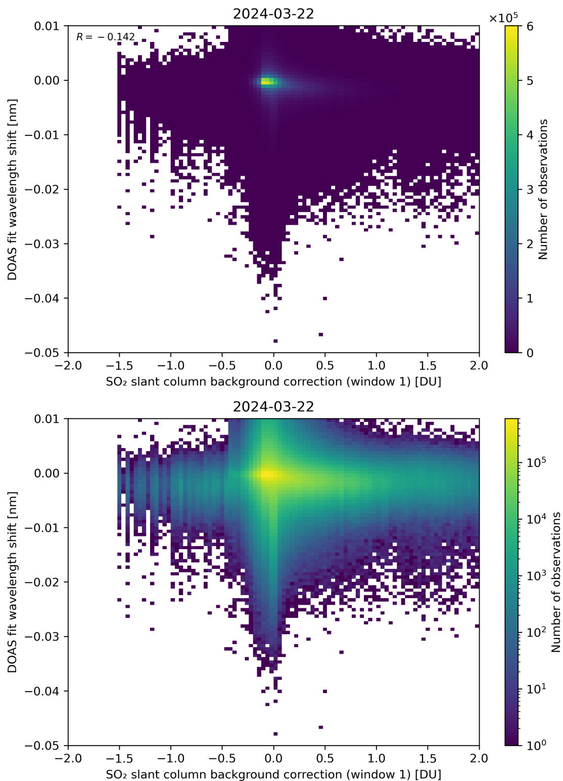
Figure 100: Scatter density plot of “SO 2 slant column background correction (window 1)” against “DOAS fit wavelength shift” for 2024-03-21 to 2024-03-22.
