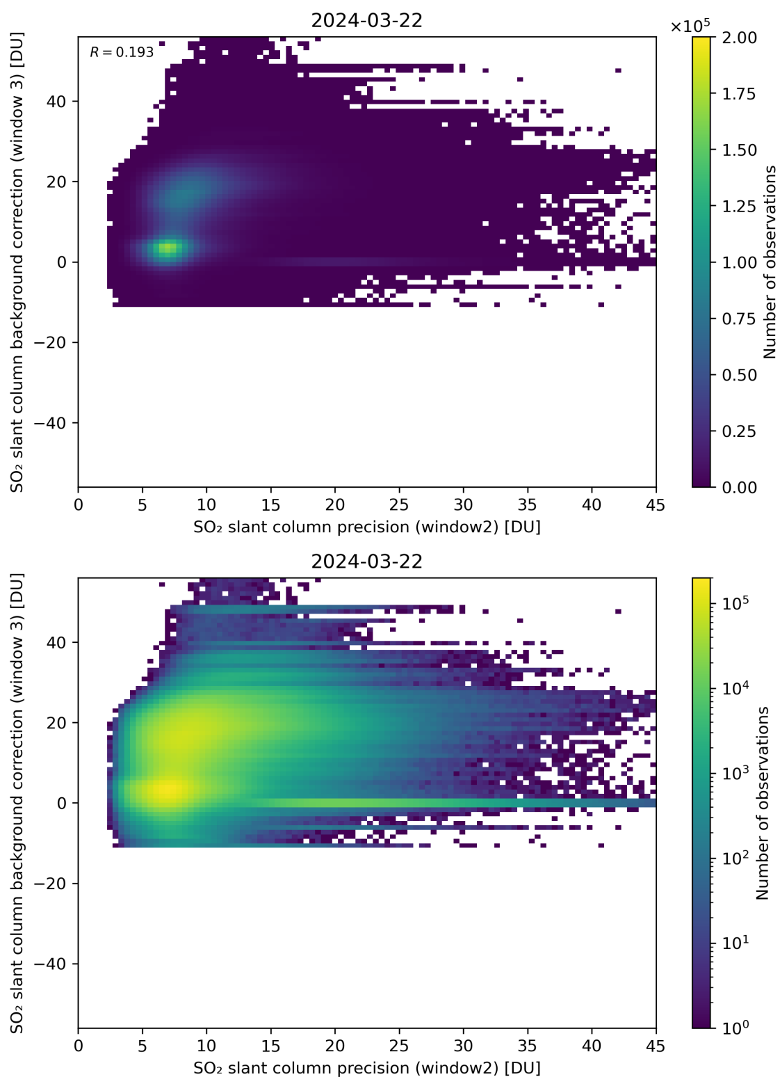
Figure 242: Scatter density plot of “SO 2 slant column precision (window2)” against “SO 2 slant column background correction (window 3)” for 2024-03-21 to 2024-03-22.
