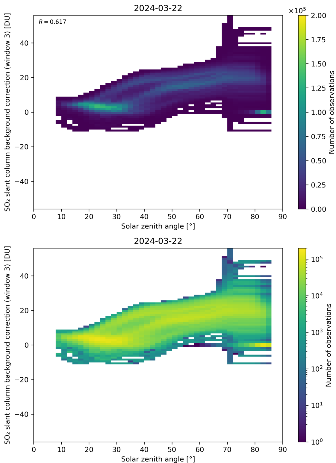
Figure 160: Scatter density plot of “Solar zenith angle” against “SO 2 slant column background correction (window 3)” for 2024-03-21 to 2024-03-22.
