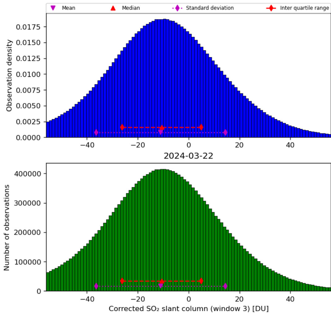
Figure 66: Histogram of “Corrected SO 2 slant column (window 3)” for 2024-03-21 to 2024-03-22
