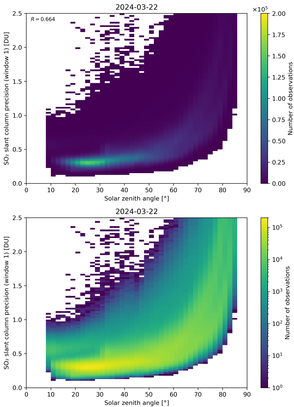
Figure 170: Scatter density plot of “Solar zenith angle” against “SO 2 slant column precision (window 1)” for 2024-03-21 to 2024-03-22.
