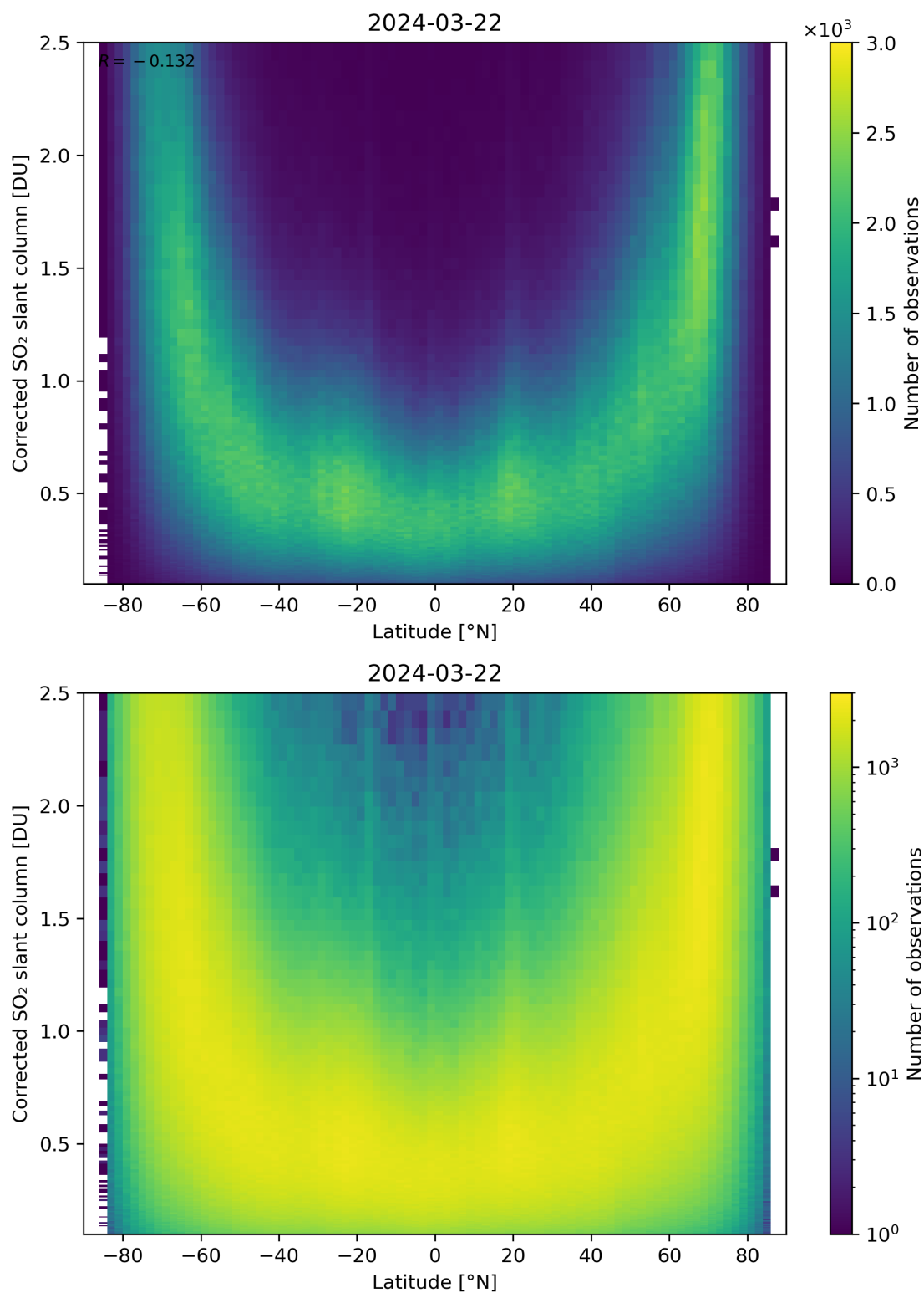
Figure 146: Scatter density plot of “Latitude” against “Corrected SO 2 slant column” for 2024-03-21 to 2024-03-22.
