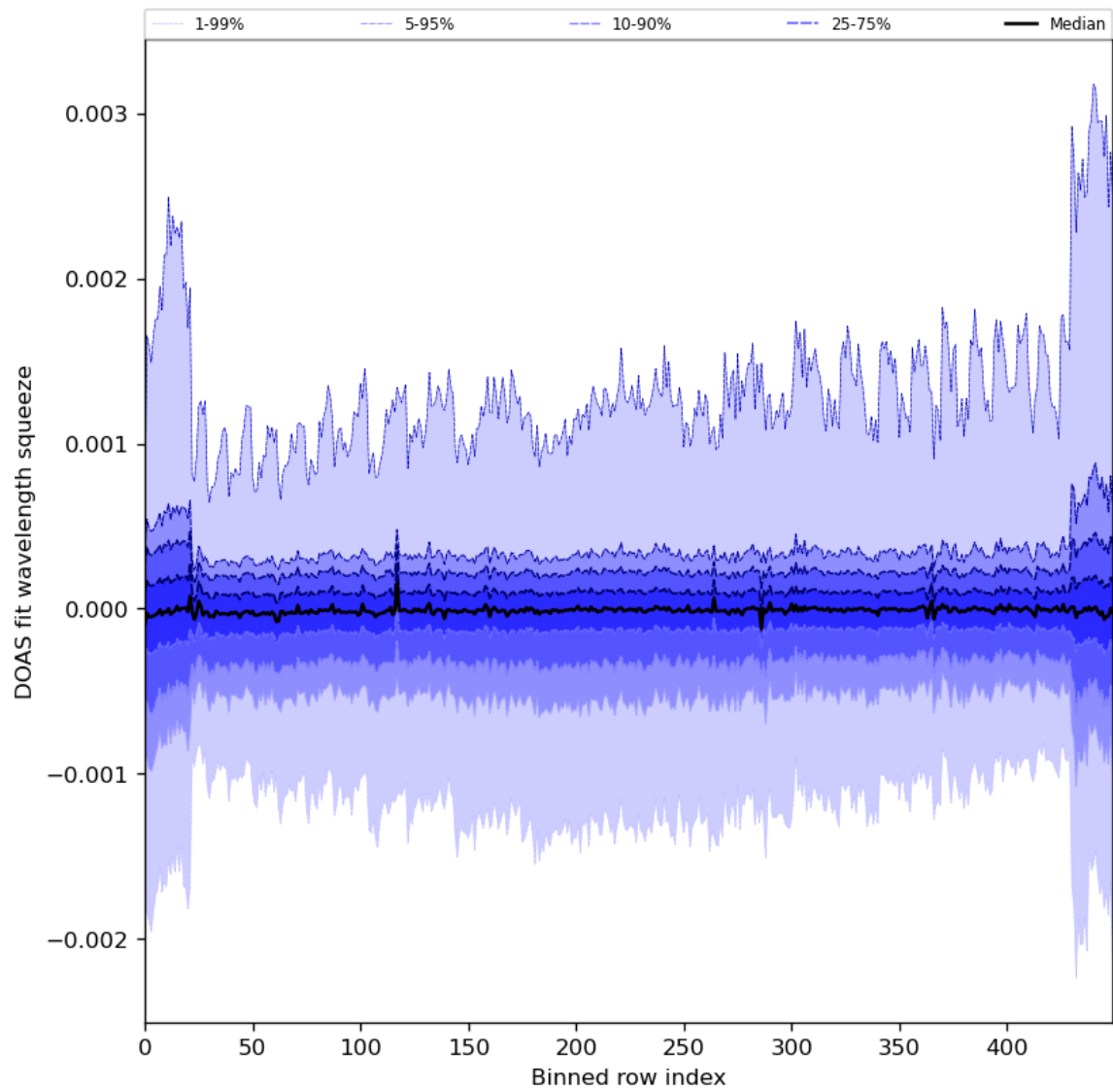
Figure 92: Along track statistics of “DOAS fit wavelength squeeze” for 2024-03-21 to 2024-03-22
