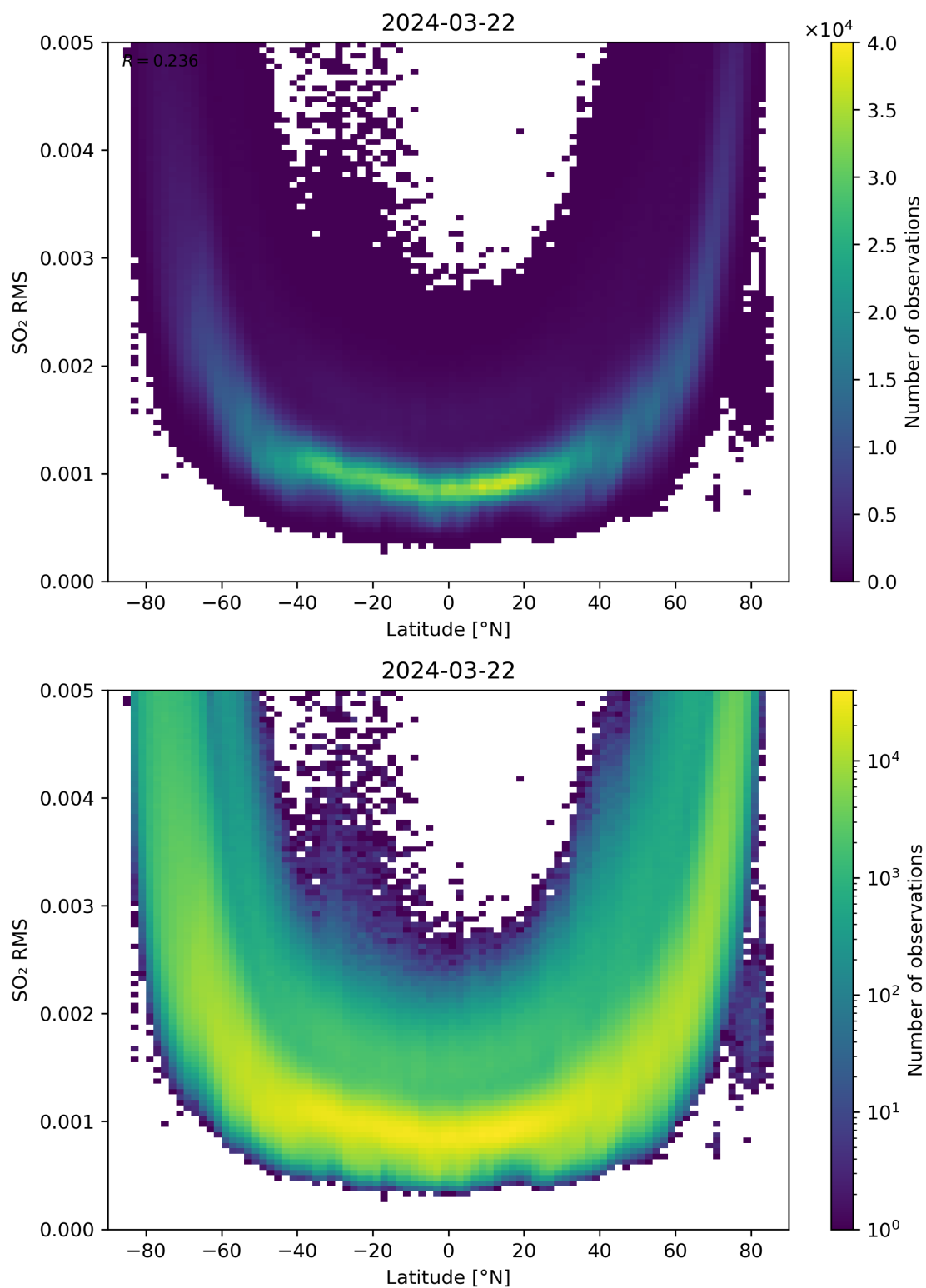
Figure 144: Scatter density plot of “Latitude” against “SO 2 RMS” for 2024-03-21 to 2024-03-22.
