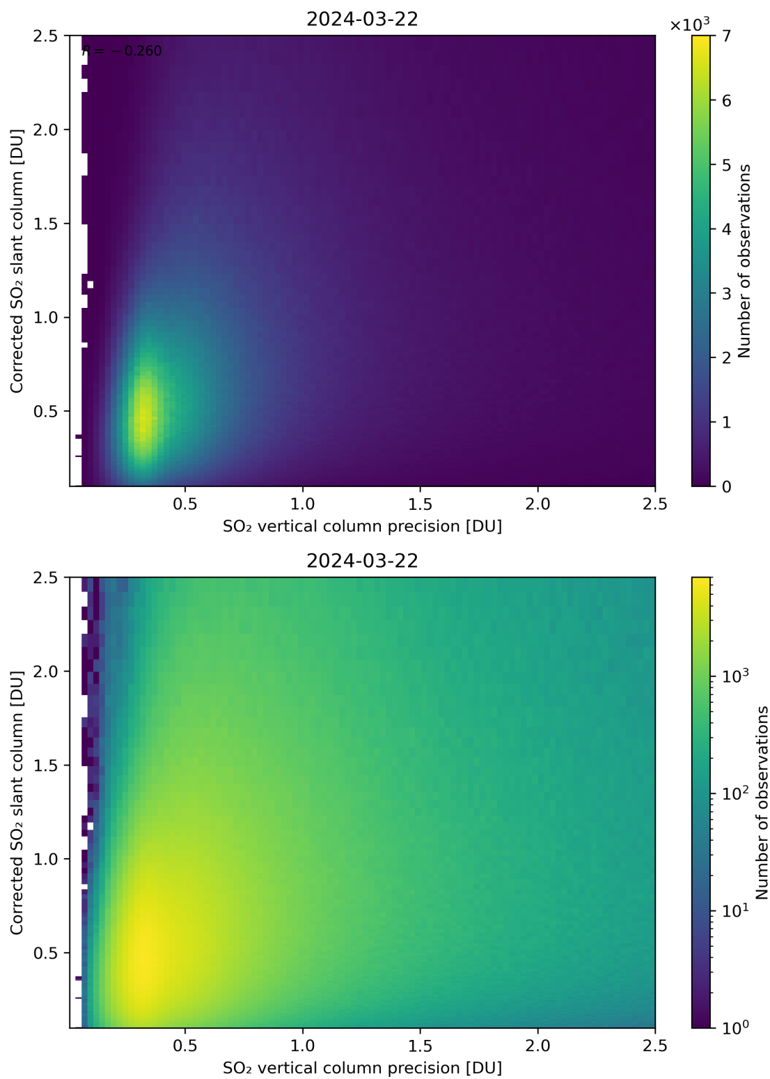
Figure 286: Scatter density plot of “SO 2 vertical column precision” against “Corrected SO 2 slant column” for 2024-03-21 to 2024-03-22.
