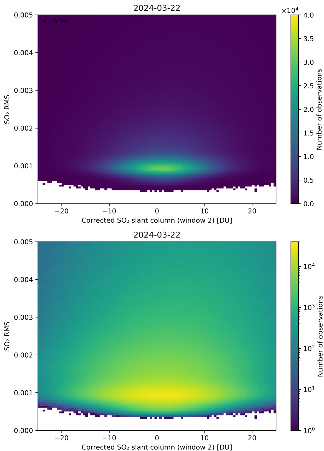
Figure 198: Scatter density plot of “Corrected SO 2 slant column (window 2)” against “SO 2 RMS” for 2024-03-21 to 2024-03-22.
