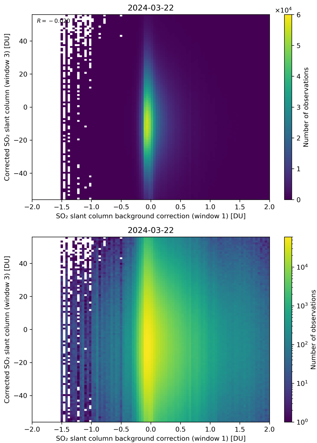
Figure 105: Scatter density plot of “SO 2 slant column background correction (window 1)” against “Corrected SO 2 slant column (window 3)” for 2024-03-21 to 2024-03-22.
