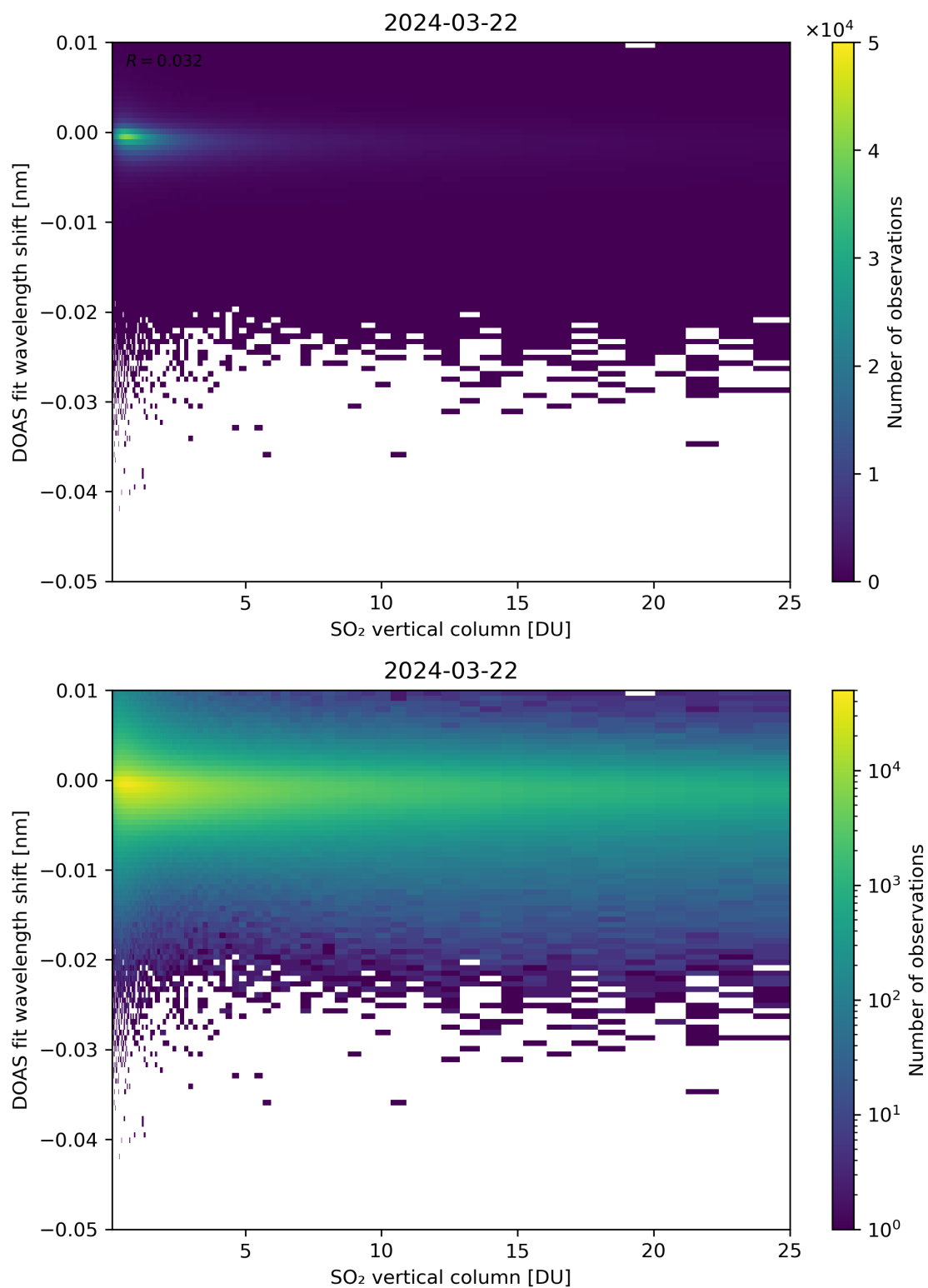
Figure 276: Scatter density plot of “SO 2 vertical column” against “DOAS fit wavelength shift” for 2024-03-21 to 2024-03-22.
