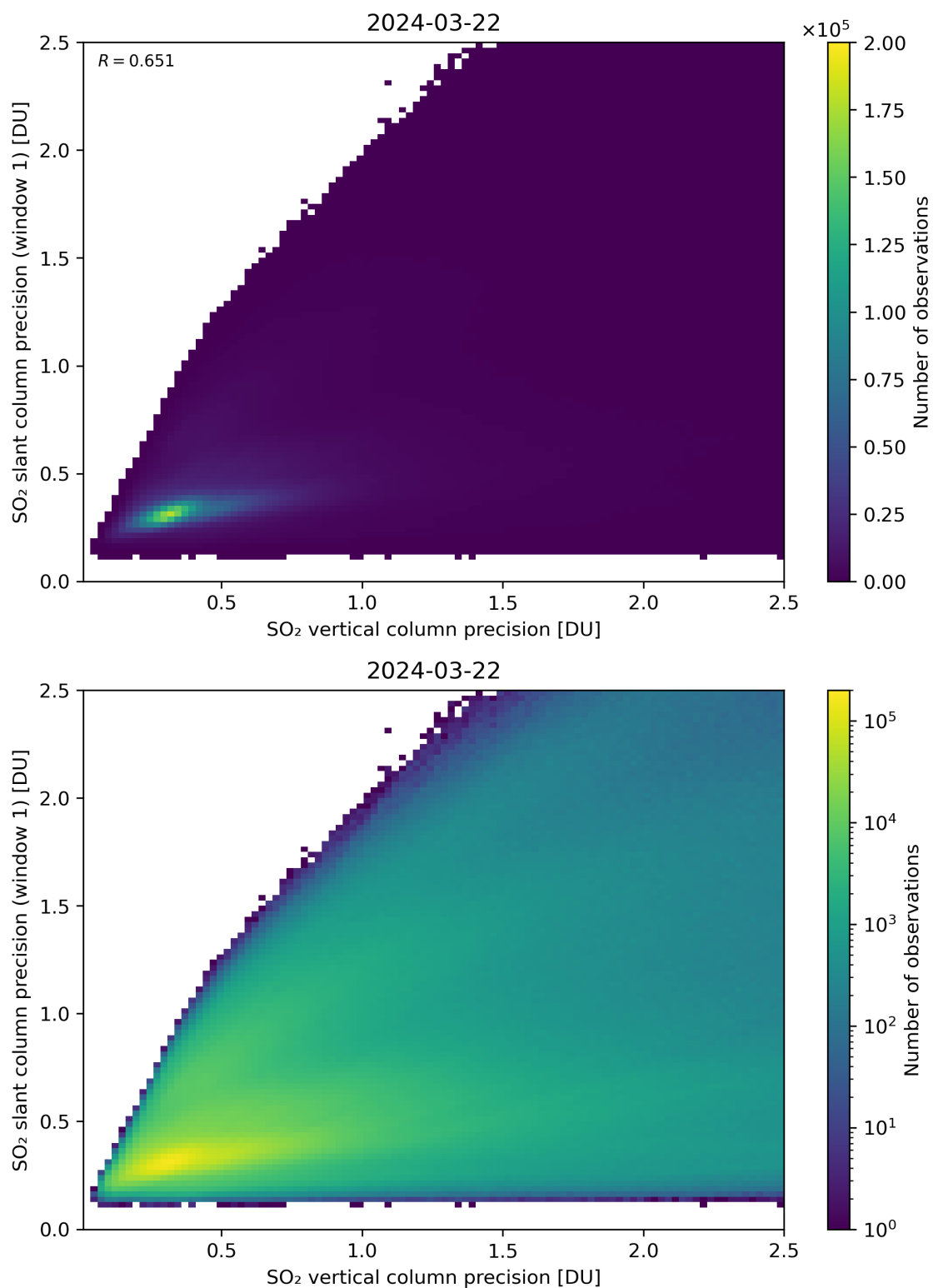
Figure 290: Scatter density plot of “SO 2 vertical column precision” against “SO 2 slant column precision (window 1)” for 2024-03-21 to 2024-03-22.
