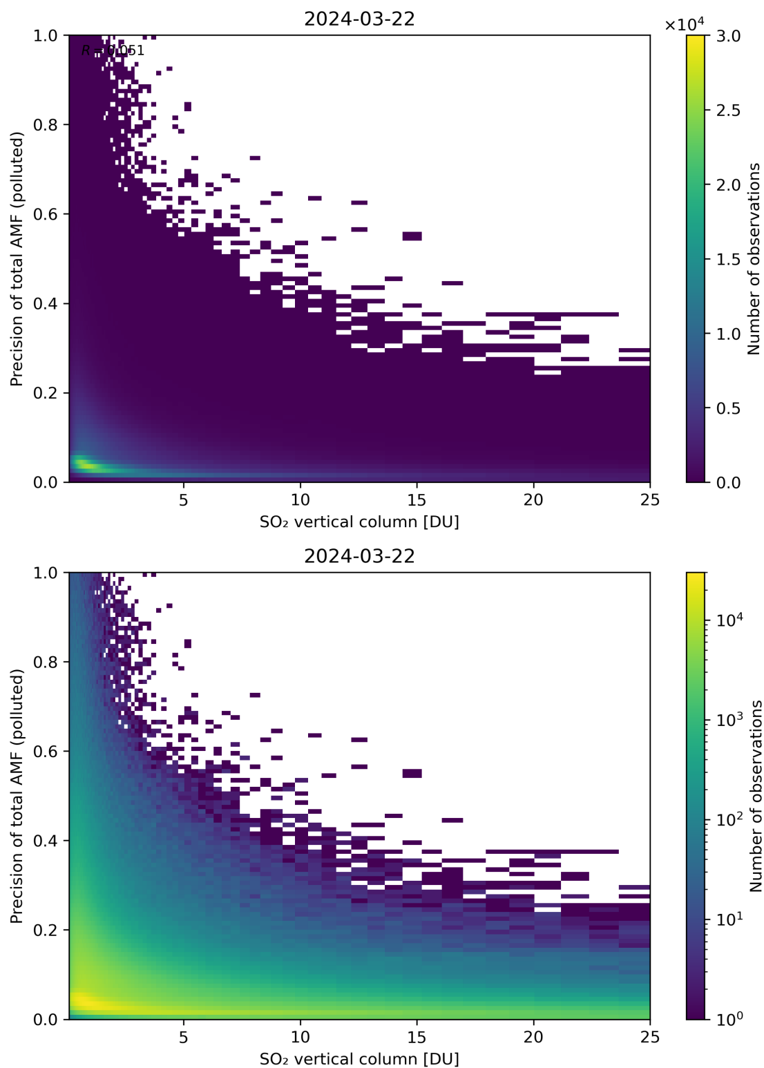
Figure 306: Scatter density plot of “SO 2 vertical column” against “Precision of total AMF (polluted)” for 2024-03-21 to 2024-03-22.
