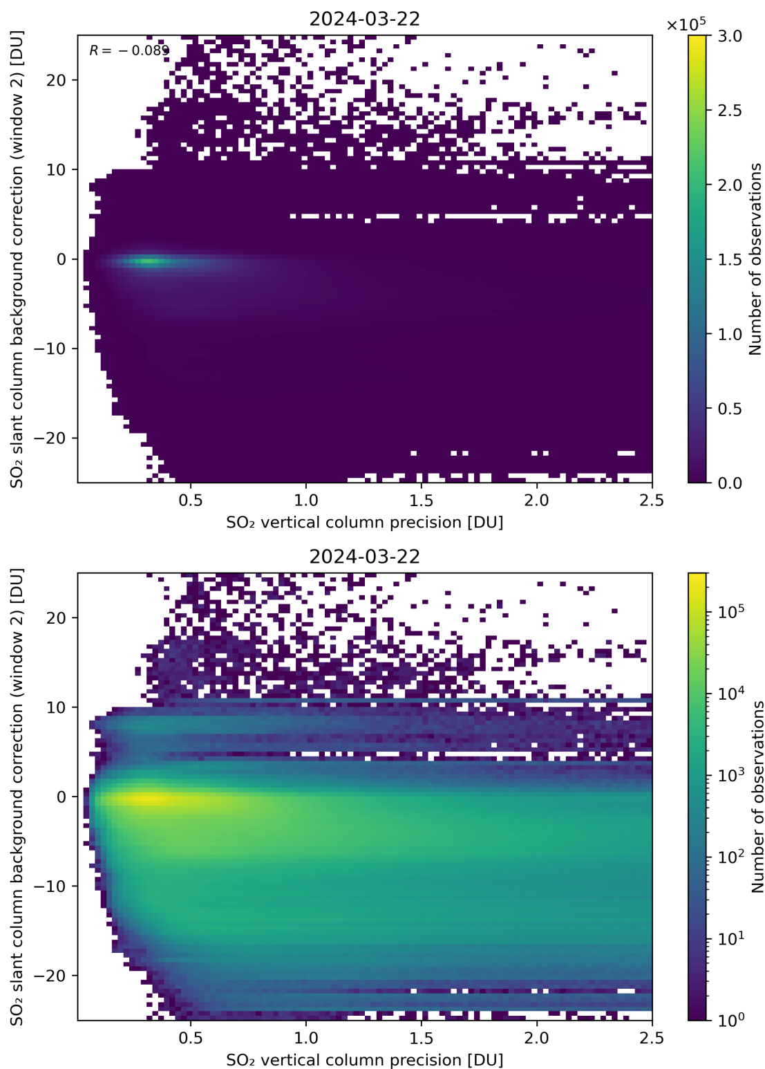
Figure 280: Scatter density plot of “SO 2 vertical column precision” against “SO 2 slant column background correction (window 2)” for 2024-03-21 to 2024-03-22.
