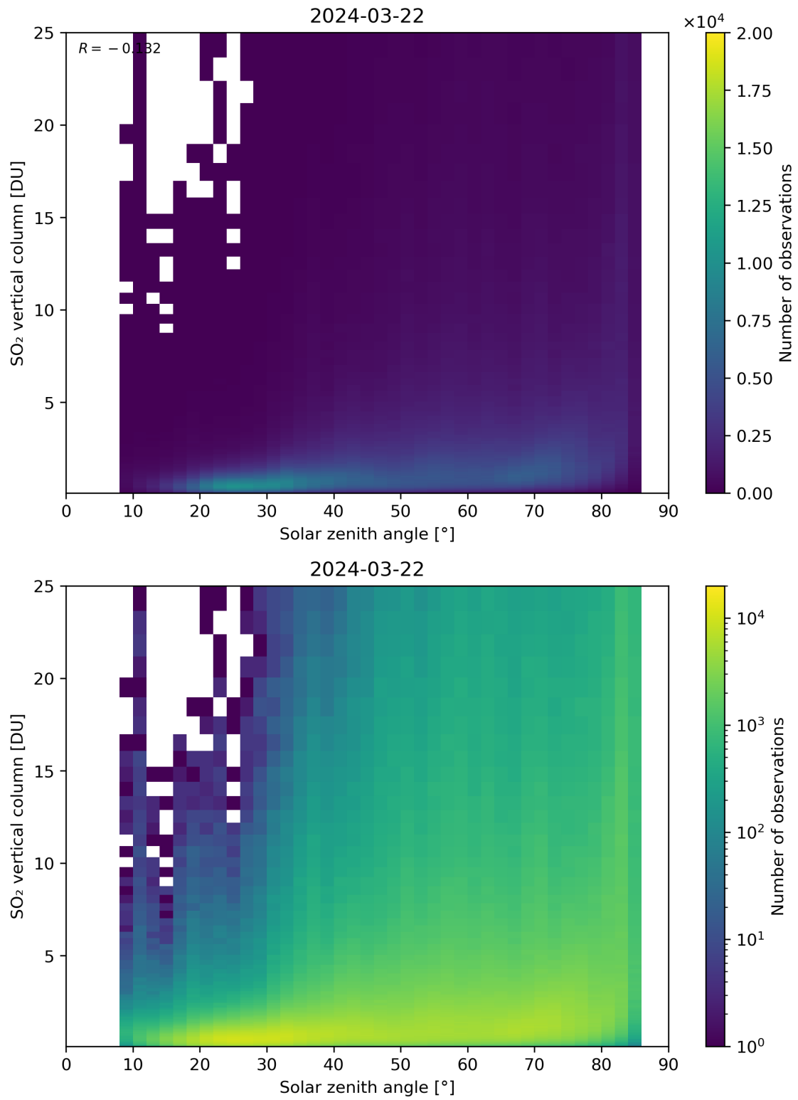
Figure 176: Scatter density plot of “Solar zenith angle” against “SO 2 vertical column” for 2024-03-21 to 2024-03-22.
