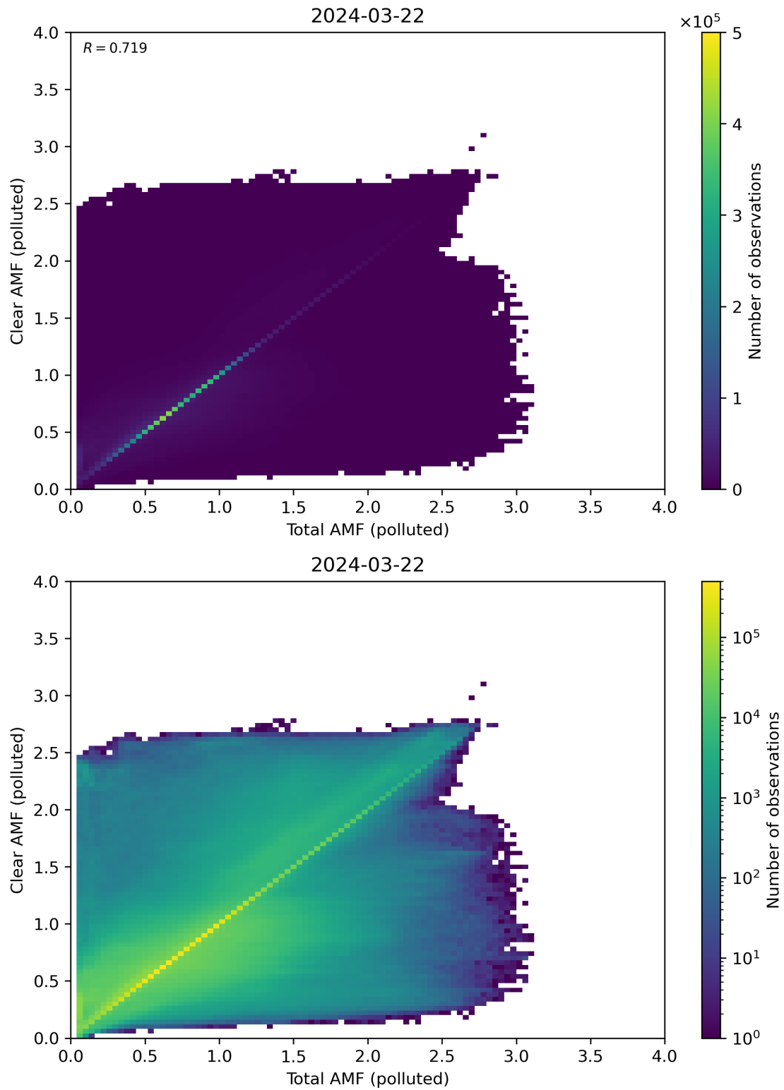
Figure 271: Scatter density plot of “Total AMF (polluted)” against “Clear AMF (polluted)” for 2024-03-21 to 2024-03-22.
