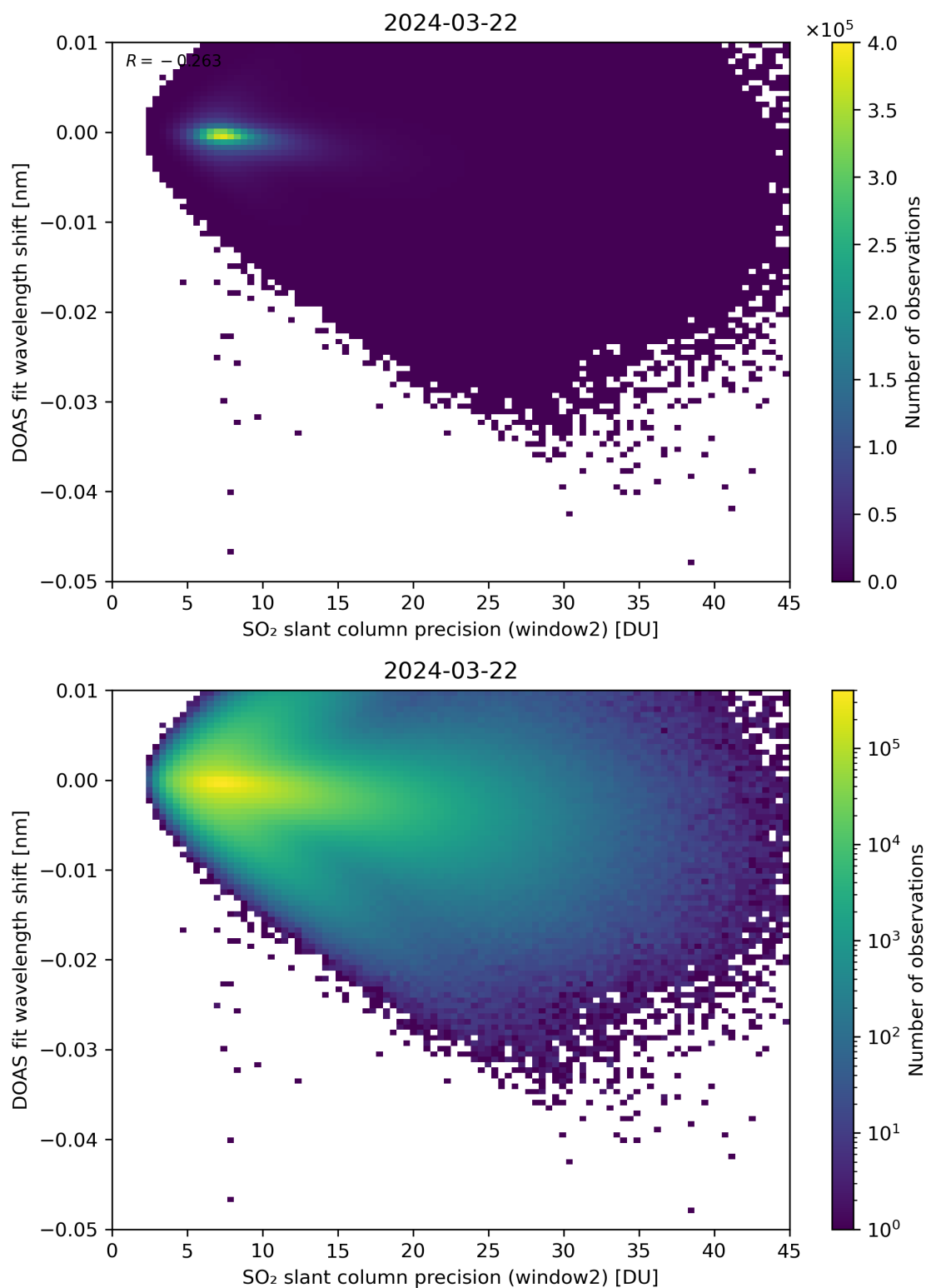
Figure 243: Scatter density plot of “SO 2 slant column precision (window2)” against “DOAS fit wavelength shift” for 2024-03-21 to 2024-03-22.
