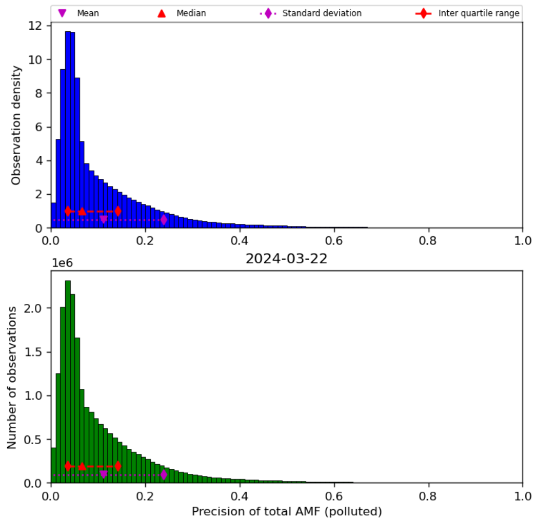
Figure 72: Histogram of “Precision of total AMF (polluted)” for 2024-03-21 to 2024-03-22
