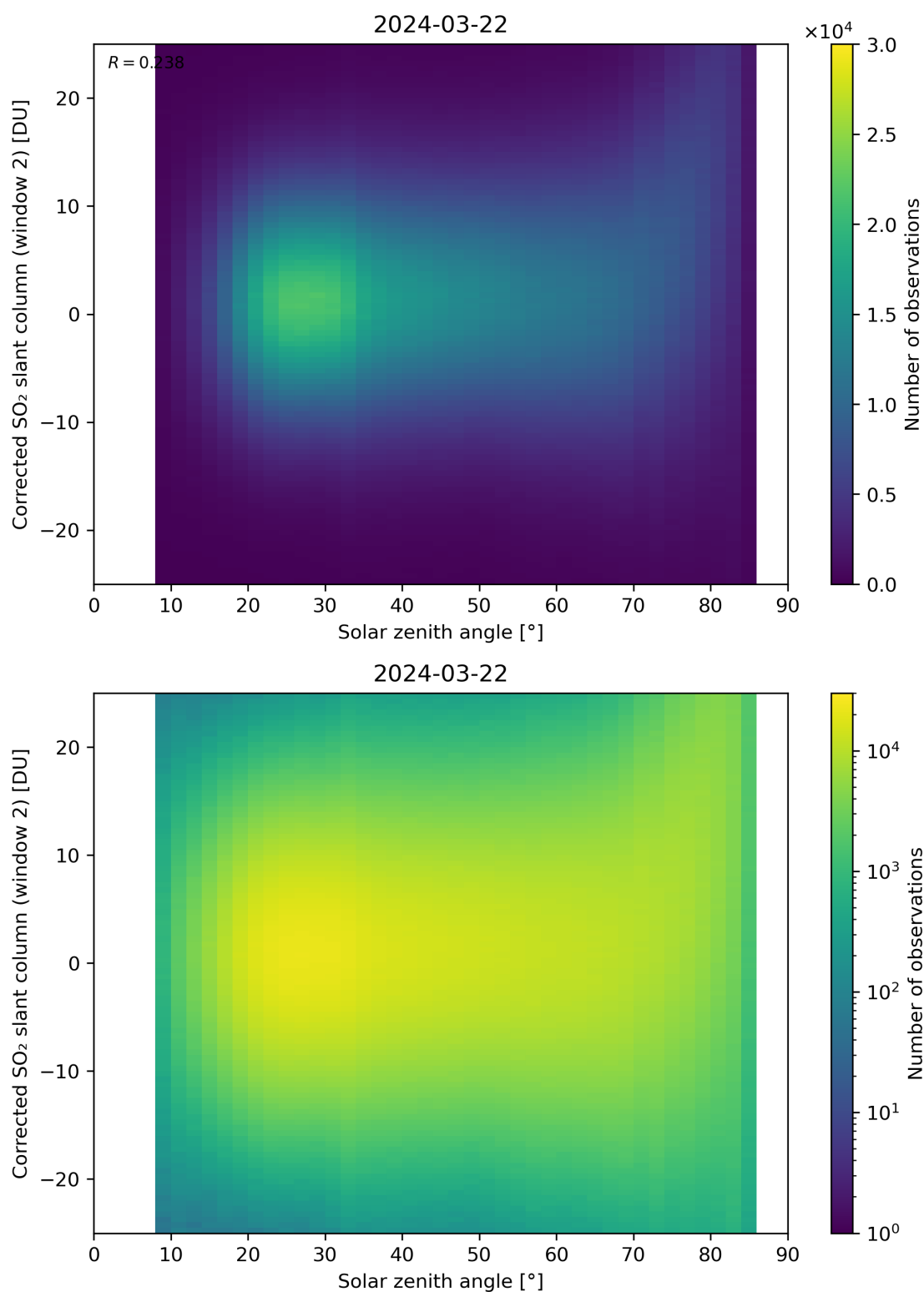
Figure 167: Scatter density plot of “Solar zenith angle” against “Corrected SO 2 slant column (window 2)” for 2024-03-21 to 2024-03-22.
