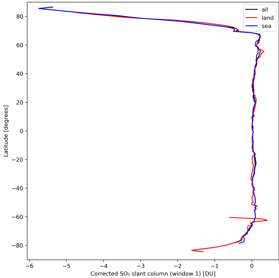
Figure 35: Zonal average of “Corrected SO 2 slant column (window 1)” for 2024-03-21 to 2024-03-22.
