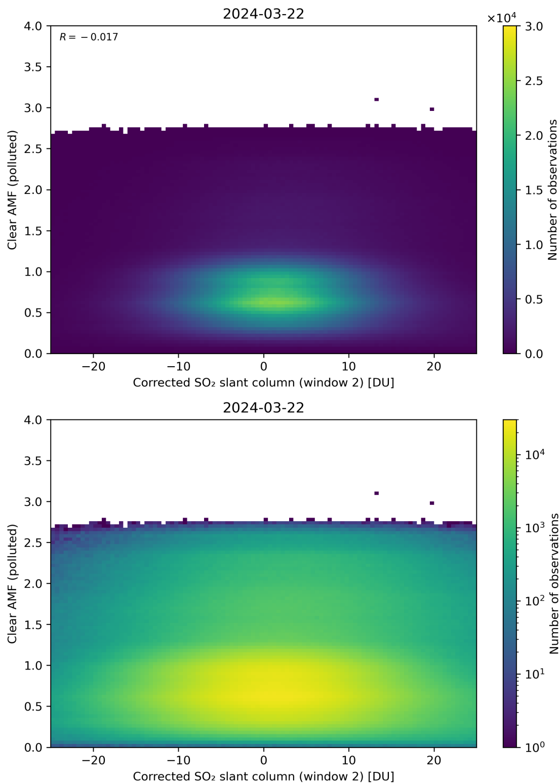
Figure 199: Scatter density plot of “Corrected SO 2 slant column (window 2)” against “Clear AMF (polluted)” for 2024-03-21 to 2024-03-22.
