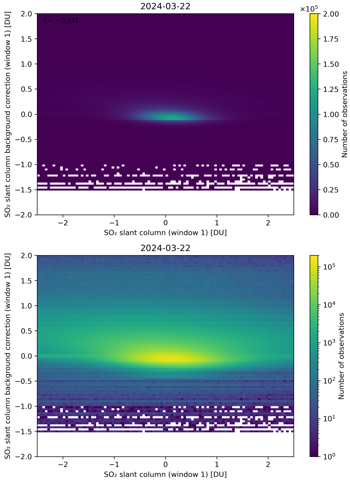
Figure 212: Scatter density plot of “SO 2 slant column (window 1)” against “SO 2 slant column background correction (window 1)” for 2024-03-21 to 2024-03-22.
