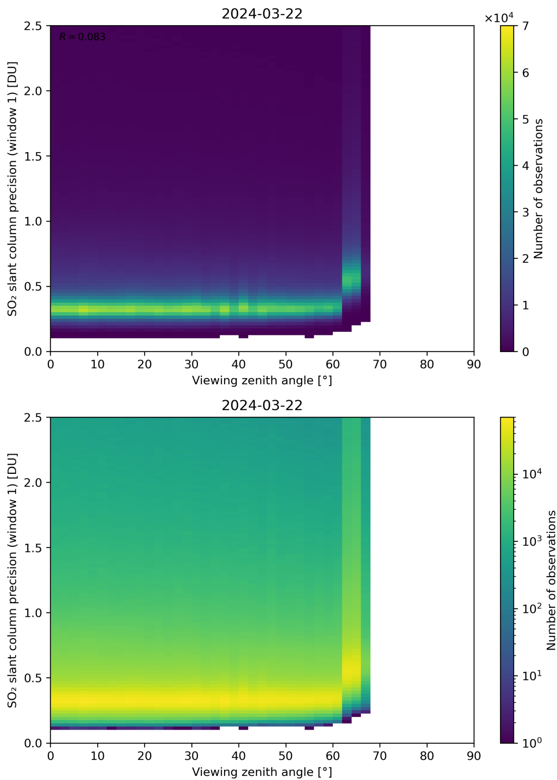
Figure 321: Scatter density plot of “Viewing zenith angle” against “SO 2 slant column precision (window 1)” for 2024-03-21 to 2024-03-22.
