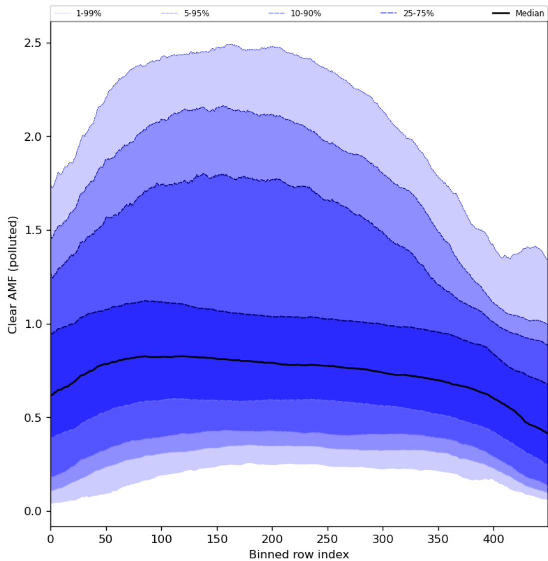
Figure 96: Along track statistics of “Clear AMF (polluted)” for 2024-03-21 to 2024-03-22
