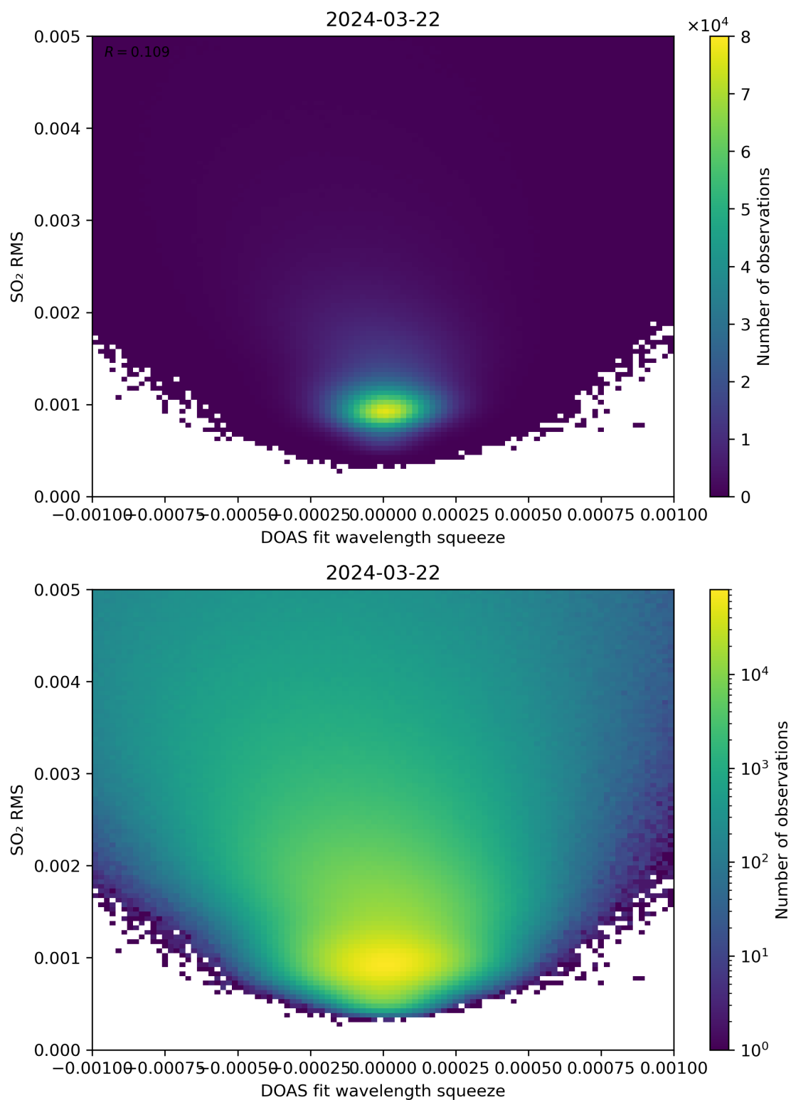
Figure 132: Scatter density plot of “DOAS fit wavelength squeeze” against “SO 2 RMS” for 2024-03-21 to 2024-03-22.
