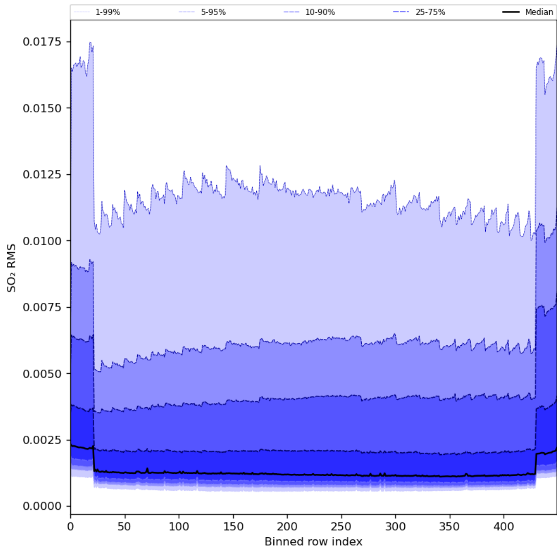
Figure 93: Along track statistics of “SO 2 RMS” for 2024-03-21 to 2024-03-22
