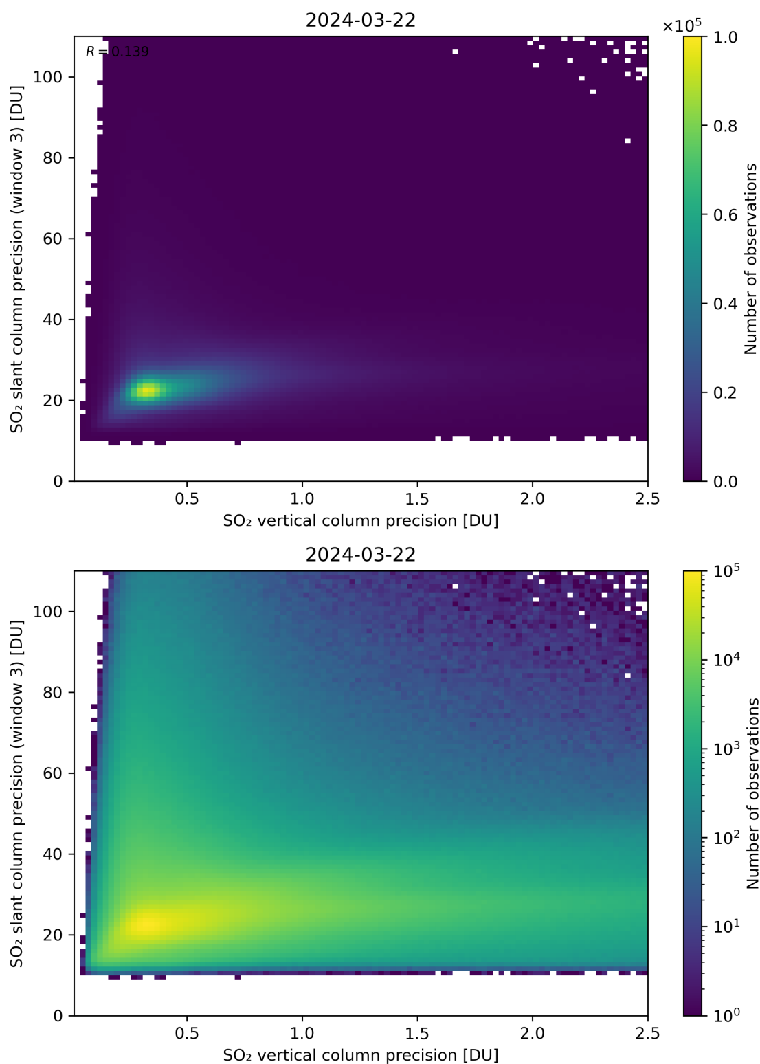
Figure 293: Scatter density plot of “SO 2 vertical column precision” against “SO 2 slant column precision (window 3)” for 2024-03-21 to 2024-03-22.
