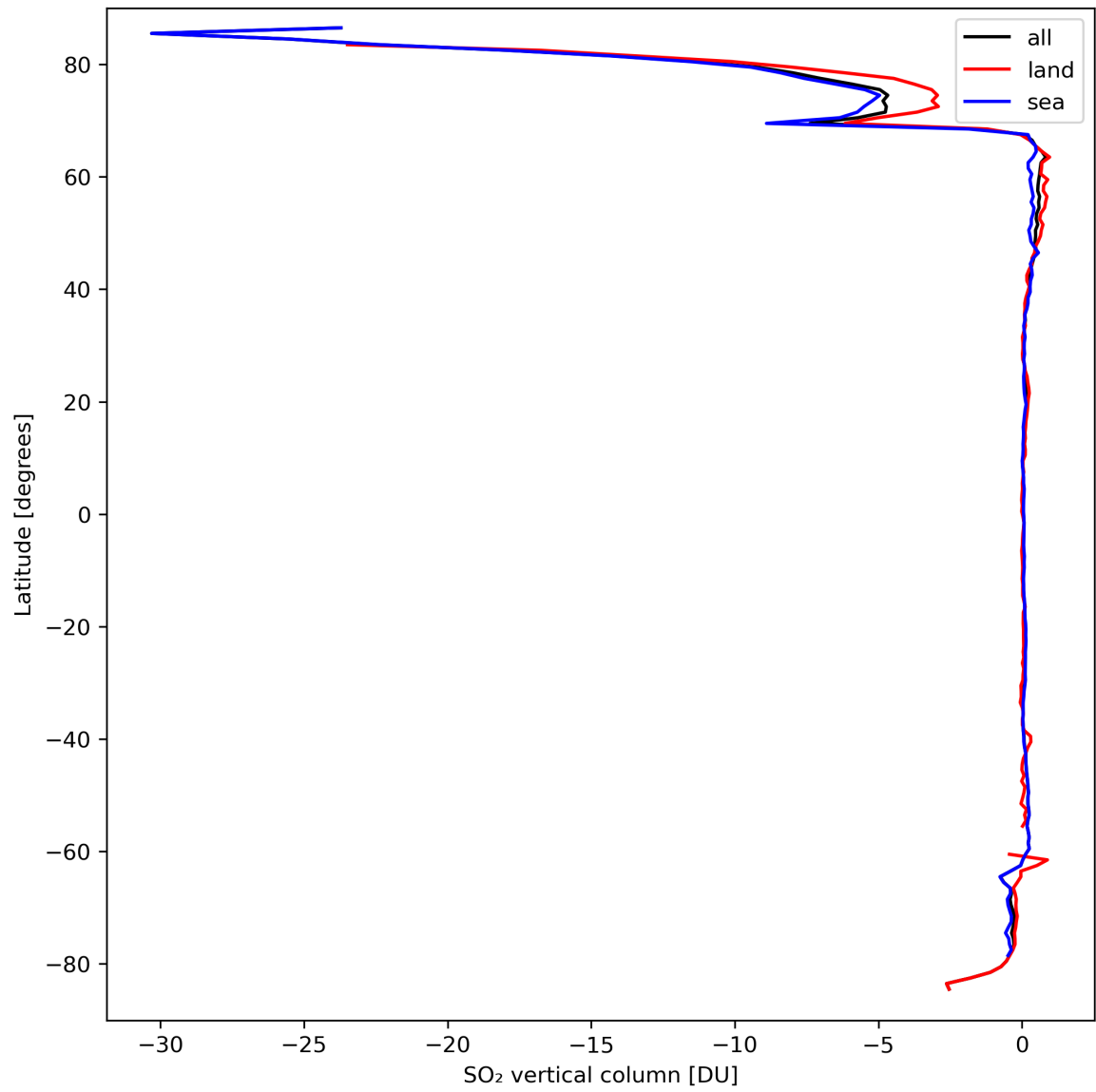
Figure 30: Zonal average of “SO 2 vertical column” for 2024-03-21 to 2024-03-22.
