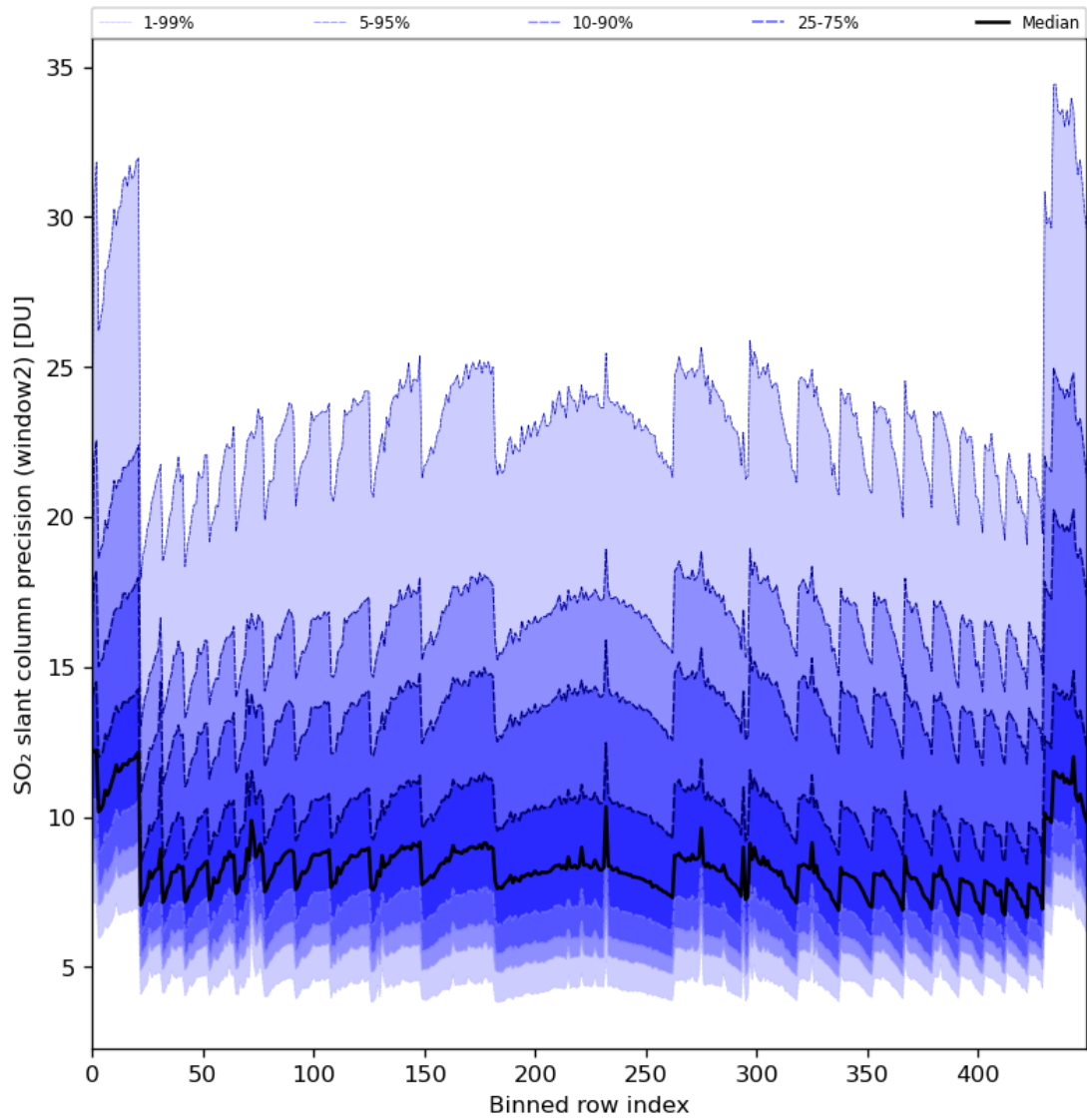
Figure 84: Along track statistics of “SO 2 slant column precision (window2)” for 2024-03-21 to 2024-03-22
