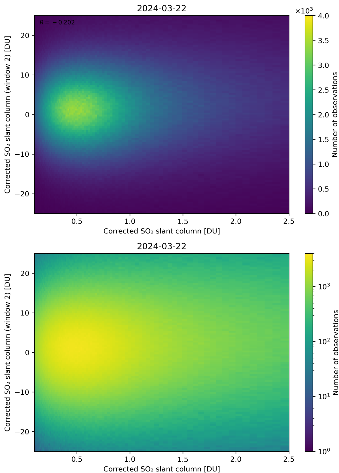
Figure 185: Scatter density plot of “Corrected SO 2 slant column” against “Corrected SO 2 slant column (window 2)” for 2024-03-21 to 2024-03-22.
