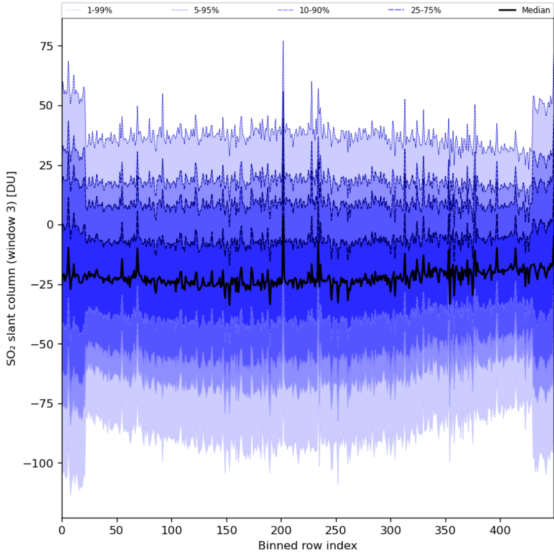
Figure 87: Along track statistics of “SO 2 slant column (window 3)” for 2024-03-21 to 2024-03-22
