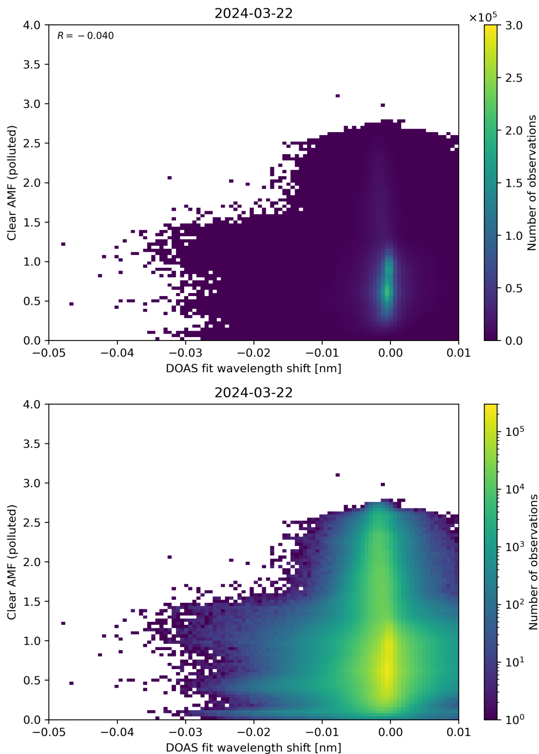
Figure 129: Scatter density plot of “DOAS fit wavelength shift” against “Clear AMF (polluted)” for 2024-03-21 to 2024-03-22.
