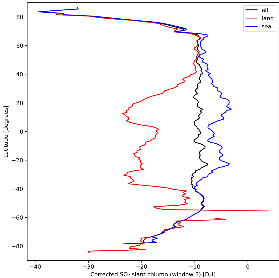
Figure 43: Zonal average of “Corrected SO 2 slant column (window 3)” for 2024-03-21 to 2024-03-22.
