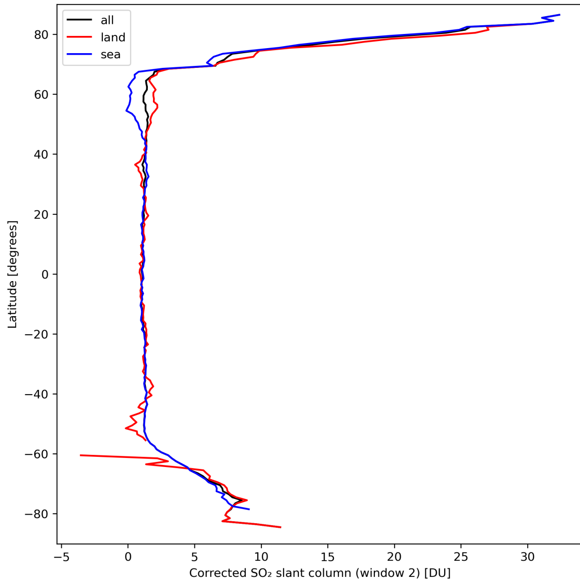
Figure 39: Zonal average of “Corrected SO 2 slant column (window 2)” for 2024-03-21 to 2024-03-22.
