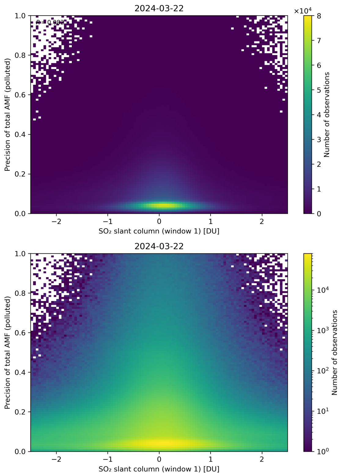
Figure 240: Scatter density plot of “SO 2 slant column (window 1)” against “Precision of total AMF (polluted)” for 2024-03-21 to 2024-03-22.
