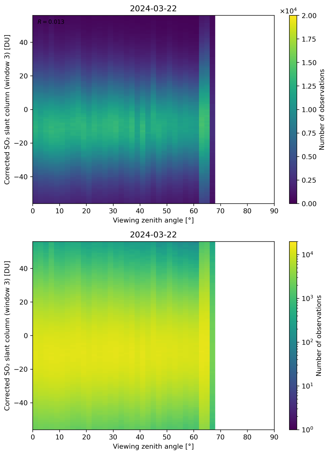
Figure 319: Scatter density plot of “Viewing zenith angle” against “Corrected SO 2 slant column (window 3)” for 2024-03-21 to 2024-03-22.
