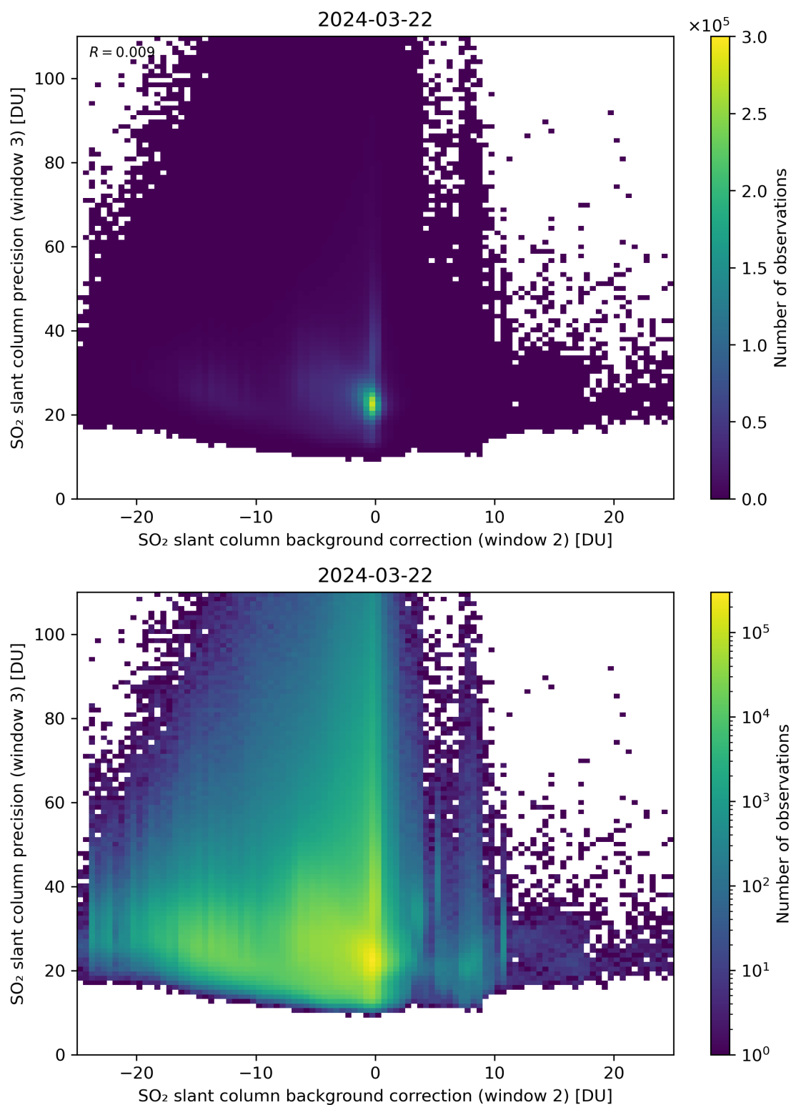
Figure 118: Scatter density plot of “SO 2 slant column background correction (window 2)” against “SO 2 slant column precision (window 3)” for 2024-03-21 to 2024-03-22.
