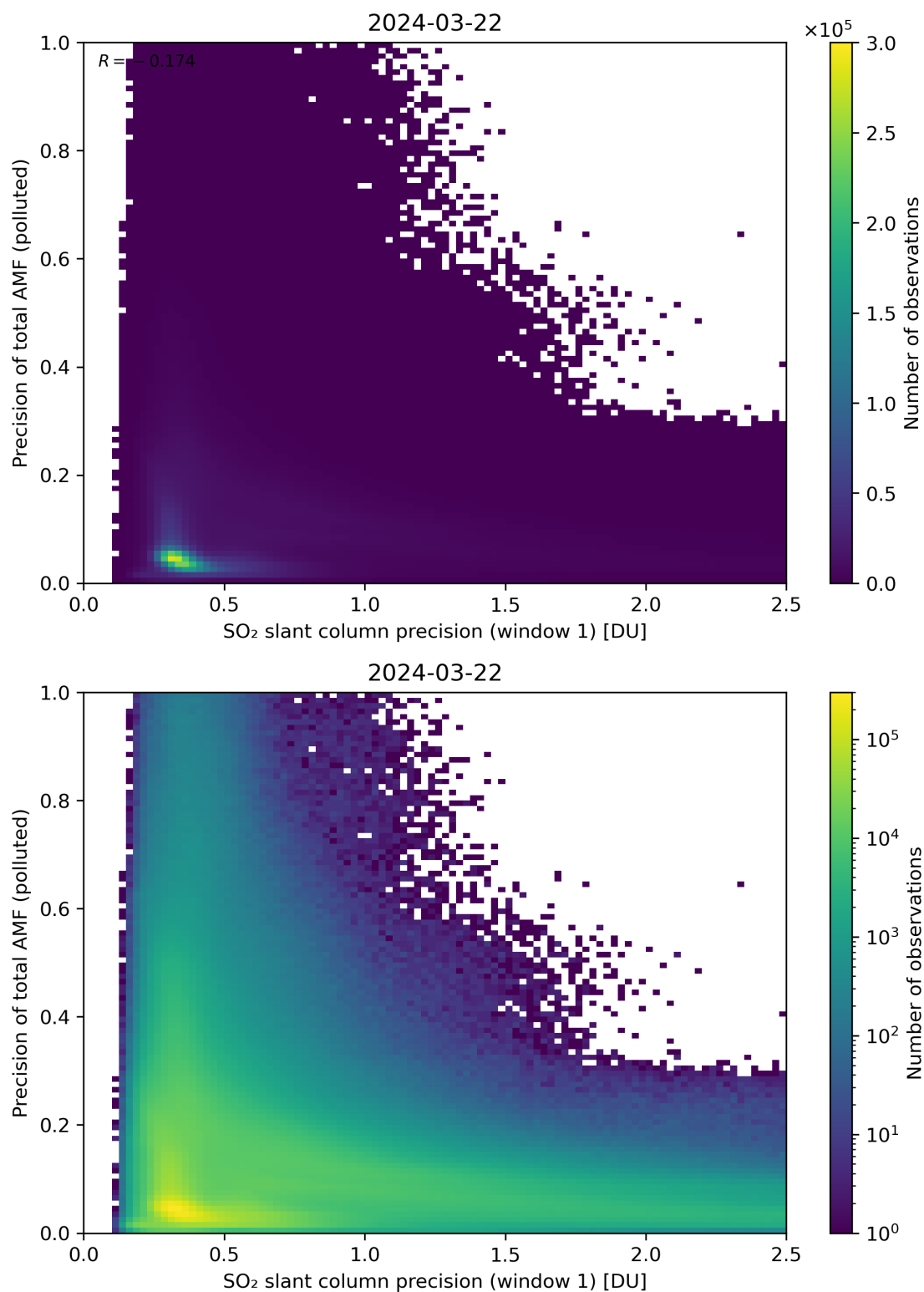
Figure 231: Scatter density plot of “SO 2 slant column precision (window 1)” against “Precision of total AMF (polluted)” for 2024-03-21 to 2024-03-22.
