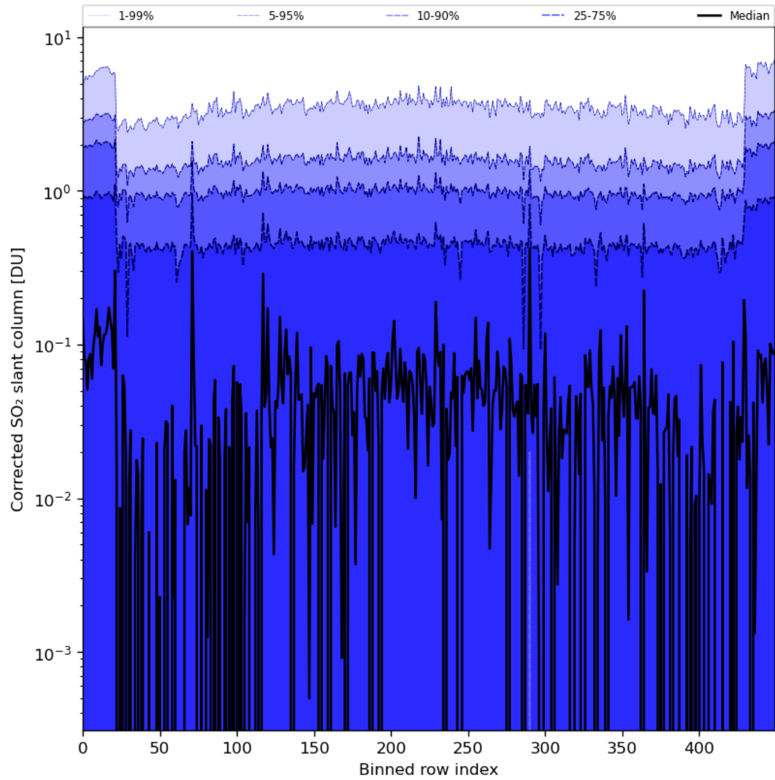
Figure 78: Along track statistics of “Corrected SO 2 slant column” for 2024-03-21 to 2024-03-22
