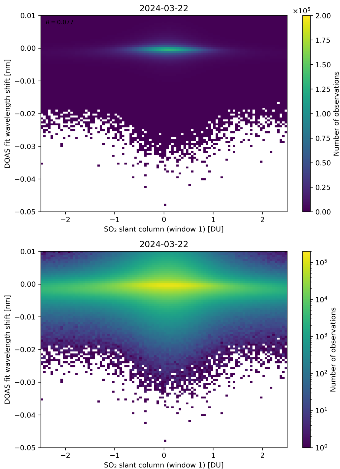
Figure 215: Scatter density plot of “SO 2 slant column (window 1)” against “DOAS fit wavelength shift” for 2024-03-21 to 2024-03-22.
