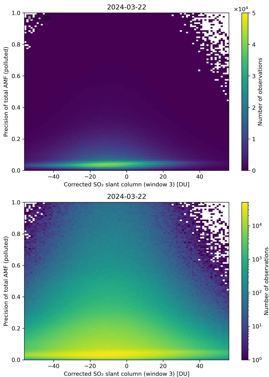
Figure 211: Scatter density plot of “Corrected SO 2 slant column (window 3)” against “Precision of total AMF (polluted)” for 2024-03-21 to 2024-03-22.
