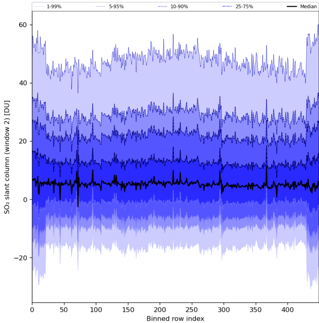
Figure 83: Along track statistics of “SO 2 slant column (window 2)” for 2024-03-21 to 2024-03-22
