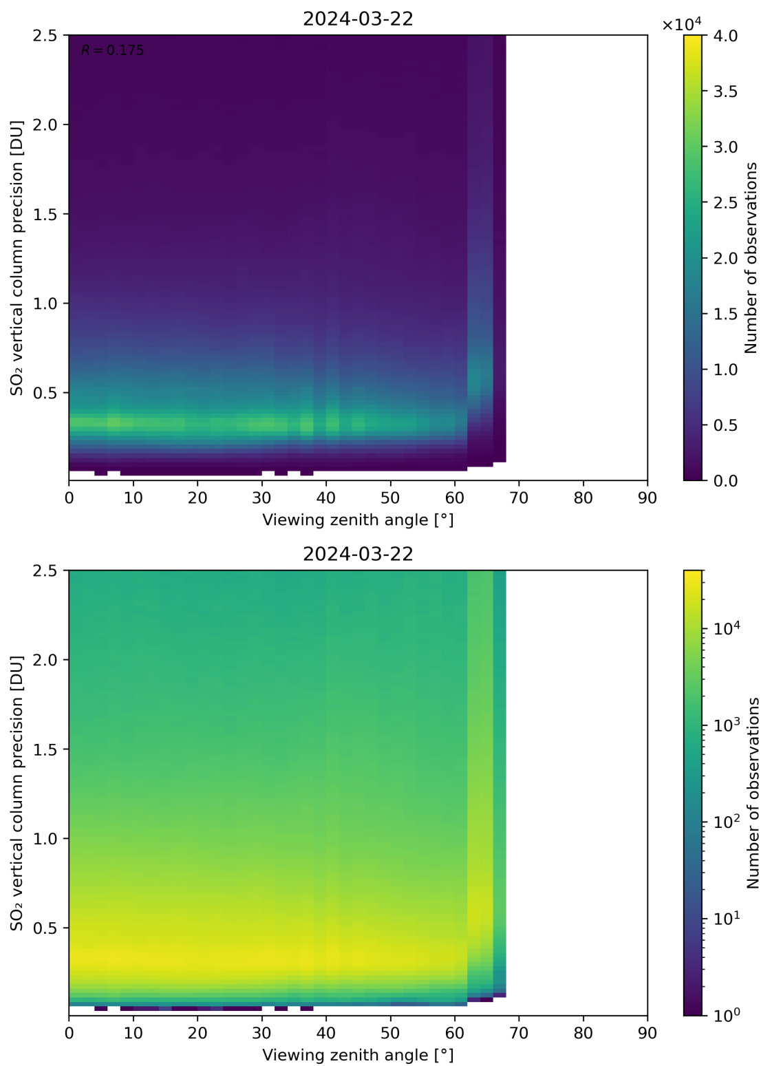
Figure 328: Scatter density plot of “Viewing zenith angle” against “SO 2 vertical column precision” for 2024-03-21 to 2024-03-22.
