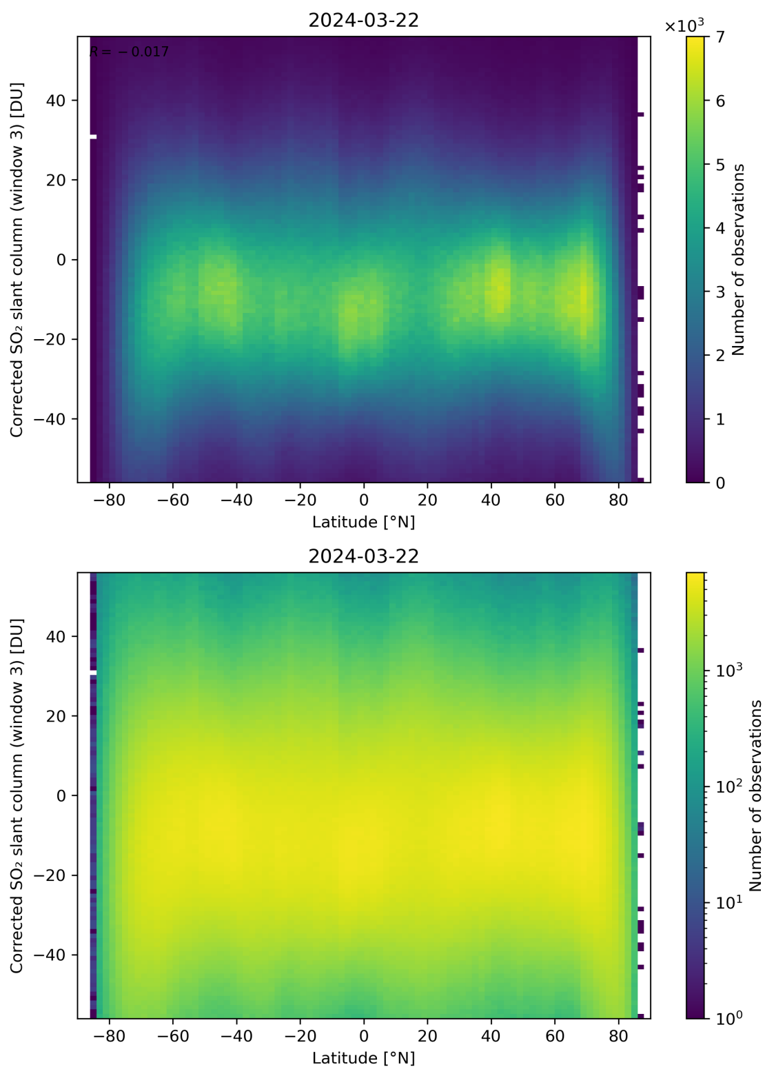
Figure 148: Scatter density plot of “Latitude” against “Corrected SO 2 slant column (window 3)” for 2024-03-21 to 2024-03-22.
