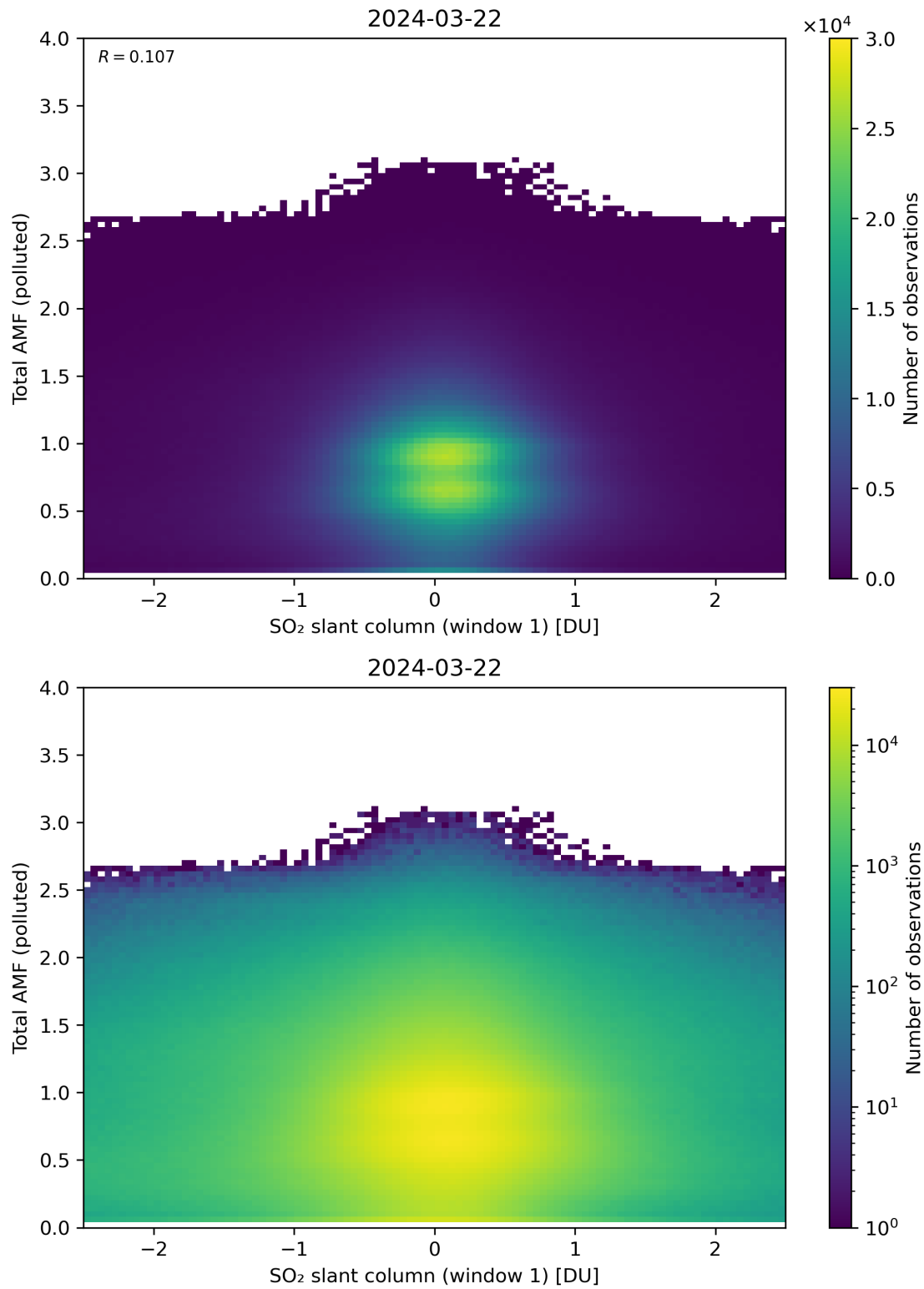
Figure 239: Scatter density plot of “SO 2 slant column (window 1)” against “Total AMF (polluted)” for 2024-03-21 to 2024-03-22.
