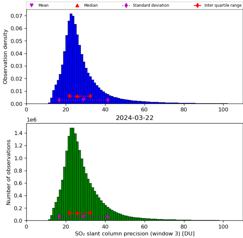
Figure 65: Histogram of “SO 2 slant column precision (window 3)” for 2024-03-21 to 2024-03-22
