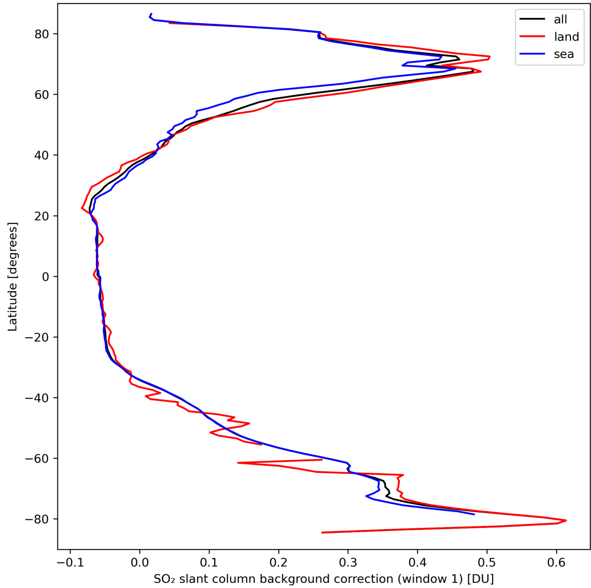
Figure 36: Zonal average of “SO 2 slant column background correction (window 1)” for 2024-03-21 to 2024-03-22.
