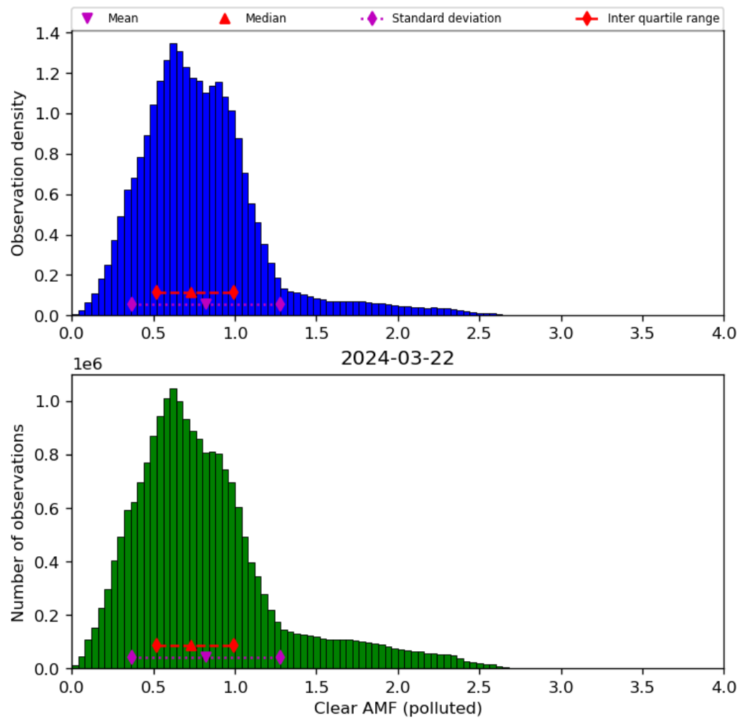
Figure 73: Histogram of “Clear AMF (polluted)” for 2024-03-21 to 2024-03-22
