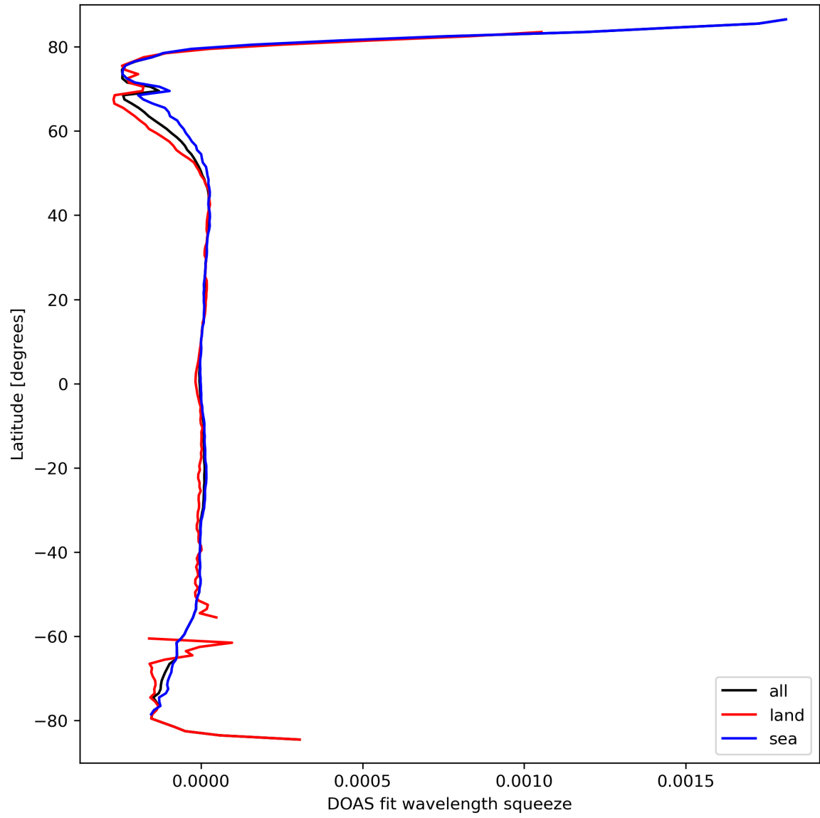
Figure 46: Zonal average of “DOAS fit wavelength squeeze” for 2024-03-21 to 2024-03-22.
