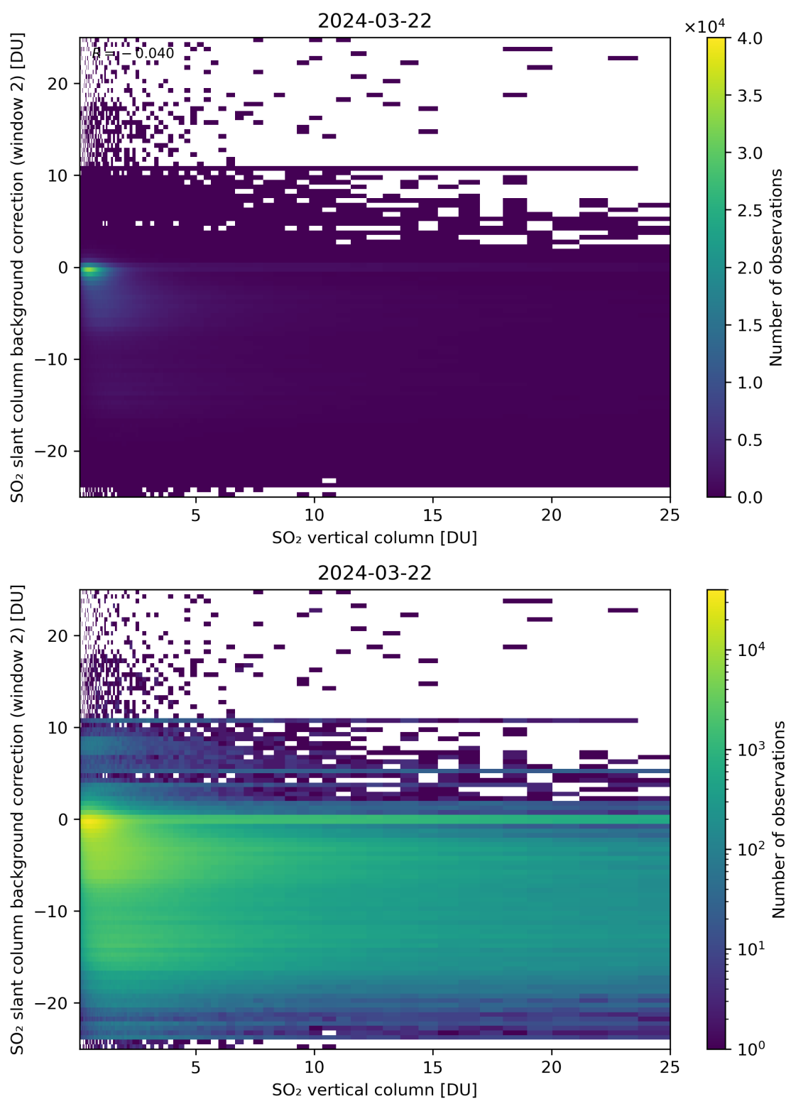
Figure 274: Scatter density plot of “SO 2 vertical column” against “SO 2 slant column background correction (window 2)” for 2024-03-21 to 2024-03-22.
