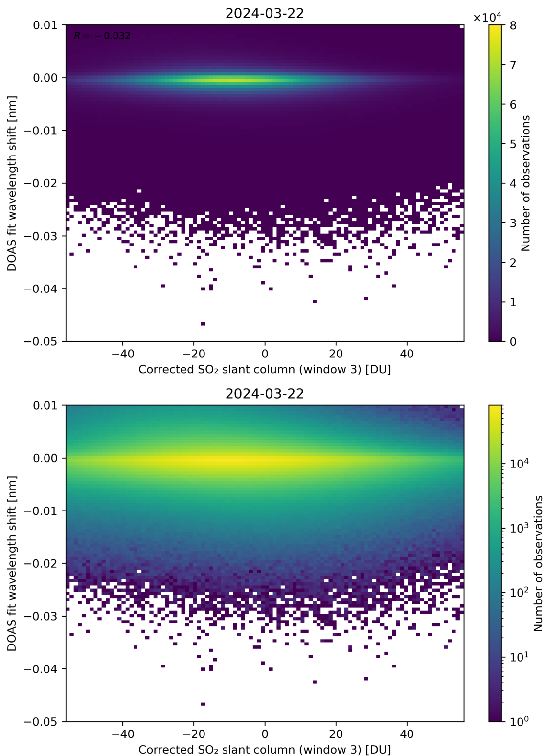
Figure 206: Scatter density plot of “Corrected SO 2 slant column (window 3)” against “DOAS fit wavelength shift” for 2024-03-21 to 2024-03-22.
