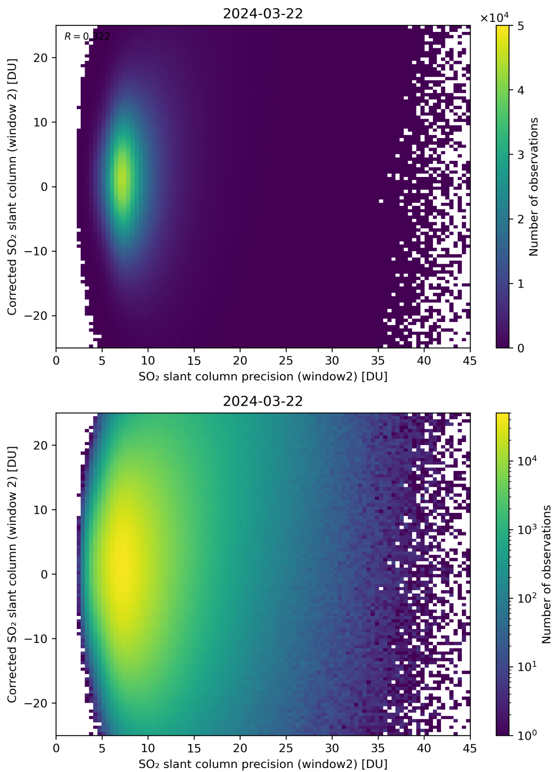
Figure 247: Scatter density plot of “SO 2 slant column precision (window2)” against “Corrected SO 2 slant column (window 2)” for 2024-03-21 to 2024-03-22.
