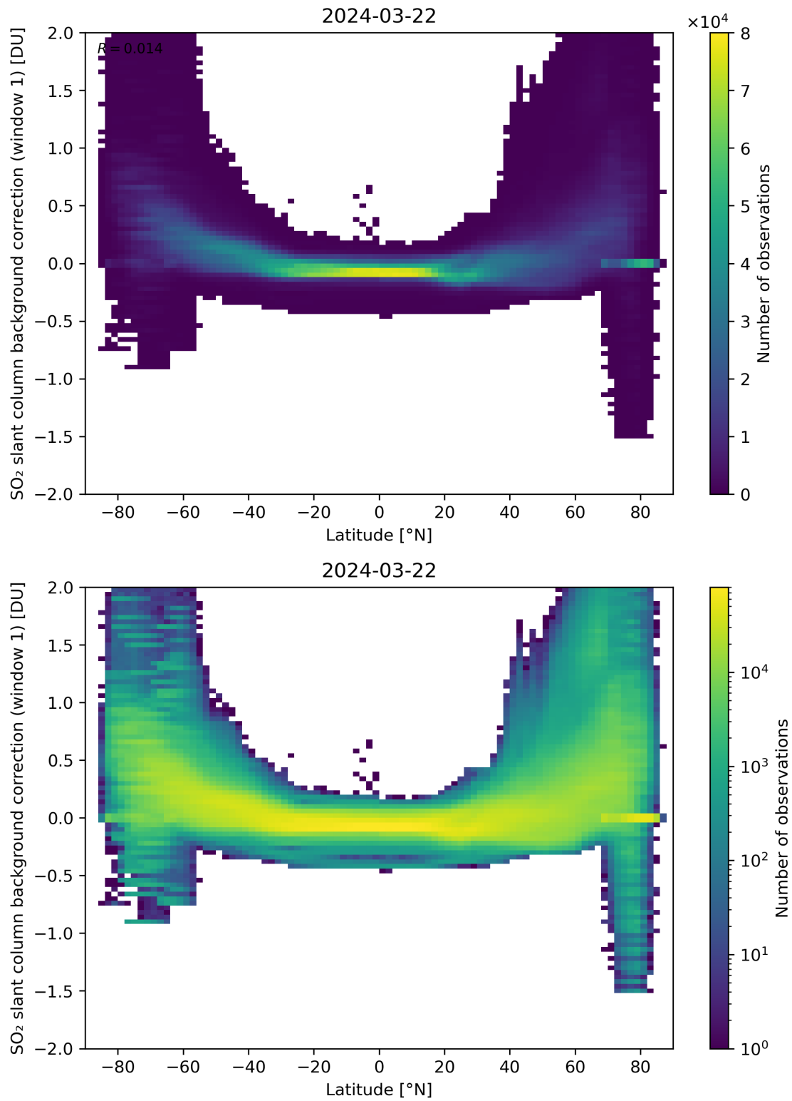
Figure 139: Scatter density plot of “Latitude” against “SO 2 slant column background correction (window 1)” for 2024-03-21 to 2024-03-22.
