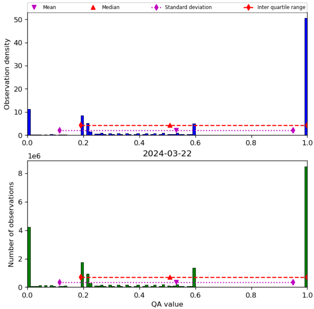
Figure 52: Histogram of “QA value” for 2024-03-21 to 2024-03-22
