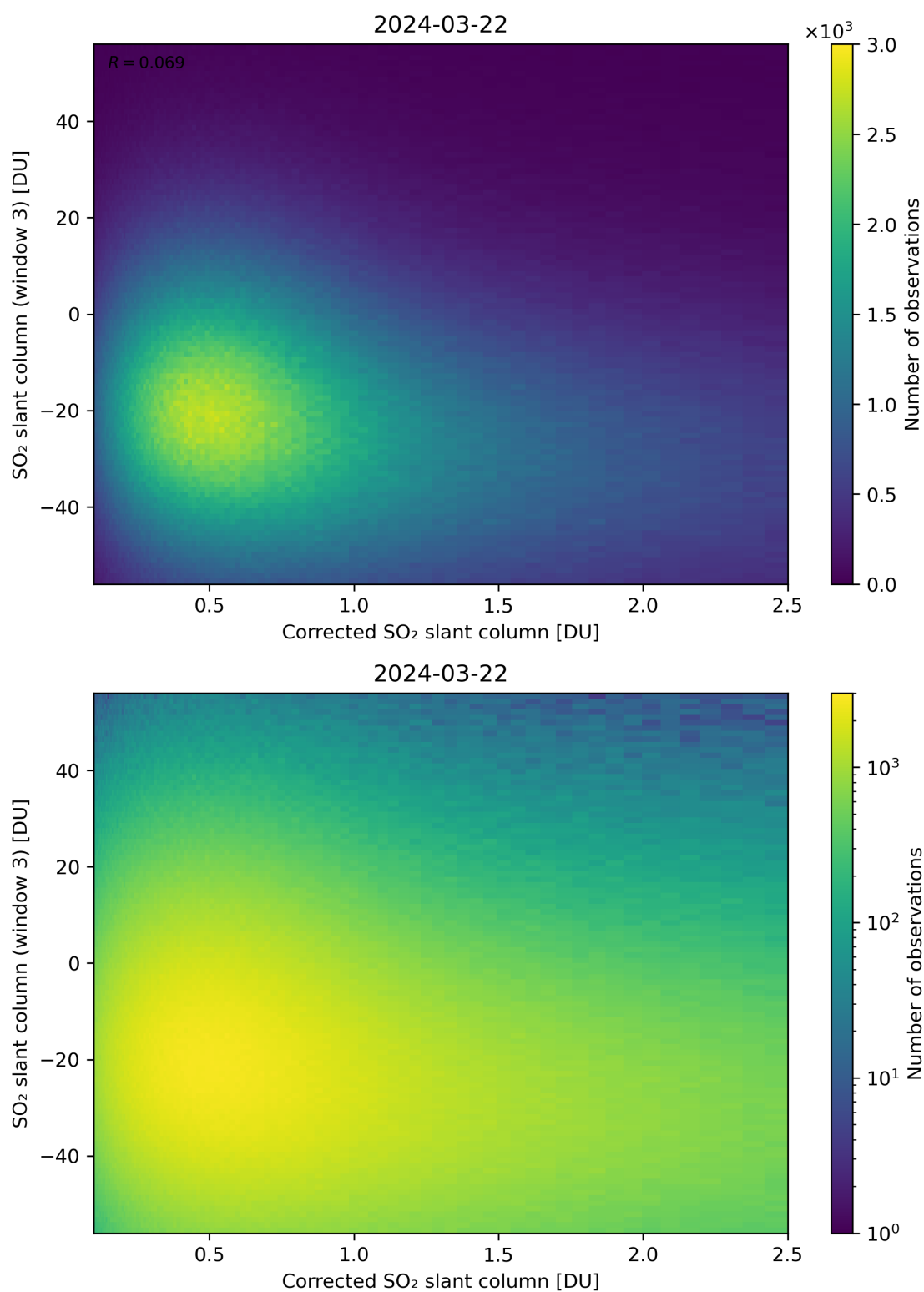
Figure 190: Scatter density plot of “Corrected SO 2 slant column” against “SO 2 slant column (window 3)” for 2024-03-21 to 2024-03-22.
