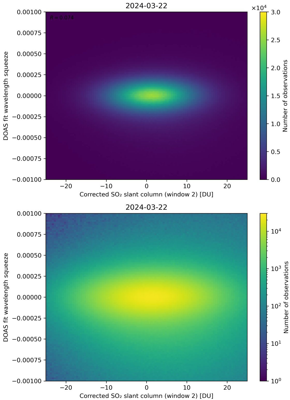
Figure 197: Scatter density plot of “Corrected SO 2 slant column (window 2)” against “DOAS fit wavelength squeeze” for 2024-03-21 to 2024-03-22.
