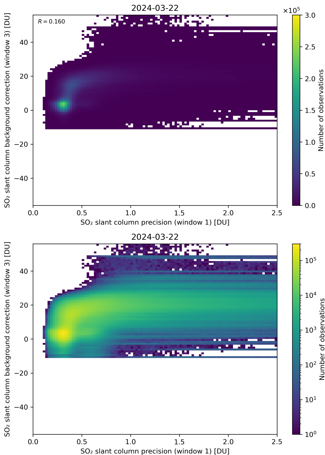
Figure 220: Scatter density plot of “SO 2 slant column precision (window 1)” against “SO 2 slant column background correction (window 3)” for 2024-03-21 to 2024-03-22.
