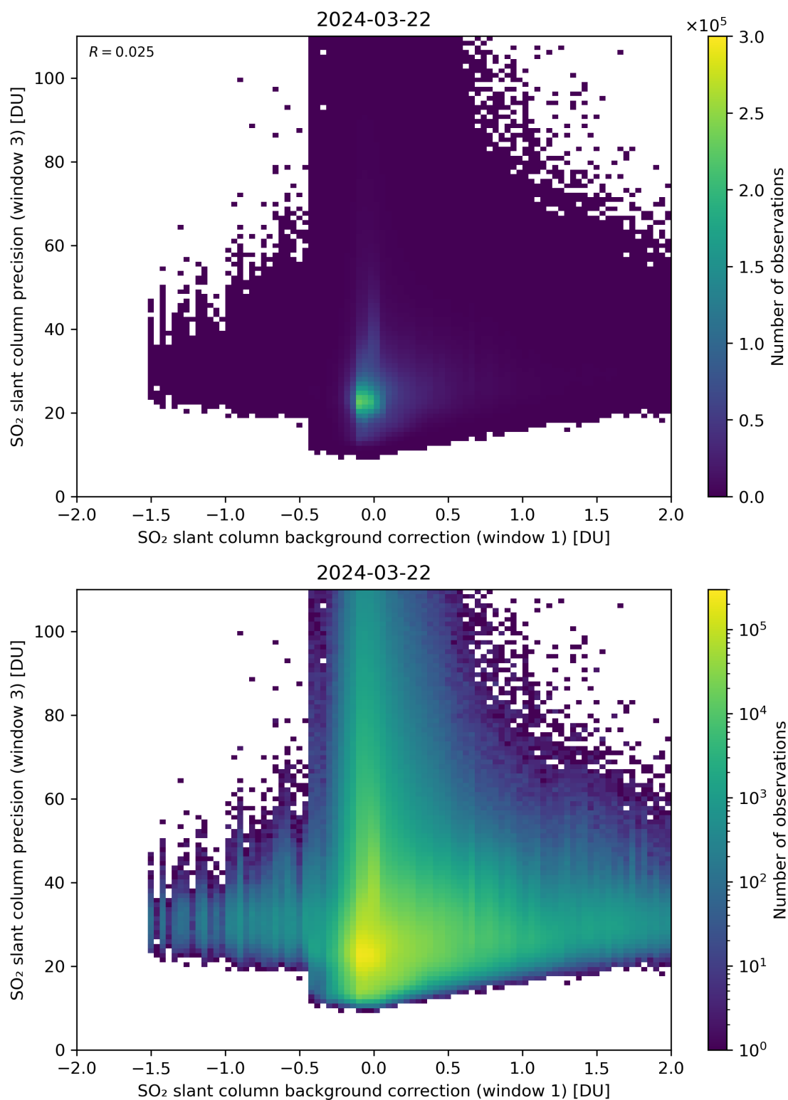
Figure 108: Scatter density plot of “SO 2 slant column background correction (window 1)” against “SO 2 slant column precision (window 3)” for 2024-03-21 to 2024-03-22.
