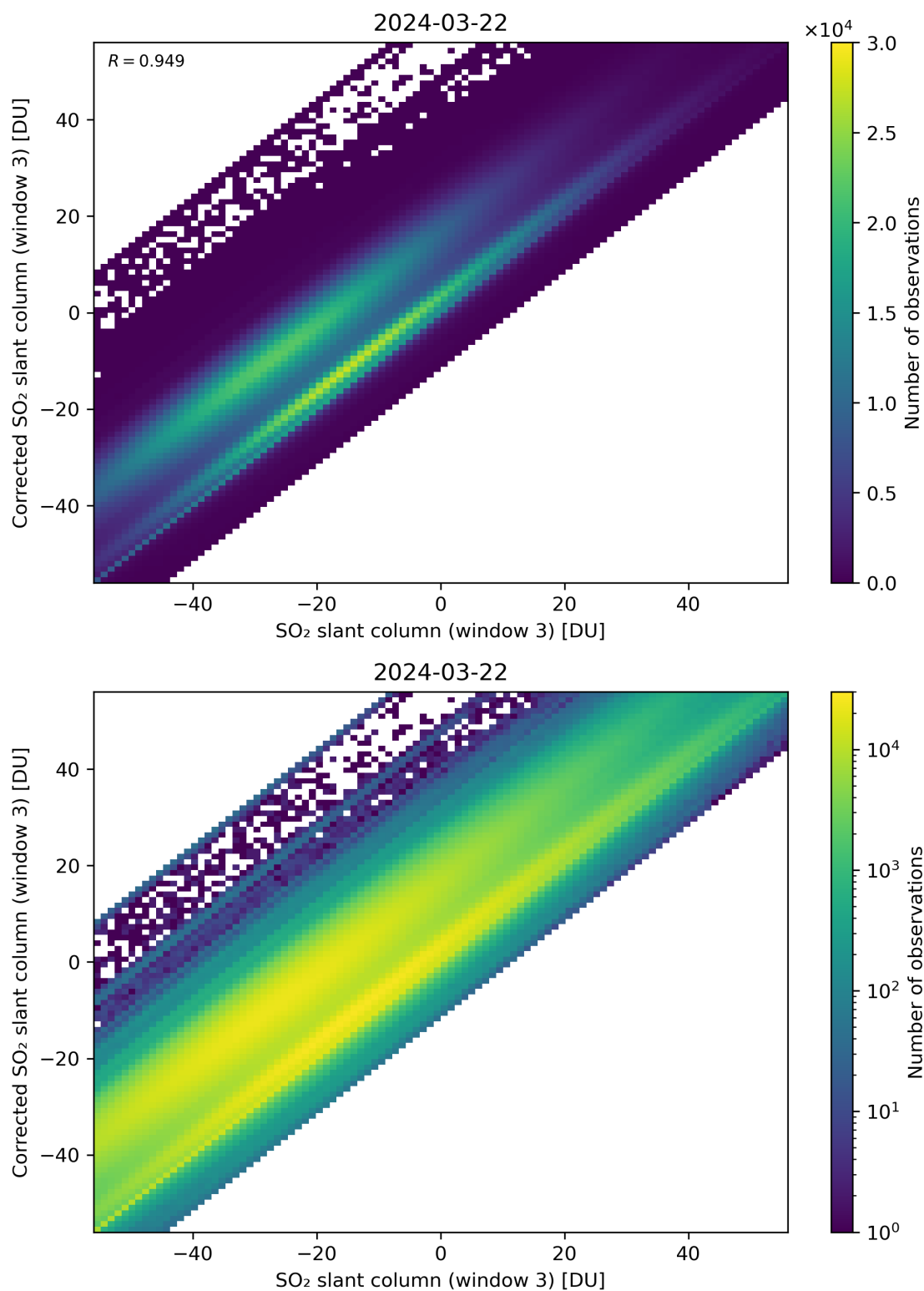
Figure 266: Scatter density plot of “SO 2 slant column (window 3)” against “Corrected SO 2 slant column (window 3)” for 2024-03-21 to 2024-03-22.
