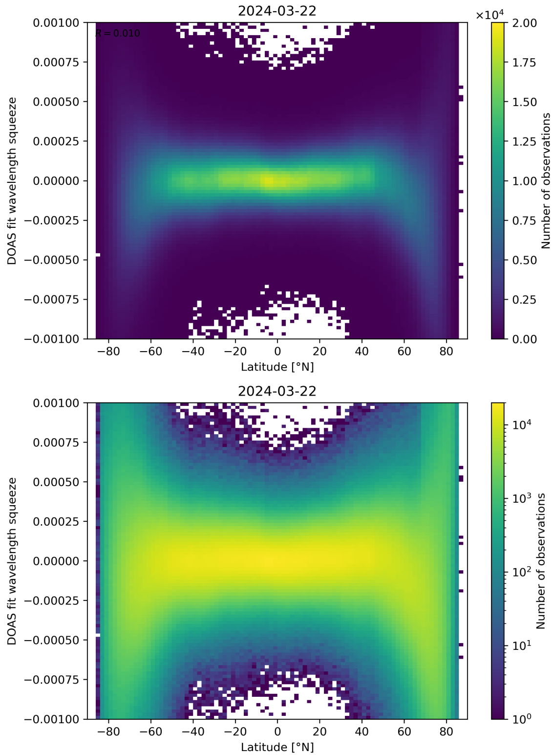
Figure 143: Scatter density plot of “Latitude” against “DOAS fit wavelength squeeze” for 2024-03-21 to 2024-03-22.
