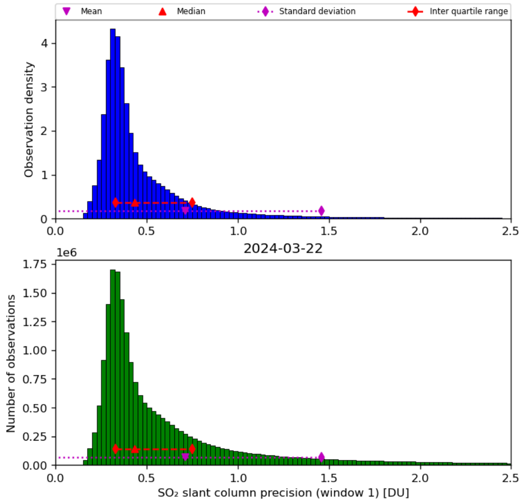
Figure 57: Histogram of “SO 2 slant column precision (window 1)” for 2024-03-21 to 2024-03-22
