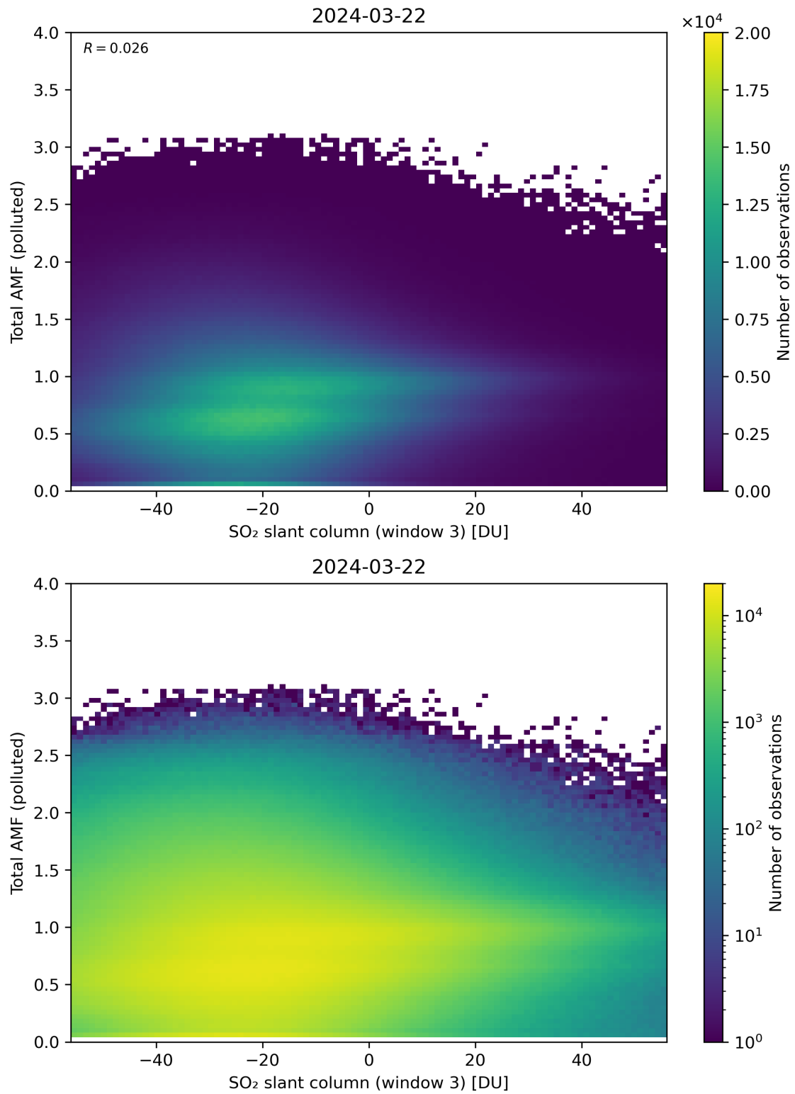
Figure 268: Scatter density plot of “SO 2 slant column (window 3)” against “Total AMF (polluted)” for 2024-03-21 to 2024-03-22.
