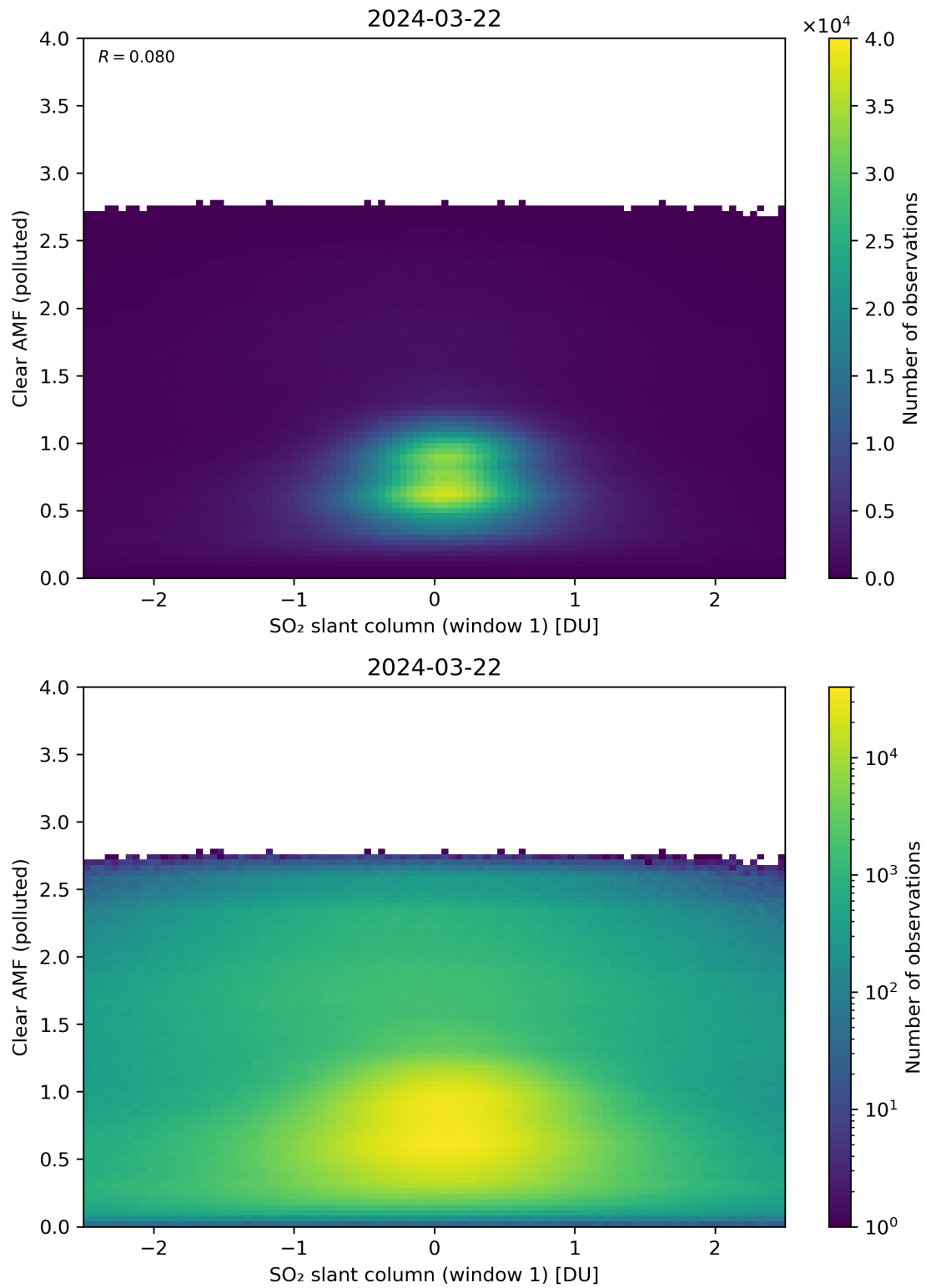
Figure 232: Scatter density plot of “SO 2 slant column (window 1)” against “Clear AMF (polluted)” for 2024-03-21 to 2024-03-22.
