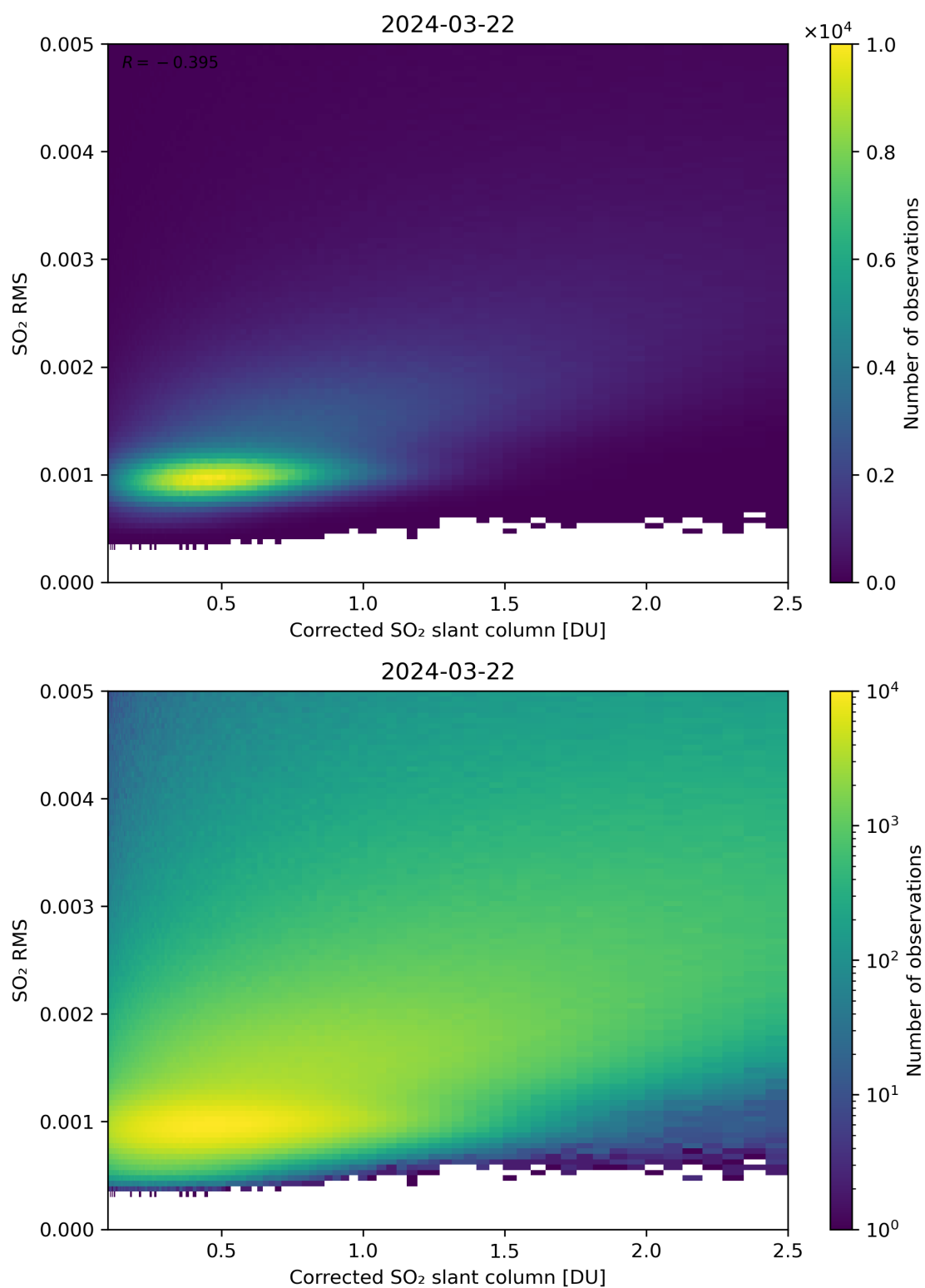
Figure 183: Scatter density plot of “Corrected SO 2 slant column” against “SO 2 RMS” for 2024-03-21 to 2024-03-22.
