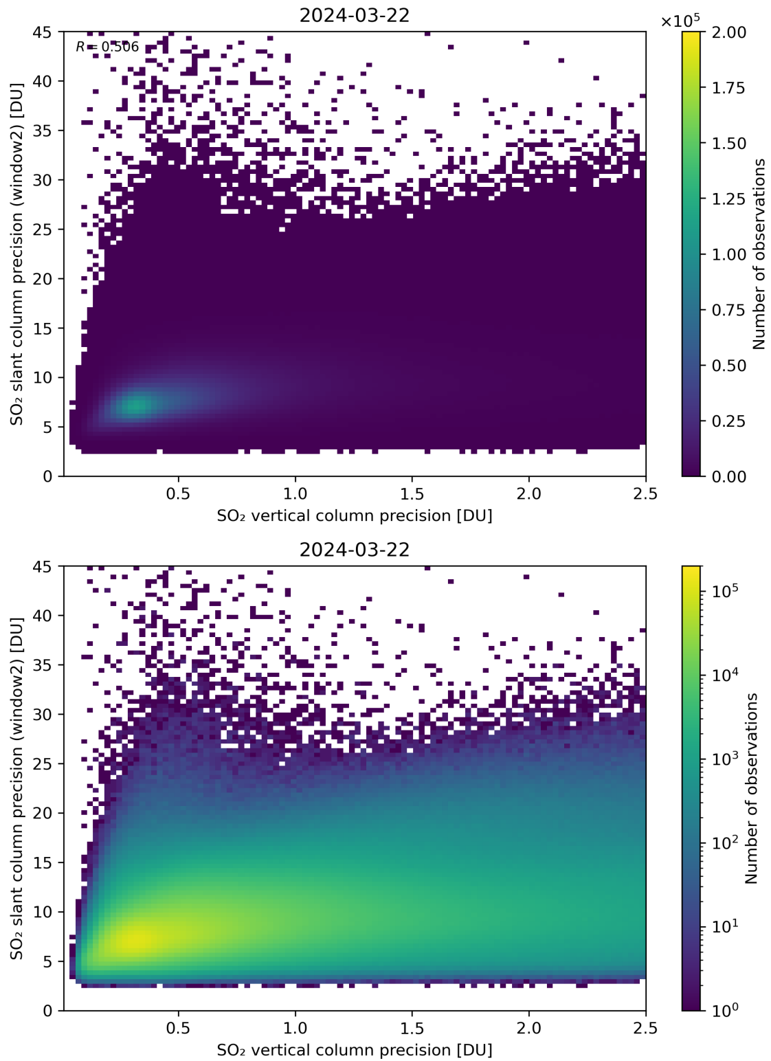
Figure 291: Scatter density plot of “SO 2 vertical column precision” against “SO 2 slant column precision (window2)” for 2024-03-21 to 2024-03-22.
