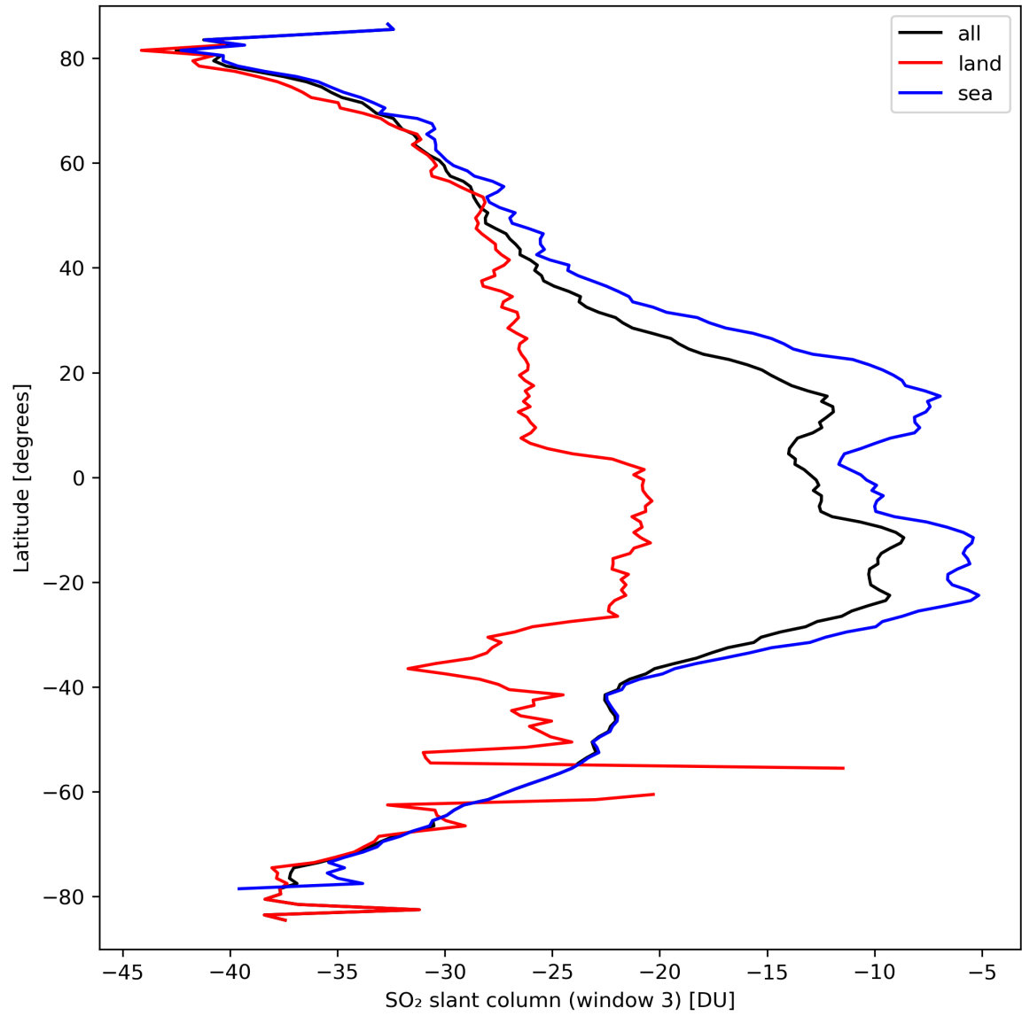
Figure 41: Zonal average of “SO 2 slant column (window 3)” for 2024-03-21 to 2024-03-22.
