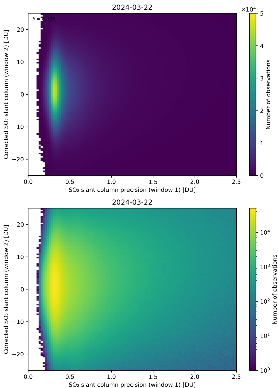
Figure 225: Scatter density plot of “SO 2 slant column precision (window 1)” against “Corrected SO 2 slant column (window 2)” for 2024-03-21 to 2024-03-22.
