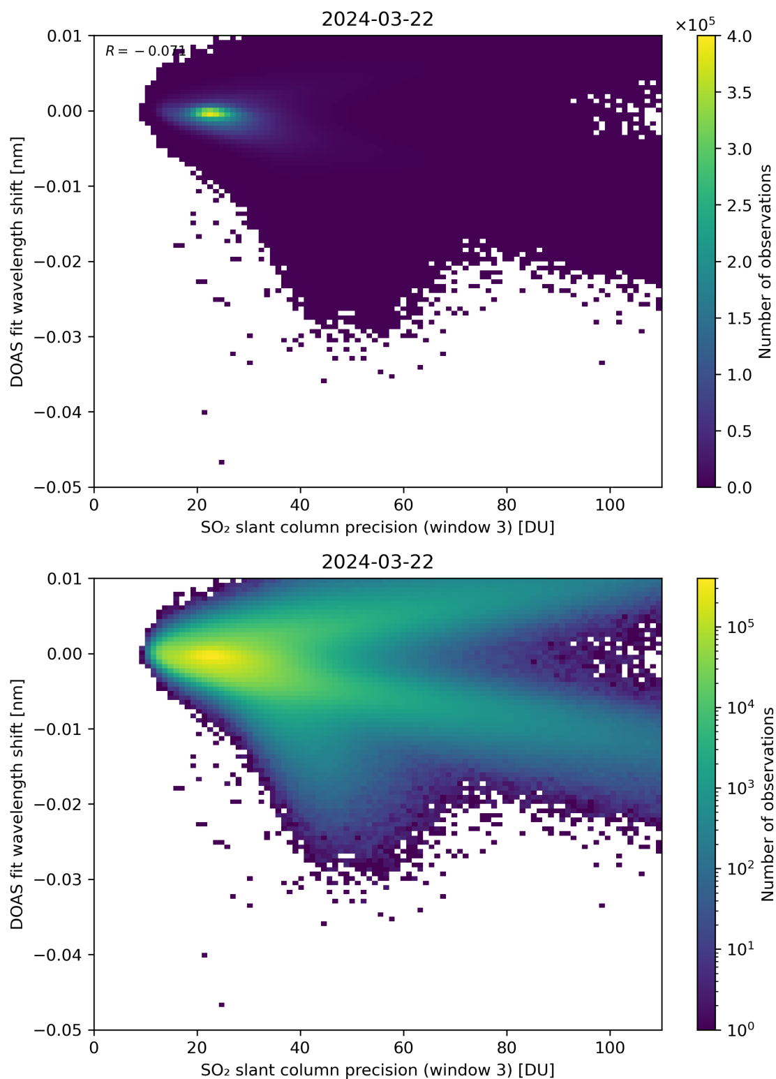
Figure 258: Scatter density plot of “SO 2 slant column precision (window 3)” against “DOAS fit wavelength shift” for 2024-03-21 to 2024-03-22.
