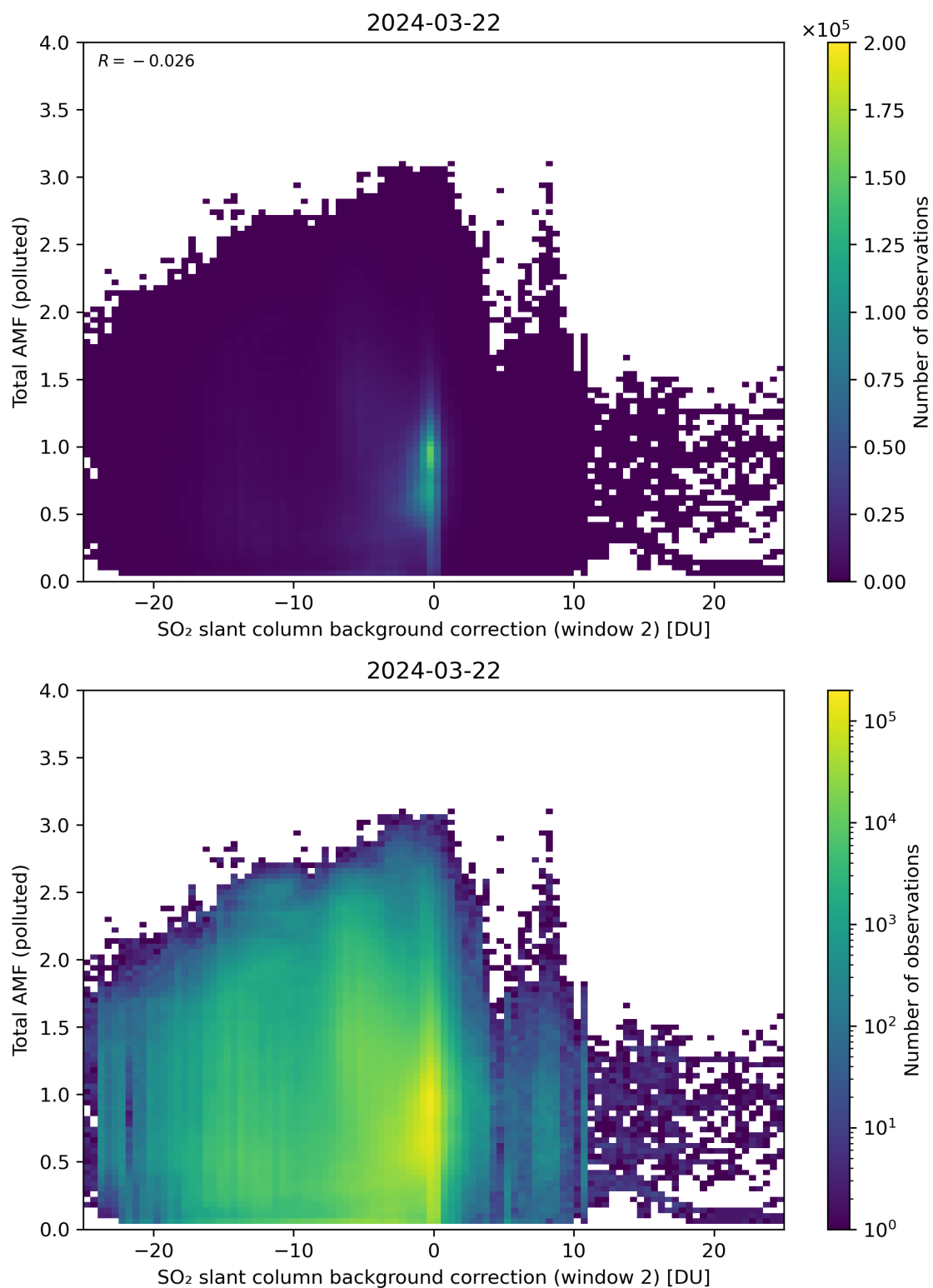
Figure 119: Scatter density plot of “SO 2 slant column background correction (window 2)” against “Total AMF (polluted)” for 2024-03-21 to 2024-03-22.
