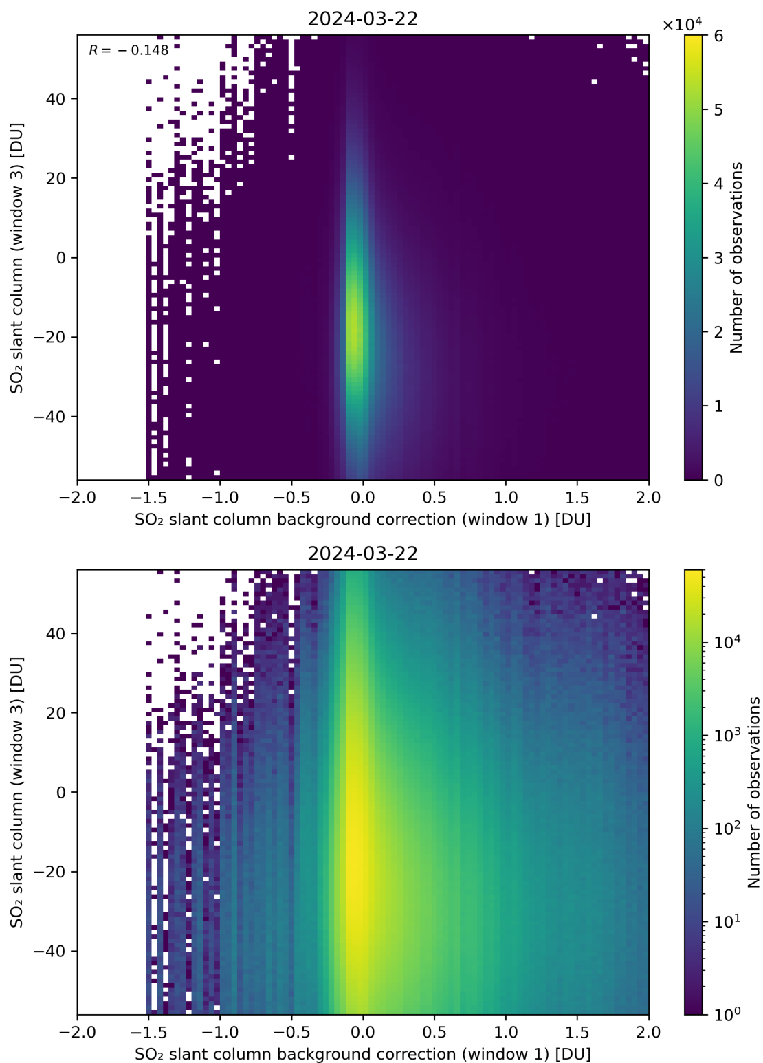
Figure 107: Scatter density plot of “SO 2 slant column background correction (window 1)” against “SO 2 slant column (window 3)” for 2024-03-21 to 2024-03-22.
