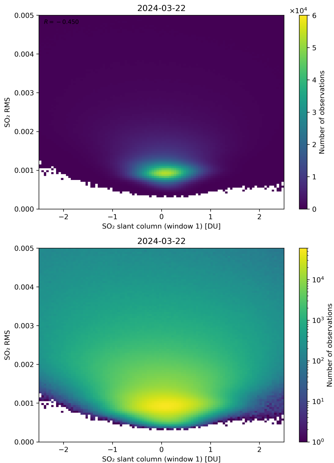
Figure 217: Scatter density plot of “SO 2 slant column (window 1)” against “SO 2 RMS” for 2024-03-21 to 2024-03-22.
