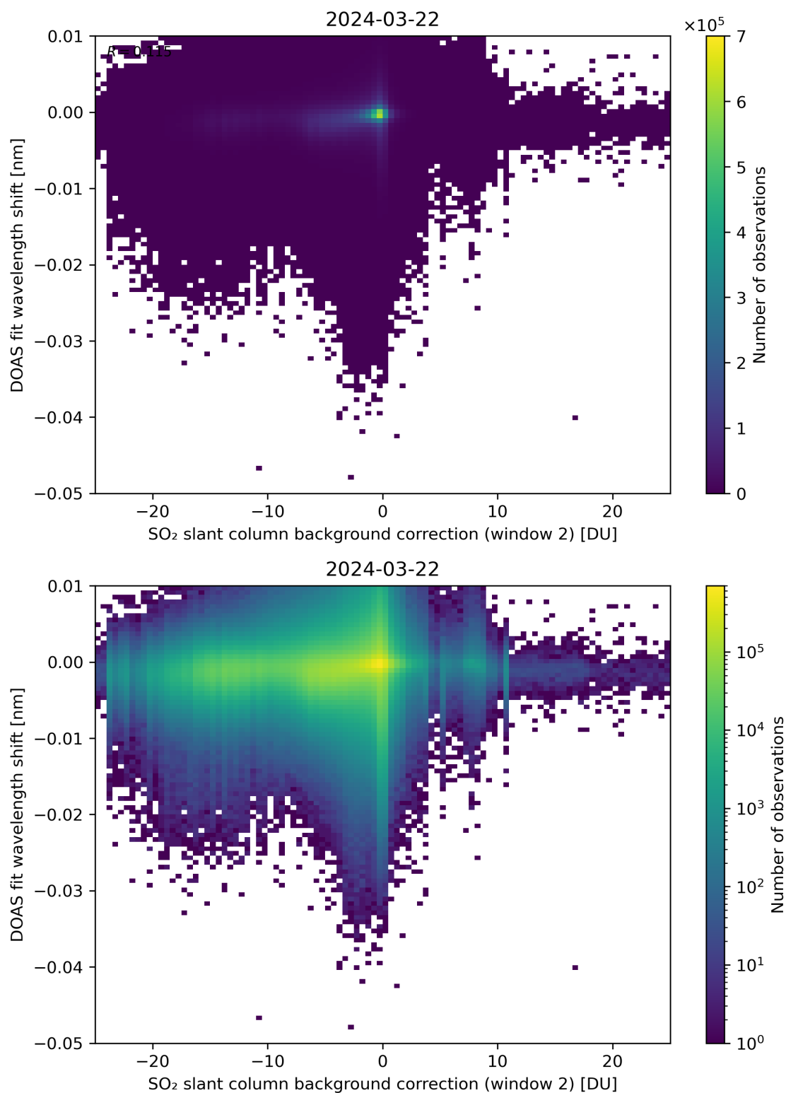
Figure 112: Scatter density plot of “SO 2 slant column background correction (window 2)” against “DOAS fit wavelength shift” for 2024-03-21 to 2024-03-22.
