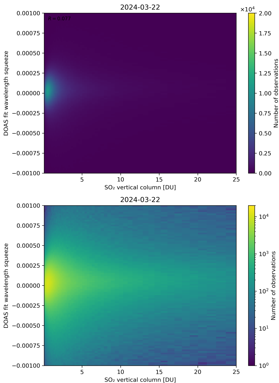
Figure 277: Scatter density plot of “SO 2 vertical column” against “DOAS fit wavelength squeeze” for 2024-03-21 to 2024-03-22.
