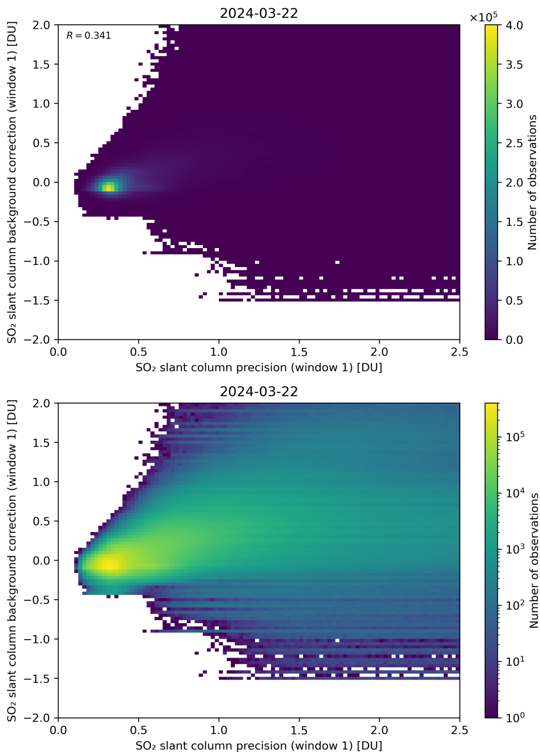
Figure 218: Scatter density plot of “SO 2 slant column precision (window 1)” against “SO 2 slant column background correction (window 1)” for 2024-03-21 to 2024-03-22.
