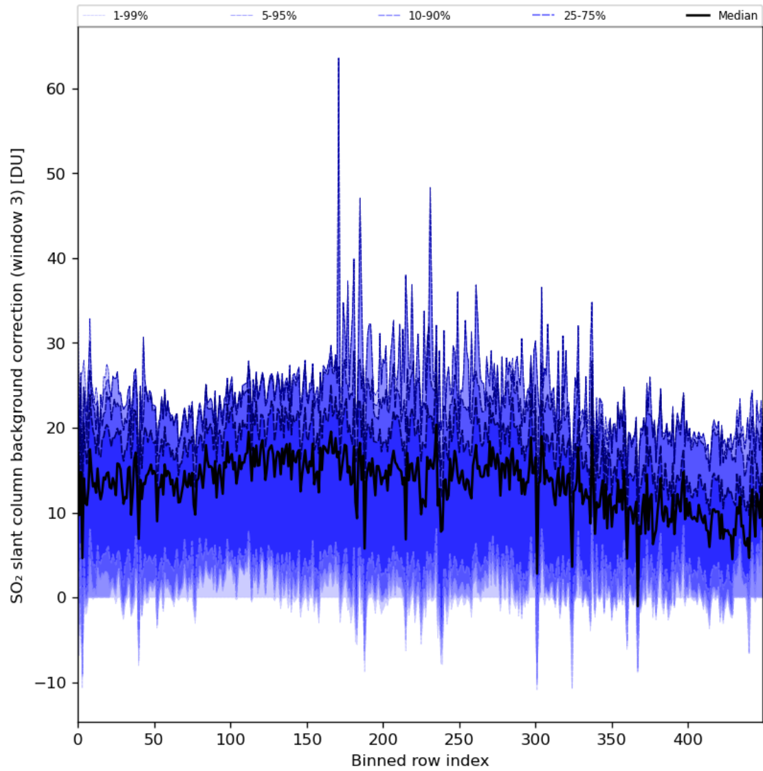
Figure 90: Along track statistics of “SO 2 slant column background correction (window 3)” for 2024-03-21 to 2024-03-22
