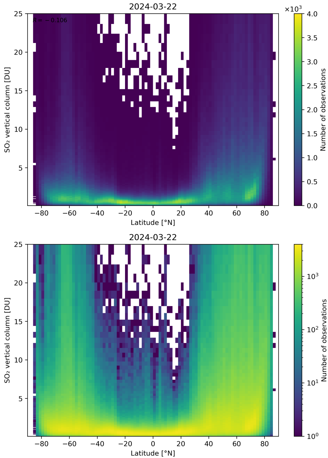
Figure 156: Scatter density plot of “Latitude” against “SO 2 vertical column” for 2024-03-21 to 2024-03-22.
