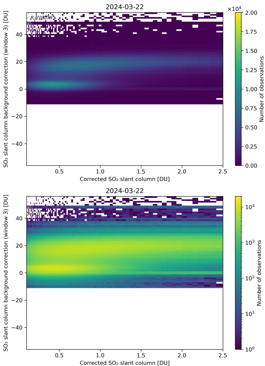
Figure 180: Scatter density plot of “Corrected SO 2 slant column” against “SO 2 slant column background correction (window 3)” for 2024-03-21 to 2024-03-22.
