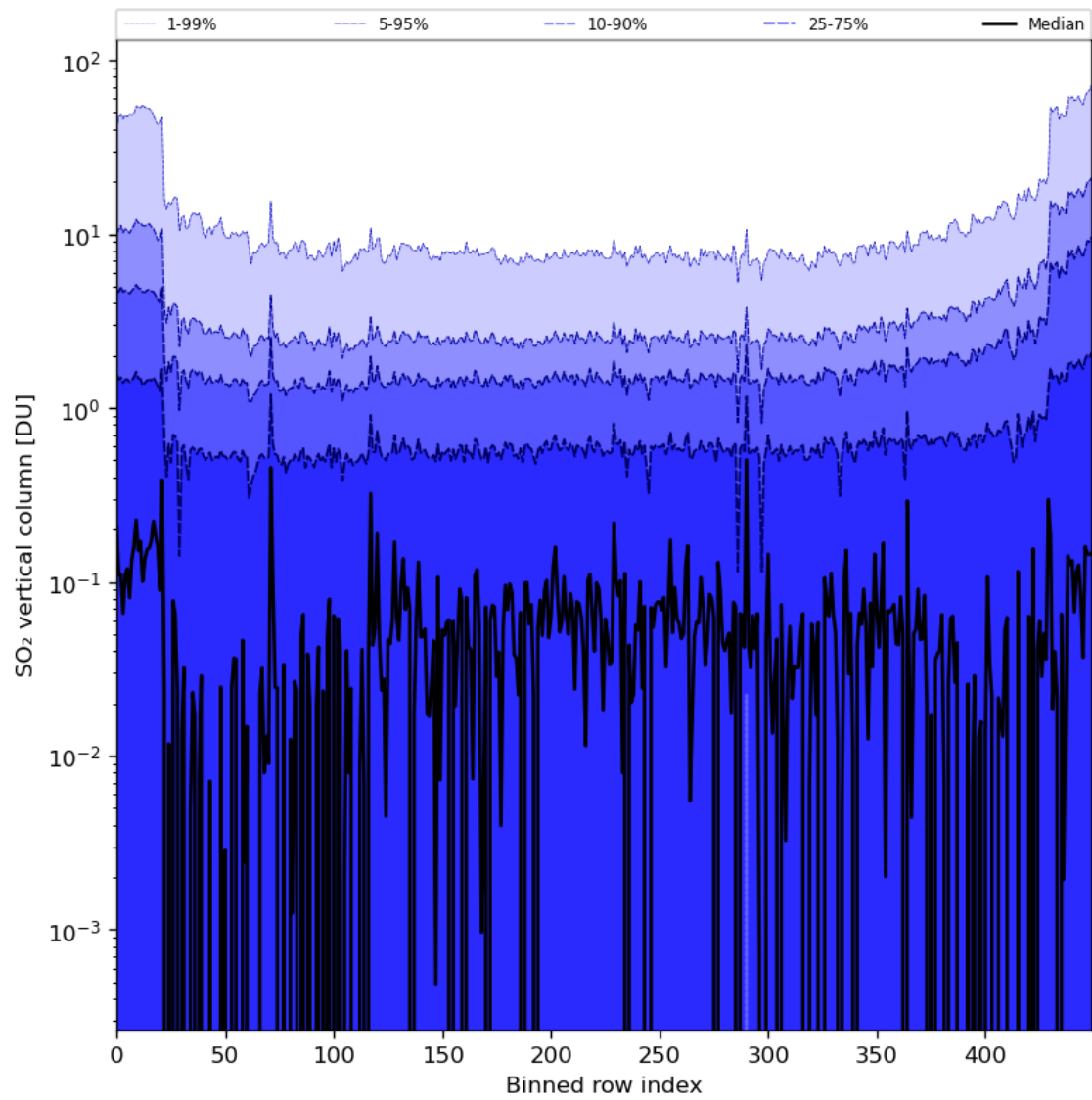
Figure 76: Along track statistics of “SO 2 vertical column” for 2024-03-21 to 2024-03-22
