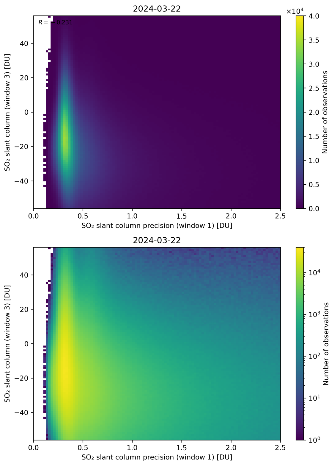
Figure 228: Scatter density plot of “SO 2 slant column precision (window 1)” against “SO 2 slant column (window 3)” for 2024-03-21 to 2024-03-22.
