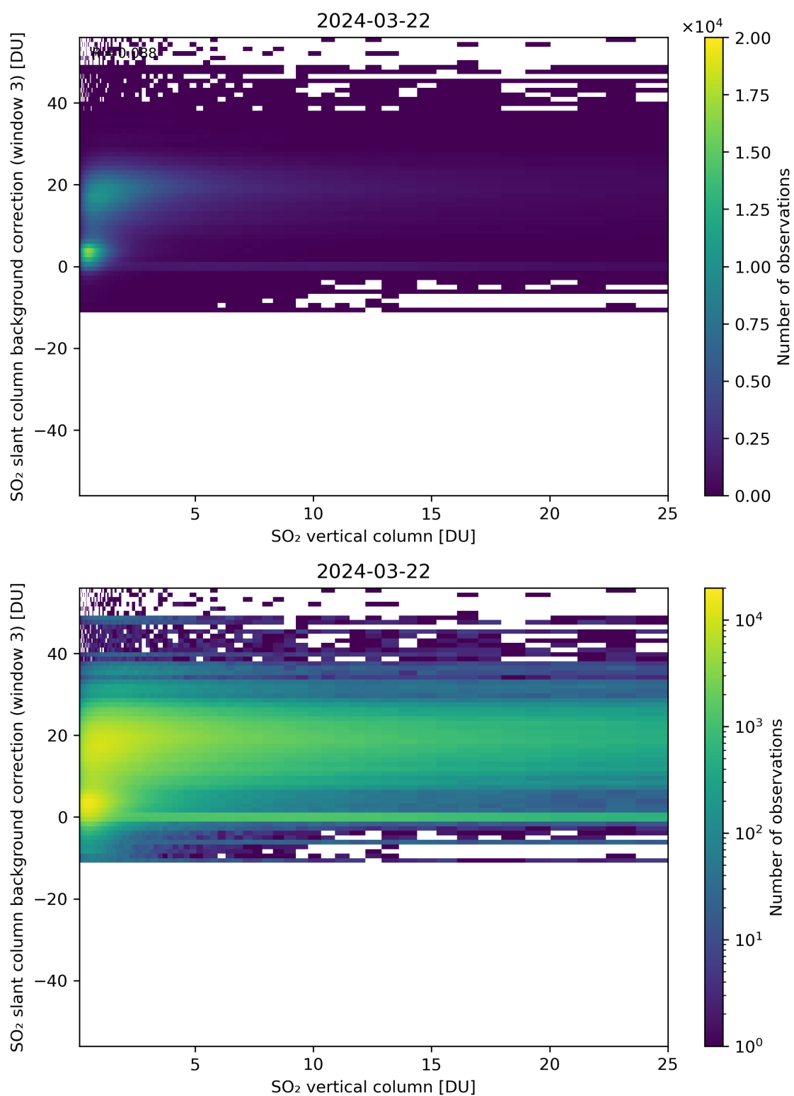
Figure 275: Scatter density plot of “SO 2 vertical column” against “SO 2 slant column background correction (window 3)” for 2024-03-21 to 2024-03-22.
