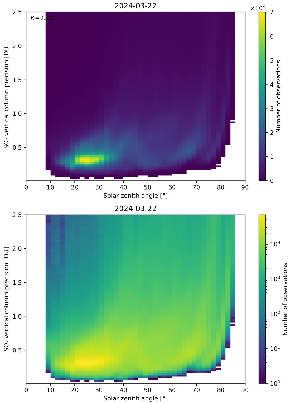
Figure 177: Scatter density plot of “Solar zenith angle” against “SO 2 vertical column precision” for 2024-03-21 to 2024-03-22.
