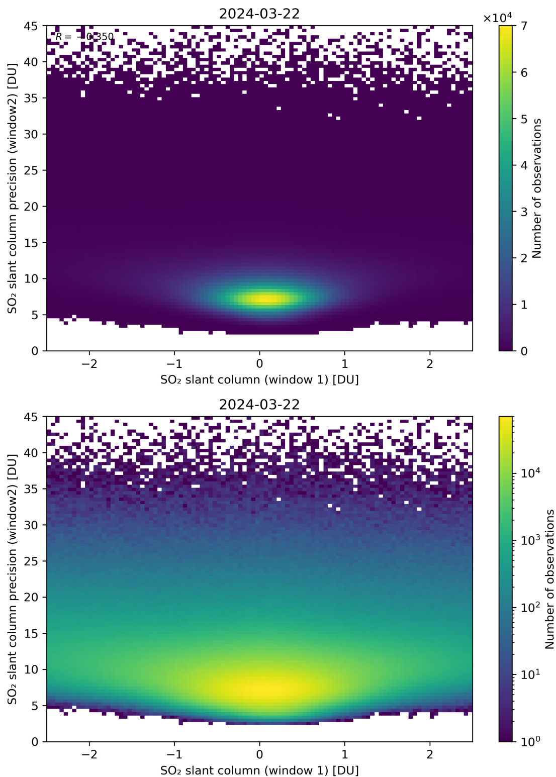
Figure 236: Scatter density plot of “SO 2 slant column (window 1)” against “SO 2 slant column precision (window2)” for 2024-03-21 to 2024-03-22.
