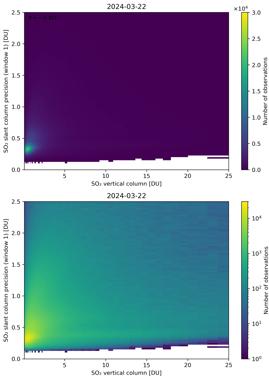
Figure 301: Scatter density plot of “SO 2 vertical column” against “SO 2 slant column precision (window 1)” for 2024-03-21 to 2024-03-22.
