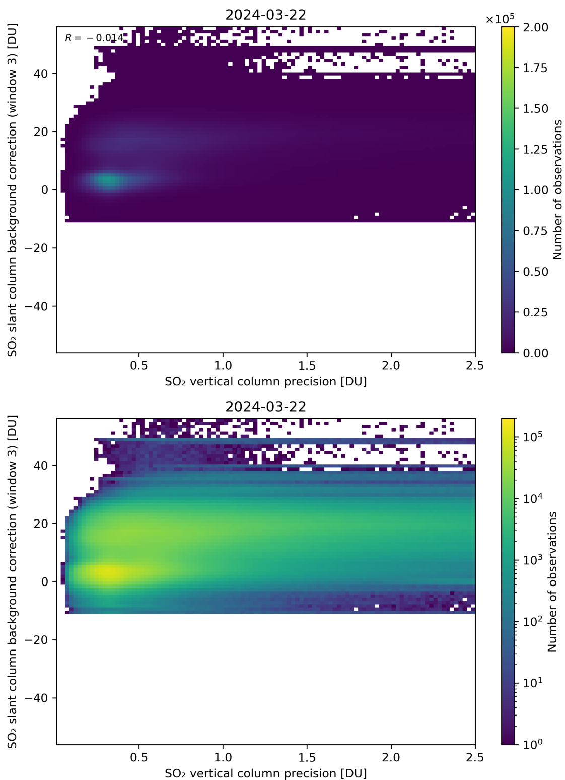
Figure 281: Scatter density plot of “SO 2 vertical column precision” against “SO 2 slant column background correction (window 3)” for 2024-03-21 to 2024-03-22.
