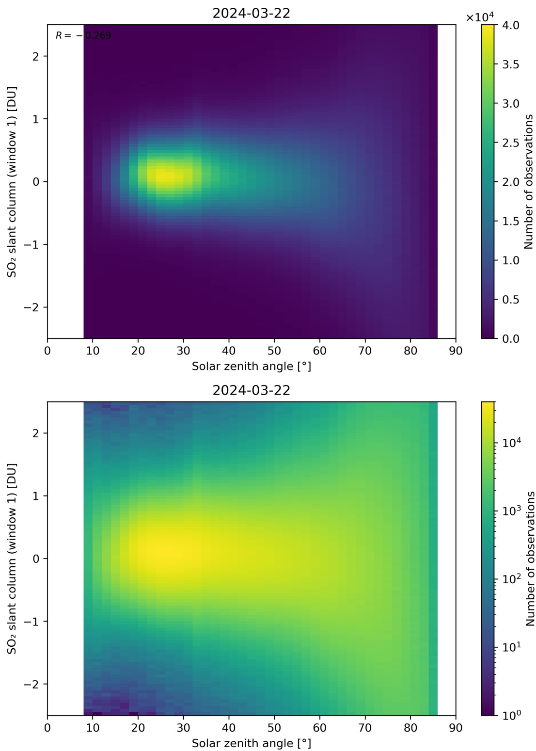
Figure 169: Scatter density plot of “Solar zenith angle” against “SO 2 slant column (window 1)” for 2024-03-21 to 2024-03-22.
