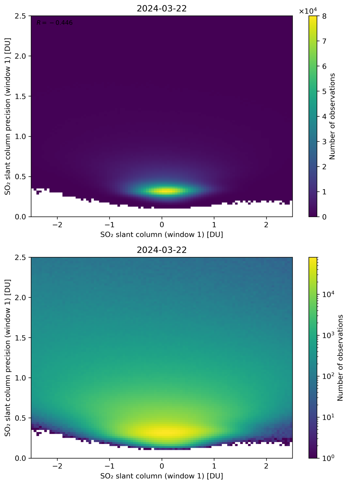
Figure 235: Scatter density plot of “SO 2 slant column (window 1)” against “SO 2 slant column precision (window 1)” for 2024-03-21 to 2024-03-22.
