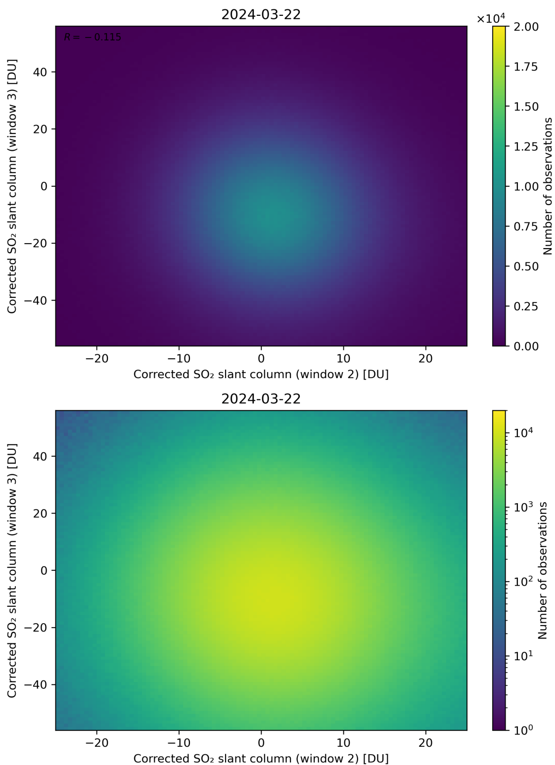
Figure 200: Scatter density plot of “Corrected SO 2 slant column (window 2)” against “Corrected SO 2 slant column (window 3)” for 2024-03-21 to 2024-03-22.
