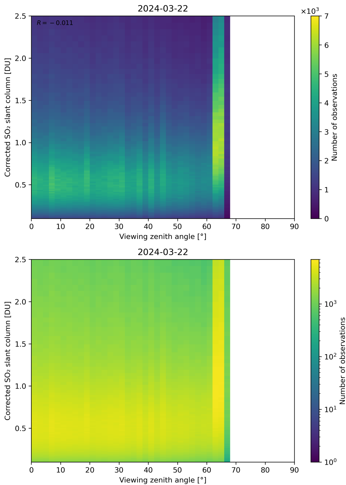
Figure 317: Scatter density plot of “Viewing zenith angle” against “Corrected SO 2 slant column” for 2024-03-21 to 2024-03-22.
