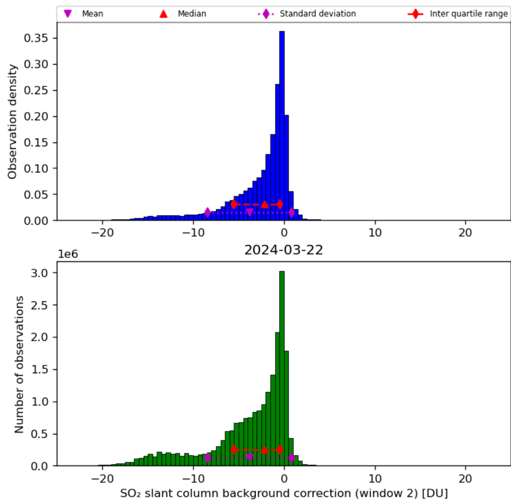
Figure 63: Histogram of “SO 2 slant column background correction (window 2)” for 2024-03-21 to 2024-03-22
