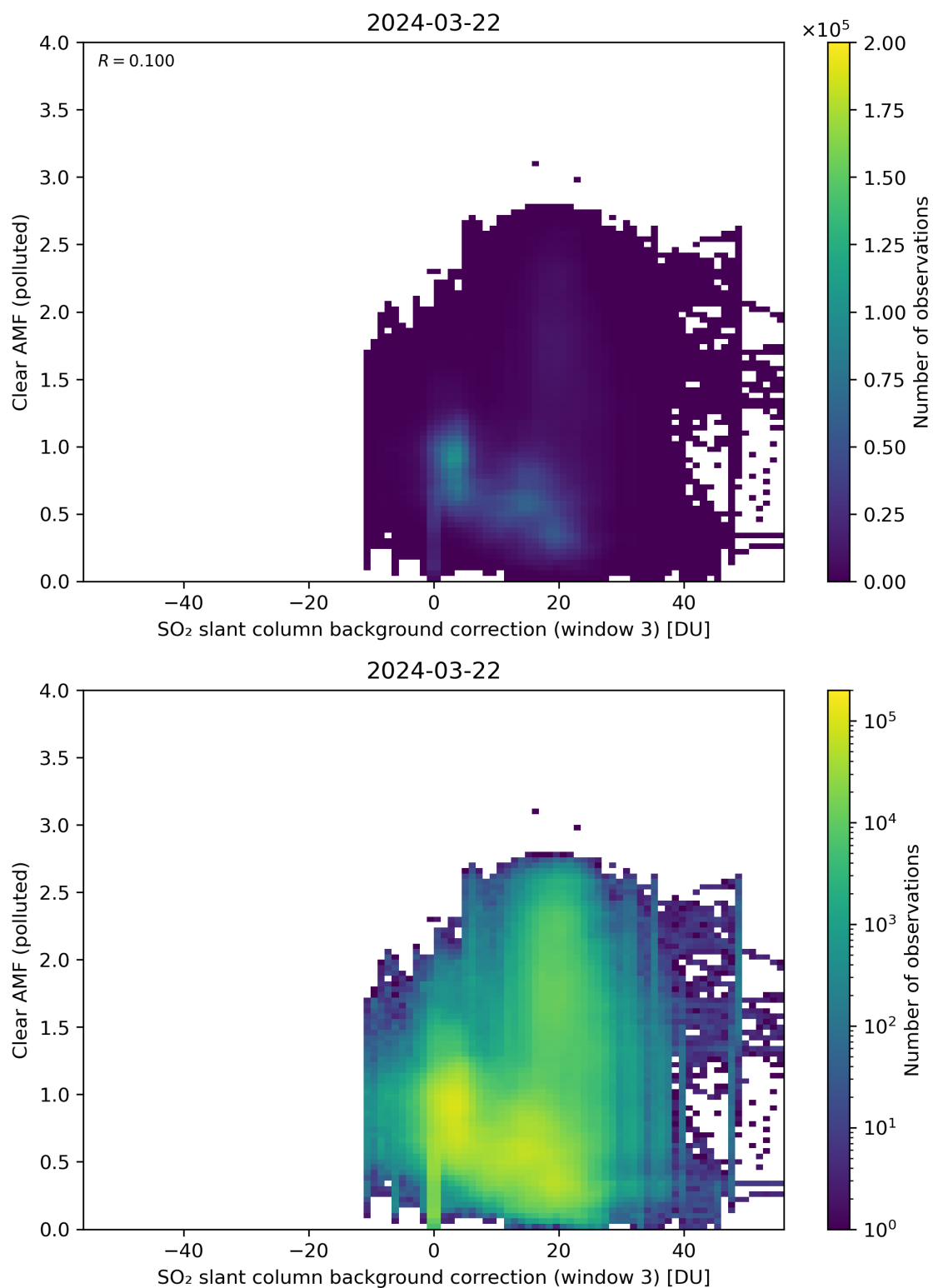
Figure 124: Scatter density plot of “SO 2 slant column background correction (window 3)” against “Clear AMF (polluted)” for 2024-03-21 to 2024-03-22.
