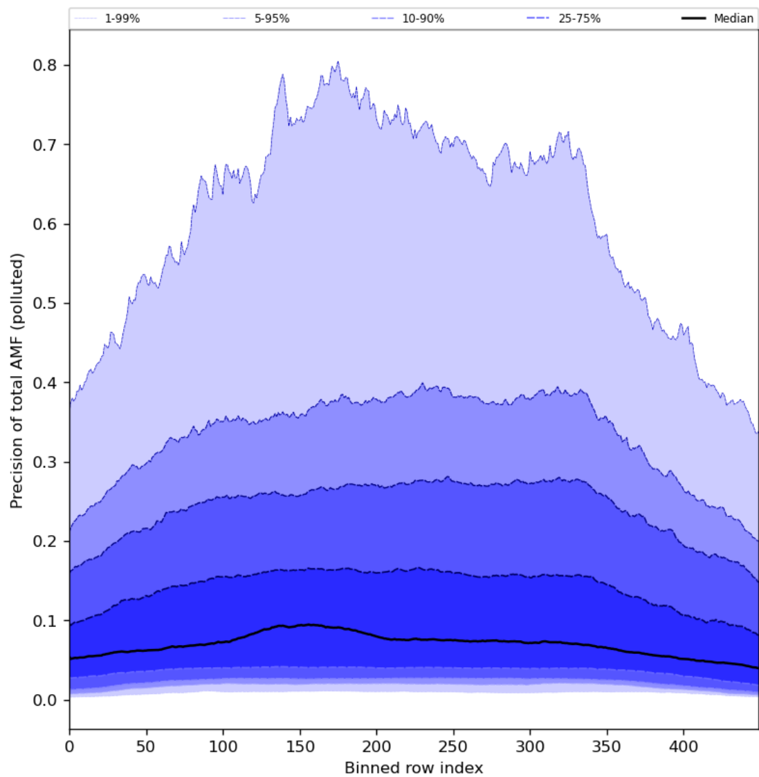
Figure 95: Along track statistics of “Precision of total AMF (polluted)” for 2024-03-21 to 2024-03-22
