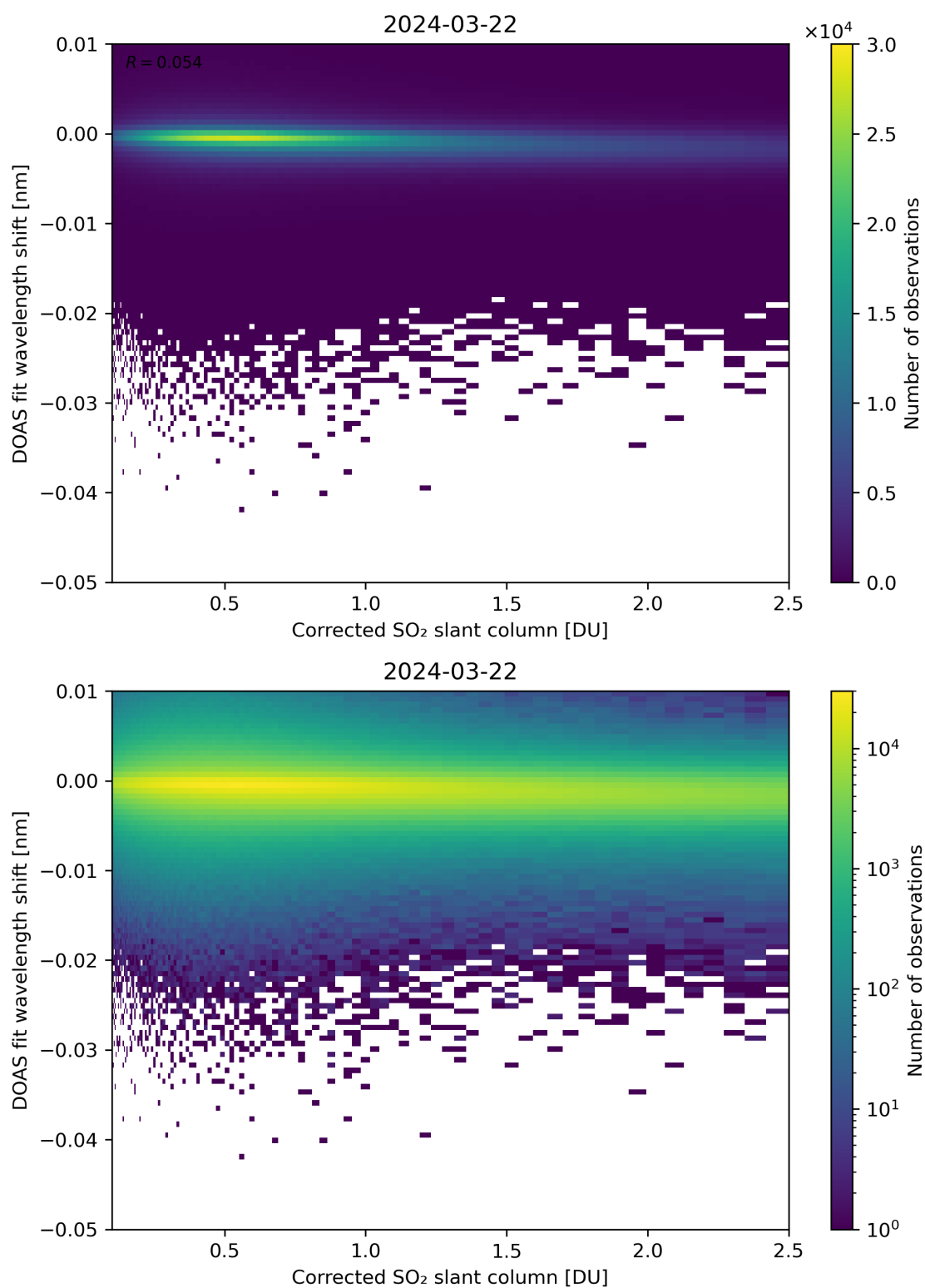
Figure 181: Scatter density plot of “Corrected SO 2 slant column” against “DOAS fit wavelength shift” for 2024-03-21 to 2024-03-22.
