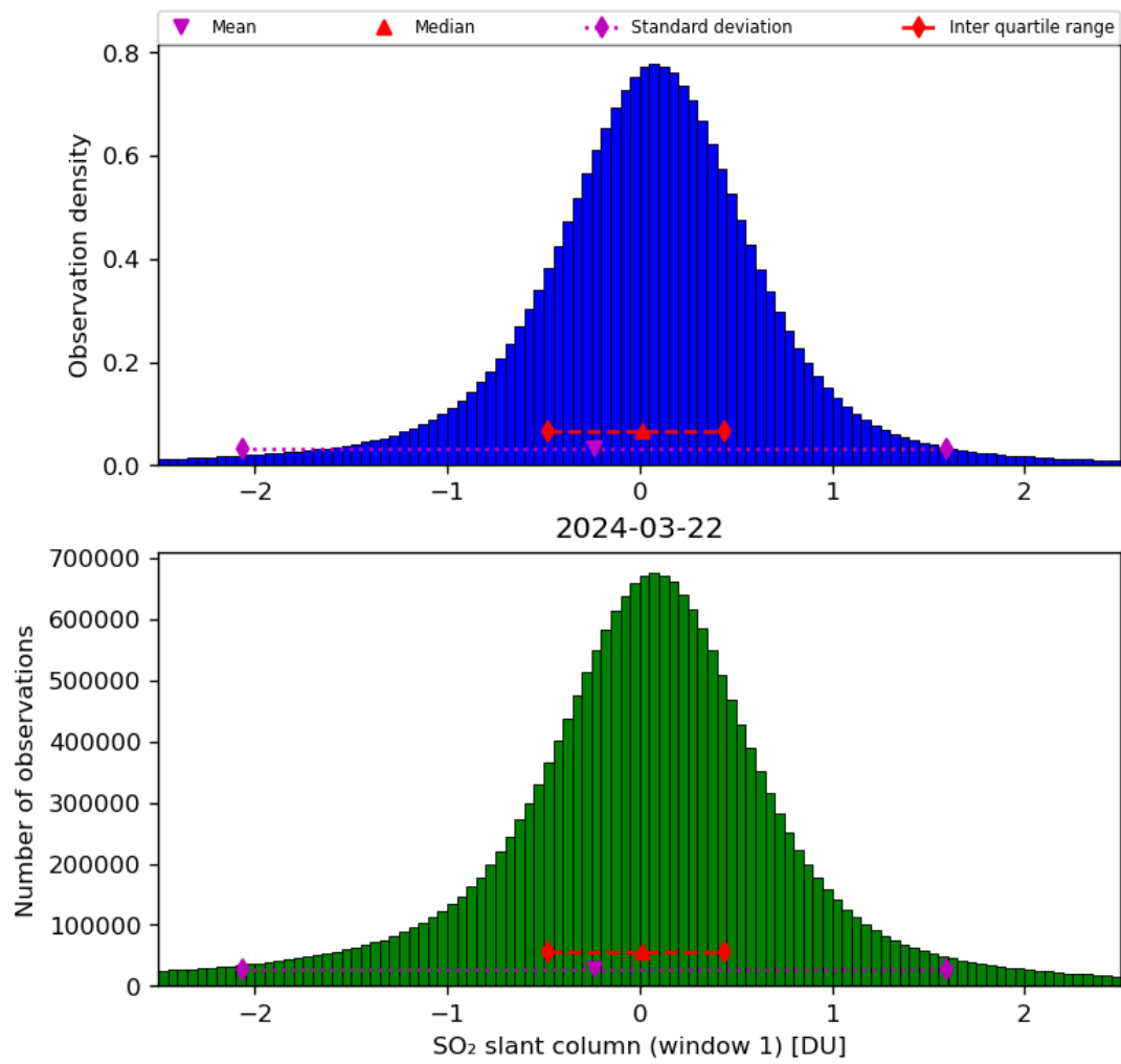
Figure 56: Histogram of “SO 2 slant column (window 1)” for 2024-03-21 to 2024-03-22
