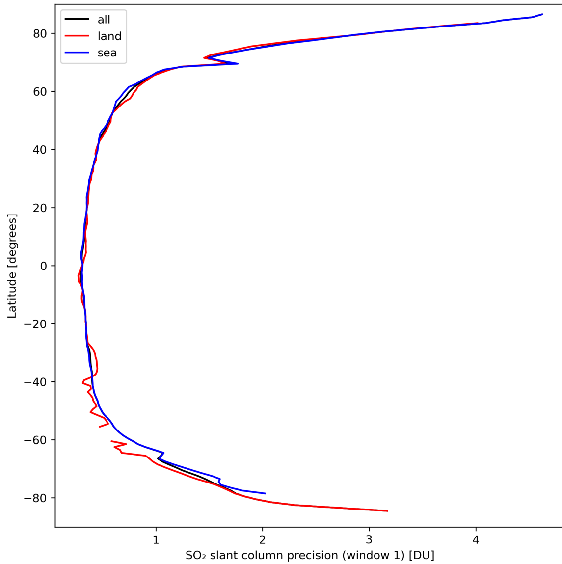
Figure 34: Zonal average of “SO 2 slant column precision (window 1)” for 2024-03-21 to 2024-03-22.
