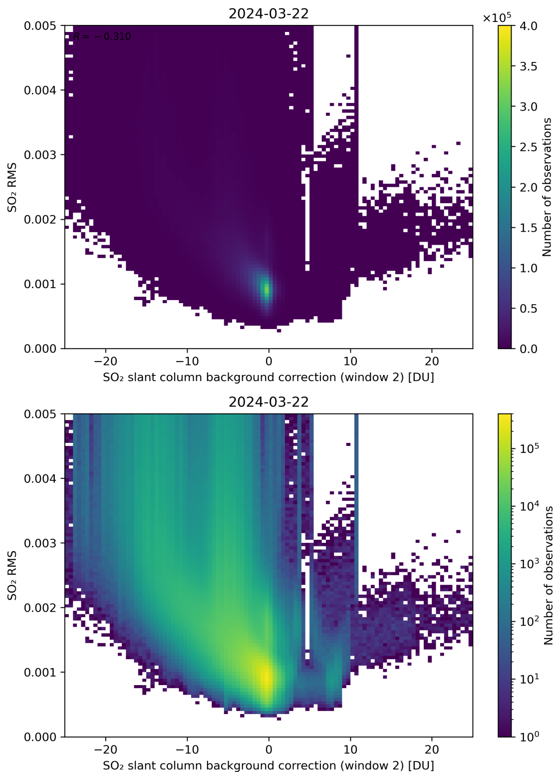
Figure 114: Scatter density plot of “SO 2 slant column background correction (window 2)” against “SO 2 RMS” for 2024-03-21 to 2024-03-22.
