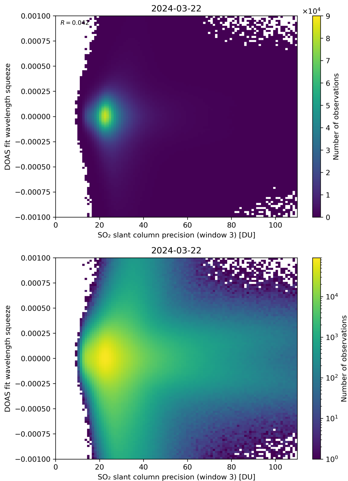
Figure 259: Scatter density plot of “SO 2 slant column precision (window 3)” against “DOAS fit wavelength squeeze” for 2024-03-21 to 2024-03-22.
