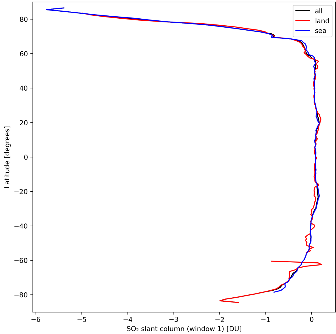
Figure 33: Zonal average of “SO 2 slant column (window 1)” for 2024-03-21 to 2024-03-22.
