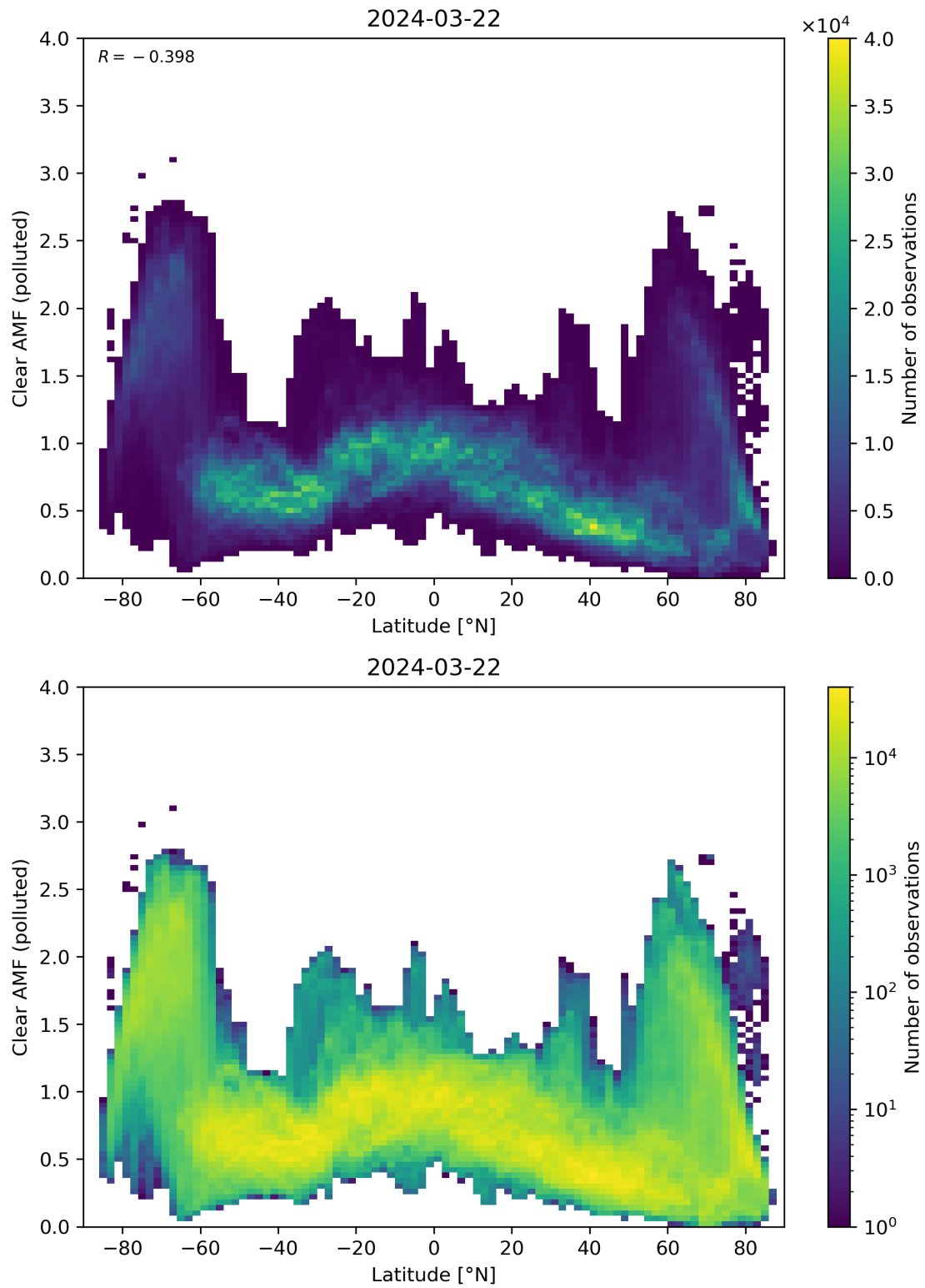
Figure 145: Scatter density plot of “Latitude” against “Clear AMF (polluted)” for 2024-03-21 to 2024-03-22.
