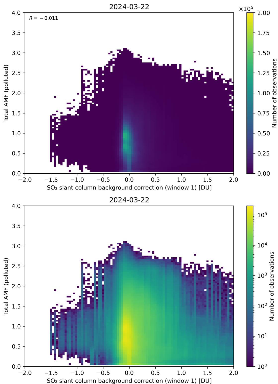
Figure 109: Scatter density plot of “SO 2 slant column background correction (window 1)” against “Total AMF (polluted)” for 2024-03-21 to 2024-03-22.
