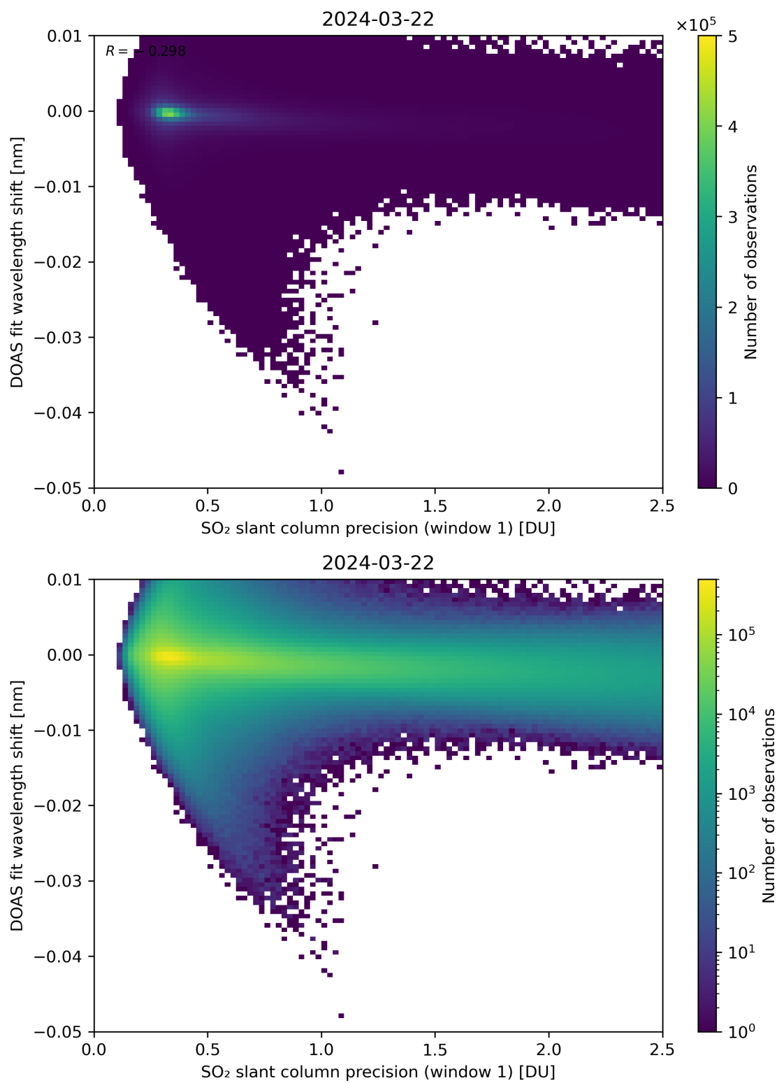
Figure 221: Scatter density plot of “SO 2 slant column precision (window 1)” against “DOAS fit wavelength shift” for 2024-03-21 to 2024-03-22.
