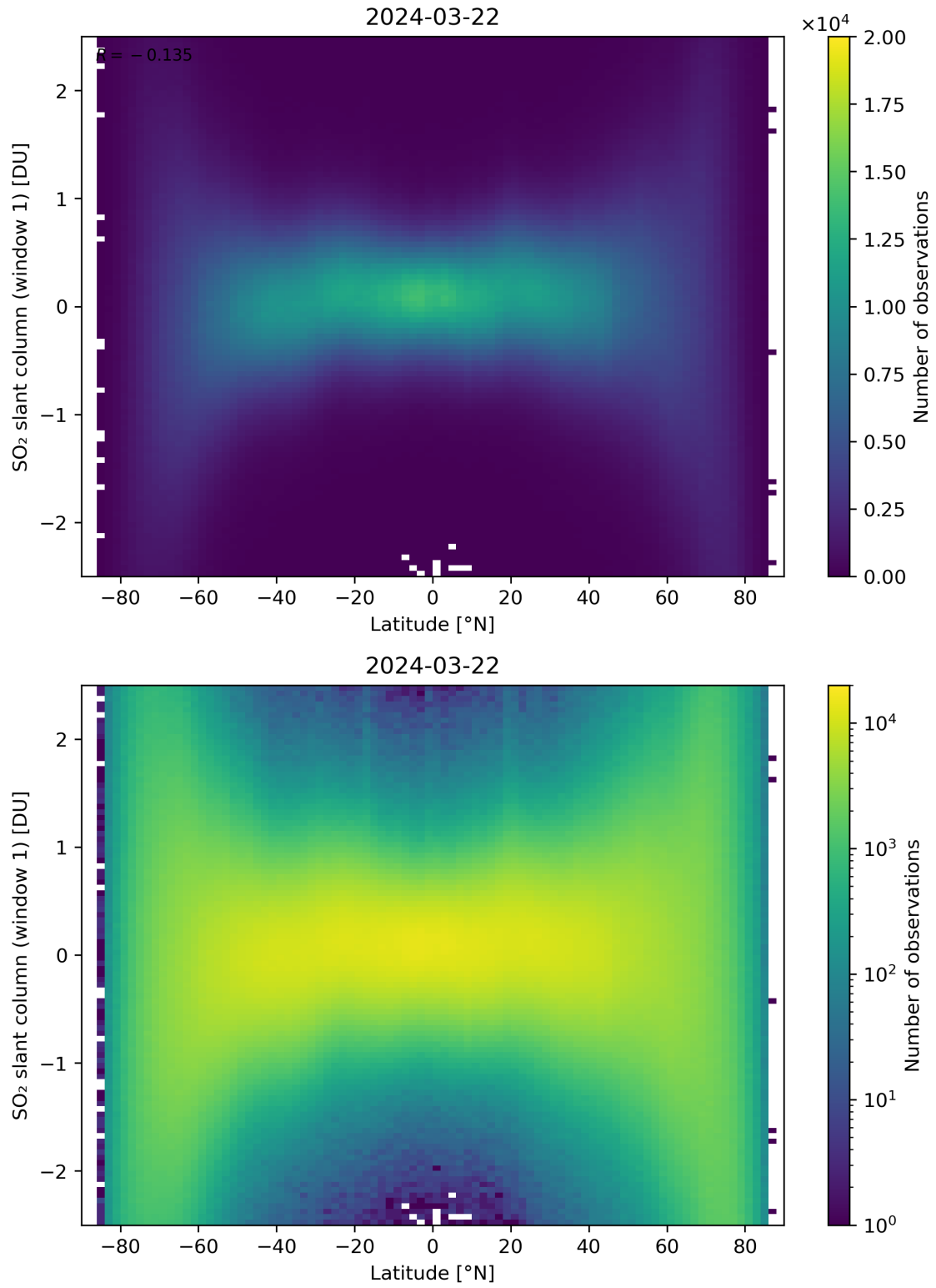
Figure 149: Scatter density plot of “Latitude” against “SO 2 slant column (window 1)” for 2024-03-21 to 2024-03-22.
