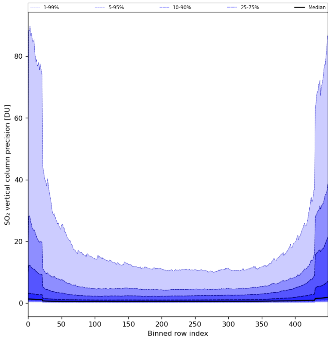
Figure 77: Along track statistics of “SO 2 vertical column precision” for 2024-03-21 to 2024-03-22
