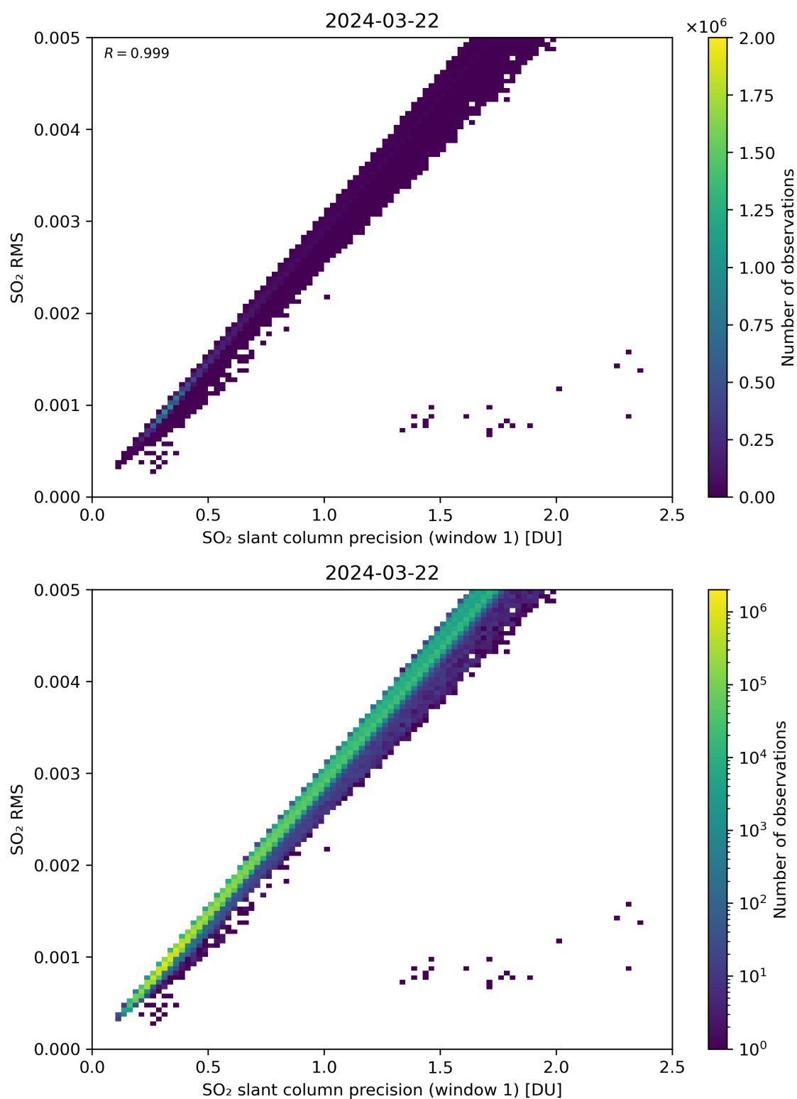
Figure 223: Scatter density plot of “SO 2 slant column precision (window 1)” against “SO 2 RMS” for 2024-03-21 to 2024-03-22.
