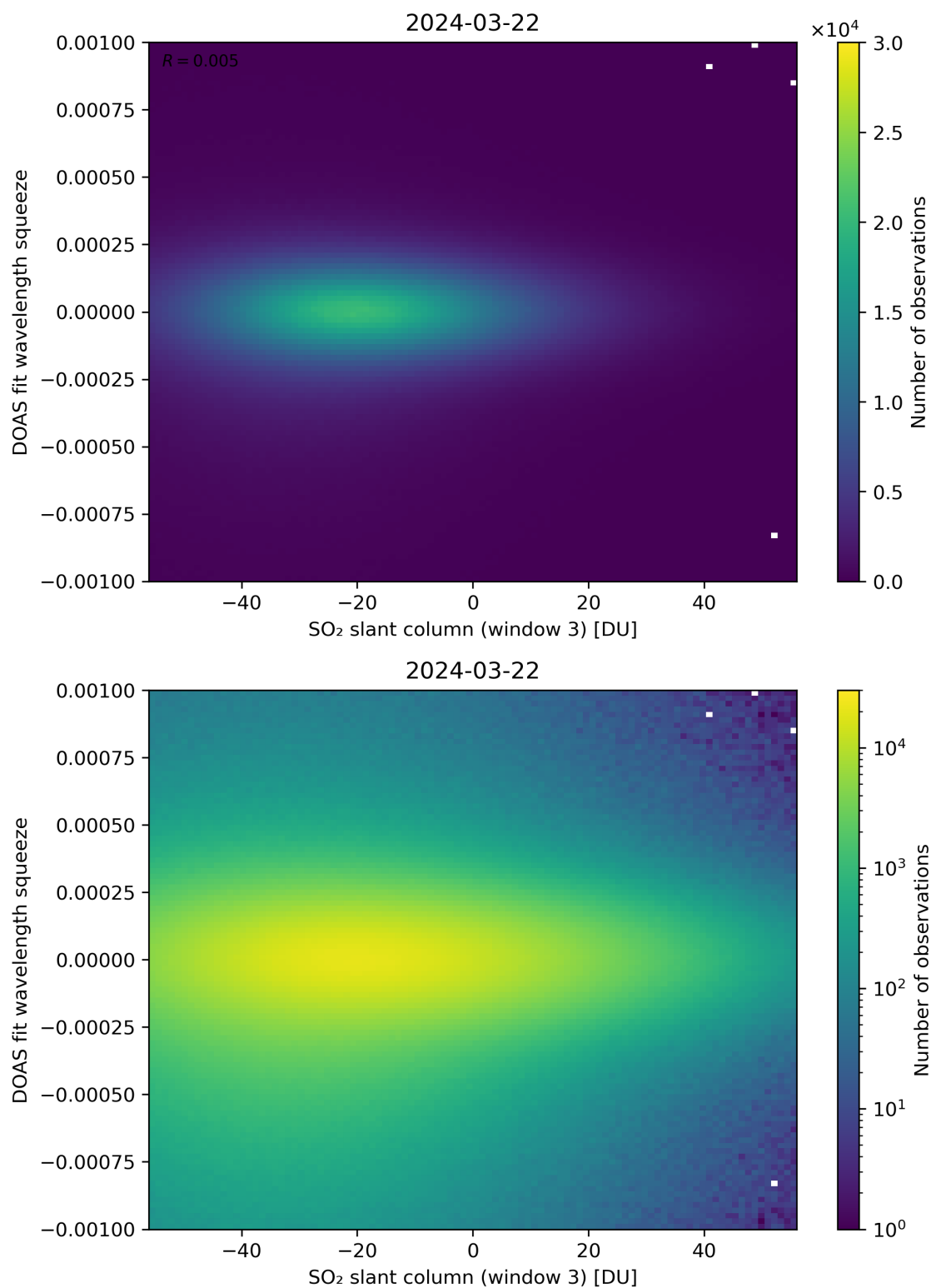
Figure 255: Scatter density plot of “SO 2 slant column (window 3)” against “DOAS fit wavelength squeeze” for 2024-03-21 to 2024-03-22.
