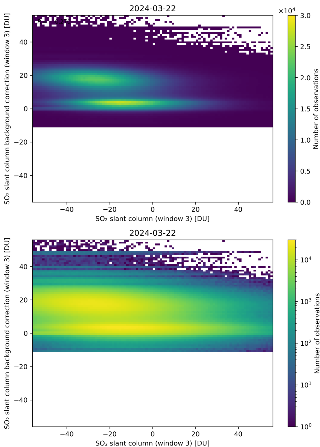
Figure 253: Scatter density plot of “SO 2 slant column (window 3)” against “SO 2 slant column background correction (window 3)” for 2024-03-21 to 2024-03-22.
