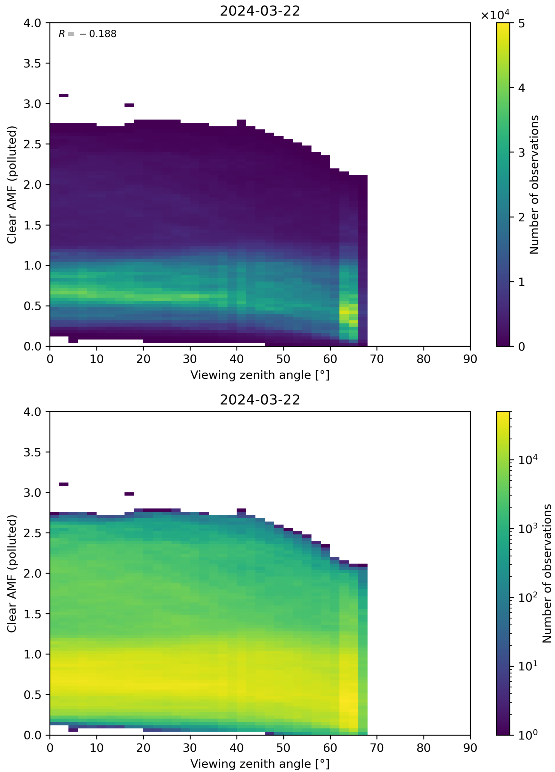
Figure 316: Scatter density plot of “Viewing zenith angle” against “Clear AMF (polluted)” for 2024-03-21 to 2024-03-22.
