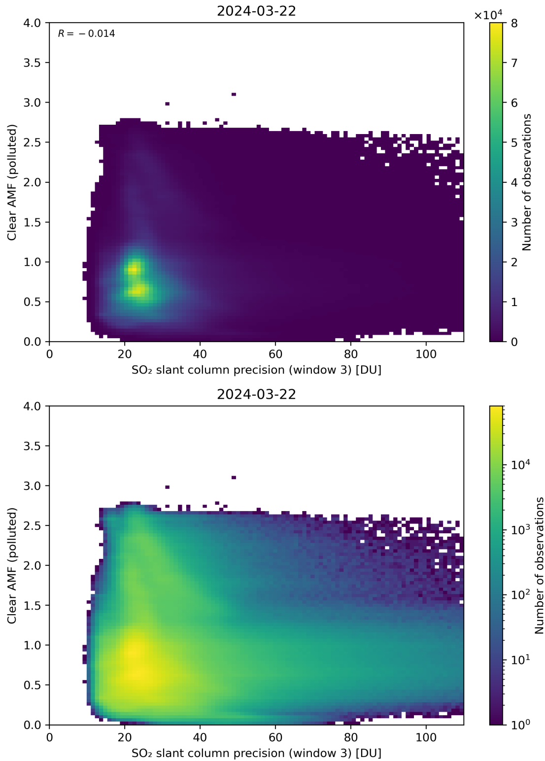
Figure 261: Scatter density plot of “SO 2 slant column precision (window 3)” against “Clear AMF (polluted)” for 2024-03-21 to 2024-03-22.
