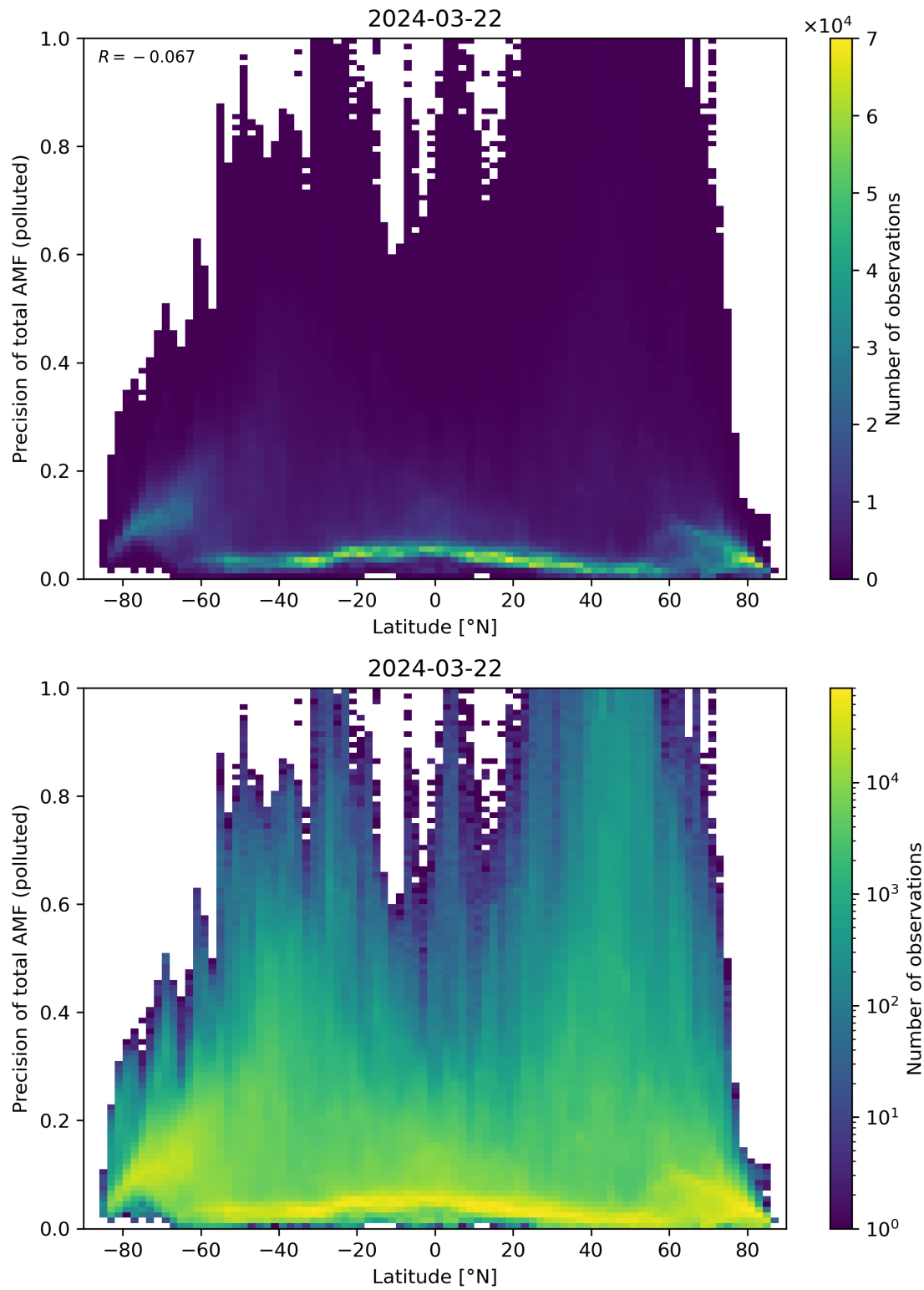
Figure 155: Scatter density plot of “Latitude” against “Precision of total AMF (polluted)” for 2024-03-21 to 2024-03-22.
