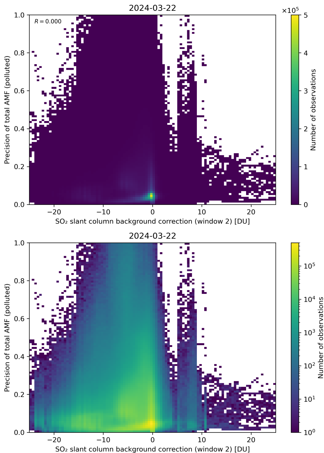
Figure 120: Scatter density plot of “SO 2 slant column background correction (window 2)” against “Precision of total AMF (polluted)” for 2024-03-21 to 2024-03-22.
