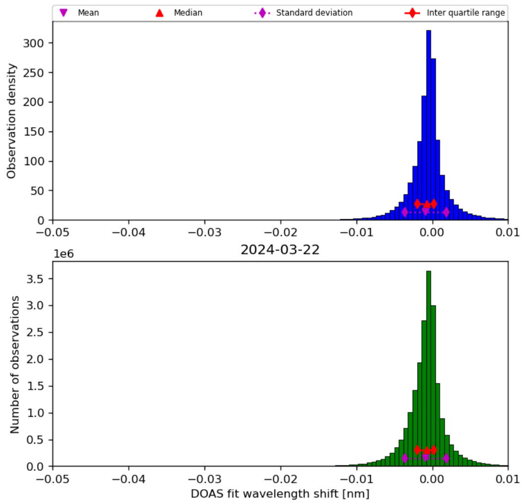
Figure 68: Histogram of “DOAS fit wavelength shift” for 2024-03-21 to 2024-03-22
