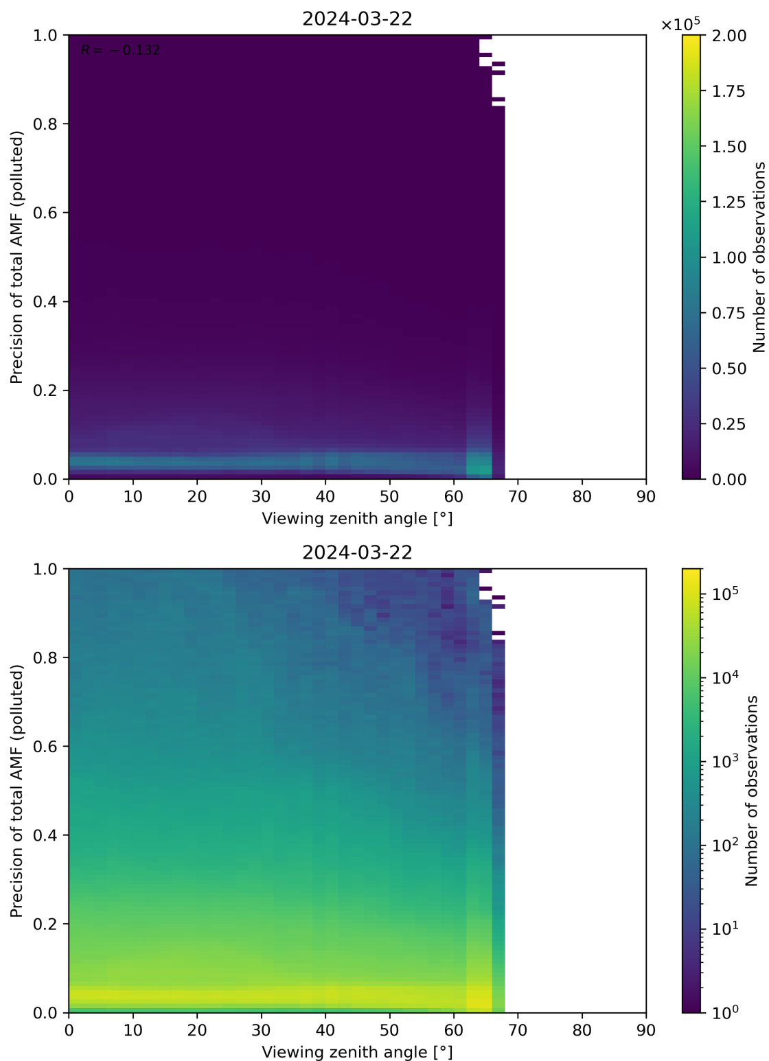
Figure 326: Scatter density plot of “Viewing zenith angle” against “Precision of total AMF (polluted)” for 2024-03-21 to 2024-03-22.
