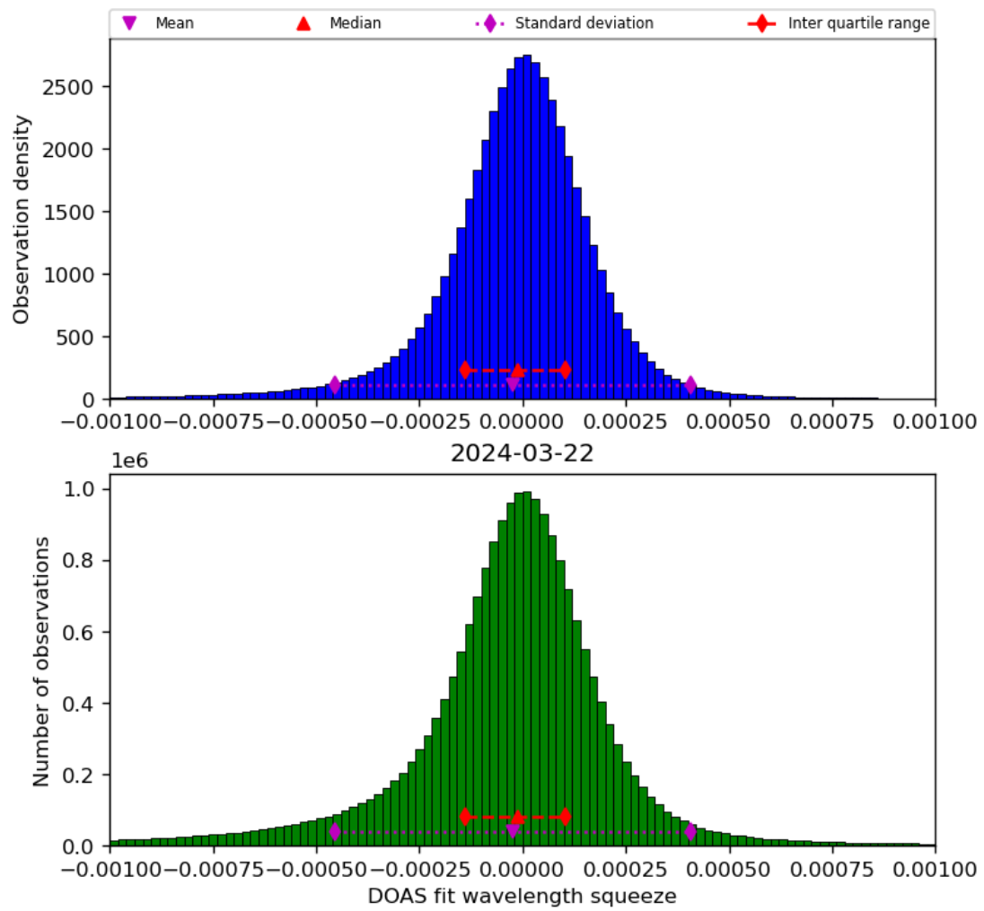
Figure 69: Histogram of “DOAS fit wavelength squeeze” for 2024-03-21 to 2024-03-22
