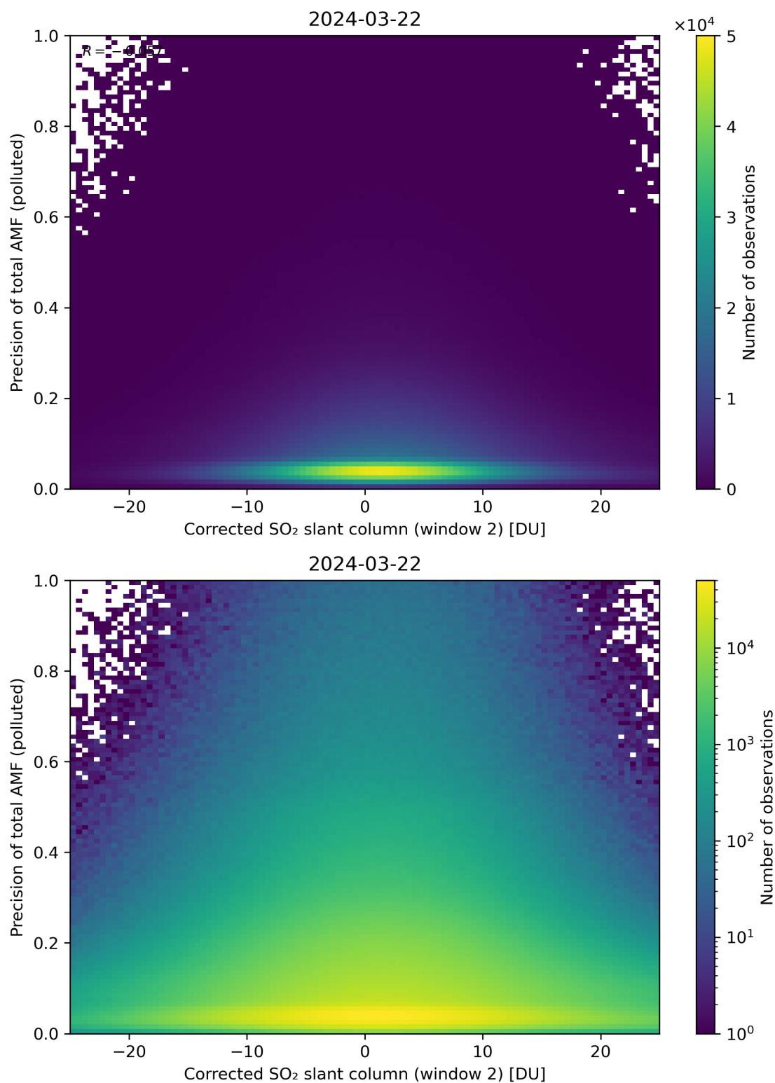
Figure 204: Scatter density plot of “Corrected SO 2 slant column (window 2)” against “Precision of total AMF (polluted)” for 2024-03-21 to 2024-03-22.
