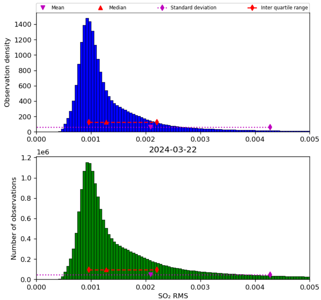
Figure 70: Histogram of “SO 2 RMS” for 2024-03-21 to 2024-03-22
