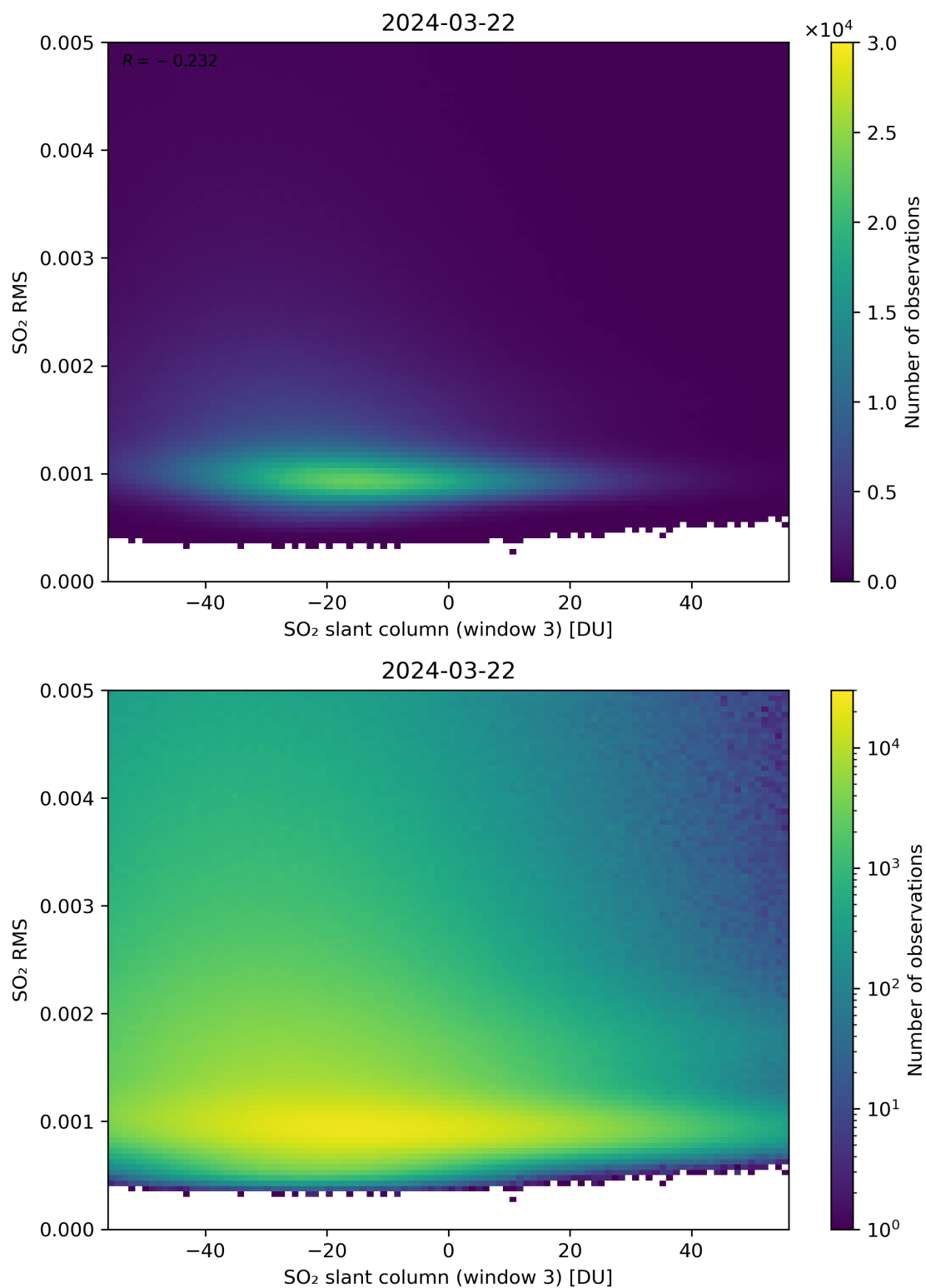
Figure 256: Scatter density plot of “SO 2 slant column (window 3)” against “SO 2 RMS” for 2024-03-21 to 2024-03-22.
