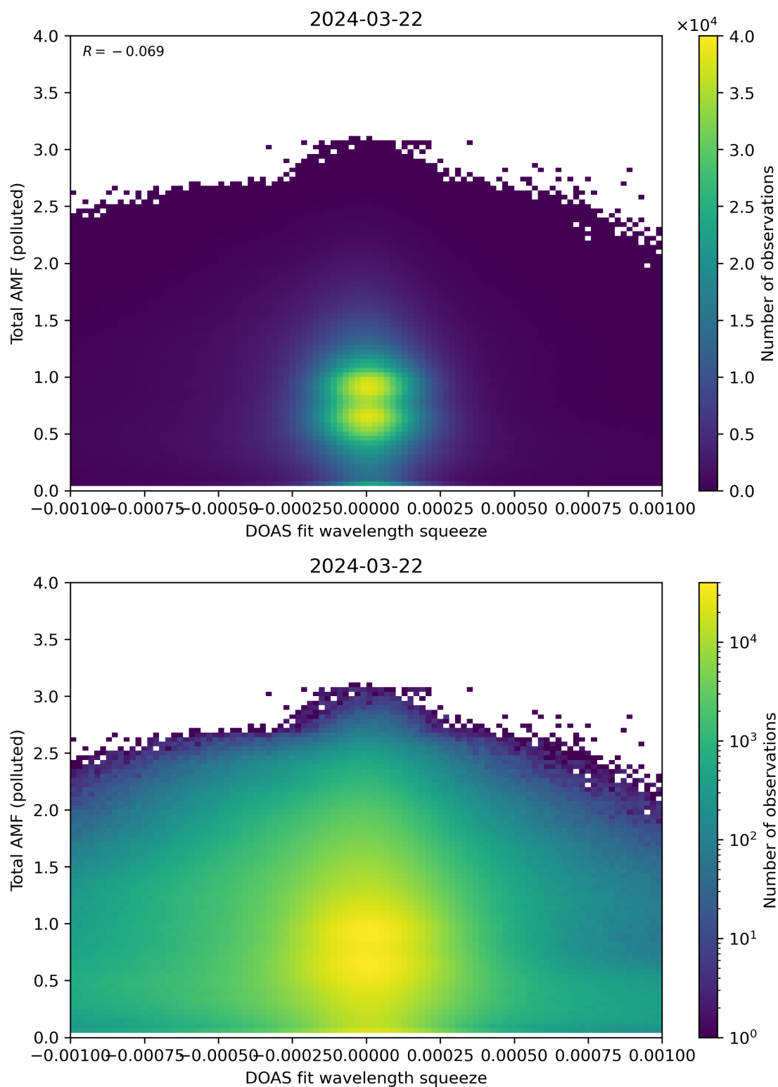
Figure 134: Scatter density plot of “DOAS fit wavelength squeeze” against “Total AMF (polluted)” for 2024-03-21 to 2024-03-22.
