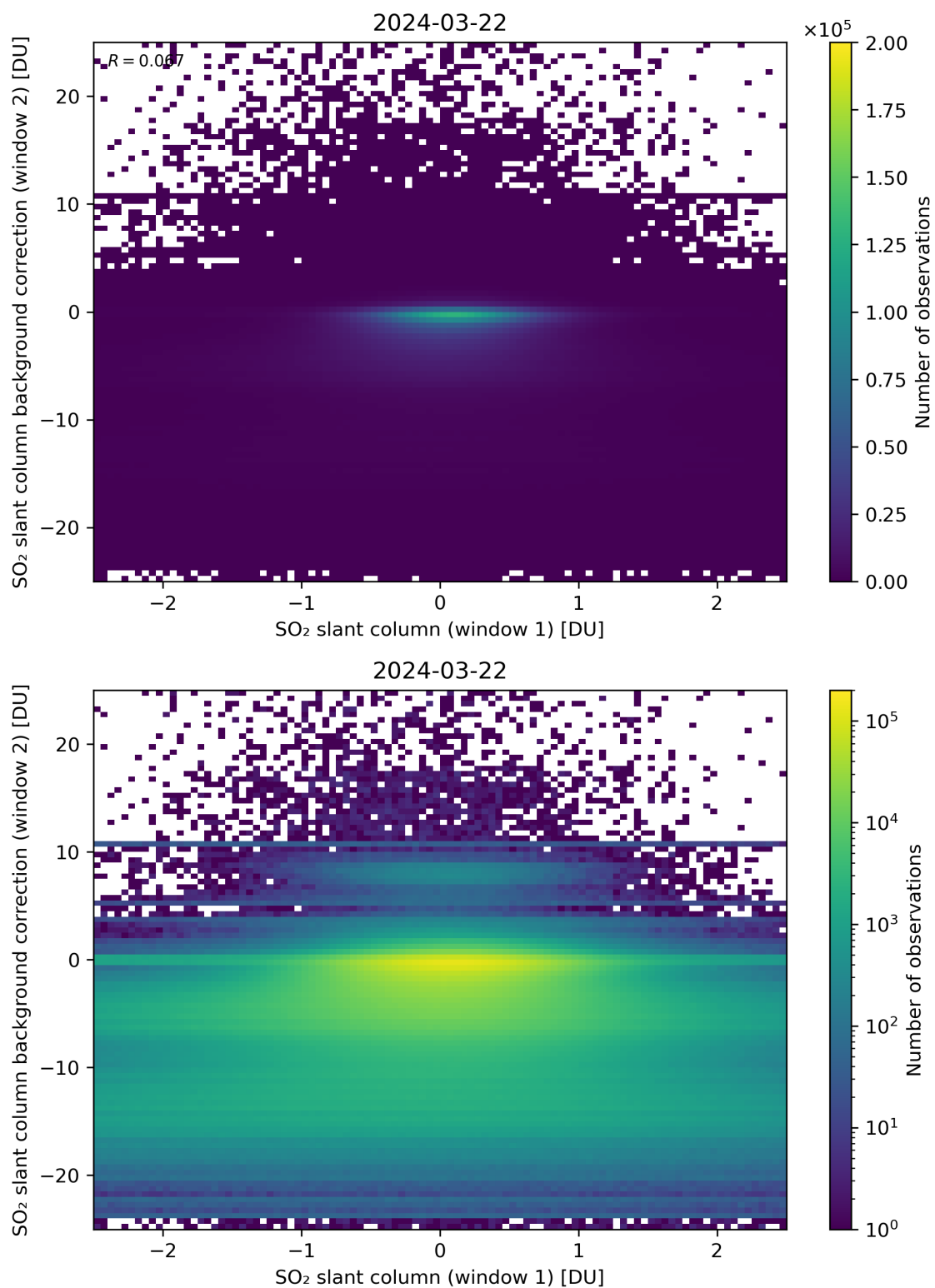
Figure 213: Scatter density plot of “SO 2 slant column (window 1)” against “SO 2 slant column background correction (window 2)” for 2024-03-21 to 2024-03-22.
