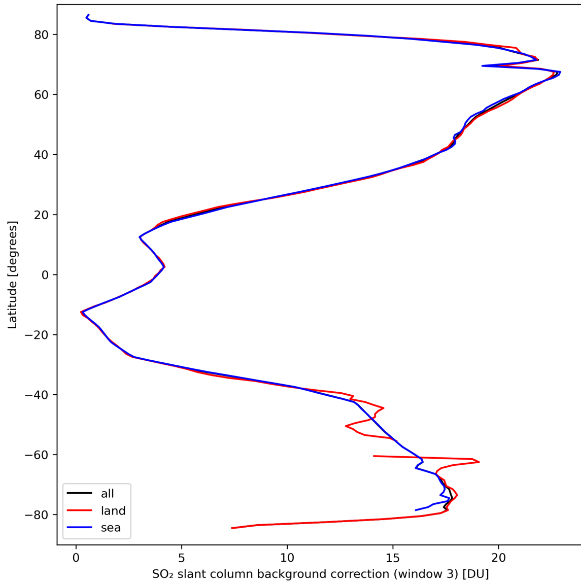
Figure 44: Zonal average of “SO 2 slant column background correction (window 3)” for 2024-03-21 to 2024-03-22.
