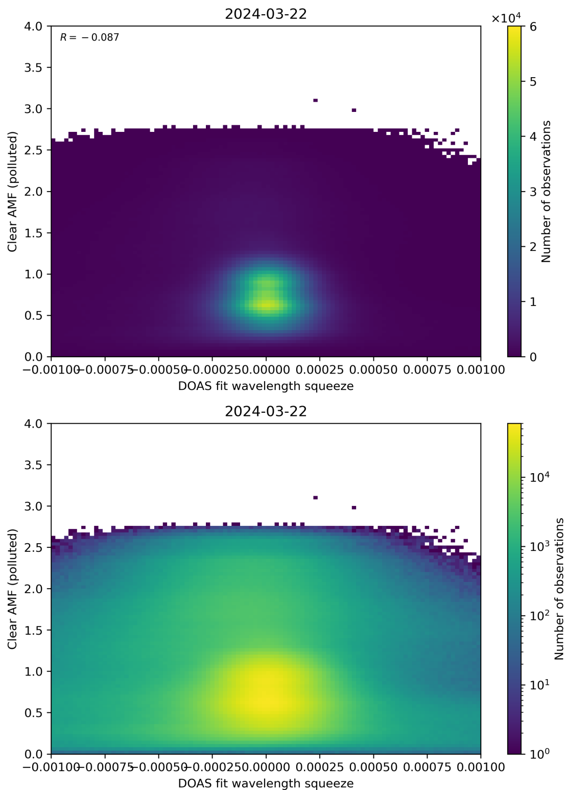
Figure 133: Scatter density plot of “DOAS fit wavelength squeeze” against “Clear AMF (polluted)” for 2024-03-21 to 2024-03-22.
