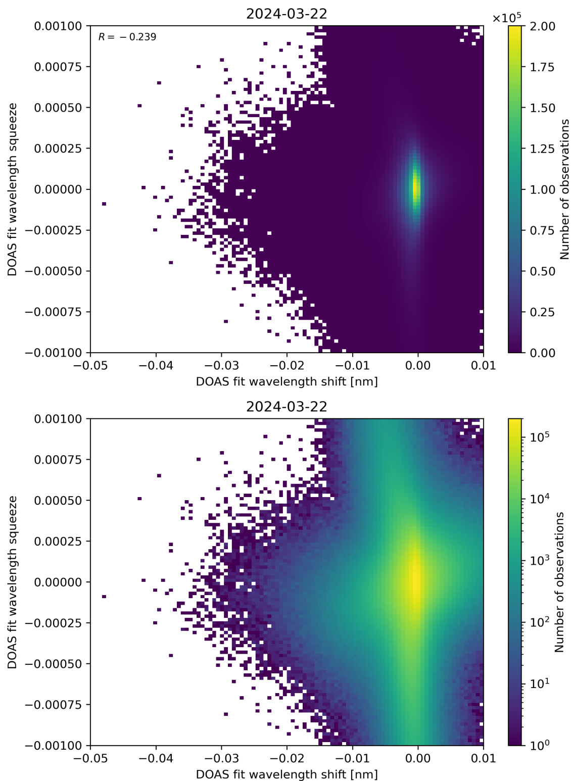
Figure 127: Scatter density plot of “DOAS fit wavelength shift” against “DOAS fit wavelength squeeze” for 2024-03-21 to 2024-03-22.
