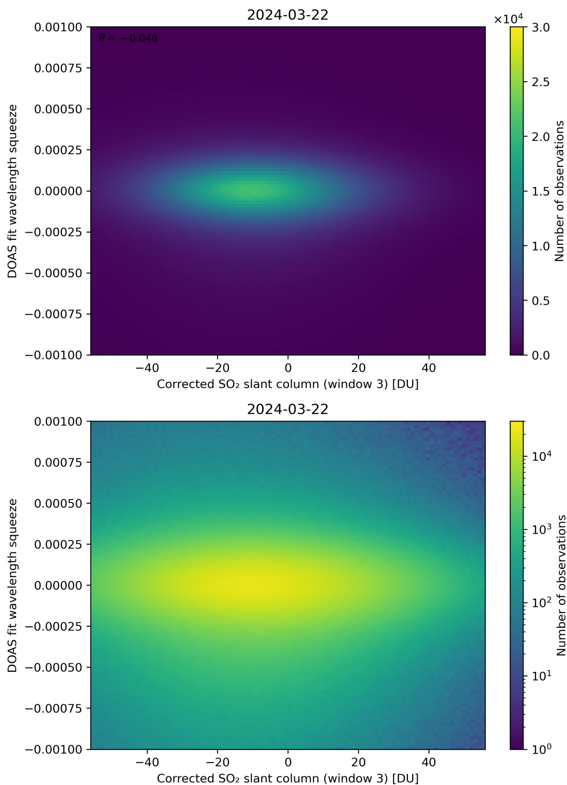
Figure 207: Scatter density plot of “Corrected SO 2 slant column (window 3)” against “DOAS fit wavelength squeeze” for 2024-03-21 to 2024-03-22.
