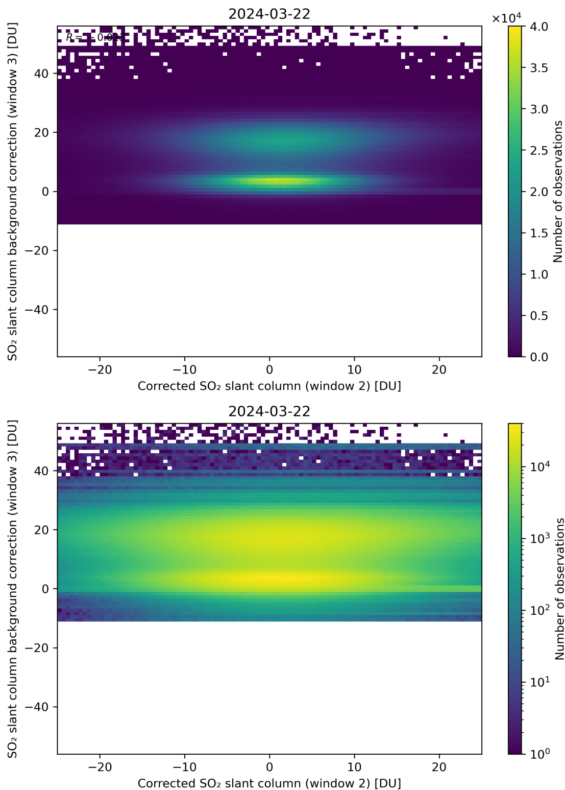
Figure 195: Scatter density plot of “Corrected SO 2 slant column (window 2)” against “SO 2 slant column background correction (window 3)” for 2024-03-21 to 2024-03-22.
