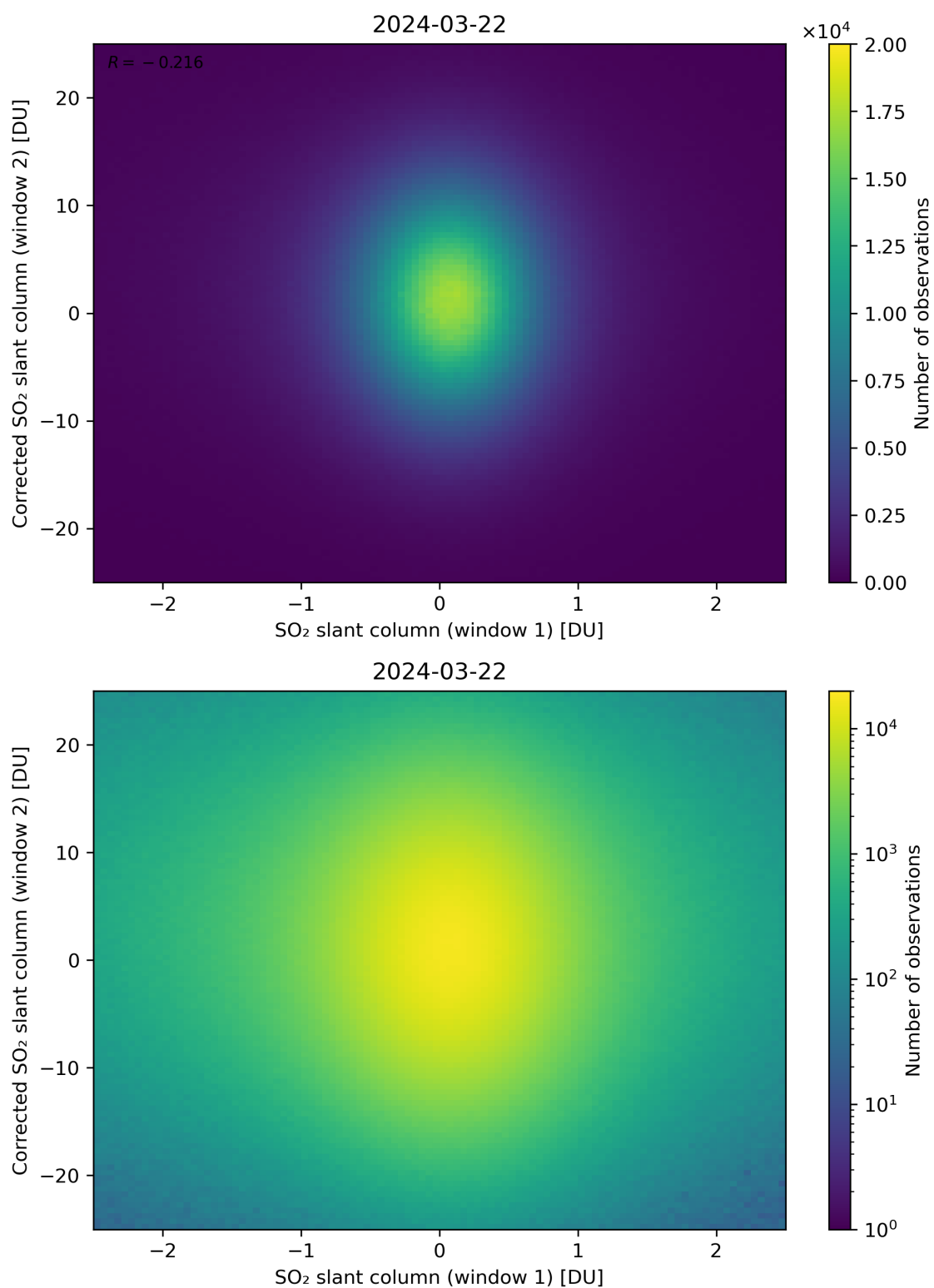
Figure 233: Scatter density plot of “SO 2 slant column (window 1)” against “Corrected SO 2 slant column (window 2)” for 2024-03-21 to 2024-03-22.
