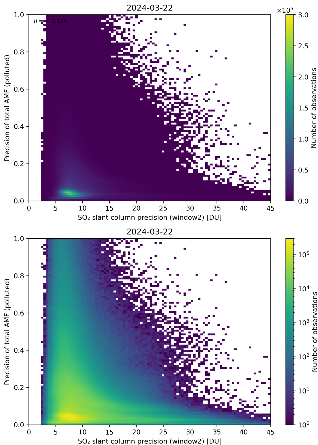
Figure 252: Scatter density plot of “SO 2 slant column precision (window2)” against “Precision of total AMF (polluted)” for 2024-03-21 to 2024-03-22.
