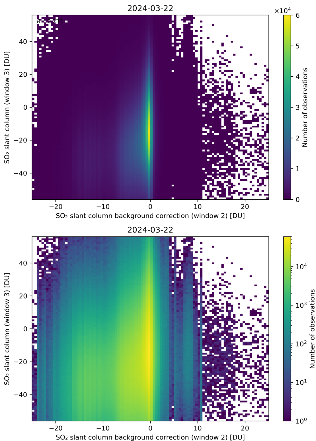
Figure 117: Scatter density plot of “SO 2 slant column background correction (window 2)” against “SO 2 slant column (window 3)” for 2024-03-21 to 2024-03-22.
