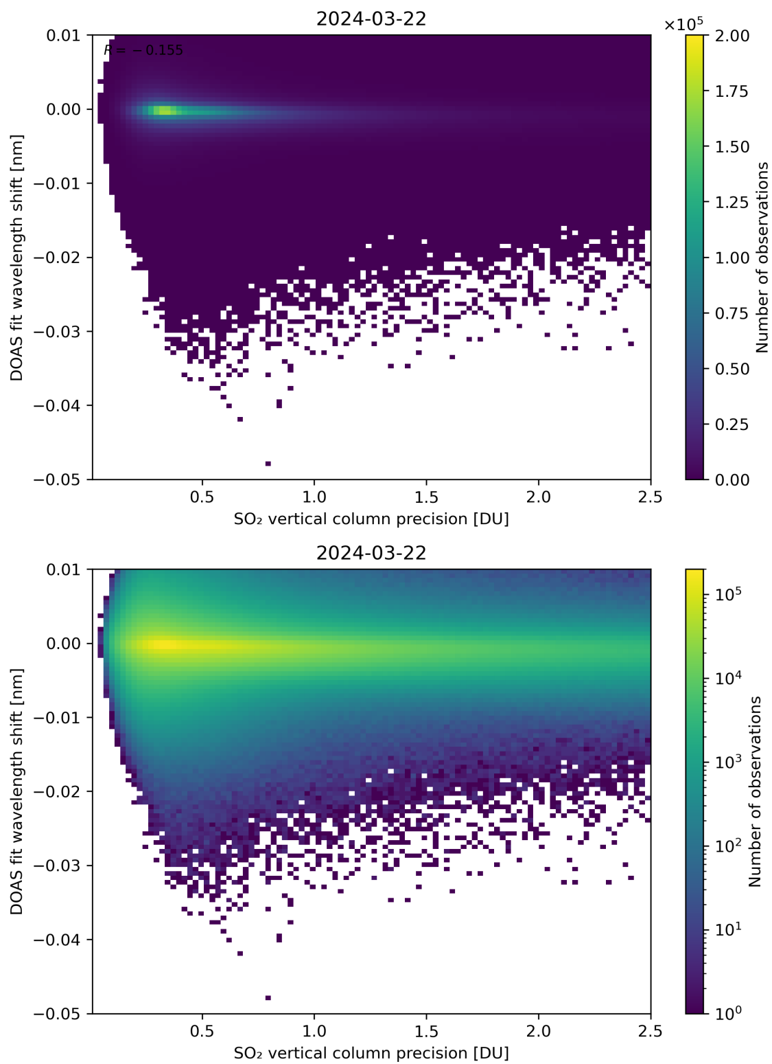
Figure 282: Scatter density plot of “SO 2 vertical column precision” against “DOAS fit wavelength shift” for 2024-03-21 to 2024-03-22.
