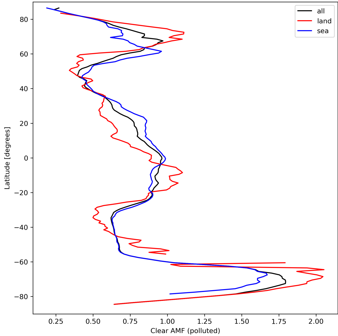
Figure 50: Zonal average of “Clear AMF (polluted)” for 2024-03-21 to 2024-03-22.
