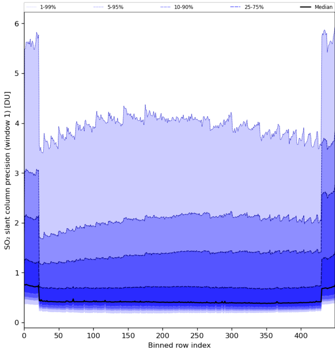
Figure 80: Along track statistics of “SO 2 slant column precision (window 1)” for 2024-03-21 to 2024-03-22
