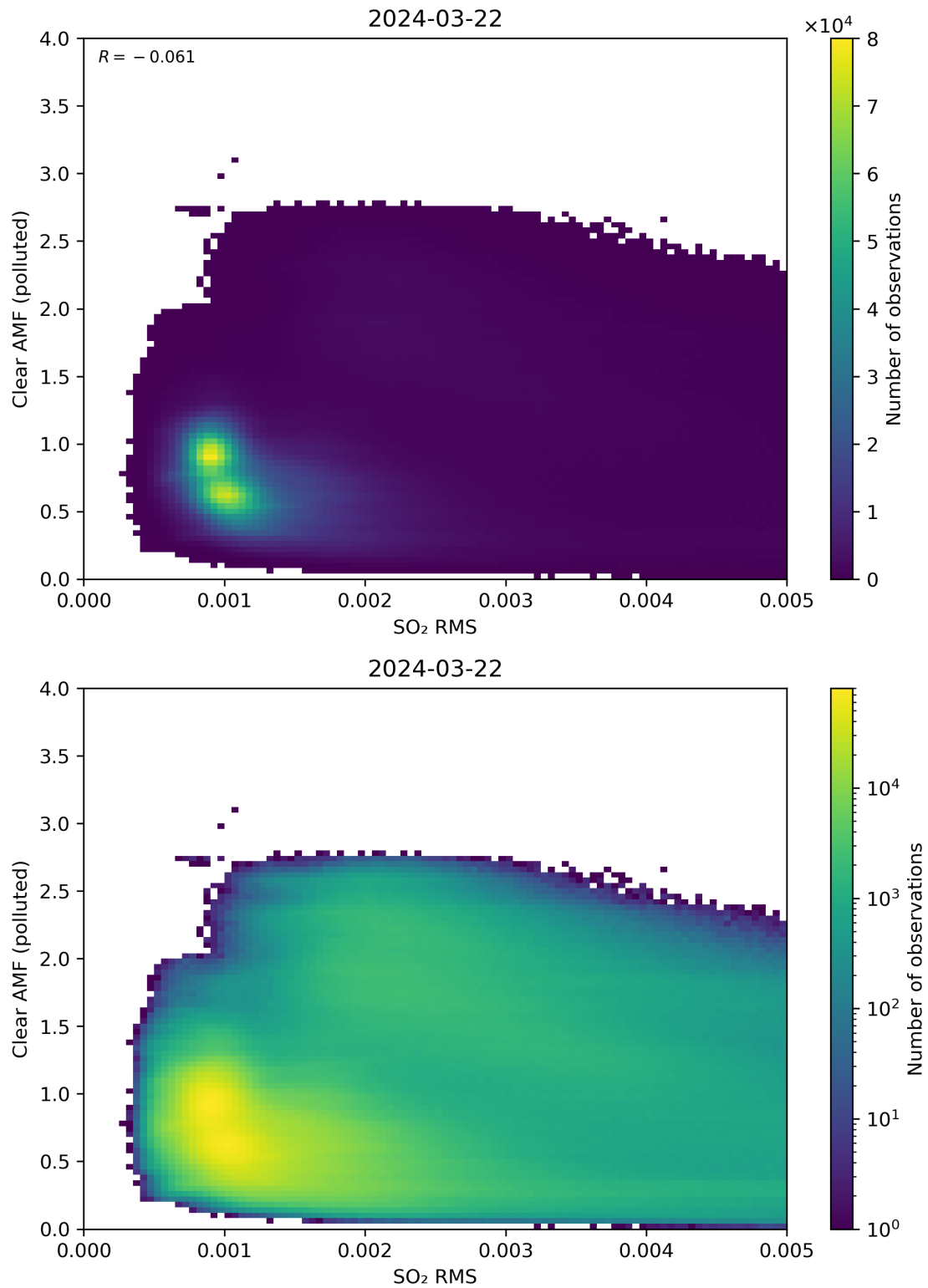
Figure 136: Scatter density plot of “SO 2 RMS” against “Clear AMF (polluted)” for 2024-03-21 to 2024-03-22.
