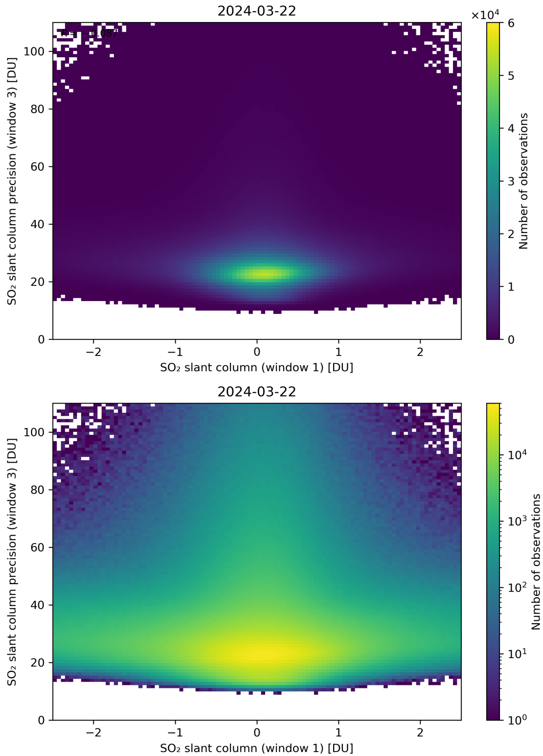
Figure 238: Scatter density plot of “SO 2 slant column (window 1)” against “SO 2 slant column precision (window 3)” for 2024-03-21 to 2024-03-22.
