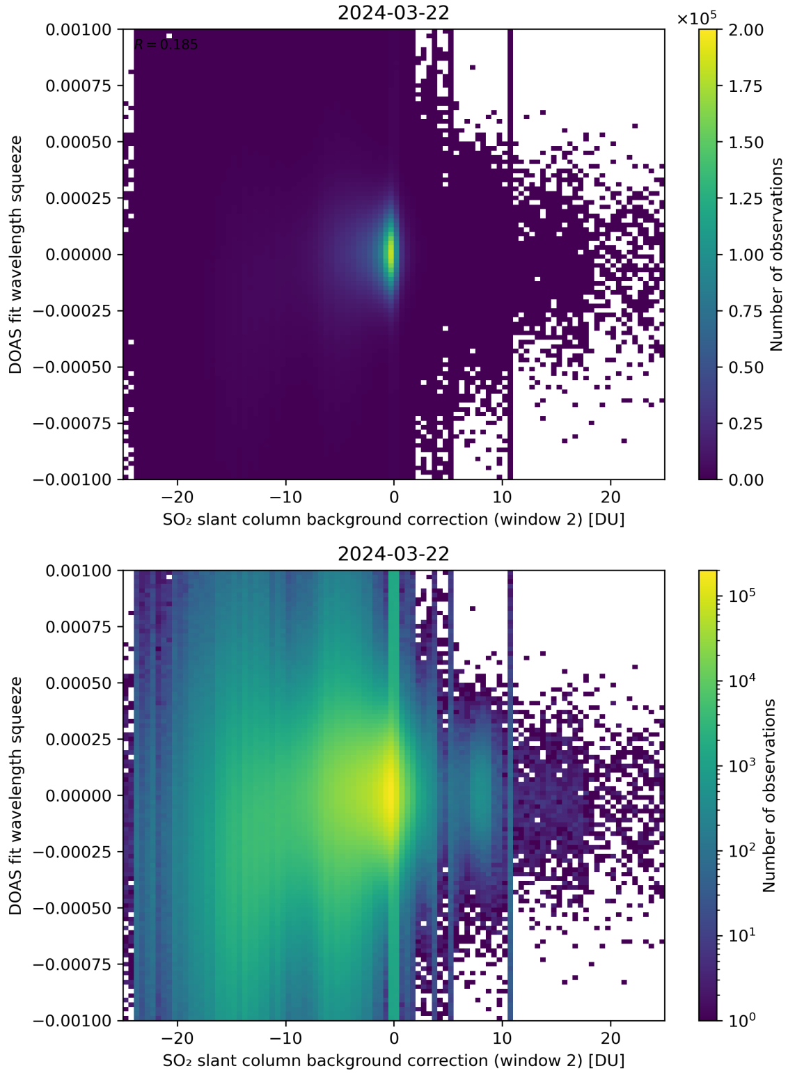
Figure 113: Scatter density plot of “SO 2 slant column background correction (window 2)” against “DOAS fit wavelength squeeze” for 2024-03-21 to 2024-03-22.
