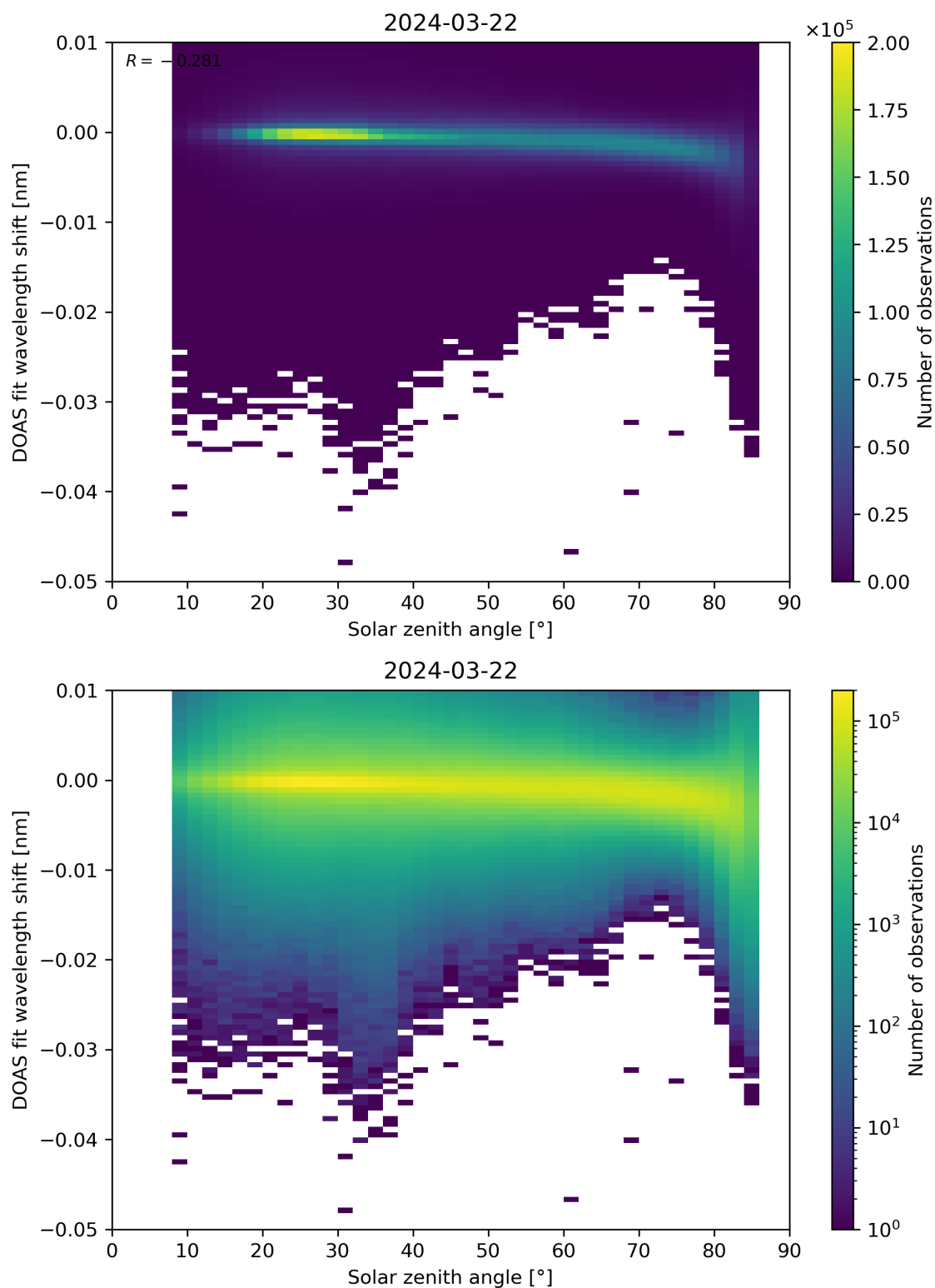
Figure 161: Scatter density plot of “Solar zenith angle” against “DOAS fit wavelength shift” for 2024-03-21 to 2024-03-22.
