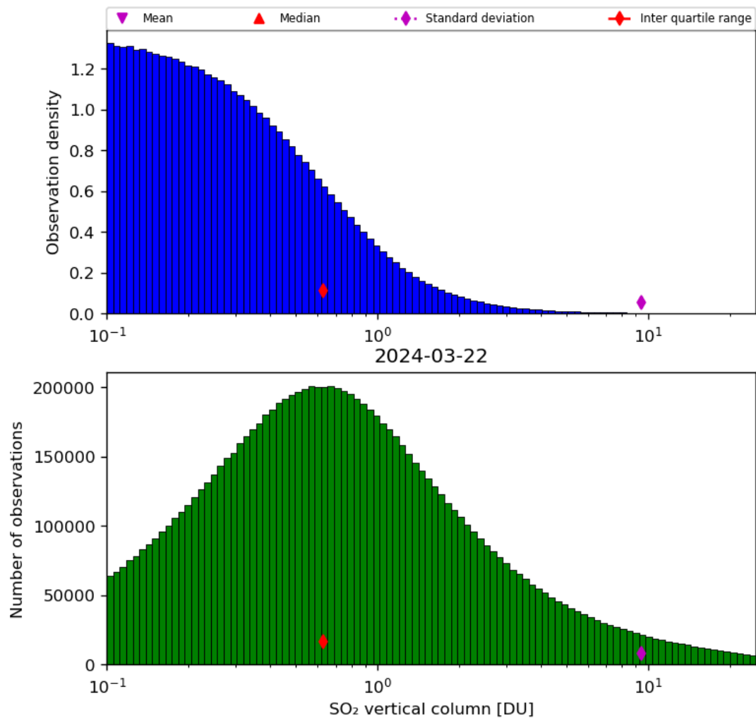
Figure 53: Histogram of “SO 2 vertical column” for 2024-03-21 to 2024-03-22
