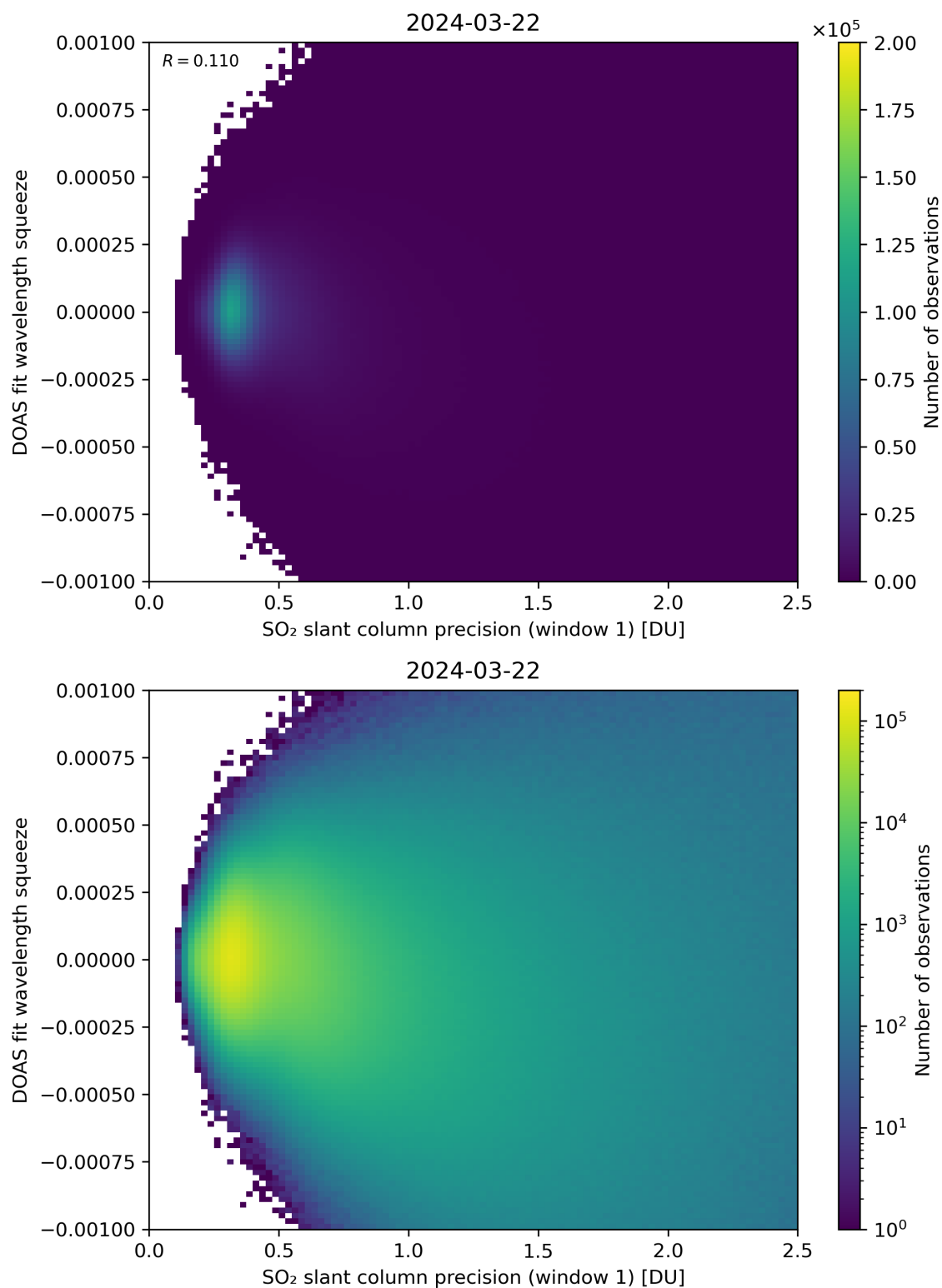
Figure 222: Scatter density plot of “SO 2 slant column precision (window 1)” against “DOAS fit wavelength squeeze” for 2024-03-21 to 2024-03-22.
