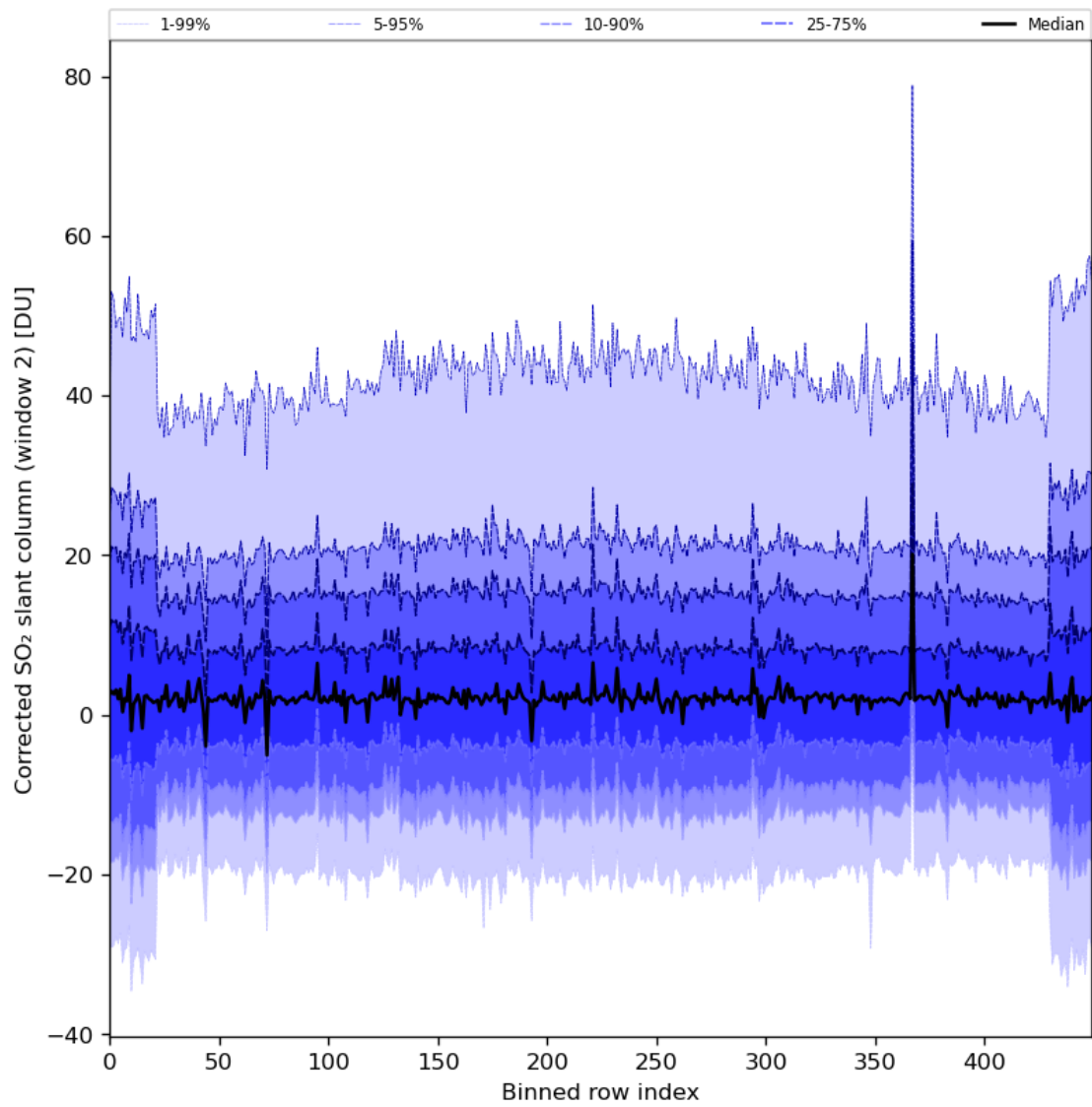
Figure 85: Along track statistics of "Corrected SO 2 slant column (window 2)" for 2024-03-21 to 2024-03-22
