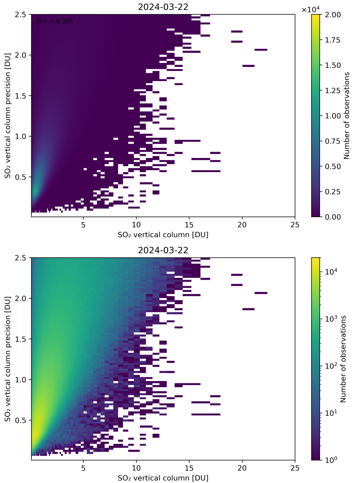
Figure 307: Scatter density plot of “SO 2 vertical column” against “SO 2 vertical column precision” for 2024-03-21 to 2024-03-22.
