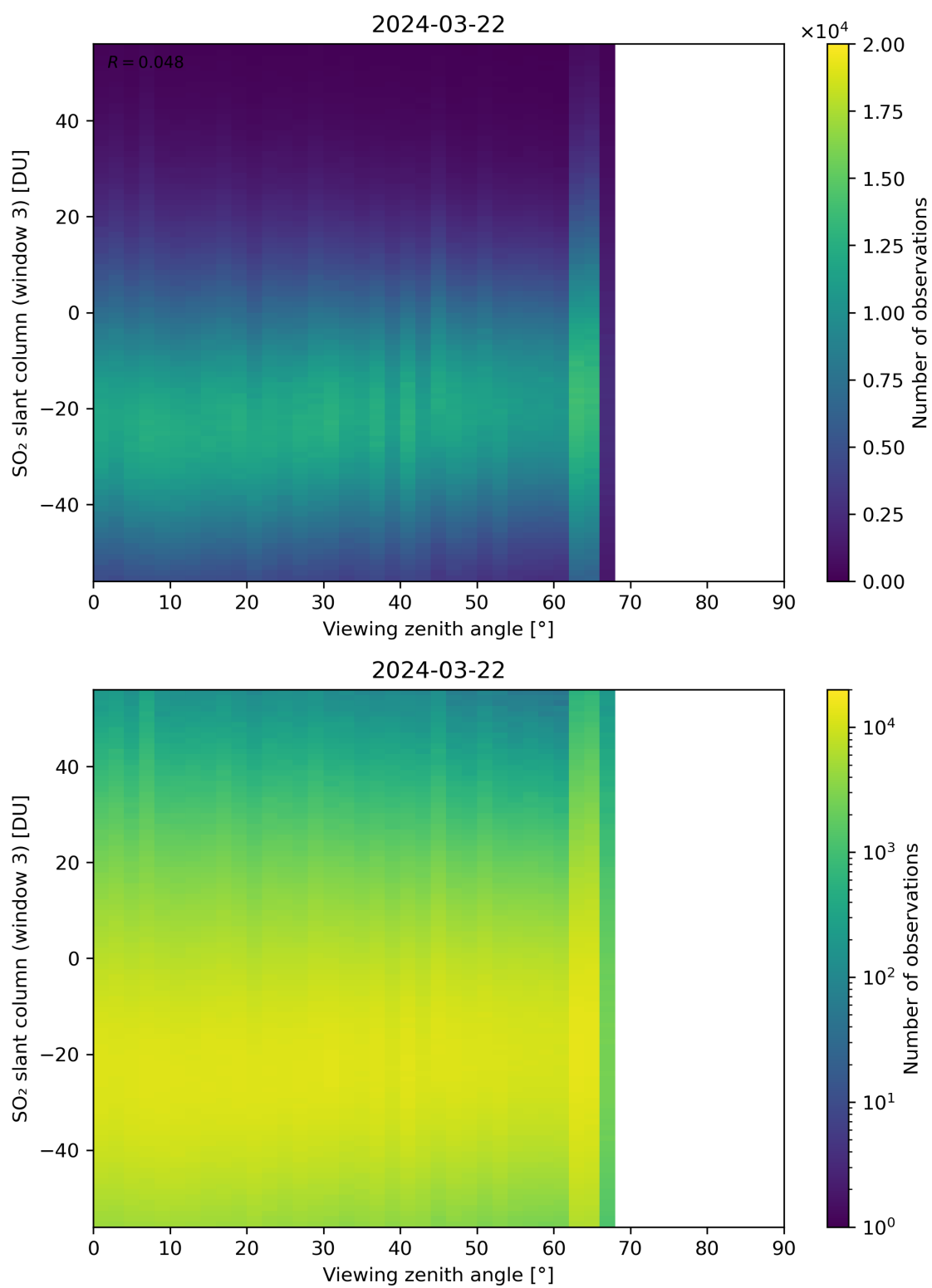
Figure 323: Scatter density plot of “Viewing zenith angle” against “SO 2 slant column (window 3)” for 2024-03-21 to 2024-03-22.
