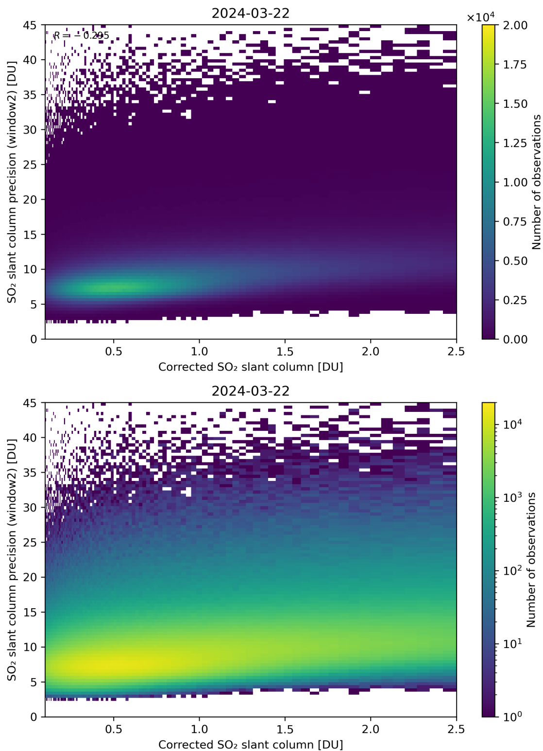
Figure 189: Scatter density plot of “Corrected SO 2 slant column” against “SO 2 slant column precision (window2)” for 2024-03-21 to 2024-03-22.
