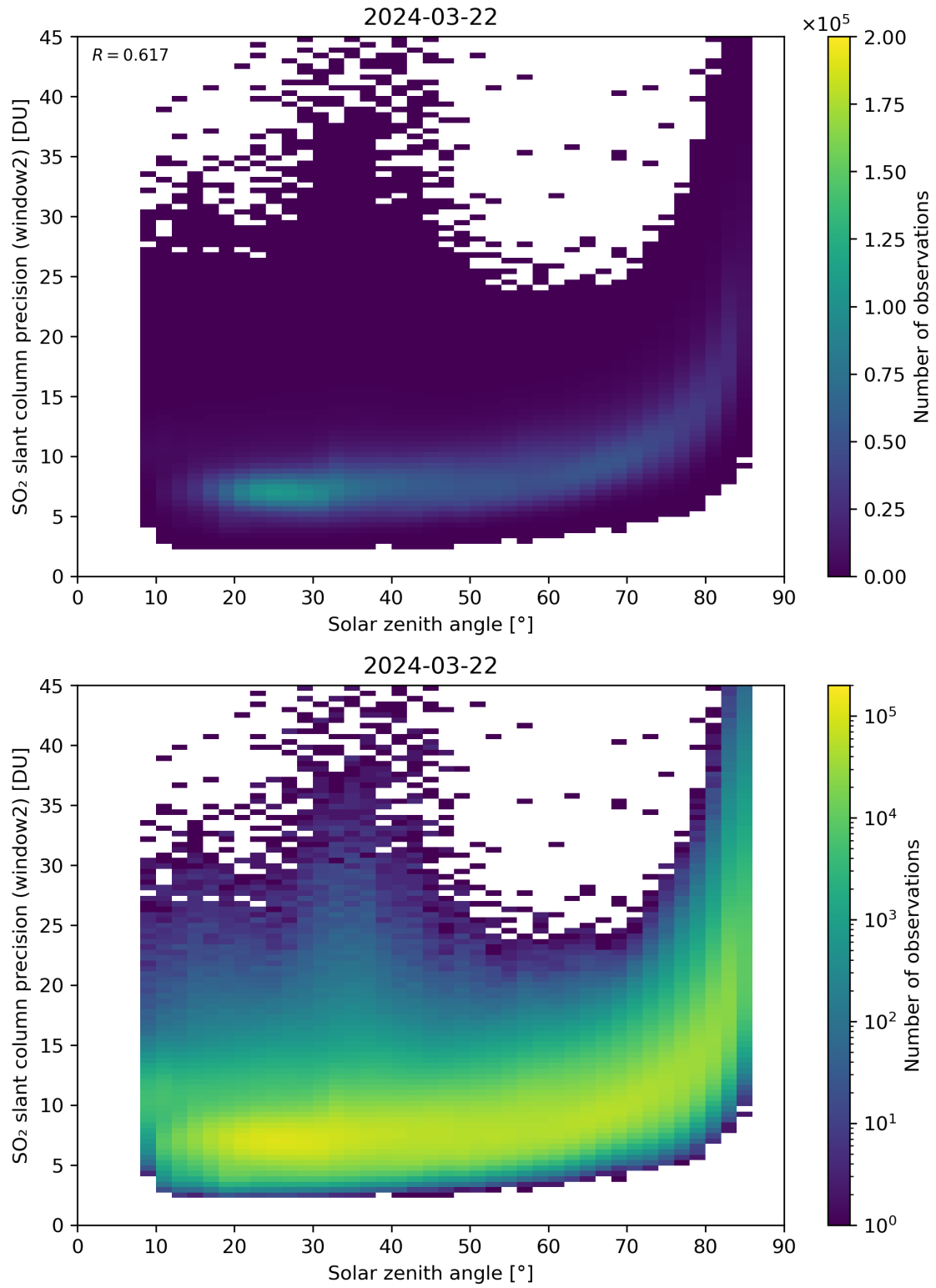
Figure 171: Scatter density plot of “Solar zenith angle” against “SO 2 slant column precision (window2)” for 2024-03-21 to 2024-03-22.
