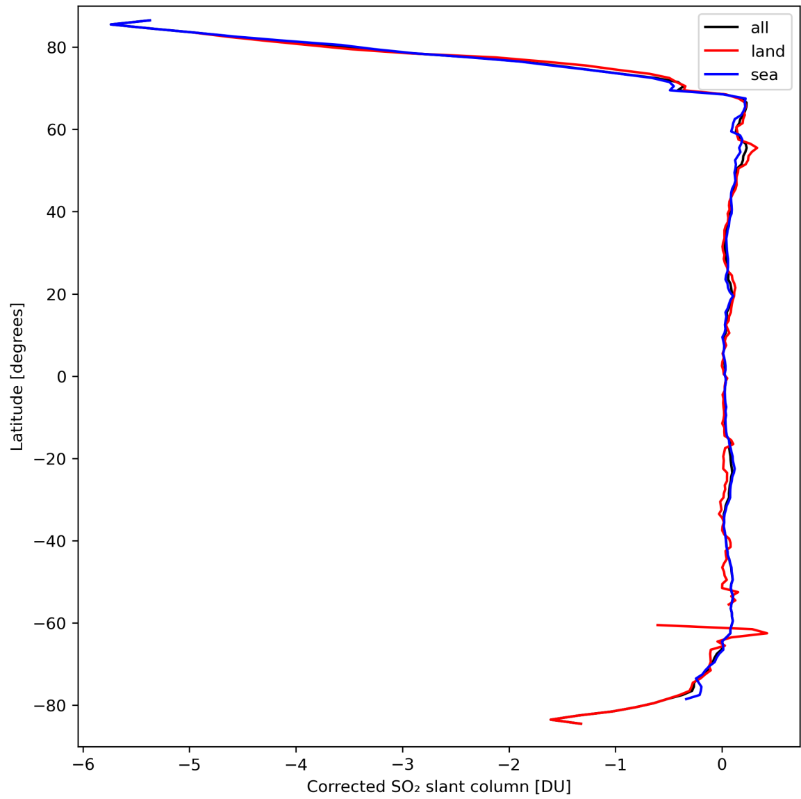
Figure 32: Zonal average of “Corrected SO 2 slant column” for 2024-03-21 to 2024-03-22.
