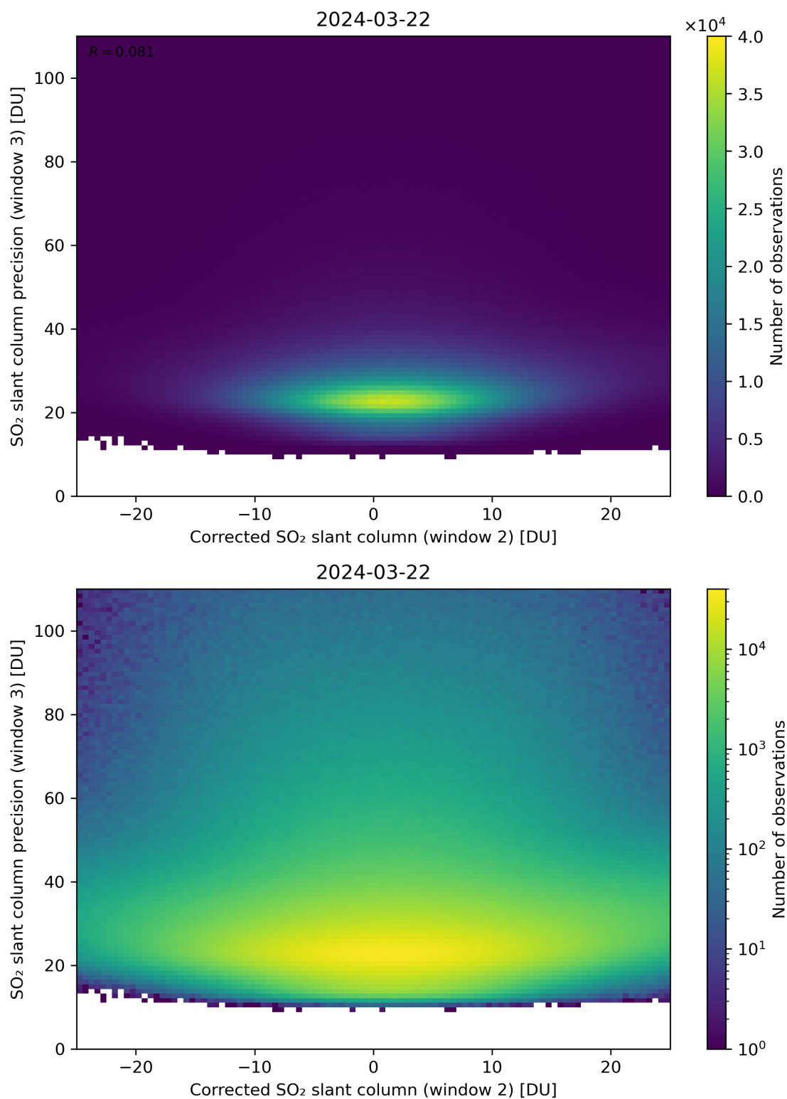
Figure 202: Scatter density plot of “Corrected SO 2 slant column (window 2)” against “SO 2 slant column precision (window 3)” for 2024-03-21 to 2024-03-22.
