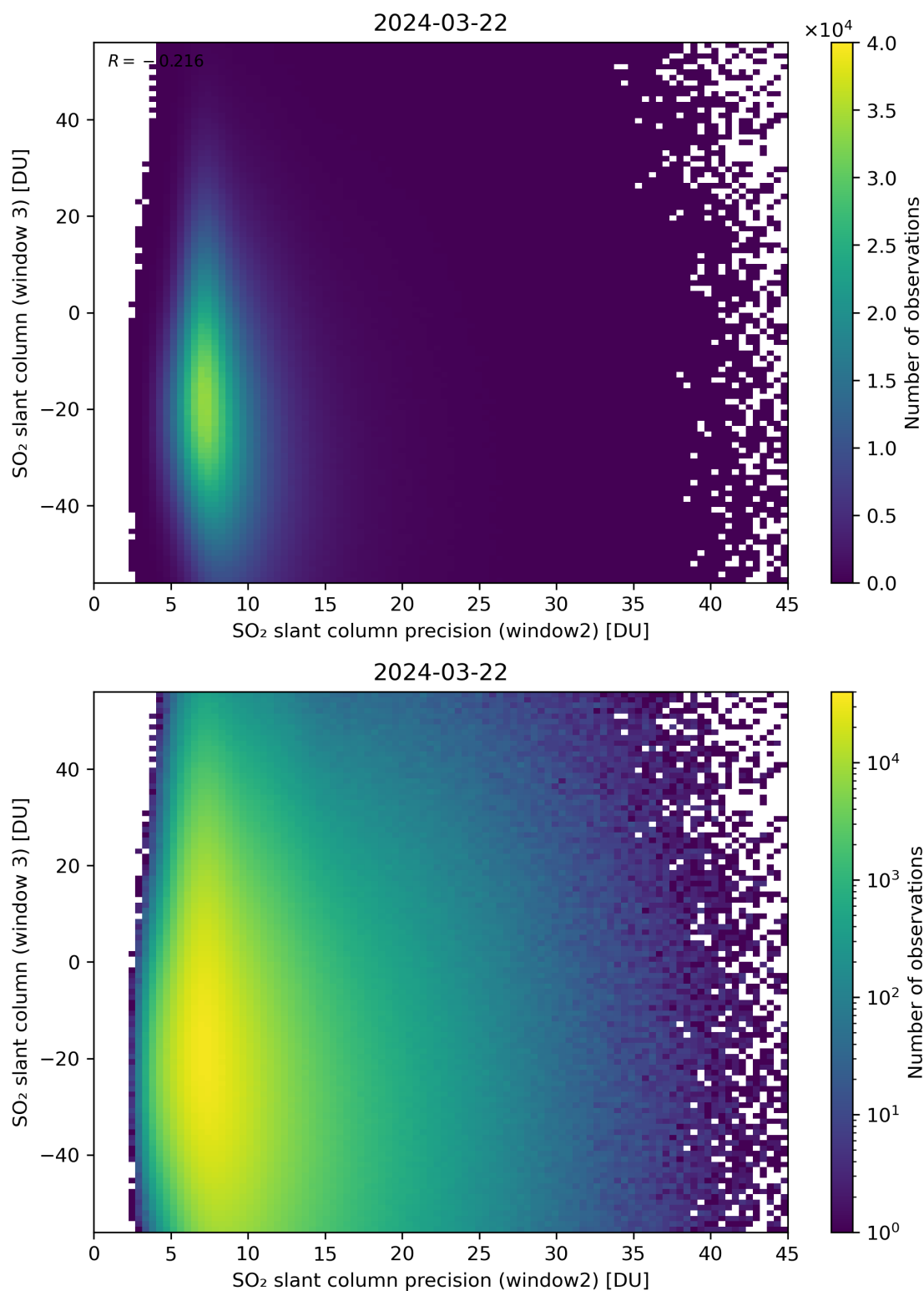
Figure 249: Scatter density plot of “SO 2 slant column precision (window2)” against “SO 2 slant column (window 3)” for 2024-03-21 to 2024-03-22.
