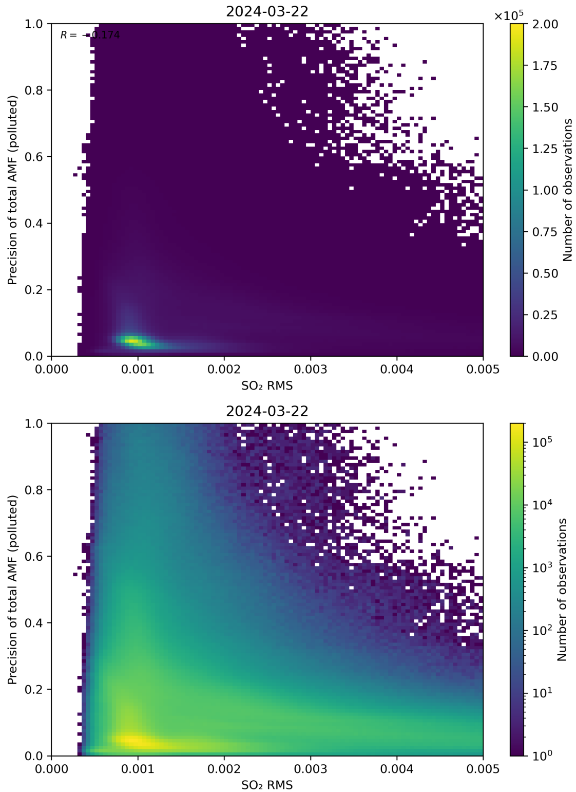
Figure 138: Scatter density plot of “SO 2 RMS” against “Precision of total AMF (polluted)” for 2024-03-21 to 2024-03-22.
