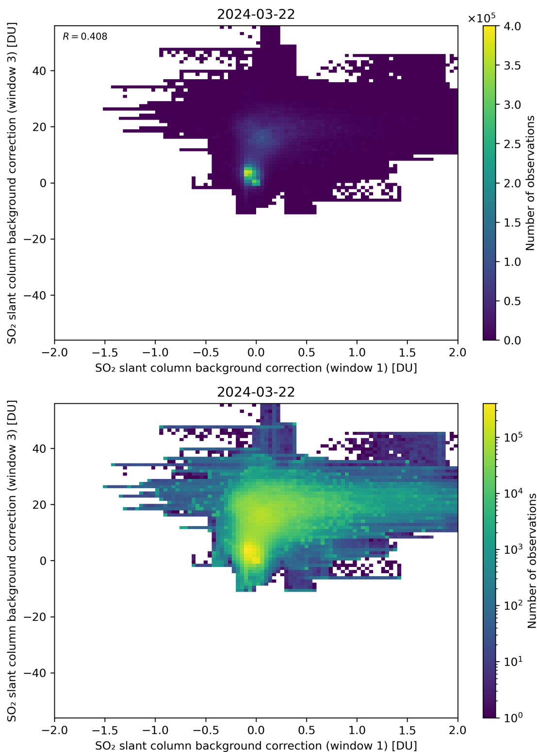
Figure 99: Scatter density plot of “SO 2 slant column background correction (window 1)” against “SO 2 slant column background correction (window 3)” for 2024-03-21 to 2024-03-22.
