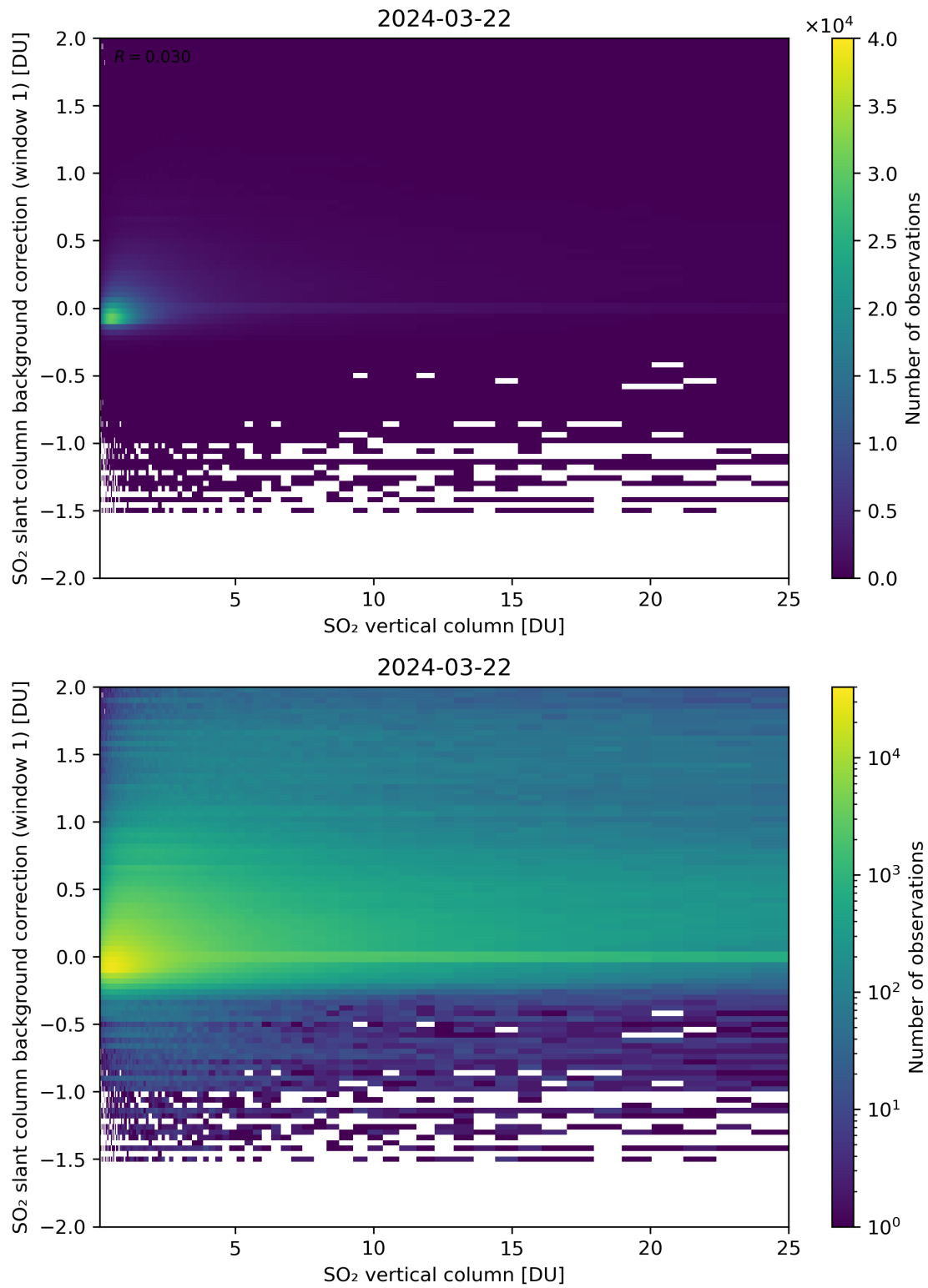
Figure 273: Scatter density plot of “SO 2 vertical column” against “SO 2 slant column background correction (window 1)” for 2024-03-21 to 2024-03-22.
