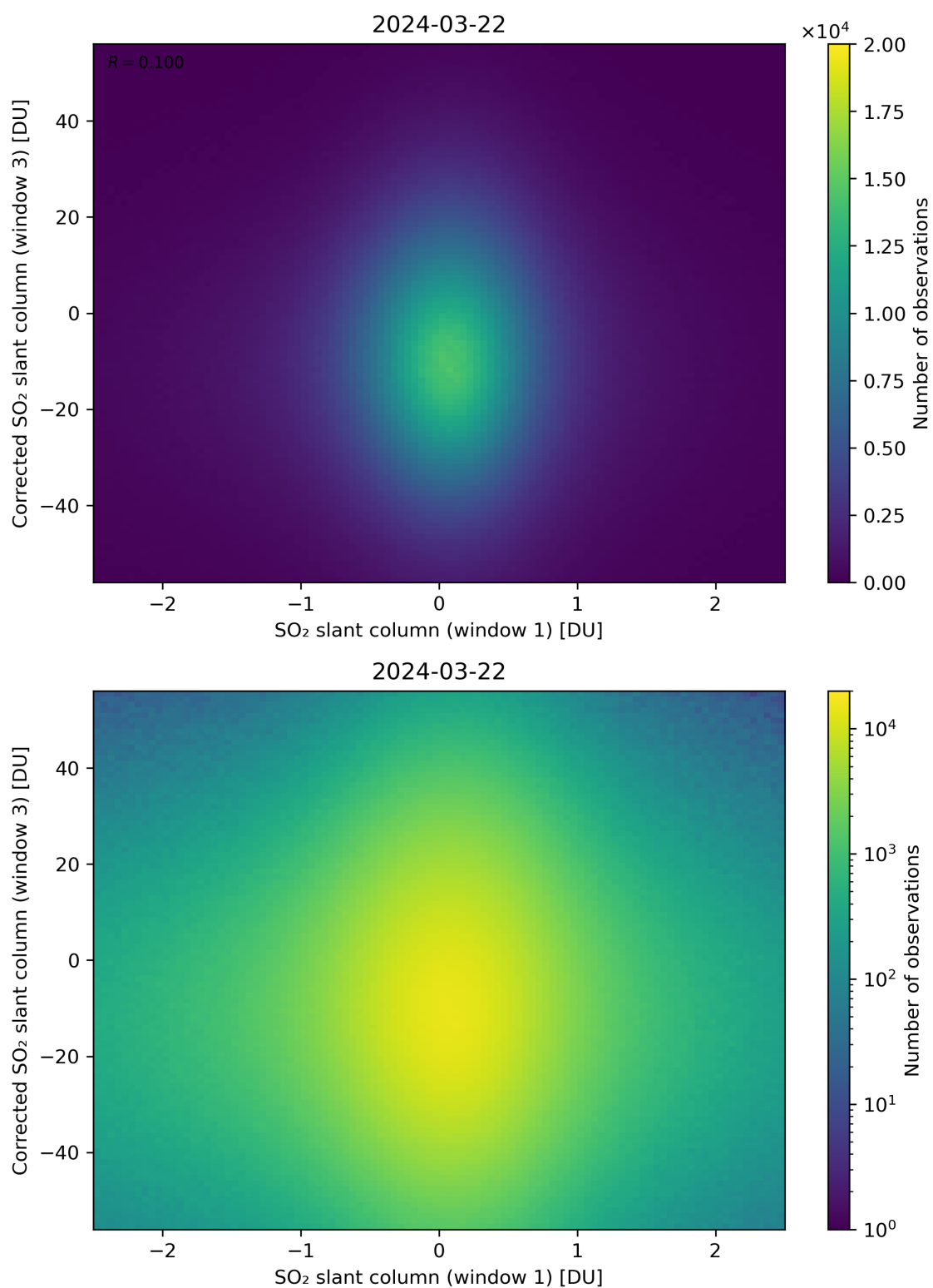
Figure 234: Scatter density plot of “SO 2 slant column (window 1)” against “Corrected SO 2 slant column (window 3)” for 2024-03-21 to 2024-03-22.
