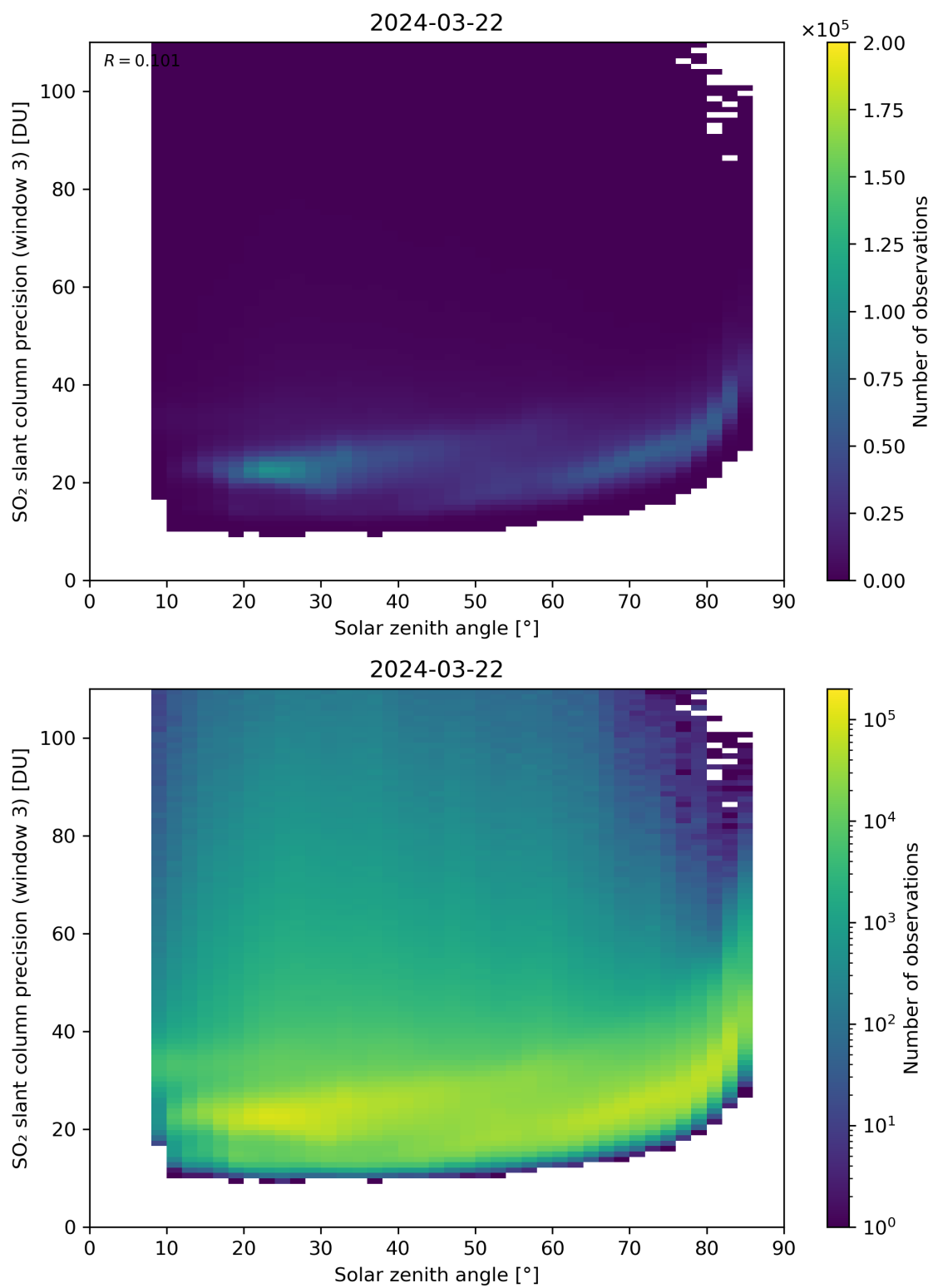
Figure 173: Scatter density plot of “Solar zenith angle” against “SO 2 slant column precision (window 3)” for 2024-03-21 to 2024-03-22.
