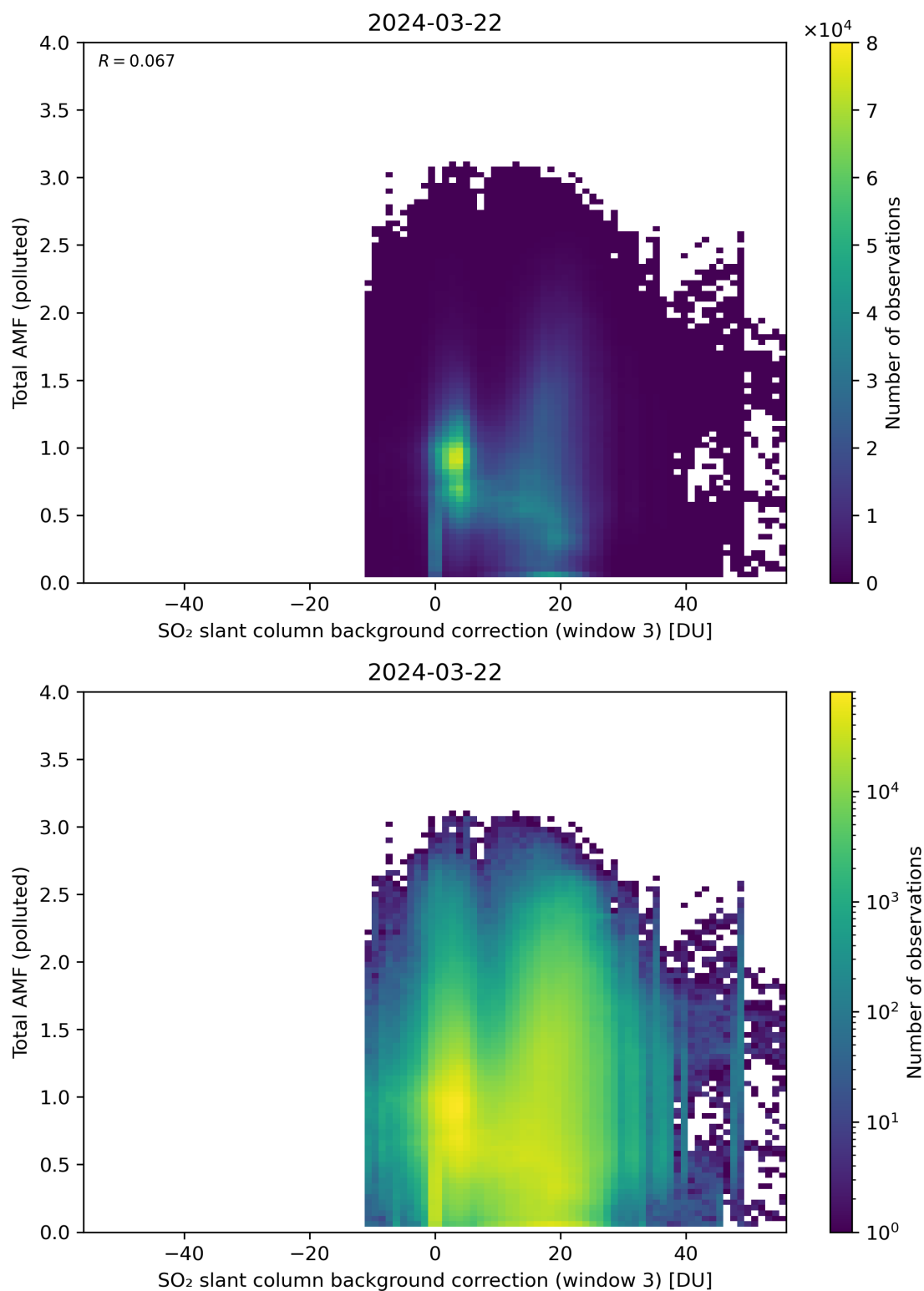
Figure 125: Scatter density plot of “SO 2 slant column background correction (window 3)” against “Total AMF (polluted)” for 2024-03-21 to 2024-03-22.
