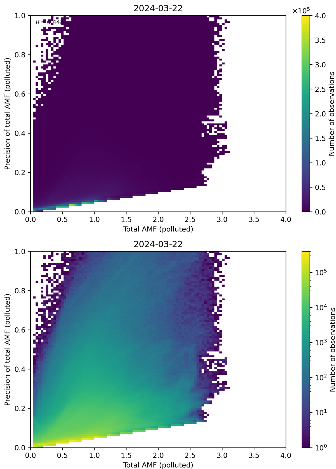
Figure 272: Scatter density plot of “Total AMF (polluted)” against “Precision of total AMF (polluted)” for 2024-03-21 to 2024-03-22.
