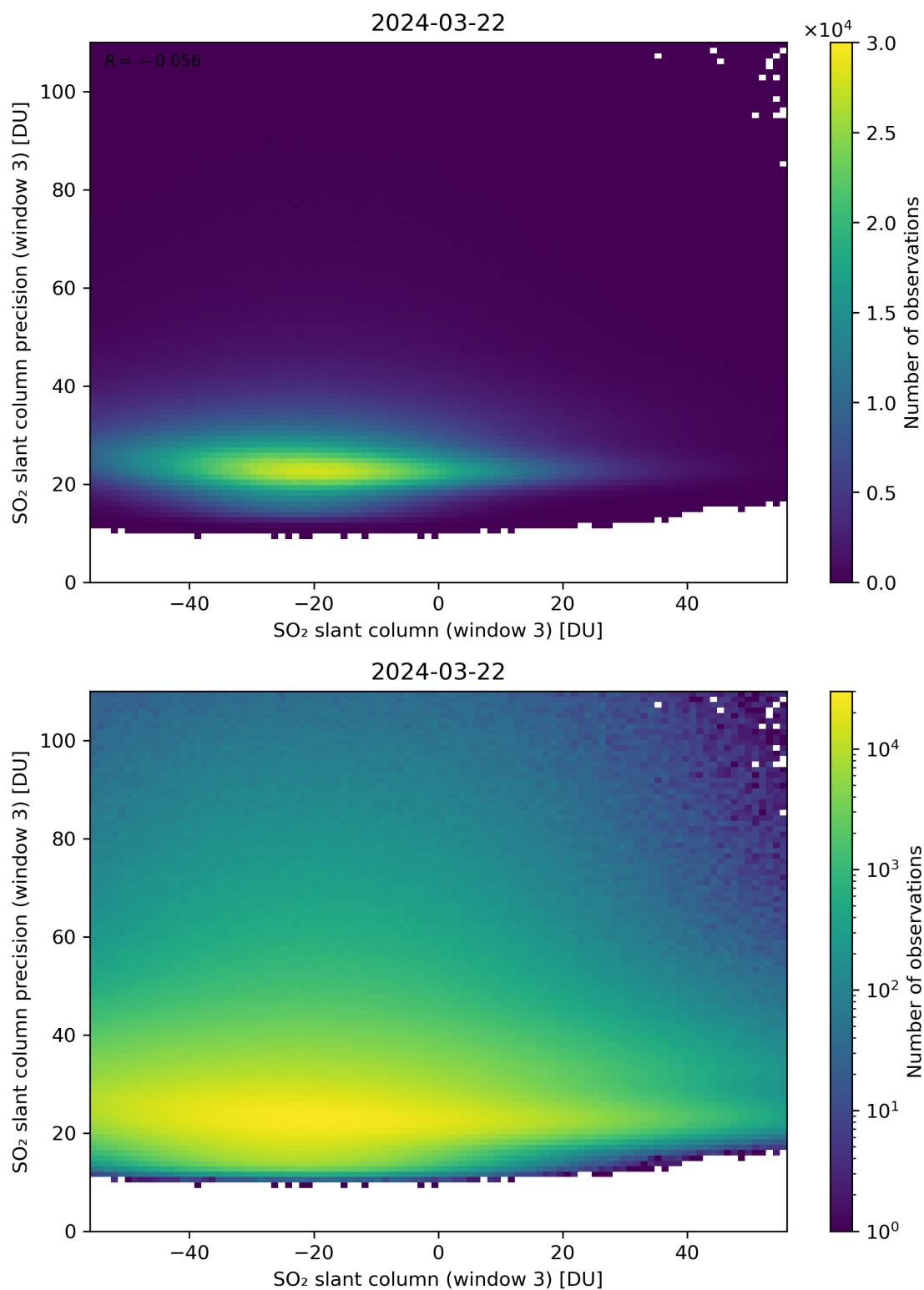
Figure 267: Scatter density plot of “SO 2 slant column (window 3)” against “SO 2 slant column precision (window 3)” for 2024-03-21 to 2024-03-22.
