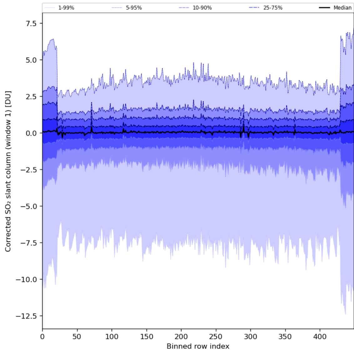
Figure 81: Along track statistics of “Corrected SO 2 slant column (window 1)” for 2024-03-21 to 2024-03-22
