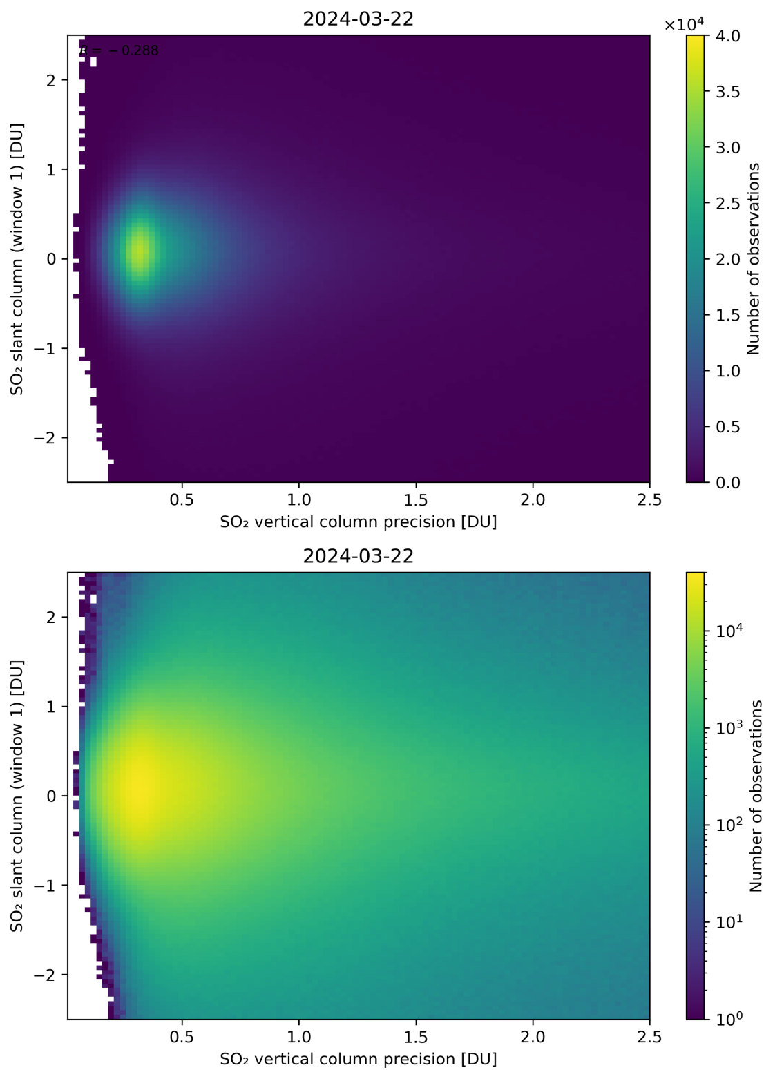
Figure 289: Scatter density plot of “SO 2 vertical column precision” against “SO 2 slant column (window 1)” for 2024-03-21 to 2024-03-22.
