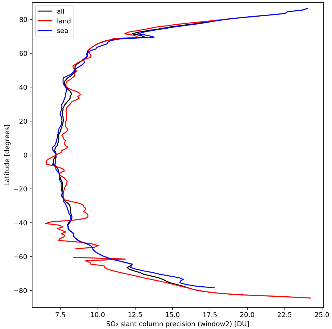
Figure 38: Zonal average of “SO 2 slant column precision (window2)” for 2024-03-21 to 2024-03-22.
