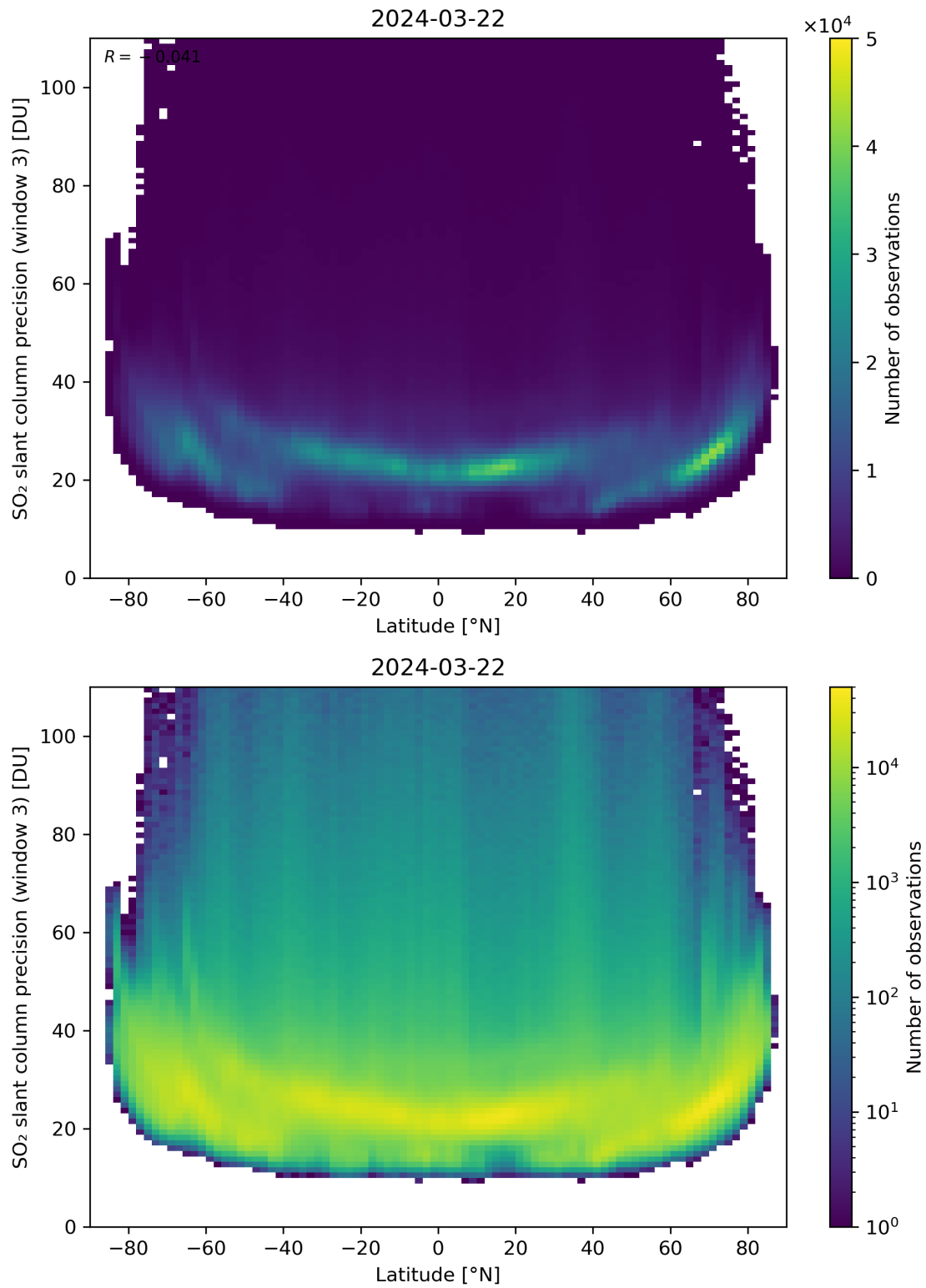
Figure 153: Scatter density plot of “Latitude” against “SO 2 slant column precision (window 3)” for 2024-03-21 to 2024-03-22.
