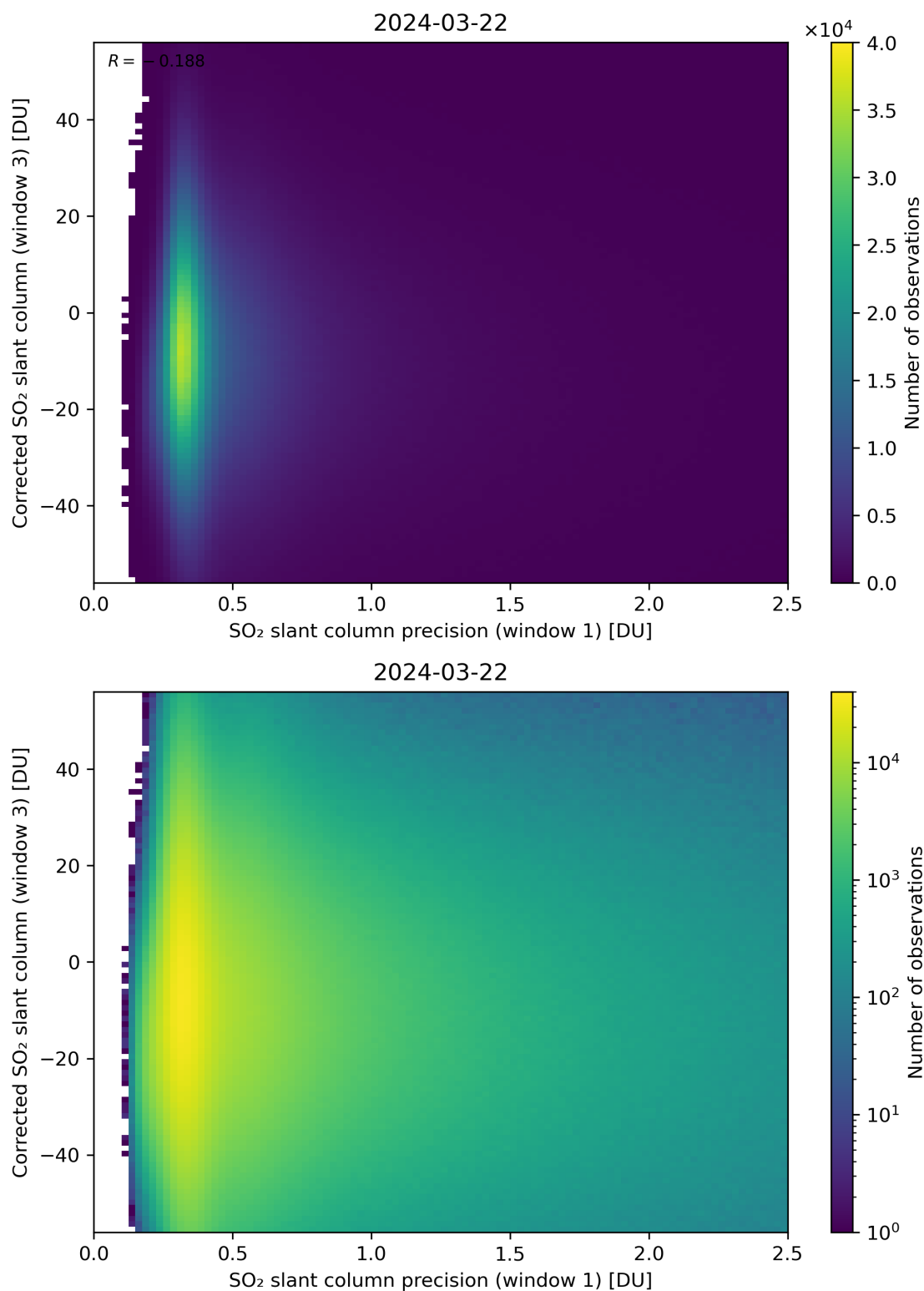
Figure 226: Scatter density plot of “SO 2 slant column precision (window 1)” against “Corrected SO 2 slant column (window 3)” for 2024-03-21 to 2024-03-22.
