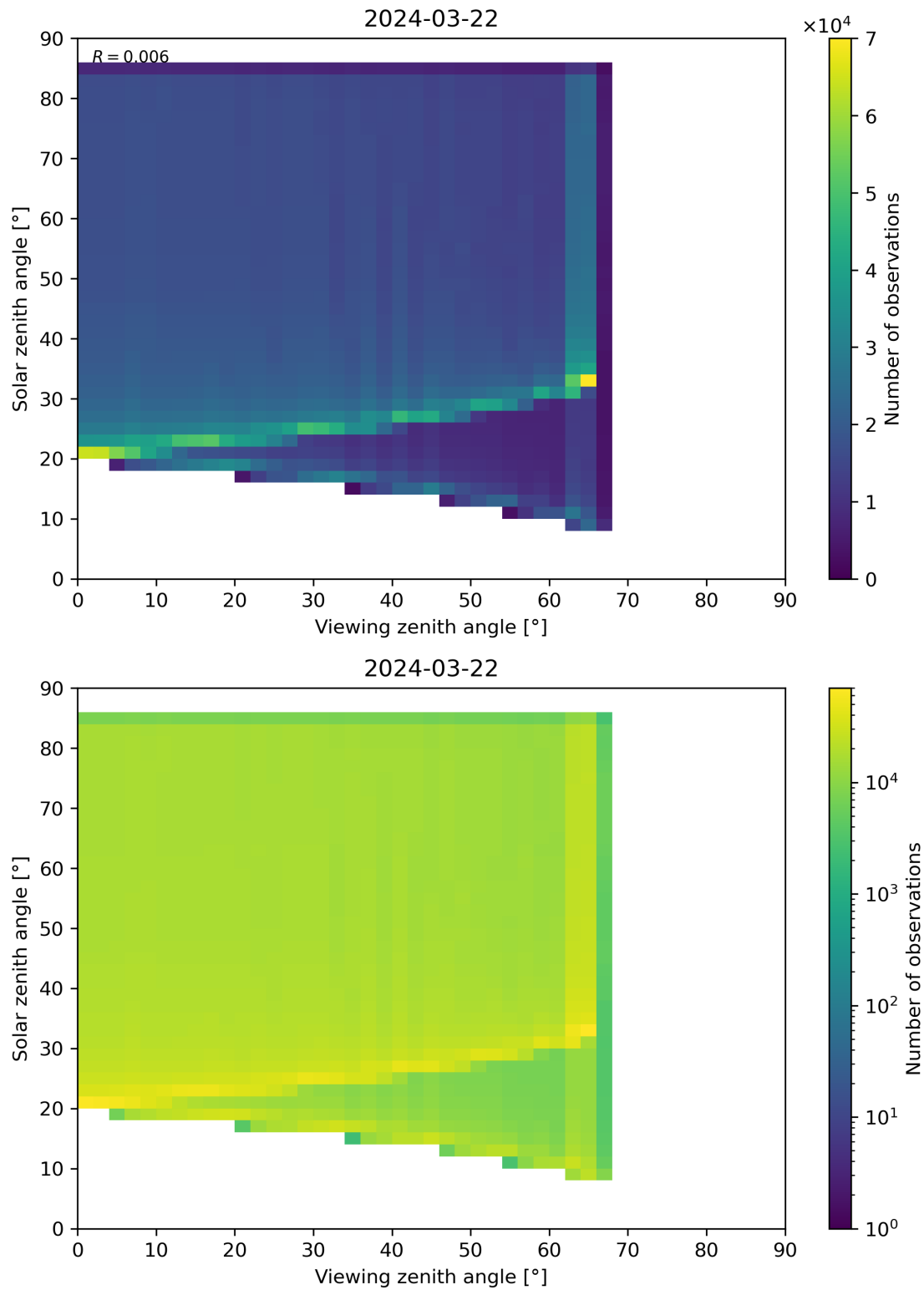
Figure 315: Scatter density plot of “Viewing zenith angle” against “Solar zenith angle” for 2024-03-21 to 2024-03-22.
