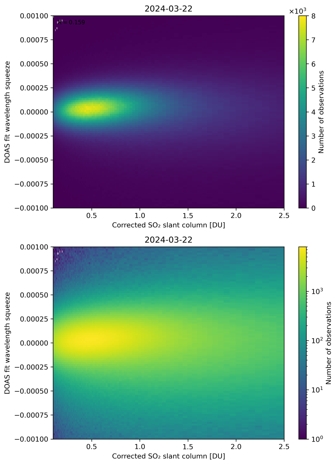
Figure 182: Scatter density plot of “Corrected SO 2 slant column” against “DOAS fit wavelength squeeze” for 2024-03-21 to 2024-03-22.
