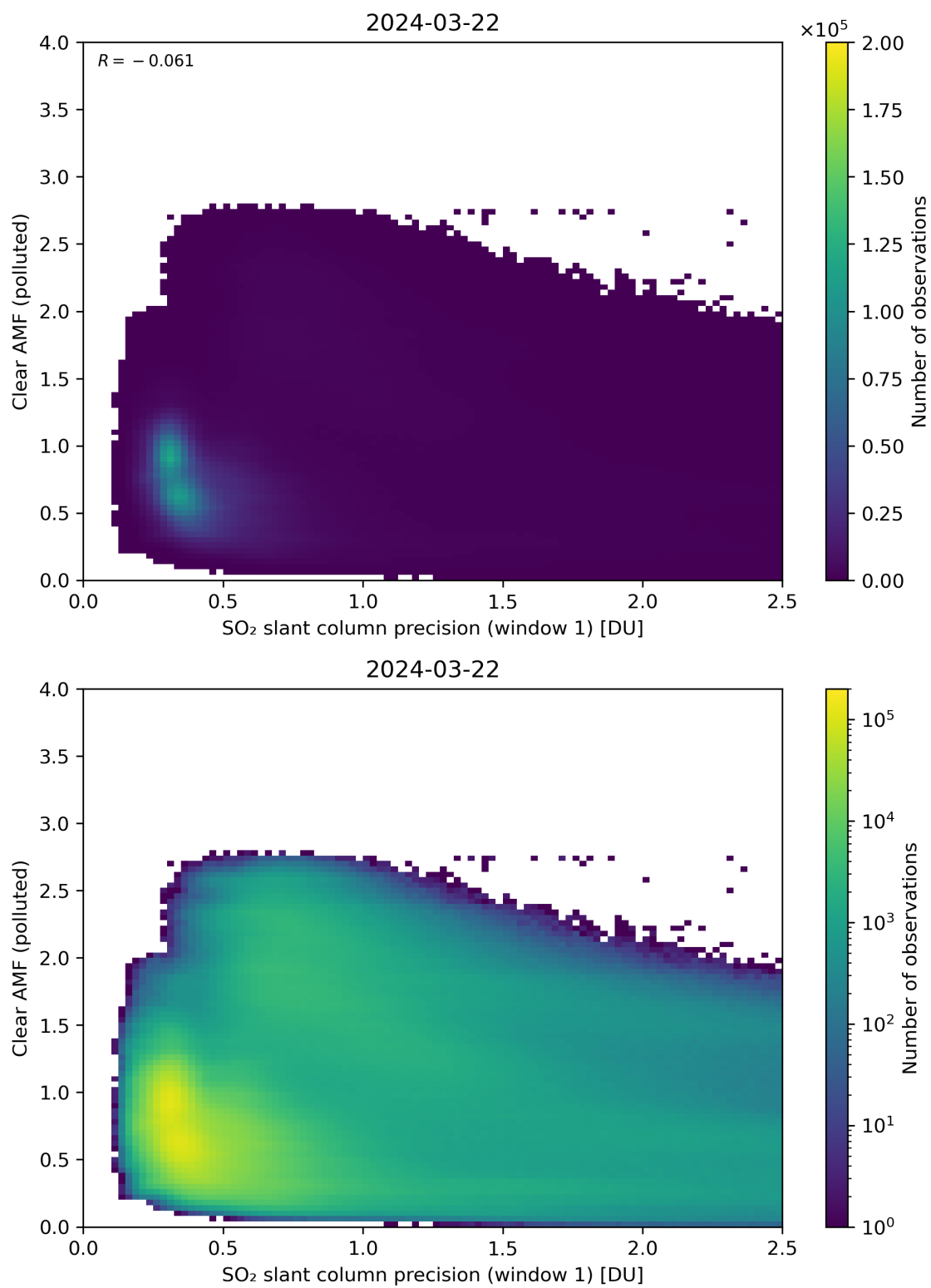
Figure 224: Scatter density plot of “SO 2 slant column precision (window 1)” against “Clear AMF (polluted)” for 2024-03-21 to 2024-03-22.
