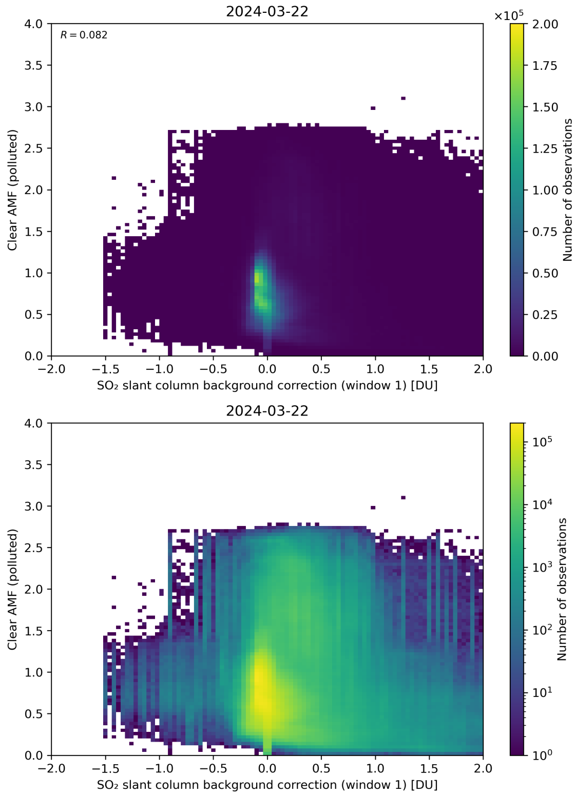
Figure 103: Scatter density plot of “SO 2 slant column background correction (window 1)” against “Clear AMF (polluted)” for 2024-03-21 to 2024-03-22.
