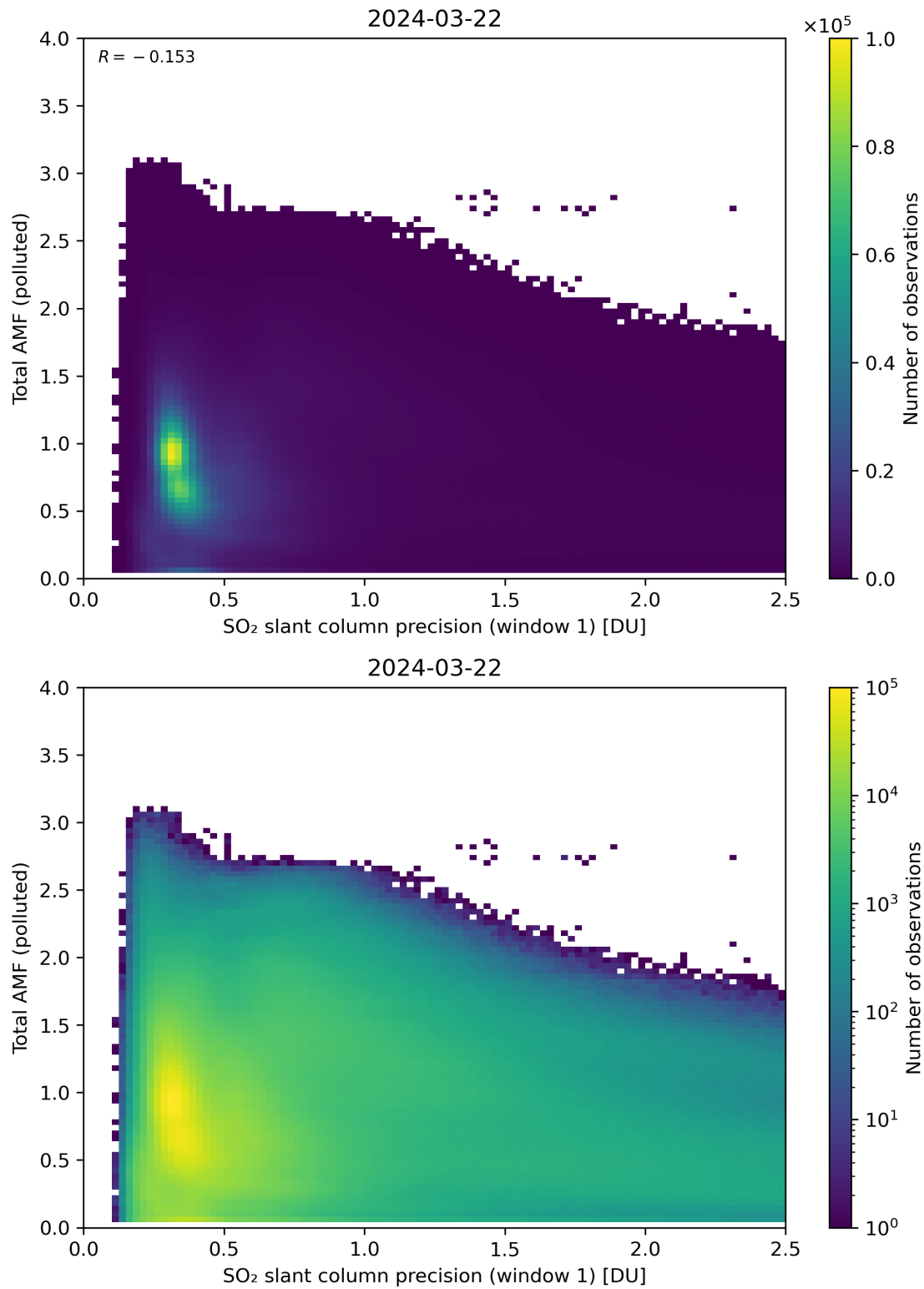
Figure 230: Scatter density plot of “SO 2 slant column precision (window 1)” against “Total AMF (polluted)” for 2024-03-21 to 2024-03-22.
