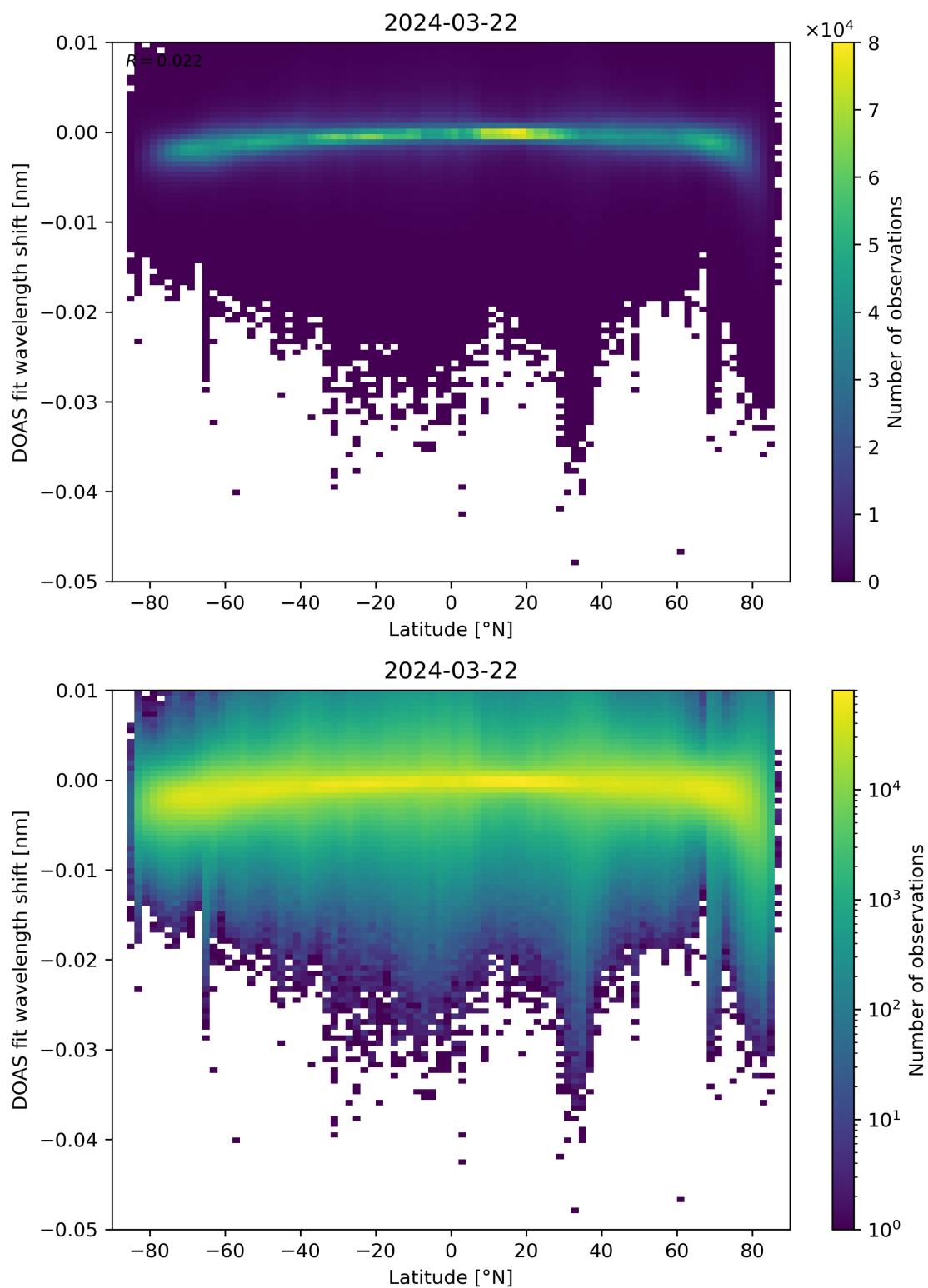
Figure 142: Scatter density plot of “Latitude” against “DOAS fit wavelength shift” for 2024-03-21 to 2024-03-22.
