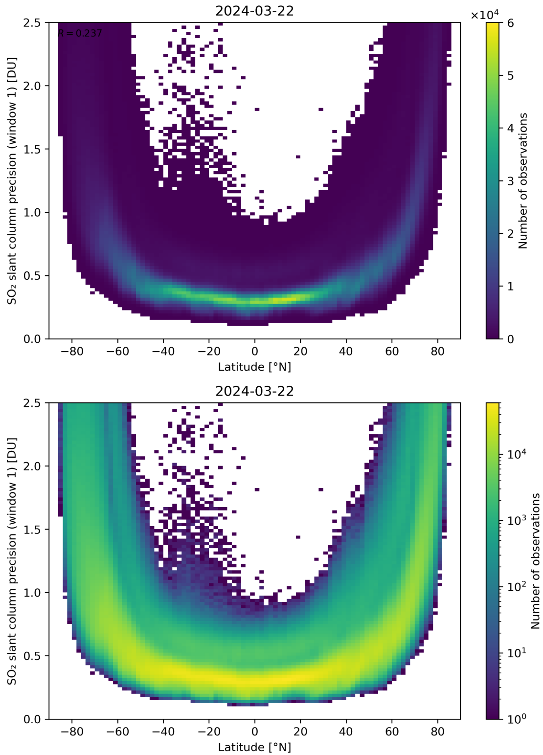
Figure 150: Scatter density plot of “Latitude” against “SO 2 slant column precision (window 1)” for 2024-03-21 to 2024-03-22.
