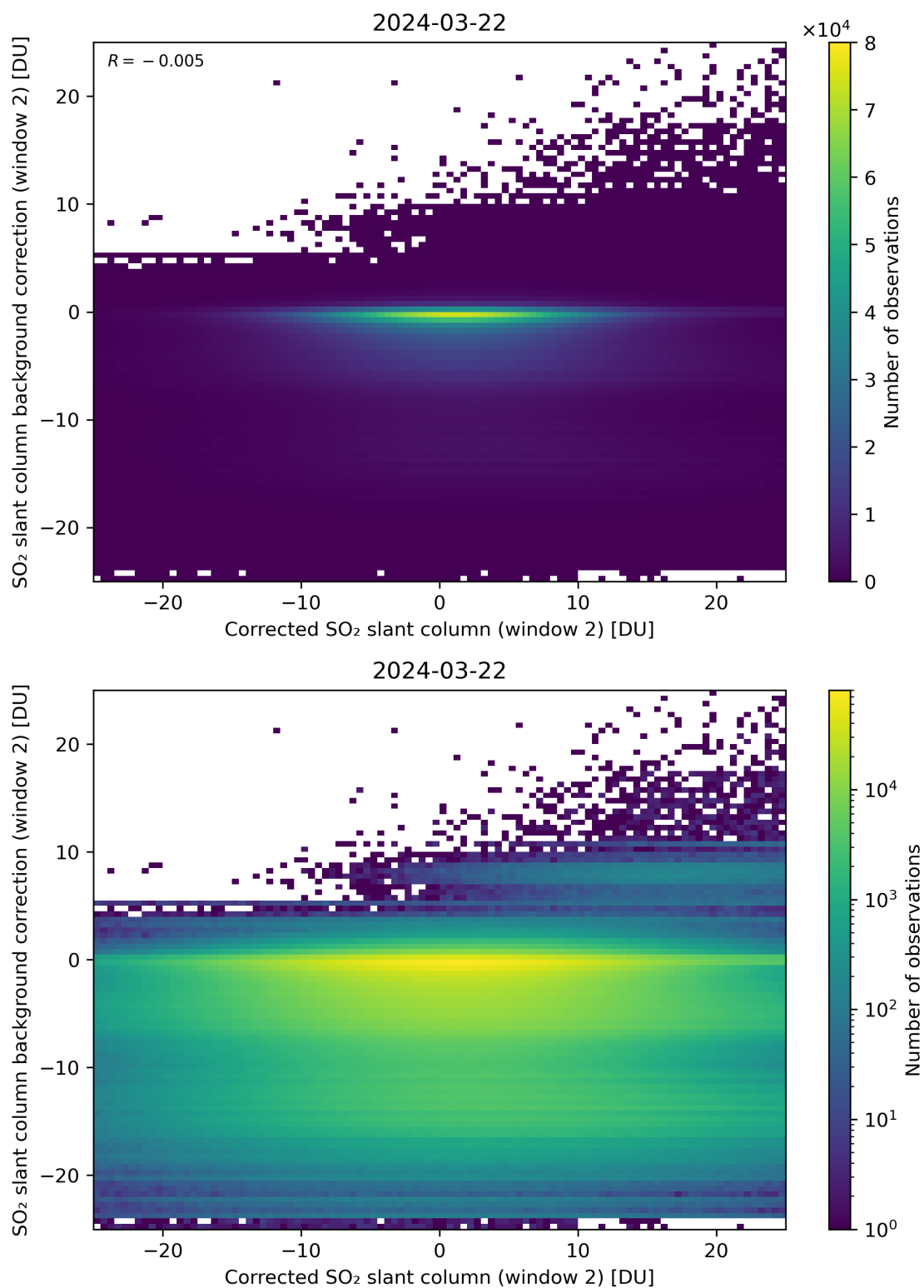
Figure 194: Scatter density plot of “Corrected SO 2 slant column (window 2)” against “SO 2 slant column background correction (window 2)” for 2024-03-21 to 2024-03-22.
