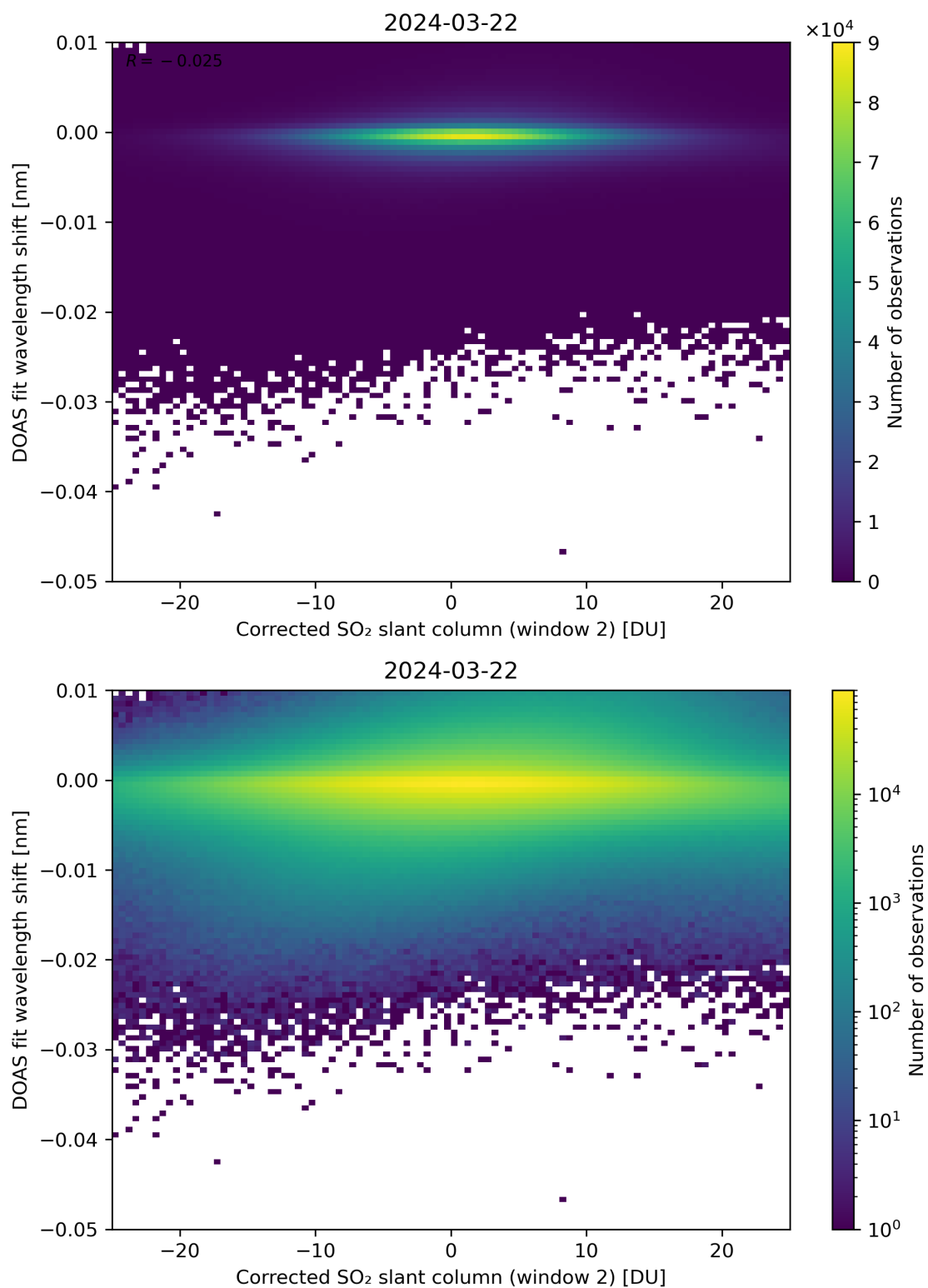
Figure 196: Scatter density plot of “Corrected SO 2 slant column (window 2)” against “DOAS fit wavelength shift” for 2024-03-21 to 2024-03-22.
