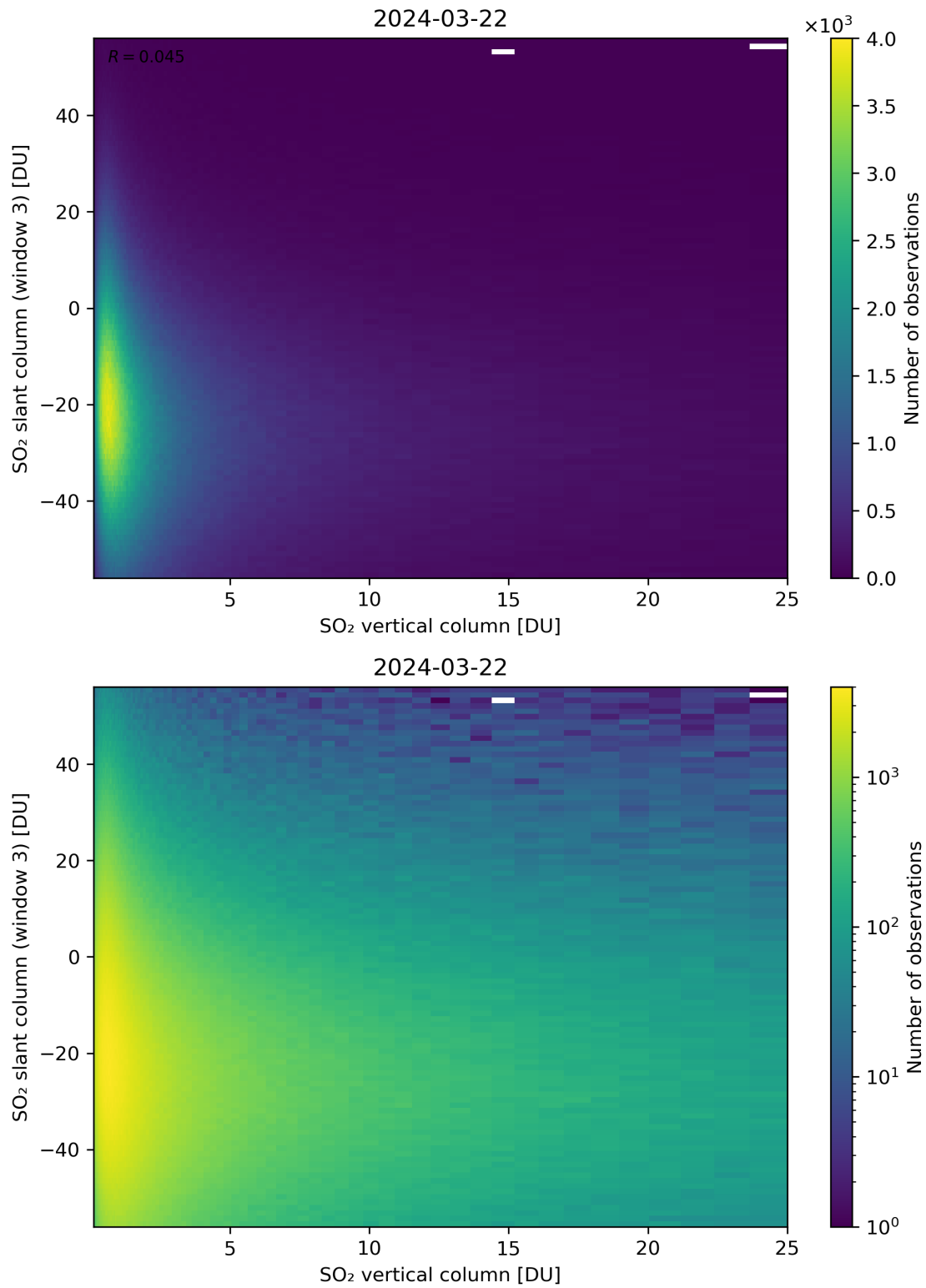
Figure 303: Scatter density plot of “SO 2 vertical column” against “SO 2 slant column (window 3)” for 2024-03-21 to 2024-03-22.
