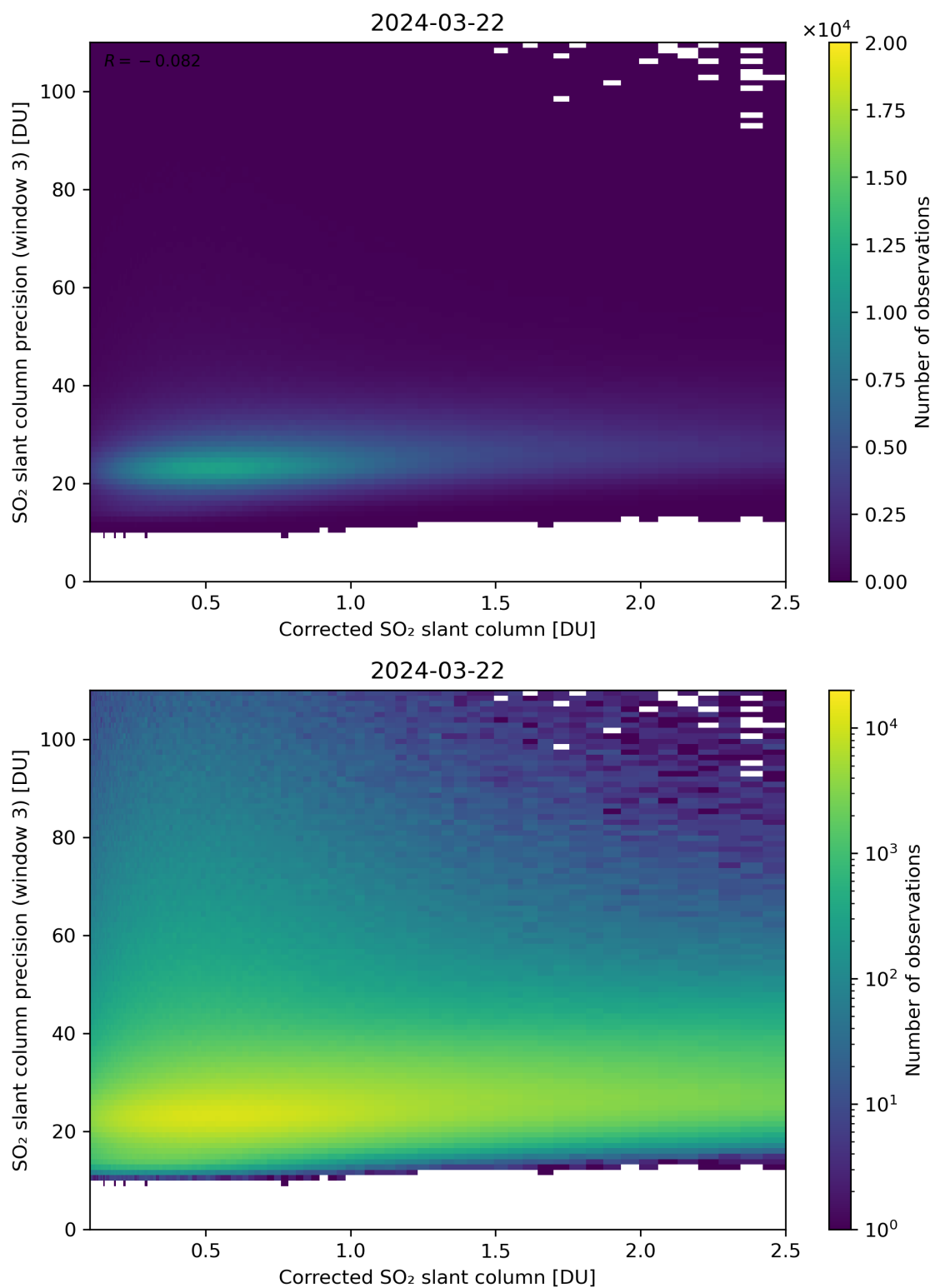
Figure 191: Scatter density plot of “Corrected SO 2 slant column” against “SO 2 slant column precision (window 3)” for 2024-03-21 to 2024-03-22.
