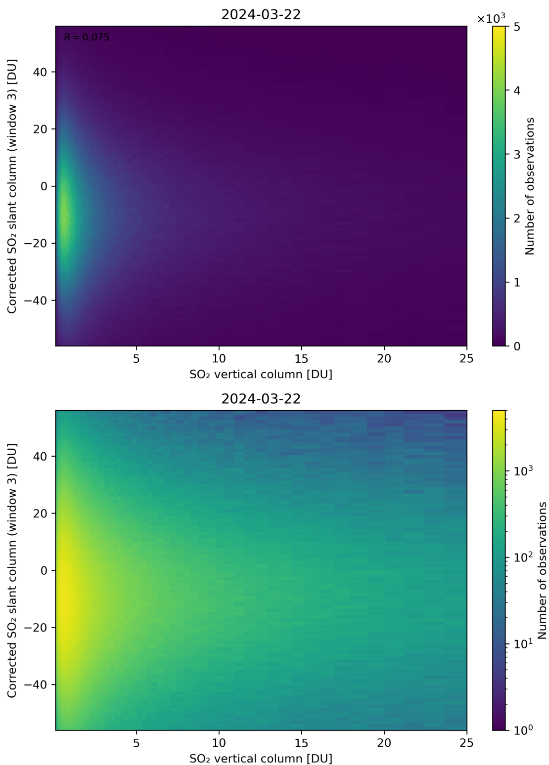
Figure 299: Scatter density plot of “SO 2 vertical column” against “Corrected SO 2 slant column (window 3)” for 2024-03-21 to 2024-03-22.
