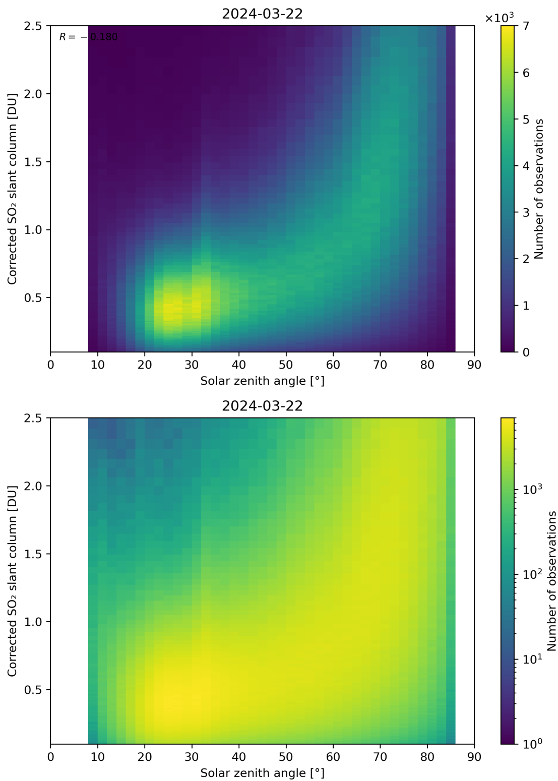
Figure 166: Scatter density plot of “Solar zenith angle” against “Corrected SO 2 slant column” for 2024-03-21 to 2024-03-22.
