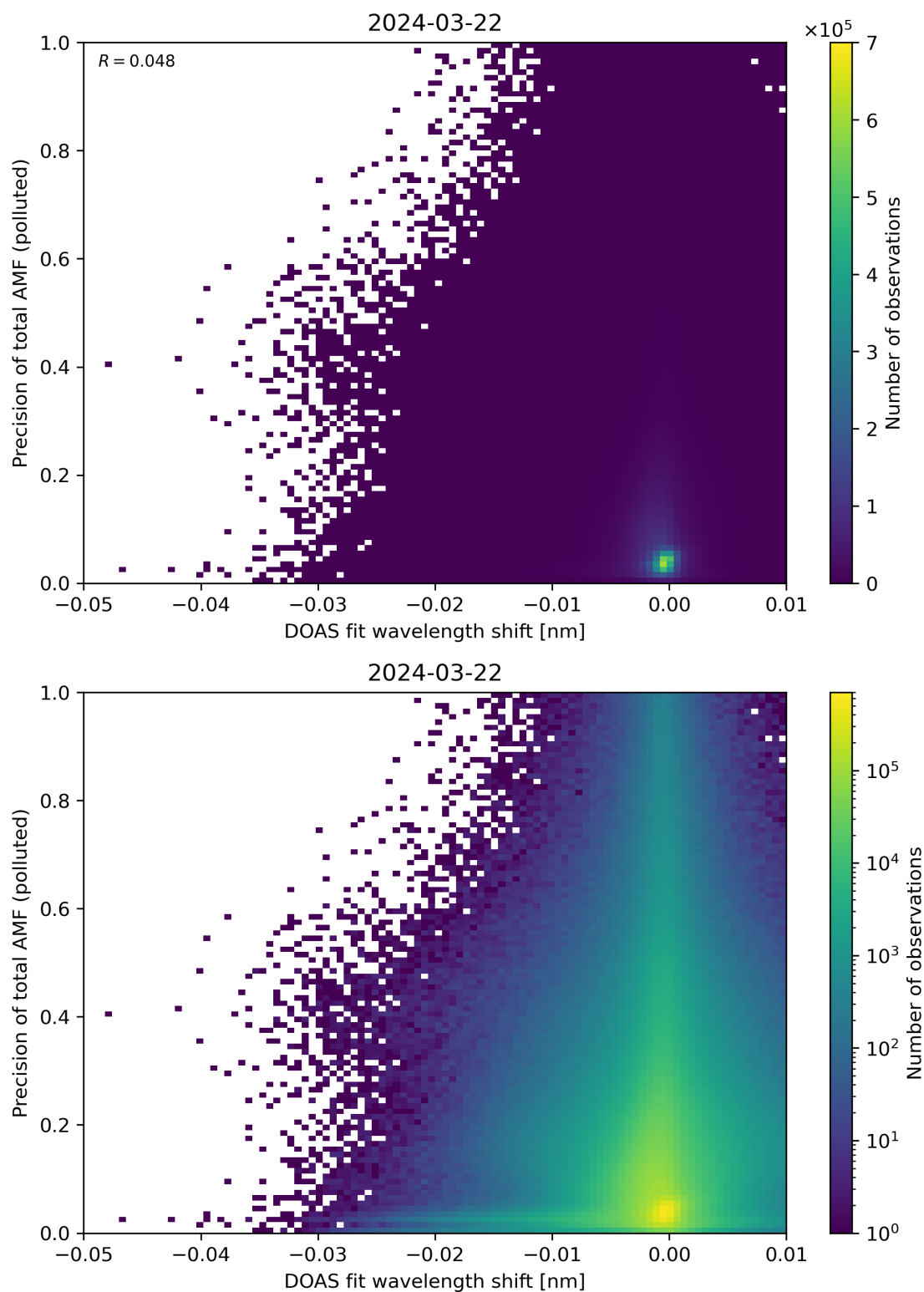
Figure 131: Scatter density plot of “DOAS fit wavelength shift” against “Precision of total AMF (polluted)” for 2024-03-21 to 2024-03-22.
