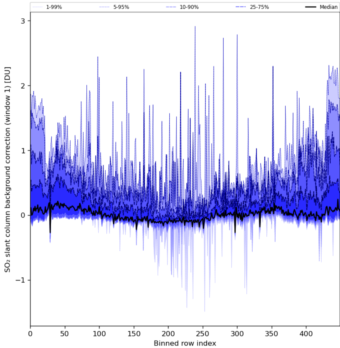
Figure 82: Along track statistics of “SO 2 slant column background correction (window 1)” for 2024-03-21 to 2024-03-22
