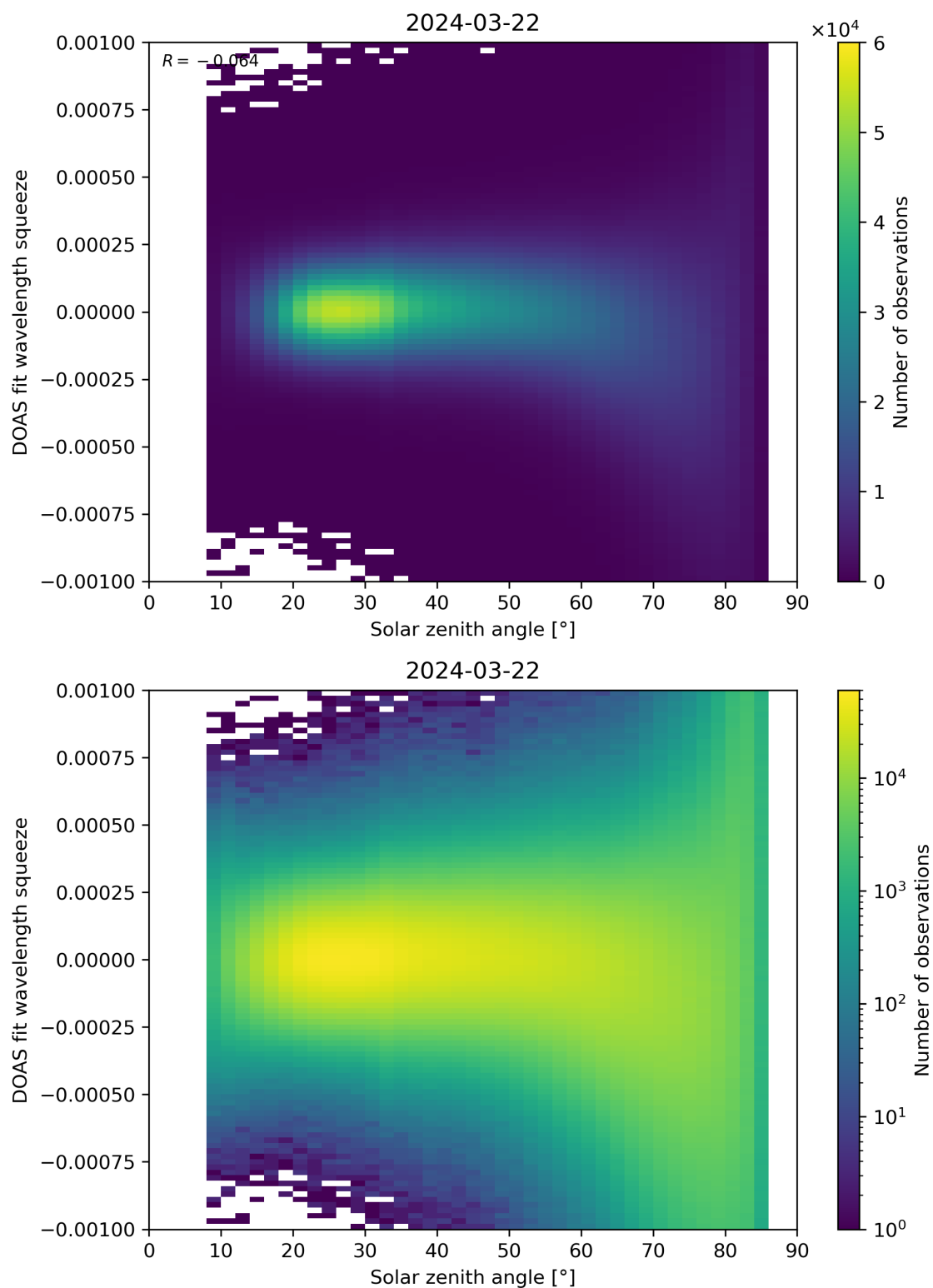
Figure 162: Scatter density plot of “Solar zenith angle” against “DOAS fit wavelength squeeze” for 2024-03-21 to 2024-03-22.
