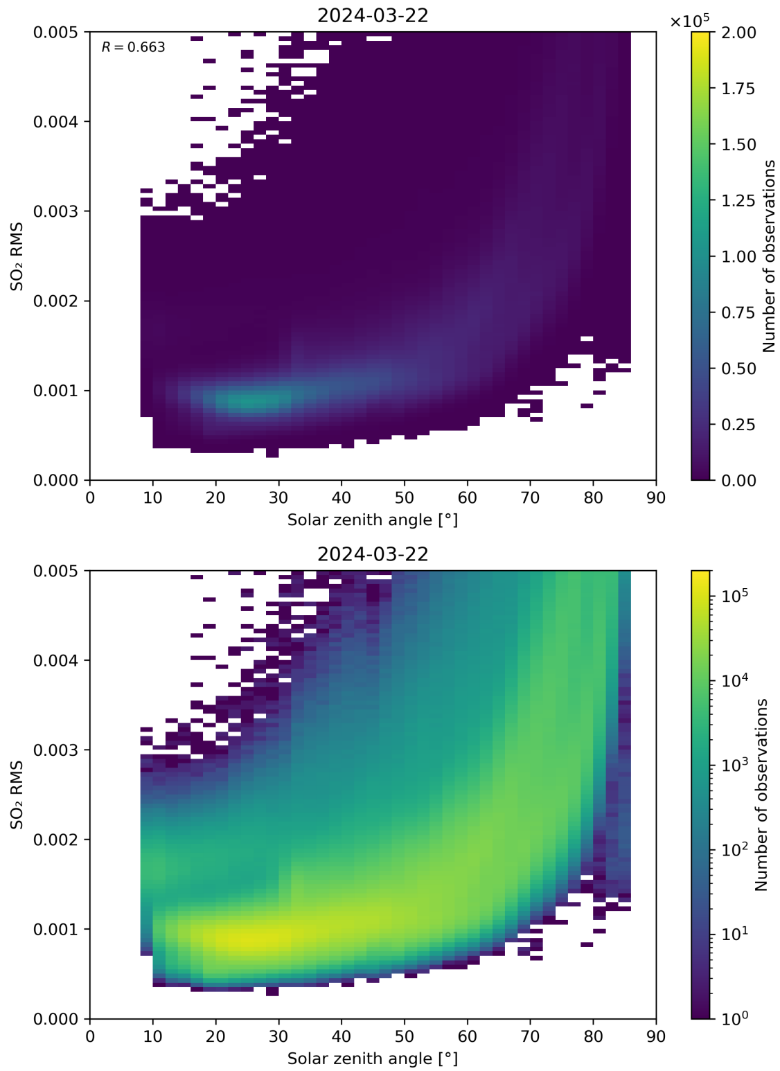
Figure 163: Scatter density plot of “Solar zenith angle” against “SO 2 RMS” for 2024-03-21 to 2024-03-22.
