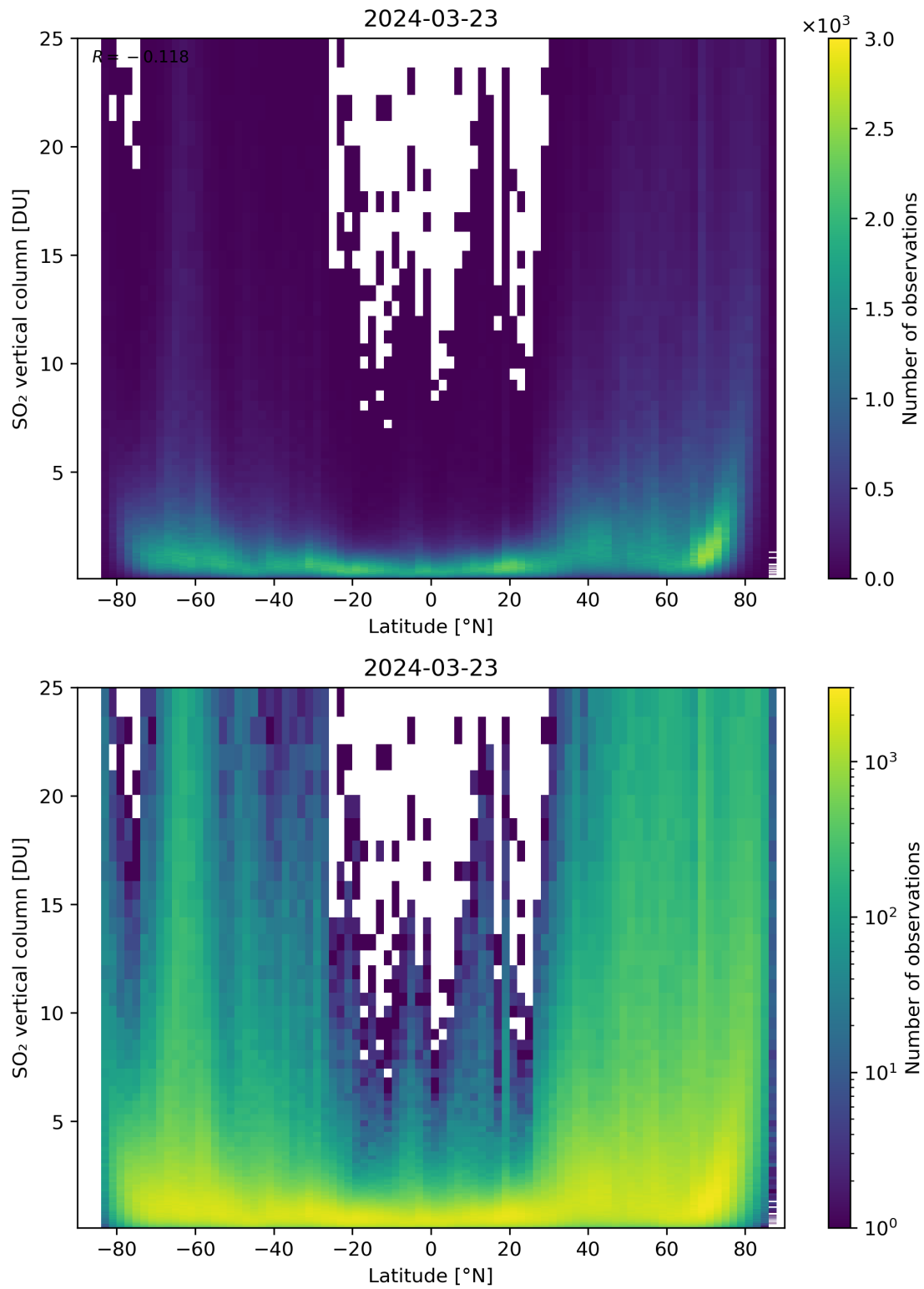
Figure 156: Scatter density plot of “Latitude” against “SO 2 vertical column” for 2024-03-23 to 2024-03-24.
