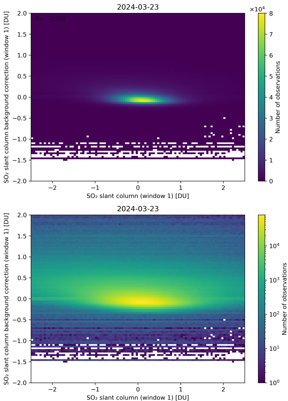
Figure 212: Scatter density plot of “SO 2 slant column (window 1)” against “SO 2 slant column background correction (window 1)” for 2024-03-23 to 2024-03-24.
