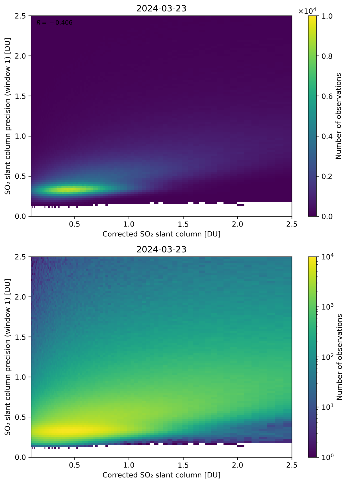
Figure 188: Scatter density plot of “Corrected SO 2 slant column” against “SO 2 slant column precision (window 1)” for 2024-03-23 to 2024-03-24.
