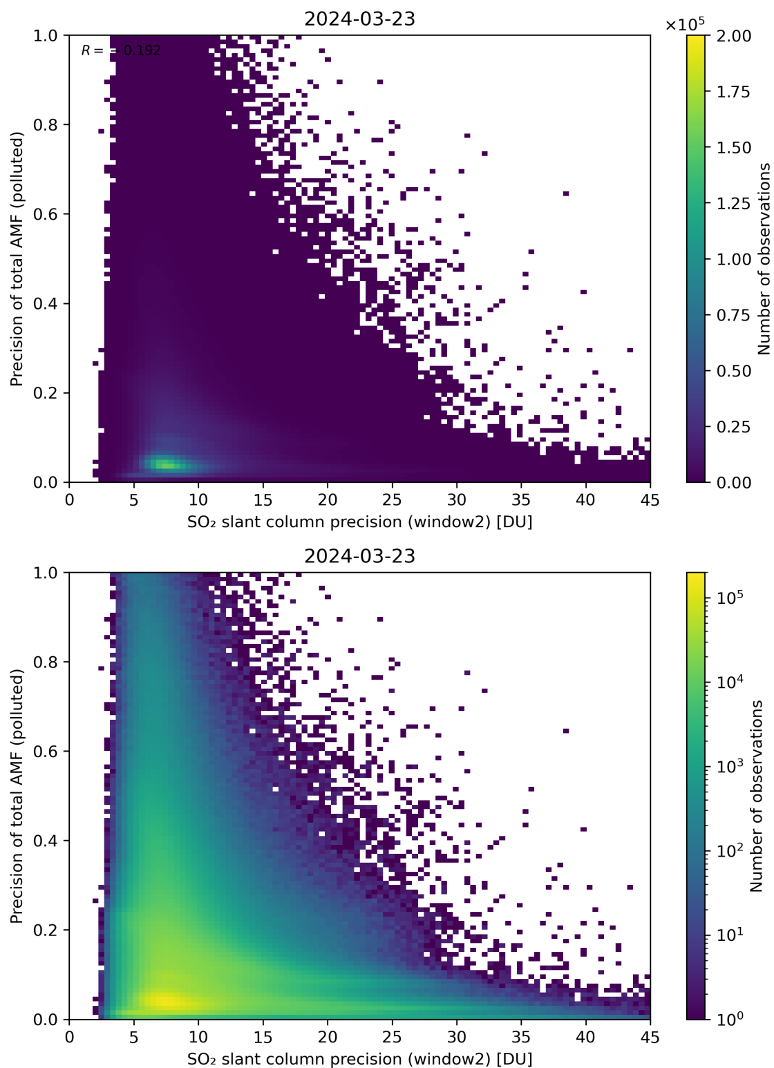
Figure 252: Scatter density plot of “SO 2 slant column precision (window2)” against “Precision of total AMF (polluted)” for 2024-03-23 to 2024-03-24.
