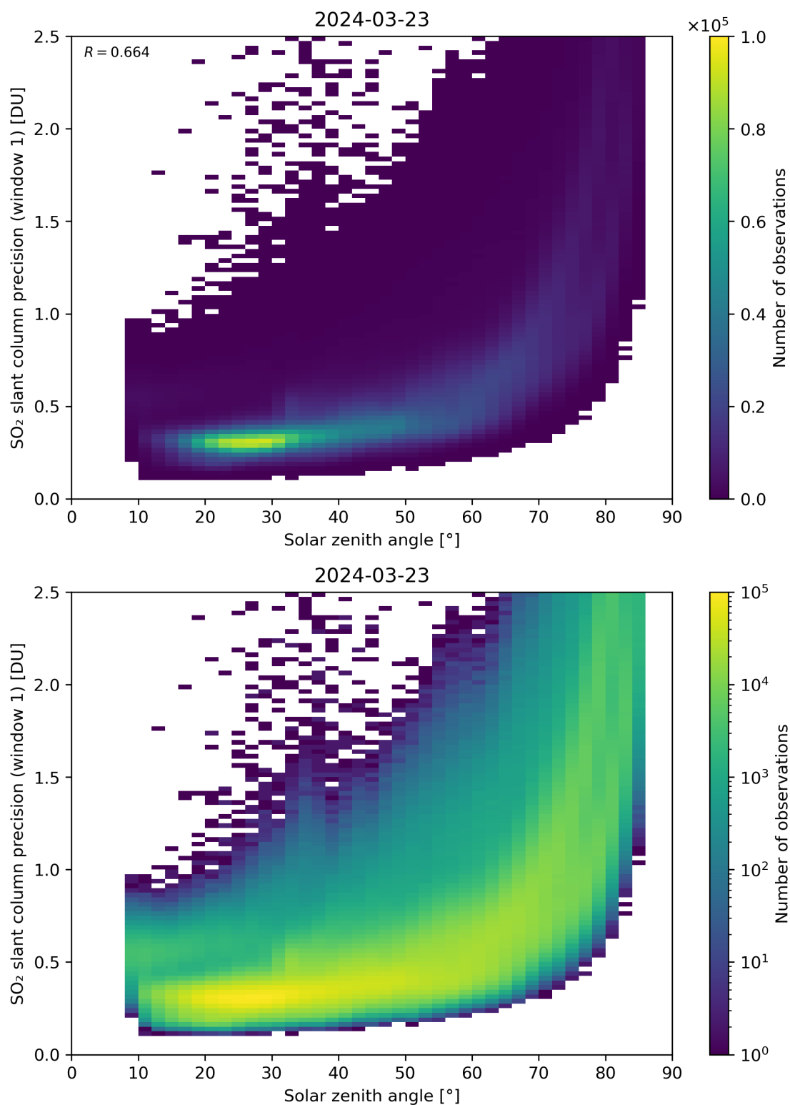
Figure 170: Scatter density plot of “Solar zenith angle” against “SO 2 slant column precision (window 1)” for 2024-03-23 to 2024-03-24.
