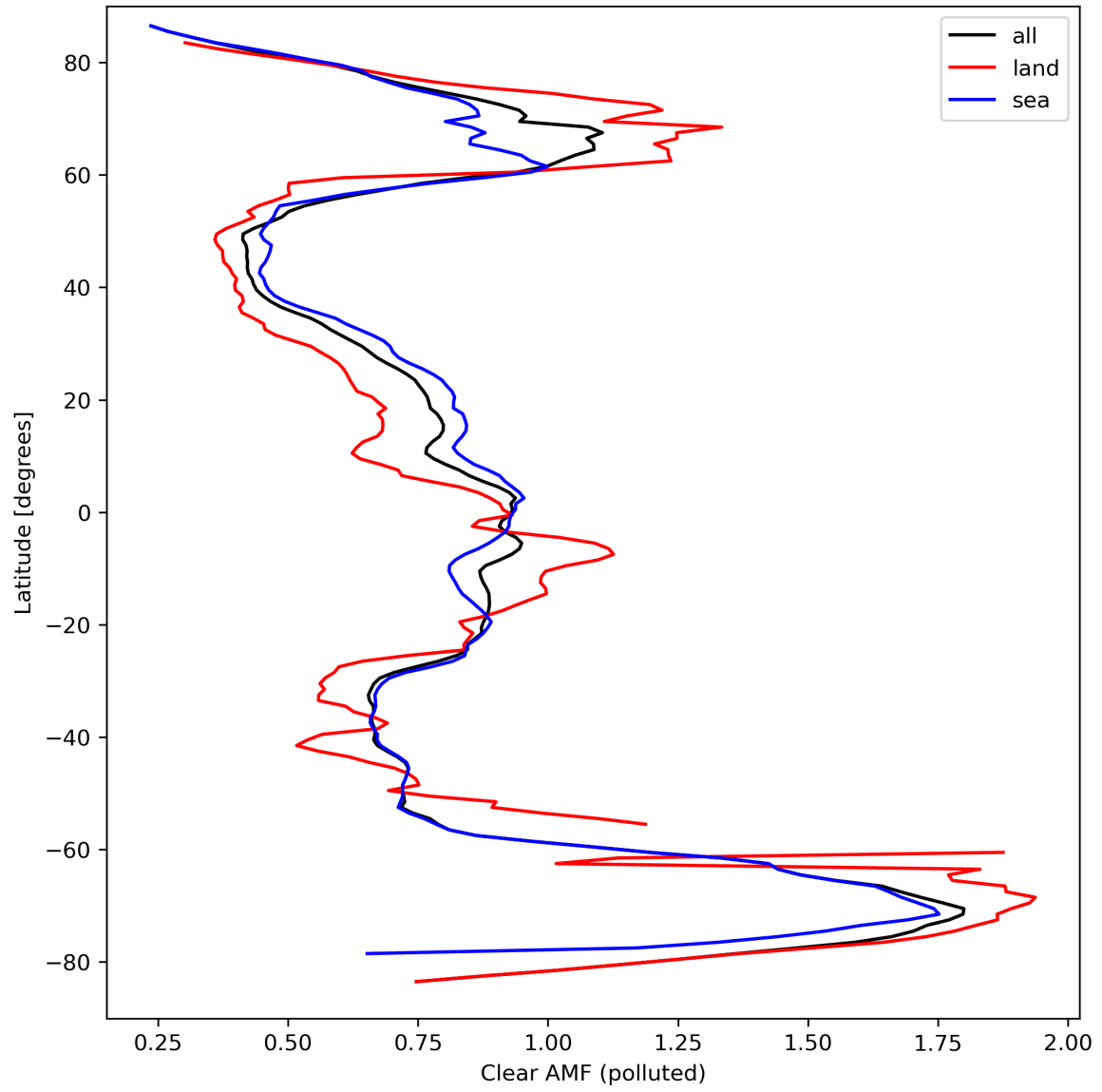
Figure 50: Zonal average of “Clear AMF (polluted)” for 2024-03-23 to 2024-03-24.
