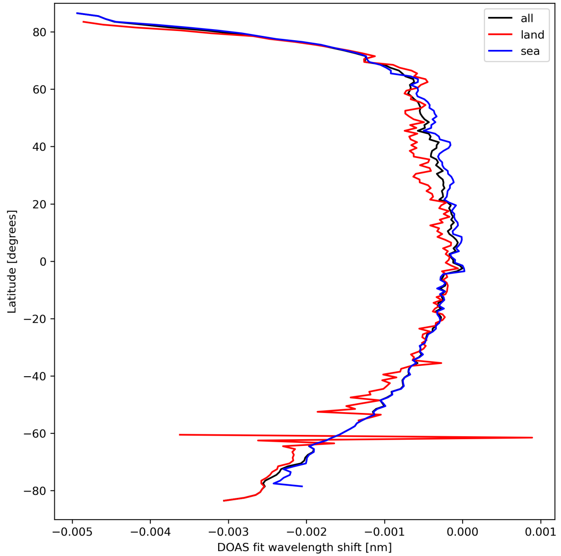
Figure 45: Zonal average of “DOAS fit wavelength shift” for 2024-03-23 to 2024-03-24.
