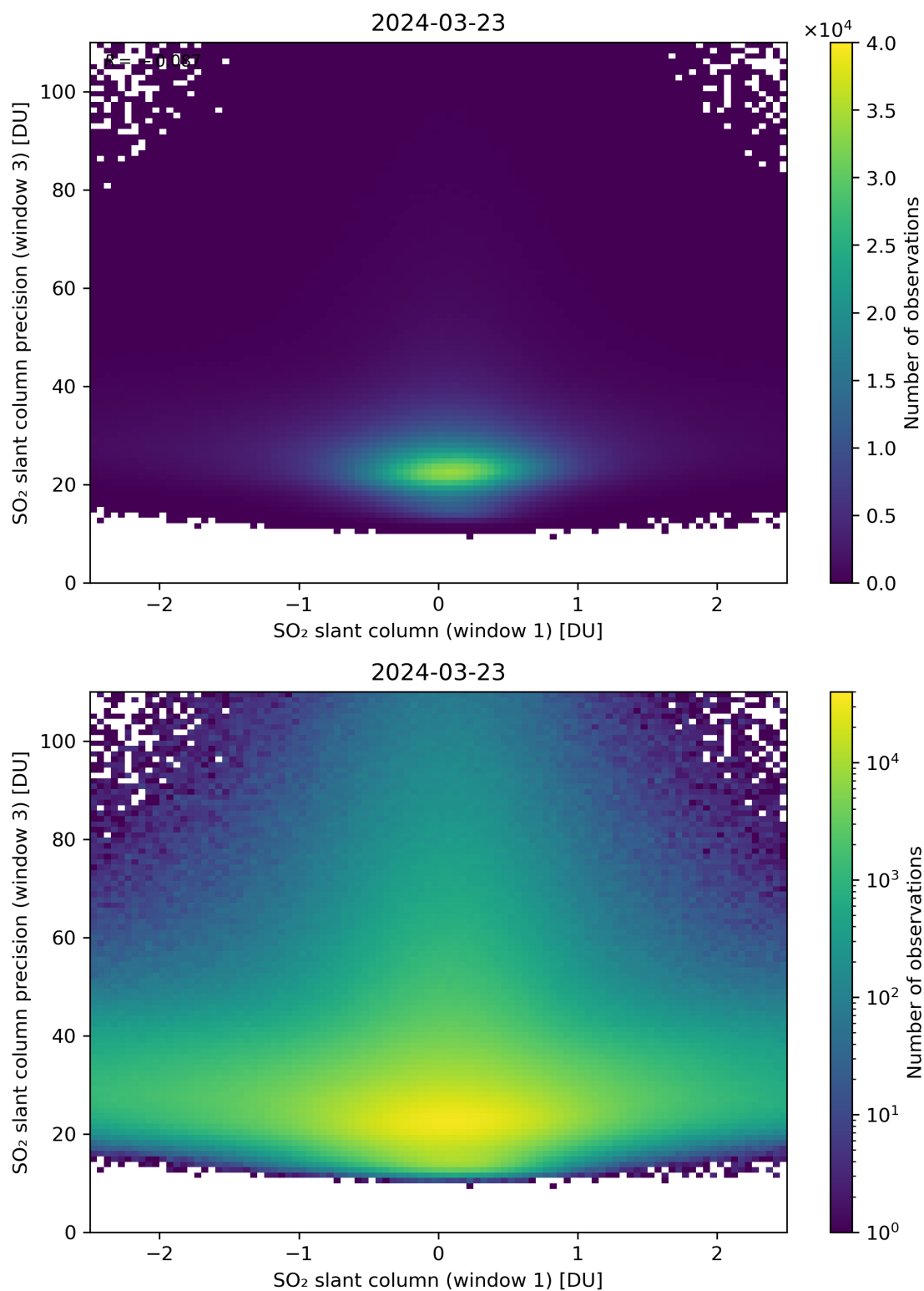
Figure 238: Scatter density plot of “SO 2 slant column (window 1)” against “SO 2 slant column precision (window 3)” for 2024-03-23 to 2024-03-24.
