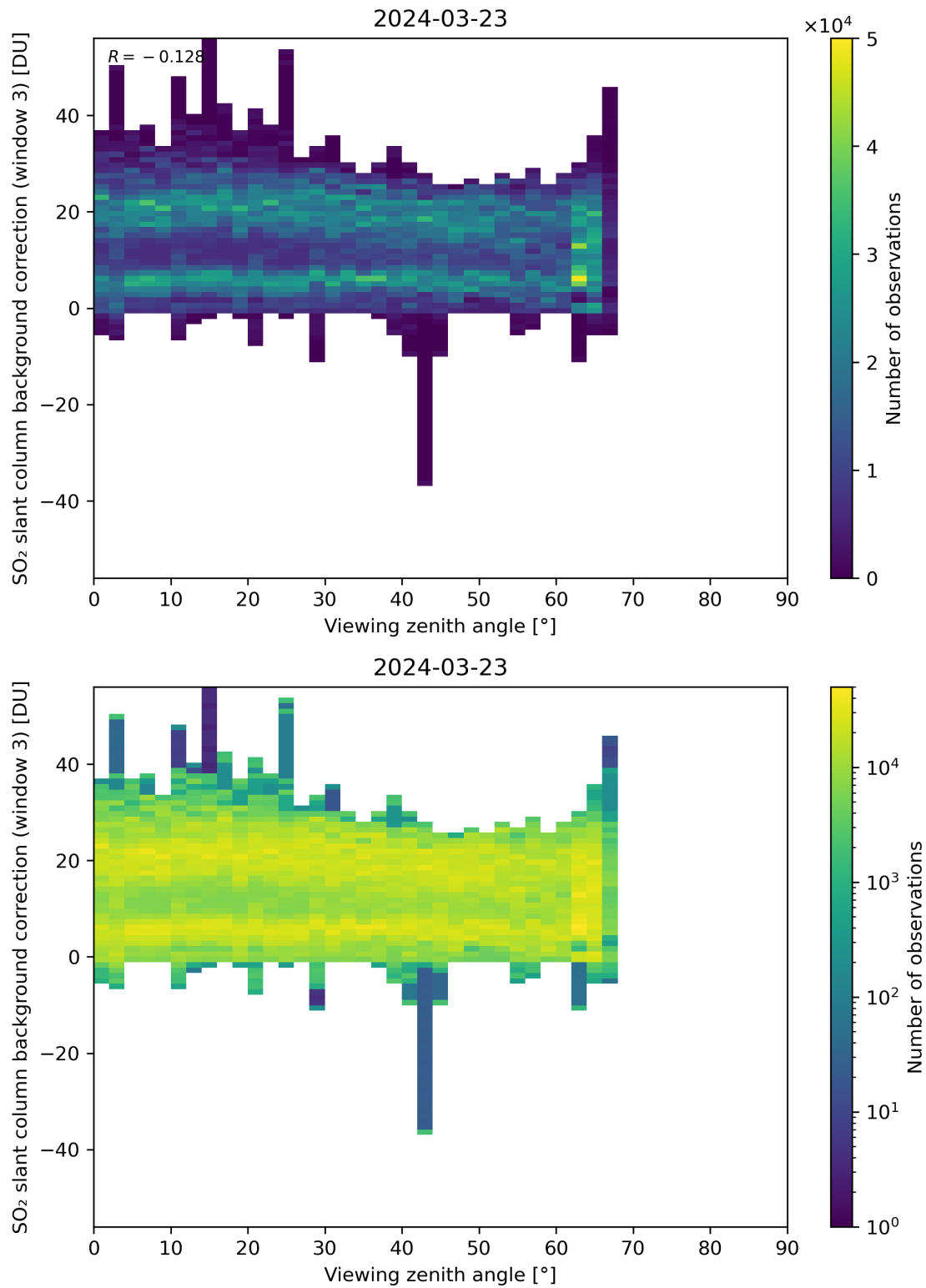
Figure 310: Scatter density plot of “Viewing zenith angle” against “SO 2 slant column background correction (window 3)” for 2024-03-23 to 2024-03-24.
