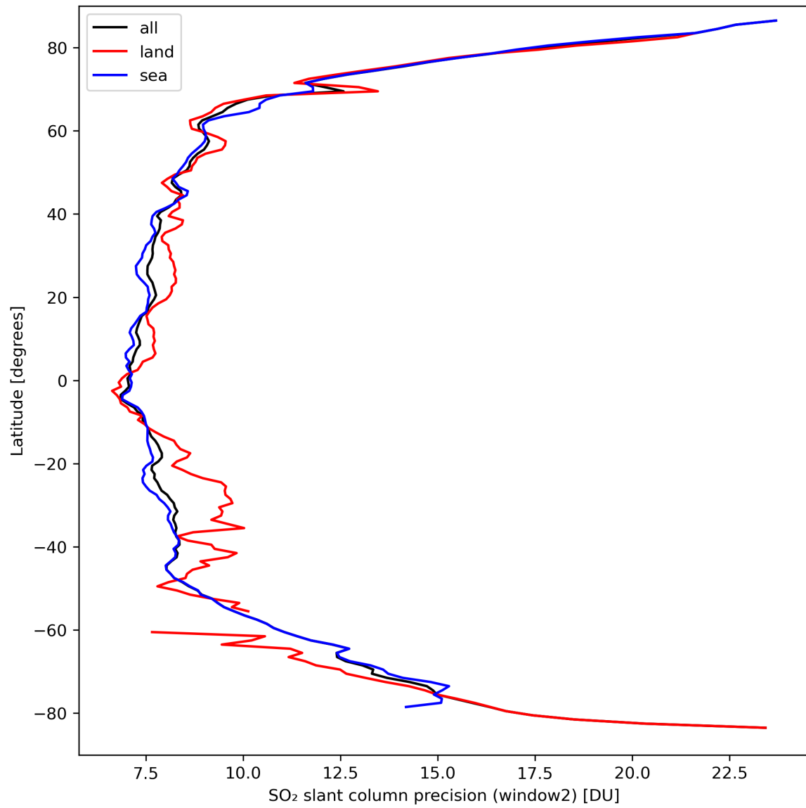
Figure 38: Zonal average of “SO 2 slant column precision (window2)” for 2024-03-23 to 2024-03-24.
