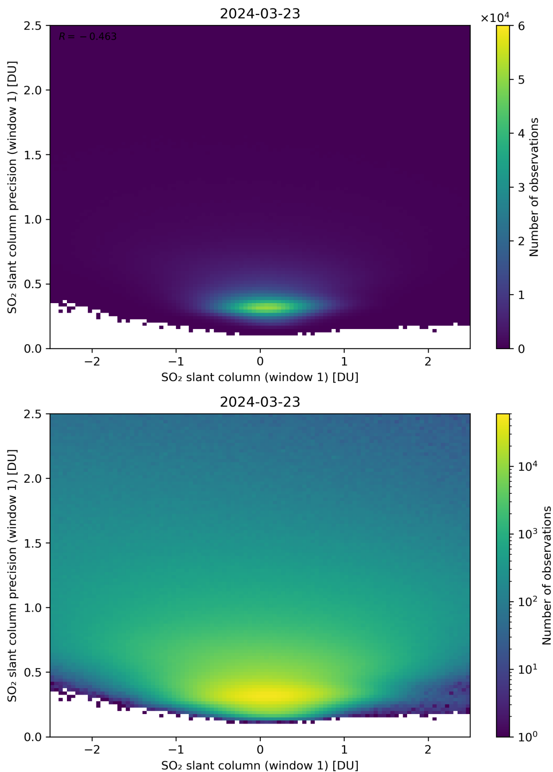
Figure 235: Scatter density plot of “SO 2 slant column (window 1)” against “SO 2 slant column precision (window 1)” for 2024-03-23 to 2024-03-24.
