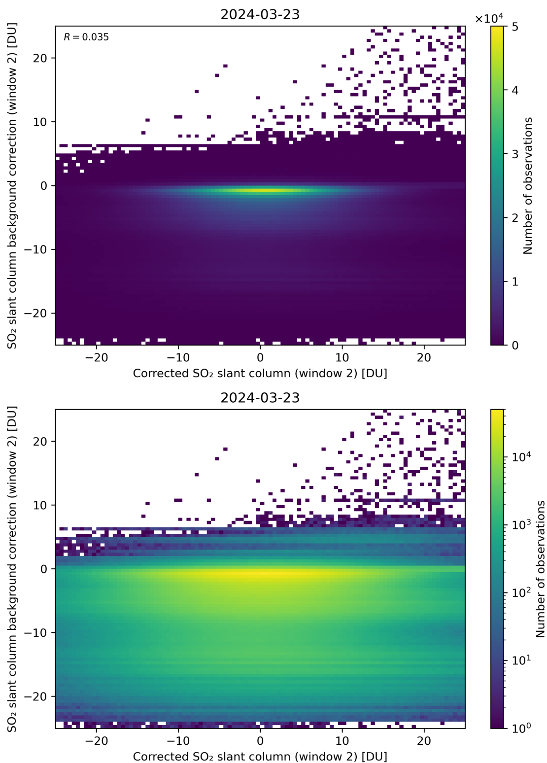
Figure 194: Scatter density plot of “Corrected SO 2 slant column (window 2)” against “SO 2 slant column background correction (window 2)” for 2024-03-23 to 2024-03-24.
