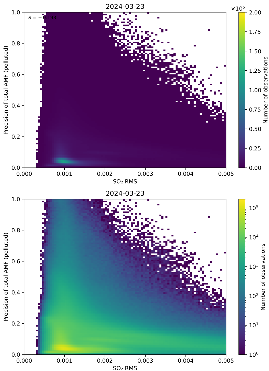
Figure 138: Scatter density plot of “SO 2 RMS” against “Precision of total AMF (polluted)” for 2024-03-23 to 2024-03-24.
