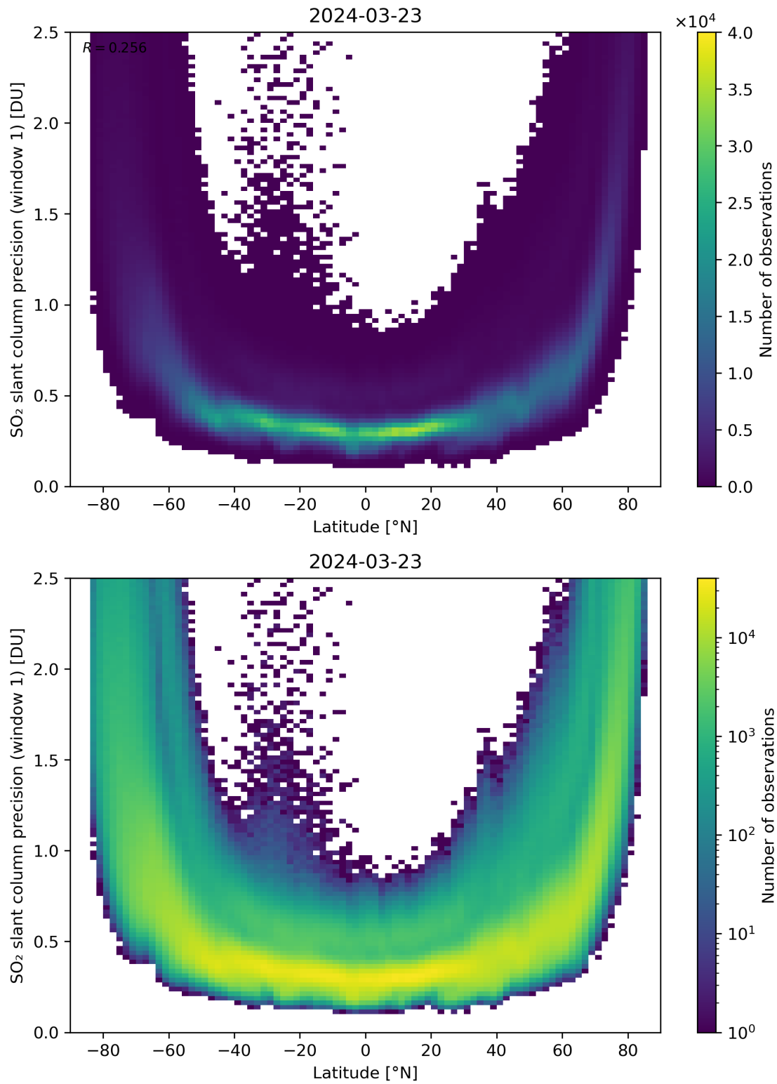
Figure 150: Scatter density plot of “Latitude” against “SO 2 slant column precision (window 1)” for 2024-03-23 to 2024-03-24.
