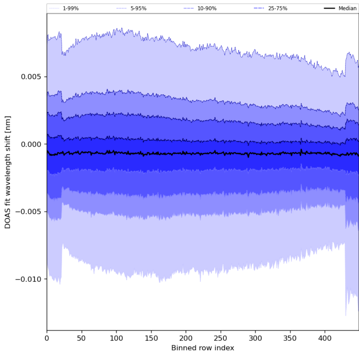
Figure 91: Along track statistics of “DOAS fit wavelength shift” for 2024-03-23 to 2024-03-24
