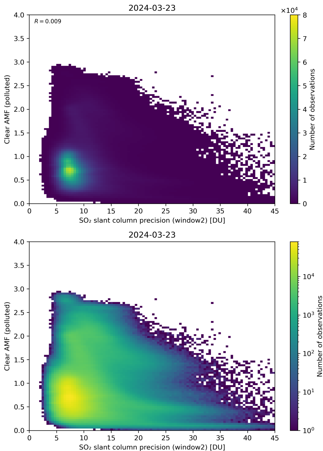
Figure 246: Scatter density plot of “SO 2 slant column precision (window2)” against “Clear AMF (polluted)” for 2024-03-23 to 2024-03-24.
