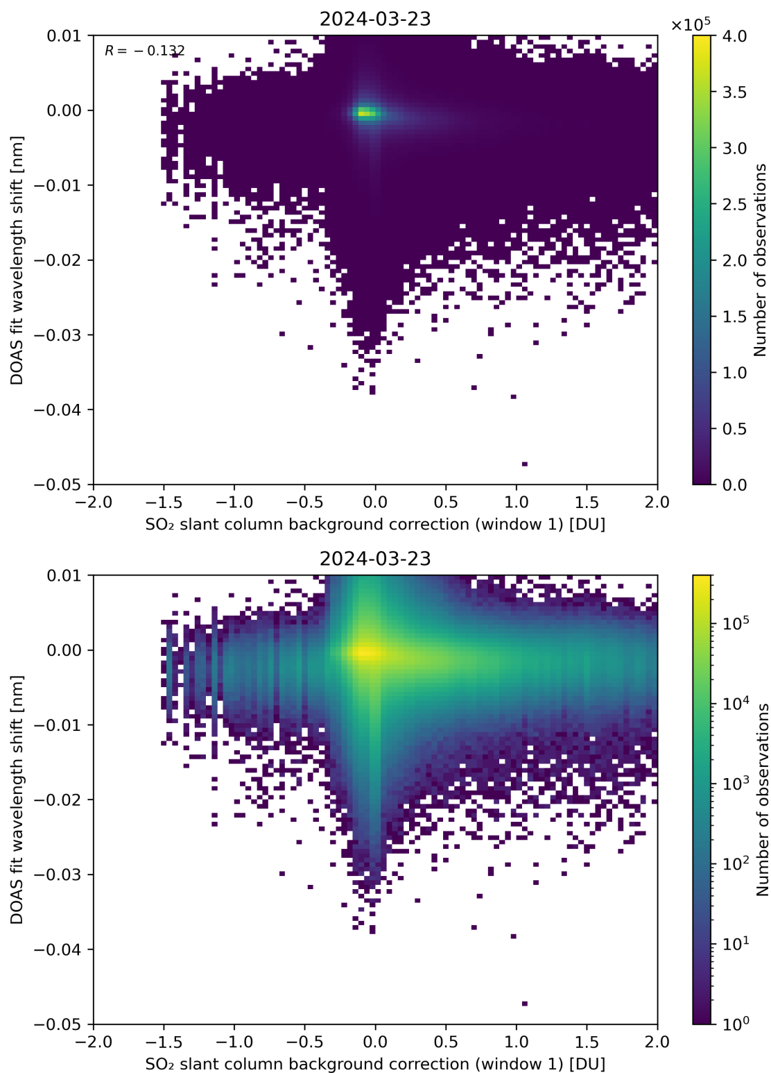
Figure 100: Scatter density plot of “SO 2 slant column background correction (window 1)” against “DOAS fit wavelength shift” for 2024-03-23 to 2024-03-24.
