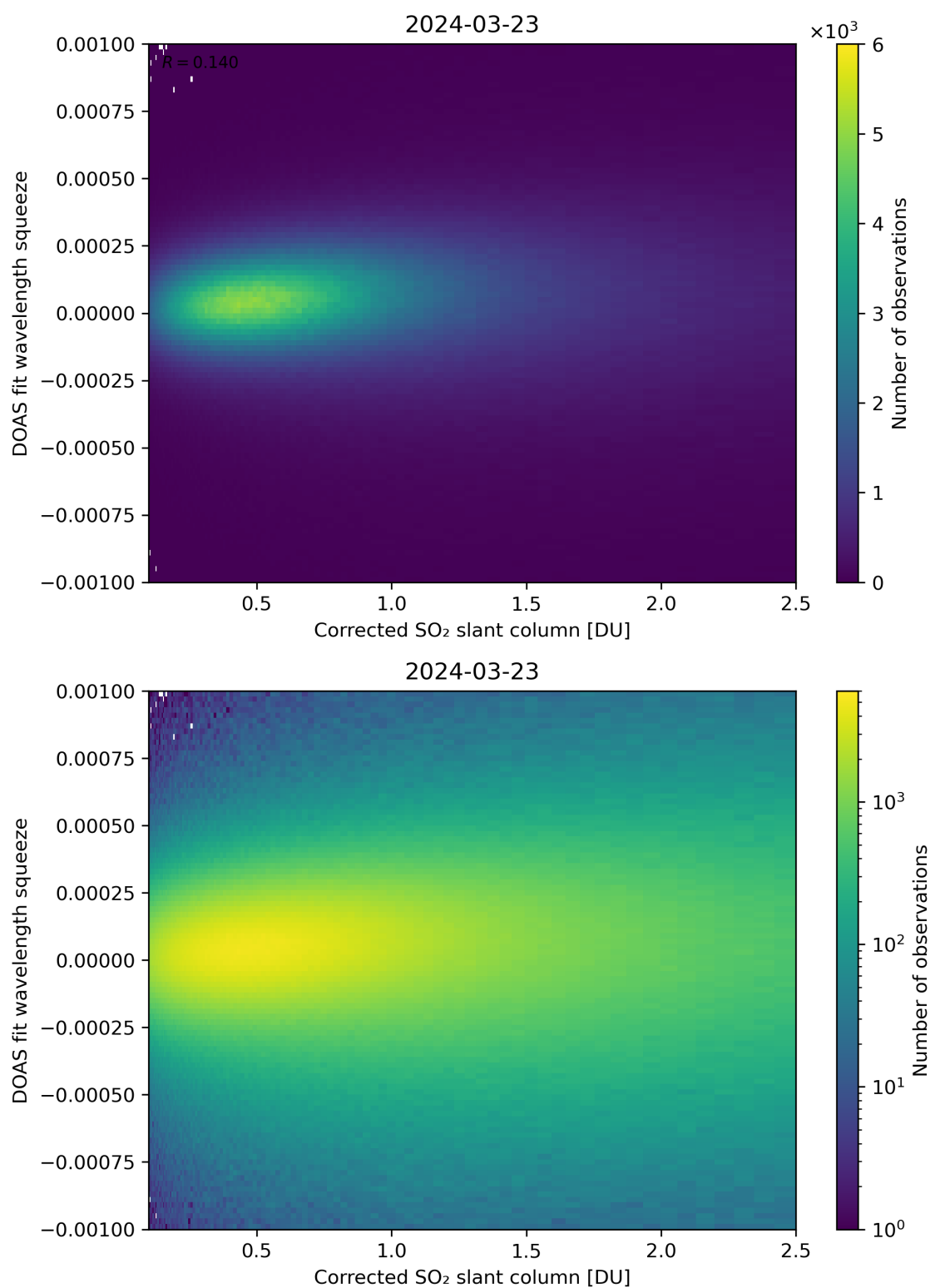
Figure 182: Scatter density plot of “Corrected SO 2 slant column” against “DOAS fit wavelength squeeze” for 2024-03-23 to 2024-03-24.
