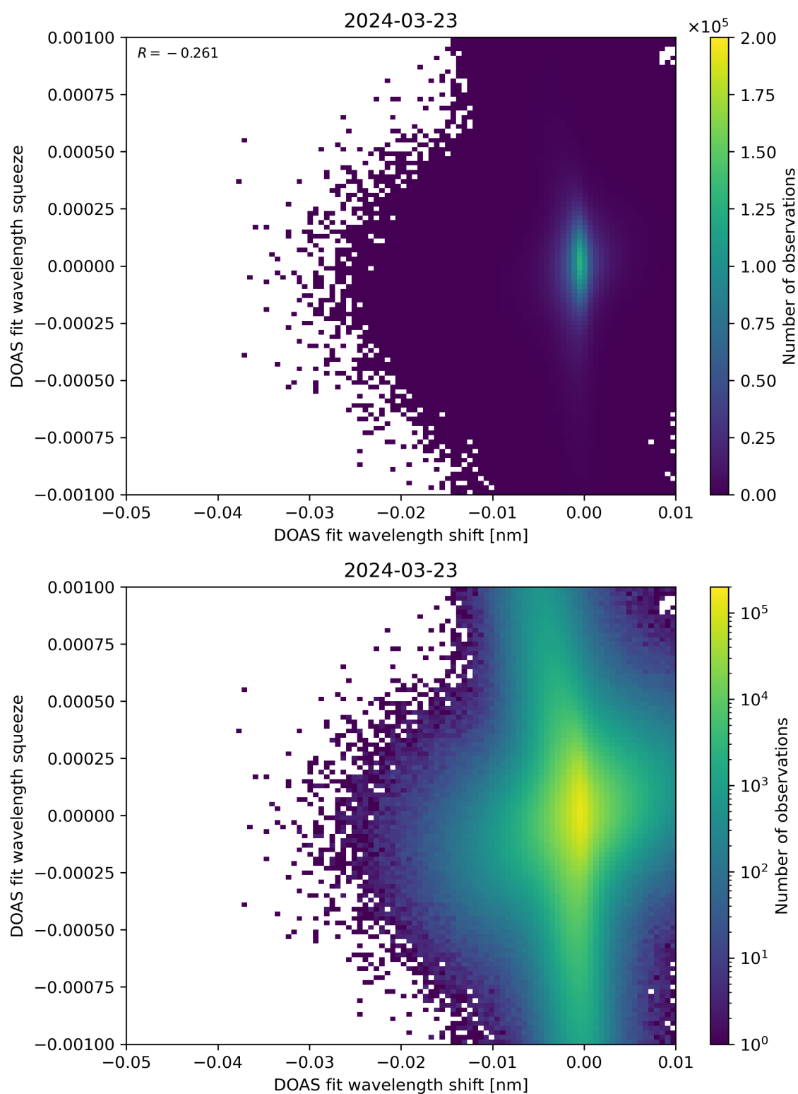
Figure 127: Scatter density plot of “DOAS fit wavelength shift” against “DOAS fit wavelength squeeze” for 2024-03-23 to 2024-03-24.
