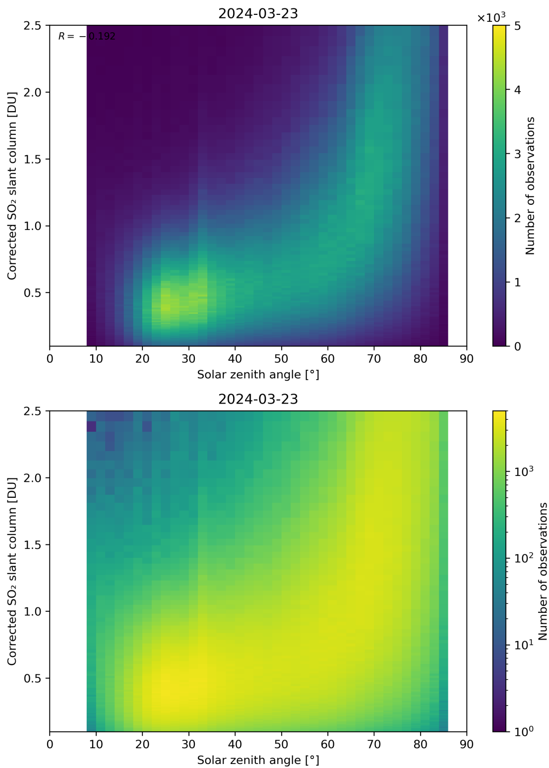
Figure 166: Scatter density plot of “Solar zenith angle” against “Corrected SO 2 slant column” for 2024-03-23 to 2024-03-24.
