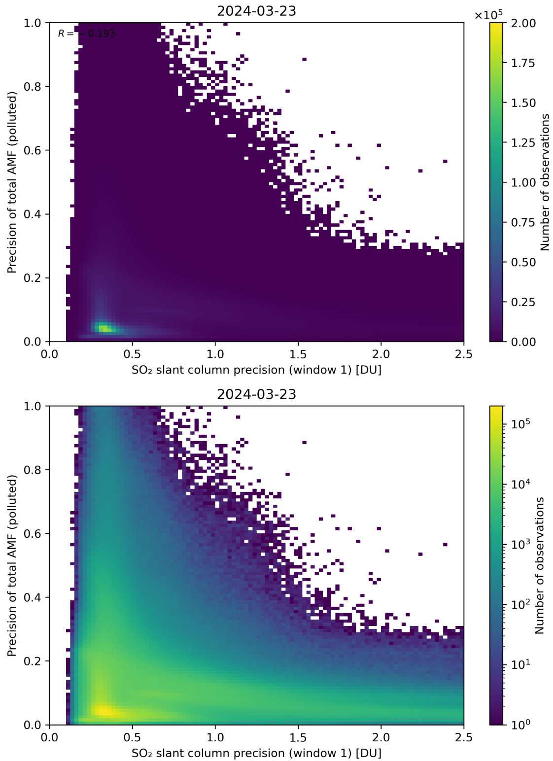
Figure 231: Scatter density plot of “SO 2 slant column precision (window 1)” against “Precision of total AMF (polluted)” for 2024-03-23 to 2024-03-24.
