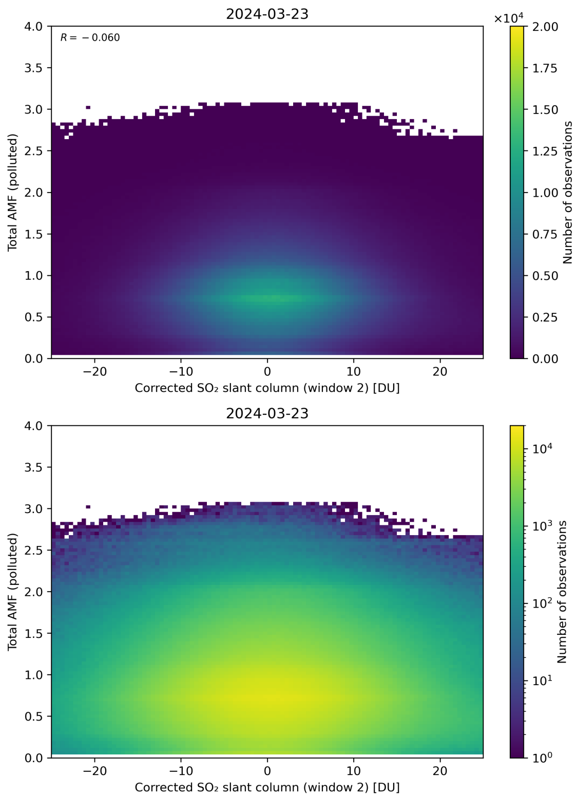
Figure 203: Scatter density plot of “Corrected SO 2 slant column (window 2)” against “Total AMF (polluted)” for 2024-03-23 to 2024-03-24.
