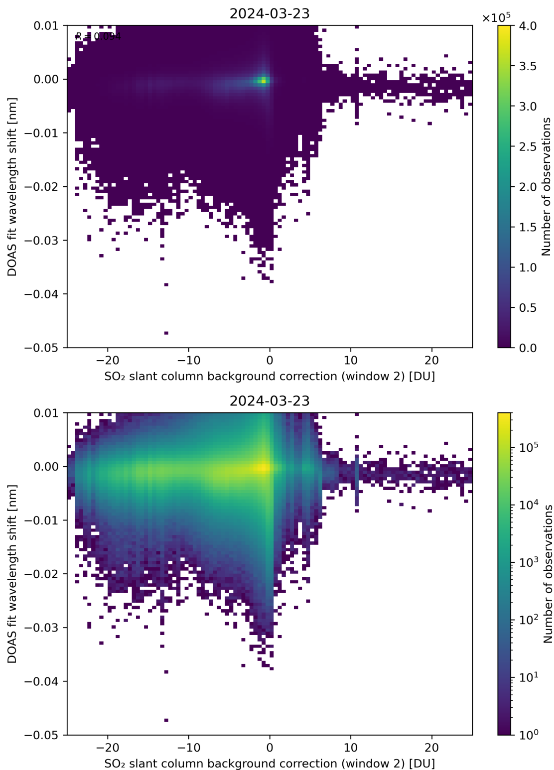
Figure 112: Scatter density plot of “SO 2 slant column background correction (window 2)” against “DOAS fit wavelength shift” for 2024-03-23 to 2024-03-24.
