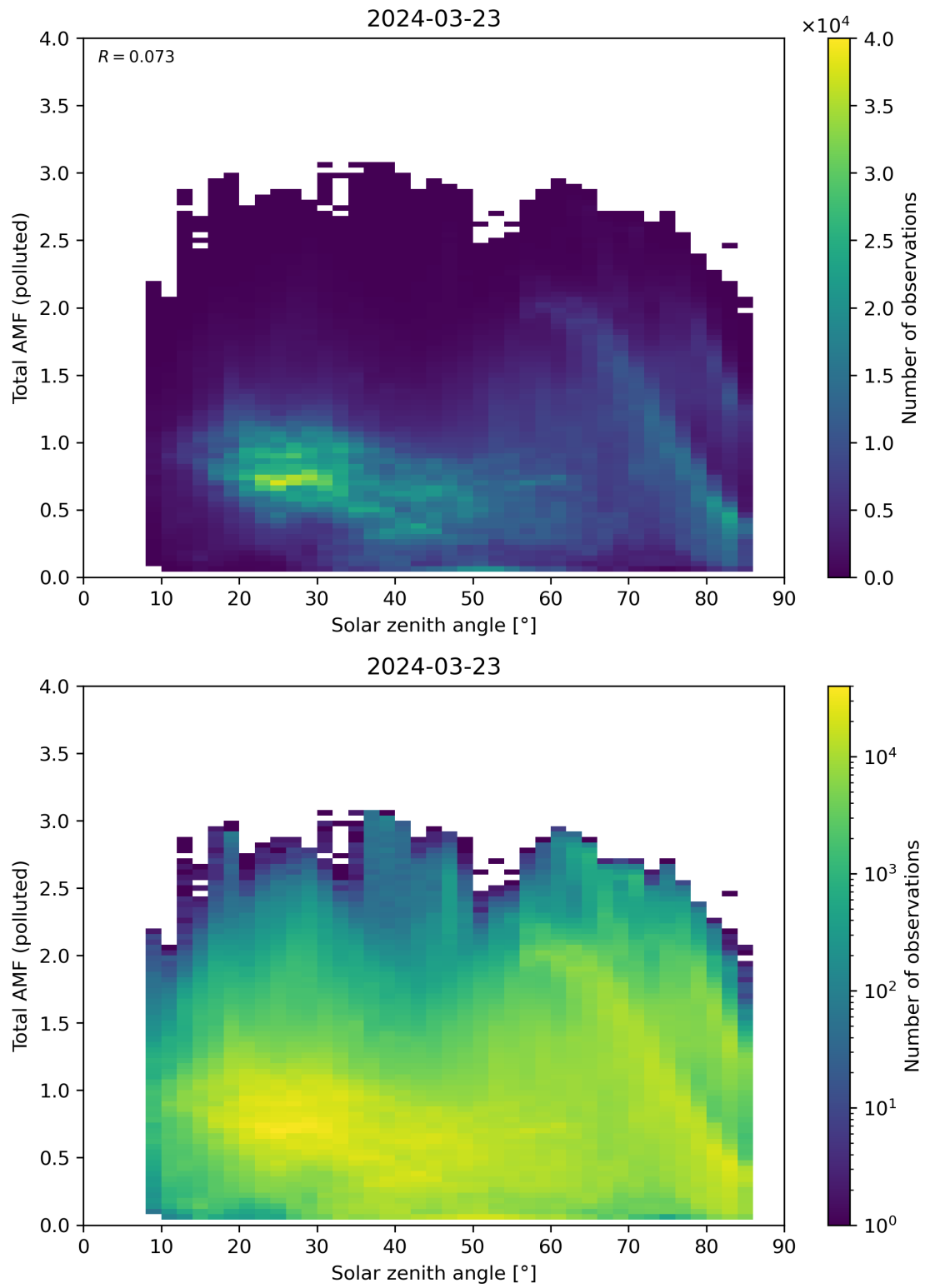
Figure 174: Scatter density plot of “Solar zenith angle” against “Total AMF (polluted)” for 2024-03-23 to 2024-03-24.
