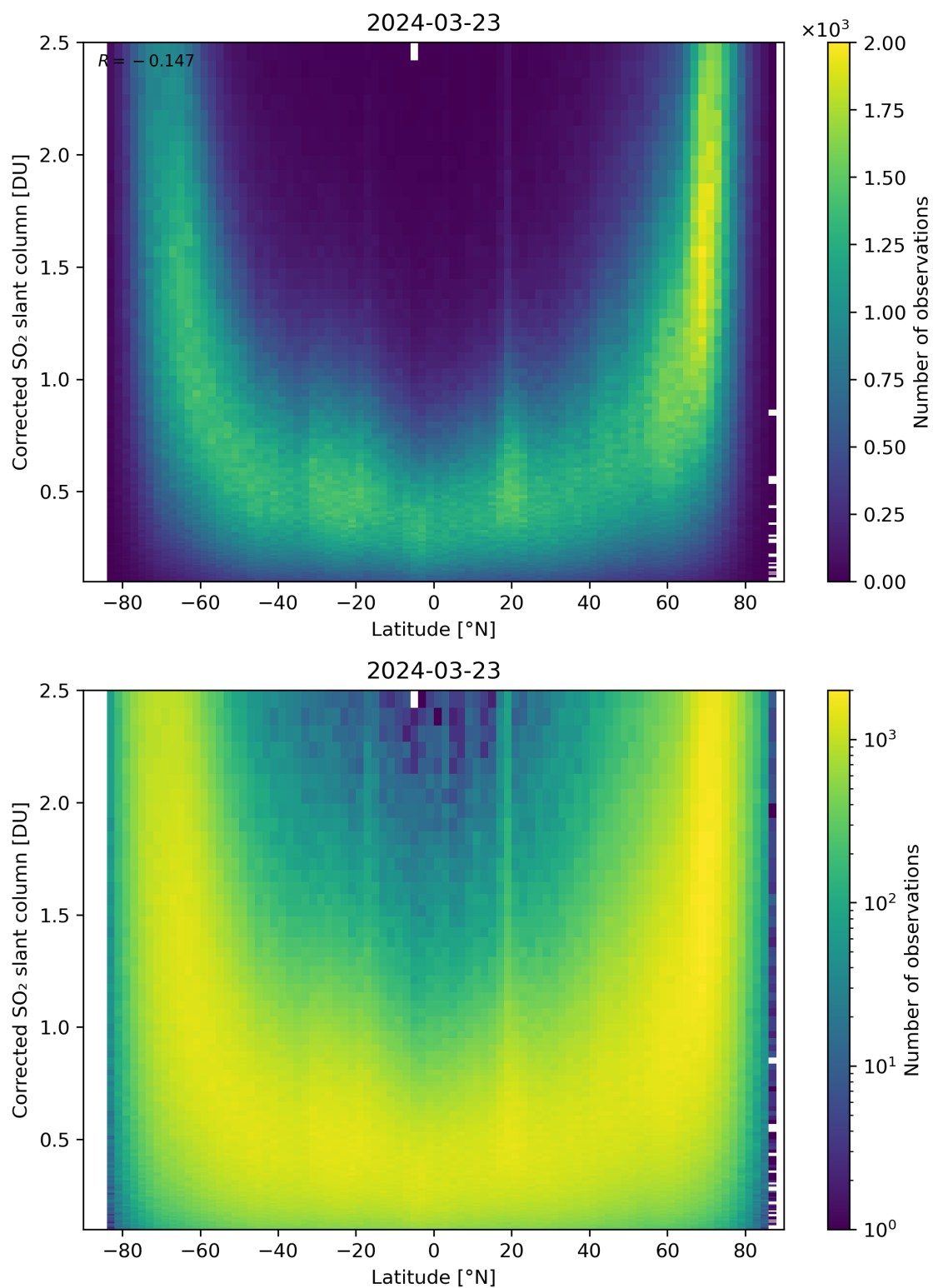
Figure 146: Scatter density plot of “Latitude” against “Corrected SO 2 slant column” for 2024-03-23 to 2024-03-24.
