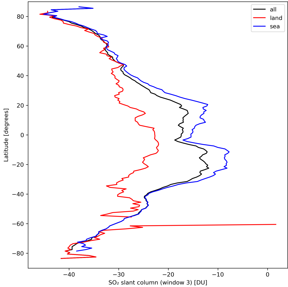
Figure 41: Zonal average of “SO 2 slant column (window 3)” for 2024-03-23 to 2024-03-24.
