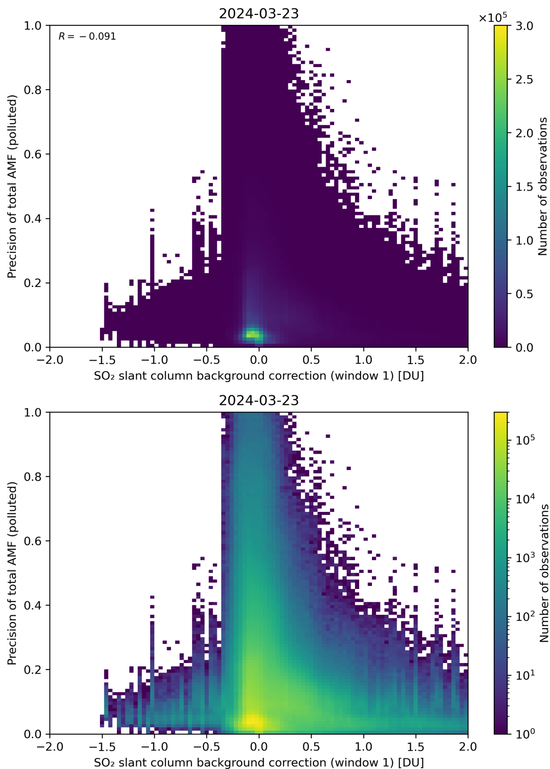
Figure 110: Scatter density plot of “SO 2 slant column background correction (window 1)” against “Precision of total AMF (polluted)” for 2024-03-23 to 2024-03-24.
