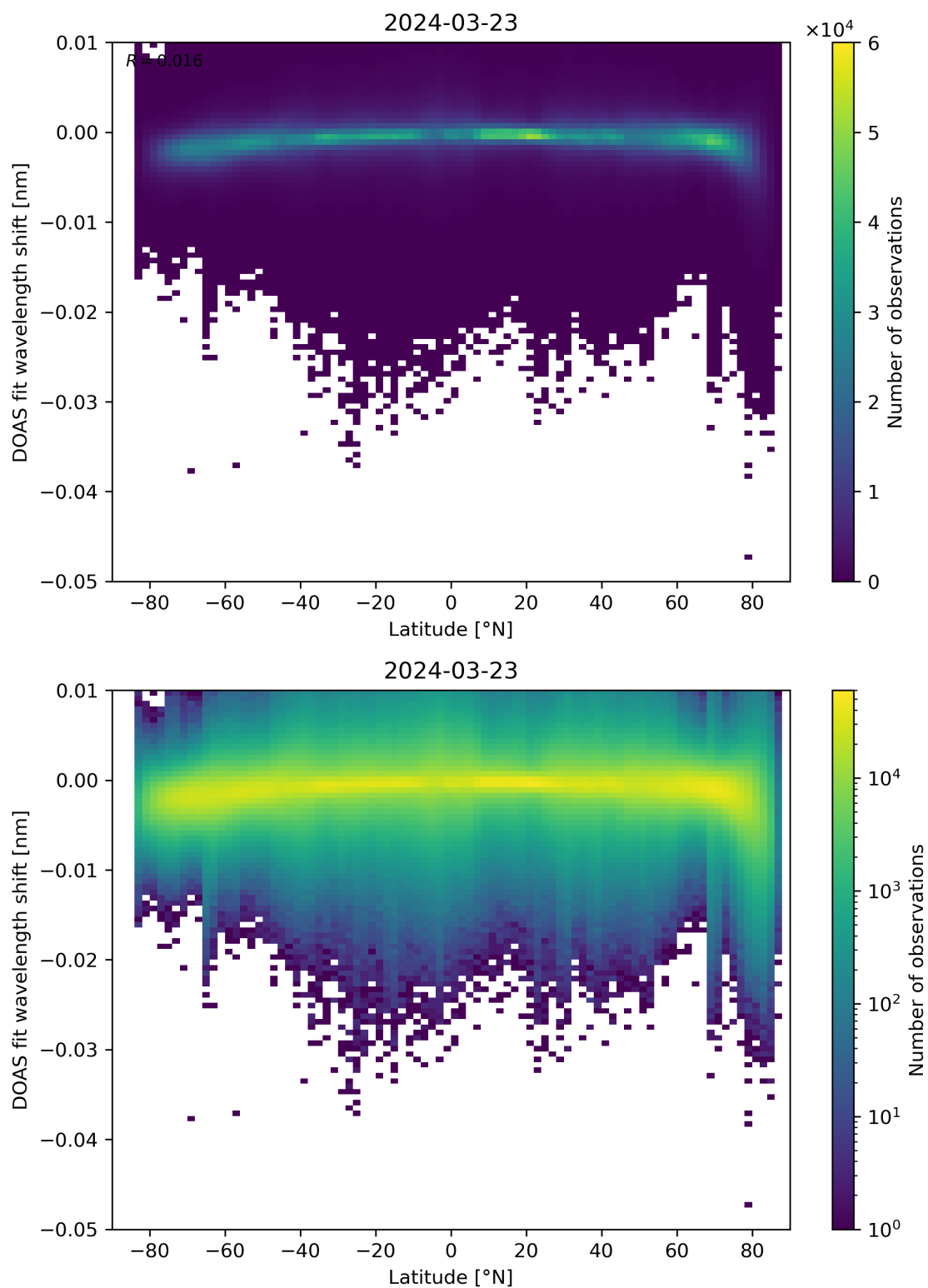
Figure 142: Scatter density plot of “Latitude” against “DOAS fit wavelength shift” for 2024-03-23 to 2024-03-24.
