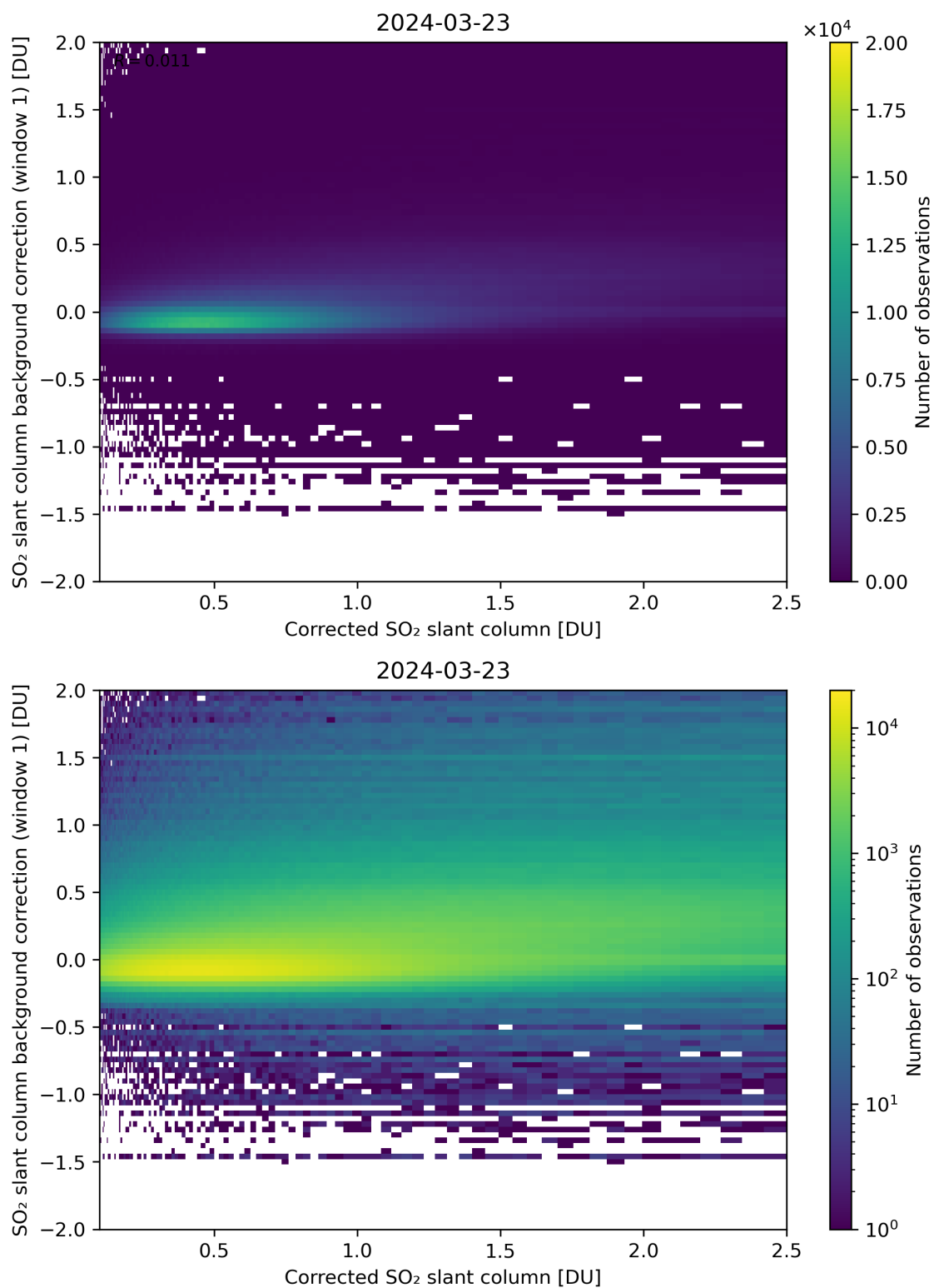
Figure 178: Scatter density plot of “Corrected SO 2 slant column” against “SO 2 slant column background correction (window 1)” for 2024-03-23 to 2024-03-24.
