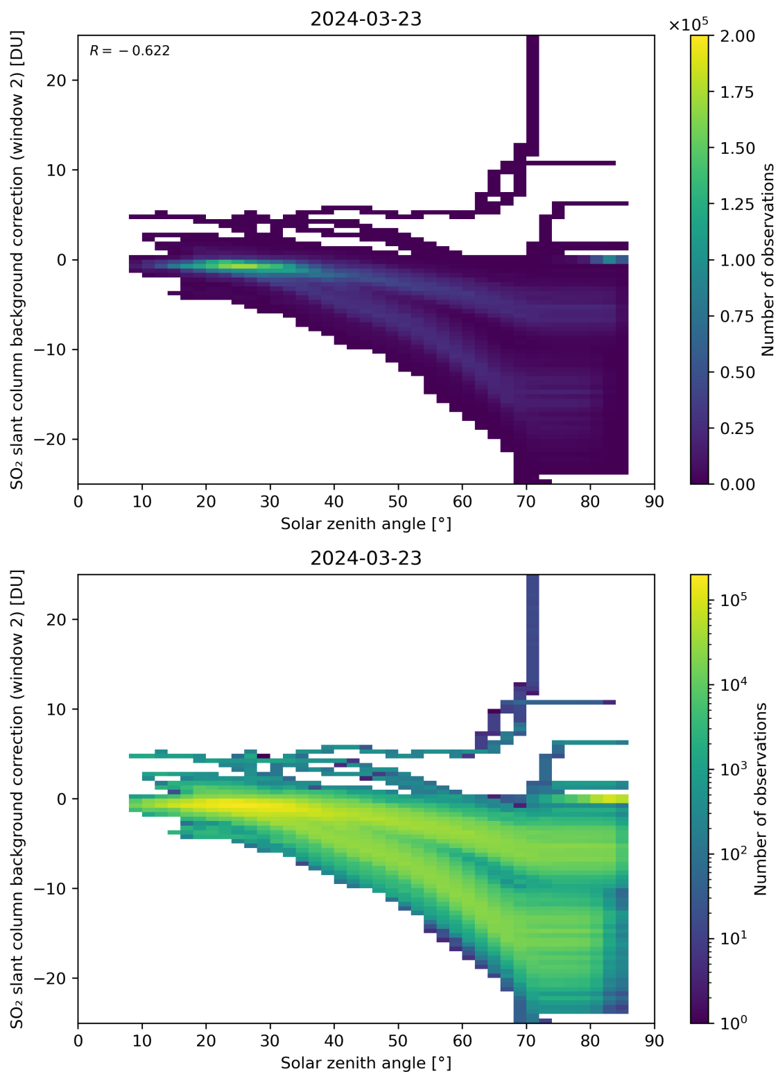
Figure 159: Scatter density plot of “Solar zenith angle” against “SO 2 slant column background correction (window 2)” for 2024-03-23 to 2024-03-24.
