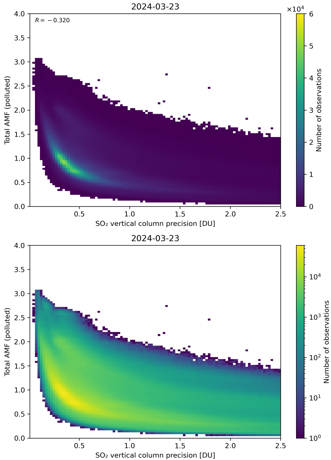
Figure 294: Scatter density plot of “SO 2 vertical column precision” against “Total AMF (polluted)” for 2024-03-23 to 2024-03-24.
