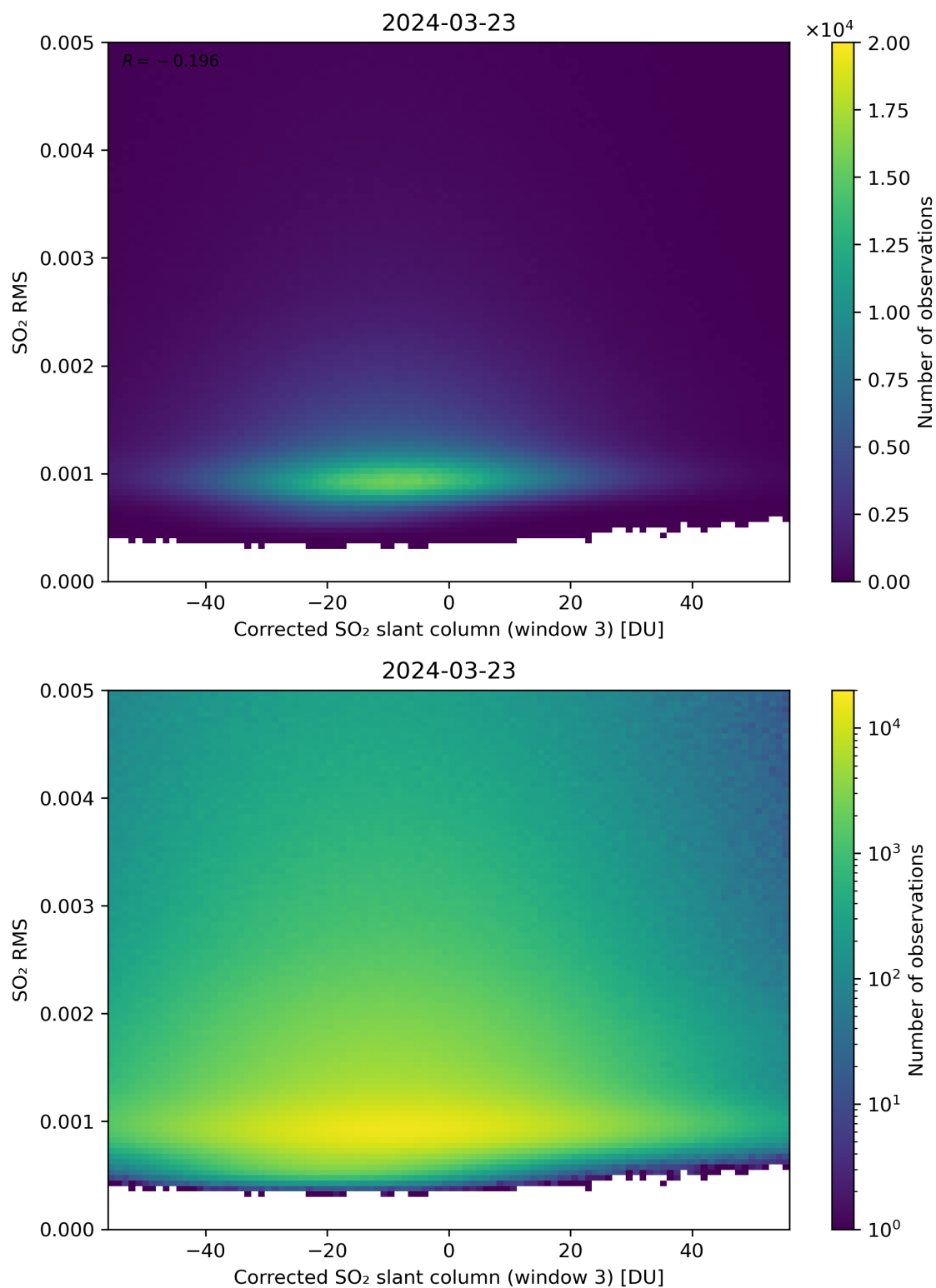
Figure 208: Scatter density plot of “Corrected SO 2 slant column (window 3)” against “SO 2 RMS” for 2024-03-23 to 2024-03-24.
