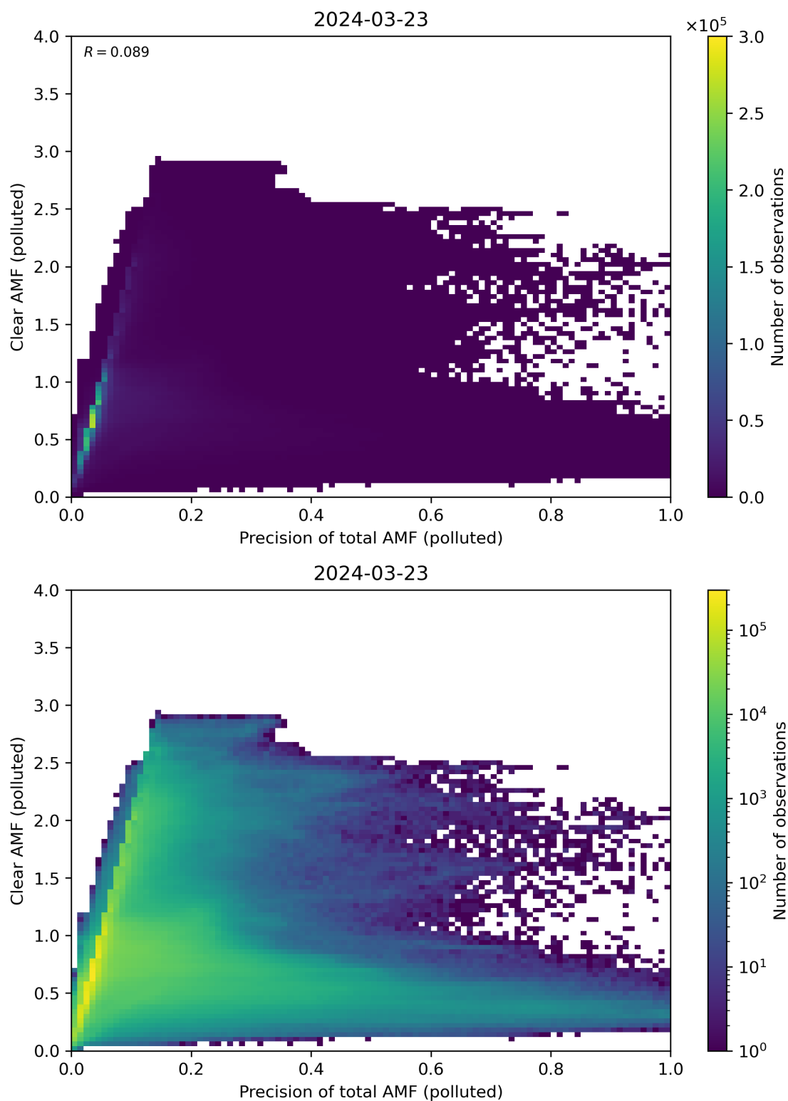
Figure 270: Scatter density plot of “Precision of total AMF (polluted)” against “Clear AMF (polluted)” for 2024-03-23 to 2024-03-24.
