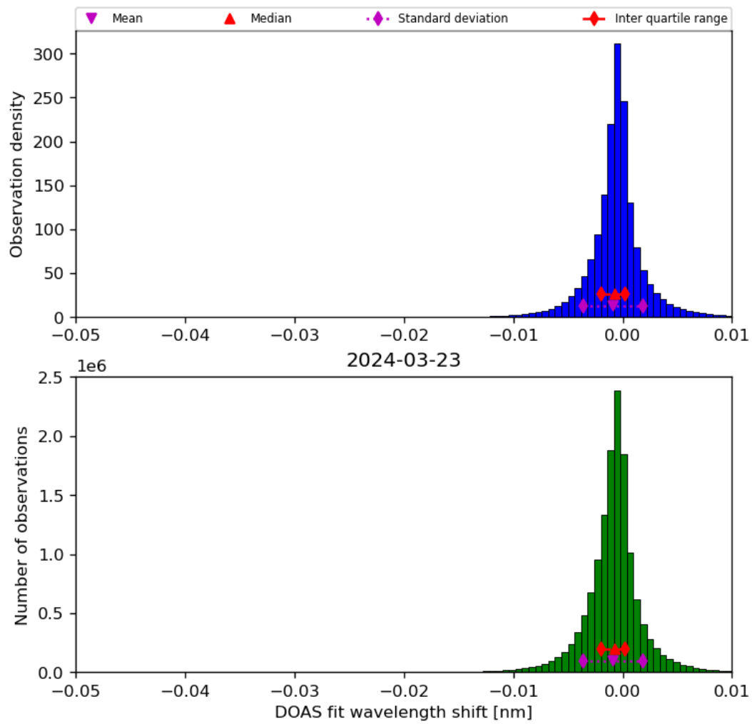
Figure 68: Histogram of “DOAS fit wavelength shift” for 2024-03-23 to 2024-03-24
