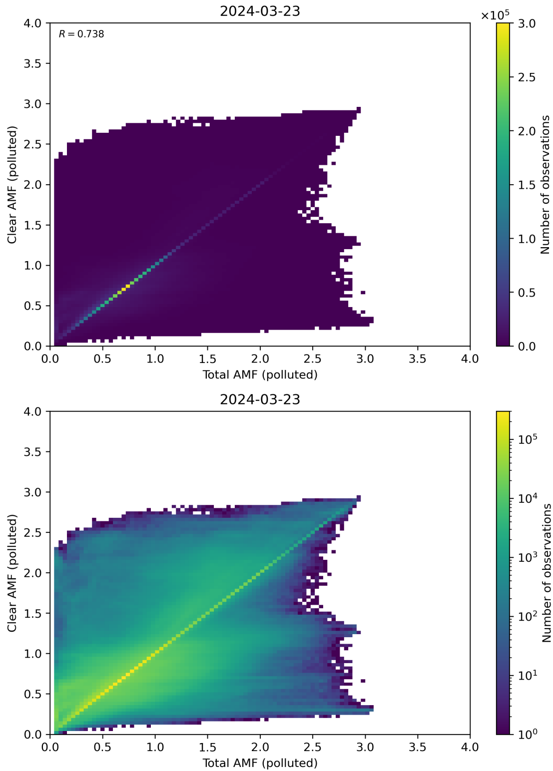
Figure 271: Scatter density plot of “Total AMF (polluted)” against “Clear AMF (polluted)” for 2024-03-23 to 2024-03-24.
