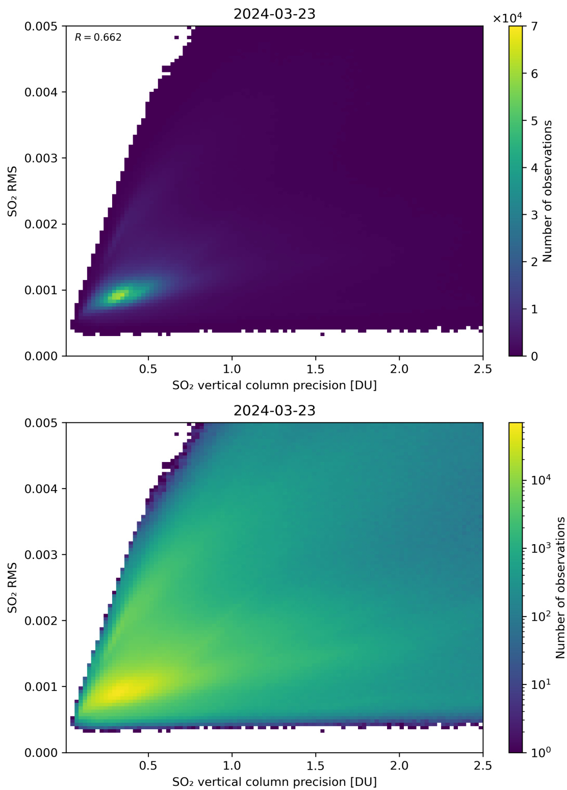
Figure 284: Scatter density plot of “SO 2 vertical column precision” against “SO 2 RMS” for 2024-03-23 to 2024-03-24.
