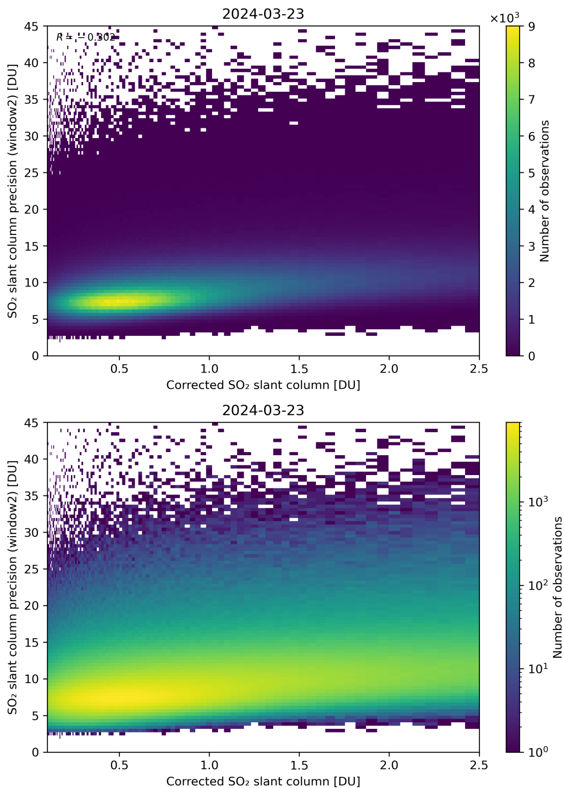
Figure 189: Scatter density plot of “Corrected SO 2 slant column” against “SO 2 slant column precision (window2)” for 2024-03-23 to 2024-03-24.
