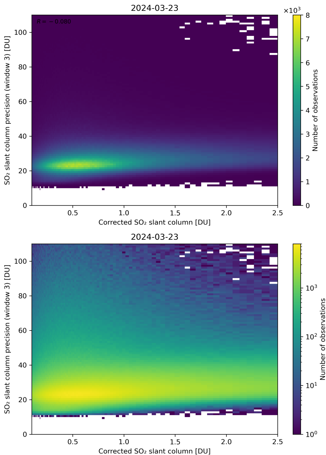
Figure 191: Scatter density plot of “Corrected SO 2 slant column” against “SO 2 slant column precision (window 3)” for 2024-03-23 to 2024-03-24.
