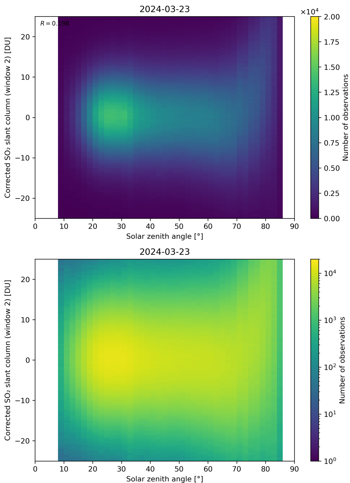
Figure 167: Scatter density plot of “Solar zenith angle” against “Corrected SO 2 slant column (window 2)” for 2024-03-23 to 2024-03-24.
