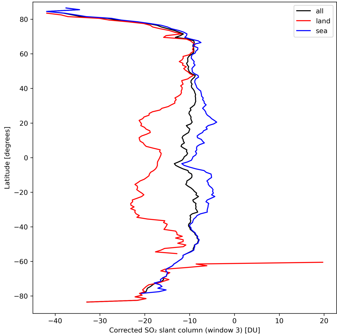
Figure 43: Zonal average of “Corrected SO 2 slant column (window 3)” for 2024-03-23 to 2024-03-24.
