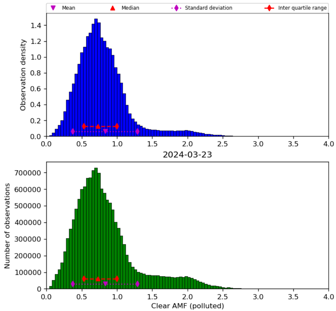
Figure 73: Histogram of “Clear AMF (polluted)” for 2024-03-23 to 2024-03-24
