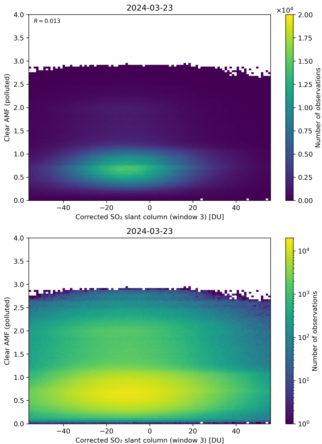
Figure 209: Scatter density plot of “Corrected SO 2 slant column (window 3)” against “Clear AMF (polluted)” for 2024-03-23 to 2024-03-24.
