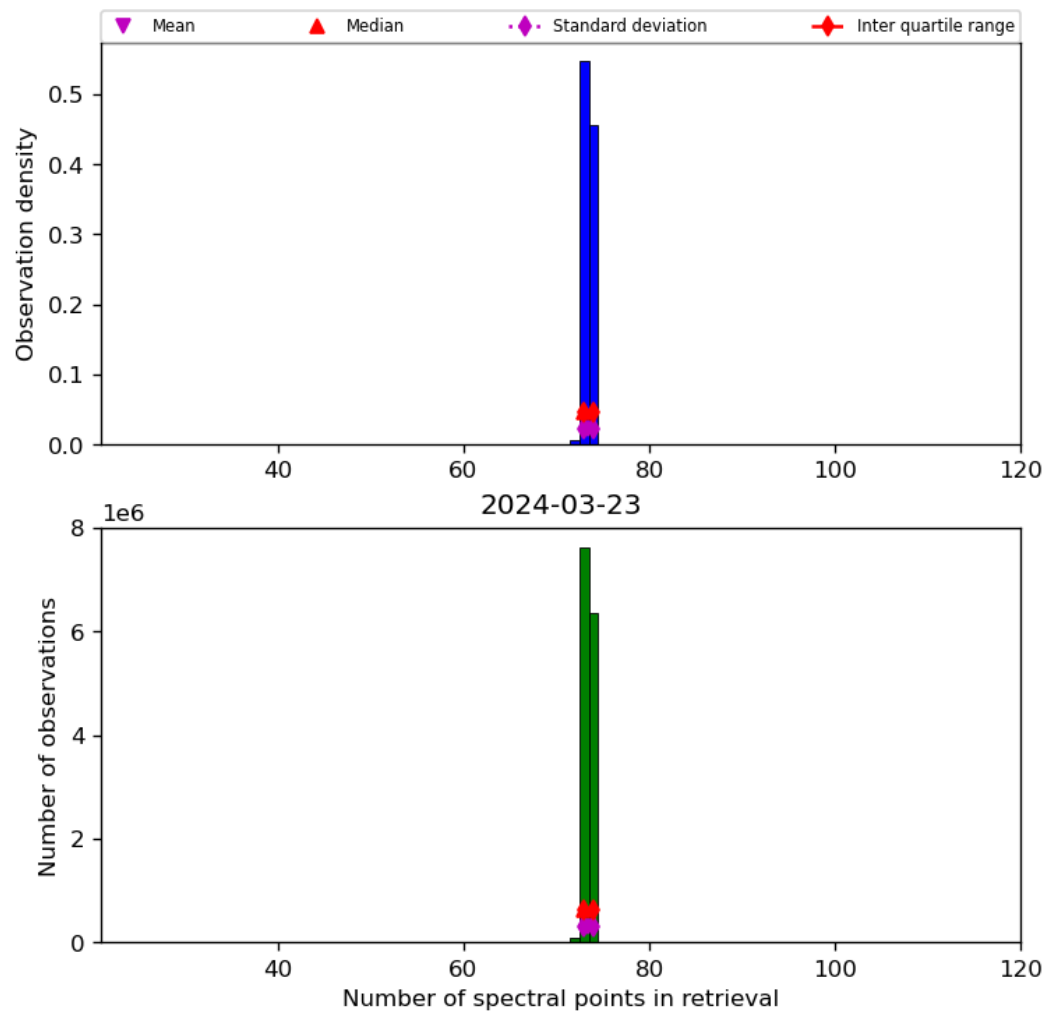
Figure 74: Histogram of “Number of spectral points in retrieval” for 2024-03-23 to 2024-03-24
