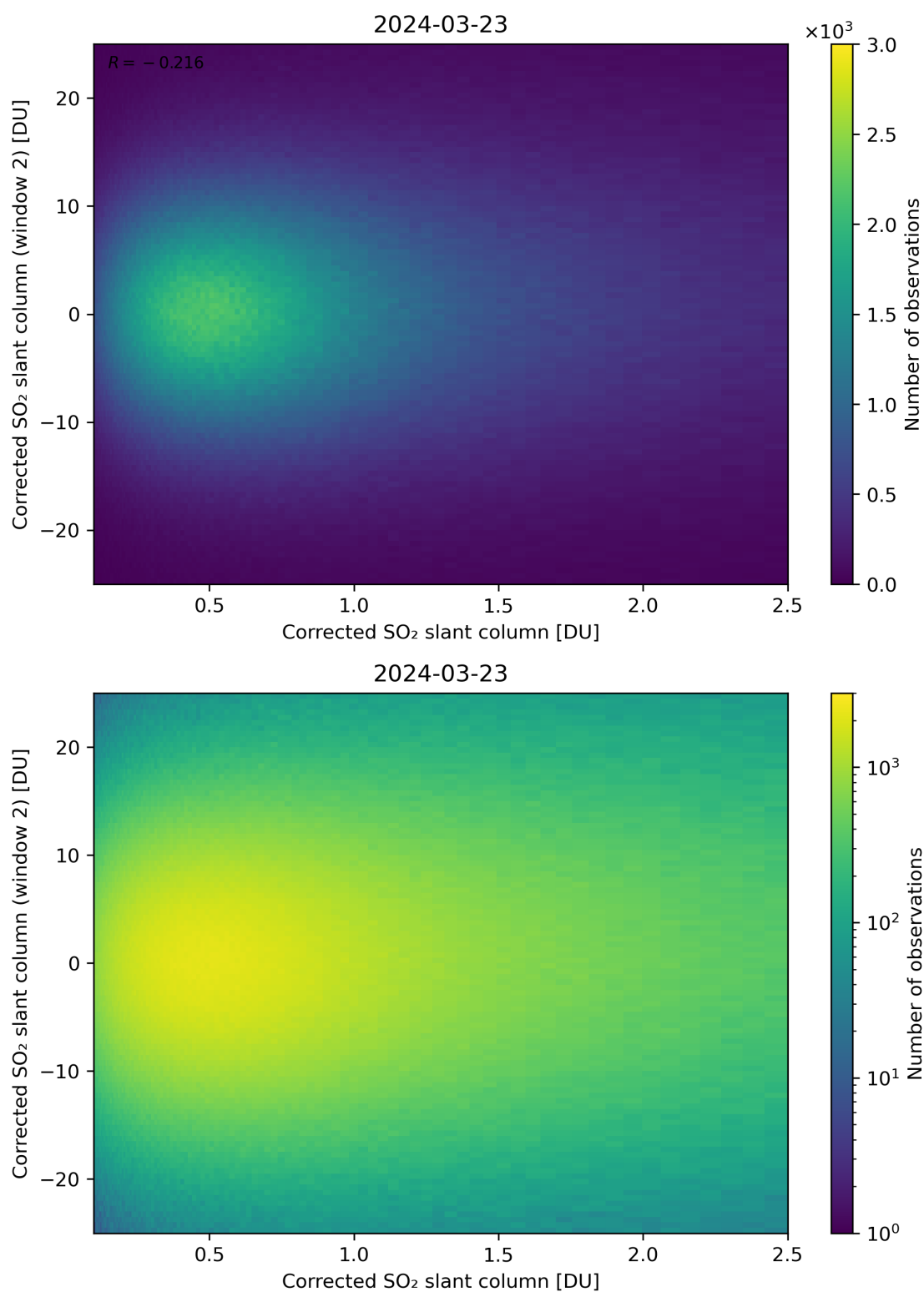
Figure 185: Scatter density plot of “Corrected SO 2 slant column” against “Corrected SO 2 slant column (window 2)” for 2024-03-23 to 2024-03-24.
