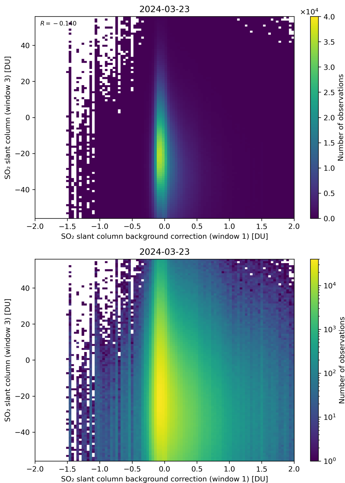
Figure 107: Scatter density plot of “SO 2 slant column background correction (window 1)” against “SO 2 slant column (window 3)” for 2024-03-23 to 2024-03-24.
