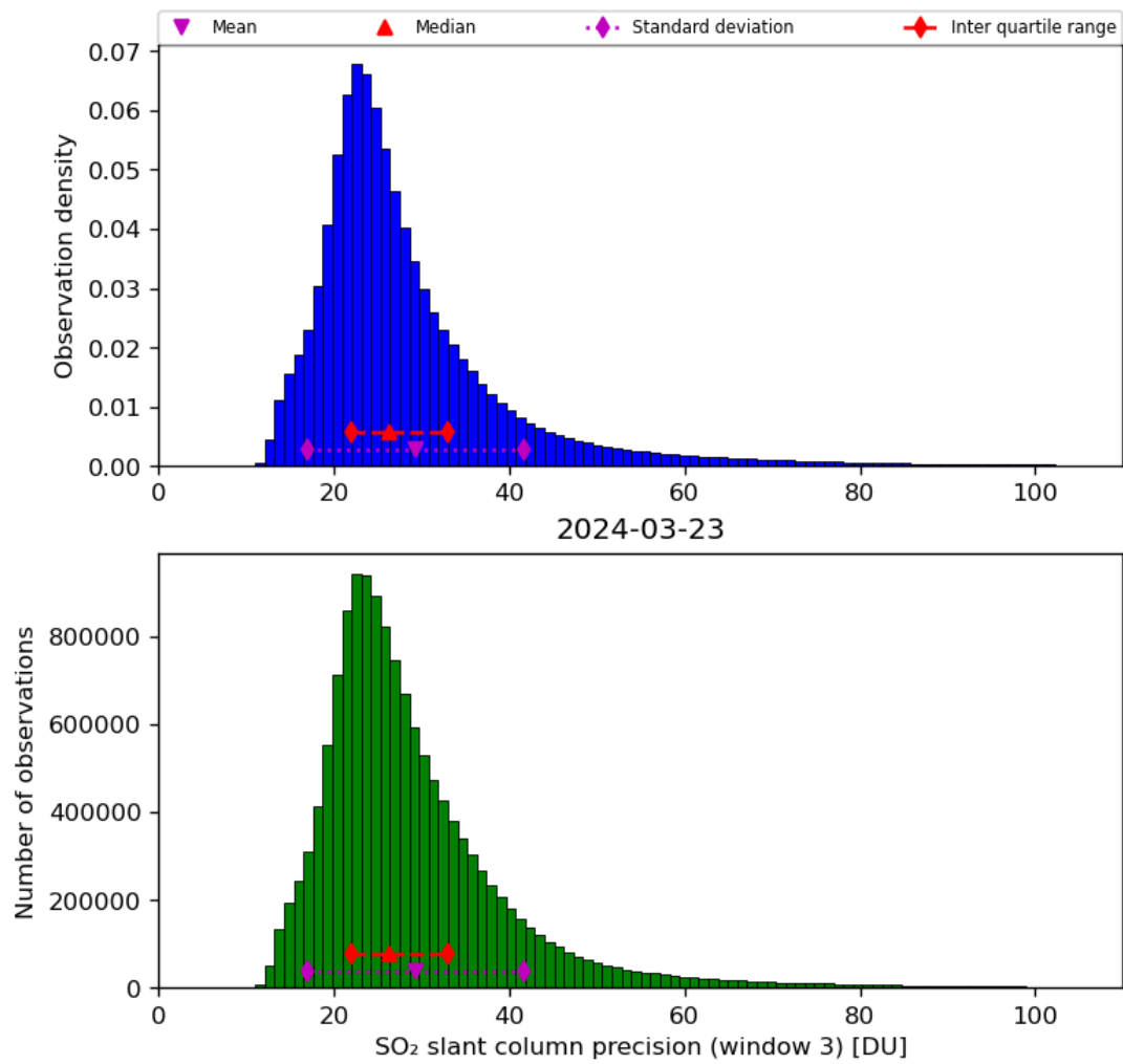
Figure 65: Histogram of “SO 2 slant column precision (window 3)” for 2024-03-23 to 2024-03-24
