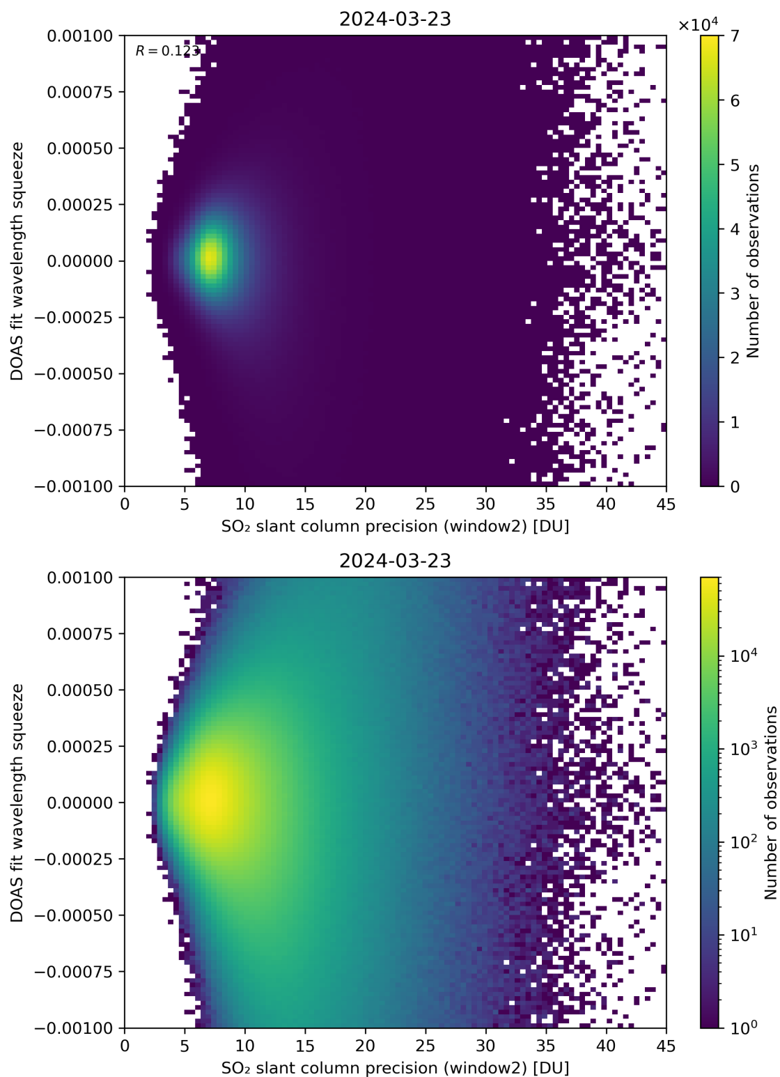
Figure 244: Scatter density plot of “SO 2 slant column precision (window2)” against “DOAS fit wavelength squeeze” for 2024-03-23 to 2024-03-24.
