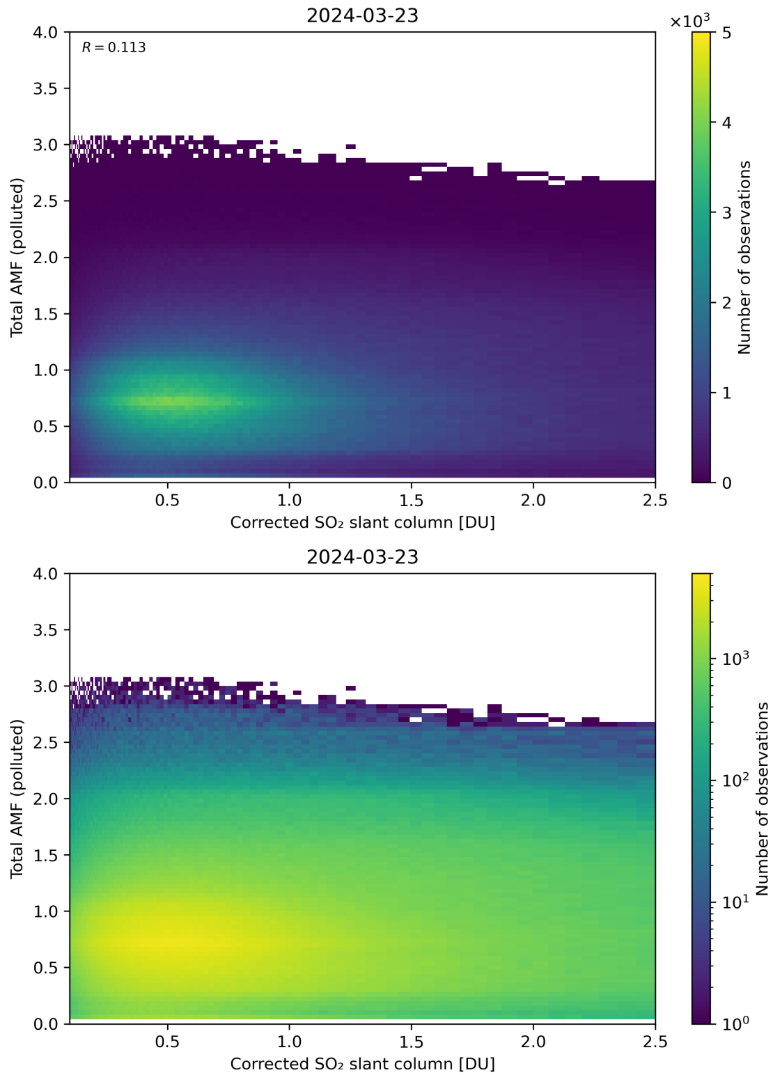
Figure 192: Scatter density plot of “Corrected SO 2 slant column” against “Total AMF (polluted)” for 2024-03-23 to 2024-03-24.
