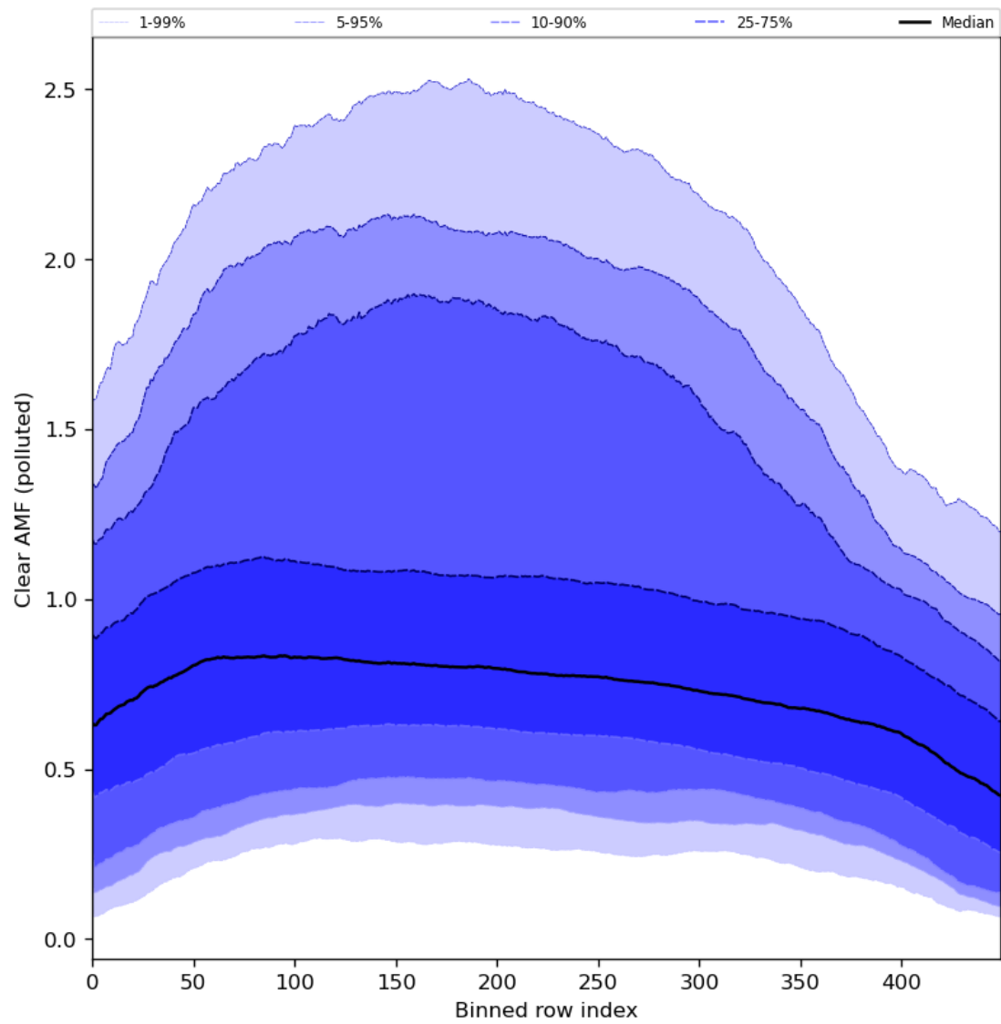
Figure 96: Along track statistics of “Clear AMF (polluted)” for 2024-03-23 to 2024-03-24
