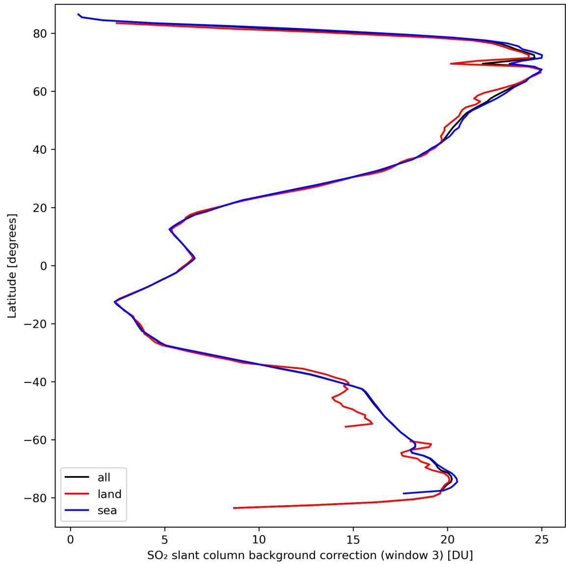
Figure 44: Zonal average of “SO 2 slant column background correction (window 3)” for 2024-03-23 to 2024-03-24.
