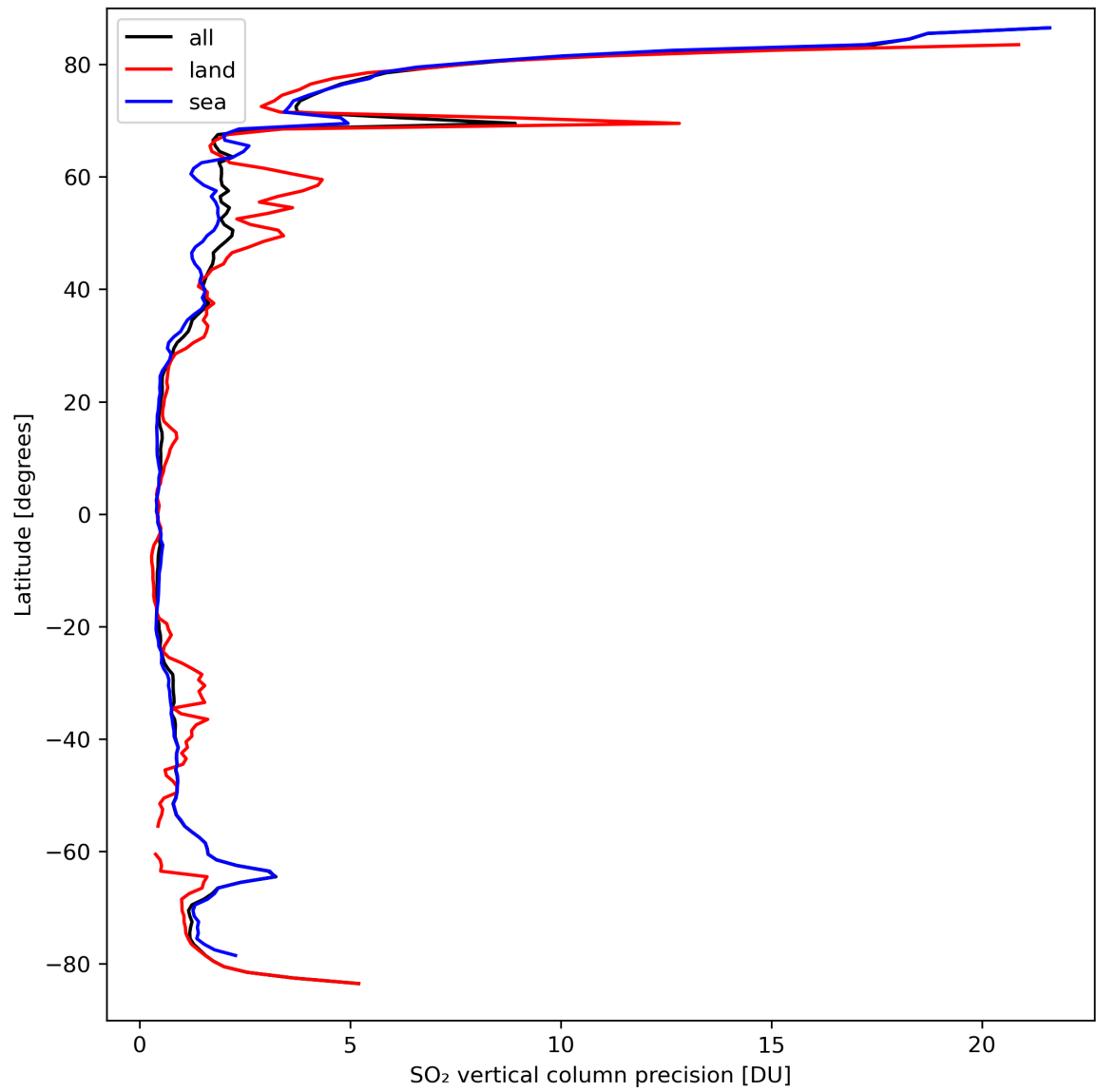
Figure 31: Zonal average of “SO 2 vertical column precision” for 2024-03-23 to 2024-03-24.
