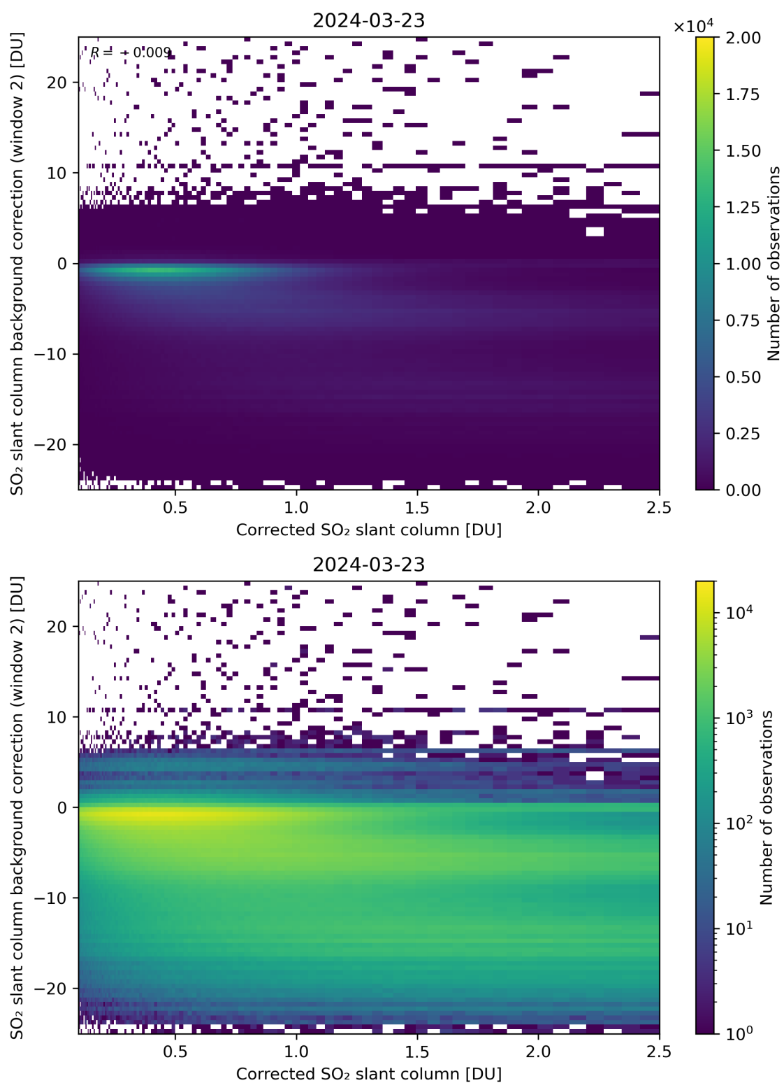
Figure 179: Scatter density plot of “Corrected SO 2 slant column” against “SO 2 slant column background correction (window 2)” for 2024-03-23 to 2024-03-24.
