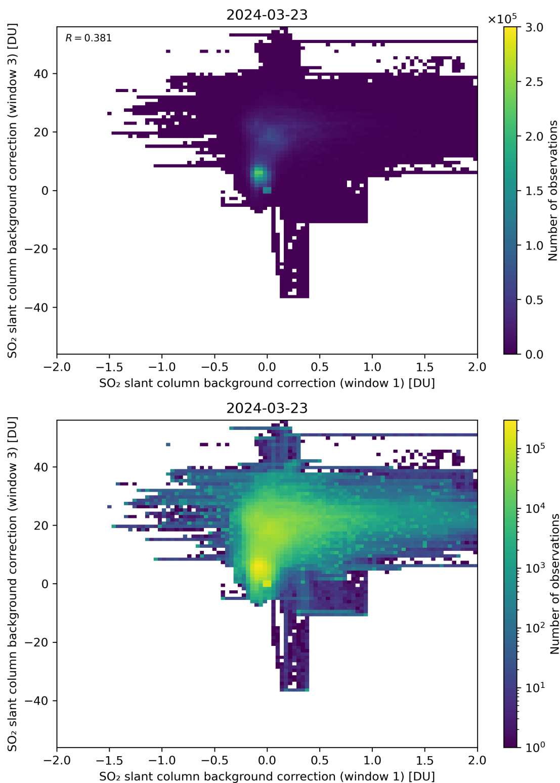
Figure 99: Scatter density plot of “SO 2 slant column background correction (window 1)” against “SO 2 slant column background correction (window 3)” for 2024-03-23 to 2024-03-24.
