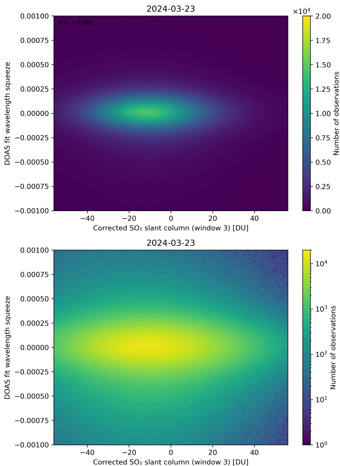
Figure 207: Scatter density plot of “Corrected SO 2 slant column (window 3)” against “DOAS fit wavelength squeeze” for 2024-03-23 to 2024-03-24.
