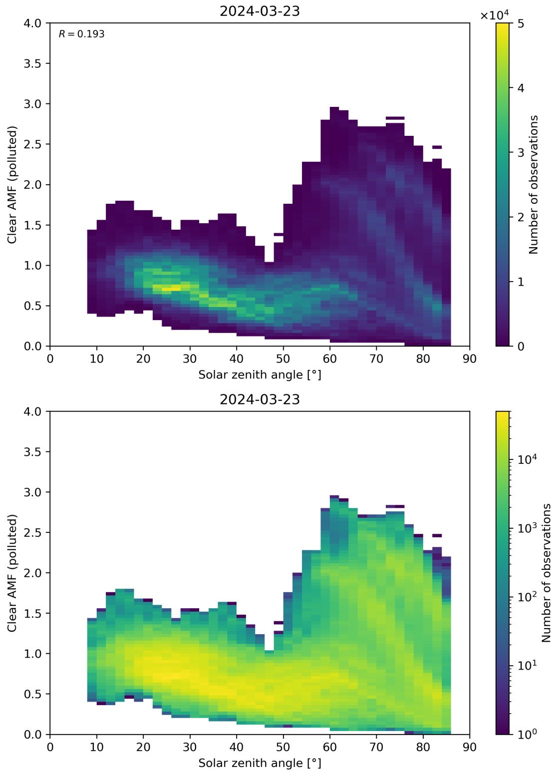
Figure 165: Scatter density plot of “Solar zenith angle” against “Clear AMF (polluted)” for 2024-03-23 to 2024-03-24.
