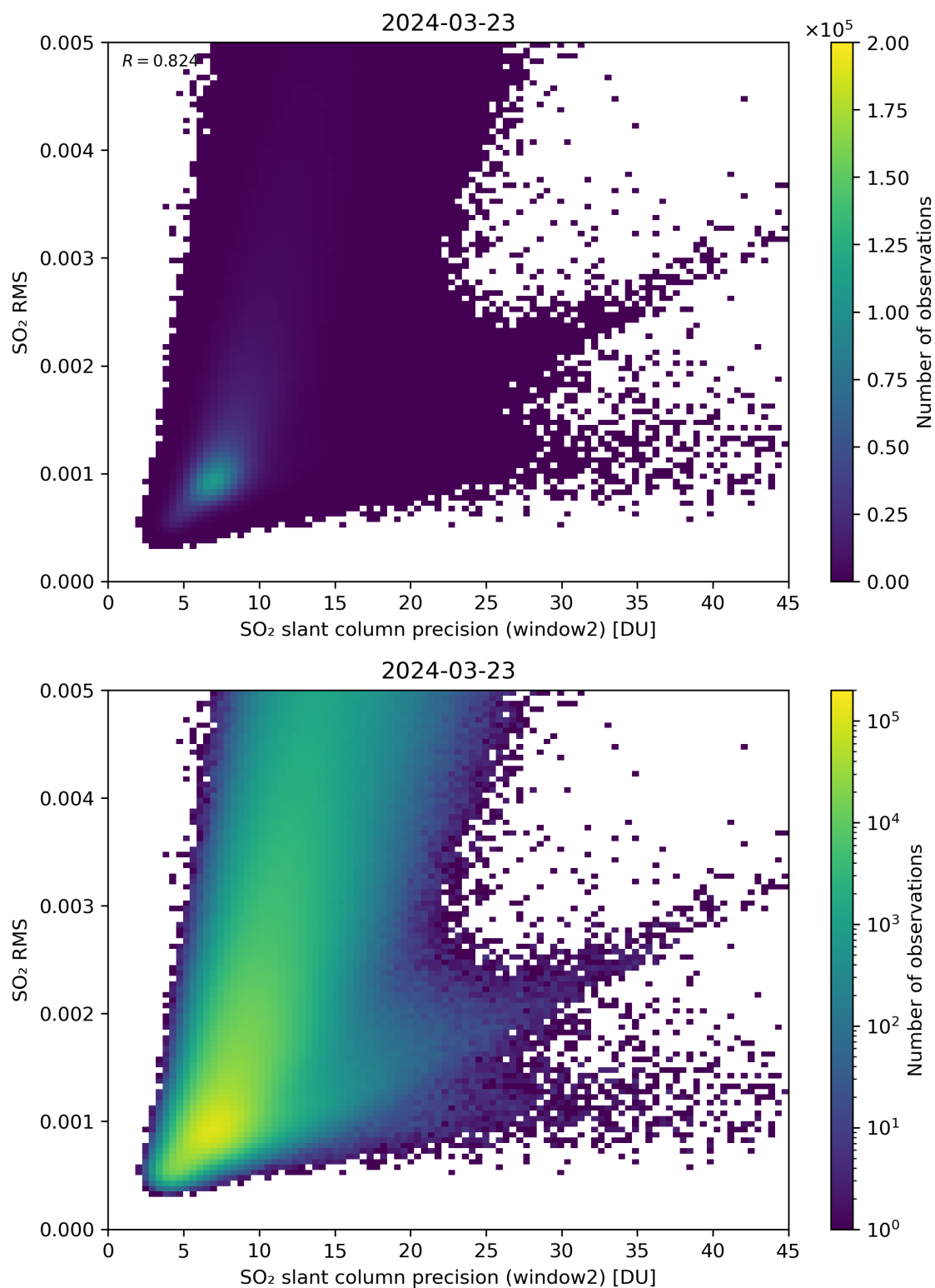
Figure 245: Scatter density plot of “SO 2 slant column precision (window2)” against “SO 2 RMS” for 2024-03-23 to 2024-03-24.
