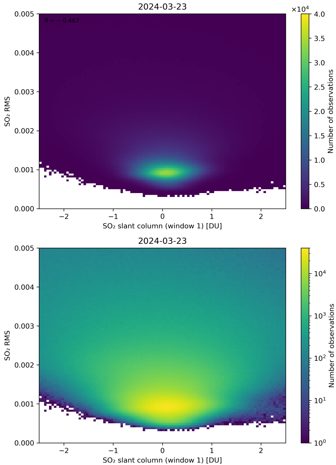
Figure 217: Scatter density plot of “SO 2 slant column (window 1)” against “SO 2 RMS” for 2024-03-23 to 2024-03-24.
