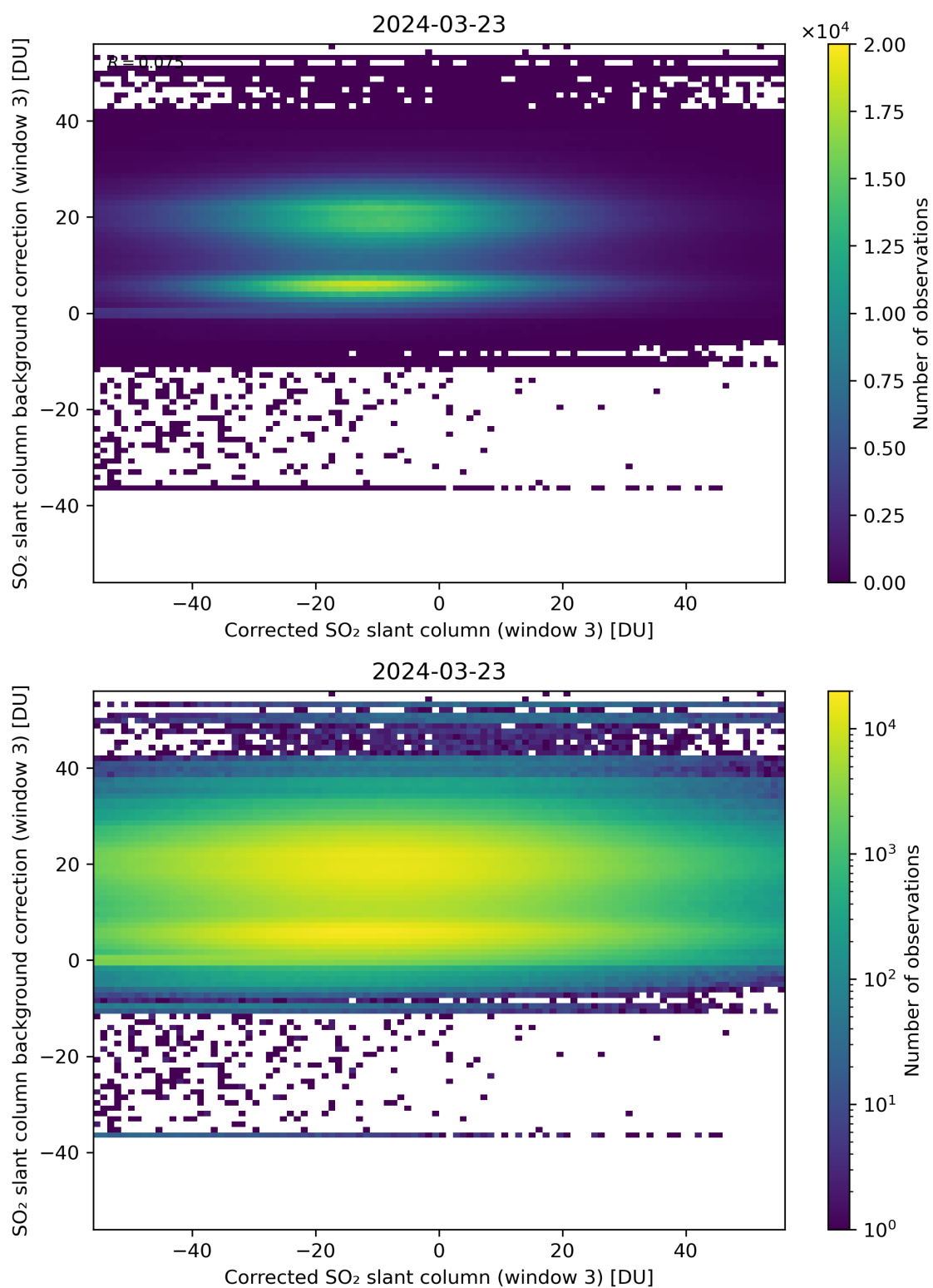
Figure 205: Scatter density plot of “Corrected SO 2 slant column (window 3)” against “SO 2 slant column background correction (window 3)” for 2024-03-23 to 2024-03-24.
