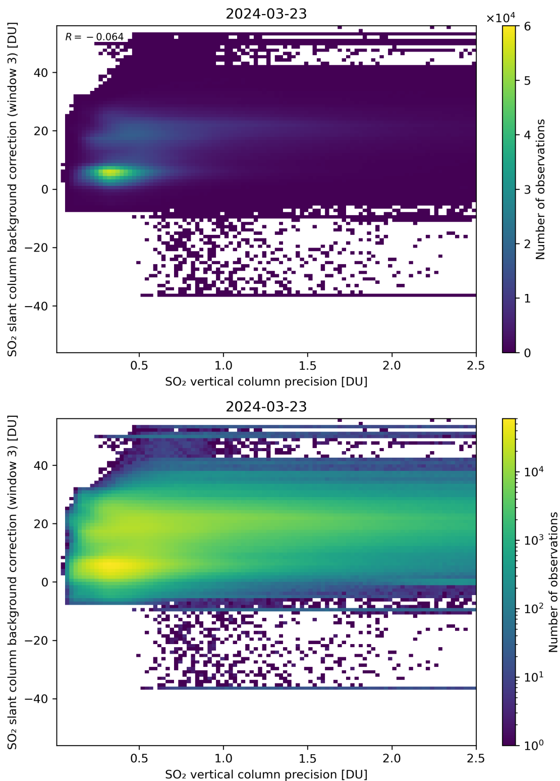
Figure 281: Scatter density plot of “SO 2 vertical column precision” against “SO 2 slant column background correction (window 3)” for 2024-03-23 to 2024-03-24.
