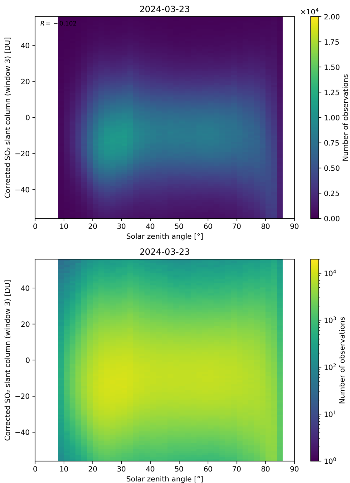
Figure 168: Scatter density plot of “Solar zenith angle” against “Corrected SO 2 slant column (window 3)” for 2024-03-23 to 2024-03-24.
