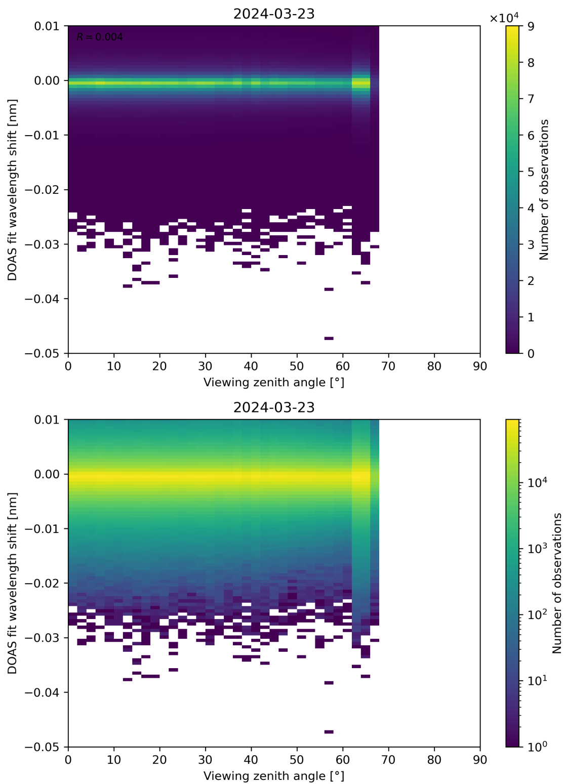
Figure 311: Scatter density plot of “Viewing zenith angle” against “DOAS fit wavelength shift” for 2024-03-23 to 2024-03-24.
