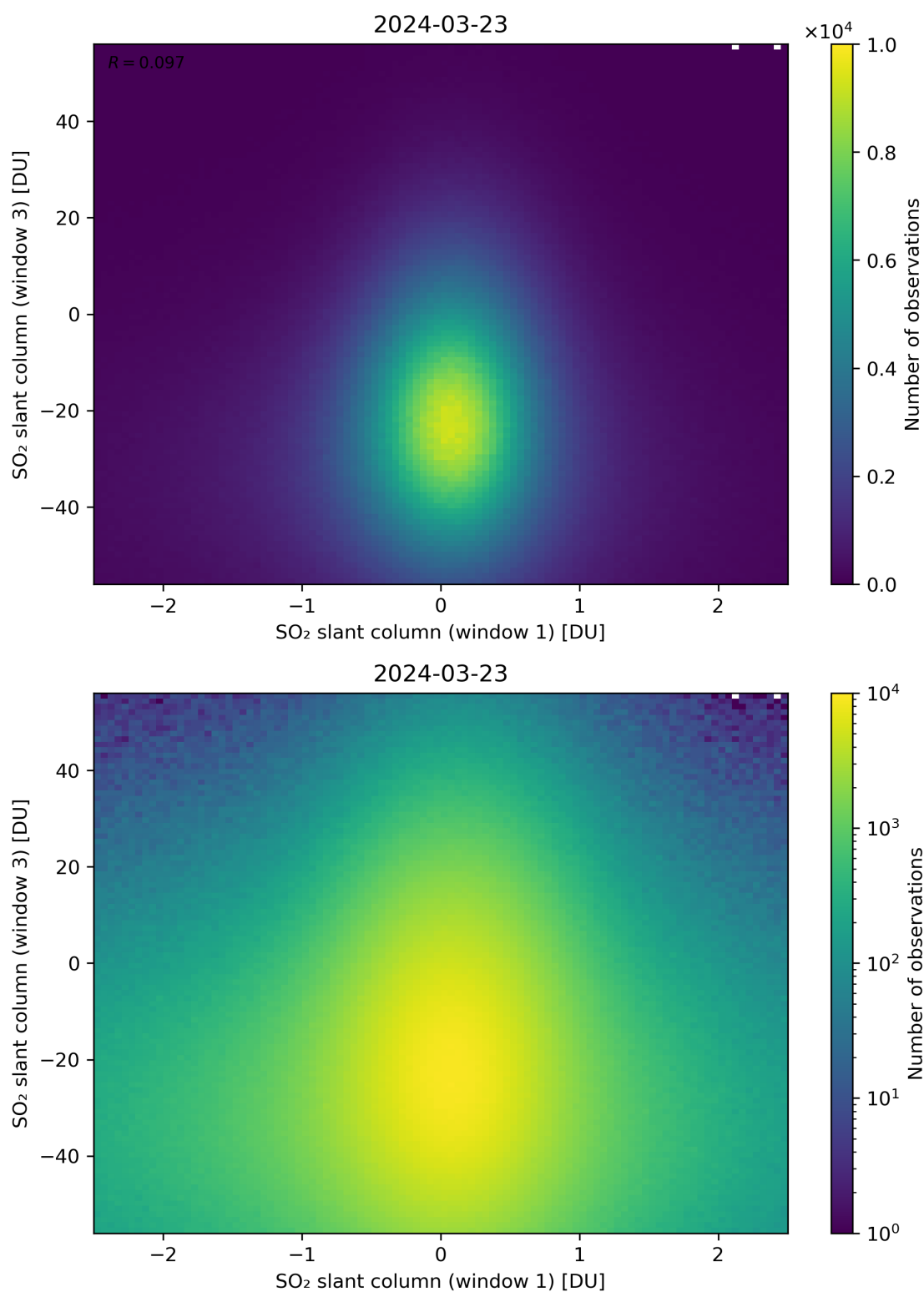
Figure 237: Scatter density plot of “SO 2 slant column (window 1)” against “SO 2 slant column (window 3)” for 2024-03-23 to 2024-03-24.
