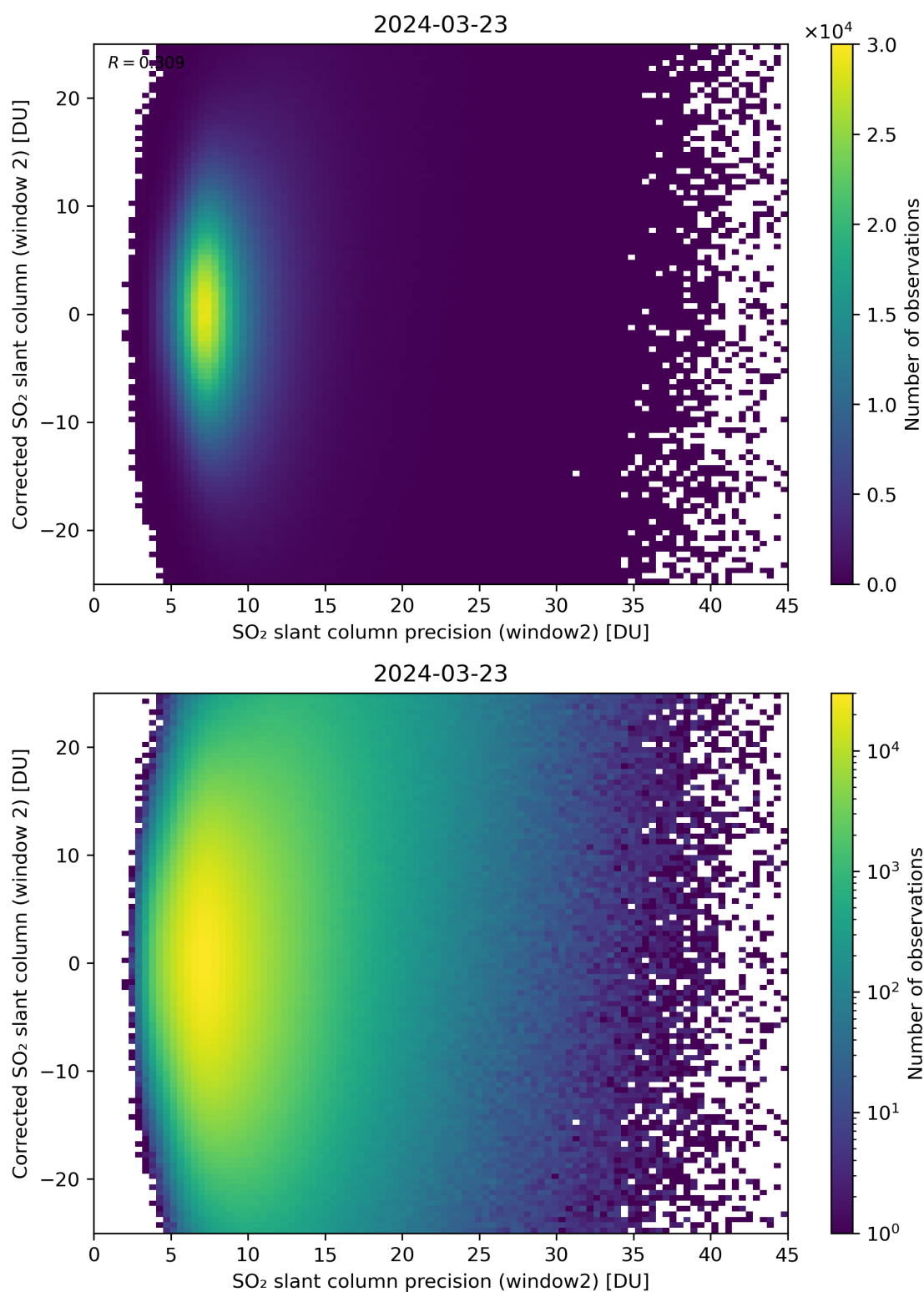
Figure 247: Scatter density plot of “SO 2 slant column precision (window2)” against “Corrected SO 2 slant column (window 2)” for 2024-03-23 to 2024-03-24.
