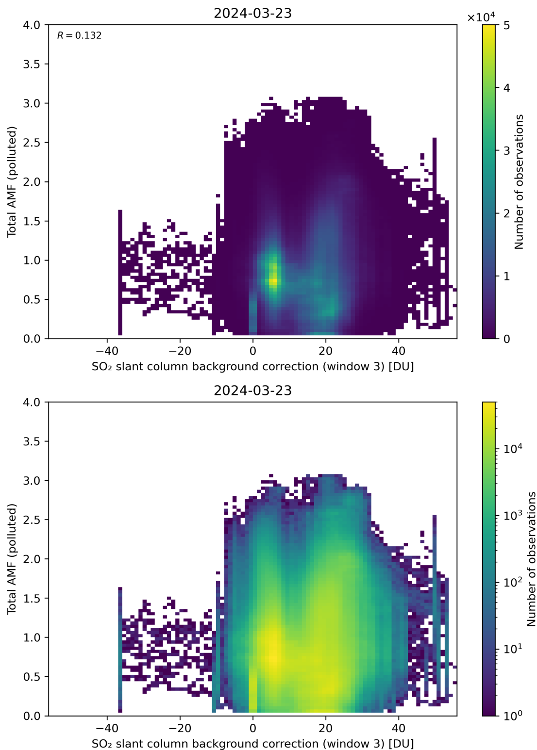
Figure 125: Scatter density plot of “SO 2 slant column background correction (window 3)” against “Total AMF (polluted)” for 2024-03-23 to 2024-03-24.
