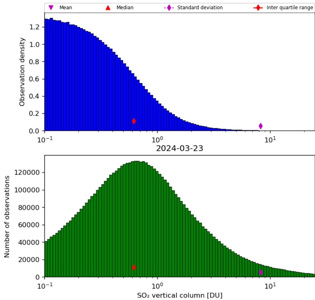
Figure 53: Histogram of “SO 2 vertical column” for 2024-03-23 to 2024-03-24
