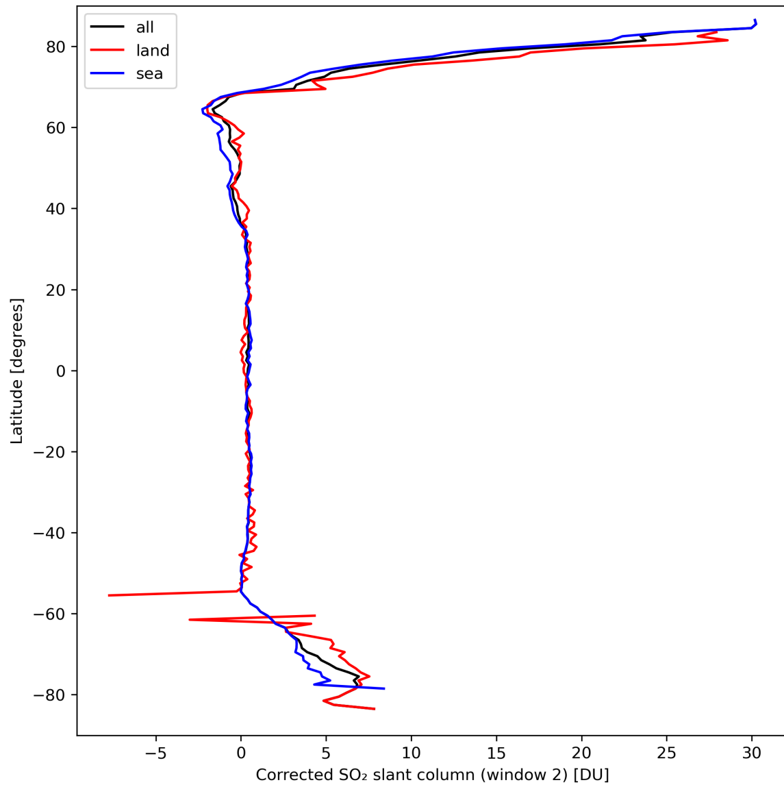
Figure 39: Zonal average of “Corrected SO 2 slant column (window 2)” for 2024-03-23 to 2024-03-24.
