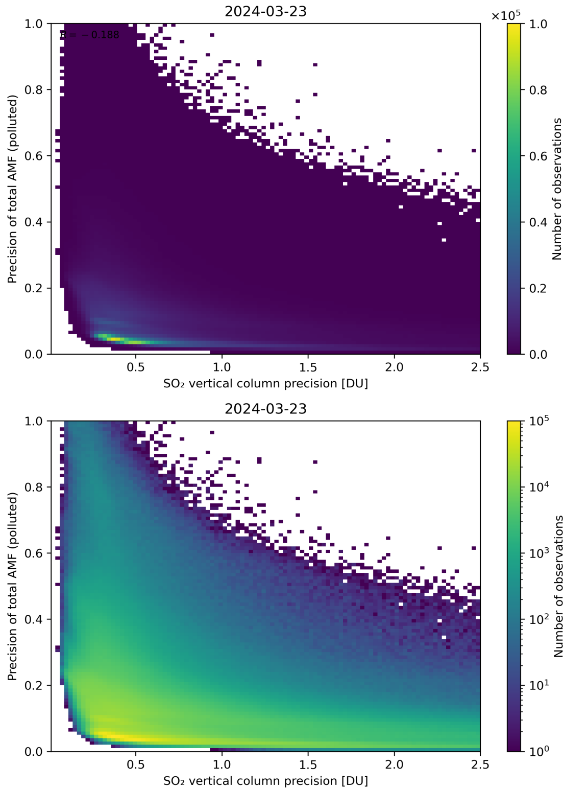
Figure 295: Scatter density plot of “SO 2 vertical column precision” against “Precision of total AMF (polluted)” for 2024-03-23 to 2024-03-24.
