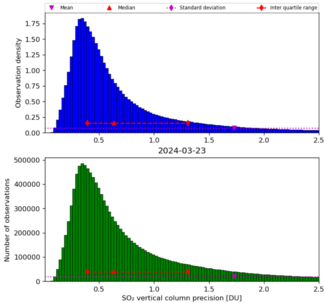
Figure 54: Histogram of “SO 2 vertical column precision” for 2024-03-23 to 2024-03-24
