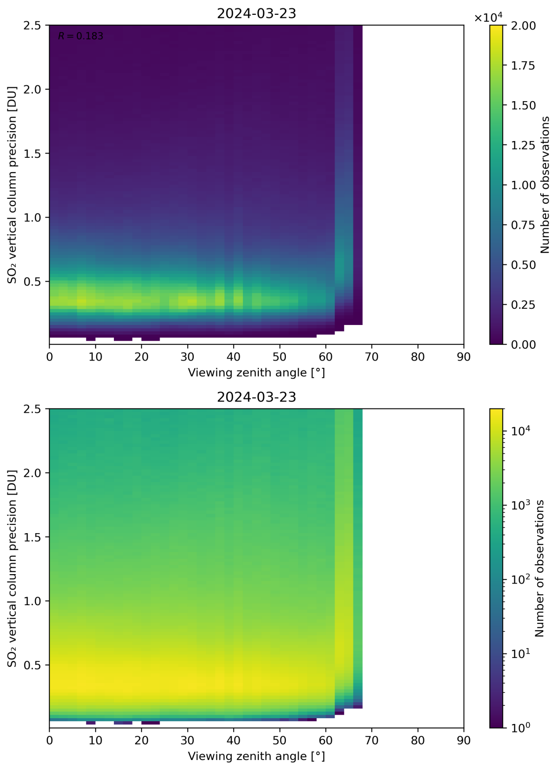
Figure 328: Scatter density plot of “Viewing zenith angle” against “SO 2 vertical column precision” for 2024-03-23 to 2024-03-24.
