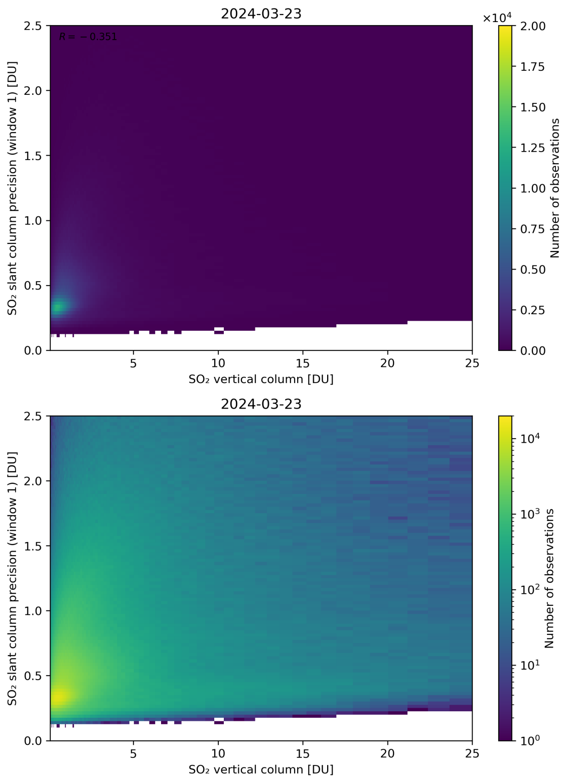
Figure 301: Scatter density plot of “SO 2 vertical column” against “SO 2 slant column precision (window 1)” for 2024-03-23 to 2024-03-24.
