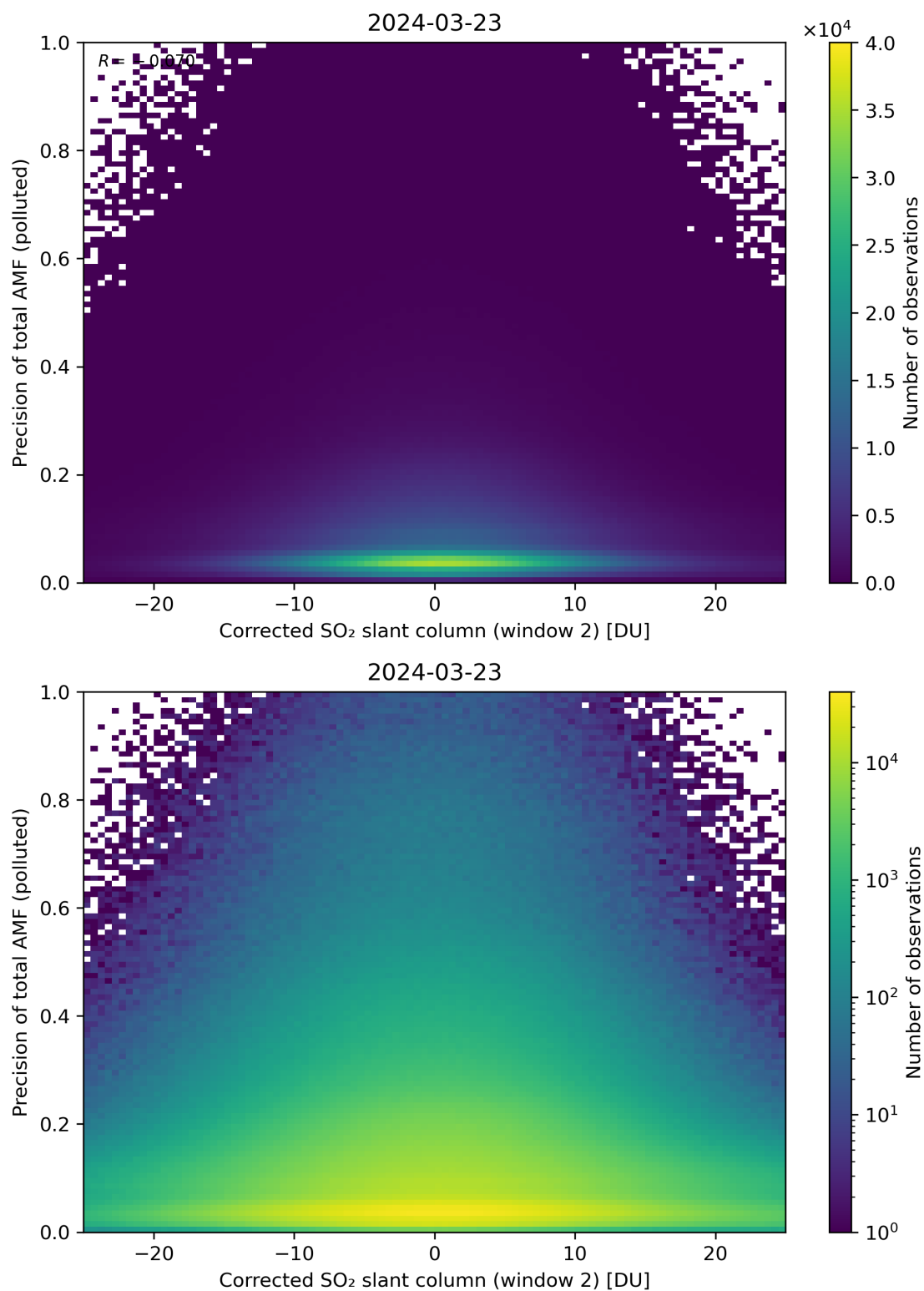
Figure 204: Scatter density plot of “Corrected SO 2 slant column (window 2)” against “Precision of total AMF (polluted)” for 2024-03-23 to 2024-03-24.
