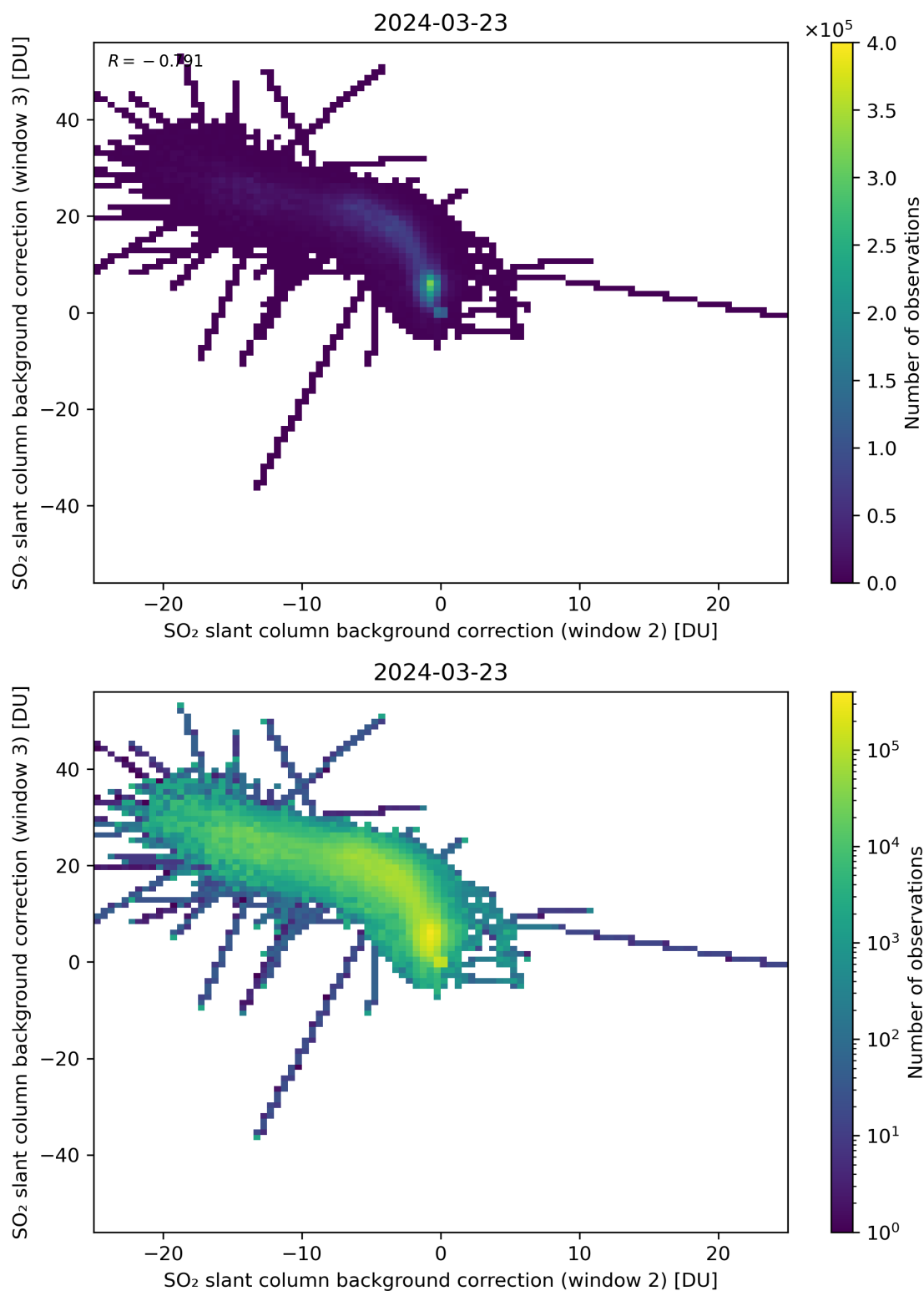
Figure 111: Scatter density plot of “SO 2 slant column background correction (window 2)” against “SO 2 slant column background correction (window 3)” for 2024-03-23 to 2024-03-24.
