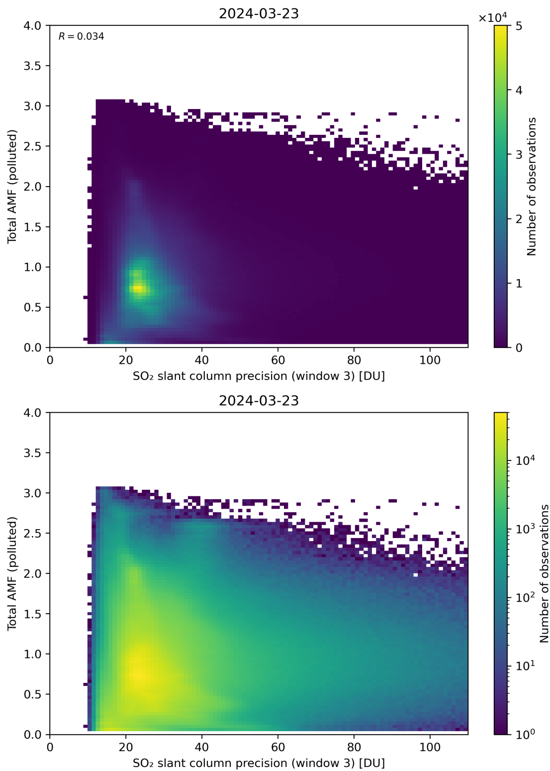
Figure 263: Scatter density plot of “SO 2 slant column precision (window 3)” against “Total AMF (polluted)” for 2024-03-23 to 2024-03-24.
