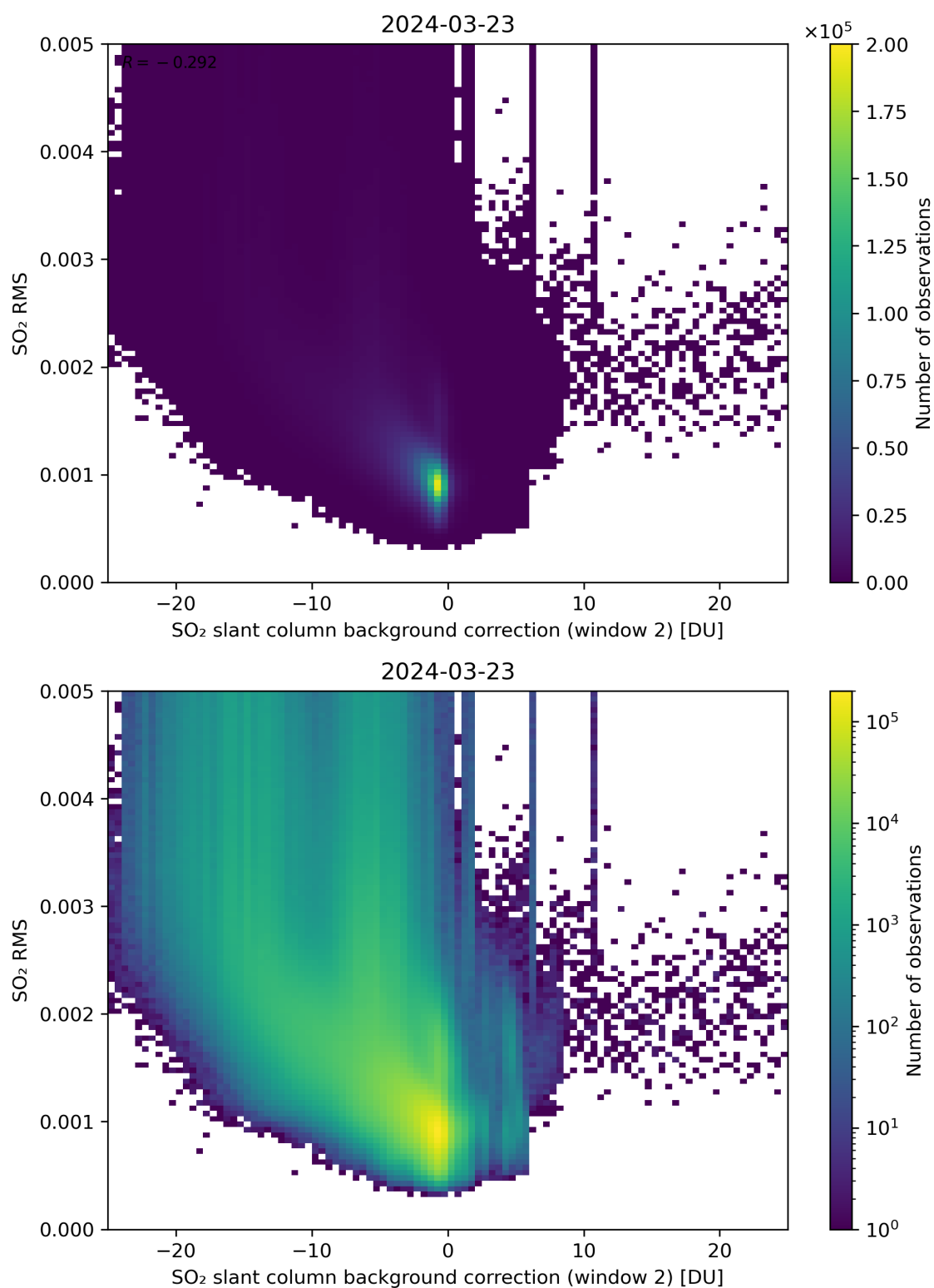
Figure 114: Scatter density plot of “SO 2 slant column background correction (window 2)” against “SO 2 RMS” for 2024-03-23 to 2024-03-24.
