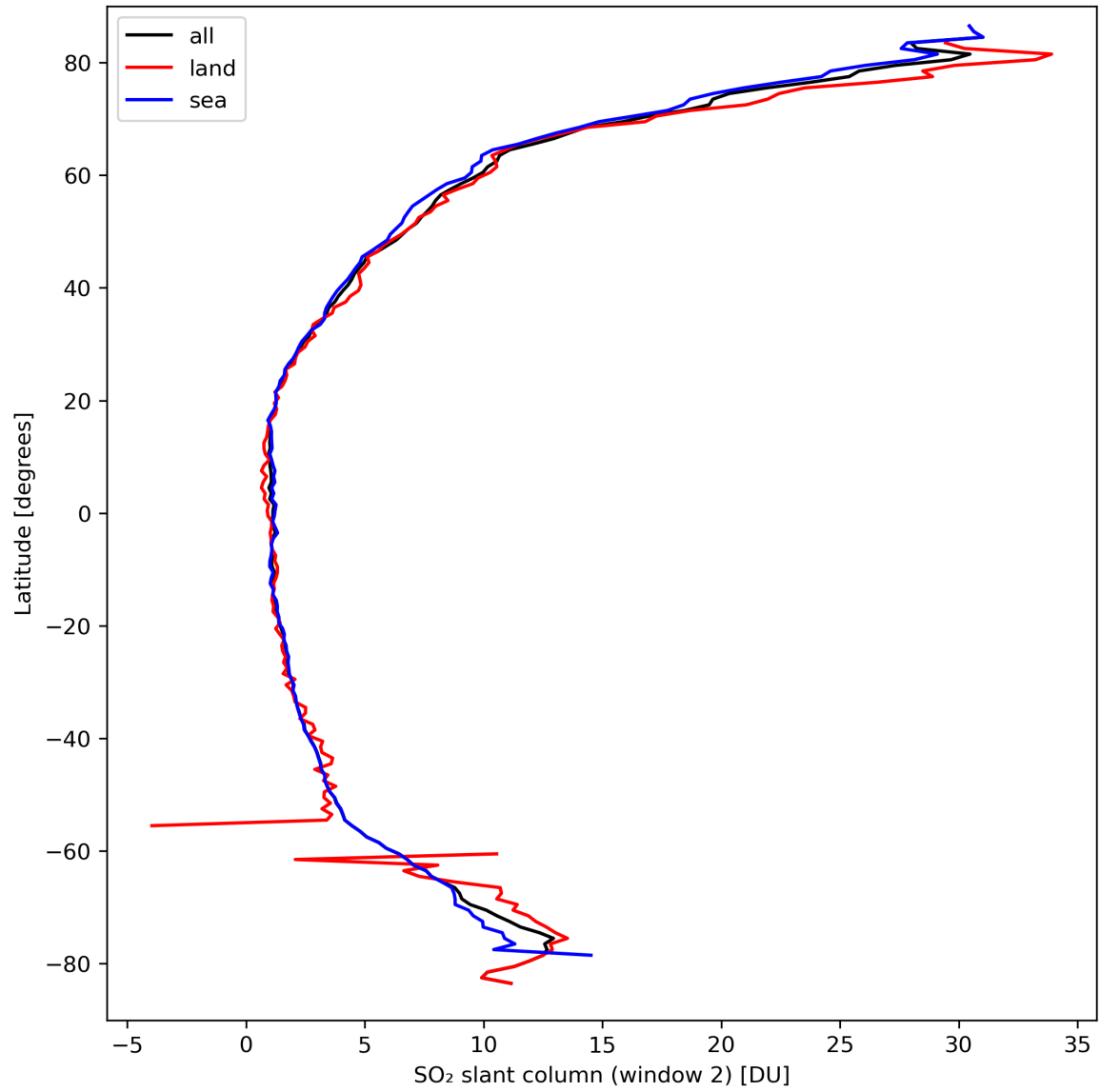
Figure 37: Zonal average of “SO 2 slant column (window 2)” for 2024-03-23 to 2024-03-24.
