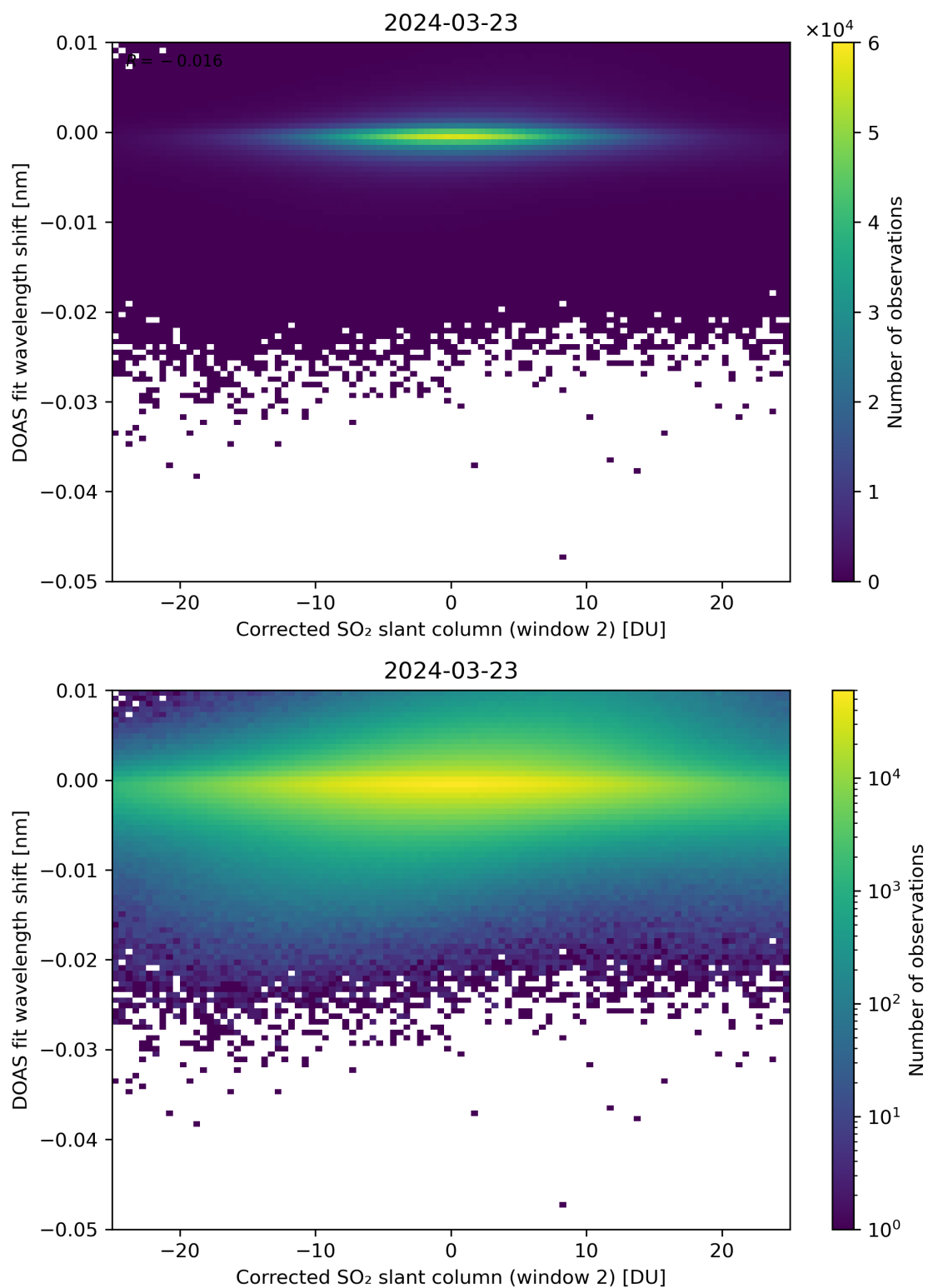
Figure 196: Scatter density plot of “Corrected SO 2 slant column (window 2)” against “DOAS fit wavelength shift” for 2024-03-23 to 2024-03-24.
