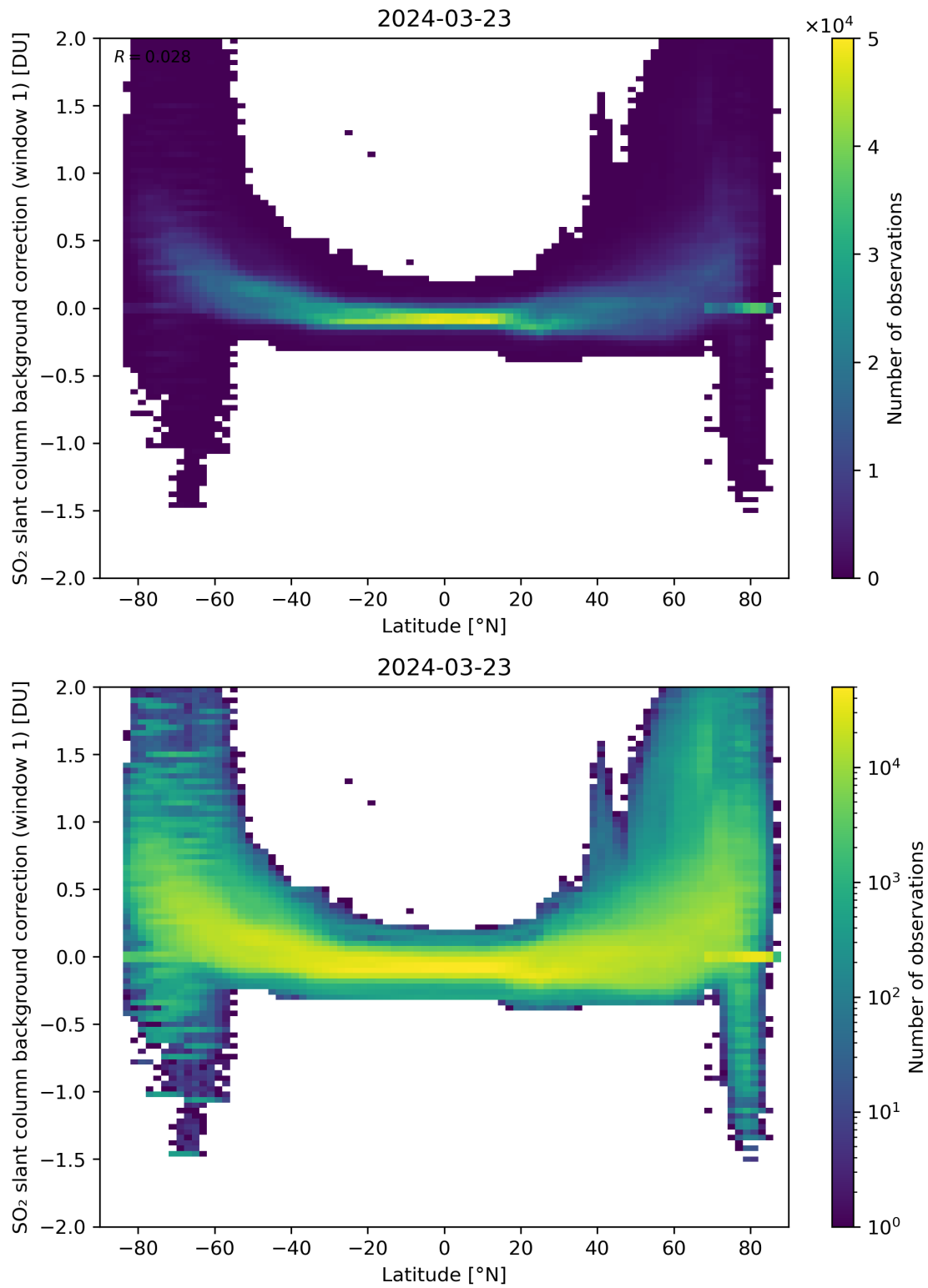
Figure 139: Scatter density plot of “Latitude” against “SO 2 slant column background correction (window 1)” for 2024-03-23 to 2024-03-24.
