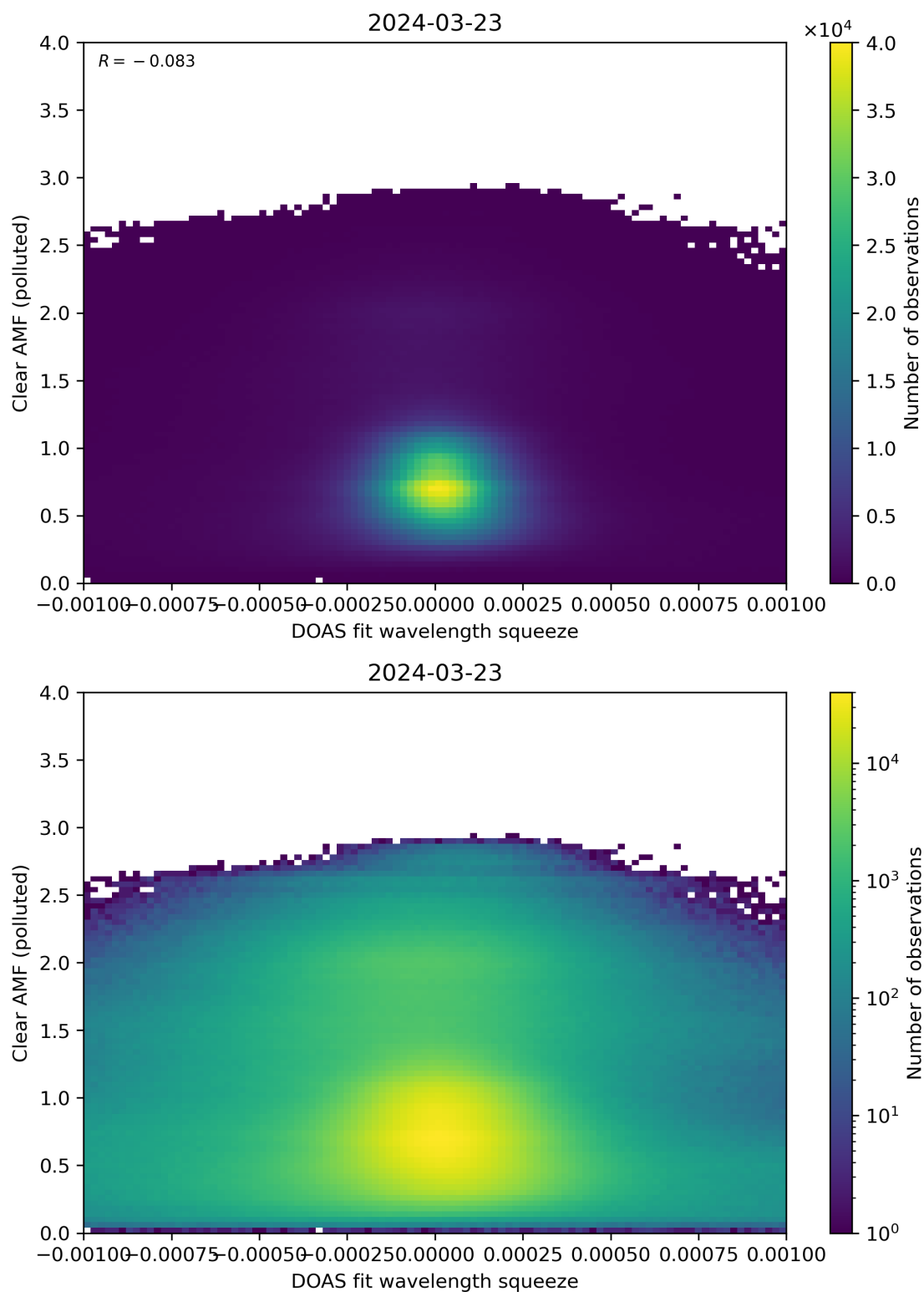
Figure 133: Scatter density plot of “DOAS fit wavelength squeeze” against “Clear AMF (polluted)” for 2024-03-23 to 2024-03-24.
