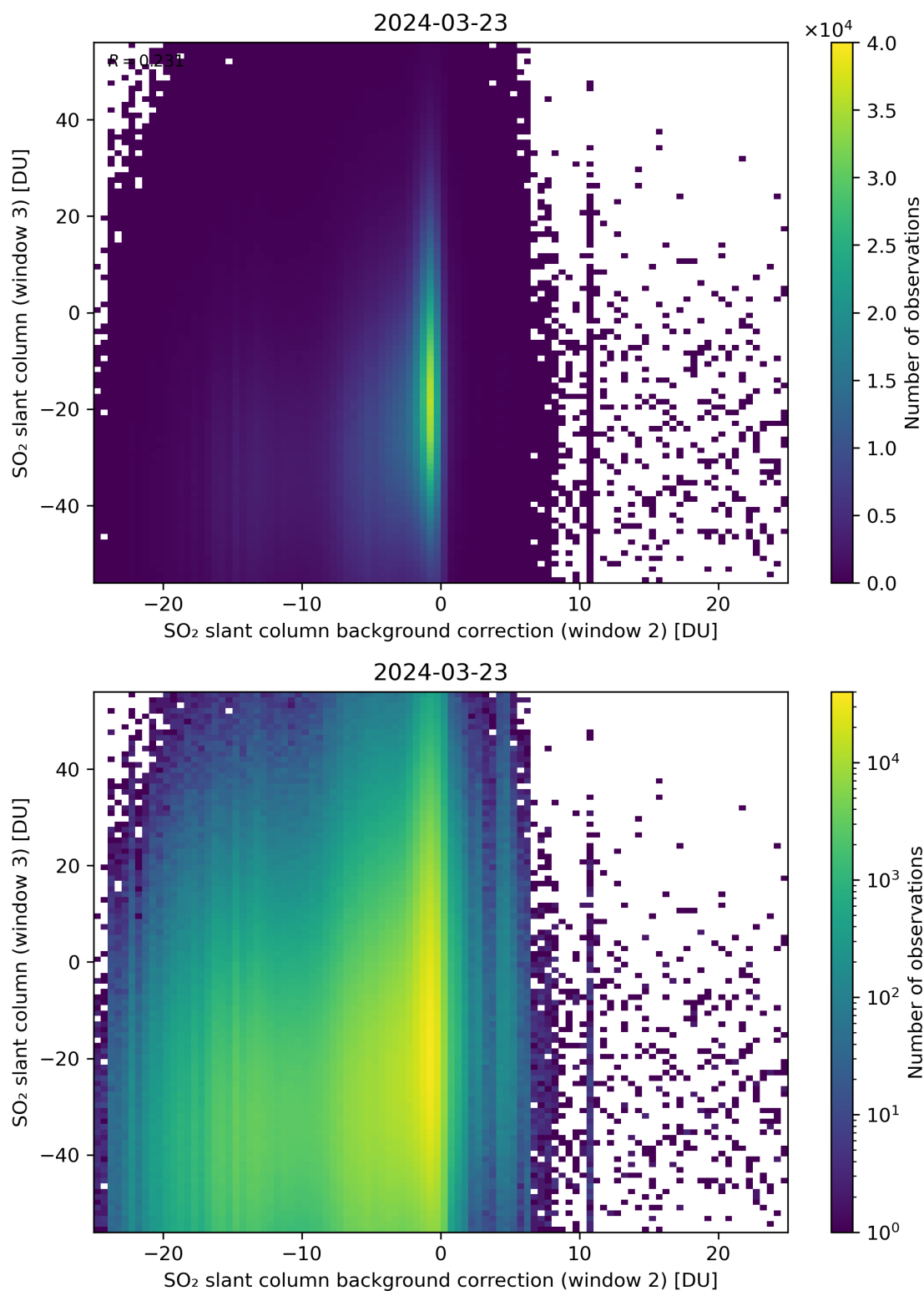
Figure 117: Scatter density plot of “SO 2 slant column background correction (window 2)” against “SO 2 slant column (window 3)” for 2024-03-23 to 2024-03-24.
