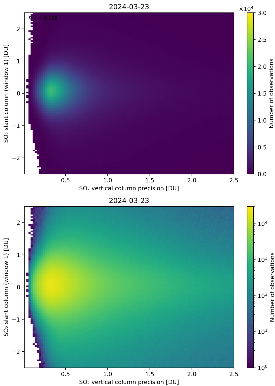
Figure 289: Scatter density plot of “SO 2 vertical column precision” against “SO 2 slant column (window 1)” for 2024-03-23 to 2024-03-24.
