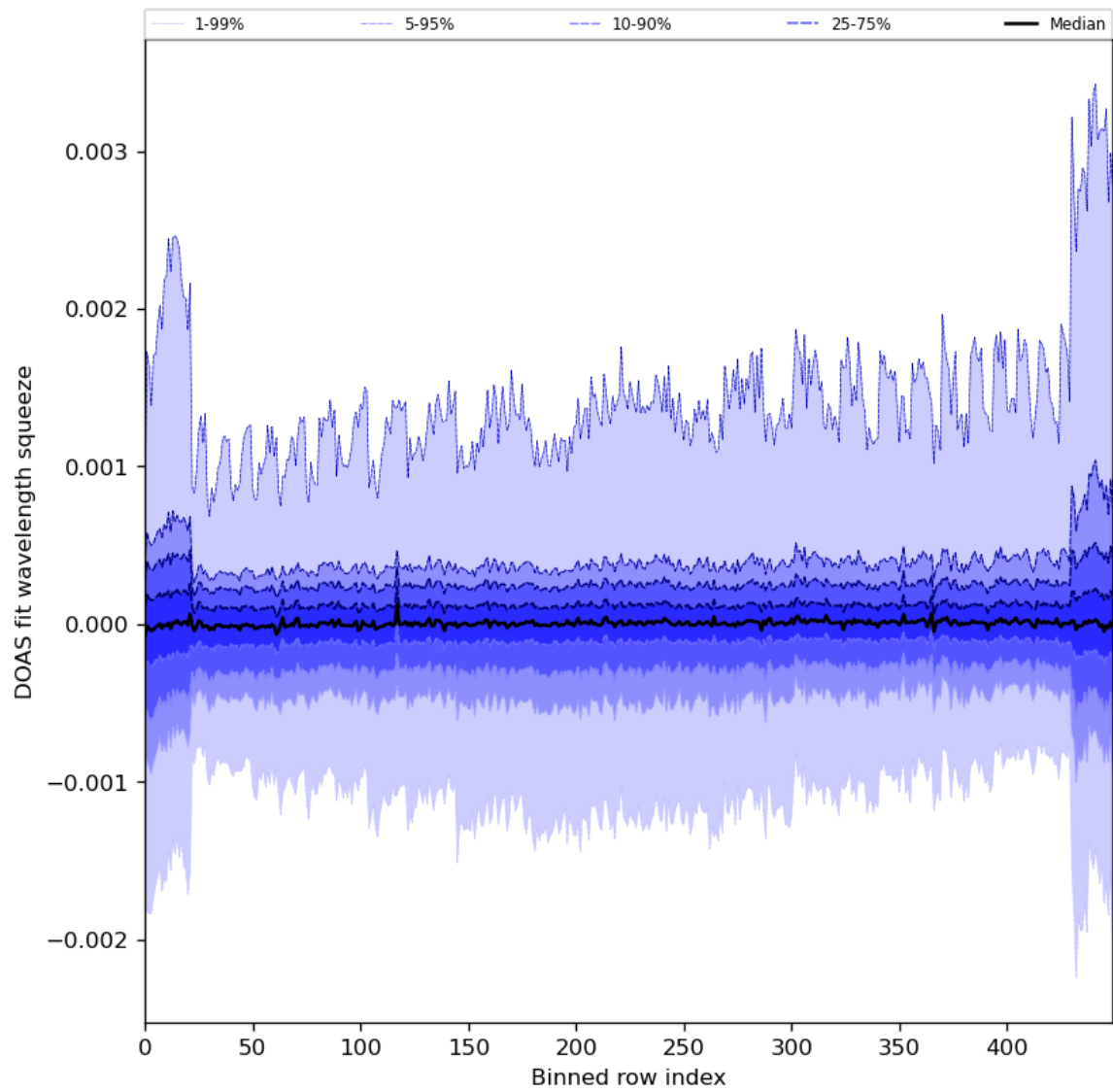
Figure 92: Along track statistics of “DOAS fit wavelength squeeze” for 2024-03-23 to 2024-03-24
