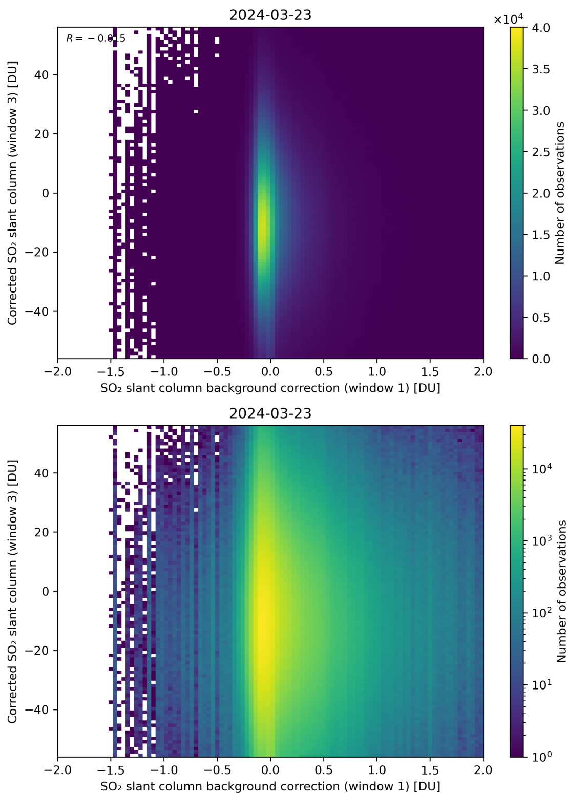
Figure 105: Scatter density plot of “SO 2 slant column background correction (window 1)” against “Corrected SO 2 slant column (window 3)” for 2024-03-23 to 2024-03-24.
