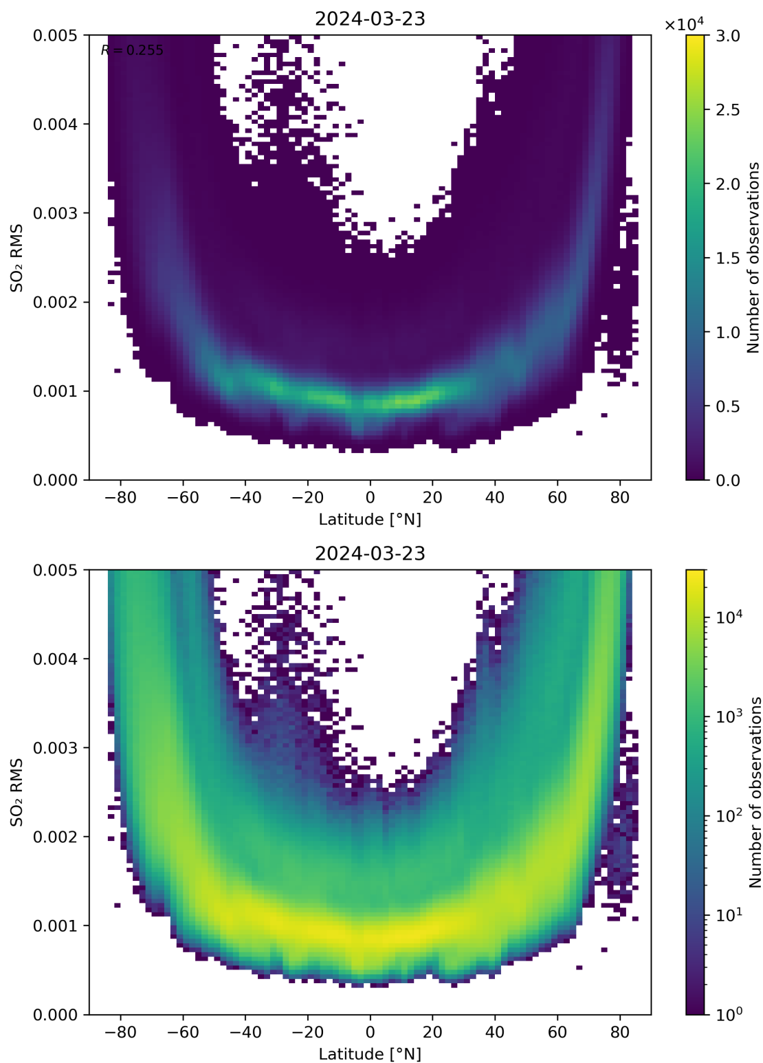
Figure 144: Scatter density plot of “Latitude” against “SO 2 RMS” for 2024-03-23 to 2024-03-24.
