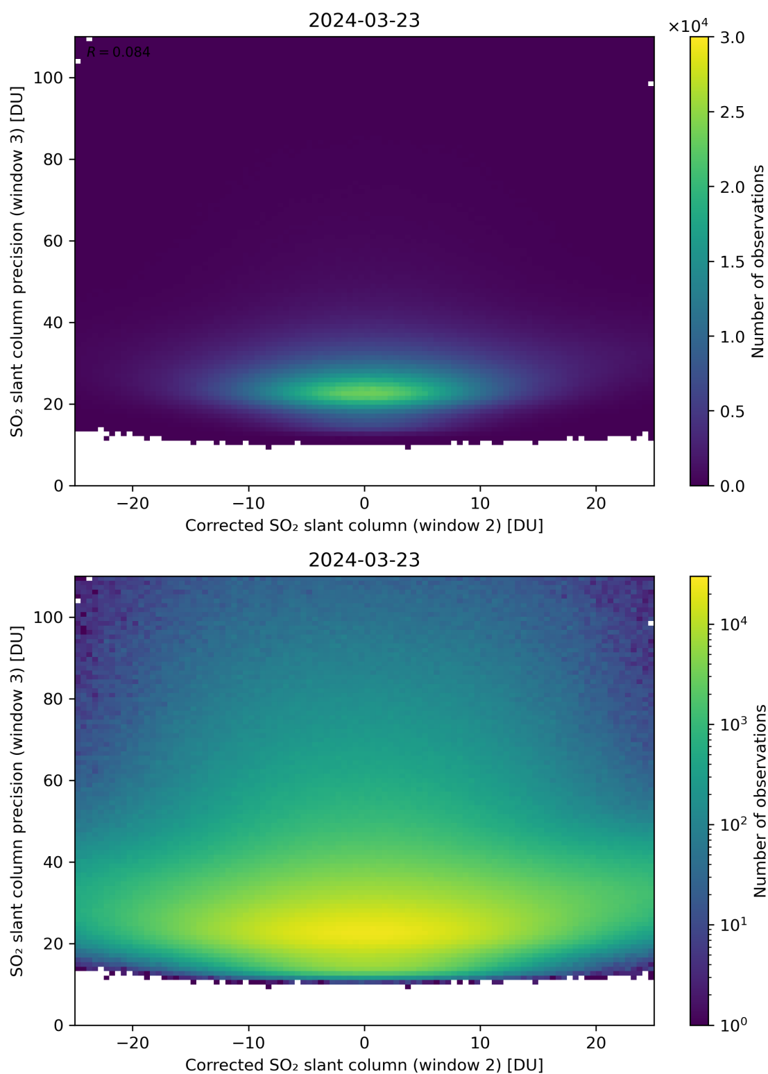
Figure 202: Scatter density plot of “Corrected SO 2 slant column (window 2)” against “SO 2 slant column precision (window 3)” for 2024-03-23 to 2024-03-24.
