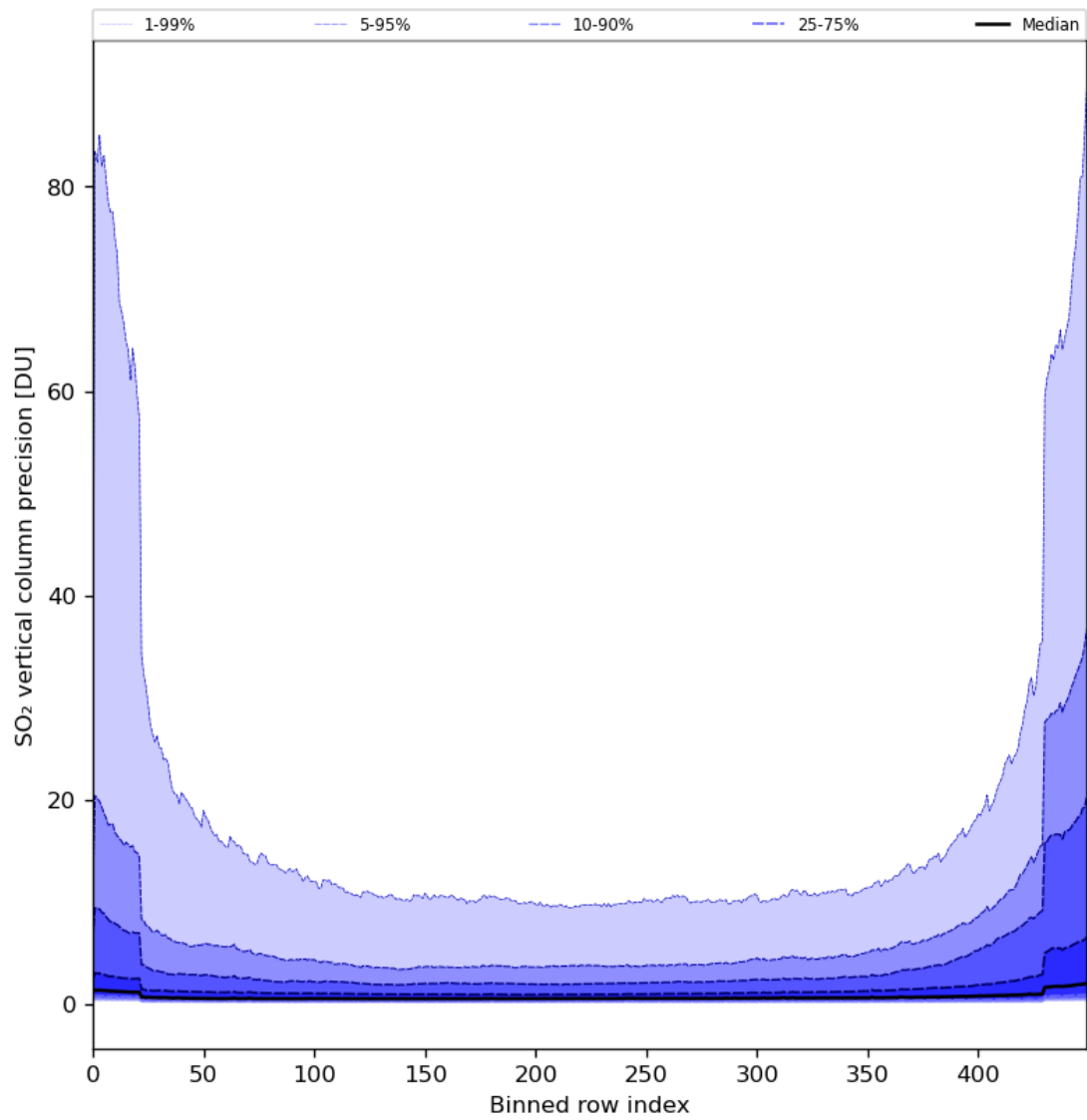
Figure 77: Along track statistics of “SO 2 vertical column precision” for 2024-03-23 to 2024-03-24
