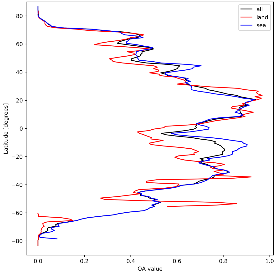
Figure 29: Zonal average of “QA value” for 2024-03-23 to 2024-03-24.
