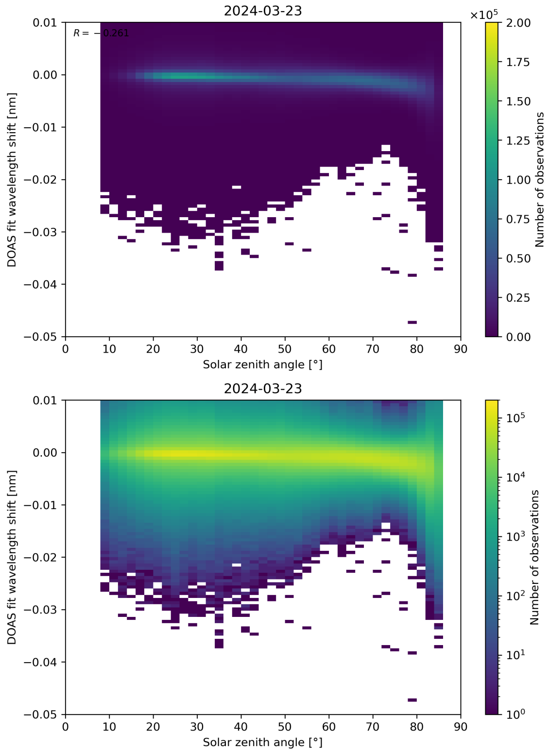
Figure 161: Scatter density plot of “Solar zenith angle” against “DOAS fit wavelength shift” for 2024-03-23 to 2024-03-24.
