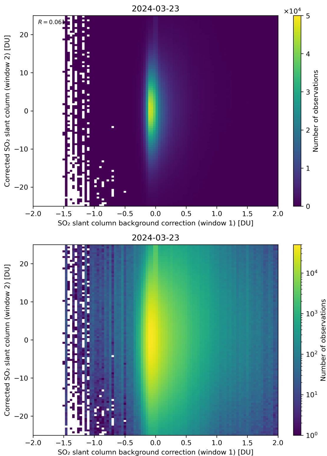
Figure 104: Scatter density plot of “SO 2 slant column background correction (window 1)” against “Corrected SO 2 slant column (window 2)” for 2024-03-23 to 2024-03-24.
