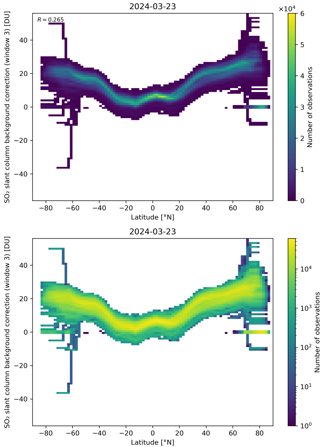
Figure 141: Scatter density plot of “Latitude” against “SO 2 slant column background correction (window 3)” for 2024-03-23 to 2024-03-24.
