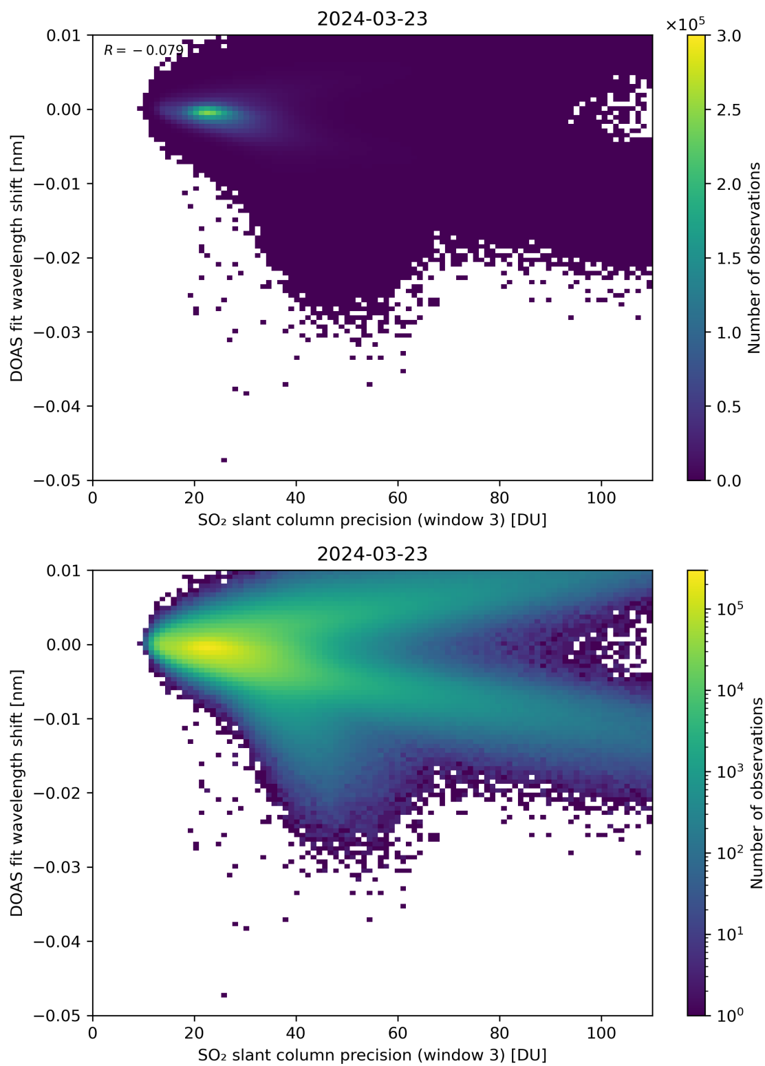
Figure 258: Scatter density plot of “SO 2 slant column precision (window 3)” against “DOAS fit wavelength shift” for 2024-03-23 to 2024-03-24.
