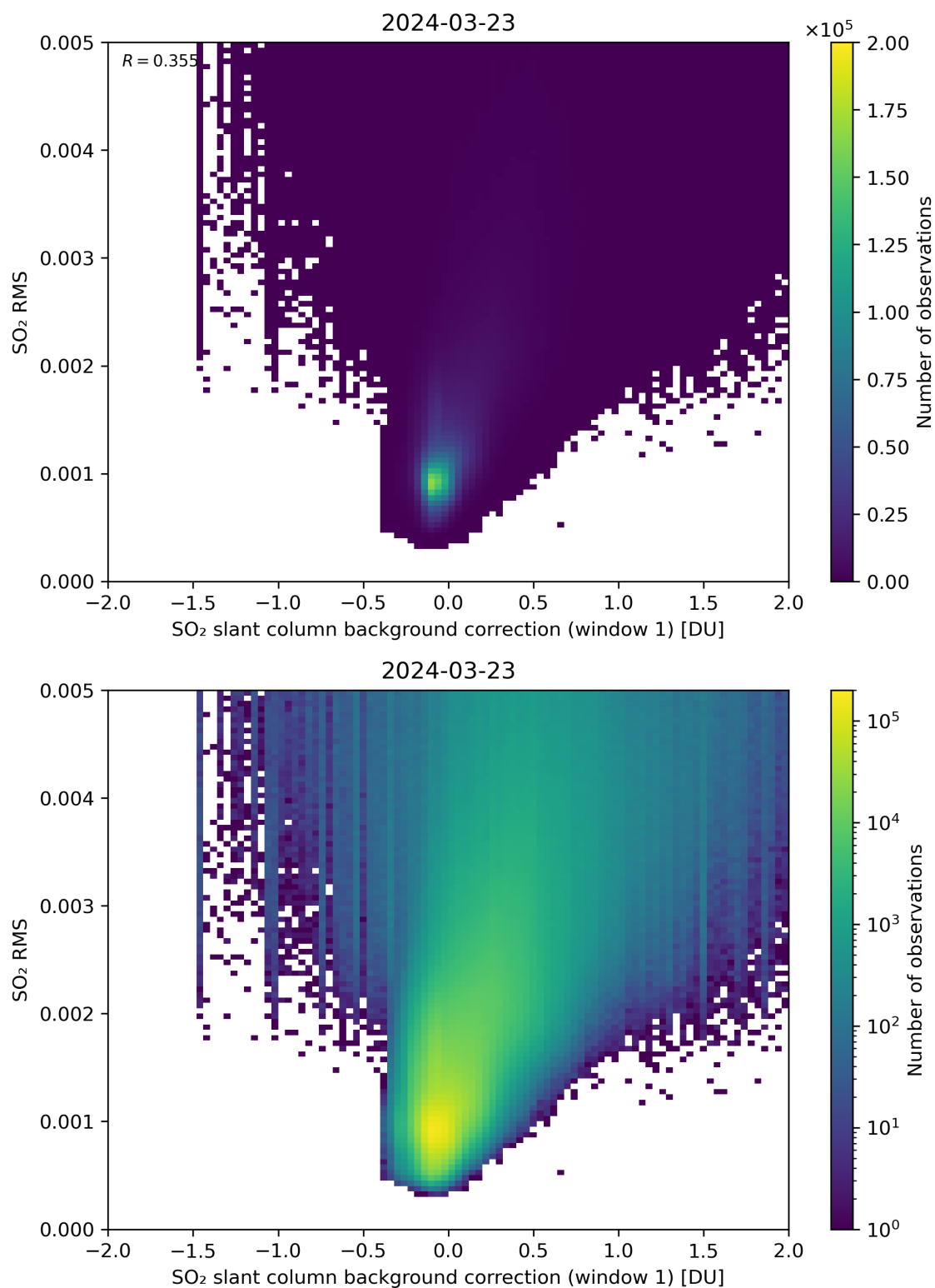
Figure 102: Scatter density plot of “SO 2 slant column background correction (window 1)” against “SO 2 RMS” for 2024-03-23 to 2024-03-24.
