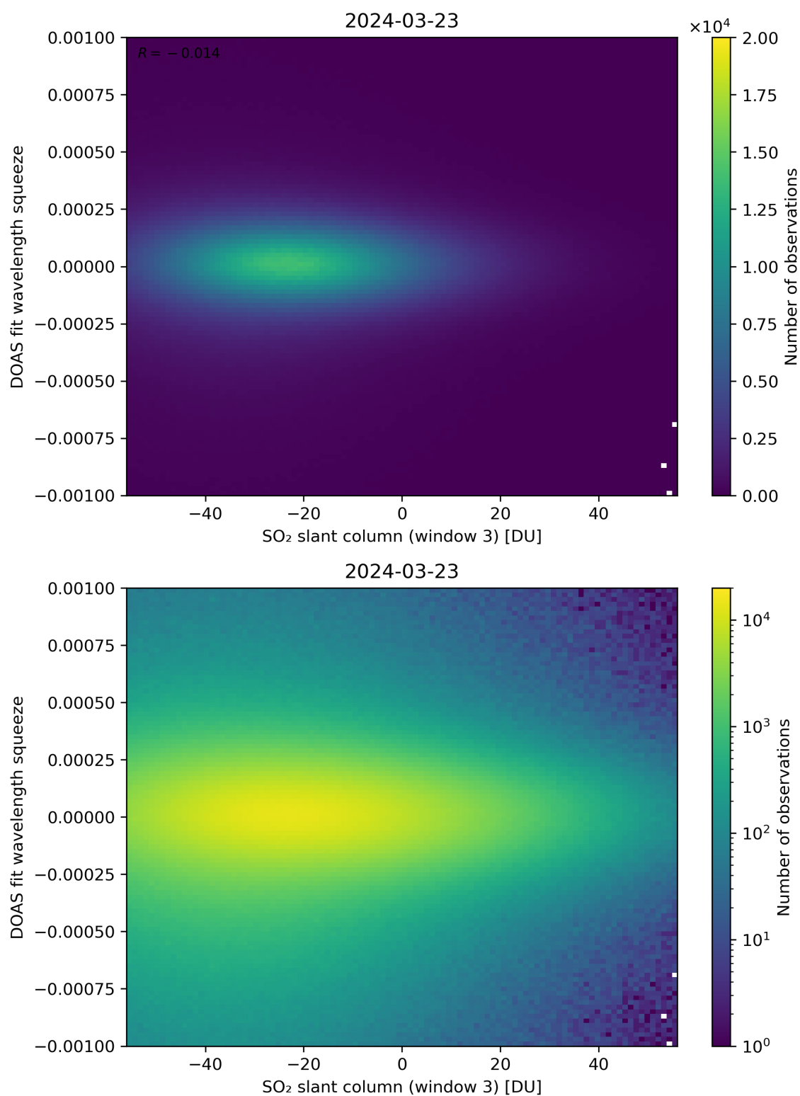
Figure 255: Scatter density plot of “SO 2 slant column (window 3)” against “DOAS fit wavelength squeeze” for 2024-03-23 to 2024-03-24.
