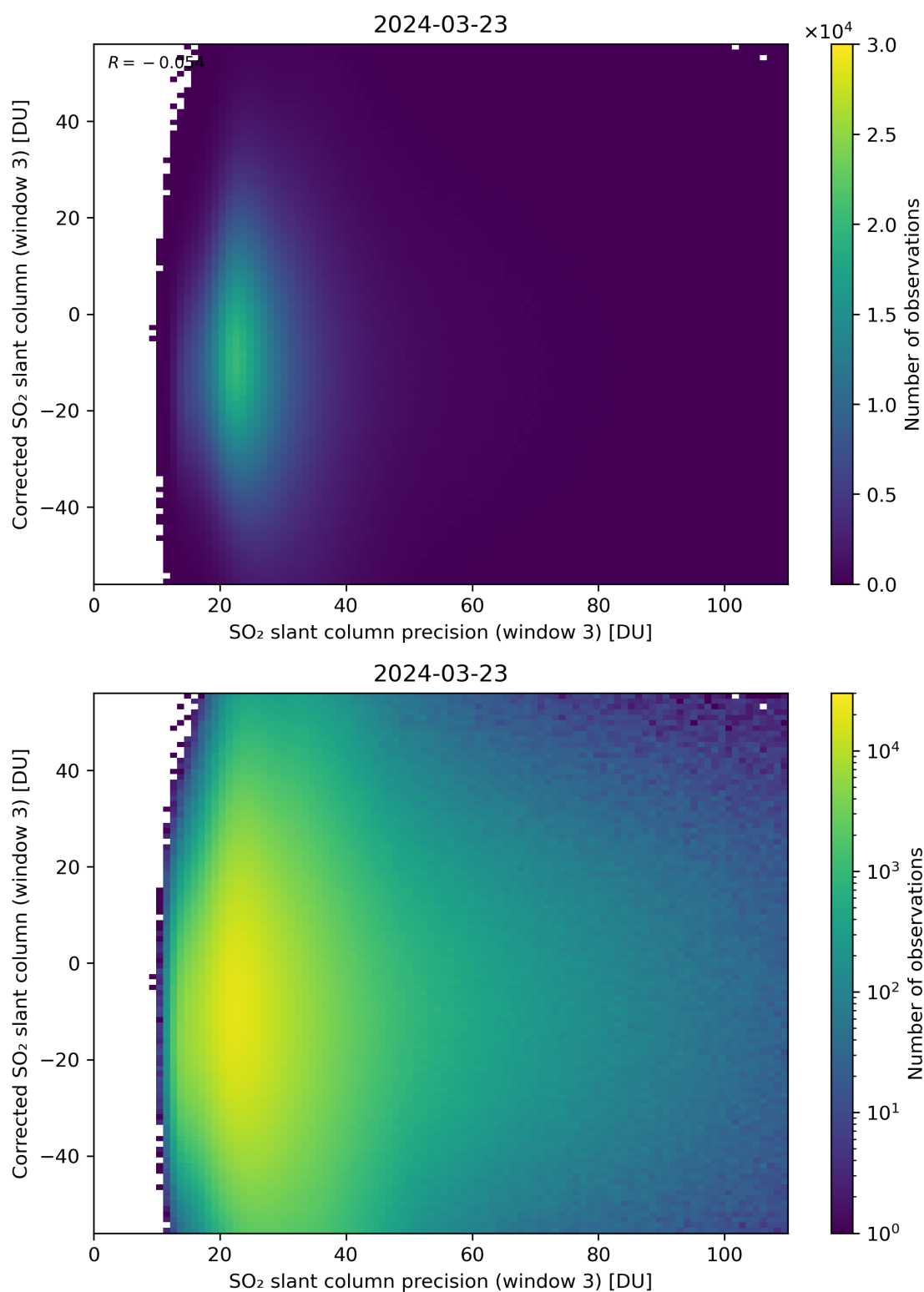
Figure 262: Scatter density plot of “SO 2 slant column precision (window 3)” against “Corrected SO 2 slant column (window 3)” for 2024-03-23 to 2024-03-24.
