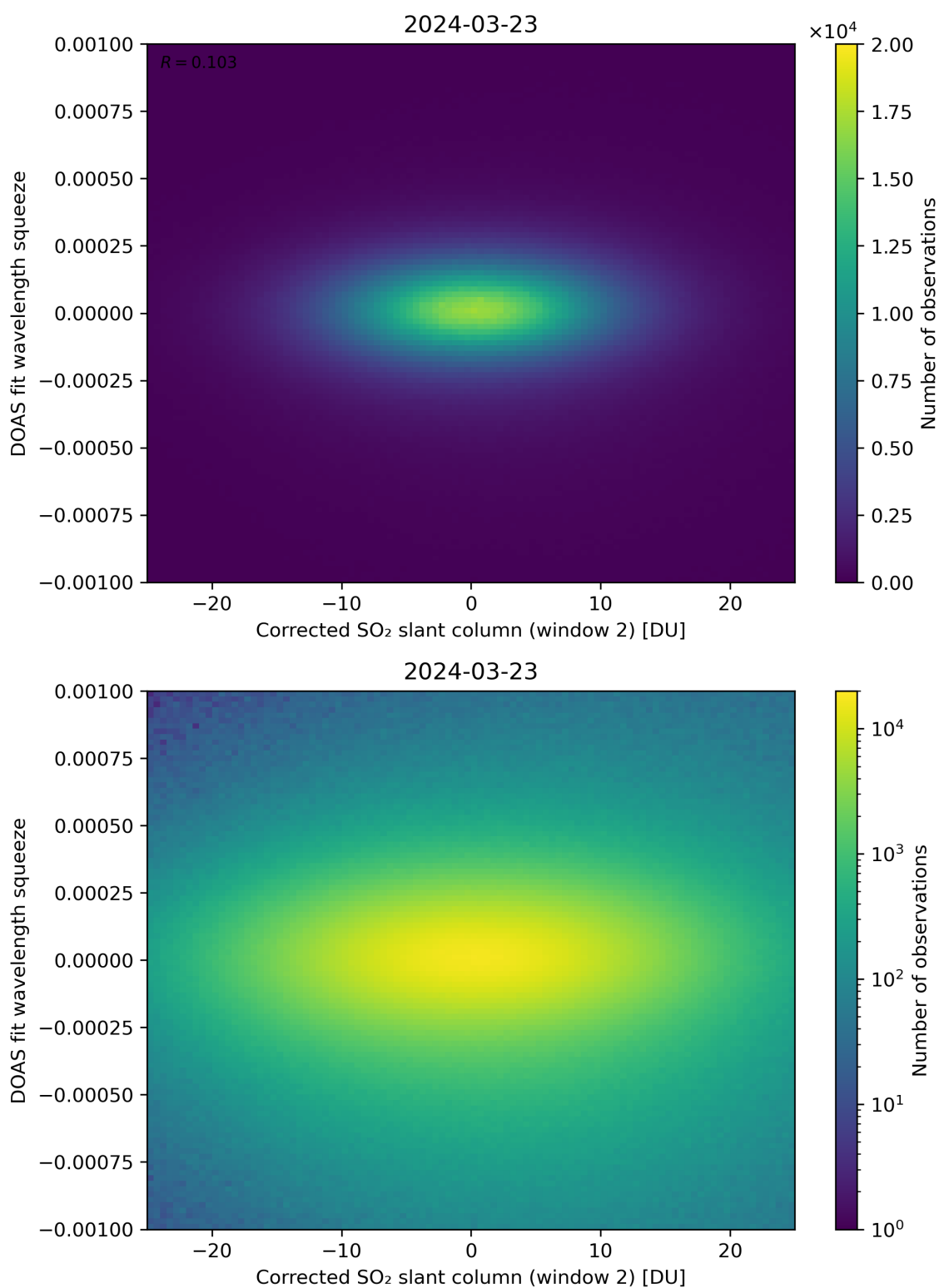
Figure 197: Scatter density plot of “Corrected SO 2 slant column (window 2)” against “DOAS fit wavelength squeeze” for 2024-03-23 to 2024-03-24.
