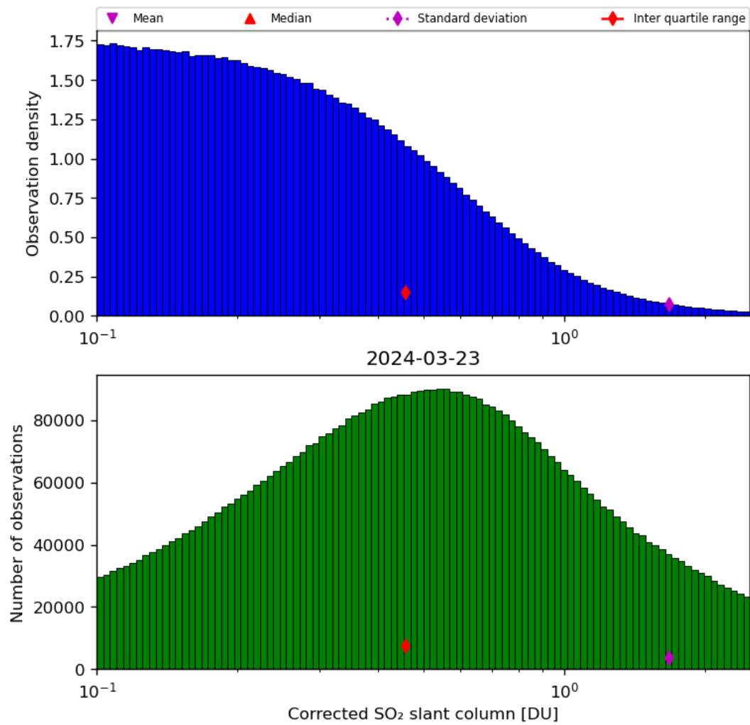
Figure 55: Histogram of “Corrected SO 2 slant column” for 2024-03-23 to 2024-03-24
