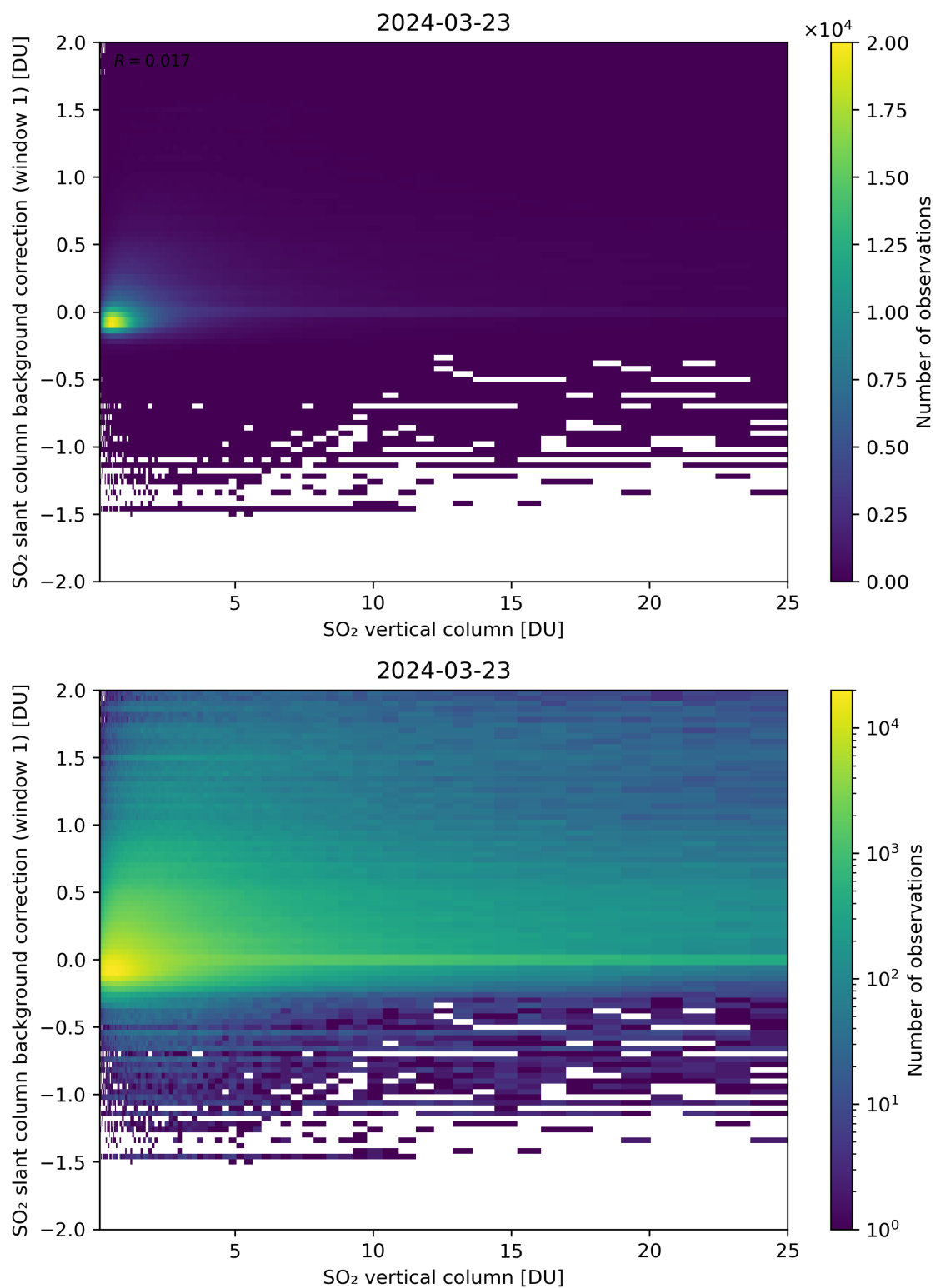
Figure 273: Scatter density plot of “SO 2 vertical column” against “SO 2 slant column background correction (window 1)” for 2024-03-23 to 2024-03-24.
