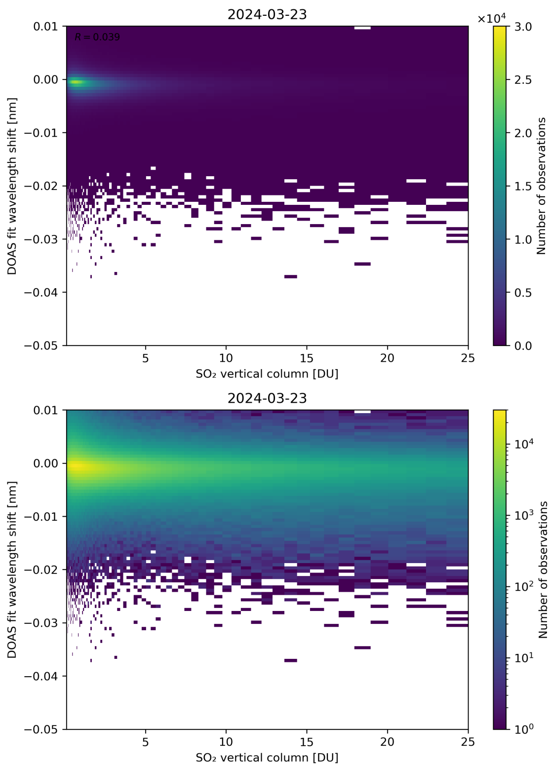
Figure 276: Scatter density plot of “SO 2 vertical column” against “DOAS fit wavelength shift” for 2024-03-23 to 2024-03-24.
