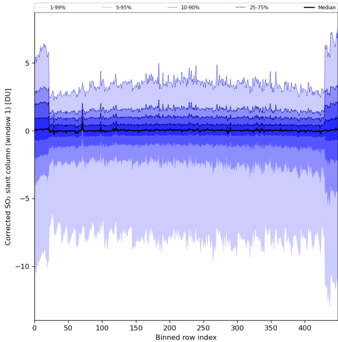
Figure 81: Along track statistics of “Corrected SO 2 slant column (window 1)” for 2024-03-23 to 2024-03-24
