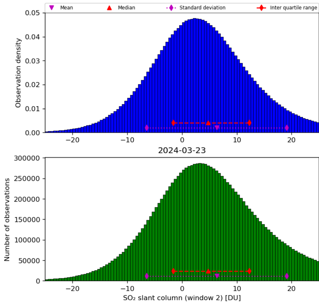
Figure 60: Histogram of “SO 2 slant column (window 2)” for 2024-03-23 to 2024-03-24
