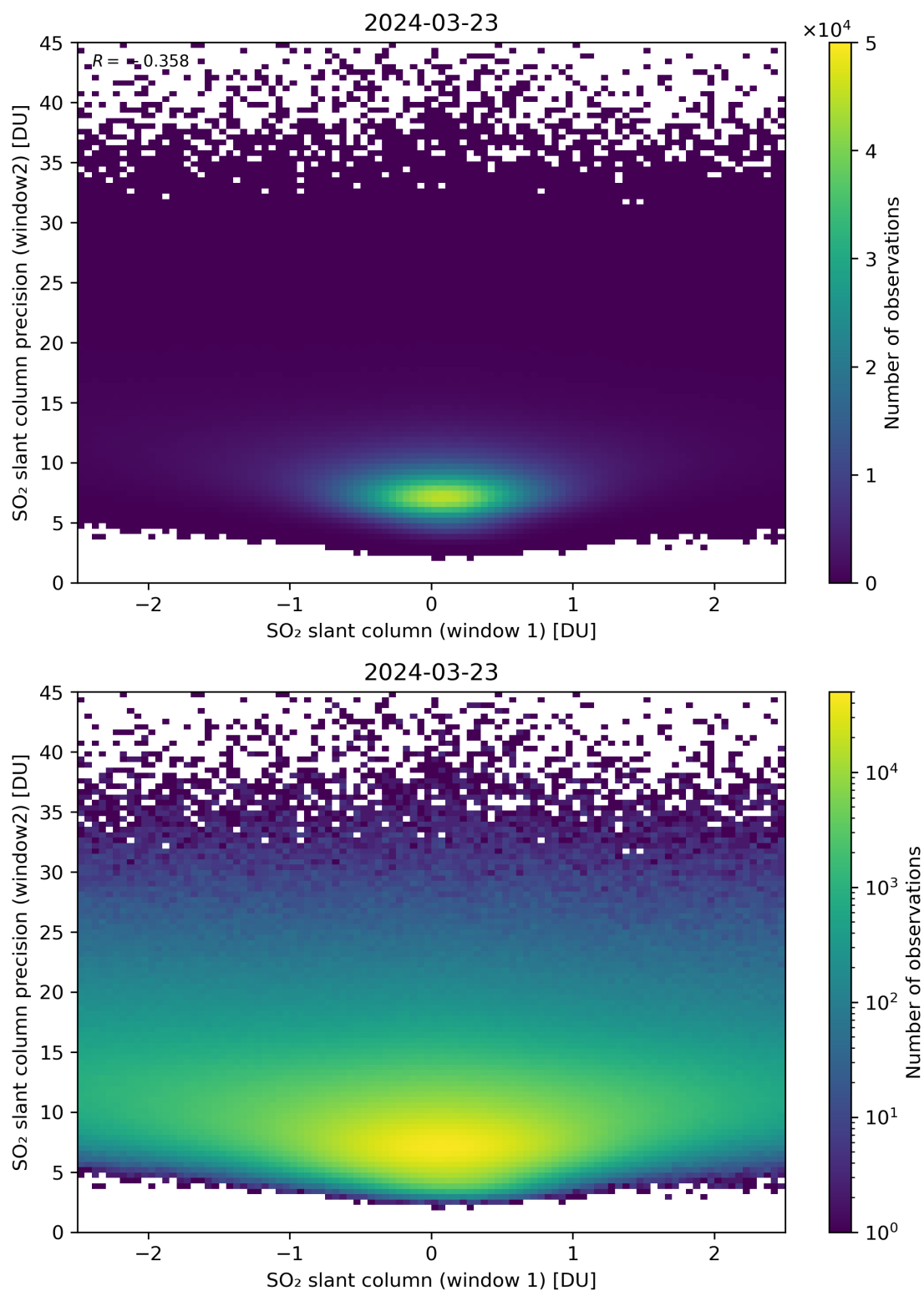
Figure 236: Scatter density plot of “SO 2 slant column (window 1)” against “SO 2 slant column precision (window2)” for 2024-03-23 to 2024-03-24.
