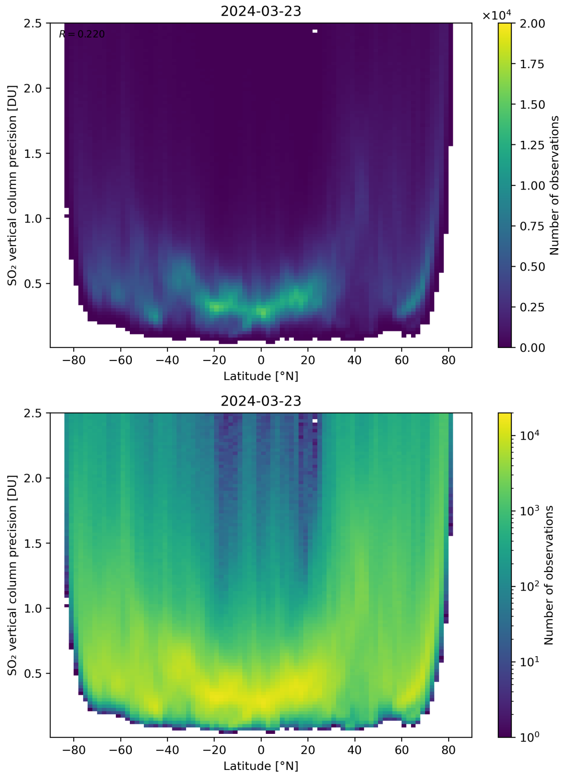
Figure 157: Scatter density plot of “Latitude” against “SO 2 vertical column precision” for 2024-03-23 to 2024-03-24.
