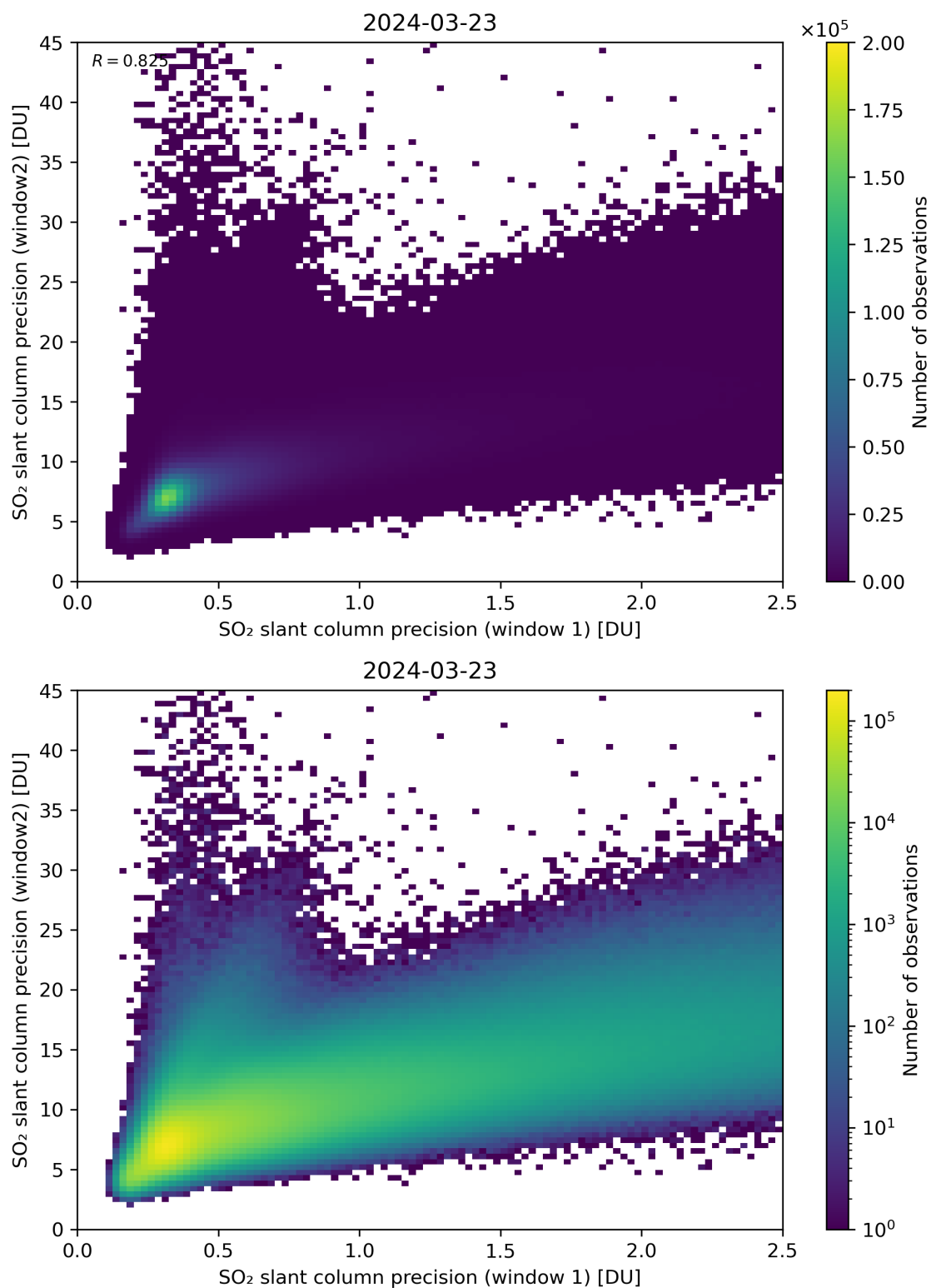
Figure 227: Scatter density plot of “SO 2 slant column precision (window 1)” against “SO 2 slant column precision (window2)” for 2024-03-23 to 2024-03-24.
