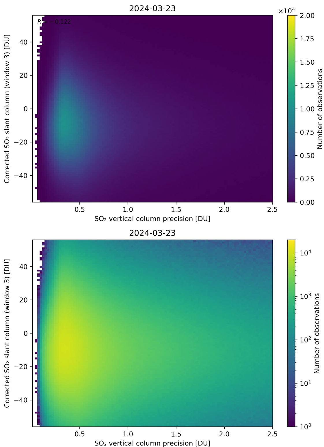
Figure 288: Scatter density plot of “SO 2 vertical column precision” against “Corrected SO 2 slant column (window 3)” for 2024-03-23 to 2024-03-24.
