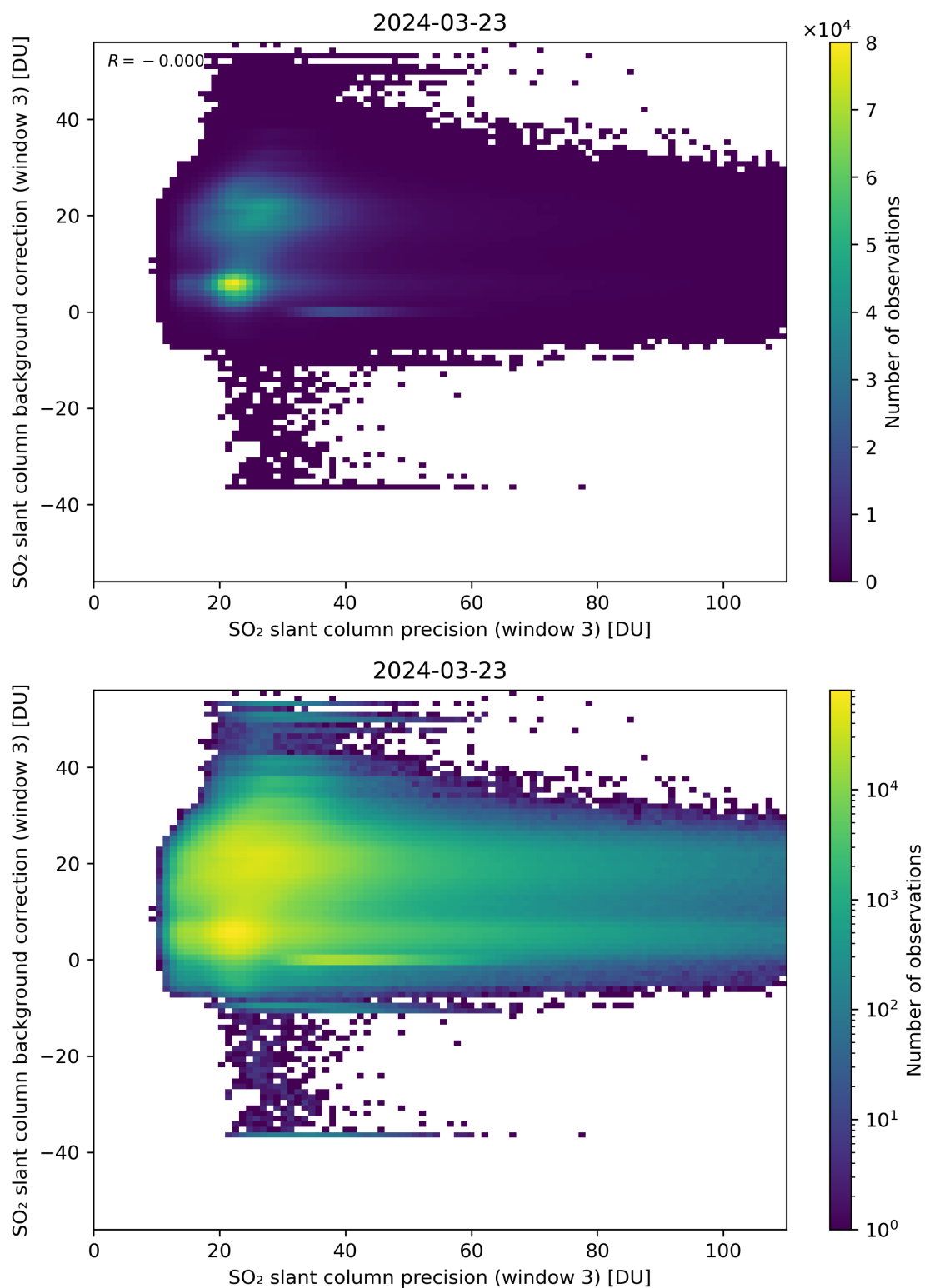
Figure 257: Scatter density plot of “SO 2 slant column precision (window 3)” against “SO 2 slant column background correction (window 3)” for 2024-03-23 to 2024-03-24.
