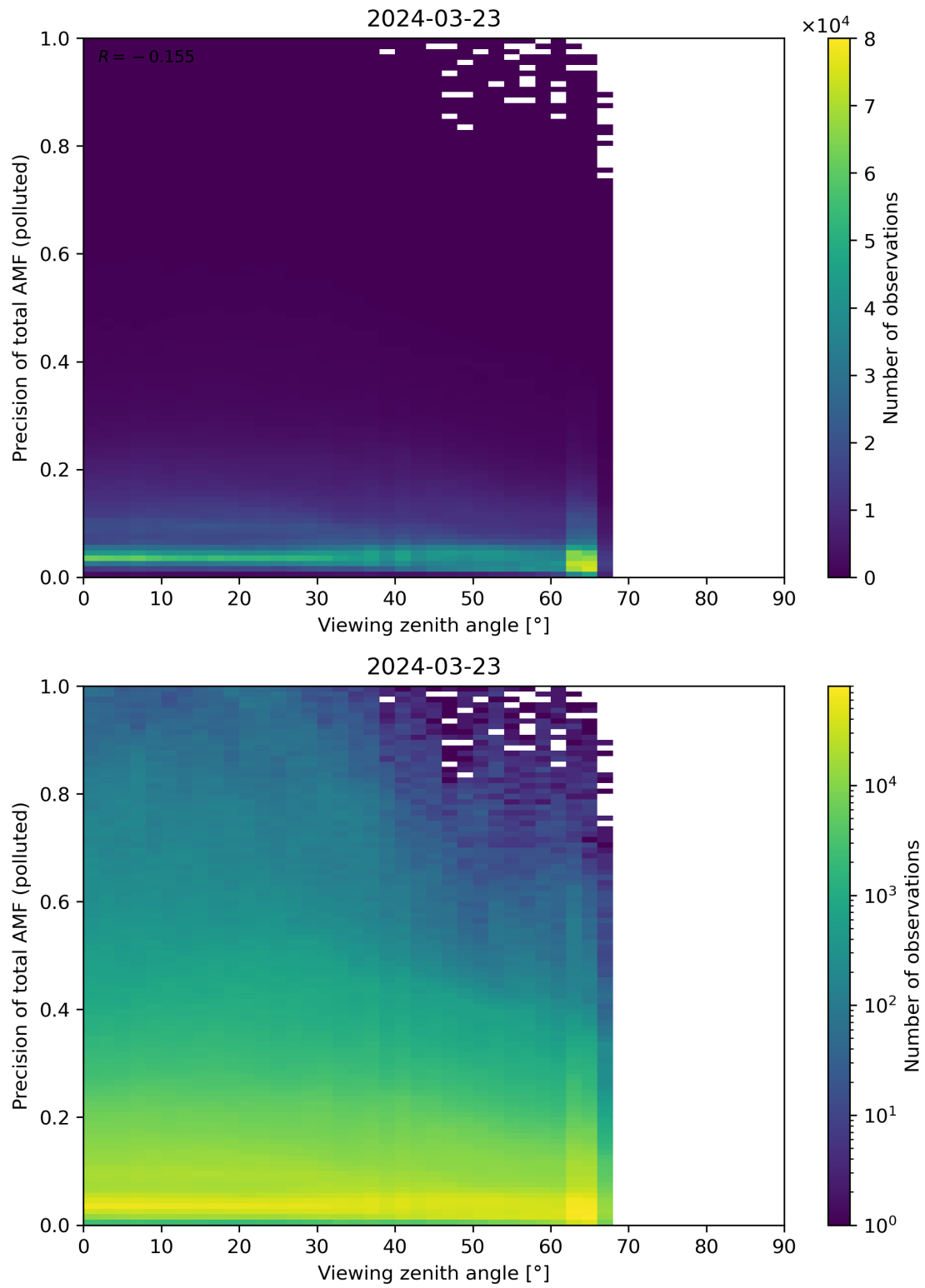
Figure 326: Scatter density plot of “Viewing zenith angle” against “Precision of total AMF (polluted)” for 2024-03-23 to 2024-03-24.
