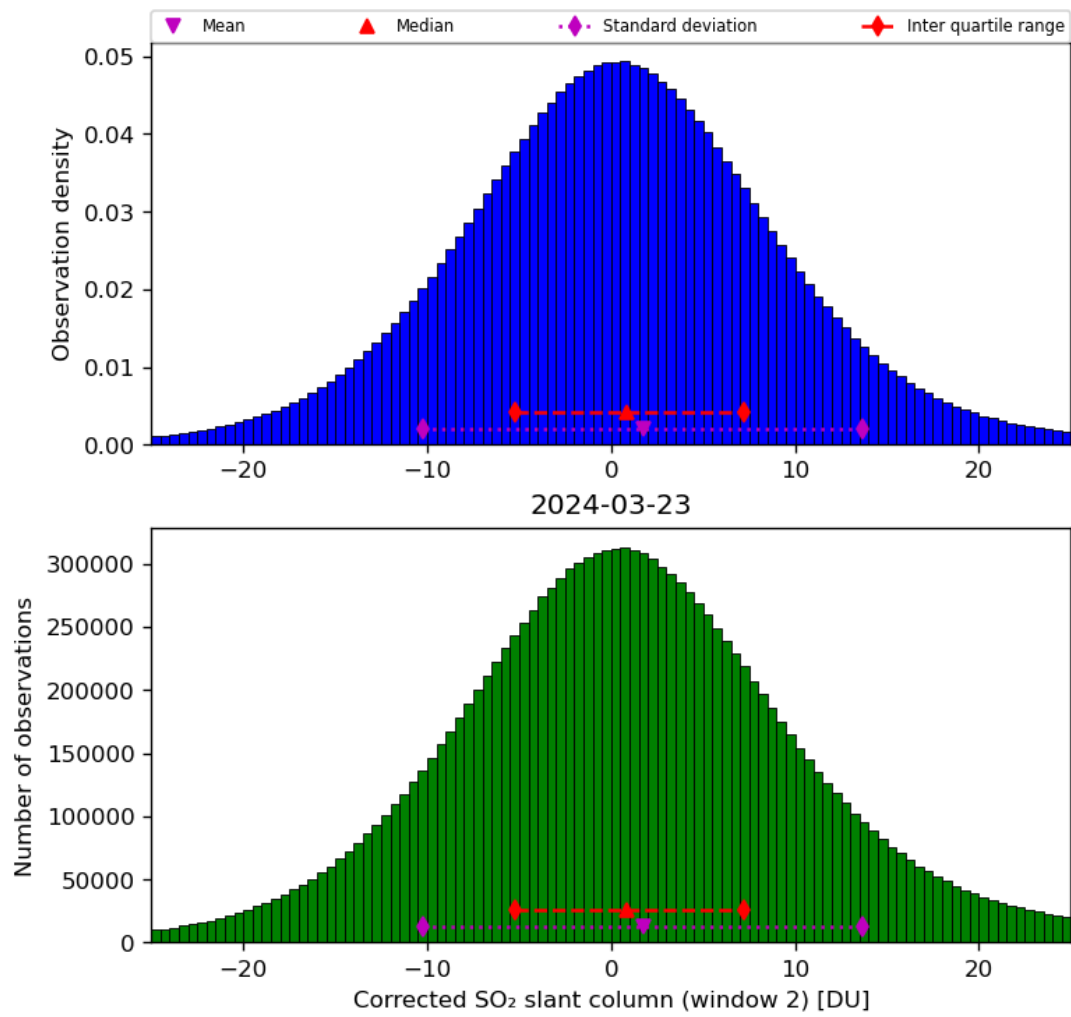
Figure 62: Histogram of “Corrected SO 2 slant column (window 2)” for 2024-03-23 to 2024-03-24
