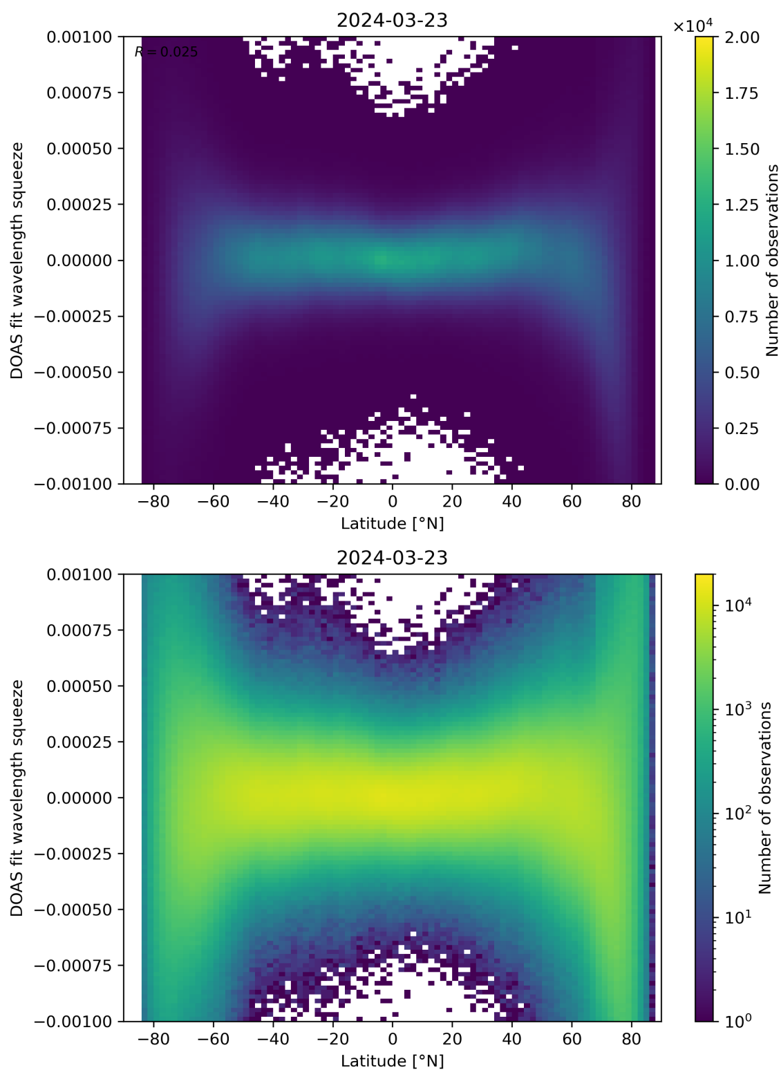
Figure 143: Scatter density plot of “Latitude” against “DOAS fit wavelength squeeze” for 2024-03-23 to 2024-03-24.
