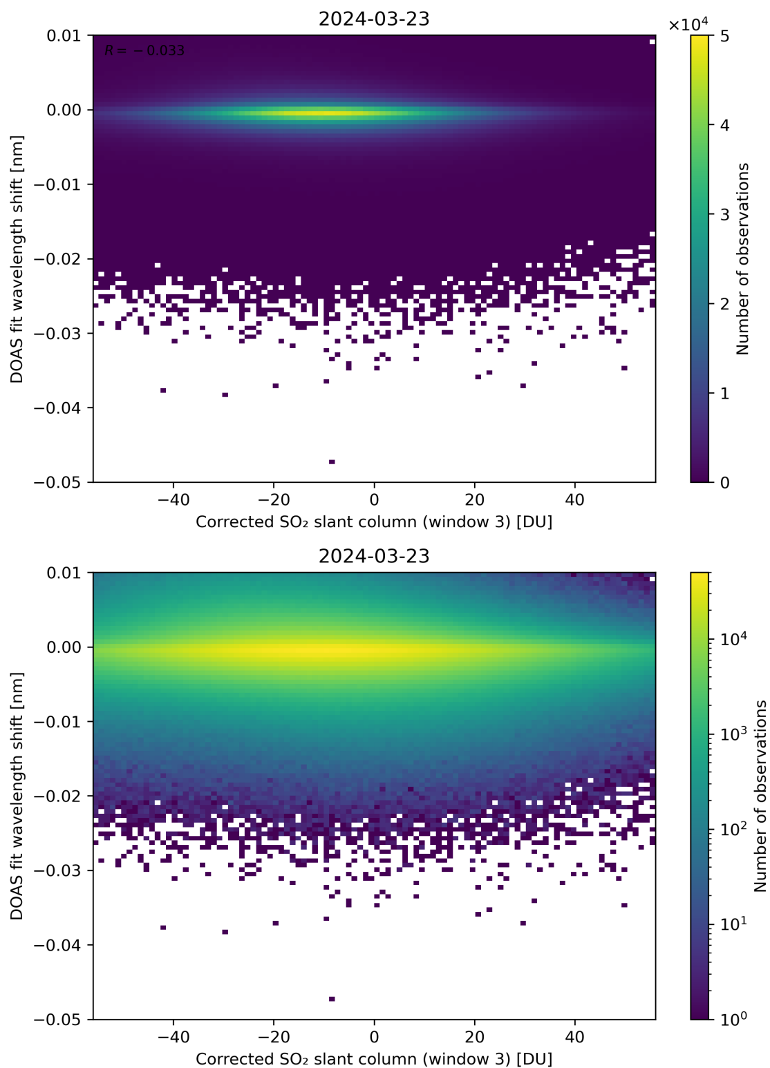
Figure 206: Scatter density plot of “Corrected SO 2 slant column (window 3)” against “DOAS fit wavelength shift” for 2024-03-23 to 2024-03-24.
