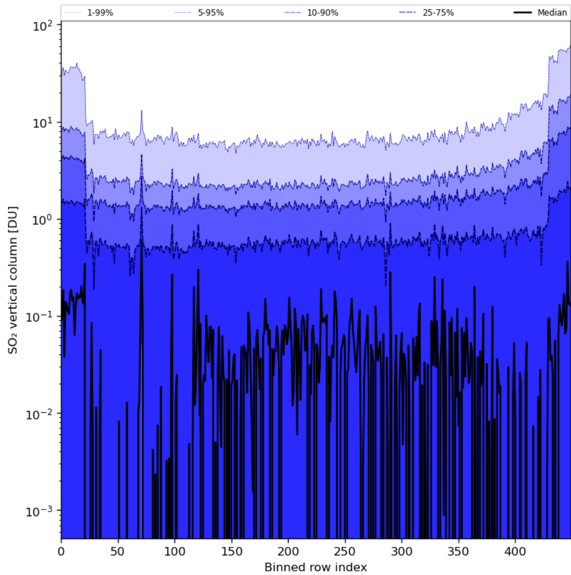
Figure 76: Along track statistics of “SO 2 vertical column” for 2024-03-23 to 2024-03-24
