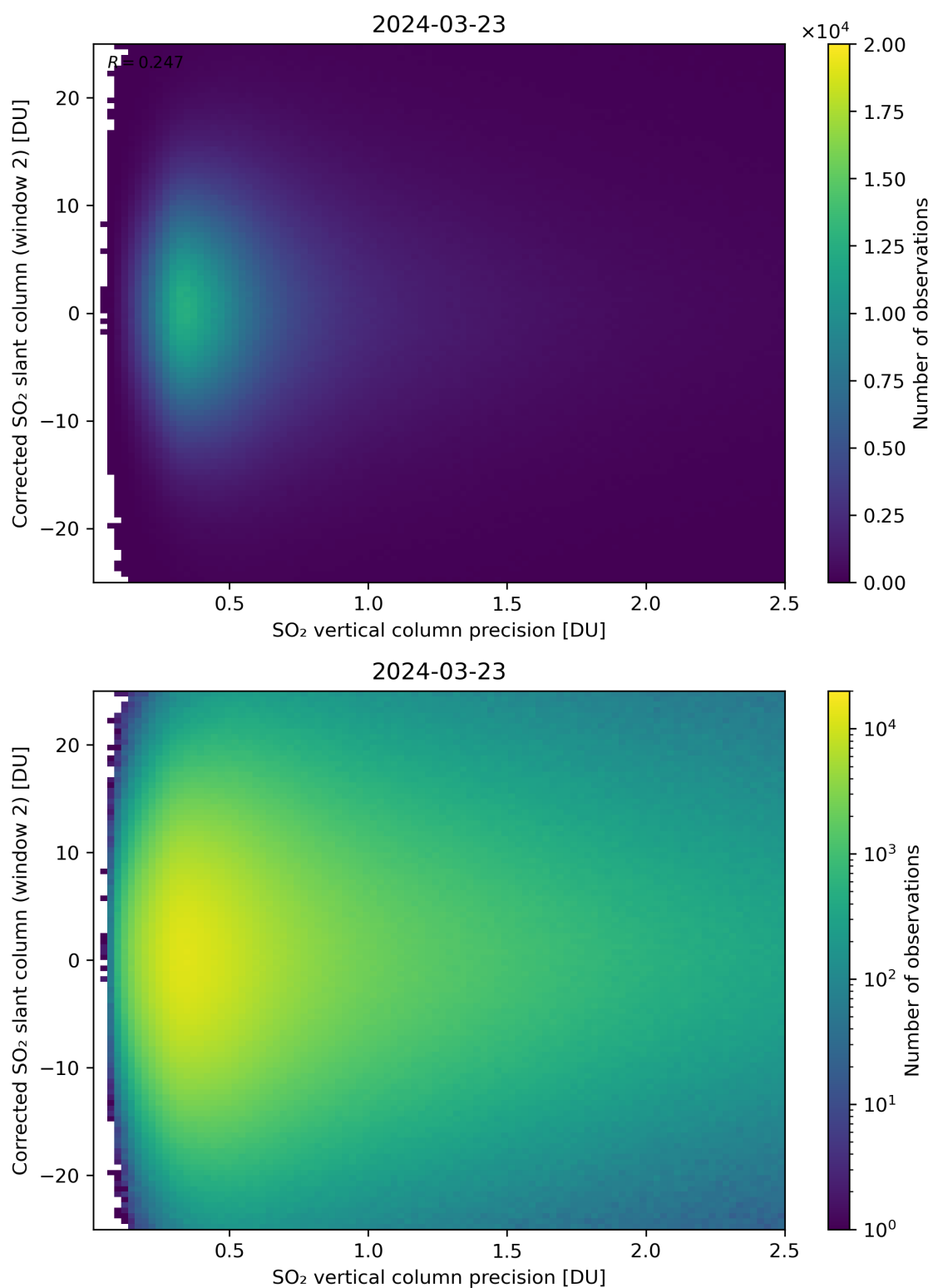
Figure 287: Scatter density plot of “SO 2 vertical column precision” against “Corrected SO 2 slant column (window 2)” for 2024-03-23 to 2024-03-24.
