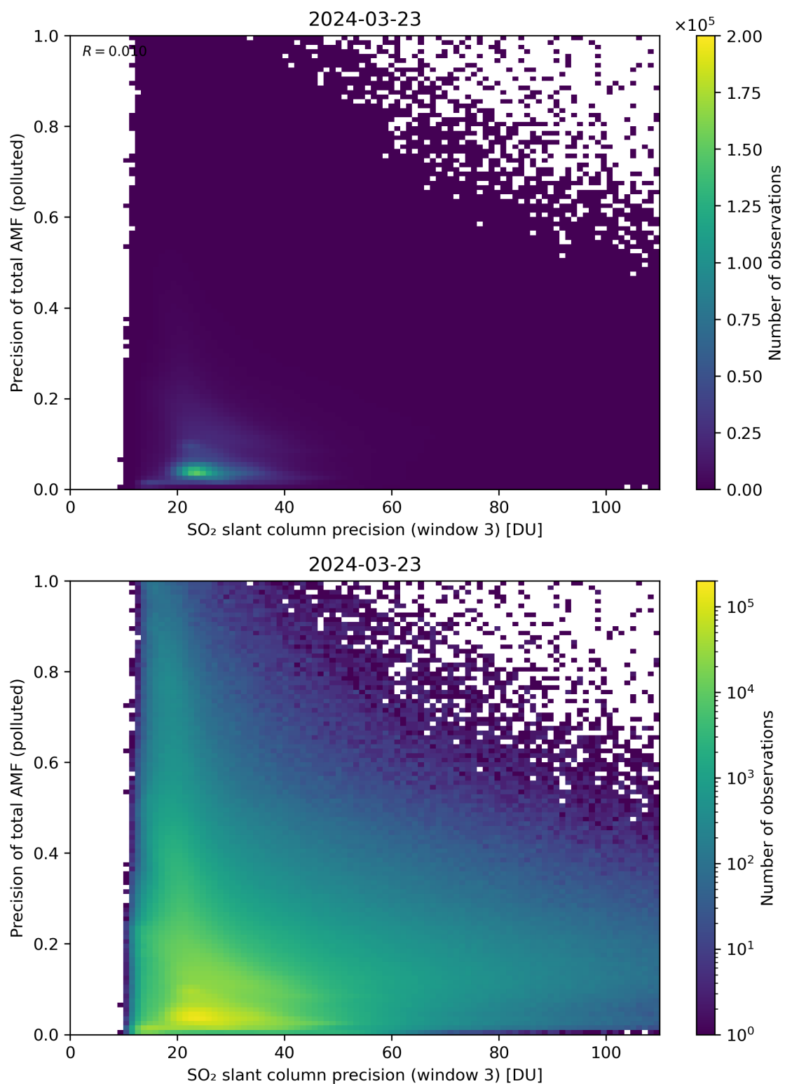
Figure 264: Scatter density plot of “SO 2 slant column precision (window 3)” against “Precision of total AMF (polluted)” for 2024-03-23 to 2024-03-24.
