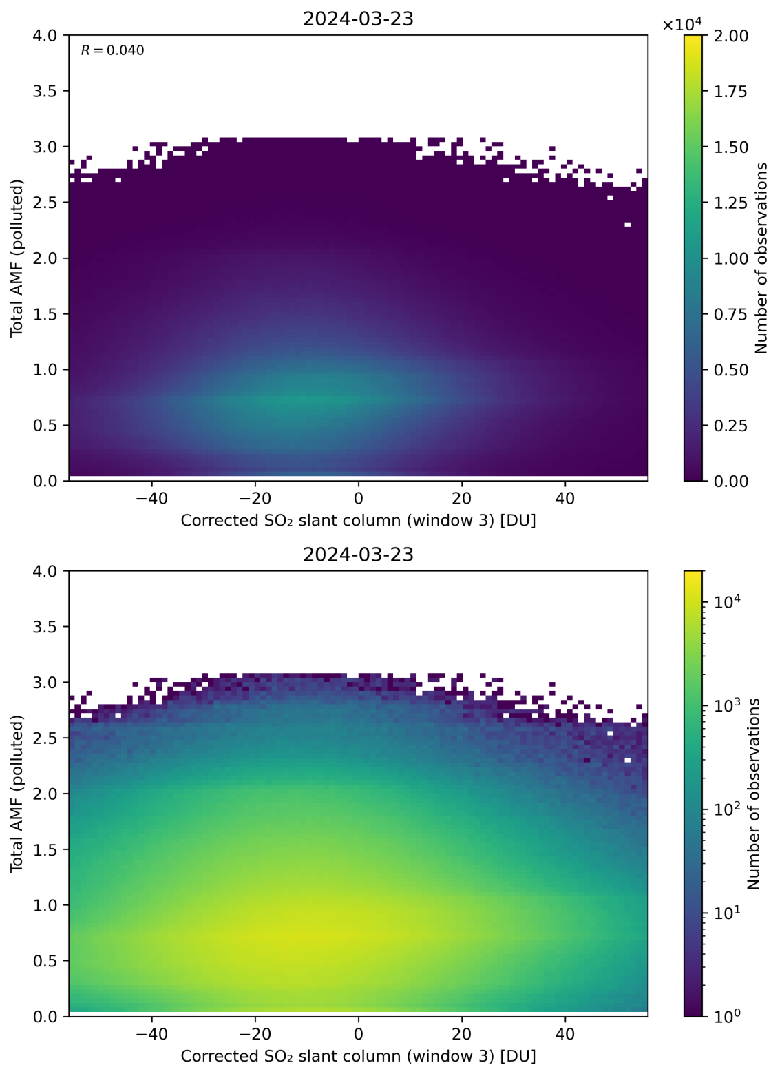
Figure 210: Scatter density plot of “Corrected SO 2 slant column (window 3)” against “Total AMF (polluted)” for 2024-03-23 to 2024-03-24.
