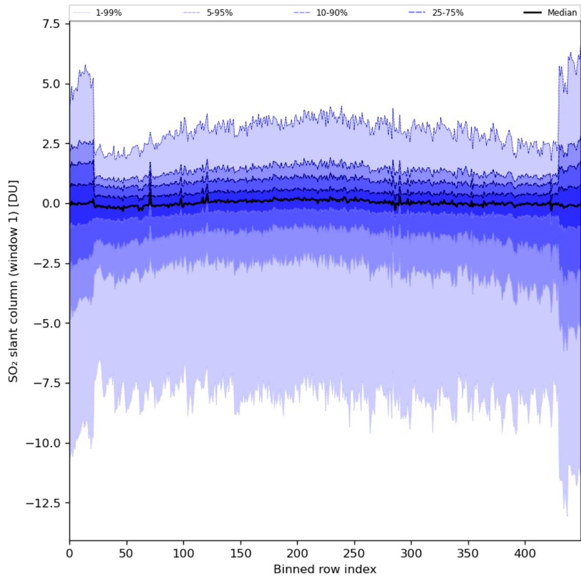
Figure 79: Along track statistics of “SO 2 slant column (window 1)” for 2024-03-23 to 2024-03-24
