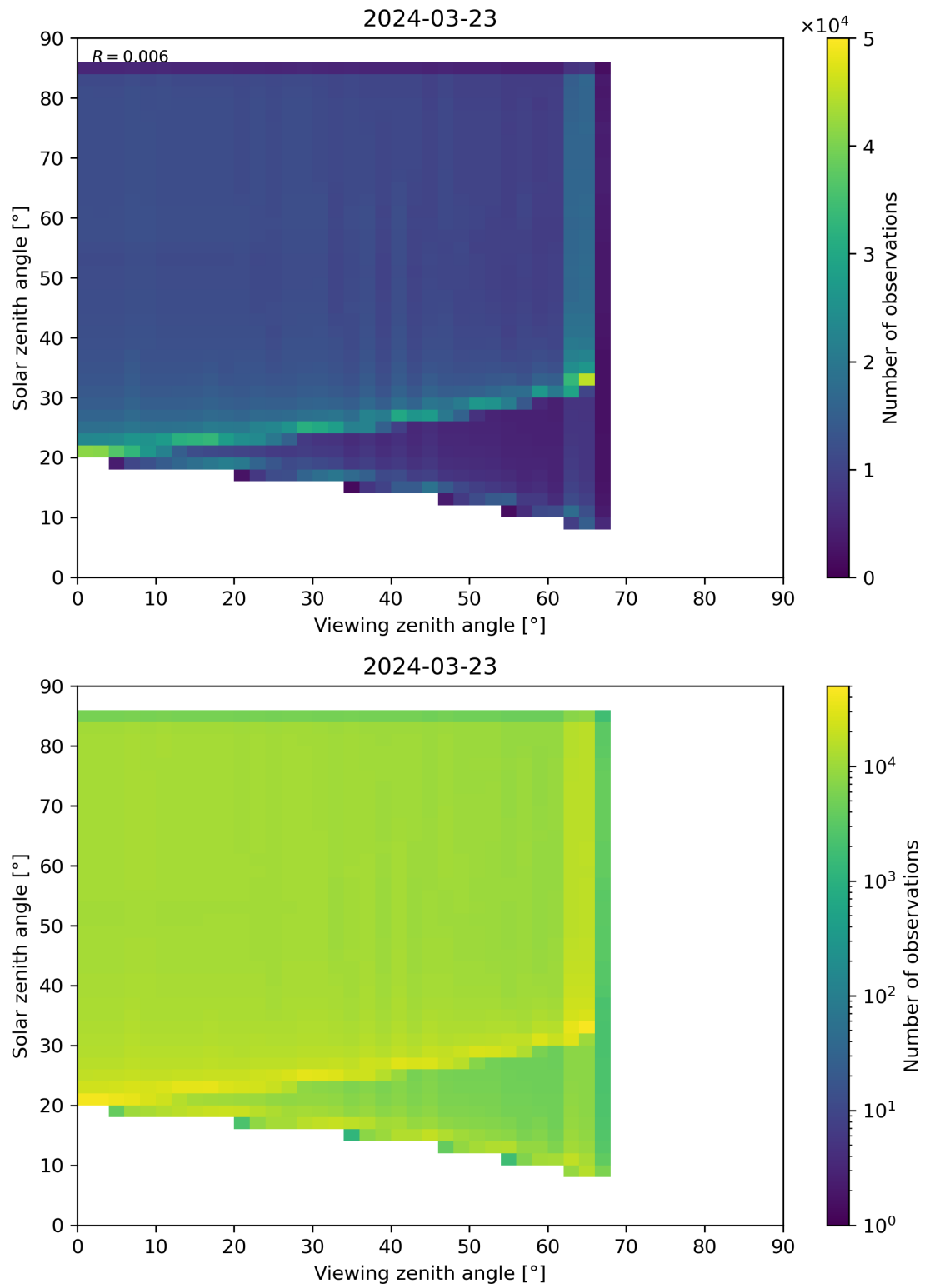
Figure 315: Scatter density plot of “Viewing zenith angle” against “Solar zenith angle” for 2024-03-23 to 2024-03-24.
