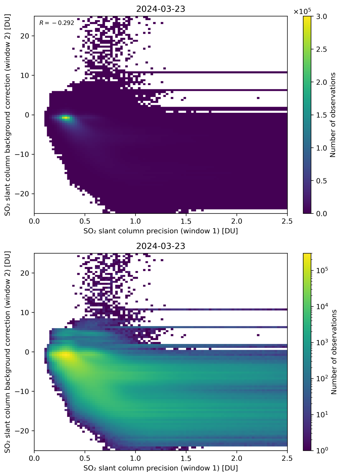
Figure 219: Scatter density plot of “SO 2 slant column precision (window 1)” against “SO 2 slant column background correction (window 2)” for 2024-03-23 to 2024-03-24.
