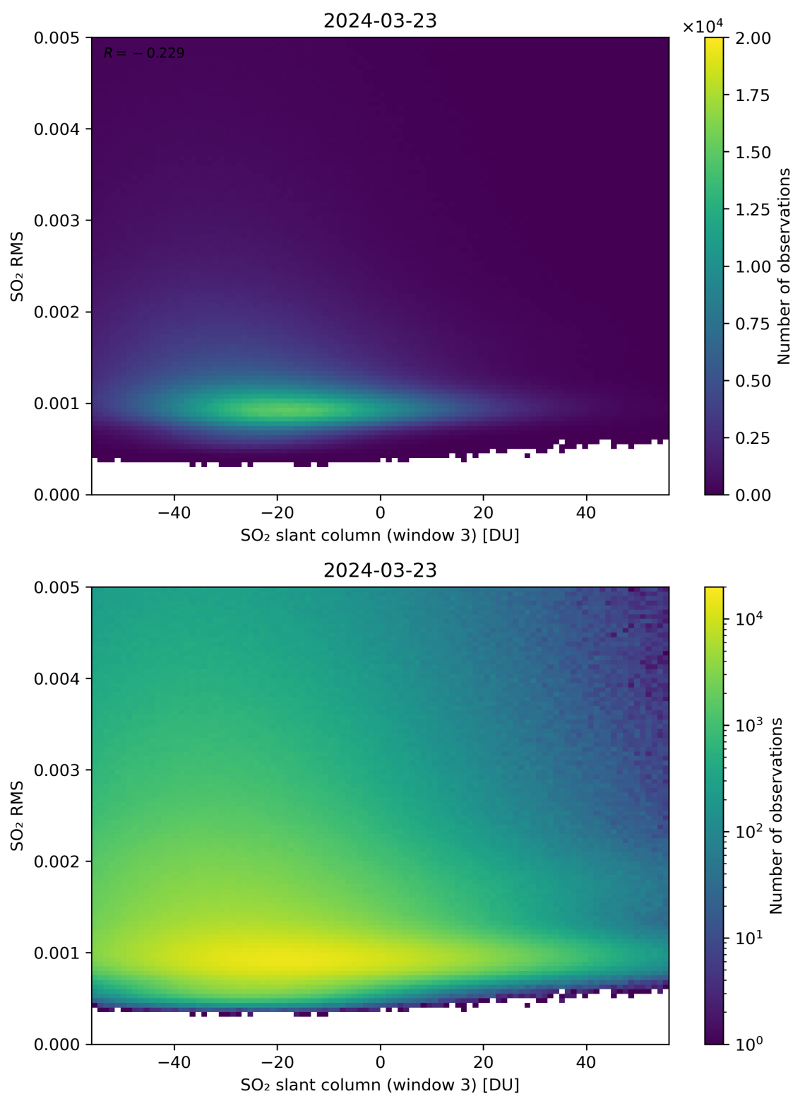
Figure 256: Scatter density plot of “SO 2 slant column (window 3)” against “SO 2 RMS” for 2024-03-23 to 2024-03-24.
