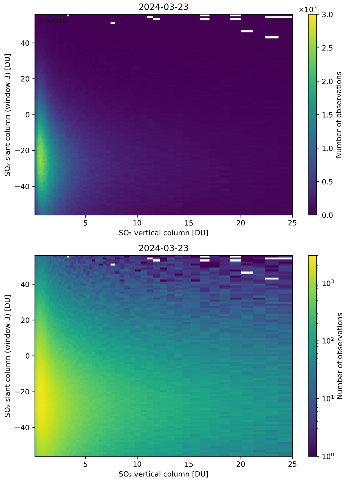
Figure 303: Scatter density plot of “SO 2 vertical column” against “SO 2 slant column (window 3)” for 2024-03-23 to 2024-03-24.
