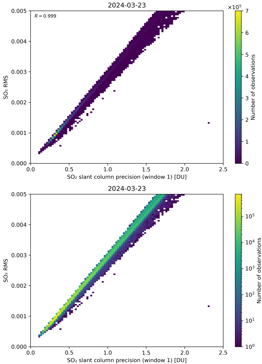
Figure 223: Scatter density plot of “SO 2 slant column precision (window 1)” against “SO 2 RMS” for 2024-03-23 to 2024-03-24.
