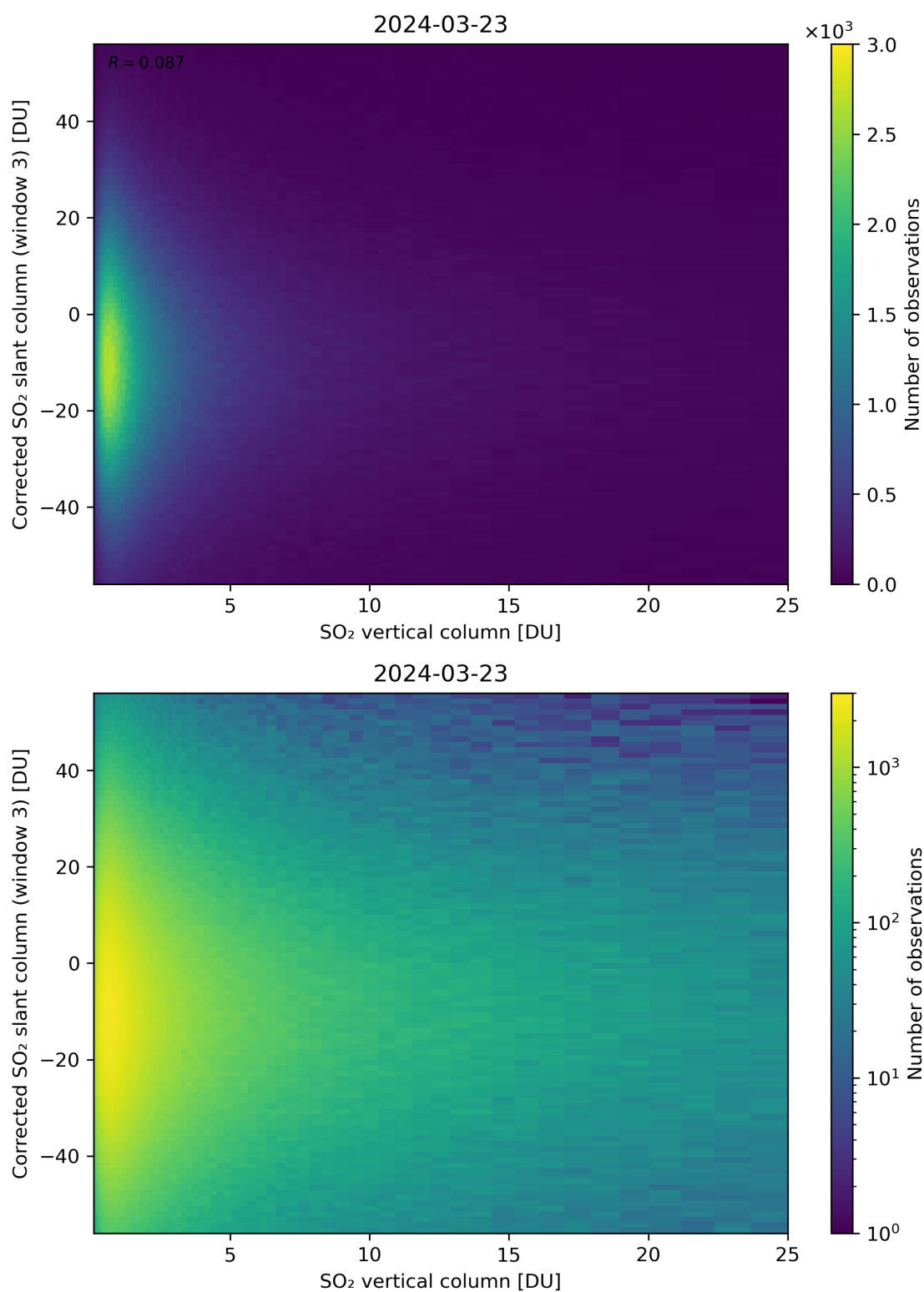
Figure 299: Scatter density plot of “SO 2 vertical column” against “Corrected SO 2 slant column (window 3)” for 2024-03-23 to 2024-03-24.
