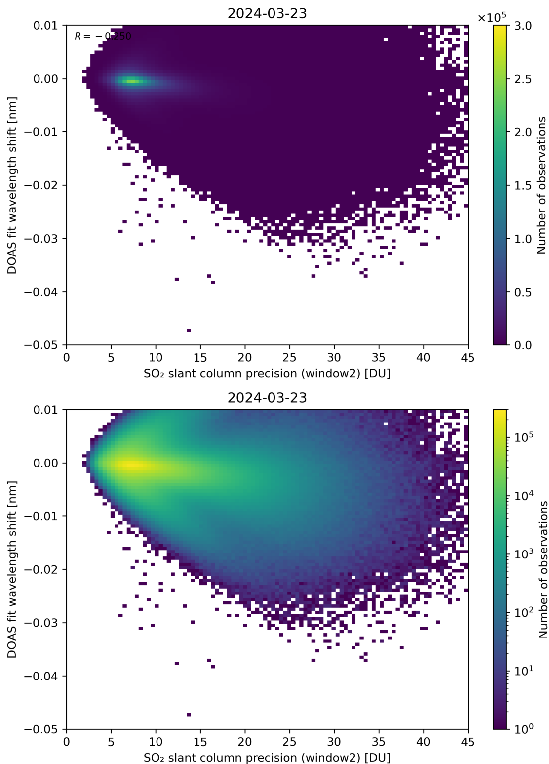
Figure 243: Scatter density plot of “SO 2 slant column precision (window2)” against “DOAS fit wavelength shift” for 2024-03-23 to 2024-03-24.
