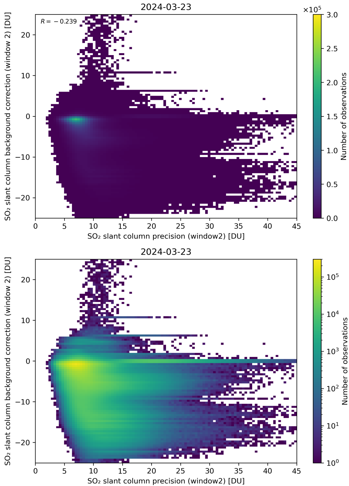
Figure 241: Scatter density plot of “SO 2 slant column precision (window2)” against “SO 2 slant column background correction (window 2)” for 2024-03-23 to 2024-03-24.
