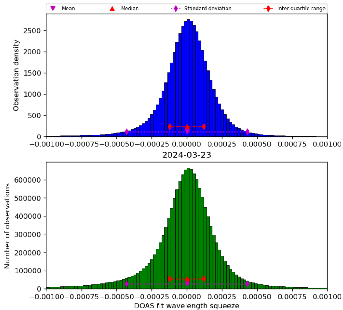
Figure 69: Histogram of “DOAS fit wavelength squeeze” for 2024-03-23 to 2024-03-24
