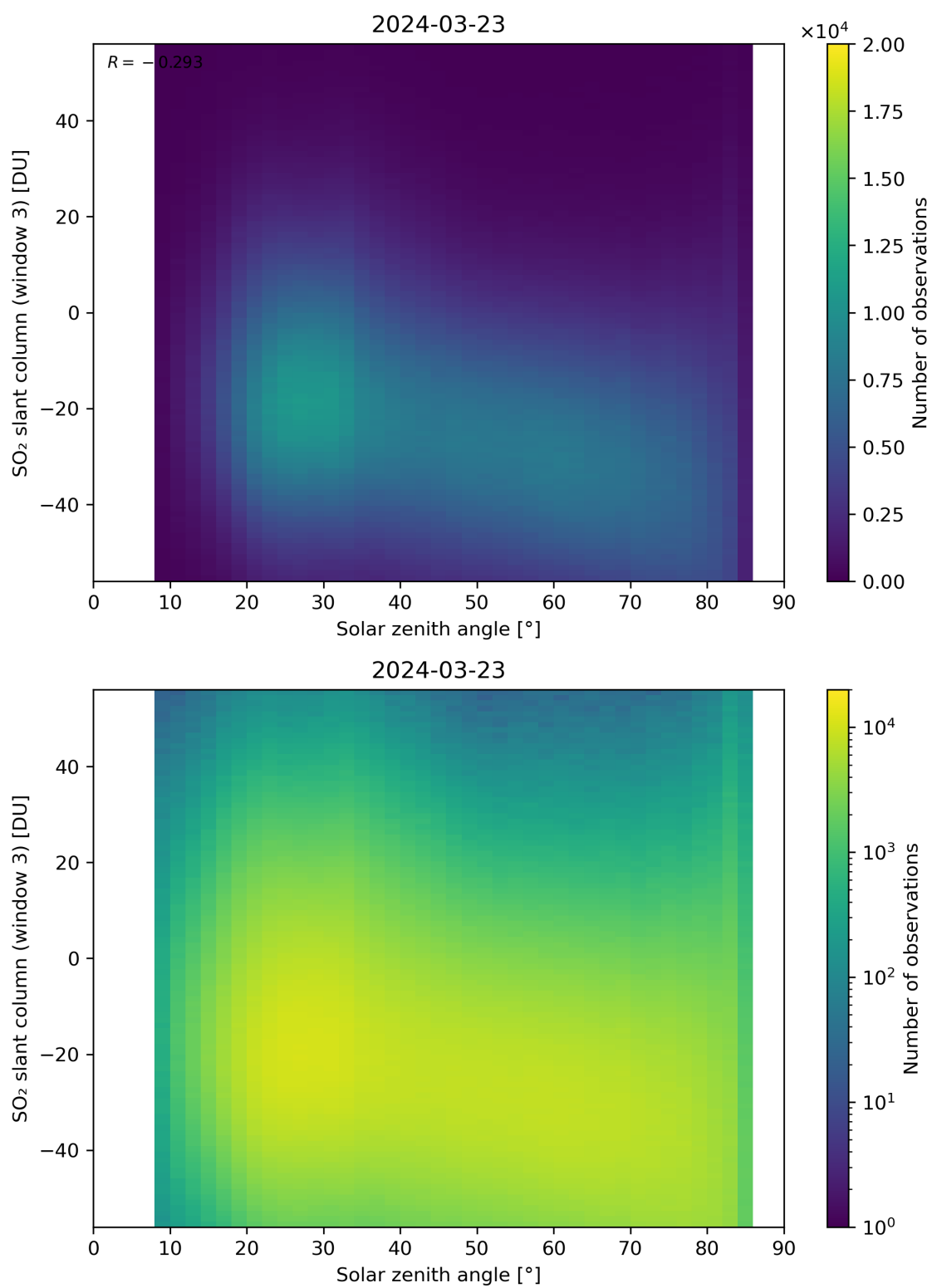
Figure 172: Scatter density plot of “Solar zenith angle” against “SO 2 slant column (window 3)” for 2024-03-23 to 2024-03-24.
