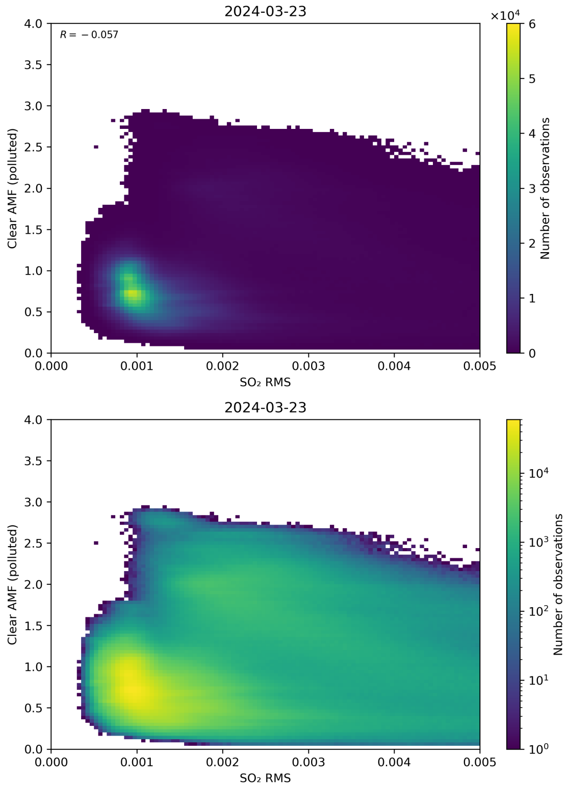
Figure 136: Scatter density plot of “SO 2 RMS” against “Clear AMF (polluted)” for 2024-03-23 to 2024-03-24.
