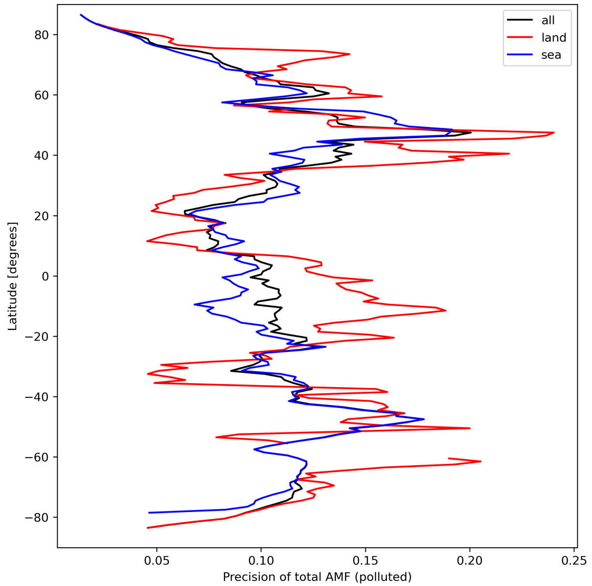
Figure 49: Zonal average of “Precision of total AMF (polluted)” for 2024-03-23 to 2024-03-24.
