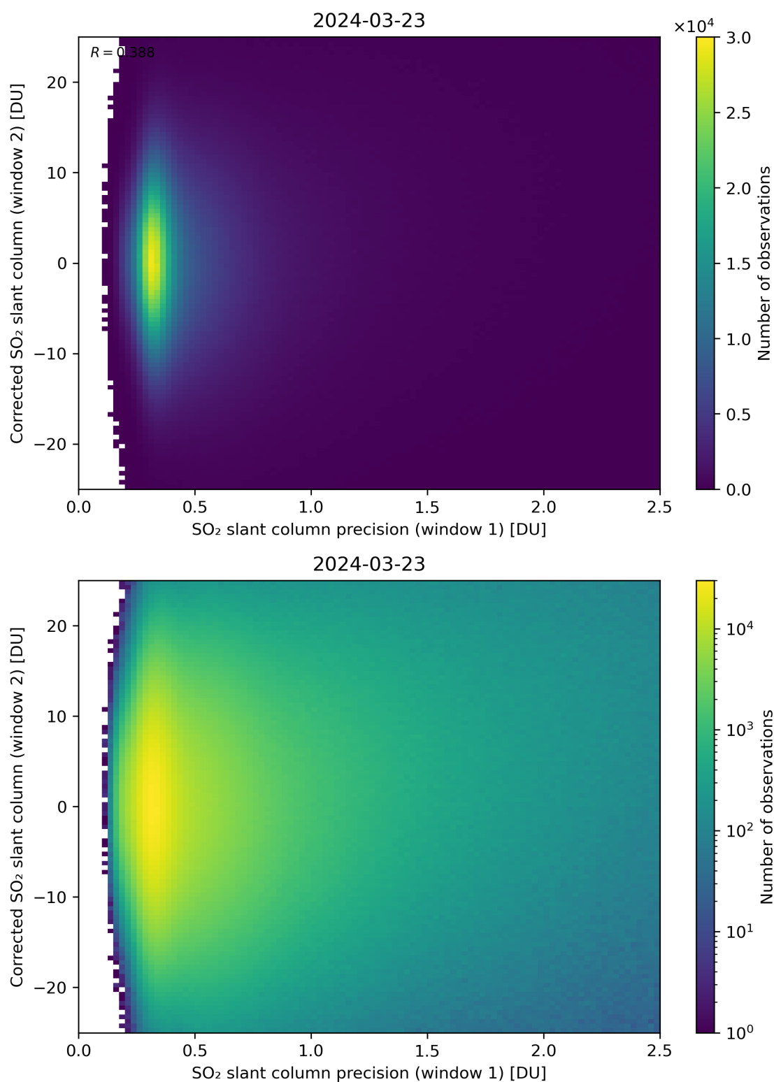
Figure 225: Scatter density plot of “SO 2 slant column precision (window 1)” against “Corrected SO 2 slant column (window 2)” for 2024-03-23 to 2024-03-24.
