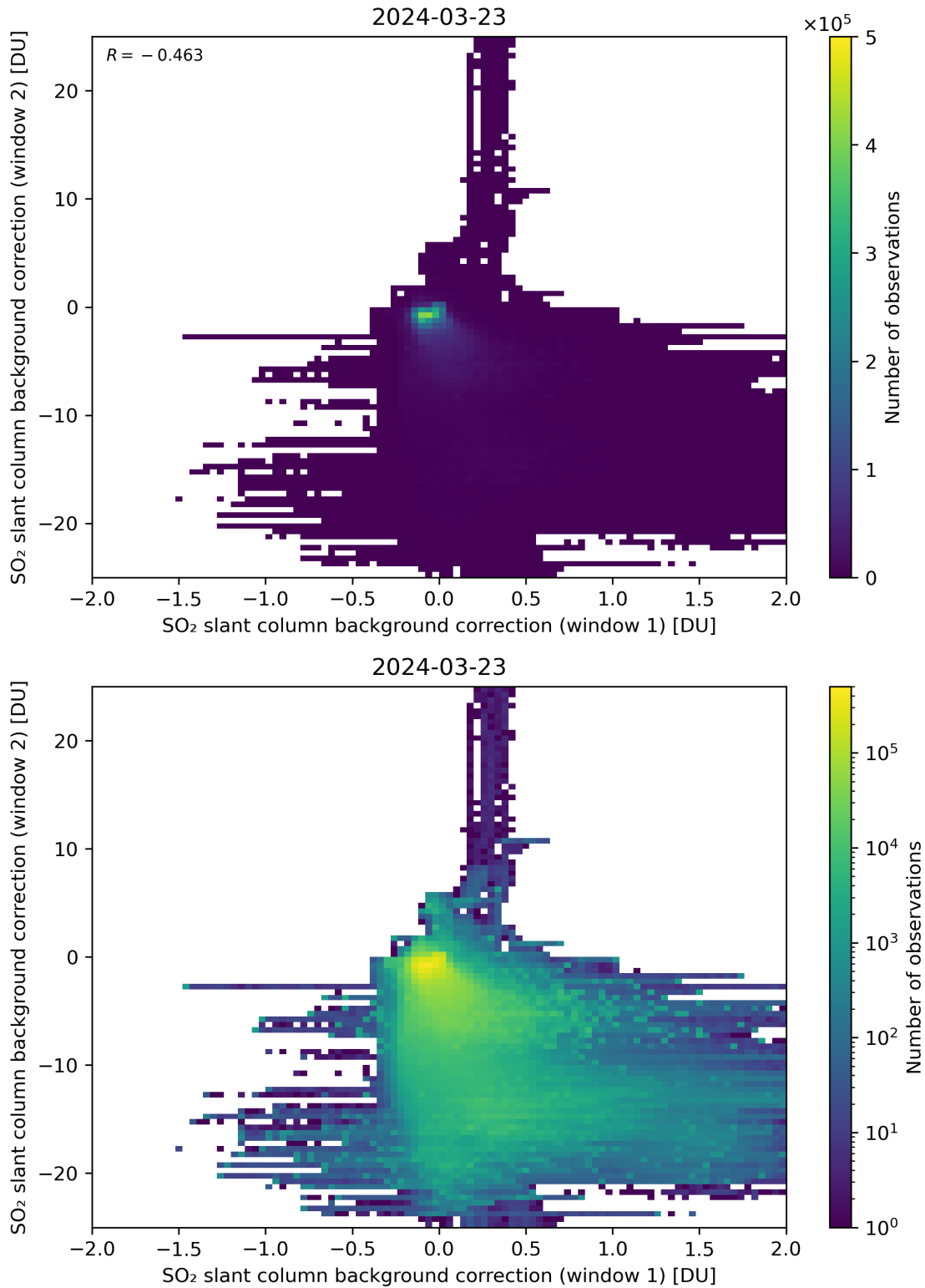
Figure 98: Scatter density plot of “SO 2 slant column background correction (window 1)” against “SO 2 slant column background correction (window 2)” for 2024-03-23 to 2024-03-24.
