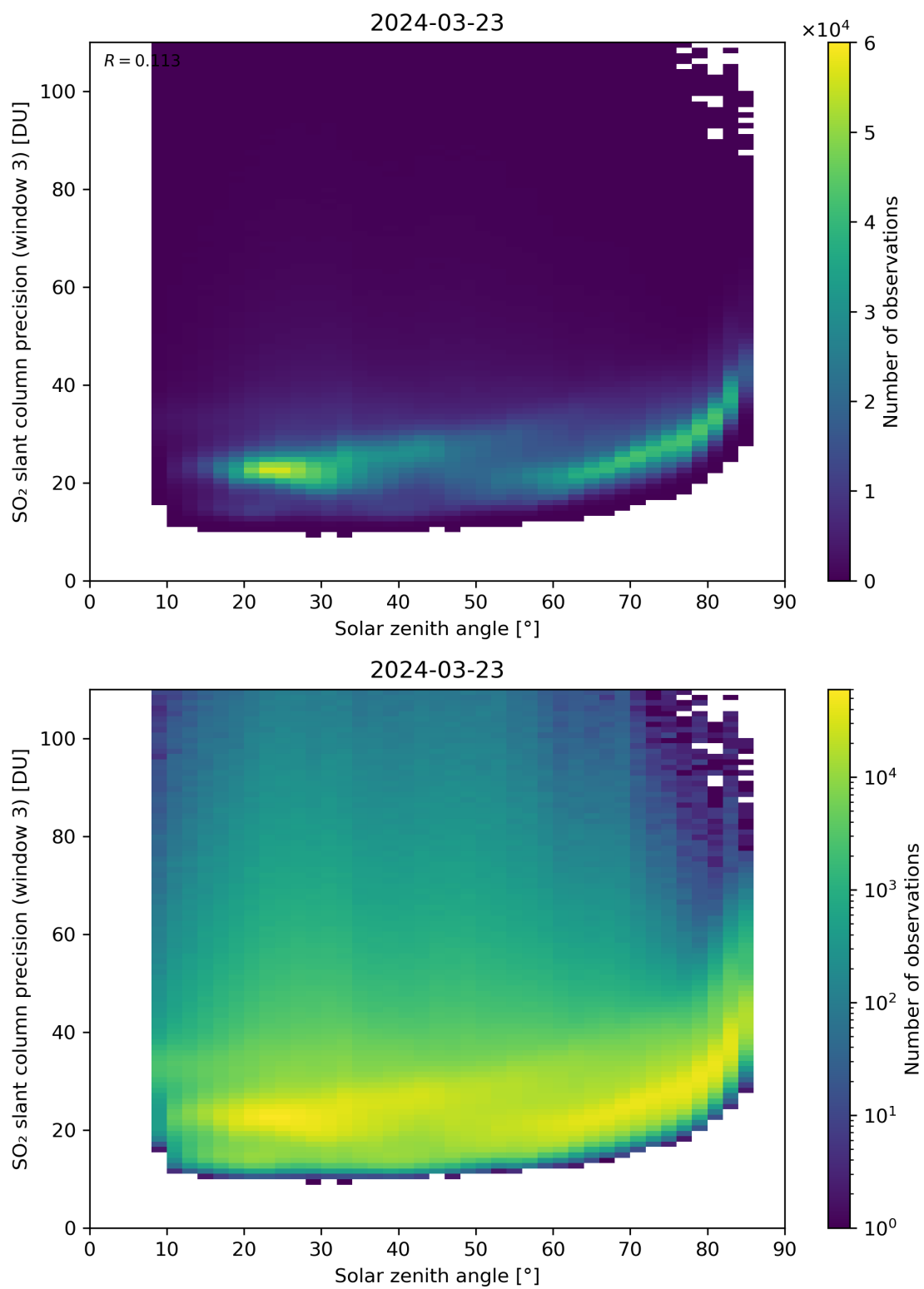
Figure 173: Scatter density plot of “Solar zenith angle” against “SO 2 slant column precision (window 3)” for 2024-03-23 to 2024-03-24.
