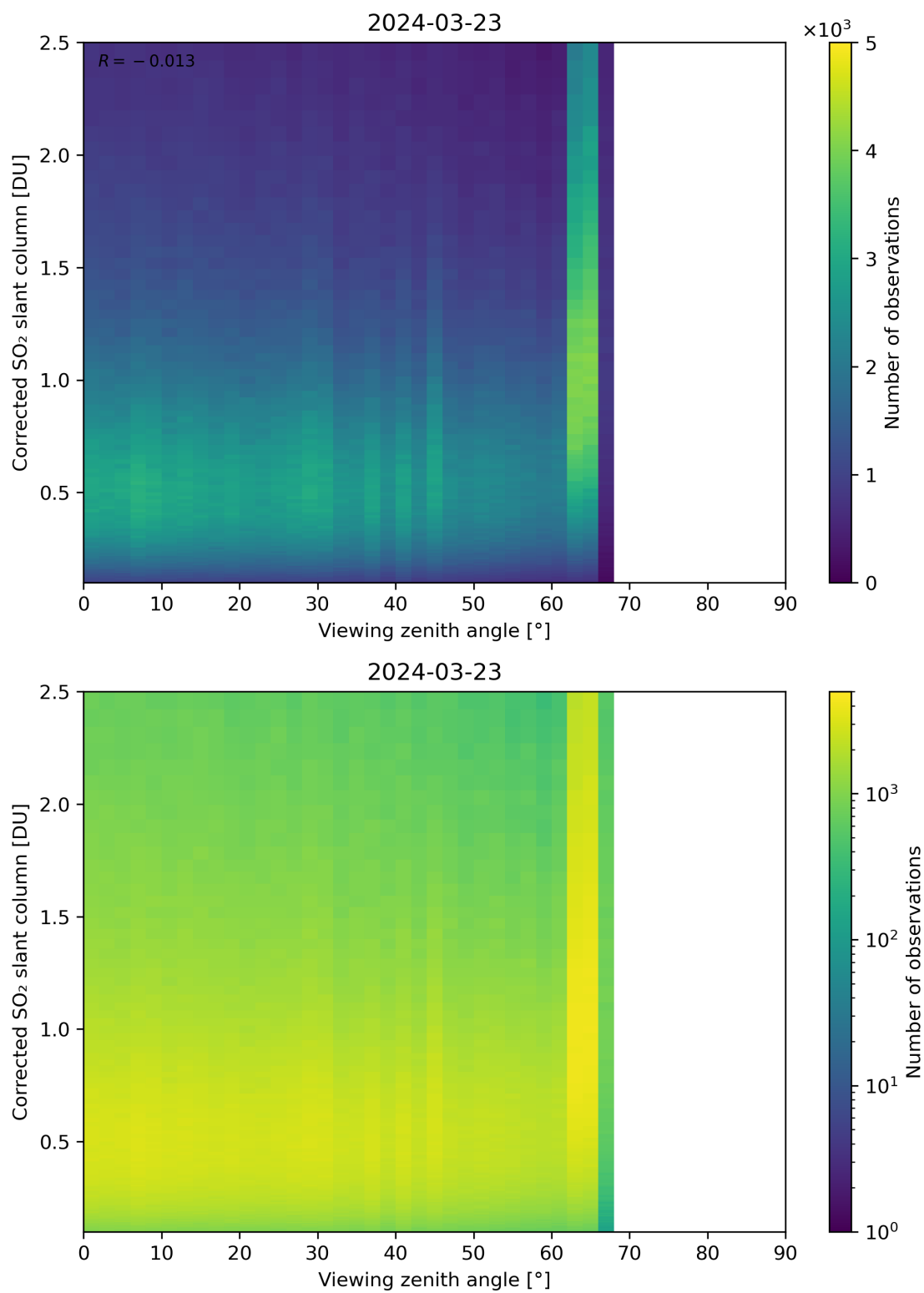
Figure 317: Scatter density plot of “Viewing zenith angle” against “Corrected SO 2 slant column” for 2024-03-23 to 2024-03-24.
