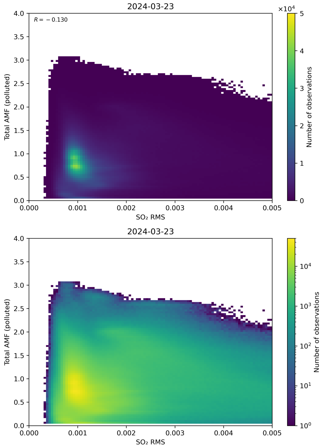
Figure 137: Scatter density plot of “SO 2 RMS” against “Total AMF (polluted)” for 2024-03-23 to 2024-03-24.
