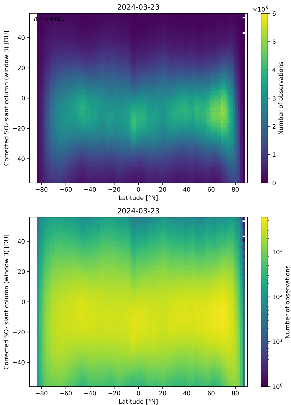
Figure 148: Scatter density plot of “Latitude” against “Corrected SO 2 slant column (window 3)” for 2024-03-23 to 2024-03-24.
