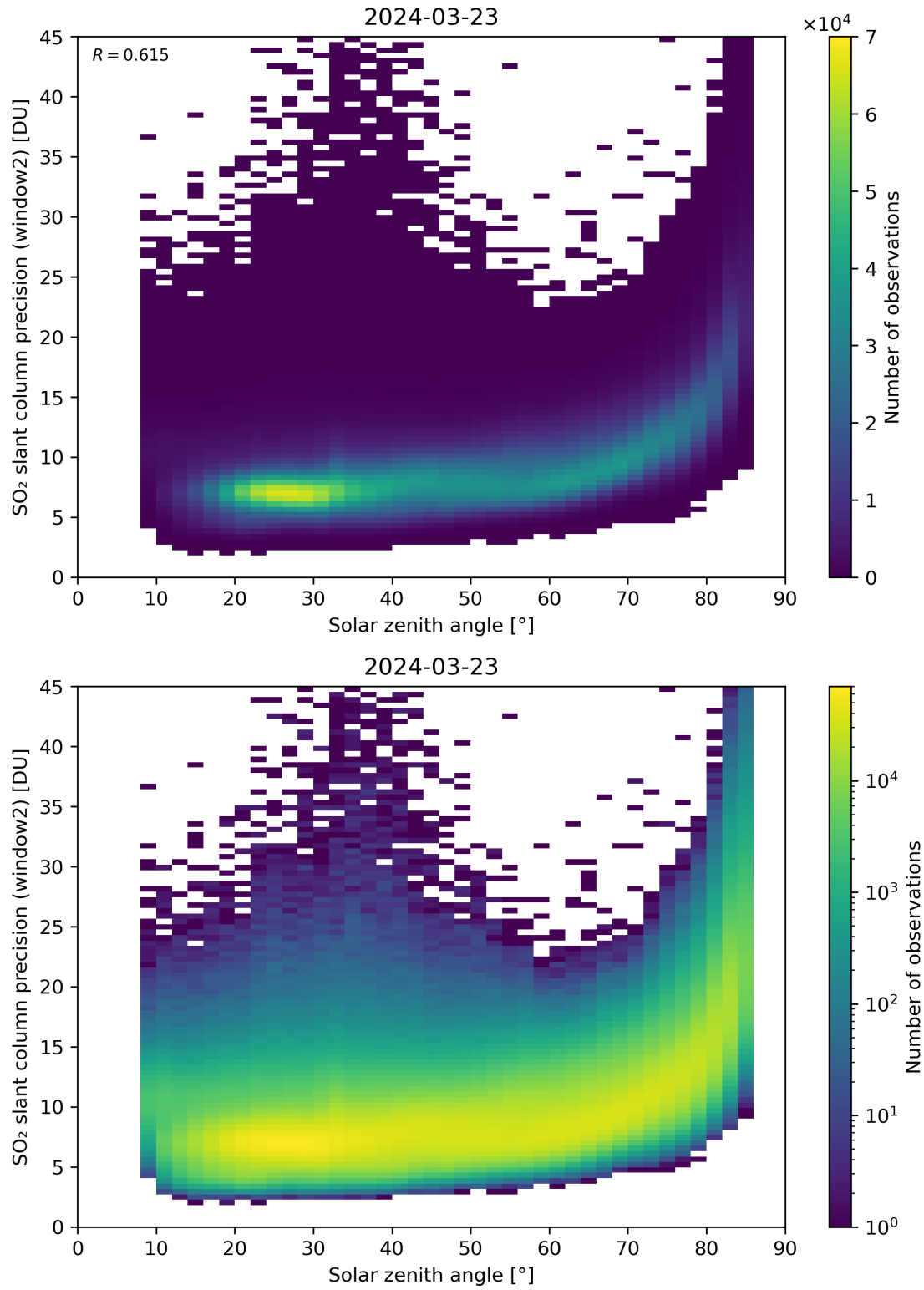
Figure 171: Scatter density plot of “Solar zenith angle” against “SO 2 slant column precision (window2)” for 2024-03-23 to 2024-03-24.
