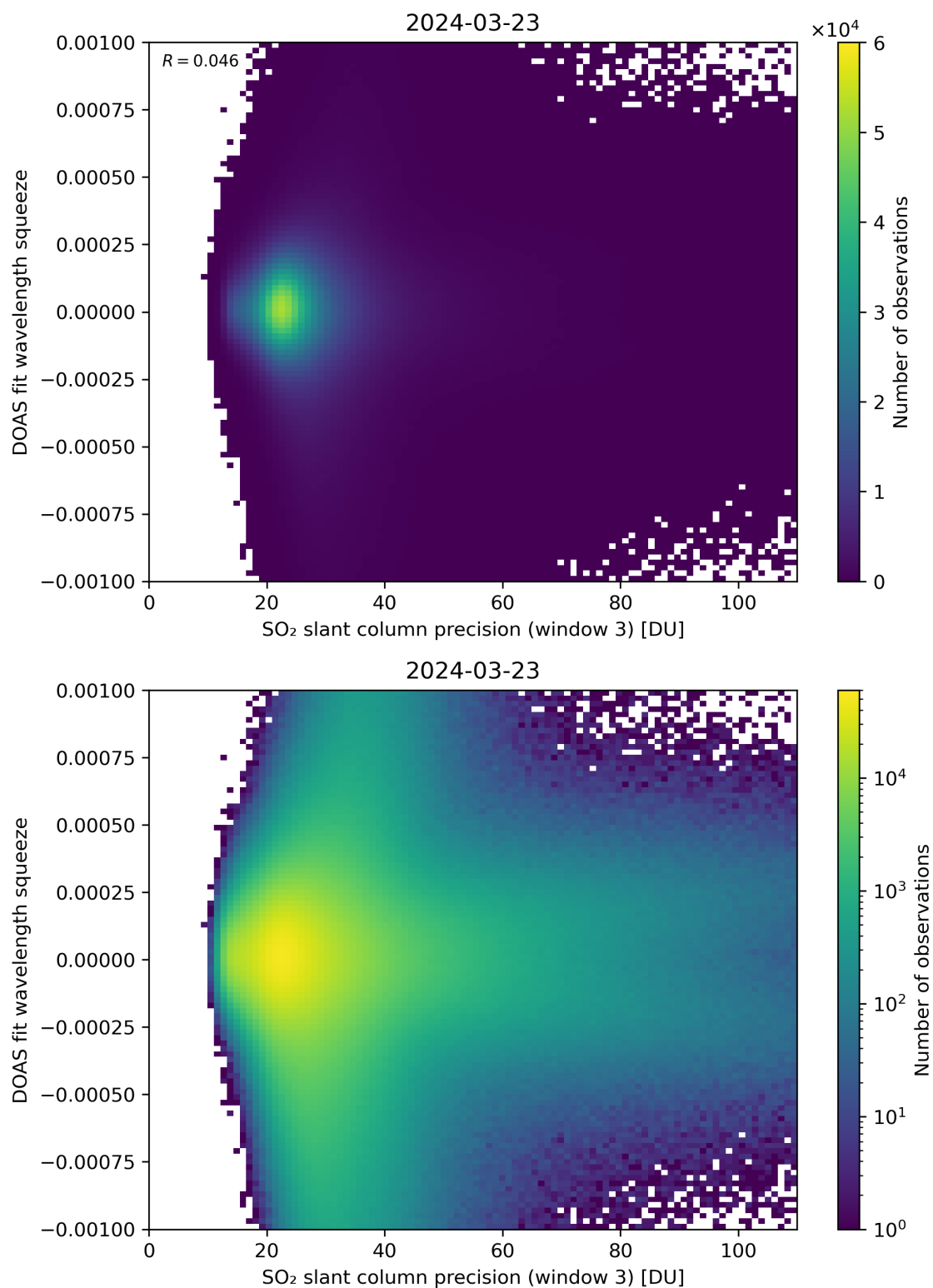
Figure 259: Scatter density plot of “SO 2 slant column precision (window 3)” against “DOAS fit wavelength squeeze” for 2024-03-23 to 2024-03-24.
