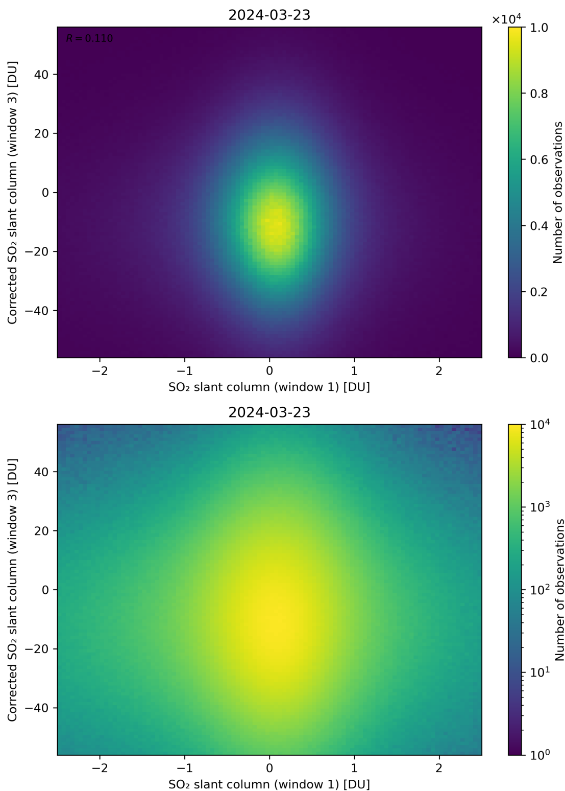
Figure 234: Scatter density plot of “SO 2 slant column (window 1)” against “Corrected SO 2 slant column (window 3)” for 2024-03-23 to 2024-03-24.
