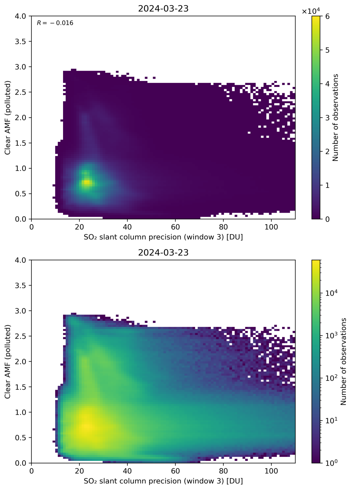
Figure 261: Scatter density plot of “SO 2 slant column precision (window 3)” against “Clear AMF (polluted)” for 2024-03-23 to 2024-03-24.
