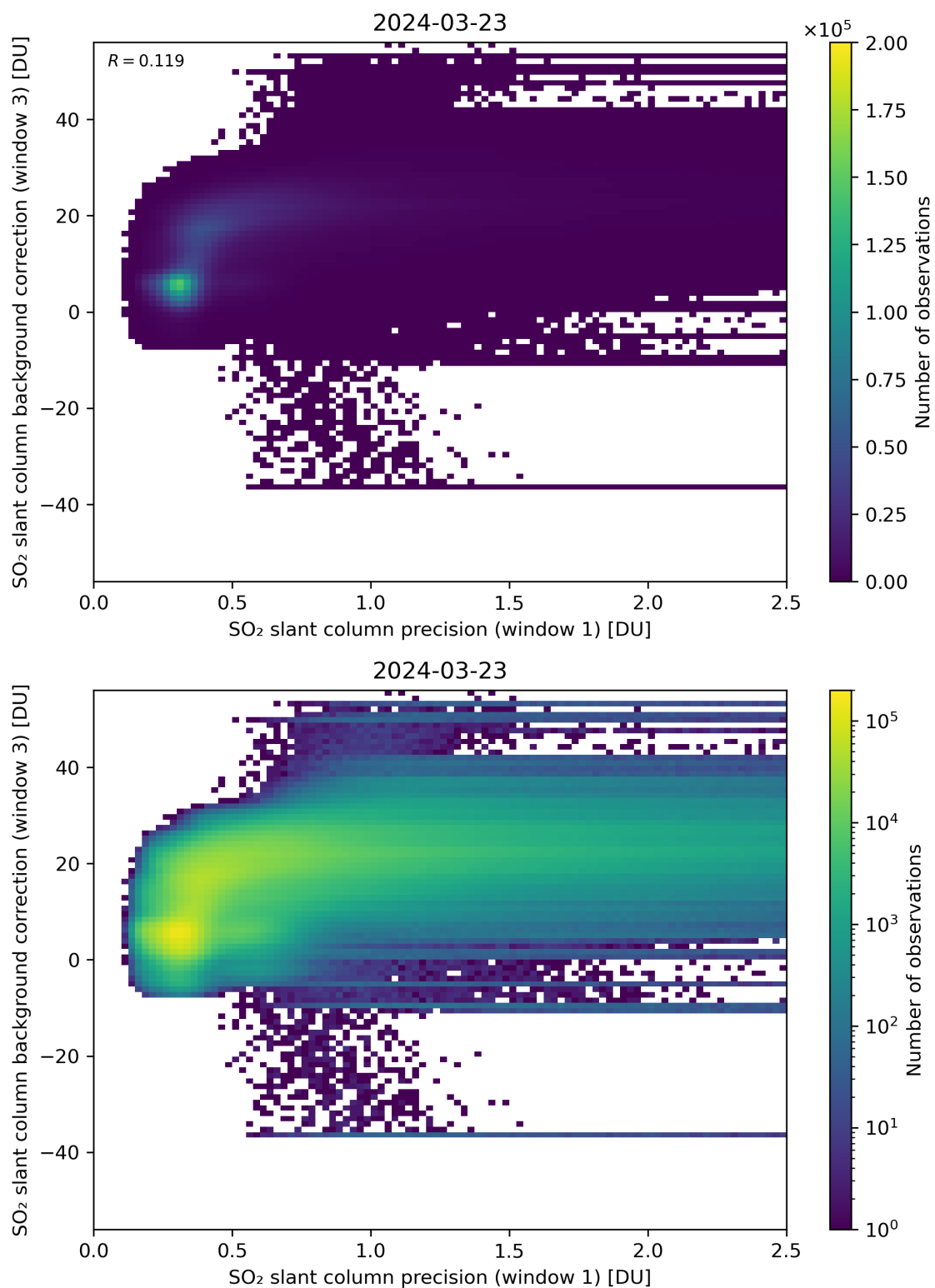
Figure 220: Scatter density plot of “SO 2 slant column precision (window 1)” against “SO 2 slant column background correction (window 3)” for 2024-03-23 to 2024-03-24.
