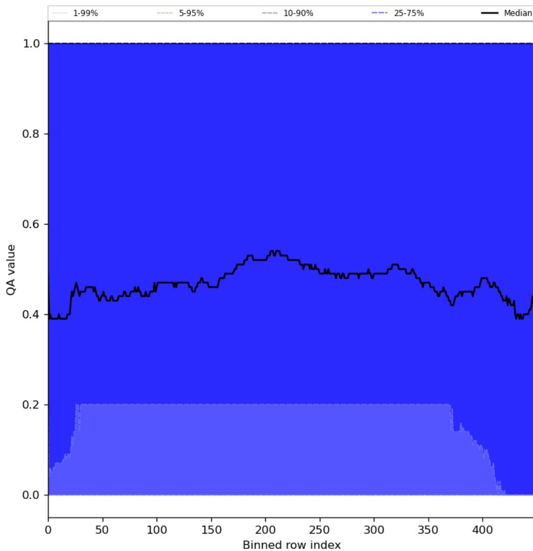
Figure 75: Along track statistics of “QA value” for 2024-03-23 to 2024-03-24
