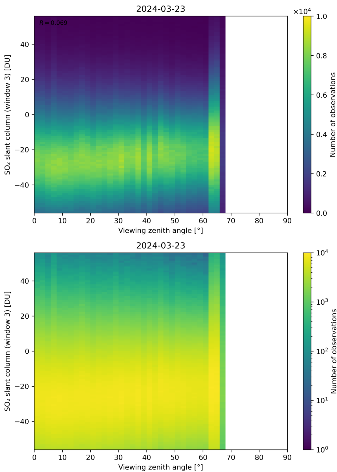
Figure 323: Scatter density plot of “Viewing zenith angle” against “SO 2 slant column (window 3)” for 2024-03-23 to 2024-03-24.
