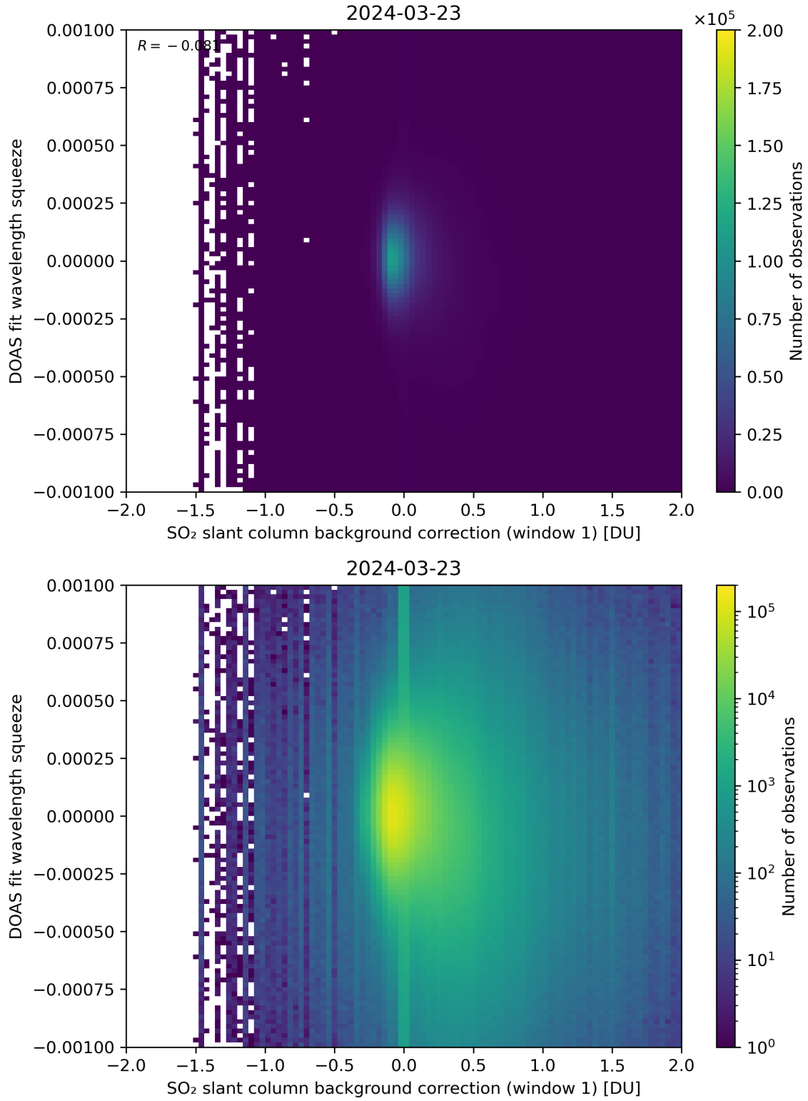
Figure 101: Scatter density plot of “SO 2 slant column background correction (window 1)” against “DOAS fit wavelength squeeze” for 2024-03-23 to 2024-03-24.
