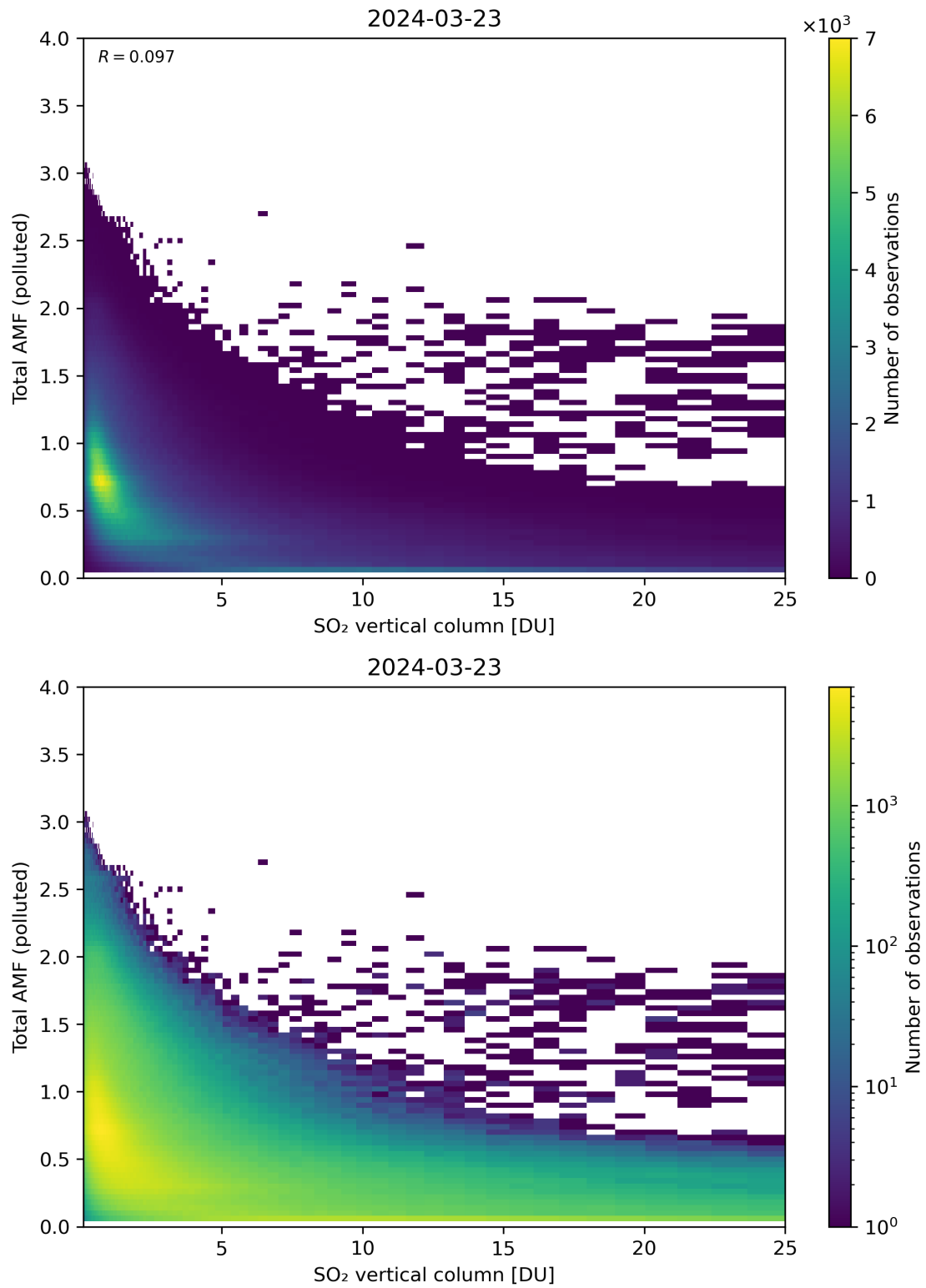
Figure 305: Scatter density plot of “SO 2 vertical column” against “Total AMF (polluted)” for 2024-03-23 to 2024-03-24.
