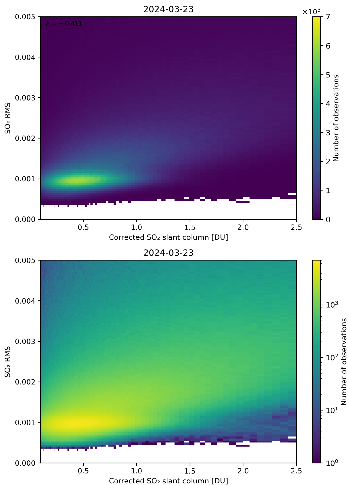
Figure 183: Scatter density plot of “Corrected SO 2 slant column” against “SO 2 RMS” for 2024-03-23 to 2024-03-24.
