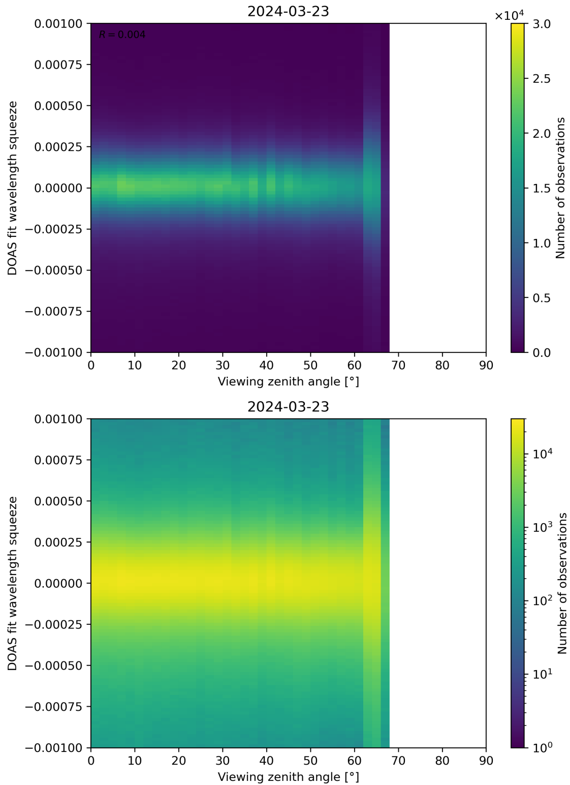
Figure 312: Scatter density plot of “Viewing zenith angle” against “DOAS fit wavelength squeeze” for 2024-03-23 to 2024-03-24.
