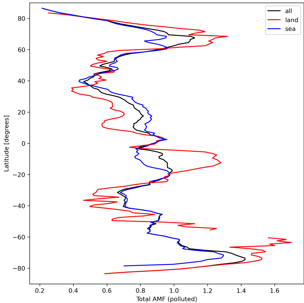
Figure 48: Zonal average of “Total AMF (polluted)” for 2024-03-23 to 2024-03-24.
