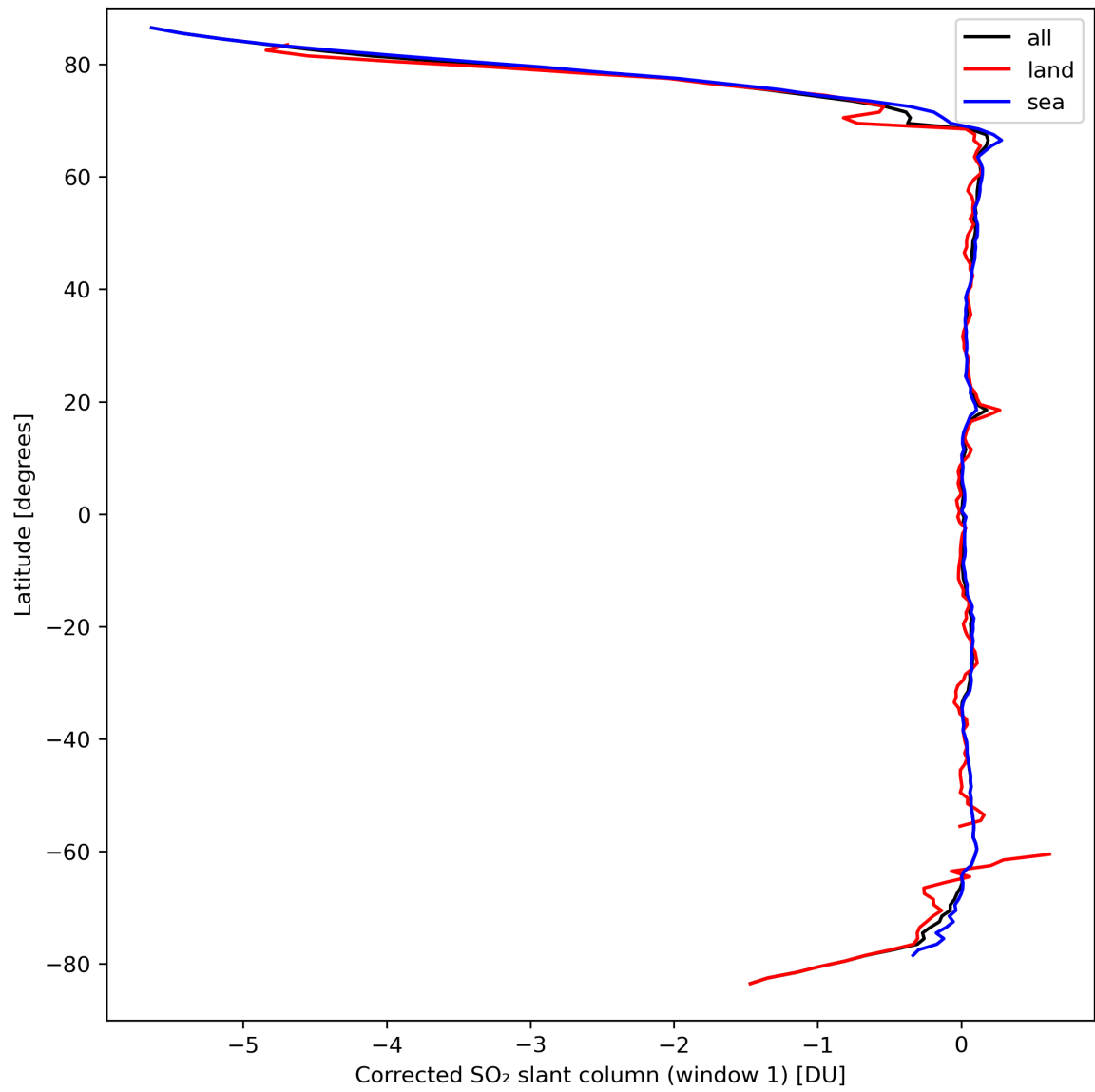
Figure 35: Zonal average of “Corrected SO 2 slant column (window 1)” for 2024-03-23 to 2024-03-24.
