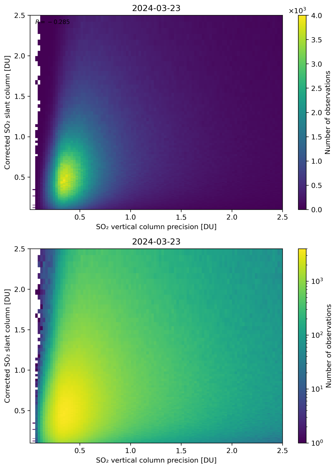
Figure 286: Scatter density plot of “SO 2 vertical column precision” against “Corrected SO 2 slant column” for 2024-03-23 to 2024-03-24.
