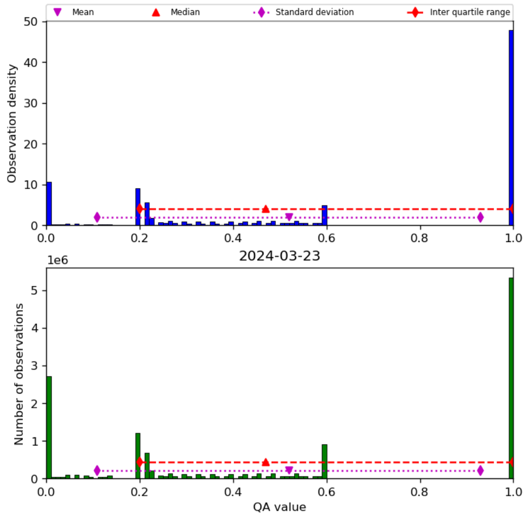
Figure 52: Histogram of “QA value” for 2024-03-23 to 2024-03-24
