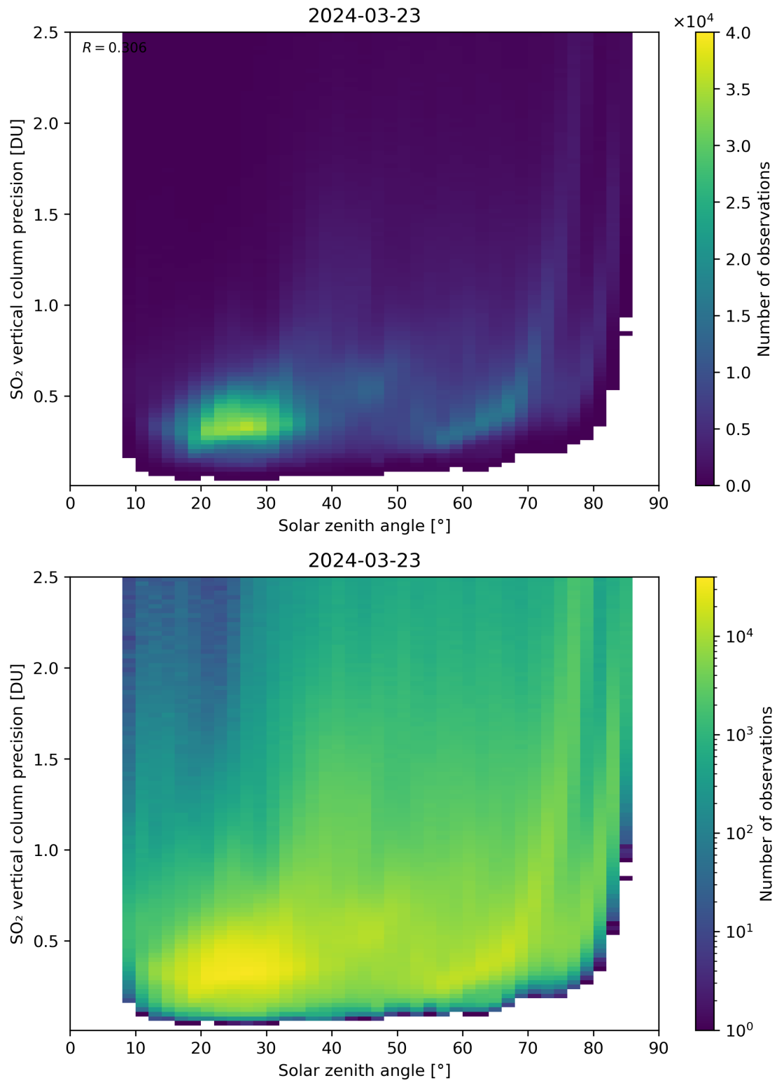
Figure 177: Scatter density plot of “Solar zenith angle” against “SO 2 vertical column precision” for 2024-03-23 to 2024-03-24.
