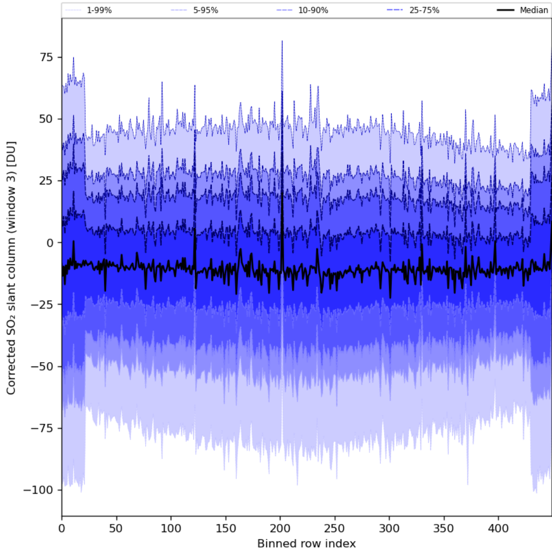
Figure 89: Along track statistics of “Corrected SO 2 slant column (window 3)” for 2024-03-23 to 2024-03-24
