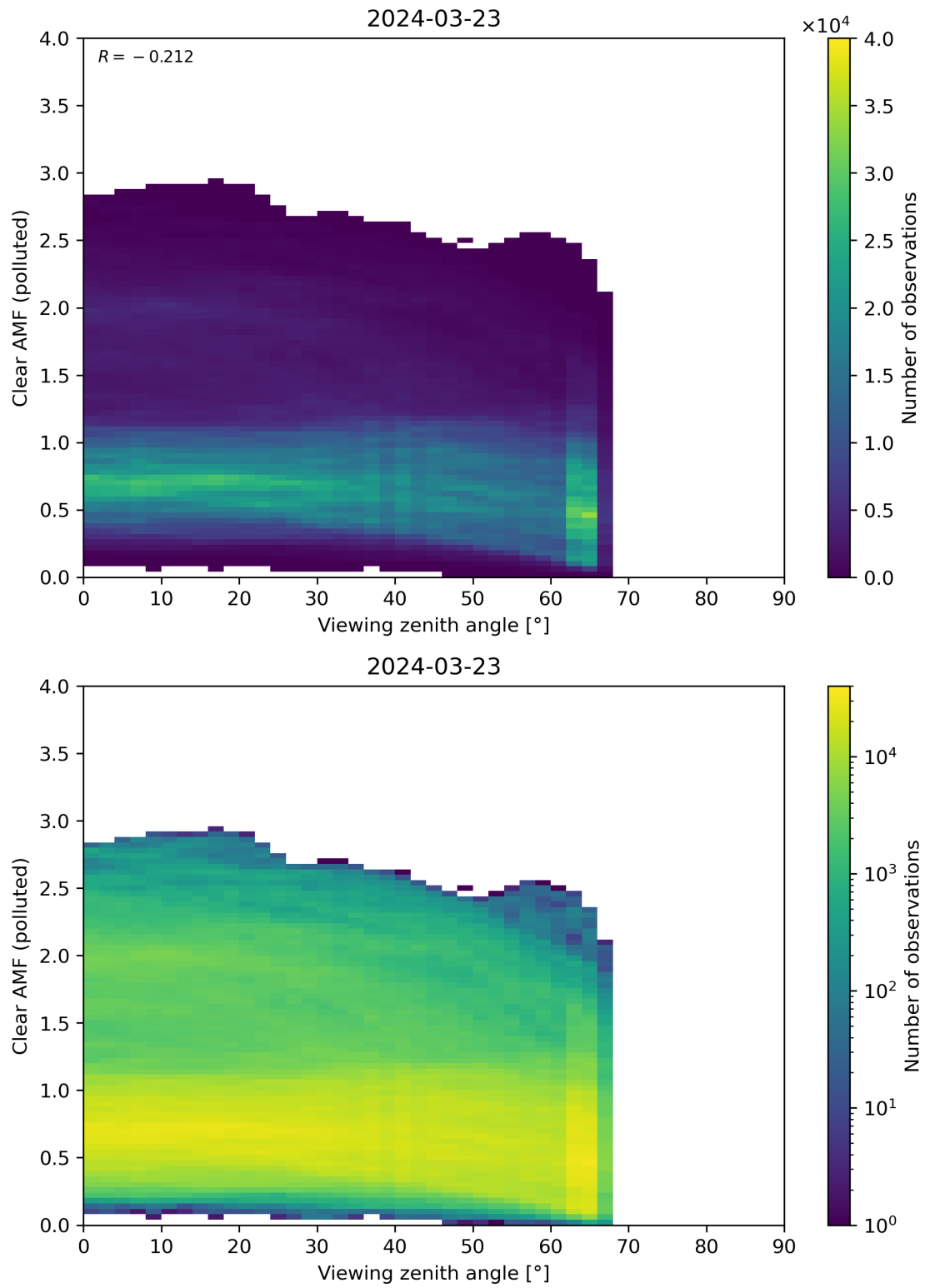
Figure 316: Scatter density plot of “Viewing zenith angle” against “Clear AMF (polluted)” for 2024-03-23 to 2024-03-24.
