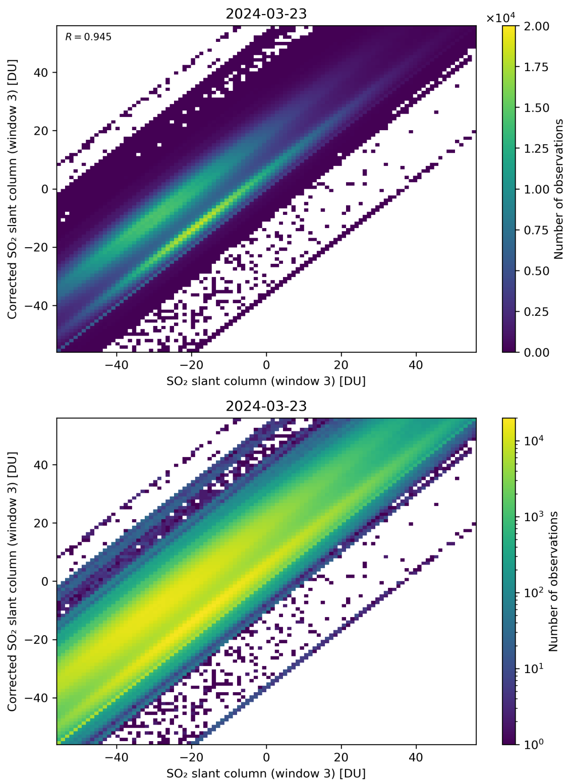
Figure 266: Scatter density plot of “SO 2 slant column (window 3)” against “Corrected SO 2 slant column (window 3)” for 2024-03-23 to 2024-03-24.
