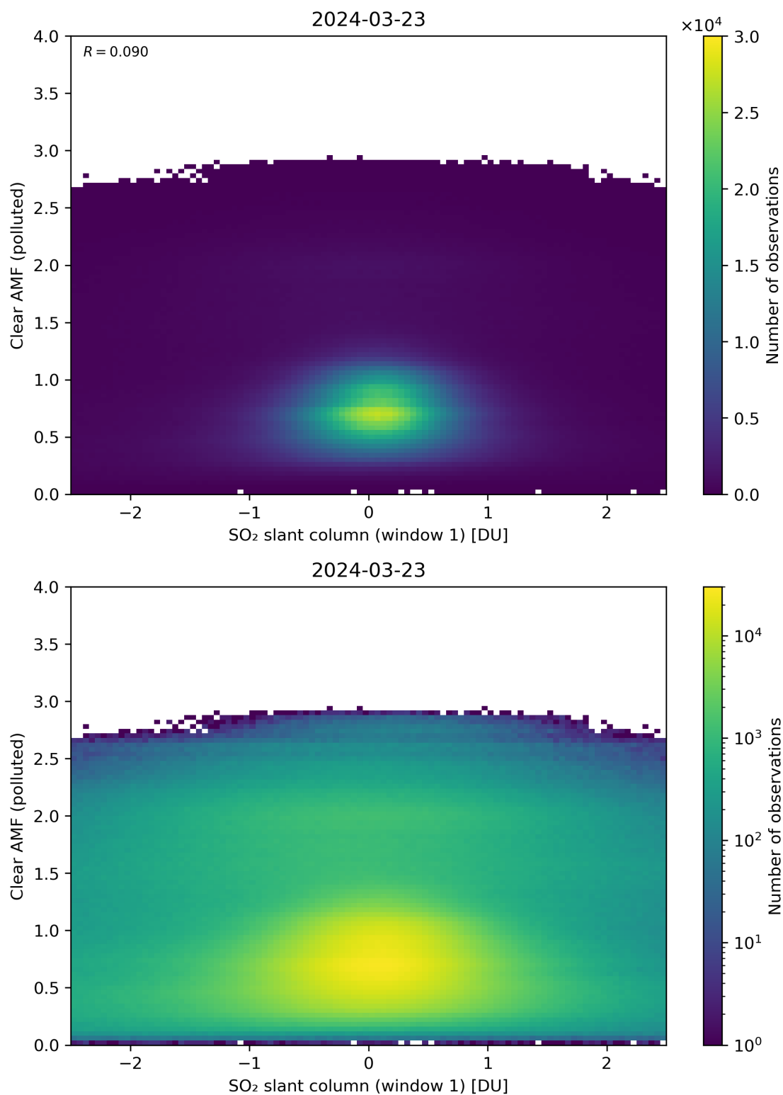
Figure 232: Scatter density plot of “SO 2 slant column (window 1)” against “Clear AMF (polluted)” for 2024-03-23 to 2024-03-24.
