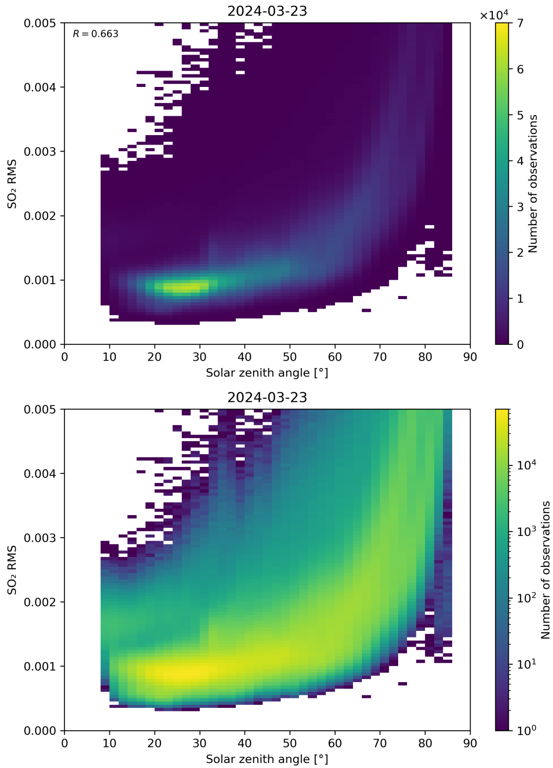
Figure 163: Scatter density plot of “Solar zenith angle” against “SO 2 RMS” for 2024-03-23 to 2024-03-24.
