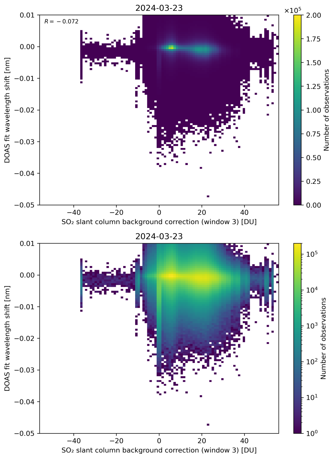
Figure 121: Scatter density plot of “SO 2 slant column background correction (window 3)” against “DOAS fit wavelength shift” for 2024-03-23 to 2024-03-24.
