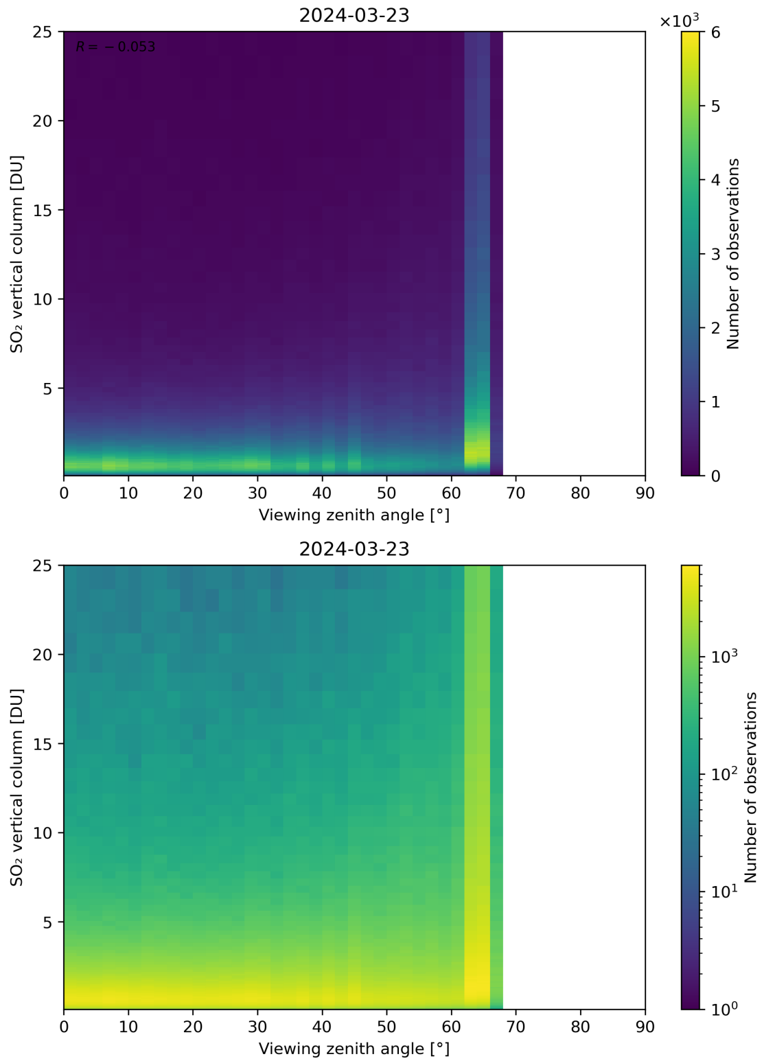
Figure 327: Scatter density plot of “Viewing zenith angle” against “SO 2 vertical column” for 2024-03-23 to 2024-03-24.
