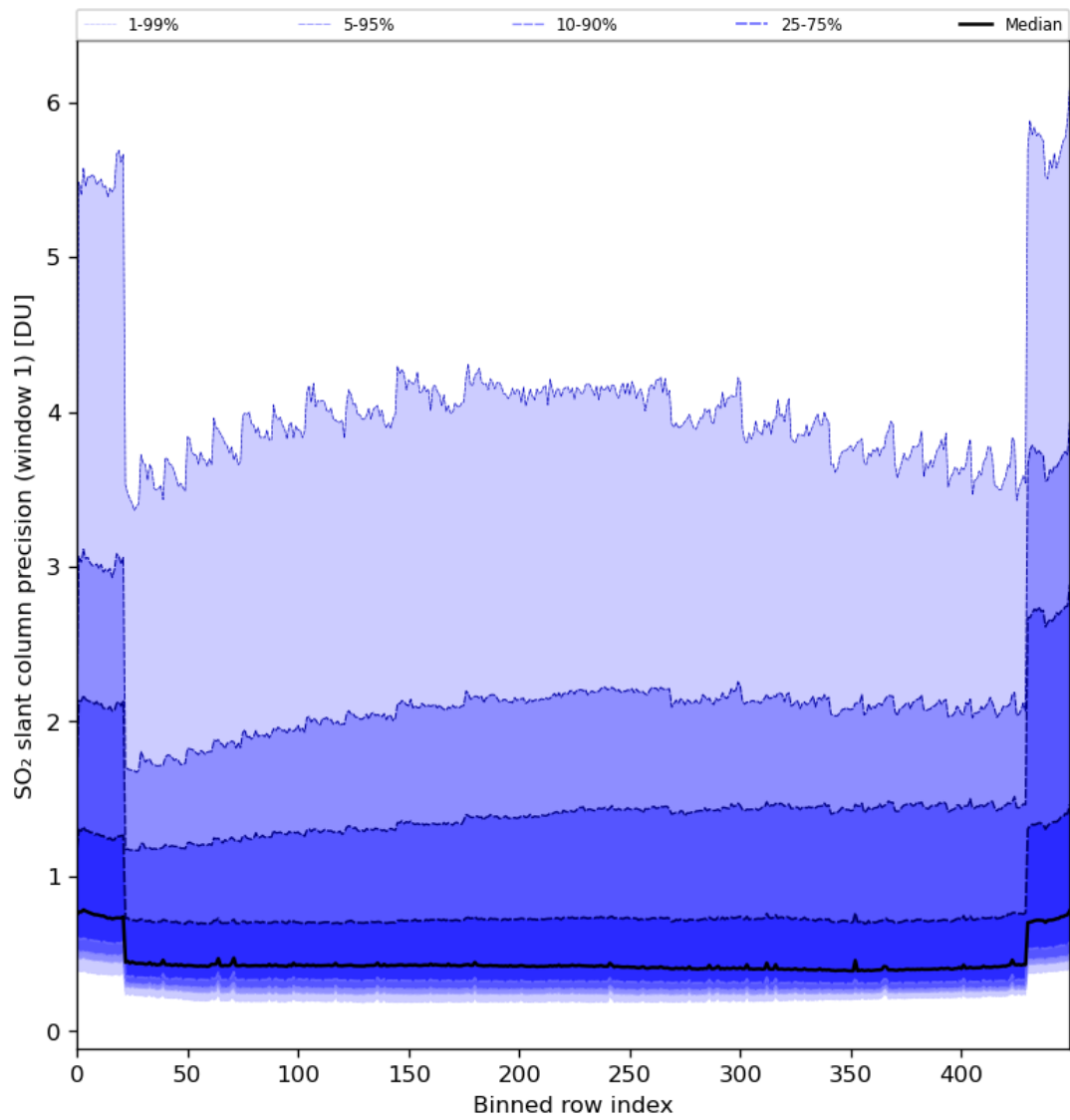
Figure 80: Along track statistics of “SO 2 slant column precision (window 1)” for 2024-03-23 to 2024-03-24
