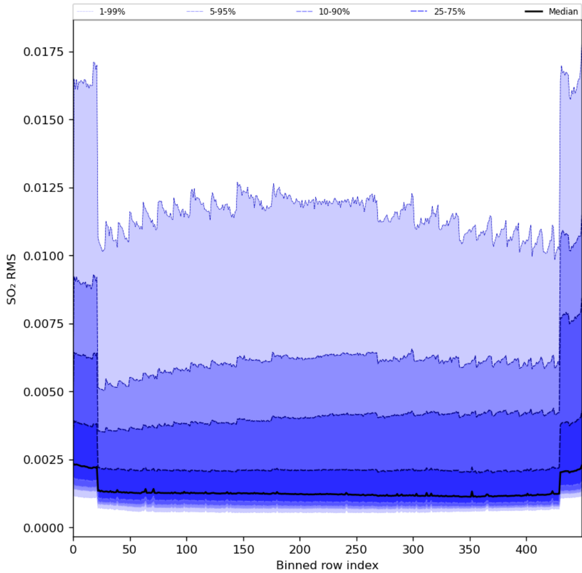
Figure 93: Along track statistics of “SO 2 RMS” for 2024-03-23 to 2024-03-24
