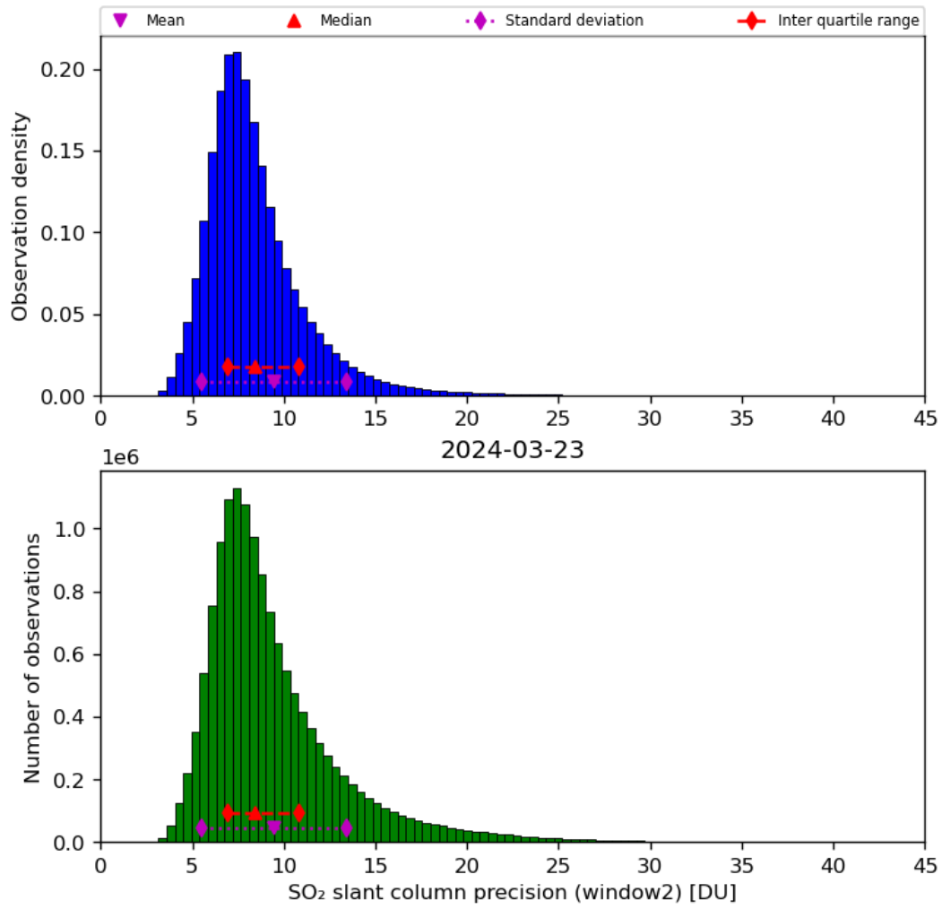
Figure 61: Histogram of “SO 2 slant column precision (window2)” for 2024-03-23 to 2024-03-24
