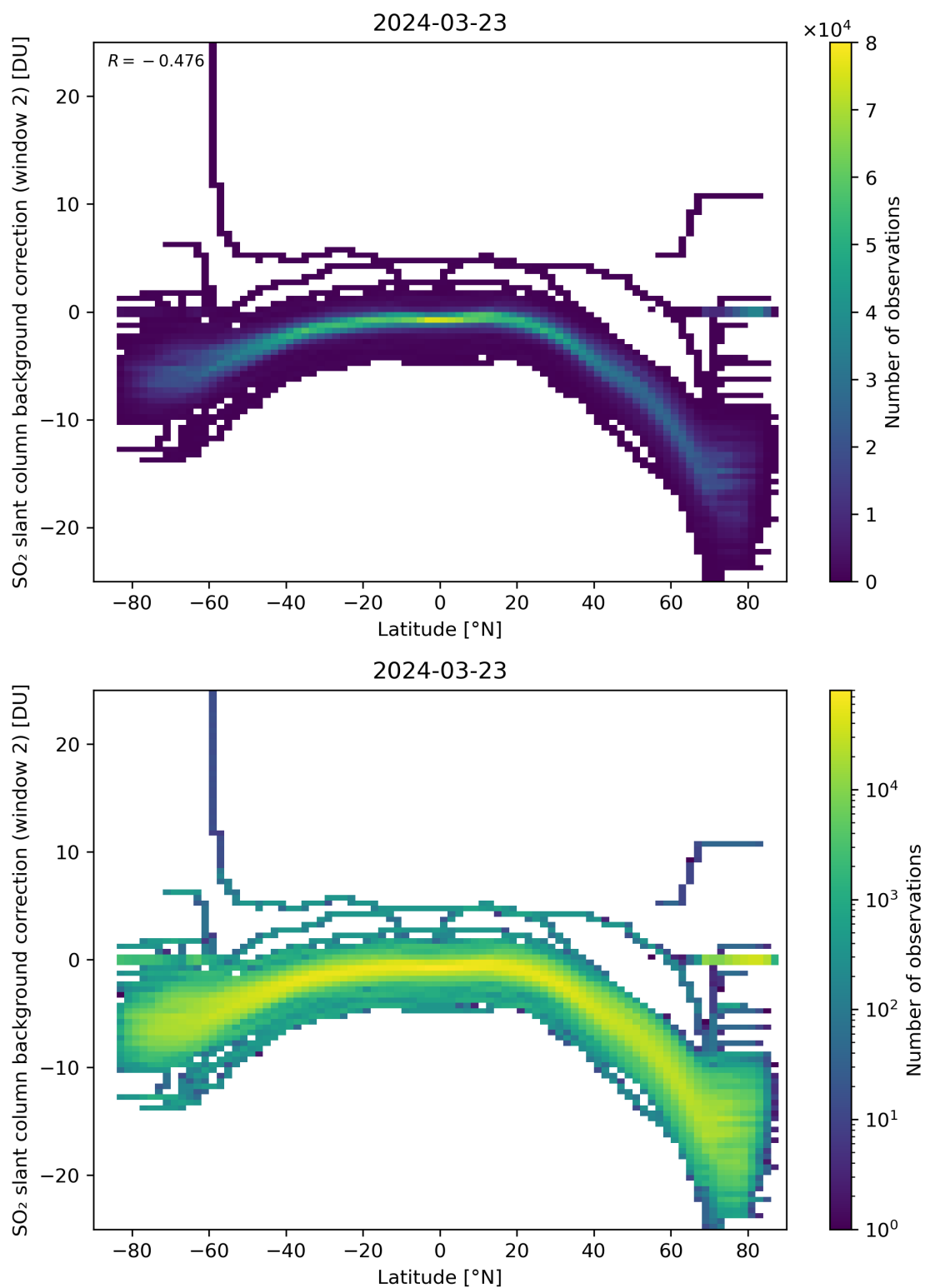
Figure 140: Scatter density plot of “Latitude” against “SO 2 slant column background correction (window 2)” for 2024-03-23 to 2024-03-24.
