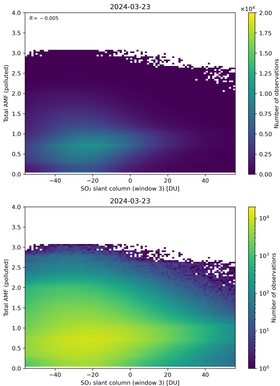
Figure 268: Scatter density plot of “SO 2 slant column (window 3)” against “Total AMF (polluted)” for 2024-03-23 to 2024-03-24.
