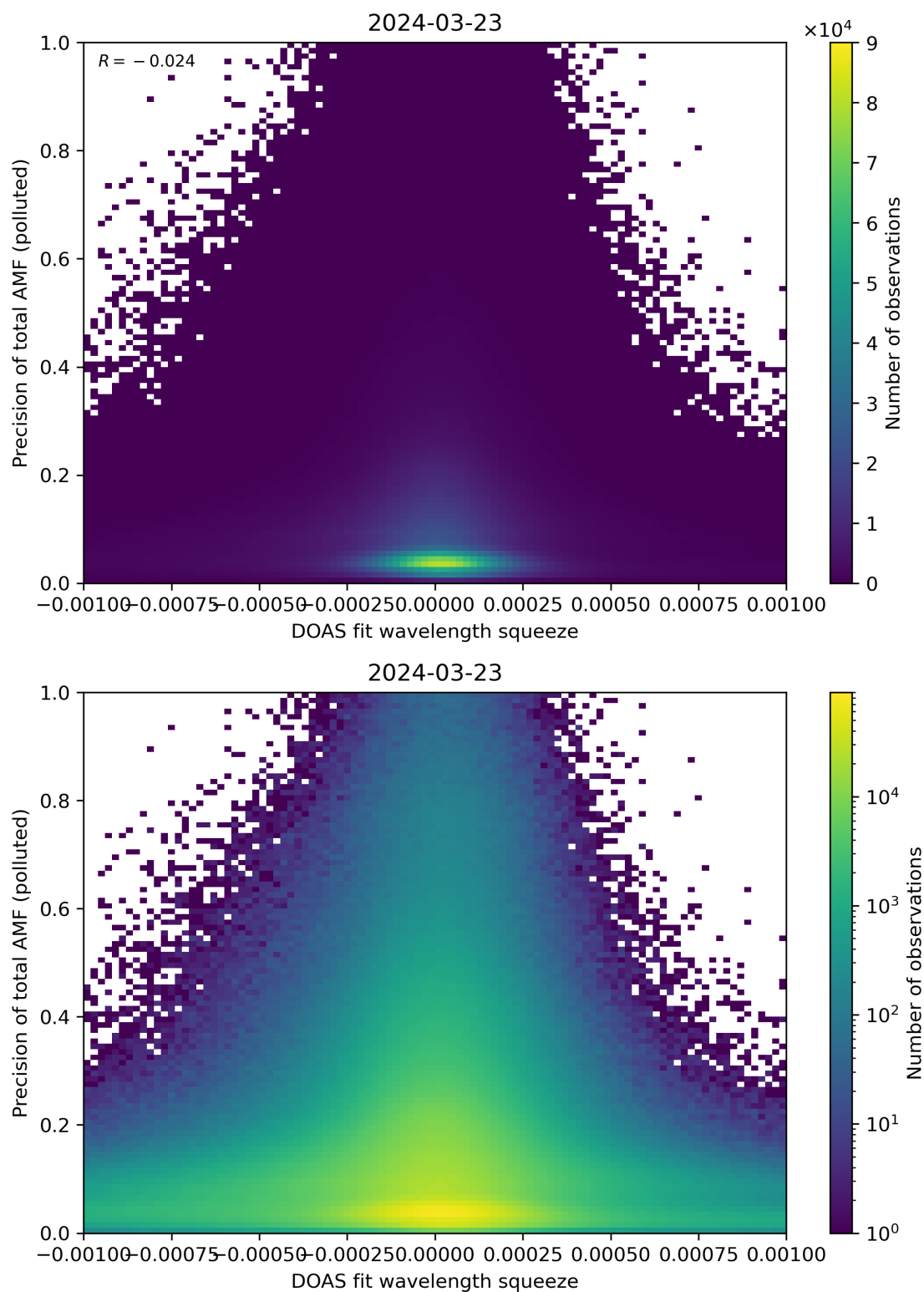
Figure 135: Scatter density plot of “DOAS fit wavelength squeeze” against “Precision of total AMF (polluted)” for 2024-03-23 to 2024-03-24.
