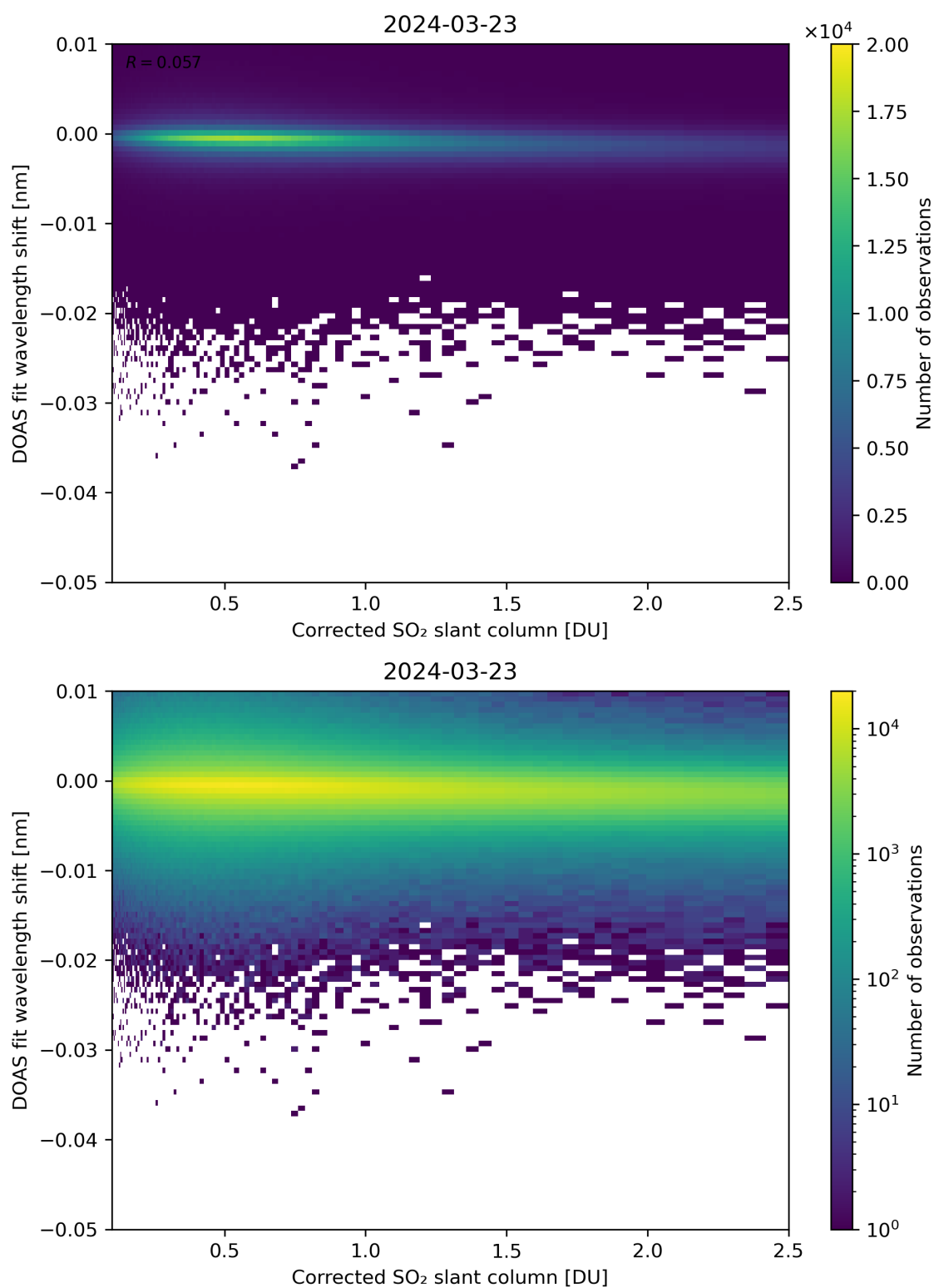
Figure 181: Scatter density plot of “Corrected SO 2 slant column” against “DOAS fit wavelength shift” for 2024-03-23 to 2024-03-24.
