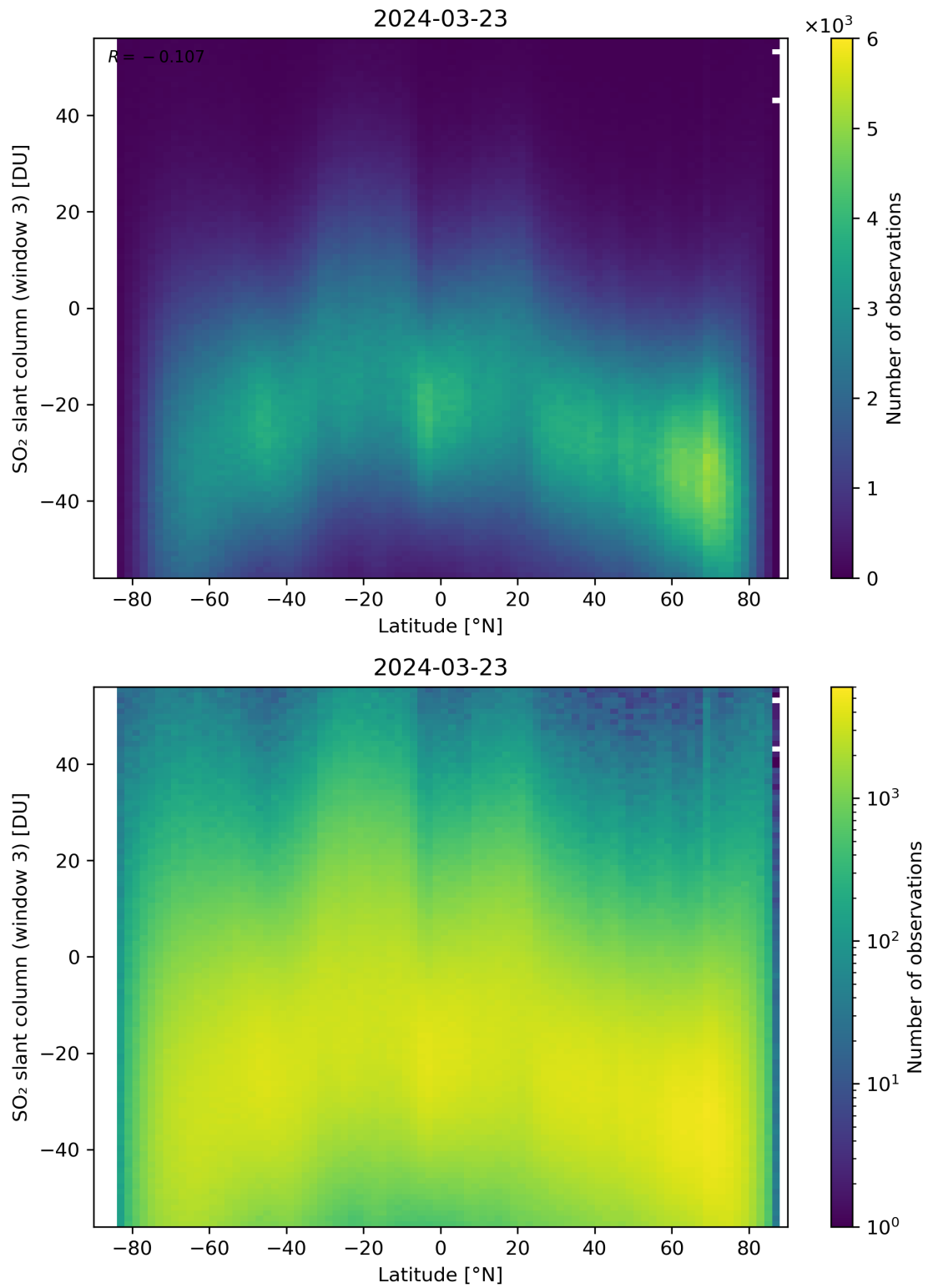
Figure 152: Scatter density plot of “Latitude” against “SO 2 slant column (window 3)” for 2024-03-23 to 2024-03-24.
