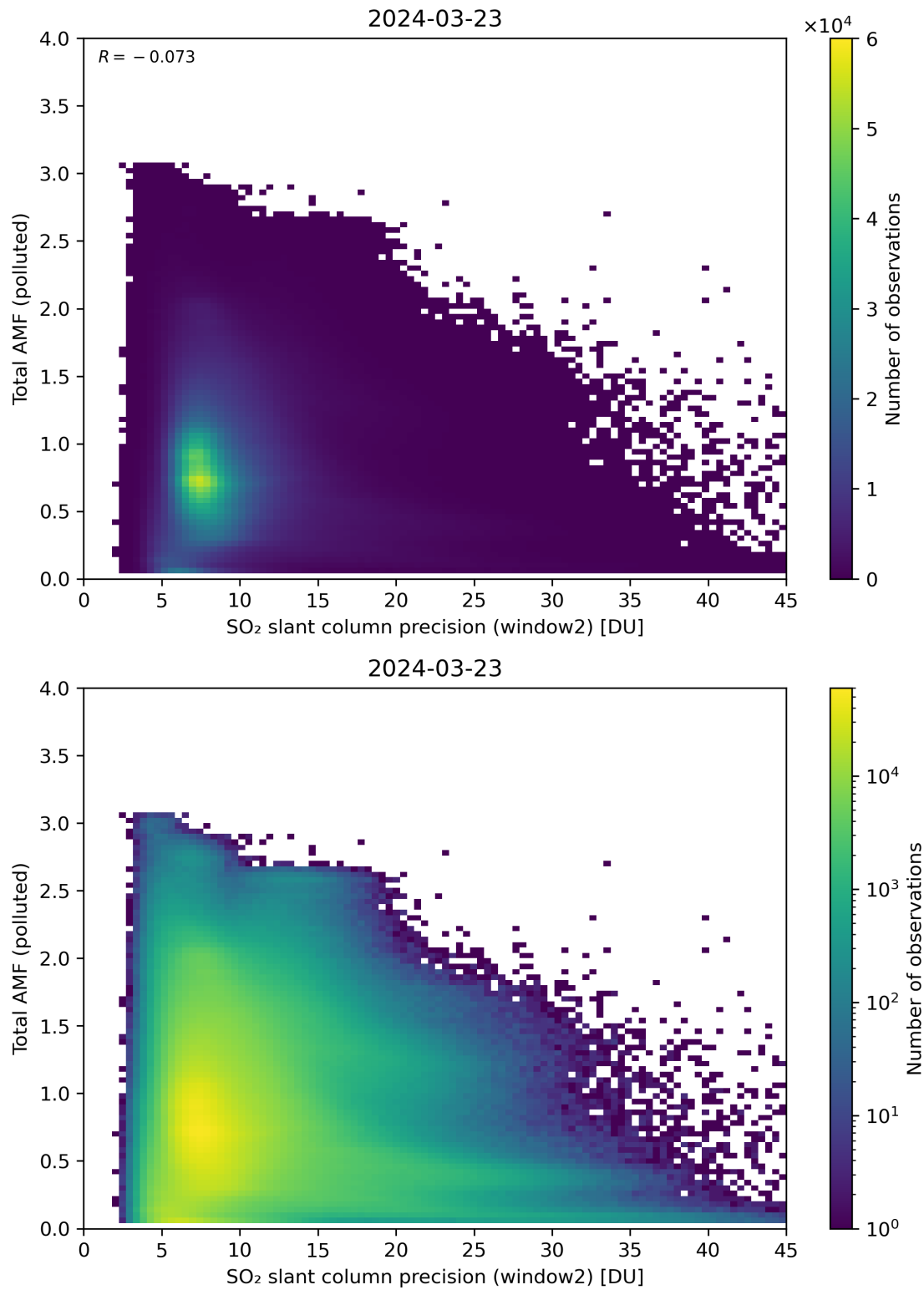
Figure 251: Scatter density plot of “SO 2 slant column precision (window2)” against “Total AMF (polluted)” for 2024-03-23 to 2024-03-24.
