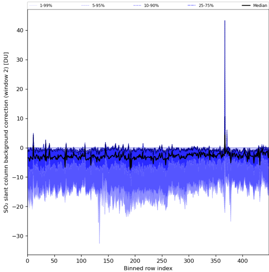
Figure 86: Along track statistics of “SO 2 slant column background correction (window 2)” for 2024-03-23 to 2024-03-24
