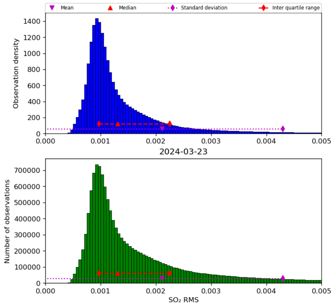
Figure 70: Histogram of “SO 2 RMS” for 2024-03-23 to 2024-03-24
