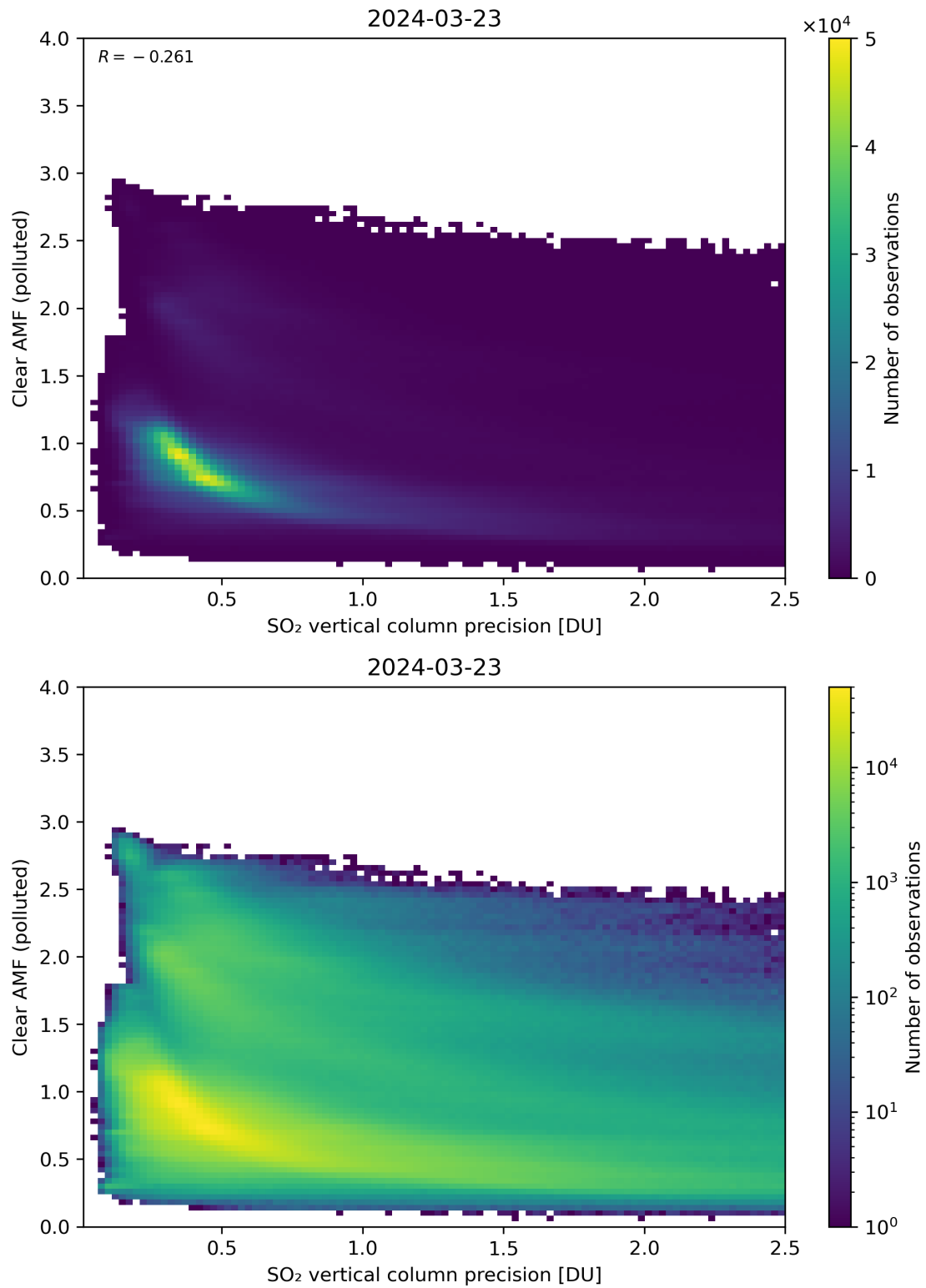
Figure 285: Scatter density plot of “SO 2 vertical column precision” against “Clear AMF (polluted)” for 2024-03-23 to 2024-03-24.
