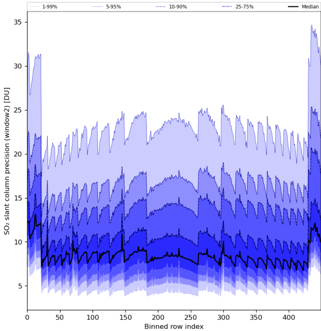
Figure 84: Along track statistics of “SO 2 slant column precision (window2)” for 2024-03-23 to 2024-03-24
