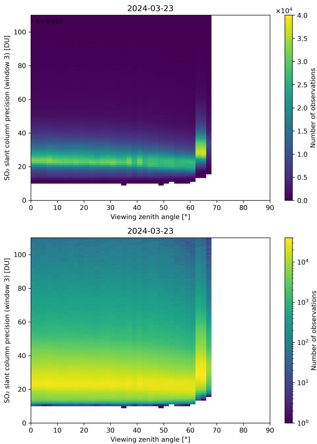
Figure 324: Scatter density plot of “Viewing zenith angle” against “SO 2 slant column precision (window 3)” for 2024-03-23 to 2024-03-24.
