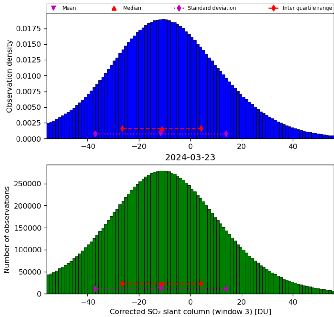
Figure 66: Histogram of "Corrected SO 2 slant column (window 3)" for 2024-03-23 to 2024-03-24
