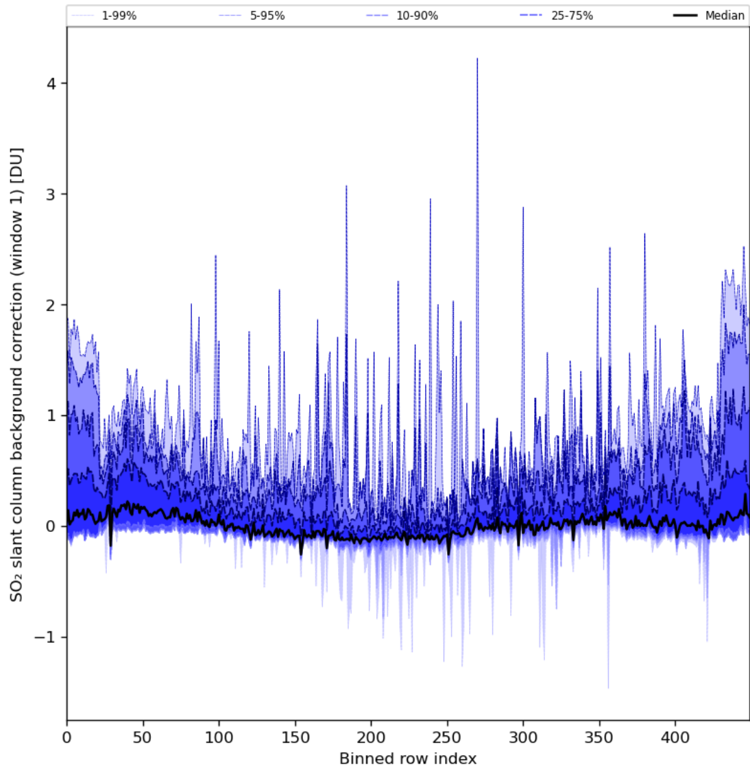
Figure 82: Along track statistics of “SO 2 slant column background correction (window 1)” for 2024-03-23 to 2024-03-24
