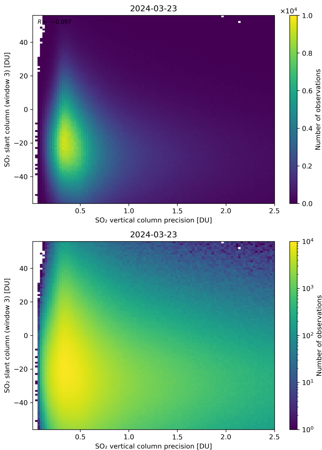
Figure 292: Scatter density plot of “SO 2 vertical column precision” against “SO 2 slant column (window 3)” for 2024-03-23 to 2024-03-24.
