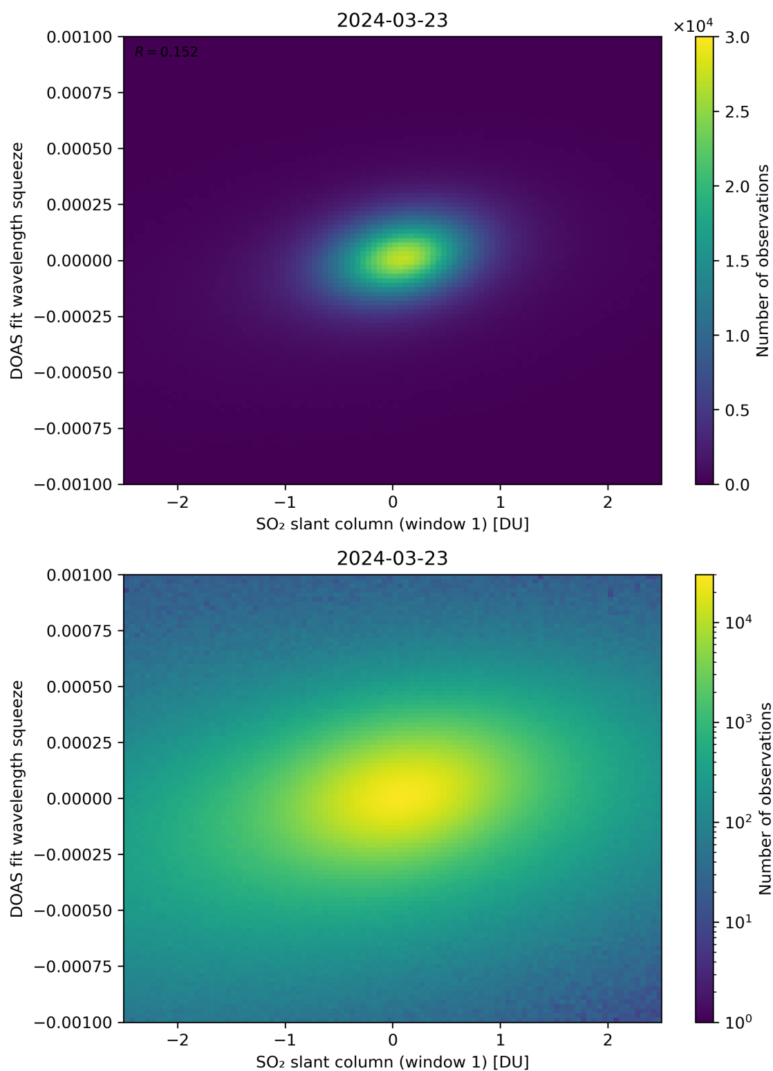
Figure 216: Scatter density plot of “SO 2 slant column (window 1)” against “DOAS fit wavelength squeeze” for 2024-03-23 to 2024-03-24.
