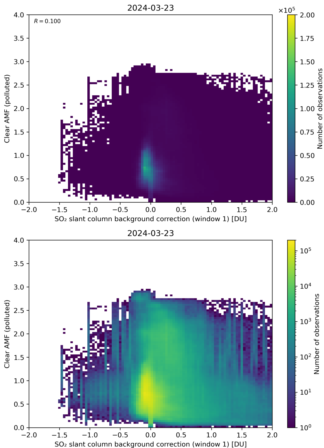
Figure 103: Scatter density plot of “SO 2 slant column background correction (window 1)” against “Clear AMF (polluted)” for 2024-03-23 to 2024-03-24.
