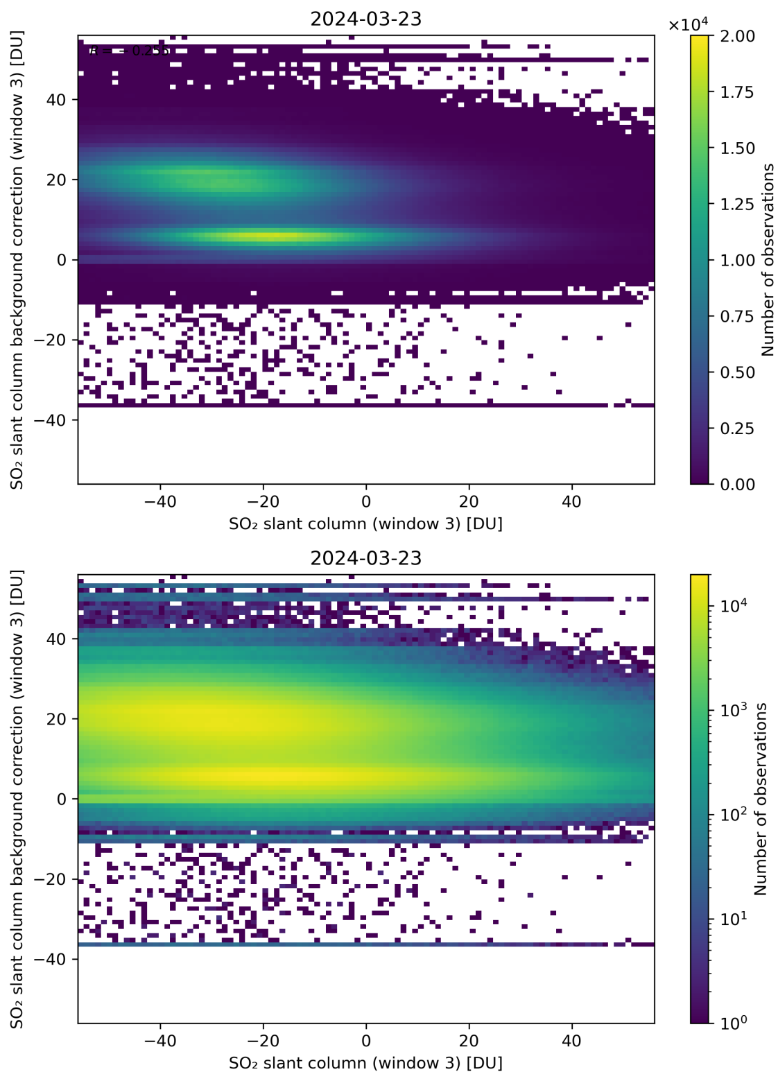
Figure 253: Scatter density plot of “SO 2 slant column (window 3)” against “SO 2 slant column background correction (window 3)” for 2024-03-23 to 2024-03-24.
