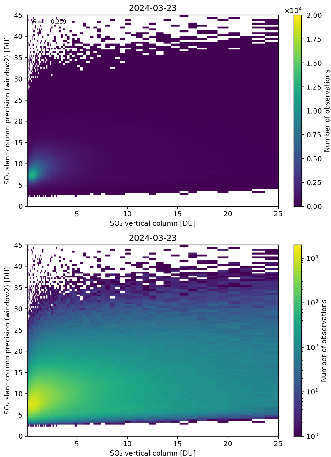
Figure 302: Scatter density plot of “SO 2 vertical column” against “SO 2 slant column precision (window2)” for 2024-03-23 to 2024-03-24.
