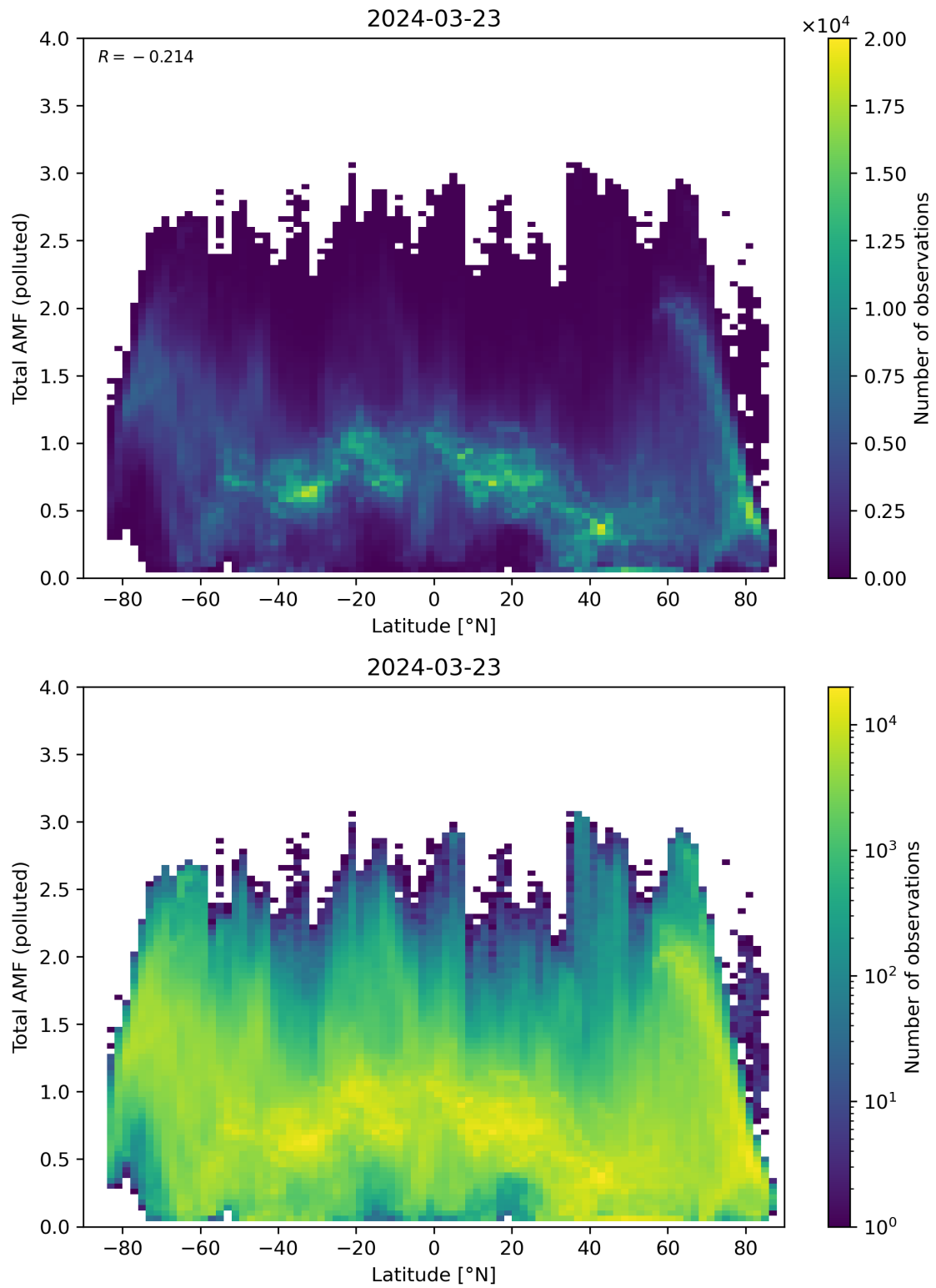
Figure 154: Scatter density plot of “Latitude” against “Total AMF (polluted)” for 2024-03-23 to 2024-03-24.
