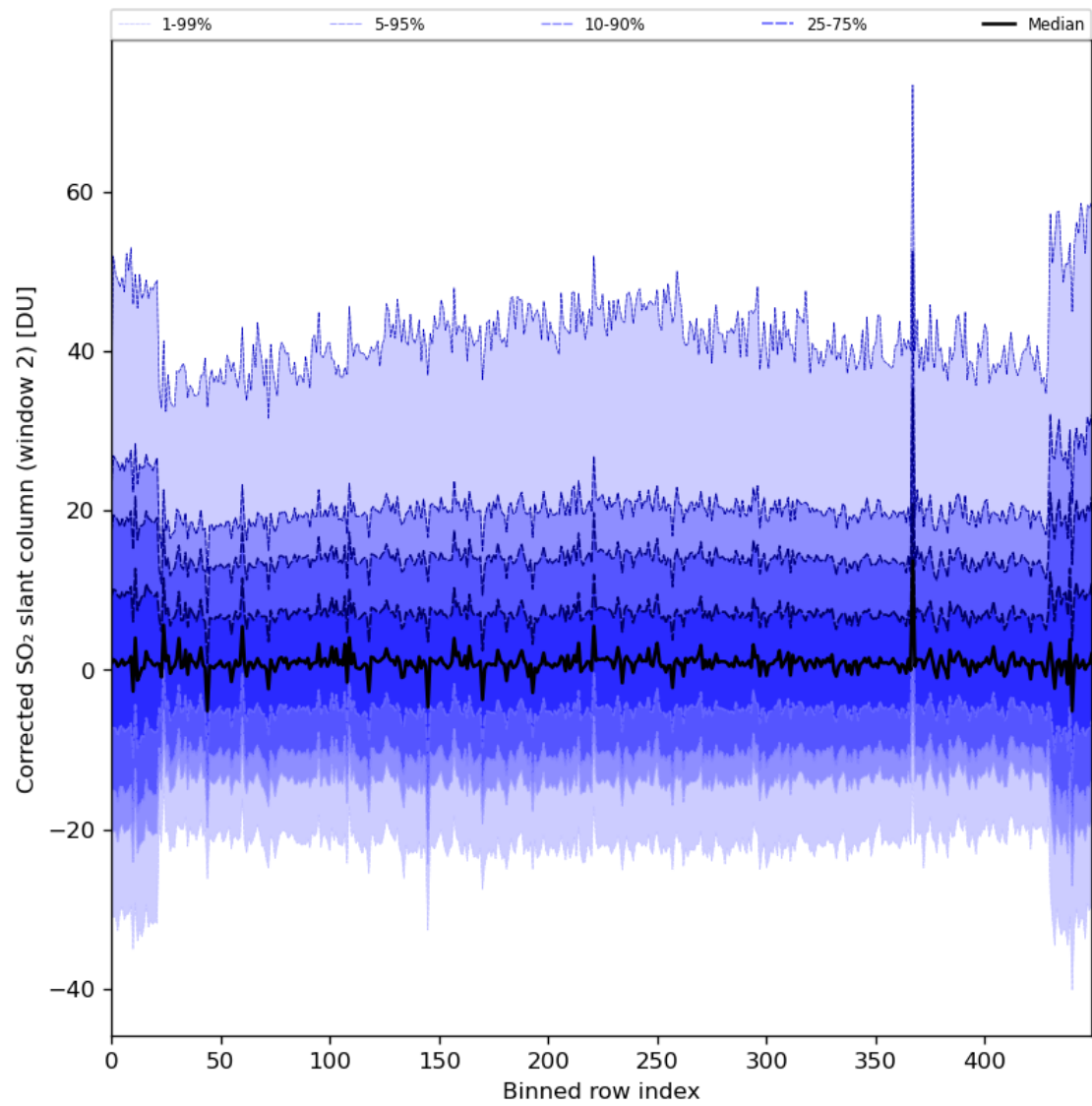
Figure 85: Along track statistics of “Corrected SO 2 slant column (window 2)” for 2024-03-23 to 2024-03-24
