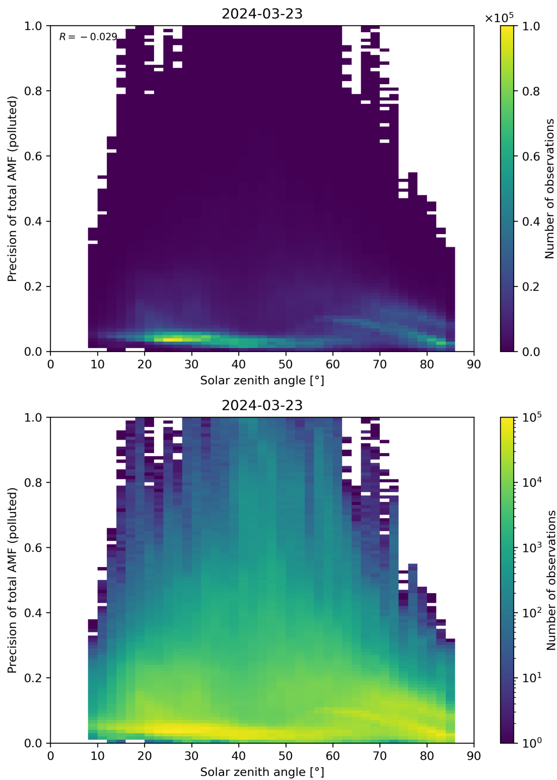
Figure 175: Scatter density plot of “Solar zenith angle” against “Precision of total AMF (polluted)” for 2024-03-23 to 2024-03-24.
