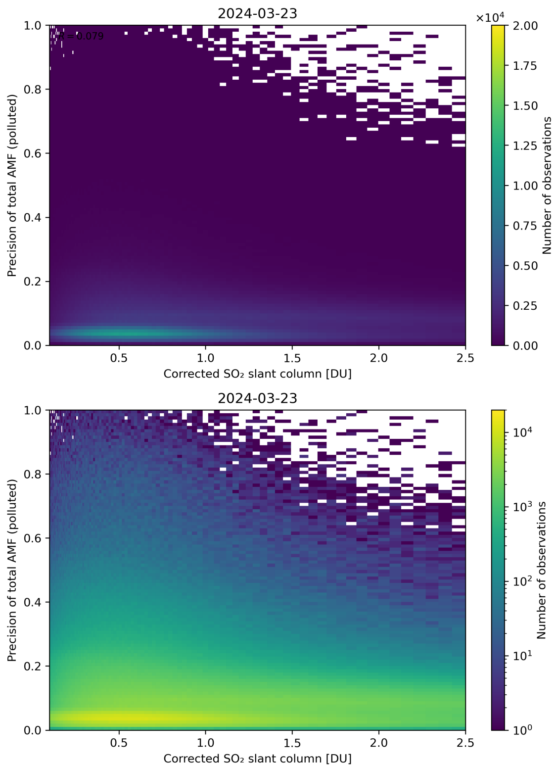
Figure 193: Scatter density plot of “Corrected SO 2 slant column” against “Precision of total AMF (polluted)” for 2024-03-23 to 2024-03-24.
