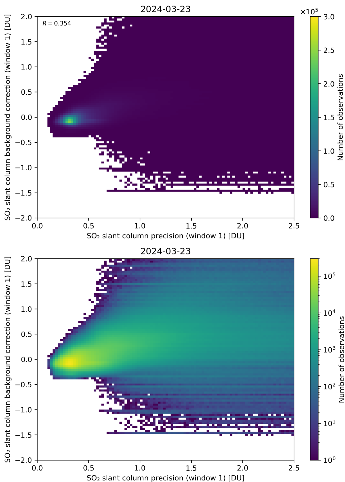
Figure 218: Scatter density plot of “SO 2 slant column precision (window 1)” against “SO 2 slant column background correction (window 1)” for 2024-03-23 to 2024-03-24.
