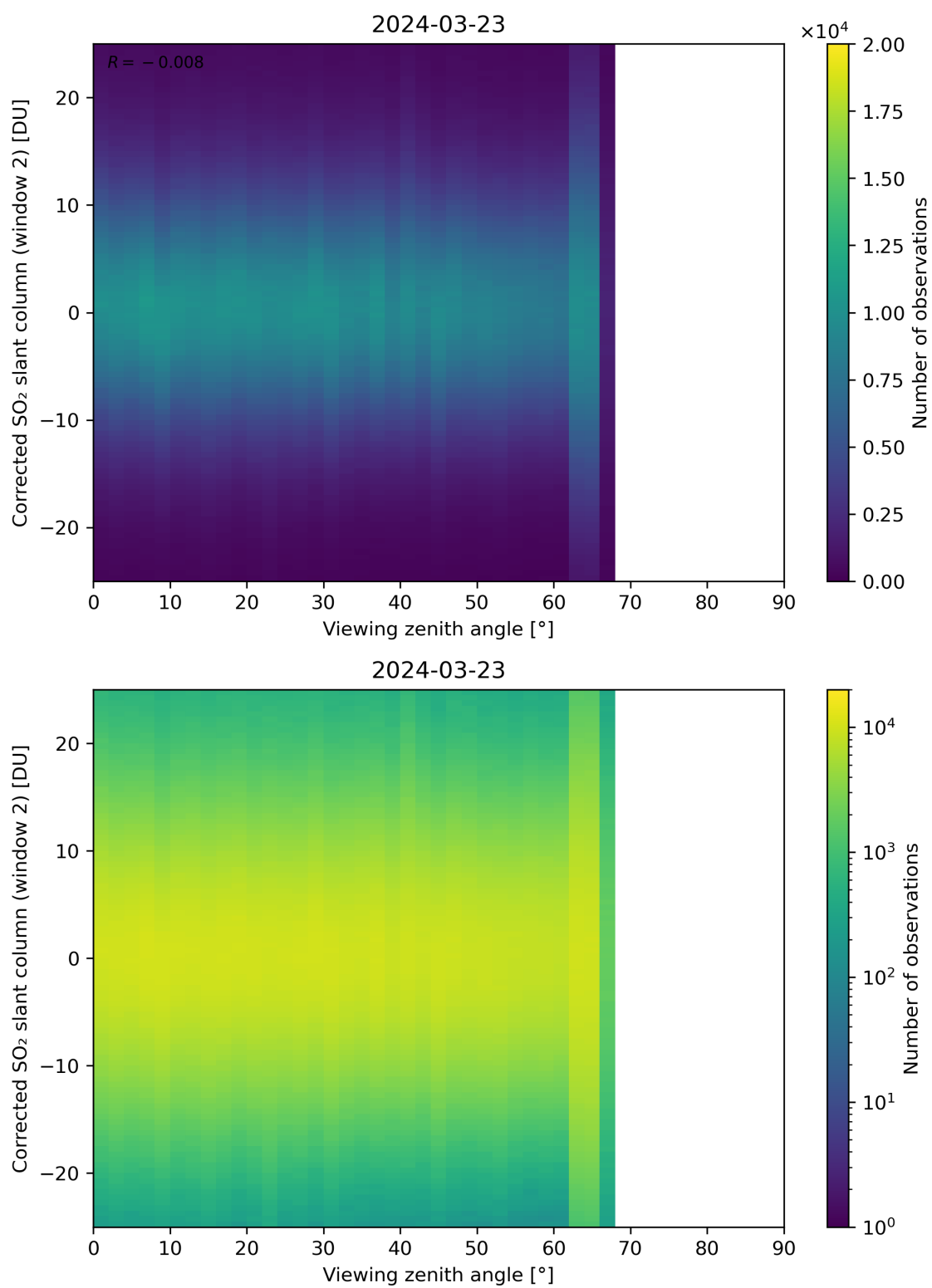
Figure 318: Scatter density plot of “Viewing zenith angle” against “Corrected SO 2 slant column (window 2)” for 2024-03-23 to 2024-03-24.
