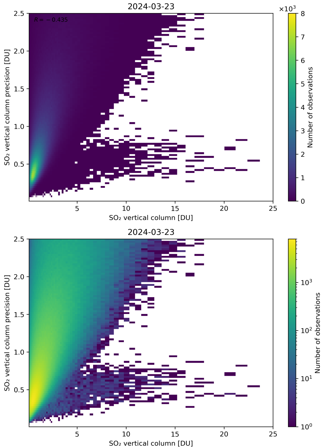
Figure 307: Scatter density plot of “SO 2 vertical column” against “SO 2 vertical column precision” for 2024-03-23 to 2024-03-24.
