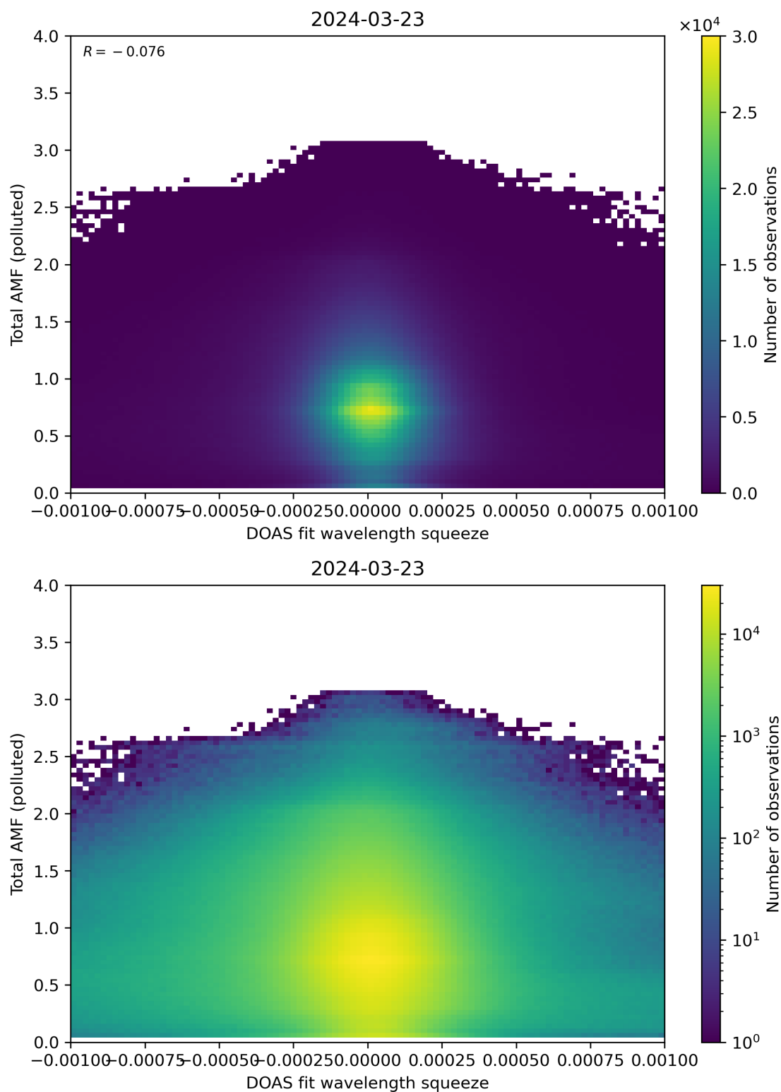
Figure 134: Scatter density plot of “DOAS fit wavelength squeeze” against “Total AMF (polluted)” for 2024-03-23 to 2024-03-24.
