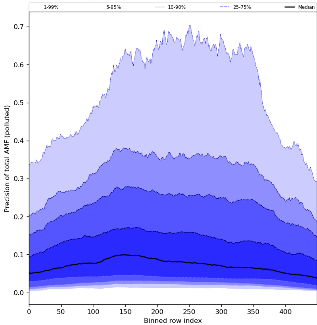
Figure 95: Along track statistics of “Precision of total AMF (polluted)” for 2024-03-23 to 2024-03-24
