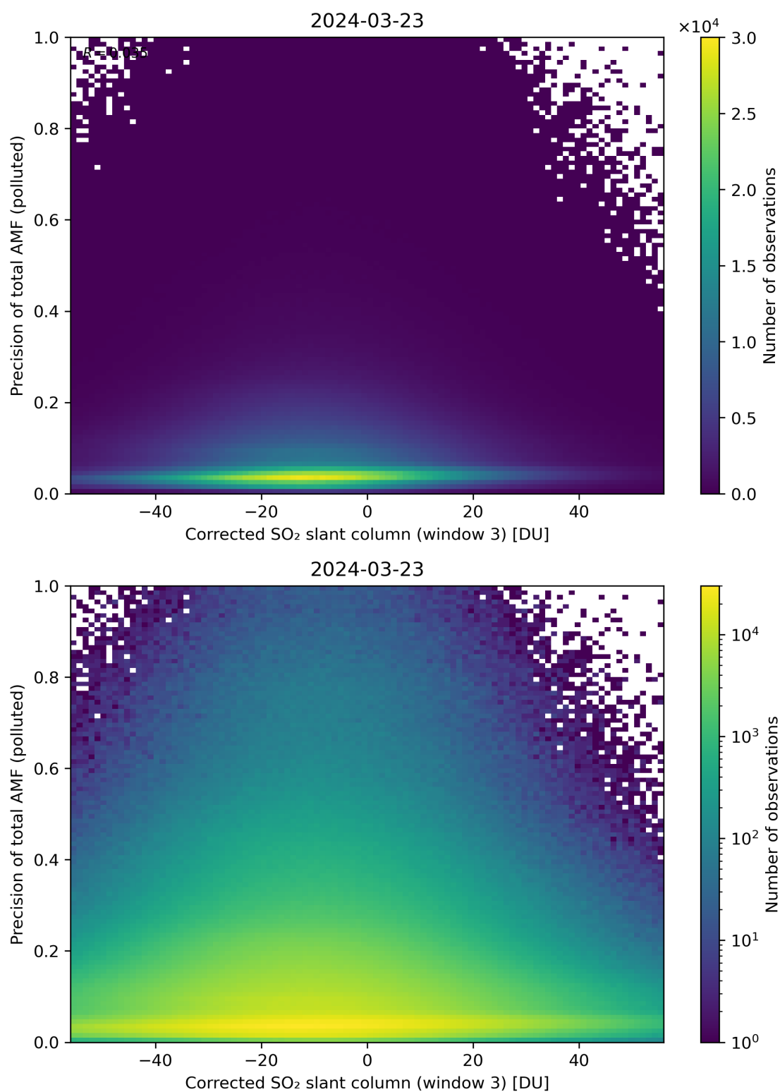
Figure 211: Scatter density plot of “Corrected SO 2 slant column (window 3)” against “Precision of total AMF (polluted)” for 2024-03-23 to 2024-03-24.
