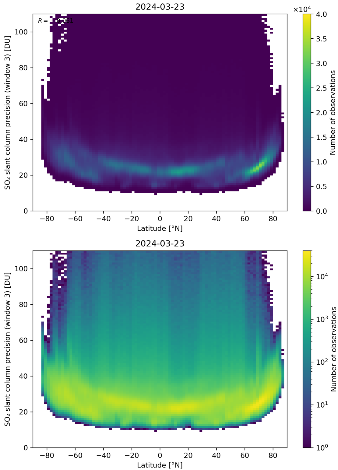
Figure 153: Scatter density plot of “Latitude” against “SO 2 slant column precision (window 3)” for 2024-03-23 to 2024-03-24.
