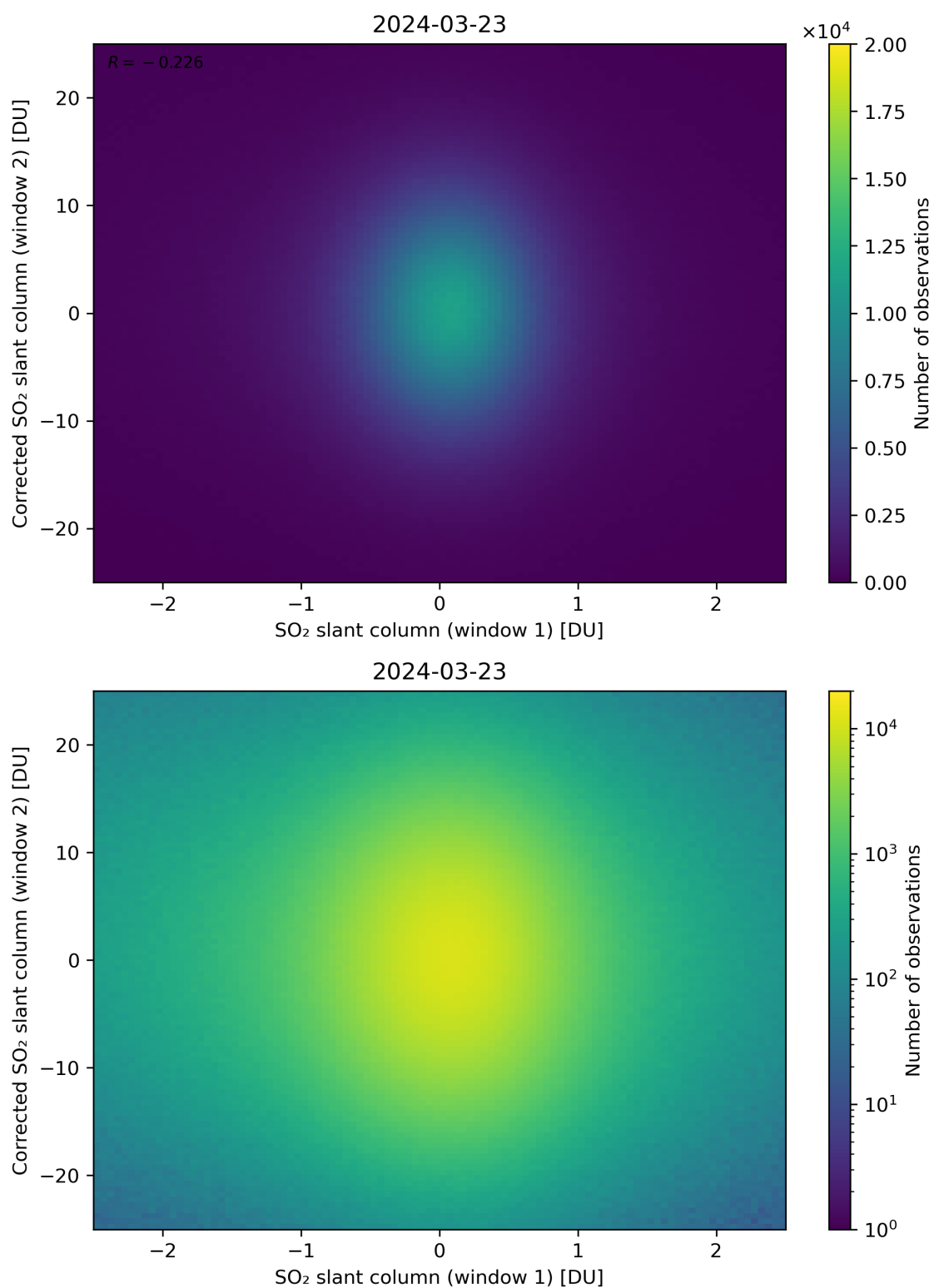
Figure 233: Scatter density plot of “SO 2 slant column (window 1)” against “Corrected SO 2 slant column (window 2)” for 2024-03-23 to 2024-03-24.
