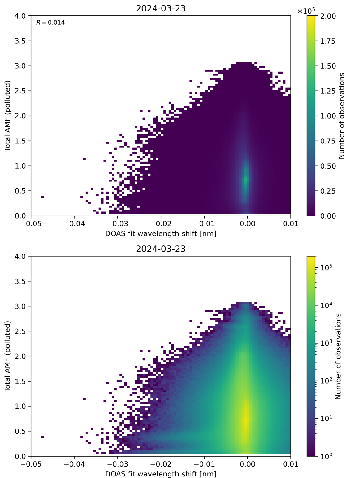
Figure 130: Scatter density plot of “DOAS fit wavelength shift” against “Total AMF (polluted)” for 2024-03-23 to 2024-03-24.
