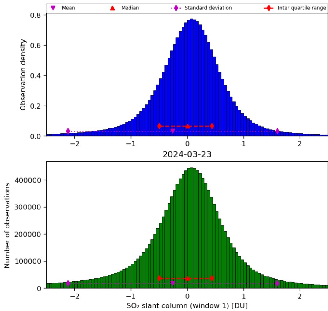
Figure 56: Histogram of “SO 2 slant column (window 1)” for 2024-03-23 to 2024-03-24
