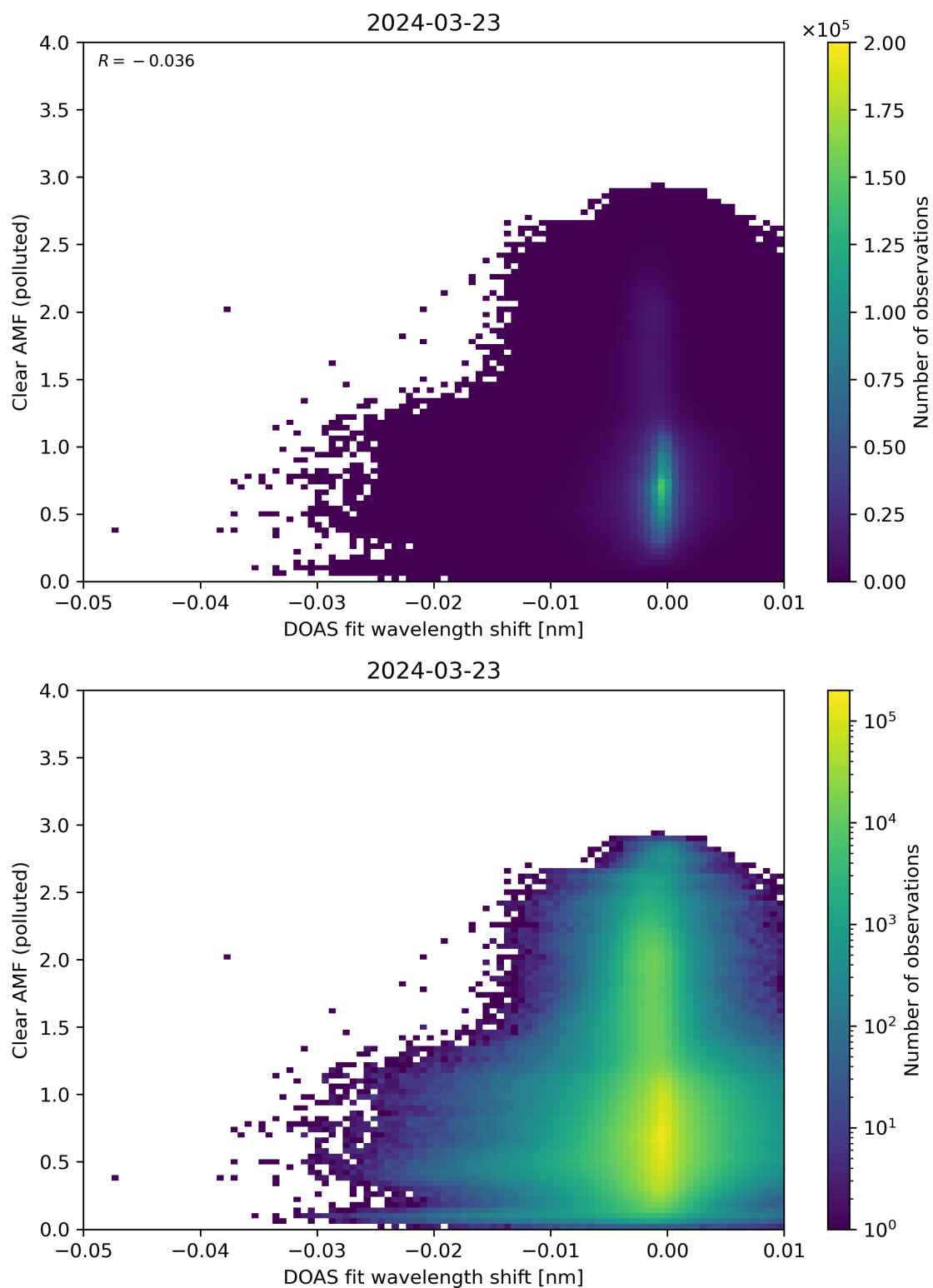
Figure 129: Scatter density plot of “DOAS fit wavelength shift” against “Clear AMF (polluted)” for 2024-03-23 to 2024-03-24.
