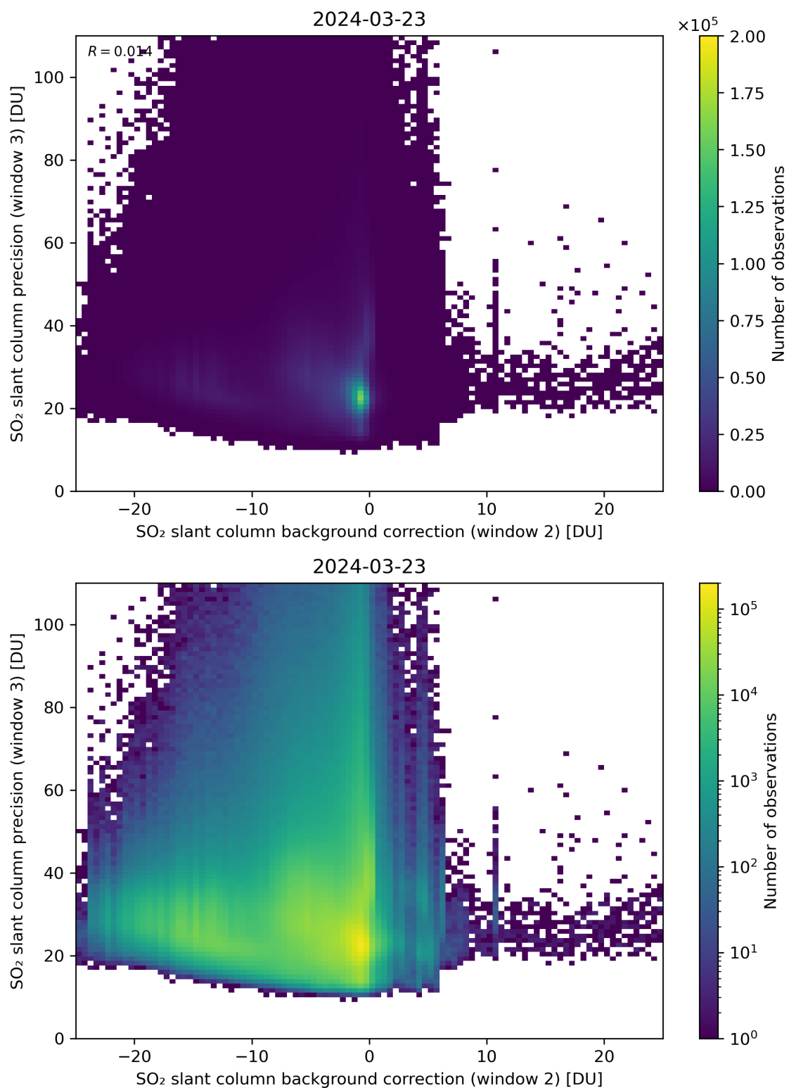
Figure 118: Scatter density plot of “SO 2 slant column background correction (window 2)” against “SO 2 slant column precision (window 3)” for 2024-03-23 to 2024-03-24.
