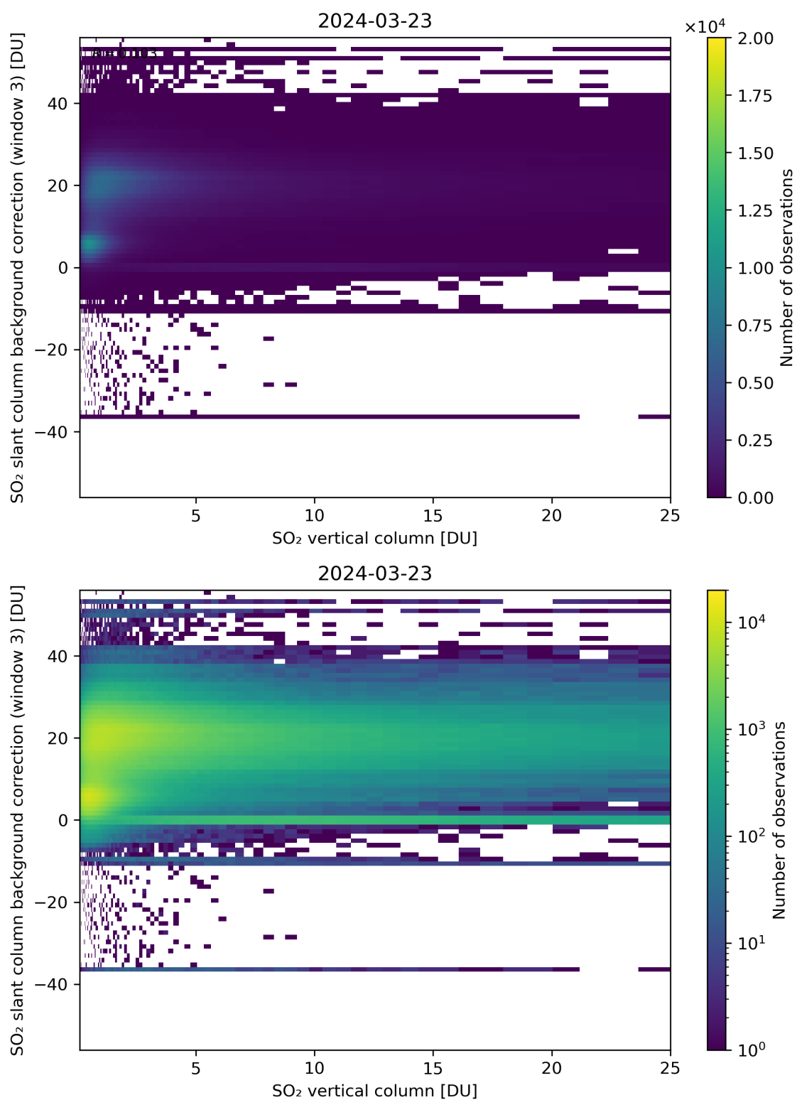
Figure 275: Scatter density plot of “SO 2 vertical column” against “SO 2 slant column background correction (window 3)” for 2024-03-23 to 2024-03-24.
