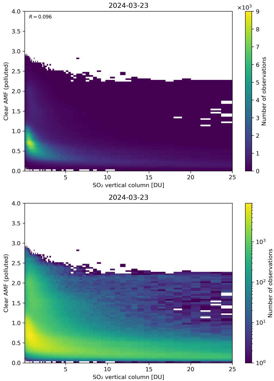
Figure 296: Scatter density plot of “SO 2 vertical column” against “Clear AMF (polluted)” for 2024-03-23 to 2024-03-24.
