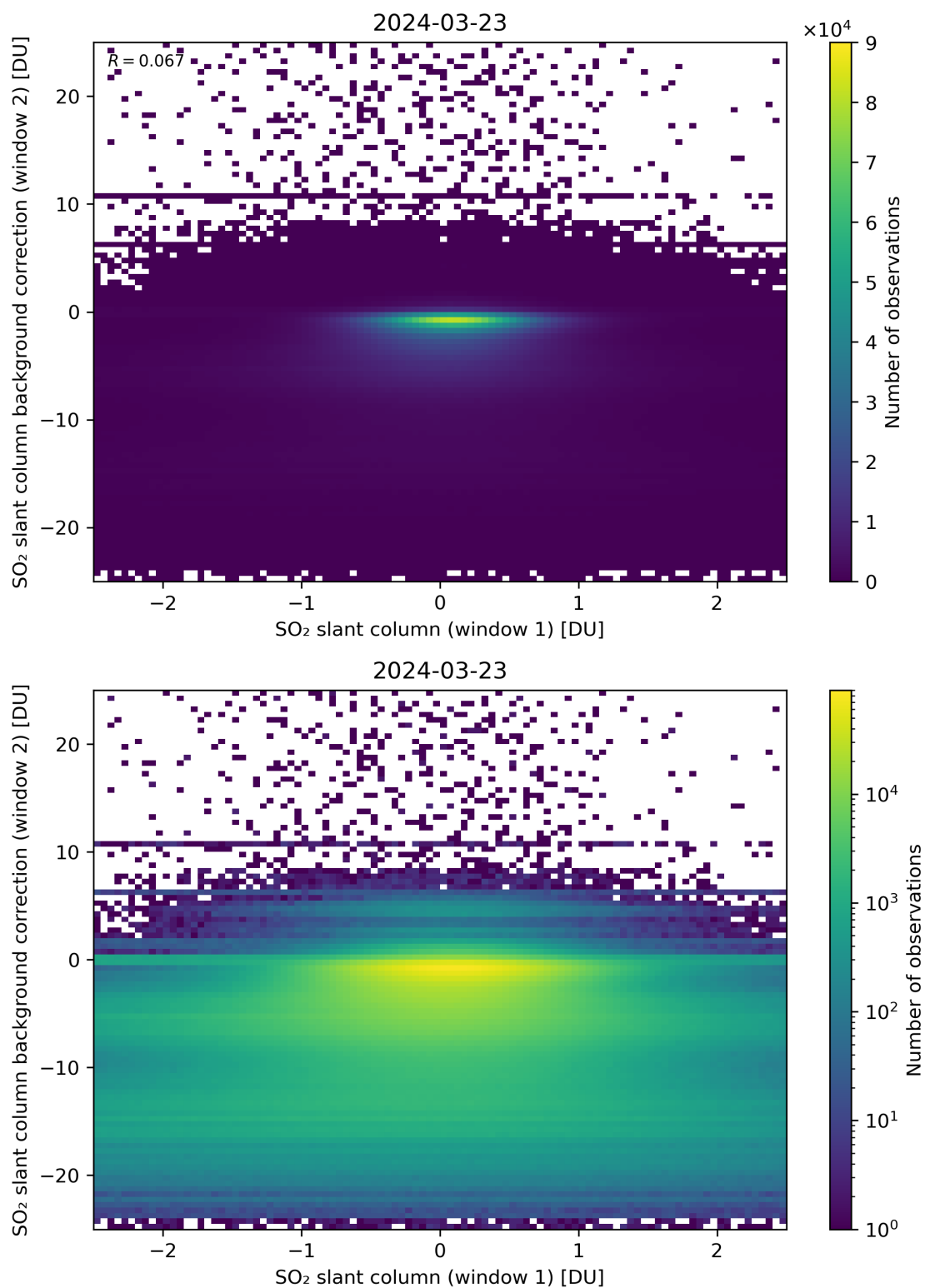
Figure 213: Scatter density plot of “SO 2 slant column (window 1)” against “SO 2 slant column background correction (window 2)” for 2024-03-23 to 2024-03-24.
