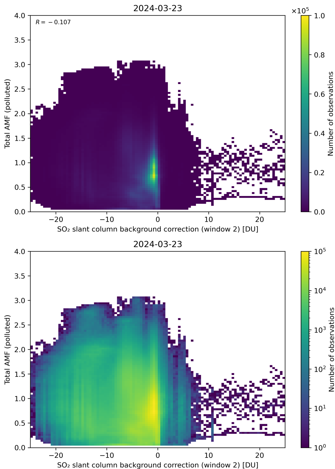
Figure 119: Scatter density plot of “SO 2 slant column background correction (window 2)” against “Total AMF (polluted)” for 2024-03-23 to 2024-03-24.
