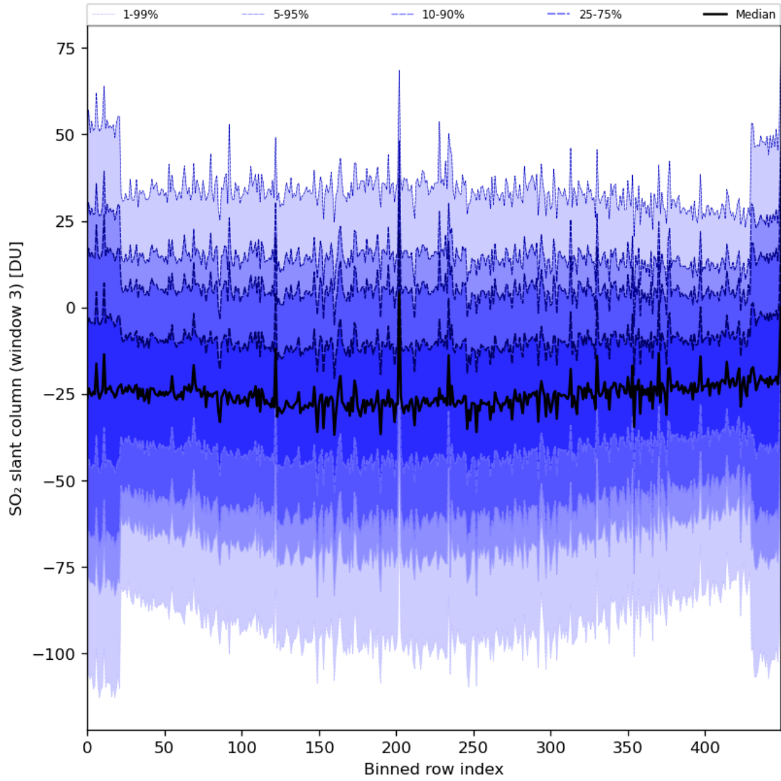
Figure 87: Along track statistics of “SO 2 slant column (window 3)” for 2024-03-23 to 2024-03-24
