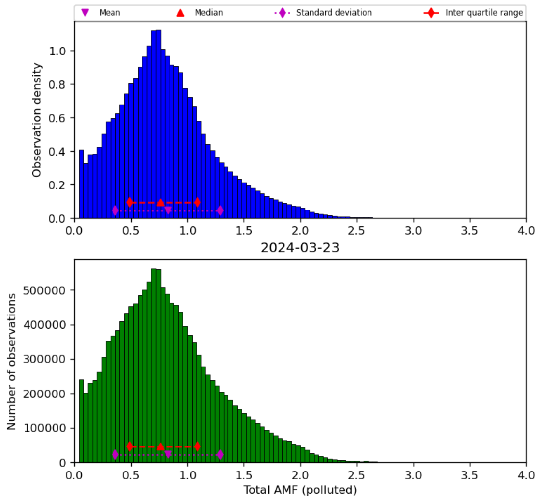
Figure 71: Histogram of “Total AMF (polluted)” for 2024-03-23 to 2024-03-24
