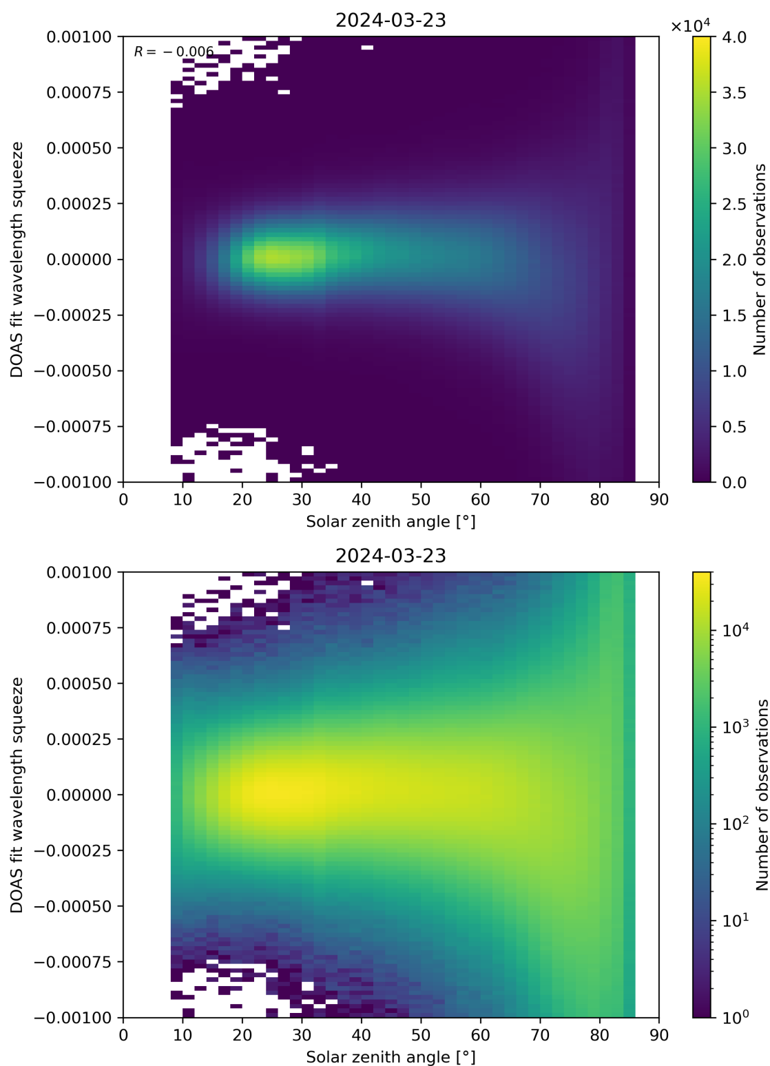
Figure 162: Scatter density plot of “Solar zenith angle” against “DOAS fit wavelength squeeze” for 2024-03-23 to 2024-03-24.
