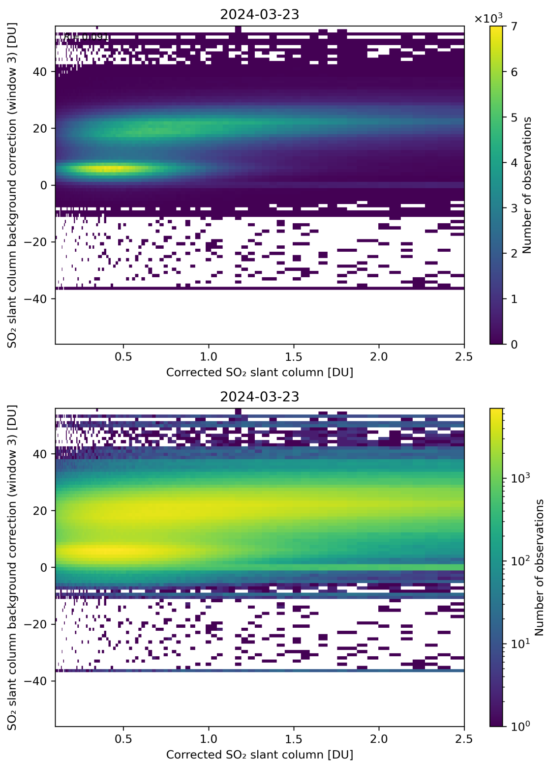
Figure 180: Scatter density plot of “Corrected SO 2 slant column” against “SO 2 slant column background correction (window 3)” for 2024-03-23 to 2024-03-24.
