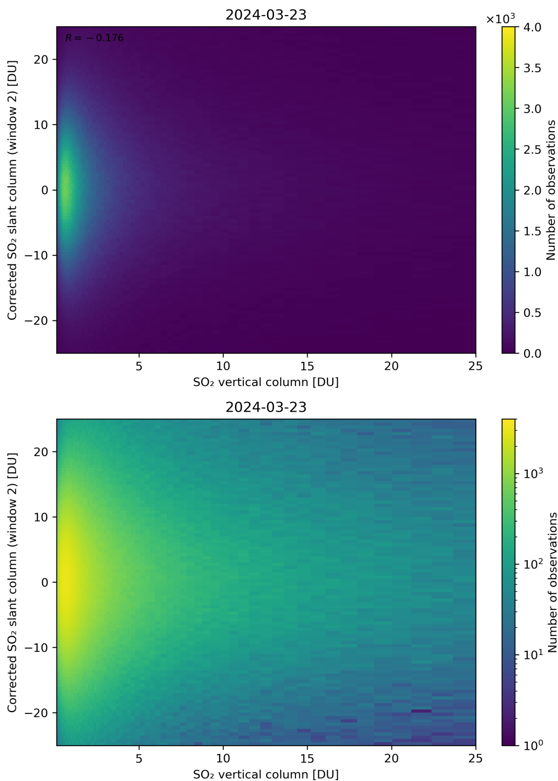
Figure 298: Scatter density plot of “SO 2 vertical column” against “Corrected SO 2 slant column (window 2)” for 2024-03-23 to 2024-03-24.
