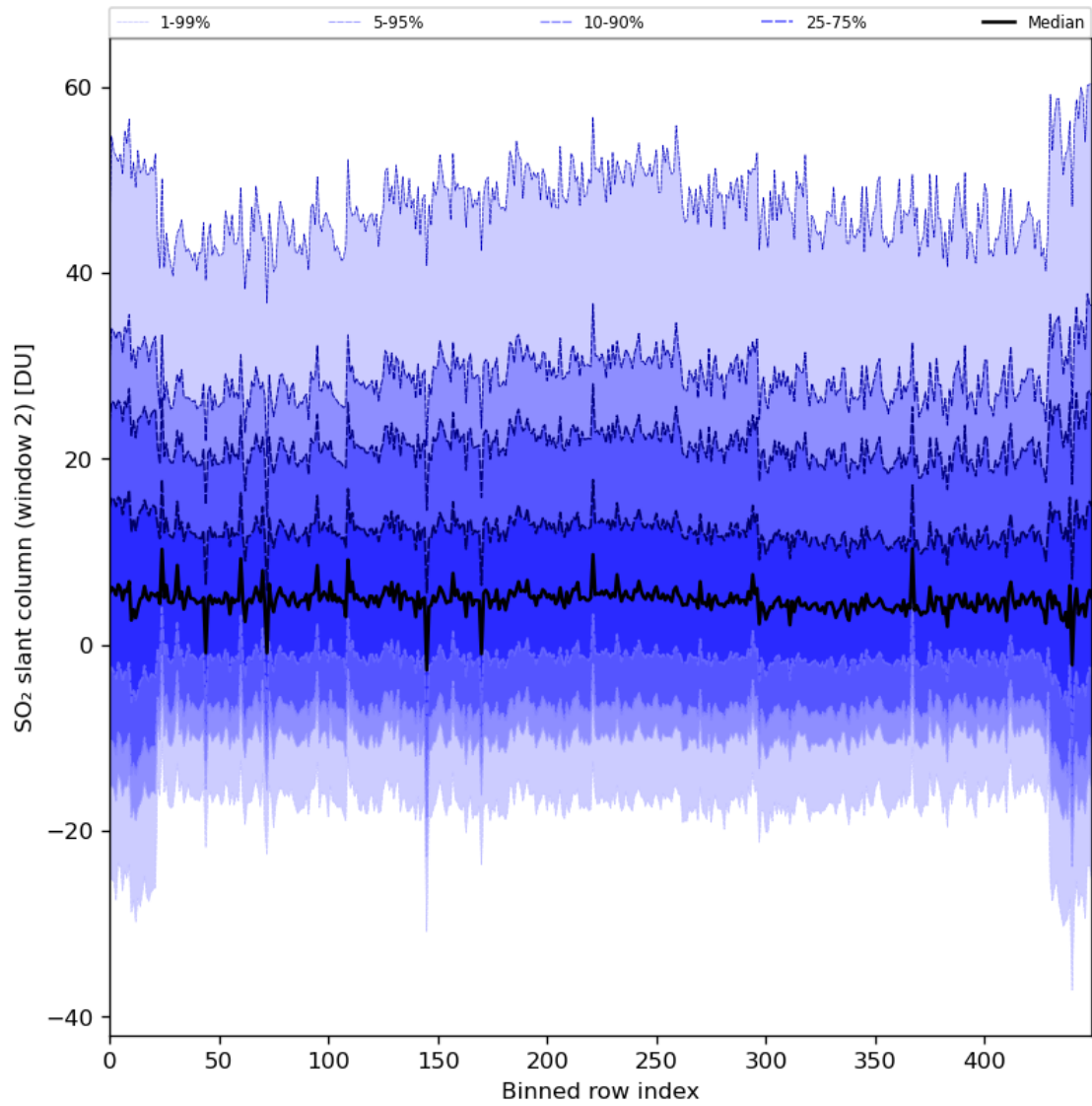
Figure 83: Along track statistics of “SO 2 slant column (window 2)” for 2024-03-23 to 2024-03-24
