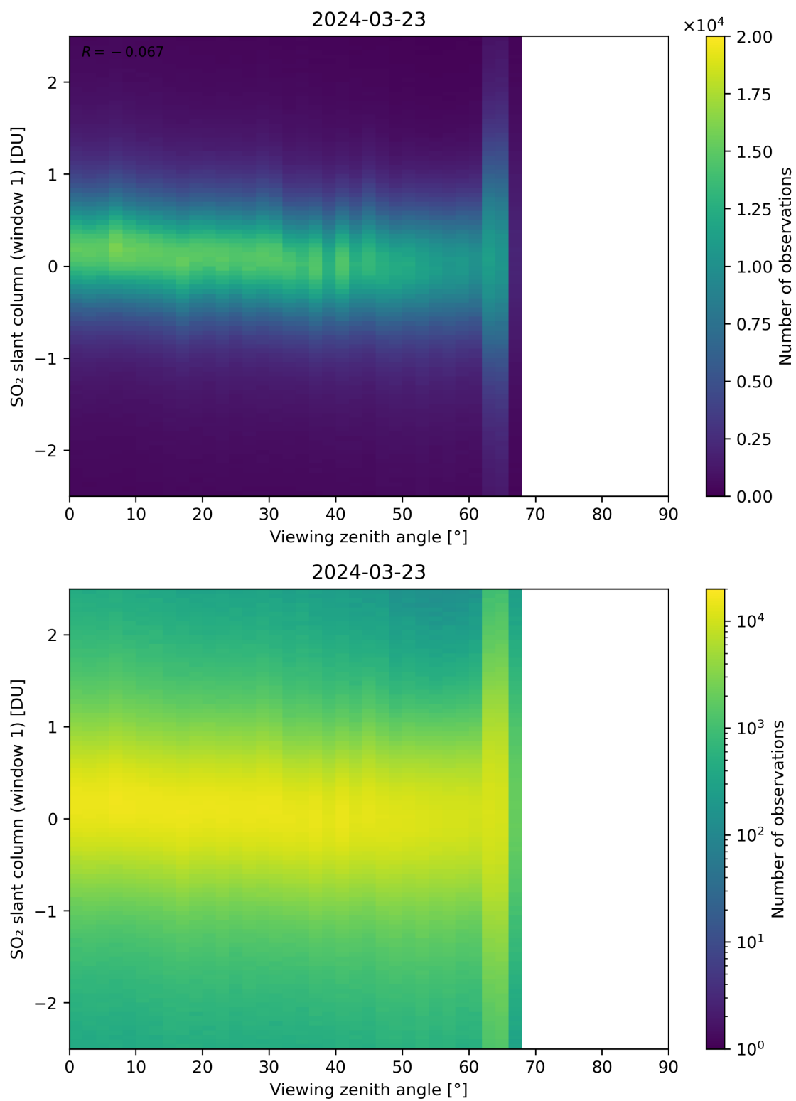
Figure 320: Scatter density plot of “Viewing zenith angle” against “SO 2 slant column (window 1)” for 2024-03-23 to 2024-03-24.
