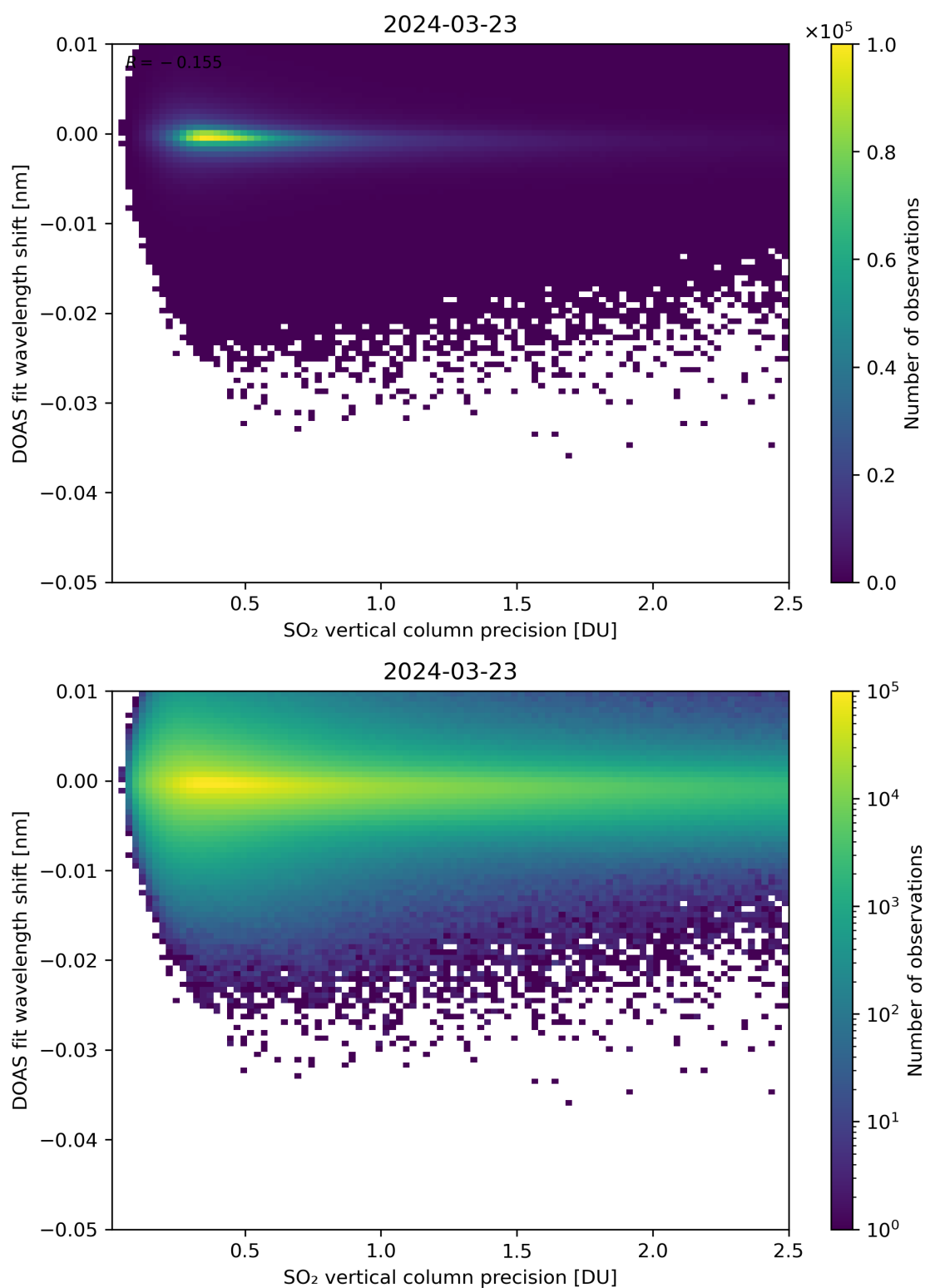
Figure 282: Scatter density plot of “SO 2 vertical column precision” against “DOAS fit wavelength shift” for 2024-03-23 to 2024-03-24.
