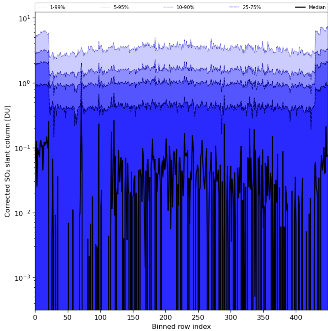
Figure 78: Along track statistics of “Corrected SO 2 slant column” for 2024-03-23 to 2024-03-24
