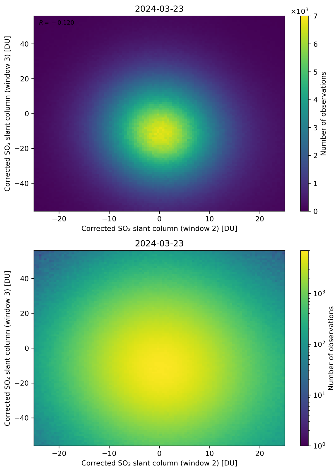
Figure 200: Scatter density plot of “Corrected SO 2 slant column (window 2)” against “Corrected SO 2 slant column (window 3)” for 2024-03-23 to 2024-03-24.
