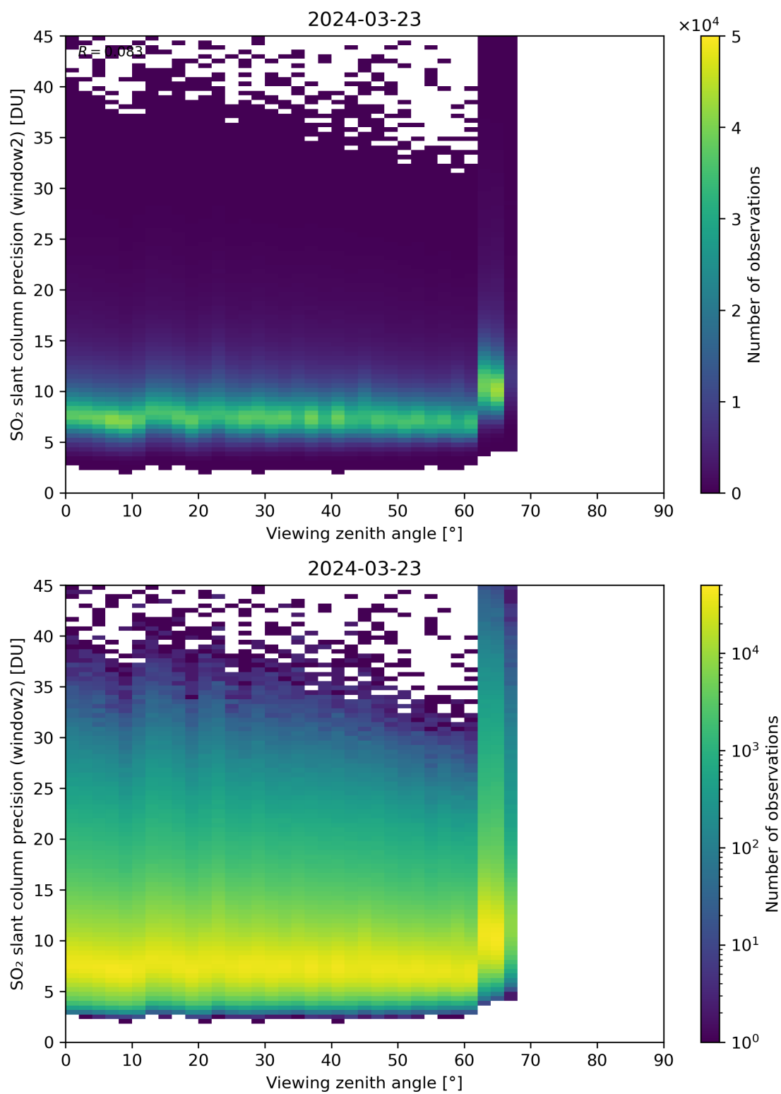
Figure 322: Scatter density plot of “Viewing zenith angle” against “SO 2 slant column precision (window2)” for 2024-03-23 to 2024-03-24.
