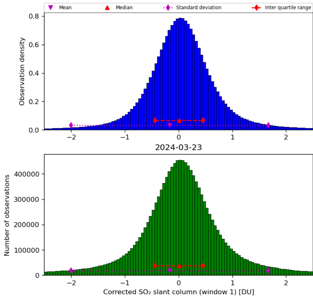
Figure 58: Histogram of “Corrected SO 2 slant column (window 1)” for 2024-03-23 to 2024-03-24
