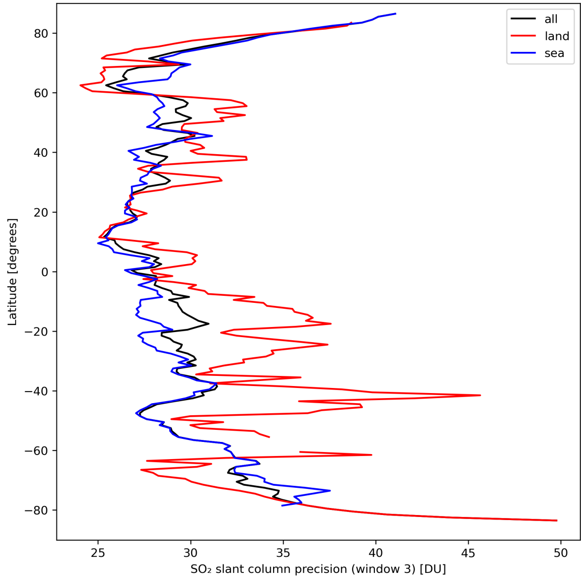
Figure 42: Zonal average of “SO 2 slant column precision (window 3)” for 2024-03-23 to 2024-03-24.
