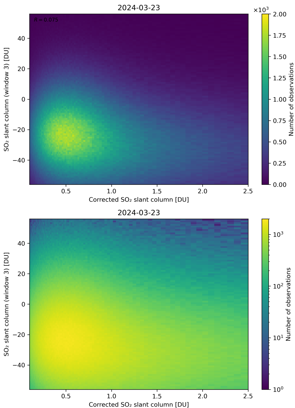
Figure 190: Scatter density plot of “Corrected SO 2 slant column” against “SO 2 slant column (window 3)” for 2024-03-23 to 2024-03-24.
