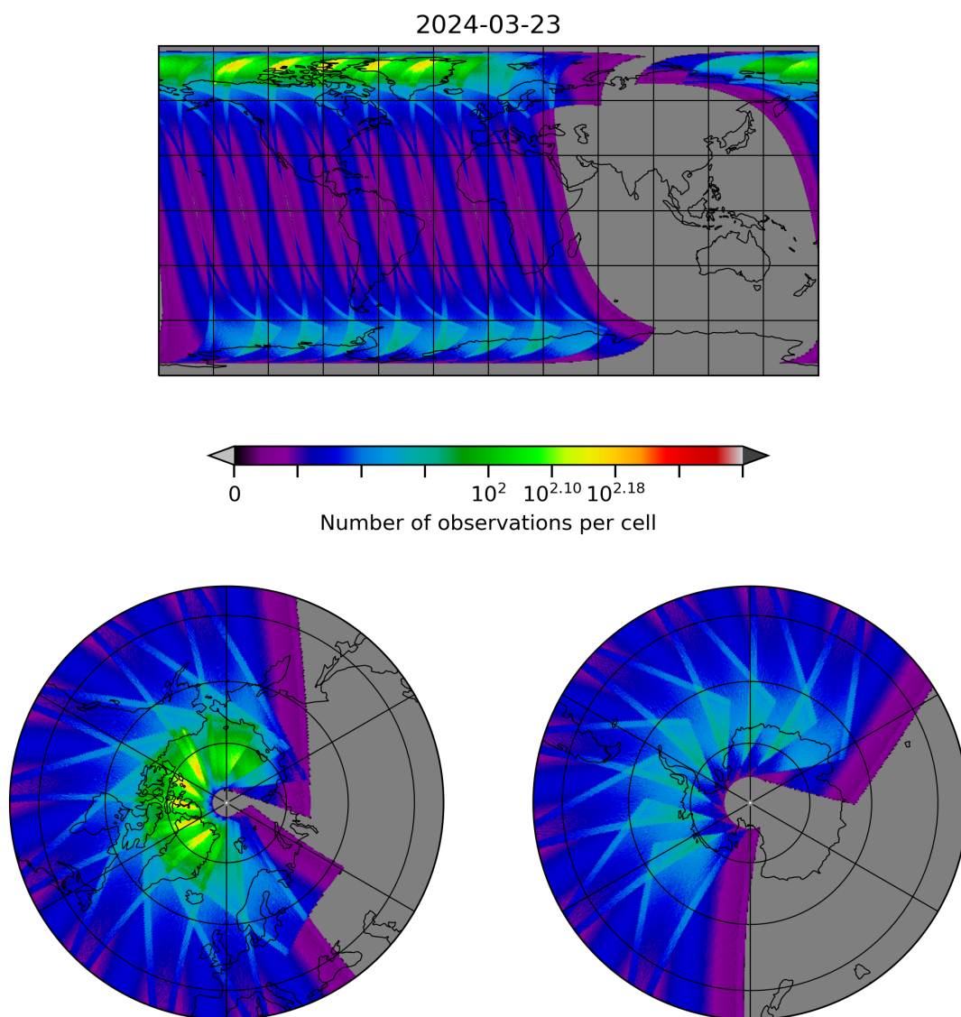
Figure 28: Map of the number of observations for 2024-03-23 to 2024-03-24
