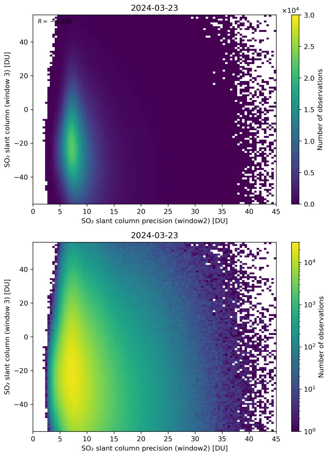
Figure 249: Scatter density plot of “SO 2 slant column precision (window2)” against “SO 2 slant column (window 3)” for 2024-03-23 to 2024-03-24.
