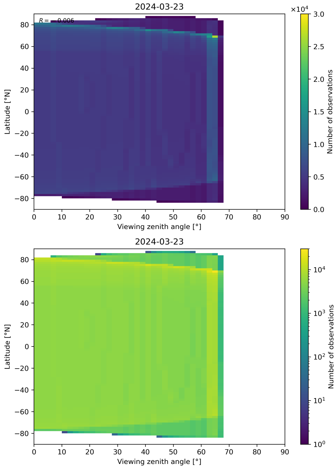
Figure 314: Scatter density plot of “Viewing zenith angle” against “Latitude” for 2024-03-23 to 2024-03-24.
