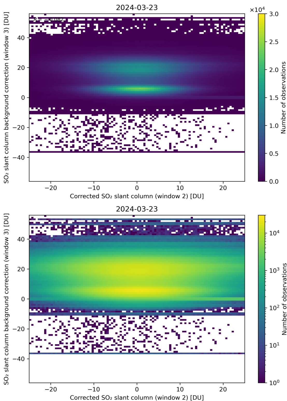
Figure 195: Scatter density plot of “Corrected SO 2 slant column (window 2)” against “SO 2 slant column background correction (window 3)” for 2024-03-23 to 2024-03-24.
