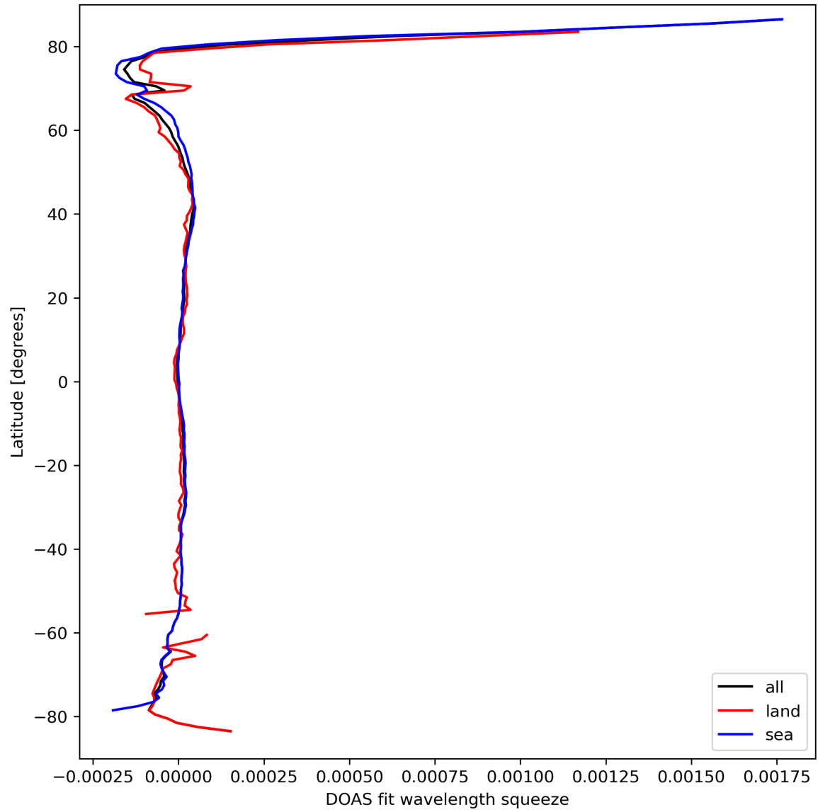
Figure 46: Zonal average of “DOAS fit wavelength squeeze” for 2024-03-23 to 2024-03-24.
