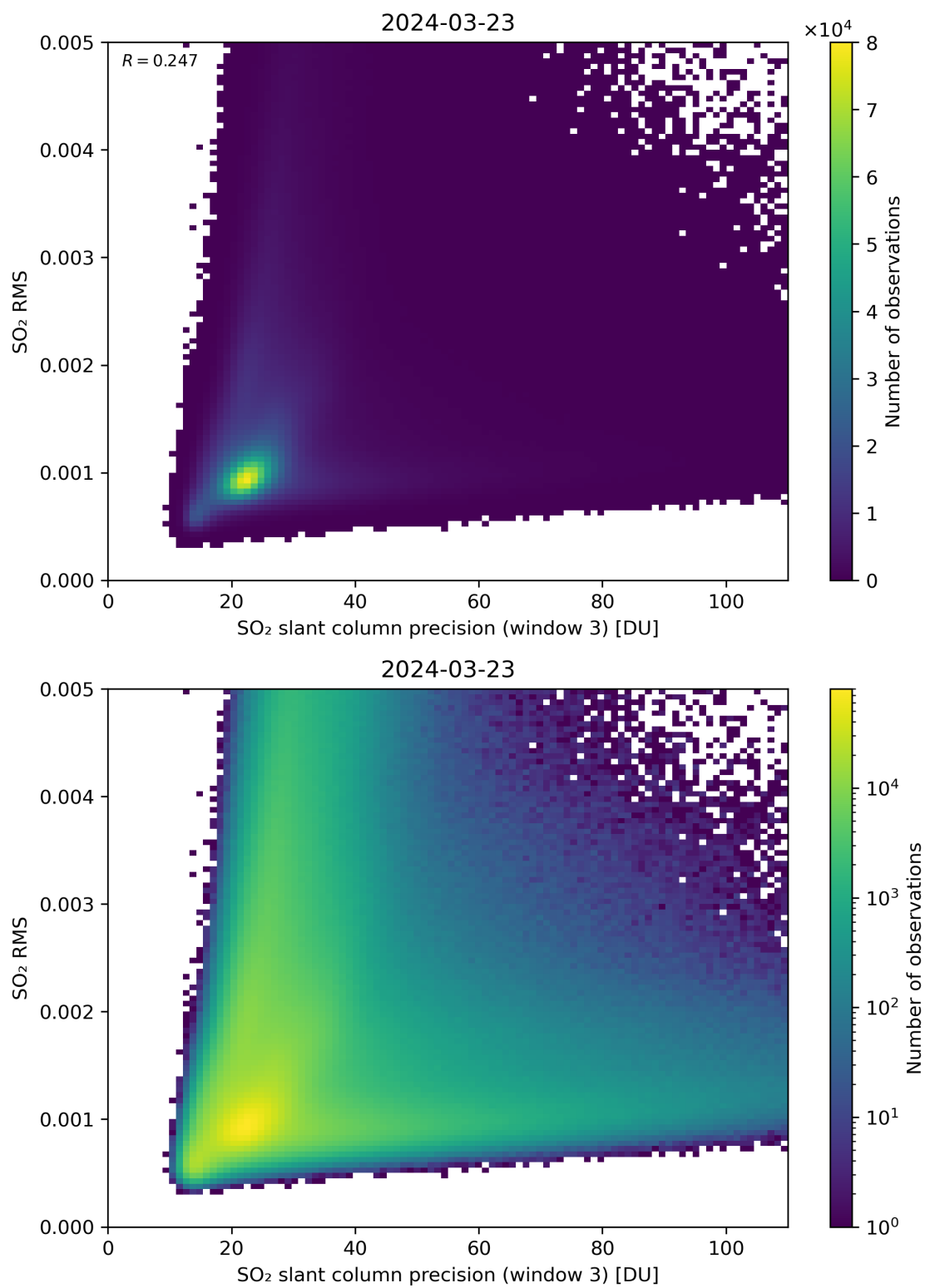
Figure 260: Scatter density plot of “SO 2 slant column precision (window 3)” against “SO 2 RMS” for 2024-03-23 to 2024-03-24.
