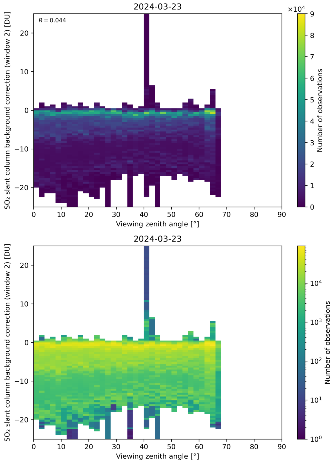
Figure 309: Scatter density plot of “Viewing zenith angle” against “SO 2 slant column background correction (window 2)” for 2024-03-23 to 2024-03-24.
