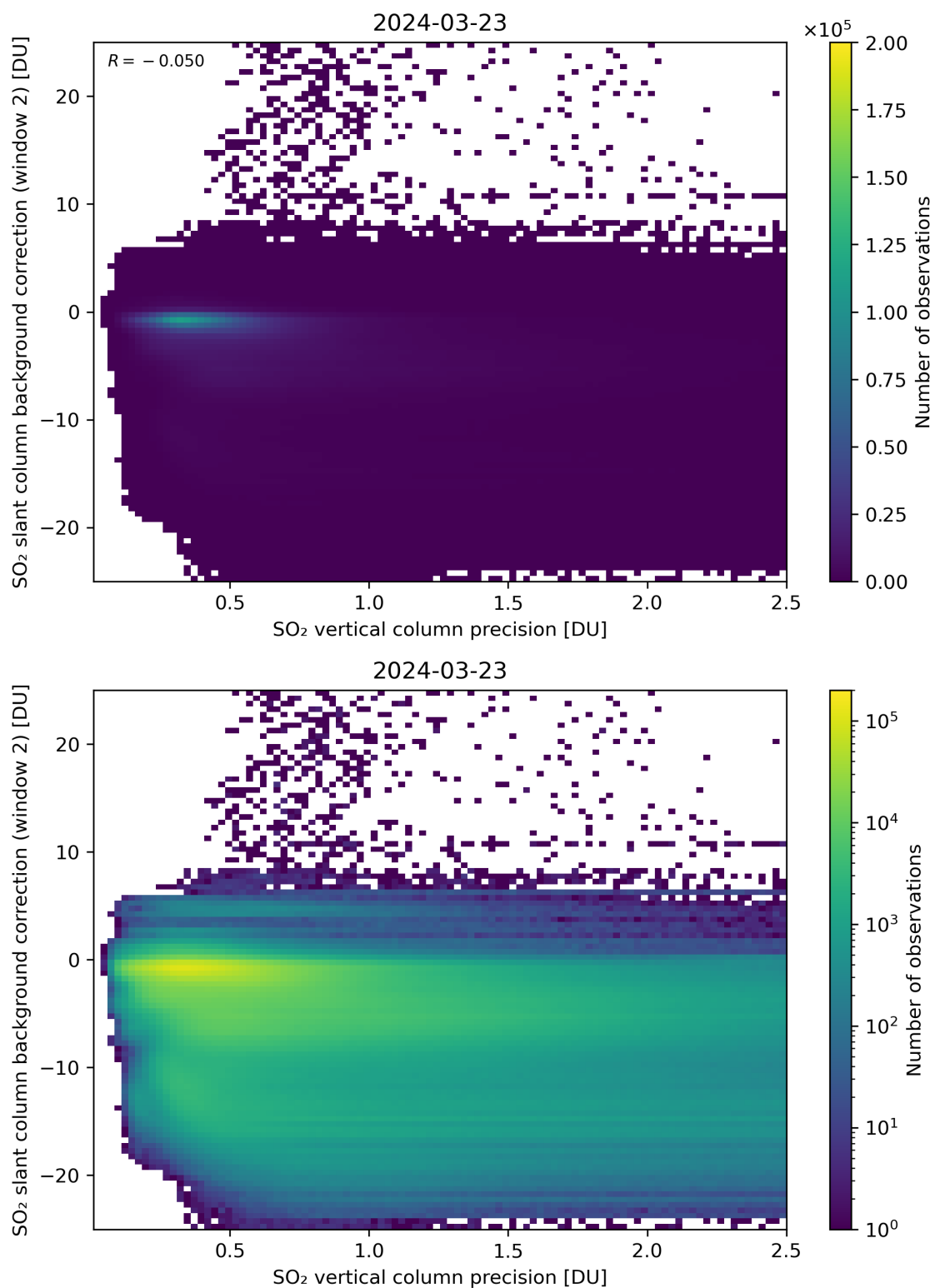
Figure 280: Scatter density plot of “SO 2 vertical column precision” against “SO 2 slant column background correction (window 2)” for 2024-03-23 to 2024-03-24.
