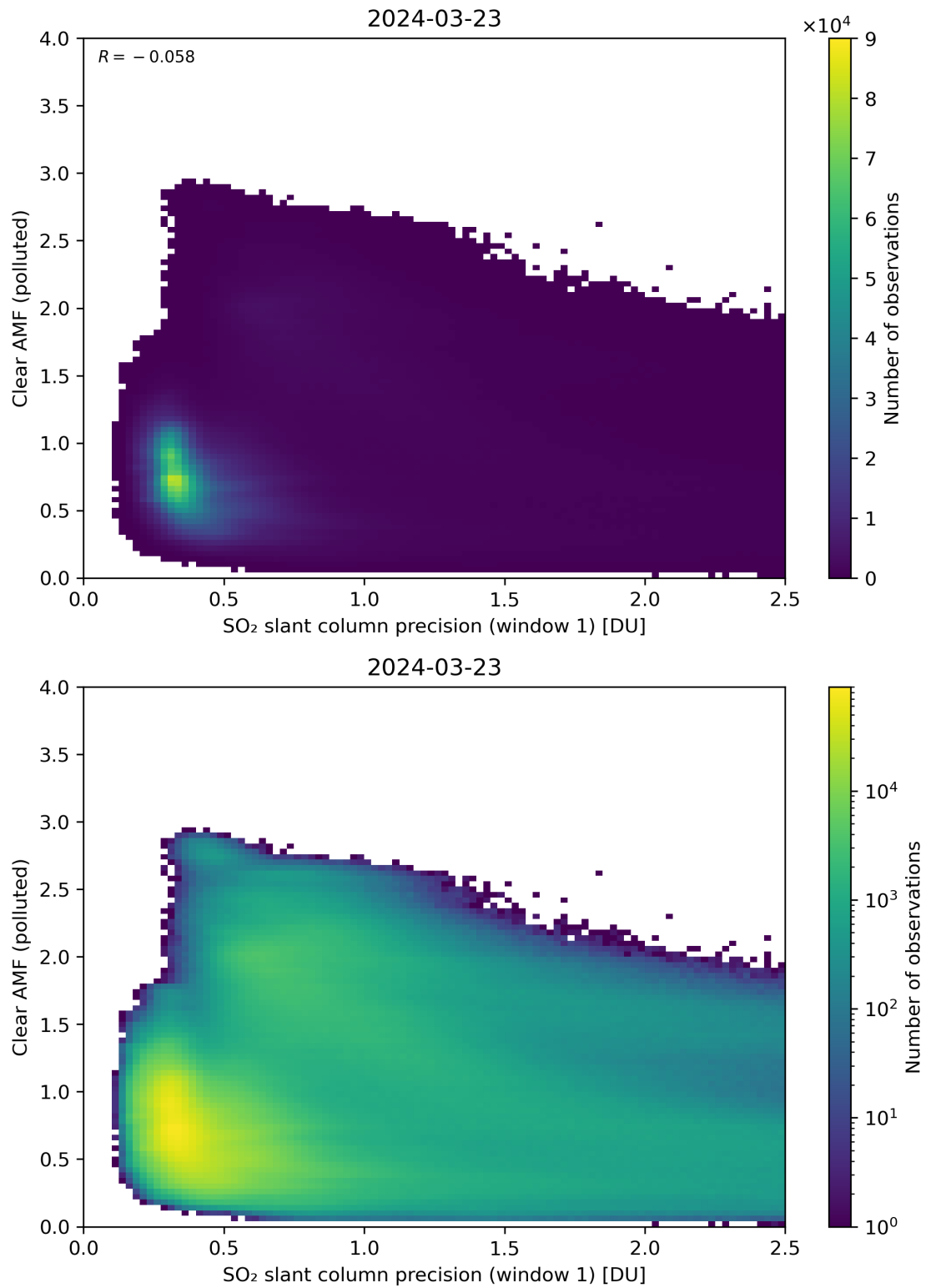
Figure 224: Scatter density plot of “SO 2 slant column precision (window 1)” against “Clear AMF (polluted)” for 2024-03-23 to 2024-03-24.
