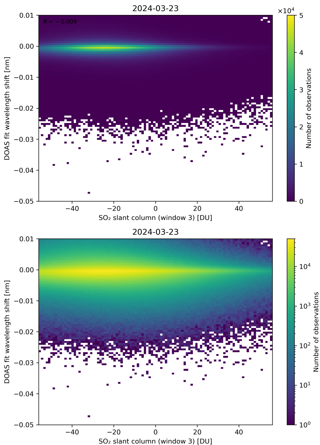
Figure 254: Scatter density plot of “SO 2 slant column (window 3)” against “DOAS fit wavelength shift” for 2024-03-23 to 2024-03-24.
