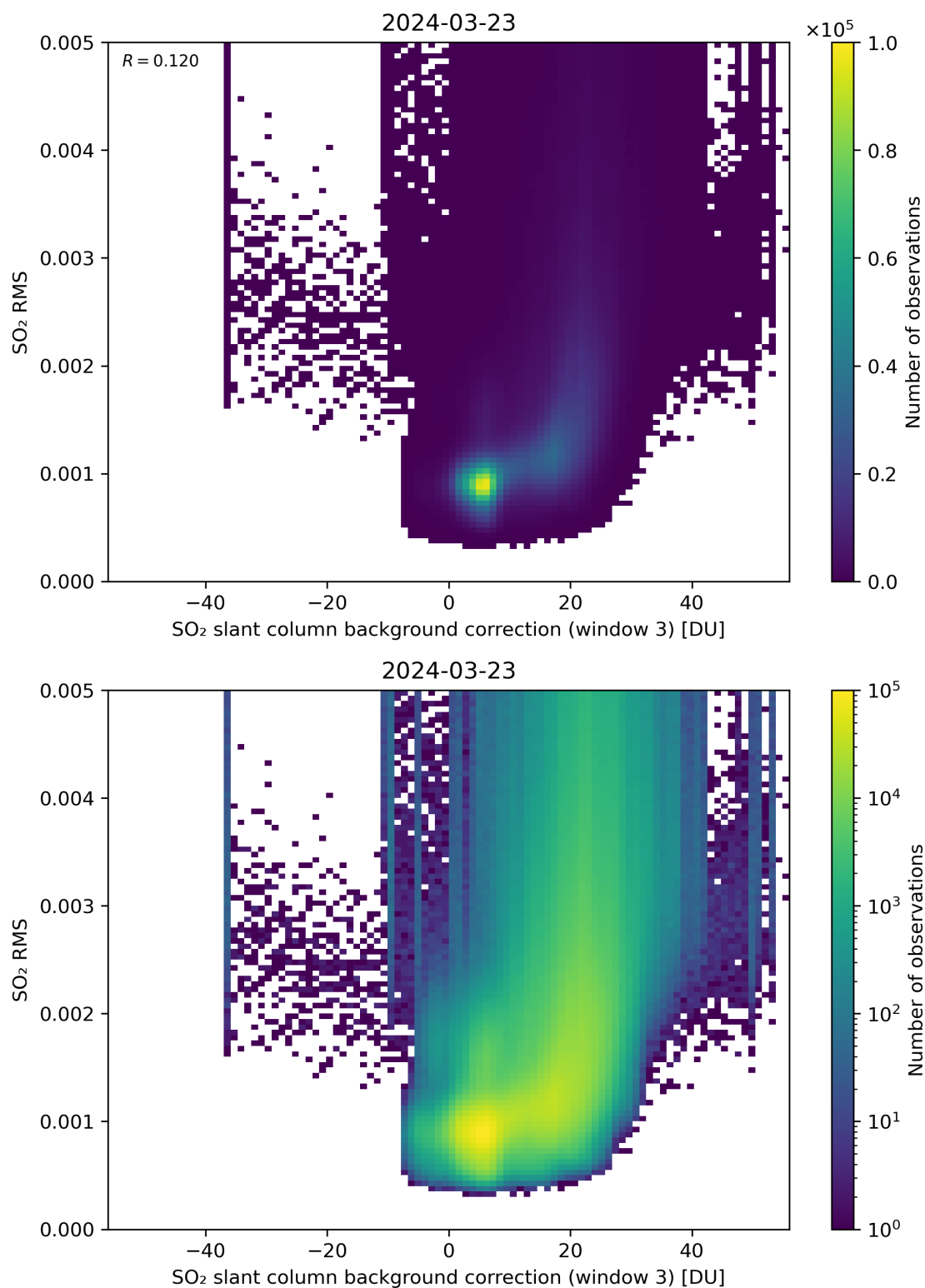
Figure 123: Scatter density plot of “SO 2 slant column background correction (window 3)” against “SO 2 RMS” for 2024-03-23 to 2024-03-24.
