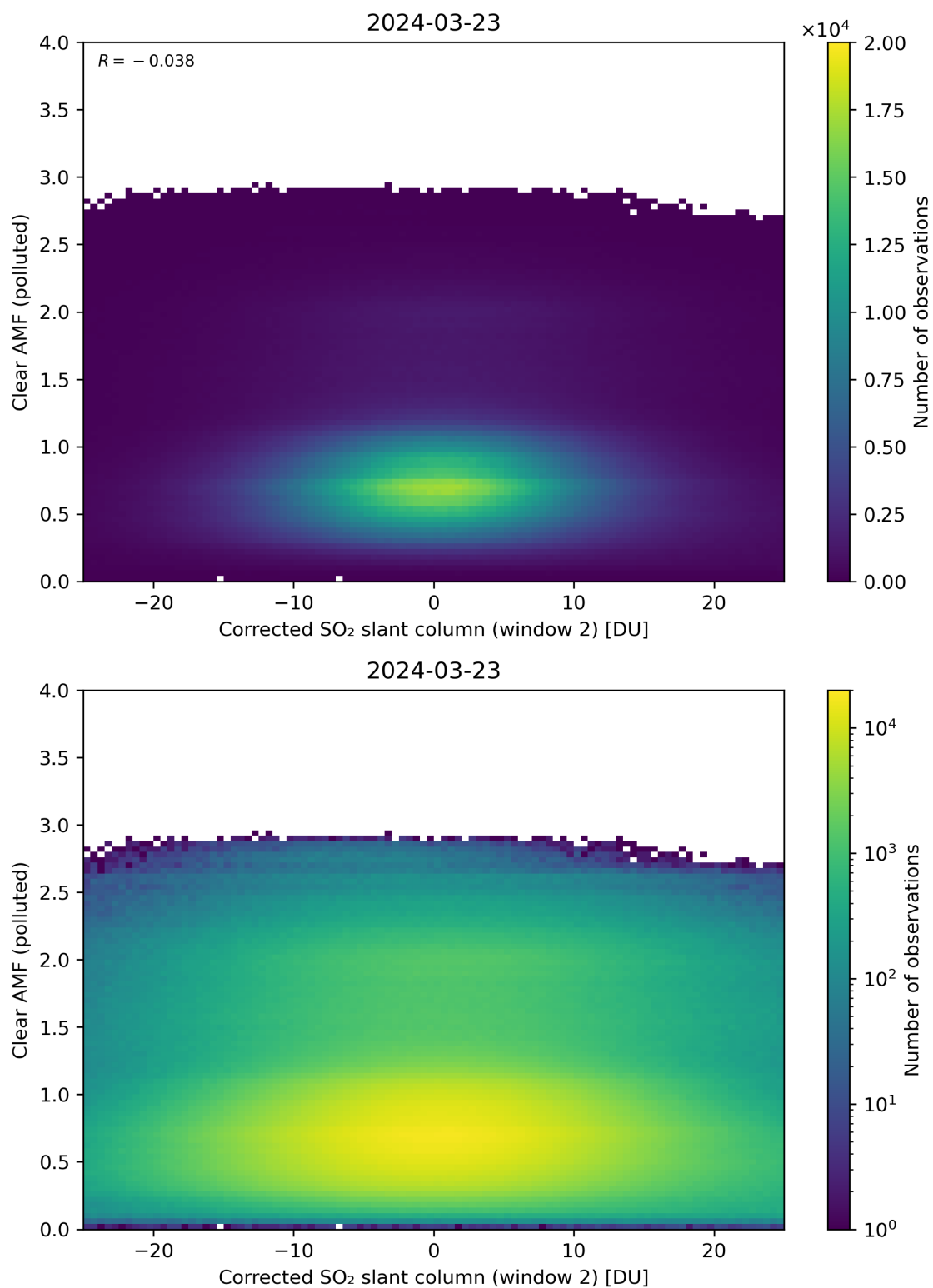
Figure 199: Scatter density plot of “Corrected SO 2 slant column (window 2)” against “Clear AMF (polluted)” for 2024-03-23 to 2024-03-24.
