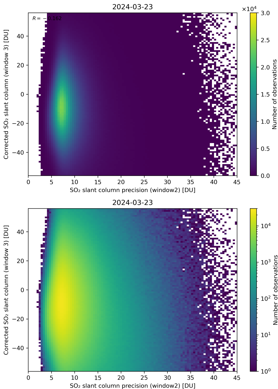
Figure 248: Scatter density plot of “SO 2 slant column precision (window2)” against “Corrected SO 2 slant column (window 3)” for 2024-03-23 to 2024-03-24.
