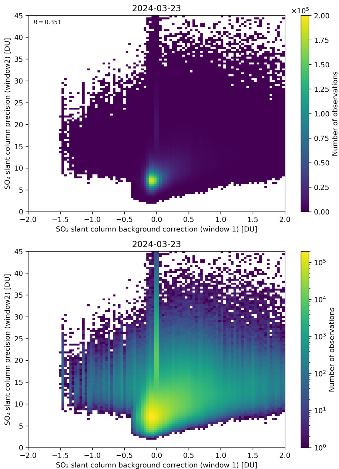
Figure 106: Scatter density plot of “SO 2 slant column background correction (window 1)” against “SO 2 slant column precision (window2)” for 2024-03-23 to 2024-03-24.
