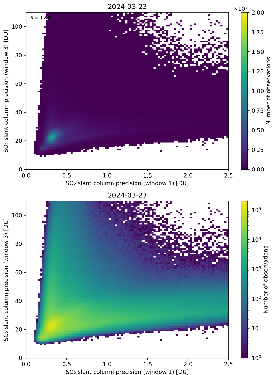
Figure 229: Scatter density plot of “SO 2 slant column precision (window 1)” against “SO 2 slant column precision (window 3)” for 2024-03-23 to 2024-03-24.
