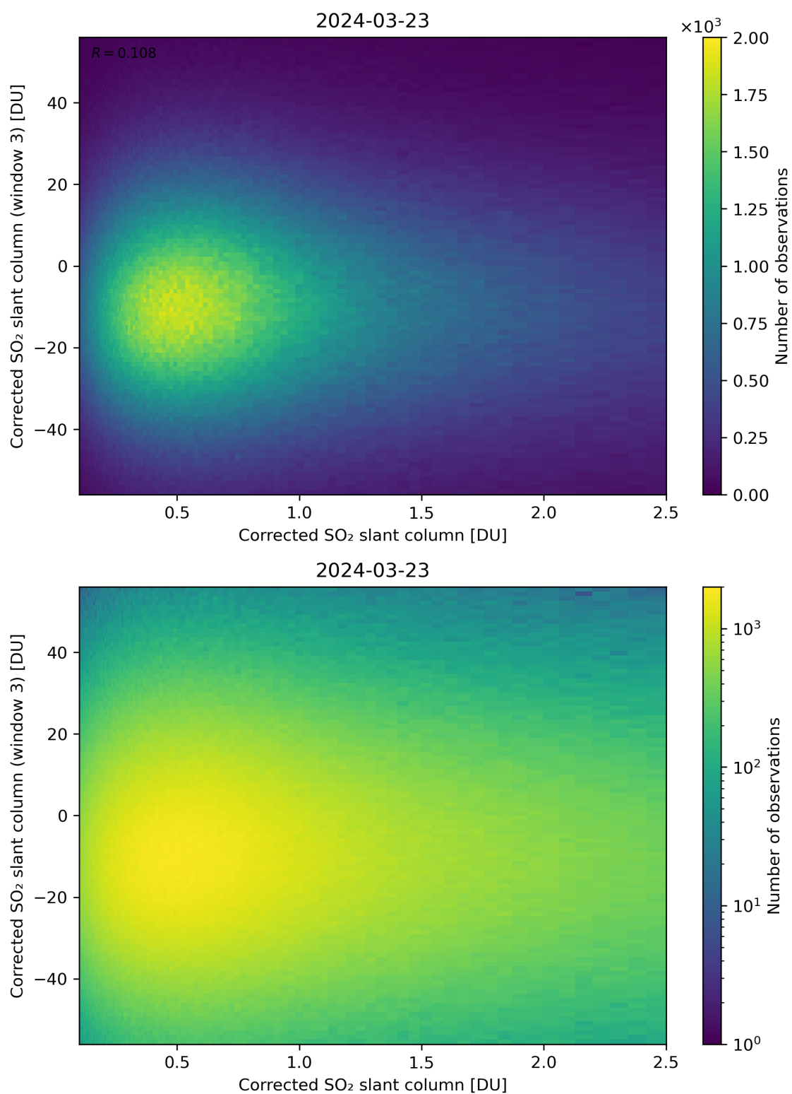
Figure 186: Scatter density plot of “Corrected SO 2 slant column” against “Corrected SO 2 slant column (window 3)” for 2024-03-23 to 2024-03-24.
