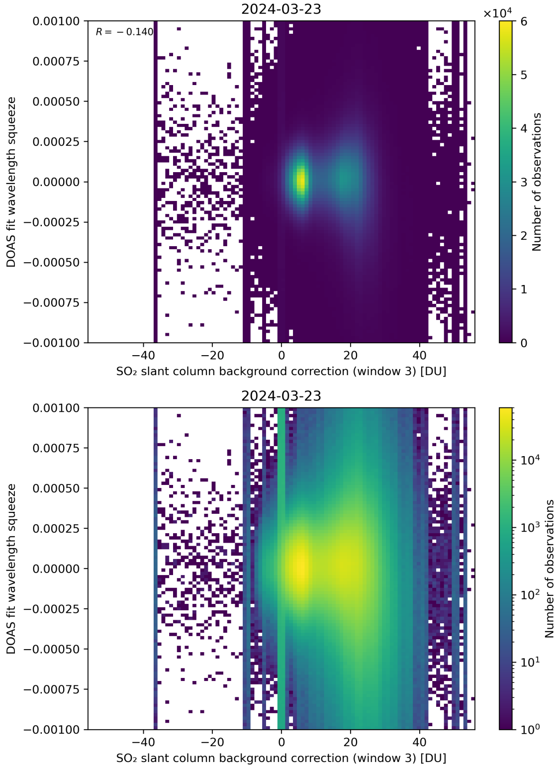
Figure 122: Scatter density plot of “SO 2 slant column background correction (window 3)” against “DOAS fit wavelength squeeze” for 2024-03-23 to 2024-03-24.
