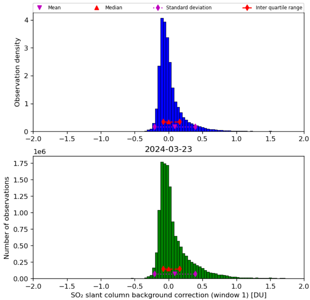
Figure 59: Histogram of “SO 2 slant column background correction (window 1)” for 2024-03-23 to 2024-03-24
