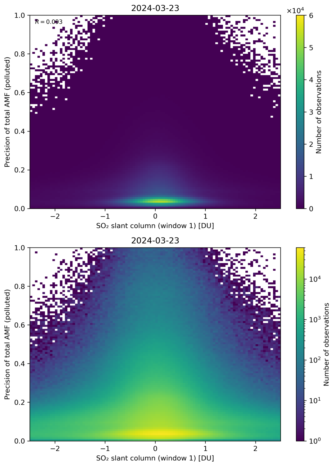
Figure 240: Scatter density plot of “SO 2 slant column (window 1)” against “Precision of total AMF (polluted)” for 2024-03-23 to 2024-03-24.
