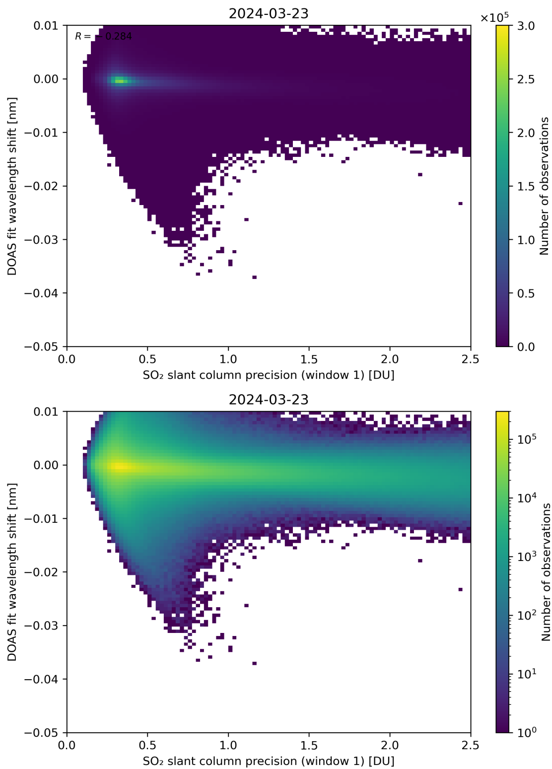
Figure 221: Scatter density plot of “SO 2 slant column precision (window 1)” against “DOAS fit wavelength shift” for 2024-03-23 to 2024-03-24.
