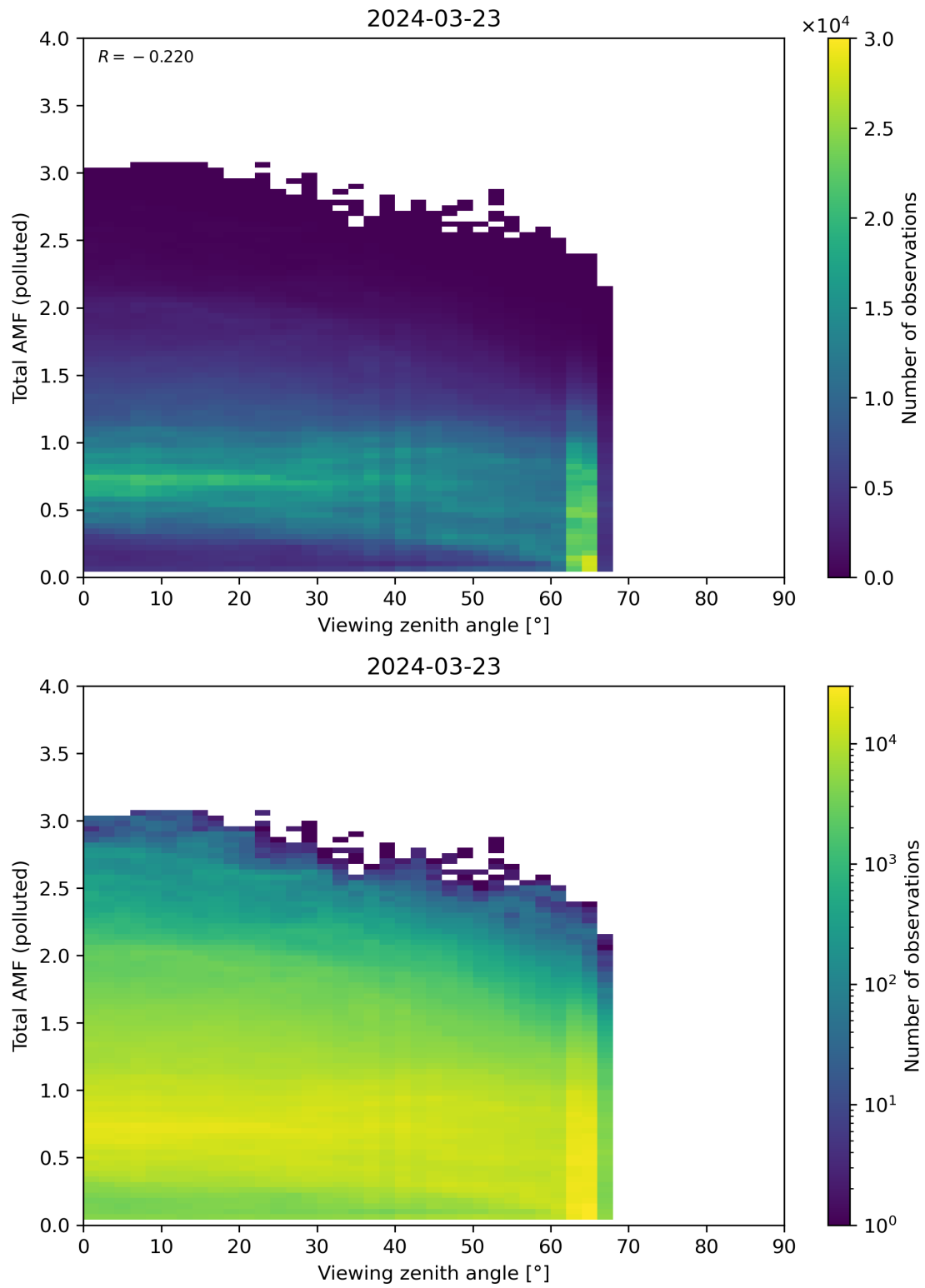
Figure 325: Scatter density plot of “Viewing zenith angle” against “Total AMF (polluted)” for 2024-03-23 to 2024-03-24.
