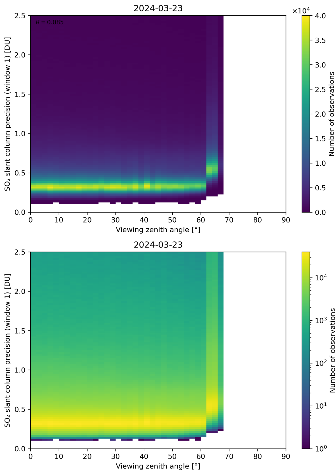
Figure 321: Scatter density plot of “Viewing zenith angle” against “SO 2 slant column precision (window 1)” for 2024-03-23 to 2024-03-24.
