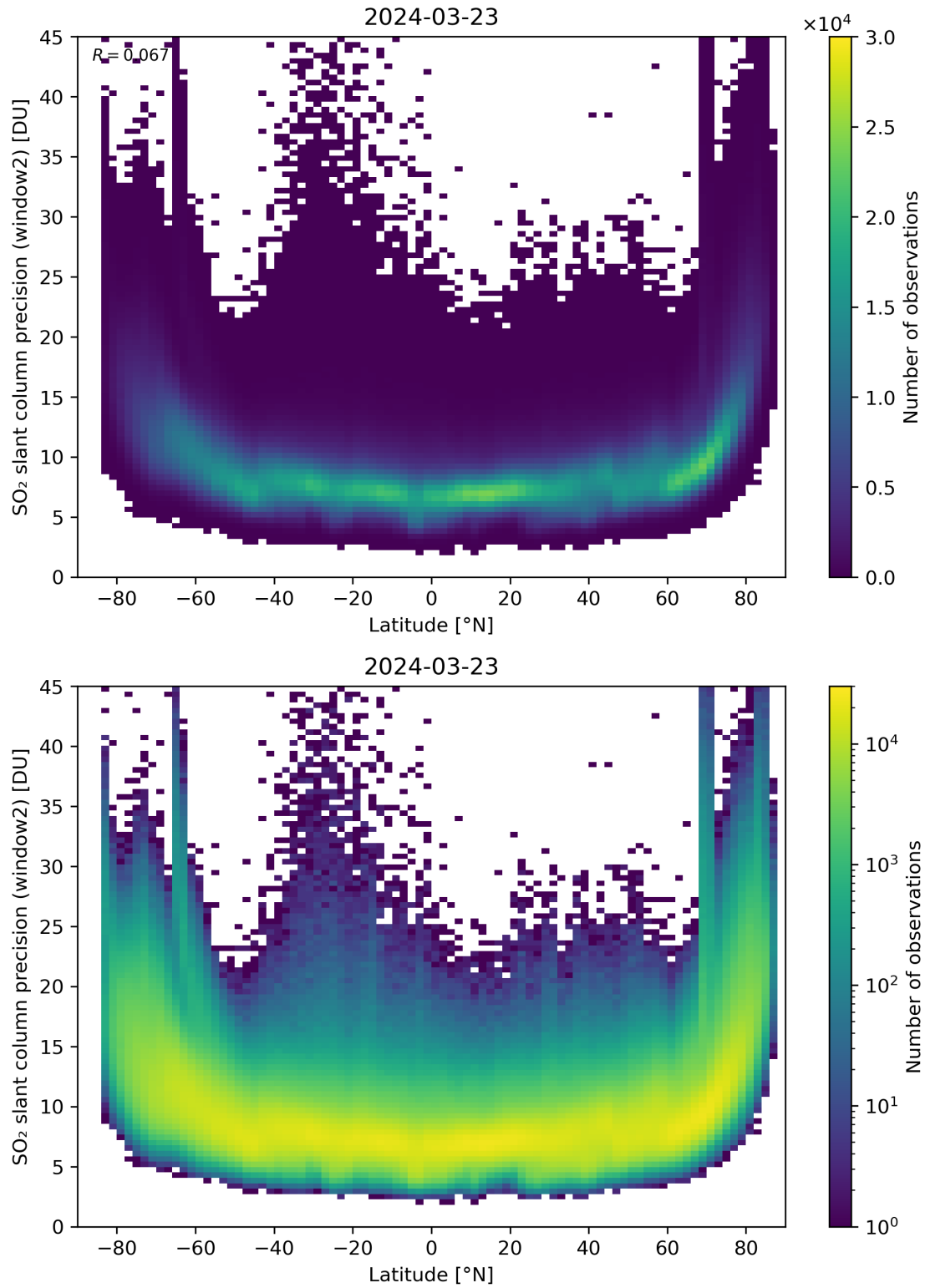
Figure 151: Scatter density plot of “Latitude” against “SO 2 slant column precision (window2)” for 2024-03-23 to 2024-03-24.
