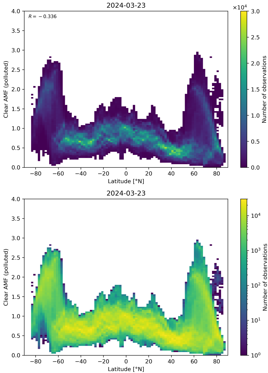
Figure 145: Scatter density plot of “Latitude” against “Clear AMF (polluted)” for 2024-03-23 to 2024-03-24.
