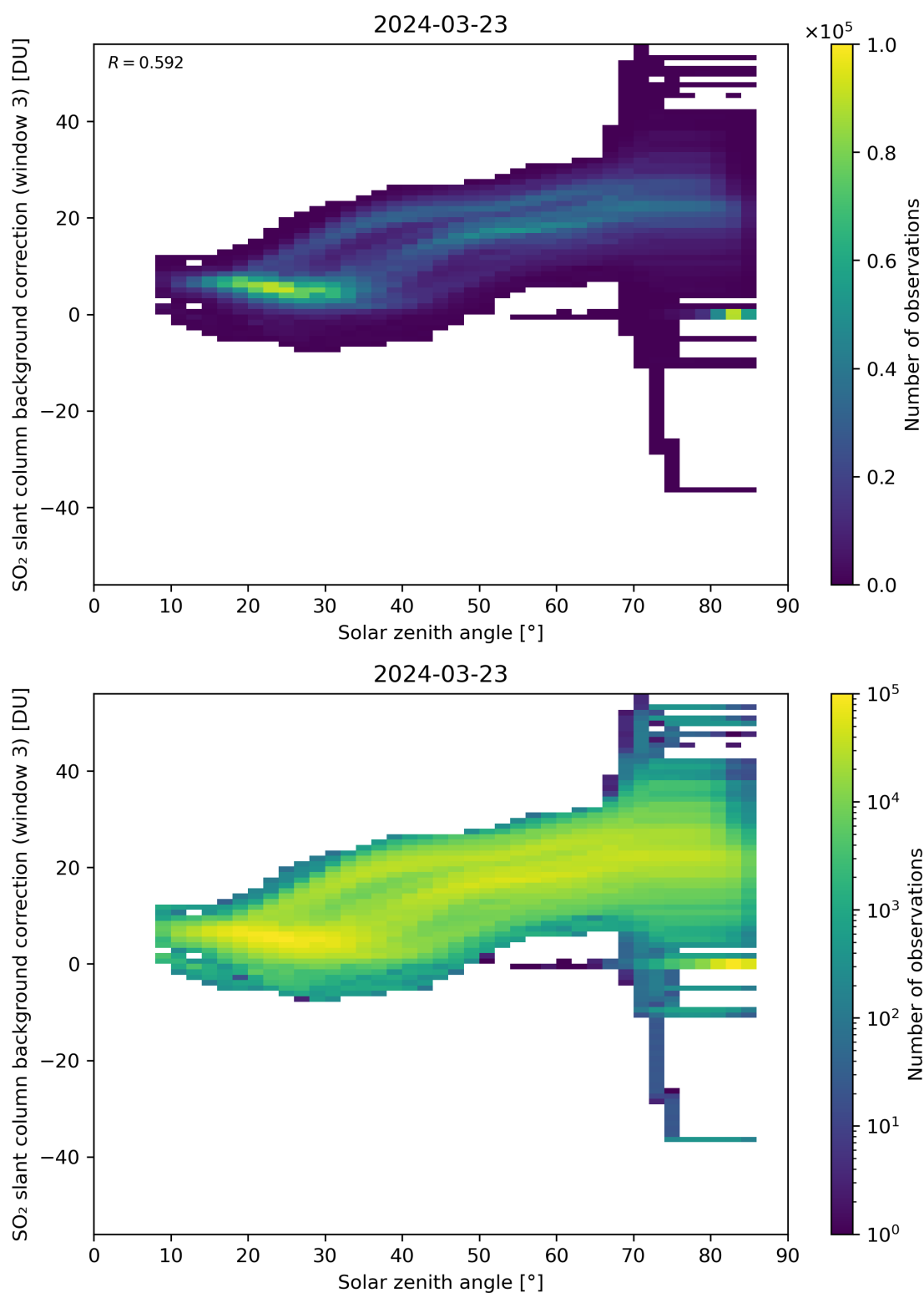
Figure 160: Scatter density plot of “Solar zenith angle” against “SO 2 slant column background correction (window 3)” for 2024-03-23 to 2024-03-24.
