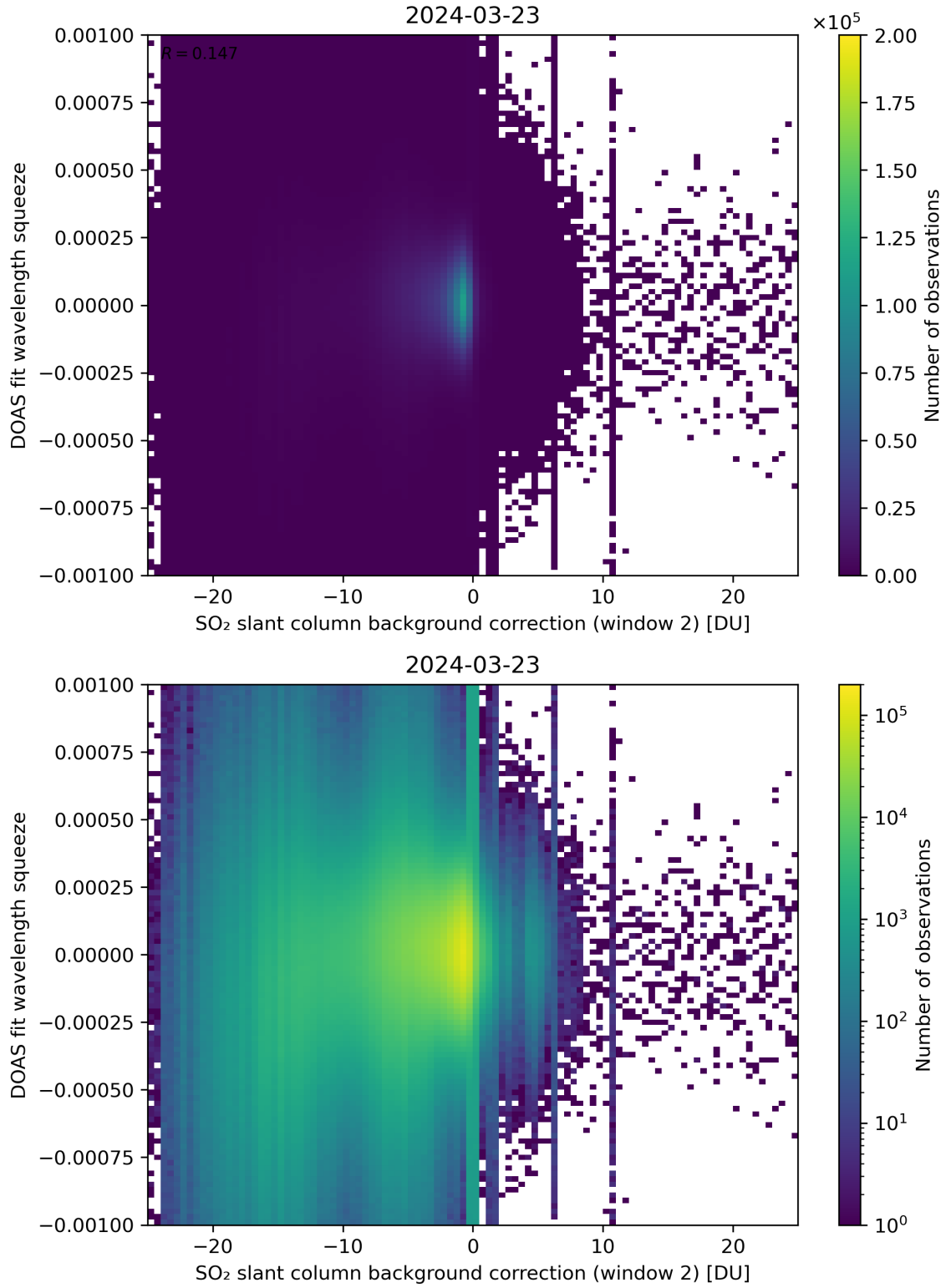
Figure 113: Scatter density plot of “SO 2 slant column background correction (window 2)” against “DOAS fit wavelength squeeze” for 2024-03-23 to 2024-03-24.
