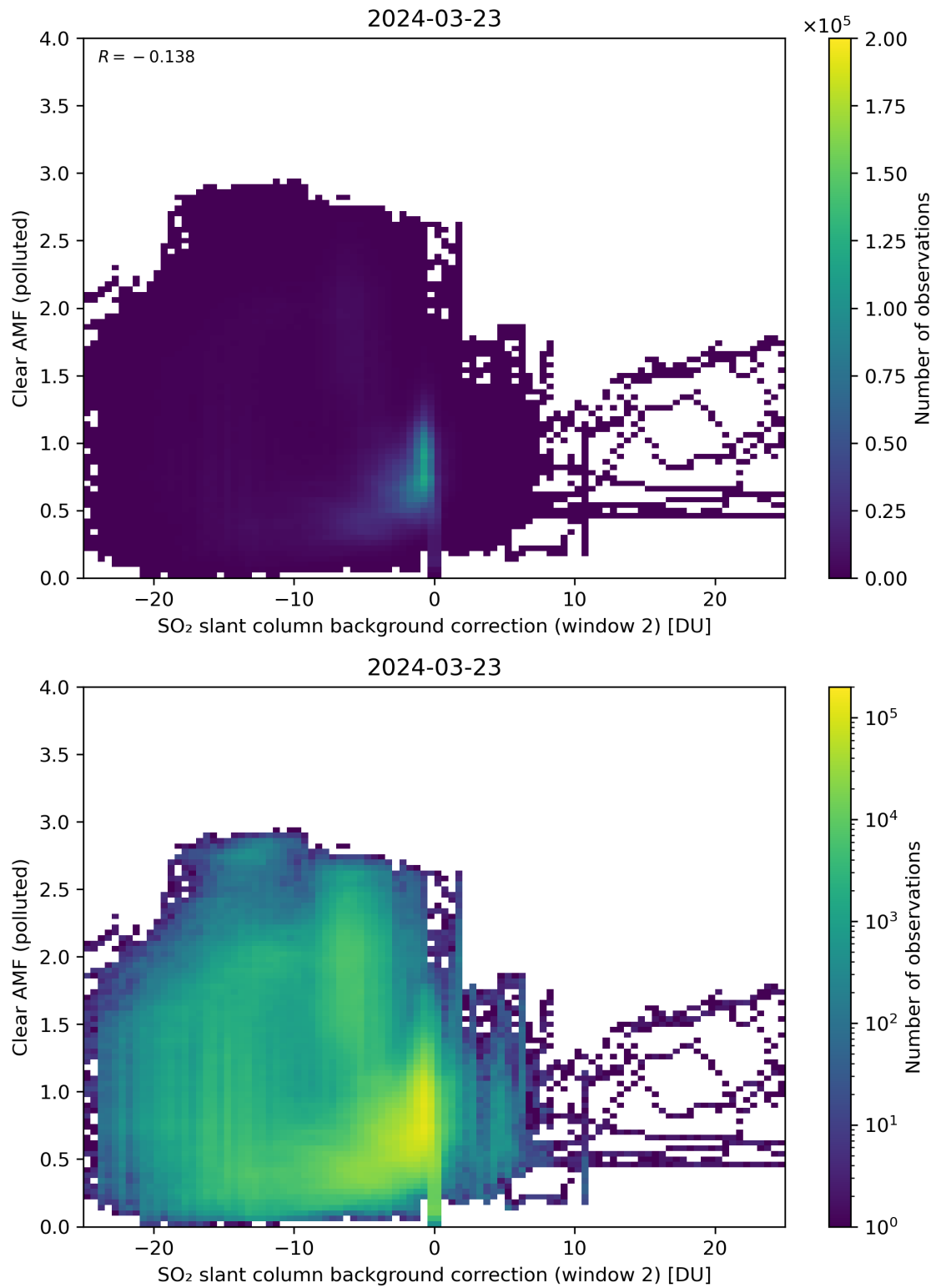
Figure 115: Scatter density plot of “SO 2 slant column background correction (window 2)” against “Clear AMF (polluted)” for 2024-03-23 to 2024-03-24.
