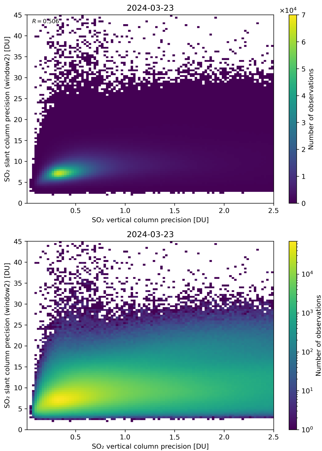
Figure 291: Scatter density plot of “SO 2 vertical column precision” against “SO 2 slant column precision (window2)” for 2024-03-23 to 2024-03-24.
