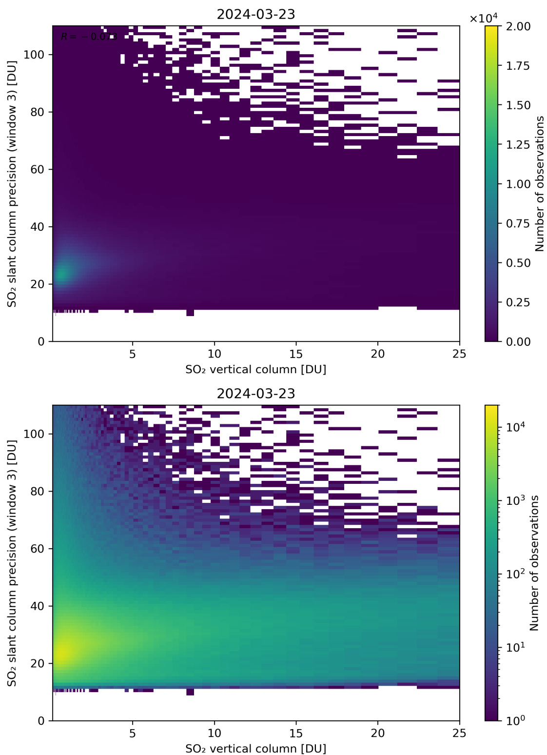
Figure 304: Scatter density plot of “SO 2 vertical column” against “SO 2 slant column precision (window 3)” for 2024-03-23 to 2024-03-24.
