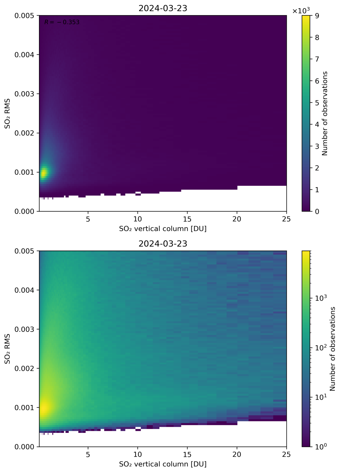
Figure 278: Scatter density plot of “SO 2 vertical column” against “SO 2 RMS” for 2024-03-23 to 2024-03-24.
