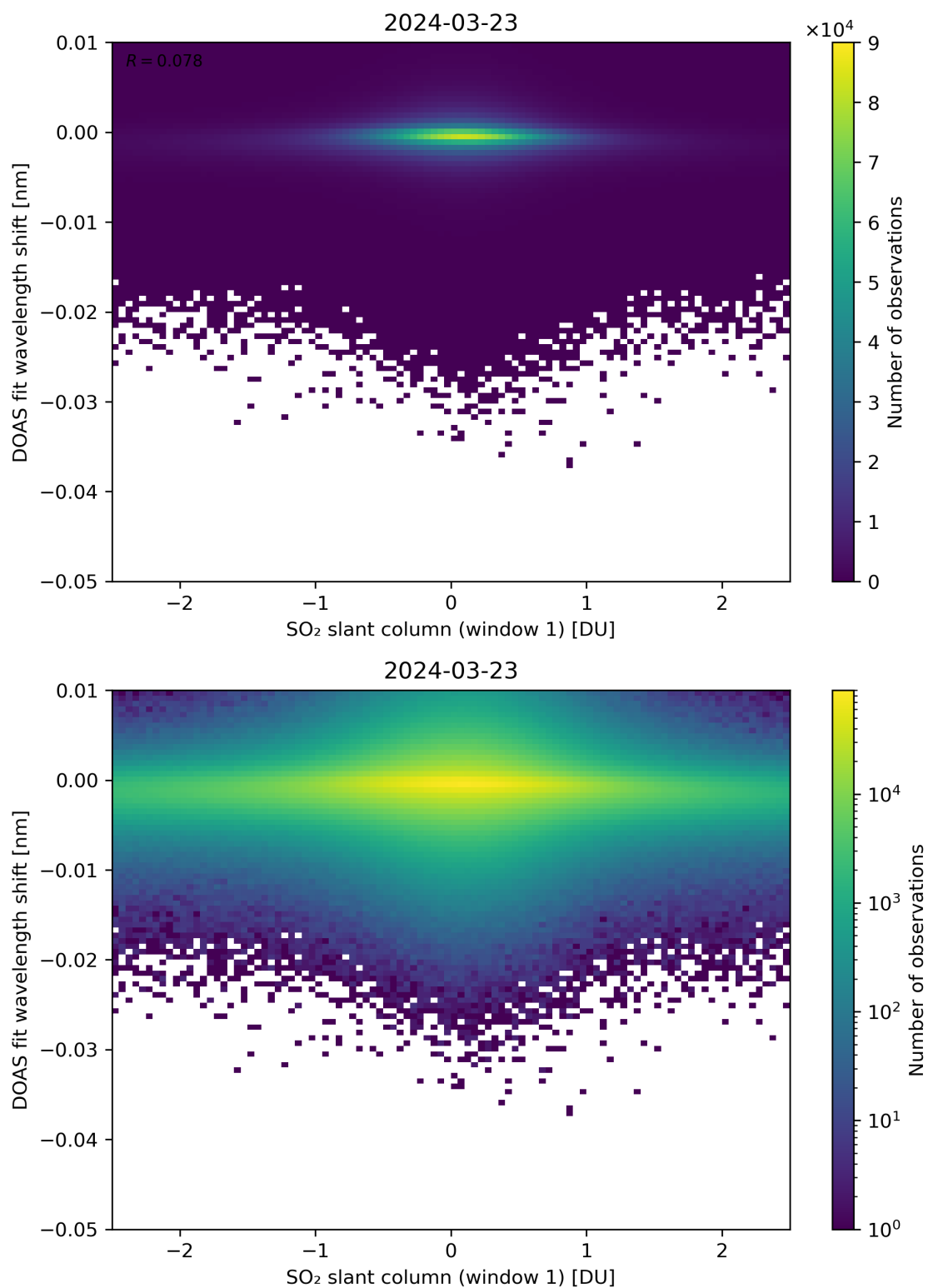
Figure 215: Scatter density plot of “SO 2 slant column (window 1)” against “DOAS fit wavelength shift” for 2024-03-23 to 2024-03-24.
