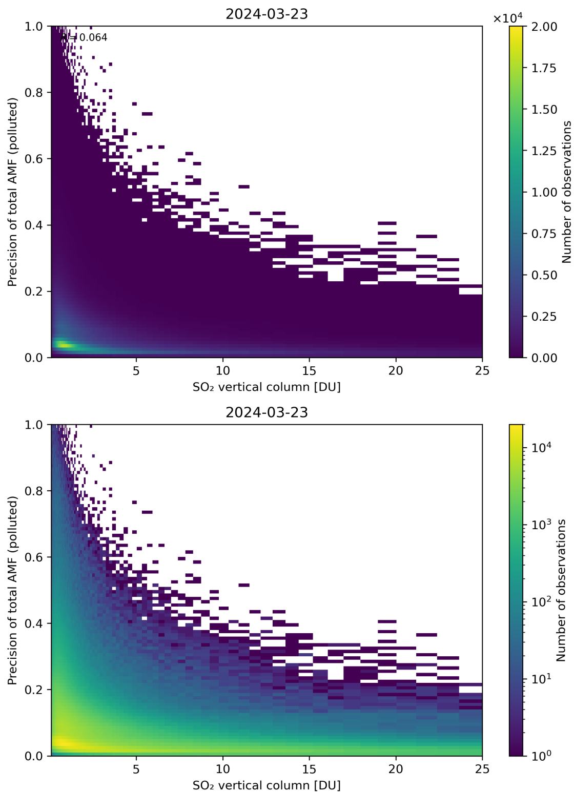
Figure 306: Scatter density plot of “SO 2 vertical column” against “Precision of total AMF (polluted)” for 2024-03-23 to 2024-03-24.
