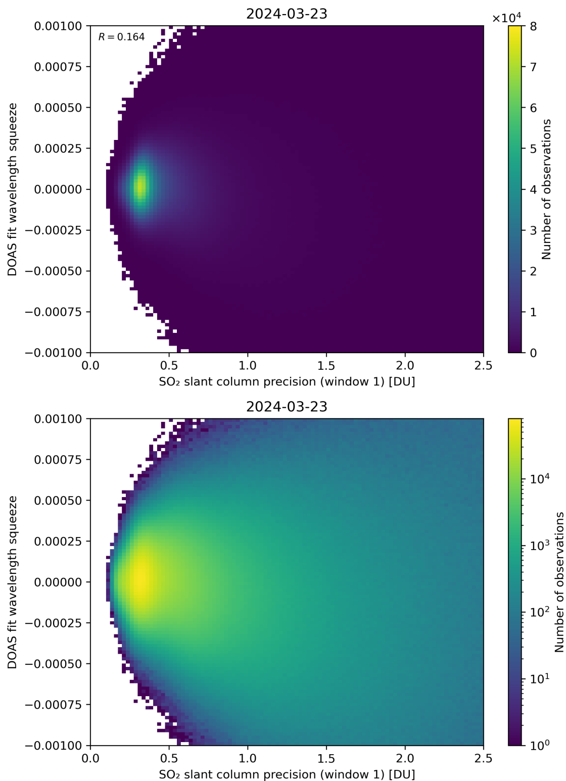
Figure 222: Scatter density plot of “SO 2 slant column precision (window 1)” against “DOAS fit wavelength squeeze” for 2024-03-23 to 2024-03-24.
