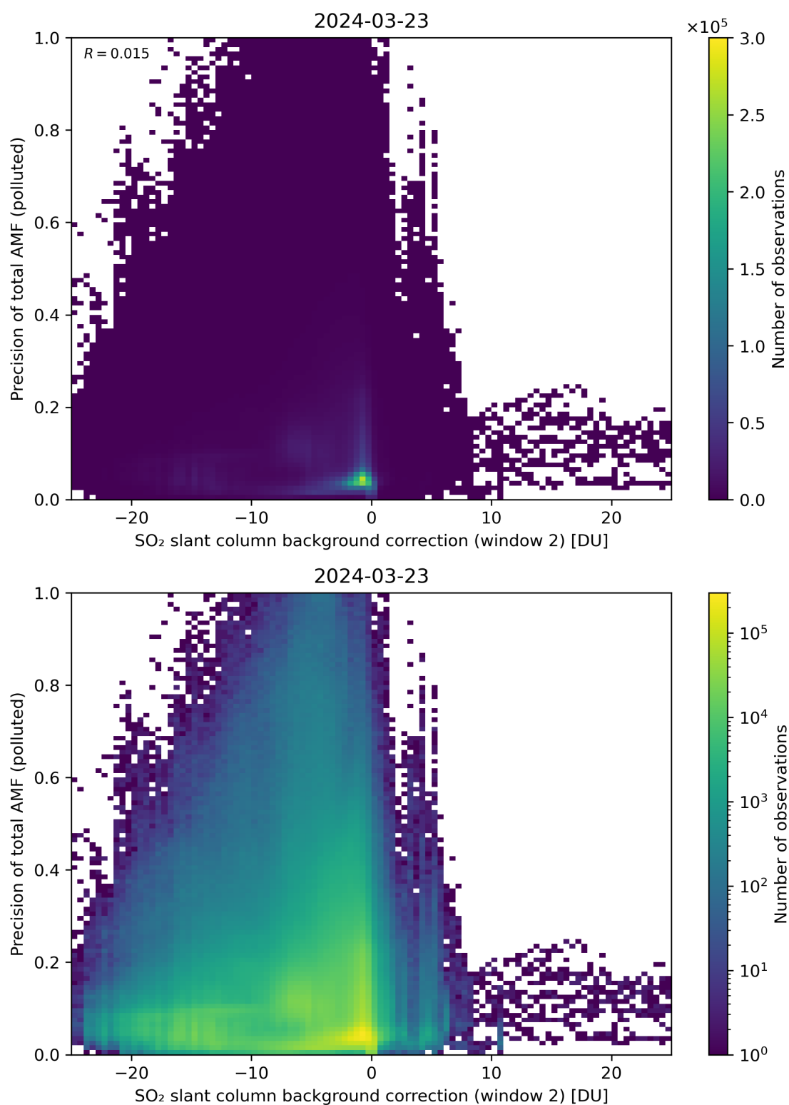
Figure 120: Scatter density plot of “SO 2 slant column background correction (window 2)” against “Precision of total AMF (polluted)” for 2024-03-23 to 2024-03-24.
