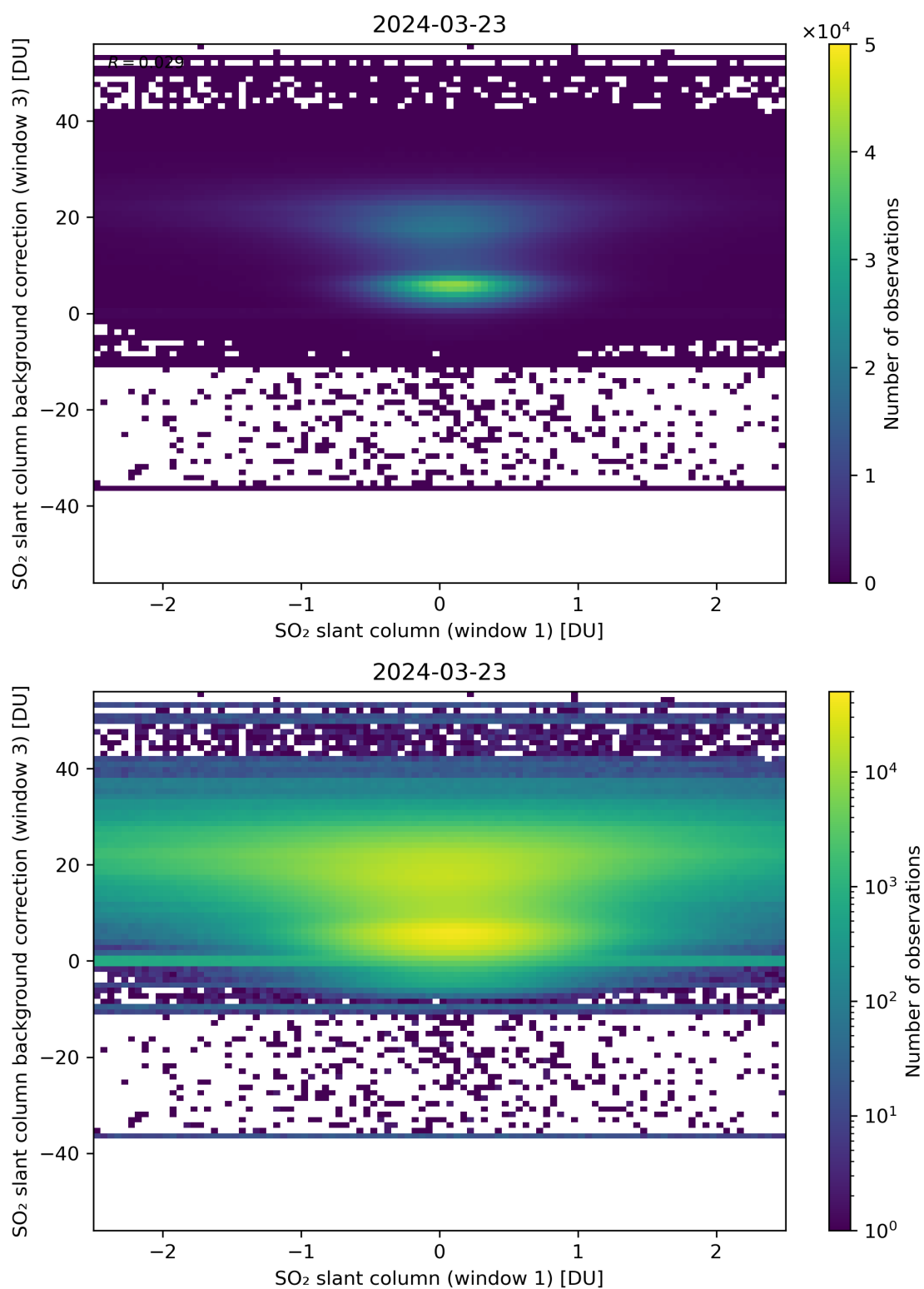
Figure 214: Scatter density plot of “SO 2 slant column (window 1)” against “SO 2 slant column background correction (window 3)” for 2024-03-23 to 2024-03-24.
