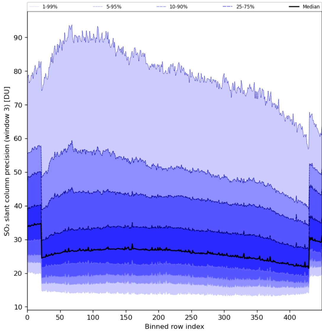
Figure 88: Along track statistics of “SO 2 slant column precision (window 3)” for 2024-03-23 to 2024-03-24
