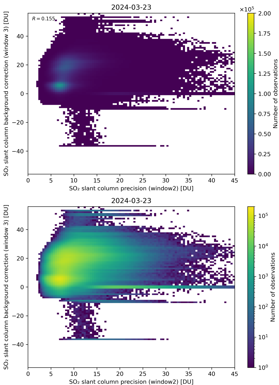
Figure 242: Scatter density plot of “SO 2 slant column precision (window2)” against “SO 2 slant column background correction (window 3)” for 2024-03-23 to 2024-03-24.
