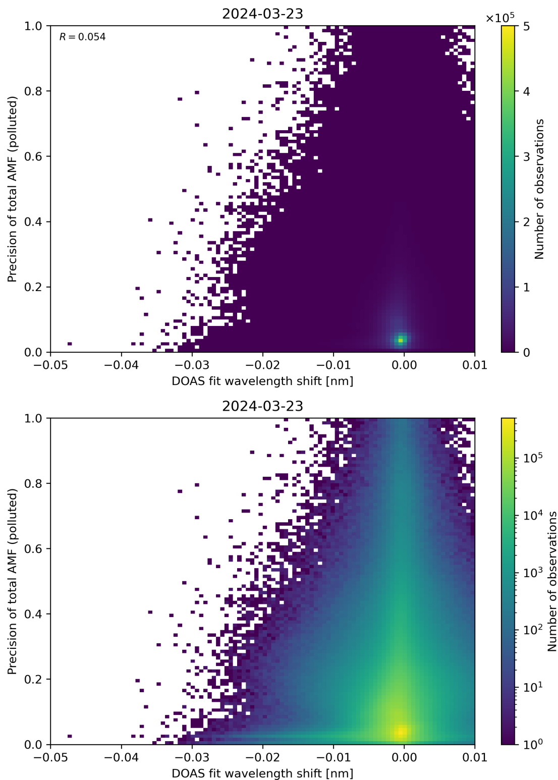
Figure 131: Scatter density plot of “DOAS fit wavelength shift” against “Precision of total AMF (polluted)” for 2024-03-23 to 2024-03-24.
