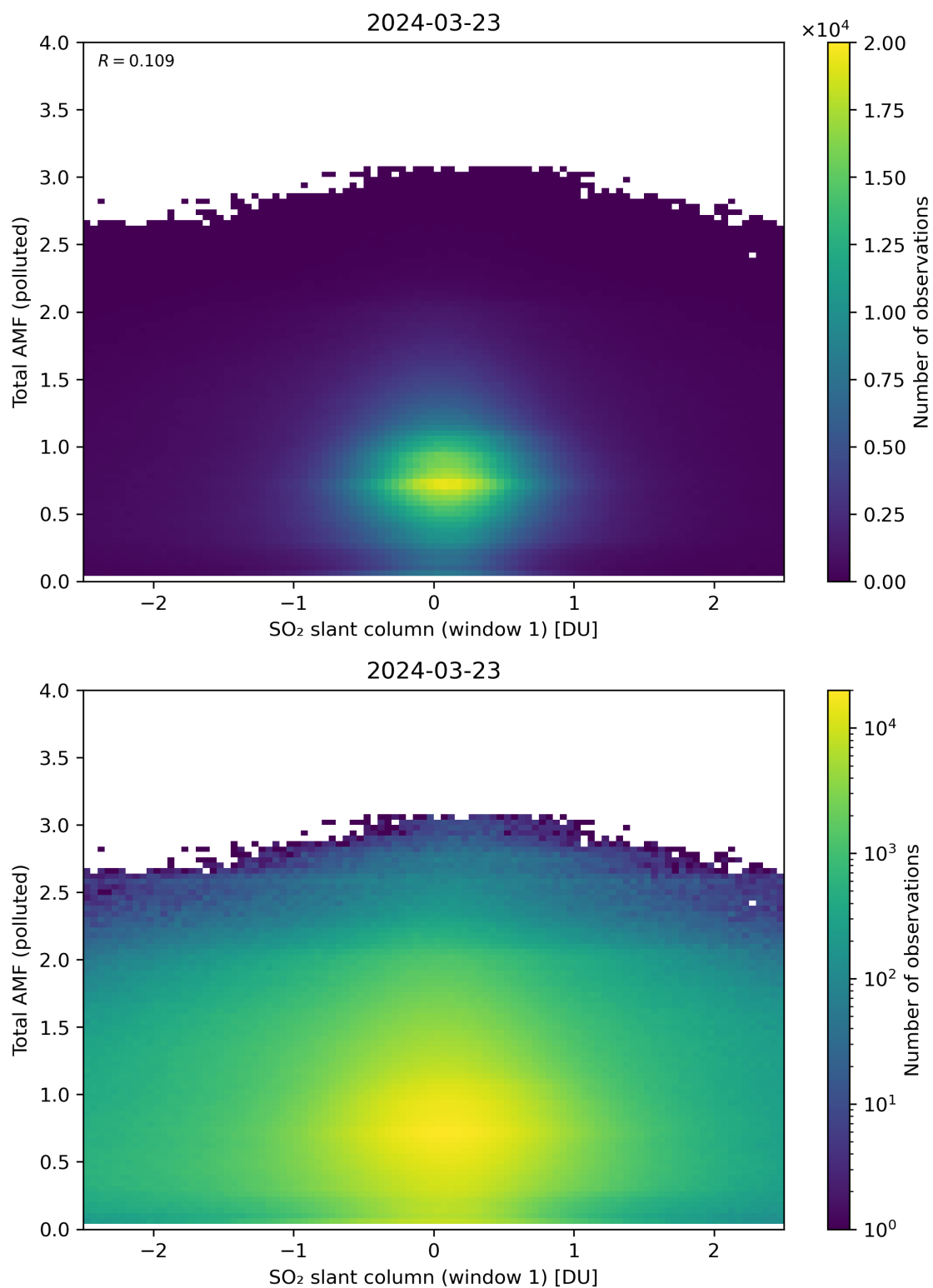
Figure 239: Scatter density plot of “SO 2 slant column (window 1)” against “Total AMF (polluted)” for 2024-03-23 to 2024-03-24.
