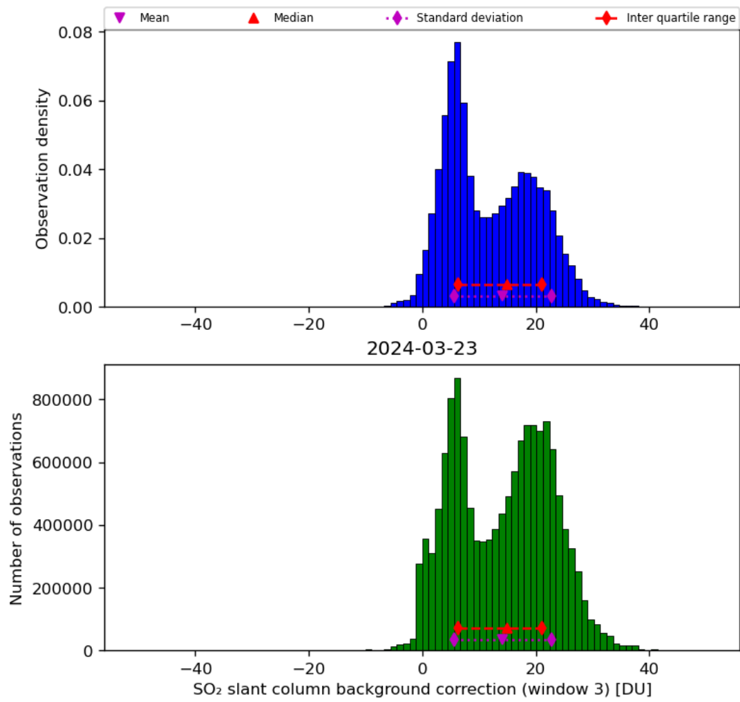
Figure 67: Histogram of “SO 2 slant column background correction (window 3)” for 2024-03-23 to 2024-03-24
