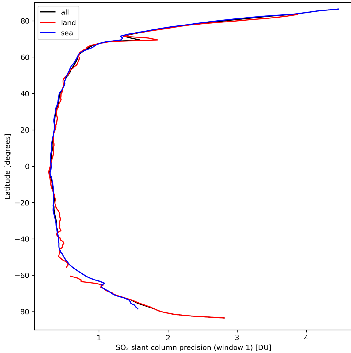
Figure 34: Zonal average of “SO 2 slant column precision (window 1)” for 2024-03-23 to 2024-03-24.
