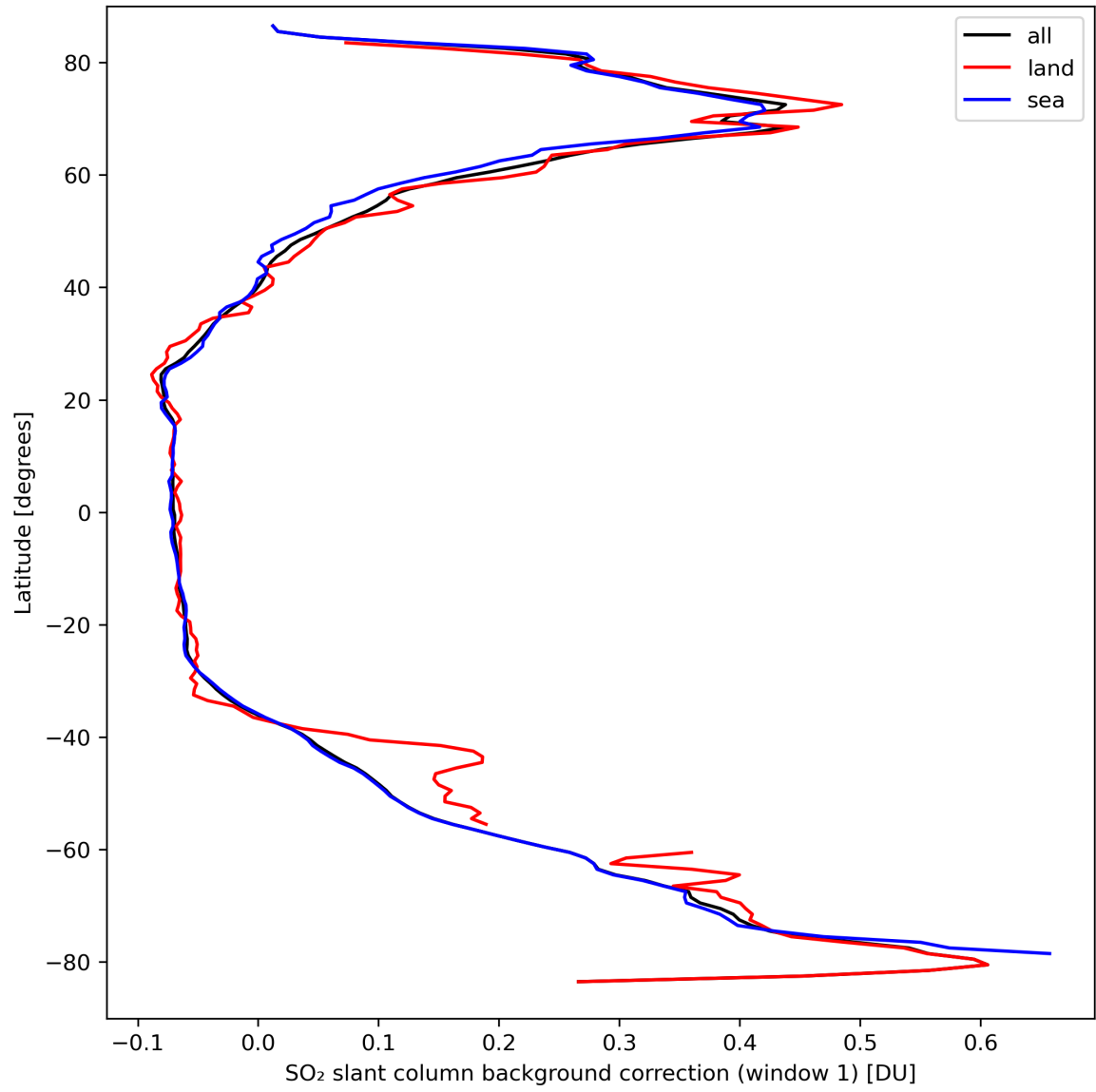
Figure 36: Zonal average of “SO 2 slant column background correction (window 1)” for 2024-03-23 to 2024-03-24.
