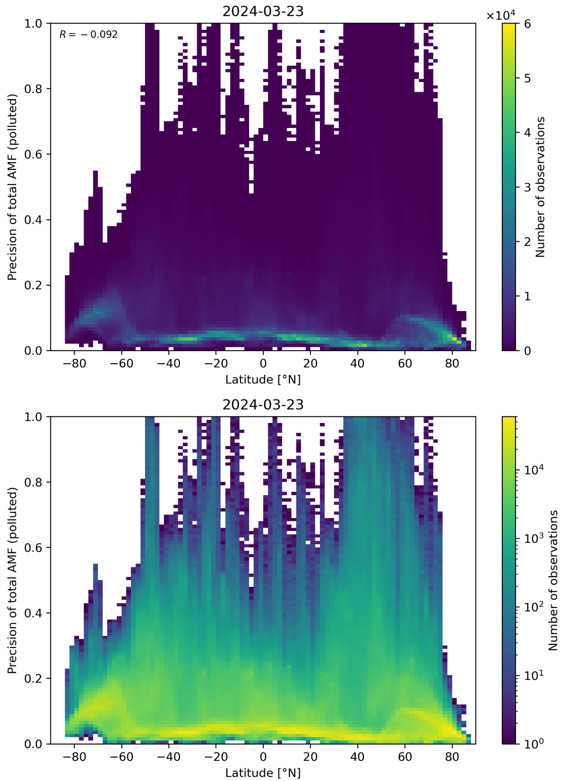
Figure 155: Scatter density plot of “Latitude” against “Precision of total AMF (polluted)” for 2024-03-23 to 2024-03-24.
