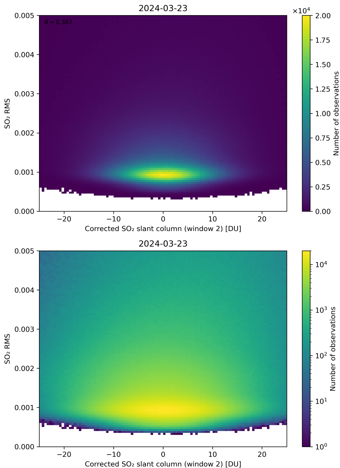
Figure 198: Scatter density plot of “Corrected SO 2 slant column (window 2)” against “SO 2 RMS” for 2024-03-23 to 2024-03-24.
