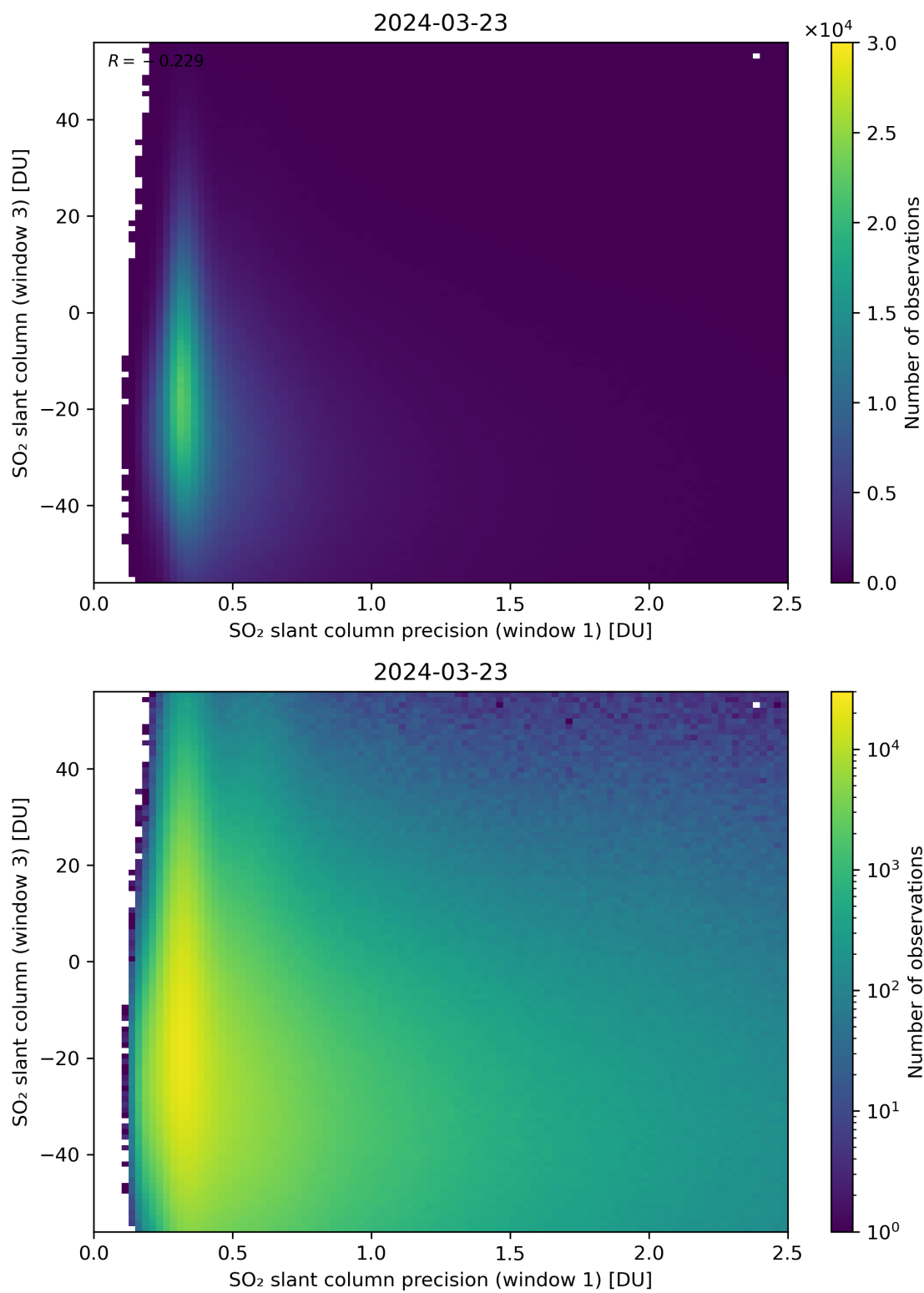
Figure 228: Scatter density plot of “SO 2 slant column precision (window 1)” against “SO 2 slant column (window 3)” for 2024-03-23 to 2024-03-24.
