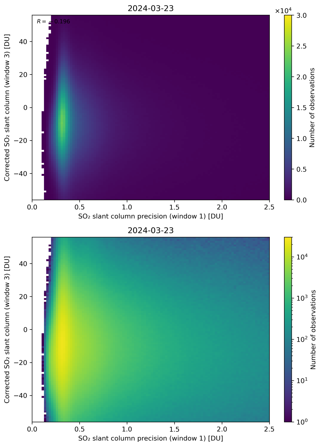
Figure 226: Scatter density plot of “SO 2 slant column precision (window 1)” against “Corrected SO 2 slant column (window 3)” for 2024-03-23 to 2024-03-24.
