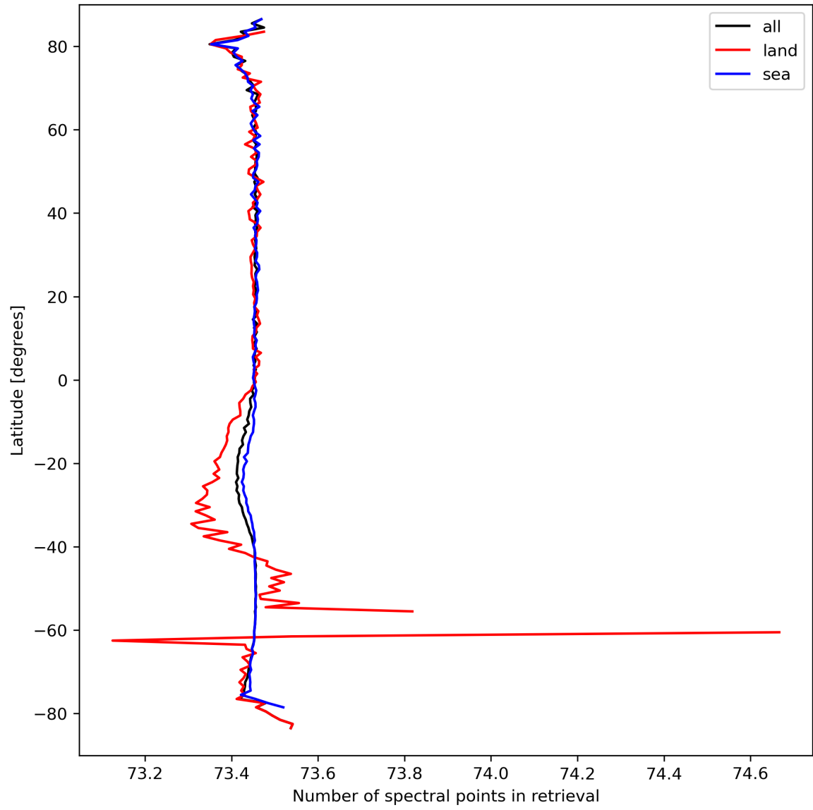
Figure 51: Zonal average of “Number of spectral points in retrieval” for 2024-03-23 to 2024-03-24.
