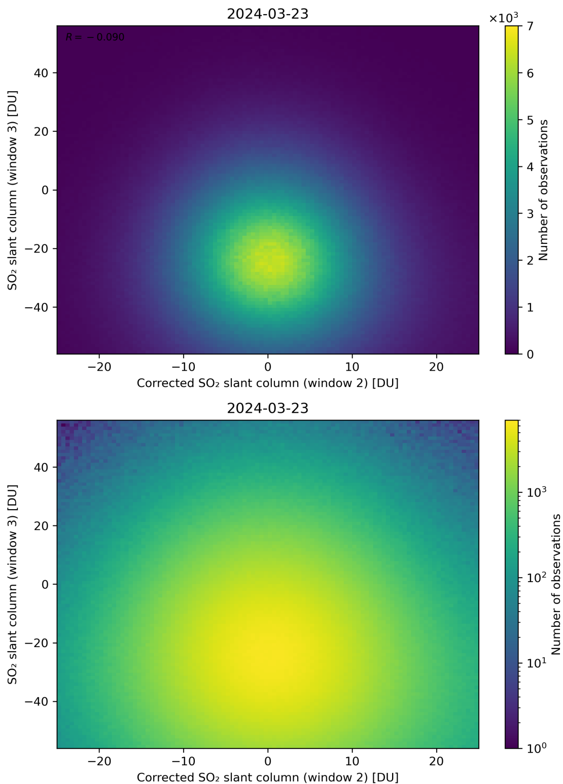
Figure 201: Scatter density plot of “Corrected SO 2 slant column (window 2)” against “SO 2 slant column (window 3)” for 2024-03-23 to 2024-03-24.
