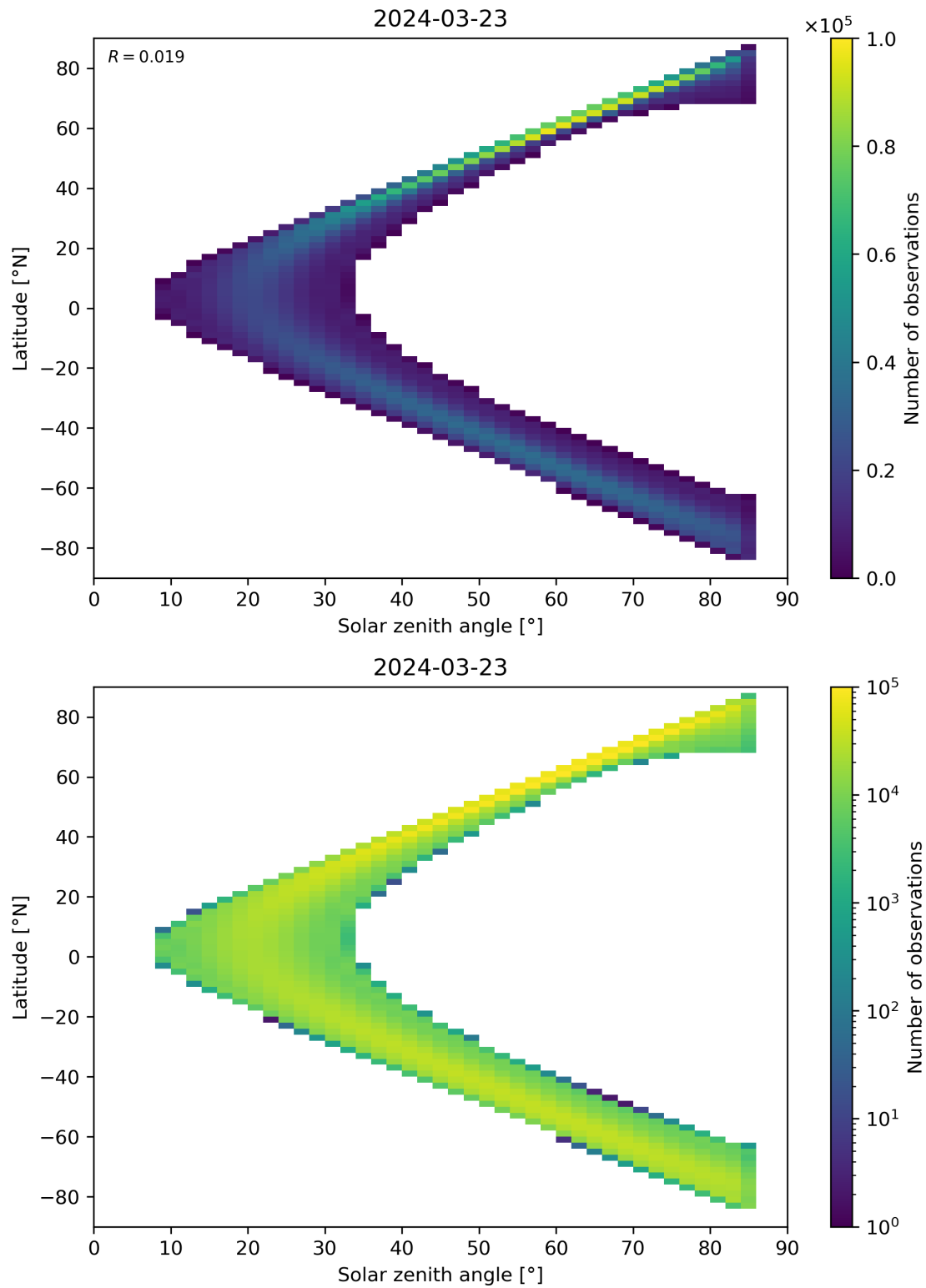
Figure 164: Scatter density plot of “Solar zenith angle” against “Latitude” for 2024-03-23 to 2024-03-24.
