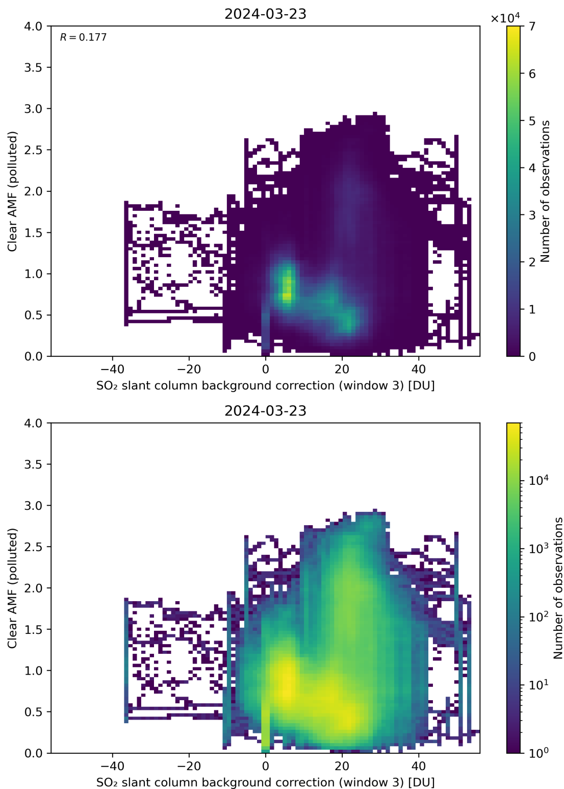
Figure 124: Scatter density plot of “SO 2 slant column background correction (window 3)” against “Clear AMF (polluted)” for 2024-03-23 to 2024-03-24.
