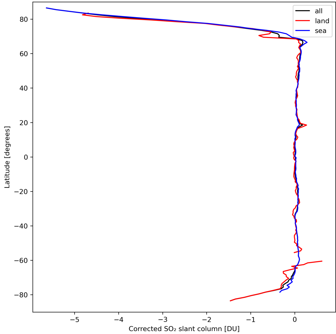
Figure 32: Zonal average of “Corrected SO 2 slant column” for 2024-03-23 to 2024-03-24.
