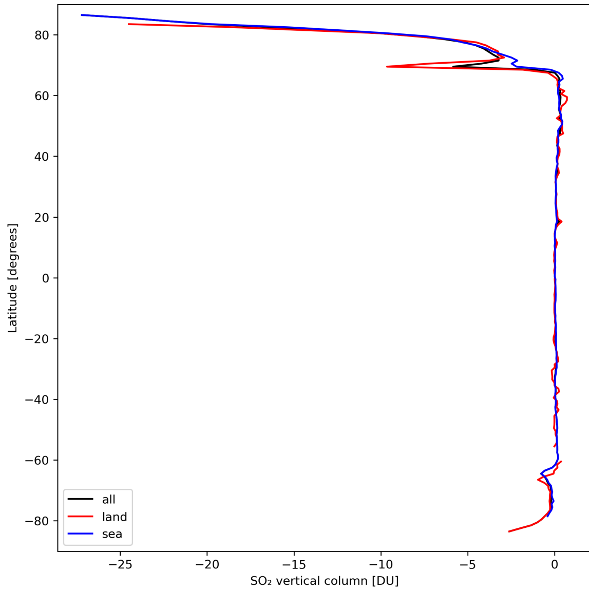
Figure 30: Zonal average of “SO 2 vertical column” for 2024-03-23 to 2024-03-24.
