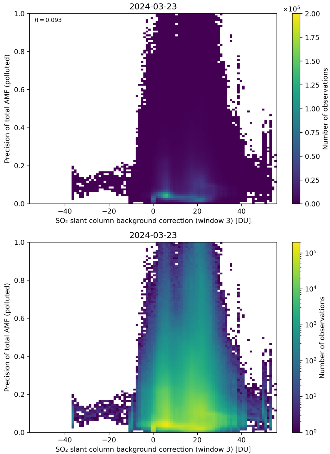
Figure 126: Scatter density plot of “SO 2 slant column background correction (window 3)” against “Precision of total AMF (polluted)” for 2024-03-23 to 2024-03-24.
