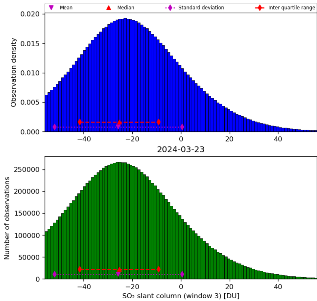
Figure 64: Histogram of “SO 2 slant column (window 3)” for 2024-03-23 to 2024-03-24
