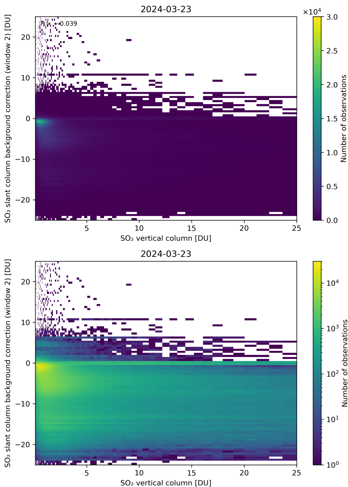
Figure 274: Scatter density plot of “SO 2 vertical column” against “SO 2 slant column background correction (window 2)” for 2024-03-23 to 2024-03-24.
