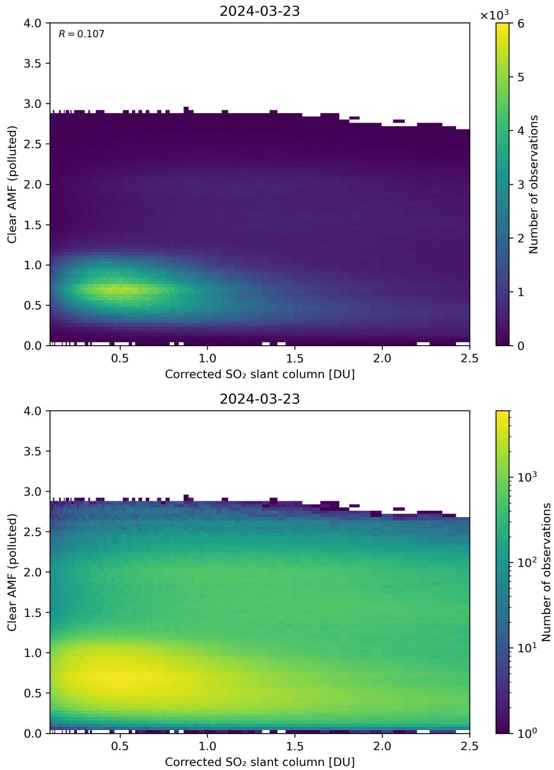
Figure 184: Scatter density plot of “Corrected SO 2 slant column” against “Clear AMF (polluted)” for 2024-03-23 to 2024-03-24.
