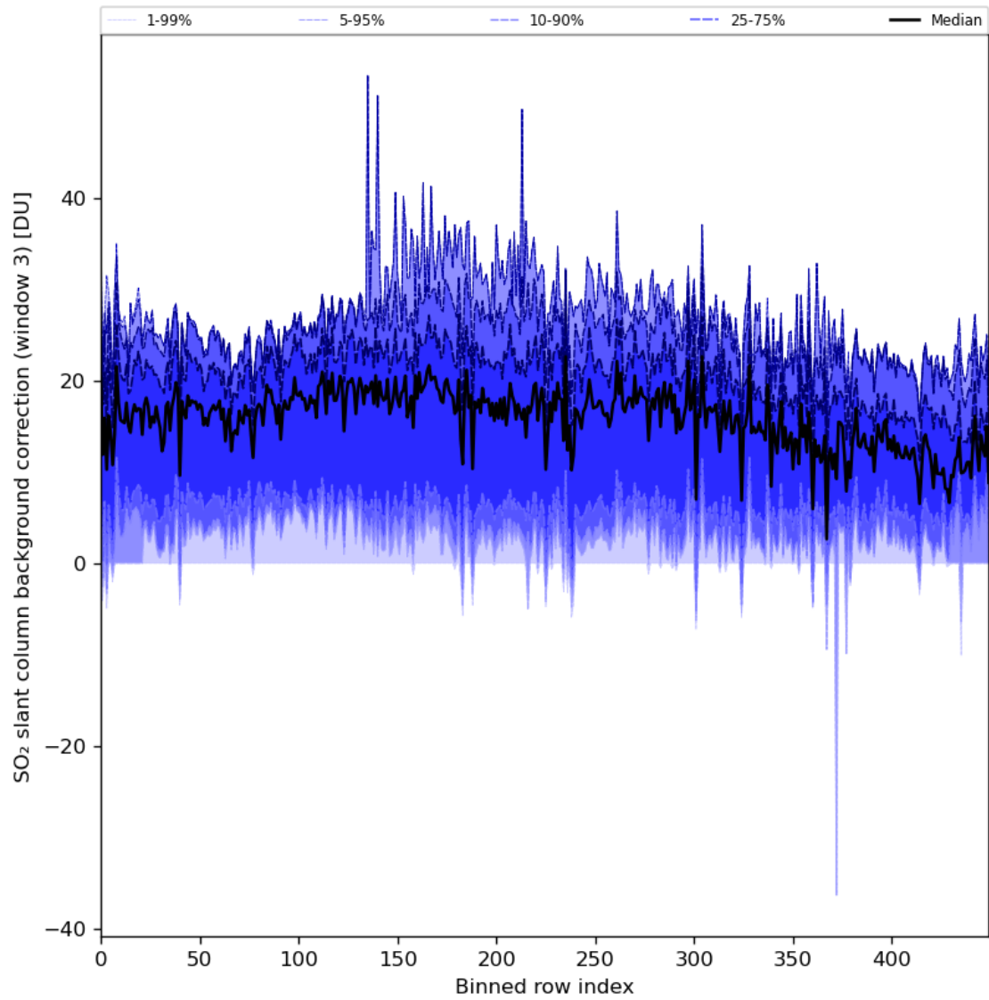
Figure 90: Along track statistics of “SO 2 slant column background correction (window 3)” for 2024-03-23 to 2024-03-24
