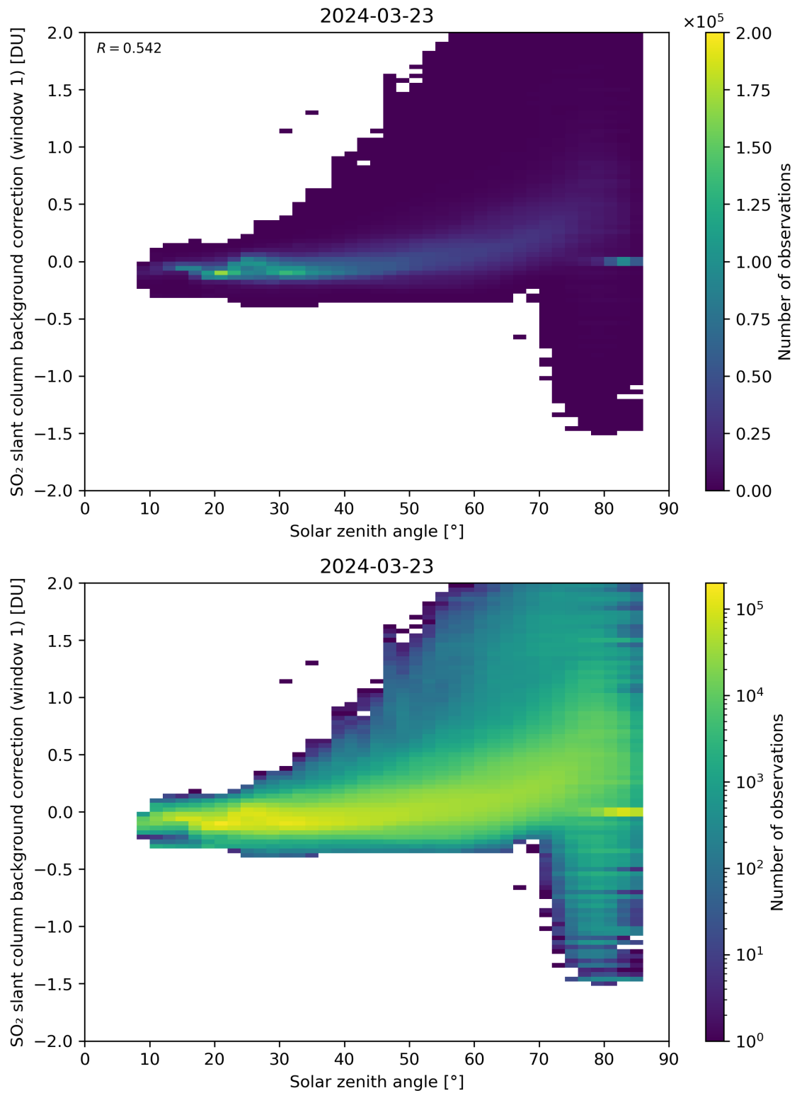
Figure 158: Scatter density plot of “Solar zenith angle” against “SO 2 slant column background correction (window 1)” for 2024-03-23 to 2024-03-24.
