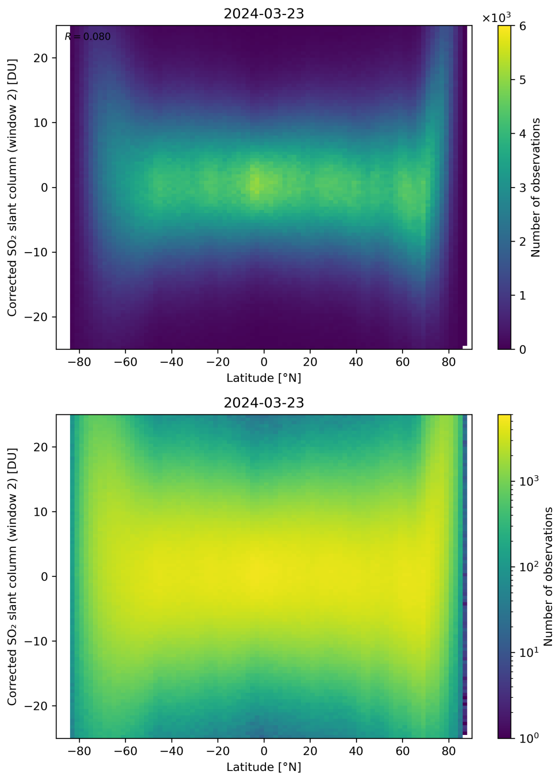
Figure 147: Scatter density plot of “Latitude” against “Corrected SO 2 slant column (window 2)” for 2024-03-23 to 2024-03-24.
