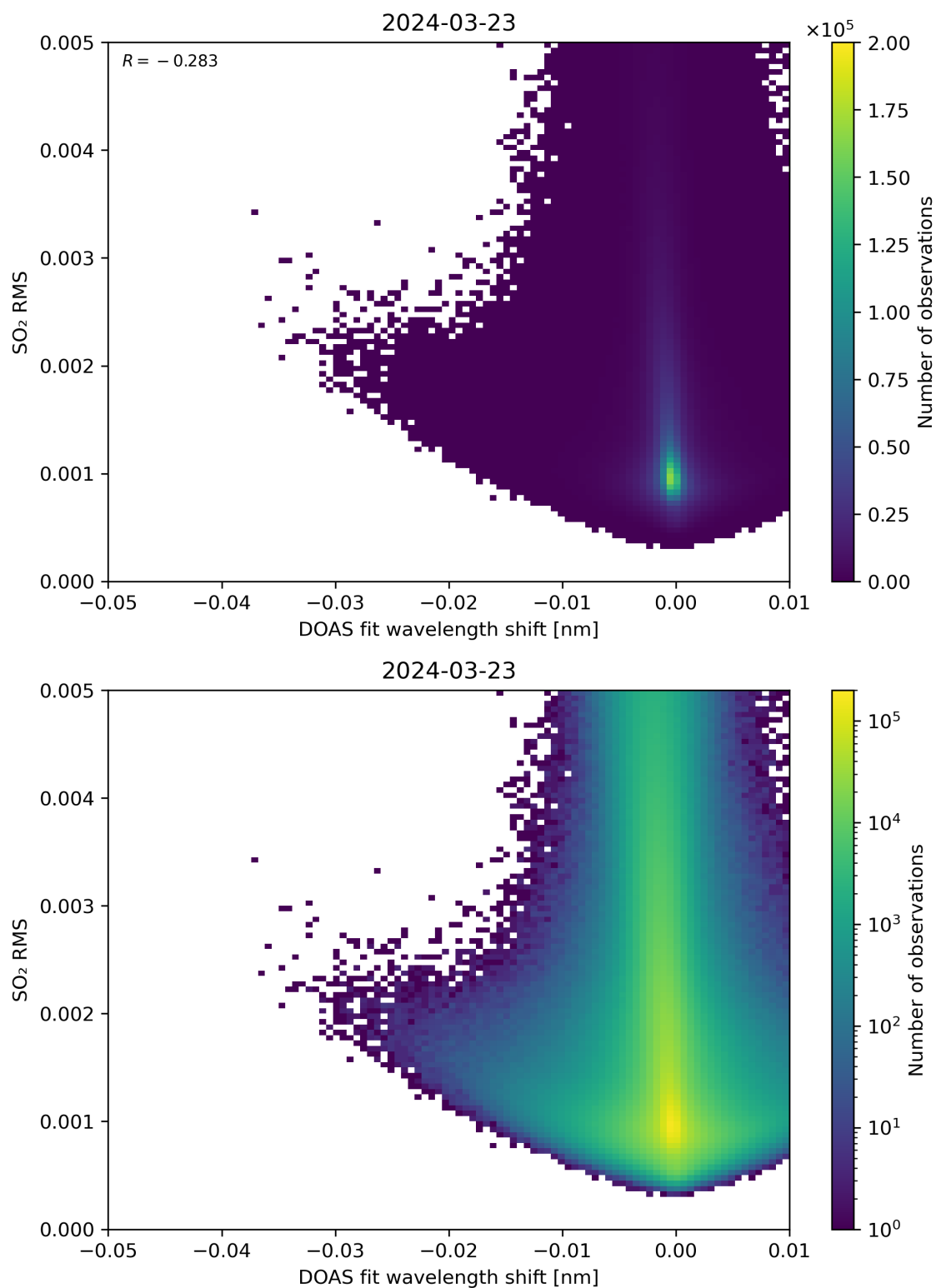
Figure 128: Scatter density plot of “DOAS fit wavelength shift” against “SO 2 RMS” for 2024-03-23 to 2024-03-24.
