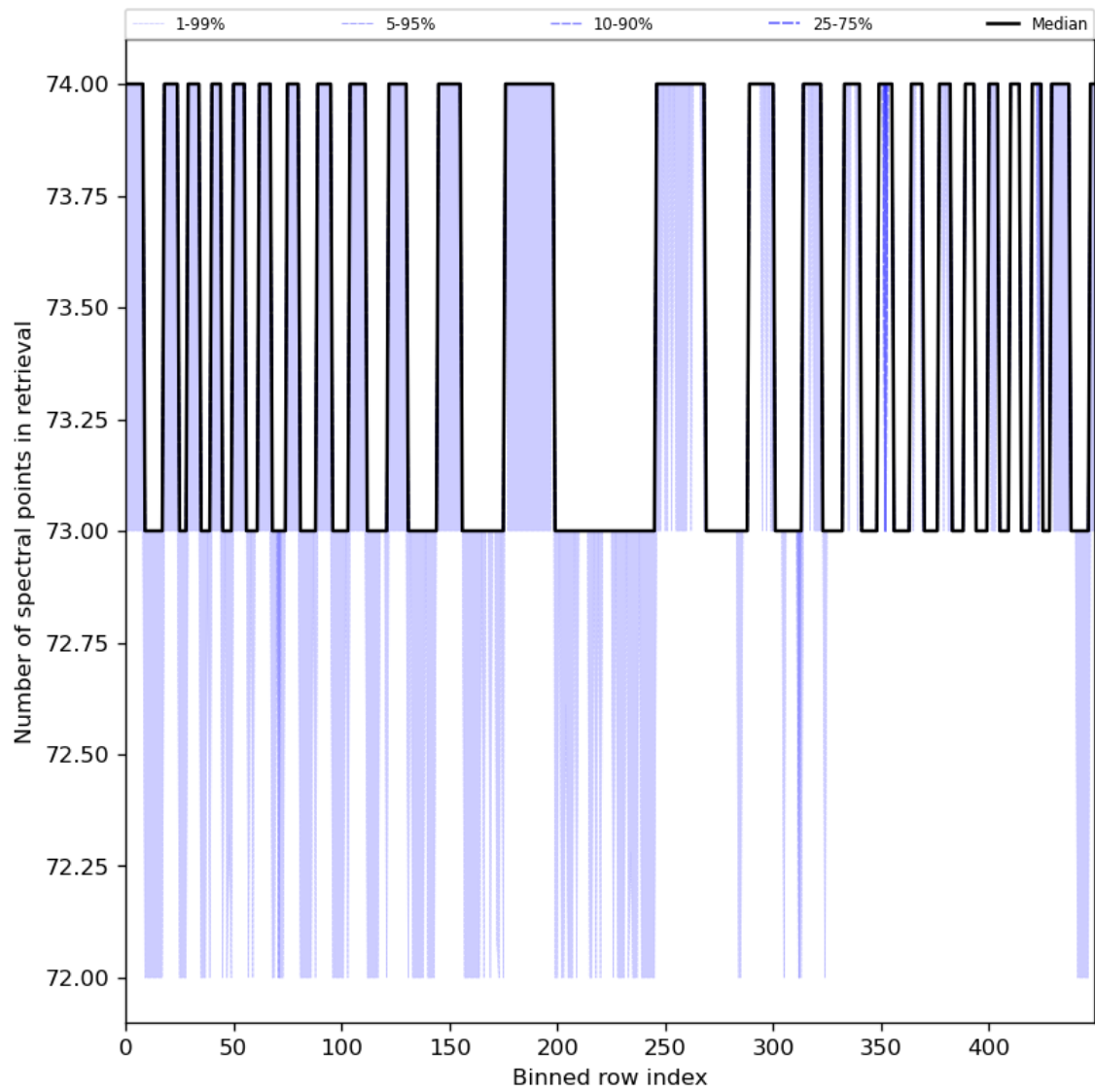
Figure 97: Along track statistics of “Number of spectral points in retrieval” for 2024-03-23 to 2024-03-24
