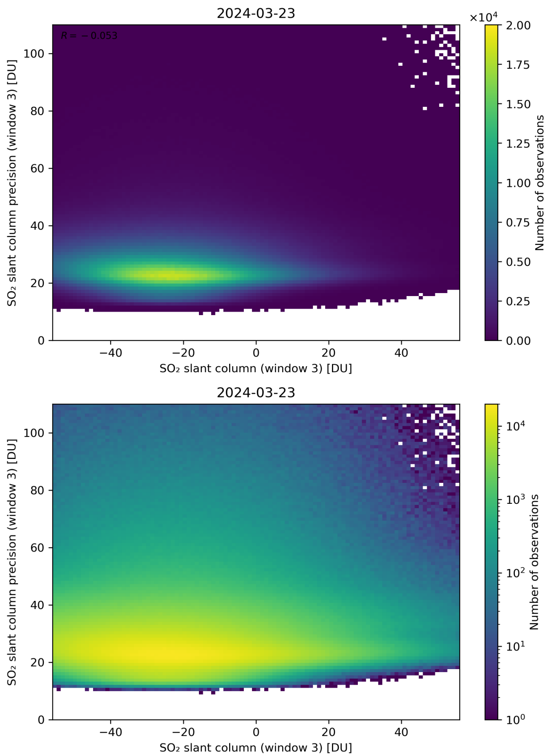
Figure 267: Scatter density plot of “SO 2 slant column (window 3)” against “SO 2 slant column precision (window 3)” for 2024-03-23 to 2024-03-24.
