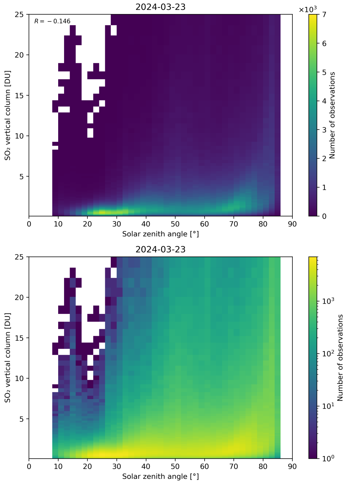
Figure 176: Scatter density plot of “Solar zenith angle” against “SO 2 vertical column” for 2024-03-23 to 2024-03-24.
