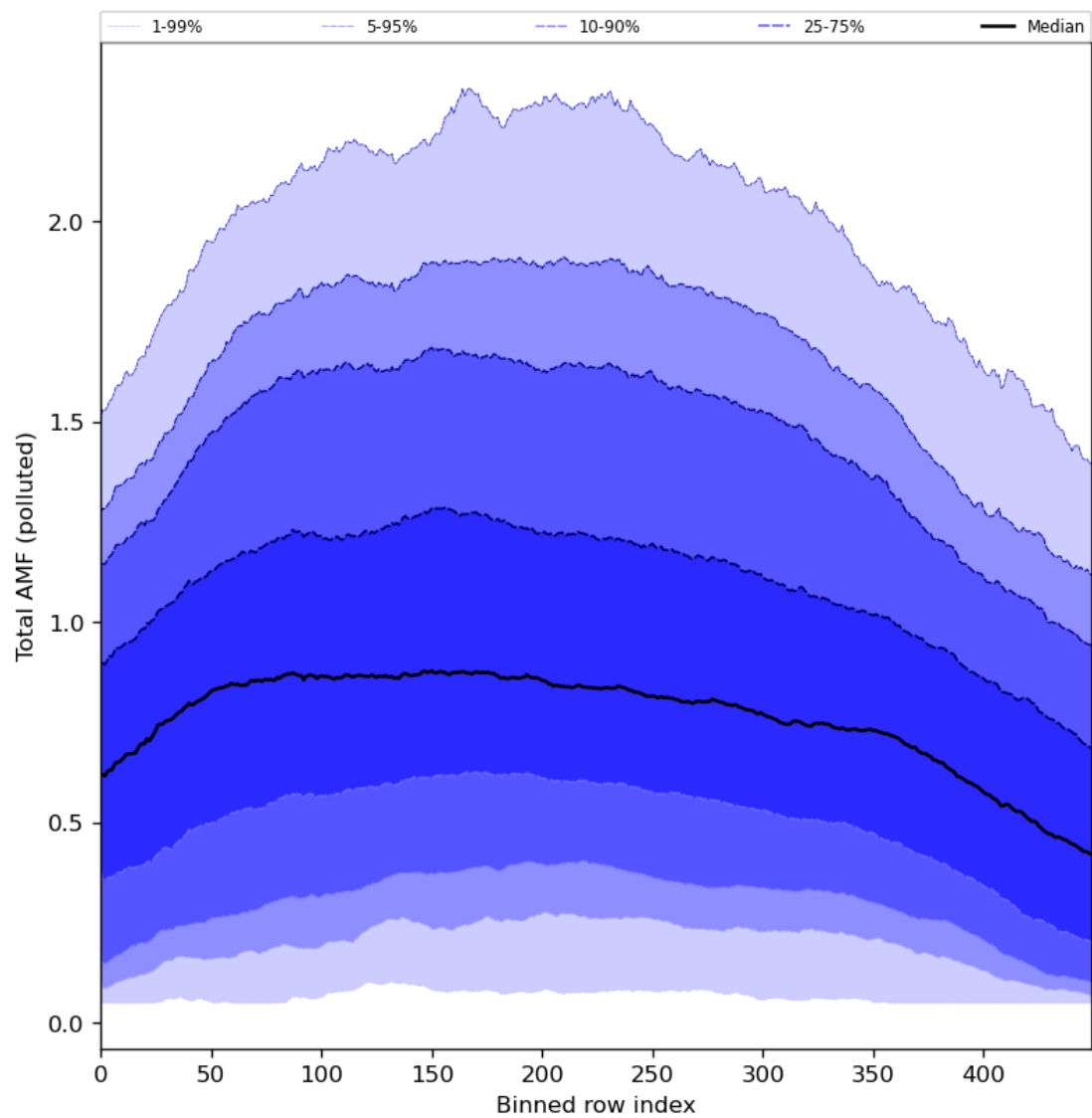
Figure 94: Along track statistics of “Total AMF (polluted)” for 2024-03-23 to 2024-03-24
