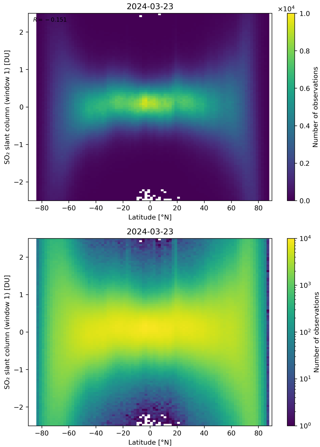
Figure 149: Scatter density plot of “Latitude” against “SO 2 slant column (window 1)” for 2024-03-23 to 2024-03-24.
