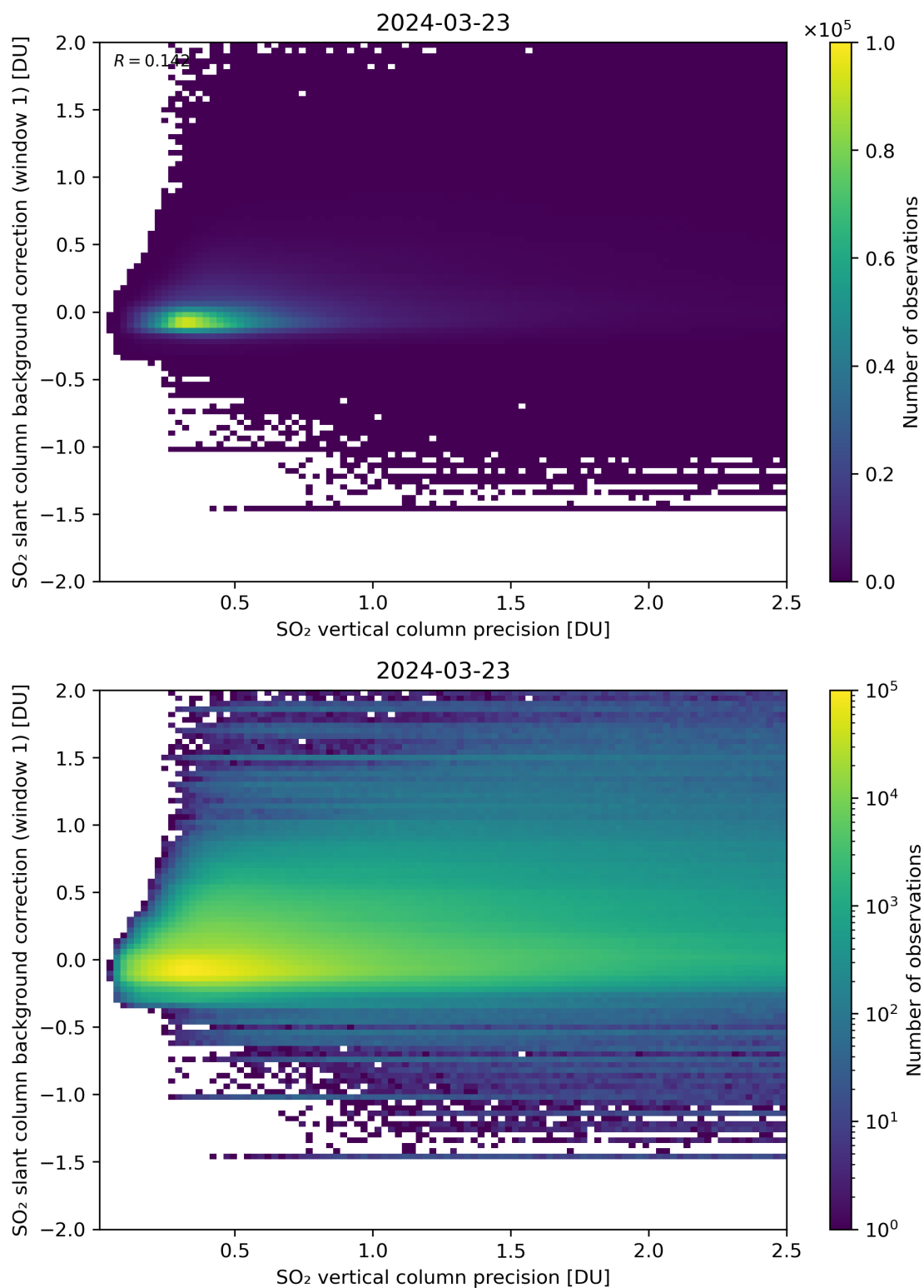
Figure 279: Scatter density plot of “SO 2 vertical column precision” against “SO 2 slant column background correction (window 1)” for 2024-03-23 to 2024-03-24.
