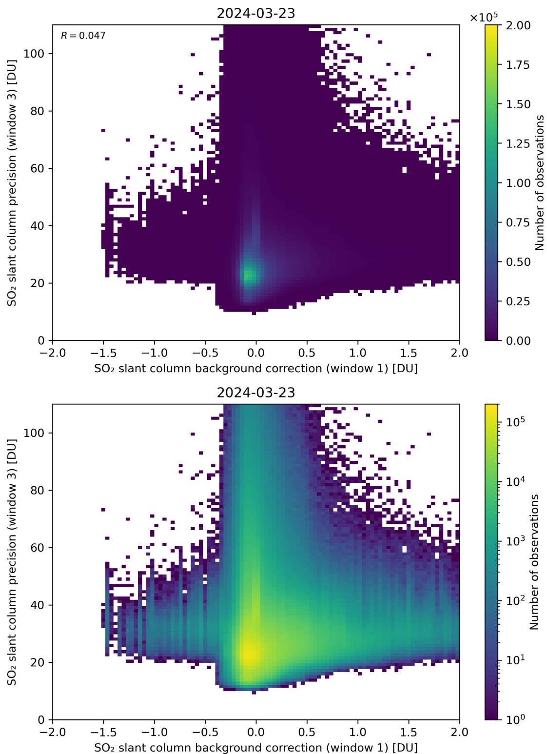
Figure 108: Scatter density plot of “SO 2 slant column background correction (window 1)” against “SO 2 slant column precision (window 3)” for 2024-03-23 to 2024-03-24.
