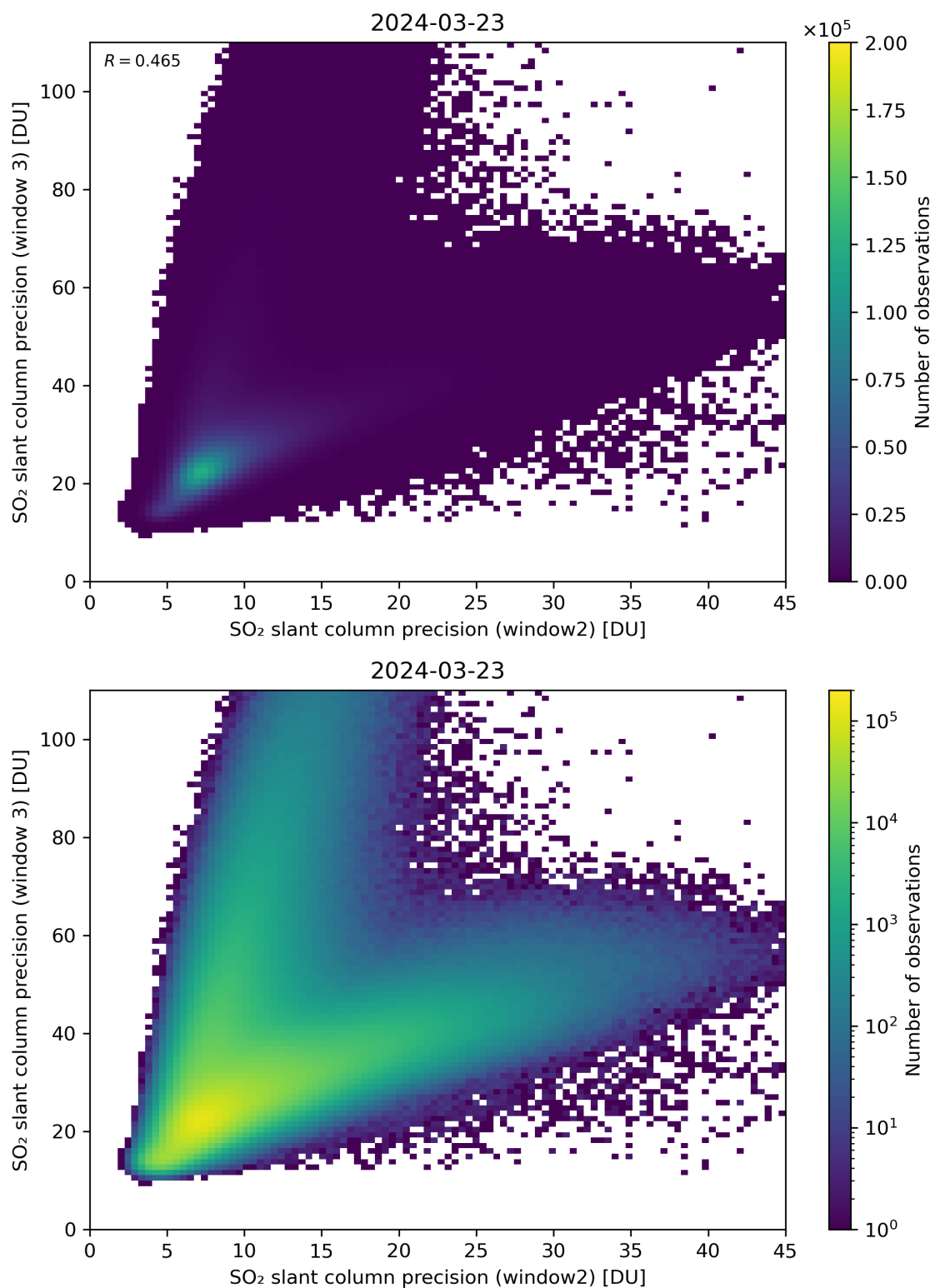
Figure 250: Scatter density plot of “SO 2 slant column precision (window2)” against “SO 2 slant column precision (window 3)” for 2024-03-23 to 2024-03-24.
