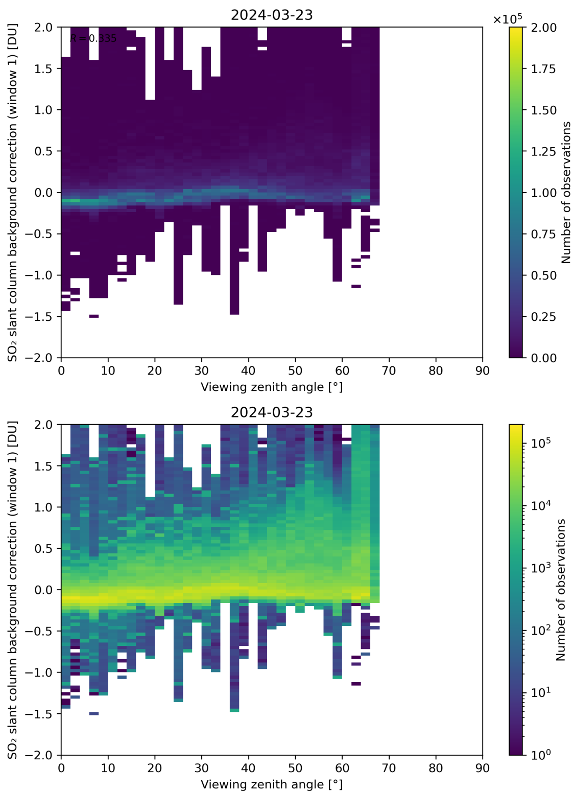
Figure 308: Scatter density plot of “Viewing zenith angle” against “SO 2 slant column background correction (window 1)” for 2024-03-23 to 2024-03-24.
