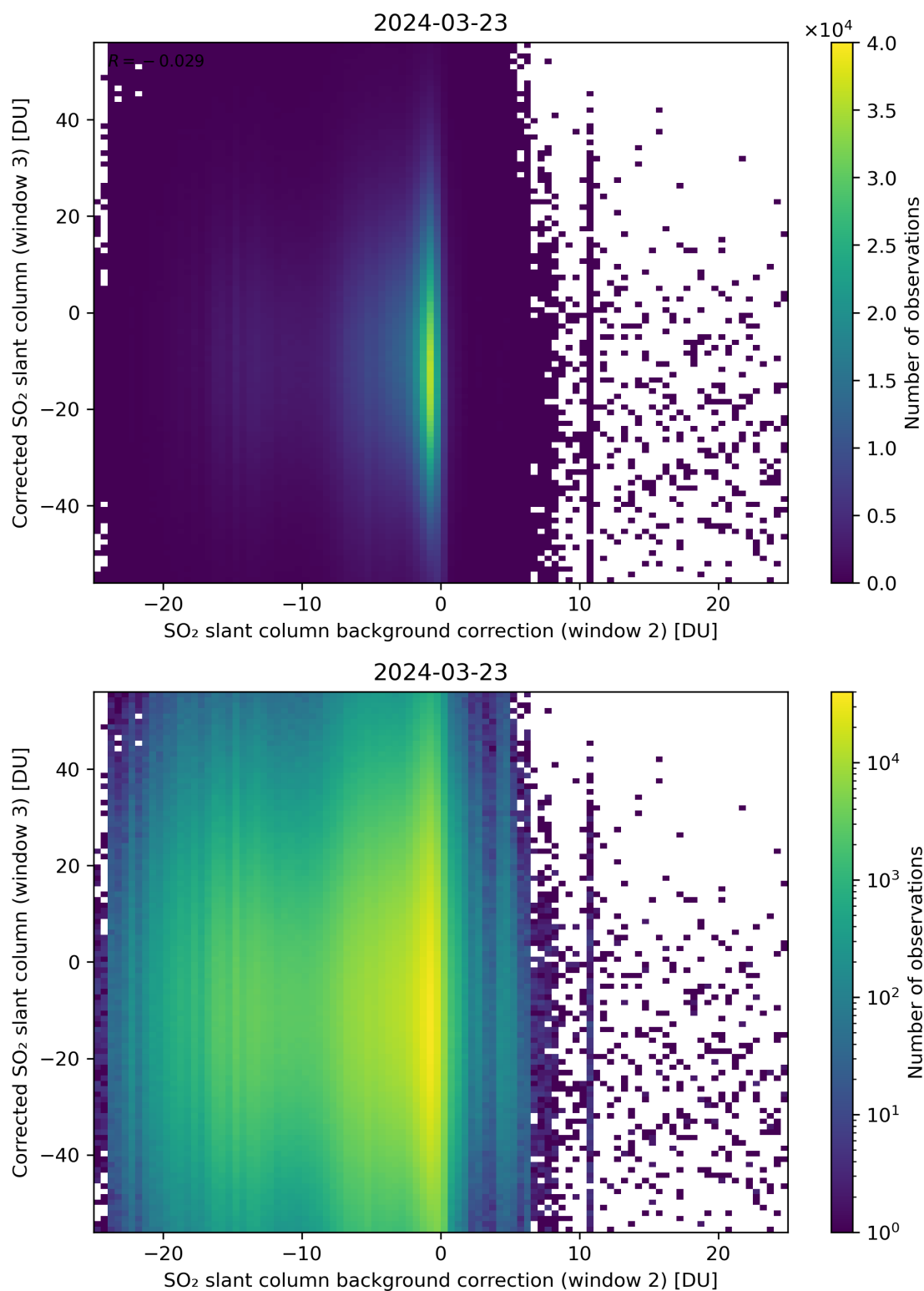
Figure 116: Scatter density plot of “SO 2 slant column background correction (window 2)” against “Corrected SO 2 slant column (window 3)” for 2024-03-23 to 2024-03-24.
