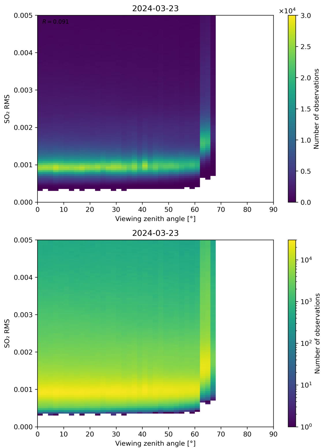
Figure 313: Scatter density plot of “Viewing zenith angle” against “SO 2 RMS” for 2024-03-23 to 2024-03-24.
