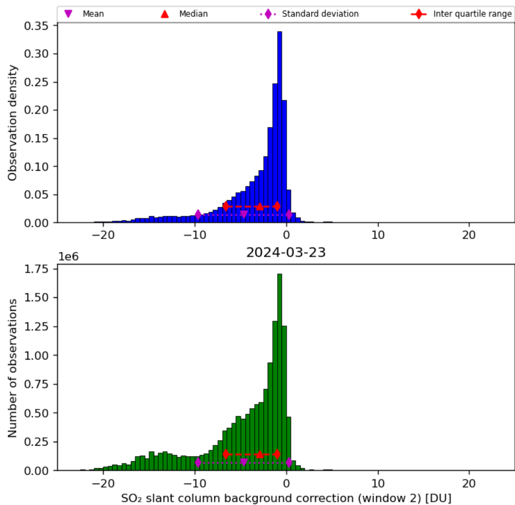
Figure 63: Histogram of “SO 2 slant column background correction (window 2)” for 2024-03-23 to 2024-03-24
