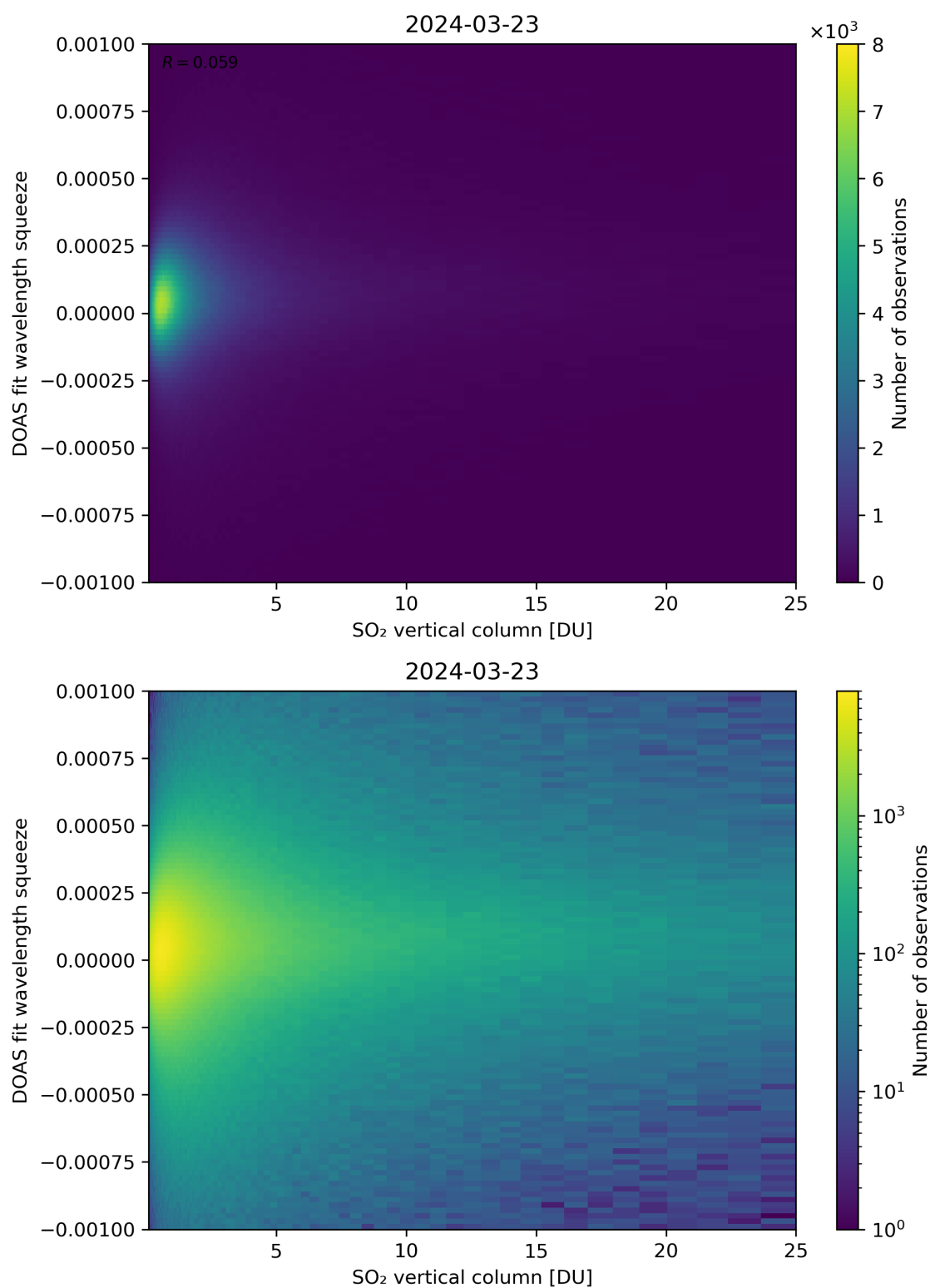
Figure 277: Scatter density plot of “SO 2 vertical column” against “DOAS fit wavelength squeeze” for 2024-03-23 to 2024-03-24.
