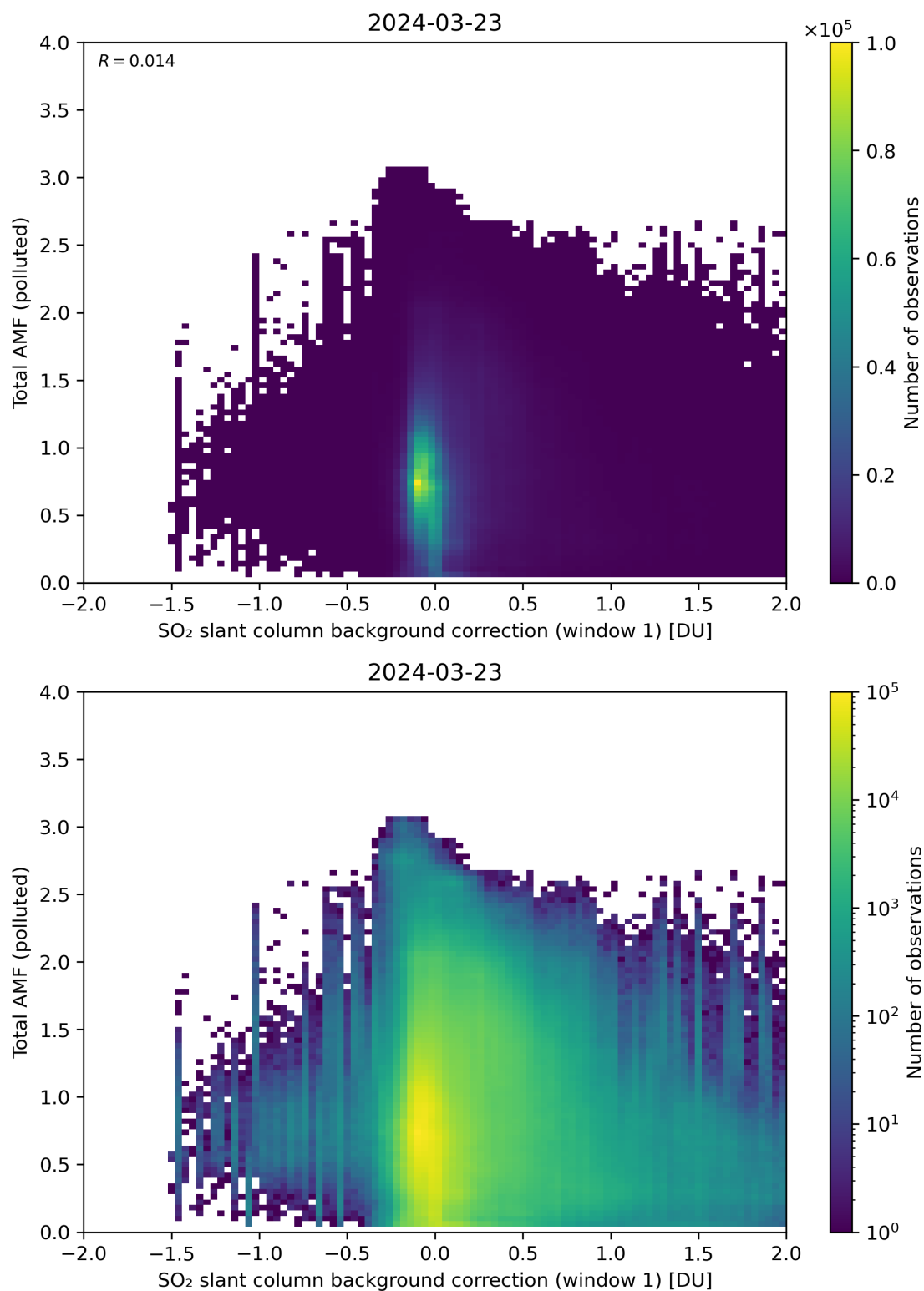
Figure 109: Scatter density plot of “SO 2 slant column background correction (window 1)” against “Total AMF (polluted)” for 2024-03-23 to 2024-03-24.
