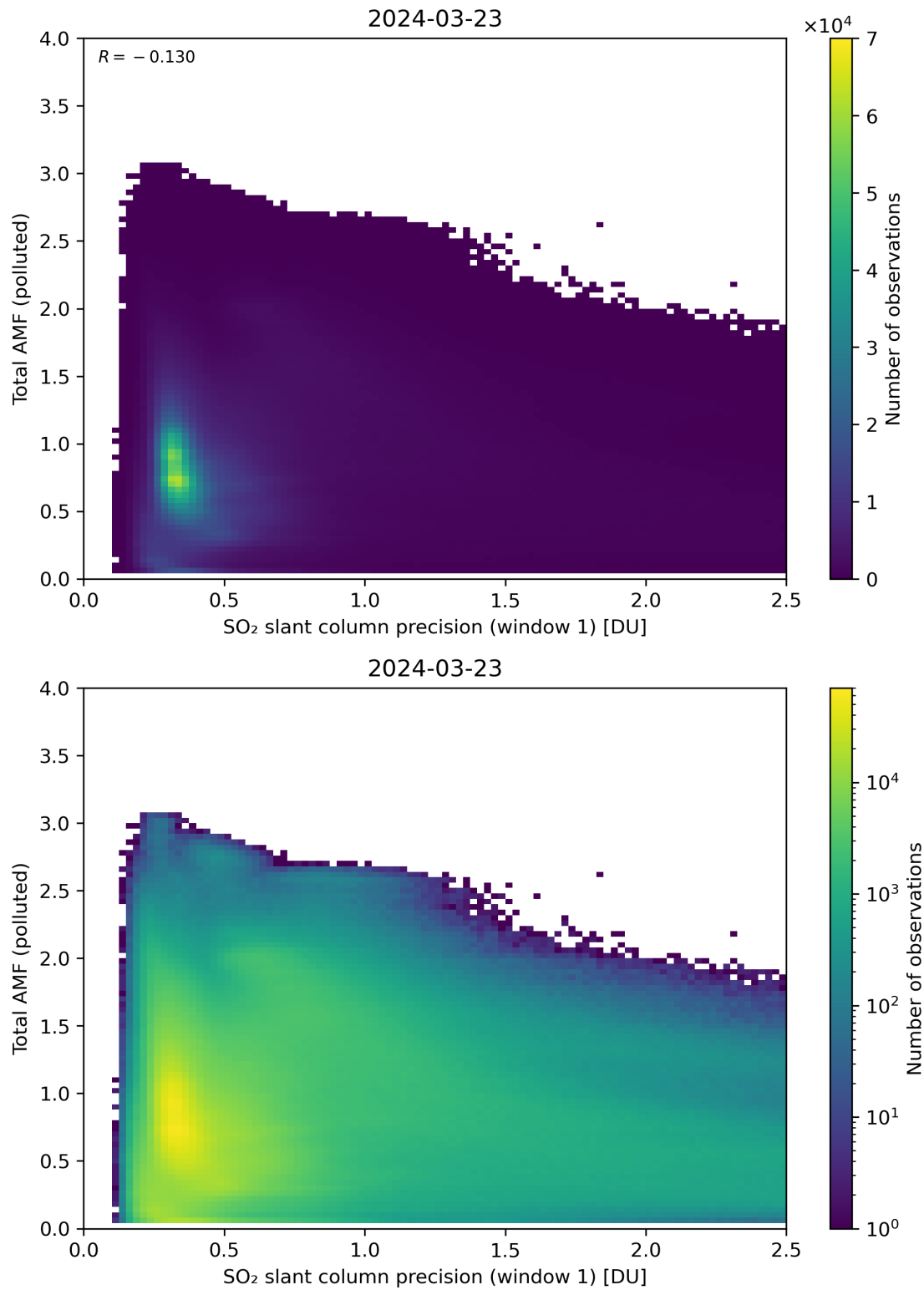
Figure 230: Scatter density plot of “SO 2 slant column precision (window 1)” against “Total AMF (polluted)” for 2024-03-23 to 2024-03-24.
