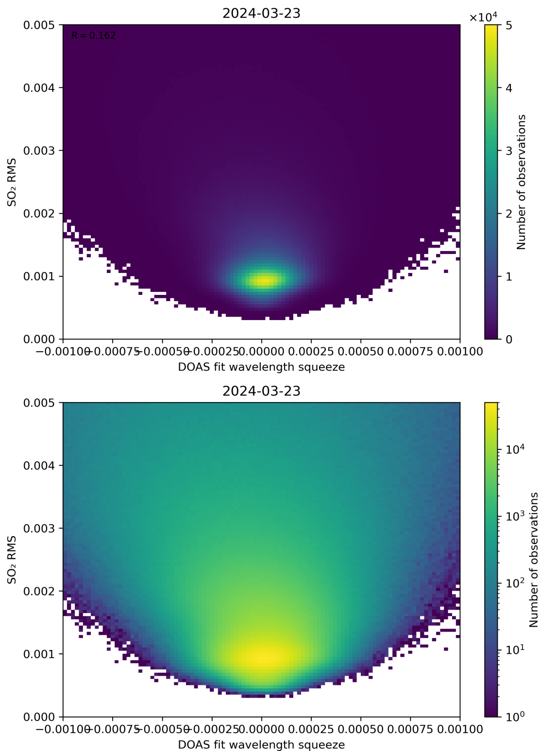
Figure 132: Scatter density plot of “DOAS fit wavelength squeeze” against “SO 2 RMS” for 2024-03-23 to 2024-03-24.
