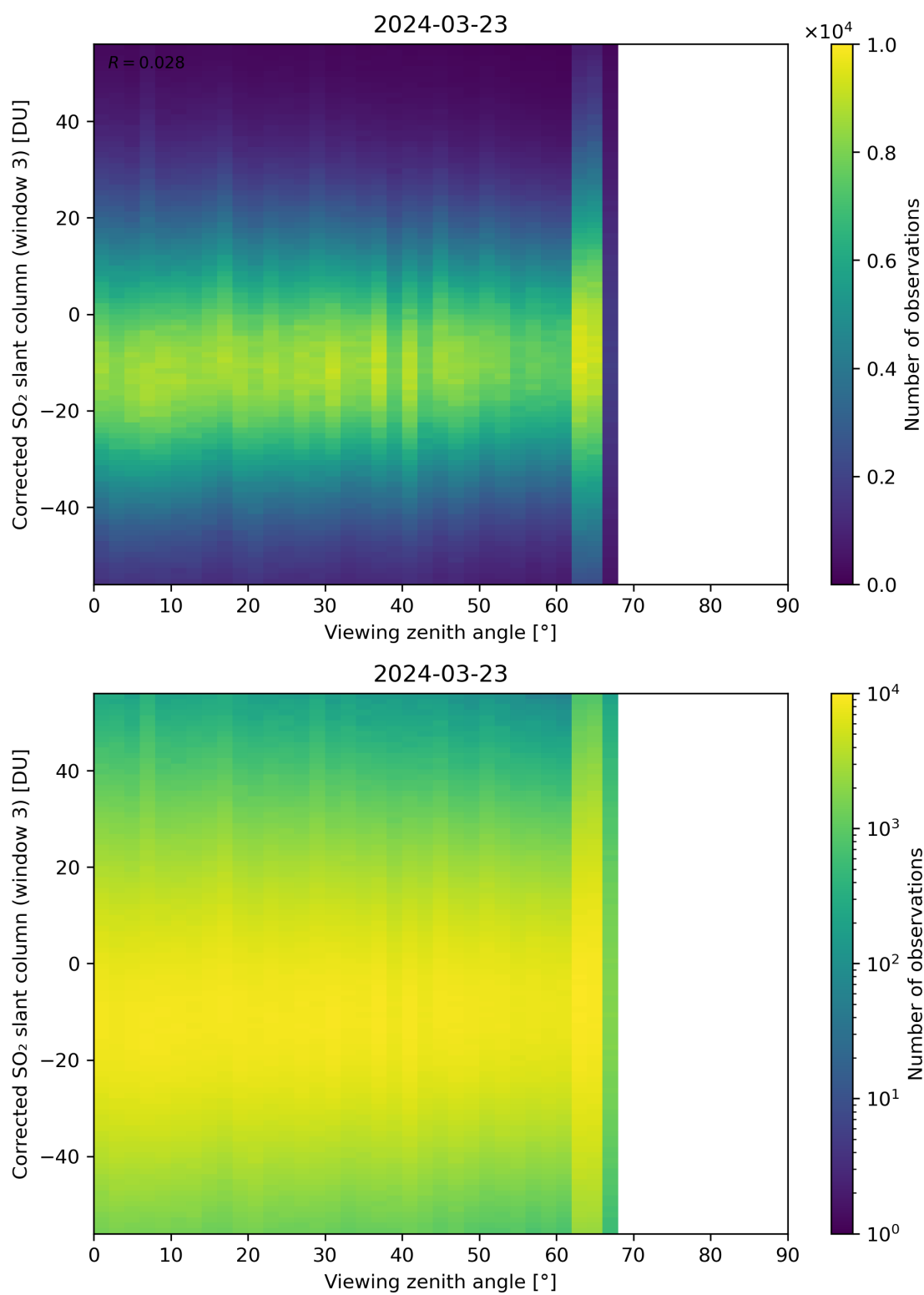
Figure 319: Scatter density plot of “Viewing zenith angle” against “Corrected SO 2 slant column (window 3)” for 2024-03-23 to 2024-03-24.
