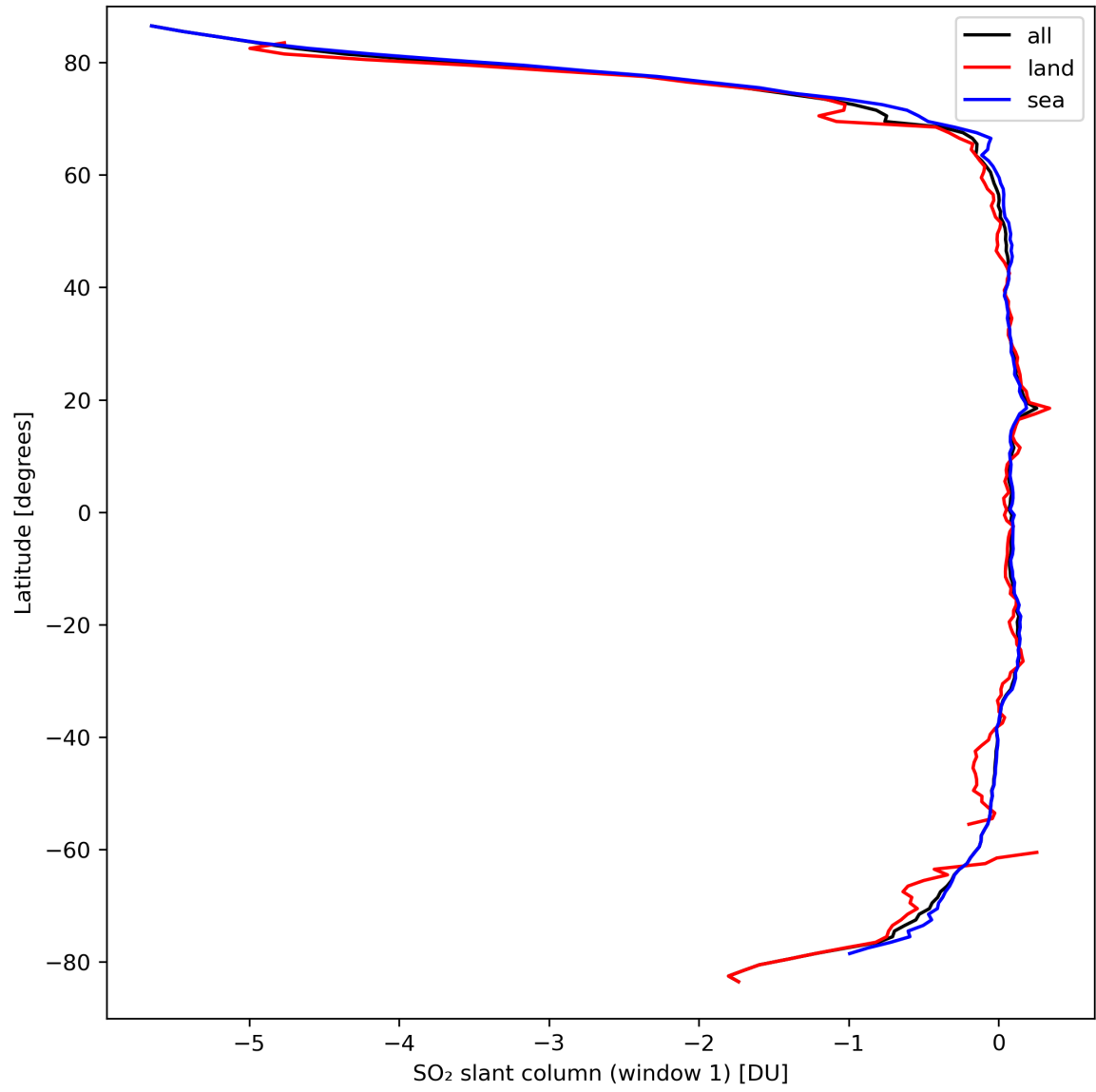
Figure 33: Zonal average of “SO 2 slant column (window 1)” for 2024-03-23 to 2024-03-24.
