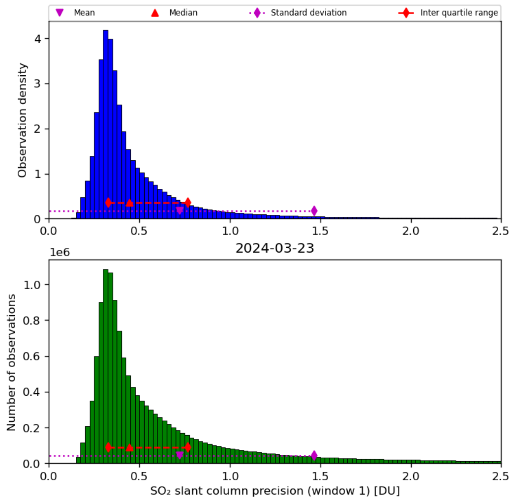
Figure 57: Histogram of “SO 2 slant column precision (window 1)” for 2024-03-23 to 2024-03-24
