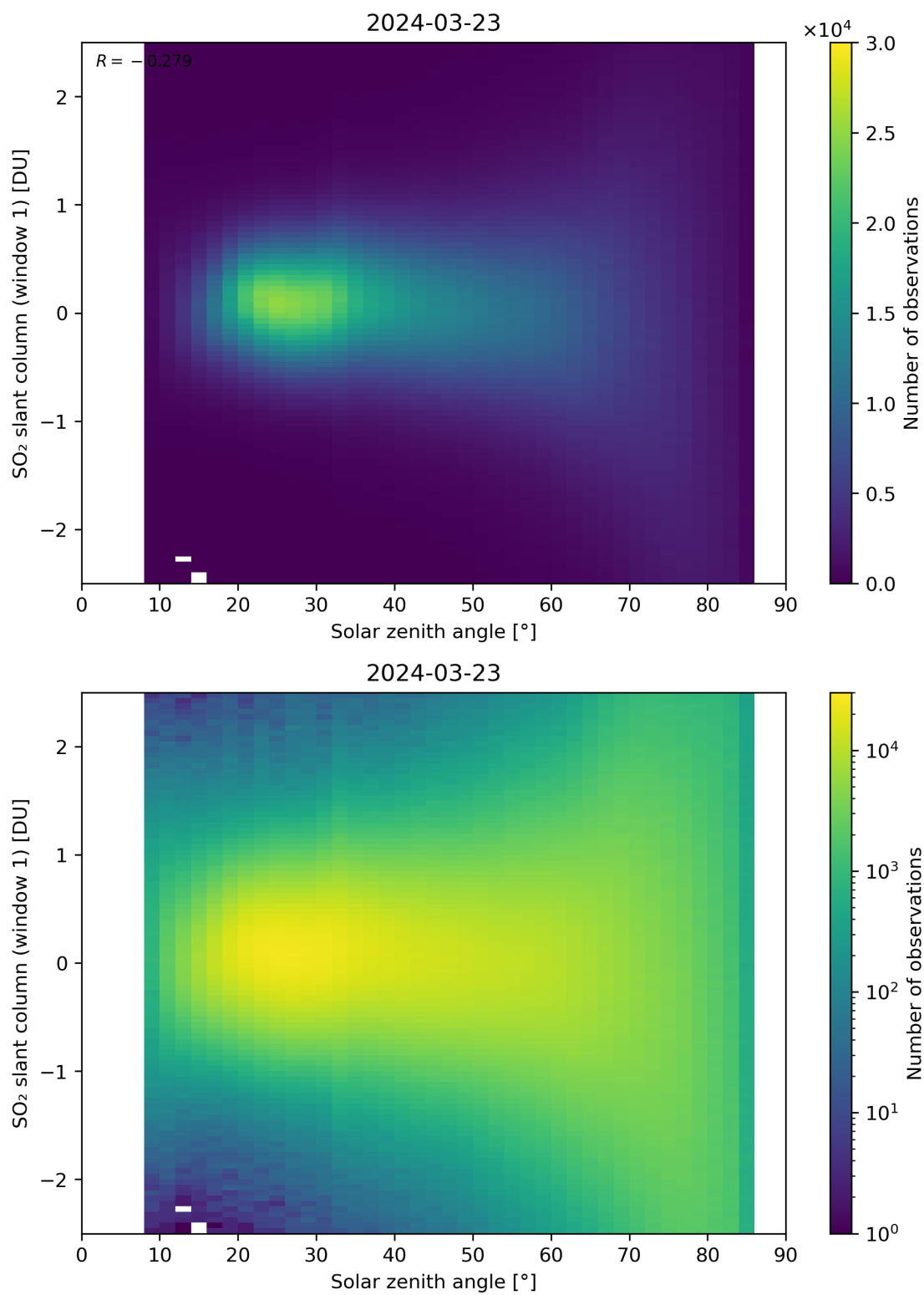
Figure 169: Scatter density plot of “Solar zenith angle” against “SO 2 slant column (window 1)” for 2024-03-23 to 2024-03-24.
