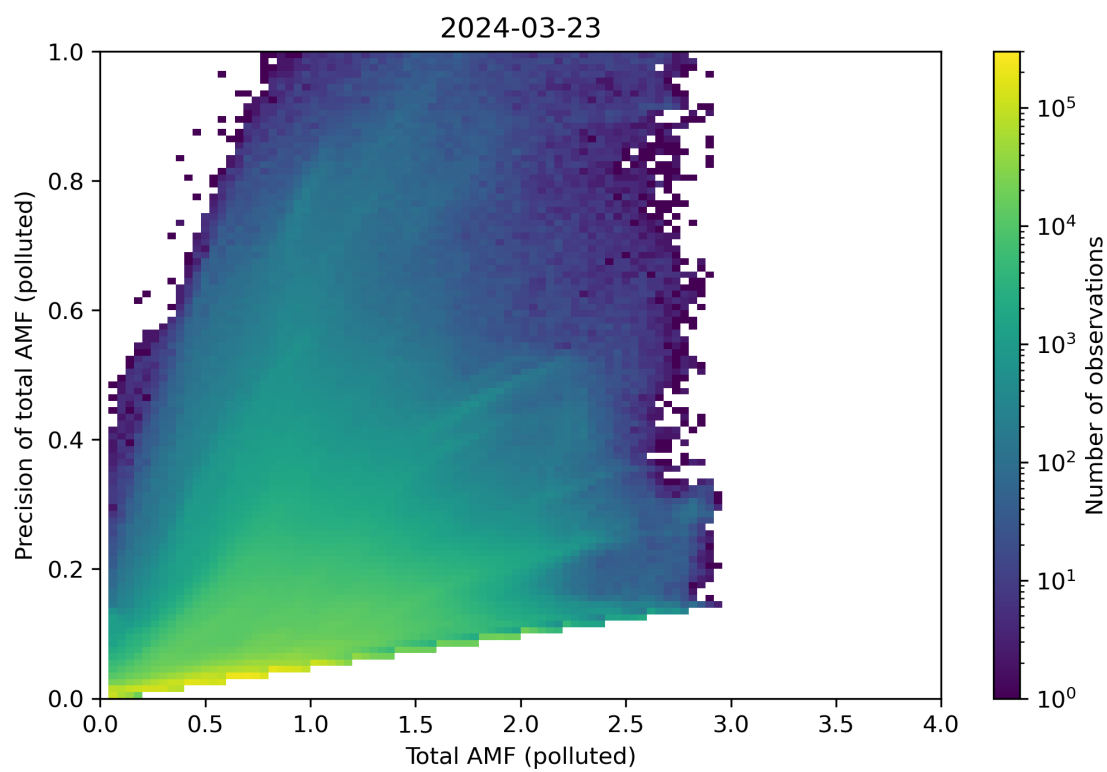
Figure 272: Scatter density plot of “Total AMF (polluted)” against “Precision of total AMF (polluted)” for 2024-03-23 to 2024-03-24.
