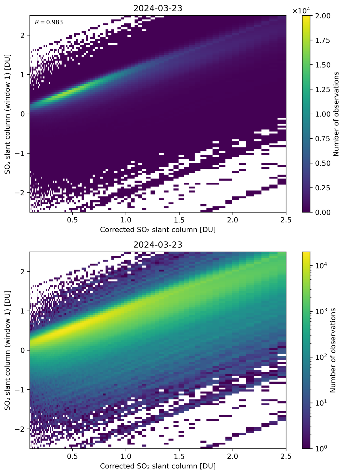
Figure 187: Scatter density plot of “Corrected SO 2 slant column” against “SO 2 slant column (window 1)” for 2024-03-23 to 2024-03-24.
