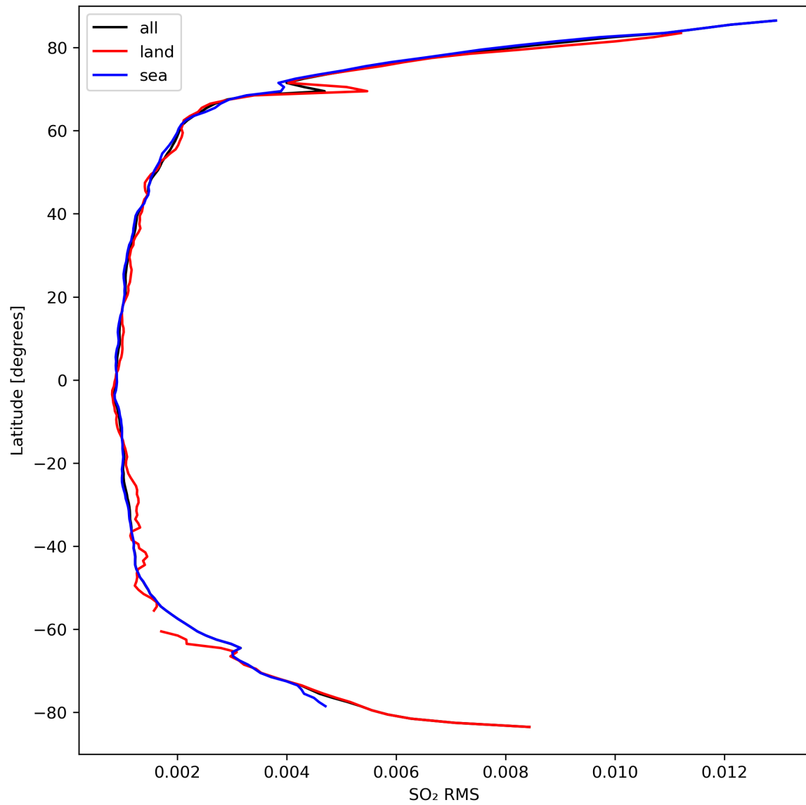
Figure 47: Zonal average of “SO 2 RMS” for 2024-03-23 to 2024-03-24.
