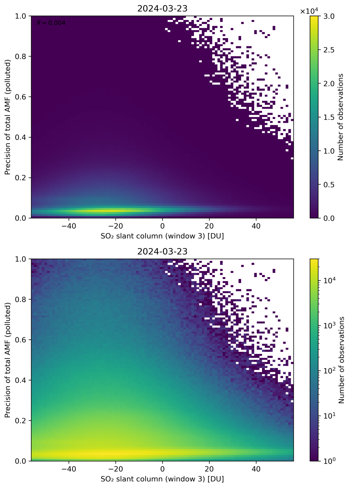
Figure 269: Scatter density plot of “SO 2 slant column (window 3)” against “Precision of total AMF (polluted)” for 2024-03-23 to 2024-03-24.
