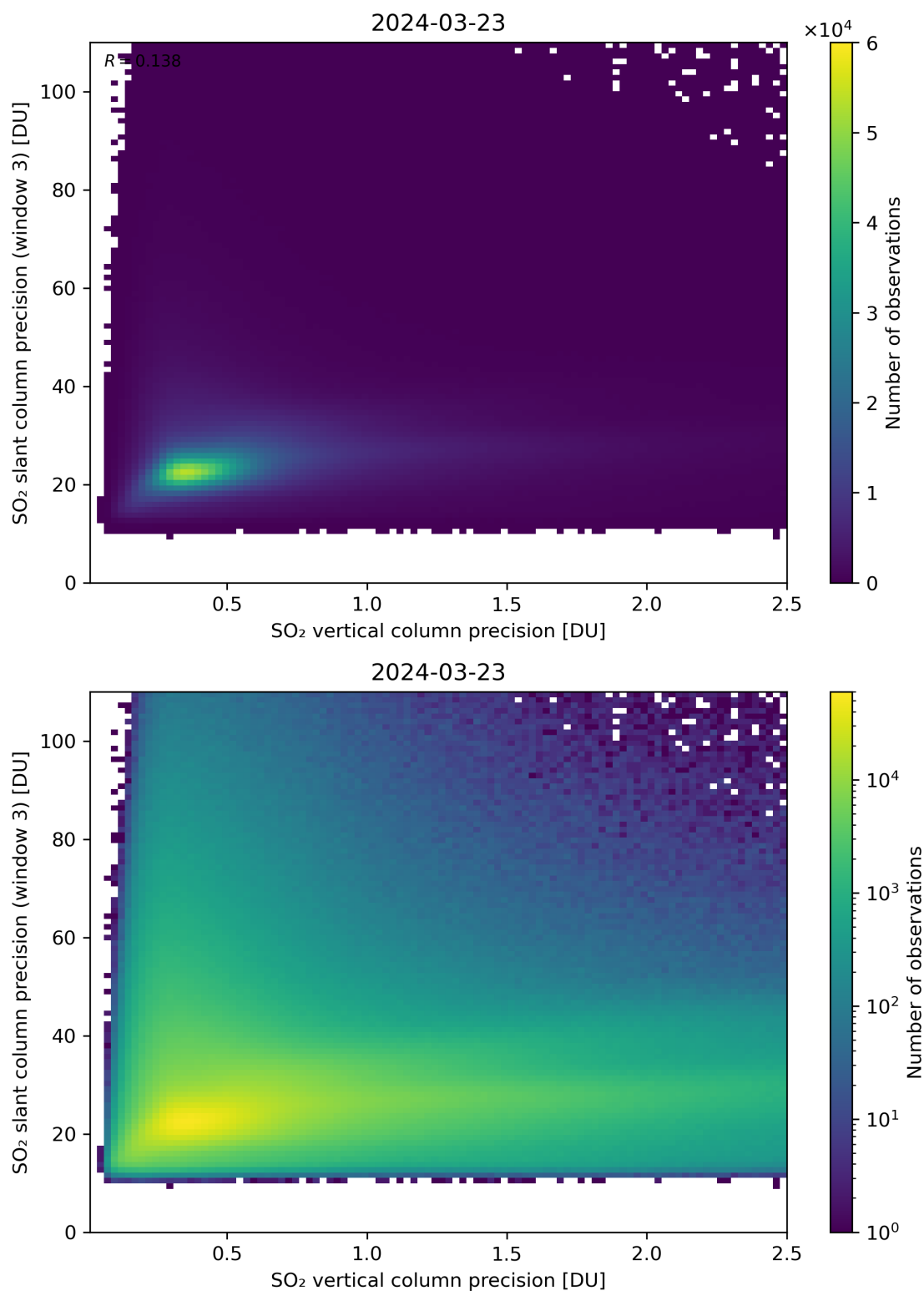
Figure 293: Scatter density plot of “SO 2 vertical column precision” against “SO 2 slant column precision (window 3)” for 2024-03-23 to 2024-03-24.
