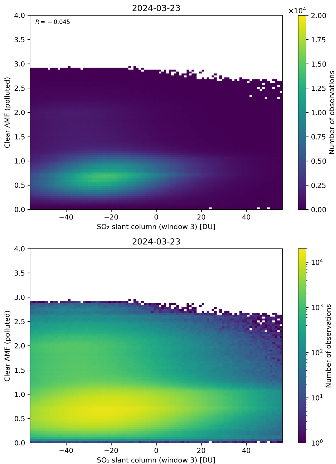
Figure 265: Scatter density plot of “SO 2 slant column (window 3)” against “Clear AMF (polluted)” for 2024-03-23 to 2024-03-24.
