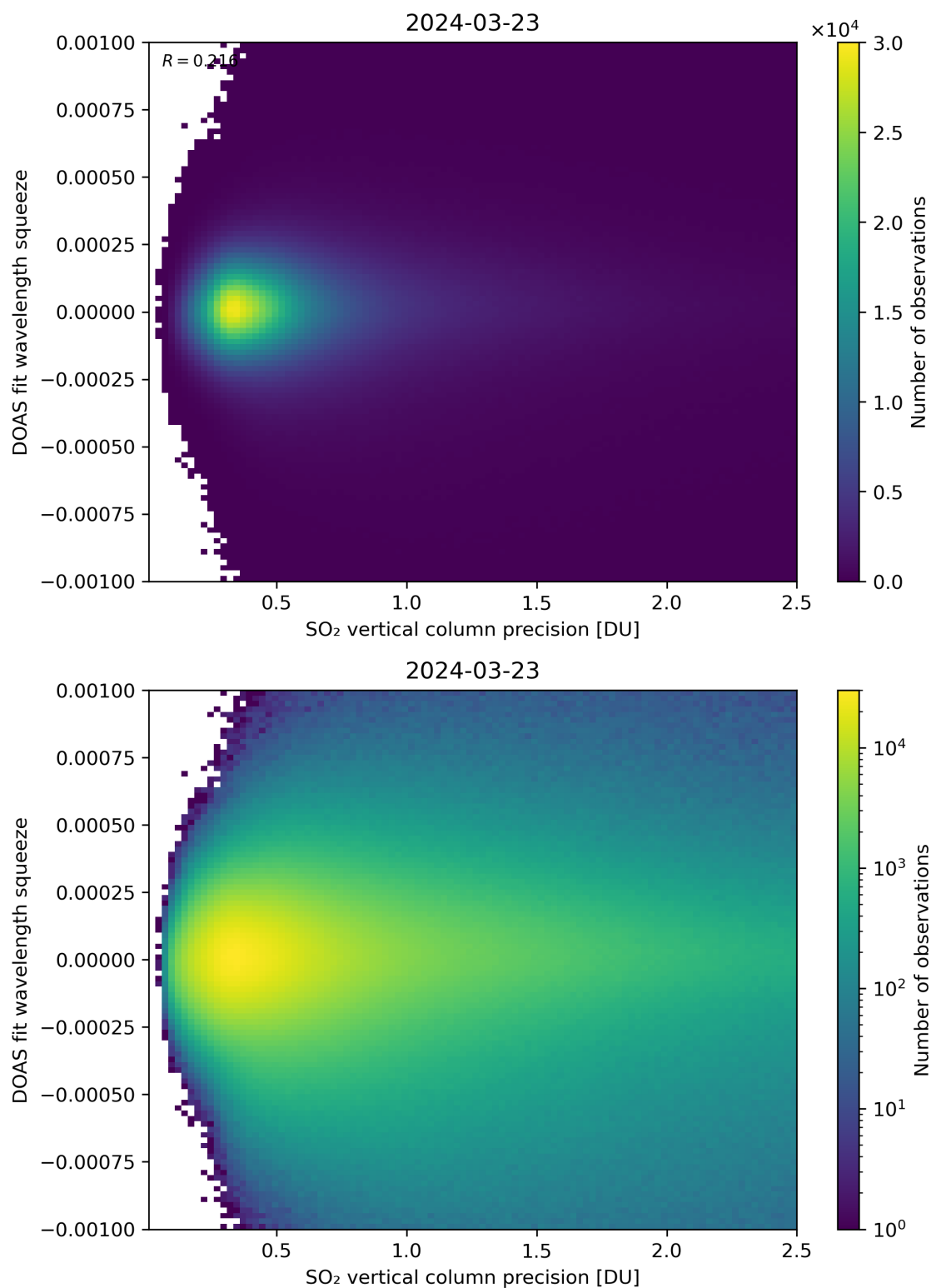
Figure 283: Scatter density plot of “SO 2 vertical column precision” against “DOAS fit wavelength squeeze” for 2024-03-23 to 2024-03-24.
