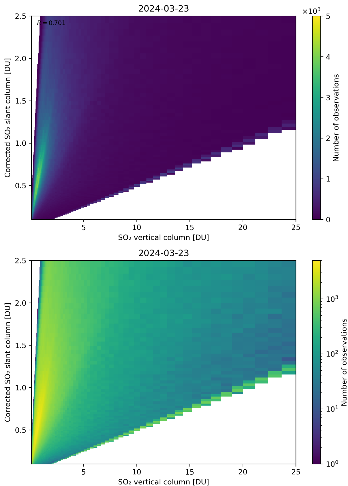
Figure 297: Scatter density plot of “SO 2 vertical column” against “Corrected SO 2 slant column” for 2024-03-23 to 2024-03-24.
