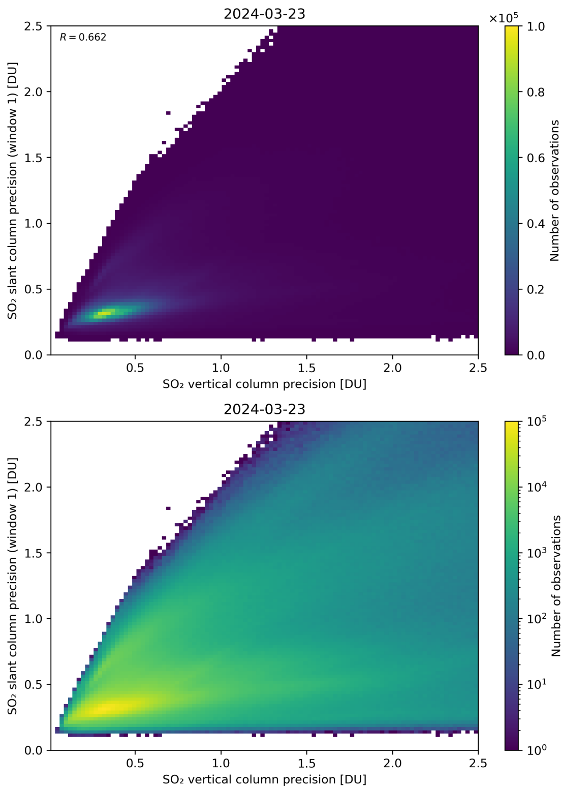
Figure 290: Scatter density plot of “SO 2 vertical column precision” against “SO 2 slant column precision (window 1)” for 2024-03-23 to 2024-03-24.
