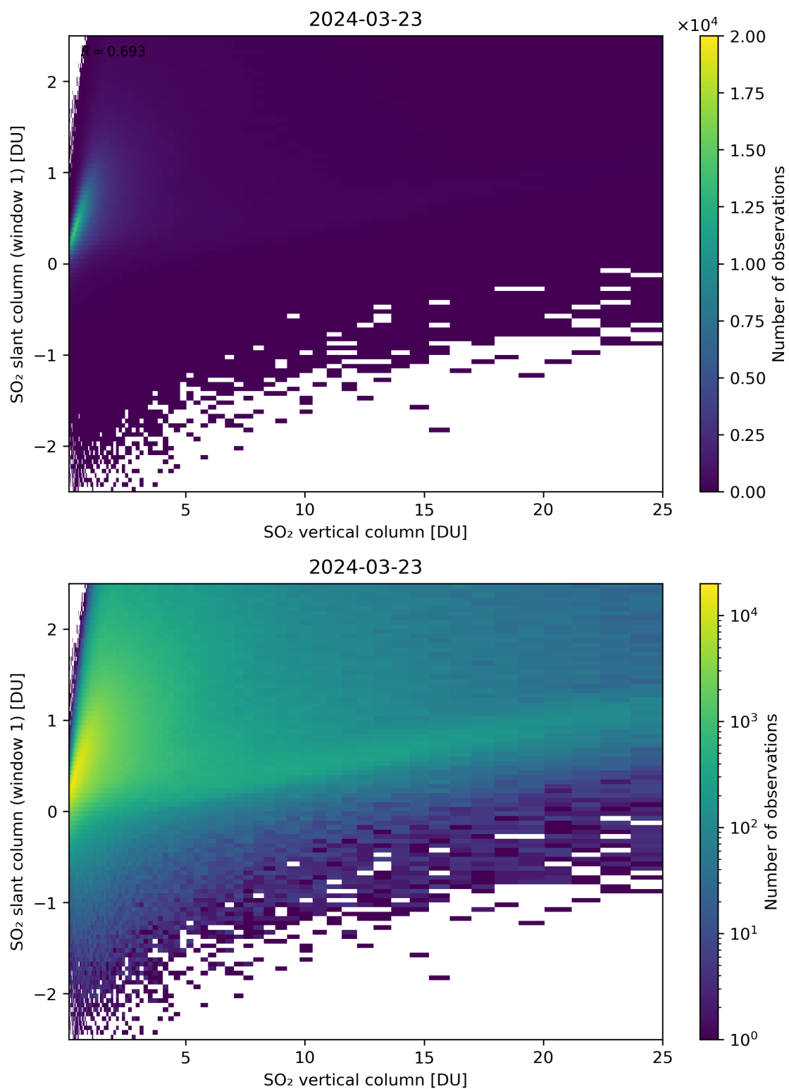
Figure 300: Scatter density plot of “SO 2 vertical column” against “SO 2 slant column (window 1)” for 2024-03-23 to 2024-03-24.
