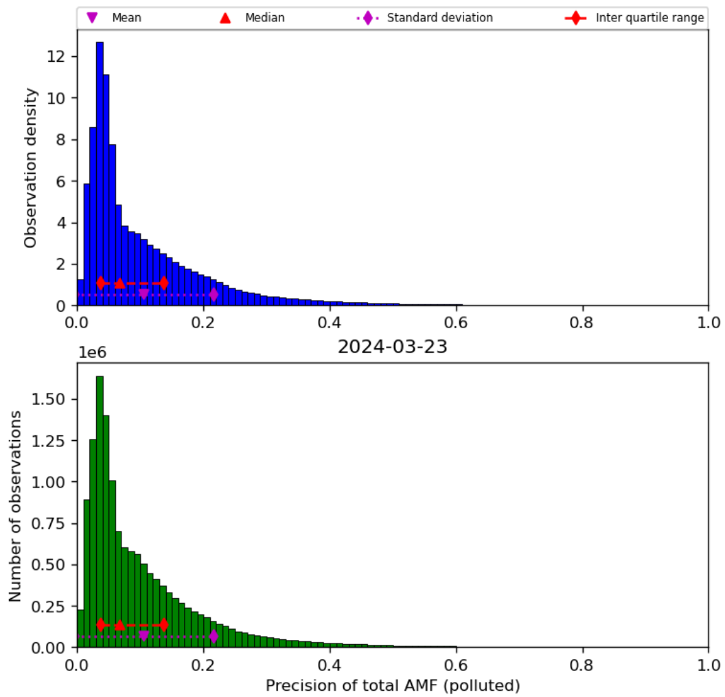
Figure 72: Histogram of “Precision of total AMF (polluted)” for 2024-03-23 to 2024-03-24
