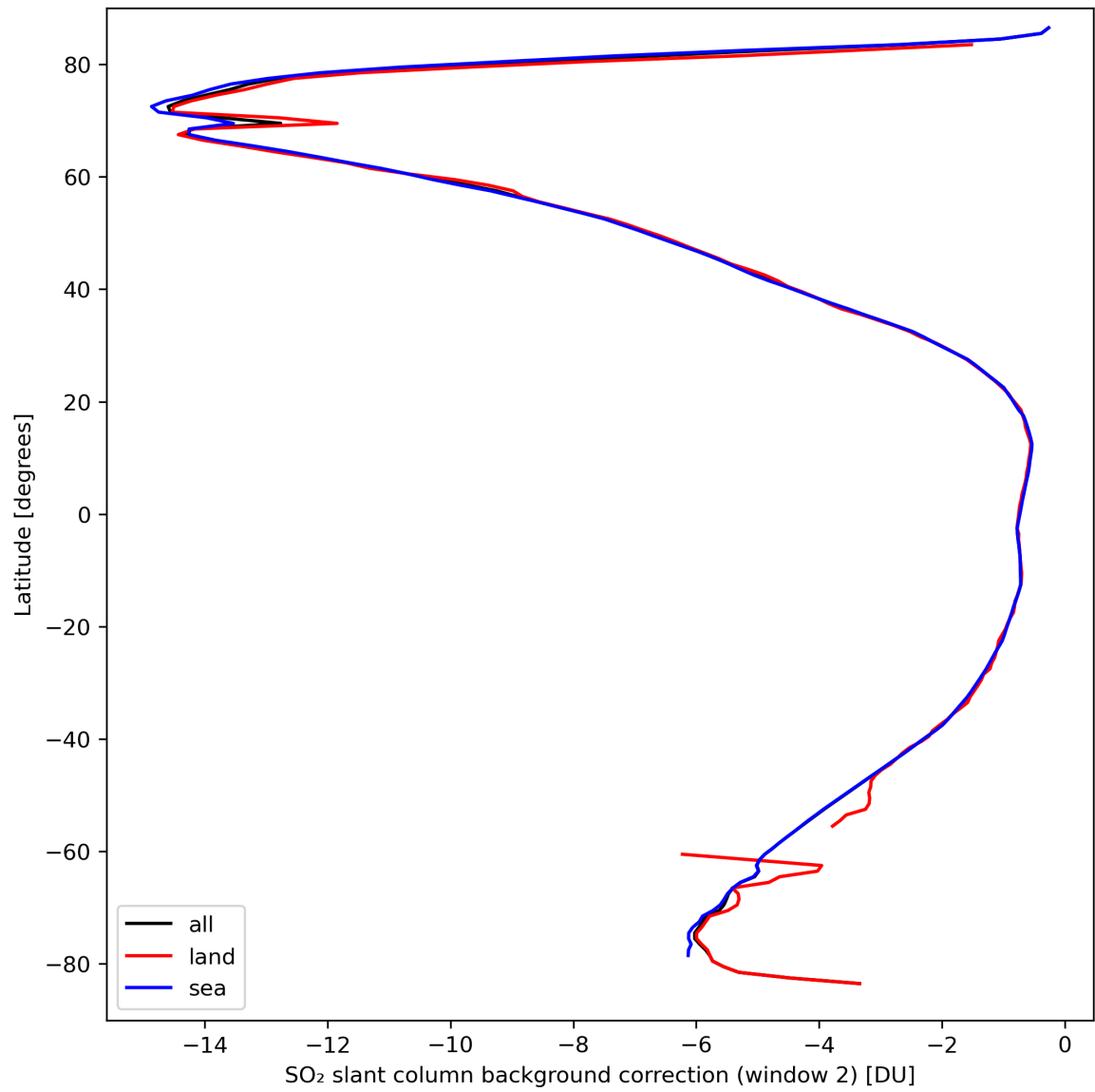
Figure 40: Zonal average of “SO 2 slant column background correction (window 2)” for 2024-03-23 to 2024-03-24.
