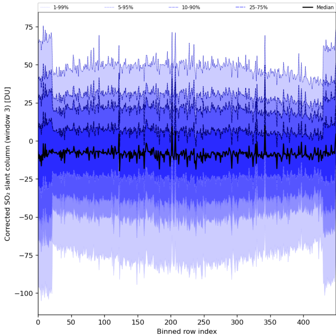
Figure 89: Along track statistics of “Corrected SO 2 slant column (window 3)” for 2024-03-23 to 2024-03-25
