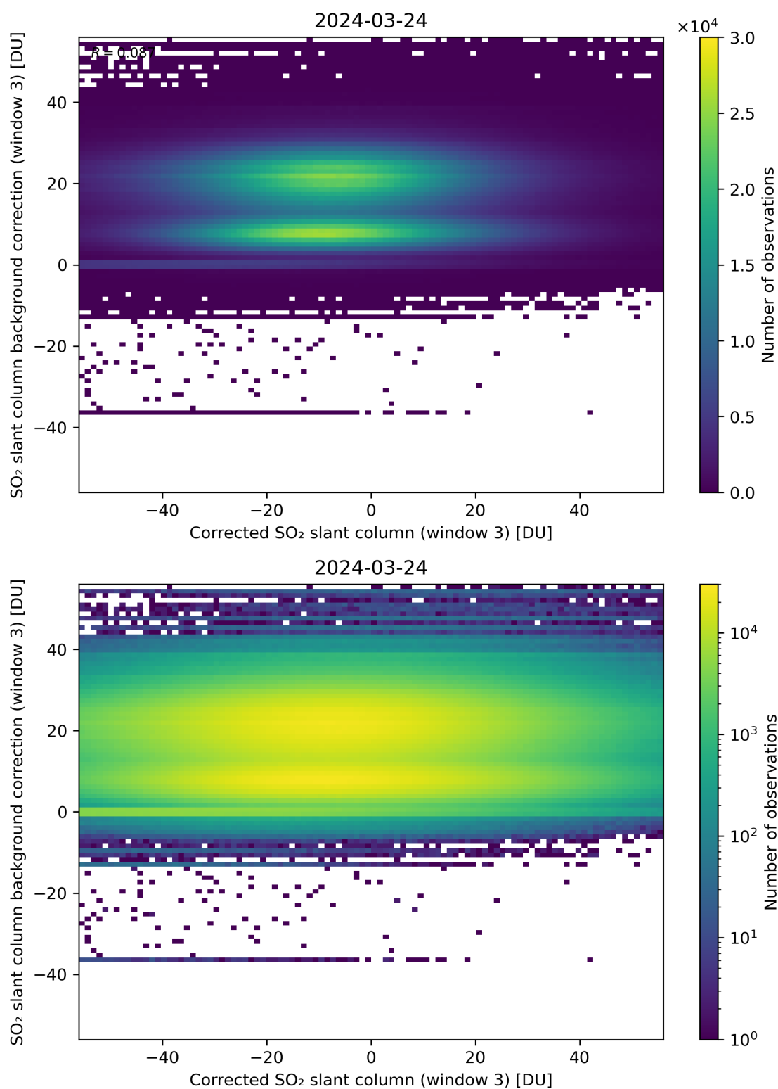
Figure 205: Scatter density plot of “Corrected SO 2 slant column (window 3)” against “SO 2 slant column background correction (window 3)” for 2024-03-23 to 2024-03-25.
