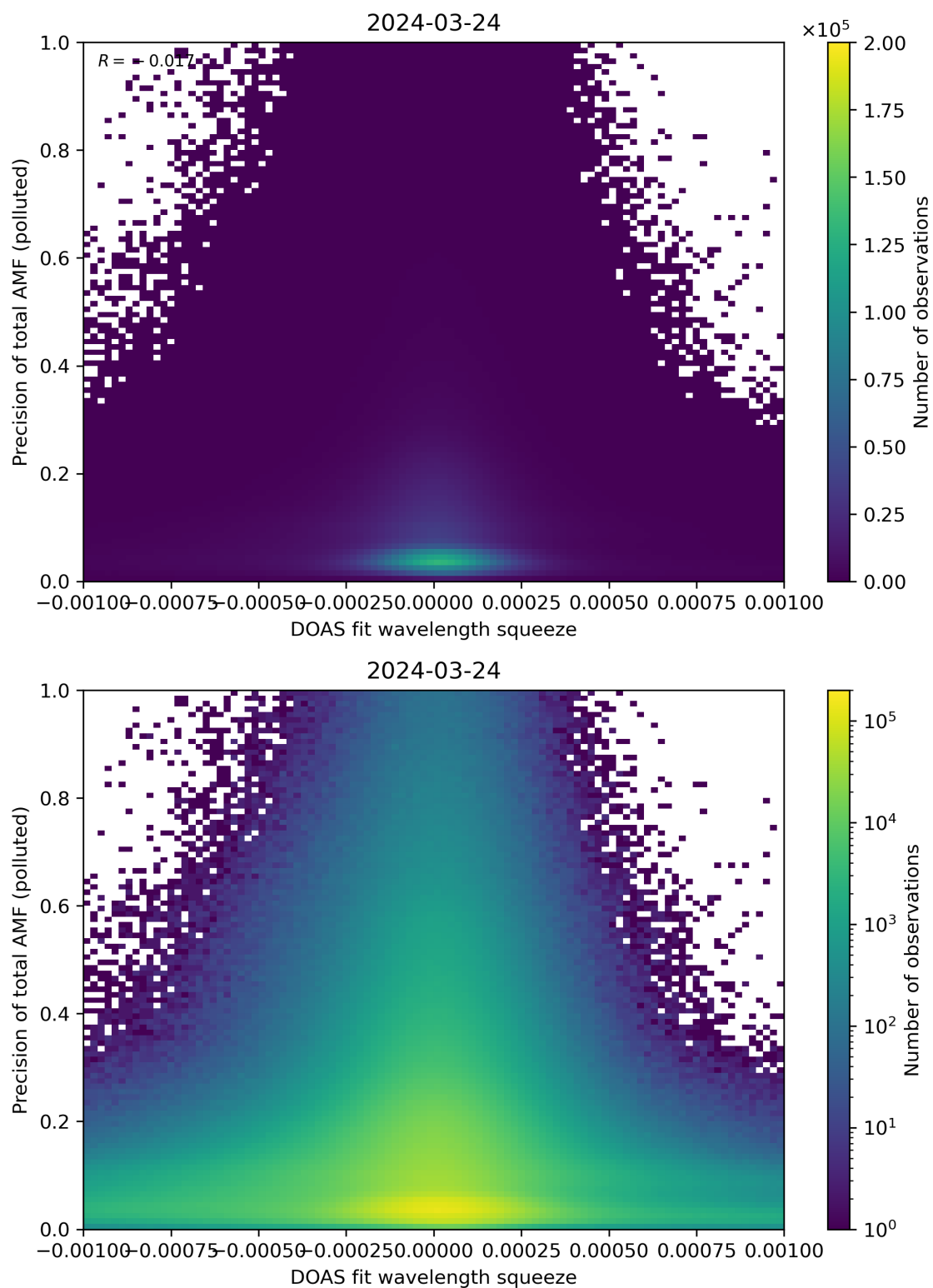
Figure 135: Scatter density plot of “DOAS fit wavelength squeeze” against “Precision of total AMF (polluted)” for 2024-03-23 to 2024-03-25.
