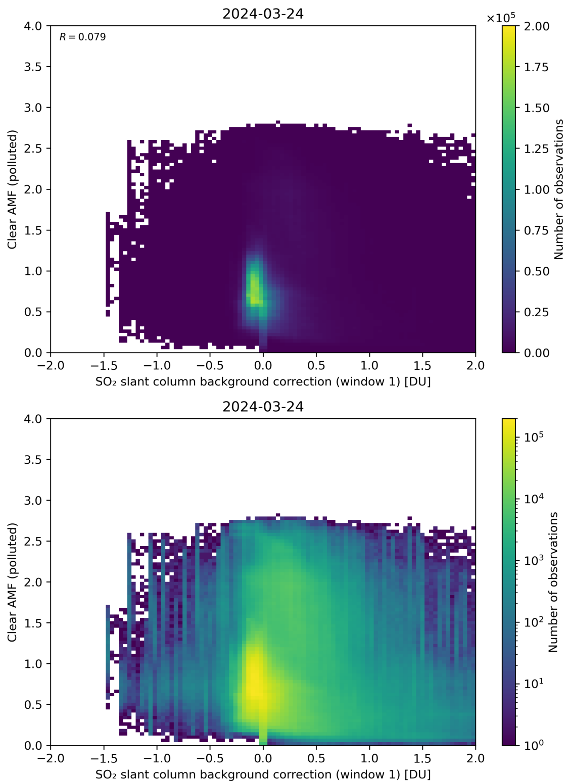
Figure 103: Scatter density plot of “SO 2 slant column background correction (window 1)” against “Clear AMF (polluted)” for 2024-03-23 to 2024-03-25.
