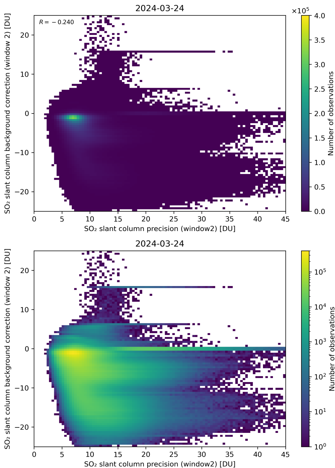
Figure 241: Scatter density plot of “SO 2 slant column precision (window2)” against “SO 2 slant column background correction (window 2)” for 2024-03-23 to 2024-03-25.
