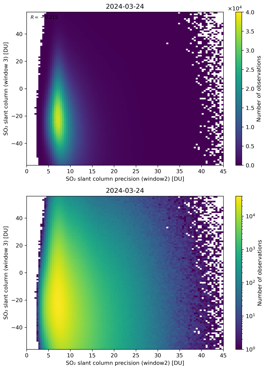
Figure 249: Scatter density plot of “SO 2 slant column precision (window2)” against “SO 2 slant column (window 3)” for 2024-03-23 to 2024-03-25.
