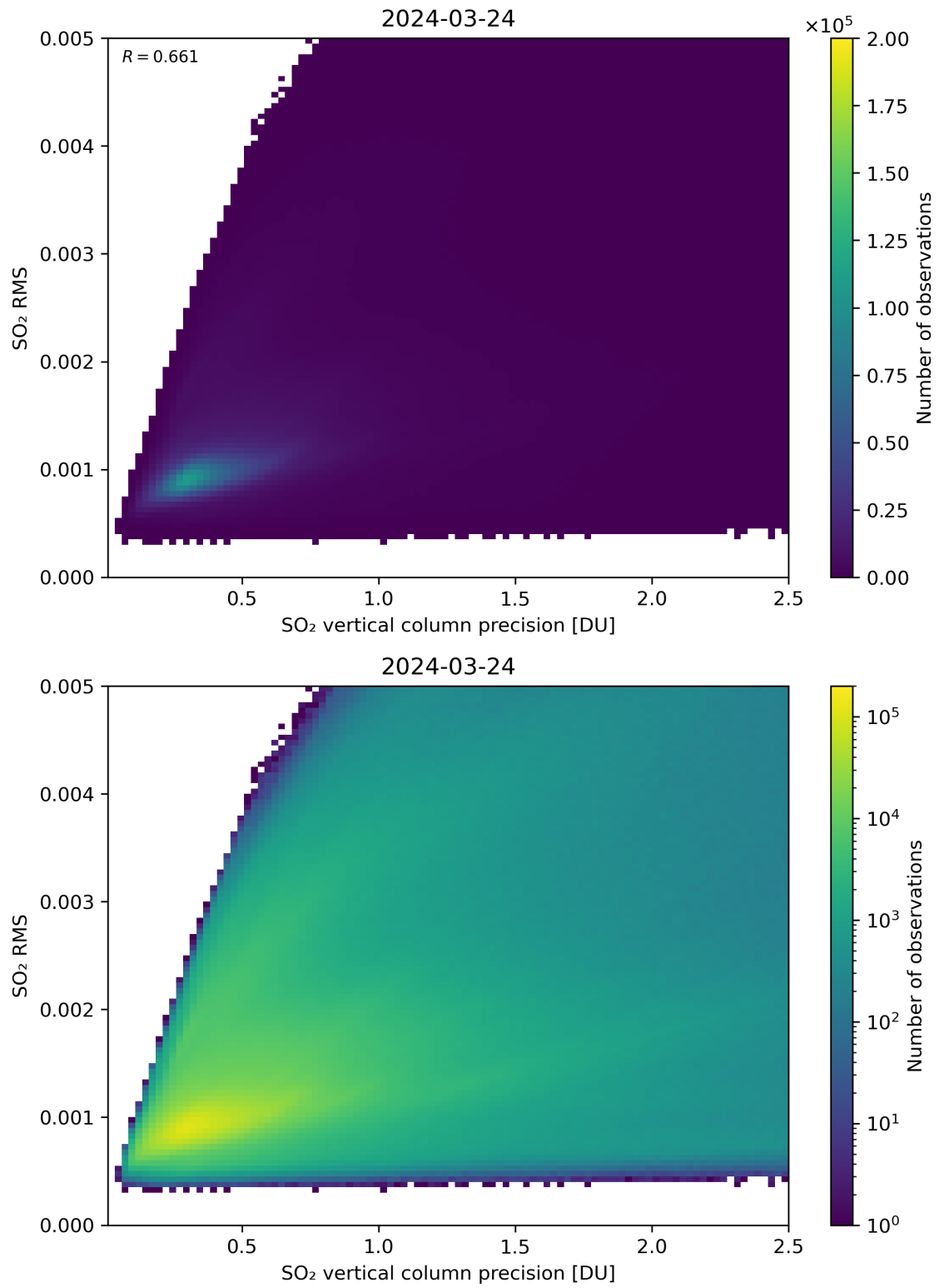
Figure 284: Scatter density plot of “SO 2 vertical column precision” against “SO 2 RMS” for 2024-03-23 to 2024-03-25.
