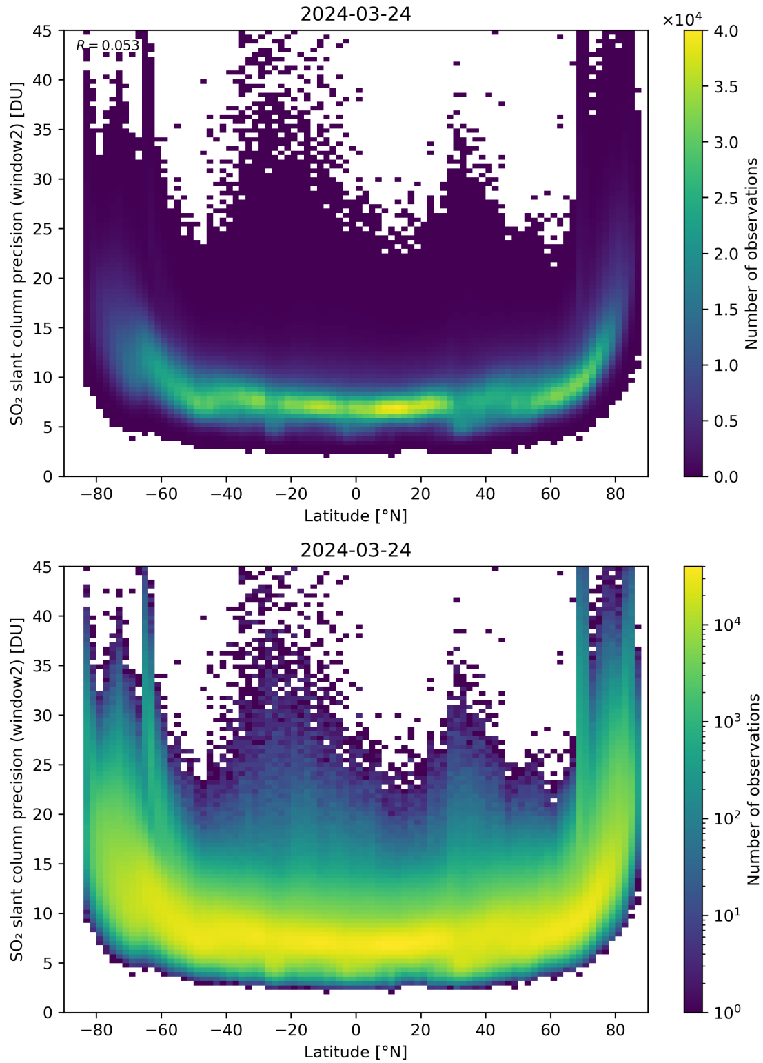
Figure 151: Scatter density plot of “Latitude” against “SO 2 slant column precision (window2)” for 2024-03-23 to 2024-03-25.
