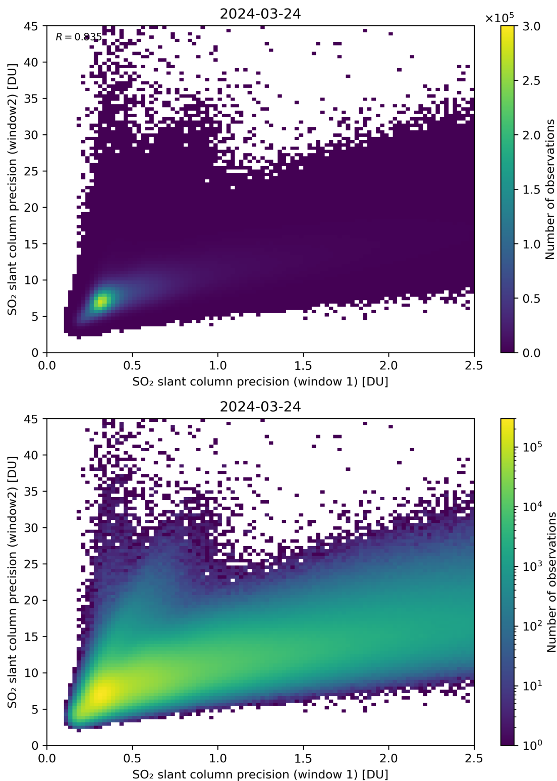
Figure 227: Scatter density plot of “SO 2 slant column precision (window 1)” against “SO 2 slant column precision (window2)” for 2024-03-23 to 2024-03-25.
