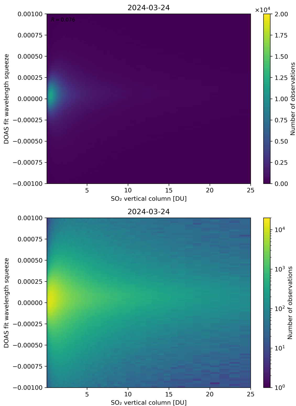
Figure 277: Scatter density plot of “SO 2 vertical column” against “DOAS fit wavelength squeeze” for 2024-03-23 to 2024-03-25.
