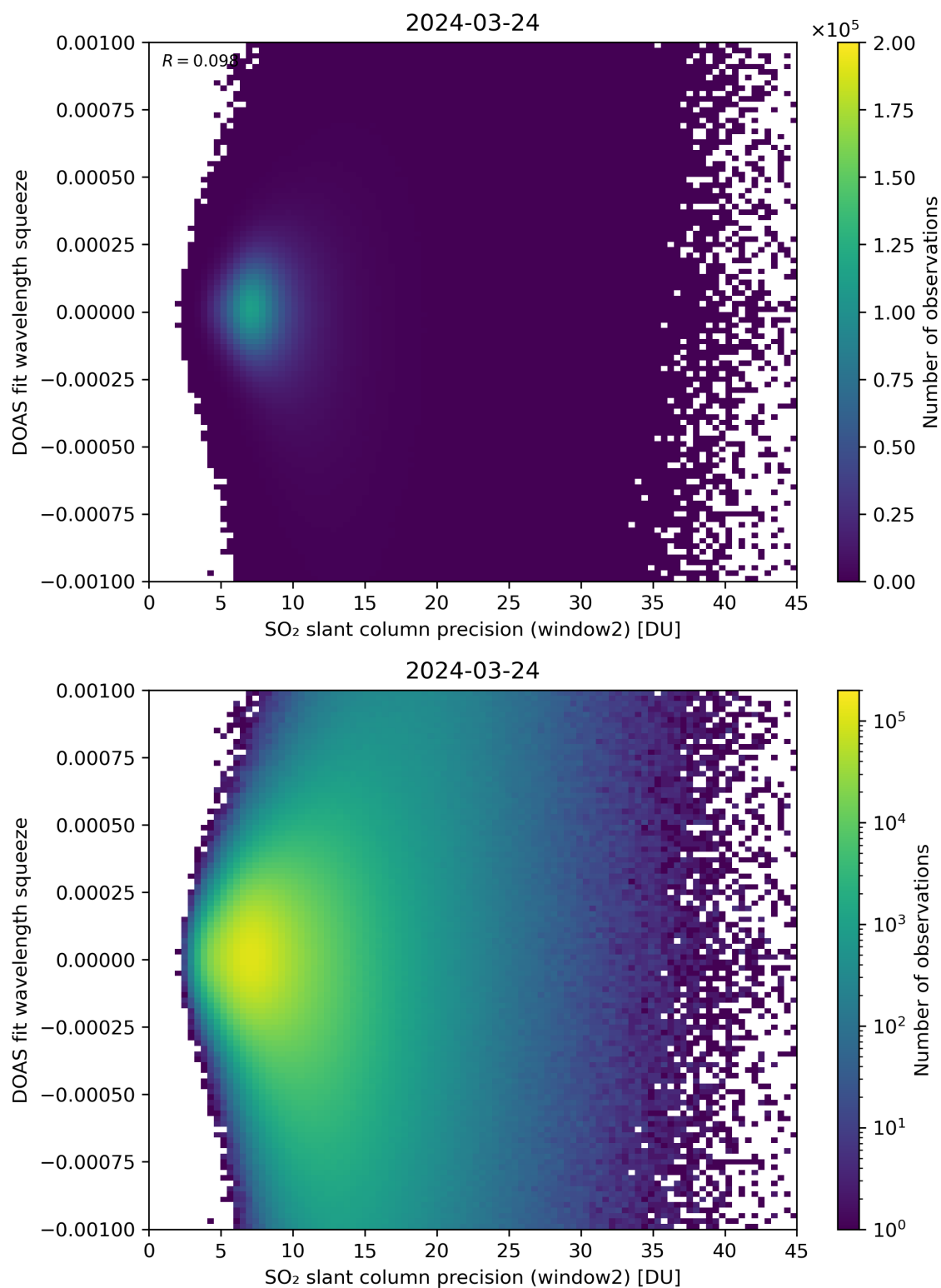
Figure 244: Scatter density plot of “SO 2 slant column precision (window2)” against “DOAS fit wavelength squeeze” for 2024-03-23 to 2024-03-25.
