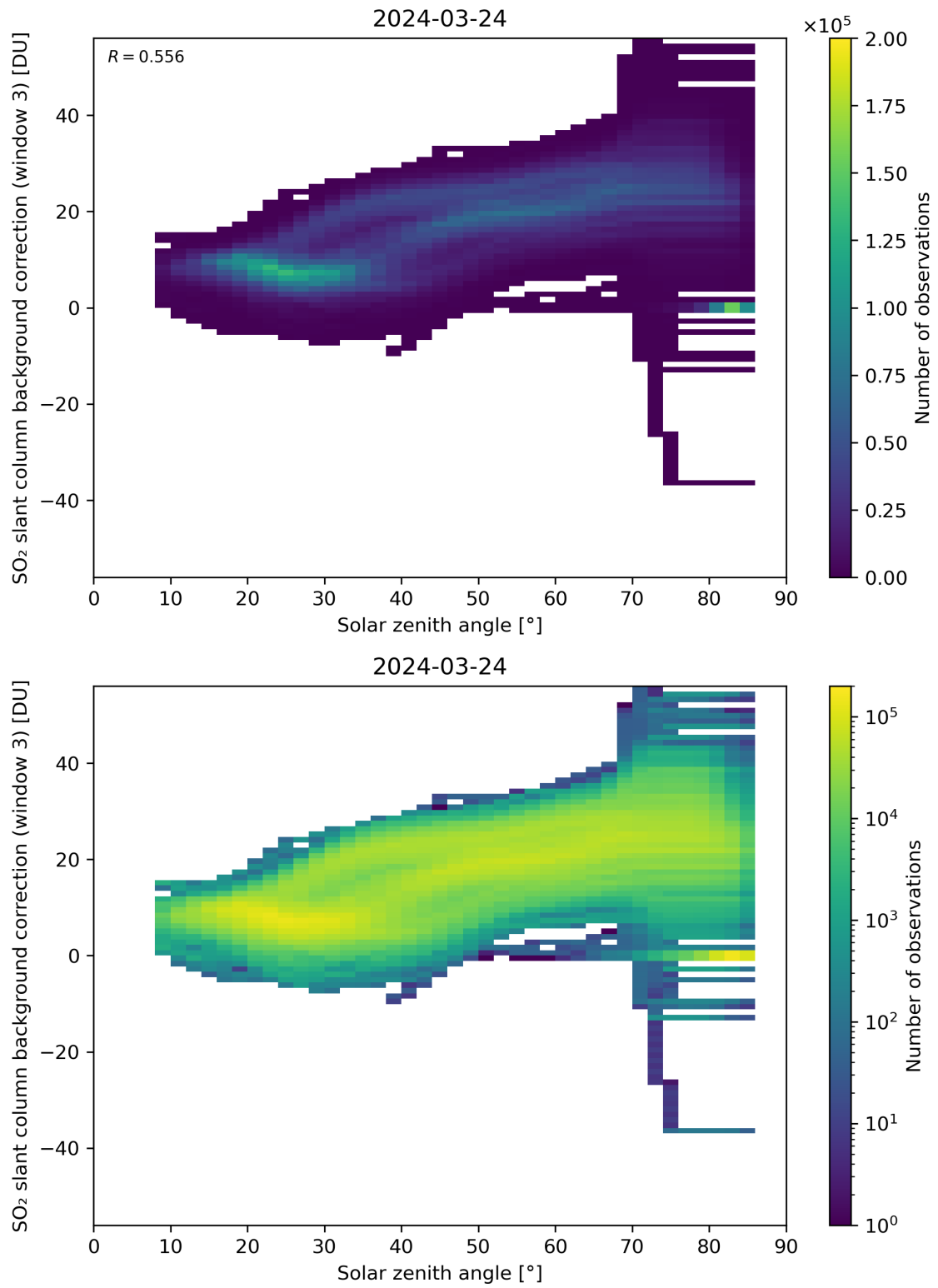
Figure 160: Scatter density plot of “Solar zenith angle” against “SO 2 slant column background correction (window 3)” for 2024-03-23 to 2024-03-25.
