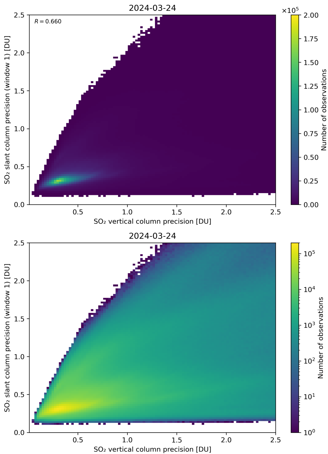
Figure 290: Scatter density plot of “SO 2 vertical column precision” against “SO 2 slant column precision (window 1)” for 2024-03-23 to 2024-03-25.
