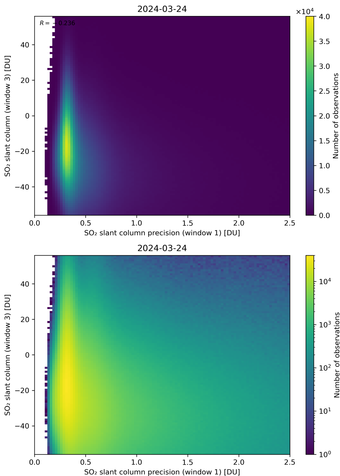
Figure 228: Scatter density plot of “SO 2 slant column precision (window 1)” against “SO 2 slant column (window 3)” for 2024-03-23 to 2024-03-25.
