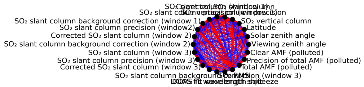
Figure 1: Map of correlation graph for 2024-03-23 to 2024-03-25.
