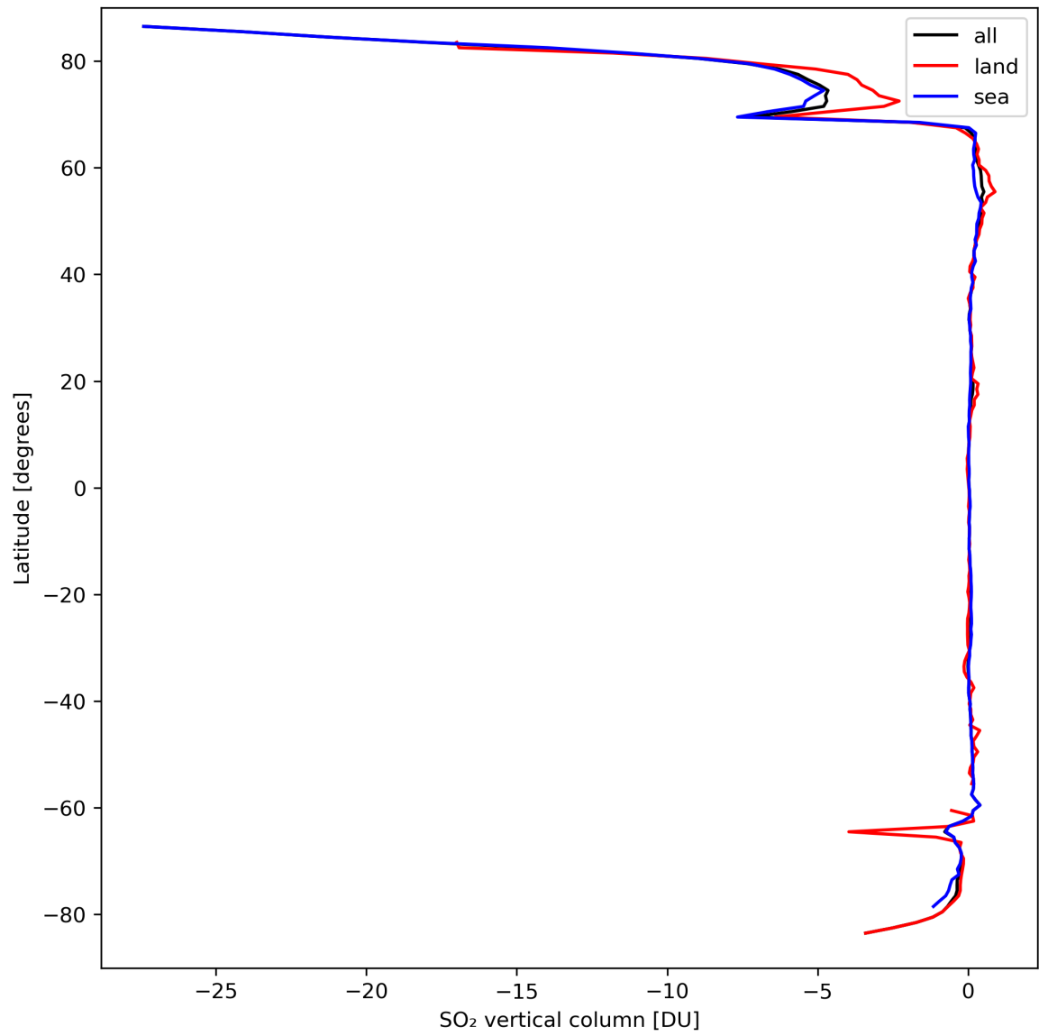
Figure 30: Zonal average of “SO 2 vertical column” for 2024-03-23 to 2024-03-25.
