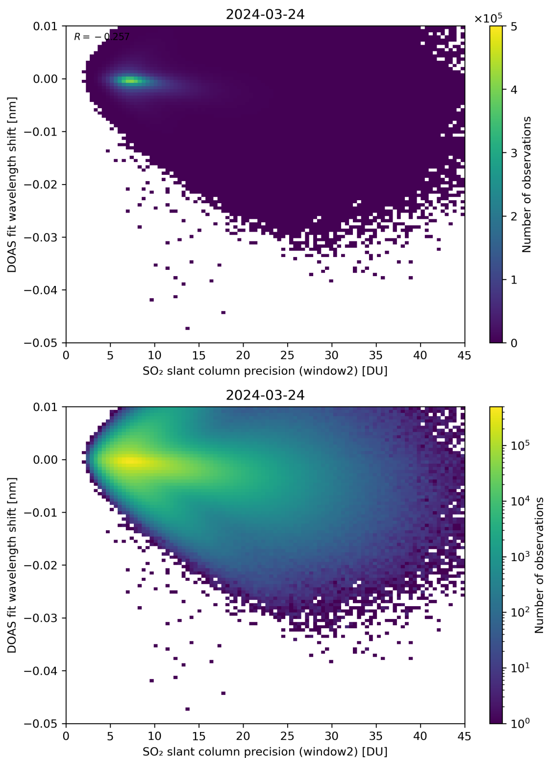
Figure 243: Scatter density plot of “SO 2 slant column precision (window2)” against “DOAS fit wavelength shift” for 2024-03-23 to 2024-03-25.
