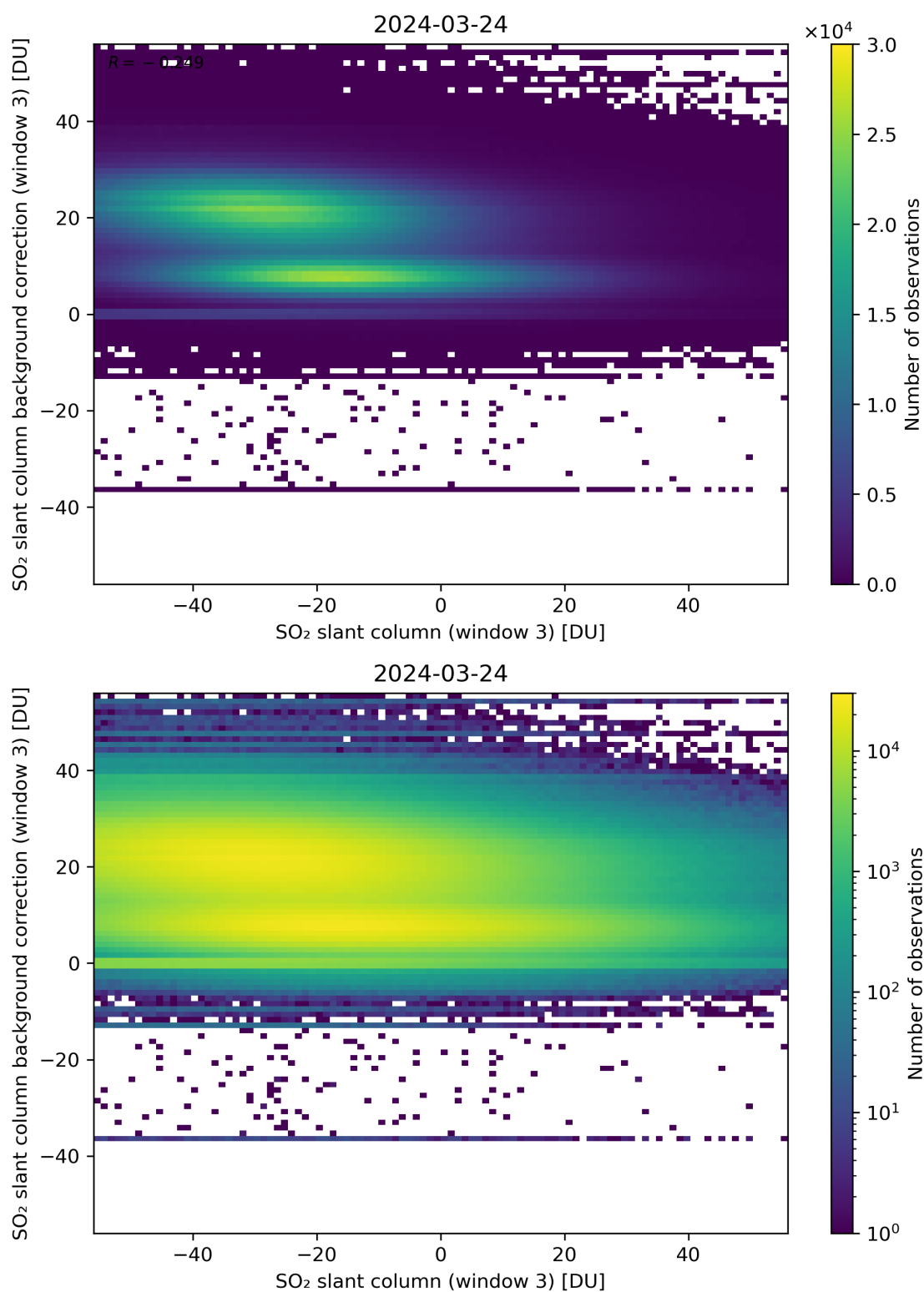
Figure 253: Scatter density plot of “SO 2 slant column (window 3)” against “SO 2 slant column background correction (window 3)” for 2024-03-23 to 2024-03-25.
