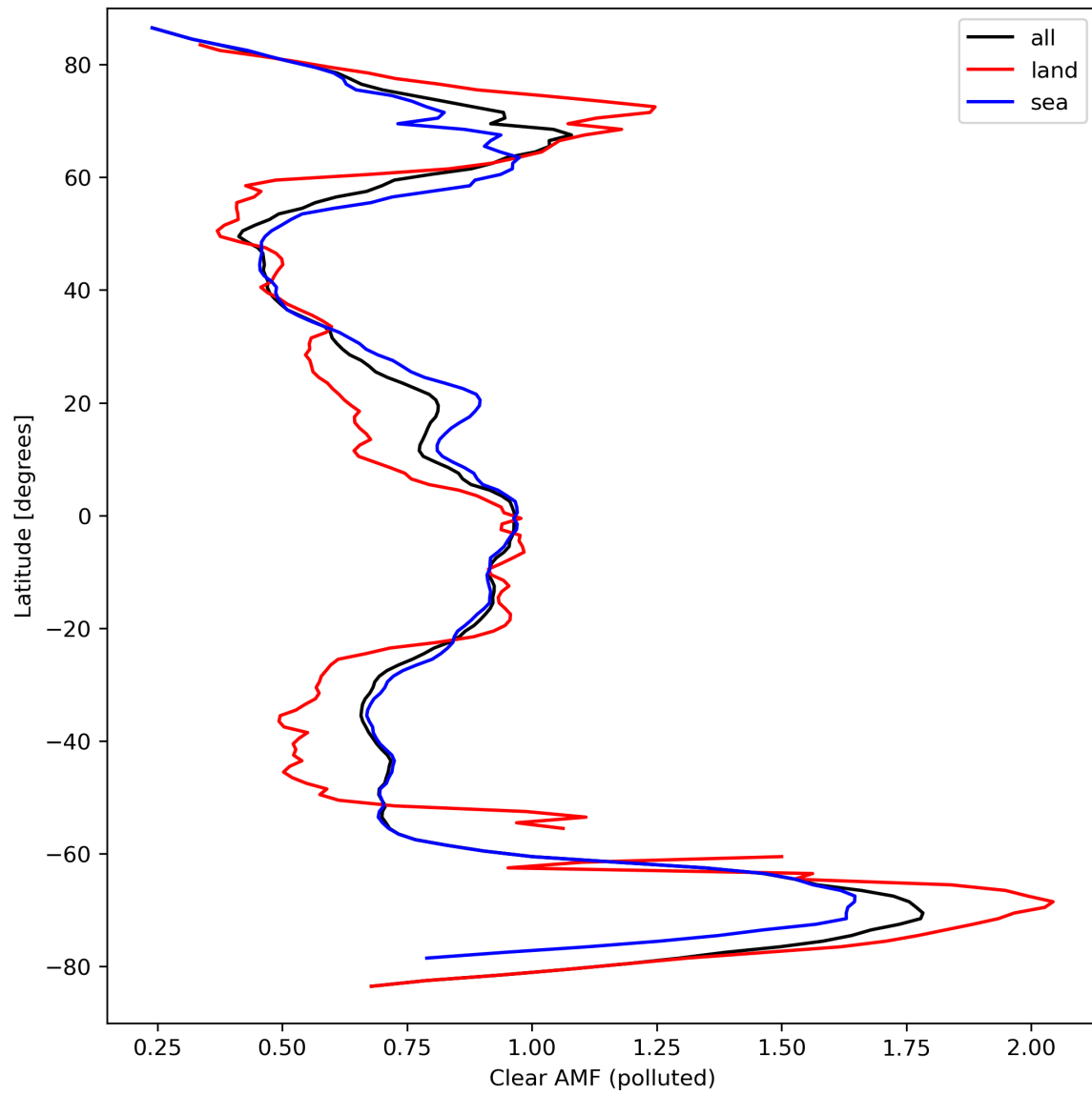
Figure 50: Zonal average of “Clear AMF (polluted)” for 2024-03-23 to 2024-03-25.
