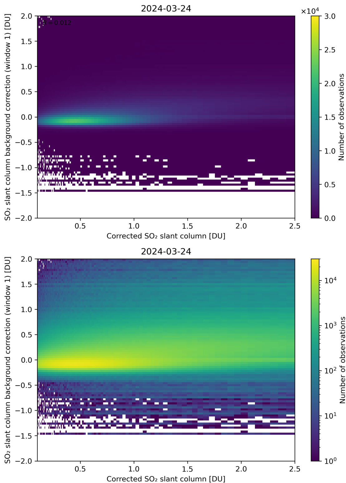
Figure 178: Scatter density plot of “Corrected SO 2 slant column” against “SO 2 slant column background correction (window 1)” for 2024-03-23 to 2024-03-25.
