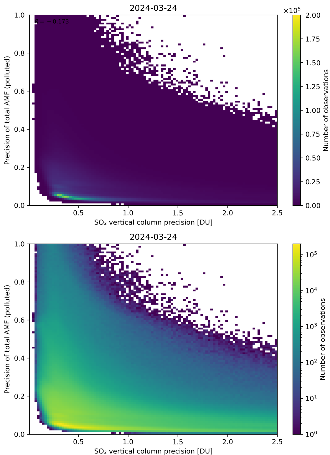
Figure 295: Scatter density plot of “SO 2 vertical column precision” against “Precision of total AMF (polluted)” for 2024-03-23 to 2024-03-25.
