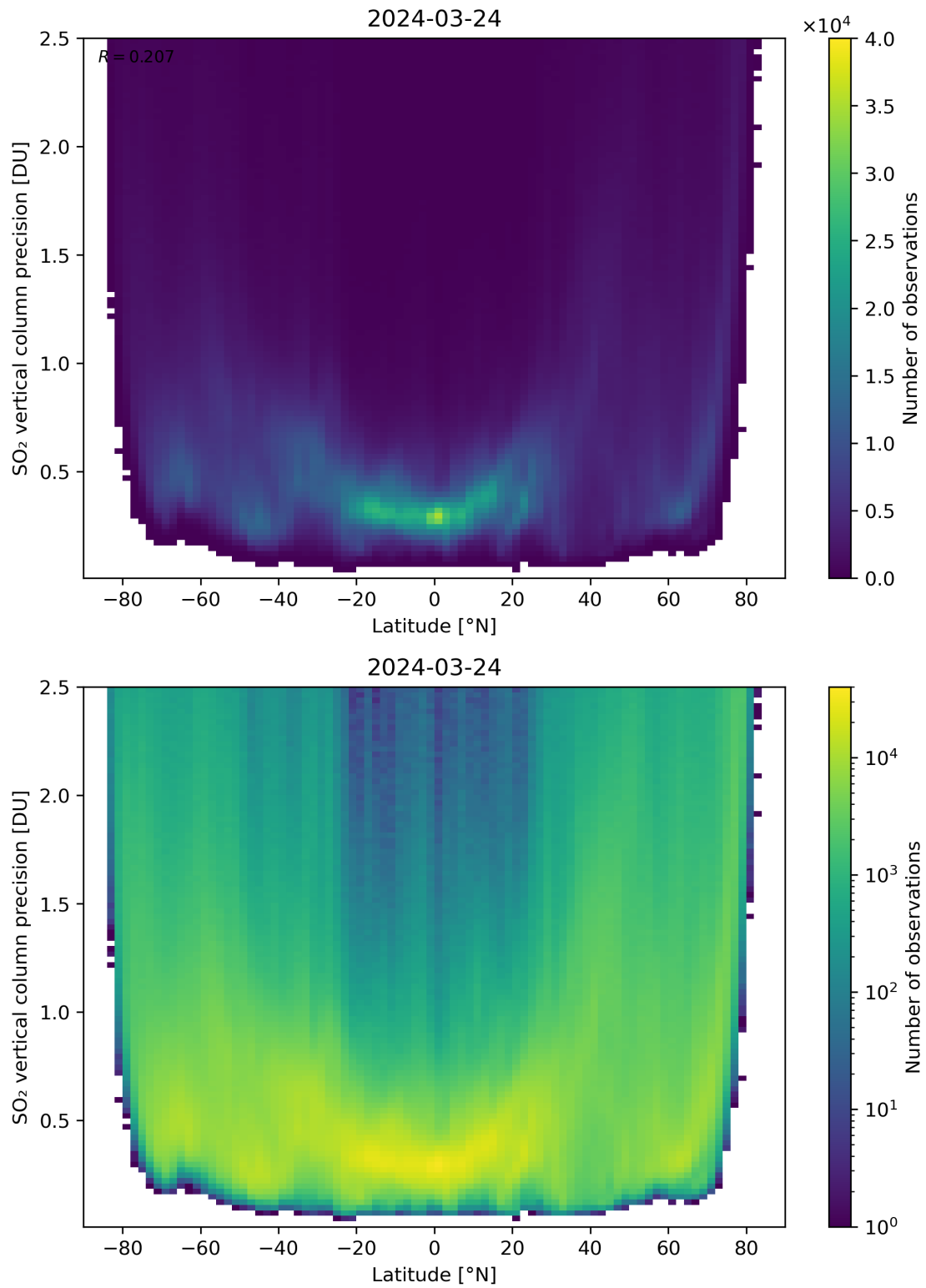
Figure 157: Scatter density plot of “Latitude” against “SO 2 vertical column precision” for 2024-03-23 to 2024-03-25.
