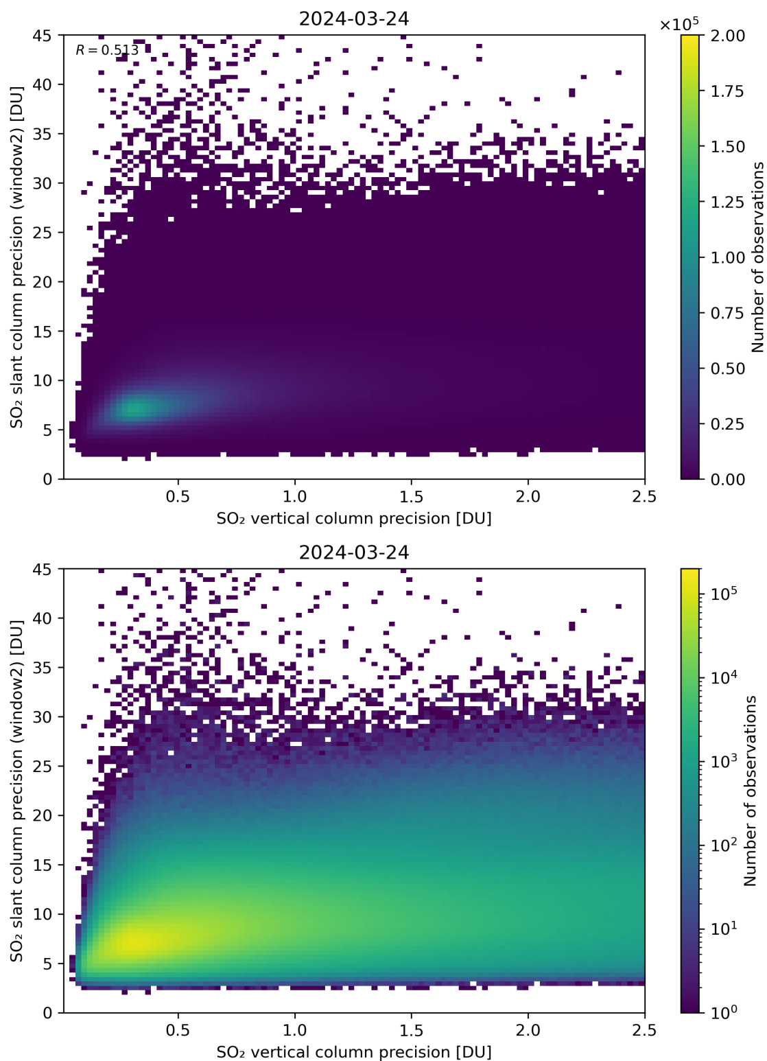
Figure 291: Scatter density plot of “SO 2 vertical column precision” against “SO 2 slant column precision (window2)” for 2024-03-23 to 2024-03-25.
