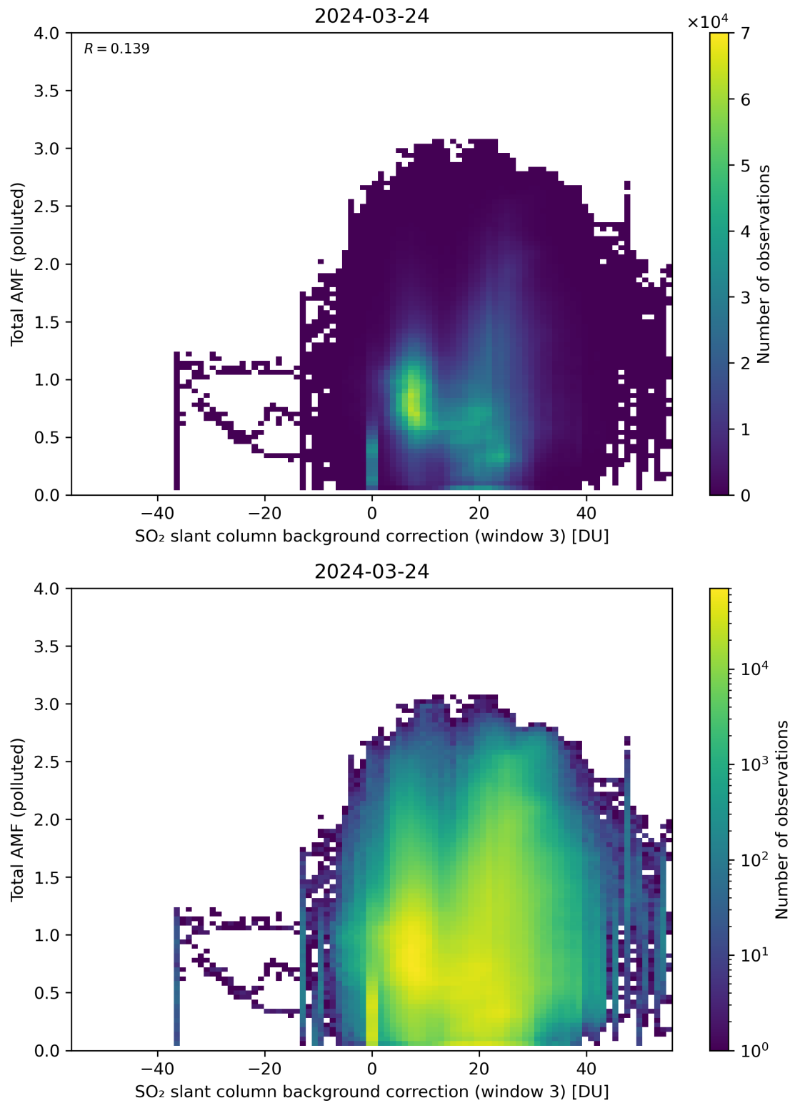
Figure 125: Scatter density plot of “SO 2 slant column background correction (window 3)” against “Total AMF (polluted)” for 2024-03-23 to 2024-03-25.
