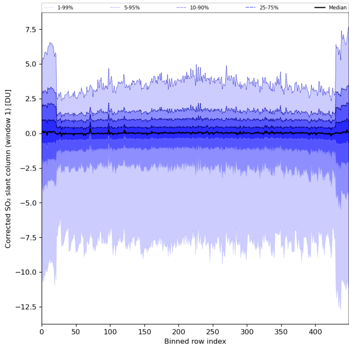
Figure 81: Along track statistics of “Corrected SO 2 slant column (window 1)” for 2024-03-23 to 2024-03-25
