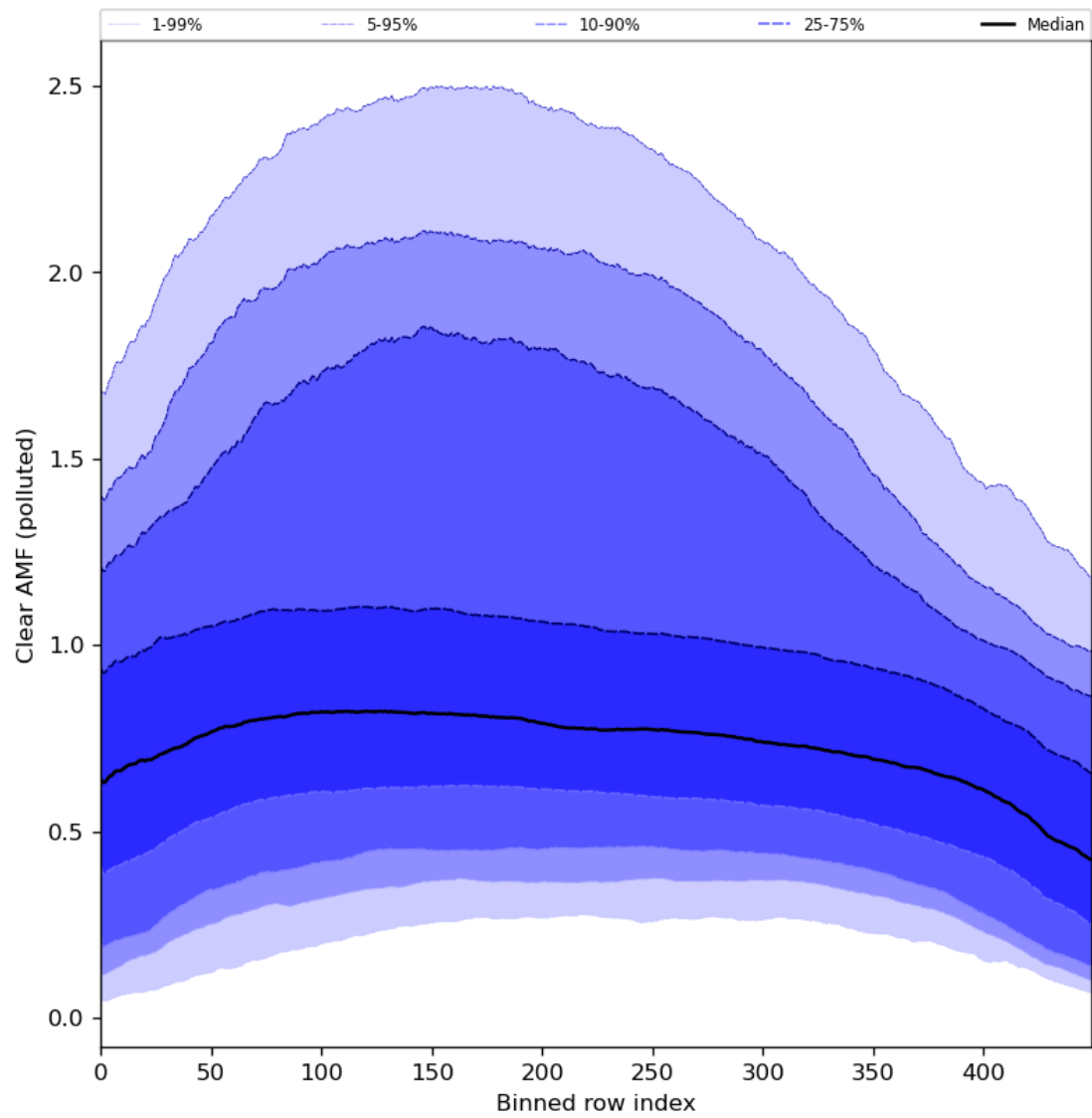
Figure 96: Along track statistics of “Clear AMF (polluted)” for 2024-03-23 to 2024-03-25
