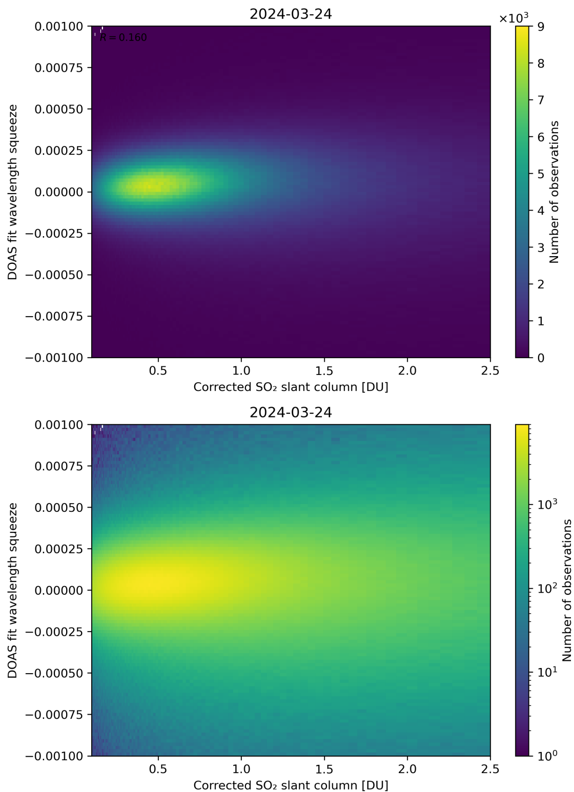
Figure 182: Scatter density plot of “Corrected SO 2 slant column” against “DOAS fit wavelength squeeze” for 2024-03-23 to 2024-03-25.
