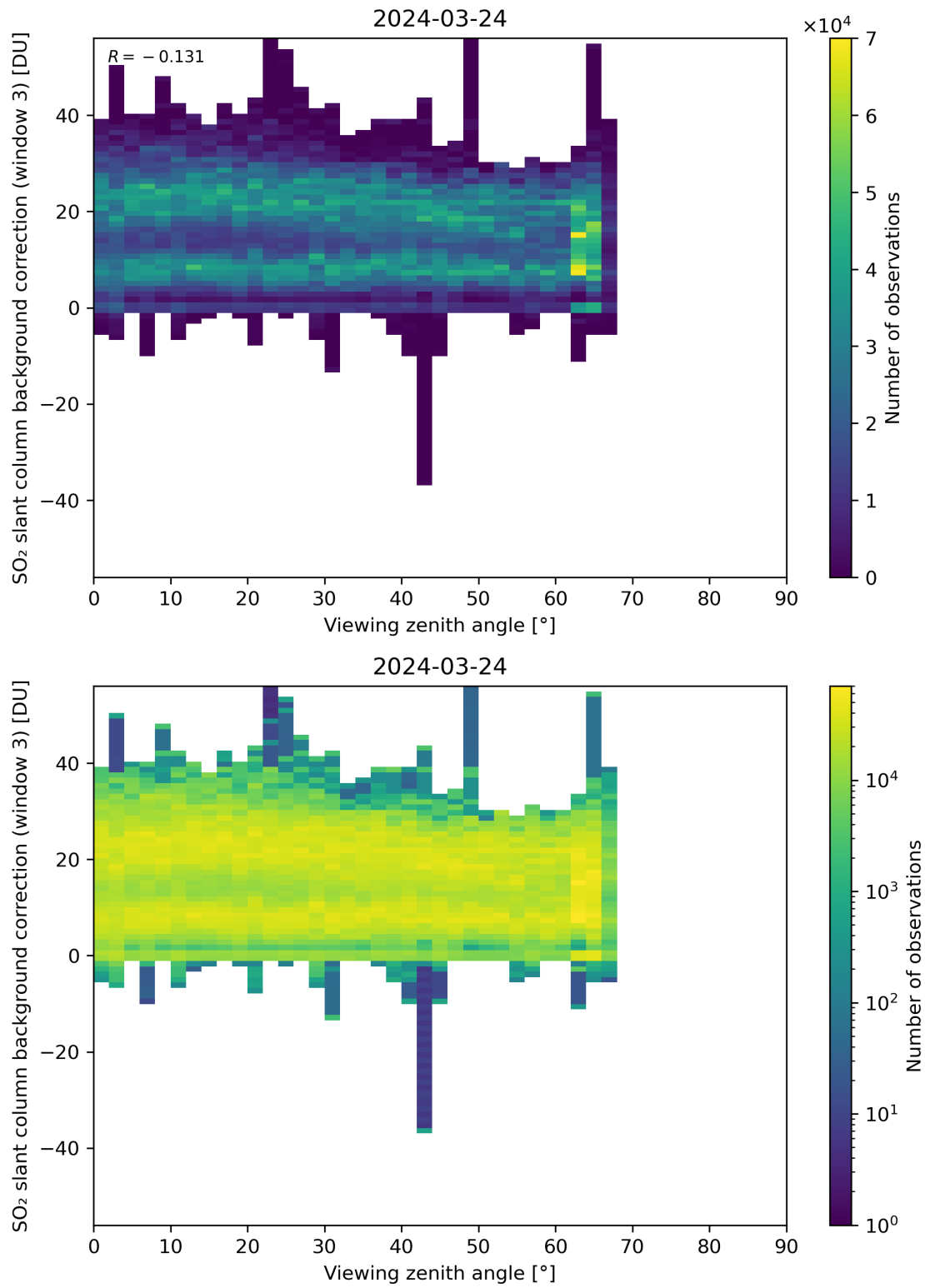
Figure 310: Scatter density plot of “Viewing zenith angle” against “SO 2 slant column background correction (window 3)” for 2024-03-23 to 2024-03-25.
