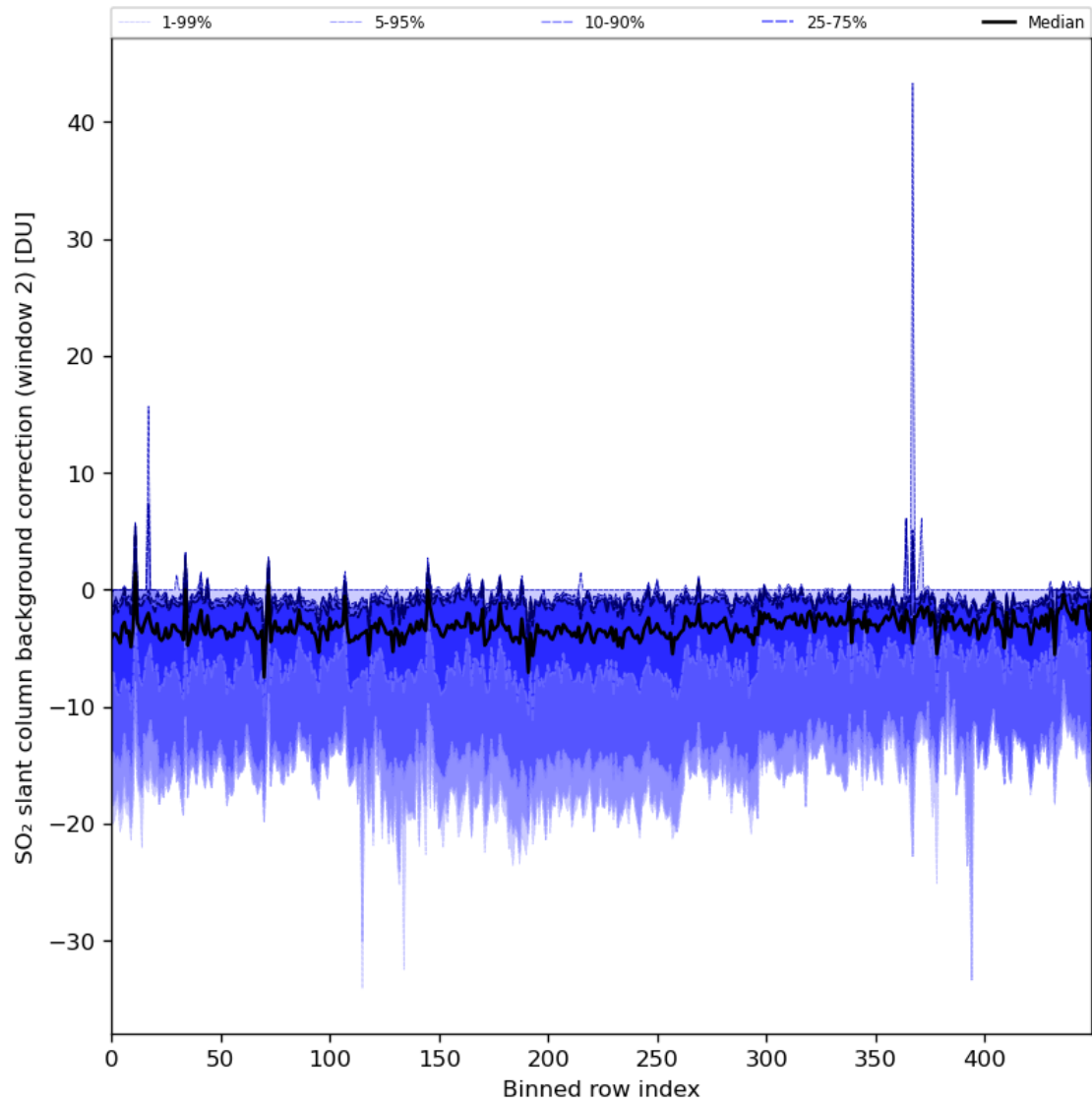
Figure 86: Along track statistics of “SO 2 slant column background correction (window 2)” for 2024-03-23 to 2024-03-25
