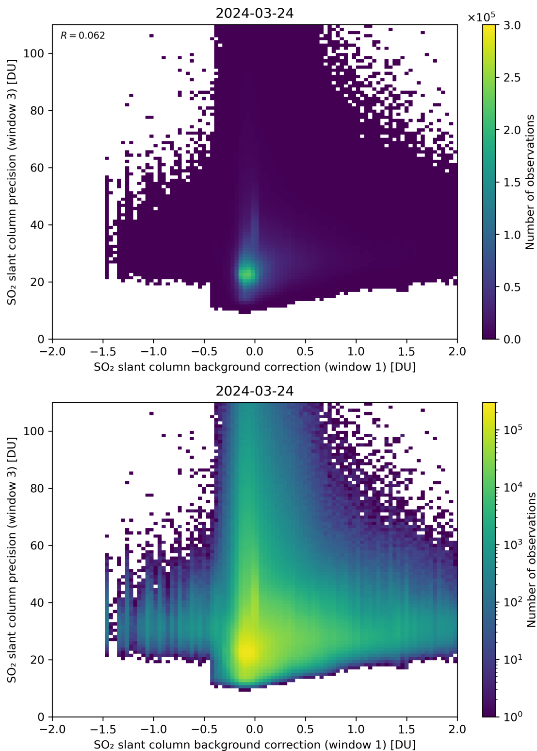
Figure 108: Scatter density plot of “SO 2 slant column background correction (window 1)” against “SO 2 slant column precision (window 3)” for 2024-03-23 to 2024-03-25.
