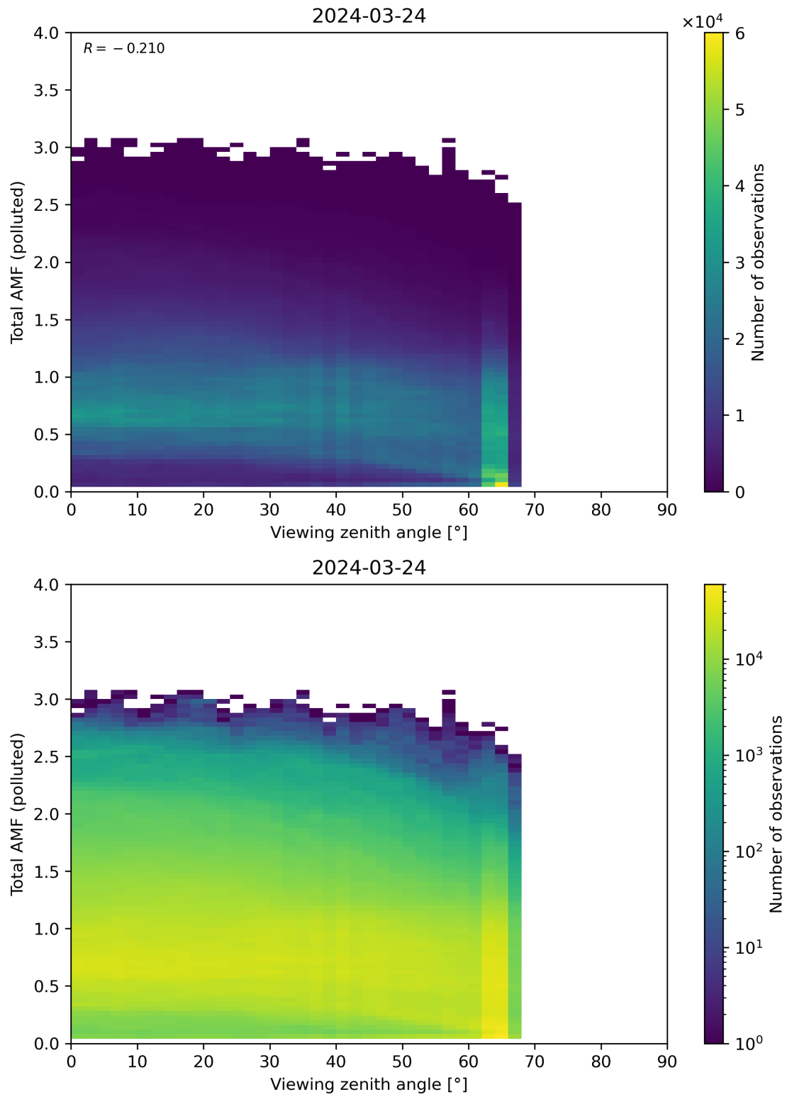
Figure 325: Scatter density plot of “Viewing zenith angle” against “Total AMF (polluted)” for 2024-03-23 to 2024-03-25.
