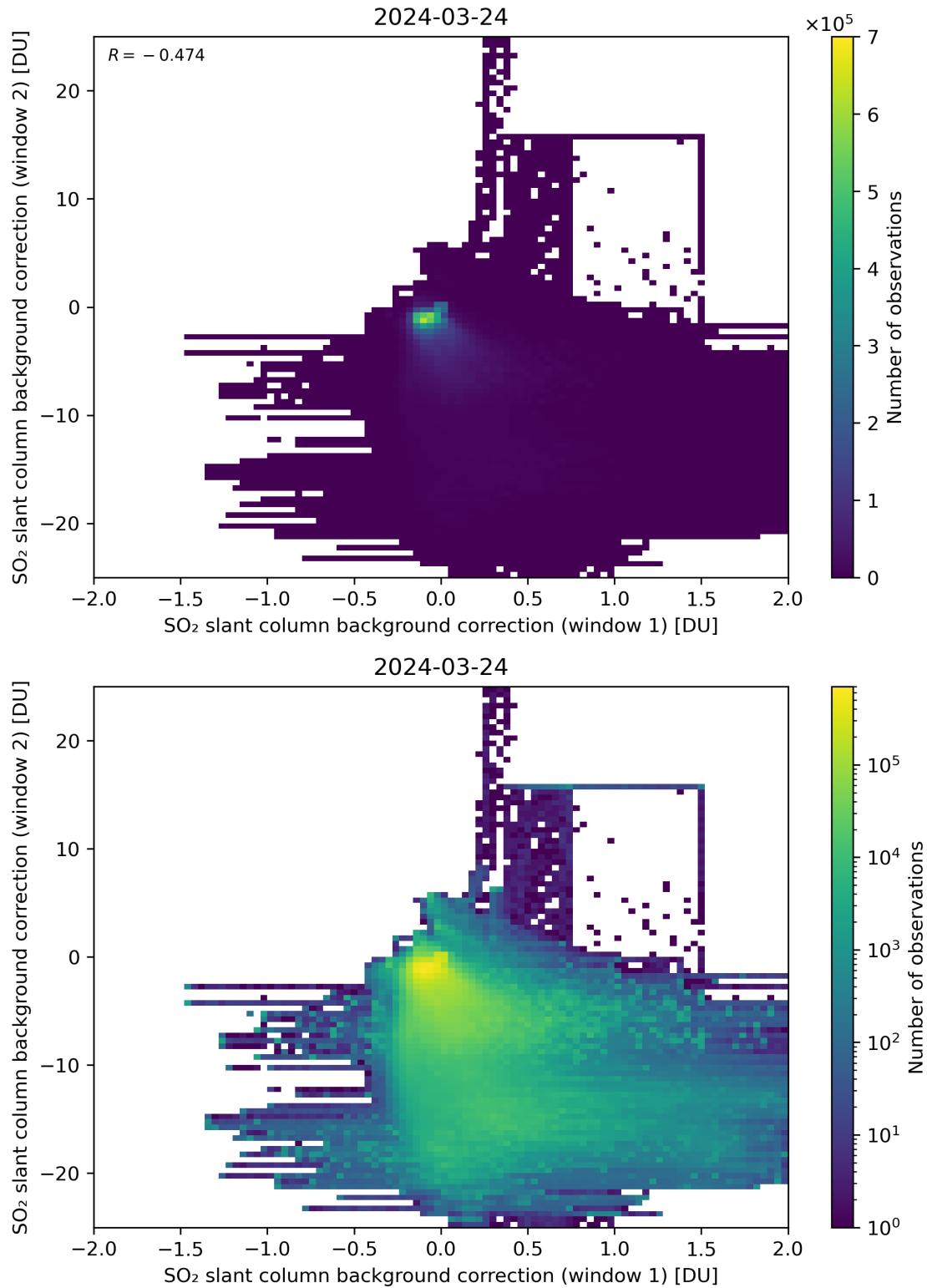
Figure 98: Scatter density plot of “SO 2 slant column background correction (window 1)” against “SO 2 slant column background correction (window 2)” for 2024-03-23 to 2024-03-25.
