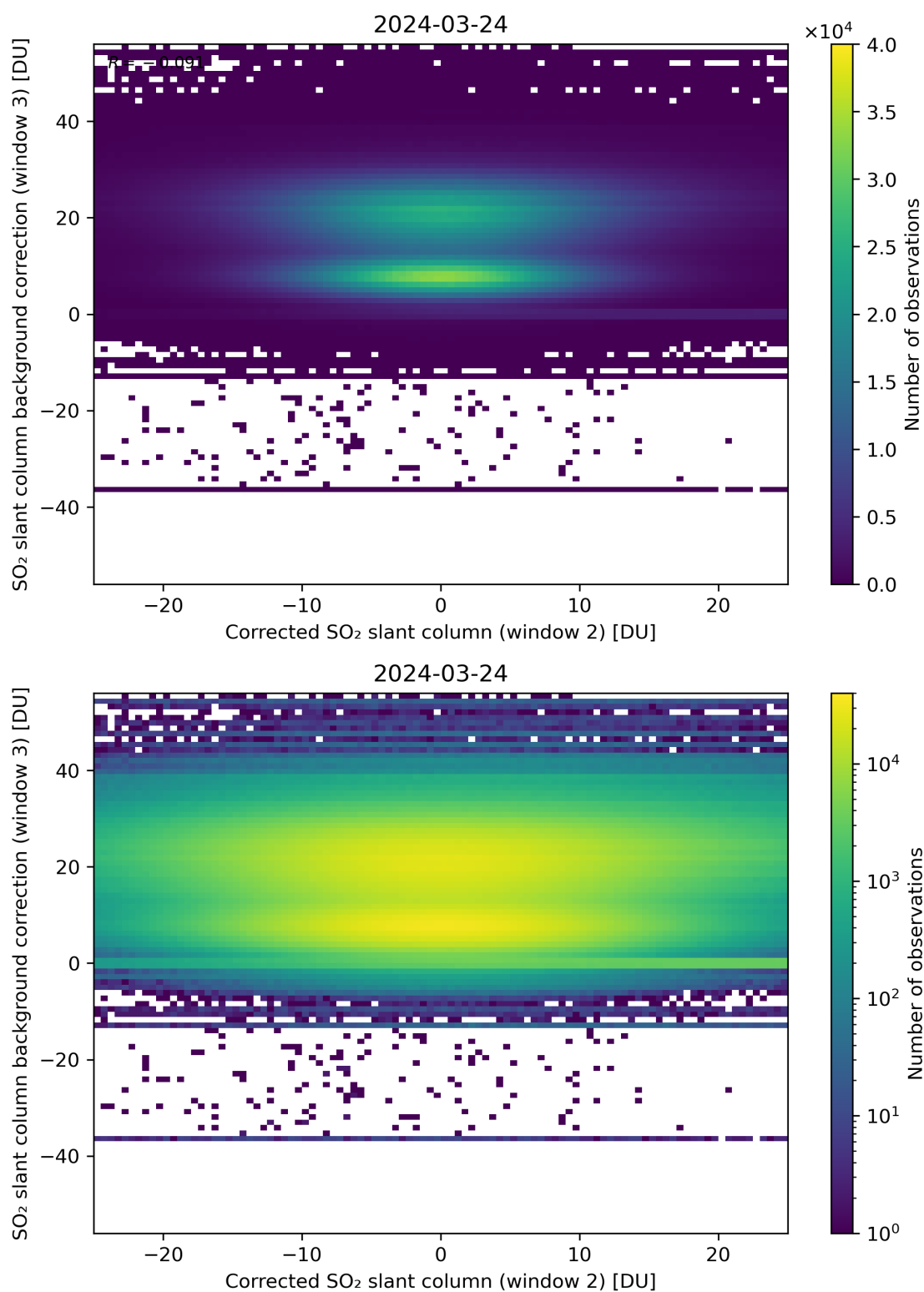
Figure 195: Scatter density plot of “Corrected SO 2 slant column (window 2)” against “SO 2 slant column background correction (window 3)” for 2024-03-23 to 2024-03-25.
