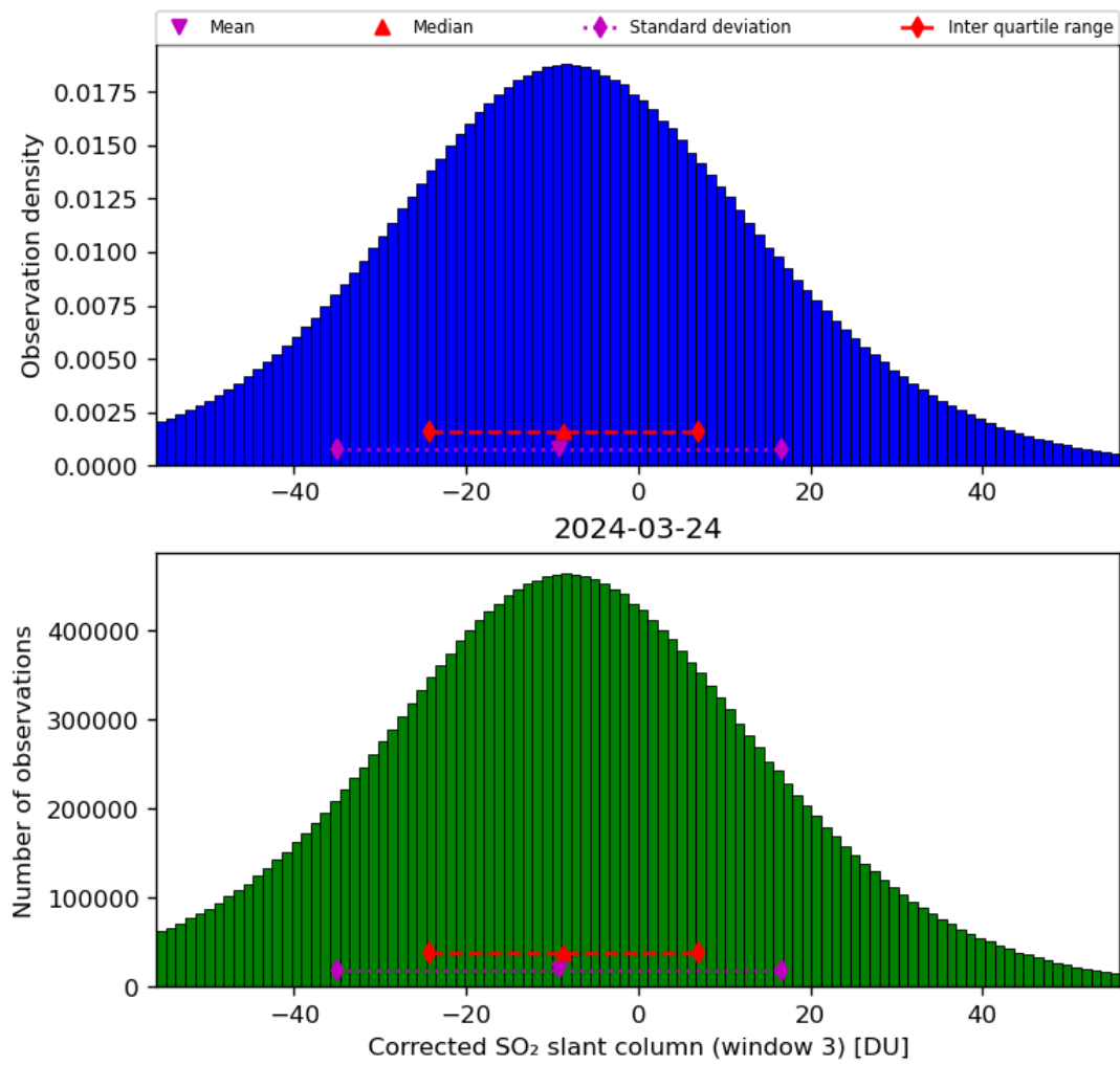
Figure 66: Histogram of “Corrected SO 2 slant column (window 3)” for 2024-03-23 to 2024-03-25
