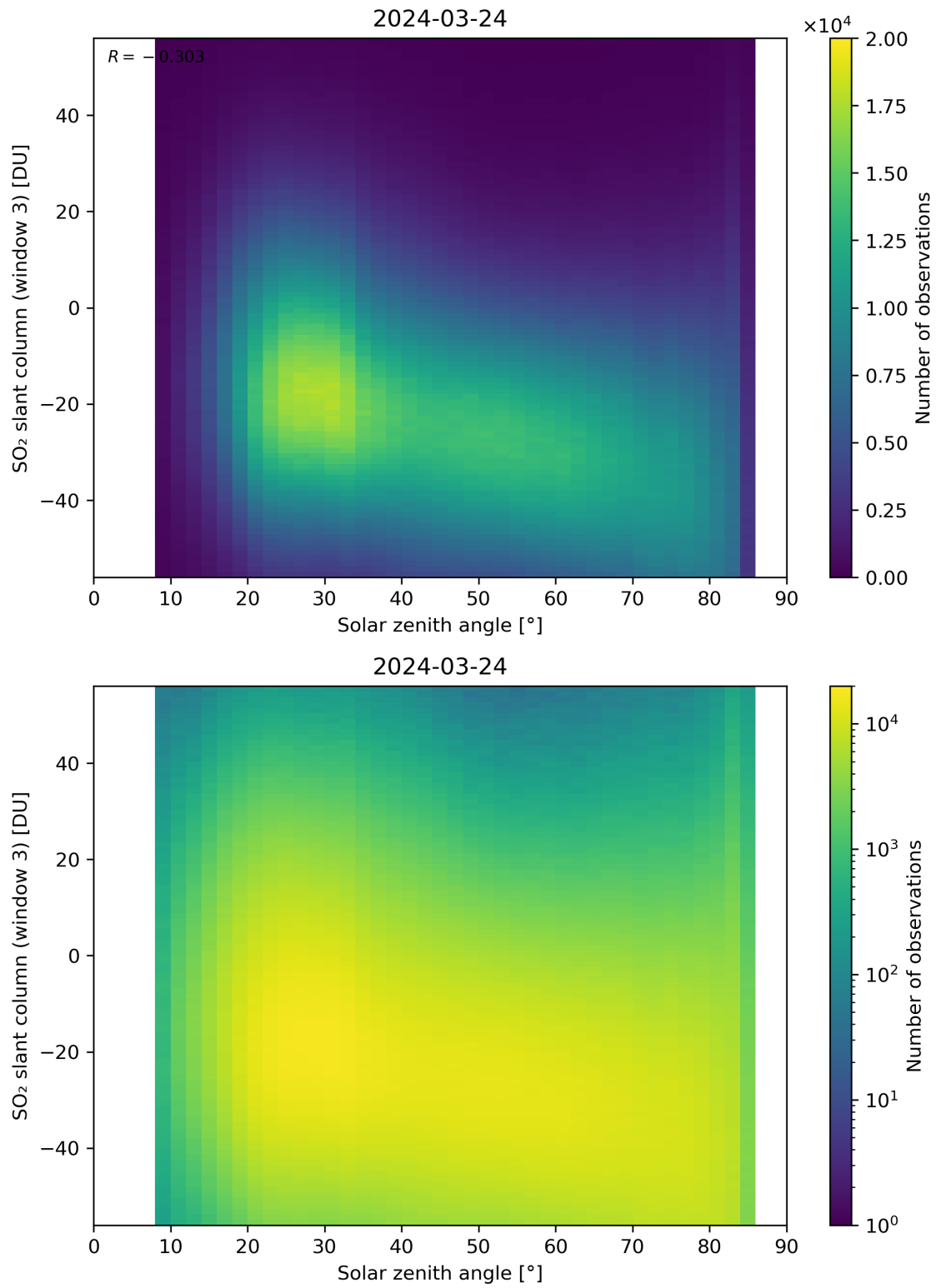
Figure 172: Scatter density plot of “Solar zenith angle” against “SO 2 slant column (window 3)” for 2024-03-23 to 2024-03-25.
