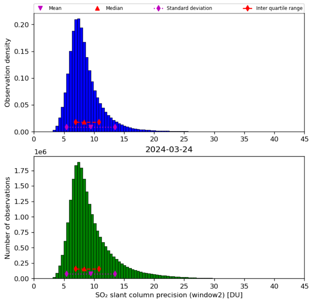
Figure 61: Histogram of “SO 2 slant column precision (window2)” for 2024-03-23 to 2024-03-25
