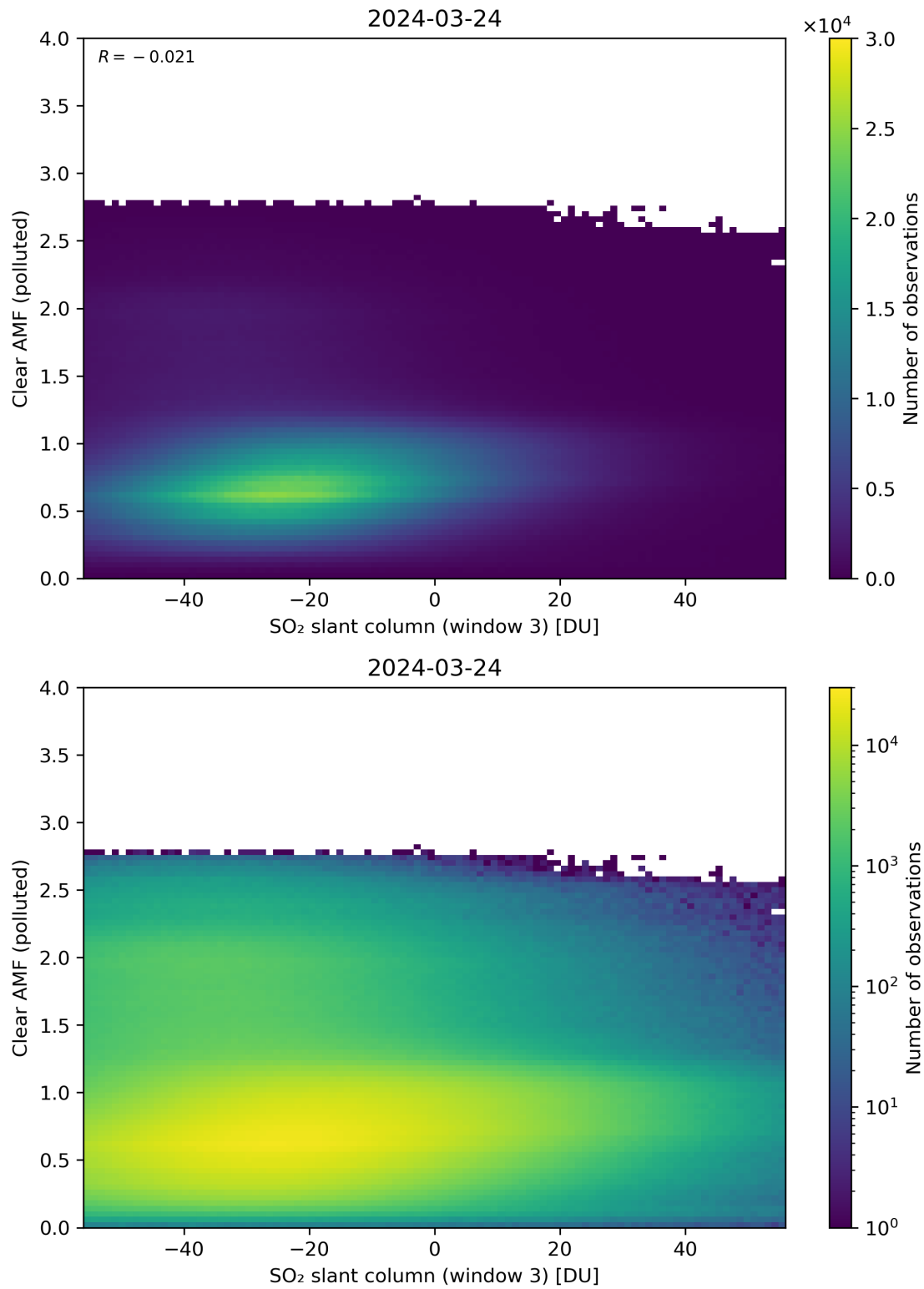
Figure 265: Scatter density plot of “SO 2 slant column (window 3)” against “Clear AMF (polluted)” for 2024-03-23 to 2024-03-25.
