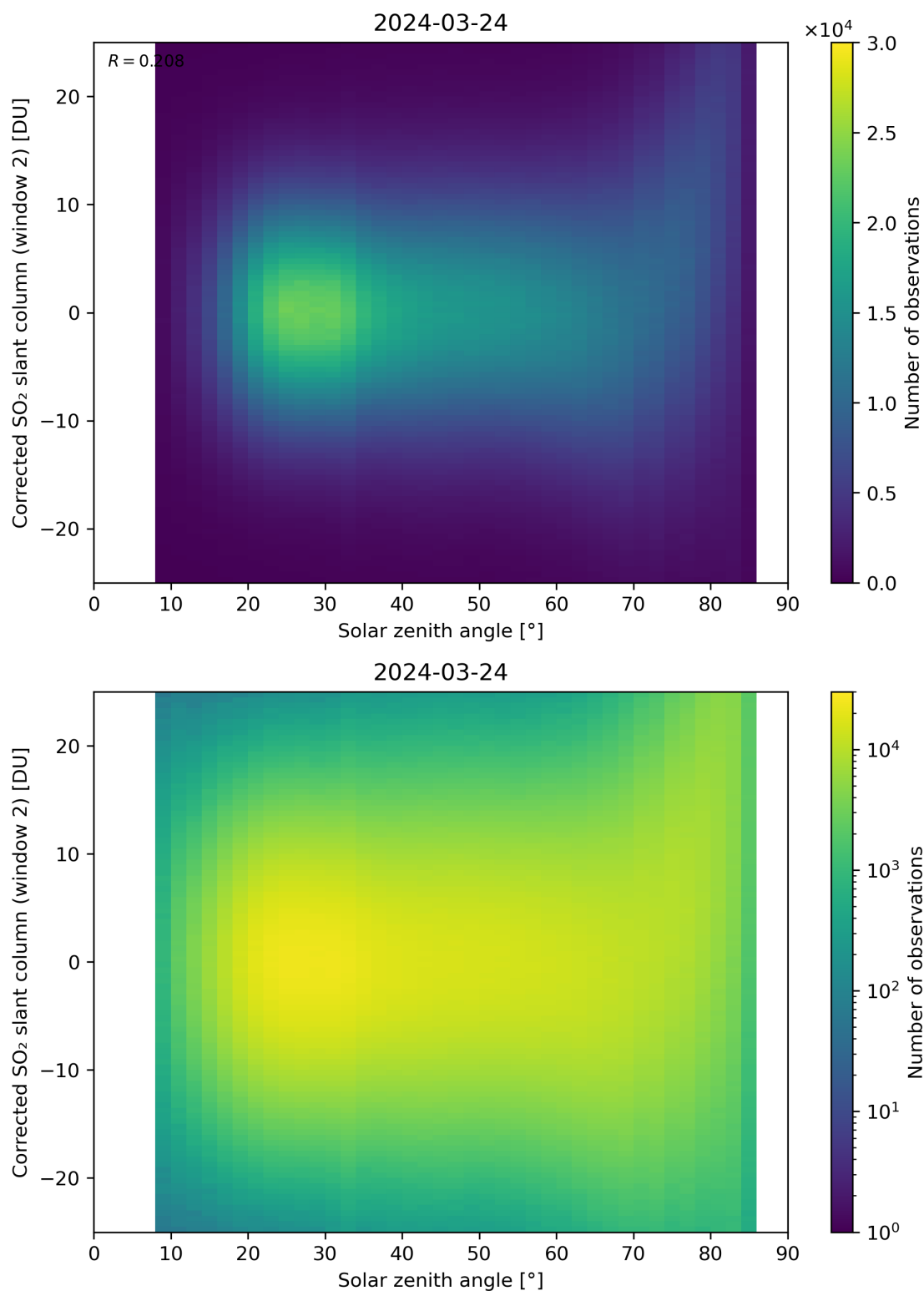
Figure 167: Scatter density plot of “Solar zenith angle” against “Corrected SO 2 slant column (window 2)” for 2024-03-23 to 2024-03-25.
