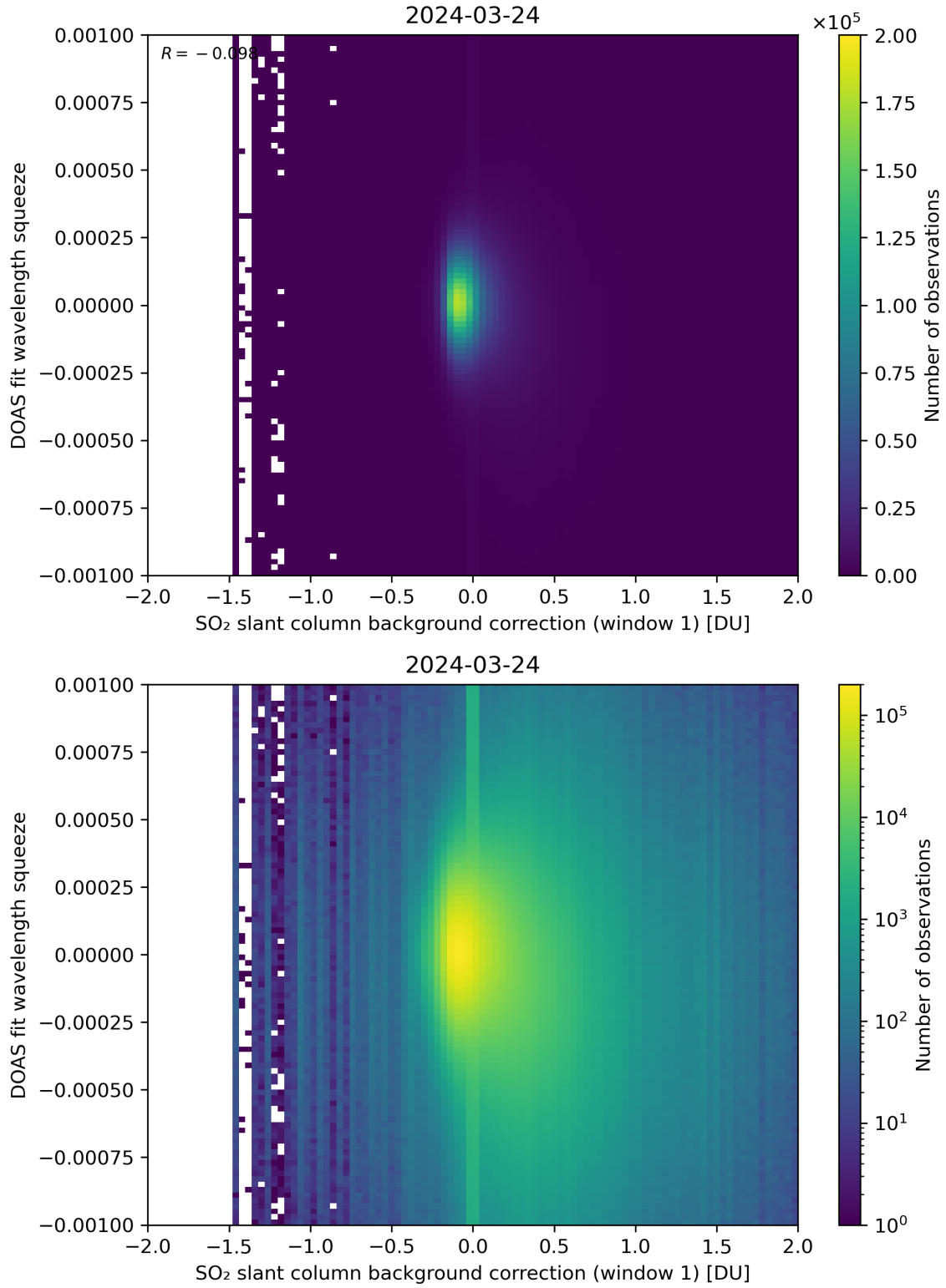
Figure 101: Scatter density plot of “SO 2 slant column background correction (window 1)” against “DOAS fit wavelength squeeze” for 2024-03-23 to 2024-03-25.
