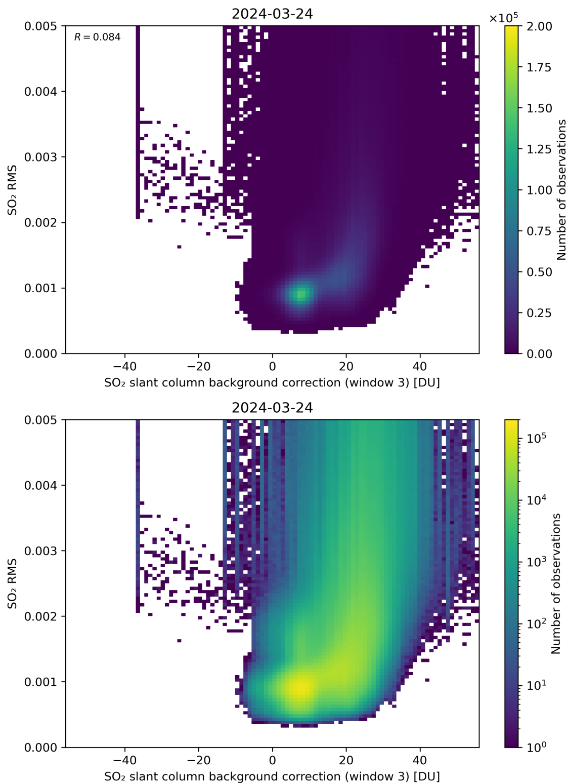
Figure 123: Scatter density plot of “SO 2 slant column background correction (window 3)” against “SO 2 RMS” for 2024-03-23 to 2024-03-25.
