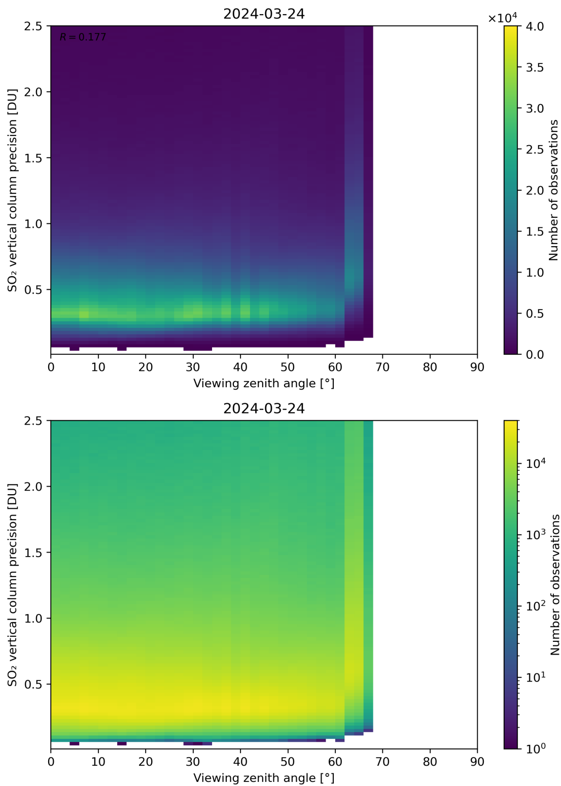
Figure 328: Scatter density plot of “Viewing zenith angle” against “SO 2 vertical column precision” for 2024-03-23 to 2024-03-25.
