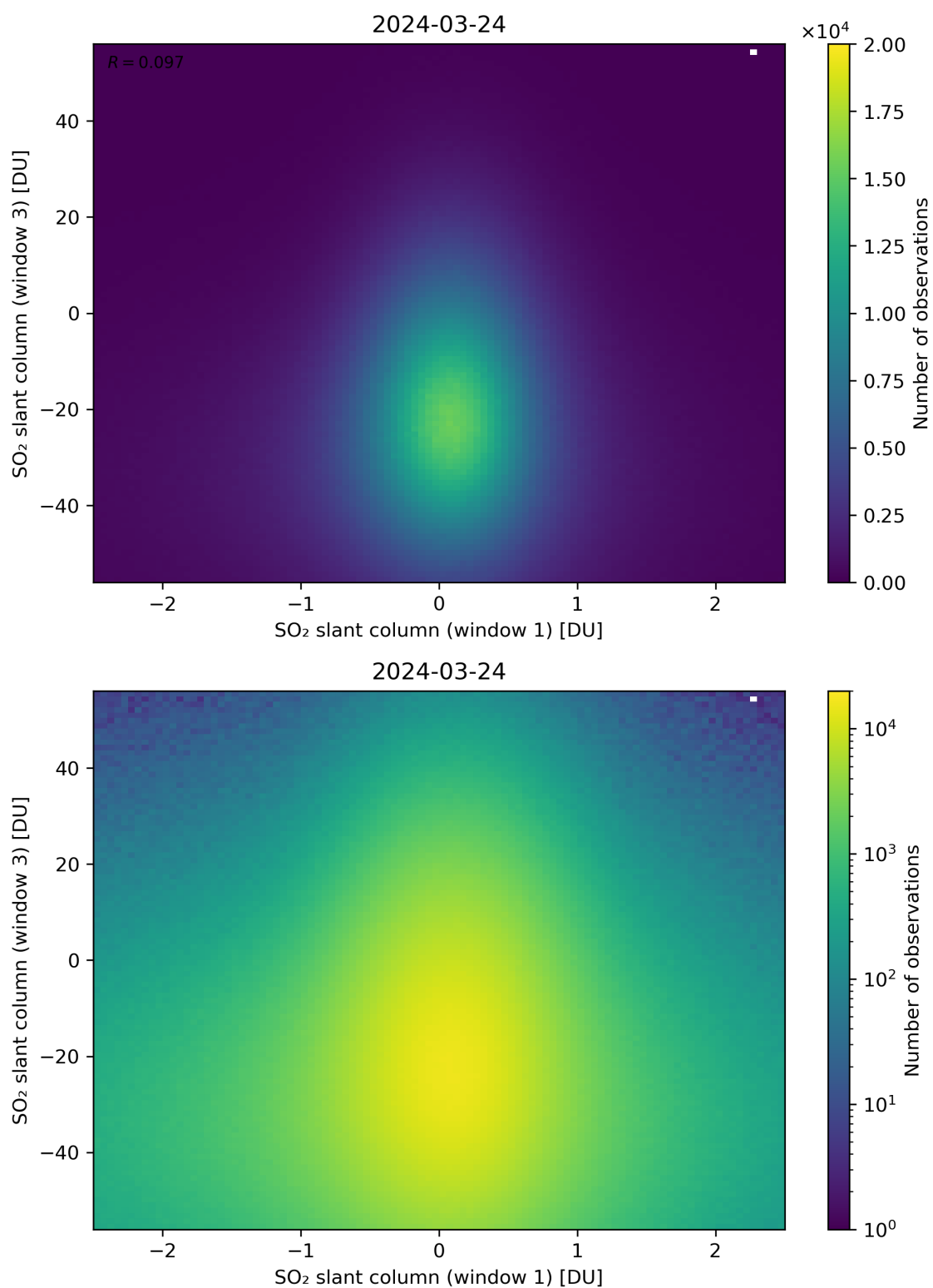
Figure 237: Scatter density plot of “SO 2 slant column (window 1)” against “SO 2 slant column (window 3)” for 2024-03-23 to 2024-03-25.
