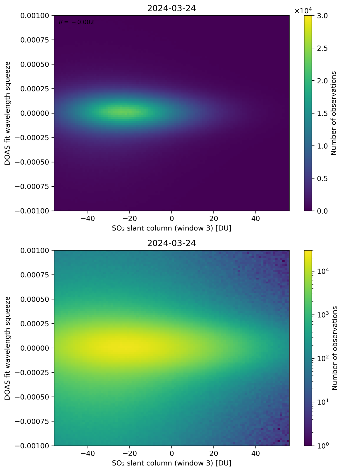
Figure 255: Scatter density plot of “SO 2 slant column (window 3)” against “DOAS fit wavelength squeeze” for 2024-03-23 to 2024-03-25.
