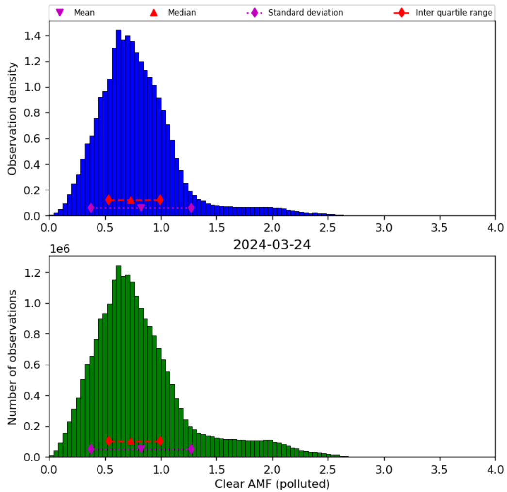
Figure 73: Histogram of “Clear AMF (polluted)” for 2024-03-23 to 2024-03-25
