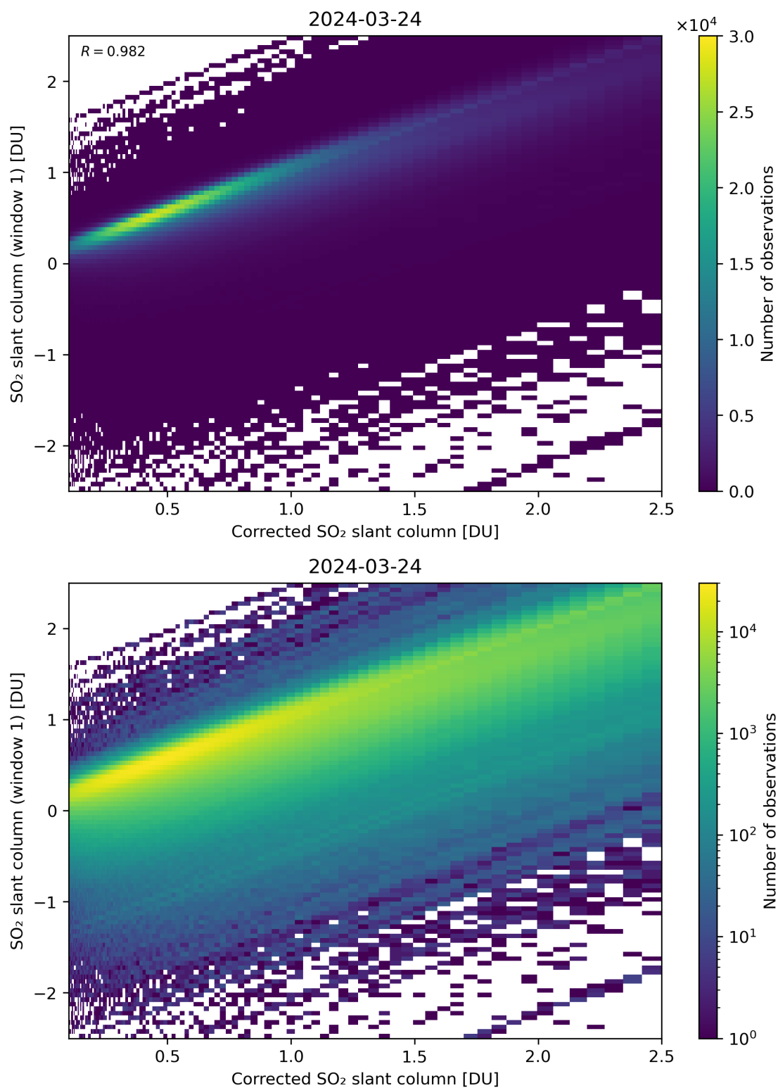
Figure 187: Scatter density plot of “Corrected SO 2 slant column” against “SO 2 slant column (window 1)” for 2024-03-23 to 2024-03-25.
