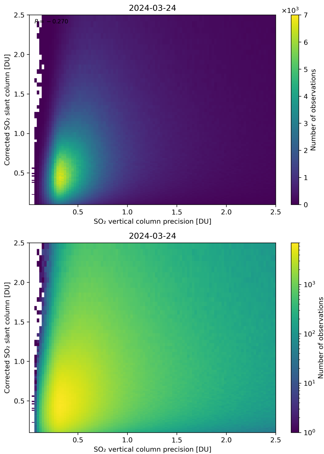
Figure 286: Scatter density plot of “SO 2 vertical column precision” against “Corrected SO 2 slant column” for 2024-03-23 to 2024-03-25.
