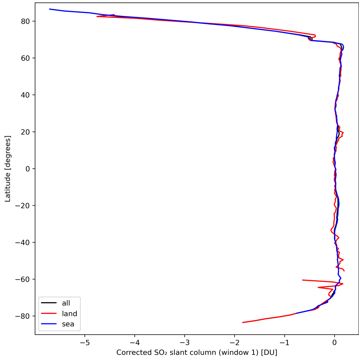
Figure 35: Zonal average of “Corrected SO 2 slant column (window 1)” for 2024-03-23 to 2024-03-25.
