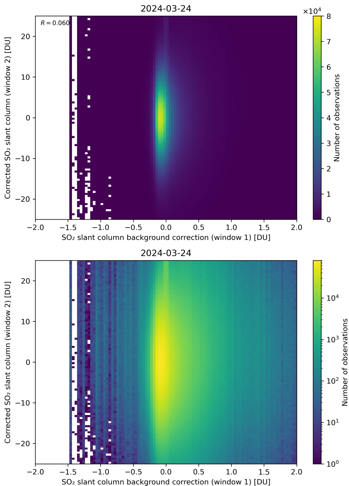
Figure 104: Scatter density plot of “SO 2 slant column background correction (window 1)” against “Corrected SO 2 slant column (window 2)” for 2024-03-23 to 2024-03-25.
