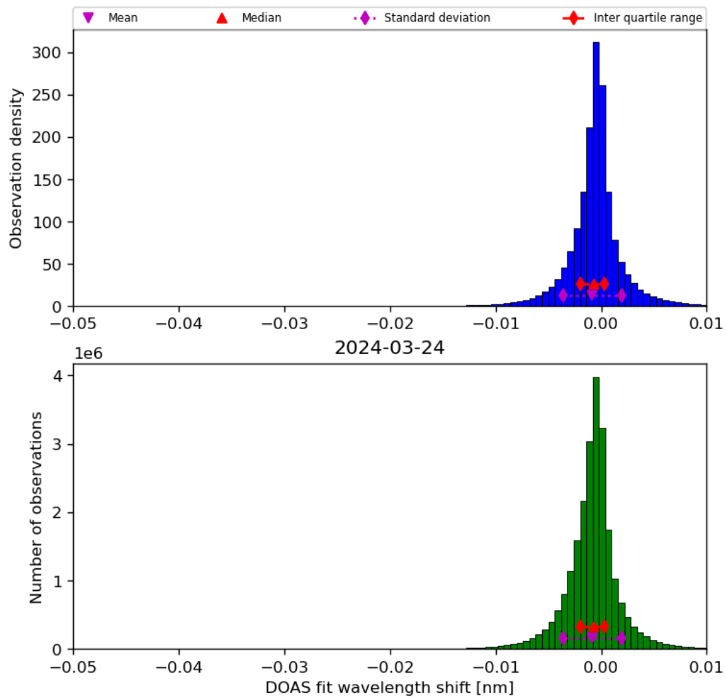
Figure 68: Histogram of “DOAS fit wavelength shift” for 2024-03-23 to 2024-03-25
