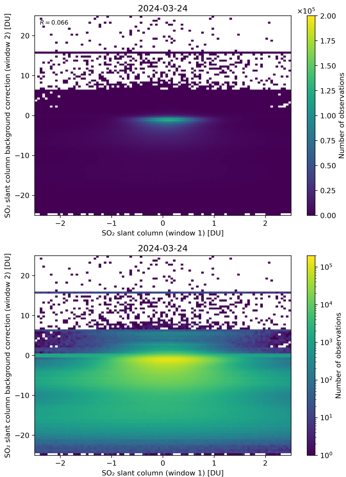
Figure 213: Scatter density plot of “SO 2 slant column (window 1)” against “SO 2 slant column background correction (window 2)” for 2024-03-23 to 2024-03-25.
