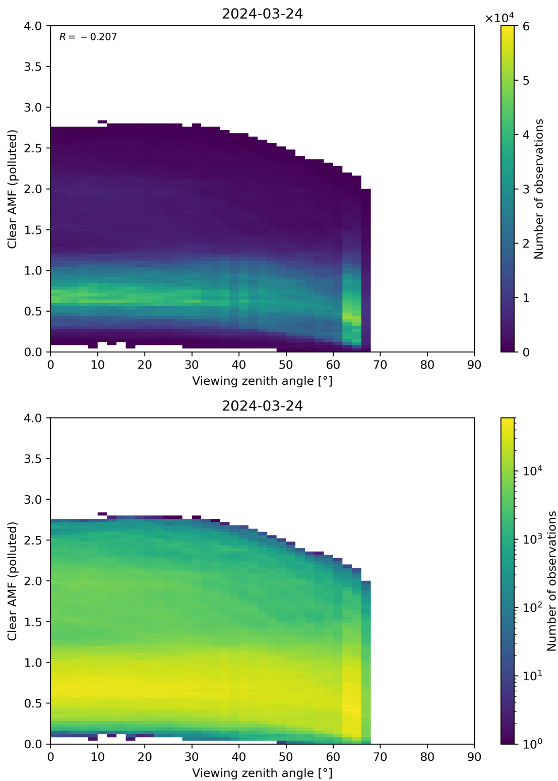
Figure 316: Scatter density plot of “Viewing zenith angle” against “Clear AMF (polluted)” for 2024-03-23 to 2024-03-25.
