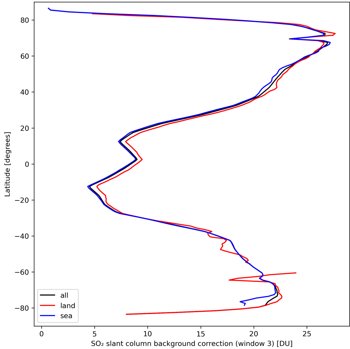
Figure 44: Zonal average of "SO 2 slant column background correction (window 3)" for 2024-03-23 to 2024-03-25.
