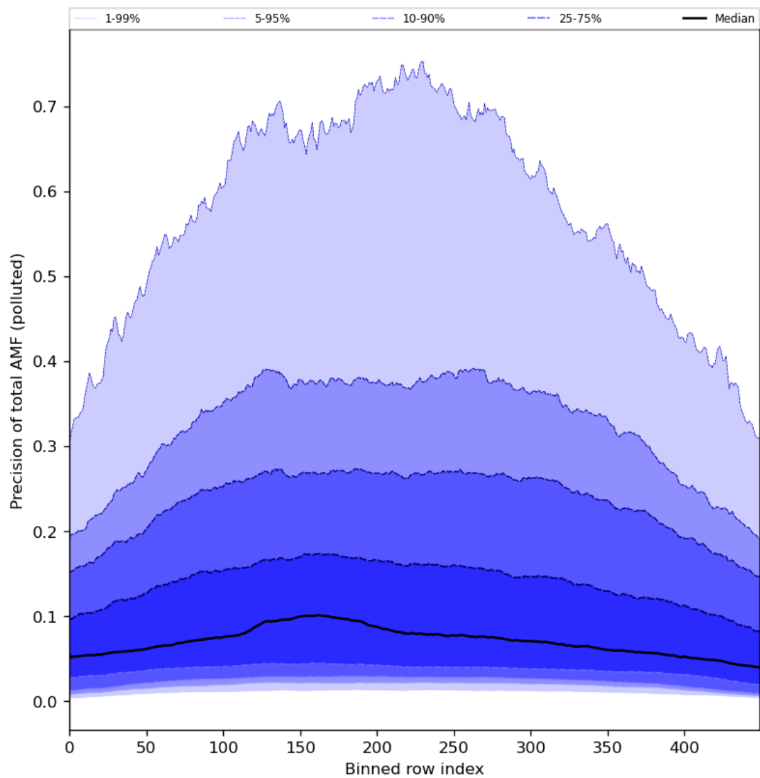
Figure 95: Along track statistics of “Precision of total AMF (polluted)” for 2024-03-23 to 2024-03-25
