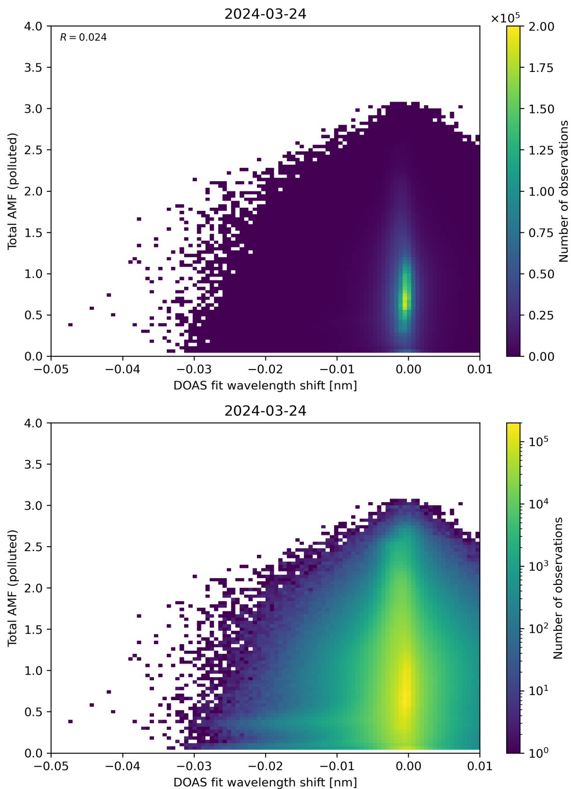
Figure 130: Scatter density plot of “DOAS fit wavelength shift” against “Total AMF (polluted)” for 2024-03-23 to 2024-03-25.
