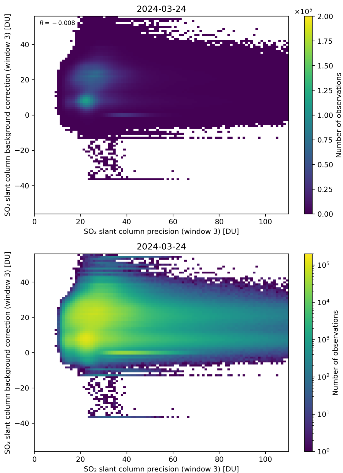
Figure 257: Scatter density plot of “SO 2 slant column precision (window 3)” against “SO 2 slant column background correction (window 3)” for 2024-03-23 to 2024-03-25.
