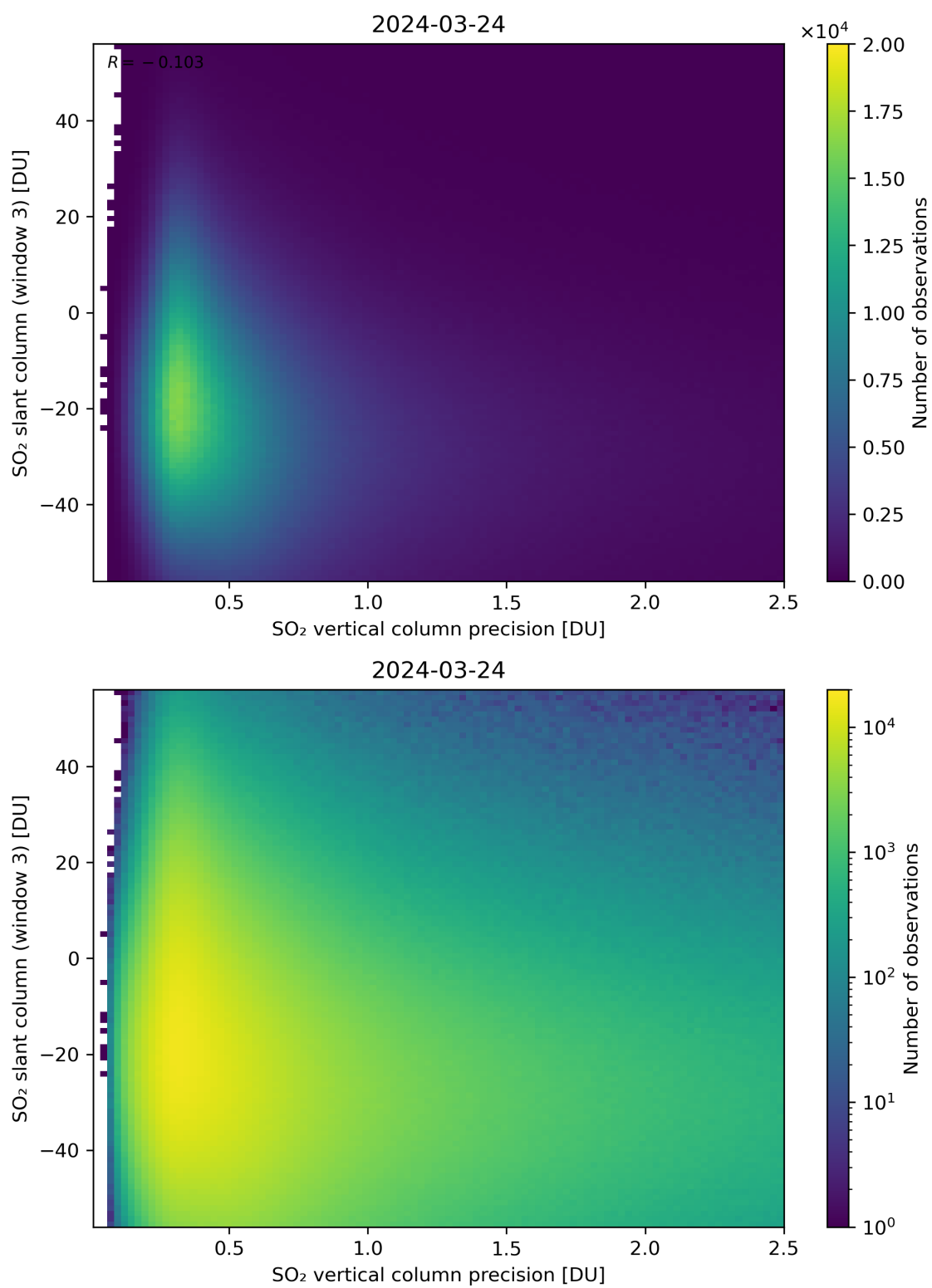
Figure 292: Scatter density plot of “SO 2 vertical column precision” against “SO 2 slant column (window 3)” for 2024-03-23 to 2024-03-25.
