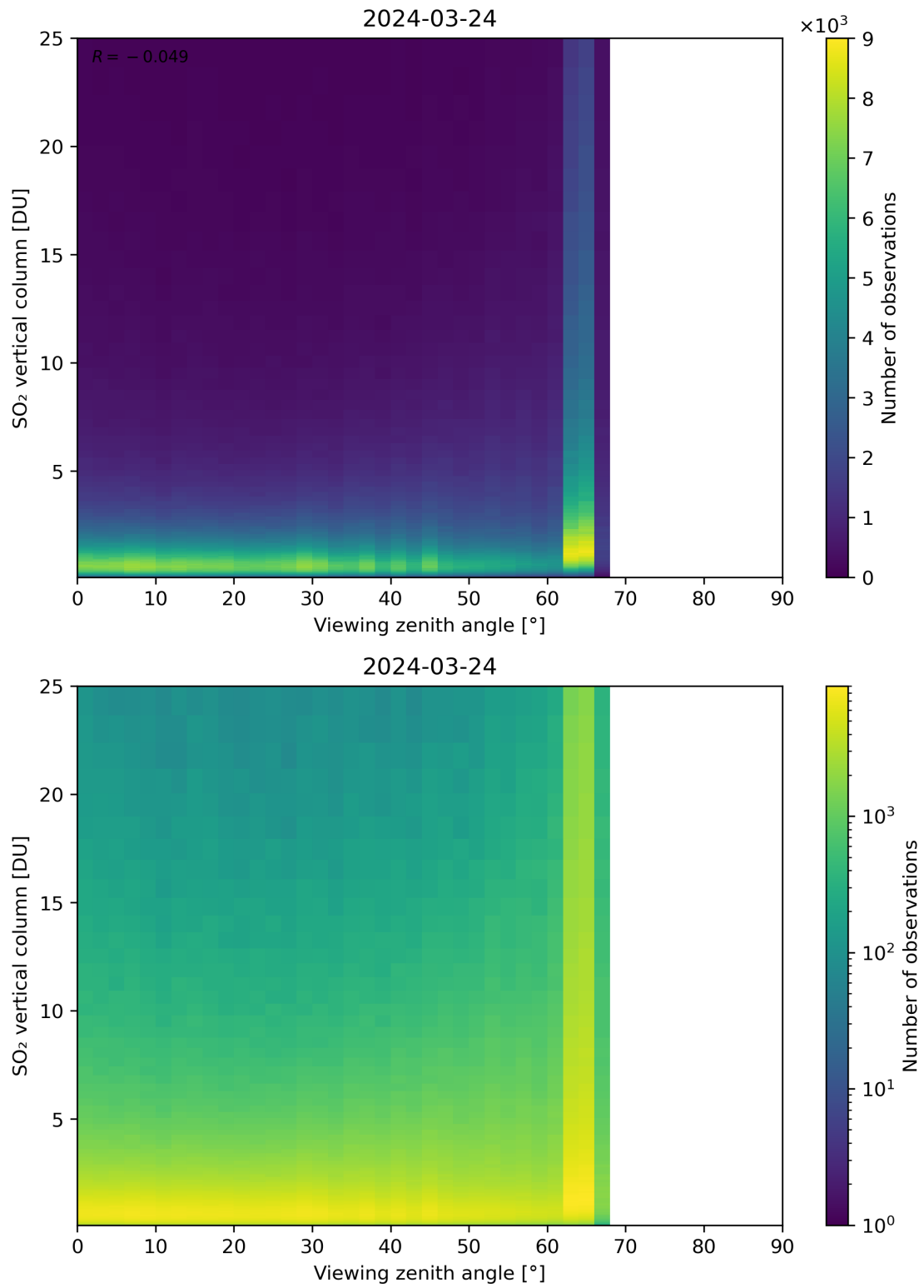
Figure 327: Scatter density plot of “Viewing zenith angle” against “SO 2 vertical column” for 2024-03-23 to 2024-03-25.
