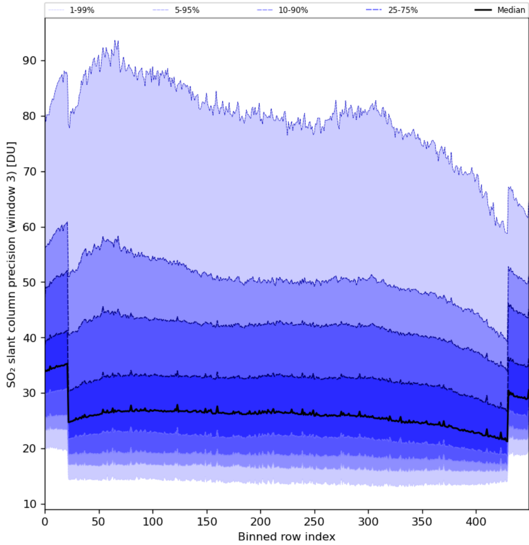
Figure 88: Along track statistics of “SO 2 slant column precision (window 3)” for 2024-03-23 to 2024-03-25
