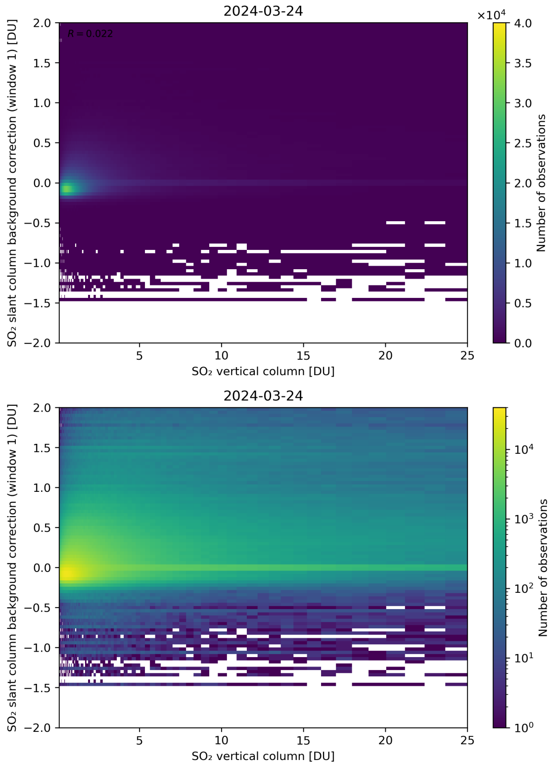
Figure 273: Scatter density plot of “SO 2 vertical column” against “SO 2 slant column background correction (window 1)” for 2024-03-23 to 2024-03-25.
