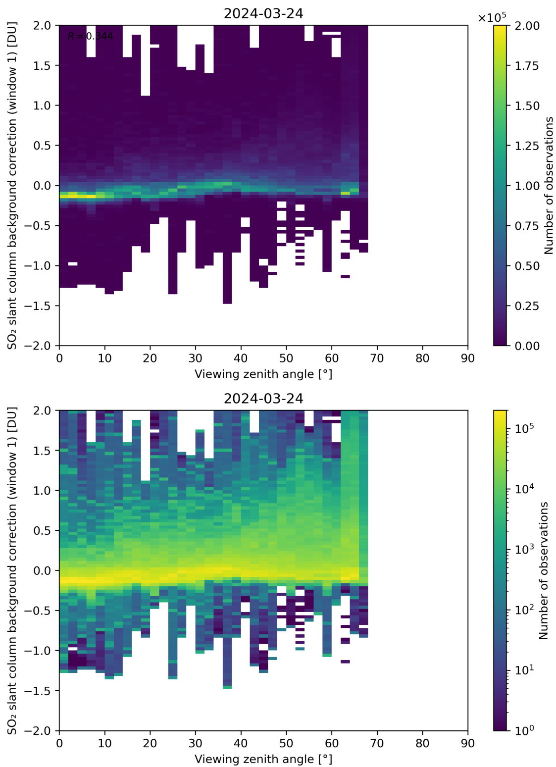
Figure 308: Scatter density plot of “Viewing zenith angle” against “SO 2 slant column background correction (window 1)” for 2024-03-23 to 2024-03-25.
