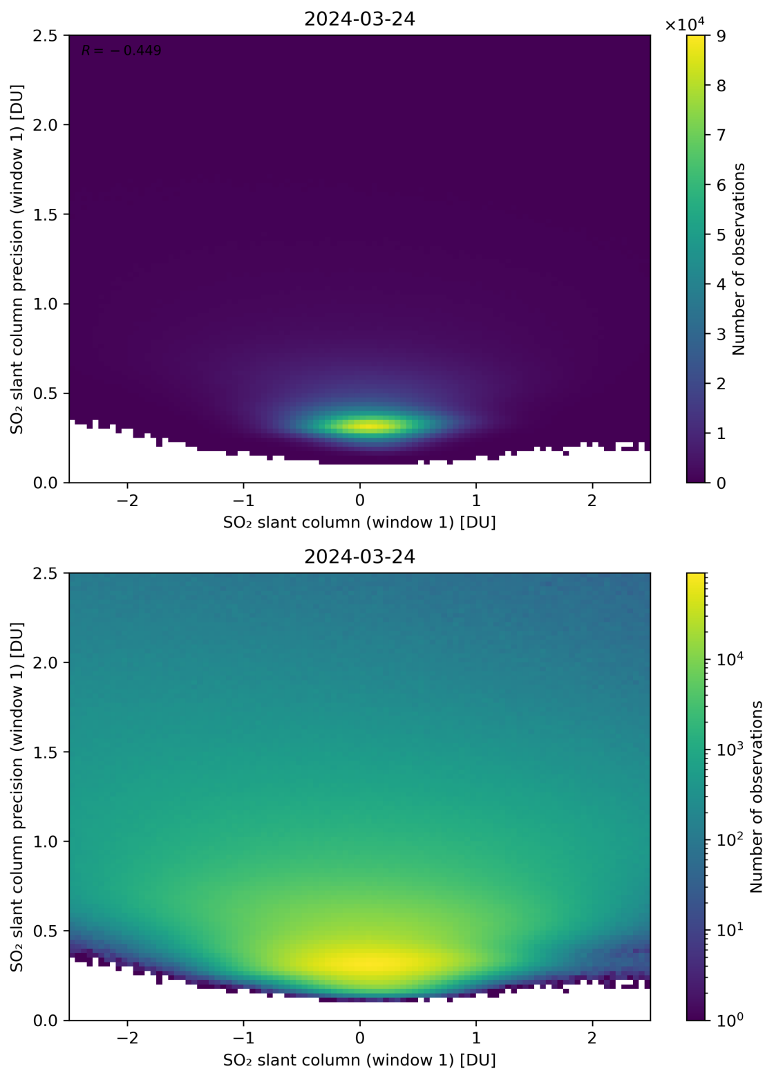
Figure 235: Scatter density plot of “SO 2 slant column (window 1)” against “SO 2 slant column precision (window 1)” for 2024-03-23 to 2024-03-25.
