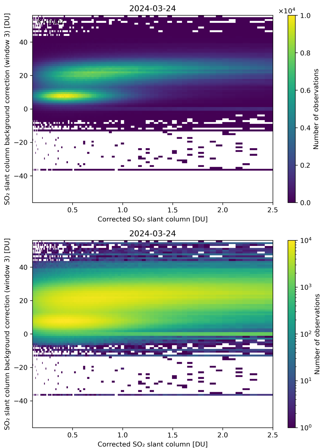
Figure 180: Scatter density plot of “Corrected SO 2 slant column” against “SO 2 slant column background correction (window 3)” for 2024-03-23 to 2024-03-25.
