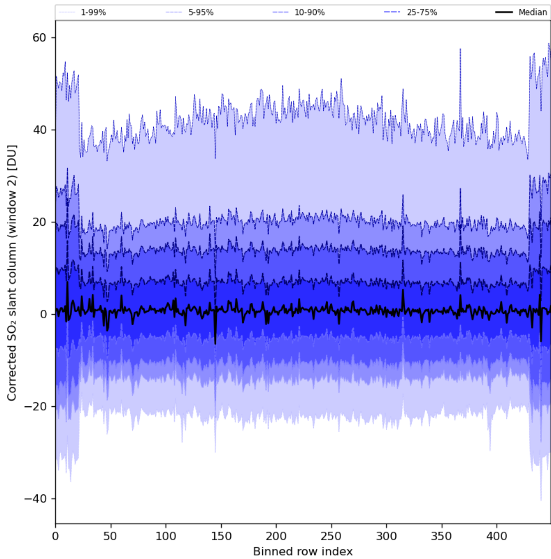
Figure 85: Along track statistics of “Corrected SO 2 slant column (window 2)” for 2024-03-23 to 2024-03-25
