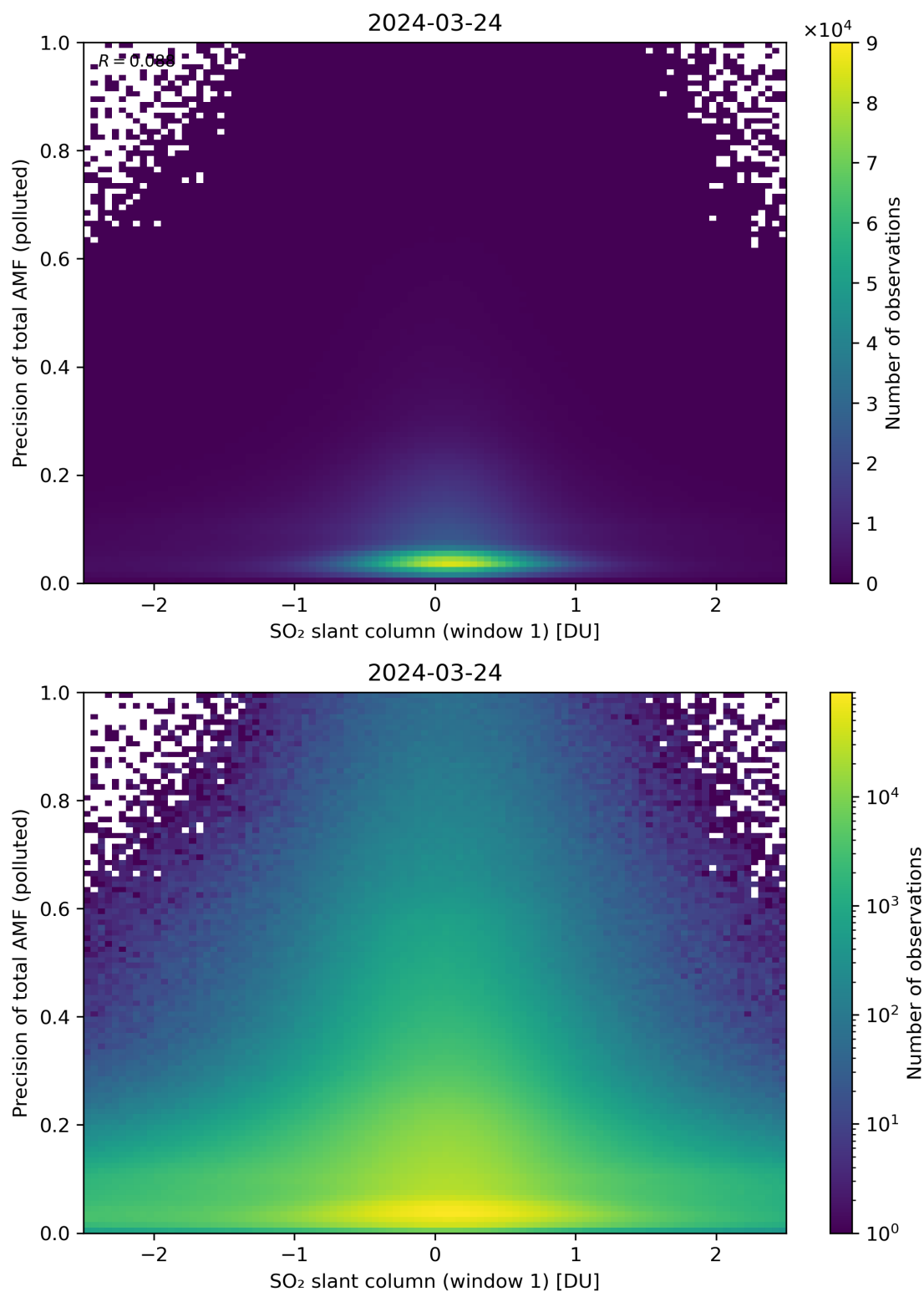
Figure 240: Scatter density plot of “SO 2 slant column (window 1)” against “Precision of total AMF (polluted)” for 2024-03-23 to 2024-03-25.
