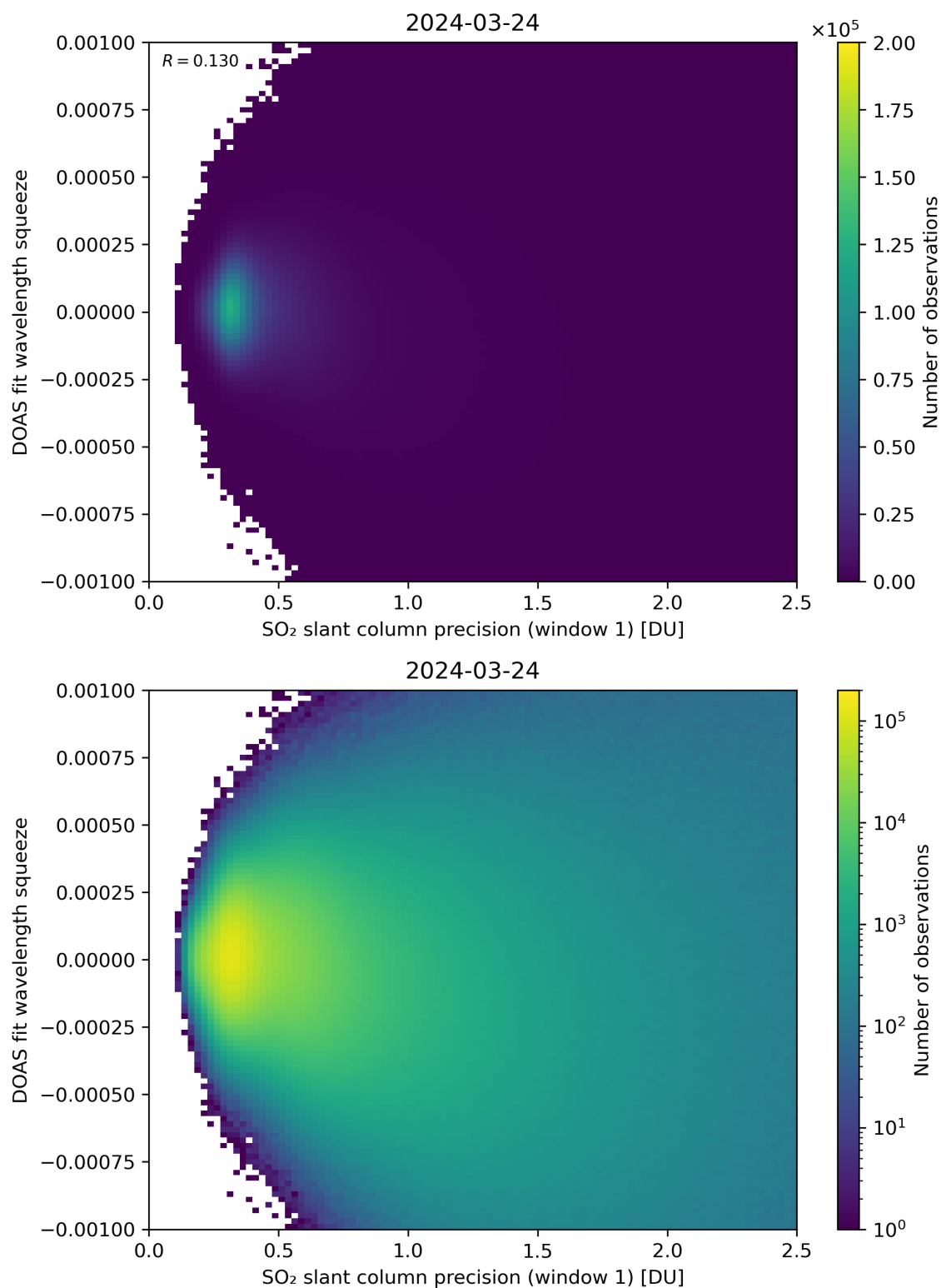
Figure 222: Scatter density plot of “SO 2 slant column precision (window 1)” against “DOAS fit wavelength squeeze” for 2024-03-23 to 2024-03-25.
