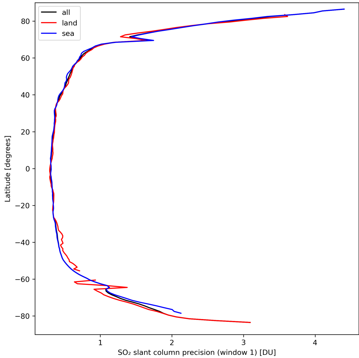
Figure 34: Zonal average of “SO 2 slant column precision (window 1)” for 2024-03-23 to 2024-03-25.
