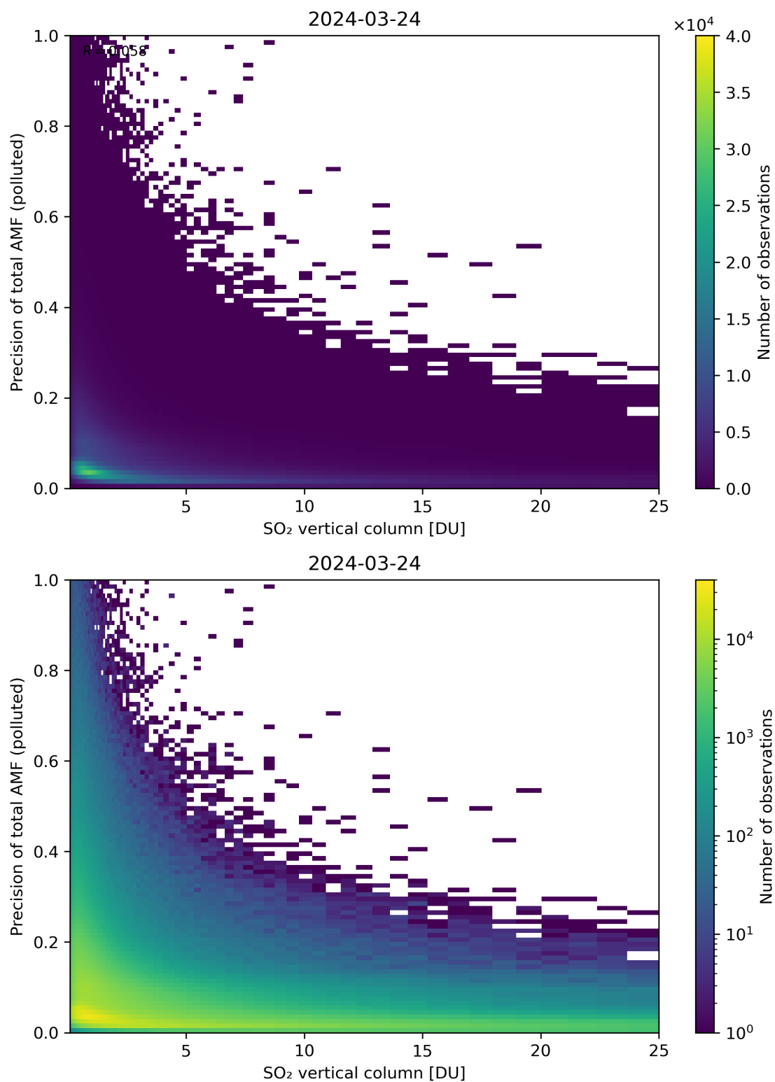
Figure 306: Scatter density plot of “SO 2 vertical column” against “Precision of total AMF (polluted)” for 2024-03-23 to 2024-03-25.
