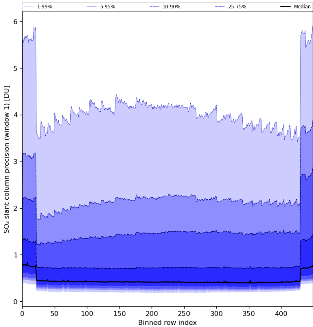
Figure 80: Along track statistics of “SO 2 slant column precision (window 1)” for 2024-03-23 to 2024-03-25
