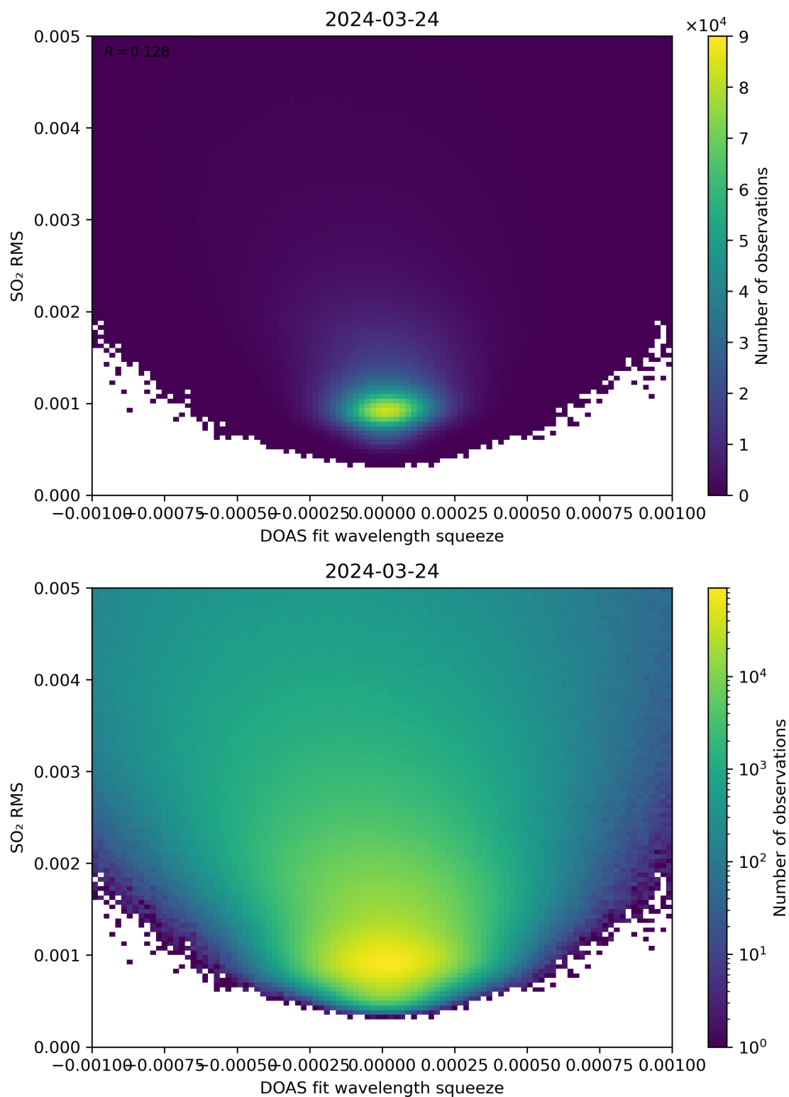
Figure 132: Scatter density plot of “DOAS fit wavelength squeeze” against “SO 2 RMS” for 2024-03-23 to 2024-03-25.
