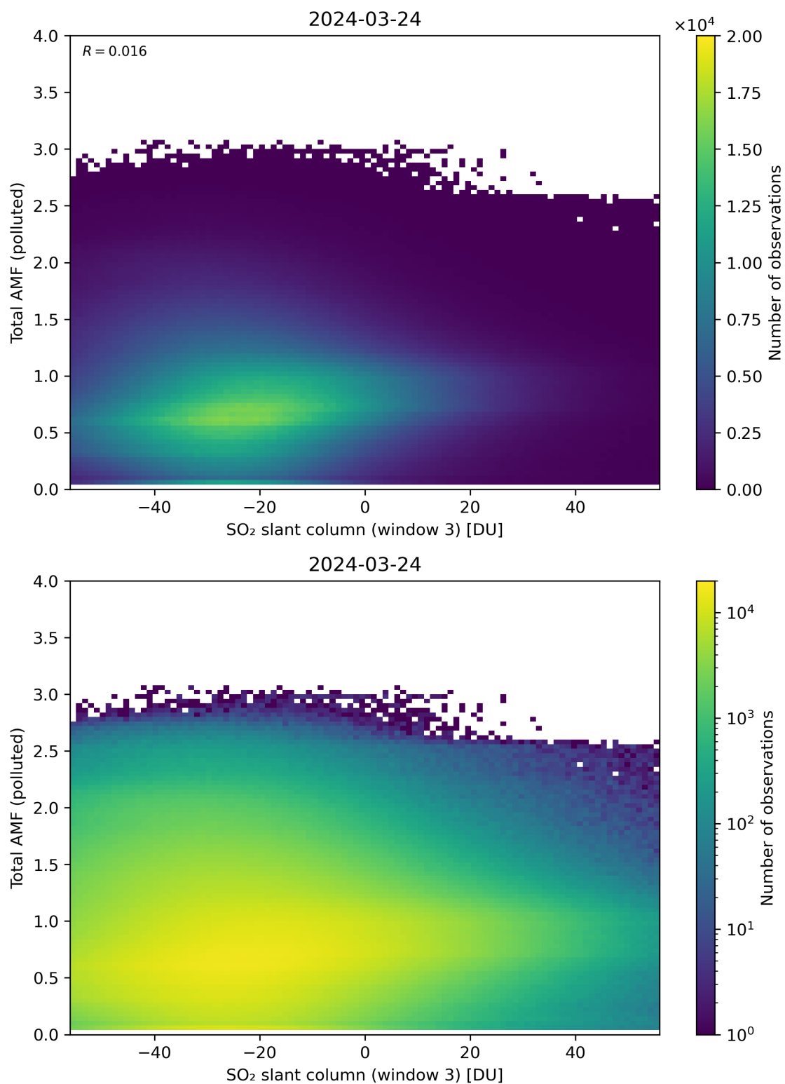
Figure 268: Scatter density plot of “SO 2 slant column (window 3)” against “Total AMF (polluted)” for 2024-03-23 to 2024-03-25.
