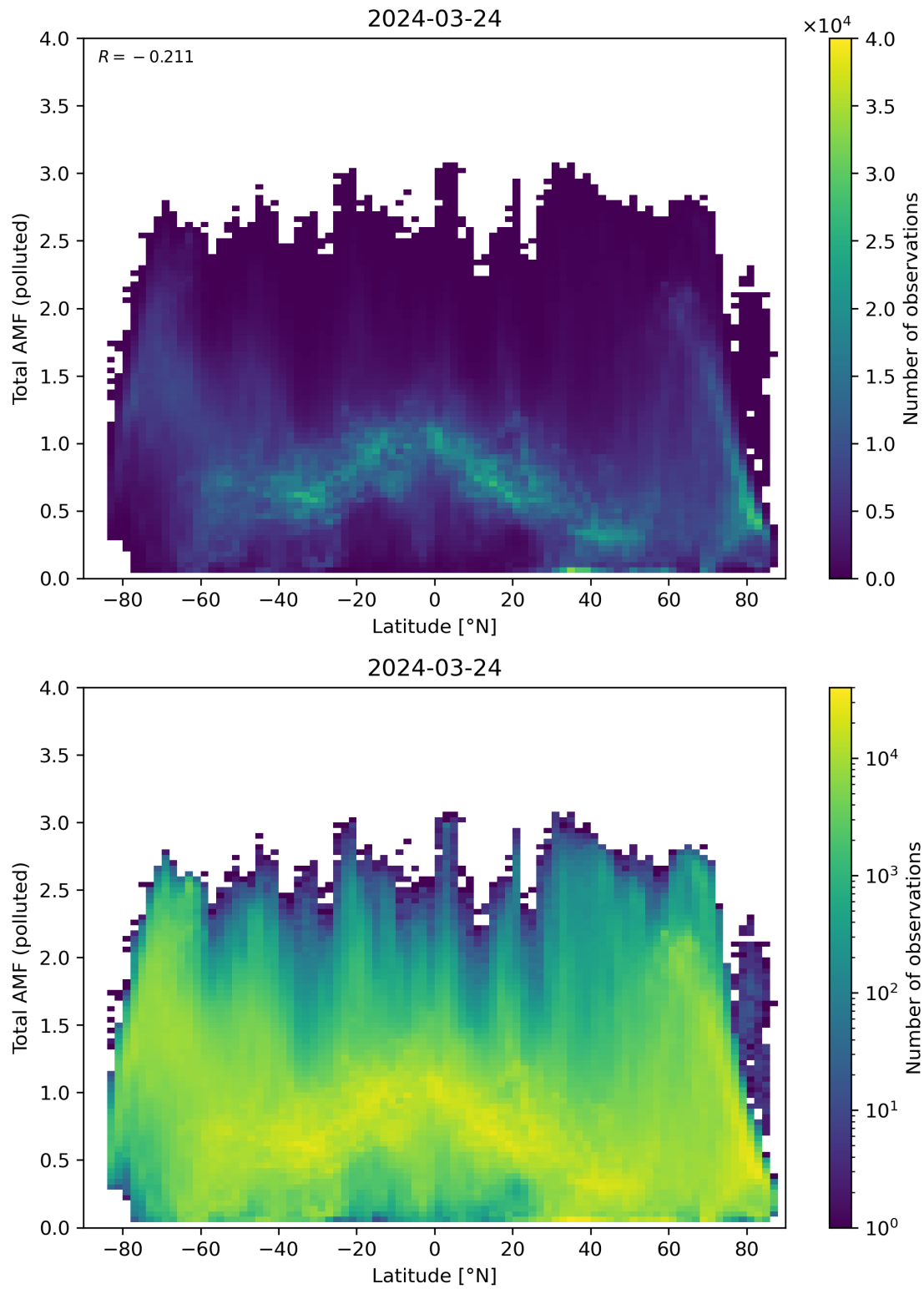
Figure 154: Scatter density plot of “Latitude” against “Total AMF (polluted)” for 2024-03-23 to 2024-03-25.
