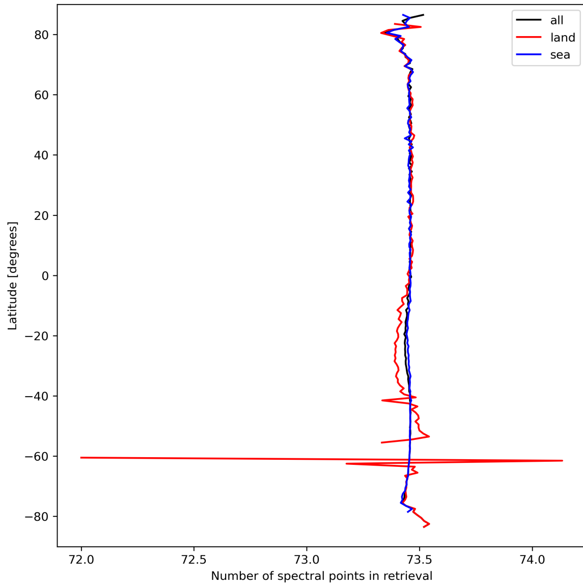
Figure 51: Zonal average of “Number of spectral points in retrieval” for 2024-03-23 to 2024-03-25.
