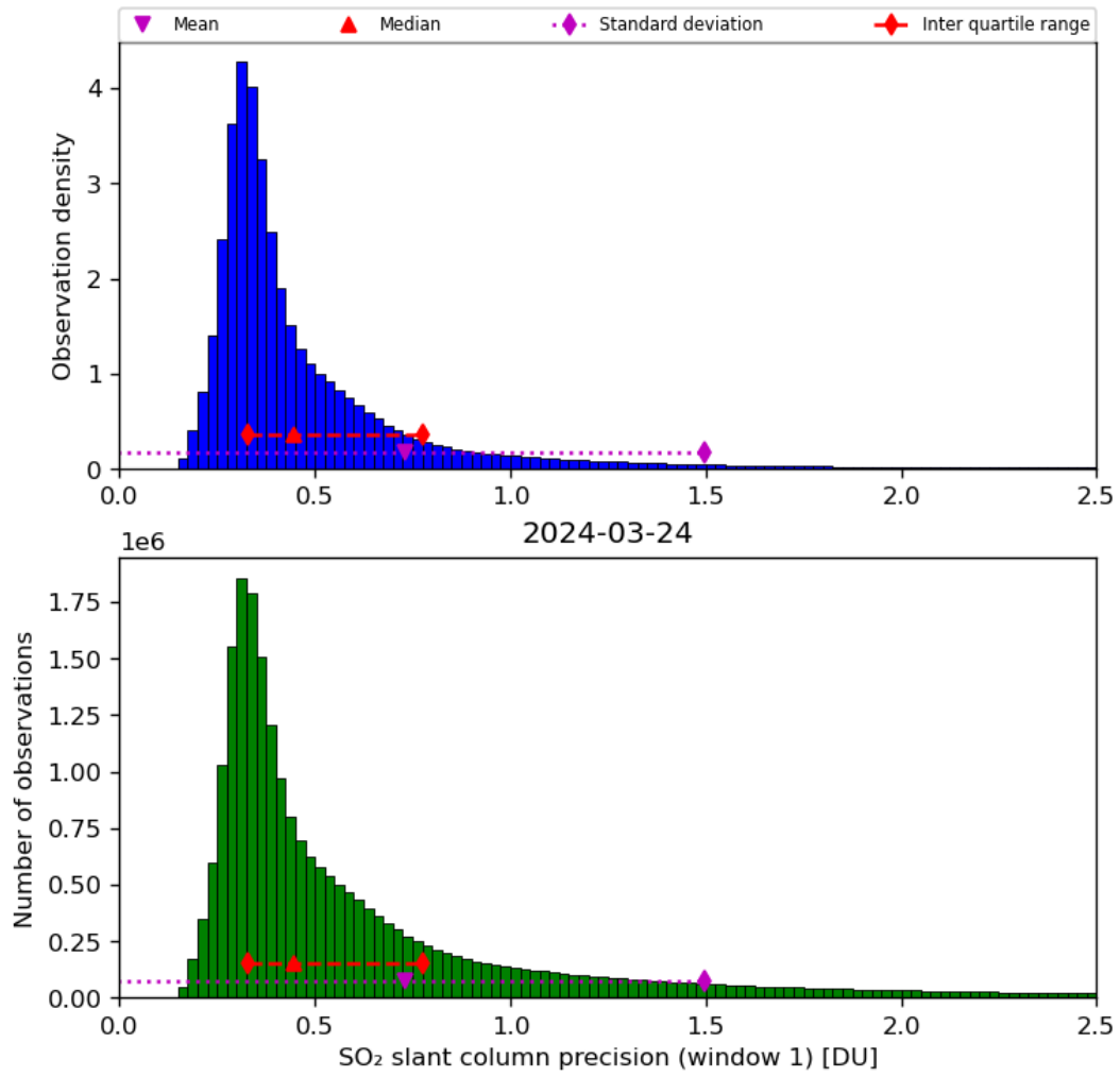
Figure 57: Histogram of “SO 2 slant column precision (window 1)” for 2024-03-23 to 2024-03-25
