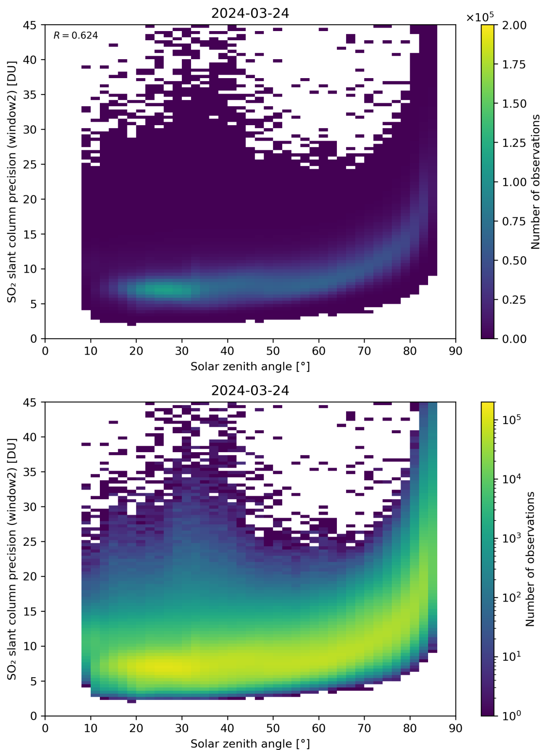
Figure 171: Scatter density plot of “Solar zenith angle” against “SO 2 slant column precision (window2)” for 2024-03-23 to 2024-03-25.
