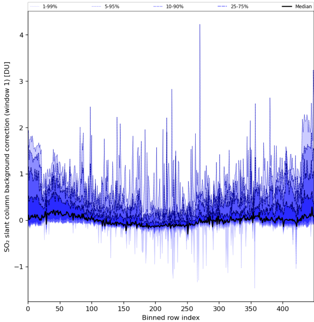
Figure 82: Along track statistics of “SO 2 slant column background correction (window 1)” for 2024-03-23 to 2024-03-25
