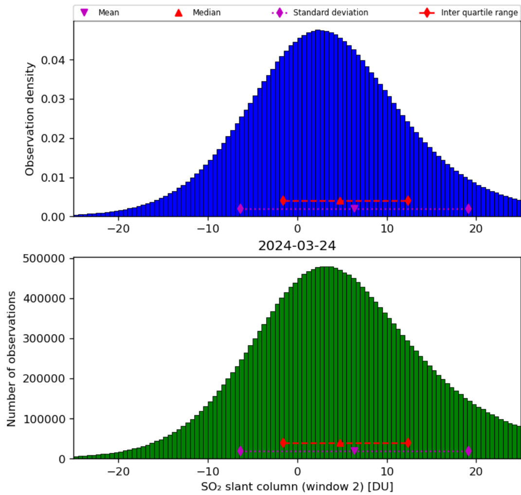
Figure 60: Histogram of “SO 2 slant column (window 2)” for 2024-03-23 to 2024-03-25
