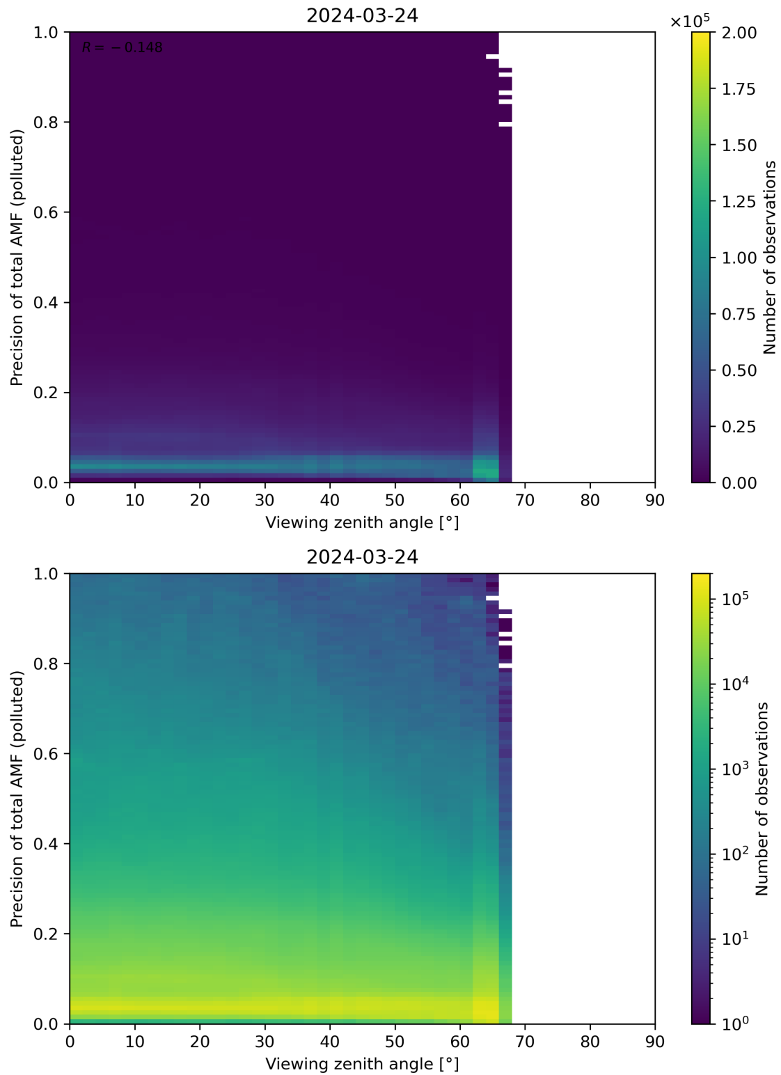
Figure 326: Scatter density plot of “Viewing zenith angle” against “Precision of total AMF (polluted)” for 2024-03-23 to 2024-03-25.
