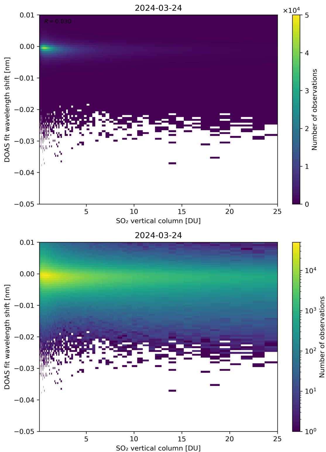
Figure 276: Scatter density plot of “SO 2 vertical column” against “DOAS fit wavelength shift” for 2024-03-23 to 2024-03-25.
