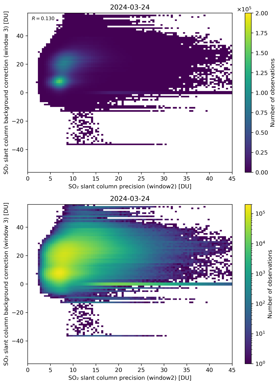
Figure 242: Scatter density plot of “SO 2 slant column precision (window2)” against “SO 2 slant column background correction (window 3)” for 2024-03-23 to 2024-03-25.
