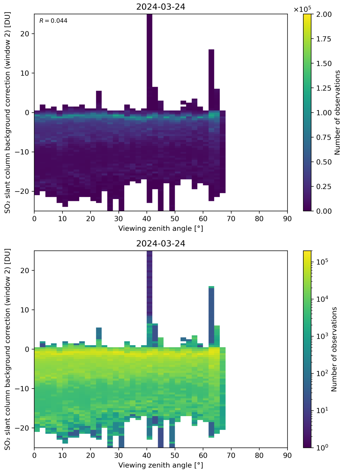
Figure 309: Scatter density plot of “Viewing zenith angle” against “SO 2 slant column background correction (window 2)” for 2024-03-23 to 2024-03-25.
