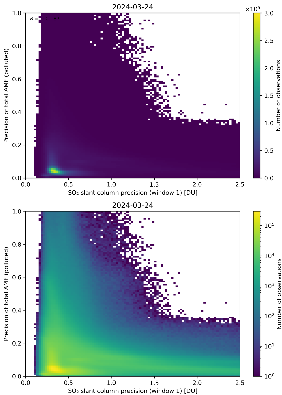
Figure 231: Scatter density plot of “SO 2 slant column precision (window 1)” against “Precision of total AMF (polluted)” for 2024-03-23 to 2024-03-25.
