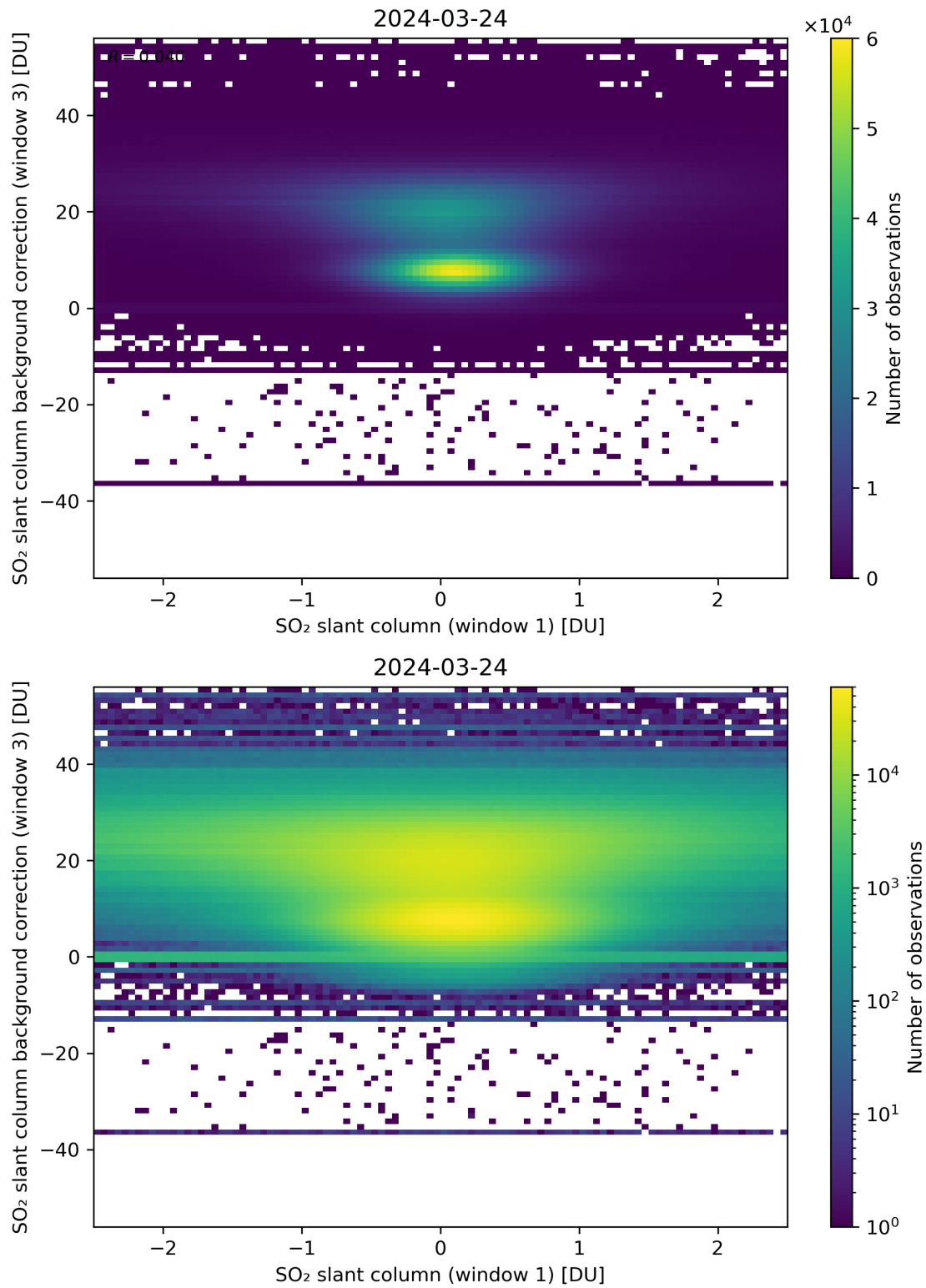
Figure 214: Scatter density plot of “SO 2 slant column (window 1)” against “SO 2 slant column background correction (window 3)” for 2024-03-23 to 2024-03-25.
