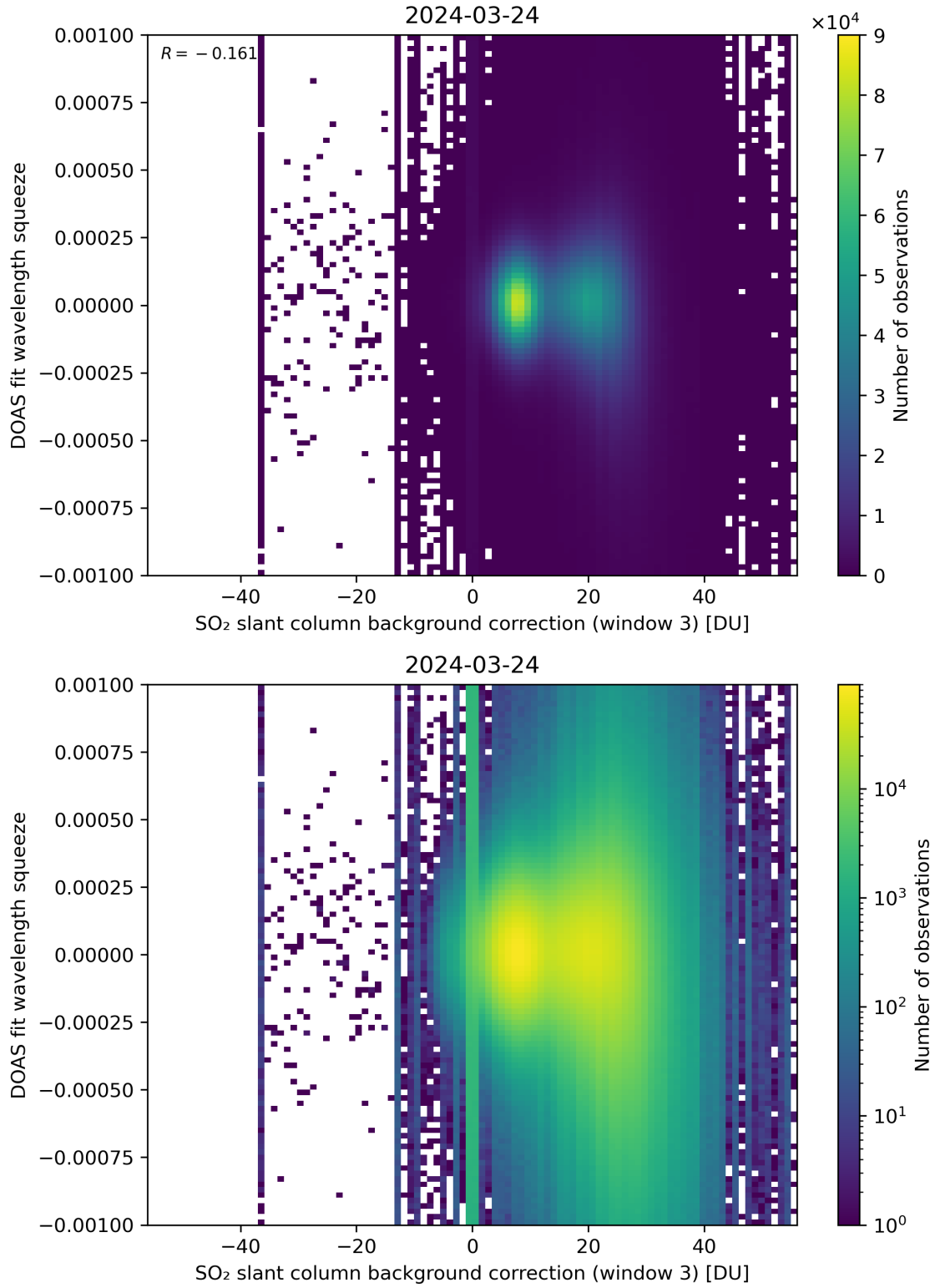
Figure 122: Scatter density plot of “SO 2 slant column background correction (window 3)” against “DOAS fit wavelength squeeze” for 2024-03-23 to 2024-03-25.
