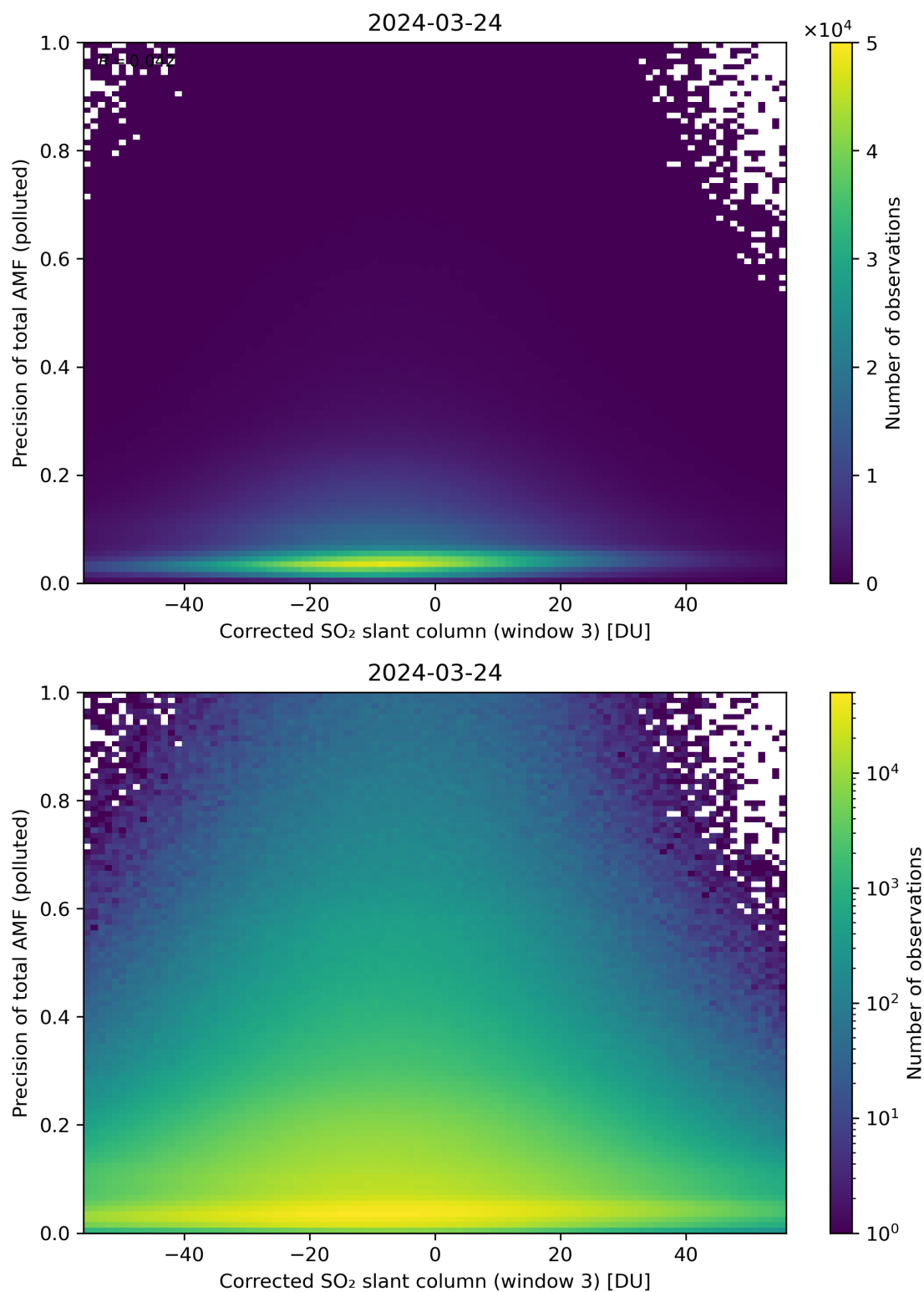
Figure 211: Scatter density plot of “Corrected SO 2 slant column (window 3)” against “Precision of total AMF (polluted)” for 2024-03-23 to 2024-03-25.
