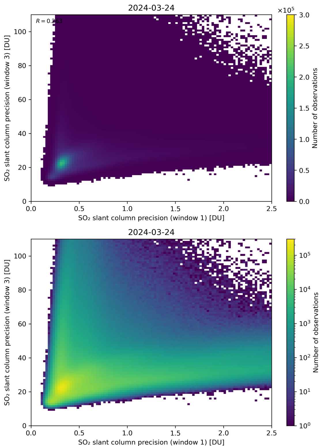
Figure 229: Scatter density plot of “SO 2 slant column precision (window 1)” against “SO 2 slant column precision (window 3)” for 2024-03-23 to 2024-03-25.
