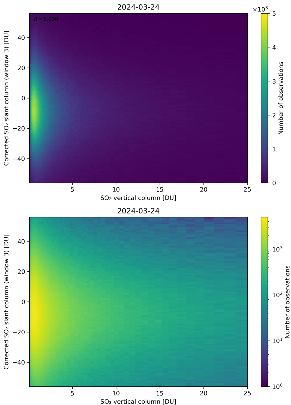
Figure 299: Scatter density plot of “SO 2 vertical column” against “Corrected SO 2 slant column (window 3)” for 2024-03-23 to 2024-03-25.
