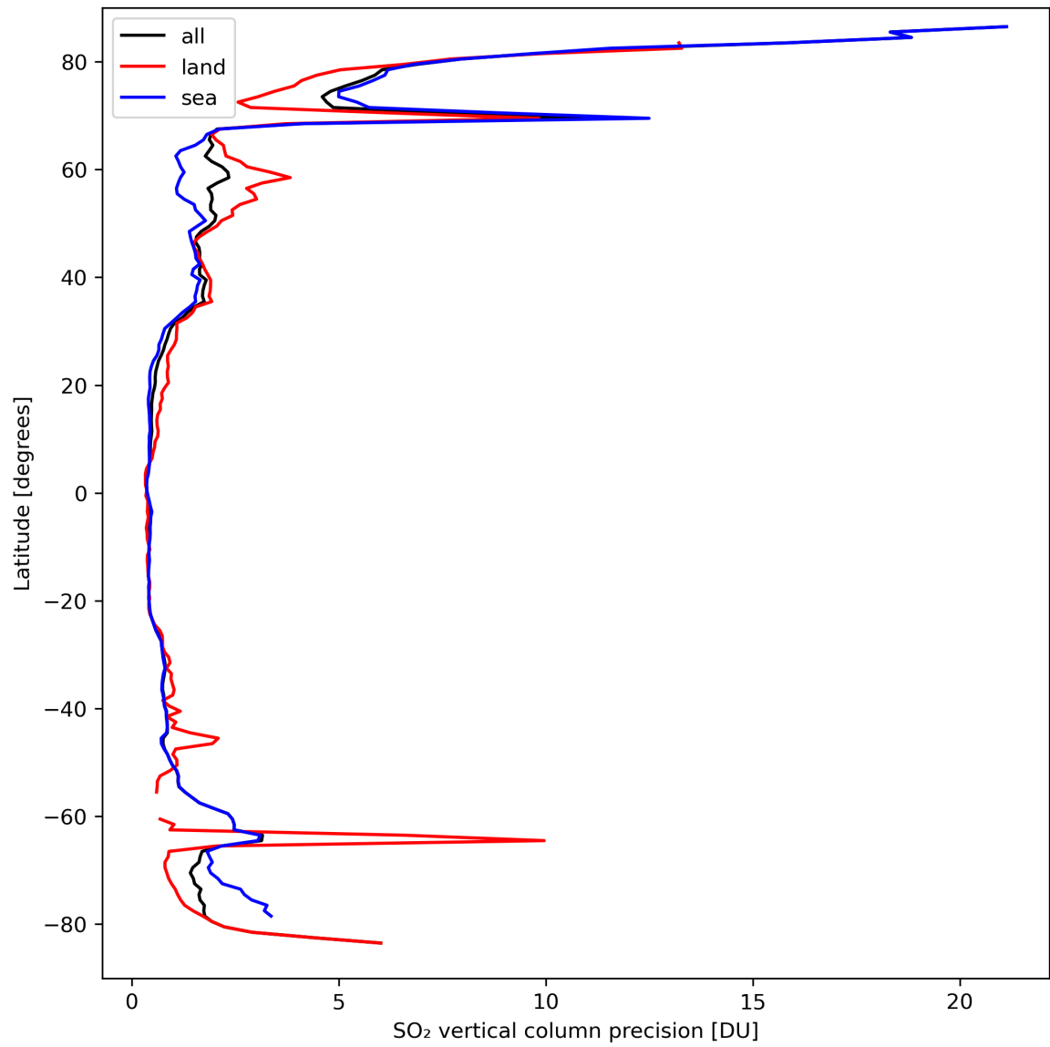
Figure 31: Zonal average of “SO 2 vertical column precision” for 2024-03-23 to 2024-03-25.
