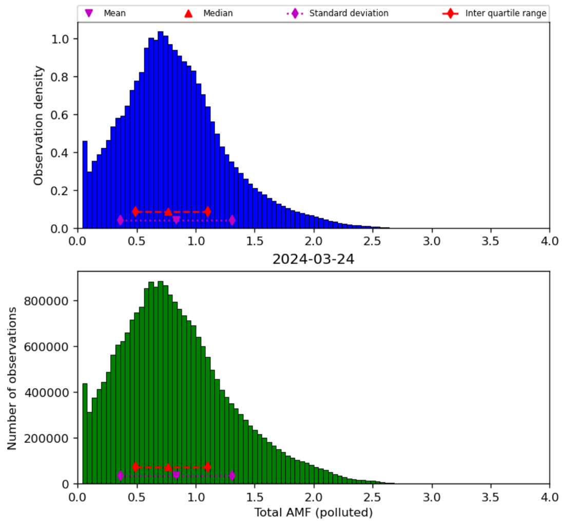
Figure 71: Histogram of “Total AMF (polluted)” for 2024-03-23 to 2024-03-25
