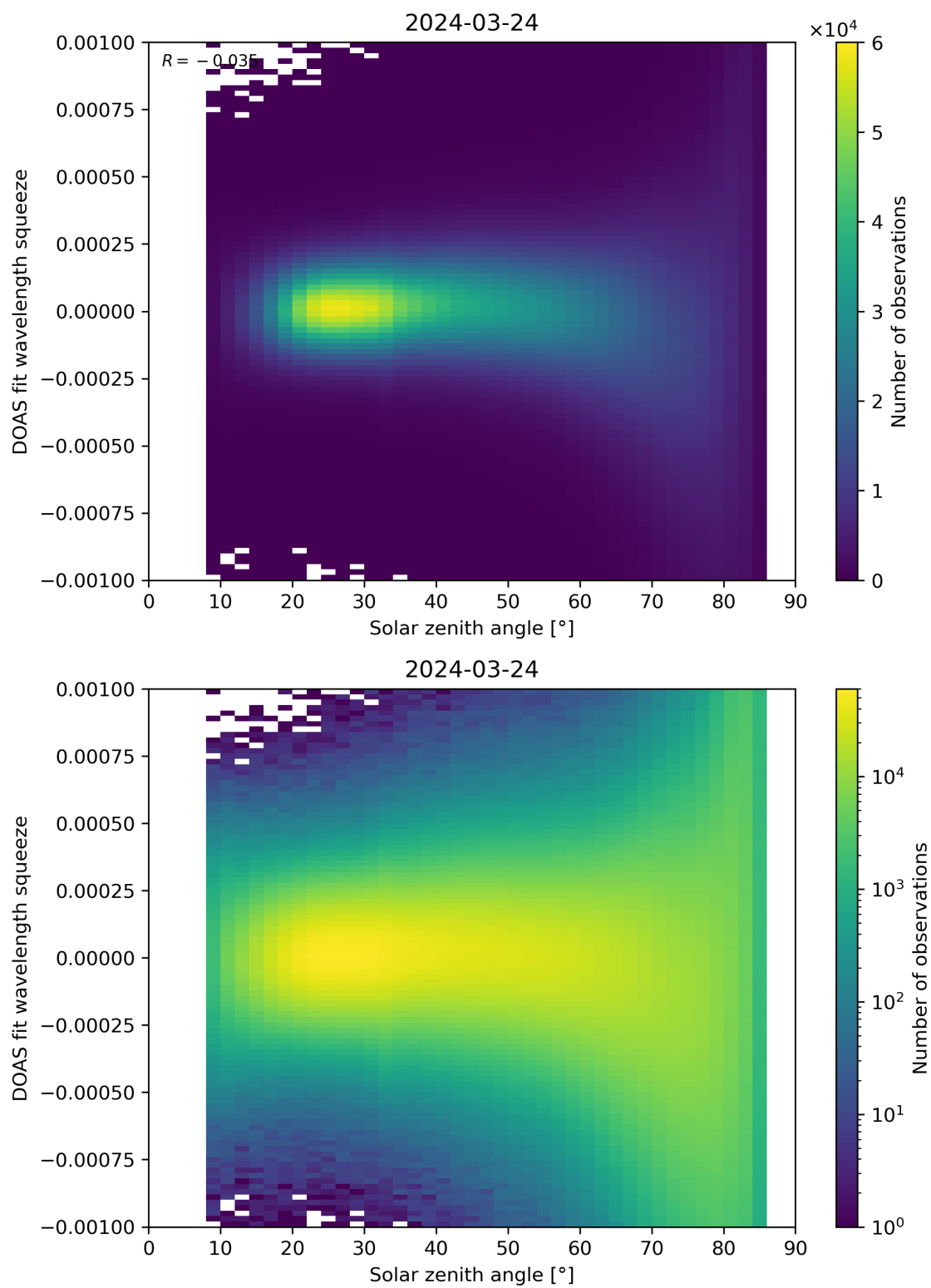
Figure 162: Scatter density plot of “Solar zenith angle” against “DOAS fit wavelength squeeze” for 2024-03-23 to 2024-03-25.
