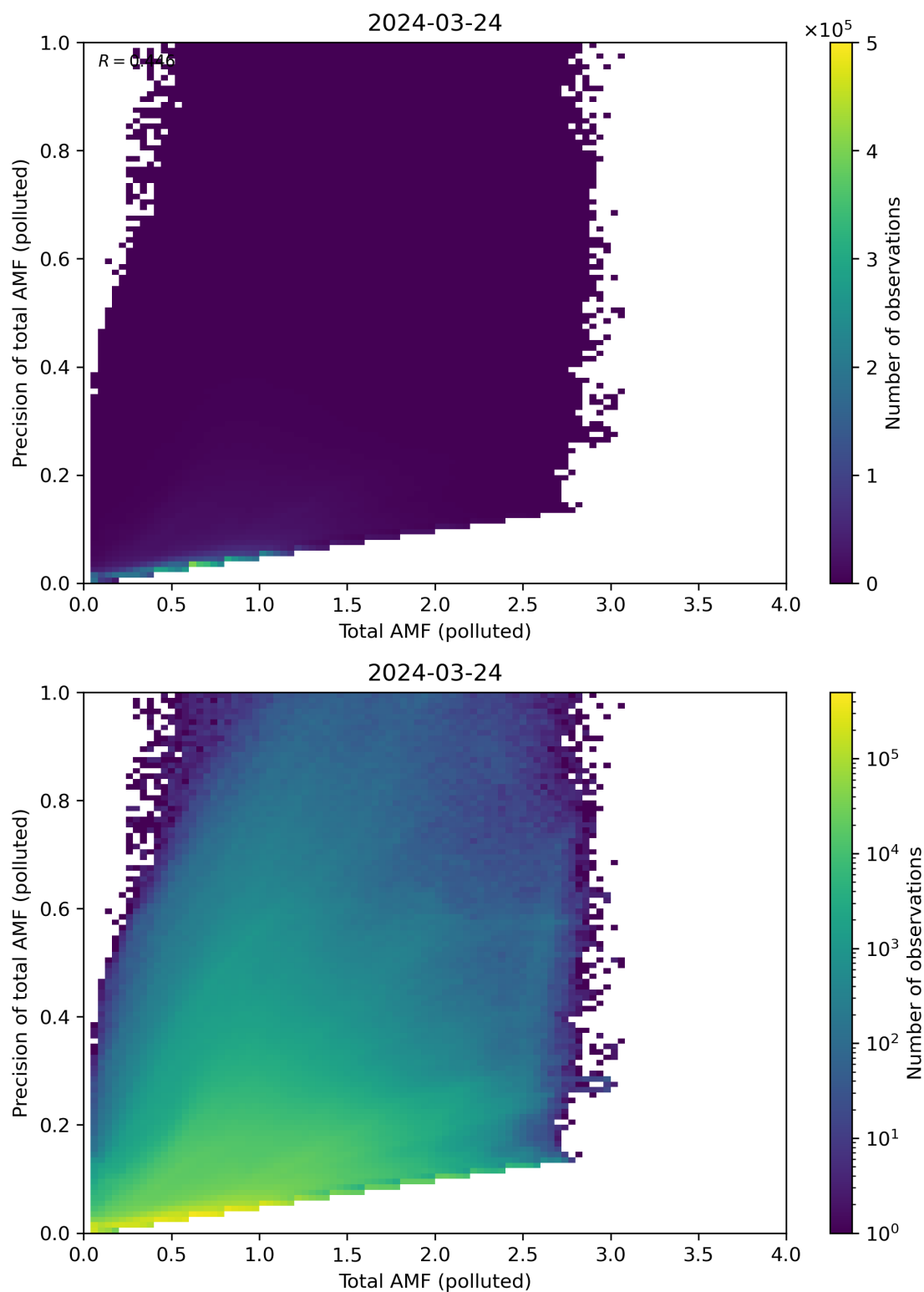
Figure 272: Scatter density plot of “Total AMF (polluted)” against “Precision of total AMF (polluted)” for 2024-03-23 to 2024-03-25.
