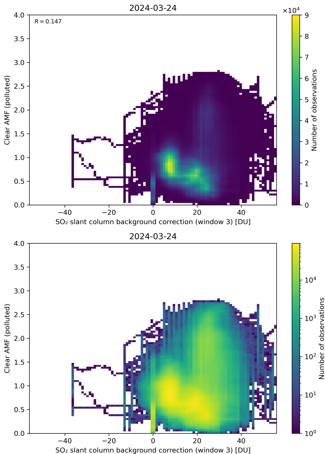
Figure 124: Scatter density plot of “SO 2 slant column background correction (window 3)” against “Clear AMF (polluted)” for 2024-03-23 to 2024-03-25.
