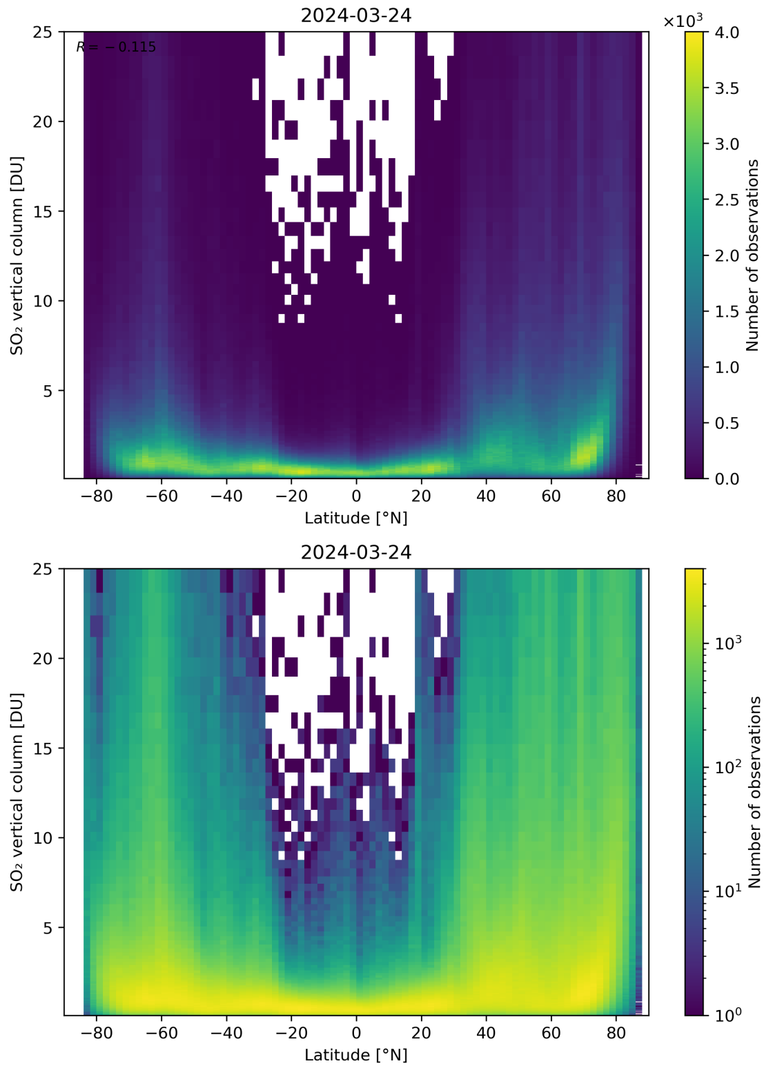
Figure 156: Scatter density plot of “Latitude” against “SO 2 vertical column” for 2024-03-23 to 2024-03-25.
