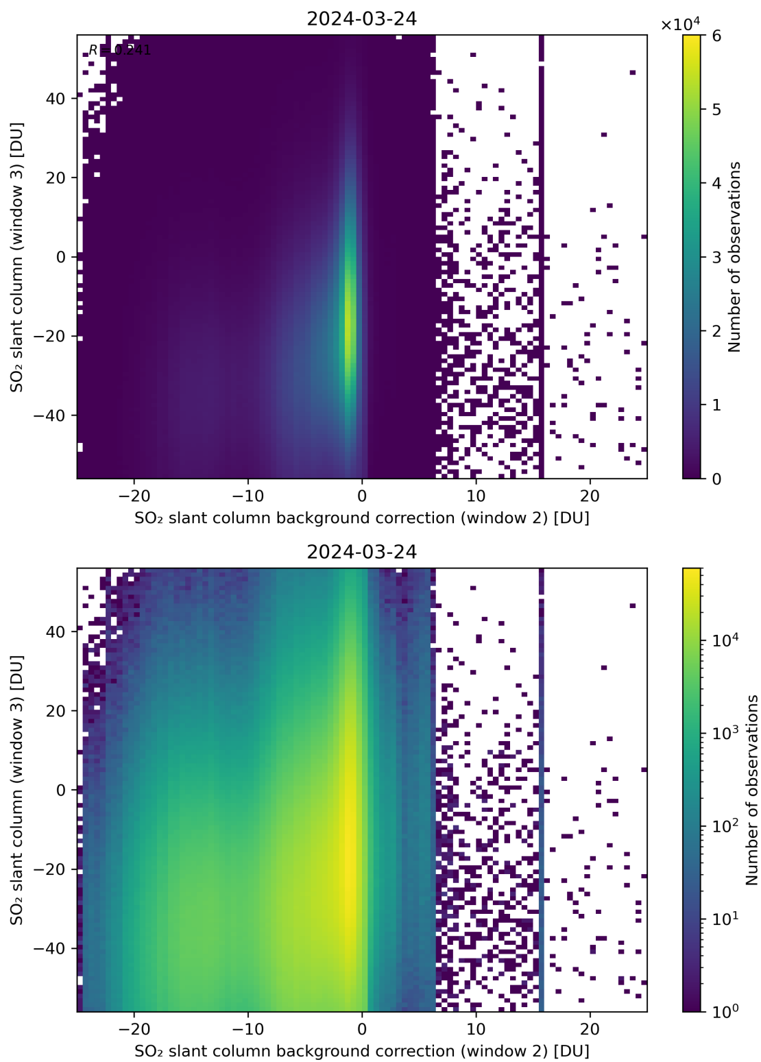
Figure 117: Scatter density plot of “SO 2 slant column background correction (window 2)” against “SO 2 slant column (window 3)” for 2024-03-23 to 2024-03-25.
