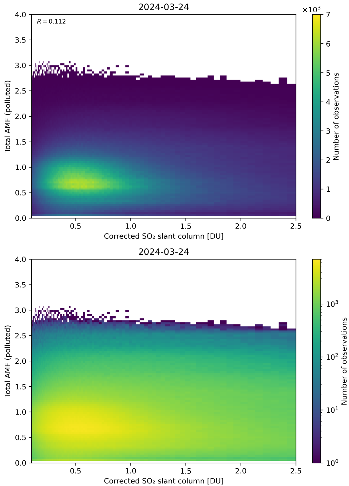
Figure 192: Scatter density plot of “Corrected SO 2 slant column” against “Total AMF (polluted)” for 2024-03-23 to 2024-03-25.
