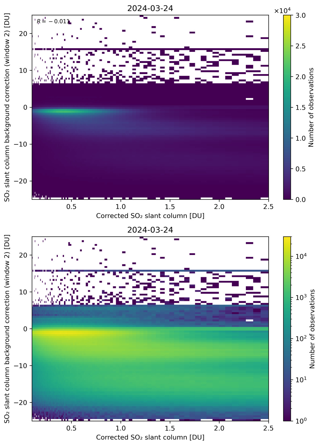
Figure 179: Scatter density plot of “Corrected SO 2 slant column” against “SO 2 slant column background correction (window 2)” for 2024-03-23 to 2024-03-25.
