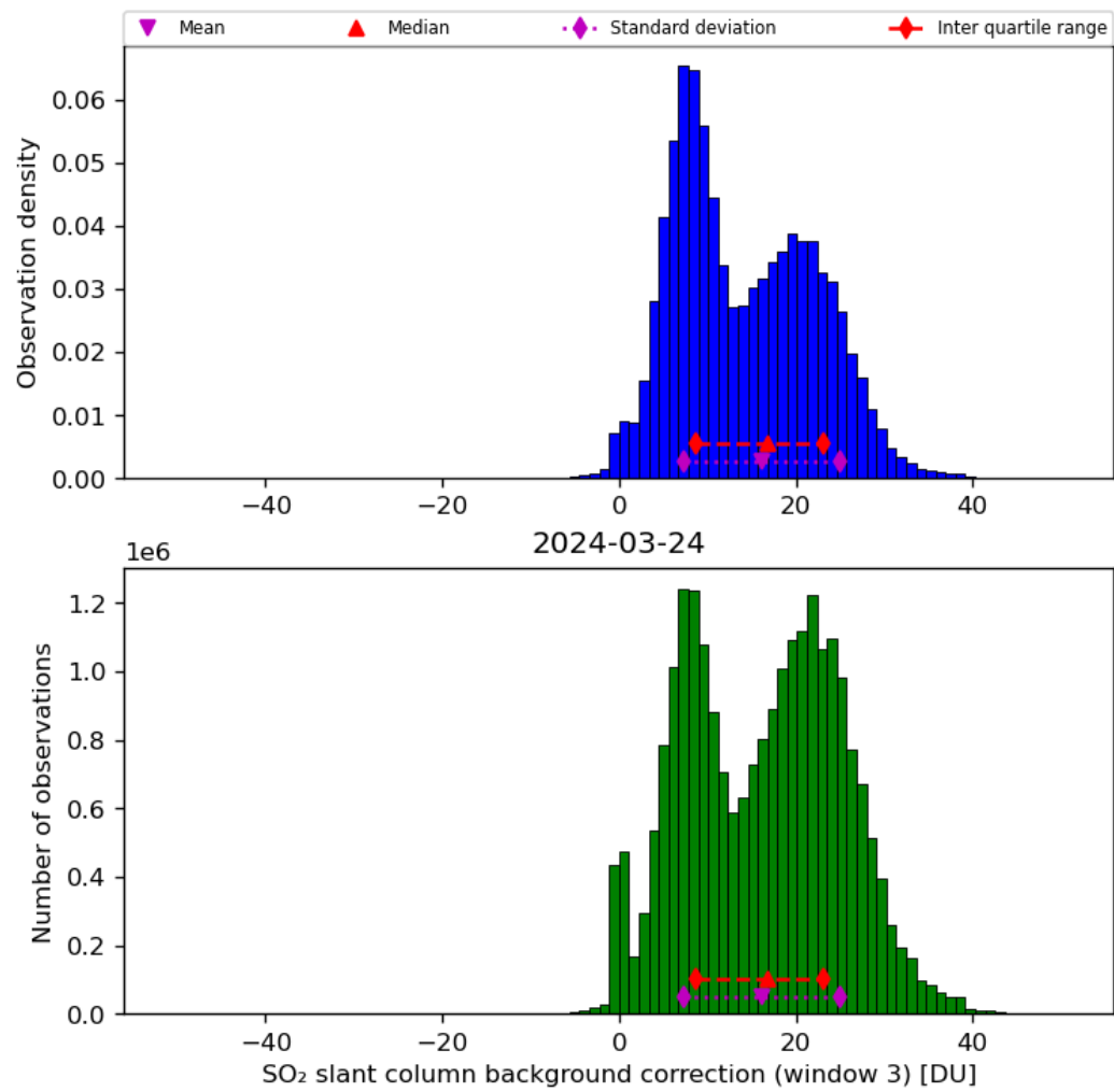
Figure 67: Histogram of “SO 2 slant column background correction (window 3)” for 2024-03-23 to 2024-03-25
