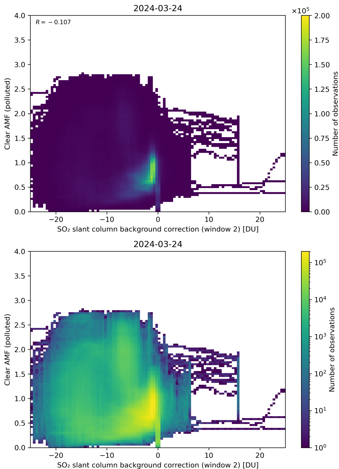
Figure 115: Scatter density plot of “SO 2 slant column background correction (window 2)” against “Clear AMF (polluted)” for 2024-03-23 to 2024-03-25.
