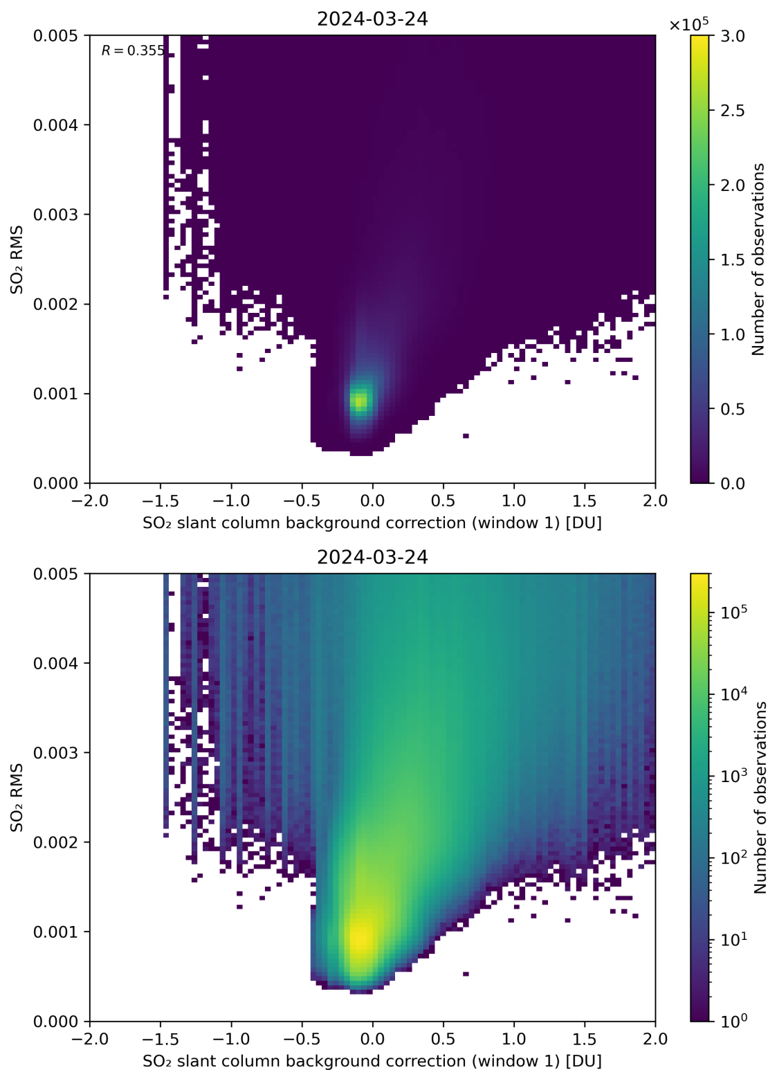
Figure 102: Scatter density plot of “SO 2 slant column background correction (window 1)” against “SO 2 RMS” for 2024-03-23 to 2024-03-25.
