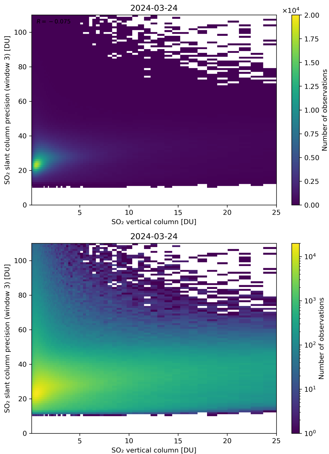
Figure 304: Scatter density plot of “SO 2 vertical column” against “SO 2 slant column precision (window 3)” for 2024-03-23 to 2024-03-25.
