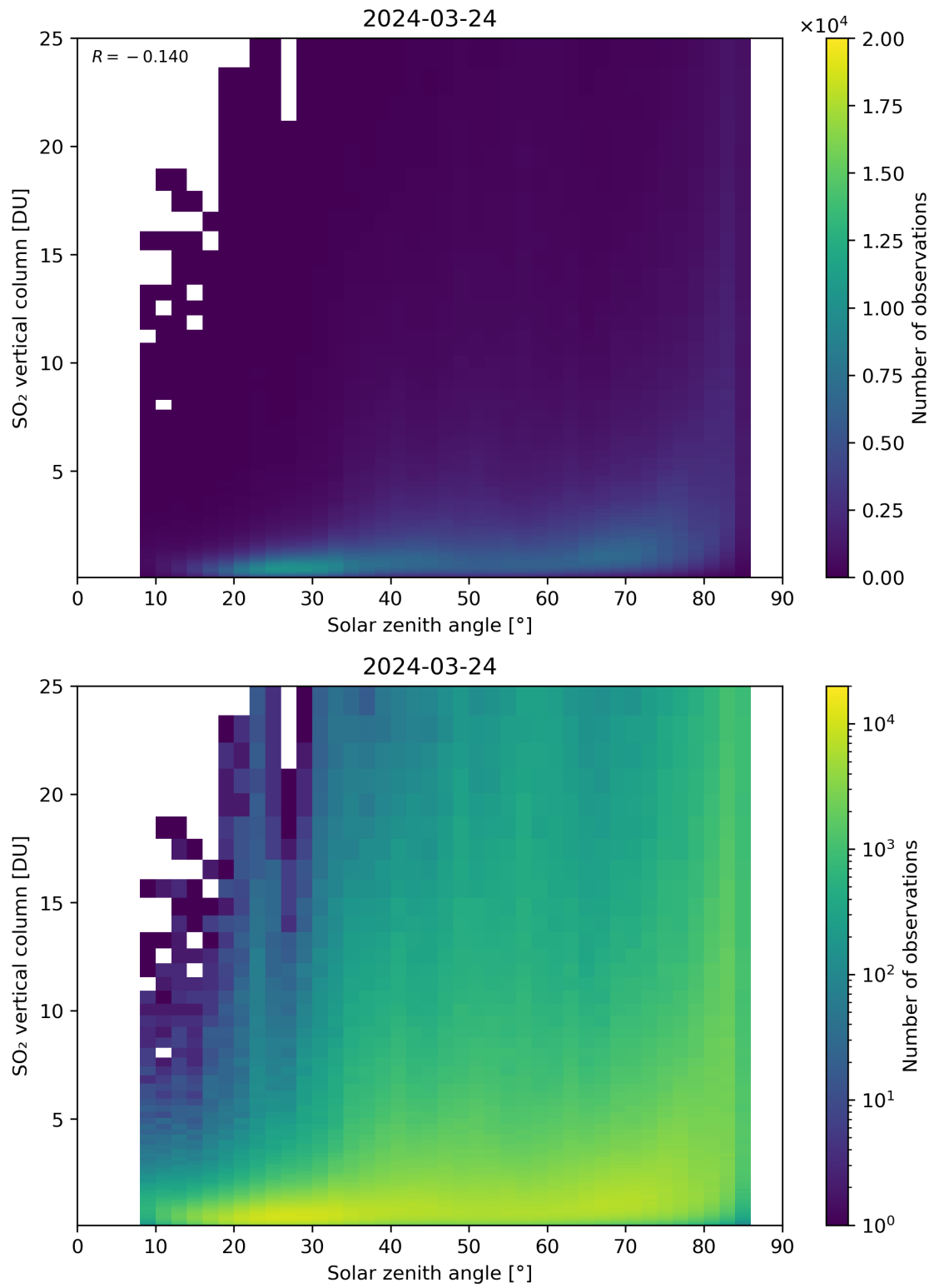
Figure 176: Scatter density plot of “Solar zenith angle” against “SO 2 vertical column” for 2024-03-23 to 2024-03-25.
