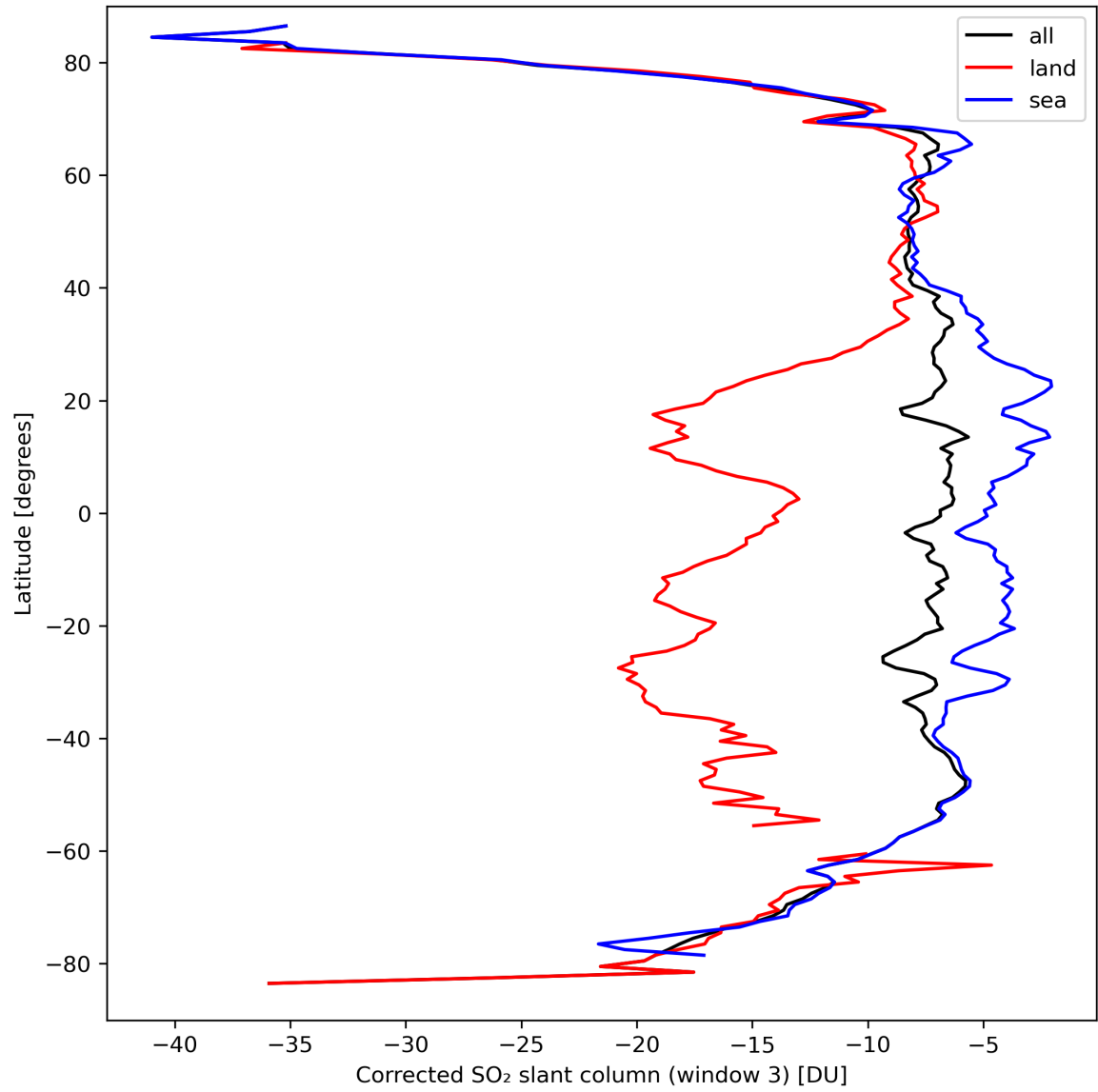
Figure 43: Zonal average of “Corrected SO 2 slant column (window 3)” for 2024-03-23 to 2024-03-25.
