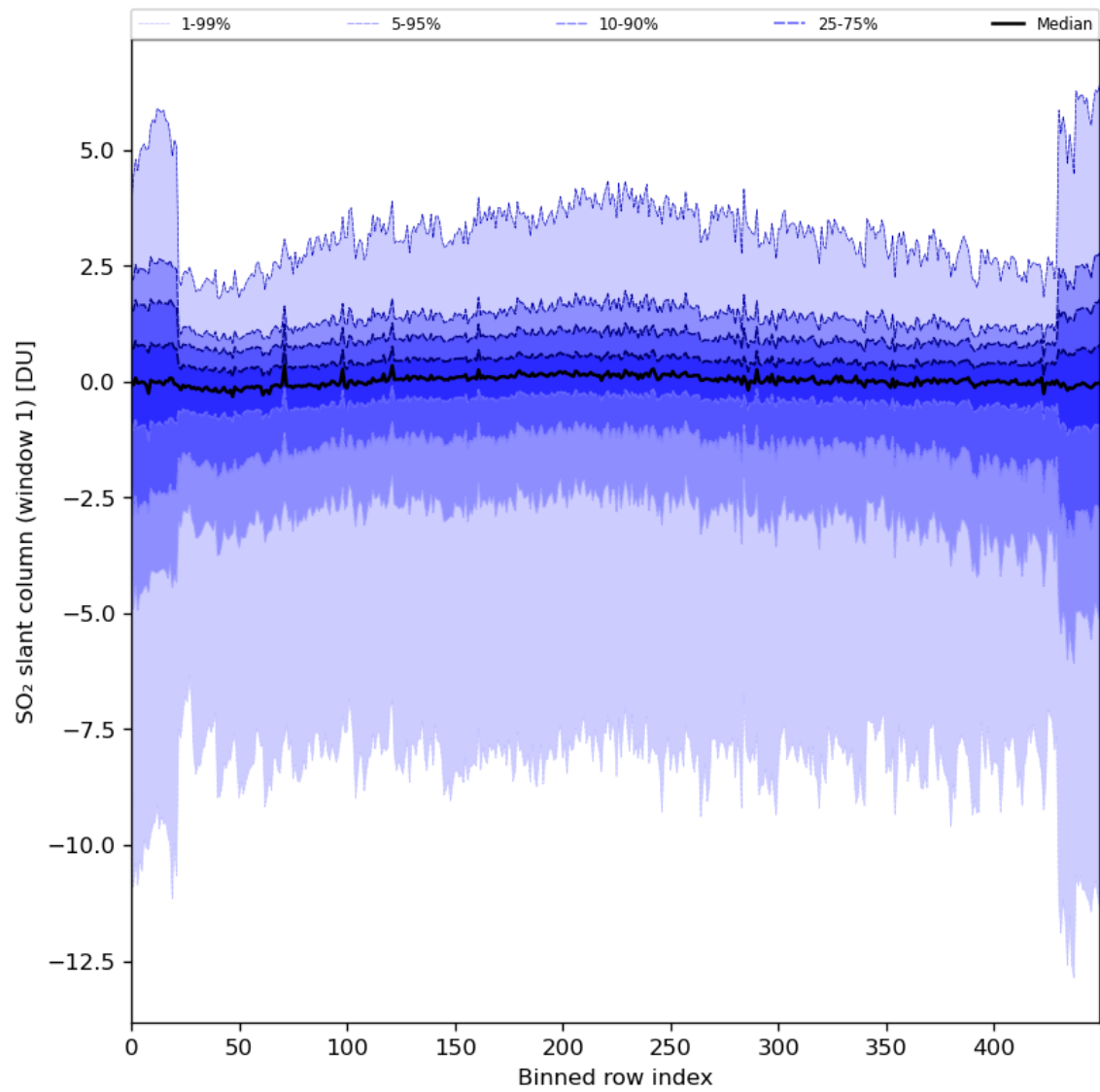
Figure 79: Along track statistics of “SO 2 slant column (window 1)” for 2024-03-23 to 2024-03-25
