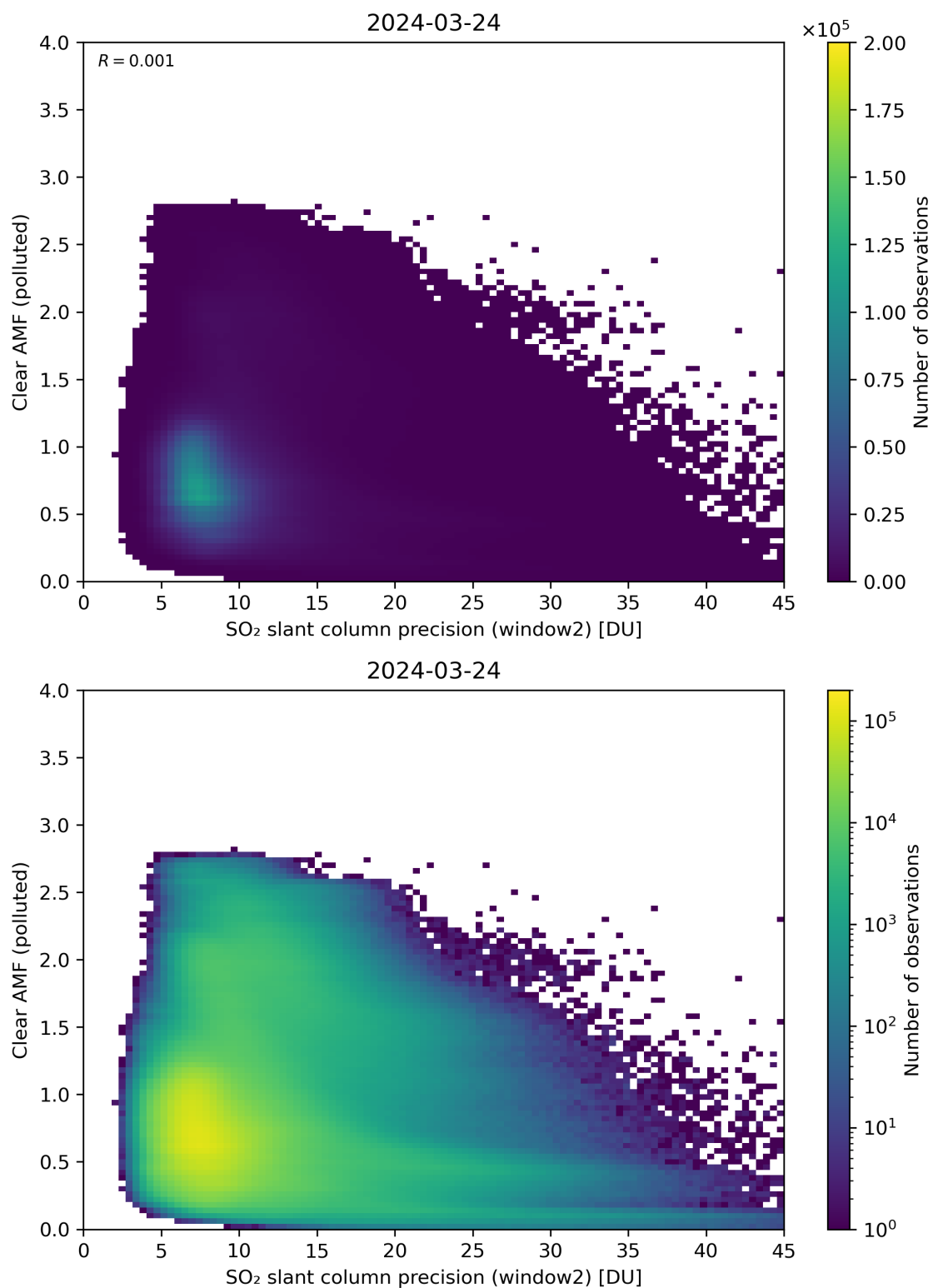
Figure 246: Scatter density plot of “SO 2 slant column precision (window2)” against “Clear AMF (polluted)” for 2024-03-23 to 2024-03-25.
