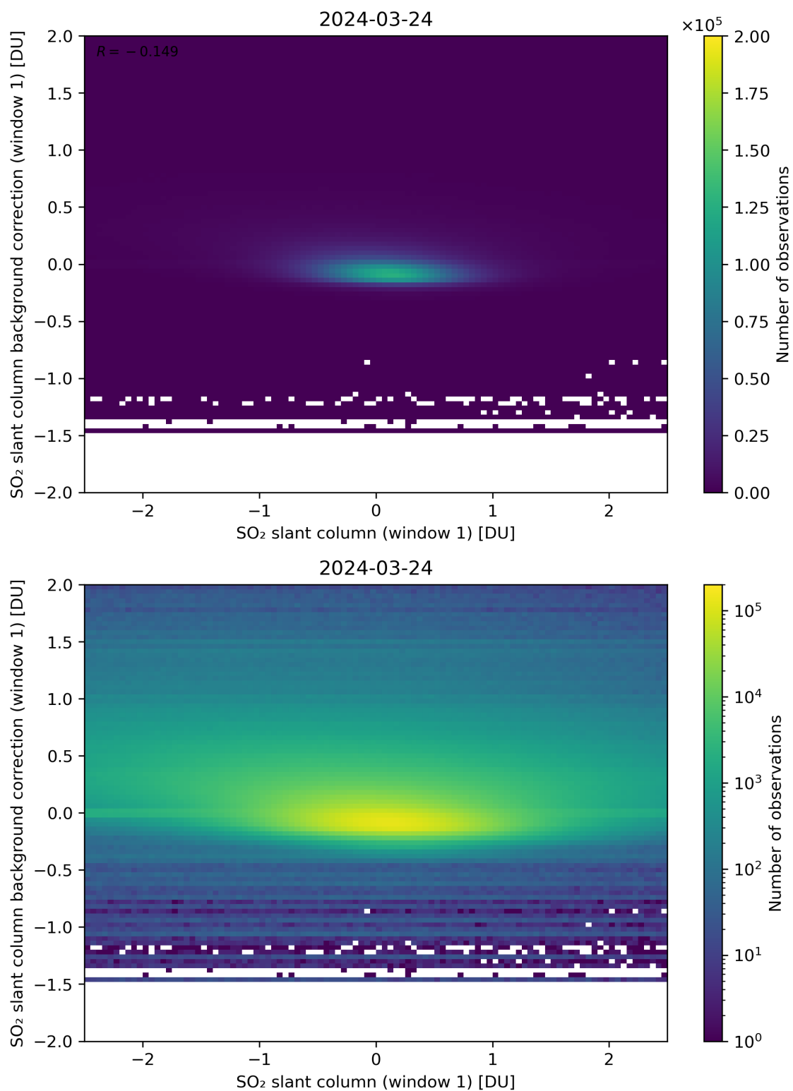
Figure 212: Scatter density plot of “SO 2 slant column (window 1)” against “SO 2 slant column background correction (window 1)” for 2024-03-23 to 2024-03-25.
