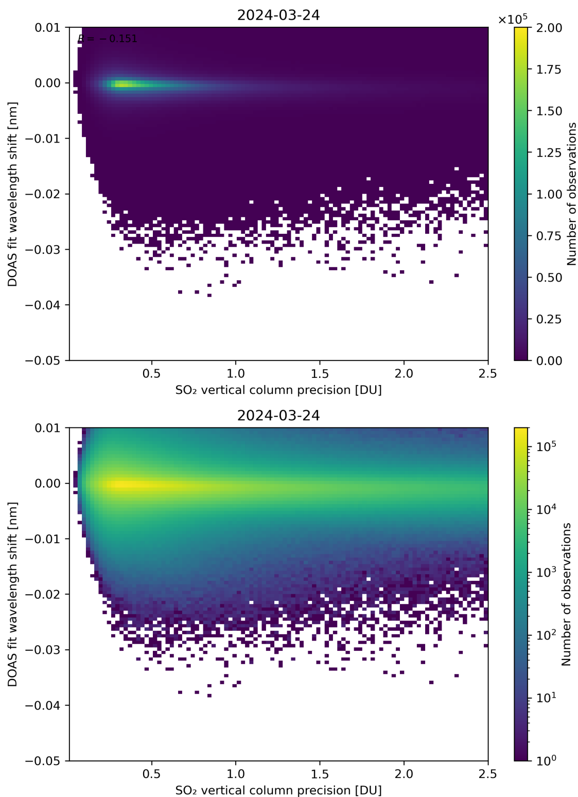
Figure 282: Scatter density plot of “SO 2 vertical column precision” against “DOAS fit wavelength shift” for 2024-03-23 to 2024-03-25.
