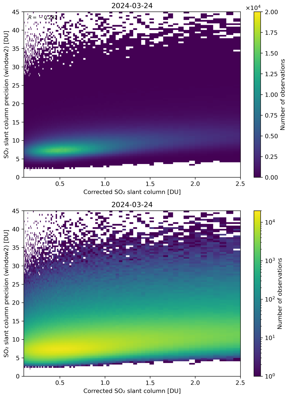
Figure 189: Scatter density plot of “Corrected SO 2 slant column” against “SO 2 slant column precision (window2)” for 2024-03-23 to 2024-03-25.
