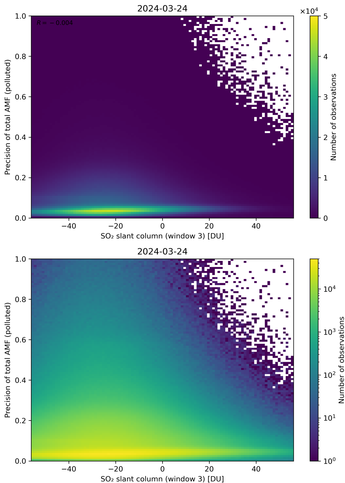
Figure 269: Scatter density plot of “SO 2 slant column (window 3)” against “Precision of total AMF (polluted)” for 2024-03-23 to 2024-03-25.
