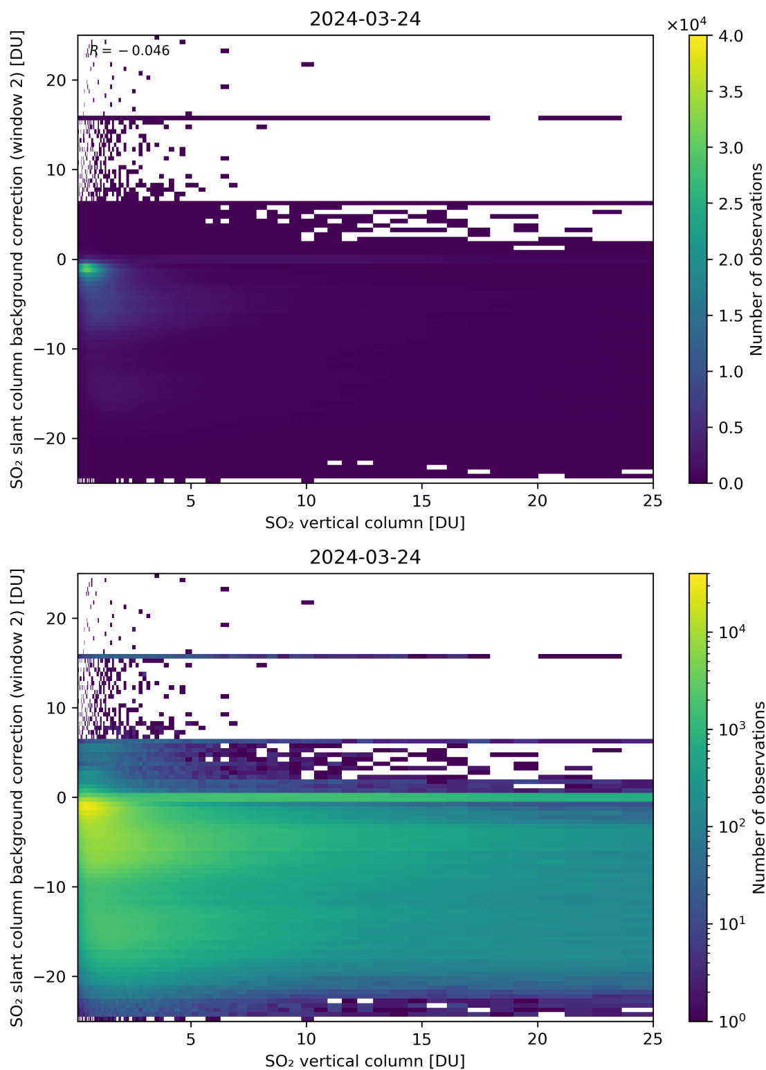
Figure 274: Scatter density plot of “SO 2 vertical column” against “SO 2 slant column background correction (window 2)” for 2024-03-23 to 2024-03-25.
