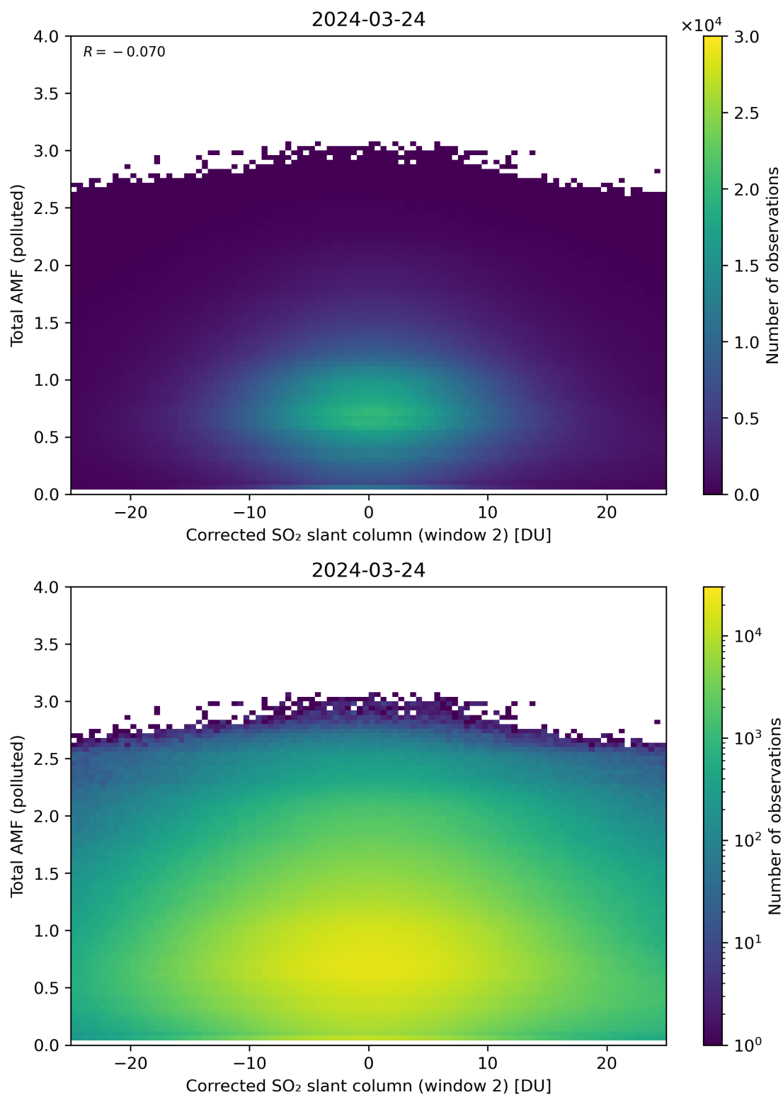
Figure 203: Scatter density plot of “Corrected SO 2 slant column (window 2)” against “Total AMF (polluted)” for 2024-03-23 to 2024-03-25.
