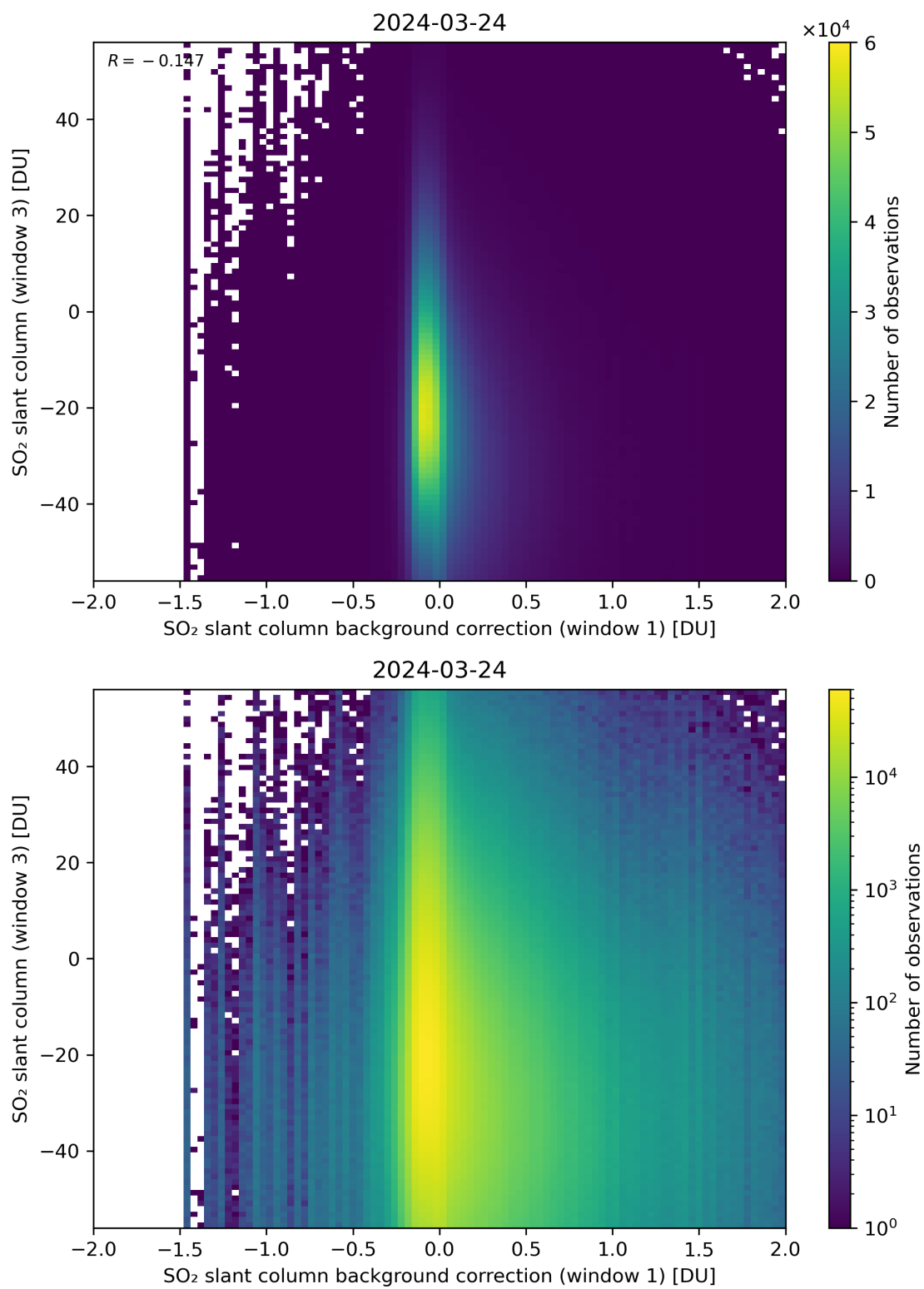
Figure 107: Scatter density plot of “SO 2 slant column background correction (window 1)” against “SO 2 slant column (window 3)” for 2024-03-23 to 2024-03-25.
