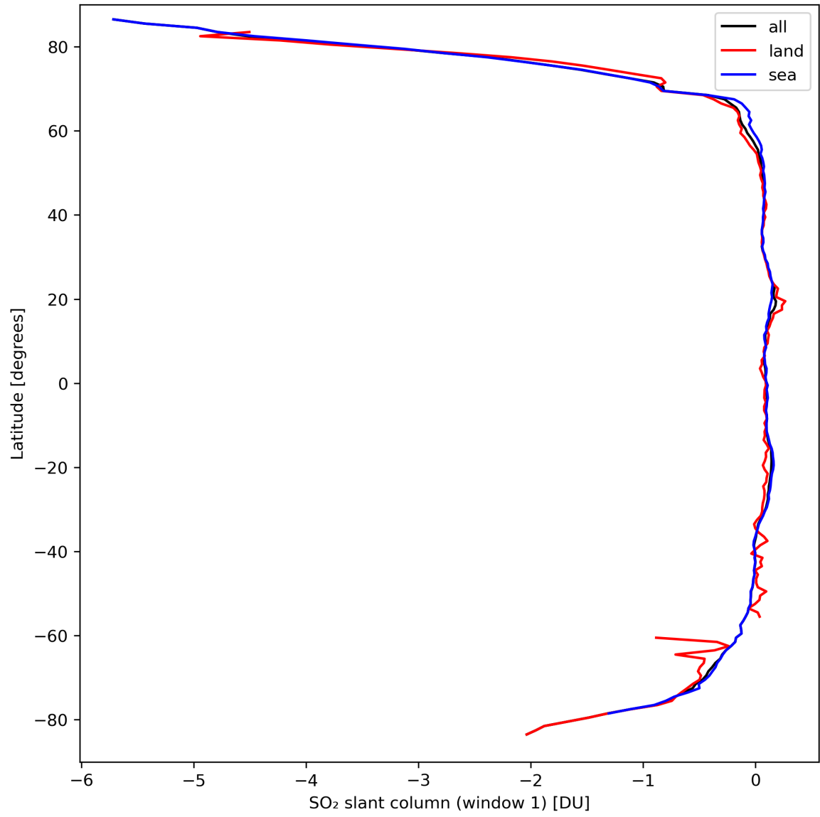
Figure 33: Zonal average of “SO 2 slant column (window 1)” for 2024-03-23 to 2024-03-25.
