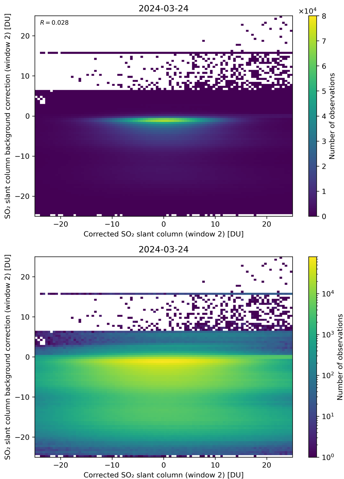
Figure 194: Scatter density plot of “Corrected SO 2 slant column (window 2)” against “SO 2 slant column background correction (window 2)” for 2024-03-23 to 2024-03-25.
