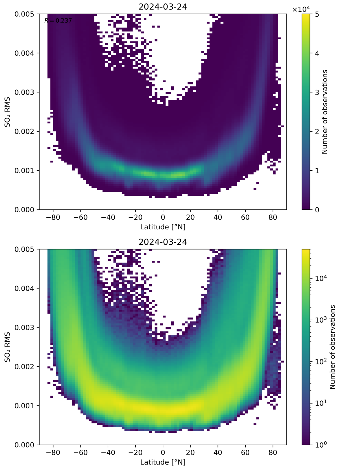
Figure 144: Scatter density plot of “Latitude” against “SO 2 RMS” for 2024-03-23 to 2024-03-25.
