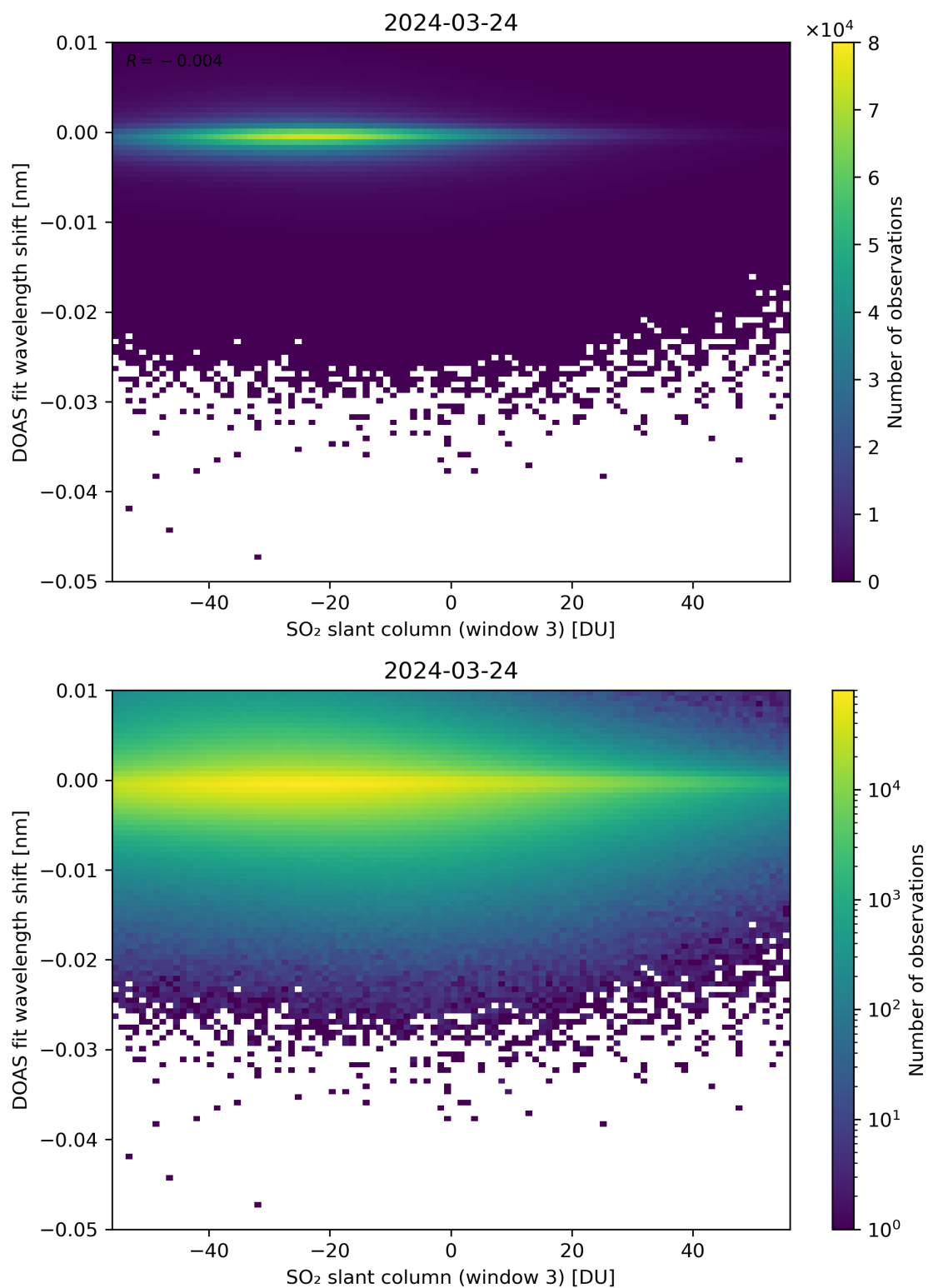
Figure 254: Scatter density plot of “SO 2 slant column (window 3)” against “DOAS fit wavelength shift” for 2024-03-23 to 2024-03-25.
