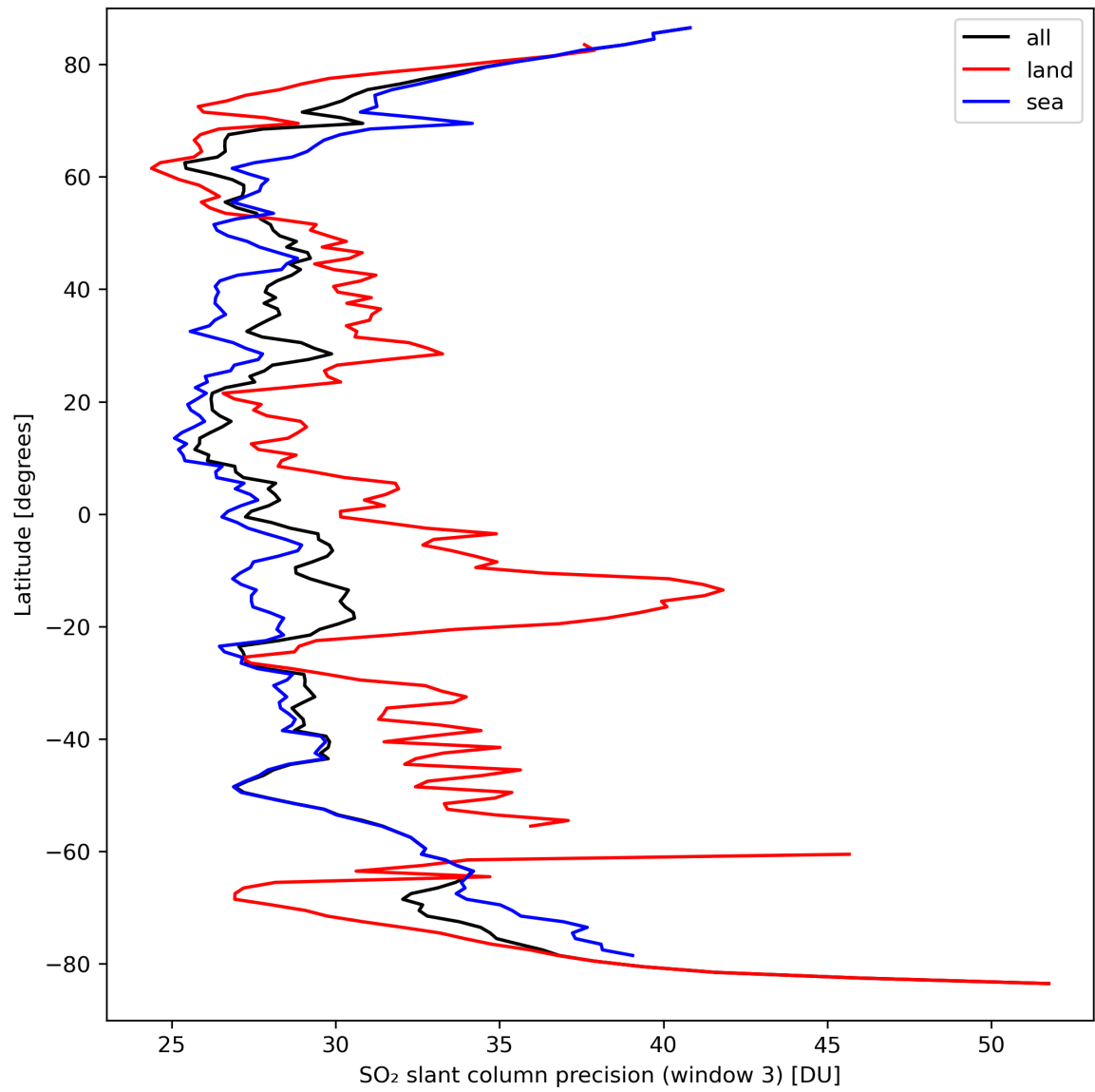
Figure 42: Zonal average of “SO 2 slant column precision (window 3)” for 2024-03-23 to 2024-03-25.
