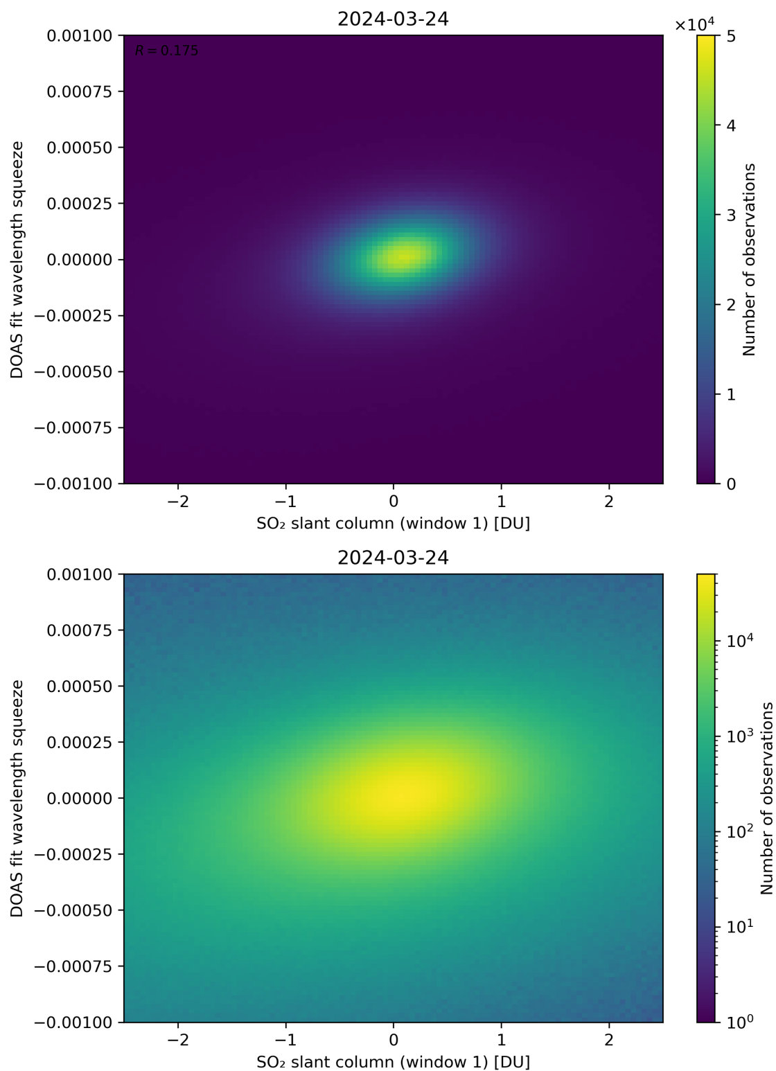
Figure 216: Scatter density plot of “SO 2 slant column (window 1)” against “DOAS fit wavelength squeeze” for 2024-03-23 to 2024-03-25.
