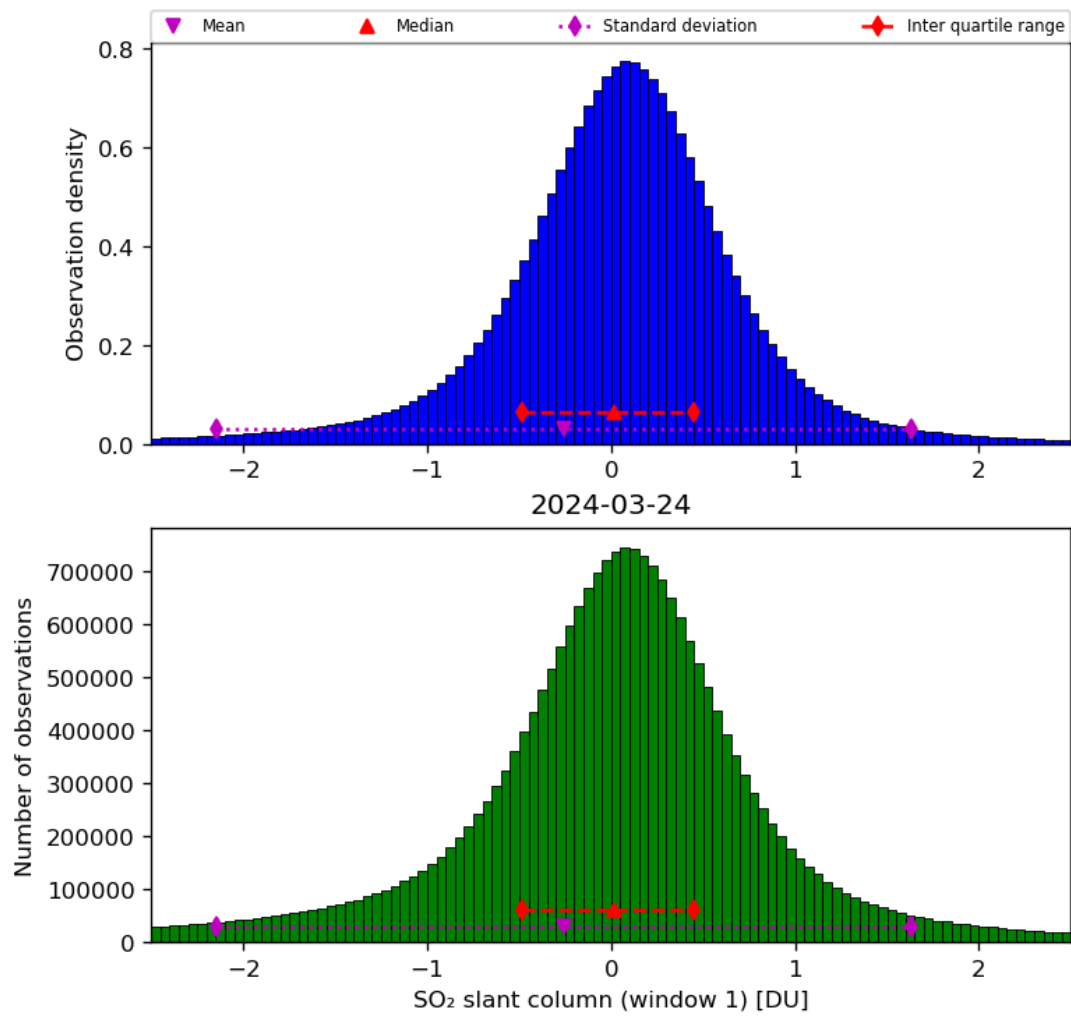
Figure 56: Histogram of “SO 2 slant column (window 1)” for 2024-03-23 to 2024-03-25
