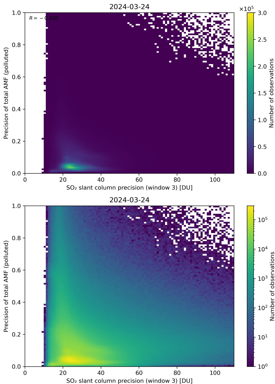
Figure 264: Scatter density plot of “SO 2 slant column precision (window 3)” against “Precision of total AMF (polluted)” for 2024-03-23 to 2024-03-25.
