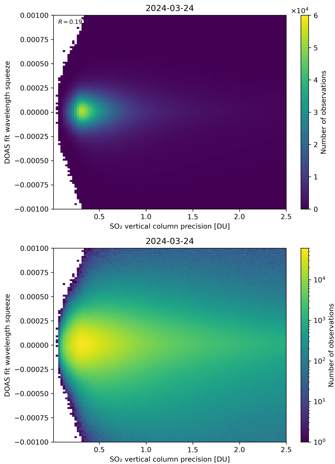
Figure 283: Scatter density plot of “SO 2 vertical column precision” against “DOAS fit wavelength squeeze” for 2024-03-23 to 2024-03-25.
