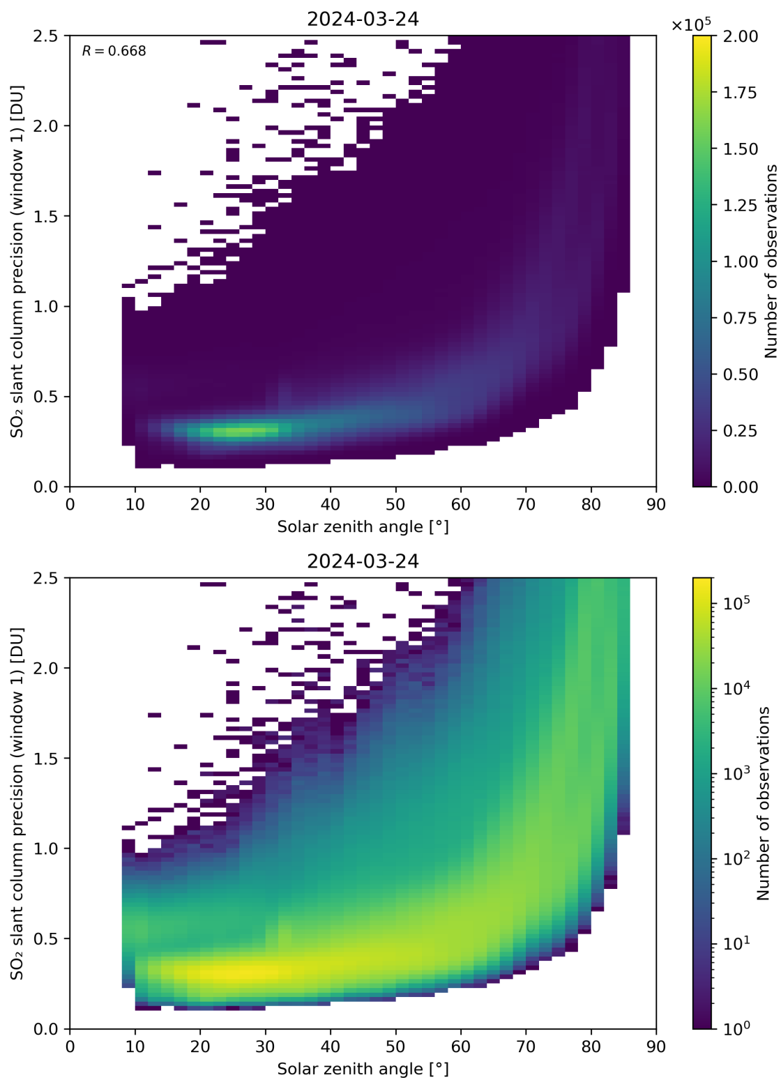
Figure 170: Scatter density plot of “Solar zenith angle” against “SO 2 slant column precision (window 1)” for 2024-03-23 to 2024-03-25.
