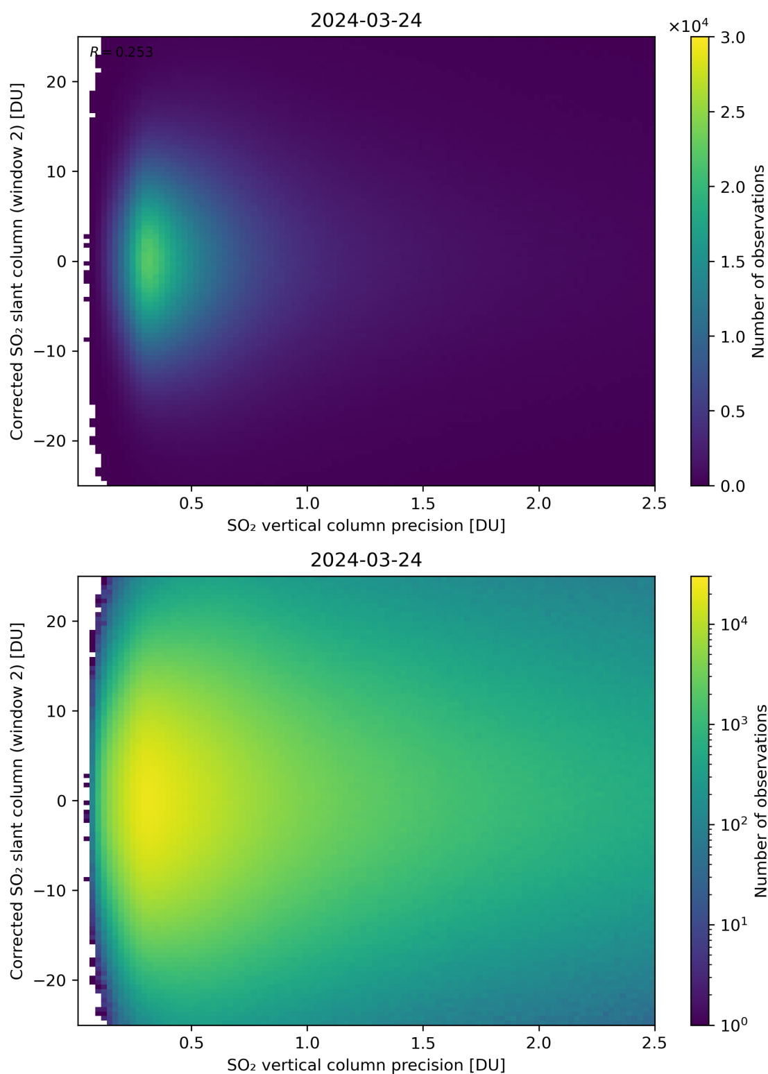
Figure 287: Scatter density plot of “SO 2 vertical column precision” against “Corrected SO 2 slant column (window 2)” for 2024-03-23 to 2024-03-25.
