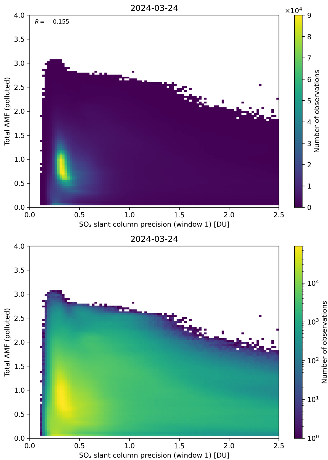
Figure 230: Scatter density plot of “SO 2 slant column precision (window 1)” against “Total AMF (polluted)” for 2024-03-23 to 2024-03-25.
