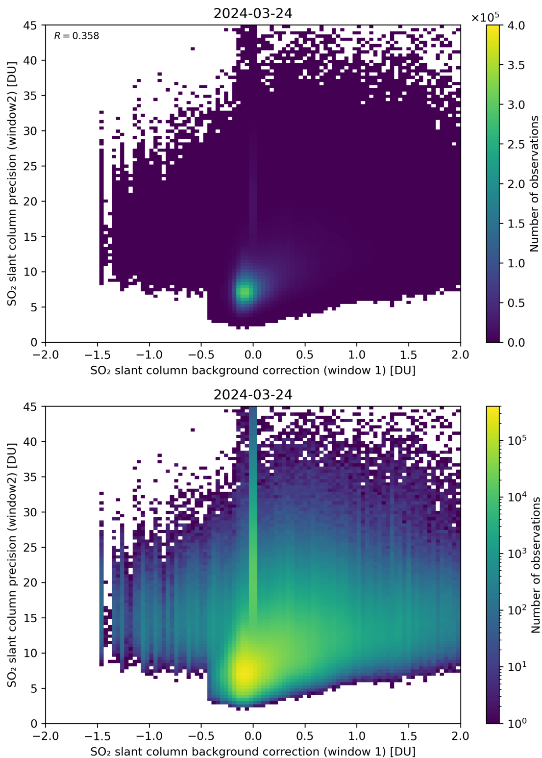
Figure 106: Scatter density plot of “SO 2 slant column background correction (window 1)” against “SO 2 slant column precision (window2)” for 2024-03-23 to 2024-03-25.
