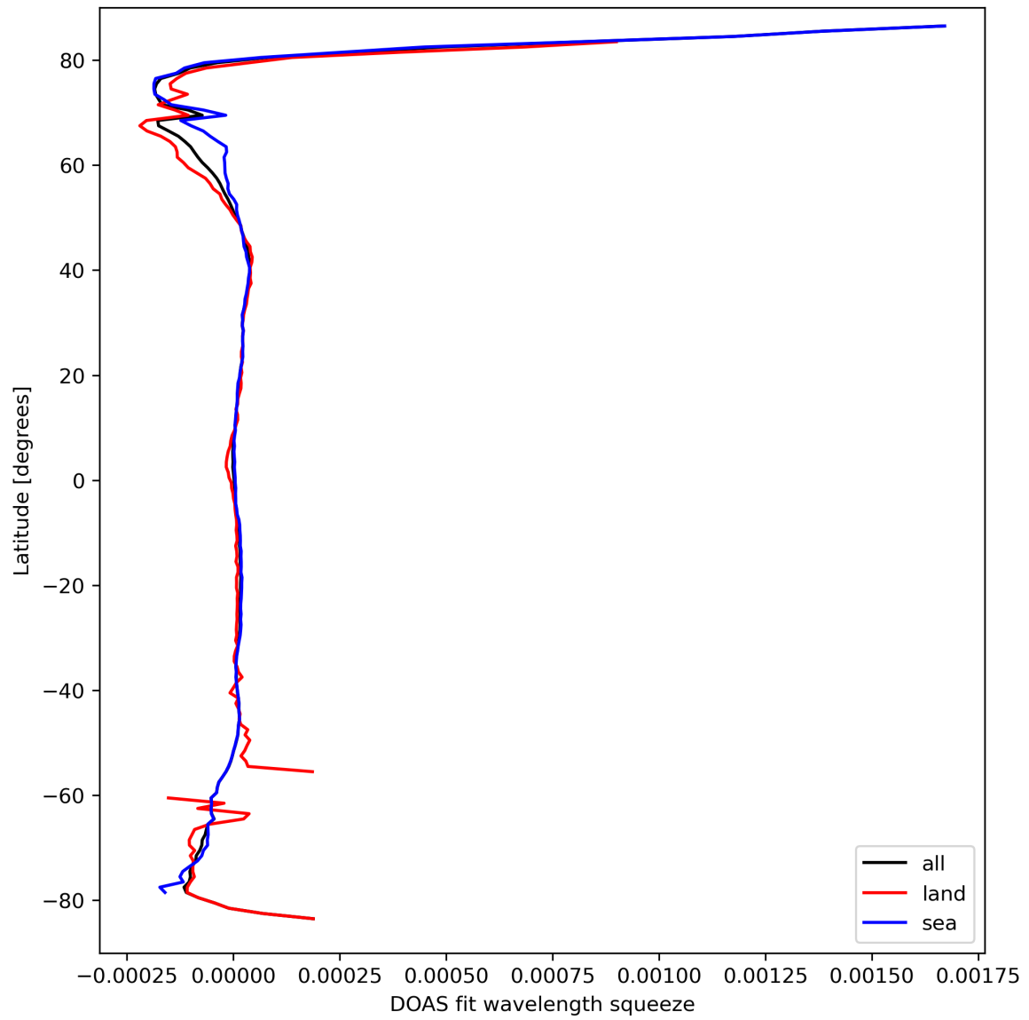
Figure 46: Zonal average of “DOAS fit wavelength squeeze” for 2024-03-23 to 2024-03-25.
