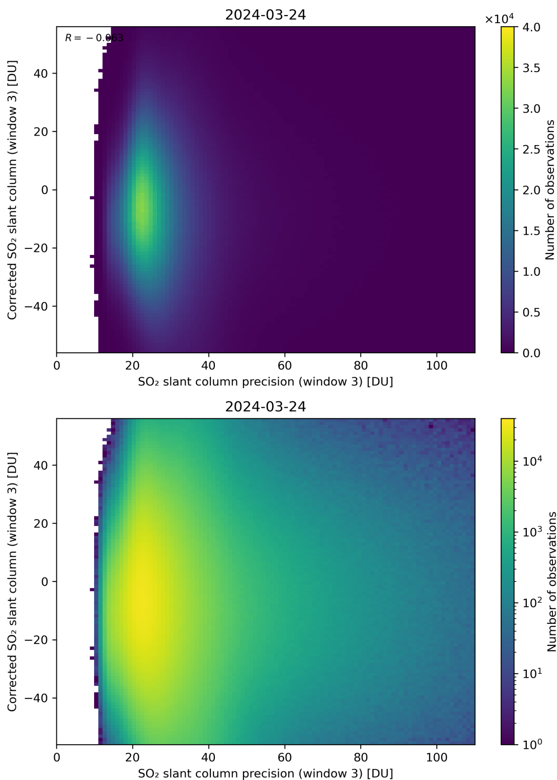
Figure 262: Scatter density plot of “SO 2 slant column precision (window 3)” against “Corrected SO 2 slant column (window 3)” for 2024-03-23 to 2024-03-25.
