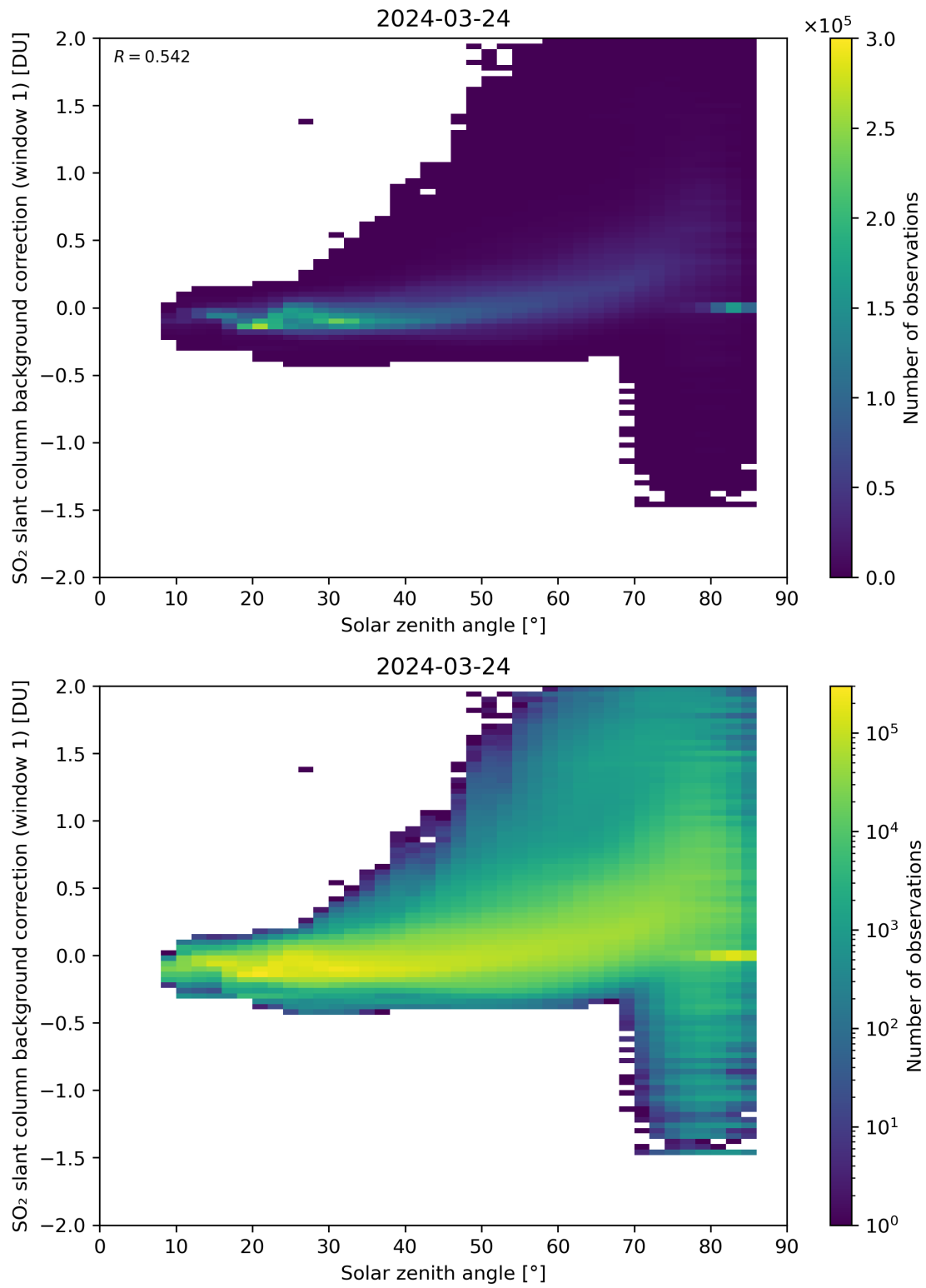
Figure 158: Scatter density plot of “Solar zenith angle” against “SO 2 slant column background correction (window 1)” for 2024-03-23 to 2024-03-25.
