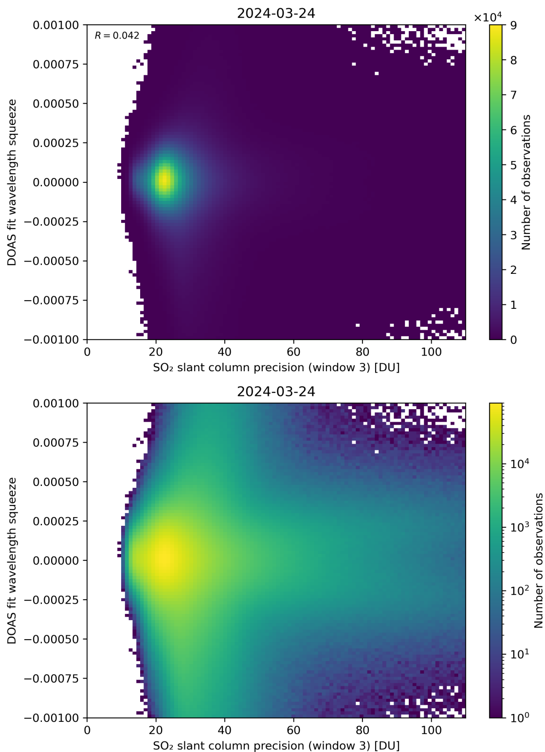
Figure 259: Scatter density plot of “SO 2 slant column precision (window 3)” against “DOAS fit wavelength squeeze” for 2024-03-23 to 2024-03-25.
