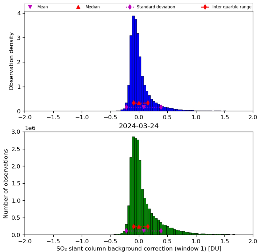
Figure 59: Histogram of “SO 2 slant column background correction (window 1)” for 2024-03-23 to 2024-03-25
