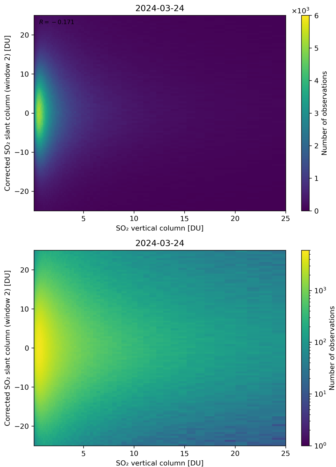
Figure 298: Scatter density plot of “SO 2 vertical column” against “Corrected SO 2 slant column (window 2)” for 2024-03-23 to 2024-03-25.
