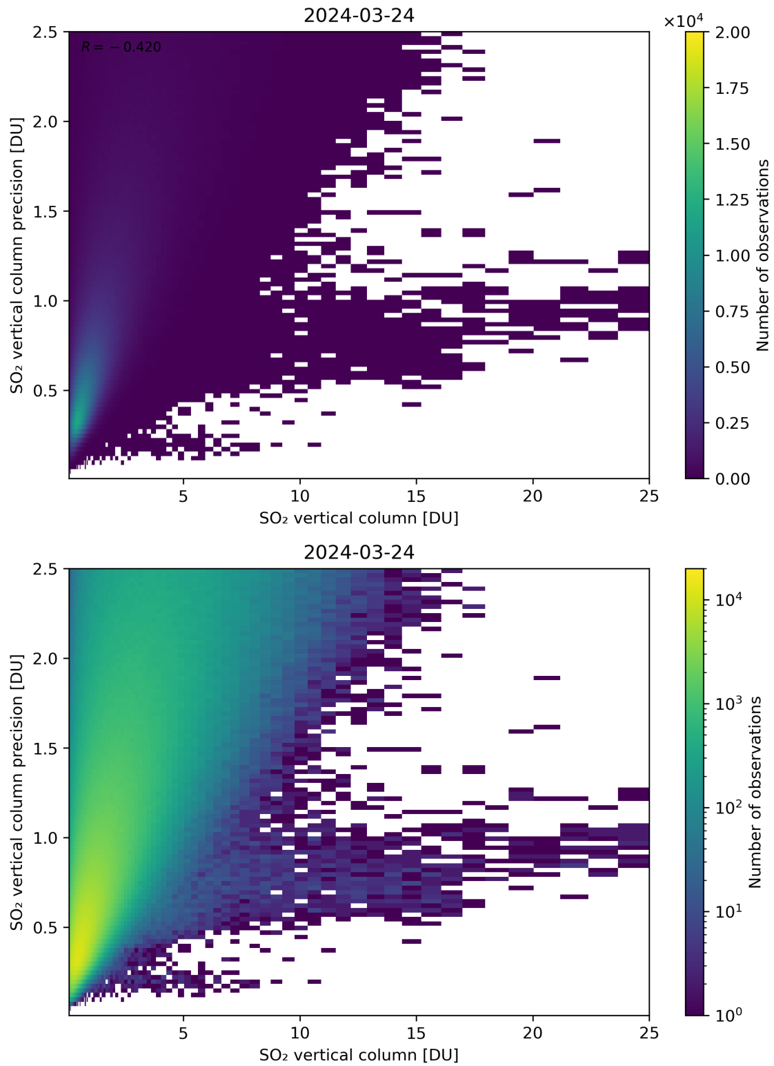
Figure 307: Scatter density plot of “SO 2 vertical column” against “SO 2 vertical column precision” for 2024-03-23 to 2024-03-25.
