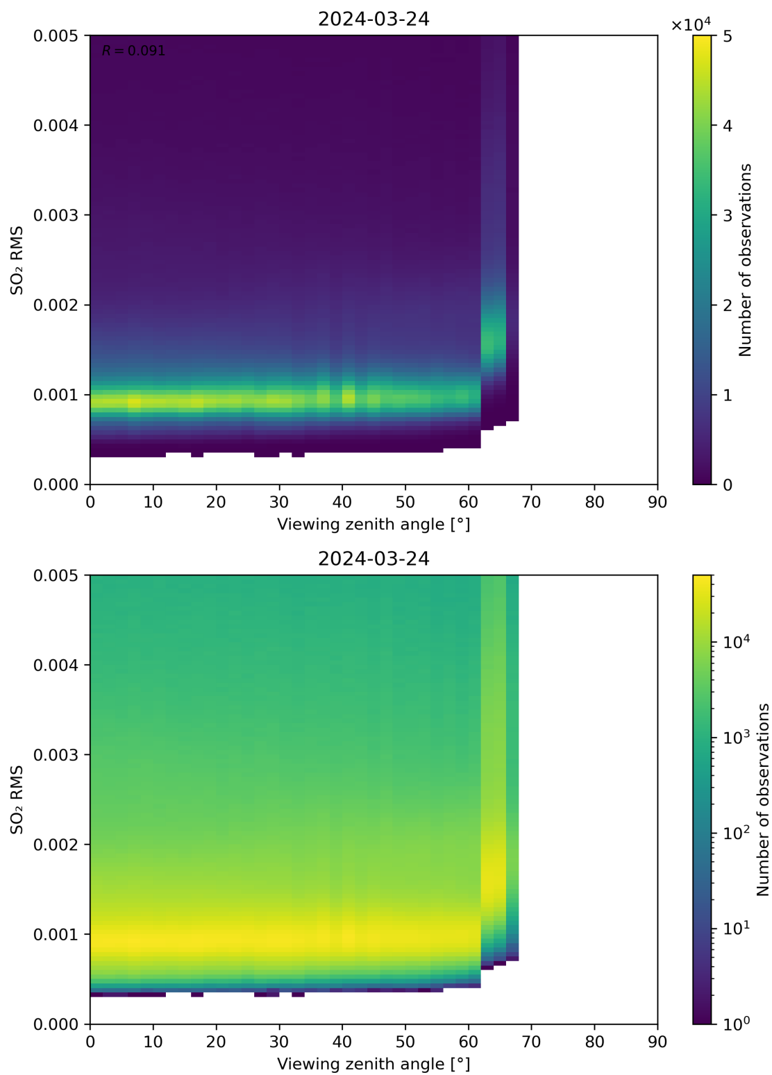
Figure 313: Scatter density plot of “Viewing zenith angle” against “SO 2 RMS” for 2024-03-23 to 2024-03-25.
