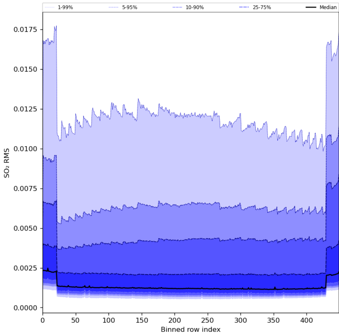
Figure 93: Along track statistics of “SO 2 RMS” for 2024-03-23 to 2024-03-25
