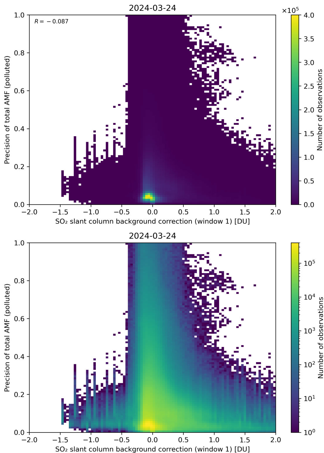
Figure 110: Scatter density plot of “SO 2 slant column background correction (window 1)” against “Precision of total AMF (polluted)” for 2024-03-23 to 2024-03-25.
