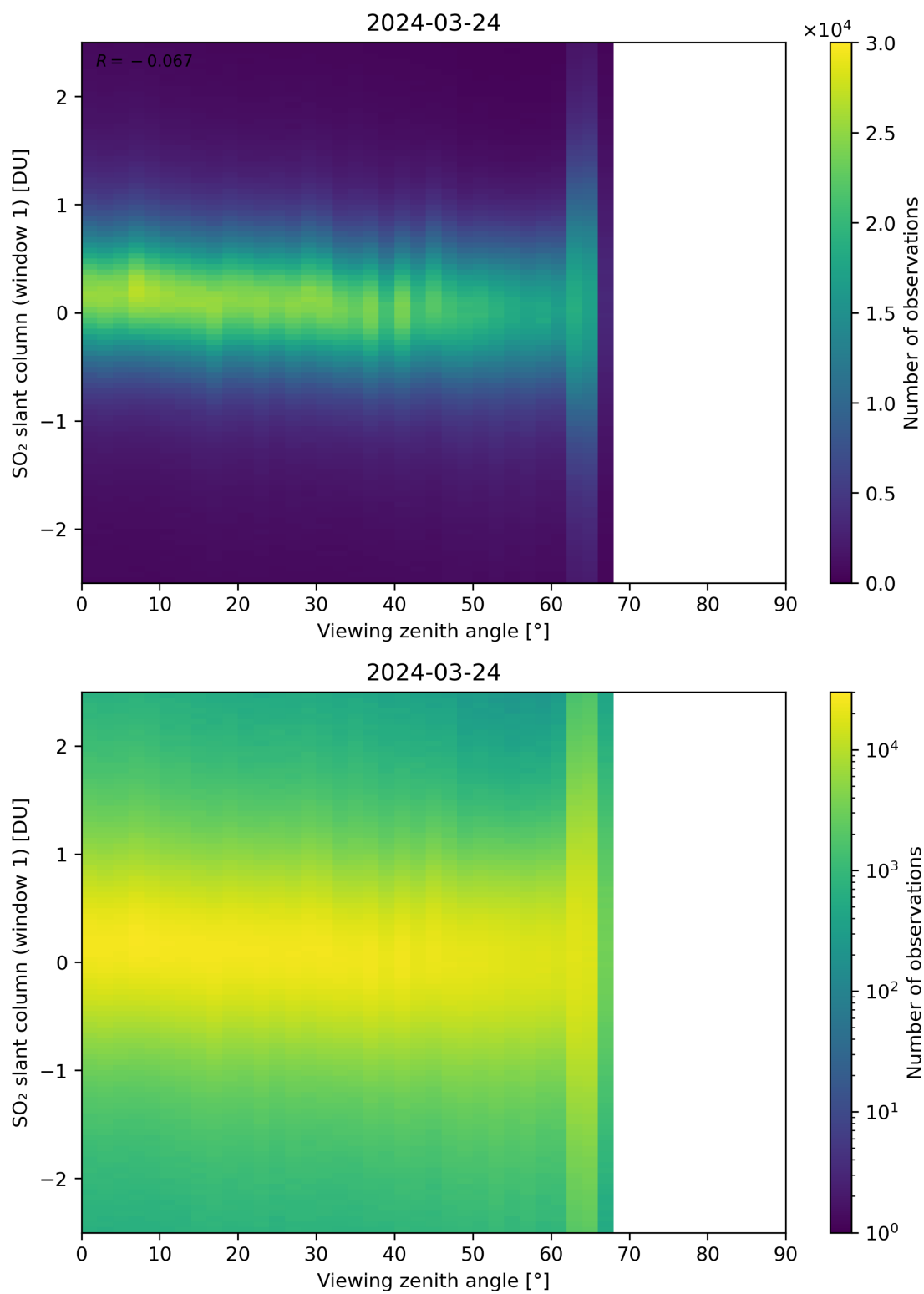
Figure 320: Scatter density plot of “Viewing zenith angle” against “SO 2 slant column (window 1)” for 2024-03-23 to 2024-03-25.
