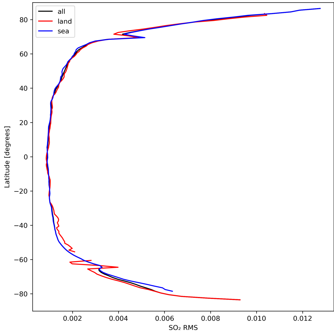
Figure 47: Zonal average of “SO 2 RMS” for 2024-03-23 to 2024-03-25.
