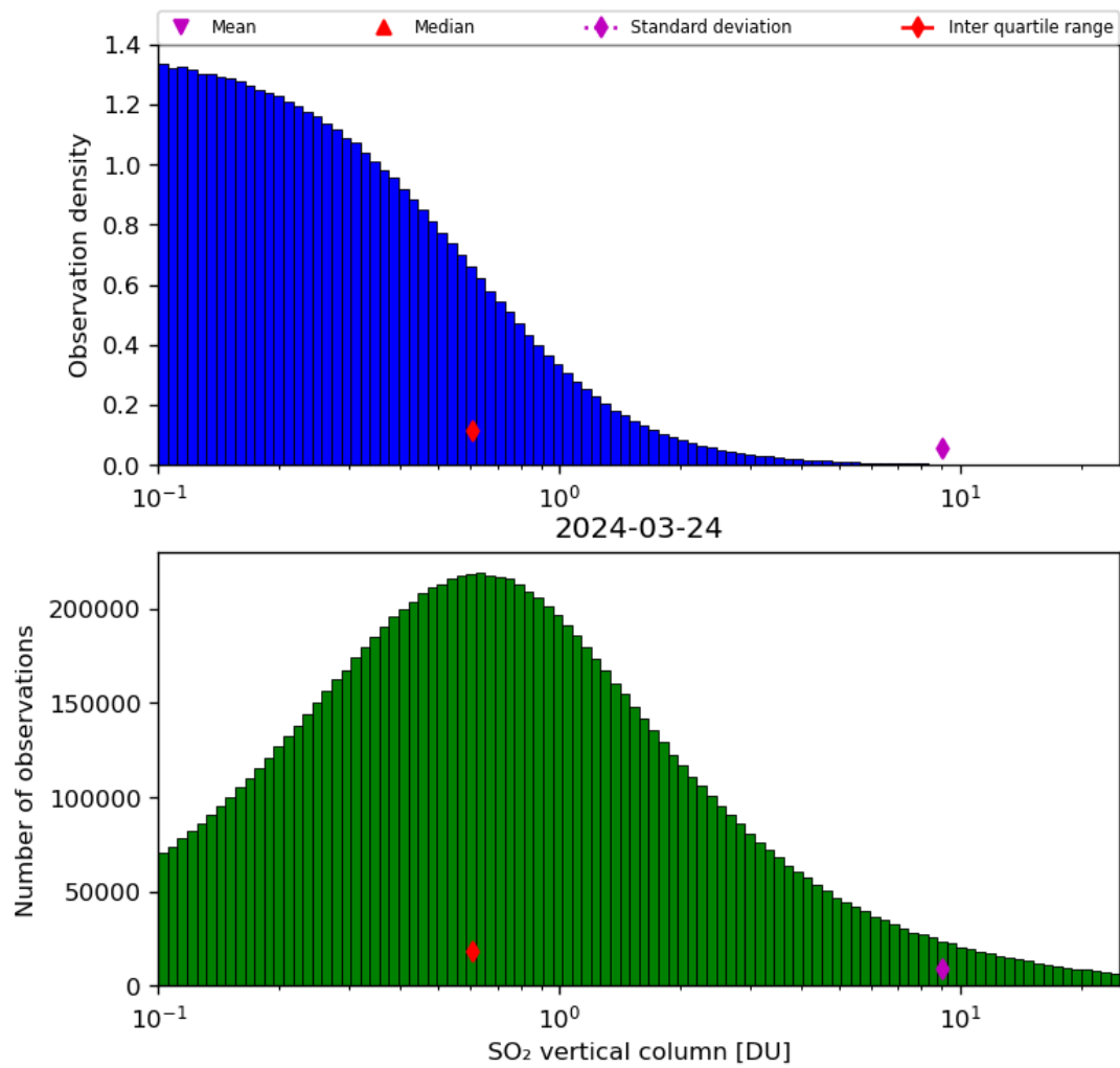
Figure 53: Histogram of “SO 2 vertical column” for 2024-03-23 to 2024-03-25
