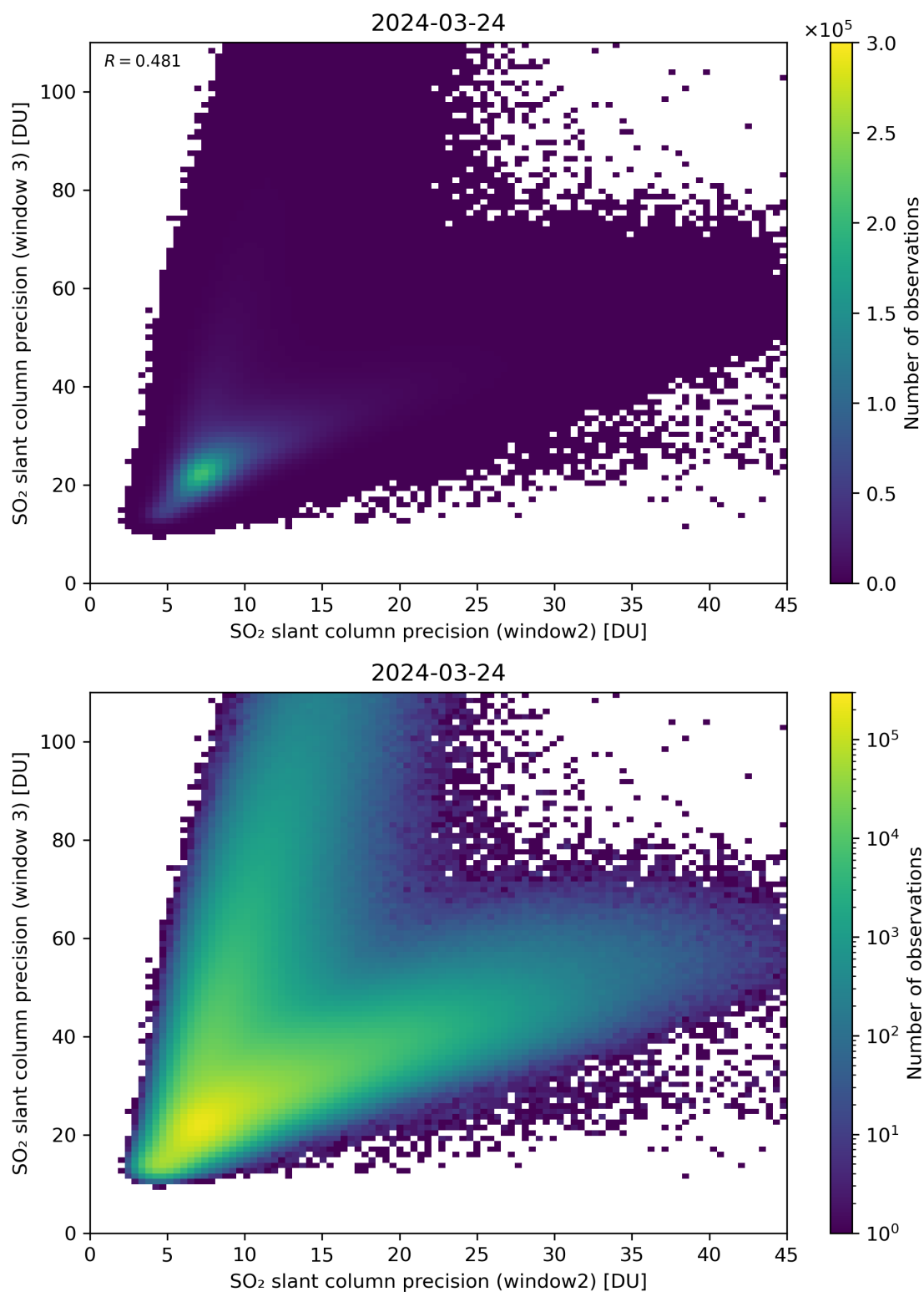
Figure 250: Scatter density plot of “SO 2 slant column precision (window2)” against “SO 2 slant column precision (window 3)” for 2024-03-23 to 2024-03-25.
