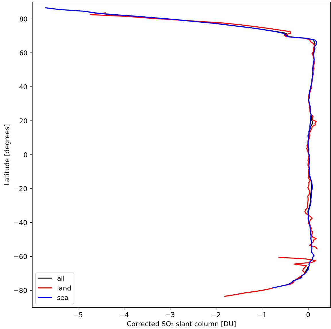
Figure 32: Zonal average of “Corrected SO 2 slant column” for 2024-03-23 to 2024-03-25.
