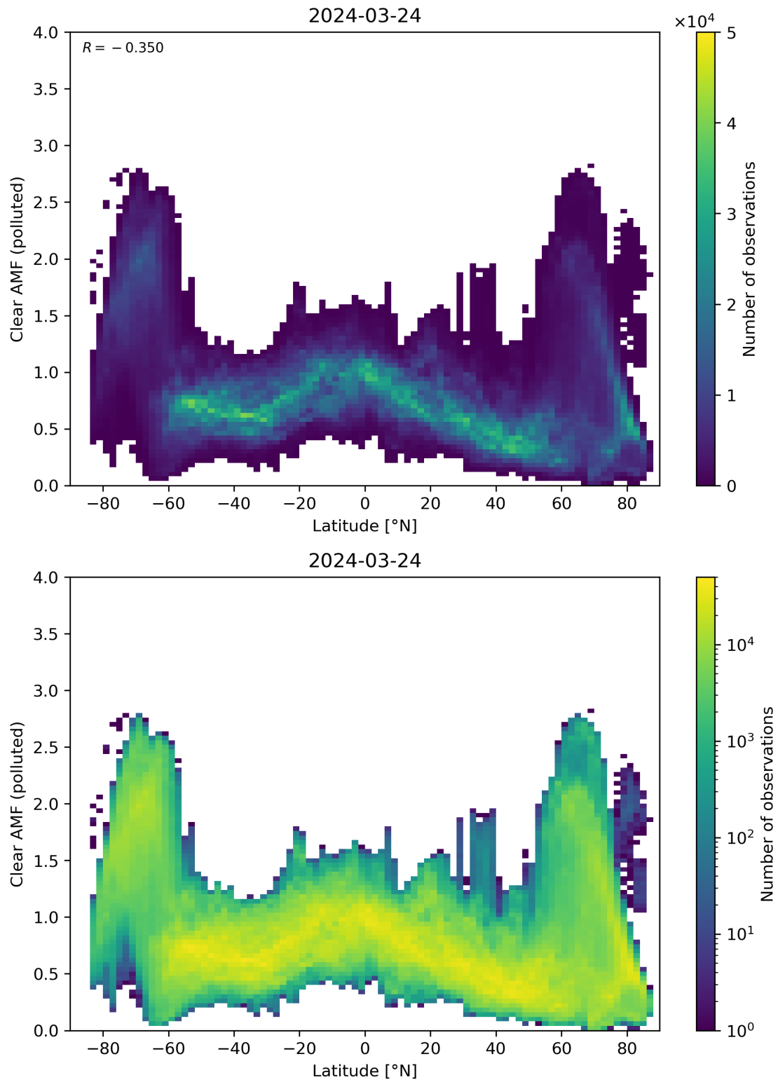
Figure 145: Scatter density plot of “Latitude” against “Clear AMF (polluted)” for 2024-03-23 to 2024-03-25.
