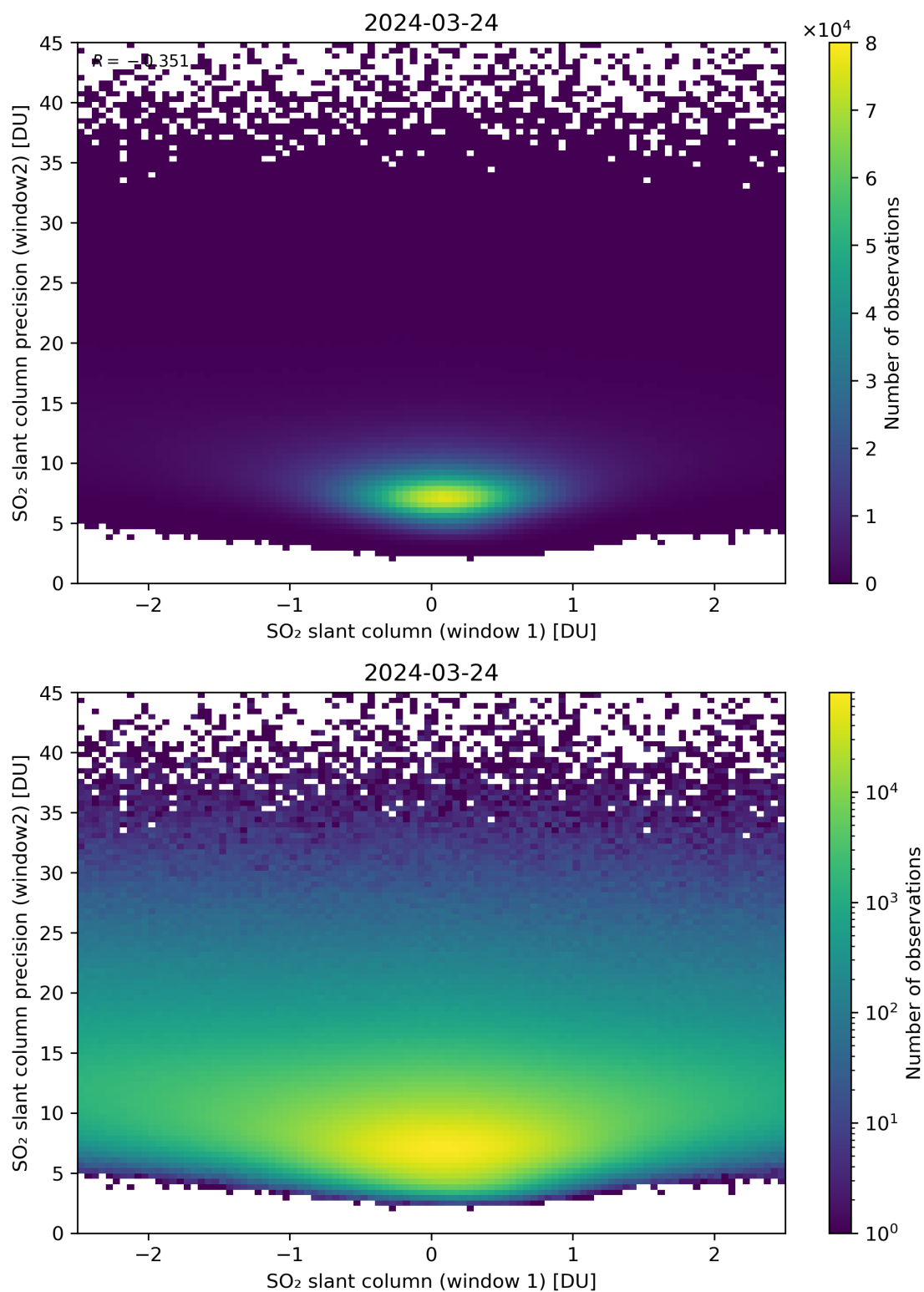
Figure 236: Scatter density plot of “SO 2 slant column (window 1)” against “SO 2 slant column precision (window2)” for 2024-03-23 to 2024-03-25.
