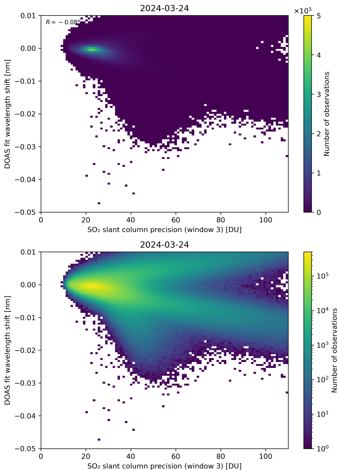
Figure 258: Scatter density plot of “SO 2 slant column precision (window 3)” against “DOAS fit wavelength shift” for 2024-03-23 to 2024-03-25.
