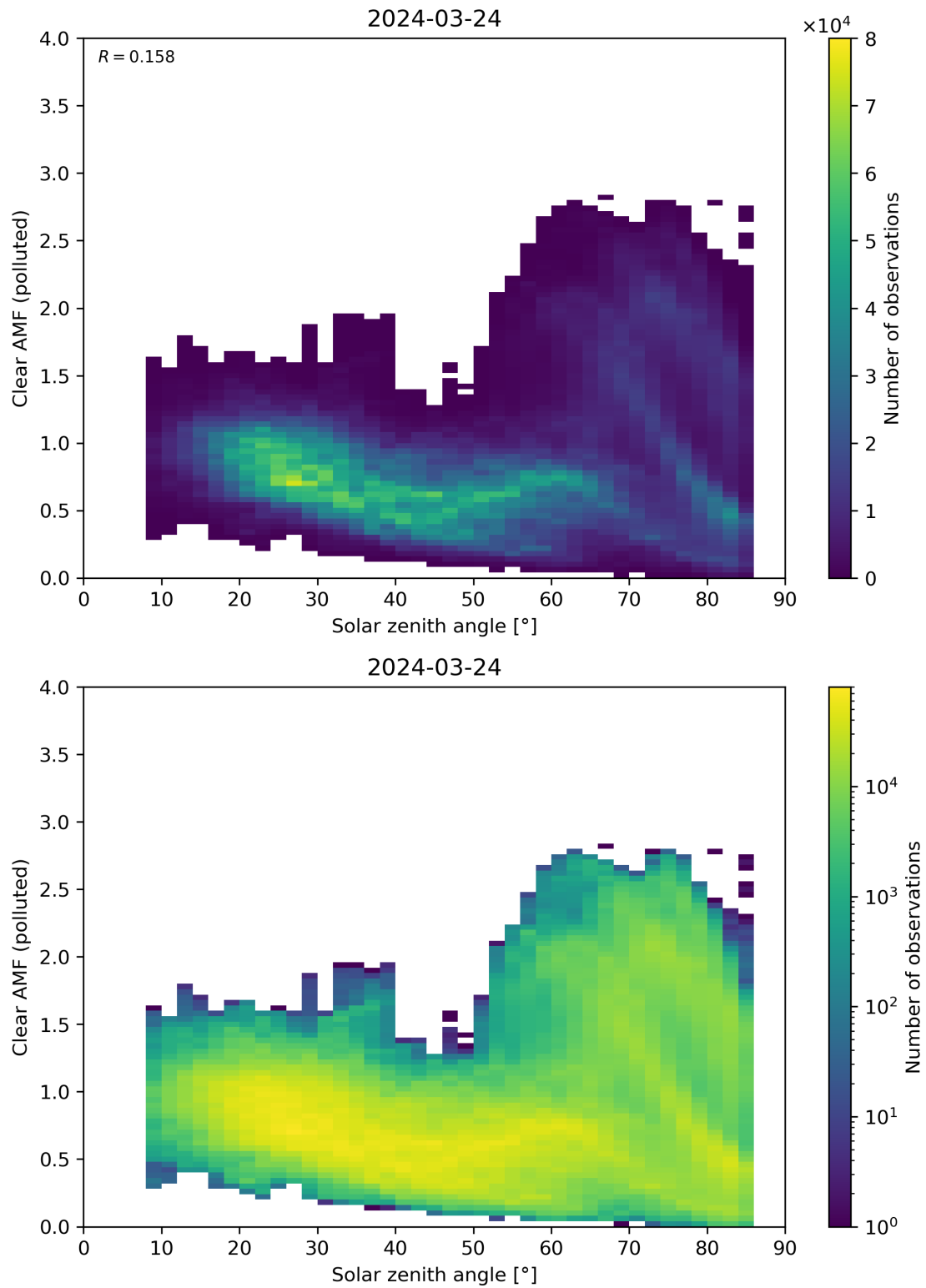
Figure 165: Scatter density plot of “Solar zenith angle” against “Clear AMF (polluted)” for 2024-03-23 to 2024-03-25.
