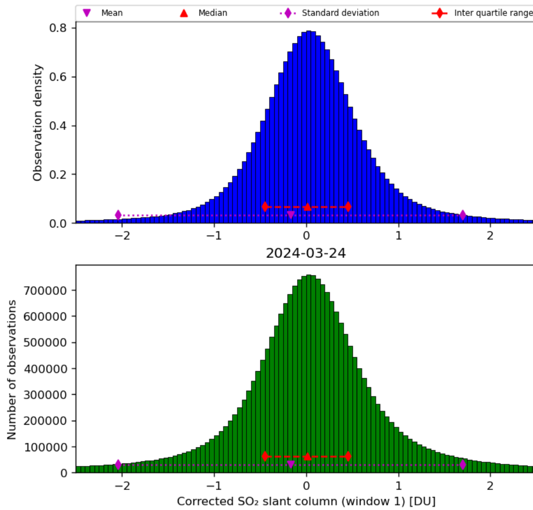
Figure 58: Histogram of “Corrected SO 2 slant column (window 1)” for 2024-03-23 to 2024-03-25
