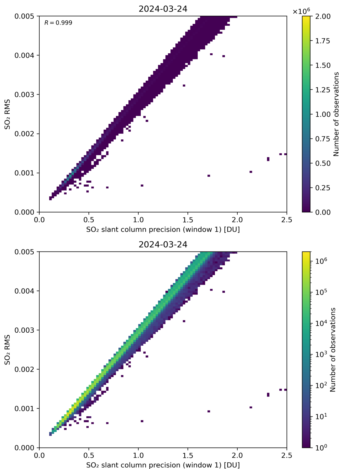
Figure 223: Scatter density plot of “SO 2 slant column precision (window 1)” against “SO 2 RMS” for 2024-03-23 to 2024-03-25.
