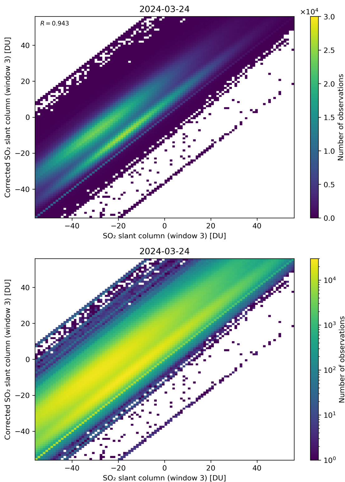
Figure 266: Scatter density plot of “SO 2 slant column (window 3)” against “Corrected SO 2 slant column (window 3)” for 2024-03-23 to 2024-03-25.
