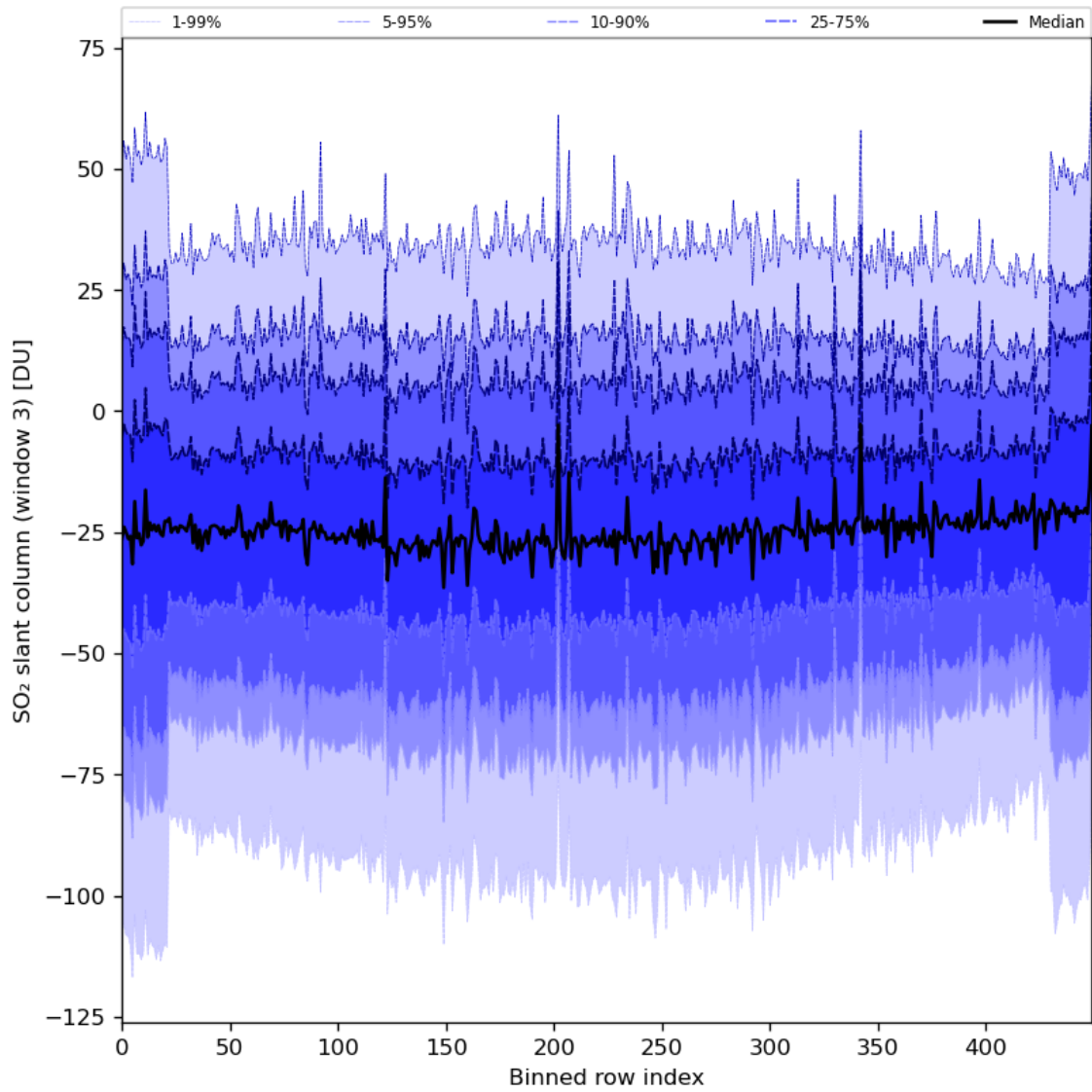
Figure 87: Along track statistics of “SO 2 slant column (window 3)” for 2024-03-23 to 2024-03-25
