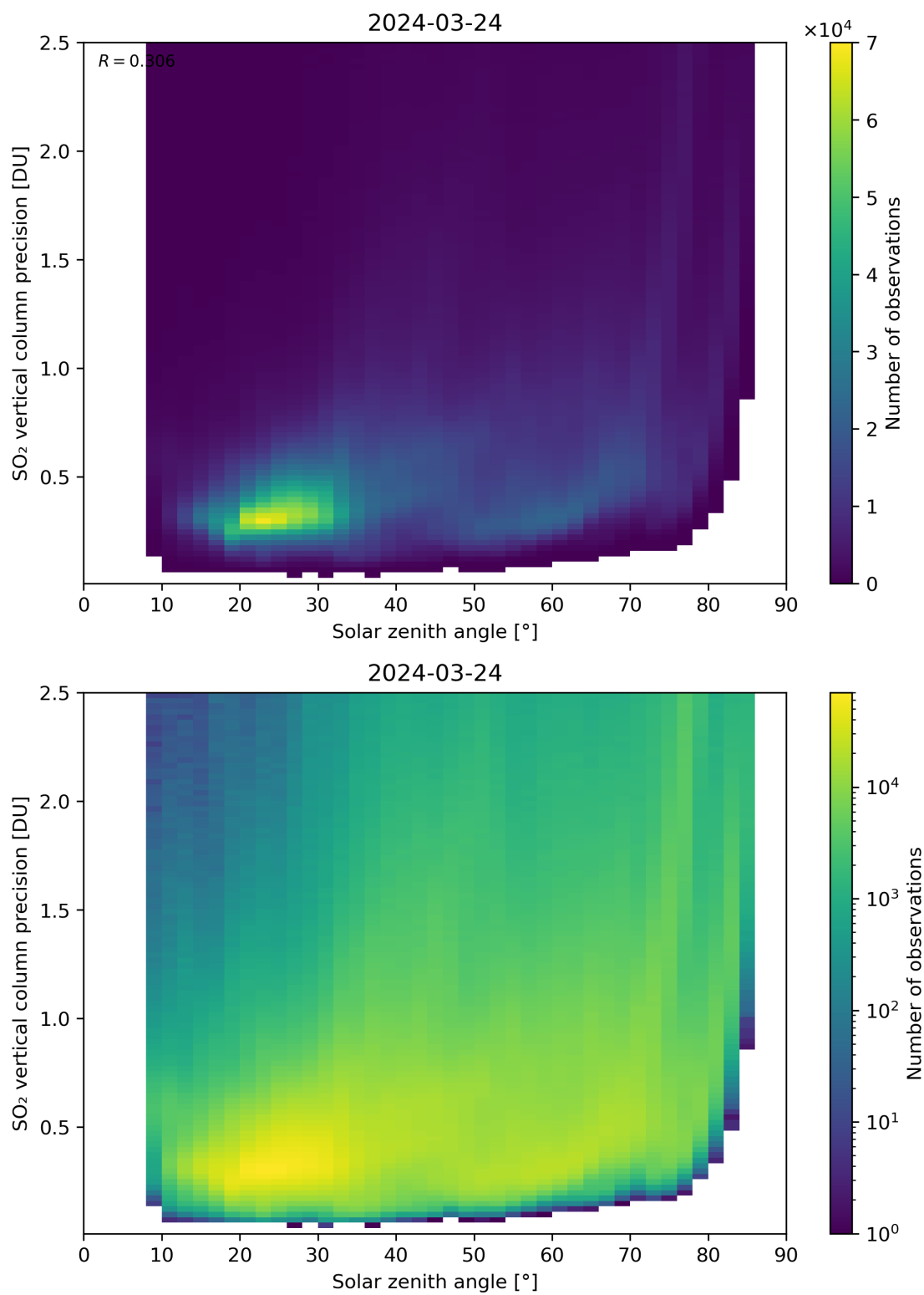
Figure 177: Scatter density plot of “Solar zenith angle” against “SO 2 vertical column precision” for 2024-03-23 to 2024-03-25.
