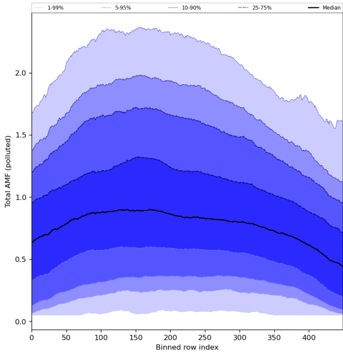
Figure 94: Along track statistics of “Total AMF (polluted)” for 2024-03-23 to 2024-03-25
