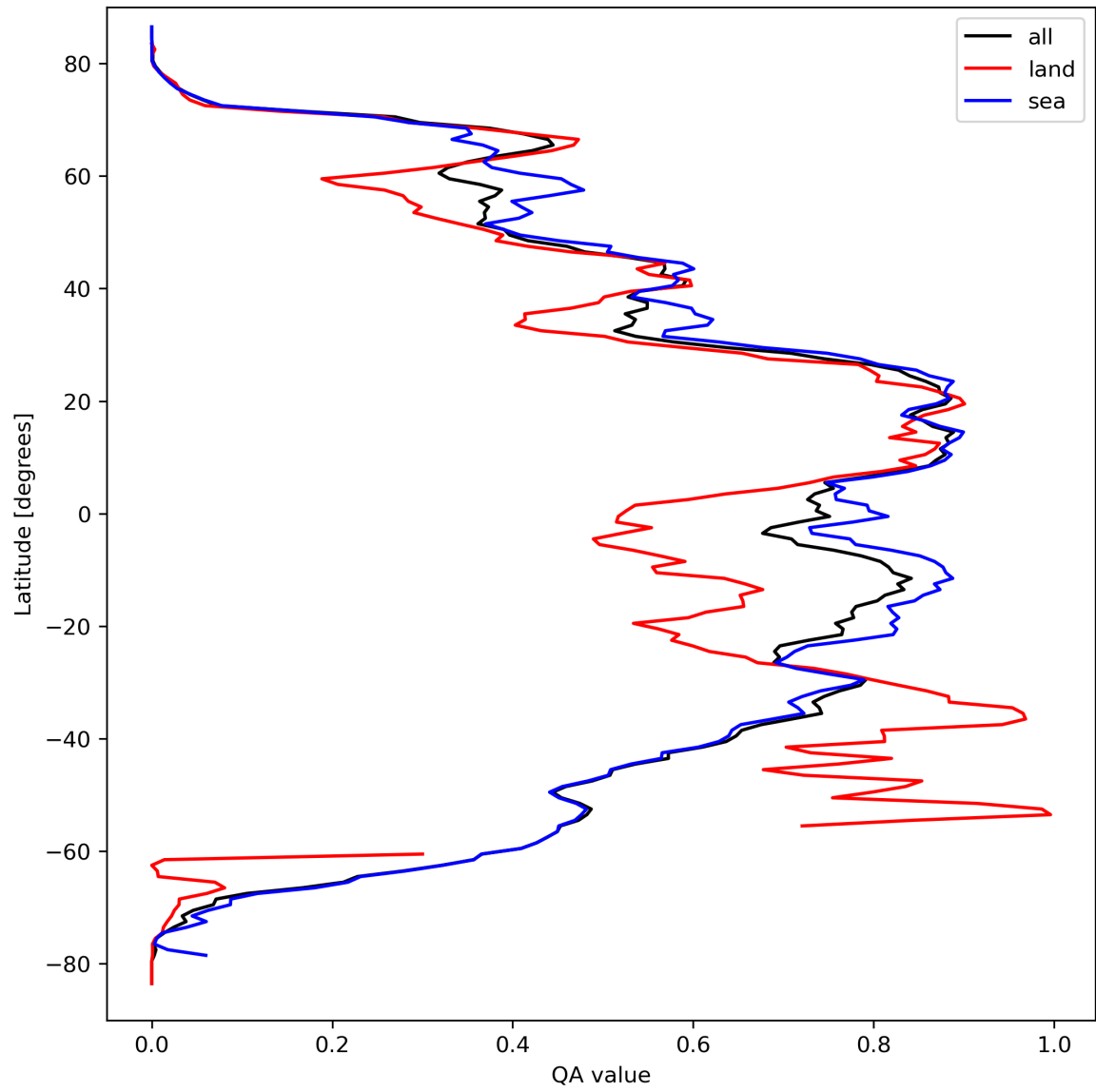
Figure 29: Zonal average of “QA value” for 2024-03-23 to 2024-03-25.
