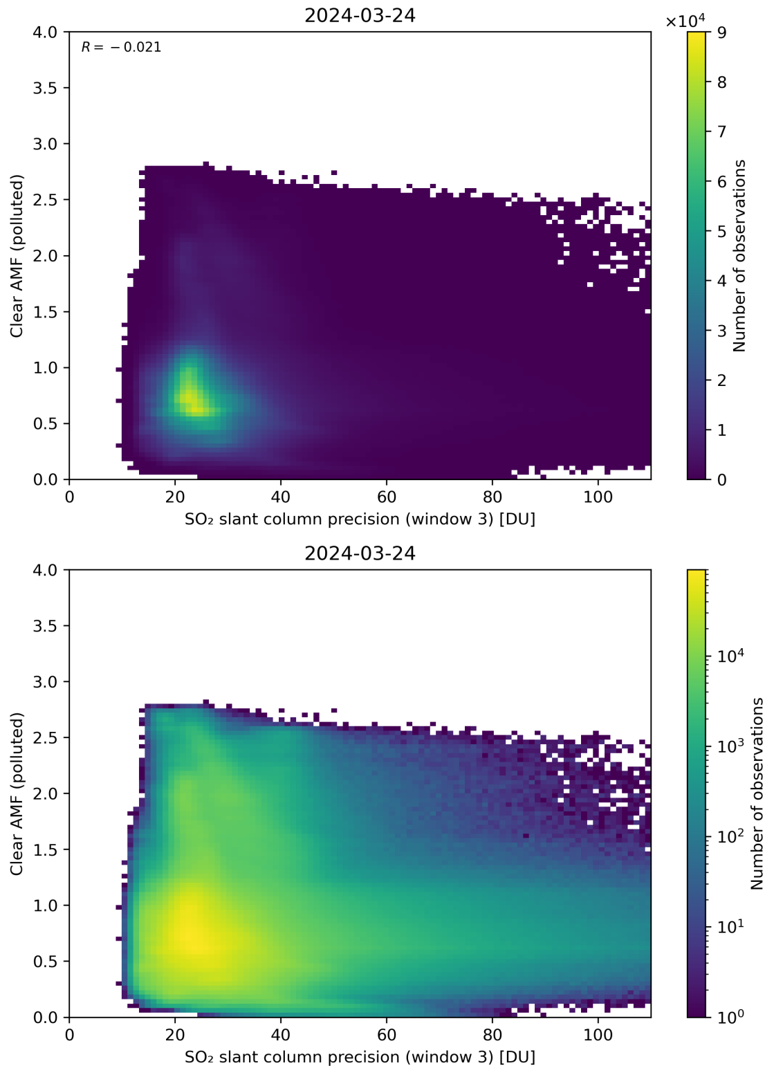
Figure 261: Scatter density plot of “SO 2 slant column precision (window 3)” against “Clear AMF (polluted)” for 2024-03-23 to 2024-03-25.
