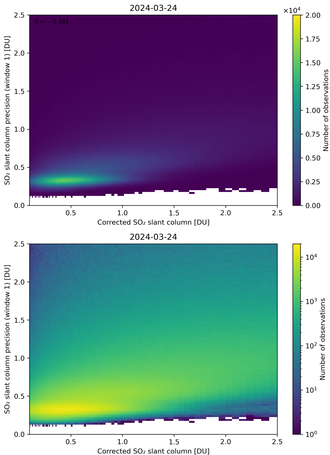
Figure 188: Scatter density plot of “Corrected SO 2 slant column” against “SO 2 slant column precision (window 1)” for 2024-03-23 to 2024-03-25.
