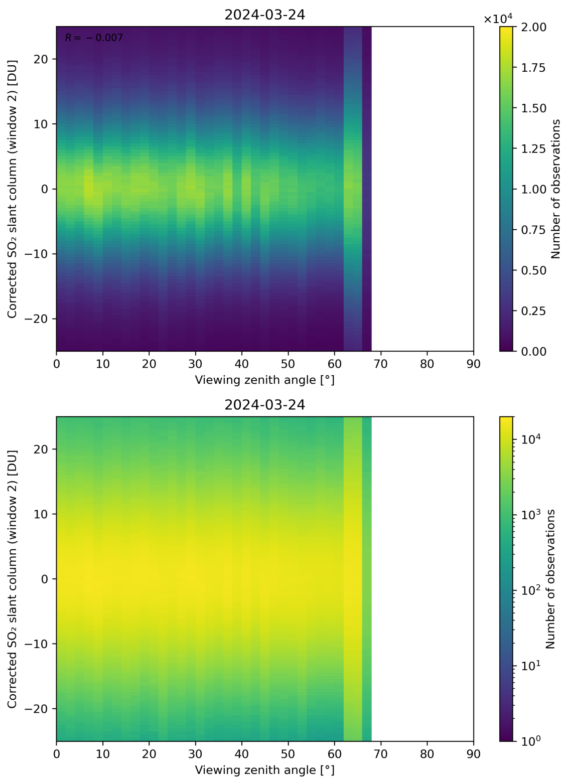
Figure 318: Scatter density plot of “Viewing zenith angle” against “Corrected SO 2 slant column (window 2)” for 2024-03-23 to 2024-03-25.
