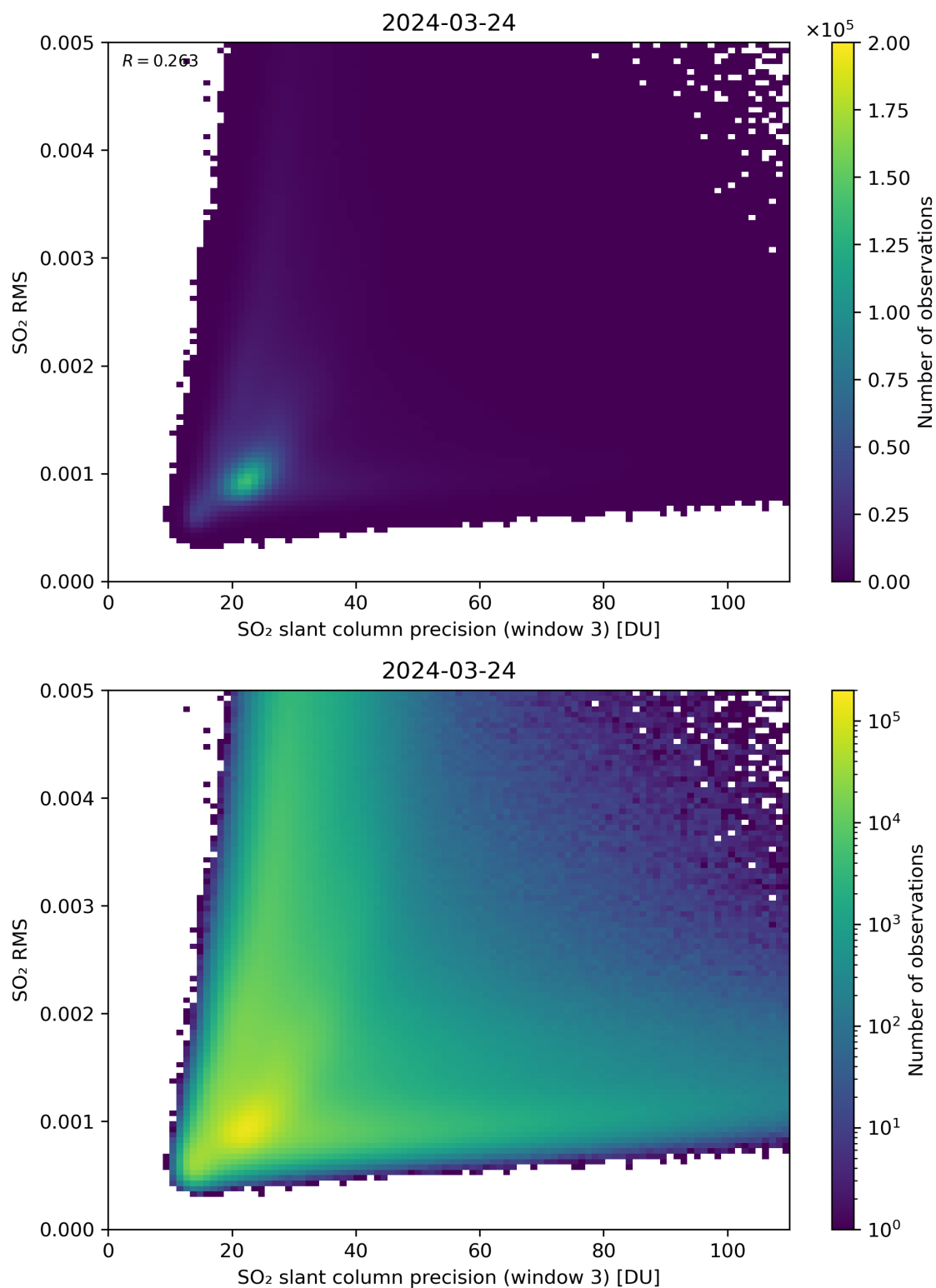
Figure 260: Scatter density plot of “SO 2 slant column precision (window 3)” against “SO 2 RMS” for 2024-03-23 to 2024-03-25.
