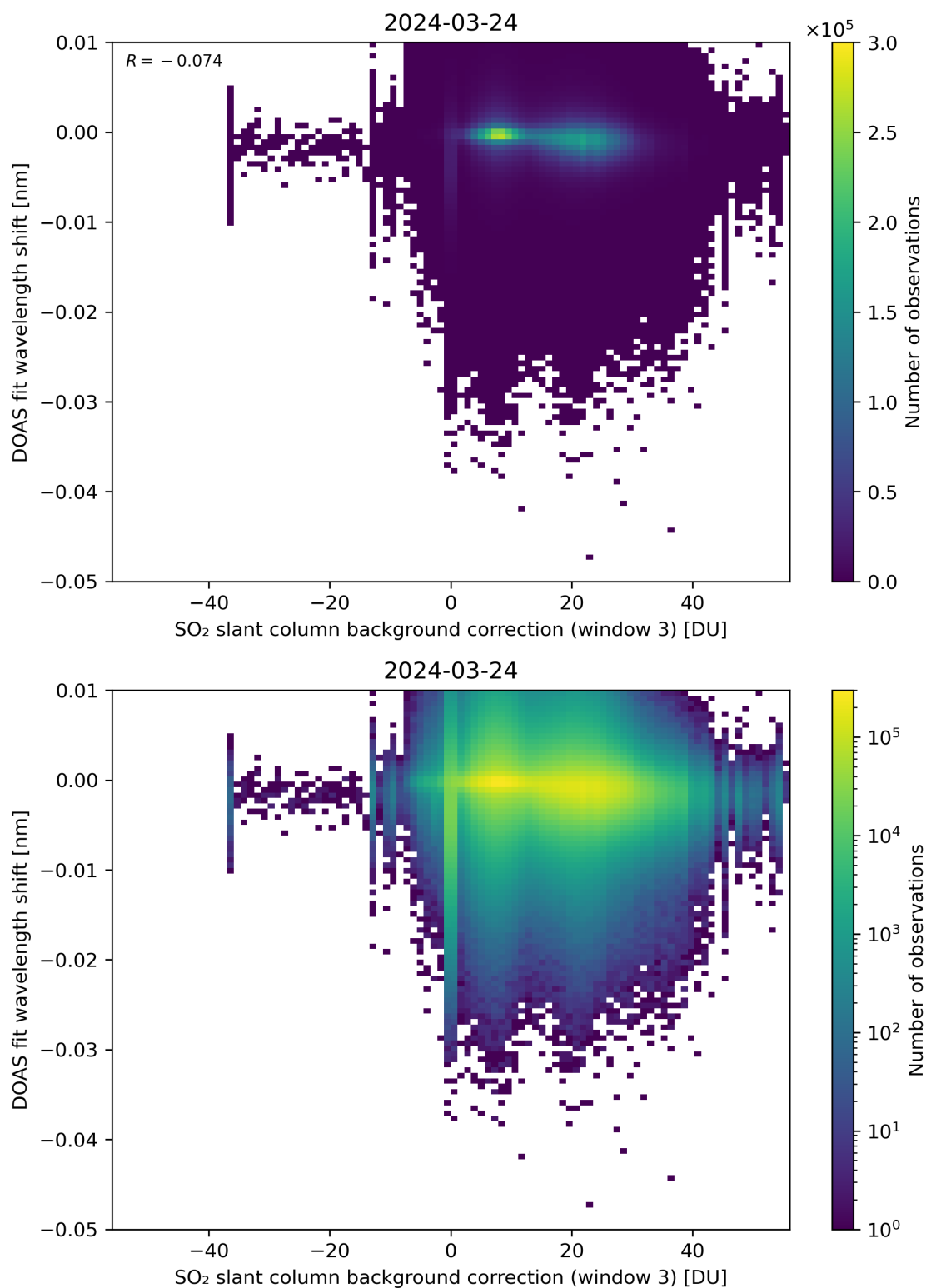
Figure 121: Scatter density plot of “SO 2 slant column background correction (window 3)” against “DOAS fit wavelength shift” for 2024-03-23 to 2024-03-25.
