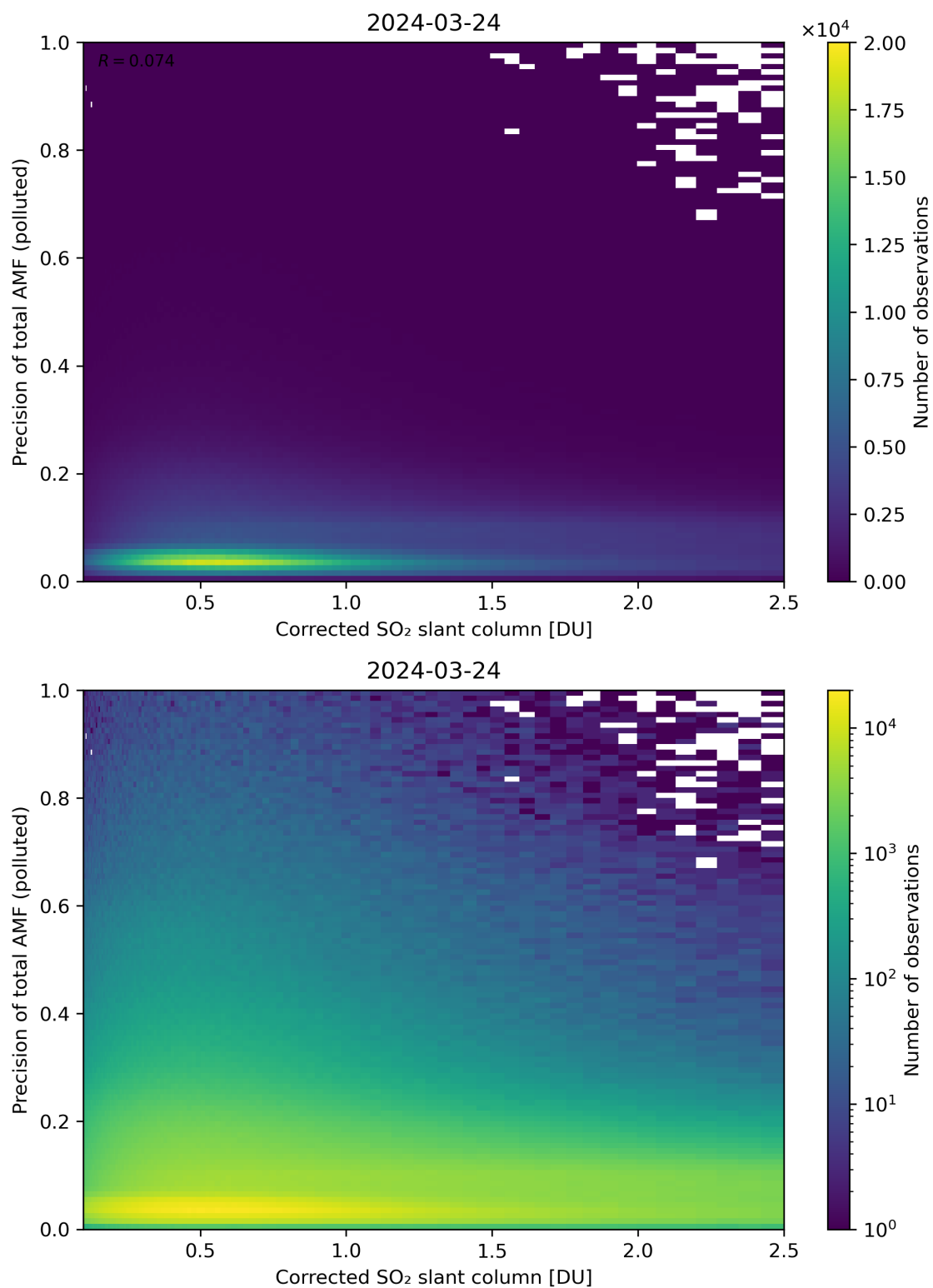
Figure 193: Scatter density plot of “Corrected SO 2 slant column” against “Precision of total AMF (polluted)” for 2024-03-23 to 2024-03-25.
