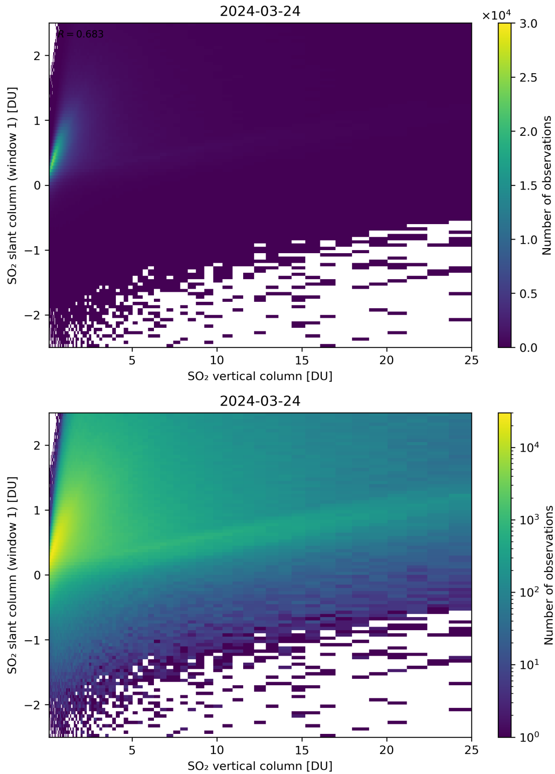
Figure 300: Scatter density plot of “SO 2 vertical column” against “SO 2 slant column (window 1)” for 2024-03-23 to 2024-03-25.
