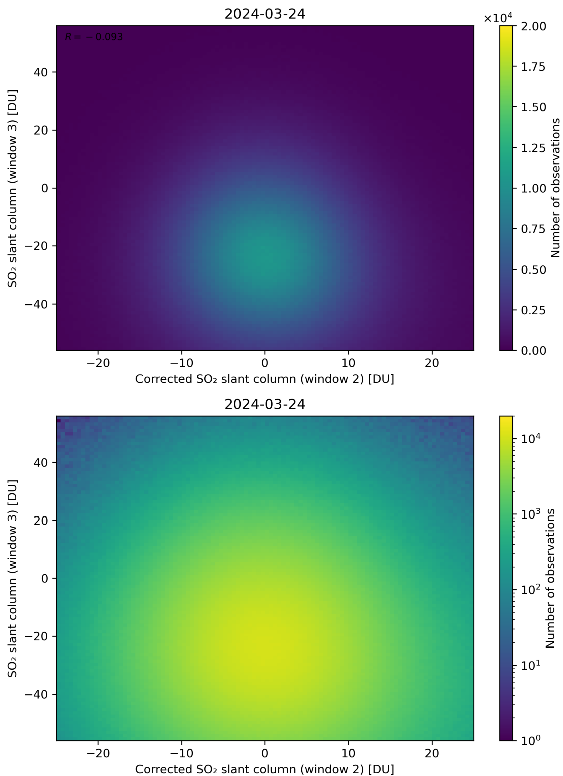
Figure 201: Scatter density plot of “Corrected SO 2 slant column (window 2)” against “SO 2 slant column (window 3)” for 2024-03-23 to 2024-03-25.
