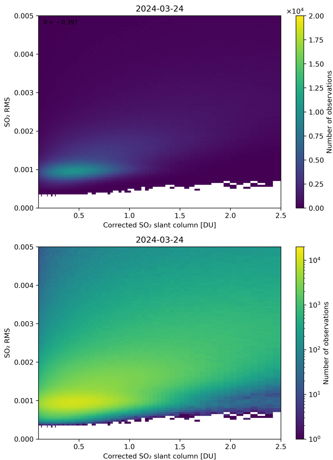
Figure 183: Scatter density plot of “Corrected SO 2 slant column” against “SO 2 RMS” for 2024-03-23 to 2024-03-25.
