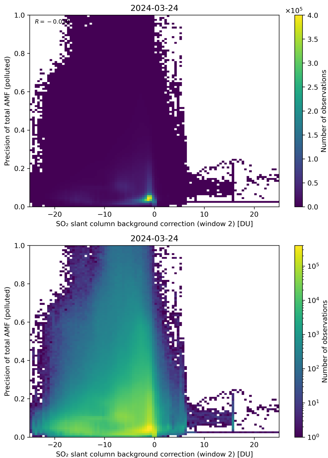
Figure 120: Scatter density plot of “SO 2 slant column background correction (window 2)” against “Precision of total AMF (polluted)” for 2024-03-23 to 2024-03-25.
