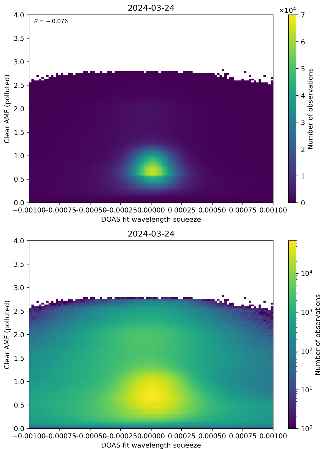
Figure 133: Scatter density plot of “DOAS fit wavelength squeeze” against “Clear AMF (polluted)” for 2024-03-23 to 2024-03-25.
