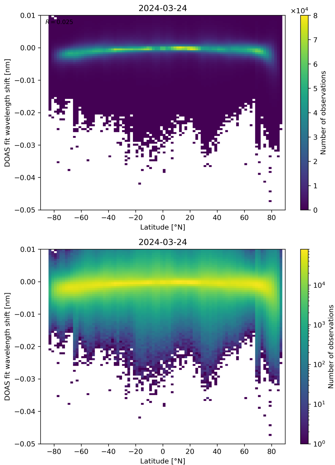
Figure 142: Scatter density plot of “Latitude” against “DOAS fit wavelength shift” for 2024-03-23 to 2024-03-25.
