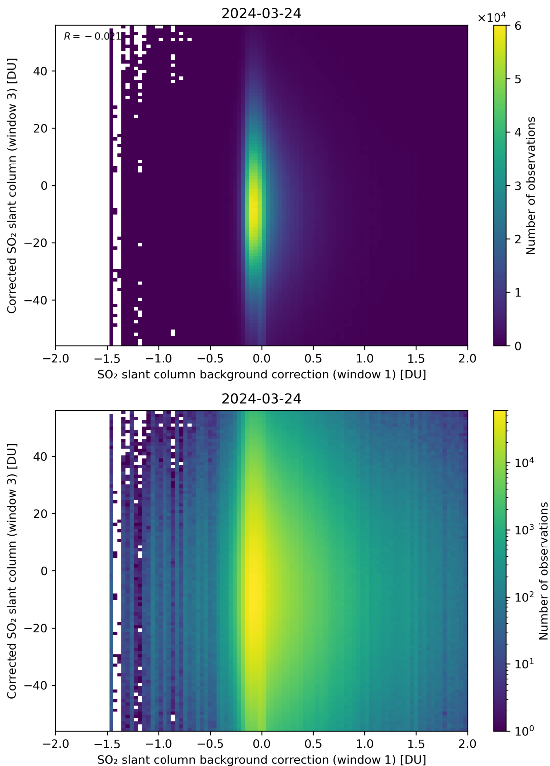
Figure 105: Scatter density plot of “SO 2 slant column background correction (window 1)” against “Corrected SO 2 slant column (window 3)” for 2024-03-23 to 2024-03-25.
