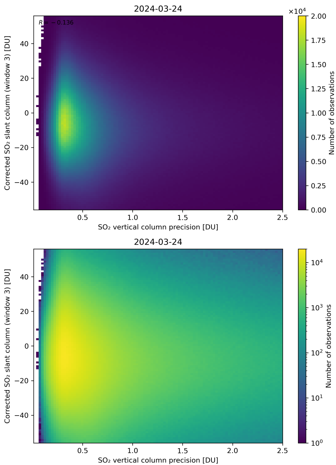
Figure 288: Scatter density plot of “SO 2 vertical column precision” against “Corrected SO 2 slant column (window 3)” for 2024-03-23 to 2024-03-25.
