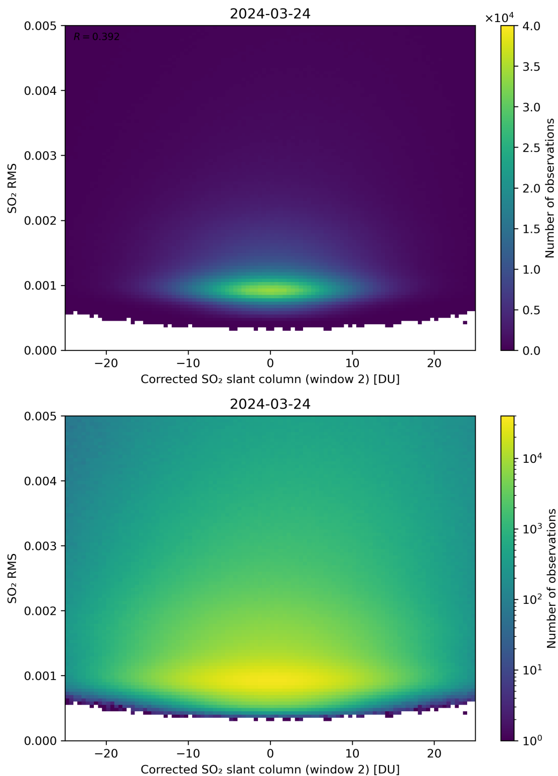
Figure 198: Scatter density plot of “Corrected SO 2 slant column (window 2)” against “SO 2 RMS” for 2024-03-23 to 2024-03-25.
