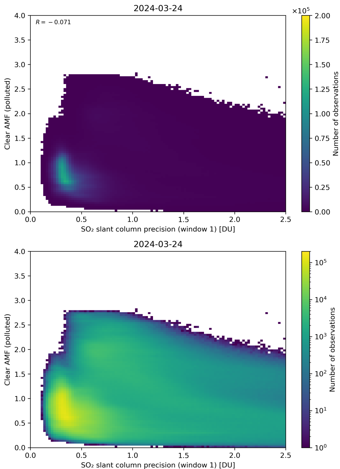
Figure 224: Scatter density plot of “SO 2 slant column precision (window 1)” against “Clear AMF (polluted)” for 2024-03-23 to 2024-03-25.
