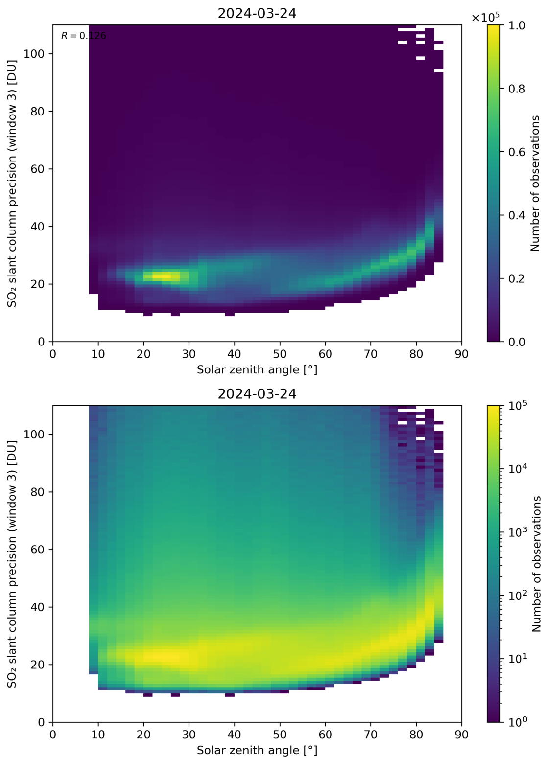
Figure 173: Scatter density plot of “Solar zenith angle” against “SO 2 slant column precision (window 3)” for 2024-03-23 to 2024-03-25.
