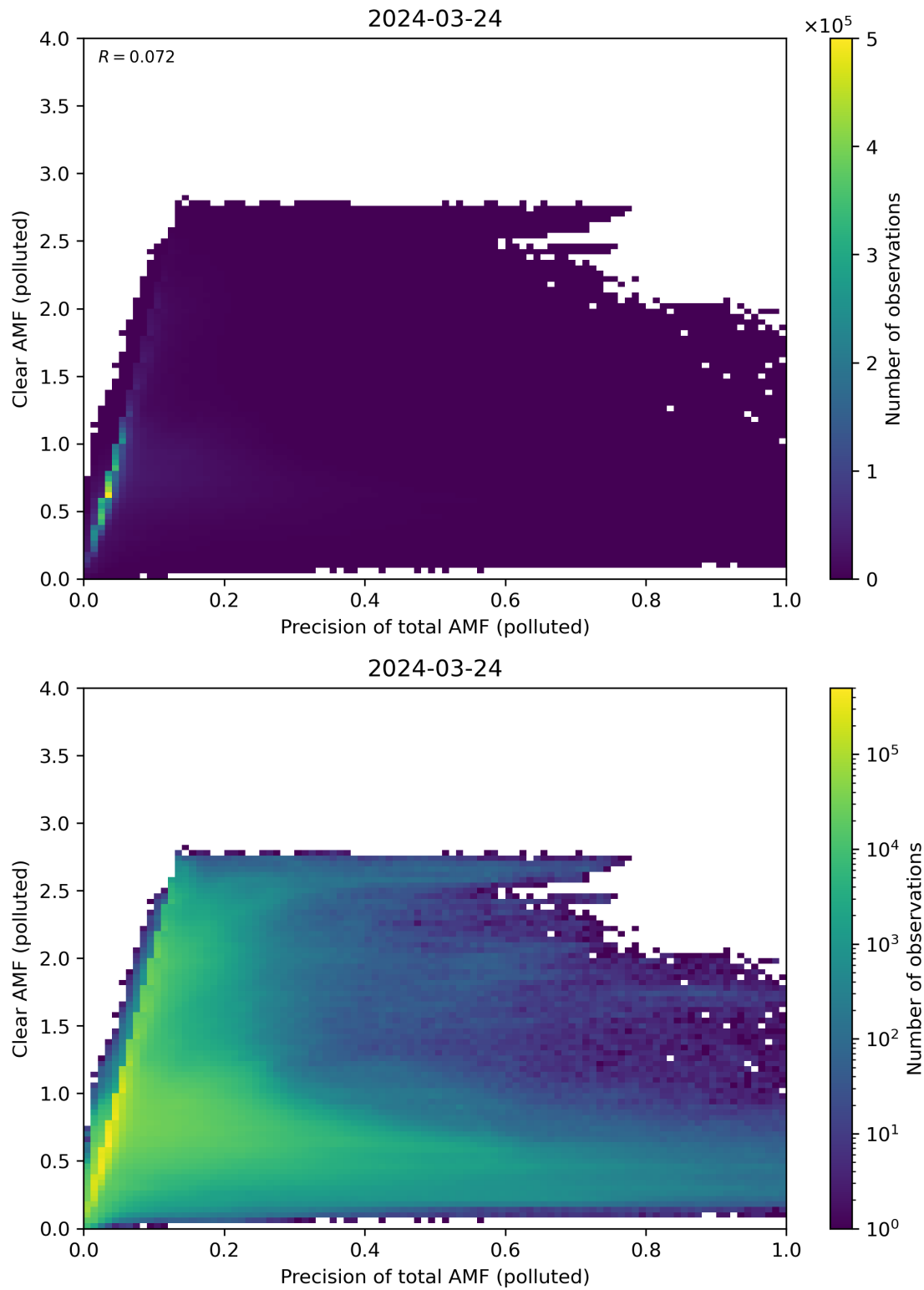
Figure 270: Scatter density plot of “Precision of total AMF (polluted)” against “Clear AMF (polluted)” for 2024-03-23 to 2024-03-25.
