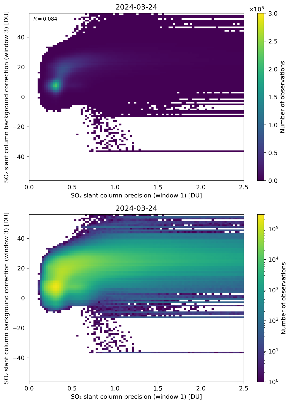
Figure 220: Scatter density plot of “SO 2 slant column precision (window 1)” against “SO 2 slant column background correction (window 3)” for 2024-03-23 to 2024-03-25.
