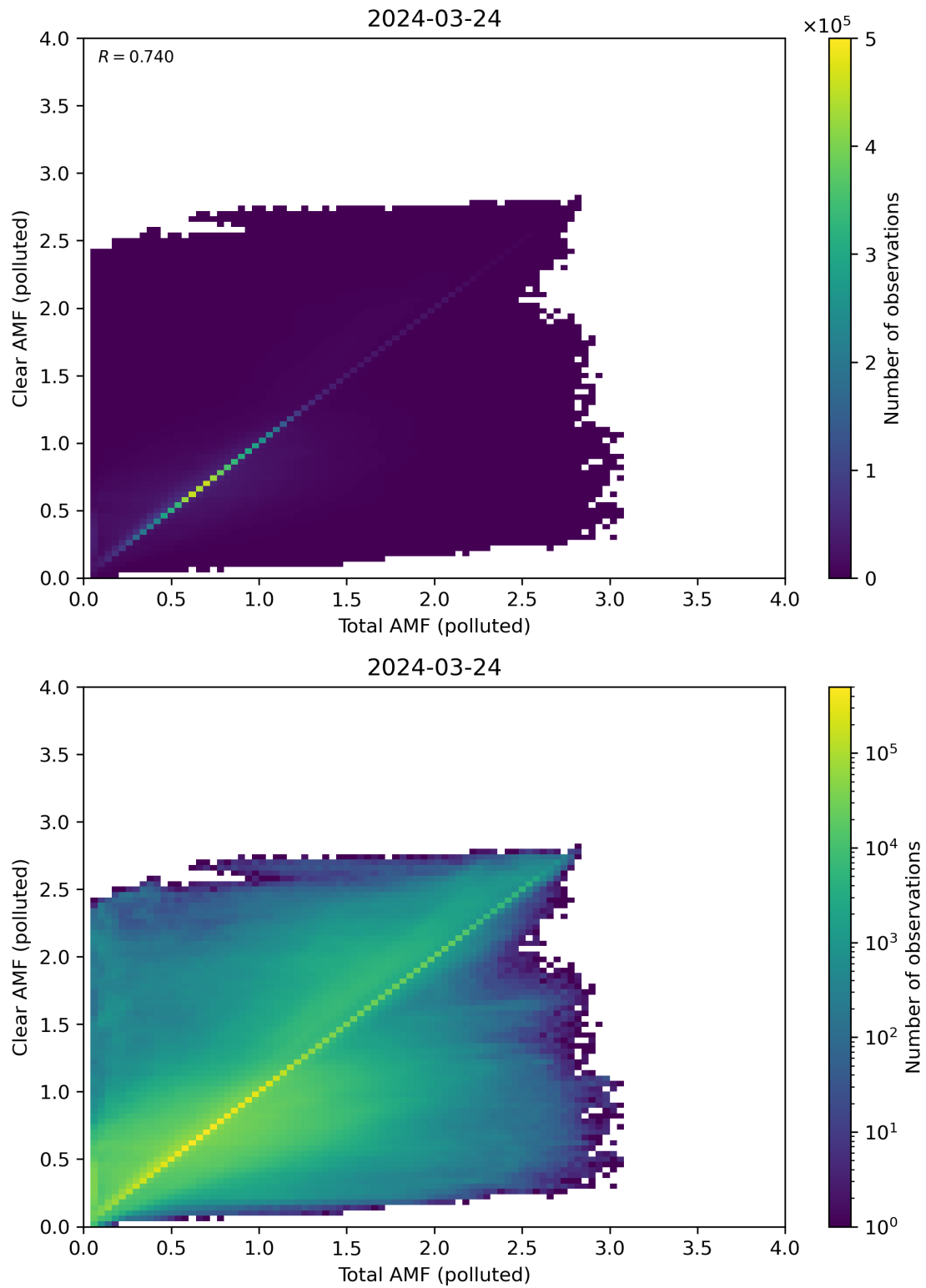
Figure 271: Scatter density plot of “Total AMF (polluted)” against “Clear AMF (polluted)” for 2024-03-23 to 2024-03-25.
