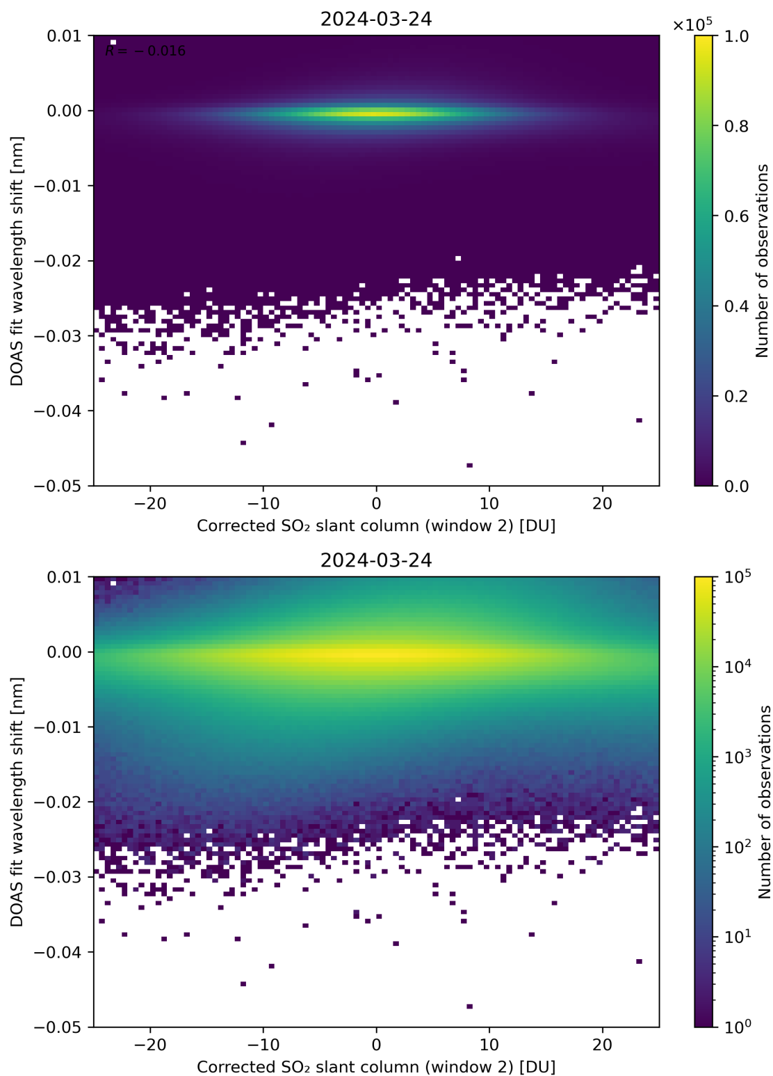
Figure 196: Scatter density plot of “Corrected SO 2 slant column (window 2)” against “DOAS fit wavelength shift” for 2024-03-23 to 2024-03-25.
