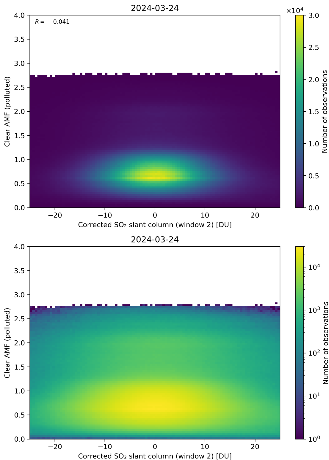
Figure 199: Scatter density plot of “Corrected SO 2 slant column (window 2)” against “Clear AMF (polluted)” for 2024-03-23 to 2024-03-25.
