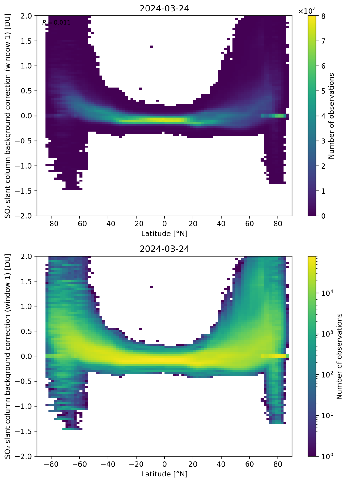
Figure 139: Scatter density plot of “Latitude” against “SO 2 slant column background correction (window 1)” for 2024-03-23 to 2024-03-25.
