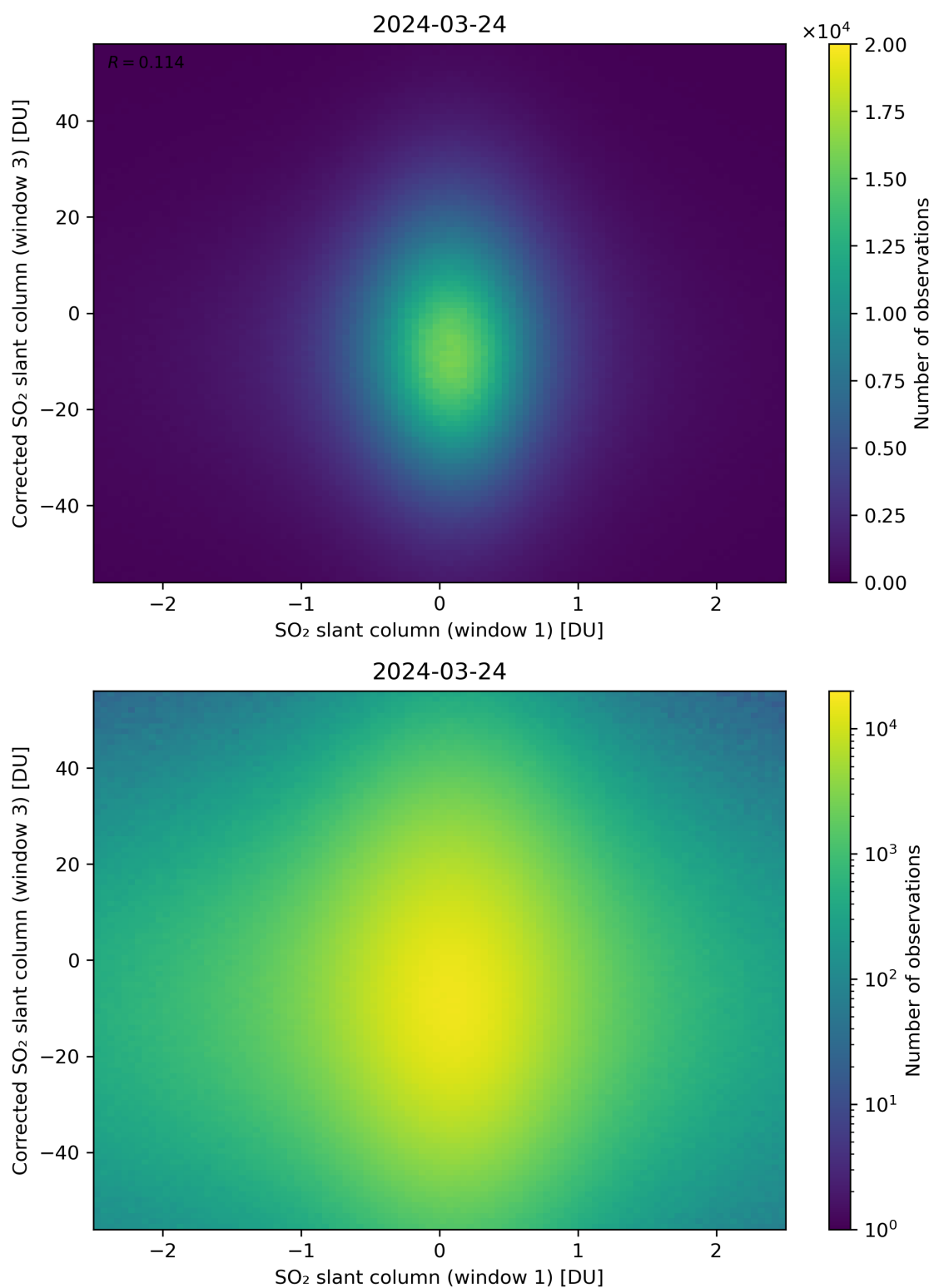
Figure 234: Scatter density plot of “SO 2 slant column (window 1)” against “Corrected SO 2 slant column (window 3)” for 2024-03-23 to 2024-03-25.
