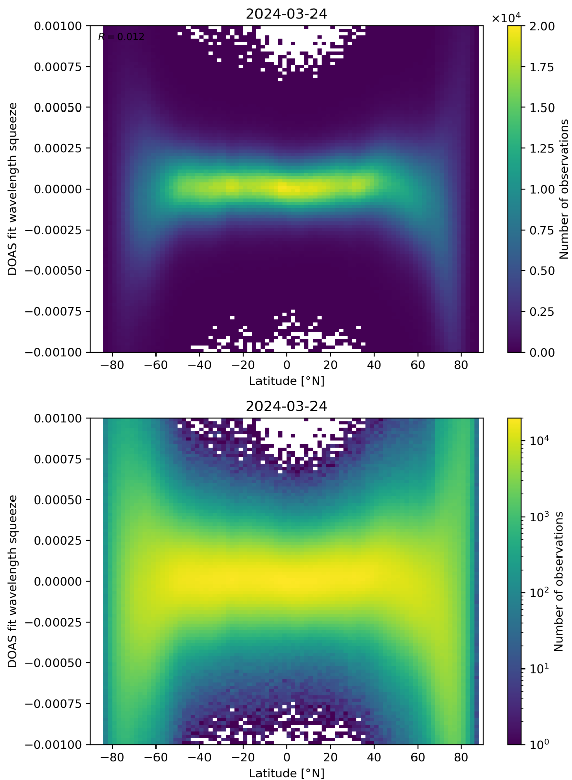
Figure 143: Scatter density plot of “Latitude” against “DOAS fit wavelength squeeze” for 2024-03-23 to 2024-03-25.
