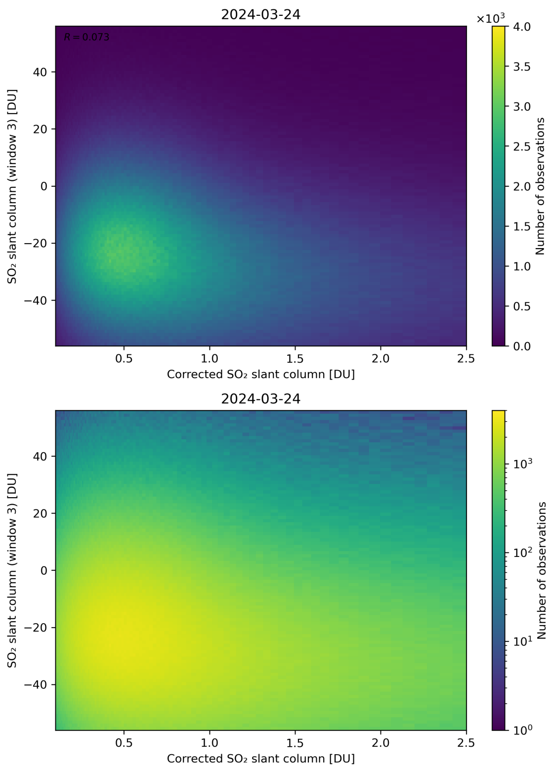
Figure 190: Scatter density plot of “Corrected SO 2 slant column” against “SO 2 slant column (window 3)” for 2024-03-23 to 2024-03-25.
