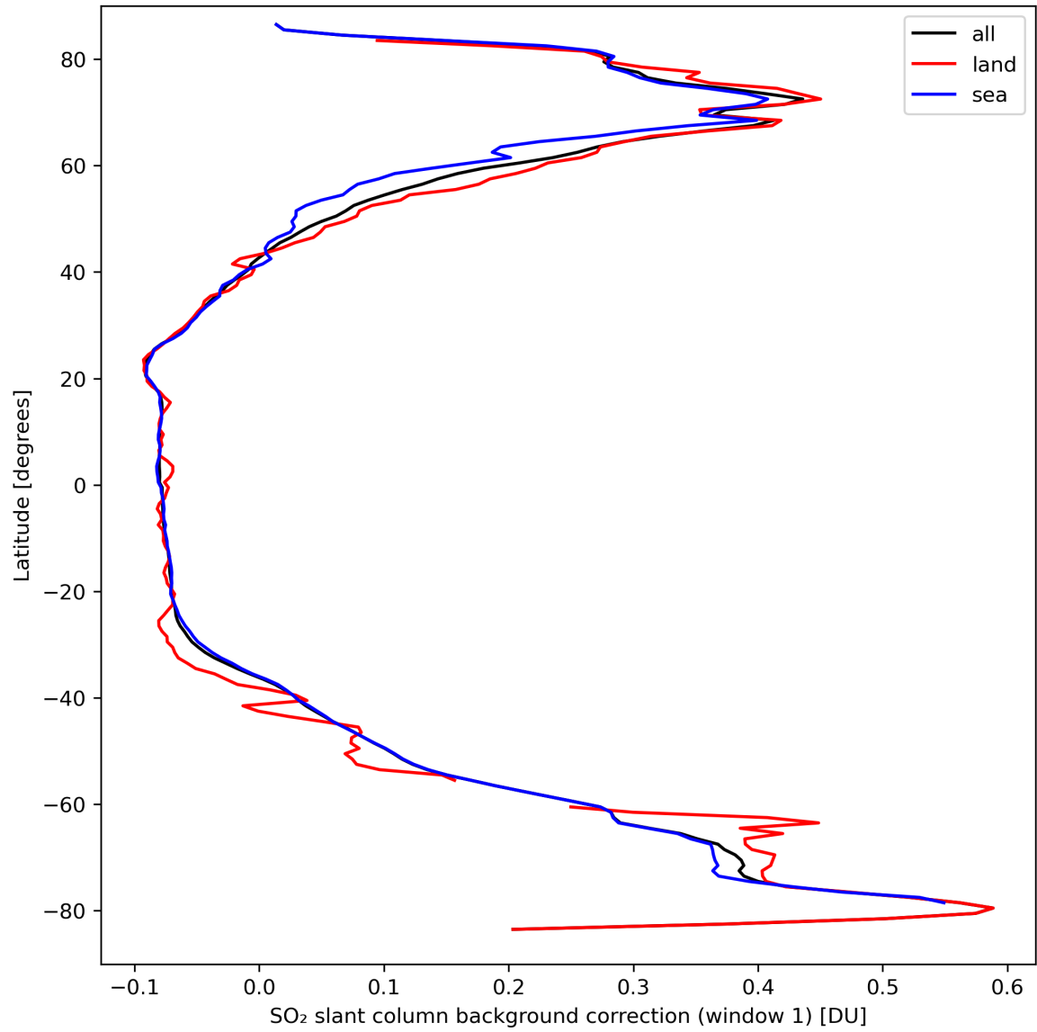
Figure 36: Zonal average of “SO 2 slant column background correction (window 1)” for 2024-03-23 to 2024-03-25.
