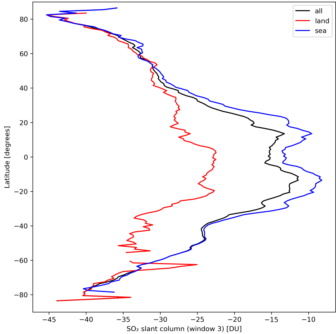
Figure 41: Zonal average of “SO 2 slant column (window 3)” for 2024-03-23 to 2024-03-25.
