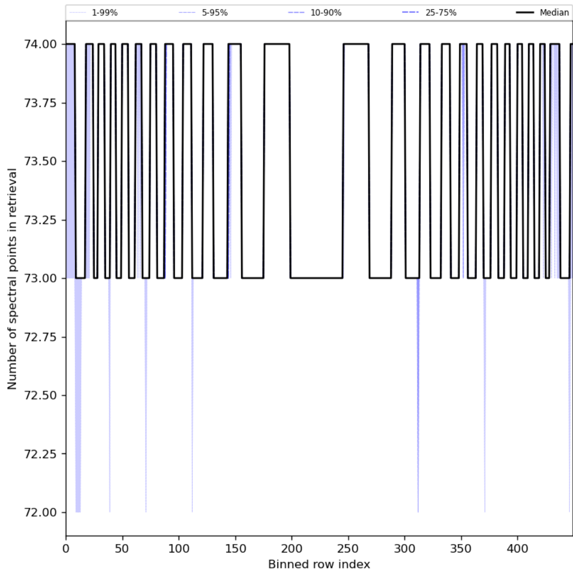
Figure 97: Along track statistics of “Number of spectral points in retrieval” for 2024-03-23 to 2024-03-25
