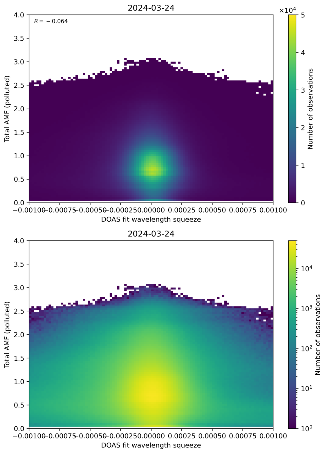
Figure 134: Scatter density plot of “DOAS fit wavelength squeeze” against “Total AMF (polluted)” for 2024-03-23 to 2024-03-25.
