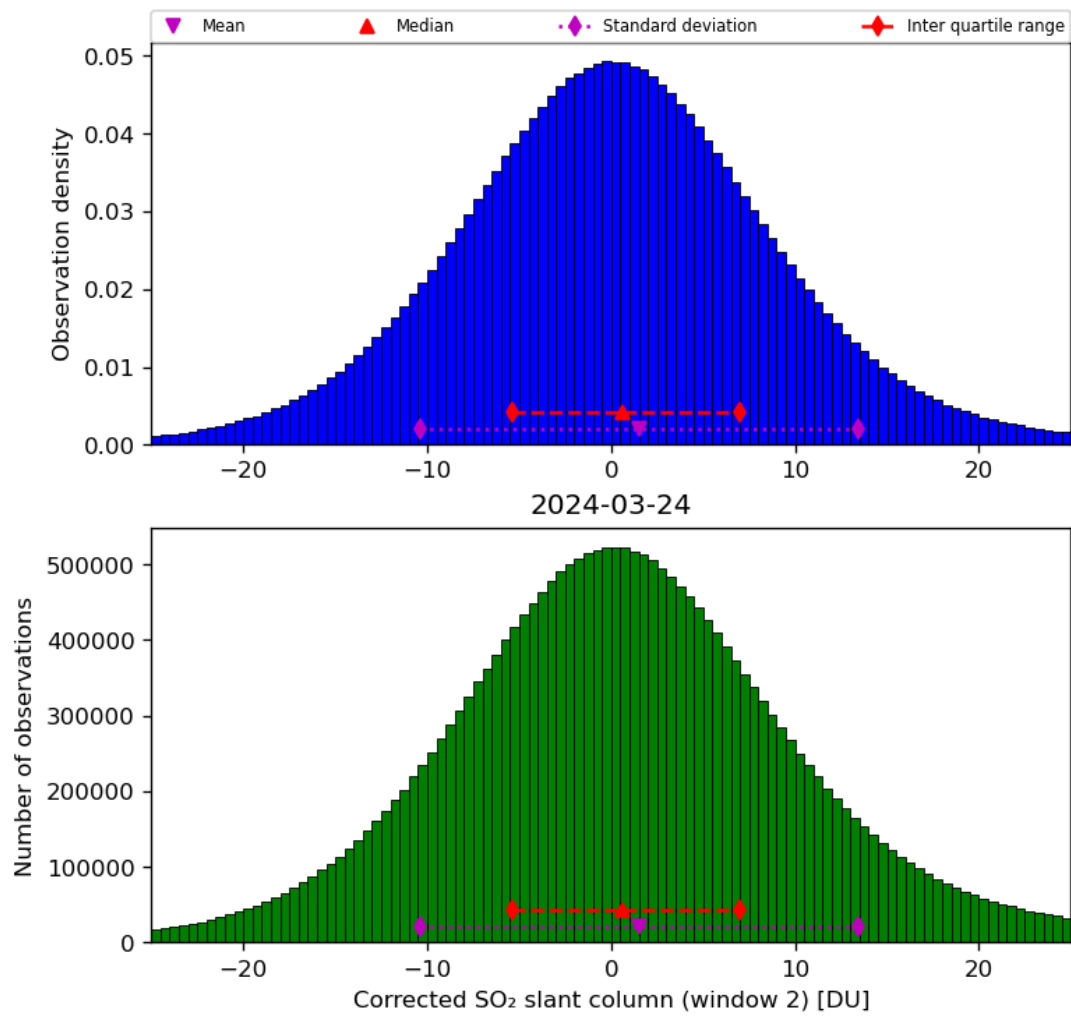
Figure 62: Histogram of “Corrected SO 2 slant column (window 2)” for 2024-03-23 to 2024-03-25
