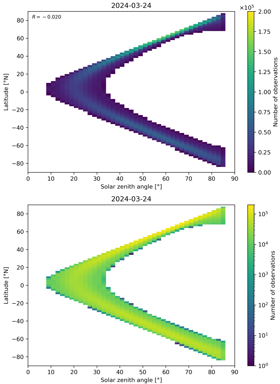
Figure 164: Scatter density plot of “Solar zenith angle” against “Latitude” for 2024-03-23 to 2024-03-25.
