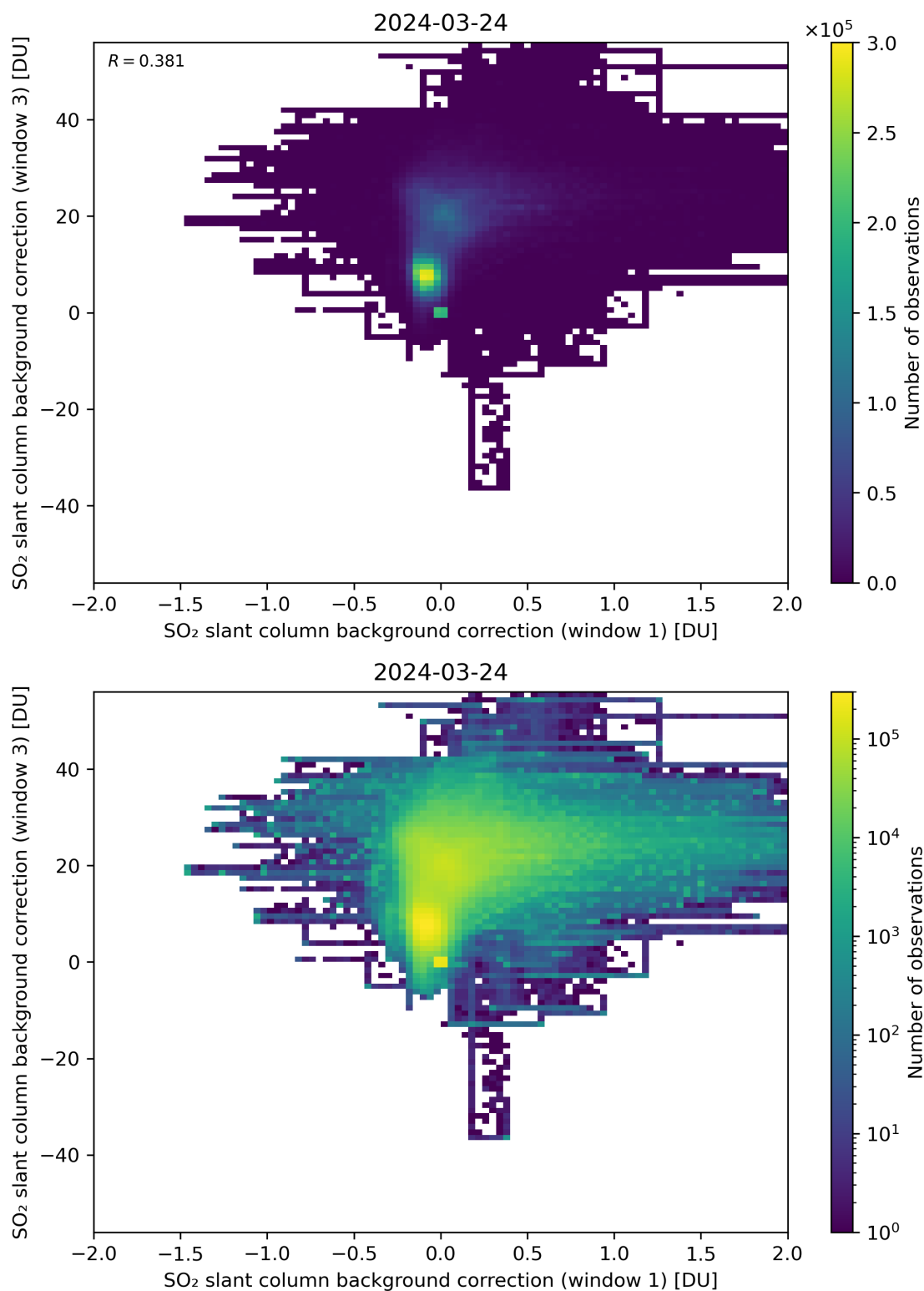
Figure 99: Scatter density plot of “SO 2 slant column background correction (window 1)” against “SO 2 slant column background correction (window 3)” for 2024-03-23 to 2024-03-25.
