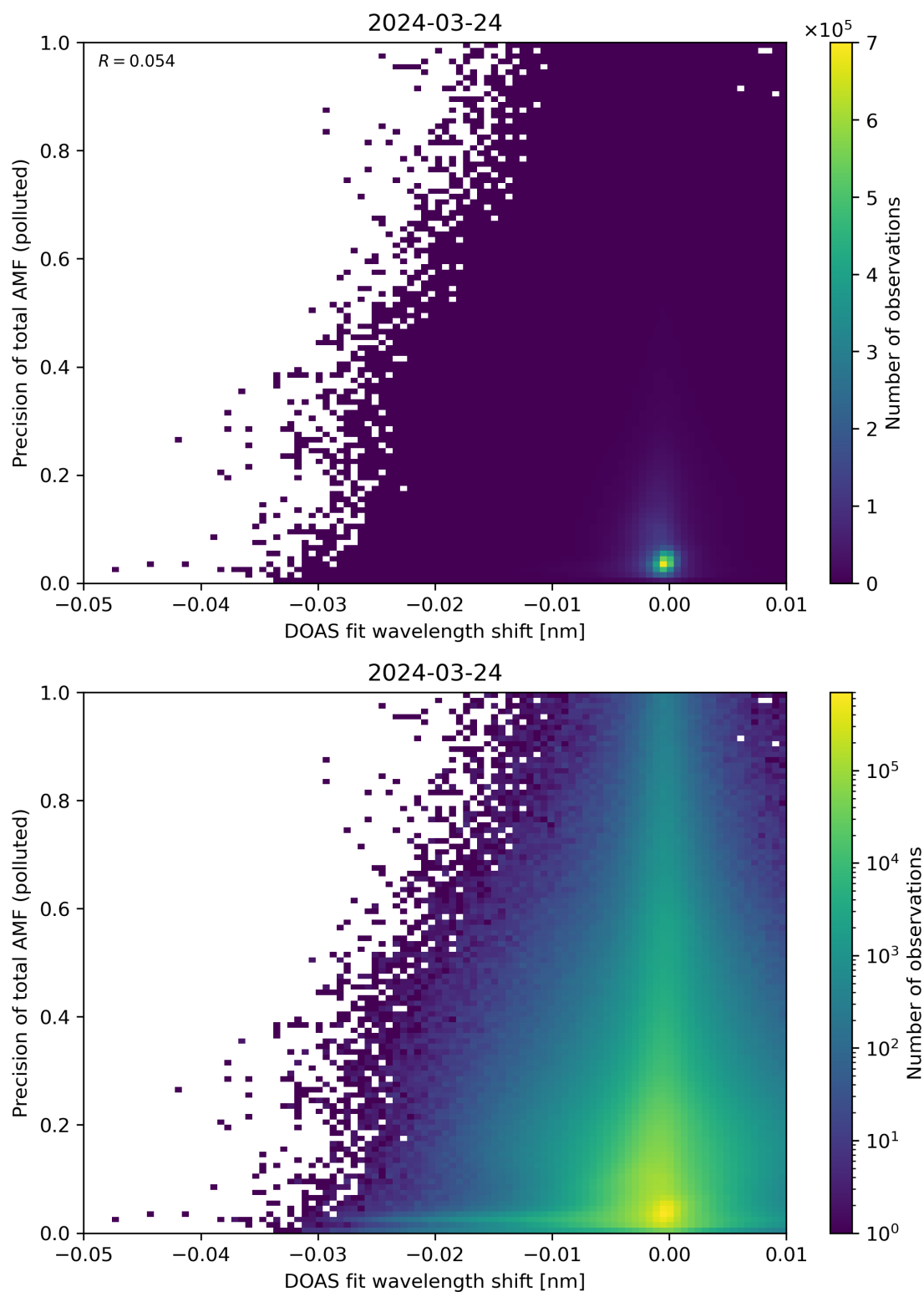
Figure 131: Scatter density plot of “DOAS fit wavelength shift” against “Precision of total AMF (polluted)” for 2024-03-23 to 2024-03-25.
