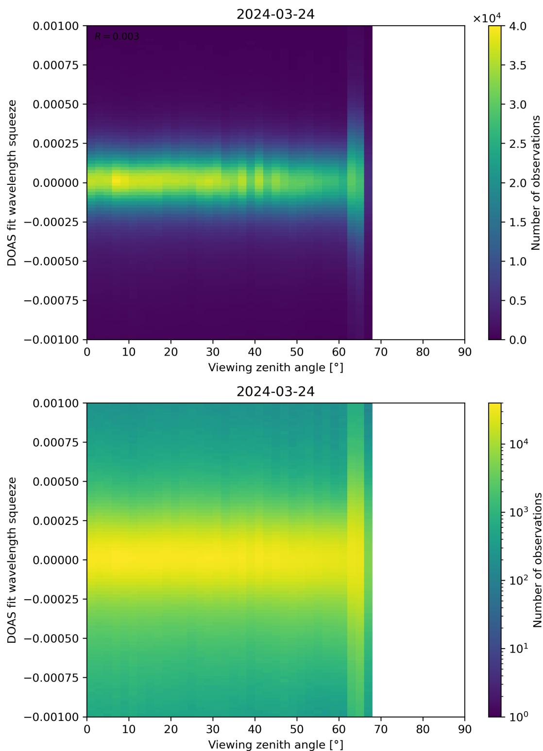
Figure 312: Scatter density plot of “Viewing zenith angle” against “DOAS fit wavelength squeeze” for 2024-03-23 to 2024-03-25.
