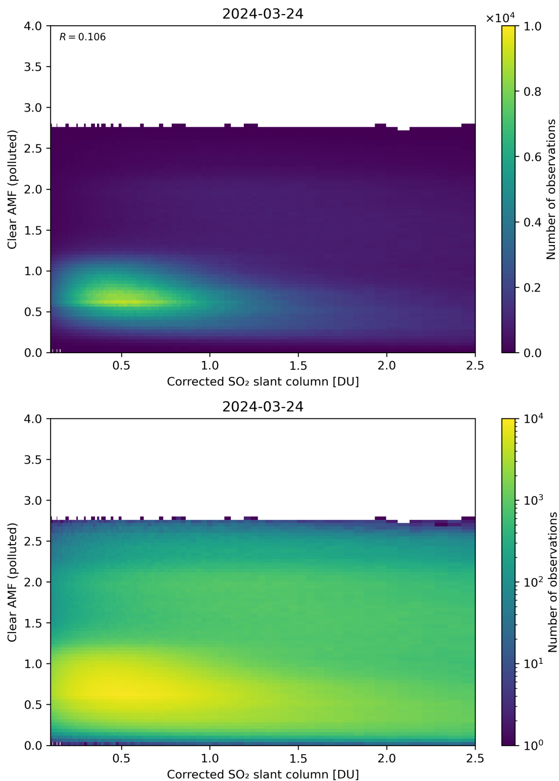
Figure 184: Scatter density plot of “Corrected SO 2 slant column” against “Clear AMF (polluted)” for 2024-03-23 to 2024-03-25.
