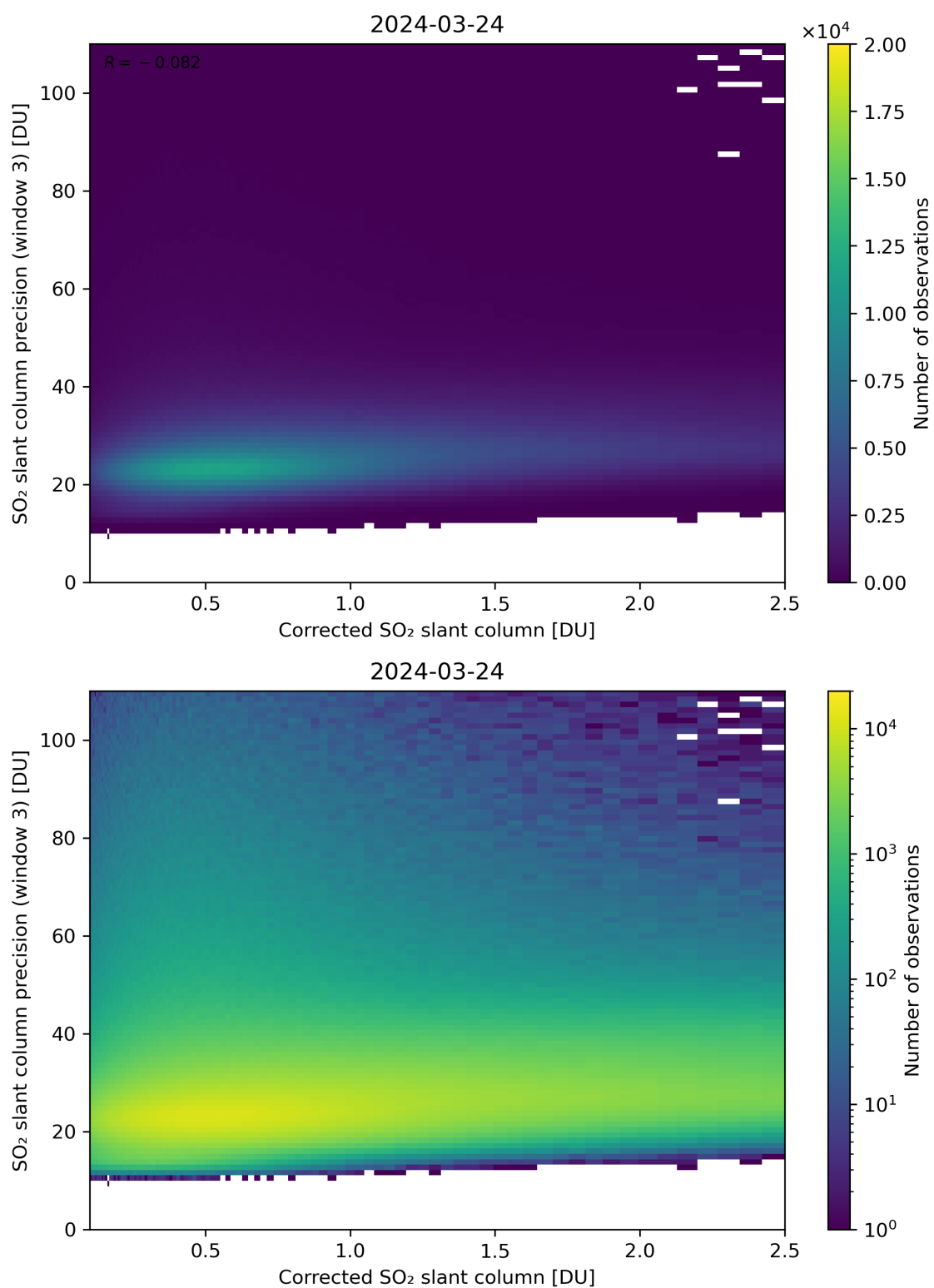
Figure 191: Scatter density plot of “Corrected SO 2 slant column” against “SO 2 slant column precision (window 3)” for 2024-03-23 to 2024-03-25.
