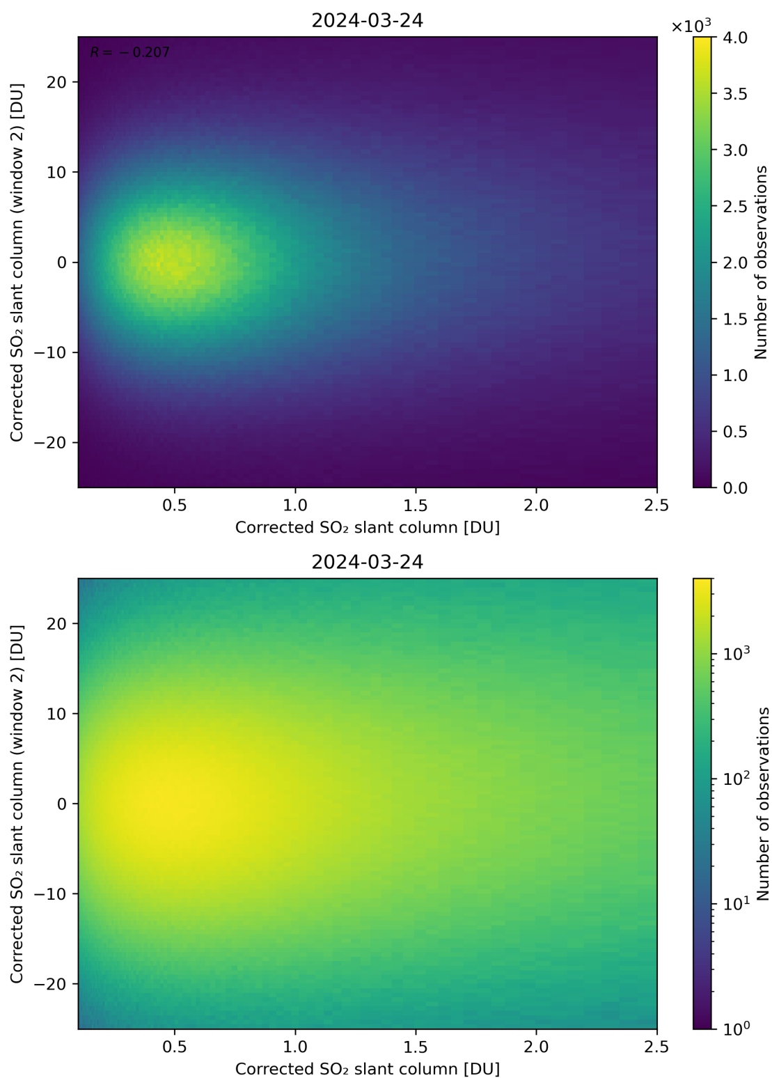
Figure 185: Scatter density plot of “Corrected SO 2 slant column” against “Corrected SO 2 slant column (window 2)” for 2024-03-23 to 2024-03-25.
