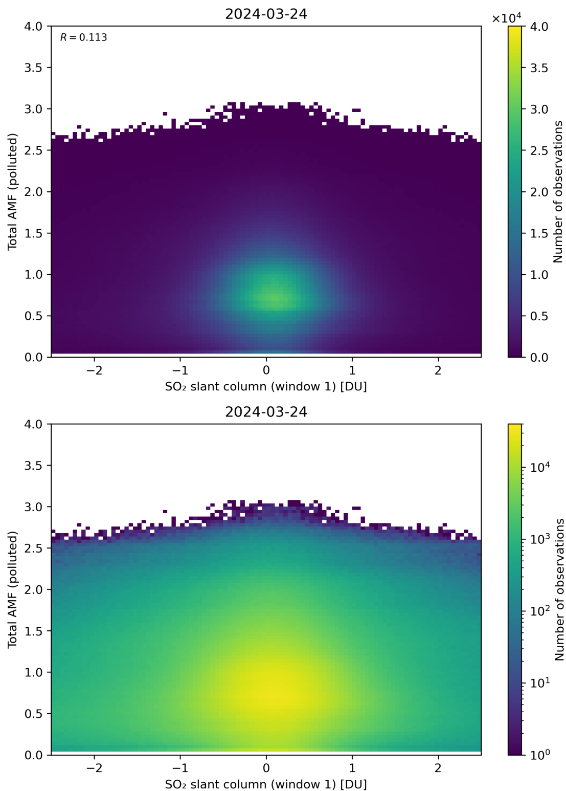
Figure 239: Scatter density plot of “SO 2 slant column (window 1)” against “Total AMF (polluted)” for 2024-03-23 to 2024-03-25.
