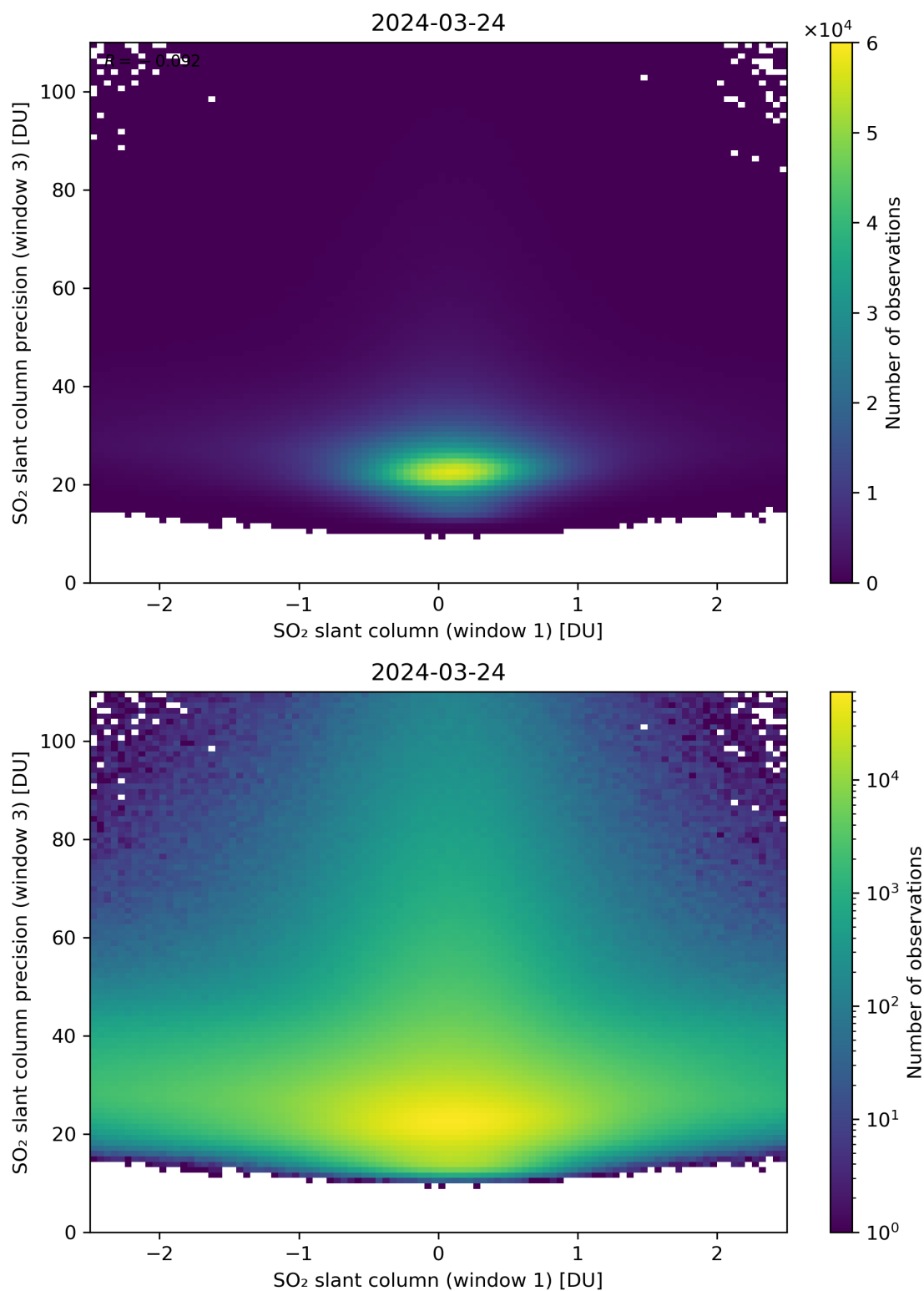
Figure 238: Scatter density plot of “SO 2 slant column (window 1)” against “SO 2 slant column precision (window 3)” for 2024-03-23 to 2024-03-25.
