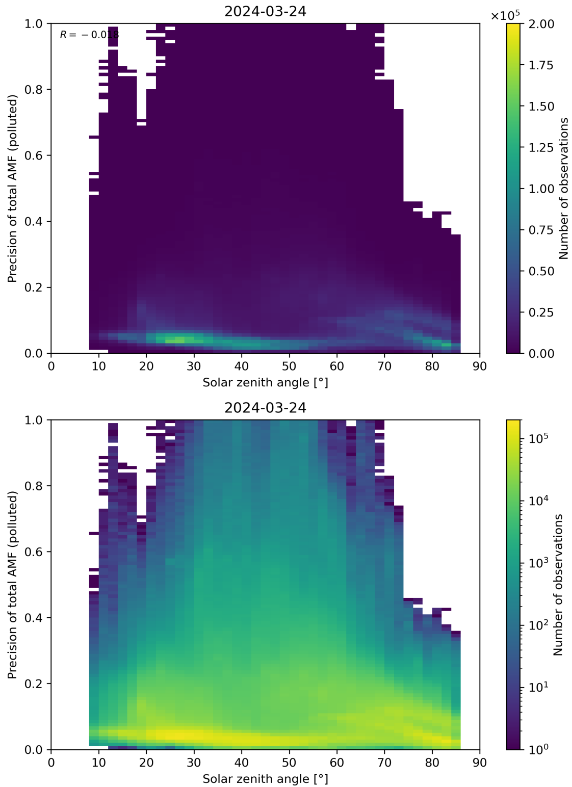
Figure 175: Scatter density plot of “Solar zenith angle” against “Precision of total AMF (polluted)” for 2024-03-23 to 2024-03-25.
