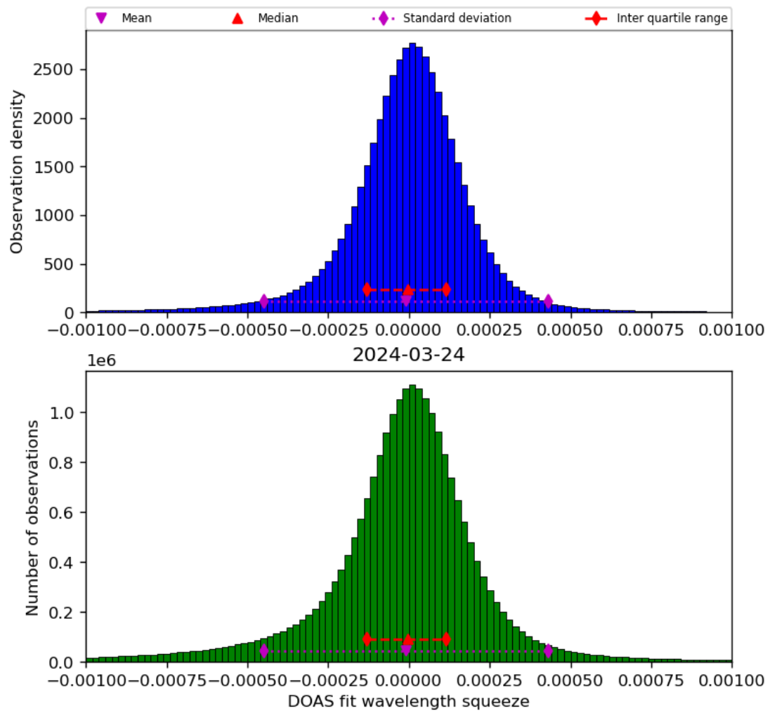
Figure 69: Histogram of “DOAS fit wavelength squeeze” for 2024-03-23 to 2024-03-25
