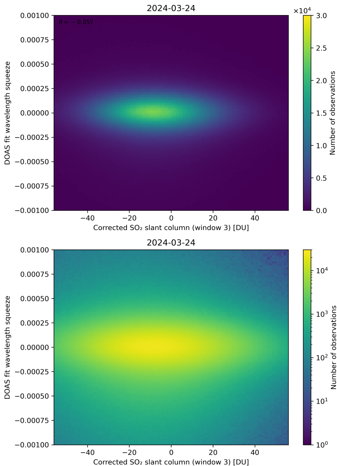
Figure 207: Scatter density plot of “Corrected SO 2 slant column (window 3)” against “DOAS fit wavelength squeeze” for 2024-03-23 to 2024-03-25.
