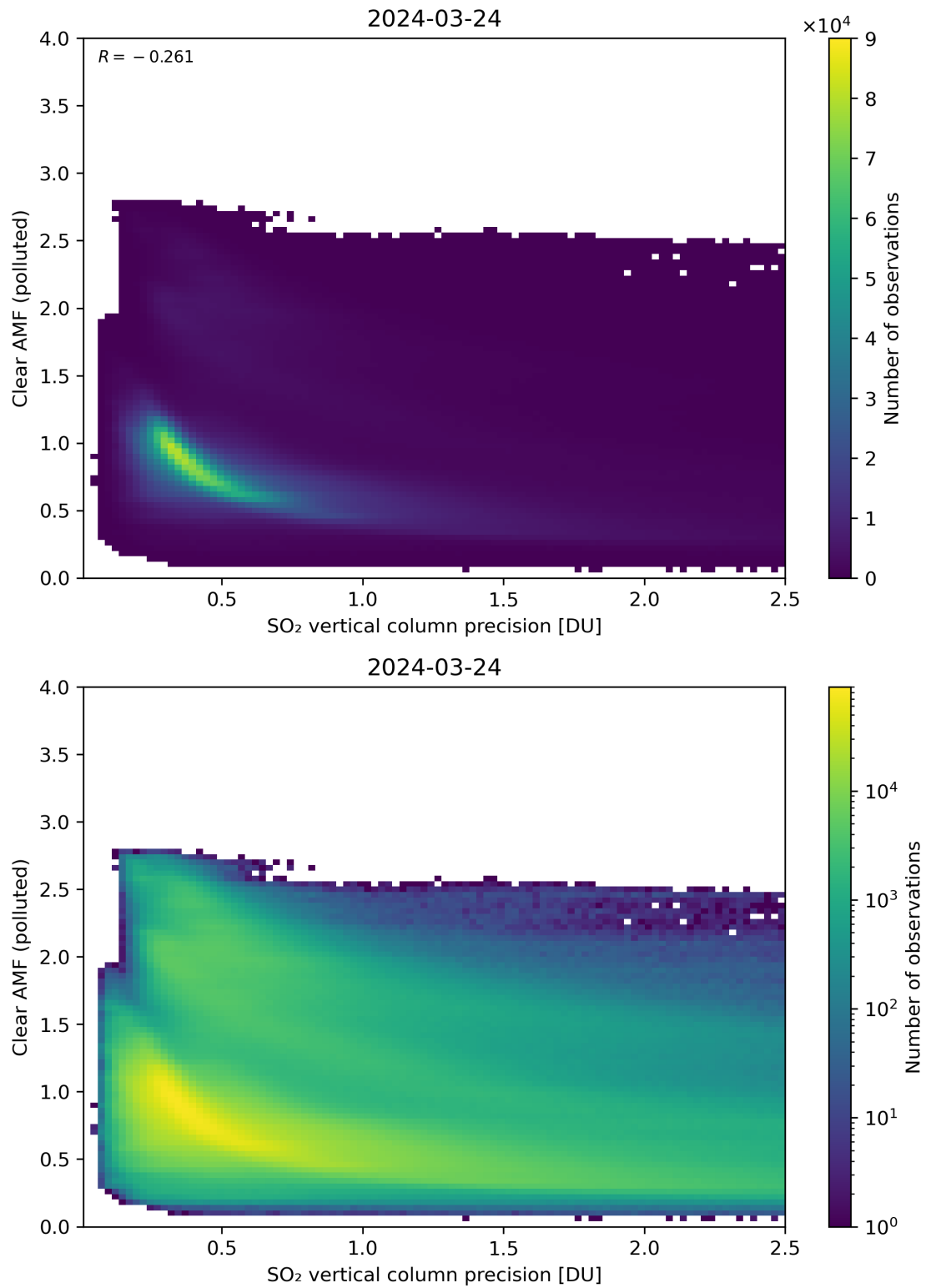
Figure 285: Scatter density plot of “SO 2 vertical column precision” against “Clear AMF (polluted)” for 2024-03-23 to 2024-03-25.
