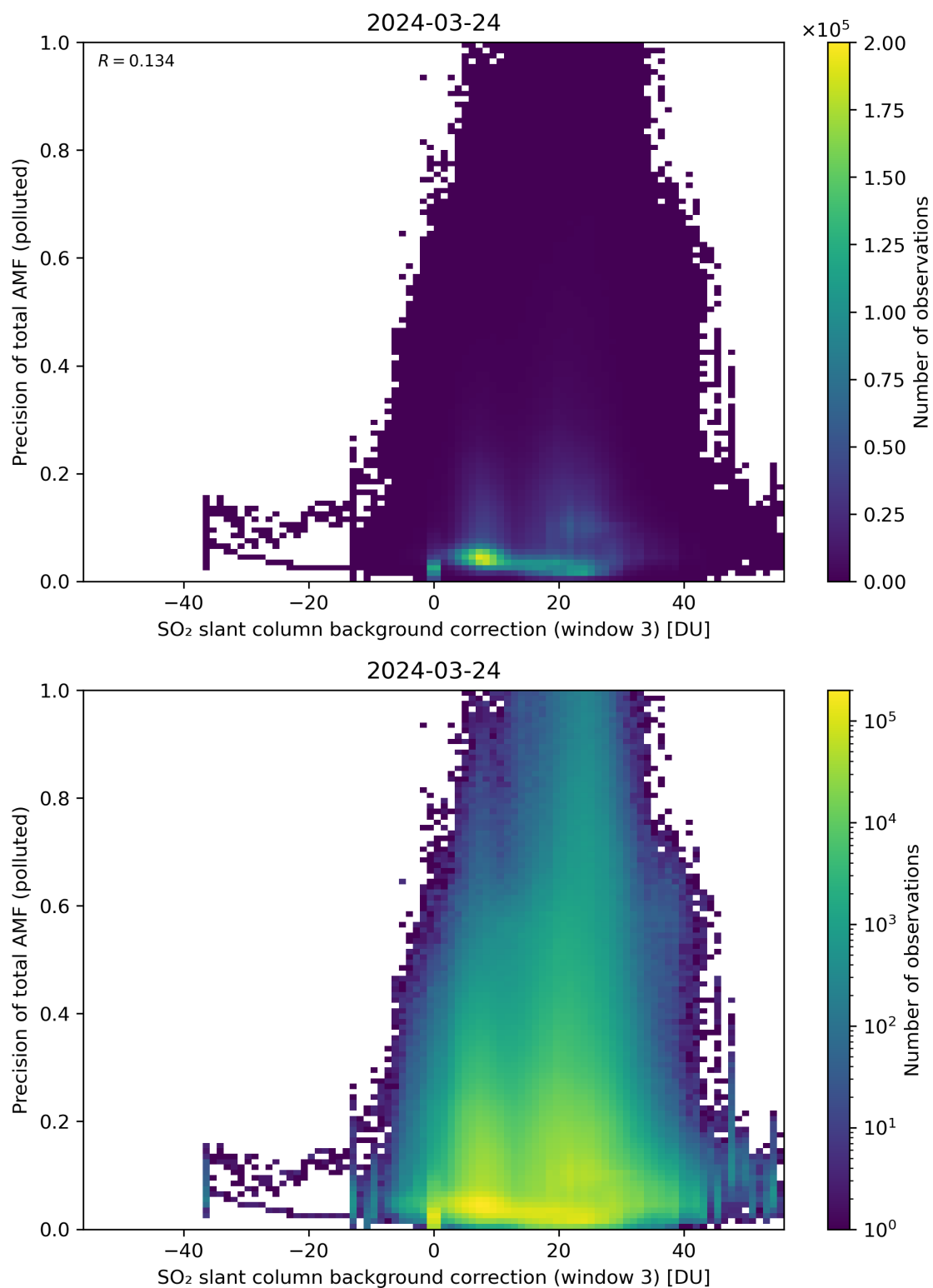
Figure 126: Scatter density plot of “SO 2 slant column background correction (window 3)” against “Precision of total AMF (polluted)” for 2024-03-23 to 2024-03-25.
