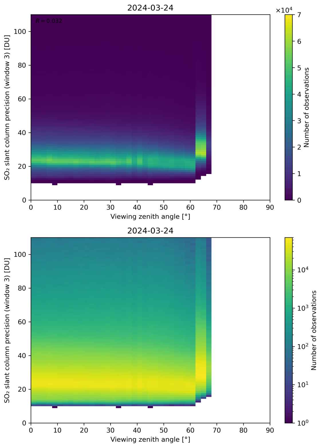
Figure 324: Scatter density plot of “Viewing zenith angle” against “SO 2 slant column precision (window 3)” for 2024-03-23 to 2024-03-25.
