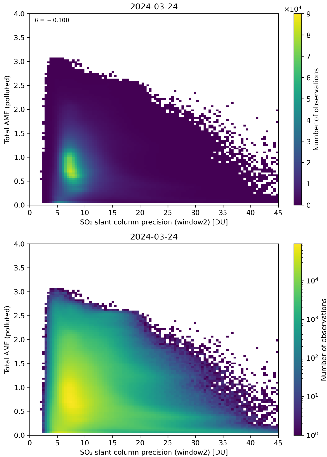
Figure 251: Scatter density plot of “SO 2 slant column precision (window2)” against “Total AMF (polluted)” for 2024-03-23 to 2024-03-25.
