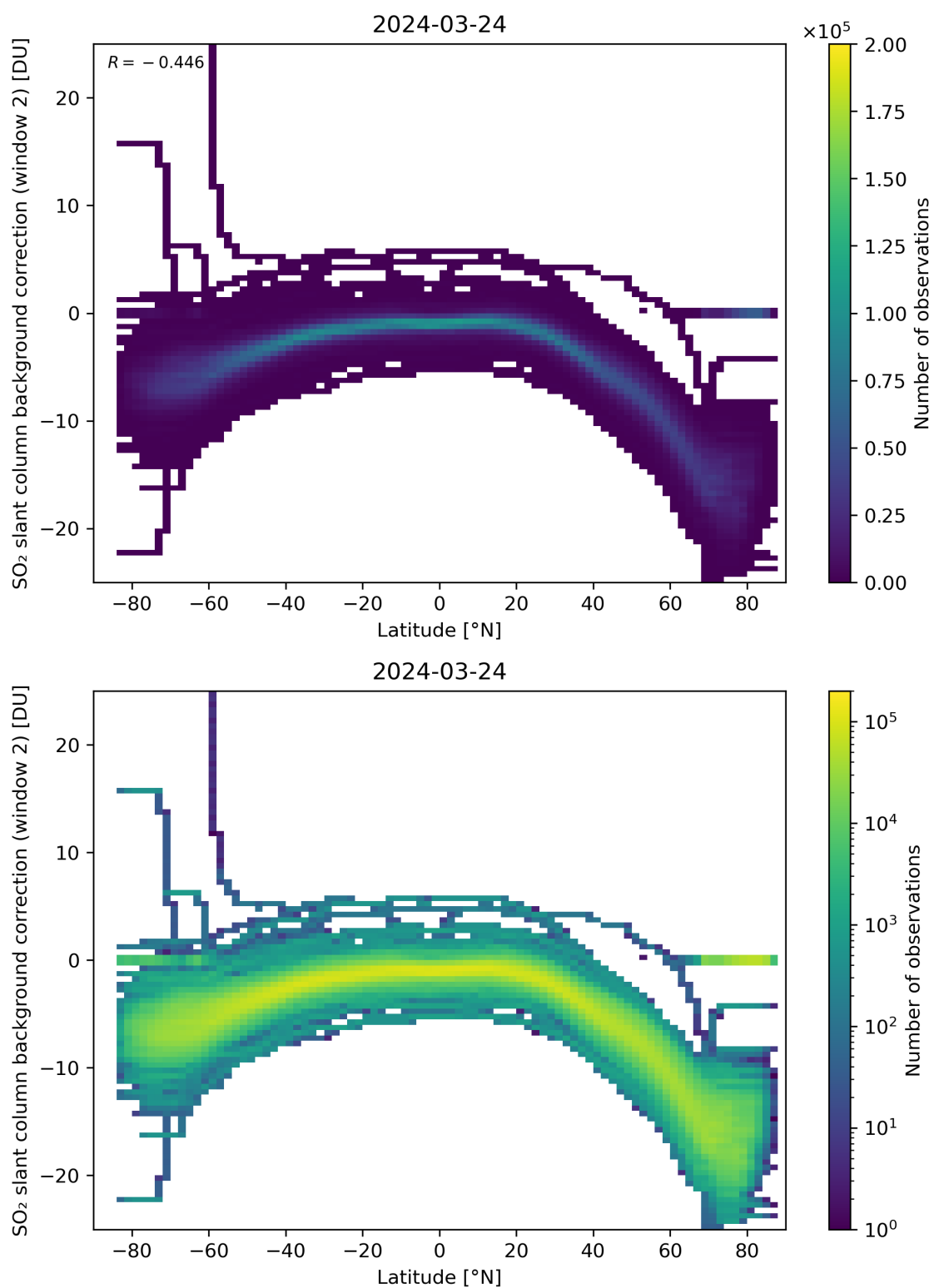
Figure 140: Scatter density plot of “Latitude” against “SO 2 slant column background correction (window 2)” for 2024-03-23 to 2024-03-25.
