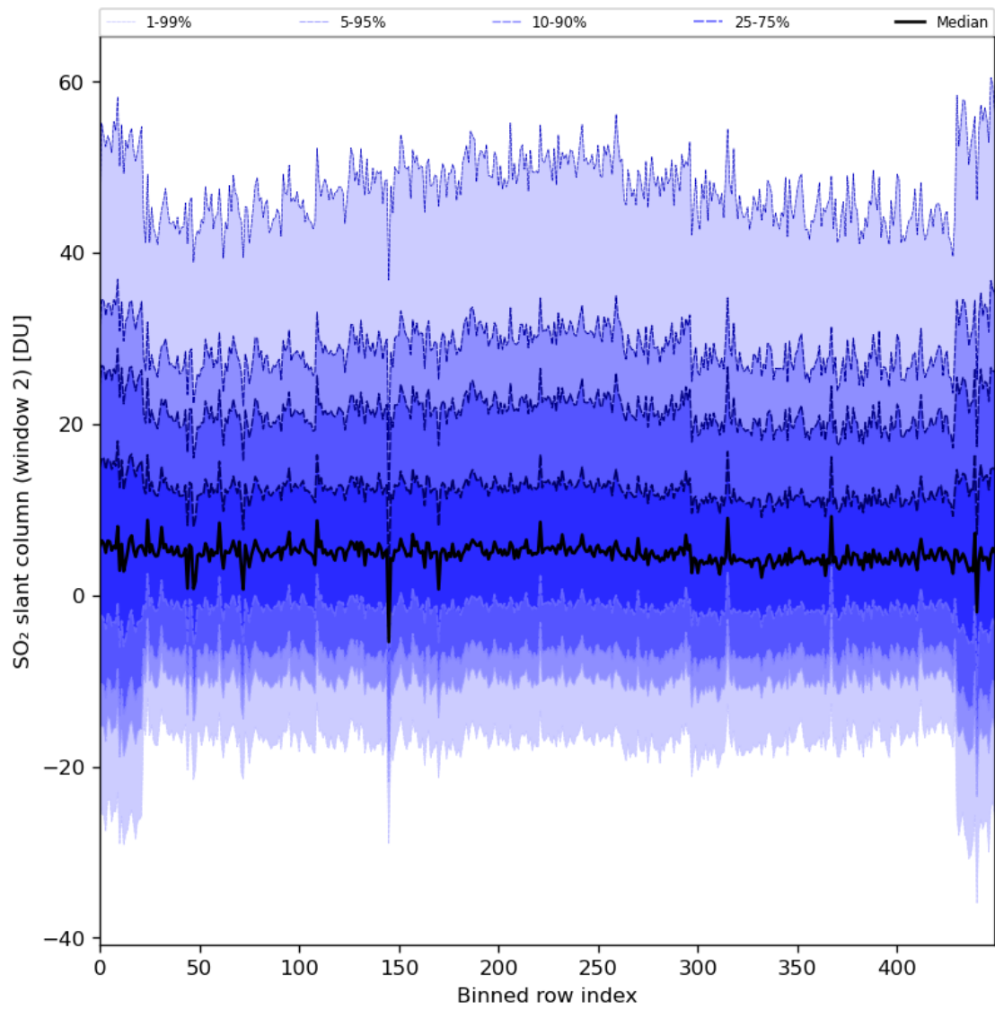
Figure 83: Along track statistics of “SO 2 slant column (window 2)” for 2024-03-23 to 2024-03-25
