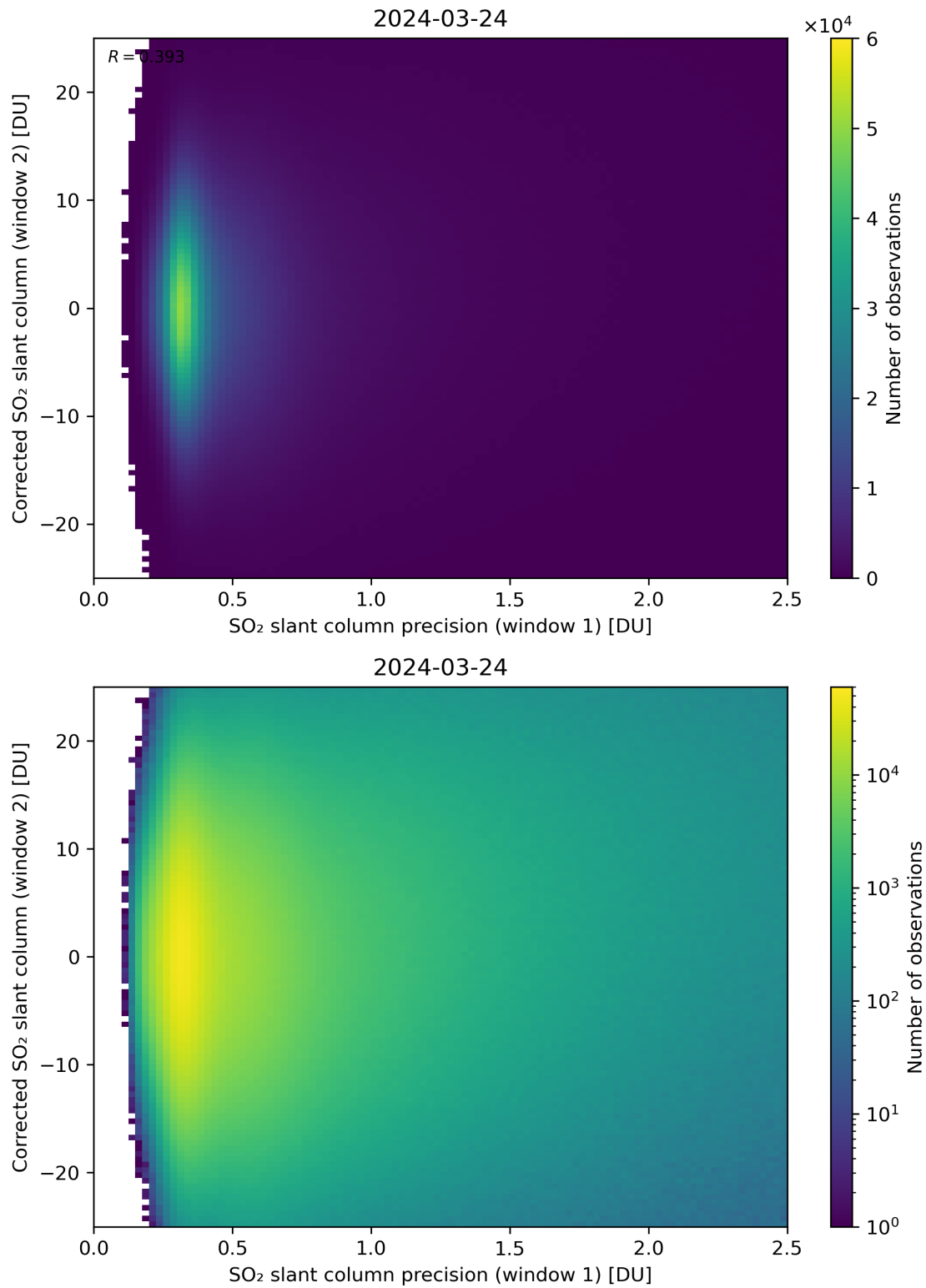
Figure 225: Scatter density plot of “SO 2 slant column precision (window 1)” against “Corrected SO 2 slant column (window 2)” for 2024-03-23 to 2024-03-25.
