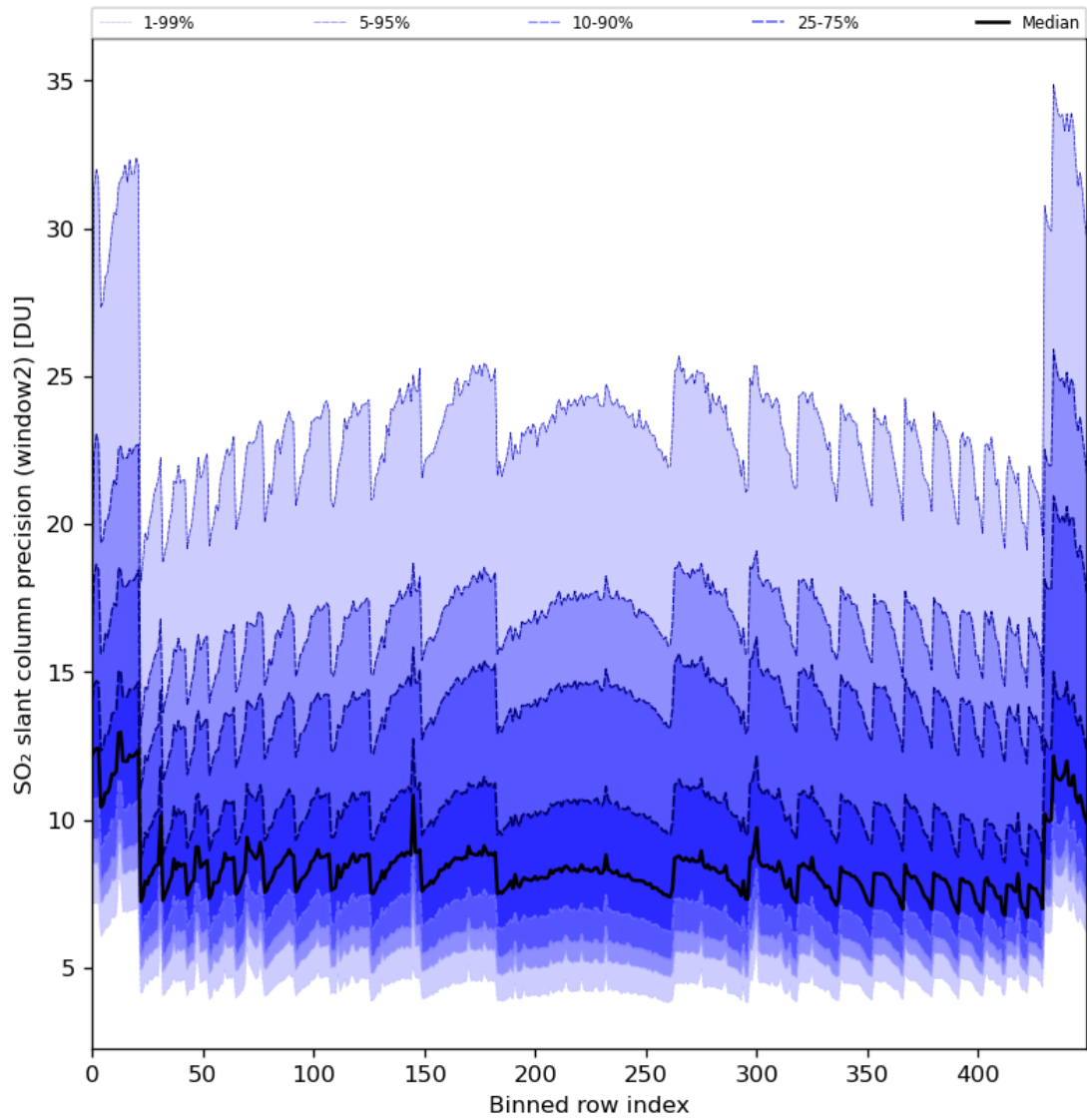
Figure 84: Along track statistics of “SO 2 slant column precision (window2)” for 2024-03-23 to 2024-03-25
