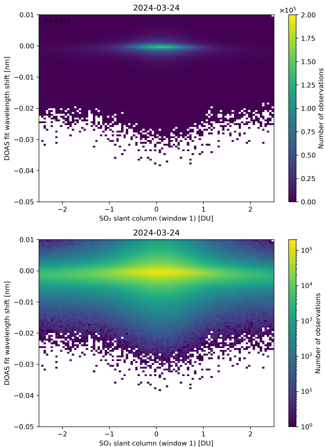
Figure 215: Scatter density plot of “SO 2 slant column (window 1)” against “DOAS fit wavelength shift” for 2024-03-23 to 2024-03-25.
