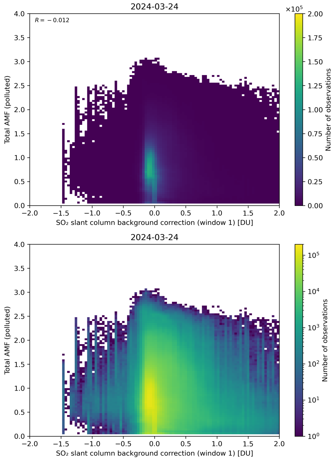
Figure 109: Scatter density plot of “SO 2 slant column background correction (window 1)” against “Total AMF (polluted)” for 2024-03-23 to 2024-03-25.
