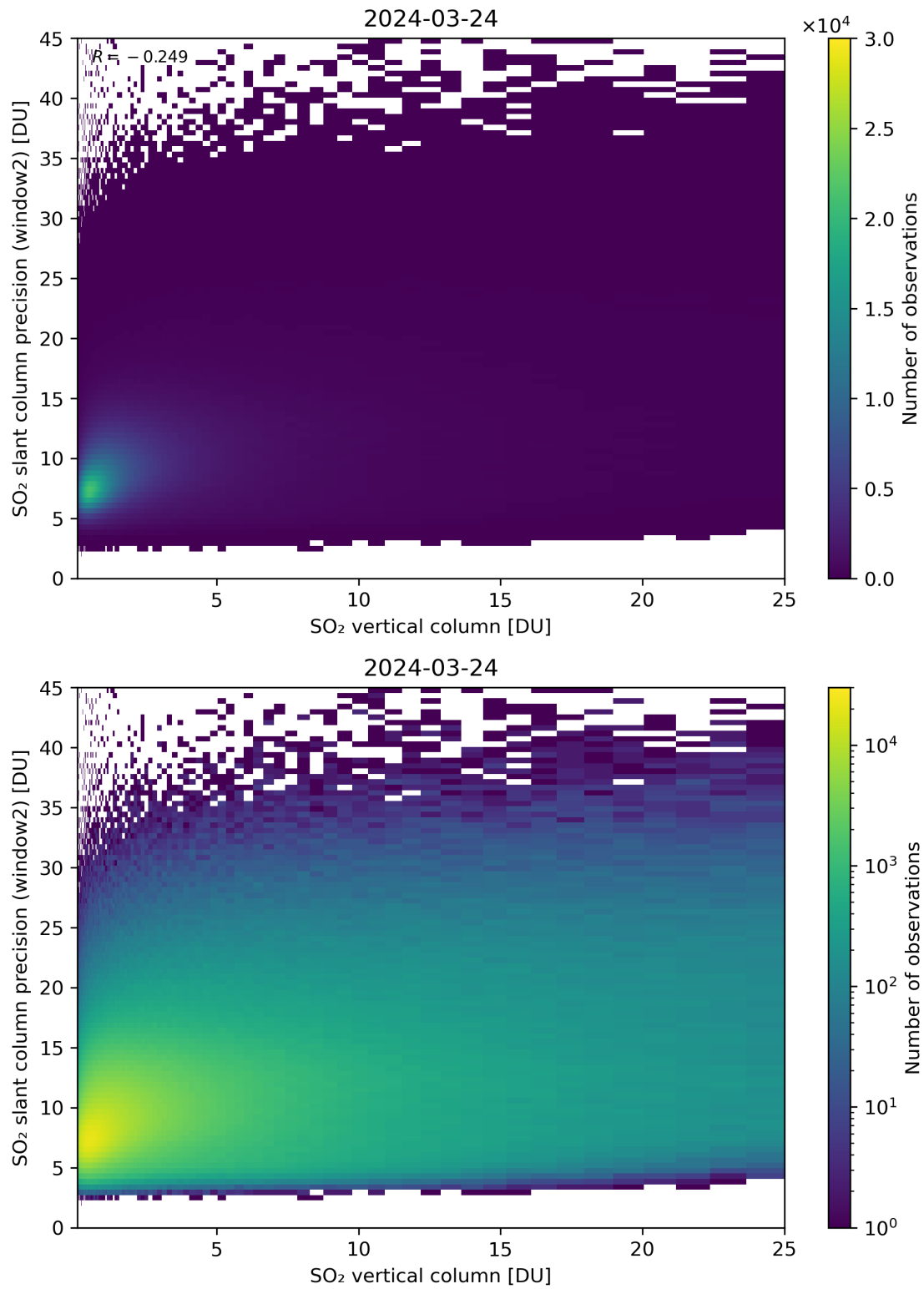
Figure 302: Scatter density plot of “SO 2 vertical column” against “SO 2 slant column precision (window2)” for 2024-03-23 to 2024-03-25.
