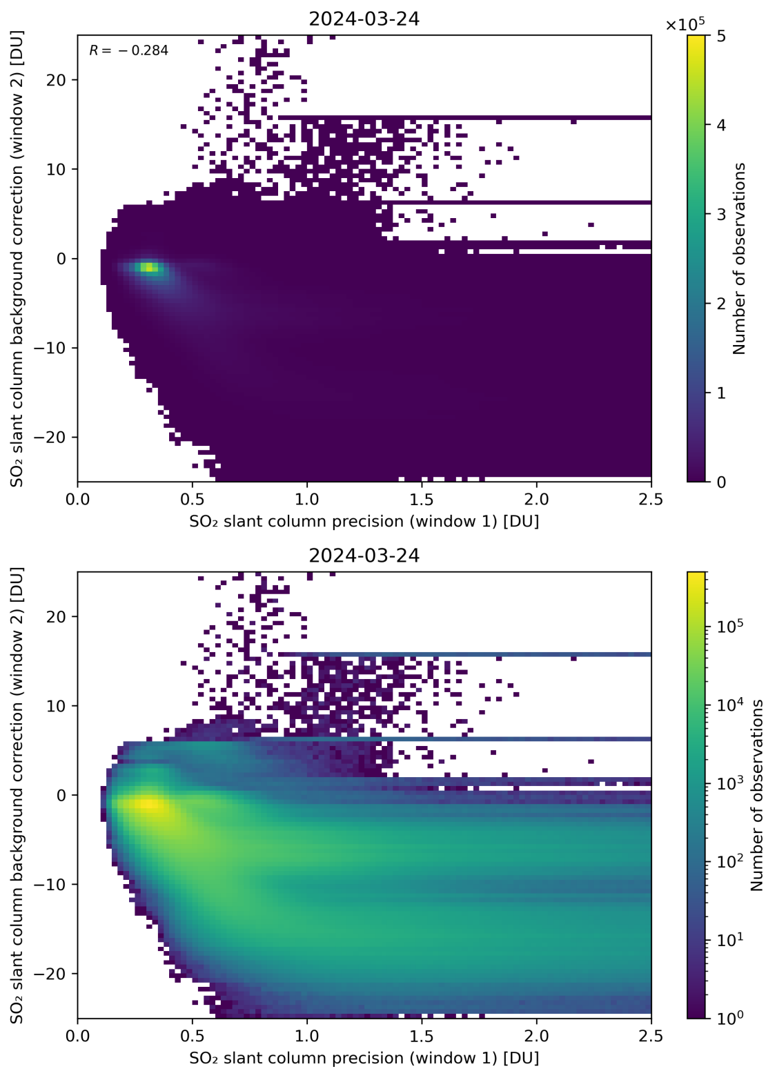
Figure 219: Scatter density plot of “SO 2 slant column precision (window 1)” against “SO 2 slant column background correction (window 2)” for 2024-03-23 to 2024-03-25.
