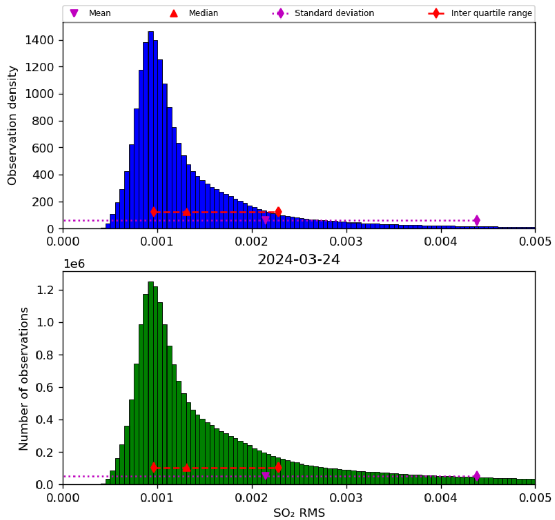
Figure 70: Histogram of “SO 2 RMS” for 2024-03-23 to 2024-03-25
