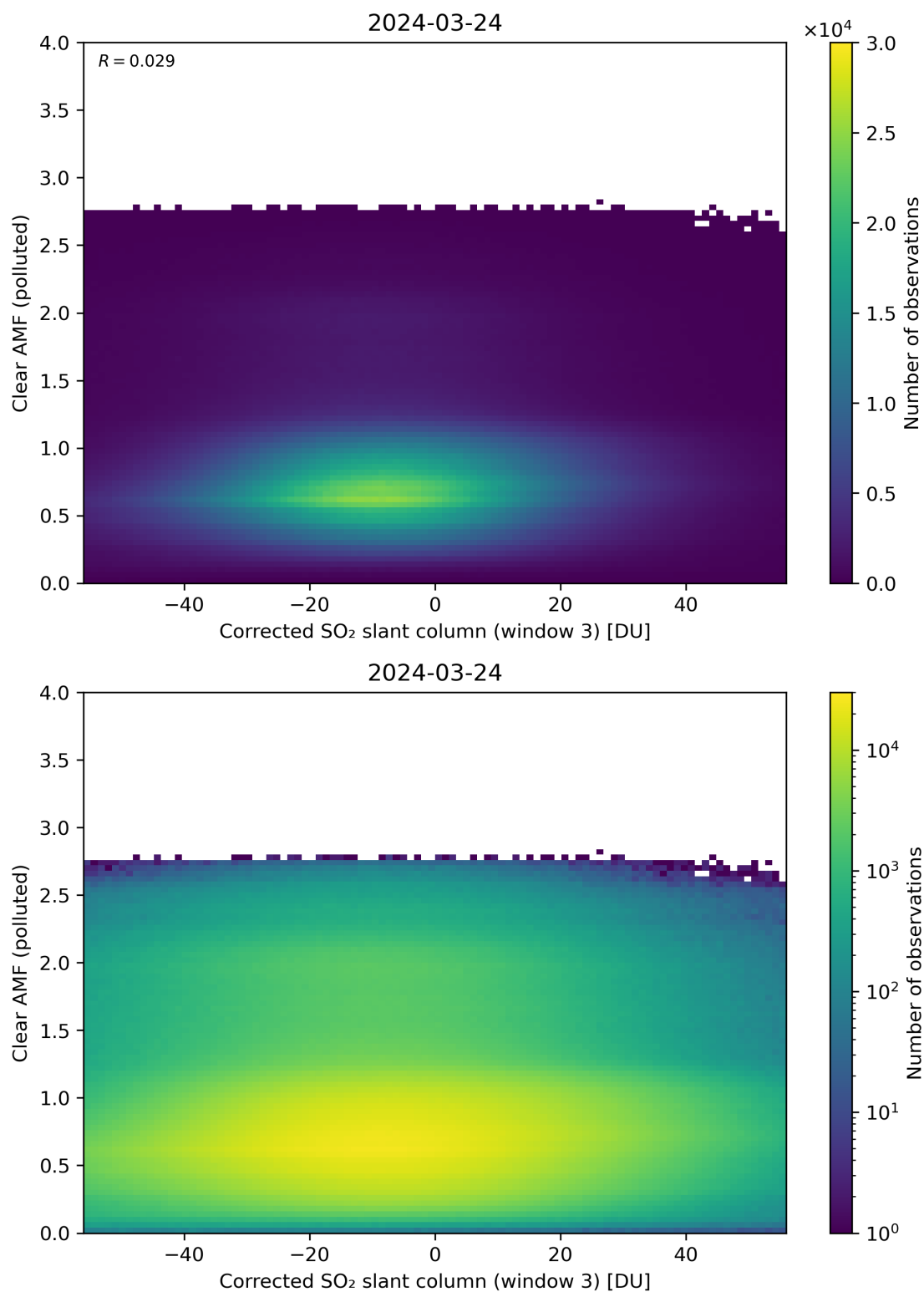
Figure 209: Scatter density plot of “Corrected SO 2 slant column (window 3)” against “Clear AMF (polluted)” for 2024-03-23 to 2024-03-25.
