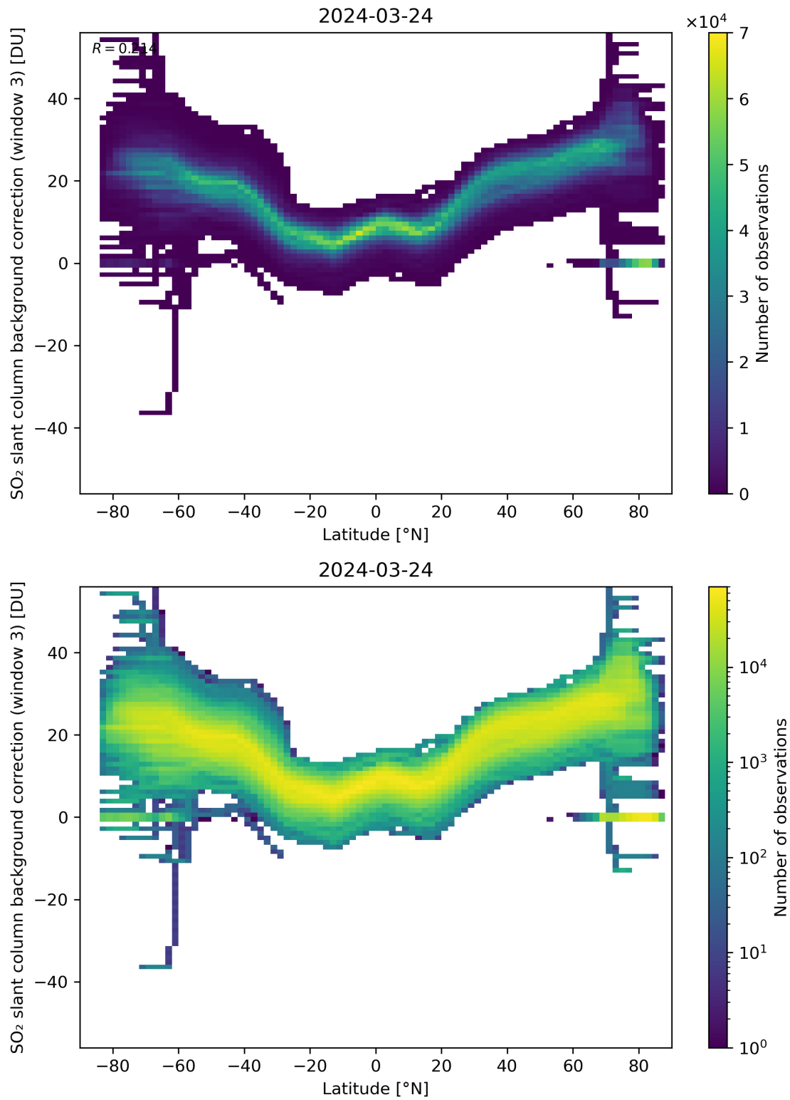
Figure 141: Scatter density plot of “Latitude” against “SO 2 slant column background correction (window 3)” for 2024-03-23 to 2024-03-25.
