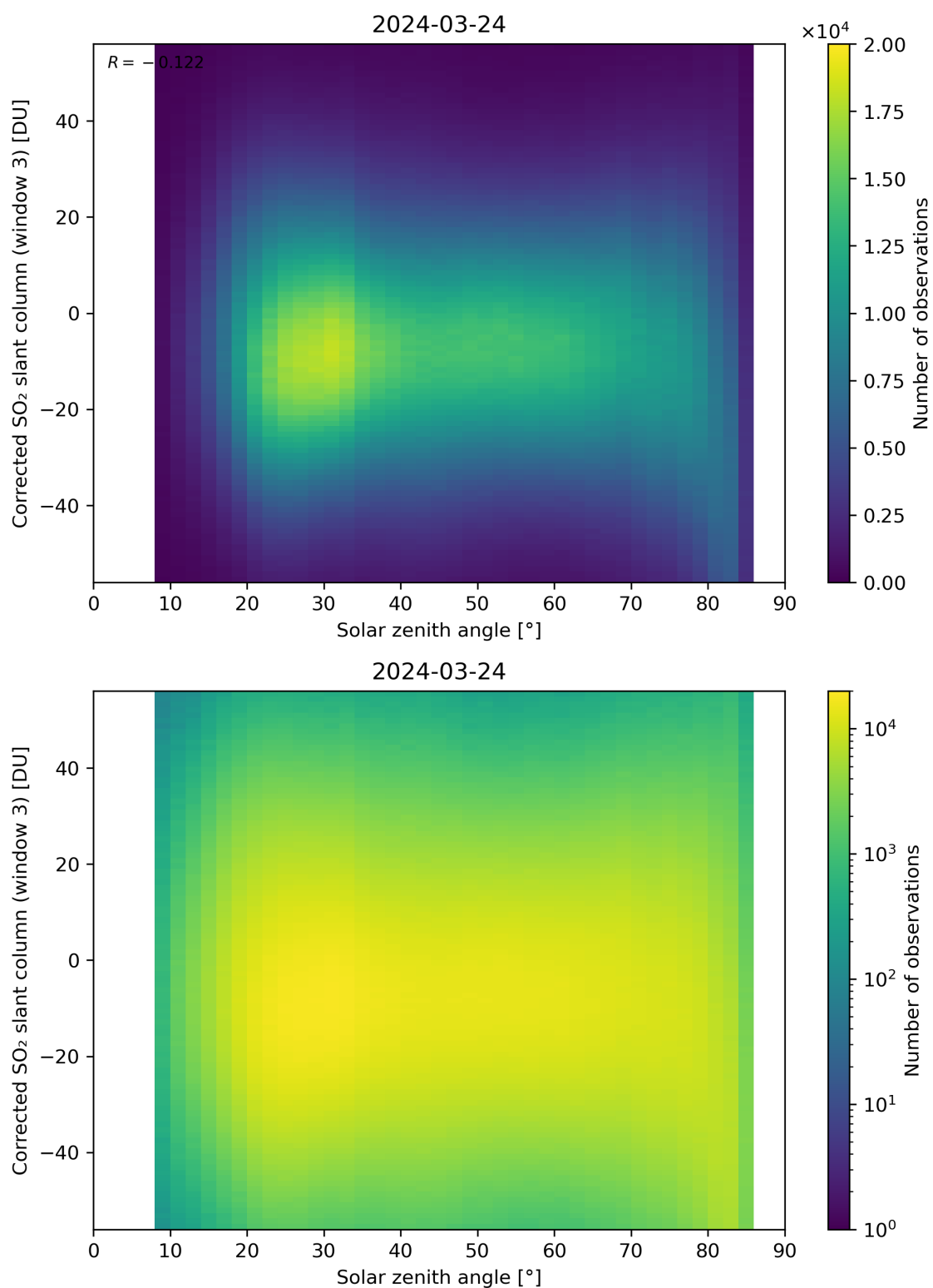
Figure 168: Scatter density plot of “Solar zenith angle” against “Corrected SO 2 slant column (window 3)” for 2024-03-23 to 2024-03-25.
