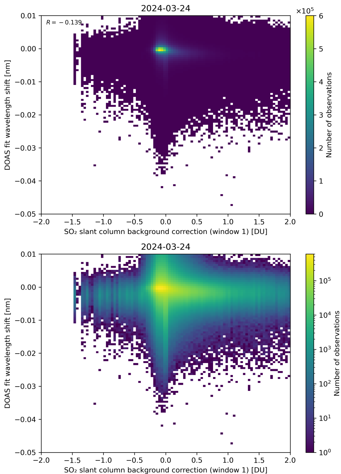
Figure 100: Scatter density plot of “SO 2 slant column background correction (window 1)” against “DOAS fit wavelength shift” for 2024-03-23 to 2024-03-25.
