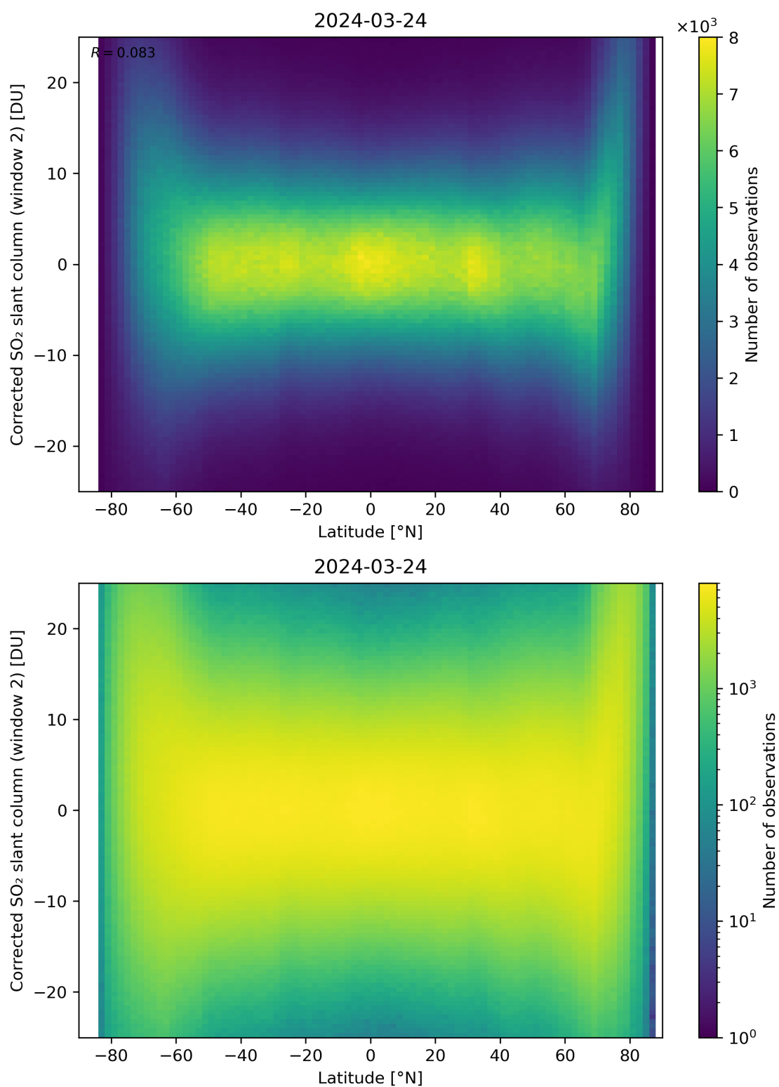
Figure 147: Scatter density plot of “Latitude” against “Corrected SO 2 slant column (window 2)” for 2024-03-23 to 2024-03-25.
