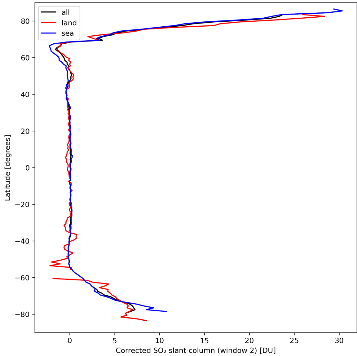
Figure 39: Zonal average of “Corrected SO 2 slant column (window 2)” for 2024-03-23 to 2024-03-25.
