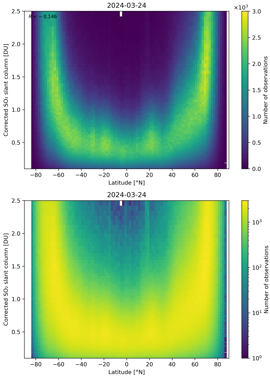
Figure 146: Scatter density plot of “Latitude” against “Corrected SO 2 slant column” for 2024-03-23 to 2024-03-25.
