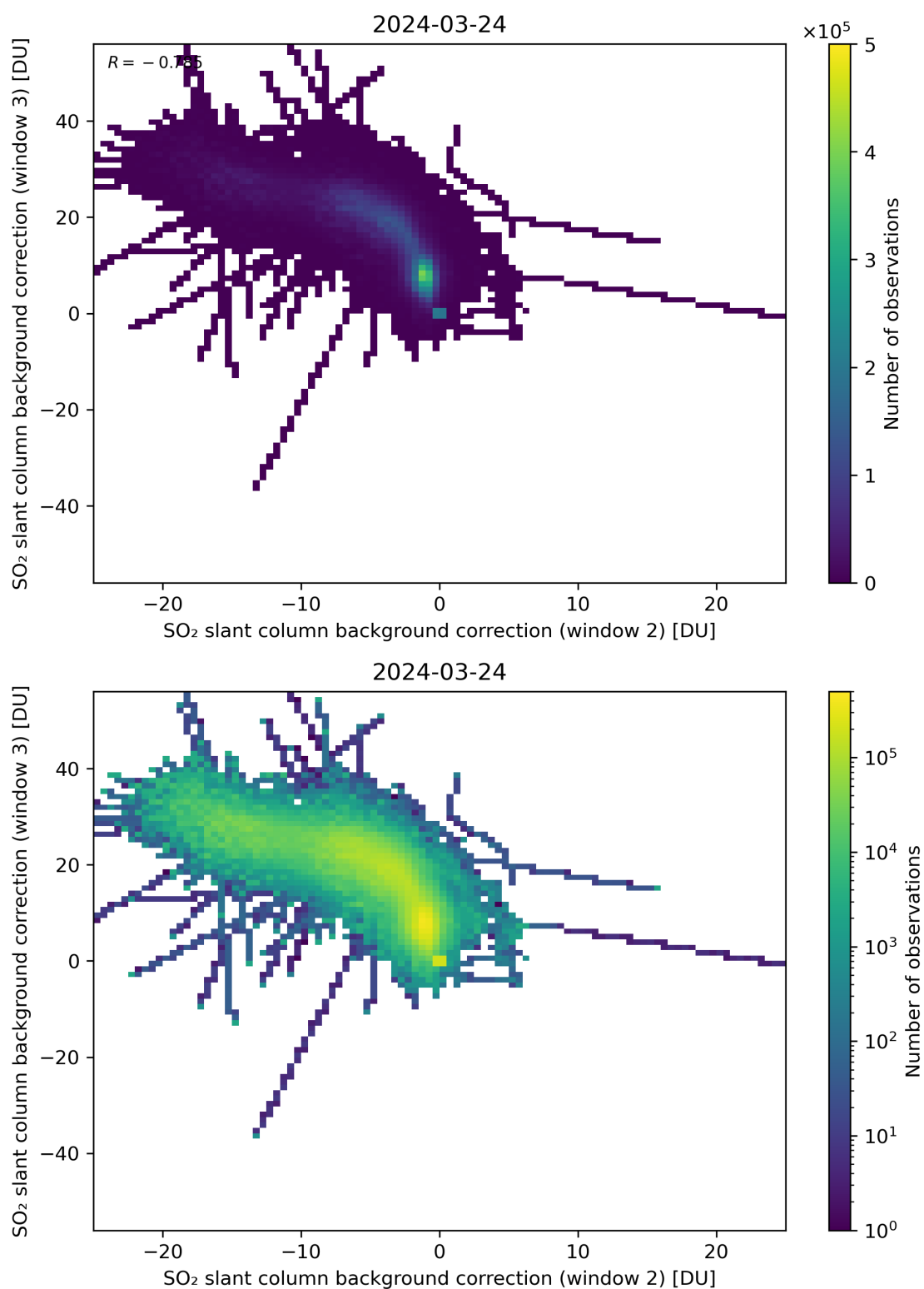
Figure 111: Scatter density plot of “SO 2 slant column background correction (window 2)” against “SO 2 slant column background correction (window 3)” for 2024-03-23 to 2024-03-25.
