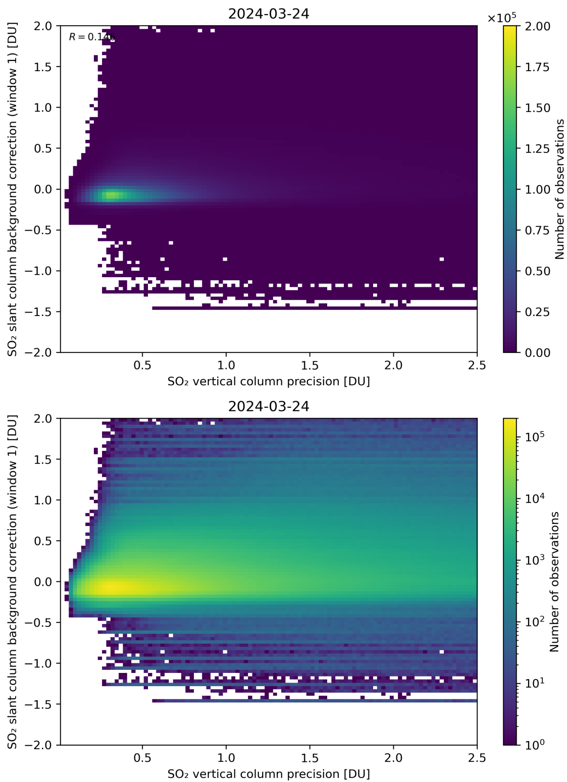
Figure 279: Scatter density plot of “SO 2 vertical column precision” against “SO 2 slant column background correction (window 1)” for 2024-03-23 to 2024-03-25.
