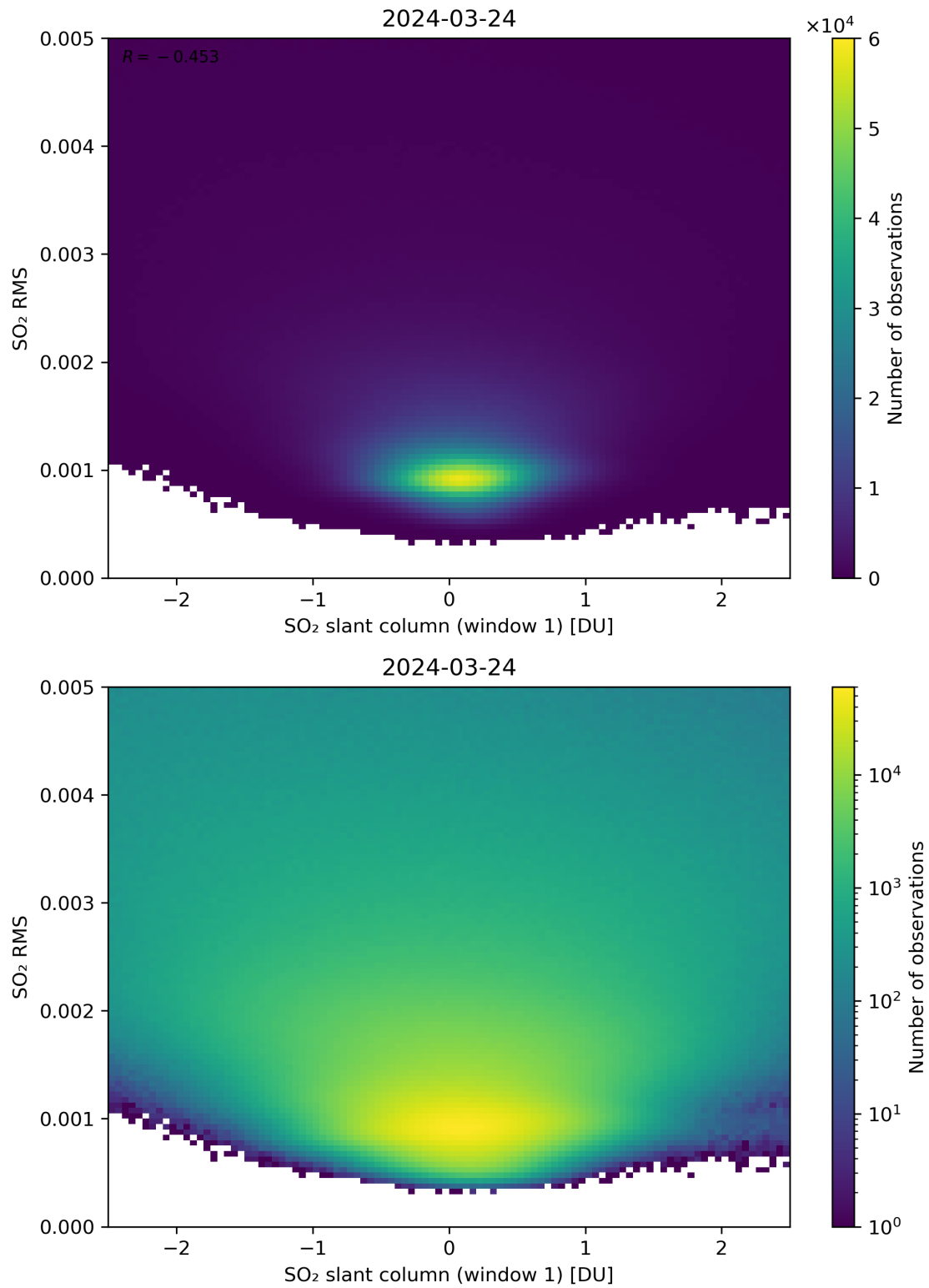
Figure 217: Scatter density plot of “SO 2 slant column (window 1)” against “SO 2 RMS” for 2024-03-23 to 2024-03-25.
