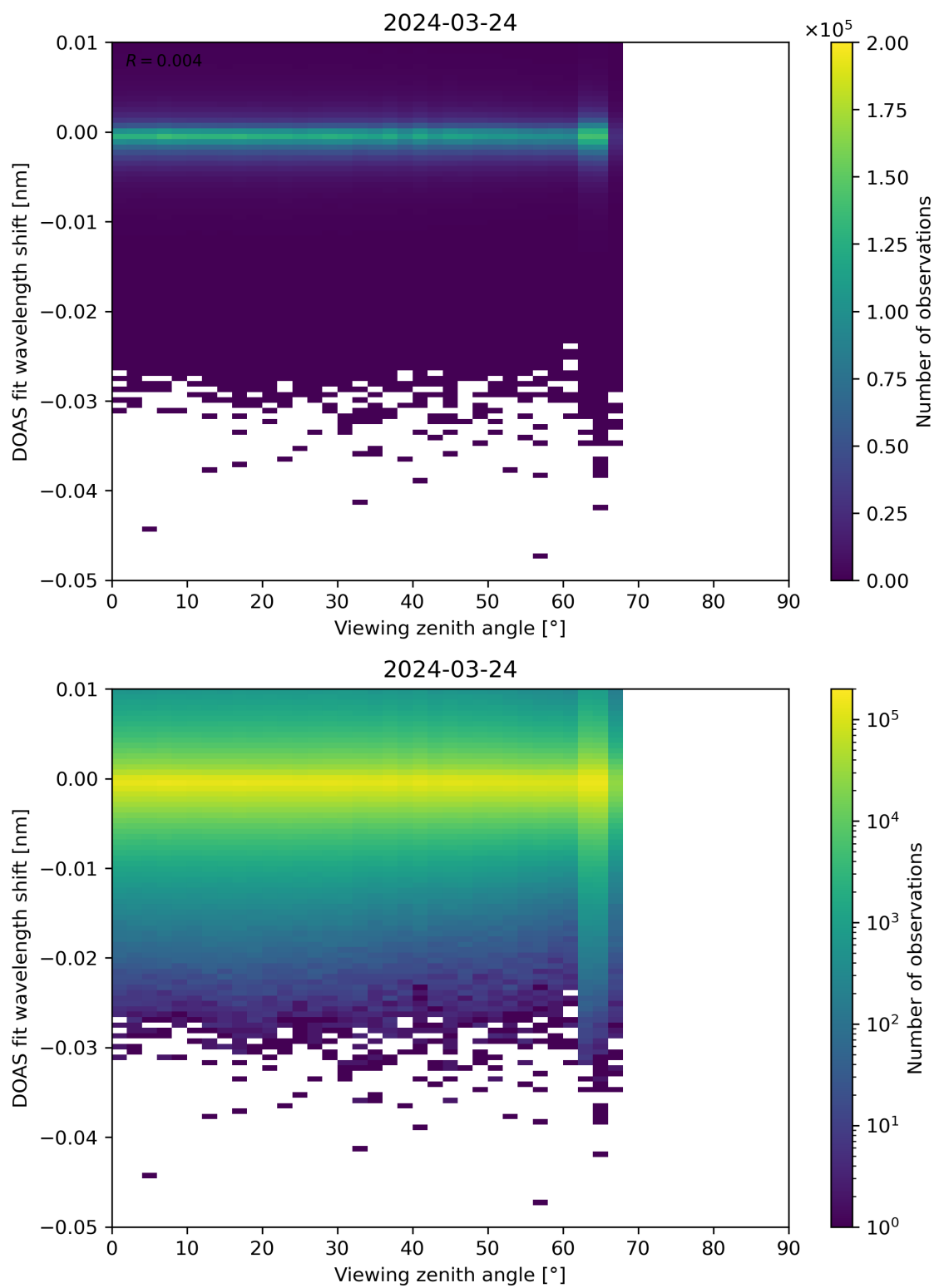
Figure 311: Scatter density plot of “Viewing zenith angle” against “DOAS fit wavelength shift” for 2024-03-23 to 2024-03-25.
