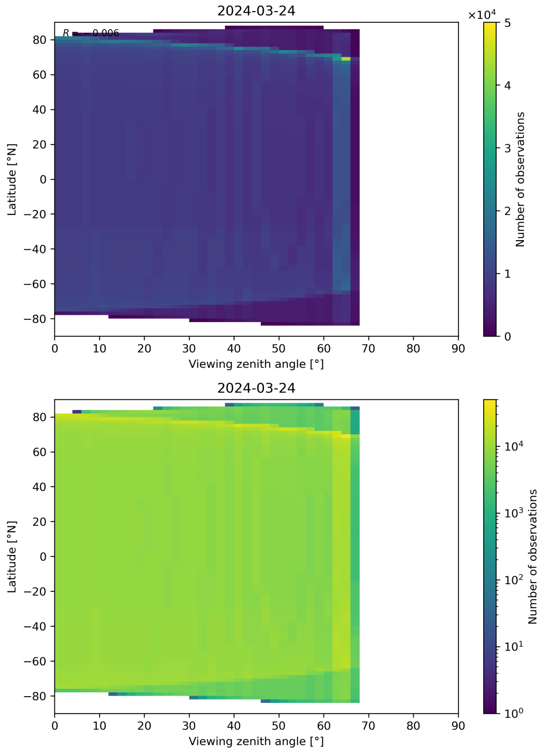
Figure 314: Scatter density plot of “Viewing zenith angle” against “Latitude” for 2024-03-23 to 2024-03-25.
