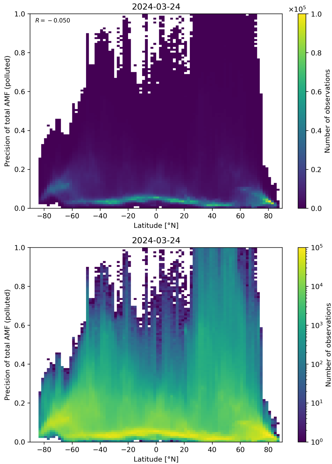
Figure 155: Scatter density plot of “Latitude” against “Precision of total AMF (polluted)” for 2024-03-23 to 2024-03-25.
