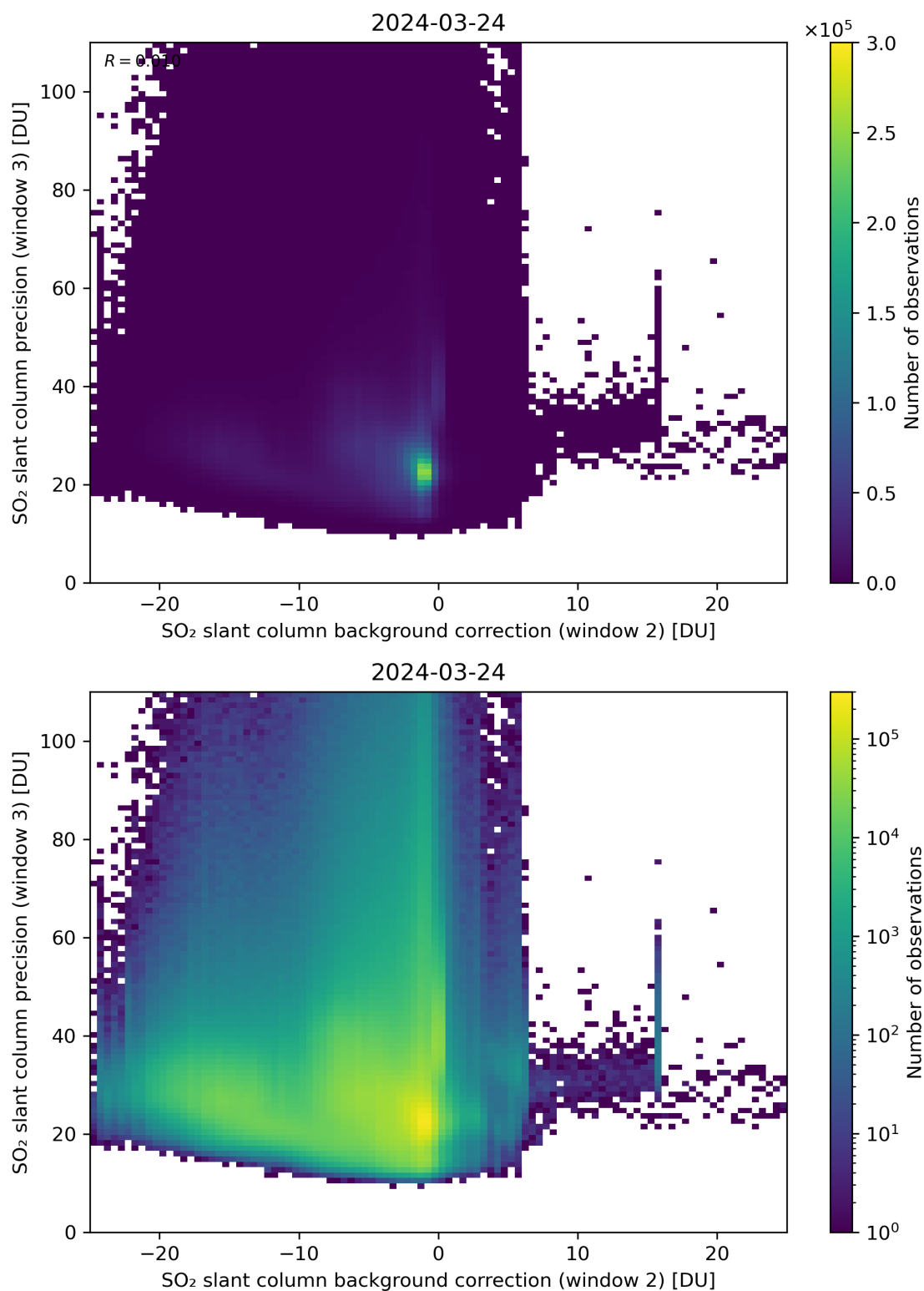
Figure 118: Scatter density plot of “SO 2 slant column background correction (window 2)” against “SO 2 slant column precision (window 3)” for 2024-03-23 to 2024-03-25.
