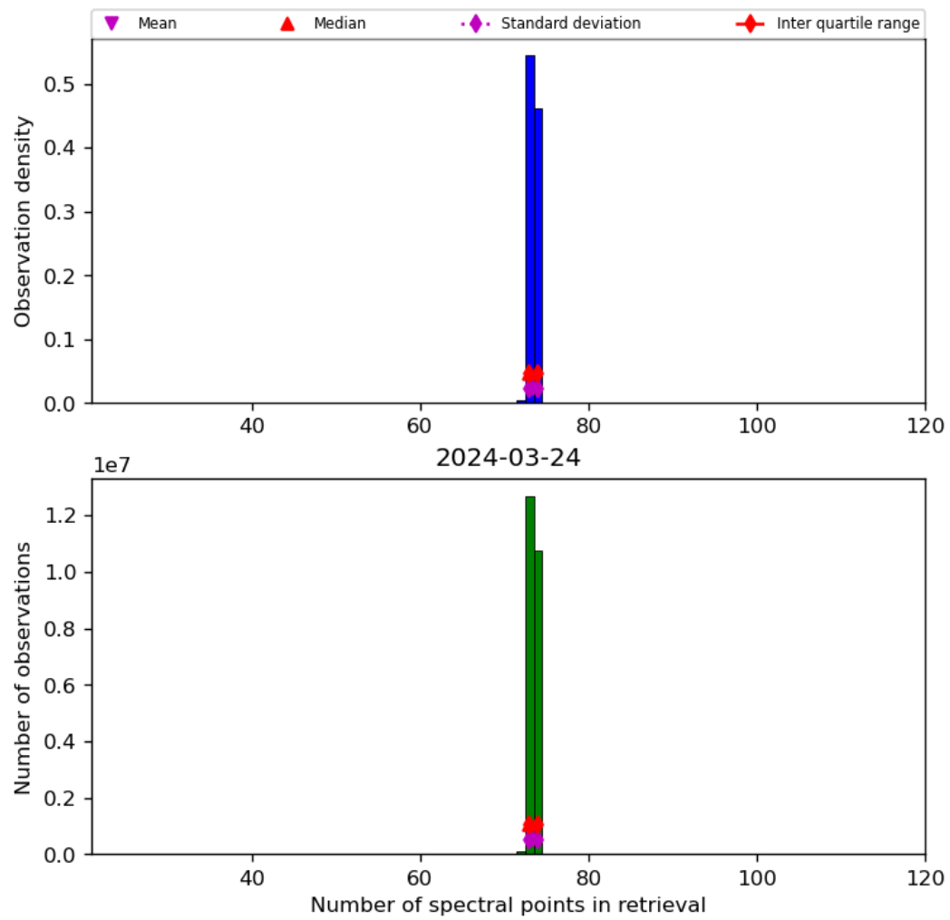
Figure 74: Histogram of “Number of spectral points in retrieval” for 2024-03-23 to 2024-03-25
