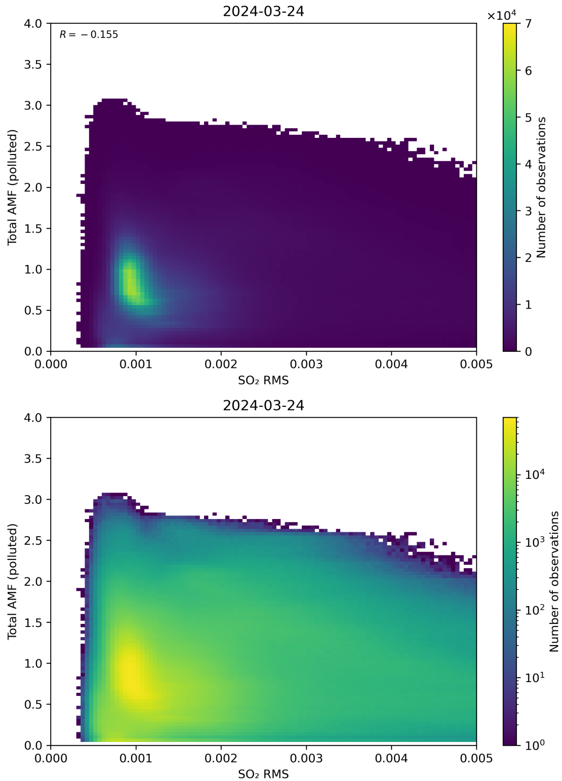
Figure 137: Scatter density plot of “SO 2 RMS” against “Total AMF (polluted)” for 2024-03-23 to 2024-03-25.
