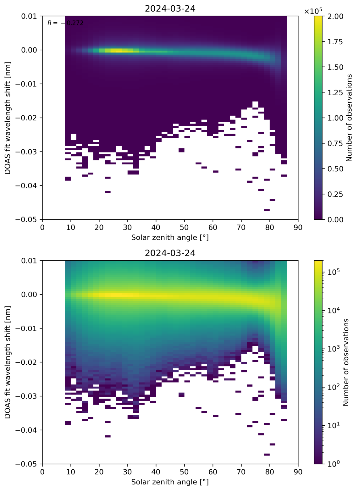
Figure 161: Scatter density plot of “Solar zenith angle” against “DOAS fit wavelength shift” for 2024-03-23 to 2024-03-25.
