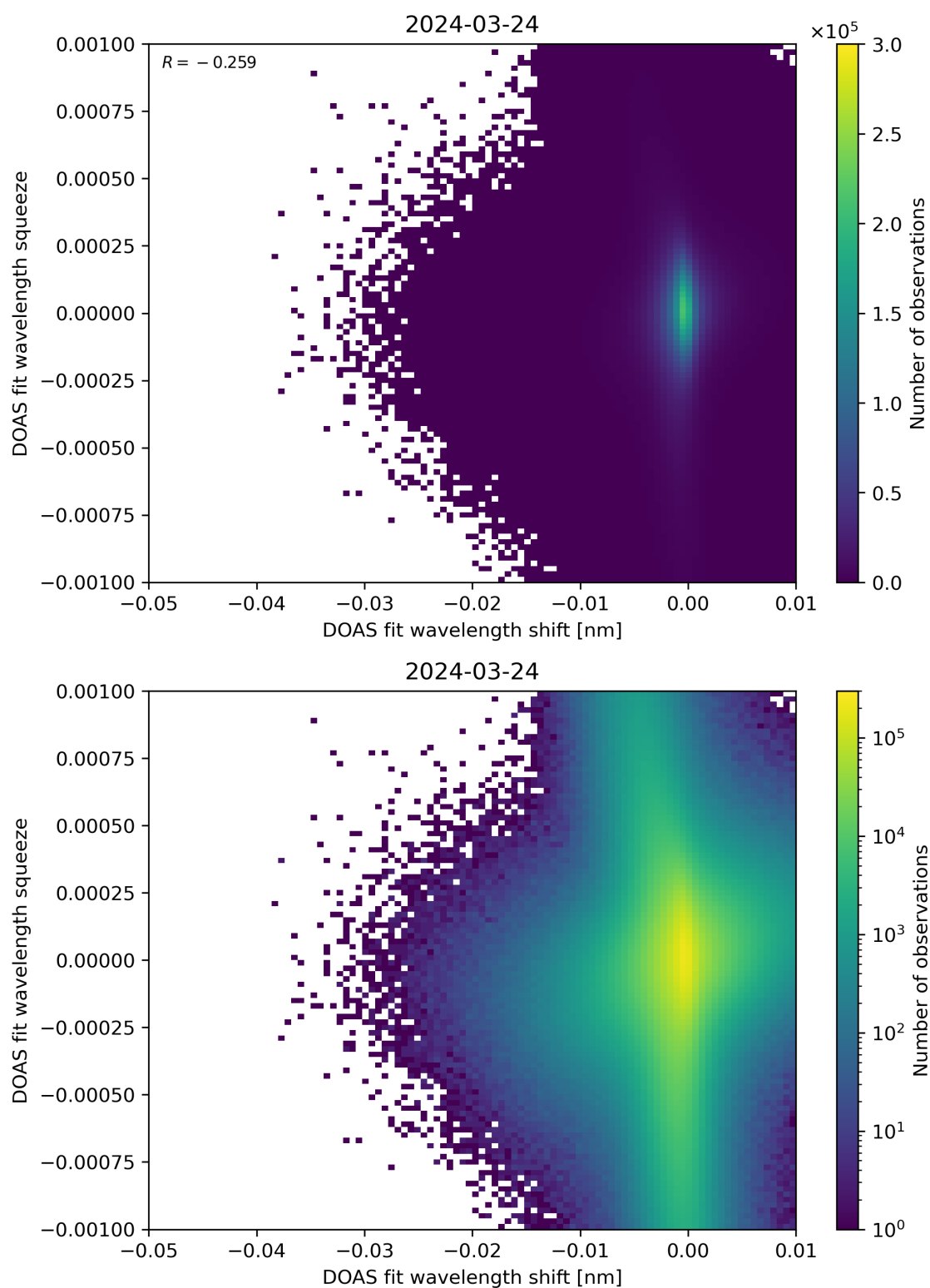
Figure 127: Scatter density plot of “DOAS fit wavelength shift” against “DOAS fit wavelength squeeze” for 2024-03-23 to 2024-03-25.
