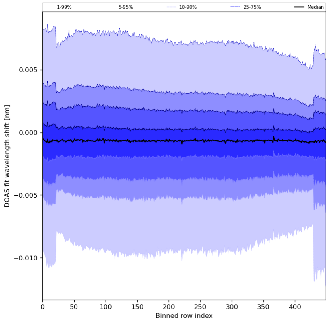
Figure 91: Along track statistics of “DOAS fit wavelength shift” for 2024-03-23 to 2024-03-25
