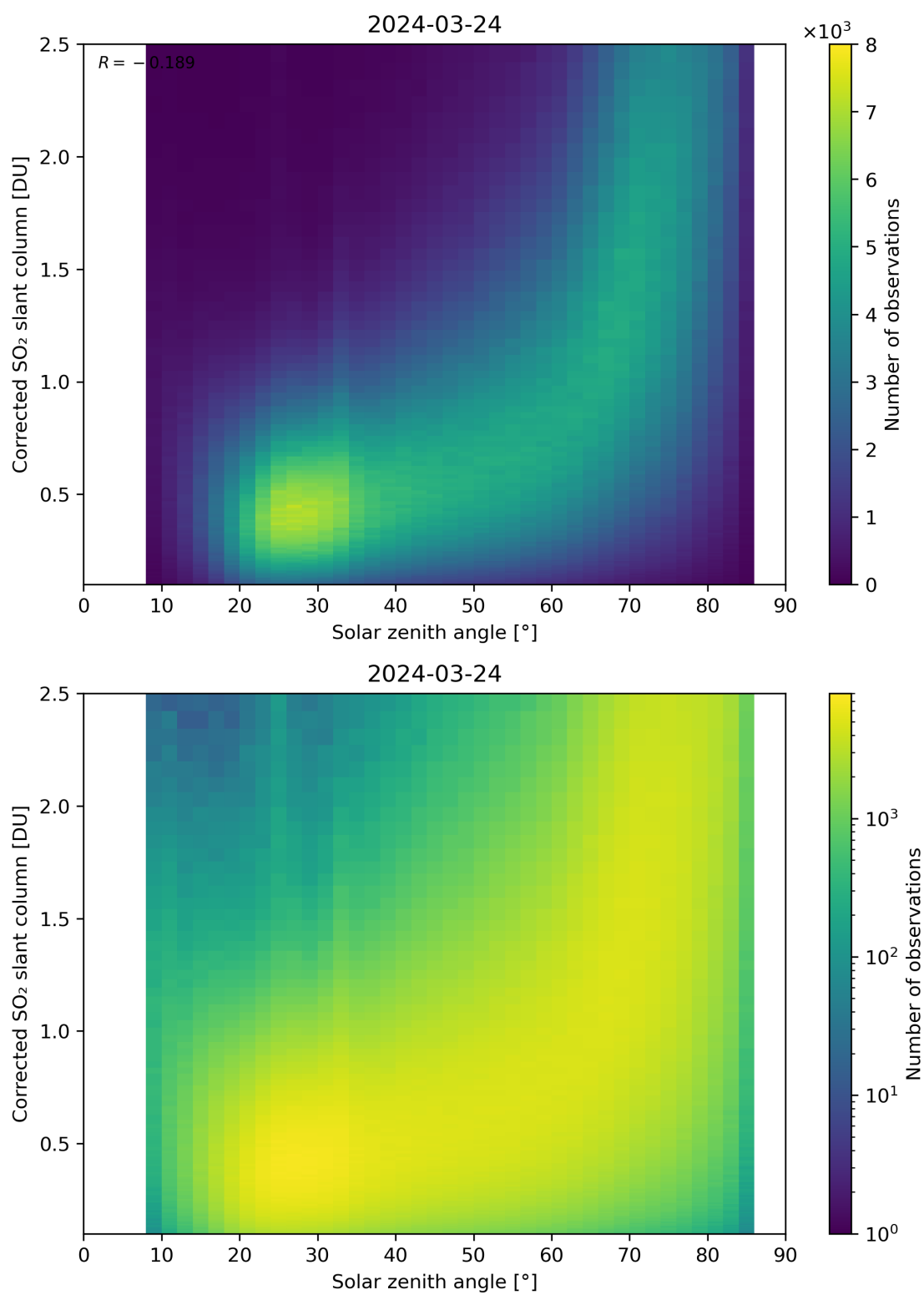
Figure 166: Scatter density plot of “Solar zenith angle” against “Corrected SO 2 slant column” for 2024-03-23 to 2024-03-25.
