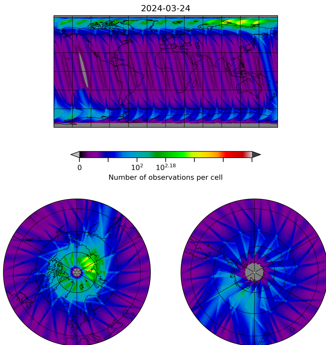
Figure 28: Map of the number of observations for 2024-03-23 to 2024-03-25
