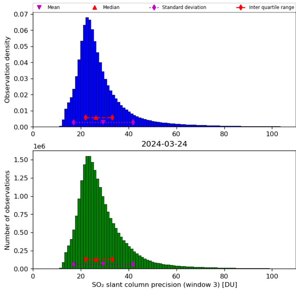
Figure 65: Histogram of “SO 2 slant column precision (window 3)” for 2024-03-23 to 2024-03-25
