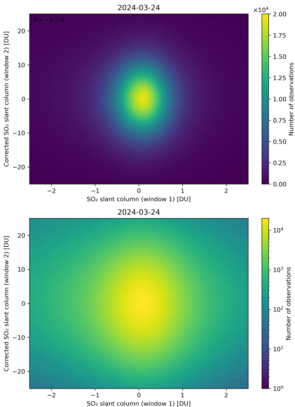
Figure 233: Scatter density plot of “SO 2 slant column (window 1)” against “Corrected SO 2 slant column (window 2)” for 2024-03-23 to 2024-03-25.
