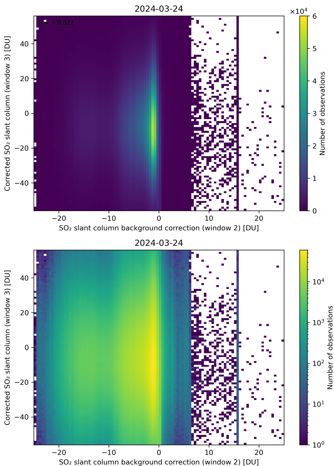
Figure 116: Scatter density plot of “SO 2 slant column background correction (window 2)” against “Corrected SO 2 slant column (window 3)” for 2024-03-23 to 2024-03-25.
