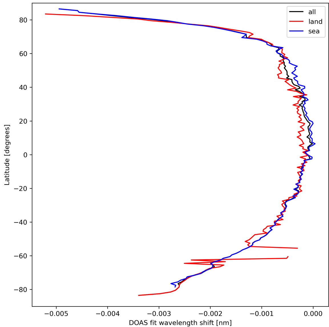
Figure 45: Zonal average of “DOAS fit wavelength shift” for 2024-03-23 to 2024-03-25.
