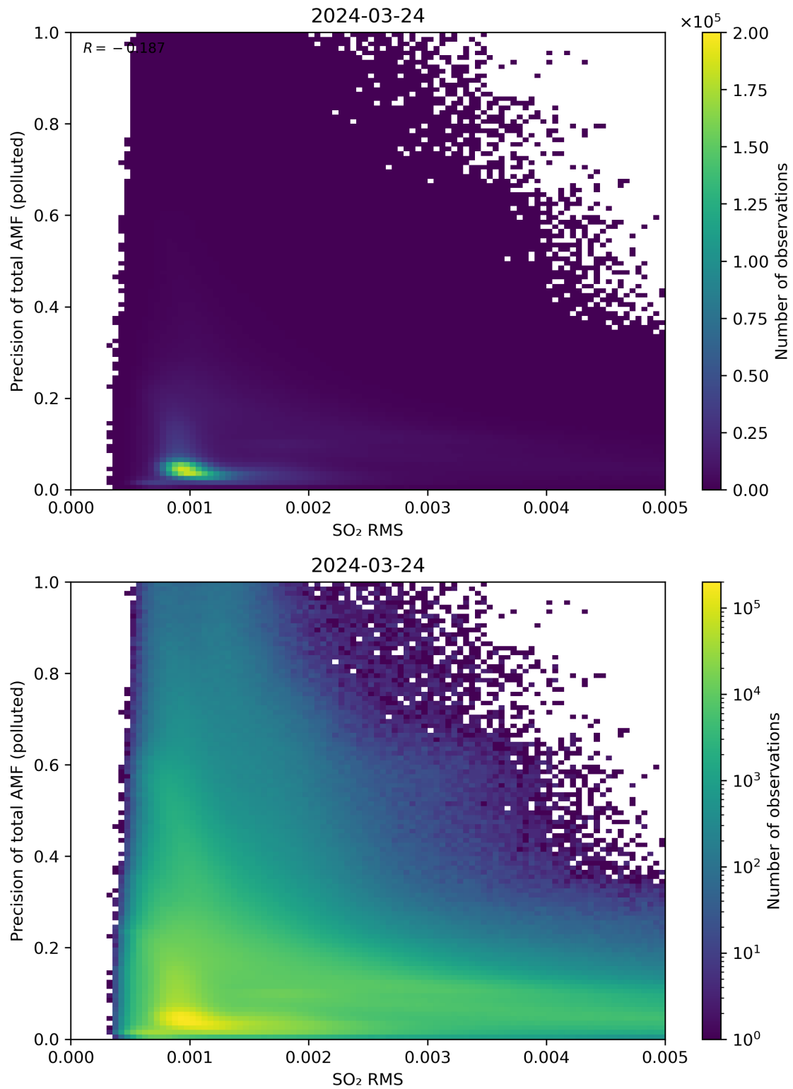
Figure 138: Scatter density plot of “SO 2 RMS” against “Precision of total AMF (polluted)” for 2024-03-23 to 2024-03-25.
