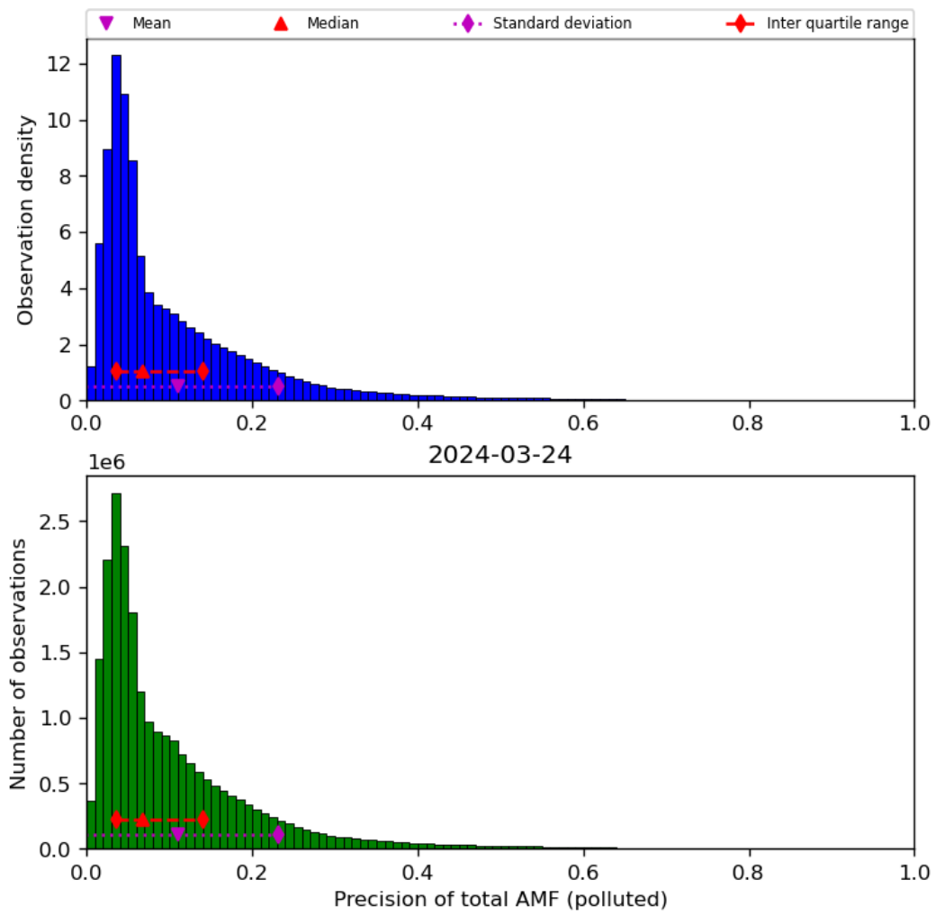
Figure 72: Histogram of “Precision of total AMF (polluted)” for 2024-03-23 to 2024-03-25
