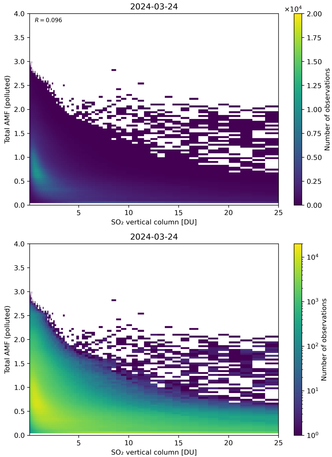
Figure 305: Scatter density plot of “SO 2 vertical column” against “Total AMF (polluted)” for 2024-03-23 to 2024-03-25.
