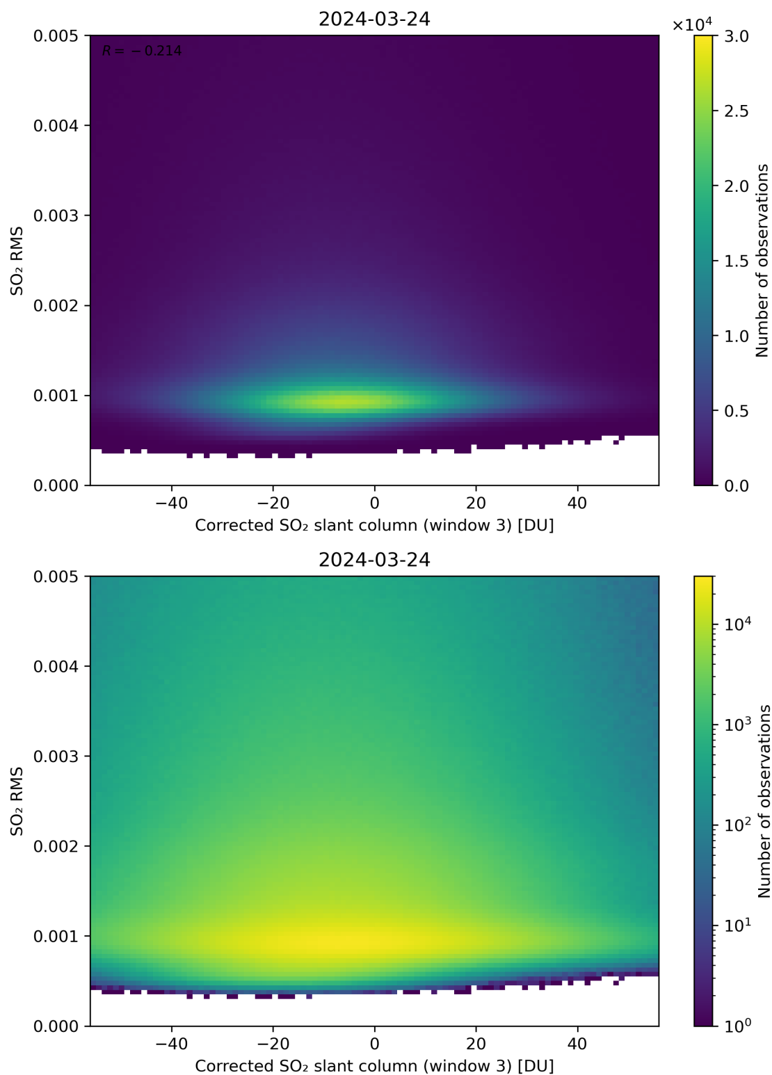
Figure 208: Scatter density plot of “Corrected SO 2 slant column (window 3)” against “SO 2 RMS” for 2024-03-23 to 2024-03-25.
