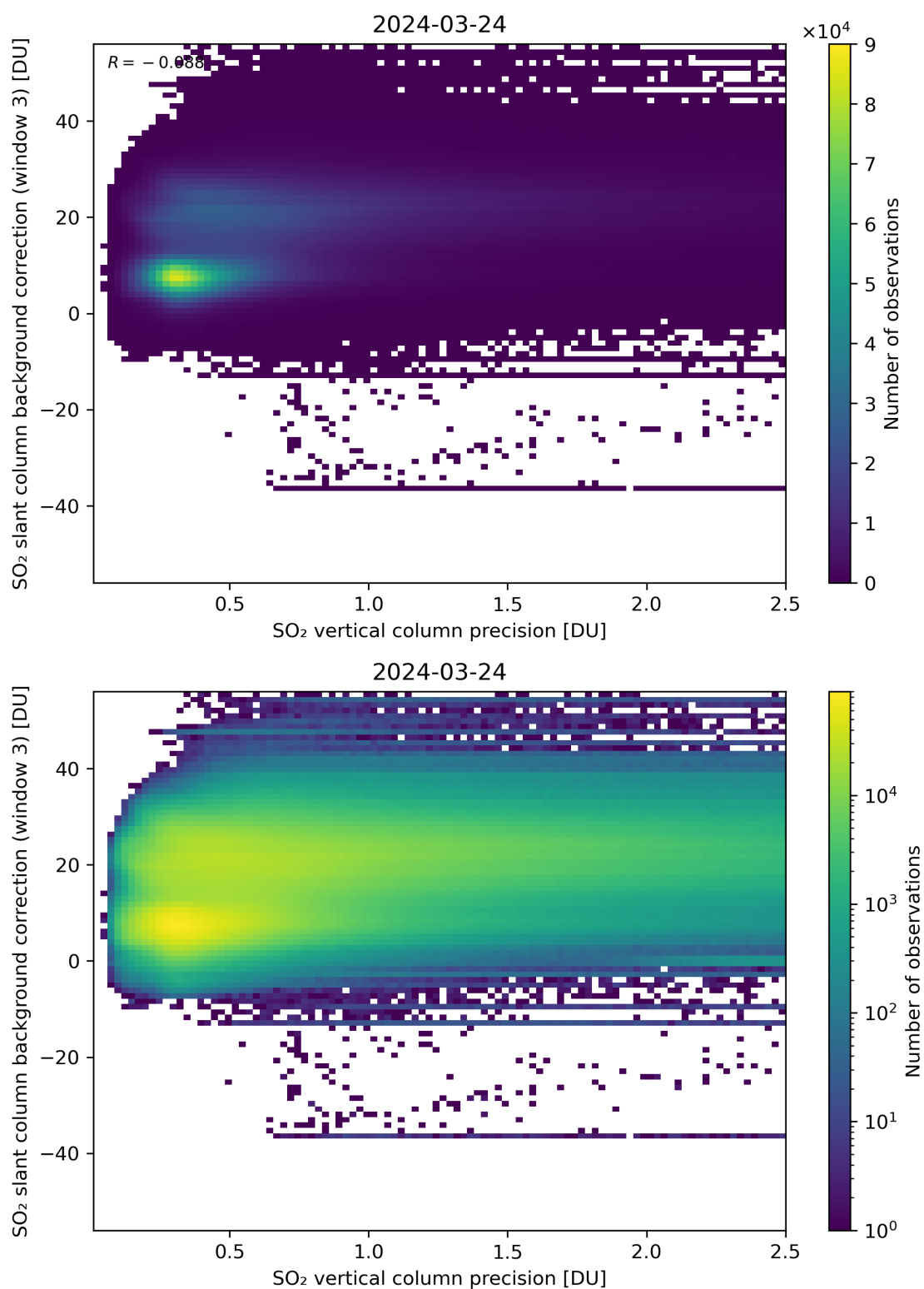
Figure 281: Scatter density plot of “SO 2 vertical column precision” against “SO 2 slant column background correction (window 3)” for 2024-03-23 to 2024-03-25.
