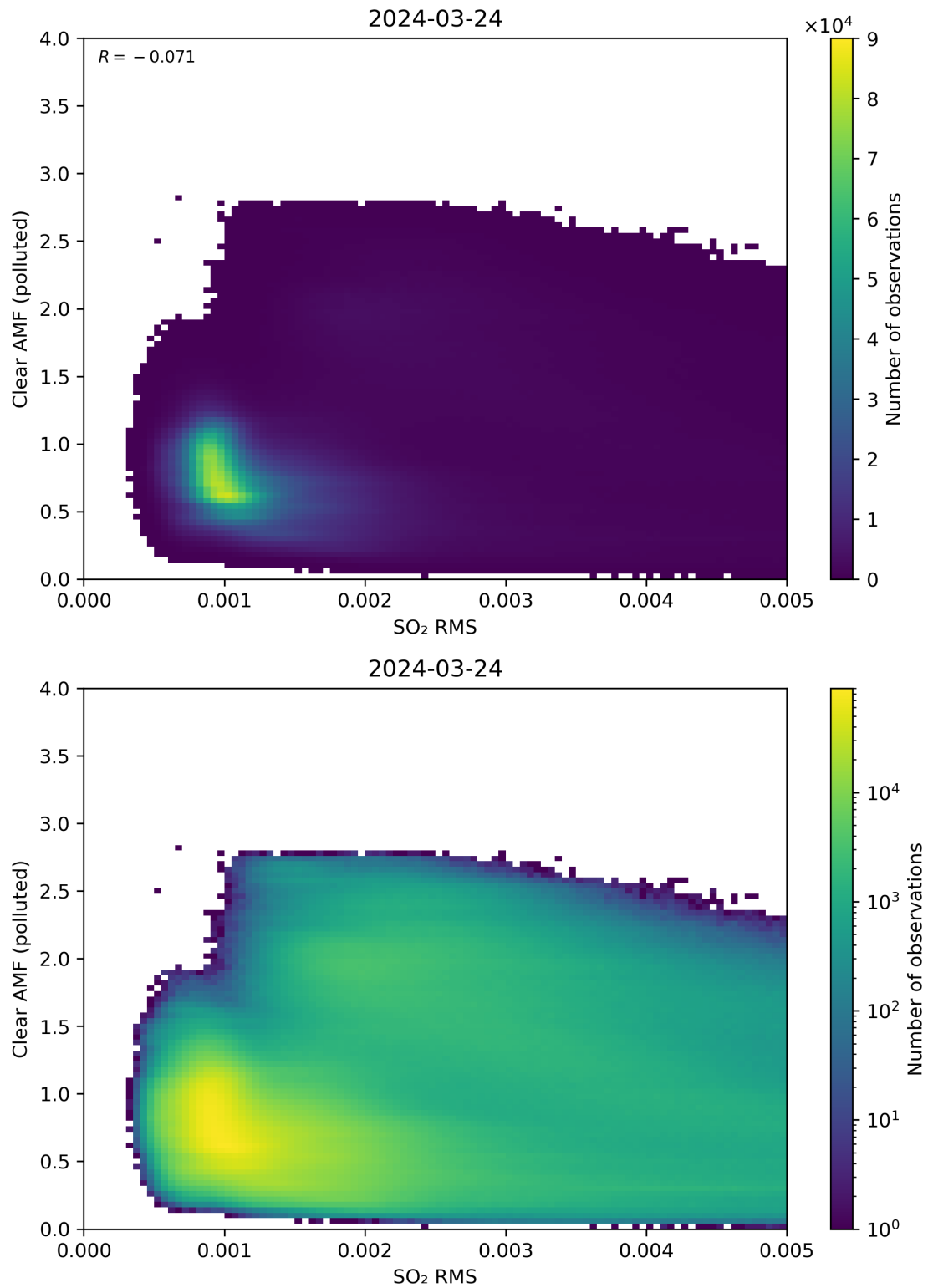
Figure 136: Scatter density plot of “SO 2 RMS” against “Clear AMF (polluted)” for 2024-03-23 to 2024-03-25.
