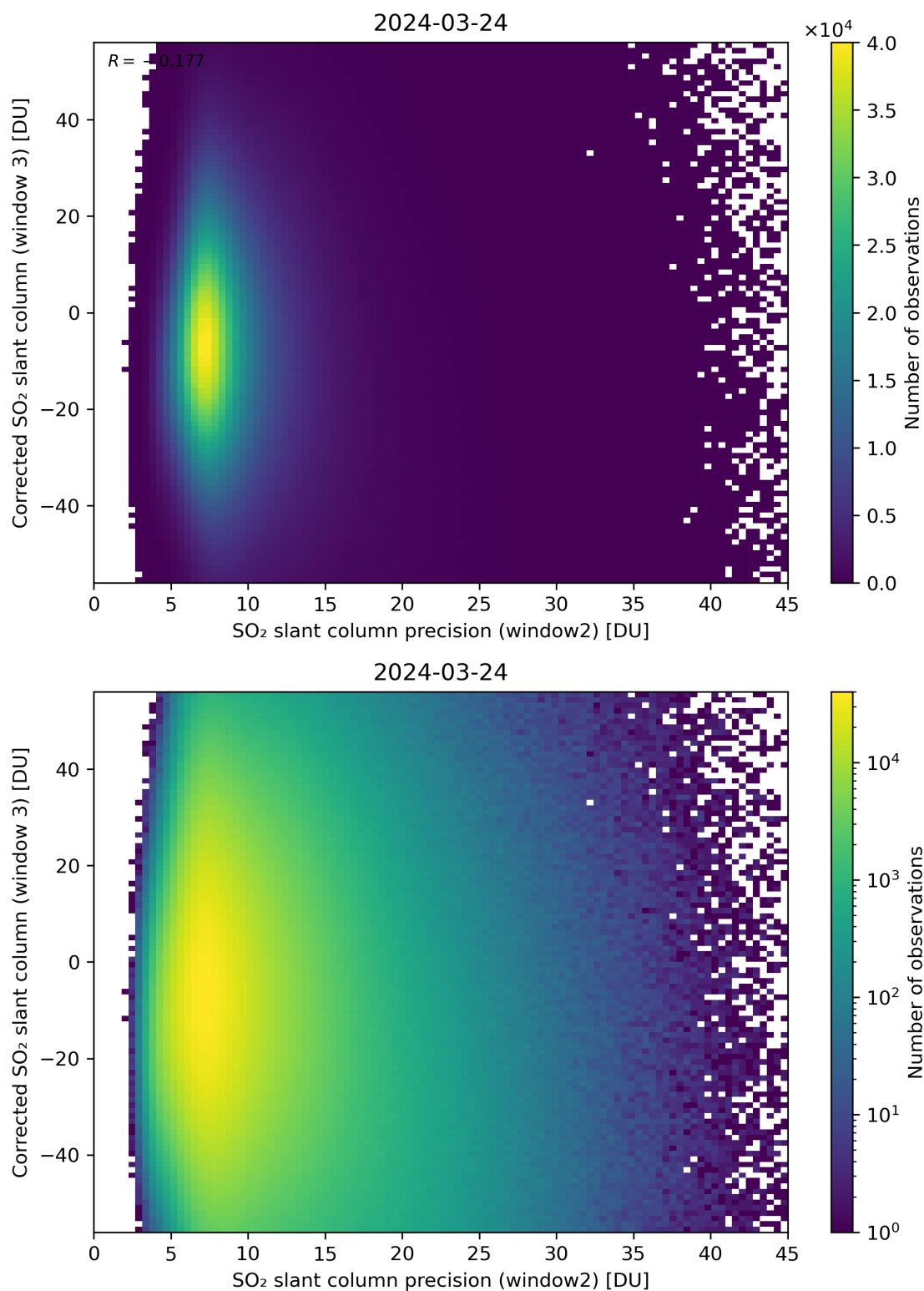
Figure 248: Scatter density plot of “SO 2 slant column precision (window2)” against “Corrected SO 2 slant column (window 3)” for 2024-03-23 to 2024-03-25.
