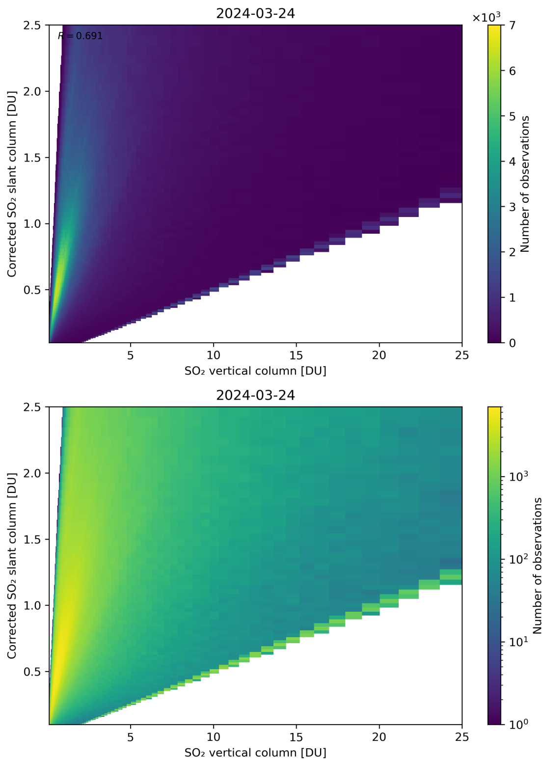
Figure 297: Scatter density plot of “SO 2 vertical column” against “Corrected SO 2 slant column” for 2024-03-23 to 2024-03-25.
