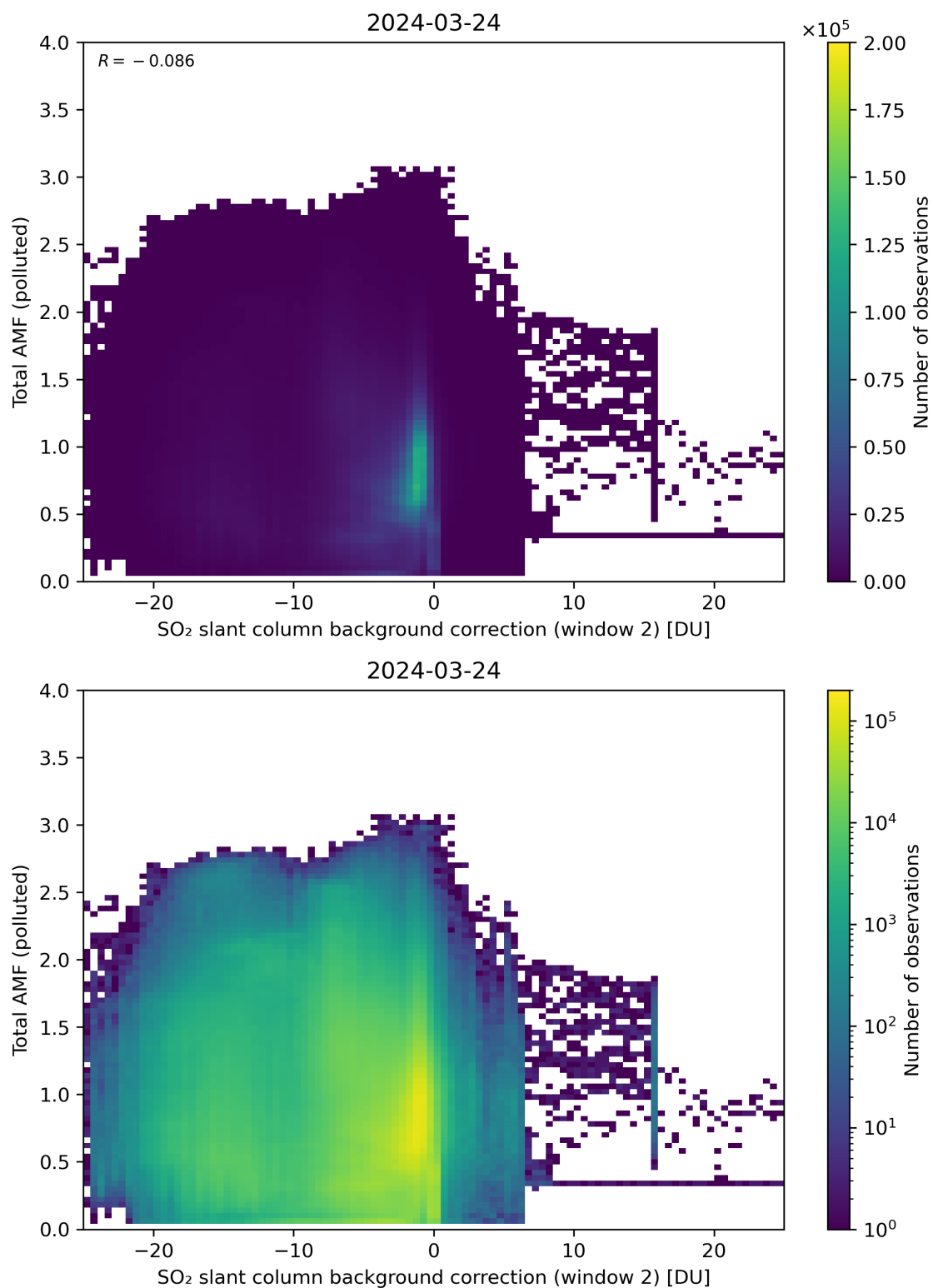
Figure 119: Scatter density plot of “SO 2 slant column background correction (window 2)” against “Total AMF (polluted)” for 2024-03-23 to 2024-03-25.
