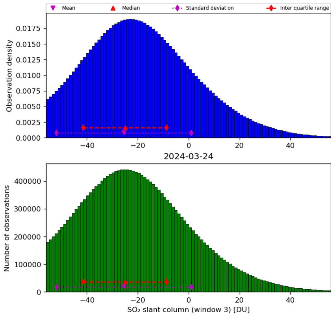
Figure 64: Histogram of “SO 2 slant column (window 3)” for 2024-03-23 to 2024-03-25
