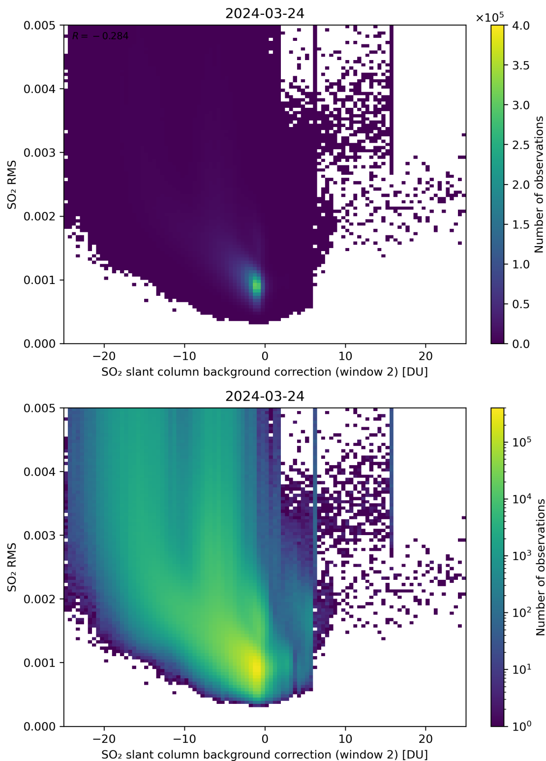
Figure 114: Scatter density plot of “SO 2 slant column background correction (window 2)” against “SO 2 RMS” for 2024-03-23 to 2024-03-25.
