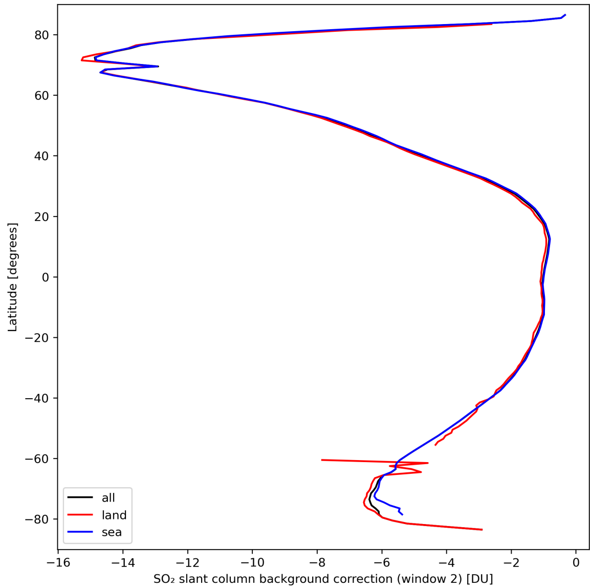
Figure 40: Zonal average of “SO 2 slant column background correction (window 2)” for 2024-03-23 to 2024-03-25.
