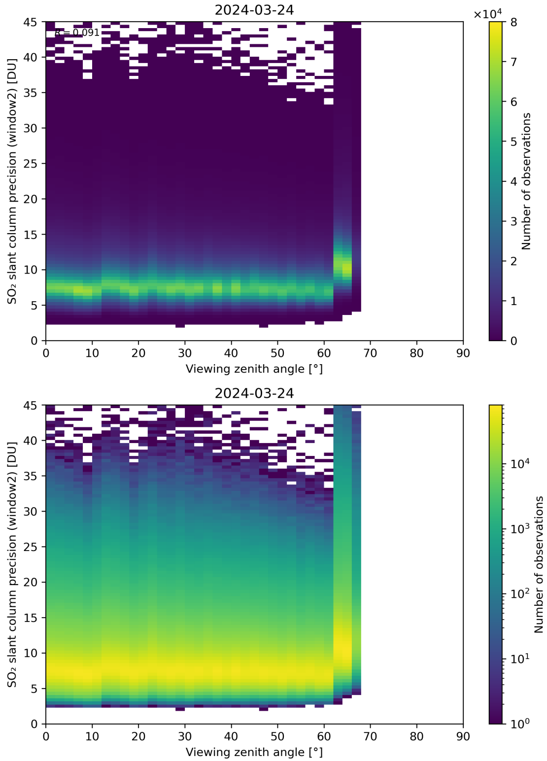
Figure 322: Scatter density plot of “Viewing zenith angle” against “SO 2 slant column precision (window2)” for 2024-03-23 to 2024-03-25.
