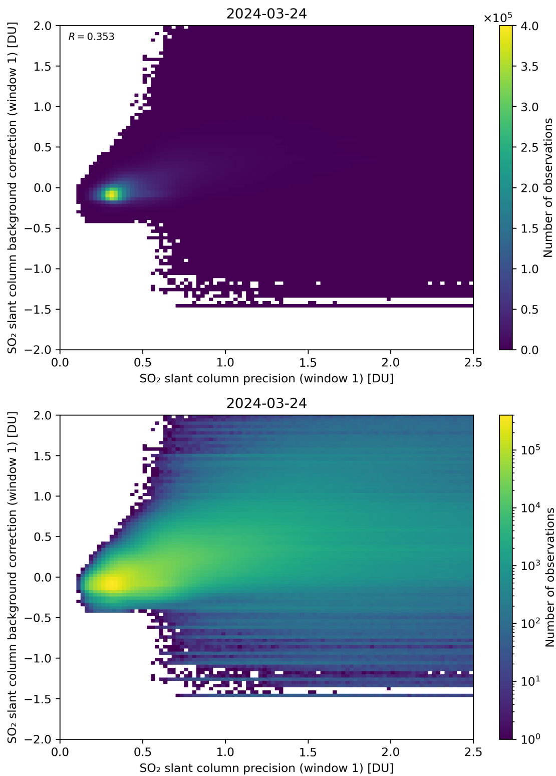
Figure 218: Scatter density plot of “SO 2 slant column precision (window 1)” against “SO 2 slant column background correction (window 1)” for 2024-03-23 to 2024-03-25.
