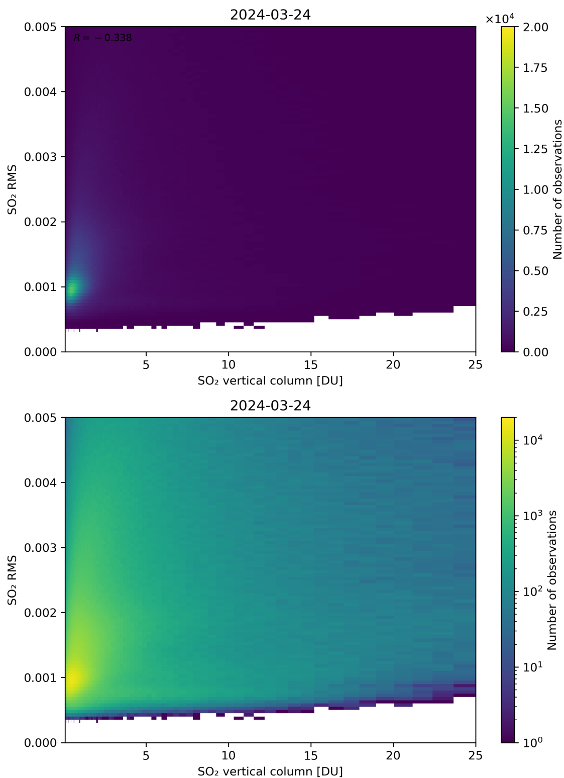
Figure 278: Scatter density plot of “SO 2 vertical column” against “SO 2 RMS” for 2024-03-23 to 2024-03-25.
