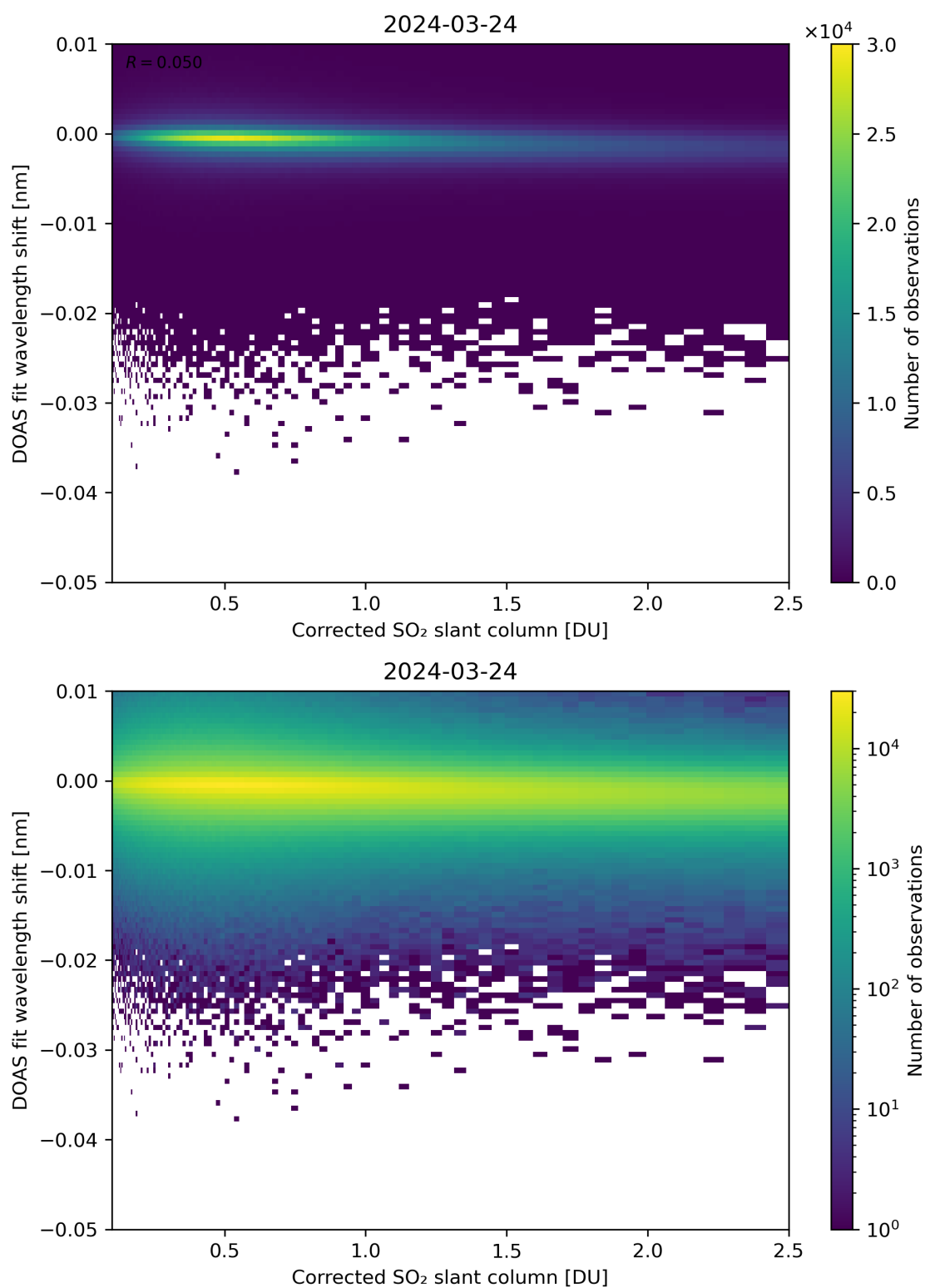
Figure 181: Scatter density plot of “Corrected SO 2 slant column” against “DOAS fit wavelength shift” for 2024-03-23 to 2024-03-25.
