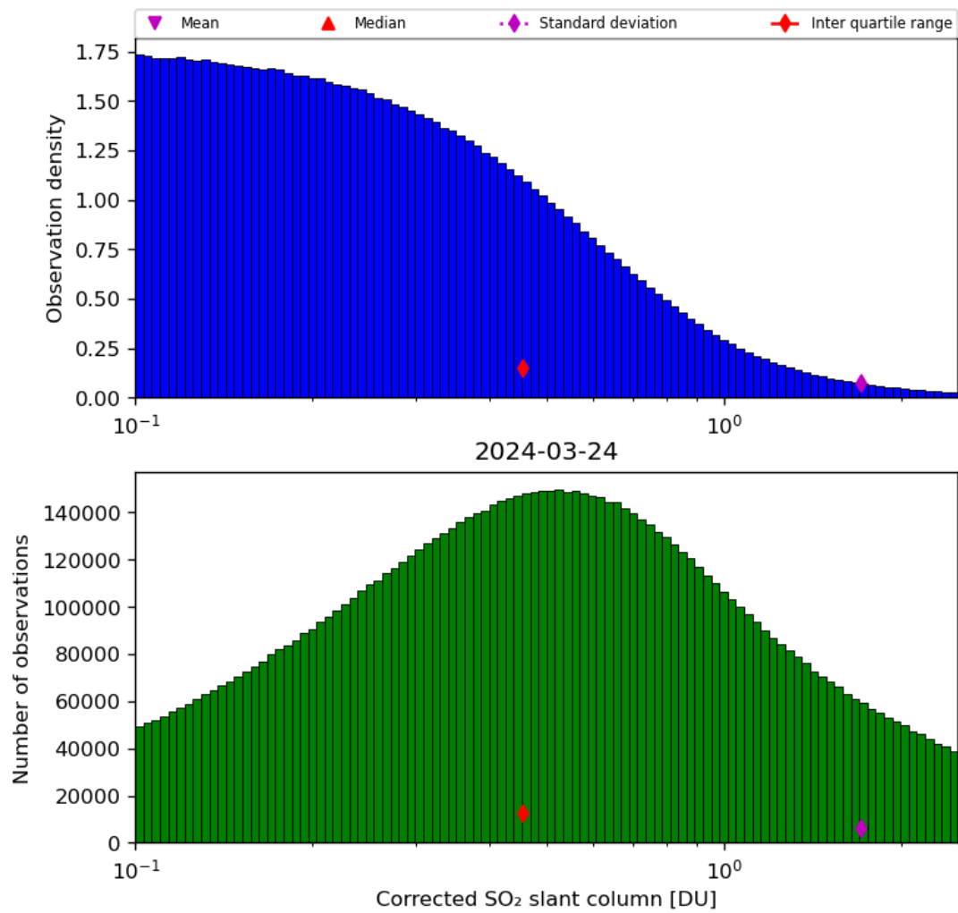
Figure 55: Histogram of “Corrected SO 2 slant column” for 2024-03-23 to 2024-03-25
