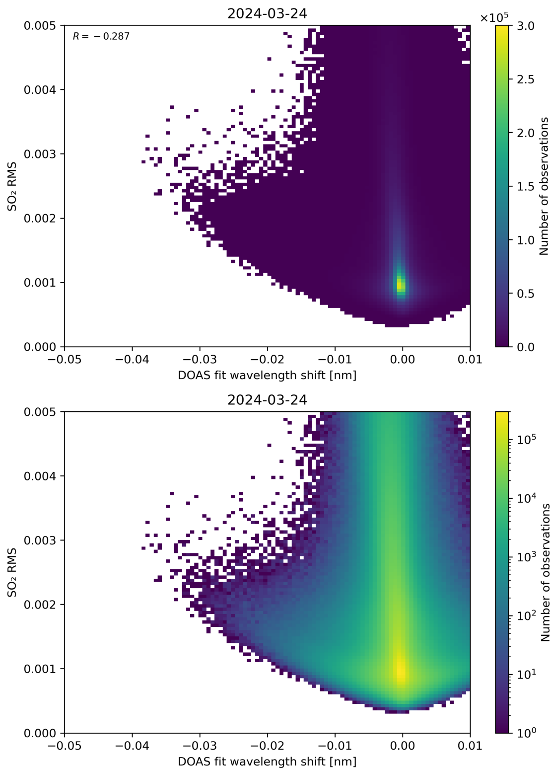
Figure 128: Scatter density plot of “DOAS fit wavelength shift” against “SO 2 RMS” for 2024-03-23 to 2024-03-25.
