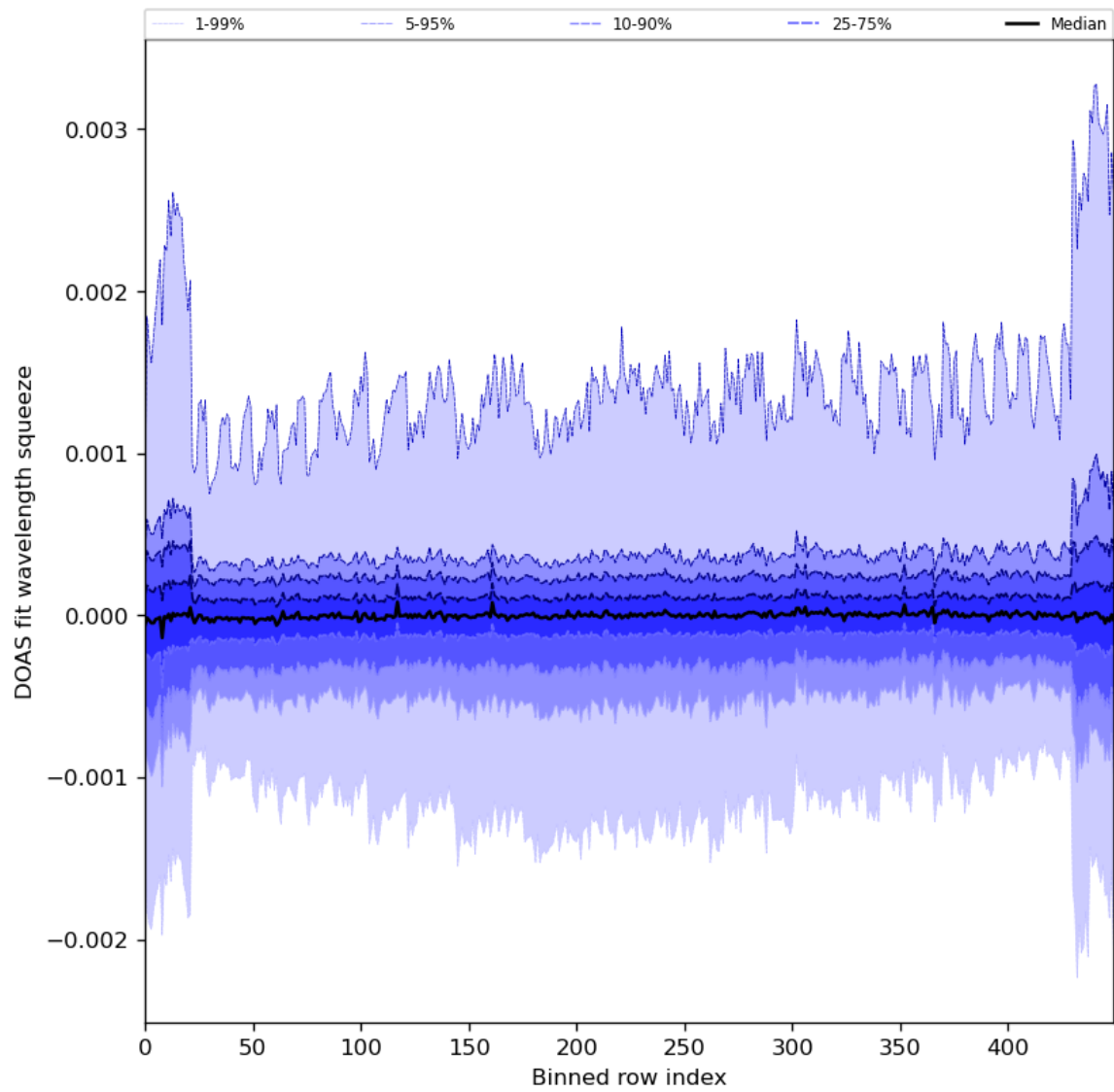
Figure 92: Along track statistics of “DOAS fit wavelength squeeze” for 2024-03-23 to 2024-03-25
