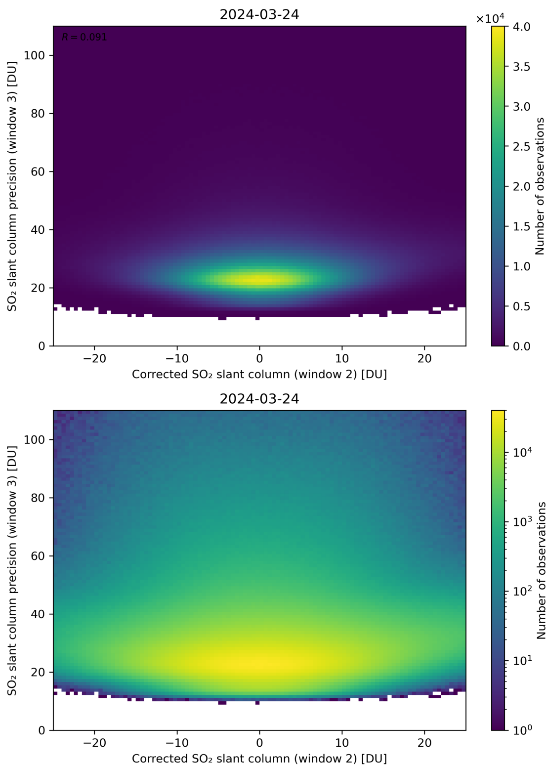
Figure 202: Scatter density plot of “Corrected SO 2 slant column (window 2)” against “SO 2 slant column precision (window 3)” for 2024-03-23 to 2024-03-25.
