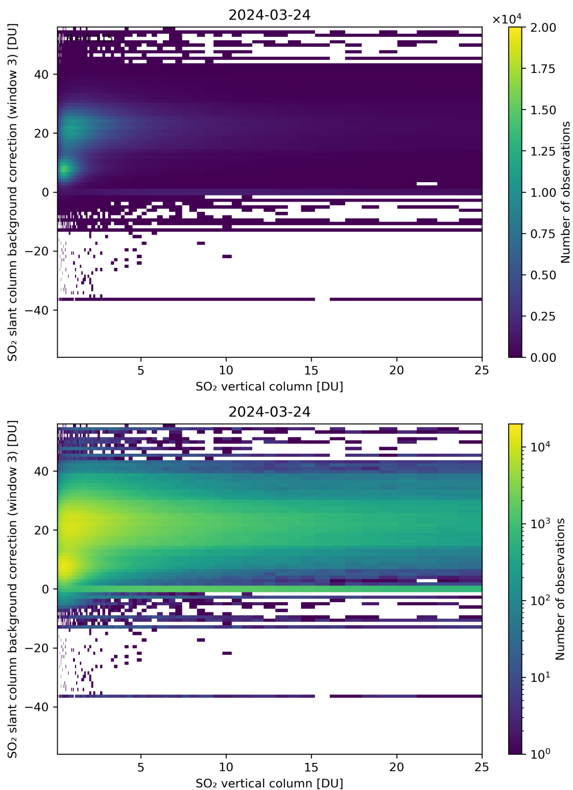
Figure 275: Scatter density plot of “SO 2 vertical column” against “SO 2 slant column background correction (window 3)” for 2024-03-23 to 2024-03-25.
