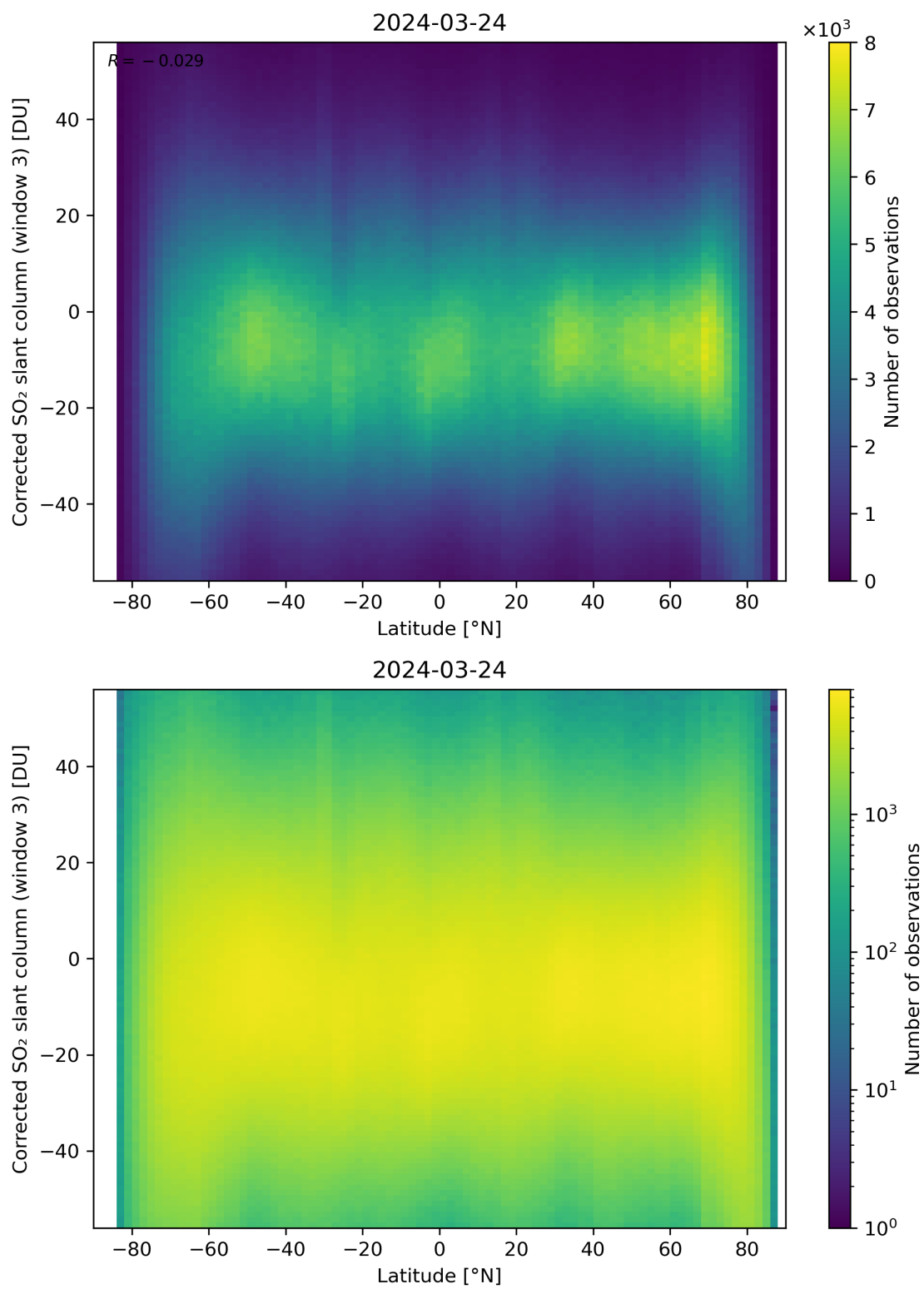
Figure 148: Scatter density plot of “Latitude” against “Corrected SO 2 slant column (window 3)” for 2024-03-23 to 2024-03-25.
