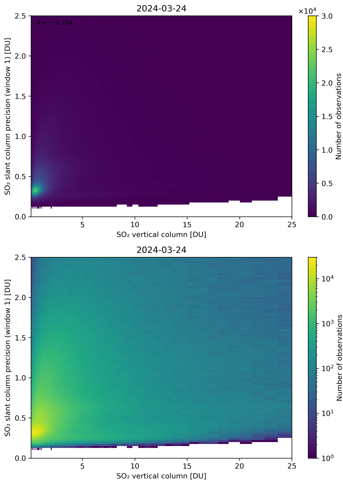
Figure 301: Scatter density plot of “SO 2 vertical column” against “SO 2 slant column precision (window 1)” for 2024-03-23 to 2024-03-25.
