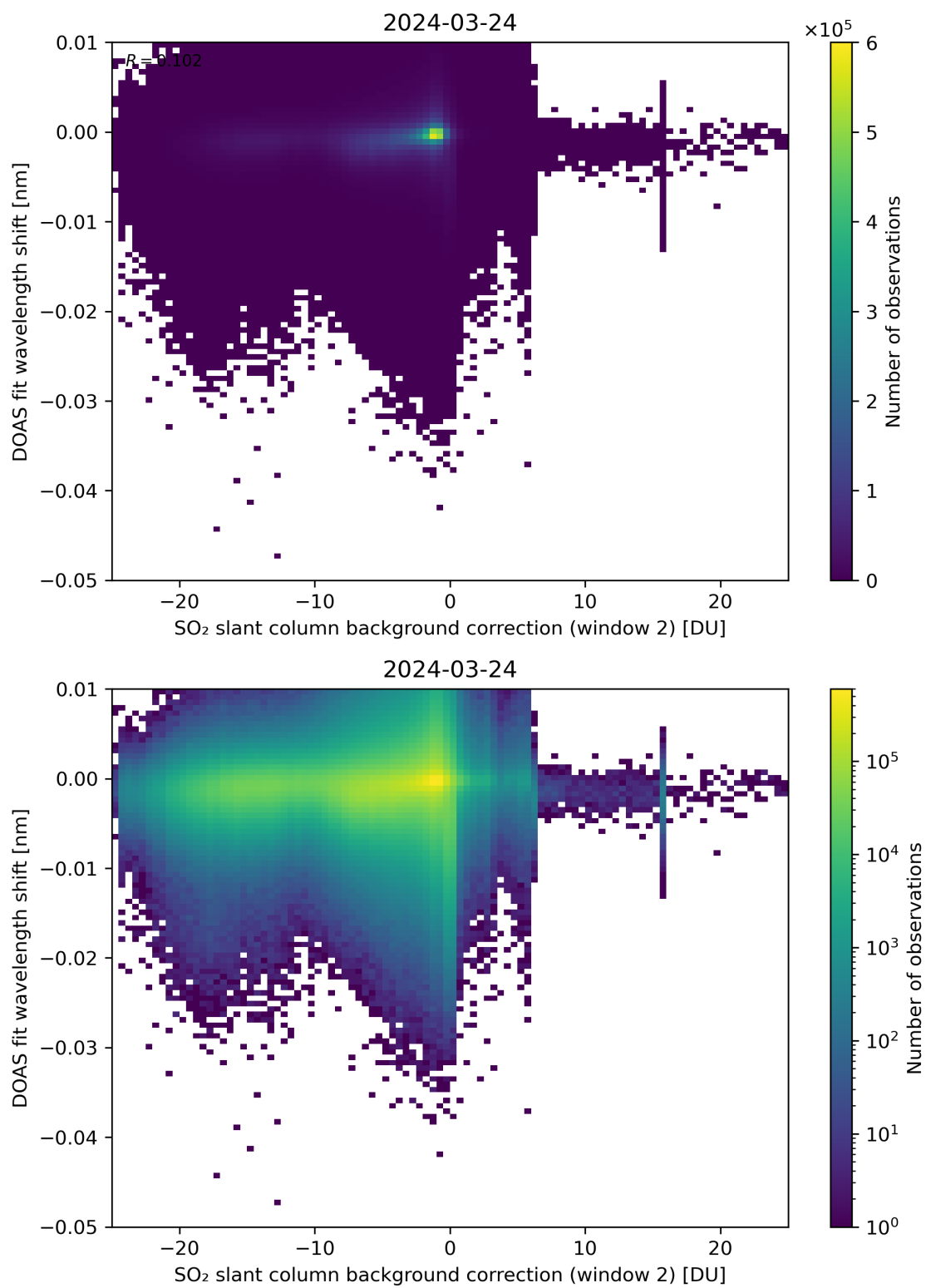
Figure 112: Scatter density plot of “SO 2 slant column background correction (window 2)” against “DOAS fit wavelength shift” for 2024-03-23 to 2024-03-25.
