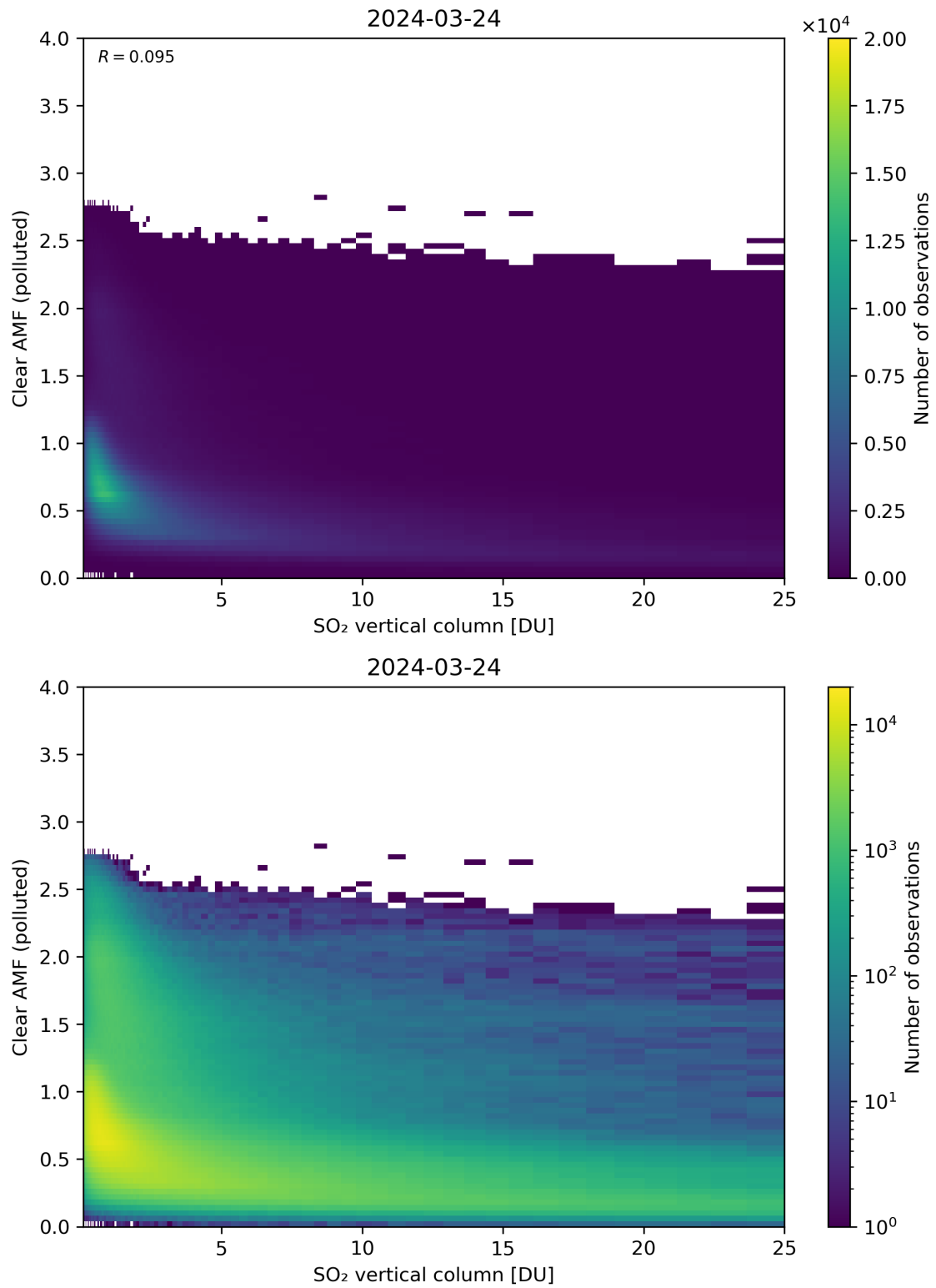
Figure 296: Scatter density plot of “SO 2 vertical column” against “Clear AMF (polluted)” for 2024-03-23 to 2024-03-25.
