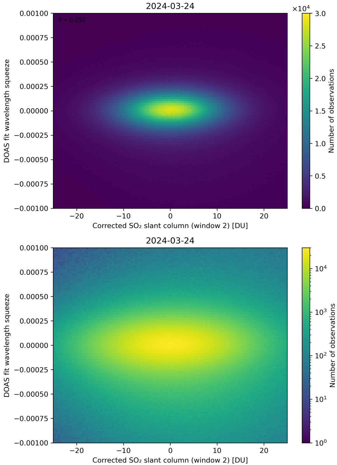
Figure 197: Scatter density plot of “Corrected SO 2 slant column (window 2)” against “DOAS fit wavelength squeeze” for 2024-03-23 to 2024-03-25.
