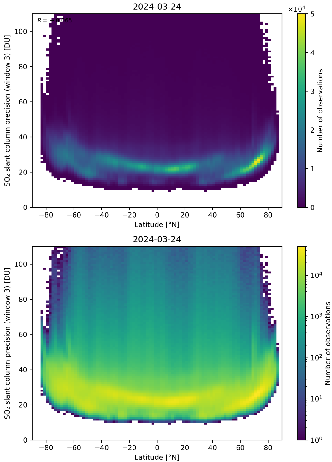
Figure 153: Scatter density plot of “Latitude” against “SO 2 slant column precision (window 3)” for 2024-03-23 to 2024-03-25.
