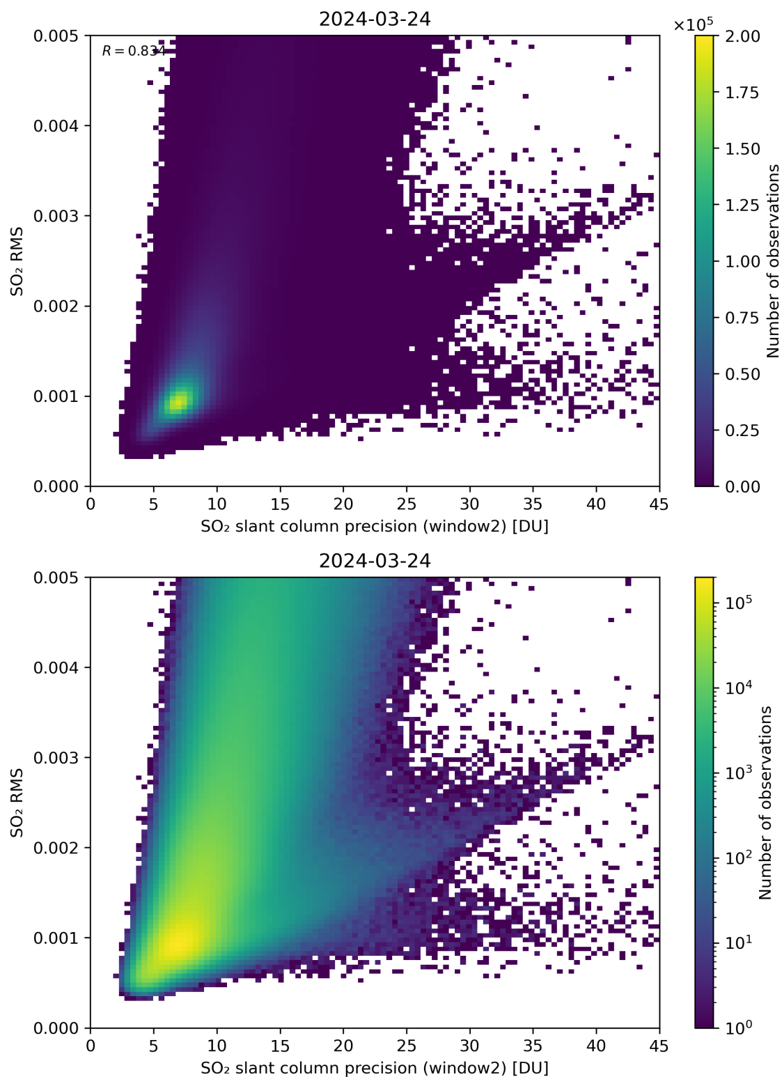
Figure 245: Scatter density plot of “SO 2 slant column precision (window2)” against “SO 2 RMS” for 2024-03-23 to 2024-03-25.
