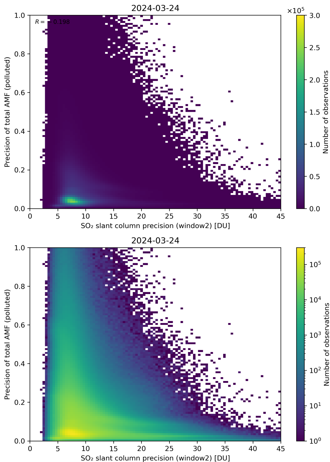
Figure 252: Scatter density plot of “SO 2 slant column precision (window2)” against “Precision of total AMF (polluted)” for 2024-03-23 to 2024-03-25.
