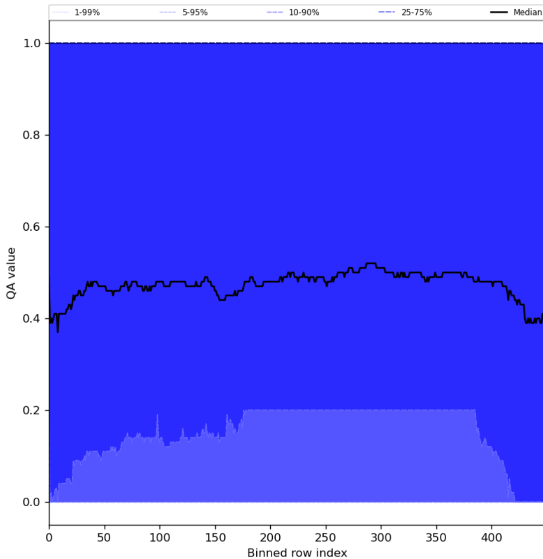
Figure 75: Along track statistics of “QA value” for 2024-03-23 to 2024-03-25
