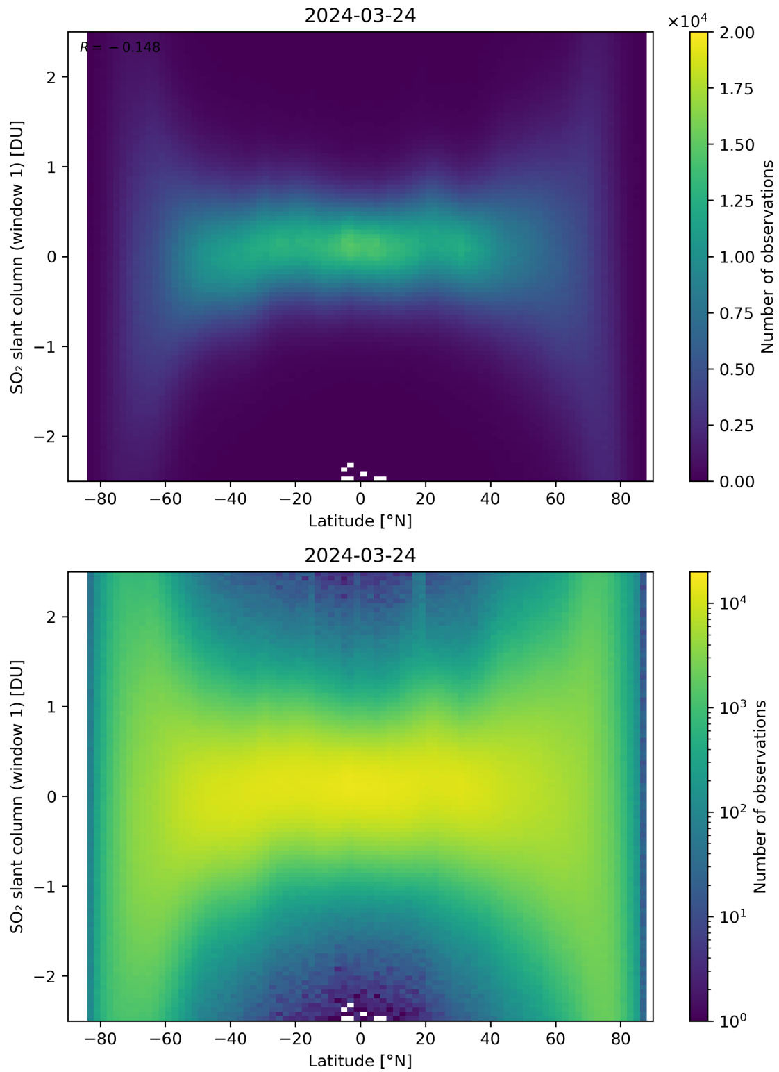
Figure 149: Scatter density plot of “Latitude” against “SO 2 slant column (window 1)” for 2024-03-23 to 2024-03-25.
