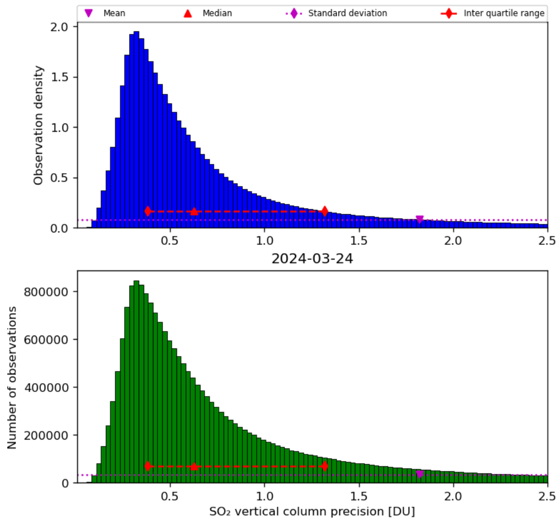
Figure 54: Histogram of “SO 2 vertical column precision” for 2024-03-23 to 2024-03-25
