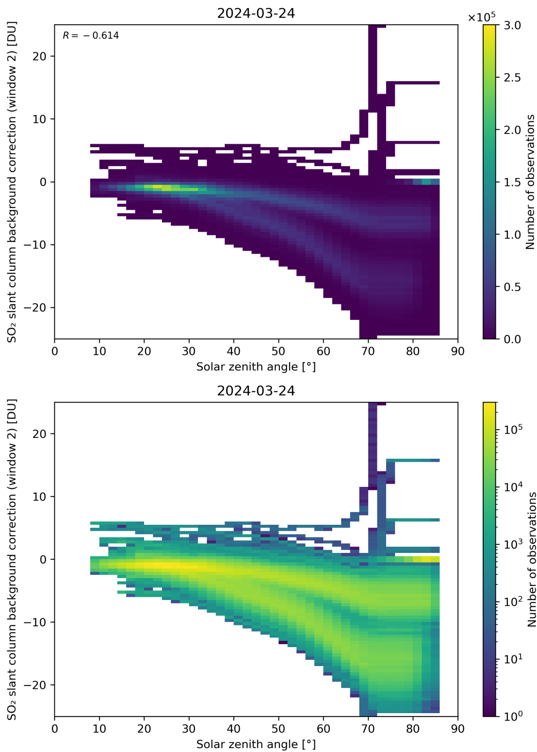
Figure 159: Scatter density plot of “Solar zenith angle” against “SO 2 slant column background correction (window 2)” for 2024-03-23 to 2024-03-25.
