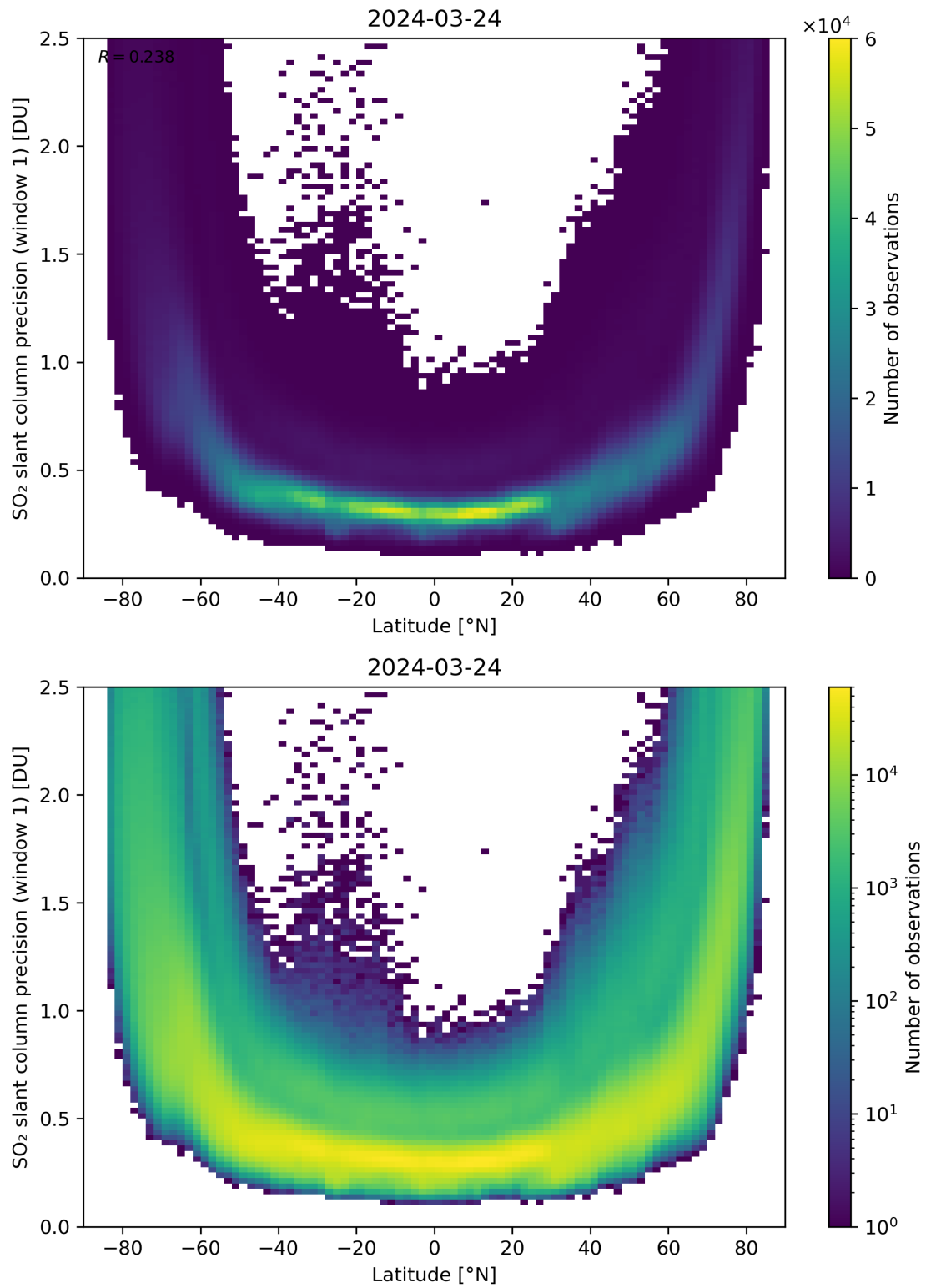
Figure 150: Scatter density plot of “Latitude” against “SO 2 slant column precision (window 1)” for 2024-03-23 to 2024-03-25.
