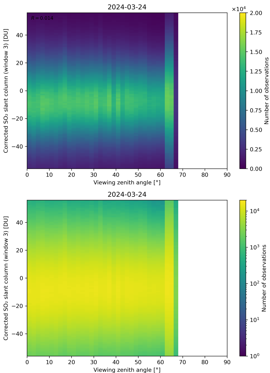
Figure 319: Scatter density plot of “Viewing zenith angle” against “Corrected SO 2 slant column (window 3)” for 2024-03-23 to 2024-03-25.
