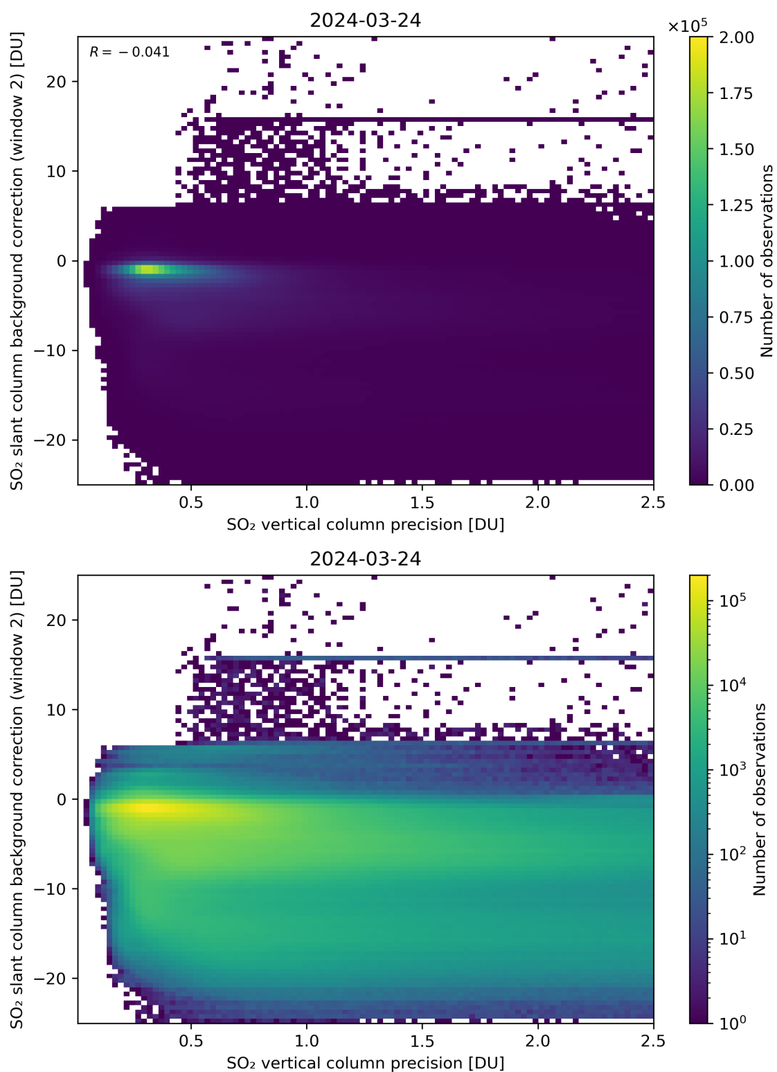
Figure 280: Scatter density plot of “SO 2 vertical column precision” against “SO 2 slant column background correction (window 2)” for 2024-03-23 to 2024-03-25.
