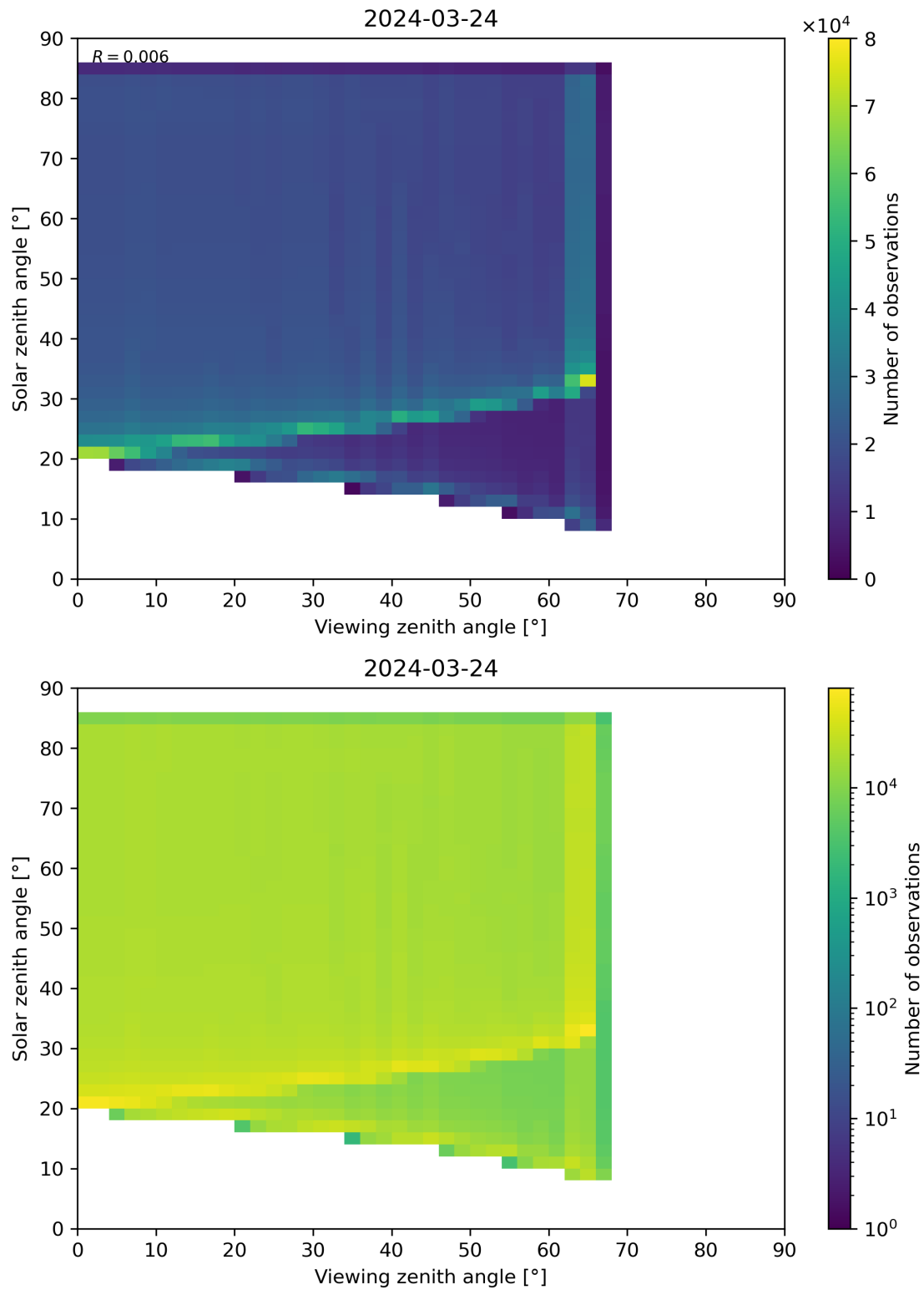
Figure 315: Scatter density plot of “Viewing zenith angle” against “Solar zenith angle” for 2024-03-23 to 2024-03-25.
