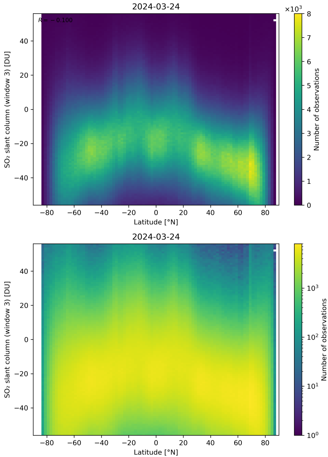
Figure 152: Scatter density plot of “Latitude” against “SO 2 slant column (window 3)” for 2024-03-23 to 2024-03-25.
