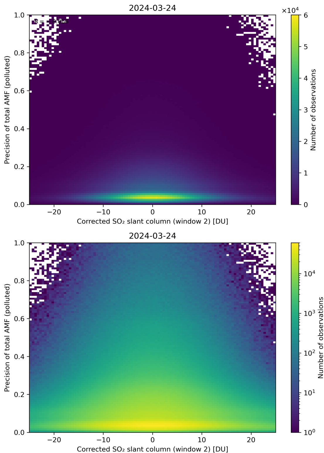
Figure 204: Scatter density plot of “Corrected SO 2 slant column (window 2)” against “Precision of total AMF (polluted)” for 2024-03-23 to 2024-03-25.
