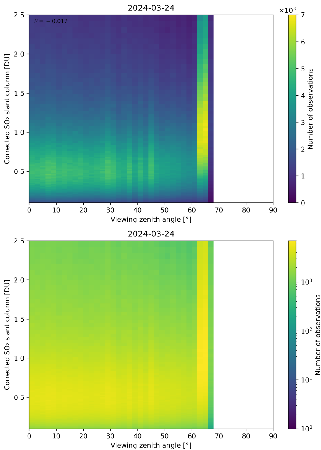
Figure 317: Scatter density plot of “Viewing zenith angle” against “Corrected SO 2 slant column” for 2024-03-23 to 2024-03-25.
