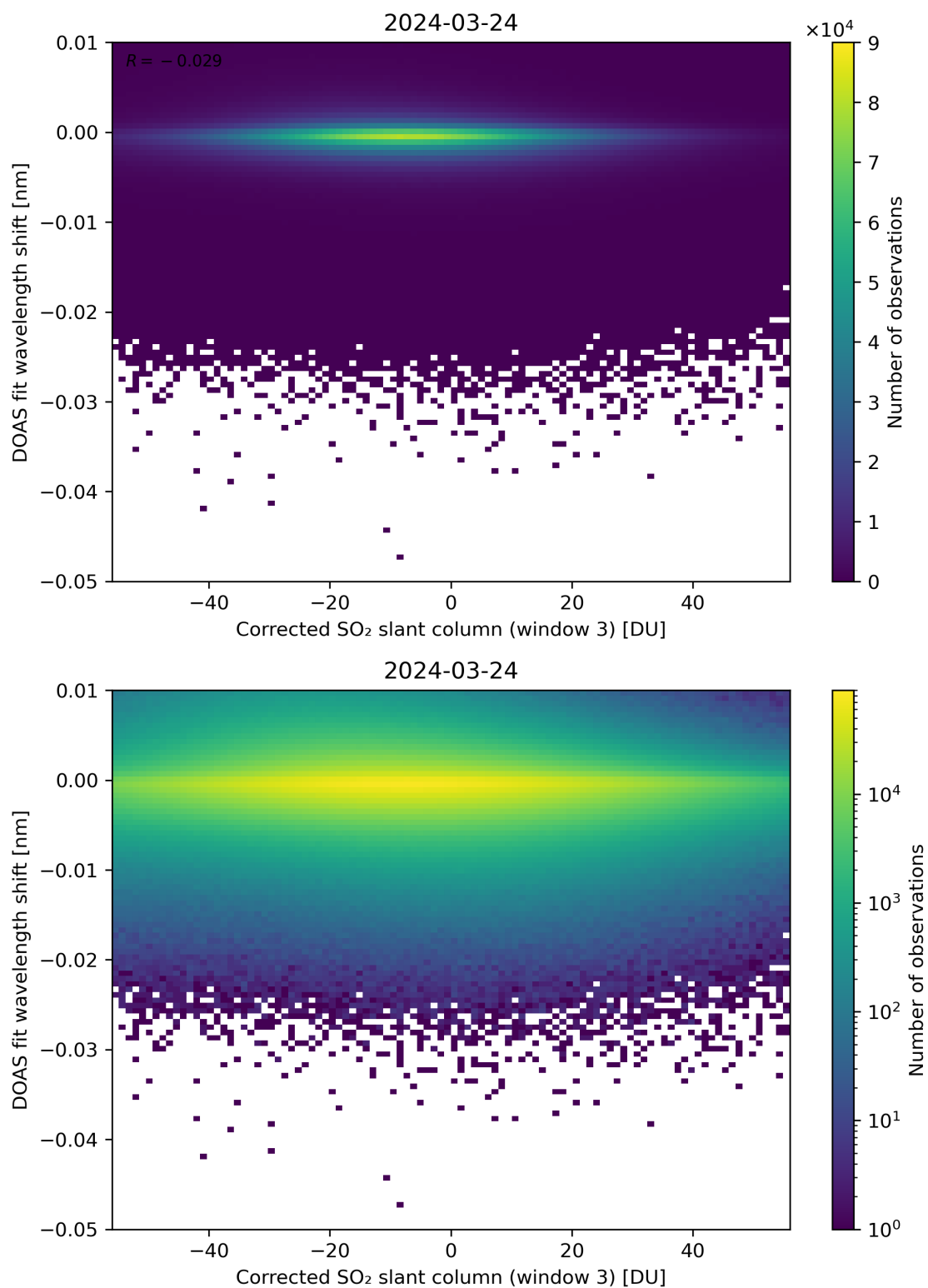
Figure 206: Scatter density plot of “Corrected SO 2 slant column (window 3)” against “DOAS fit wavelength shift” for 2024-03-23 to 2024-03-25.
