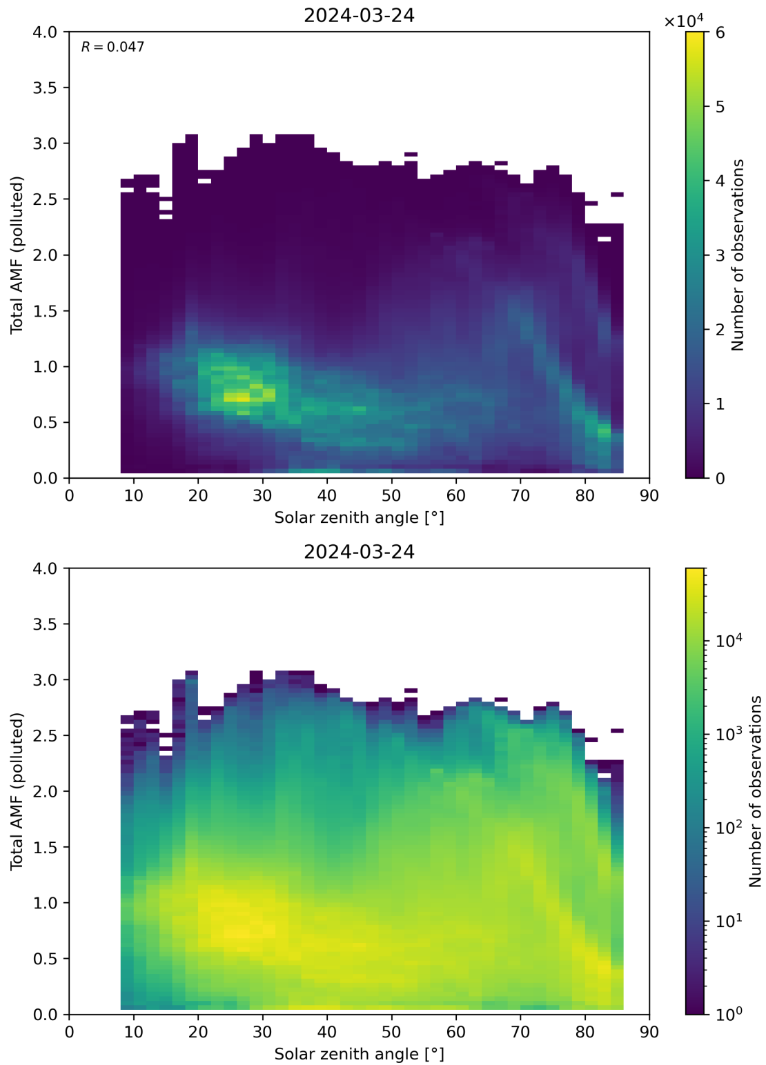
Figure 174: Scatter density plot of “Solar zenith angle” against “Total AMF (polluted)” for 2024-03-23 to 2024-03-25.
