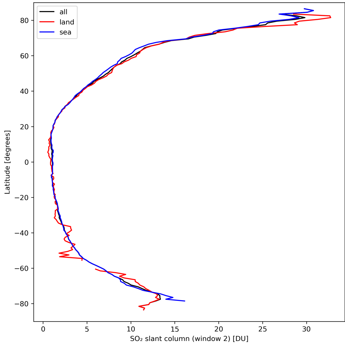
Figure 37: Zonal average of “SO 2 slant column (window 2)” for 2024-03-23 to 2024-03-25.
