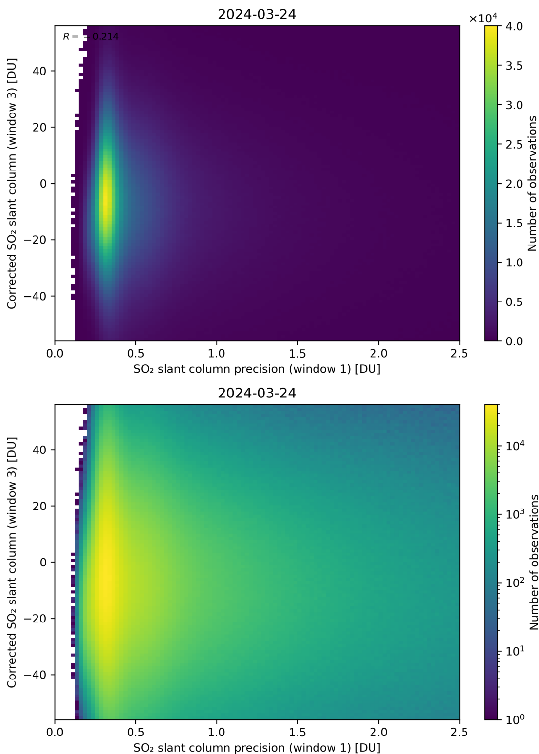
Figure 226: Scatter density plot of “SO 2 slant column precision (window 1)” against “Corrected SO 2 slant column (window 3)” for 2024-03-23 to 2024-03-25.
