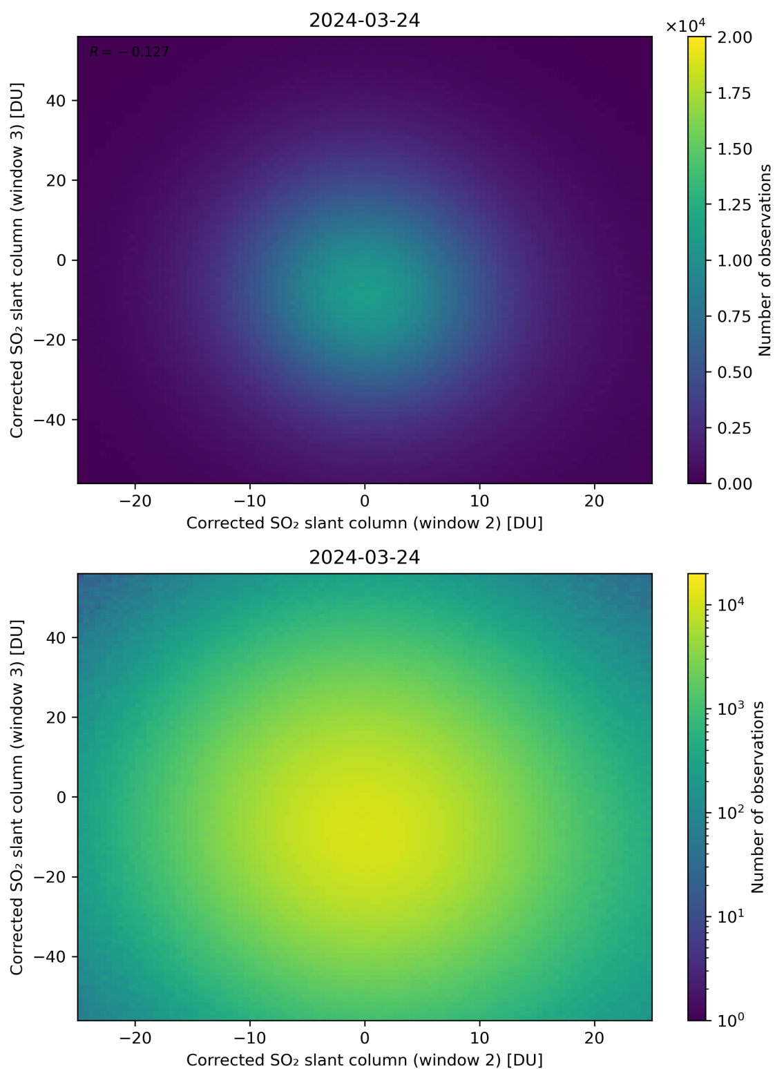
Figure 200: Scatter density plot of “Corrected SO 2 slant column (window 2)” against “Corrected SO 2 slant column (window 3)” for 2024-03-23 to 2024-03-25.
