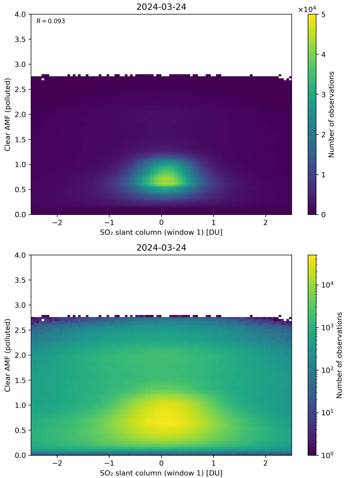
Figure 232: Scatter density plot of “SO 2 slant column (window 1)” against “Clear AMF (polluted)” for 2024-03-23 to 2024-03-25.
