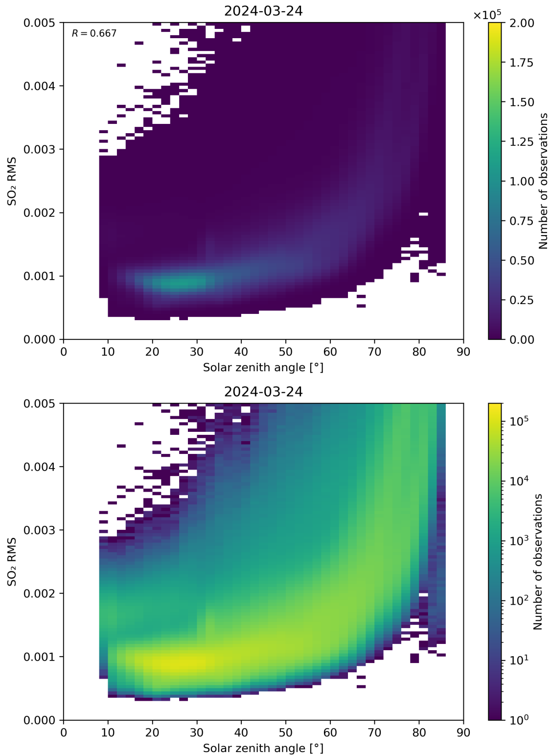
Figure 163: Scatter density plot of “Solar zenith angle” against “SO 2 RMS” for 2024-03-23 to 2024-03-25.
