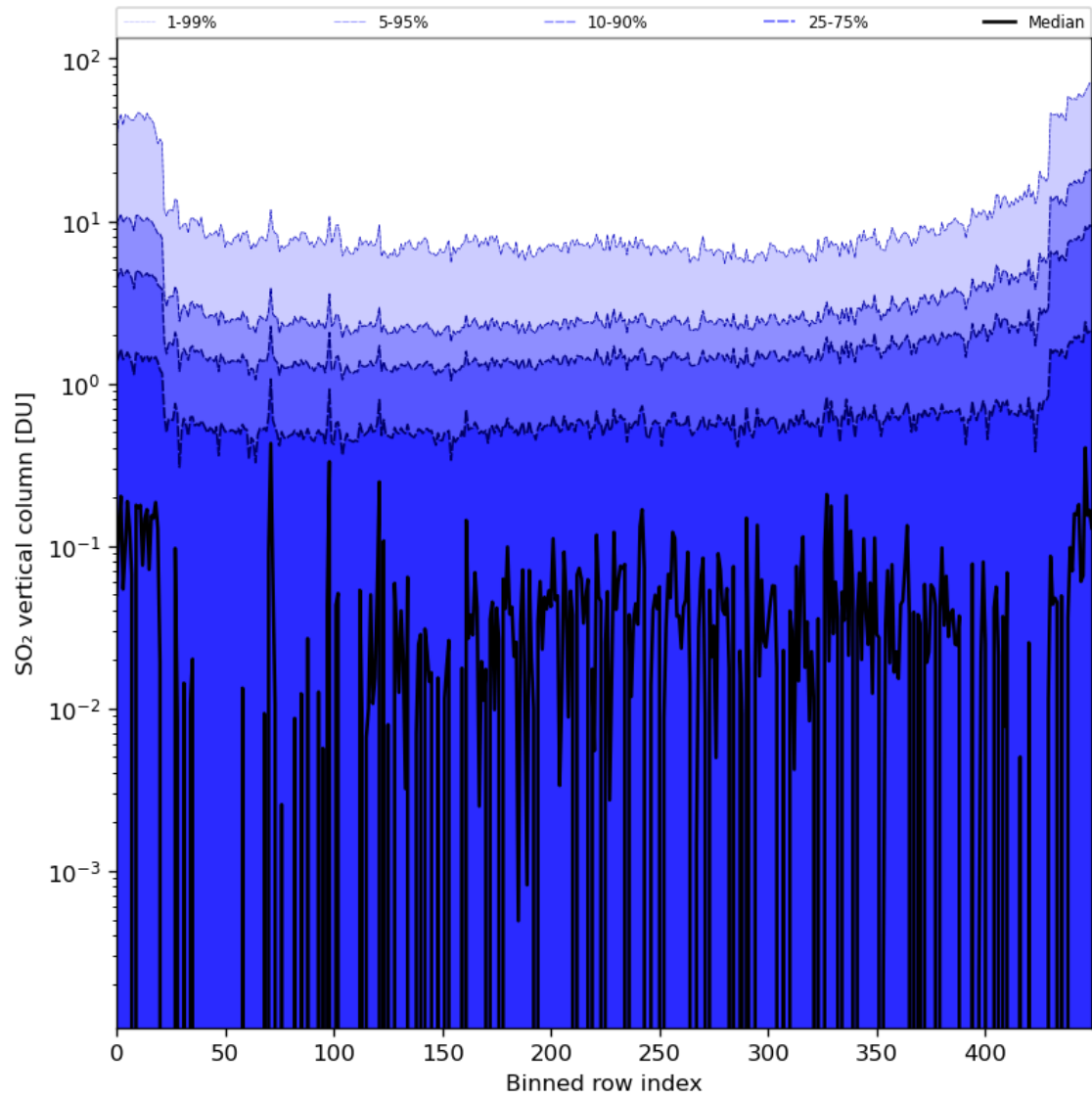
Figure 76: Along track statistics of “SO 2 vertical column” for 2024-03-23 to 2024-03-25
