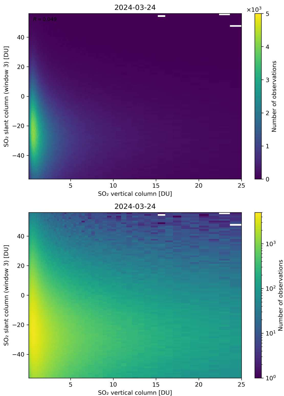
Figure 303: Scatter density plot of “SO 2 vertical column” against “SO 2 slant column (window 3)” for 2024-03-23 to 2024-03-25.
