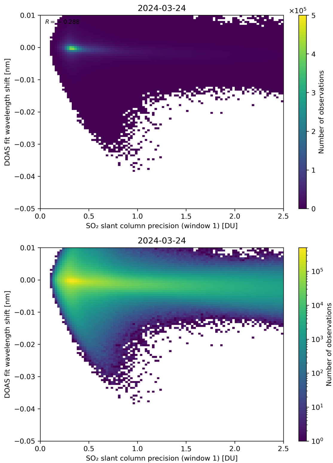
Figure 221: Scatter density plot of “SO 2 slant column precision (window 1)” against “DOAS fit wavelength shift” for 2024-03-23 to 2024-03-25.
