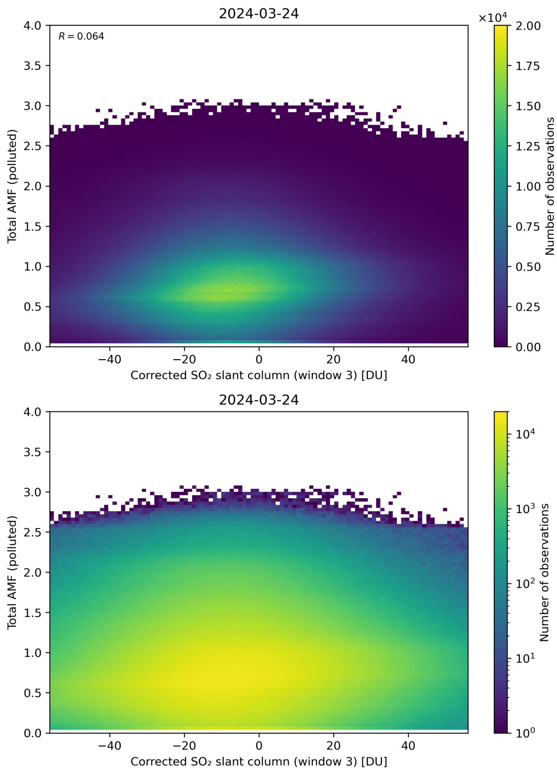
Figure 210: Scatter density plot of “Corrected SO 2 slant column (window 3)” against “Total AMF (polluted)” for 2024-03-23 to 2024-03-25.
