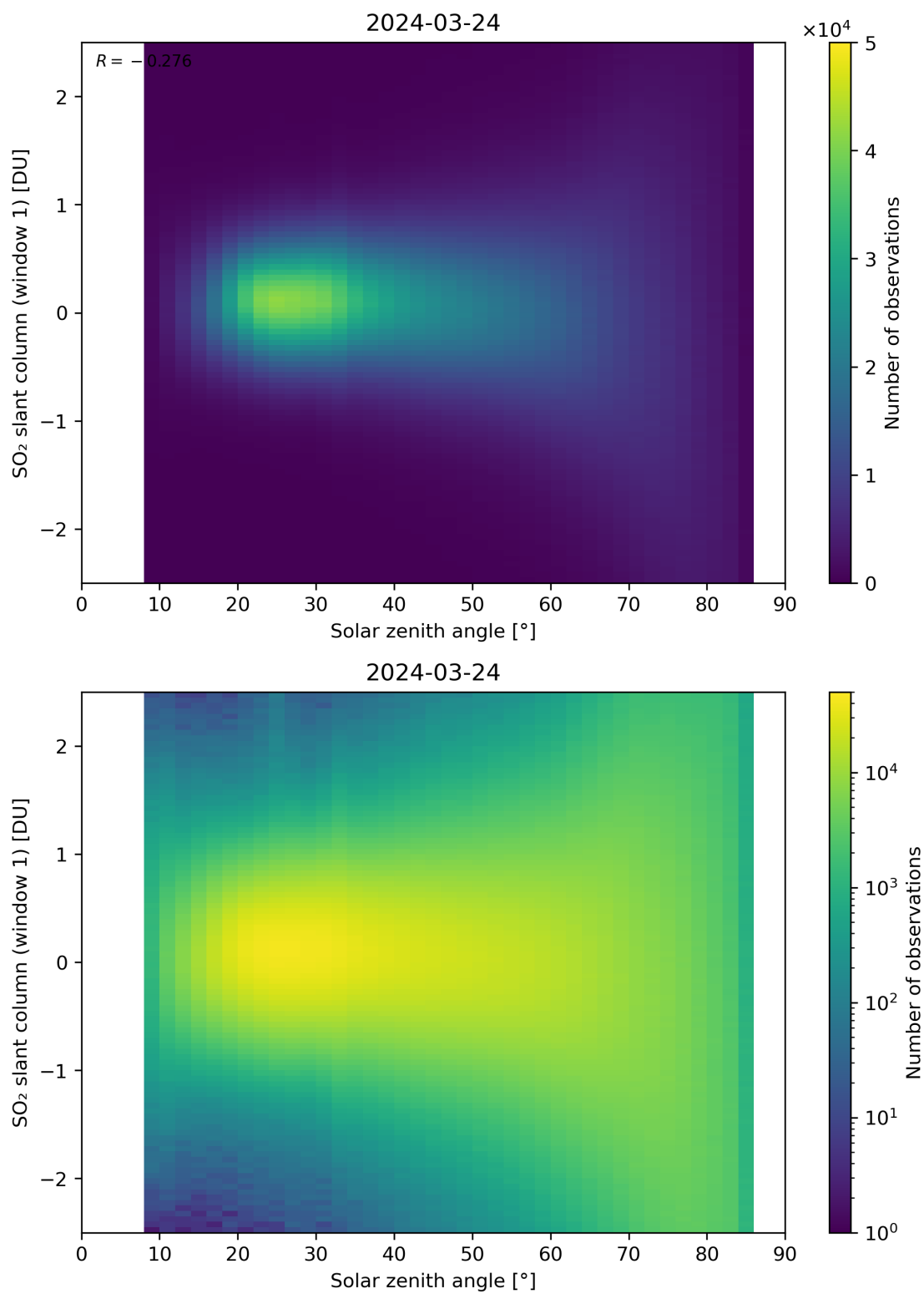
Figure 169: Scatter density plot of “Solar zenith angle” against “SO 2 slant column (window 1)” for 2024-03-23 to 2024-03-25.
