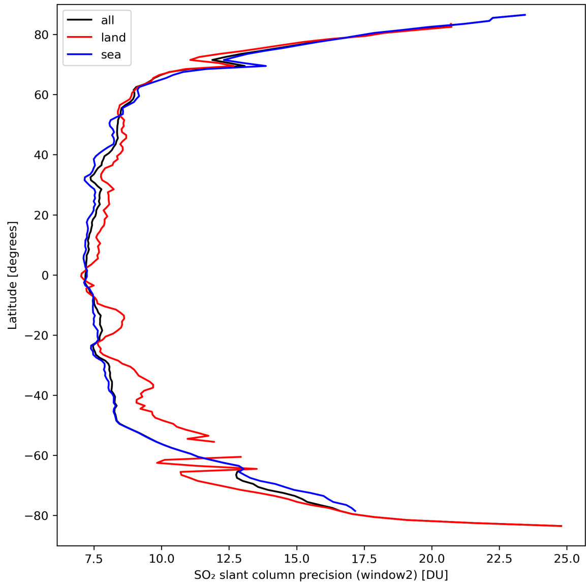
Figure 38: Zonal average of “SO 2 slant column precision (window2)” for 2024-03-23 to 2024-03-25.
