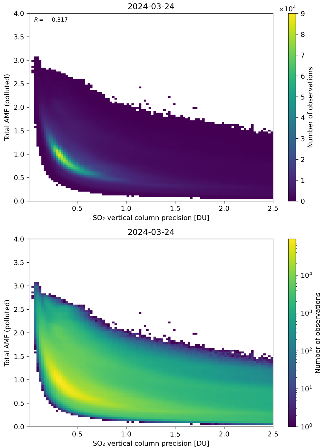
Figure 294: Scatter density plot of “SO 2 vertical column precision” against “Total AMF (polluted)” for 2024-03-23 to 2024-03-25.
