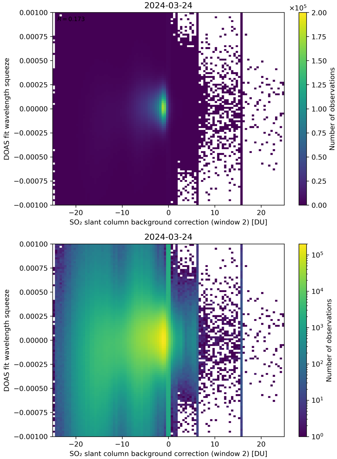
Figure 113: Scatter density plot of “SO 2 slant column background correction (window 2)” against “DOAS fit wavelength squeeze” for 2024-03-23 to 2024-03-25.
