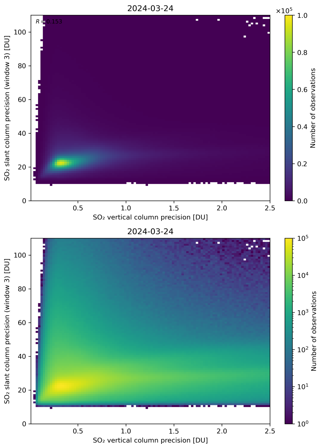
Figure 293: Scatter density plot of “SO 2 vertical column precision” against “SO 2 slant column precision (window 3)” for 2024-03-23 to 2024-03-25.
