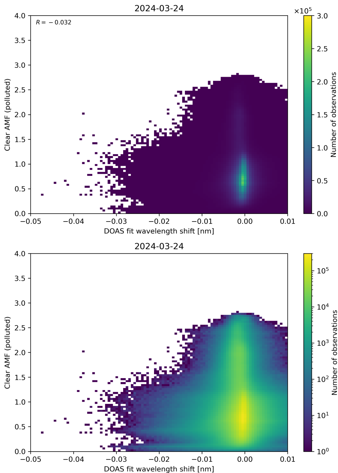
Figure 129: Scatter density plot of “DOAS fit wavelength shift” against “Clear AMF (polluted)” for 2024-03-23 to 2024-03-25.
