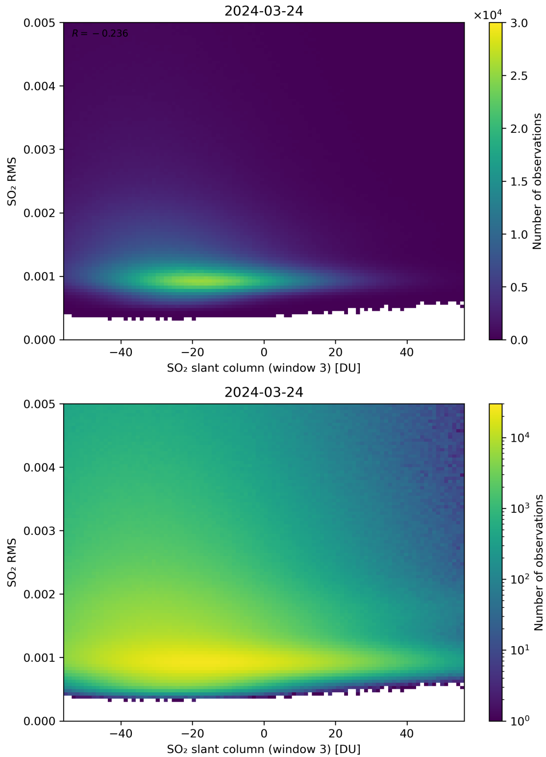
Figure 256: Scatter density plot of “SO 2 slant column (window 3)” against “SO 2 RMS” for 2024-03-23 to 2024-03-25.
