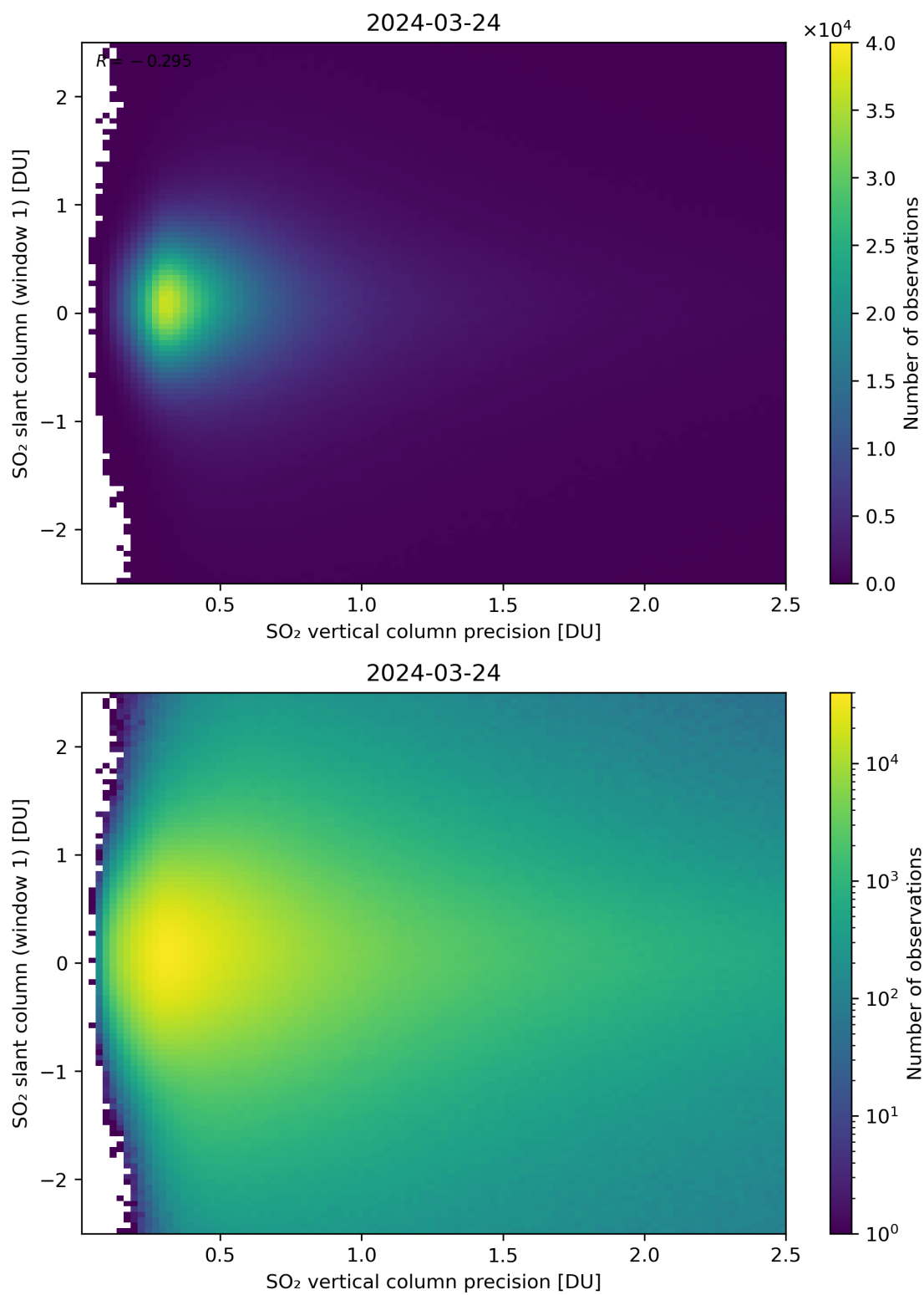
Figure 289: Scatter density plot of “SO 2 vertical column precision” against “SO 2 slant column (window 1)” for 2024-03-23 to 2024-03-25.
