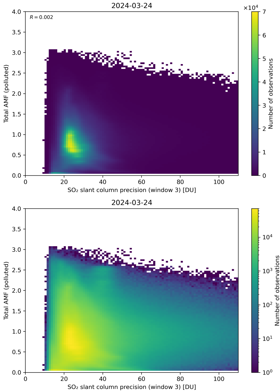
Figure 263: Scatter density plot of “SO 2 slant column precision (window 3)” against “Total AMF (polluted)” for 2024-03-23 to 2024-03-25.
