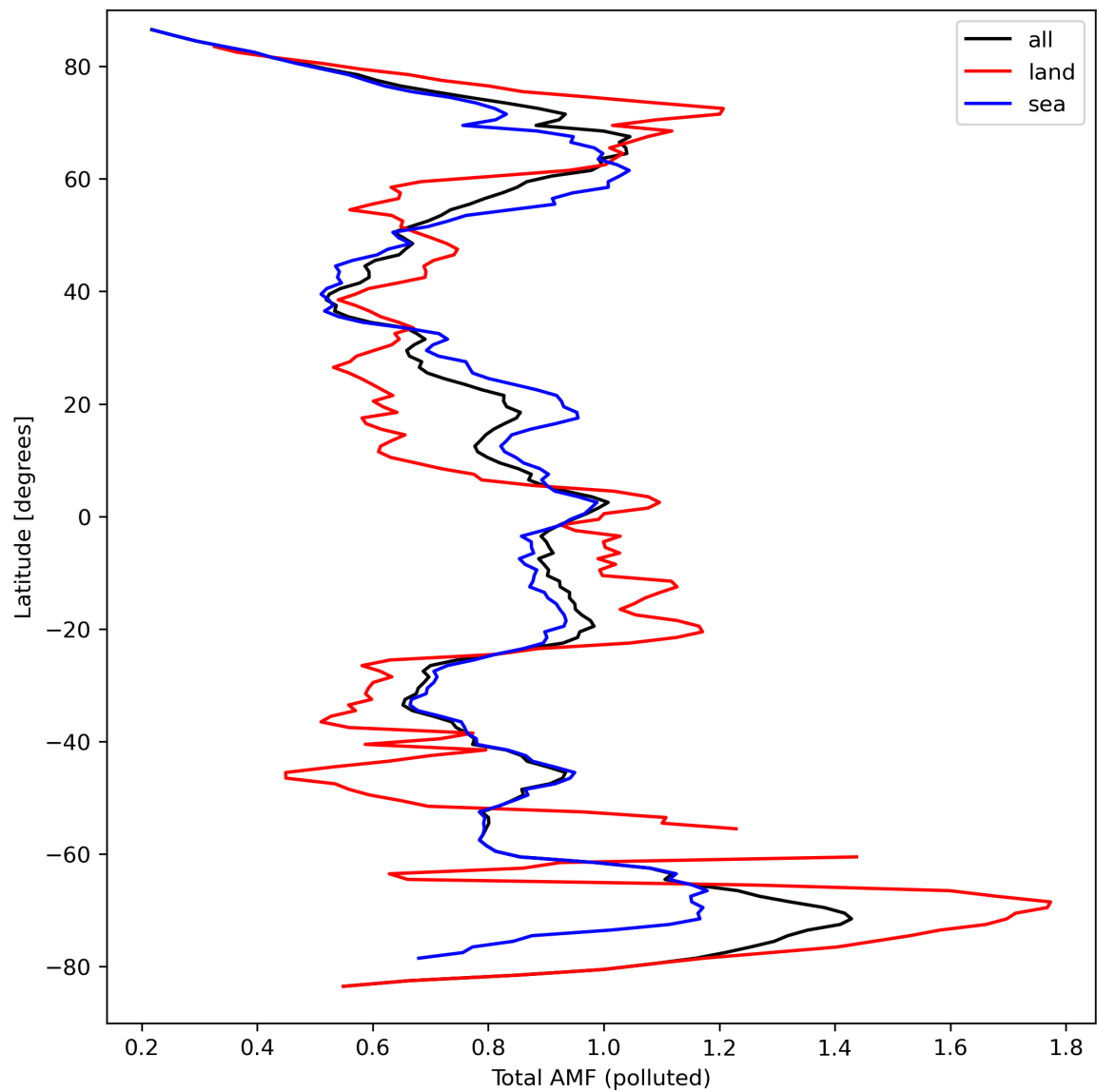
Figure 48: Zonal average of “Total AMF (polluted)” for 2024-03-23 to 2024-03-25.
