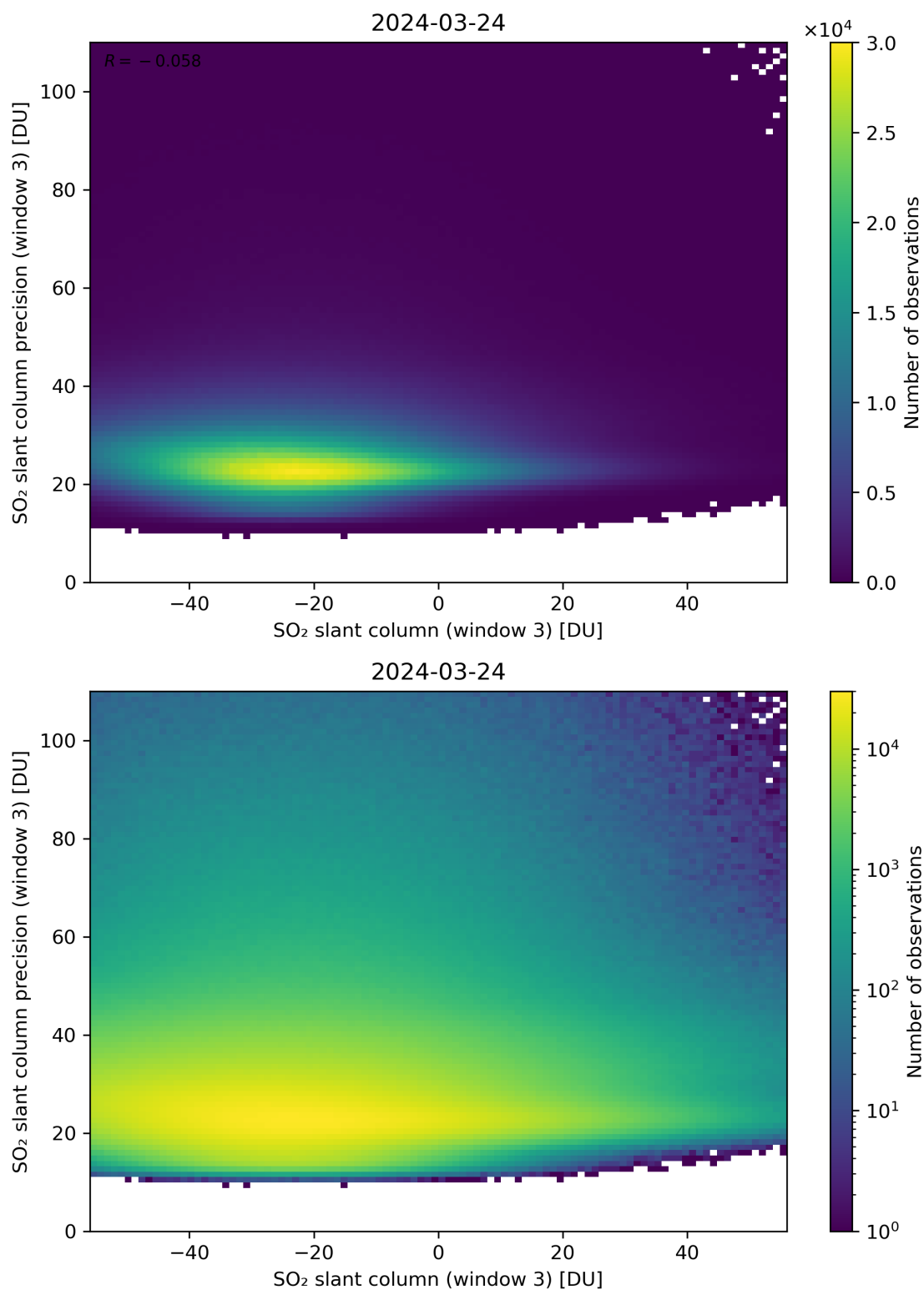
Figure 267: Scatter density plot of “SO 2 slant column (window 3)” against “SO 2 slant column precision (window 3)” for 2024-03-23 to 2024-03-25.
