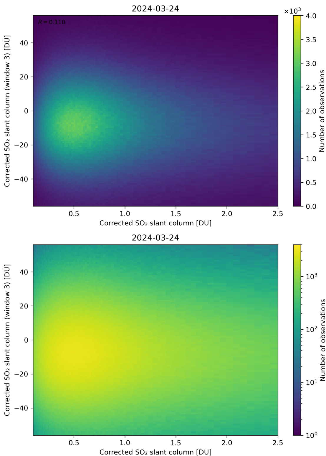
Figure 186: Scatter density plot of “Corrected SO 2 slant column” against “Corrected SO 2 slant column (window 3)” for 2024-03-23 to 2024-03-25.
