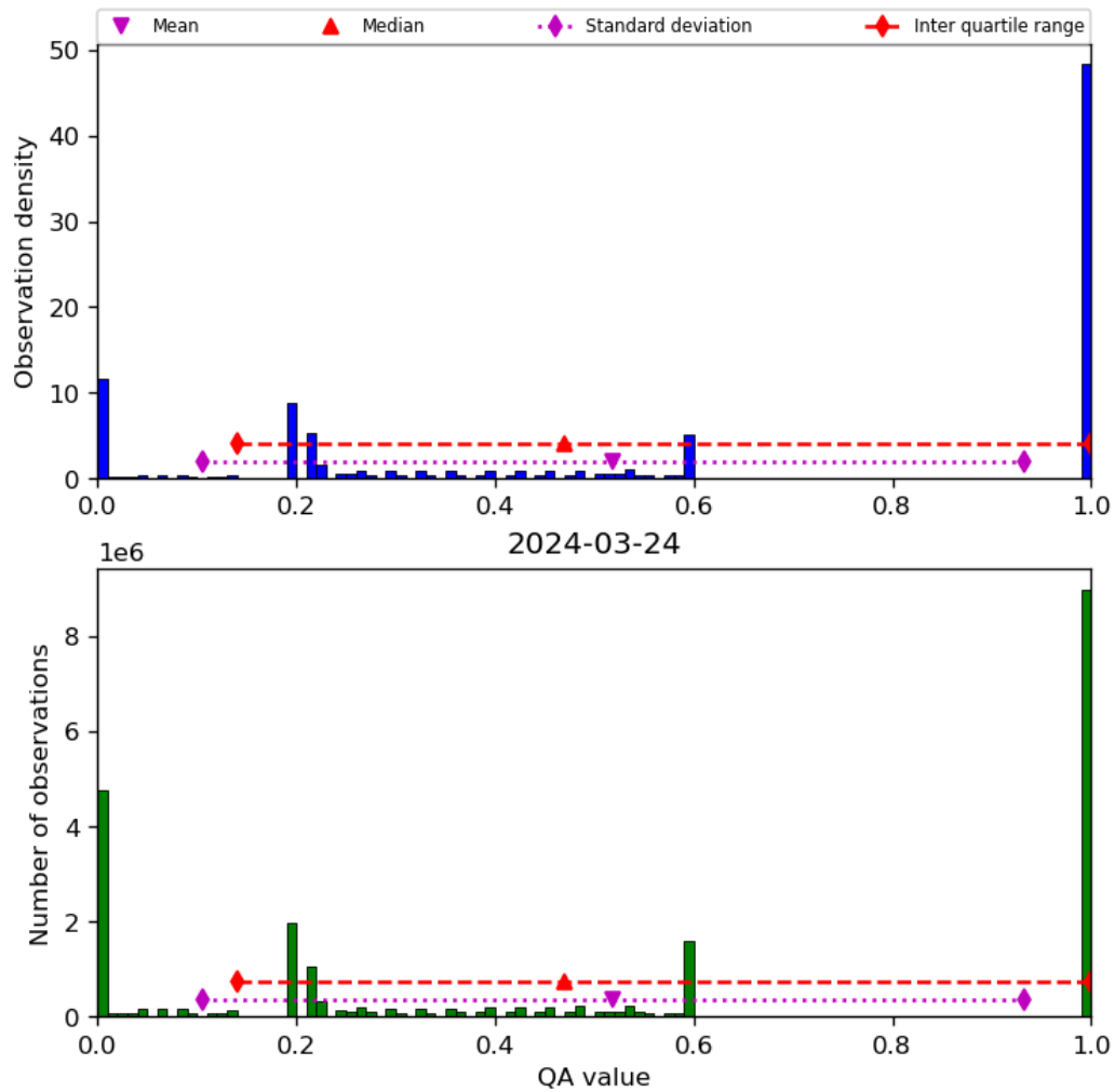
Figure 52: Histogram of “QA value” for 2024-03-23 to 2024-03-25
