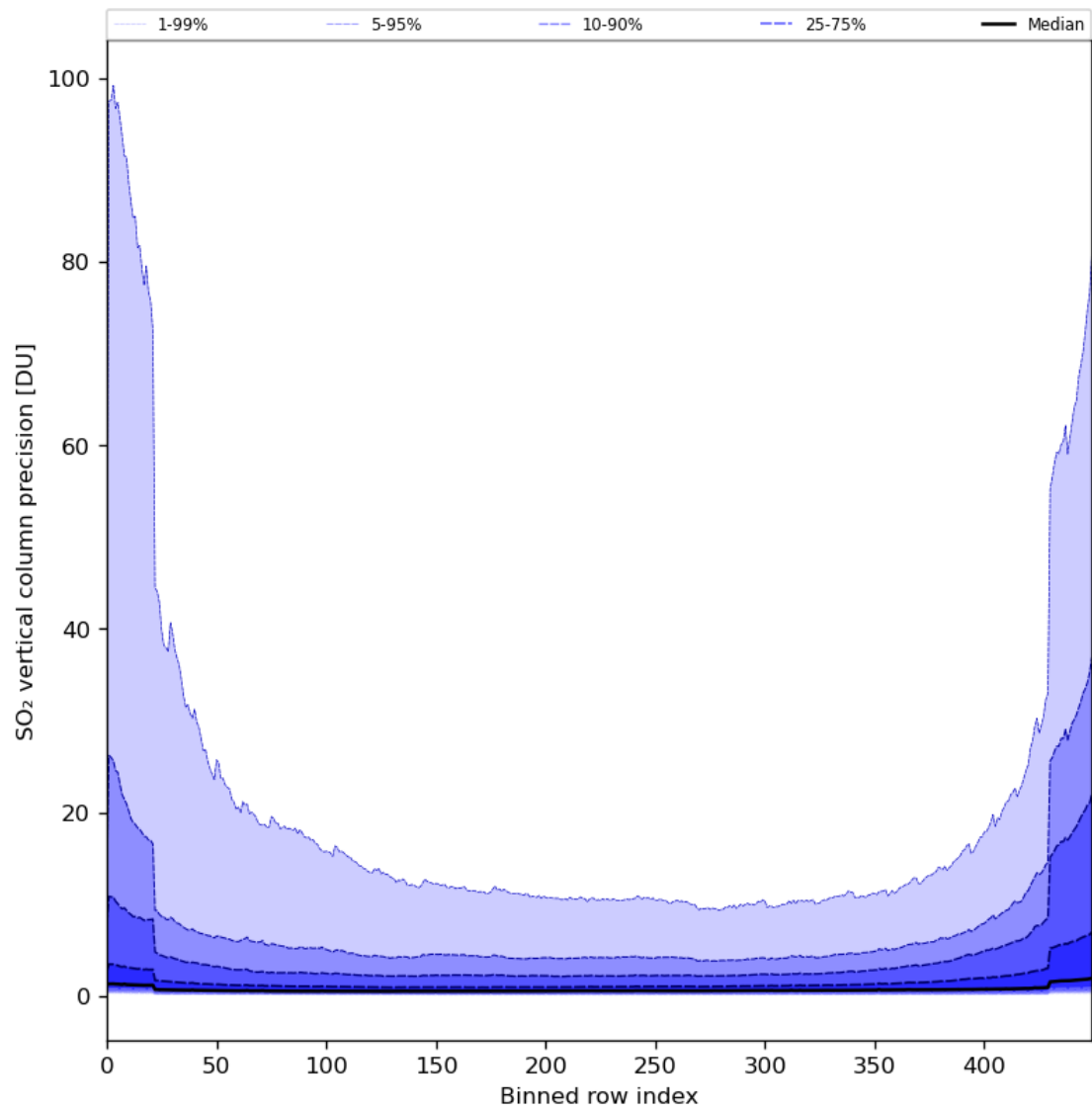
Figure 77: Along track statistics of “SO 2 vertical column precision” for 2024-03-23 to 2024-03-25
