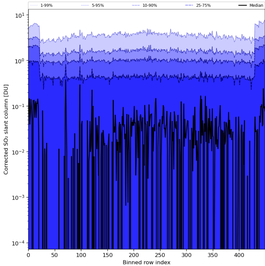
Figure 78: Along track statistics of “Corrected SO 2 slant column” for 2024-03-23 to 2024-03-25
