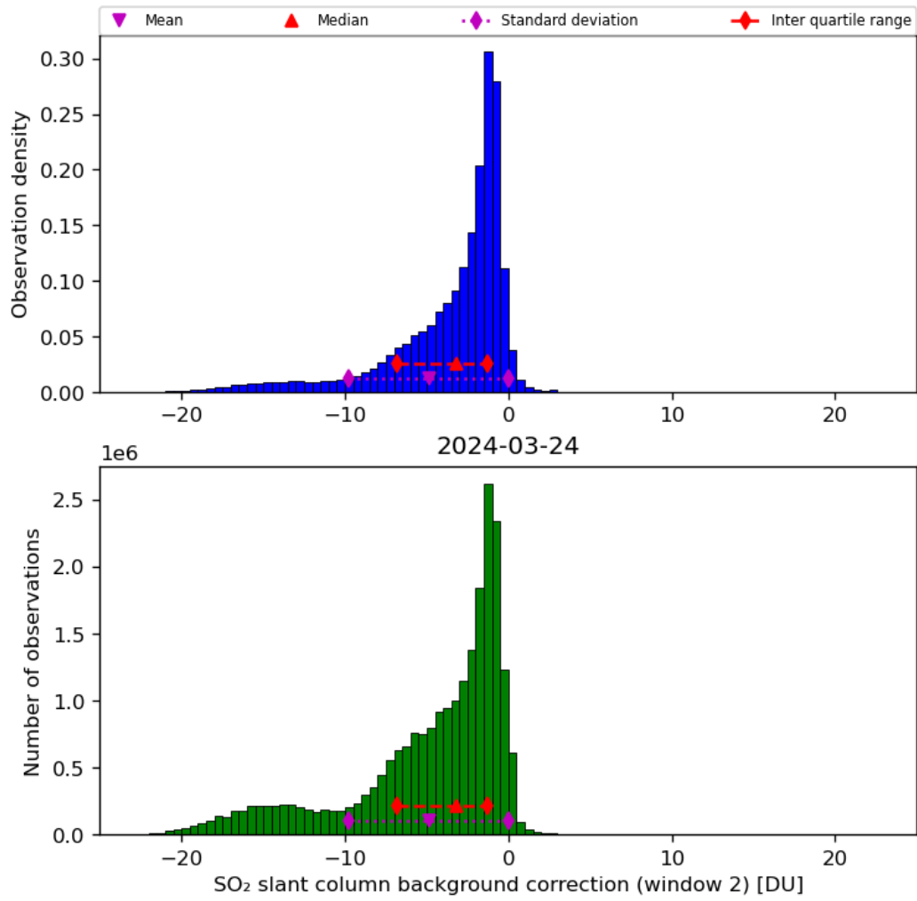
Figure 63: Histogram of “SO 2 slant column background correction (window 2)” for 2024-03-23 to 2024-03-25
