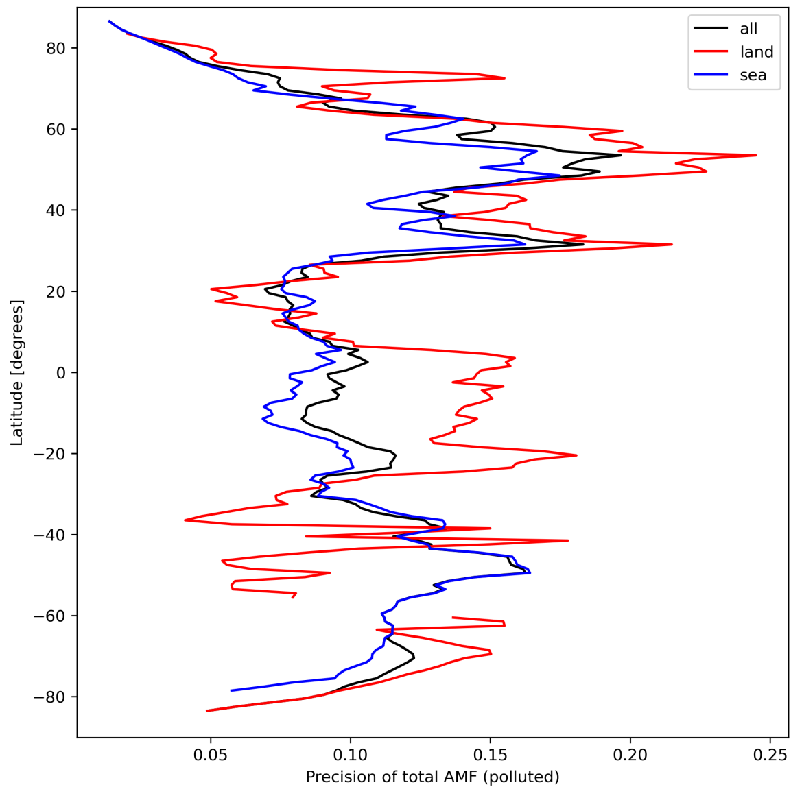
Figure 49: Zonal average of “Precision of total AMF (polluted)” for 2024-03-23 to 2024-03-25.
