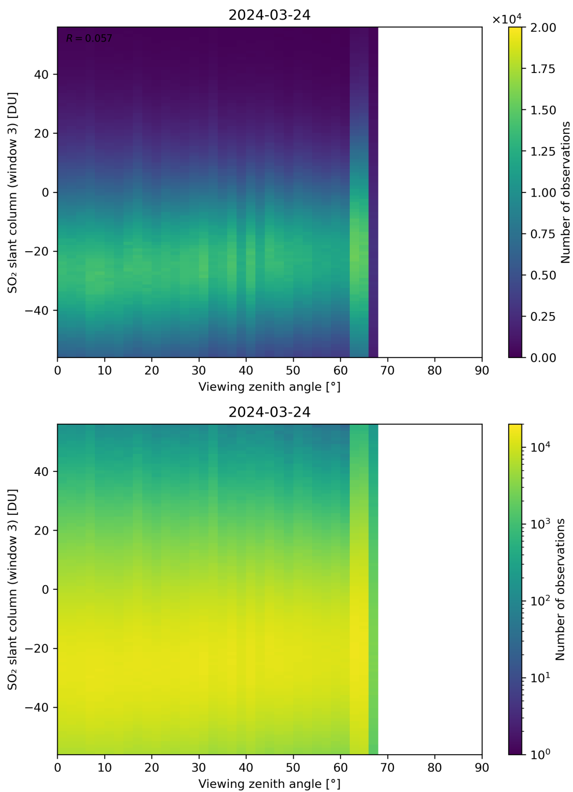
Figure 323: Scatter density plot of “Viewing zenith angle” against “SO 2 slant column (window 3)” for 2024-03-23 to 2024-03-25.
