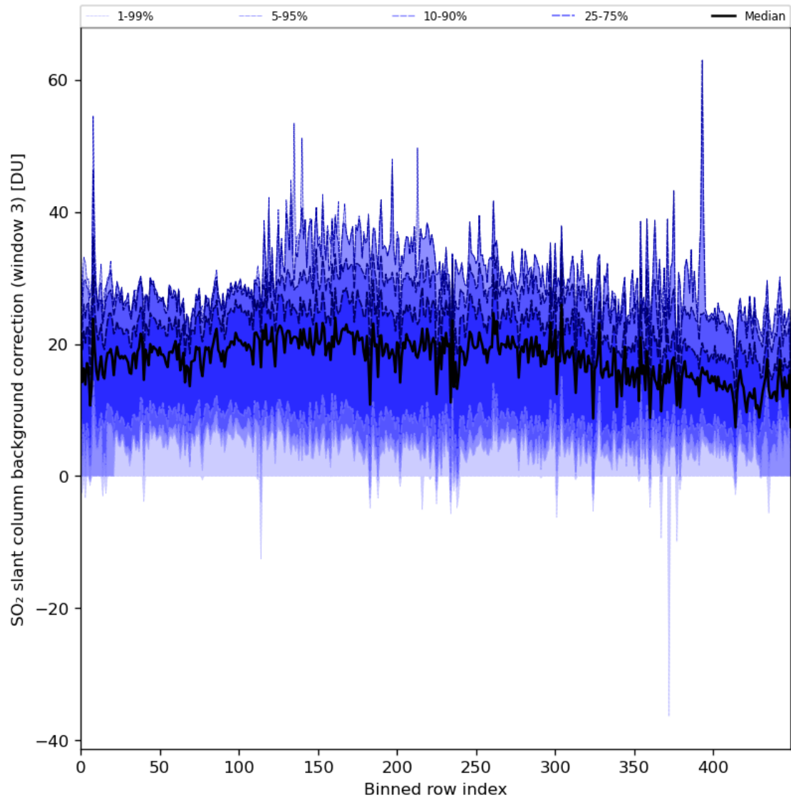
Figure 90: Along track statistics of “SO 2 slant column background correction (window 3)” for 2024-03-23 to 2024-03-25
