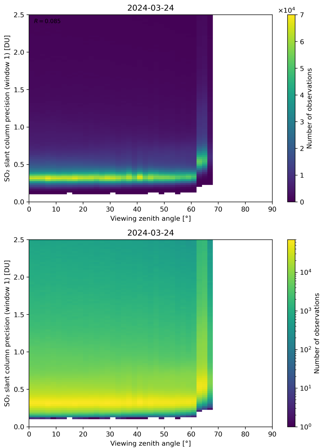
Figure 321: Scatter density plot of “Viewing zenith angle” against “SO 2 slant column precision (window 1)” for 2024-03-23 to 2024-03-25.
