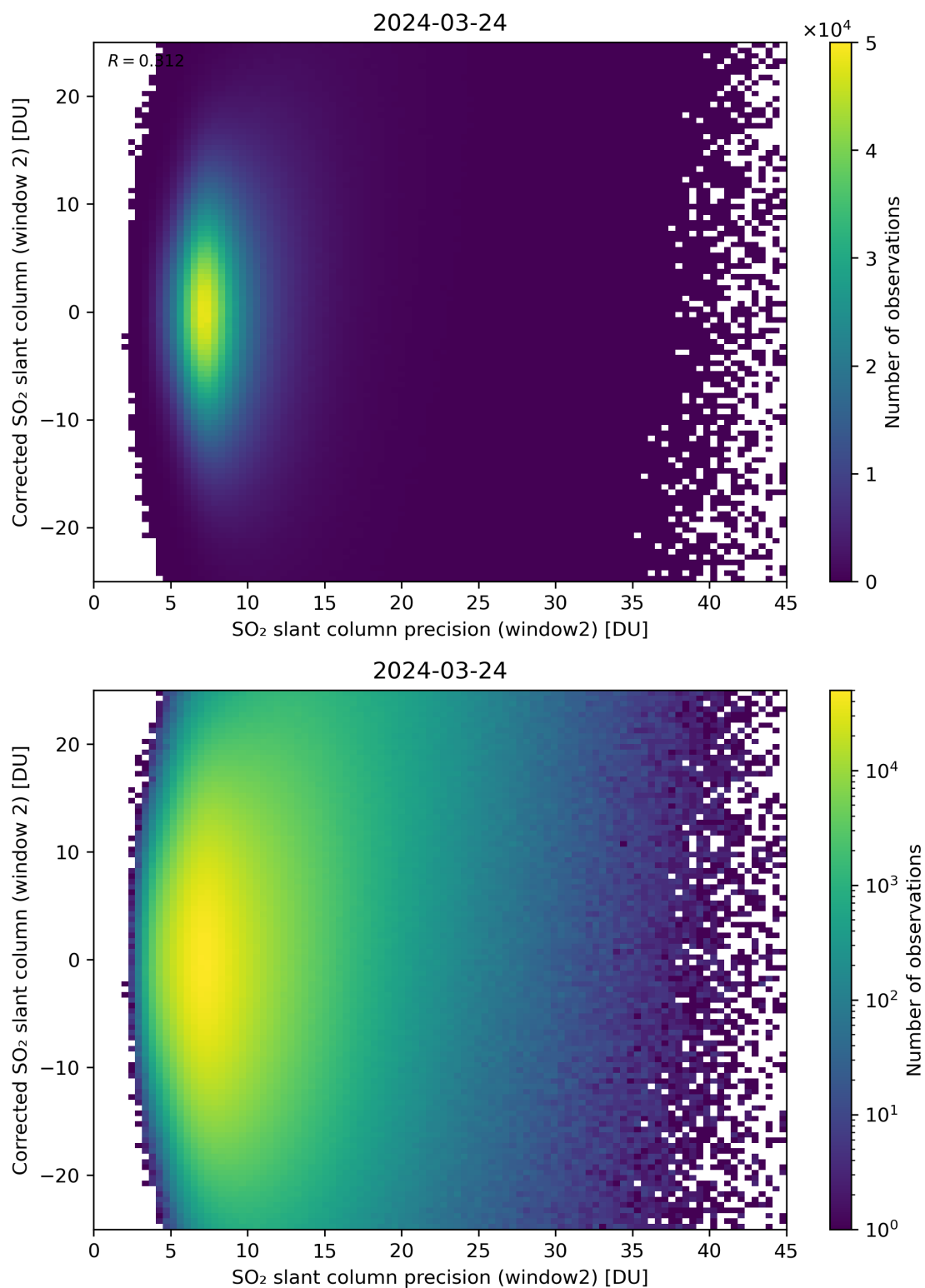
Figure 247: Scatter density plot of “SO 2 slant column precision (window2)” against “Corrected SO 2 slant column (window 2)” for 2024-03-23 to 2024-03-25.
