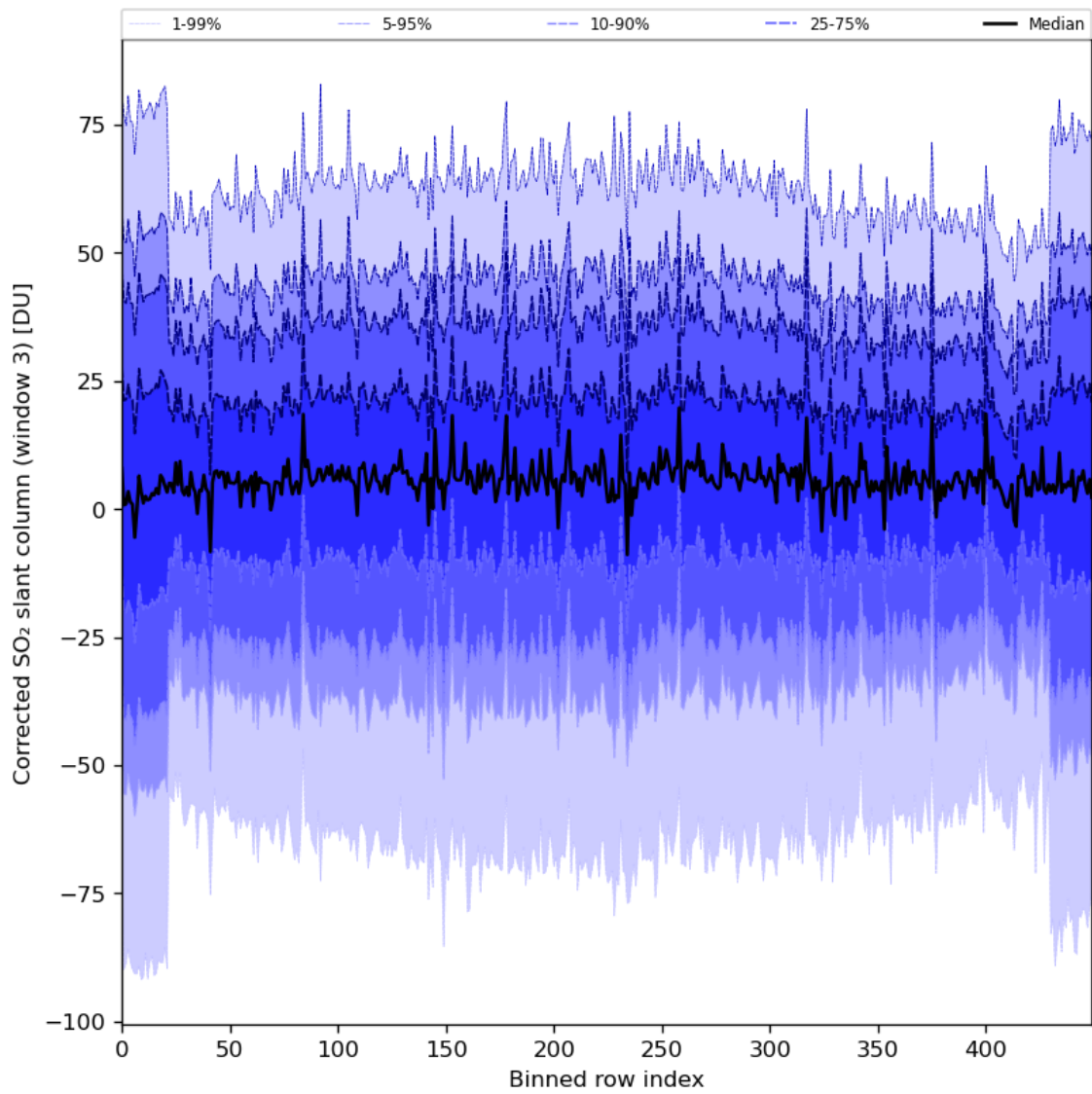
Figure 89: Along track statistics of “Corrected SO 2 slant column (window 3)” for 2024-03-25 to 2024-03-27
