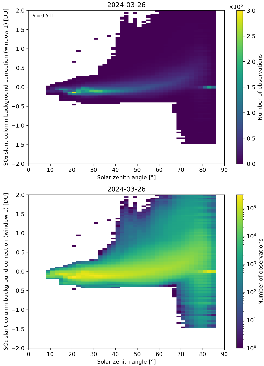
Figure 158: Scatter density plot of “Solar zenith angle” against “SO 2 slant column background correction (window 1)” for 2024-03-25 to 2024-03-27.
