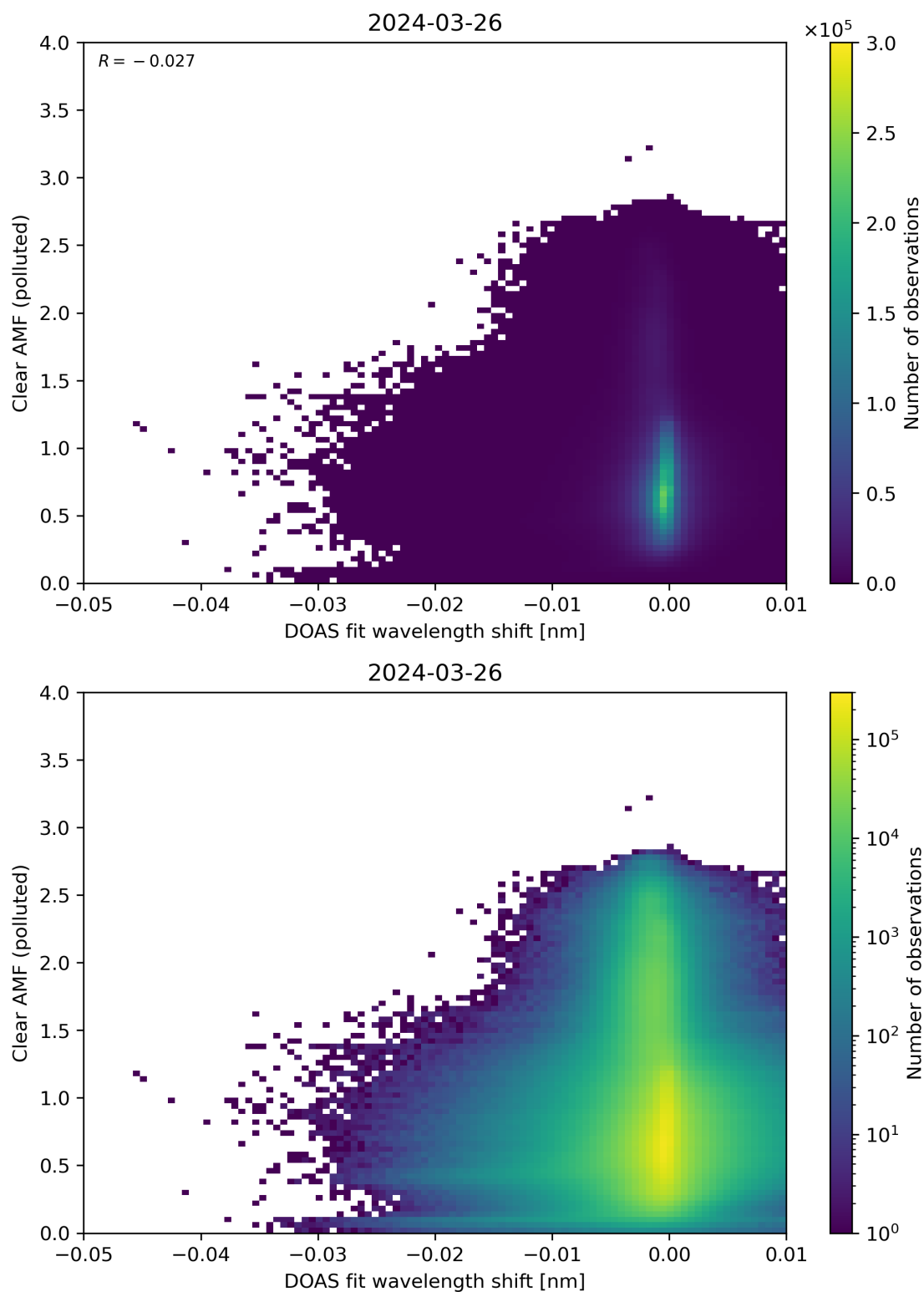
Figure 129: Scatter density plot of “DOAS fit wavelength shift” against “Clear AMF (polluted)” for 2024-03-25 to 2024-03-27.
