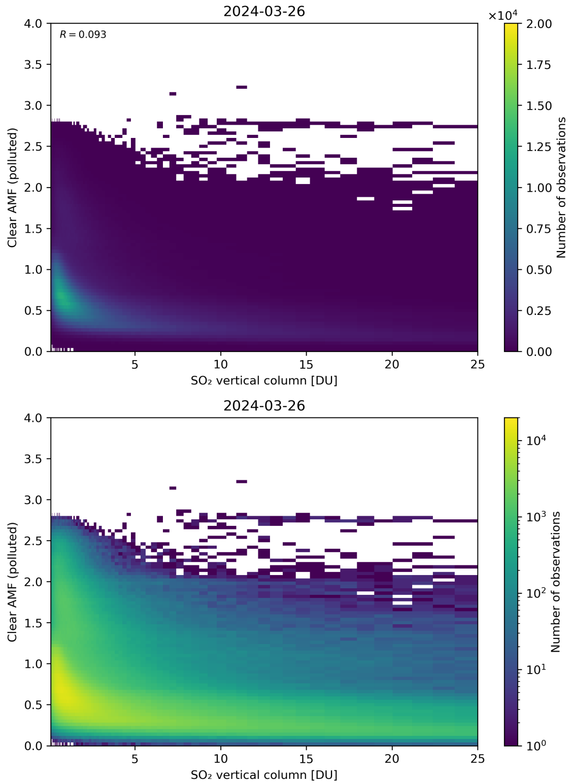
Figure 296: Scatter density plot of “SO 2 vertical column” against “Clear AMF (polluted)” for 2024-03-25 to 2024-03-27.
