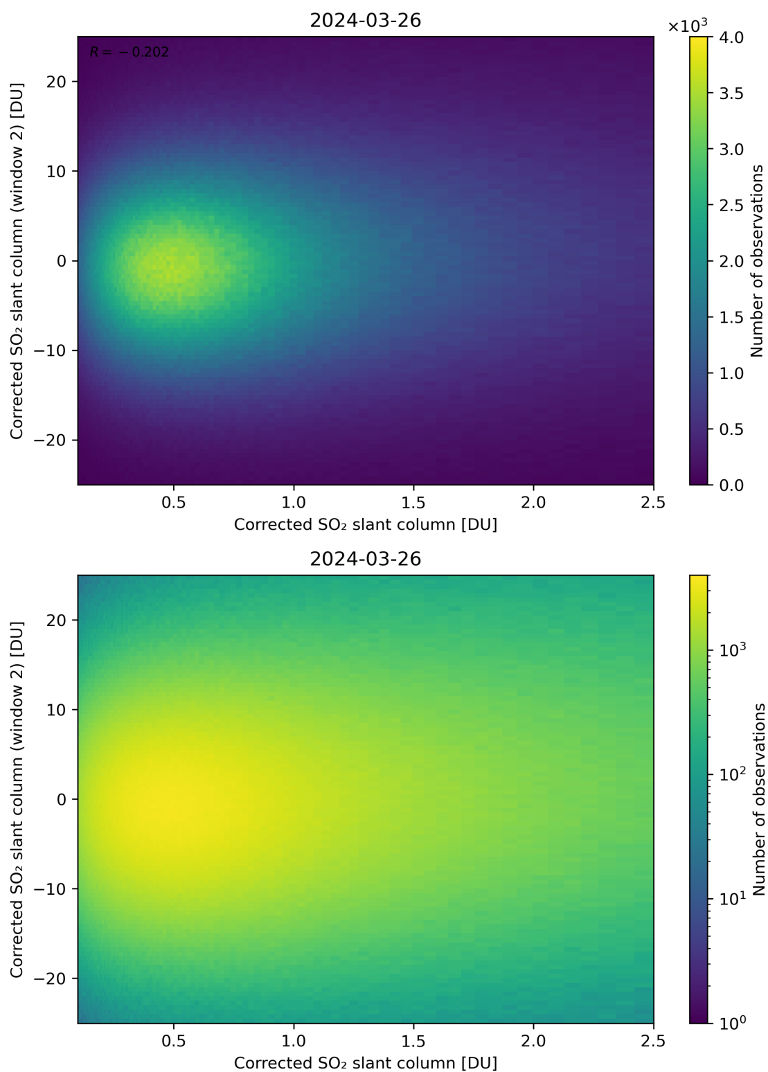
Figure 185: Scatter density plot of “Corrected SO 2 slant column” against “Corrected SO 2 slant column (window 2)” for 2024-03-25 to 2024-03-27.
