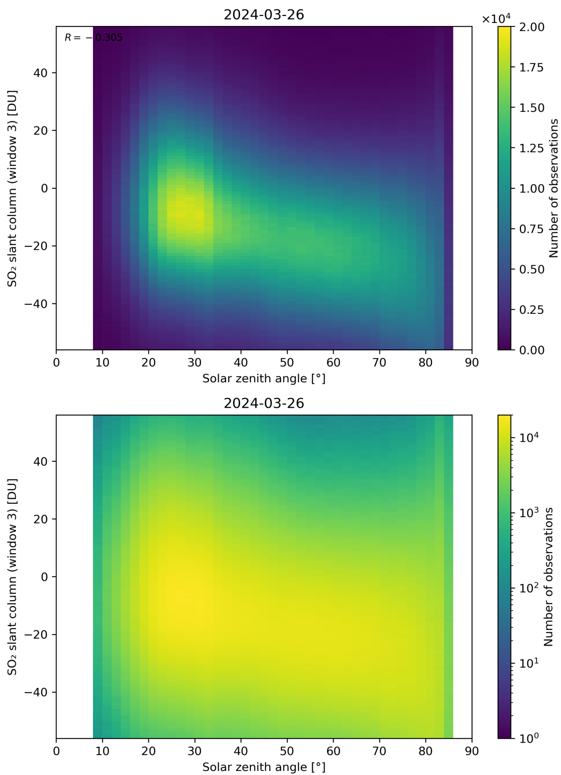
Figure 172: Scatter density plot of “Solar zenith angle” against “SO 2 slant column (window 3)” for 2024-03-25 to 2024-03-27.
