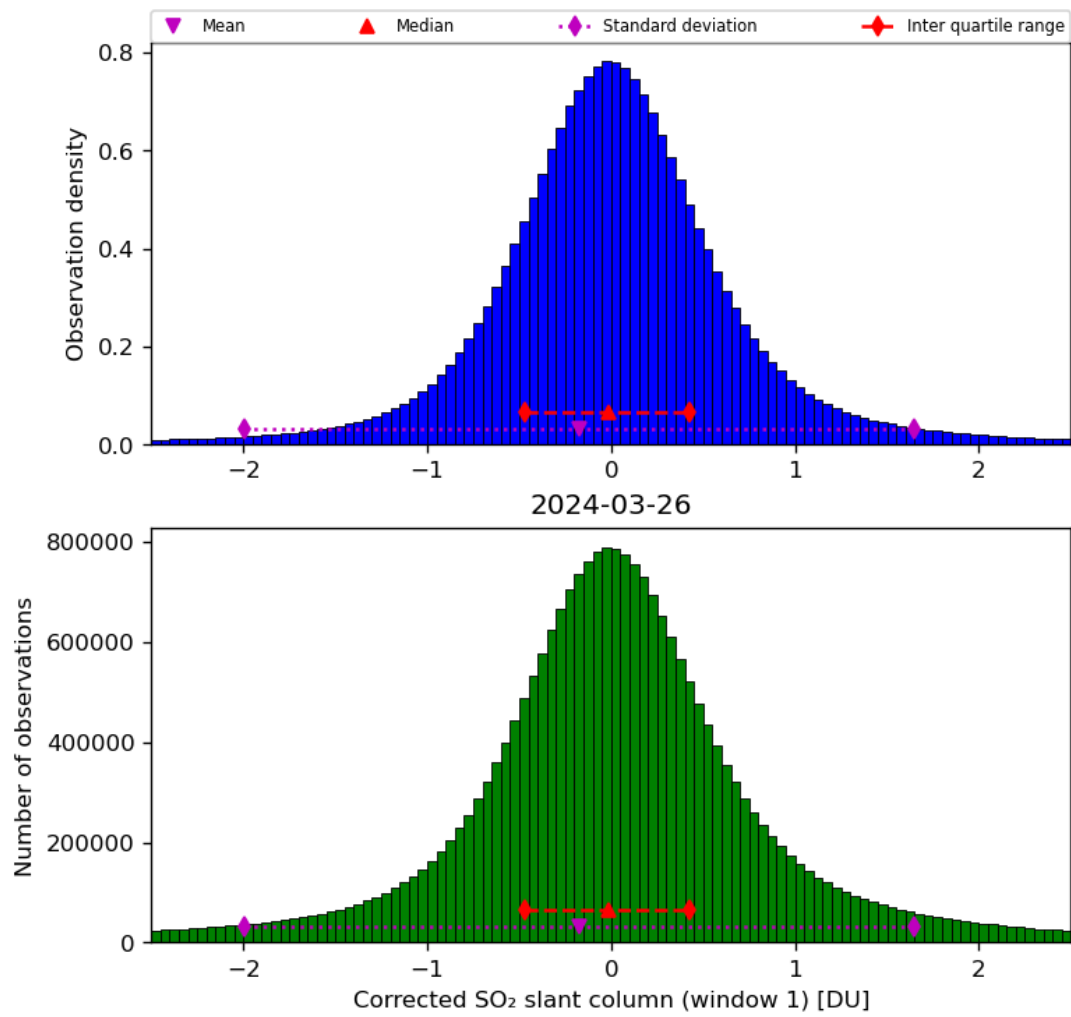
Figure 58: Histogram of “Corrected SO 2 slant column (window 1)” for 2024-03-25 to 2024-03-27
