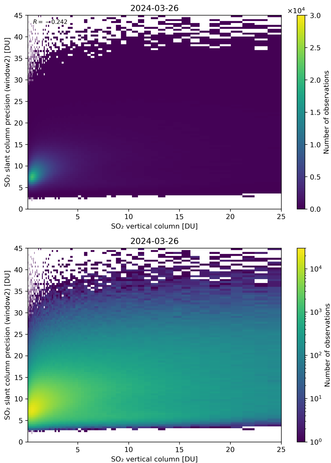
Figure 302: Scatter density plot of “SO 2 vertical column” against “SO 2 slant column precision (window2)” for 2024-03-25 to 2024-03-27.
