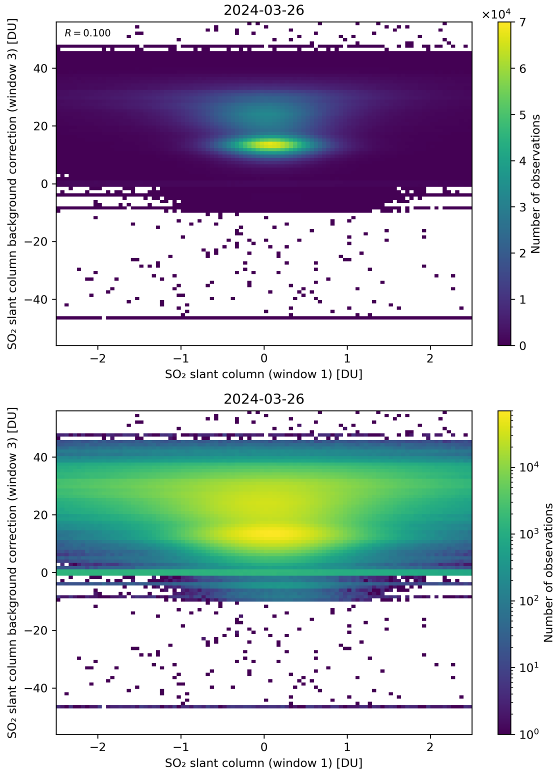
Figure 214: Scatter density plot of “SO 2 slant column (window 1)” against “SO 2 slant column background correction (window 3)” for 2024-03-25 to 2024-03-27.
