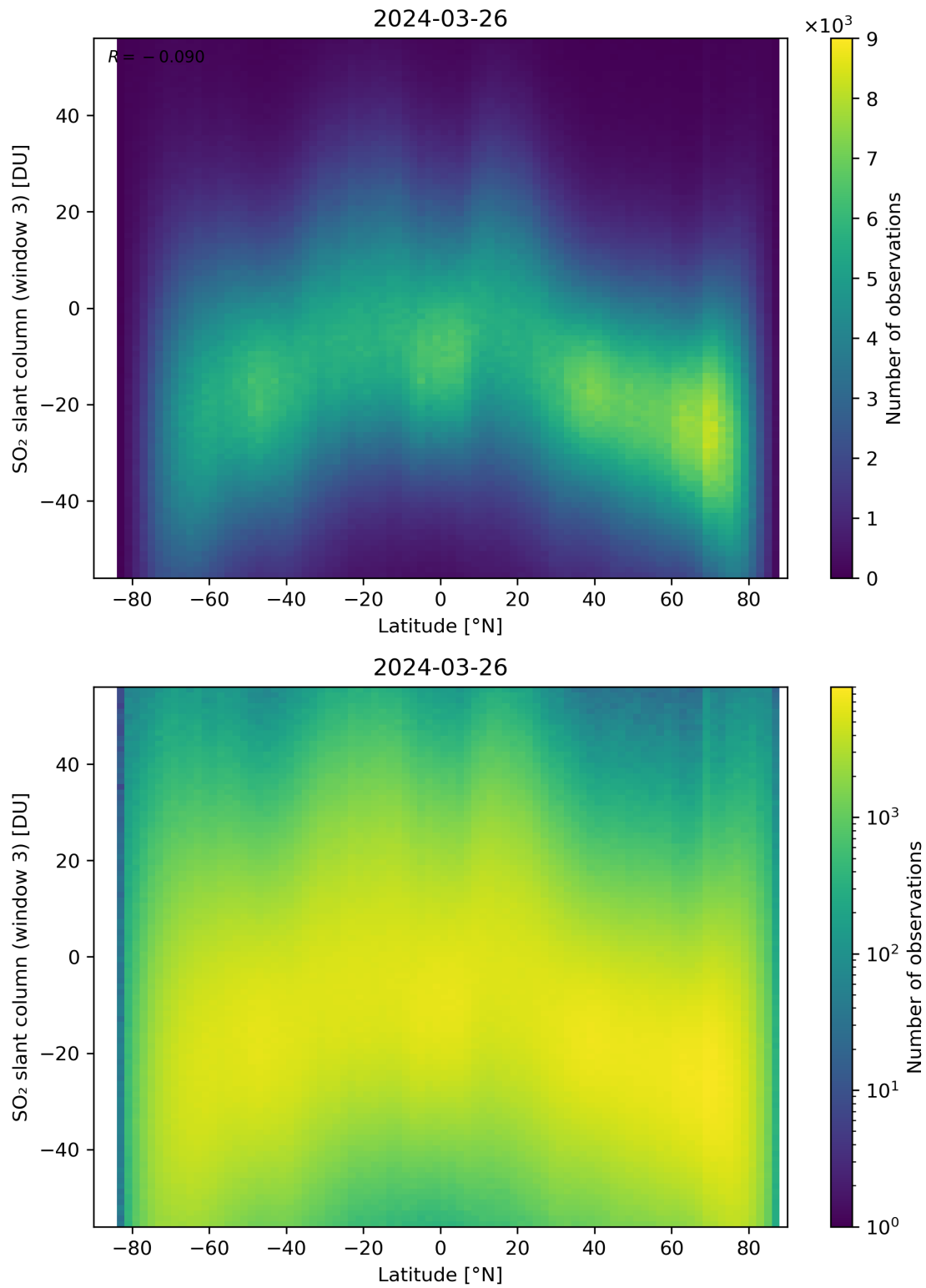
Figure 152: Scatter density plot of “Latitude” against “SO 2 slant column (window 3)” for 2024-03-25 to 2024-03-27.
