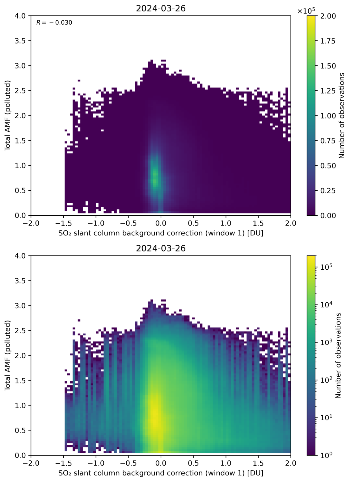
Figure 109: Scatter density plot of “SO 2 slant column background correction (window 1)” against “Total AMF (polluted)” for 2024-03-25 to 2024-03-27.
