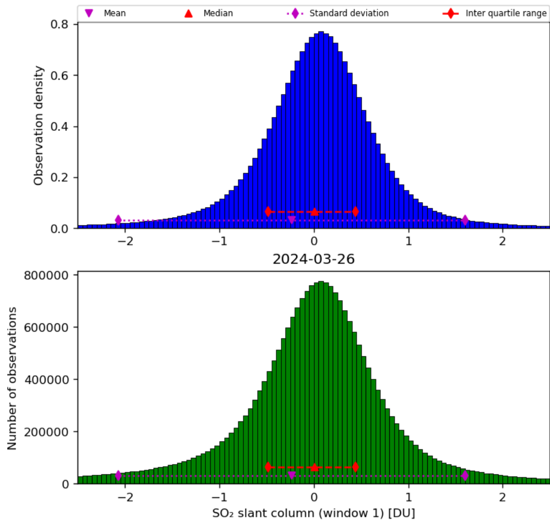
Figure 56: Histogram of “SO 2 slant column (window 1)” for 2024-03-25 to 2024-03-27
