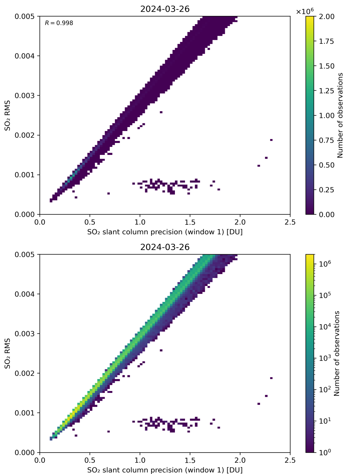
Figure 223: Scatter density plot of “SO 2 slant column precision (window 1)” against “SO 2 RMS” for 2024-03-25 to 2024-03-27.
