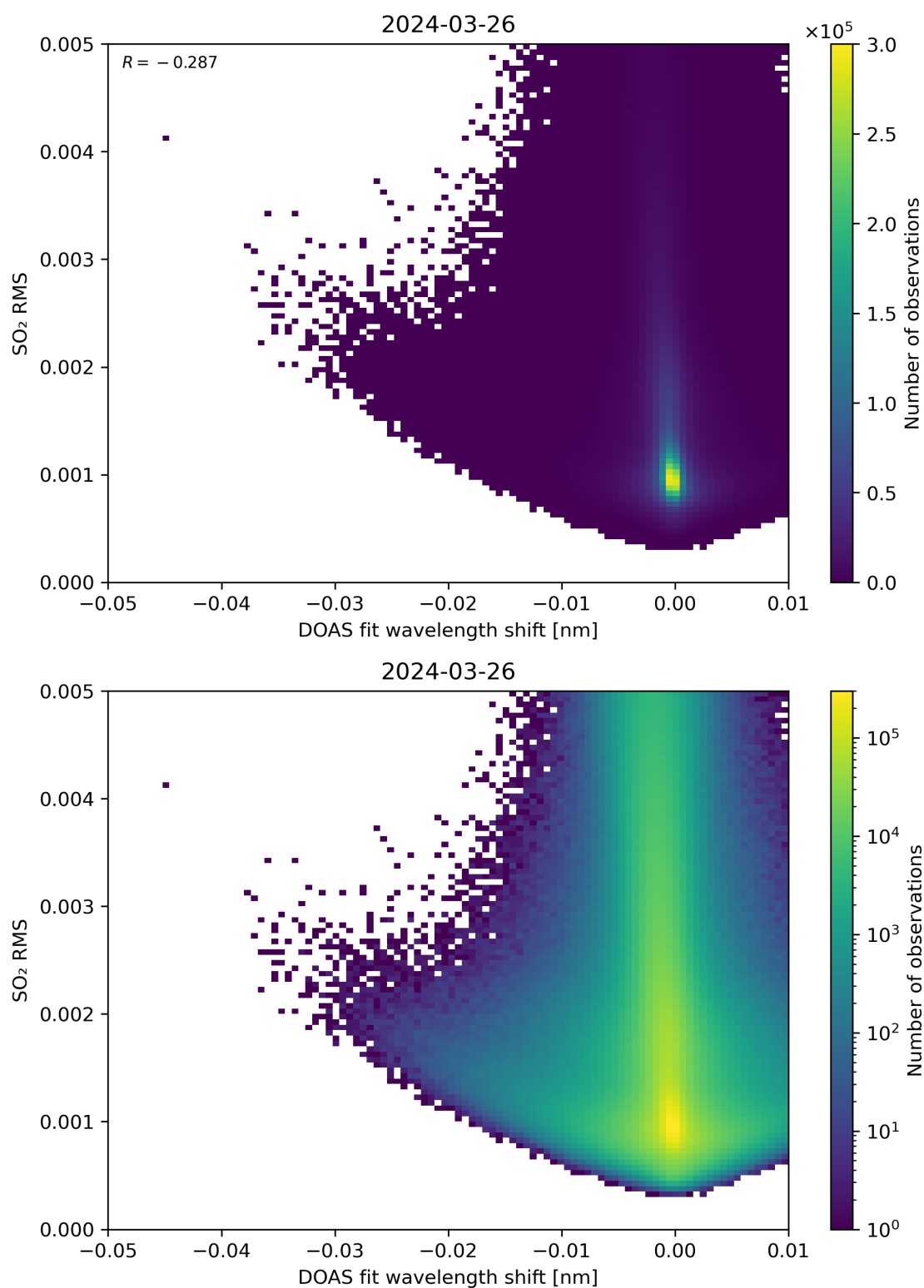
Figure 128: Scatter density plot of “DOAS fit wavelength shift” against “SO 2 RMS” for 2024-03-25 to 2024-03-27.
