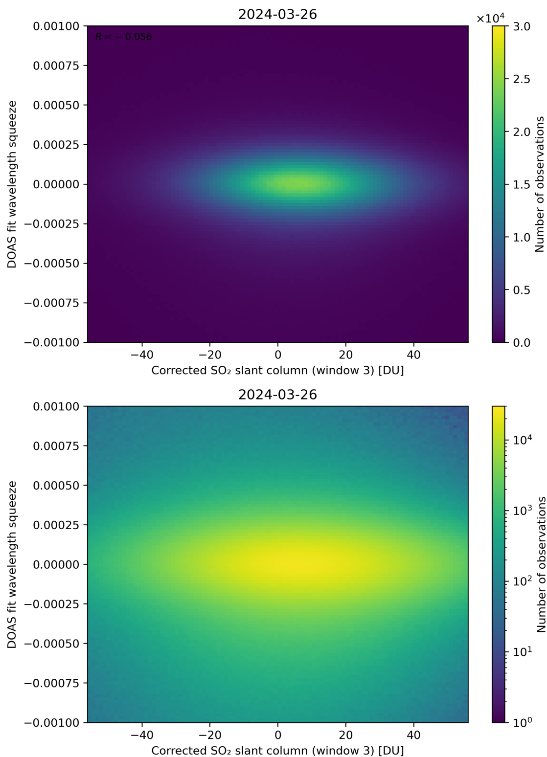
Figure 207: Scatter density plot of “Corrected SO 2 slant column (window 3)” against “DOAS fit wavelength squeeze” for 2024-03-25 to 2024-03-27.
