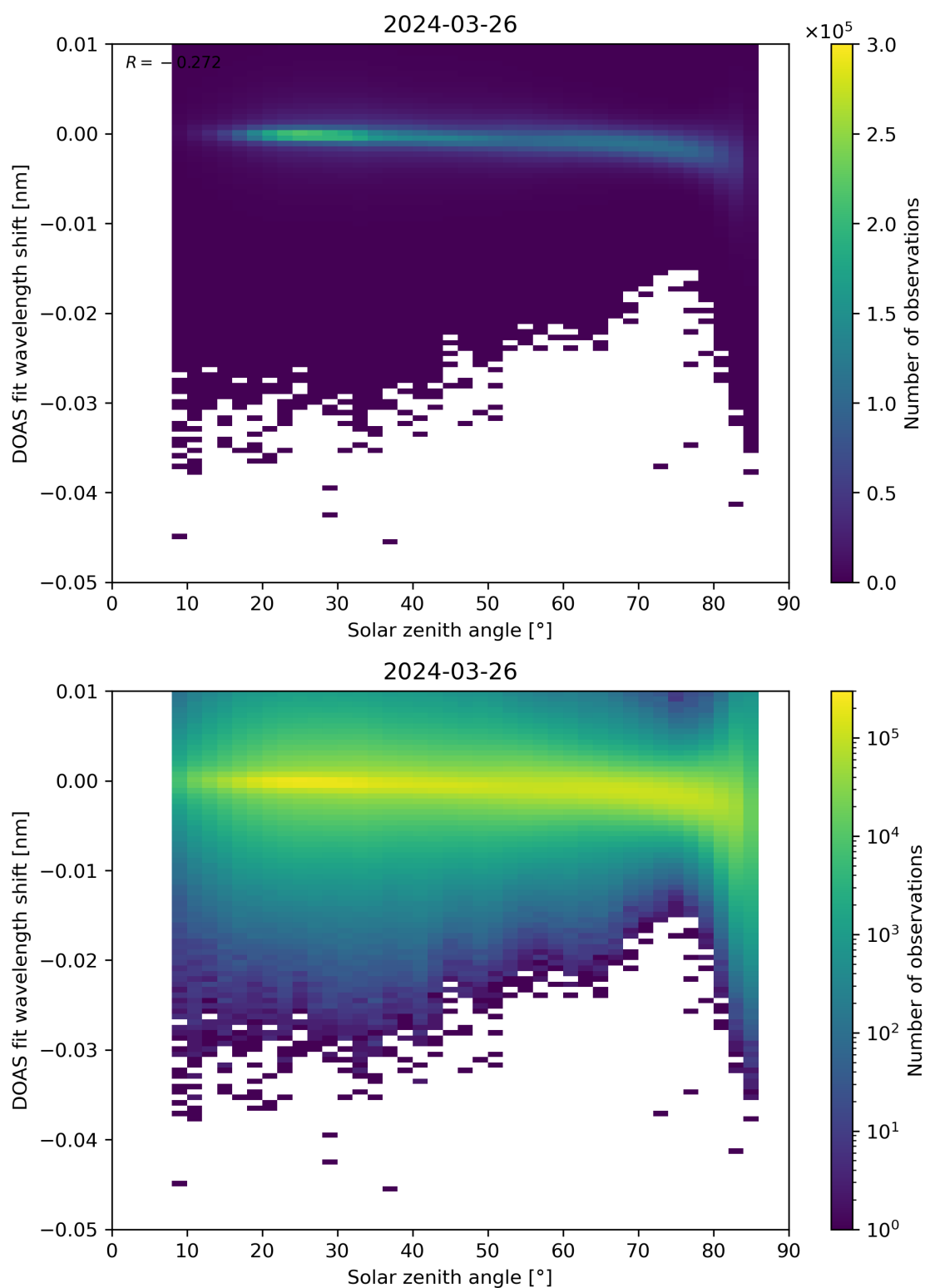
Figure 161: Scatter density plot of “Solar zenith angle” against “DOAS fit wavelength shift” for 2024-03-25 to 2024-03-27.
