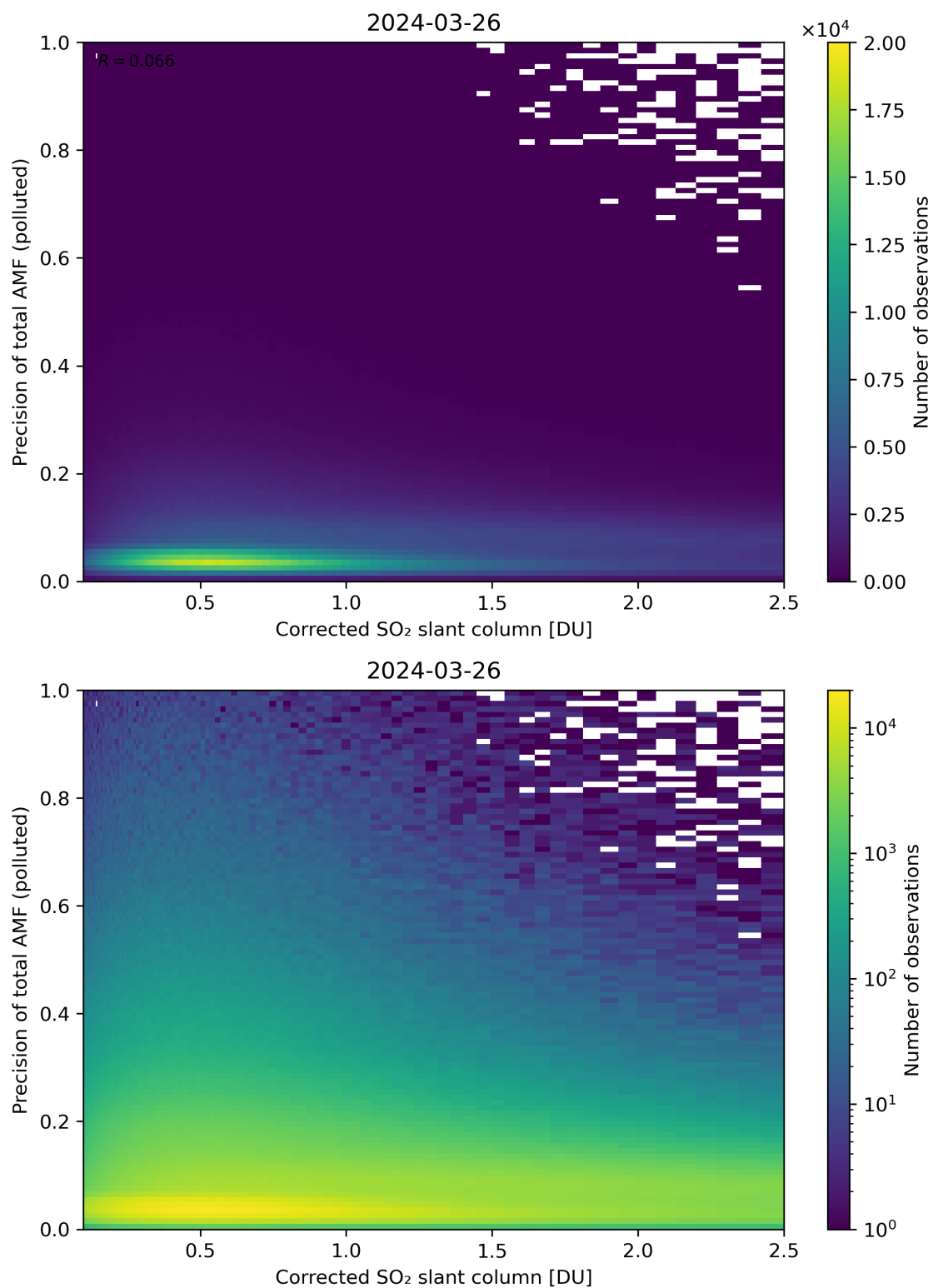
Figure 193: Scatter density plot of “Corrected SO 2 slant column” against “Precision of total AMF (polluted)” for 2024-03-25 to 2024-03-27.
