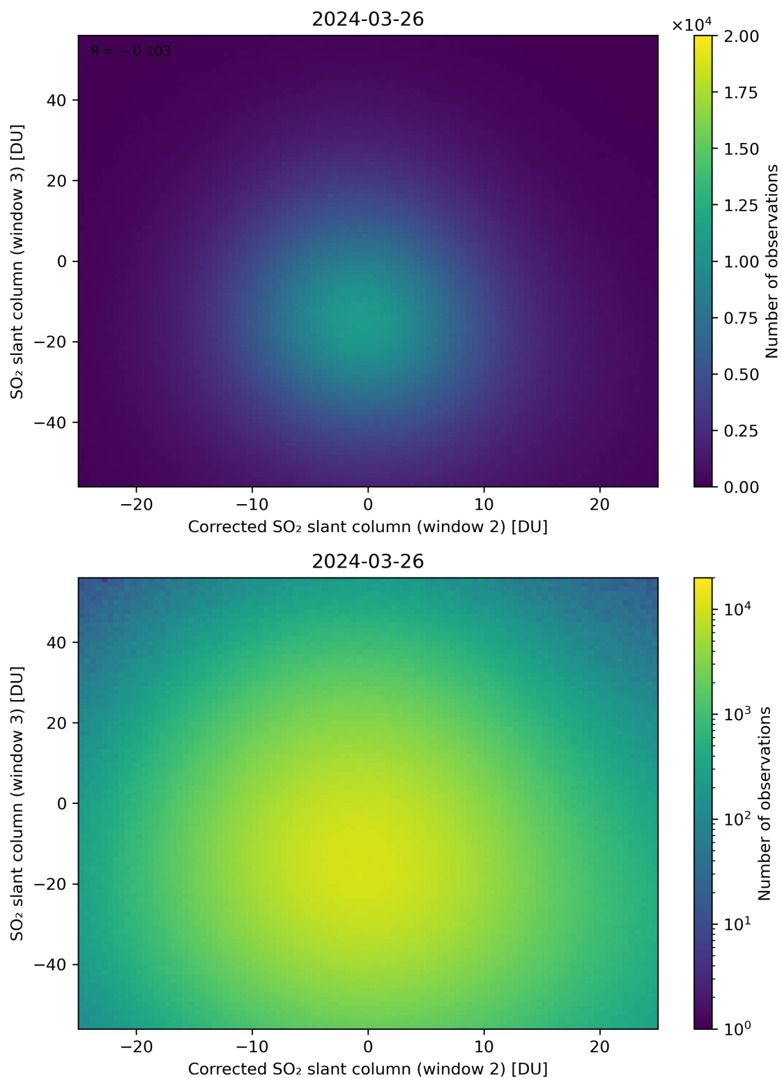
Figure 201: Scatter density plot of “Corrected SO 2 slant column (window 2)” against “SO 2 slant column (window 3)” for 2024-03-25 to 2024-03-27.
