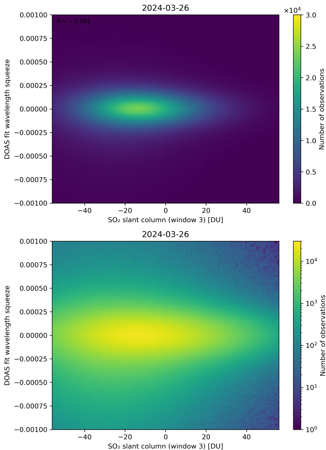
Figure 255: Scatter density plot of “SO 2 slant column (window 3)” against “DOAS fit wavelength squeeze” for 2024-03-25 to 2024-03-27.
