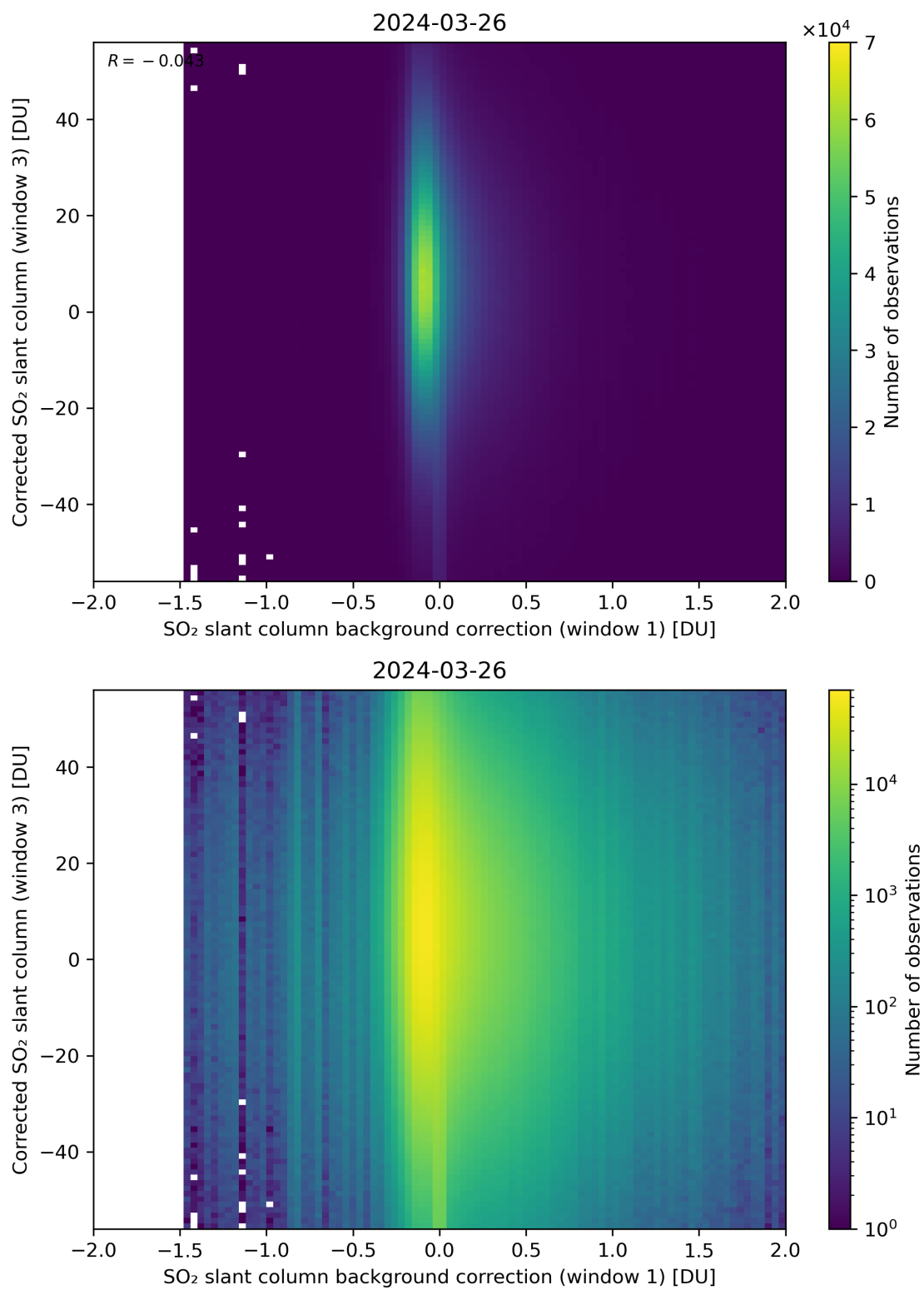
Figure 105: Scatter density plot of “SO 2 slant column background correction (window 1)” against “Corrected SO 2 slant column (window 3)” for 2024-03-25 to 2024-03-27.
