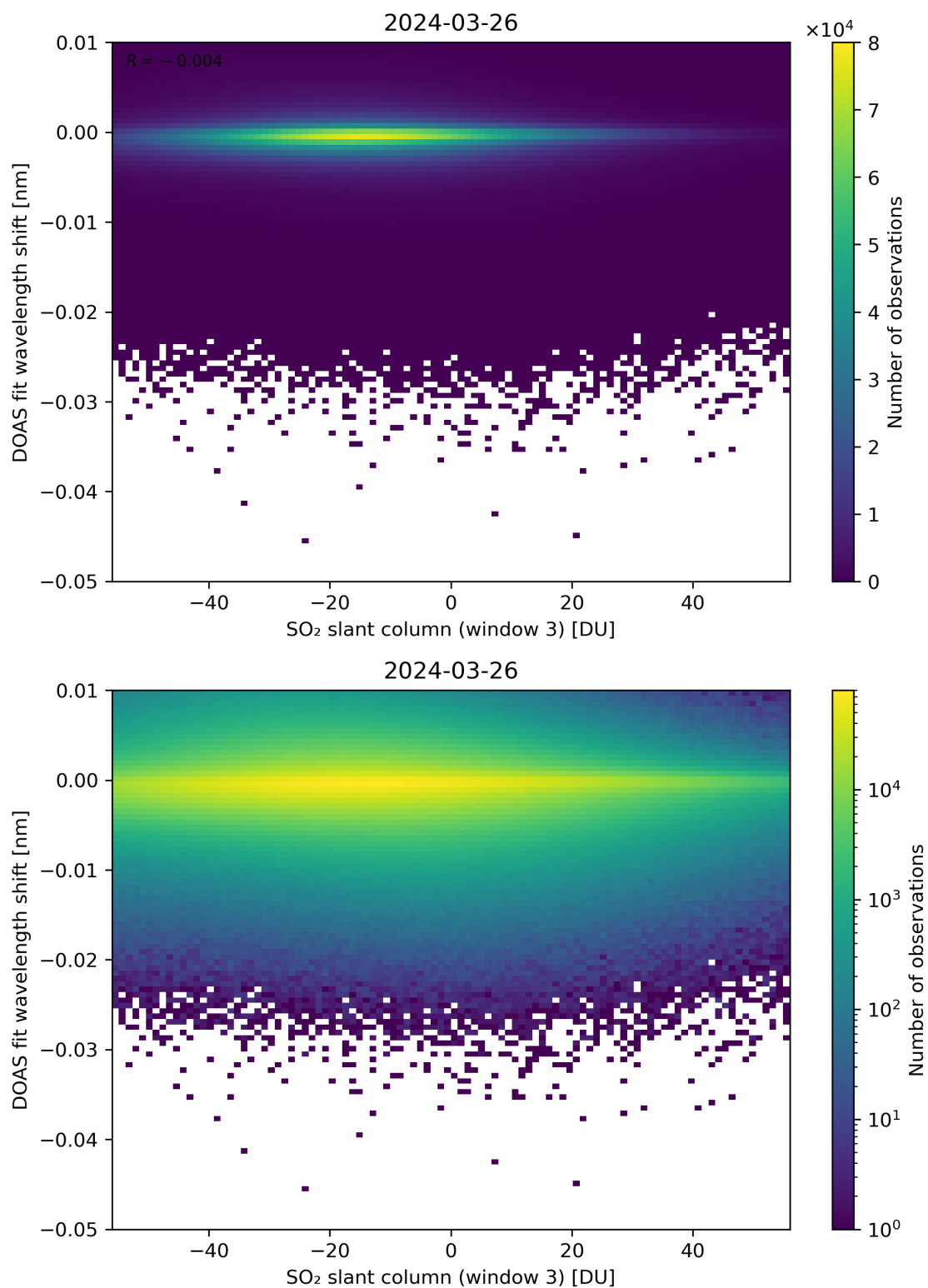
Figure 254: Scatter density plot of “SO 2 slant column (window 3)” against “DOAS fit wavelength shift” for 2024-03-25 to 2024-03-27.
