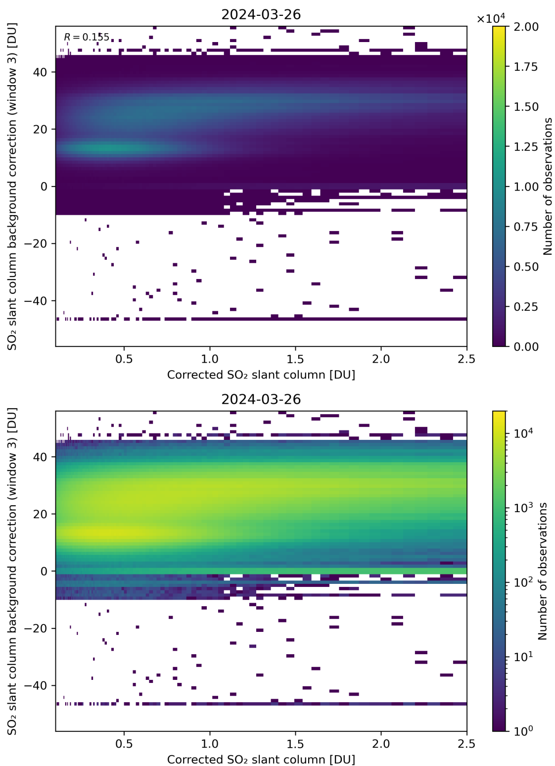
Figure 180: Scatter density plot of “Corrected SO 2 slant column” against “SO 2 slant column background correction (window 3)” for 2024-03-25 to 2024-03-27.
