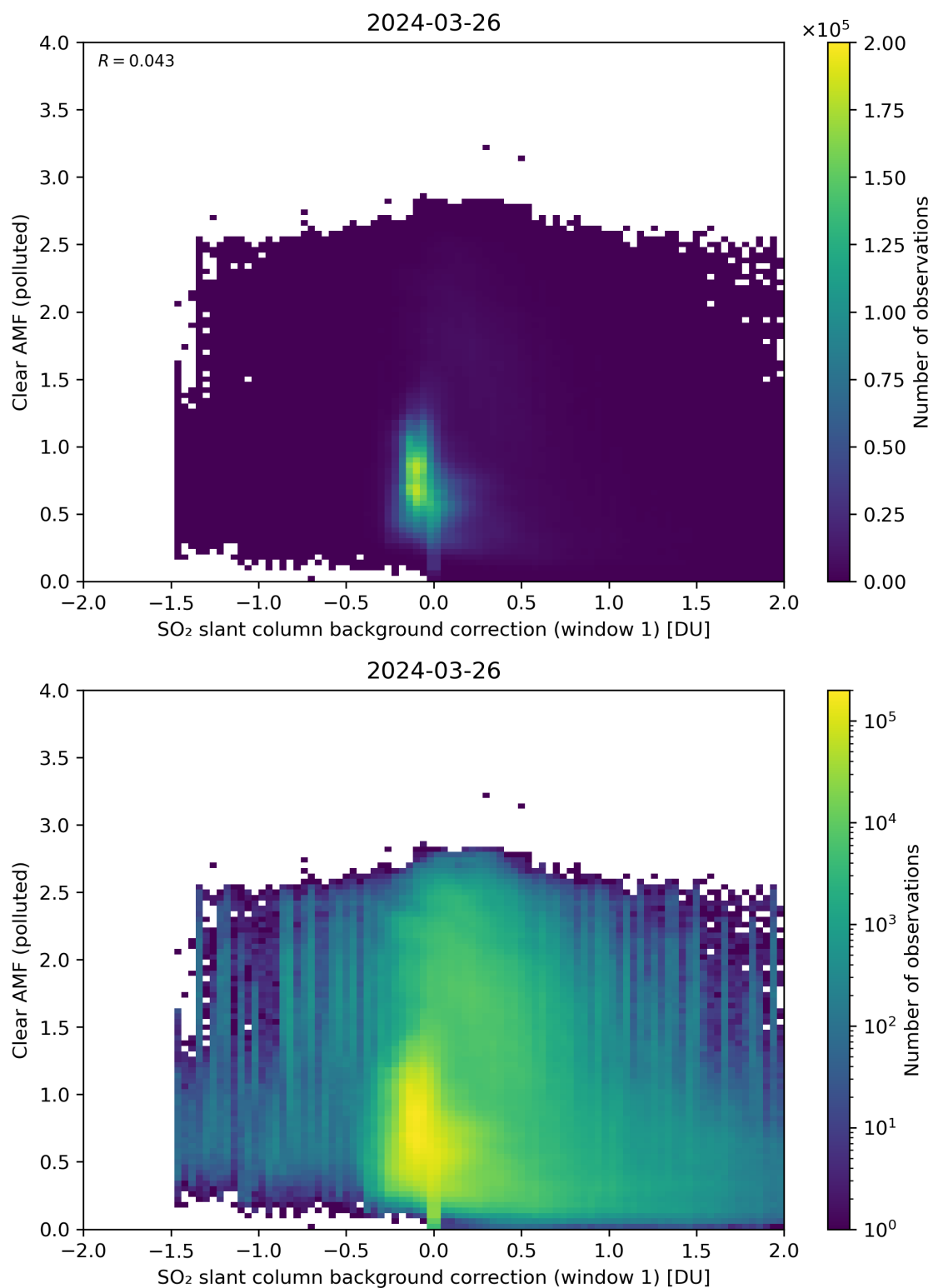
Figure 103: Scatter density plot of “SO 2 slant column background correction (window 1)” against “Clear AMF (polluted)” for 2024-03-25 to 2024-03-27.
