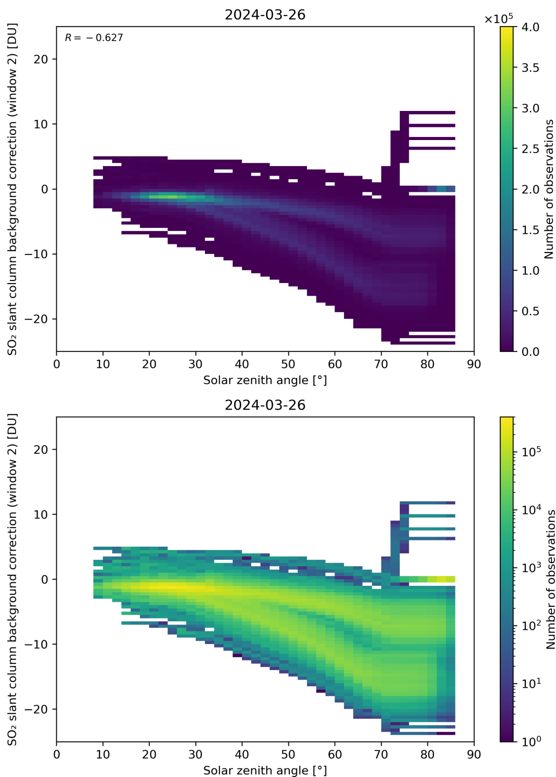
Figure 159: Scatter density plot of “Solar zenith angle” against “SO 2 slant column background correction (window 2)” for 2024-03-25 to 2024-03-27.
