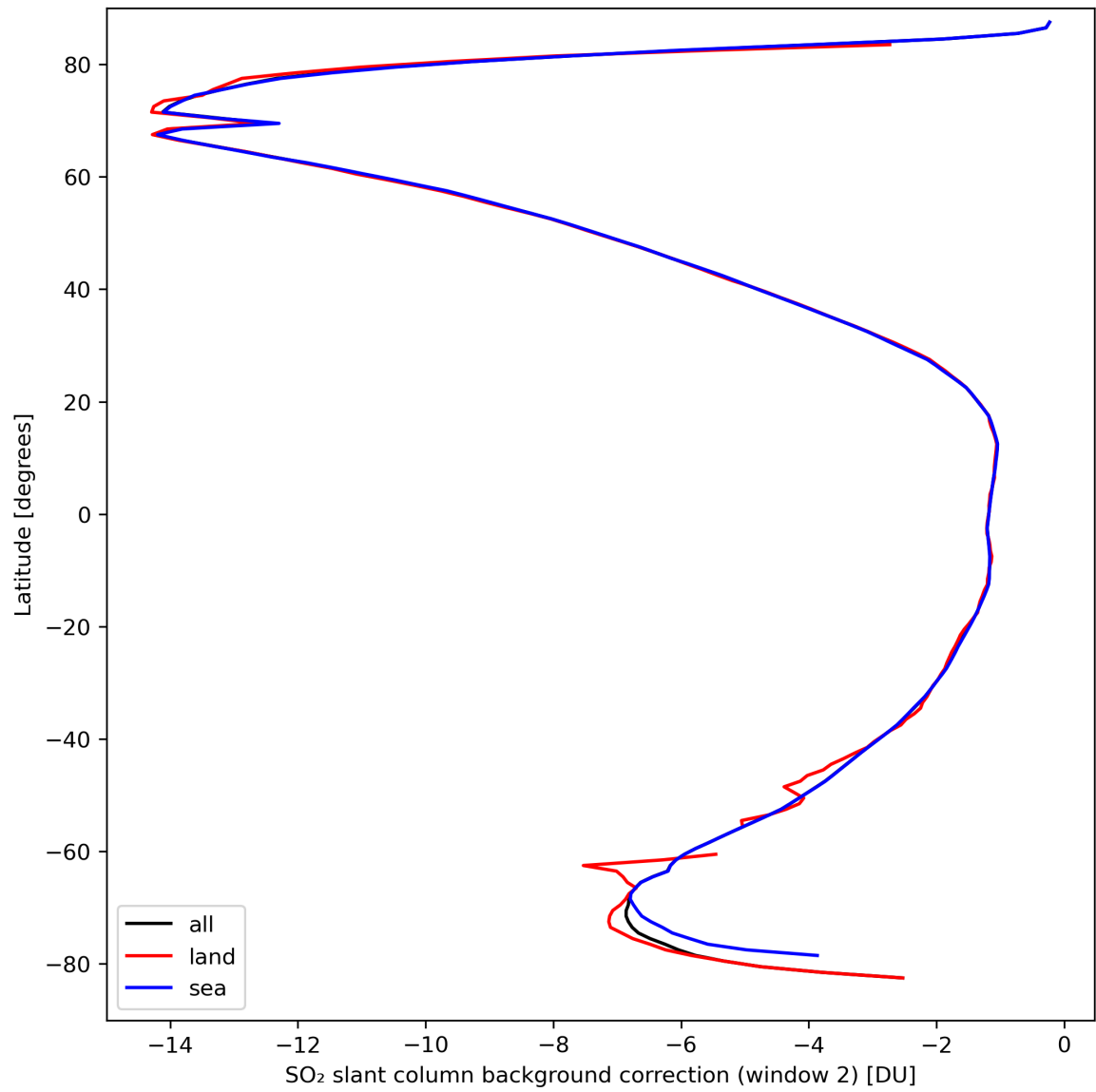
Figure 40: Zonal average of “SO 2 slant column background correction (window 2)” for 2024-03-25 to 2024-03-27.
