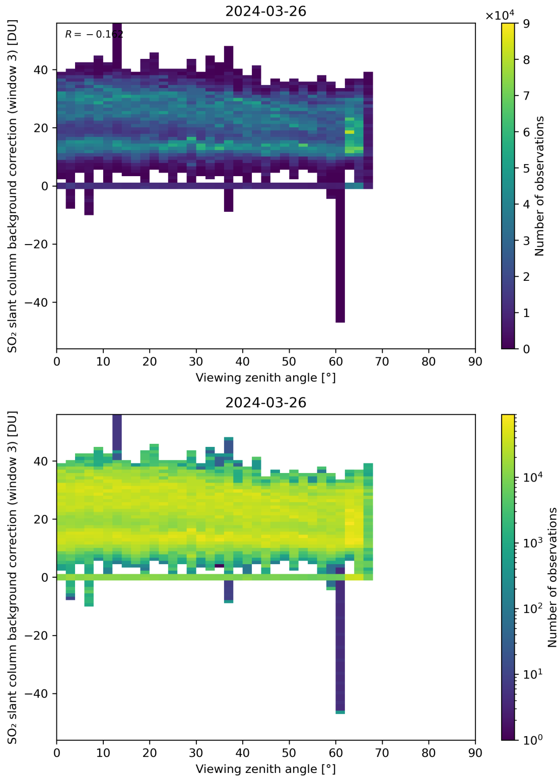
Figure 310: Scatter density plot of “Viewing zenith angle” against “SO 2 slant column background correction (window 3)” for 2024-03-25 to 2024-03-27.
