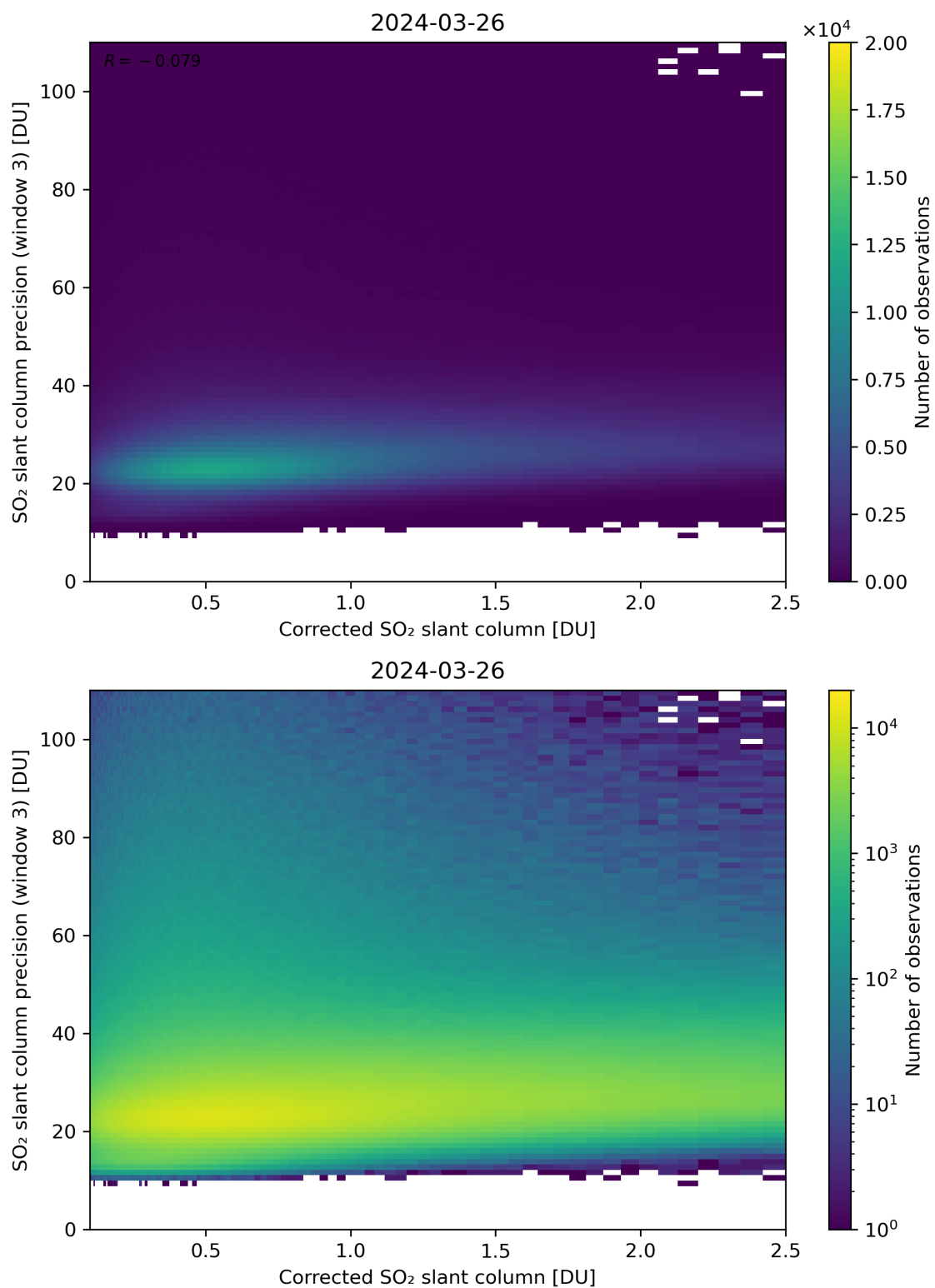
Figure 191: Scatter density plot of “Corrected SO 2 slant column” against “SO 2 slant column precision (window 3)” for 2024-03-25 to 2024-03-27.
