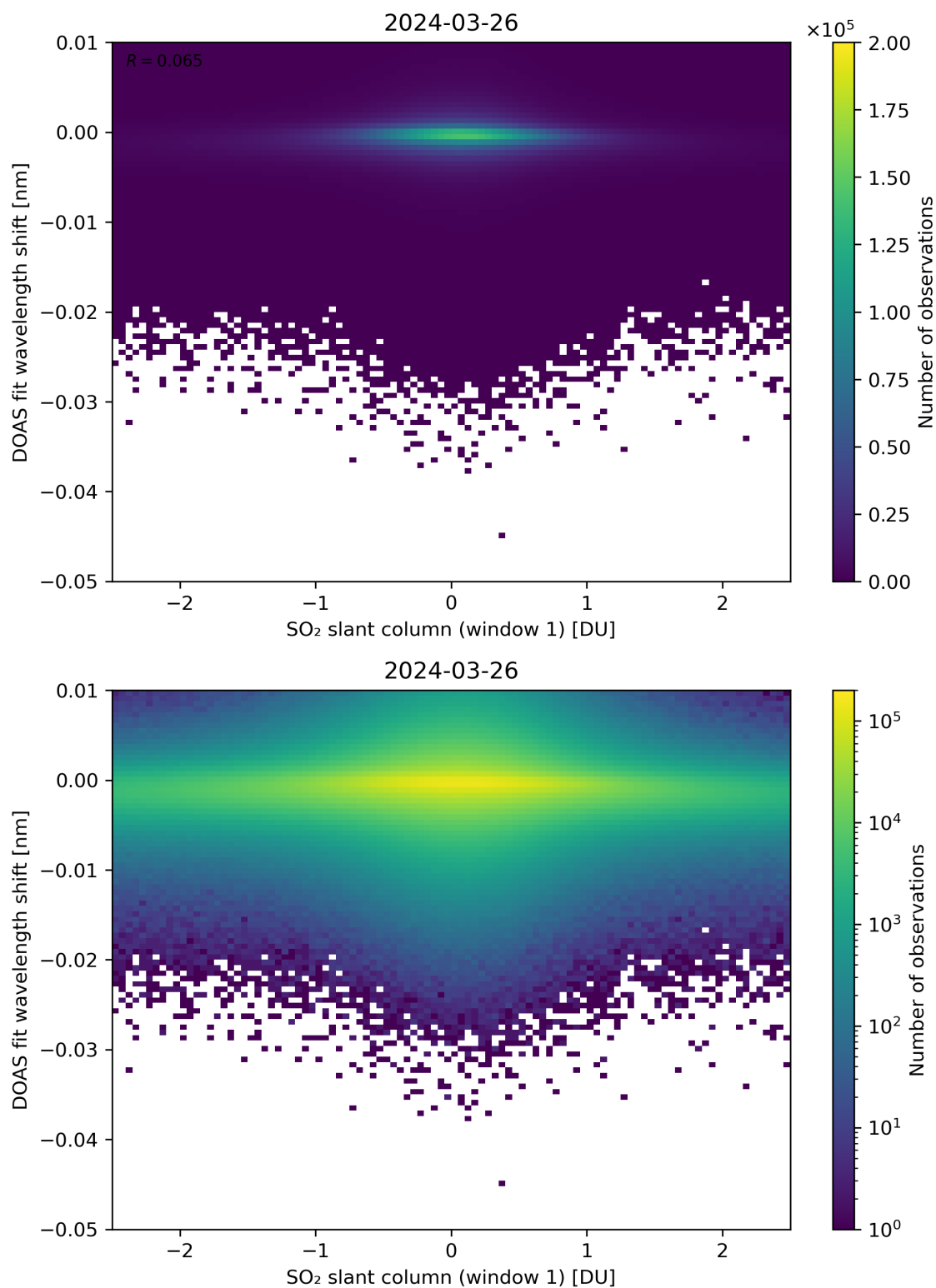
Figure 215: Scatter density plot of “SO 2 slant column (window 1)” against “DOAS fit wavelength shift” for 2024-03-25 to 2024-03-27.
