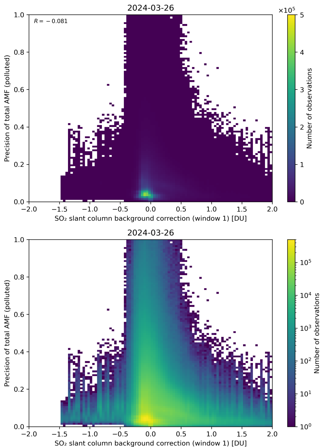
Figure 110: Scatter density plot of “SO 2 slant column background correction (window 1)” against “Precision of total AMF (polluted)” for 2024-03-25 to 2024-03-27.
