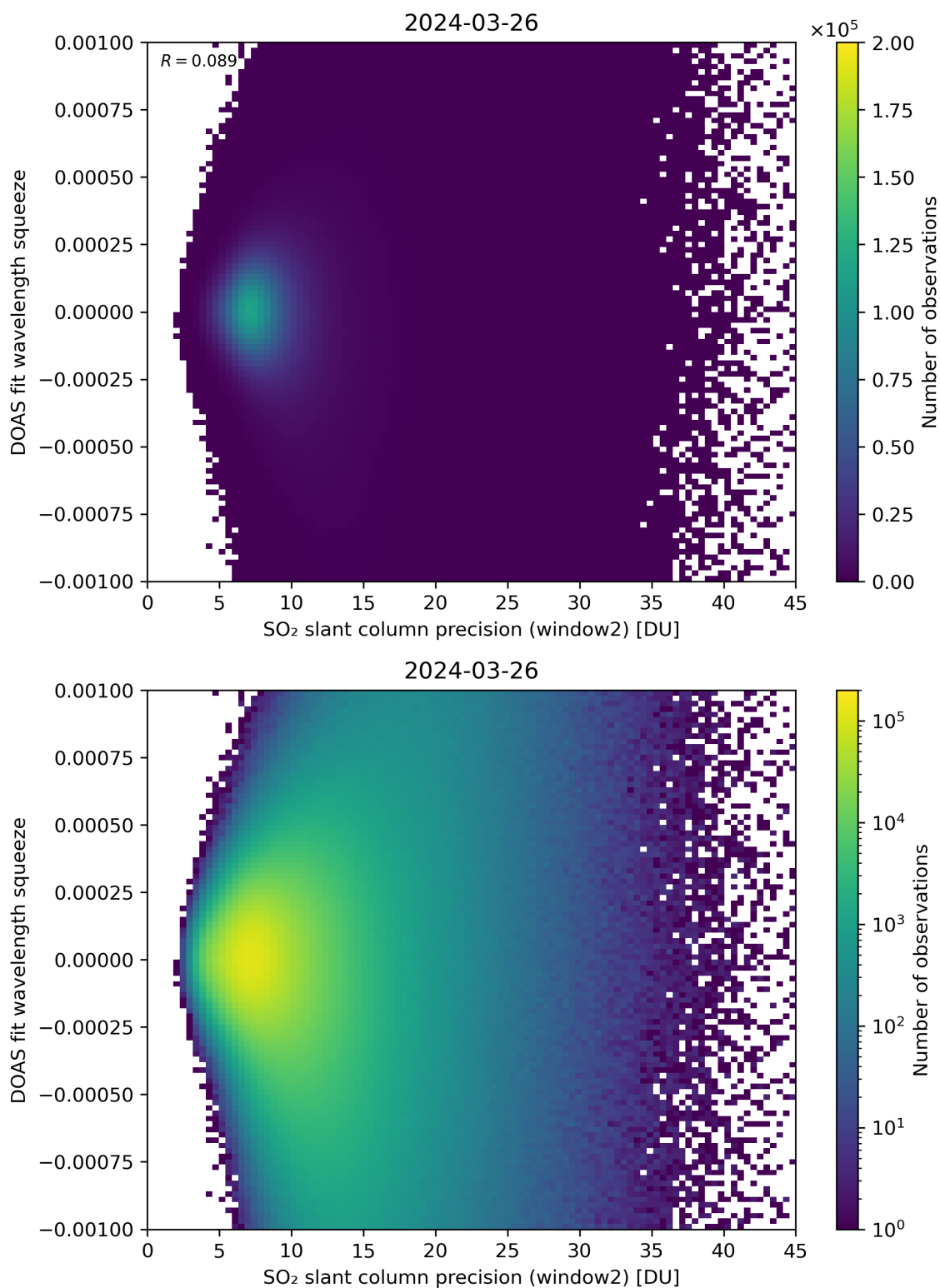
Figure 244: Scatter density plot of “SO 2 slant column precision (window2)” against “DOAS fit wavelength squeeze” for 2024-03-25 to 2024-03-27.
