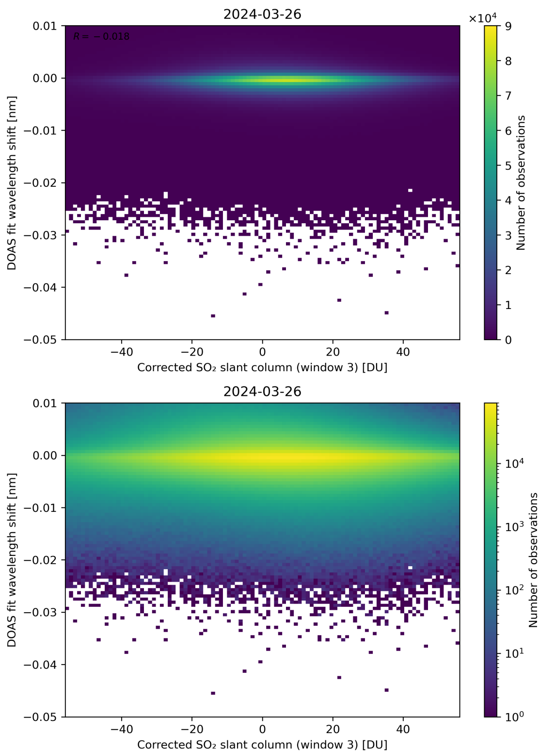
Figure 206: Scatter density plot of “Corrected SO 2 slant column (window 3)” against “DOAS fit wavelength shift” for 2024-03-25 to 2024-03-27.
