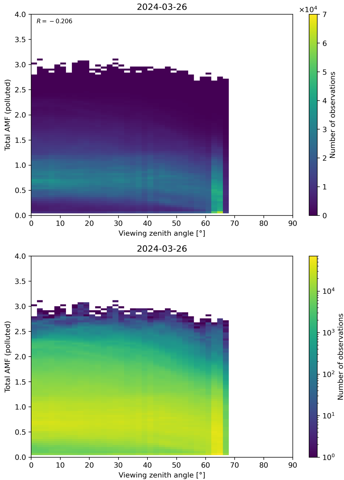
Figure 325: Scatter density plot of “Viewing zenith angle” against “Total AMF (polluted)” for 2024-03-25 to 2024-03-27.
