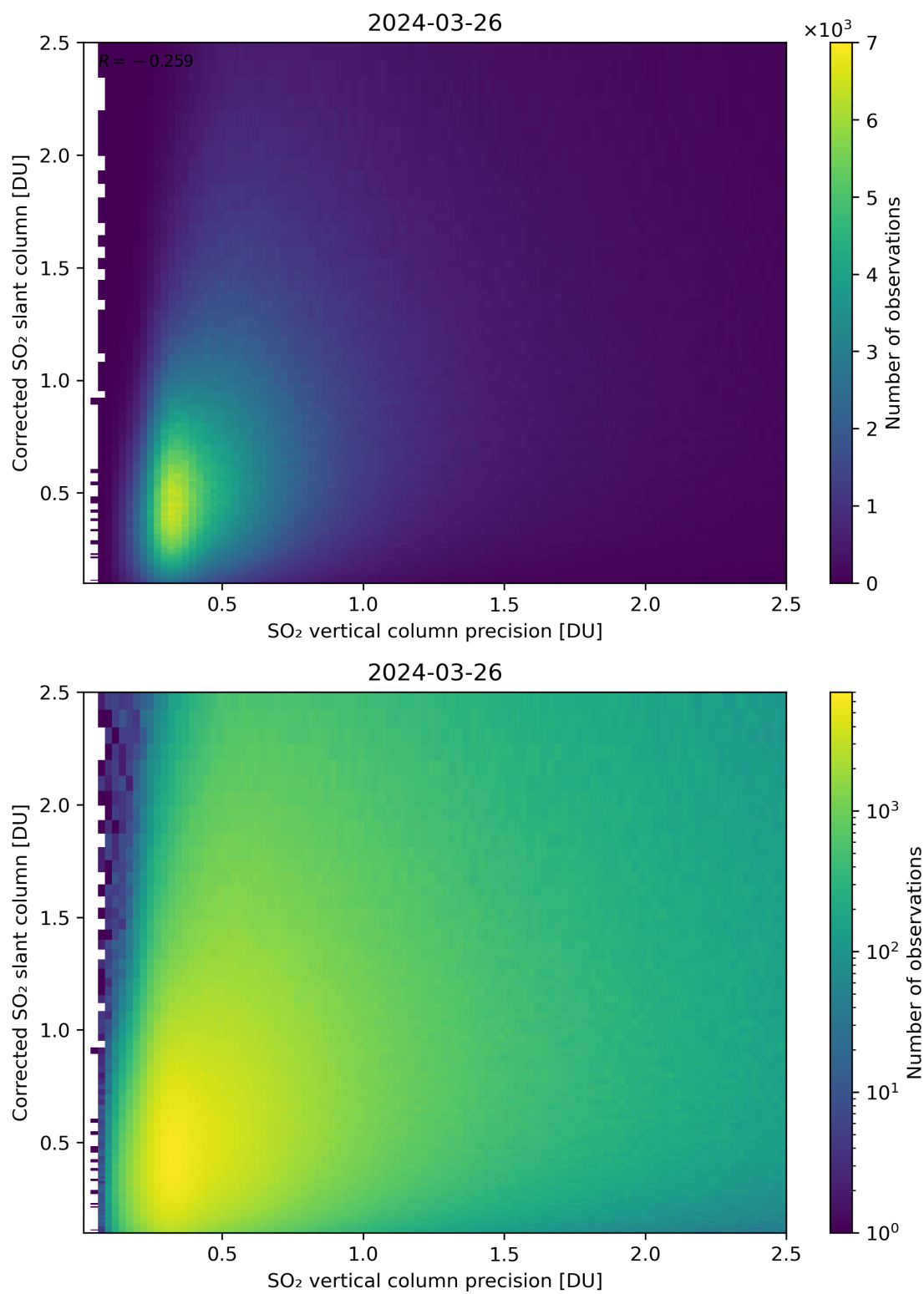
Figure 286: Scatter density plot of “SO 2 vertical column precision” against “Corrected SO 2 slant column” for 2024-03-25 to 2024-03-27.
