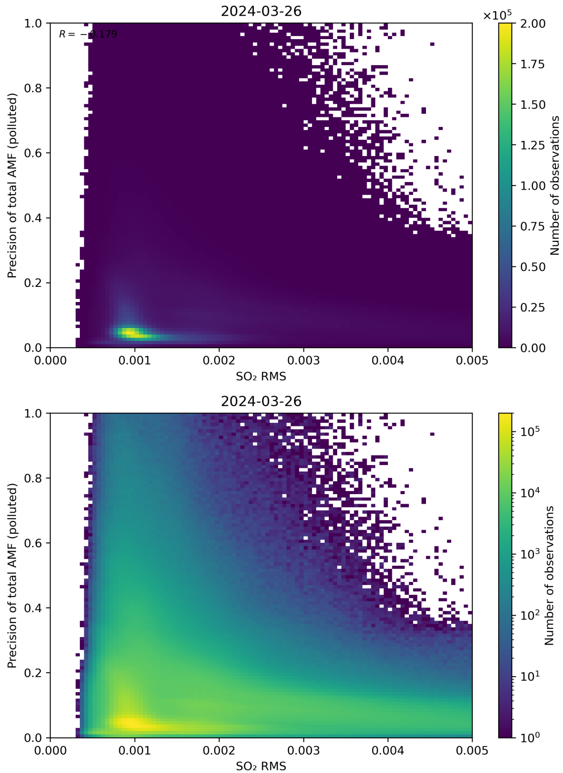
Figure 138: Scatter density plot of “SO 2 RMS” against “Precision of total AMF (polluted)” for 2024-03-25 to 2024-03-27.
