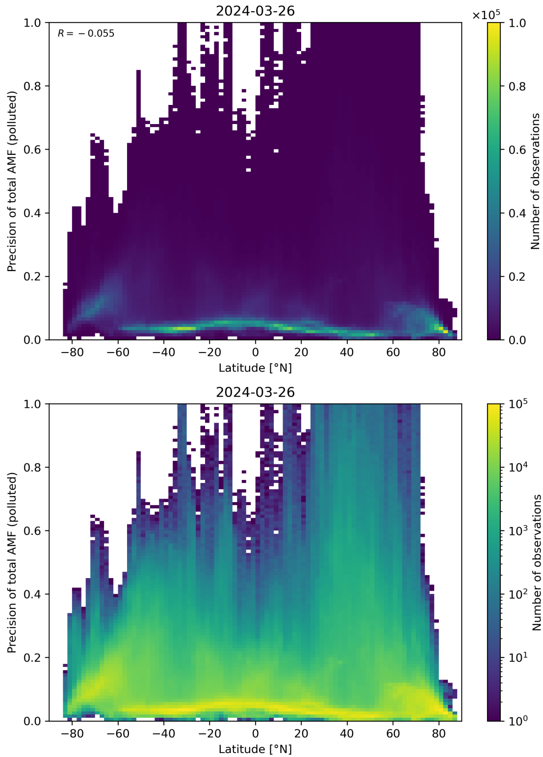
Figure 155: Scatter density plot of “Latitude” against “Precision of total AMF (polluted)” for 2024-03-25 to 2024-03-27.
