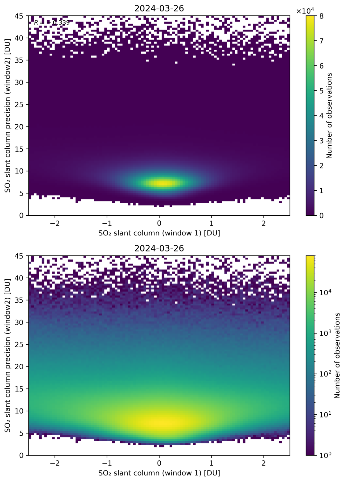
Figure 236: Scatter density plot of “SO 2 slant column (window 1)” against “SO 2 slant column precision (window2)” for 2024-03-25 to 2024-03-27.
