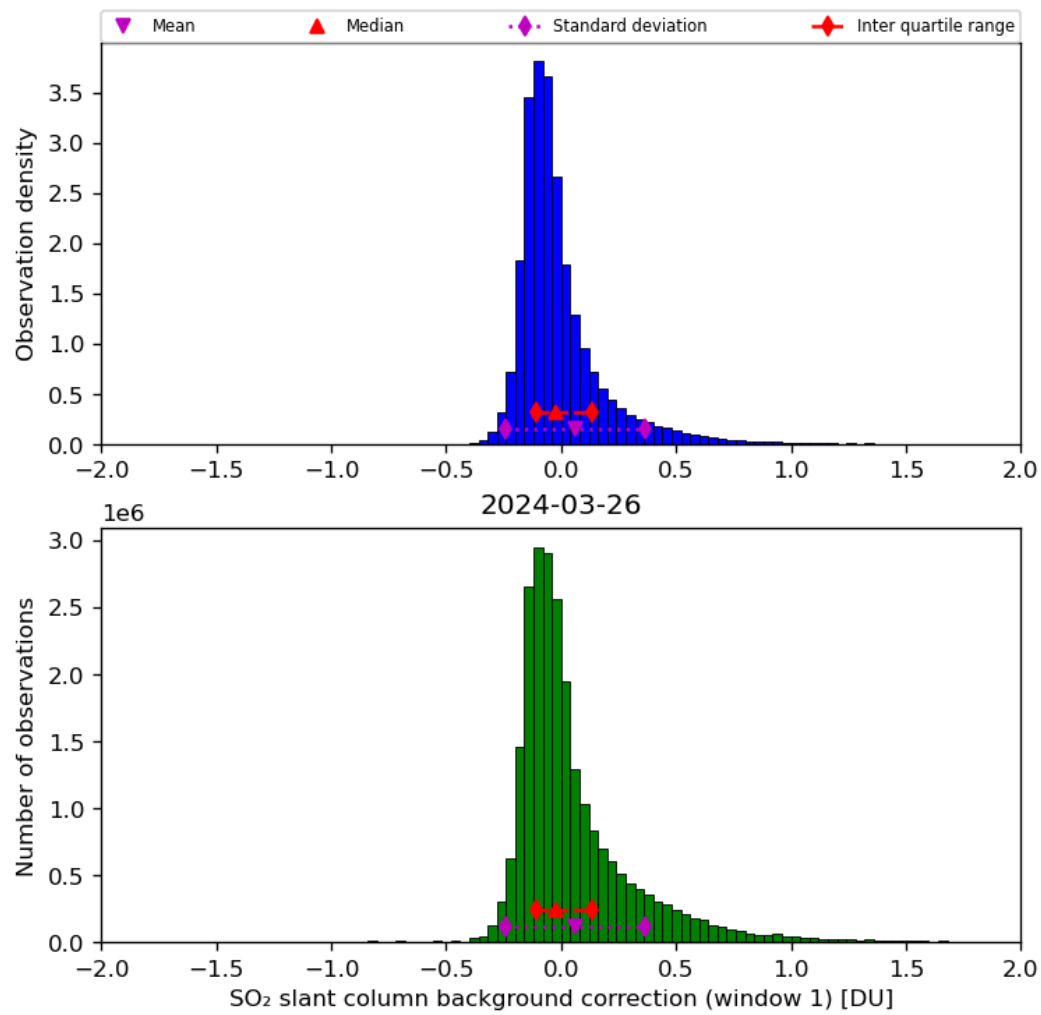
Figure 59: Histogram of “SO 2 slant column background correction (window 1)” for 2024-03-25 to 2024-03-27
