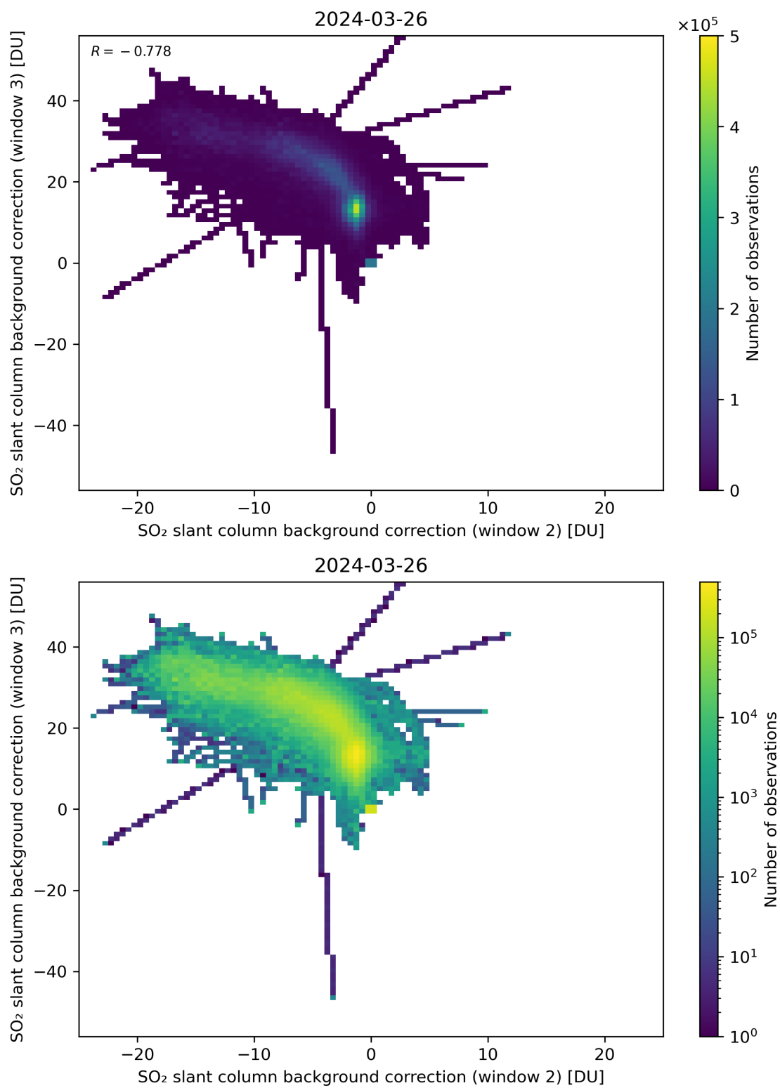
Figure 111: Scatter density plot of “SO 2 slant column background correction (window 2)” against “SO 2 slant column background correction (window 3)” for 2024-03-25 to 2024-03-27.
