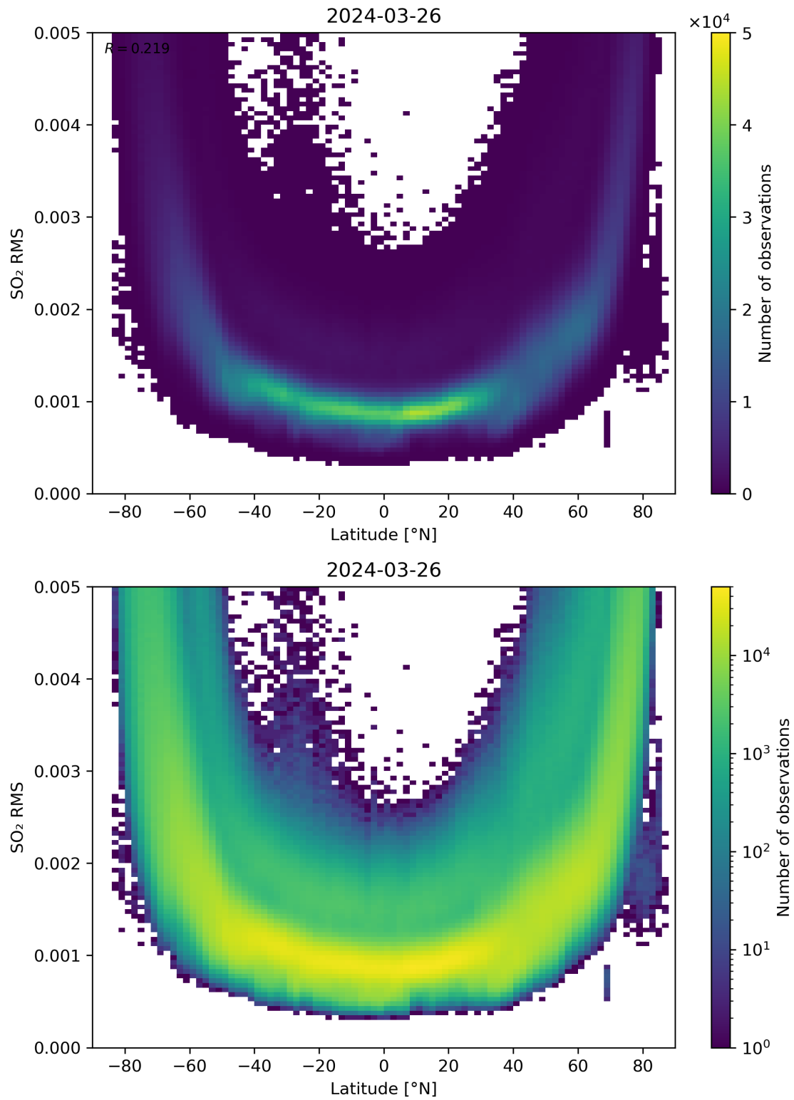
Figure 144: Scatter density plot of “Latitude” against “SO 2 RMS” for 2024-03-25 to 2024-03-27.
