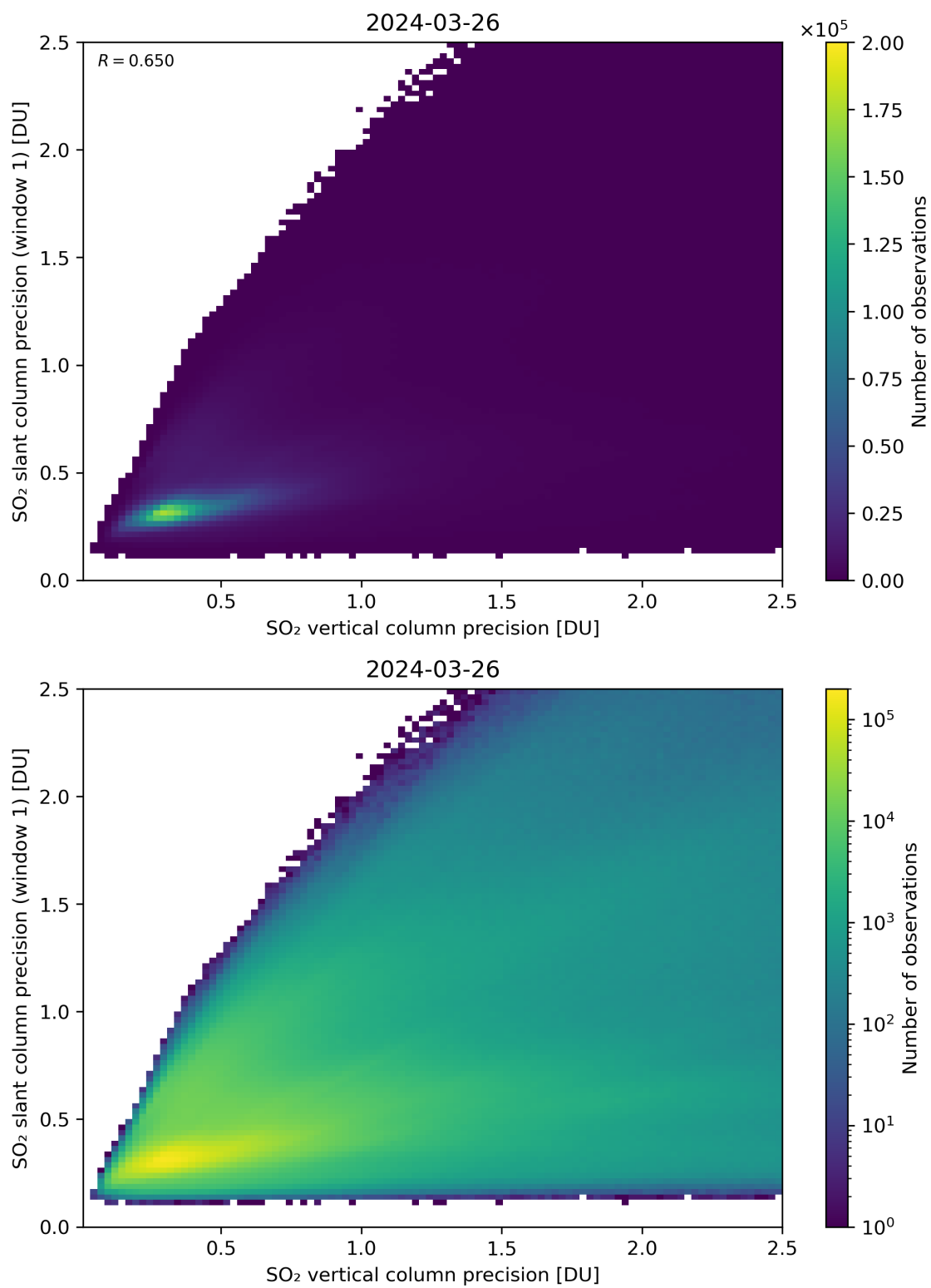
Figure 290: Scatter density plot of “SO 2 vertical column precision” against “SO 2 slant column precision (window 1)” for 2024-03-25 to 2024-03-27.
