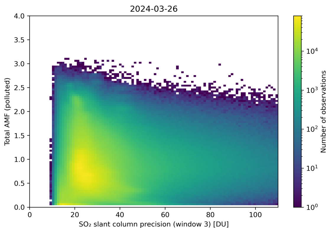
Figure 263: Scatter density plot of “SO 2 slant column precision (window 3)” against “Total AMF (polluted)” for 2024-03-25 to 2024-03-27.
