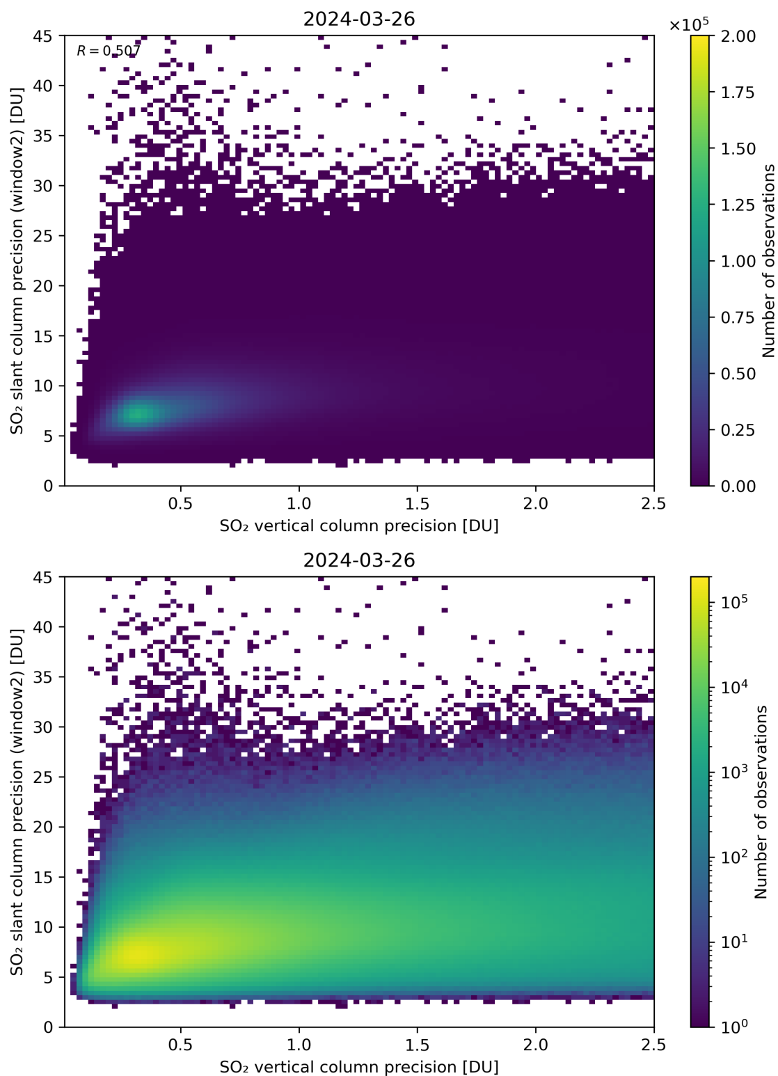
Figure 291: Scatter density plot of “SO 2 vertical column precision” against “SO 2 slant column precision (window2)” for 2024-03-25 to 2024-03-27.
