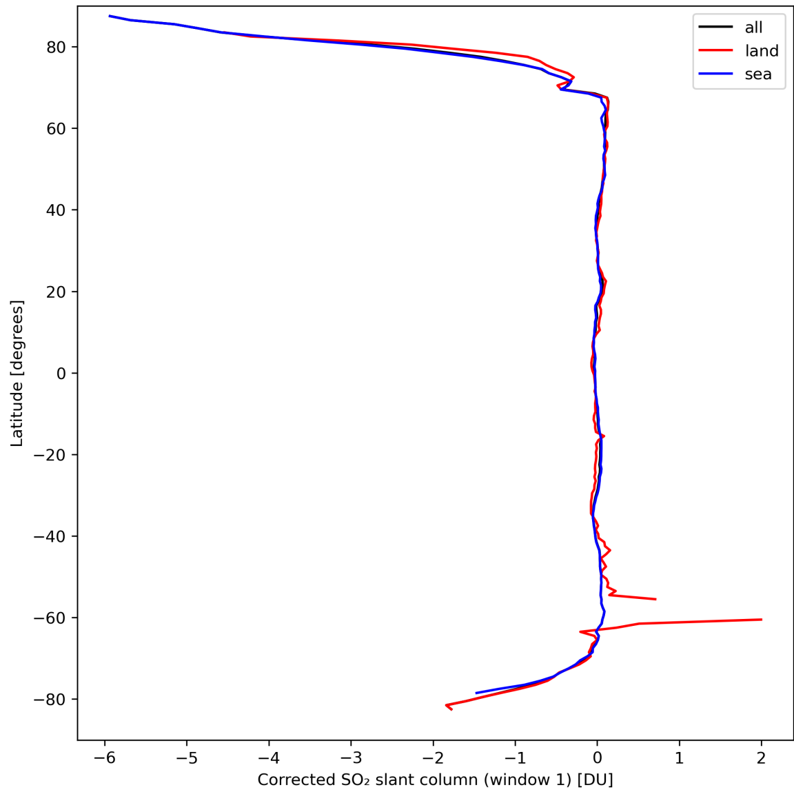
Figure 35: Zonal average of “Corrected SO 2 slant column (window 1)” for 2024-03-25 to 2024-03-27.
