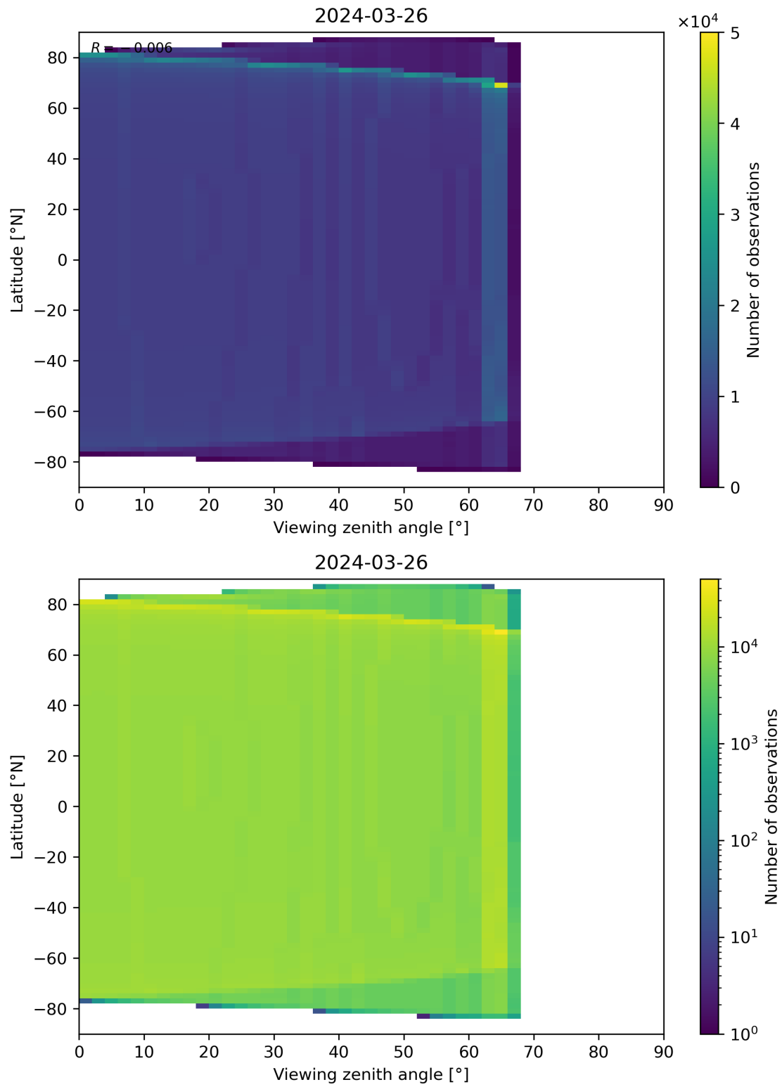
Figure 314: Scatter density plot of “Viewing zenith angle” against “Latitude” for 2024-03-25 to 2024-03-27.
