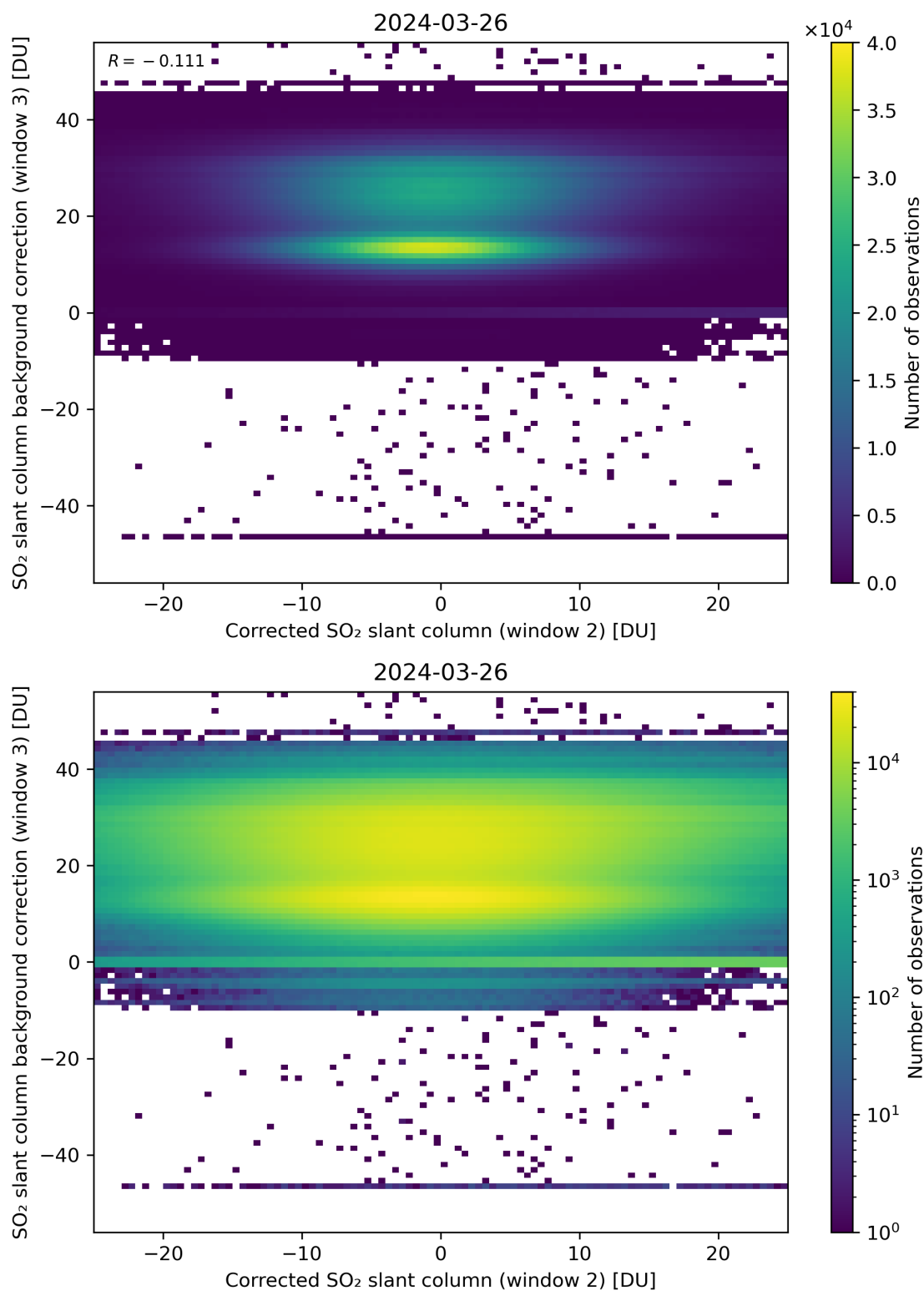
Figure 195: Scatter density plot of “Corrected SO 2 slant column (window 2)” against “SO 2 slant column background correction (window 3)” for 2024-03-25 to 2024-03-27.
