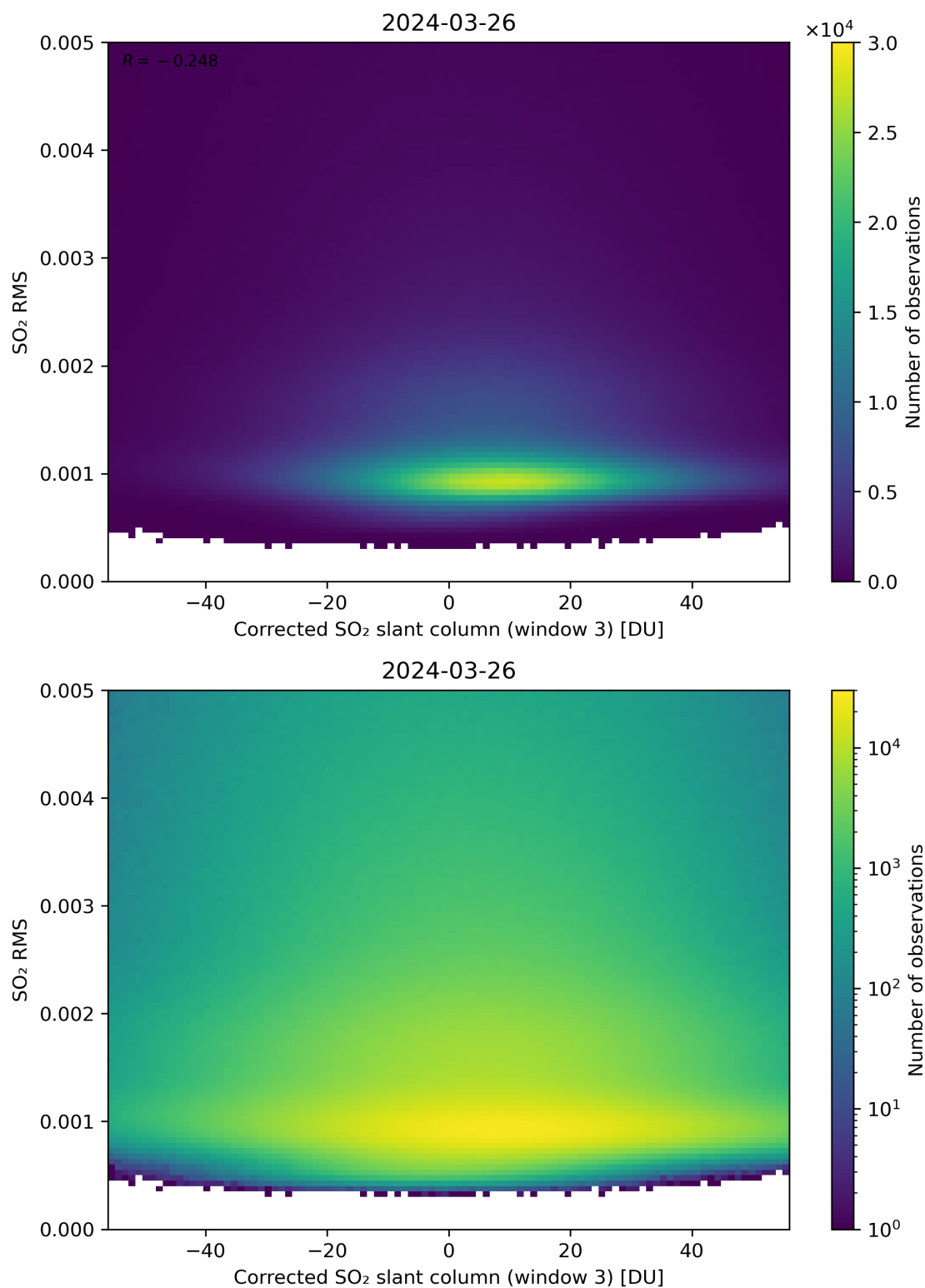
Figure 208: Scatter density plot of “Corrected SO 2 slant column (window 3)” against “SO 2 RMS” for 2024-03-25 to 2024-03-27.
