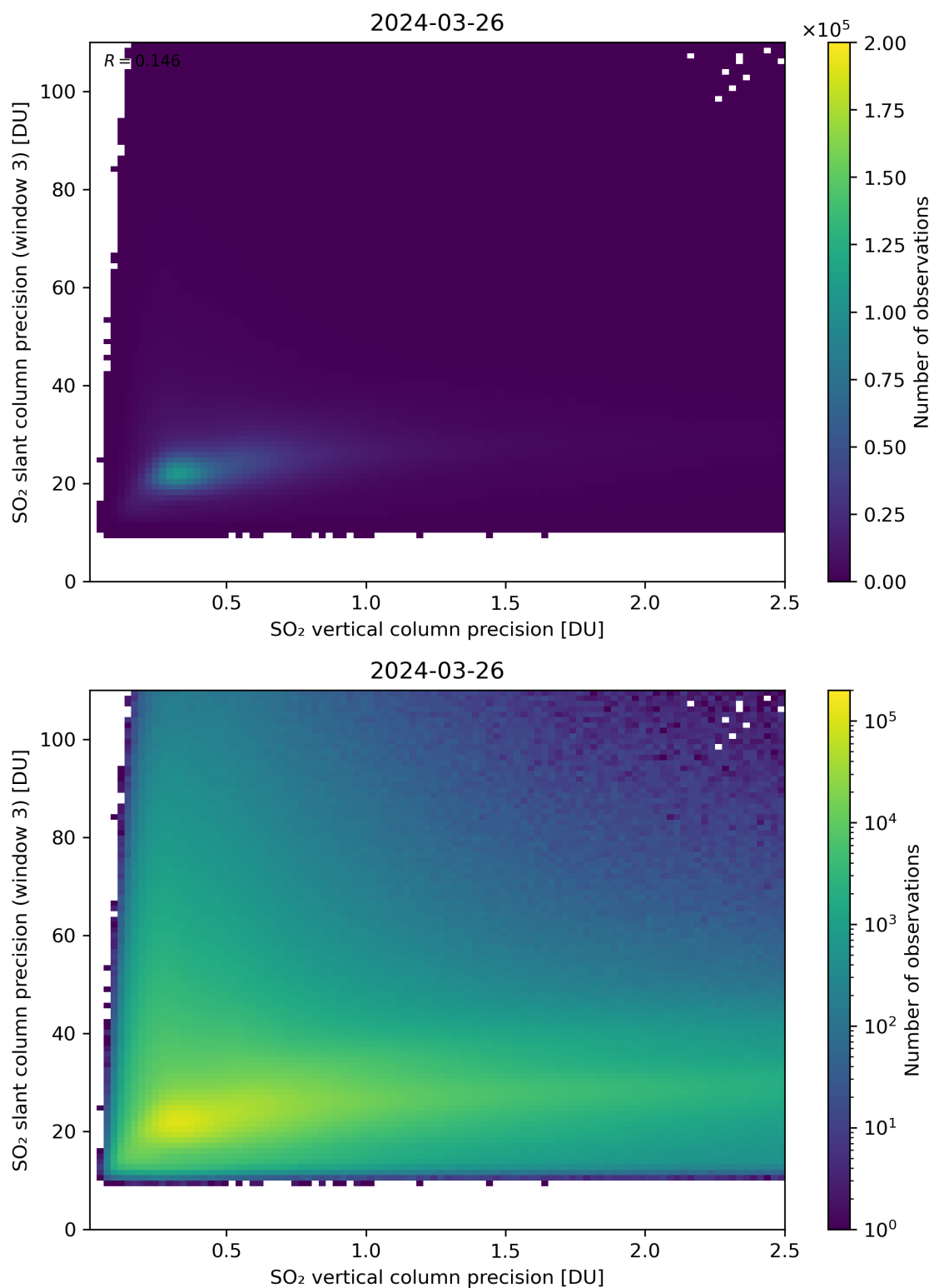
Figure 293: Scatter density plot of “SO 2 vertical column precision” against “SO 2 slant column precision (window 3)” for 2024-03-25 to 2024-03-27.
