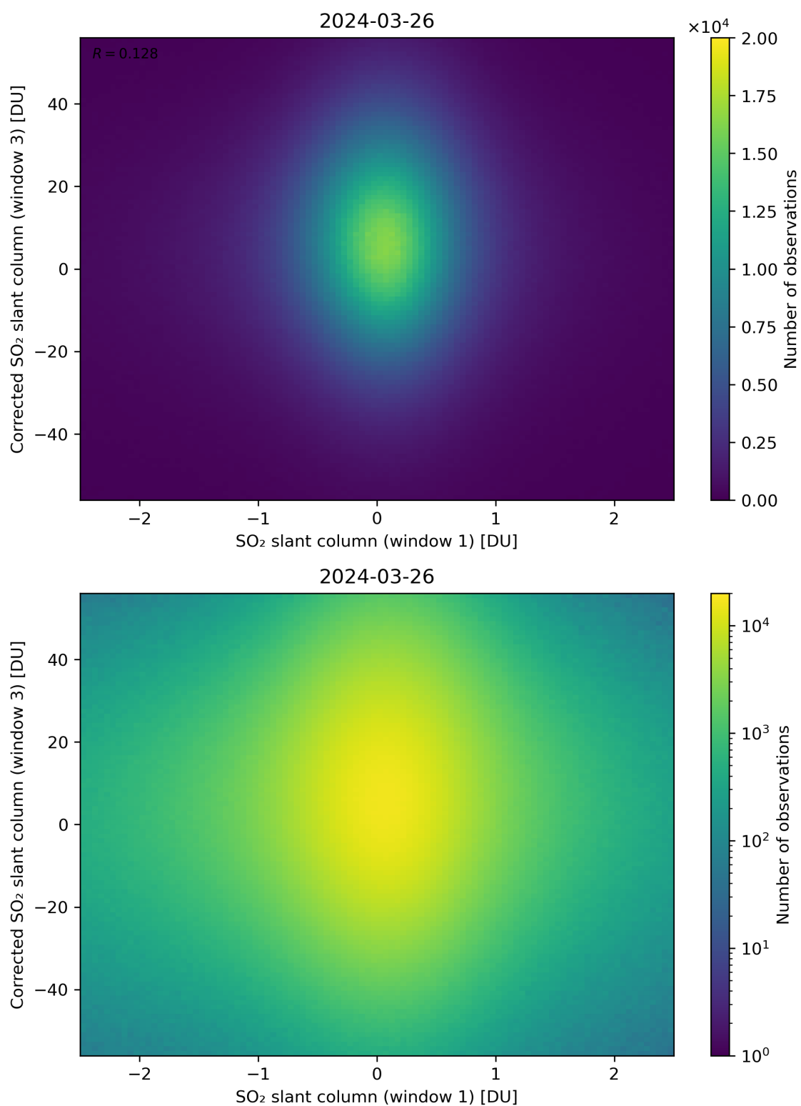
Figure 234: Scatter density plot of “SO 2 slant column (window 1)” against “Corrected SO 2 slant column (window 3)” for 2024-03-25 to 2024-03-27.
