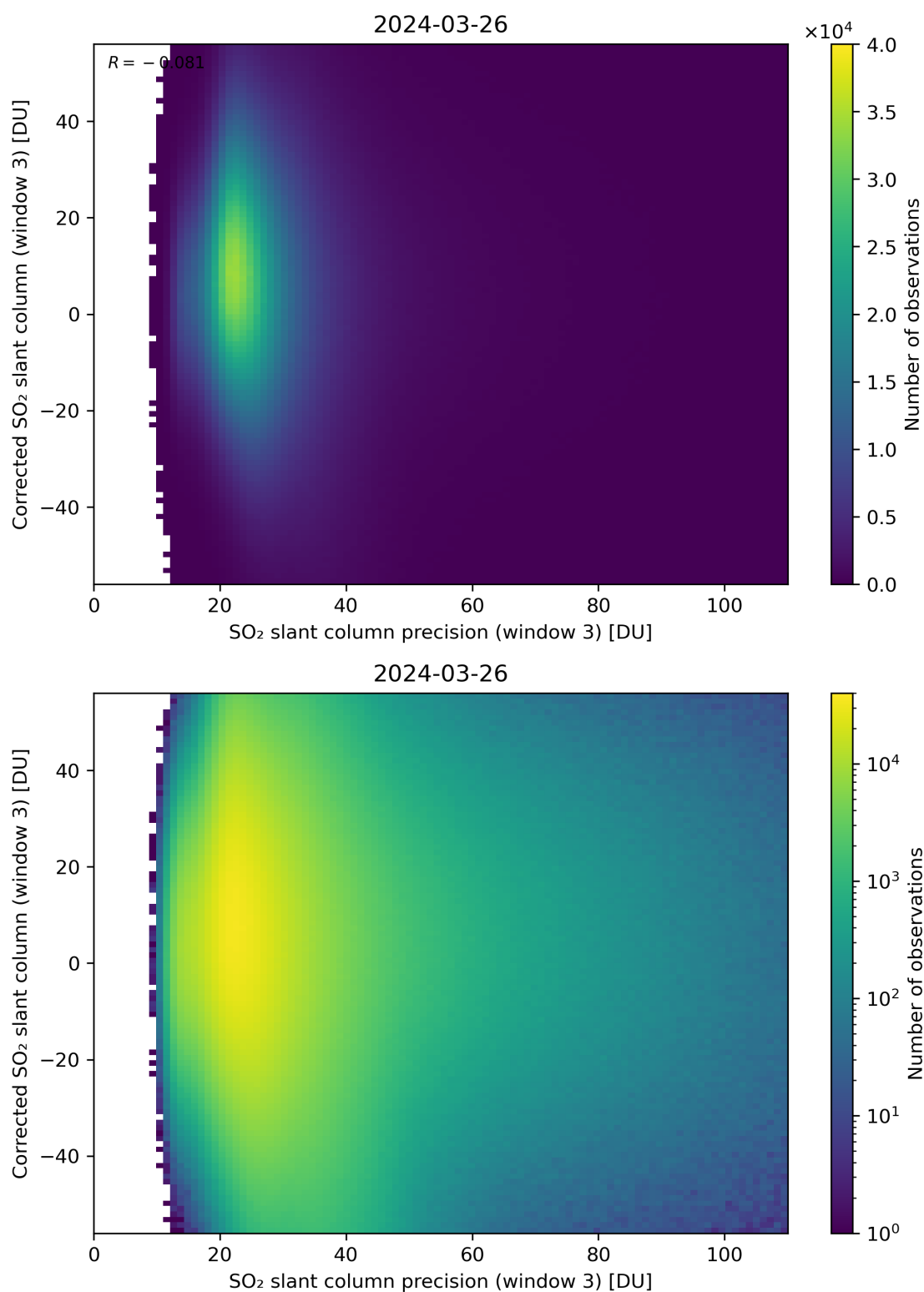
Figure 262: Scatter density plot of “SO 2 slant column precision (window 3)” against “Corrected SO 2 slant column (window 3)” for 2024-03-25 to 2024-03-27.
