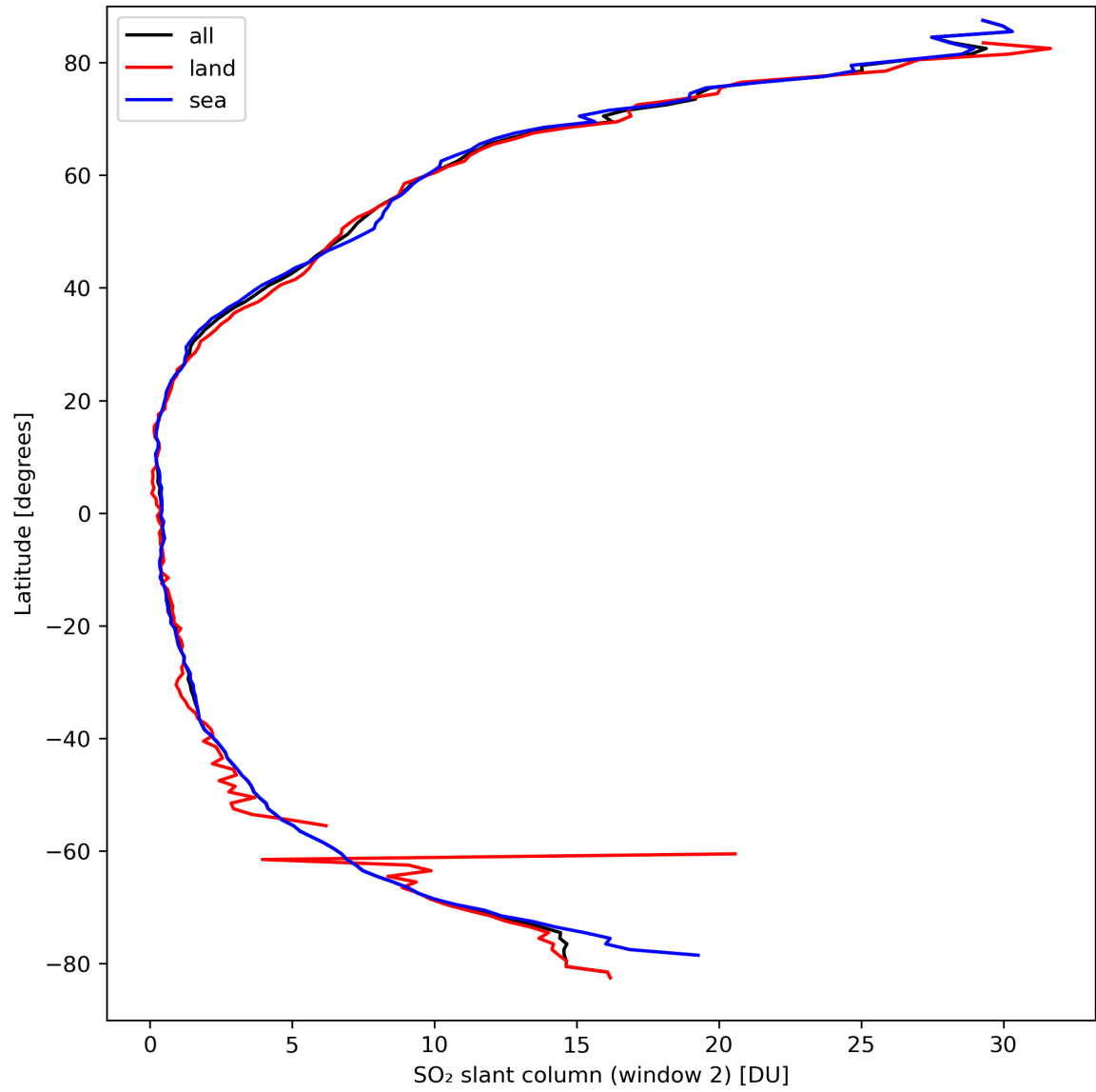
Figure 37: Zonal average of “SO 2 slant column (window 2)” for 2024-03-25 to 2024-03-27.
