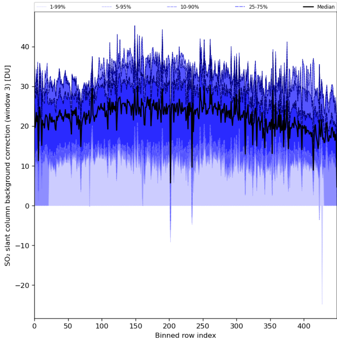
Figure 90: Along track statistics of “SO 2 slant column background correction (window 3)” for 2024-03-25 to 2024-03-27
