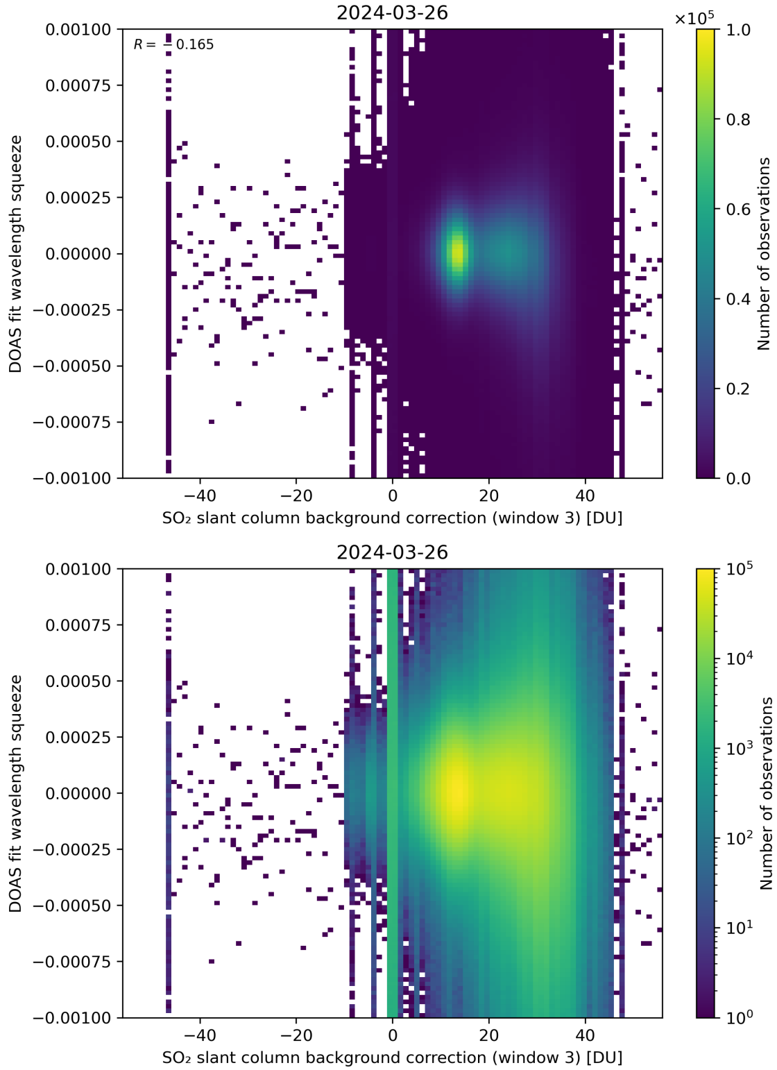
Figure 122: Scatter density plot of “SO 2 slant column background correction (window 3)” against “DOAS fit wavelength squeeze” for 2024-03-25 to 2024-03-27.
