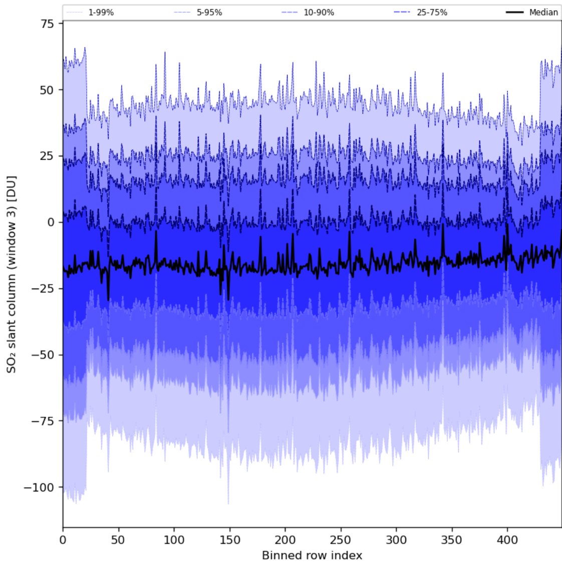
Figure 87: Along track statistics of “SO 2 slant column (window 3)” for 2024-03-25 to 2024-03-27
