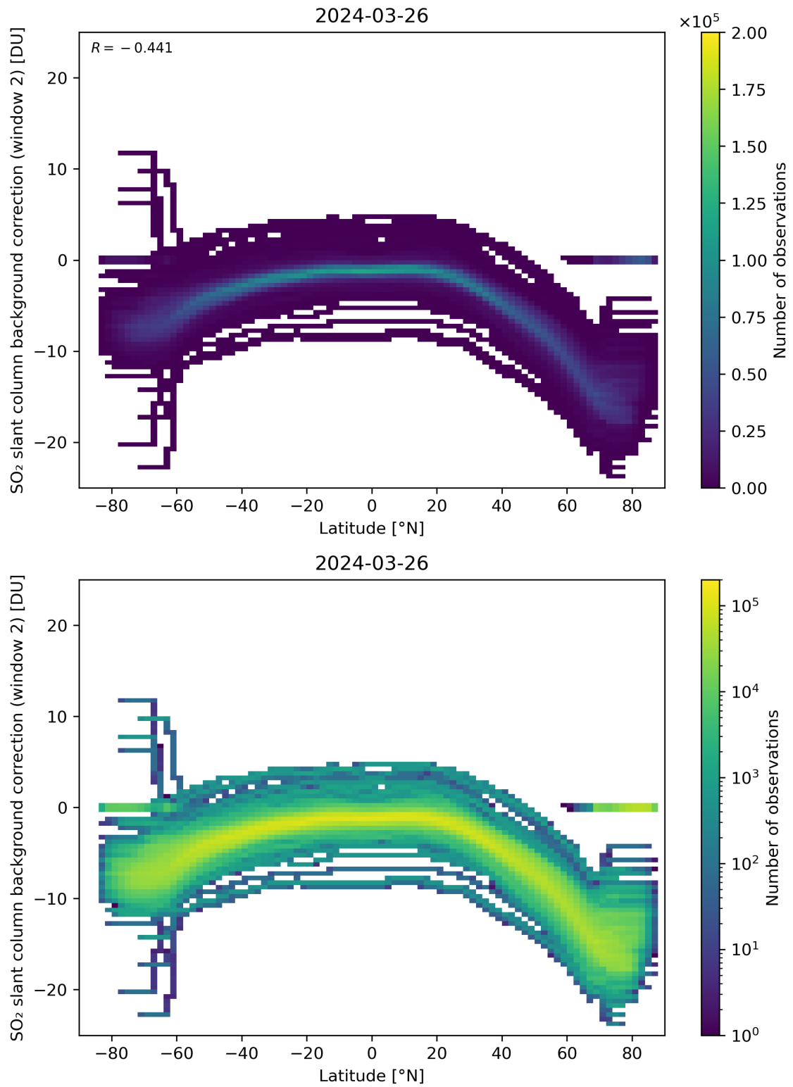
Figure 140: Scatter density plot of “Latitude” against “SO 2 slant column background correction (window 2)” for 2024-03-25 to 2024-03-27.
