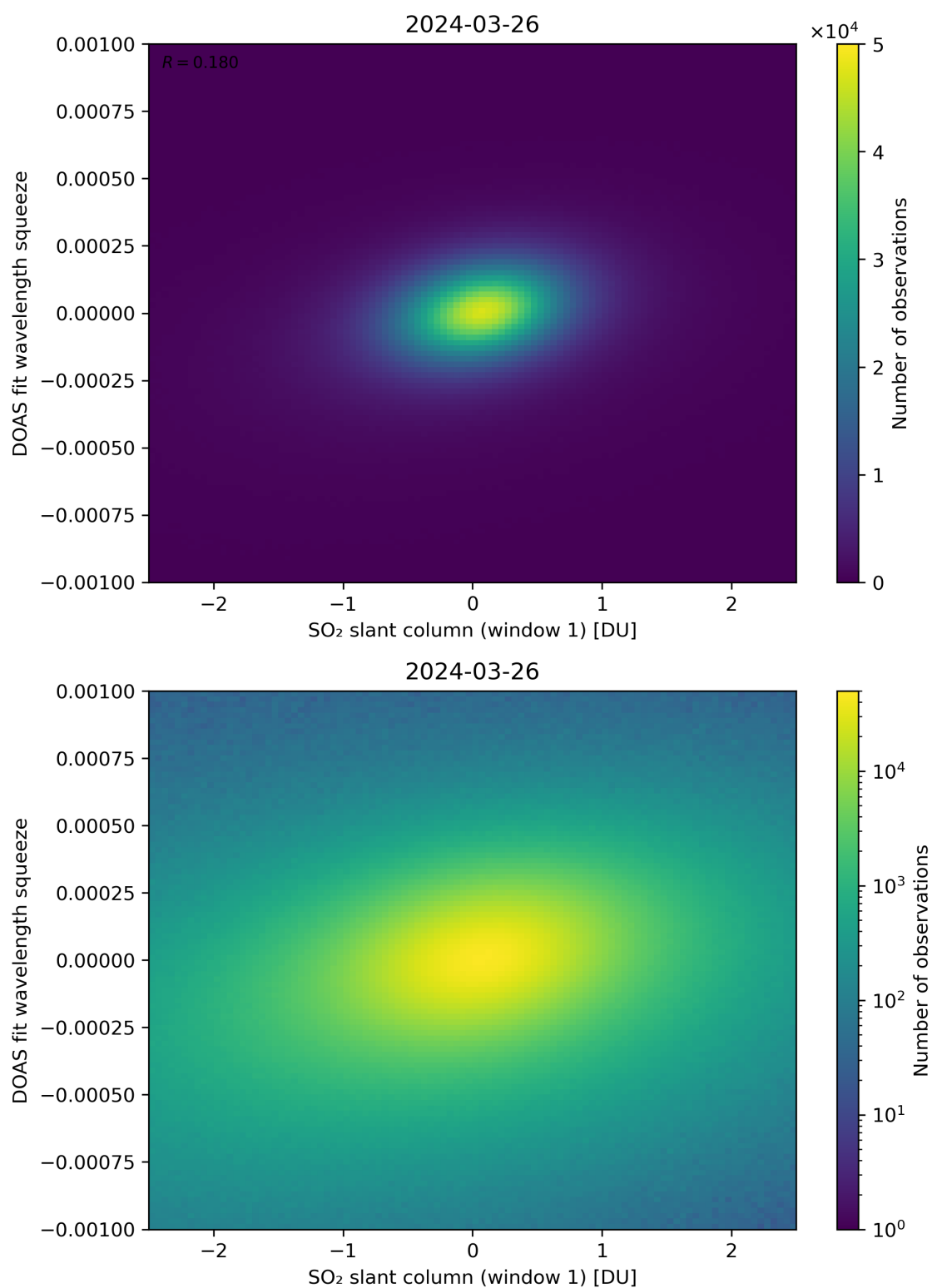
Figure 216: Scatter density plot of “SO 2 slant column (window 1)” against “DOAS fit wavelength squeeze” for 2024-03-25 to 2024-03-27.
