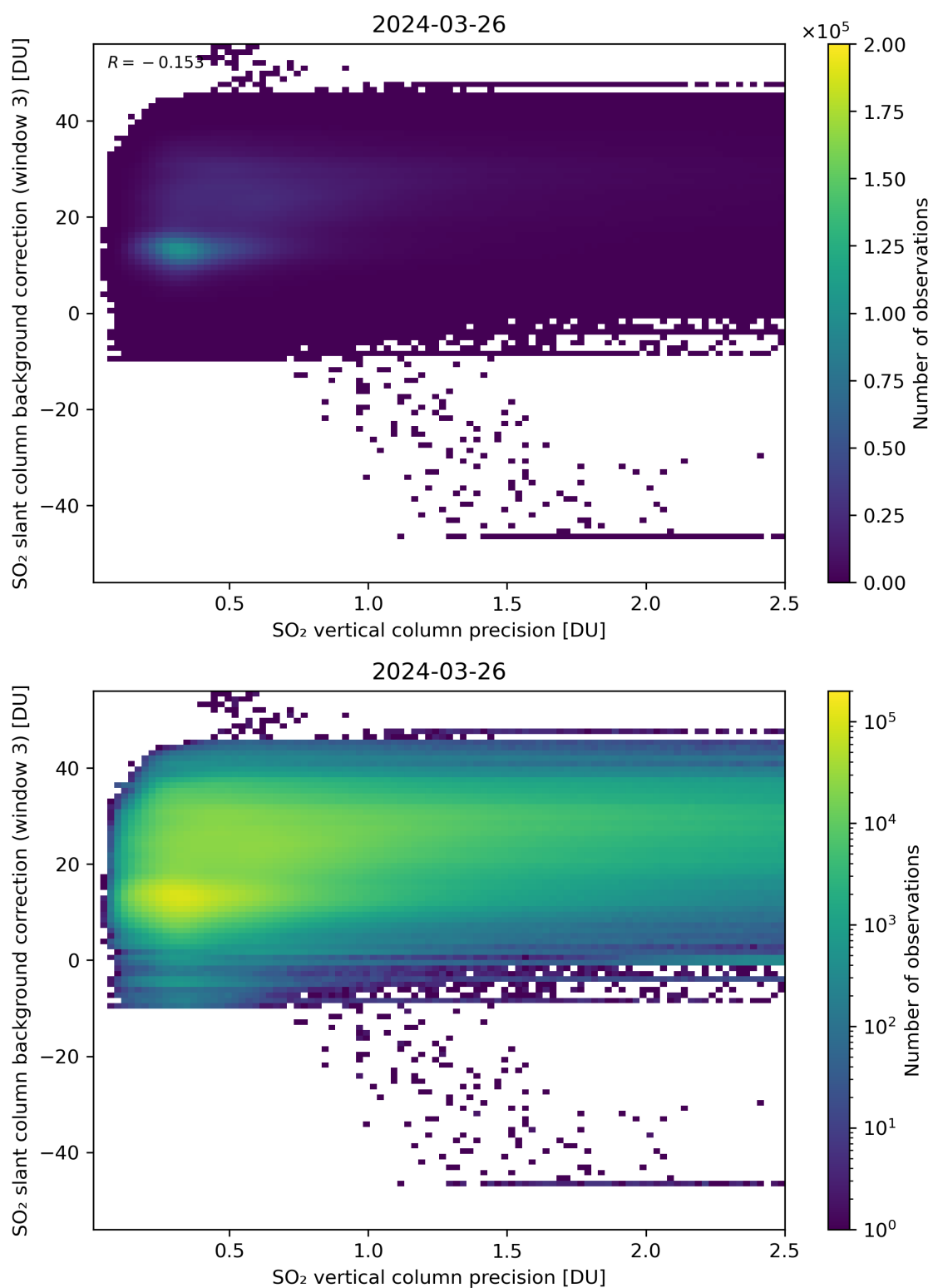
Figure 281: Scatter density plot of “SO 2 vertical column precision” against “SO 2 slant column background correction (window 3)” for 2024-03-25 to 2024-03-27.
