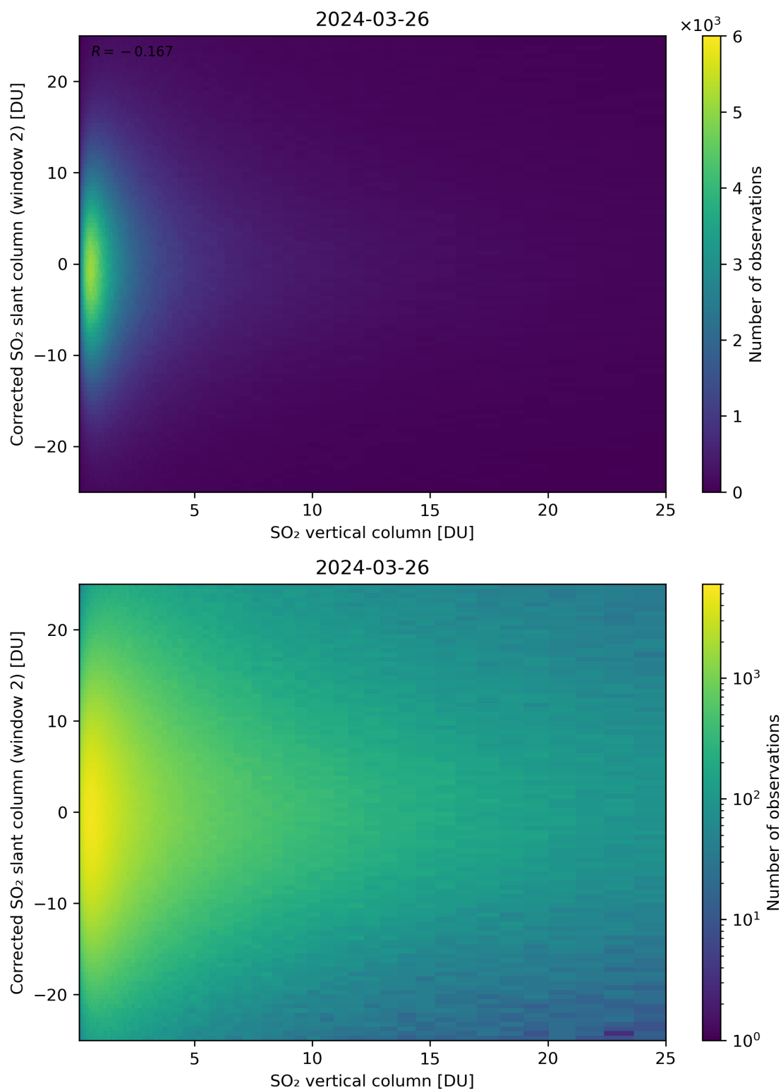
Figure 298: Scatter density plot of “SO 2 vertical column” against “Corrected SO 2 slant column (window 2)” for 2024-03-25 to 2024-03-27.
