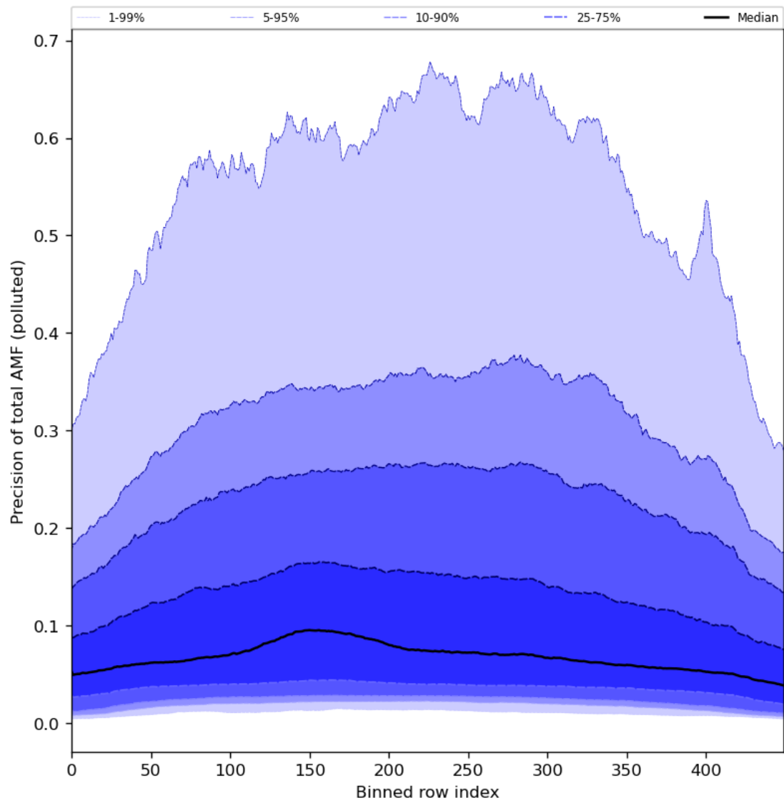
Figure 95: Along track statistics of “Precision of total AMF (polluted)” for 2024-03-25 to 2024-03-27
