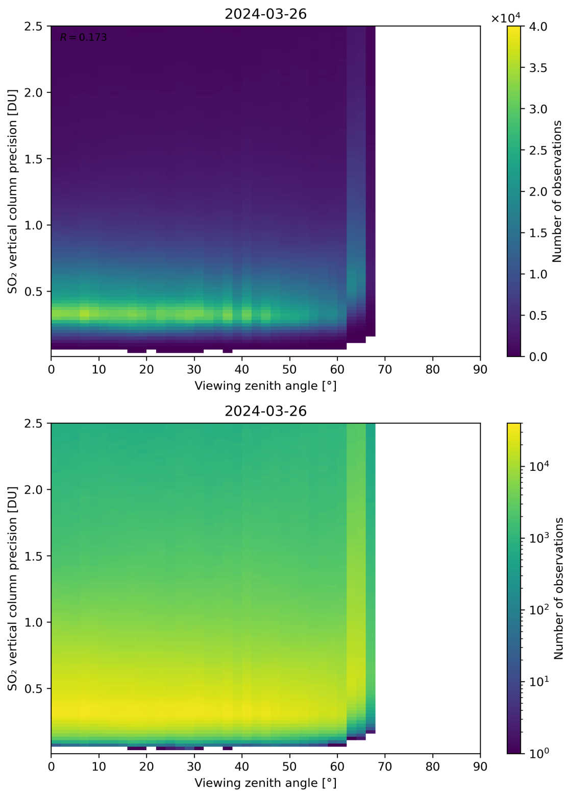
Figure 328: Scatter density plot of “Viewing zenith angle” against “SO 2 vertical column precision” for 2024-03-25 to 2024-03-27.
