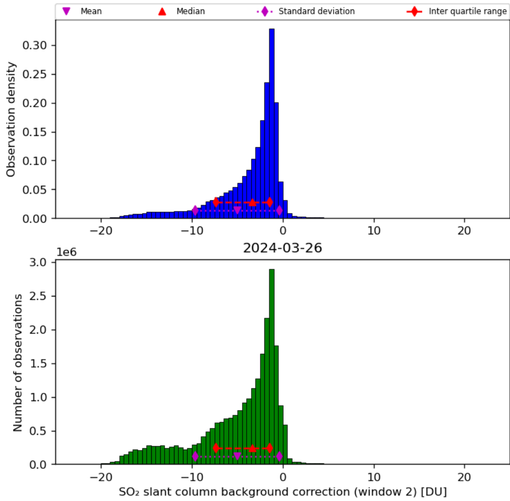
Figure 63: Histogram of “SO 2 slant column background correction (window 2)” for 2024-03-25 to 2024-03-27
