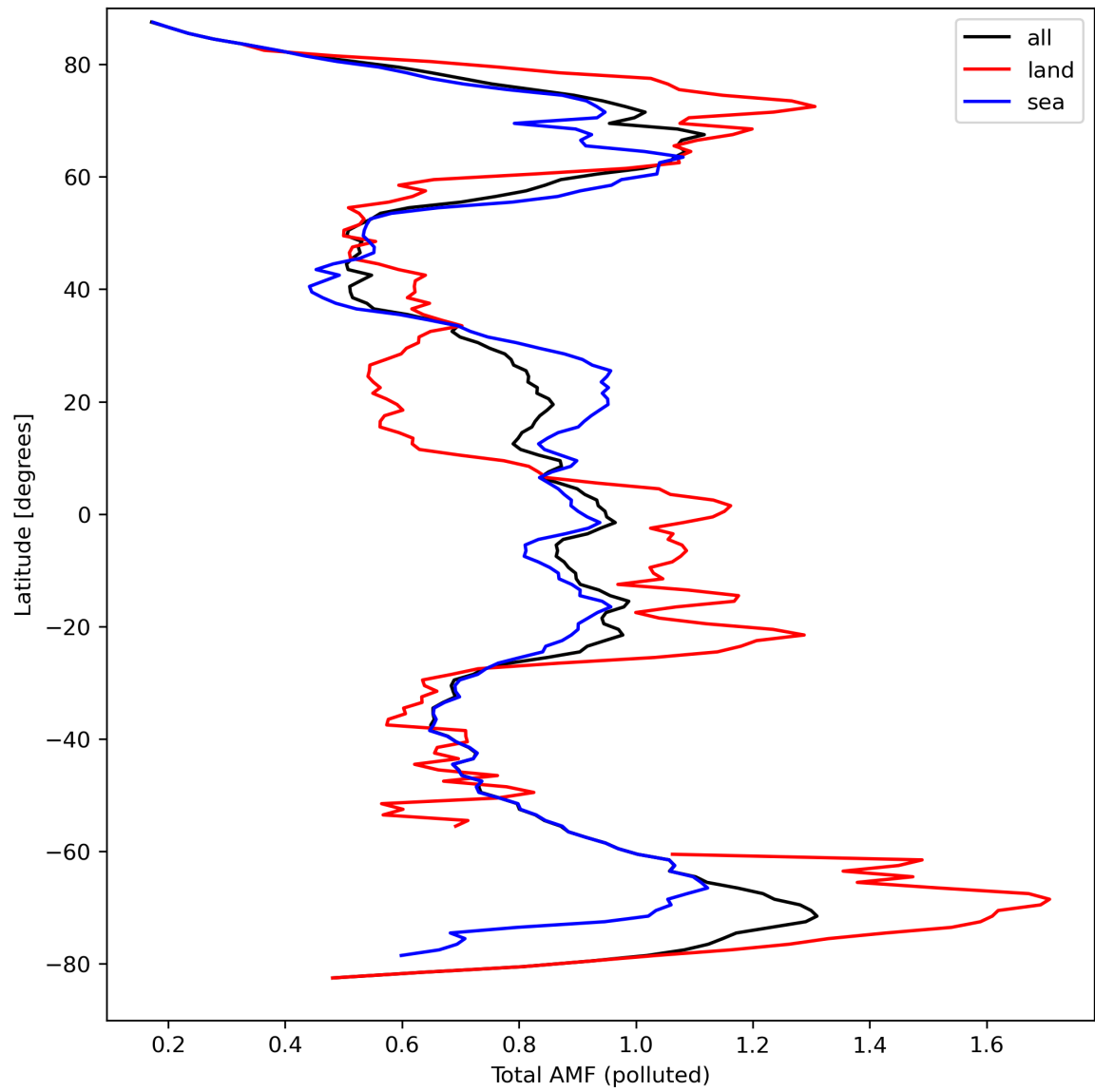
Figure 48: Zonal average of “Total AMF (polluted)” for 2024-03-25 to 2024-03-27.
