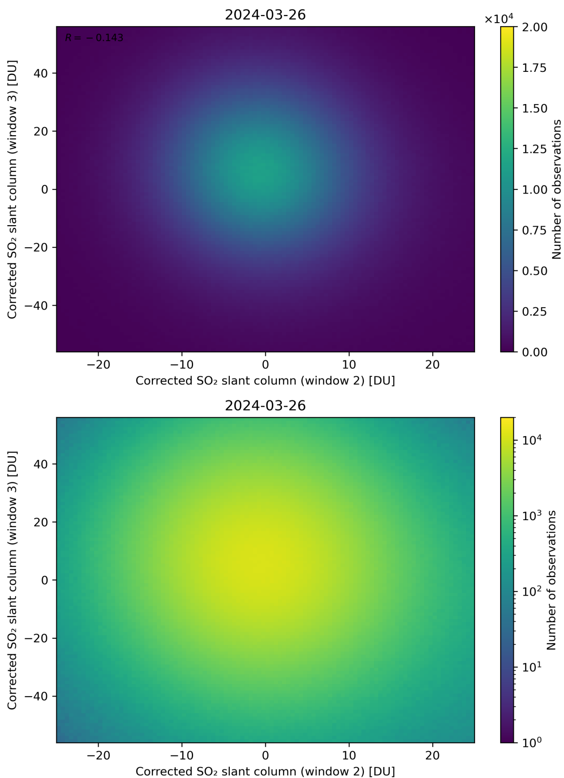
Figure 200: Scatter density plot of “Corrected SO 2 slant column (window 2)” against “Corrected SO 2 slant column (window 3)” for 2024-03-25 to 2024-03-27.
