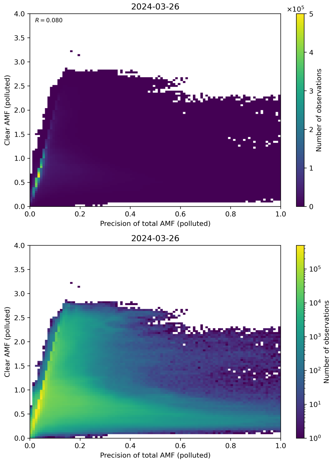
Figure 270: Scatter density plot of “Precision of total AMF (polluted)” against “Clear AMF (polluted)” for 2024-03-25 to 2024-03-27.
