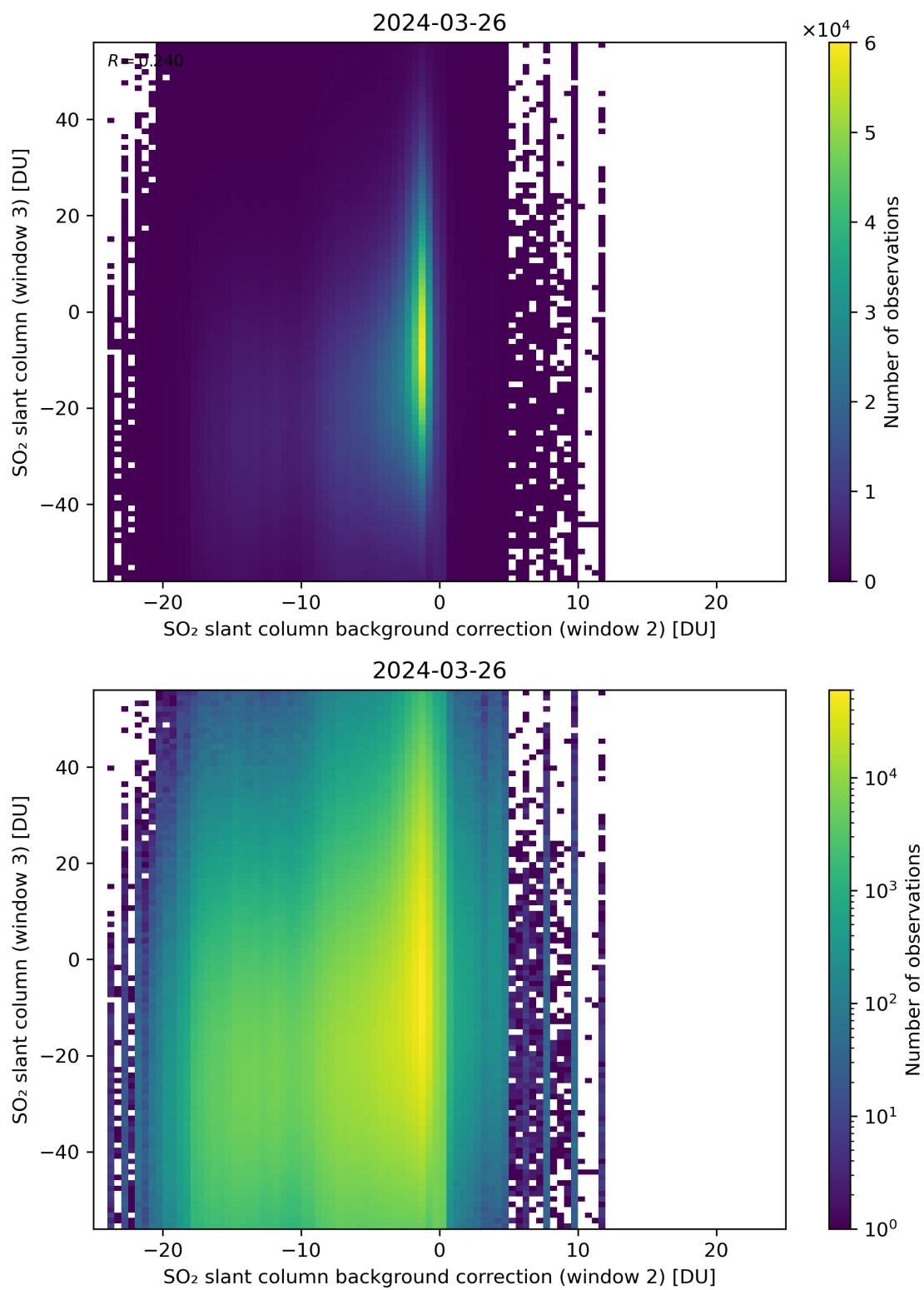
Figure 117: Scatter density plot of “SO 2 slant column background correction (window 2)” against “SO 2 slant column (window 3)” for 2024-03-25 to 2024-03-27.
