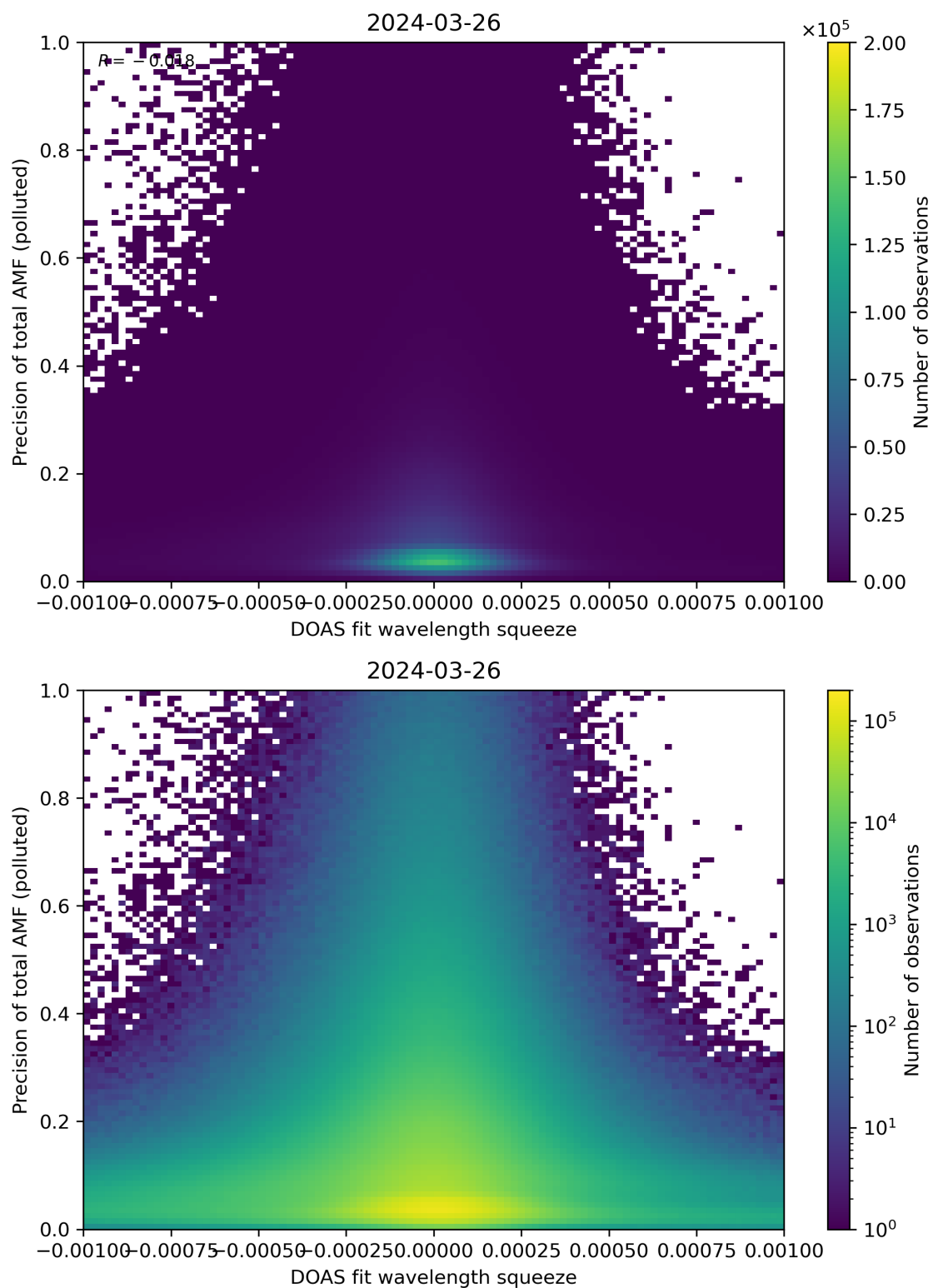
Figure 135: Scatter density plot of “DOAS fit wavelength squeeze” against “Precision of total AMF (polluted)” for 2024-03-25 to 2024-03-27.
