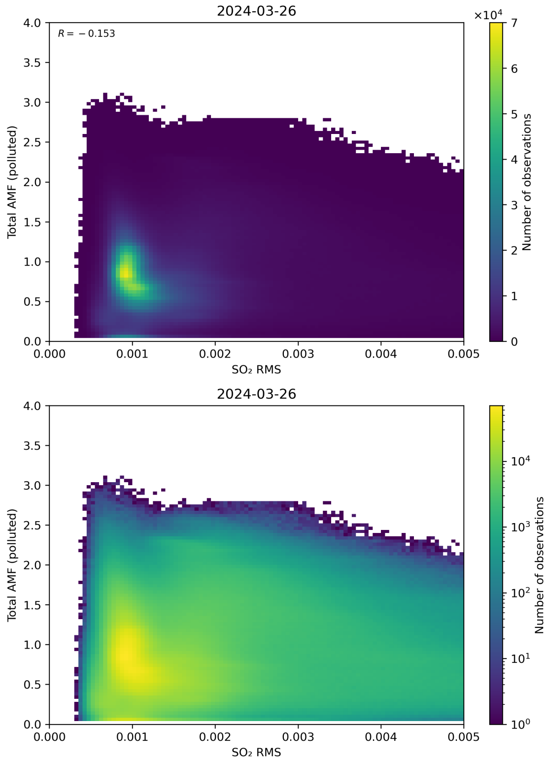
Figure 137: Scatter density plot of “SO 2 RMS” against “Total AMF (polluted)” for 2024-03-25 to 2024-03-27.
