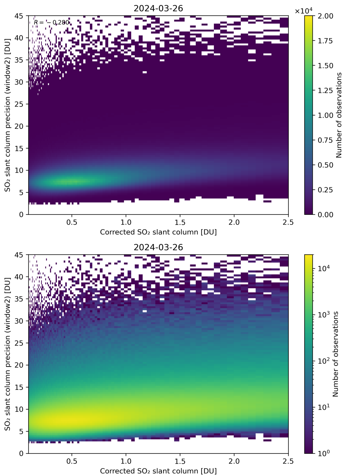
Figure 189: Scatter density plot of “Corrected SO 2 slant column” against “SO 2 slant column precision (window2)” for 2024-03-25 to 2024-03-27.
