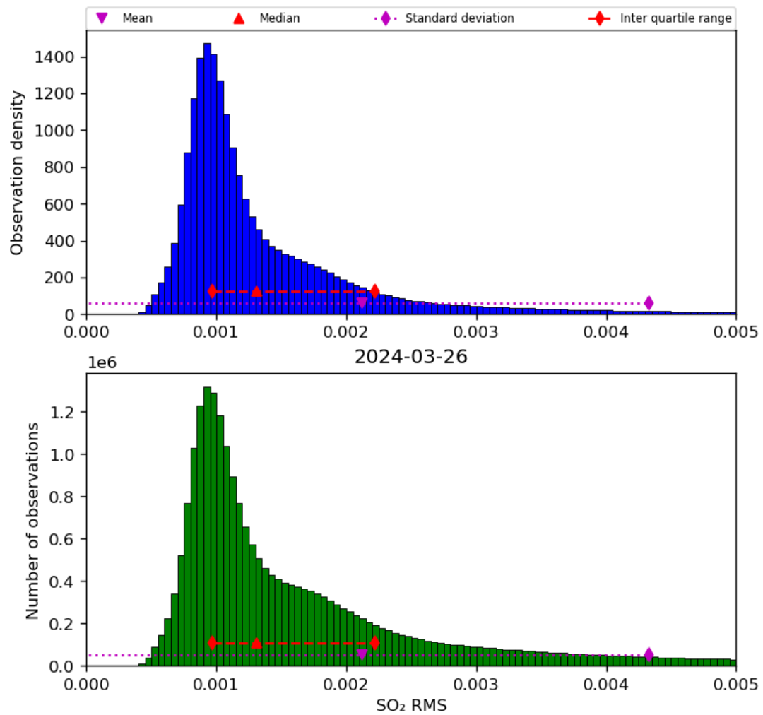
Figure 70: Histogram of “SO 2 RMS” for 2024-03-25 to 2024-03-27
