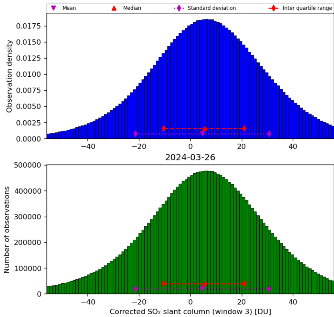
Figure 66: Histogram of “Corrected SO 2 slant column (window 3)” for 2024-03-25 to 2024-03-27
