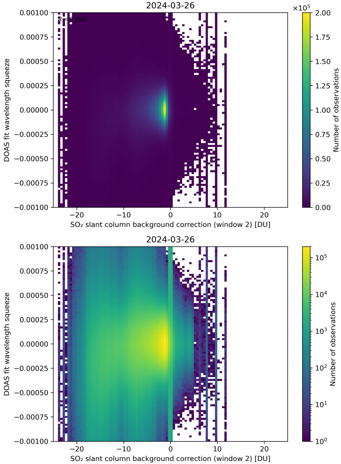
Figure 113: Scatter density plot of “SO 2 slant column background correction (window 2)” against “DOAS fit wavelength squeeze” for 2024-03-25 to 2024-03-27.
