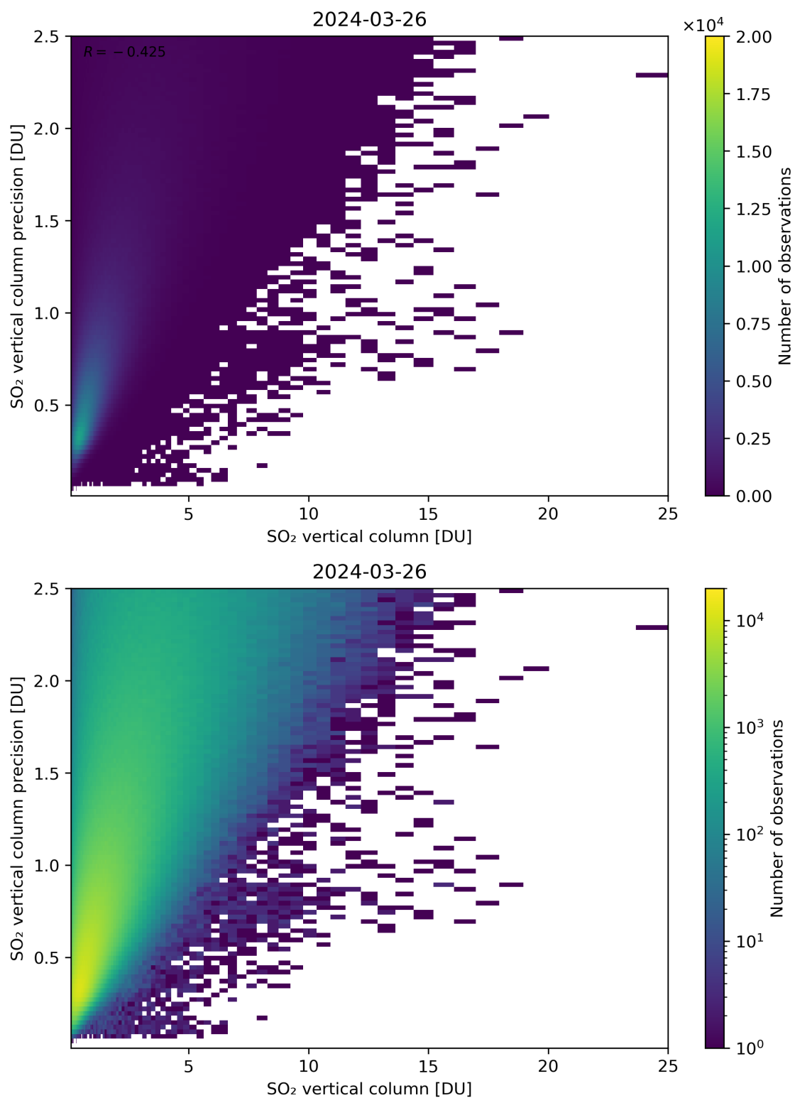
Figure 307: Scatter density plot of “SO 2 vertical column” against “SO 2 vertical column precision” for 2024-03-25 to 2024-03-27.
