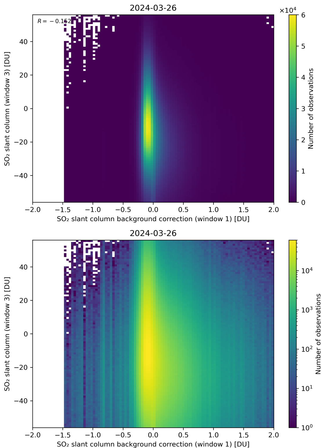
Figure 107: Scatter density plot of “SO 2 slant column background correction (window 1)” against “SO 2 slant column (window 3)” for 2024-03-25 to 2024-03-27.
