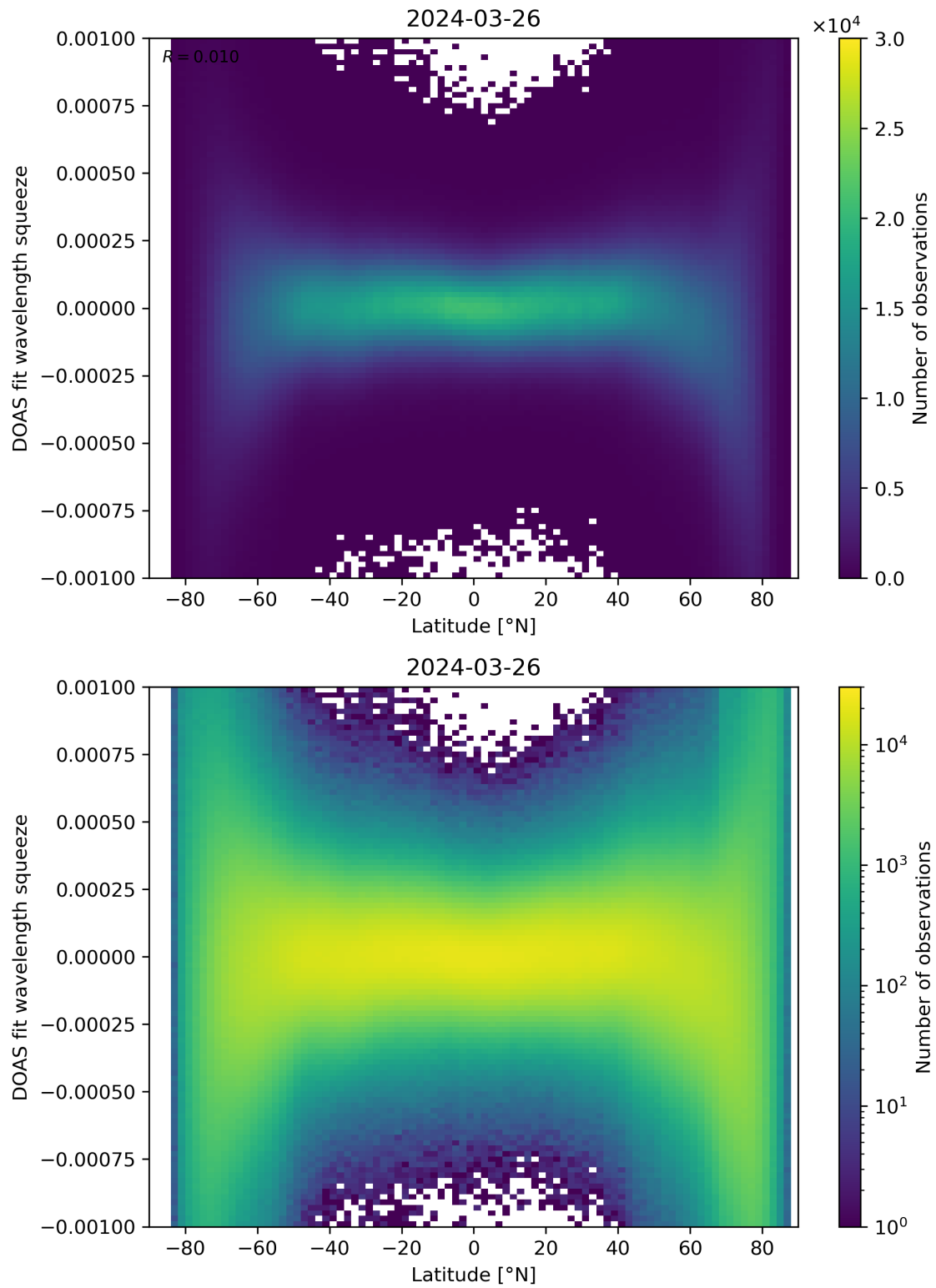
Figure 143: Scatter density plot of “Latitude” against “DOAS fit wavelength squeeze” for 2024-03-25 to 2024-03-27.
