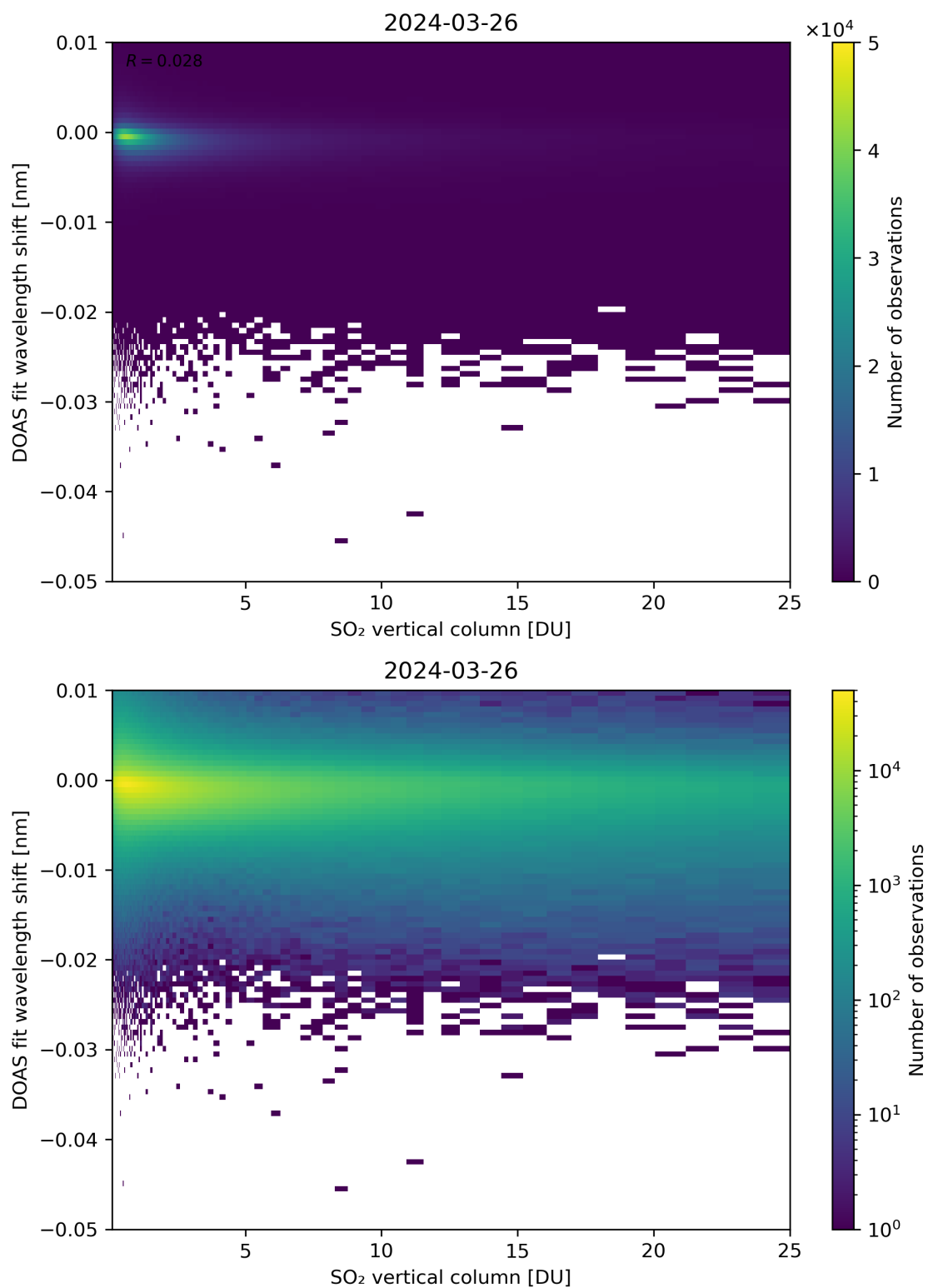
Figure 276: Scatter density plot of “SO 2 vertical column” against “DOAS fit wavelength shift” for 2024-03-25 to 2024-03-27.
