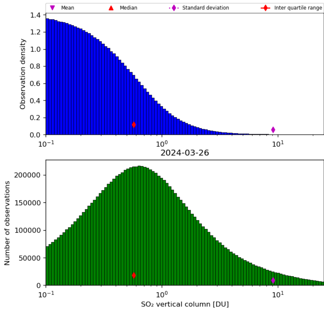
Figure 53: Histogram of “SO 2 vertical column” for 2024-03-25 to 2024-03-27
