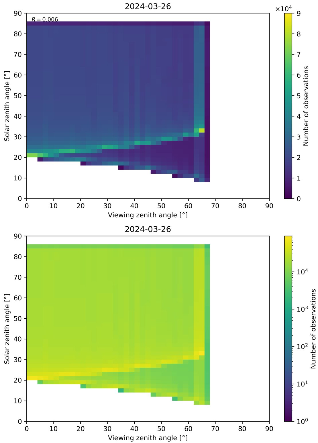
Figure 315: Scatter density plot of “Viewing zenith angle” against “Solar zenith angle” for 2024-03-25 to 2024-03-27.
