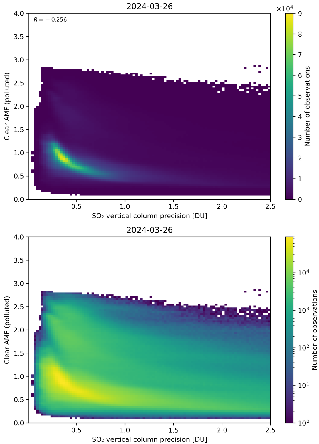
Figure 285: Scatter density plot of “SO 2 vertical column precision” against “Clear AMF (polluted)” for 2024-03-25 to 2024-03-27.
