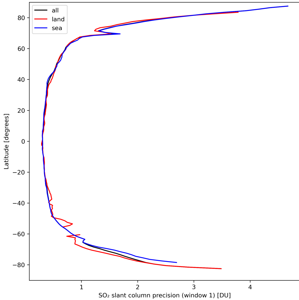
Figure 34: Zonal average of “SO 2 slant column precision (window 1)” for 2024-03-25 to 2024-03-27.
