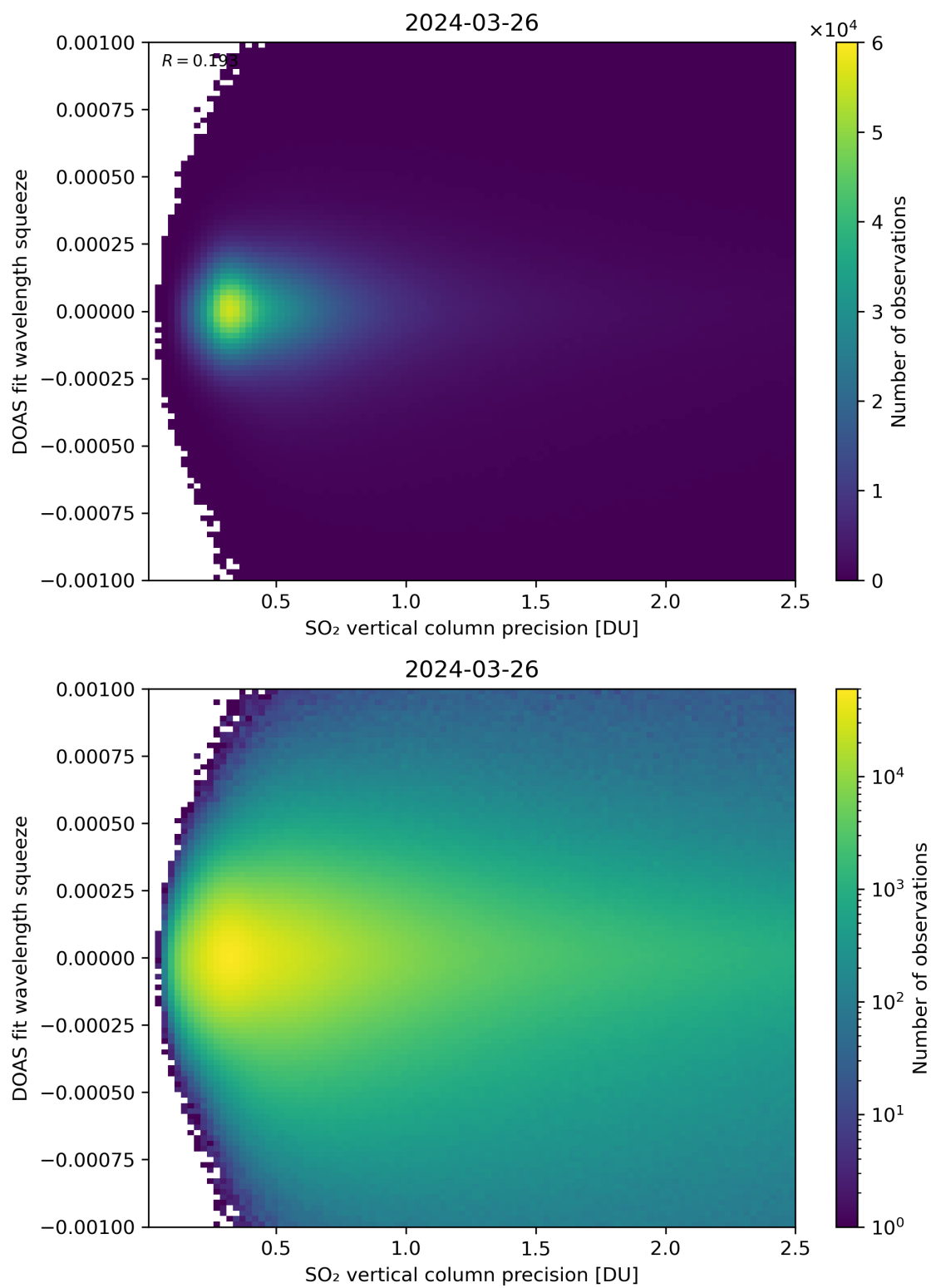
Figure 283: Scatter density plot of “SO 2 vertical column precision” against “DOAS fit wavelength squeeze” for 2024-03-25 to 2024-03-27.
