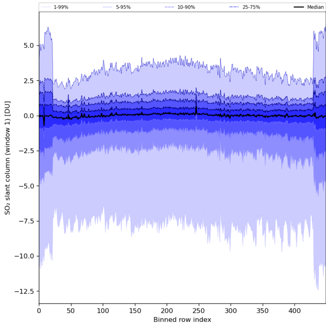
Figure 79: Along track statistics of “SO 2 slant column (window 1)” for 2024-03-25 to 2024-03-27
