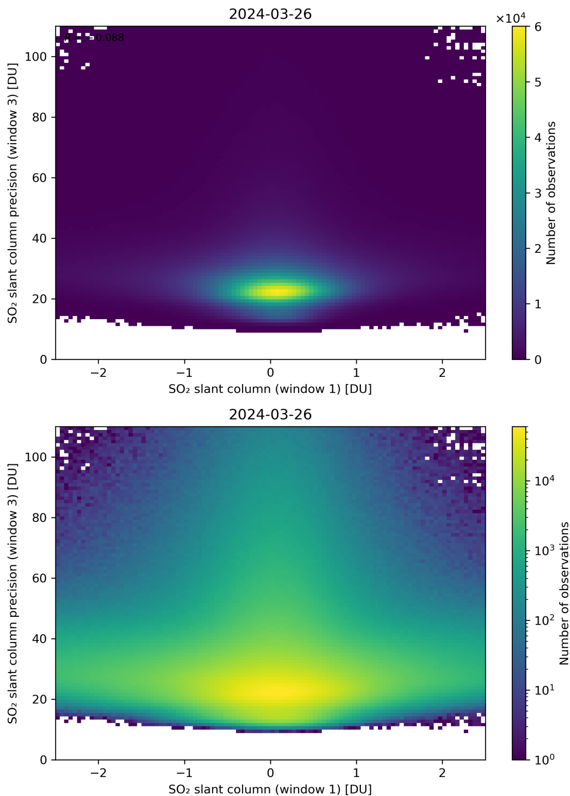
Figure 238: Scatter density plot of “SO 2 slant column (window 1)” against “SO 2 slant column precision (window 3)” for 2024-03-25 to 2024-03-27.
