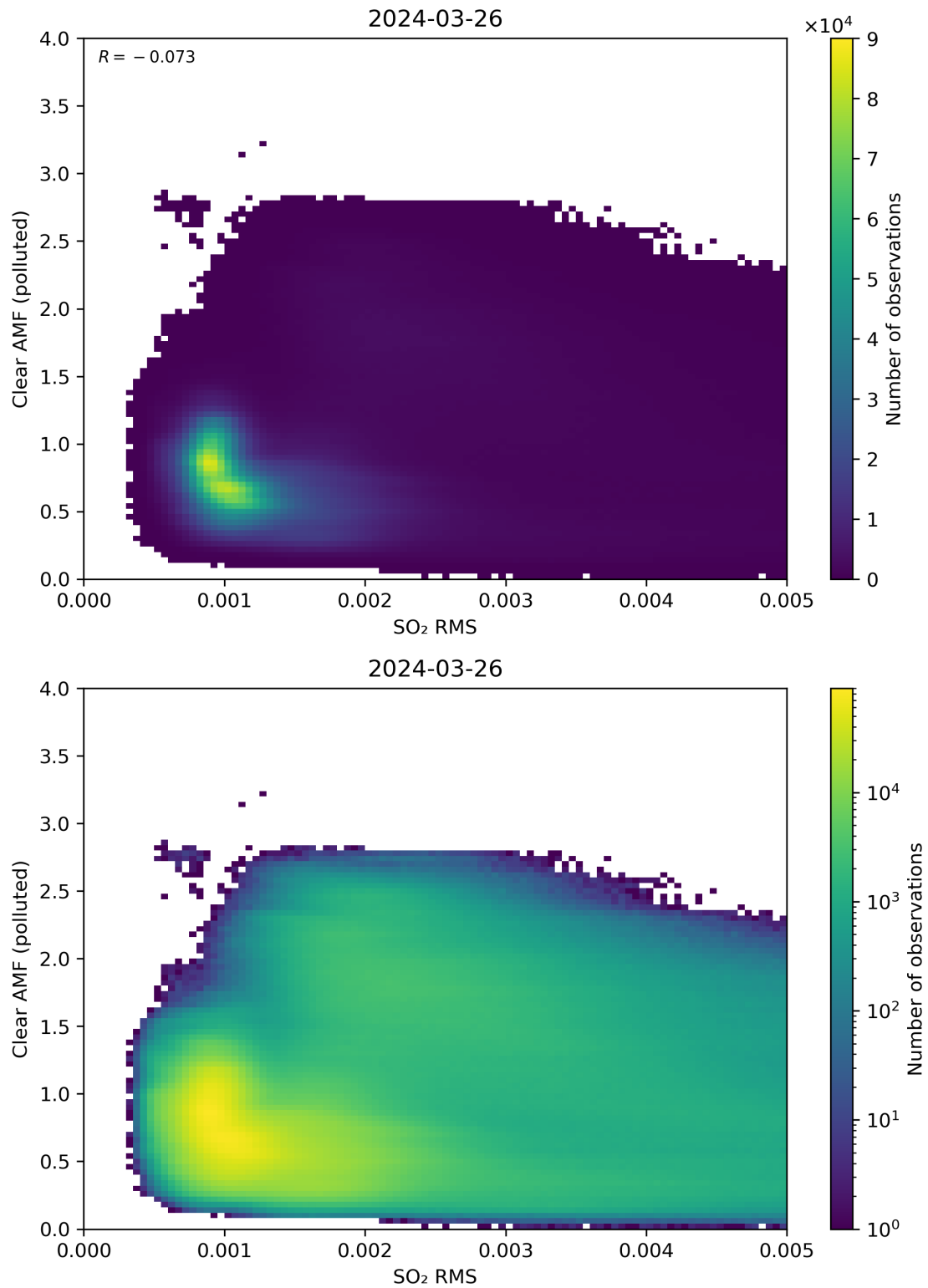
Figure 136: Scatter density plot of “SO 2 RMS” against “Clear AMF (polluted)” for 2024-03-25 to 2024-03-27.
