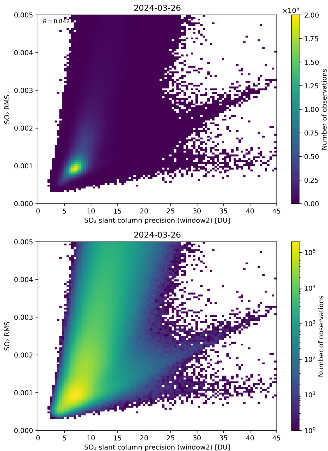
Figure 245: Scatter density plot of “SO 2 slant column precision (window2)” against “SO 2 RMS” for 2024-03-25 to 2024-03-27.
