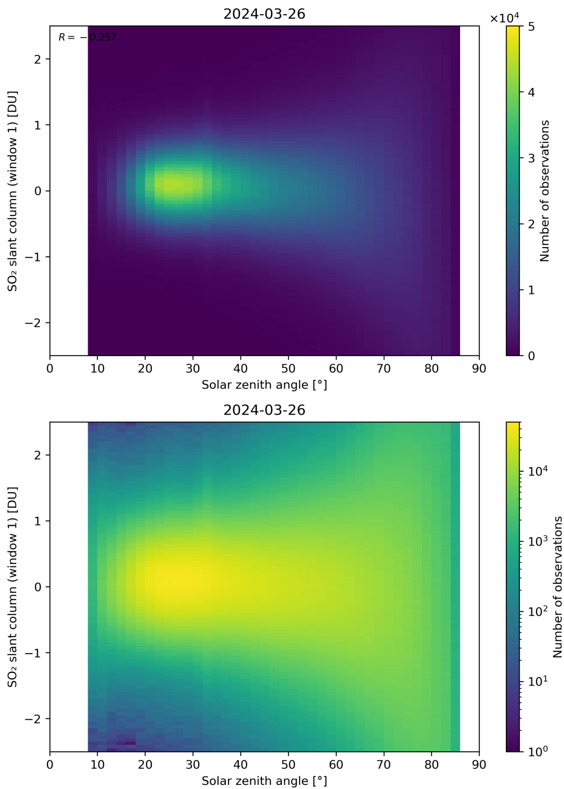
Figure 169: Scatter density plot of “Solar zenith angle” against “SO 2 slant column (window 1)” for 2024-03-25 to 2024-03-27.
