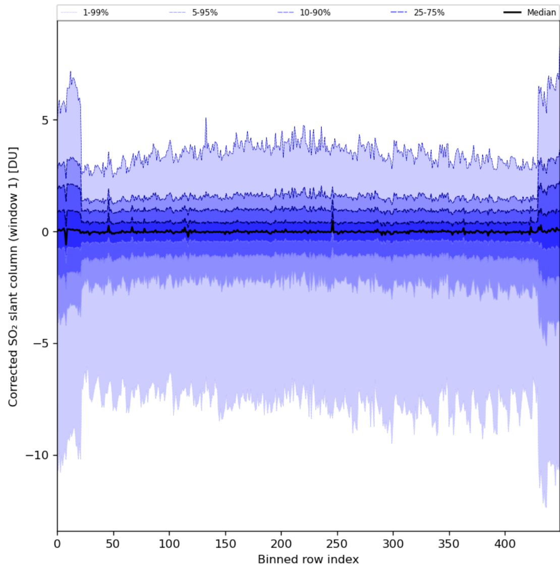
Figure 81: Along track statistics of “Corrected SO 2 slant column (window 1)” for 2024-03-25 to 2024-03-27
