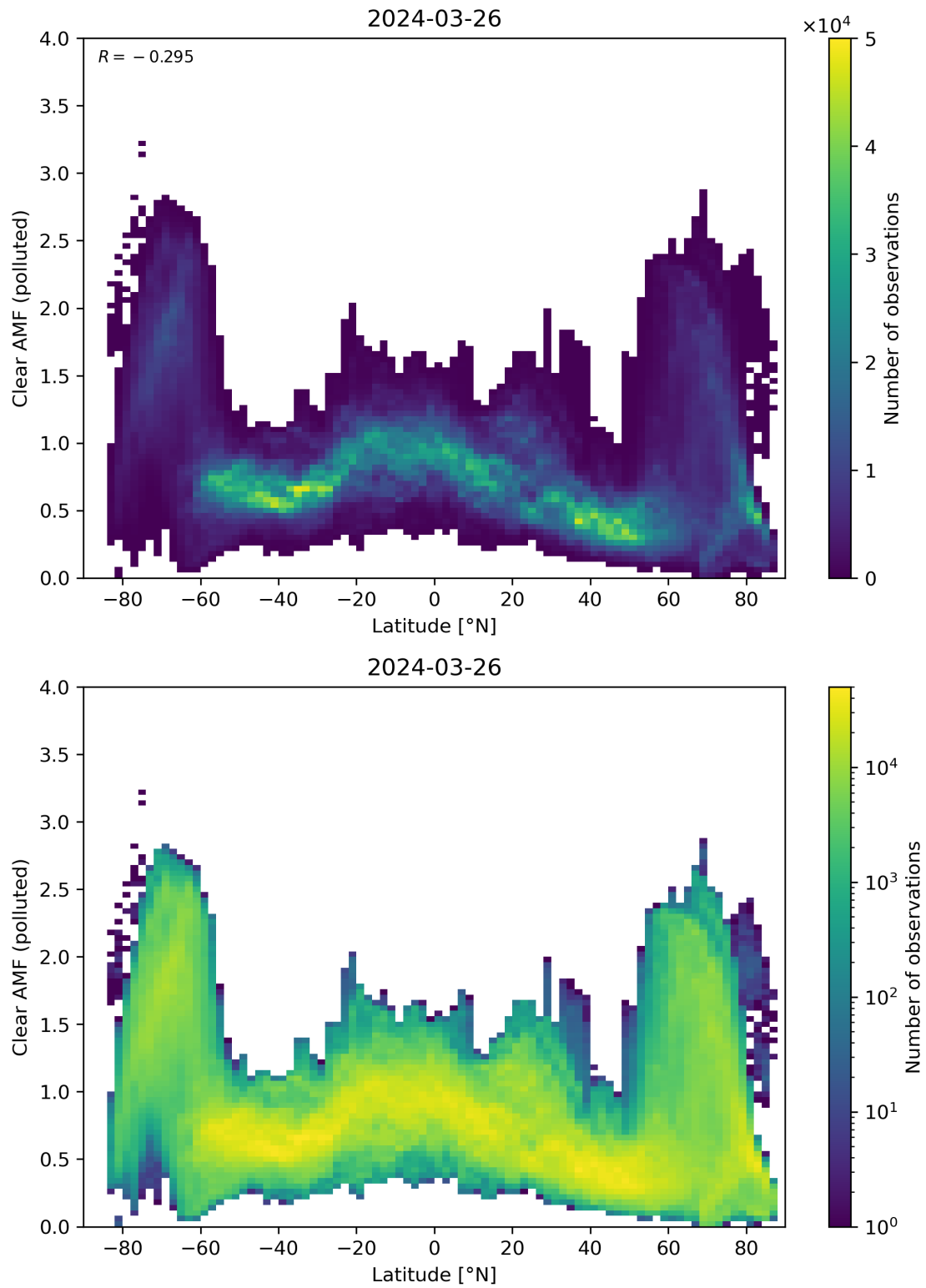
Figure 145: Scatter density plot of “Latitude” against “Clear AMF (polluted)” for 2024-03-25 to 2024-03-27.
