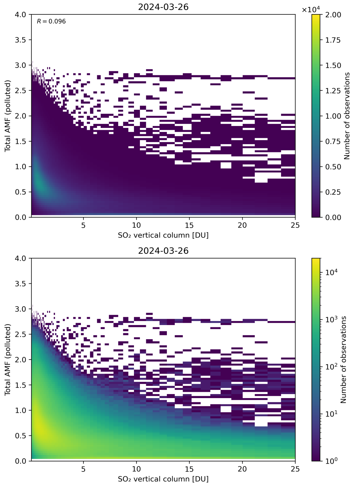
Figure 305: Scatter density plot of “SO 2 vertical column” against “Total AMF (polluted)” for 2024-03-25 to 2024-03-27.
