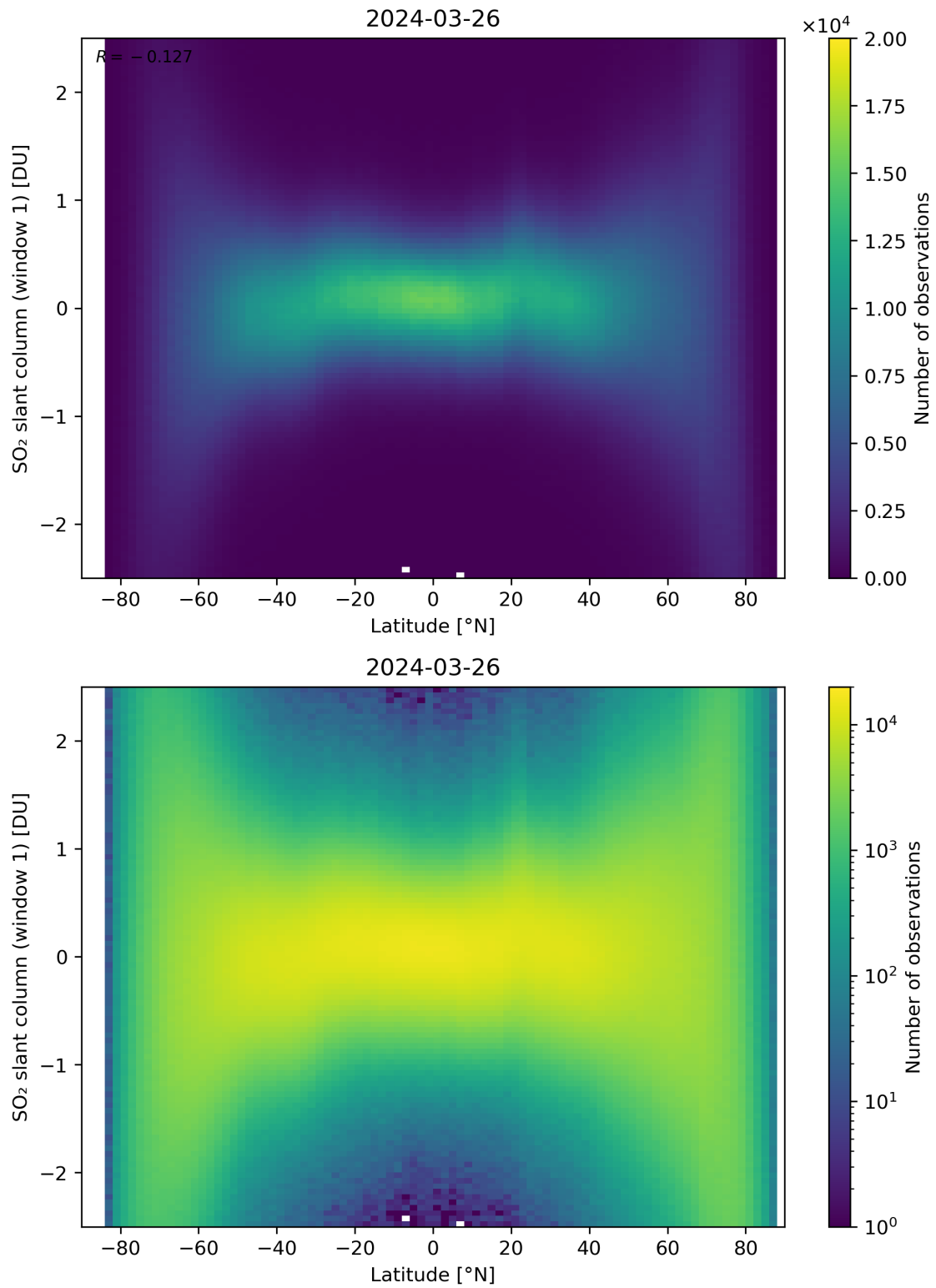
Figure 149: Scatter density plot of “Latitude” against “SO 2 slant column (window 1)” for 2024-03-25 to 2024-03-27.
