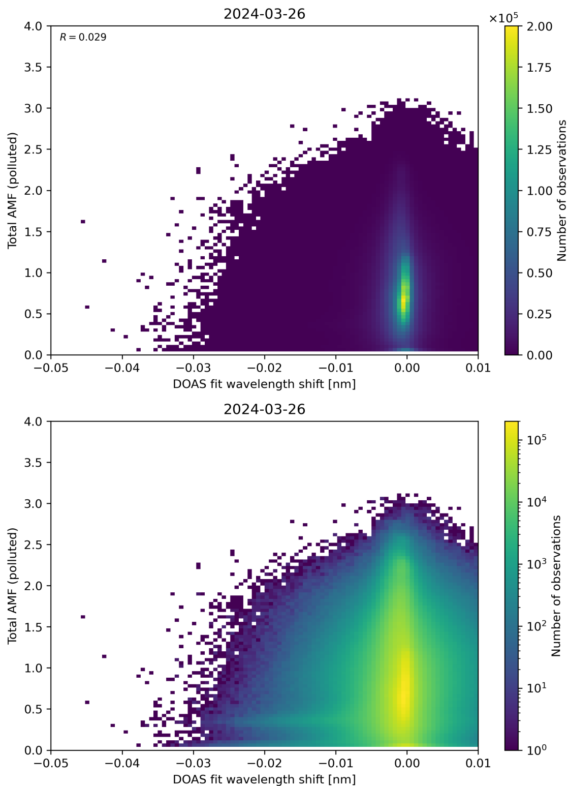
Figure 130: Scatter density plot of “DOAS fit wavelength shift” against “Total AMF (polluted)” for 2024-03-25 to 2024-03-27.
