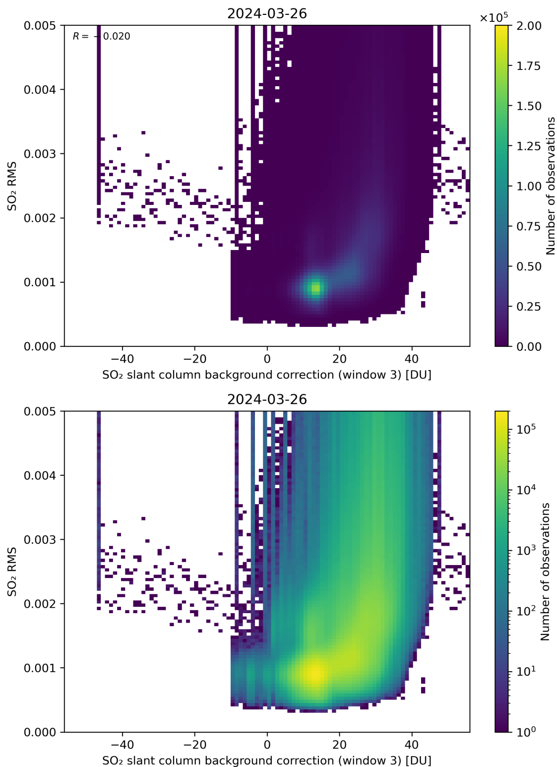
Figure 123: Scatter density plot of “SO 2 slant column background correction (window 3)” against “SO 2 RMS” for 2024-03-25 to 2024-03-27.
