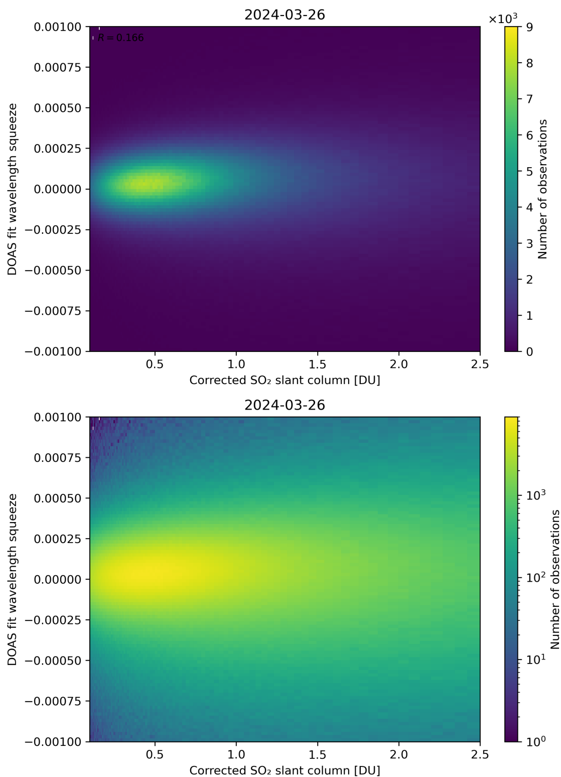
Figure 182: Scatter density plot of “Corrected SO 2 slant column” against “DOAS fit wavelength squeeze” for 2024-03-25 to 2024-03-27.
