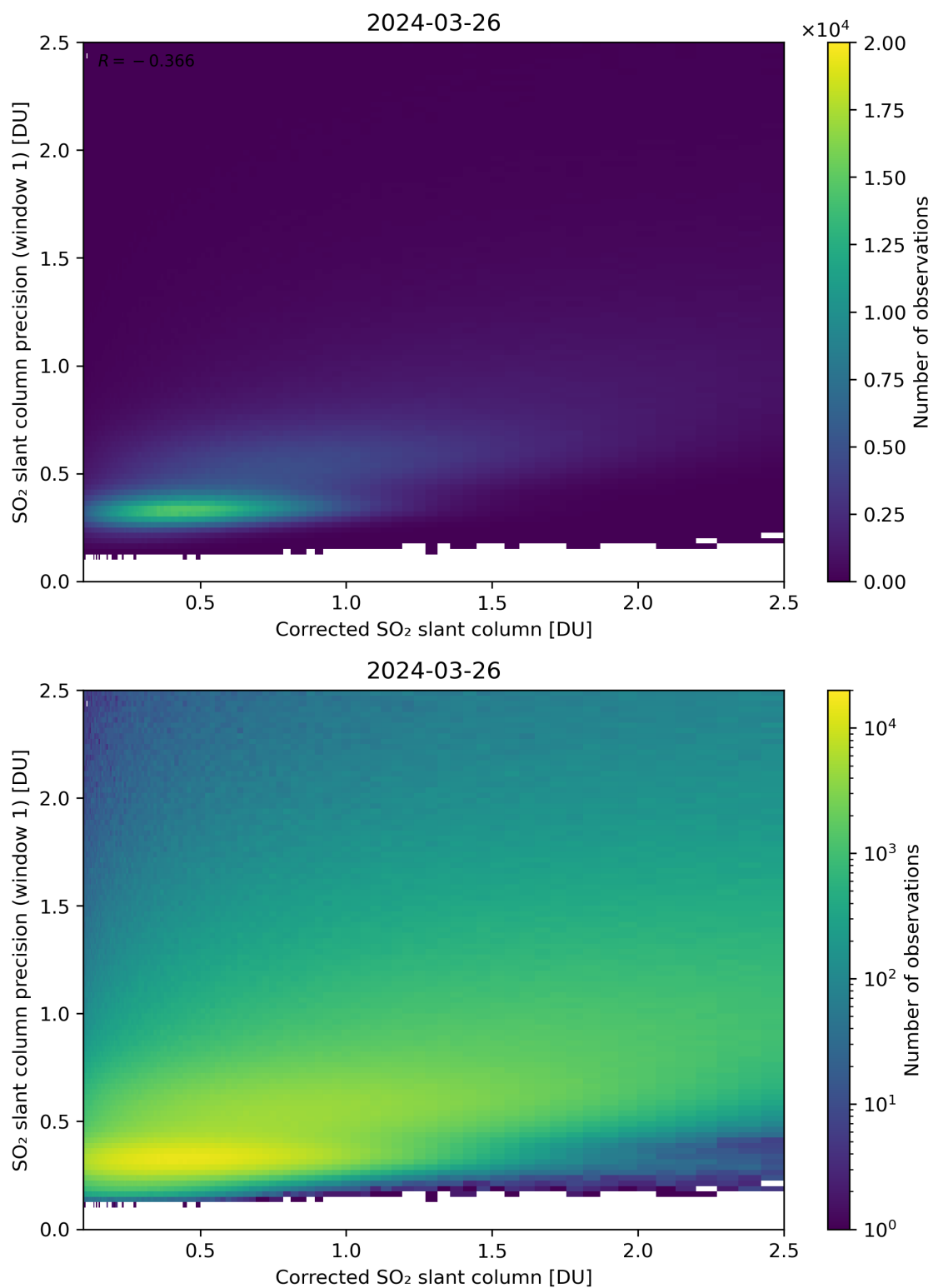
Figure 188: Scatter density plot of “Corrected SO 2 slant column” against “SO 2 slant column precision (window 1)” for 2024-03-25 to 2024-03-27.
