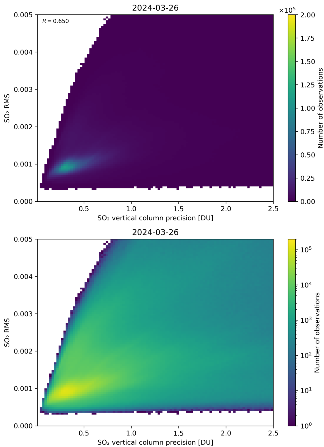
Figure 284: Scatter density plot of “SO 2 vertical column precision” against “SO 2 RMS” for 2024-03-25 to 2024-03-27.
