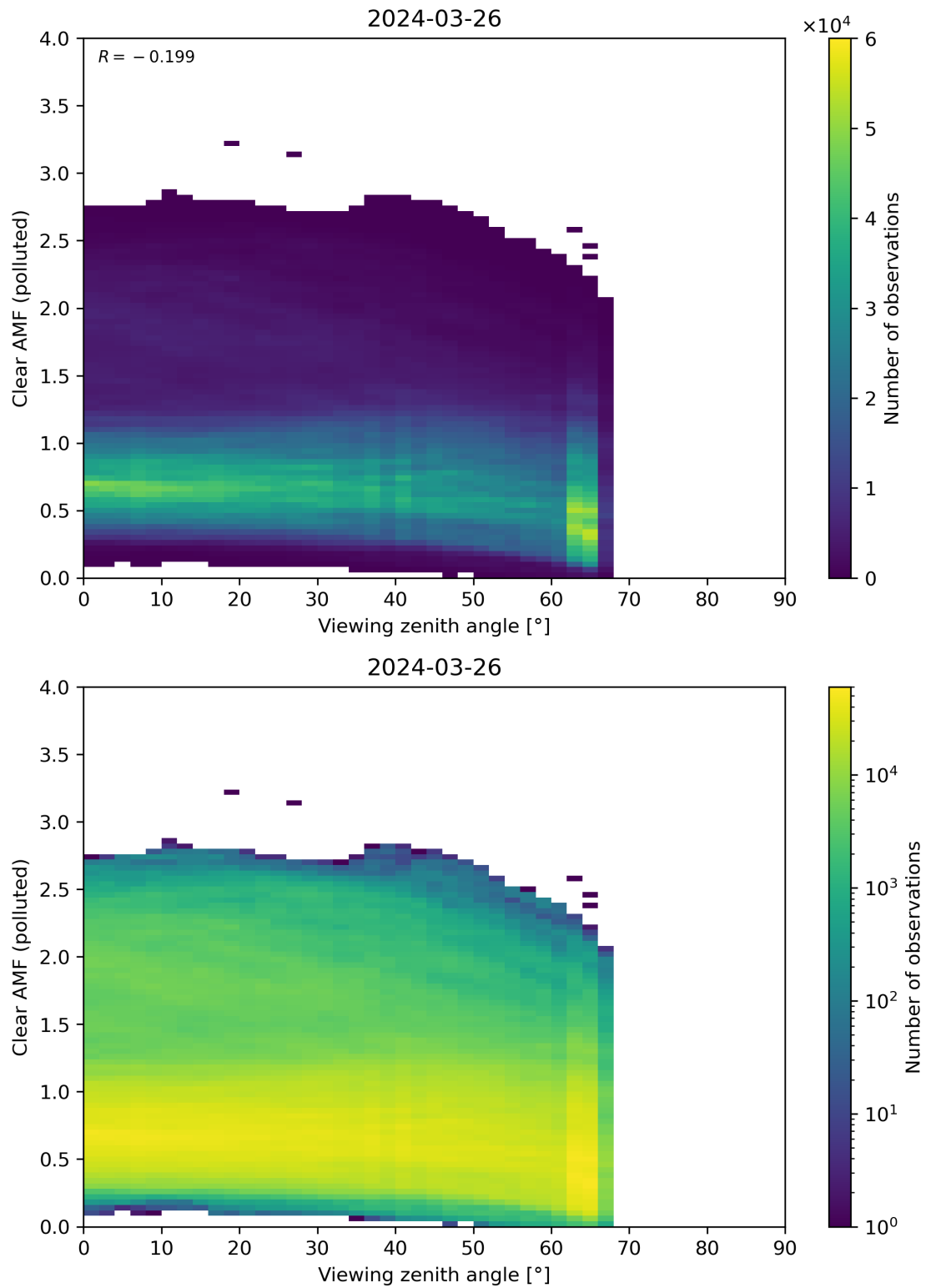
Figure 316: Scatter density plot of “Viewing zenith angle” against “Clear AMF (polluted)” for 2024-03-25 to 2024-03-27.
