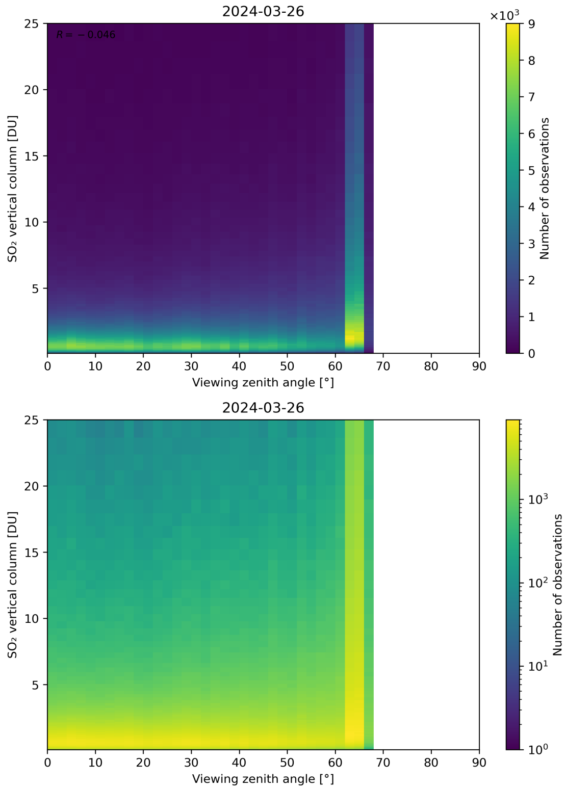
Figure 327: Scatter density plot of “Viewing zenith angle” against “SO 2 vertical column” for 2024-03-25 to 2024-03-27.
