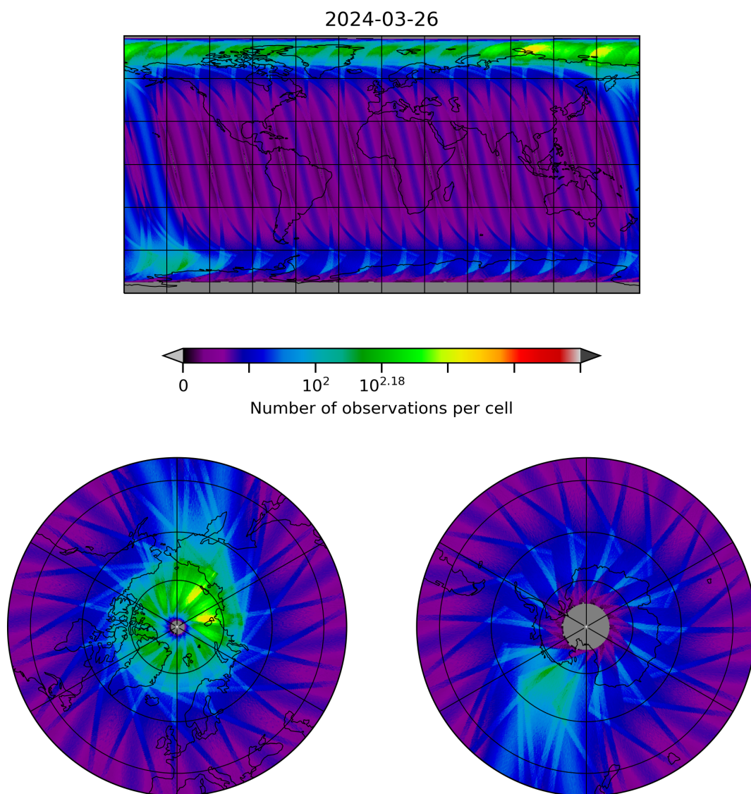
Figure 28: Map of the number of observations for 2024-03-25 to 2024-03-27
