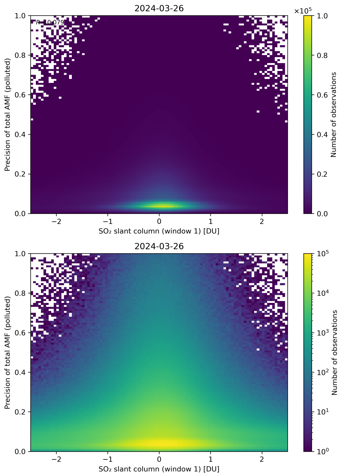
Figure 240: Scatter density plot of “SO 2 slant column (window 1)” against “Precision of total AMF (polluted)” for 2024-03-25 to 2024-03-27.
