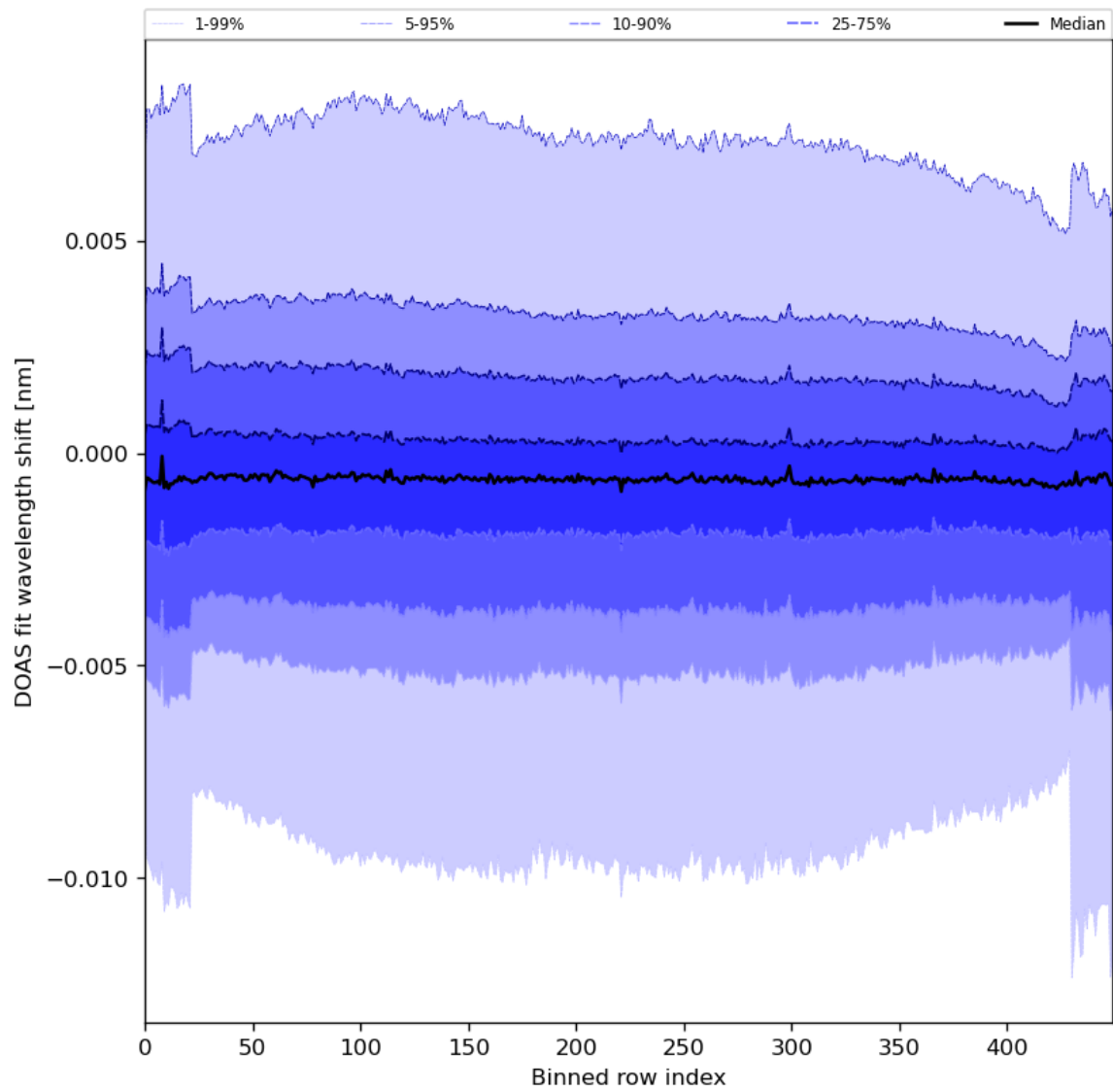
Figure 91: Along track statistics of “DOAS fit wavelength shift” for 2024-03-25 to 2024-03-27
