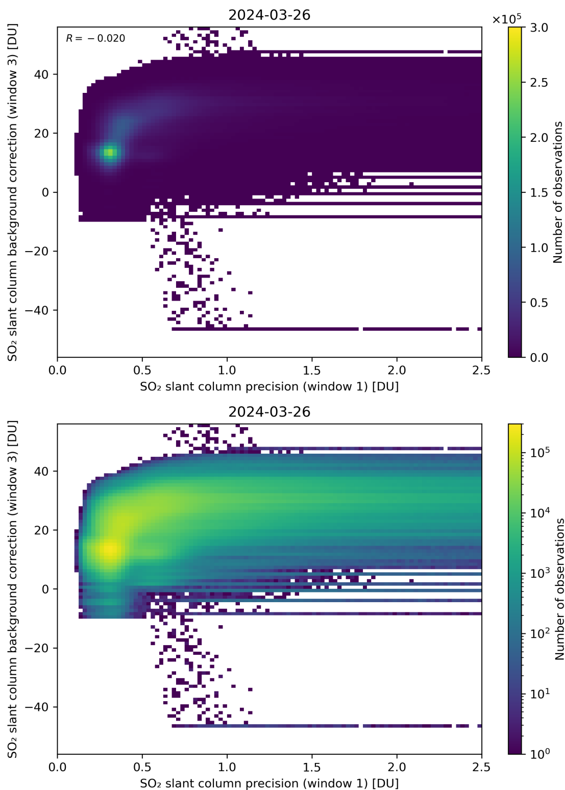
Figure 220: Scatter density plot of “SO 2 slant column precision (window 1)” against “SO 2 slant column background correction (window 3)” for 2024-03-25 to 2024-03-27.
