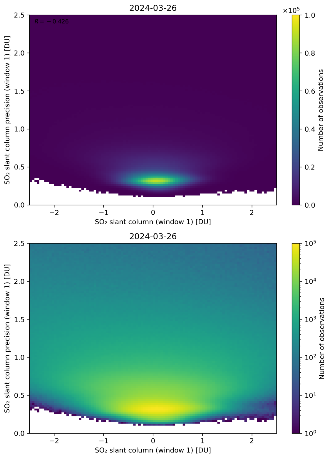
Figure 235: Scatter density plot of “SO 2 slant column (window 1)” against “SO 2 slant column precision (window 1)” for 2024-03-25 to 2024-03-27.
