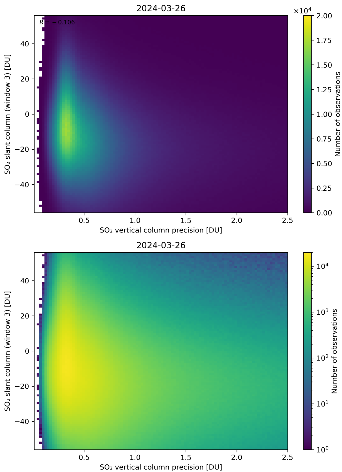
Figure 292: Scatter density plot of “SO 2 vertical column precision” against “SO 2 slant column (window 3)” for 2024-03-25 to 2024-03-27.
