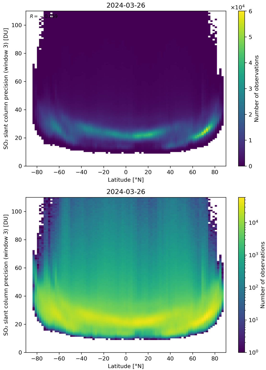
Figure 153: Scatter density plot of “Latitude” against “SO 2 slant column precision (window 3)” for 2024-03-25 to 2024-03-27.
