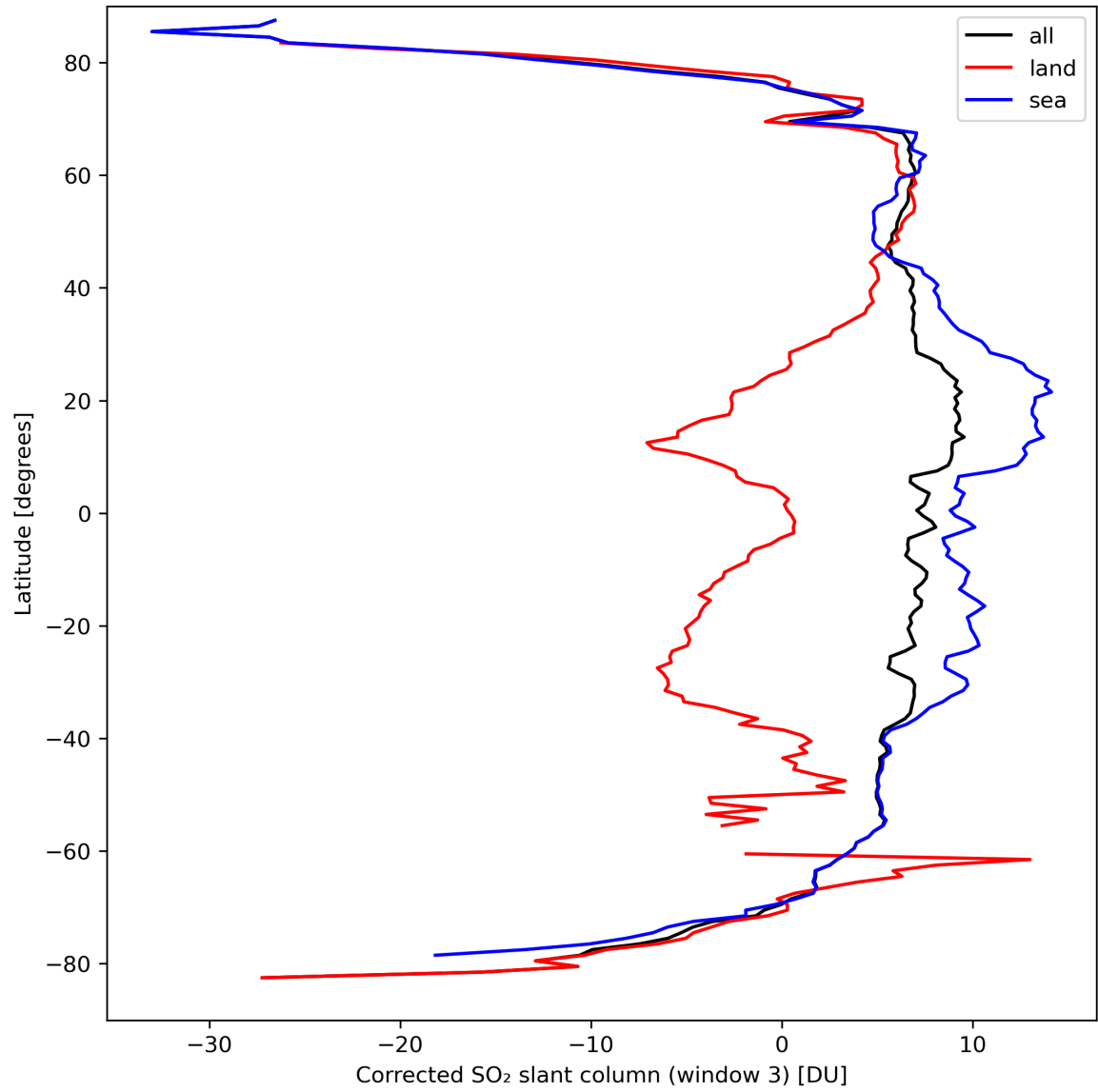
Figure 43: Zonal average of “Corrected SO 2 slant column (window 3)” for 2024-03-25 to 2024-03-27.
