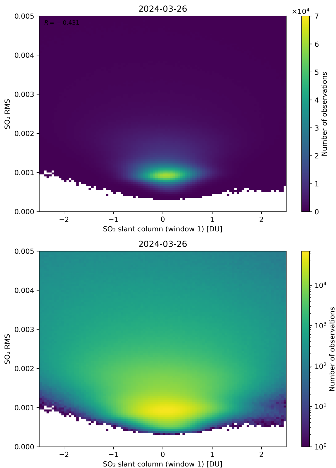
Figure 217: Scatter density plot of “SO 2 slant column (window 1)” against “SO 2 RMS” for 2024-03-25 to 2024-03-27.
