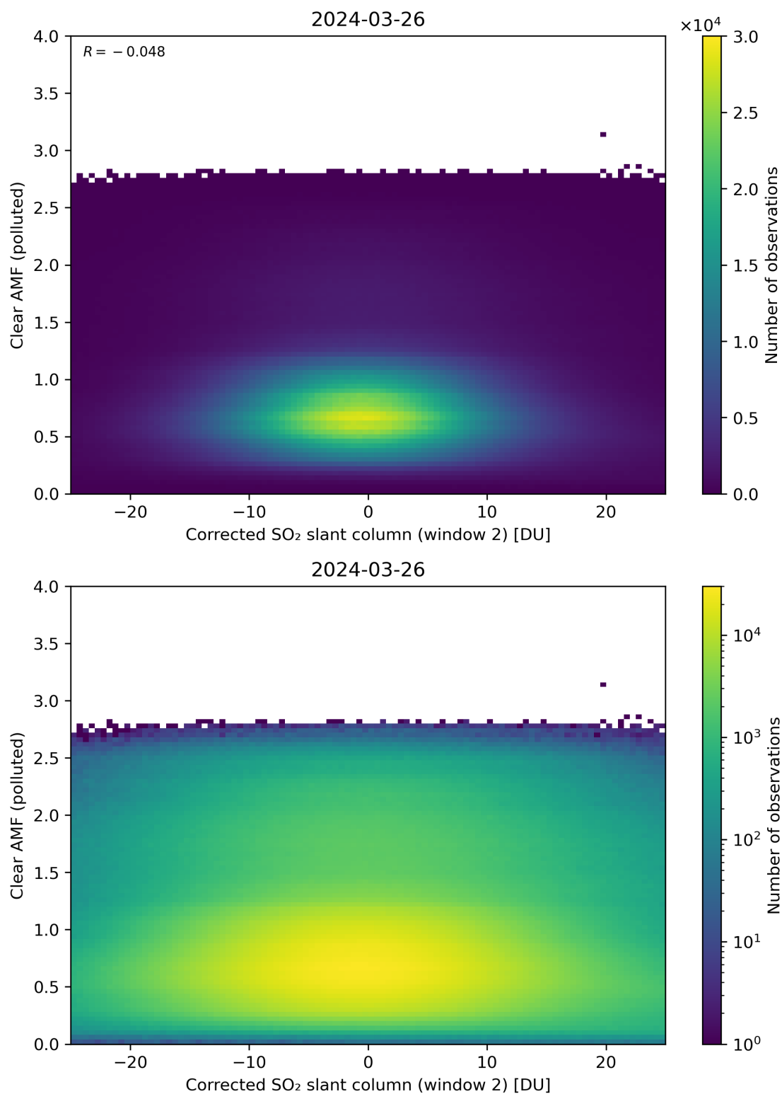
Figure 199: Scatter density plot of “Corrected SO 2 slant column (window 2)” against “Clear AMF (polluted)” for 2024-03-25 to 2024-03-27.
