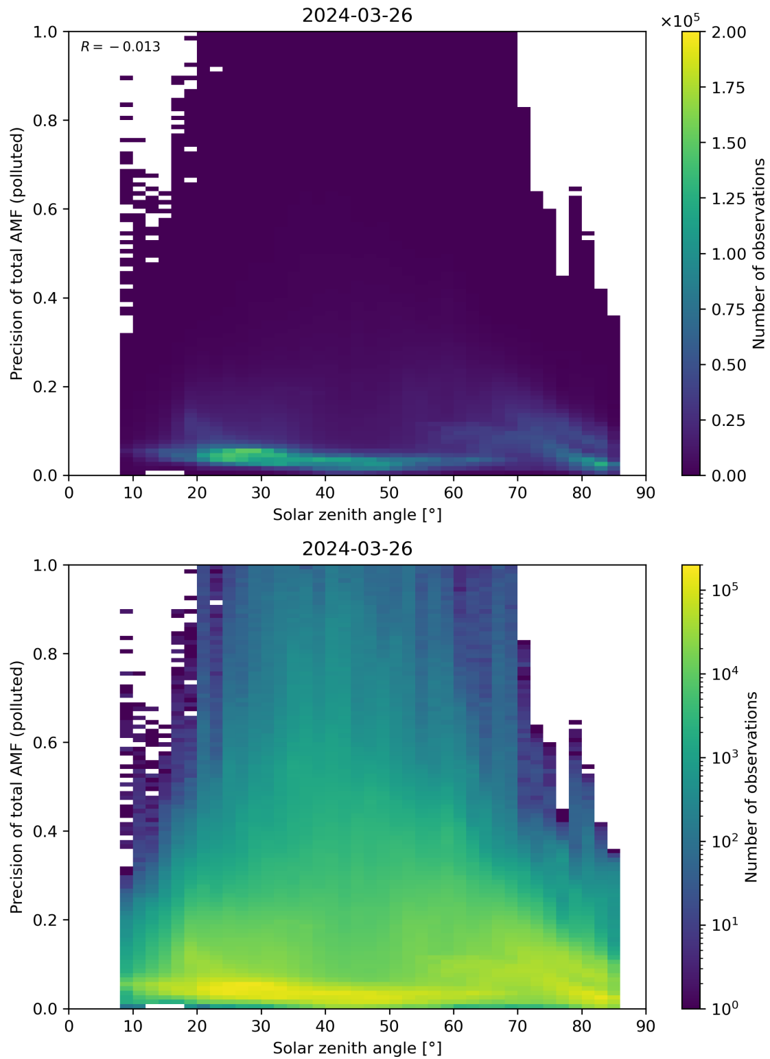
Figure 175: Scatter density plot of “Solar zenith angle” against “Precision of total AMF (polluted)” for 2024-03-25 to 2024-03-27.
