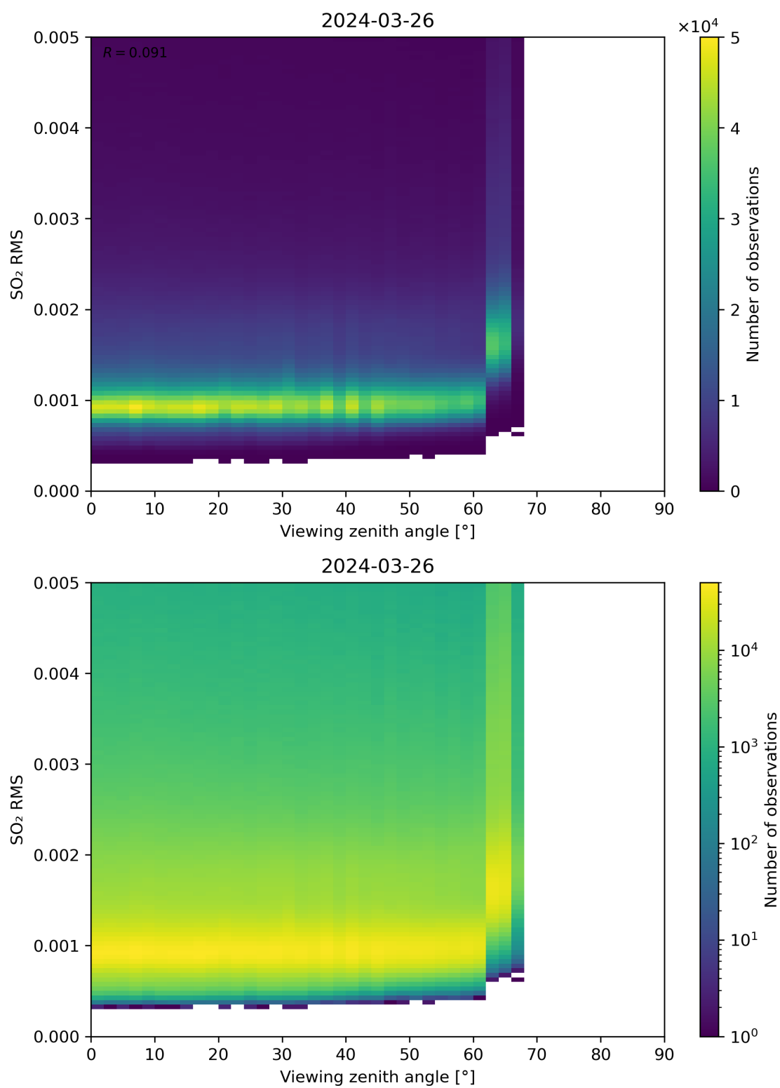
Figure 313: Scatter density plot of “Viewing zenith angle” against “SO 2 RMS” for 2024-03-25 to 2024-03-27.
