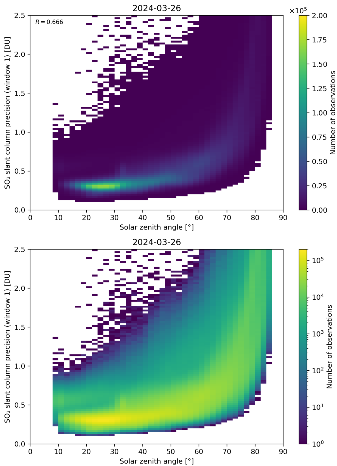
Figure 170: Scatter density plot of “Solar zenith angle” against “SO 2 slant column precision (window 1)” for 2024-03-25 to 2024-03-27.
