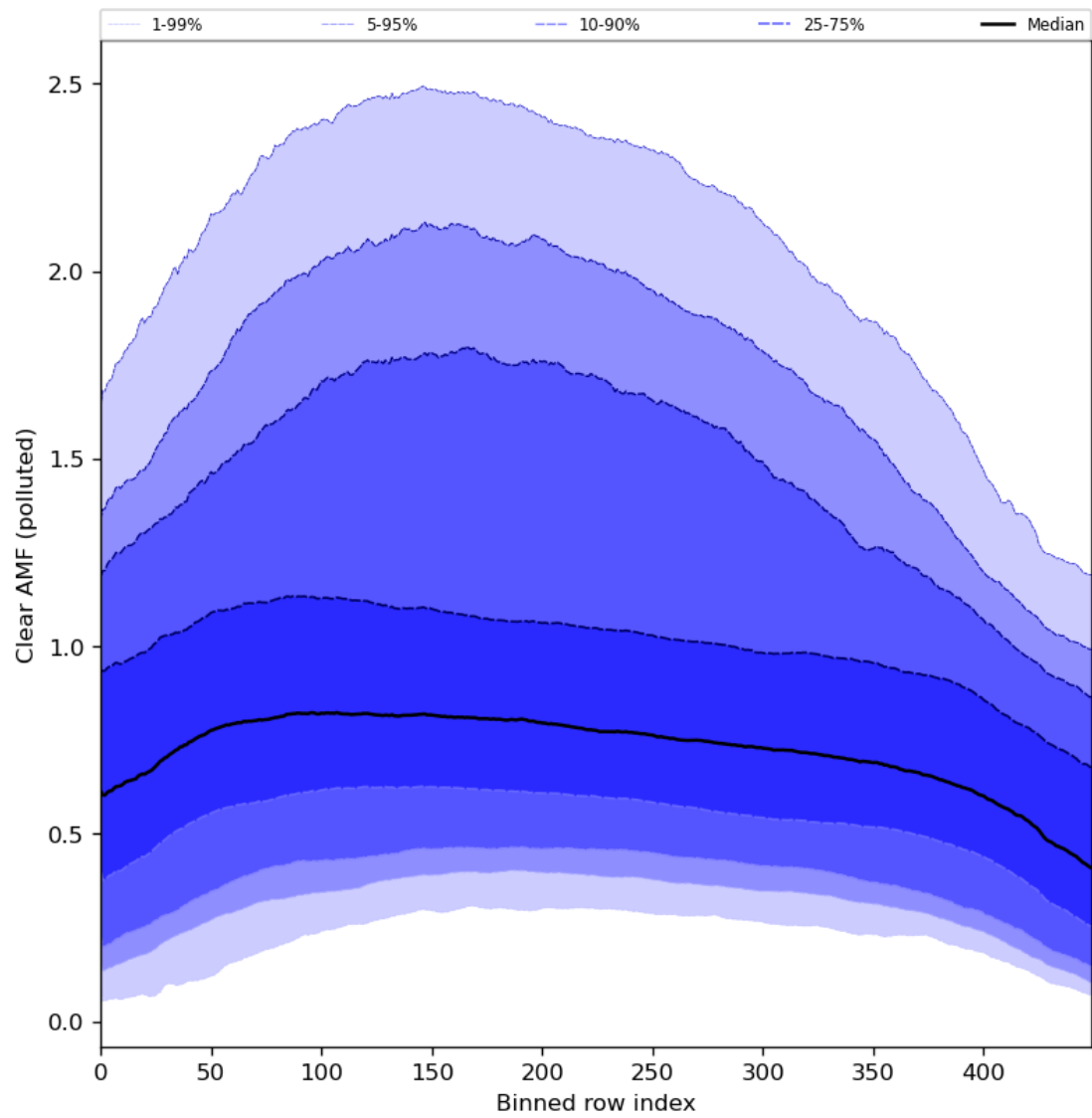
Figure 96: Along track statistics of “Clear AMF (polluted)” for 2024-03-25 to 2024-03-27
