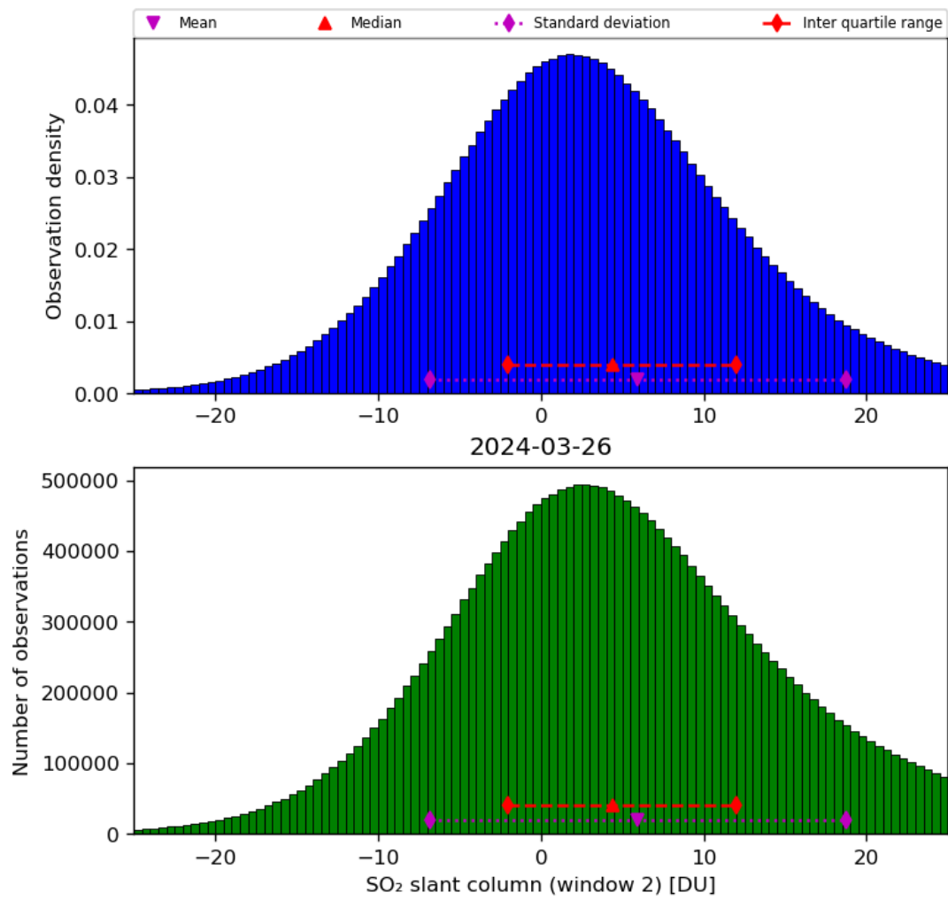
Figure 60: Histogram of “SO 2 slant column (window 2)” for 2024-03-25 to 2024-03-27
