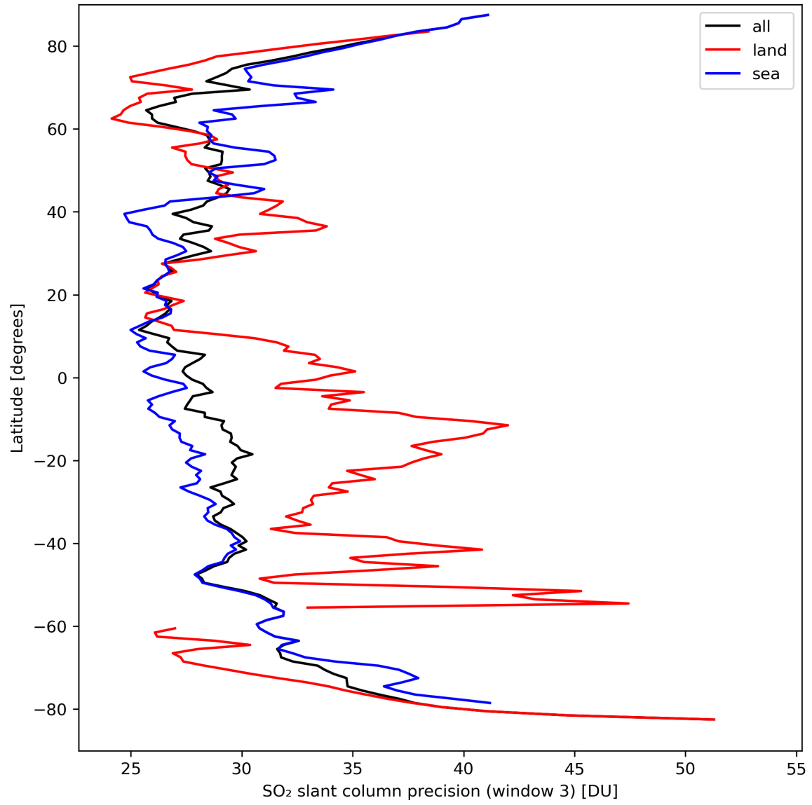
Figure 42: Zonal average of “SO 2 slant column precision (window 3)” for 2024-03-25 to 2024-03-27.
