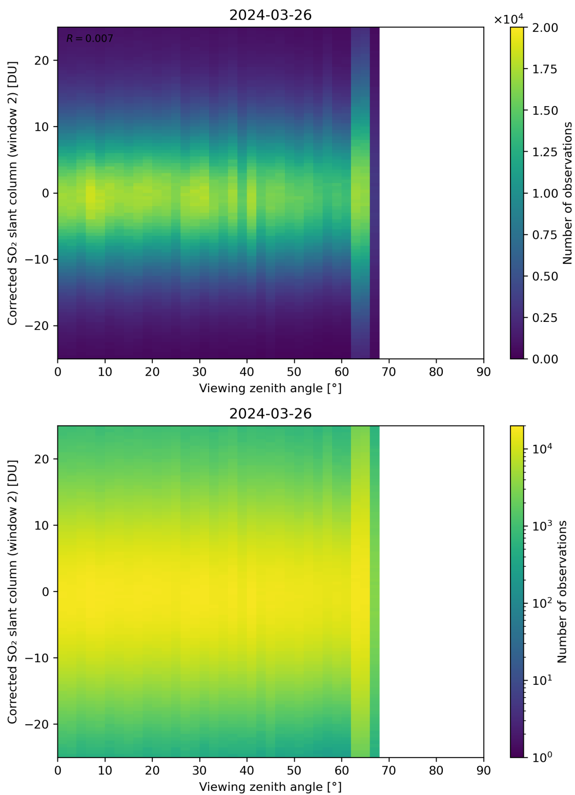
Figure 318: Scatter density plot of “Viewing zenith angle” against “Corrected SO 2 slant column (window 2)” for 2024-03-25 to 2024-03-27.
