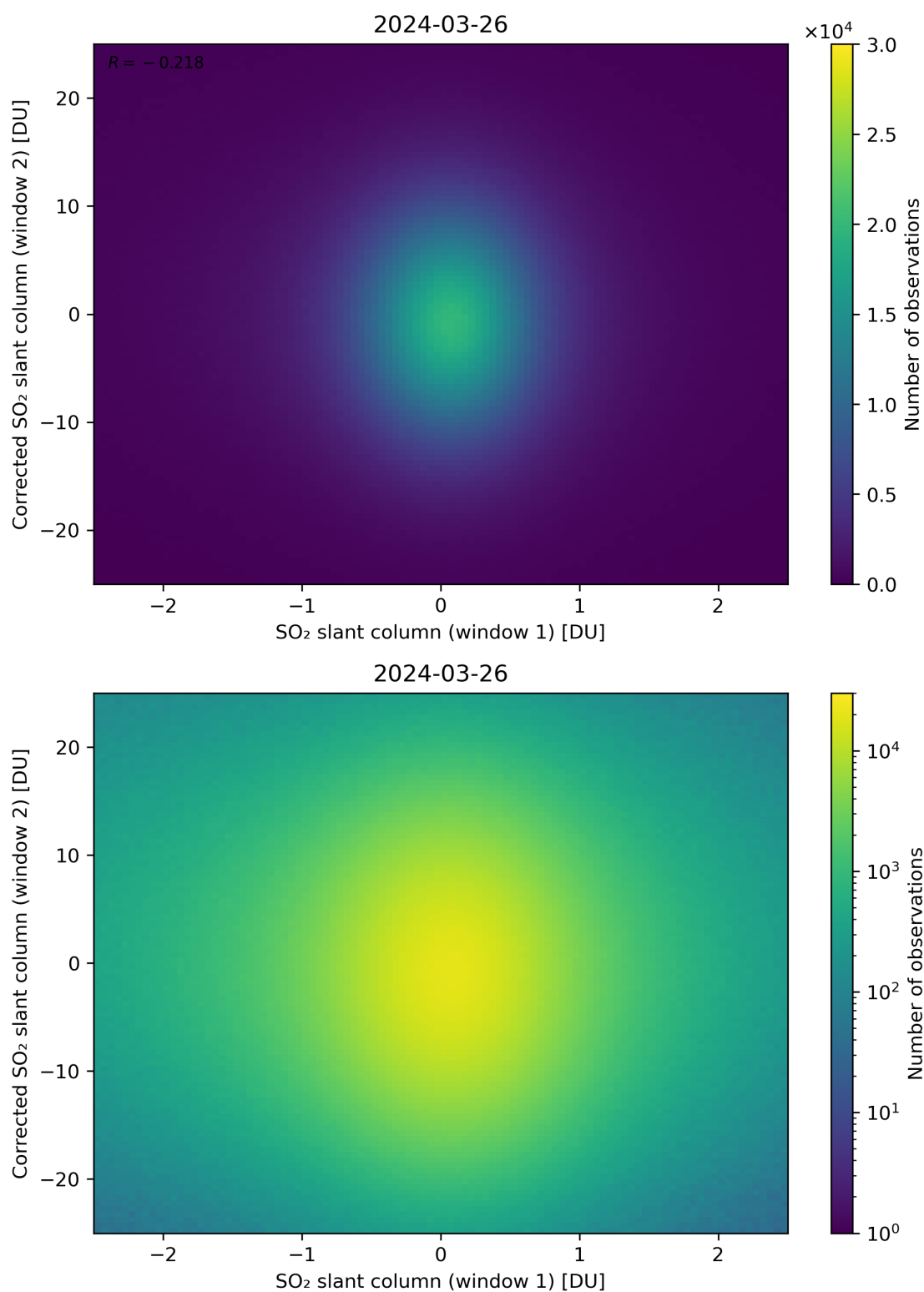
Figure 233: Scatter density plot of “SO 2 slant column (window 1)” against “Corrected SO 2 slant column (window 2)” for 2024-03-25 to 2024-03-27.
