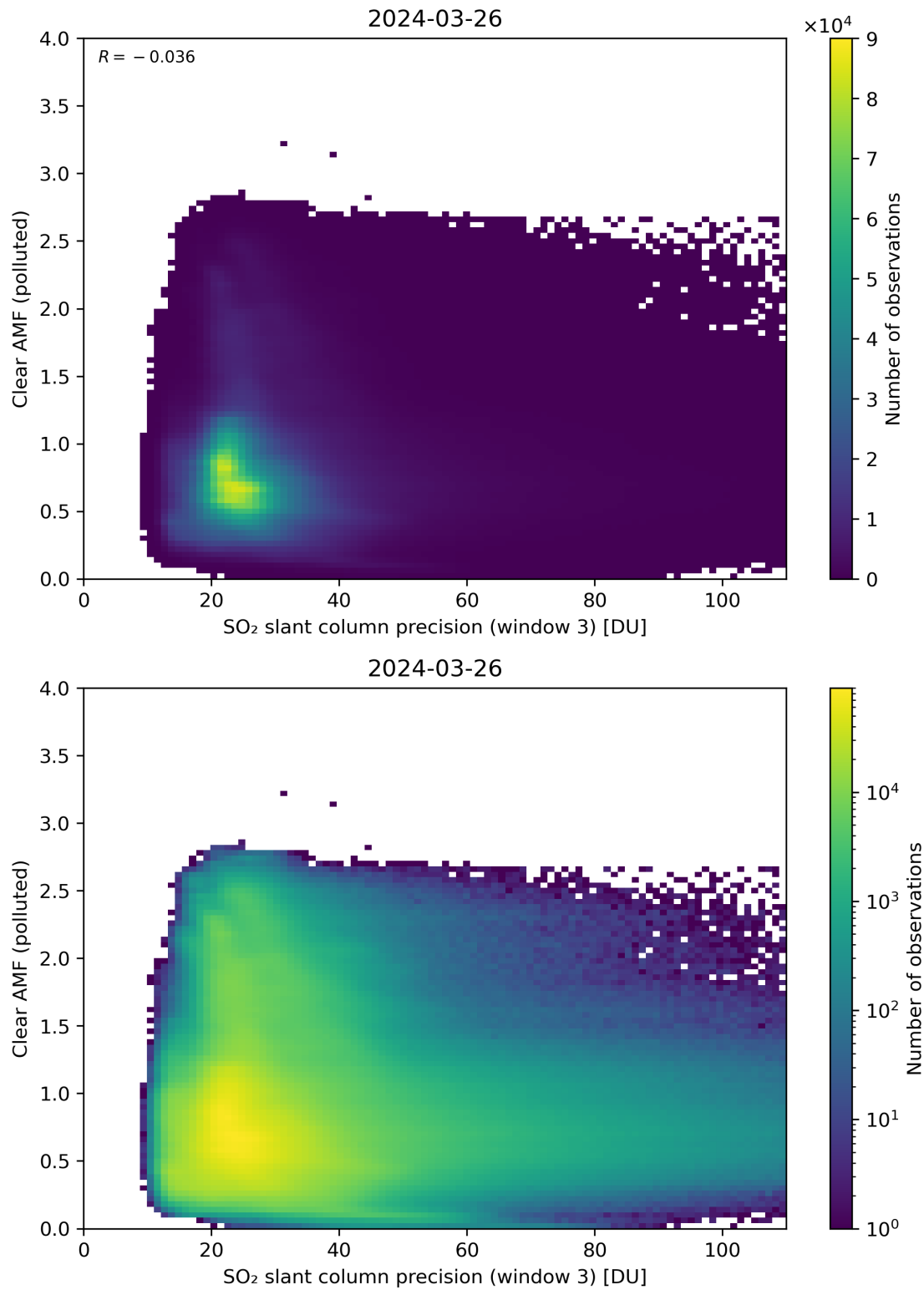
Figure 261: Scatter density plot of “SO 2 slant column precision (window 3)” against “Clear AMF (polluted)” for 2024-03-25 to 2024-03-27.
