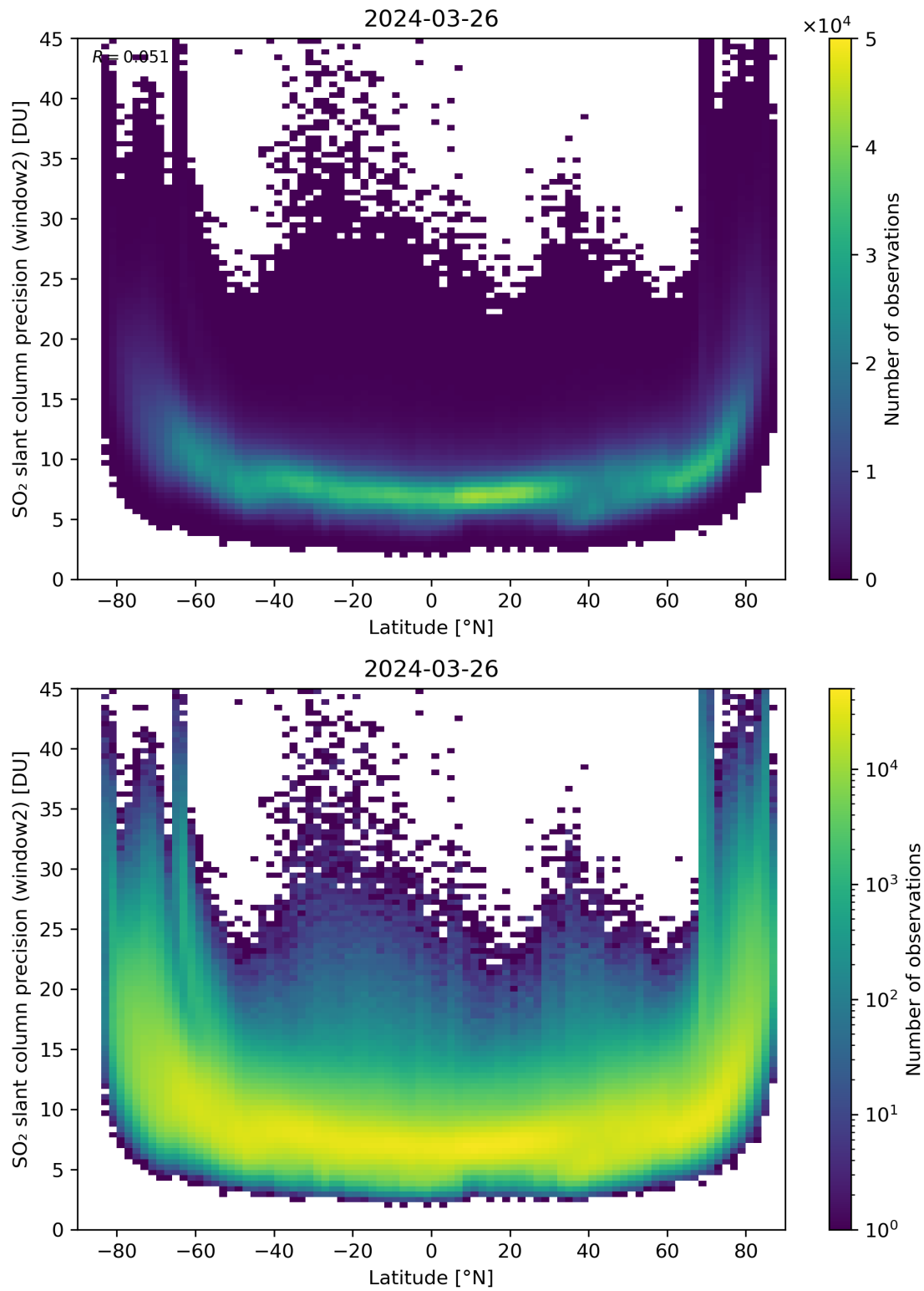
Figure 151: Scatter density plot of “Latitude” against “SO 2 slant column precision (window2)” for 2024-03-25 to 2024-03-27.
