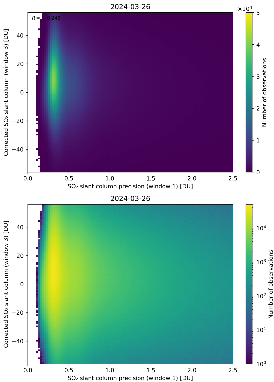
Figure 226: Scatter density plot of “SO 2 slant column precision (window 1)” against “Corrected SO 2 slant column (window 3)” for 2024-03-25 to 2024-03-27.
