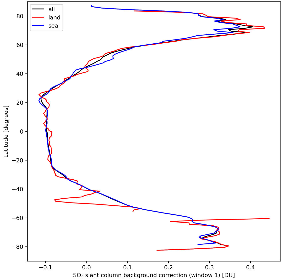
Figure 36: Zonal average of “SO 2 slant column background correction (window 1)” for 2024-03-25 to 2024-03-27.
