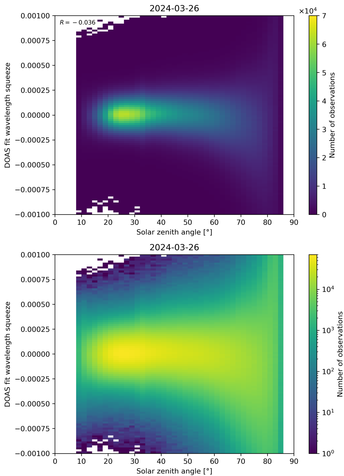
Figure 162: Scatter density plot of “Solar zenith angle” against “DOAS fit wavelength squeeze” for 2024-03-25 to 2024-03-27.
