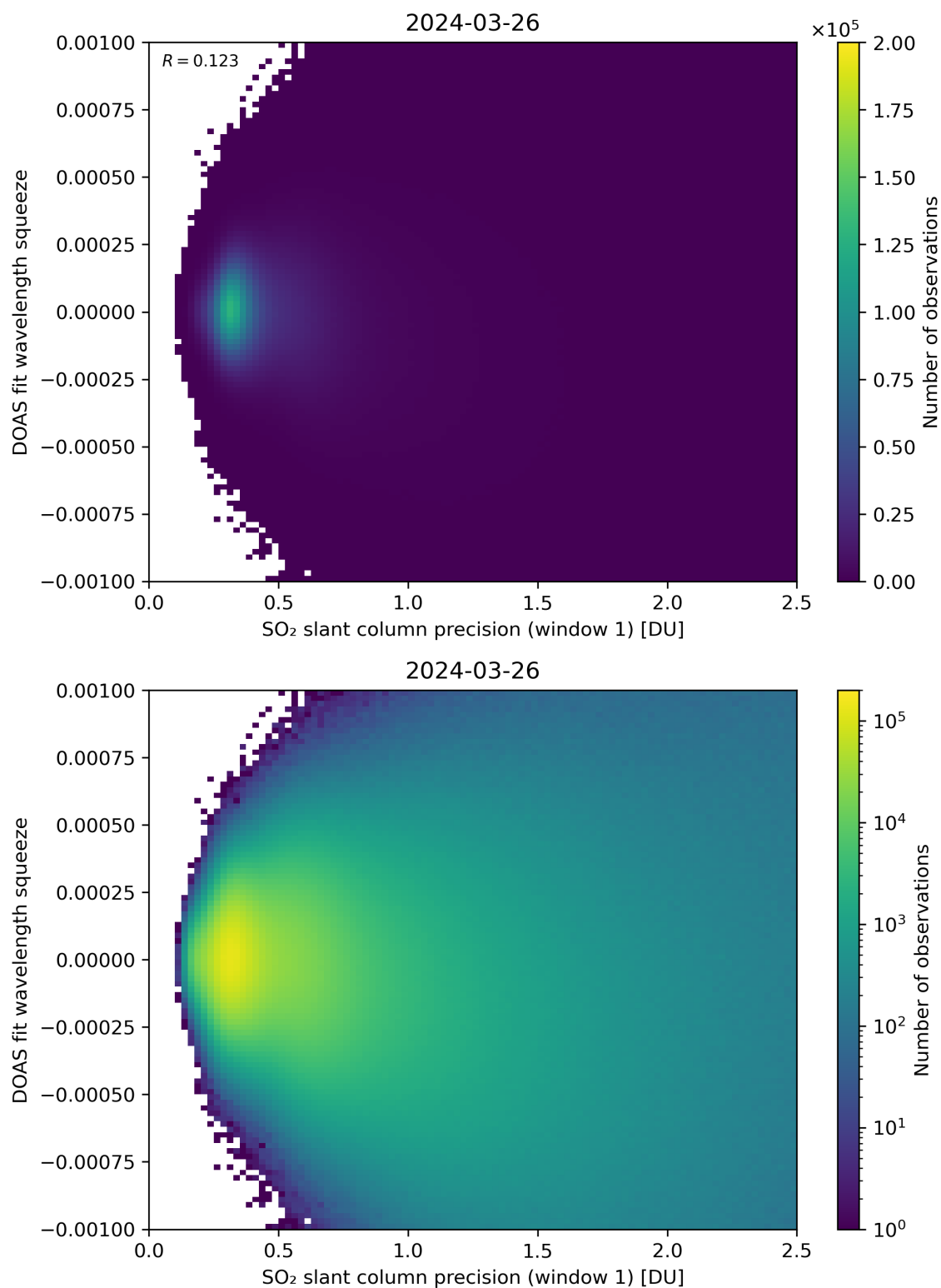
Figure 222: Scatter density plot of “SO 2 slant column precision (window 1)” against “DOAS fit wavelength squeeze” for 2024-03-25 to 2024-03-27.
