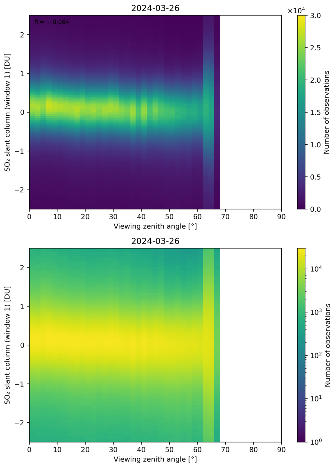
Figure 320: Scatter density plot of “Viewing zenith angle” against “SO 2 slant column (window 1)” for 2024-03-25 to 2024-03-27.
