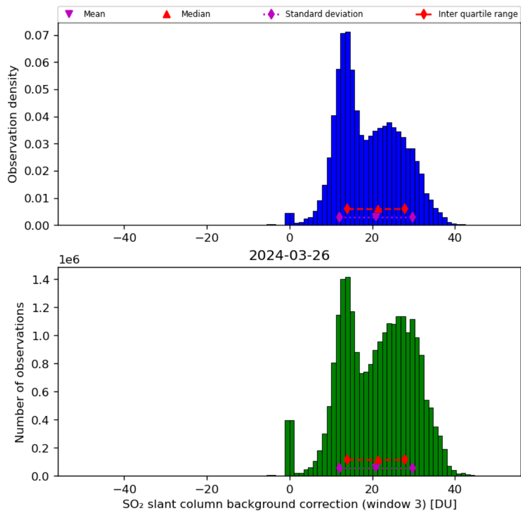
Figure 67: Histogram of “SO 2 slant column background correction (window 3)” for 2024-03-25 to 2024-03-27
