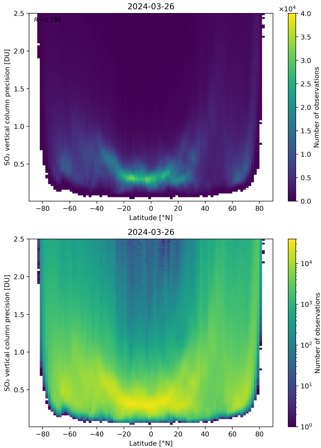
Figure 157: Scatter density plot of “Latitude” against “SO 2 vertical column precision” for 2024-03-25 to 2024-03-27.
