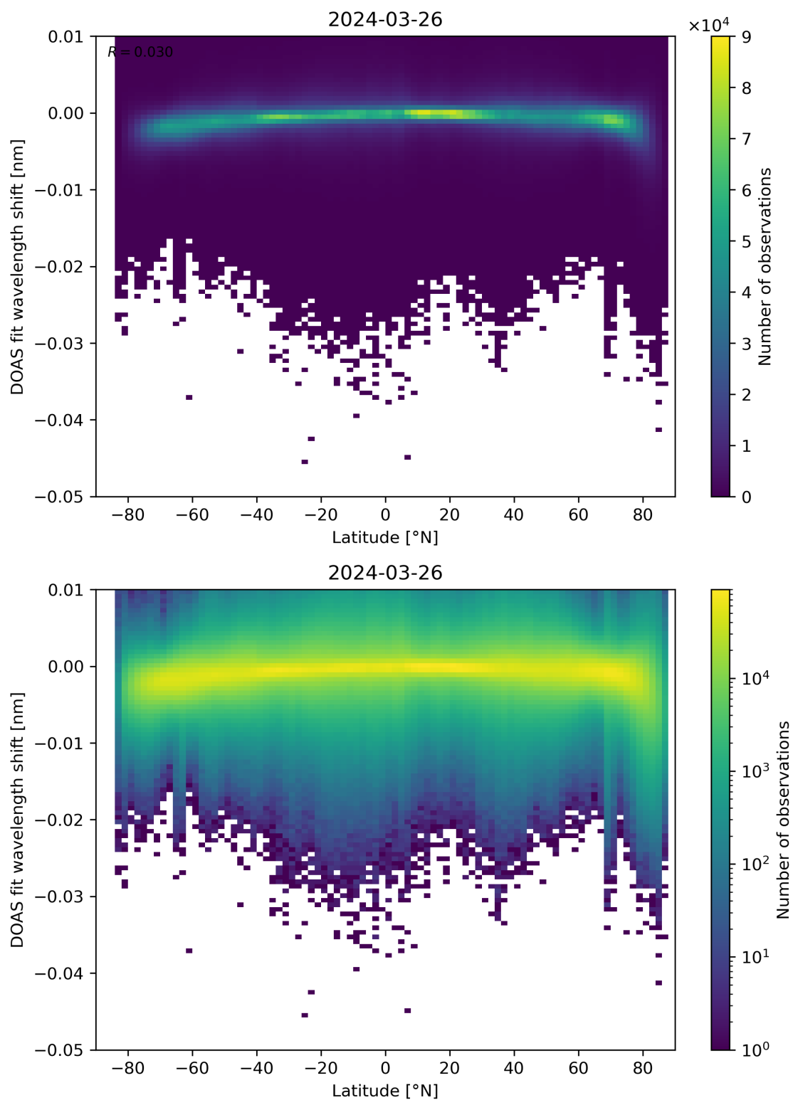
Figure 142: Scatter density plot of “Latitude” against “DOAS fit wavelength shift” for 2024-03-25 to 2024-03-27.
