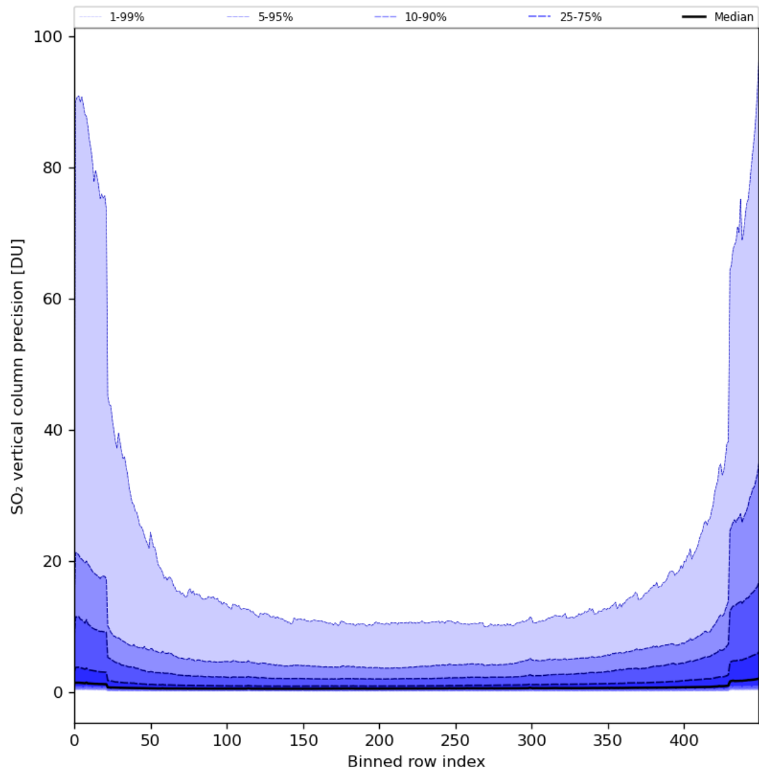
Figure 77: Along track statistics of “SO 2 vertical column precision” for 2024-03-25 to 2024-03-27
