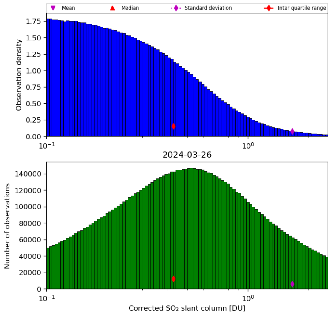
Figure 55: Histogram of “Corrected SO 2 slant column” for 2024-03-25 to 2024-03-27
