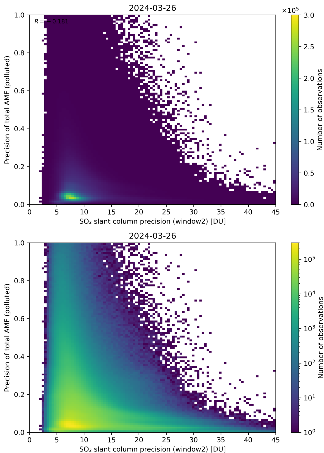
Figure 252: Scatter density plot of “SO 2 slant column precision (window2)” against “Precision of total AMF (polluted)” for 2024-03-25 to 2024-03-27.
