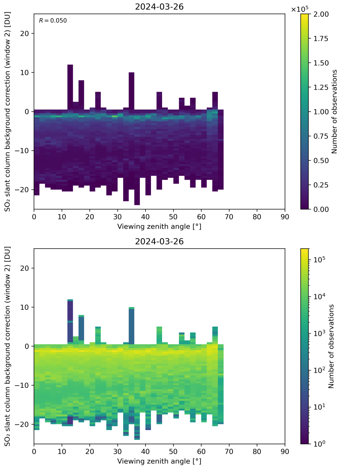
Figure 309: Scatter density plot of “Viewing zenith angle” against “SO 2 slant column background correction (window 2)” for 2024-03-25 to 2024-03-27.
