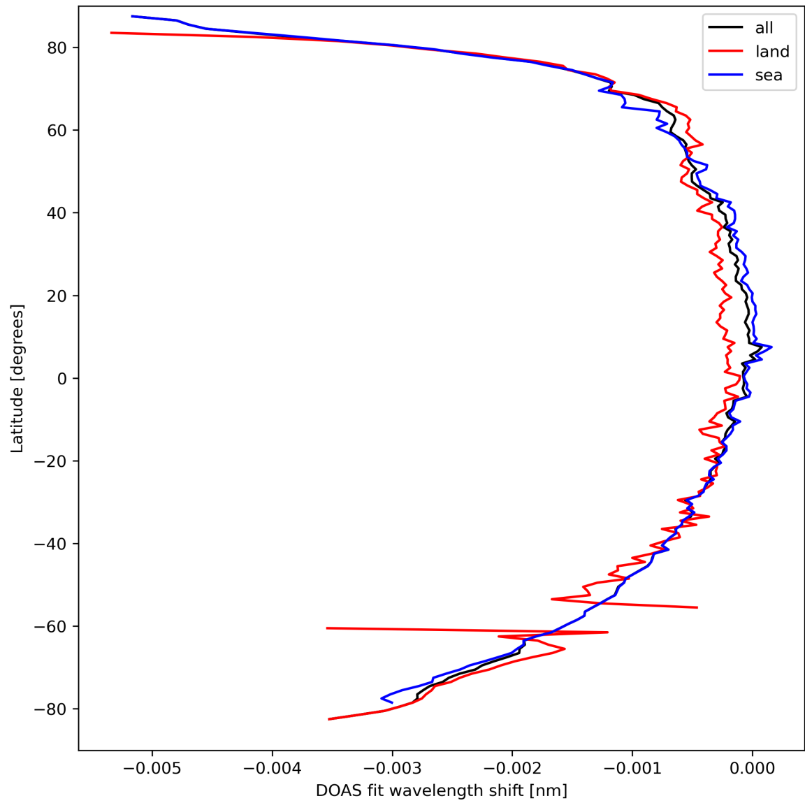
Figure 45: Zonal average of “DOAS fit wavelength shift” for 2024-03-25 to 2024-03-27.
