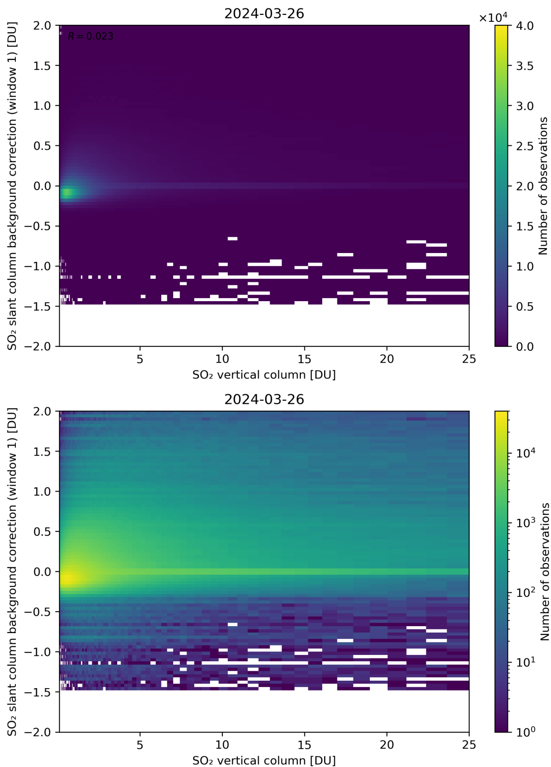
Figure 273: Scatter density plot of “SO 2 vertical column” against “SO 2 slant column background correction (window 1)” for 2024-03-25 to 2024-03-27.
