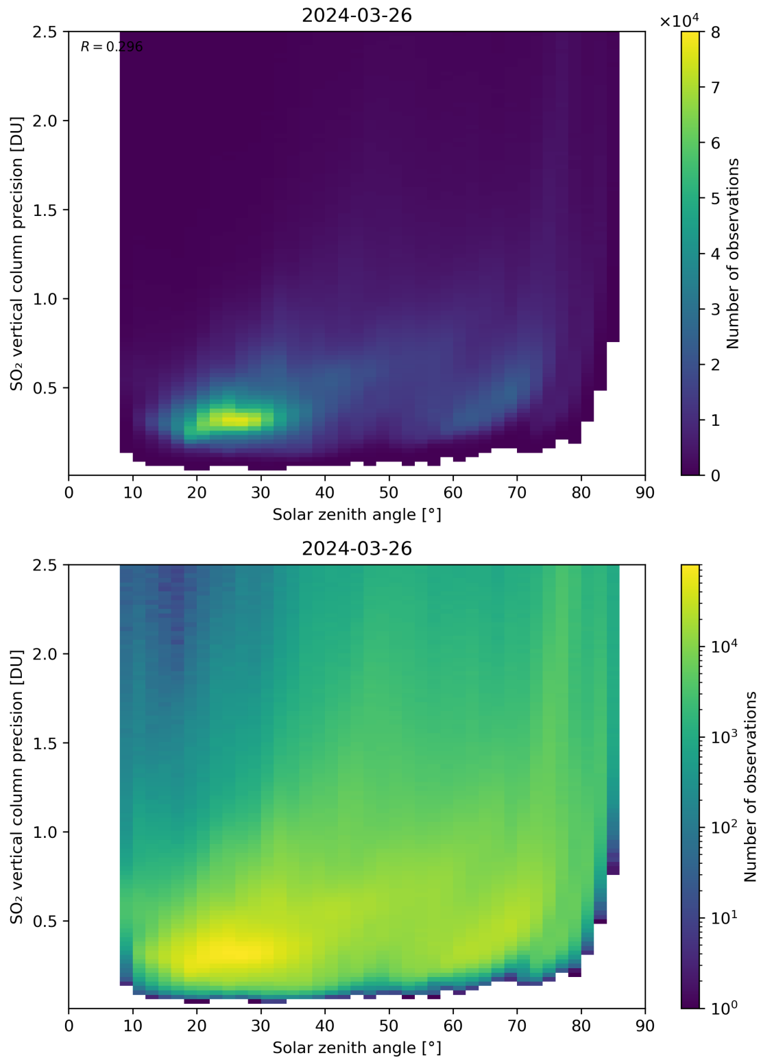
Figure 177: Scatter density plot of “Solar zenith angle” against “SO 2 vertical column precision” for 2024-03-25 to 2024-03-27.
