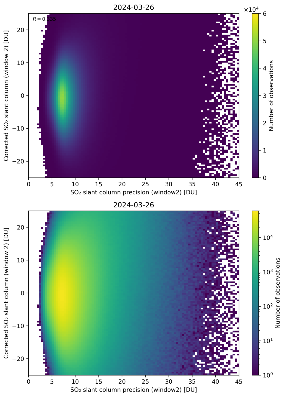
Figure 247: Scatter density plot of “SO 2 slant column precision (window2)” against “Corrected SO 2 slant column (window 2)” for 2024-03-25 to 2024-03-27.
