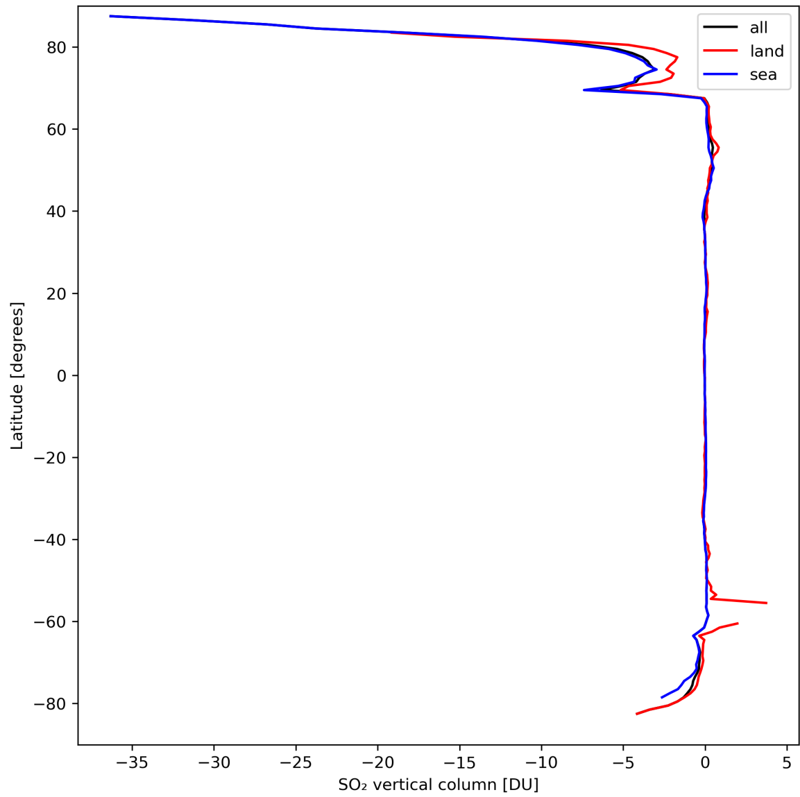
Figure 30: Zonal average of “SO 2 vertical column” for 2024-03-25 to 2024-03-27.
