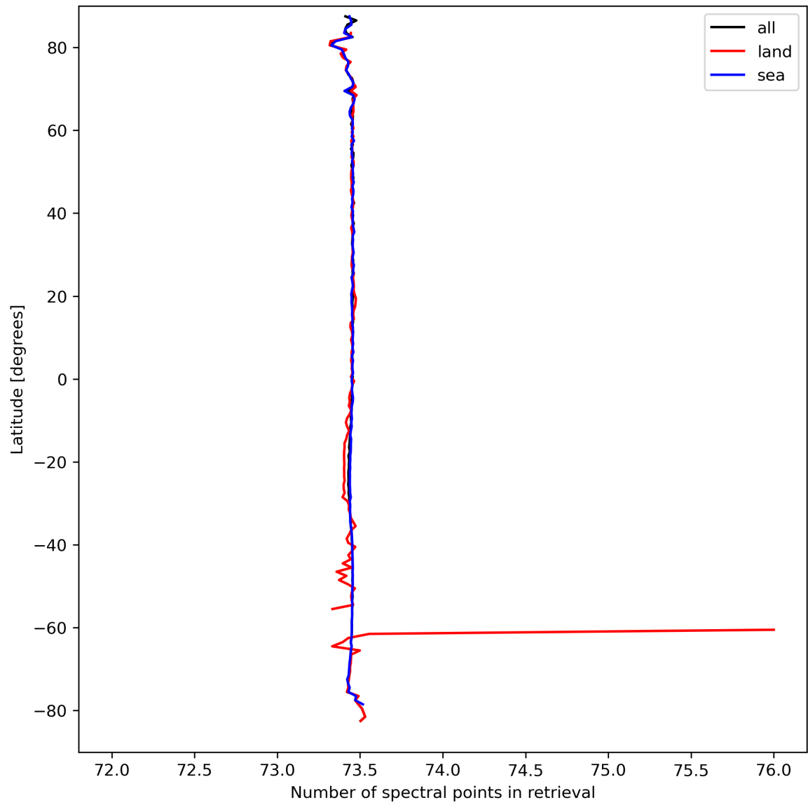
Figure 51: Zonal average of “Number of spectral points in retrieval” for 2024-03-25 to 2024-03-27.
