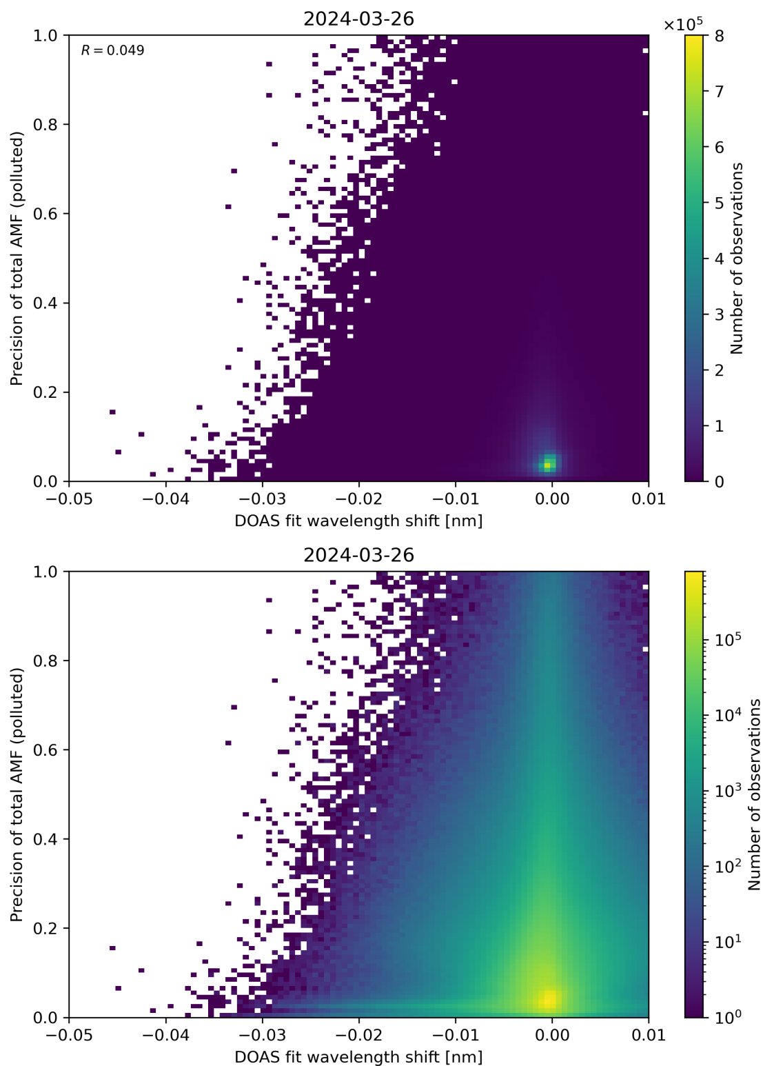
Figure 131: Scatter density plot of “DOAS fit wavelength shift” against “Precision of total AMF (polluted)” for 2024-03-25 to 2024-03-27.
