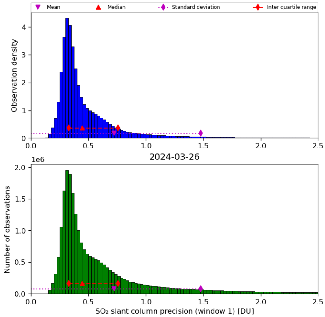
Figure 57: Histogram of “SO 2 slant column precision (window 1)” for 2024-03-25 to 2024-03-27
