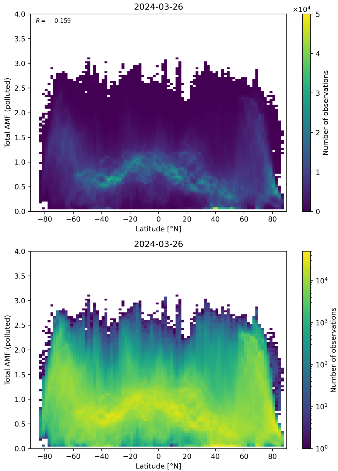
Figure 154: Scatter density plot of “Latitude” against “Total AMF (polluted)” for 2024-03-25 to 2024-03-27.
