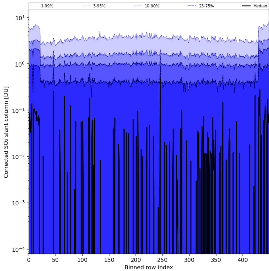
Figure 78: Along track statistics of “Corrected SO 2 slant column” for 2024-03-25 to 2024-03-27
