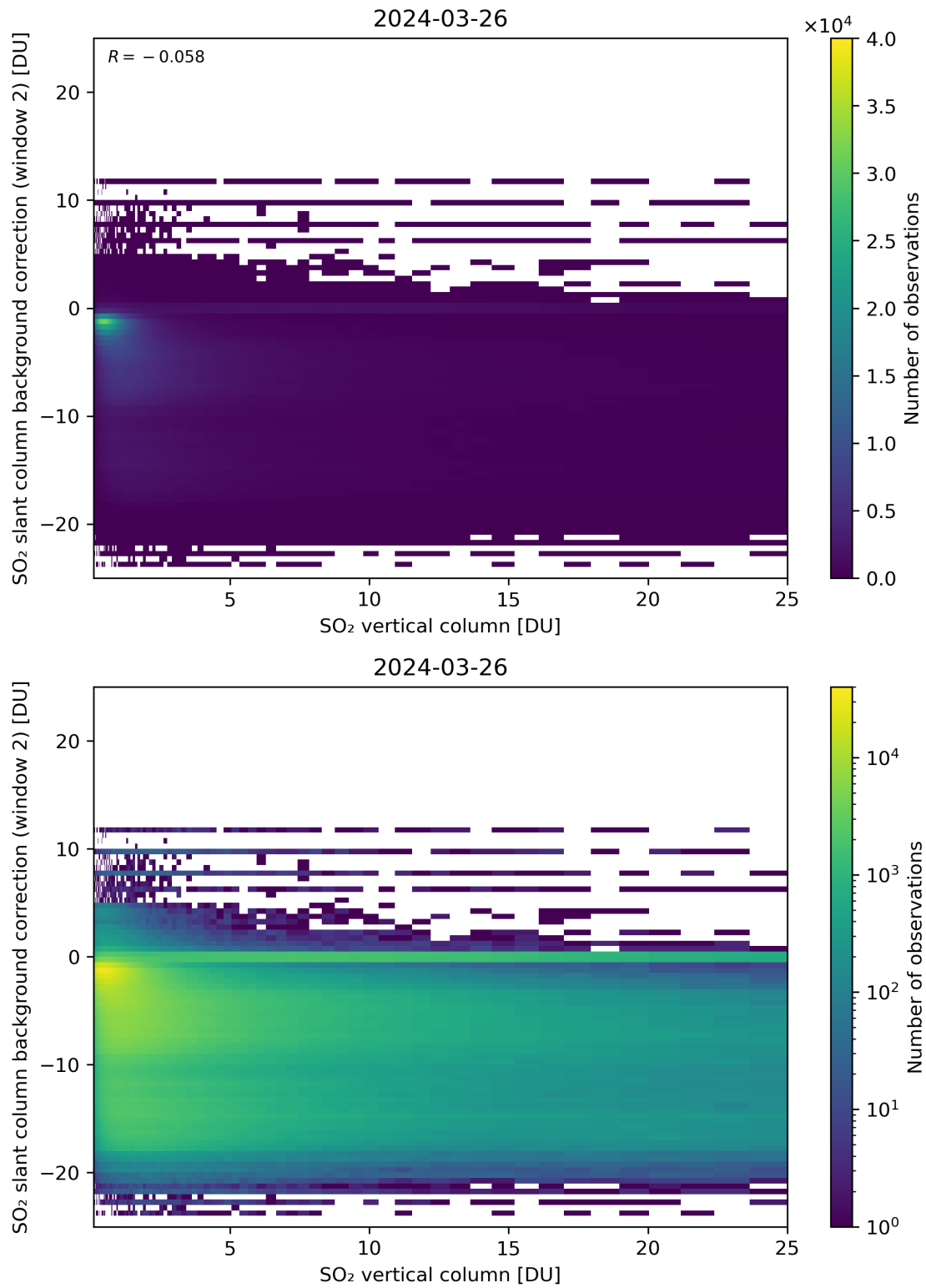
Figure 274: Scatter density plot of “SO 2 vertical column” against “SO 2 slant column background correction (window 2)” for 2024-03-25 to 2024-03-27.
