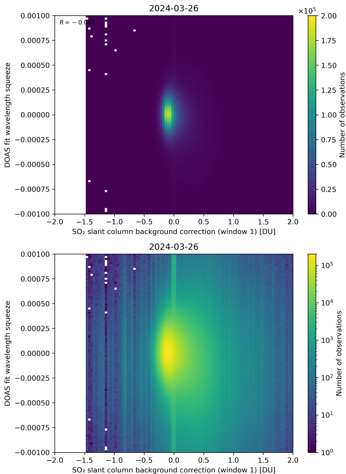
Figure 101: Scatter density plot of “SO 2 slant column background correction (window 1)” against “DOAS fit wavelength squeeze” for 2024-03-25 to 2024-03-27.
