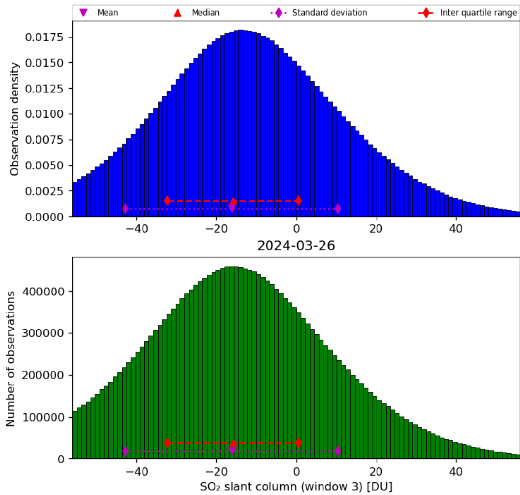
Figure 64: Histogram of “SO 2 slant column (window 3)” for 2024-03-25 to 2024-03-27
