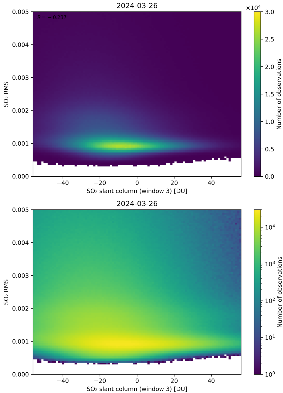
Figure 256: Scatter density plot of “SO 2 slant column (window 3)” against “SO 2 RMS” for 2024-03-25 to 2024-03-27.
