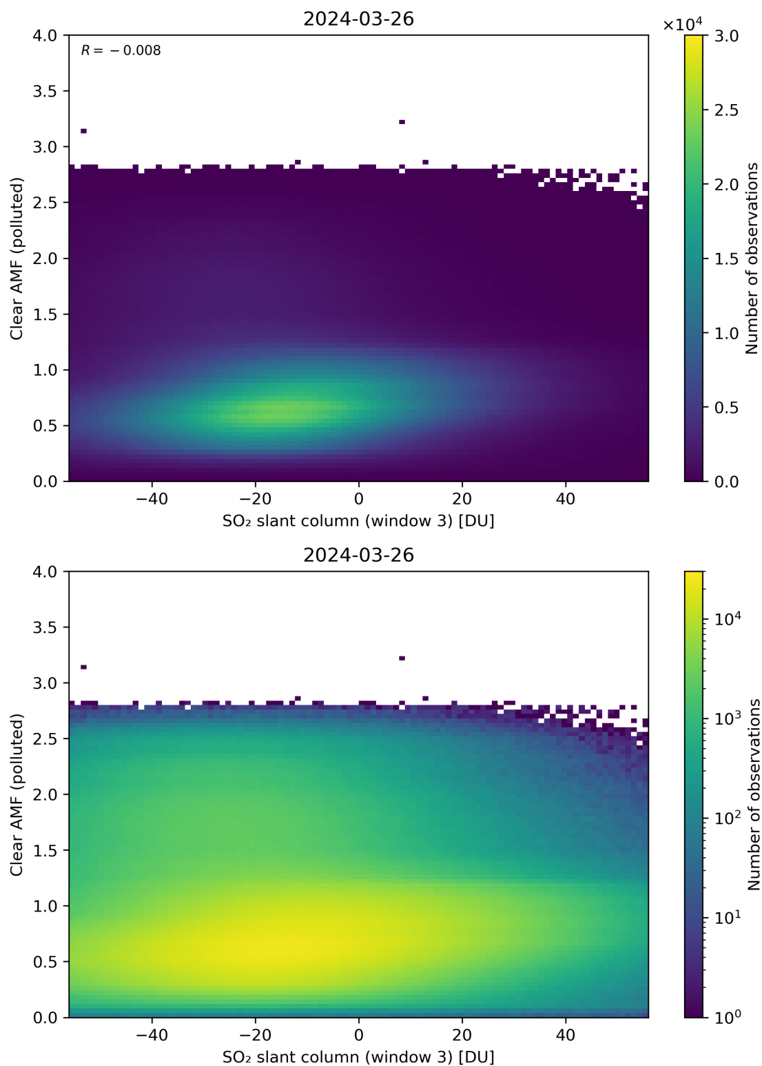
Figure 265: Scatter density plot of “SO 2 slant column (window 3)” against “Clear AMF (polluted)” for 2024-03-25 to 2024-03-27.
