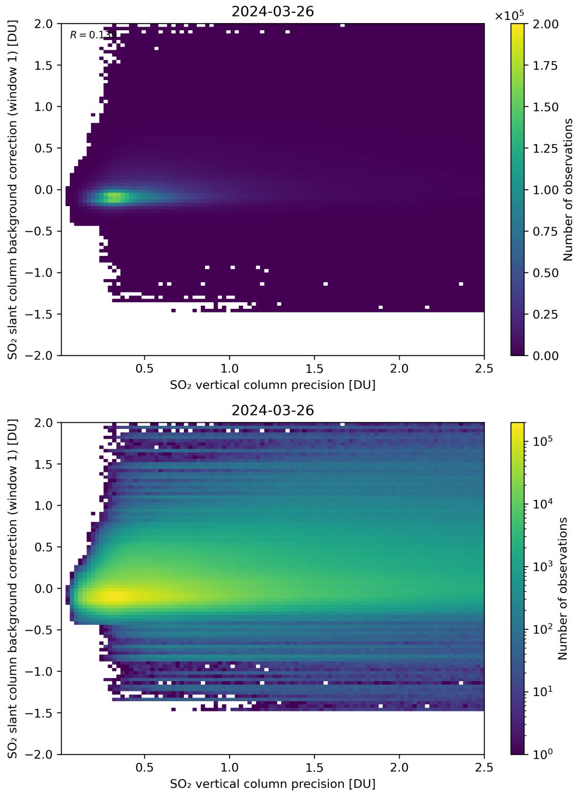
Figure 279: Scatter density plot of “SO 2 vertical column precision” against “SO 2 slant column background correction (window 1)” for 2024-03-25 to 2024-03-27.
