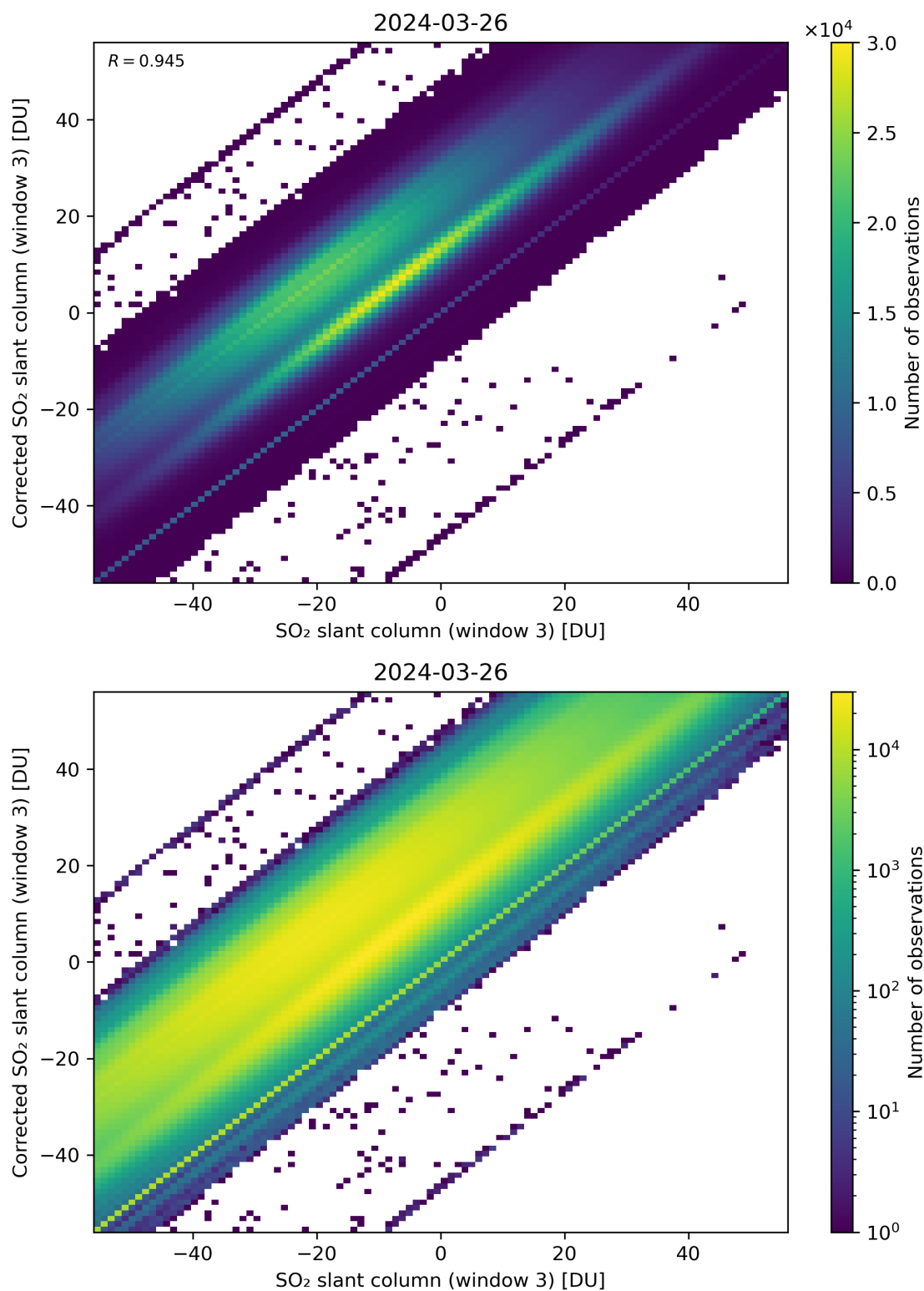
Figure 266: Scatter density plot of “SO 2 slant column (window 3)” against “Corrected SO 2 slant column (window 3)” for 2024-03-25 to 2024-03-27.
