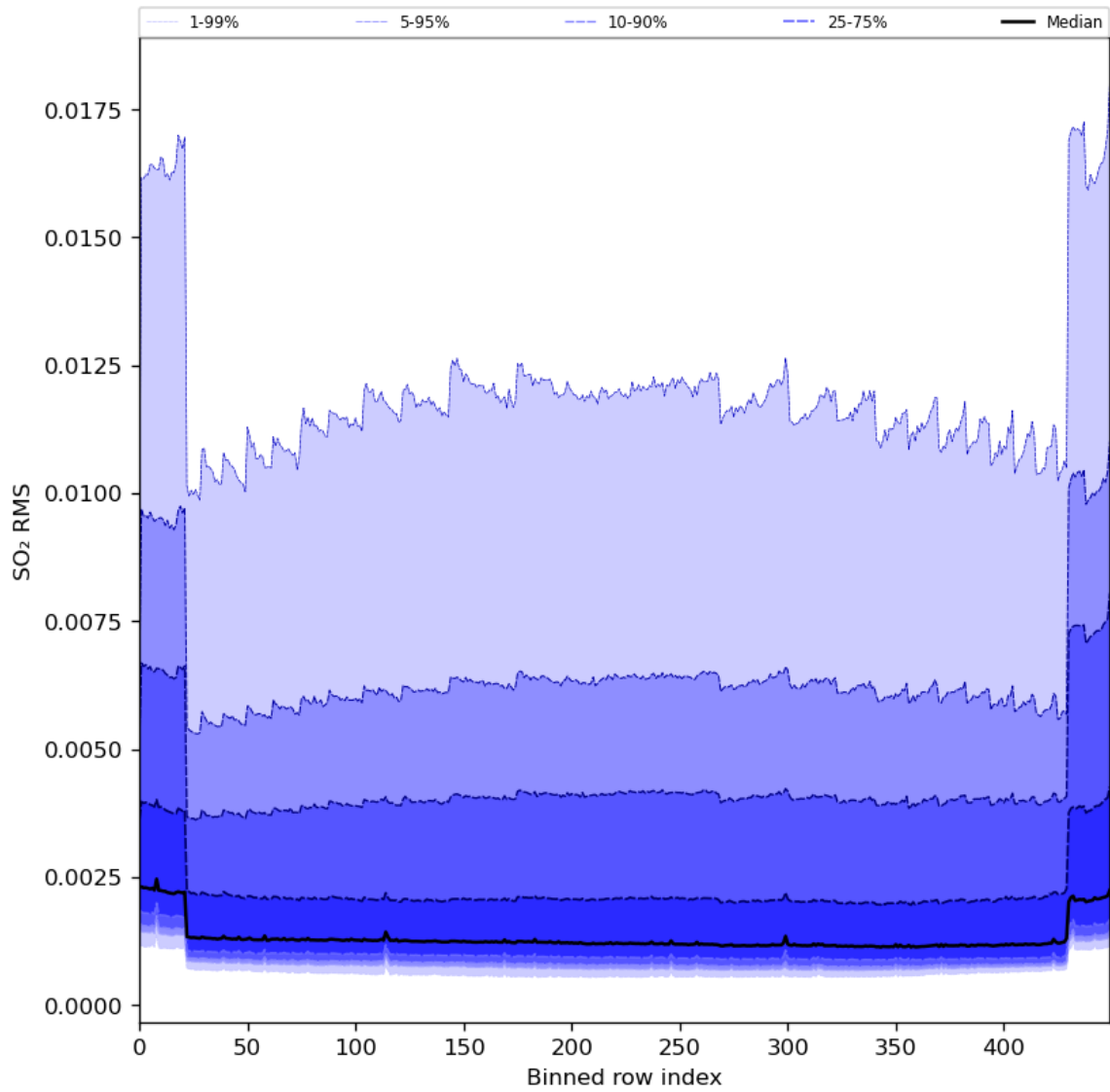
Figure 93: Along track statistics of “SO 2 RMS” for 2024-03-25 to 2024-03-27
