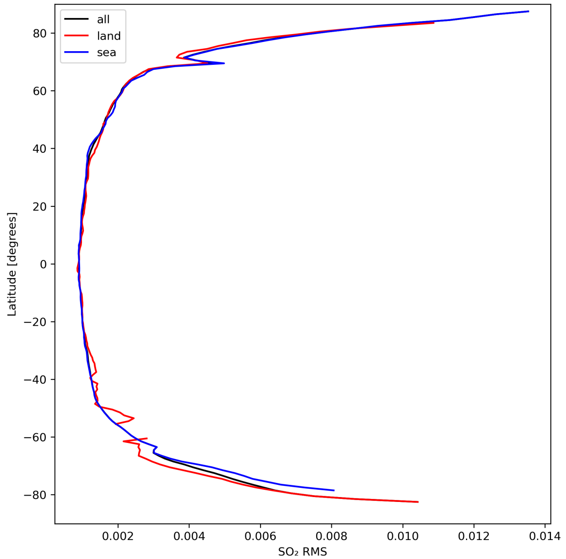
Figure 47: Zonal average of “SO 2 RMS” for 2024-03-25 to 2024-03-27.
