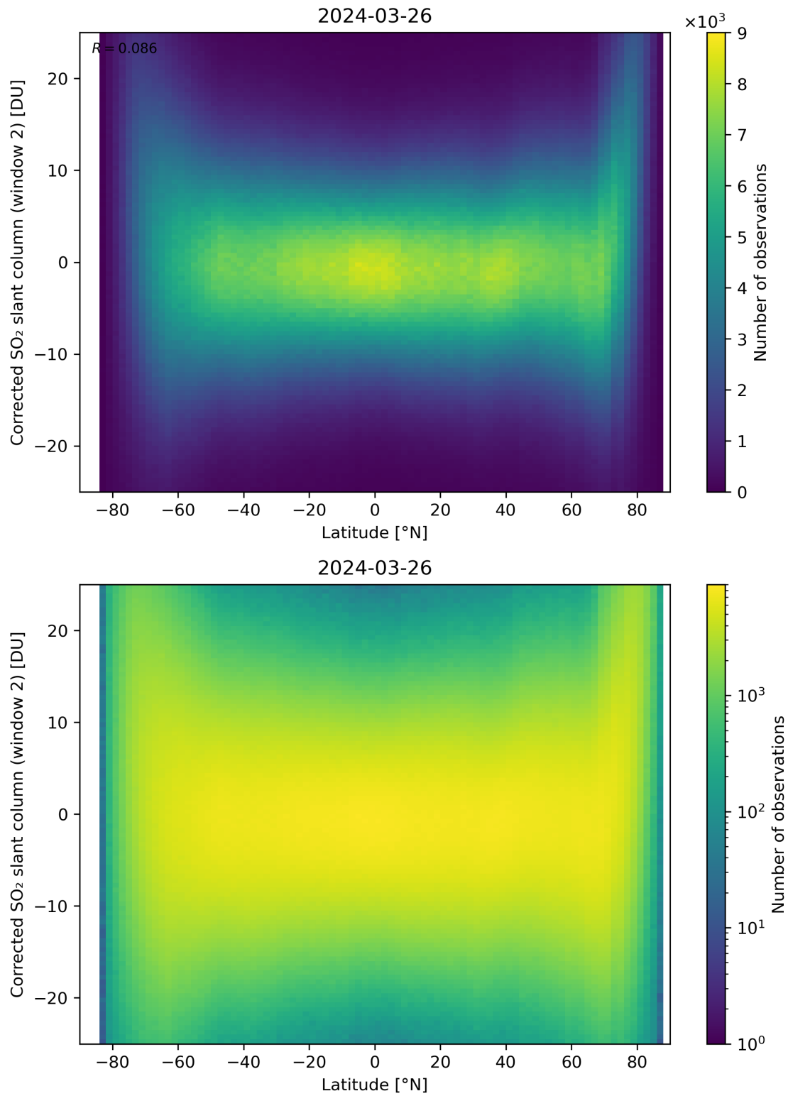
Figure 147: Scatter density plot of “Latitude” against “Corrected SO 2 slant column (window 2)” for 2024-03-25 to 2024-03-27.
