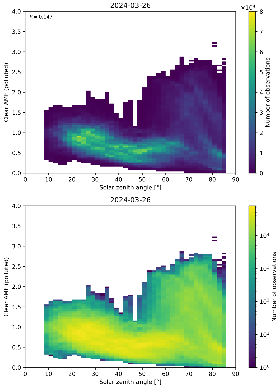
Figure 165: Scatter density plot of “Solar zenith angle” against “Clear AMF (polluted)” for 2024-03-25 to 2024-03-27.
