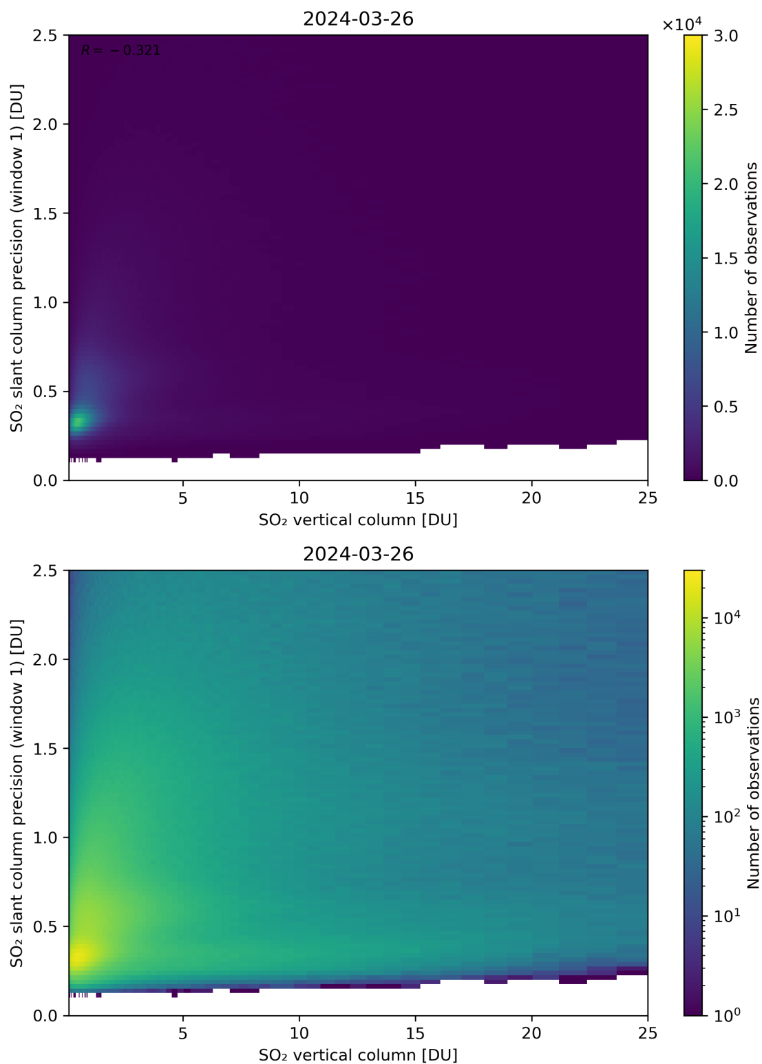
Figure 301: Scatter density plot of “SO 2 vertical column” against “SO 2 slant column precision (window 1)” for 2024-03-25 to 2024-03-27.
