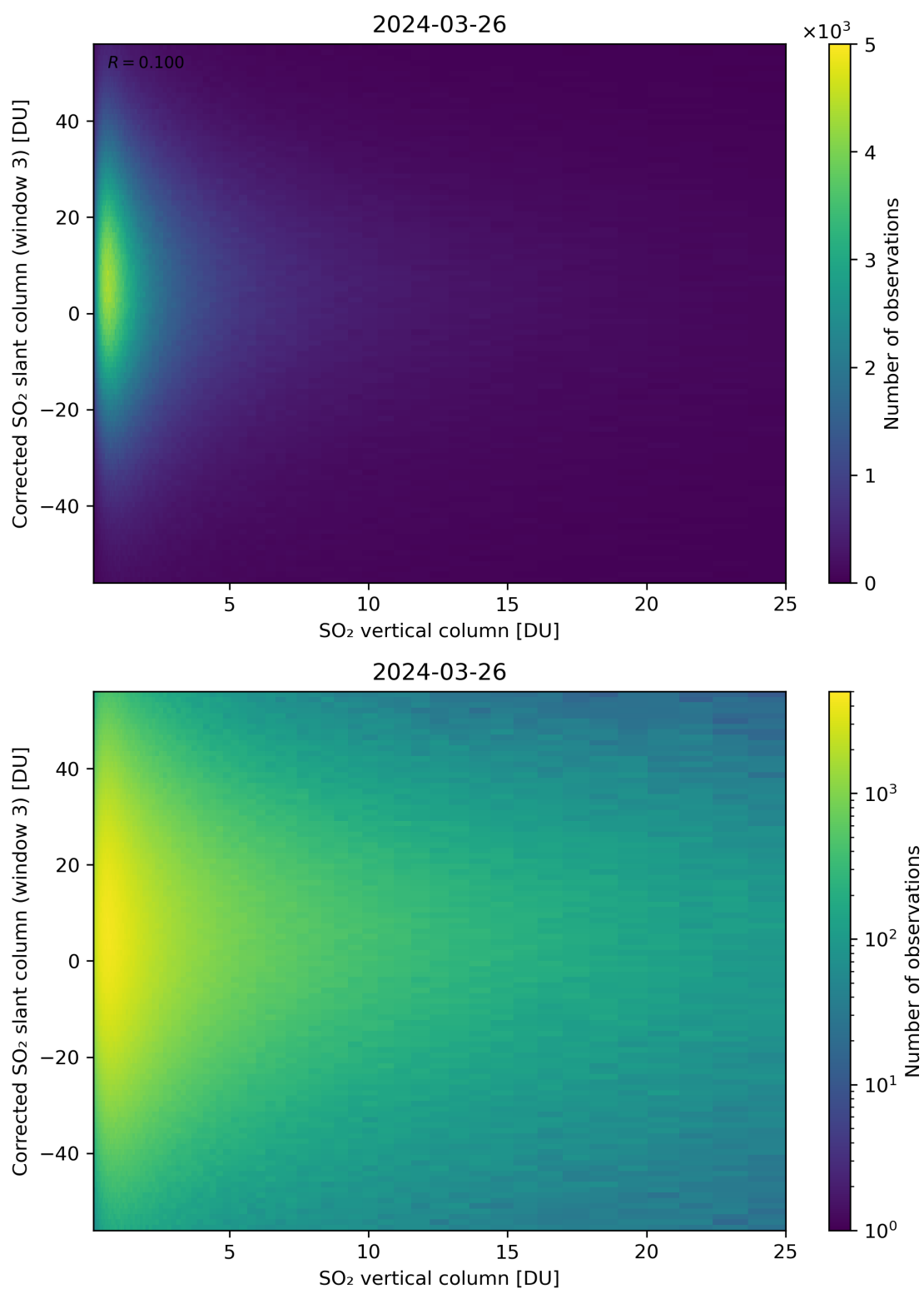
Figure 299: Scatter density plot of “SO 2 vertical column” against “Corrected SO 2 slant column (window 3)” for 2024-03-25 to 2024-03-27.
