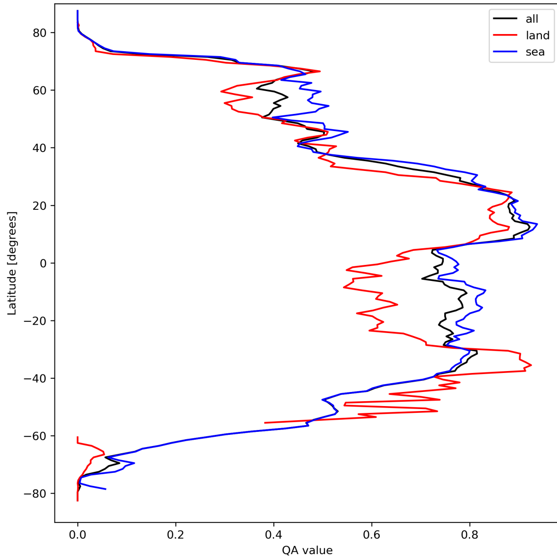
Figure 29: Zonal average of “QA value” for 2024-03-25 to 2024-03-27.
