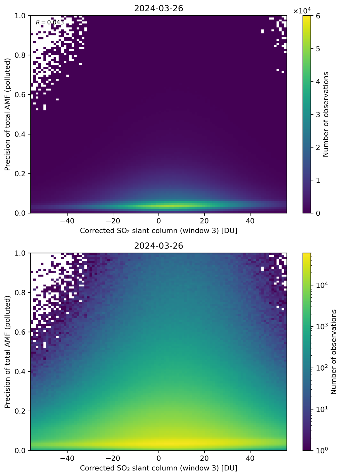
Figure 211: Scatter density plot of “Corrected SO 2 slant column (window 3)” against “Precision of total AMF (polluted)” for 2024-03-25 to 2024-03-27.
