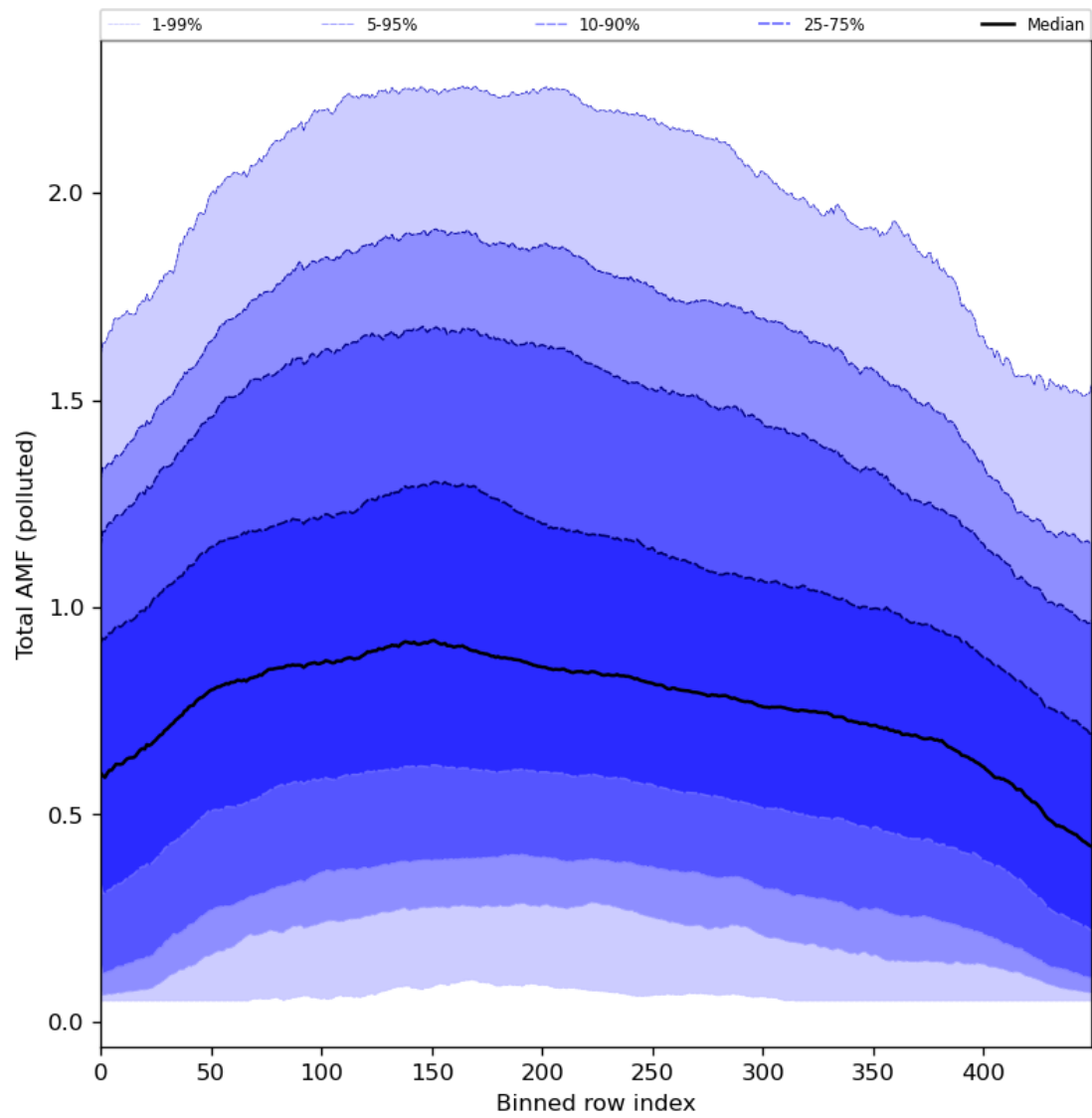
Figure 94: Along track statistics of “Total AMF (polluted)” for 2024-03-25 to 2024-03-27
