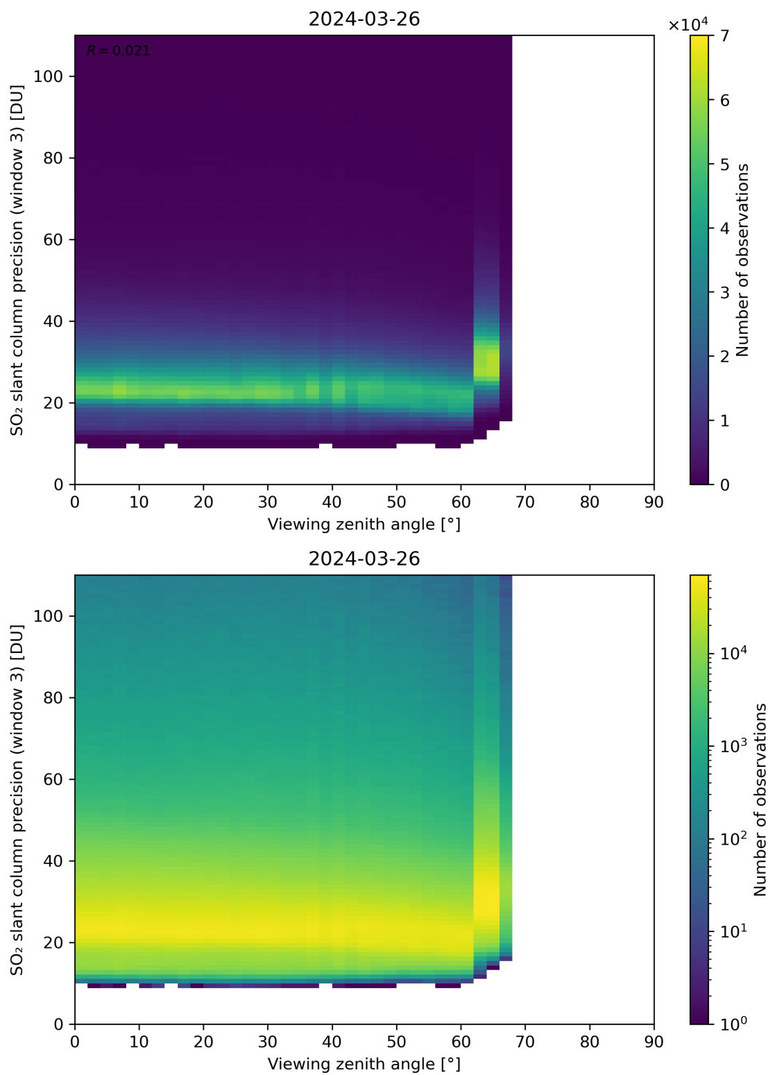
Figure 324: Scatter density plot of “Viewing zenith angle” against “SO 2 slant column precision (window 3)” for 2024-03-25 to 2024-03-27.
