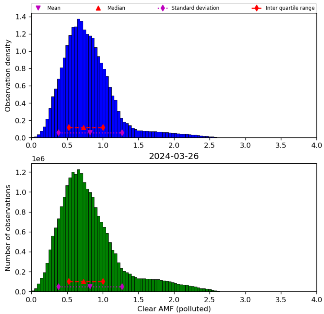
Figure 73: Histogram of “Clear AMF (polluted)” for 2024-03-25 to 2024-03-27
