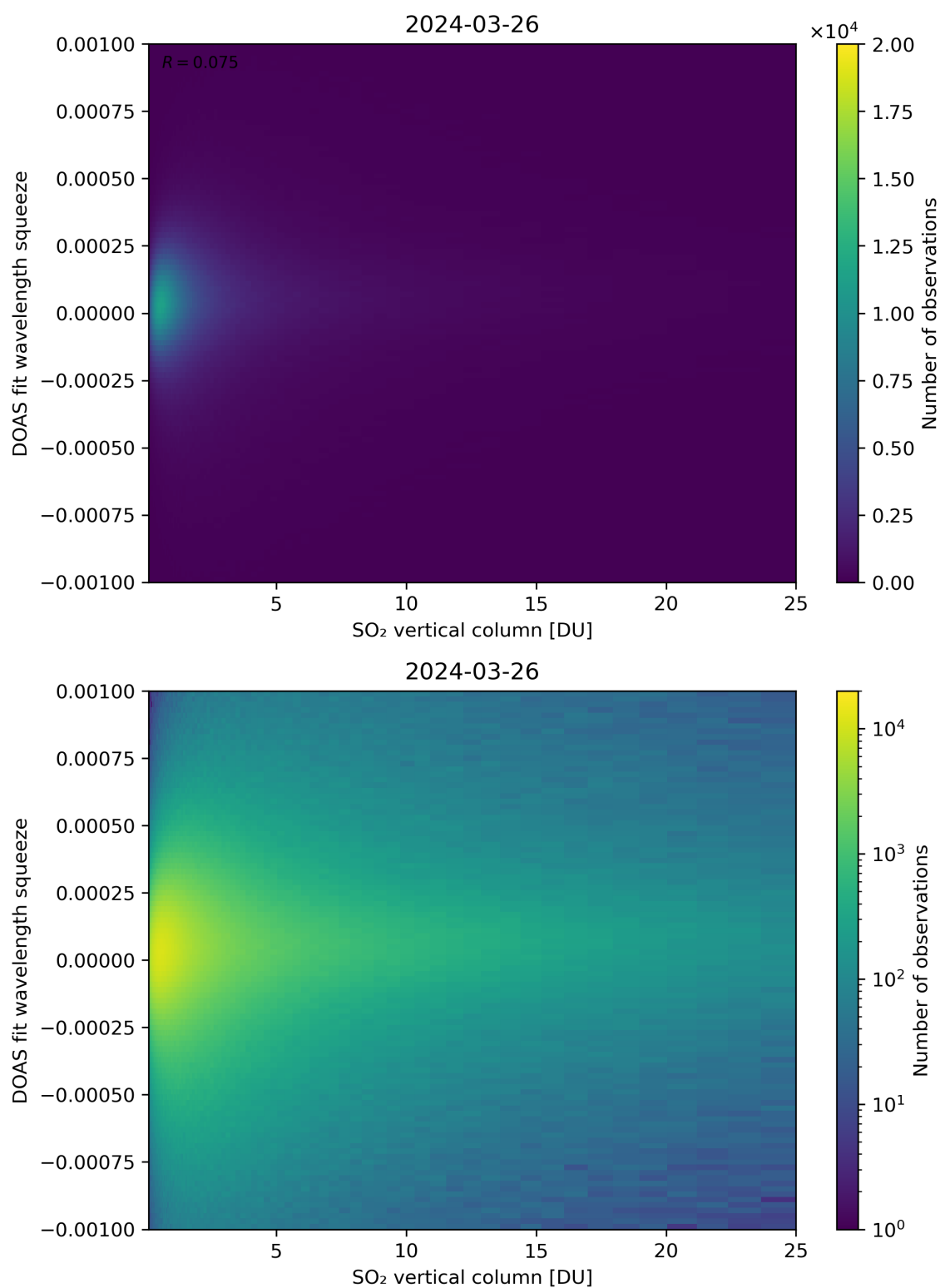
Figure 277: Scatter density plot of “SO 2 vertical column” against “DOAS fit wavelength squeeze” for 2024-03-25 to 2024-03-27.
