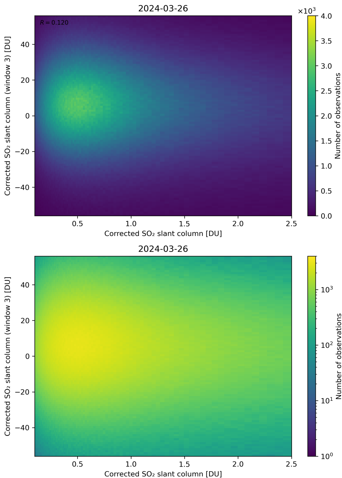
Figure 186: Scatter density plot of “Corrected SO 2 slant column” against “Corrected SO 2 slant column (window 3)” for 2024-03-25 to 2024-03-27.
