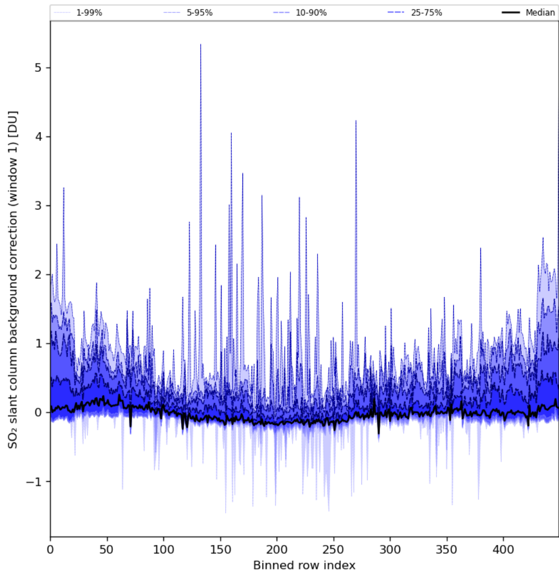
Figure 82: Along track statistics of “SO 2 slant column background correction (window 1)” for 2024-03-25 to 2024-03-27
