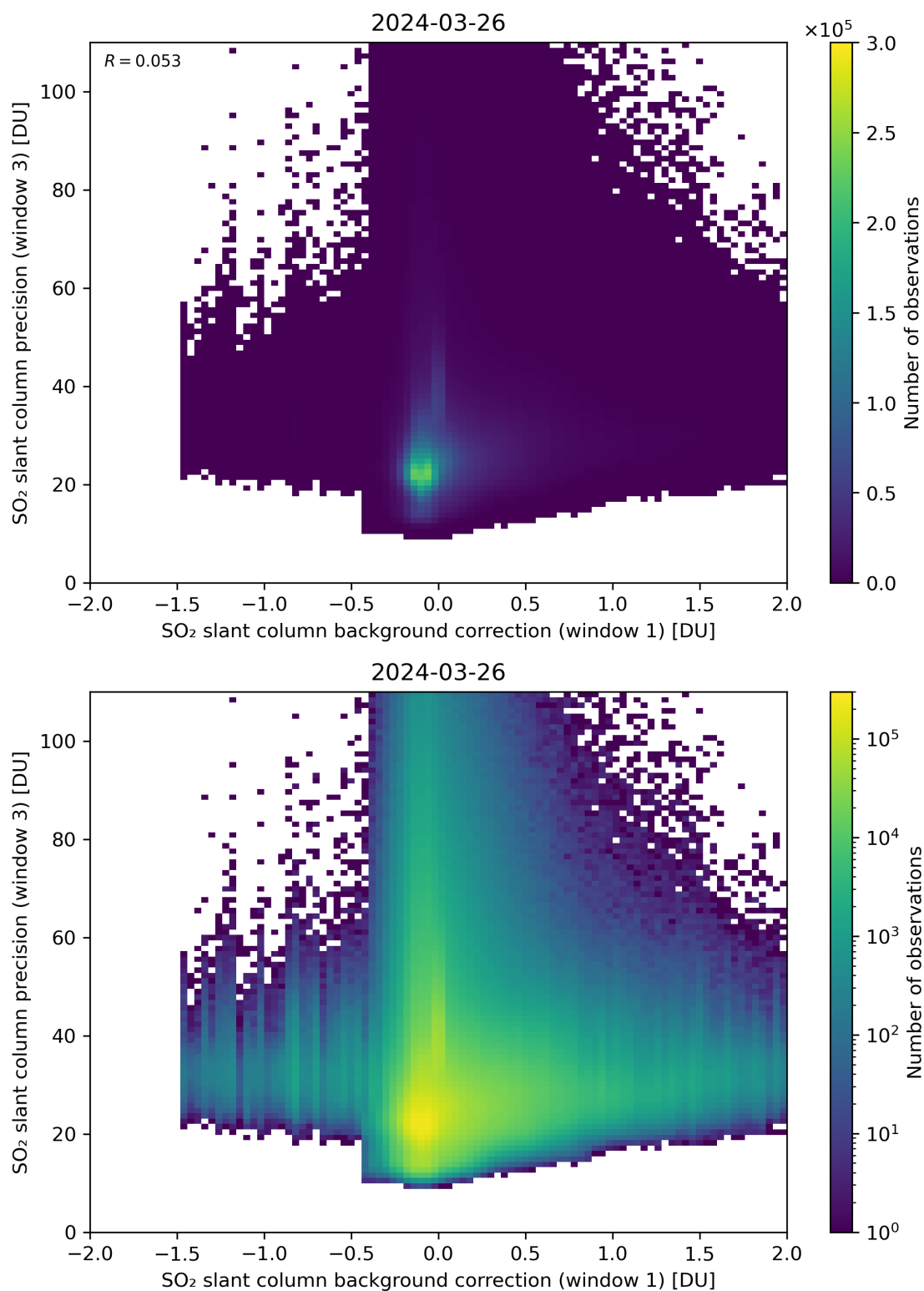
Figure 108: Scatter density plot of “SO 2 slant column background correction (window 1)” against “SO 2 slant column precision (window 3)” for 2024-03-25 to 2024-03-27.
