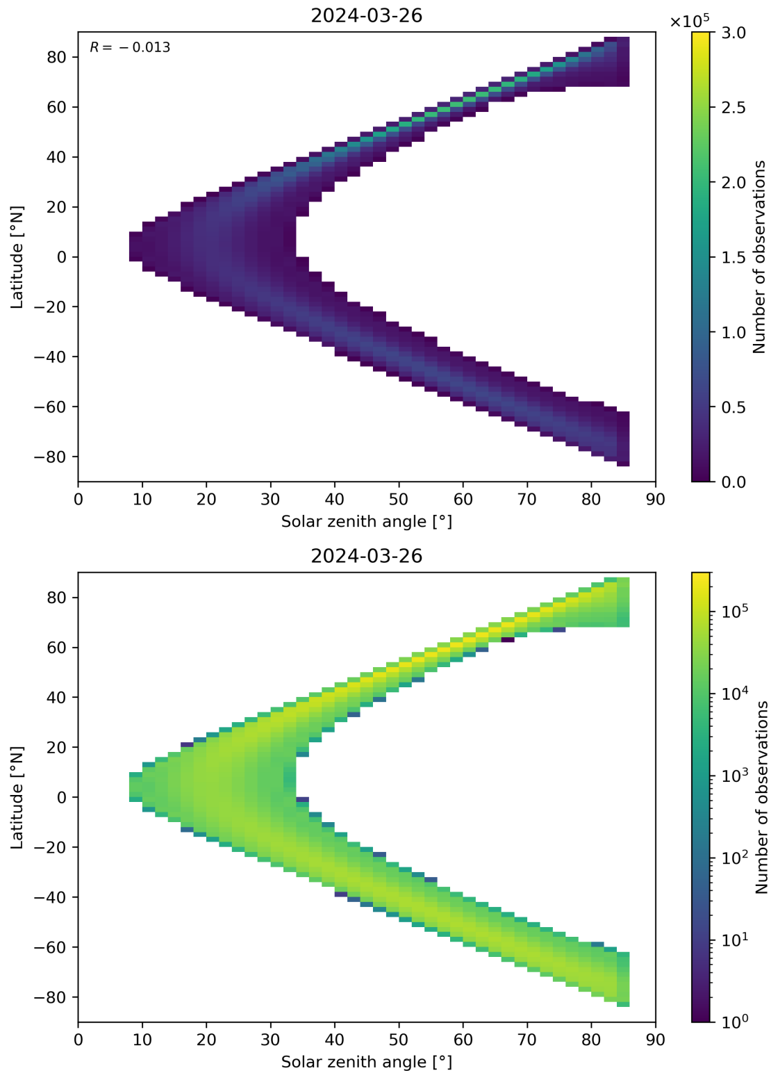
Figure 164: Scatter density plot of “Solar zenith angle” against “Latitude” for 2024-03-25 to 2024-03-27.
