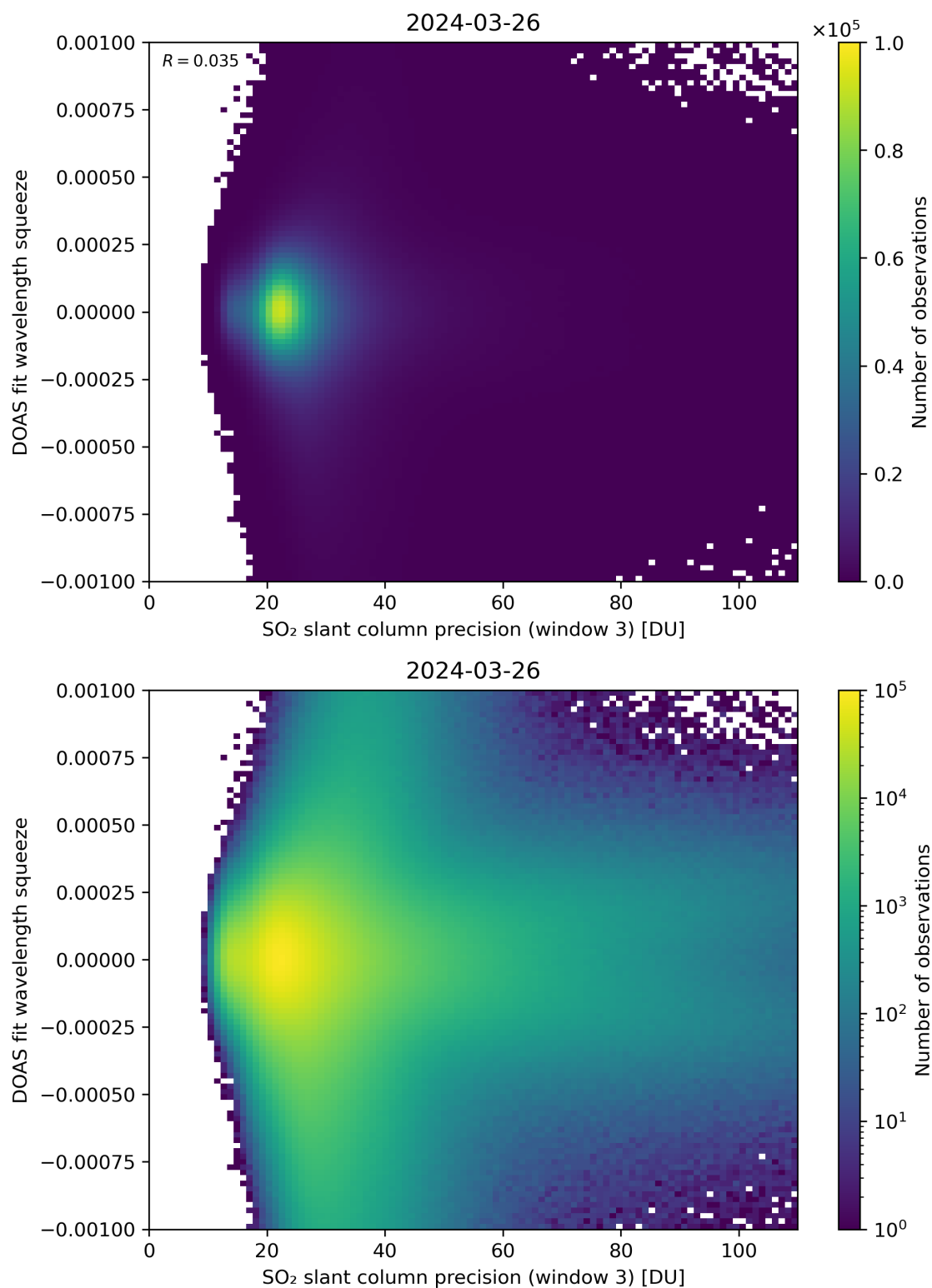
Figure 259: Scatter density plot of “SO 2 slant column precision (window 3)” against “DOAS fit wavelength squeeze” for 2024-03-25 to 2024-03-27.
