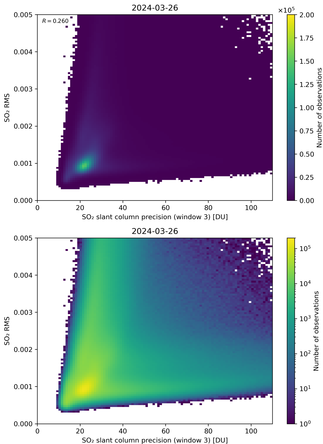
Figure 260: Scatter density plot of “SO 2 slant column precision (window 3)” against “SO 2 RMS” for 2024-03-25 to 2024-03-27.
