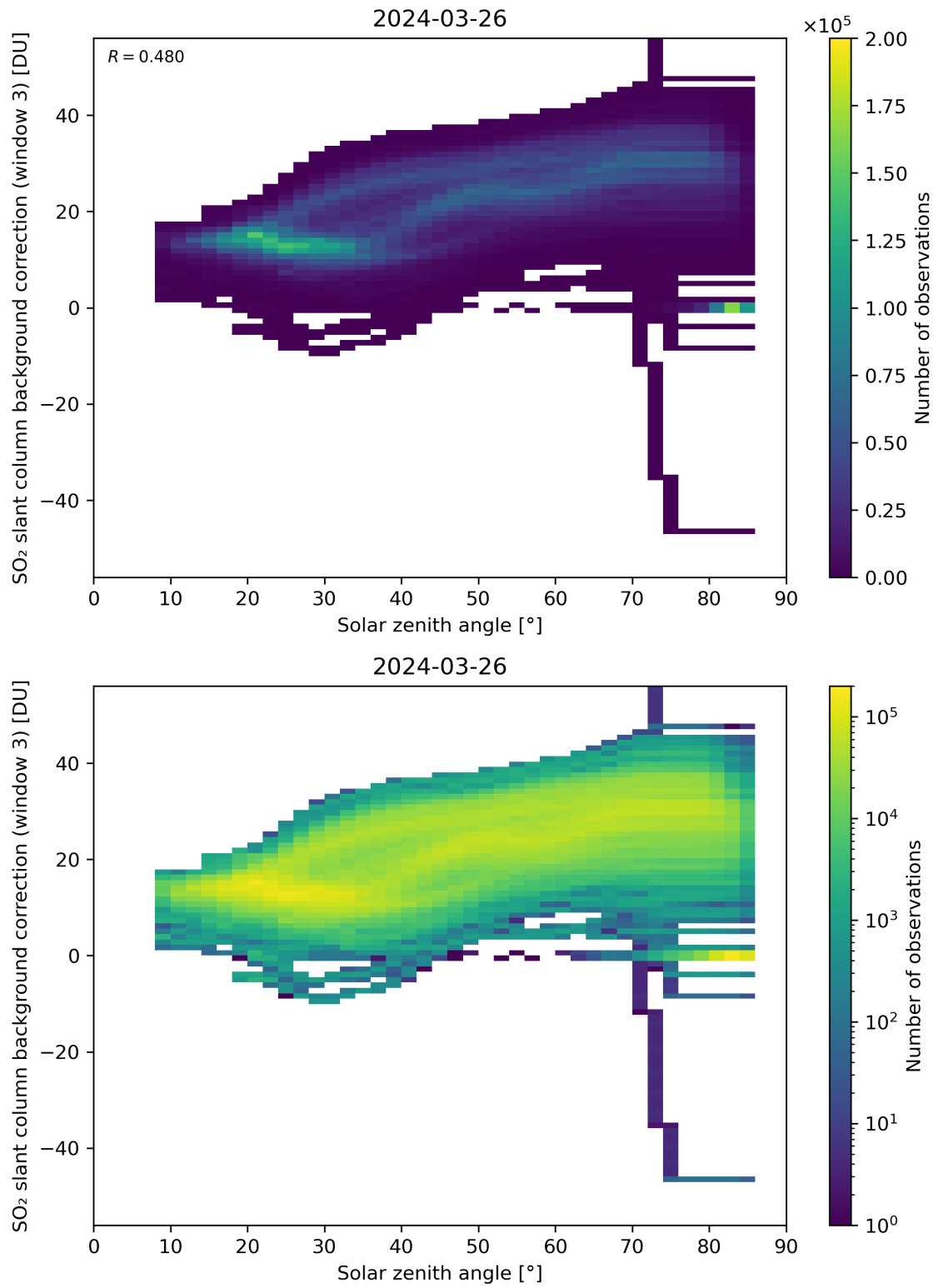
Figure 160: Scatter density plot of “Solar zenith angle” against “SO 2 slant column background correction (window 3)” for 2024-03-25 to 2024-03-27.
