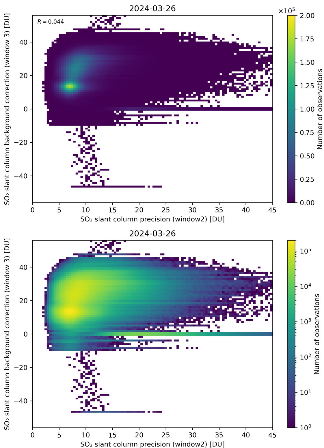
Figure 242: Scatter density plot of “SO 2 slant column precision (window2)” against “SO 2 slant column background correction (window 3)” for 2024-03-25 to 2024-03-27.
