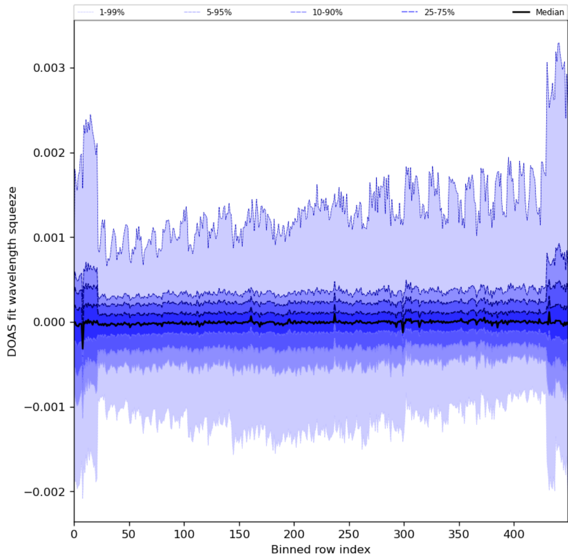
Figure 92: Along track statistics of “DOAS fit wavelength squeeze” for 2024-03-25 to 2024-03-27
