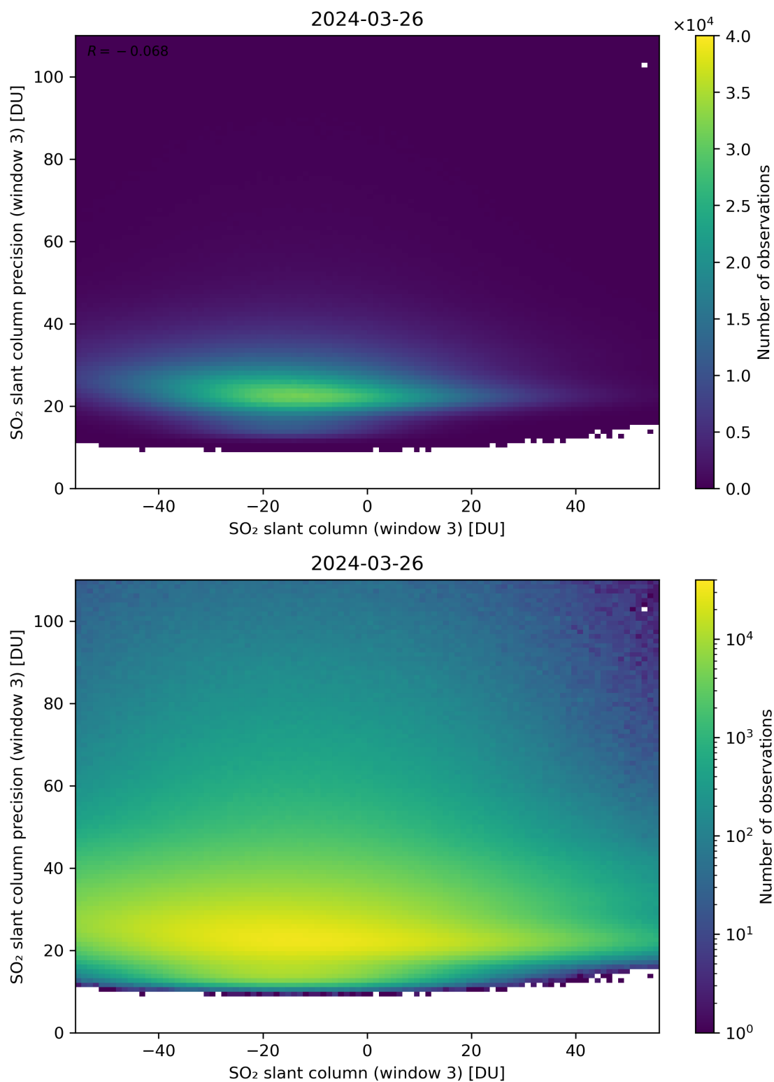
Figure 267: Scatter density plot of “SO 2 slant column (window 3)” against “SO 2 slant column precision (window 3)” for 2024-03-25 to 2024-03-27.
