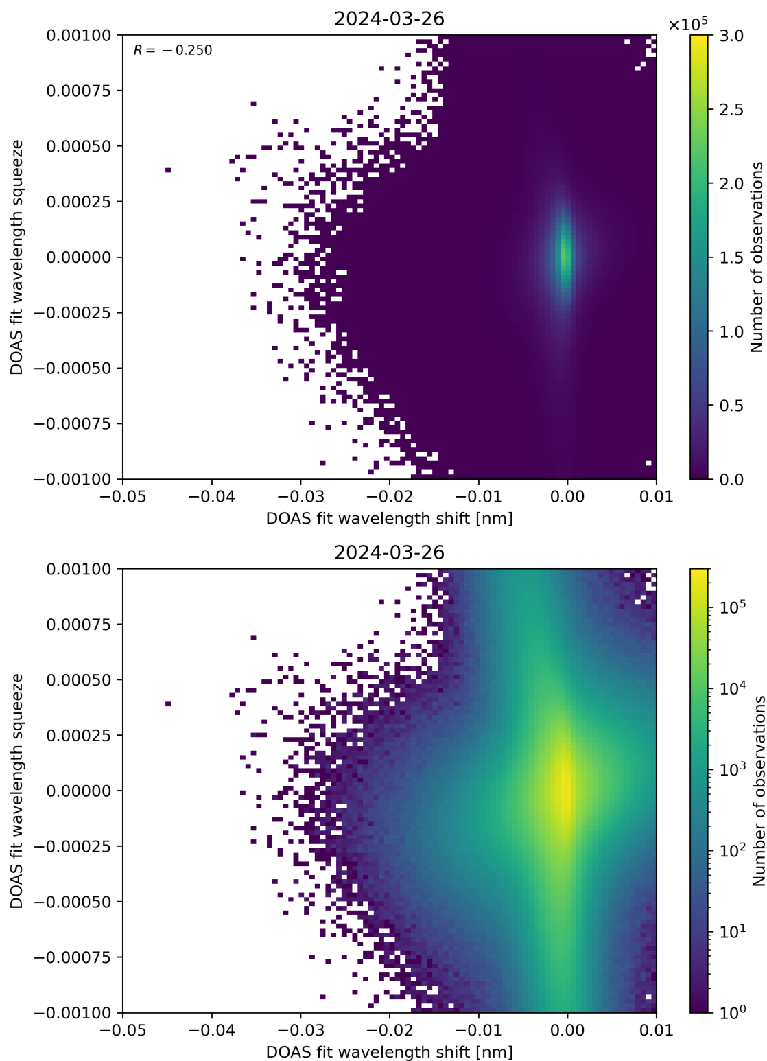
Figure 127: Scatter density plot of “DOAS fit wavelength shift” against “DOAS fit wavelength squeeze” for 2024-03-25 to 2024-03-27.
