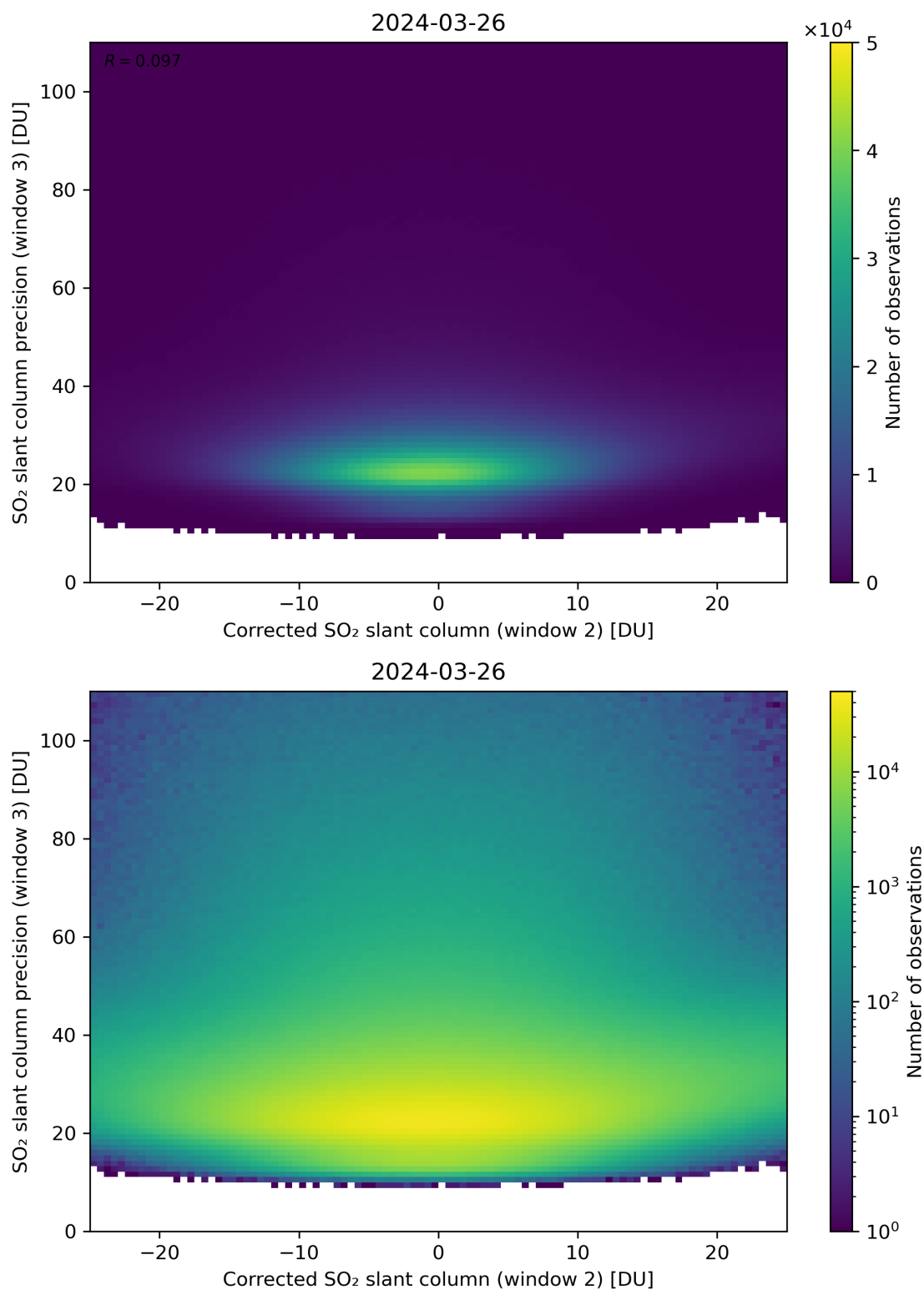
Figure 202: Scatter density plot of “Corrected SO 2 slant column (window 2)” against “SO 2 slant column precision (window 3)” for 2024-03-25 to 2024-03-27.
