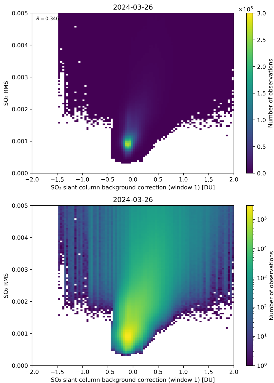
Figure 102: Scatter density plot of “SO 2 slant column background correction (window 1)” against “SO 2 RMS” for 2024-03-25 to 2024-03-27.
