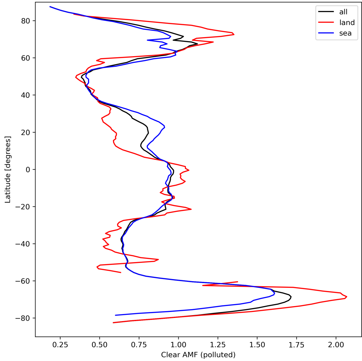
Figure 50: Zonal average of “Clear AMF (polluted)” for 2024-03-25 to 2024-03-27.
