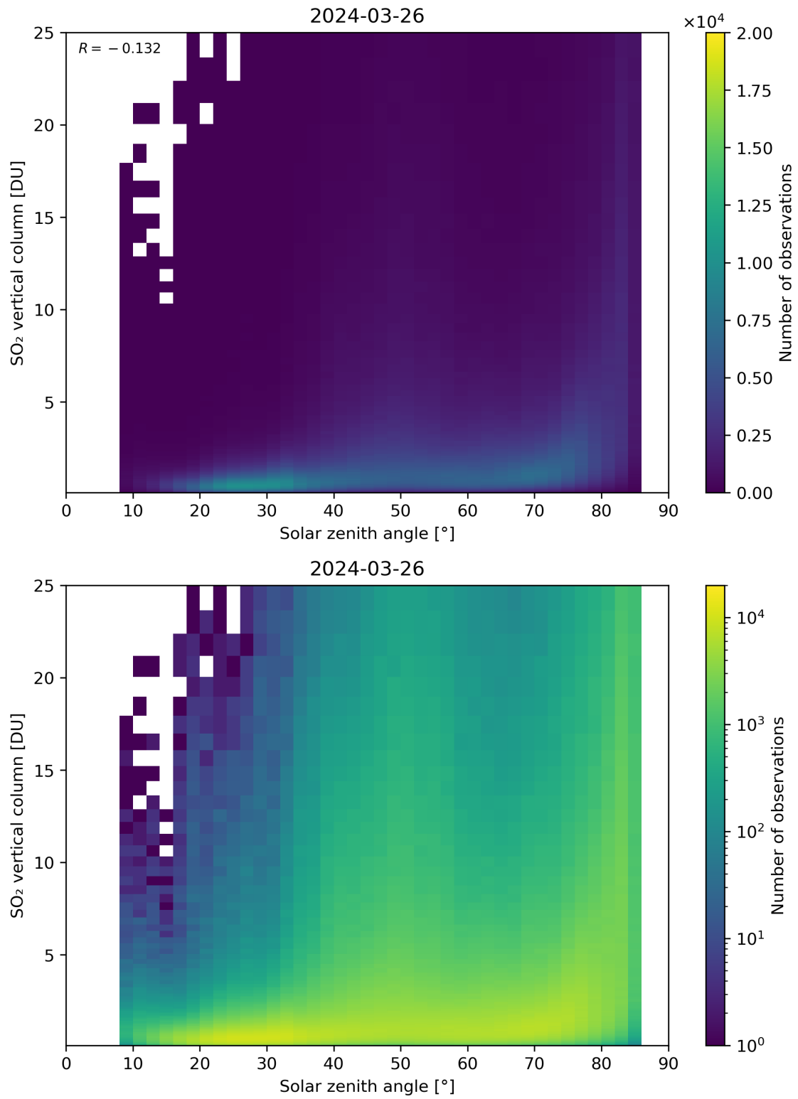
Figure 176: Scatter density plot of “Solar zenith angle” against “SO 2 vertical column” for 2024-03-25 to 2024-03-27.
