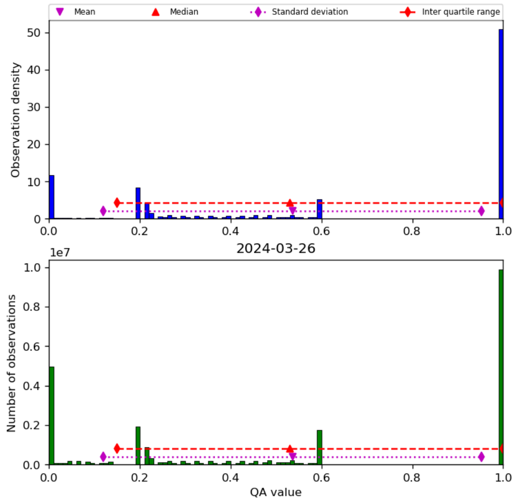
Figure 52: Histogram of “QA value” for 2024-03-25 to 2024-03-27
