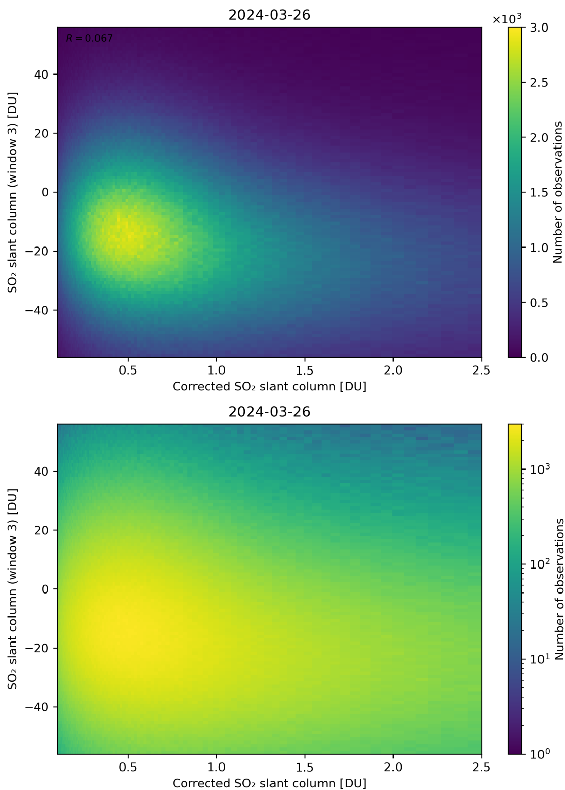
Figure 190: Scatter density plot of “Corrected SO 2 slant column” against “SO 2 slant column (window 3)” for 2024-03-25 to 2024-03-27.
