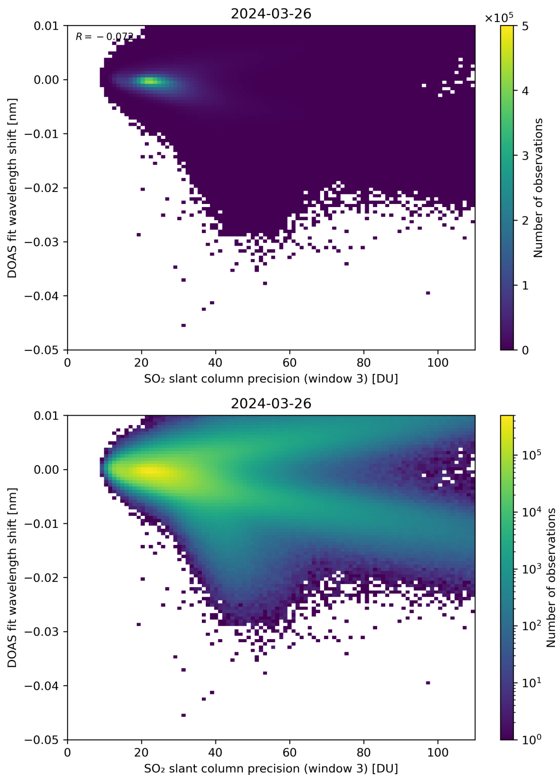
Figure 258: Scatter density plot of “SO 2 slant column precision (window 3)” against “DOAS fit wavelength shift” for 2024-03-25 to 2024-03-27.
