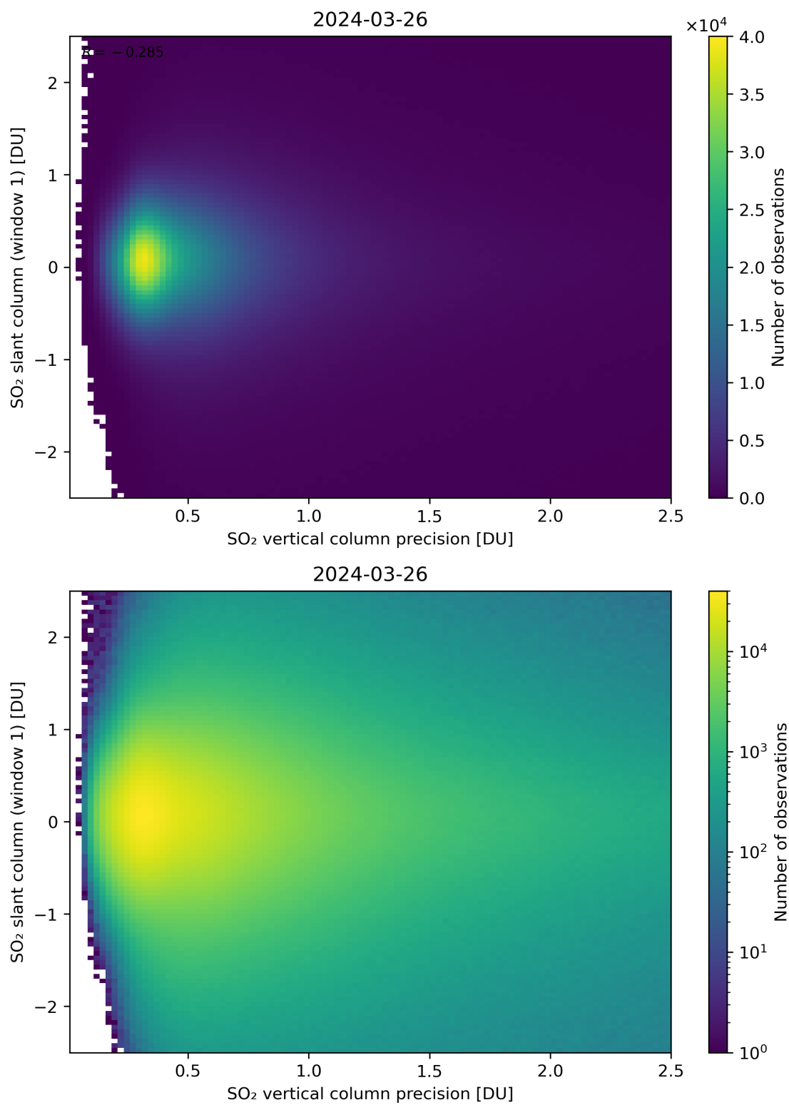
Figure 289: Scatter density plot of “SO 2 vertical column precision” against “SO 2 slant column (window 1)” for 2024-03-25 to 2024-03-27.
