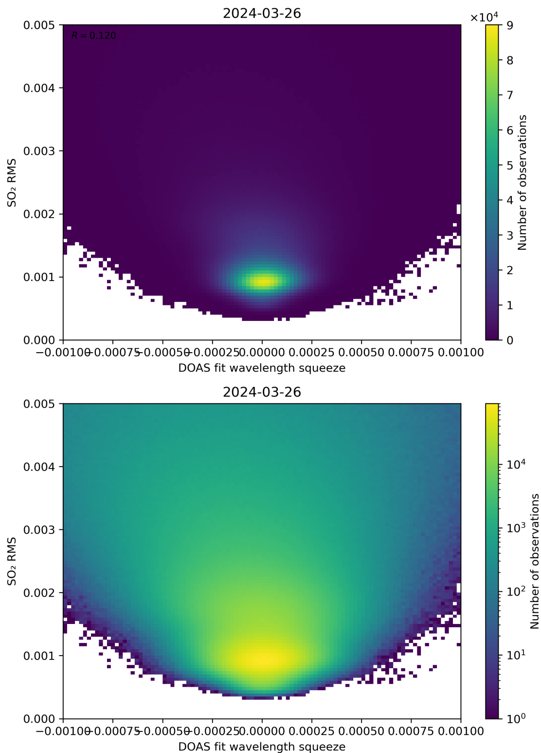
Figure 132: Scatter density plot of “DOAS fit wavelength squeeze” against “SO 2 RMS” for 2024-03-25 to 2024-03-27.
