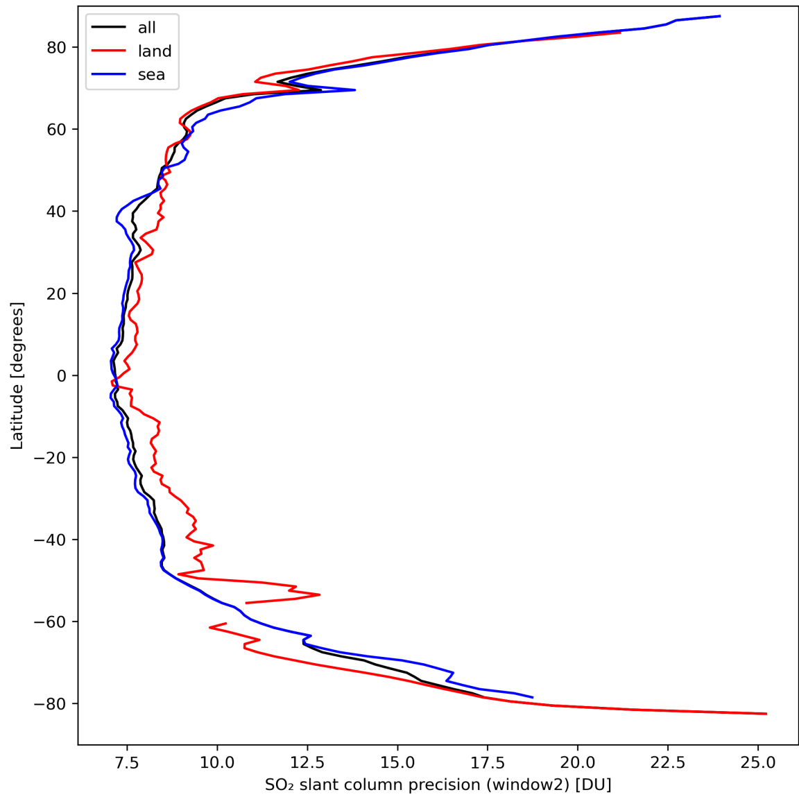
Figure 38: Zonal average of “SO 2 slant column precision (window2)” for 2024-03-25 to 2024-03-27.
