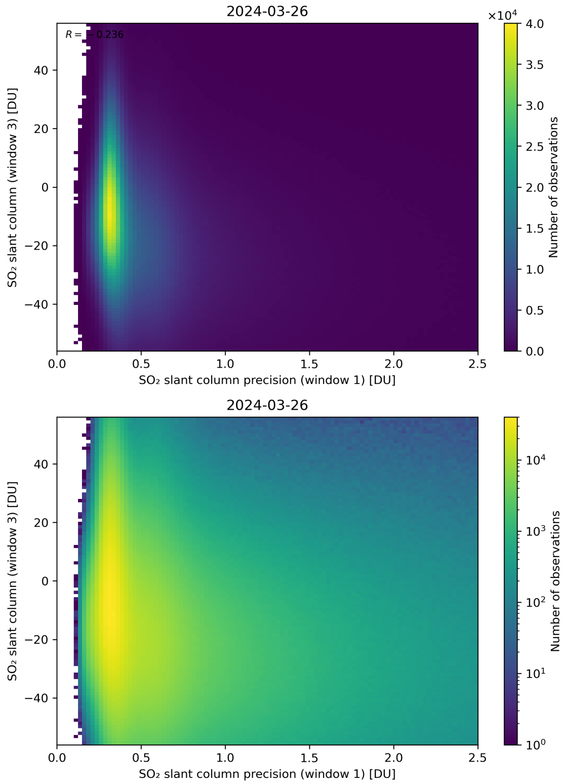
Figure 228: Scatter density plot of “SO 2 slant column precision (window 1)” against “SO 2 slant column (window 3)” for 2024-03-25 to 2024-03-27.
