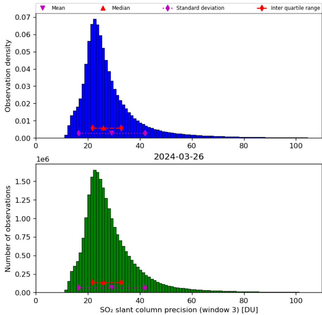
Figure 65: Histogram of “SO 2 slant column precision (window 3)” for 2024-03-25 to 2024-03-27
