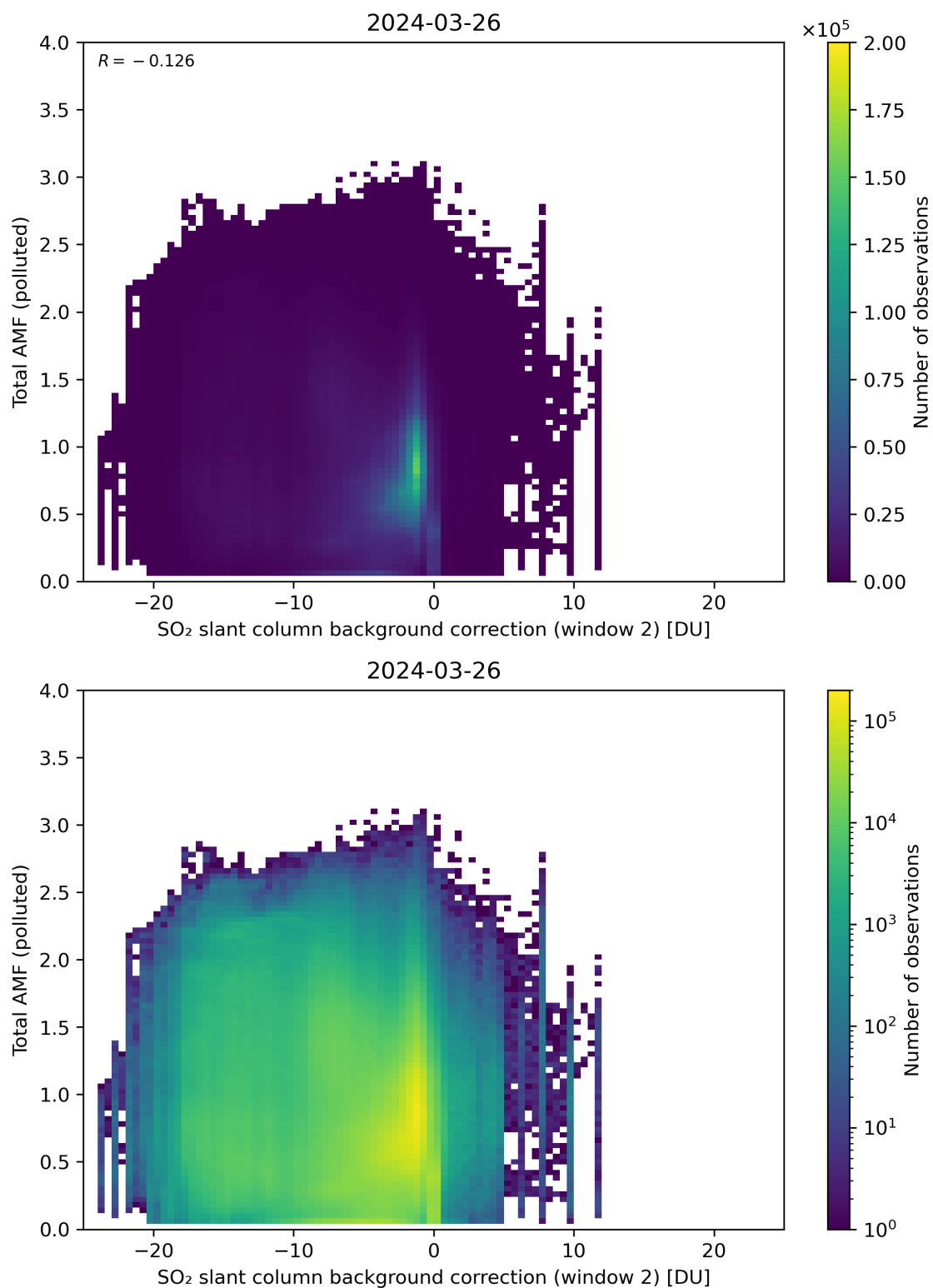
Figure 119: Scatter density plot of “SO 2 slant column background correction (window 2)” against “Total AMF (polluted)” for 2024-03-25 to 2024-03-27.
