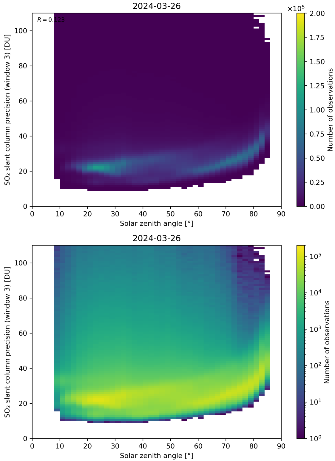
Figure 173: Scatter density plot of “Solar zenith angle” against “SO 2 slant column precision (window 3)” for 2024-03-25 to 2024-03-27.
