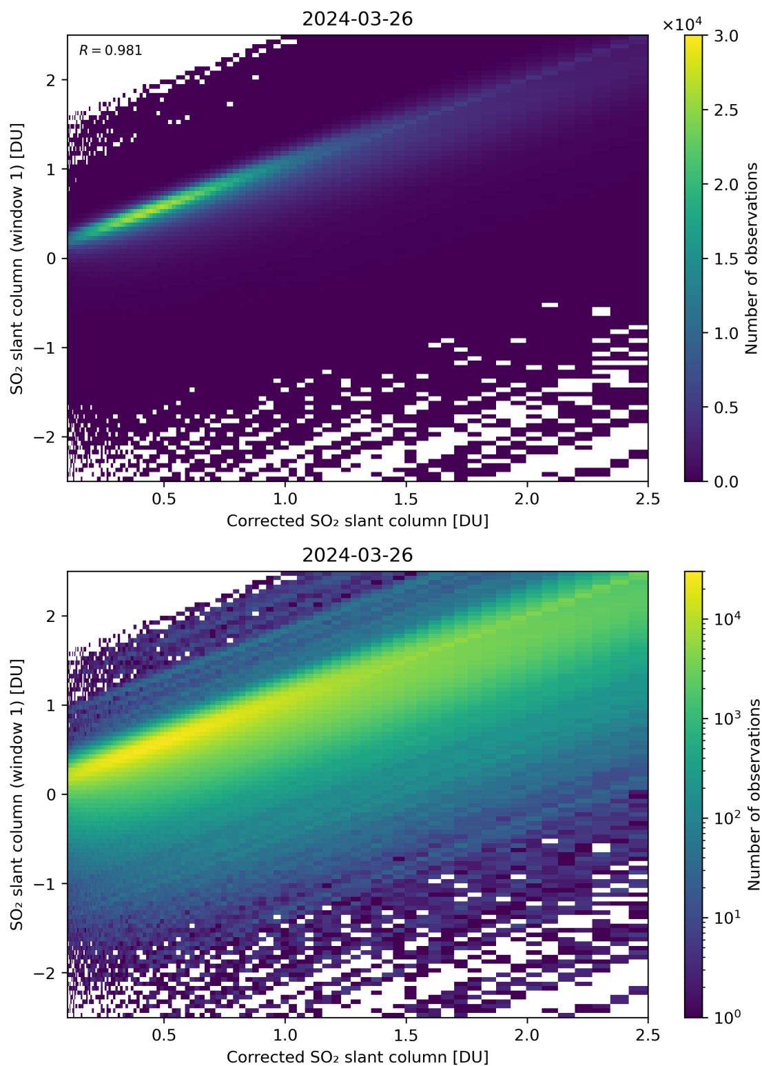
Figure 187: Scatter density plot of “Corrected SO 2 slant column” against “SO 2 slant column (window 1)” for 2024-03-25 to 2024-03-27.
