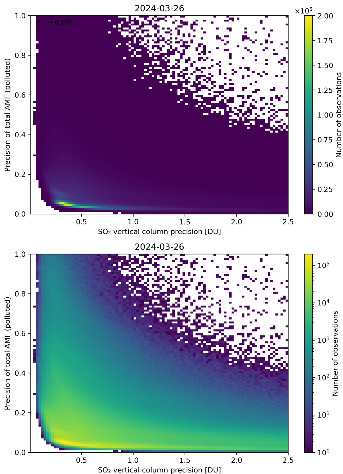
Figure 295: Scatter density plot of “SO 2 vertical column precision” against “Precision of total AMF (polluted)” for 2024-03-25 to 2024-03-27.
