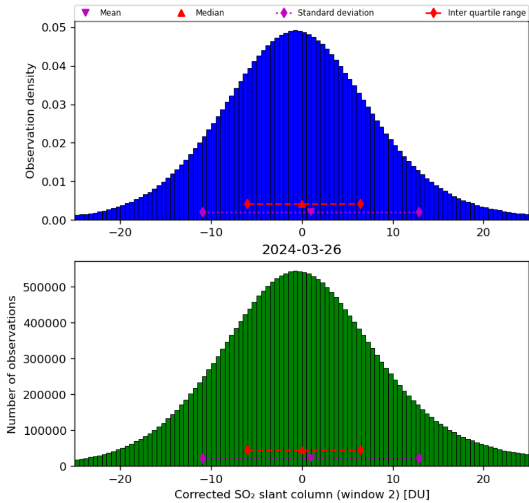
Figure 62: Histogram of “Corrected SO 2 slant column (window 2)” for 2024-03-25 to 2024-03-27
