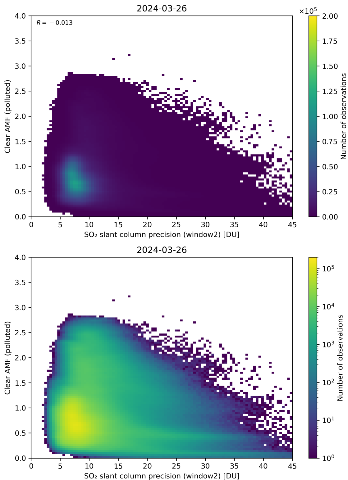
Figure 246: Scatter density plot of “SO 2 slant column precision (window2)” against “Clear AMF (polluted)” for 2024-03-25 to 2024-03-27.
