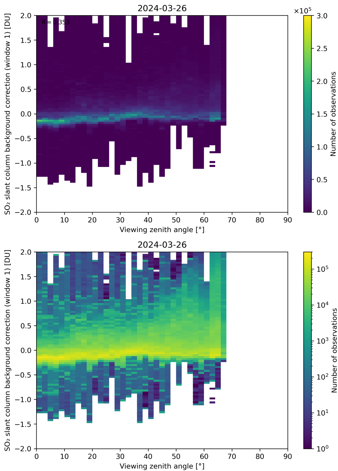
Figure 308: Scatter density plot of “Viewing zenith angle” against “SO 2 slant column background correction (window 1)” for 2024-03-25 to 2024-03-27.
