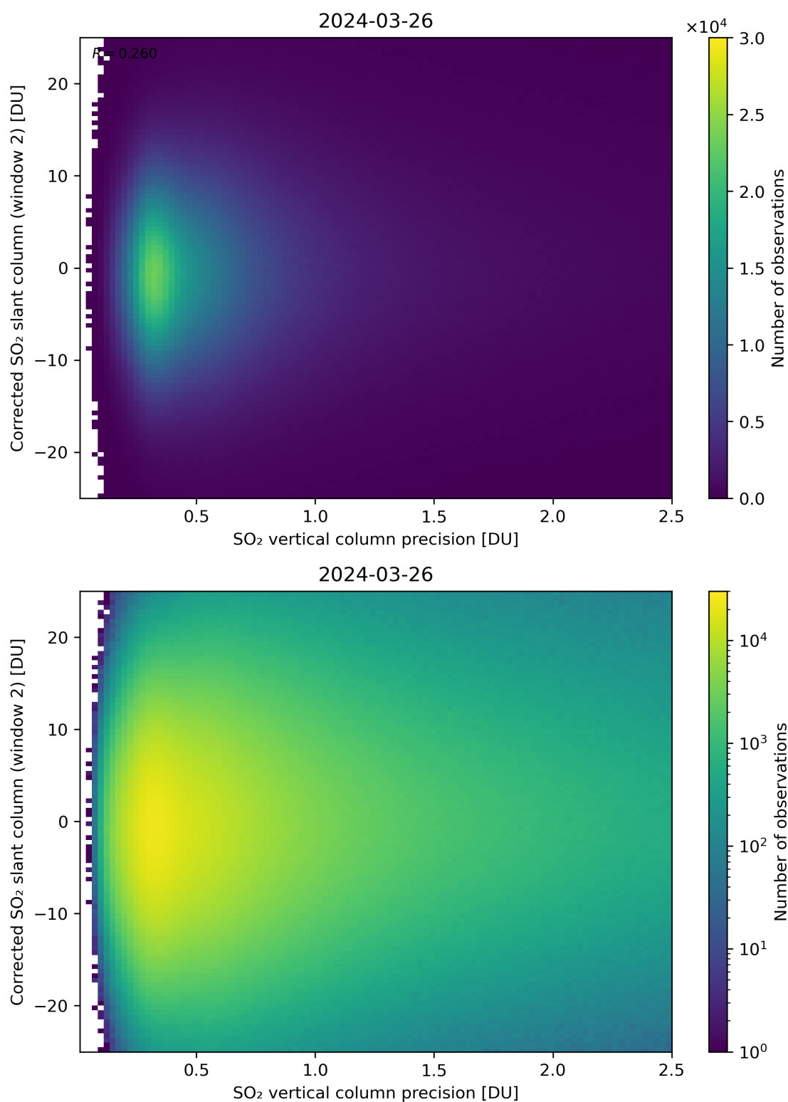
Figure 287: Scatter density plot of “SO 2 vertical column precision” against “Corrected SO 2 slant column (window 2)” for 2024-03-25 to 2024-03-27.
