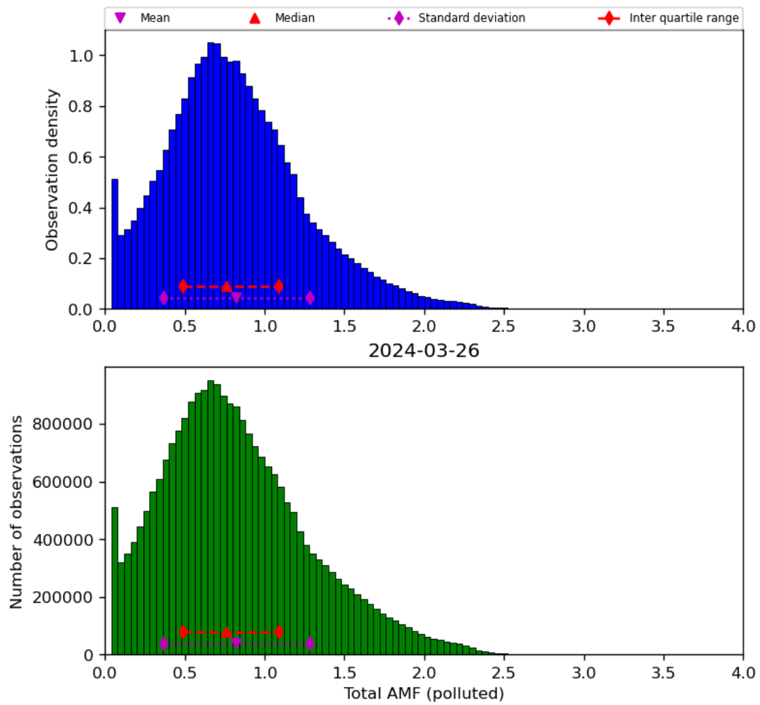
Figure 71: Histogram of “Total AMF (polluted)” for 2024-03-25 to 2024-03-27
