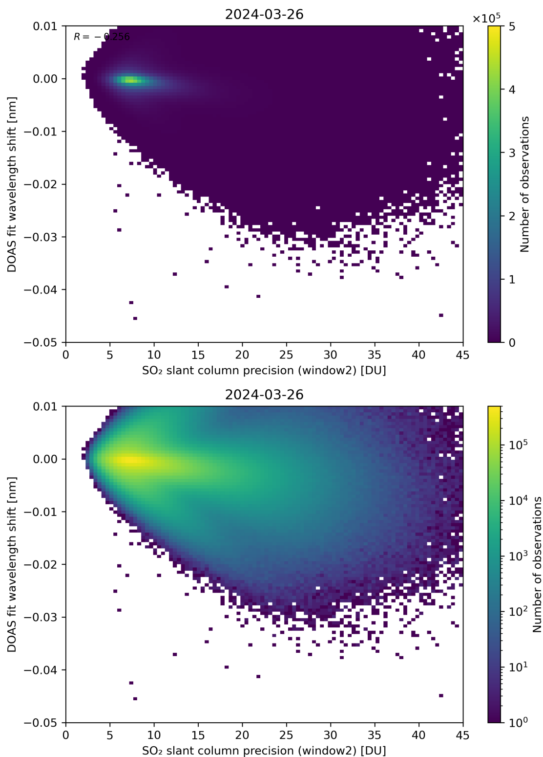
Figure 243: Scatter density plot of “SO 2 slant column precision (window2)” against “DOAS fit wavelength shift” for 2024-03-25 to 2024-03-27.
