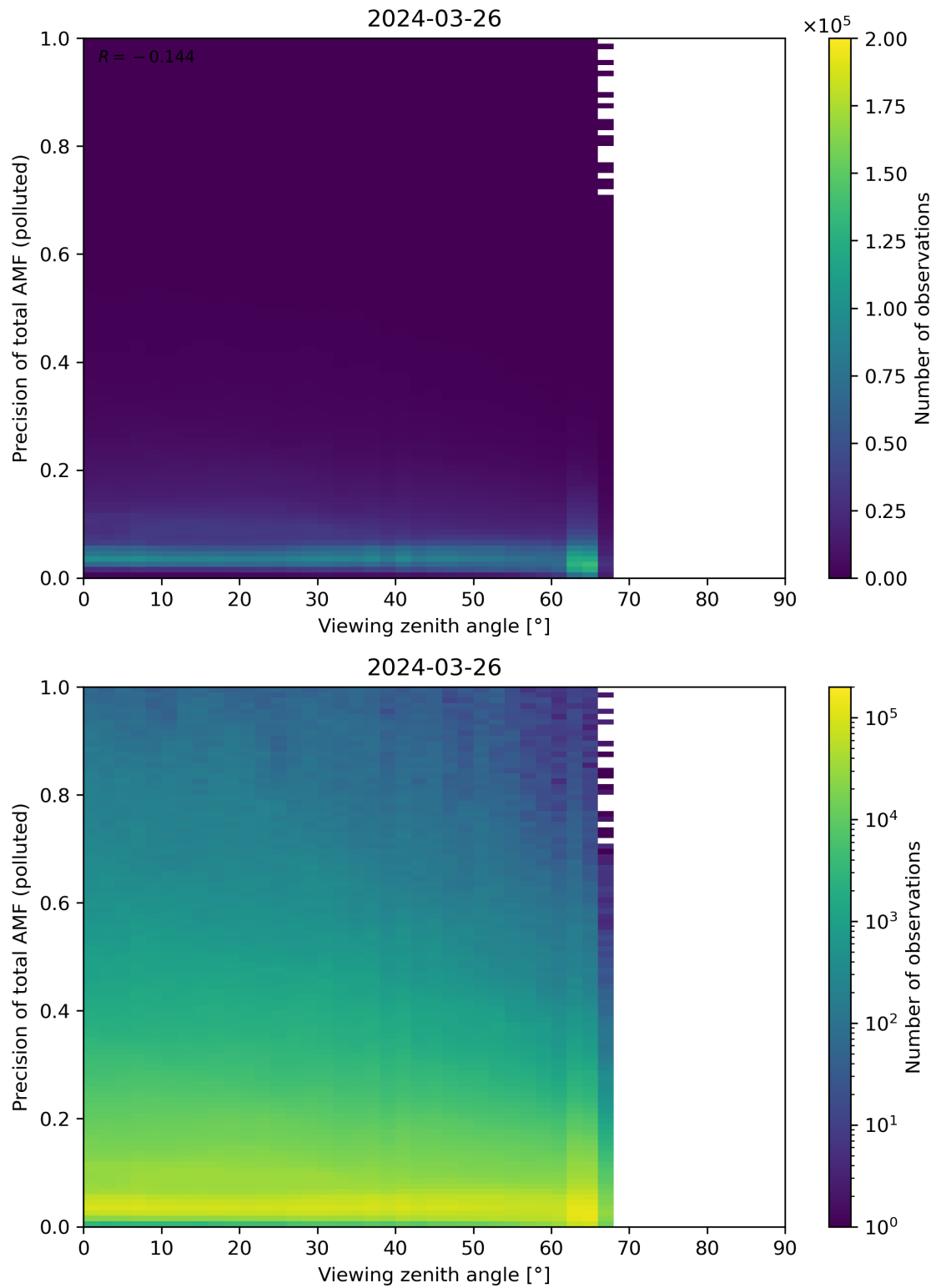
Figure 326: Scatter density plot of “Viewing zenith angle” against “Precision of total AMF (polluted)” for 2024-03-25 to 2024-03-27.
