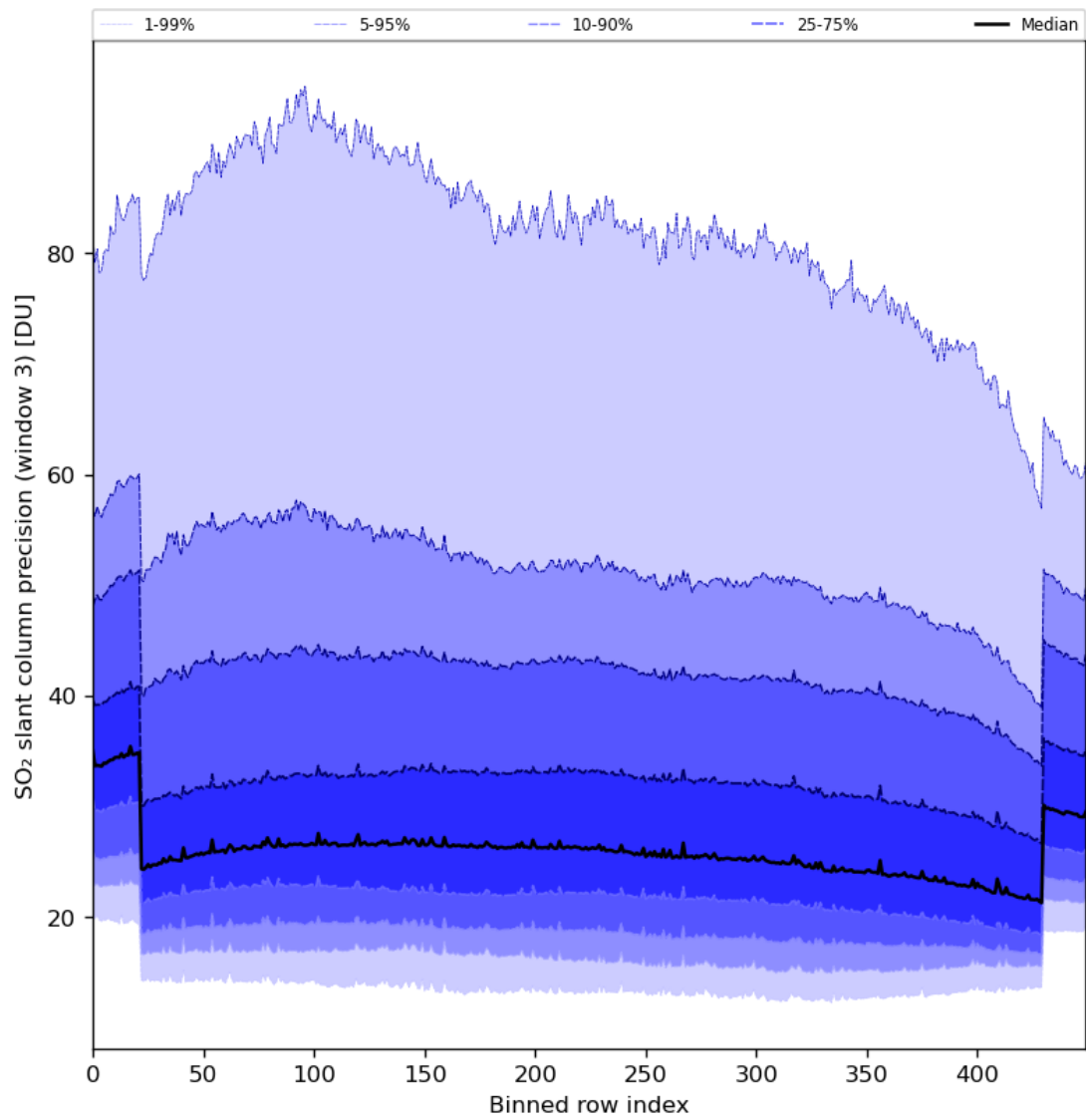
Figure 88: Along track statistics of “SO 2 slant column precision (window 3)” for 2024-03-25 to 2024-03-27
