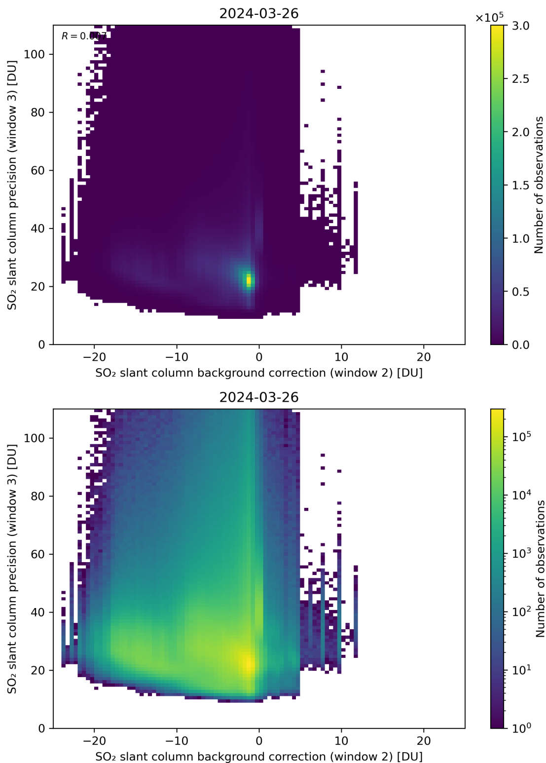
Figure 118: Scatter density plot of “SO 2 slant column background correction (window 2)” against “SO 2 slant column precision (window 3)” for 2024-03-25 to 2024-03-27.
