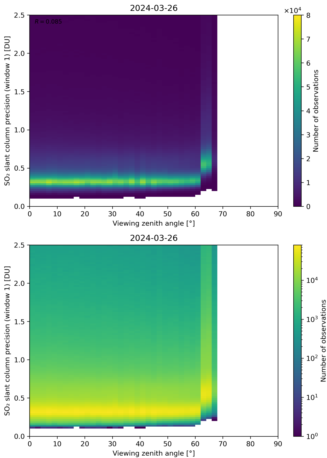
Figure 321: Scatter density plot of “Viewing zenith angle” against “SO 2 slant column precision (window 1)” for 2024-03-25 to 2024-03-27.
