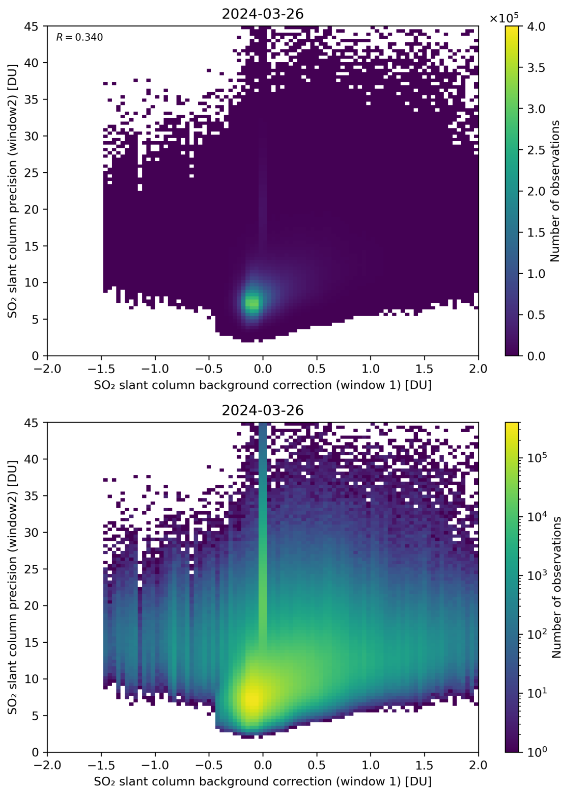
Figure 106: Scatter density plot of “SO 2 slant column background correction (window 1)” against “SO 2 slant column precision (window2)” for 2024-03-25 to 2024-03-27.
