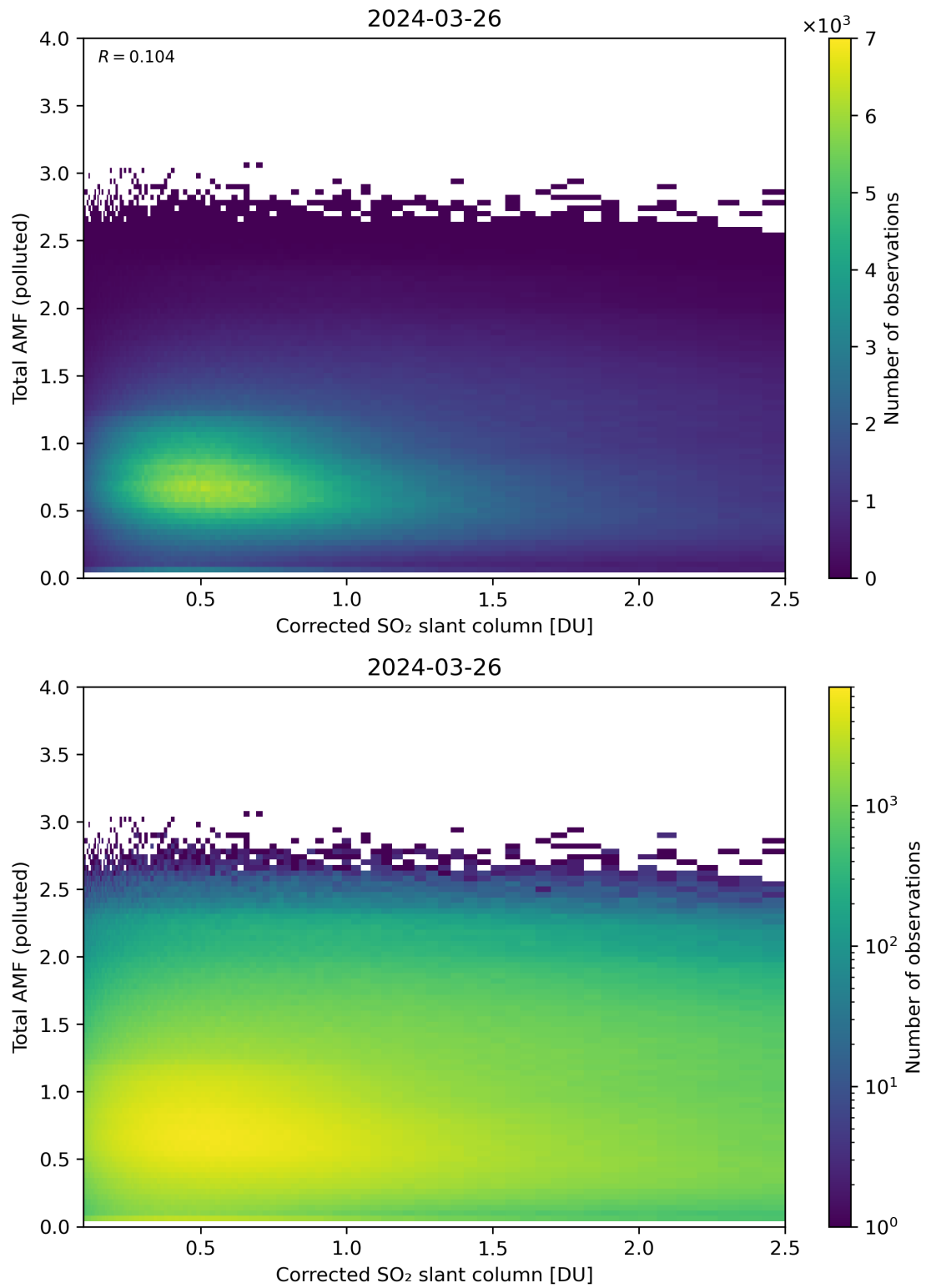
Figure 192: Scatter density plot of “Corrected SO 2 slant column” against “Total AMF (polluted)” for 2024-03-25 to 2024-03-27.
