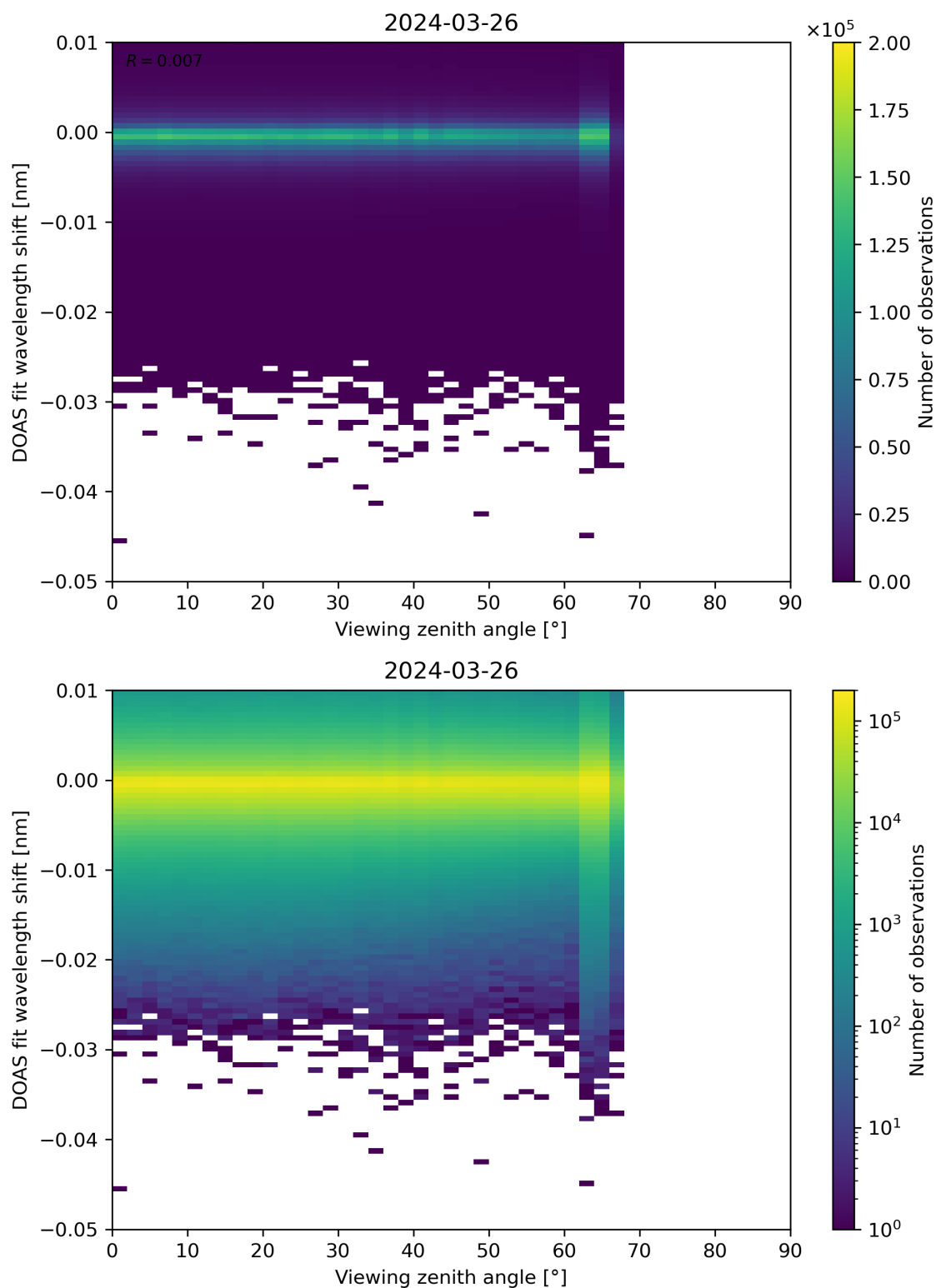
Figure 311: Scatter density plot of “Viewing zenith angle” against “DOAS fit wavelength shift” for 2024-03-25 to 2024-03-27.
