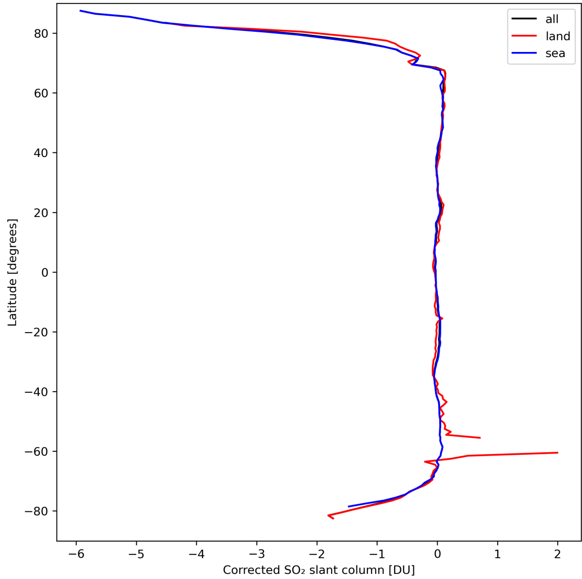
Figure 32: Zonal average of “Corrected SO 2 slant column” for 2024-03-25 to 2024-03-27.
