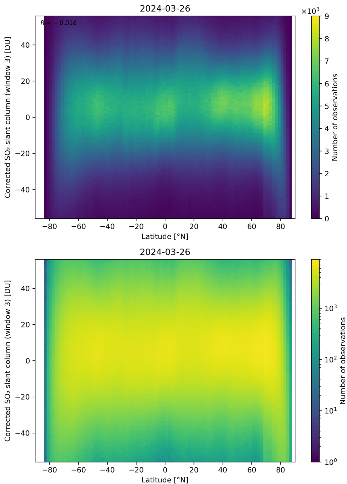
Figure 148: Scatter density plot of “Latitude” against “Corrected SO 2 slant column (window 3)” for 2024-03-25 to 2024-03-27.
