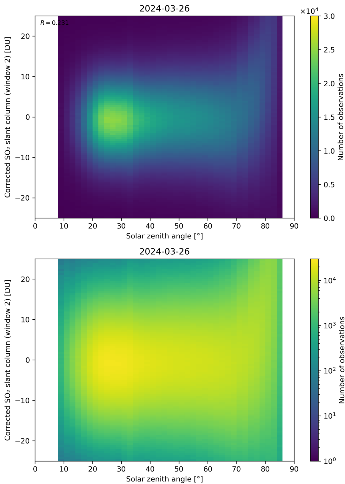
Figure 167: Scatter density plot of “Solar zenith angle” against “Corrected SO 2 slant column (window 2)” for 2024-03-25 to 2024-03-27.
