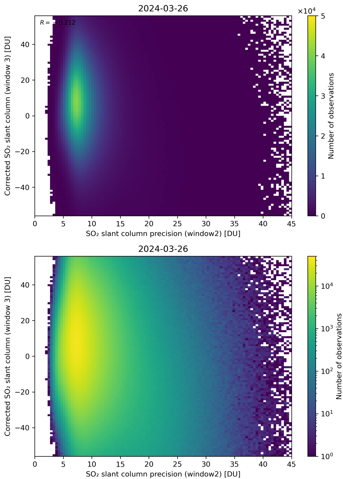
Figure 248: Scatter density plot of “SO 2 slant column precision (window2)” against “Corrected SO 2 slant column (window 3)” for 2024-03-25 to 2024-03-27.
