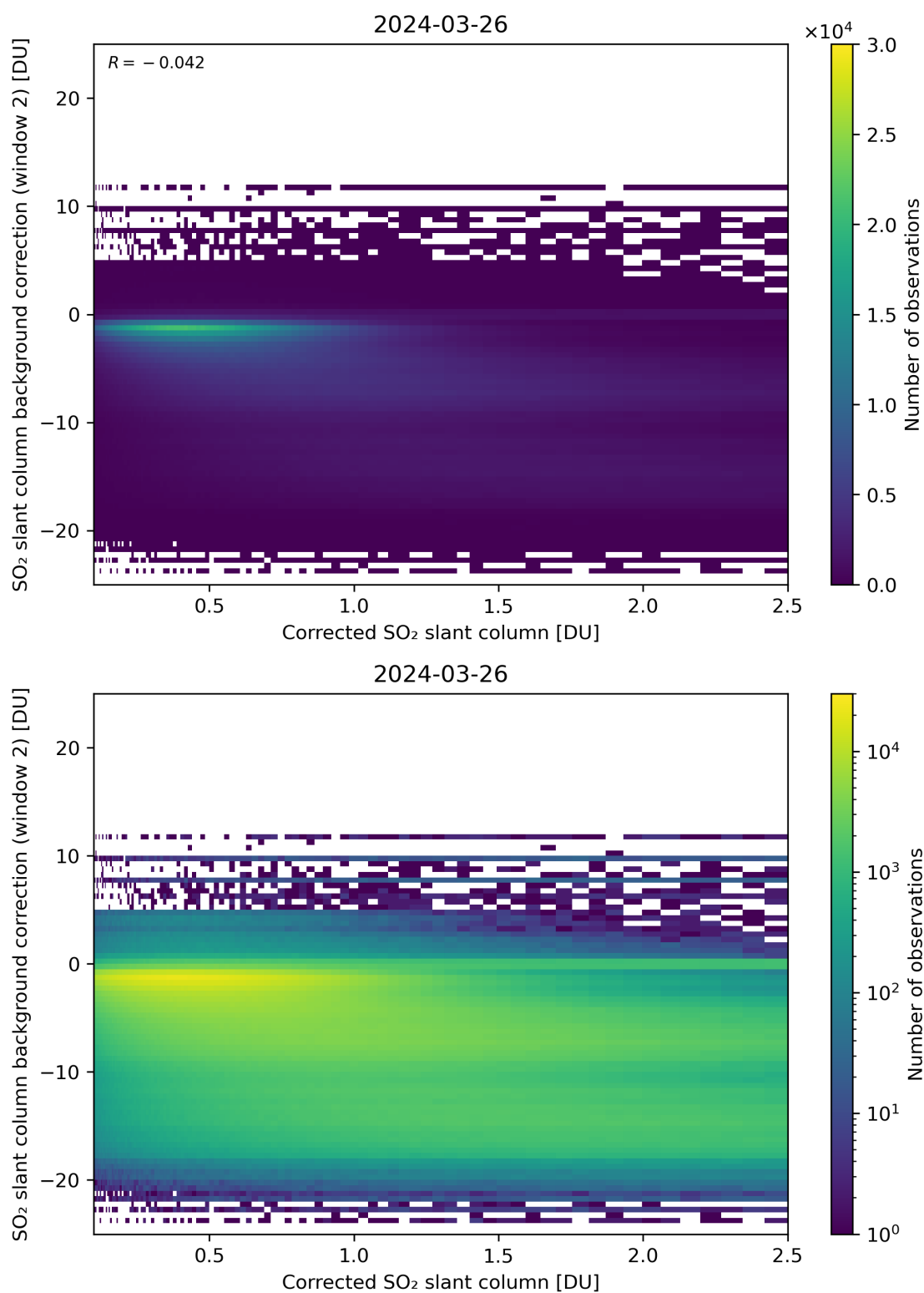
Figure 179: Scatter density plot of “Corrected SO 2 slant column” against “SO 2 slant column background correction (window 2)” for 2024-03-25 to 2024-03-27.
