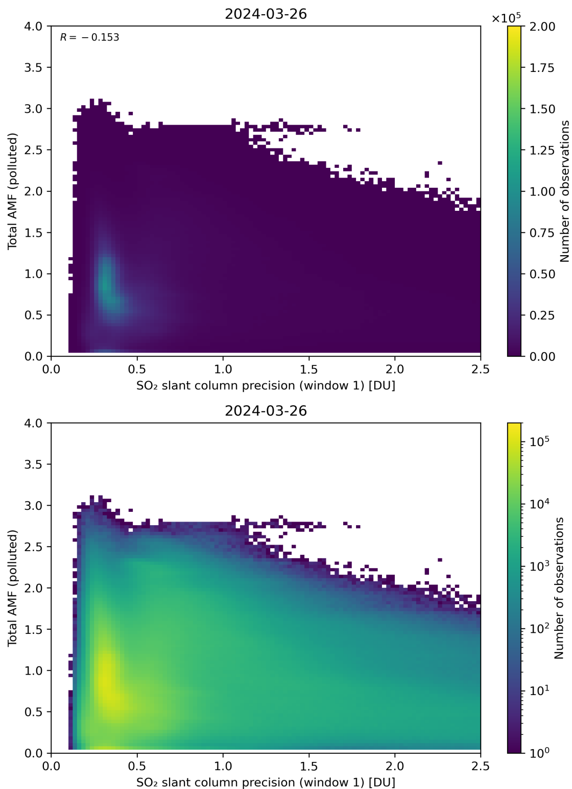
Figure 230: Scatter density plot of “SO 2 slant column precision (window 1)” against “Total AMF (polluted)” for 2024-03-25 to 2024-03-27.
