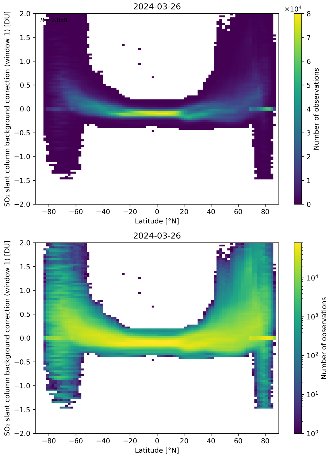
Figure 139: Scatter density plot of “Latitude” against “SO 2 slant column background correction (window 1)” for 2024-03-25 to 2024-03-27.
