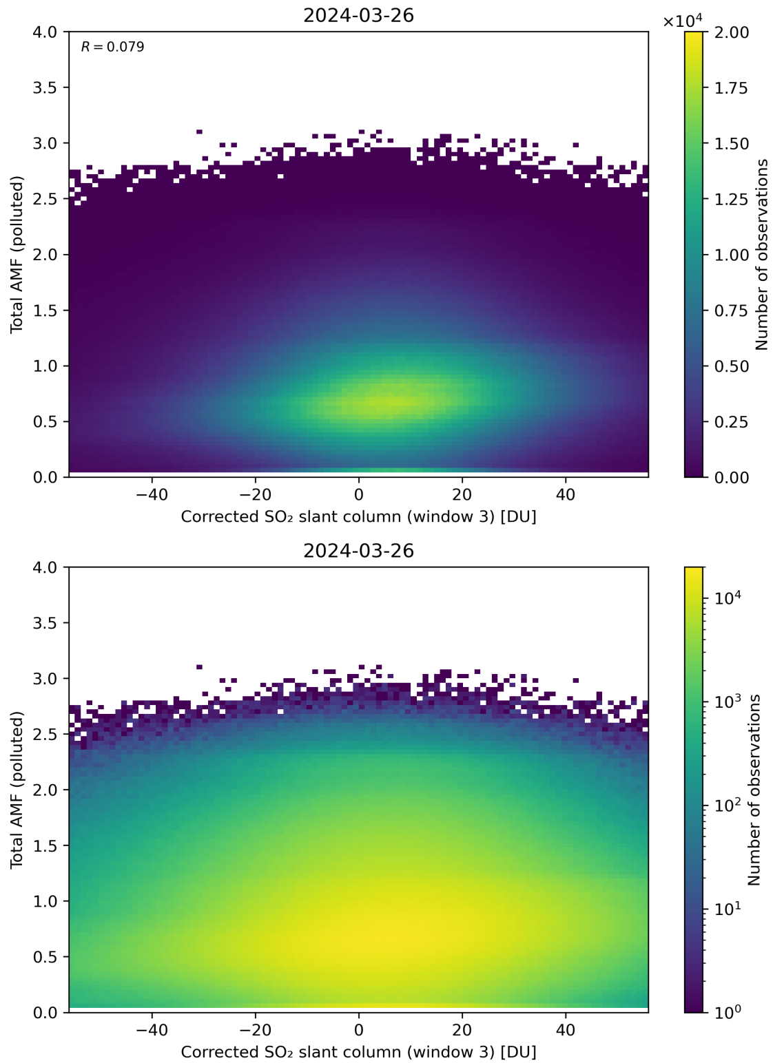
Figure 210: Scatter density plot of “Corrected SO 2 slant column (window 3)” against “Total AMF (polluted)” for 2024-03-25 to 2024-03-27.
