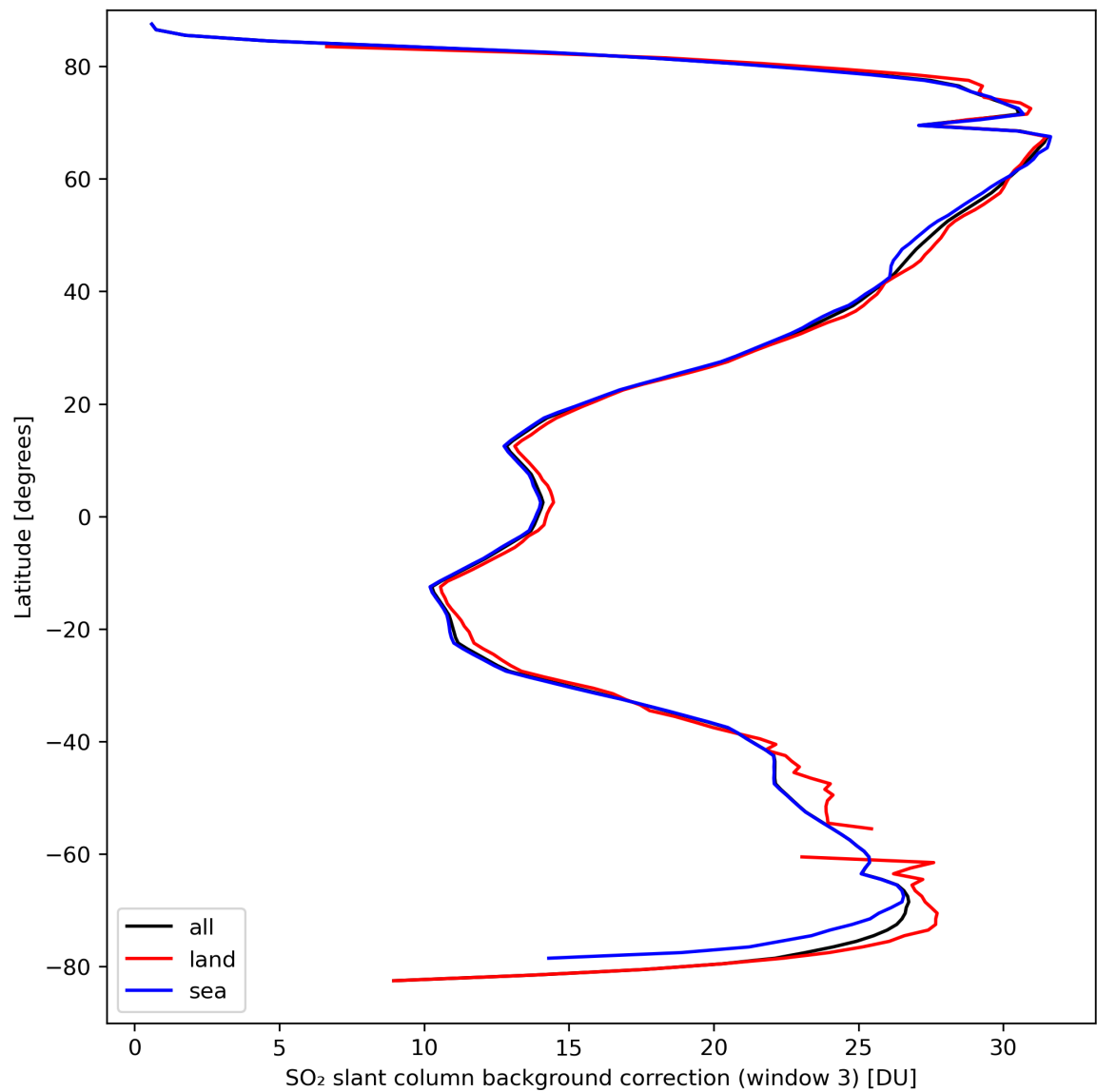
Figure 44: Zonal average of “SO 2 slant column background correction (window 3)” for 2024-03-25 to 2024-03-27.
