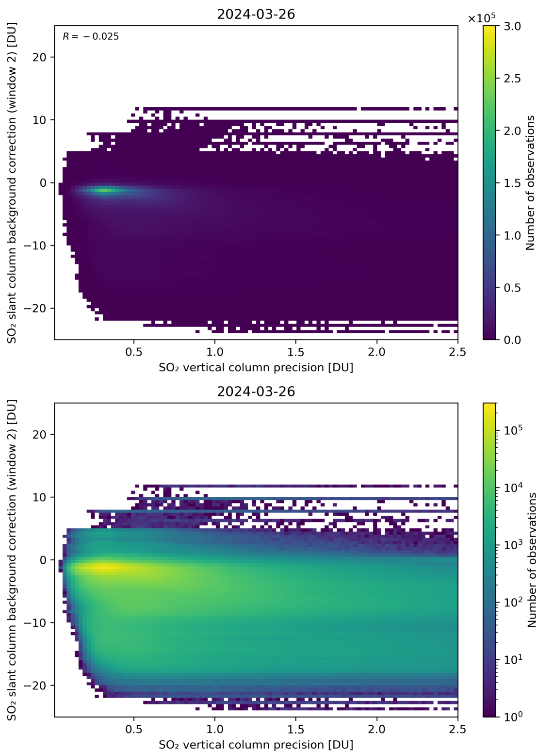
Figure 280: Scatter density plot of “SO 2 vertical column precision” against “SO 2 slant column background correction (window 2)” for 2024-03-25 to 2024-03-27.
