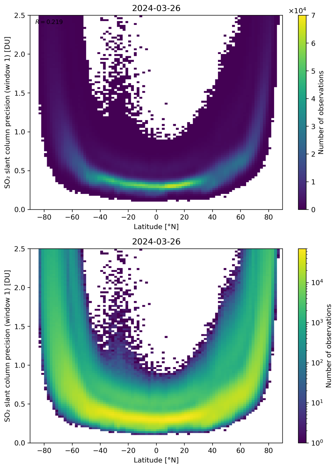
Figure 150: Scatter density plot of “Latitude” against “SO 2 slant column precision (window 1)” for 2024-03-25 to 2024-03-27.
