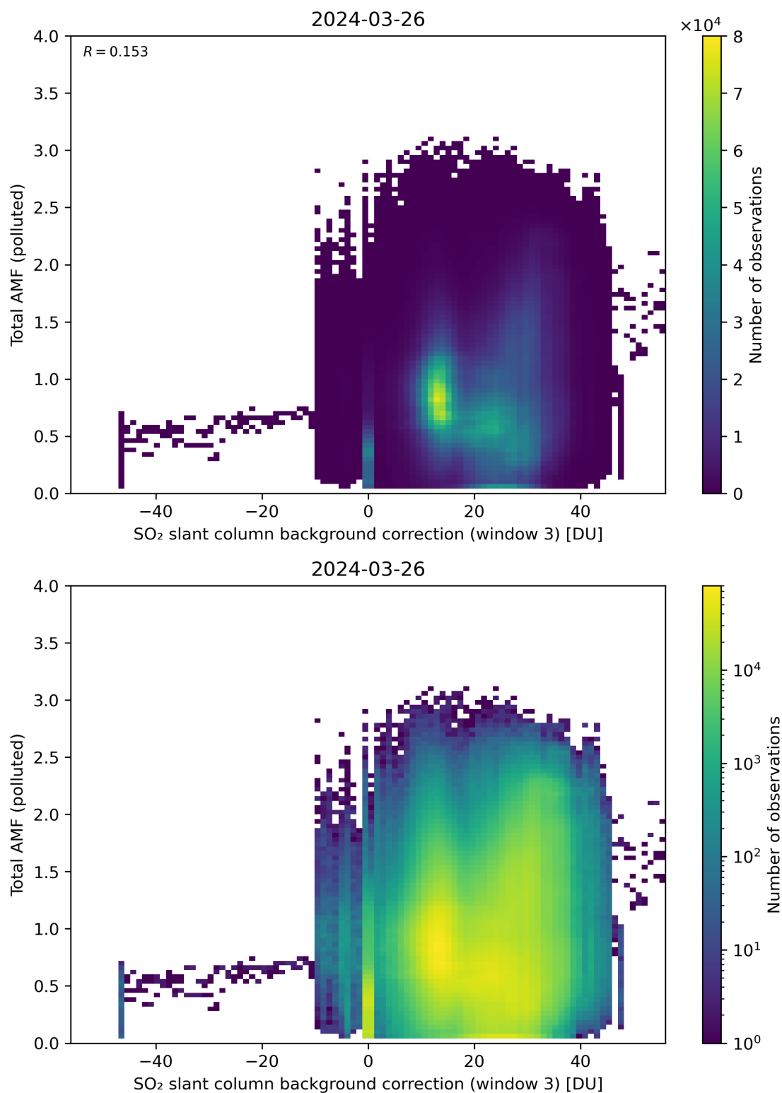
Figure 125: Scatter density plot of “SO 2 slant column background correction (window 3)” against “Total AMF (polluted)” for 2024-03-25 to 2024-03-27.
