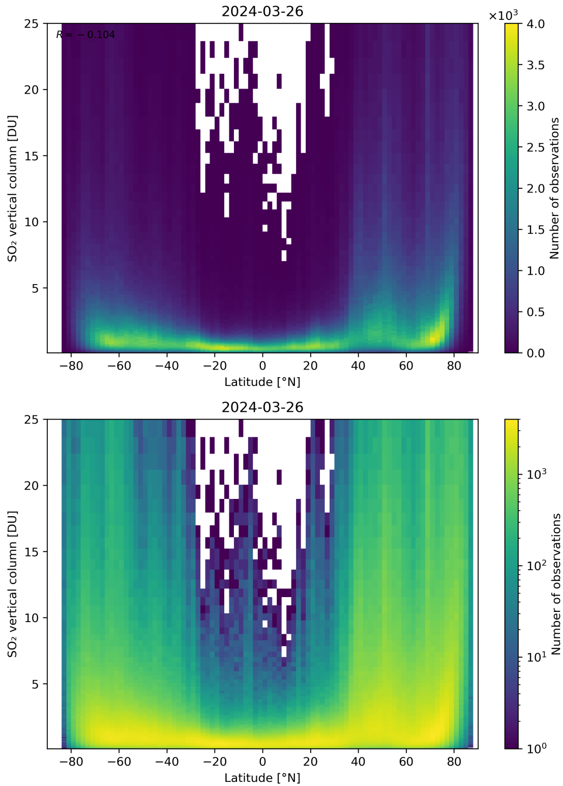
Figure 156: Scatter density plot of “Latitude” against “SO 2 vertical column” for 2024-03-25 to 2024-03-27.
