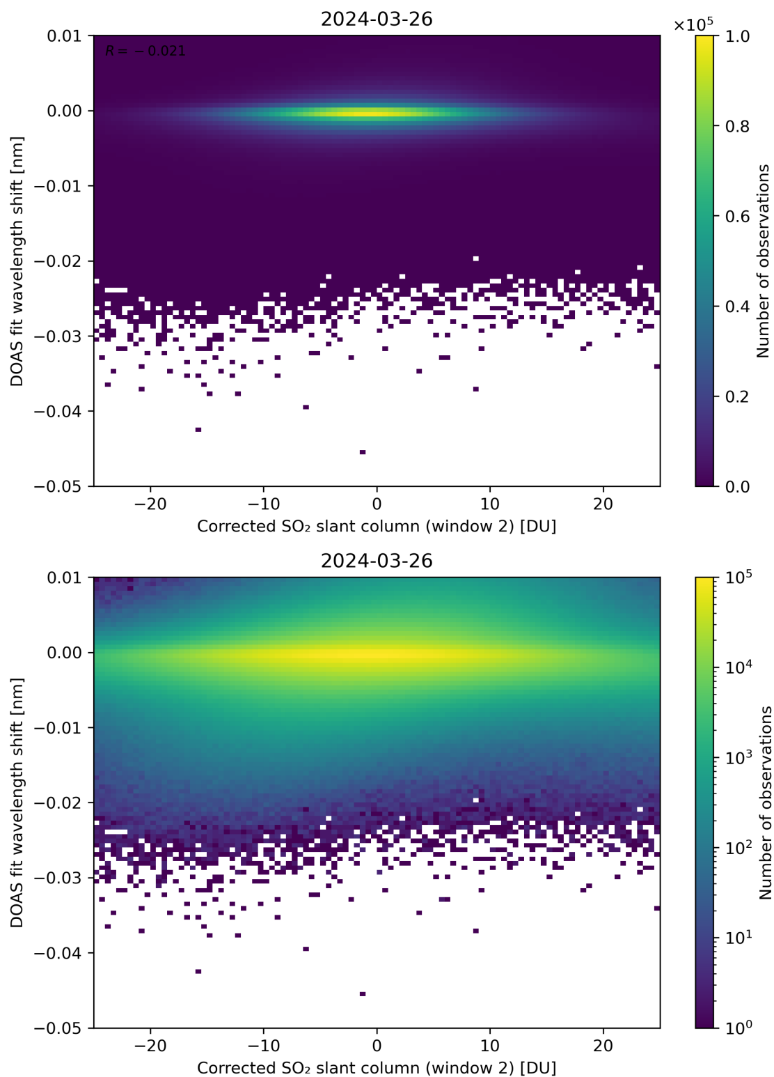
Figure 196: Scatter density plot of “Corrected SO 2 slant column (window 2)” against “DOAS fit wavelength shift” for 2024-03-25 to 2024-03-27.
