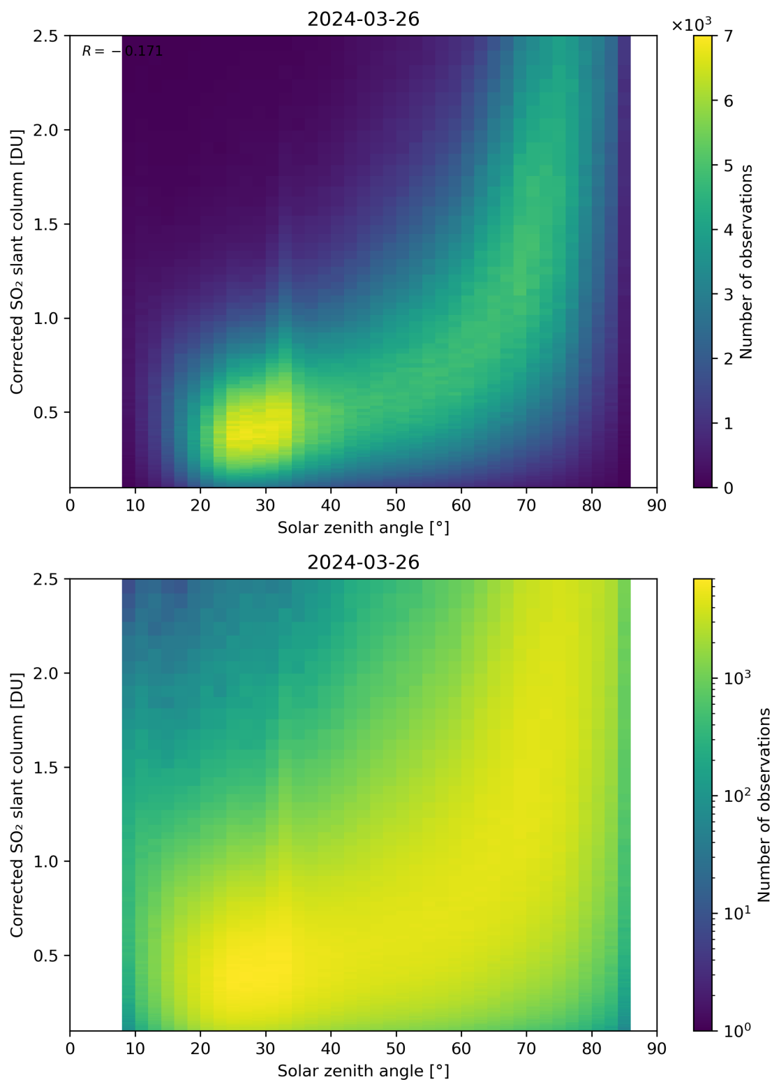
Figure 166: Scatter density plot of “Solar zenith angle” against “Corrected SO 2 slant column” for 2024-03-25 to 2024-03-27.
