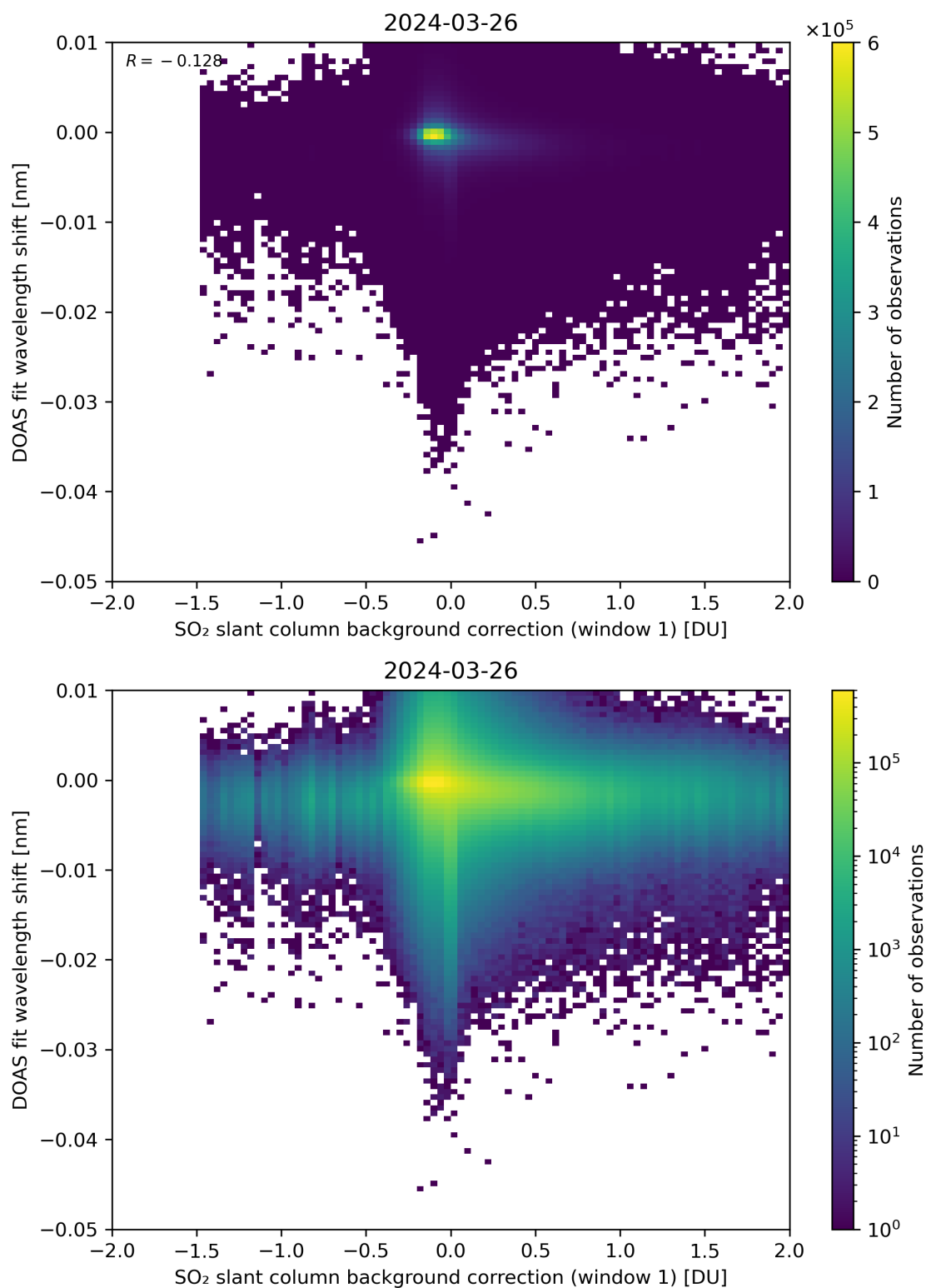
Figure 100: Scatter density plot of “SO 2 slant column background correction (window 1)” against “DOAS fit wavelength shift” for 2024-03-25 to 2024-03-27.
