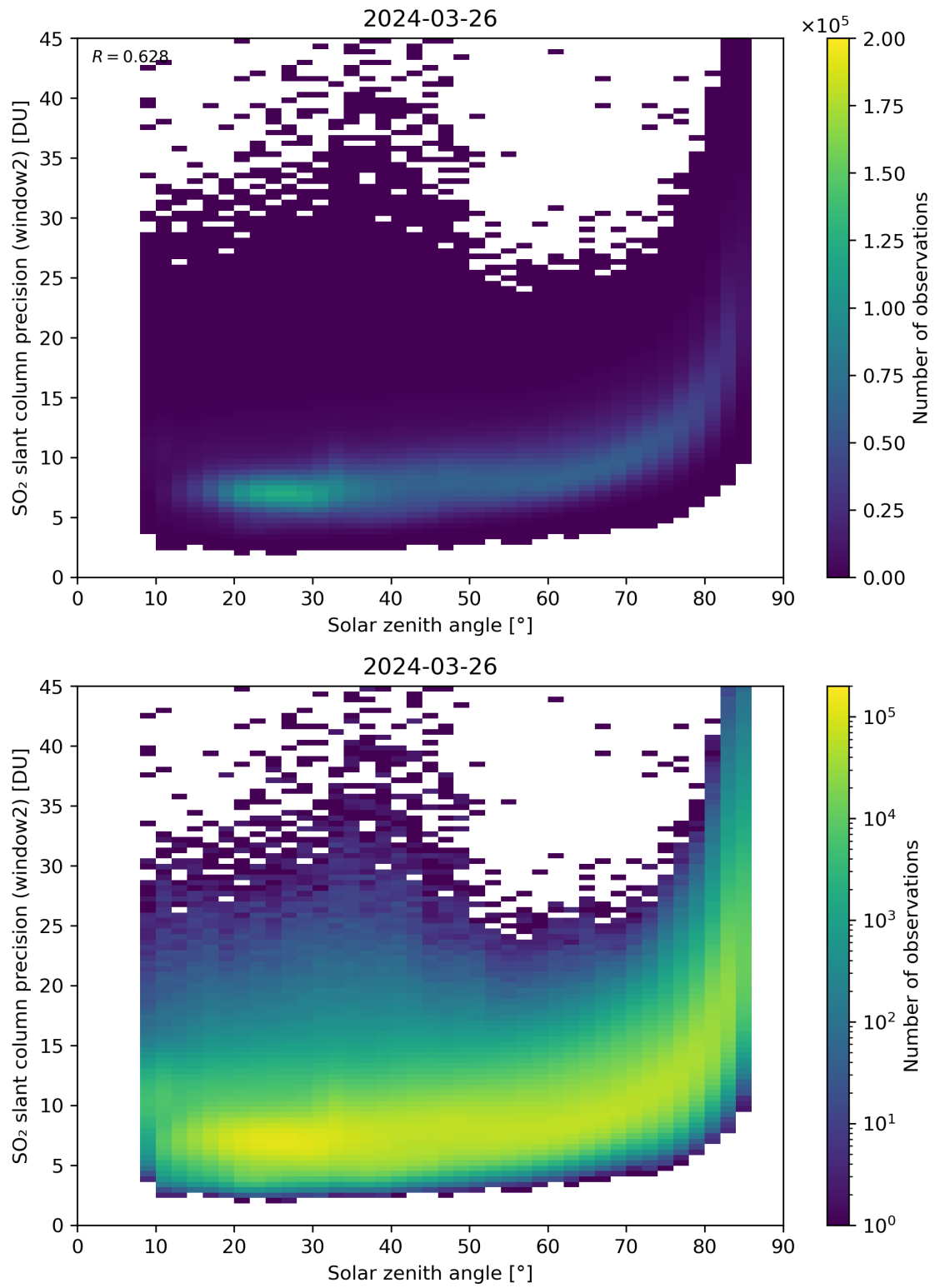
Figure 171: Scatter density plot of “Solar zenith angle” against “SO 2 slant column precision (window2)” for 2024-03-25 to 2024-03-27.
