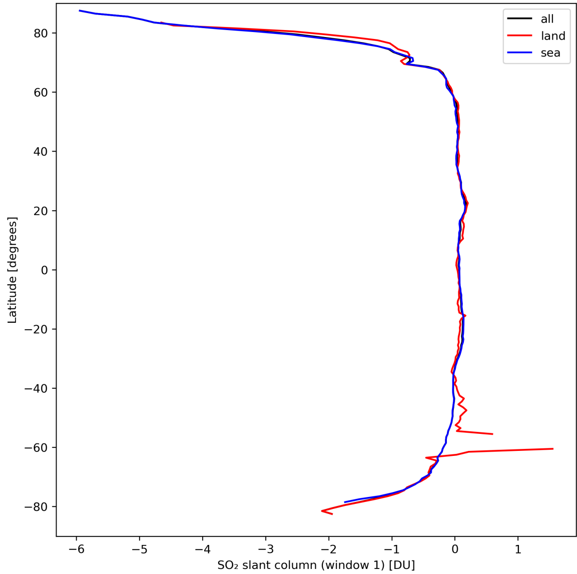
Figure 33: Zonal average of “SO 2 slant column (window 1)” for 2024-03-25 to 2024-03-27.
