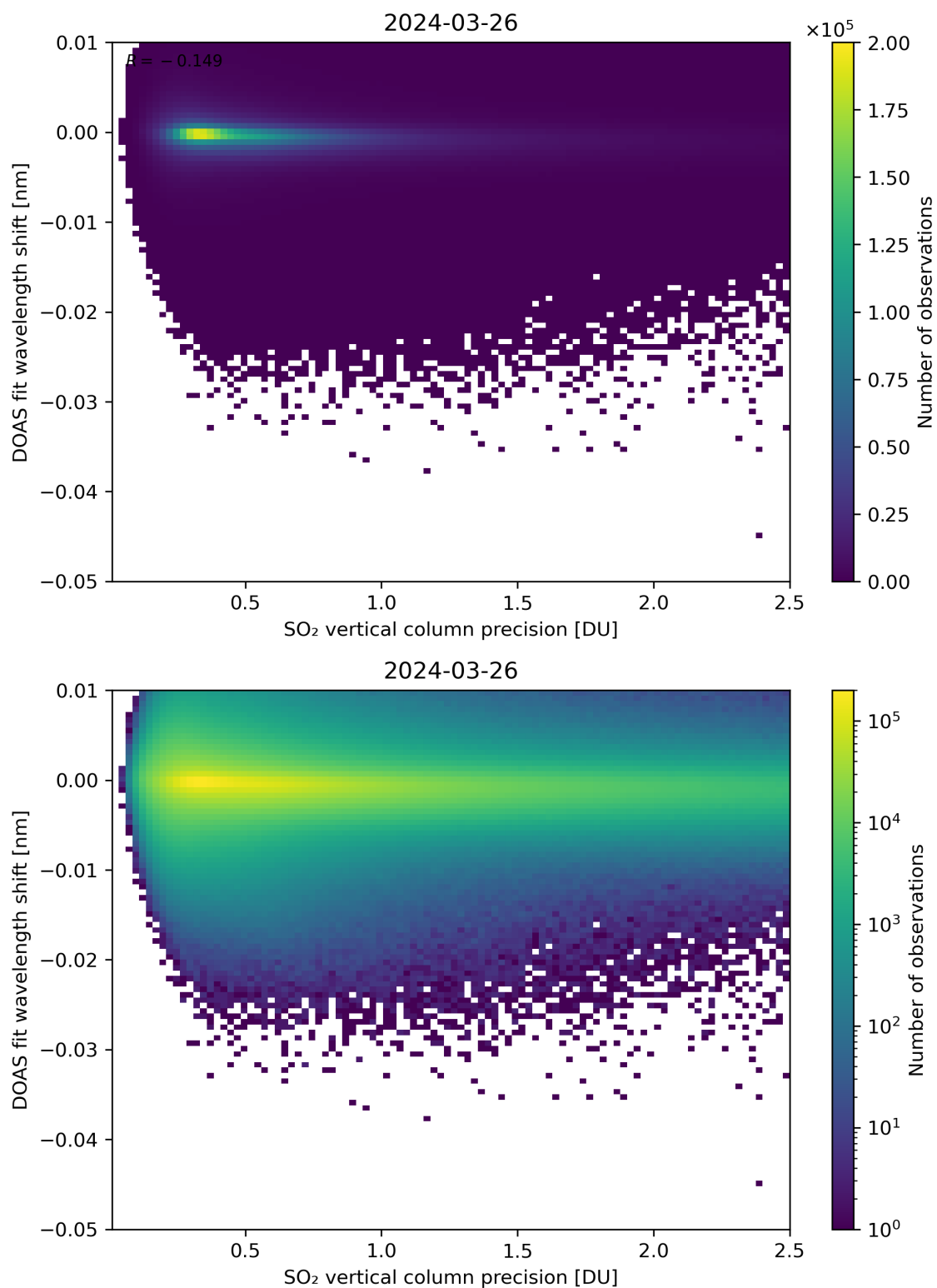
Figure 282: Scatter density plot of “SO 2 vertical column precision” against “DOAS fit wavelength shift” for 2024-03-25 to 2024-03-27.
