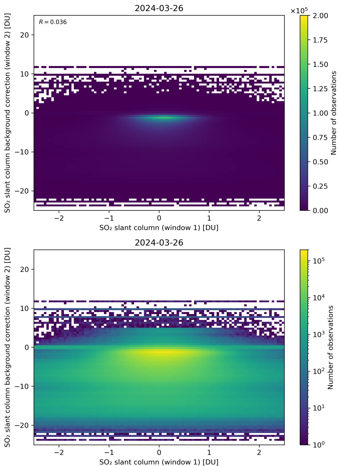
Figure 213: Scatter density plot of “SO 2 slant column (window 1)” against “SO 2 slant column background correction (window 2)” for 2024-03-25 to 2024-03-27.
