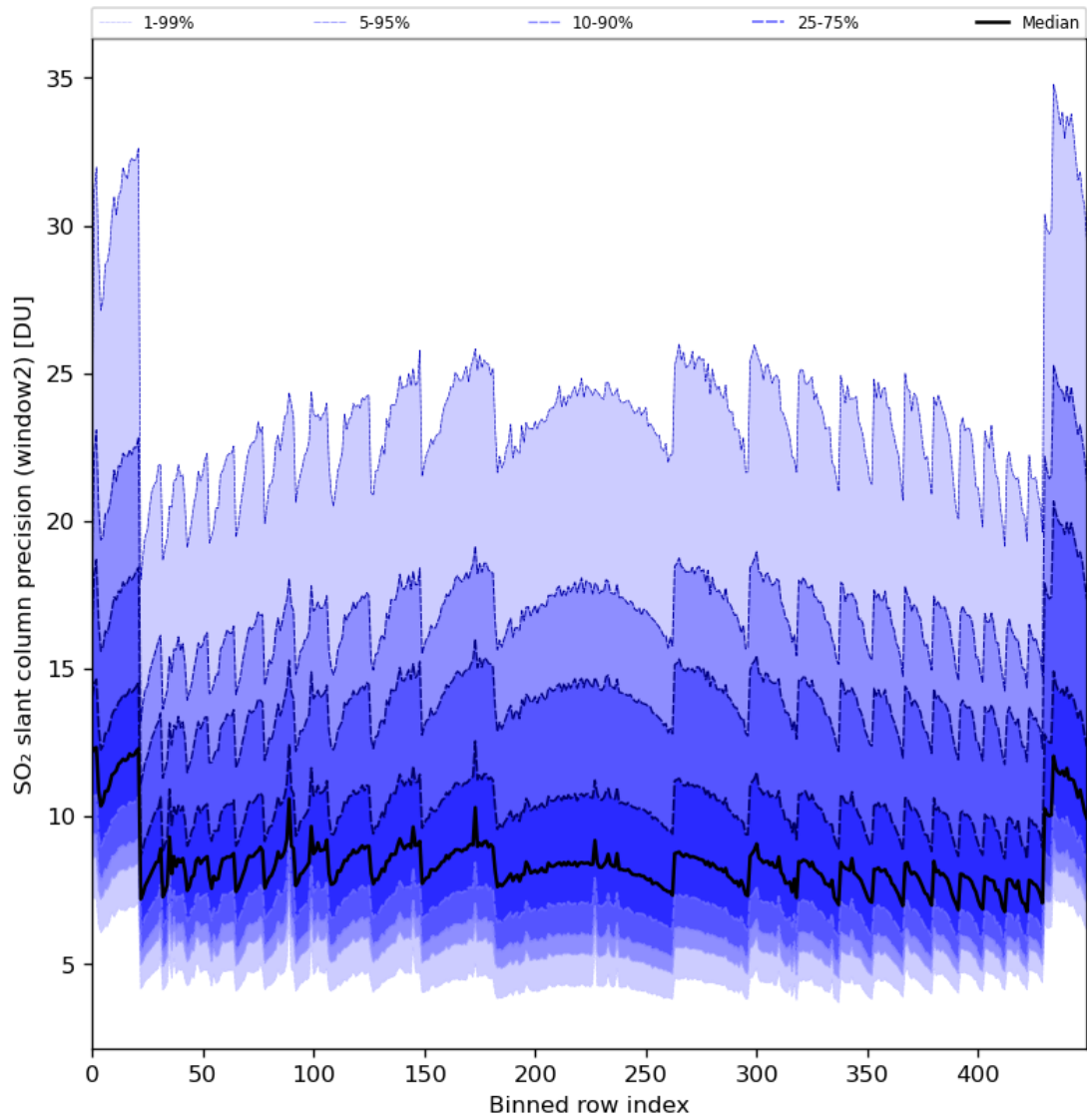
Figure 84: Along track statistics of “SO 2 slant column precision (window2)” for 2024-03-25 to 2024-03-27
