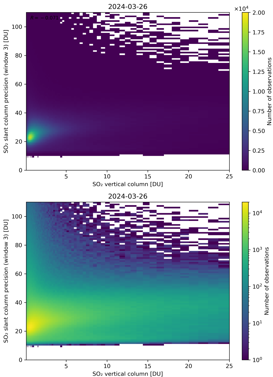
Figure 304: Scatter density plot of “SO 2 vertical column” against “SO 2 slant column precision (window 3)” for 2024-03-25 to 2024-03-27.
