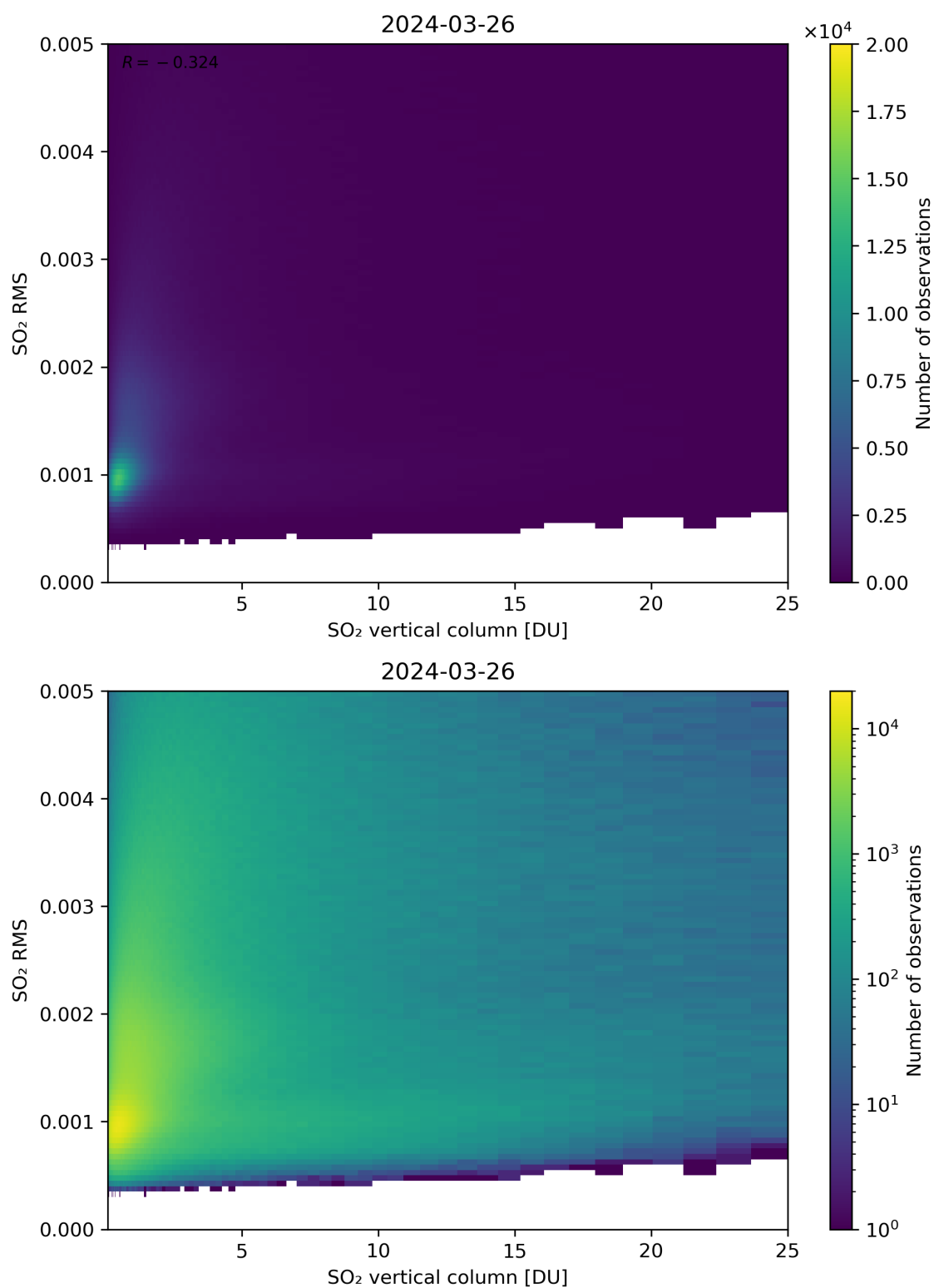
Figure 278: Scatter density plot of “SO 2 vertical column” against “SO 2 RMS” for 2024-03-25 to 2024-03-27.
