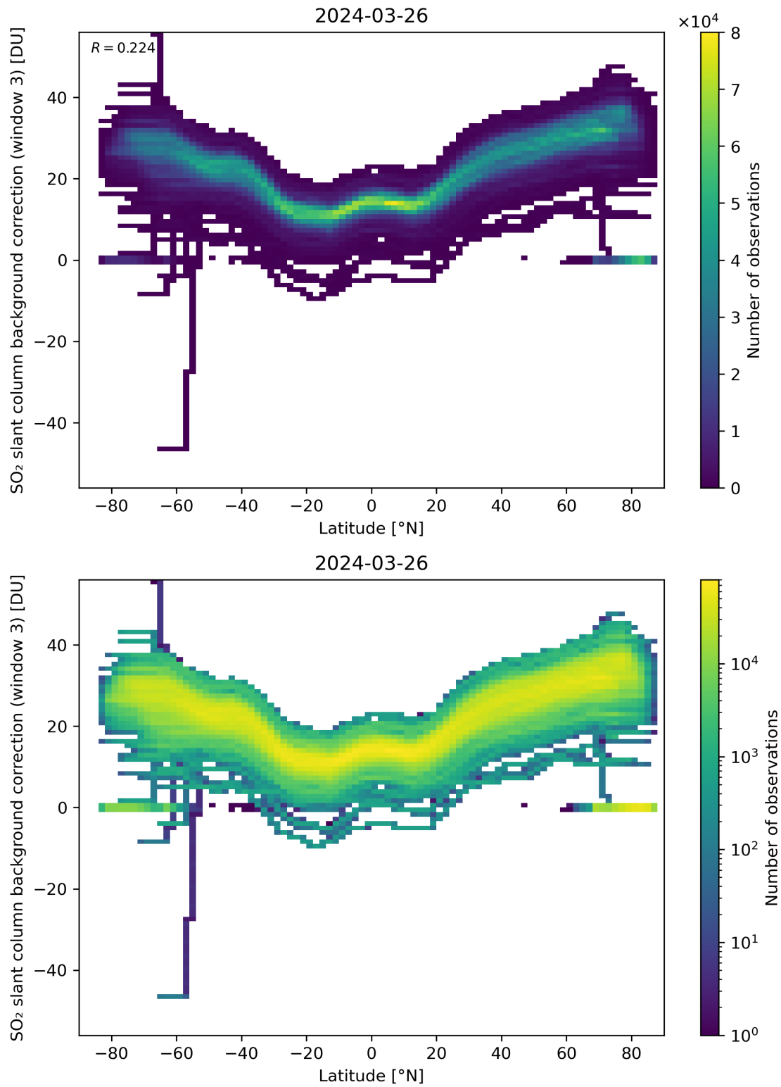
Figure 141: Scatter density plot of “Latitude” against “SO 2 slant column background correction (window 3)” for 2024-03-25 to 2024-03-27.
