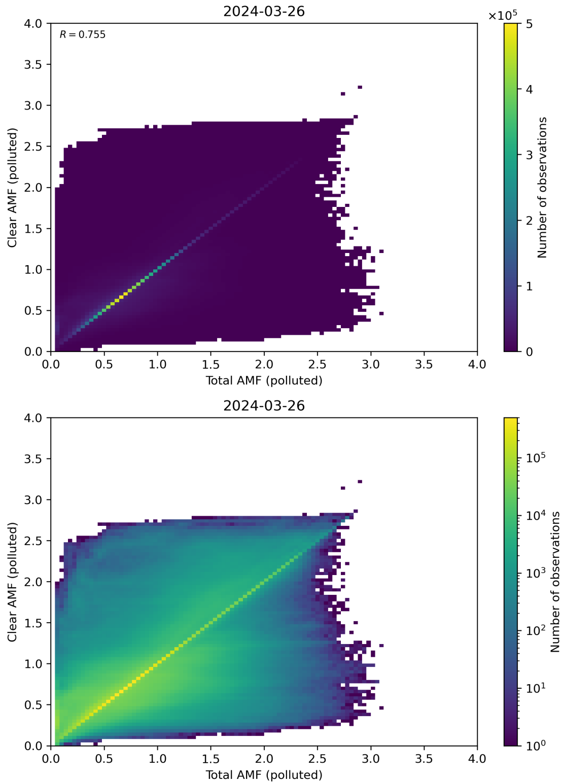
Figure 271: Scatter density plot of “Total AMF (polluted)” against “Clear AMF (polluted)” for 2024-03-25 to 2024-03-27.
