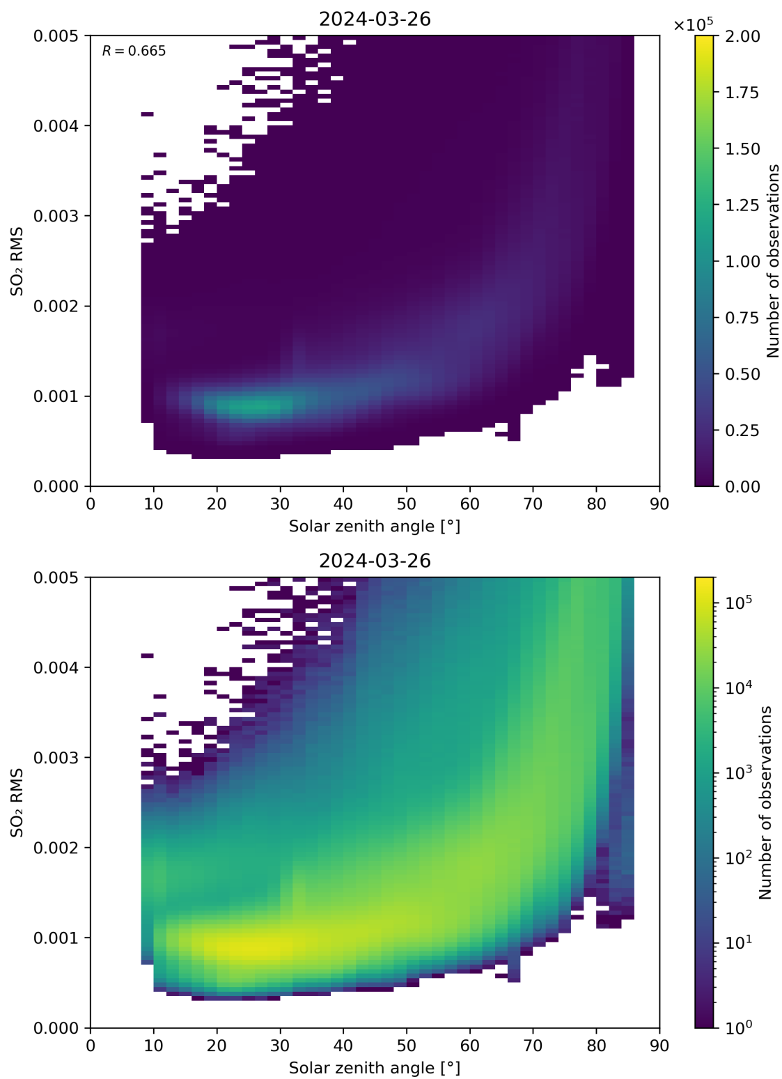
Figure 163: Scatter density plot of “Solar zenith angle” against “SO 2 RMS” for 2024-03-25 to 2024-03-27.
