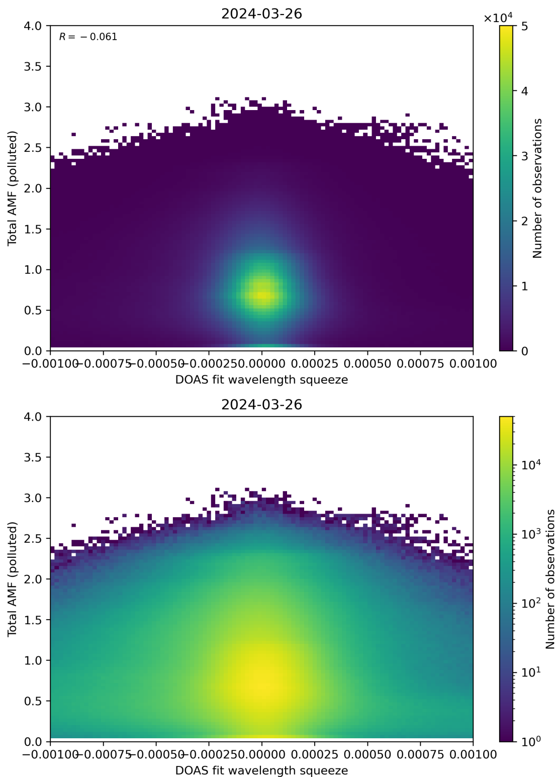
Figure 134: Scatter density plot of “DOAS fit wavelength squeeze” against “Total AMF (polluted)” for 2024-03-25 to 2024-03-27.
