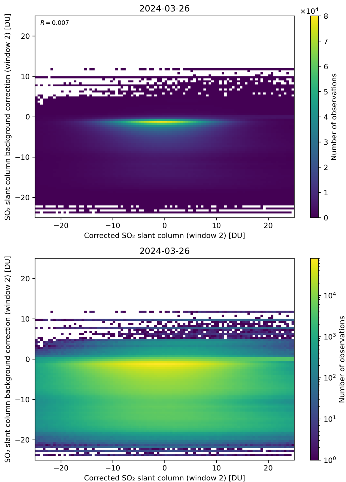
Figure 194: Scatter density plot of “Corrected SO 2 slant column (window 2)” against “SO 2 slant column background correction (window 2)” for 2024-03-25 to 2024-03-27.
