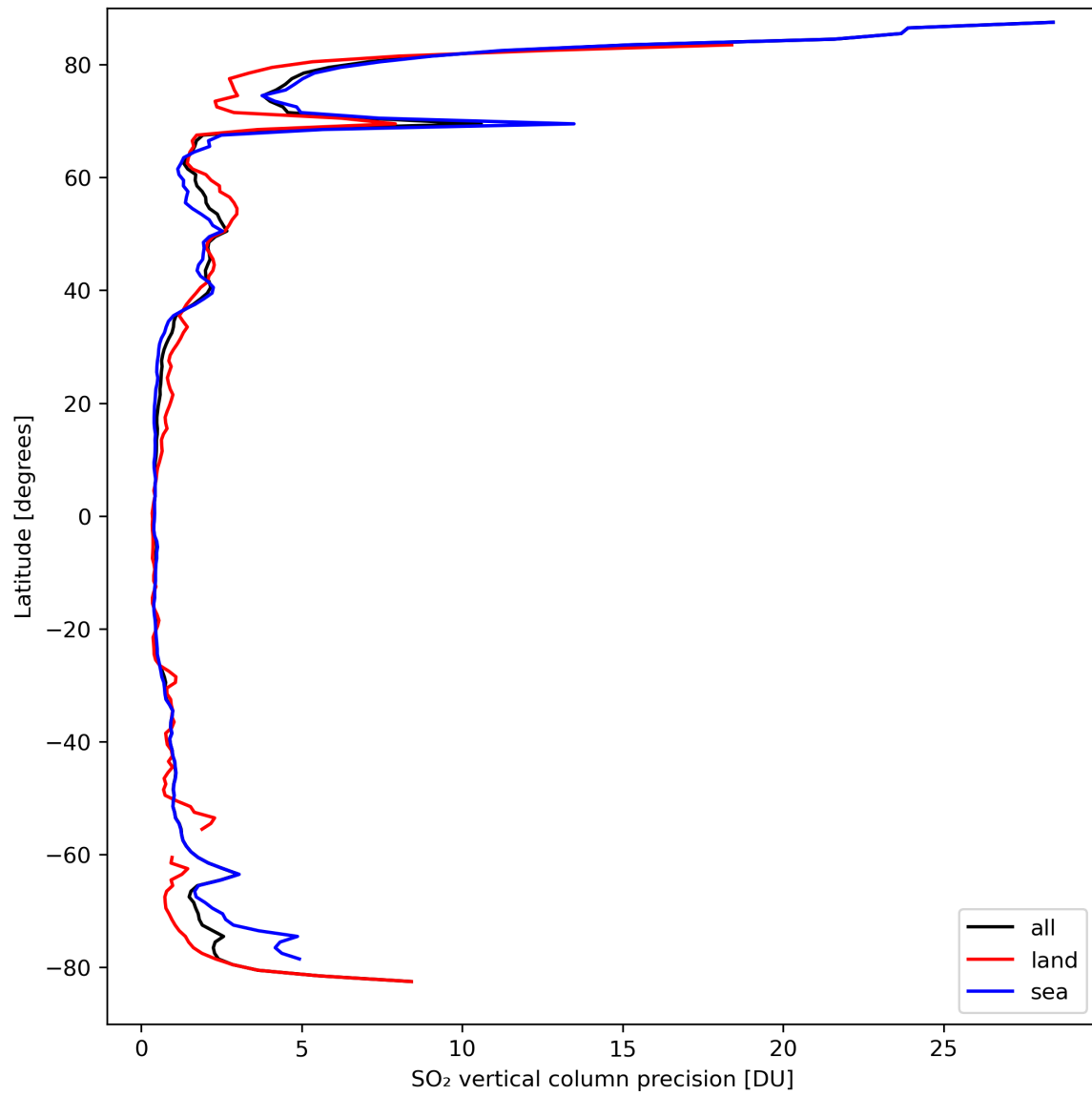
Figure 31: Zonal average of “SO 2 vertical column precision” for 2024-03-25 to 2024-03-27.
