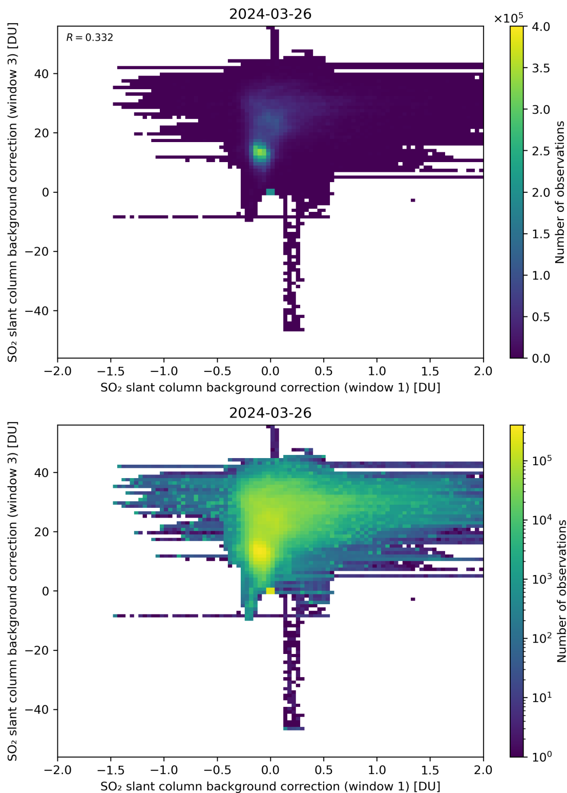
Figure 99: Scatter density plot of “SO 2 slant column background correction (window 1)” against “SO 2 slant column background correction (window 3)” for 2024-03-25 to 2024-03-27.
