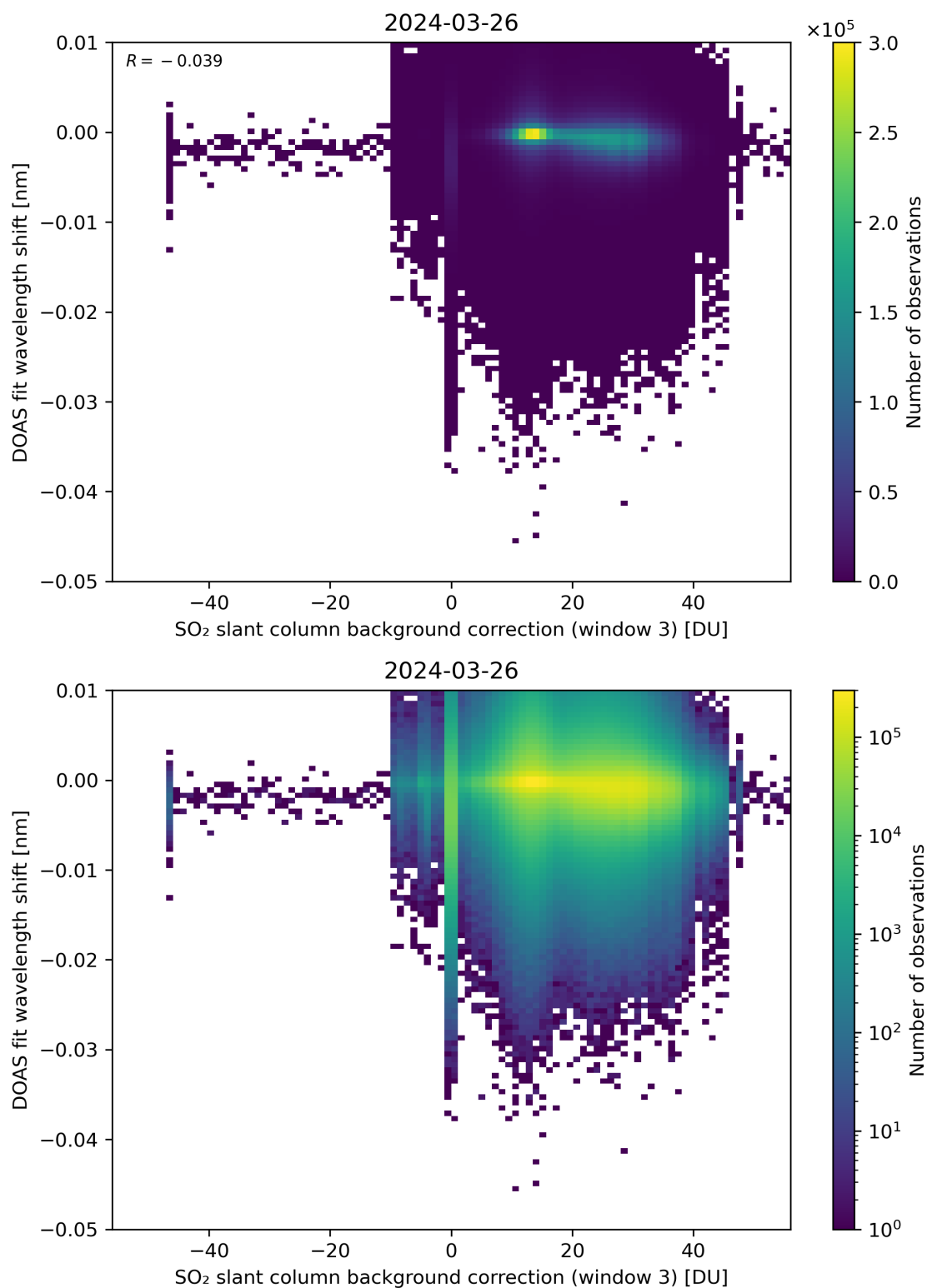
Figure 121: Scatter density plot of “SO 2 slant column background correction (window 3)” against “DOAS fit wavelength shift” for 2024-03-25 to 2024-03-27.
