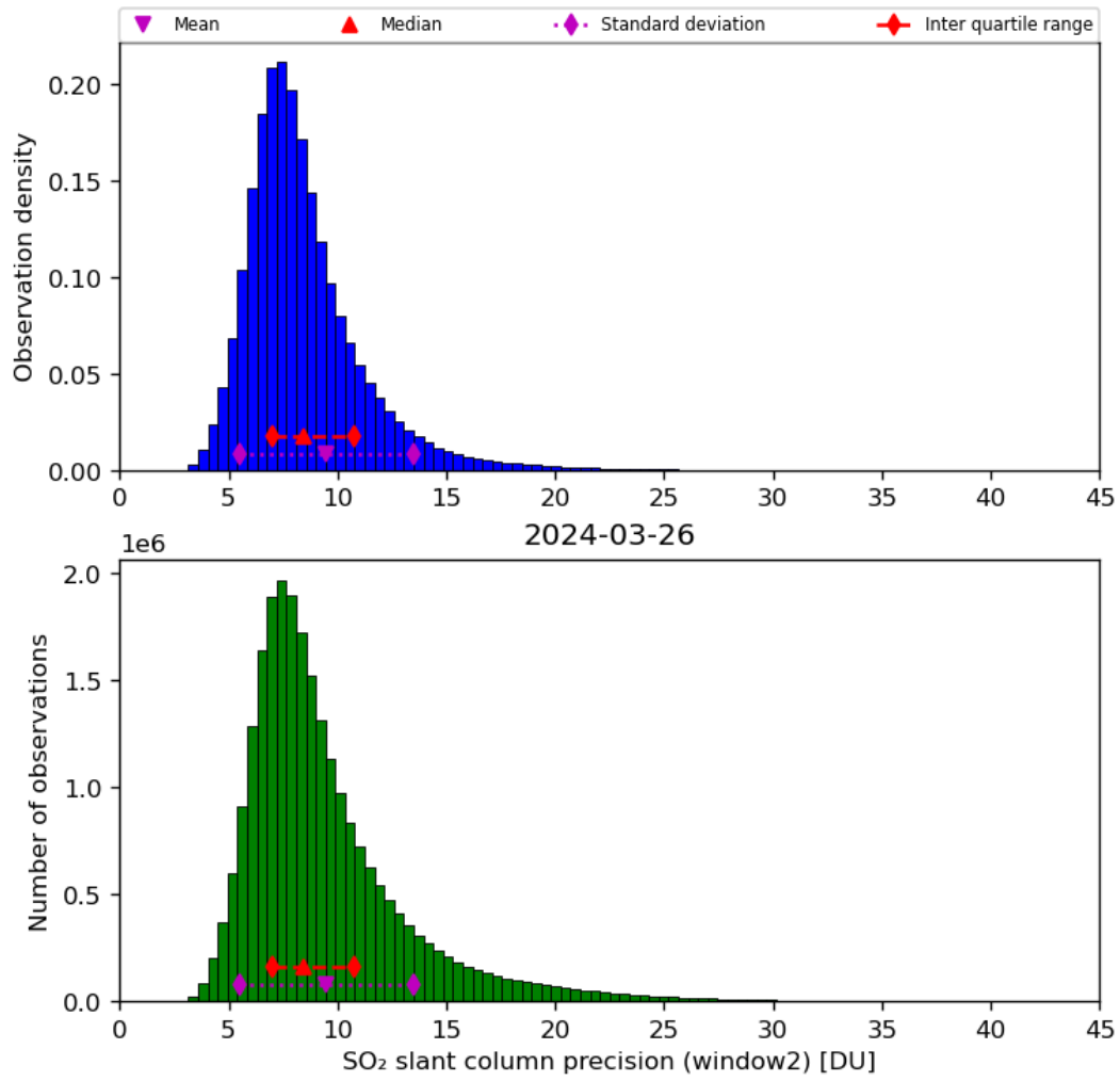
Figure 61: Histogram of “SO 2 slant column precision (window2)” for 2024-03-25 to 2024-03-27
