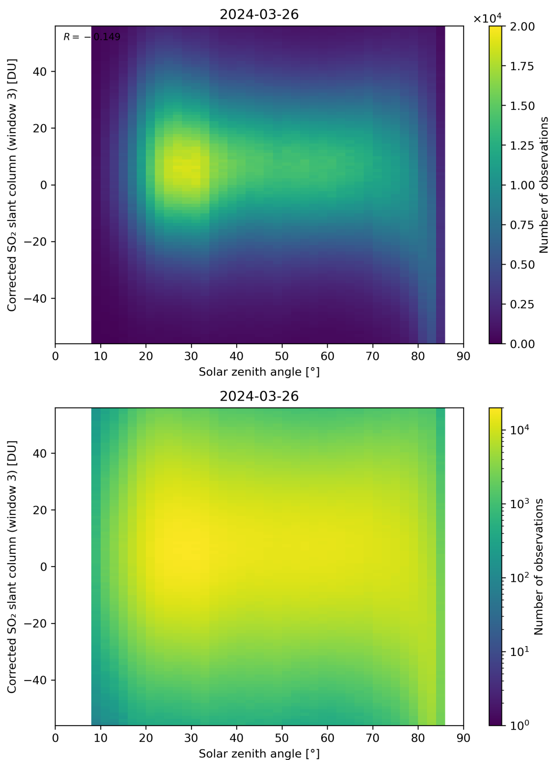
Figure 168: Scatter density plot of “Solar zenith angle” against “Corrected SO 2 slant column (window 3)” for 2024-03-25 to 2024-03-27.
