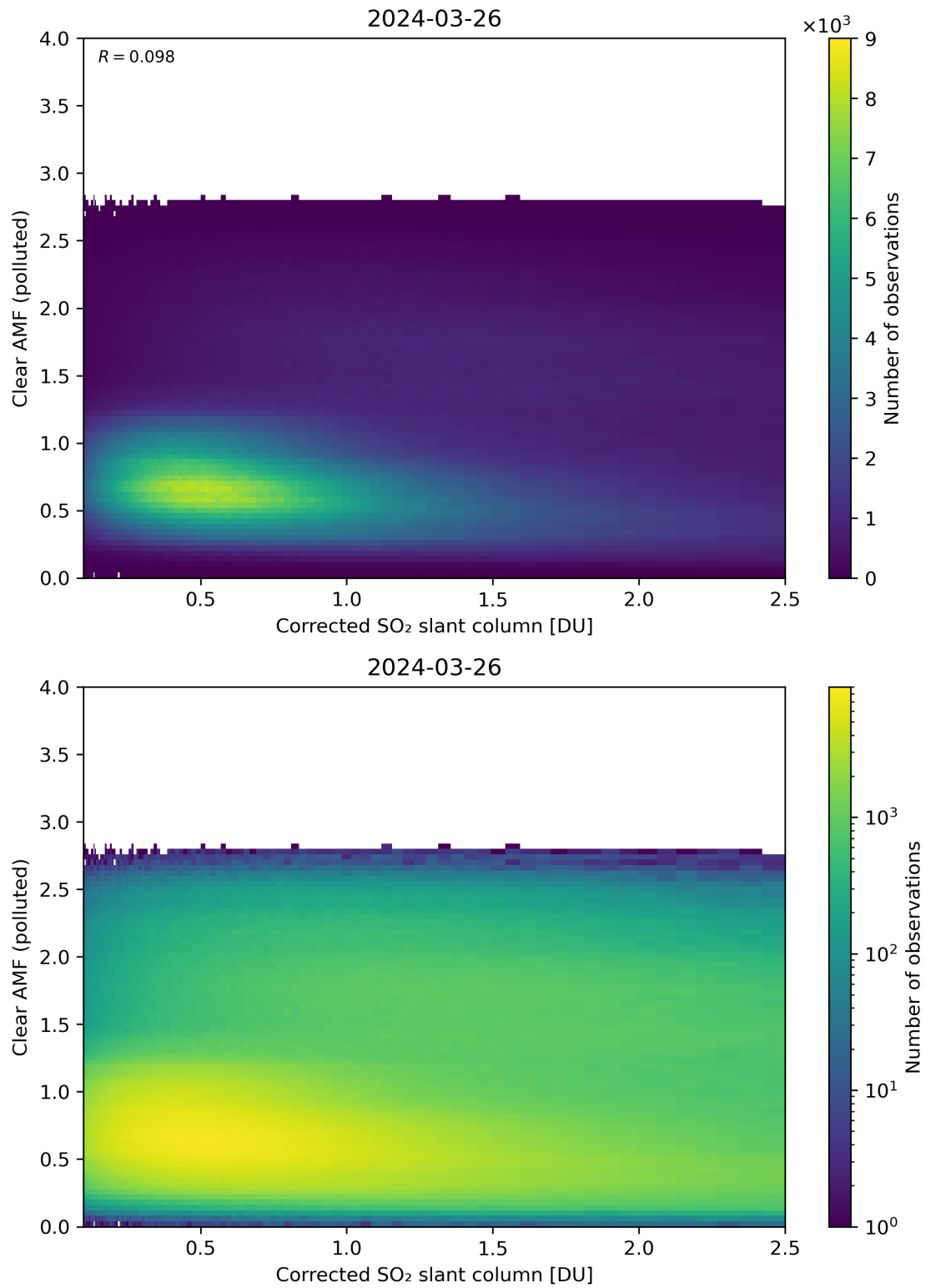
Figure 184: Scatter density plot of “Corrected SO 2 slant column” against “Clear AMF (polluted)” for 2024-03-25 to 2024-03-27.
