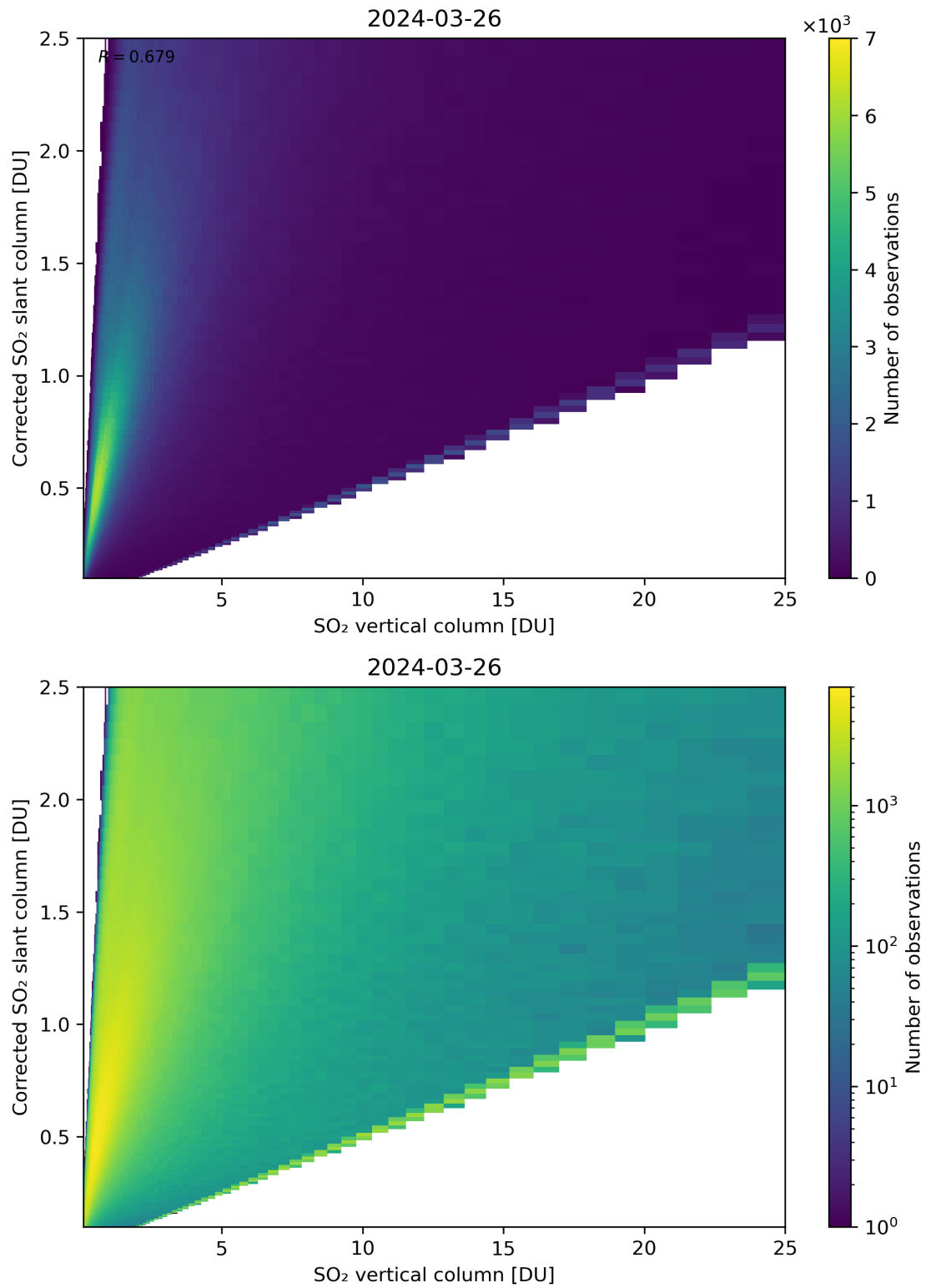
Figure 297: Scatter density plot of “SO 2 vertical column” against “Corrected SO 2 slant column” for 2024-03-25 to 2024-03-27.
