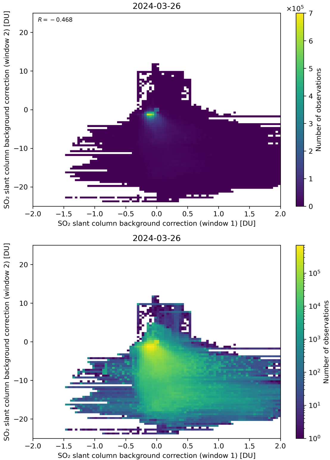
Figure 98: Scatter density plot of “SO 2 slant column background correction (window 1)” against “SO 2 slant column background correction (window 2)” for 2024-03-25 to 2024-03-27.
