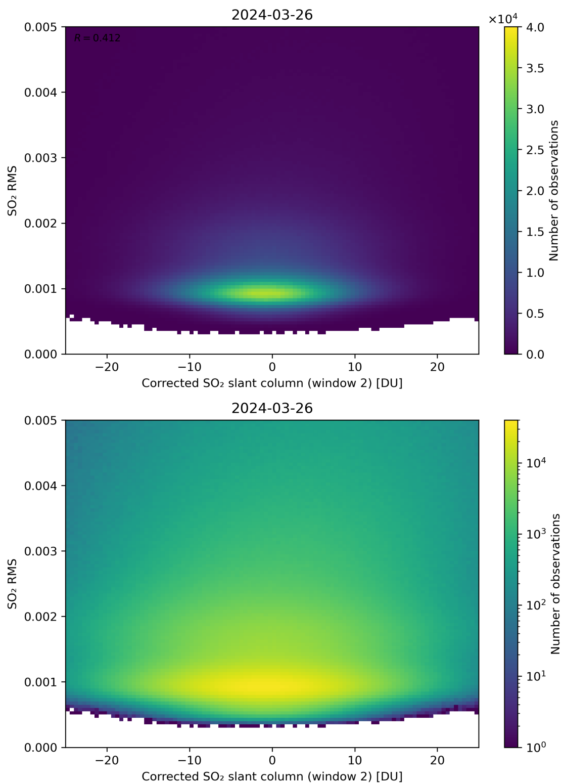
Figure 198: Scatter density plot of “Corrected SO 2 slant column (window 2)” against “SO 2 RMS” for 2024-03-25 to 2024-03-27.
