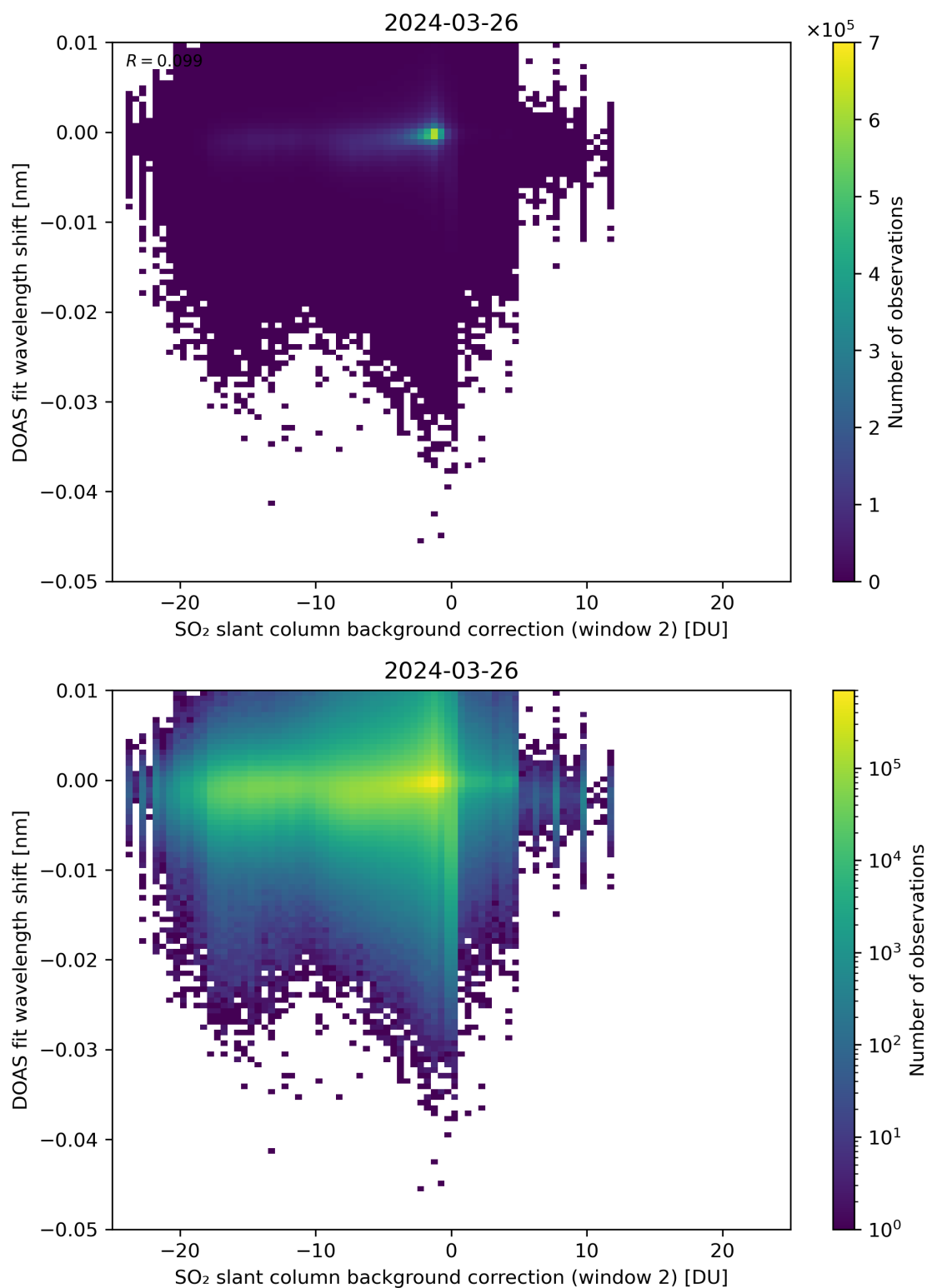
Figure 112: Scatter density plot of “SO 2 slant column background correction (window 2)” against “DOAS fit wavelength shift” for 2024-03-25 to 2024-03-27.
