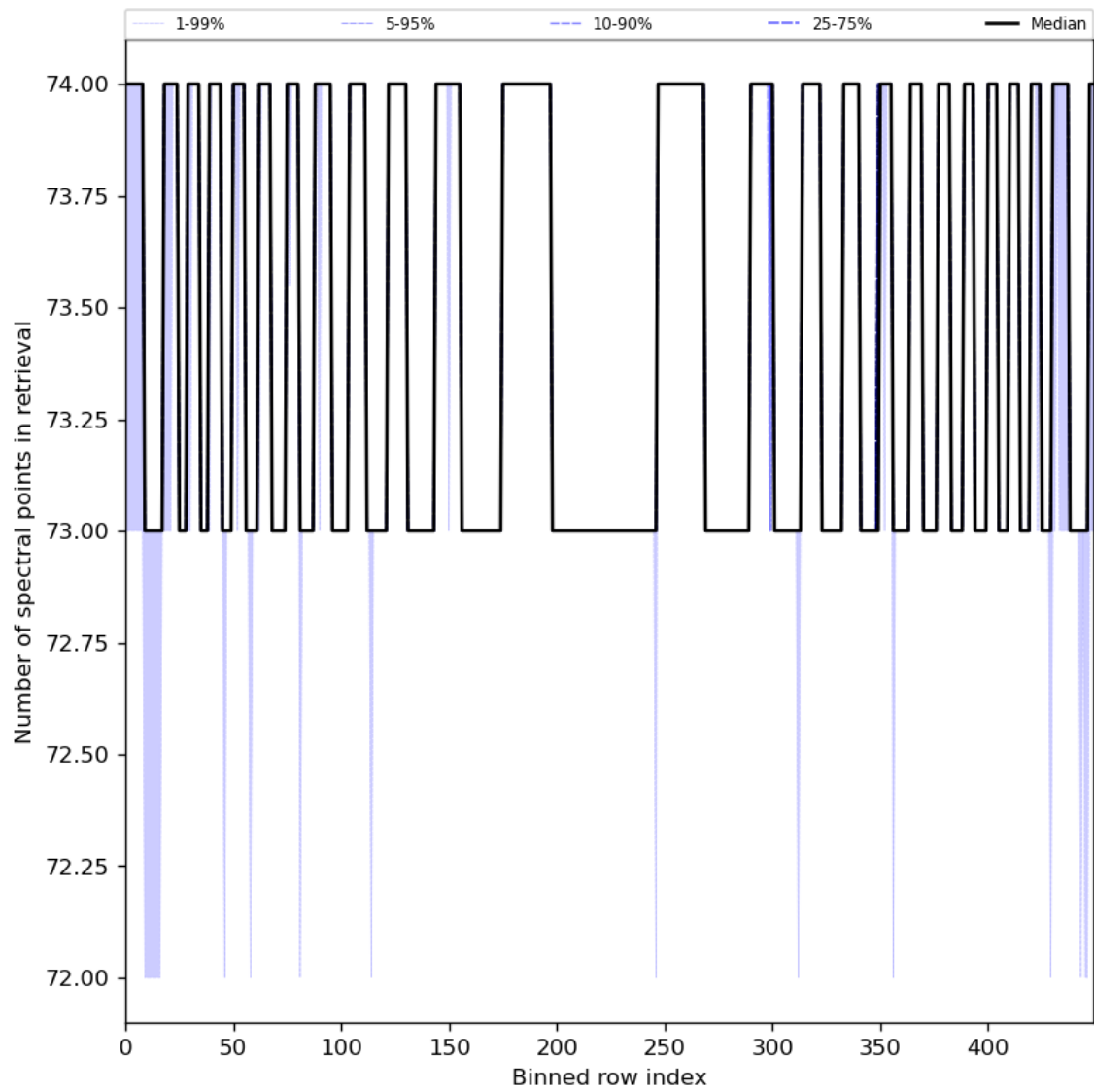
Figure 97: Along track statistics of “Number of spectral points in retrieval” for 2024-03-25 to 2024-03-27
