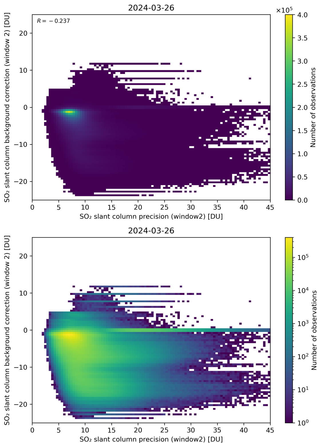
Figure 241: Scatter density plot of “SO 2 slant column precision (window2)” against “SO 2 slant column background correction (window 2)” for 2024-03-25 to 2024-03-27.
