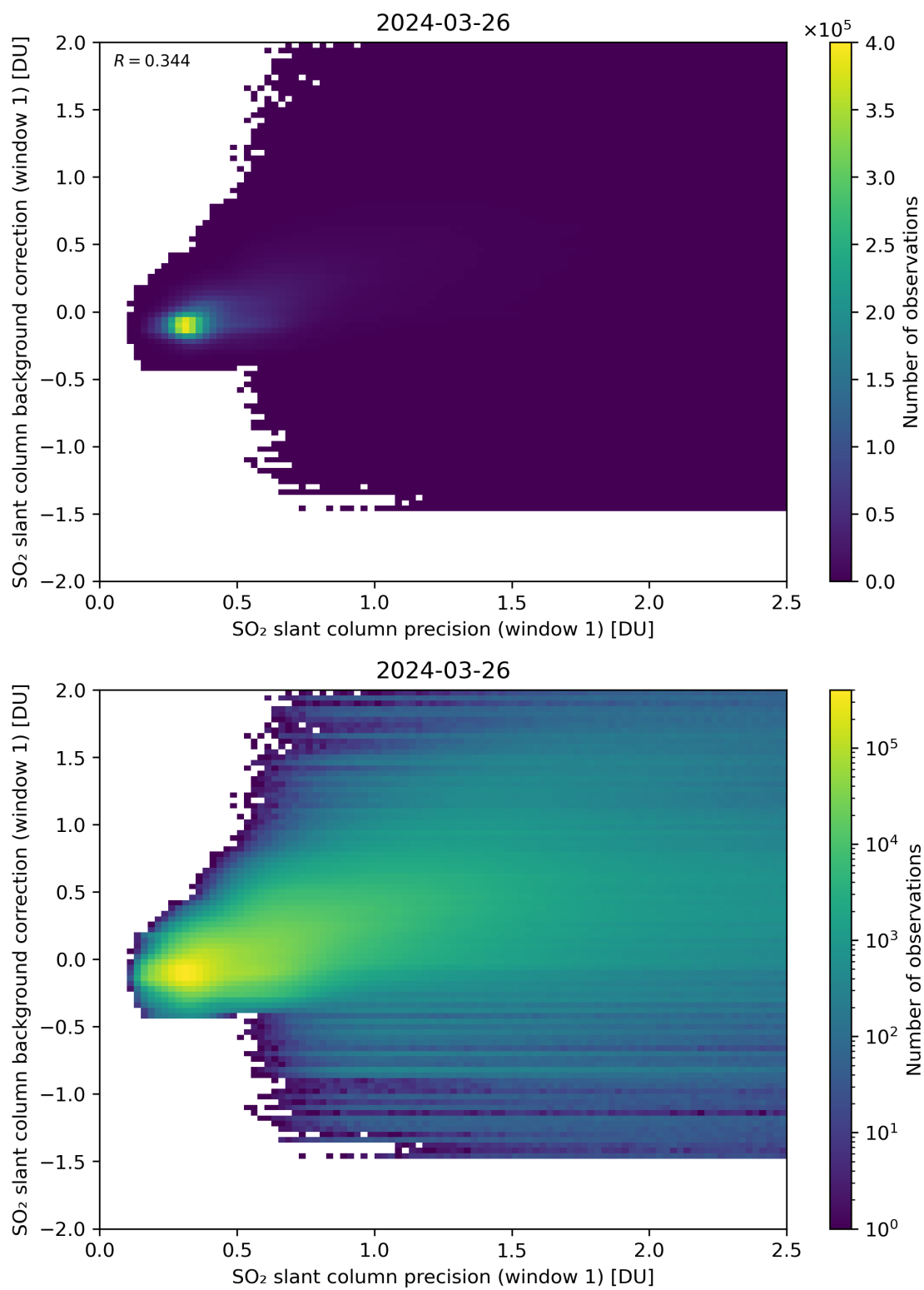
Figure 218: Scatter density plot of “SO 2 slant column precision (window 1)” against “SO 2 slant column background correction (window 1)” for 2024-03-25 to 2024-03-27.
