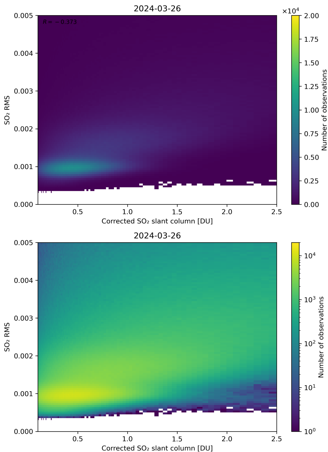
Figure 183: Scatter density plot of “Corrected SO 2 slant column” against “SO 2 RMS” for 2024-03-25 to 2024-03-27.
