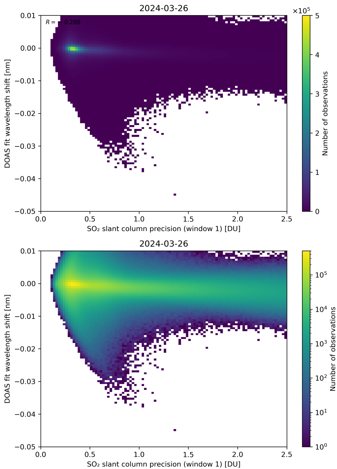
Figure 221: Scatter density plot of “SO 2 slant column precision (window 1)” against “DOAS fit wavelength shift” for 2024-03-25 to 2024-03-27.
