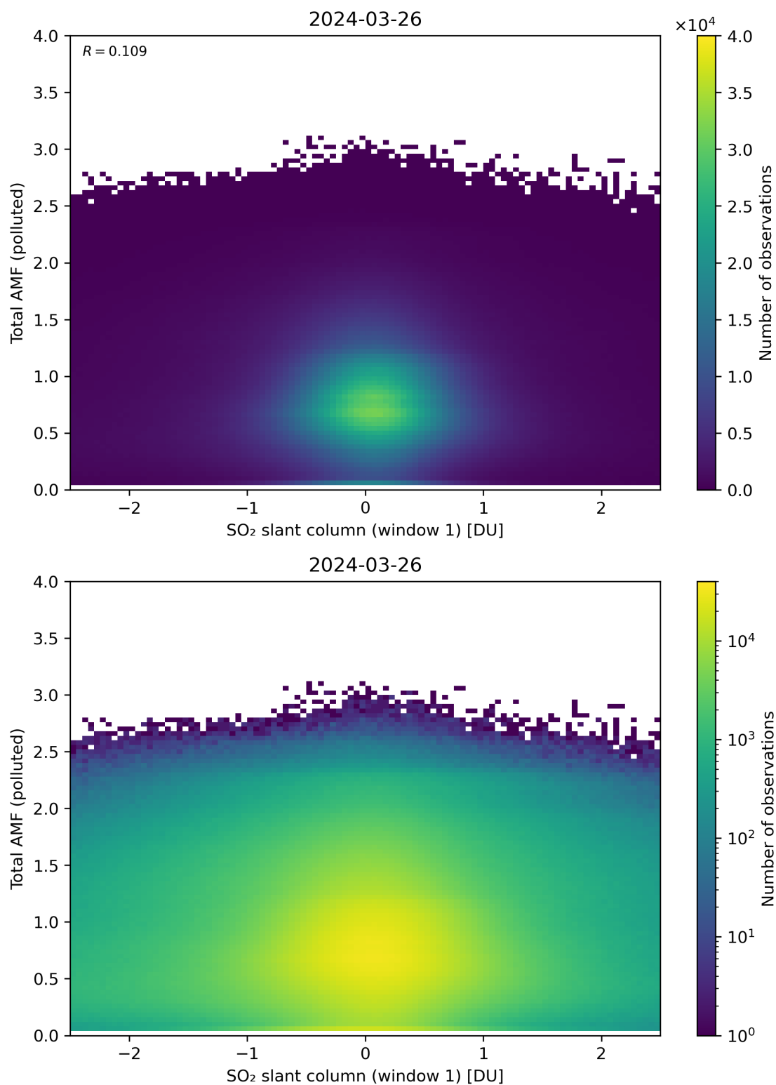
Figure 239: Scatter density plot of “SO 2 slant column (window 1)” against “Total AMF (polluted)” for 2024-03-25 to 2024-03-27.
