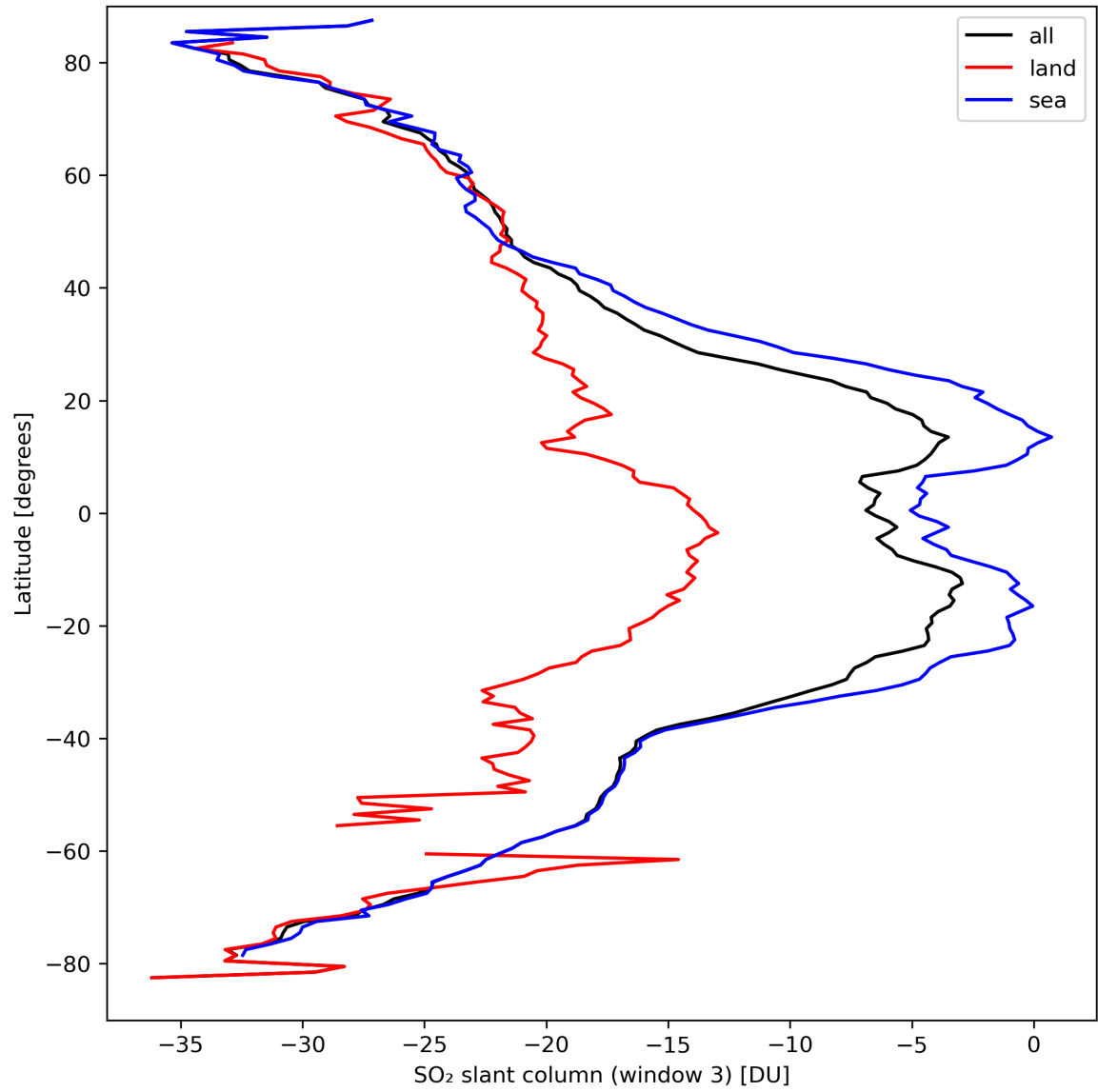
Figure 41: Zonal average of “SO 2 slant column (window 3)” for 2024-03-25 to 2024-03-27.
