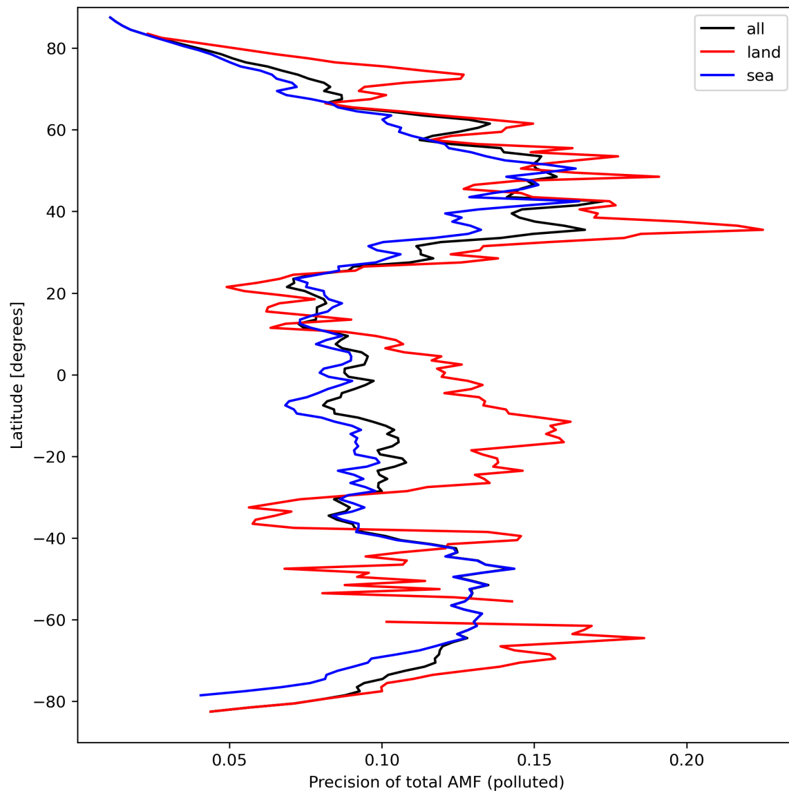
Figure 49: Zonal average of “Precision of total AMF (polluted)” for 2024-03-25 to 2024-03-27.
