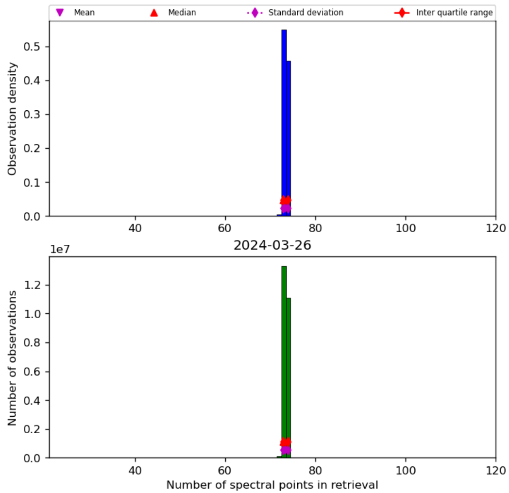
Figure 74: Histogram of “Number of spectral points in retrieval” for 2024-03-25 to 2024-03-27
