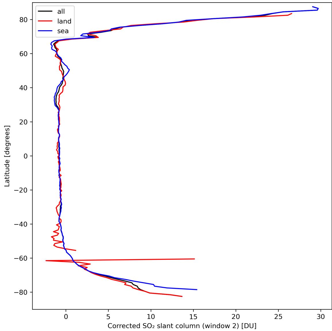
Figure 39: Zonal average of “Corrected SO 2 slant column (window 2)” for 2024-03-25 to 2024-03-27.
