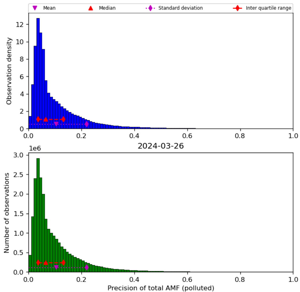
Figure 72: Histogram of “Precision of total AMF (polluted)” for 2024-03-25 to 2024-03-27
