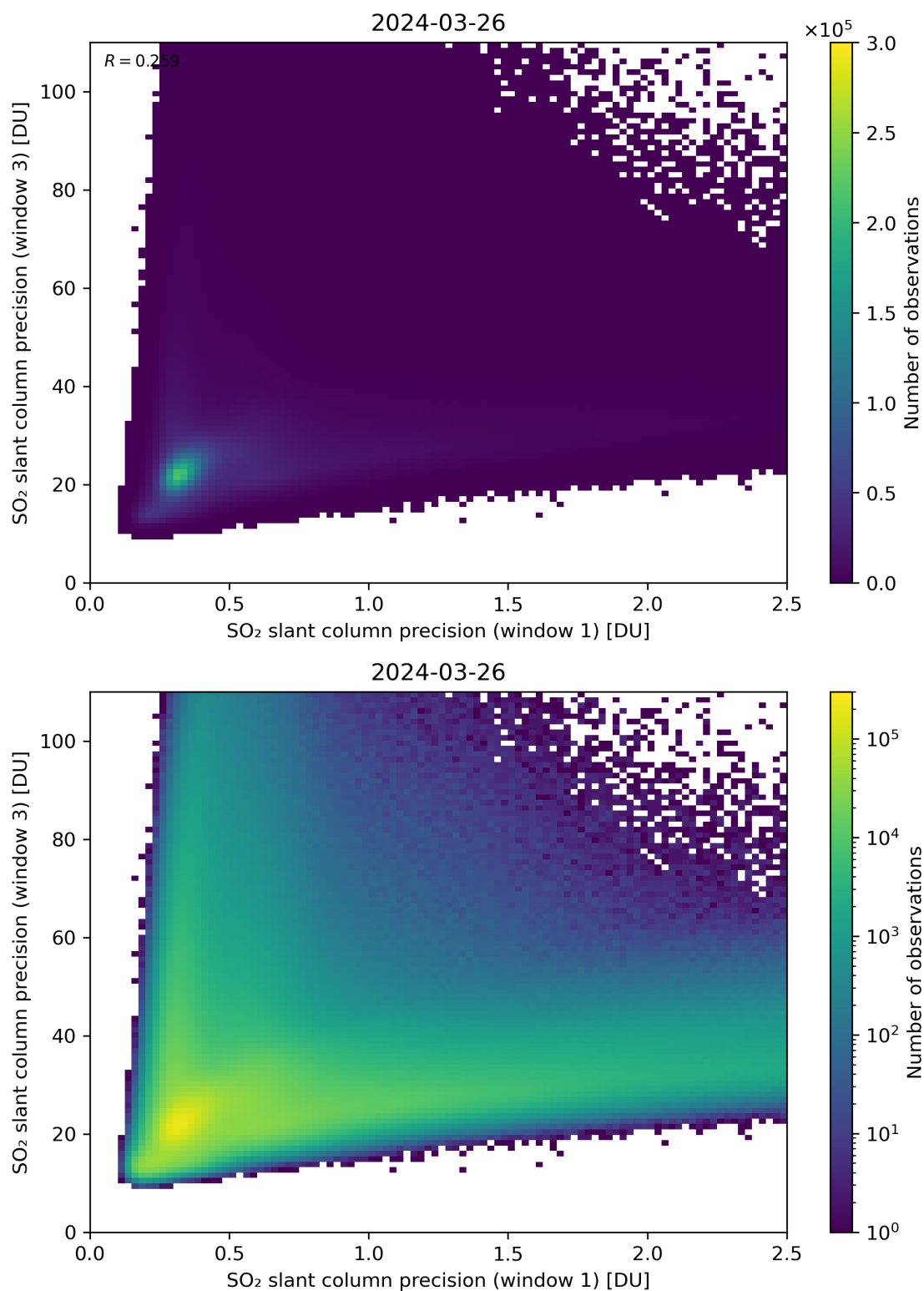
Figure 229: Scatter density plot of “SO 2 slant column precision (window 1)” against “SO 2 slant column precision (window 3)” for 2024-03-25 to 2024-03-27.
