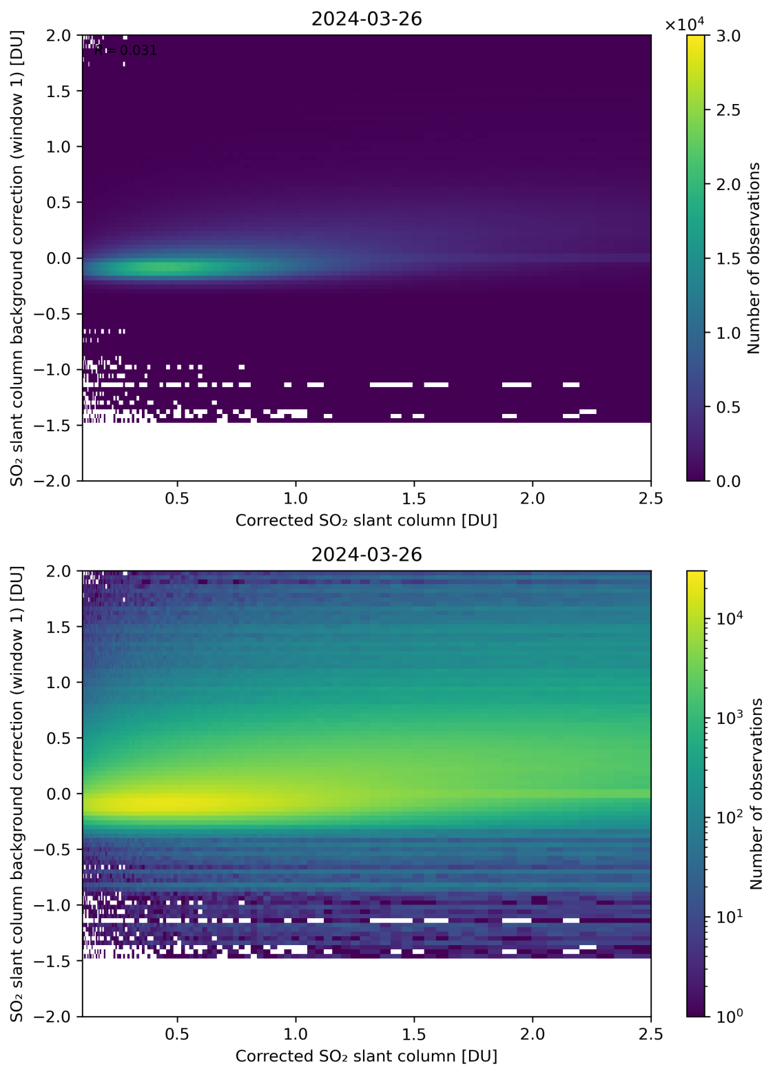
Figure 178: Scatter density plot of “Corrected SO 2 slant column” against “SO 2 slant column background correction (window 1)” for 2024-03-25 to 2024-03-27.
