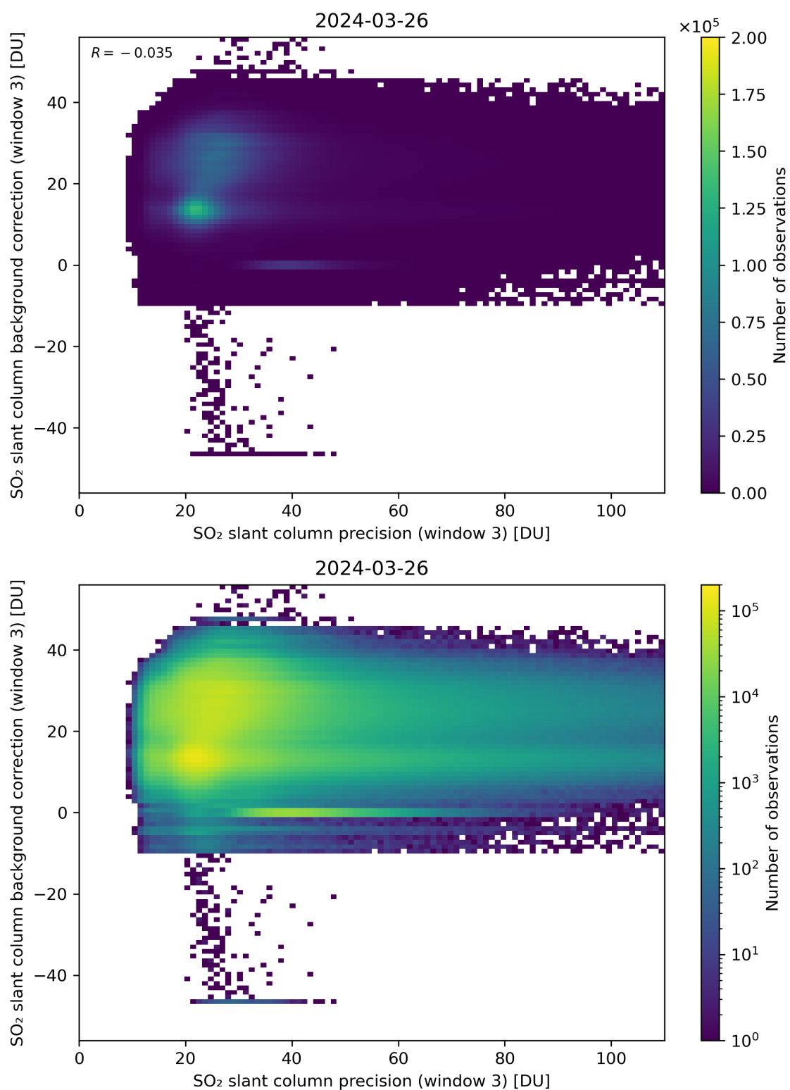
Figure 257: Scatter density plot of “SO 2 slant column precision (window 3)” against “SO 2 slant column background correction (window 3)” for 2024-03-25 to 2024-03-27.
