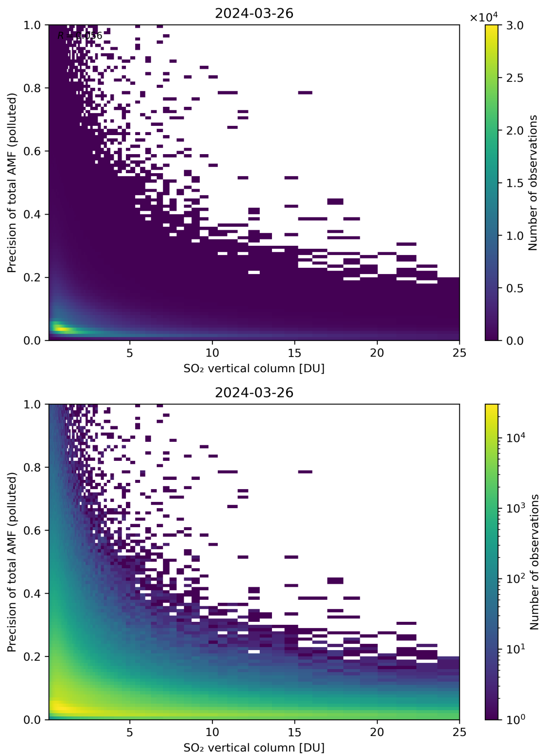
Figure 306: Scatter density plot of “SO 2 vertical column” against “Precision of total AMF (polluted)” for 2024-03-25 to 2024-03-27.
