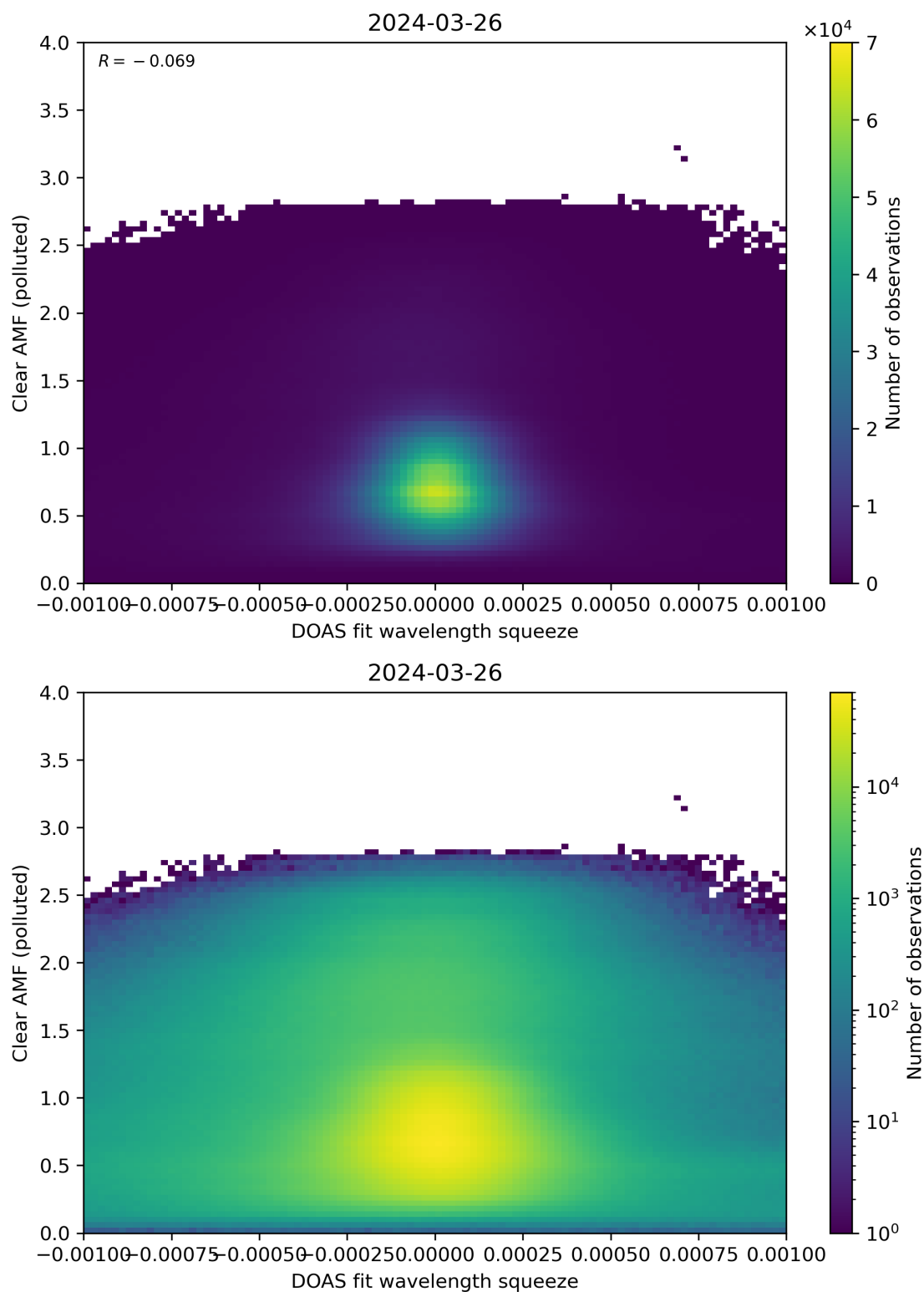
Figure 133: Scatter density plot of “DOAS fit wavelength squeeze” against “Clear AMF (polluted)” for 2024-03-25 to 2024-03-27.
