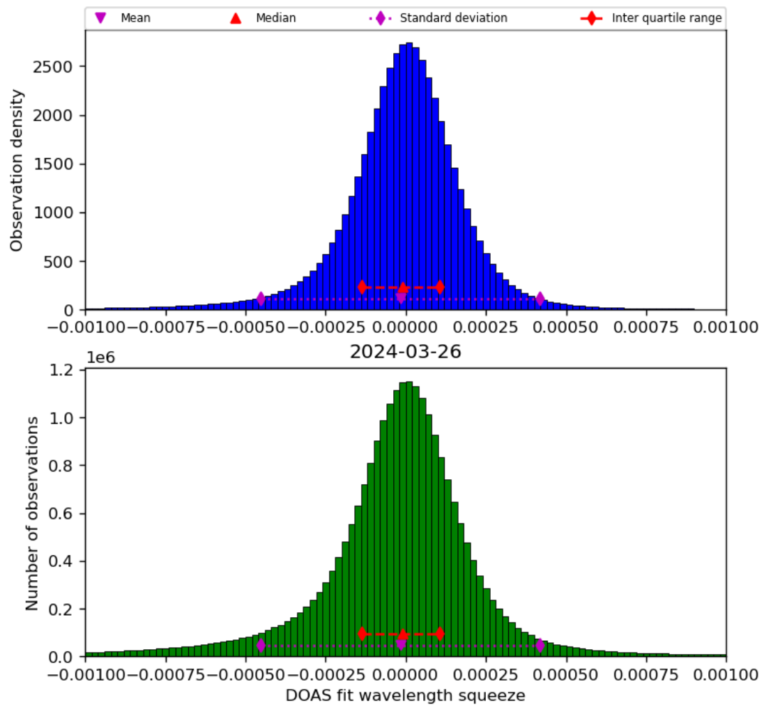
Figure 69: Histogram of “DOAS fit wavelength squeeze” for 2024-03-25 to 2024-03-27
