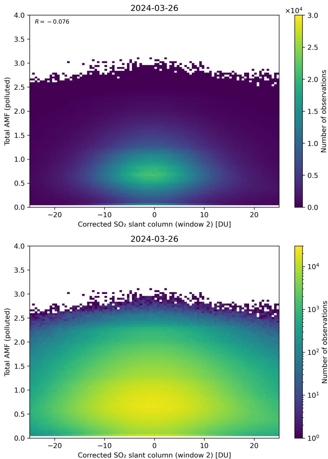
Figure 203: Scatter density plot of “Corrected SO 2 slant column (window 2)” against “Total AMF (polluted)” for 2024-03-25 to 2024-03-27.
