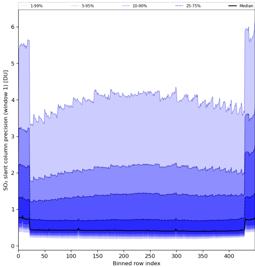
Figure 80: Along track statistics of “SO 2 slant column precision (window 1)” for 2024-03-25 to 2024-03-27
