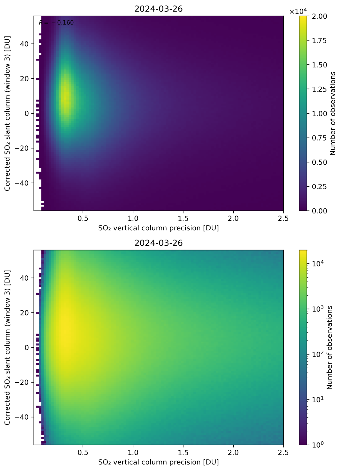
Figure 288: Scatter density plot of “SO 2 vertical column precision” against “Corrected SO 2 slant column (window 3)” for 2024-03-25 to 2024-03-27.
