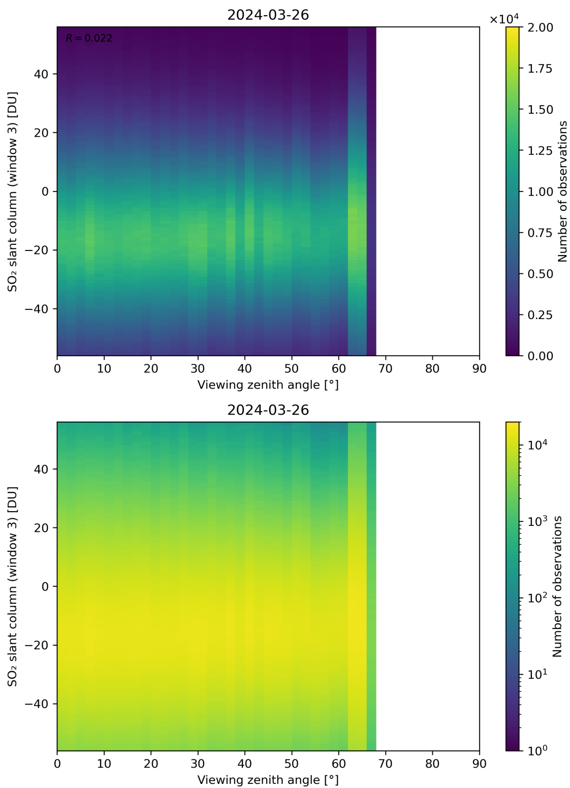
Figure 323: Scatter density plot of “Viewing zenith angle” against “SO 2 slant column (window 3)” for 2024-03-25 to 2024-03-27.
