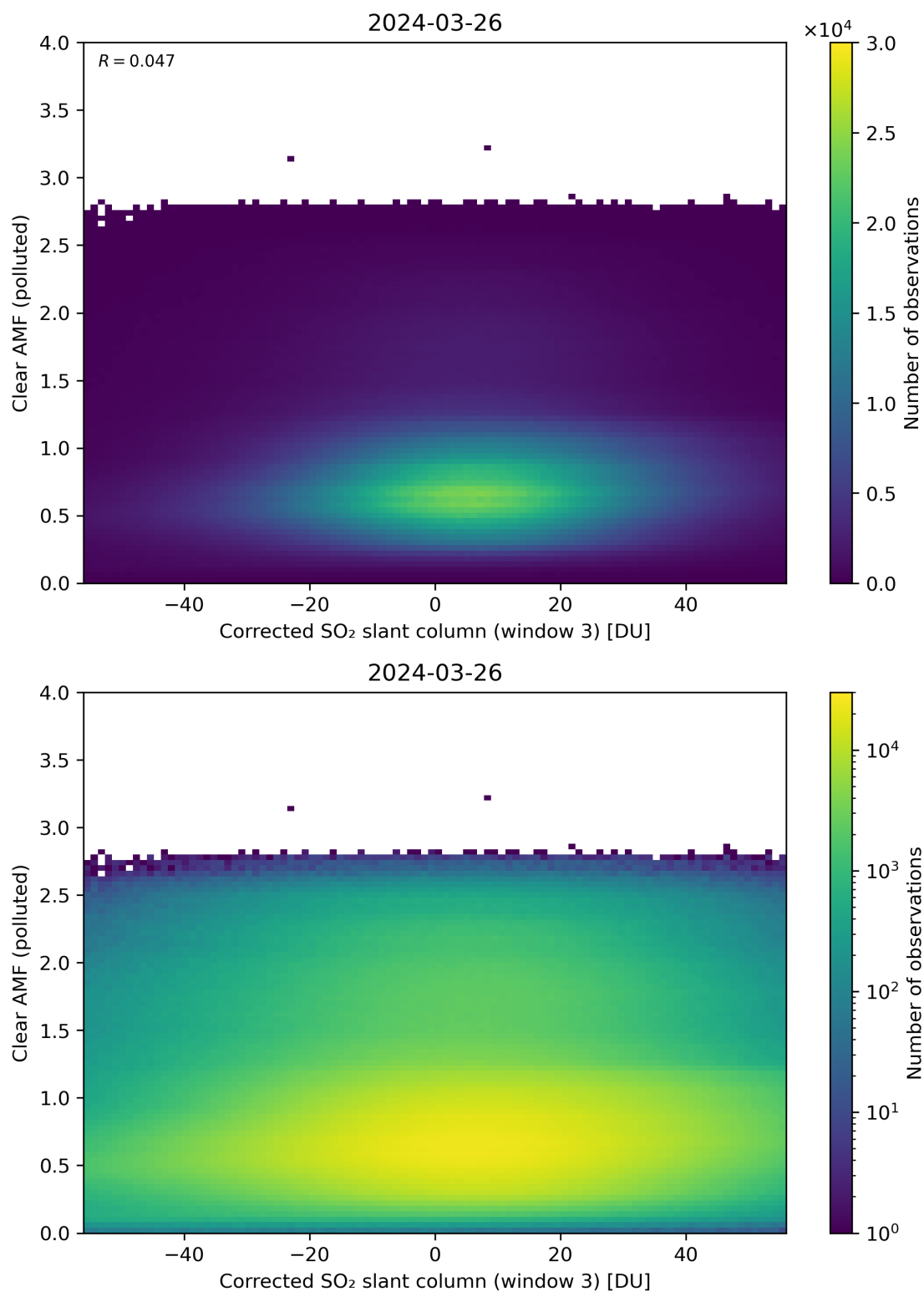
Figure 209: Scatter density plot of “Corrected SO 2 slant column (window 3)” against “Clear AMF (polluted)” for 2024-03-25 to 2024-03-27.
