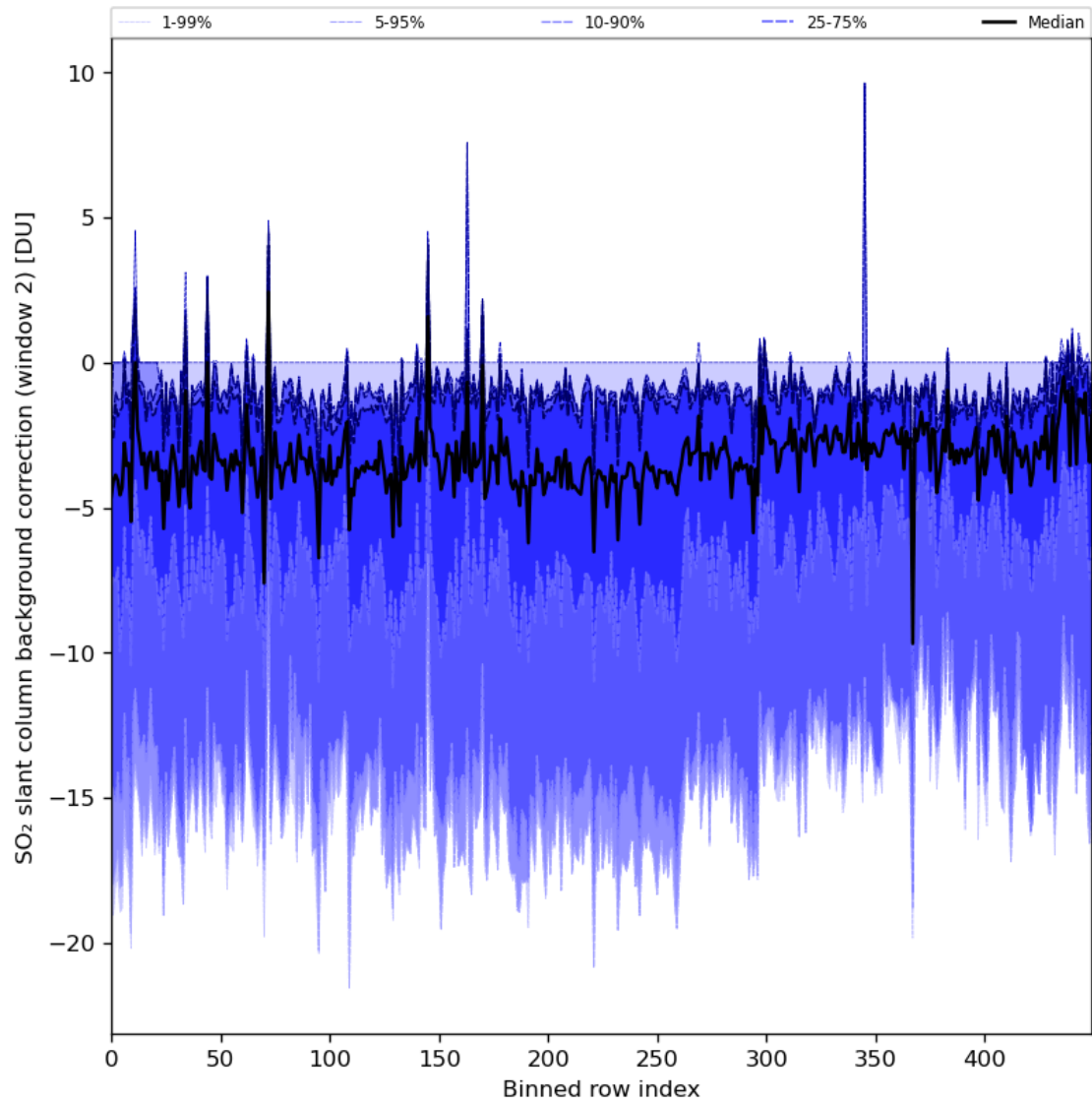
Figure 86: Along track statistics of “SO 2 slant column background correction (window 2)” for 2024-03-25 to 2024-03-27
