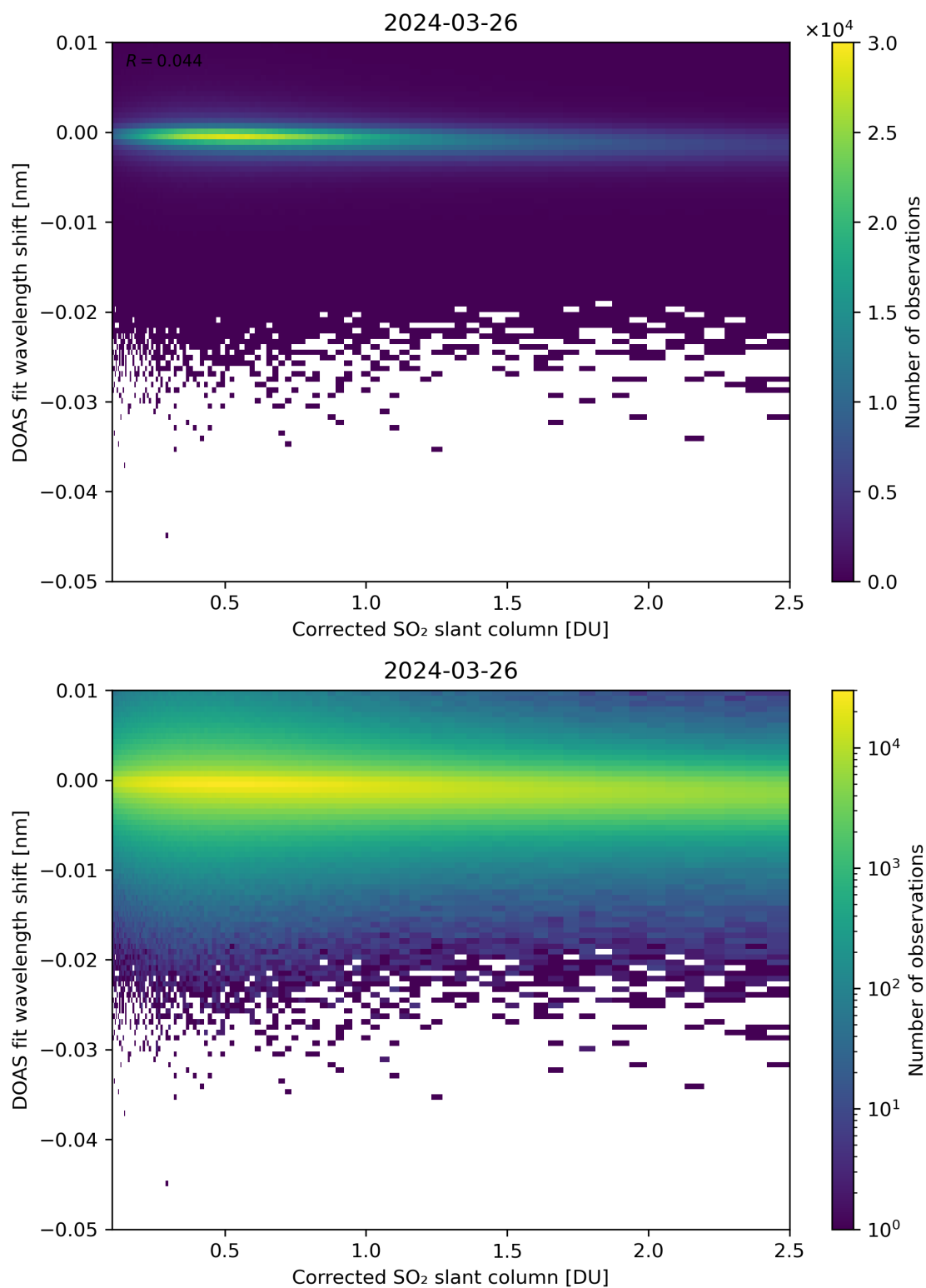
Figure 181: Scatter density plot of “Corrected SO 2 slant column” against “DOAS fit wavelength shift” for 2024-03-25 to 2024-03-27.
