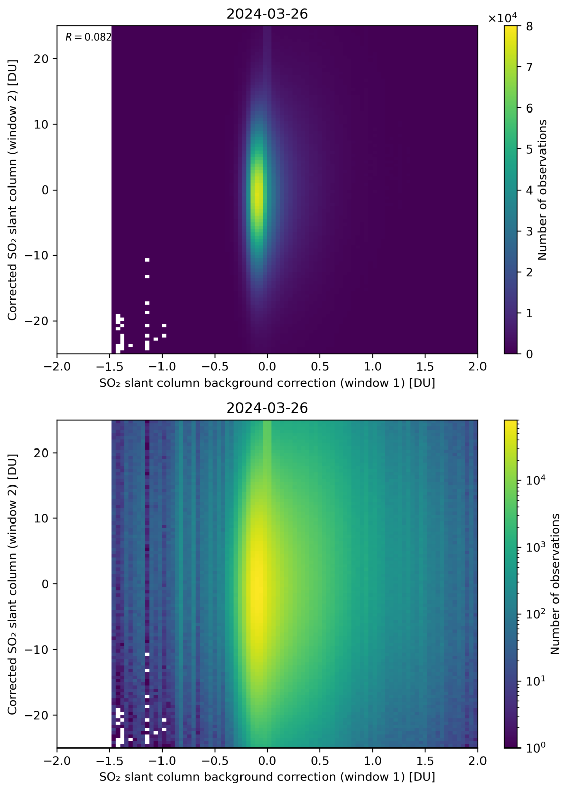
Figure 104: Scatter density plot of “SO 2 slant column background correction (window 1)” against “Corrected SO 2 slant column (window 2)” for 2024-03-25 to 2024-03-27.
