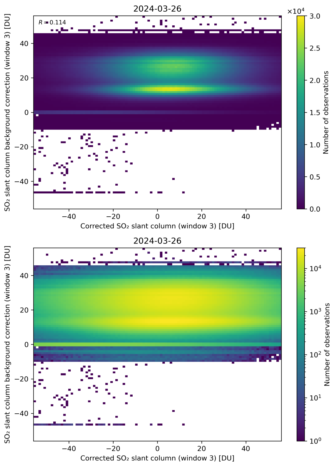
Figure 205: Scatter density plot of “Corrected SO 2 slant column (window 3)” against “SO 2 slant column background correction (window 3)” for 2024-03-25 to 2024-03-27.
