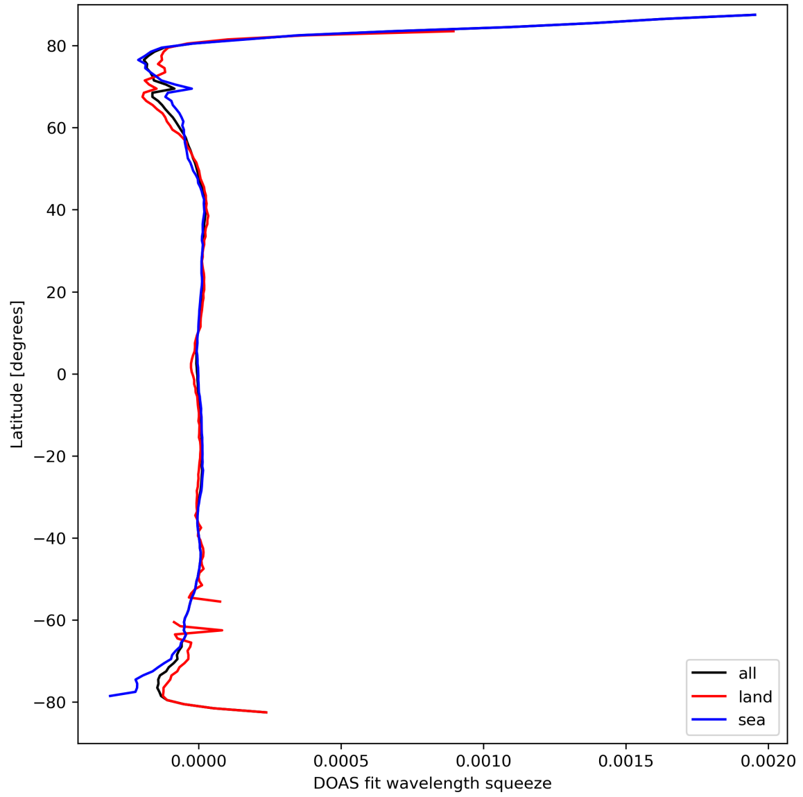
Figure 46: Zonal average of “DOAS fit wavelength squeeze” for 2024-03-25 to 2024-03-27.
