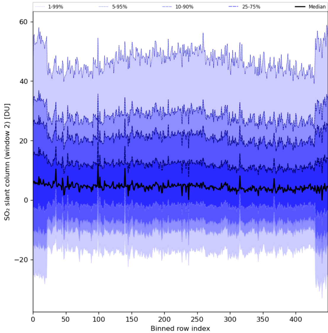
Figure 83: Along track statistics of “SO 2 slant column (window 2)” for 2024-03-25 to 2024-03-27
