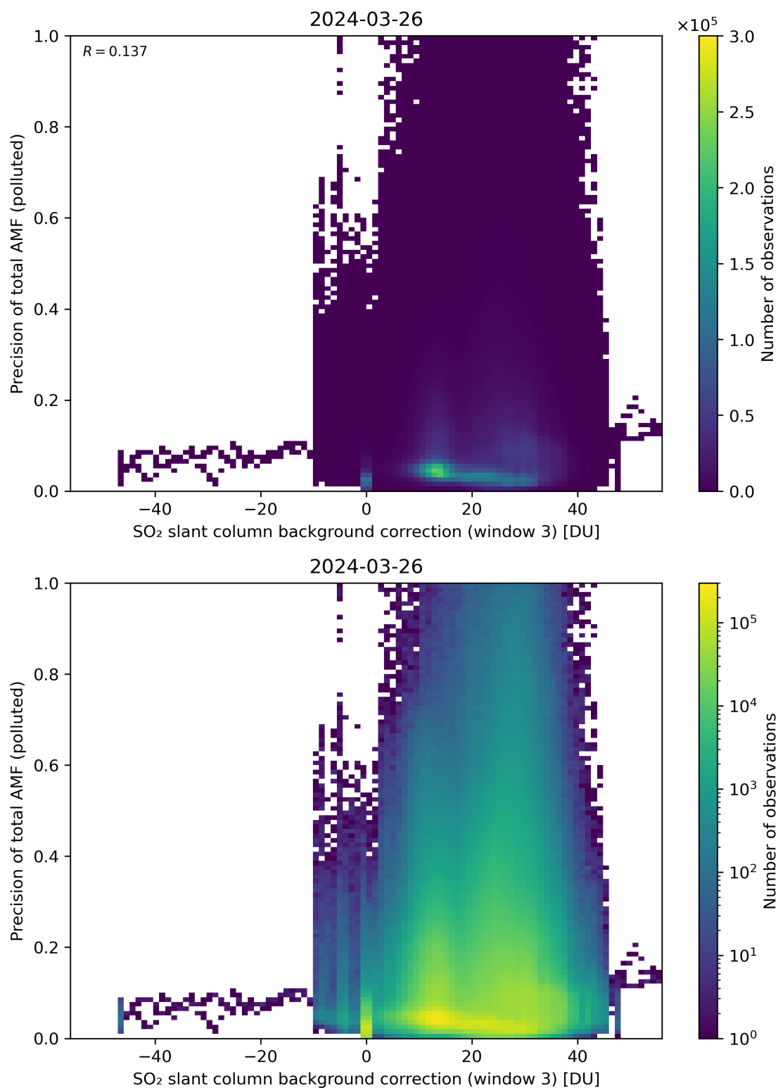
Figure 126: Scatter density plot of “SO 2 slant column background correction (window 3)” against “Precision of total AMF (polluted)” for 2024-03-25 to 2024-03-27.
