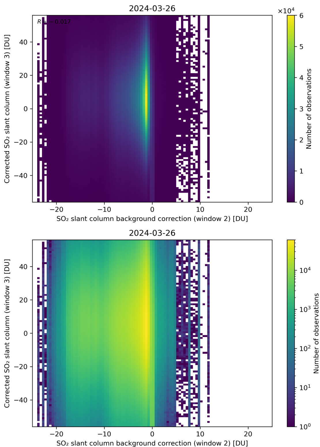
Figure 116: Scatter density plot of “SO 2 slant column background correction (window 2)” against “Corrected SO 2 slant column (window 3)” for 2024-03-25 to 2024-03-27.
