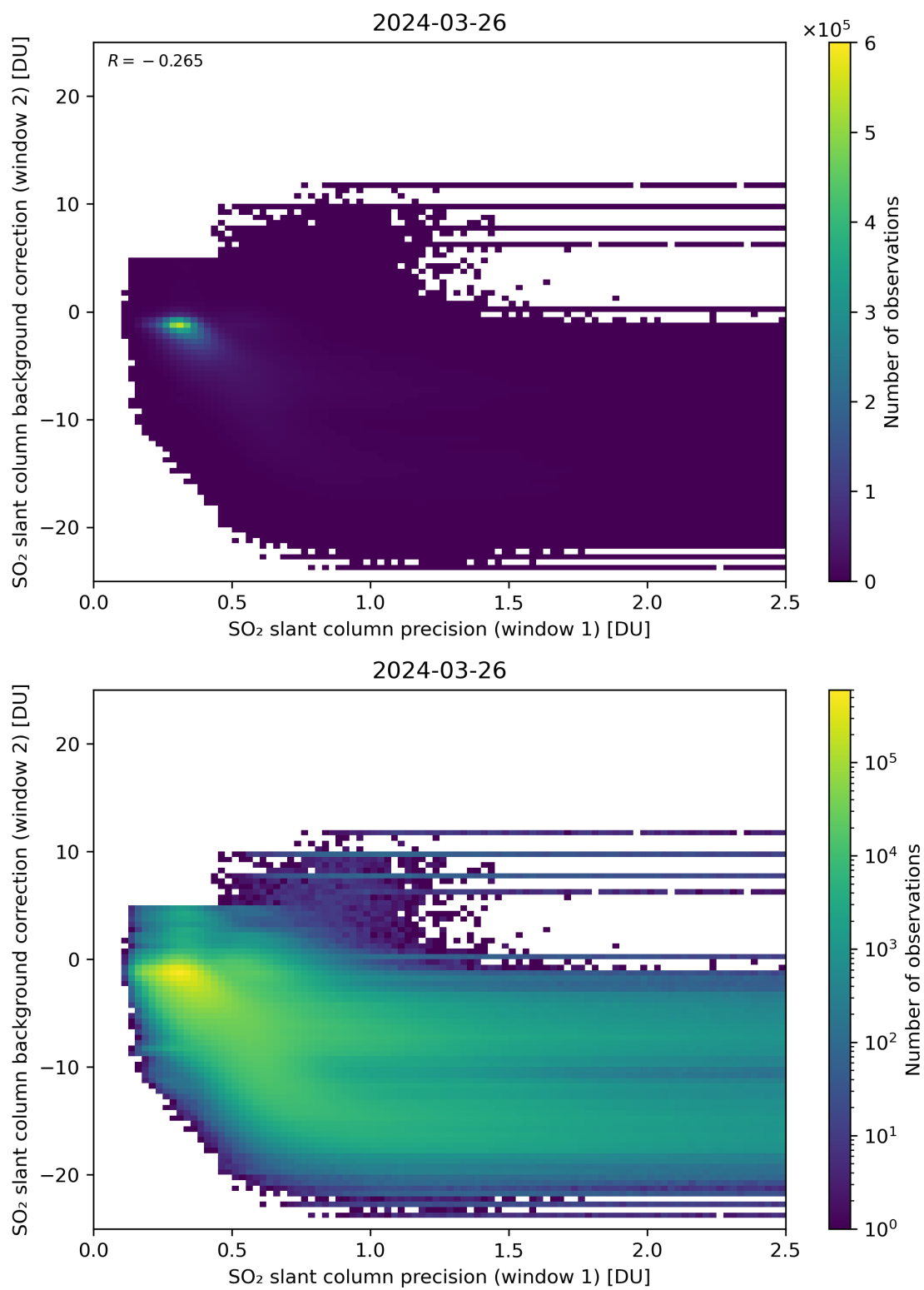
Figure 219: Scatter density plot of “SO 2 slant column precision (window 1)” against “SO 2 slant column background correction (window 2)” for 2024-03-25 to 2024-03-27.
