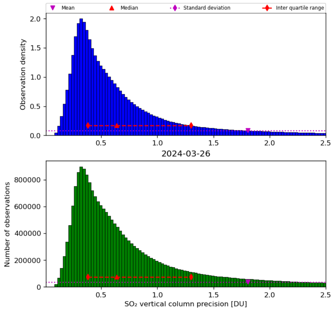
Figure 54: Histogram of “SO 2 vertical column precision” for 2024-03-25 to 2024-03-27
