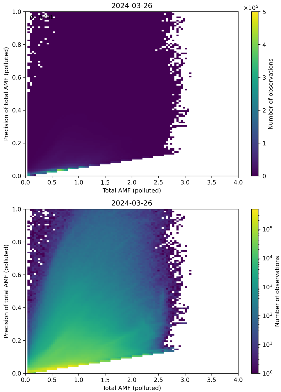
Figure 272: Scatter density plot of “Total AMF (polluted)” against “Precision of total AMF (polluted)” for 2024-03-25 to 2024-03-27.
