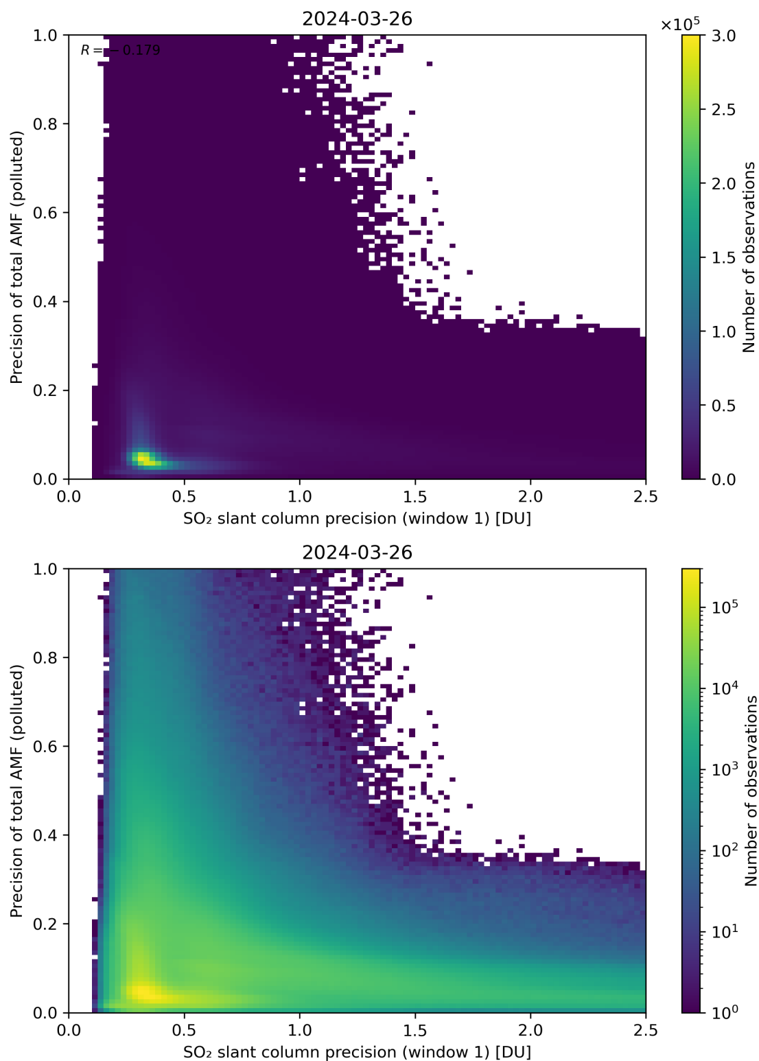
Figure 231: Scatter density plot of “SO 2 slant column precision (window 1)” against “Precision of total AMF (polluted)” for 2024-03-25 to 2024-03-27.
