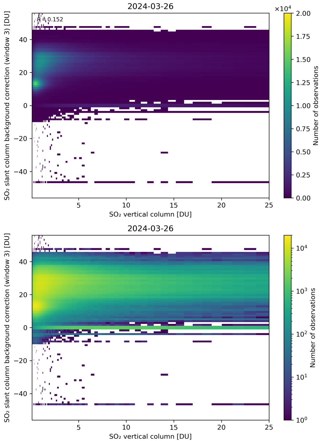
Figure 275: Scatter density plot of “SO 2 vertical column” against “SO 2 slant column background correction (window 3)” for 2024-03-25 to 2024-03-27.
