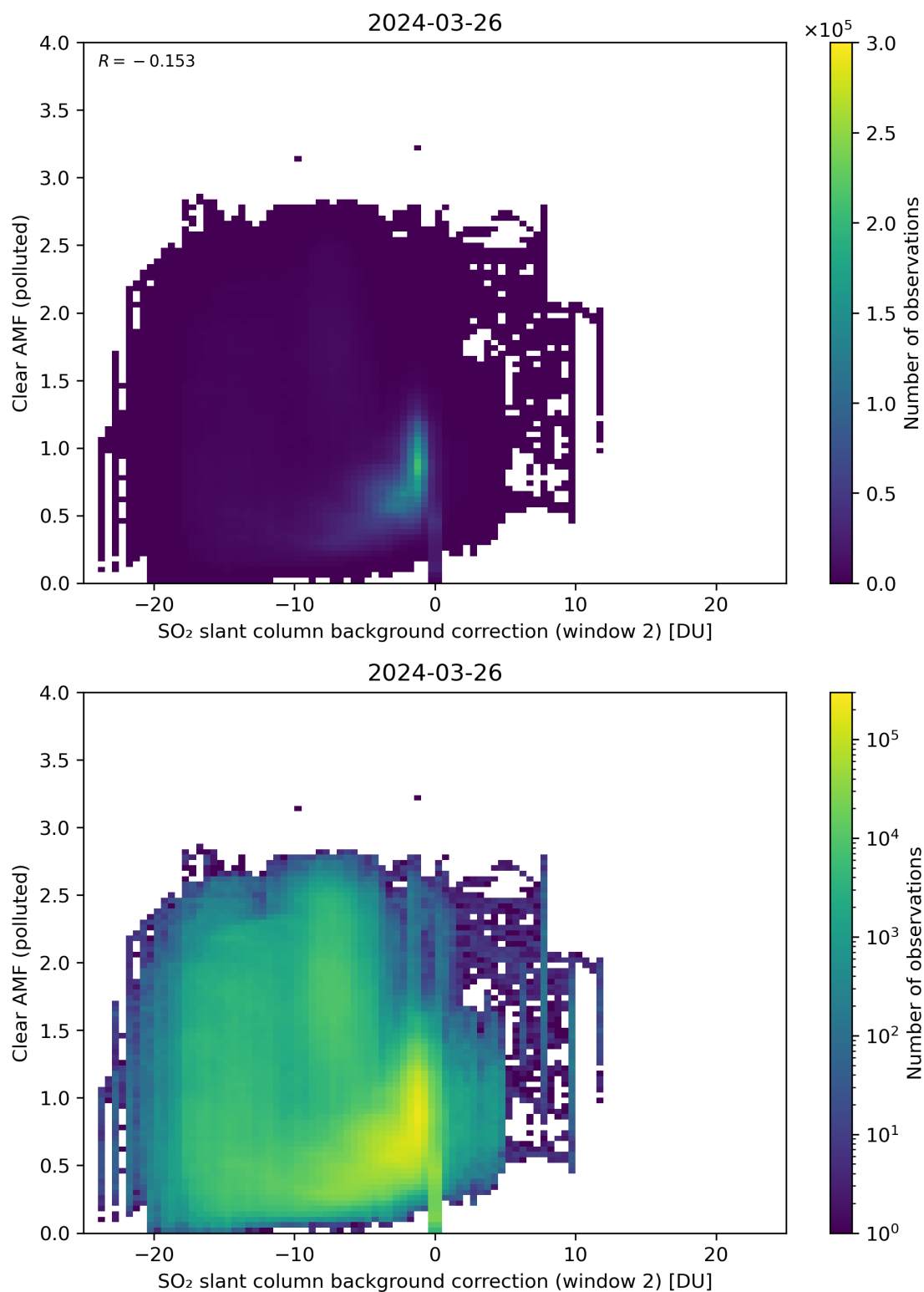
Figure 115: Scatter density plot of “SO 2 slant column background correction (window 2)” against “Clear AMF (polluted)” for 2024-03-25 to 2024-03-27.
