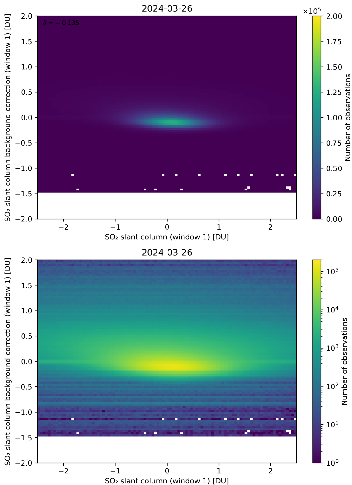
Figure 212: Scatter density plot of “SO 2 slant column (window 1)” against “SO 2 slant column background correction (window 1)” for 2024-03-25 to 2024-03-27.
