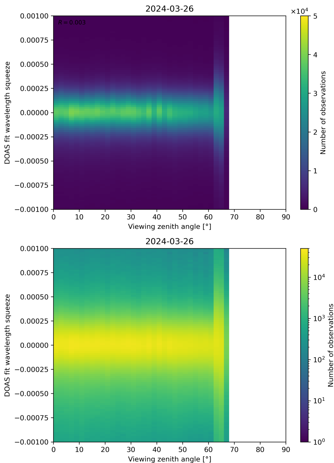
Figure 312: Scatter density plot of “Viewing zenith angle” against “DOAS fit wavelength squeeze” for 2024-03-25 to 2024-03-27.
