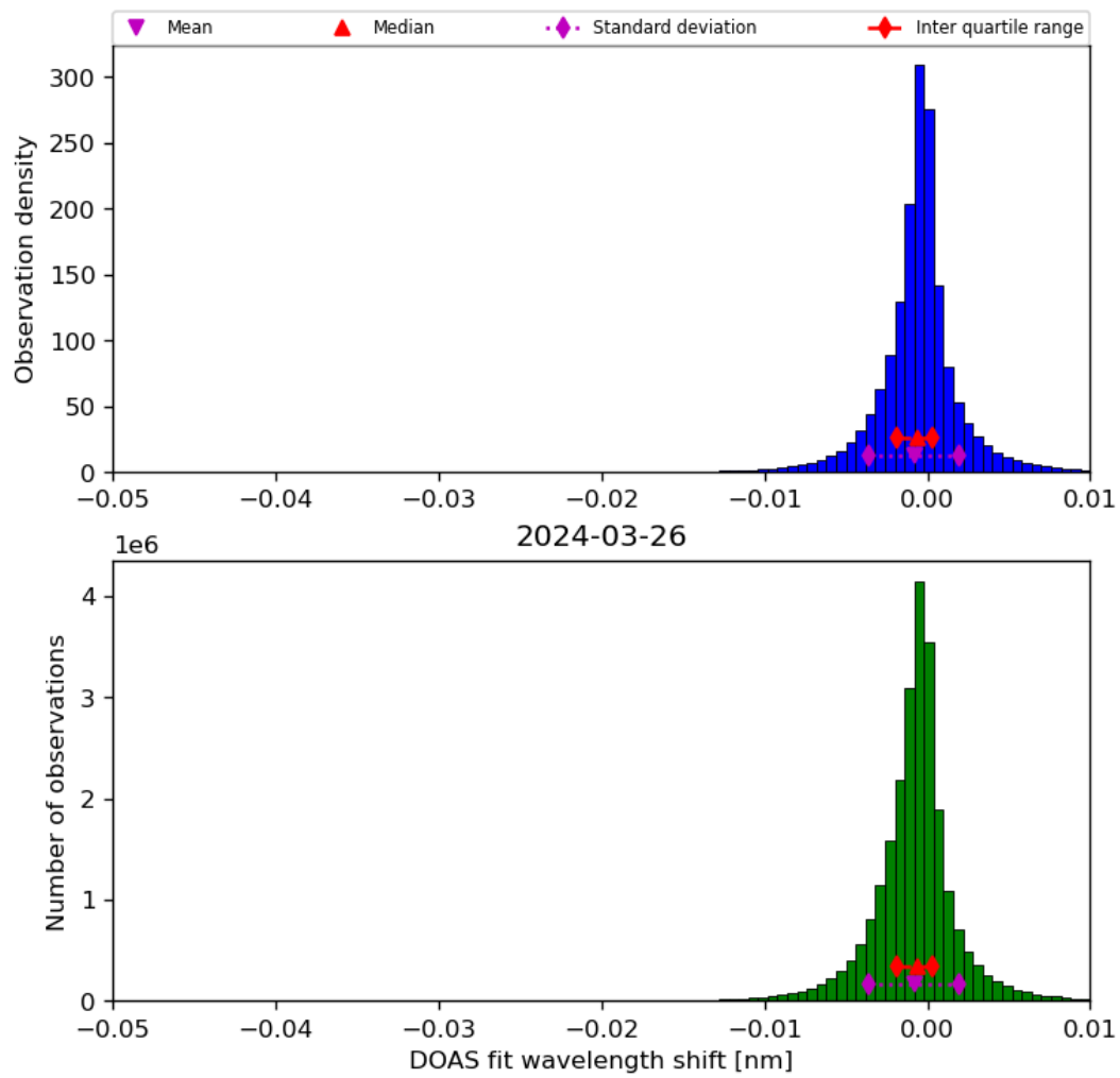
Figure 68: Histogram of “DOAS fit wavelength shift” for 2024-03-25 to 2024-03-27
