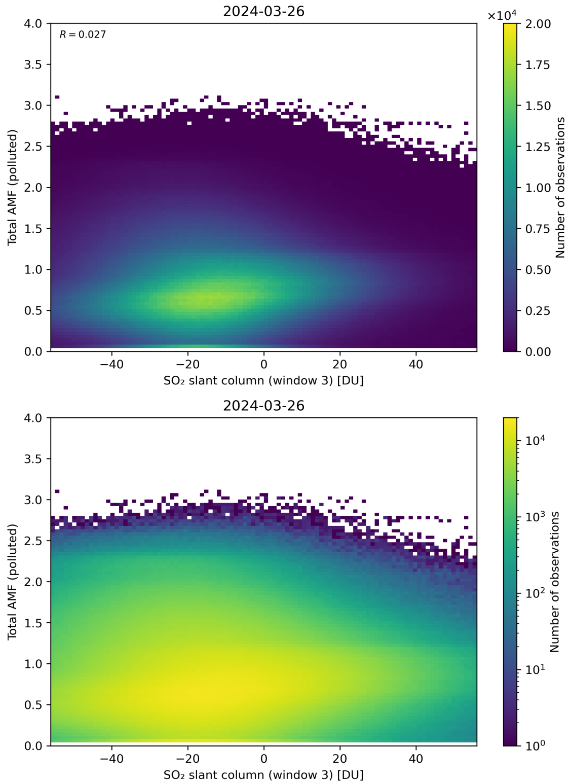
Figure 268: Scatter density plot of “SO 2 slant column (window 3)” against “Total AMF (polluted)” for 2024-03-25 to 2024-03-27.
