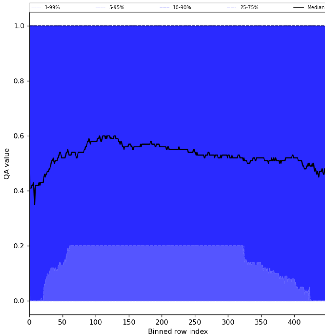
Figure 75: Along track statistics of “QA value” for 2024-03-25 to 2024-03-27
