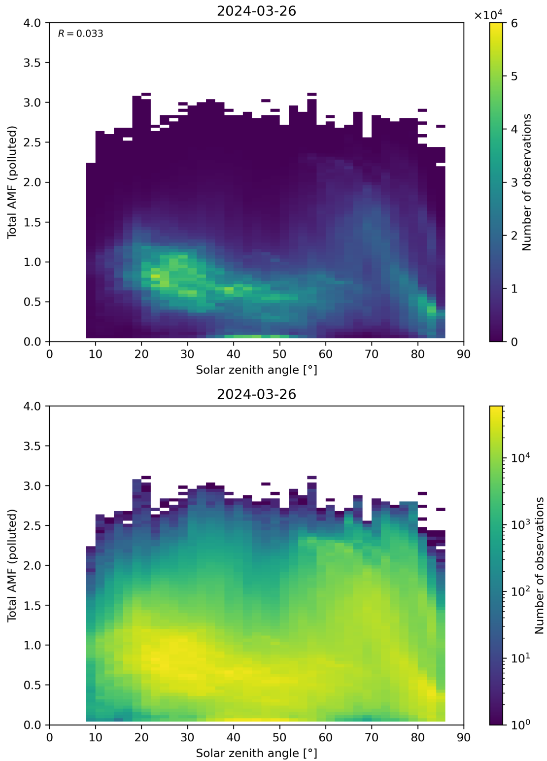
Figure 174: Scatter density plot of “Solar zenith angle” against “Total AMF (polluted)” for 2024-03-25 to 2024-03-27.
