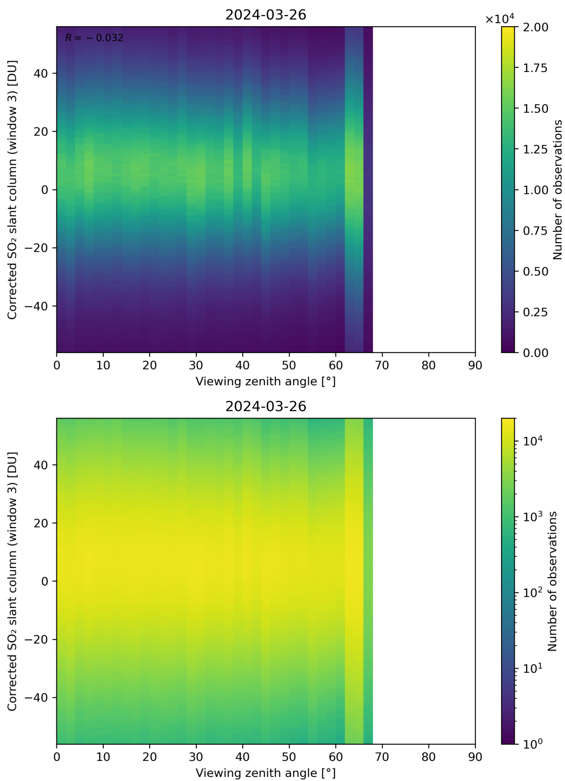
Figure 319: Scatter density plot of “Viewing zenith angle” against “Corrected SO 2 slant column (window 3)” for 2024-03-25 to 2024-03-27.
