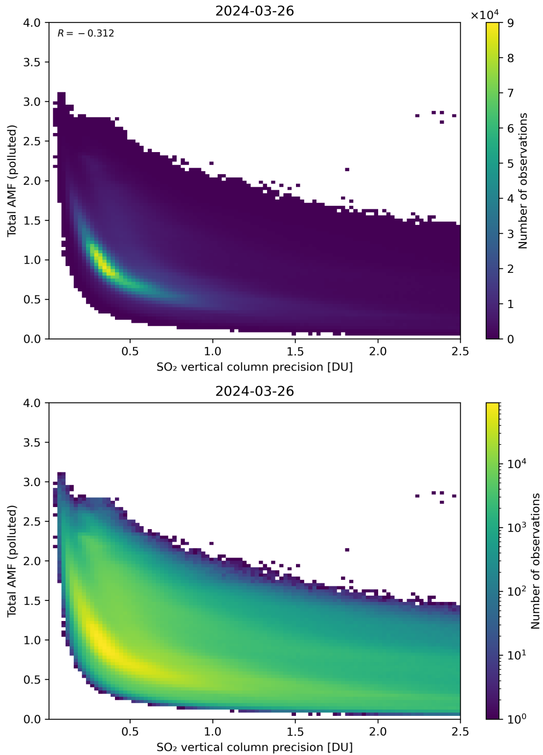
Figure 294: Scatter density plot of “SO 2 vertical column precision” against “Total AMF (polluted)” for 2024-03-25 to 2024-03-27.
