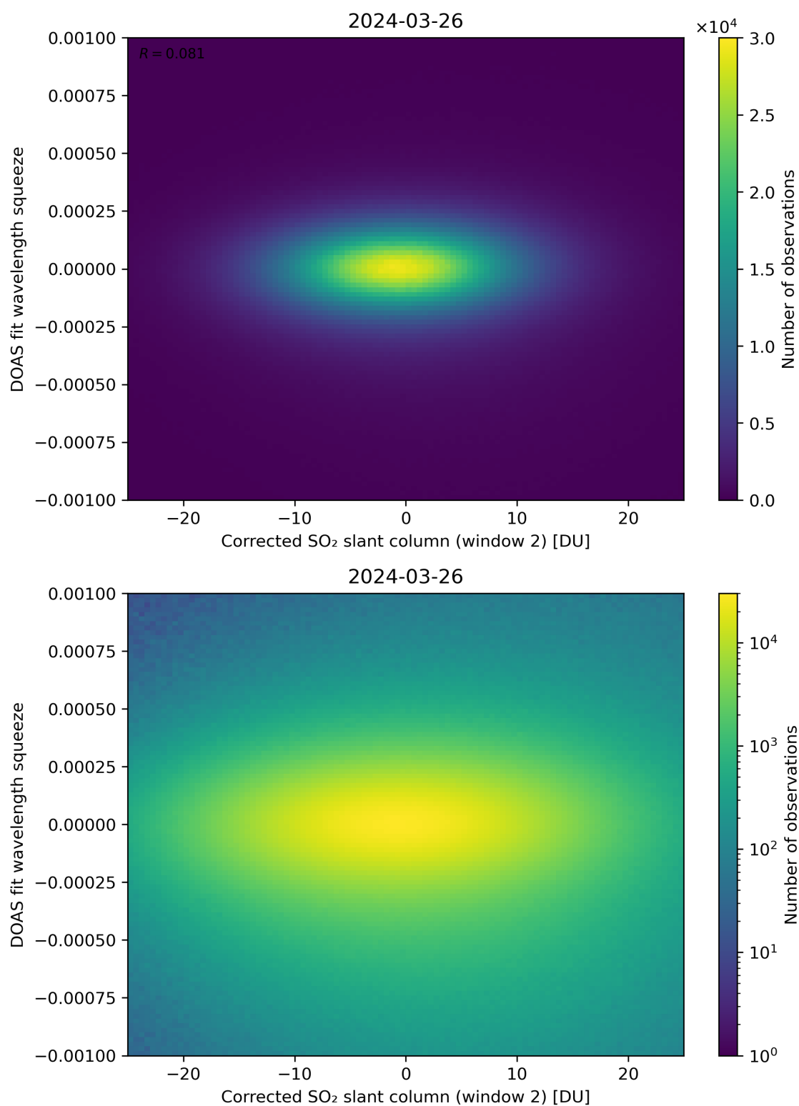
Figure 197: Scatter density plot of “Corrected SO 2 slant column (window 2)” against “DOAS fit wavelength squeeze” for 2024-03-25 to 2024-03-27.
