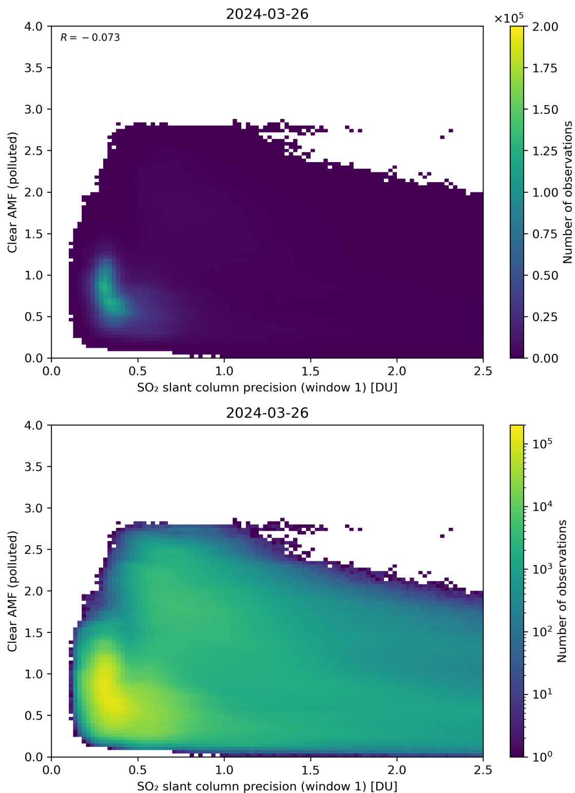
Figure 224: Scatter density plot of “SO 2 slant column precision (window 1)” against “Clear AMF (polluted)” for 2024-03-25 to 2024-03-27.
