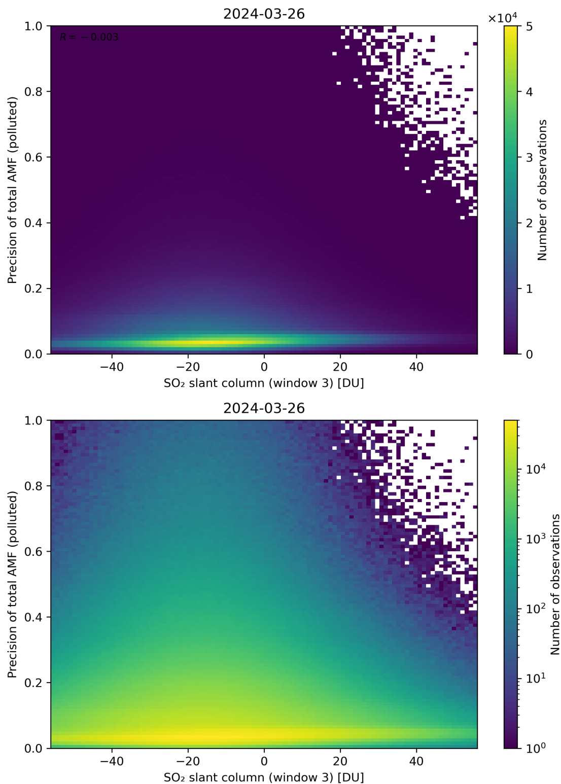
Figure 269: Scatter density plot of “SO 2 slant column (window 3)” against “Precision of total AMF (polluted)” for 2024-03-25 to 2024-03-27.
