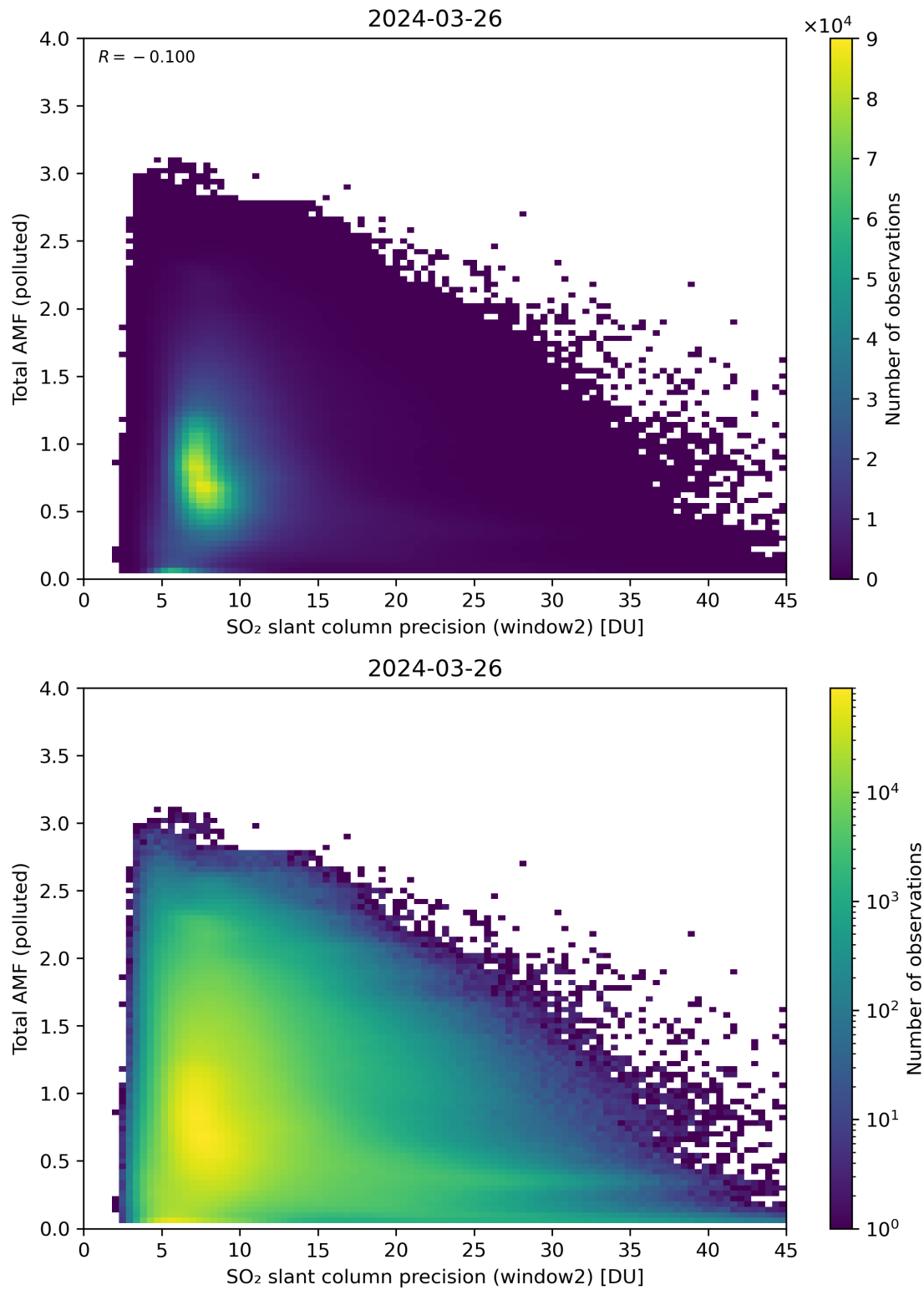
Figure 251: Scatter density plot of “SO 2 slant column precision (window2)” against “Total AMF (polluted)” for 2024-03-25 to 2024-03-27.
