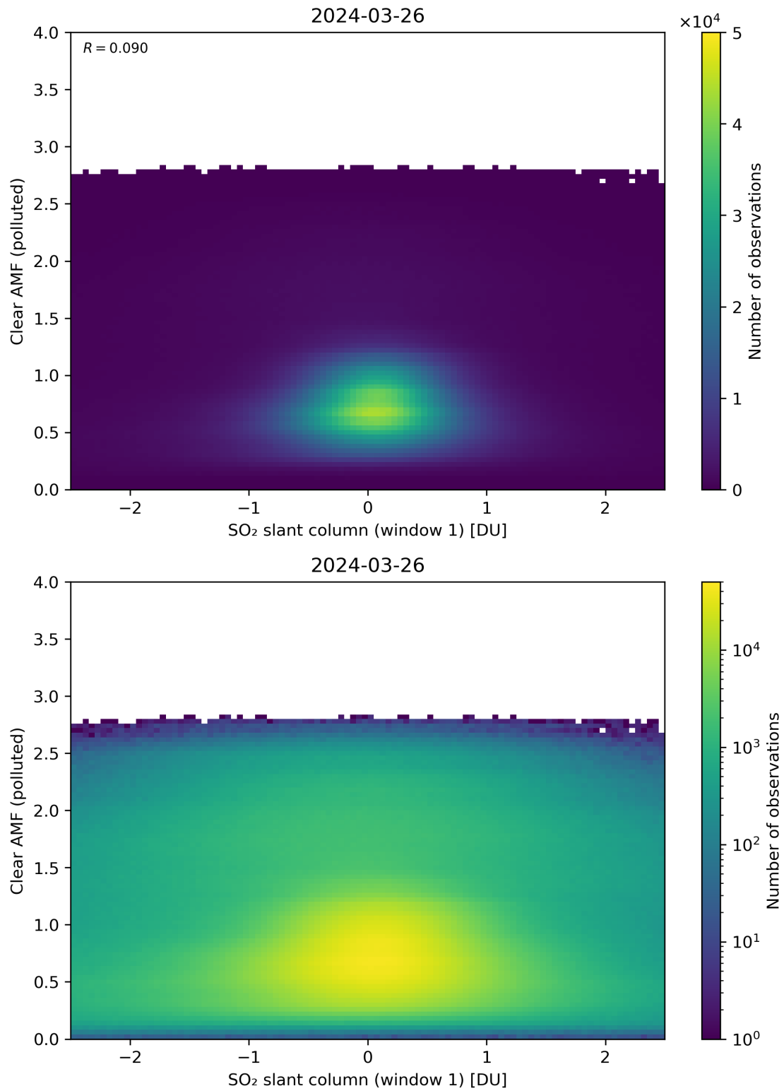
Figure 232: Scatter density plot of “SO 2 slant column (window 1)” against “Clear AMF (polluted)” for 2024-03-25 to 2024-03-27.
