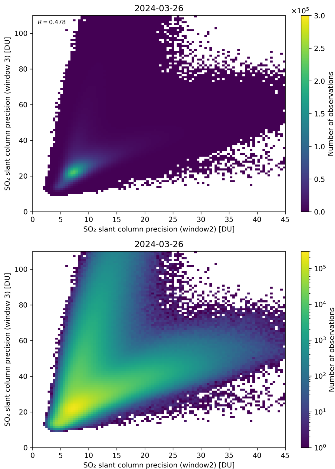
Figure 250: Scatter density plot of “SO 2 slant column precision (window2)” against “SO 2 slant column precision (window 3)” for 2024-03-25 to 2024-03-27.
