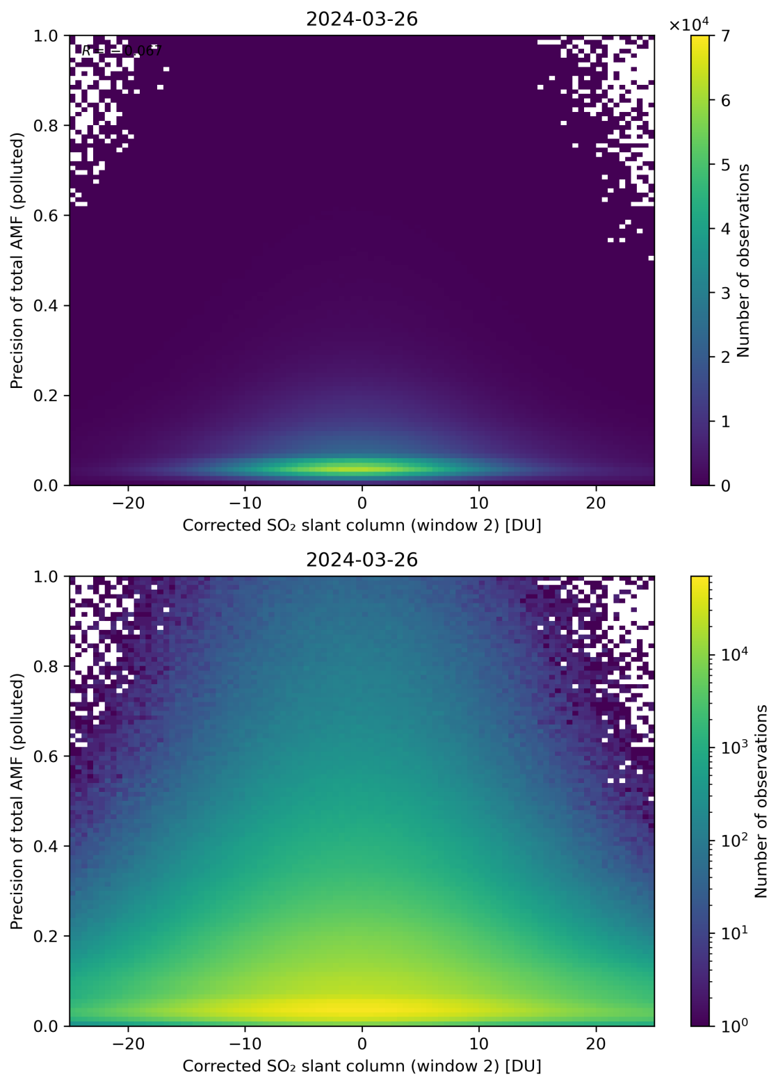
Figure 204: Scatter density plot of “Corrected SO 2 slant column (window 2)” against “Precision of total AMF (polluted)” for 2024-03-25 to 2024-03-27.
