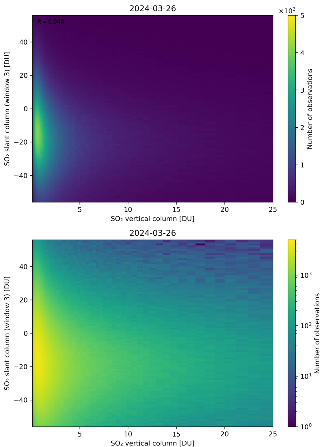
Figure 303: Scatter density plot of “SO 2 vertical column” against “SO 2 slant column (window 3)” for 2024-03-25 to 2024-03-27.
