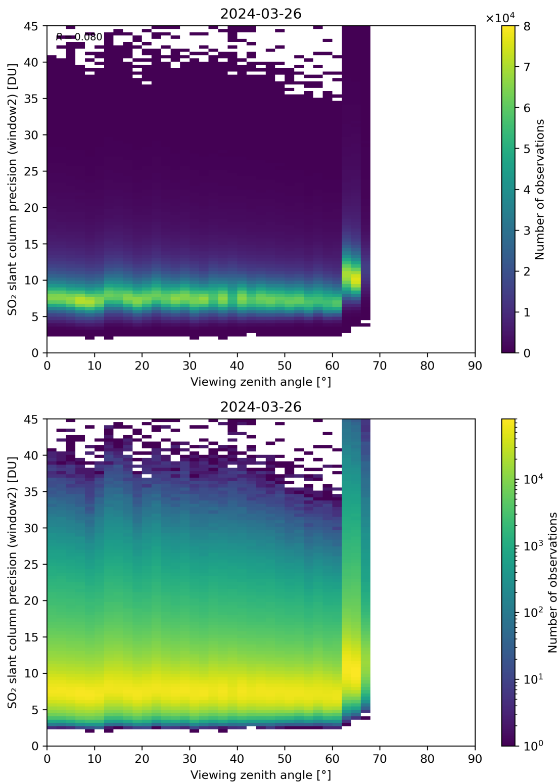
Figure 322: Scatter density plot of “Viewing zenith angle” against “SO 2 slant column precision (window2)” for 2024-03-25 to 2024-03-27.
