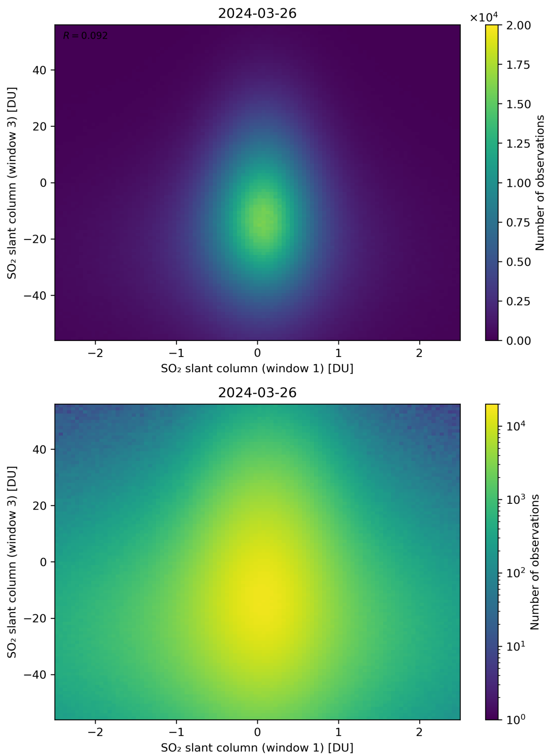
Figure 237: Scatter density plot of “SO 2 slant column (window 1)” against “SO 2 slant column (window 3)” for 2024-03-25 to 2024-03-27.
