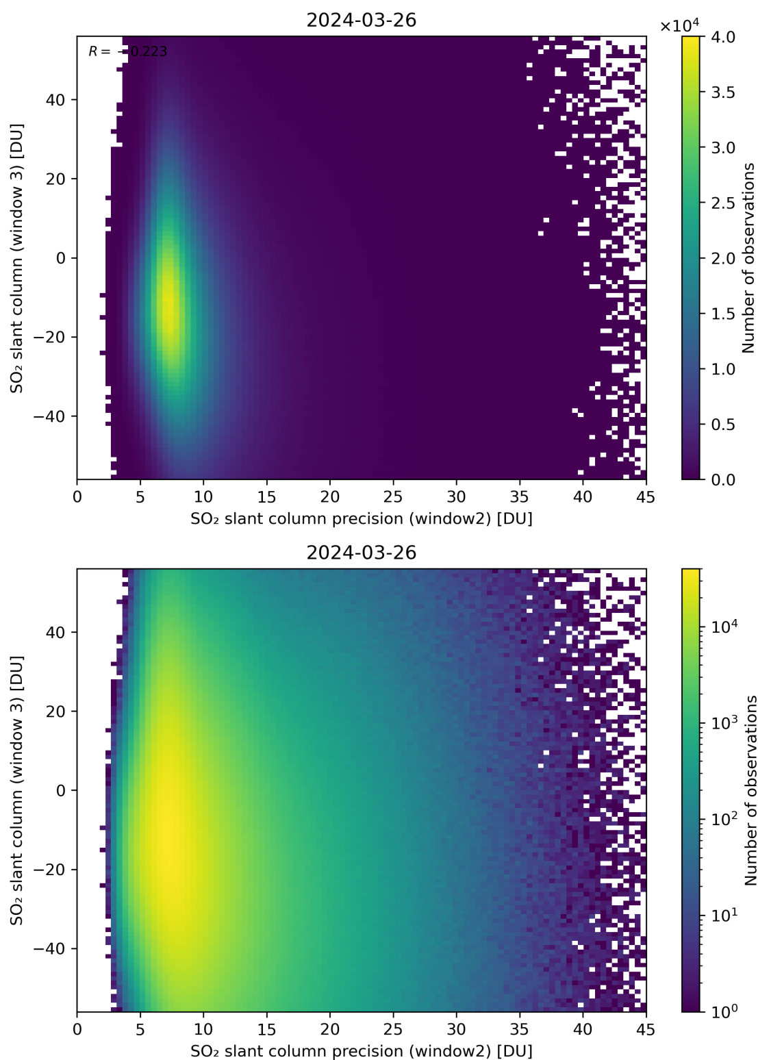
Figure 249: Scatter density plot of “SO 2 slant column precision (window2)” against “SO 2 slant column (window 3)” for 2024-03-25 to 2024-03-27.
