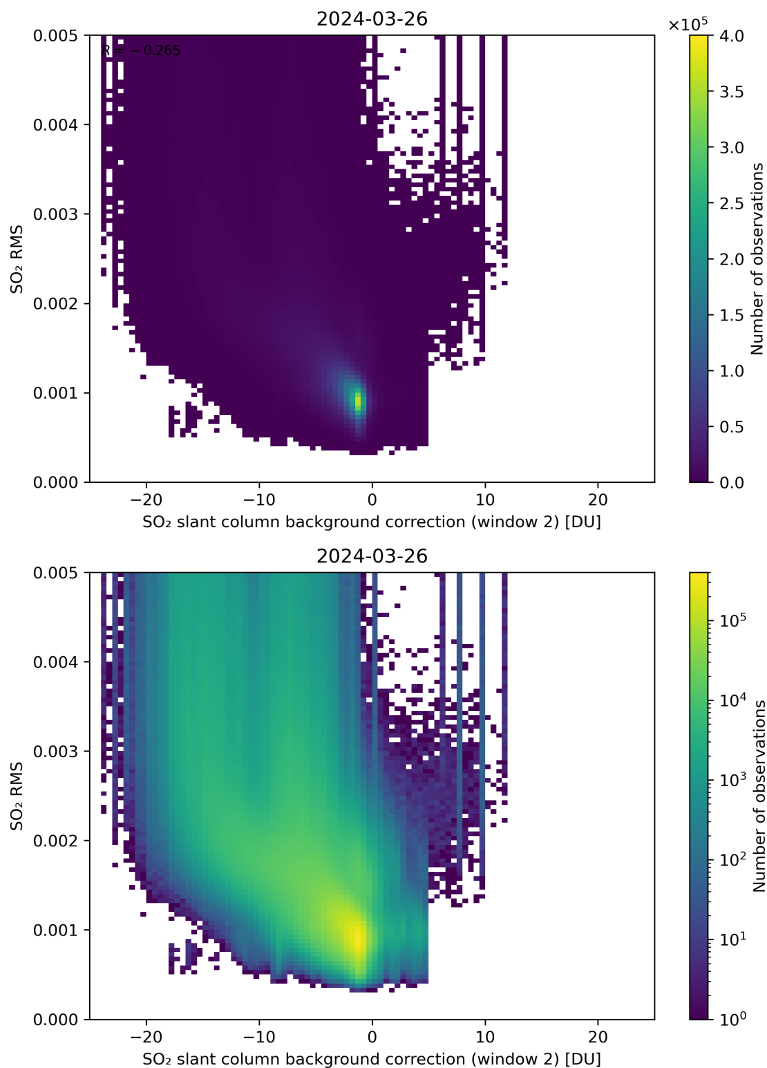
Figure 114: Scatter density plot of “SO 2 slant column background correction (window 2)” against “SO 2 RMS” for 2024-03-25 to 2024-03-27.
