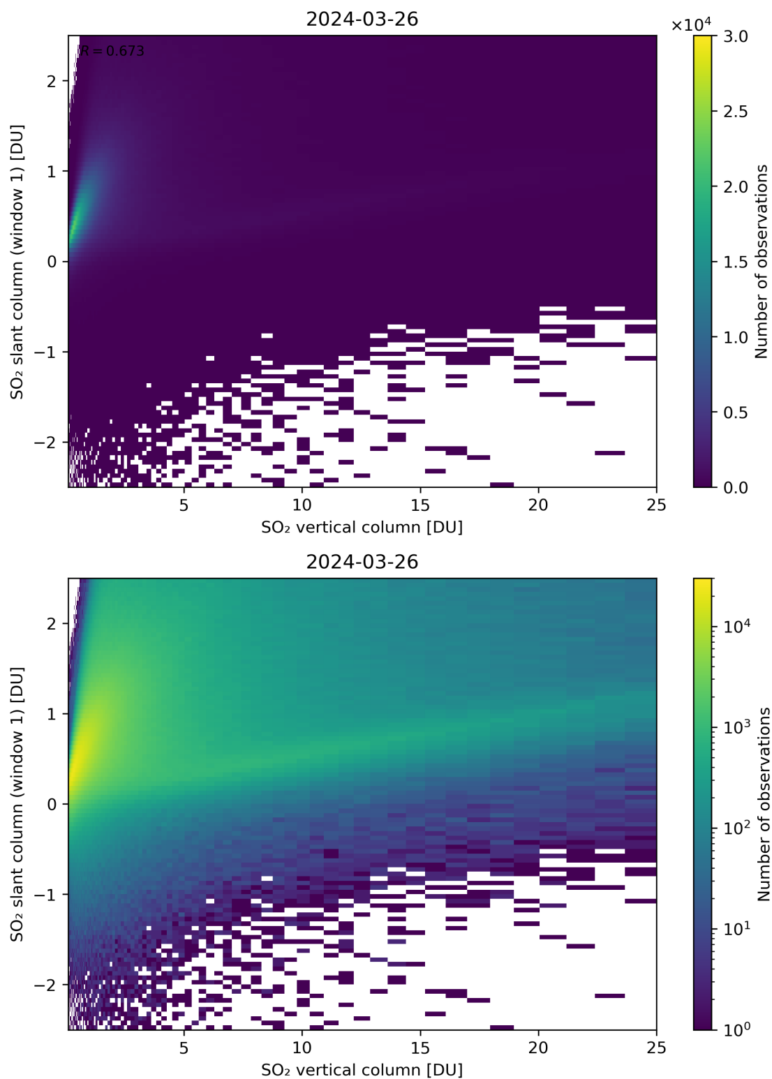
Figure 300: Scatter density plot of “SO 2 vertical column” against “SO 2 slant column (window 1)” for 2024-03-25 to 2024-03-27.
