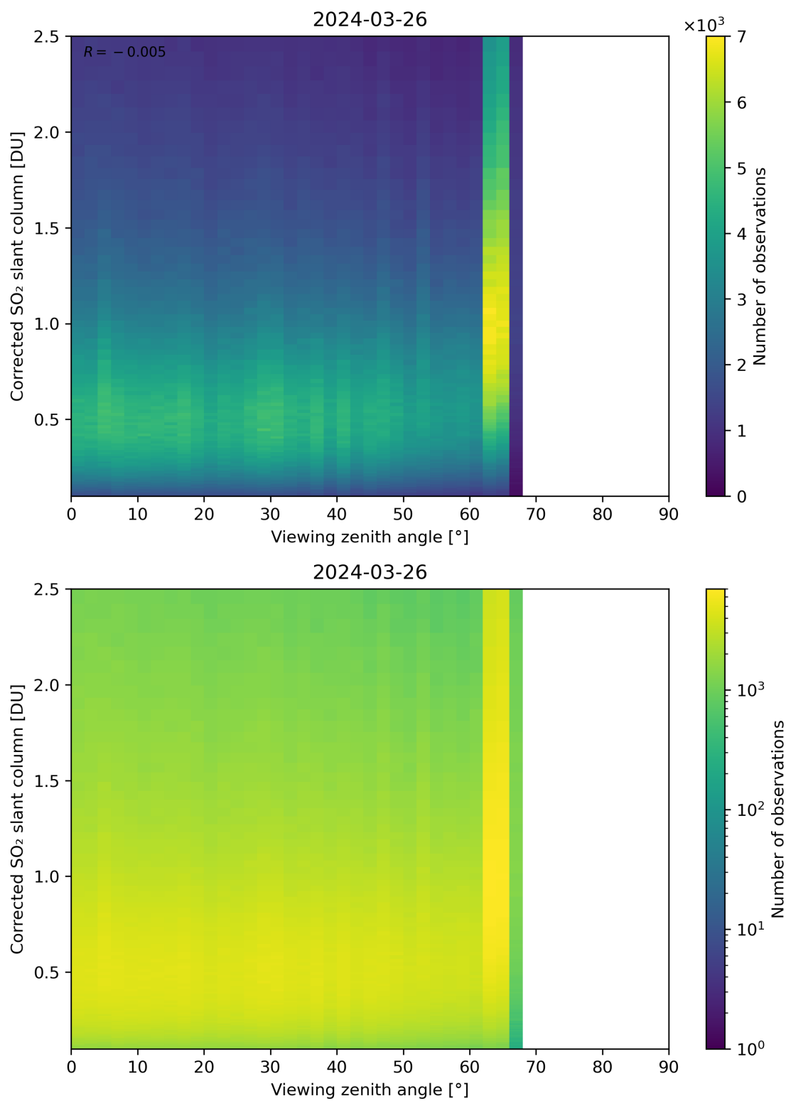
Figure 317: Scatter density plot of “Viewing zenith angle” against “Corrected SO 2 slant column” for 2024-03-25 to 2024-03-27.
