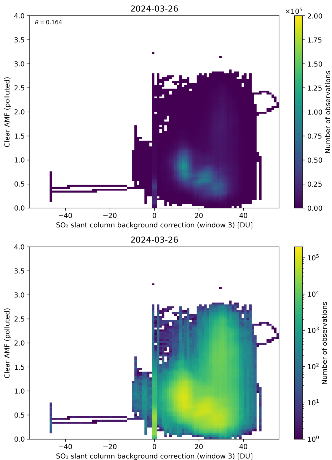
Figure 124: Scatter density plot of “SO 2 slant column background correction (window 3)” against “Clear AMF (polluted)” for 2024-03-25 to 2024-03-27.
