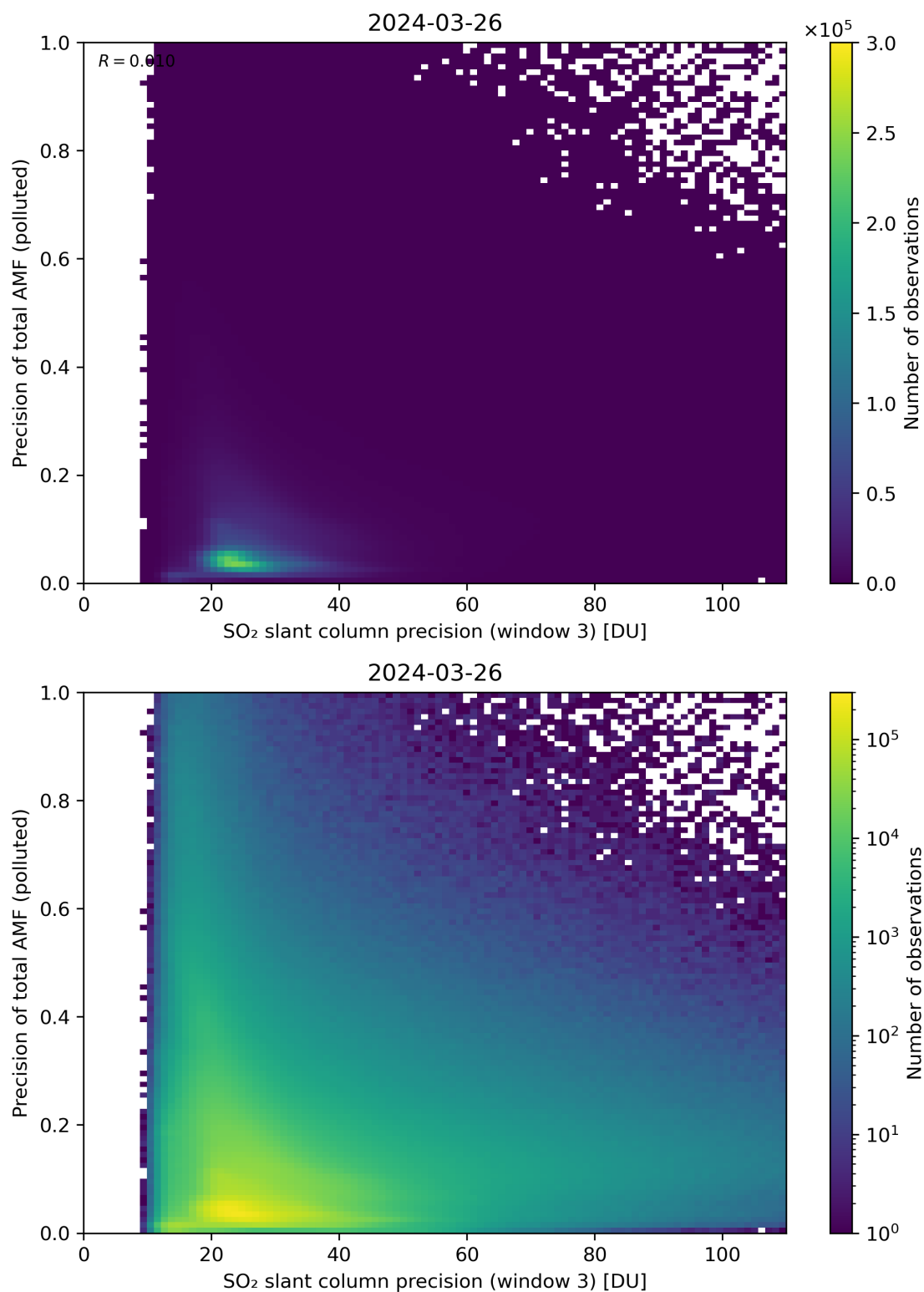
Figure 264: Scatter density plot of “SO 2 slant column precision (window 3)” against “Precision of total AMF (polluted)” for 2024-03-25 to 2024-03-27.
