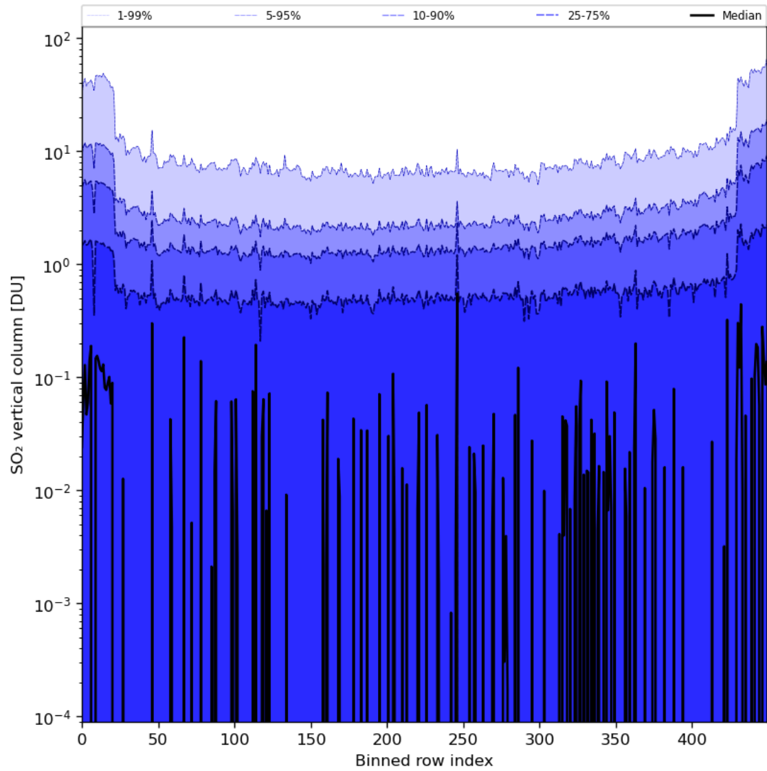
Figure 76: Along track statistics of “SO 2 vertical column” for 2024-03-25 to 2024-03-27
