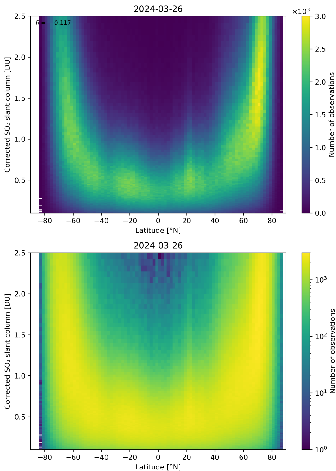
Figure 146: Scatter density plot of “Latitude” against “Corrected SO 2 slant column” for 2024-03-25 to 2024-03-27.
