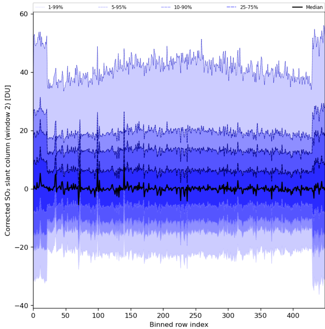
Figure 85: Along track statistics of “Corrected SO 2 slant column (window 2)” for 2024-03-25 to 2024-03-27
