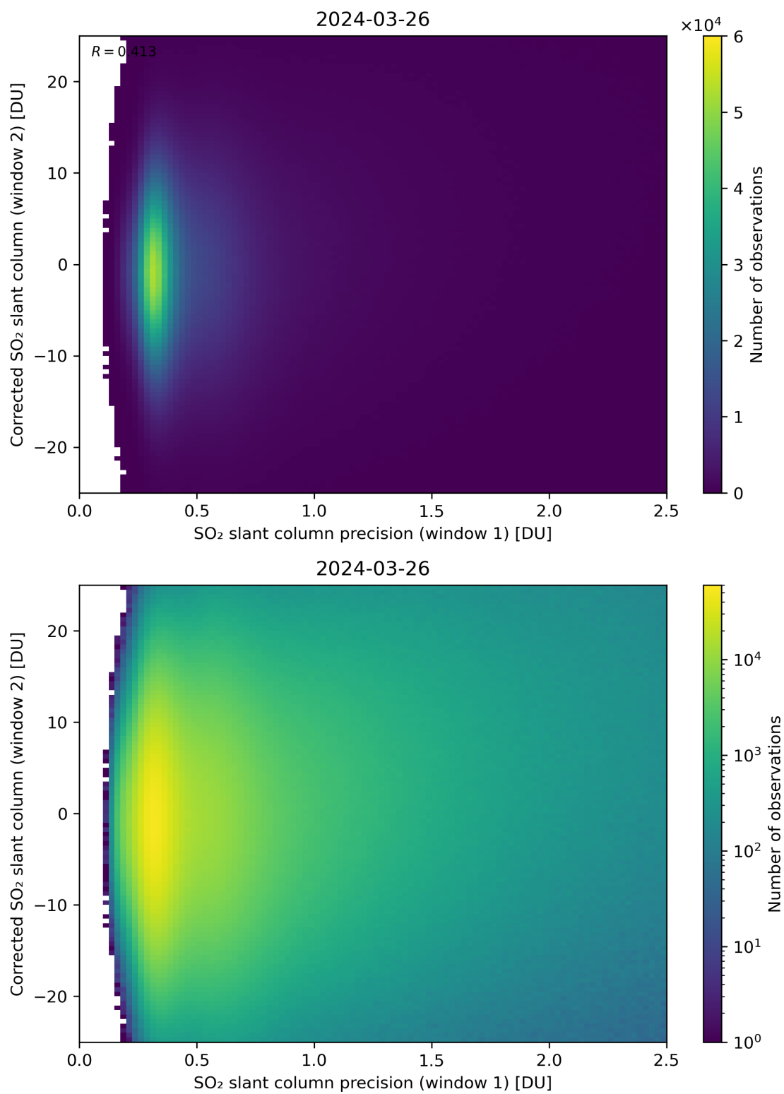
Figure 225: Scatter density plot of “SO 2 slant column precision (window 1)” against “Corrected SO 2 slant column (window 2)” for 2024-03-25 to 2024-03-27.
