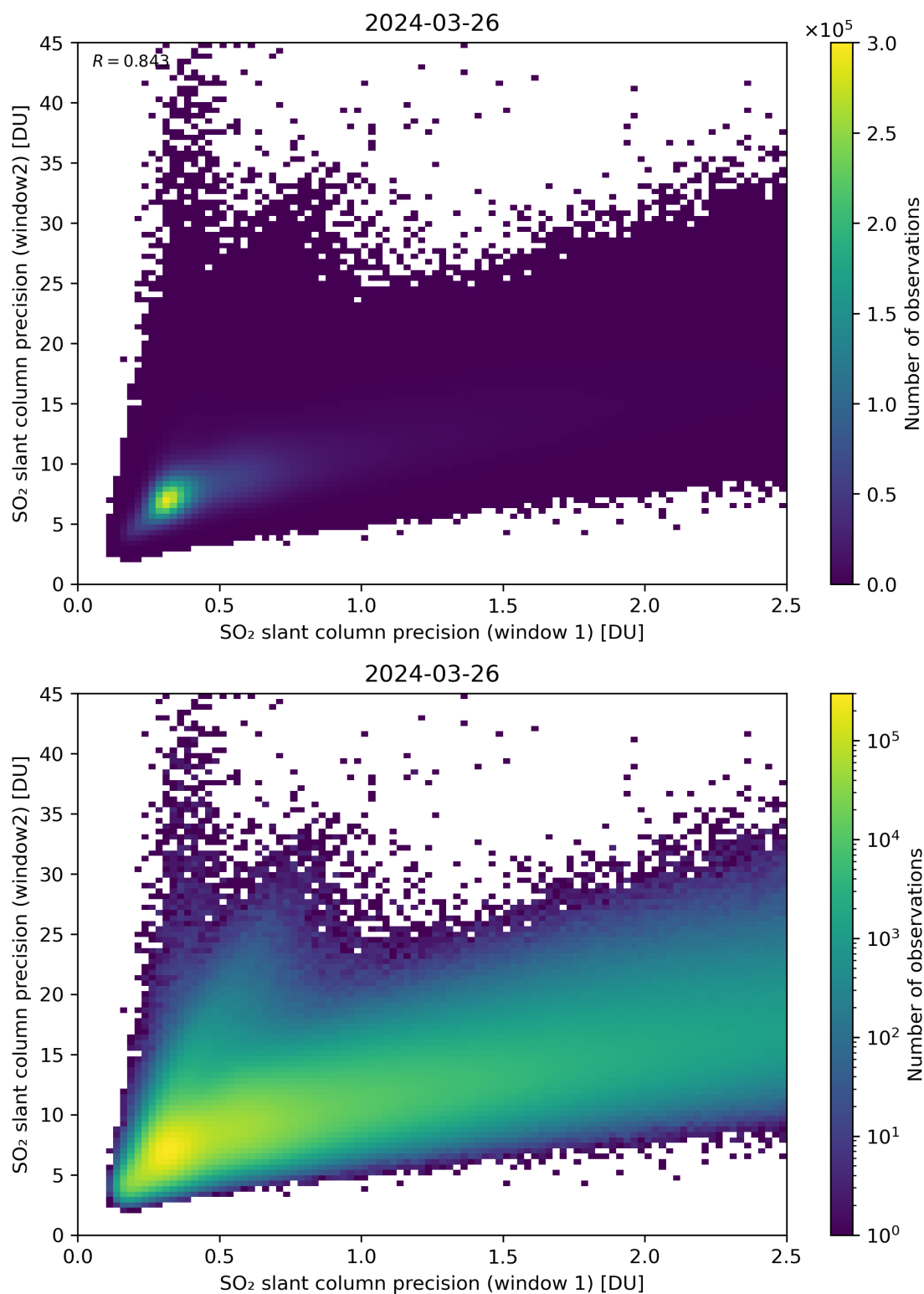
Figure 227: Scatter density plot of “SO 2 slant column precision (window 1)” against “SO 2 slant column precision (window2)” for 2024-03-25 to 2024-03-27.
