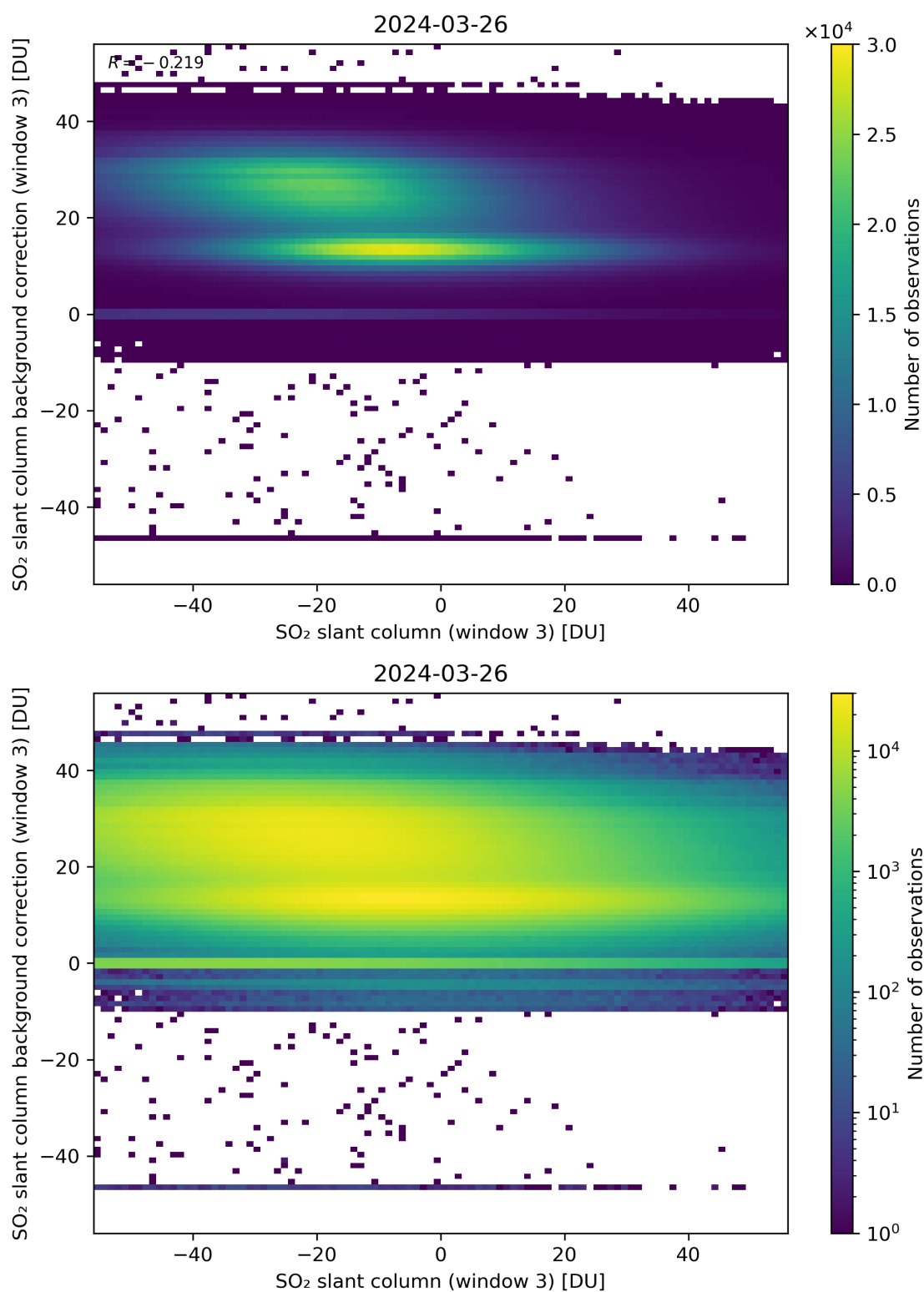
Figure 253: Scatter density plot of “SO 2 slant column (window 3)” against “SO 2 slant column background correction (window 3)” for 2024-03-25 to 2024-03-27.
