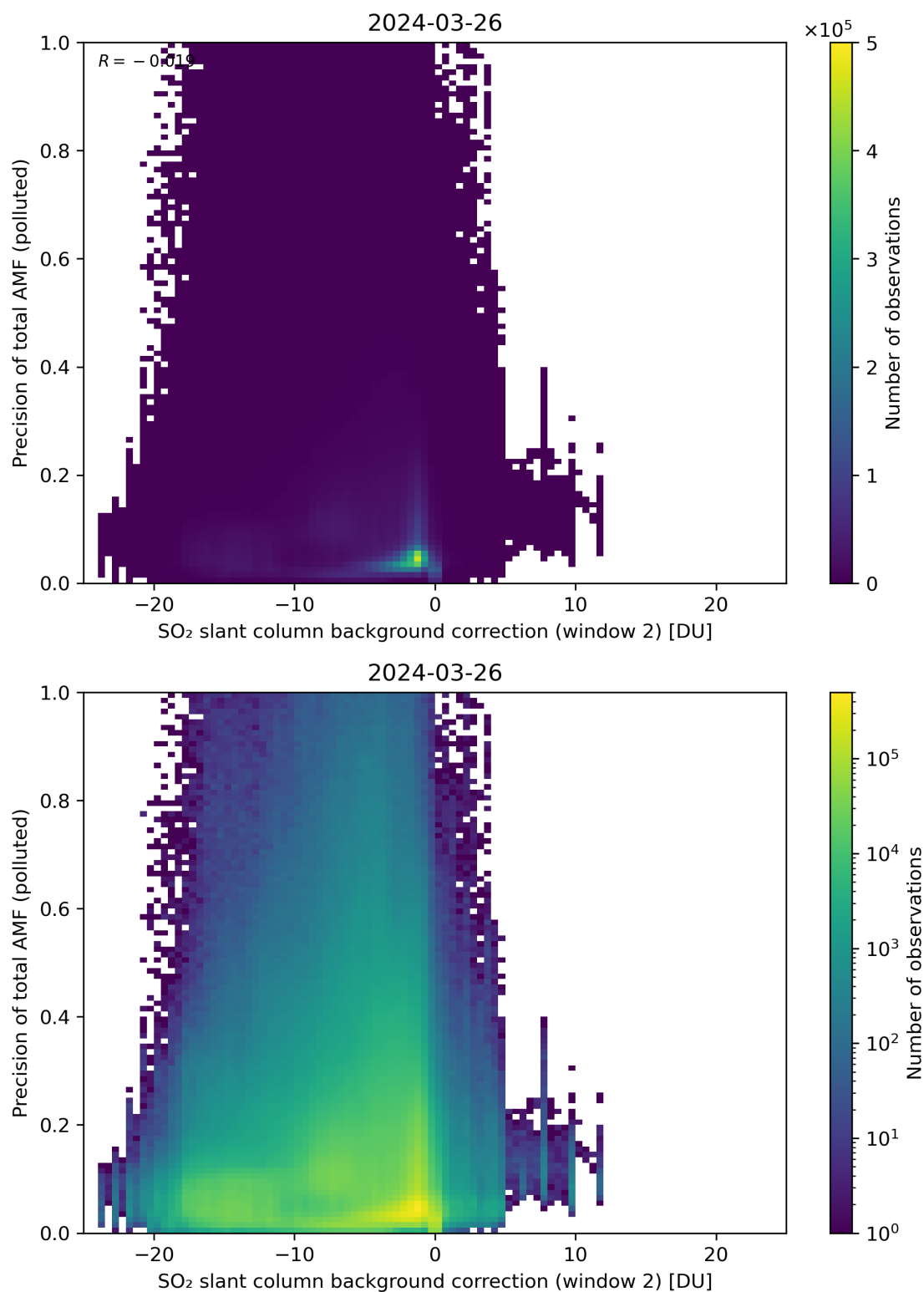
Figure 120: Scatter density plot of “SO 2 slant column background correction (window 2)” against “Precision of total AMF (polluted)” for 2024-03-25 to 2024-03-27.
