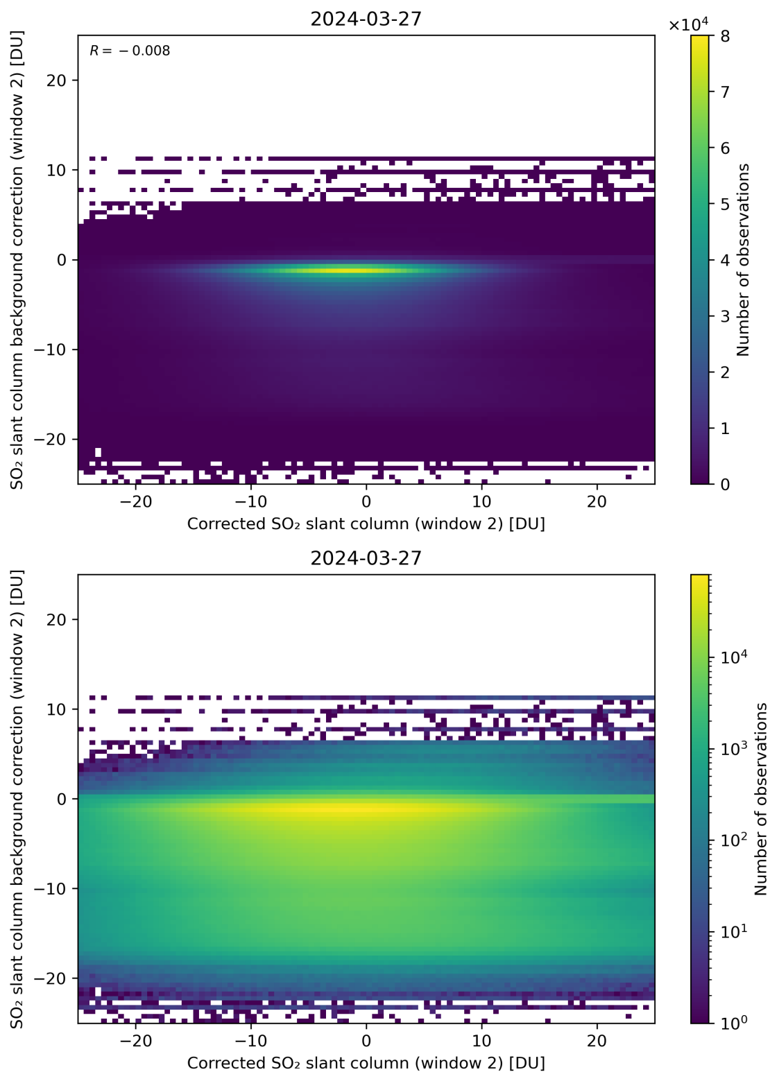
Figure 194: Scatter density plot of “Corrected SO 2 slant column (window 2)” against “SO 2 slant column background correction (window 2)” for 2024-03-26 to 2024-03-28.
