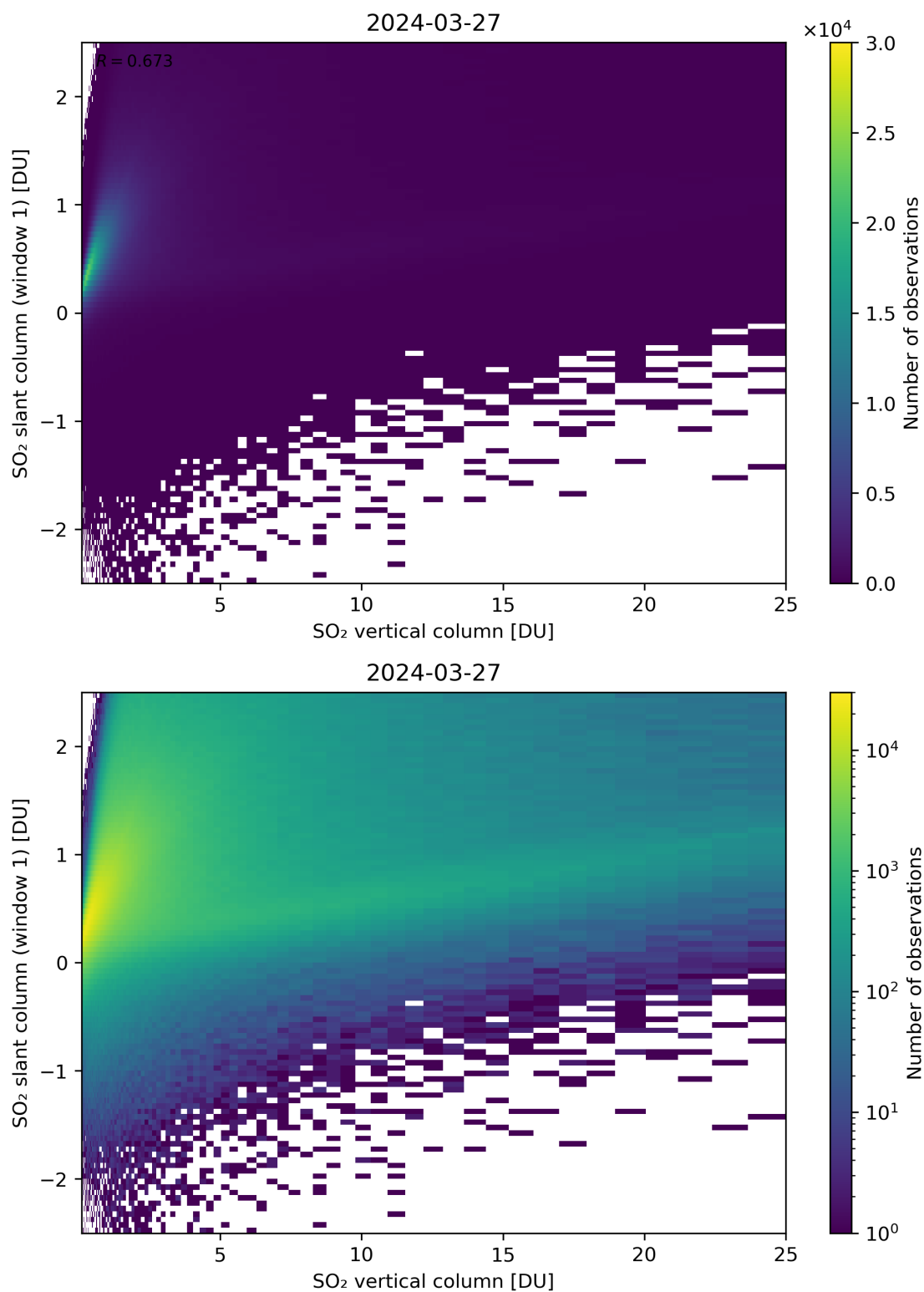
Figure 300: Scatter density plot of “SO 2 vertical column” against “SO 2 slant column (window 1)” for 2024-03-26 to 2024-03-28.
