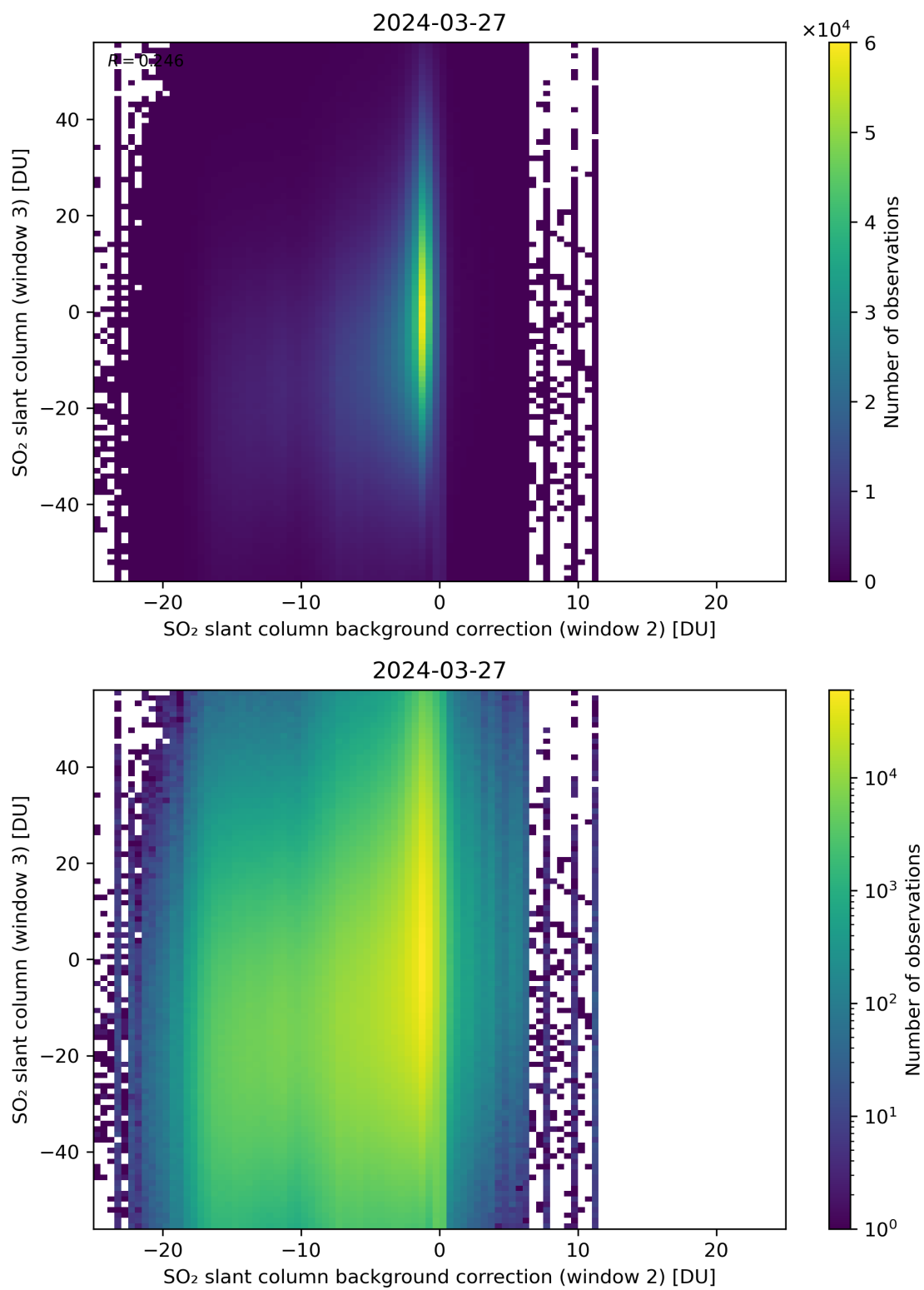
Figure 117: Scatter density plot of “SO 2 slant column background correction (window 2)” against “SO 2 slant column (window 3)” for 2024-03-26 to 2024-03-28.
