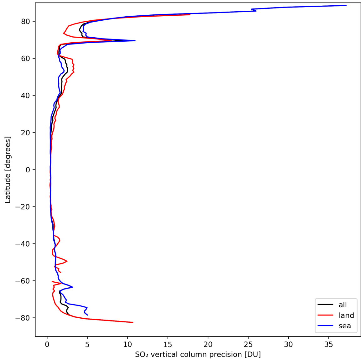
Figure 31: Zonal average of “SO 2 vertical column precision” for 2024-03-26 to 2024-03-28.
