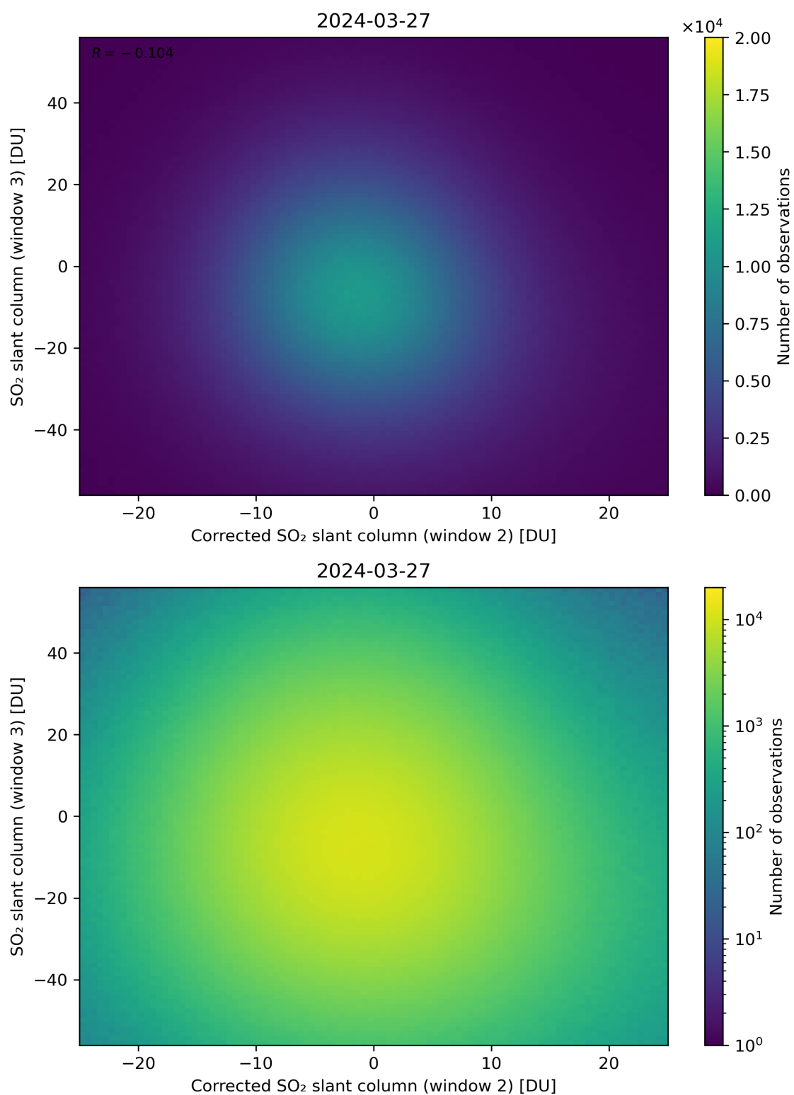
Figure 201: Scatter density plot of “Corrected SO 2 slant column (window 2)” against “SO 2 slant column (window 3)” for 2024-03-26 to 2024-03-28.
