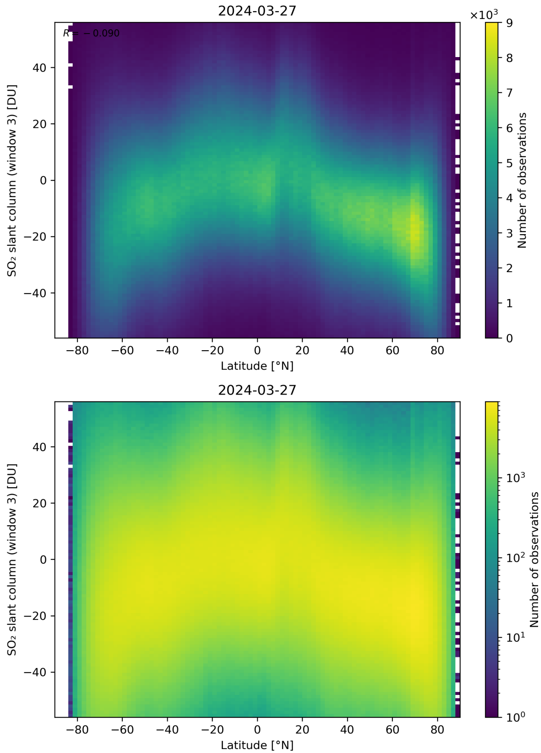
Figure 152: Scatter density plot of “Latitude” against “SO 2 slant column (window 3)” for 2024-03-26 to 2024-03-28.
