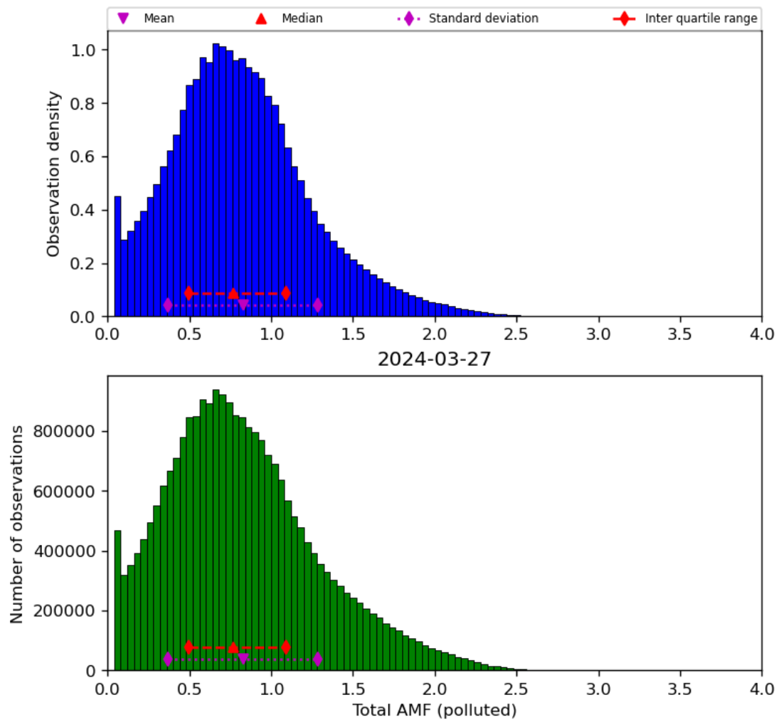
Figure 71: Histogram of “Total AMF (polluted)” for 2024-03-26 to 2024-03-28
