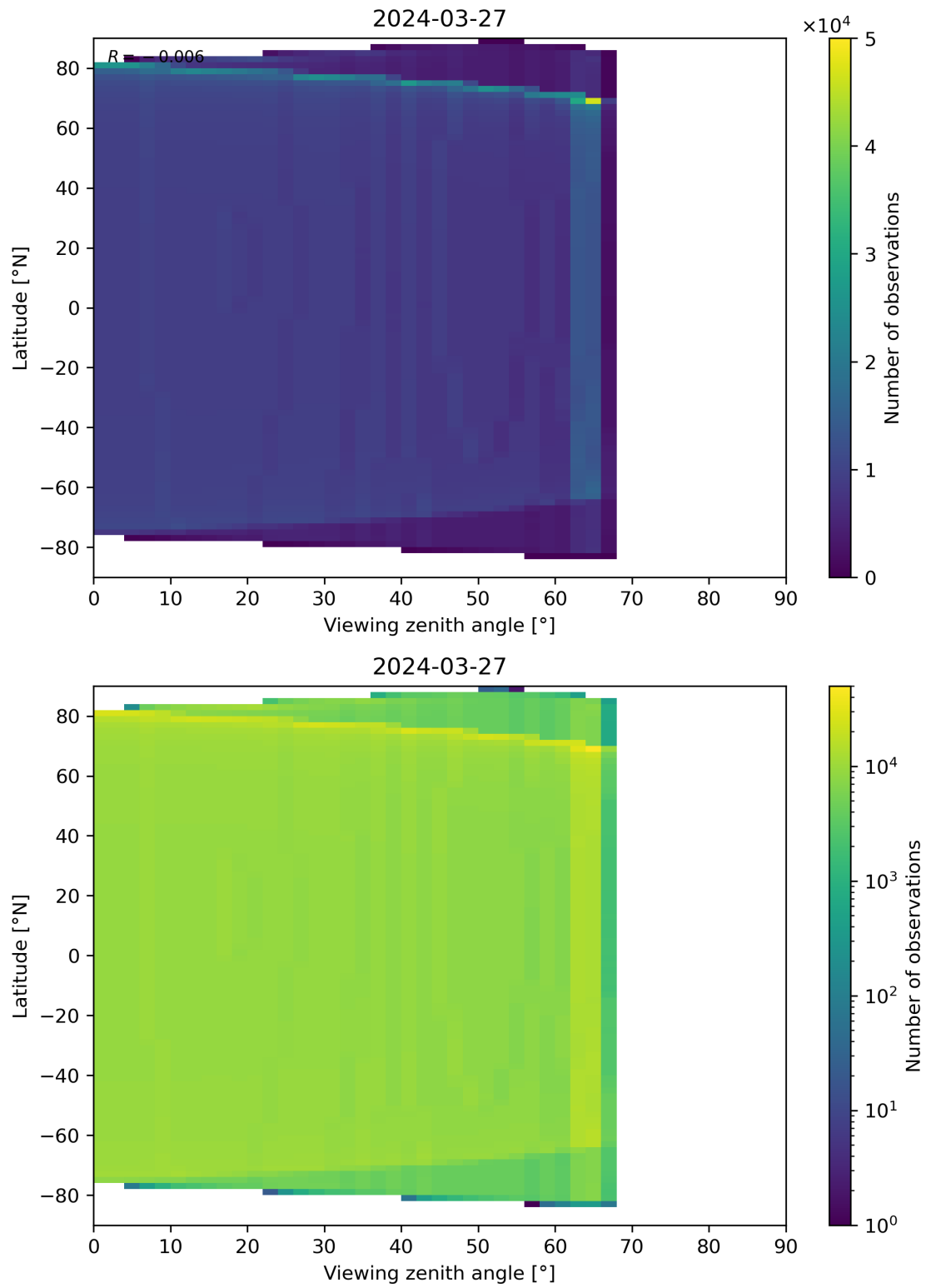
Figure 314: Scatter density plot of “Viewing zenith angle” against “Latitude” for 2024-03-26 to 2024-03-28.
