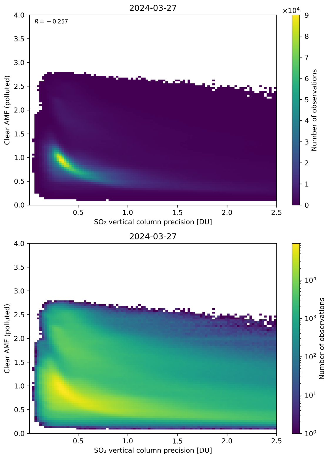
Figure 285: Scatter density plot of “SO 2 vertical column precision” against “Clear AMF (polluted)” for 2024-03-26 to 2024-03-28.
