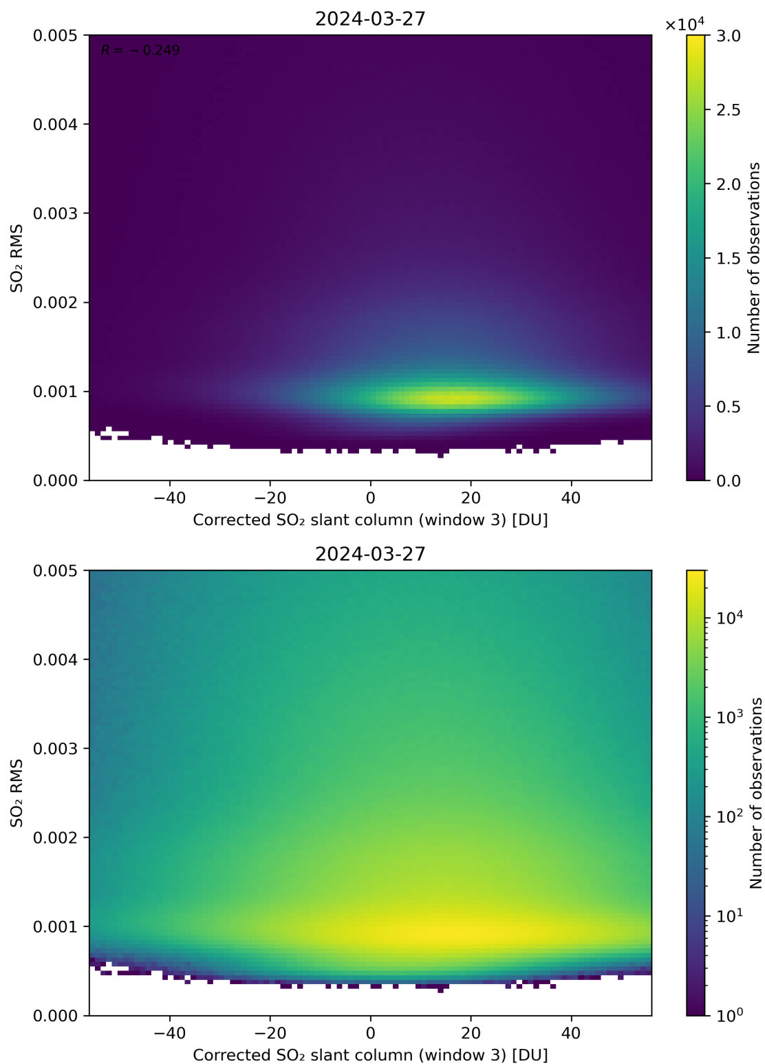
Figure 208: Scatter density plot of “Corrected SO 2 slant column (window 3)” against “SO 2 RMS” for 2024-03-26 to 2024-03-28.
