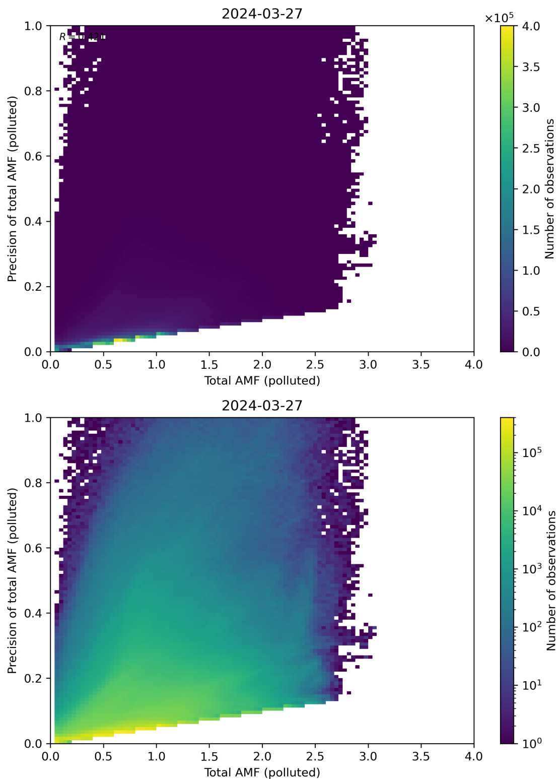
Figure 272: Scatter density plot of “Total AMF (polluted)” against “Precision of total AMF (polluted)” for 2024-03-26 to 2024-03-28.
