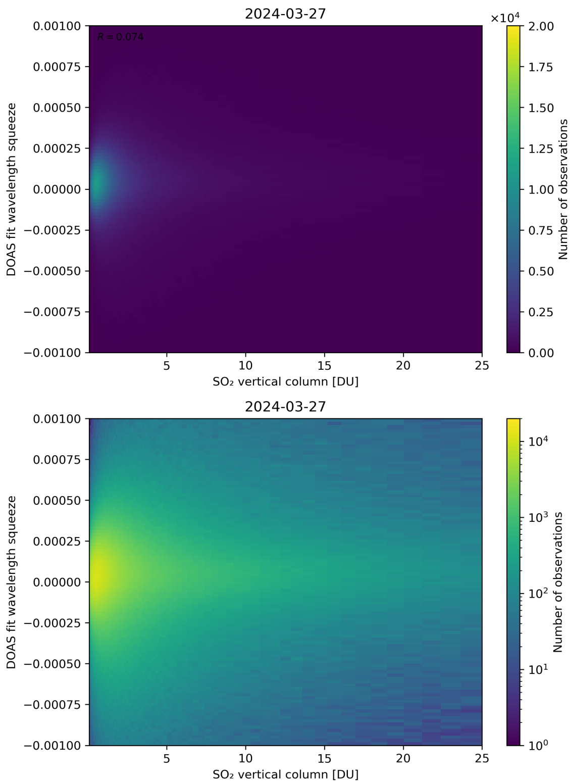
Figure 277: Scatter density plot of “SO 2 vertical column” against “DOAS fit wavelength squeeze” for 2024-03-26 to 2024-03-28.
