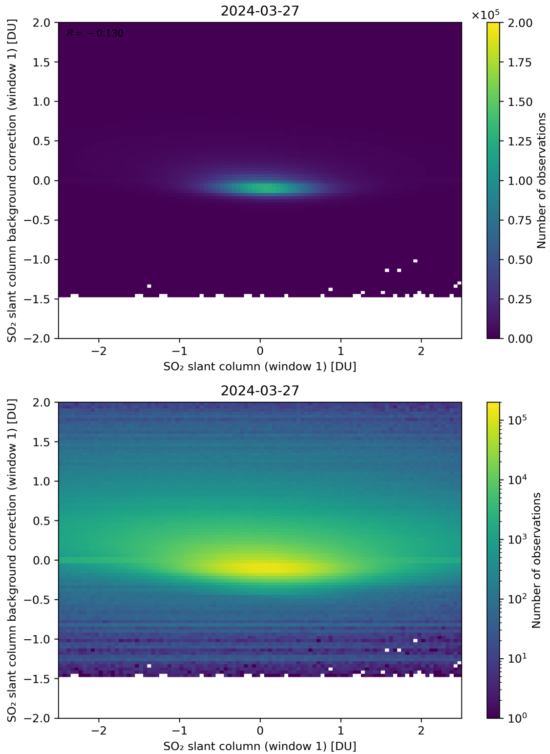
Figure 212: Scatter density plot of “SO 2 slant column (window 1)” against “SO 2 slant column background correction (window 1)” for 2024-03-26 to 2024-03-28.
