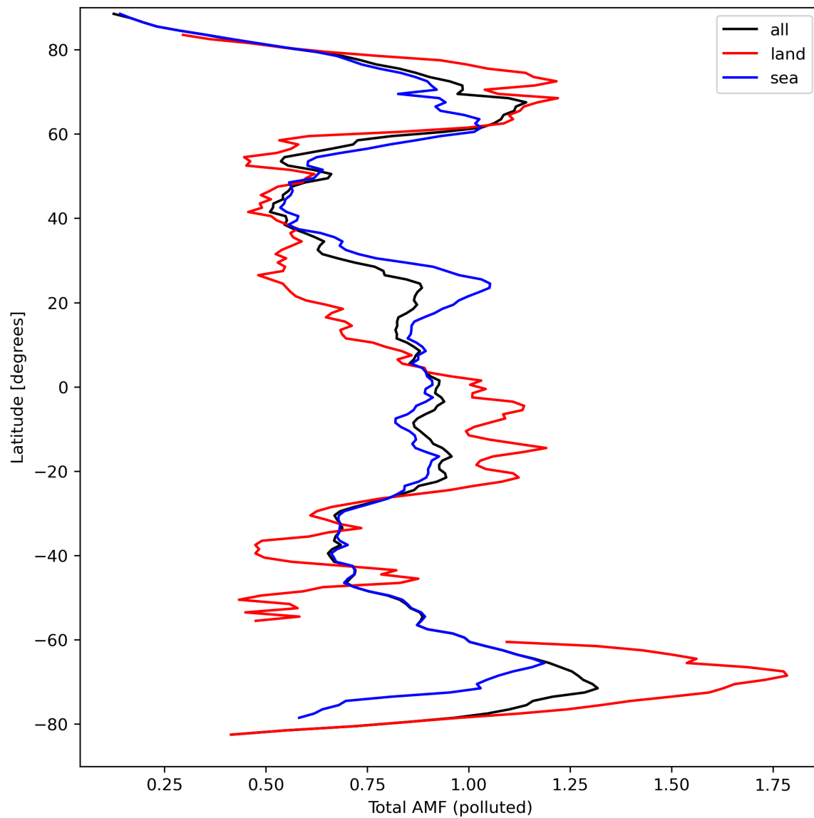
Figure 48: Zonal average of “Total AMF (polluted)” for 2024-03-26 to 2024-03-28.
