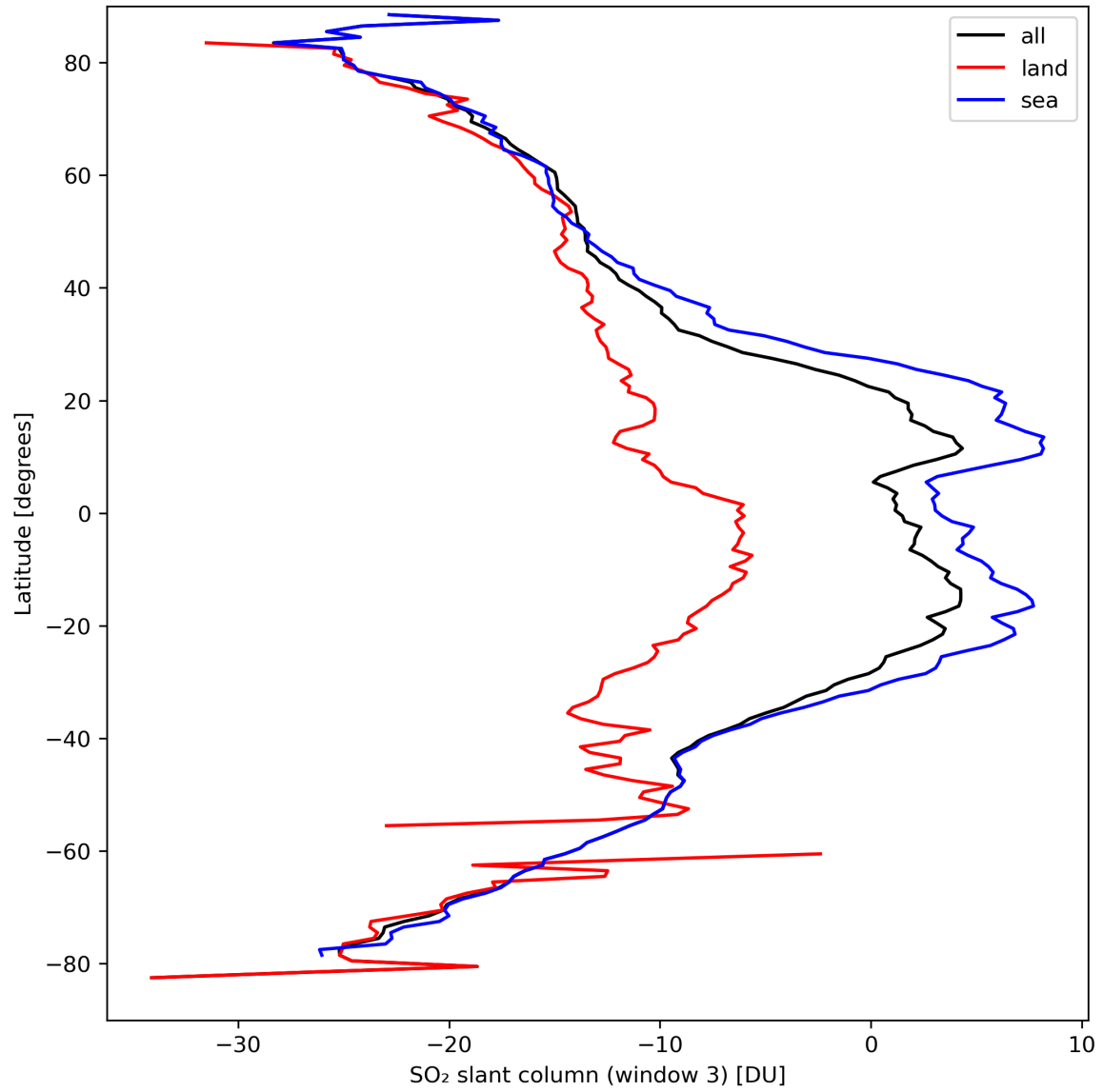
Figure 41: Zonal average of “SO 2 slant column (window 3)” for 2024-03-26 to 2024-03-28.
