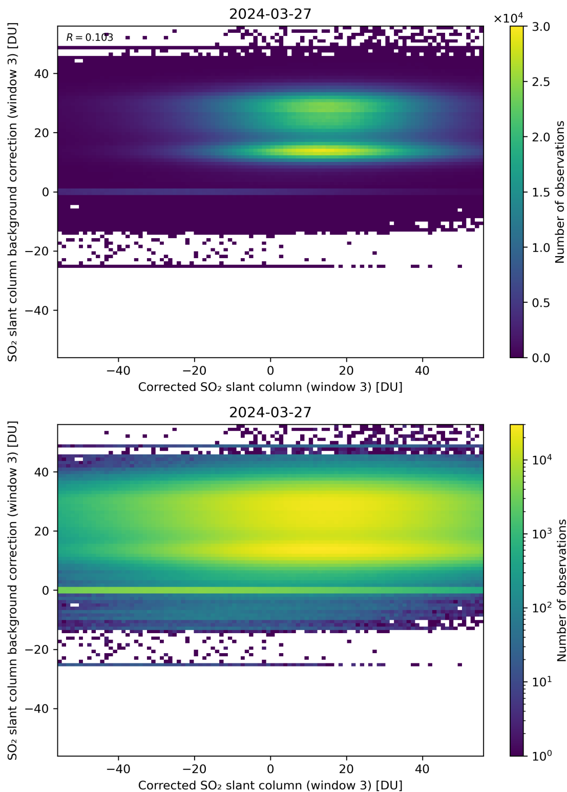
Figure 205: Scatter density plot of “Corrected SO 2 slant column (window 3)” against “SO 2 slant column background correction (window 3)” for 2024-03-26 to 2024-03-28.
