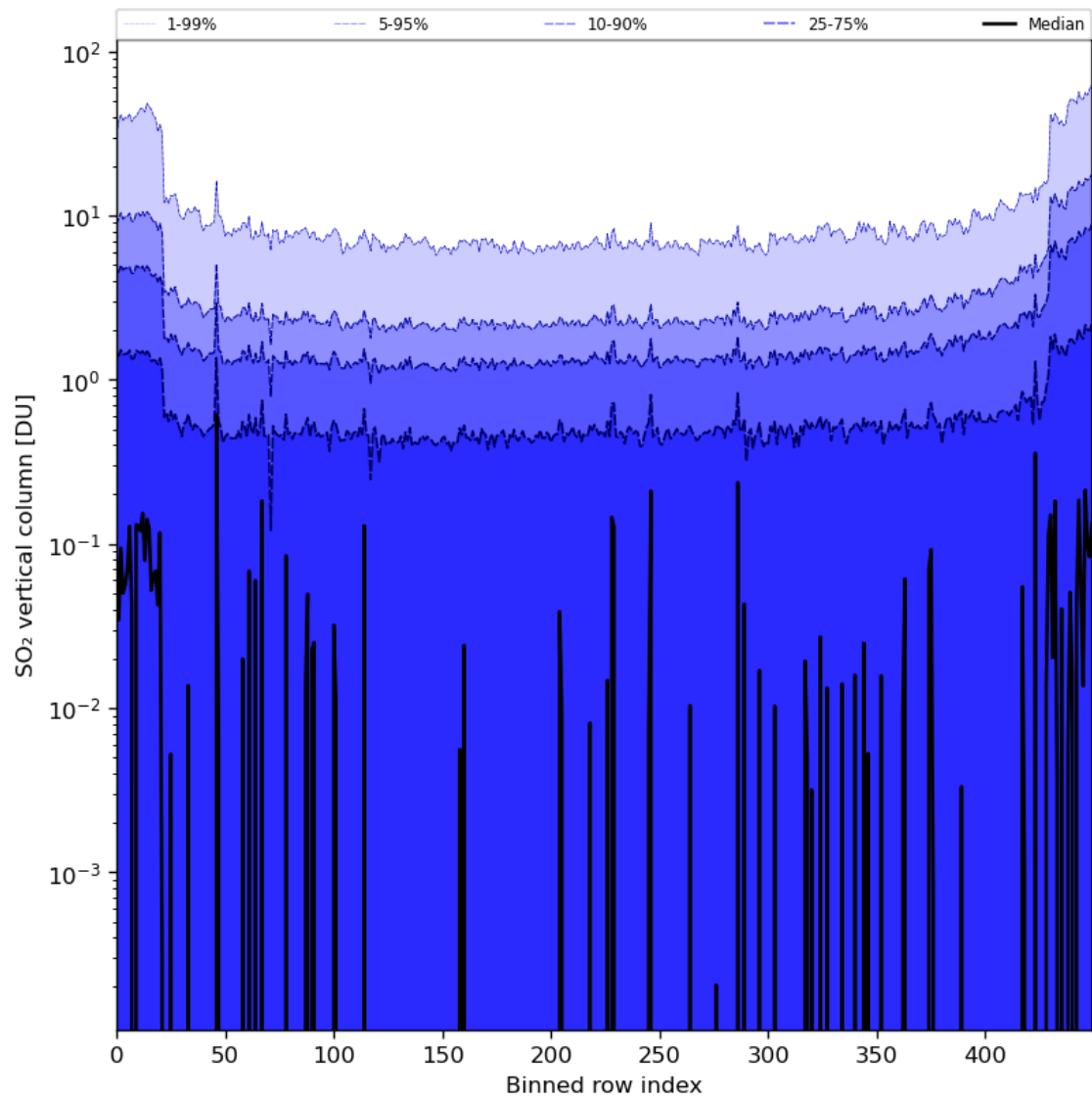
Figure 76: Along track statistics of “SO 2 vertical column” for 2024-03-26 to 2024-03-28
