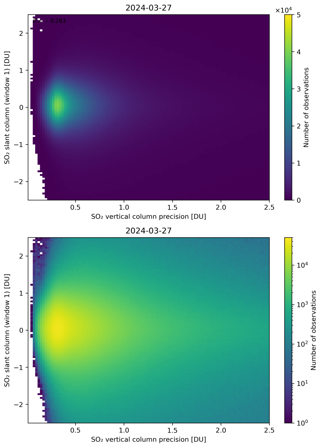
Figure 289: Scatter density plot of “SO 2 vertical column precision” against “SO 2 slant column (window 1)” for 2024-03-26 to 2024-03-28.
