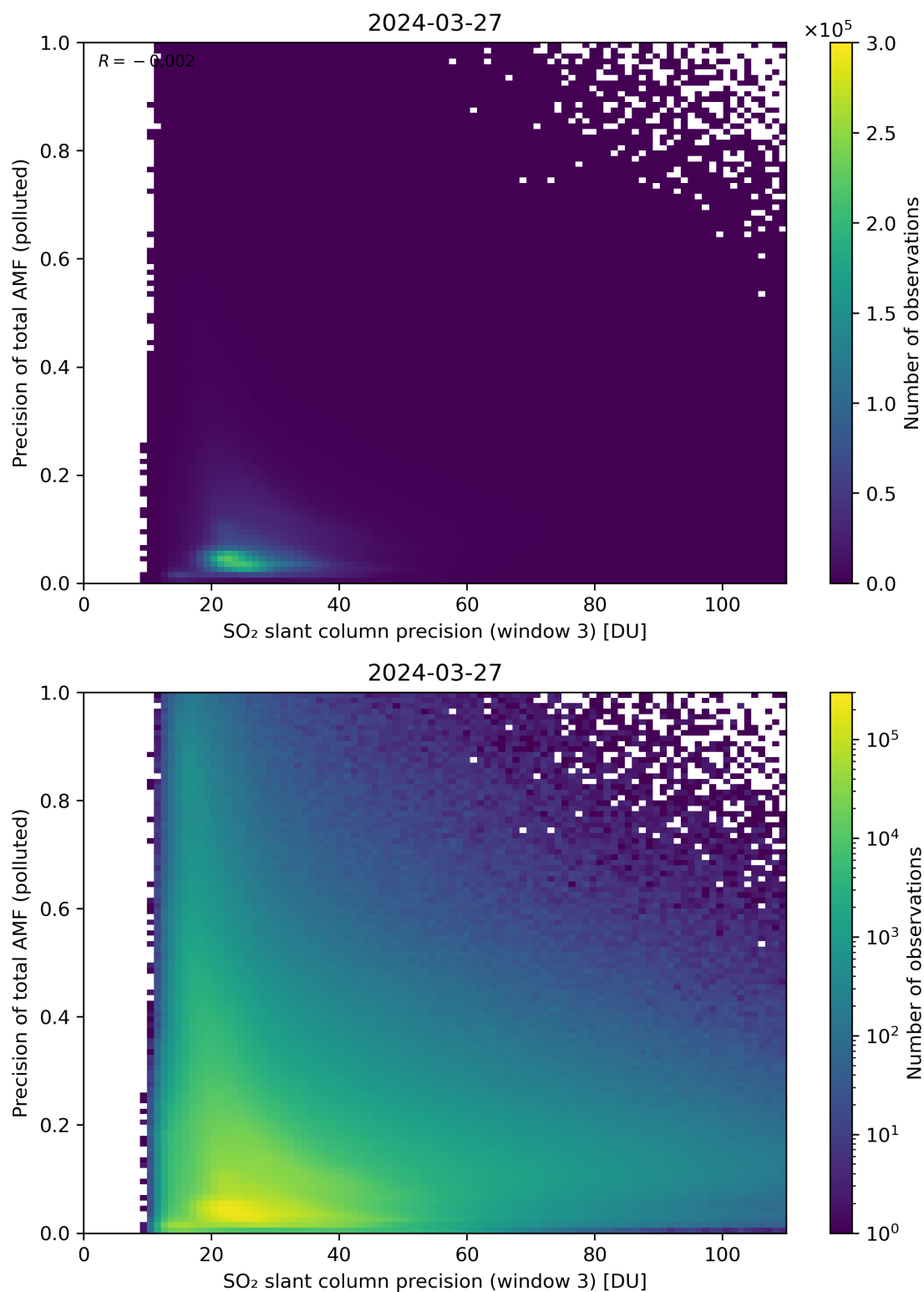
Figure 264: Scatter density plot of “SO 2 slant column precision (window 3)” against “Precision of total AMF (polluted)” for 2024-03-26 to 2024-03-28.
