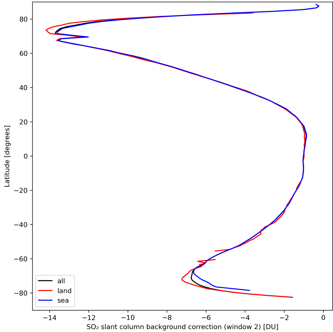
Figure 40: Zonal average of “SO 2 slant column background correction (window 2)” for 2024-03-26 to 2024-03-28.
