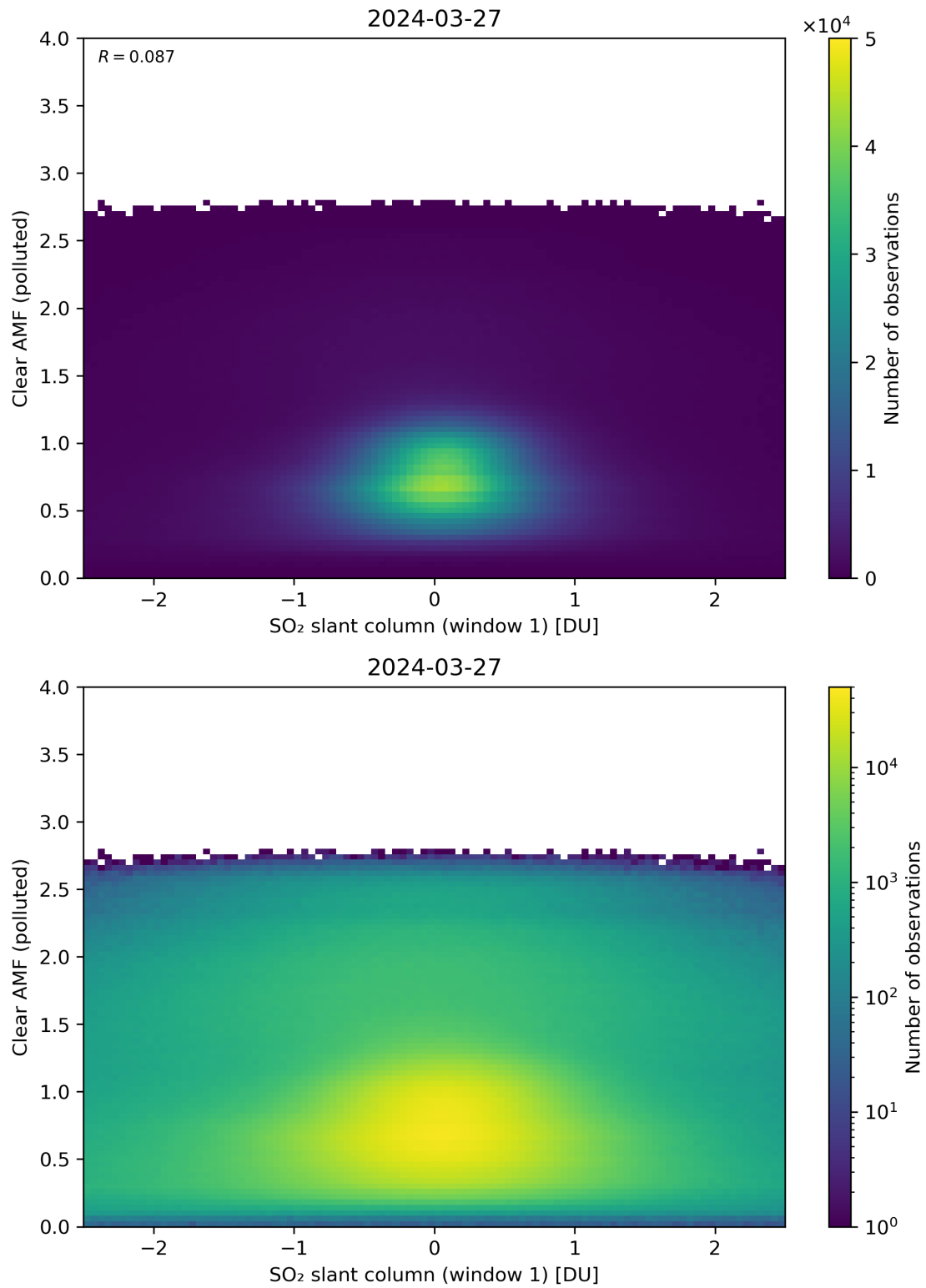
Figure 232: Scatter density plot of “SO 2 slant column (window 1)” against “Clear AMF (polluted)” for 2024-03-26 to 2024-03-28.
