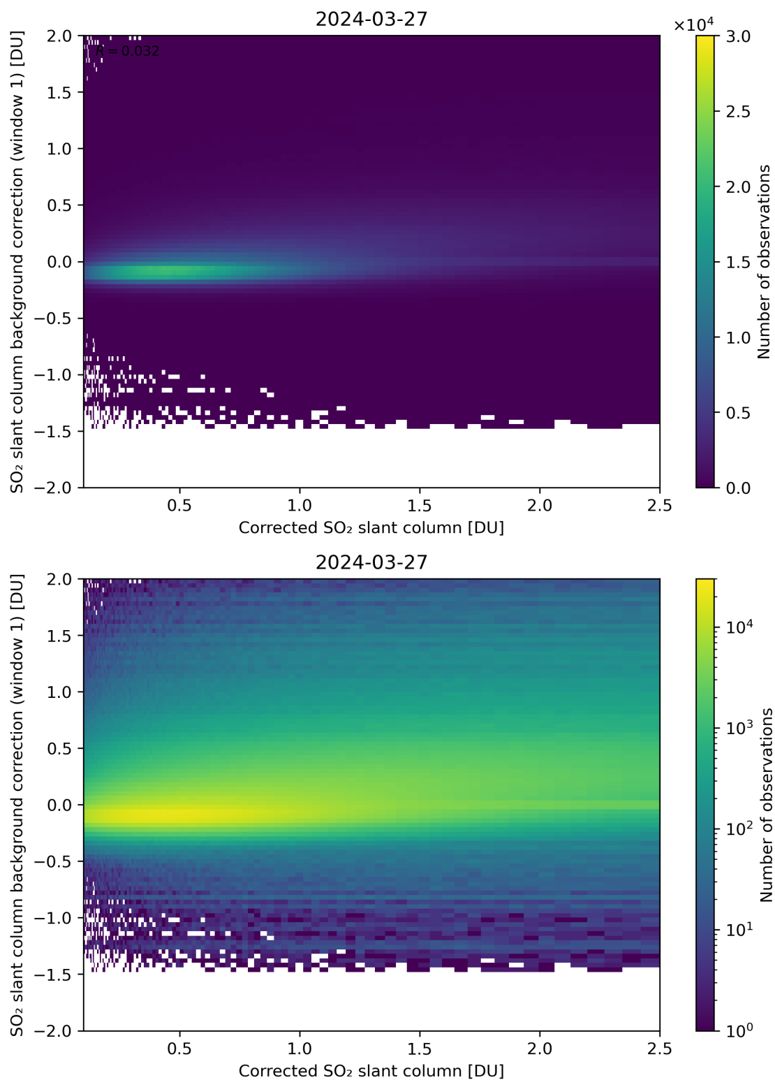
Figure 178: Scatter density plot of “Corrected SO 2 slant column” against “SO 2 slant column background correction (window 1)” for 2024-03-26 to 2024-03-28.
