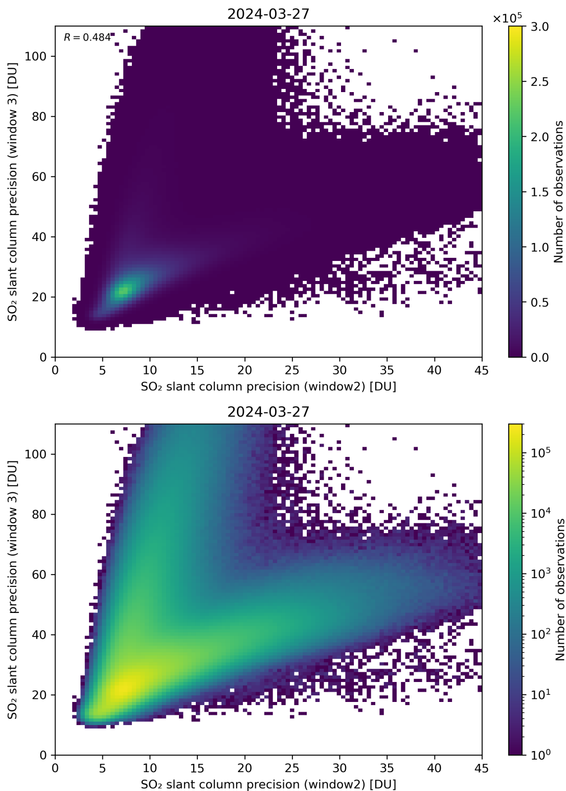
Figure 250: Scatter density plot of “SO 2 slant column precision (window2)” against “SO 2 slant column precision (window 3)” for 2024-03-26 to 2024-03-28.
