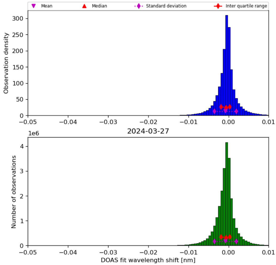
Figure 68: Histogram of “DOAS fit wavelength shift” for 2024-03-26 to 2024-03-28
