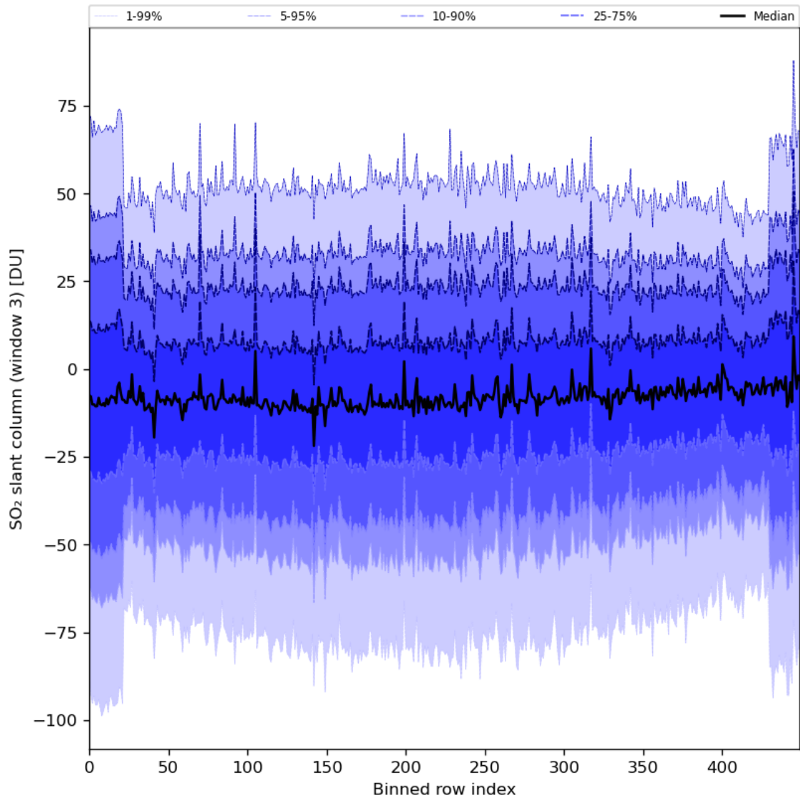
Figure 87: Along track statistics of “SO 2 slant column (window 3)” for 2024-03-26 to 2024-03-28
