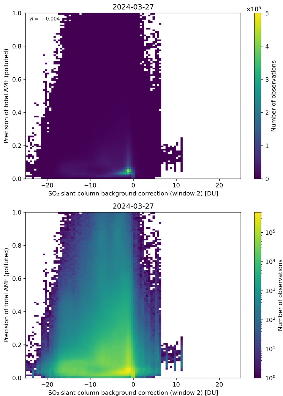
Figure 120: Scatter density plot of “SO 2 slant column background correction (window 2)” against “Precision of total AMF (polluted)” for 2024-03-26 to 2024-03-28.
