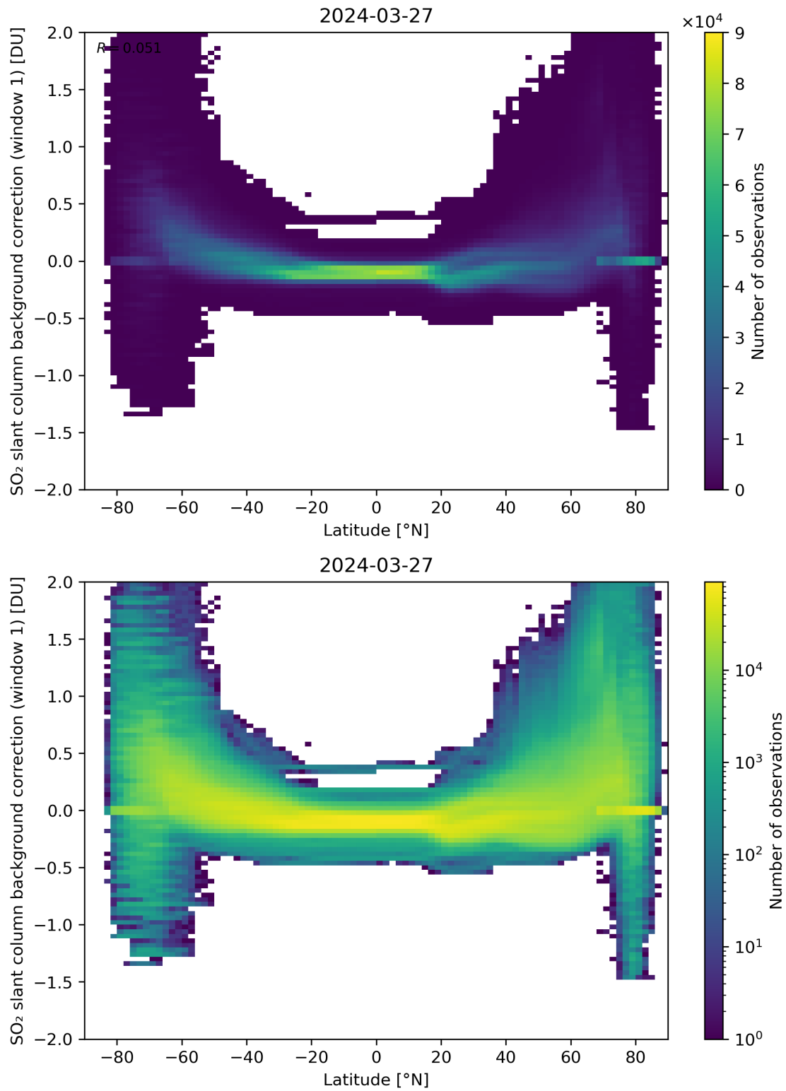
Figure 139: Scatter density plot of “Latitude” against “SO 2 slant column background correction (window 1)” for 2024-03-26 to 2024-03-28.
