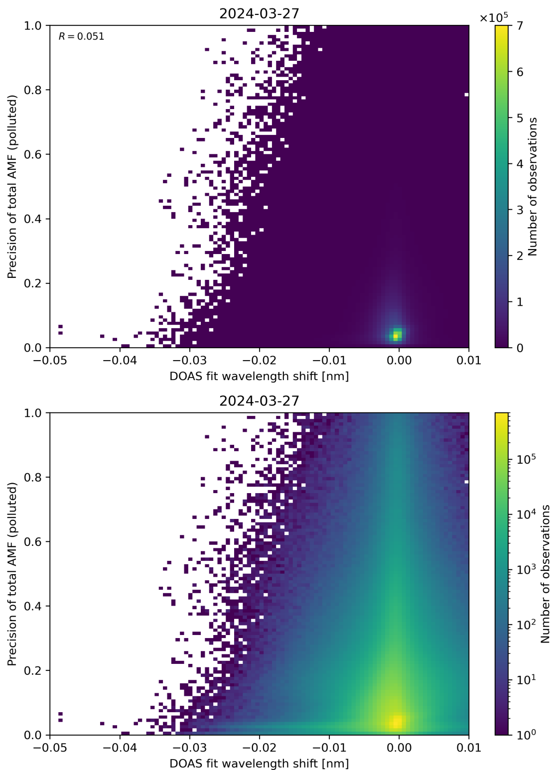
Figure 131: Scatter density plot of “DOAS fit wavelength shift” against “Precision of total AMF (polluted)” for 2024-03-26 to 2024-03-28.
