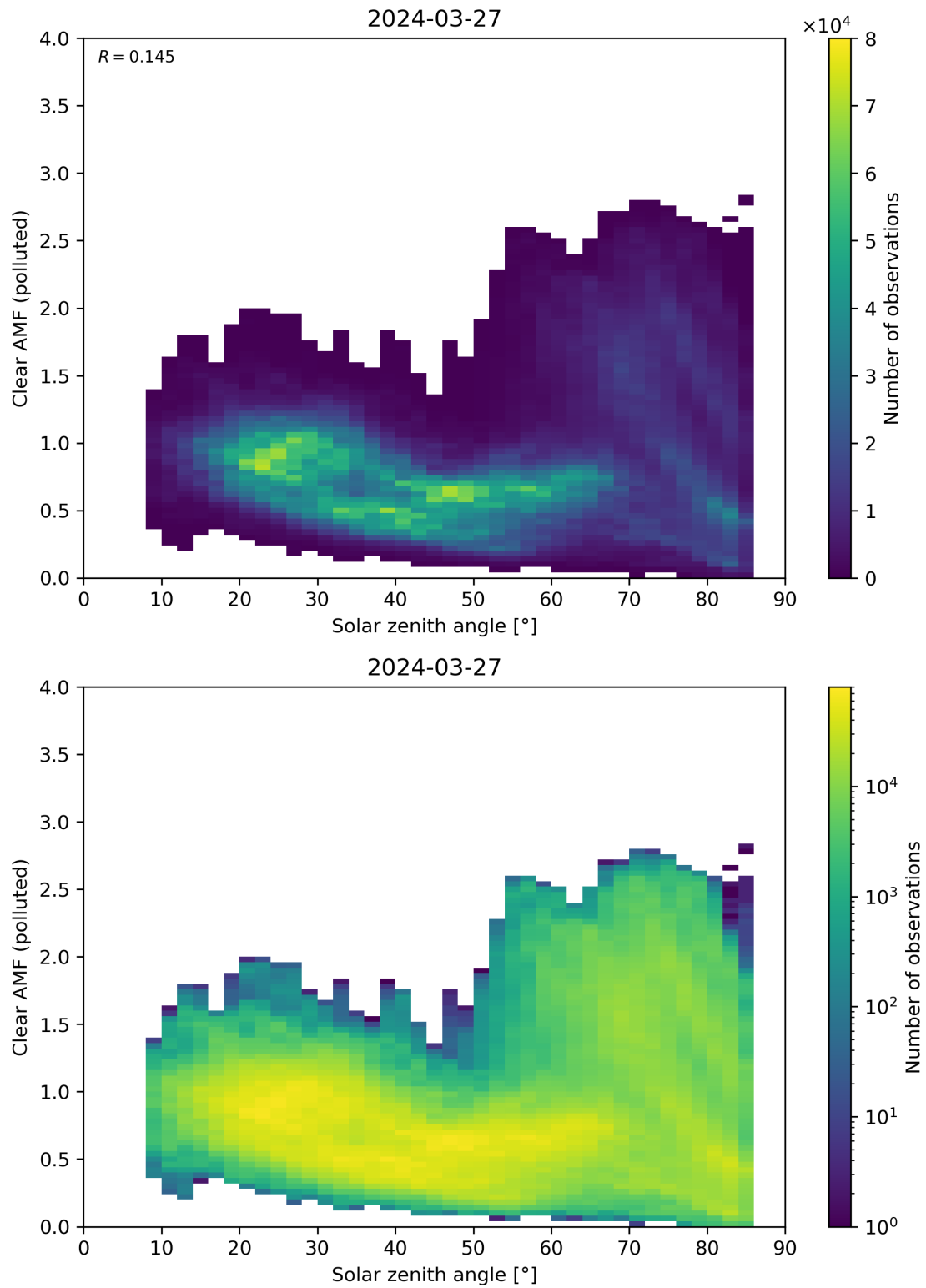
Figure 165: Scatter density plot of “Solar zenith angle” against “Clear AMF (polluted)” for 2024-03-26 to 2024-03-28.
