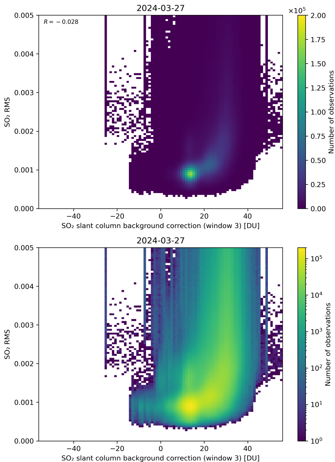
Figure 123: Scatter density plot of “SO 2 slant column background correction (window 3)” against “SO 2 RMS” for 2024-03-26 to 2024-03-28.
