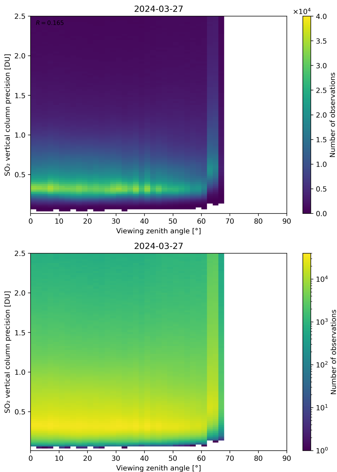
Figure 328: Scatter density plot of “Viewing zenith angle” against “SO 2 vertical column precision” for 2024-03-26 to 2024-03-28.
