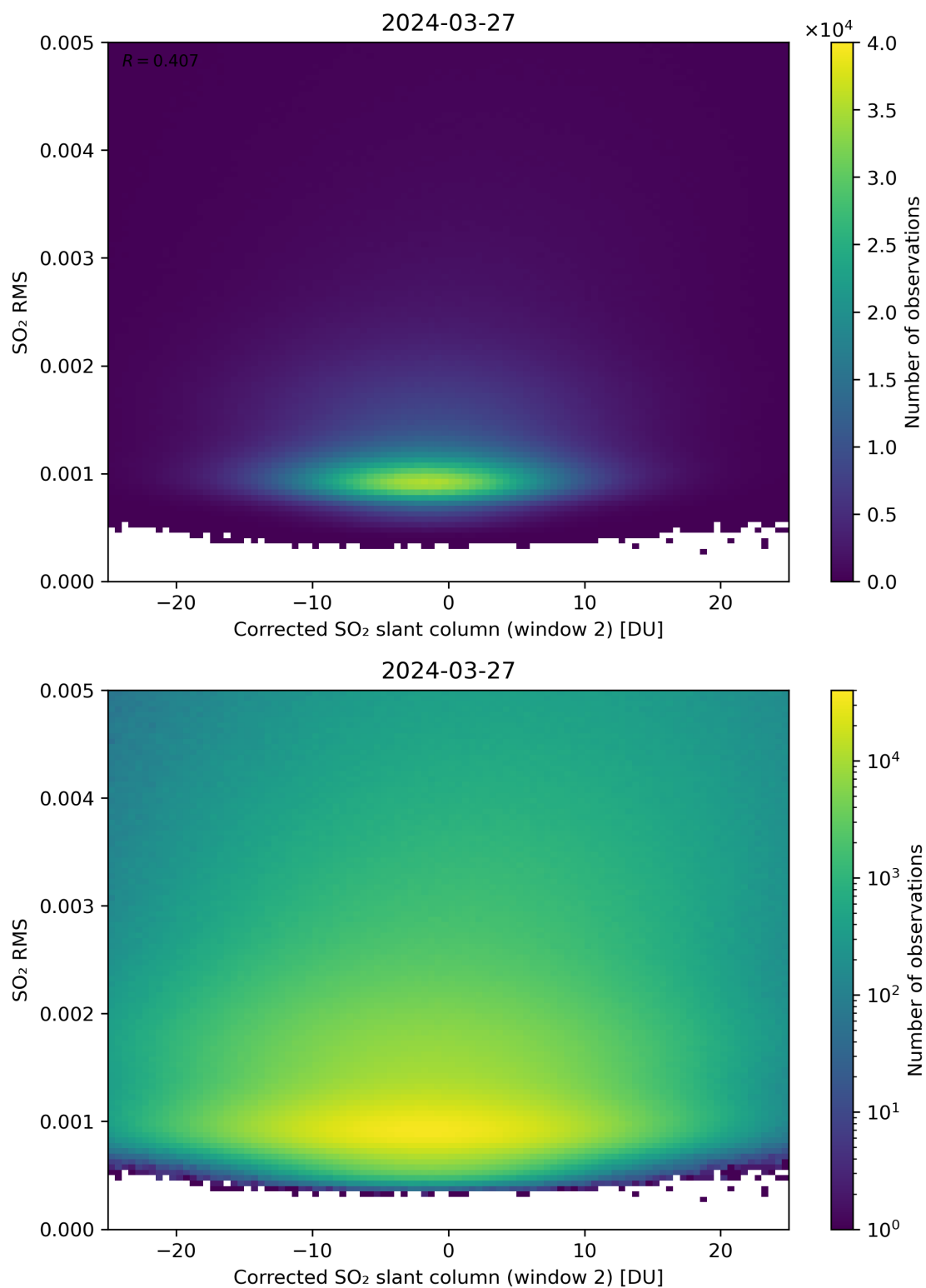
Figure 198: Scatter density plot of “Corrected SO 2 slant column (window 2)” against “SO 2 RMS” for 2024-03-26 to 2024-03-28.
