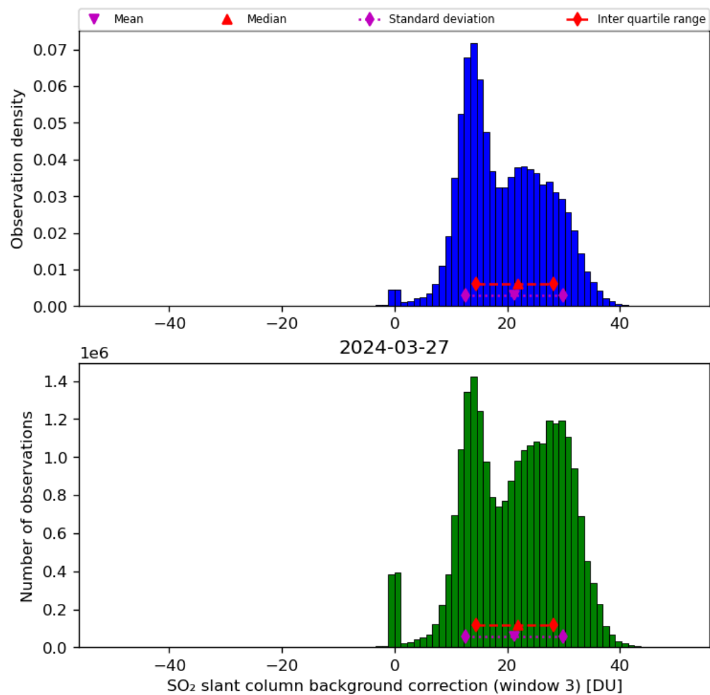
Figure 67: Histogram of “SO 2 slant column background correction (window 3)” for 2024-03-26 to 2024-03-28
