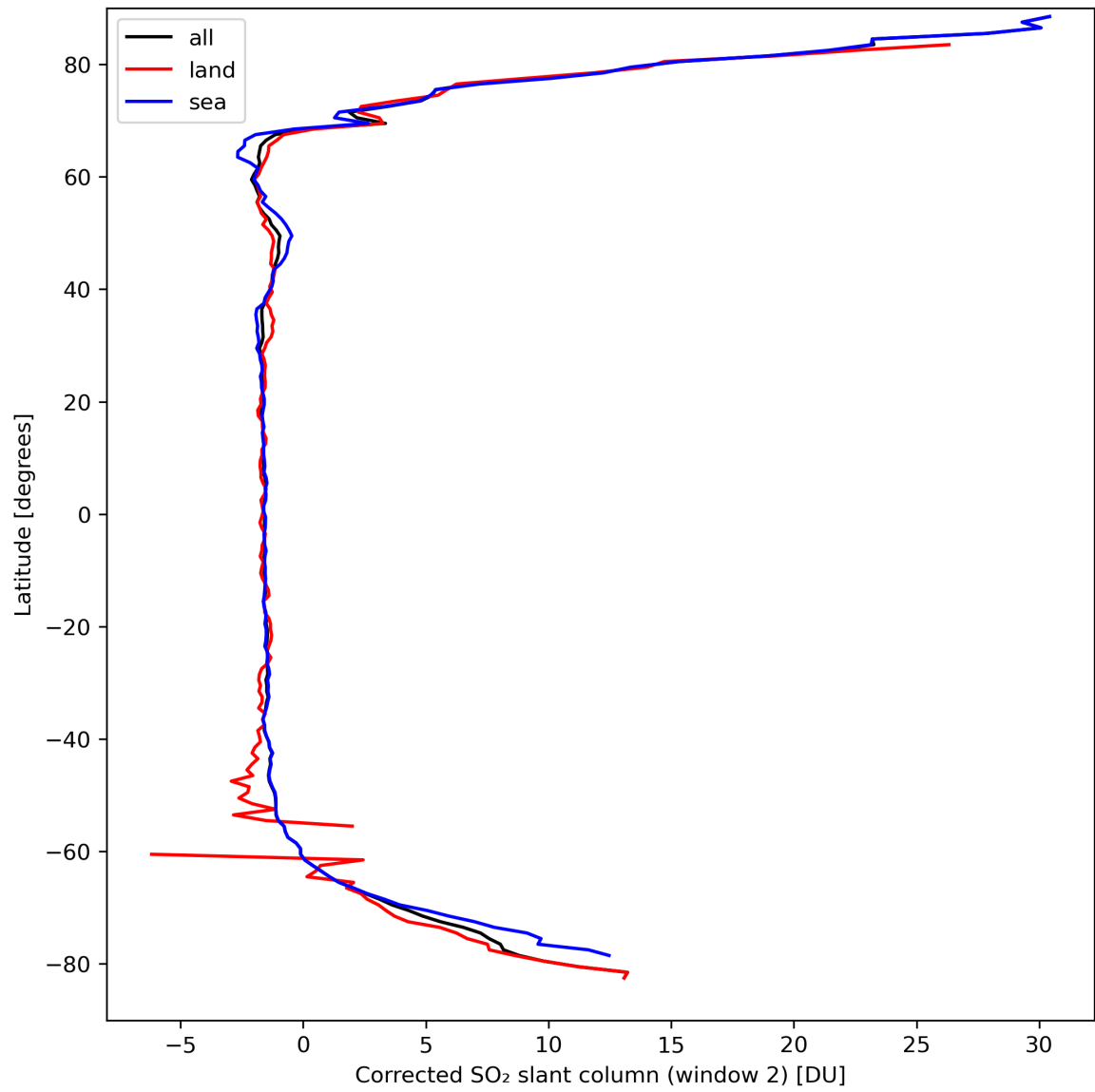
Figure 39: Zonal average of “Corrected SO 2 slant column (window 2)” for 2024-03-26 to 2024-03-28.
