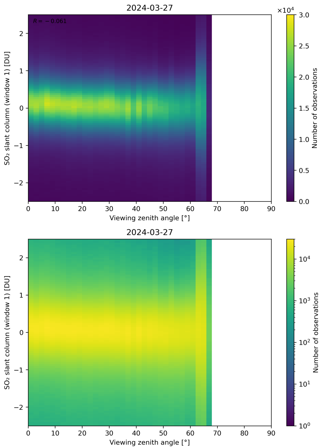
Figure 320: Scatter density plot of “Viewing zenith angle” against “SO 2 slant column (window 1)” for 2024-03-26 to 2024-03-28.
