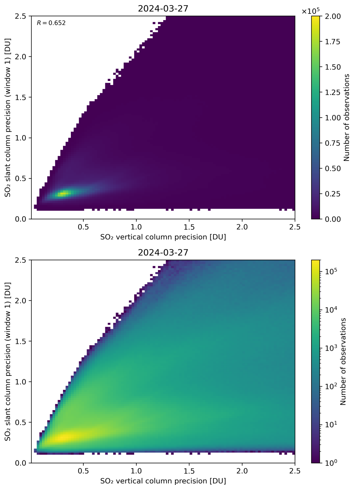
Figure 290: Scatter density plot of “SO 2 vertical column precision” against “SO 2 slant column precision (window 1)” for 2024-03-26 to 2024-03-28.
