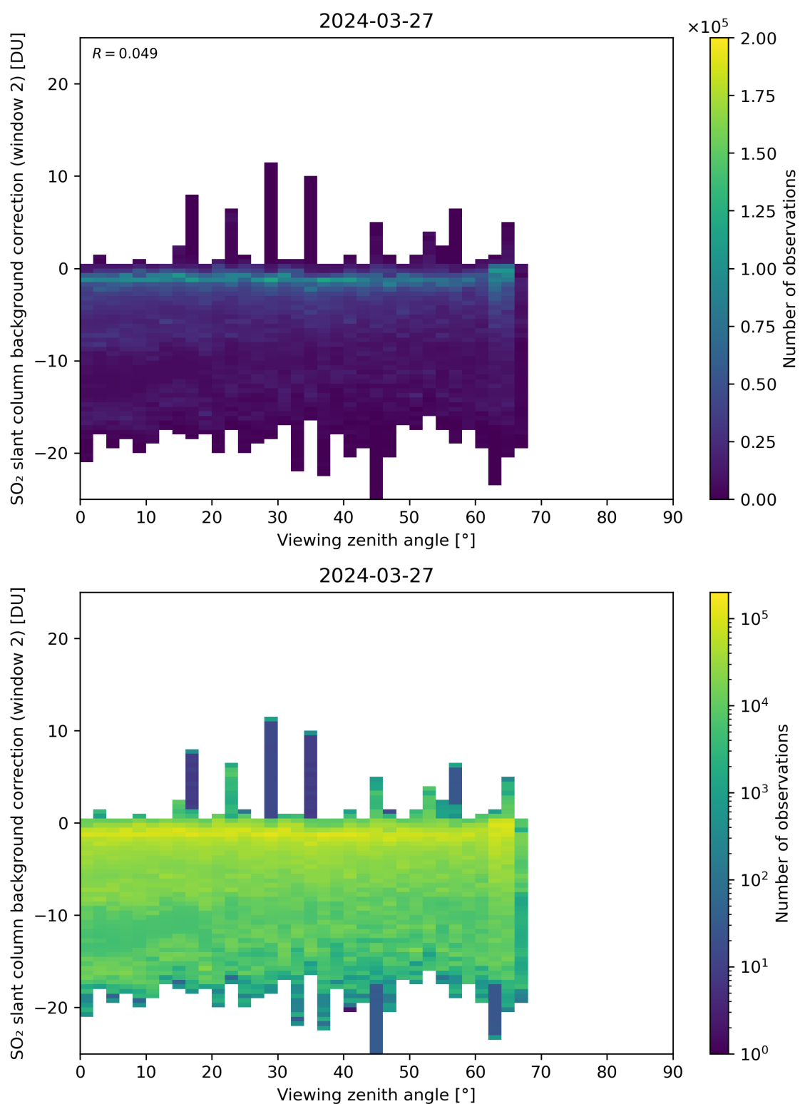
Figure 309: Scatter density plot of “Viewing zenith angle” against “SO 2 slant column background correction (window 2)” for 2024-03-26 to 2024-03-28.
