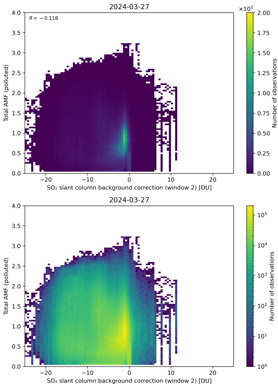
Figure 119: Scatter density plot of “SO 2 slant column background correction (window 2)” against “Total AMF (polluted)” for 2024-03-26 to 2024-03-28.
