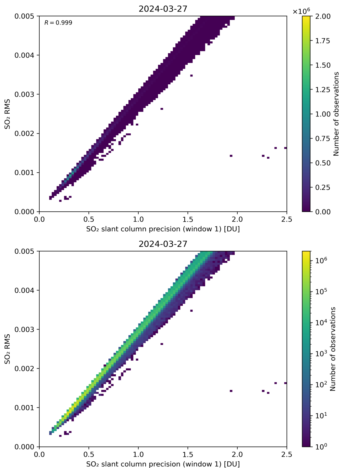
Figure 223: Scatter density plot of “SO 2 slant column precision (window 1)” against “SO 2 RMS” for 2024-03-26 to 2024-03-28.
