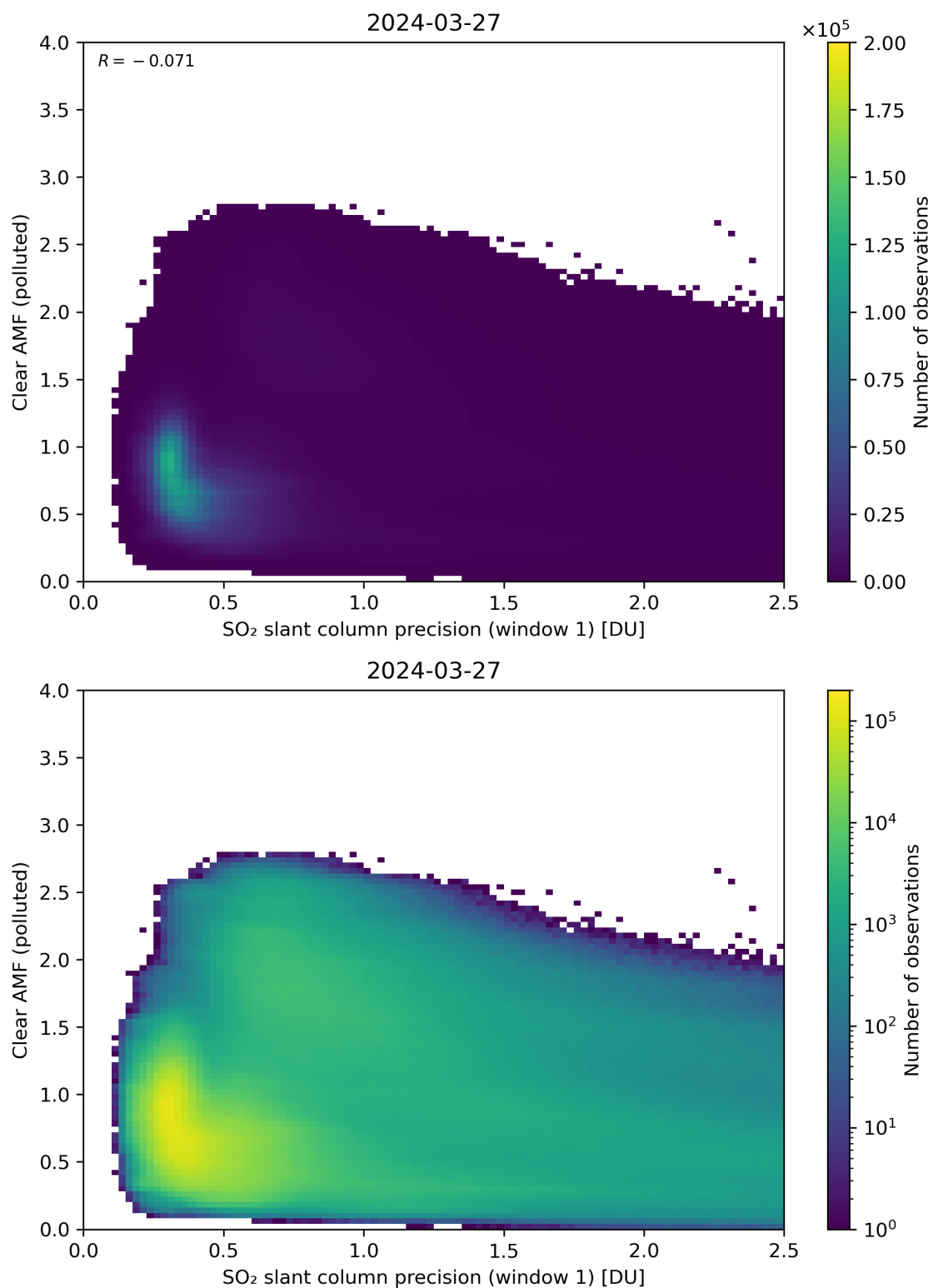
Figure 224: Scatter density plot of “SO 2 slant column precision (window 1)” against “Clear AMF (polluted)” for 2024-03-26 to 2024-03-28.
