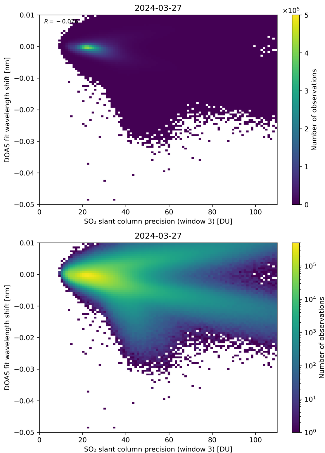
Figure 258: Scatter density plot of “SO 2 slant column precision (window 3)” against “DOAS fit wavelength shift” for 2024-03-26 to 2024-03-28.
