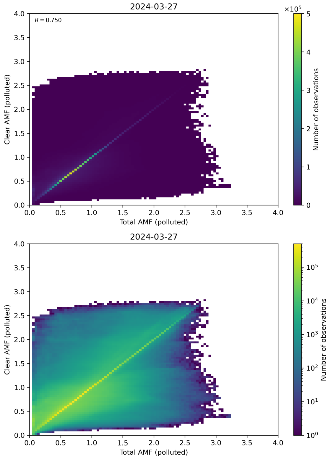
Figure 271: Scatter density plot of “Total AMF (polluted)” against “Clear AMF (polluted)” for 2024-03-26 to 2024-03-28.
