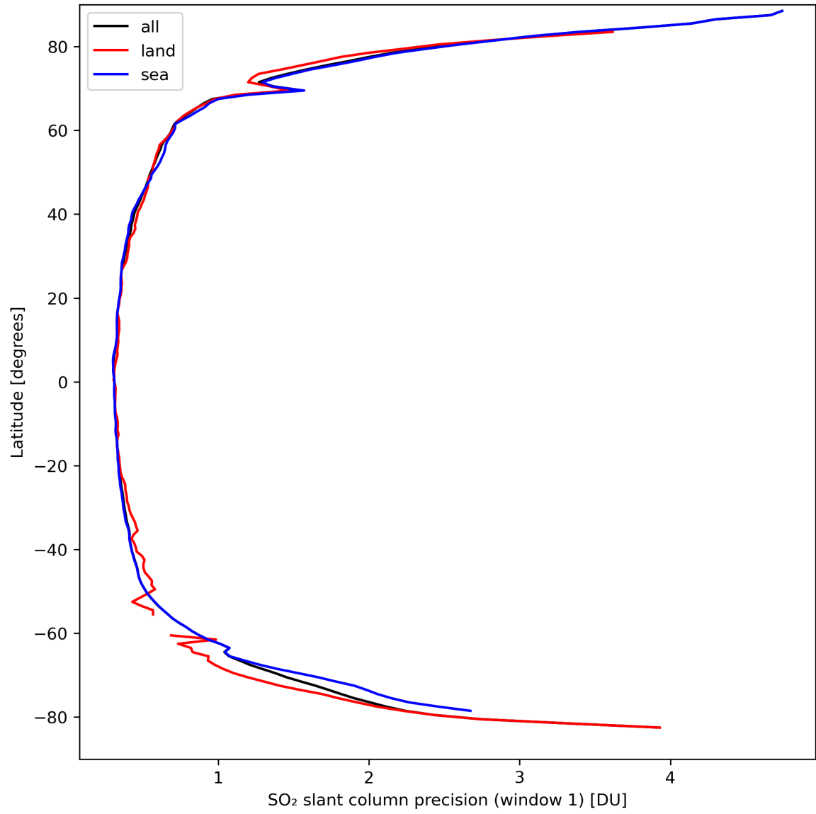
Figure 34: Zonal average of “SO 2 slant column precision (window 1)” for 2024-03-26 to 2024-03-28.
