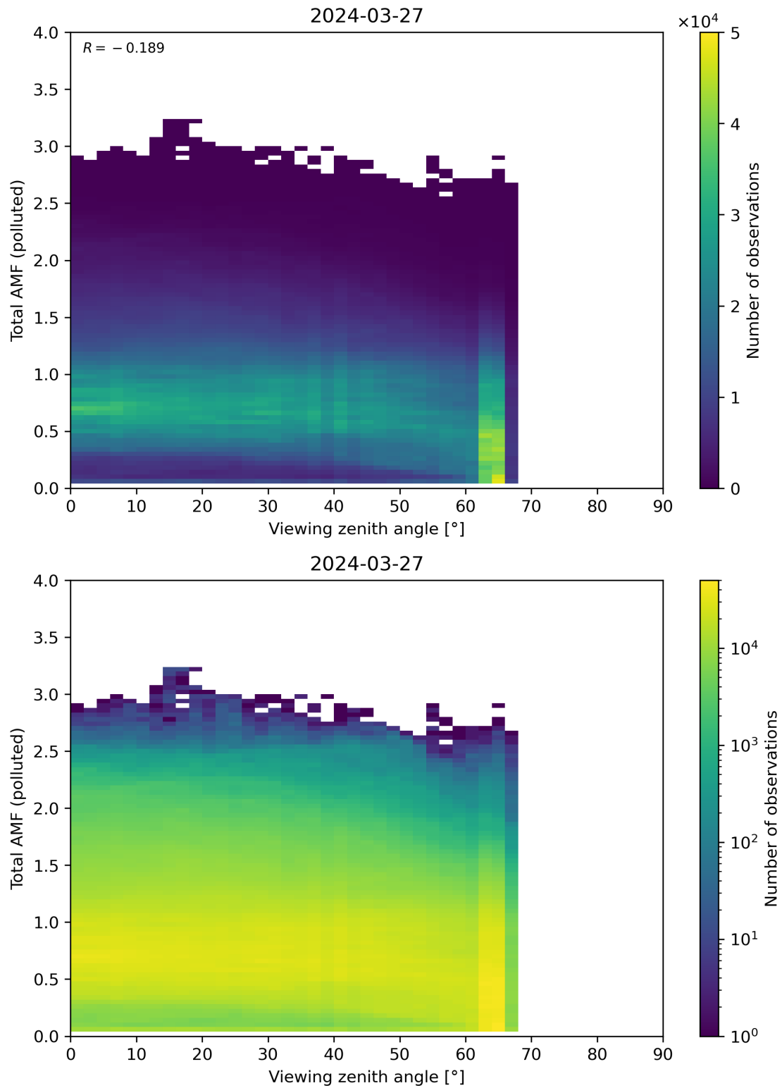
Figure 325: Scatter density plot of “Viewing zenith angle” against “Total AMF (polluted)” for 2024-03-26 to 2024-03-28.
