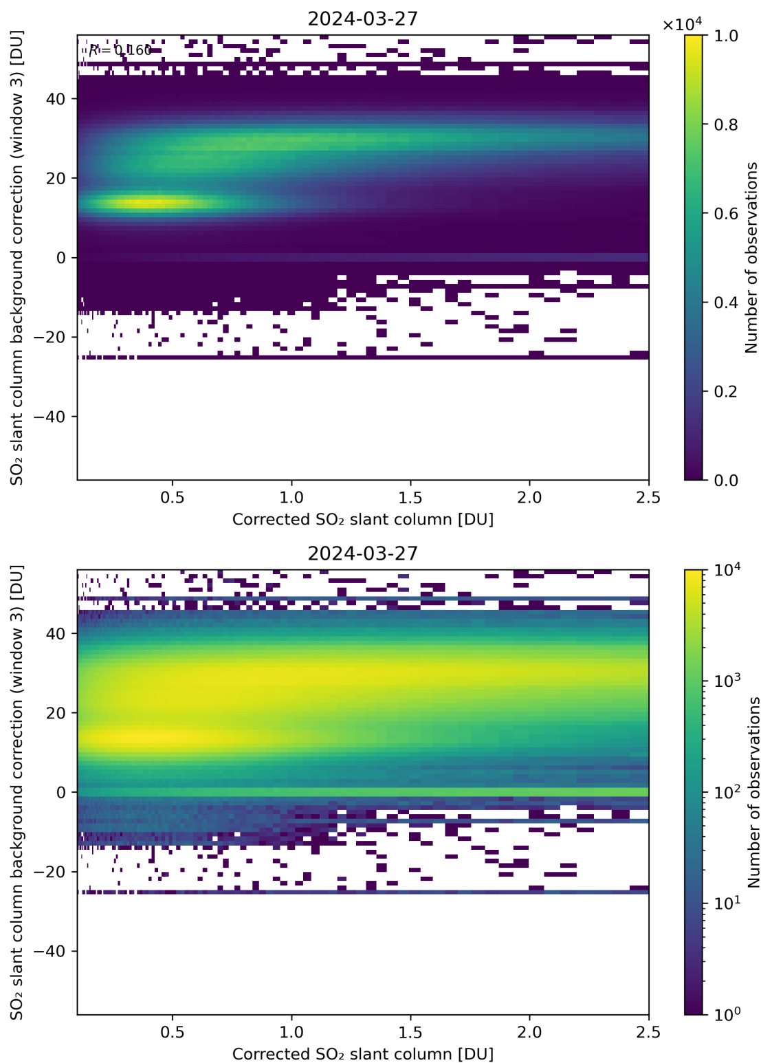
Figure 180: Scatter density plot of “Corrected SO 2 slant column” against “SO 2 slant column background correction (window 3)” for 2024-03-26 to 2024-03-28.
