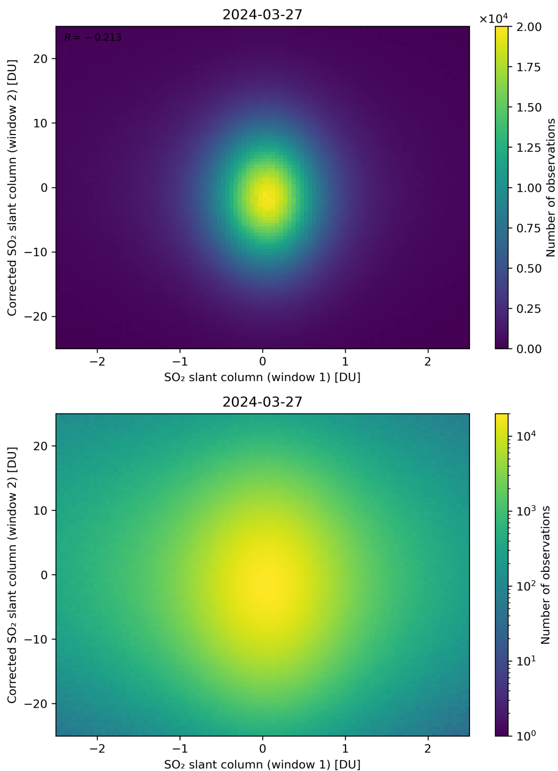
Figure 233: Scatter density plot of “SO 2 slant column (window 1)” against “Corrected SO 2 slant column (window 2)” for 2024-03-26 to 2024-03-28.
