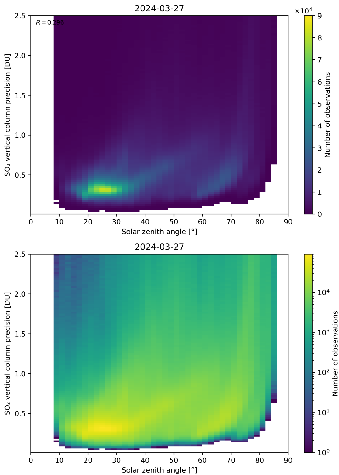
Figure 177: Scatter density plot of “Solar zenith angle” against “SO 2 vertical column precision” for 2024-03-26 to 2024-03-28.
