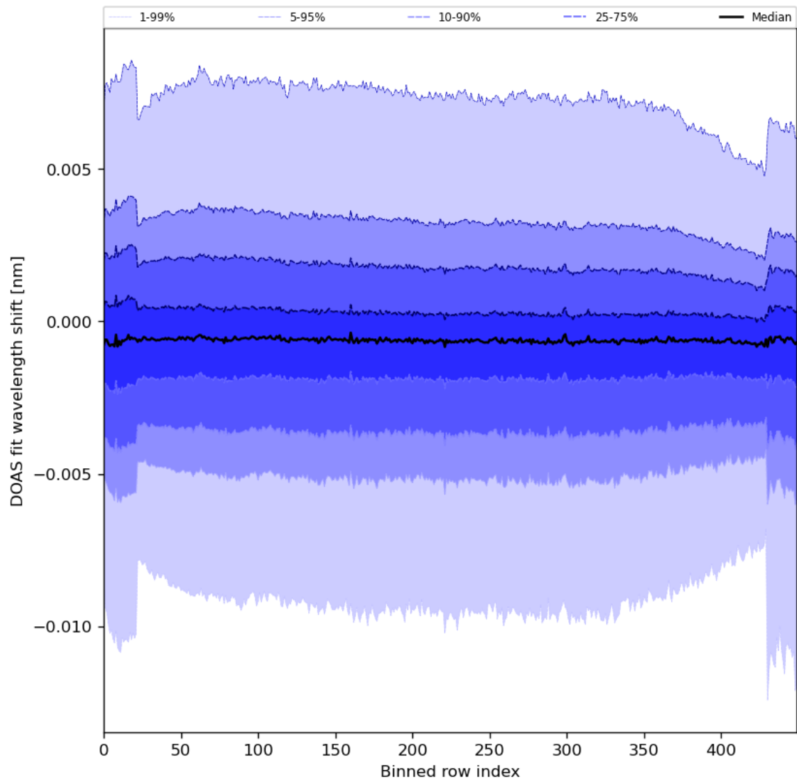
Figure 91: Along track statistics of “DOAS fit wavelength shift” for 2024-03-26 to 2024-03-28
