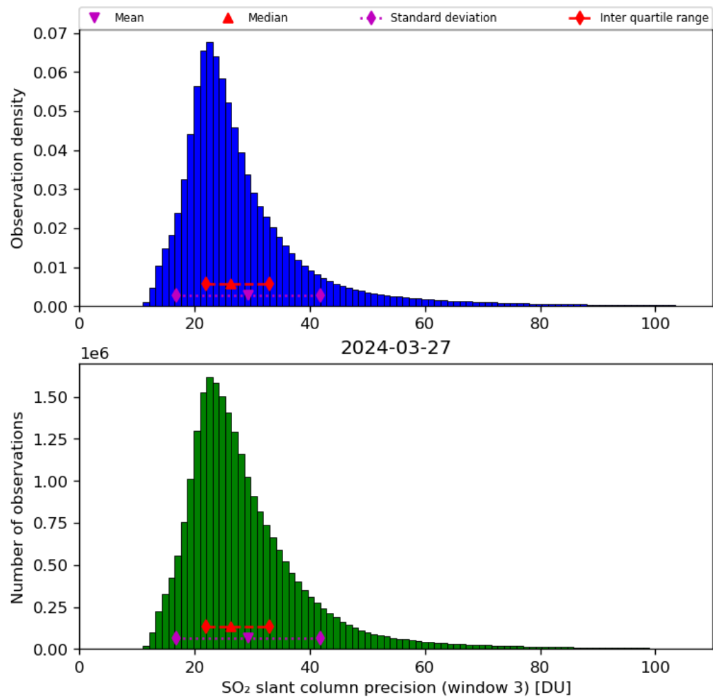
Figure 65: Histogram of “SO 2 slant column precision (window 3)” for 2024-03-26 to 2024-03-28
