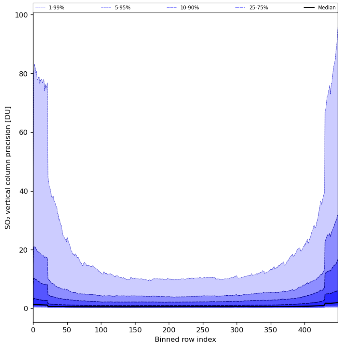
Figure 77: Along track statistics of “SO 2 vertical column precision” for 2024-03-26 to 2024-03-28
