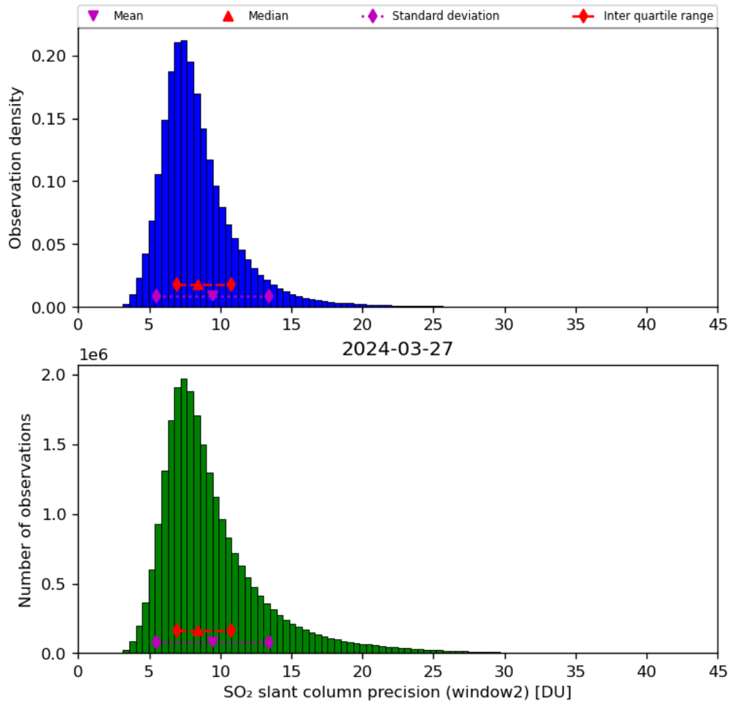
Figure 61: Histogram of “SO 2 slant column precision (window2)” for 2024-03-26 to 2024-03-28
