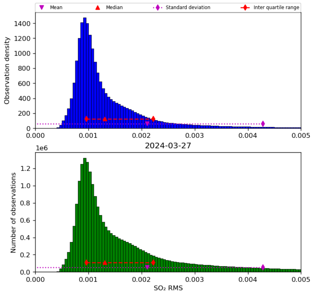
Figure 70: Histogram of “SO 2 RMS” for 2024-03-26 to 2024-03-28
