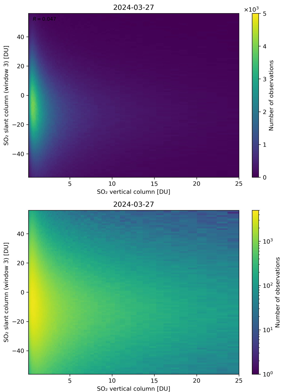
Figure 303: Scatter density plot of “SO 2 vertical column” against “SO 2 slant column (window 3)” for 2024-03-26 to 2024-03-28.
