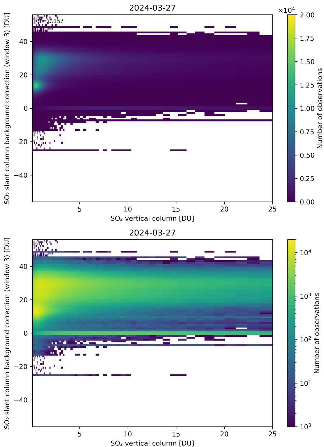
Figure 275: Scatter density plot of “SO 2 vertical column” against “SO 2 slant column background correction (window 3)” for 2024-03-26 to 2024-03-28.
