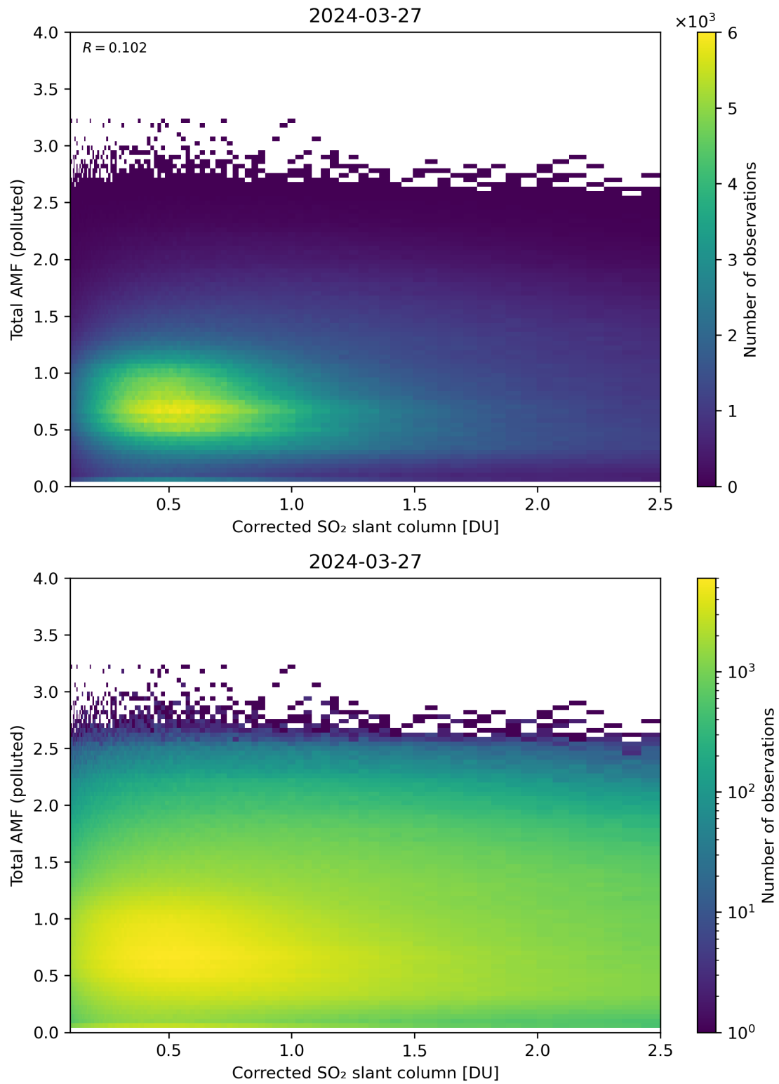
Figure 192: Scatter density plot of “Corrected SO 2 slant column” against “Total AMF (polluted)” for 2024-03-26 to 2024-03-28.
