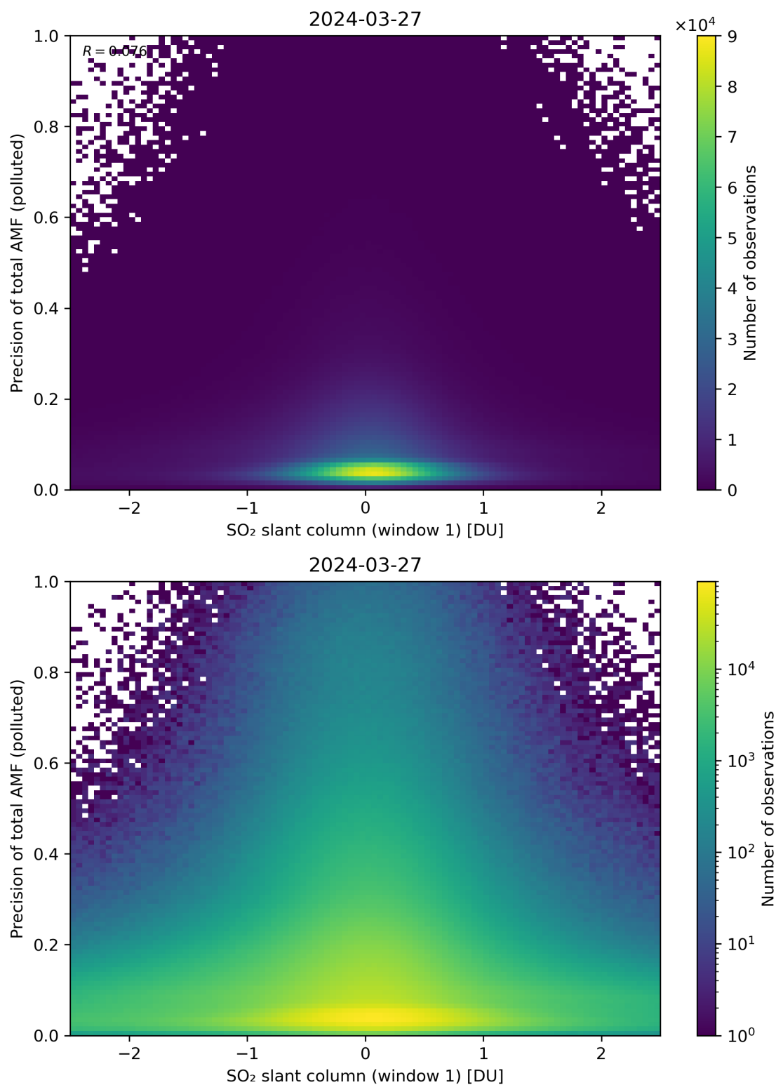
Figure 240: Scatter density plot of “SO 2 slant column (window 1)” against “Precision of total AMF (polluted)” for 2024-03-26 to 2024-03-28.
