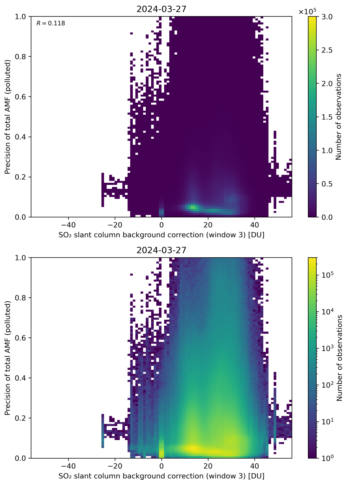
Figure 126: Scatter density plot of “SO 2 slant column background correction (window 3)” against “Precision of total AMF (polluted)” for 2024-03-26 to 2024-03-28.
