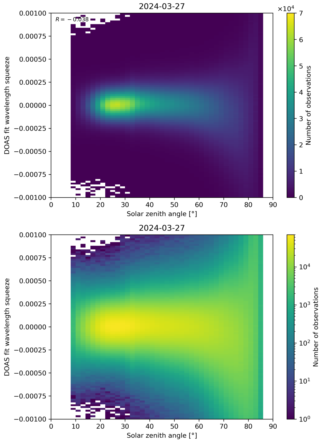
Figure 162: Scatter density plot of “Solar zenith angle” against “DOAS fit wavelength squeeze” for 2024-03-26 to 2024-03-28.
