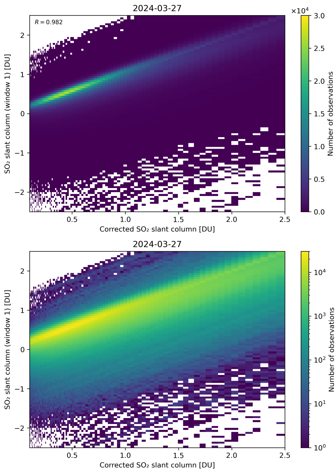
Figure 187: Scatter density plot of “Corrected SO 2 slant column” against “SO 2 slant column (window 1)” for 2024-03-26 to 2024-03-28.
