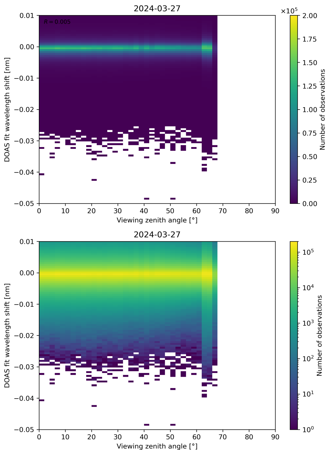
Figure 311: Scatter density plot of “Viewing zenith angle” against “DOAS fit wavelength shift” for 2024-03-26 to 2024-03-28.
