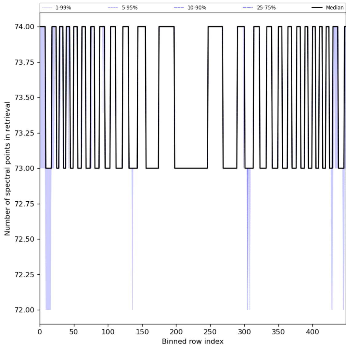
Figure 97: Along track statistics of “Number of spectral points in retrieval” for 2024-03-26 to 2024-03-28
