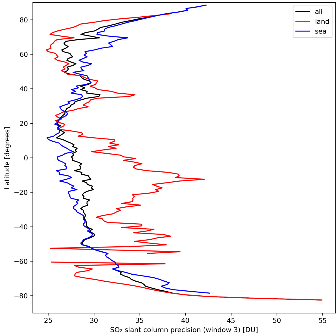
Figure 42: Zonal average of “SO 2 slant column precision (window 3)” for 2024-03-26 to 2024-03-28.
