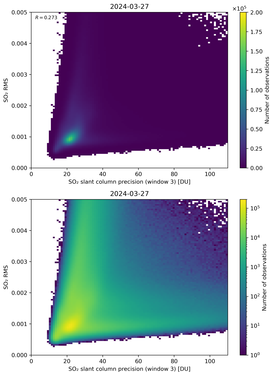
Figure 260: Scatter density plot of “SO 2 slant column precision (window 3)” against “SO 2 RMS” for 2024-03-26 to 2024-03-28.
