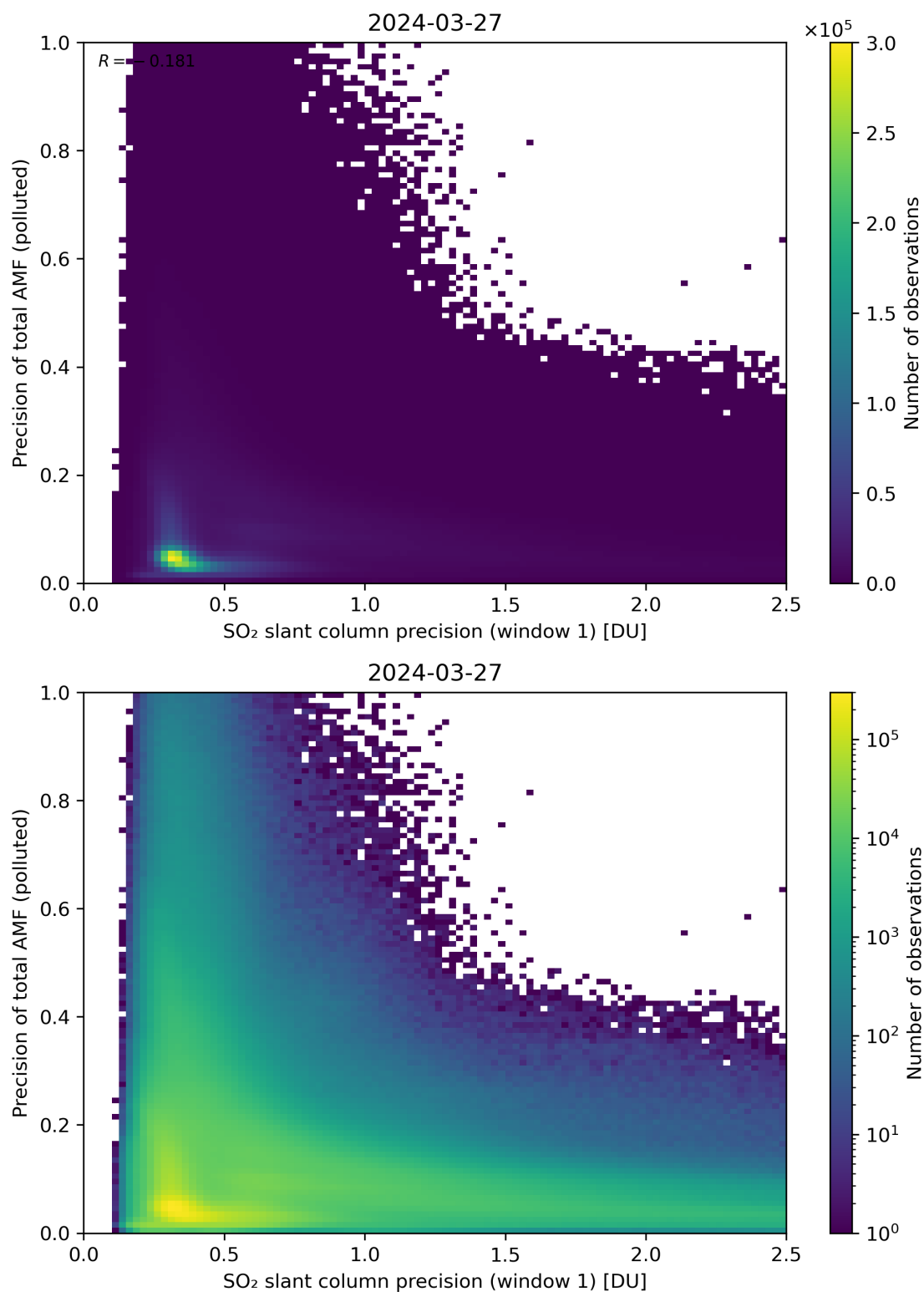
Figure 231: Scatter density plot of “SO 2 slant column precision (window 1)” against “Precision of total AMF (polluted)” for 2024-03-26 to 2024-03-28.
