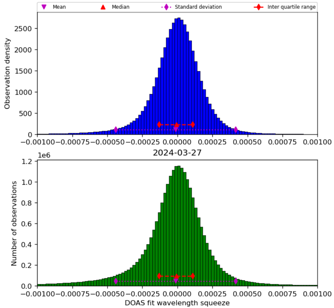
Figure 69: Histogram of “DOAS fit wavelength squeeze” for 2024-03-26 to 2024-03-28
