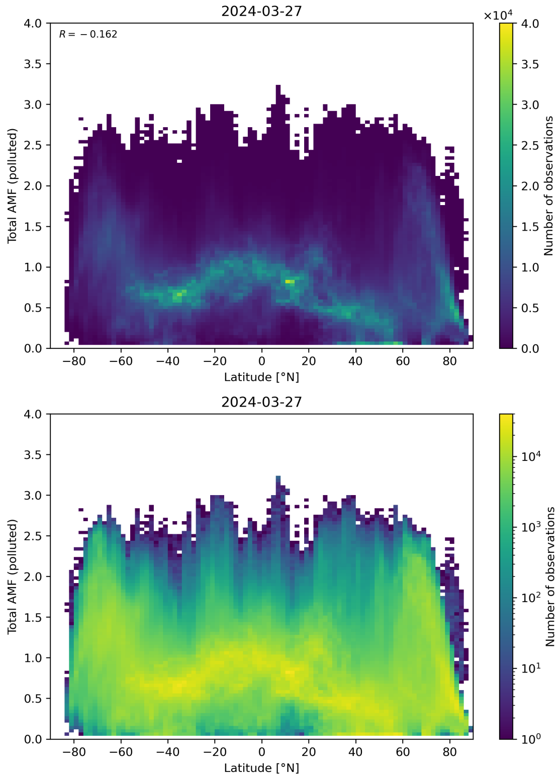
Figure 154: Scatter density plot of “Latitude” against “Total AMF (polluted)” for 2024-03-26 to 2024-03-28.
