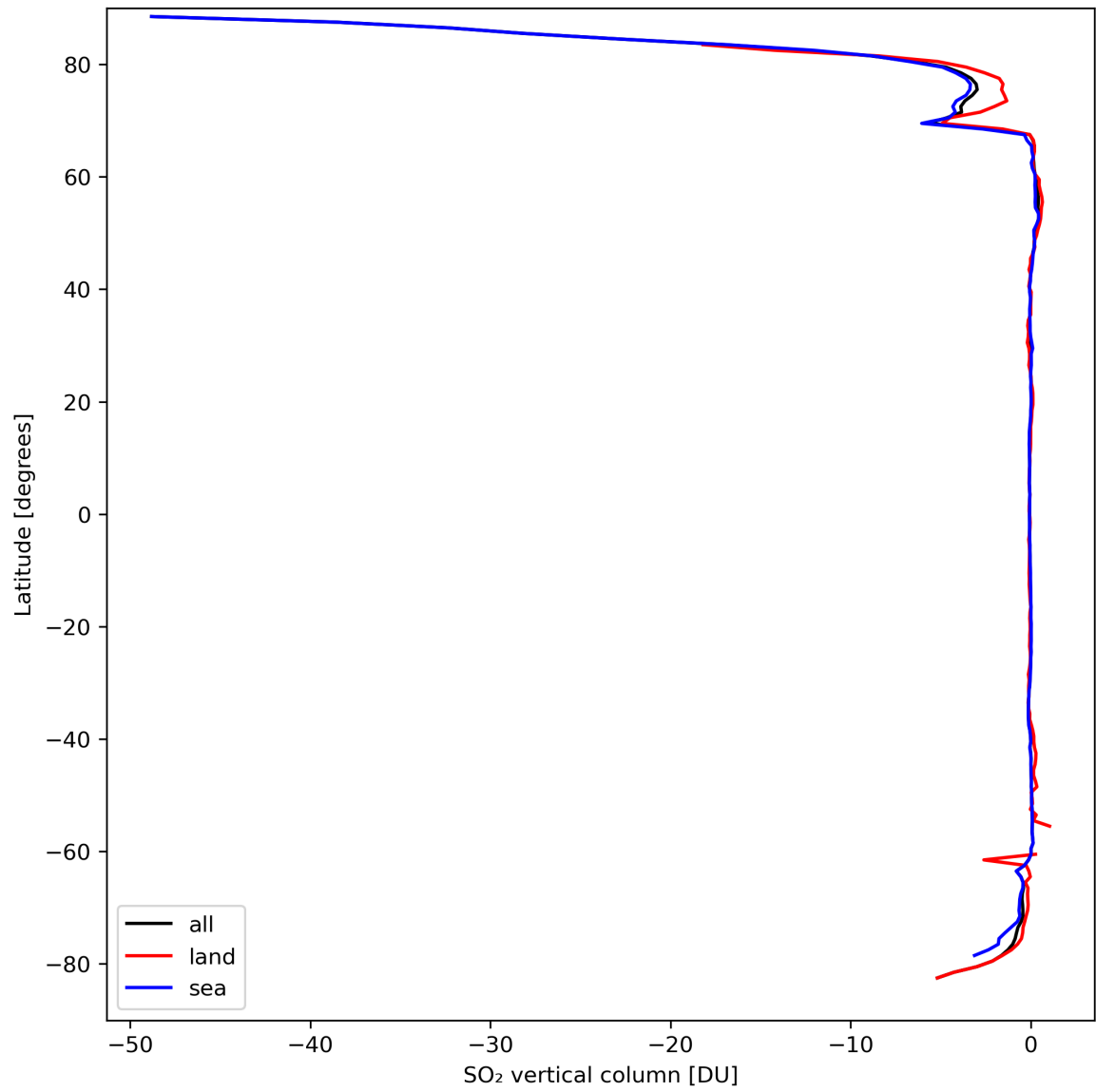
Figure 30: Zonal average of “SO 2 vertical column” for 2024-03-26 to 2024-03-28.
