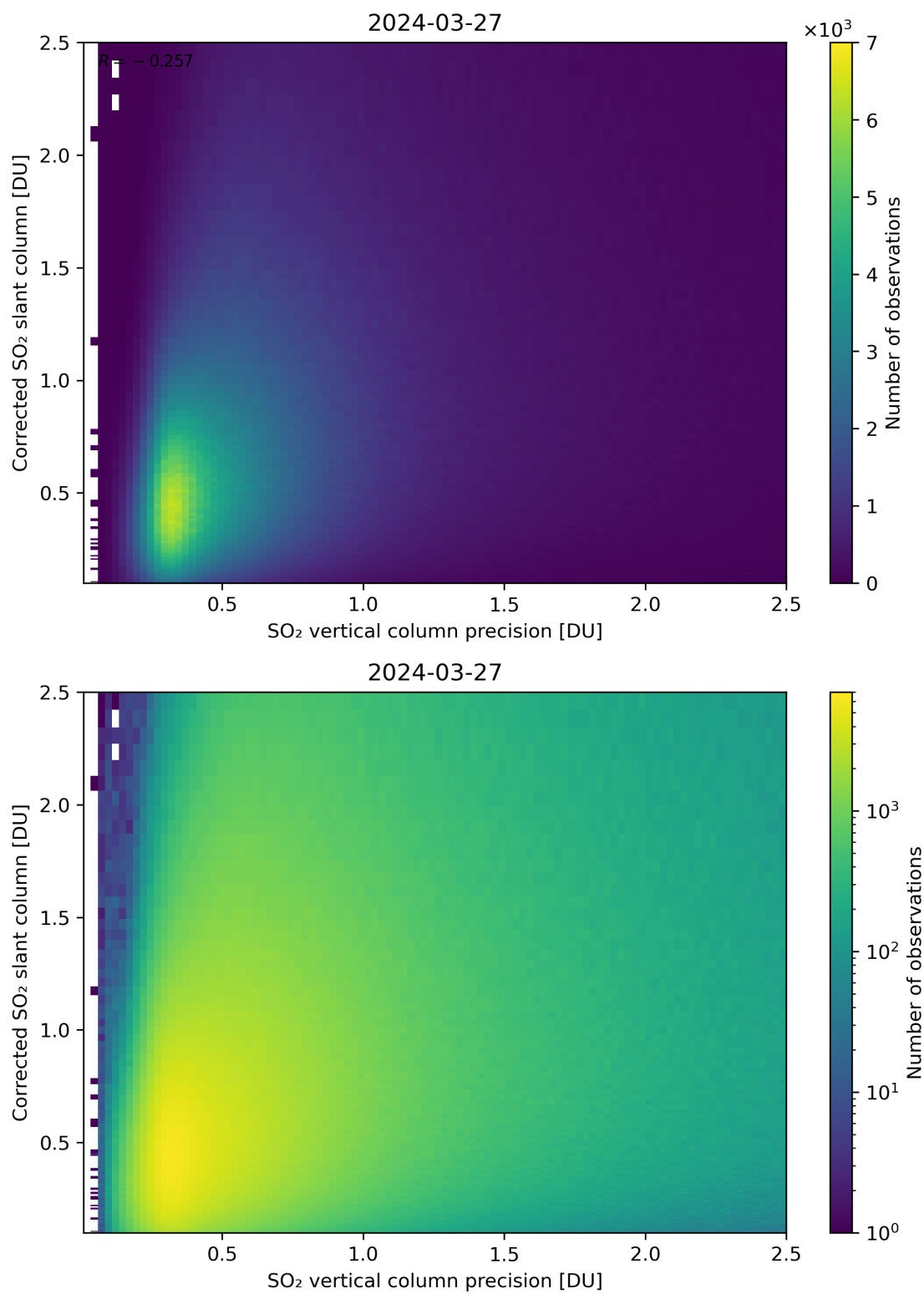
Figure 286: Scatter density plot of “SO 2 vertical column precision” against “Corrected SO 2 slant column” for 2024-03-26 to 2024-03-28.
