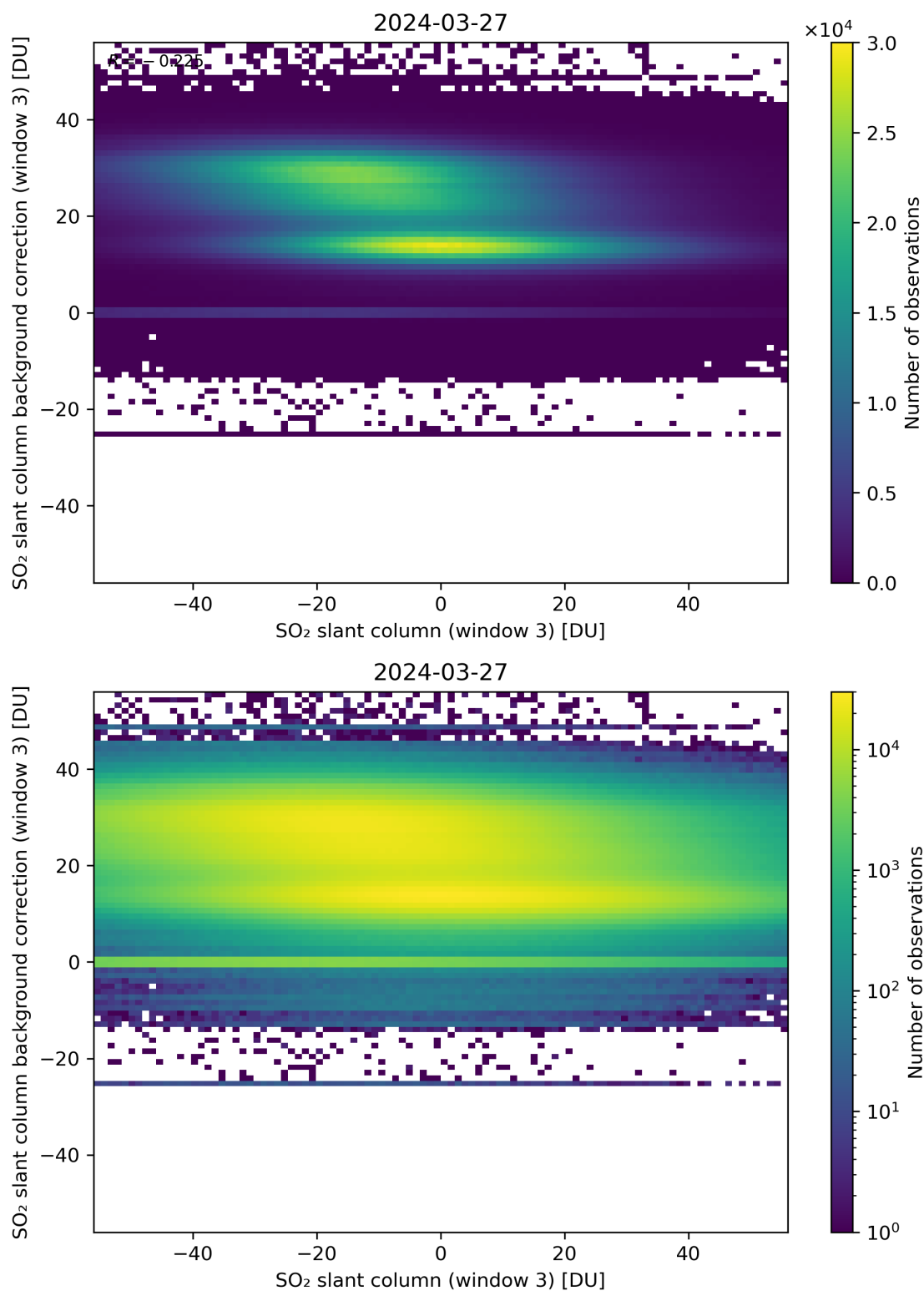
Figure 253: Scatter density plot of “SO 2 slant column (window 3)” against “SO 2 slant column background correction (window 3)” for 2024-03-26 to 2024-03-28.
