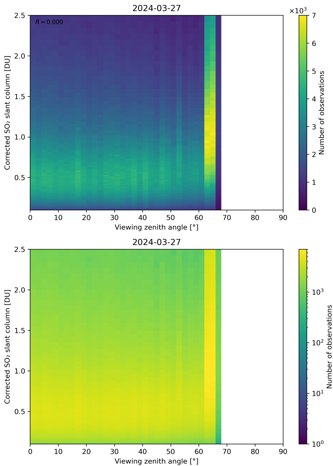
Figure 317: Scatter density plot of “Viewing zenith angle” against “Corrected SO 2 slant column” for 2024-03-26 to 2024-03-28.
