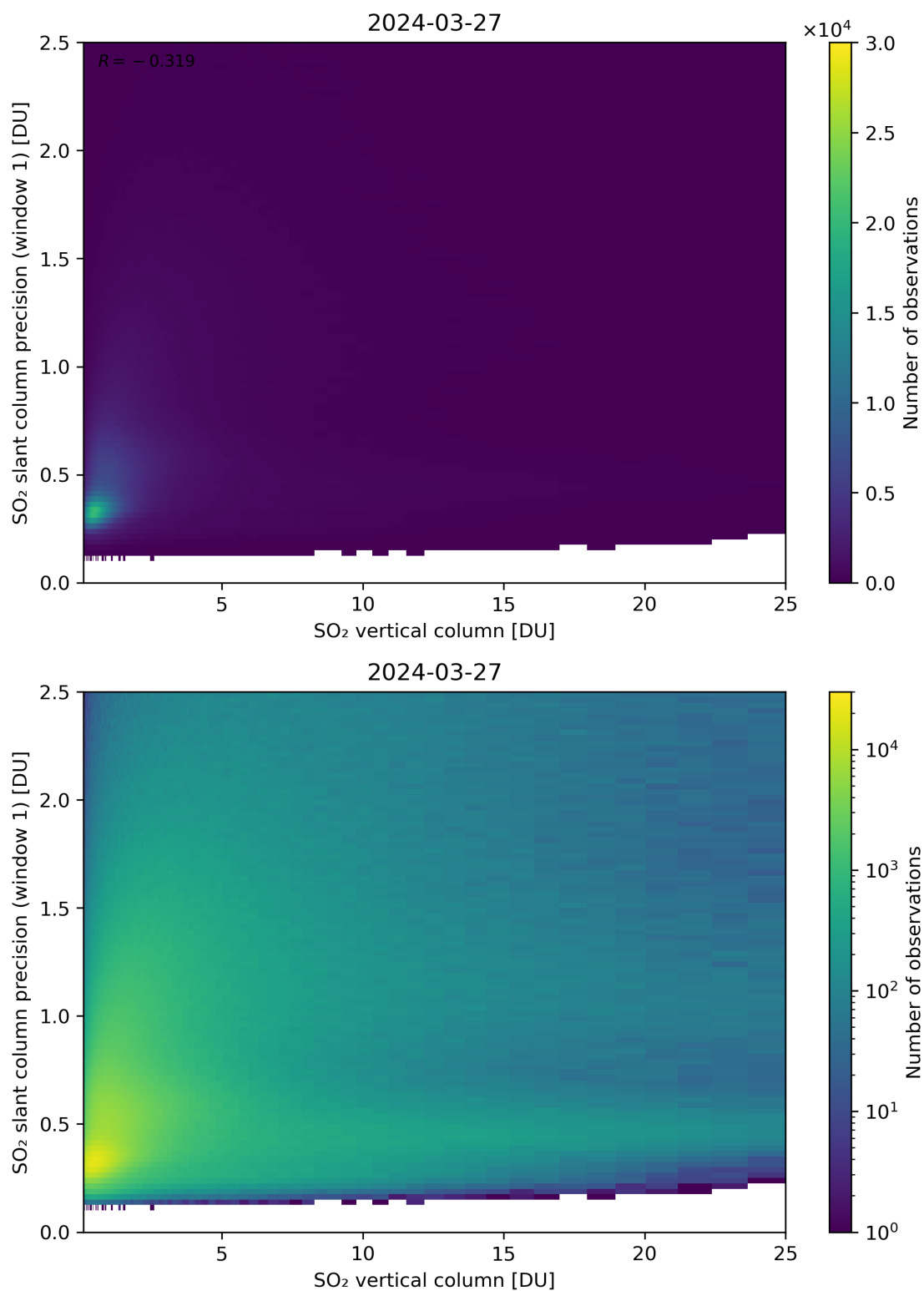
Figure 301: Scatter density plot of “SO 2 vertical column” against “SO 2 slant column precision (window 1)” for 2024-03-26 to 2024-03-28.
