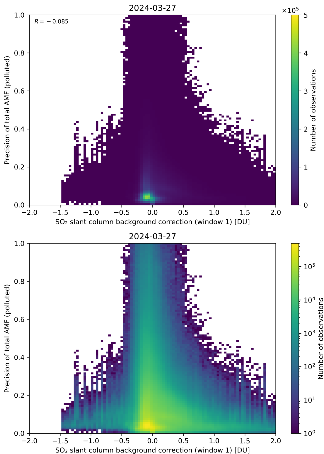
Figure 110: Scatter density plot of “SO 2 slant column background correction (window 1)” against “Precision of total AMF (polluted)” for 2024-03-26 to 2024-03-28.
