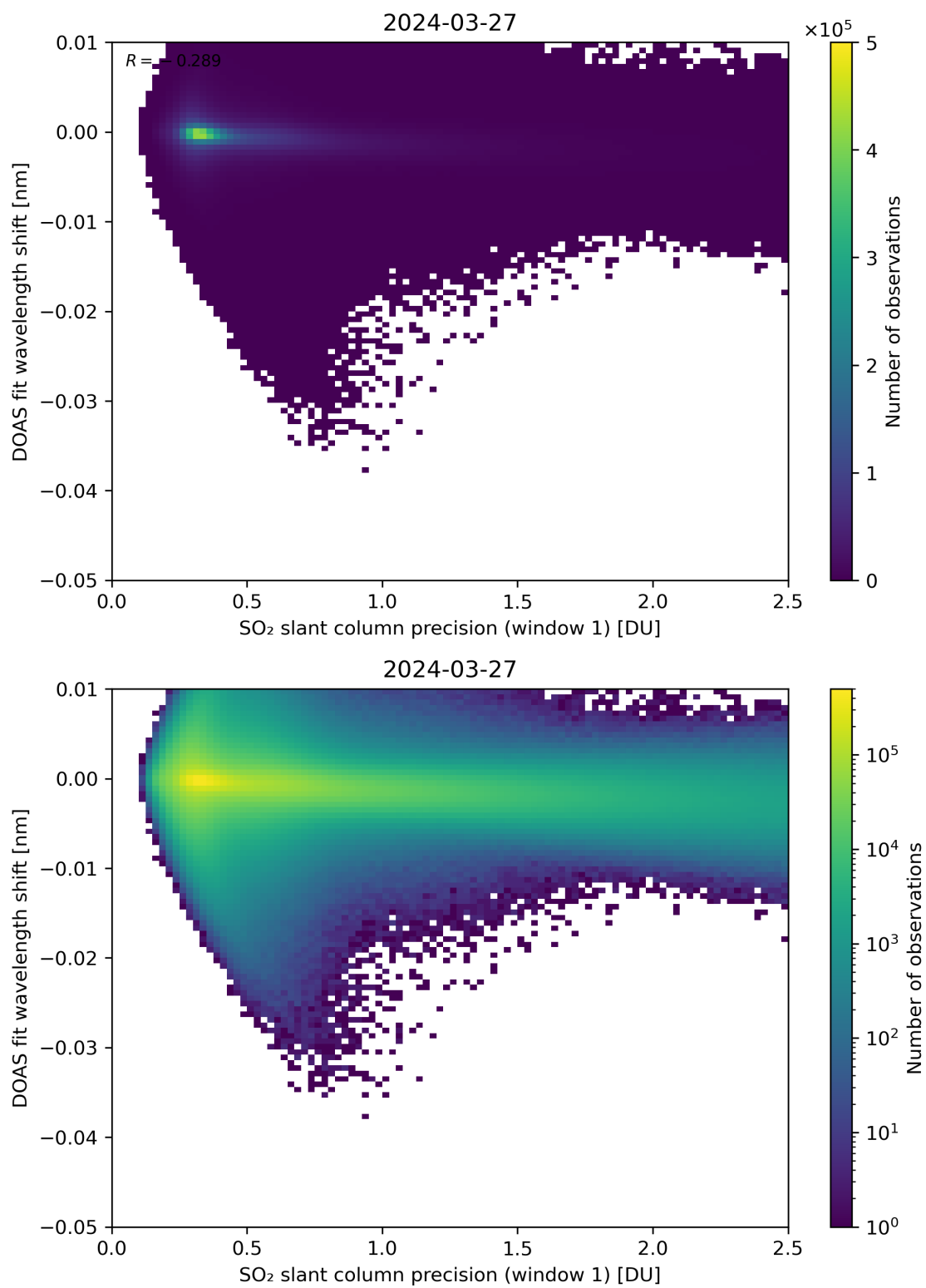
Figure 221: Scatter density plot of “SO 2 slant column precision (window 1)” against “DOAS fit wavelength shift” for 2024-03-26 to 2024-03-28.
