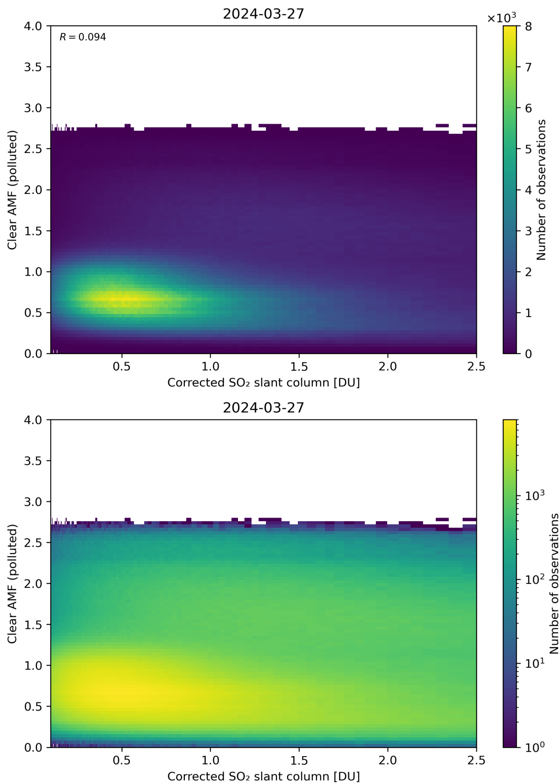
Figure 184: Scatter density plot of “Corrected SO 2 slant column” against “Clear AMF (polluted)” for 2024-03-26 to 2024-03-28.
