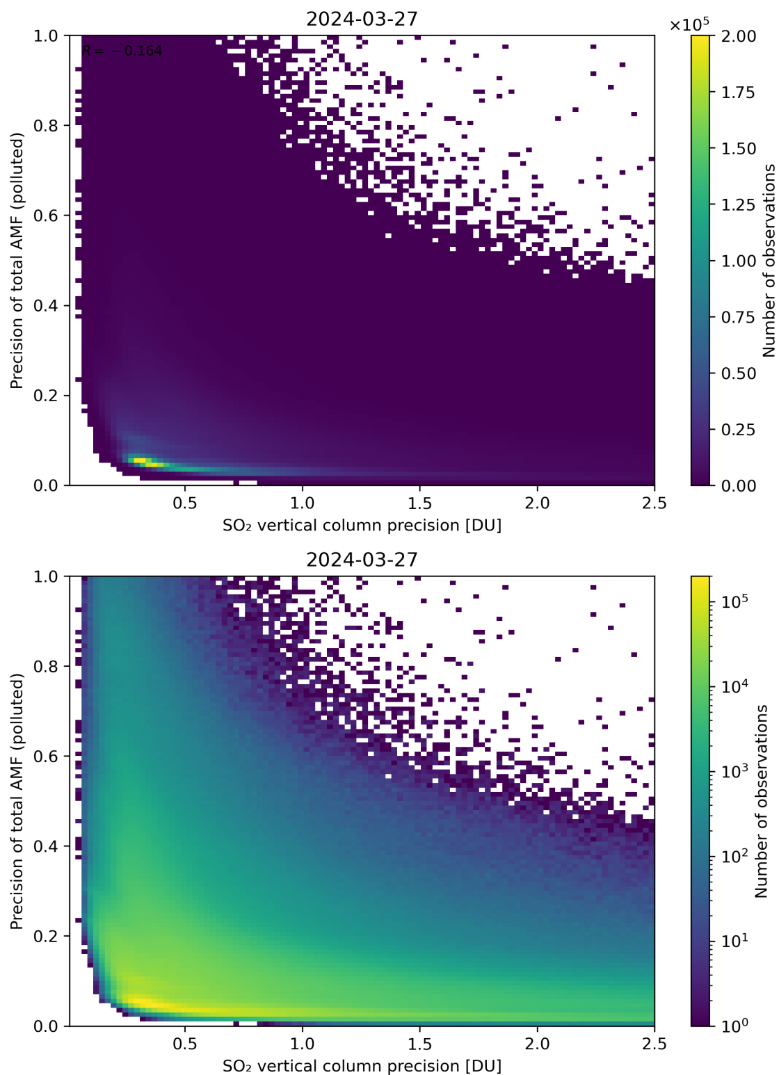
Figure 295: Scatter density plot of “SO 2 vertical column precision” against “Precision of total AMF (polluted)” for 2024-03-26 to 2024-03-28.
