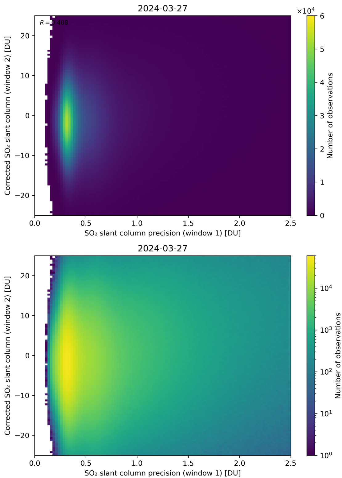
Figure 225: Scatter density plot of “SO 2 slant column precision (window 1)” against “Corrected SO 2 slant column (window 2)” for 2024-03-26 to 2024-03-28.
