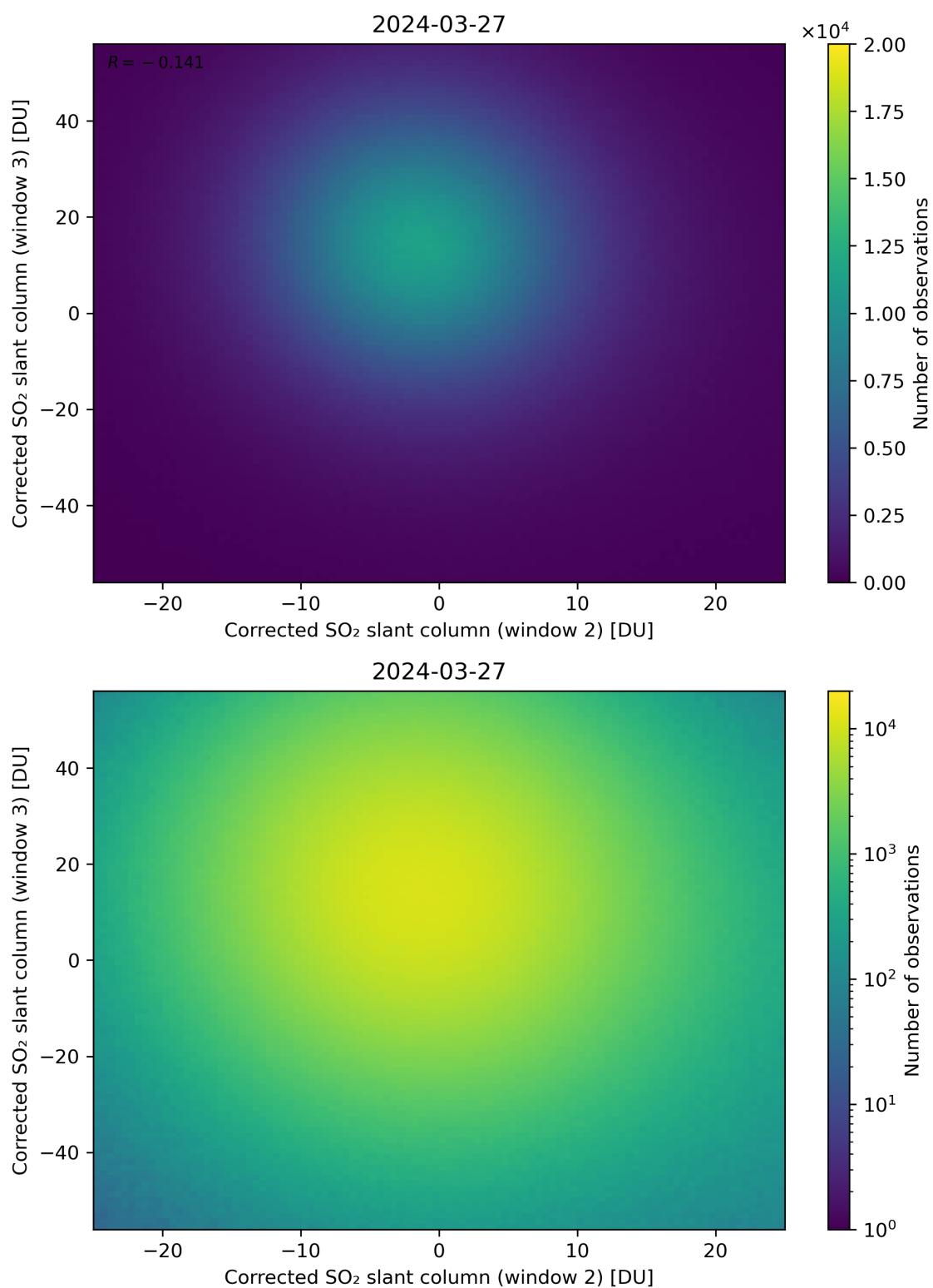
Figure 200: Scatter density plot of “Corrected SO 2 slant column (window 2)” against “Corrected SO 2 slant column (window 3)” for 2024-03-26 to 2024-03-28.
