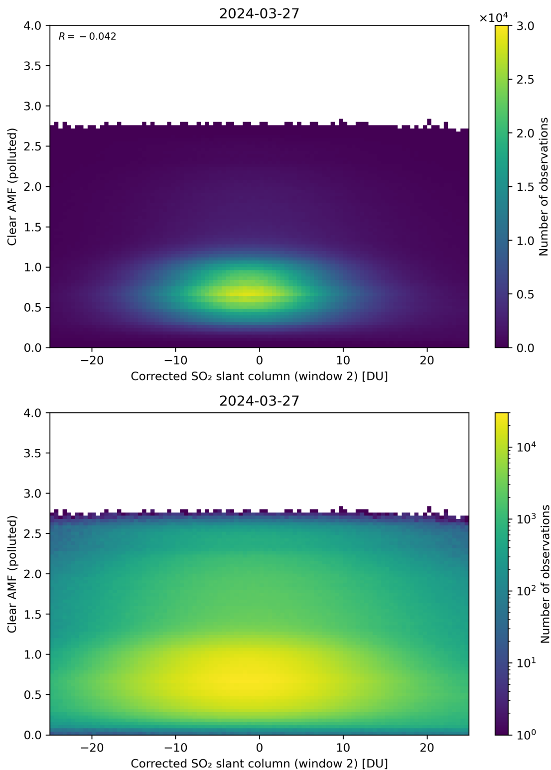
Figure 199: Scatter density plot of “Corrected SO 2 slant column (window 2)” against “Clear AMF (polluted)” for 2024-03-26 to 2024-03-28.
