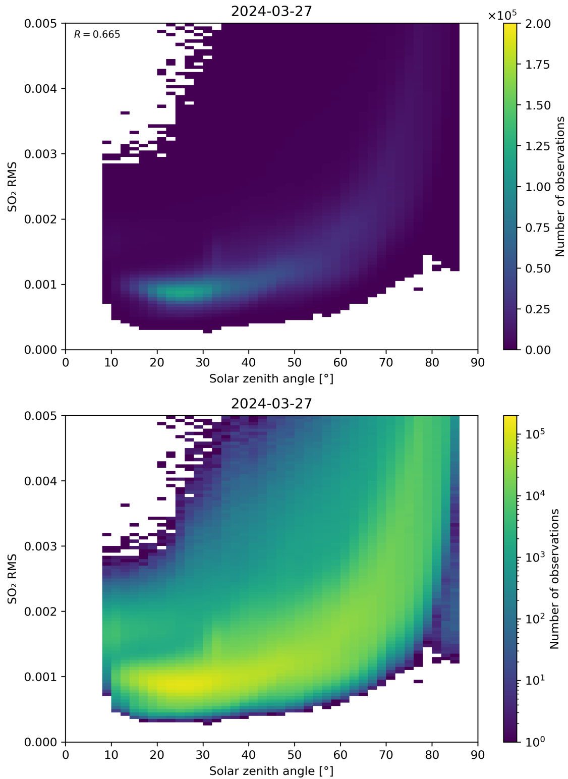
Figure 163: Scatter density plot of “Solar zenith angle” against “SO 2 RMS” for 2024-03-26 to 2024-03-28.
