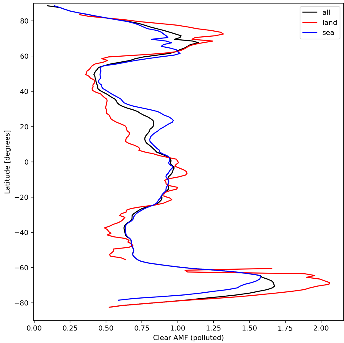
Figure 50: Zonal average of “Clear AMF (polluted)” for 2024-03-26 to 2024-03-28.
