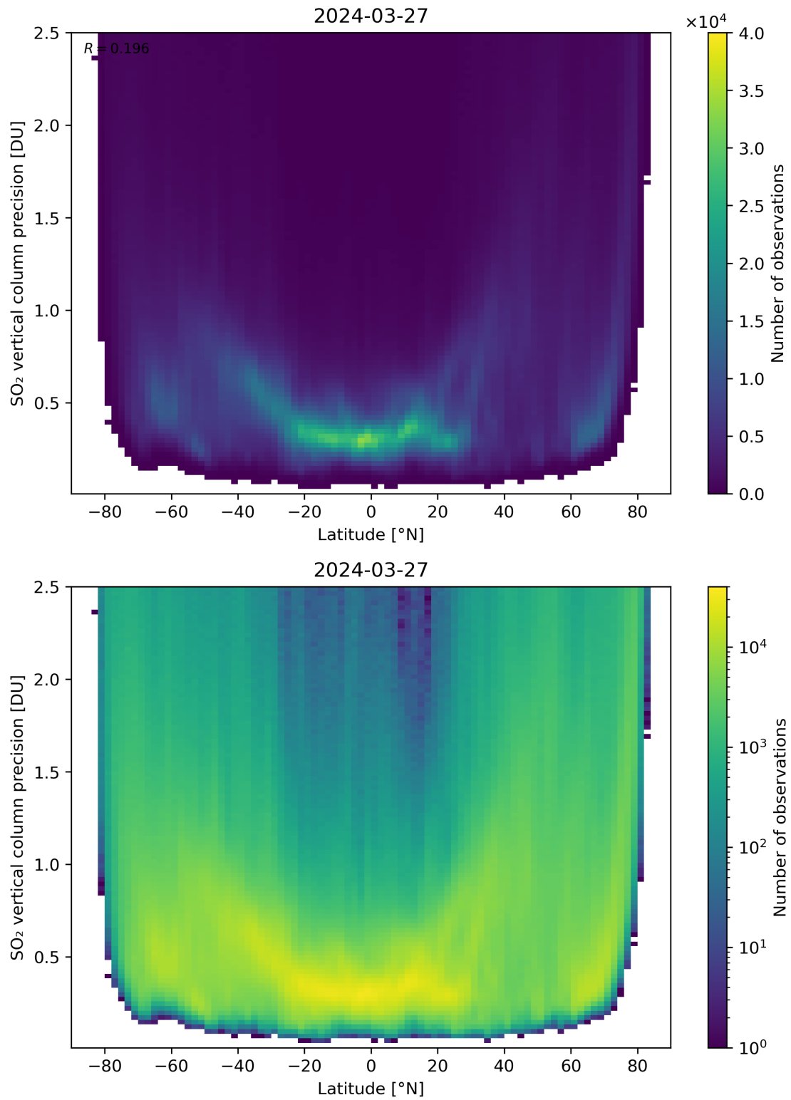
Figure 157: Scatter density plot of “Latitude” against “SO 2 vertical column precision” for 2024-03-26 to 2024-03-28.
