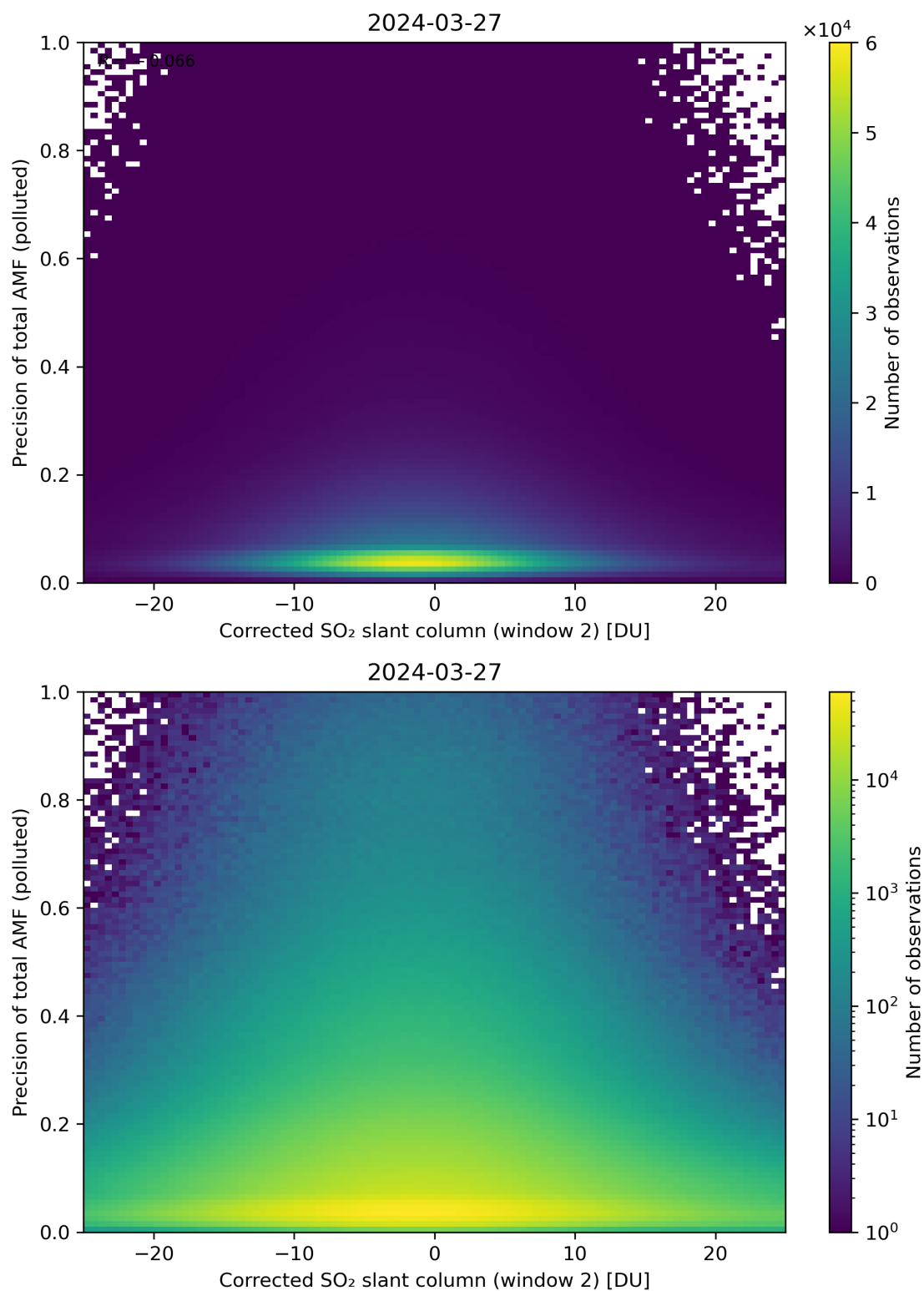
Figure 204: Scatter density plot of “Corrected SO 2 slant column (window 2)” against “Precision of total AMF (polluted)” for 2024-03-26 to 2024-03-28.
