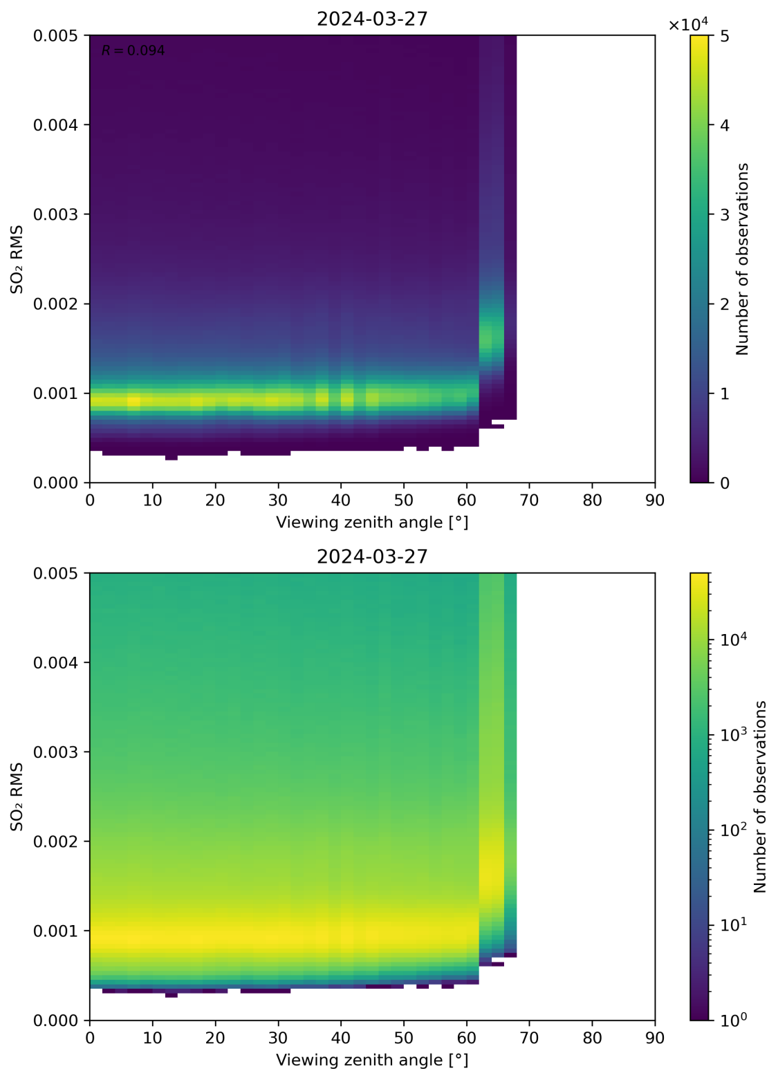
Figure 313: Scatter density plot of “Viewing zenith angle” against “SO 2 RMS” for 2024-03-26 to 2024-03-28.
