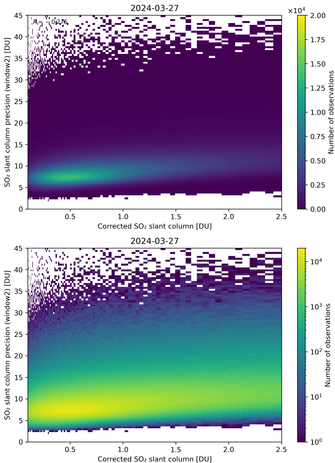
Figure 189: Scatter density plot of “Corrected SO 2 slant column” against “SO 2 slant column precision (window2)” for 2024-03-26 to 2024-03-28.
