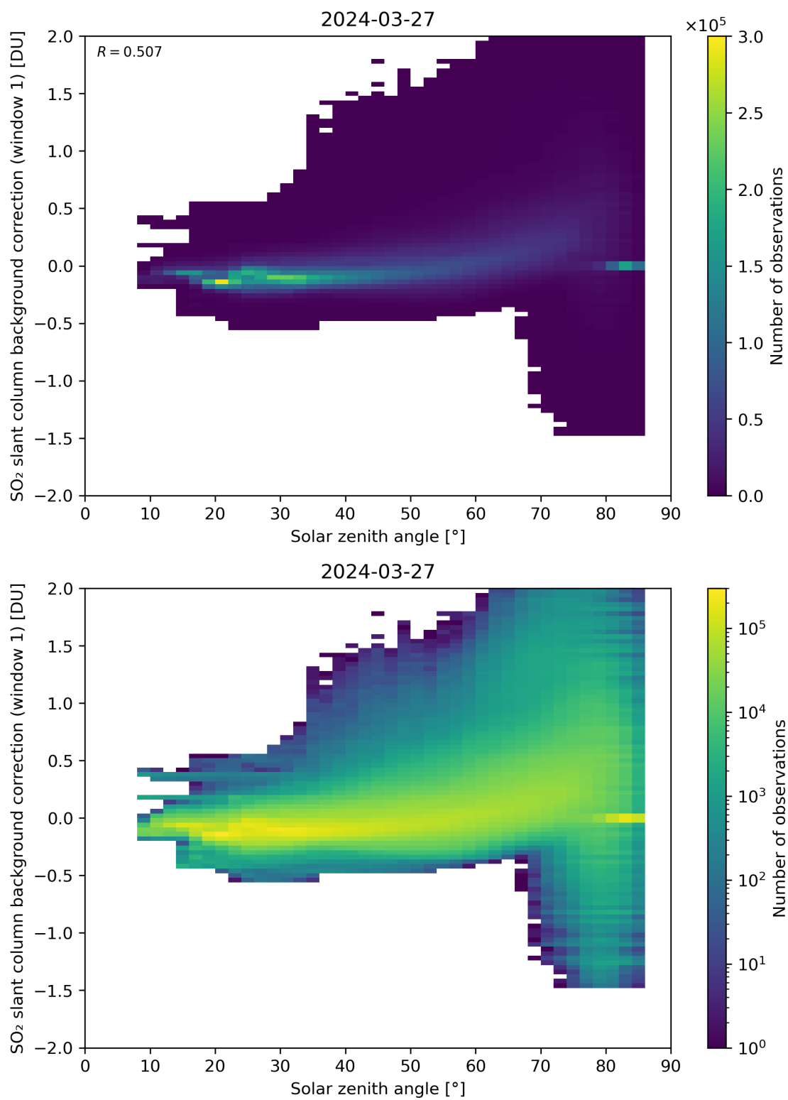
Figure 158: Scatter density plot of “Solar zenith angle” against “SO 2 slant column background correction (window 1)” for 2024-03-26 to 2024-03-28.
