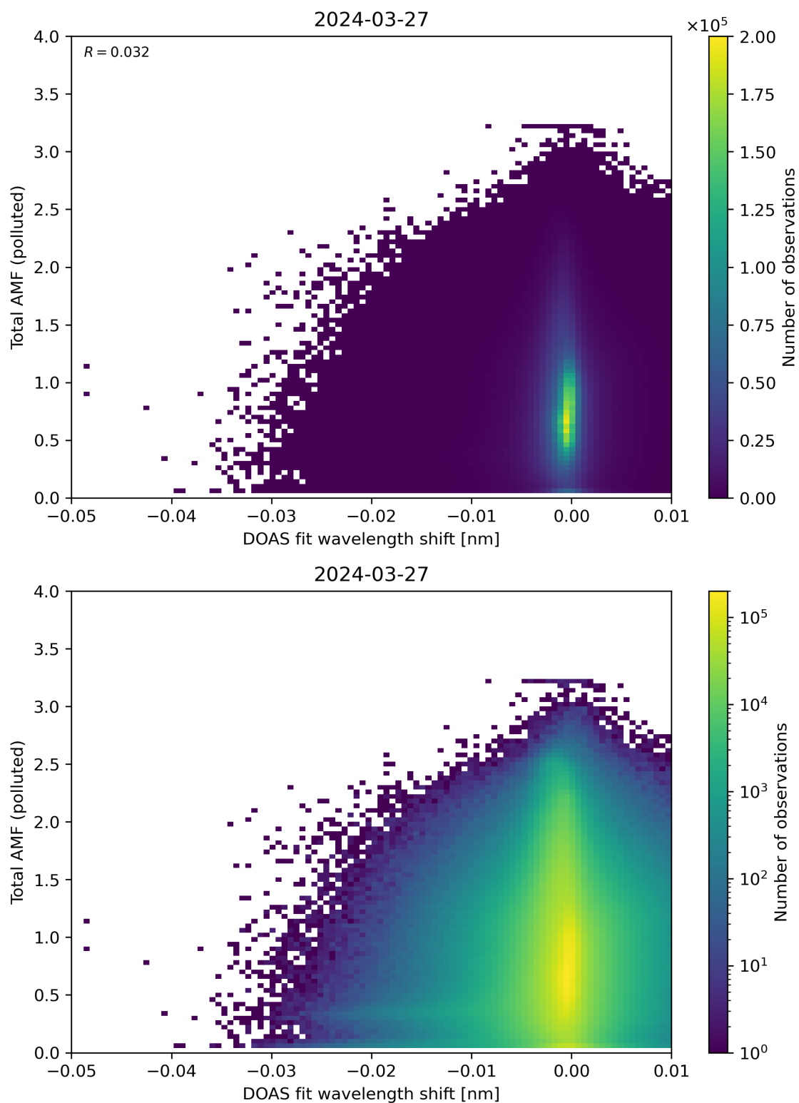
Figure 130: Scatter density plot of “DOAS fit wavelength shift” against “Total AMF (polluted)” for 2024-03-26 to 2024-03-28.
