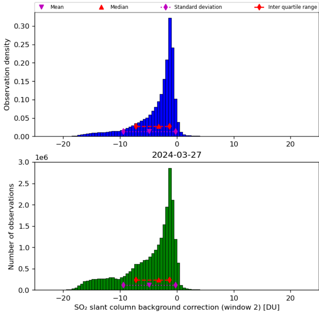
Figure 63: Histogram of “SO 2 slant column background correction (window 2)” for 2024-03-26 to 2024-03-28
