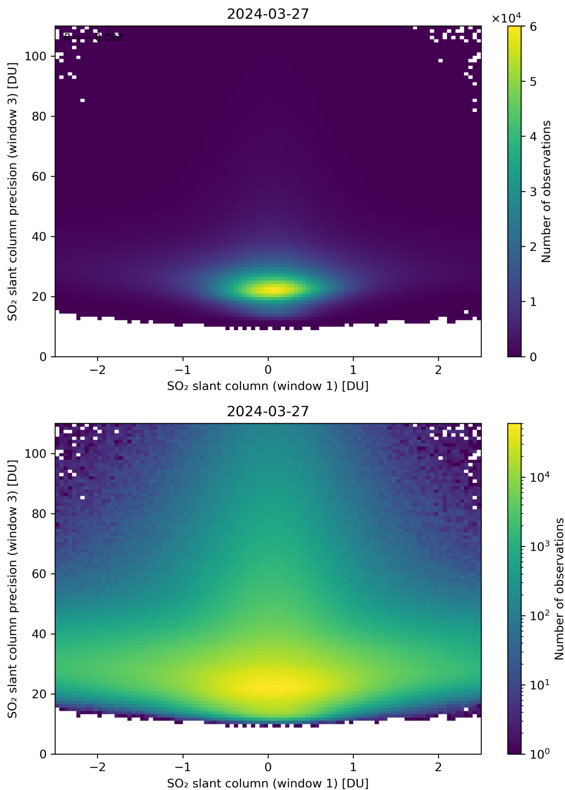
Figure 238: Scatter density plot of “SO 2 slant column (window 1)” against “SO 2 slant column precision (window 3)” for 2024-03-26 to 2024-03-28.
