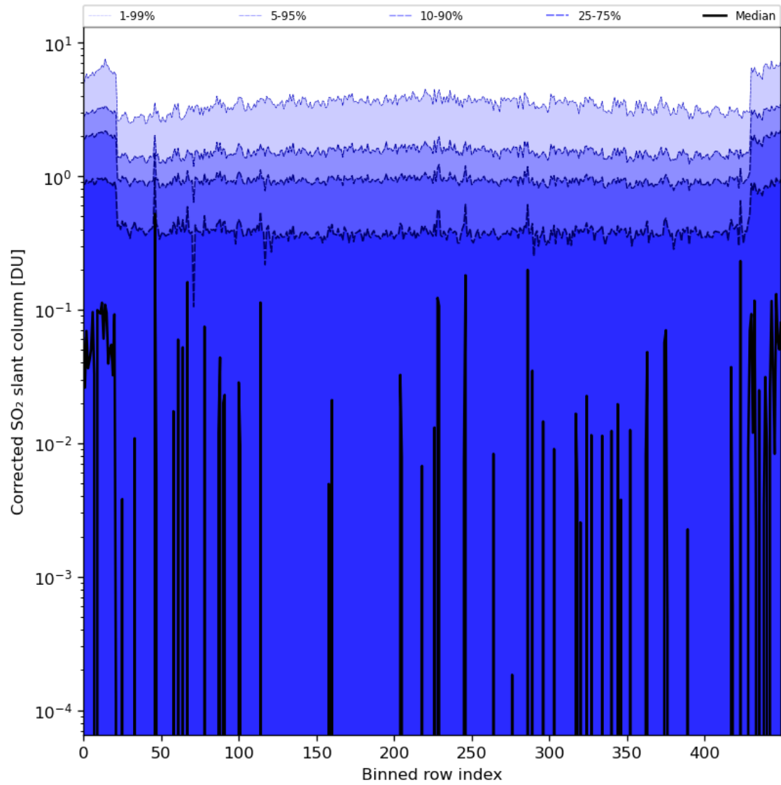
Figure 78: Along track statistics of “Corrected SO 2 slant column” for 2024-03-26 to 2024-03-28
