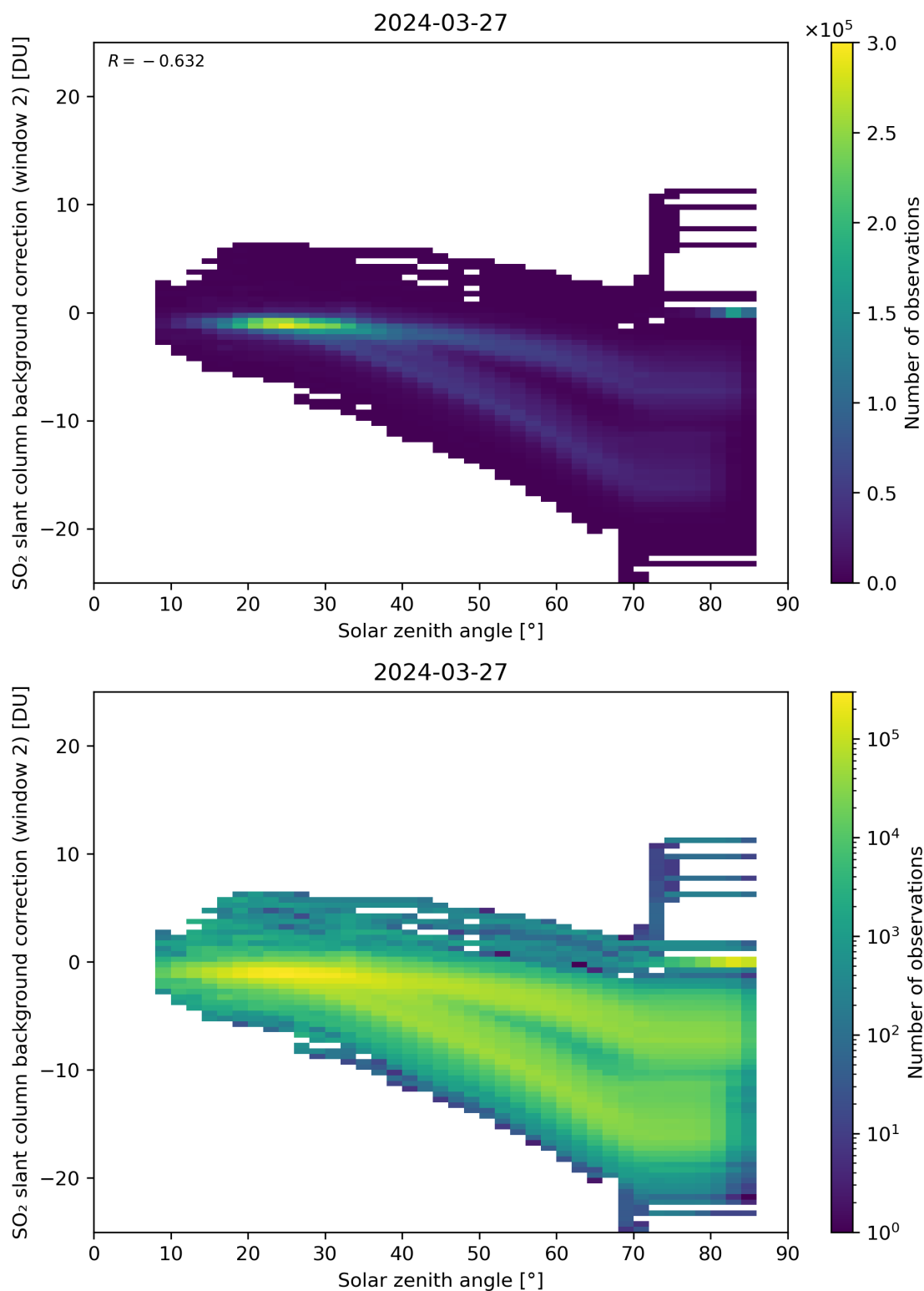
Figure 159: Scatter density plot of “Solar zenith angle” against “SO 2 slant column background correction (window 2)” for 2024-03-26 to 2024-03-28.
