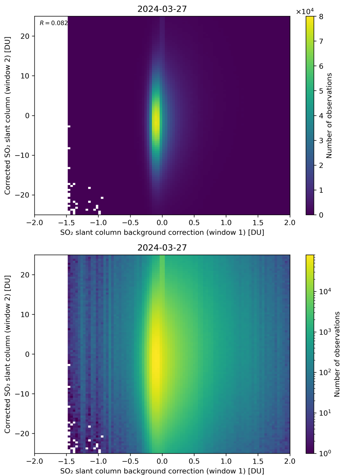
Figure 104: Scatter density plot of “SO 2 slant column background correction (window 1)” against “Corrected SO 2 slant column (window 2)” for 2024-03-26 to 2024-03-28.
