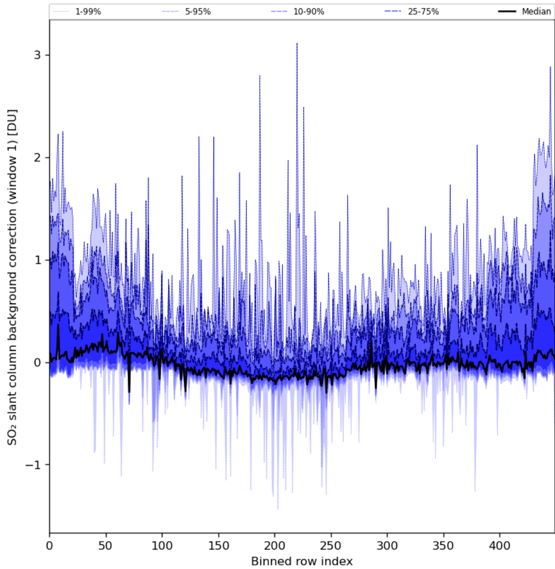
Figure 82: Along track statistics of “SO 2 slant column background correction (window 1)” for 2024-03-26 to 2024-03-28
