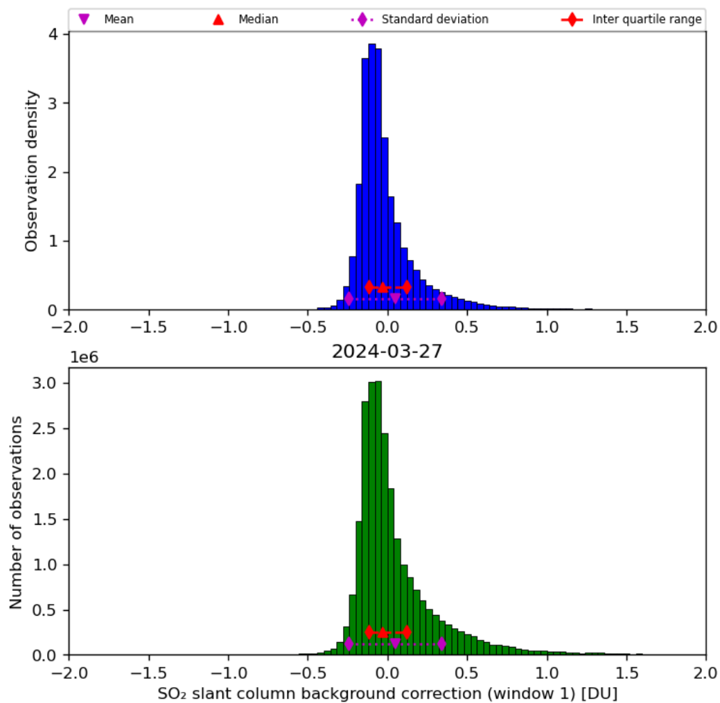
Figure 59: Histogram of “SO 2 slant column background correction (window 1)” for 2024-03-26 to 2024-03-28
