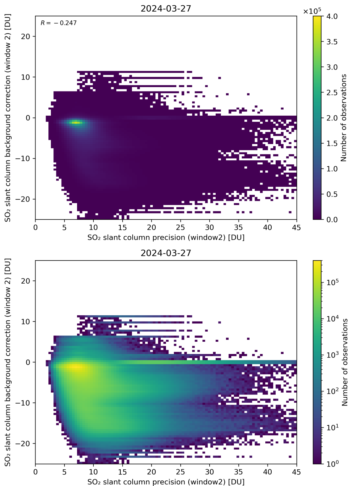
Figure 241: Scatter density plot of “SO 2 slant column precision (window2)” against “SO 2 slant column background correction (window 2)” for 2024-03-26 to 2024-03-28.
