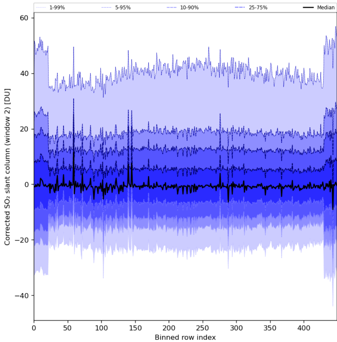
Figure 85: Along track statistics of “Corrected SO 2 slant column (window 2)” for 2024-03-26 to 2024-03-28
