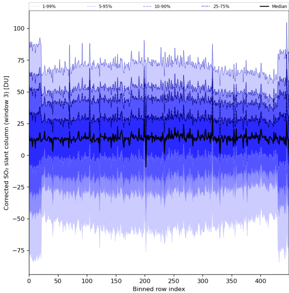
Figure 89: Along track statistics of “Corrected SO 2 slant column (window 3)” for 2024-03-26 to 2024-03-28
