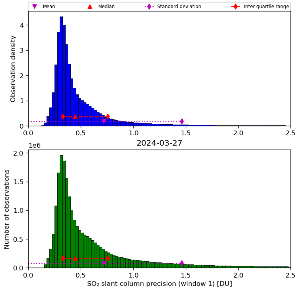
Figure 57: Histogram of “SO 2 slant column precision (window 1)” for 2024-03-26 to 2024-03-28
