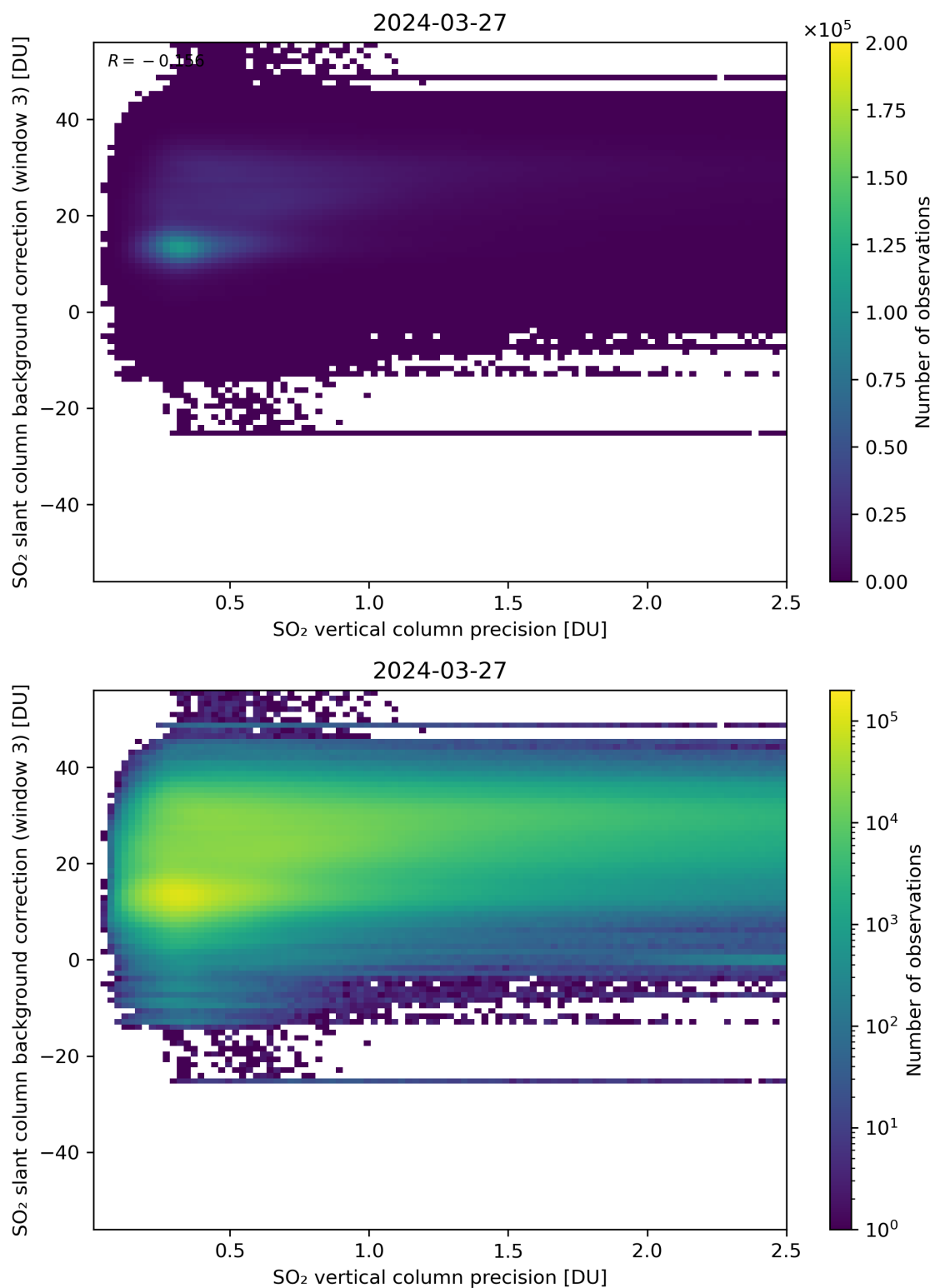
Figure 281: Scatter density plot of “SO 2 vertical column precision” against “SO 2 slant column background correction (window 3)” for 2024-03-26 to 2024-03-28.
