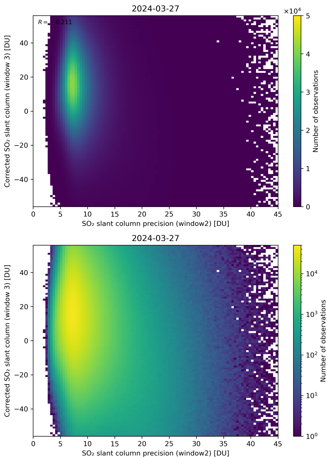
Figure 248: Scatter density plot of “SO 2 slant column precision (window2)” against “Corrected SO 2 slant column (window 3)” for 2024-03-26 to 2024-03-28.
