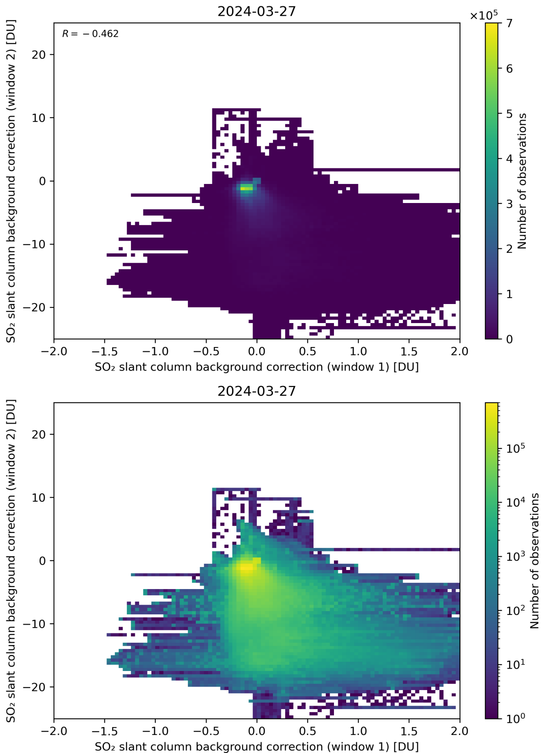
Figure 98: Scatter density plot of “SO 2 slant column background correction (window 1)” against “SO 2 slant column background correction (window 2)” for 2024-03-26 to 2024-03-28.
