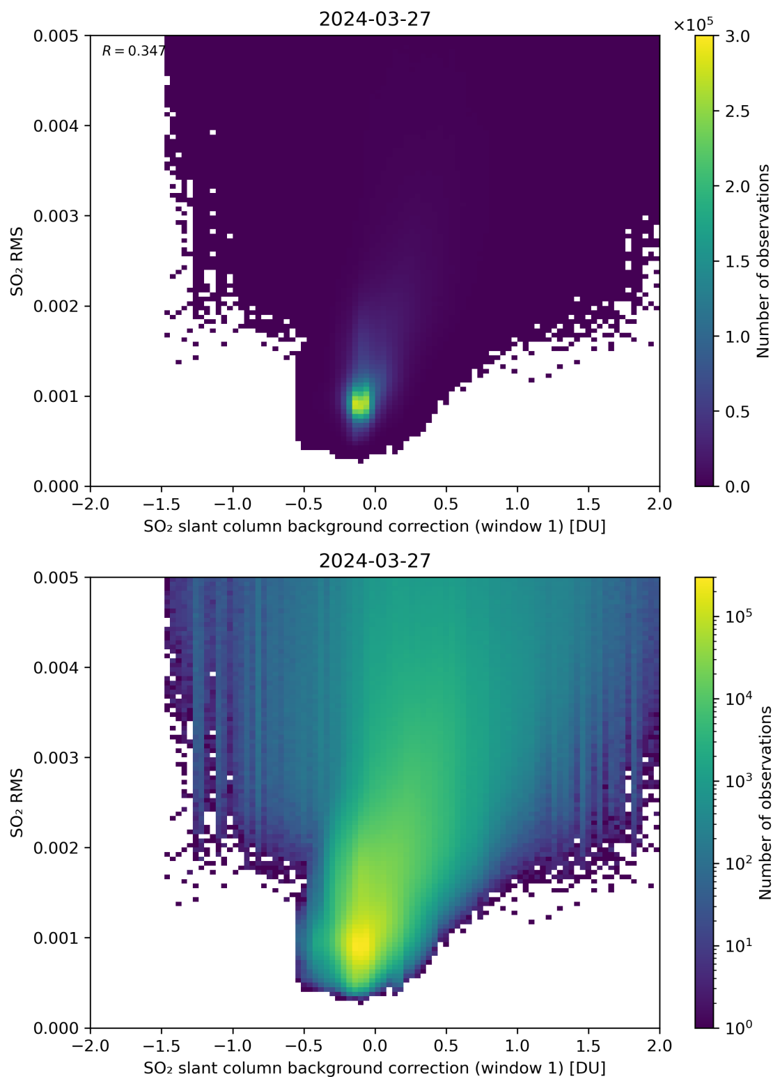
Figure 102: Scatter density plot of “SO 2 slant column background correction (window 1)” against “SO 2 RMS” for 2024-03-26 to 2024-03-28.
