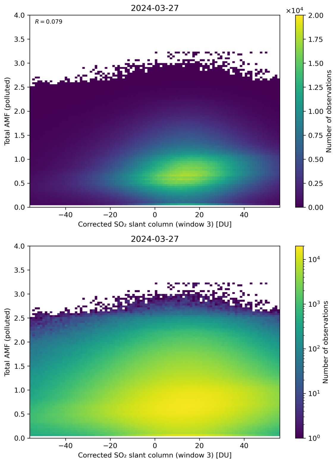
Figure 210: Scatter density plot of “Corrected SO 2 slant column (window 3)” against “Total AMF (polluted)” for 2024-03-26 to 2024-03-28.
