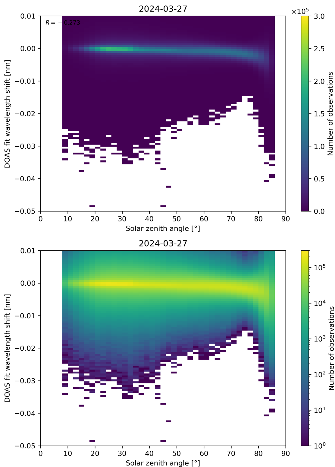
Figure 161: Scatter density plot of “Solar zenith angle” against “DOAS fit wavelength shift” for 2024-03-26 to 2024-03-28.
