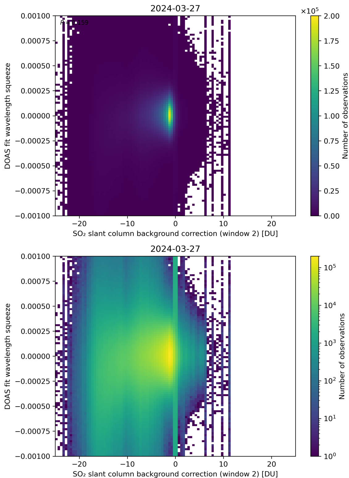
Figure 113: Scatter density plot of "SO 2 slant column background correction (window 2)" against "DOAS fit wavelength squeeze" for 2024-03-26 to 2024-03-28.
