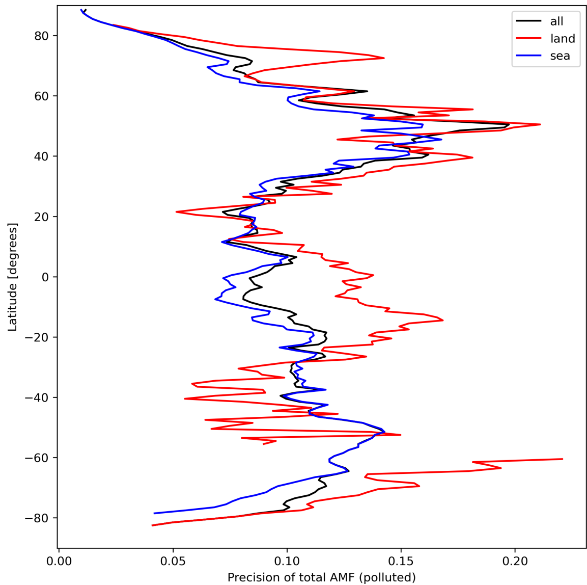
Figure 49: Zonal average of “Precision of total AMF (polluted)” for 2024-03-26 to 2024-03-28.
