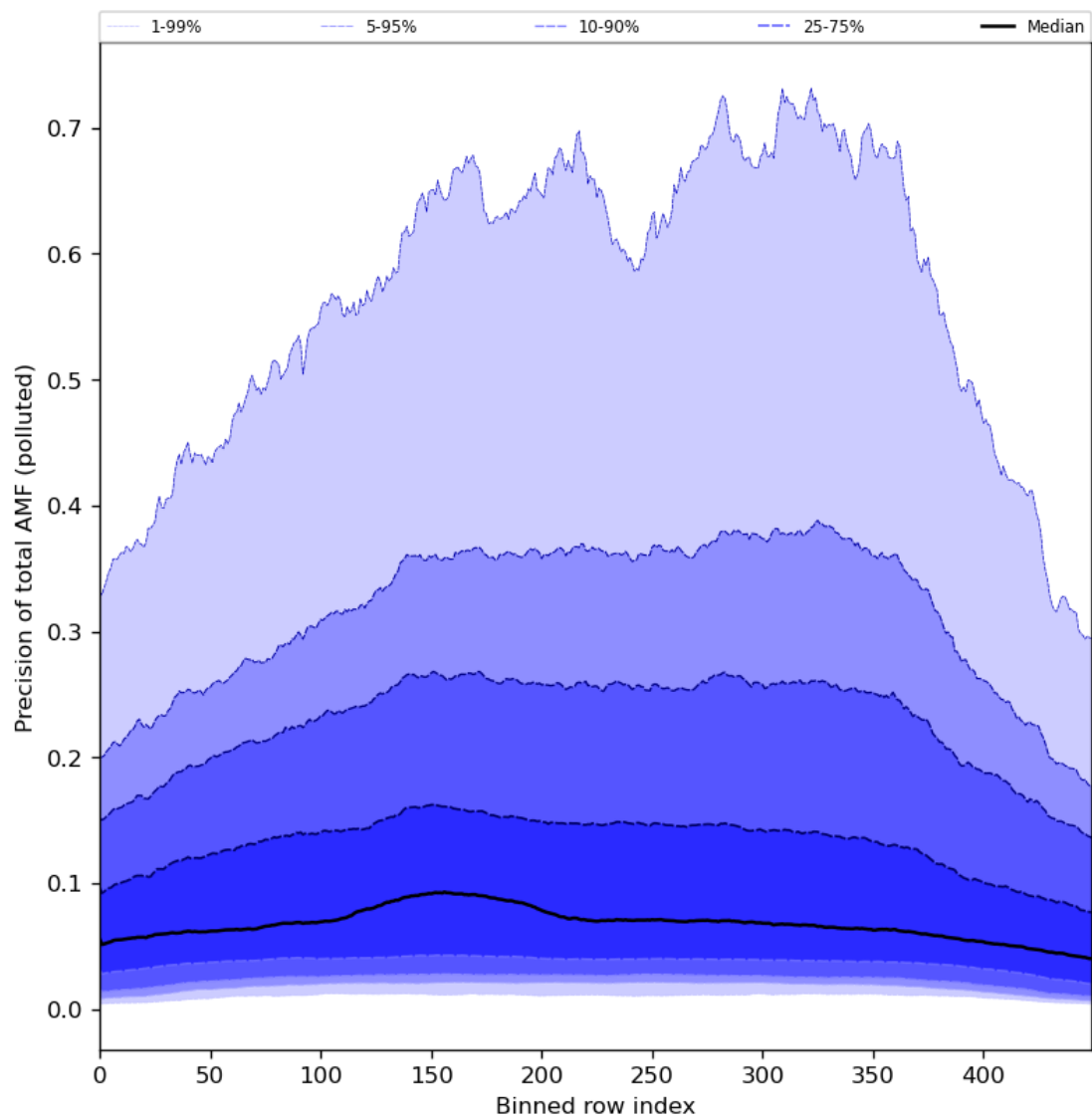
Figure 95: Along track statistics of “Precision of total AMF (polluted)” for 2024-03-26 to 2024-03-28
