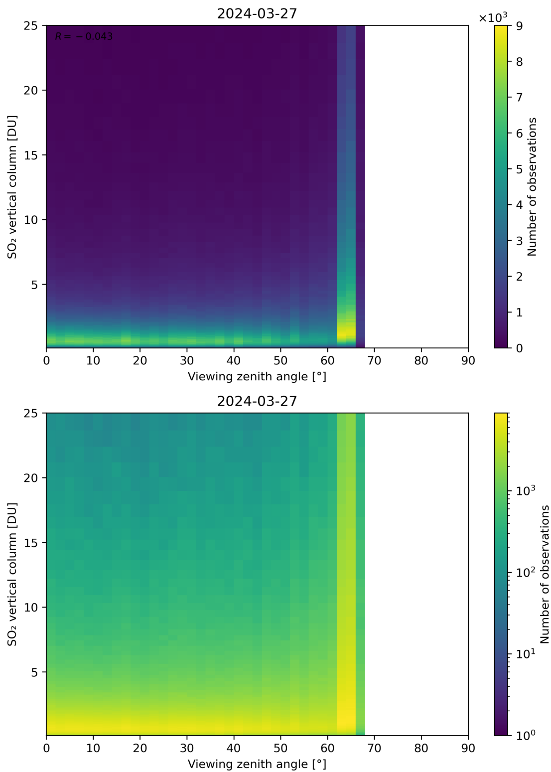
Figure 327: Scatter density plot of “Viewing zenith angle” against “SO 2 vertical column” for 2024-03-26 to 2024-03-28.
