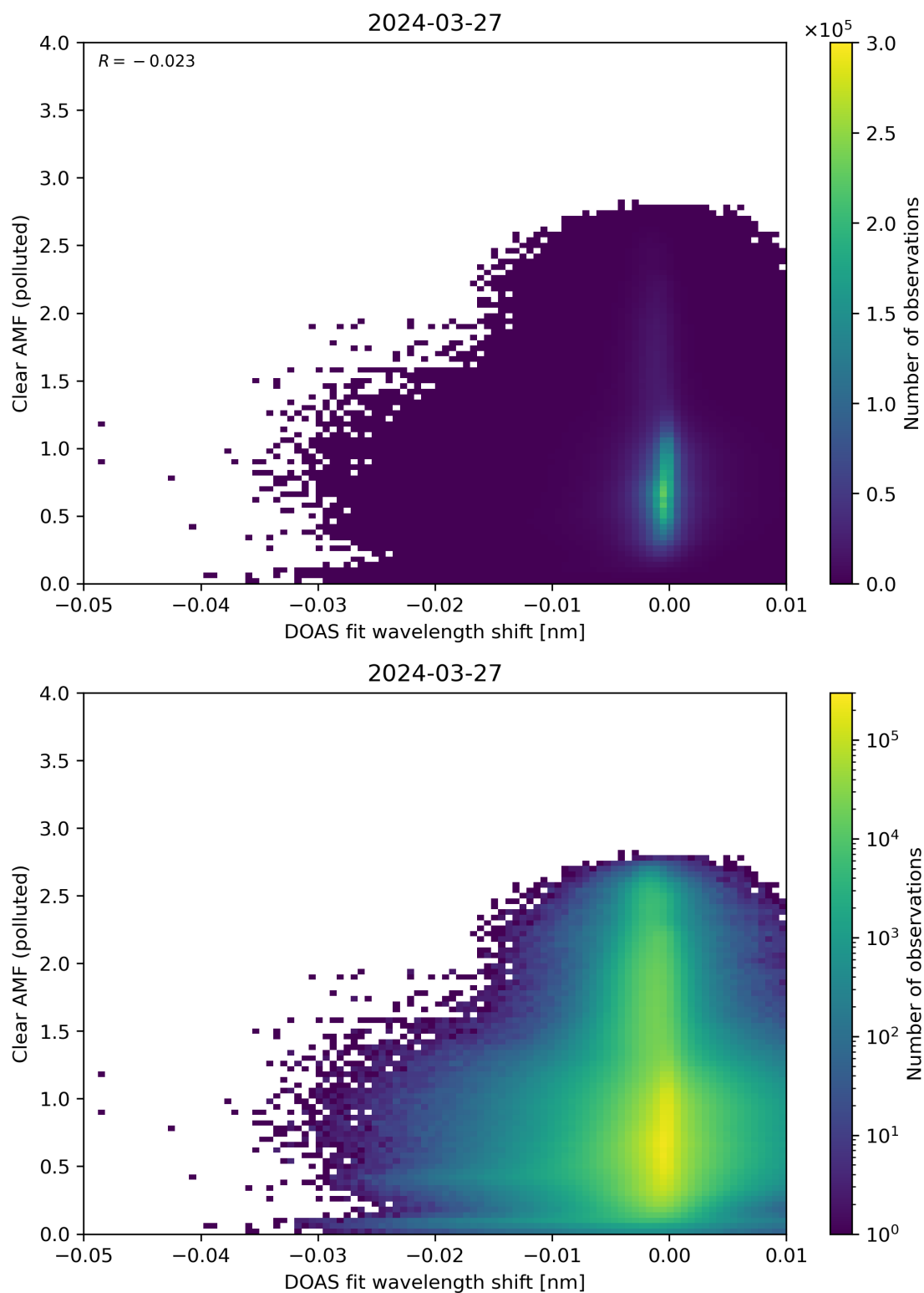
Figure 129: Scatter density plot of “DOAS fit wavelength shift” against “Clear AMF (polluted)” for 2024-03-26 to 2024-03-28.
