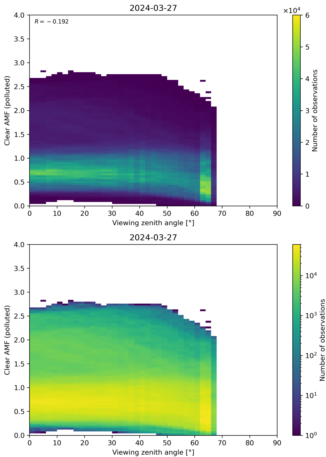
Figure 316: Scatter density plot of “Viewing zenith angle” against “Clear AMF (polluted)” for 2024-03-26 to 2024-03-28.
