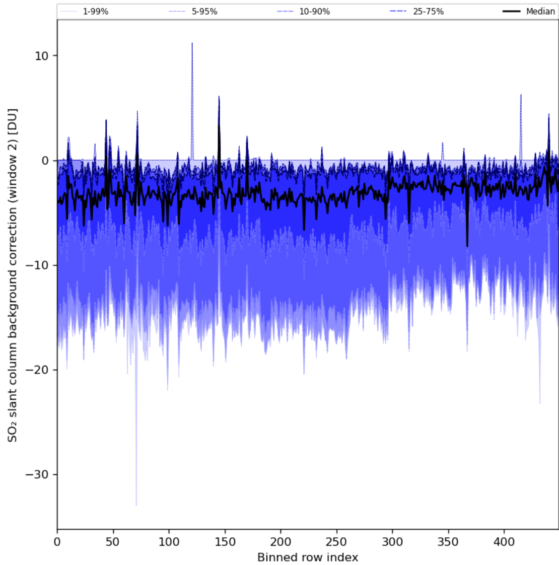
Figure 86: Along track statistics of “SO 2 slant column background correction (window 2)” for 2024-03-26 to 2024-03-28
