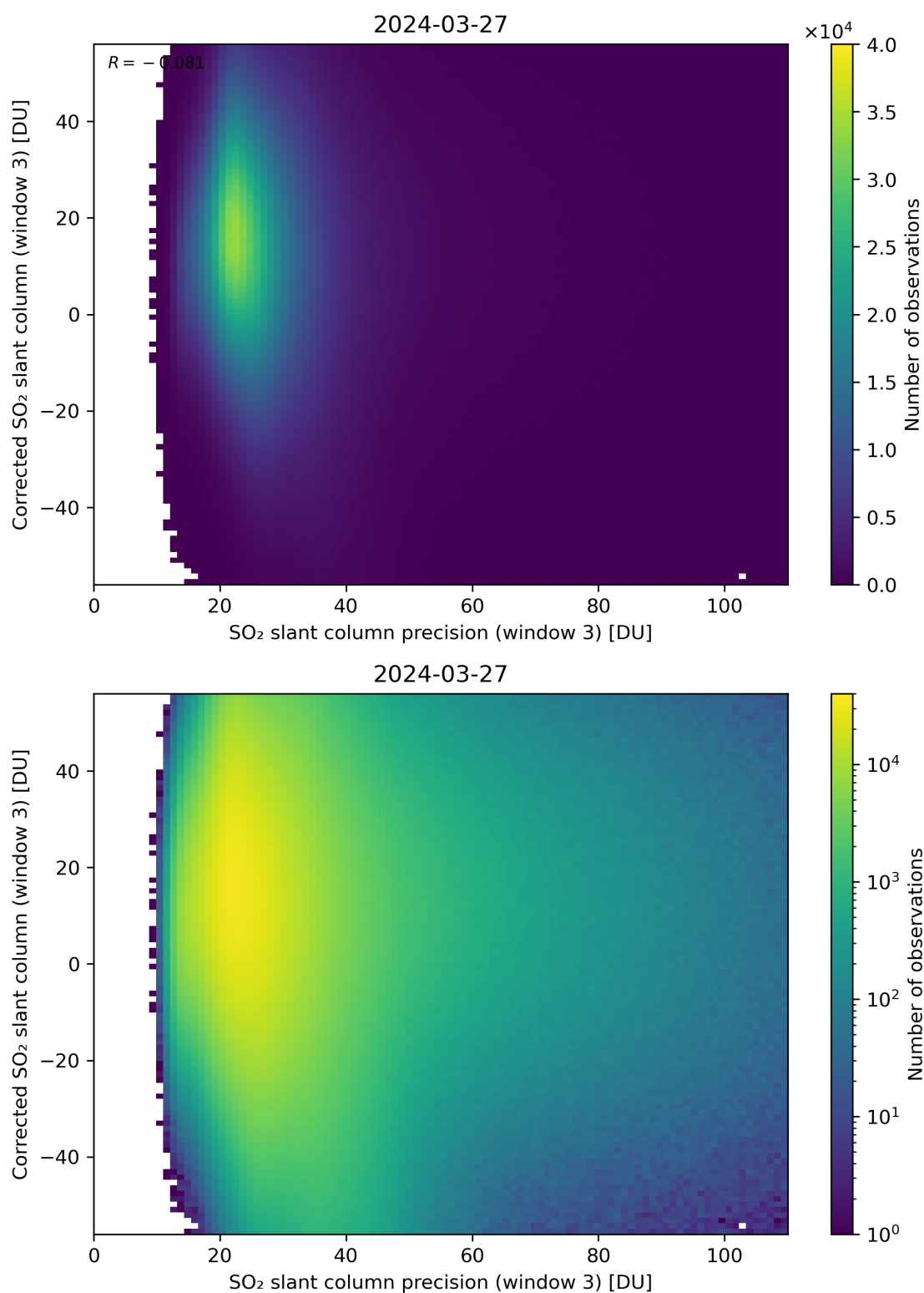
Figure 262: Scatter density plot of “SO 2 slant column precision (window 3)” against “Corrected SO 2 slant column (window 3)” for 2024-03-26 to 2024-03-28.
