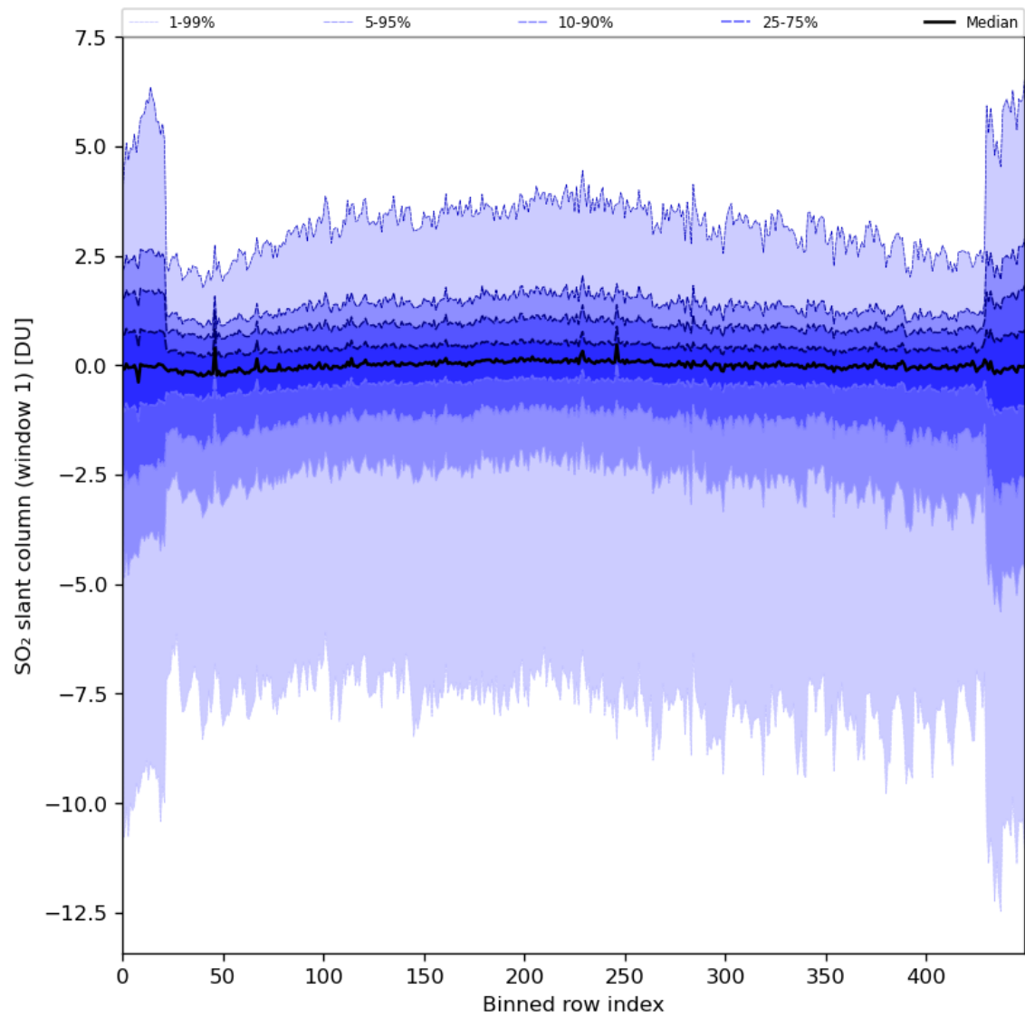
Figure 79: Along track statistics of “SO 2 slant column (window 1)” for 2024-03-26 to 2024-03-28
