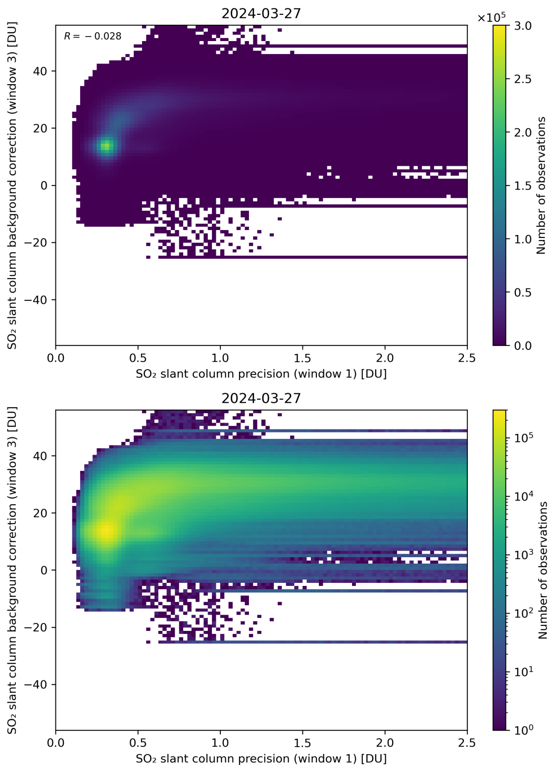
Figure 220: Scatter density plot of “SO 2 slant column precision (window 1)” against “SO 2 slant column background correction (window 3)” for 2024-03-26 to 2024-03-28.
