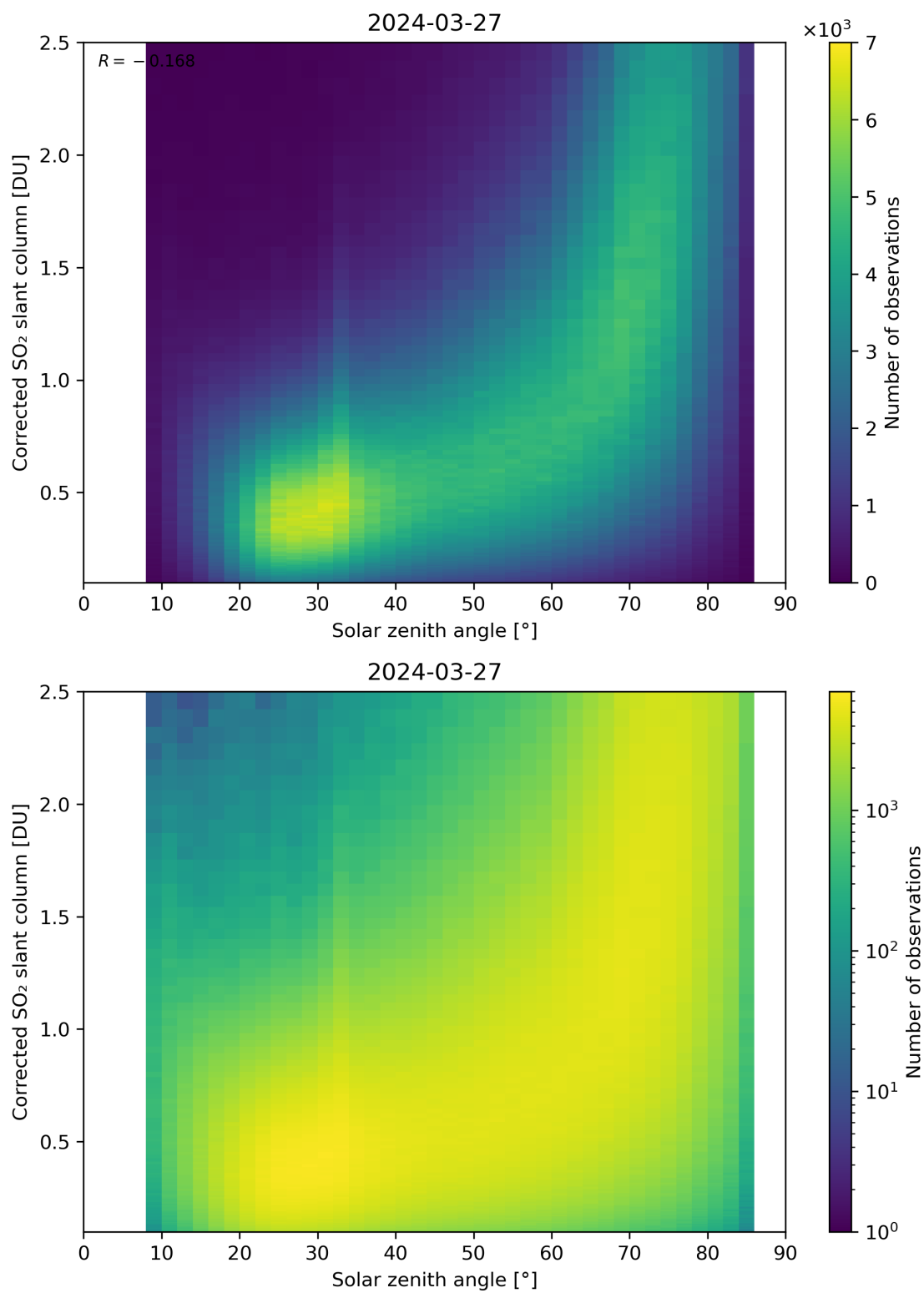
Figure 166: Scatter density plot of “Solar zenith angle” against “Corrected SO 2 slant column” for 2024-03-26 to 2024-03-28.
