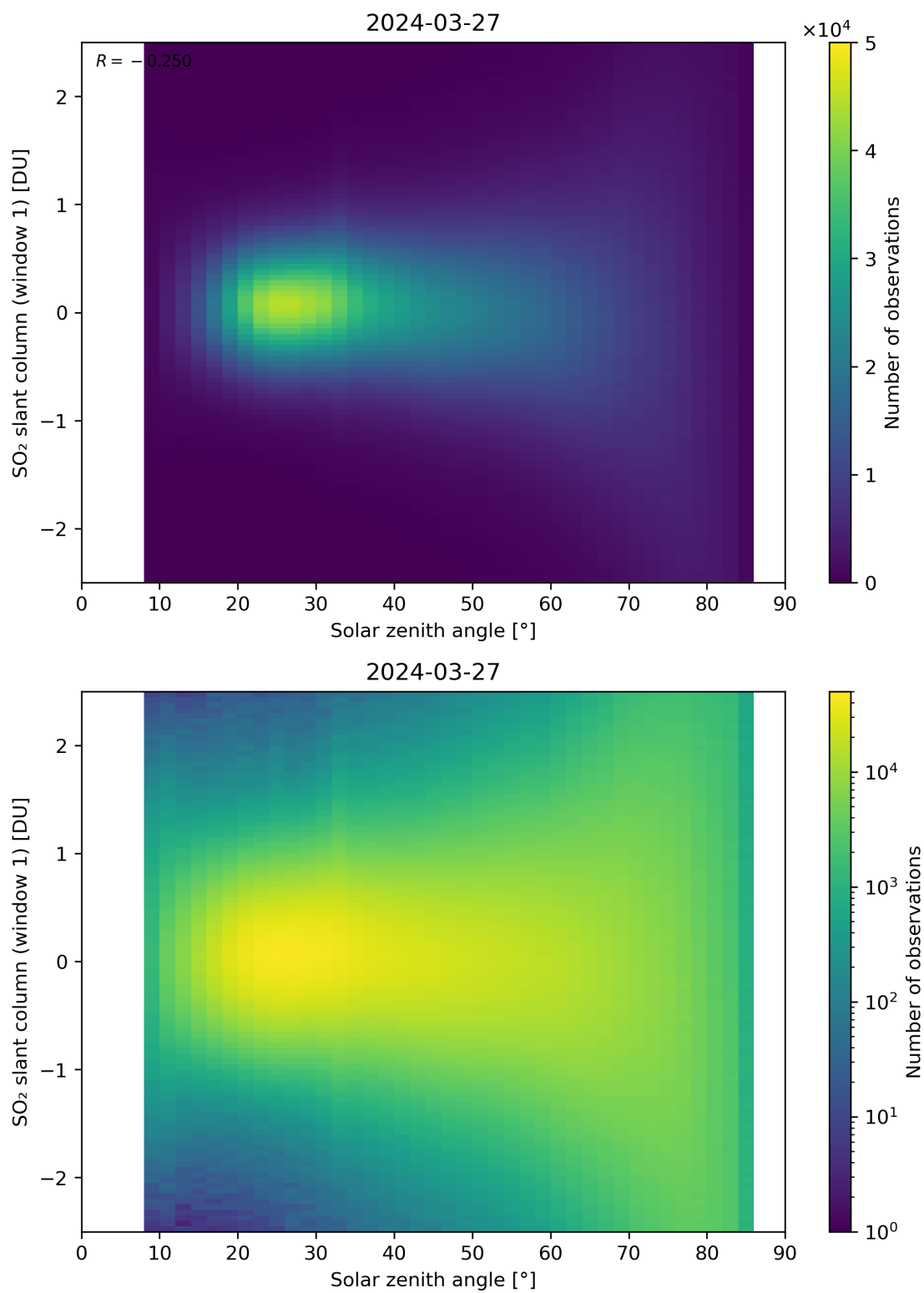
Figure 169: Scatter density plot of “Solar zenith angle” against “SO 2 slant column (window 1)” for 2024-03-26 to 2024-03-28.
