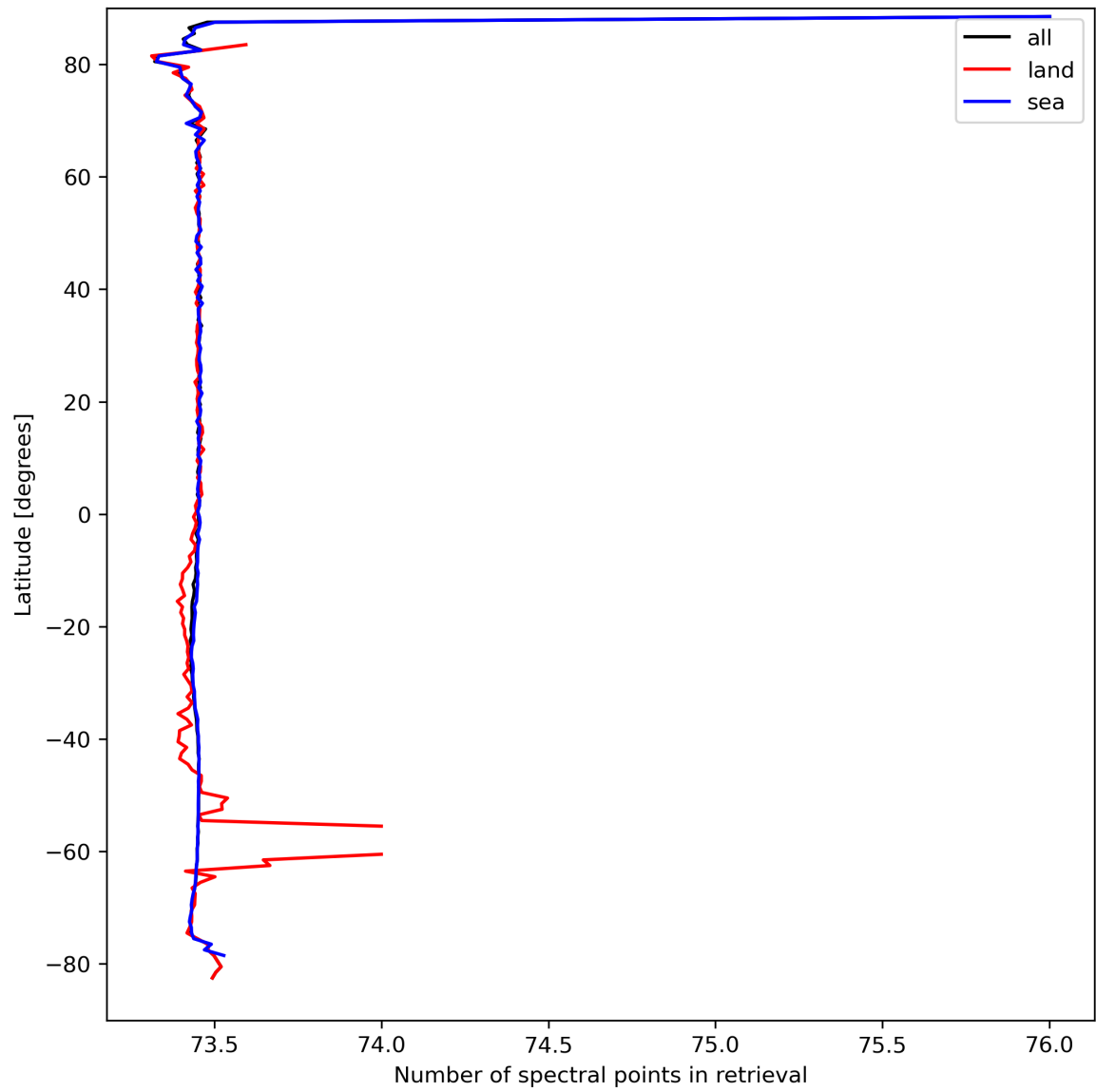
Figure 51: Zonal average of “Number of spectral points in retrieval” for 2024-03-26 to 2024-03-28.
