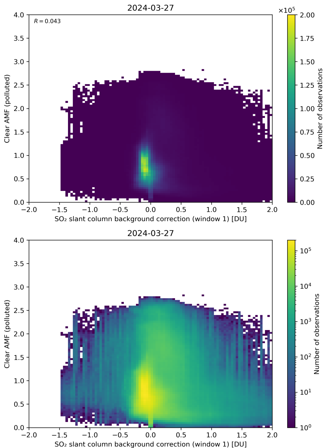
Figure 103: Scatter density plot of “SO 2 slant column background correction (window 1)” against “Clear AMF (polluted)” for 2024-03-26 to 2024-03-28.
