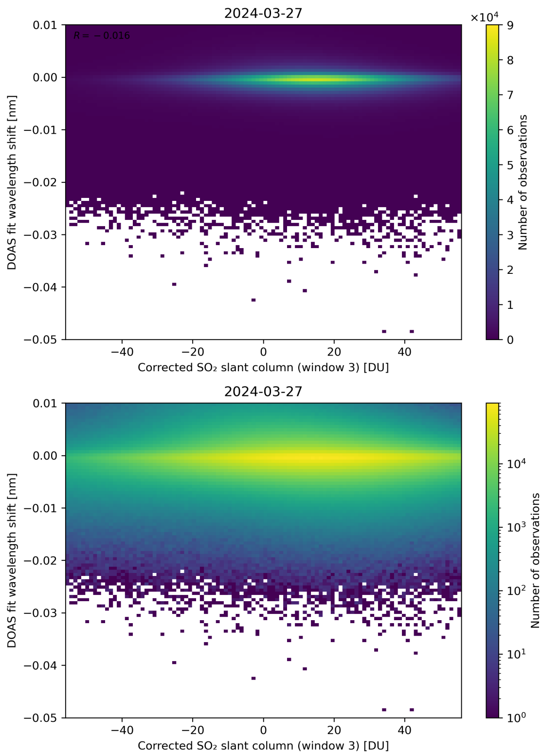
Figure 206: Scatter density plot of “Corrected SO 2 slant column (window 3)” against “DOAS fit wavelength shift” for 2024-03-26 to 2024-03-28.
