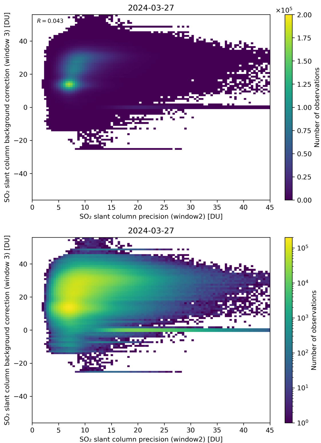
Figure 242: Scatter density plot of “SO 2 slant column precision (window2)” against “SO 2 slant column background correction (window 3)” for 2024-03-26 to 2024-03-28.
