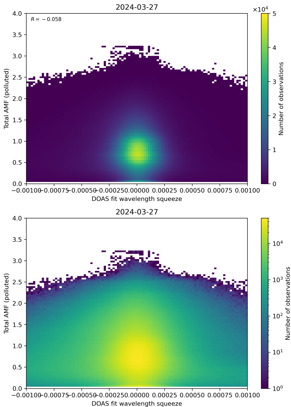
Figure 134: Scatter density plot of “DOAS fit wavelength squeeze” against “Total AMF (polluted)” for 2024-03-26 to 2024-03-28.
