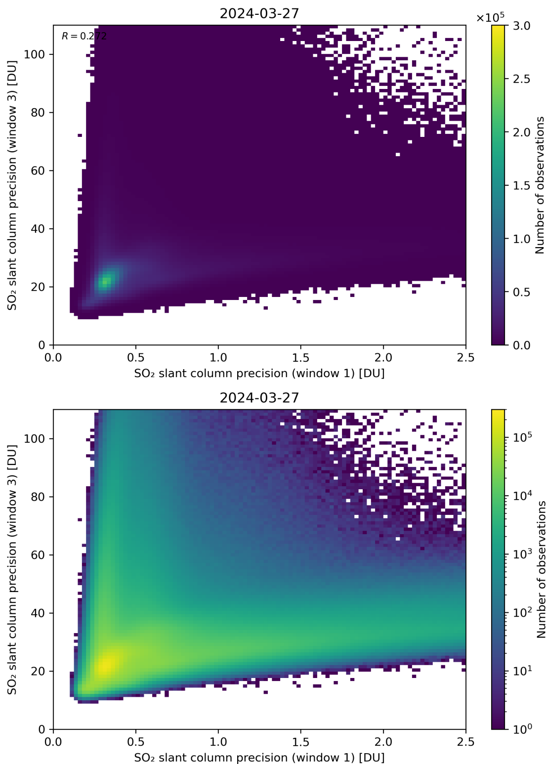
Figure 229: Scatter density plot of “SO 2 slant column precision (window 1)” against “SO 2 slant column precision (window 3)” for 2024-03-26 to 2024-03-28.
