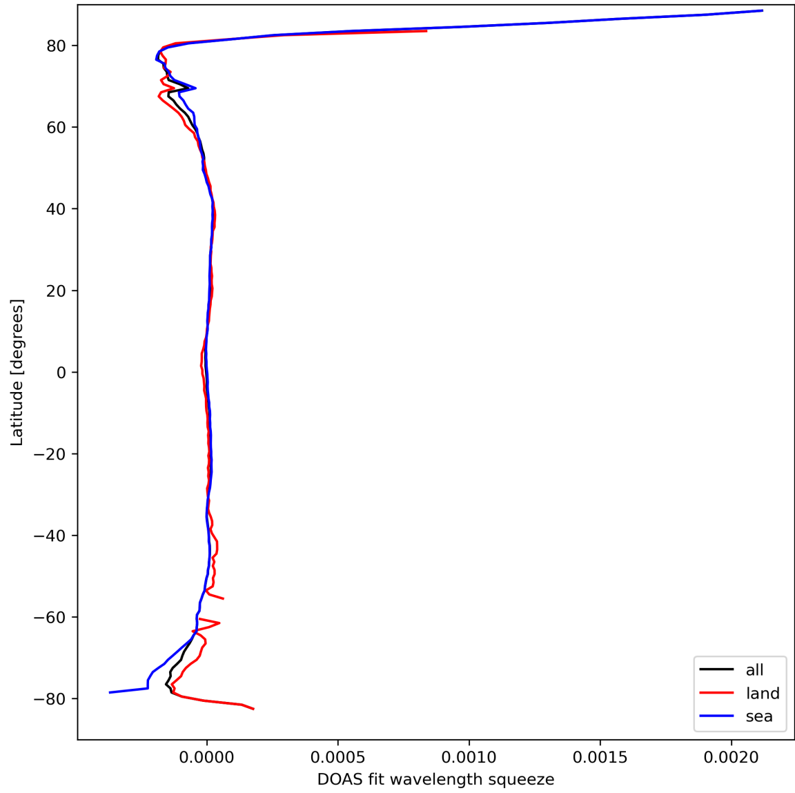
Figure 46: Zonal average of “DOAS fit wavelength squeeze” for 2024-03-26 to 2024-03-28.
