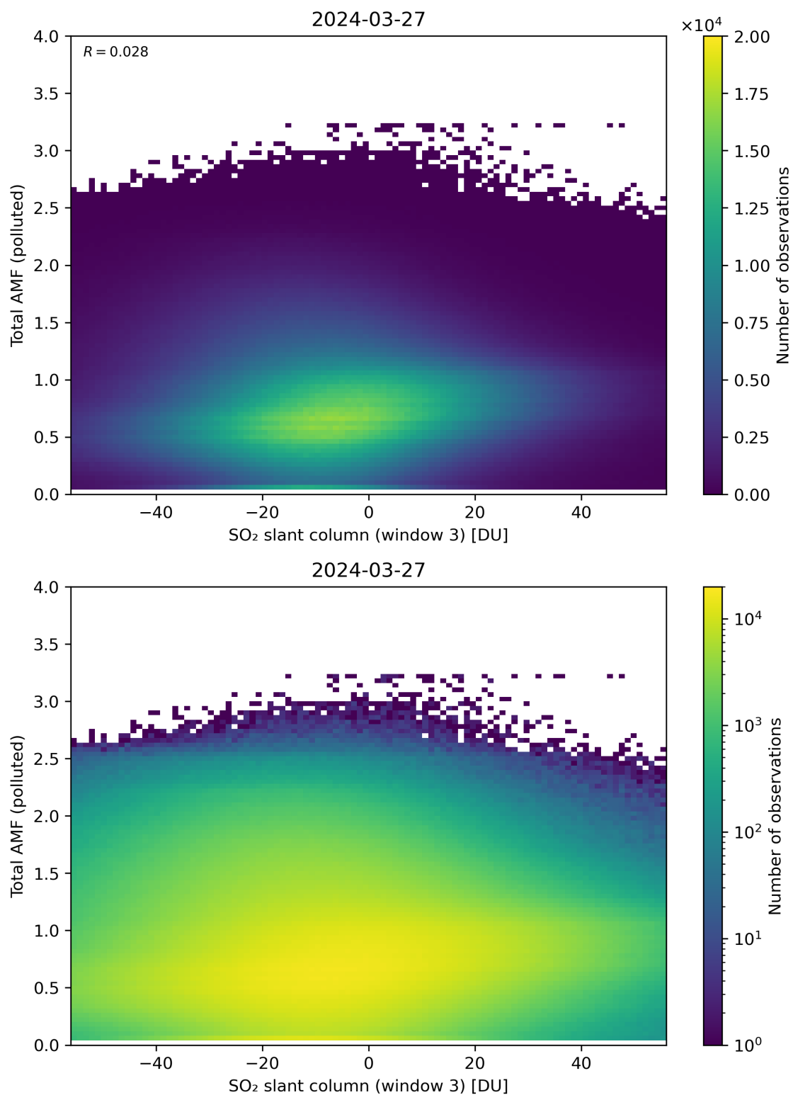
Figure 268: Scatter density plot of “SO 2 slant column (window 3)” against “Total AMF (polluted)” for 2024-03-26 to 2024-03-28.
