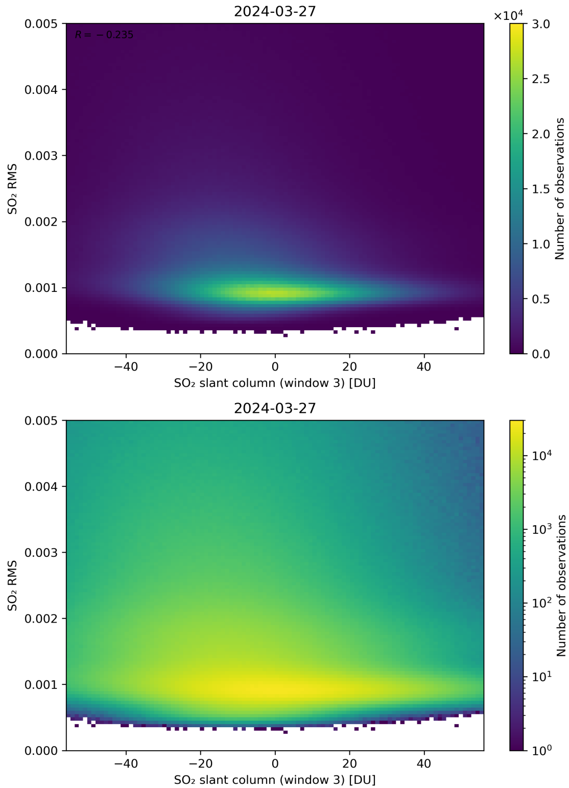
Figure 256: Scatter density plot of “SO 2 slant column (window 3)” against “SO 2 RMS” for 2024-03-26 to 2024-03-28.
