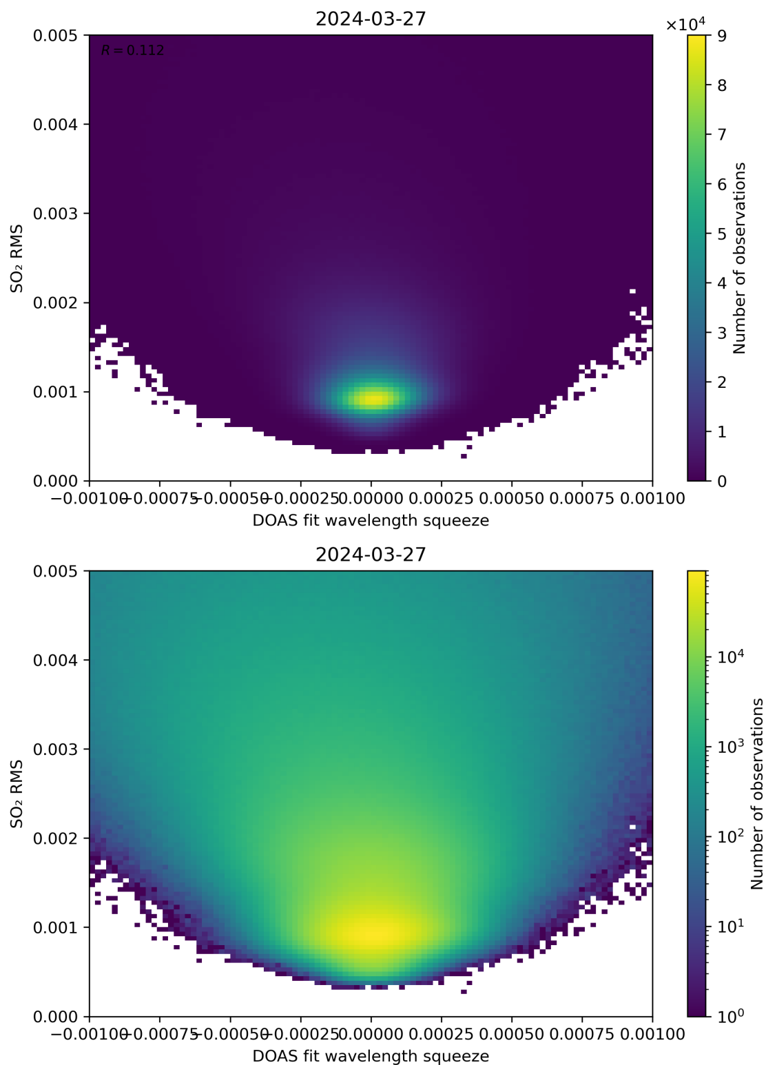
Figure 132: Scatter density plot of “DOAS fit wavelength squeeze” against “SO 2 RMS” for 2024-03-26 to 2024-03-28.
