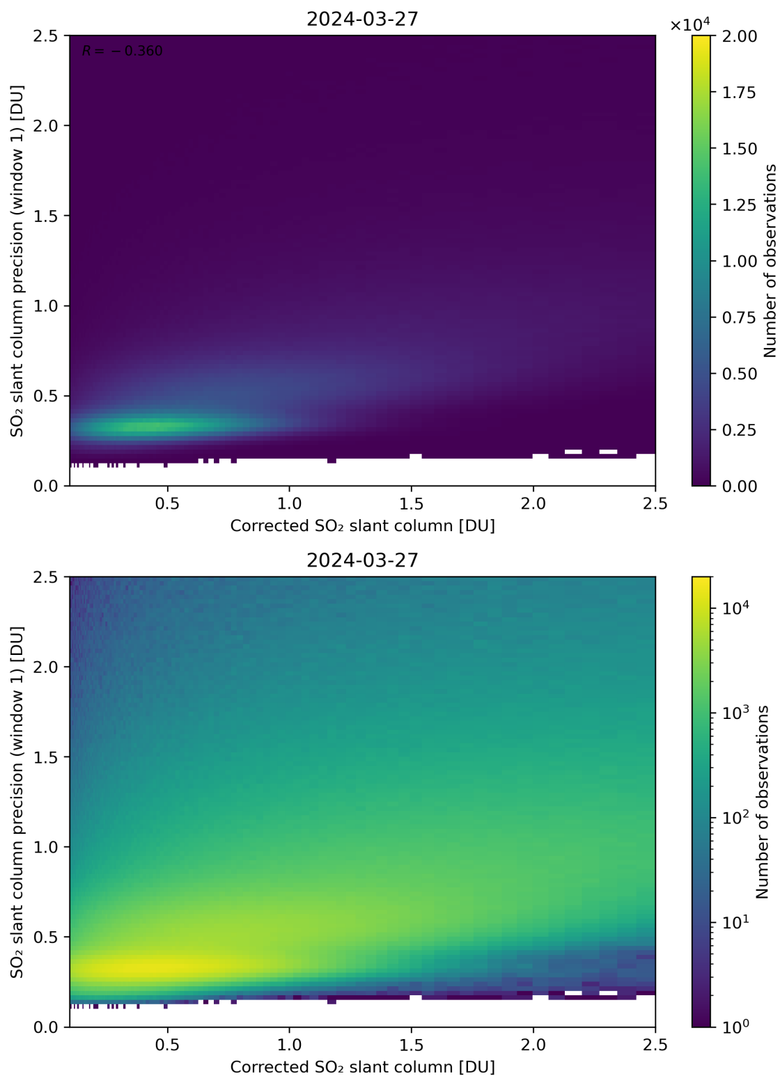
Figure 188: Scatter density plot of “Corrected SO 2 slant column” against “SO 2 slant column precision (window 1)” for 2024-03-26 to 2024-03-28.
