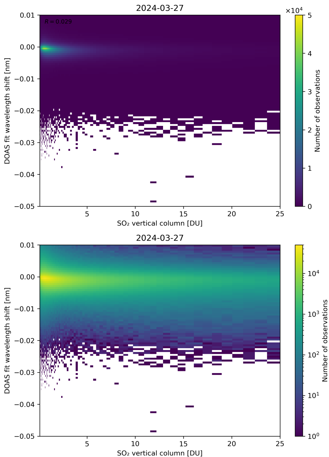
Figure 276: Scatter density plot of “SO 2 vertical column” against “DOAS fit wavelength shift” for 2024-03-26 to 2024-03-28.
