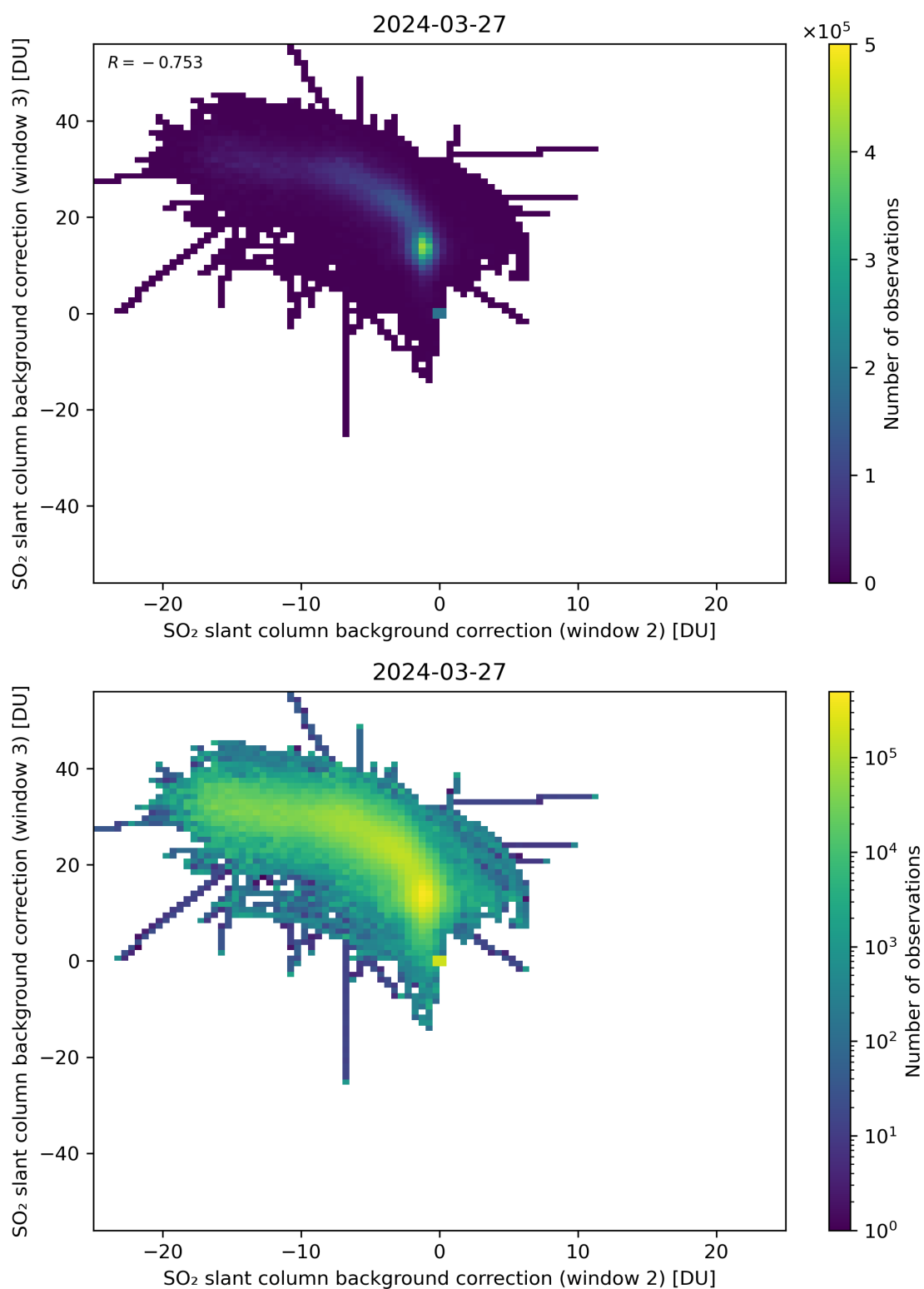
Figure 111: Scatter density plot of “SO 2 slant column background correction (window 2)” against “SO 2 slant column background correction (window 3)” for 2024-03-26 to 2024-03-28.
