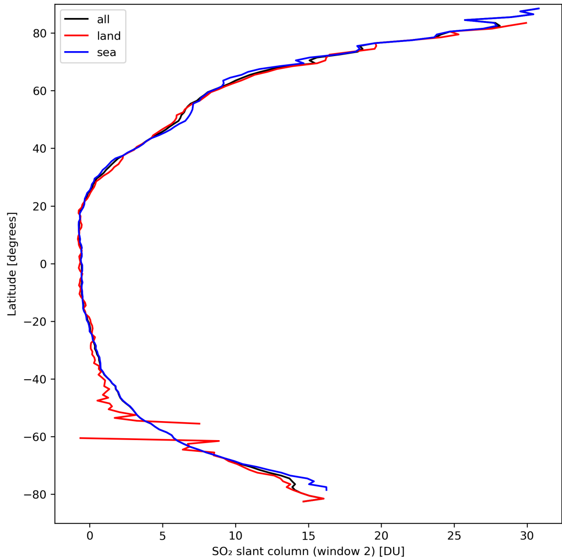
Figure 37: Zonal average of “SO 2 slant column (window 2)” for 2024-03-26 to 2024-03-28.
