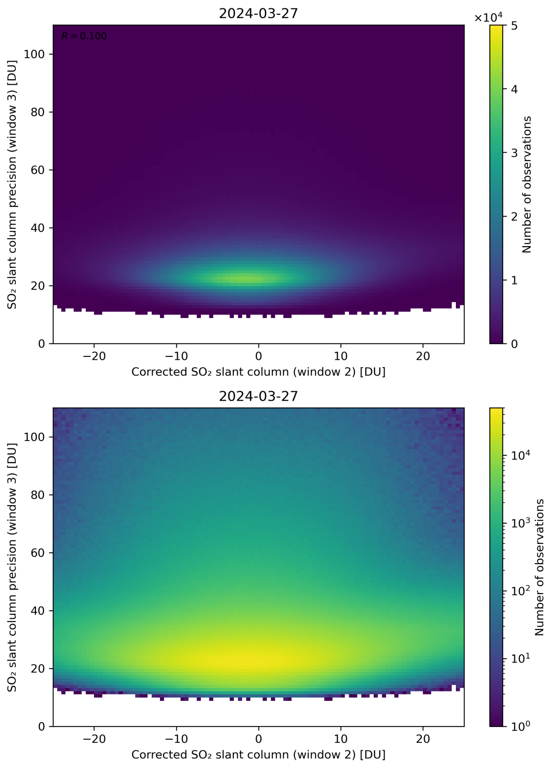
Figure 202: Scatter density plot of “Corrected SO 2 slant column (window 2)” against “SO 2 slant column precision (window 3)” for 2024-03-26 to 2024-03-28.
