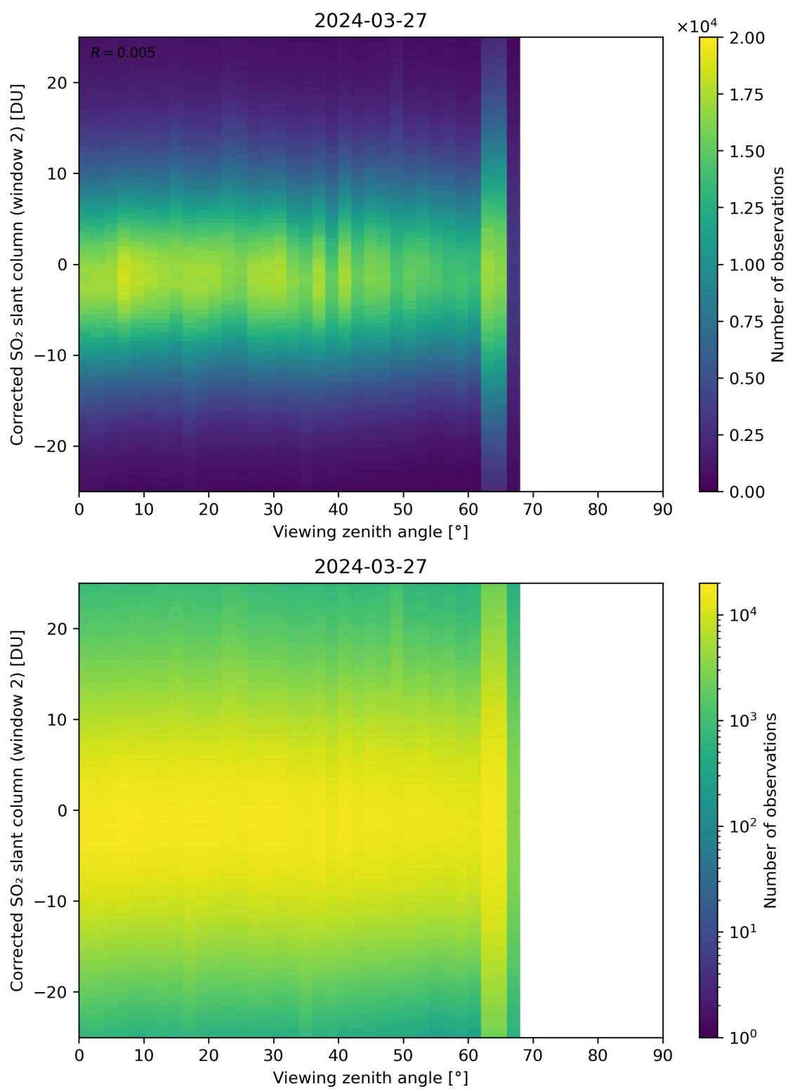
Figure 318: Scatter density plot of “Viewing zenith angle” against “Corrected SO 2 slant column (window 2)” for 2024-03-26 to 2024-03-28.
