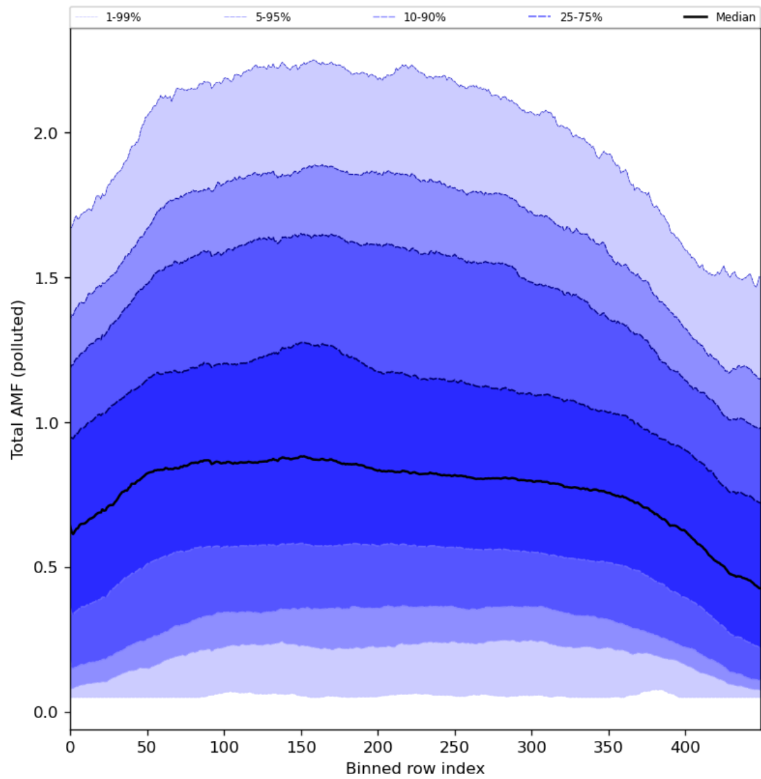
Figure 94: Along track statistics of “Total AMF (polluted)” for 2024-03-26 to 2024-03-28
