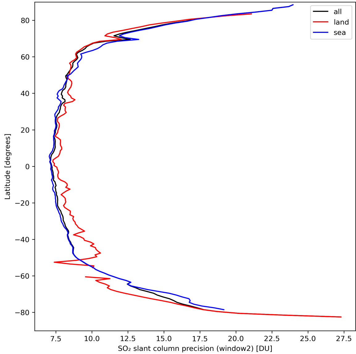
Figure 38: Zonal average of “SO 2 slant column precision (window2)” for 2024-03-26 to 2024-03-28.
