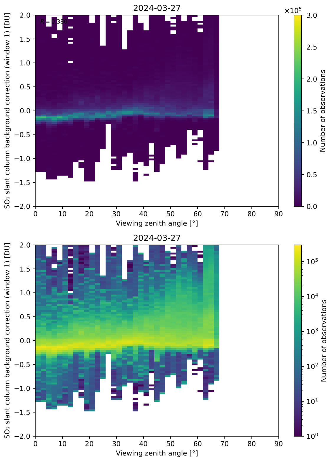
Figure 308: Scatter density plot of “Viewing zenith angle” against “SO 2 slant column background correction (window 1)” for 2024-03-26 to 2024-03-28.
