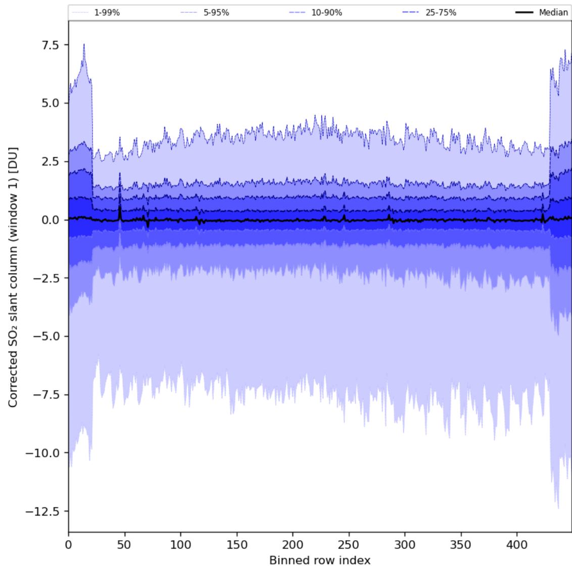
Figure 81: Along track statistics of “Corrected SO 2 slant column (window 1)” for 2024-03-26 to 2024-03-28
