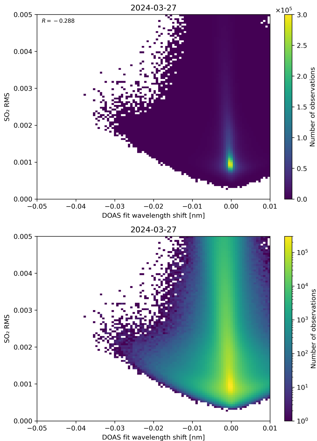
Figure 128: Scatter density plot of “DOAS fit wavelength shift” against “SO 2 RMS” for 2024-03-26 to 2024-03-28.
