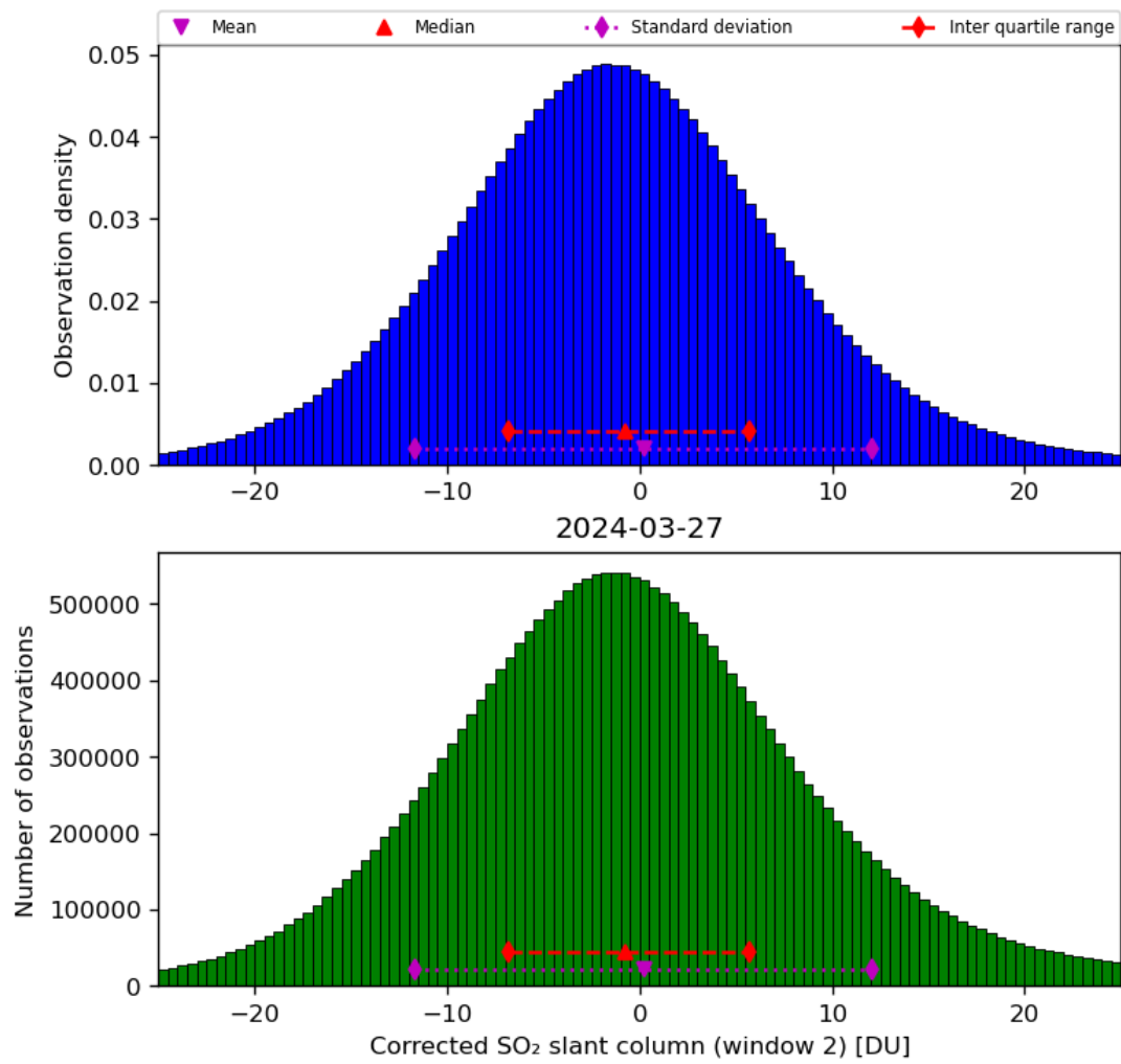
Figure 62: Histogram of “Corrected SO 2 slant column (window 2)” for 2024-03-26 to 2024-03-28
