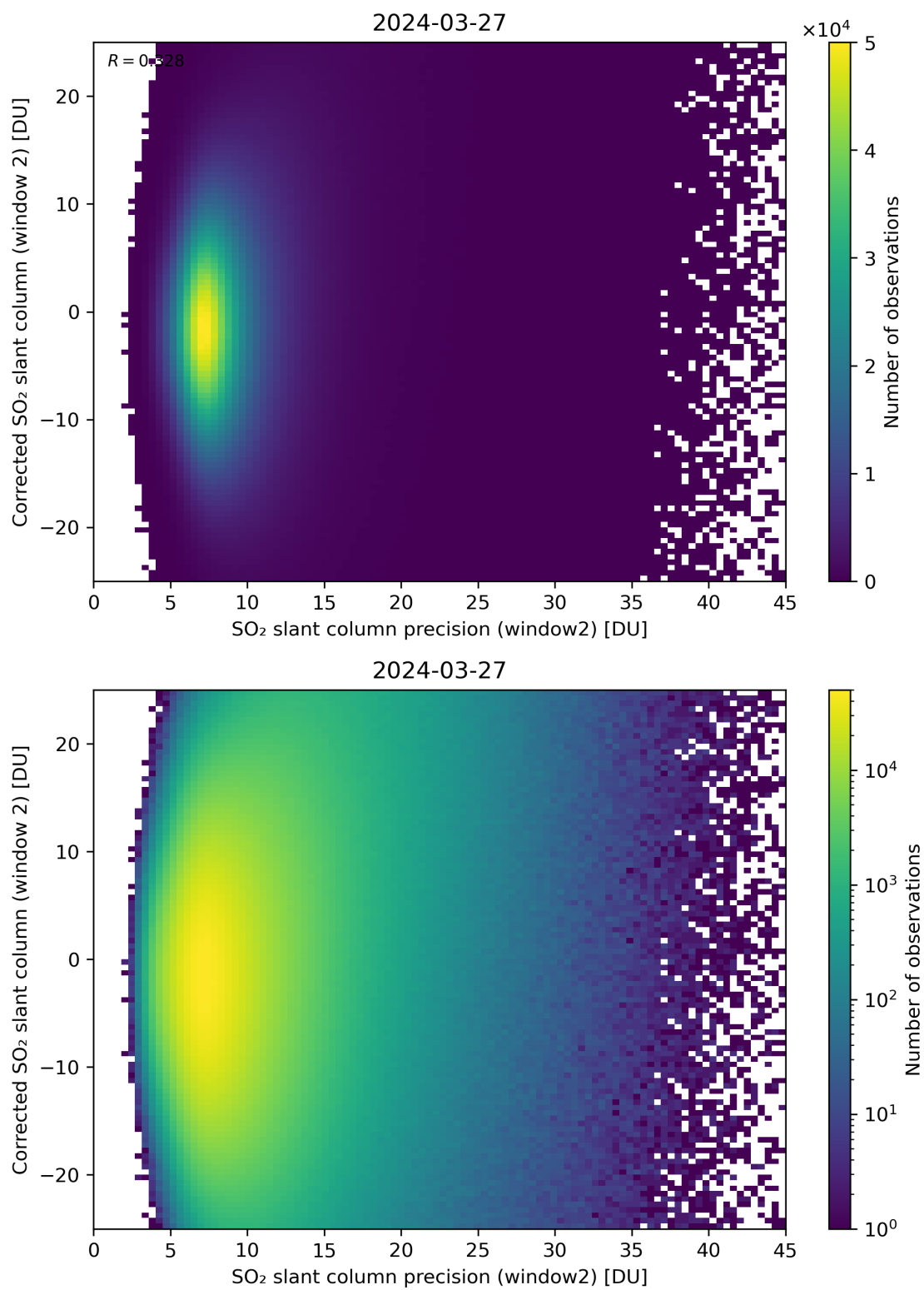
Figure 247: Scatter density plot of “SO 2 slant column precision (window2)” against “Corrected SO 2 slant column (window 2)” for 2024-03-26 to 2024-03-28.
