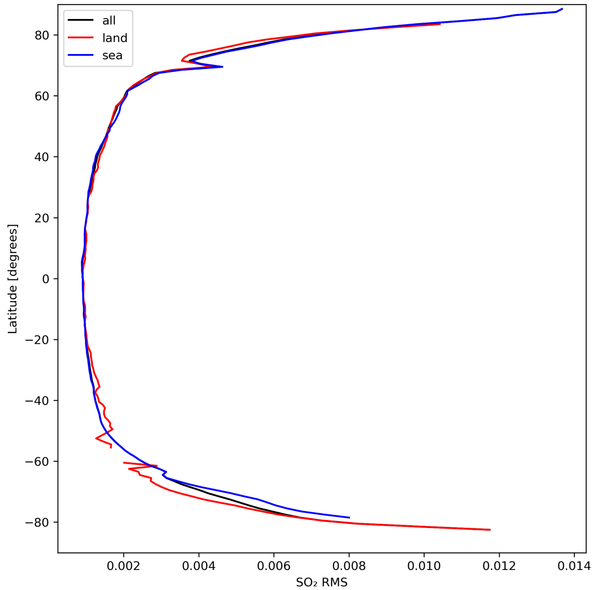
Figure 47: Zonal average of “SO 2 RMS” for 2024-03-26 to 2024-03-28.
