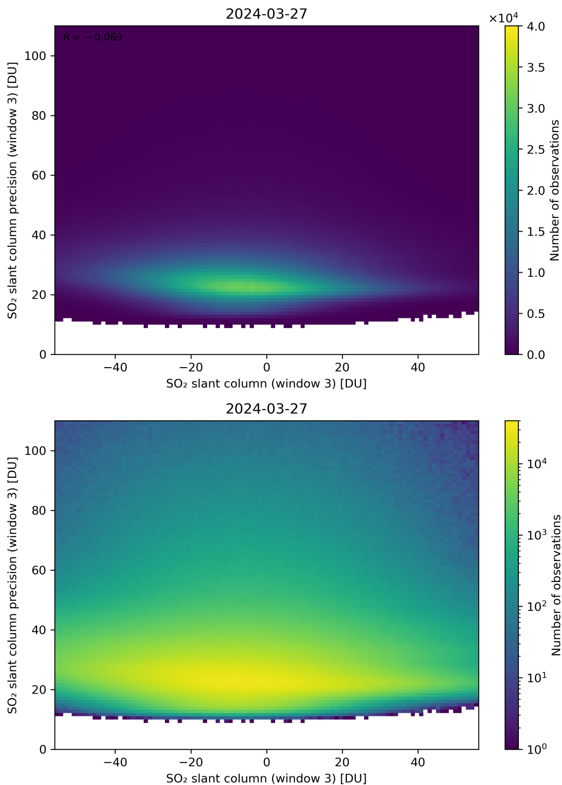
Figure 267: Scatter density plot of “SO 2 slant column (window 3)” against “SO 2 slant column precision (window 3)” for 2024-03-26 to 2024-03-28.
