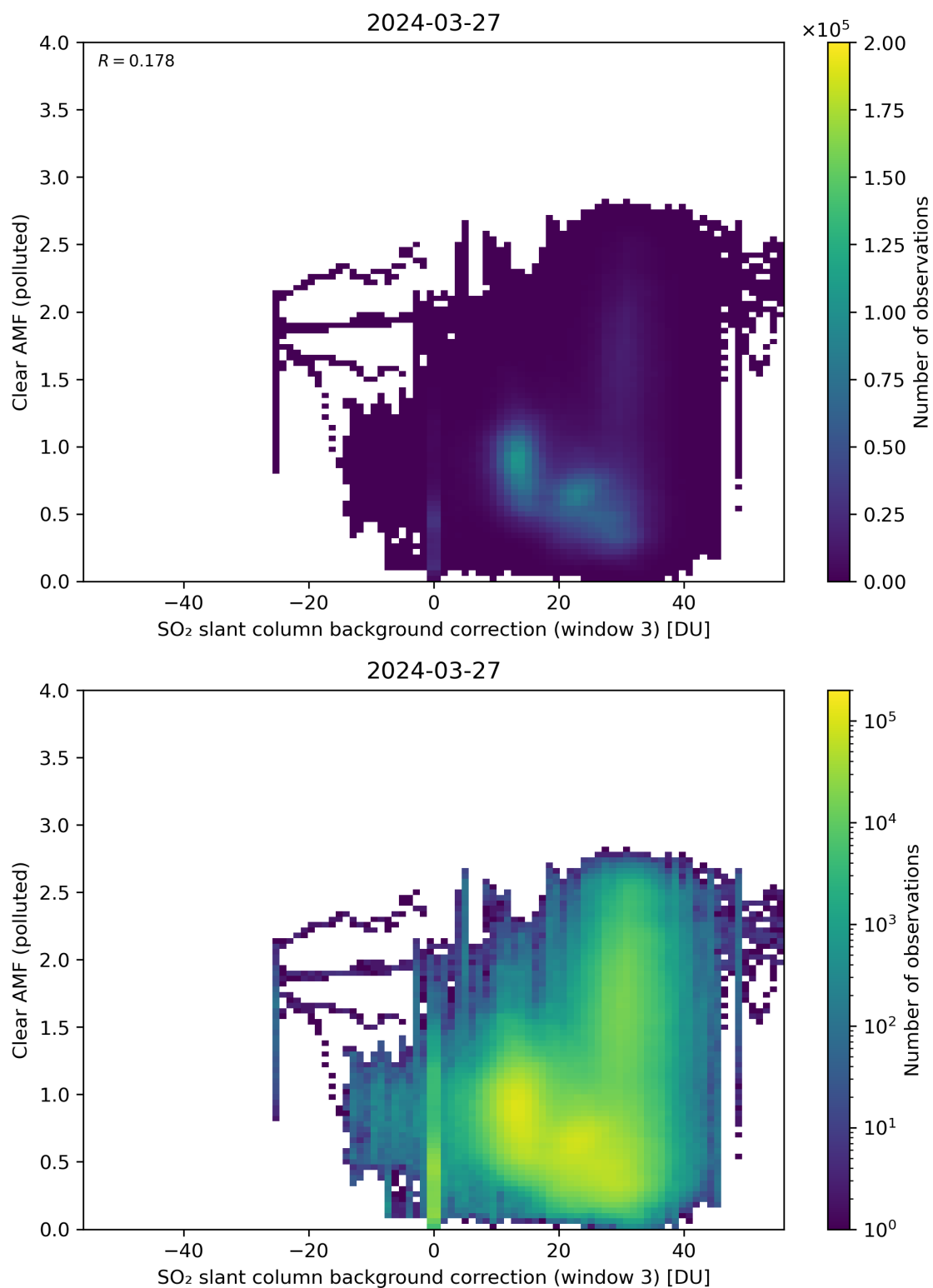
Figure 124: Scatter density plot of “SO 2 slant column background correction (window 3)” against “Clear AMF (polluted)” for 2024-03-26 to 2024-03-28.
