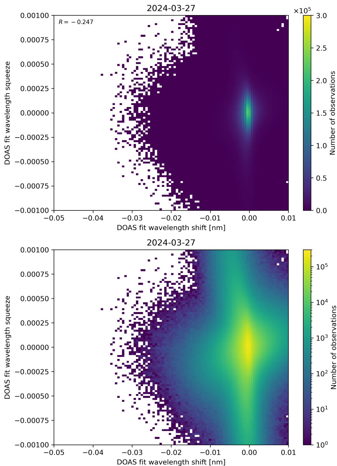
Figure 127: Scatter density plot of “DOAS fit wavelength shift” against “DOAS fit wavelength squeeze” for 2024-03-26 to 2024-03-28.
