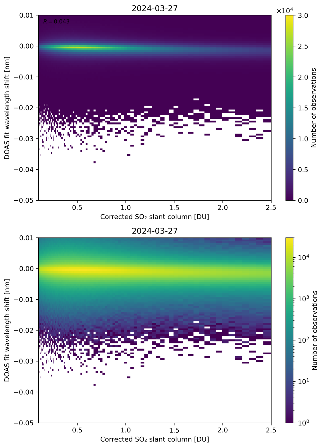
Figure 181: Scatter density plot of “Corrected SO 2 slant column” against “DOAS fit wavelength shift” for 2024-03-26 to 2024-03-28.
