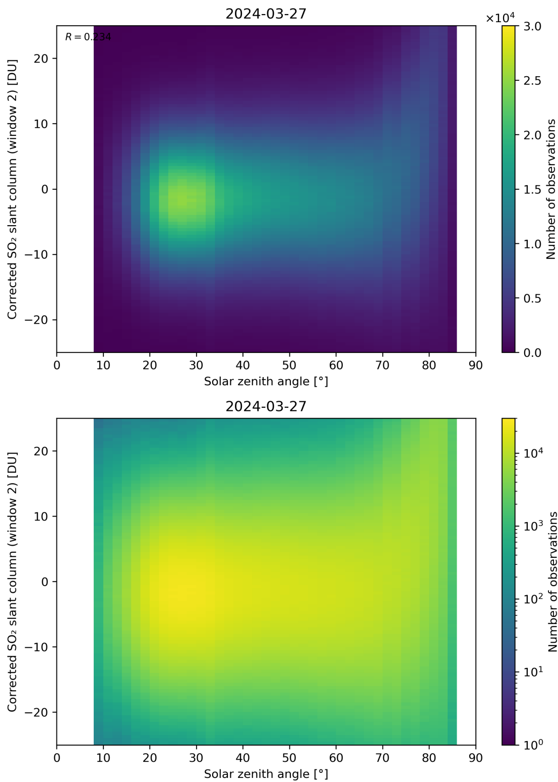
Figure 167: Scatter density plot of “Solar zenith angle” against “Corrected SO 2 slant column (window 2)” for 2024-03-26 to 2024-03-28.
