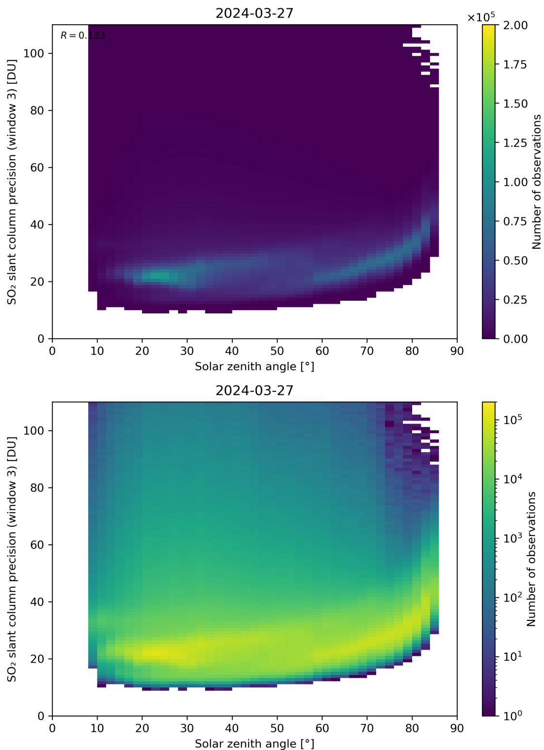
Figure 173: Scatter density plot of “Solar zenith angle” against “SO 2 slant column precision (window 3)” for 2024-03-26 to 2024-03-28.
