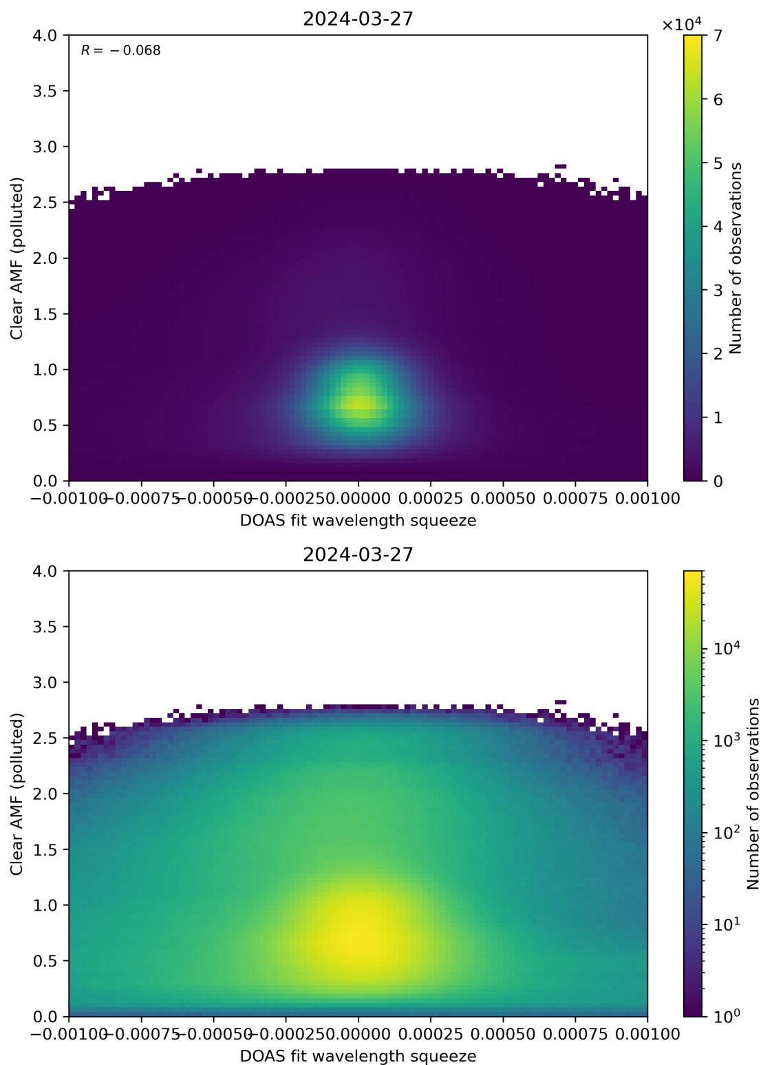
Figure 133: Scatter density plot of “DOAS fit wavelength squeeze” against “Clear AMF (polluted)” for 2024-03-26 to 2024-03-28.
