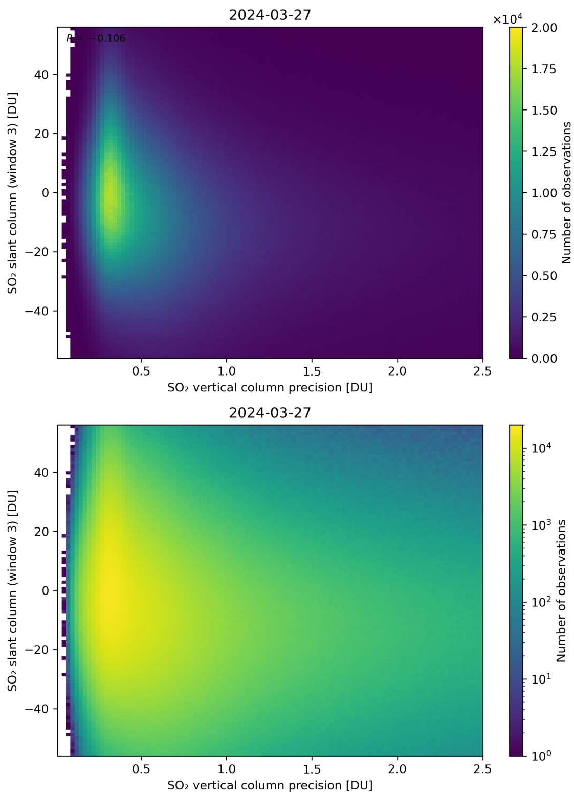
Figure 292: Scatter density plot of “SO 2 vertical column precision” against “SO 2 slant column (window 3)” for 2024-03-26 to 2024-03-28.
