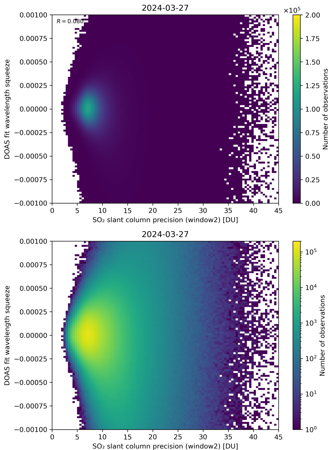
Figure 244: Scatter density plot of “SO 2 slant column precision (window2)” against “DOAS fit wavelength squeeze” for 2024-03-26 to 2024-03-28.
