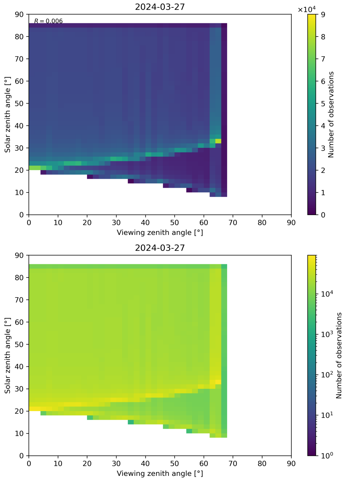
Figure 315: Scatter density plot of “Viewing zenith angle” against “Solar zenith angle” for 2024-03-26 to 2024-03-28.
