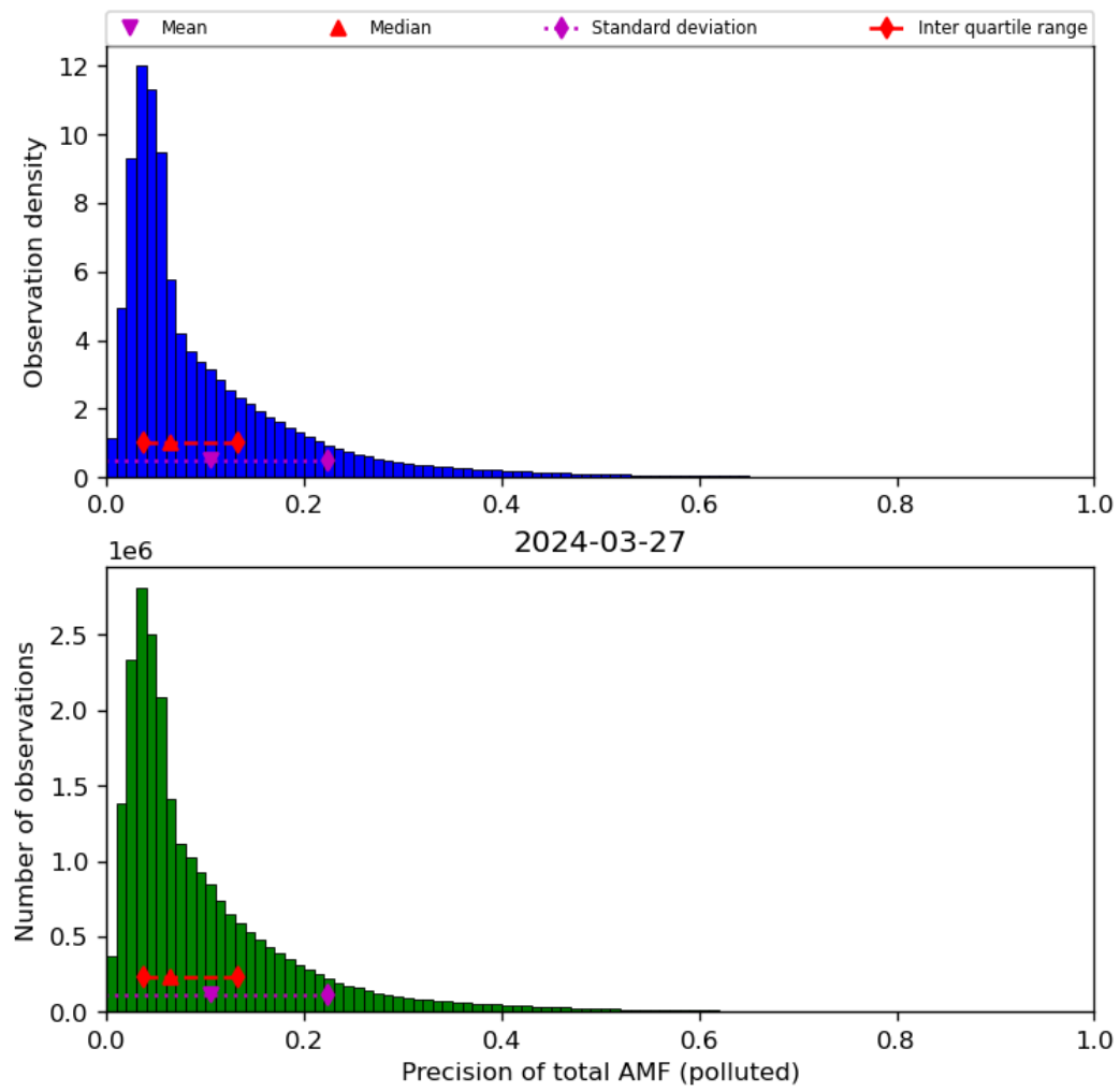
Figure 72: Histogram of “Precision of total AMF (polluted)” for 2024-03-26 to 2024-03-28
