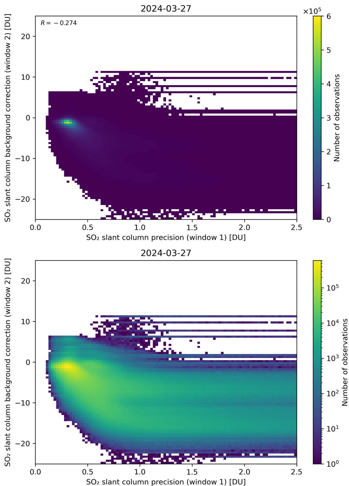
Figure 219: Scatter density plot of “SO 2 slant column precision (window 1)” against “SO 2 slant column background correction (window 2)” for 2024-03-26 to 2024-03-28.
