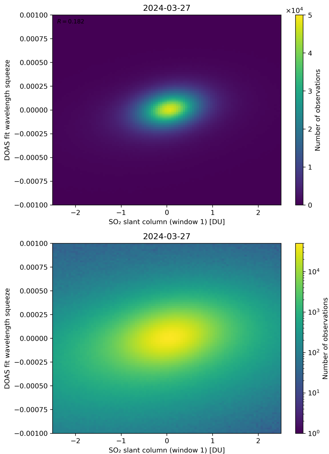
Figure 216: Scatter density plot of “SO 2 slant column (window 1)” against “DOAS fit wavelength squeeze” for 2024-03-26 to 2024-03-28.
