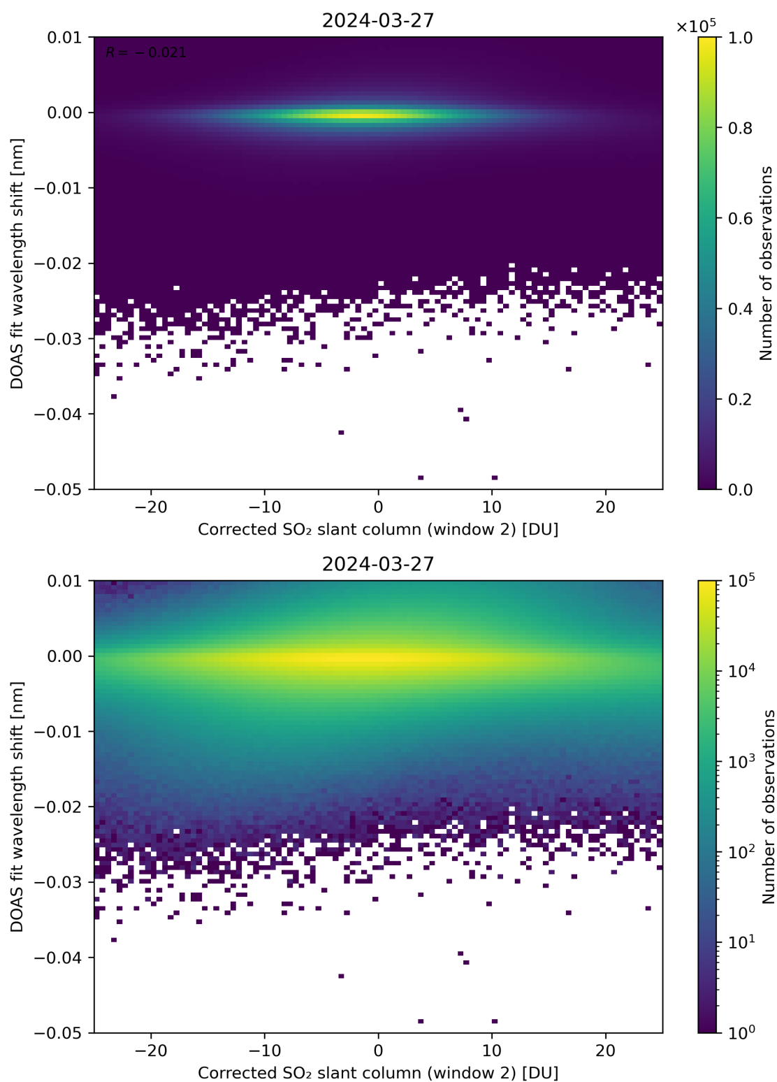
Figure 196: Scatter density plot of “Corrected SO 2 slant column (window 2)” against “DOAS fit wavelength shift” for 2024-03-26 to 2024-03-28.
