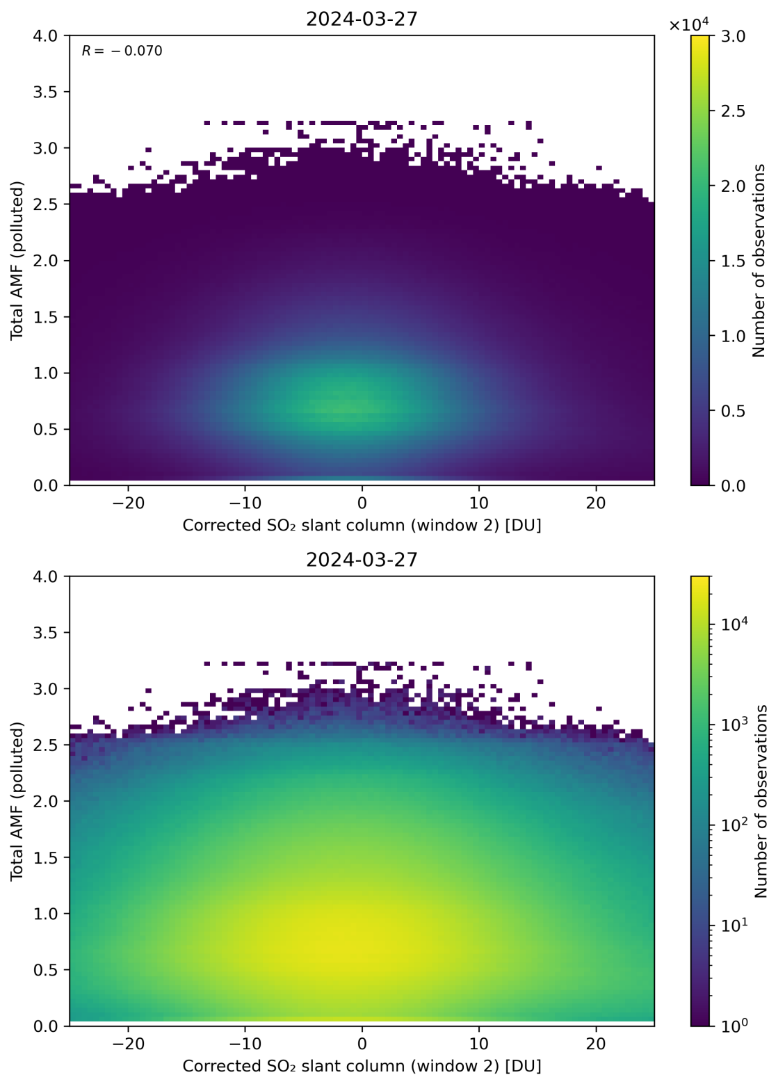
Figure 203: Scatter density plot of “Corrected SO 2 slant column (window 2)” against “Total AMF (polluted)” for 2024-03-26 to 2024-03-28.
