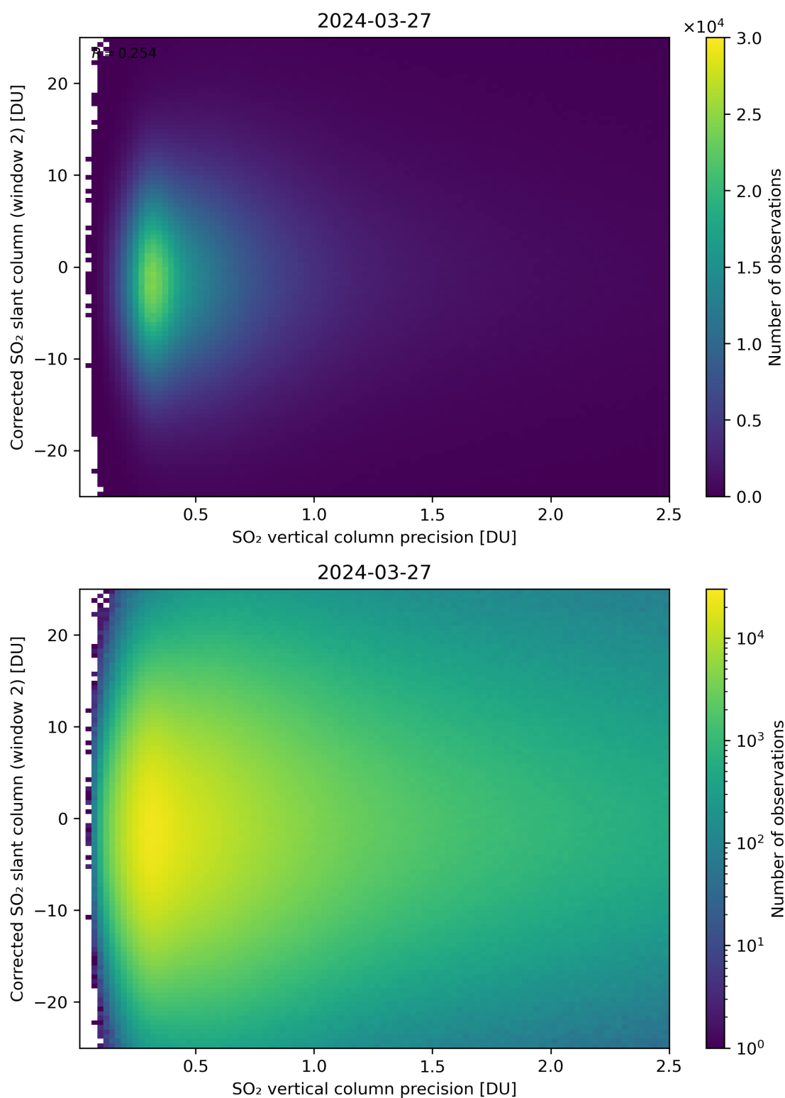
Figure 287: Scatter density plot of “SO 2 vertical column precision” against “Corrected SO 2 slant column (window 2)” for 2024-03-26 to 2024-03-28.
