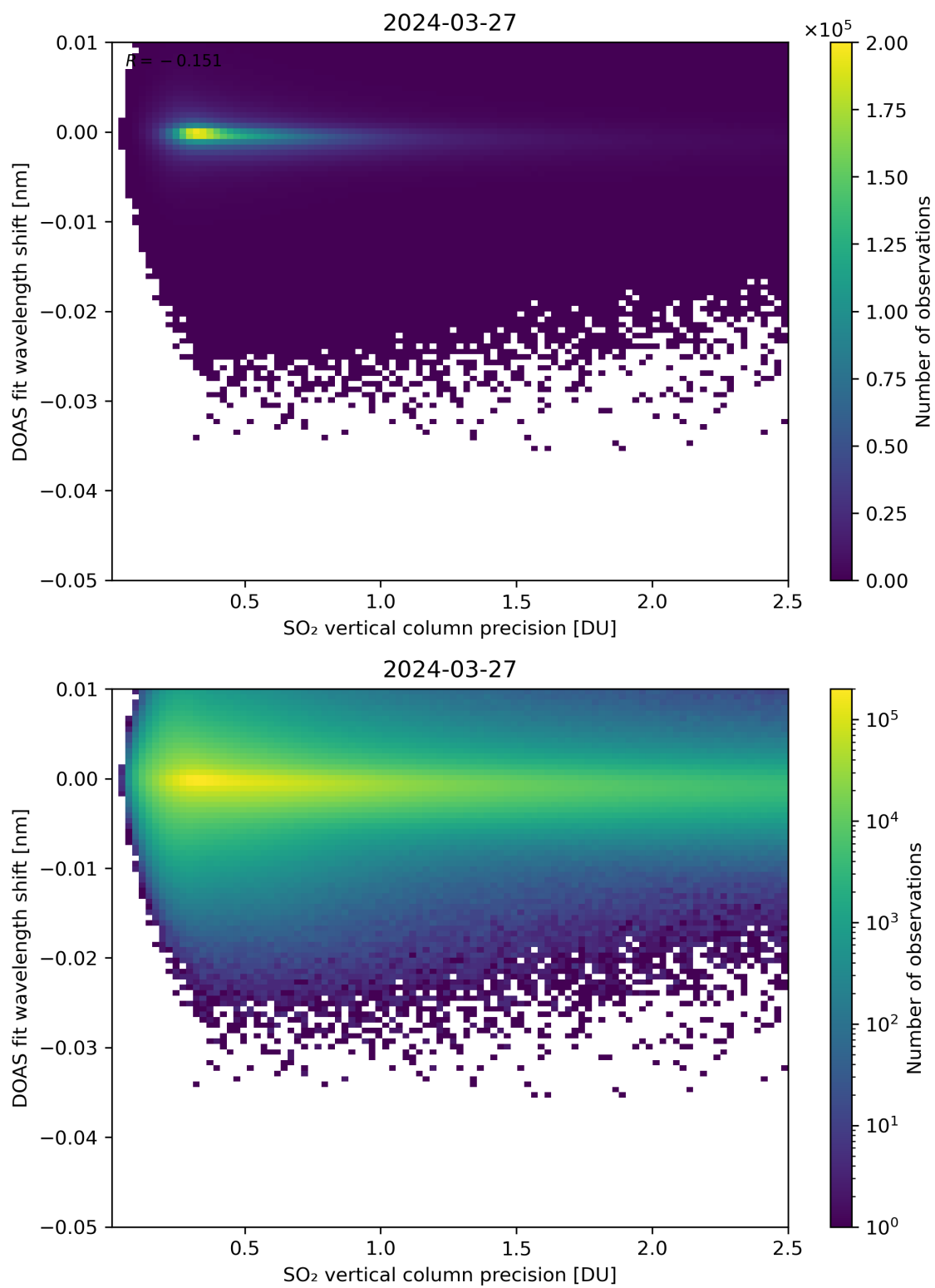
Figure 282: Scatter density plot of “SO 2 vertical column precision” against “DOAS fit wavelength shift” for 2024-03-26 to 2024-03-28.
