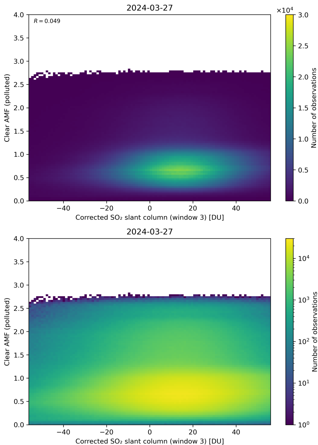
Figure 209: Scatter density plot of “Corrected SO 2 slant column (window 3)” against “Clear AMF (polluted)” for 2024-03-26 to 2024-03-28.
