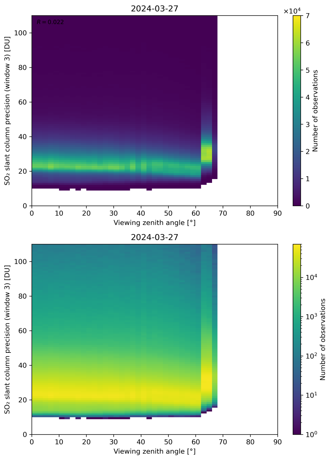
Figure 324: Scatter density plot of “Viewing zenith angle” against “SO 2 slant column precision (window 3)” for 2024-03-26 to 2024-03-28.
