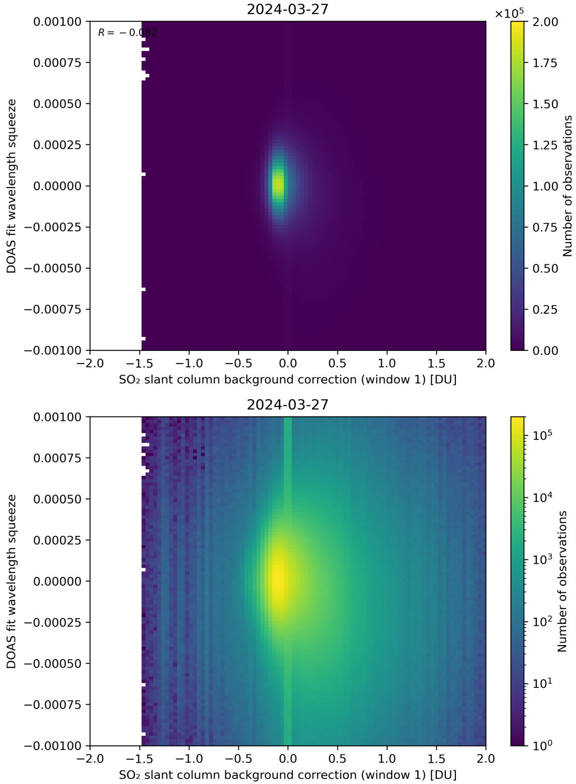
Figure 101: Scatter density plot of “SO 2 slant column background correction (window 1)” against “DOAS fit wavelength squeeze” for 2024-03-26 to 2024-03-28.
