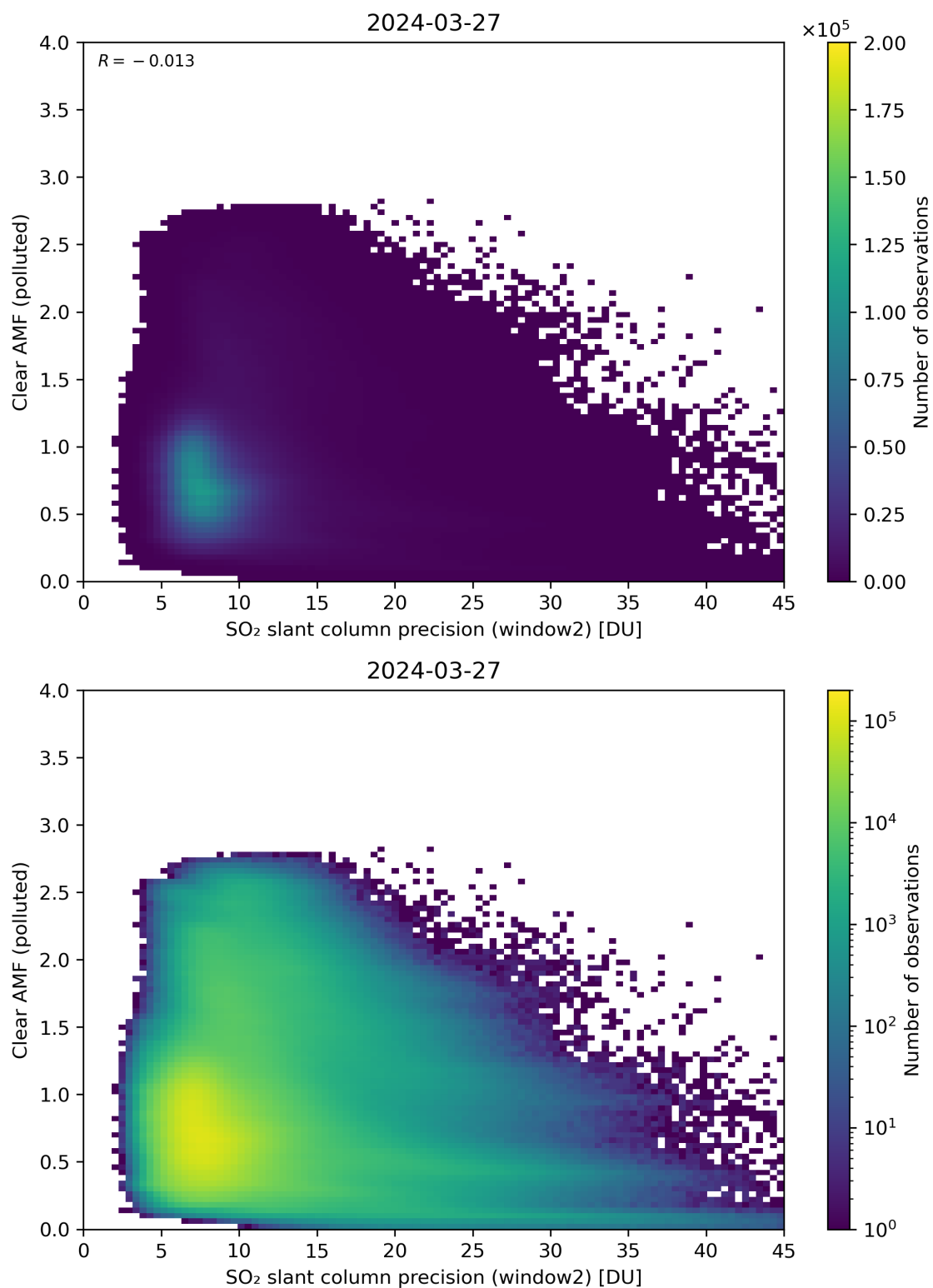
Figure 246: Scatter density plot of “SO 2 slant column precision (window2)” against “Clear AMF (polluted)” for 2024-03-26 to 2024-03-28.
