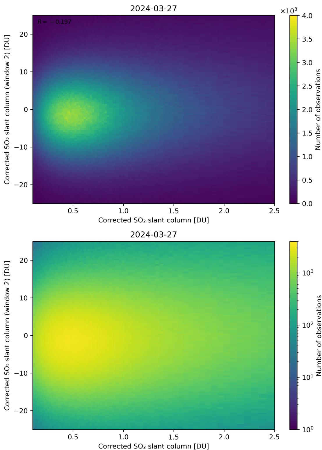
Figure 185: Scatter density plot of “Corrected SO 2 slant column” against “Corrected SO 2 slant column (window 2)” for 2024-03-26 to 2024-03-28.
