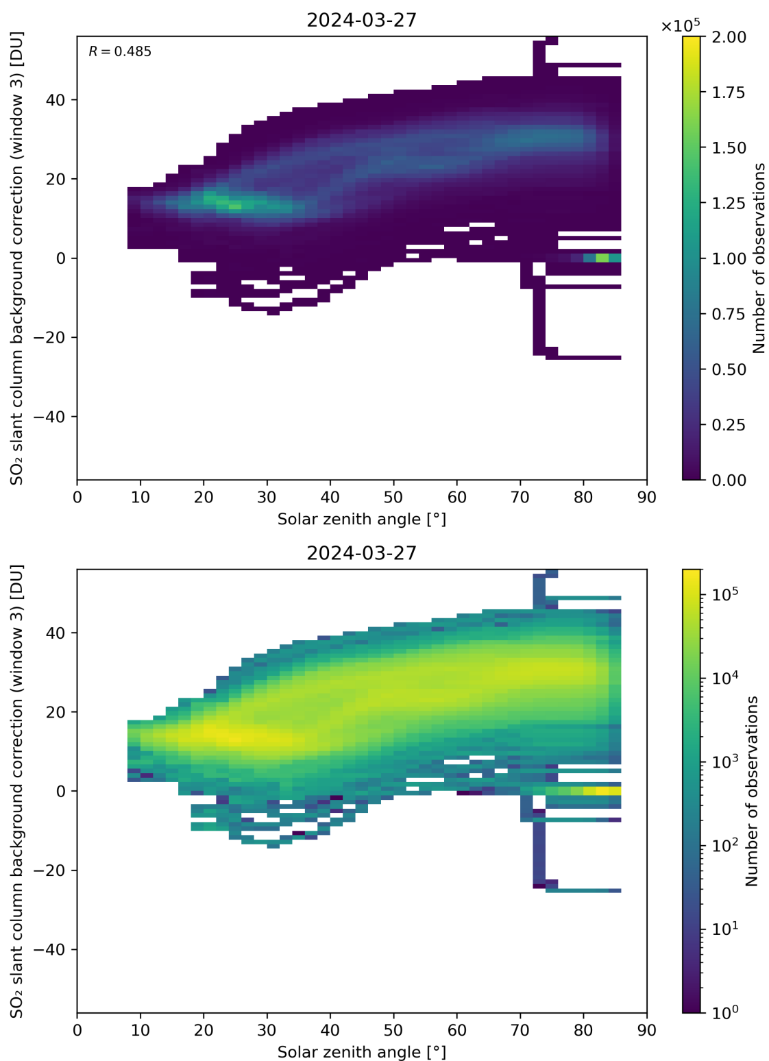
Figure 160: Scatter density plot of “Solar zenith angle” against “SO 2 slant column background correction (window 3)” for 2024-03-26 to 2024-03-28.
