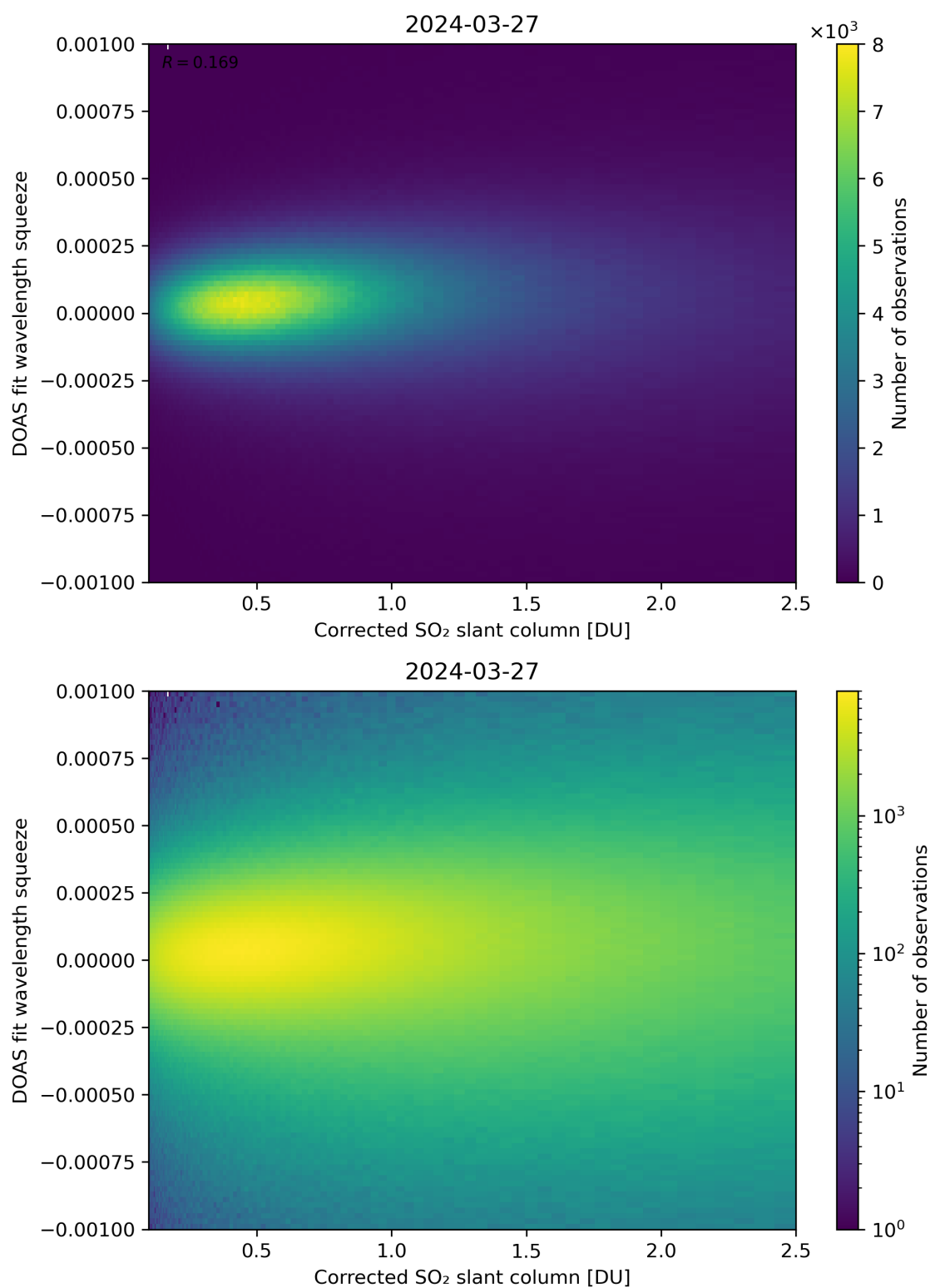
Figure 182: Scatter density plot of “Corrected SO 2 slant column” against “DOAS fit wavelength squeeze” for 2024-03-26 to 2024-03-28.
