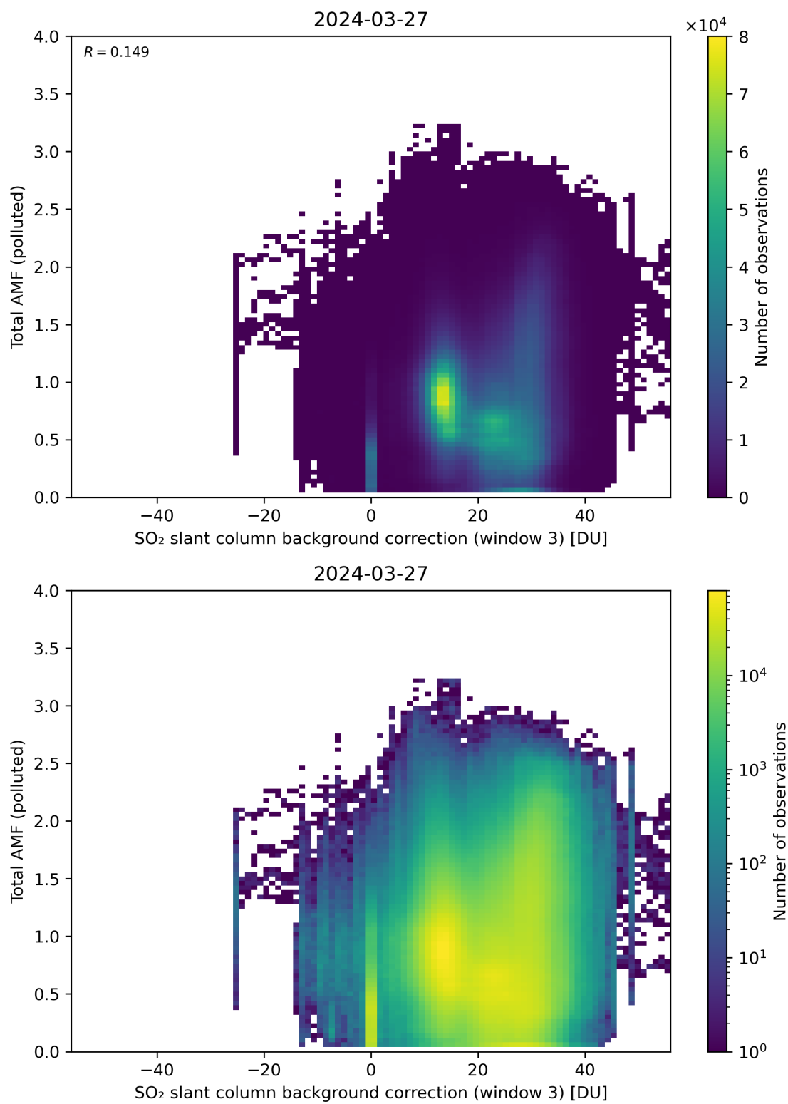
Figure 125: Scatter density plot of “SO 2 slant column background correction (window 3)” against “Total AMF (polluted)” for 2024-03-26 to 2024-03-28.
