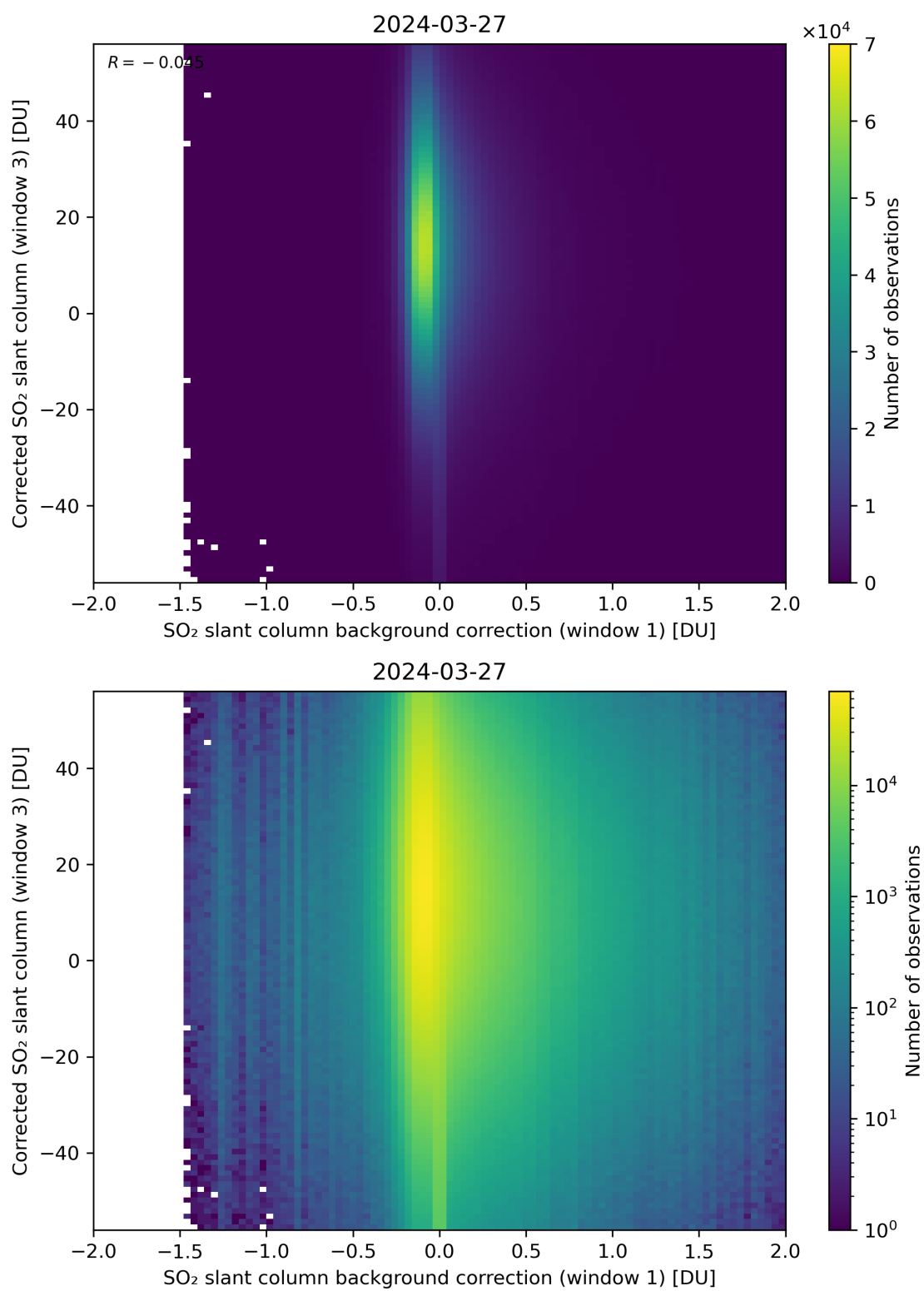
Figure 105: Scatter density plot of “SO 2 slant column background correction (window 1)” against “Corrected SO 2 slant column (window 3)” for 2024-03-26 to 2024-03-28.
