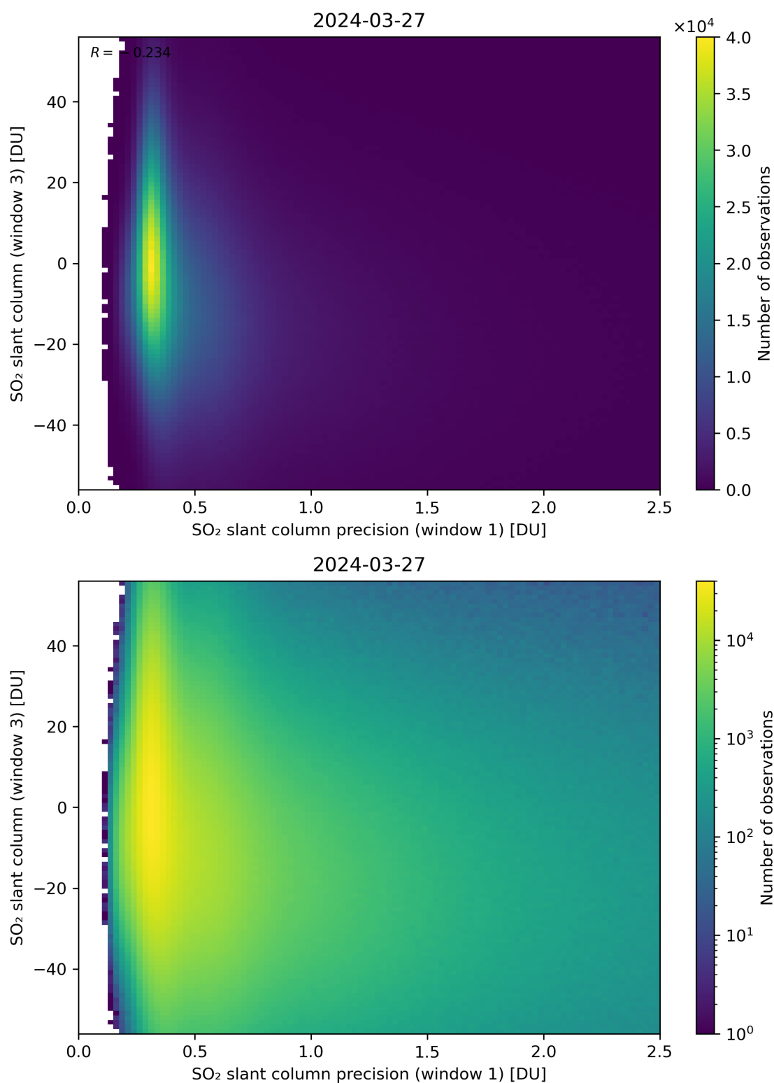
Figure 228: Scatter density plot of “SO 2 slant column precision (window 1)” against “SO 2 slant column (window 3)” for 2024-03-26 to 2024-03-28.
