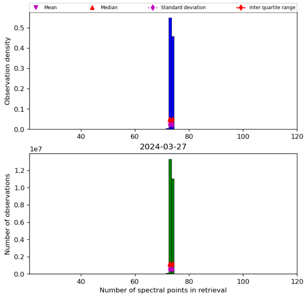
Figure 74: Histogram of “Number of spectral points in retrieval” for 2024-03-26 to 2024-03-28
