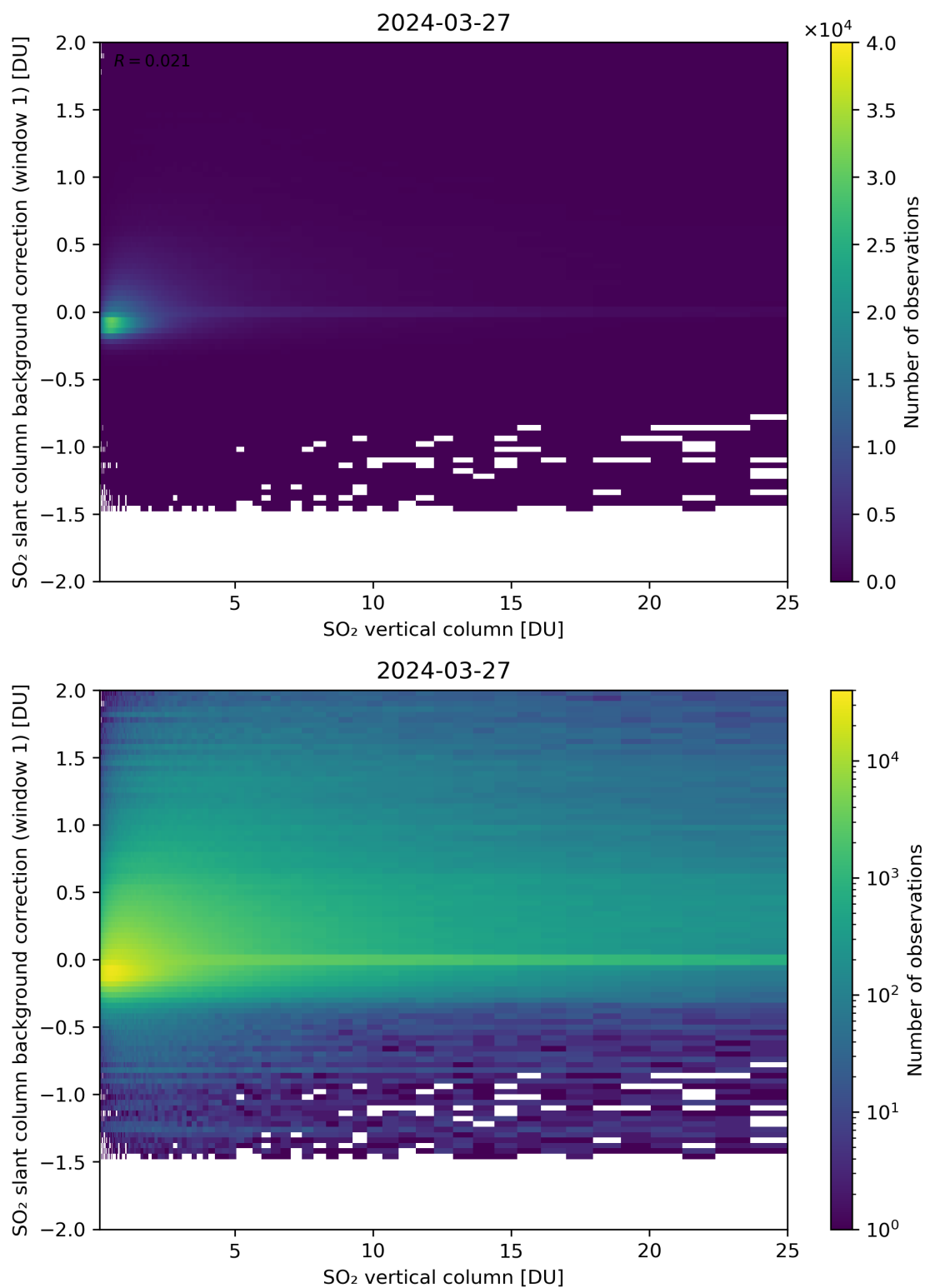
Figure 273: Scatter density plot of “SO 2 vertical column” against “SO 2 slant column background correction (window 1)” for 2024-03-26 to 2024-03-28.
