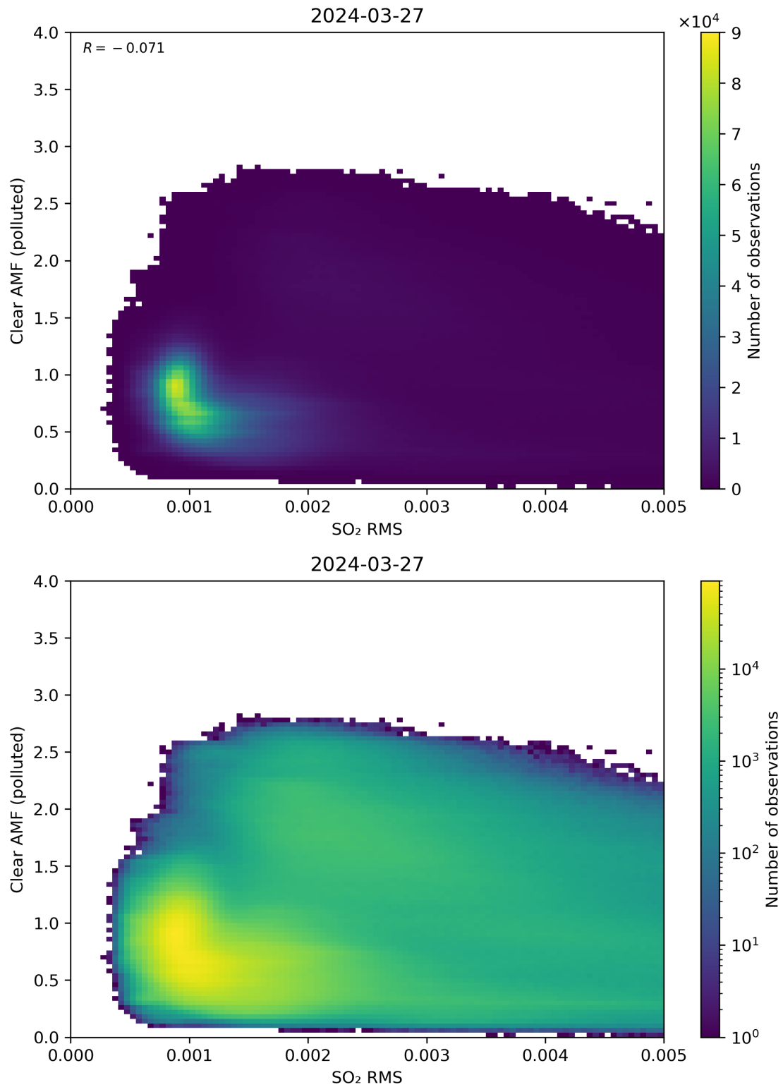
Figure 136: Scatter density plot of “SO 2 RMS” against “Clear AMF (polluted)” for 2024-03-26 to 2024-03-28.
