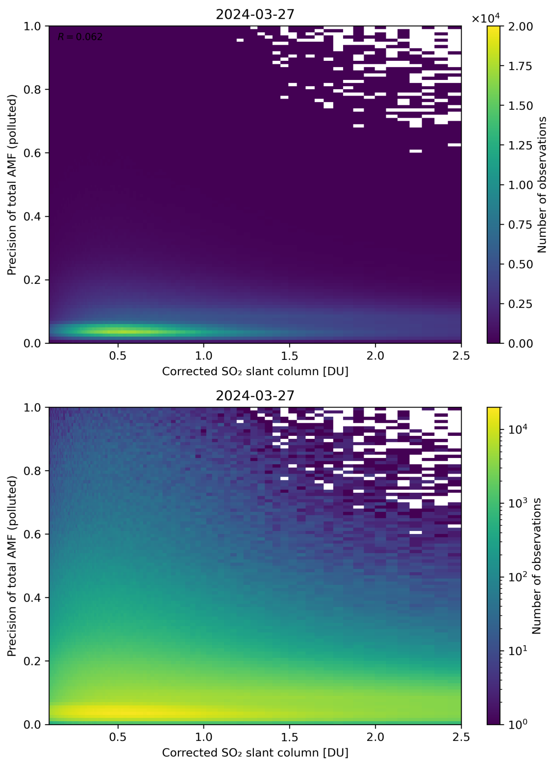
Figure 193: Scatter density plot of “Corrected SO 2 slant column” against “Precision of total AMF (polluted)” for 2024-03-26 to 2024-03-28.
