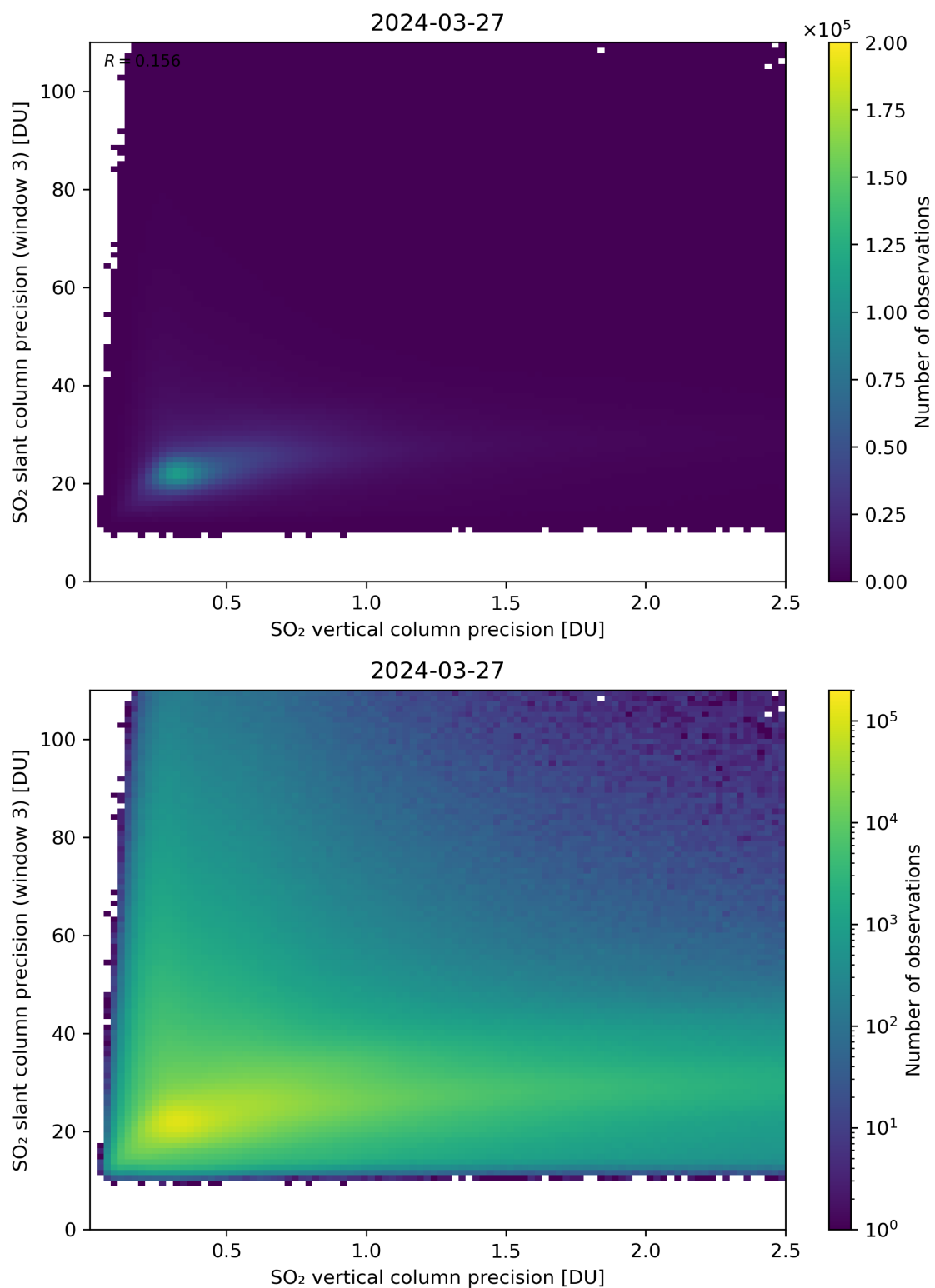
Figure 293: Scatter density plot of “SO 2 vertical column precision” against “SO 2 slant column precision (window 3)” for 2024-03-26 to 2024-03-28.
