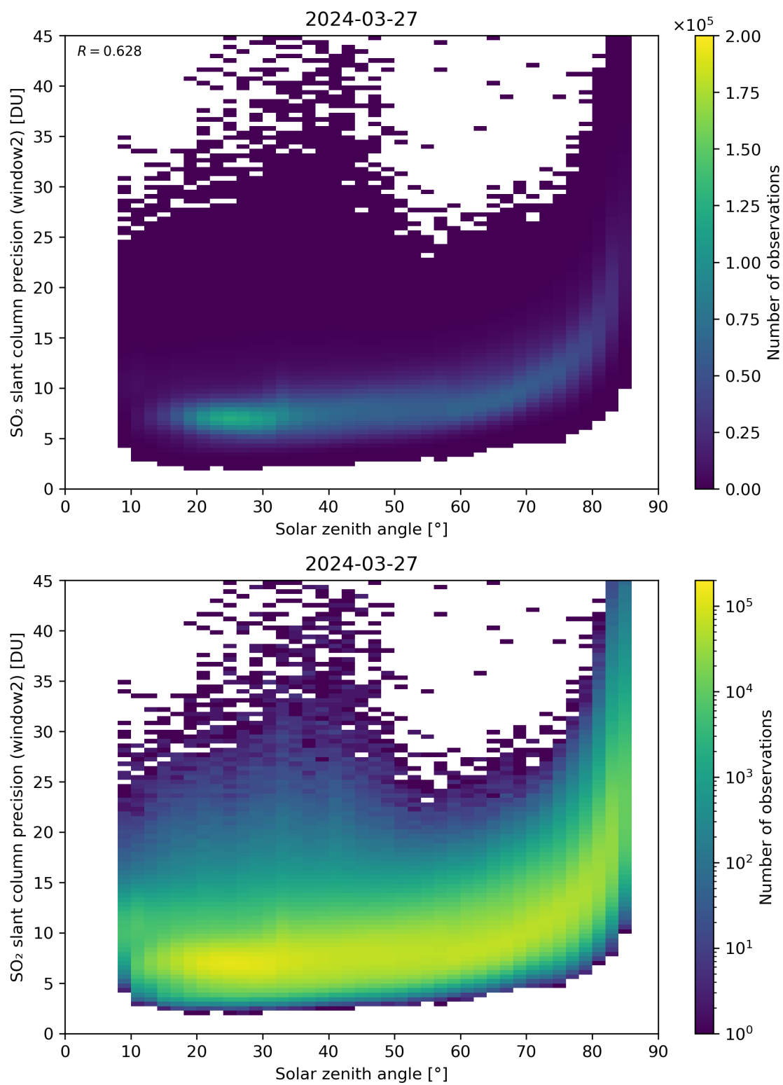
Figure 171: Scatter density plot of “Solar zenith angle” against “SO 2 slant column precision (window2)” for 2024-03-26 to 2024-03-28.
