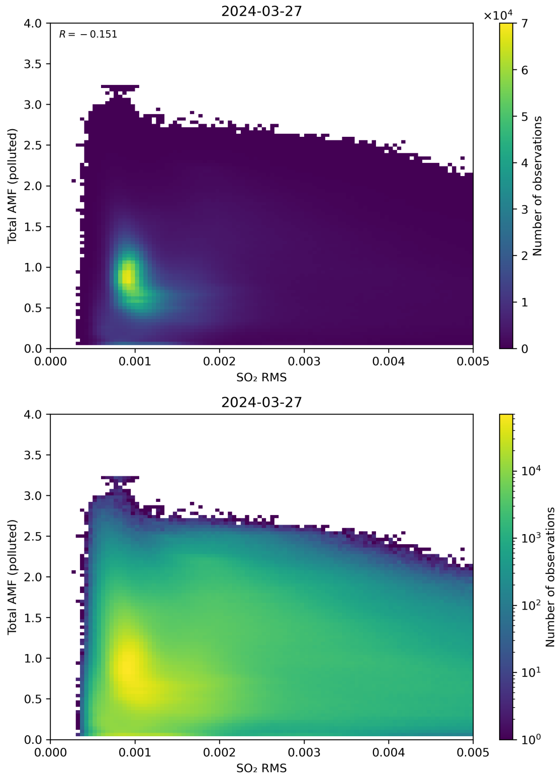
Figure 137: Scatter density plot of “SO 2 RMS” against “Total AMF (polluted)” for 2024-03-26 to 2024-03-28.
