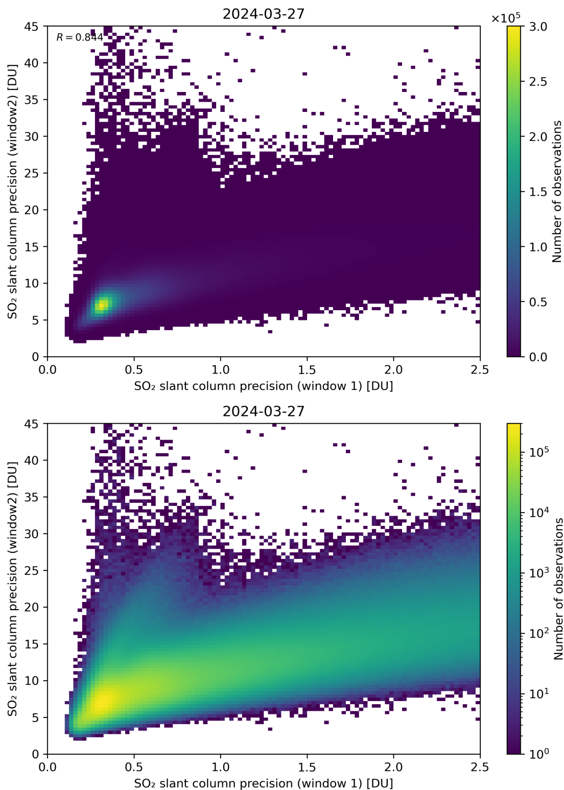
Figure 227: Scatter density plot of “SO 2 slant column precision (window 1)” against “SO 2 slant column precision (window2)” for 2024-03-26 to 2024-03-28.
