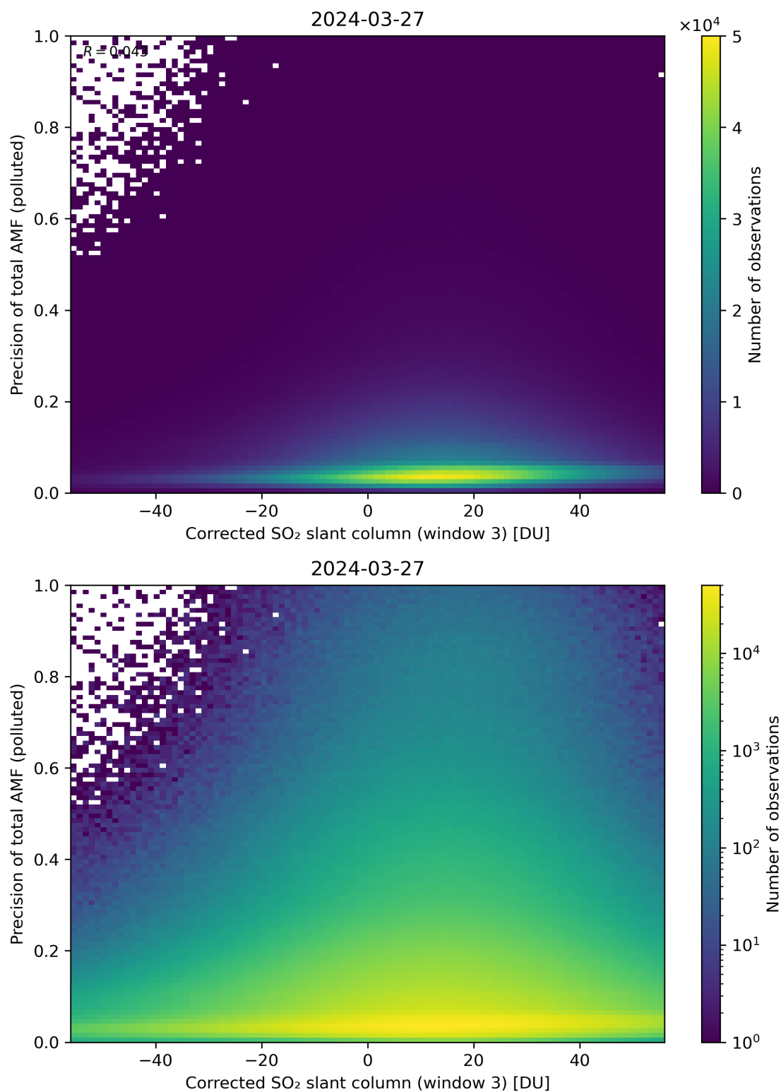
Figure 211: Scatter density plot of “Corrected SO 2 slant column (window 3)” against “Precision of total AMF (polluted)” for 2024-03-26 to 2024-03-28.
