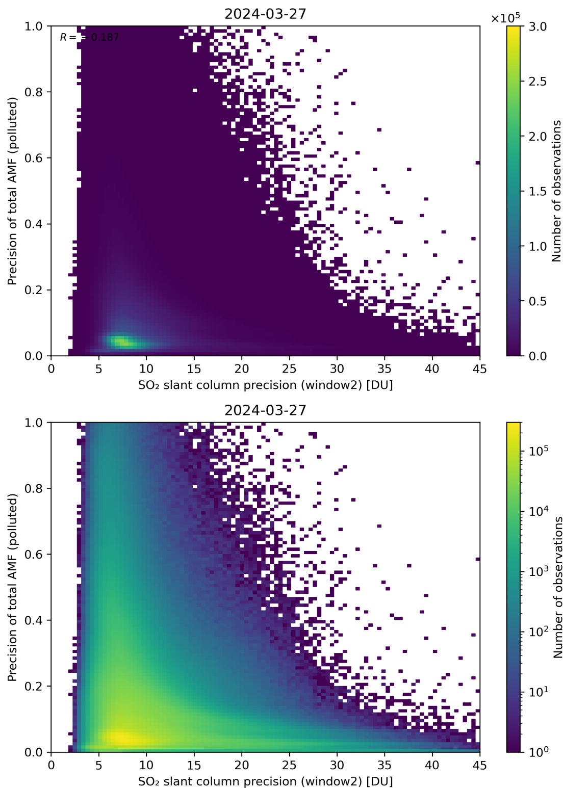
Figure 252: Scatter density plot of “SO 2 slant column precision (window2)” against “Precision of total AMF (polluted)” for 2024-03-26 to 2024-03-28.
