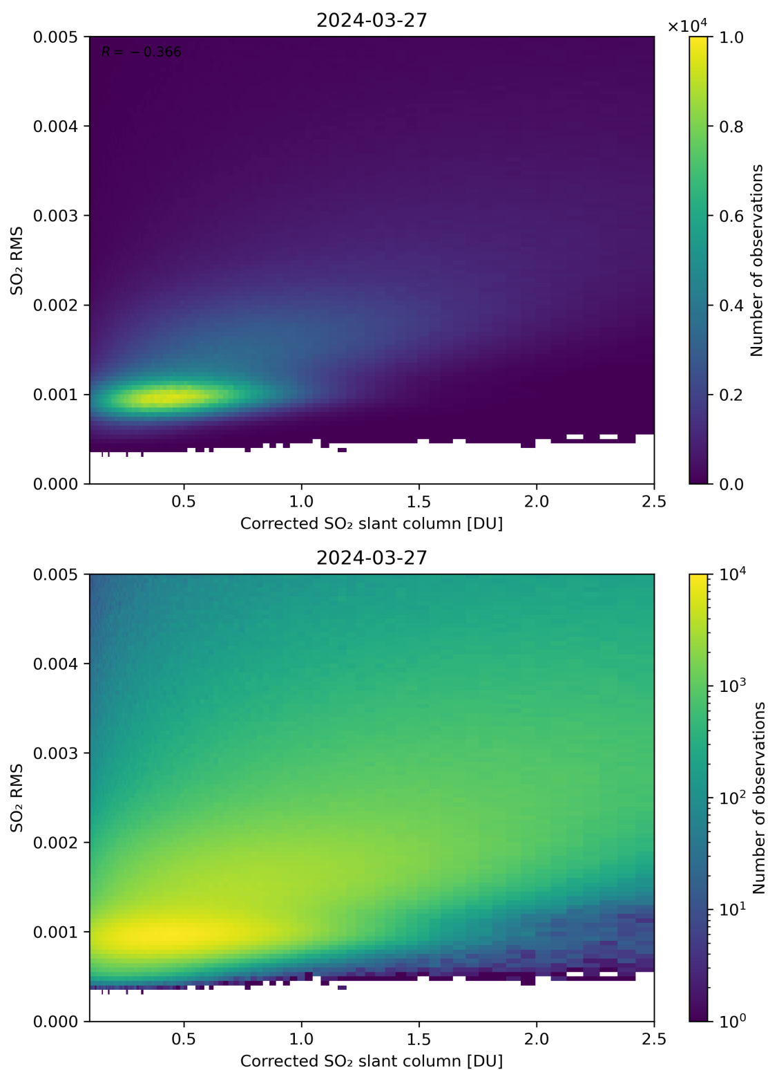
Figure 183: Scatter density plot of “Corrected SO 2 slant column” against “SO 2 RMS” for 2024-03-26 to 2024-03-28.
