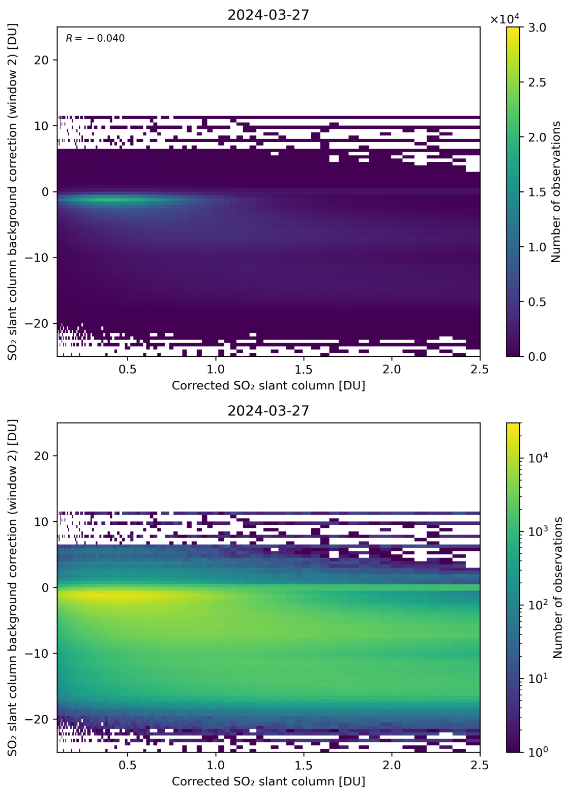
Figure 179: Scatter density plot of “Corrected SO 2 slant column” against “SO 2 slant column background correction (window 2)” for 2024-03-26 to 2024-03-28.
