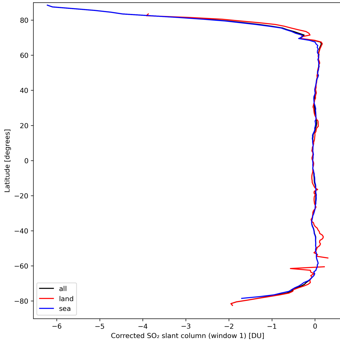
Figure 35: Zonal average of “Corrected SO 2 slant column (window 1)” for 2024-03-26 to 2024-03-28.
