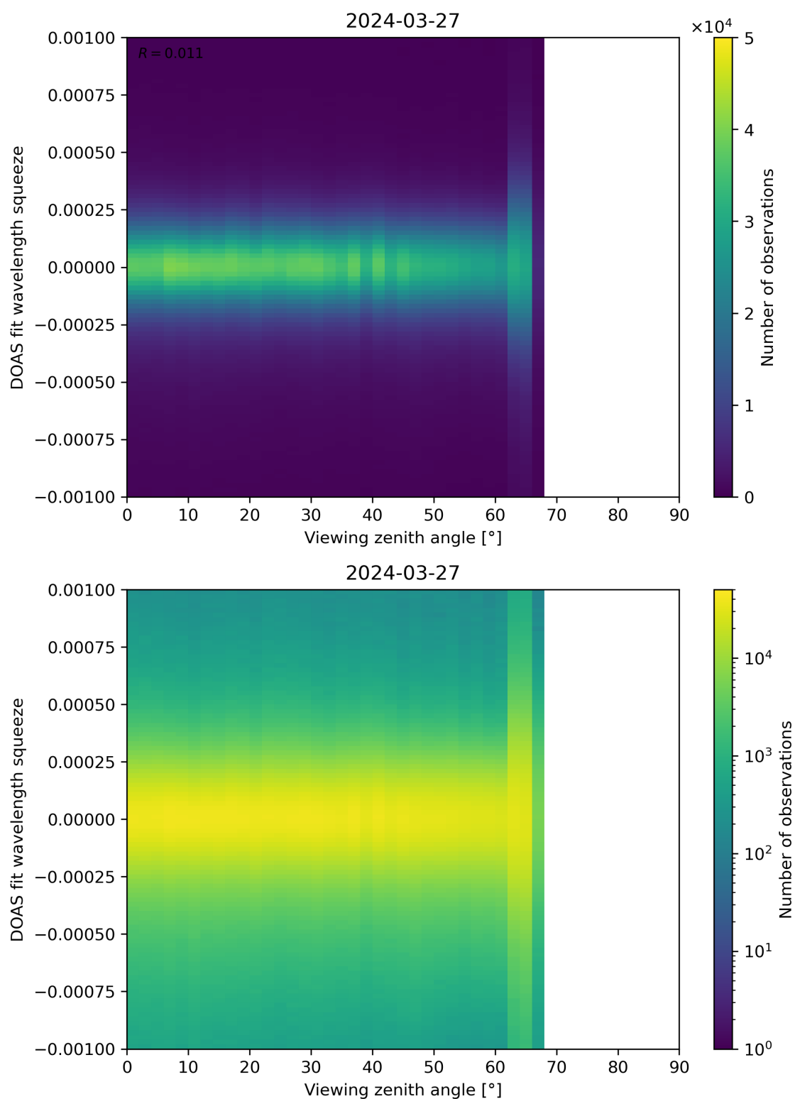
Figure 312: Scatter density plot of “Viewing zenith angle” against “DOAS fit wavelength squeeze” for 2024-03-26 to 2024-03-28.
