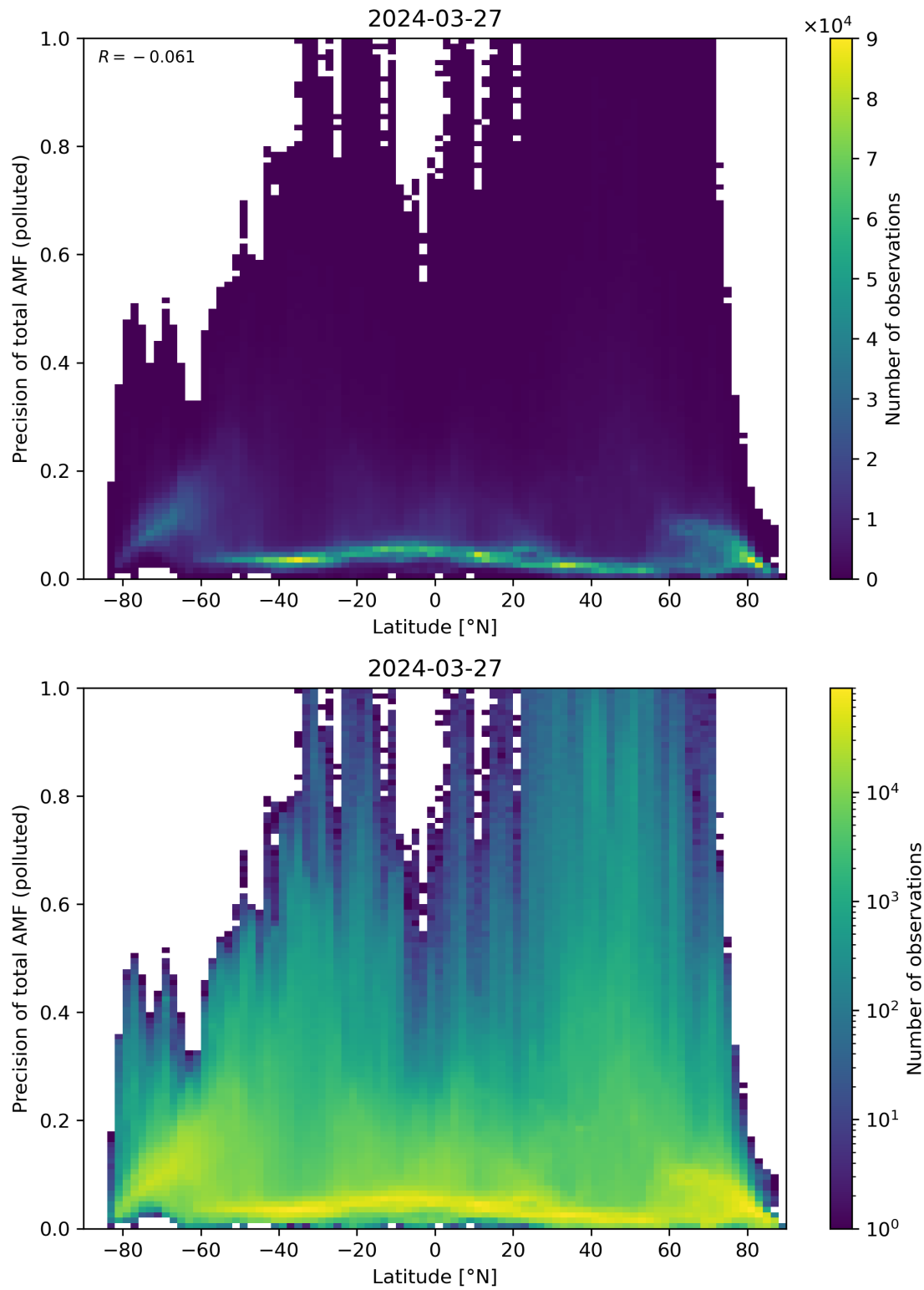
Figure 155: Scatter density plot of “Latitude” against “Precision of total AMF (polluted)” for 2024-03-26 to 2024-03-28.
