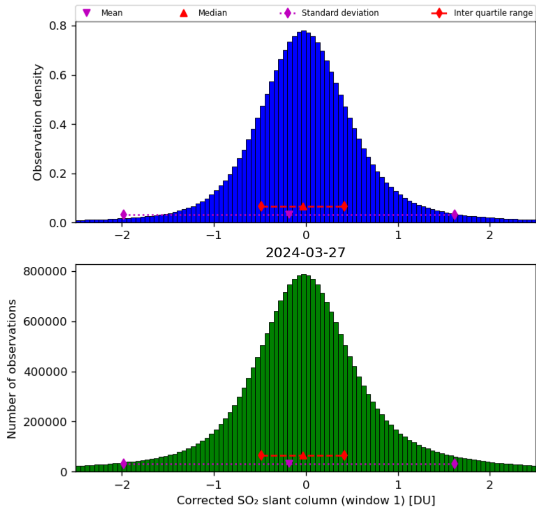
Figure 58: Histogram of “Corrected SO 2 slant column (window 1)” for 2024-03-26 to 2024-03-28
