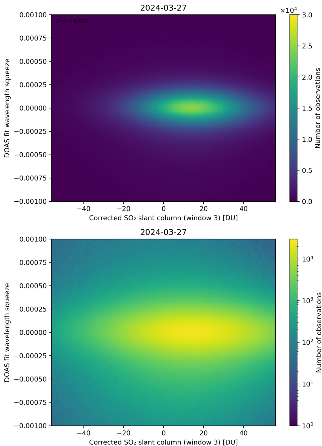
Figure 207: Scatter density plot of “Corrected SO 2 slant column (window 3)” against “DOAS fit wavelength squeeze” for 2024-03-26 to 2024-03-28.
