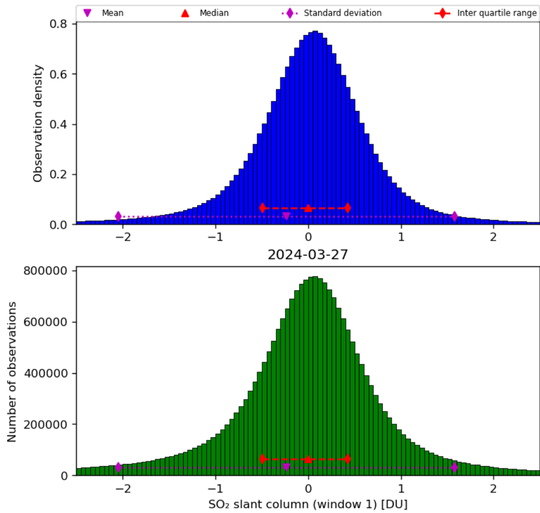
Figure 56: Histogram of “SO 2 slant column (window 1)” for 2024-03-26 to 2024-03-28
