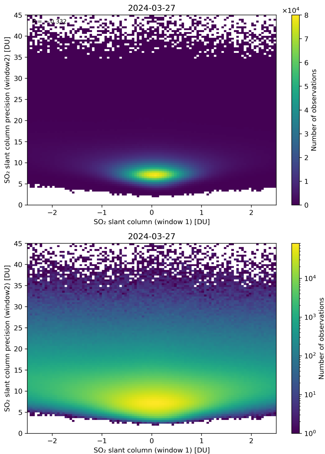
Figure 236: Scatter density plot of “SO 2 slant column (window 1)” against “SO 2 slant column precision (window2)” for 2024-03-26 to 2024-03-28.
