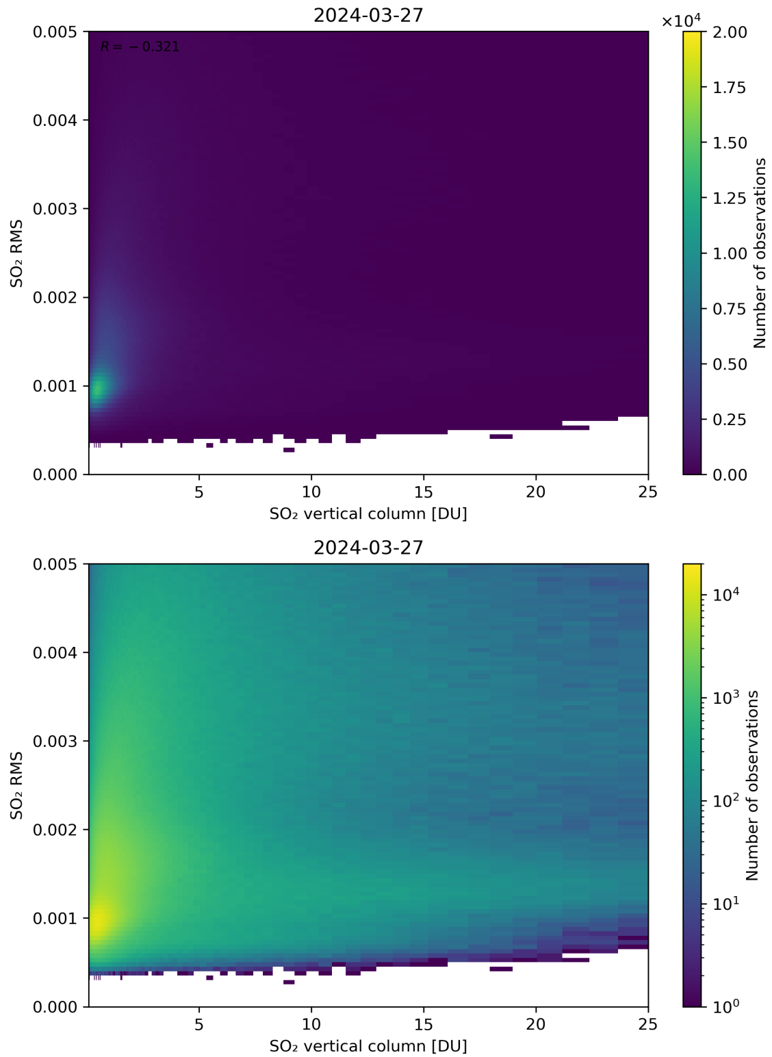
Figure 278: Scatter density plot of “SO 2 vertical column” against “SO 2 RMS” for 2024-03-26 to 2024-03-28.
