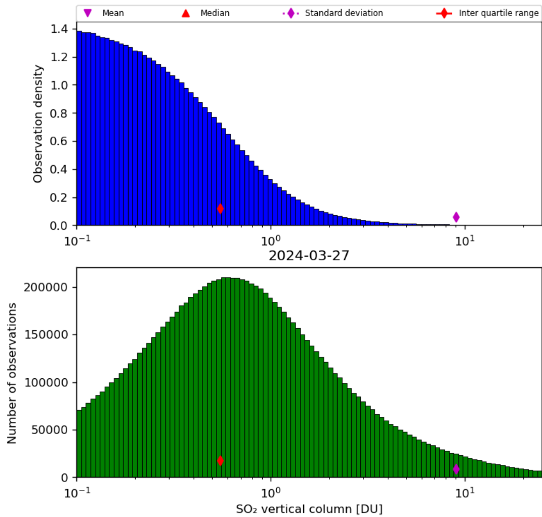
Figure 53: Histogram of “SO 2 vertical column” for 2024-03-26 to 2024-03-28
