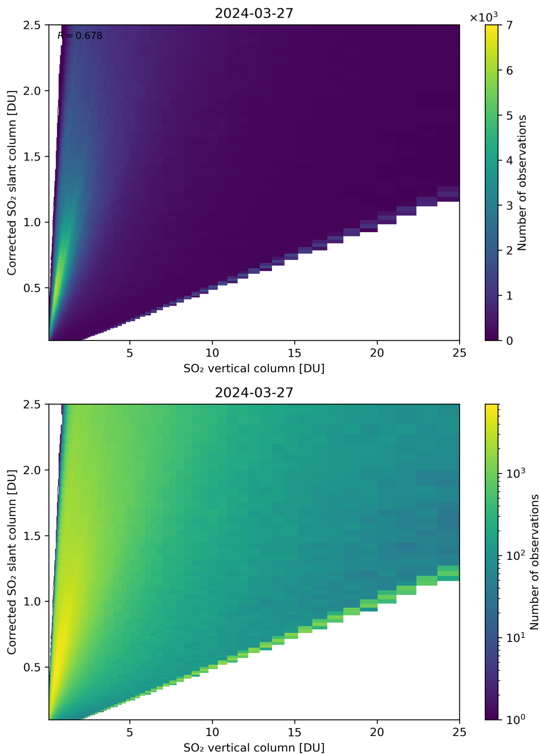
Figure 297: Scatter density plot of “SO 2 vertical column” against “Corrected SO 2 slant column” for 2024-03-26 to 2024-03-28.
