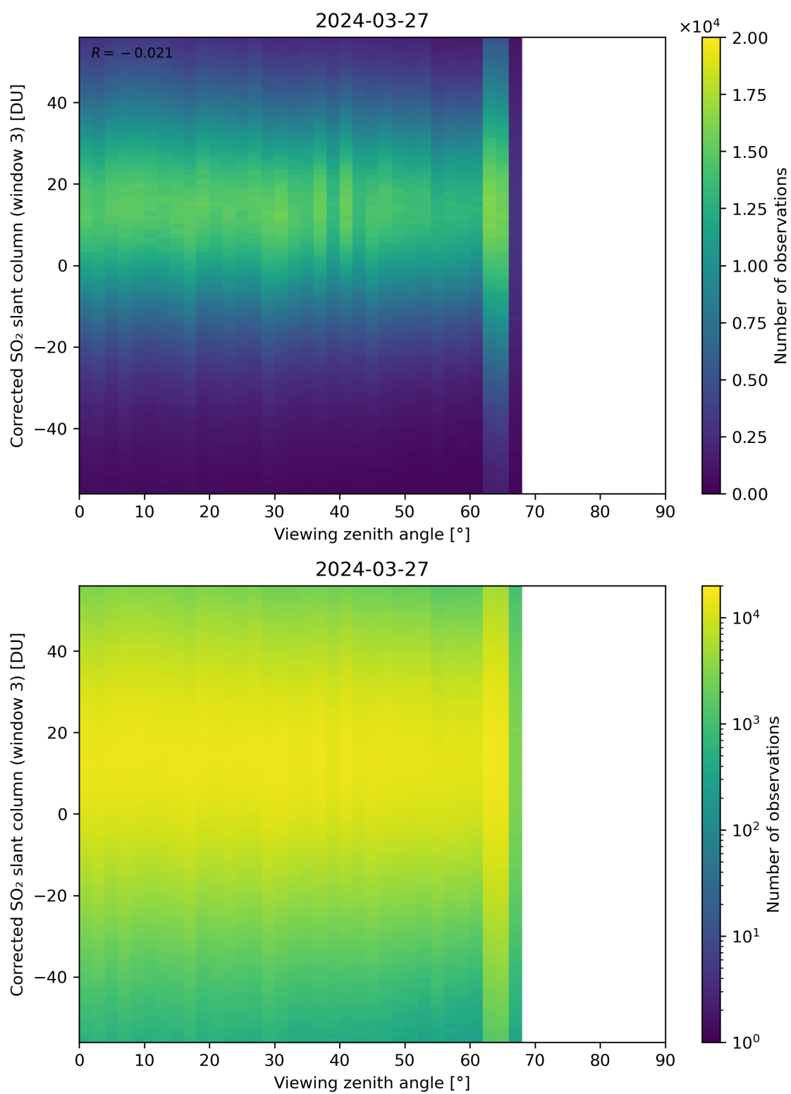
Figure 319: Scatter density plot of “Viewing zenith angle” against “Corrected SO 2 slant column (window 3)” for 2024-03-26 to 2024-03-28.
