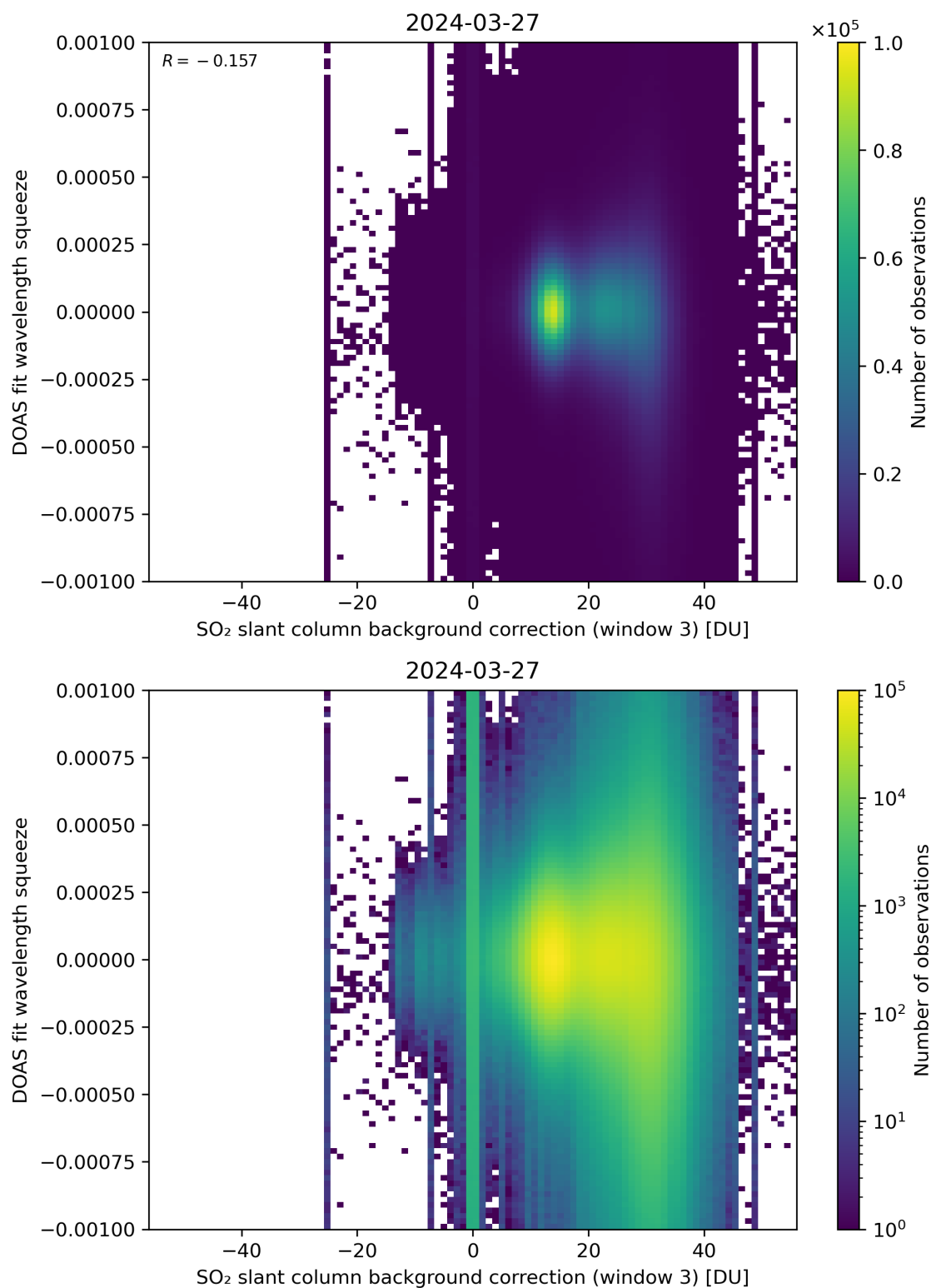
Figure 122: Scatter density plot of “SO 2 slant column background correction (window 3)” against “DOAS fit wavelength squeeze” for 2024-03-26 to 2024-03-28.
