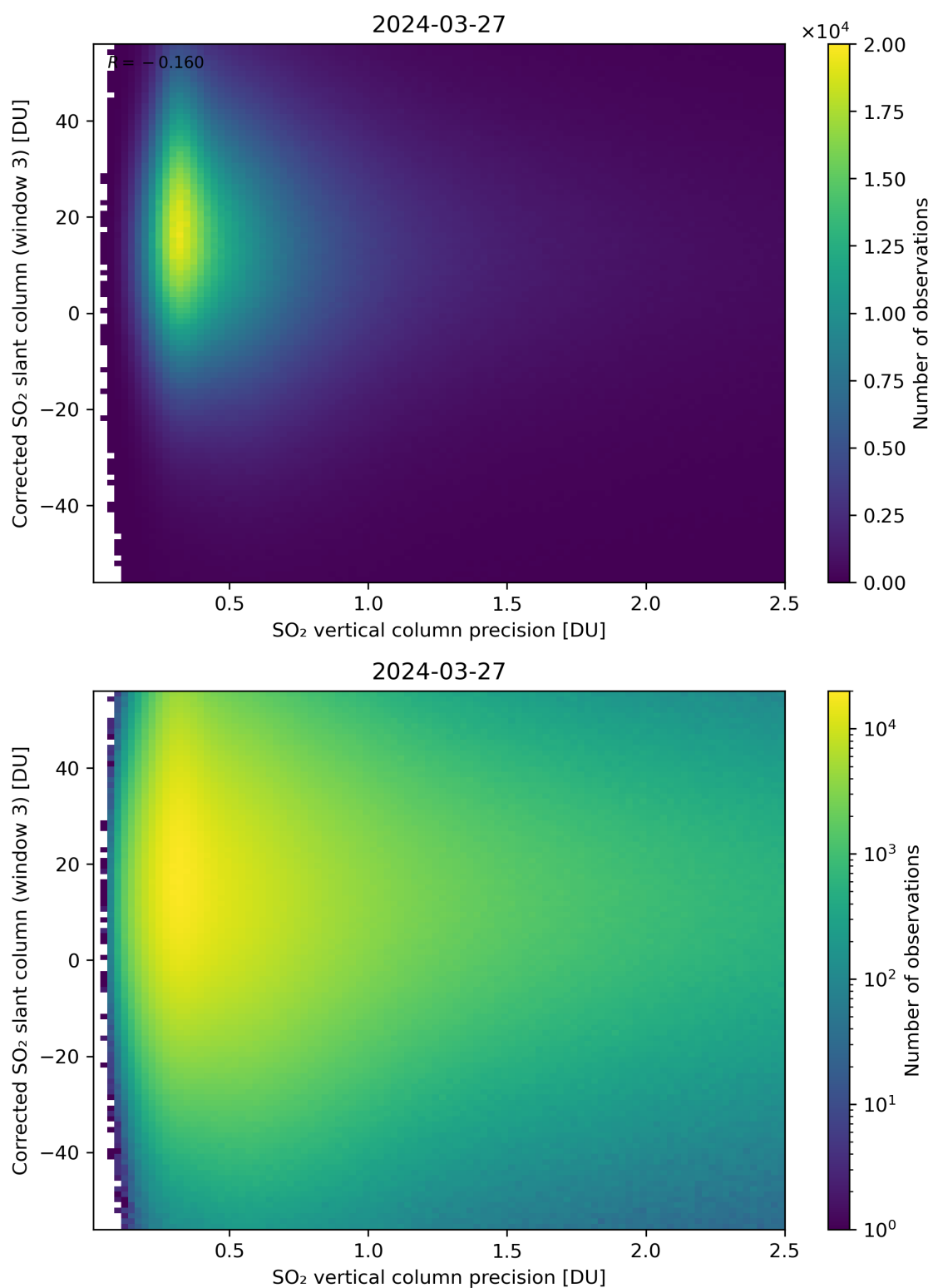
Figure 288: Scatter density plot of “SO 2 vertical column precision” against “Corrected SO 2 slant column (window 3)” for 2024-03-26 to 2024-03-28.
