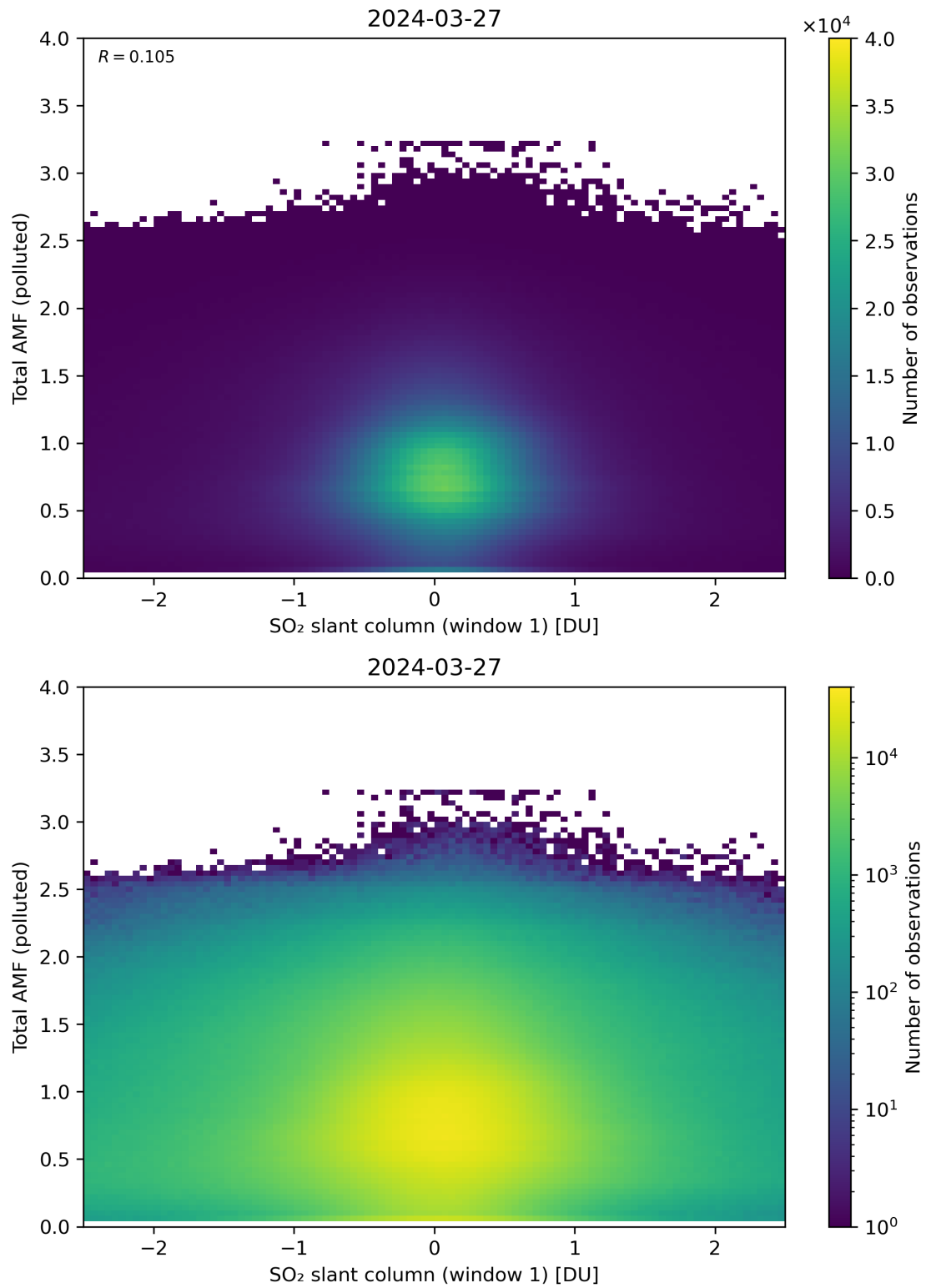
Figure 239: Scatter density plot of “SO 2 slant column (window 1)” against “Total AMF (polluted)” for 2024-03-26 to 2024-03-28.
