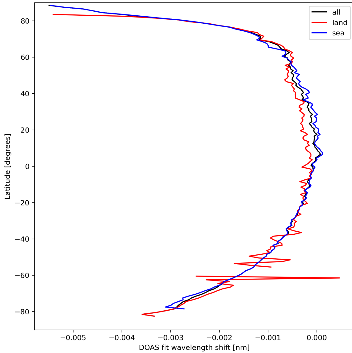
Figure 45: Zonal average of “DOAS fit wavelength shift” for 2024-03-26 to 2024-03-28.
