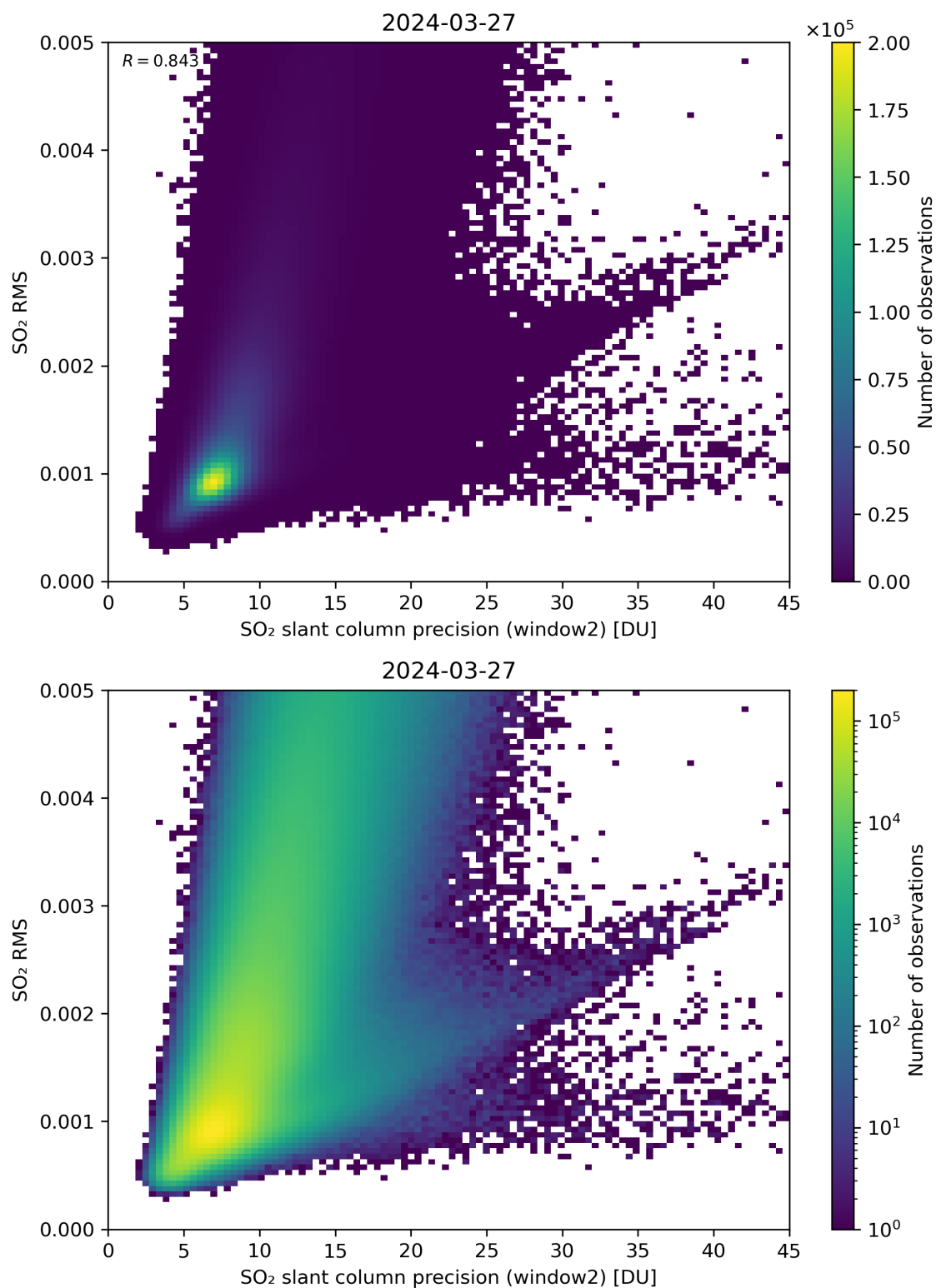
Figure 245: Scatter density plot of “SO 2 slant column precision (window2)” against “SO 2 RMS” for 2024-03-26 to 2024-03-28.
