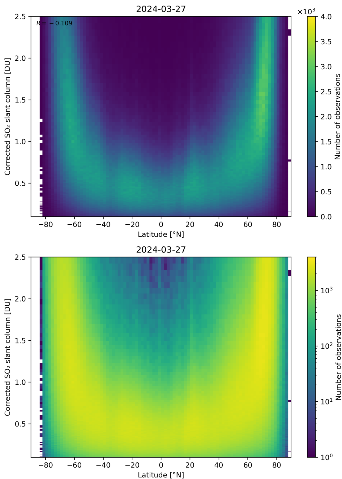
Figure 146: Scatter density plot of “Latitude” against “Corrected SO 2 slant column” for 2024-03-26 to 2024-03-28.
