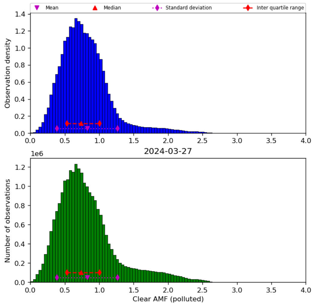
Figure 73: Histogram of “Clear AMF (polluted)” for 2024-03-26 to 2024-03-28
