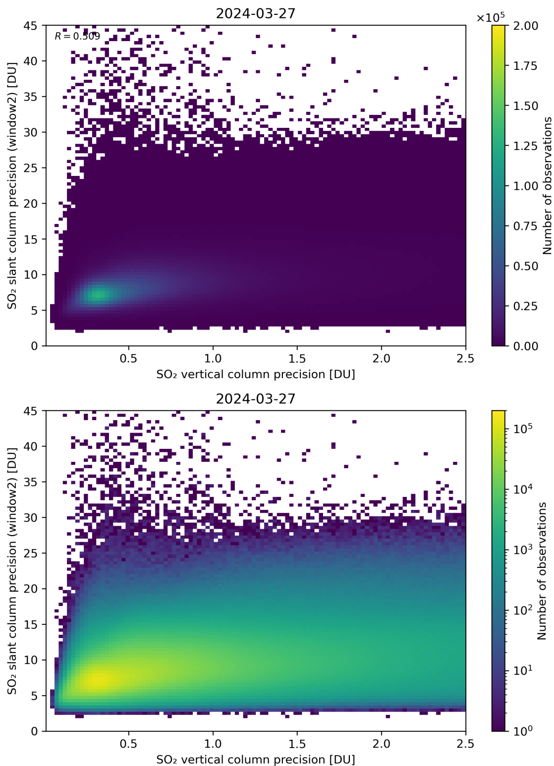
Figure 291: Scatter density plot of “SO 2 vertical column precision” against “SO 2 slant column precision (window2)” for 2024-03-26 to 2024-03-28.
