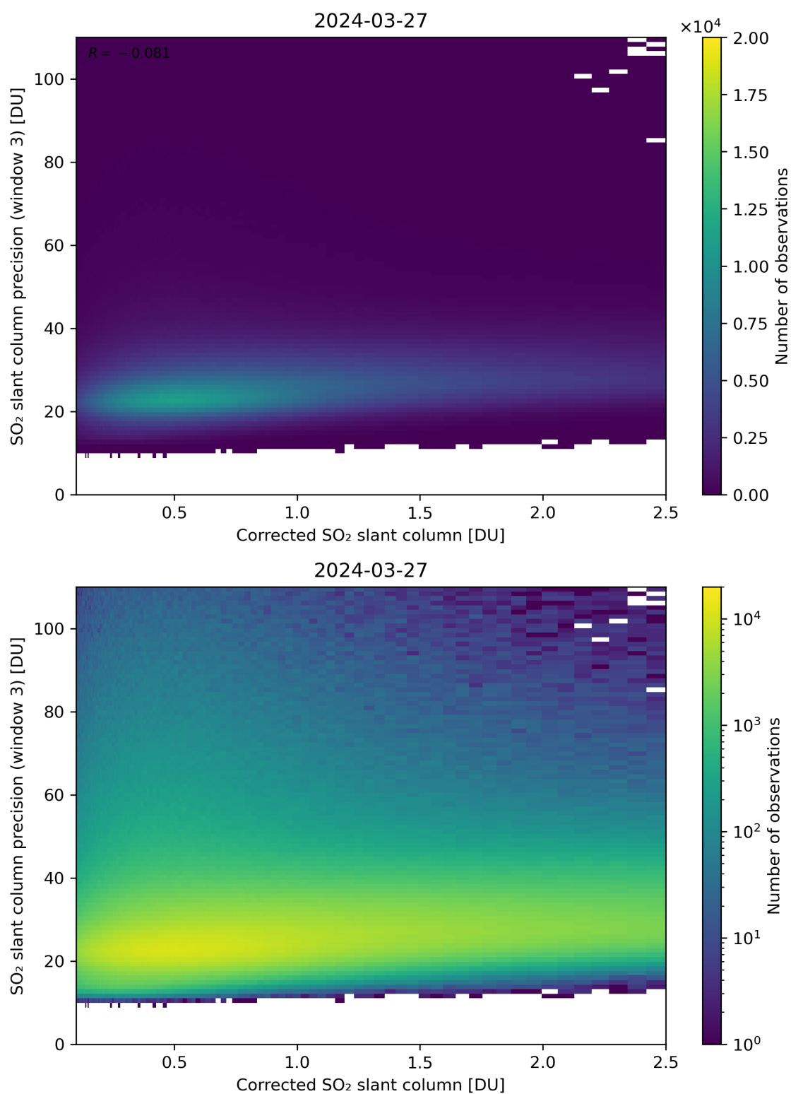
Figure 191: Scatter density plot of “Corrected SO 2 slant column” against “SO 2 slant column precision (window 3)” for 2024-03-26 to 2024-03-28.
