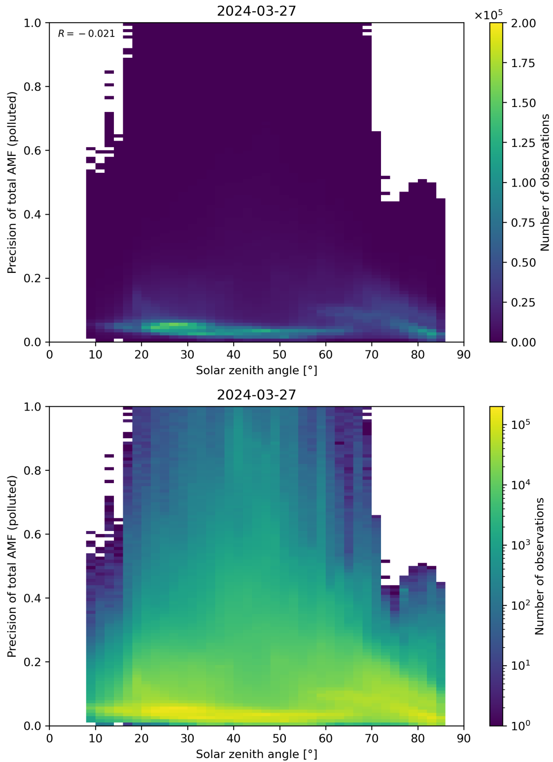
Figure 175: Scatter density plot of “Solar zenith angle” against “Precision of total AMF (polluted)” for 2024-03-26 to 2024-03-28.
