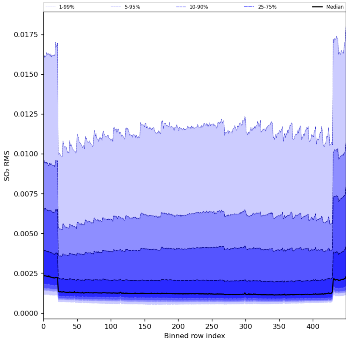
Figure 93: Along track statistics of “SO 2 RMS” for 2024-03-26 to 2024-03-28
