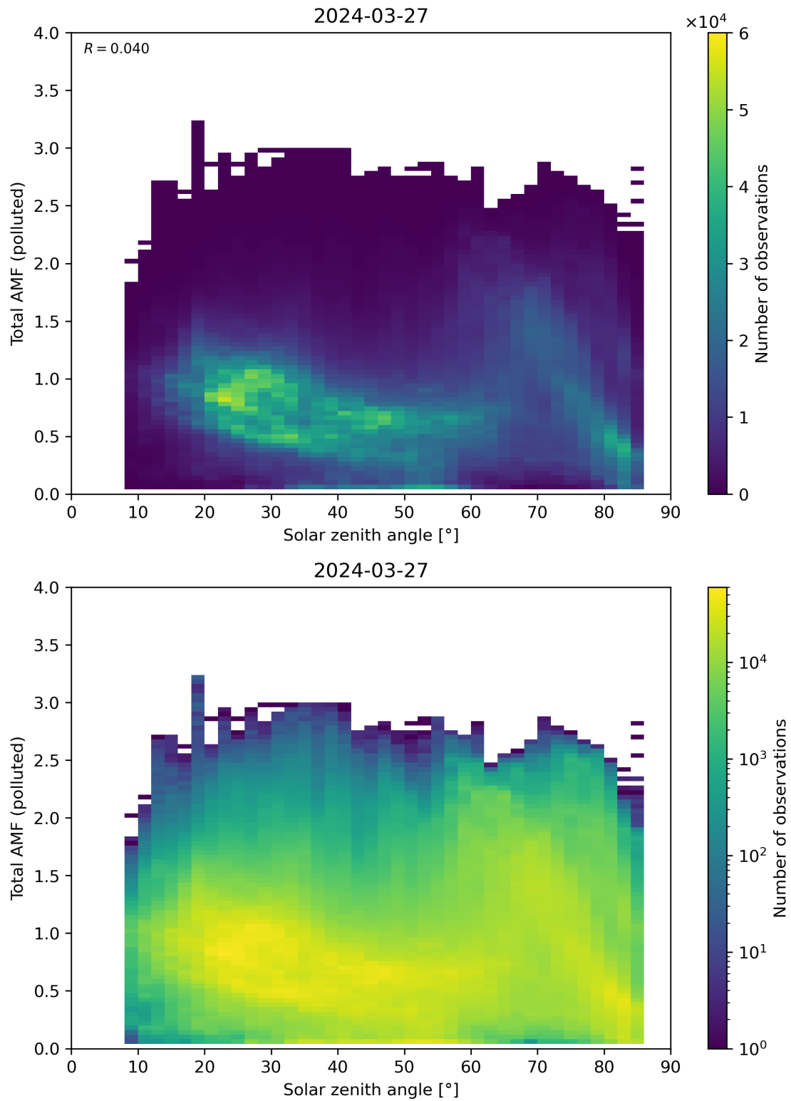
Figure 174: Scatter density plot of “Solar zenith angle” against “Total AMF (polluted)” for 2024-03-26 to 2024-03-28.
