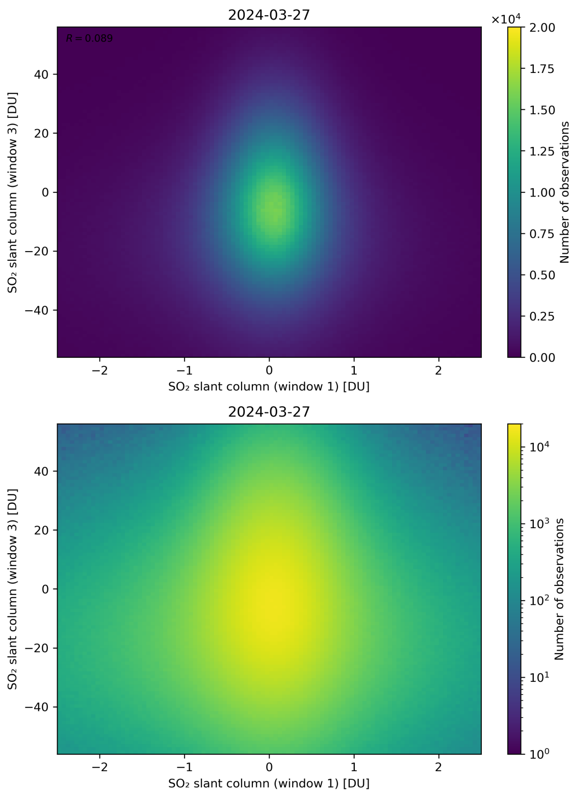
Figure 237: Scatter density plot of “SO 2 slant column (window 1)” against “SO 2 slant column (window 3)” for 2024-03-26 to 2024-03-28.
