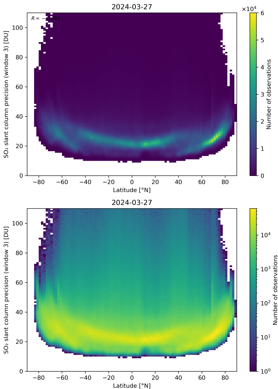
Figure 153: Scatter density plot of “Latitude” against “SO 2 slant column precision (window 3)” for 2024-03-26 to 2024-03-28.
