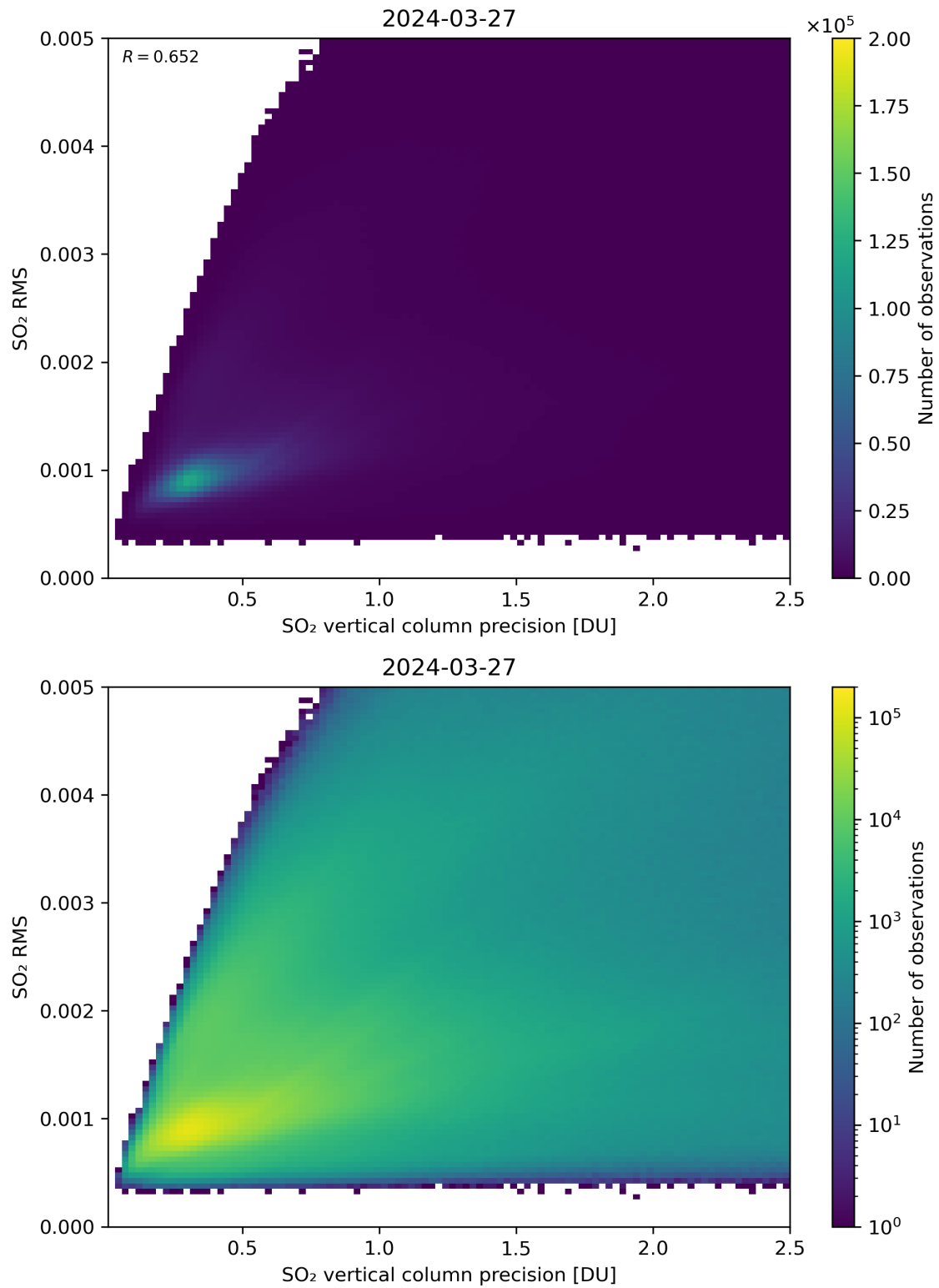
Figure 284: Scatter density plot of “SO 2 vertical column precision” against “SO 2 RMS” for 2024-03-26 to 2024-03-28.
