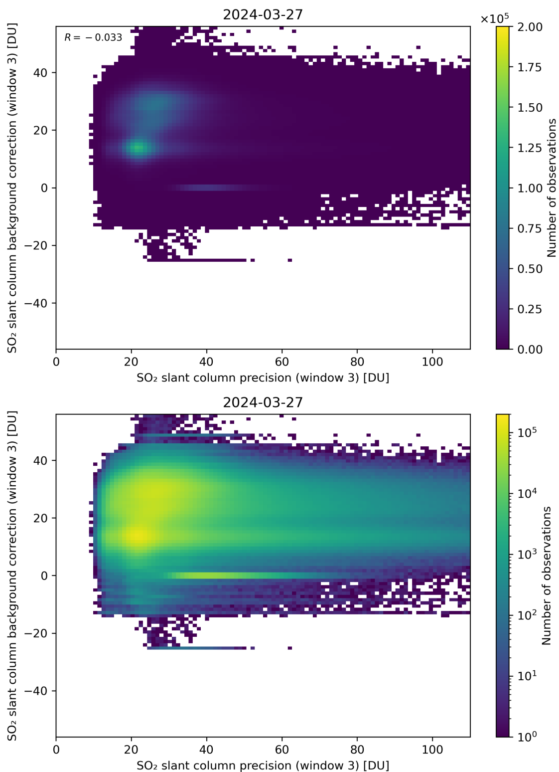
Figure 257: Scatter density plot of “SO 2 slant column precision (window 3)” against “SO 2 slant column background correction (window 3)” for 2024-03-26 to 2024-03-28.
