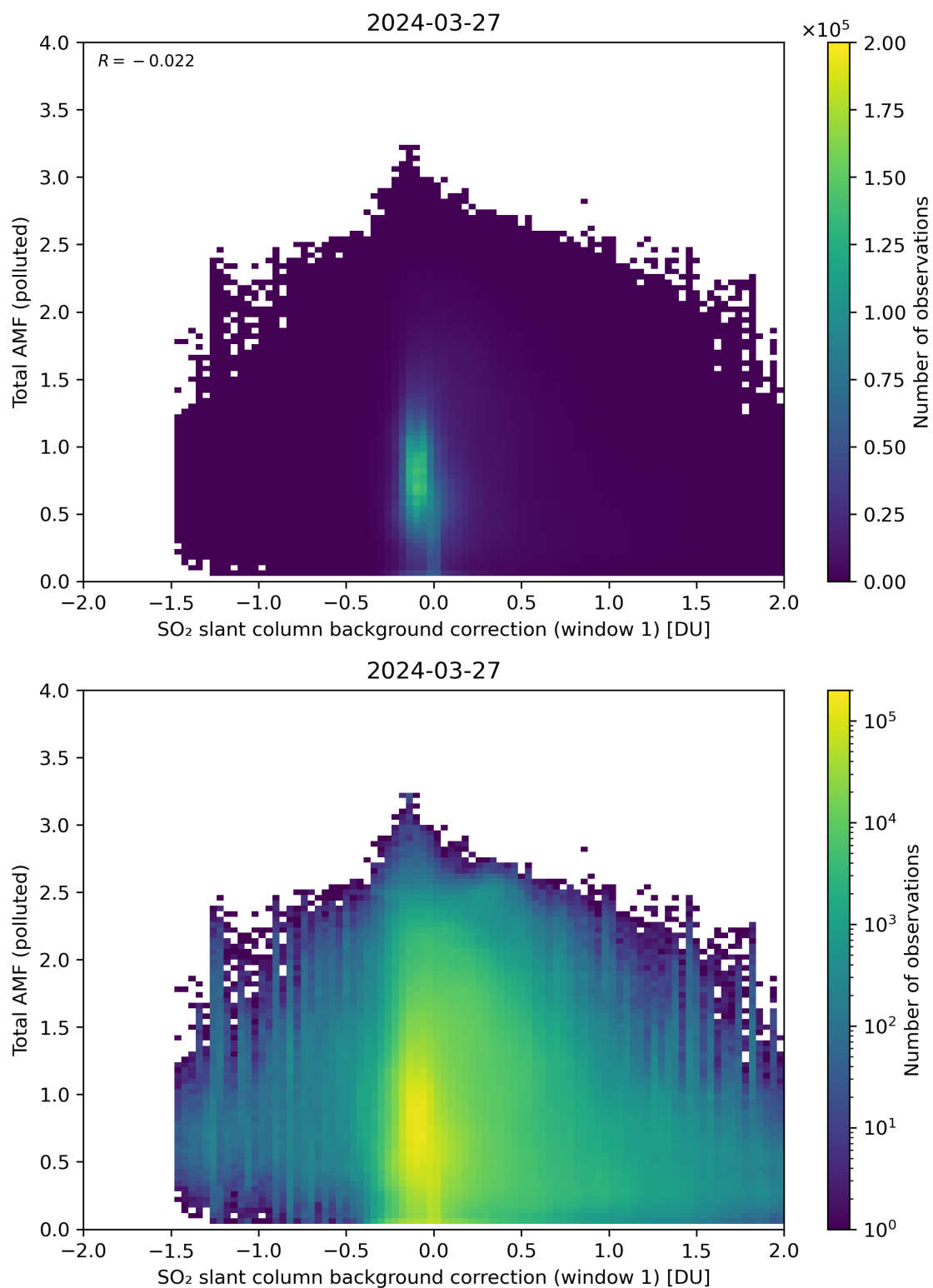
Figure 109: Scatter density plot of “SO 2 slant column background correction (window 1)” against “Total AMF (polluted)” for 2024-03-26 to 2024-03-28.
