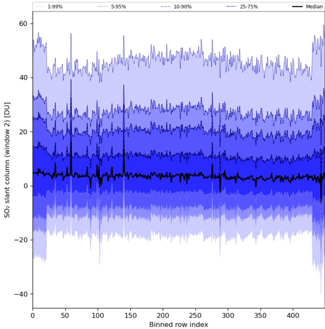
Figure 83: Along track statistics of “SO 2 slant column (window 2)” for 2024-03-26 to 2024-03-28
