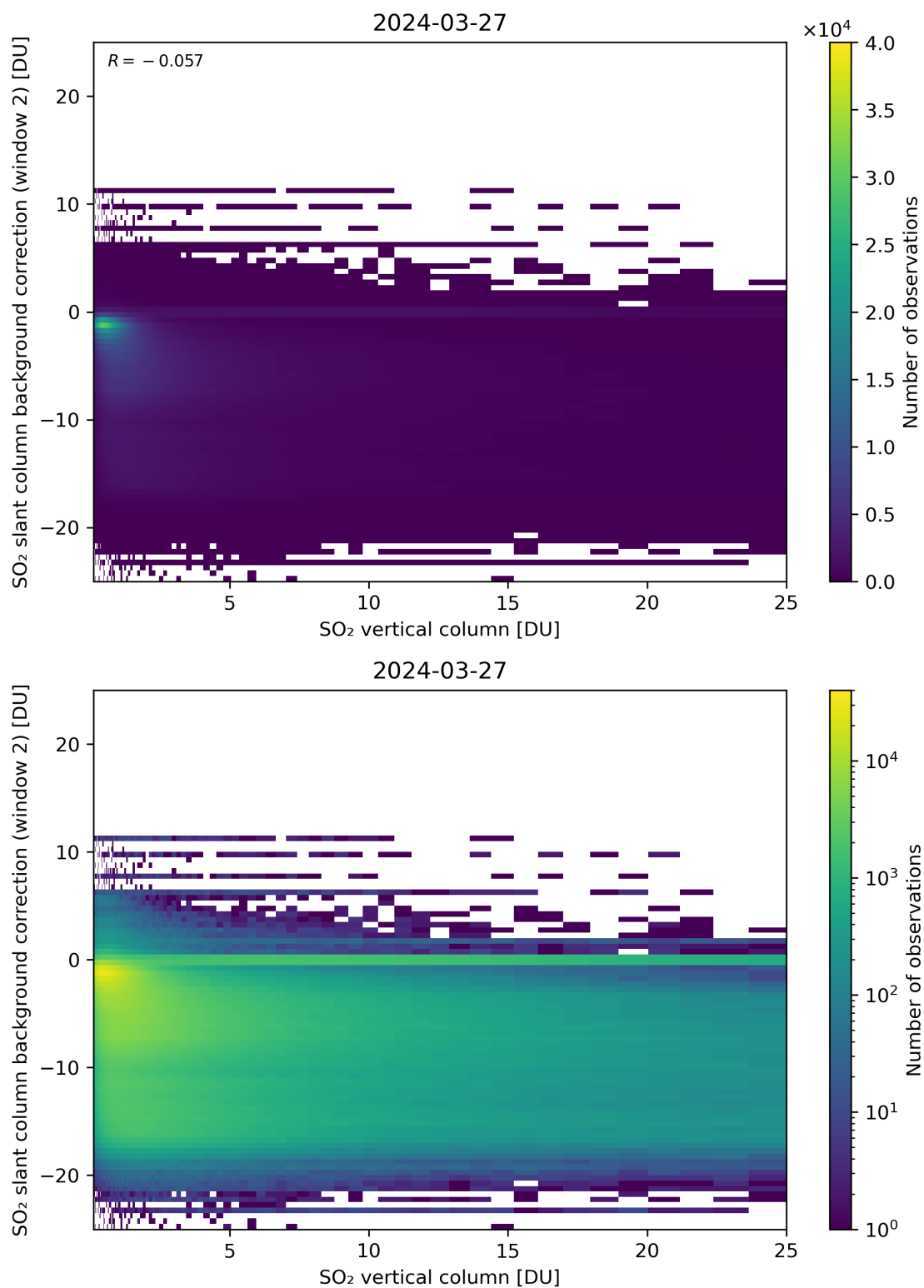
Figure 274: Scatter density plot of “SO 2 vertical column” against “SO 2 slant column background correction (window 2)” for 2024-03-26 to 2024-03-28.
