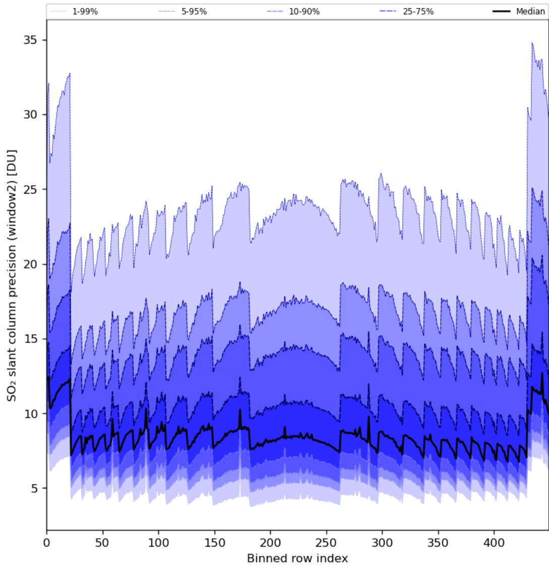
Figure 84: Along track statistics of “SO 2 slant column precision (window2)” for 2024-03-26 to 2024-03-28
