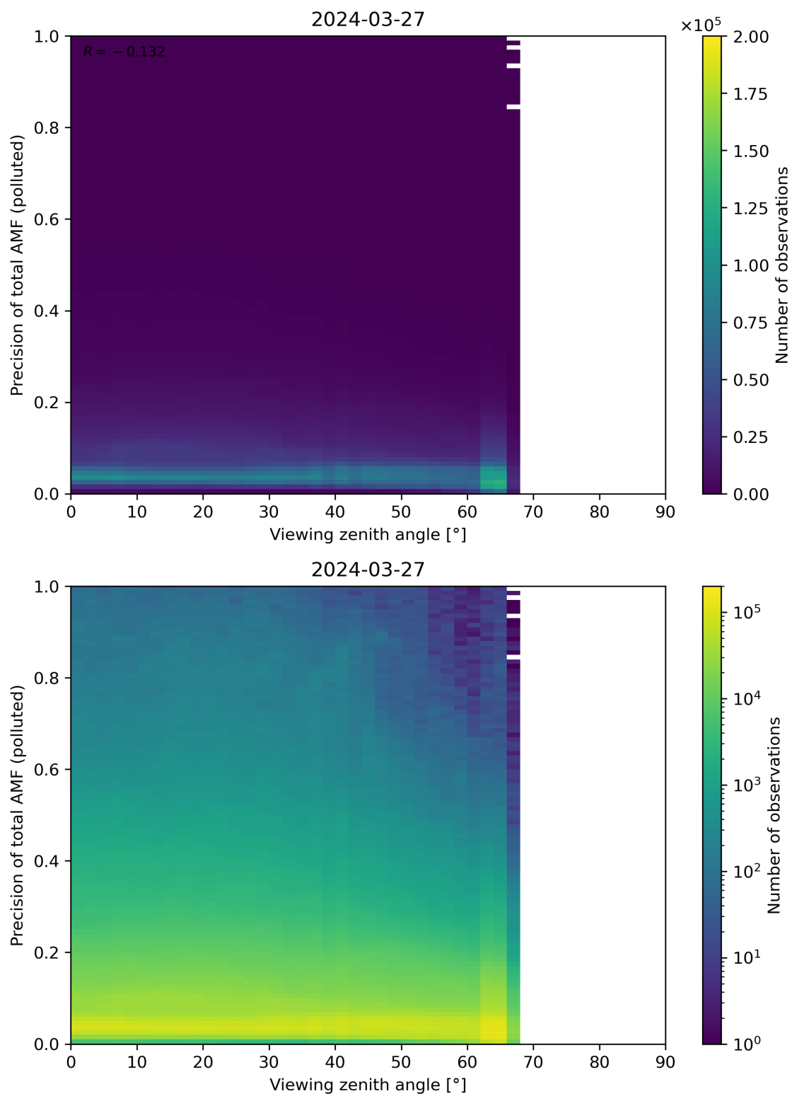
Figure 326: Scatter density plot of “Viewing zenith angle” against “Precision of total AMF (polluted)” for 2024-03-26 to 2024-03-28.
