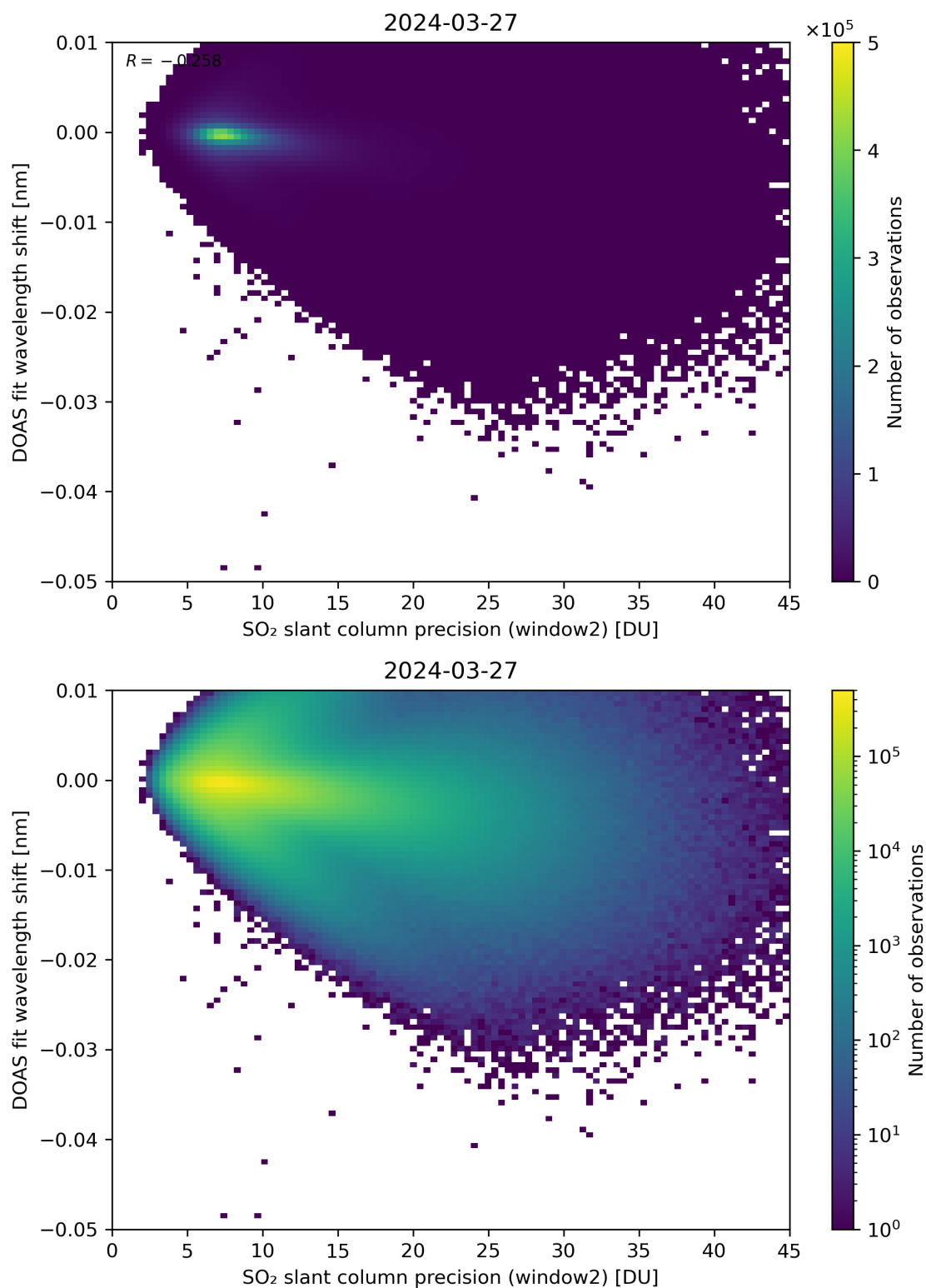
Figure 243: Scatter density plot of “SO 2 slant column precision (window2)” against “DOAS fit wavelength shift” for 2024-03-26 to 2024-03-28.
