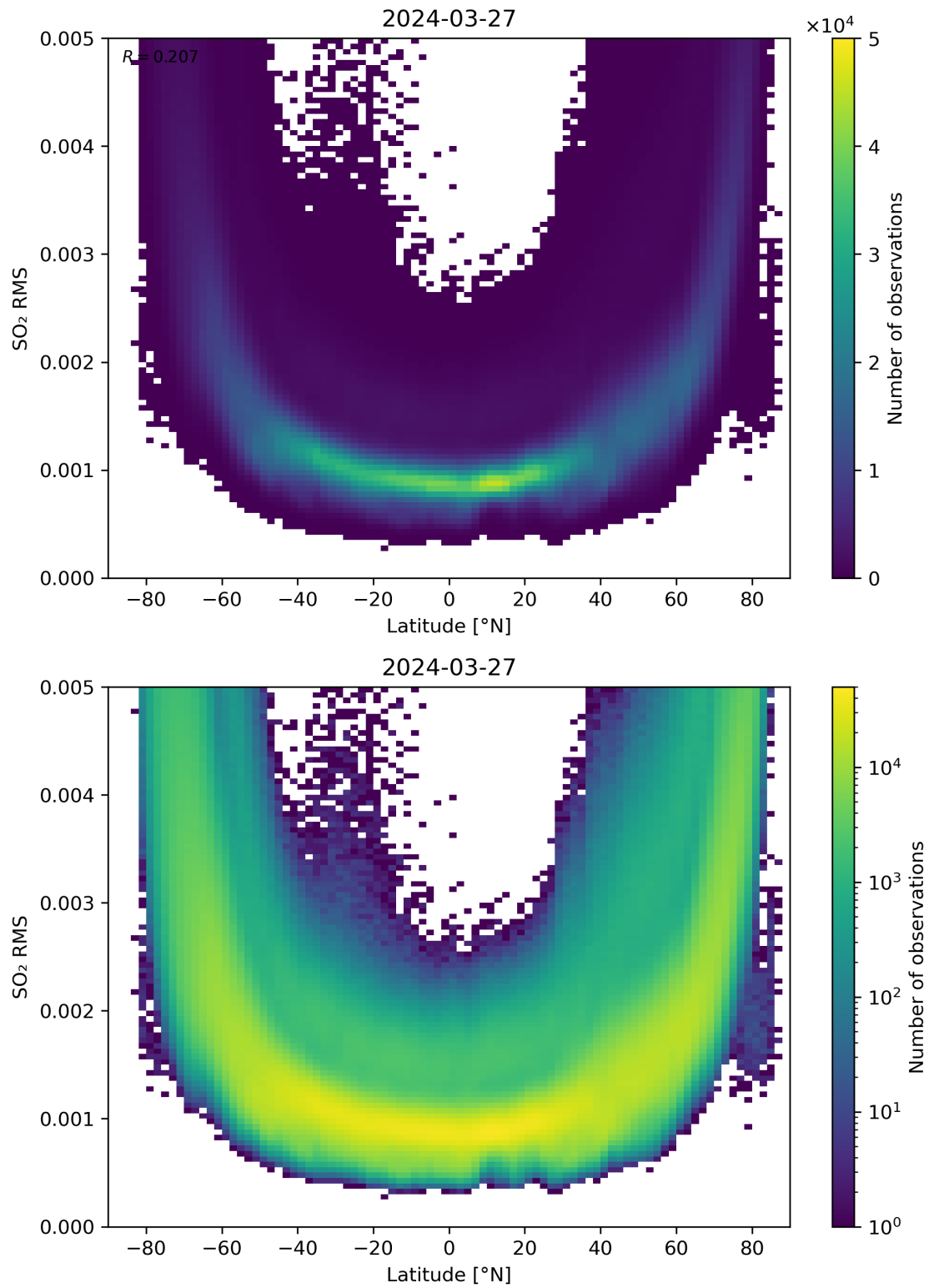
Figure 144: Scatter density plot of “Latitude” against “SO 2 RMS” for 2024-03-26 to 2024-03-28.
