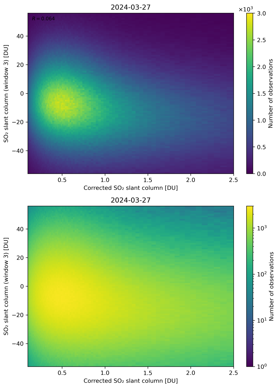
Figure 190: Scatter density plot of “Corrected SO 2 slant column” against “SO 2 slant column (window 3)” for 2024-03-26 to 2024-03-28.
