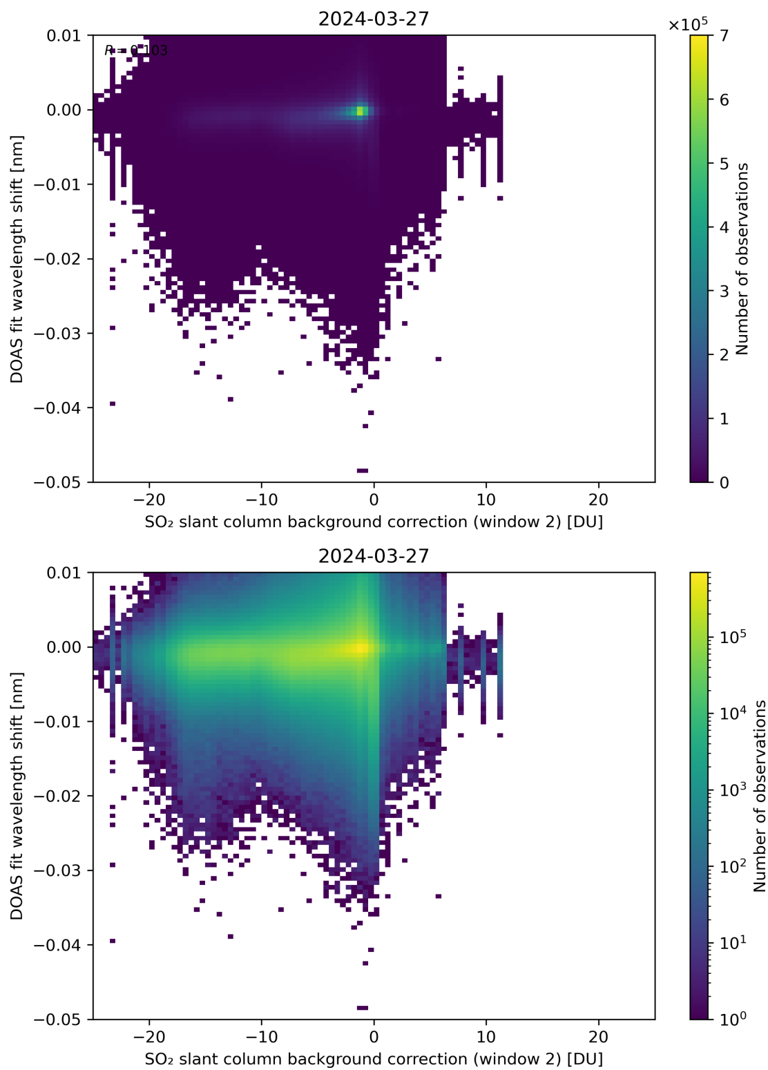
Figure 112: Scatter density plot of “SO 2 slant column background correction (window 2)” against “DOAS fit wavelength shift” for 2024-03-26 to 2024-03-28.
