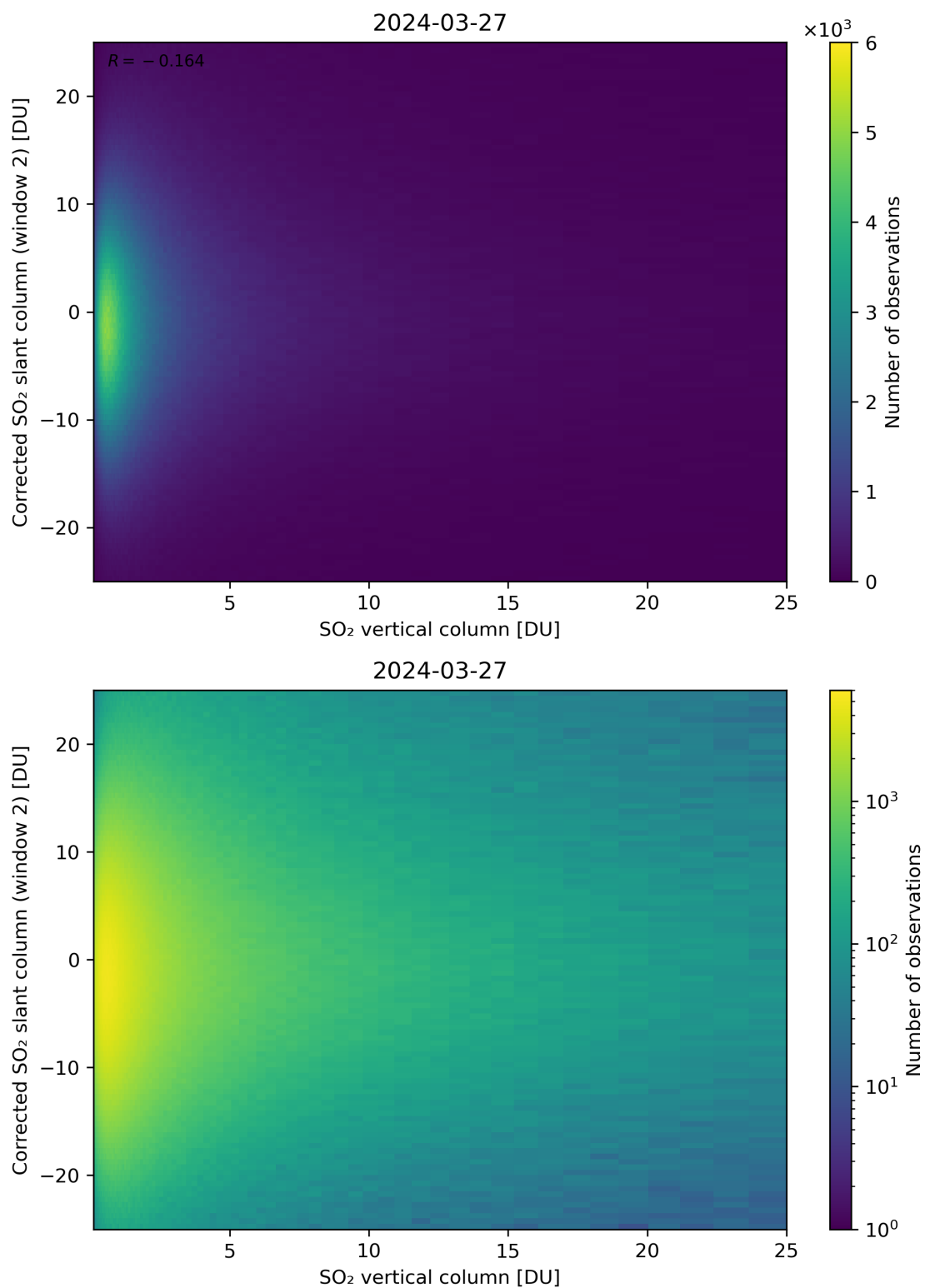
Figure 298: Scatter density plot of “SO 2 vertical column” against “Corrected SO 2 slant column (window 2)” for 2024-03-26 to 2024-03-28.
