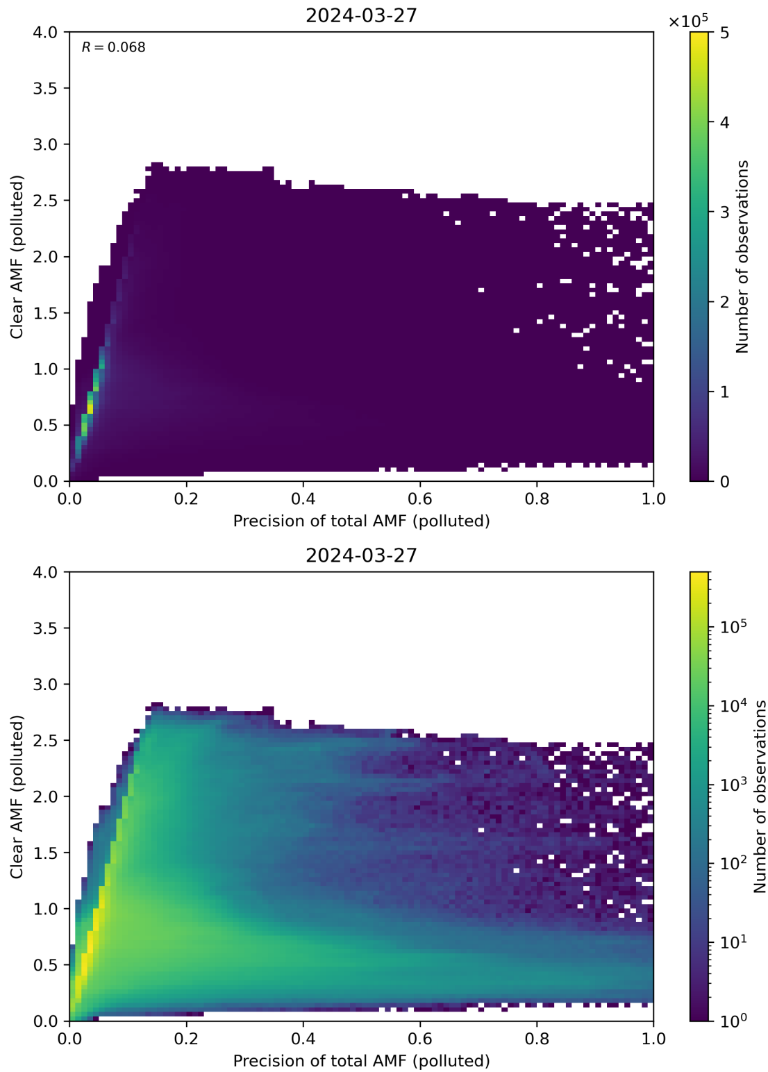
Figure 270: Scatter density plot of “Precision of total AMF (polluted)” against “Clear AMF (polluted)” for 2024-03-26 to 2024-03-28.
