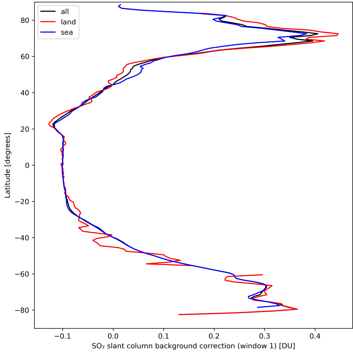
Figure 36: Zonal average of “SO 2 slant column background correction (window 1)” for 2024-03-26 to 2024-03-28.
