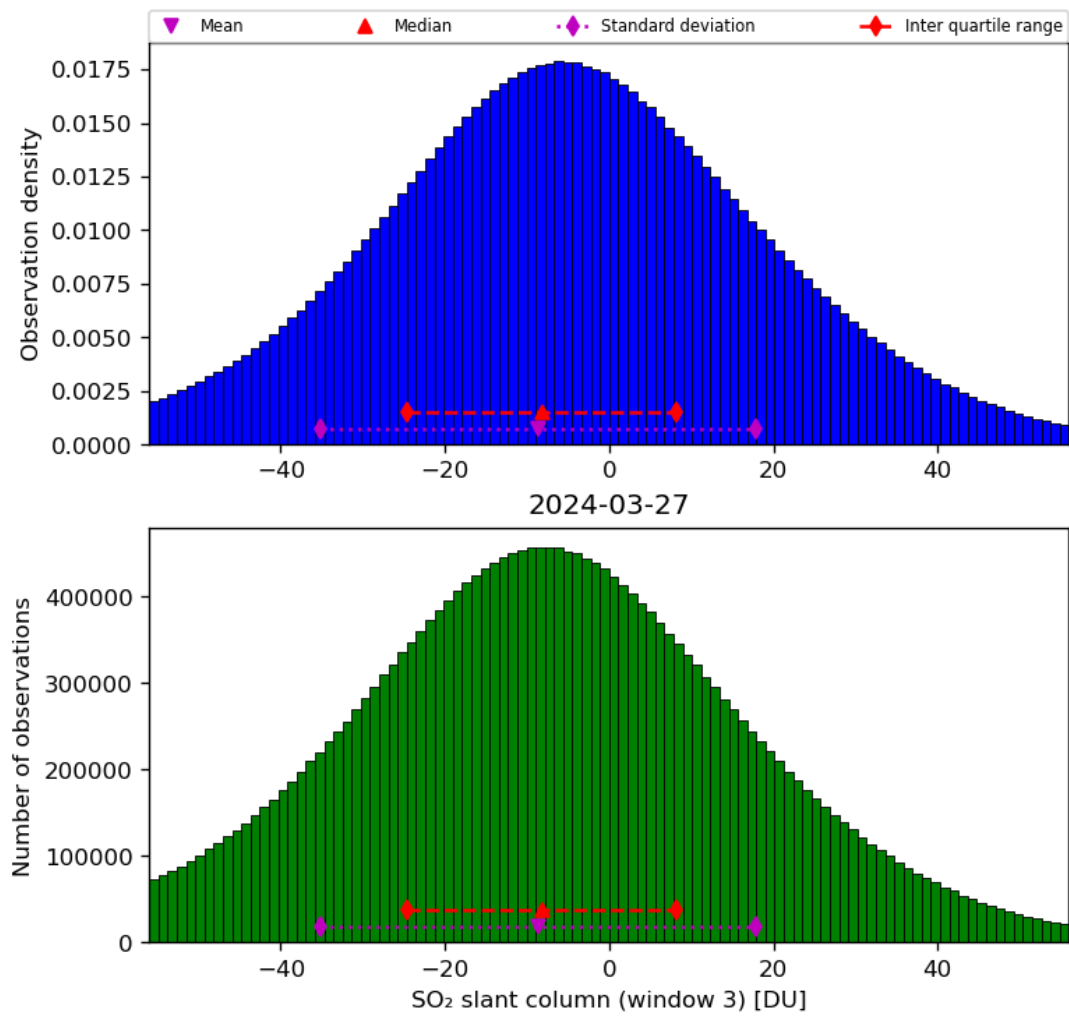
Figure 64: Histogram of “SO 2 slant column (window 3)” for 2024-03-26 to 2024-03-28
