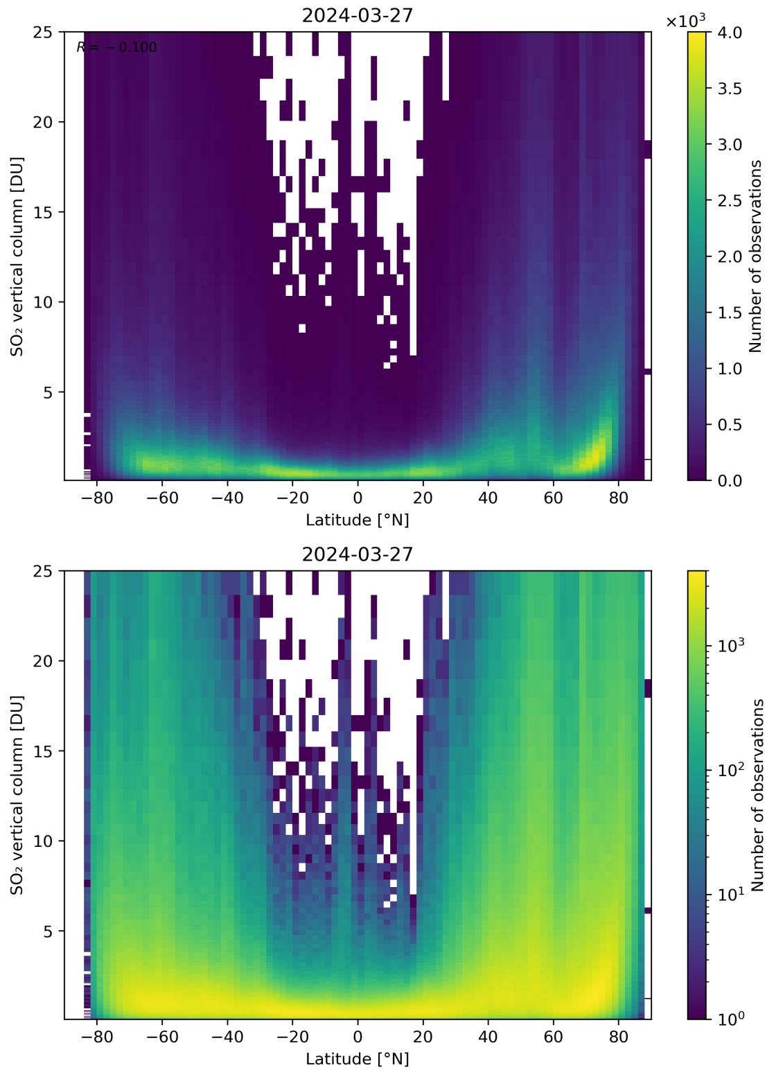
Figure 156: Scatter density plot of “Latitude” against “SO 2 vertical column” for 2024-03-26 to 2024-03-28.
