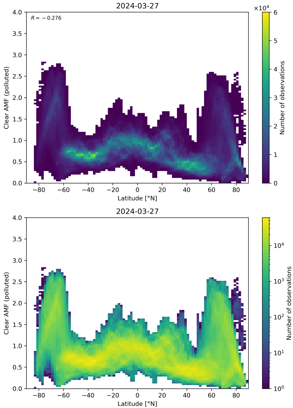
Figure 145: Scatter density plot of “Latitude” against “Clear AMF (polluted)” for 2024-03-26 to 2024-03-28.
