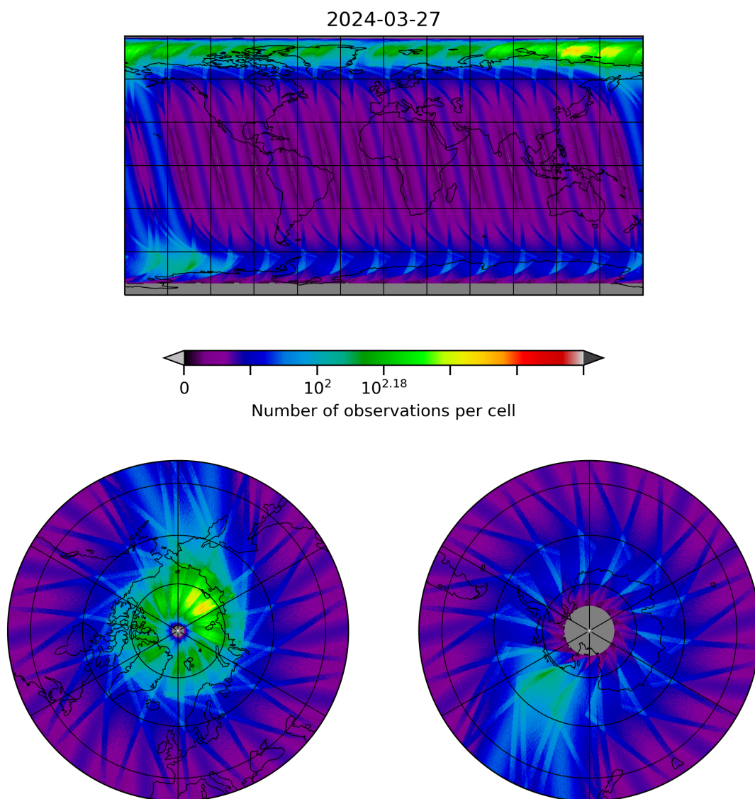
Figure 28: Map of the number of observations for 2024-03-26 to 2024-03-28
