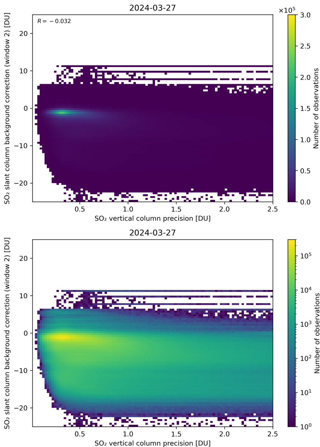
Figure 280: Scatter density plot of “SO 2 vertical column precision” against “SO 2 slant column background correction (window 2)” for 2024-03-26 to 2024-03-28.
