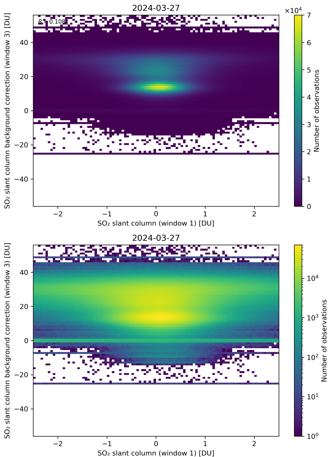
Figure 214: Scatter density plot of “SO 2 slant column (window 1)” against “SO 2 slant column background correction (window 3)” for 2024-03-26 to 2024-03-28.
