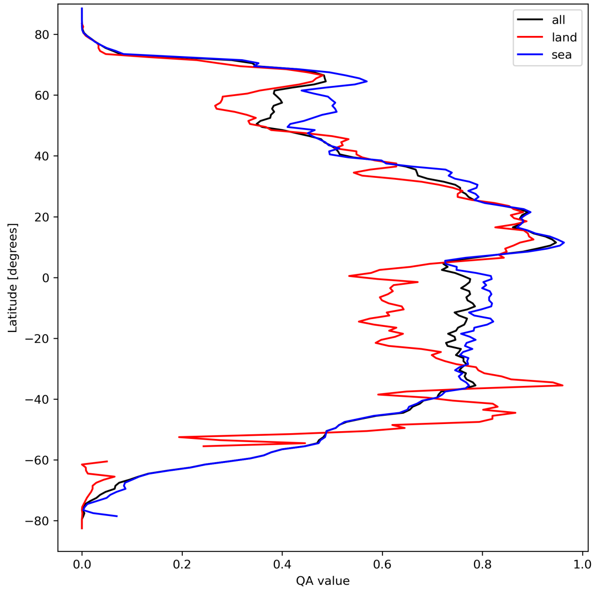
Figure 29: Zonal average of “QA value” for 2024-03-26 to 2024-03-28.
