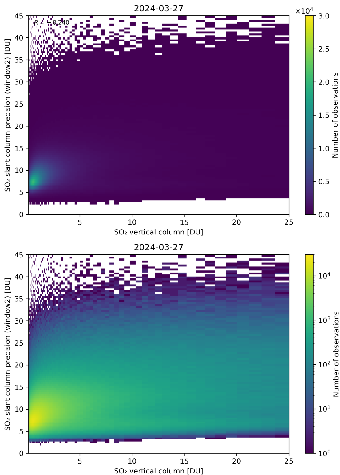
Figure 302: Scatter density plot of “SO 2 vertical column” against “SO 2 slant column precision (window2)” for 2024-03-26 to 2024-03-28.
