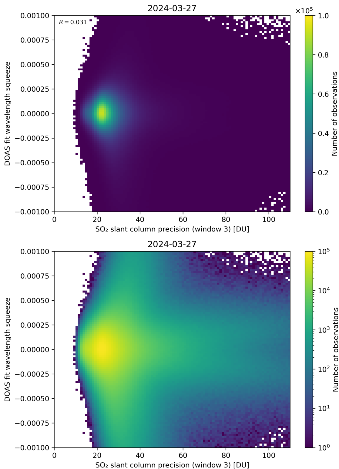
Figure 259: Scatter density plot of “SO 2 slant column precision (window 3)” against “DOAS fit wavelength squeeze” for 2024-03-26 to 2024-03-28.
