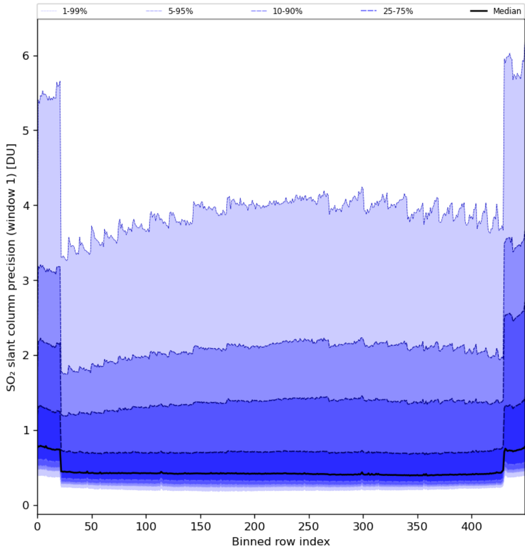
Figure 80: Along track statistics of “SO 2 slant column precision (window 1)” for 2024-03-26 to 2024-03-28
