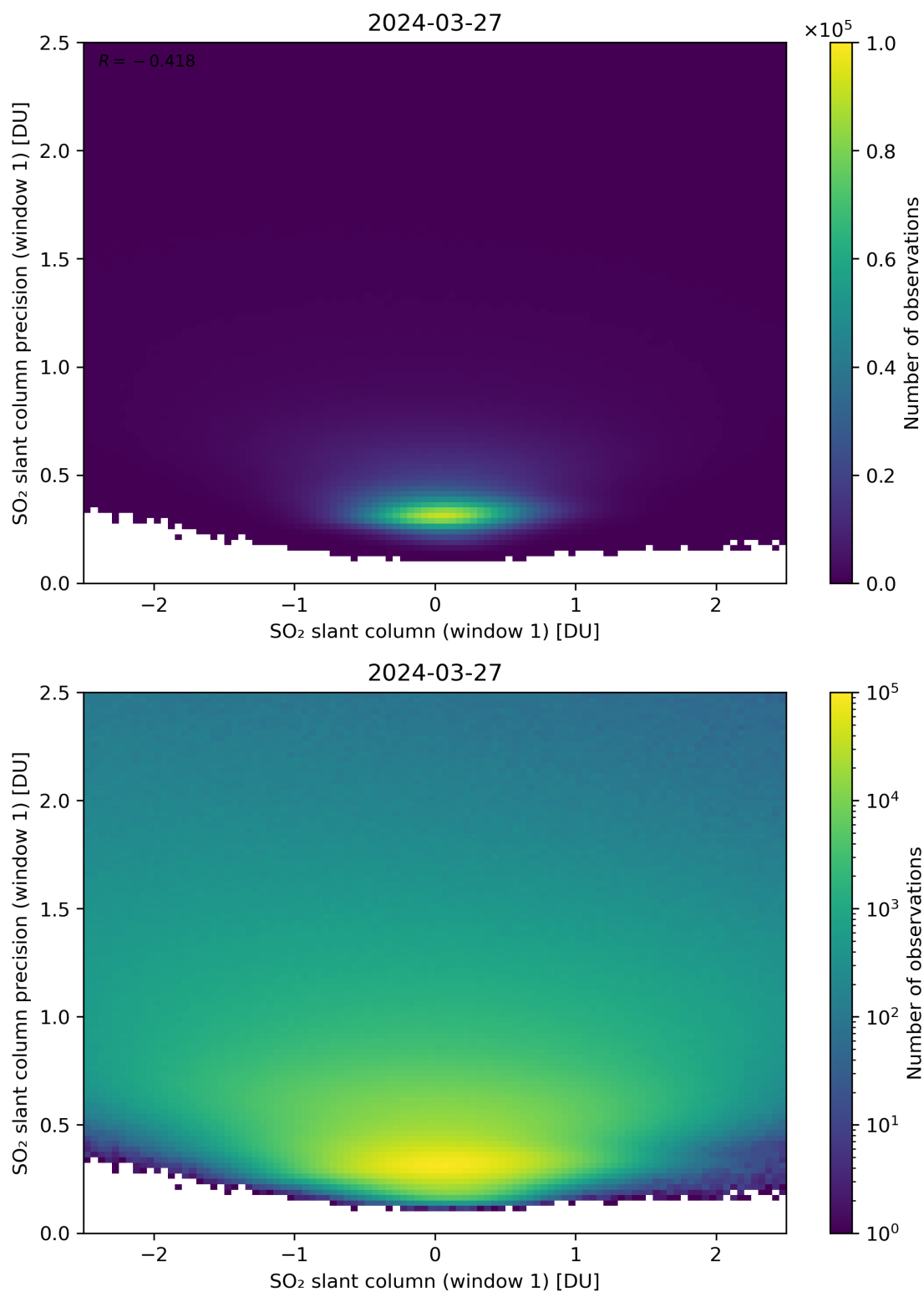
Figure 235: Scatter density plot of “SO 2 slant column (window 1)” against “SO 2 slant column precision (window 1)” for 2024-03-26 to 2024-03-28.
