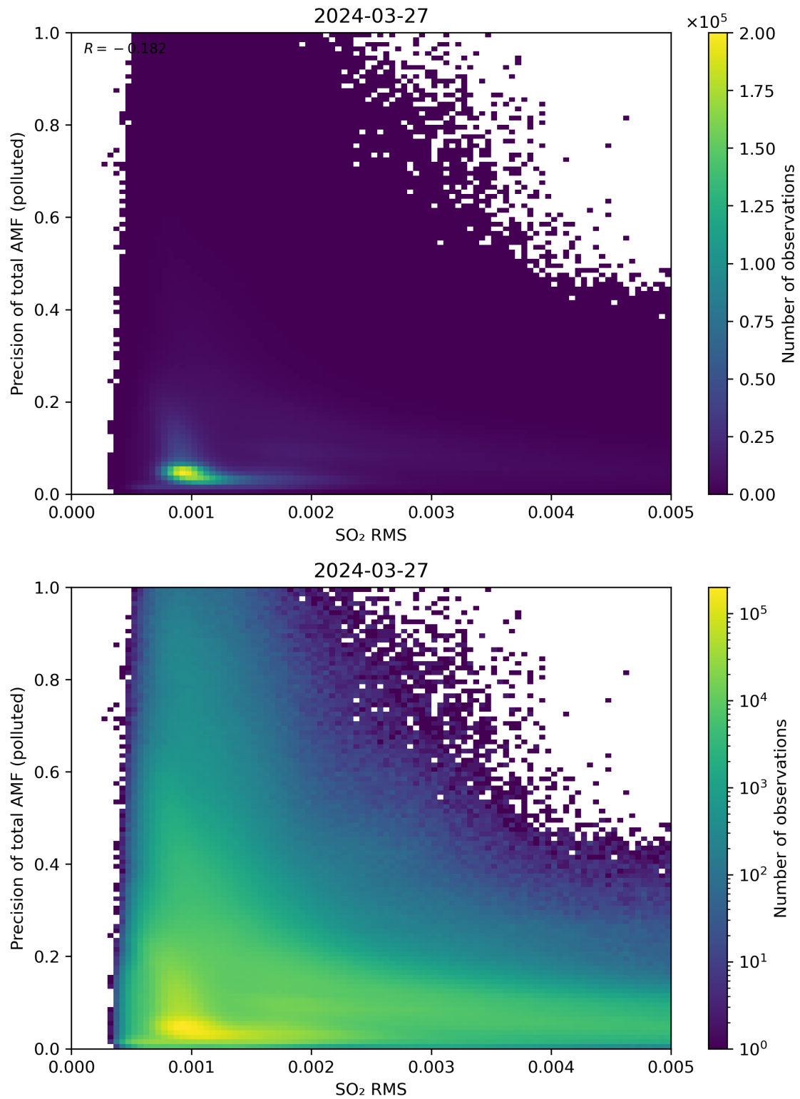
Figure 138: Scatter density plot of “SO 2 RMS” against “Precision of total AMF (polluted)” for 2024-03-26 to 2024-03-28.
