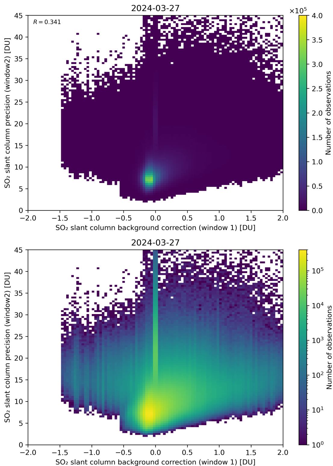
Figure 106: Scatter density plot of “SO 2 slant column background correction (window 1)” against “SO 2 slant column precision (window2)” for 2024-03-26 to 2024-03-28.
