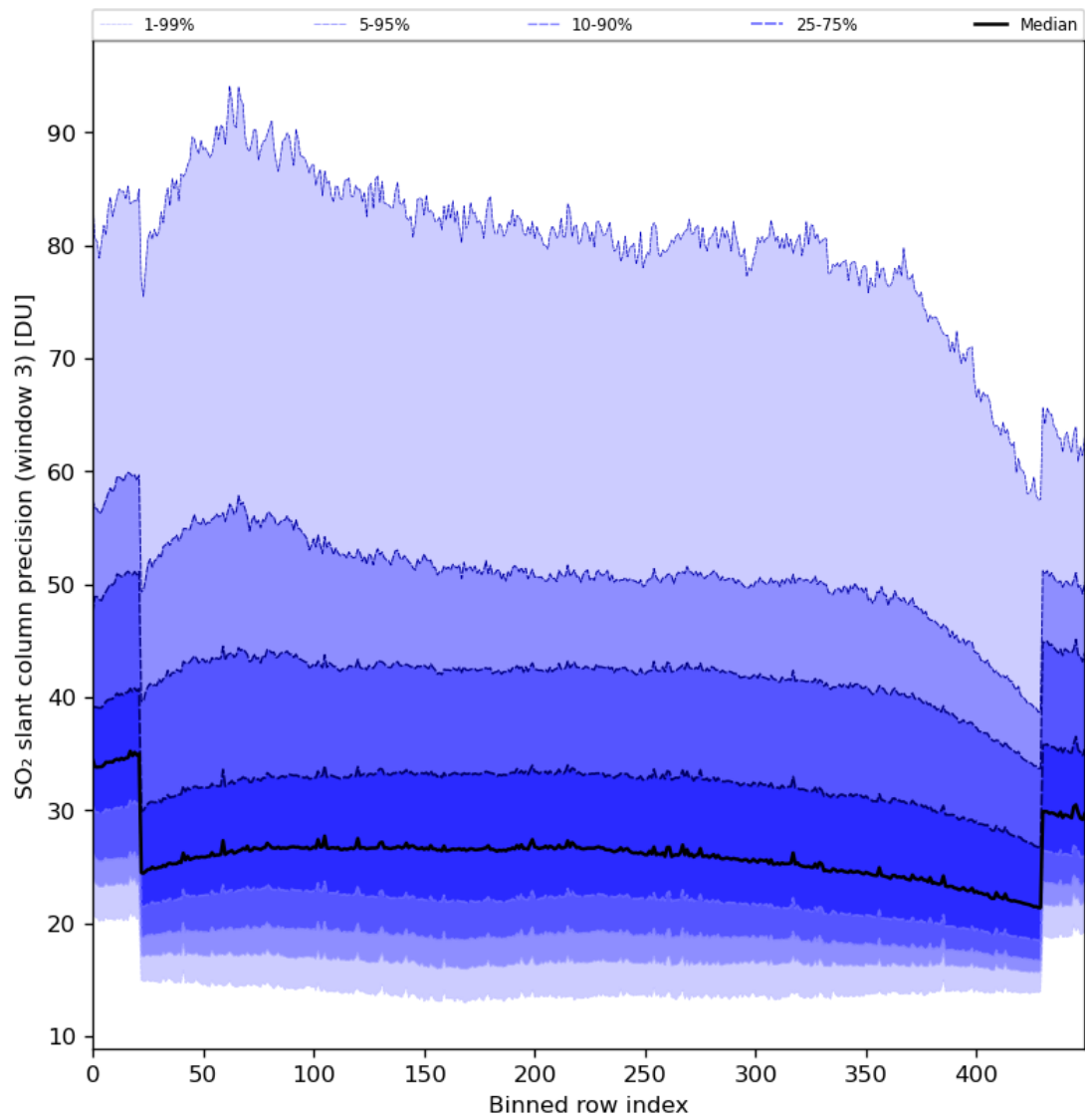
Figure 88: Along track statistics of “SO 2 slant column precision (window 3)” for 2024-03-26 to 2024-03-28
