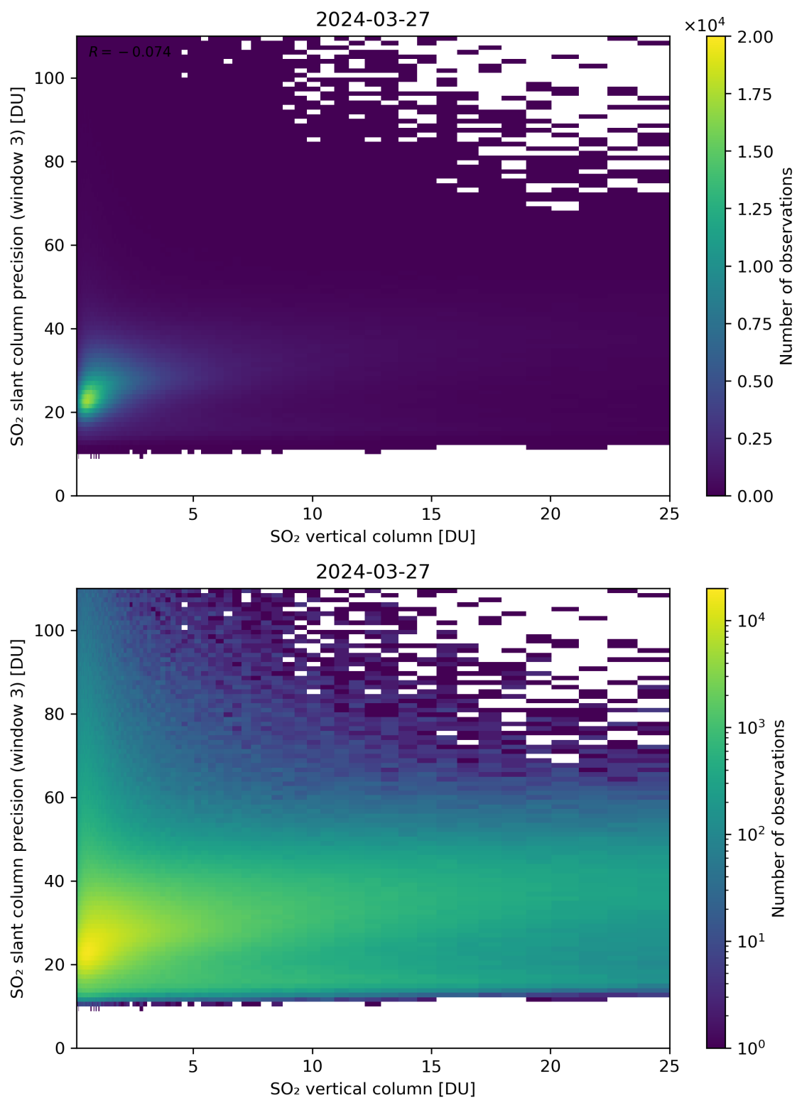
Figure 304: Scatter density plot of “SO 2 vertical column” against “SO 2 slant column precision (window 3)” for 2024-03-26 to 2024-03-28.
