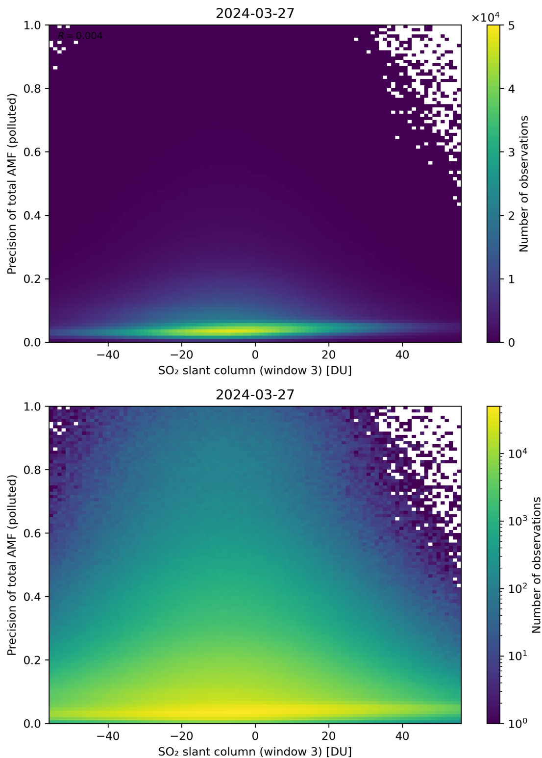
Figure 269: Scatter density plot of “SO 2 slant column (window 3)” against “Precision of total AMF (polluted)” for 2024-03-26 to 2024-03-28.
