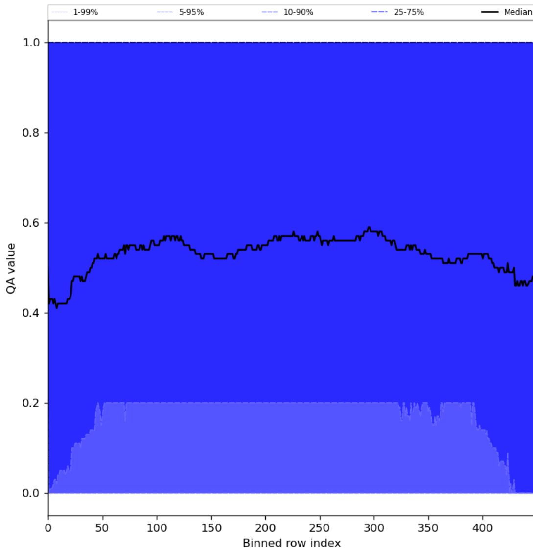
Figure 75: Along track statistics of “QA value” for 2024-03-26 to 2024-03-28
