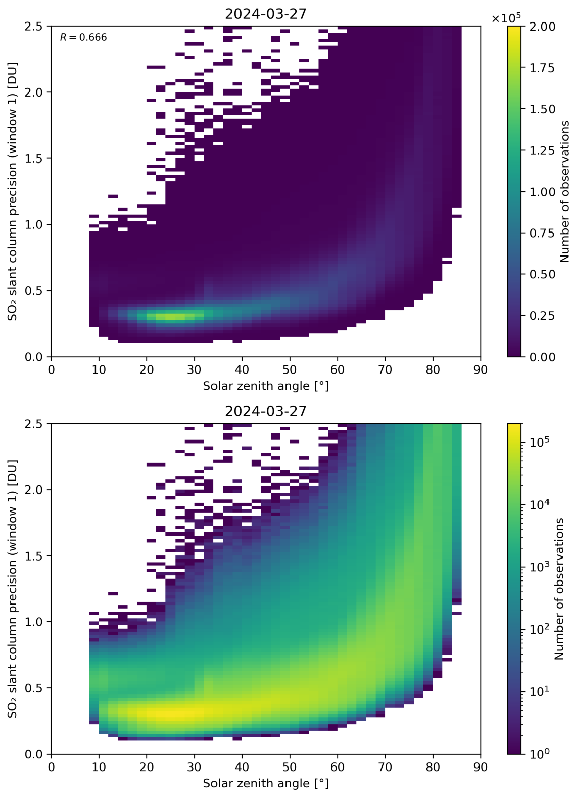
Figure 170: Scatter density plot of “Solar zenith angle” against “SO 2 slant column precision (window 1)” for 2024-03-26 to 2024-03-28.
