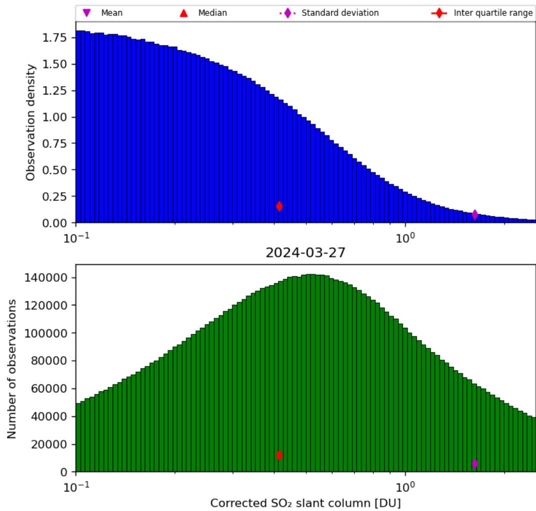
Figure 55: Histogram of “Corrected SO 2 slant column” for 2024-03-26 to 2024-03-28
