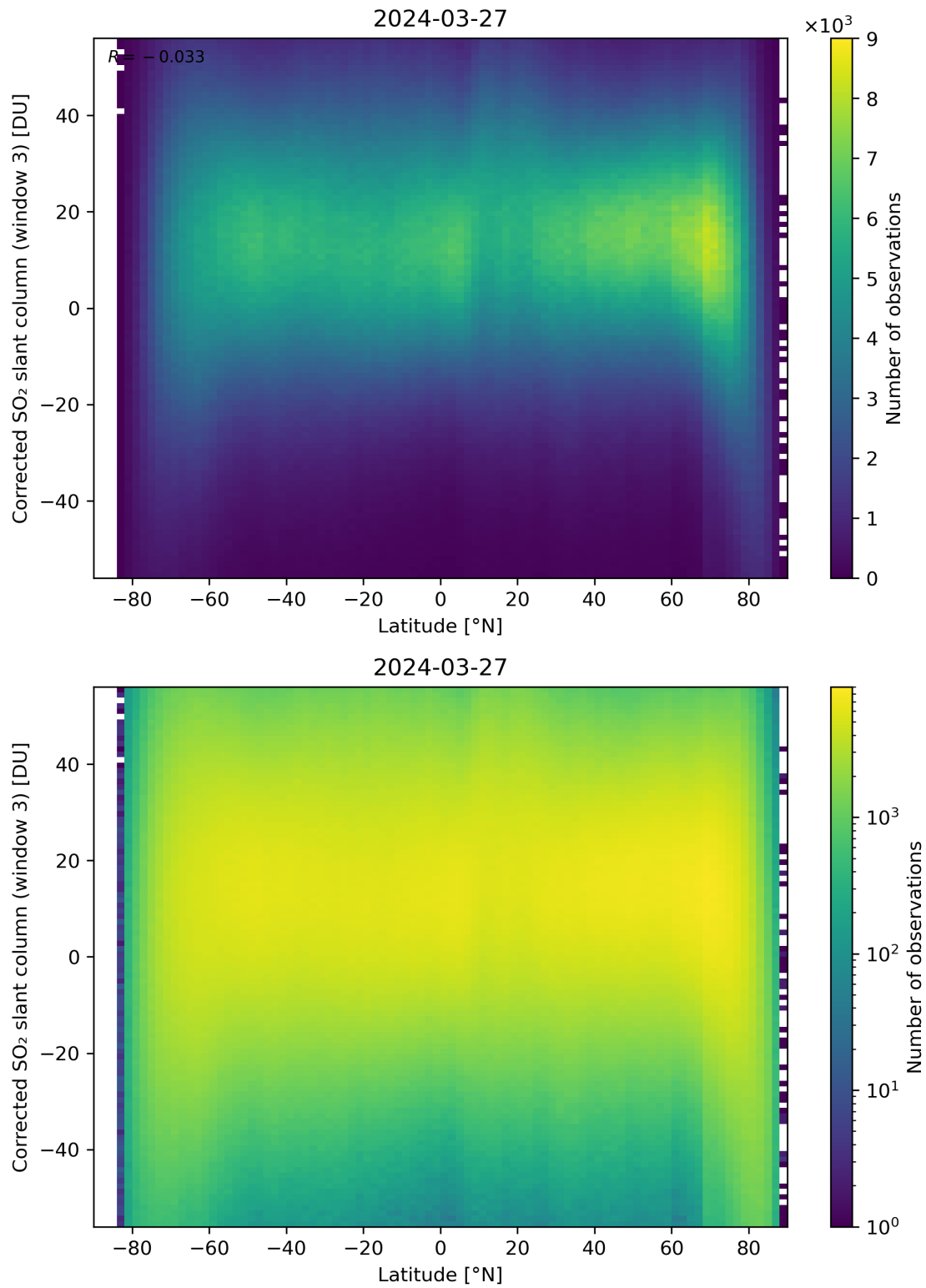
Figure 148: Scatter density plot of “Latitude” against “Corrected SO 2 slant column (window 3)” for 2024-03-26 to 2024-03-28.
