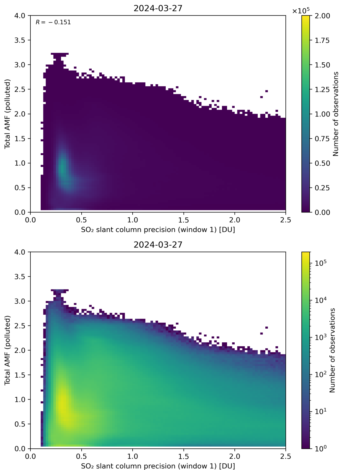
Figure 230: Scatter density plot of “SO 2 slant column precision (window 1)” against “Total AMF (polluted)” for 2024-03-26 to 2024-03-28.
