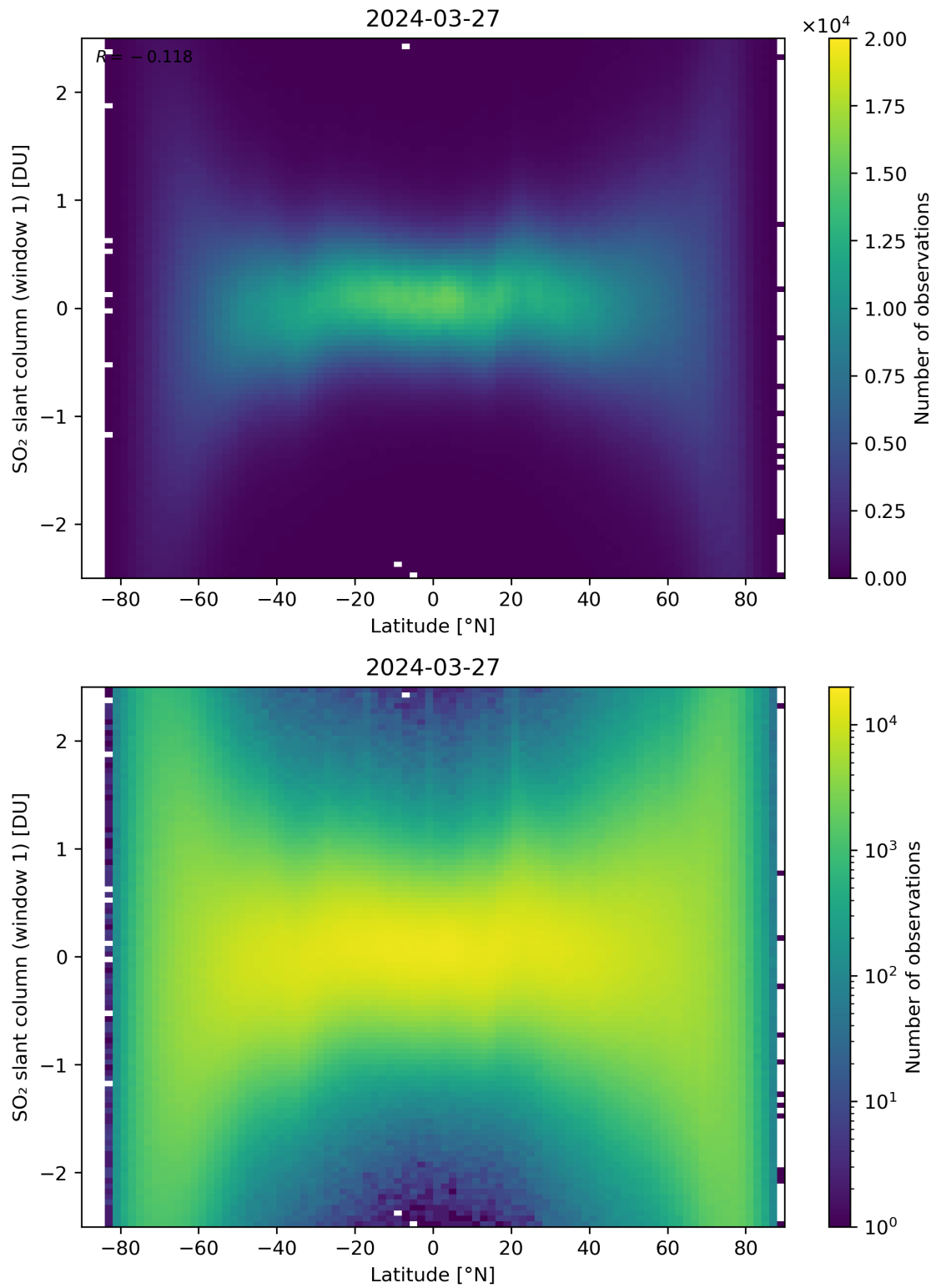
Figure 149: Scatter density plot of “Latitude” against “SO 2 slant column (window 1)” for 2024-03-26 to 2024-03-28.
