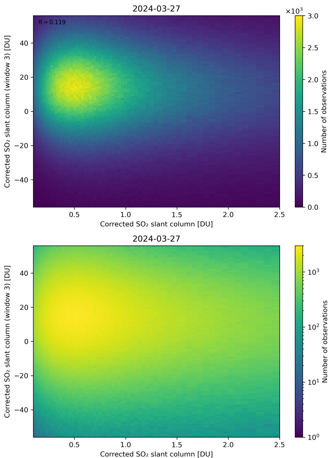
Figure 186: Scatter density plot of “Corrected SO 2 slant column” against “Corrected SO 2 slant column (window 3)” for 2024-03-26 to 2024-03-28.
