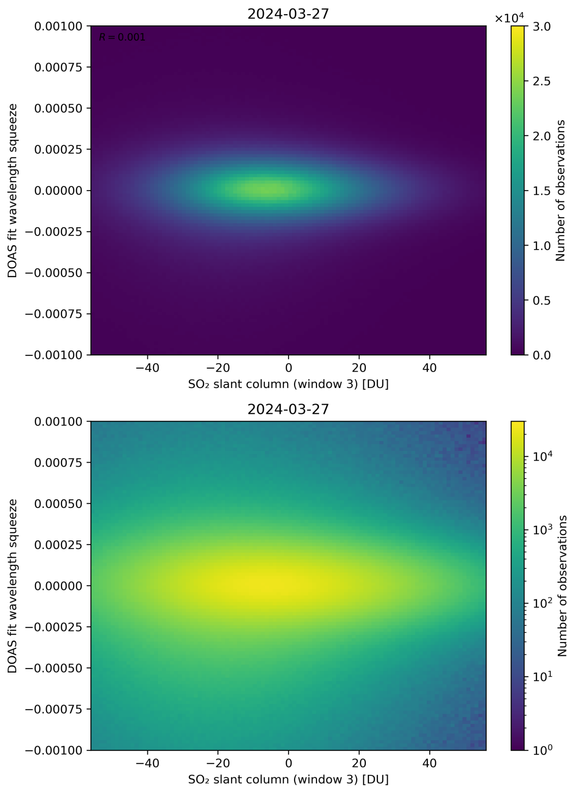
Figure 255: Scatter density plot of “SO 2 slant column (window 3)” against “DOAS fit wavelength squeeze” for 2024-03-26 to 2024-03-28.
