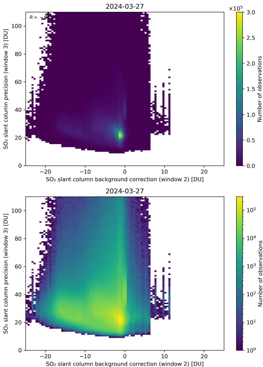
Figure 118: Scatter density plot of “SO 2 slant column background correction (window 2)” against “SO 2 slant column precision (window 3)” for 2024-03-26 to 2024-03-28.
