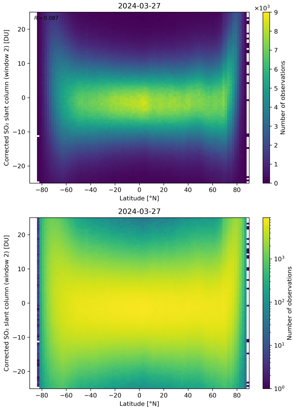
Figure 147: Scatter density plot of “Latitude” against “Corrected SO 2 slant column (window 2)” for 2024-03-26 to 2024-03-28.
