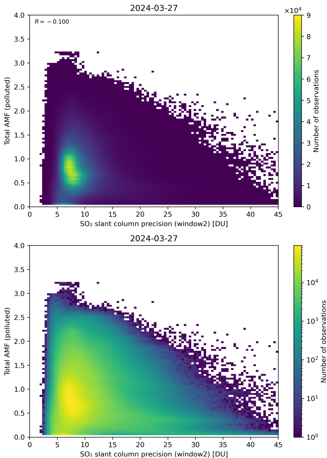
Figure 251: Scatter density plot of “SO 2 slant column precision (window2)” against “Total AMF (polluted)” for 2024-03-26 to 2024-03-28.
