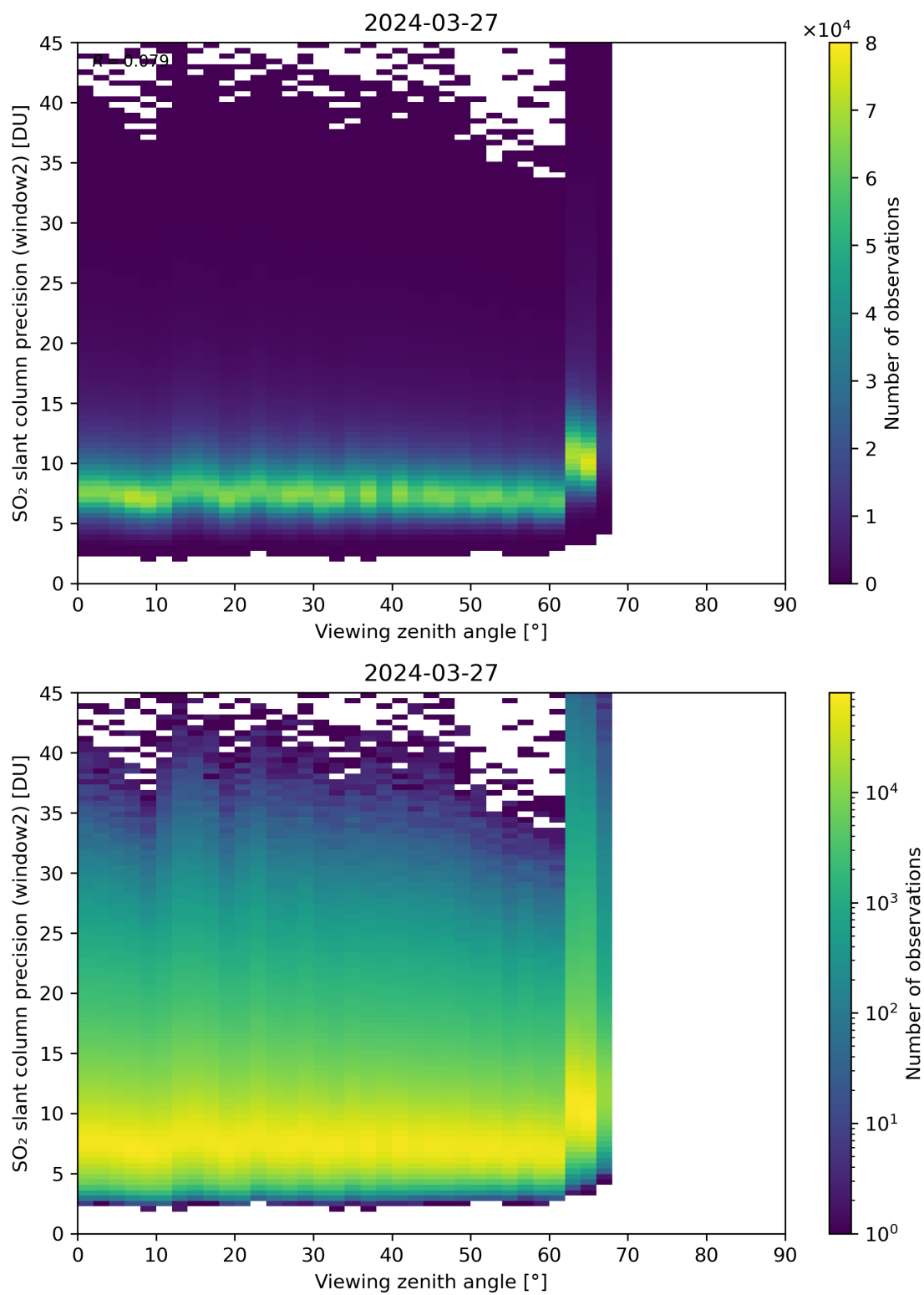
Figure 322: Scatter density plot of “Viewing zenith angle” against “SO 2 slant column precision (window2)” for 2024-03-26 to 2024-03-28.
