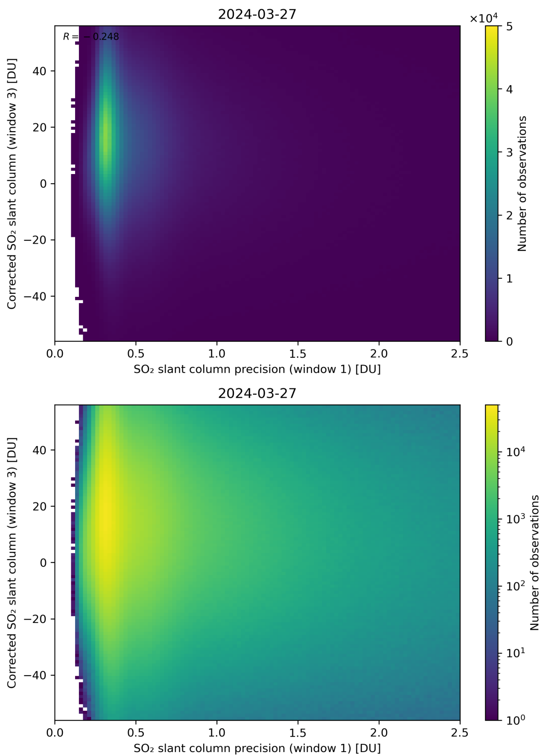
Figure 226: Scatter density plot of “SO 2 slant column precision (window 1)” against “Corrected SO 2 slant column (window 3)” for 2024-03-26 to 2024-03-28.
