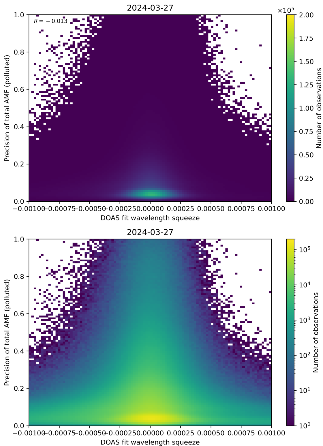
Figure 135: Scatter density plot of “DOAS fit wavelength squeeze” against “Precision of total AMF (polluted)” for 2024-03-26 to 2024-03-28.
