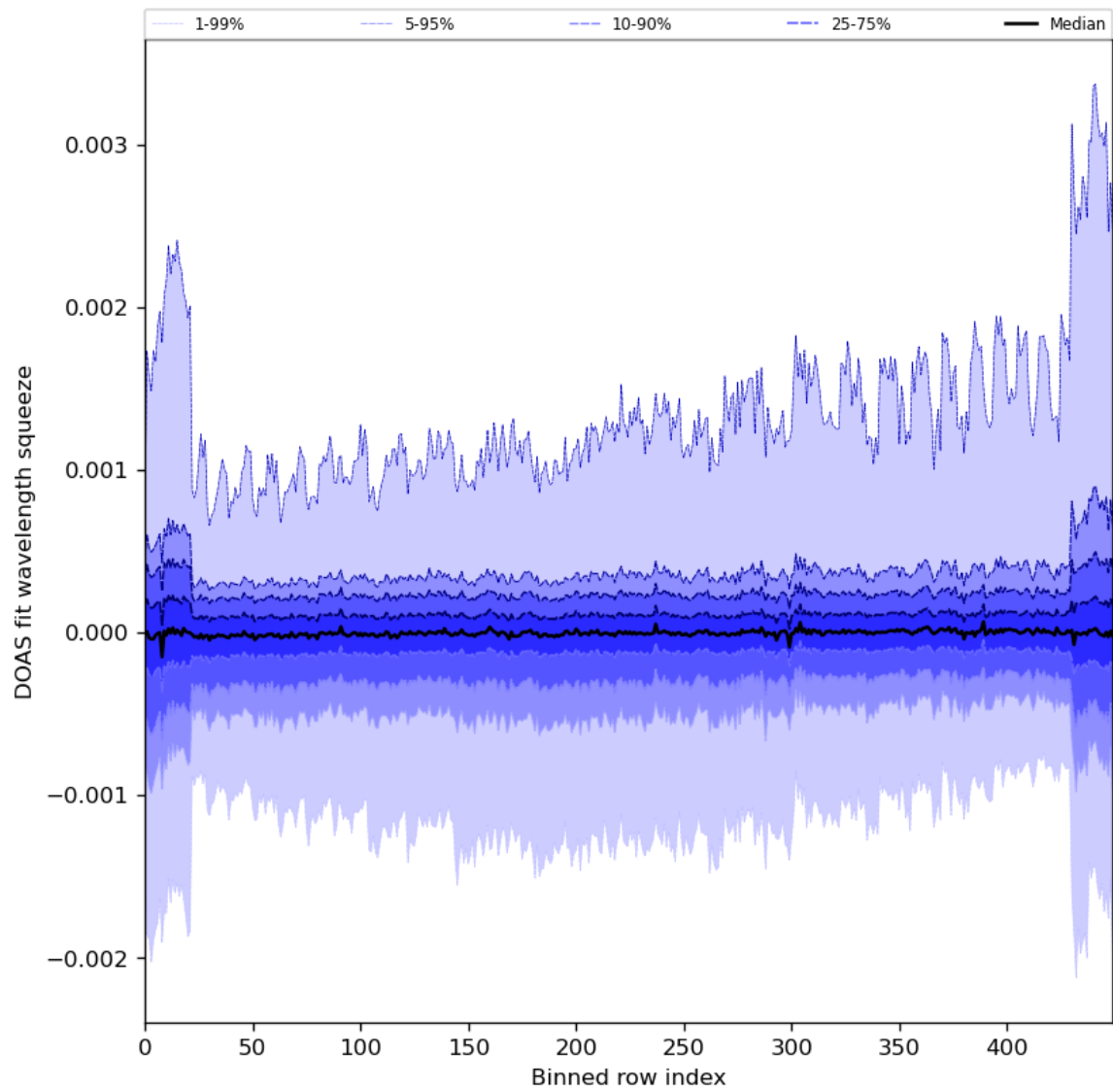
Figure 92: Along track statistics of “DOAS fit wavelength squeeze” for 2024-03-26 to 2024-03-28
