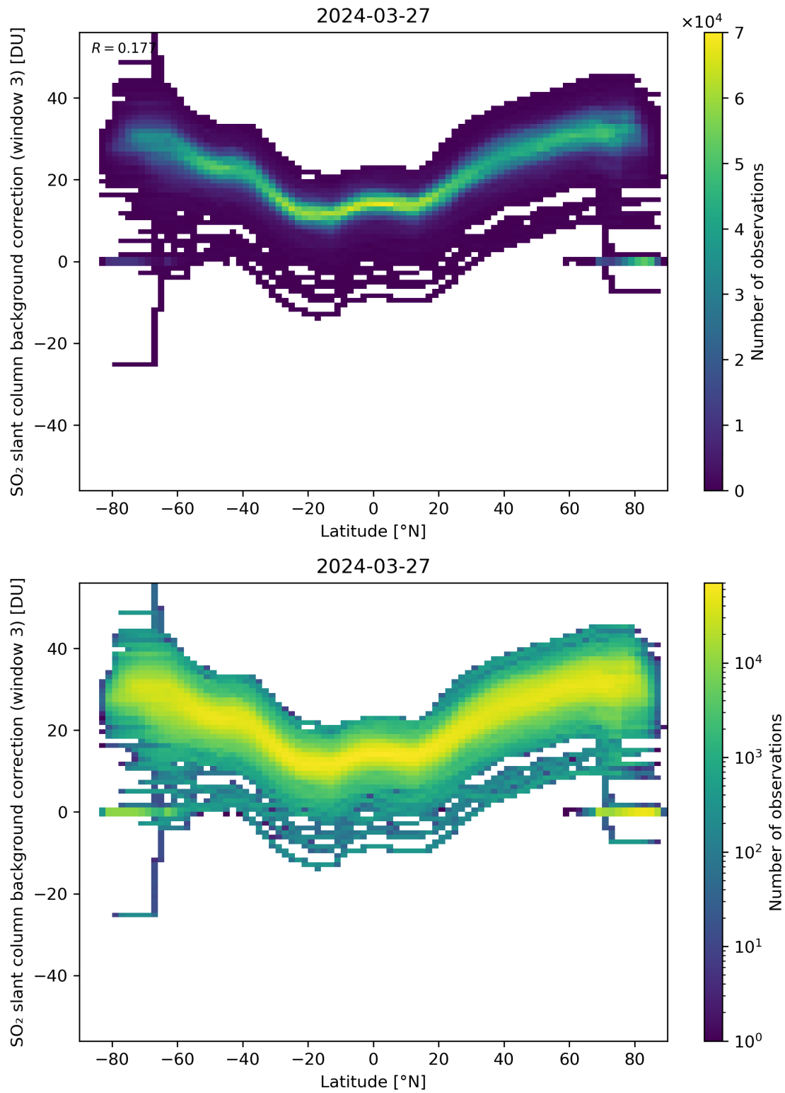
Figure 141: Scatter density plot of “Latitude” against “SO 2 slant column background correction (window 3)” for 2024-03-26 to 2024-03-28.
