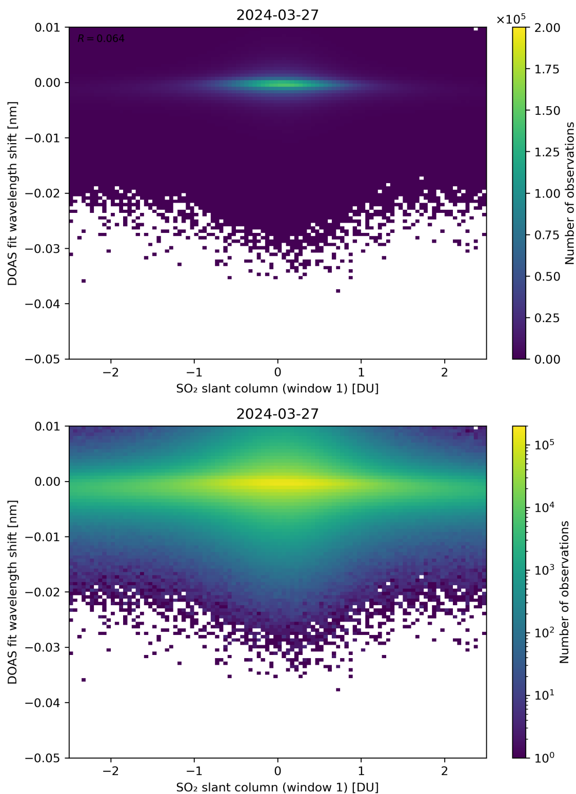
Figure 215: Scatter density plot of “SO 2 slant column (window 1)” against “DOAS fit wavelength shift” for 2024-03-26 to 2024-03-28.
