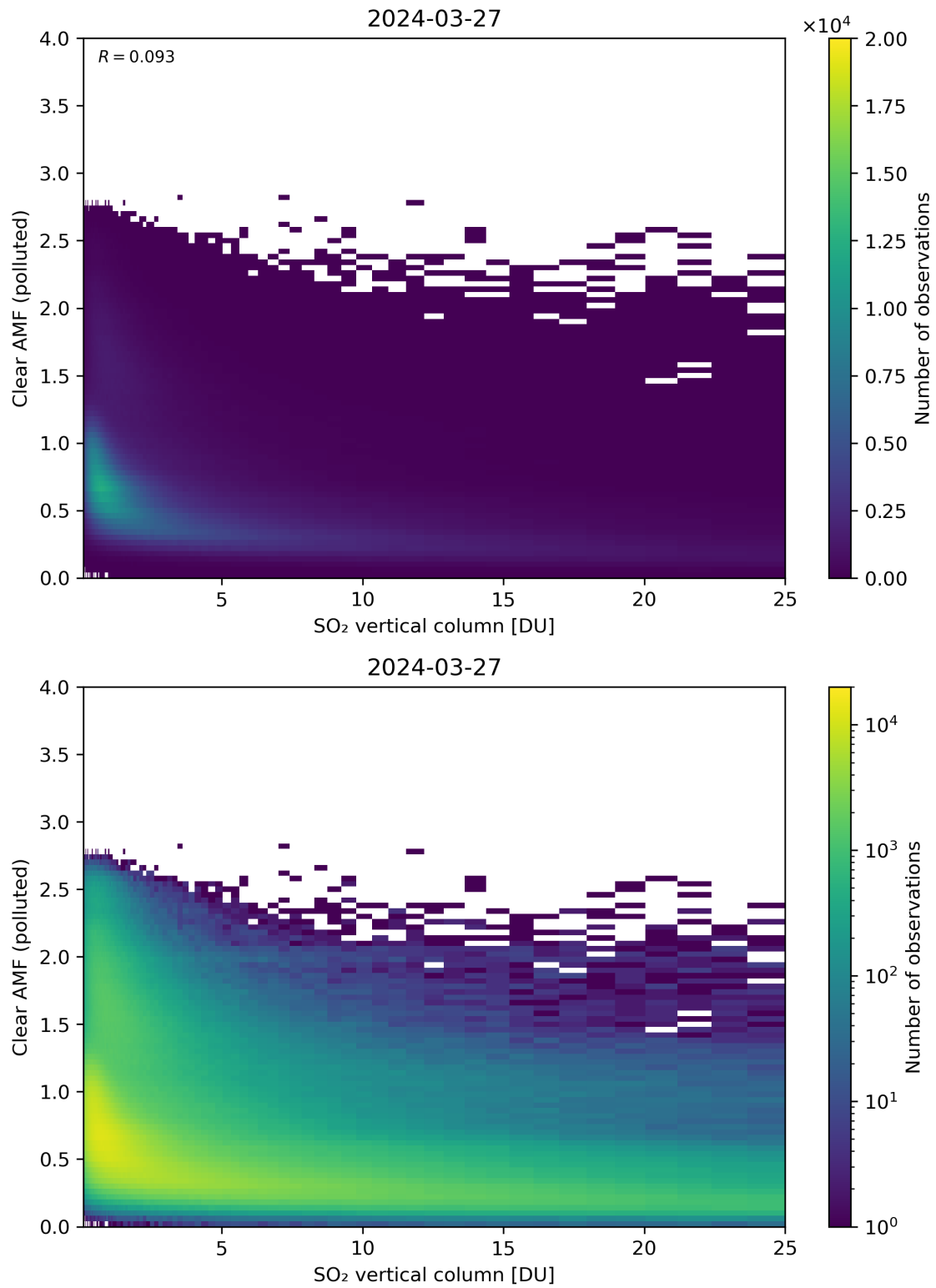
Figure 296: Scatter density plot of “SO 2 vertical column” against “Clear AMF (polluted)” for 2024-03-26 to 2024-03-28.
