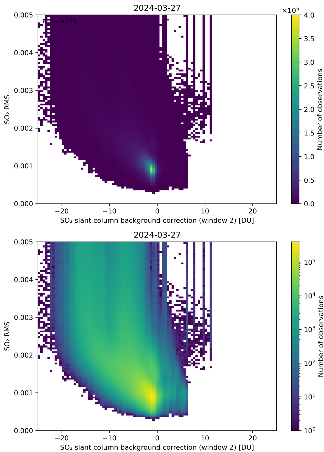
Figure 114: Scatter density plot of “SO 2 slant column background correction (window 2)” against “SO 2 RMS” for 2024-03-26 to 2024-03-28.
