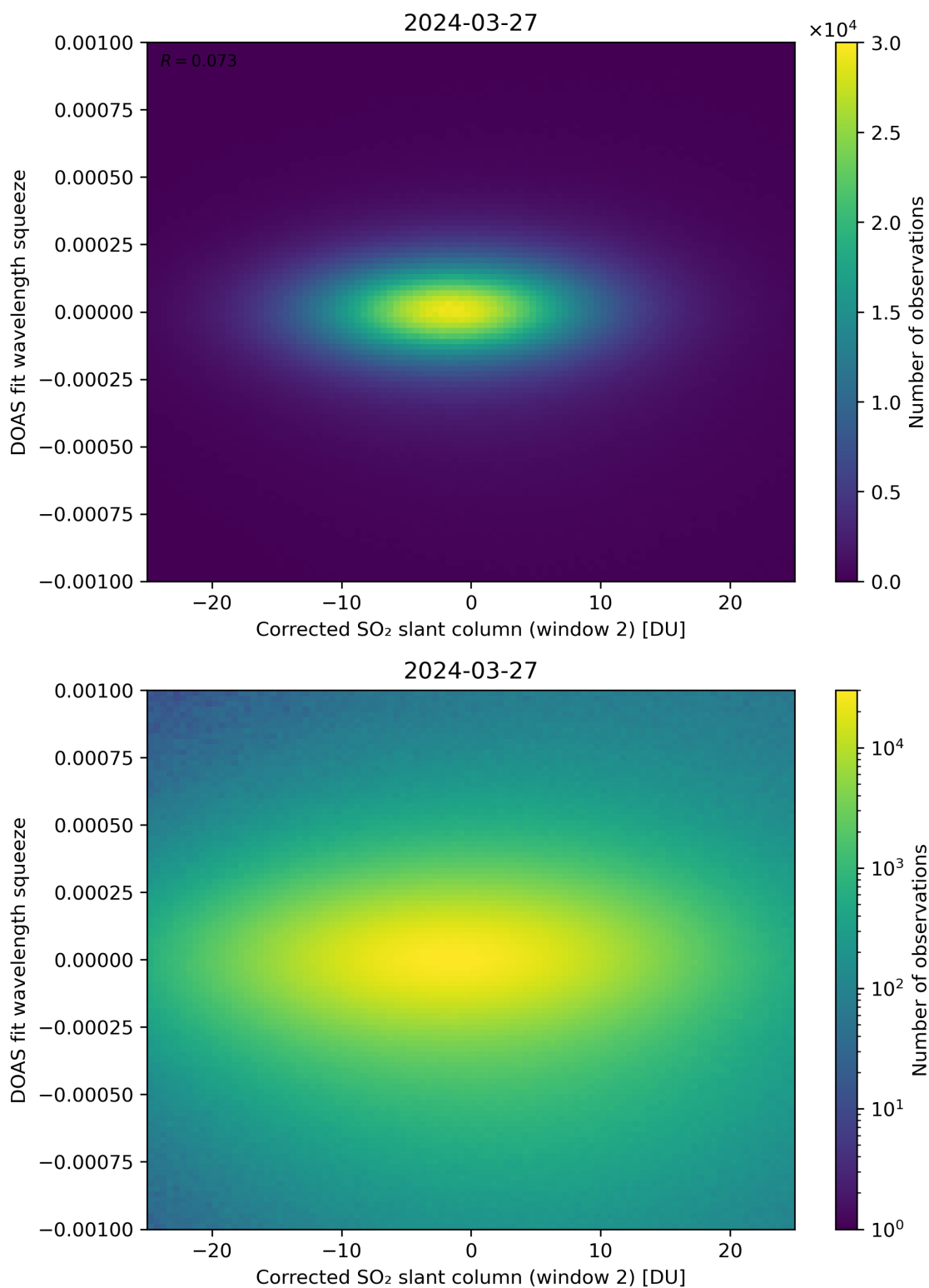
Figure 197: Scatter density plot of “Corrected SO 2 slant column (window 2)” against “DOAS fit wavelength squeeze” for 2024-03-26 to 2024-03-28.
