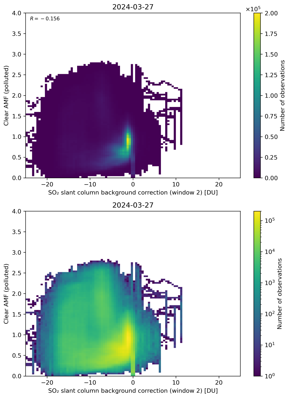
Figure 115: Scatter density plot of “SO 2 slant column background correction (window 2)” against “Clear AMF (polluted)” for 2024-03-26 to 2024-03-28.
