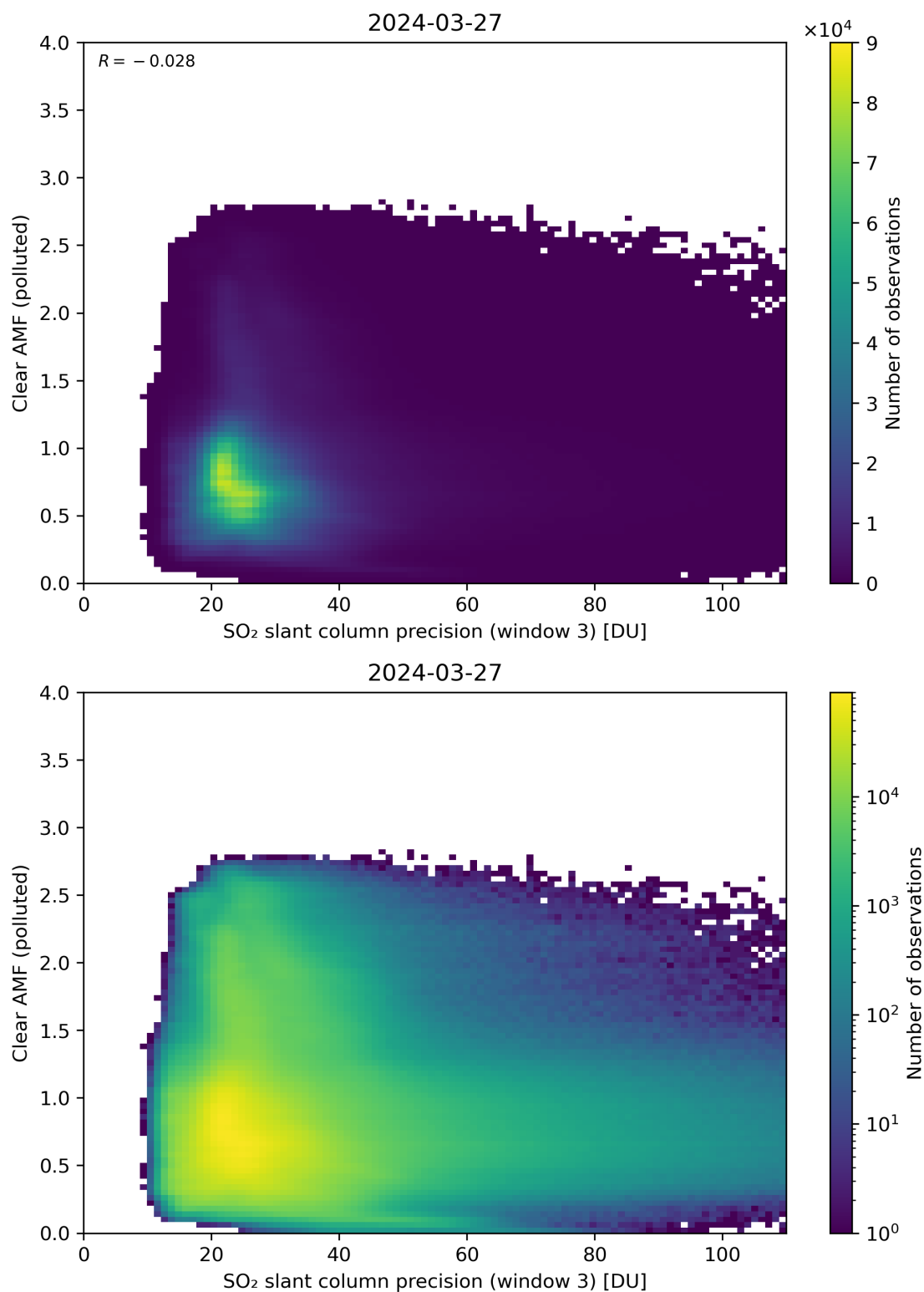
Figure 261: Scatter density plot of “SO 2 slant column precision (window 3)” against “Clear AMF (polluted)” for 2024-03-26 to 2024-03-28.
