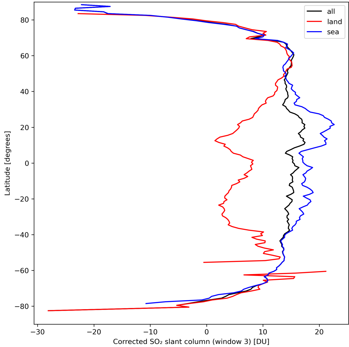
Figure 43: Zonal average of “Corrected SO 2 slant column (window 3)” for 2024-03-26 to 2024-03-28.
