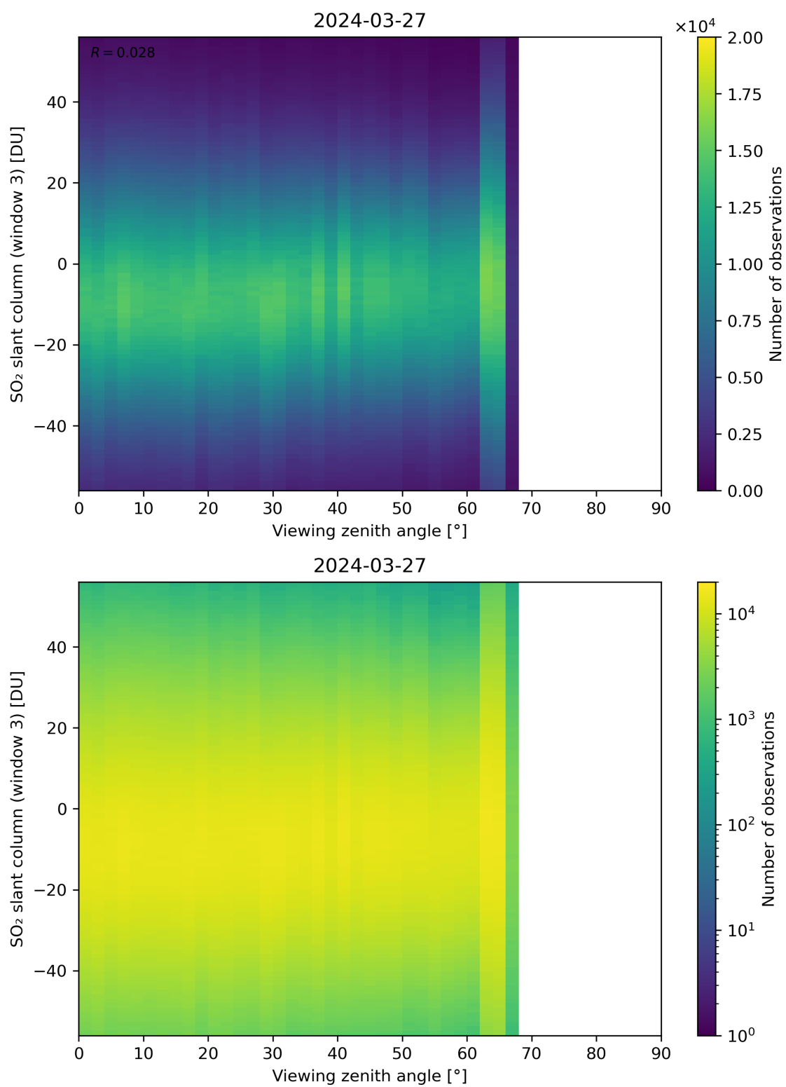
Figure 323: Scatter density plot of “Viewing zenith angle” against “SO 2 slant column (window 3)” for 2024-03-26 to 2024-03-28.
