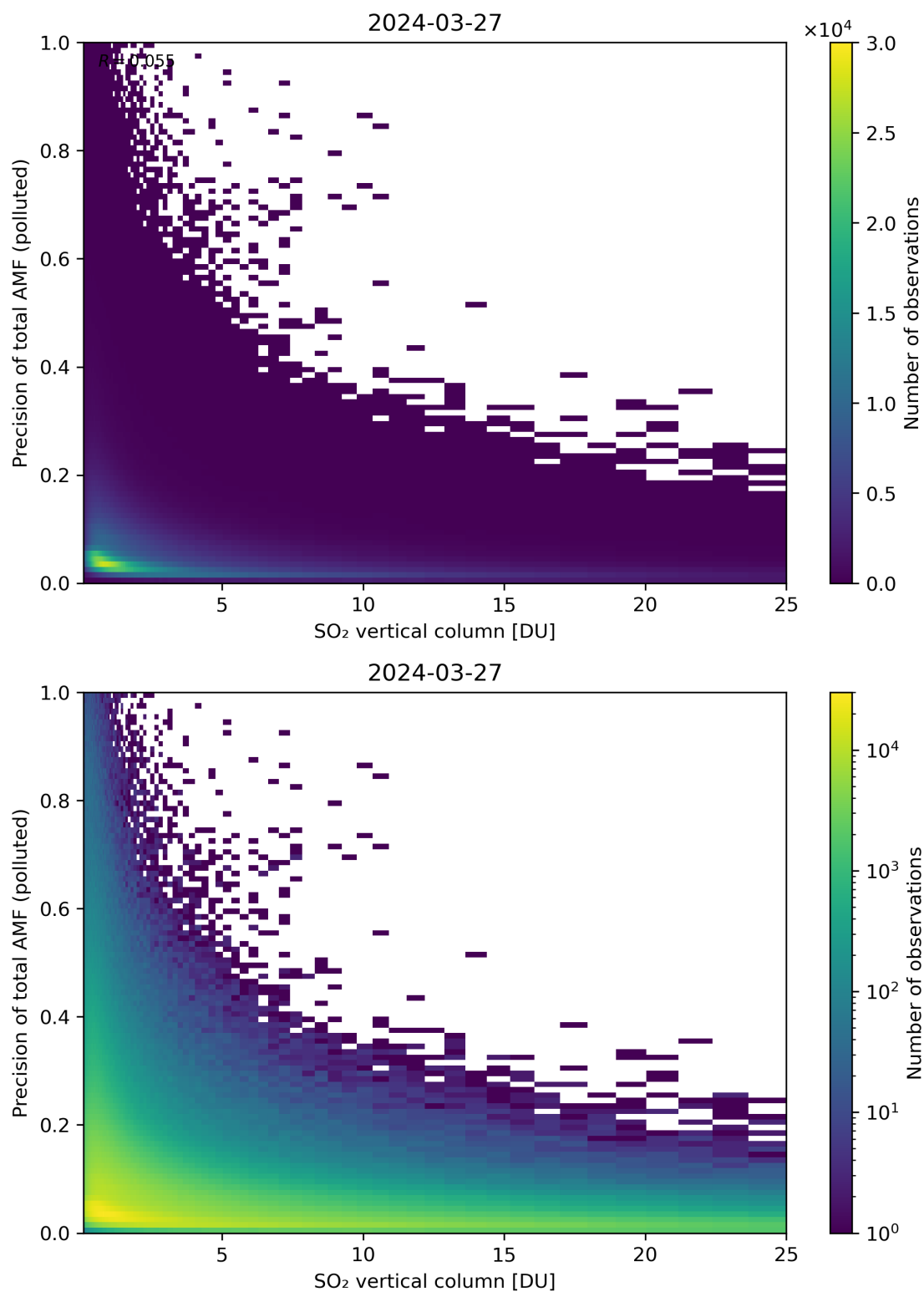
Figure 306: Scatter density plot of “SO 2 vertical column” against “Precision of total AMF (polluted)” for 2024-03-26 to 2024-03-28.
