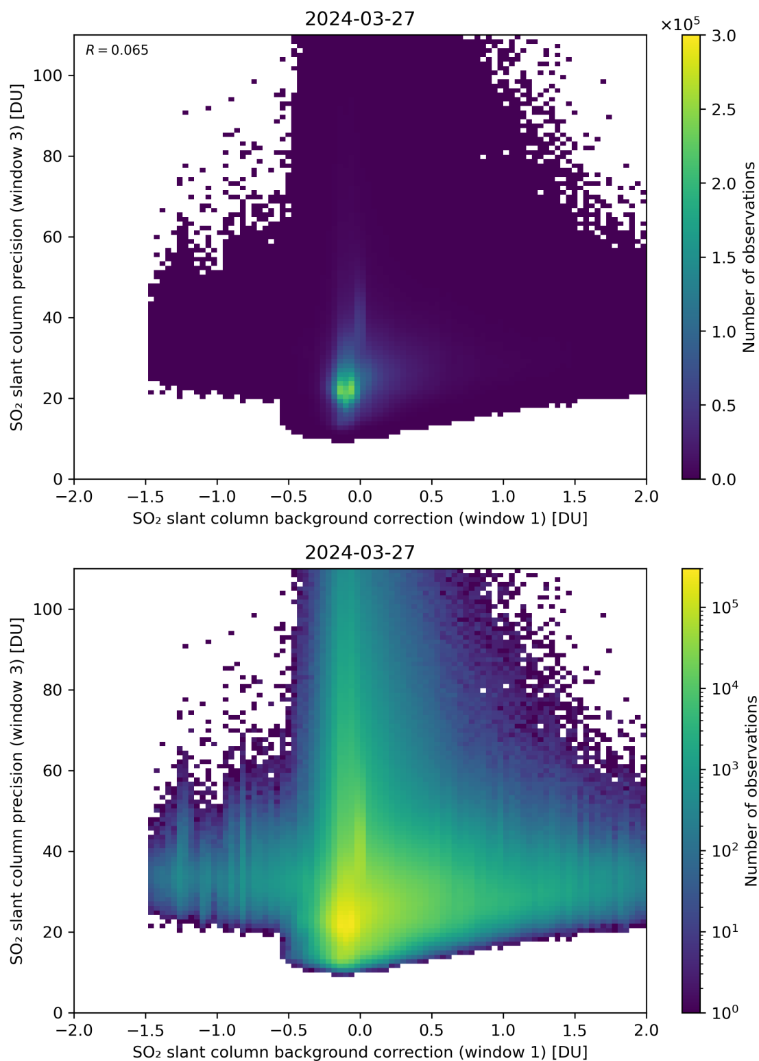
Figure 108: Scatter density plot of “SO 2 slant column background correction (window 1)” against “SO 2 slant column precision (window 3)” for 2024-03-26 to 2024-03-28.
