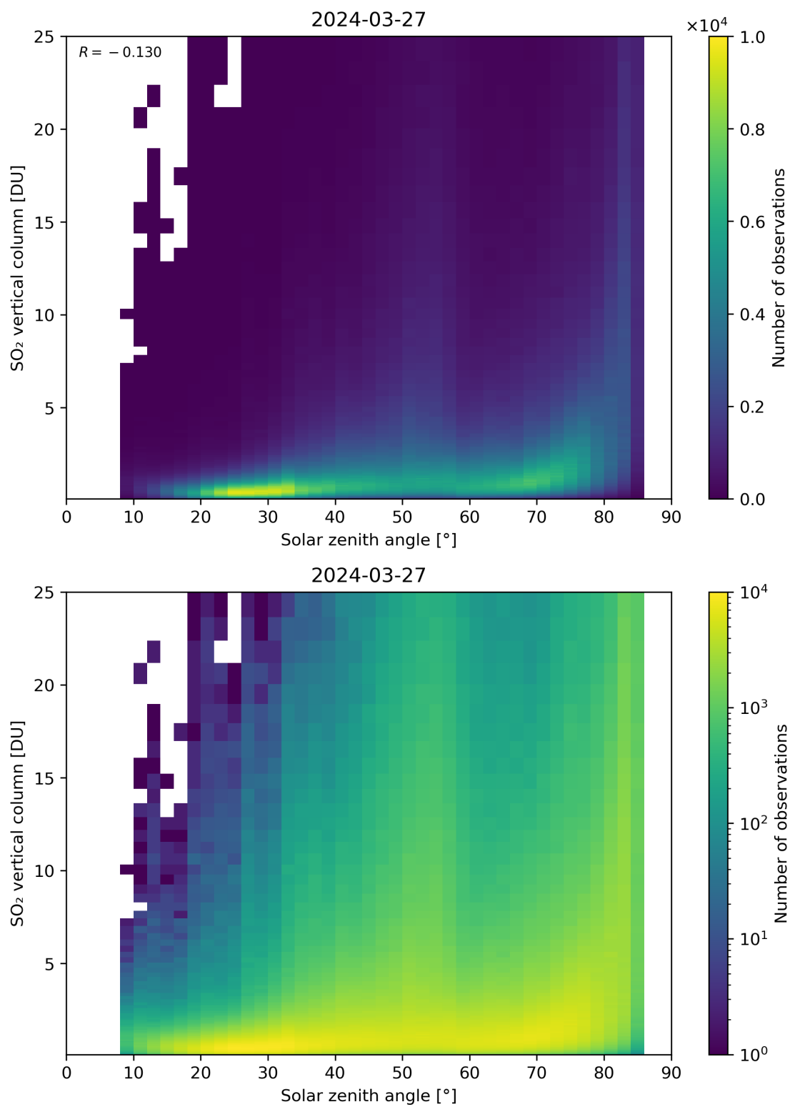
Figure 176: Scatter density plot of “Solar zenith angle” against “SO 2 vertical column” for 2024-03-26 to 2024-03-28.
