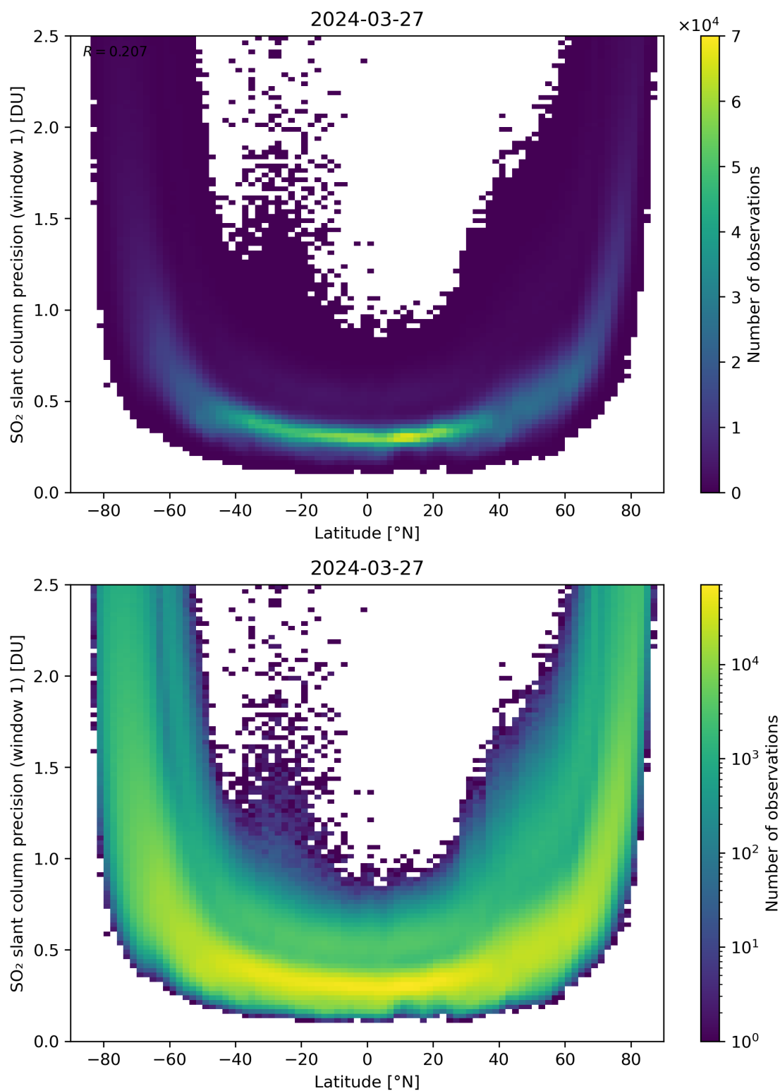
Figure 150: Scatter density plot of “Latitude” against “SO 2 slant column precision (window 1)” for 2024-03-26 to 2024-03-28.
