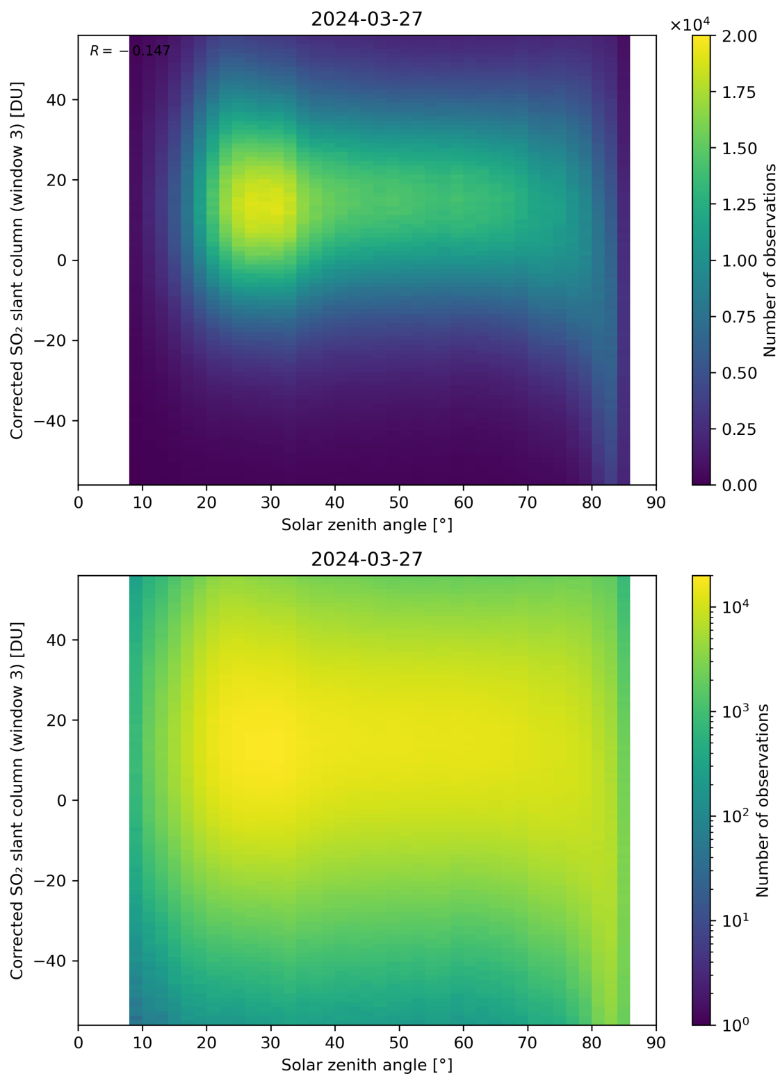
Figure 168: Scatter density plot of “Solar zenith angle” against “Corrected SO 2 slant column (window 3)” for 2024-03-26 to 2024-03-28.
