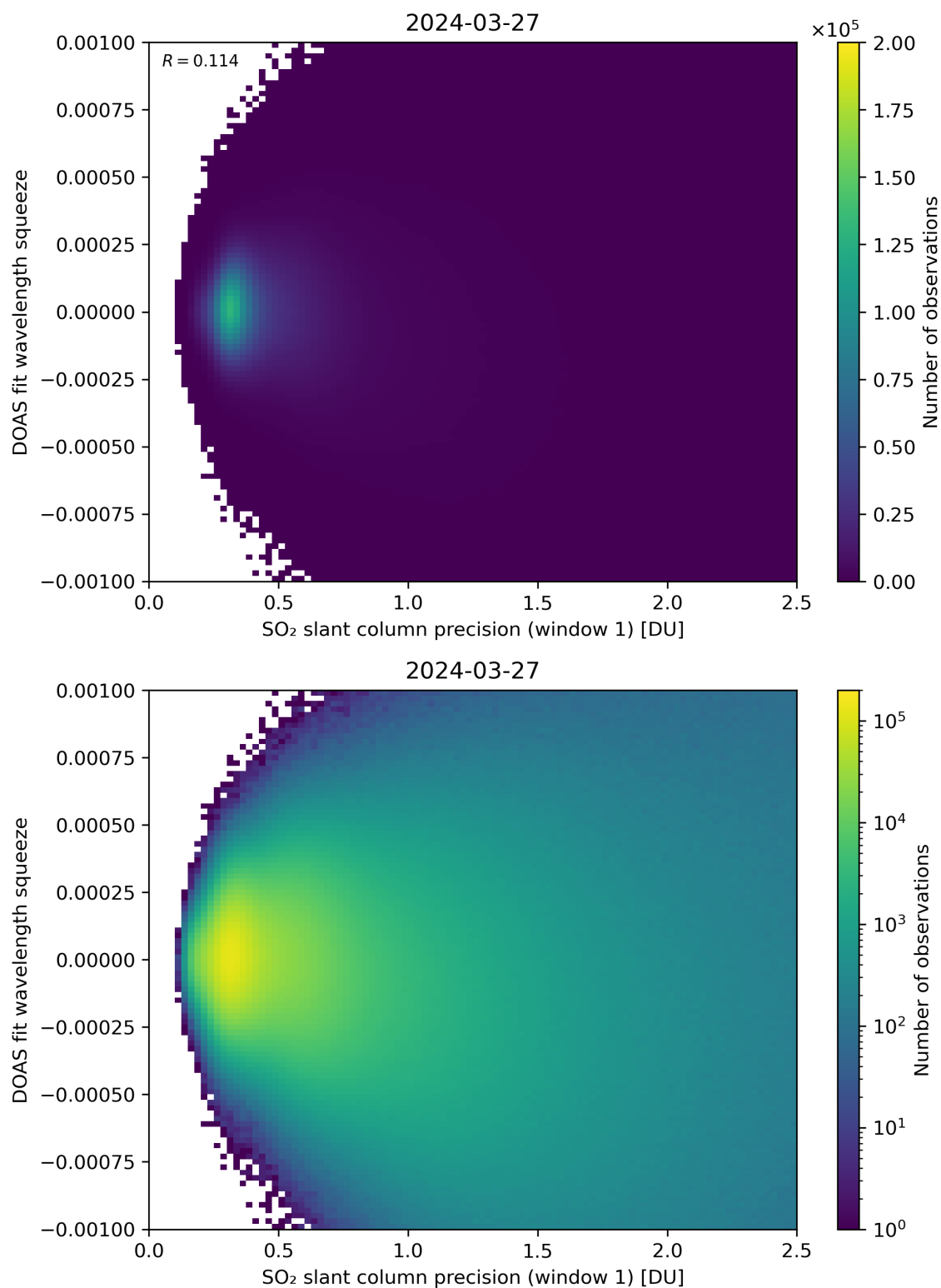
Figure 222: Scatter density plot of “SO 2 slant column precision (window 1)” against “DOAS fit wavelength squeeze” for 2024-03-26 to 2024-03-28.
