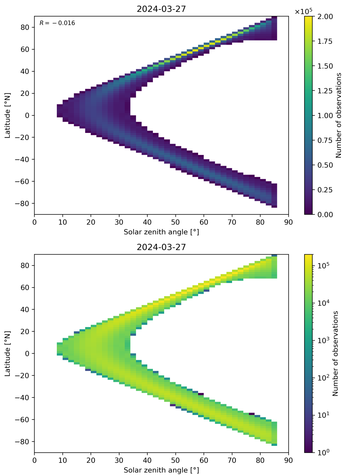
Figure 164: Scatter density plot of “Solar zenith angle” against “Latitude” for 2024-03-26 to 2024-03-28.
