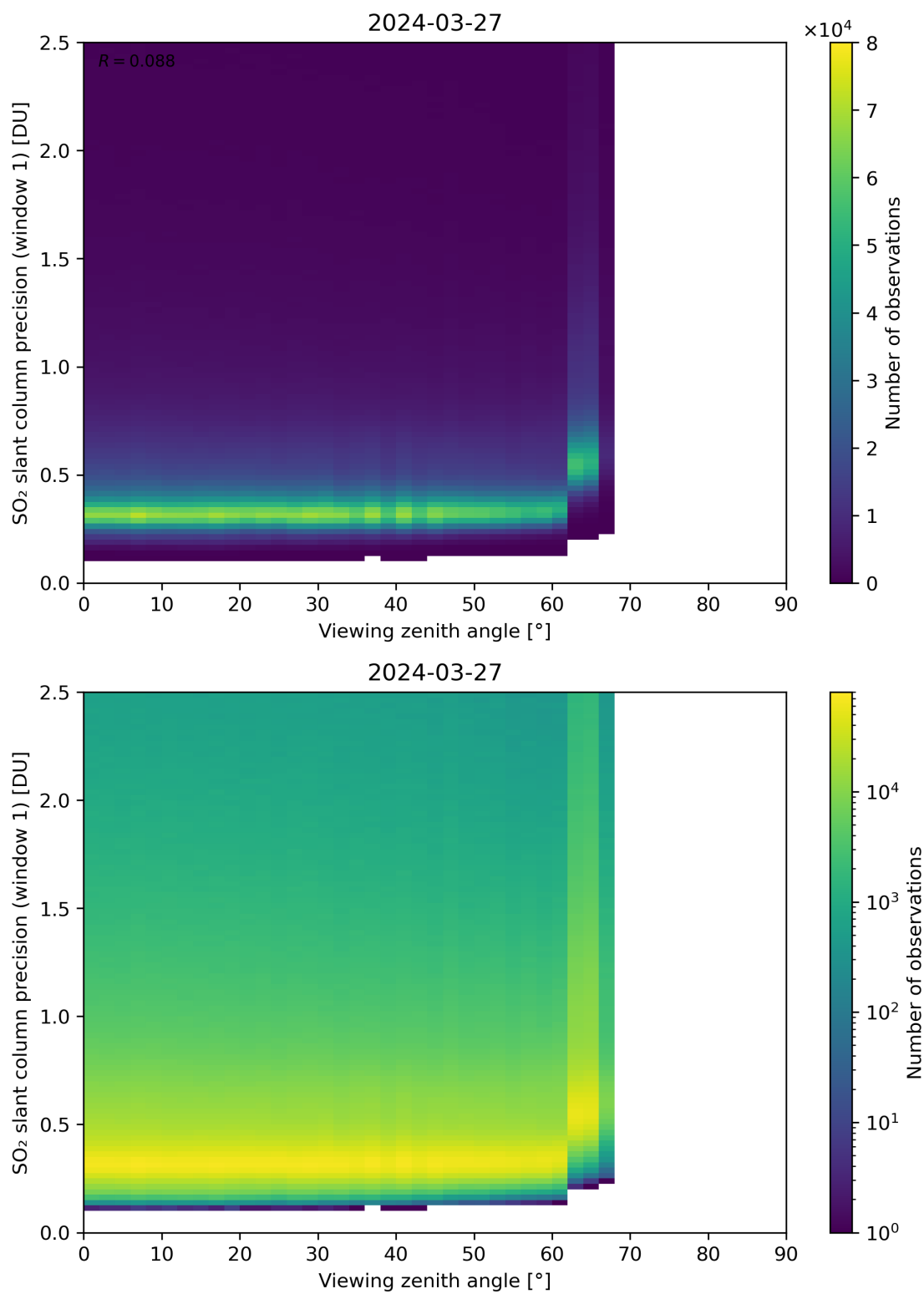
Figure 321: Scatter density plot of “Viewing zenith angle” against “SO 2 slant column precision (window 1)” for 2024-03-26 to 2024-03-28.
