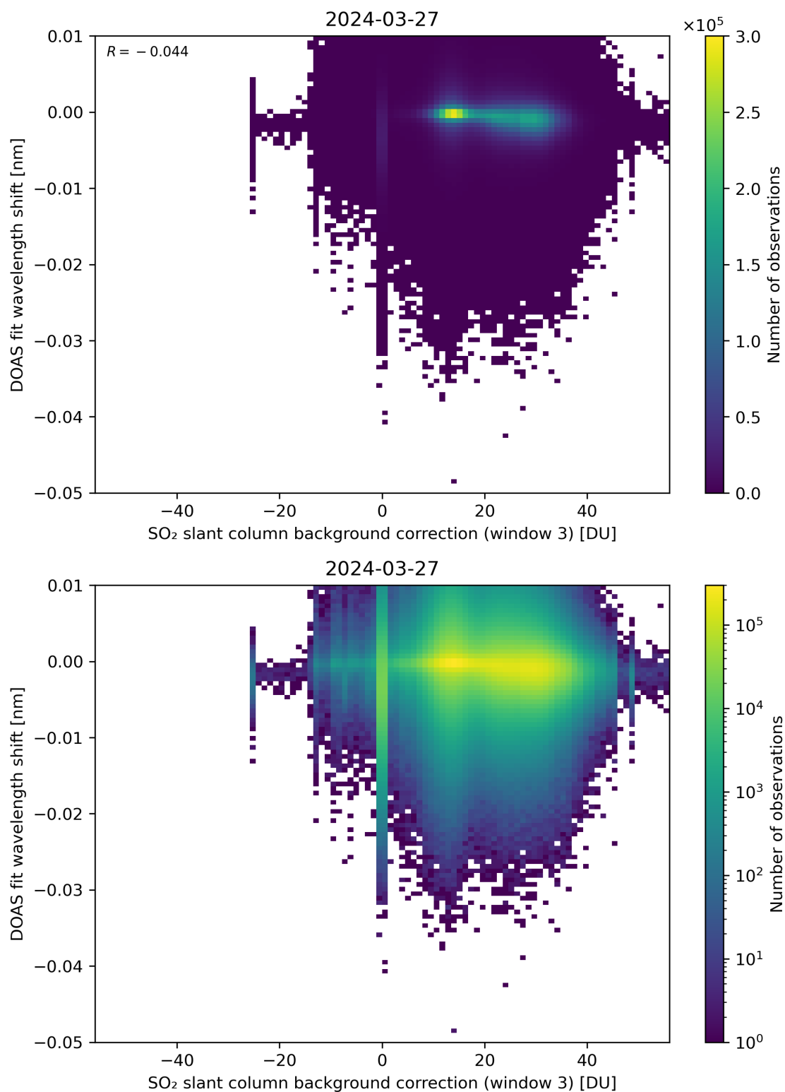
Figure 121: Scatter density plot of “SO 2 slant column background correction (window 3)” against “DOAS fit wavelength shift” for 2024-03-26 to 2024-03-28.
