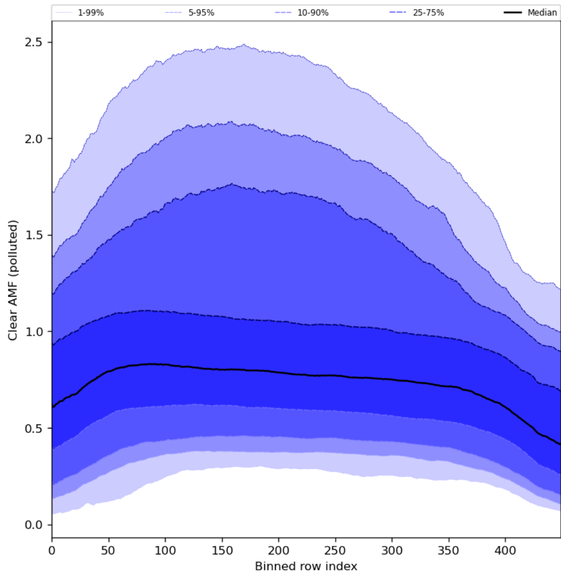
Figure 96: Along track statistics of “Clear AMF (polluted)” for 2024-03-26 to 2024-03-28
