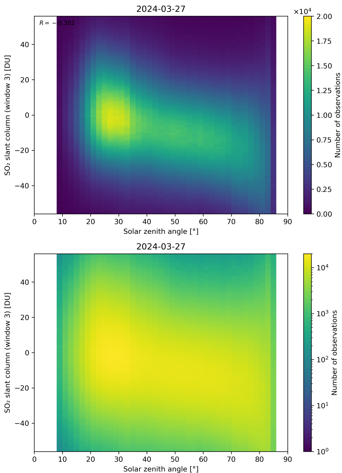
Figure 172: Scatter density plot of “Solar zenith angle” against “SO 2 slant column (window 3)” for 2024-03-26 to 2024-03-28.
