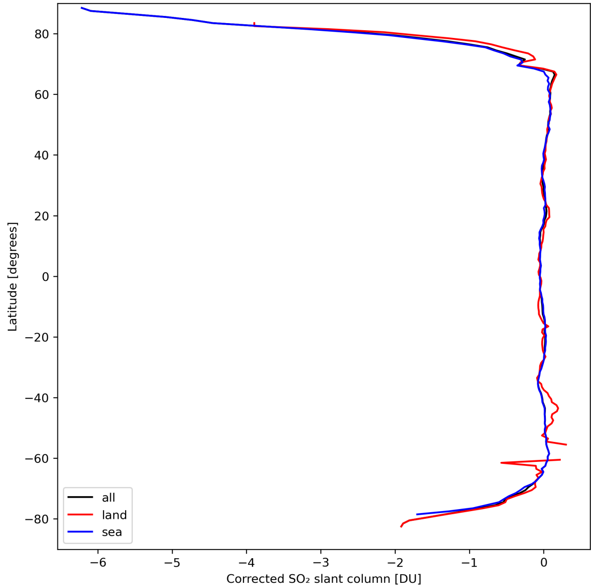
Figure 32: Zonal average of “Corrected SO 2 slant column” for 2024-03-26 to 2024-03-28.
