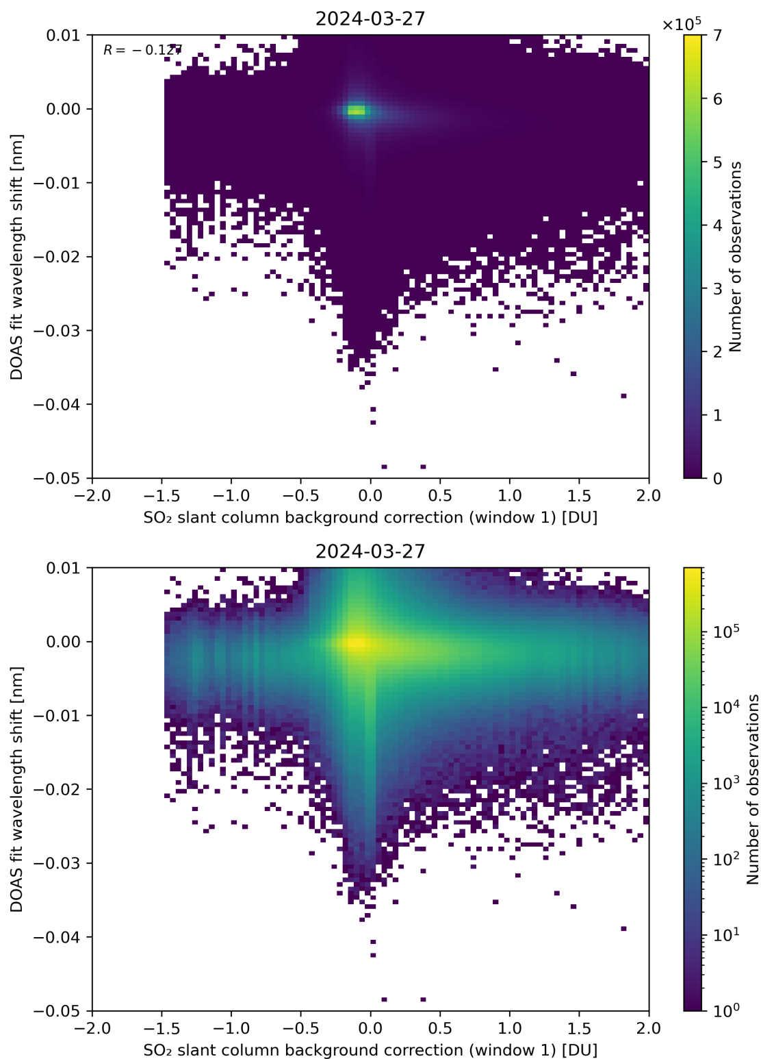
Figure 100: Scatter density plot of “SO 2 slant column background correction (window 1)” against “DOAS fit wavelength shift” for 2024-03-26 to 2024-03-28.
