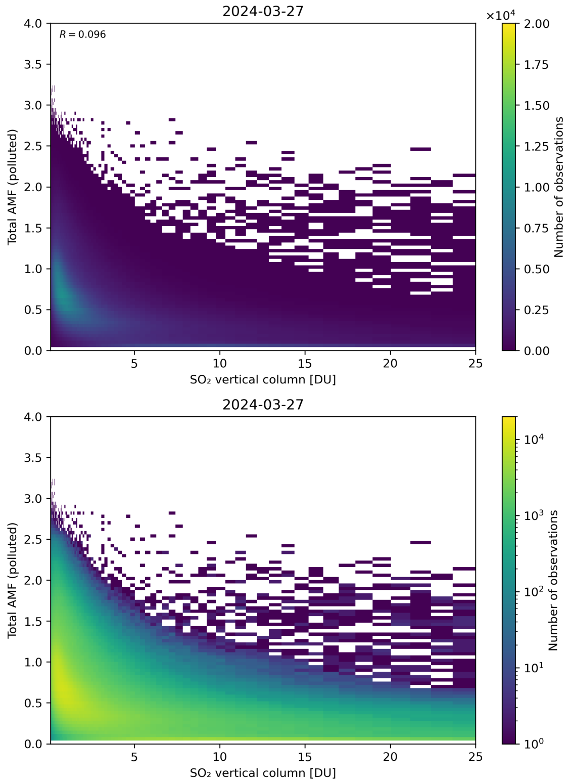
Figure 305: Scatter density plot of “SO 2 vertical column” against “Total AMF (polluted)” for 2024-03-26 to 2024-03-28.
