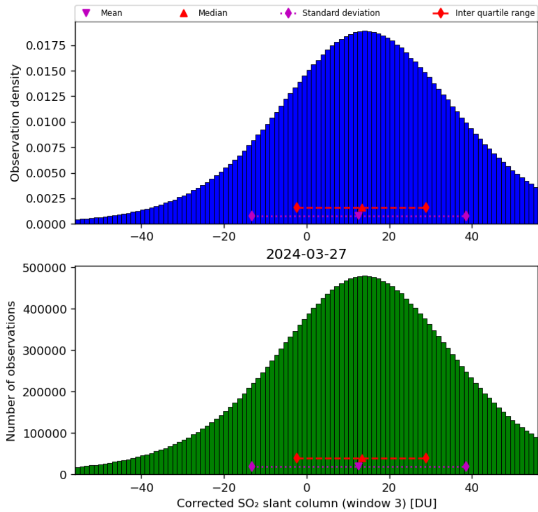
Figure 66: Histogram of “Corrected SO 2 slant column (window 3)” for 2024-03-26 to 2024-03-28
