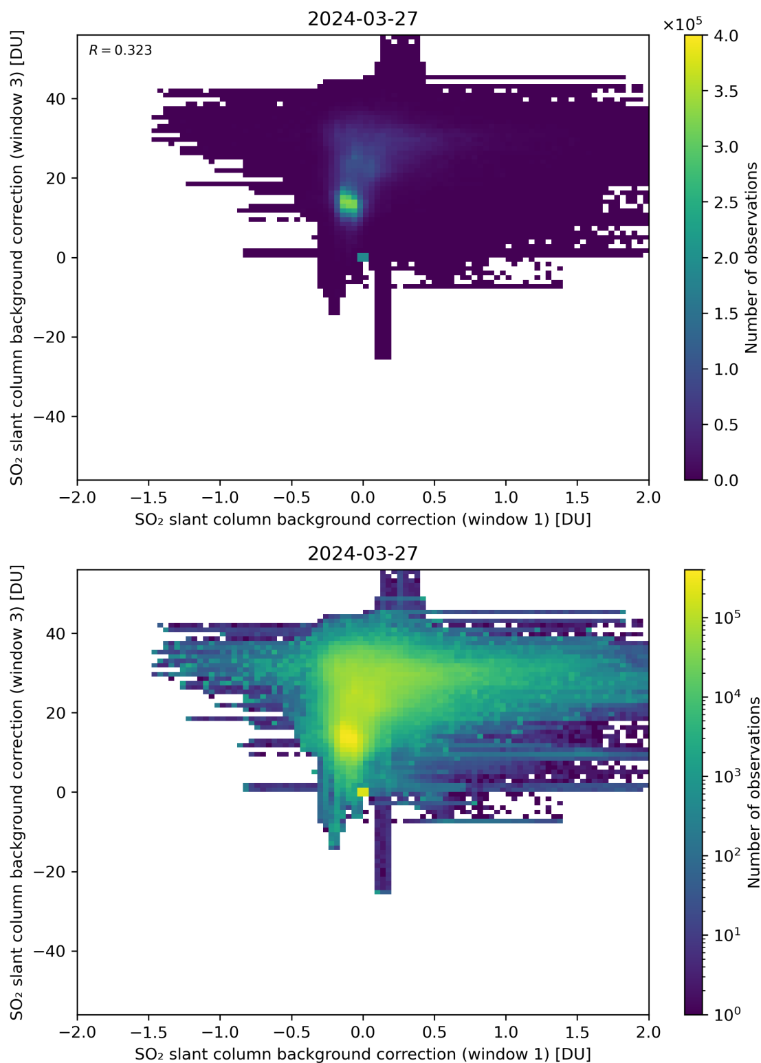
Figure 99: Scatter density plot of “SO 2 slant column background correction (window 1)” against “SO 2 slant column background correction (window 3)” for 2024-03-26 to 2024-03-28.
