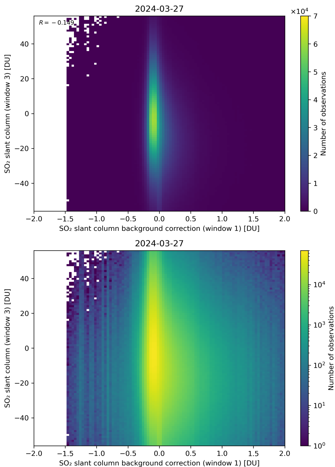
Figure 107: Scatter density plot of “SO 2 slant column background correction (window 1)” against “SO 2 slant column (window 3)” for 2024-03-26 to 2024-03-28.
