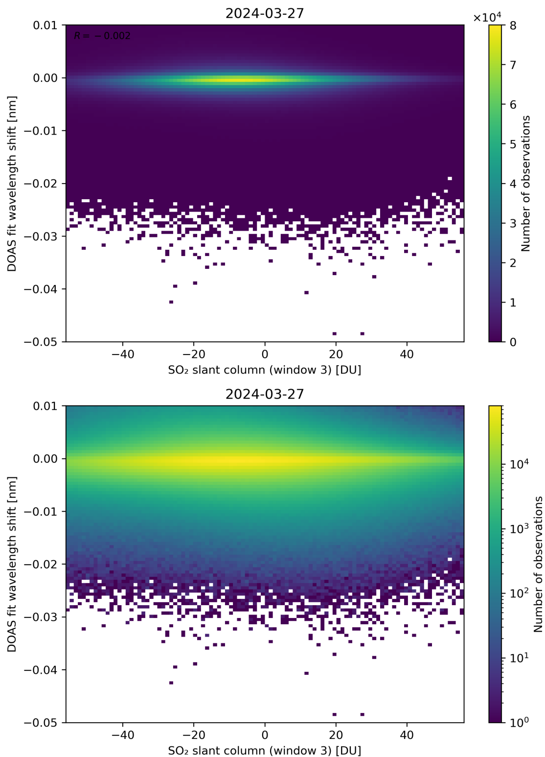
Figure 254: Scatter density plot of “SO 2 slant column (window 3)” against “DOAS fit wavelength shift” for 2024-03-26 to 2024-03-28.
