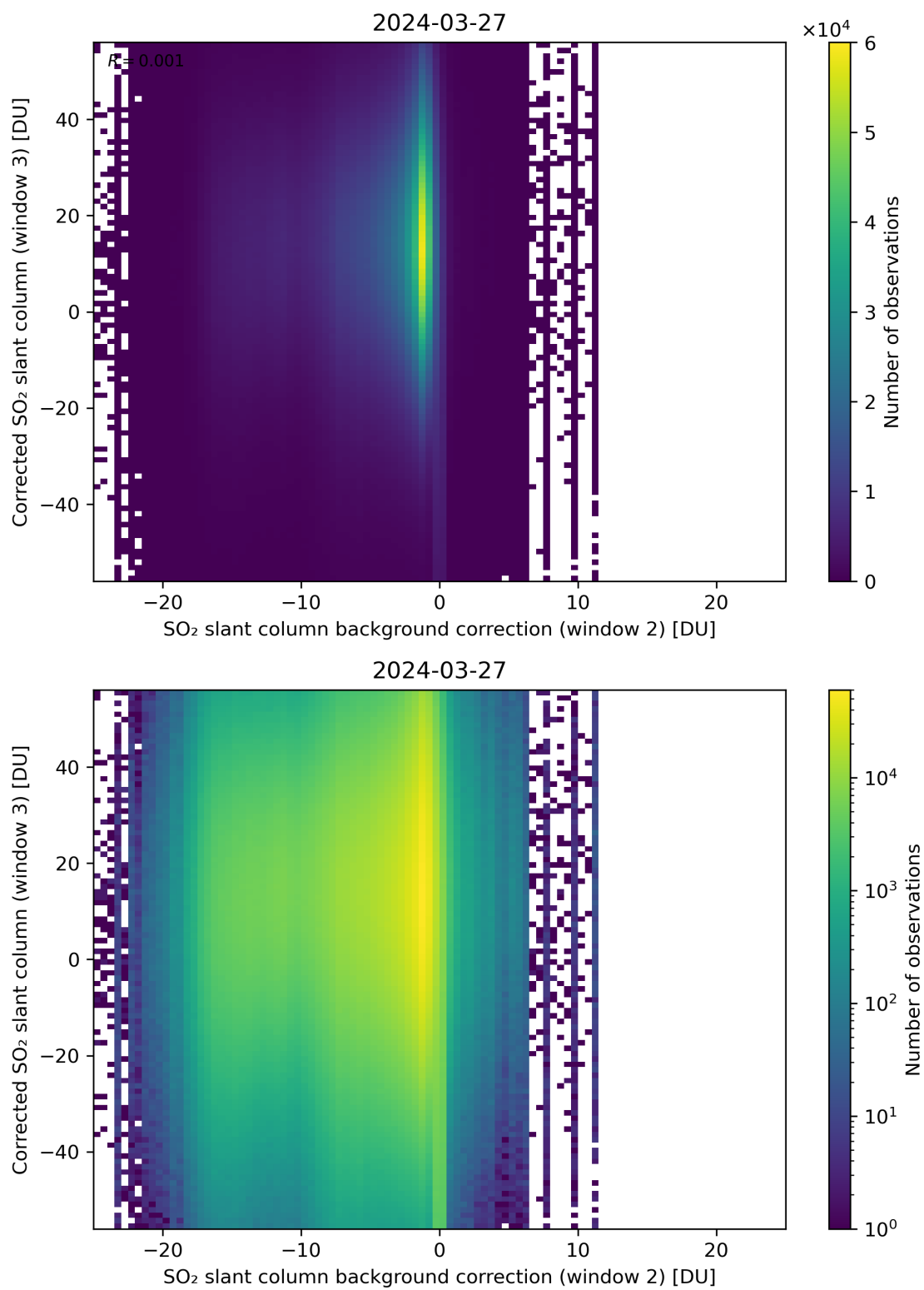
Figure 116: Scatter density plot of “SO 2 slant column background correction (window 2)” against “Corrected SO 2 slant column (window 3)” for 2024-03-26 to 2024-03-28.
