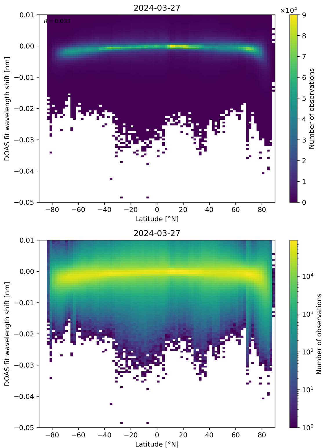
Figure 142: Scatter density plot of “Latitude” against “DOAS fit wavelength shift” for 2024-03-26 to 2024-03-28.
