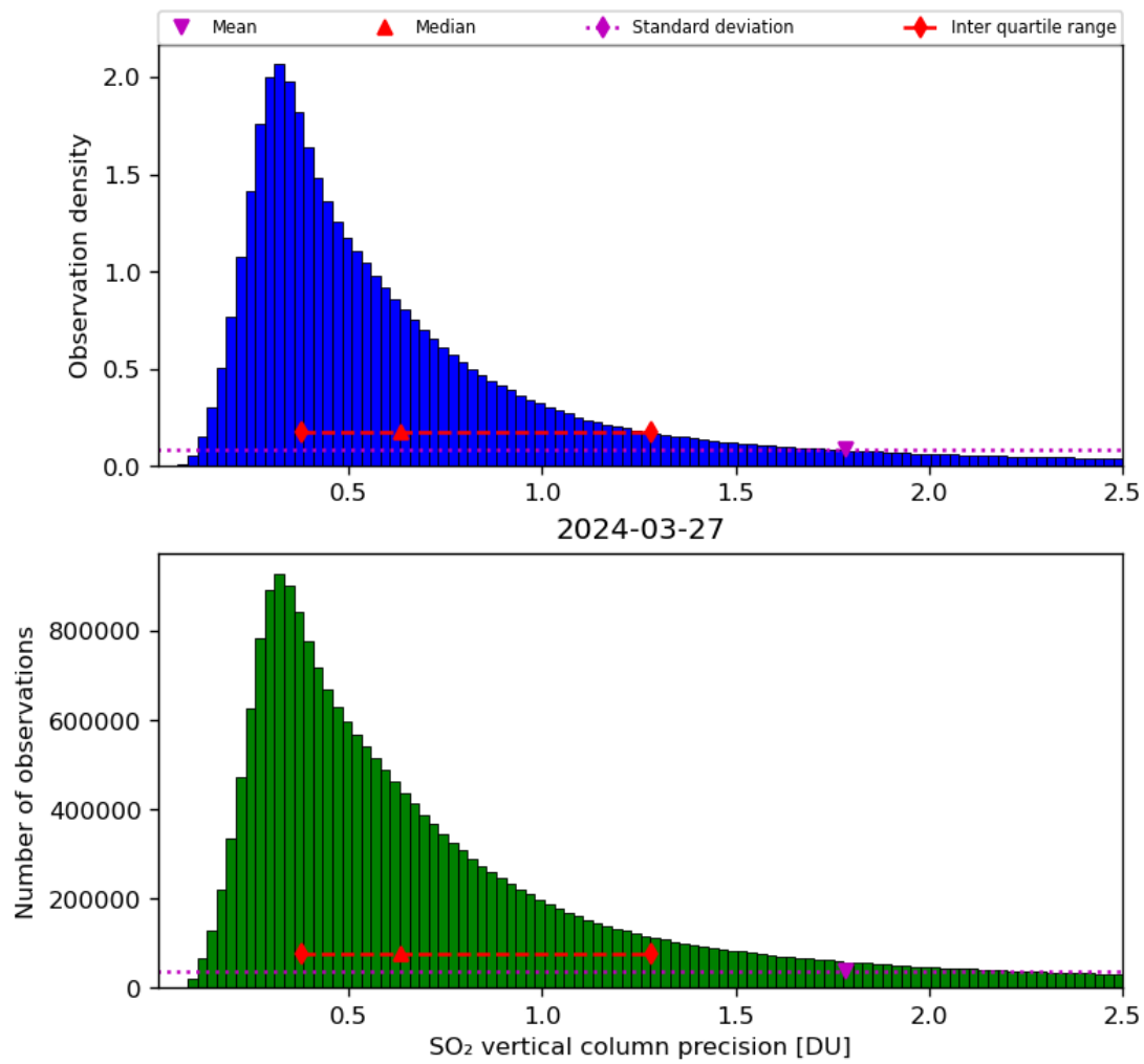
Figure 54: Histogram of “SO 2 vertical column precision” for 2024-03-26 to 2024-03-28
