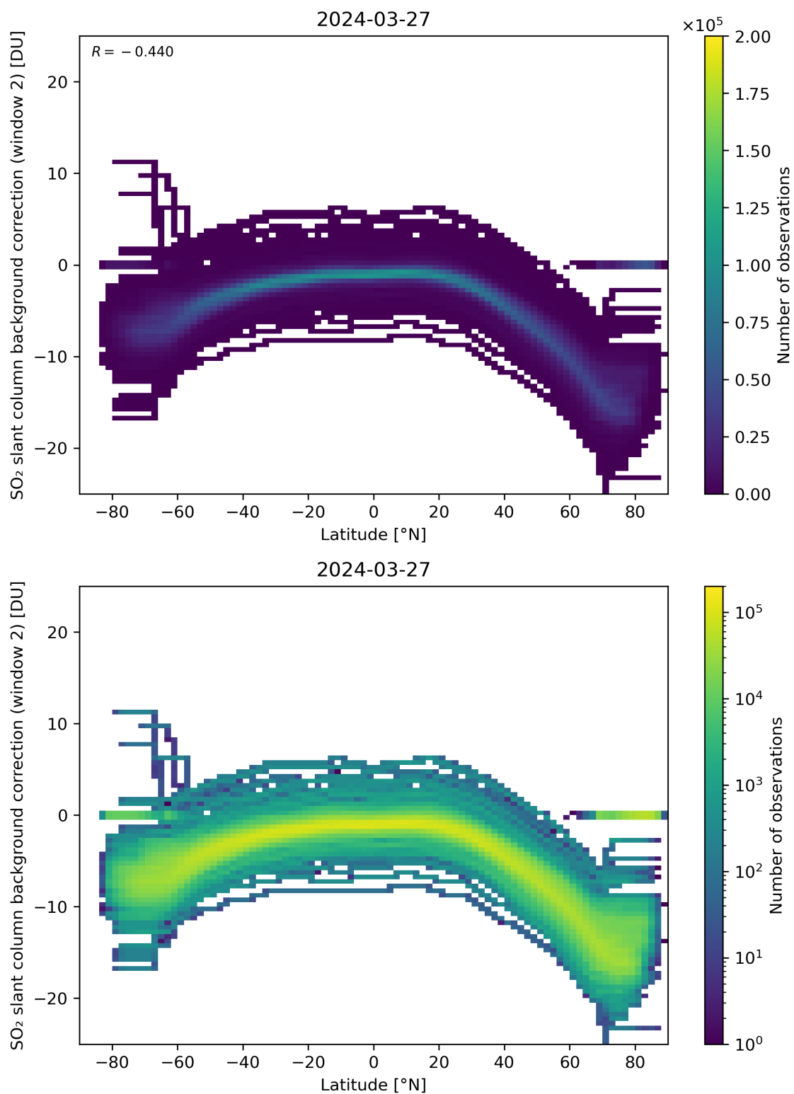
Figure 140: Scatter density plot of “Latitude” against “SO 2 slant column background correction (window 2)” for 2024-03-26 to 2024-03-28.
