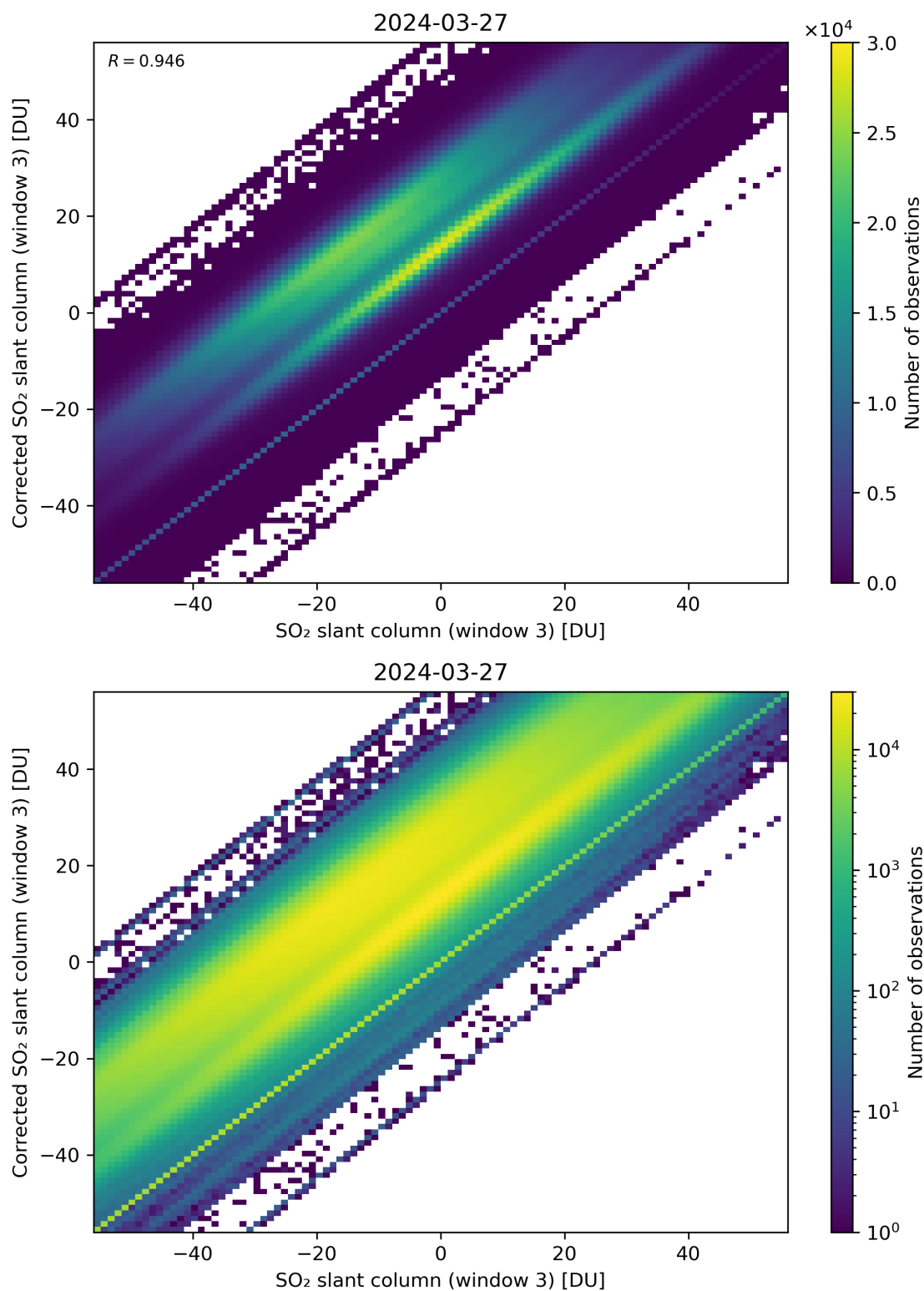
Figure 266: Scatter density plot of “SO 2 slant column (window 3)” against “Corrected SO 2 slant column (window 3)” for 2024-03-26 to 2024-03-28.
