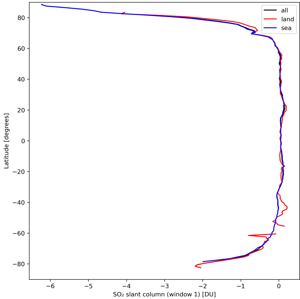
Figure 33: Zonal average of “SO 2 slant column (window 1)” for 2024-03-26 to 2024-03-28.
