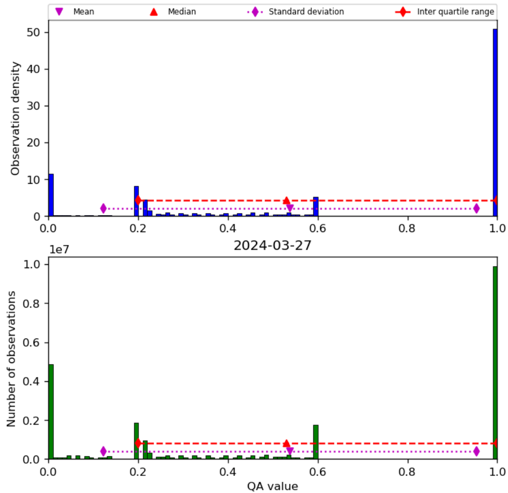
Figure 52: Histogram of “QA value” for 2024-03-26 to 2024-03-28
