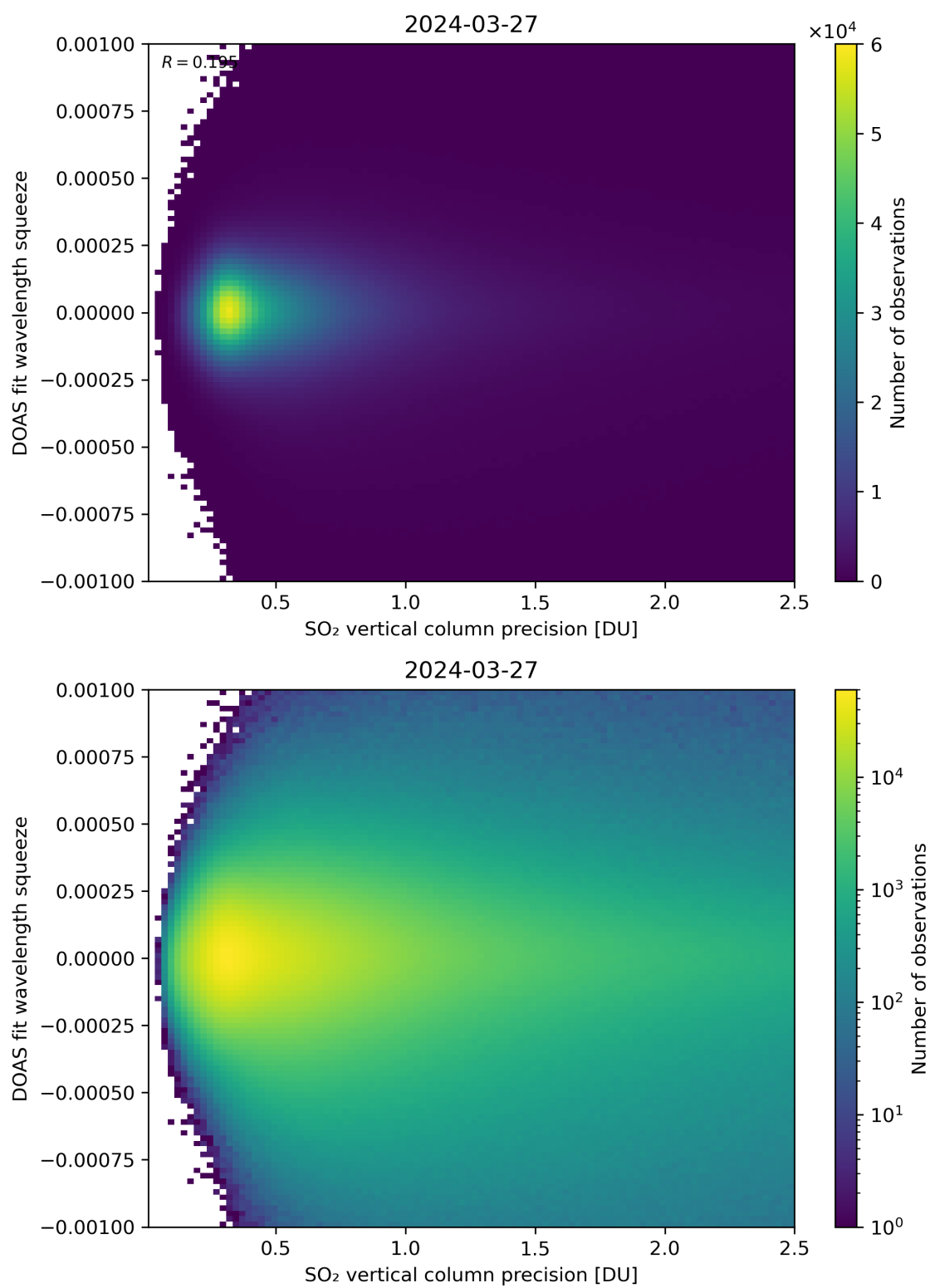
Figure 283: Scatter density plot of “SO 2 vertical column precision” against “DOAS fit wavelength squeeze” for 2024-03-26 to 2024-03-28.
