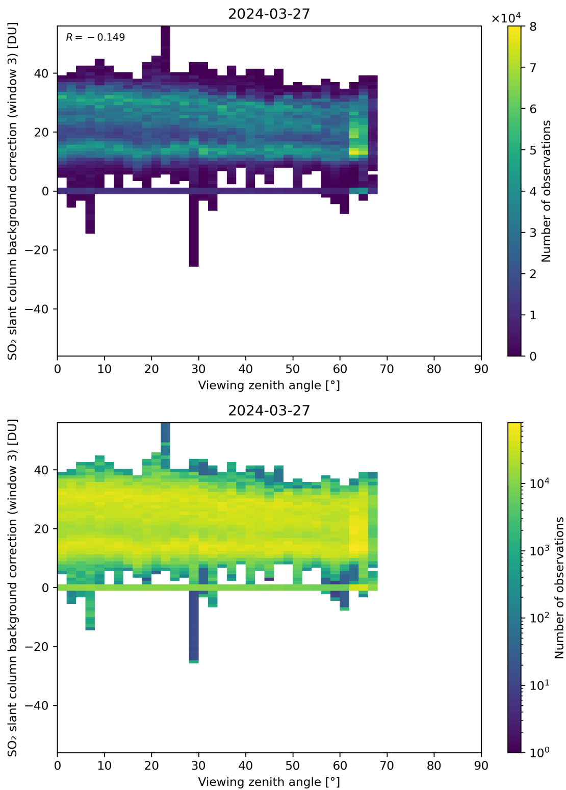
Figure 310: Scatter density plot of “Viewing zenith angle” against “SO 2 slant column background correction (window 3)” for 2024-03-26 to 2024-03-28.
