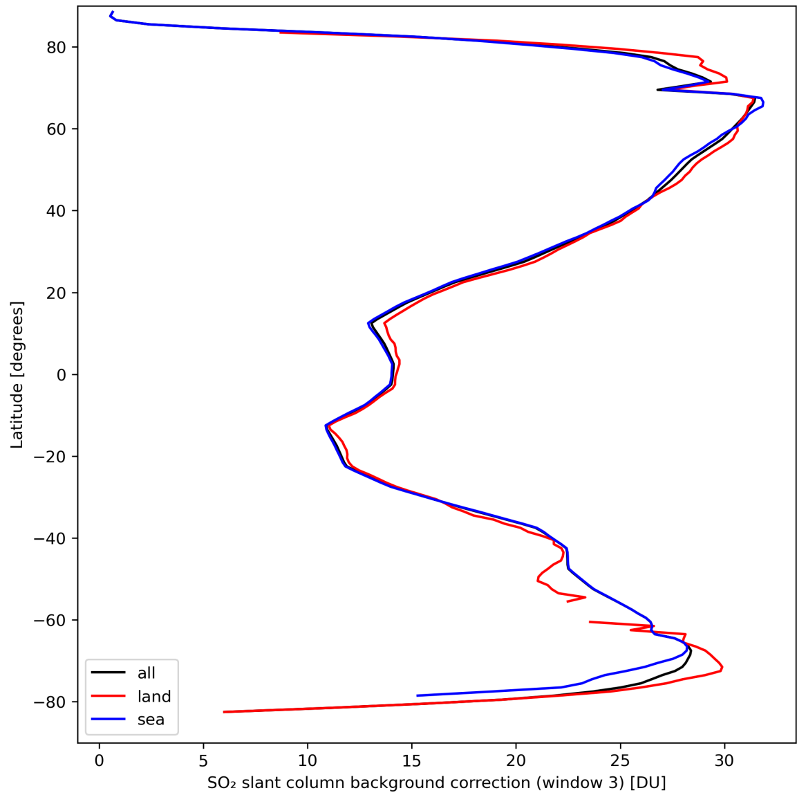
Figure 44: Zonal average of “SO 2 slant column background correction (window 3)” for 2024-03-26 to 2024-03-28.
