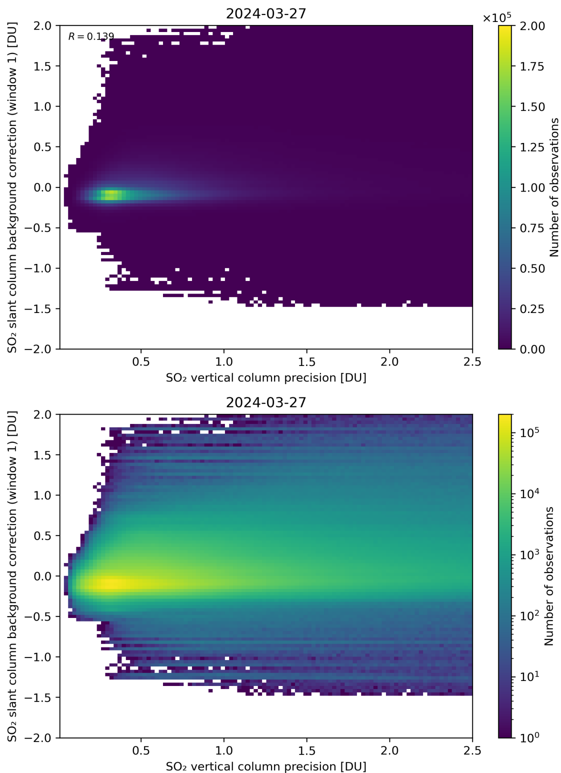
Figure 279: Scatter density plot of “SO 2 vertical column precision” against “SO 2 slant column background correction (window 1)” for 2024-03-26 to 2024-03-28.
