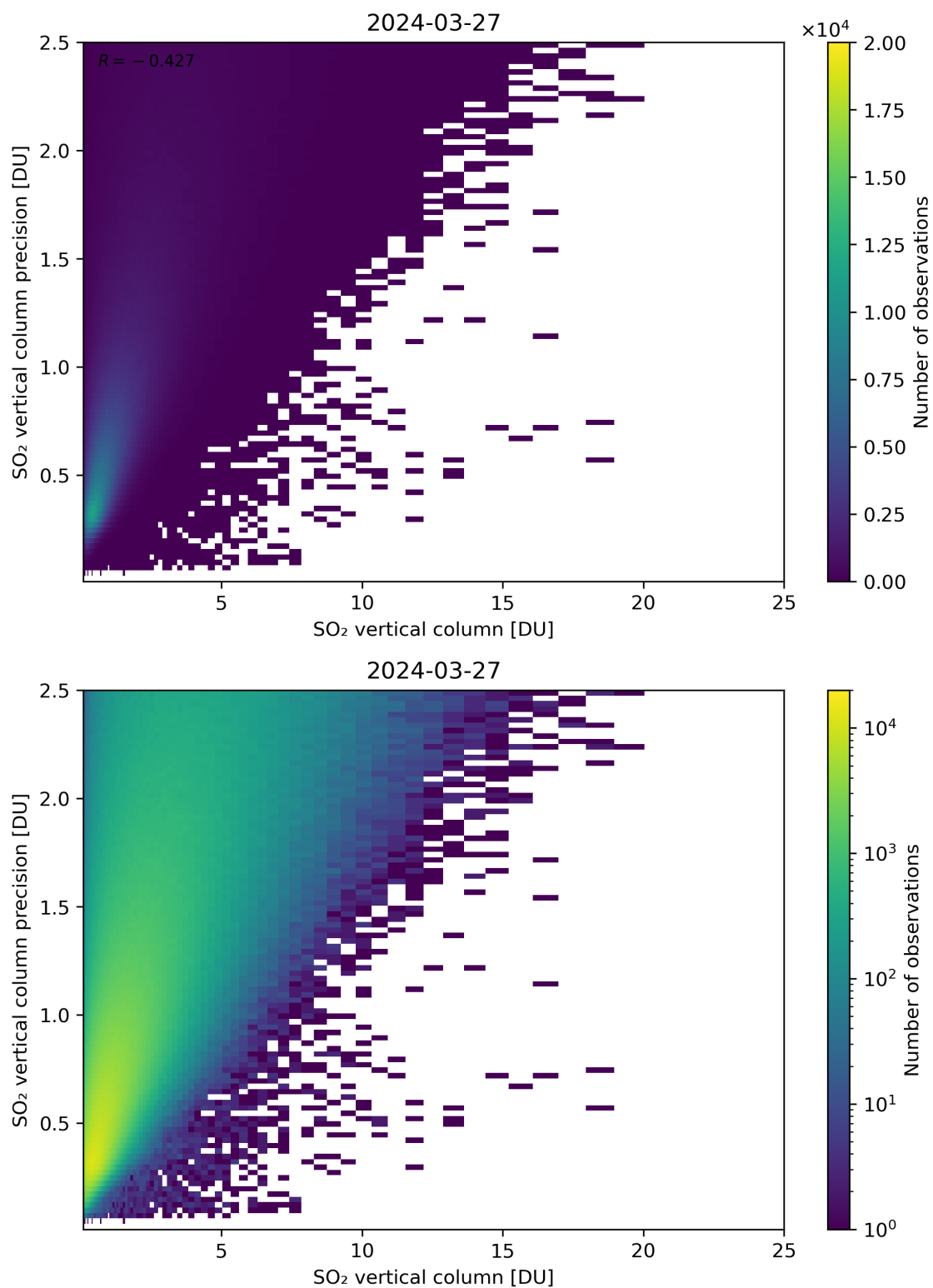
Figure 307: Scatter density plot of “SO 2 vertical column” against “SO 2 vertical column precision” for 2024-03-26 to 2024-03-28.
