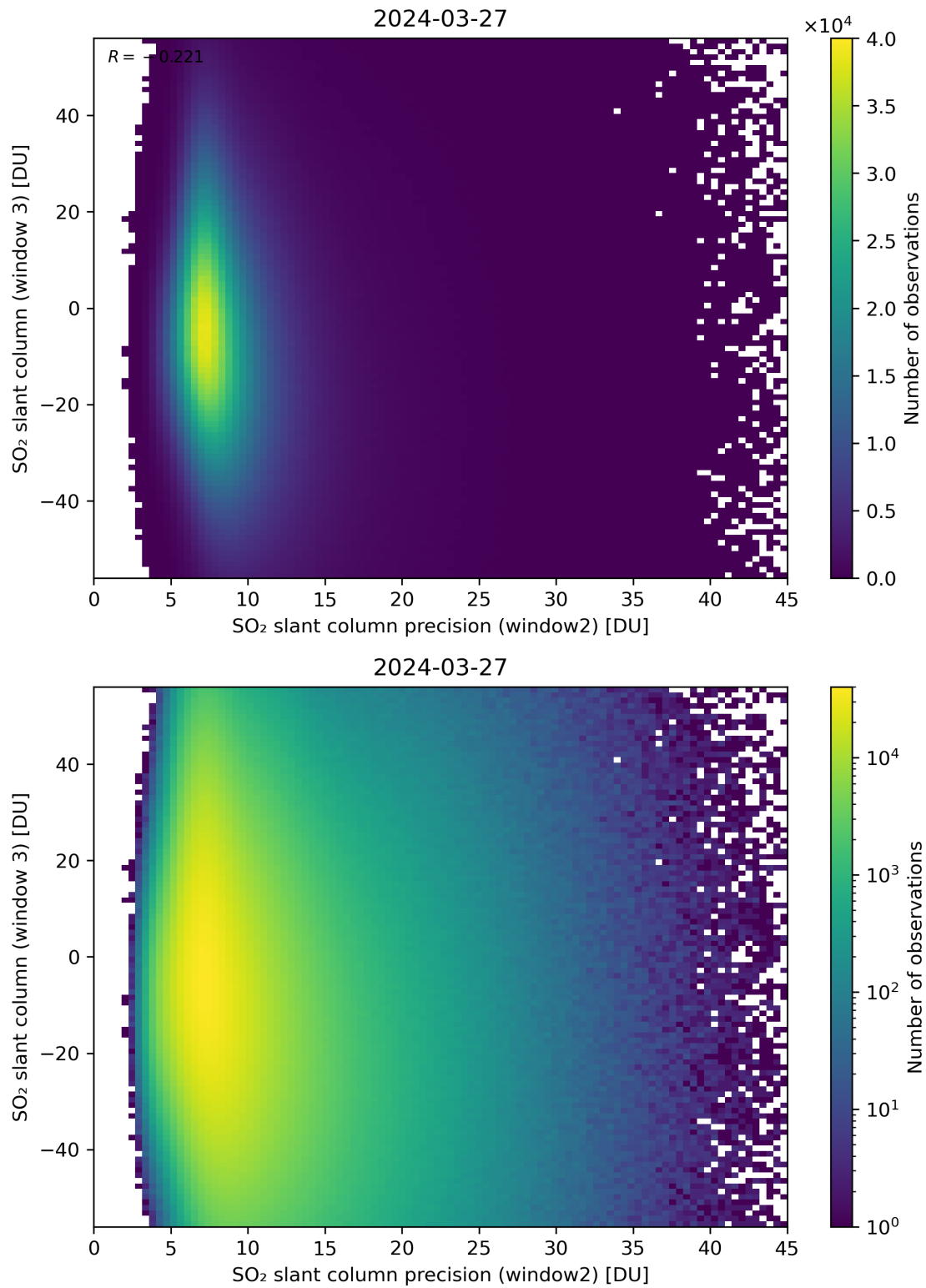
Figure 249: Scatter density plot of “SO 2 slant column precision (window2)” against “SO 2 slant column (window 3)” for 2024-03-26 to 2024-03-28.
