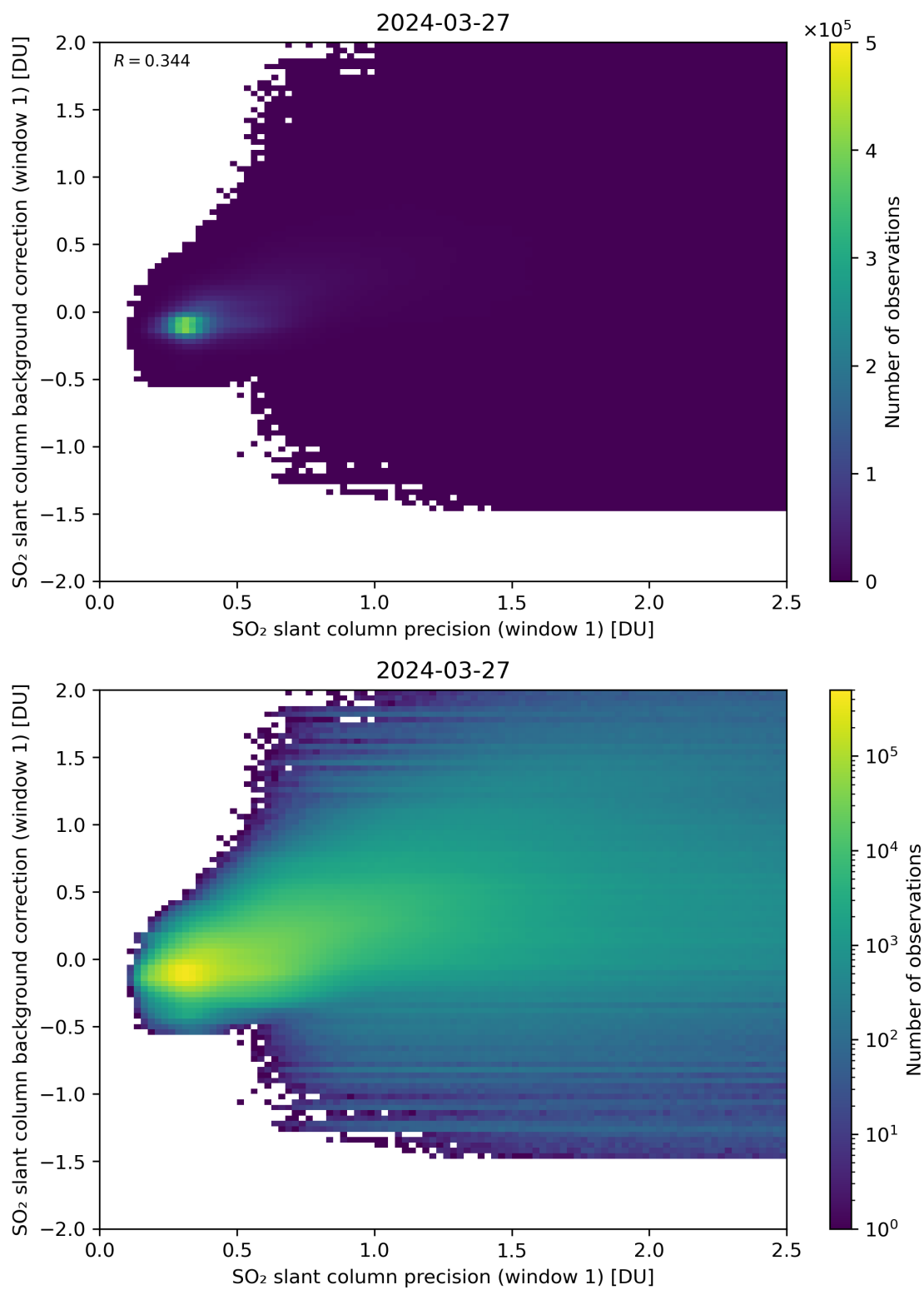
Figure 218: Scatter density plot of “SO 2 slant column precision (window 1)” against “SO 2 slant column background correction (window 1)” for 2024-03-26 to 2024-03-28.
