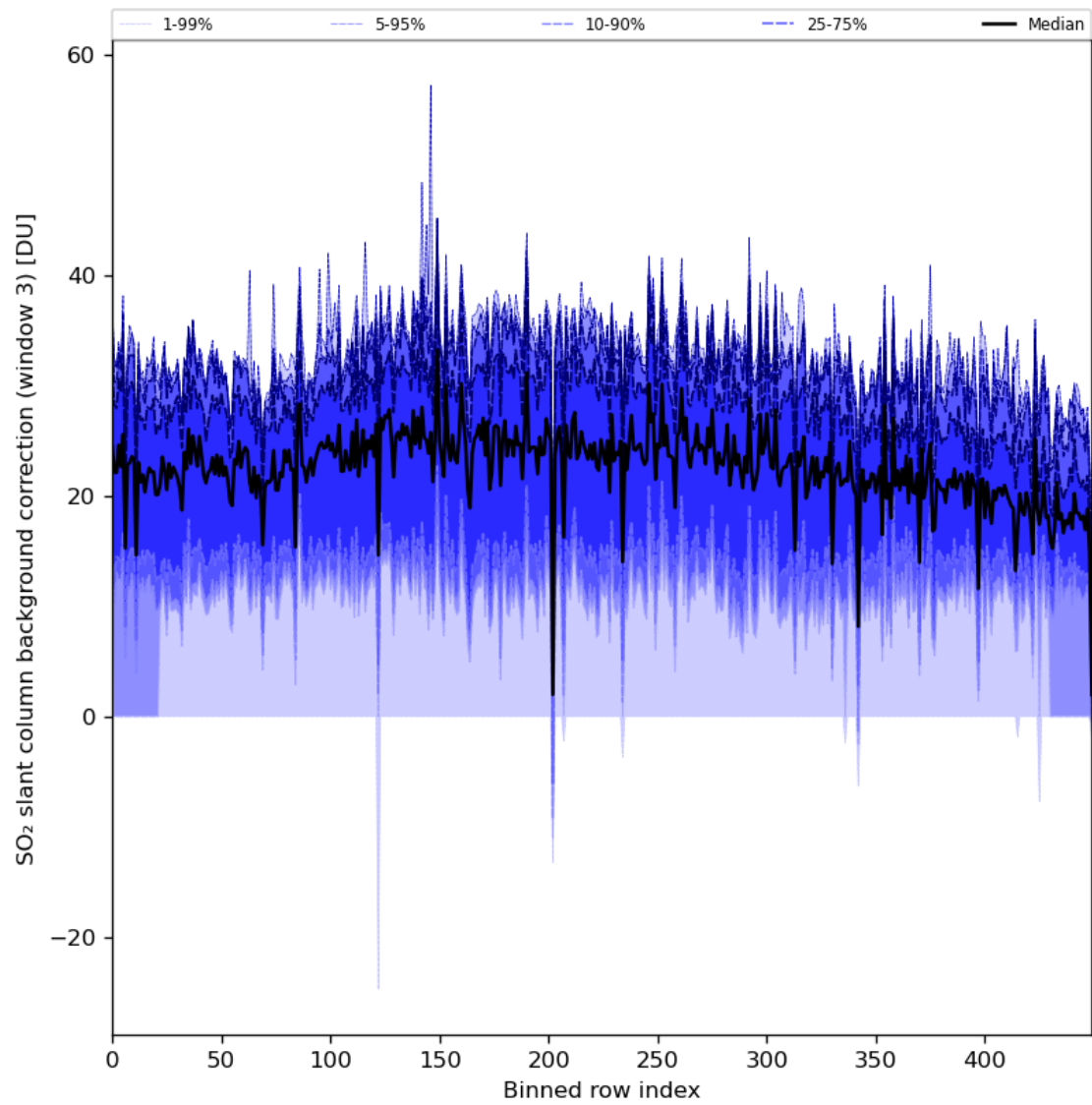
Figure 90: Along track statistics of “SO 2 slant column background correction (window 3)” for 2024-03-26 to 2024-03-28
