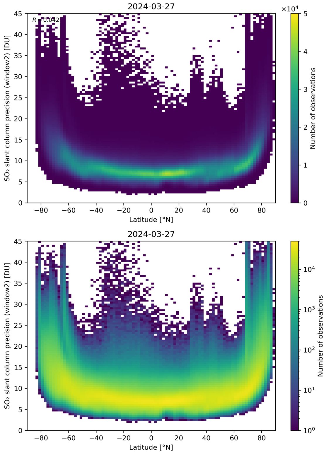
Figure 151: Scatter density plot of “Latitude” against “SO 2 slant column precision (window2)” for 2024-03-26 to 2024-03-28.
