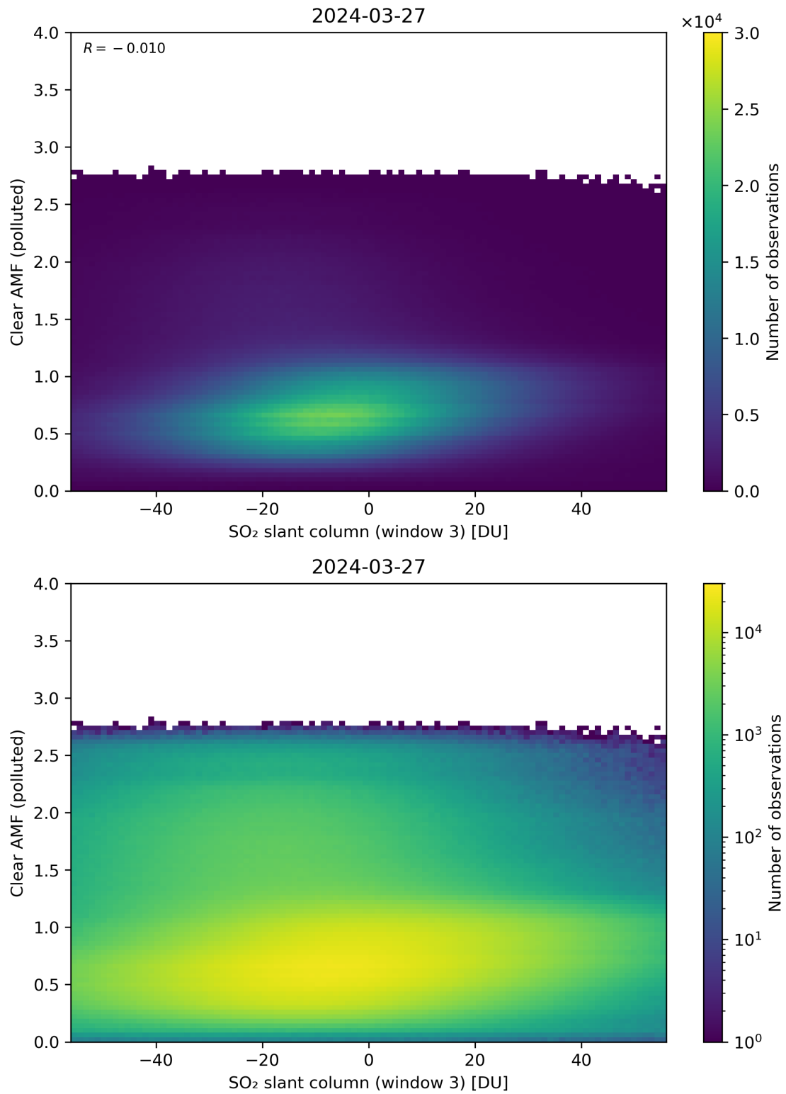
Figure 265: Scatter density plot of “SO 2 slant column (window 3)” against “Clear AMF (polluted)” for 2024-03-26 to 2024-03-28.
