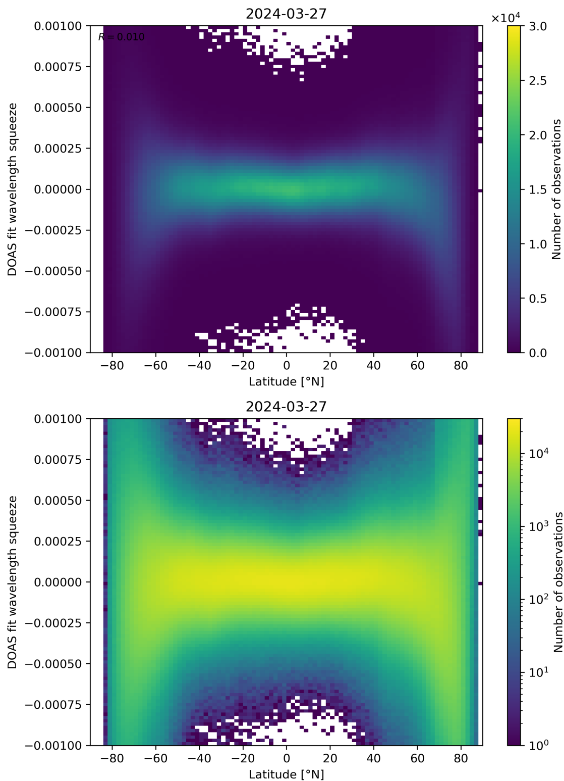
Figure 143: Scatter density plot of “Latitude” against “DOAS fit wavelength squeeze” for 2024-03-26 to 2024-03-28.
