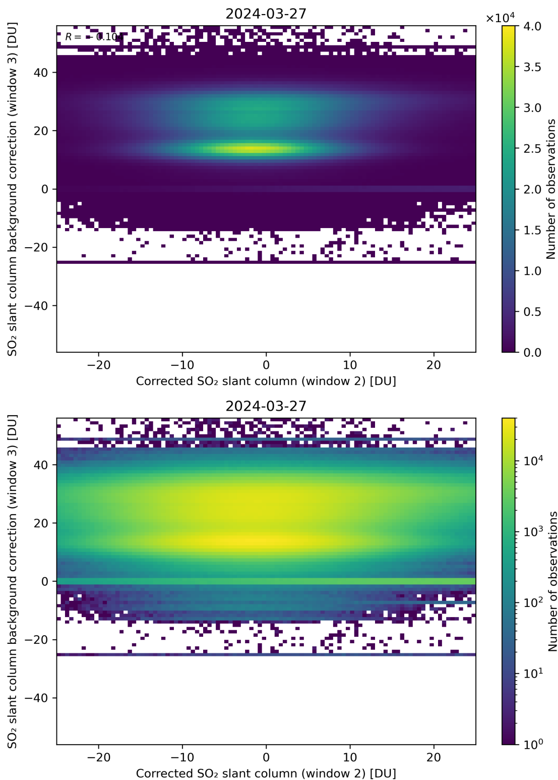
Figure 195: Scatter density plot of “Corrected SO 2 slant column (window 2)” against “SO 2 slant column background correction (window 3)” for 2024-03-26 to 2024-03-28.
