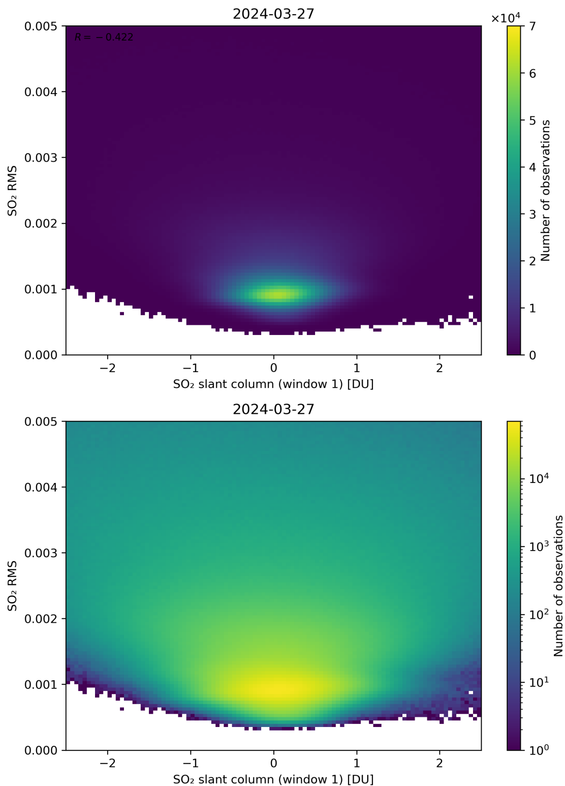
Figure 217: Scatter density plot of “SO 2 slant column (window 1)” against “SO 2 RMS” for 2024-03-26 to 2024-03-28.
