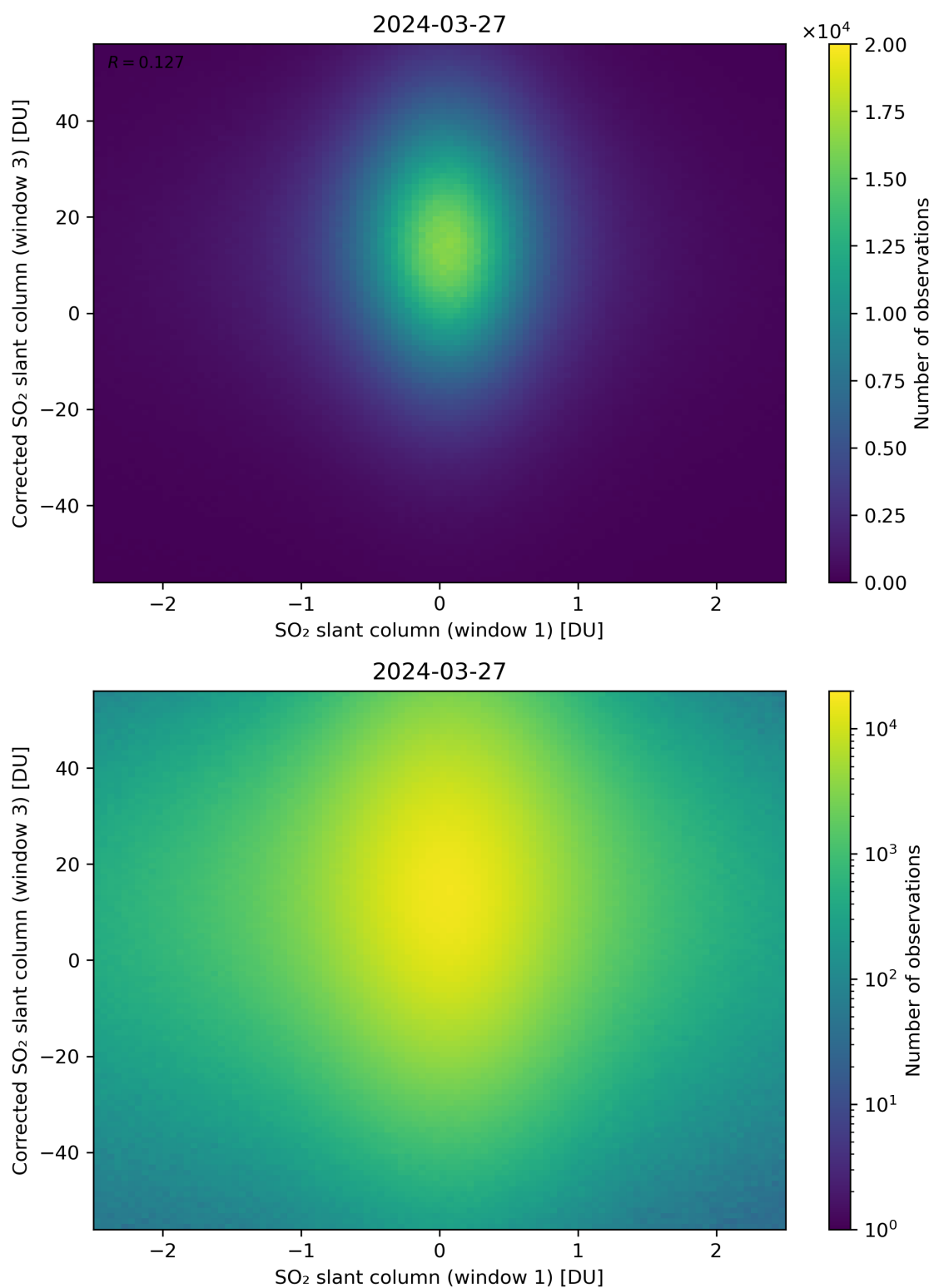
Figure 234: Scatter density plot of “SO 2 slant column (window 1)” against “Corrected SO 2 slant column (window 3)” for 2024-03-26 to 2024-03-28.
