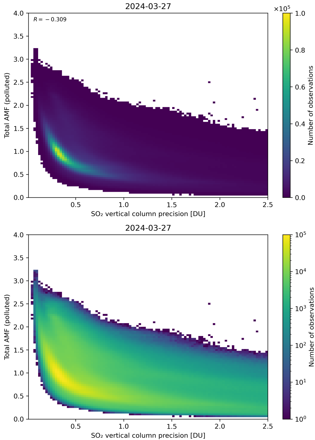
Figure 294: Scatter density plot of “SO 2 vertical column precision” against “Total AMF (polluted)” for 2024-03-26 to 2024-03-28.
