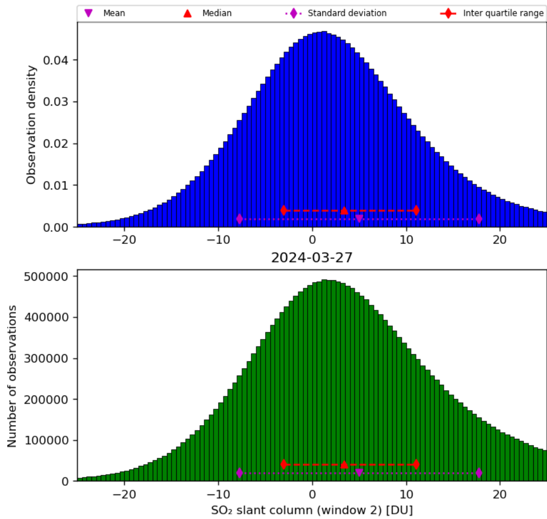
Figure 60: Histogram of “SO 2 slant column (window 2)” for 2024-03-26 to 2024-03-28
