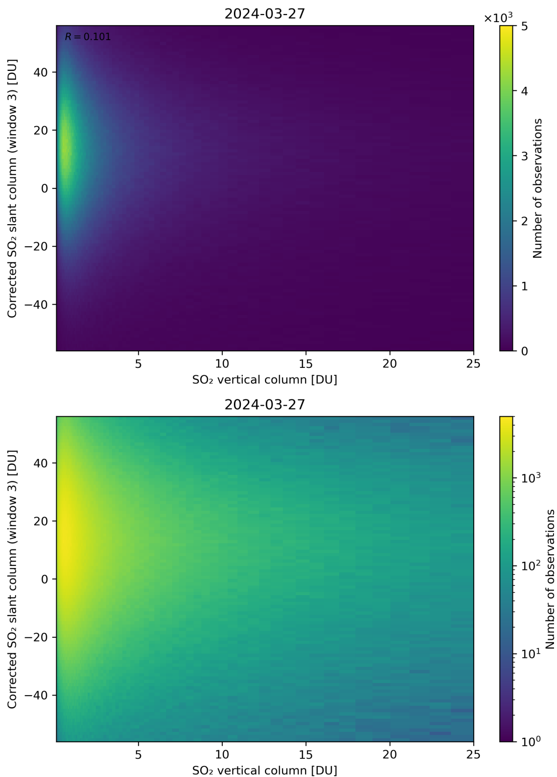
Figure 299: Scatter density plot of “SO 2 vertical column” against “Corrected SO 2 slant column (window 3)” for 2024-03-26 to 2024-03-28.
