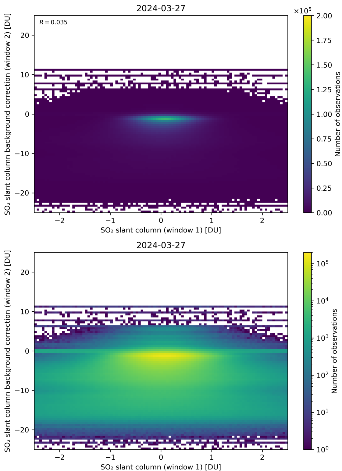
Figure 213: Scatter density plot of “SO 2 slant column (window 1)” against “SO 2 slant column background correction (window 2)” for 2024-03-26 to 2024-03-28.
