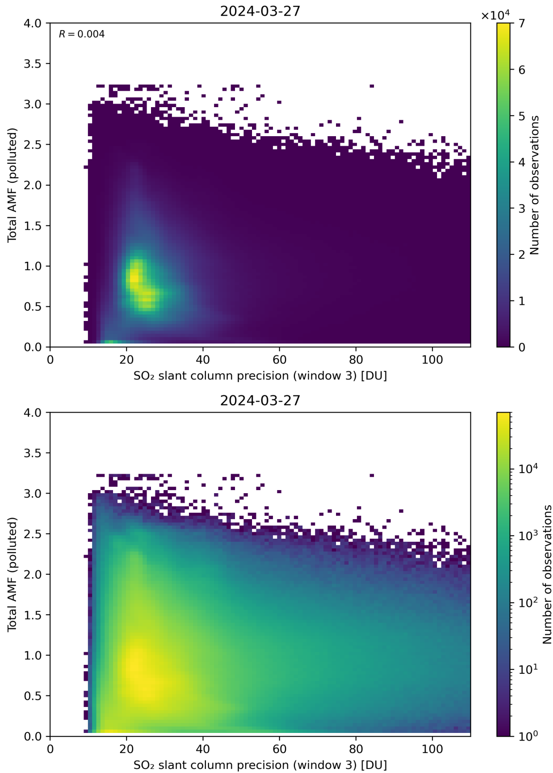
Figure 263: Scatter density plot of “SO 2 slant column precision (window 3)” against “Total AMF (polluted)” for 2024-03-26 to 2024-03-28.
