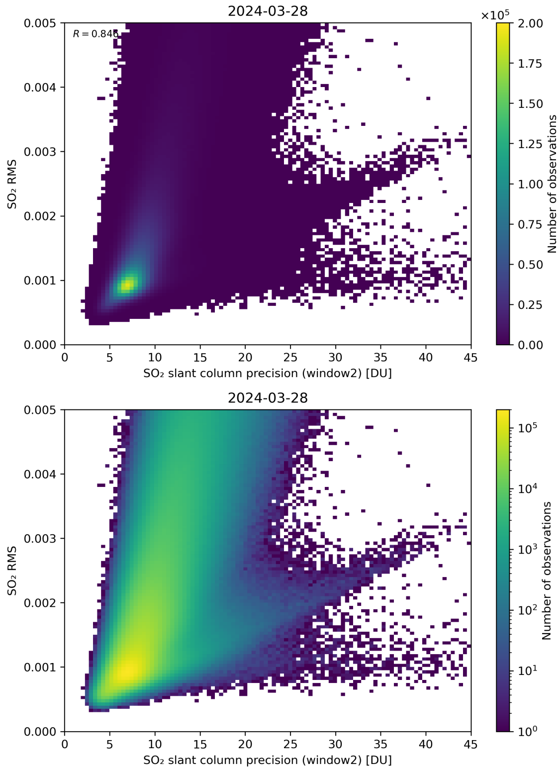
Figure 245: Scatter density plot of “SO 2 slant column precision (window2)” against “SO 2 RMS” for 2024-03-27 to 2024-03-29.
