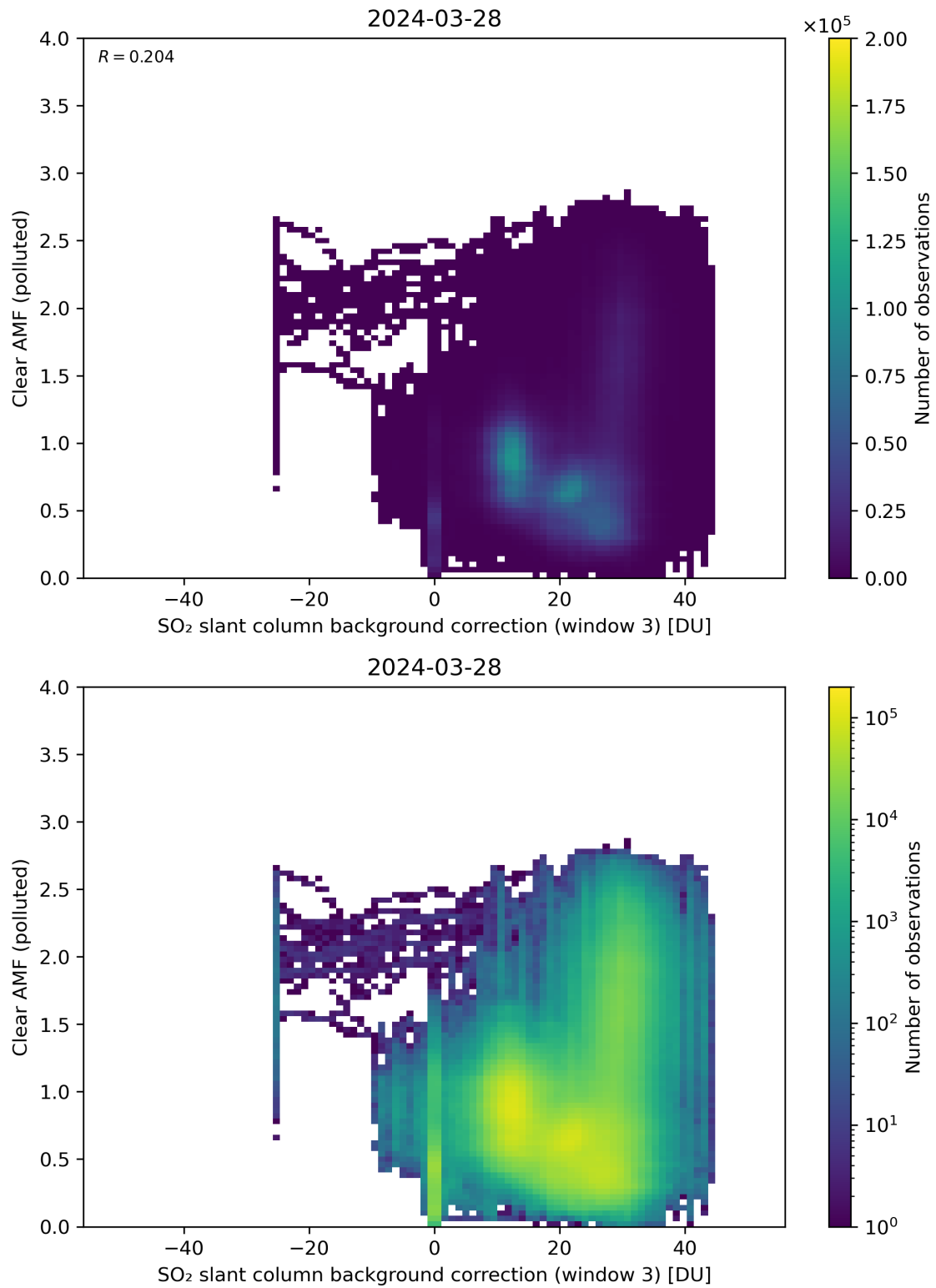
Figure 124: Scatter density plot of “SO 2 slant column background correction (window 3)” against “Clear AMF (polluted)” for 2024-03-27 to 2024-03-29.
