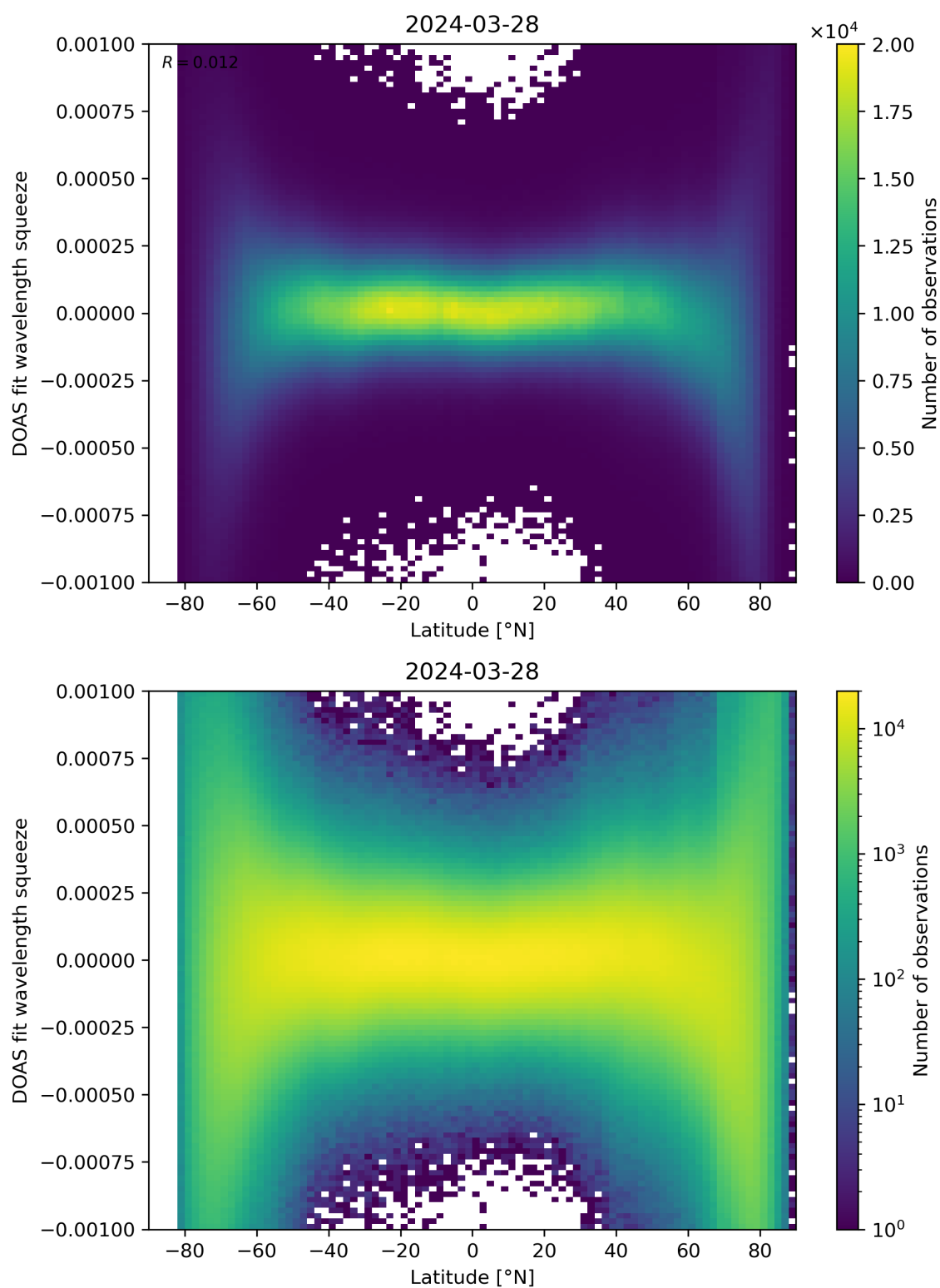
Figure 143: Scatter density plot of “Latitude” against “DOAS fit wavelength squeeze” for 2024-03-27 to 2024-03-29.
