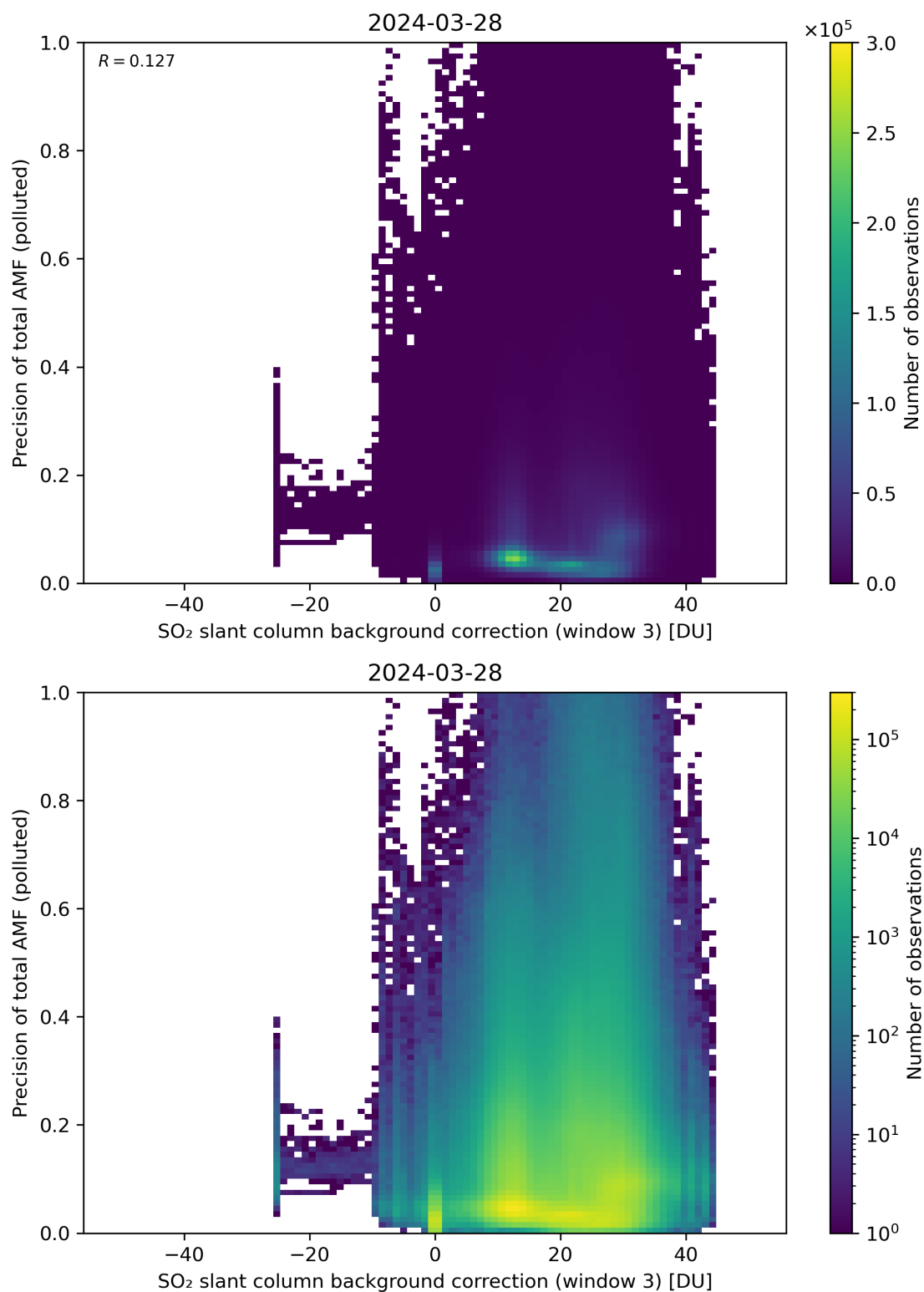
Figure 126: Scatter density plot of “SO 2 slant column background correction (window 3)” against “Precision of total AMF (polluted)” for 2024-03-27 to 2024-03-29.
