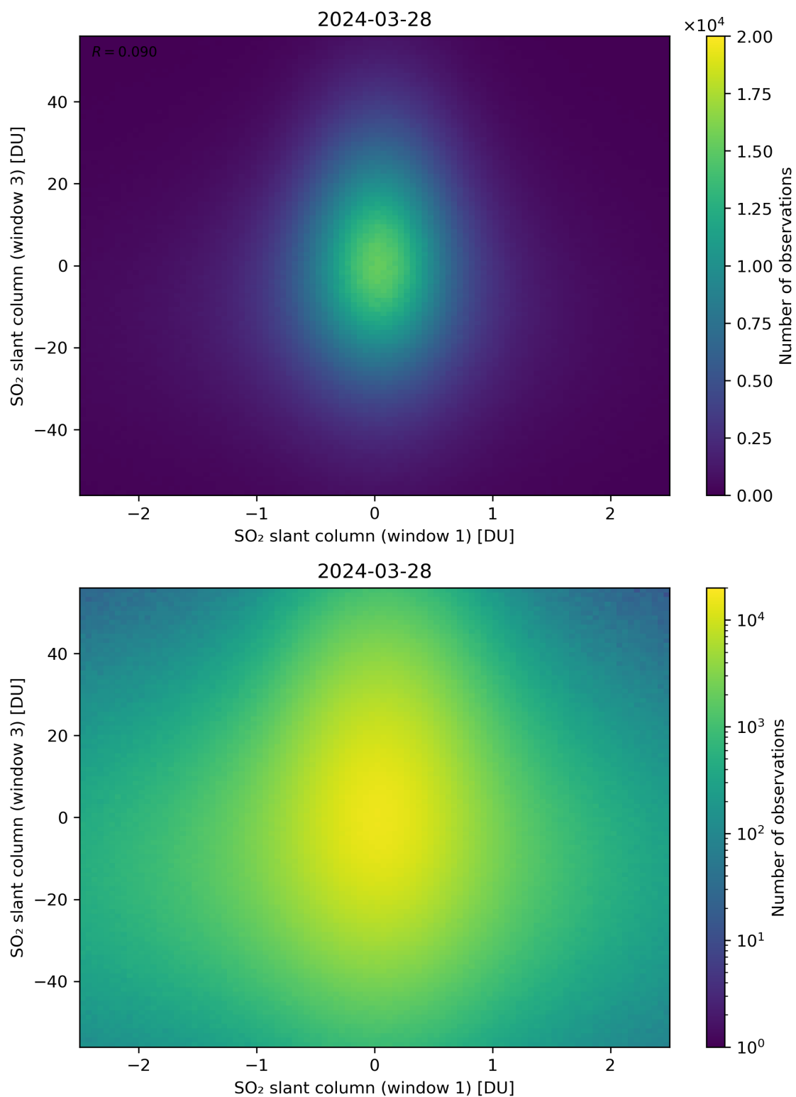
Figure 237: Scatter density plot of “SO 2 slant column (window 1)” against “SO 2 slant column (window 3)” for 2024-03-27 to 2024-03-29.
