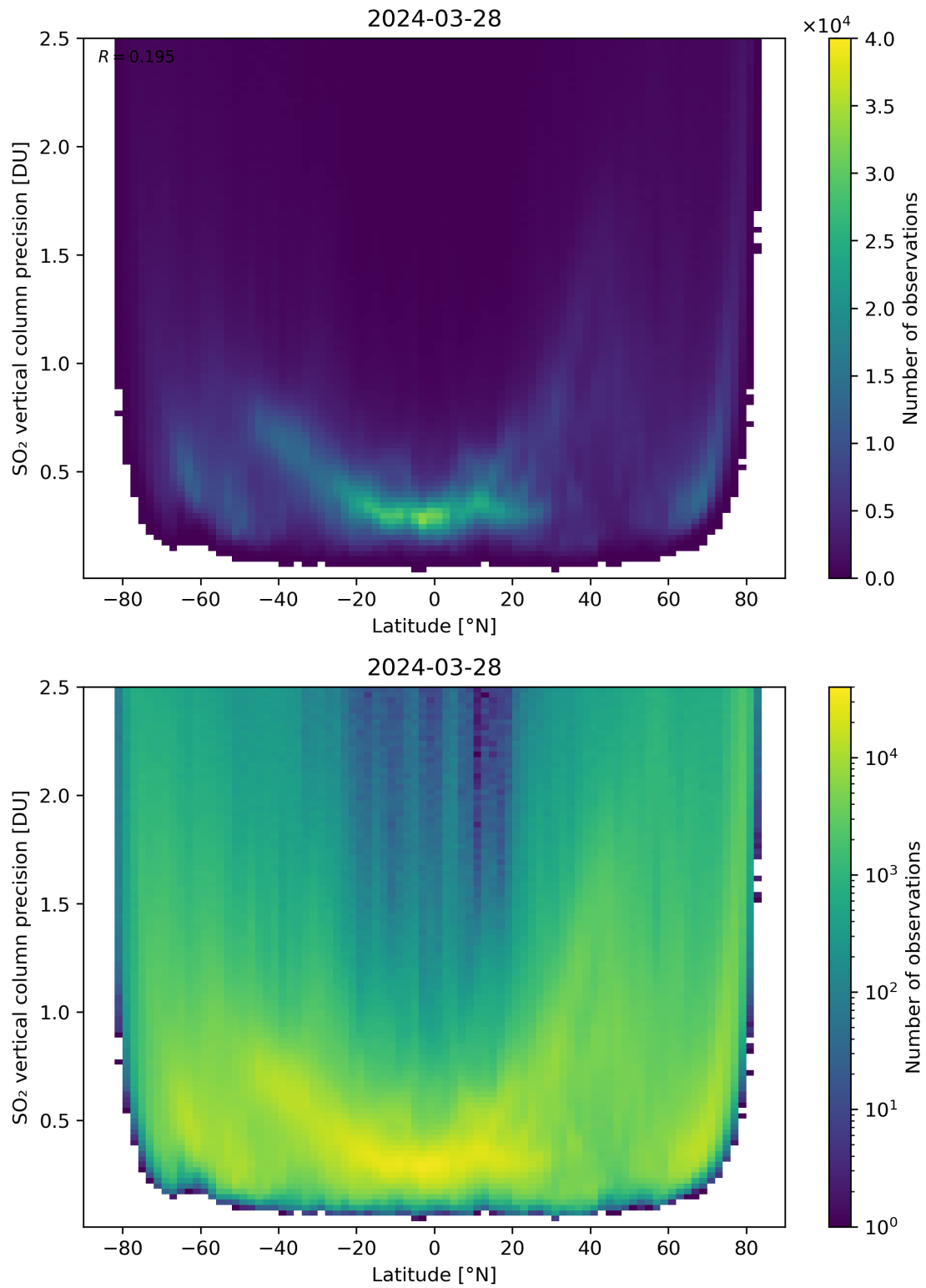
Figure 157: Scatter density plot of “Latitude” against “SO 2 vertical column precision” for 2024-03-27 to 2024-03-29.
