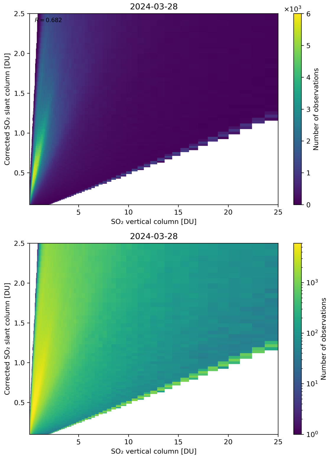
Figure 297: Scatter density plot of “SO 2 vertical column” against “Corrected SO 2 slant column” for 2024-03-27 to 2024-03-29.
