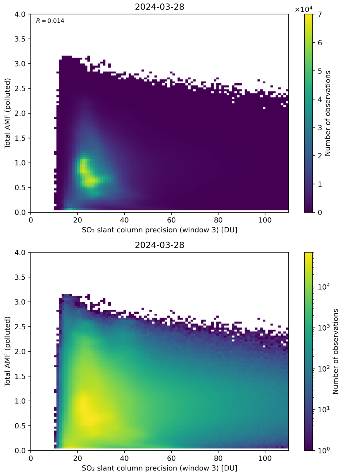
Figure 263: Scatter density plot of “SO 2 slant column precision (window 3)” against “Total AMF (polluted)” for 2024-03-27 to 2024-03-29.
