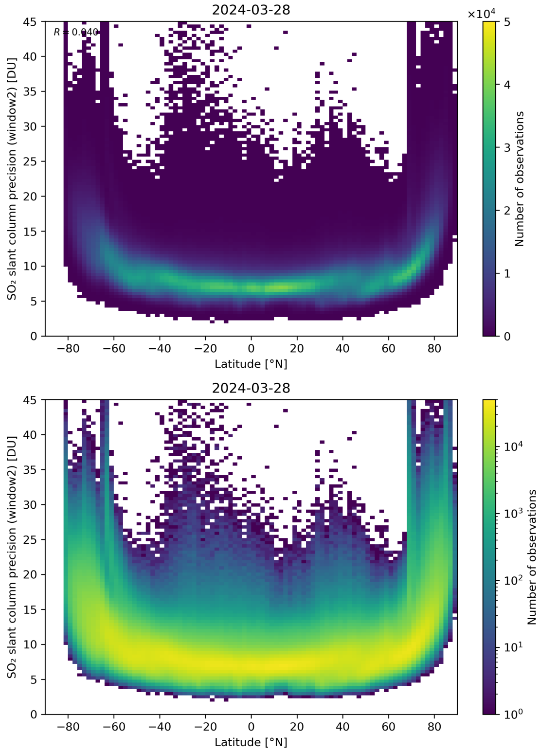
Figure 151: Scatter density plot of “Latitude” against “SO 2 slant column precision (window2)” for 2024-03-27 to 2024-03-29.
