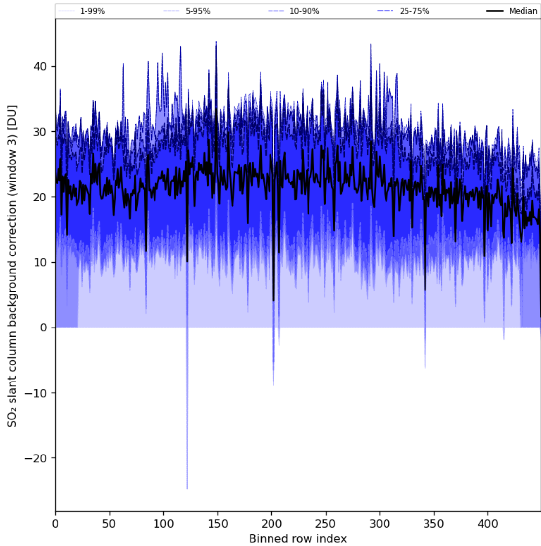
Figure 90: Along track statistics of “SO 2 slant column background correction (window 3)” for 2024-03-27 to 2024-03-29
