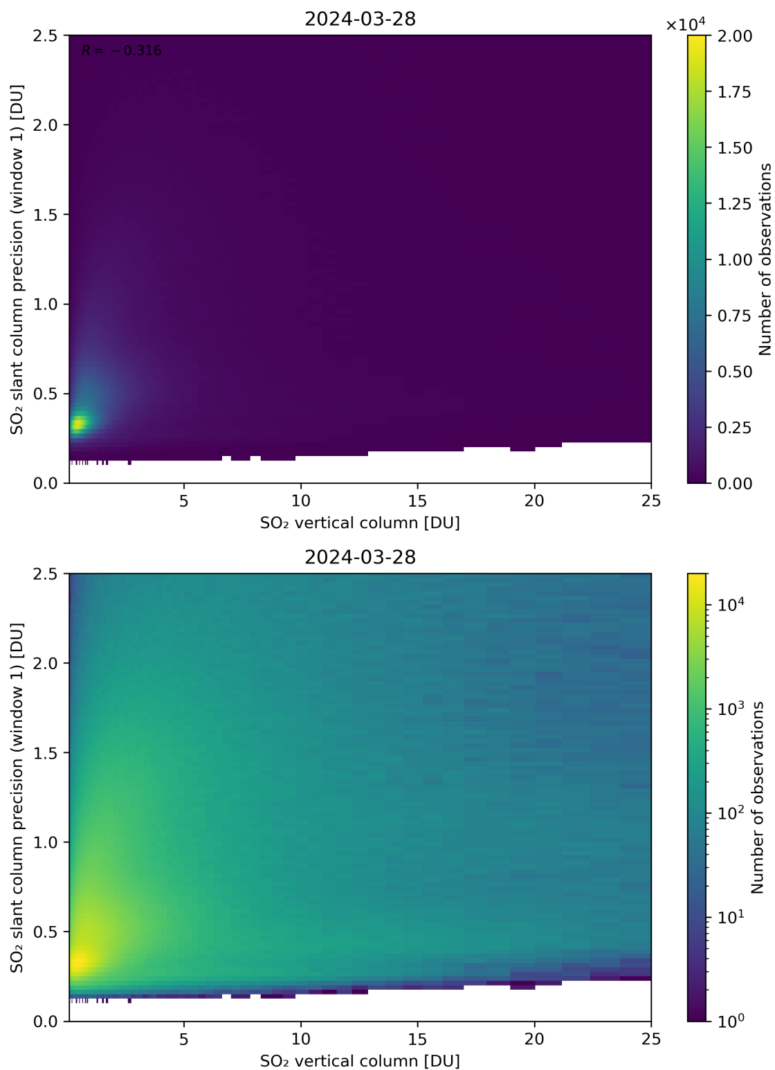
Figure 301: Scatter density plot of “SO 2 vertical column” against “SO 2 slant column precision (window 1)” for 2024-03-27 to 2024-03-29.
