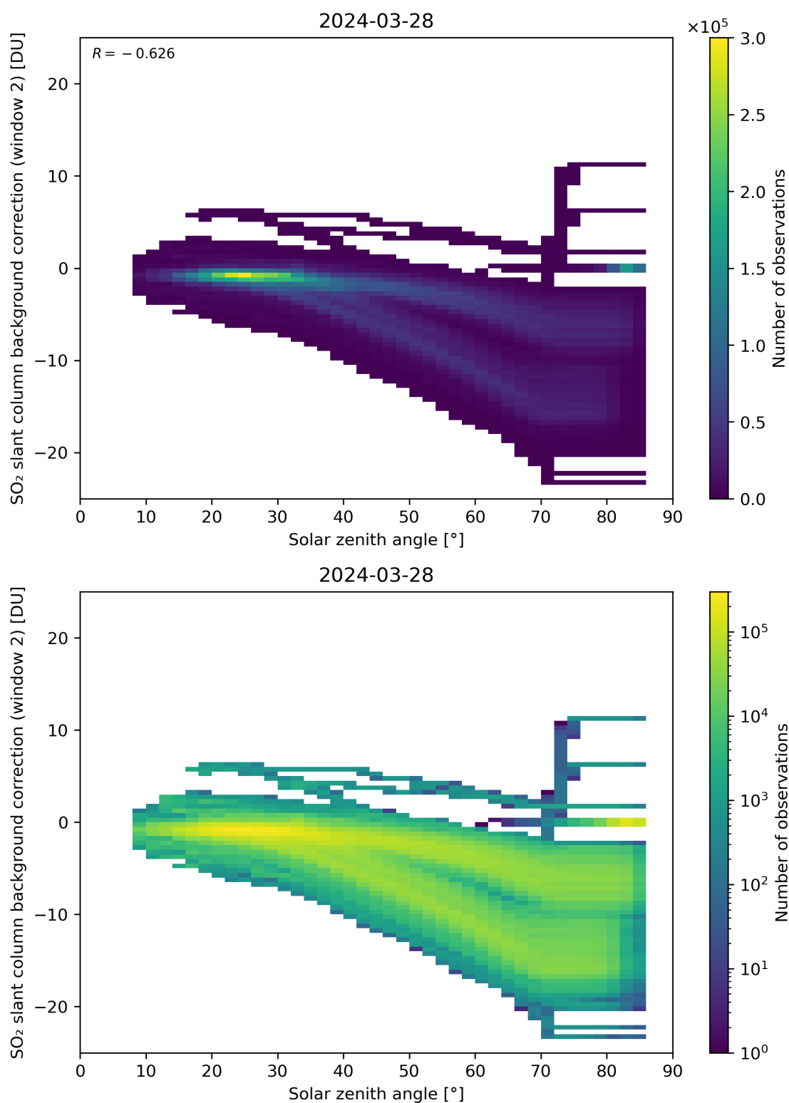
Figure 159: Scatter density plot of “Solar zenith angle” against “SO 2 slant column background correction (window 2)” for 2024-03-27 to 2024-03-29.
