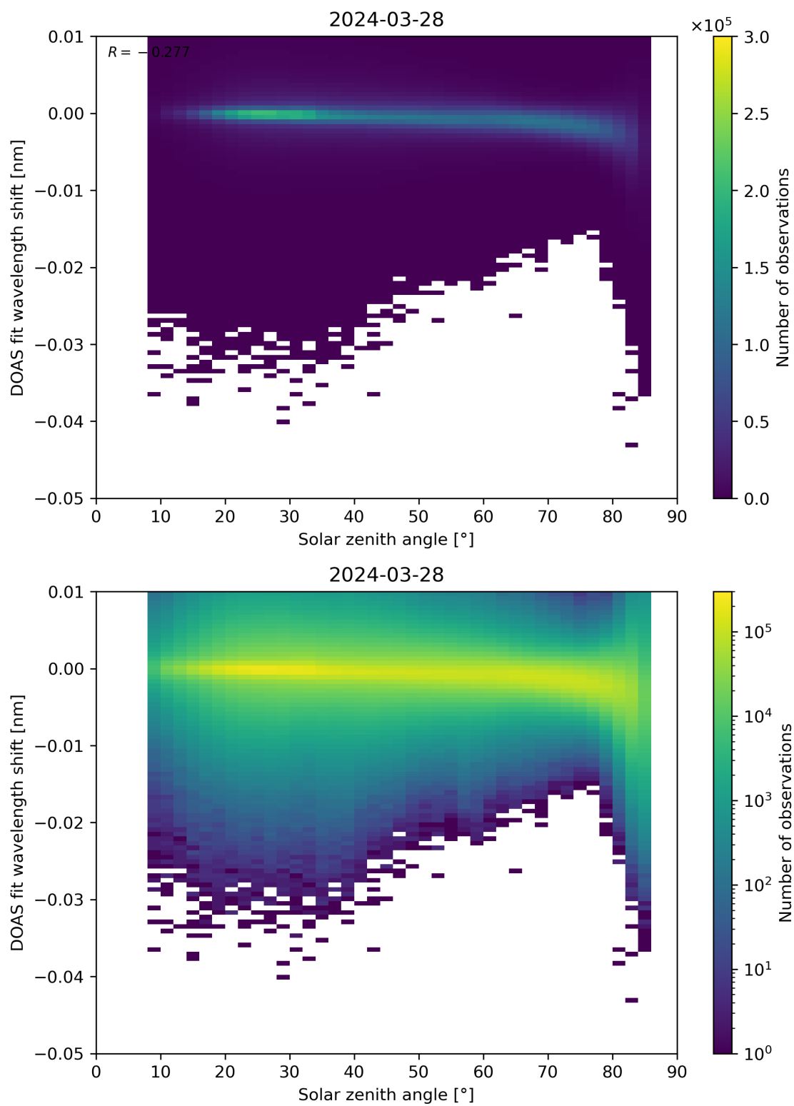
Figure 161: Scatter density plot of “Solar zenith angle” against “DOAS fit wavelength shift” for 2024-03-27 to 2024-03-29.
