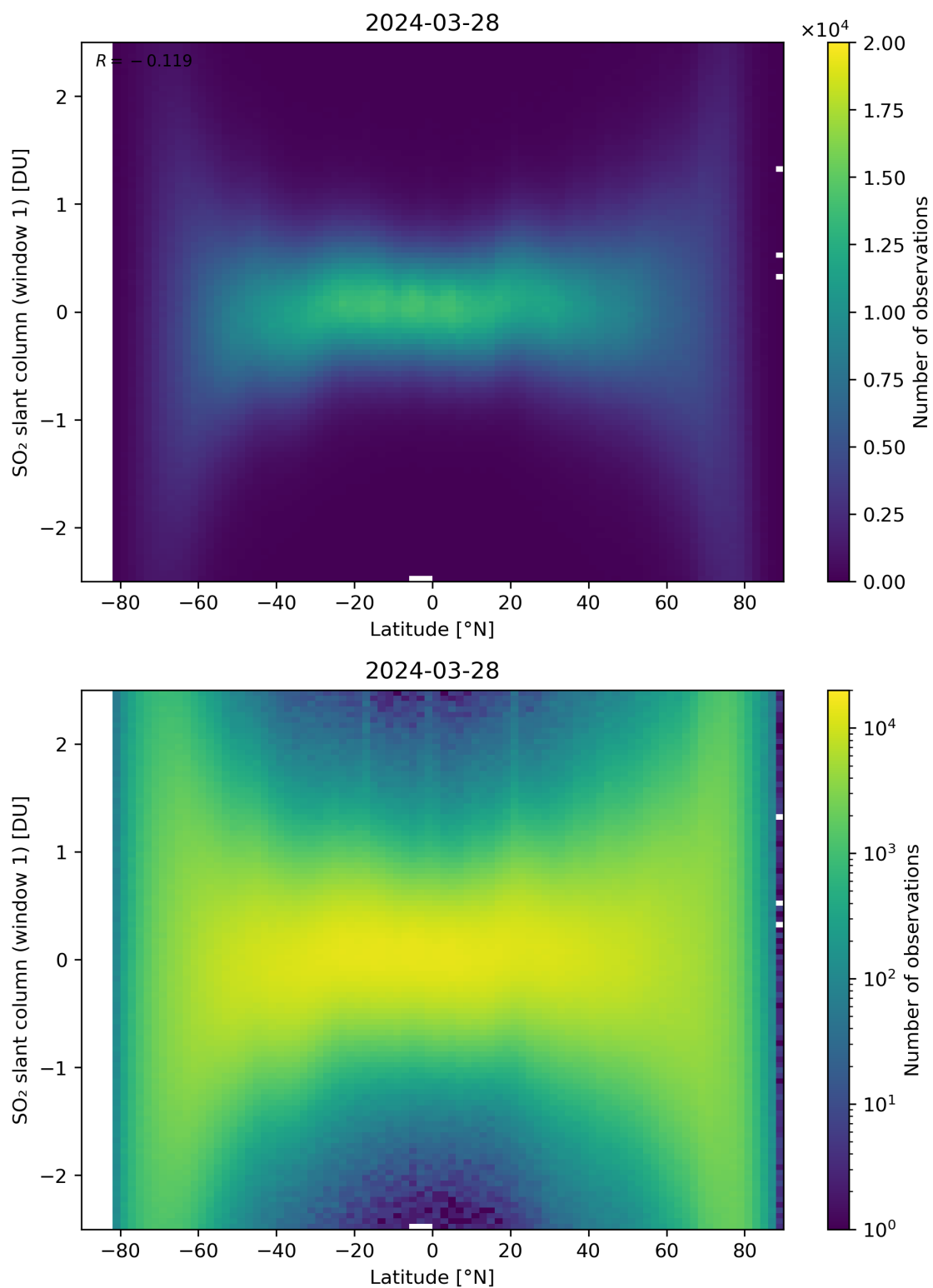
Figure 149: Scatter density plot of “Latitude” against “SO 2 slant column (window 1)” for 2024-03-27 to 2024-03-29.
