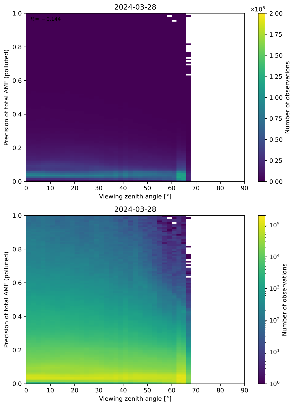
Figure 326: Scatter density plot of “Viewing zenith angle” against “Precision of total AMF (polluted)” for 2024-03-27 to 2024-03-29.
