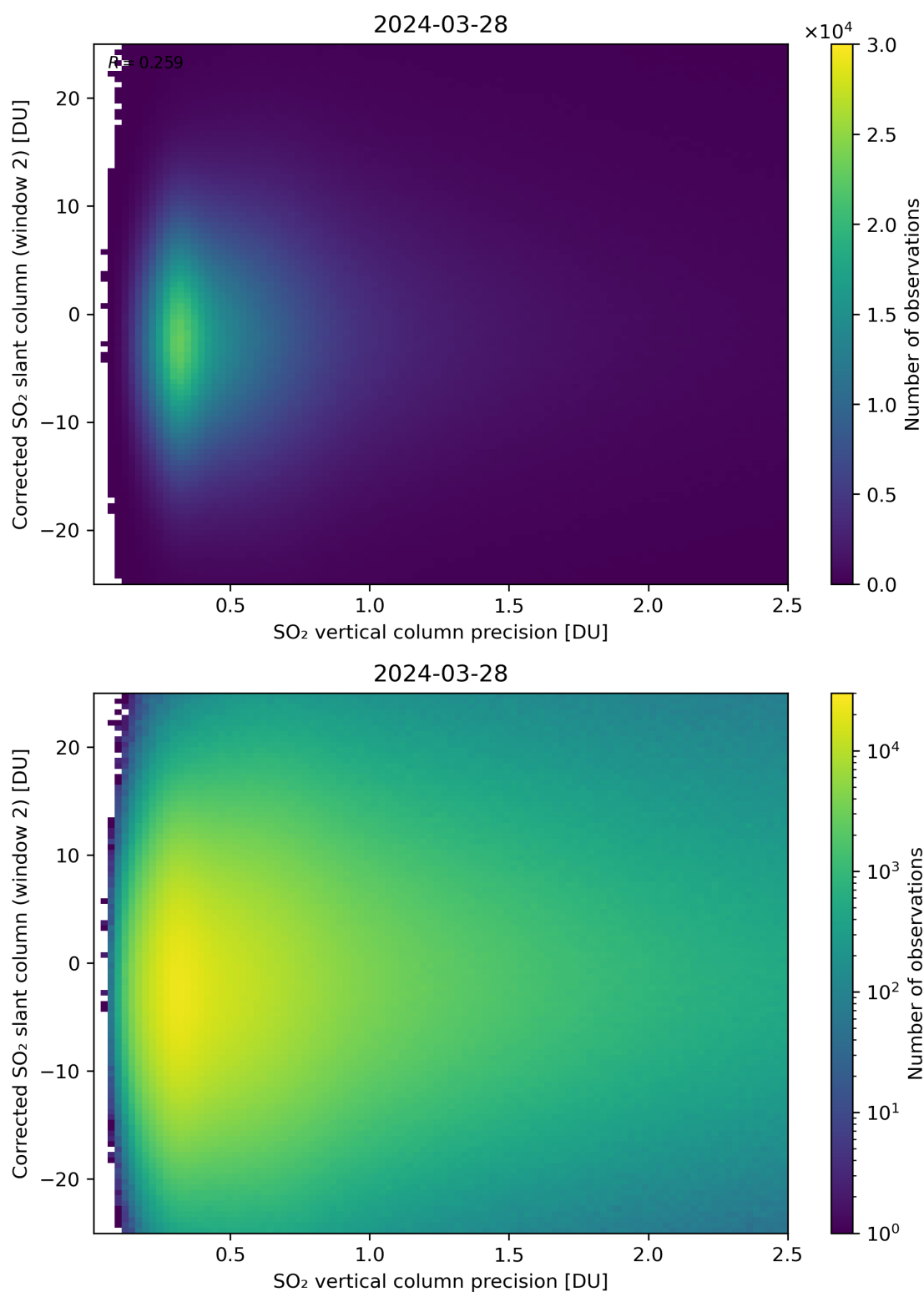
Figure 287: Scatter density plot of “SO 2 vertical column precision” against “Corrected SO 2 slant column (window 2)” for 2024-03-27 to 2024-03-29.
