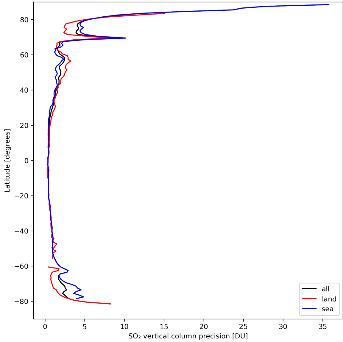
Figure 31: Zonal average of “SO 2 vertical column precision” for 2024-03-27 to 2024-03-29.
