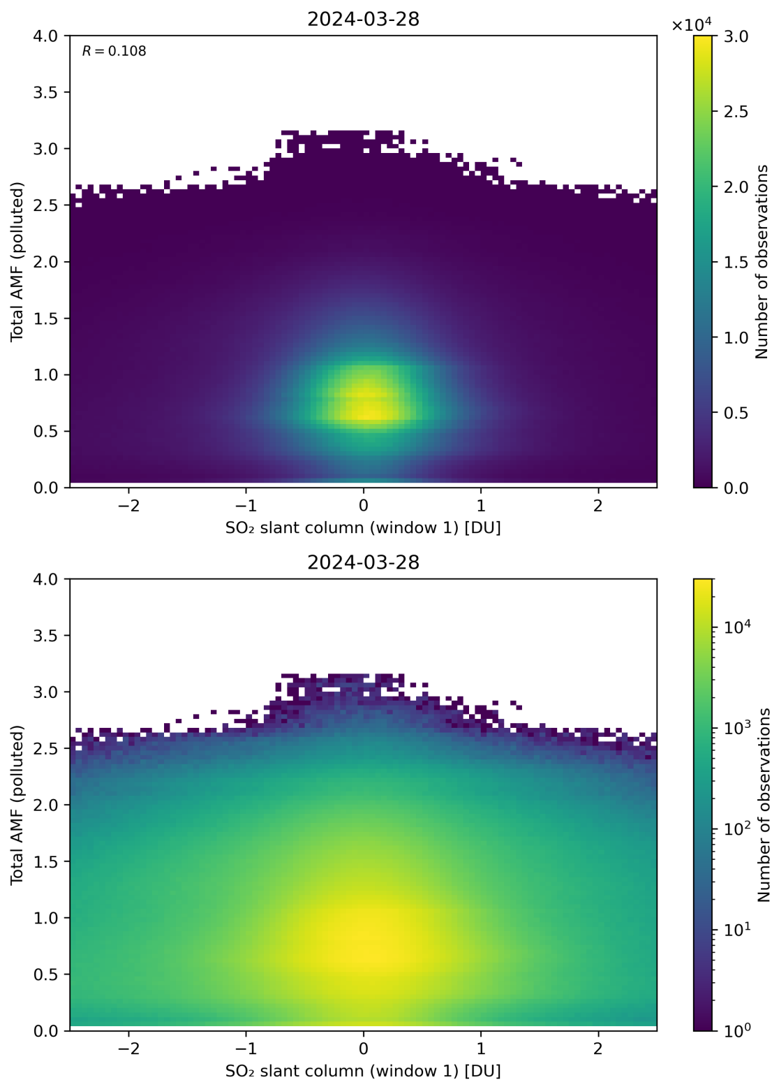
Figure 239: Scatter density plot of “SO 2 slant column (window 1)” against “Total AMF (polluted)” for 2024-03-27 to 2024-03-29.
