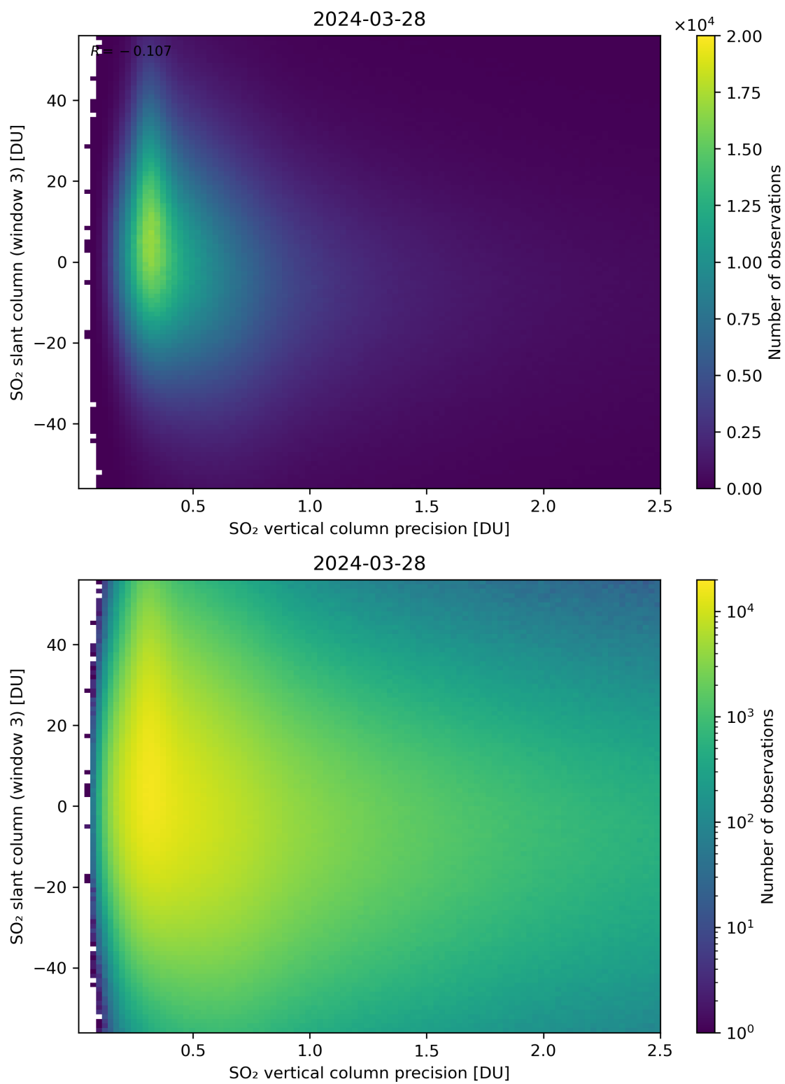
Figure 292: Scatter density plot of “SO 2 vertical column precision” against “SO 2 slant column (window 3)” for 2024-03-27 to 2024-03-29.
