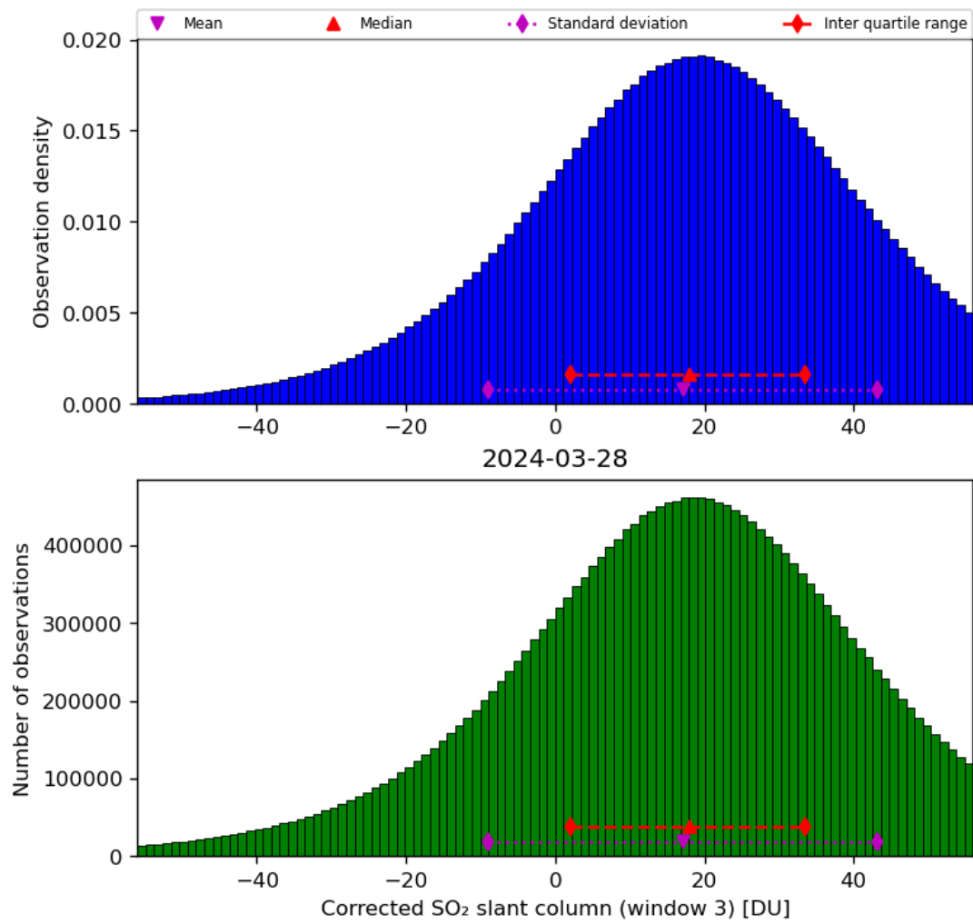
Figure 66: Histogram of “Corrected SO 2 slant column (window 3)” for 2024-03-27 to 2024-03-29
