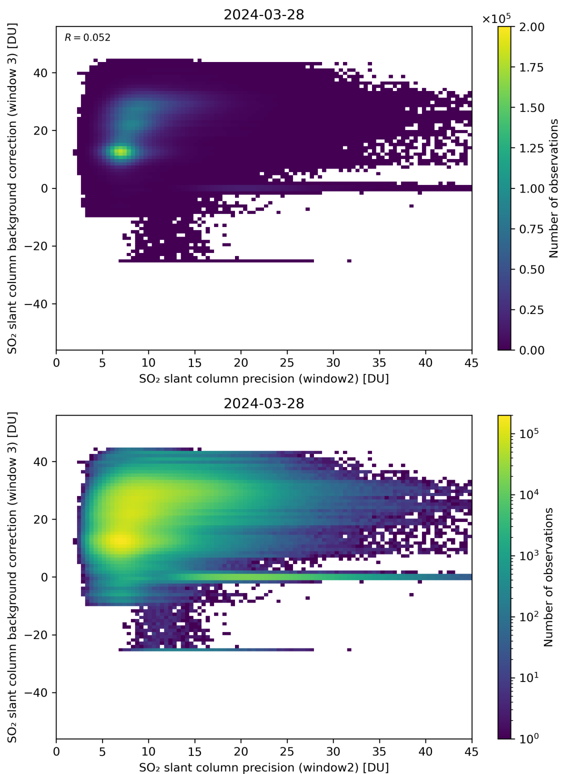
Figure 242: Scatter density plot of “SO 2 slant column precision (window2)” against “SO 2 slant column background correction (window 3)” for 2024-03-27 to 2024-03-29.
