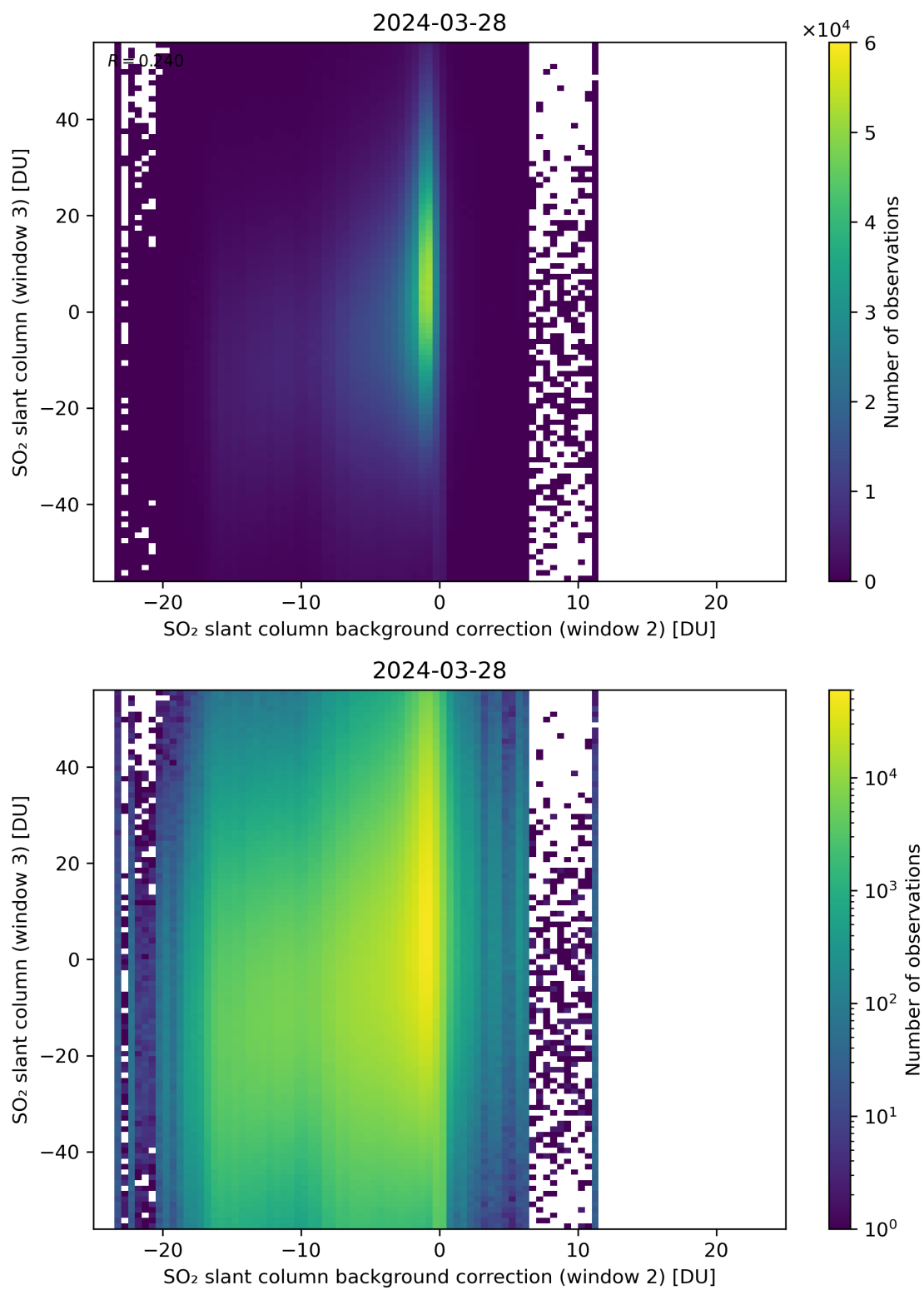
Figure 117: Scatter density plot of “SO 2 slant column background correction (window 2)” against “SO 2 slant column (window 3)” for 2024-03-27 to 2024-03-29.
