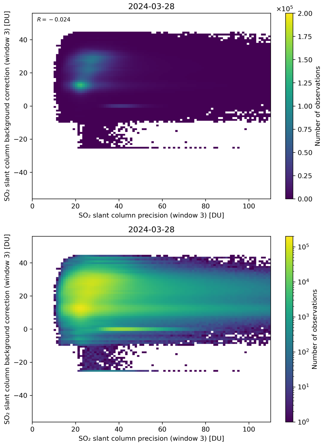
Figure 257: Scatter density plot of “SO 2 slant column precision (window 3)” against “SO 2 slant column background correction (window 3)” for 2024-03-27 to 2024-03-29.
