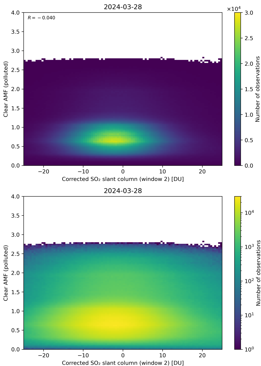
Figure 199: Scatter density plot of “Corrected SO 2 slant column (window 2)” against “Clear AMF (polluted)” for 2024-03-27 to 2024-03-29.
