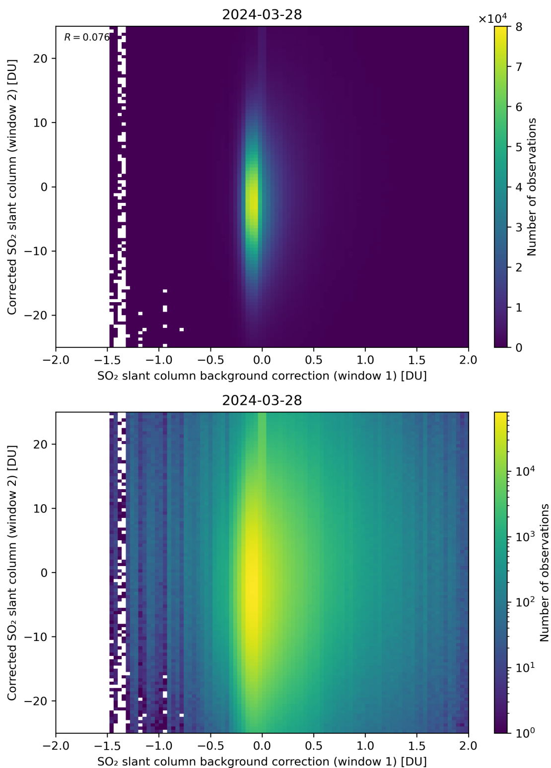
Figure 104: Scatter density plot of “SO 2 slant column background correction (window 1)” against “Corrected SO 2 slant column (window 2)” for 2024-03-27 to 2024-03-29.
