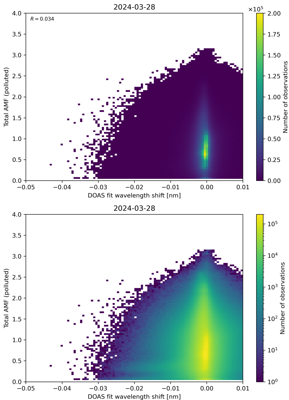
Figure 130: Scatter density plot of “DOAS fit wavelength shift” against “Total AMF (polluted)” for 2024-03-27 to 2024-03-29.
