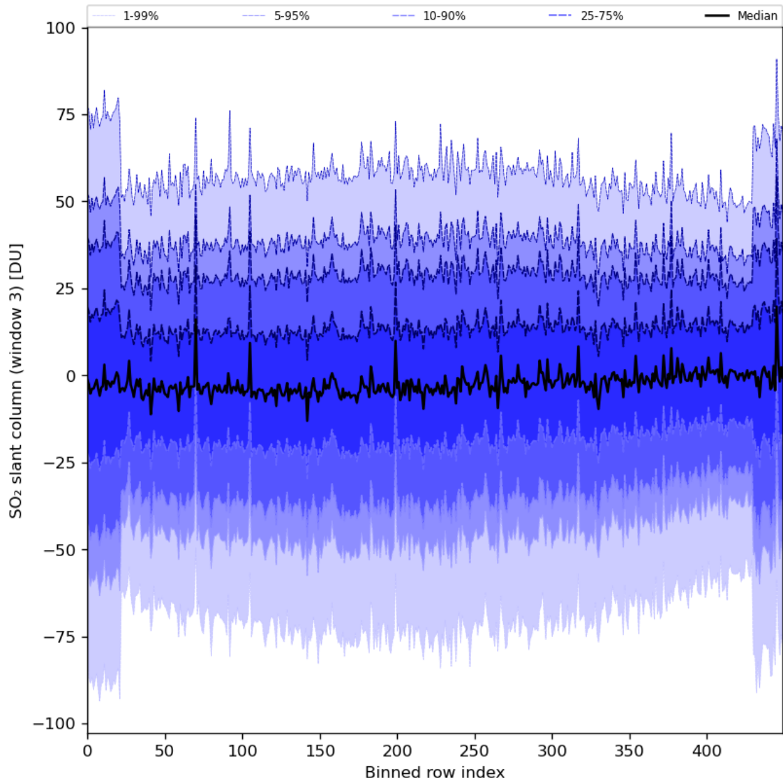
Figure 87: Along track statistics of “SO 2 slant column (window 3)” for 2024-03-27 to 2024-03-29
