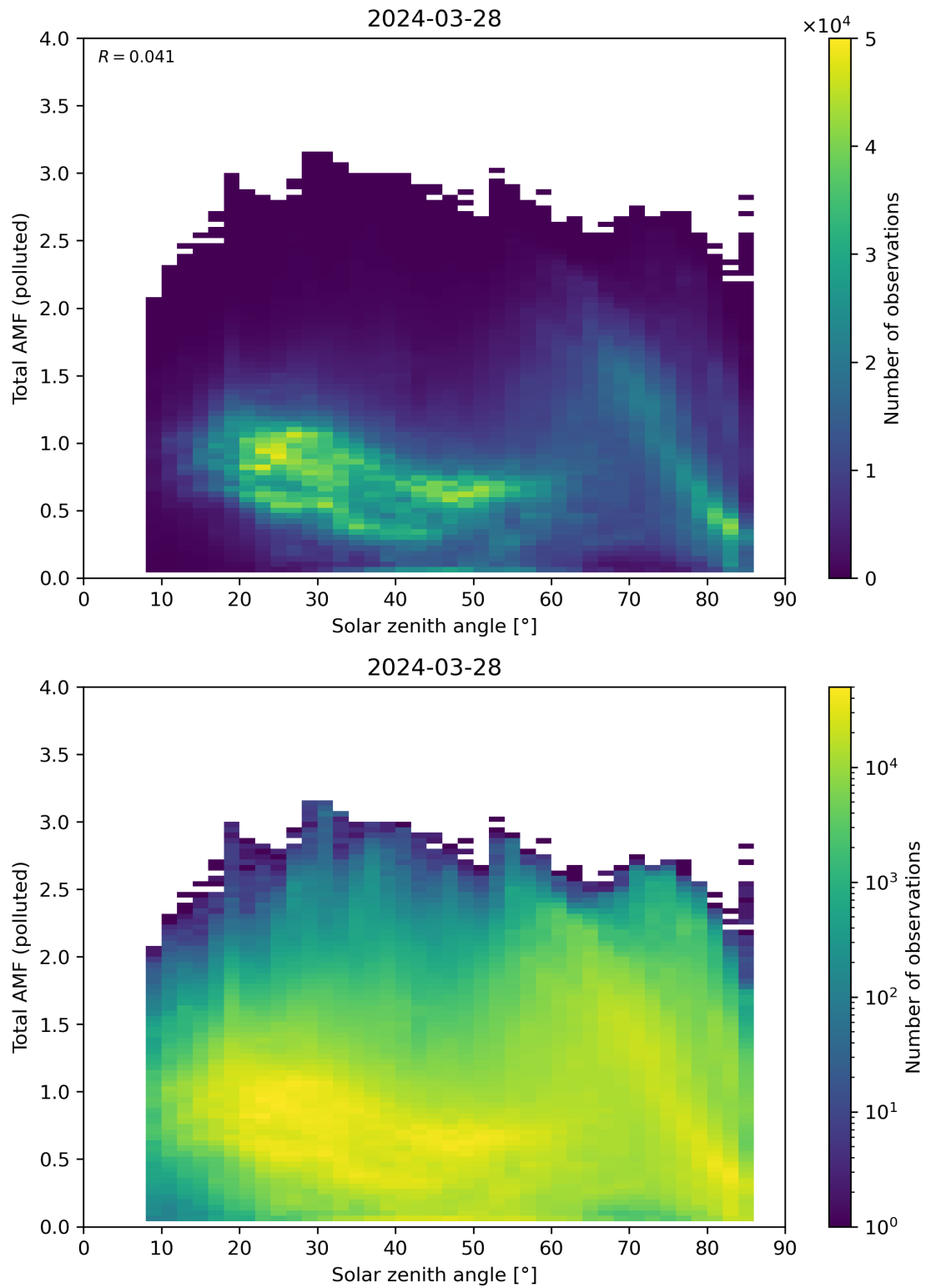
Figure 174: Scatter density plot of “Solar zenith angle” against “Total AMF (polluted)” for 2024-03-27 to 2024-03-29.
