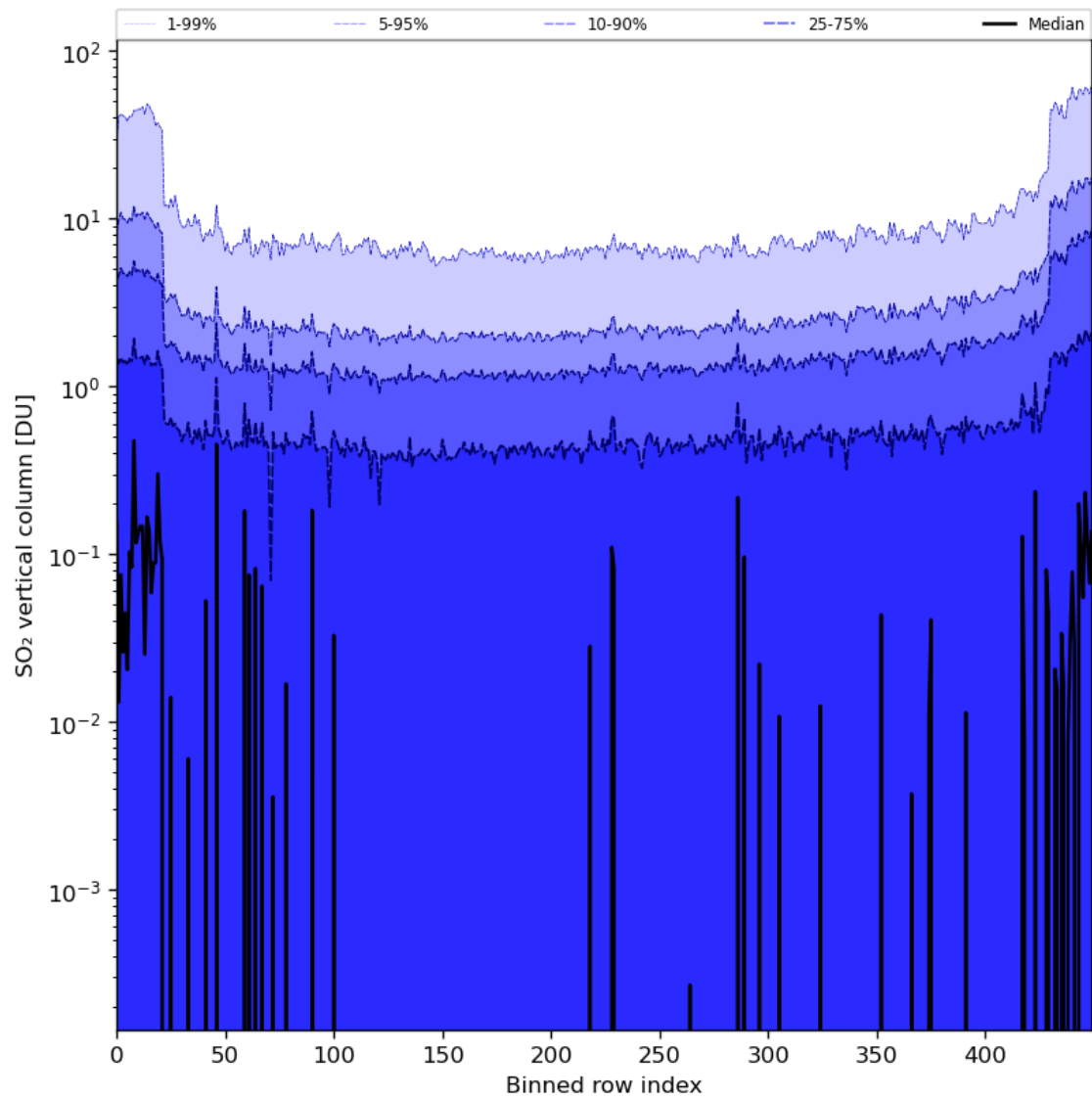
Figure 76: Along track statistics of “SO 2 vertical column” for 2024-03-27 to 2024-03-29
