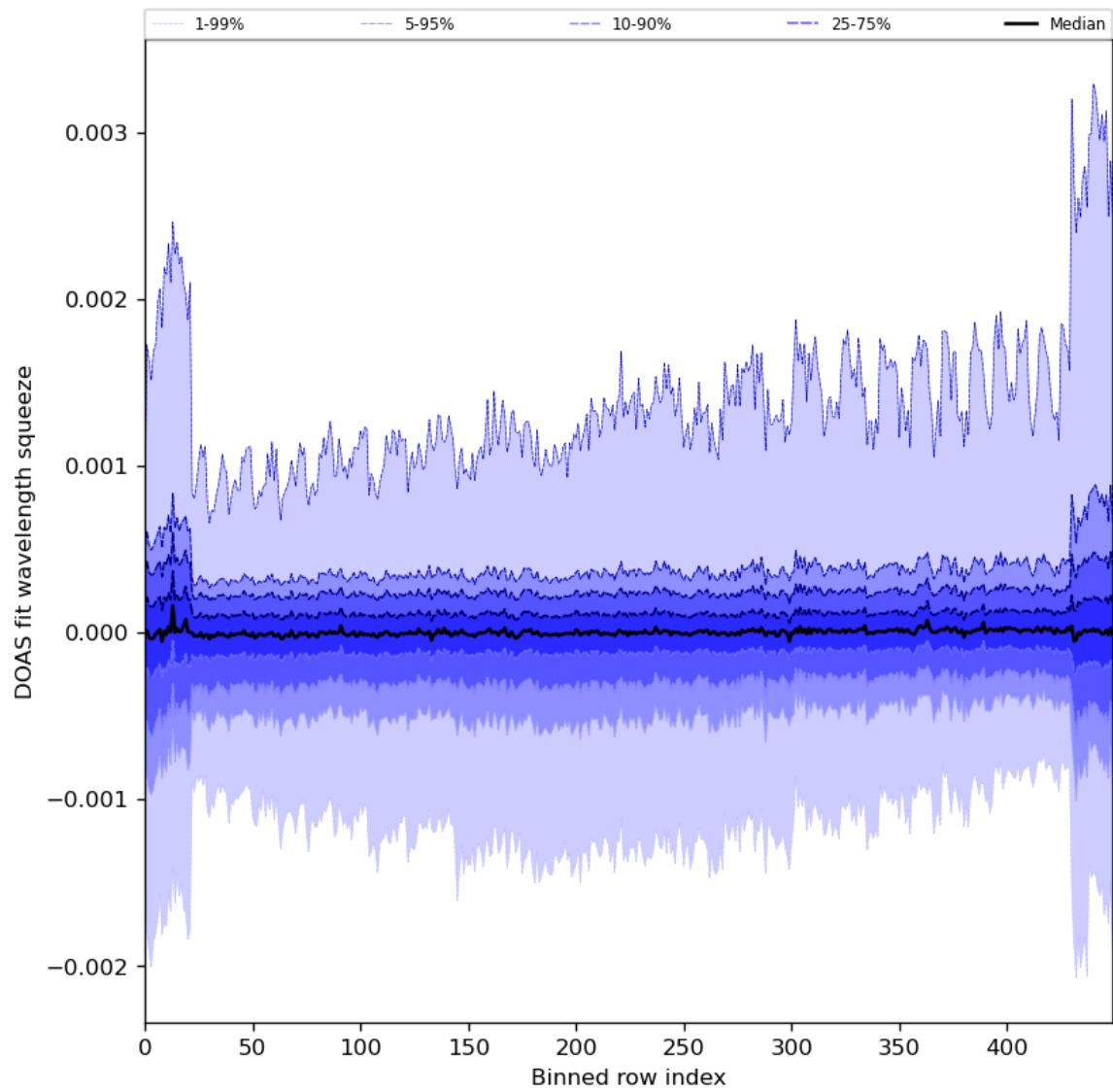
Figure 92: Along track statistics of “DOAS fit wavelength squeeze” for 2024-03-27 to 2024-03-29
