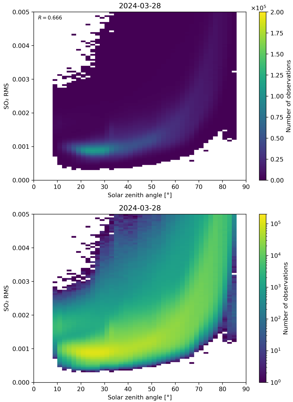
Figure 163: Scatter density plot of “Solar zenith angle” against “SO 2 RMS” for 2024-03-27 to 2024-03-29.
