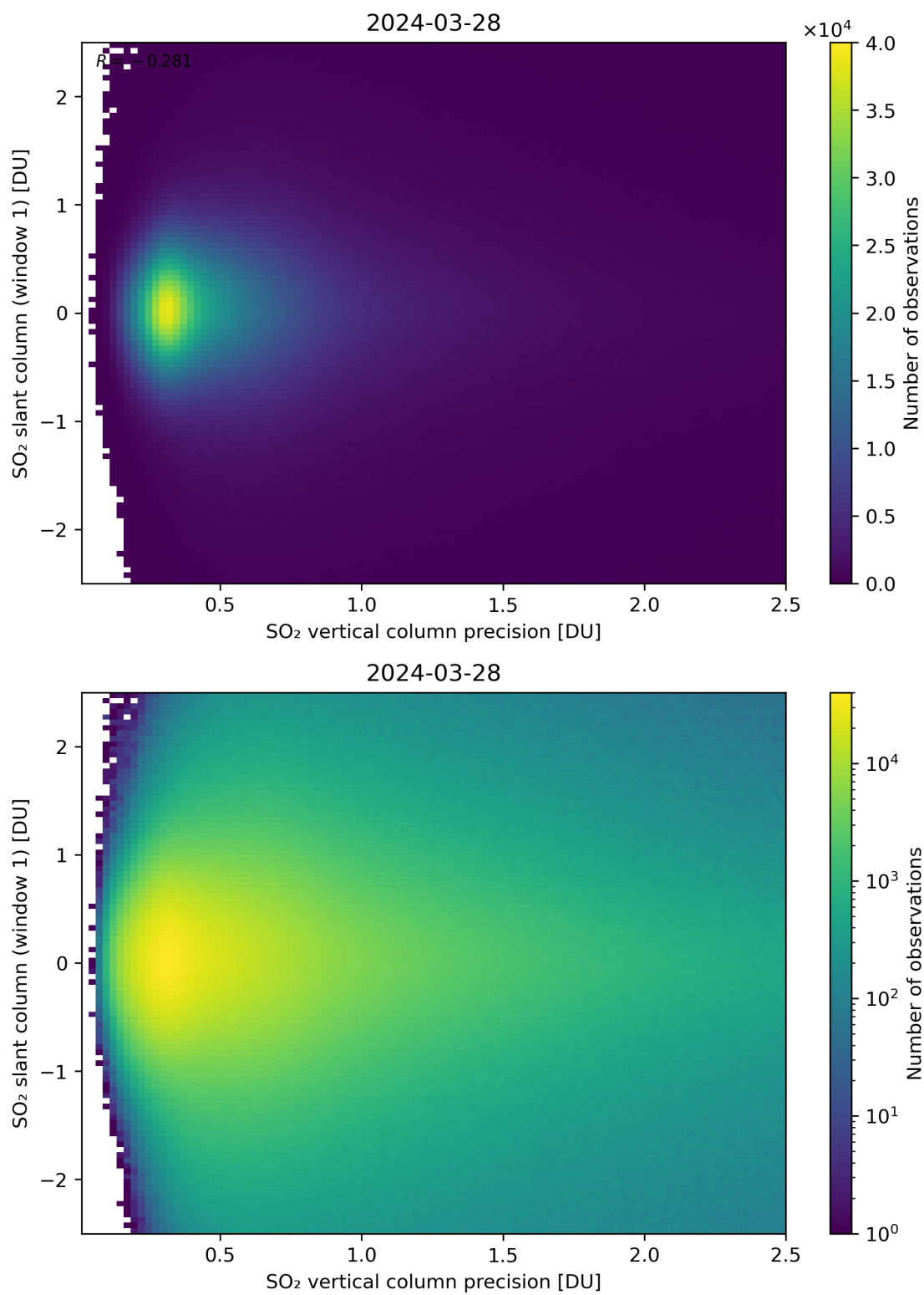
Figure 289: Scatter density plot of “SO 2 vertical column precision” against “SO 2 slant column (window 1)” for 2024-03-27 to 2024-03-29.
