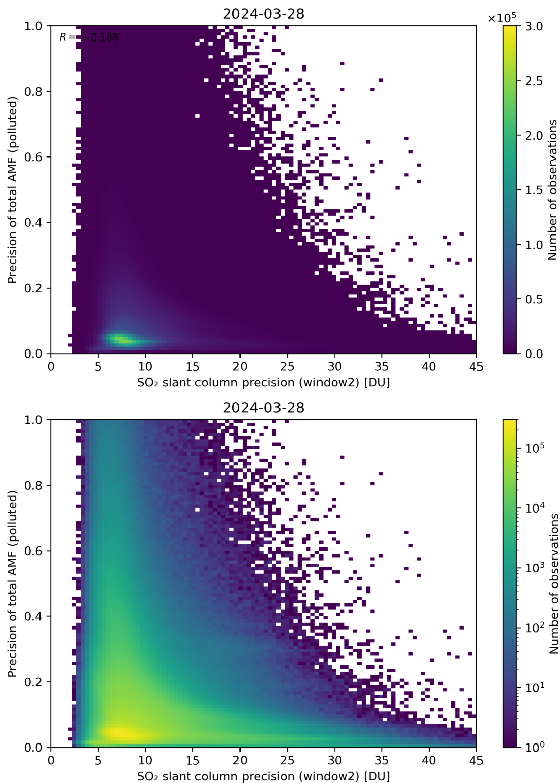
Figure 252: Scatter density plot of “SO 2 slant column precision (window2)” against “Precision of total AMF (polluted)” for 2024-03-27 to 2024-03-29.
