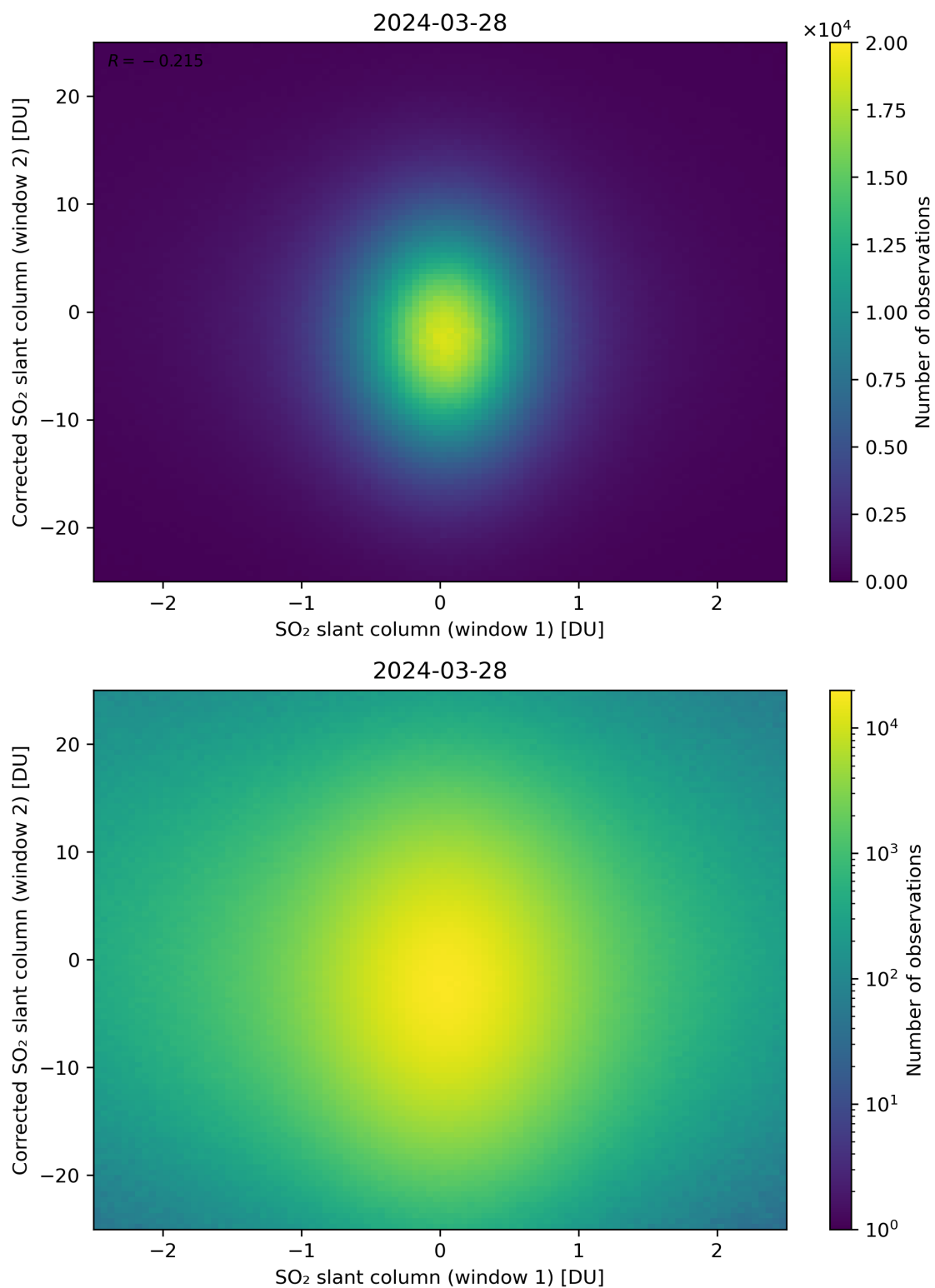
Figure 233: Scatter density plot of “SO 2 slant column (window 1)” against “Corrected SO 2 slant column (window 2)” for 2024-03-27 to 2024-03-29.
