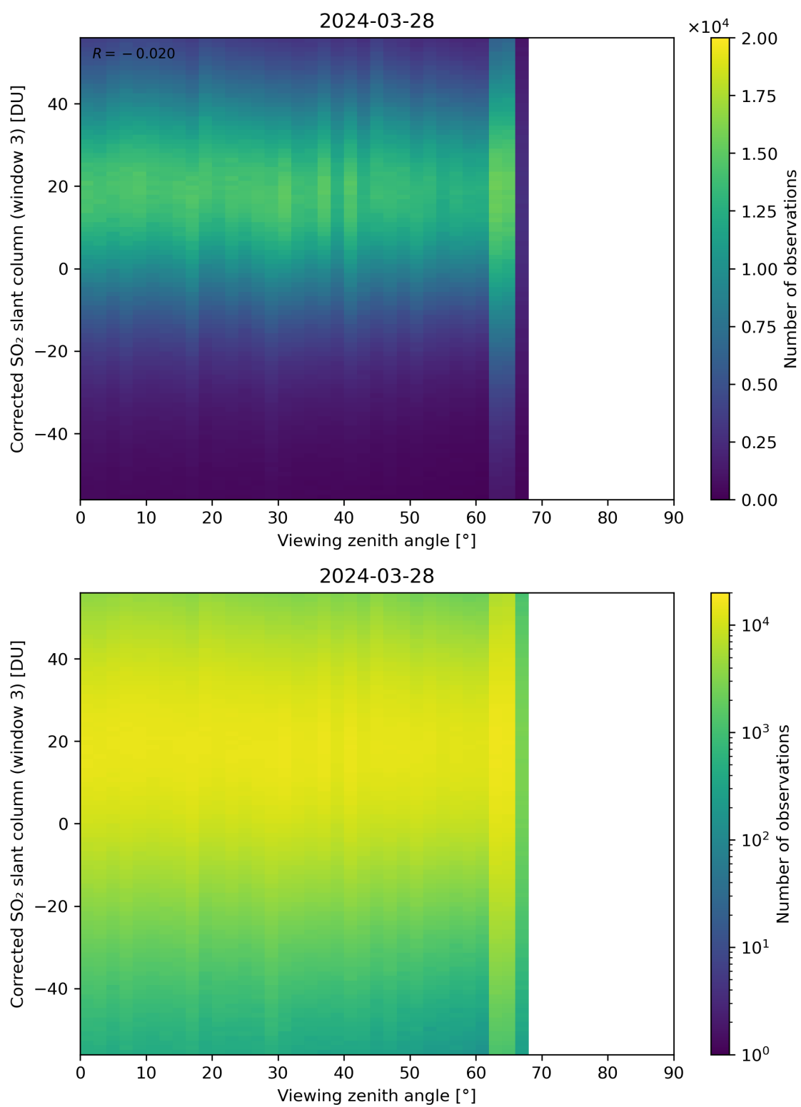
Figure 319: Scatter density plot of “Viewing zenith angle” against “Corrected SO 2 slant column (window 3)” for 2024-03-27 to 2024-03-29.
