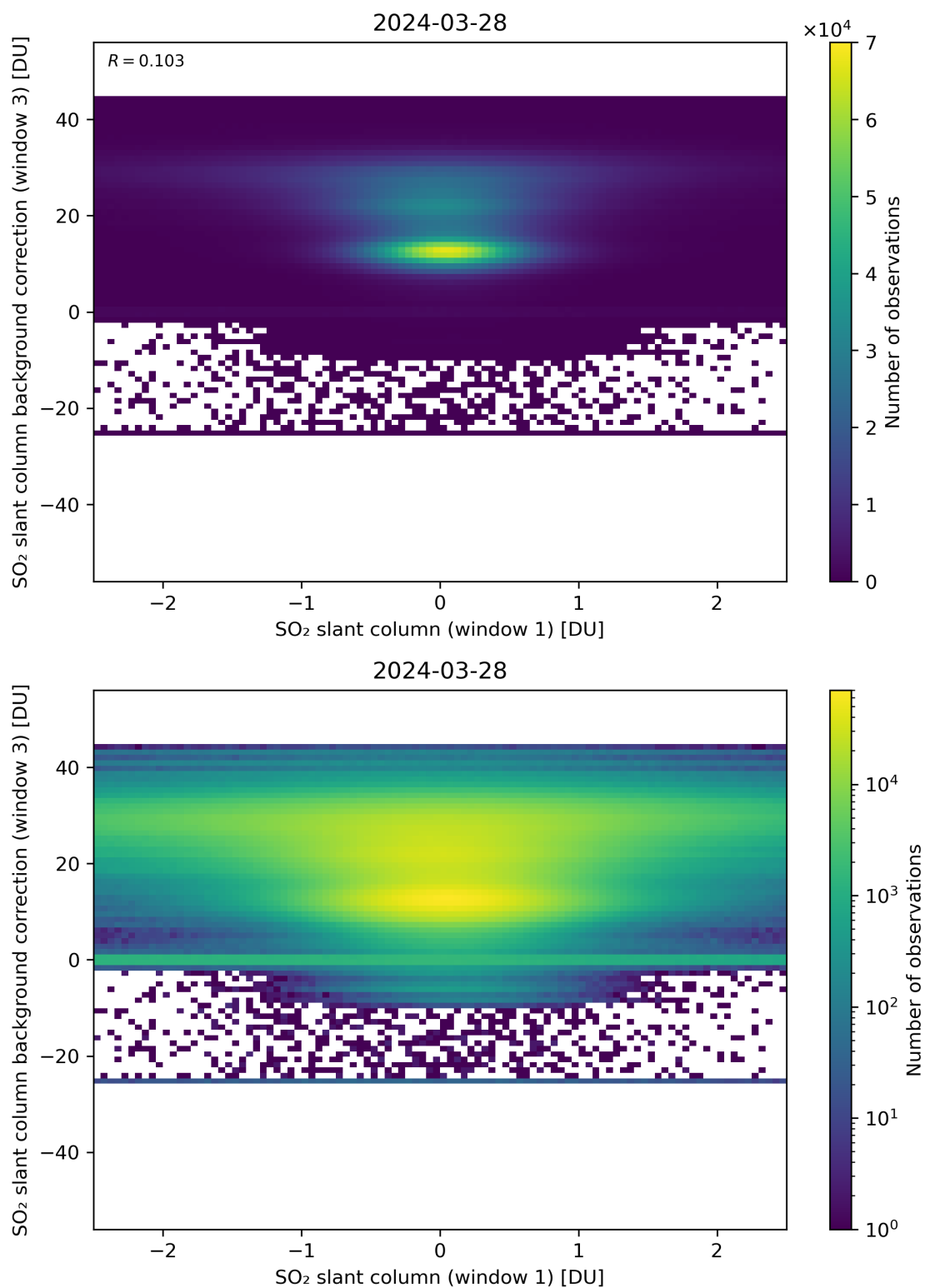
Figure 214: Scatter density plot of “SO 2 slant column (window 1)” against “SO 2 slant column background correction (window 3)” for 2024-03-27 to 2024-03-29.
