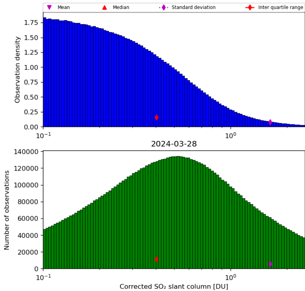
Figure 55: Histogram of “Corrected SO 2 slant column” for 2024-03-27 to 2024-03-29
