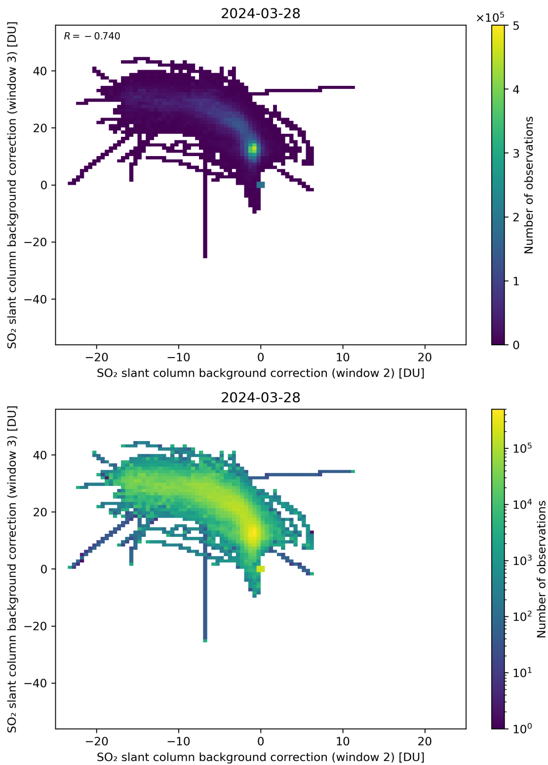
Figure 111: Scatter density plot of “SO 2 slant column background correction (window 2)” against “SO 2 slant column background correction (window 3)” for 2024-03-27 to 2024-03-29.
