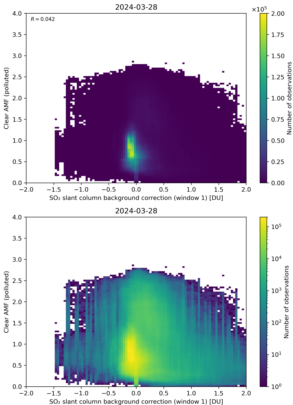
Figure 103: Scatter density plot of “SO 2 slant column background correction (window 1)” against “Clear AMF (polluted)” for 2024-03-27 to 2024-03-29.
