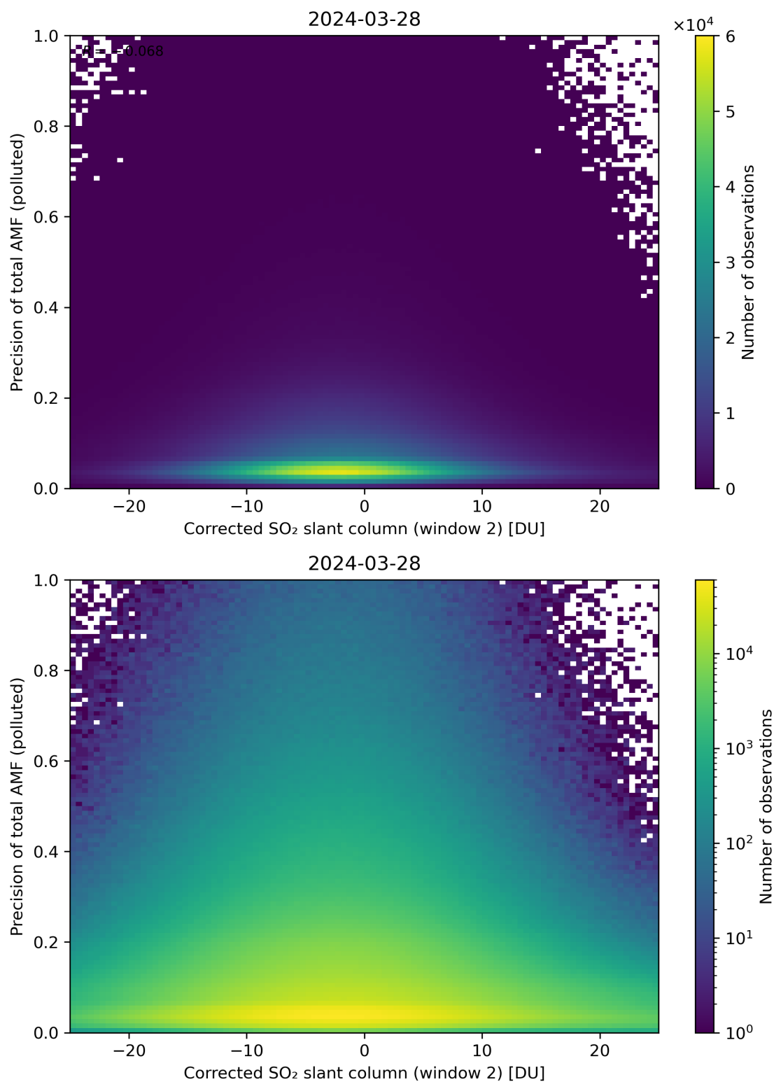
Figure 204: Scatter density plot of “Corrected SO 2 slant column (window 2)” against “Precision of total AMF (polluted)” for 2024-03-27 to 2024-03-29.
