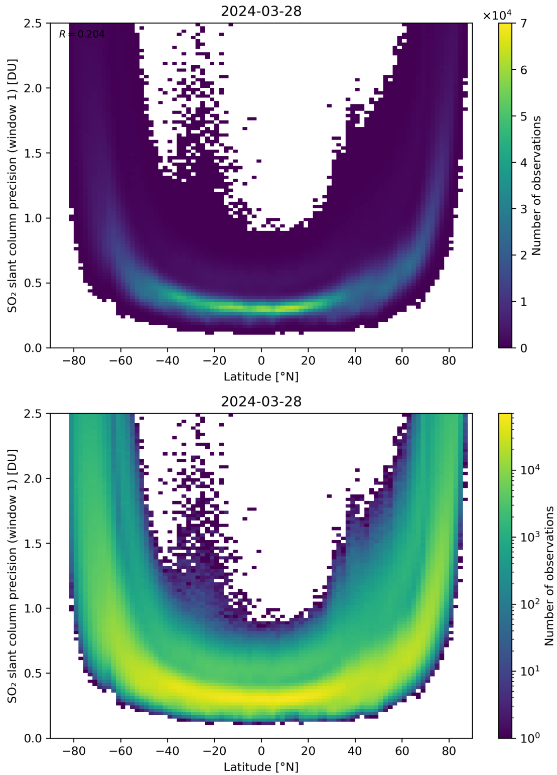
Figure 150: Scatter density plot of “Latitude” against “SO 2 slant column precision (window 1)” for 2024-03-27 to 2024-03-29.
