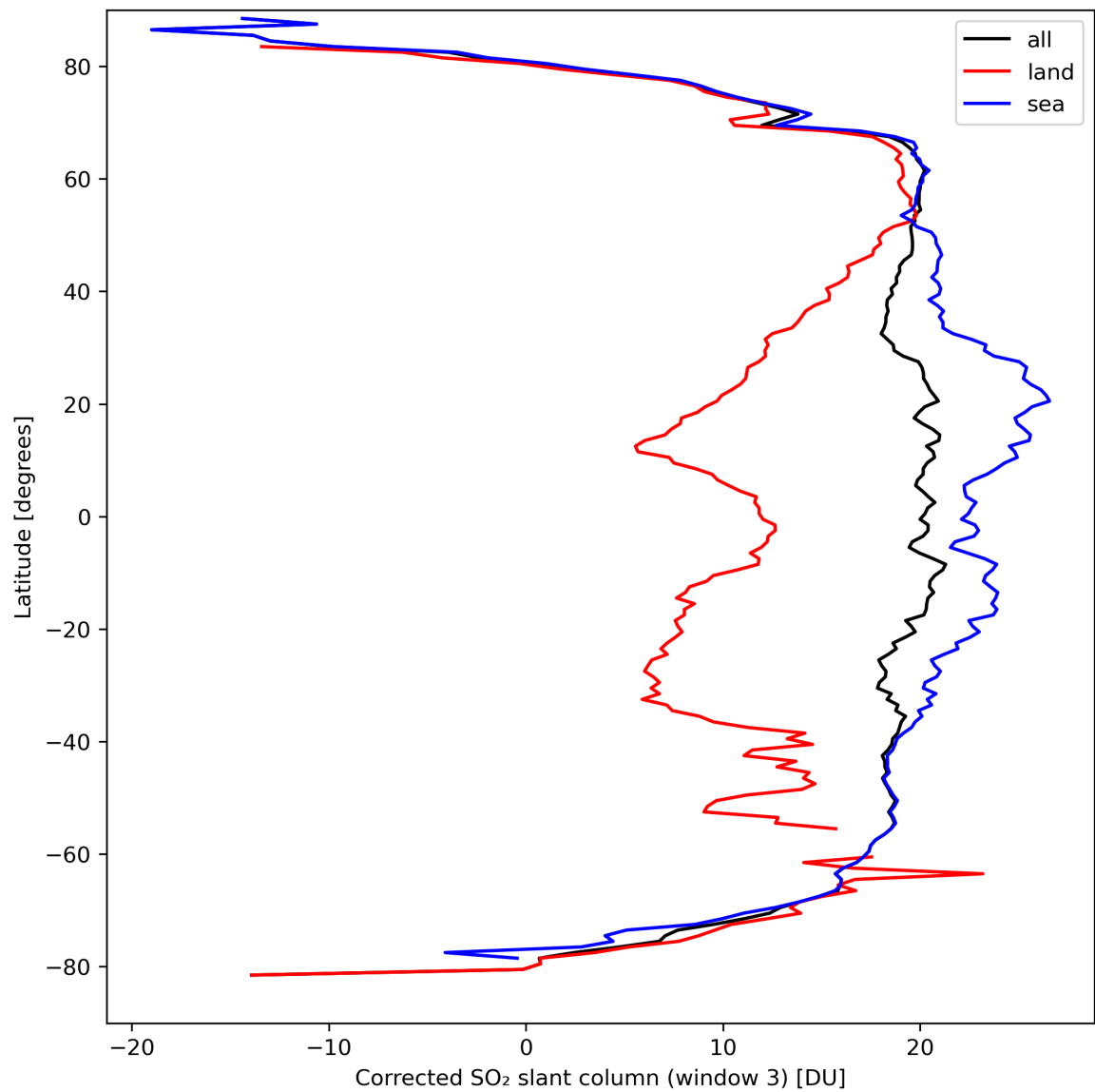
Figure 43: Zonal average of “Corrected SO 2 slant column (window 3)” for 2024-03-27 to 2024-03-29.
