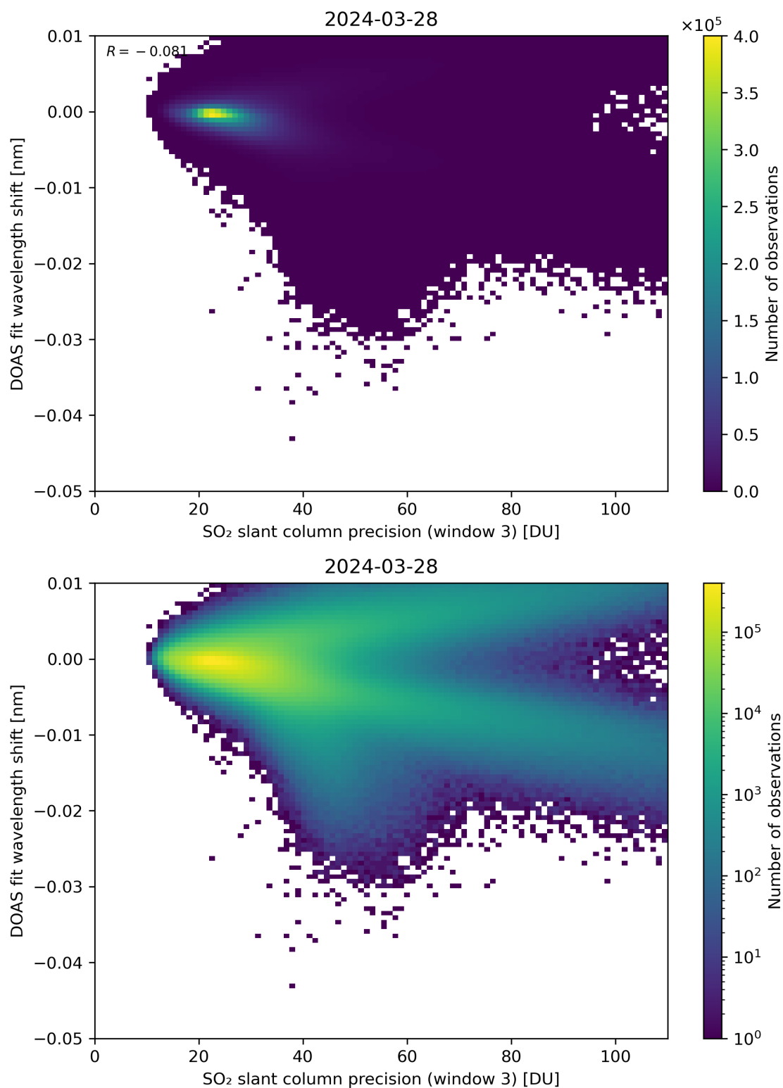
Figure 258: Scatter density plot of “SO 2 slant column precision (window 3)” against “DOAS fit wavelength shift” for 2024-03-27 to 2024-03-29.
