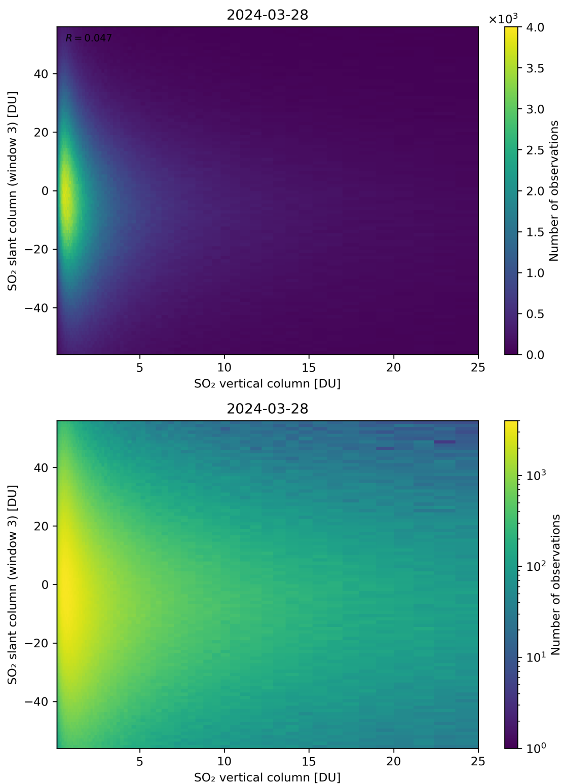
Figure 303: Scatter density plot of “SO 2 vertical column” against “SO 2 slant column (window 3)” for 2024-03-27 to 2024-03-29.
