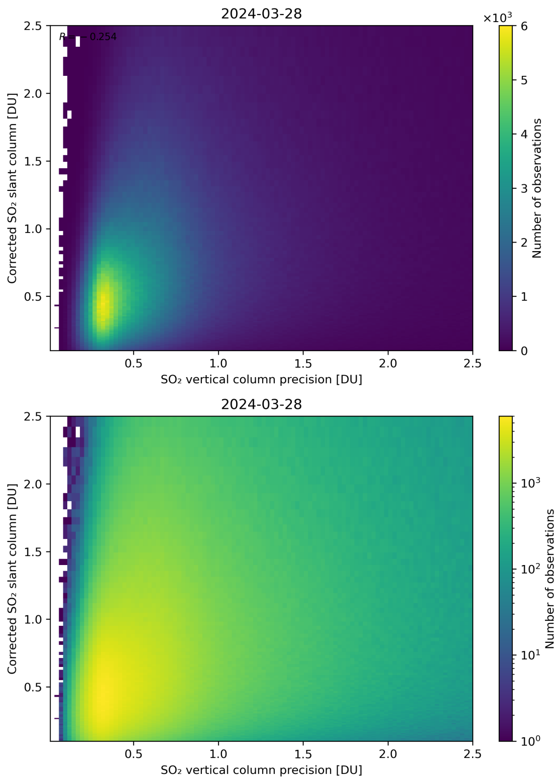
Figure 286: Scatter density plot of “SO 2 vertical column precision” against “Corrected SO 2 slant column” for 2024-03-27 to 2024-03-29.
