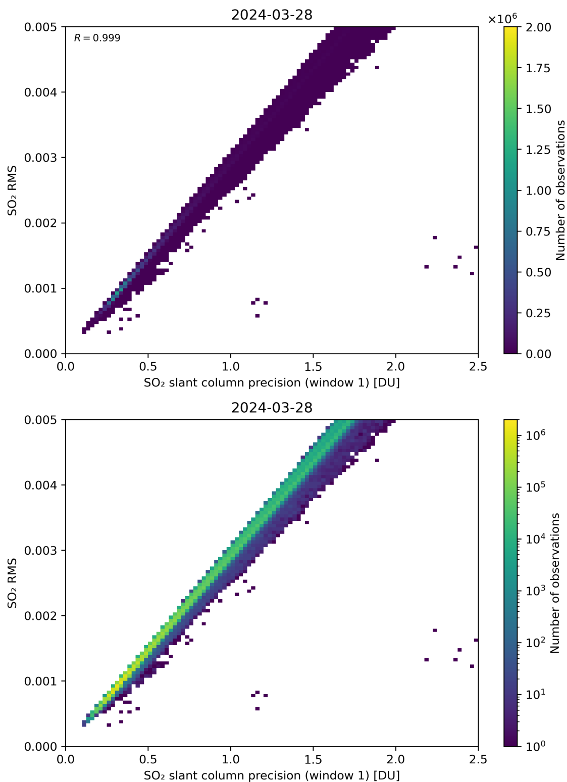
Figure 223: Scatter density plot of “SO 2 slant column precision (window 1)” against “SO 2 RMS” for 2024-03-27 to 2024-03-29.
