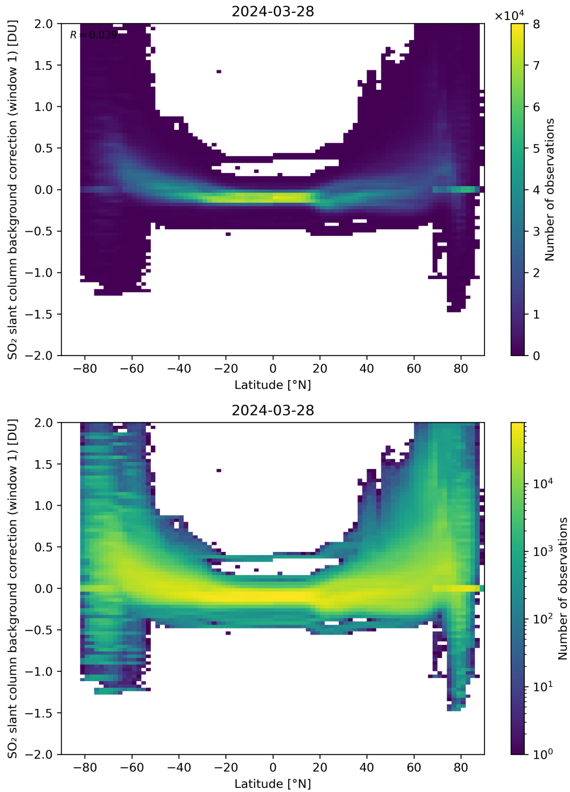
Figure 139: Scatter density plot of “Latitude” against “SO 2 slant column background correction (window 1)” for 2024-03-27 to 2024-03-29.
