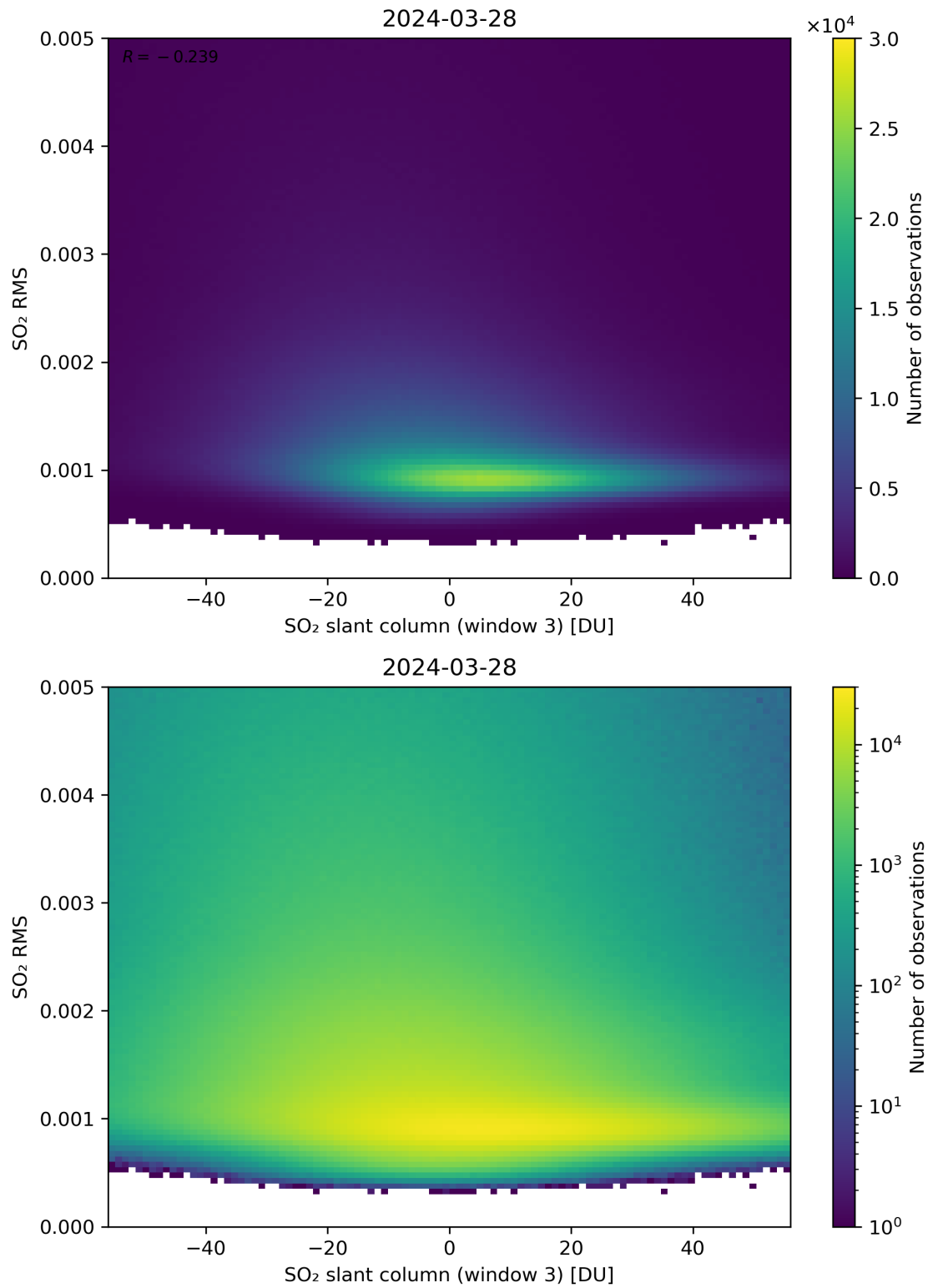
Figure 256: Scatter density plot of “SO 2 slant column (window 3)” against “SO 2 RMS” for 2024-03-27 to 2024-03-29.
