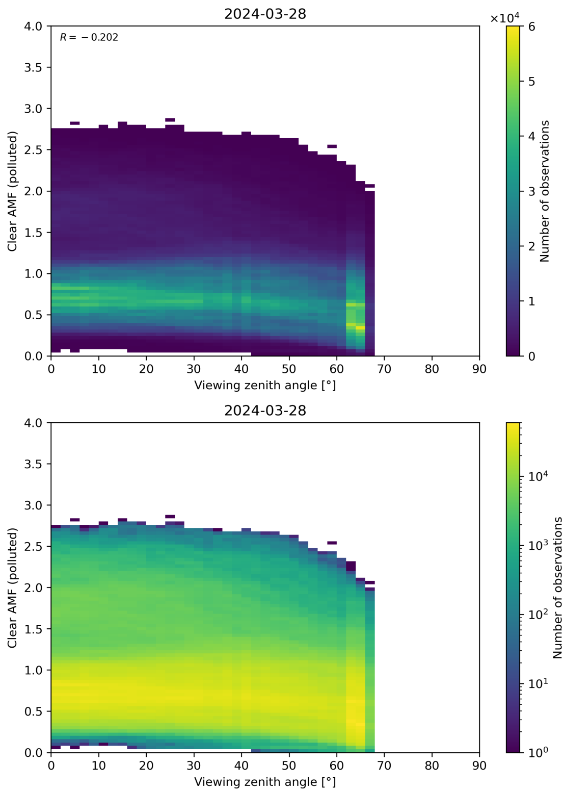
Figure 316: Scatter density plot of “Viewing zenith angle” against “Clear AMF (polluted)” for 2024-03-27 to 2024-03-29.
