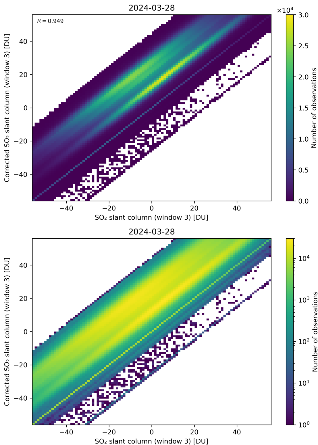
Figure 266: Scatter density plot of “SO 2 slant column (window 3)” against “Corrected SO 2 slant column (window 3)” for 2024-03-27 to 2024-03-29.
