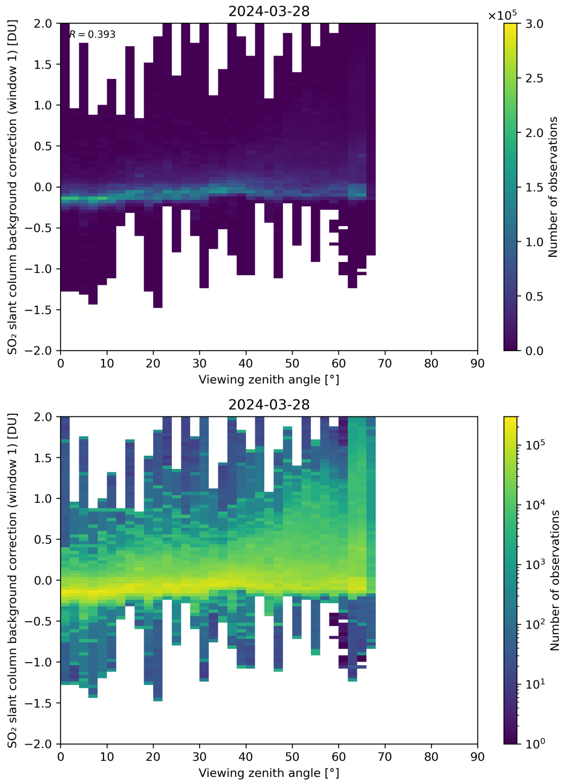
Figure 308: Scatter density plot of “Viewing zenith angle” against “SO 2 slant column background correction (window 1)” for 2024-03-27 to 2024-03-29.
