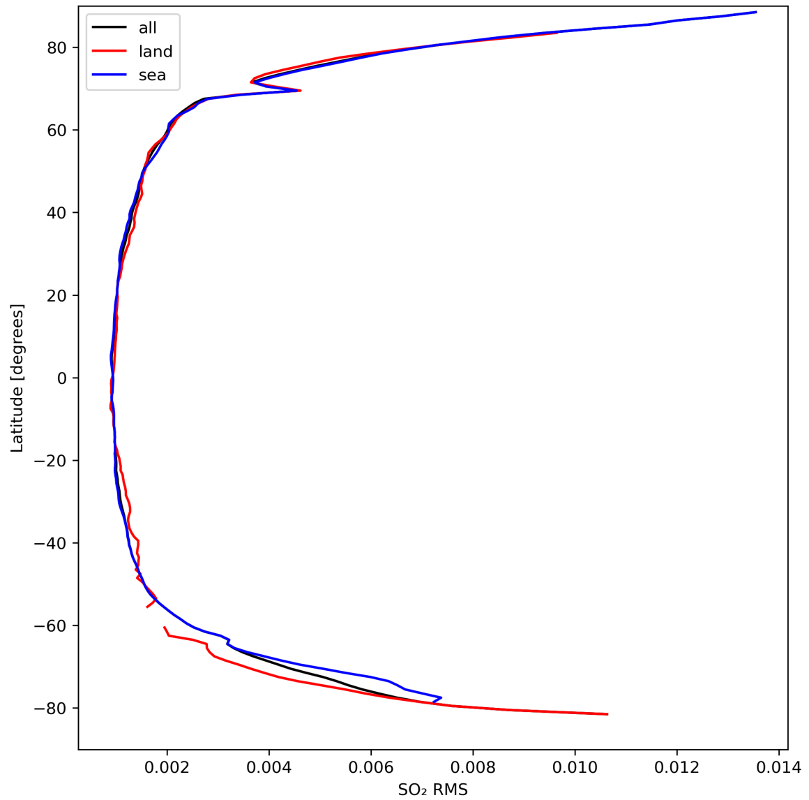
Figure 47: Zonal average of “SO 2 RMS” for 2024-03-27 to 2024-03-29.
