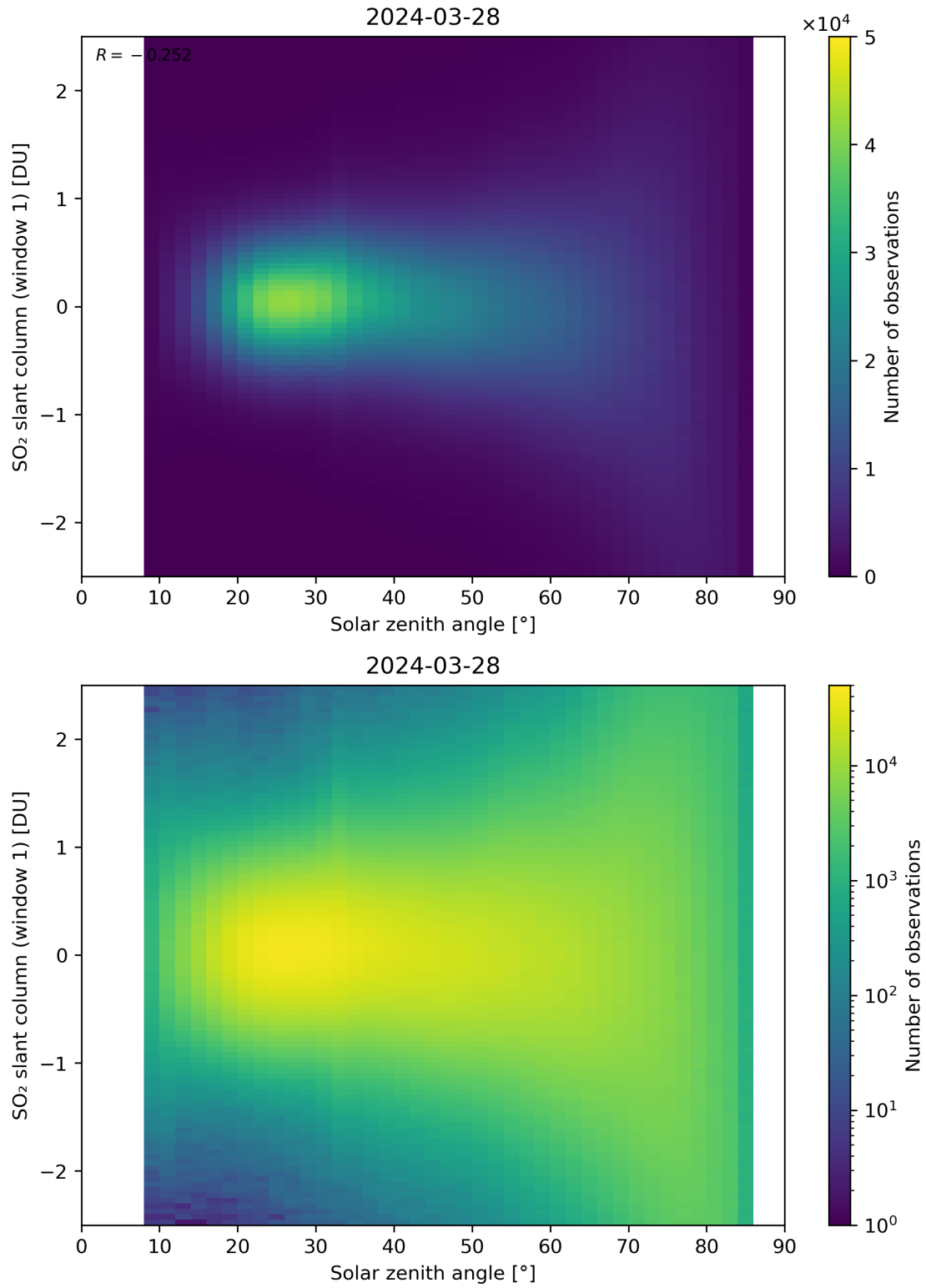
Figure 169: Scatter density plot of “Solar zenith angle” against “SO 2 slant column (window 1)” for 2024-03-27 to 2024-03-29.
