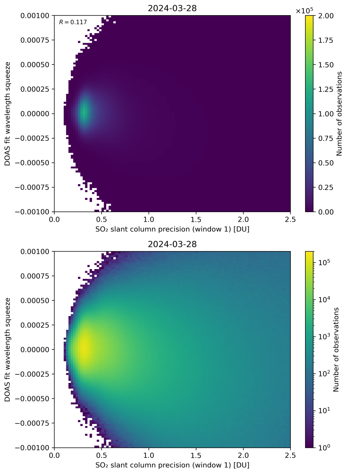
Figure 222: Scatter density plot of “SO 2 slant column precision (window 1)” against “DOAS fit wavelength squeeze” for 2024-03-27 to 2024-03-29.
