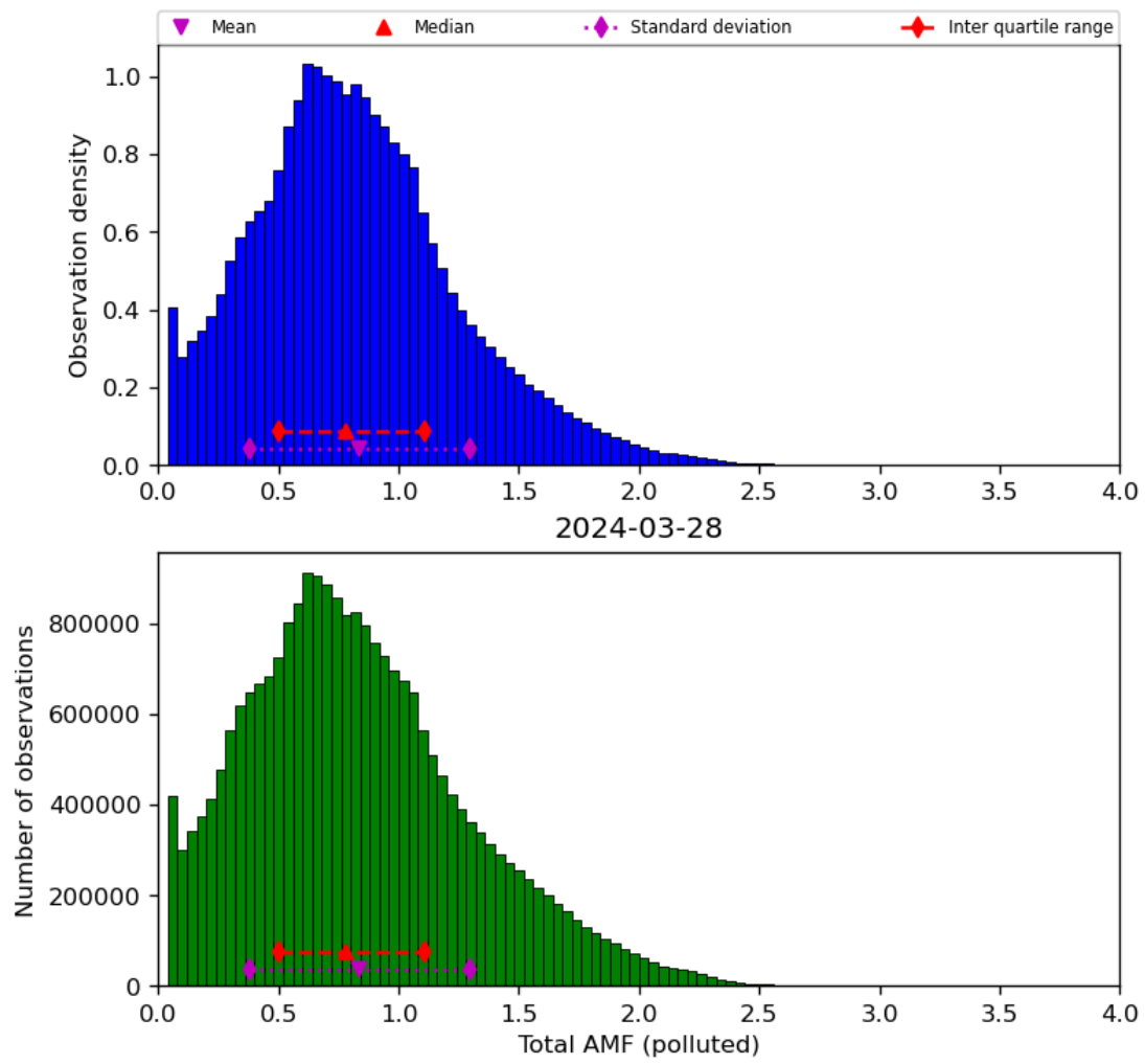
Figure 71: Histogram of “Total AMF (polluted)” for 2024-03-27 to 2024-03-29
