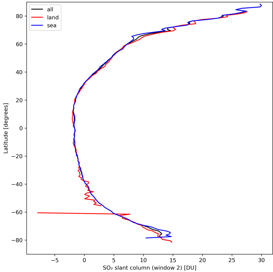
Figure 37: Zonal average of “SO 2 slant column (window 2)” for 2024-03-27 to 2024-03-29.
