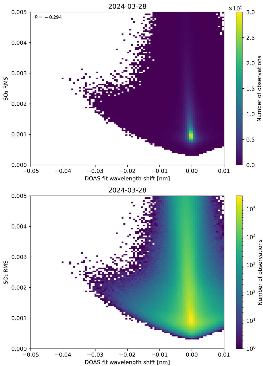
Figure 128: Scatter density plot of “DOAS fit wavelength shift” against “SO 2 RMS” for 2024-03-27 to 2024-03-29.
