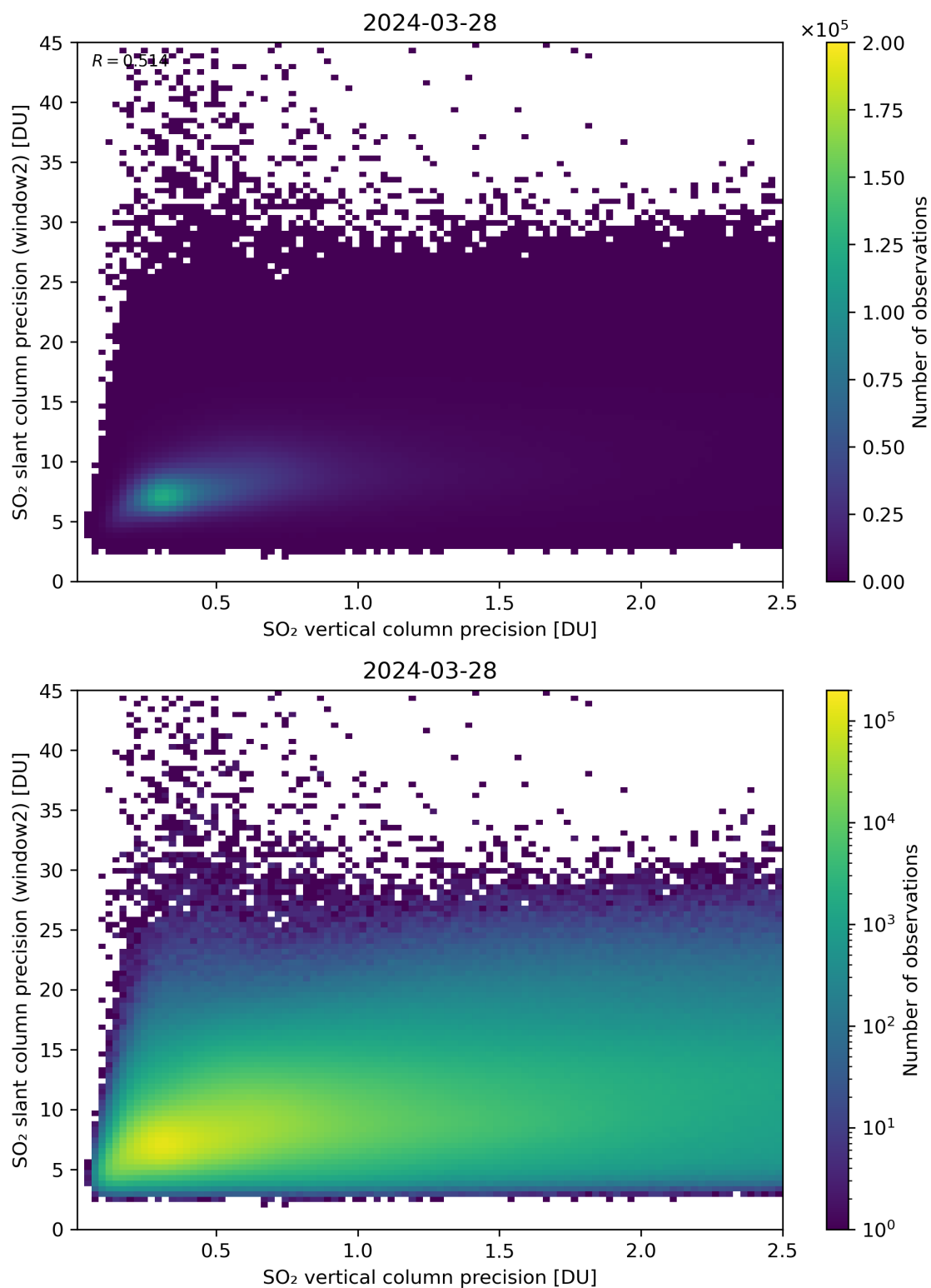
Figure 291: Scatter density plot of “SO 2 vertical column precision” against “SO 2 slant column precision (window2)” for 2024-03-27 to 2024-03-29.
