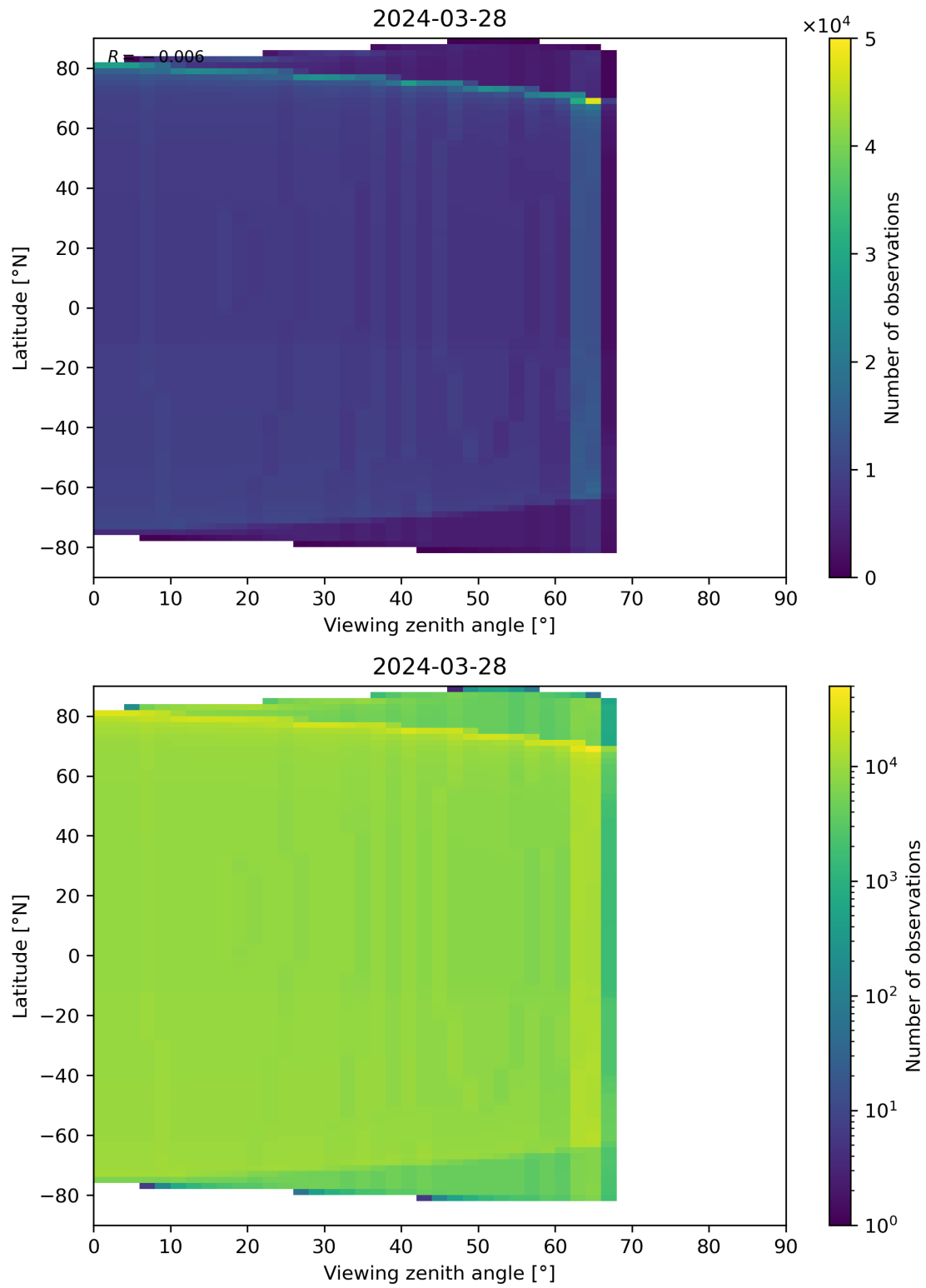
Figure 314: Scatter density plot of “Viewing zenith angle” against “Latitude” for 2024-03-27 to 2024-03-29.
