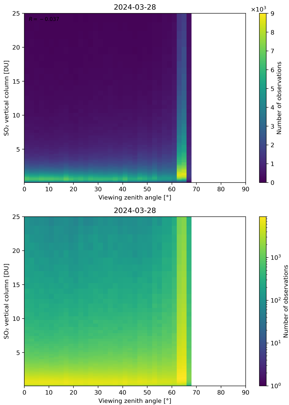
Figure 327: Scatter density plot of “Viewing zenith angle” against “SO 2 vertical column” for 2024-03-27 to 2024-03-29.
