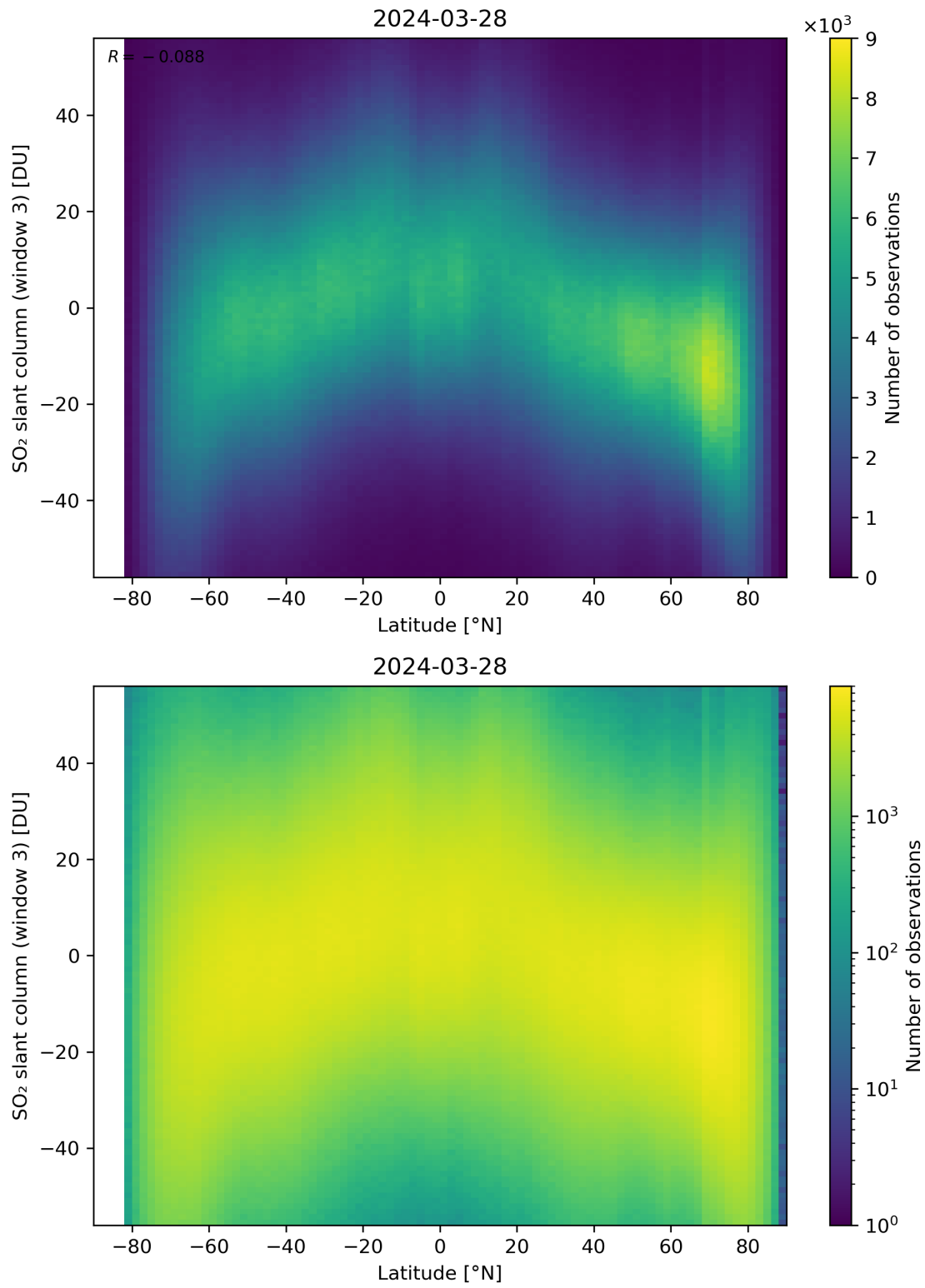
Figure 152: Scatter density plot of “Latitude” against “SO 2 slant column (window 3)” for 2024-03-27 to 2024-03-29.
