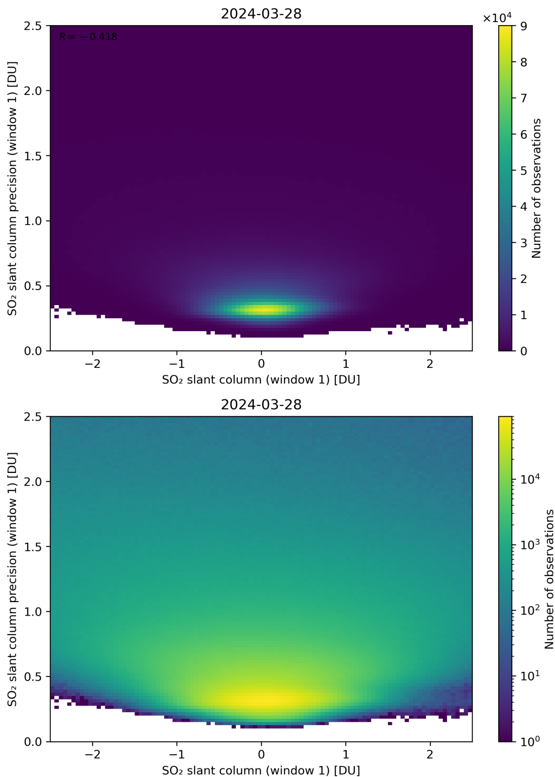
Figure 235: Scatter density plot of “SO 2 slant column (window 1)” against “SO 2 slant column precision (window 1)” for 2024-03-27 to 2024-03-29.
