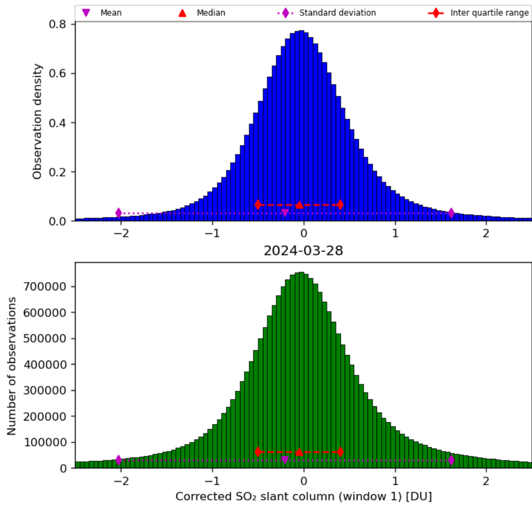
Figure 58: Histogram of “Corrected SO 2 slant column (window 1)” for 2024-03-27 to 2024-03-29
