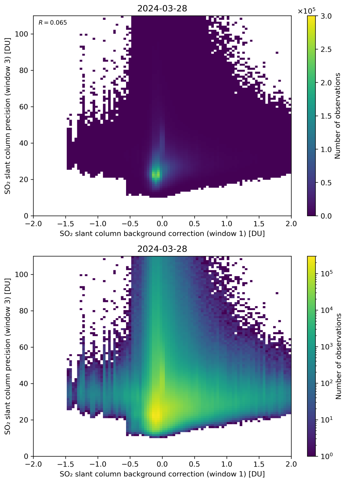
Figure 108: Scatter density plot of “SO 2 slant column background correction (window 1)” against “SO 2 slant column precision (window 3)” for 2024-03-27 to 2024-03-29.
