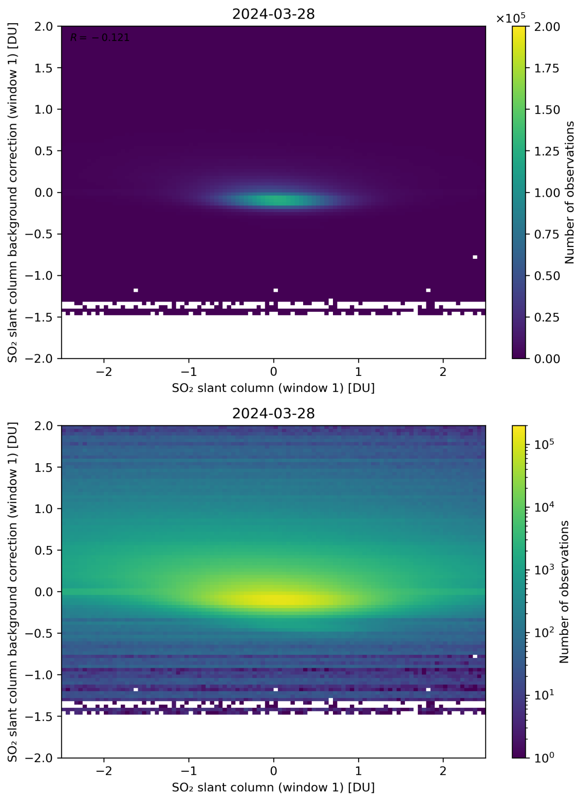
Figure 212: Scatter density plot of “SO 2 slant column (window 1)” against “SO 2 slant column background correction (window 1)” for 2024-03-27 to 2024-03-29.
