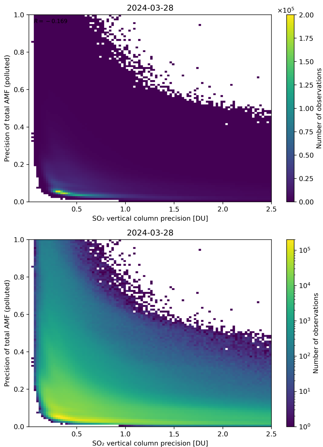
Figure 295: Scatter density plot of “SO 2 vertical column precision” against “Precision of total AMF (polluted)” for 2024-03-27 to 2024-03-29.
