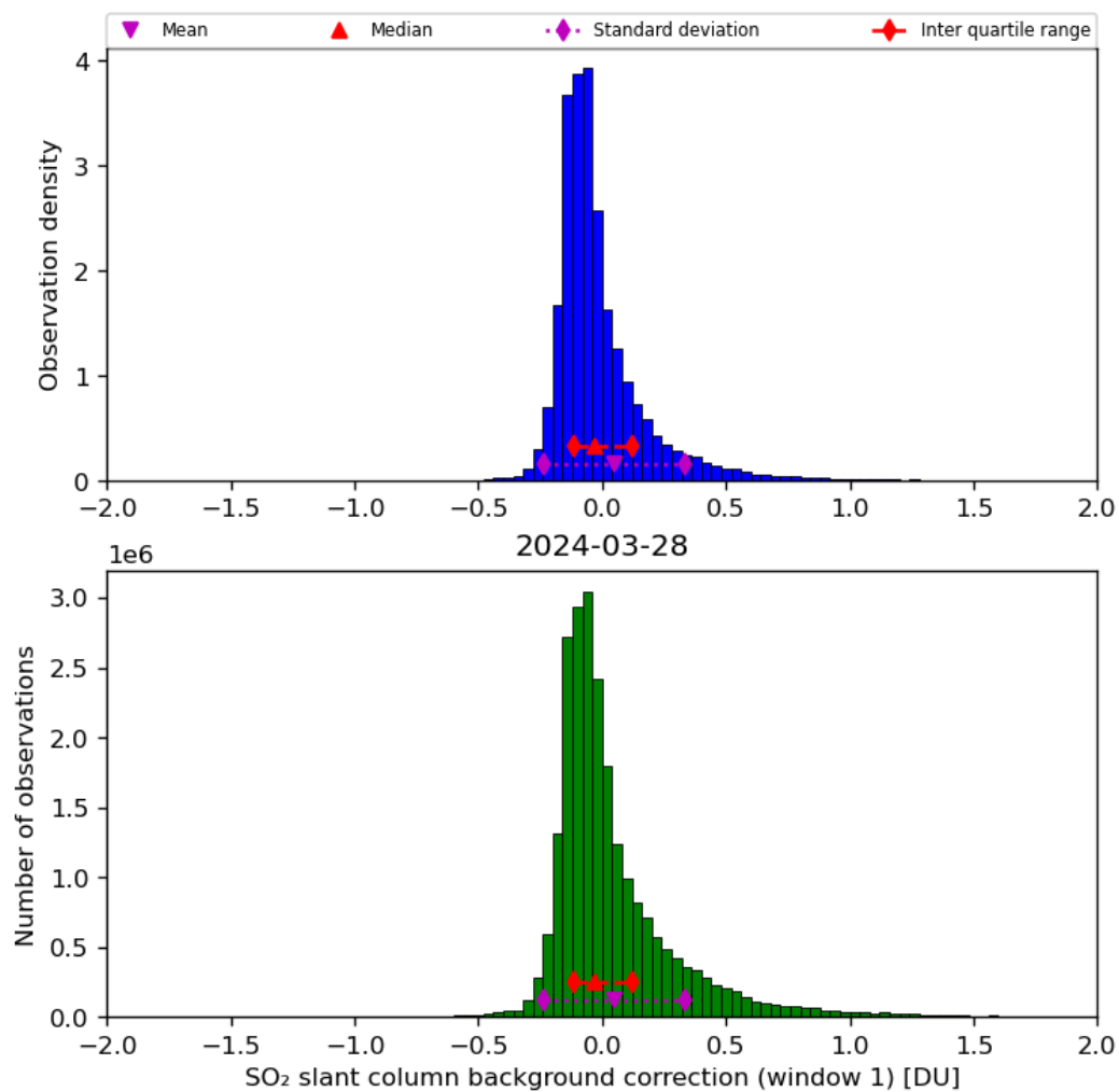
Figure 59: Histogram of “SO 2 slant column background correction (window 1)” for 2024-03-27 to 2024-03-29
