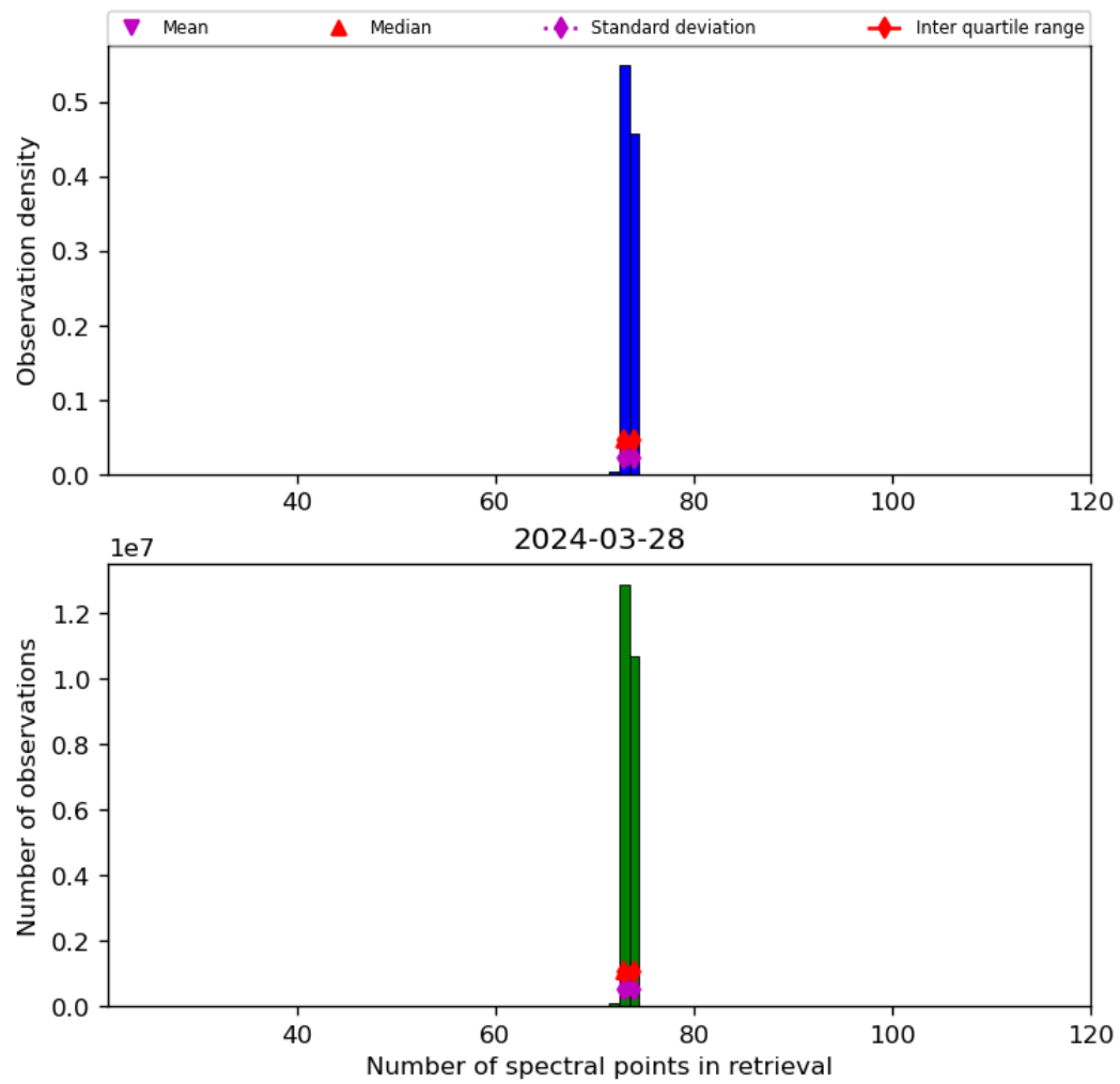
Figure 74: Histogram of “Number of spectral points in retrieval” for 2024-03-27 to 2024-03-29
