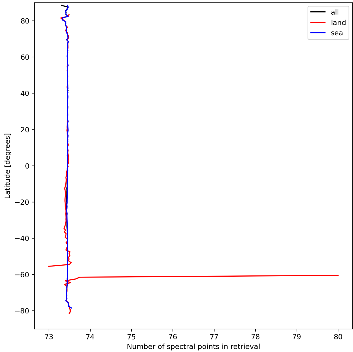
Figure 51: Zonal average of “Number of spectral points in retrieval” for 2024-03-27 to 2024-03-29.
