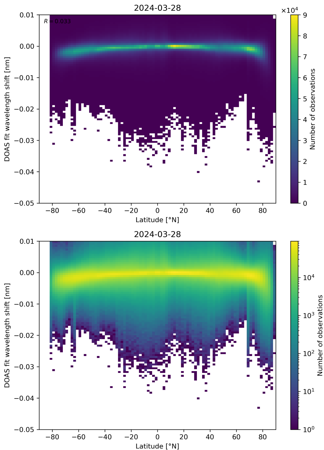
Figure 142: Scatter density plot of “Latitude” against “DOAS fit wavelength shift” for 2024-03-27 to 2024-03-29.
