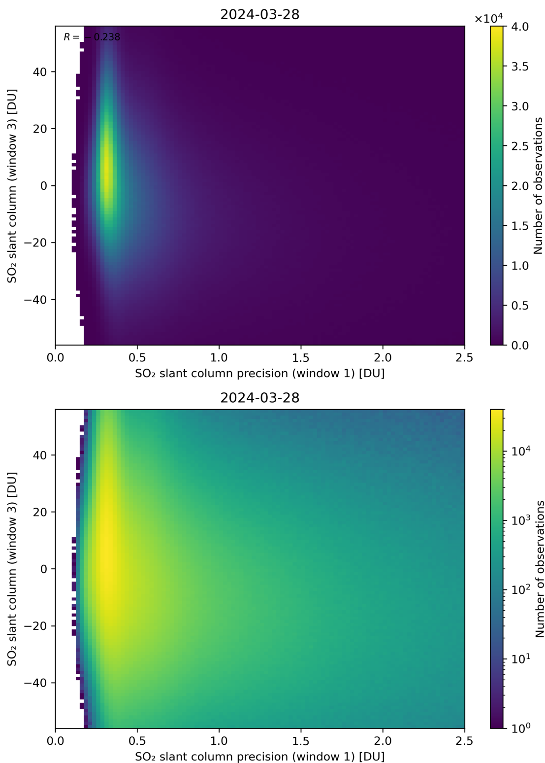
Figure 228: Scatter density plot of “SO 2 slant column precision (window 1)” against “SO 2 slant column (window 3)” for 2024-03-27 to 2024-03-29.
