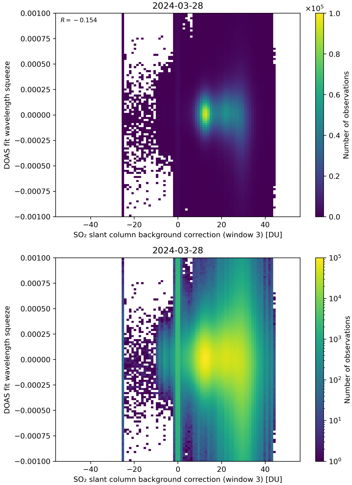
Figure 122: Scatter density plot of “SO 2 slant column background correction (window 3)” against “DOAS fit wavelength squeeze” for 2024-03-27 to 2024-03-29.
