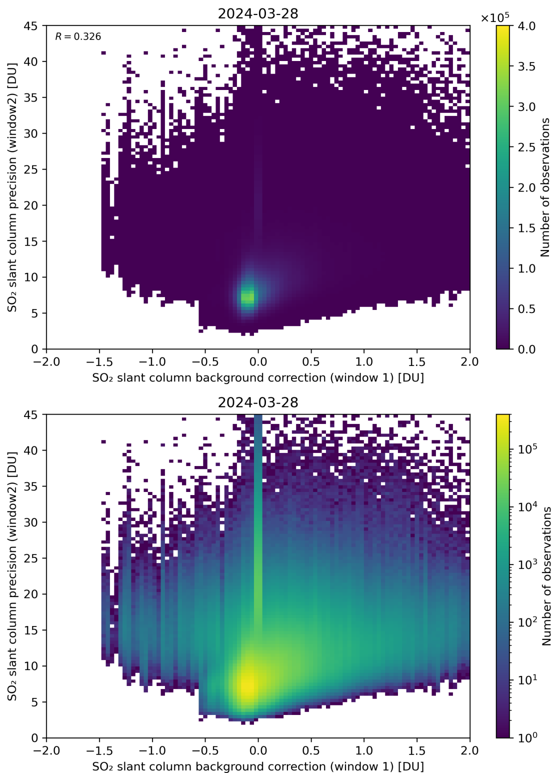
Figure 106: Scatter density plot of “SO 2 slant column background correction (window 1)” against “SO 2 slant column precision (window2)” for 2024-03-27 to 2024-03-29.
