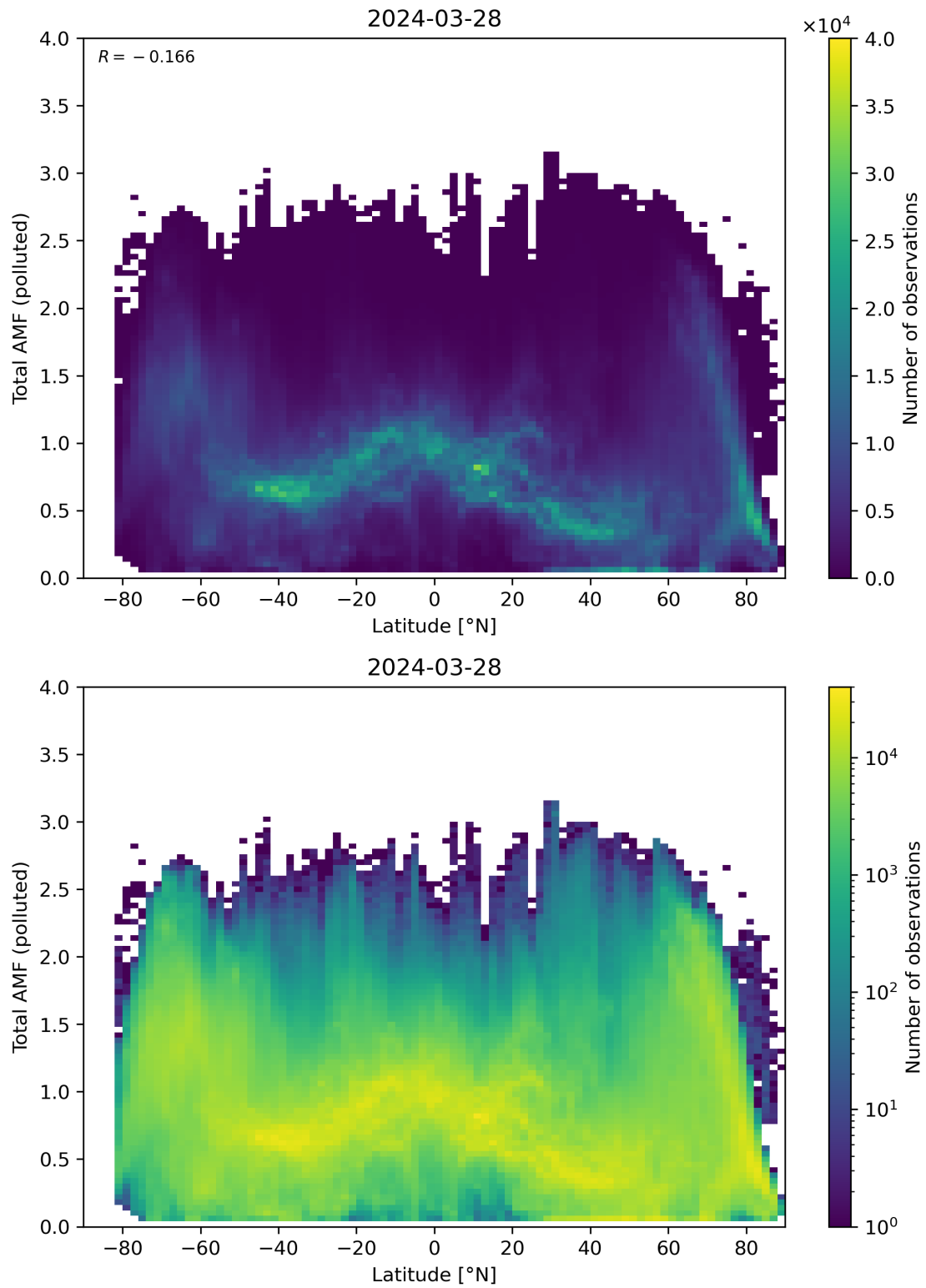
Figure 154: Scatter density plot of “Latitude” against “Total AMF (polluted)” for 2024-03-27 to 2024-03-29.
