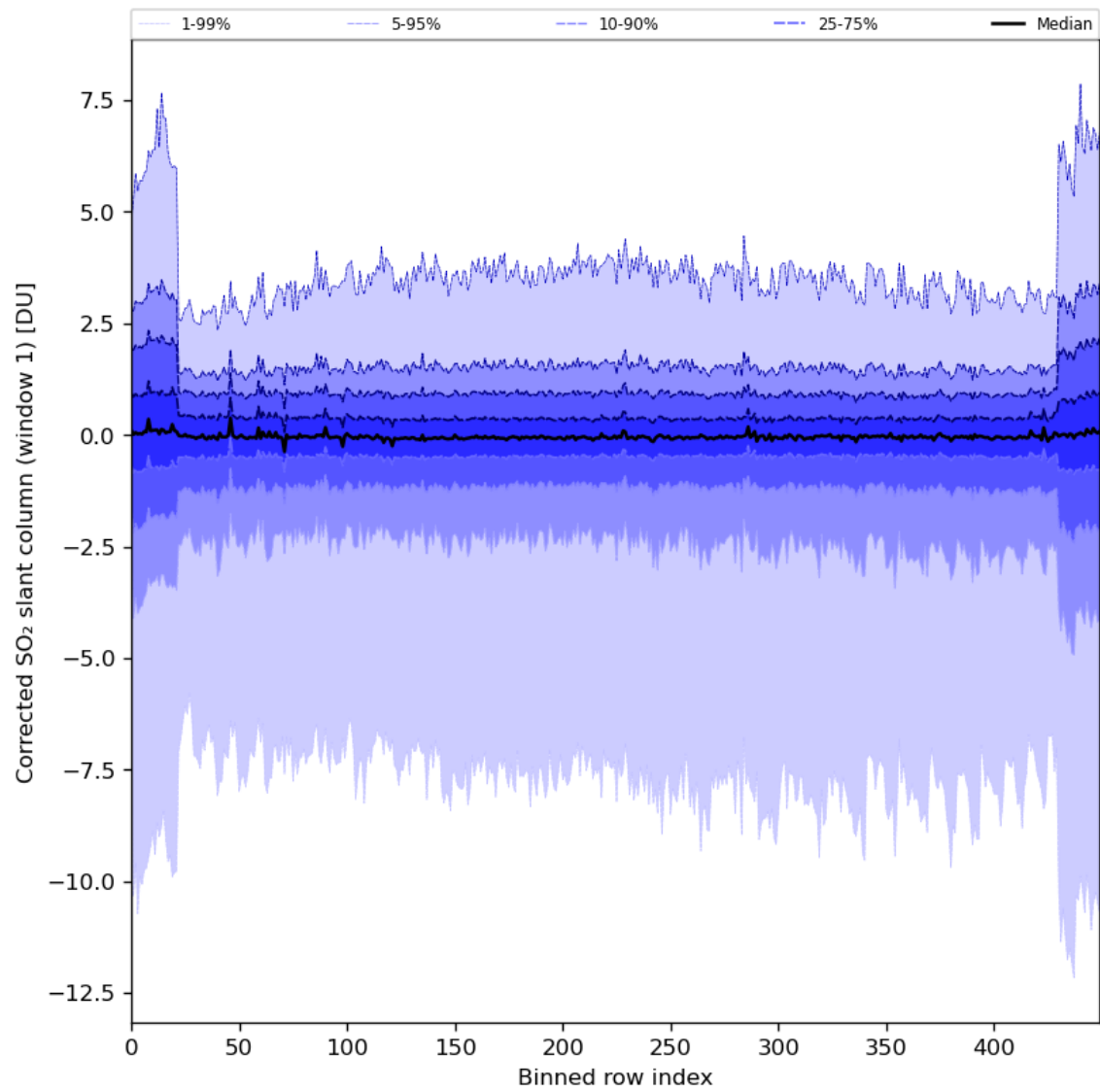
Figure 81: Along track statistics of “Corrected SO 2 slant column (window 1)” for 2024-03-27 to 2024-03-29
