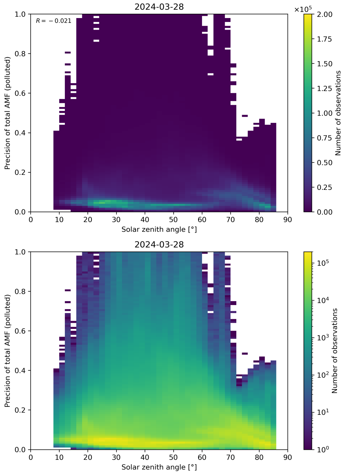
Figure 175: Scatter density plot of “Solar zenith angle” against “Precision of total AMF (polluted)” for 2024-03-27 to 2024-03-29.
