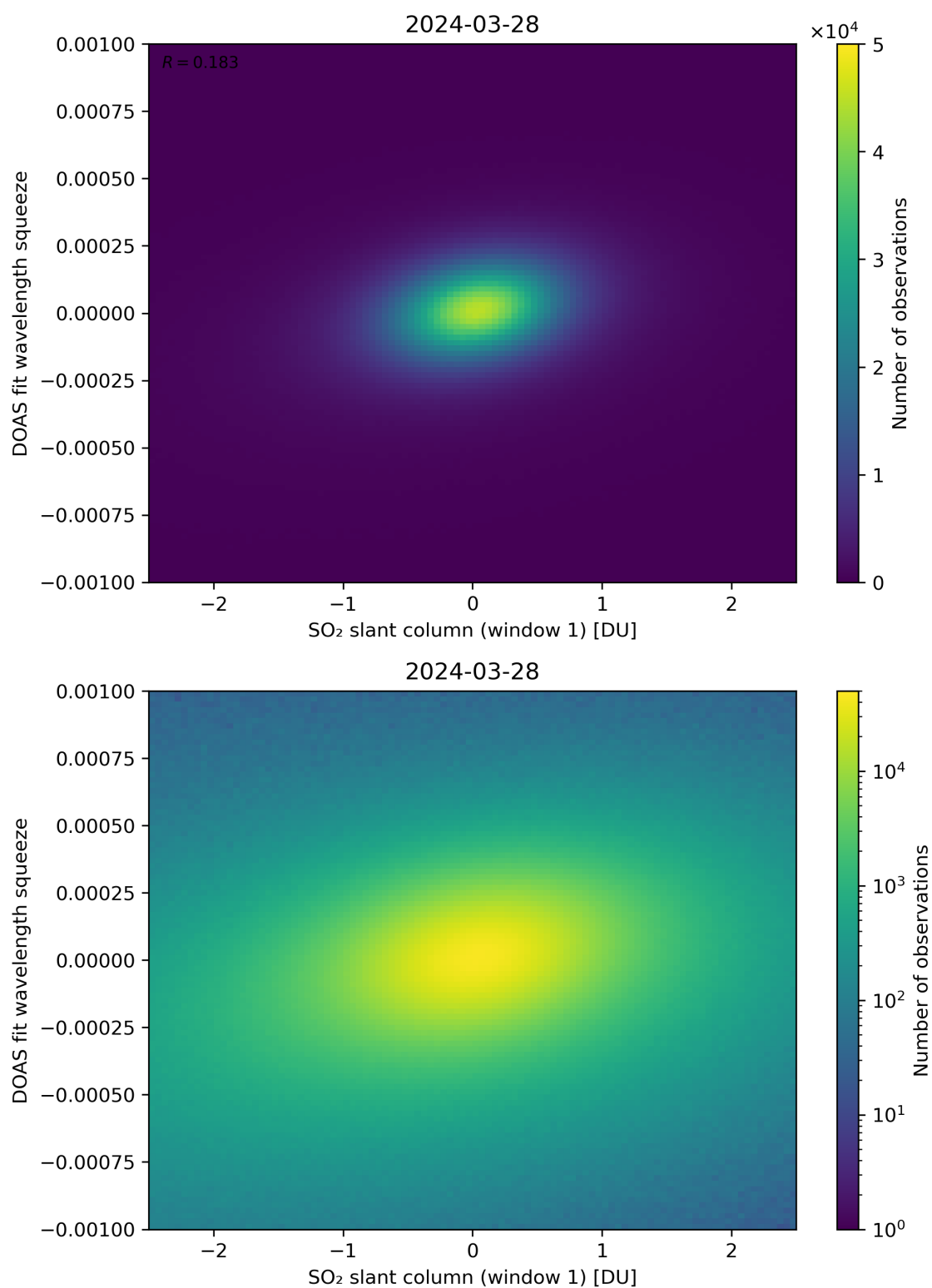
Figure 216: Scatter density plot of “SO 2 slant column (window 1)” against “DOAS fit wavelength squeeze” for 2024-03-27 to 2024-03-29.
