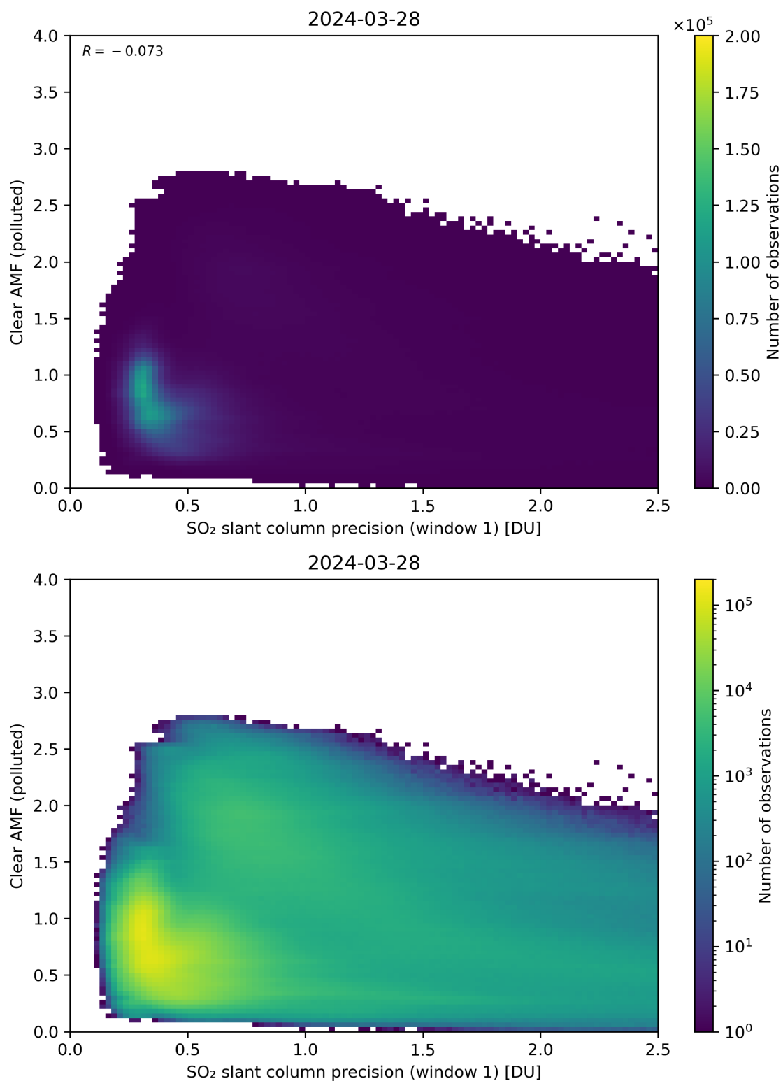
Figure 224: Scatter density plot of “SO 2 slant column precision (window 1)” against “Clear AMF (polluted)” for 2024-03-27 to 2024-03-29.
