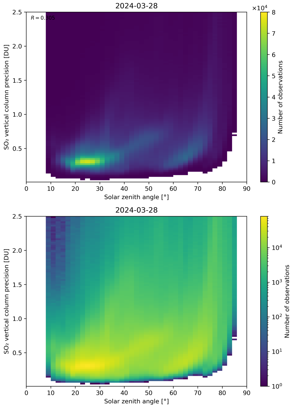
Figure 177: Scatter density plot of “Solar zenith angle” against “SO 2 vertical column precision” for 2024-03-27 to 2024-03-29.
