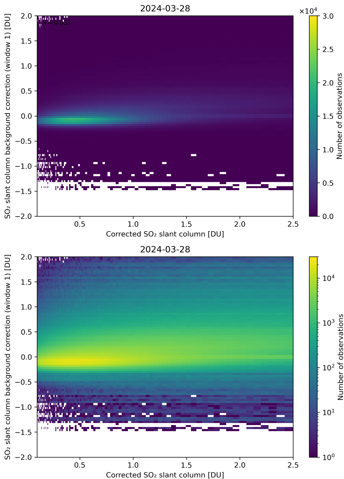
Figure 178: Scatter density plot of “Corrected SO 2 slant column” against “SO 2 slant column background correction (window 1)” for 2024-03-27 to 2024-03-29.
