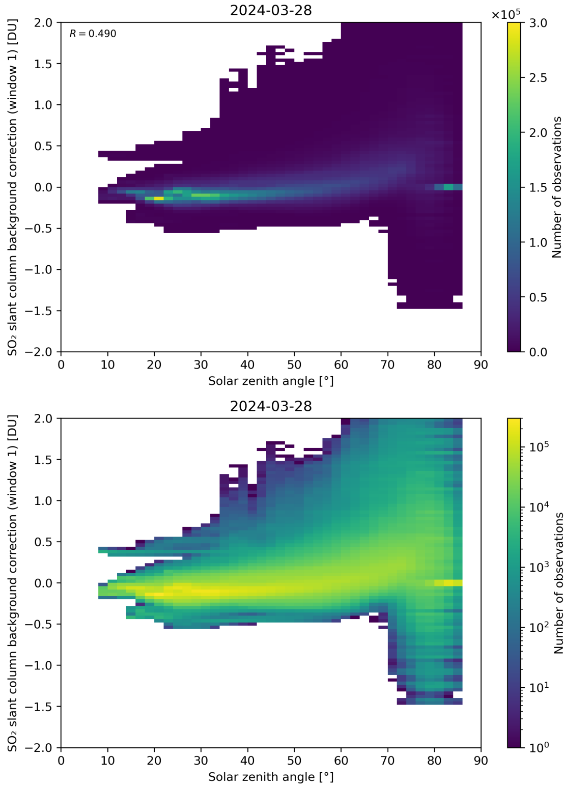
Figure 158: Scatter density plot of “Solar zenith angle” against “SO 2 slant column background correction (window 1)” for 2024-03-27 to 2024-03-29.
