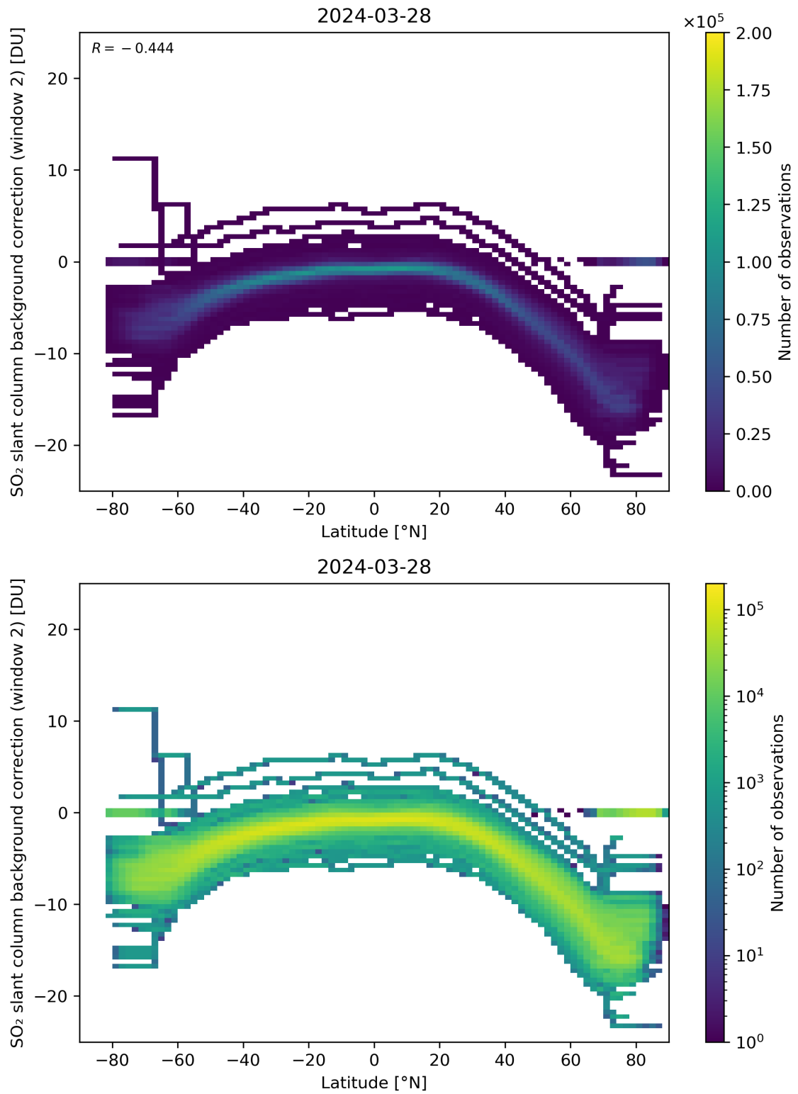
Figure 140: Scatter density plot of “Latitude” against “SO 2 slant column background correction (window 2)” for 2024-03-27 to 2024-03-29.
