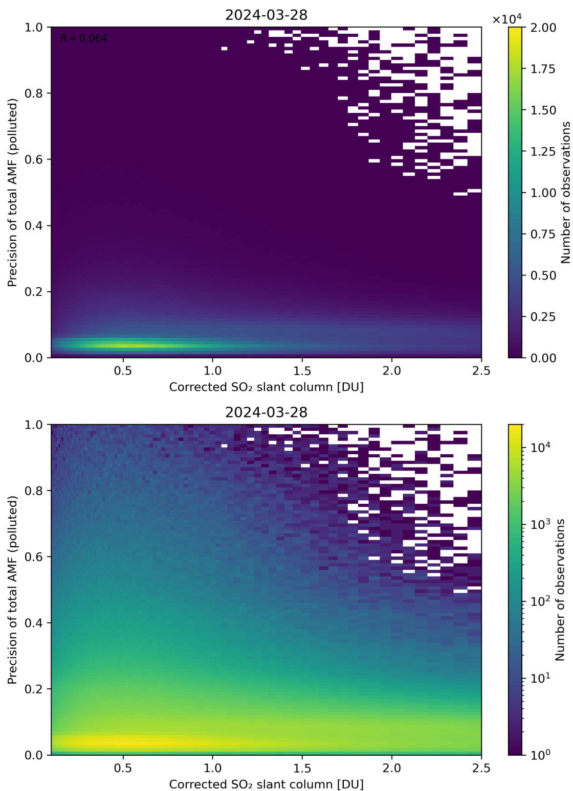
Figure 193: Scatter density plot of “Corrected SO 2 slant column” against “Precision of total AMF (polluted)” for 2024-03-27 to 2024-03-29.
