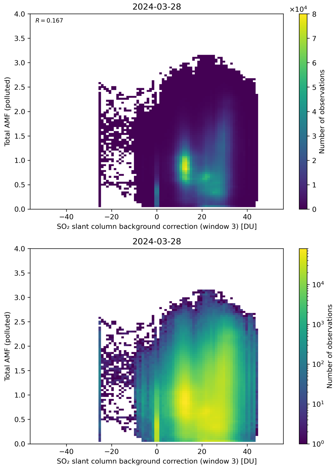
Figure 125: Scatter density plot of “SO 2 slant column background correction (window 3)” against “Total AMF (polluted)” for 2024-03-27 to 2024-03-29.
