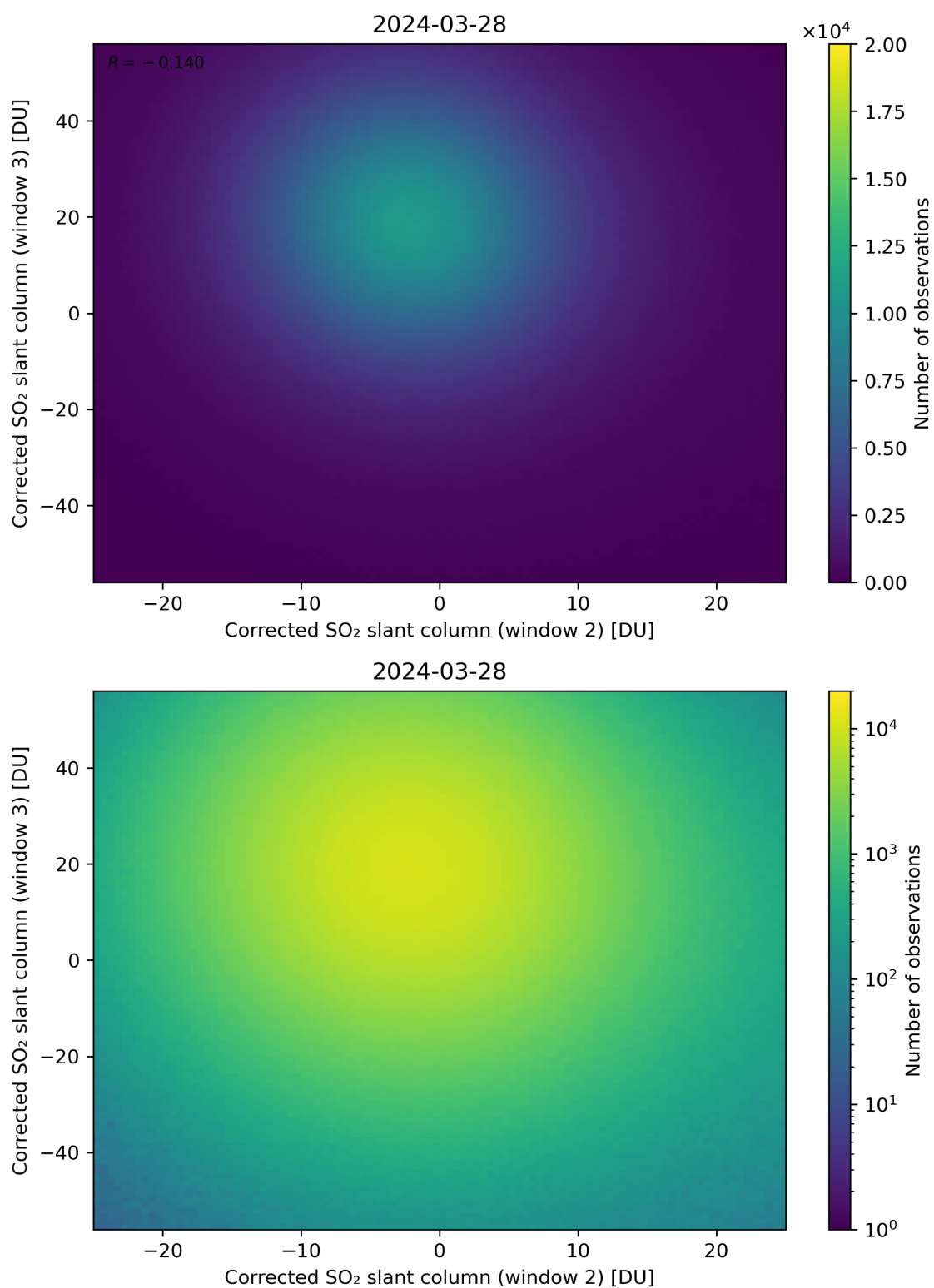
Figure 200: Scatter density plot of “Corrected SO 2 slant column (window 2)” against “Corrected SO 2 slant column (window 3)” for 2024-03-27 to 2024-03-29.
