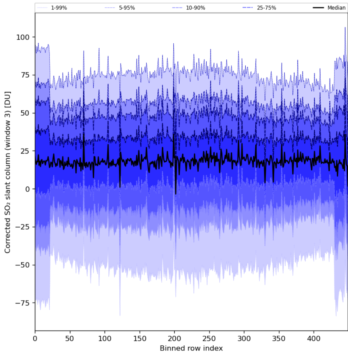
Figure 89: Along track statistics of “Corrected SO 2 slant column (window 3)” for 2024-03-27 to 2024-03-29
