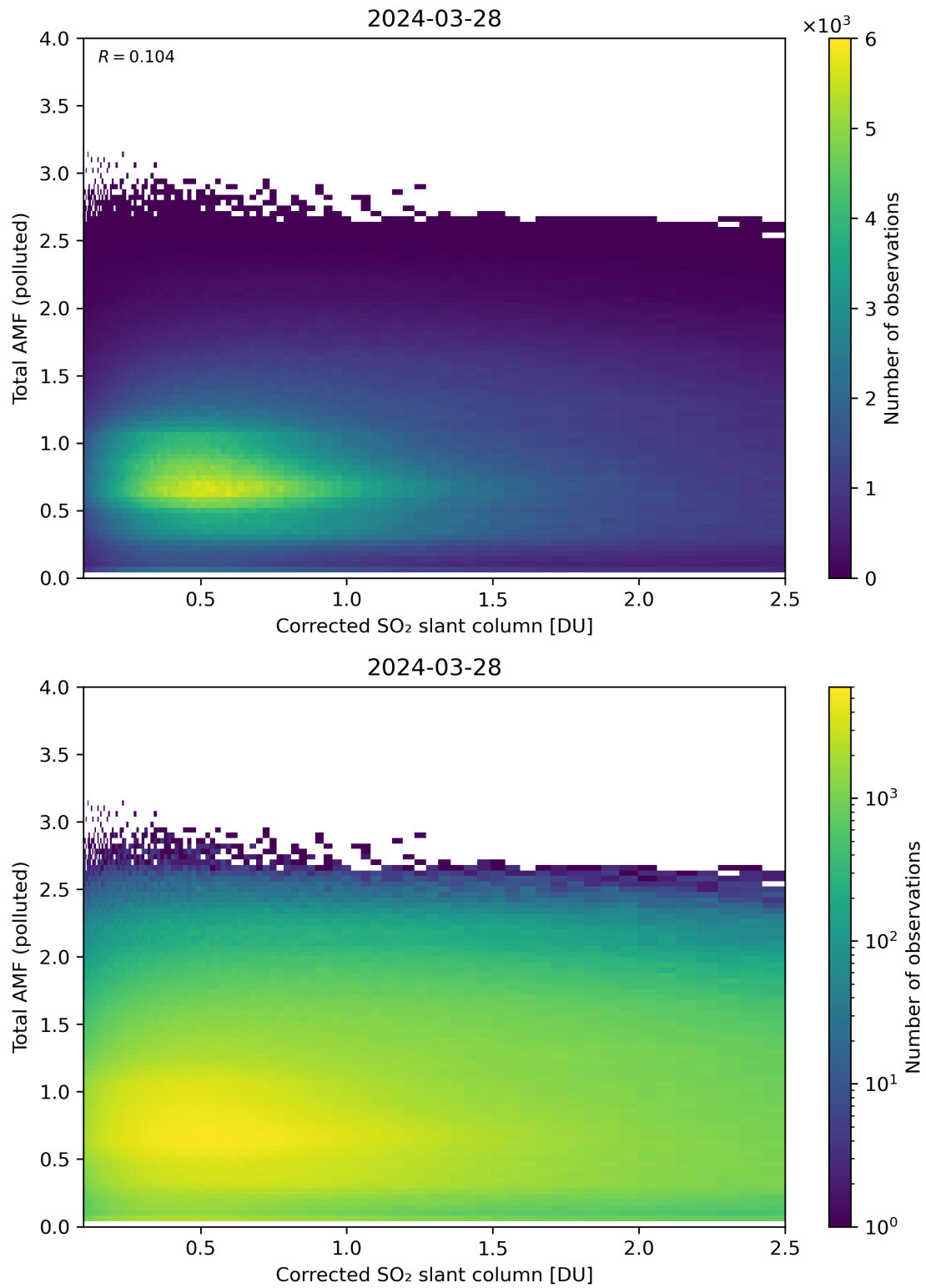
Figure 192: Scatter density plot of “Corrected SO 2 slant column” against “Total AMF (polluted)” for 2024-03-27 to 2024-03-29.
