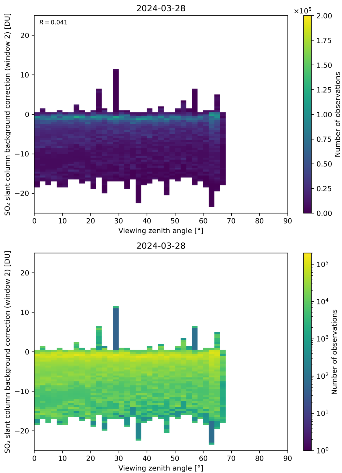
Figure 309: Scatter density plot of “Viewing zenith angle” against “SO 2 slant column background correction (window 2)” for 2024-03-27 to 2024-03-29.
