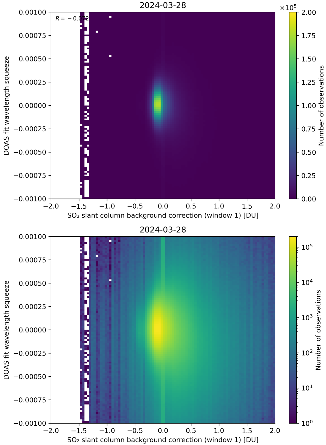
Figure 101: Scatter density plot of “SO 2 slant column background correction (window 1)” against “DOAS fit wavelength squeeze” for 2024-03-27 to 2024-03-29.
