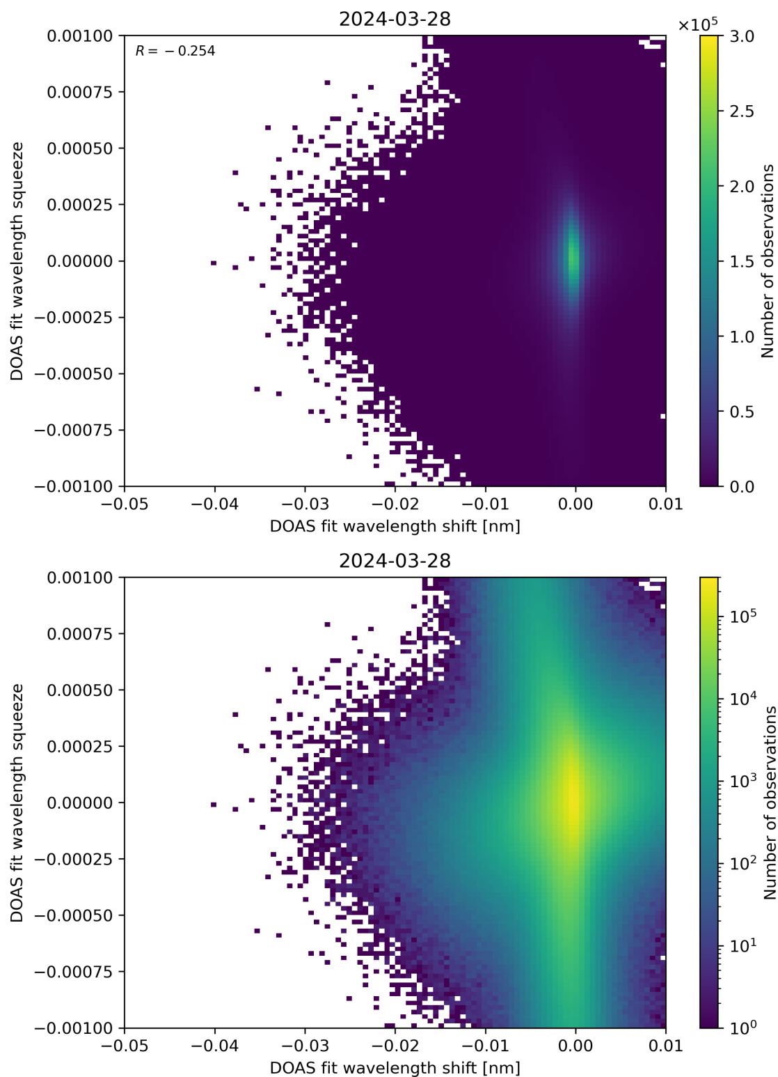
Figure 127: Scatter density plot of “DOAS fit wavelength shift” against “DOAS fit wavelength squeeze” for 2024-03-27 to 2024-03-29.
