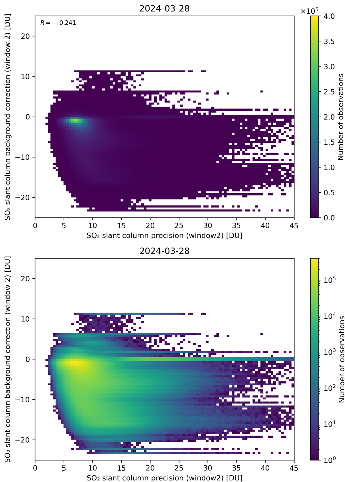
Figure 241: Scatter density plot of “SO 2 slant column precision (window2)” against “SO 2 slant column background correction (window 2)” for 2024-03-27 to 2024-03-29.
