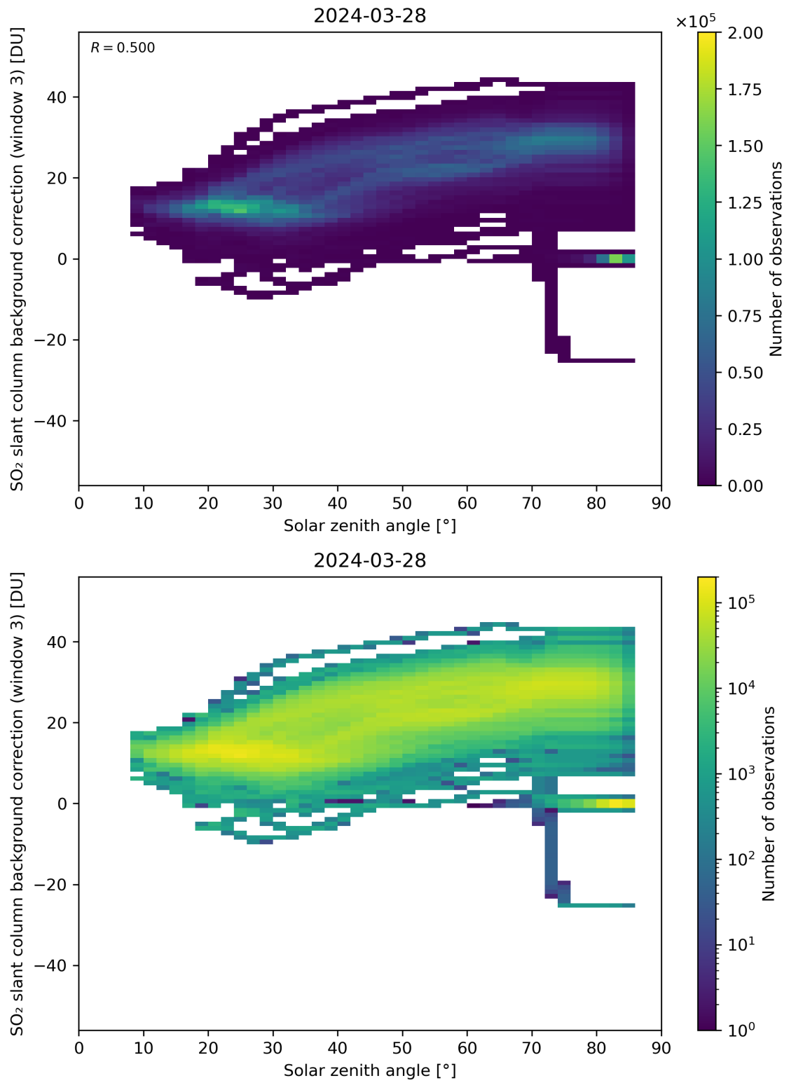
Figure 160: Scatter density plot of “Solar zenith angle” against “SO 2 slant column background correction (window 3)” for 2024-03-27 to 2024-03-29.
