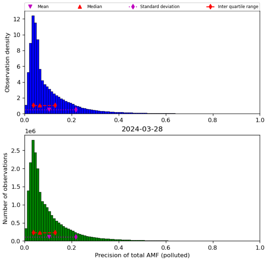
Figure 72: Histogram of “Precision of total AMF (polluted)” for 2024-03-27 to 2024-03-29
