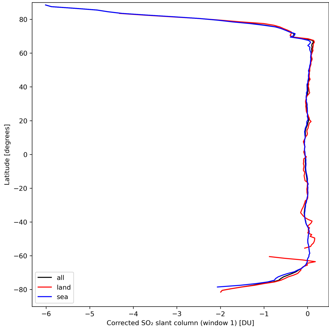
Figure 35: Zonal average of “Corrected SO 2 slant column (window 1)” for 2024-03-27 to 2024-03-29.
