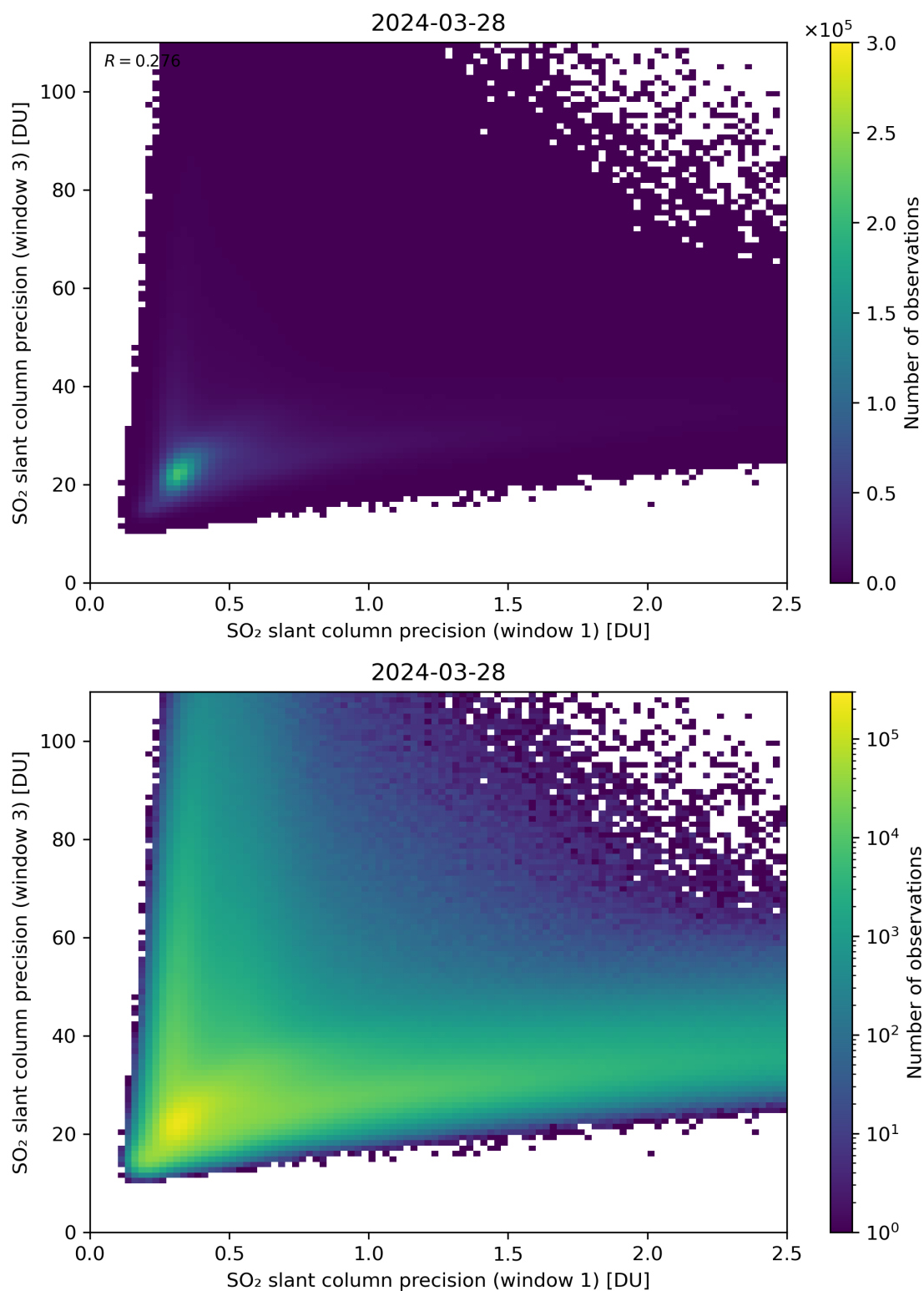
Figure 229: Scatter density plot of “SO 2 slant column precision (window 1)” against “SO 2 slant column precision (window 3)” for 2024-03-27 to 2024-03-29.
