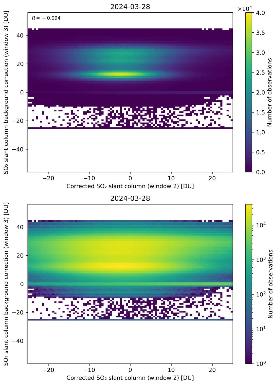
Figure 195: Scatter density plot of “Corrected SO 2 slant column (window 2)” against “SO 2 slant column background correction (window 3)” for 2024-03-27 to 2024-03-29.
