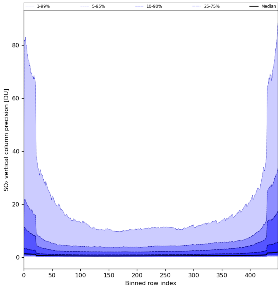
Figure 77: Along track statistics of “SO 2 vertical column precision” for 2024-03-27 to 2024-03-29
