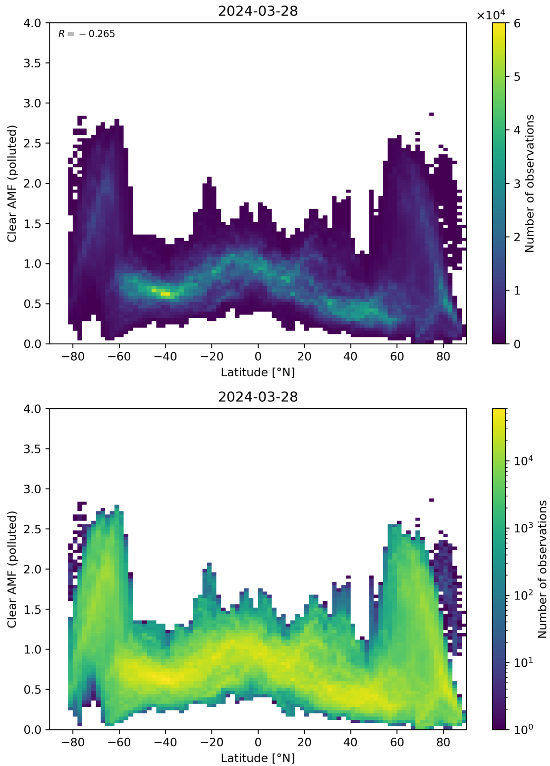
Figure 145: Scatter density plot of “Latitude” against “Clear AMF (polluted)” for 2024-03-27 to 2024-03-29.
