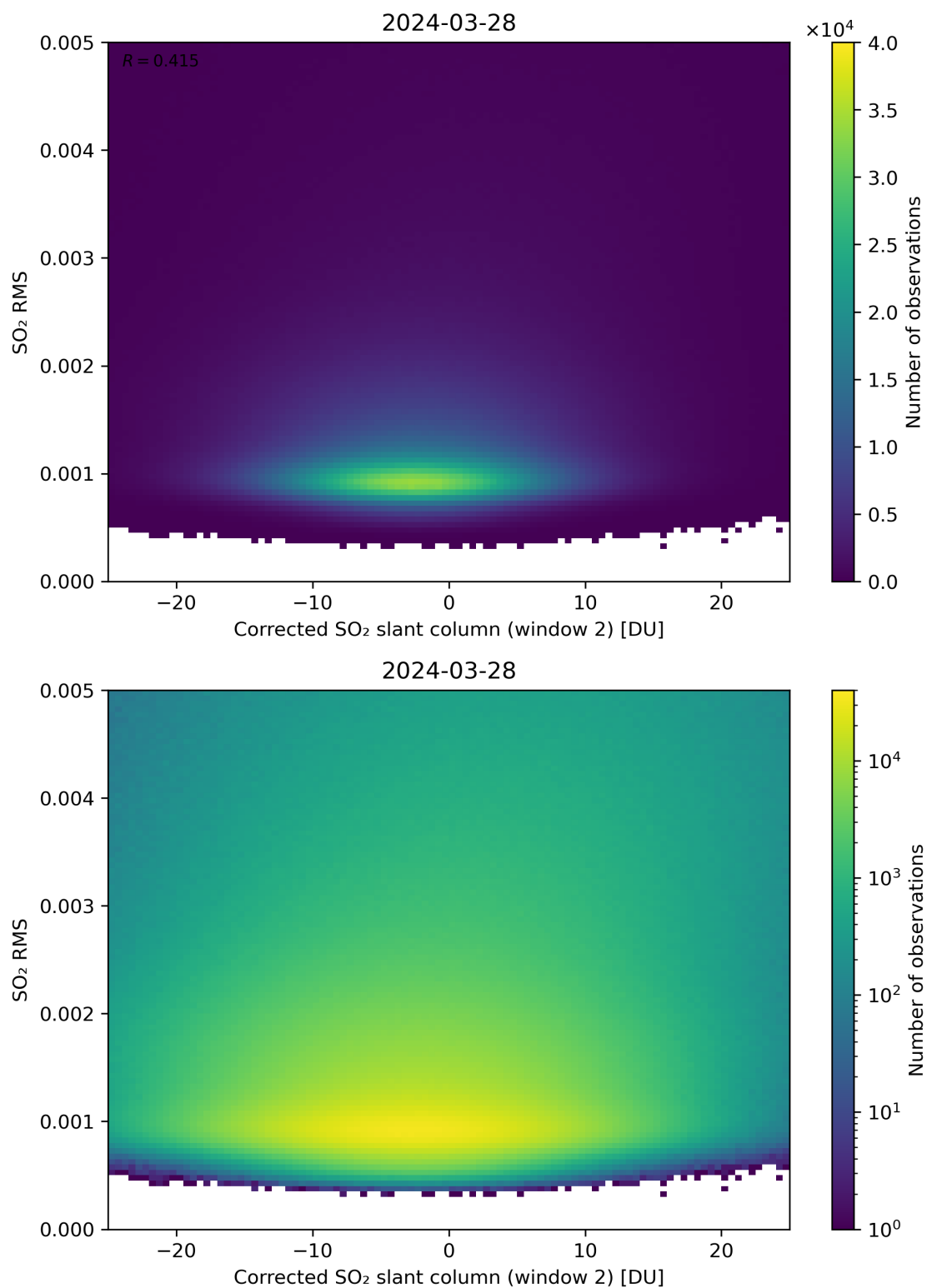
Figure 198: Scatter density plot of “Corrected SO 2 slant column (window 2)” against “SO 2 RMS” for 2024-03-27 to 2024-03-29.
