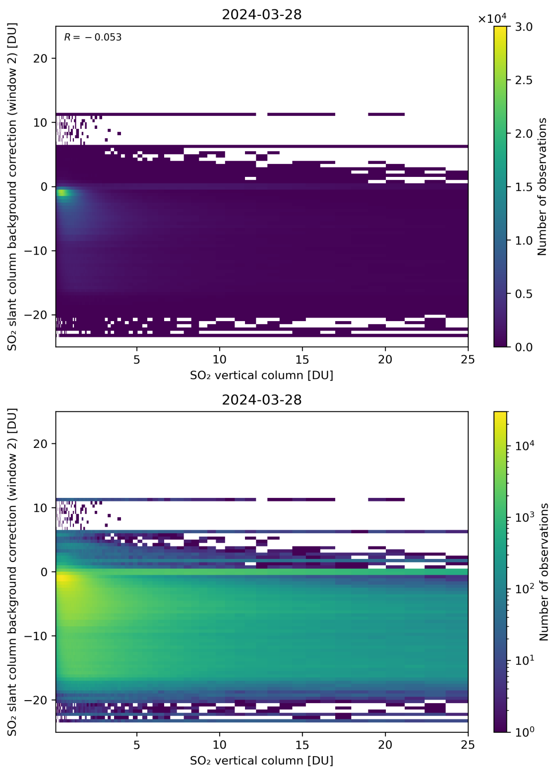
Figure 274: Scatter density plot of “SO 2 vertical column” against “SO 2 slant column background correction (window 2)” for 2024-03-27 to 2024-03-29.
