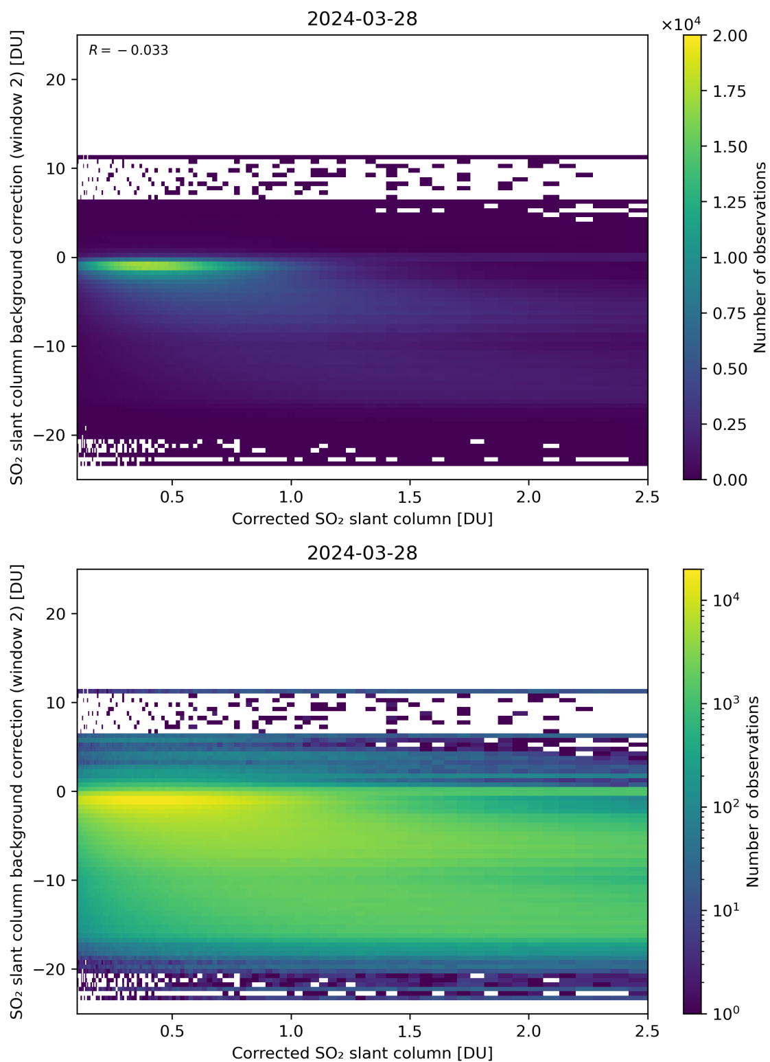
Figure 179: Scatter density plot of “Corrected SO 2 slant column” against “SO 2 slant column background correction (window 2)” for 2024-03-27 to 2024-03-29.
