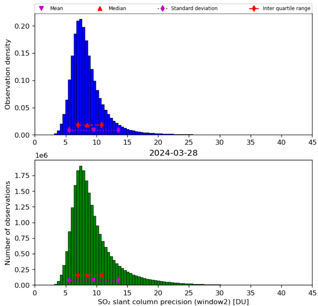
Figure 61: Histogram of “SO 2 slant column precision (window2)” for 2024-03-27 to 2024-03-29
