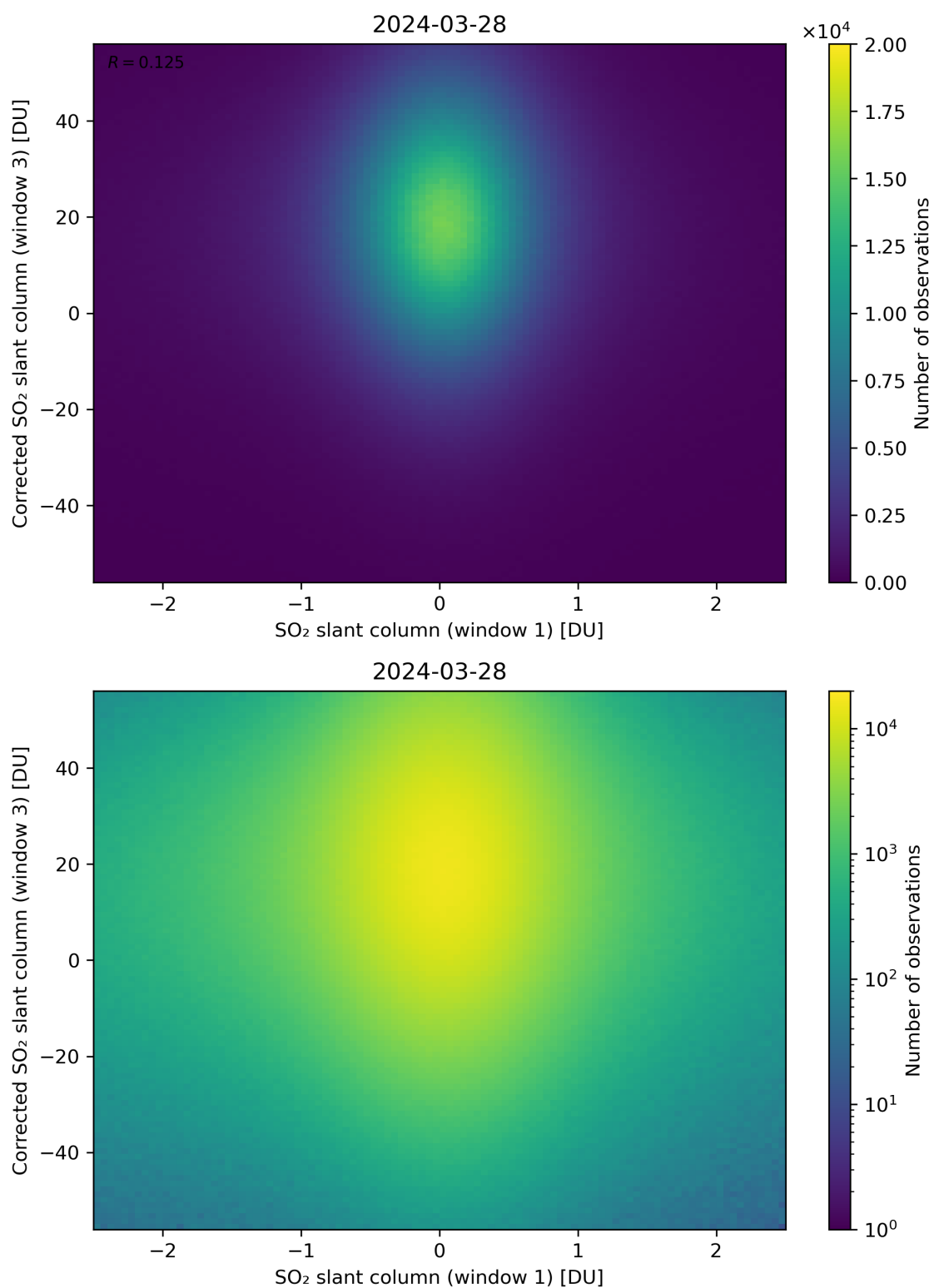
Figure 234: Scatter density plot of “SO 2 slant column (window 1)” against “Corrected SO 2 slant column (window 3)” for 2024-03-27 to 2024-03-29.
