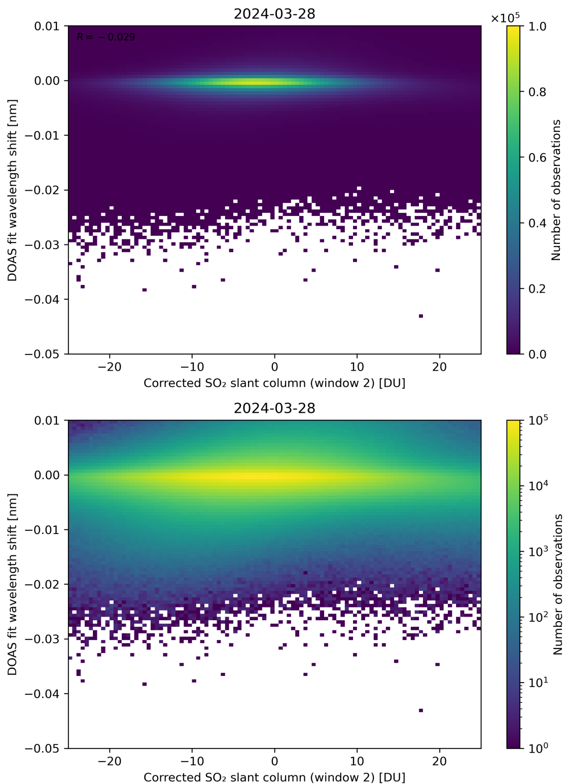
Figure 196: Scatter density plot of “Corrected SO 2 slant column (window 2)” against “DOAS fit wavelength shift” for 2024-03-27 to 2024-03-29.
