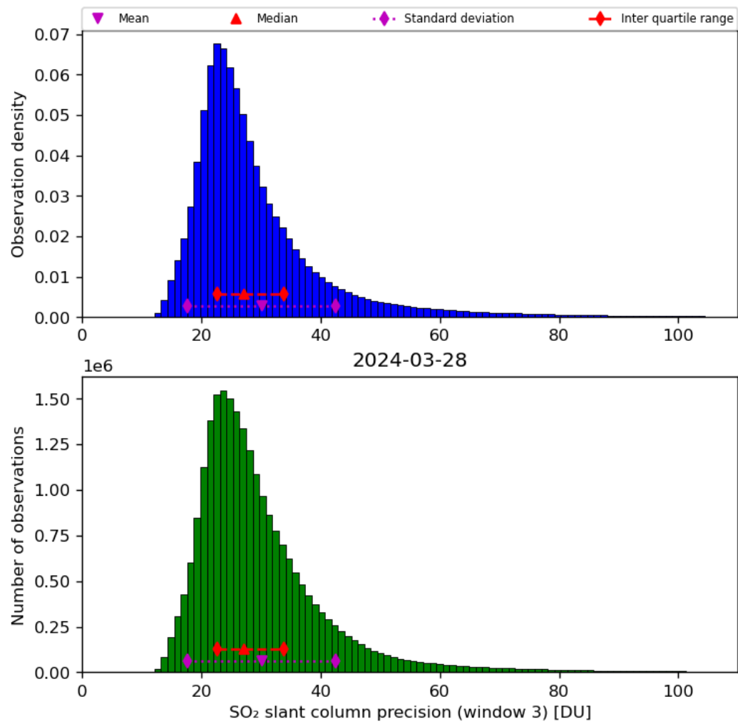
Figure 65: Histogram of “SO 2 slant column precision (window 3)” for 2024-03-27 to 2024-03-29
