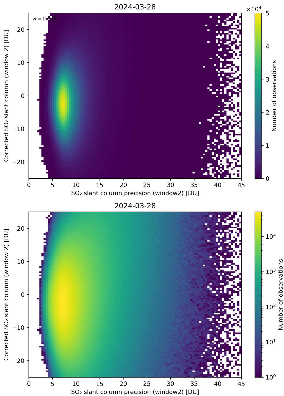
Figure 247: Scatter density plot of “SO 2 slant column precision (window2)” against “Corrected SO 2 slant column (window 2)” for 2024-03-27 to 2024-03-29.
