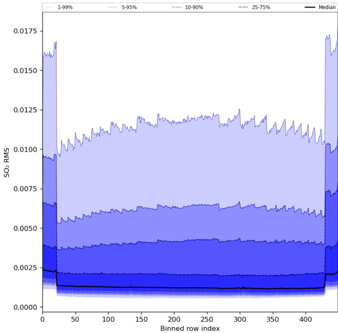
Figure 93: Along track statistics of “SO 2 RMS” for 2024-03-27 to 2024-03-29
