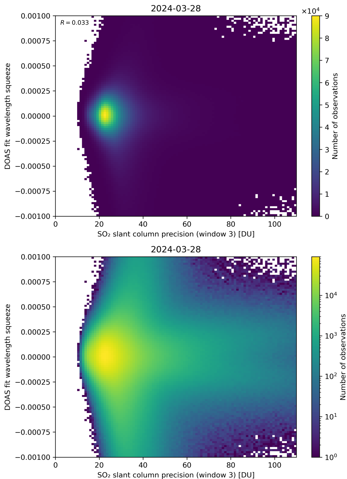
Figure 259: Scatter density plot of “SO 2 slant column precision (window 3)” against “DOAS fit wavelength squeeze” for 2024-03-27 to 2024-03-29.
