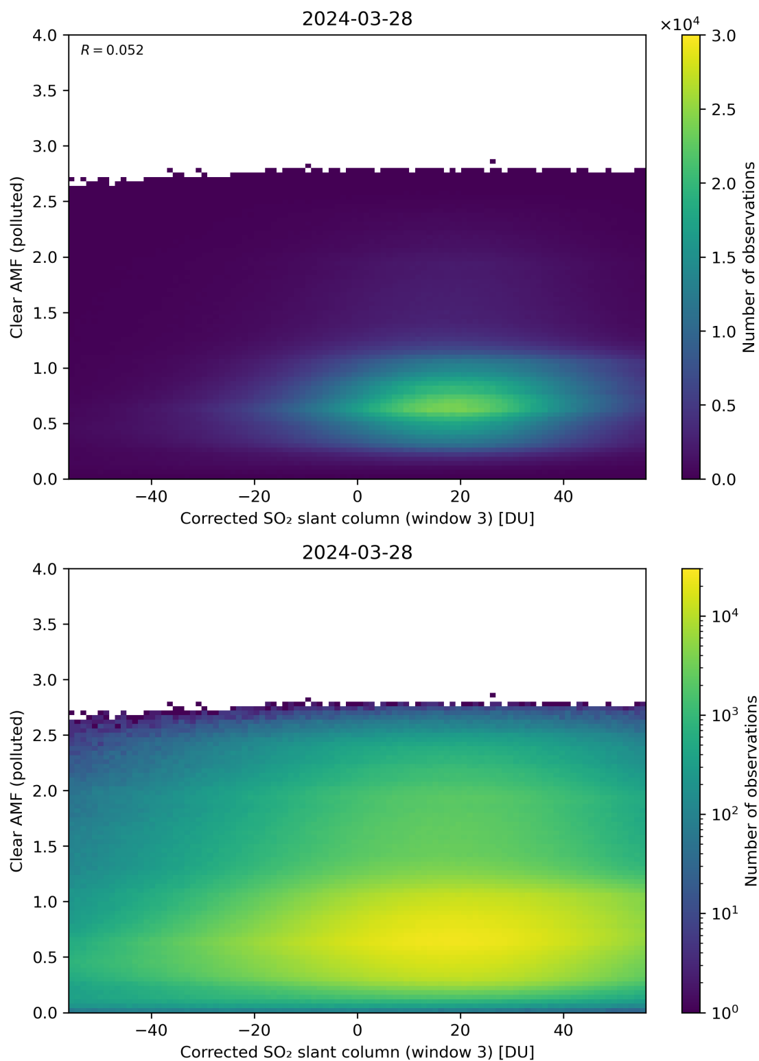
Figure 209: Scatter density plot of “Corrected SO 2 slant column (window 3)” against “Clear AMF (polluted)” for 2024-03-27 to 2024-03-29.
