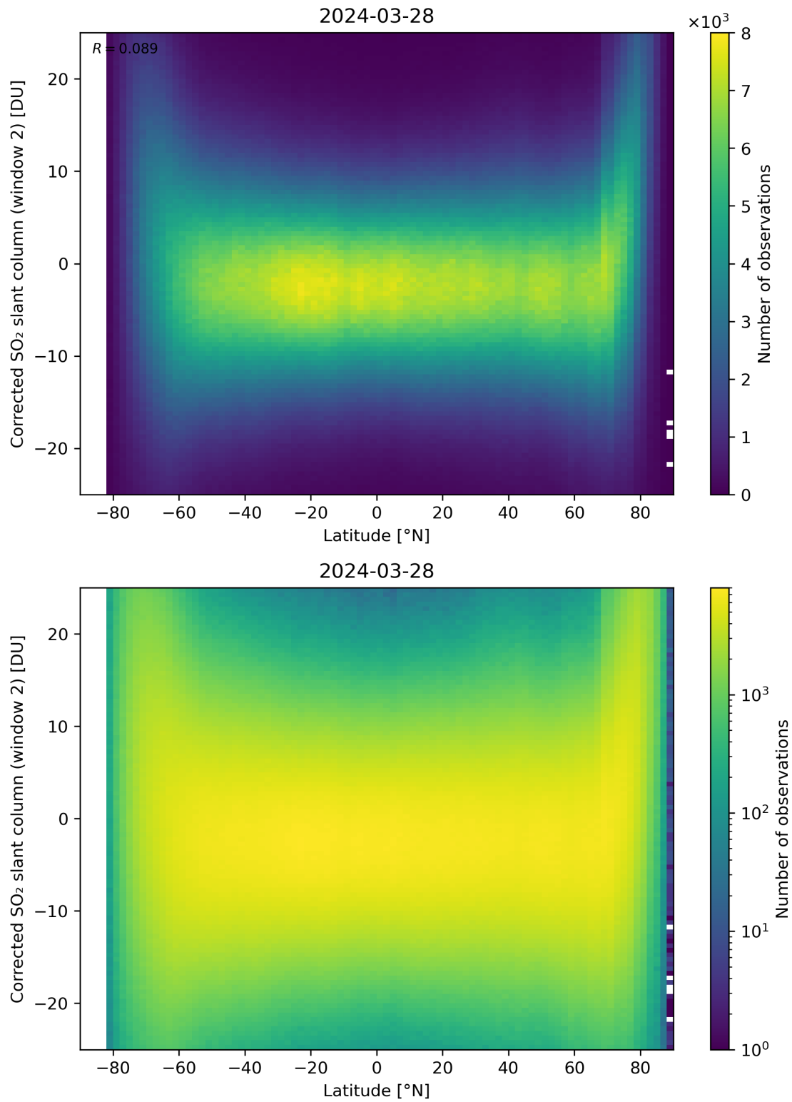
Figure 147: Scatter density plot of “Latitude” against “Corrected SO 2 slant column (window 2)” for 2024-03-27 to 2024-03-29.
