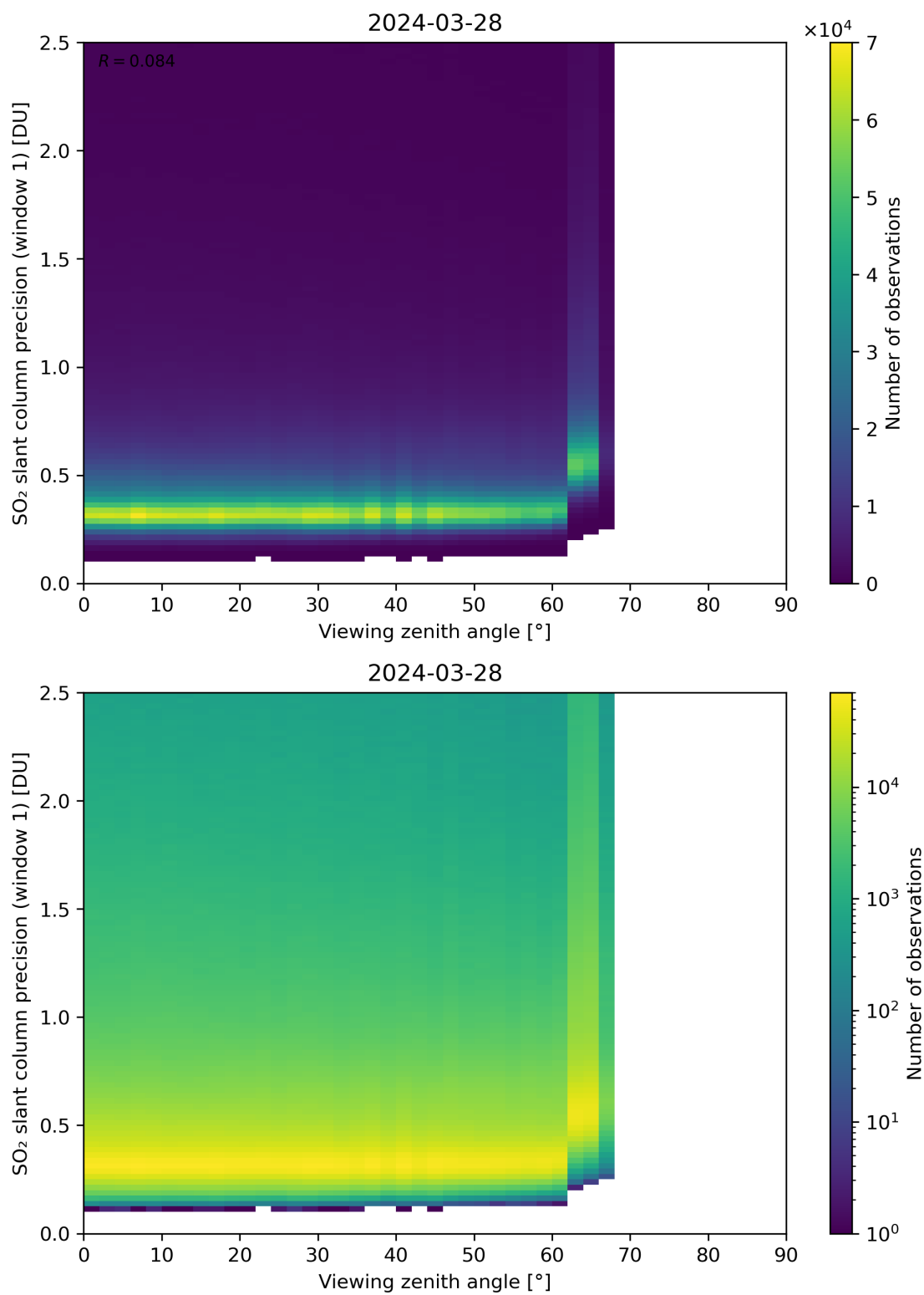
Figure 321: Scatter density plot of “Viewing zenith angle” against “SO 2 slant column precision (window 1)” for 2024-03-27 to 2024-03-29.
