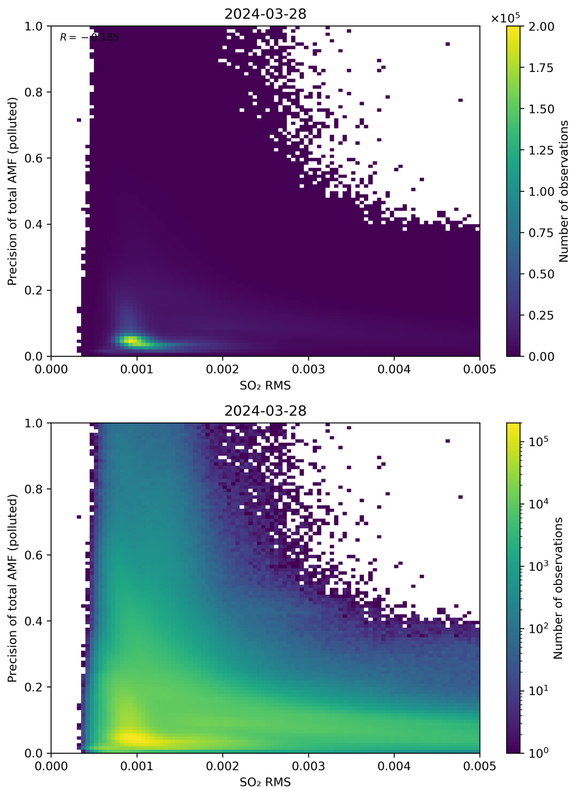
Figure 138: Scatter density plot of “SO 2 RMS” against “Precision of total AMF (polluted)” for 2024-03-27 to 2024-03-29.
