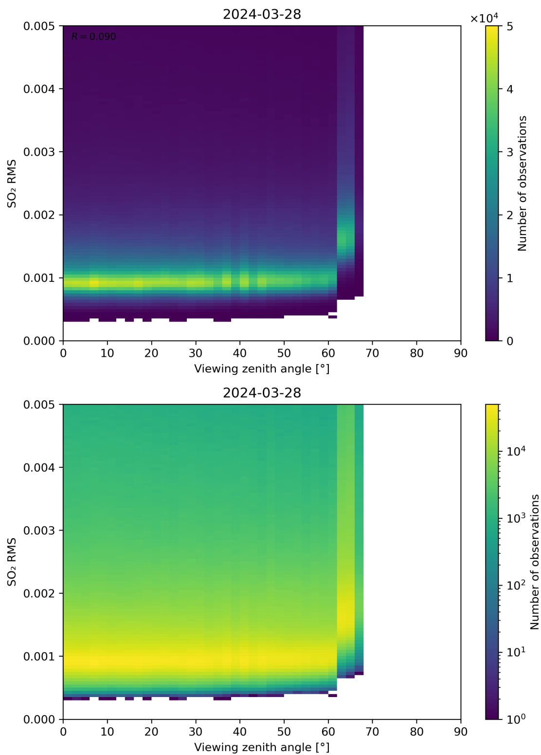
Figure 313: Scatter density plot of “Viewing zenith angle” against “SO 2 RMS” for 2024-03-27 to 2024-03-29.
