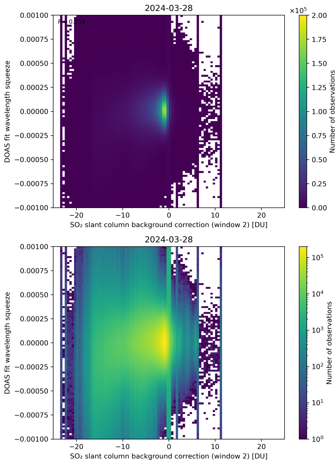
Figure 113: Scatter density plot of “SO 2 slant column background correction (window 2)” against “DOAS fit wavelength squeeze” for 2024-03-27 to 2024-03-29.
