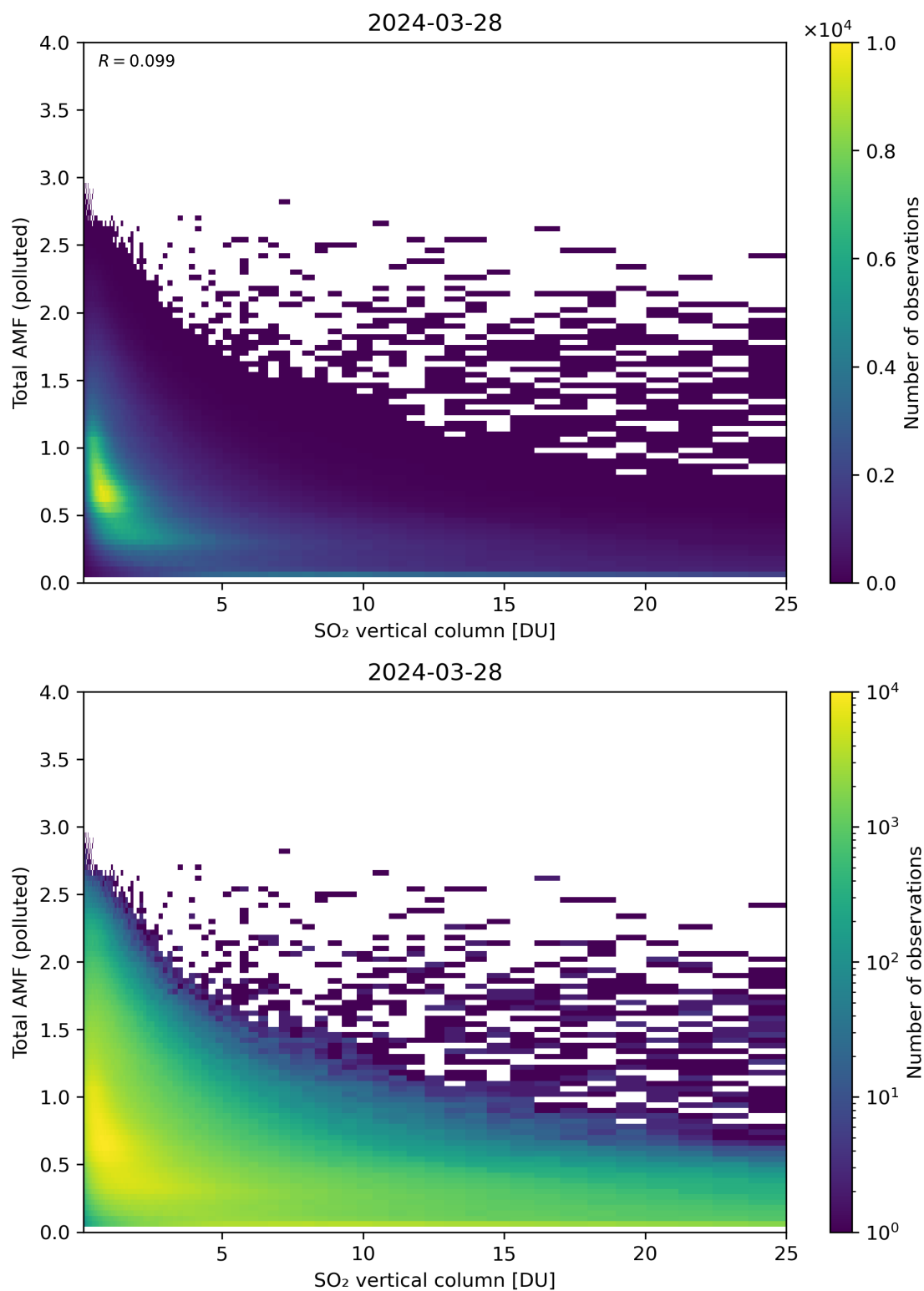
Figure 305: Scatter density plot of “SO 2 vertical column” against “Total AMF (polluted)” for 2024-03-27 to 2024-03-29.
