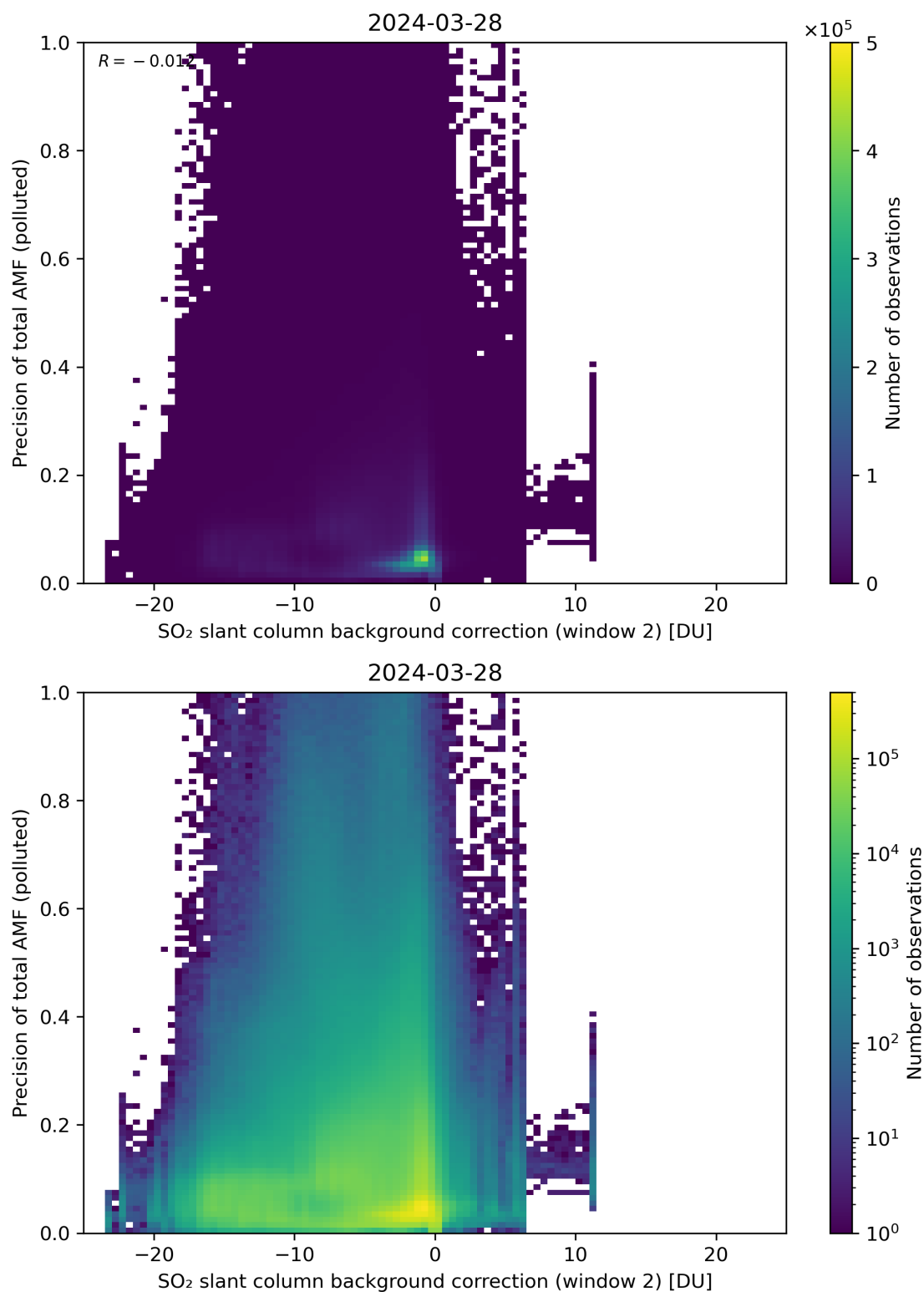
Figure 120: Scatter density plot of “SO 2 slant column background correction (window 2)” against “Precision of total AMF (polluted)” for 2024-03-27 to 2024-03-29.
