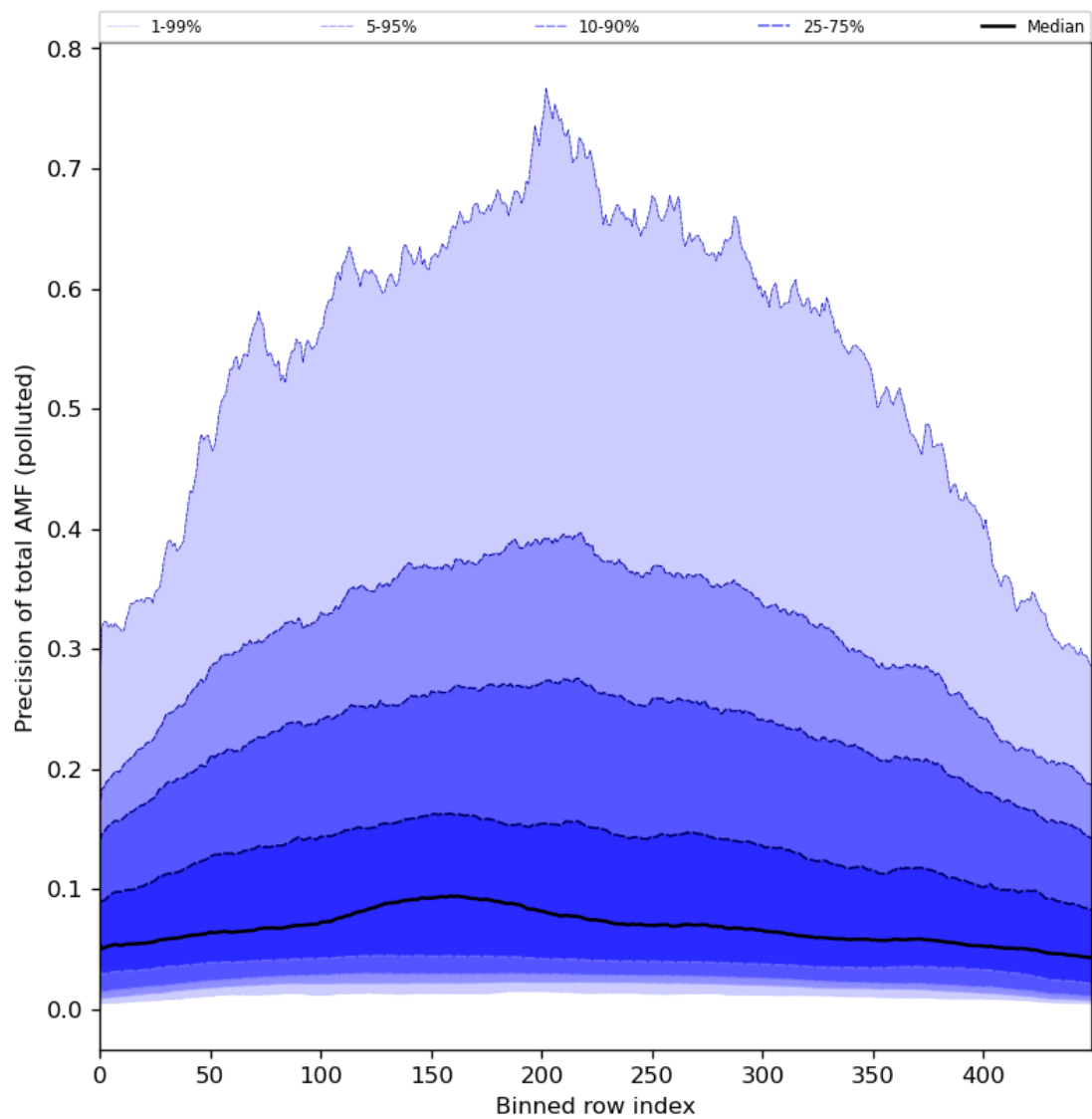
Figure 95: Along track statistics of “Precision of total AMF (polluted)” for 2024-03-27 to 2024-03-29
