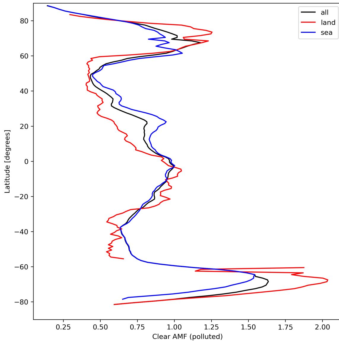
Figure 50: Zonal average of “Clear AMF (polluted)” for 2024-03-27 to 2024-03-29.
