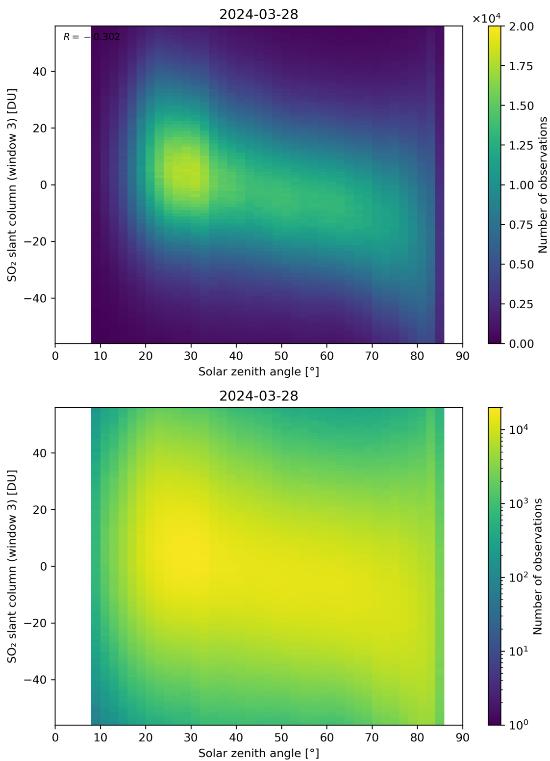
Figure 172: Scatter density plot of “Solar zenith angle” against “SO 2 slant column (window 3)” for 2024-03-27 to 2024-03-29.
