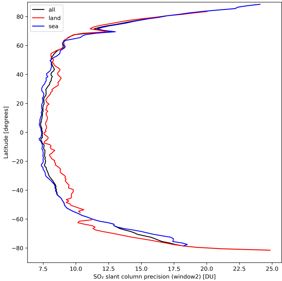
Figure 38: Zonal average of “SO 2 slant column precision (window2)” for 2024-03-27 to 2024-03-29.
