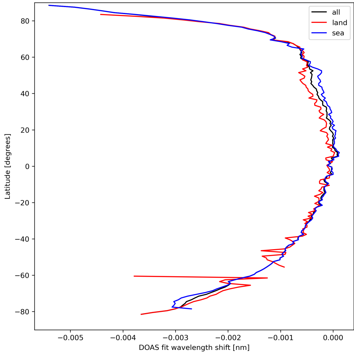
Figure 45: Zonal average of “DOAS fit wavelength shift” for 2024-03-27 to 2024-03-29.
