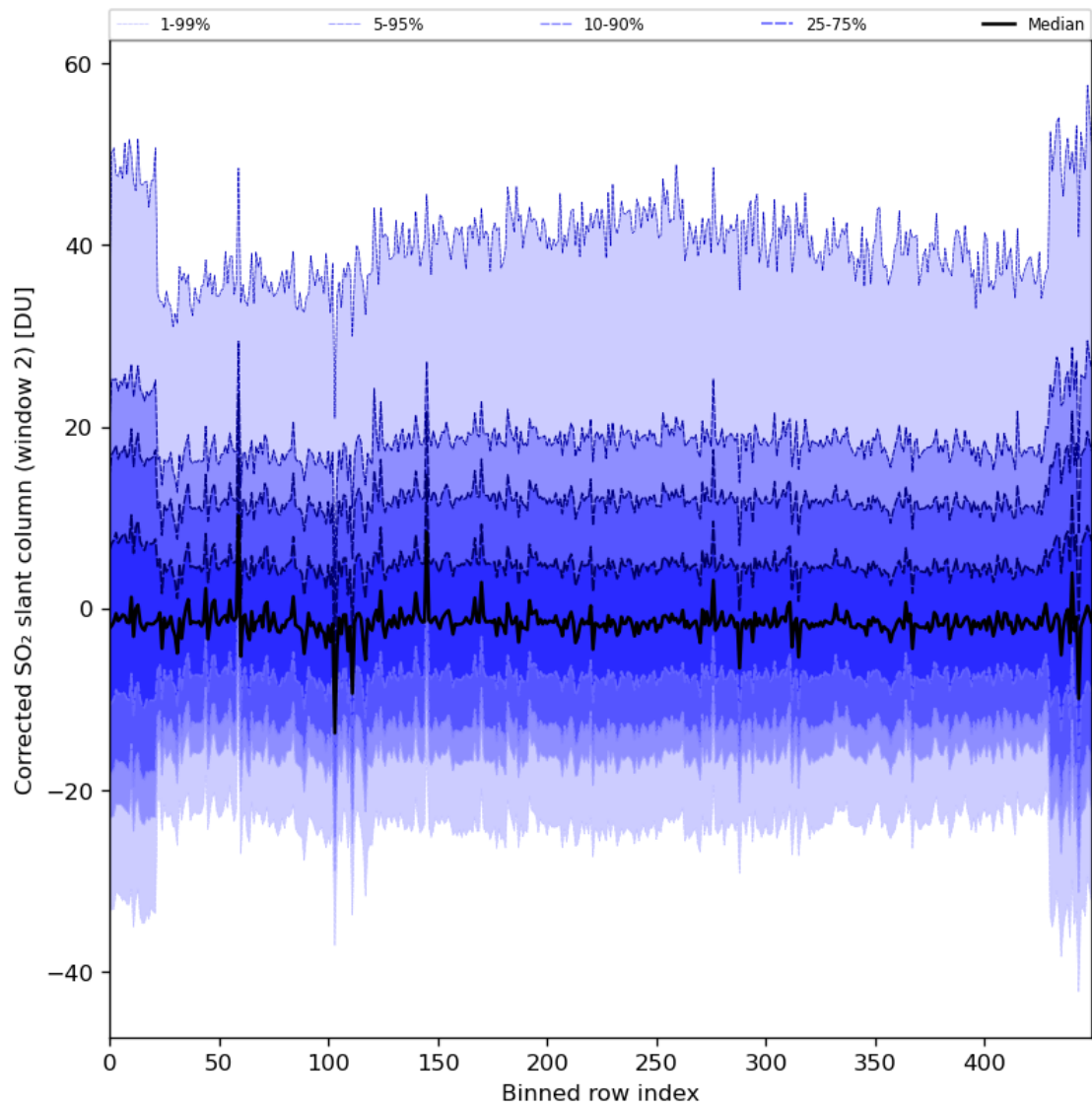
Figure 85: Along track statistics of “Corrected SO 2 slant column (window 2)” for 2024-03-27 to 2024-03-29
