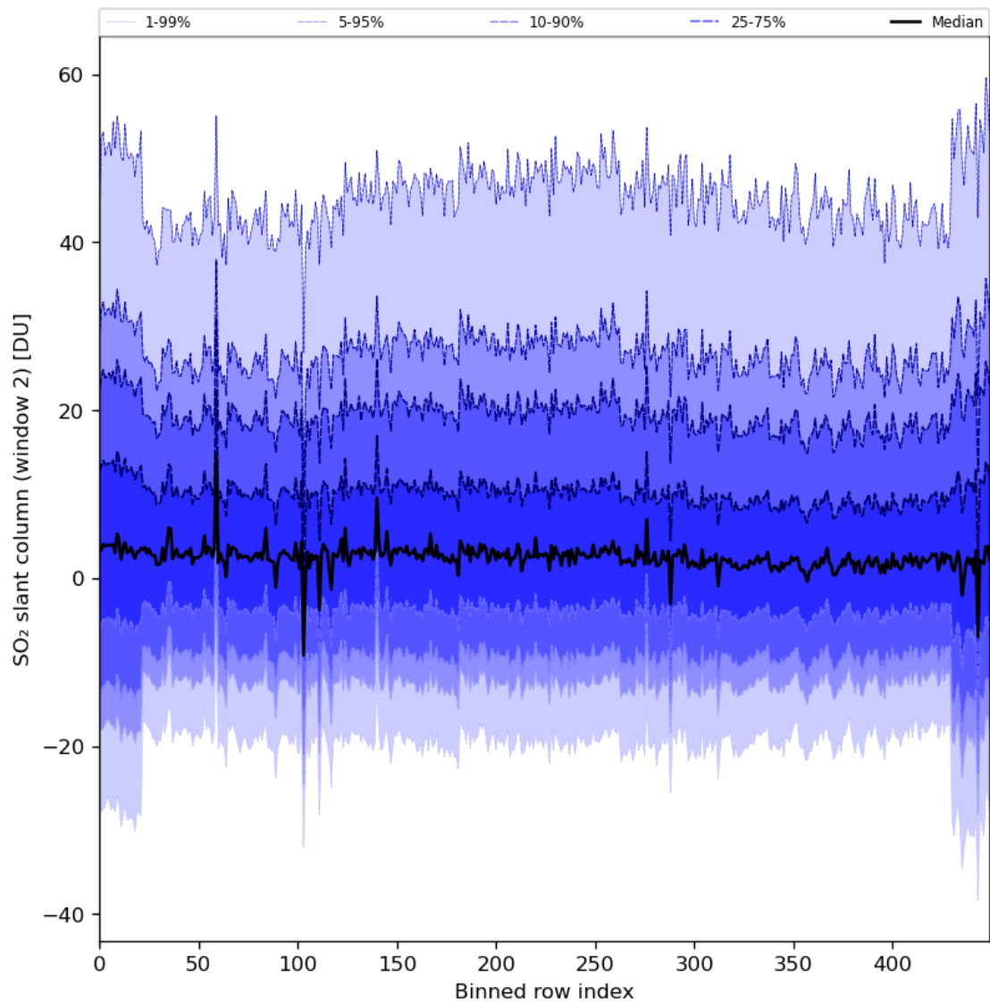
Figure 83: Along track statistics of “SO 2 slant column (window 2)” for 2024-03-27 to 2024-03-29
