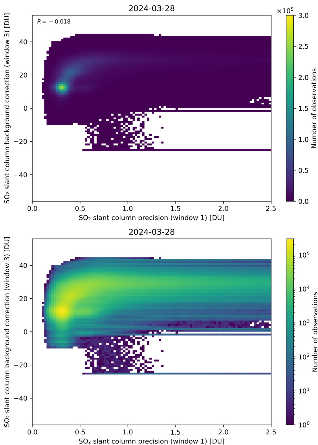
Figure 220: Scatter density plot of “SO 2 slant column precision (window 1)” against “SO 2 slant column background correction (window 3)” for 2024-03-27 to 2024-03-29.
