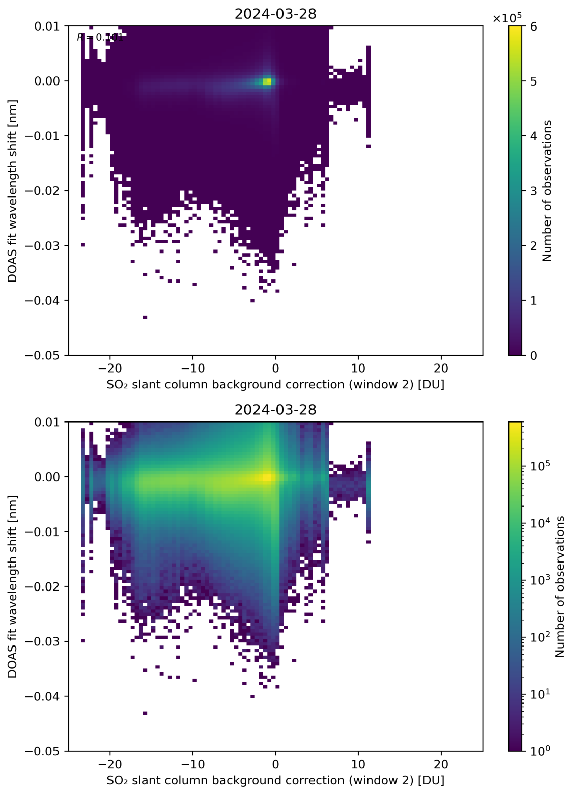
Figure 112: Scatter density plot of “SO 2 slant column background correction (window 2)” against “DOAS fit wavelength shift” for 2024-03-27 to 2024-03-29.
