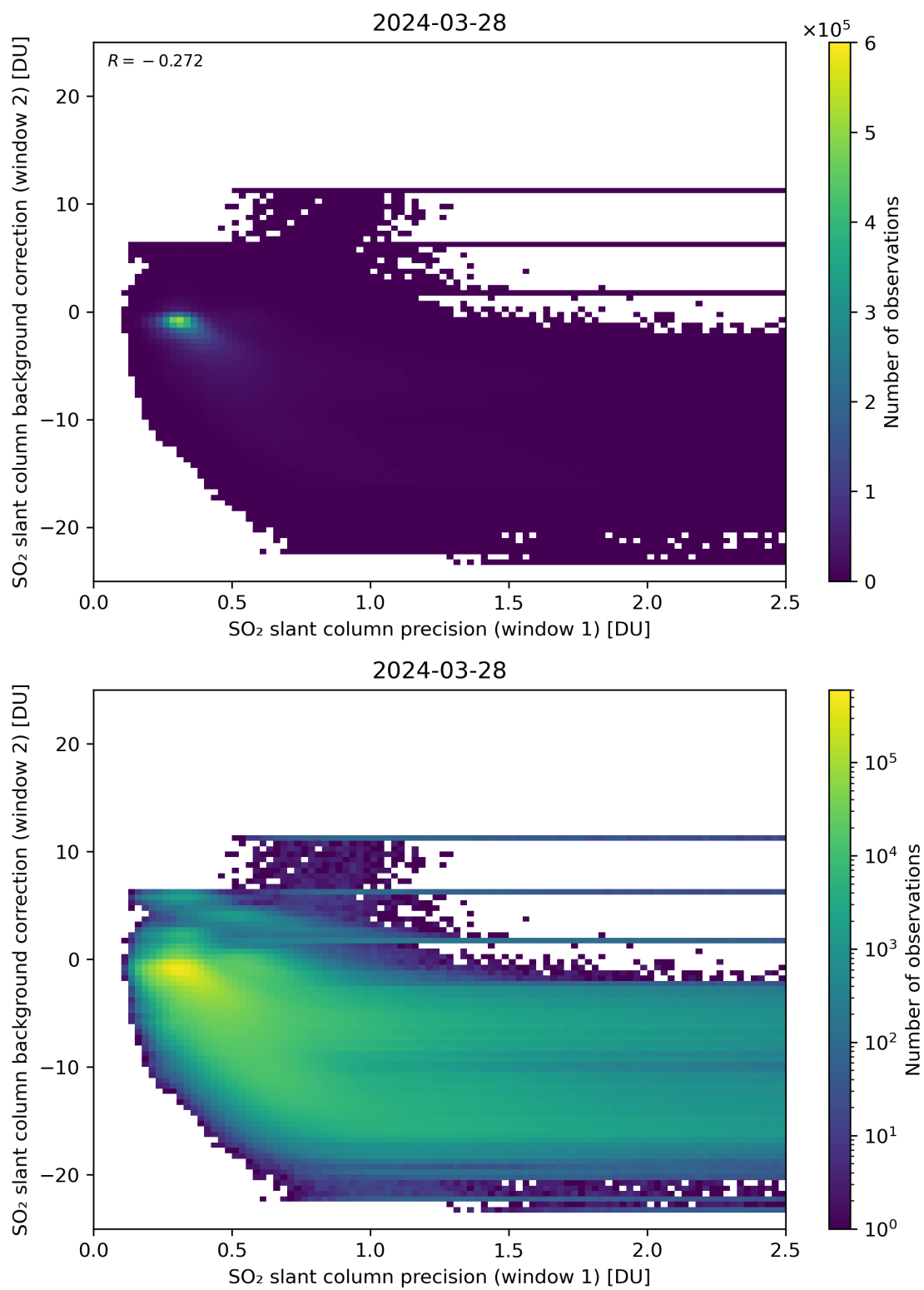
Figure 219: Scatter density plot of “SO 2 slant column precision (window 1)” against “SO 2 slant column background correction (window 2)” for 2024-03-27 to 2024-03-29.
