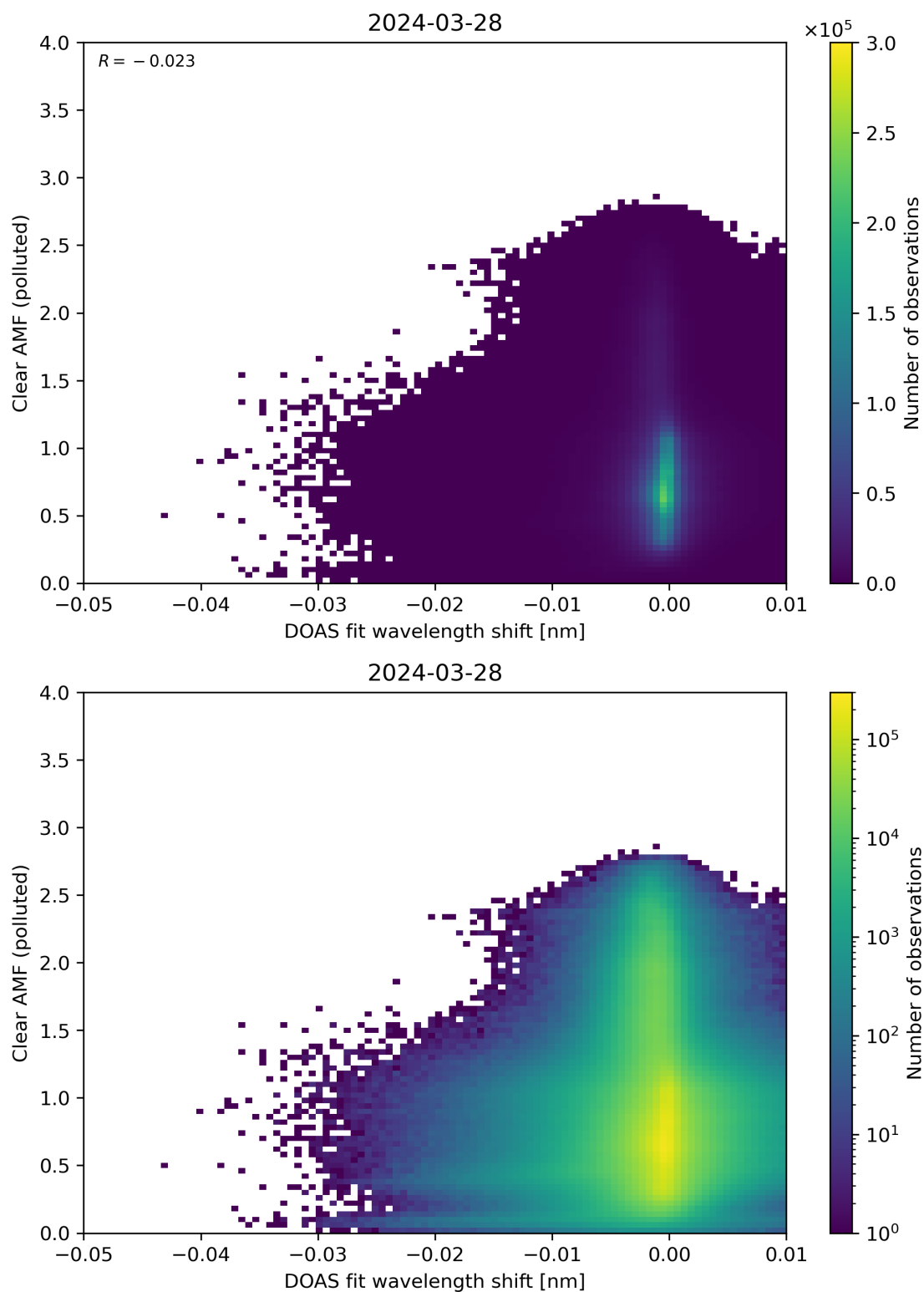
Figure 129: Scatter density plot of “DOAS fit wavelength shift” against “Clear AMF (polluted)” for 2024-03-27 to 2024-03-29.
