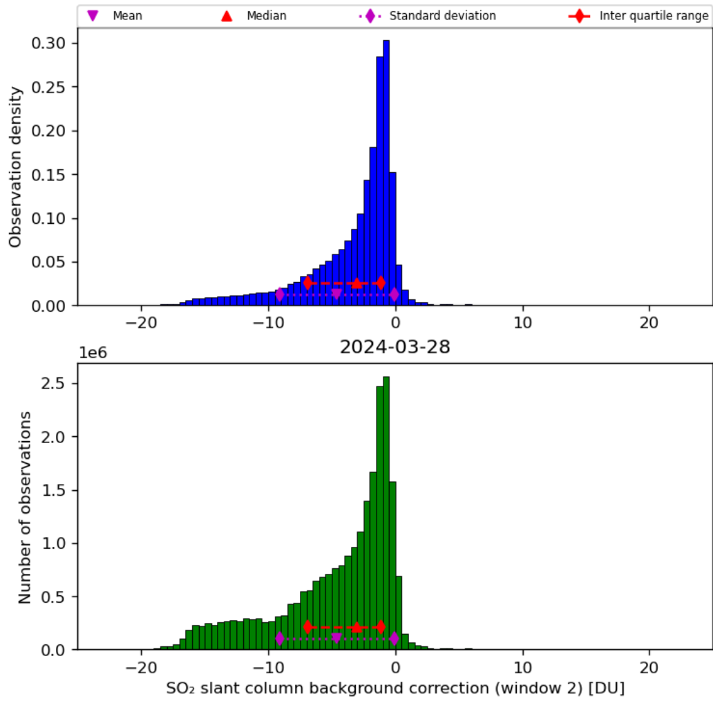
Figure 63: Histogram of “SO 2 slant column background correction (window 2)” for 2024-03-27 to 2024-03-29
