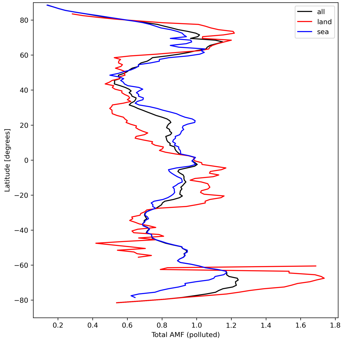
Figure 48: Zonal average of “Total AMF (polluted)” for 2024-03-27 to 2024-03-29.
