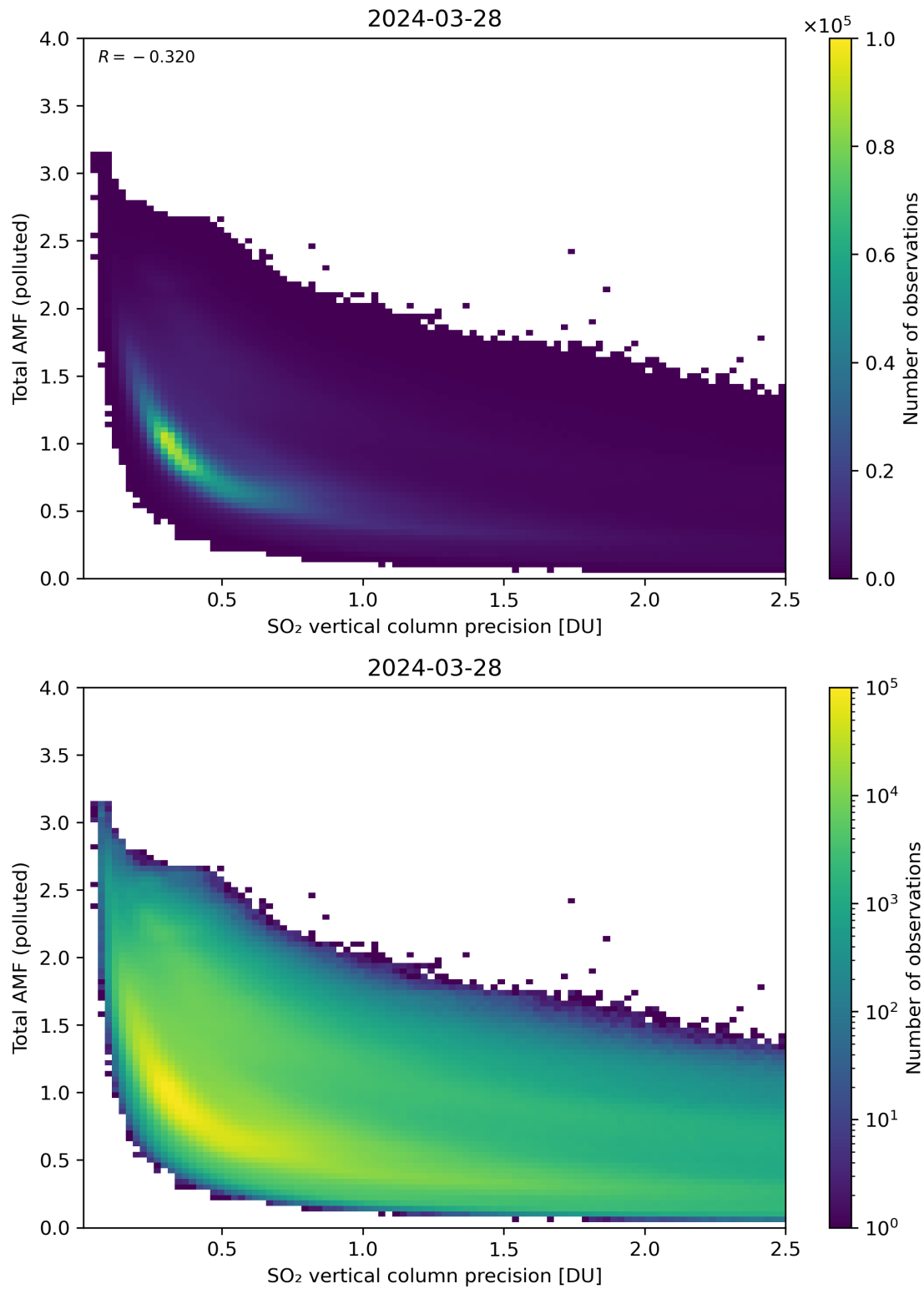
Figure 294: Scatter density plot of “SO 2 vertical column precision” against “Total AMF (polluted)” for 2024-03-27 to 2024-03-29.
