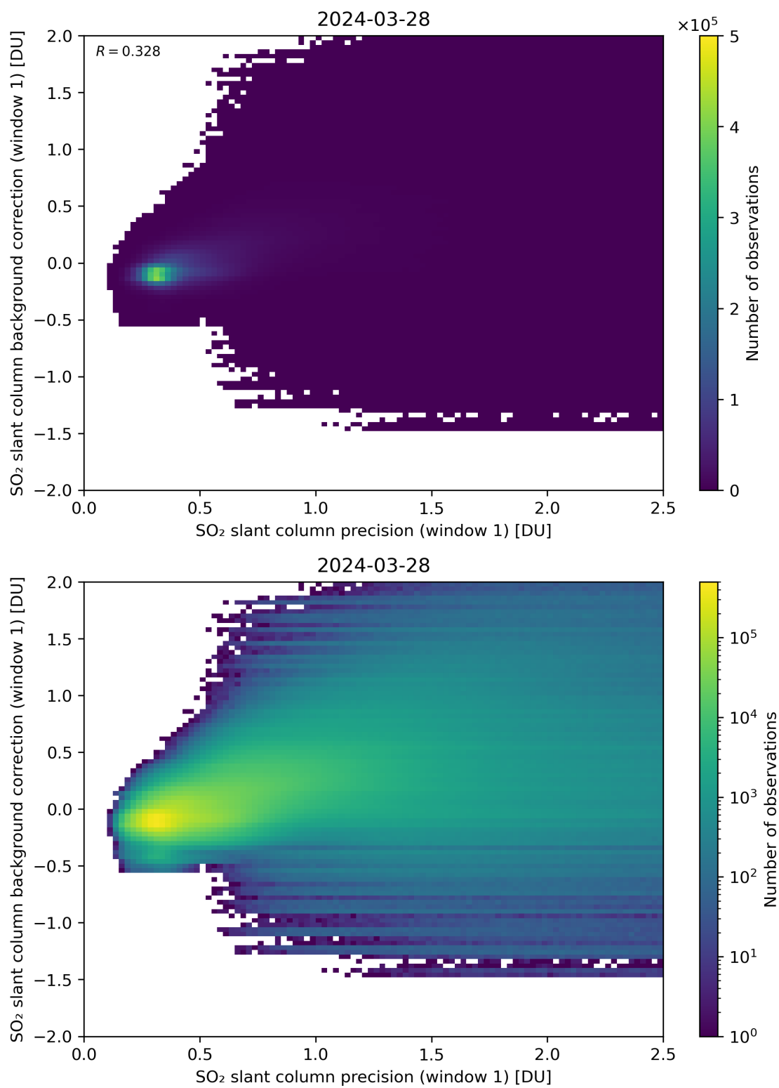
Figure 218: Scatter density plot of “SO 2 slant column precision (window 1)” against “SO 2 slant column background correction (window 1)” for 2024-03-27 to 2024-03-29.
