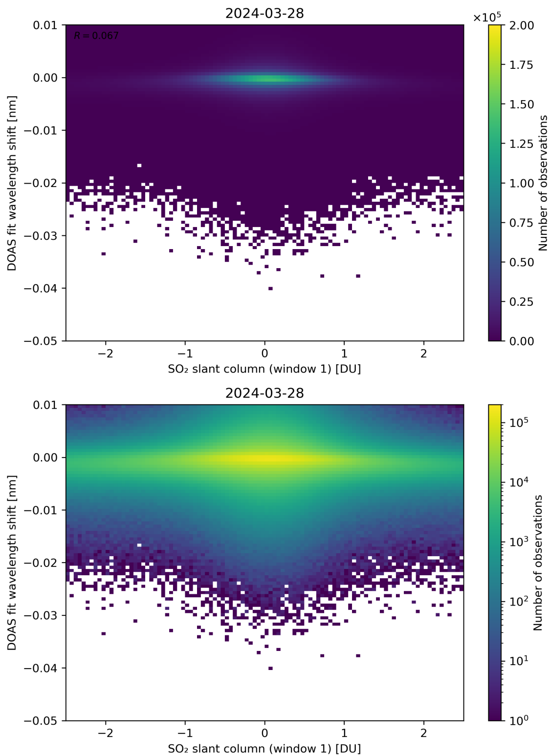
Figure 215: Scatter density plot of “SO 2 slant column (window 1)” against “DOAS fit wavelength shift” for 2024-03-27 to 2024-03-29.
