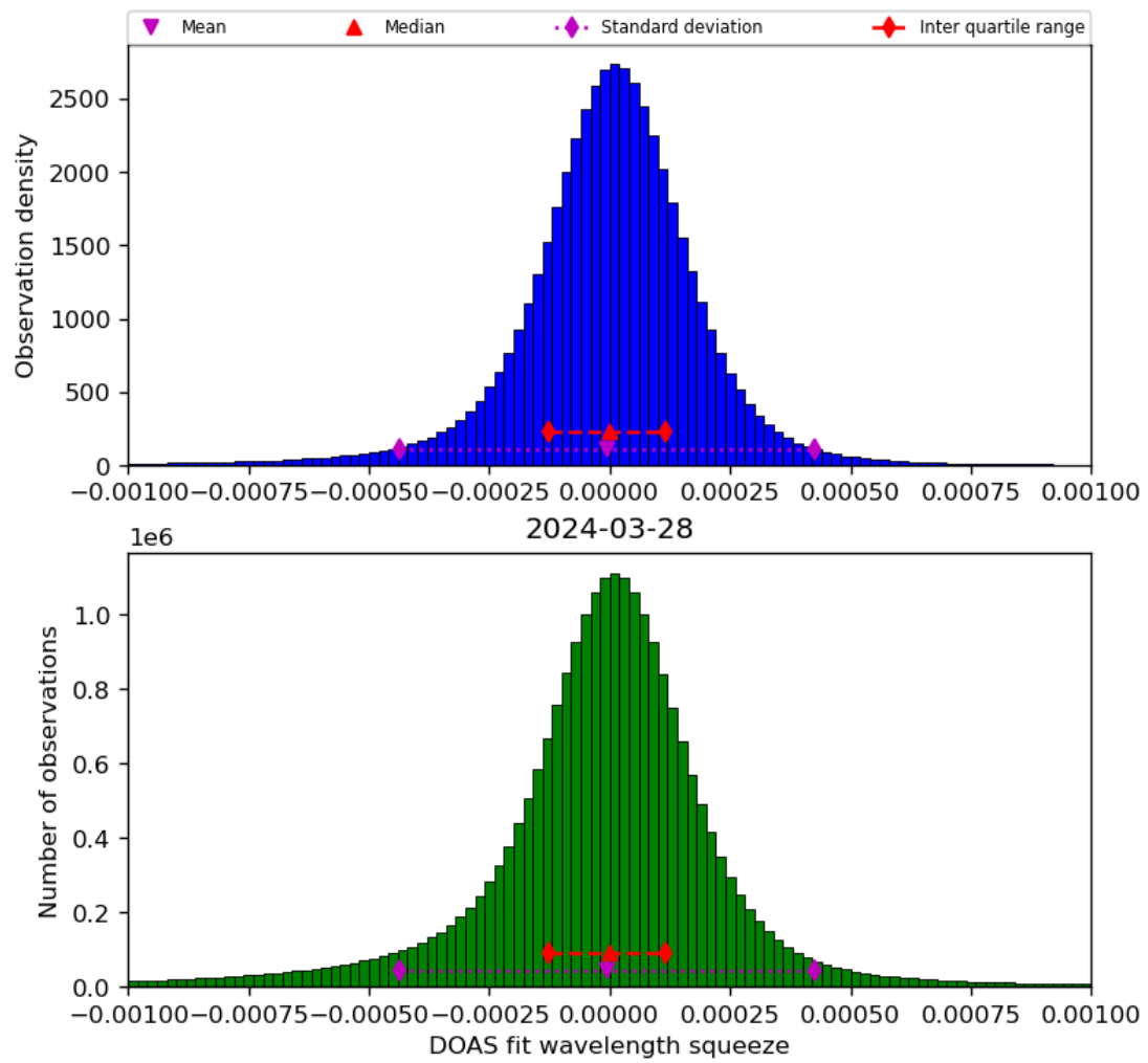
Figure 69: Histogram of “DOAS fit wavelength squeeze” for 2024-03-27 to 2024-03-29
