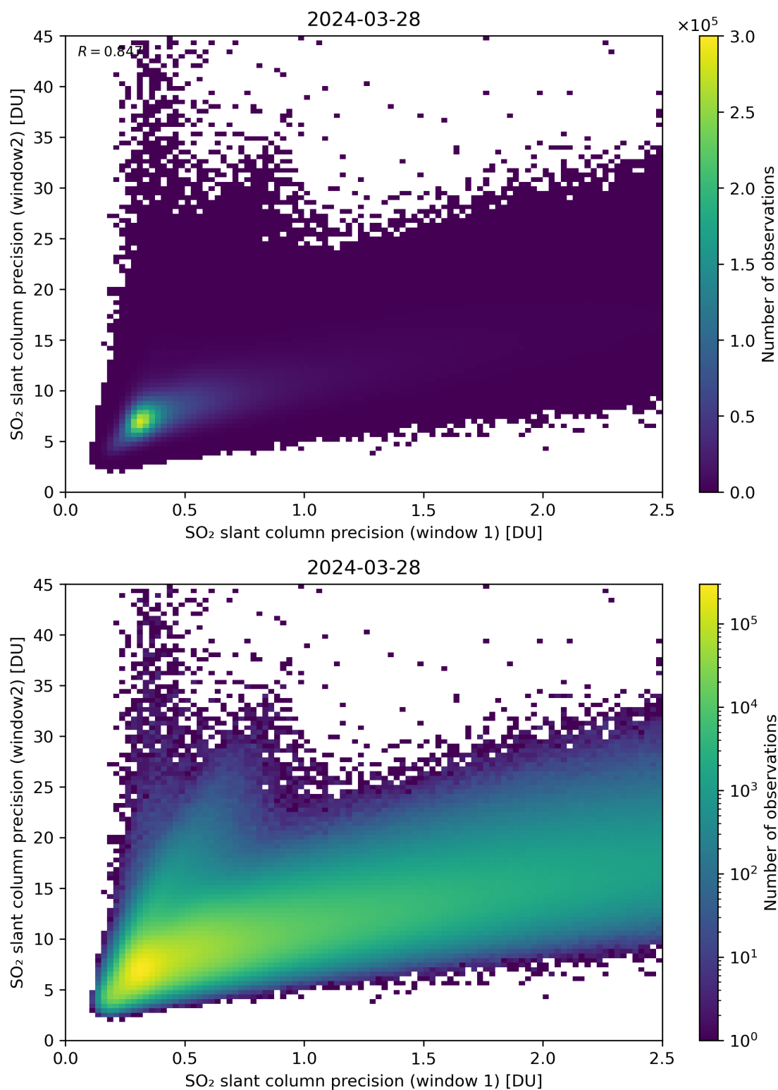
Figure 227: Scatter density plot of “SO 2 slant column precision (window 1)” against “SO 2 slant column precision (window2)” for 2024-03-27 to 2024-03-29.
