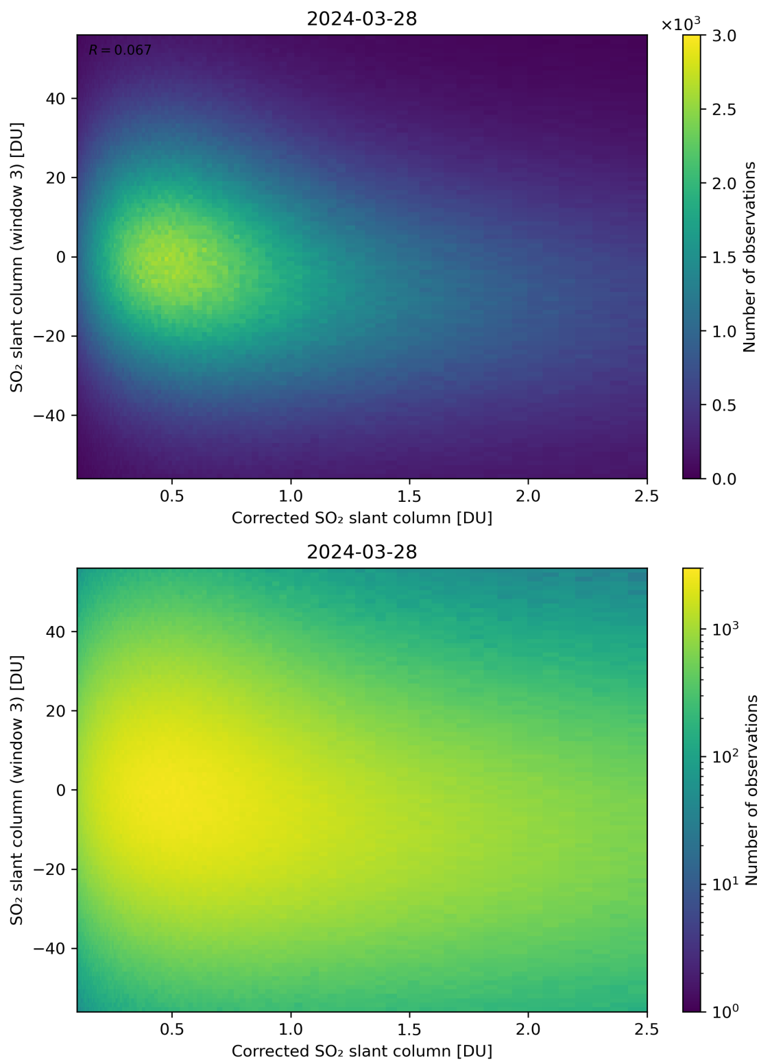
Figure 190: Scatter density plot of “Corrected SO 2 slant column” against “SO 2 slant column (window 3)” for 2024-03-27 to 2024-03-29.
