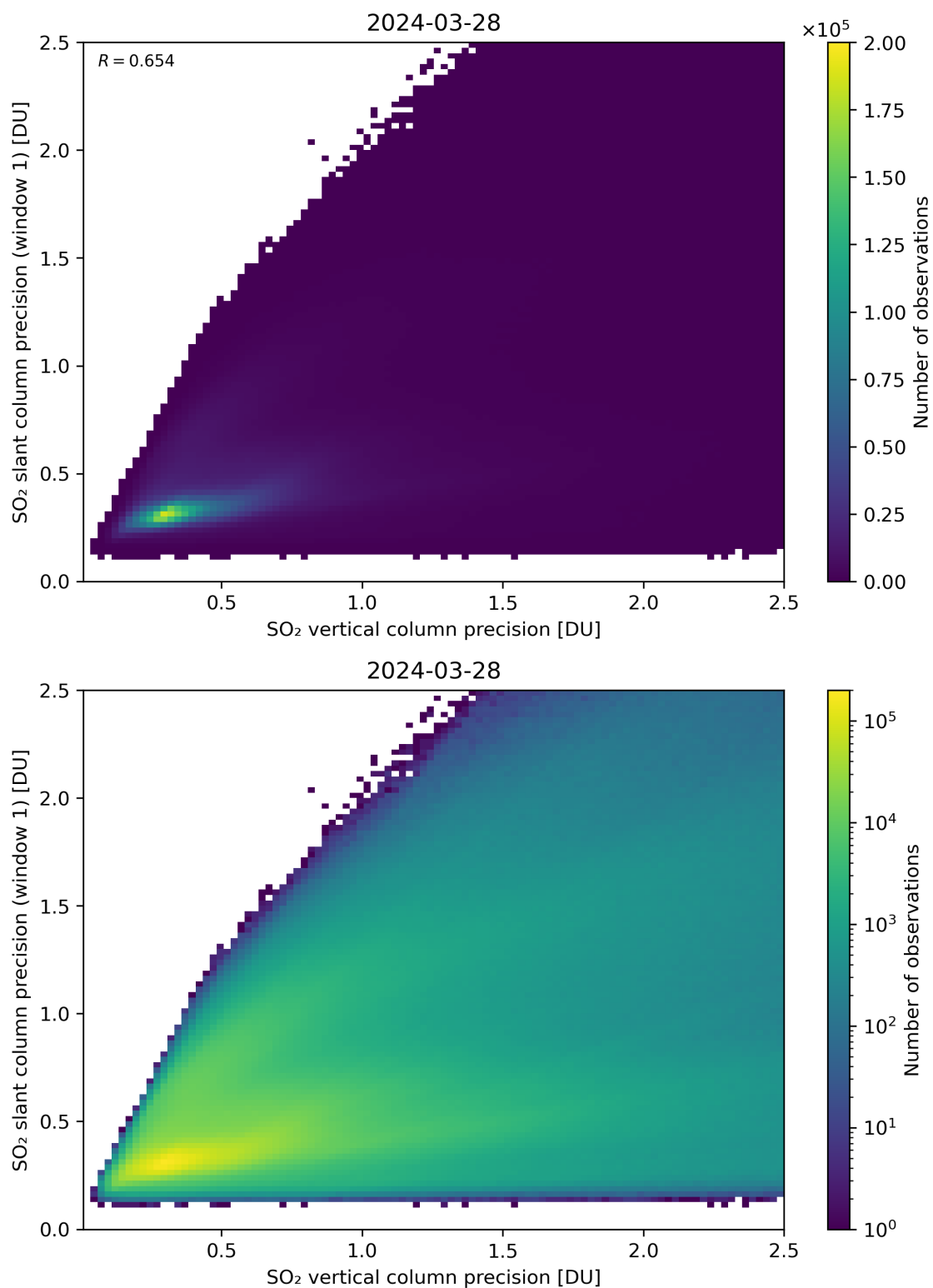
Figure 290: Scatter density plot of “SO 2 vertical column precision” against “SO 2 slant column precision (window 1)” for 2024-03-27 to 2024-03-29.
