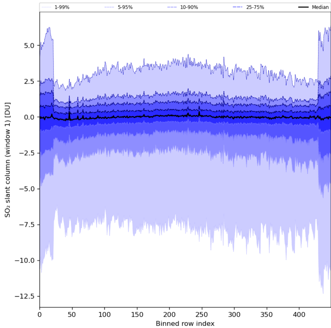
Figure 79: Along track statistics of “SO 2 slant column (window 1)” for 2024-03-27 to 2024-03-29
