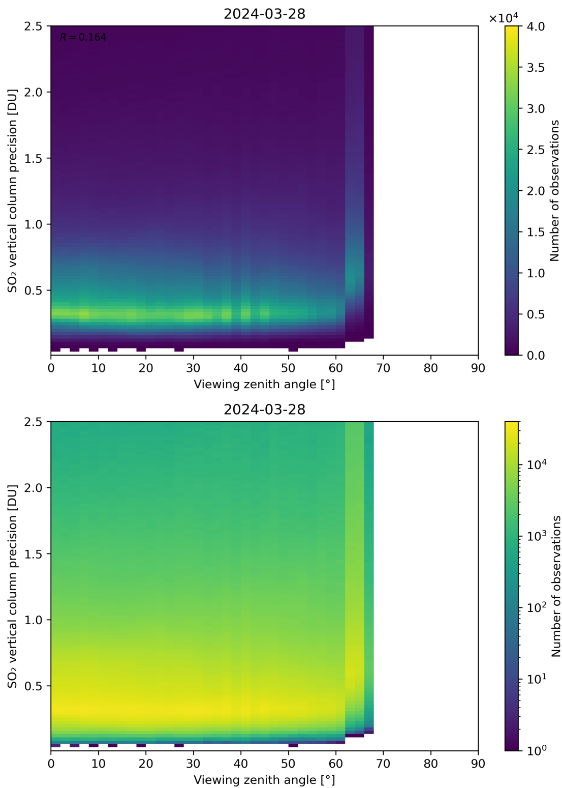
Figure 328: Scatter density plot of “Viewing zenith angle” against “SO 2 vertical column precision” for 2024-03-27 to 2024-03-29.
