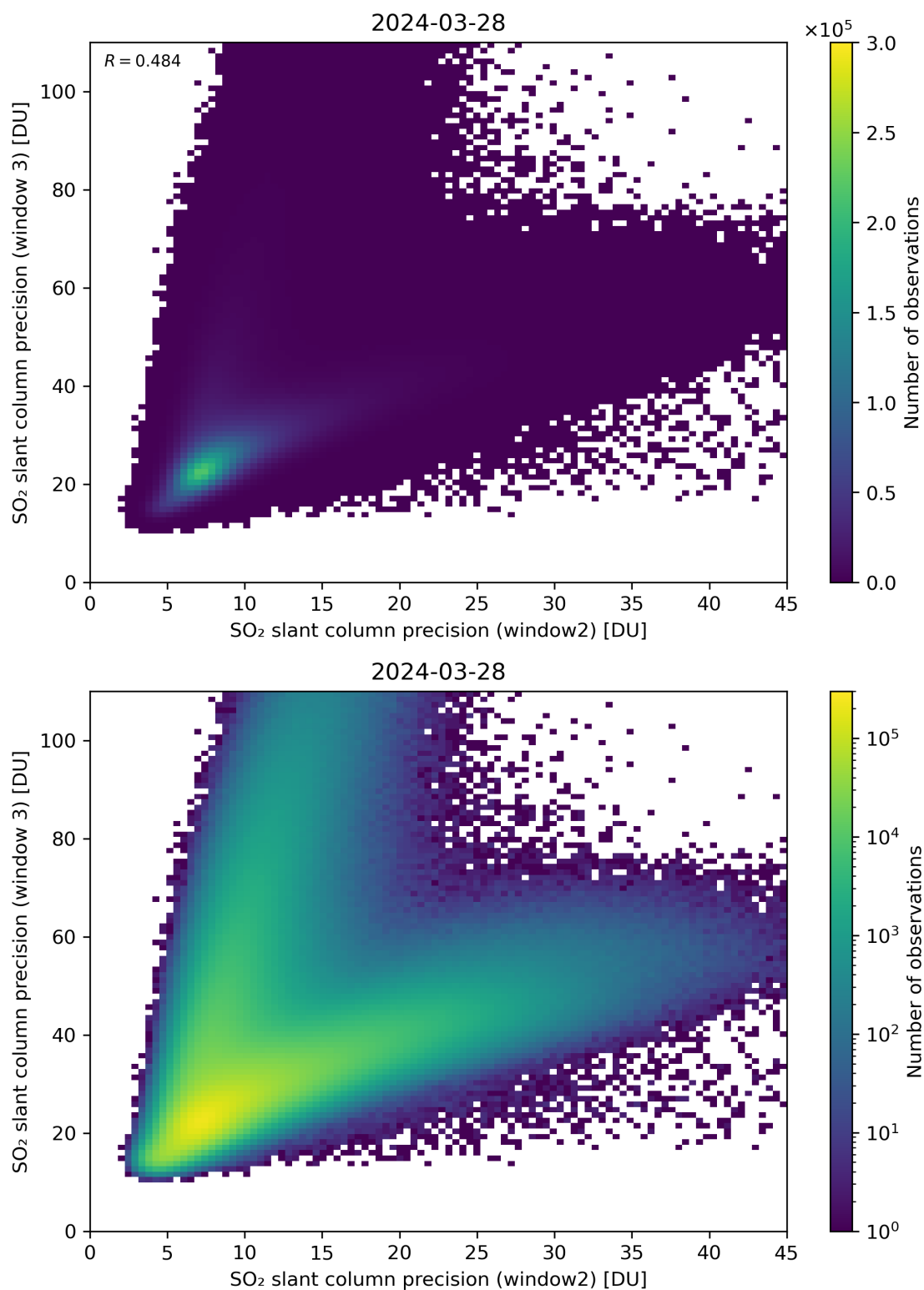
Figure 250: Scatter density plot of “SO 2 slant column precision (window2)” against “SO 2 slant column precision (window 3)” for 2024-03-27 to 2024-03-29.
