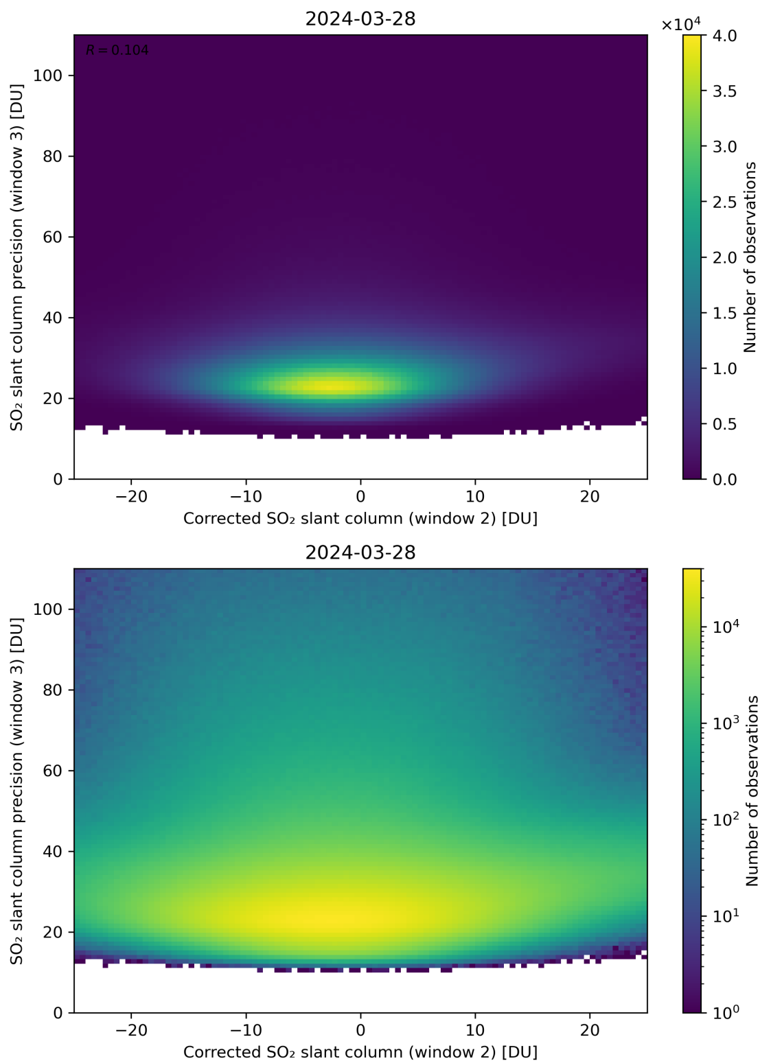
Figure 202: Scatter density plot of “Corrected SO 2 slant column (window 2)” against “SO 2 slant column precision (window 3)” for 2024-03-27 to 2024-03-29.
