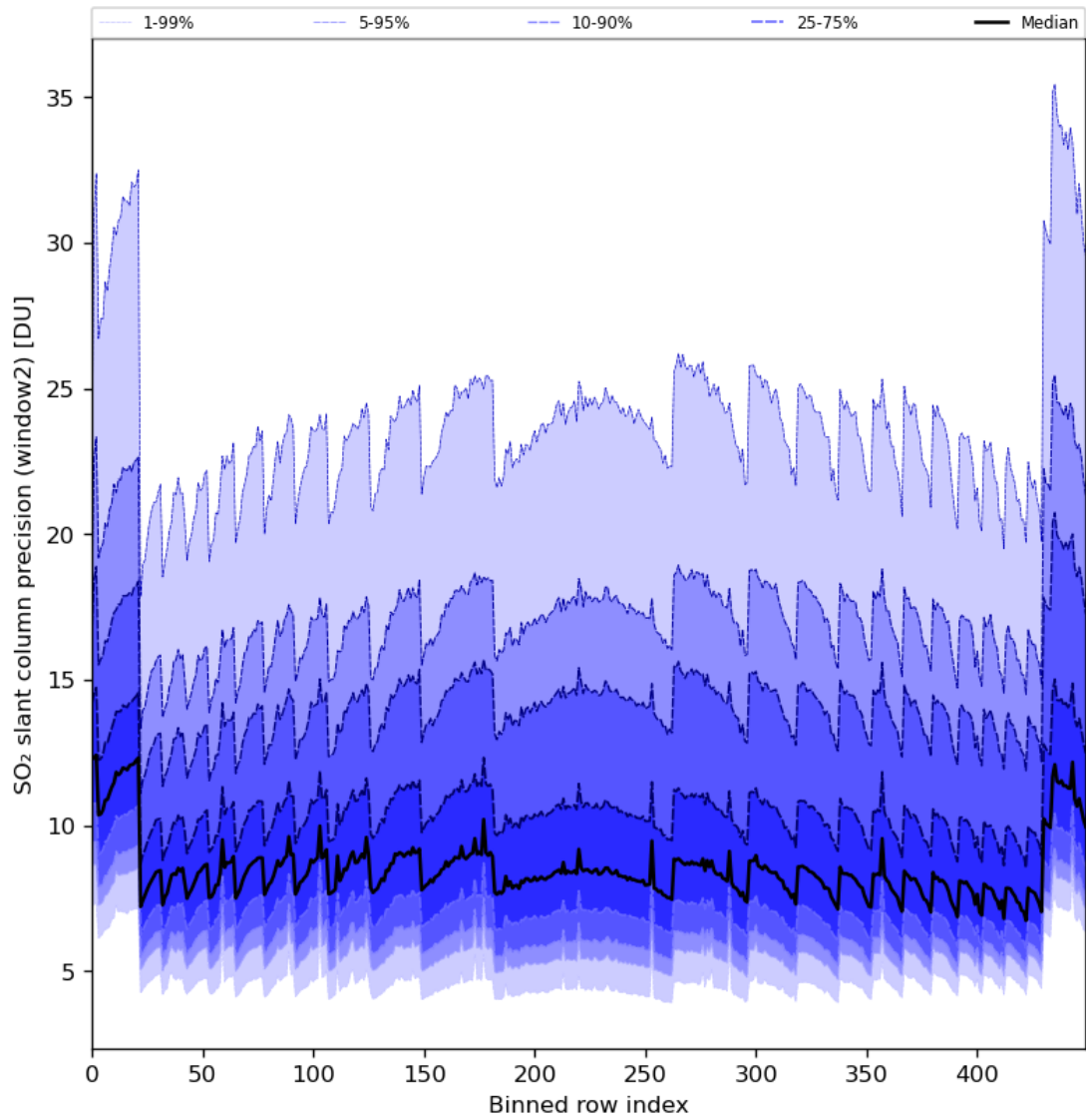
Figure 84: Along track statistics of “SO 2 slant column precision (window2)” for 2024-03-27 to 2024-03-29
