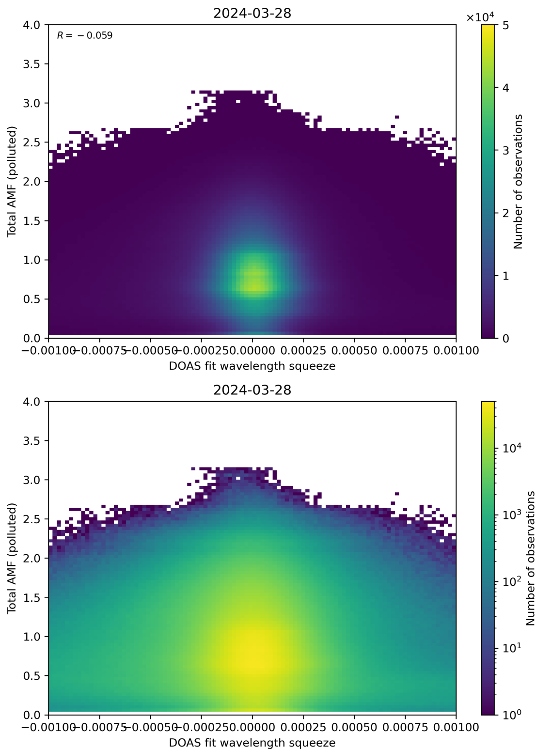
Figure 134: Scatter density plot of “DOAS fit wavelength squeeze” against “Total AMF (polluted)” for 2024-03-27 to 2024-03-29.
