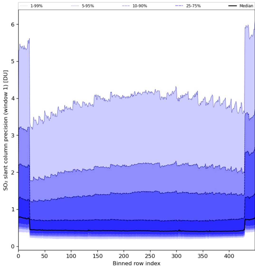
Figure 80: Along track statistics of “SO 2 slant column precision (window 1)” for 2024-03-27 to 2024-03-29
