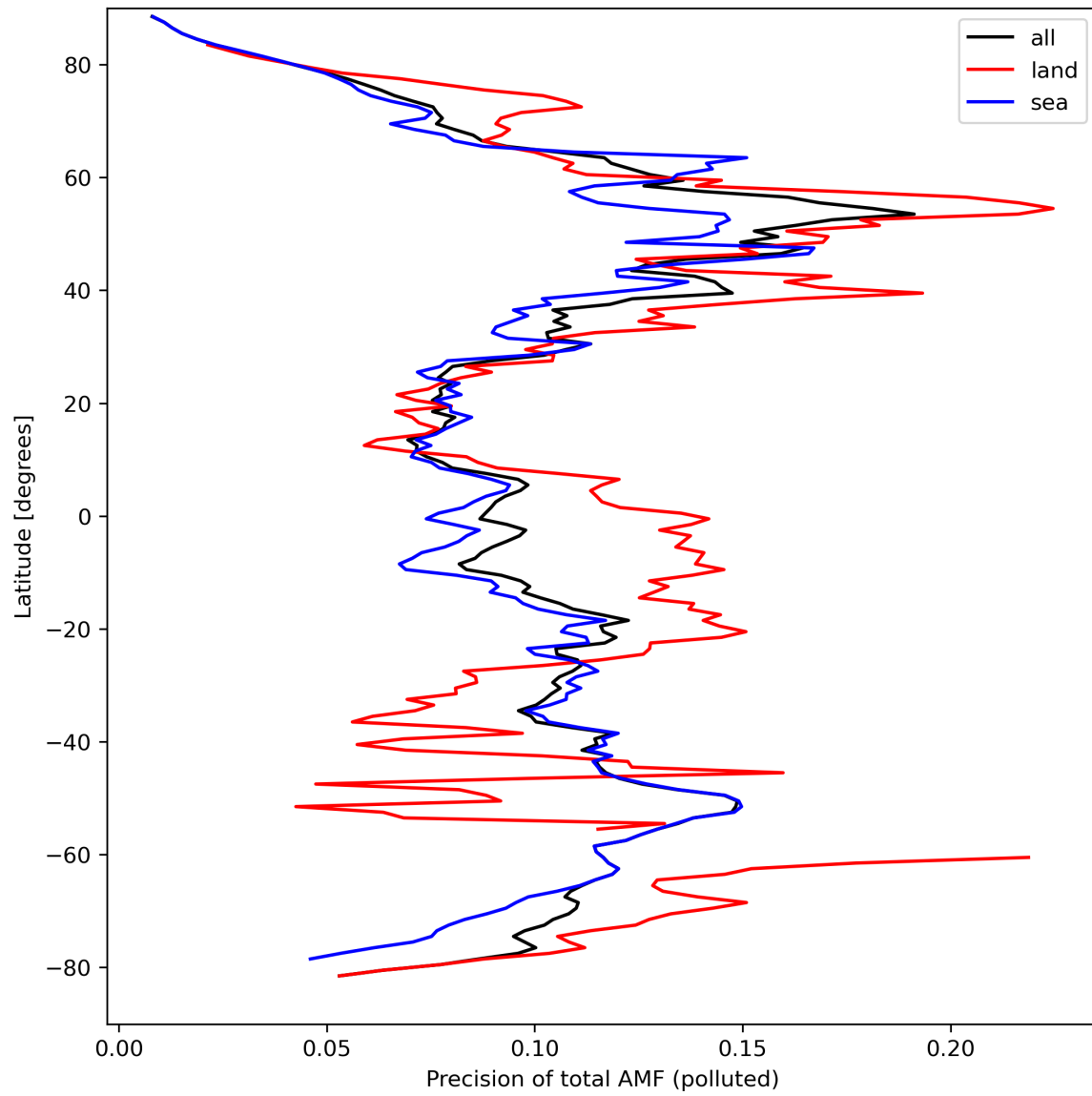
Figure 49: Zonal average of “Precision of total AMF (polluted)” for 2024-03-27 to 2024-03-29.
