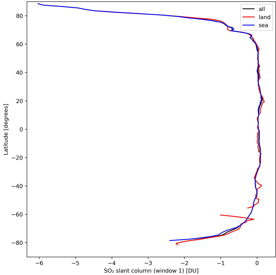
Figure 33: Zonal average of “SO 2 slant column (window 1)” for 2024-03-27 to 2024-03-29.
