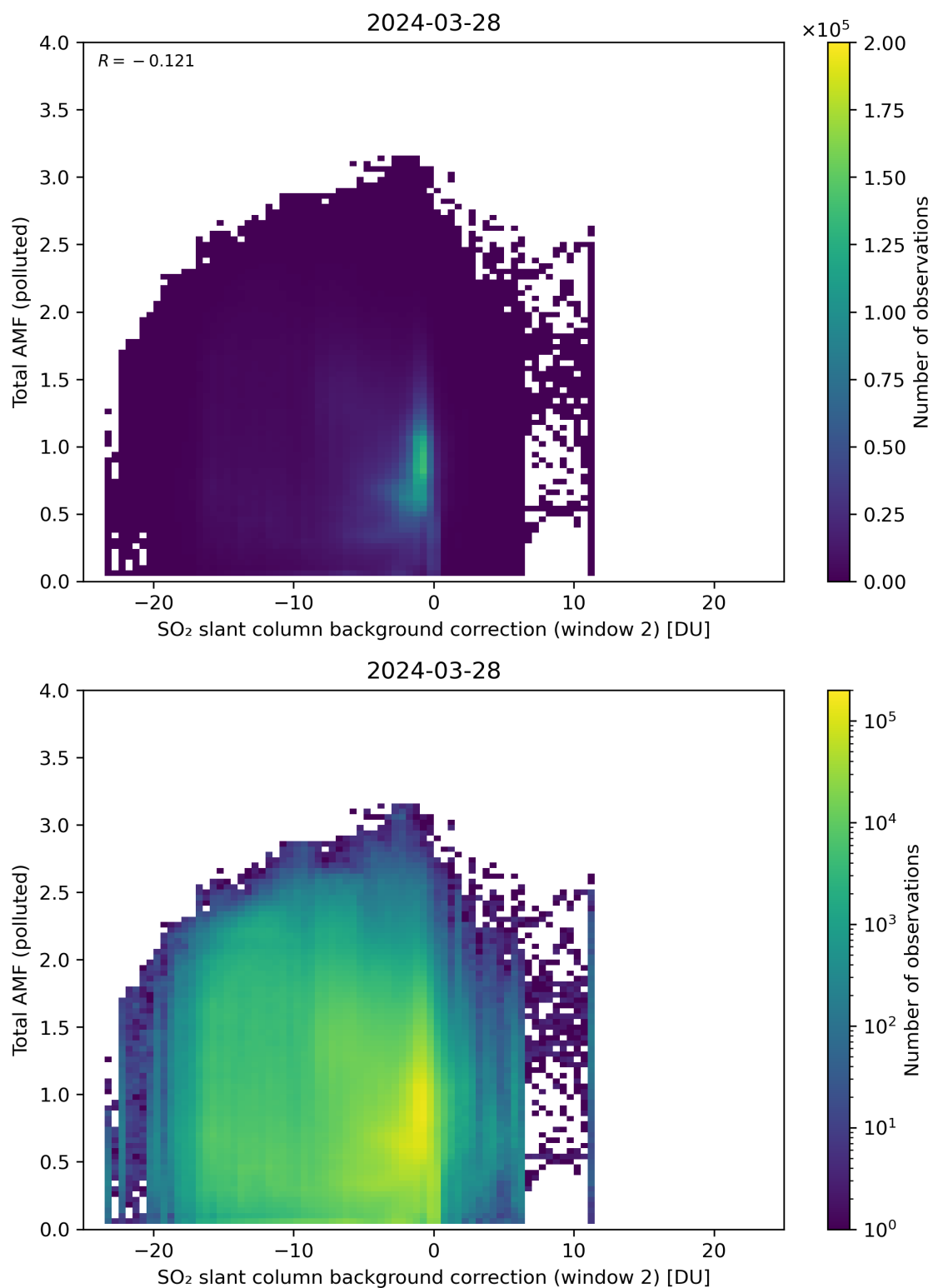
Figure 119: Scatter density plot of “SO 2 slant column background correction (window 2)” against “Total AMF (polluted)” for 2024-03-27 to 2024-03-29.
