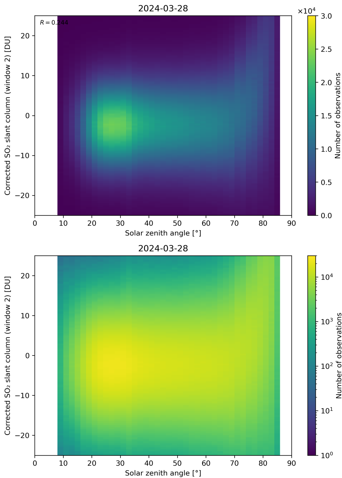
Figure 167: Scatter density plot of “Solar zenith angle” against “Corrected SO 2 slant column (window 2)” for 2024-03-27 to 2024-03-29.
