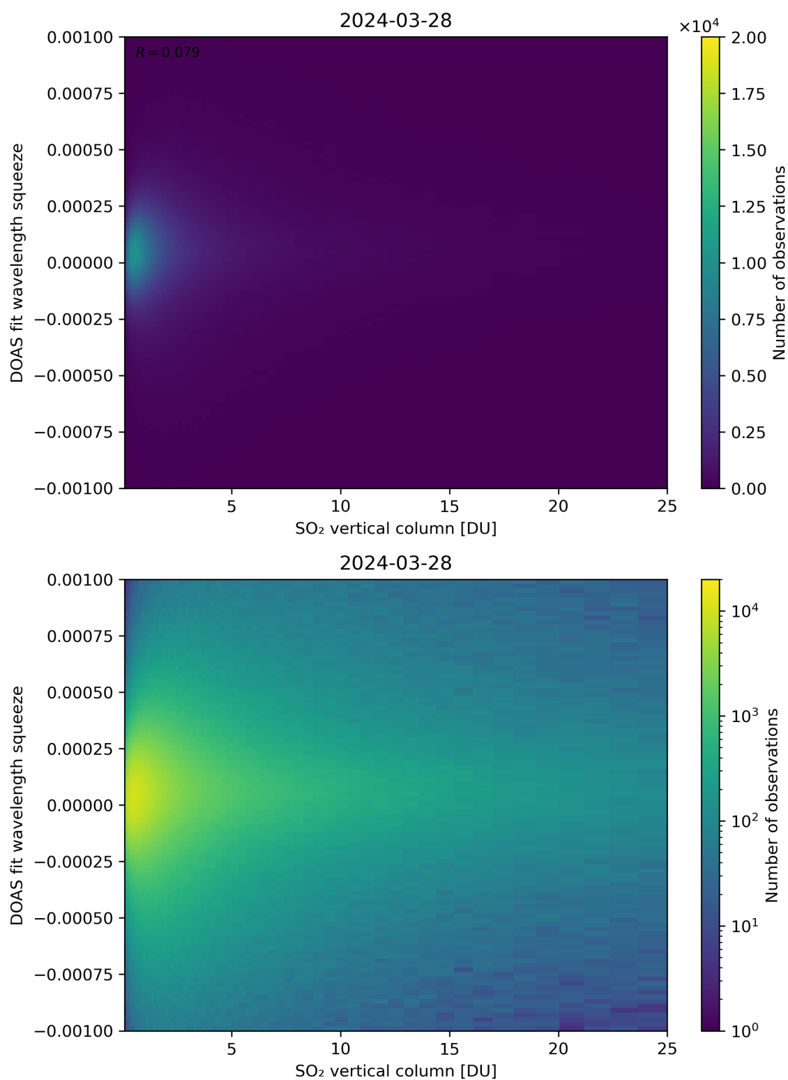
Figure 277: Scatter density plot of “SO 2 vertical column” against “DOAS fit wavelength squeeze” for 2024-03-27 to 2024-03-29.
