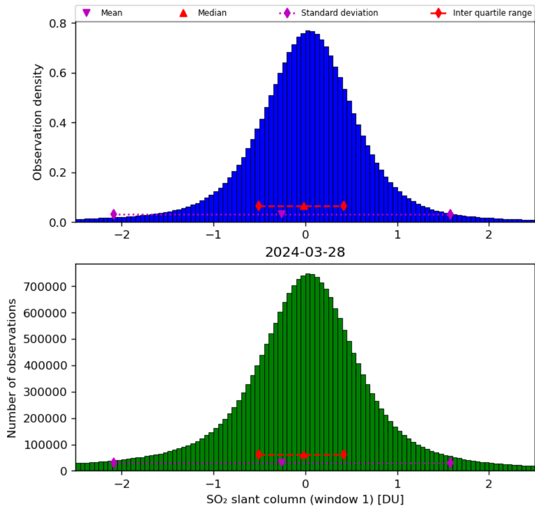
Figure 56: Histogram of “SO 2 slant column (window 1)” for 2024-03-27 to 2024-03-29
