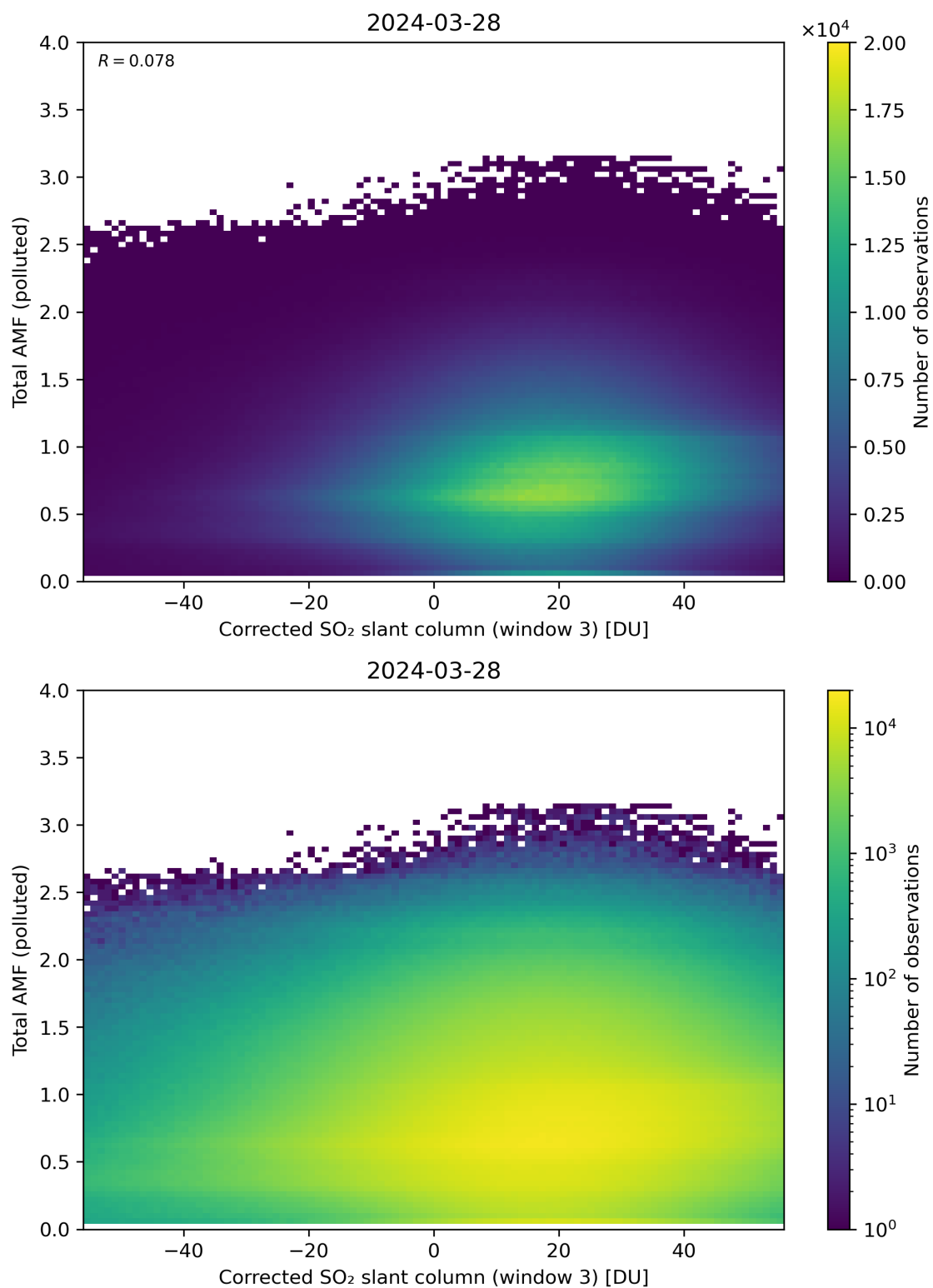
Figure 210: Scatter density plot of “Corrected SO 2 slant column (window 3)” against “Total AMF (polluted)” for 2024-03-27 to 2024-03-29.
