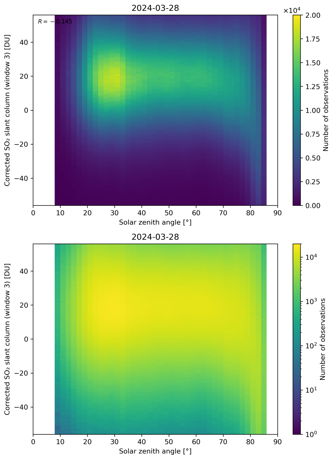
Figure 168: Scatter density plot of “Solar zenith angle” against “Corrected SO 2 slant column (window 3)” for 2024-03-27 to 2024-03-29.
