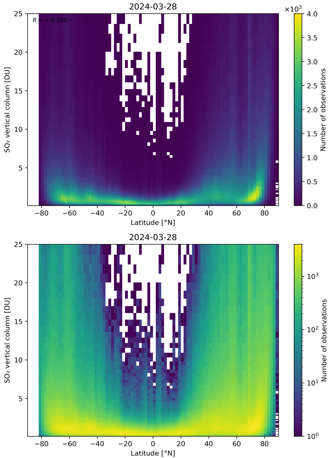
Figure 156: Scatter density plot of “Latitude” against “SO 2 vertical column” for 2024-03-27 to 2024-03-29.
