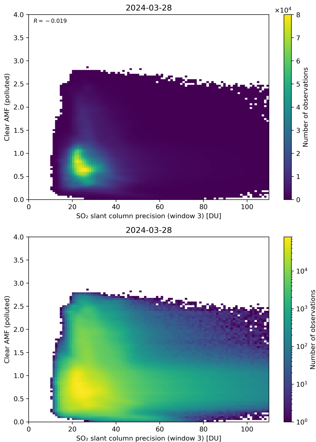
Figure 261: Scatter density plot of “SO 2 slant column precision (window 3)” against “Clear AMF (polluted)” for 2024-03-27 to 2024-03-29.
