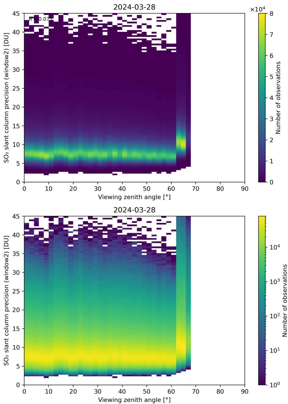
Figure 322: Scatter density plot of “Viewing zenith angle” against “SO 2 slant column precision (window2)” for 2024-03-27 to 2024-03-29.
