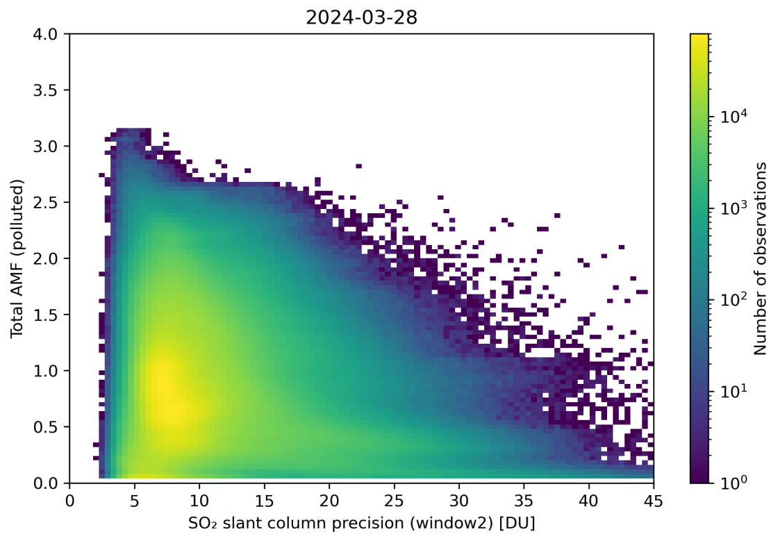
Figure 251: Scatter density plot of “SO 2 slant column precision (window2)” against “Total AMF (polluted)” for 2024-03-27 to 2024-03-29.
