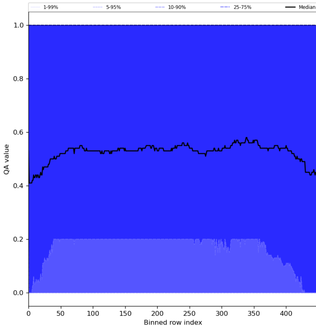
Figure 75: Along track statistics of “QA value” for 2024-03-27 to 2024-03-29
