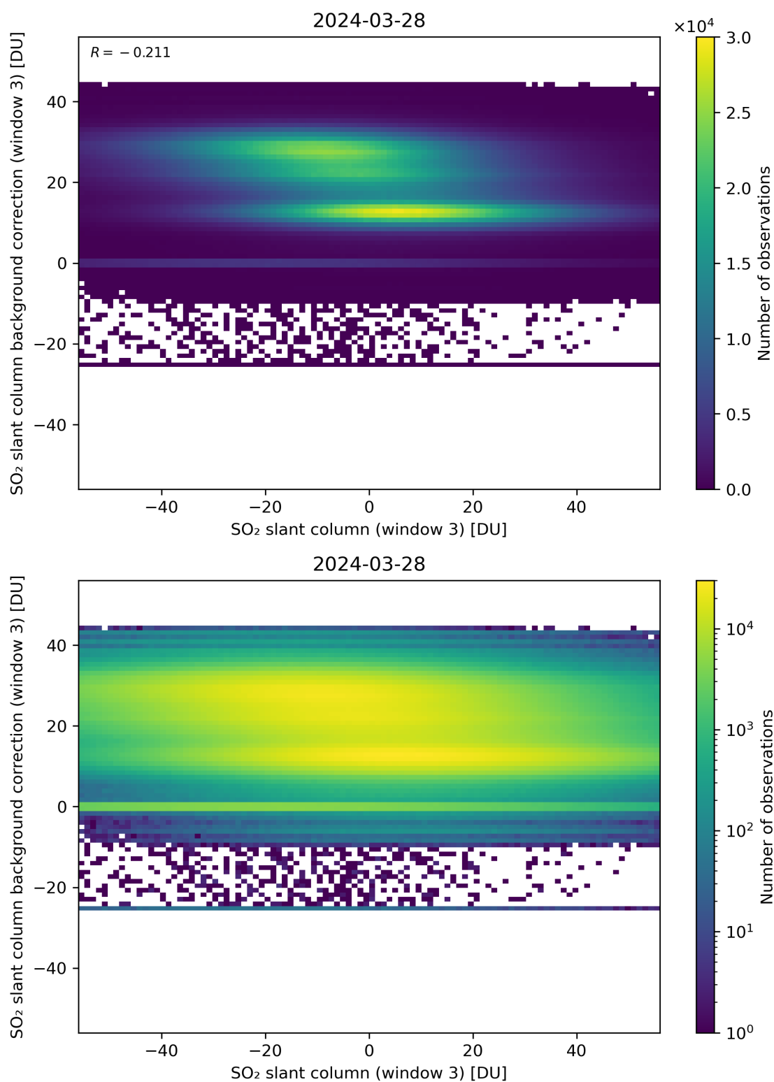
Figure 253: Scatter density plot of “SO 2 slant column (window 3)” against “SO 2 slant column background correction (window 3)” for 2024-03-27 to 2024-03-29.
