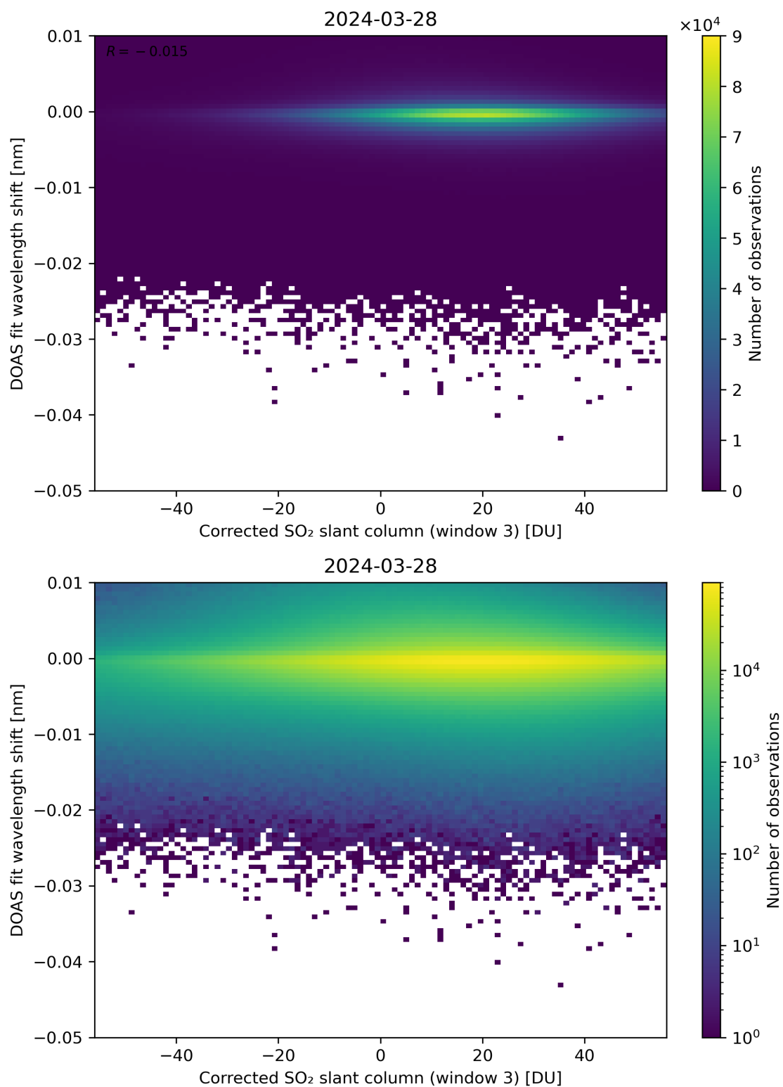
Figure 206: Scatter density plot of “Corrected SO 2 slant column (window 3)” against “DOAS fit wavelength shift” for 2024-03-27 to 2024-03-29.
