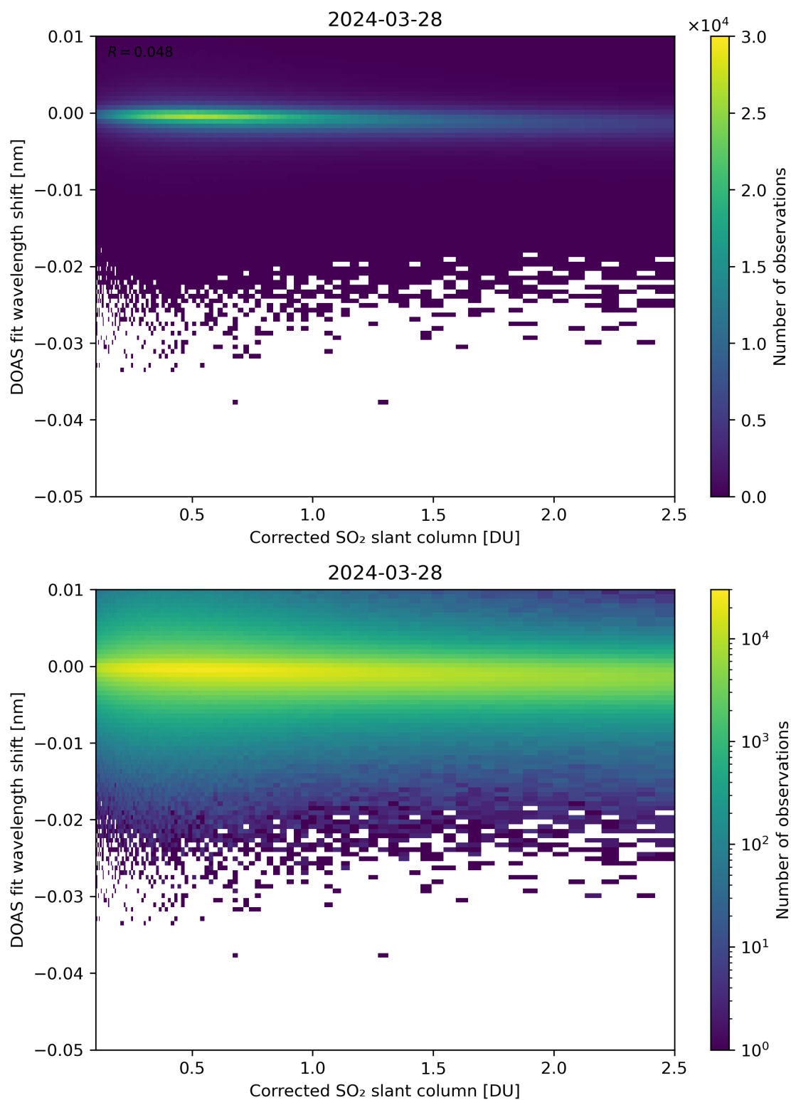
Figure 181: Scatter density plot of “Corrected SO 2 slant column” against “DOAS fit wavelength shift” for 2024-03-27 to 2024-03-29.
