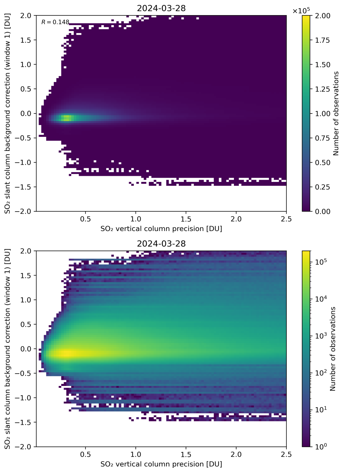
Figure 279: Scatter density plot of “SO 2 vertical column precision” against “SO 2 slant column background correction (window 1)” for 2024-03-27 to 2024-03-29.
