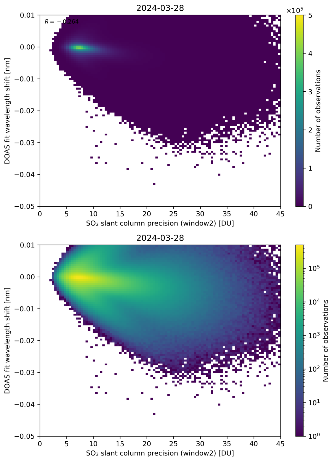
Figure 243: Scatter density plot of “SO 2 slant column precision (window2)” against “DOAS fit wavelength shift” for 2024-03-27 to 2024-03-29.
