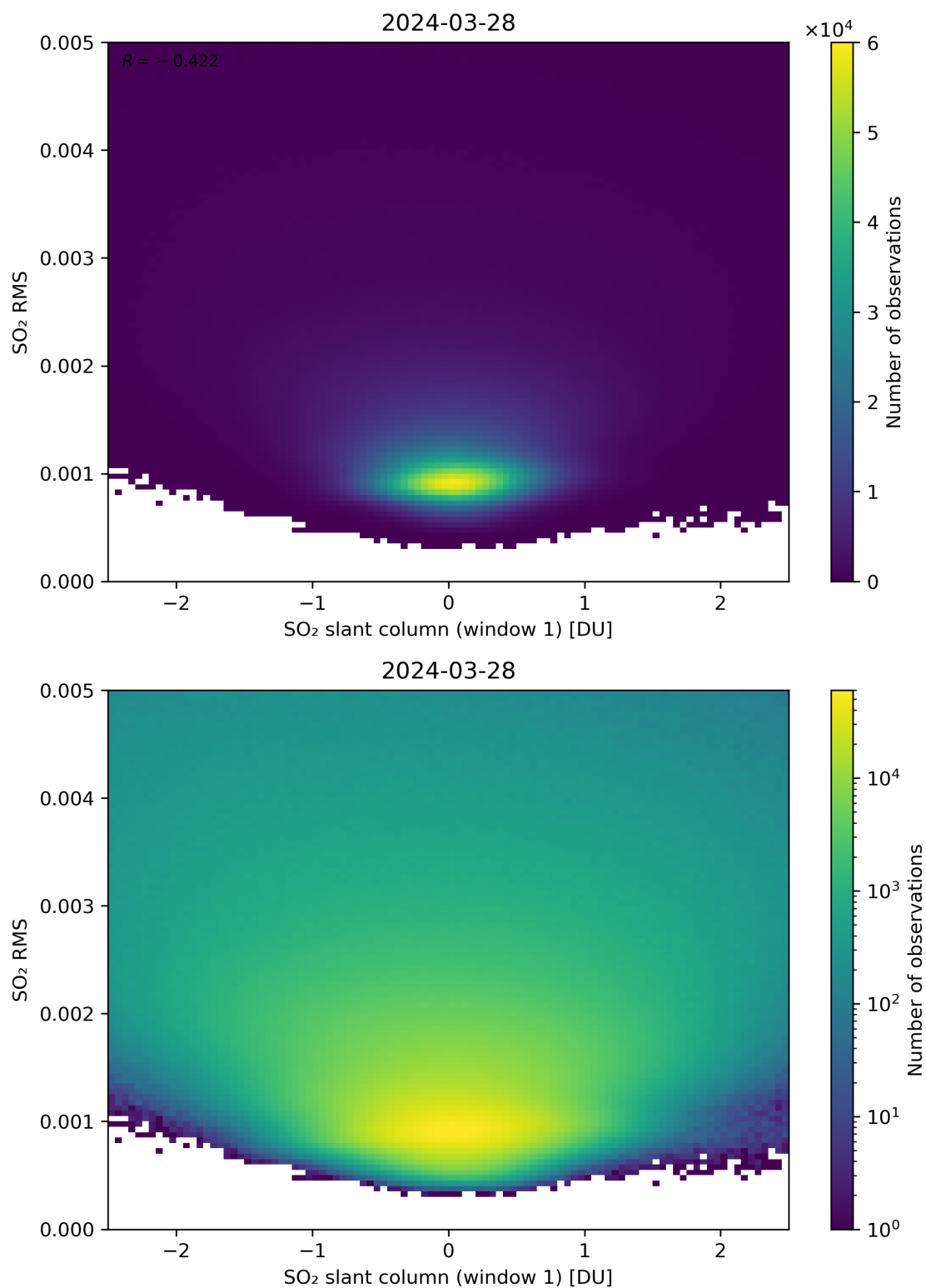
Figure 217: Scatter density plot of “SO 2 slant column (window 1)” against “SO 2 RMS” for 2024-03-27 to 2024-03-29.
