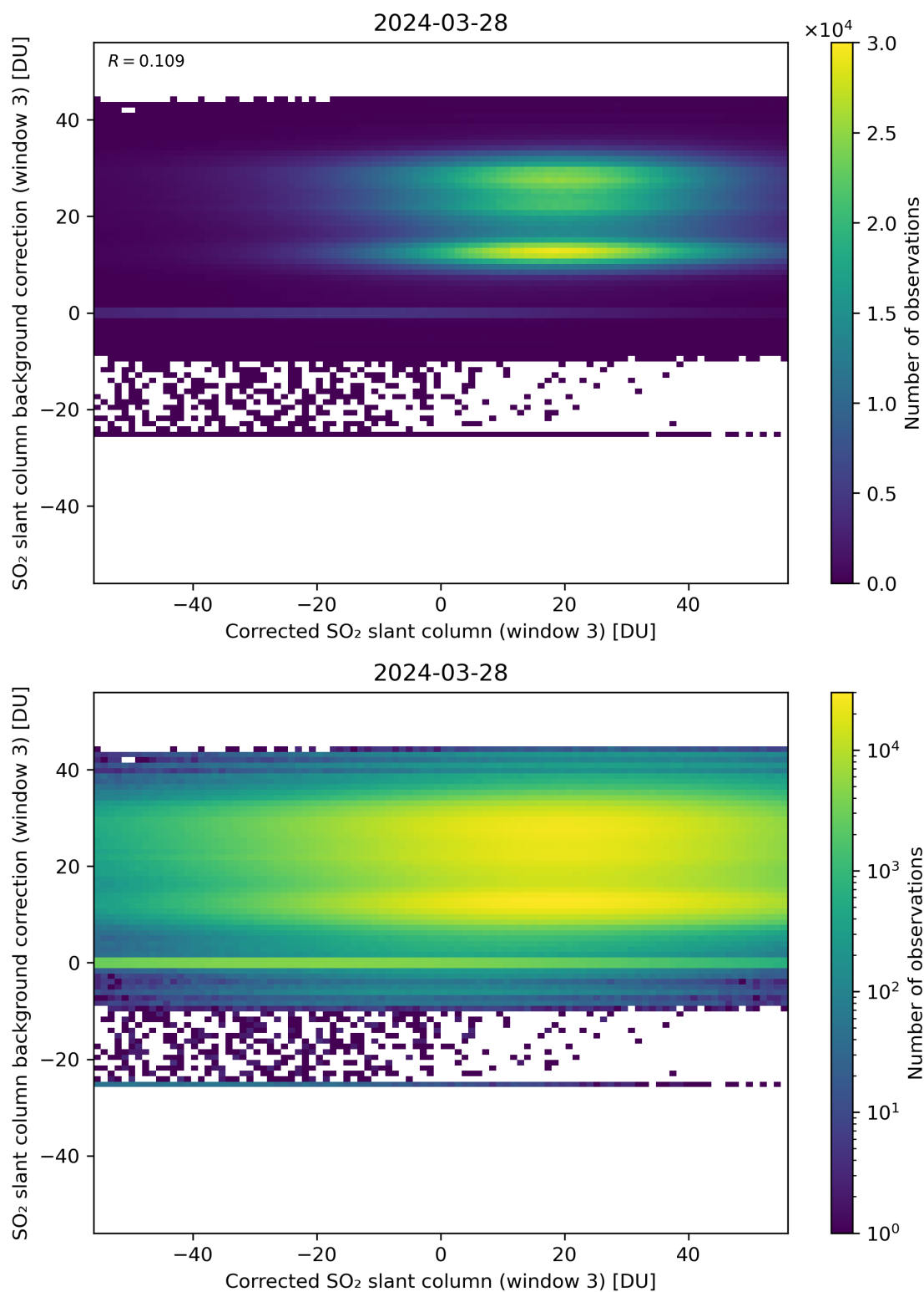
Figure 205: Scatter density plot of “Corrected SO 2 slant column (window 3)” against “SO 2 slant column background correction (window 3)” for 2024-03-27 to 2024-03-29.
