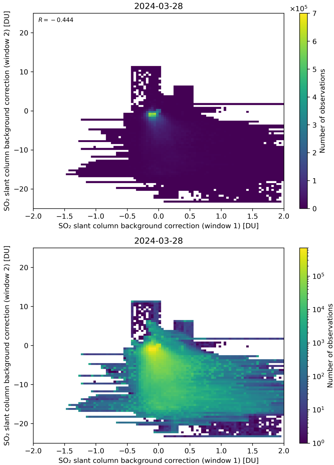
Figure 98: Scatter density plot of “SO 2 slant column background correction (window 1)” against “SO 2 slant column background correction (window 2)” for 2024-03-27 to 2024-03-29.
