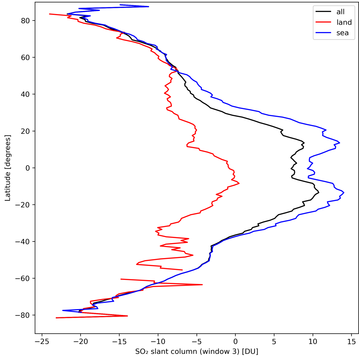
Figure 41: Zonal average of “SO 2 slant column (window 3)” for 2024-03-27 to 2024-03-29.
