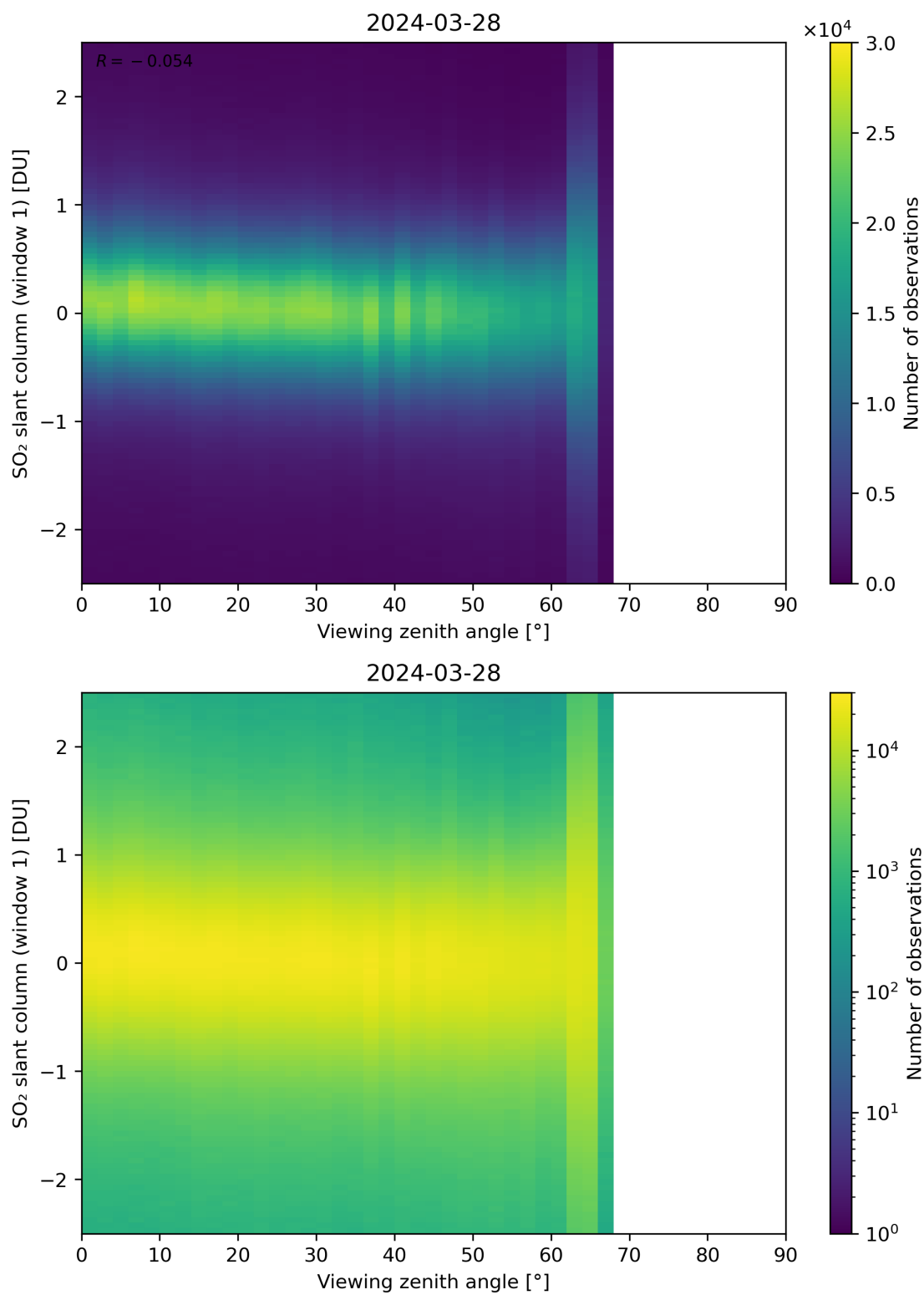
Figure 320: Scatter density plot of “Viewing zenith angle” against “SO 2 slant column (window 1)” for 2024-03-27 to 2024-03-29.
