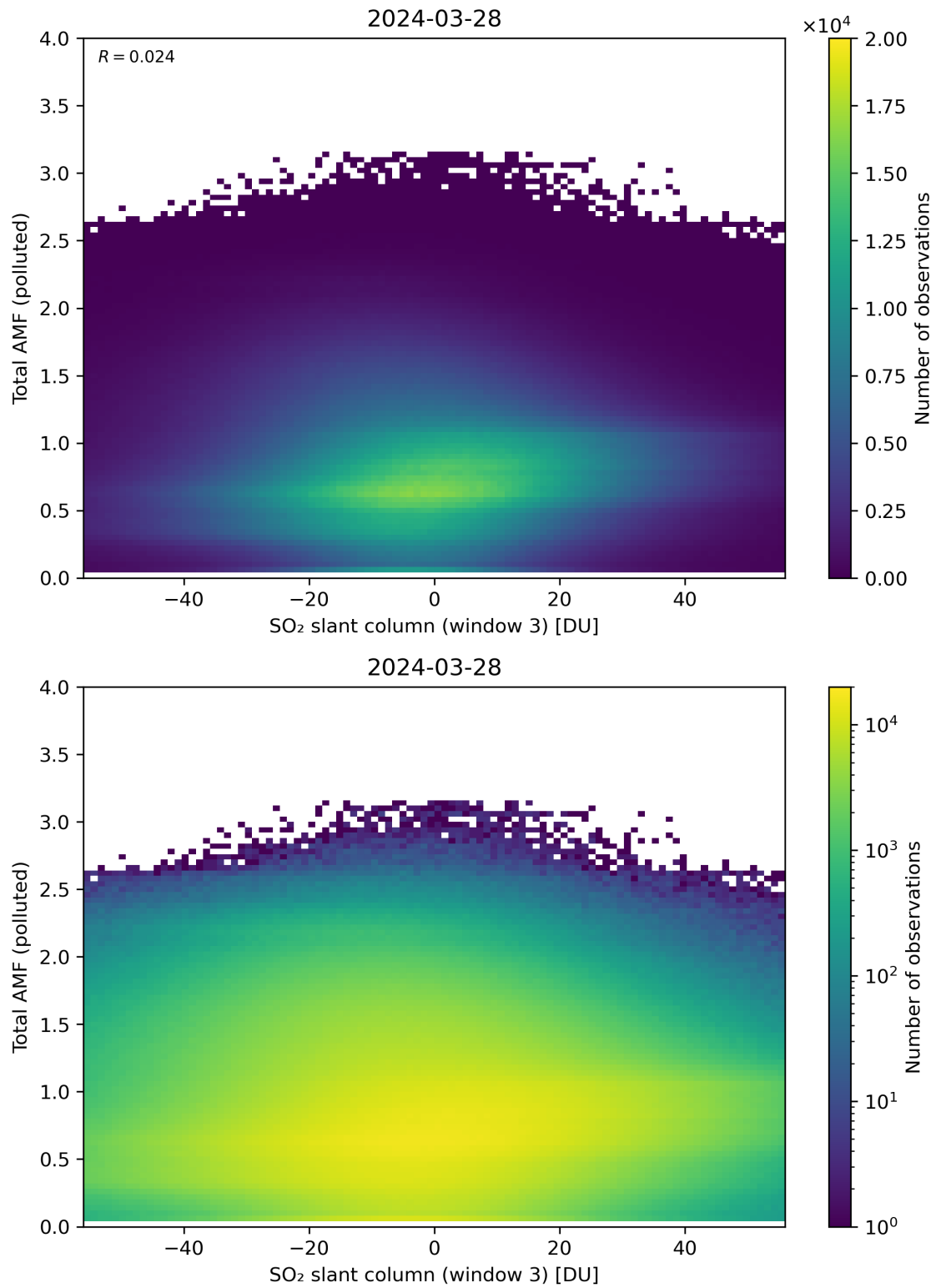
Figure 268: Scatter density plot of “SO 2 slant column (window 3)” against “Total AMF (polluted)” for 2024-03-27 to 2024-03-29.
