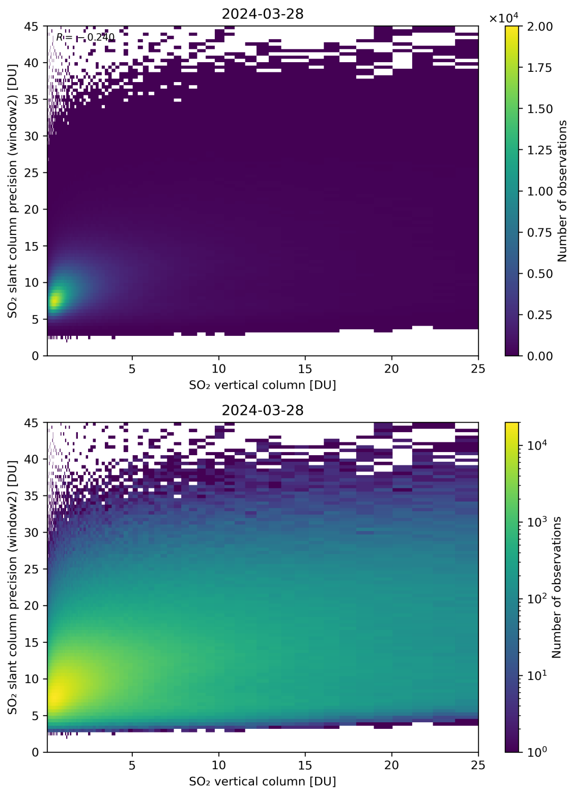
Figure 302: Scatter density plot of “SO 2 vertical column” against “SO 2 slant column precision (window2)” for 2024-03-27 to 2024-03-29.
