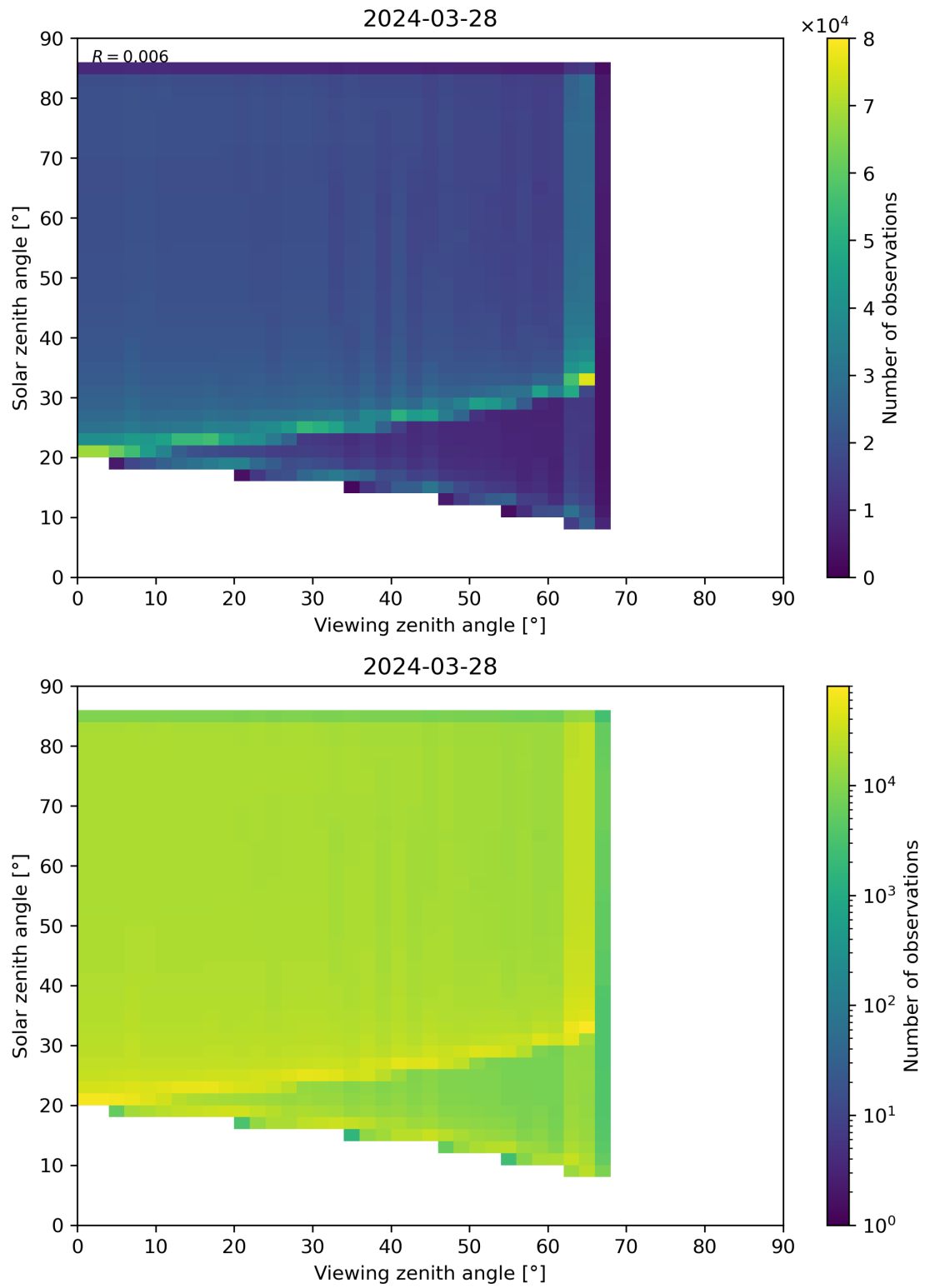
Figure 315: Scatter density plot of “Viewing zenith angle” against “Solar zenith angle” for 2024-03-27 to 2024-03-29.
