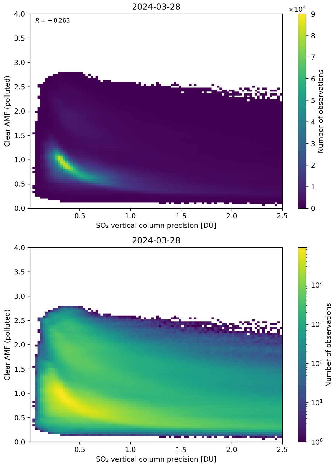
Figure 285: Scatter density plot of “SO 2 vertical column precision” against “Clear AMF (polluted)” for 2024-03-27 to 2024-03-29.
