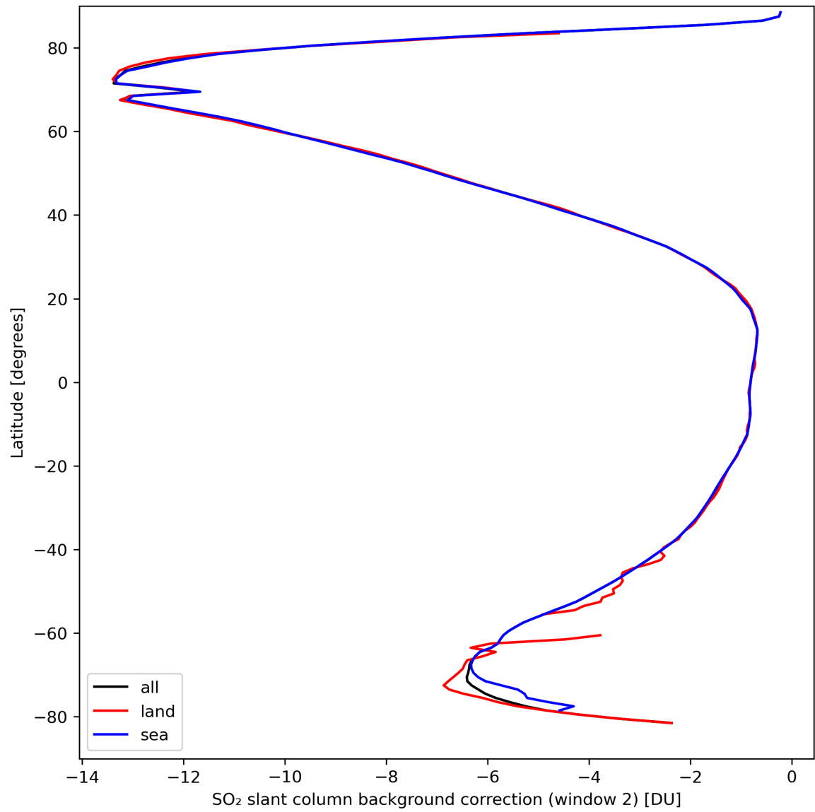
Figure 40: Zonal average of “SO 2 slant column background correction (window 2)” for 2024-03-27 to 2024-03-29.
