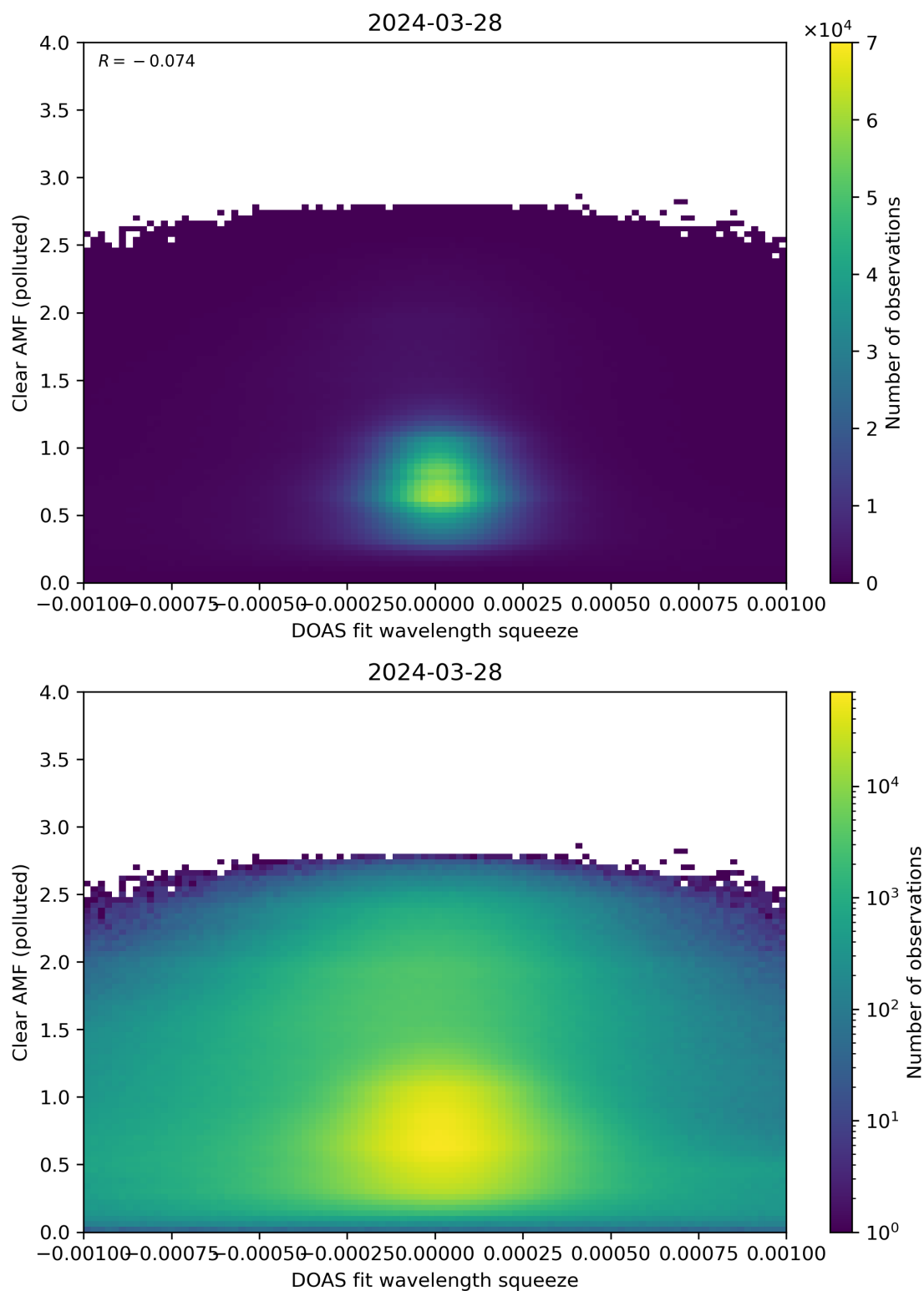
Figure 133: Scatter density plot of “DOAS fit wavelength squeeze” against “Clear AMF (polluted)” for 2024-03-27 to 2024-03-29.
