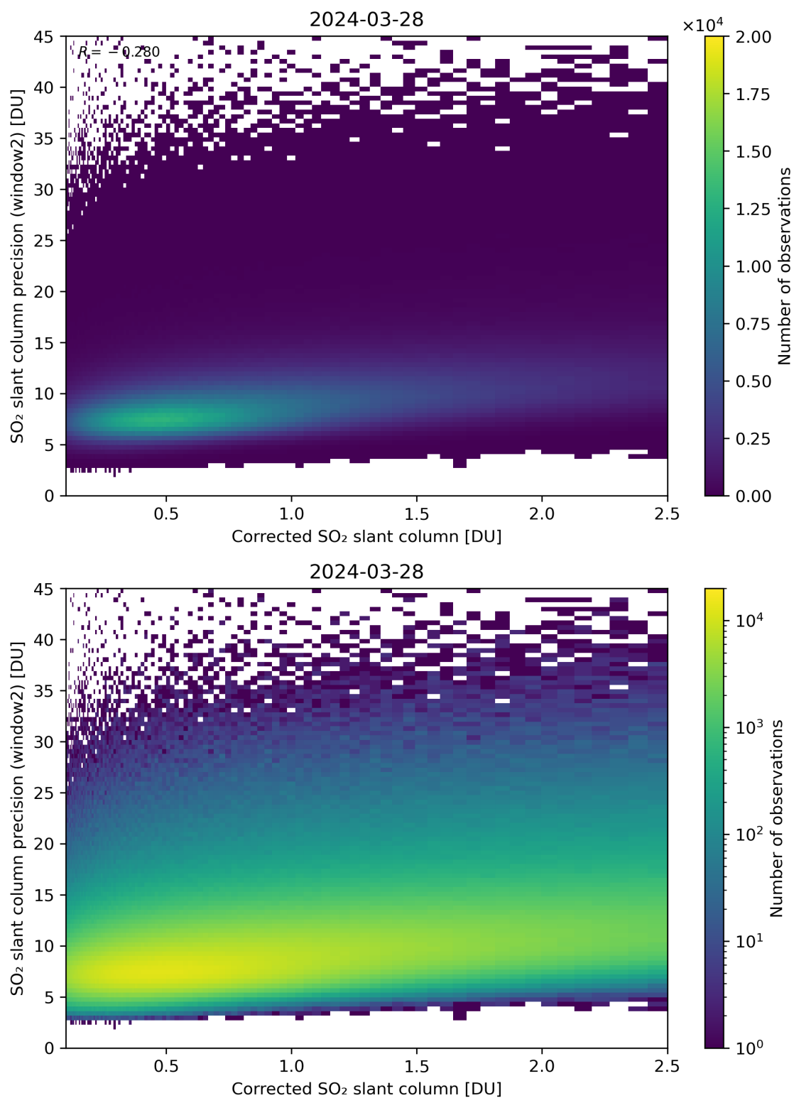
Figure 189: Scatter density plot of “Corrected SO 2 slant column” against “SO 2 slant column precision (window2)” for 2024-03-27 to 2024-03-29.
