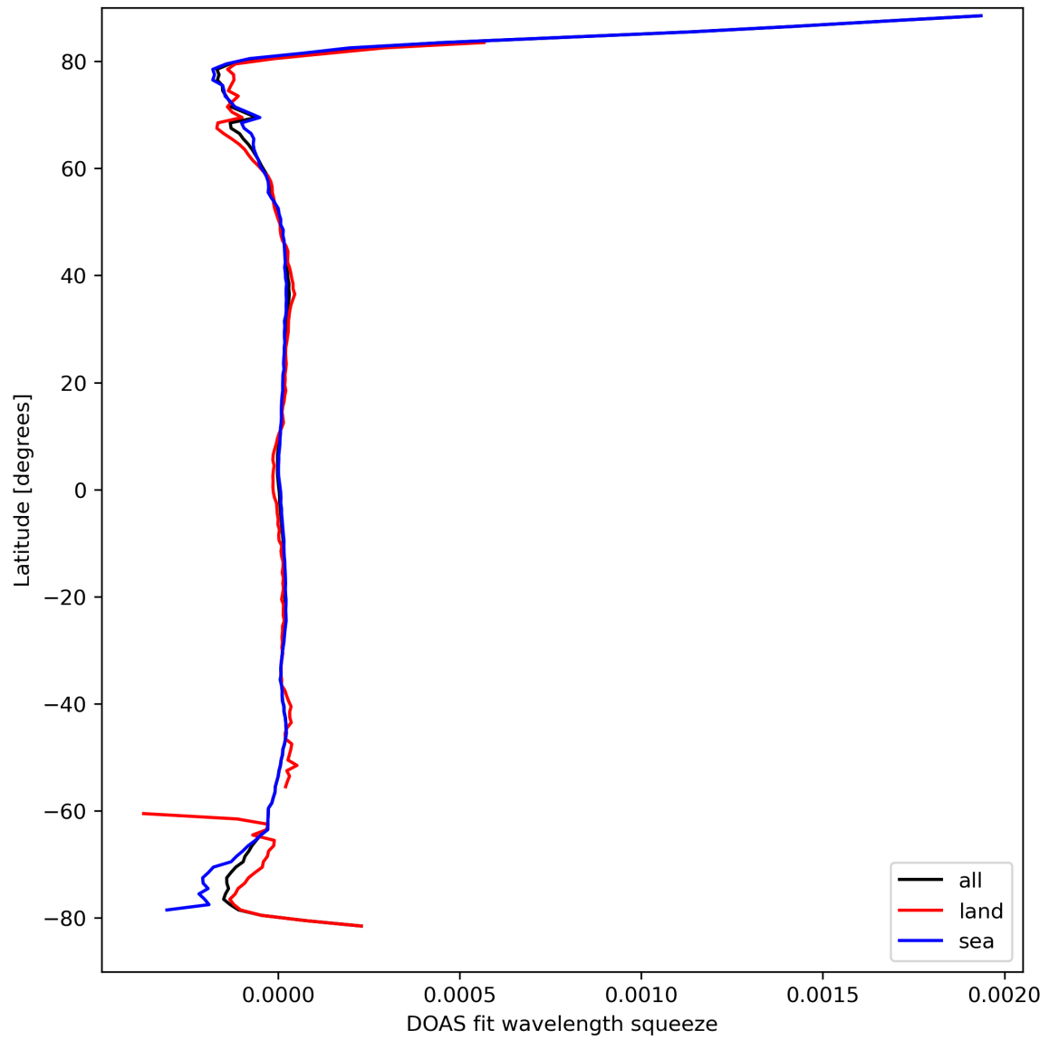
Figure 46: Zonal average of “DOAS fit wavelength squeeze” for 2024-03-27 to 2024-03-29.
