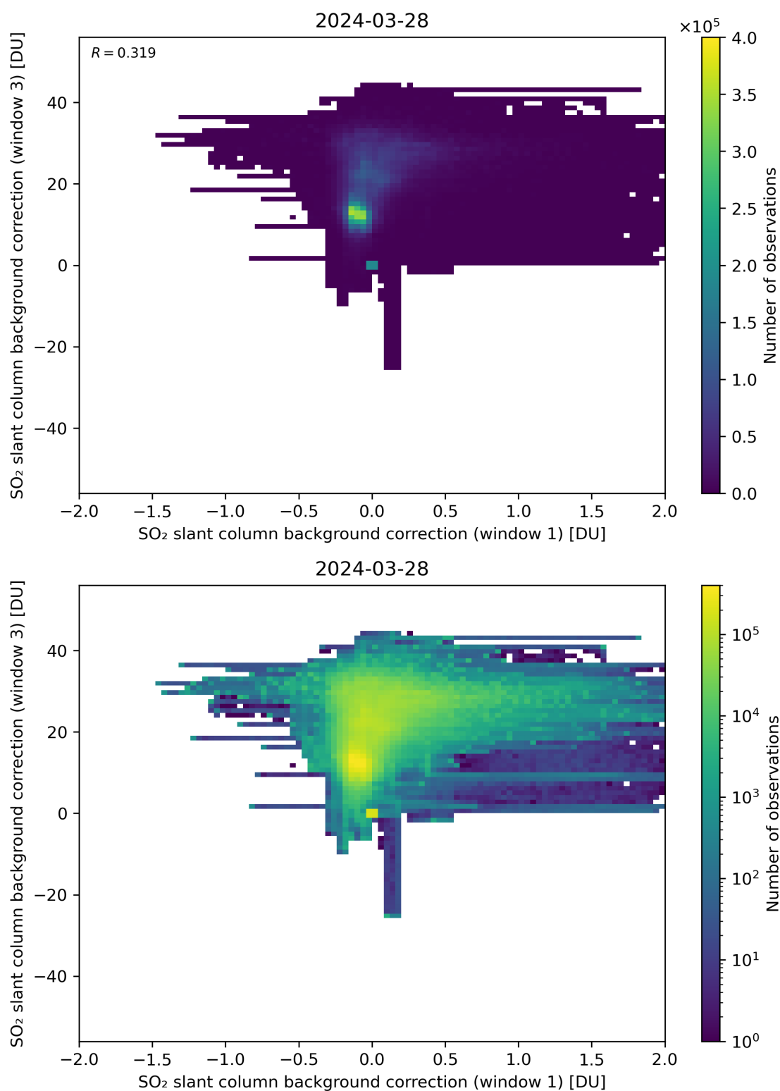
Figure 99: Scatter density plot of “SO 2 slant column background correction (window 1)” against “SO 2 slant column background correction (window 3)” for 2024-03-27 to 2024-03-29.
