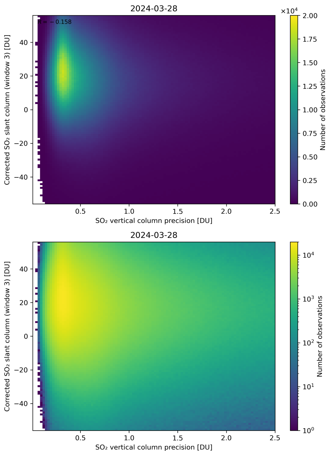
Figure 288: Scatter density plot of “SO 2 vertical column precision” against “Corrected SO 2 slant column (window 3)” for 2024-03-27 to 2024-03-29.
