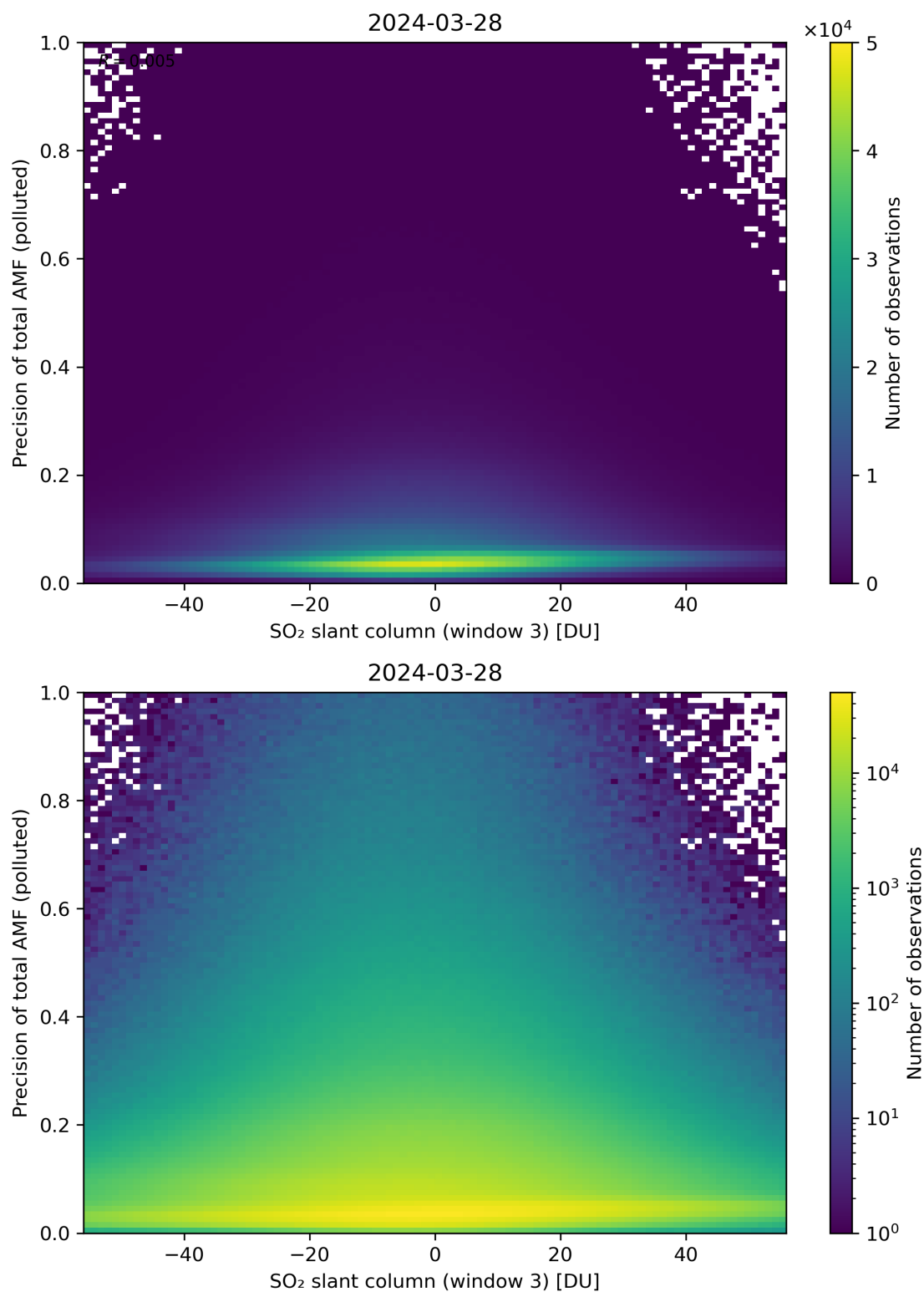
Figure 269: Scatter density plot of “SO 2 slant column (window 3)” against “Precision of total AMF (polluted)” for 2024-03-27 to 2024-03-29.
