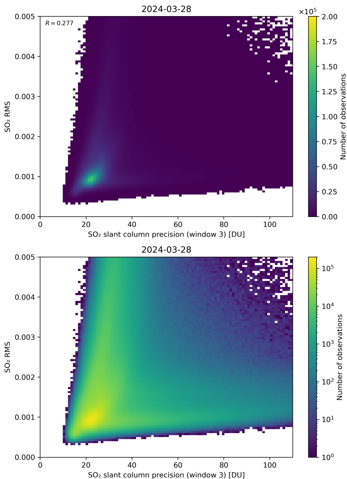
Figure 260: Scatter density plot of “SO 2 slant column precision (window 3)” against “SO 2 RMS” for 2024-03-27 to 2024-03-29.
