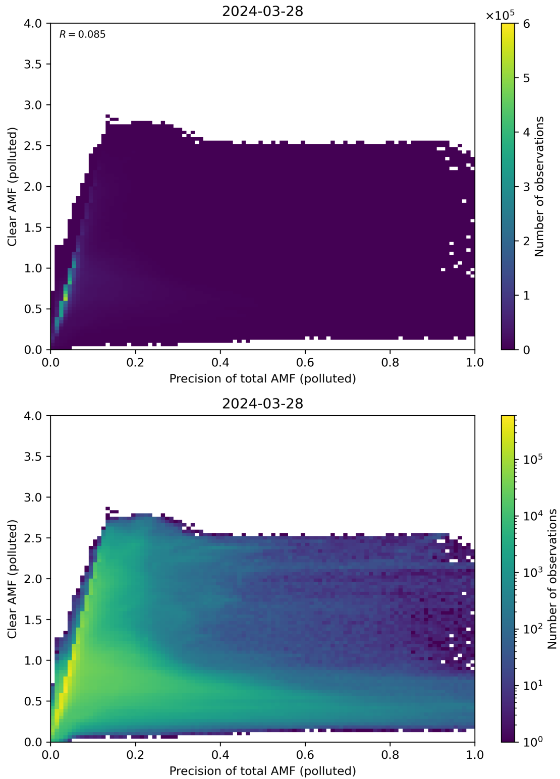
Figure 270: Scatter density plot of “Precision of total AMF (polluted)” against “Clear AMF (polluted)” for 2024-03-27 to 2024-03-29.
