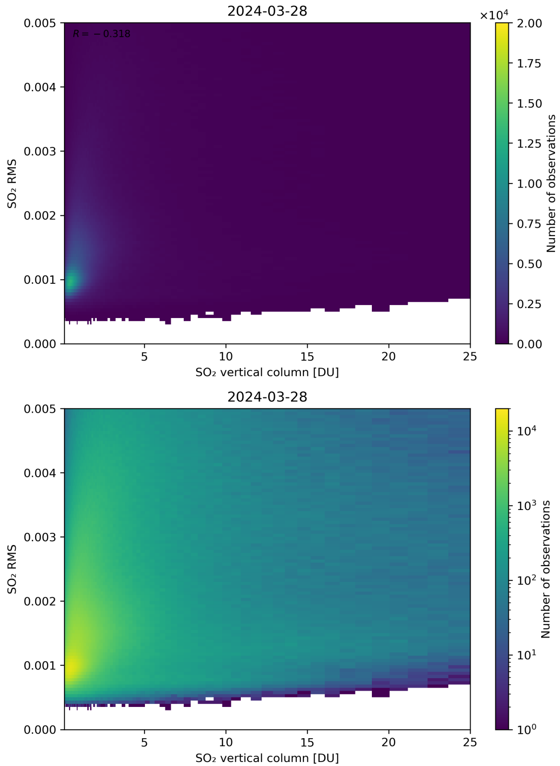
Figure 278: Scatter density plot of “SO 2 vertical column” against “SO 2 RMS” for 2024-03-27 to 2024-03-29.
