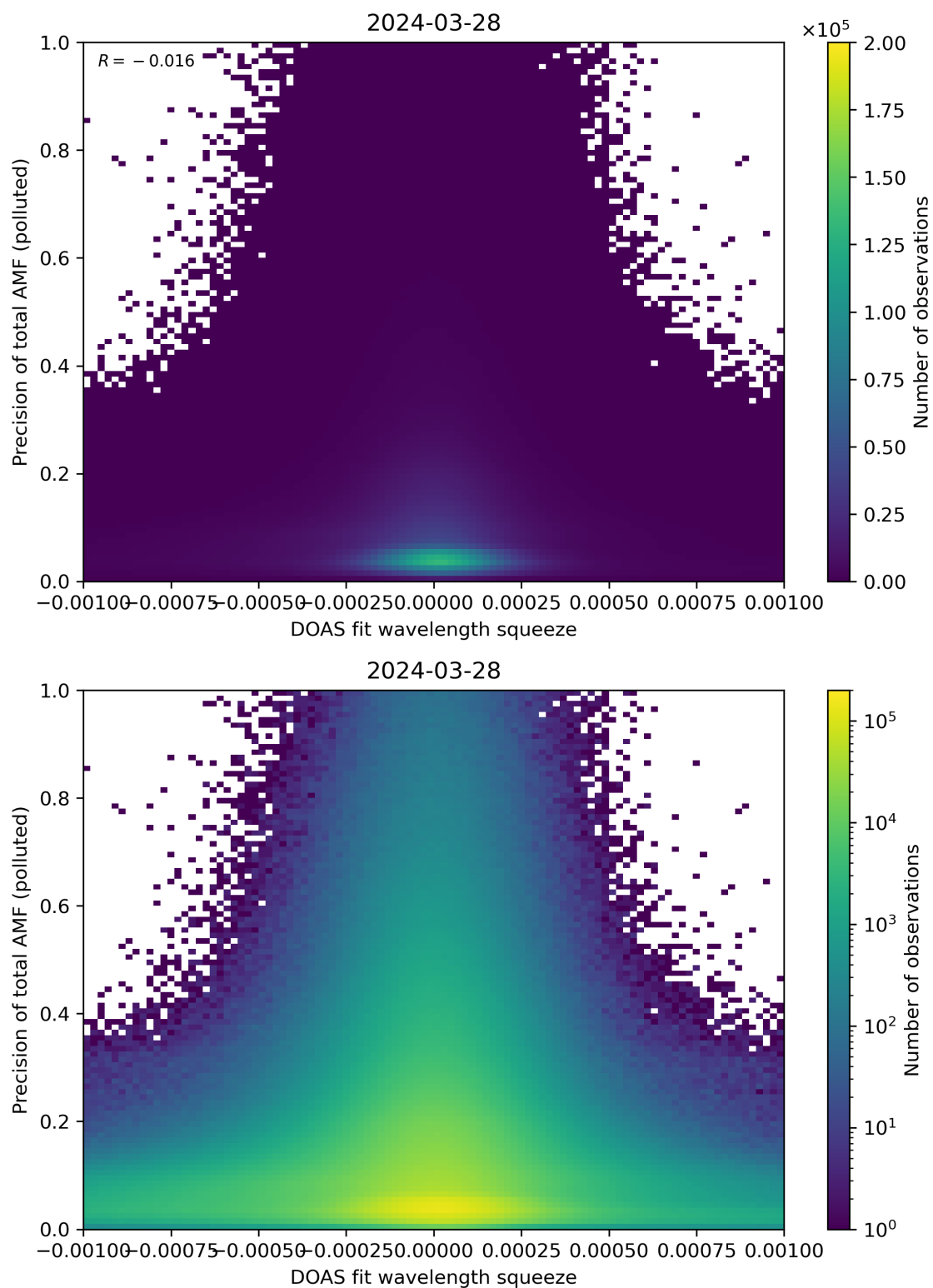
Figure 135: Scatter density plot of “DOAS fit wavelength squeeze” against “Precision of total AMF (polluted)” for 2024-03-27 to 2024-03-29.
