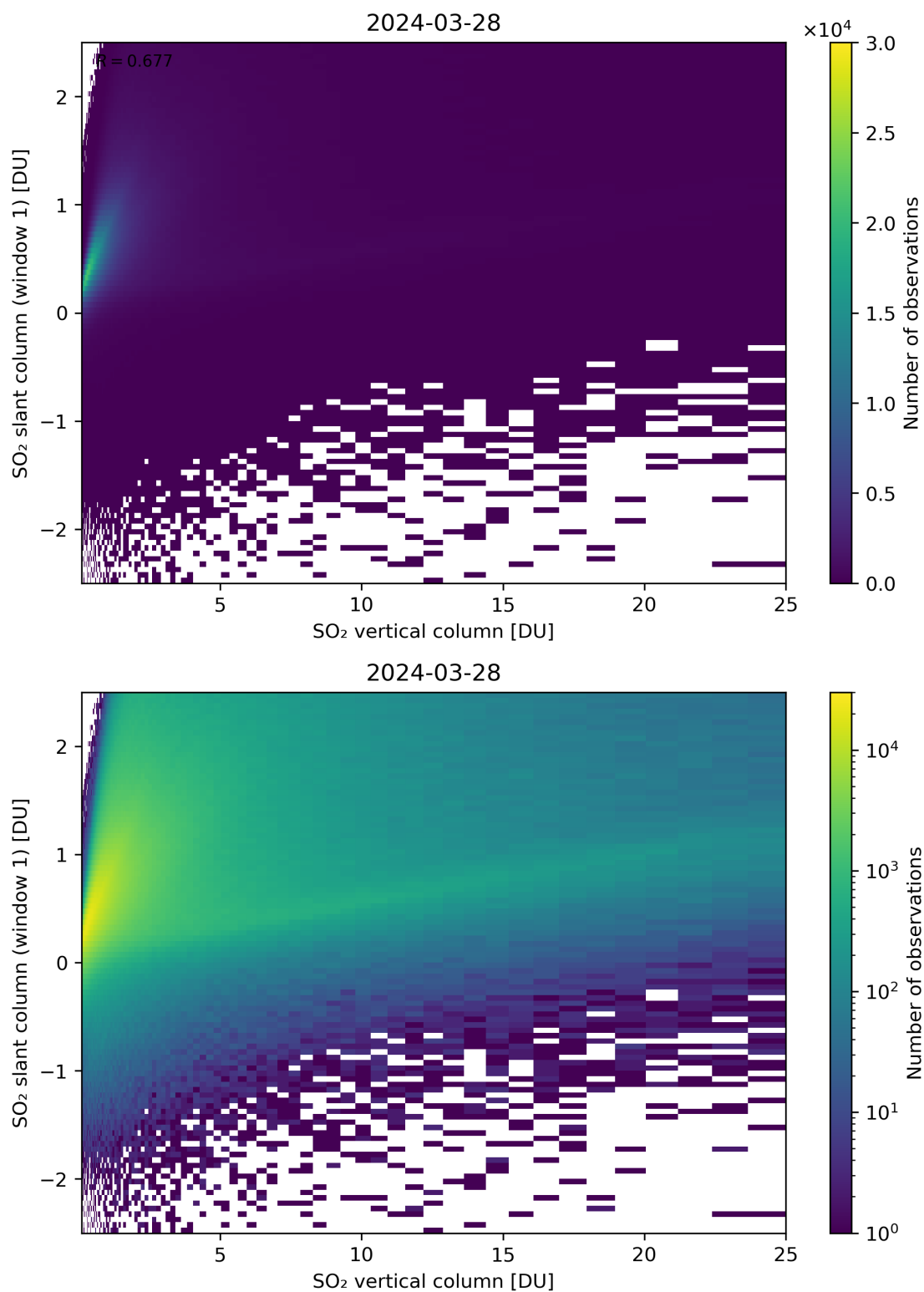
Figure 300: Scatter density plot of “SO 2 vertical column” against “SO 2 slant column (window 1)” for 2024-03-27 to 2024-03-29.
