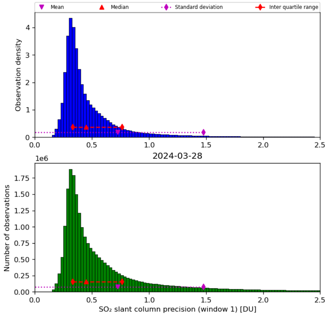
Figure 57: Histogram of “SO 2 slant column precision (window 1)” for 2024-03-27 to 2024-03-29
