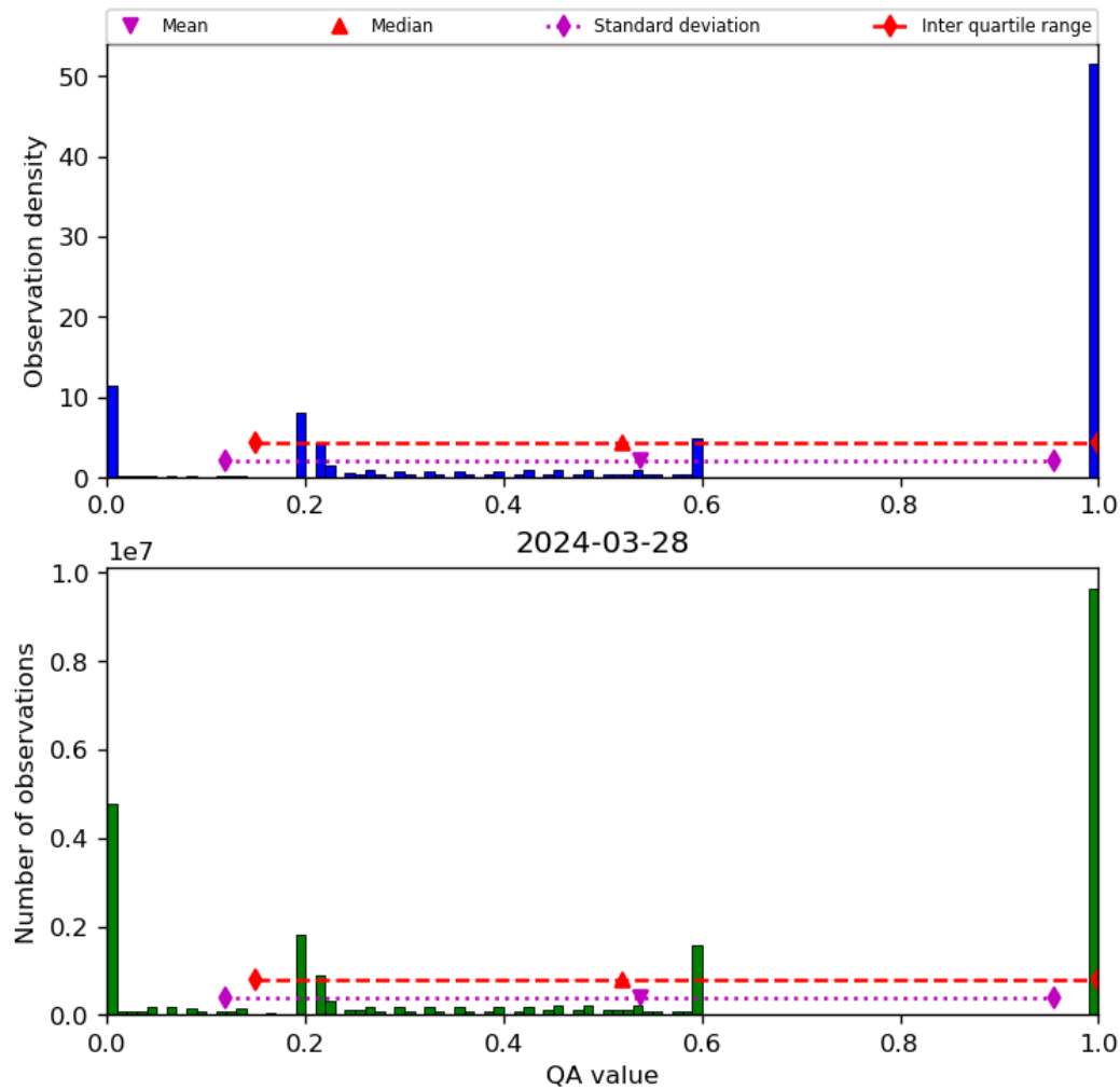
Figure 52: Histogram of “QA value” for 2024-03-27 to 2024-03-29
