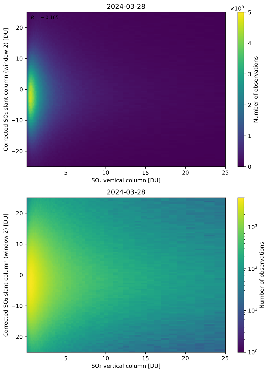
Figure 298: Scatter density plot of “SO 2 vertical column” against “Corrected SO 2 slant column (window 2)” for 2024-03-27 to 2024-03-29.
