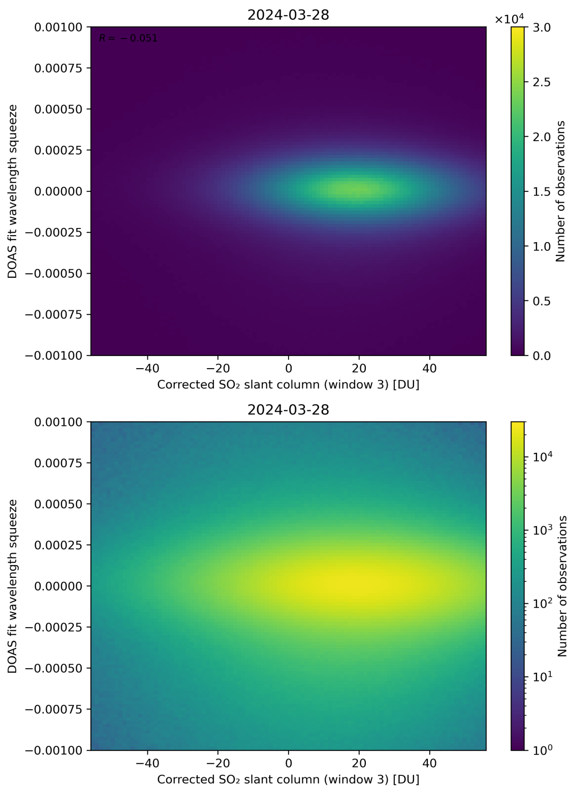
Figure 207: Scatter density plot of “Corrected SO 2 slant column (window 3)” against “DOAS fit wavelength squeeze” for 2024-03-27 to 2024-03-29.
