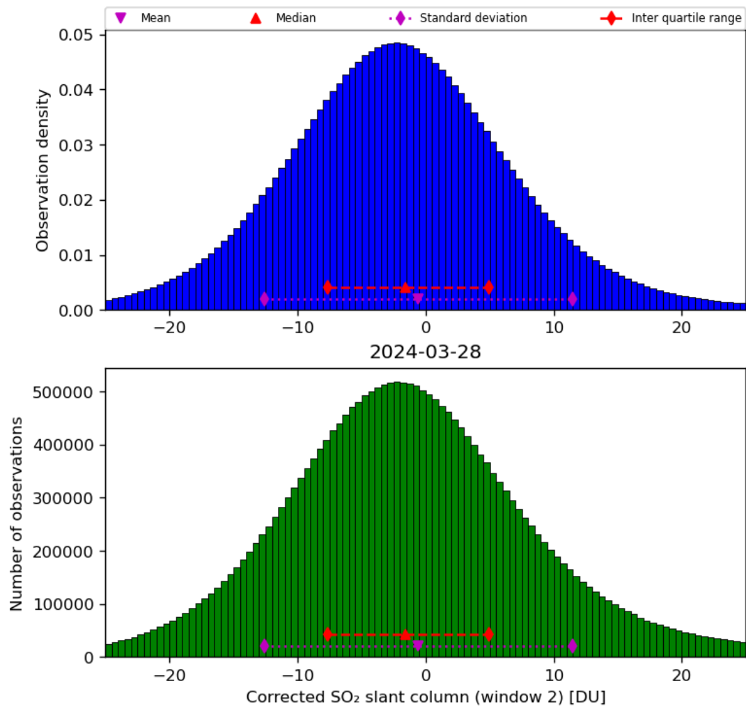
Figure 62: Histogram of “Corrected SO 2 slant column (window 2)” for 2024-03-27 to 2024-03-29
