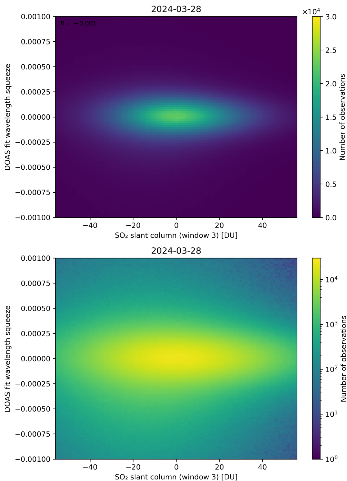
Figure 255: Scatter density plot of “SO 2 slant column (window 3)” against “DOAS fit wavelength squeeze” for 2024-03-27 to 2024-03-29.
