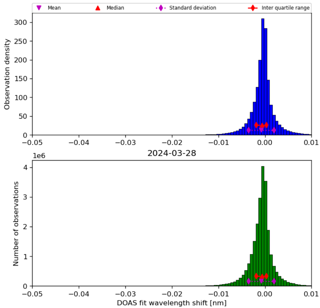
Figure 68: Histogram of “DOAS fit wavelength shift” for 2024-03-27 to 2024-03-29
