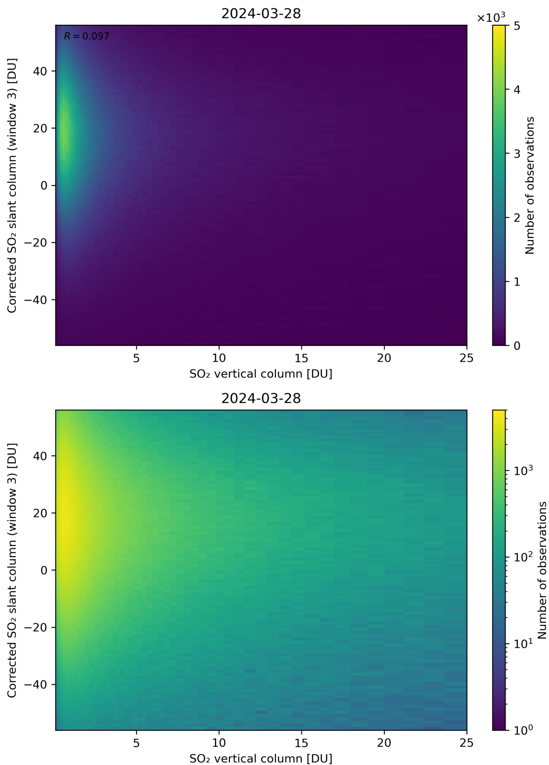
Figure 299: Scatter density plot of “SO 2 vertical column” against “Corrected SO 2 slant column (window 3)” for 2024-03-27 to 2024-03-29.
