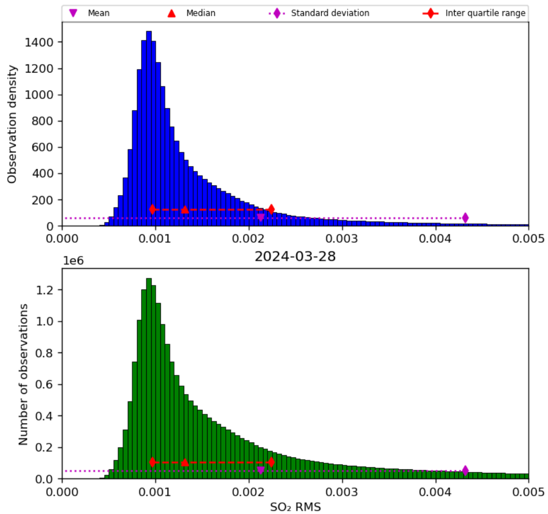
Figure 70: Histogram of “SO 2 RMS” for 2024-03-27 to 2024-03-29
