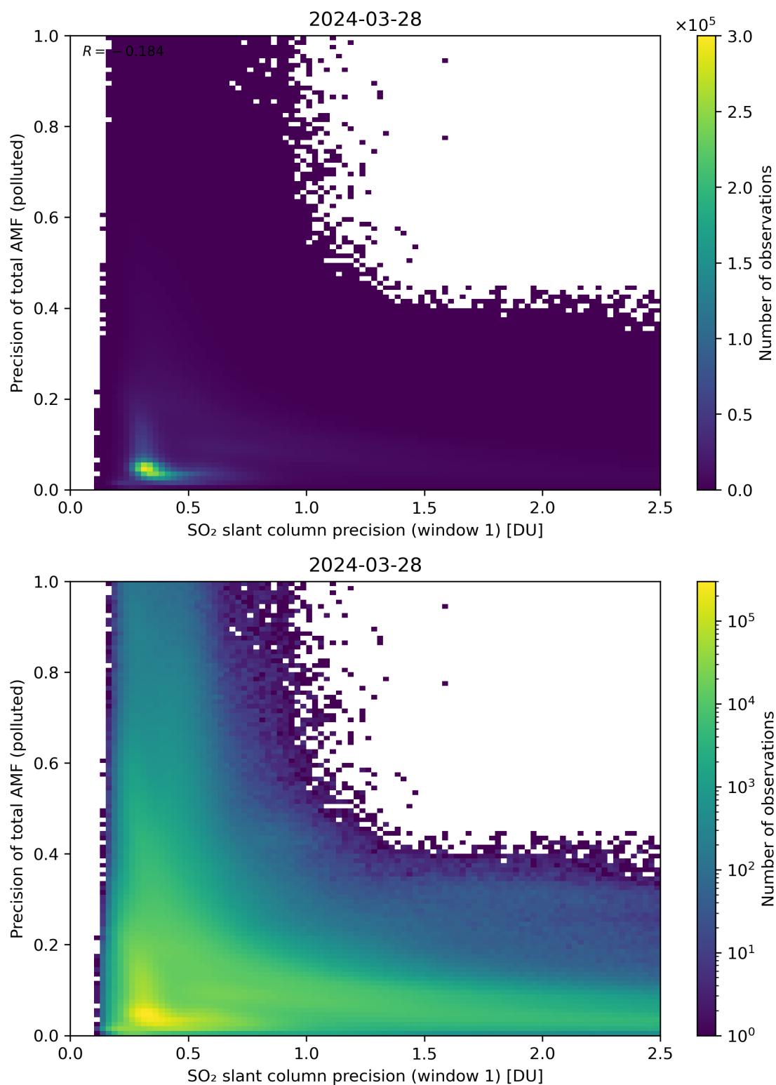
Figure 231: Scatter density plot of “SO 2 slant column precision (window 1)” against “Precision of total AMF (polluted)” for 2024-03-27 to 2024-03-29.
