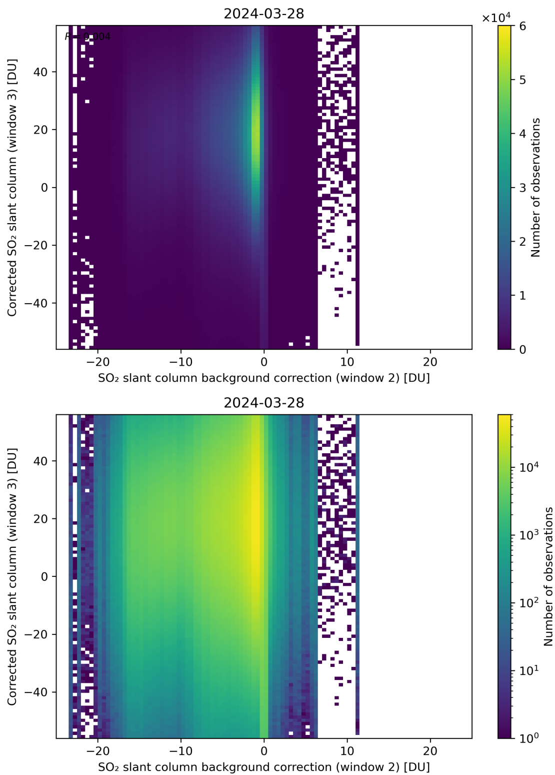
Figure 116: Scatter density plot of “SO 2 slant column background correction (window 2)” against “Corrected SO 2 slant column (window 3)” for 2024-03-27 to 2024-03-29.
