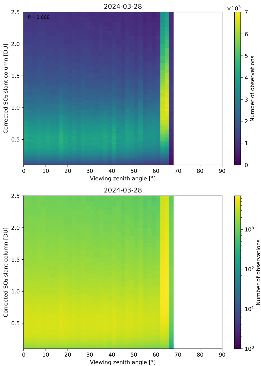
Figure 317: Scatter density plot of “Viewing zenith angle” against “Corrected SO 2 slant column” for 2024-03-27 to 2024-03-29.
