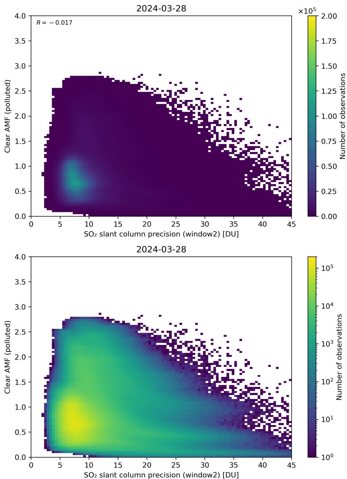
Figure 246: Scatter density plot of “SO 2 slant column precision (window2)” against “Clear AMF (polluted)” for 2024-03-27 to 2024-03-29.
