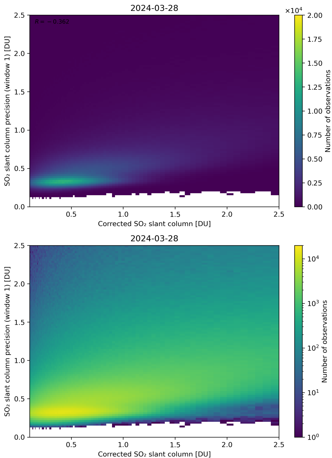
Figure 188: Scatter density plot of “Corrected SO 2 slant column” against “SO 2 slant column precision (window 1)” for 2024-03-27 to 2024-03-29.
