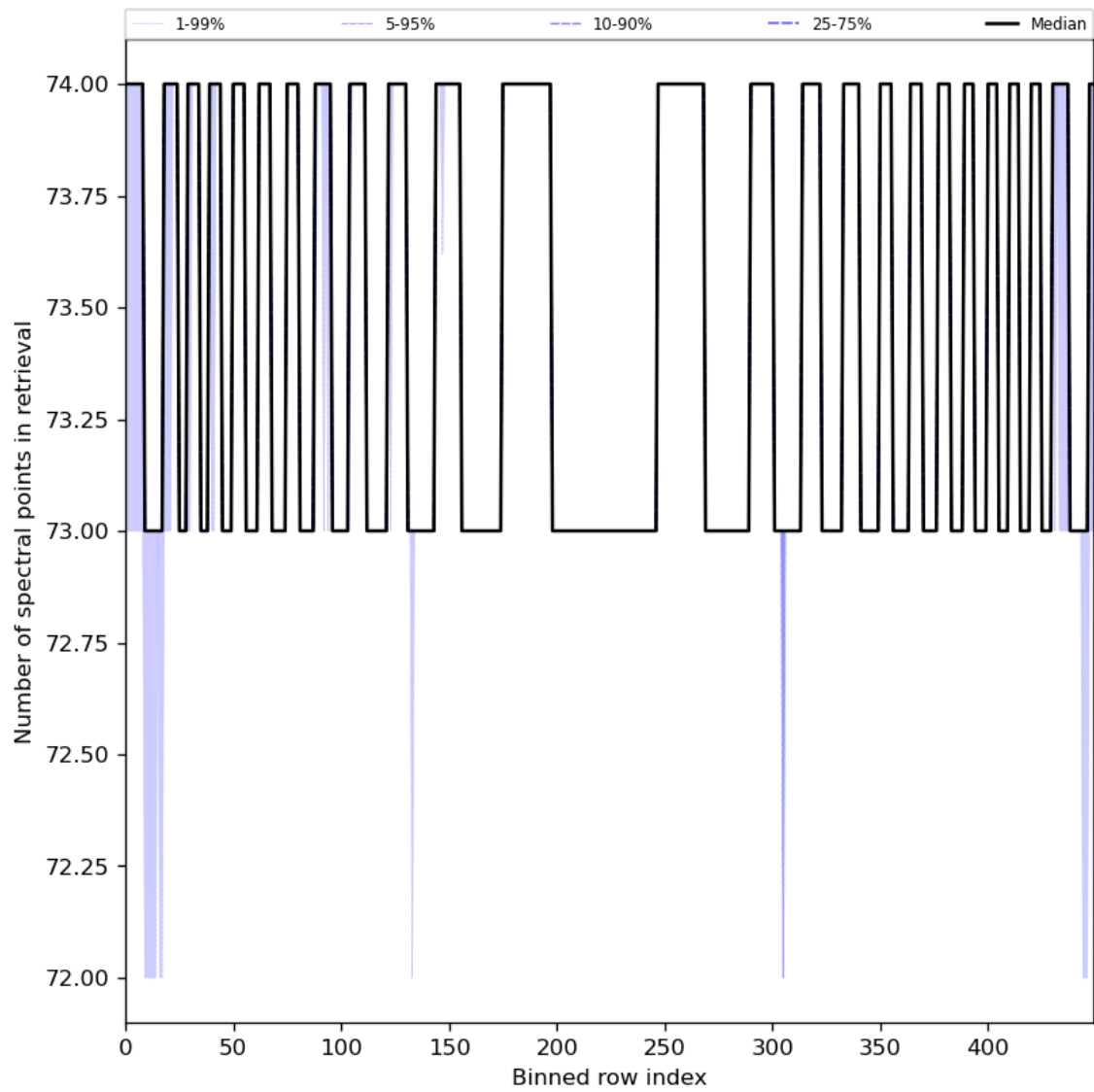
Figure 97: Along track statistics of “Number of spectral points in retrieval” for 2024-03-27 to 2024-03-29
