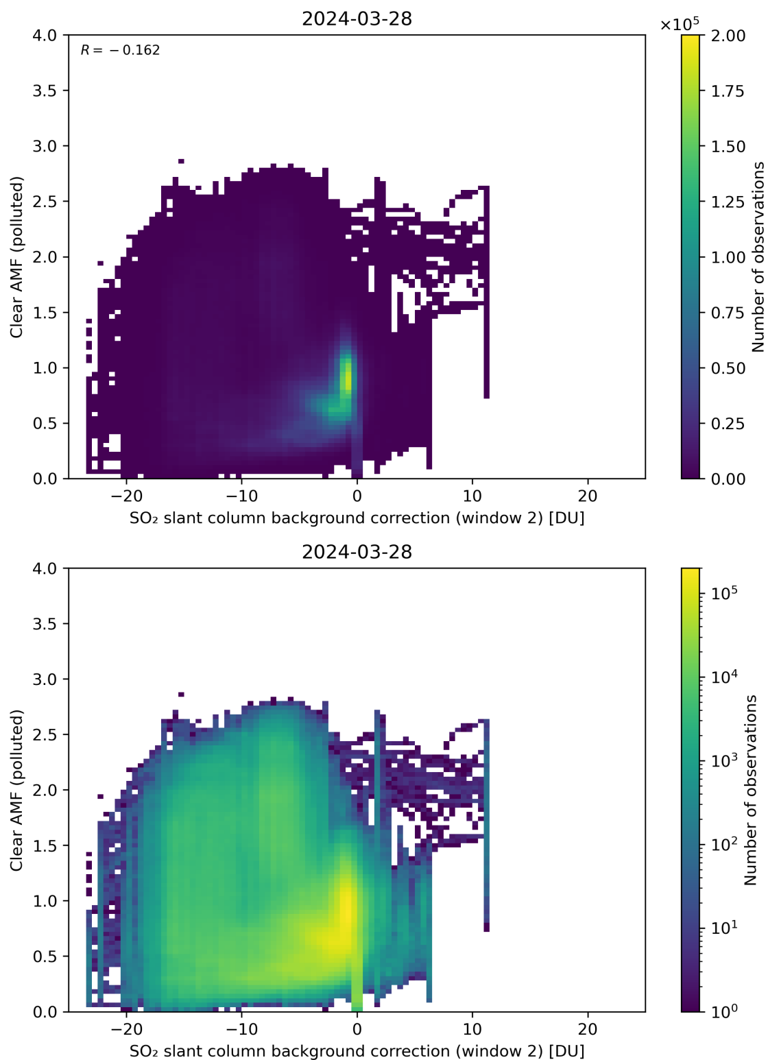
Figure 115: Scatter density plot of “SO 2 slant column background correction (window 2)” against “Clear AMF (polluted)” for 2024-03-27 to 2024-03-29.
