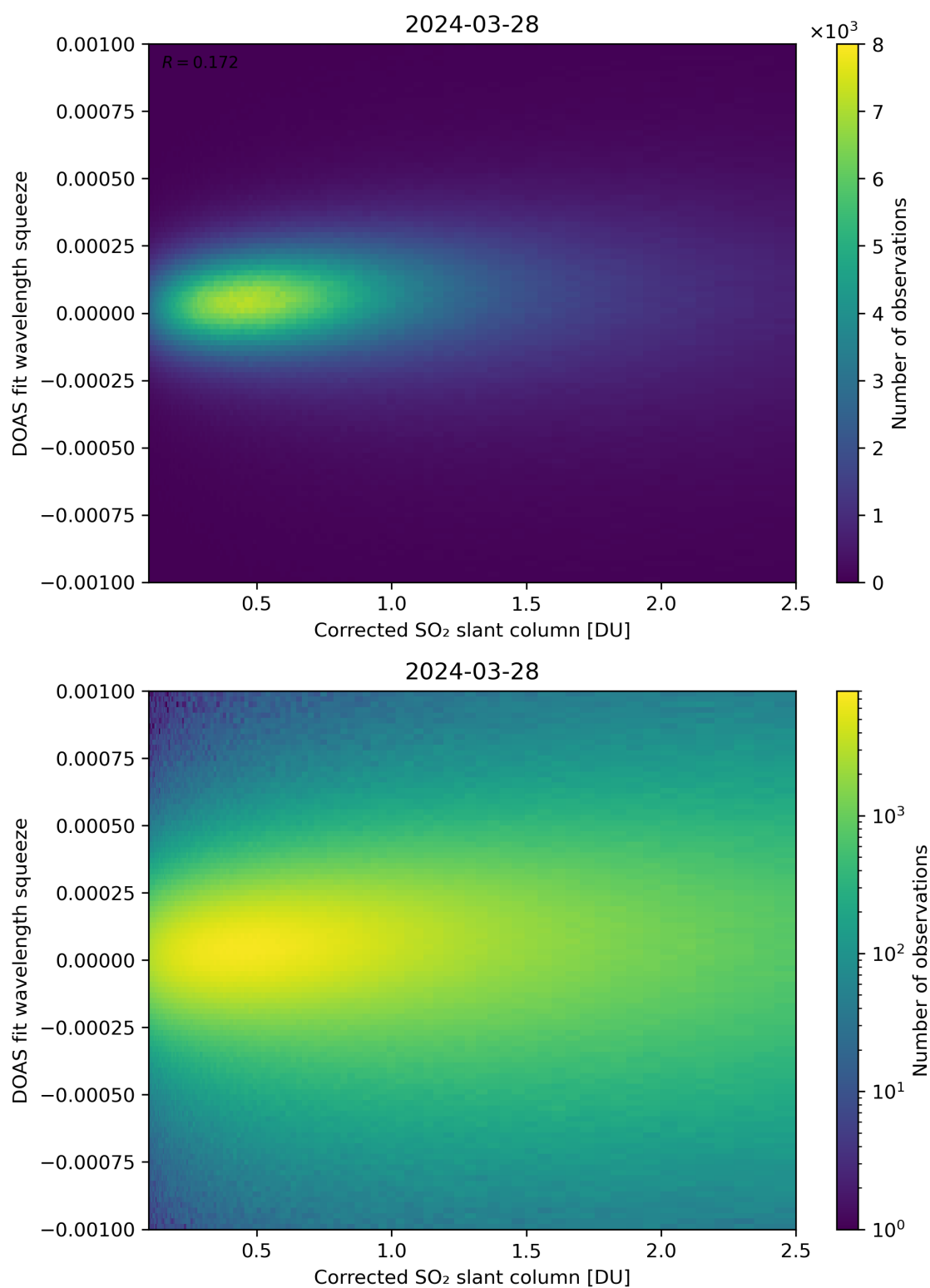
Figure 182: Scatter density plot of “Corrected SO 2 slant column” against “DOAS fit wavelength squeeze” for 2024-03-27 to 2024-03-29.
