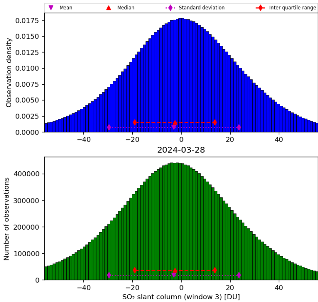
Figure 64: Histogram of “SO 2 slant column (window 3)” for 2024-03-27 to 2024-03-29
