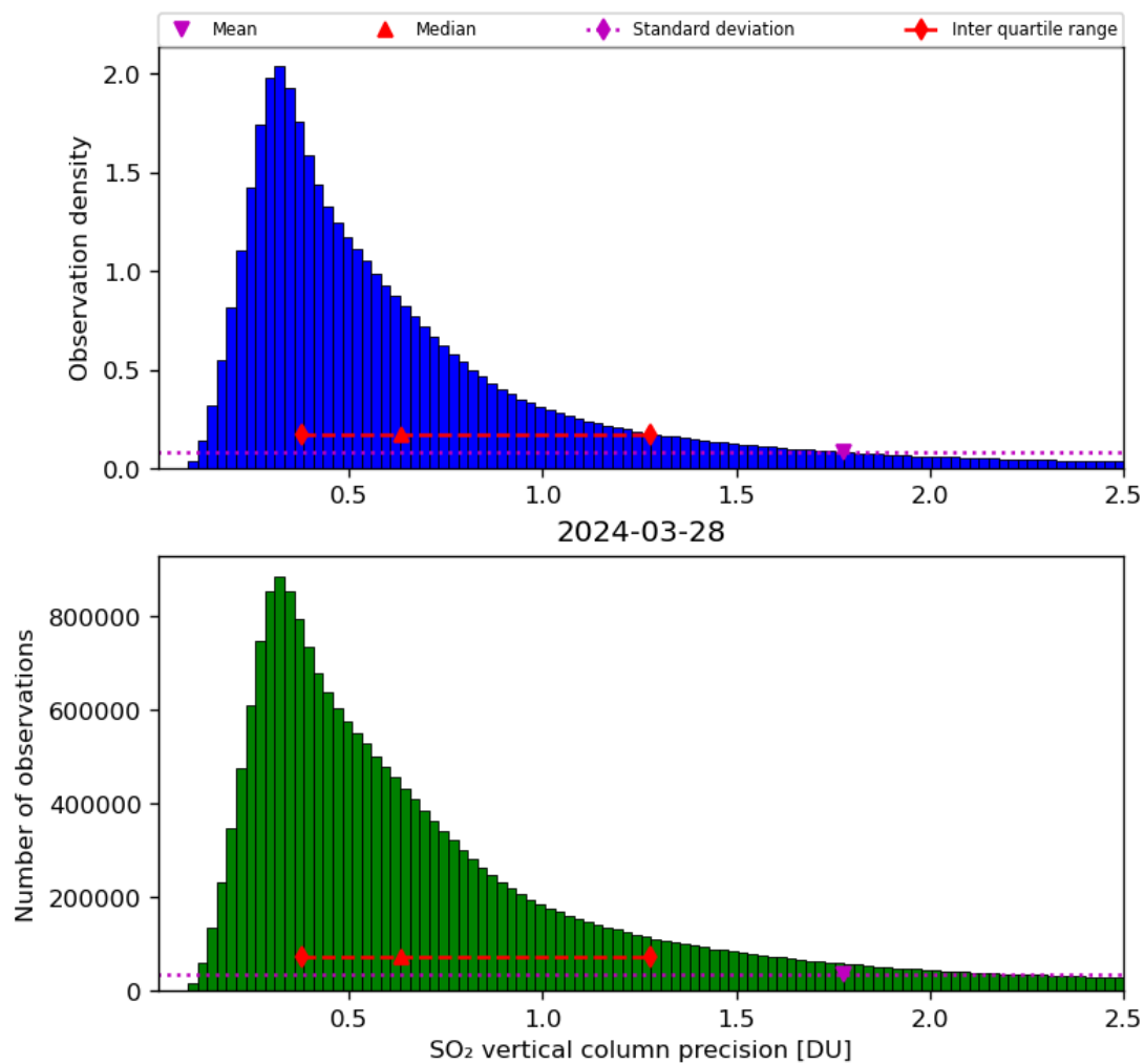
Figure 54: Histogram of “SO 2 vertical column precision” for 2024-03-27 to 2024-03-29
