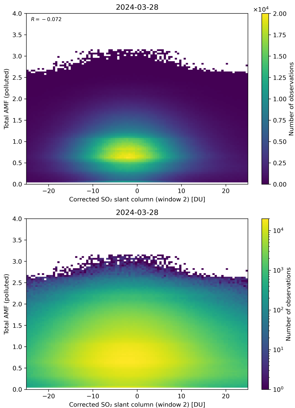
Figure 203: Scatter density plot of “Corrected SO 2 slant column (window 2)” against “Total AMF (polluted)” for 2024-03-27 to 2024-03-29.
