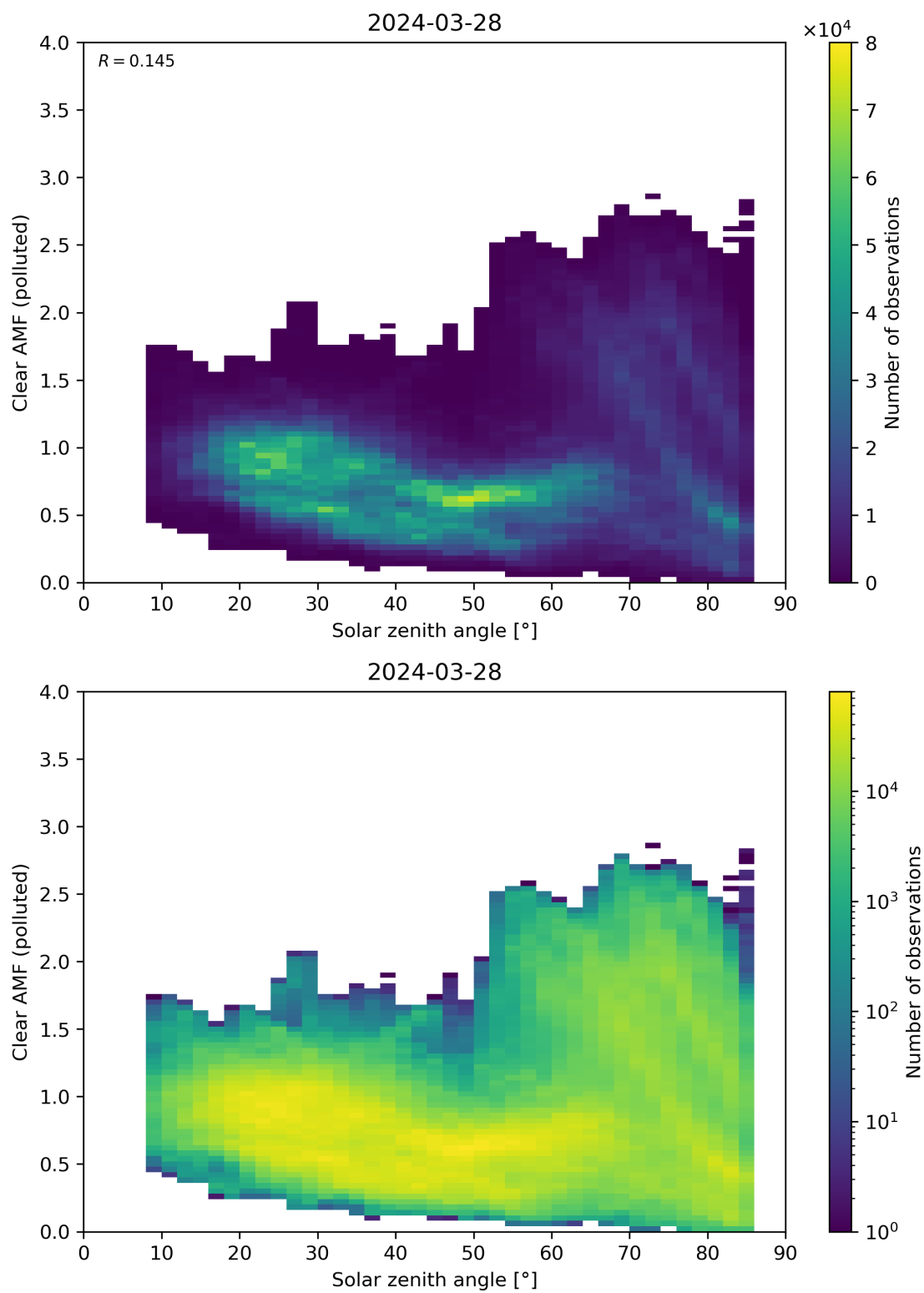
Figure 165: Scatter density plot of “Solar zenith angle” against “Clear AMF (polluted)” for 2024-03-27 to 2024-03-29.
