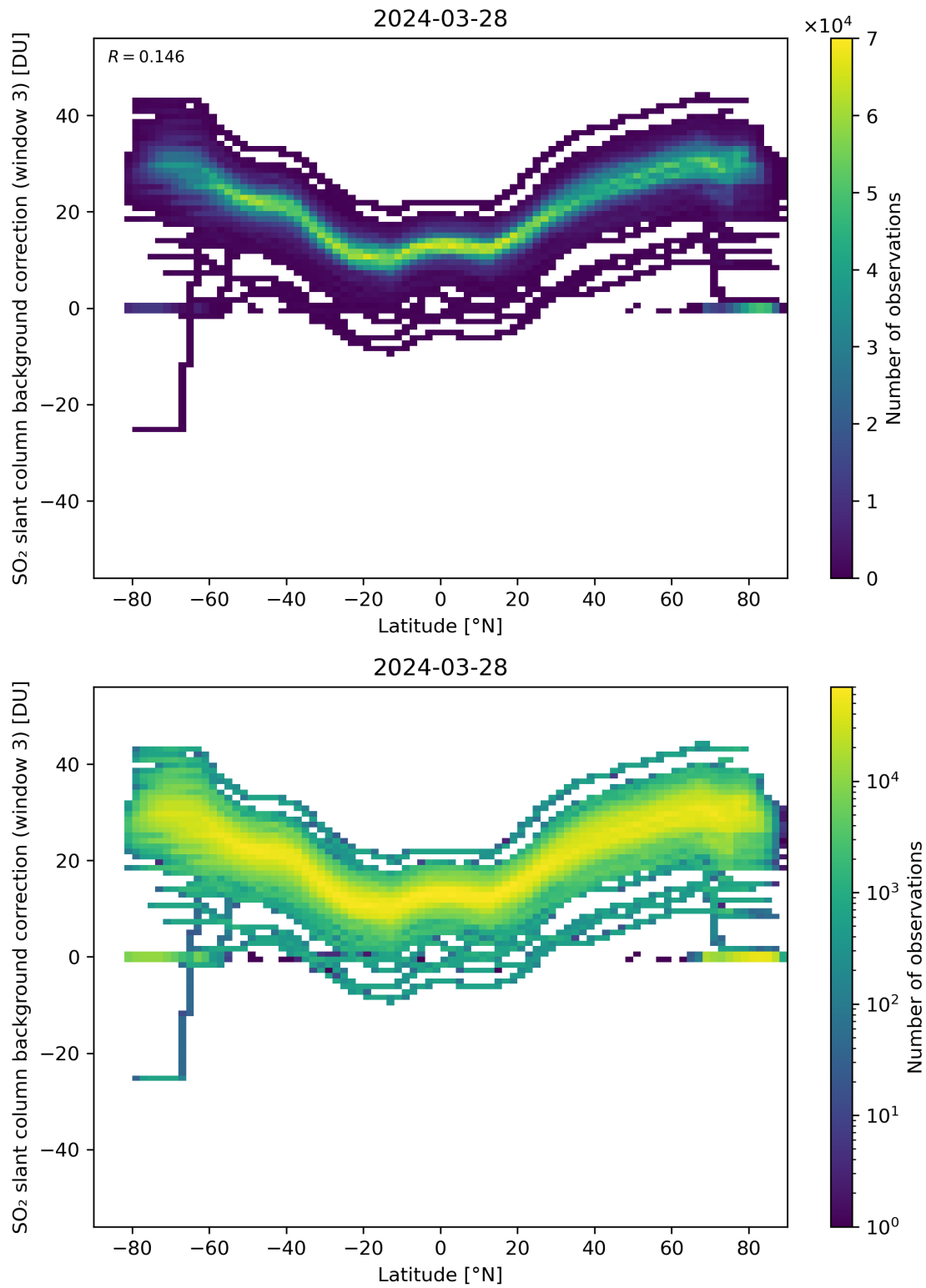
Figure 141: Scatter density plot of “Latitude” against “SO 2 slant column background correction (window 3)” for 2024-03-27 to 2024-03-29.
