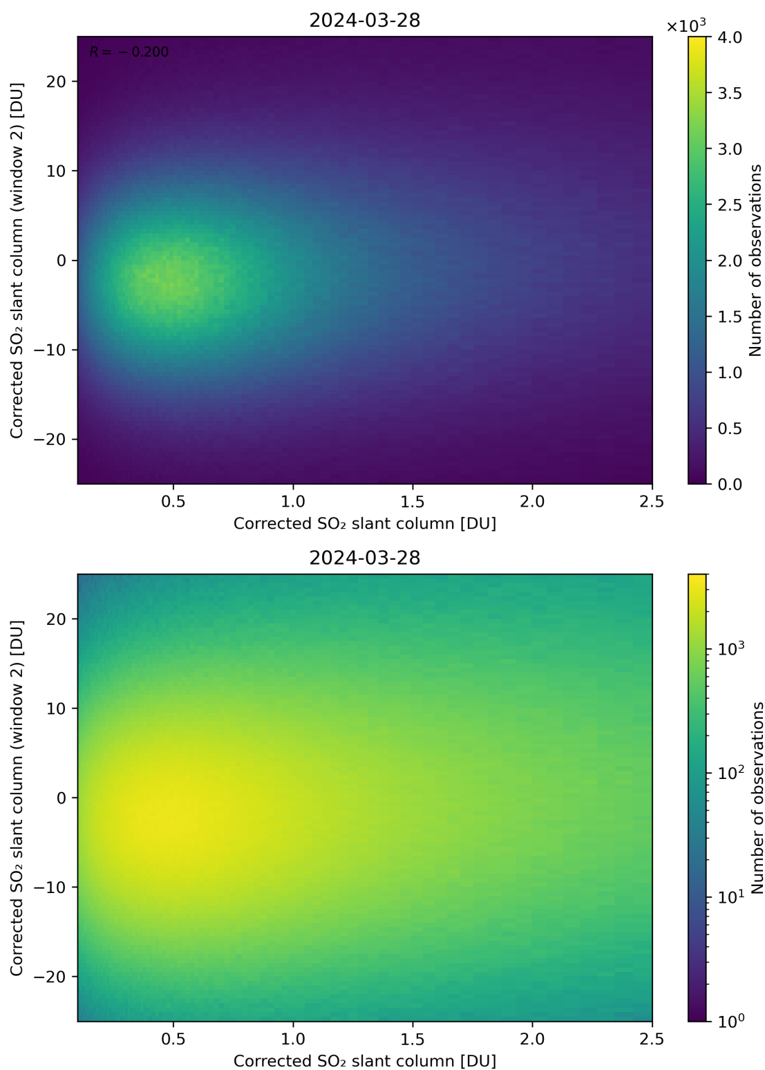
Figure 185: Scatter density plot of “Corrected SO 2 slant column” against “Corrected SO 2 slant column (window 2)” for 2024-03-27 to 2024-03-29.
