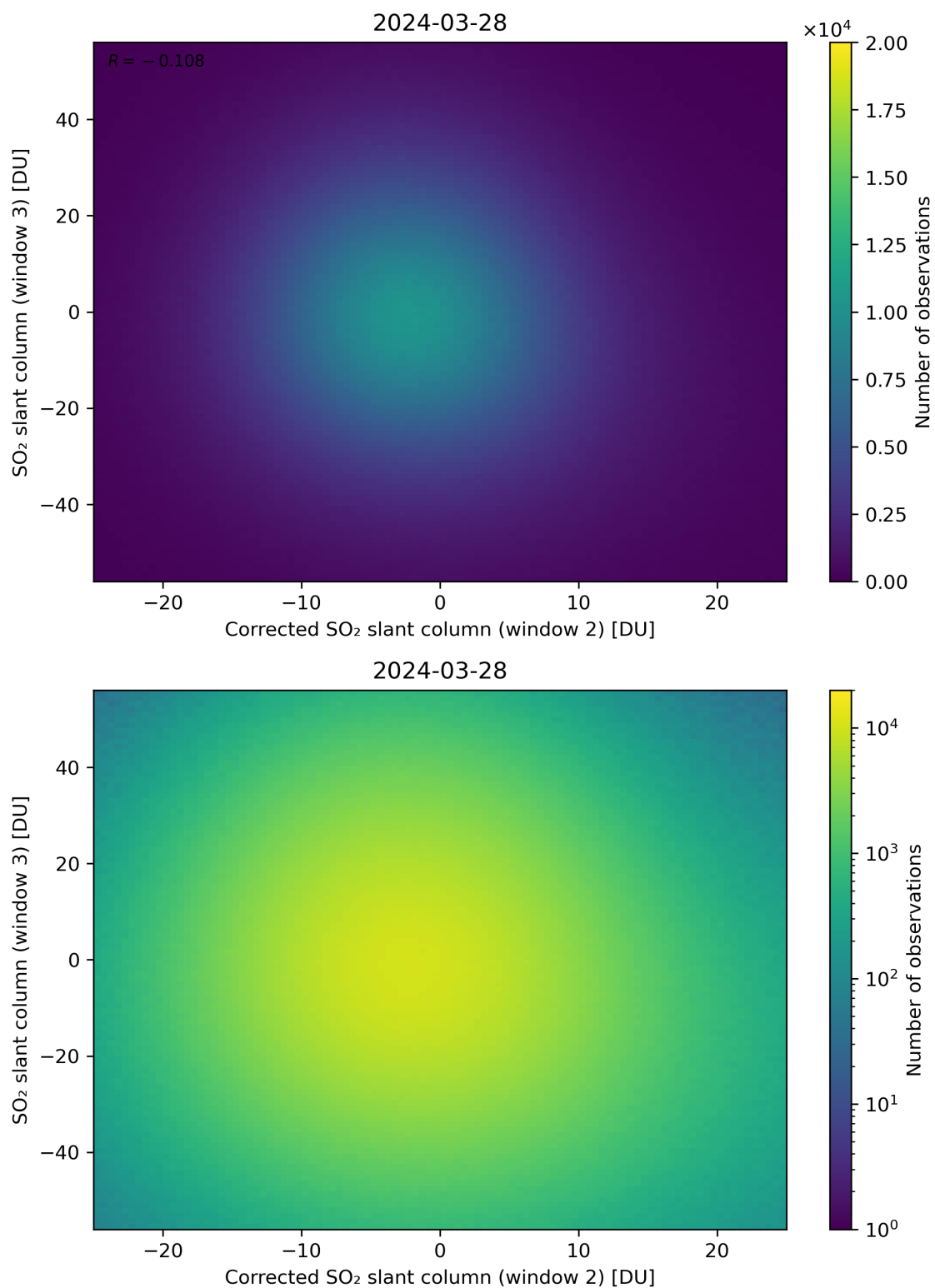
Figure 201: Scatter density plot of “Corrected SO 2 slant column (window 2)” against “SO 2 slant column (window 3)” for 2024-03-27 to 2024-03-29.
