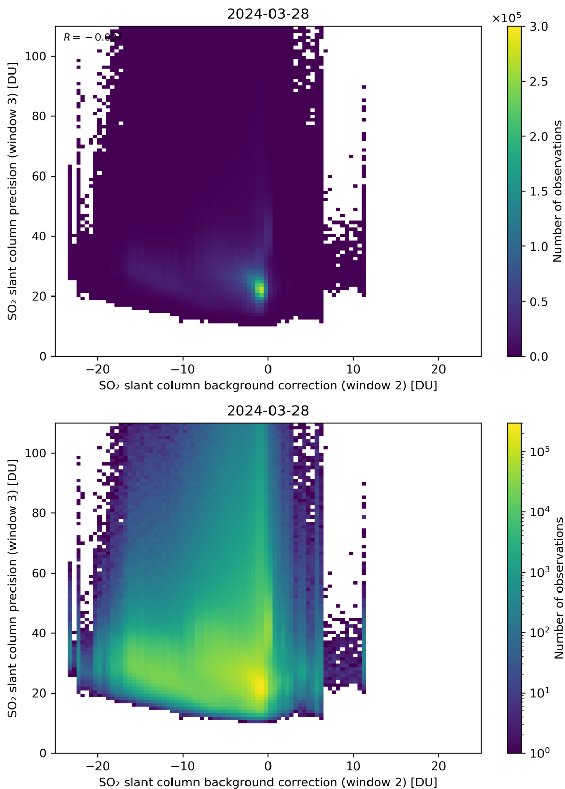
Figure 118: Scatter density plot of “SO 2 slant column background correction (window 2)” against “SO 2 slant column precision (window 3)” for 2024-03-27 to 2024-03-29.
