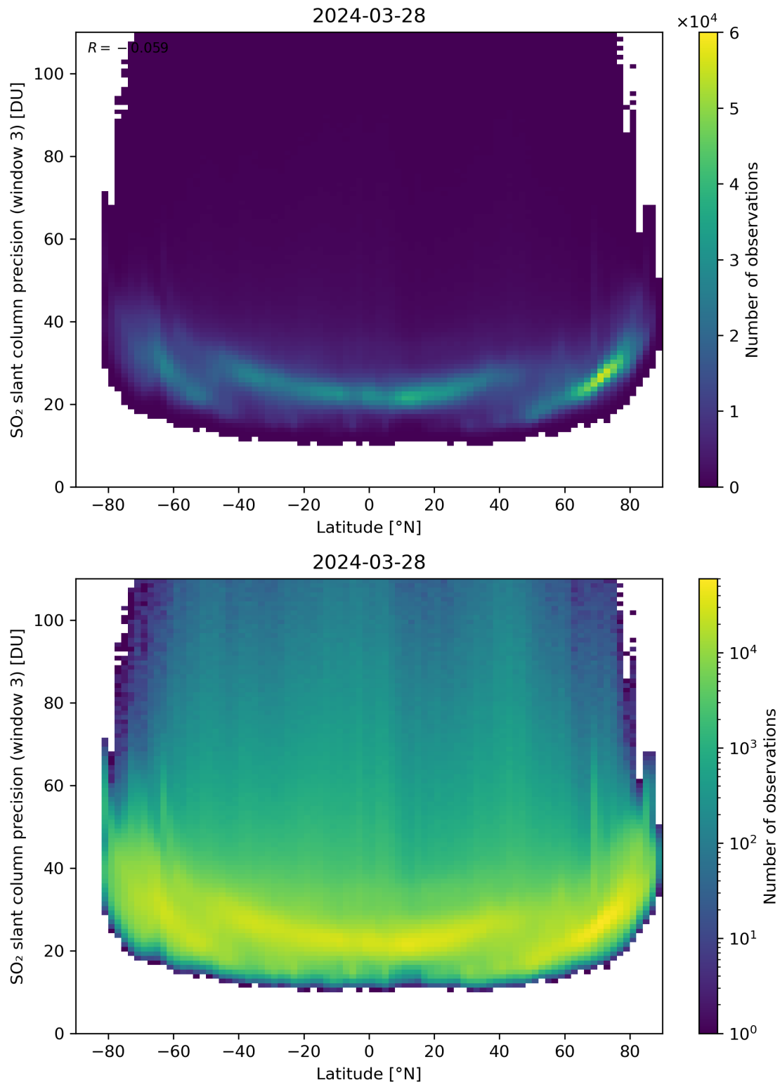
Figure 153: Scatter density plot of “Latitude” against “SO 2 slant column precision (window 3)” for 2024-03-27 to 2024-03-29.
