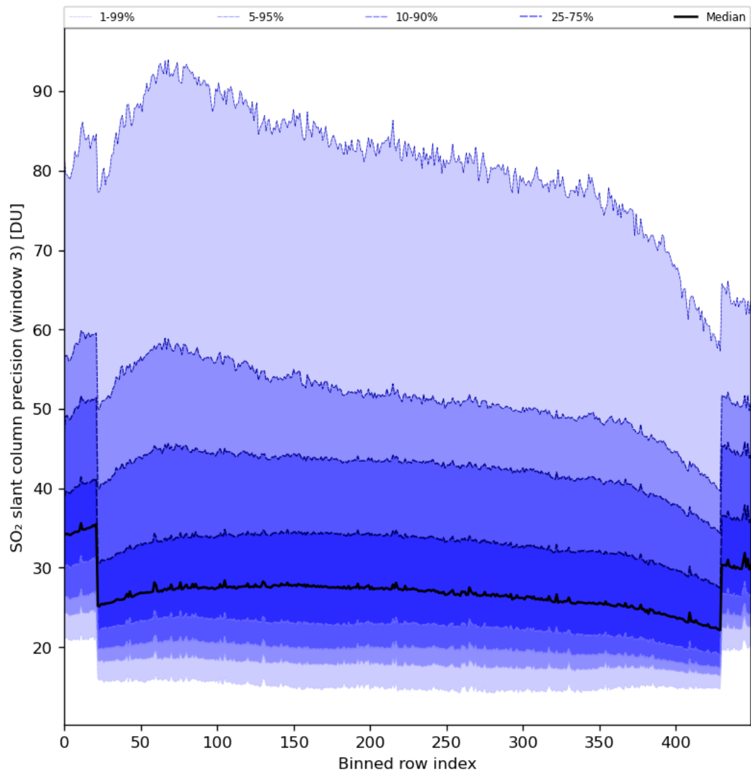
Figure 88: Along track statistics of “SO 2 slant column precision (window 3)” for 2024-03-27 to 2024-03-29
