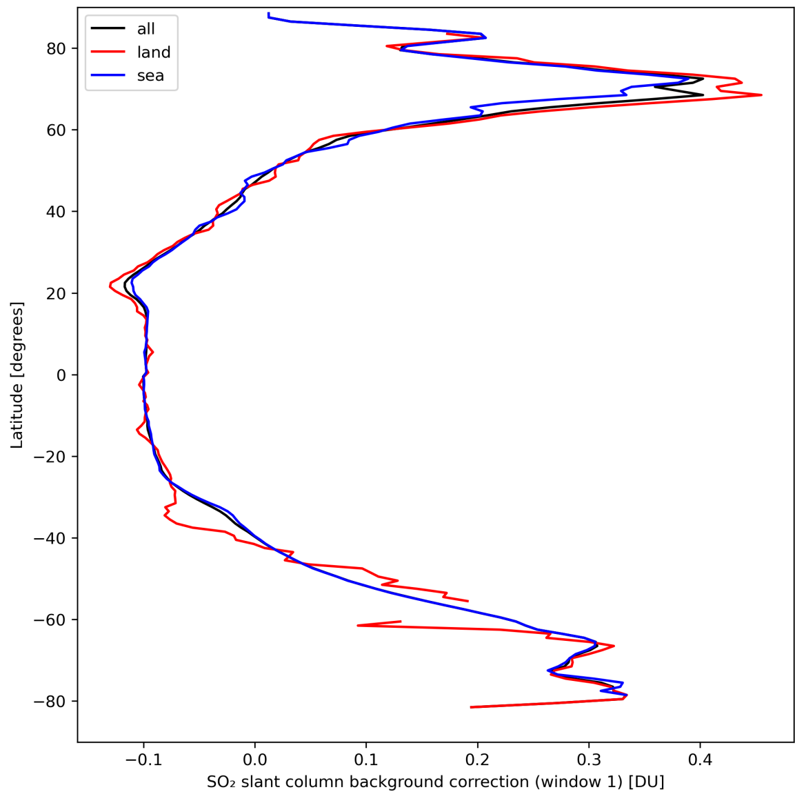
Figure 36: Zonal average of “SO 2 slant column background correction (window 1)” for 2024-03-27 to 2024-03-29.
