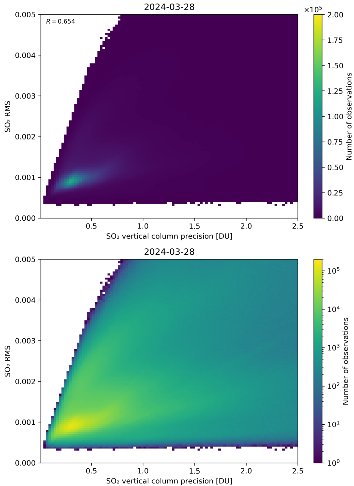
Figure 284: Scatter density plot of “SO 2 vertical column precision” against “SO 2 RMS” for 2024-03-27 to 2024-03-29.
