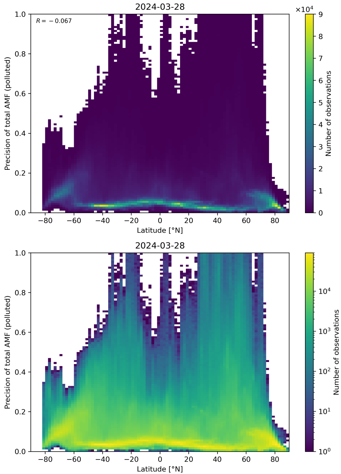
Figure 155: Scatter density plot of “Latitude” against “Precision of total AMF (polluted)” for 2024-03-27 to 2024-03-29.
