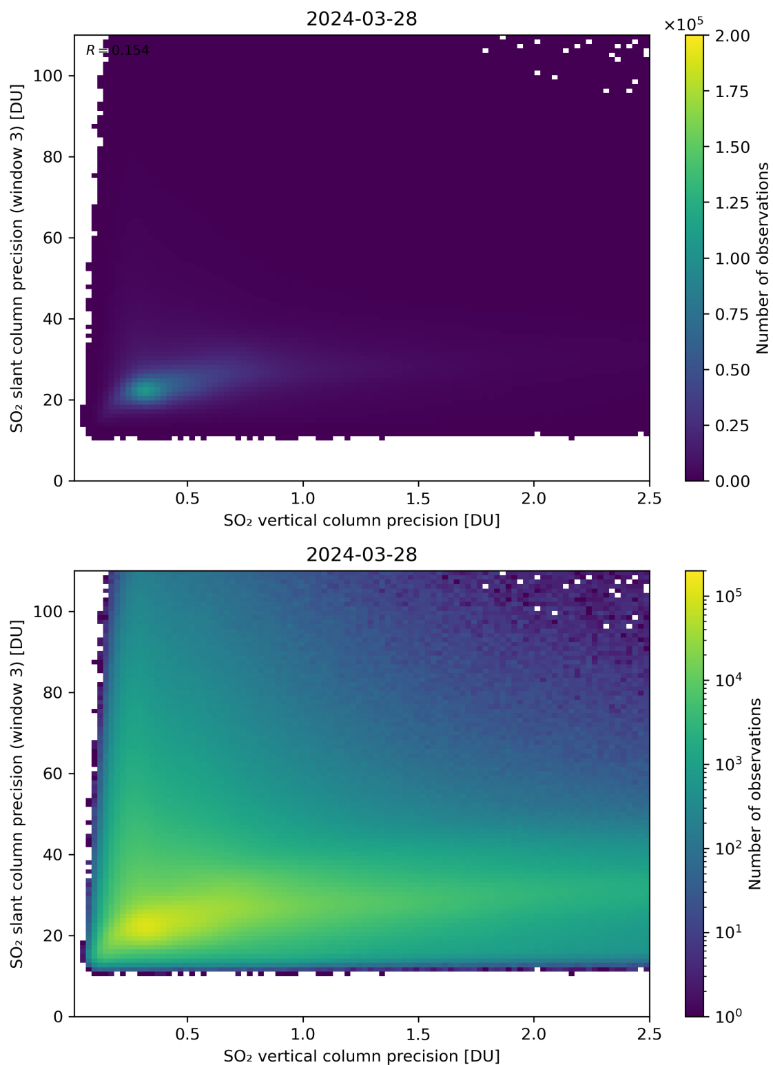
Figure 293: Scatter density plot of “SO 2 vertical column precision” against “SO 2 slant column precision (window 3)” for 2024-03-27 to 2024-03-29.
