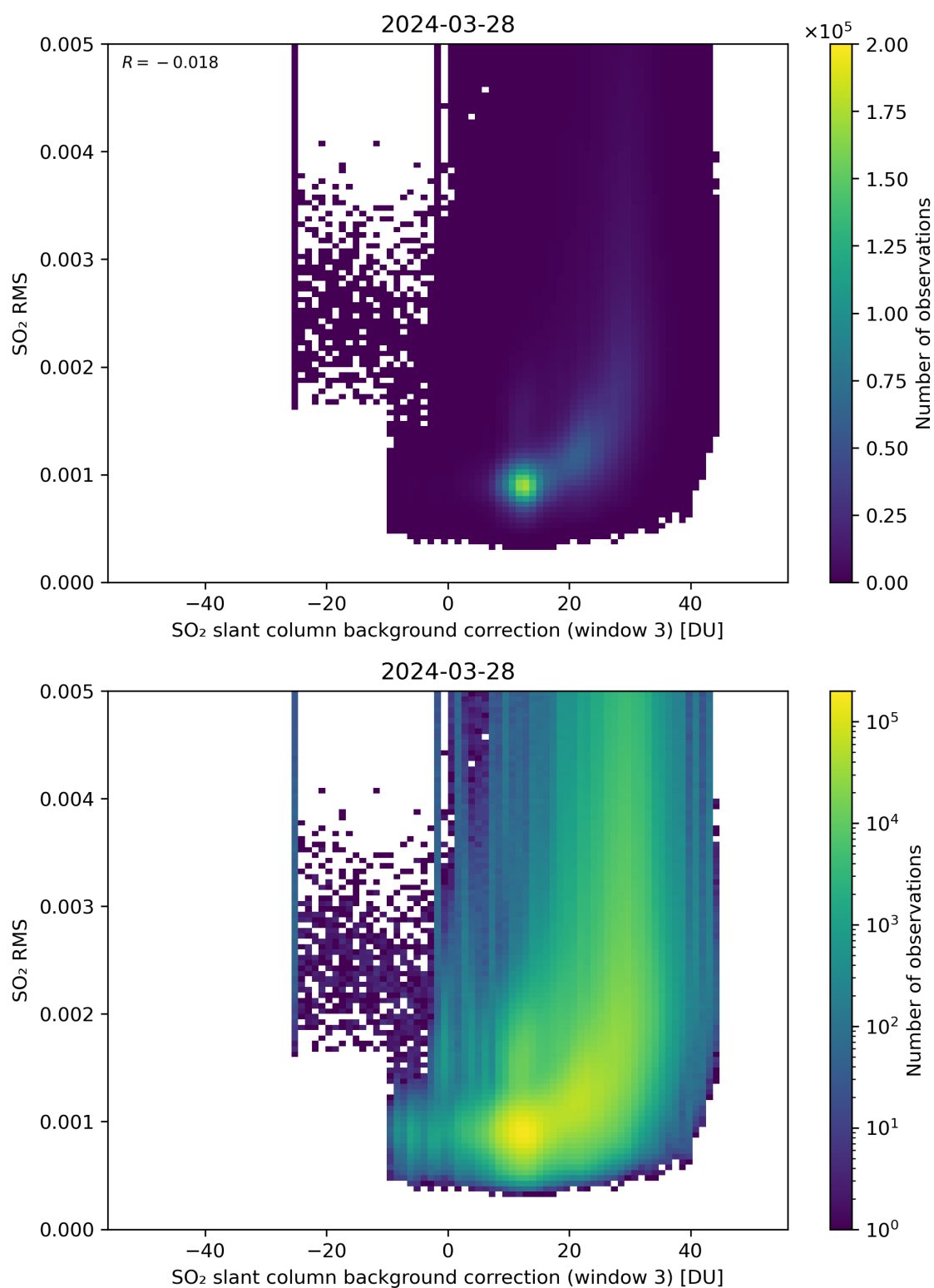
Figure 123: Scatter density plot of “SO 2 slant column background correction (window 3)” against “SO 2 RMS” for 2024-03-27 to 2024-03-29.
