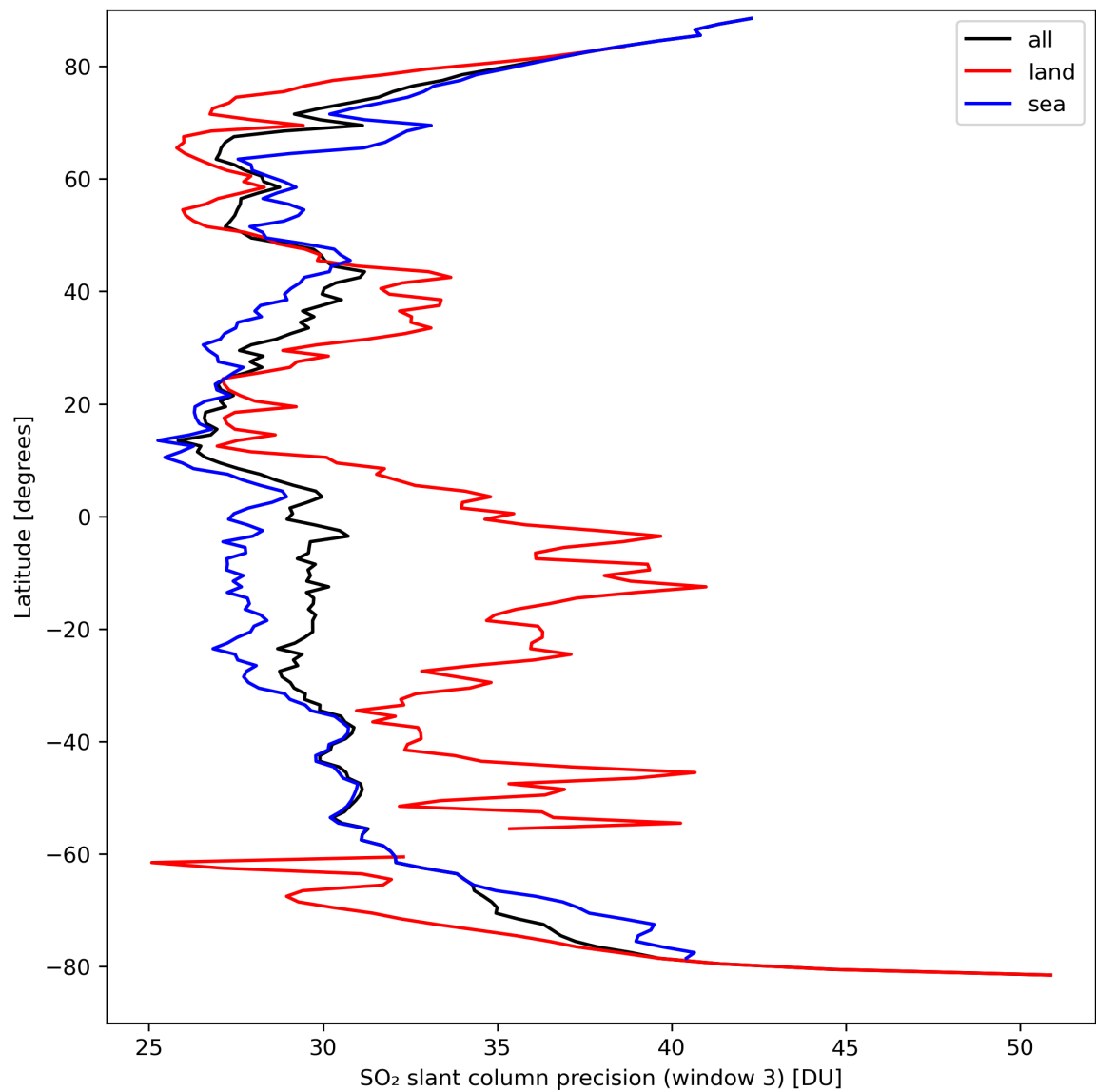
Figure 42: Zonal average of “SO 2 slant column precision (window 3)” for 2024-03-27 to 2024-03-29.
