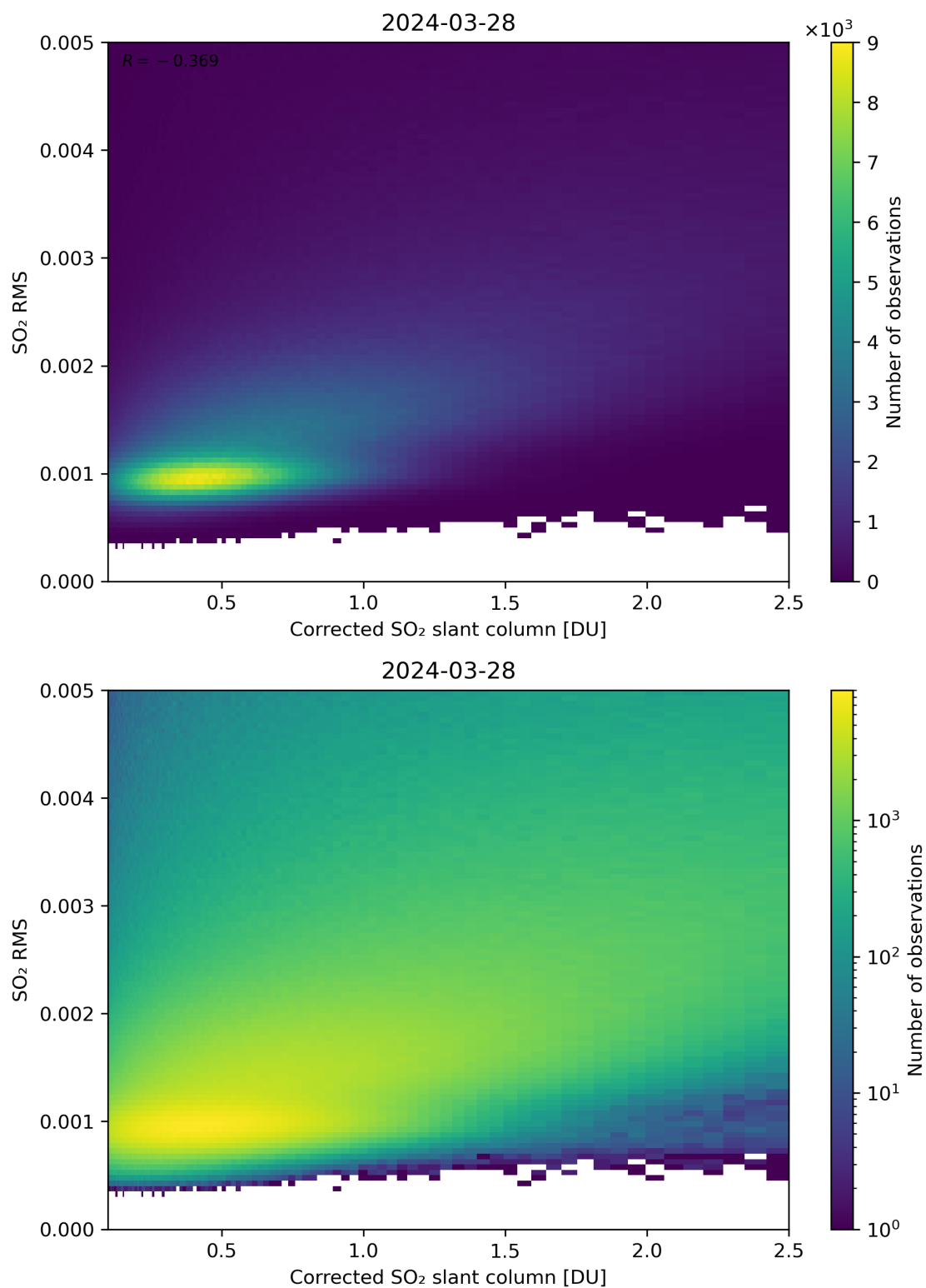
Figure 183: Scatter density plot of “Corrected SO 2 slant column” against “SO 2 RMS” for 2024-03-27 to 2024-03-29.
