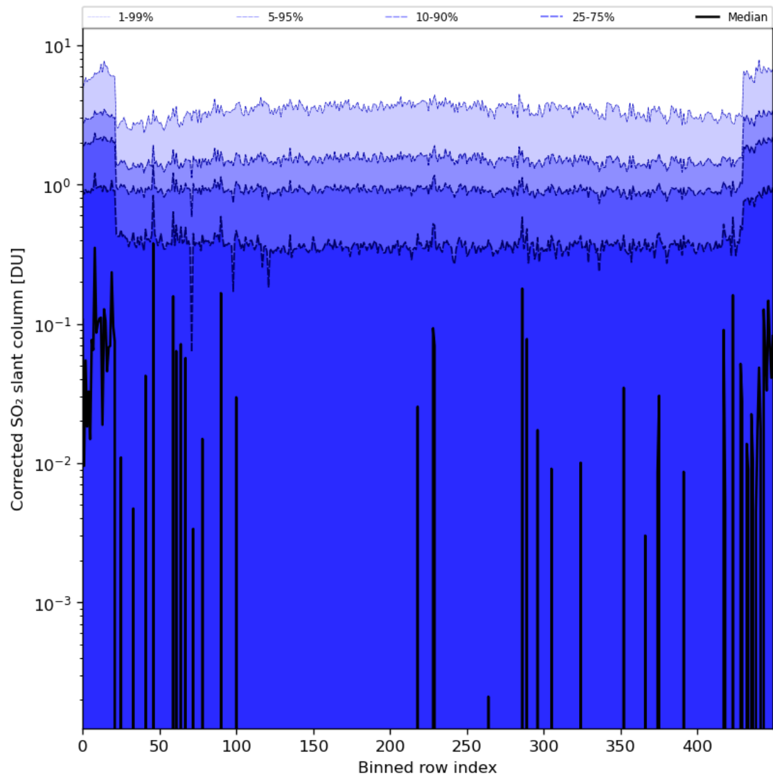
Figure 78: Along track statistics of “Corrected SO 2 slant column” for 2024-03-27 to 2024-03-29
