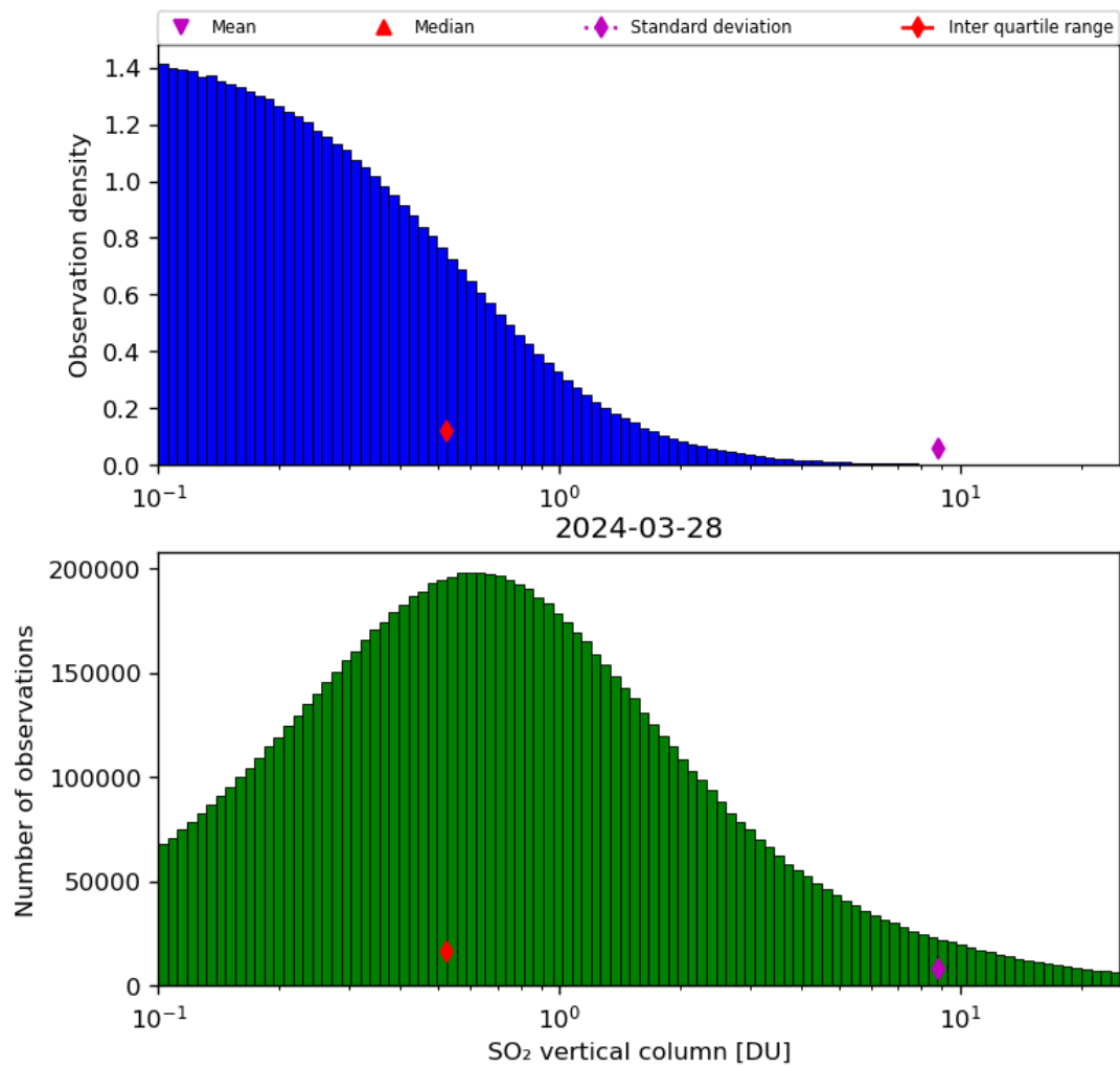
Figure 53: Histogram of “SO 2 vertical column” for 2024-03-27 to 2024-03-29
