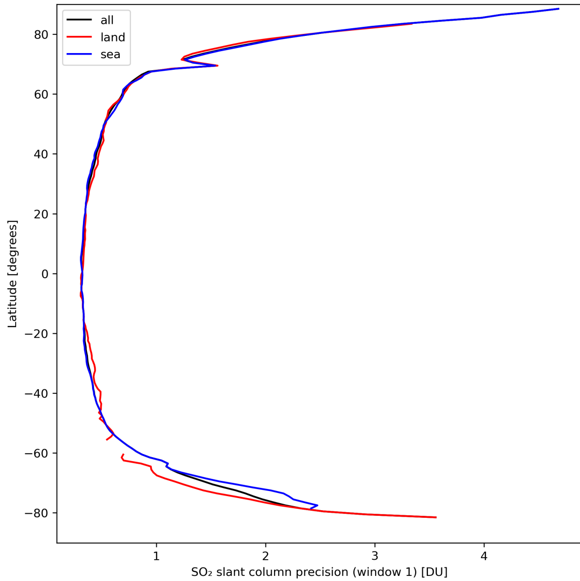
Figure 34: Zonal average of “SO 2 slant column precision (window 1)” for 2024-03-27 to 2024-03-29.
