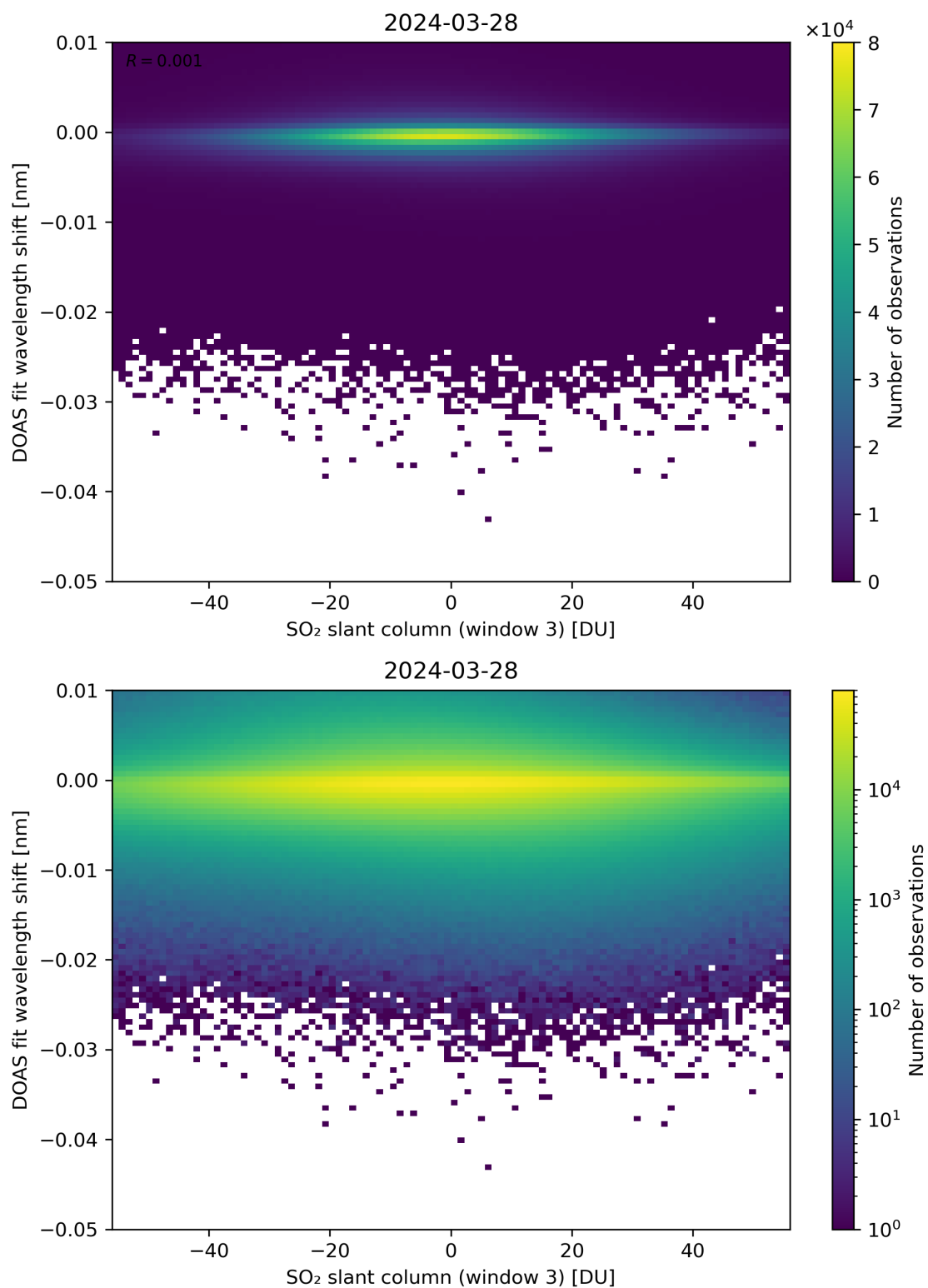
Figure 254: Scatter density plot of “SO 2 slant column (window 3)” against “DOAS fit wavelength shift” for 2024-03-27 to 2024-03-29.
