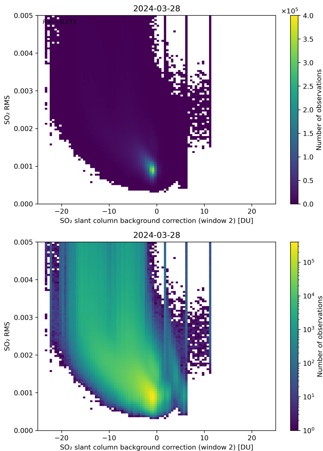
Figure 114: Scatter density plot of “SO 2 slant column background correction (window 2)” against “SO 2 RMS” for 2024-03-27 to 2024-03-29.
