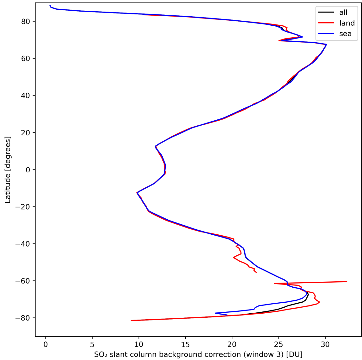
Figure 44: Zonal average of “SO 2 slant column background correction (window 3)” for 2024-03-27 to 2024-03-29.
