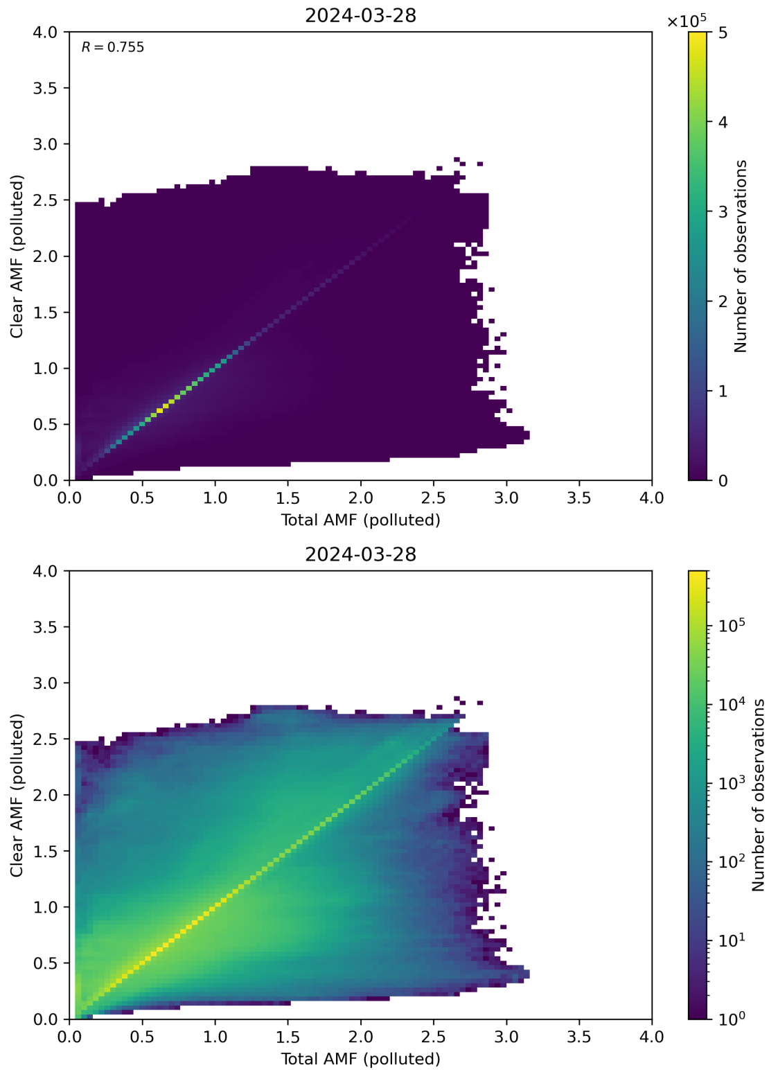
Figure 271: Scatter density plot of “Total AMF (polluted)” against “Clear AMF (polluted)” for 2024-03-27 to 2024-03-29.
