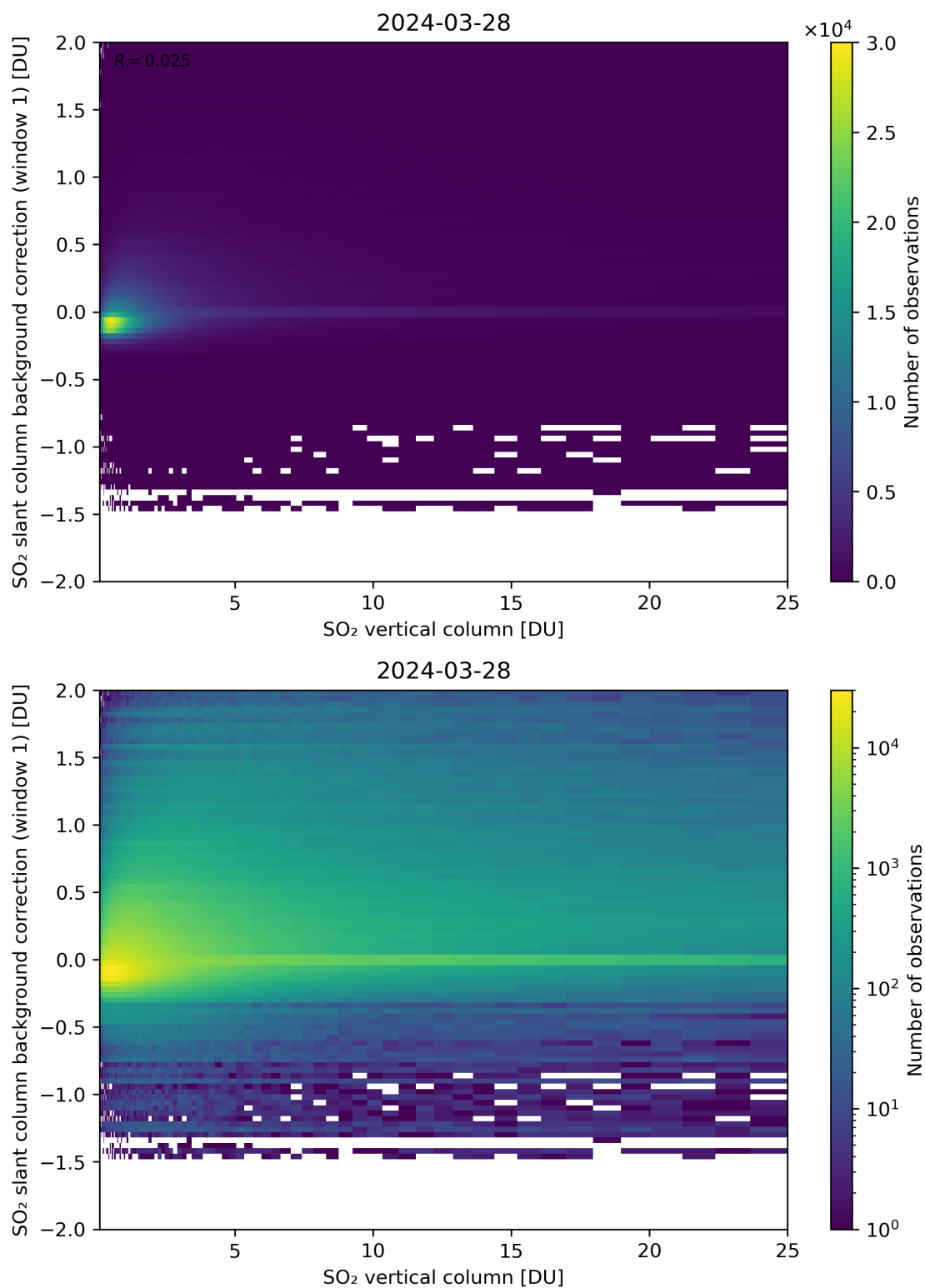
Figure 273: Scatter density plot of “SO 2 vertical column” against “SO 2 slant column background correction (window 1)” for 2024-03-27 to 2024-03-29.
