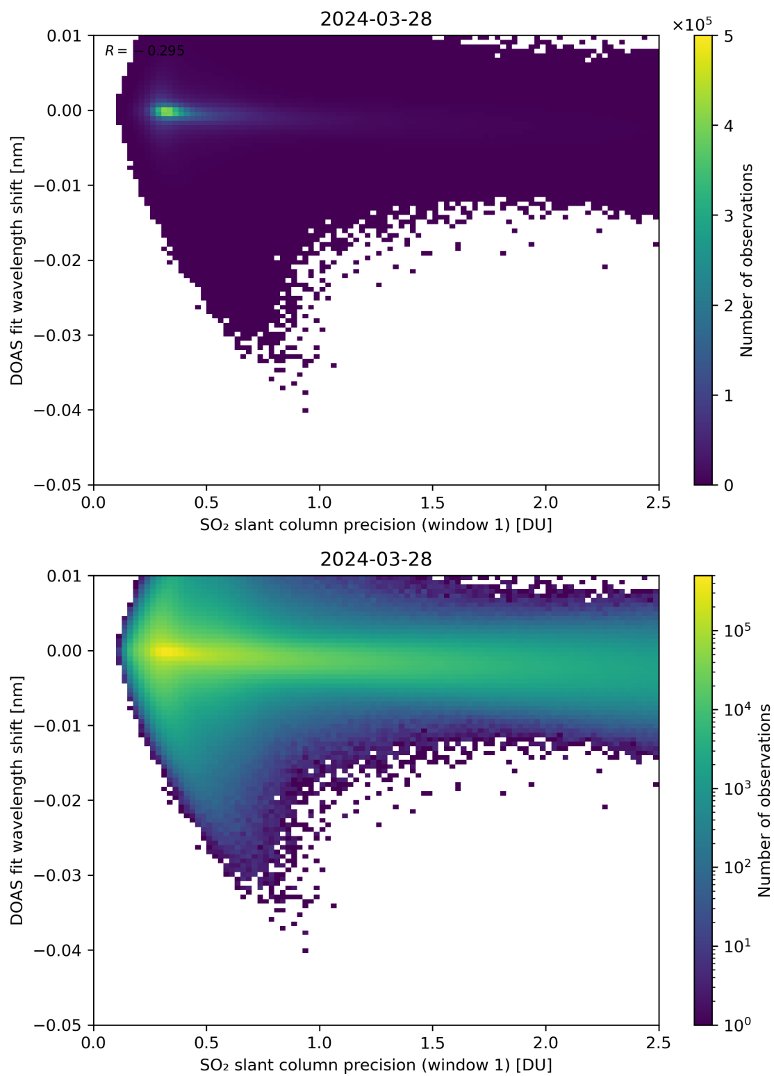
Figure 221: Scatter density plot of “SO 2 slant column precision (window 1)” against “DOAS fit wavelength shift” for 2024-03-27 to 2024-03-29.
