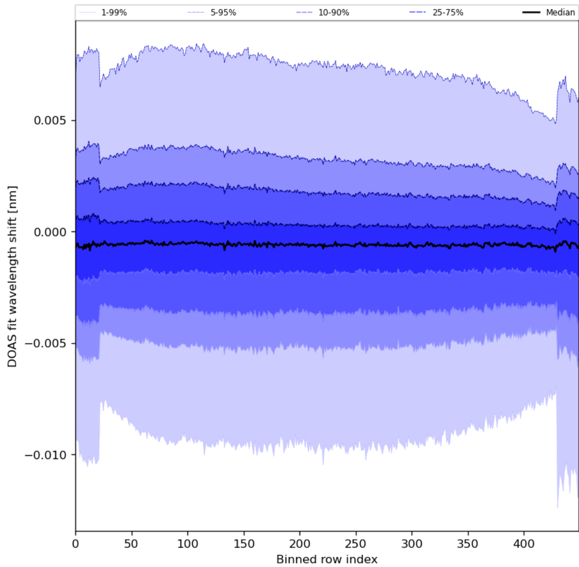
Figure 91: Along track statistics of “DOAS fit wavelength shift” for 2024-03-27 to 2024-03-29
