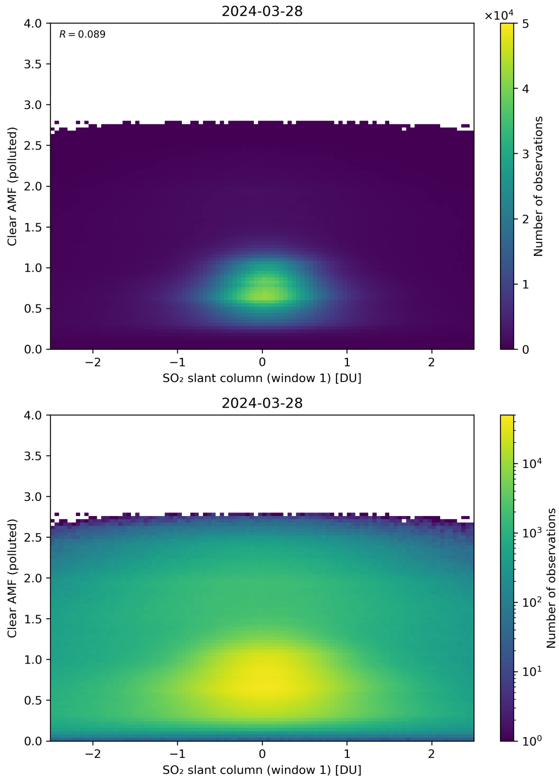
Figure 232: Scatter density plot of “SO 2 slant column (window 1)” against “Clear AMF (polluted)” for 2024-03-27 to 2024-03-29.
