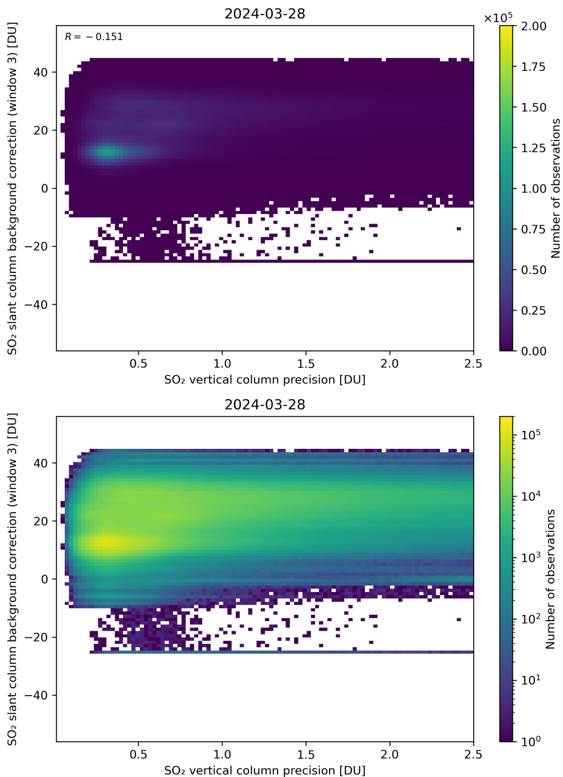
Figure 281: Scatter density plot of “SO 2 vertical column precision” against “SO 2 slant column background correction (window 3)” for 2024-03-27 to 2024-03-29.
