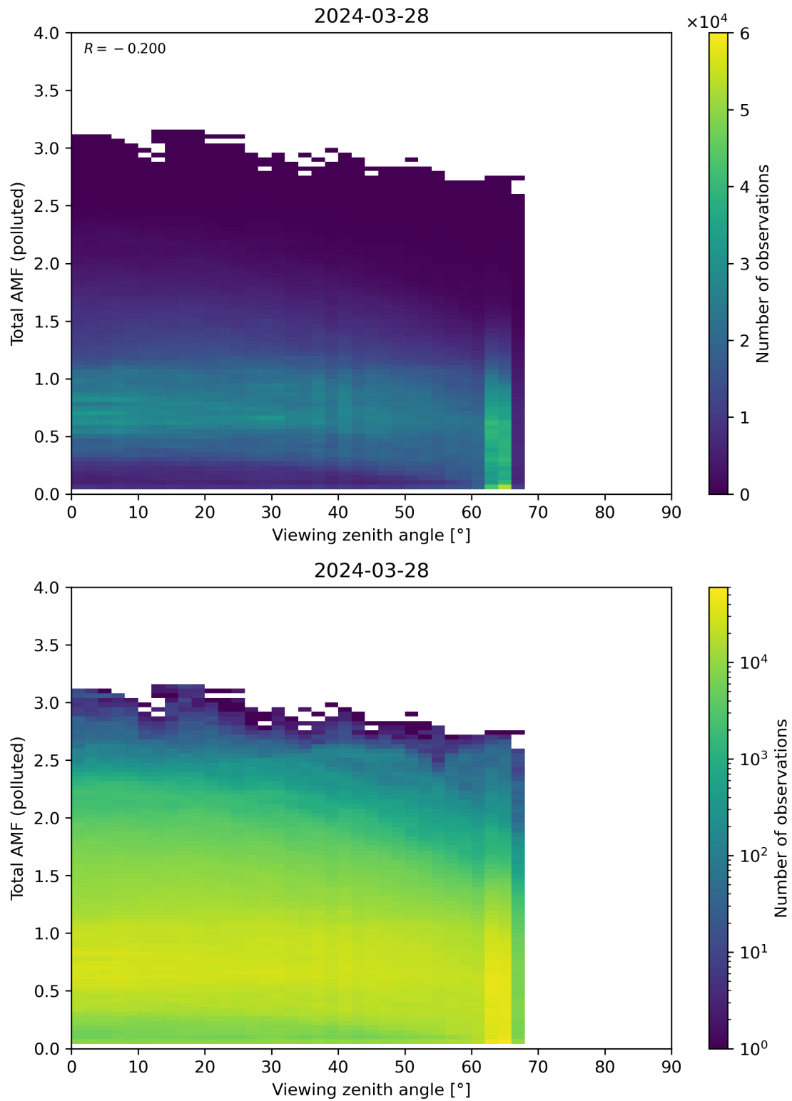
Figure 325: Scatter density plot of “Viewing zenith angle” against “Total AMF (polluted)” for 2024-03-27 to 2024-03-29.
