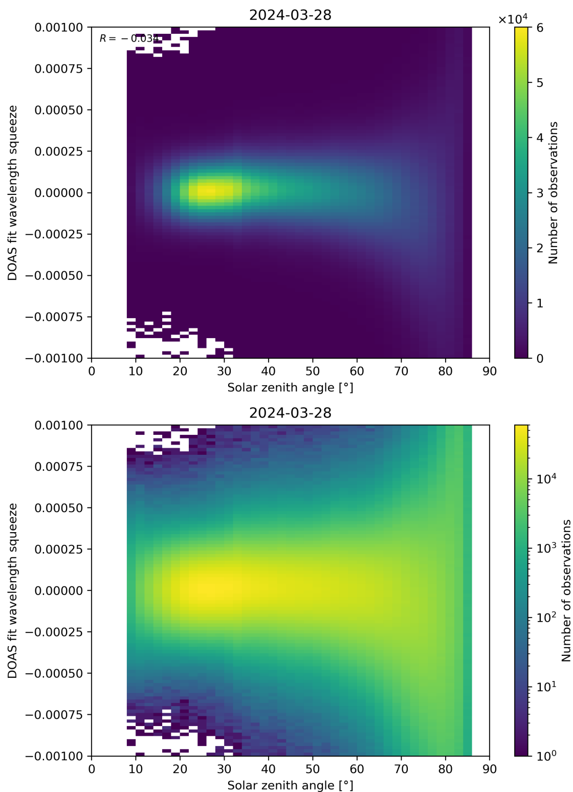
Figure 162: Scatter density plot of “Solar zenith angle” against “DOAS fit wavelength squeeze” for 2024-03-27 to 2024-03-29.
