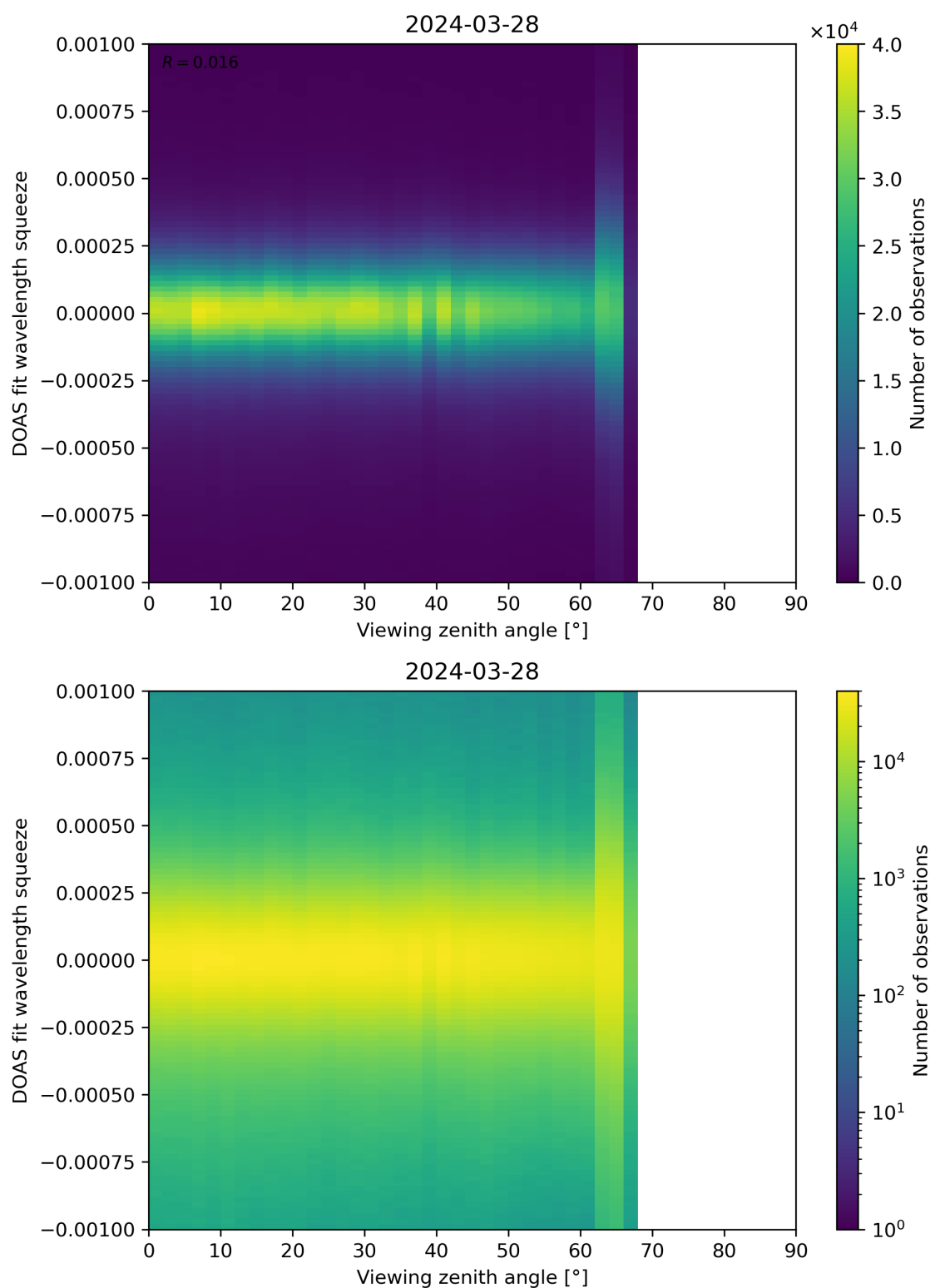
Figure 312: Scatter density plot of “Viewing zenith angle” against “DOAS fit wavelength squeeze” for 2024-03-27 to 2024-03-29.
