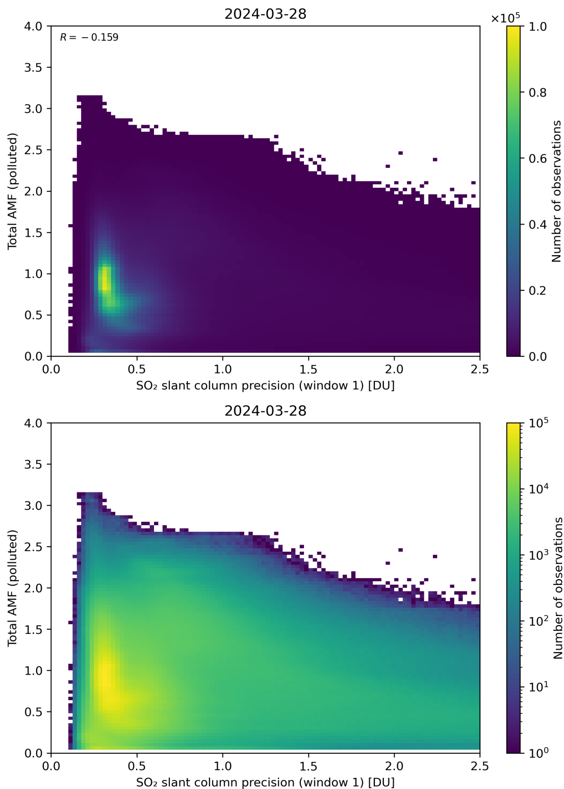
Figure 230: Scatter density plot of “SO 2 slant column precision (window 1)” against “Total AMF (polluted)” for 2024-03-27 to 2024-03-29.
