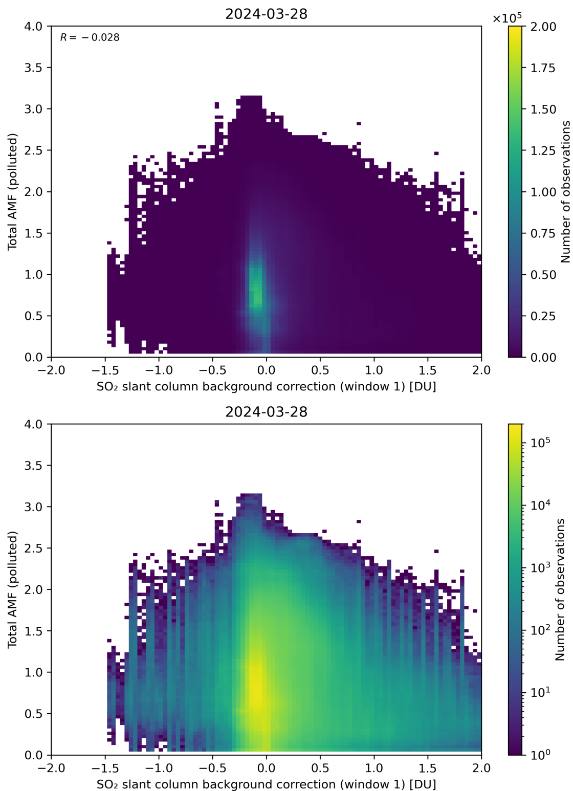
Figure 109: Scatter density plot of “SO 2 slant column background correction (window 1)” against “Total AMF (polluted)” for 2024-03-27 to 2024-03-29.
