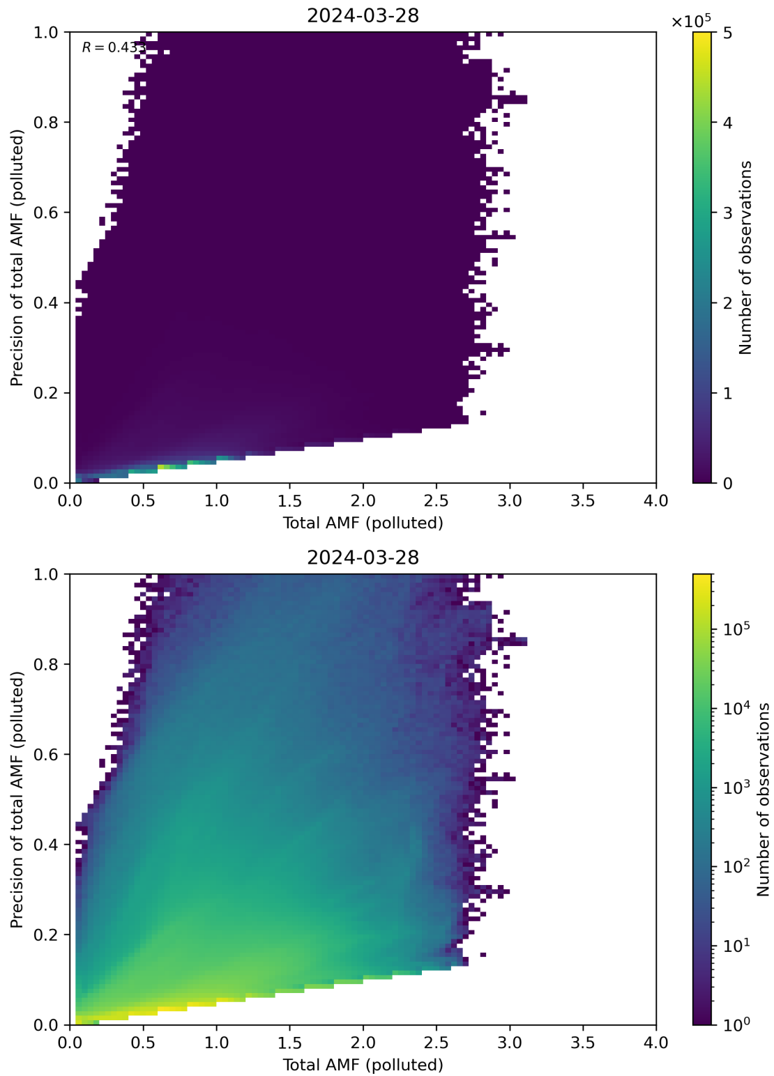
Figure 272: Scatter density plot of “Total AMF (polluted)” against “Precision of total AMF (polluted)” for 2024-03-27 to 2024-03-29.
