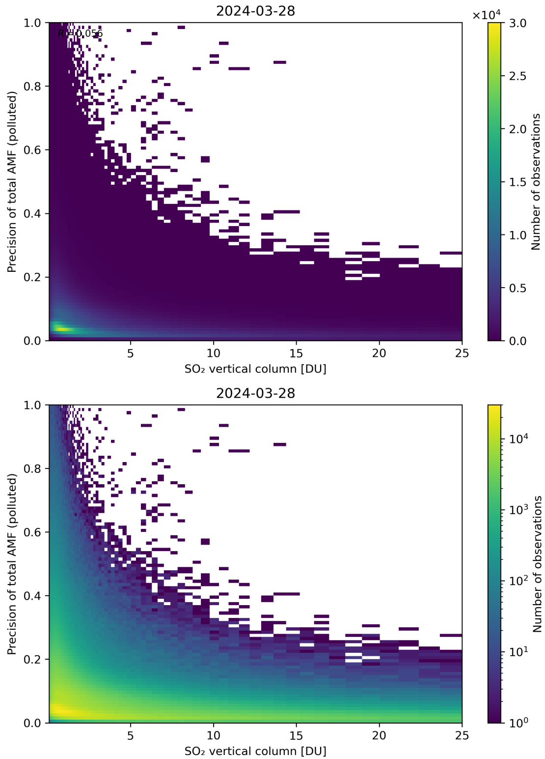
Figure 306: Scatter density plot of “SO 2 vertical column” against “Precision of total AMF (polluted)” for 2024-03-27 to 2024-03-29.
