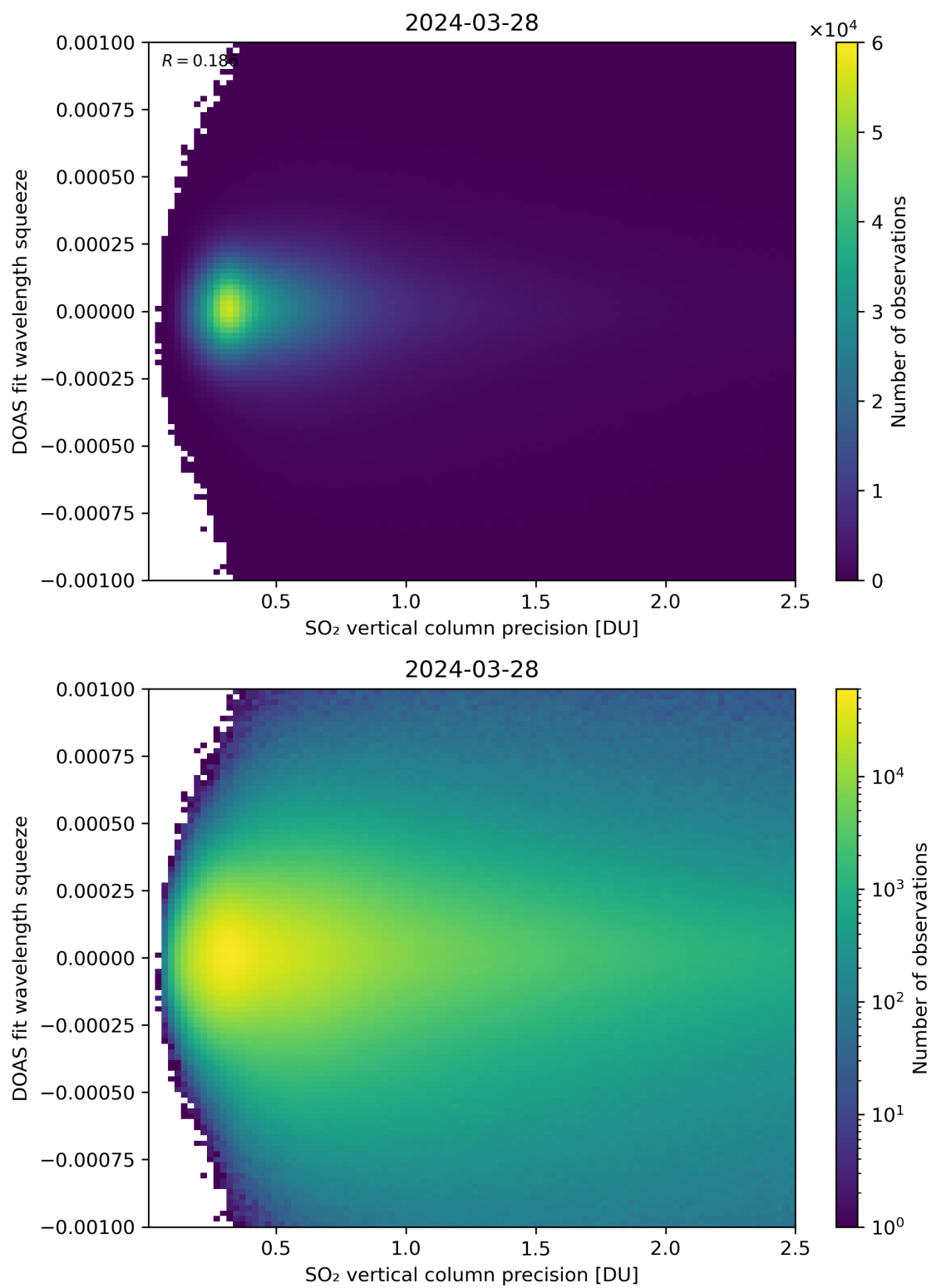
Figure 283: Scatter density plot of “SO 2 vertical column precision” against “DOAS fit wavelength squeeze” for 2024-03-27 to 2024-03-29.
