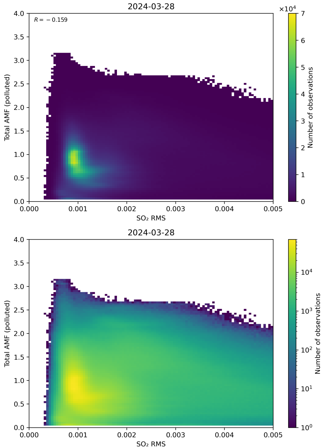
Figure 137: Scatter density plot of “SO 2 RMS” against “Total AMF (polluted)” for 2024-03-27 to 2024-03-29.
