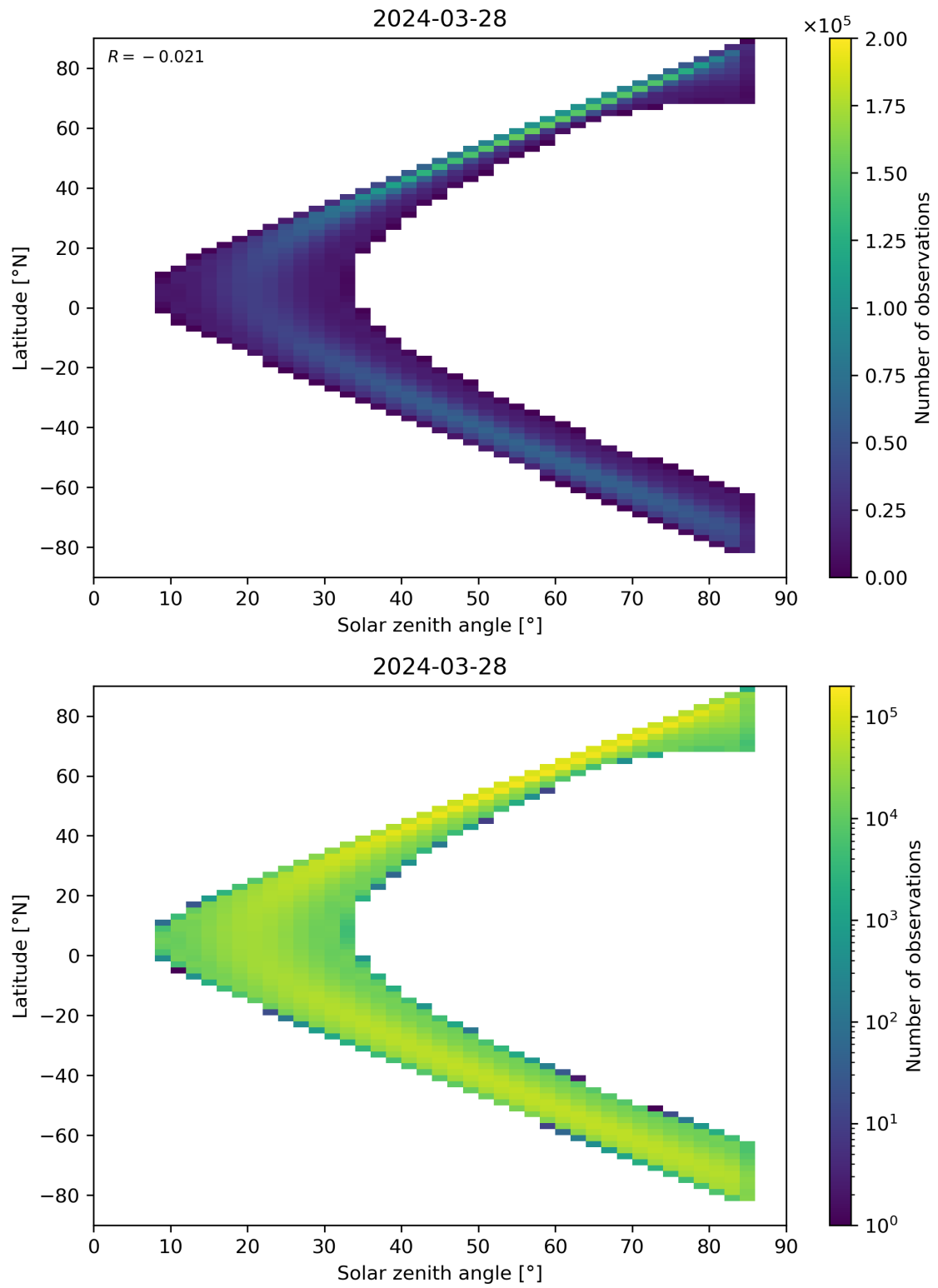
Figure 164: Scatter density plot of “Solar zenith angle” against “Latitude” for 2024-03-27 to 2024-03-29.
