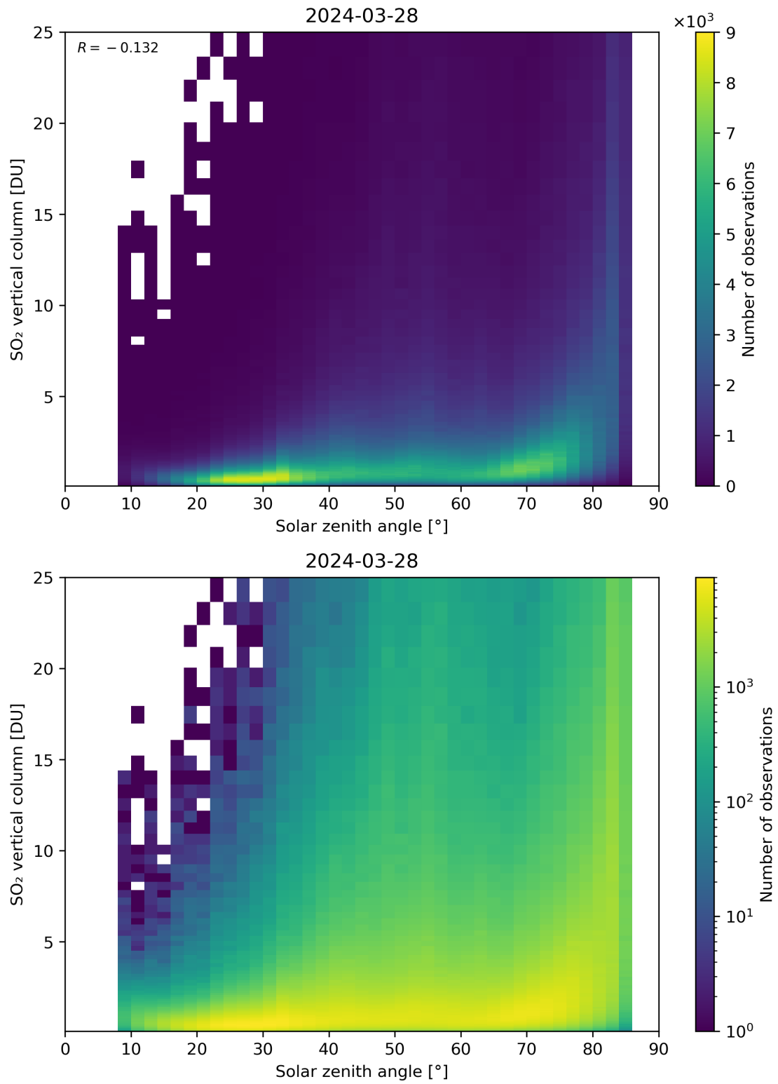
Figure 176: Scatter density plot of “Solar zenith angle” against “SO 2 vertical column” for 2024-03-27 to 2024-03-29.
