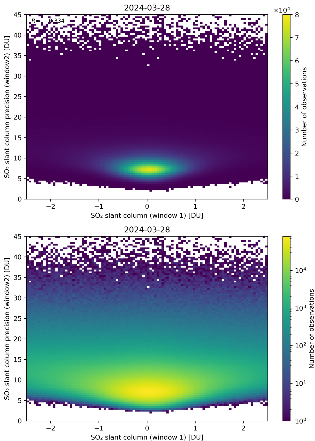
Figure 236: Scatter density plot of “SO 2 slant column (window 1)” against “SO 2 slant column precision (window2)” for 2024-03-27 to 2024-03-29.
