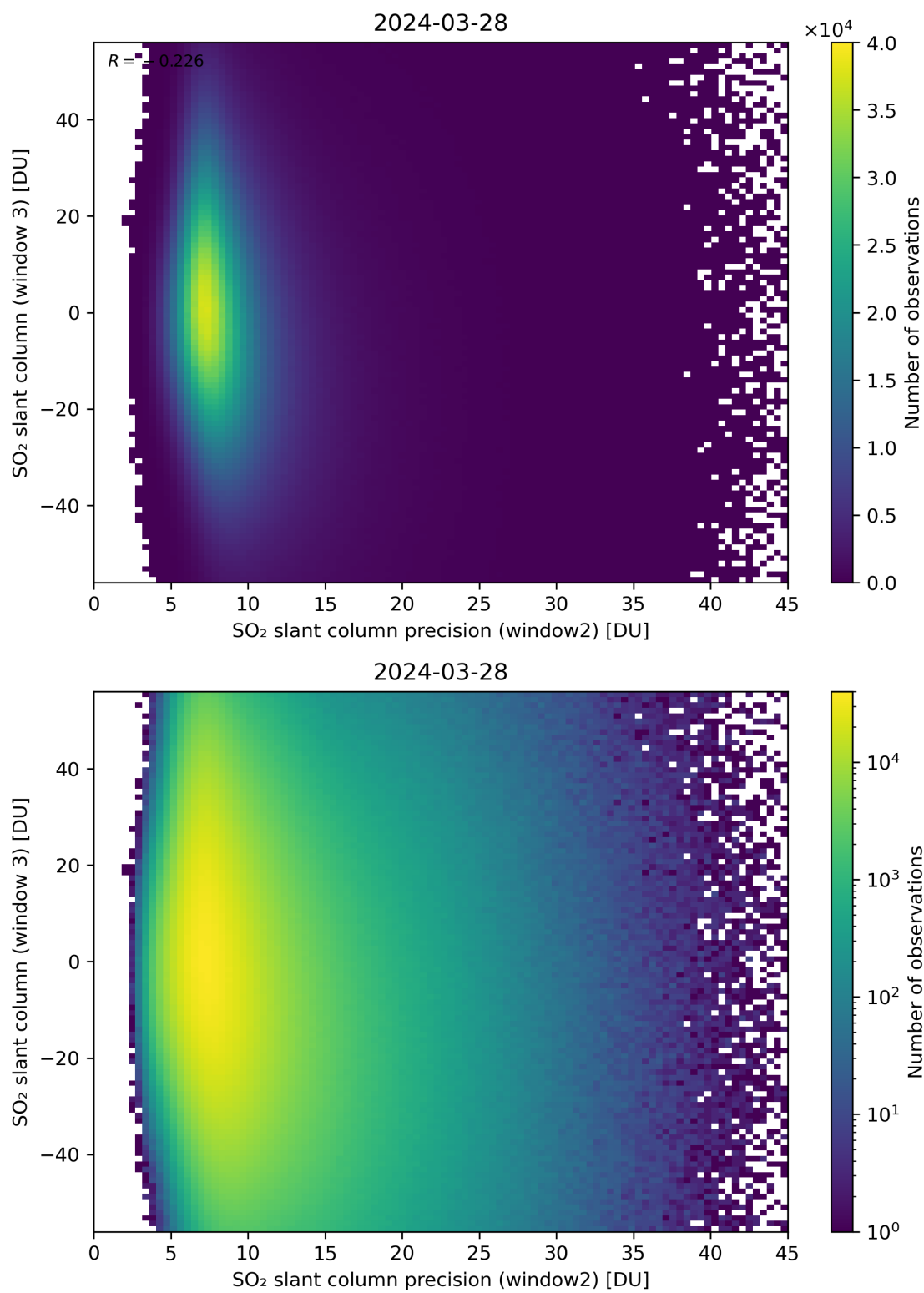
Figure 249: Scatter density plot of “SO 2 slant column precision (window2)” against “SO 2 slant column (window 3)” for 2024-03-27 to 2024-03-29.
