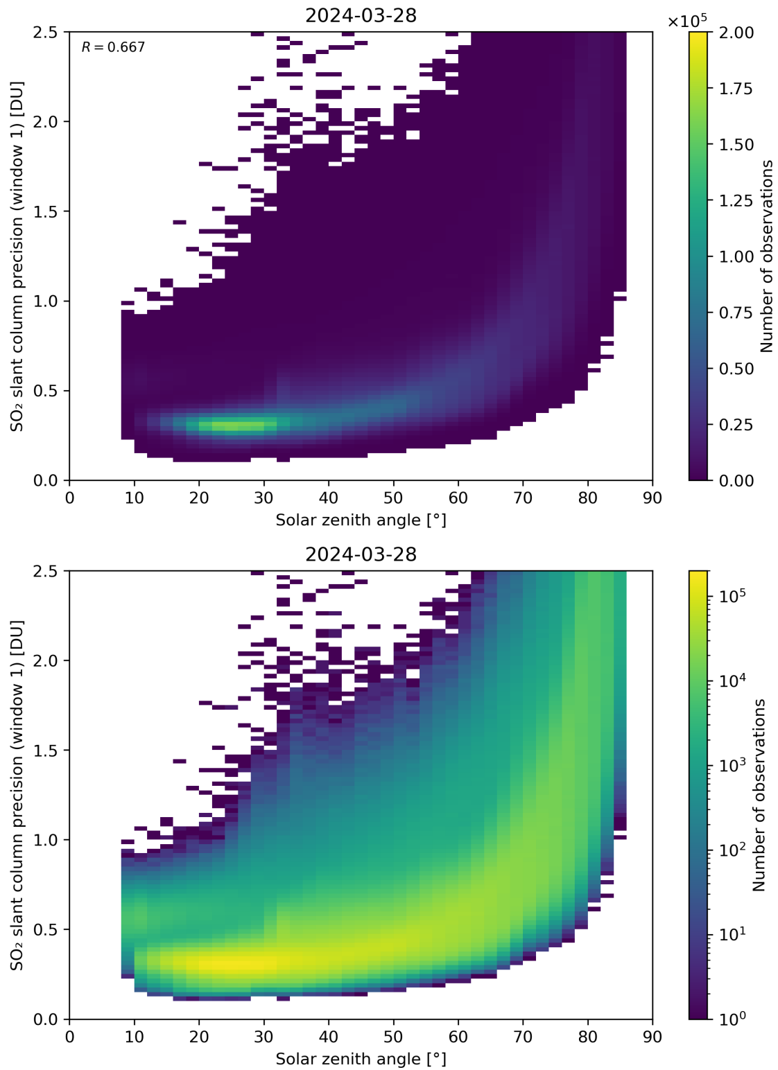
Figure 170: Scatter density plot of “Solar zenith angle” against “SO 2 slant column precision (window 1)” for 2024-03-27 to 2024-03-29.
