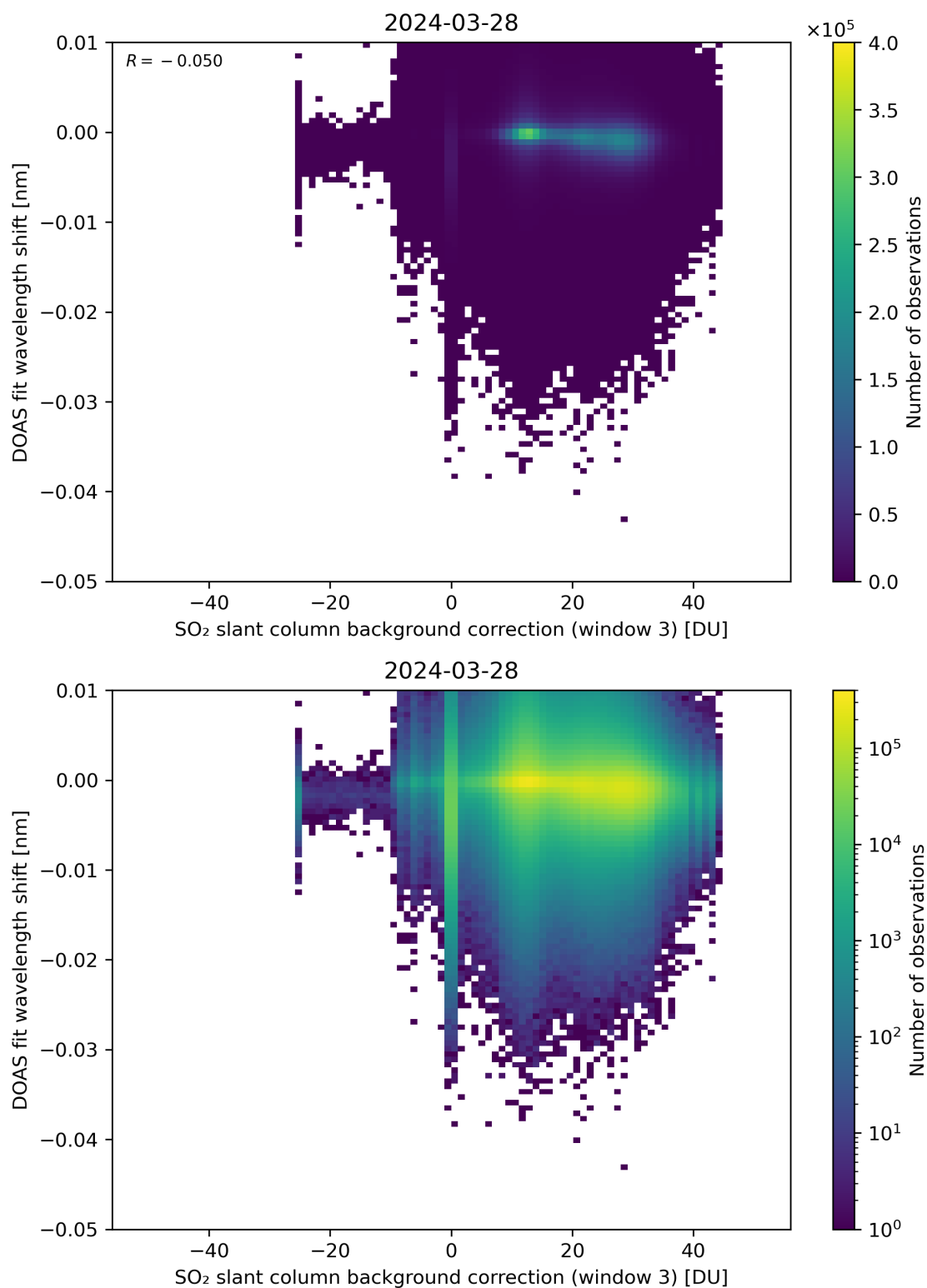
Figure 121: Scatter density plot of “SO 2 slant column background correction (window 3)” against “DOAS fit wavelength shift” for 2024-03-27 to 2024-03-29.
