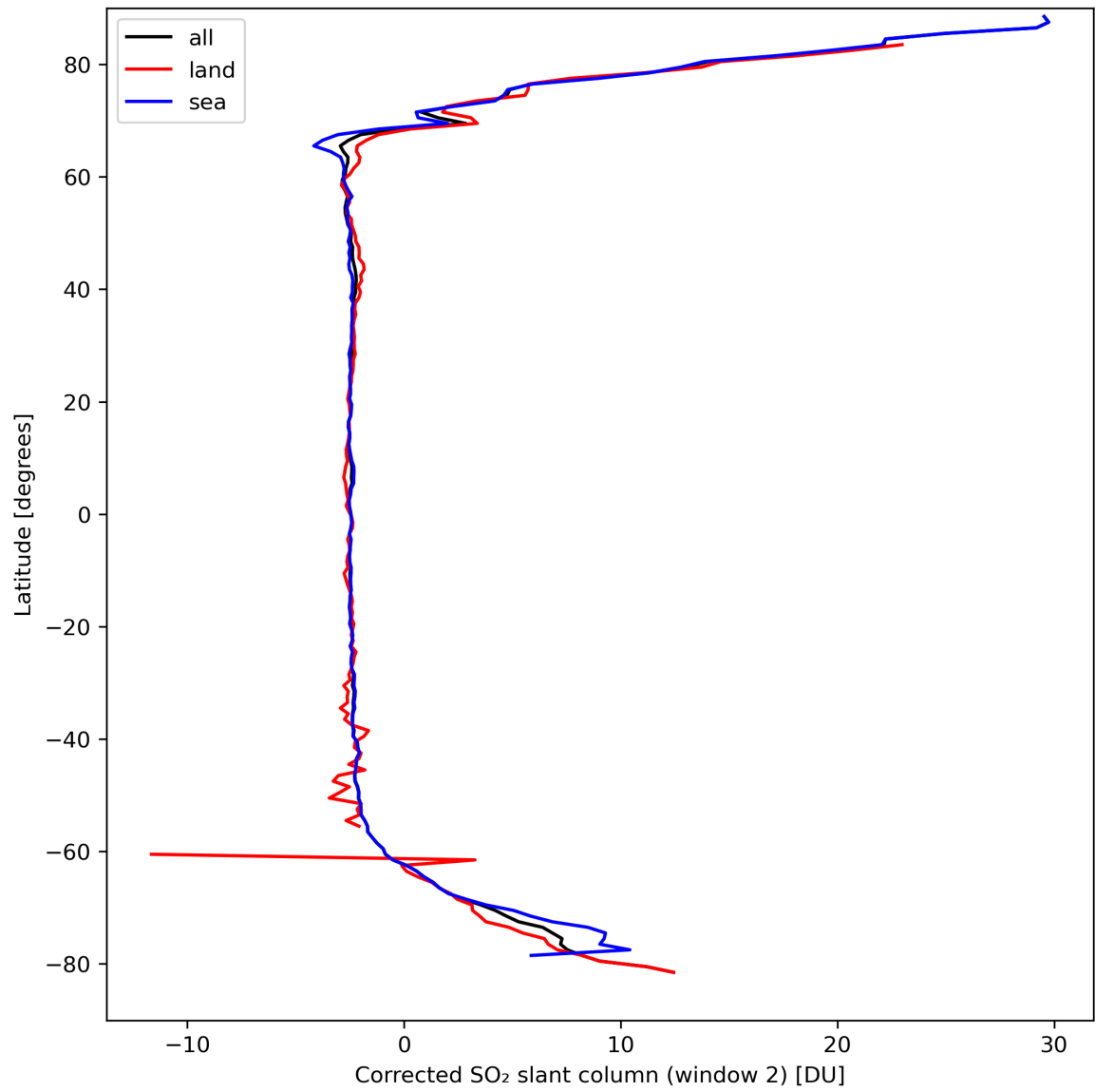
Figure 39: Zonal average of “Corrected SO 2 slant column (window 2)” for 2024-03-27 to 2024-03-29.
