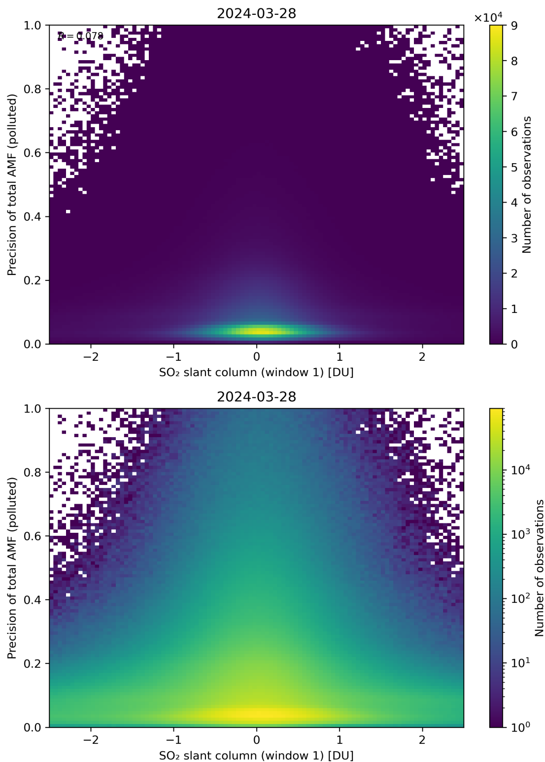
Figure 240: Scatter density plot of “SO 2 slant column (window 1)” against “Precision of total AMF (polluted)” for 2024-03-27 to 2024-03-29.
