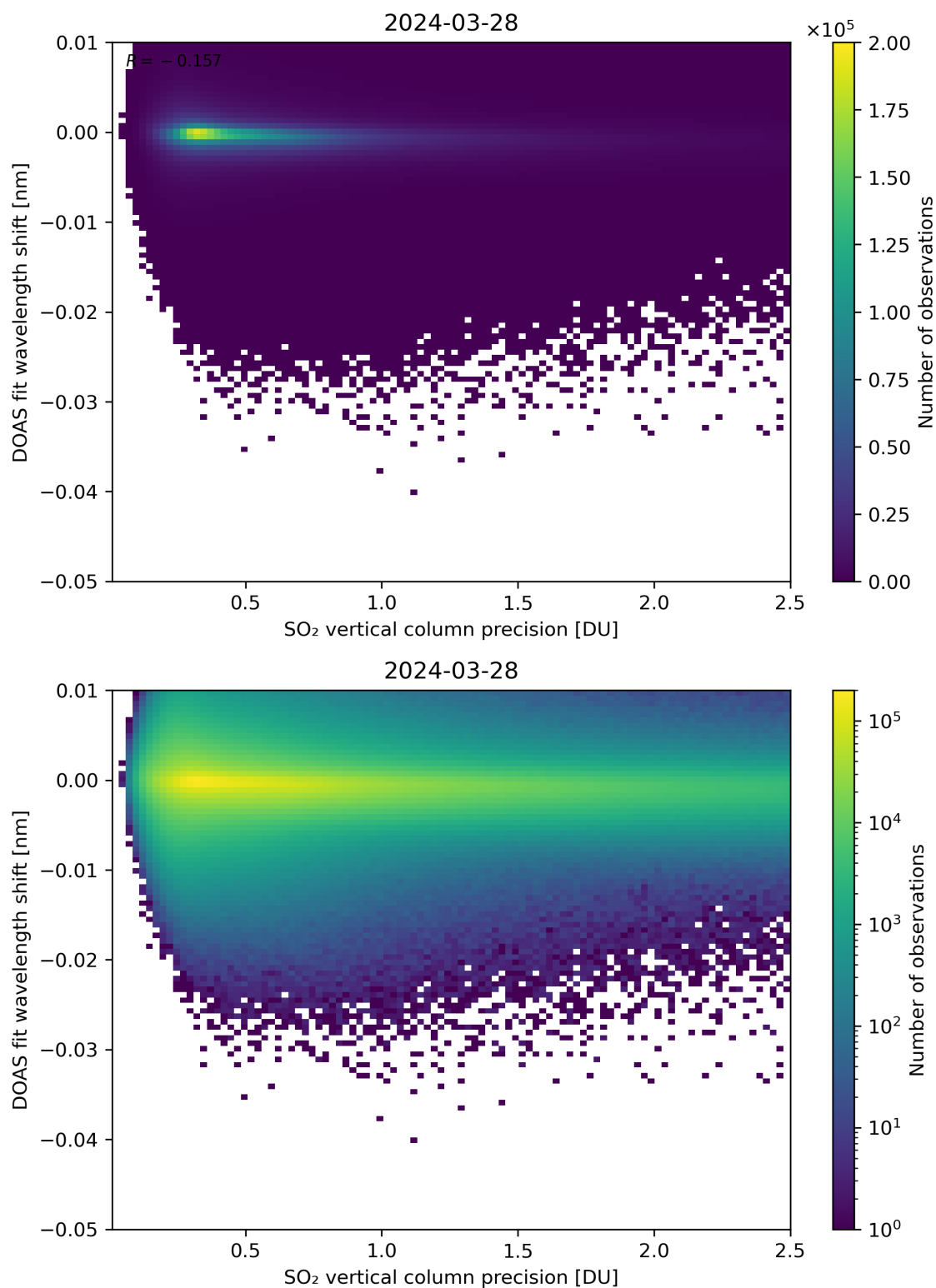
Figure 282: Scatter density plot of “SO 2 vertical column precision” against “DOAS fit wavelength shift” for 2024-03-27 to 2024-03-29.
