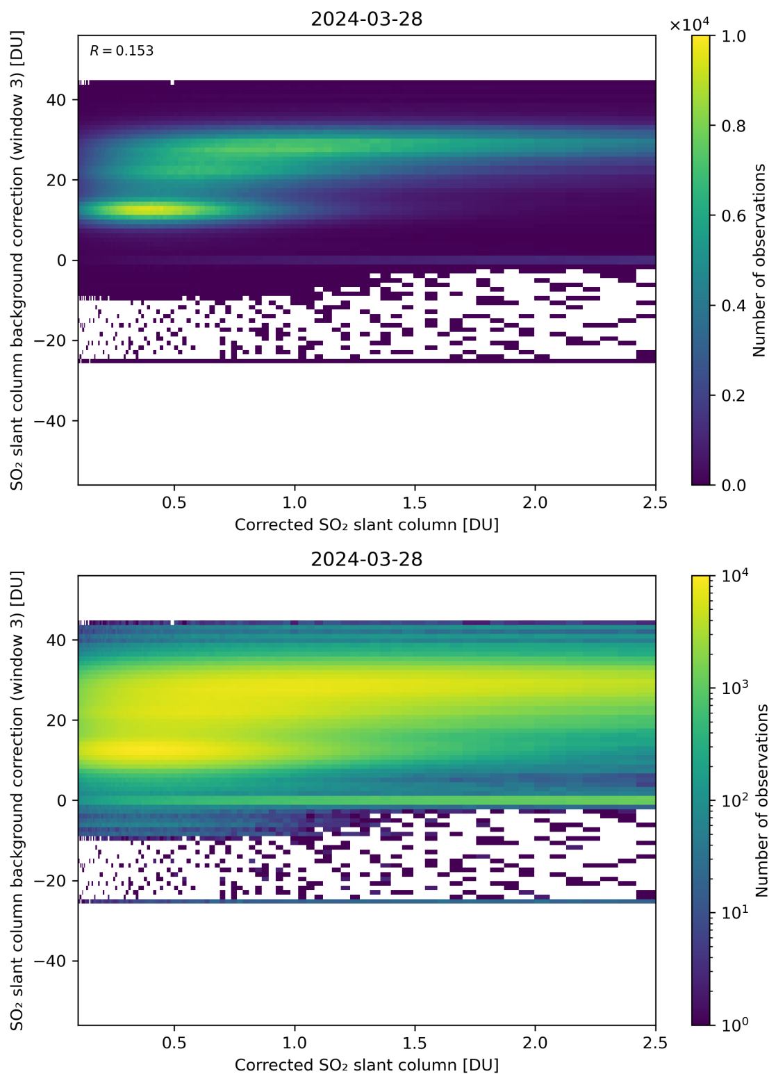
Figure 180: Scatter density plot of “Corrected SO 2 slant column” against “SO 2 slant column background correction (window 3)” for 2024-03-27 to 2024-03-29.
