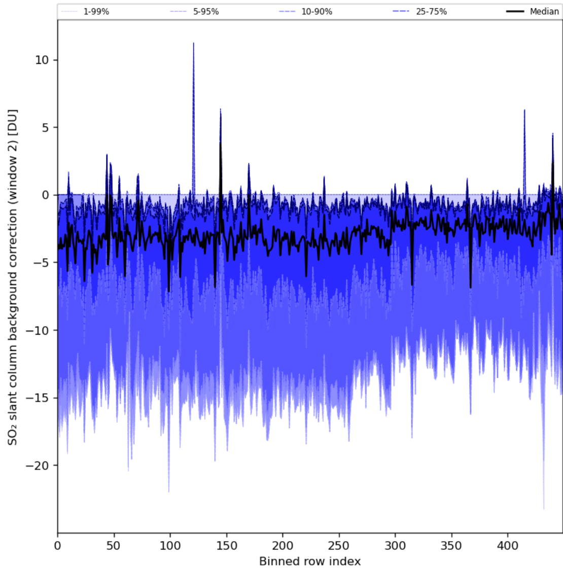
Figure 86: Along track statistics of “SO 2 slant column background correction (window 2)” for 2024-03-27 to 2024-03-29
