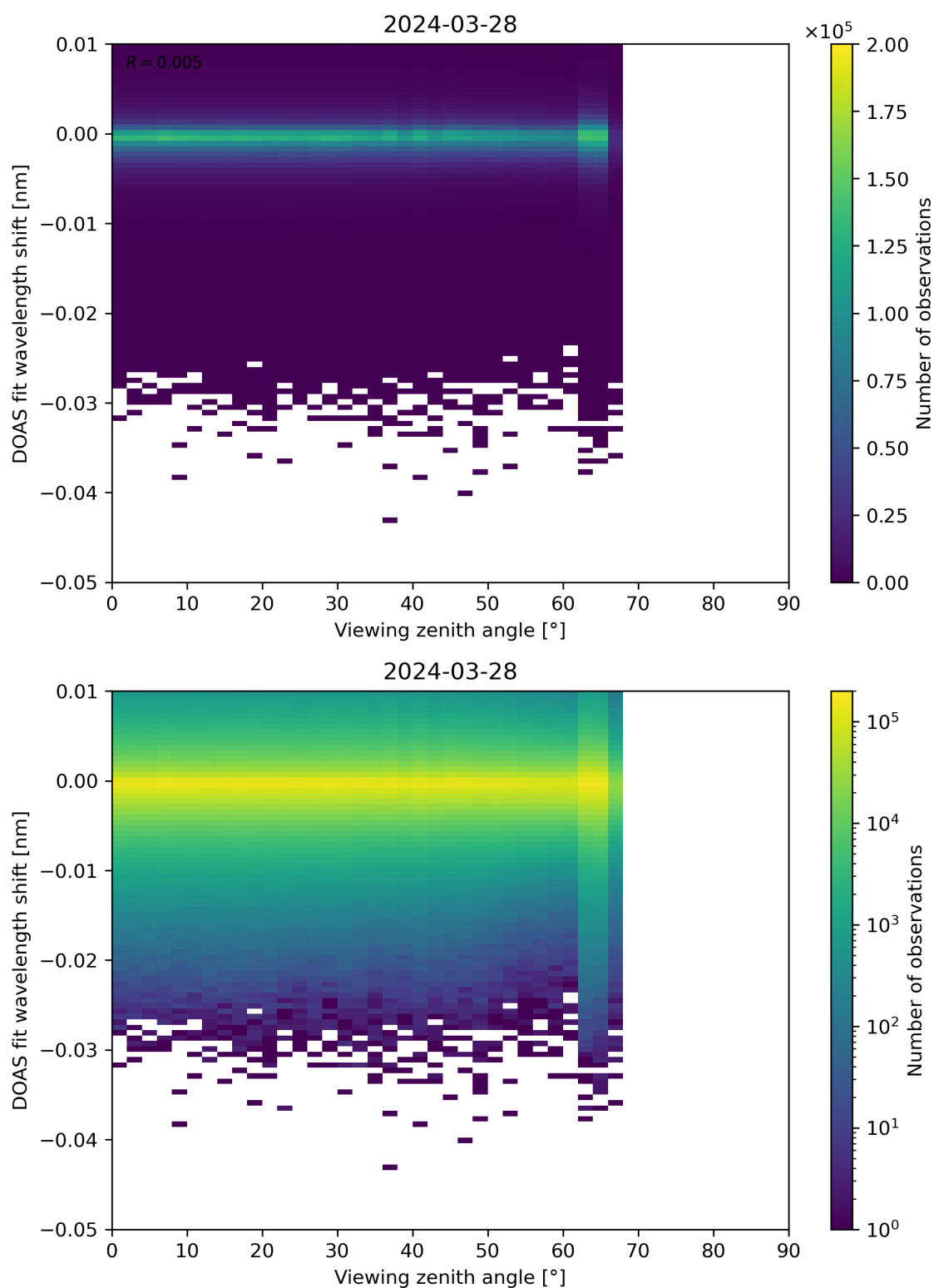
Figure 311: Scatter density plot of “Viewing zenith angle” against “DOAS fit wavelength shift” for 2024-03-27 to 2024-03-29.
