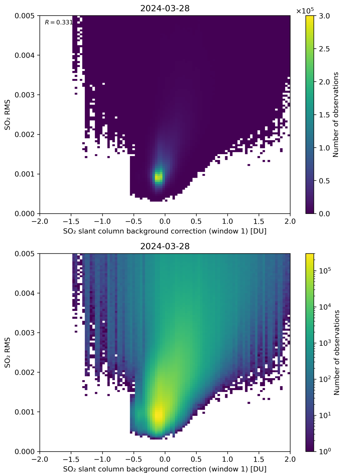
Figure 102: Scatter density plot of “SO 2 slant column background correction (window 1)” against “SO 2 RMS” for 2024-03-27 to 2024-03-29.
