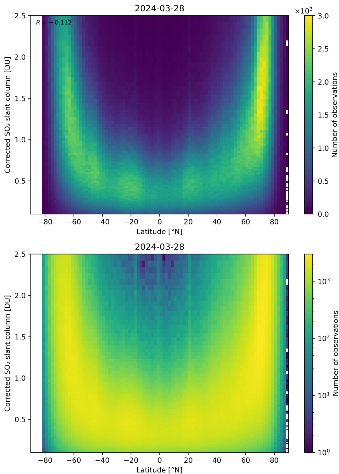
Figure 146: Scatter density plot of “Latitude” against “Corrected SO 2 slant column” for 2024-03-27 to 2024-03-29.
