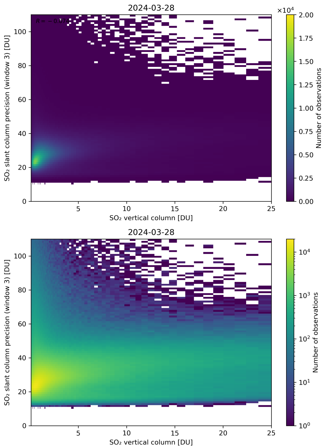
Figure 304: Scatter density plot of “SO 2 vertical column” against “SO 2 slant column precision (window 3)” for 2024-03-27 to 2024-03-29.
