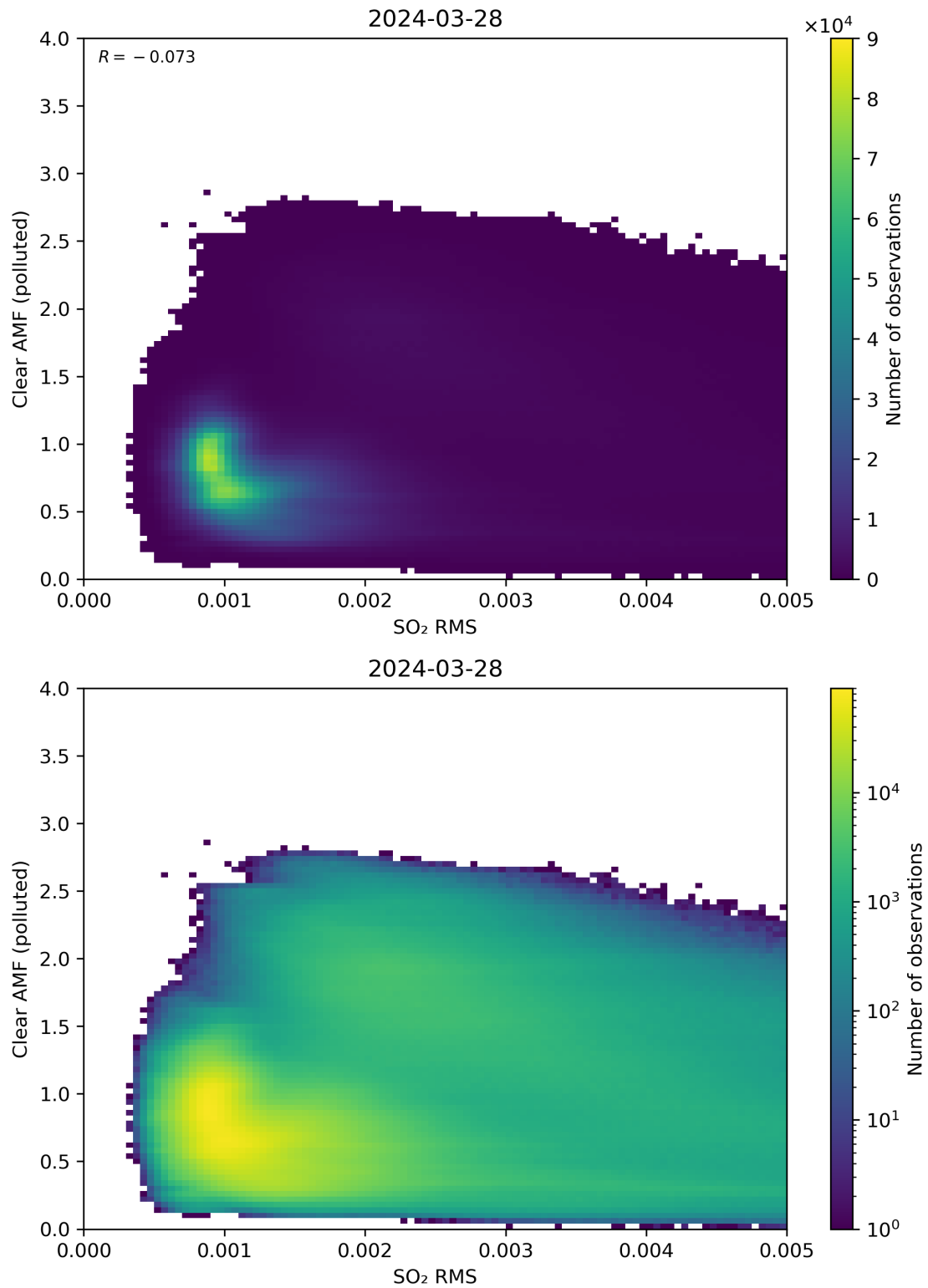
Figure 136: Scatter density plot of “SO 2 RMS” against “Clear AMF (polluted)” for 2024-03-27 to 2024-03-29.
