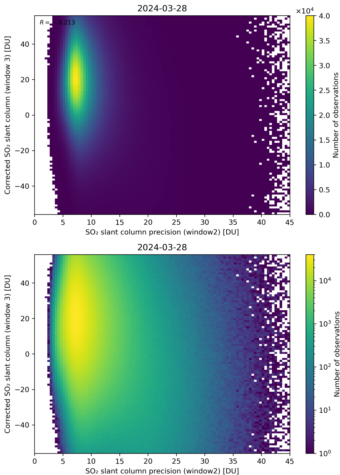
Figure 248: Scatter density plot of “SO 2 slant column precision (window2)” against “Corrected SO 2 slant column (window 3)” for 2024-03-27 to 2024-03-29.
