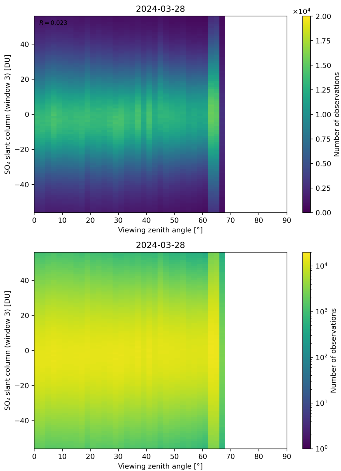
Figure 323: Scatter density plot of “Viewing zenith angle” against “SO 2 slant column (window 3)” for 2024-03-27 to 2024-03-29.
