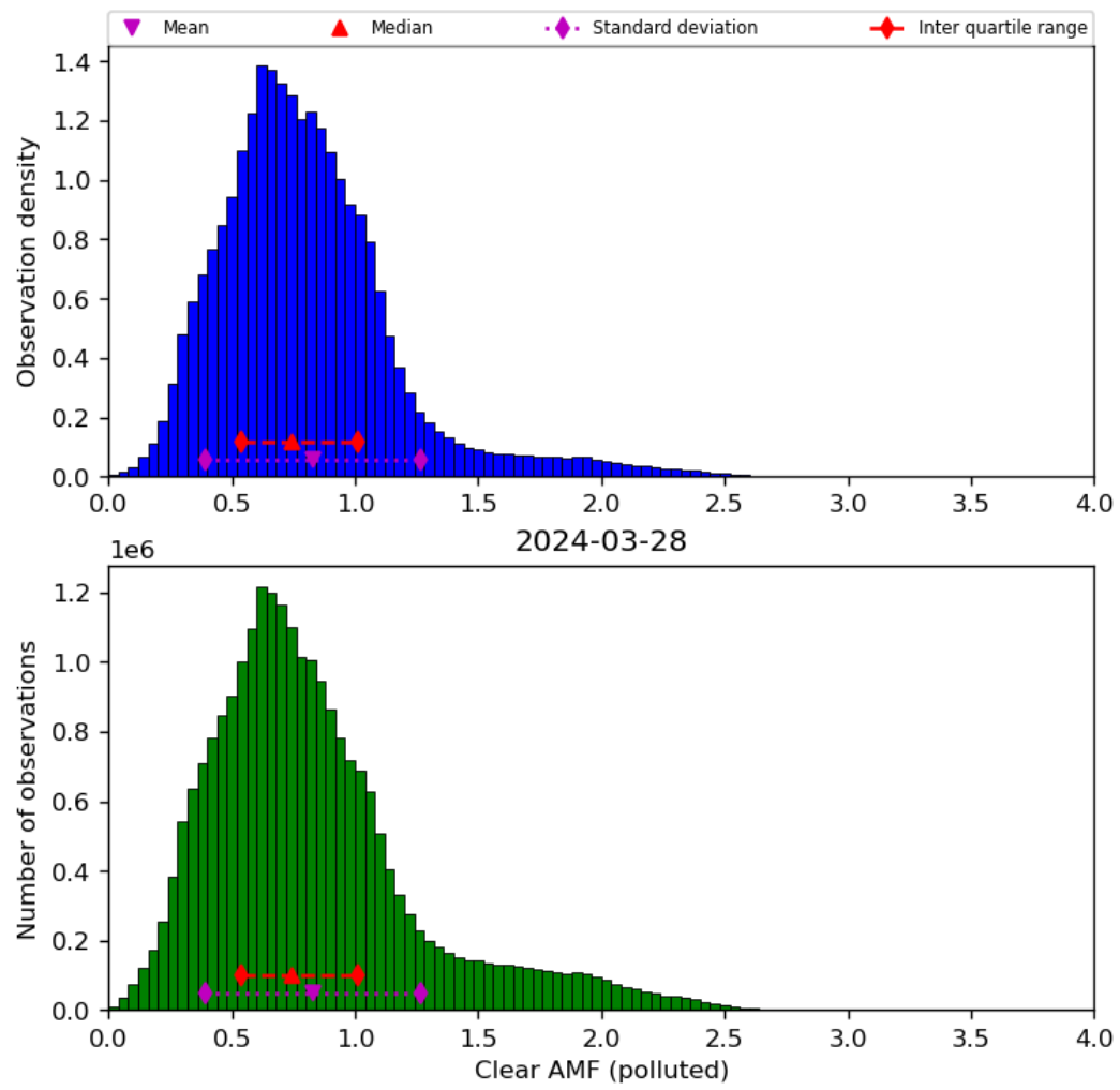
Figure 73: Histogram of “Clear AMF (polluted)” for 2024-03-27 to 2024-03-29
