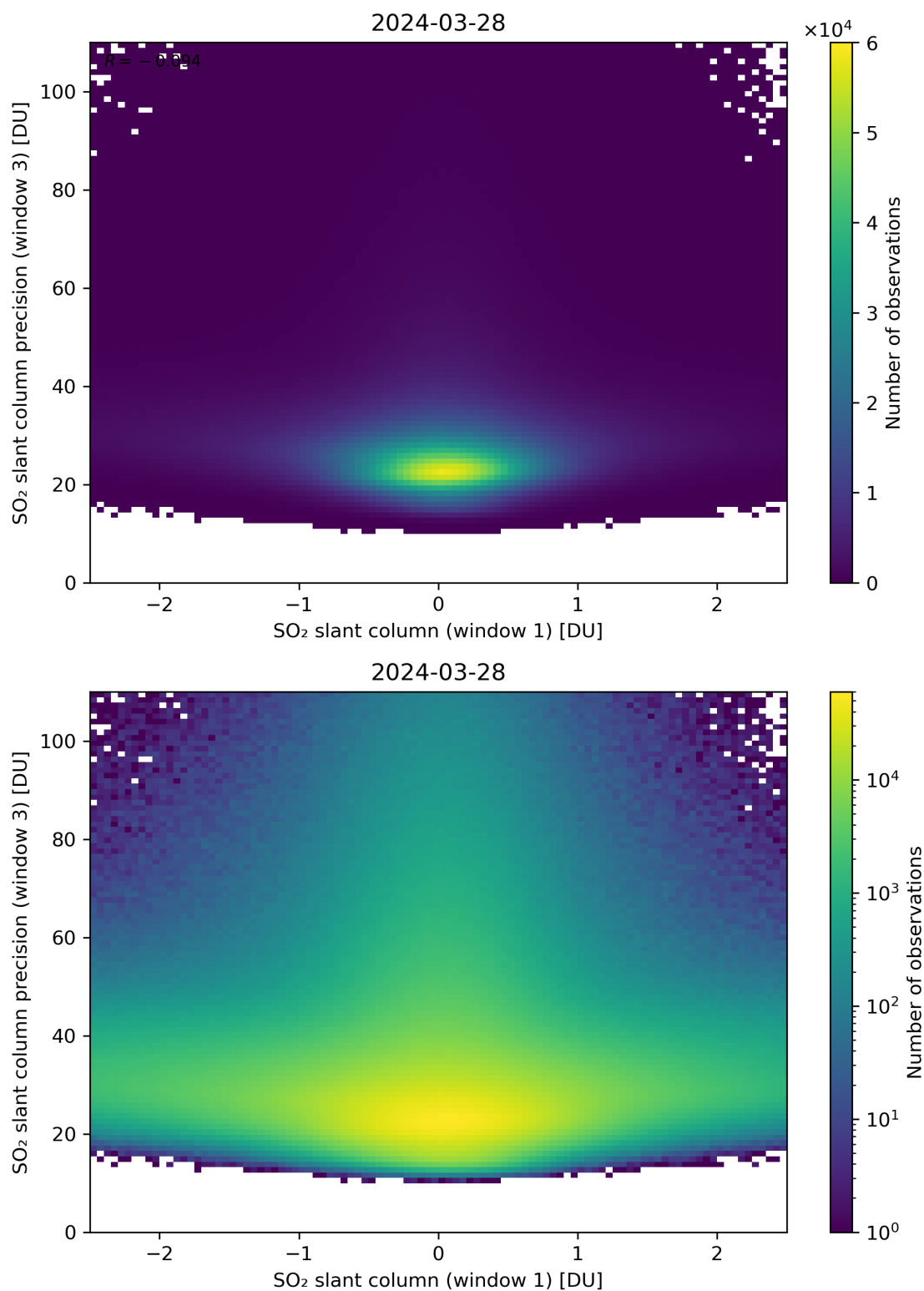
Figure 238: Scatter density plot of “SO 2 slant column (window 1)” against “SO 2 slant column precision (window 3)” for 2024-03-27 to 2024-03-29.
