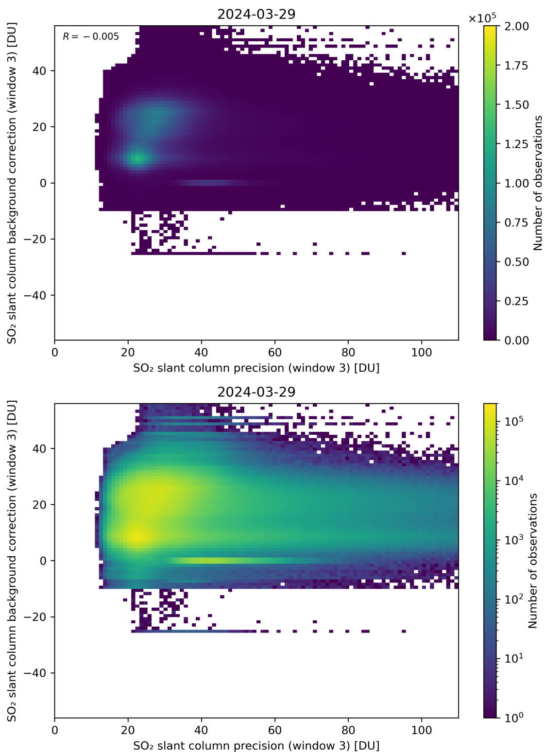
Figure 257: Scatter density plot of “SO 2 slant column precision (window 3)” against “SO 2 slant column background correction (window 3)” for 2024-03-28 to 2024-03-30.
