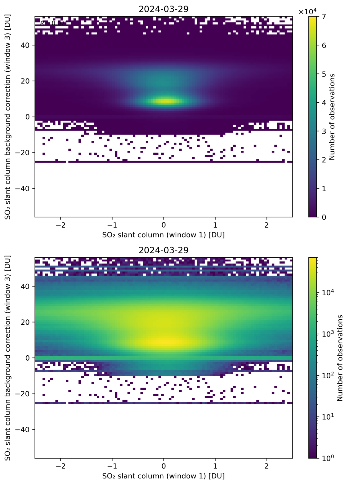
Figure 214: Scatter density plot of “SO 2 slant column (window 1)” against “SO 2 slant column background correction (window 3)” for 2024-03-28 to 2024-03-30.
