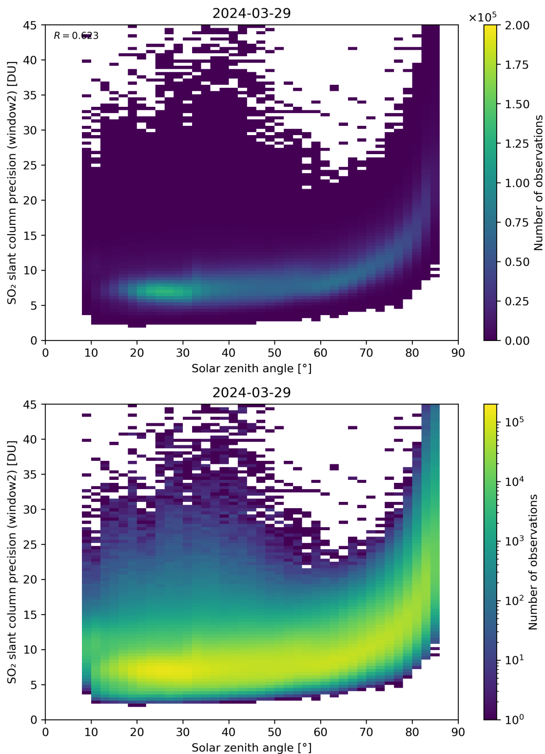
Figure 171: Scatter density plot of “Solar zenith angle” against “SO 2 slant column precision (window2)” for 2024-03-28 to 2024-03-30.
