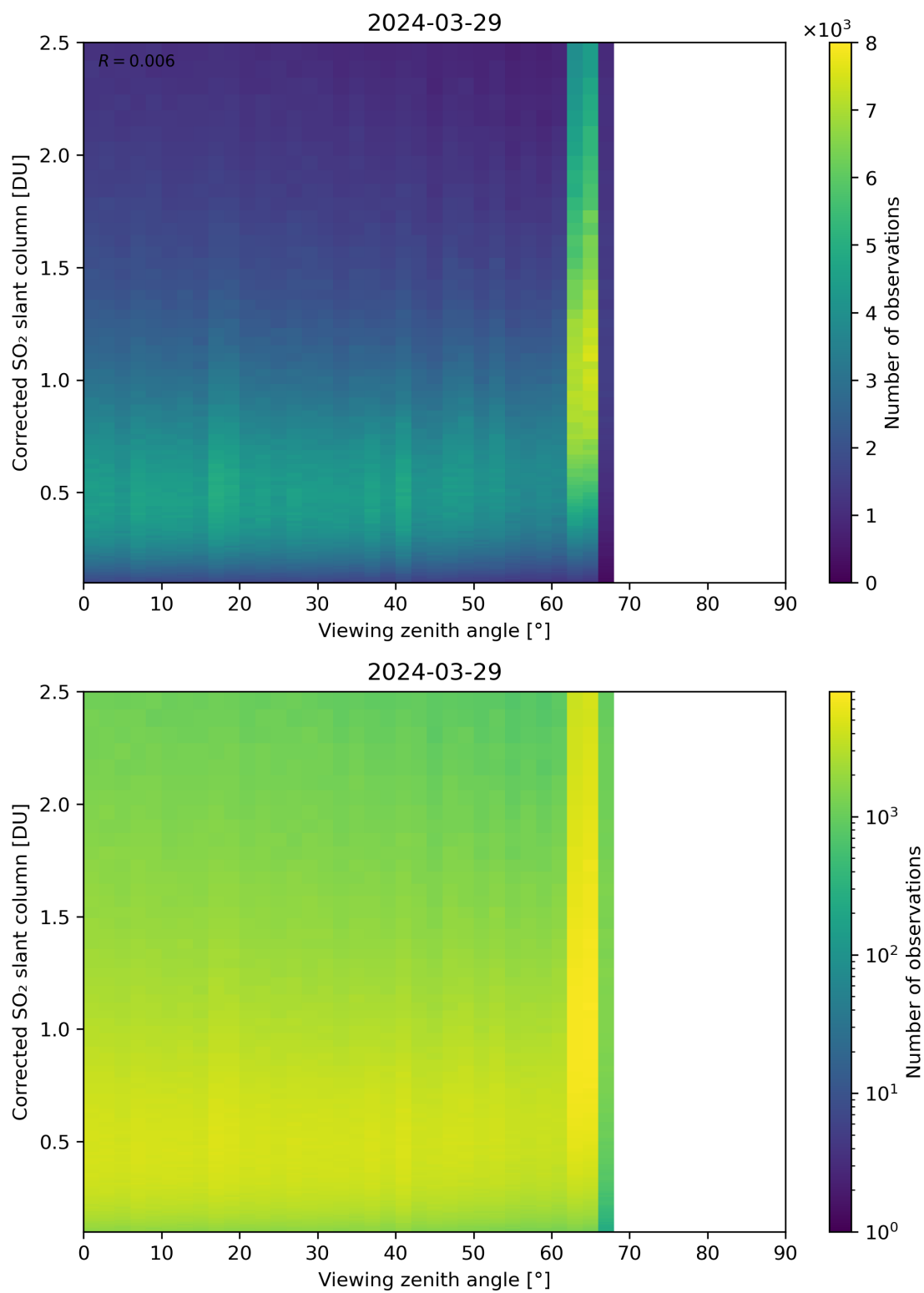
Figure 317: Scatter density plot of “Viewing zenith angle” against “Corrected SO 2 slant column” for 2024-03-28 to 2024-03-30.
