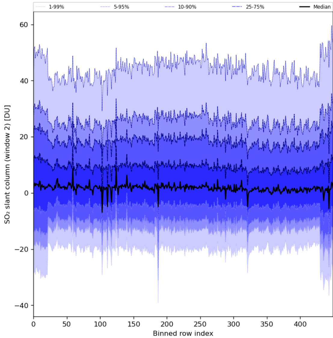
Figure 83: Along track statistics of “SO 2 slant column (window 2)” for 2024-03-28 to 2024-03-30
