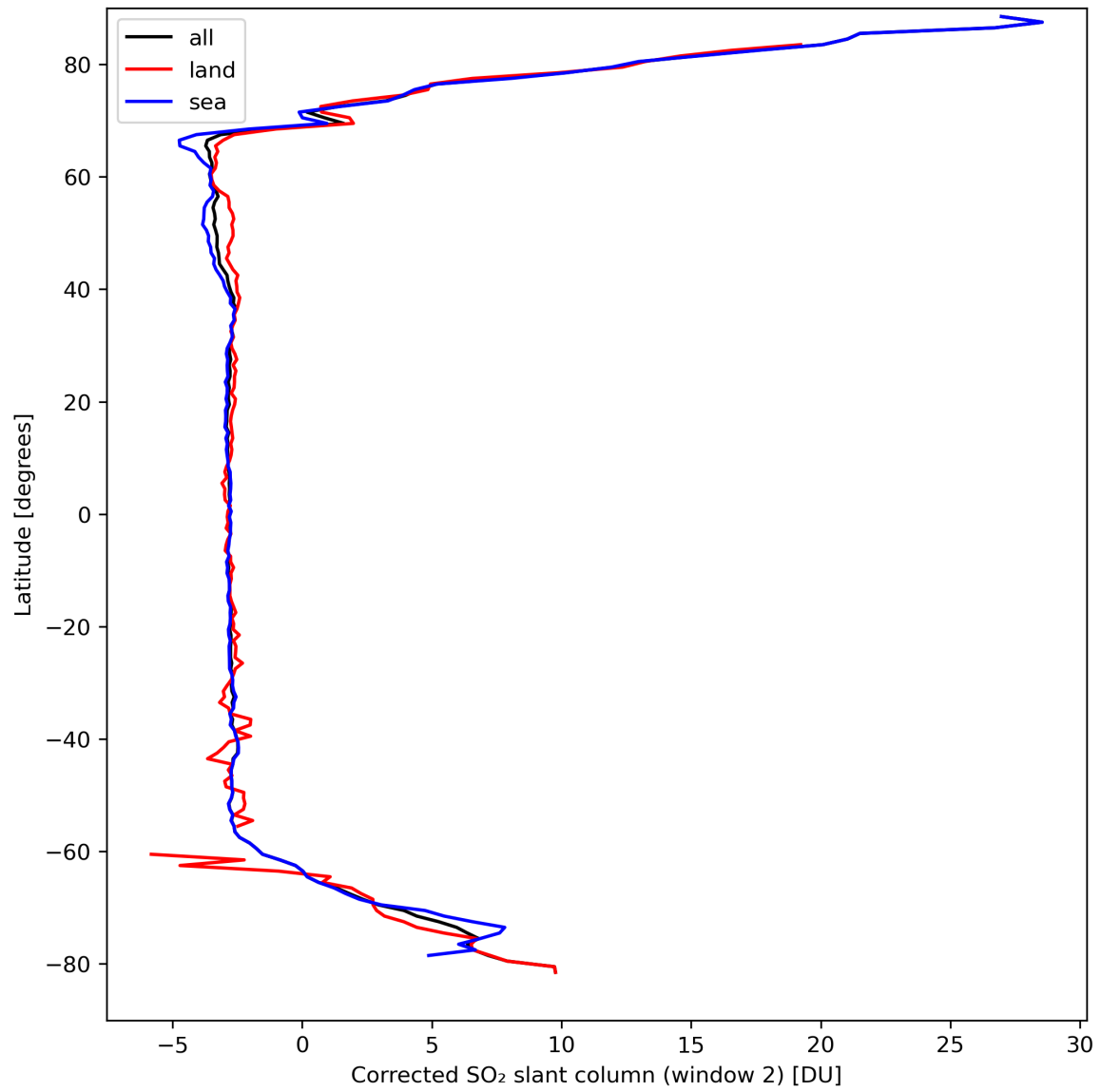
Figure 39: Zonal average of “Corrected SO 2 slant column (window 2)” for 2024-03-28 to 2024-03-30.
