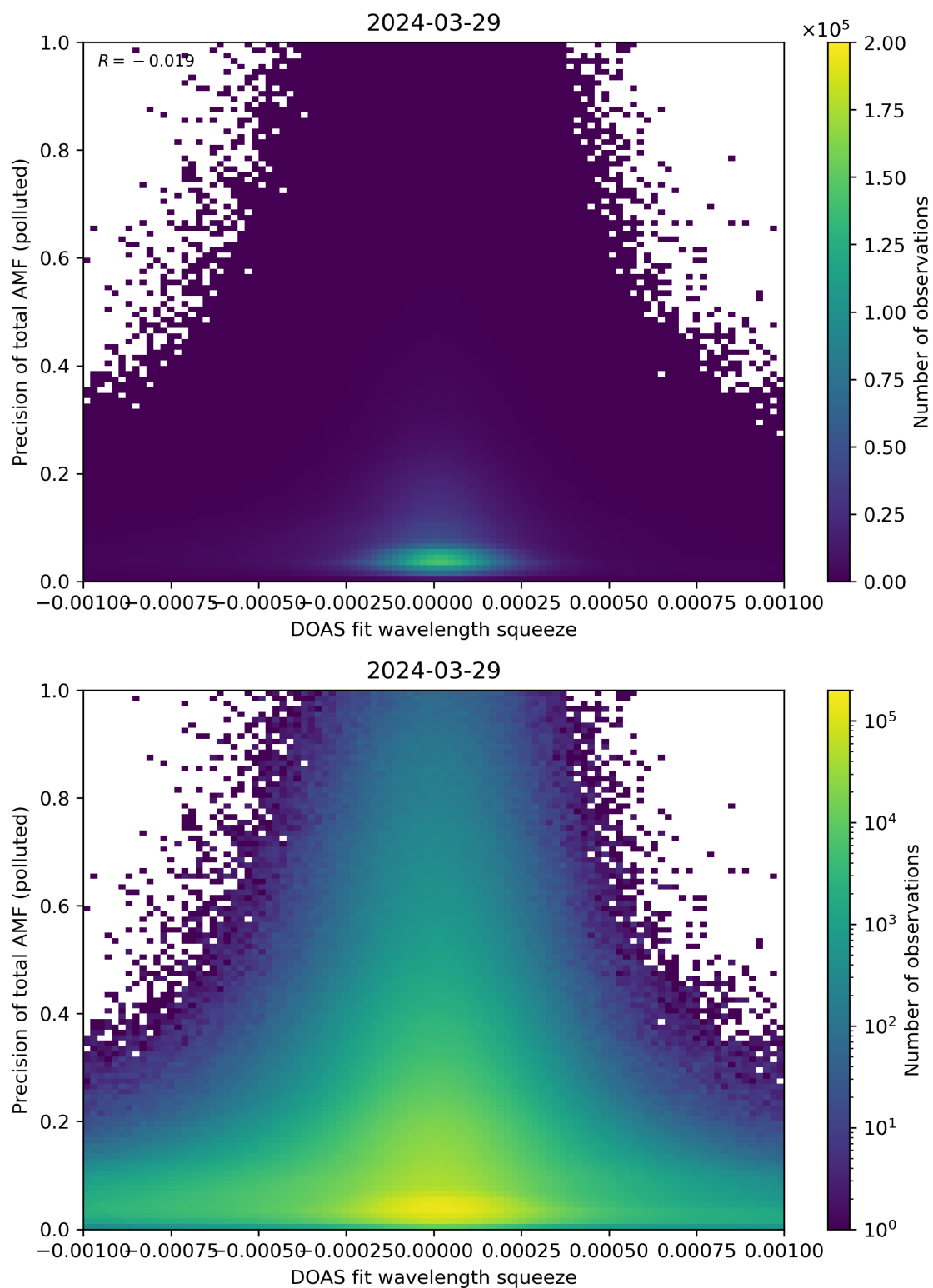
Figure 135: Scatter density plot of “DOAS fit wavelength squeeze” against “Precision of total AMF (polluted)” for 2024-03-28 to 2024-03-30.
