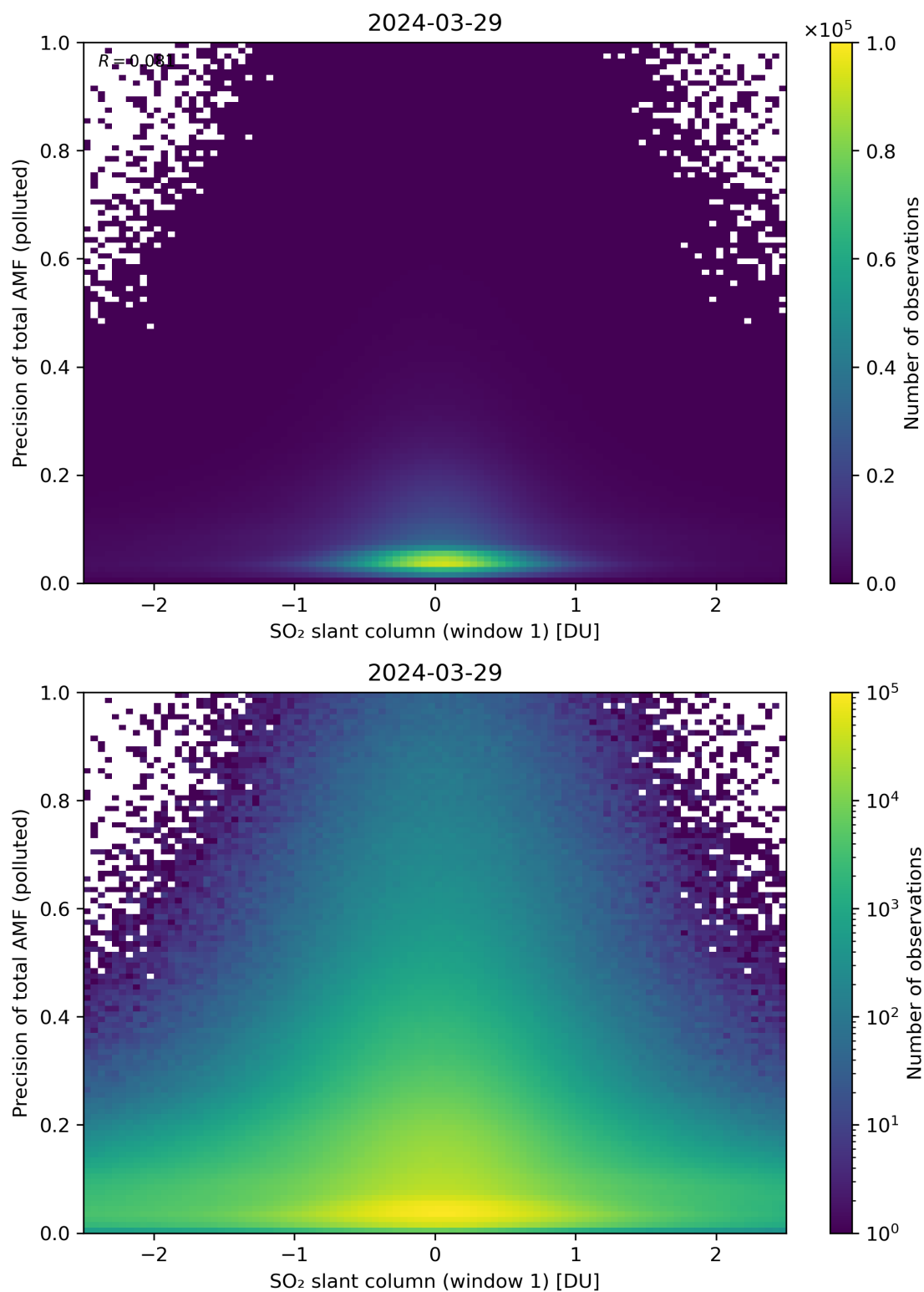
Figure 240: Scatter density plot of “SO 2 slant column (window 1)” against “Precision of total AMF (polluted)” for 2024-03-28 to 2024-03-30.
