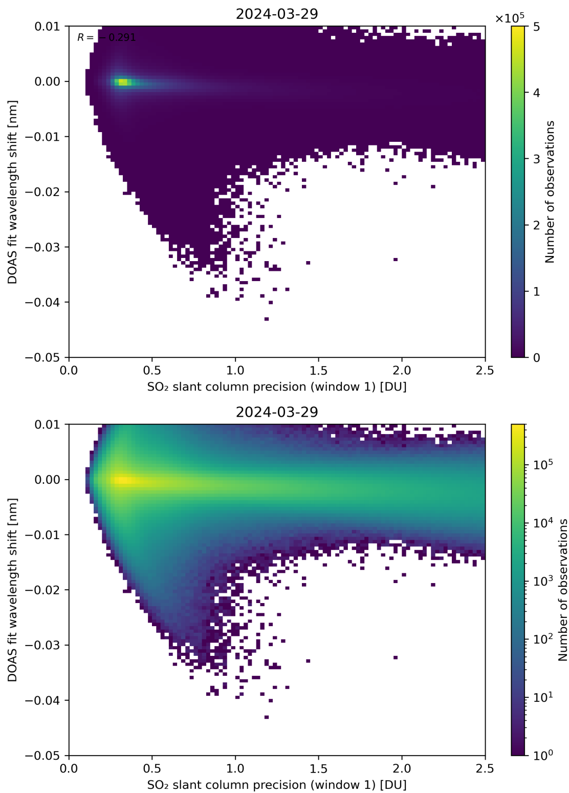
Figure 221: Scatter density plot of “SO 2 slant column precision (window 1)” against “DOAS fit wavelength shift” for 2024-03-28 to 2024-03-30.
