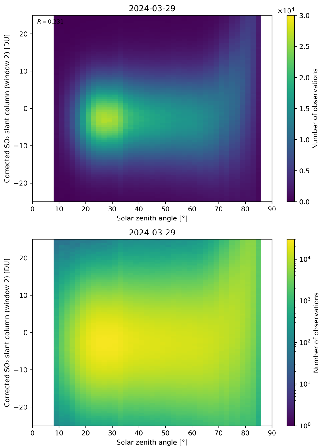
Figure 167: Scatter density plot of “Solar zenith angle” against “Corrected SO 2 slant column (window 2)” for 2024-03-28 to 2024-03-30.
