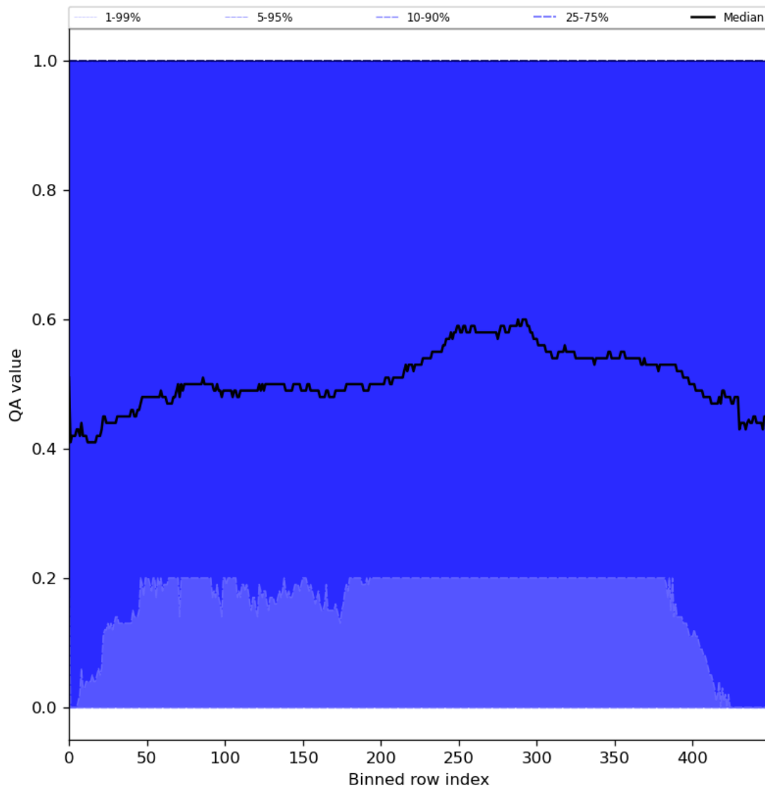
Figure 75: Along track statistics of “QA value” for 2024-03-28 to 2024-03-30
