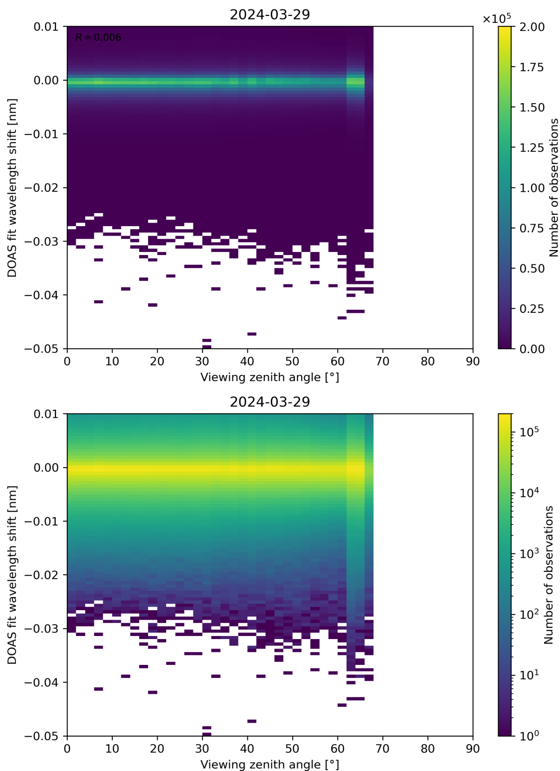
Figure 311: Scatter density plot of “Viewing zenith angle” against “DOAS fit wavelength shift” for 2024-03-28 to 2024-03-30.
