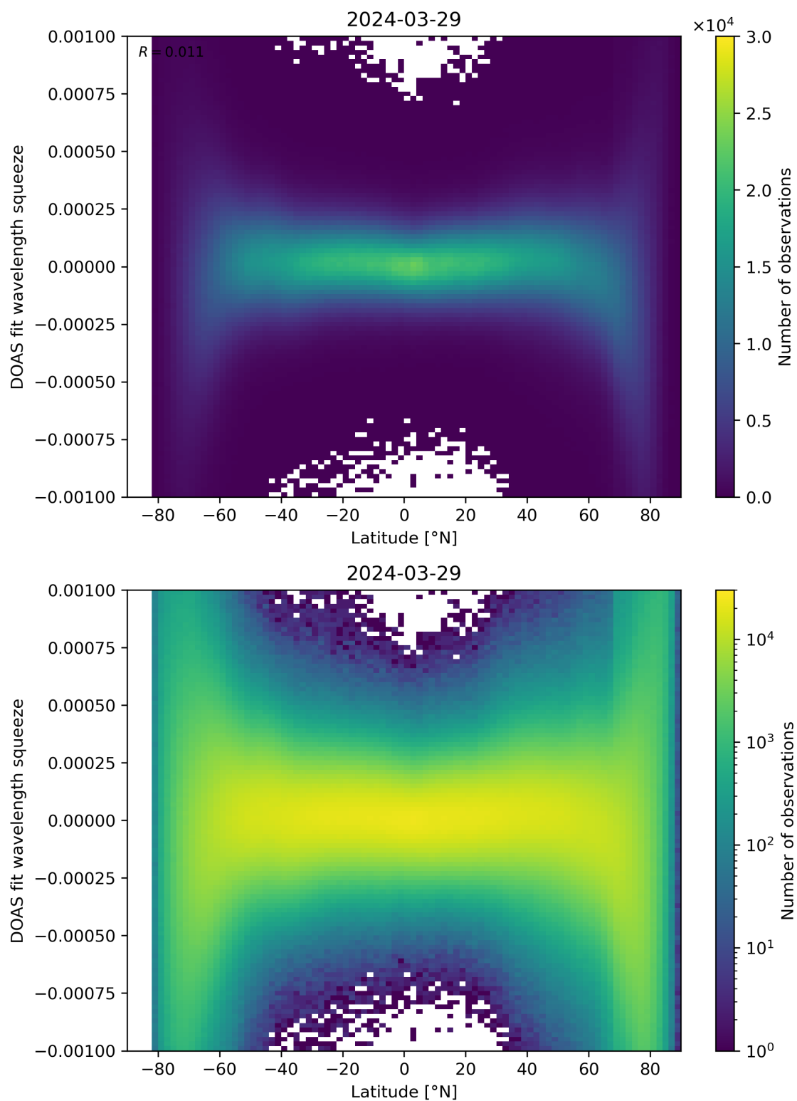
Figure 143: Scatter density plot of “Latitude” against “DOAS fit wavelength squeeze” for 2024-03-28 to 2024-03-30.
