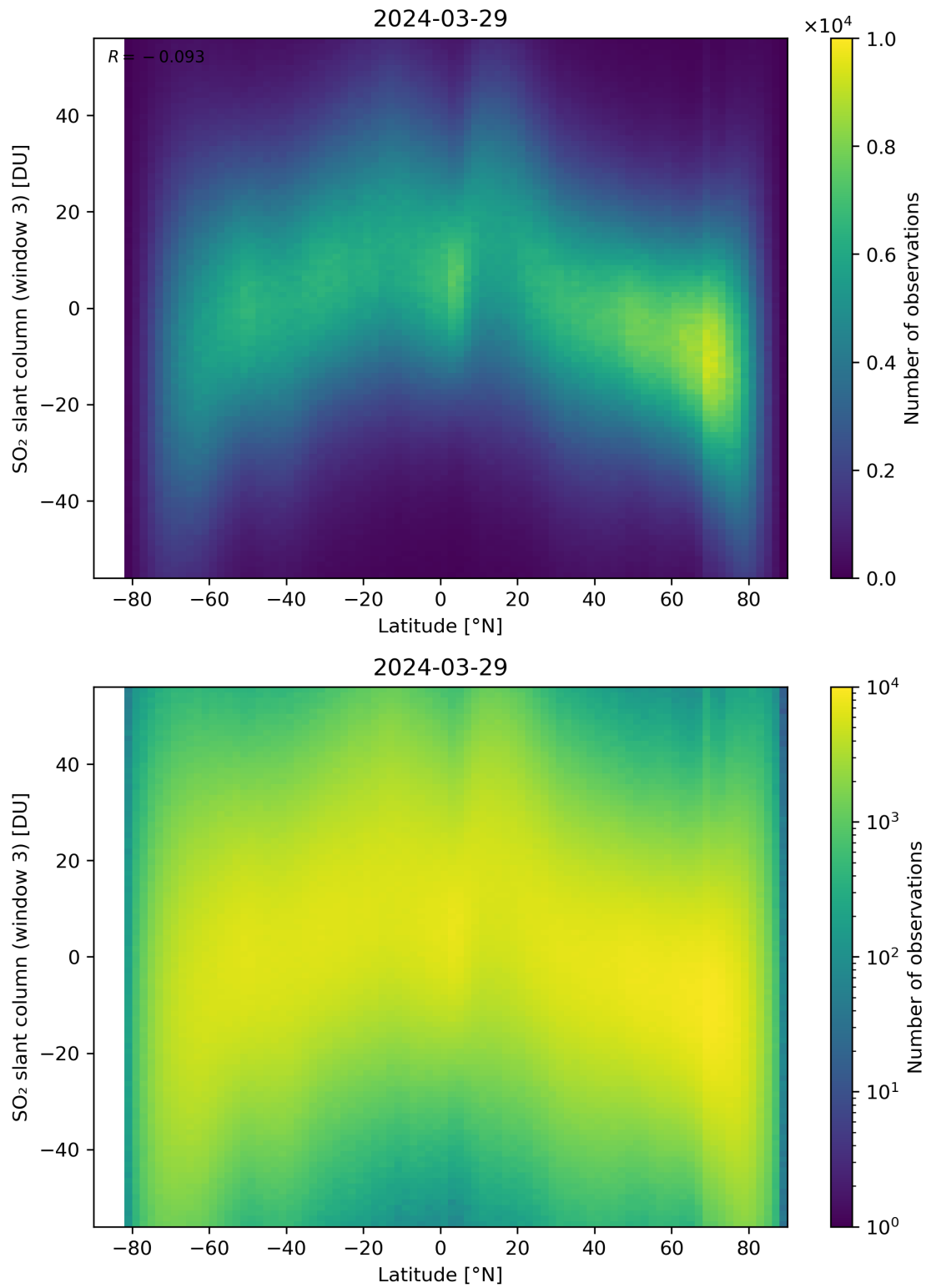
Figure 152: Scatter density plot of “Latitude” against “SO 2 slant column (window 3)” for 2024-03-28 to 2024-03-30.
