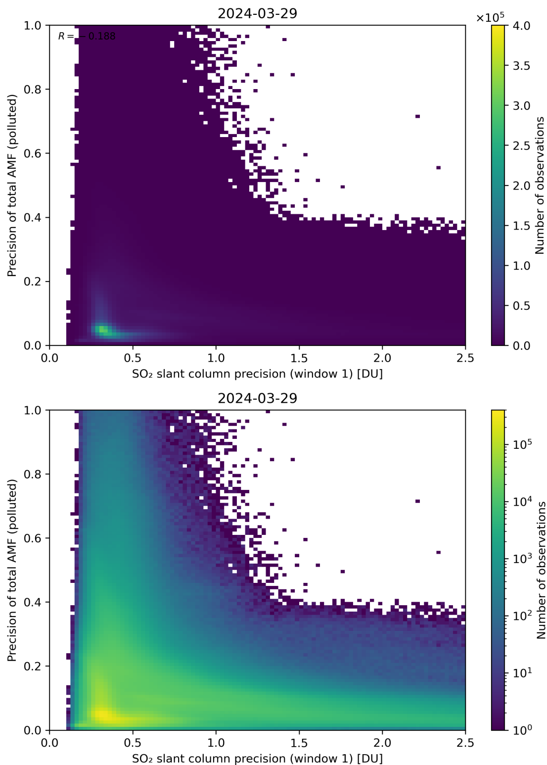
Figure 231: Scatter density plot of “SO 2 slant column precision (window 1)” against “Precision of total AMF (polluted)” for 2024-03-28 to 2024-03-30.
