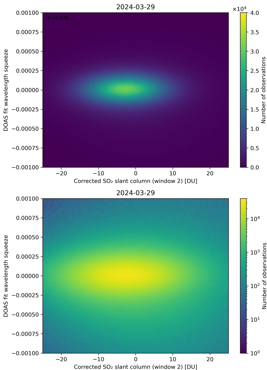
Figure 197: Scatter density plot of “Corrected SO 2 slant column (window 2)” against “DOAS fit wavelength squeeze” for 2024-03-28 to 2024-03-30.
