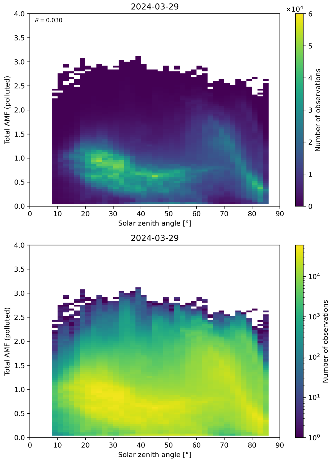
Figure 174: Scatter density plot of “Solar zenith angle” against “Total AMF (polluted)” for 2024-03-28 to 2024-03-30.
