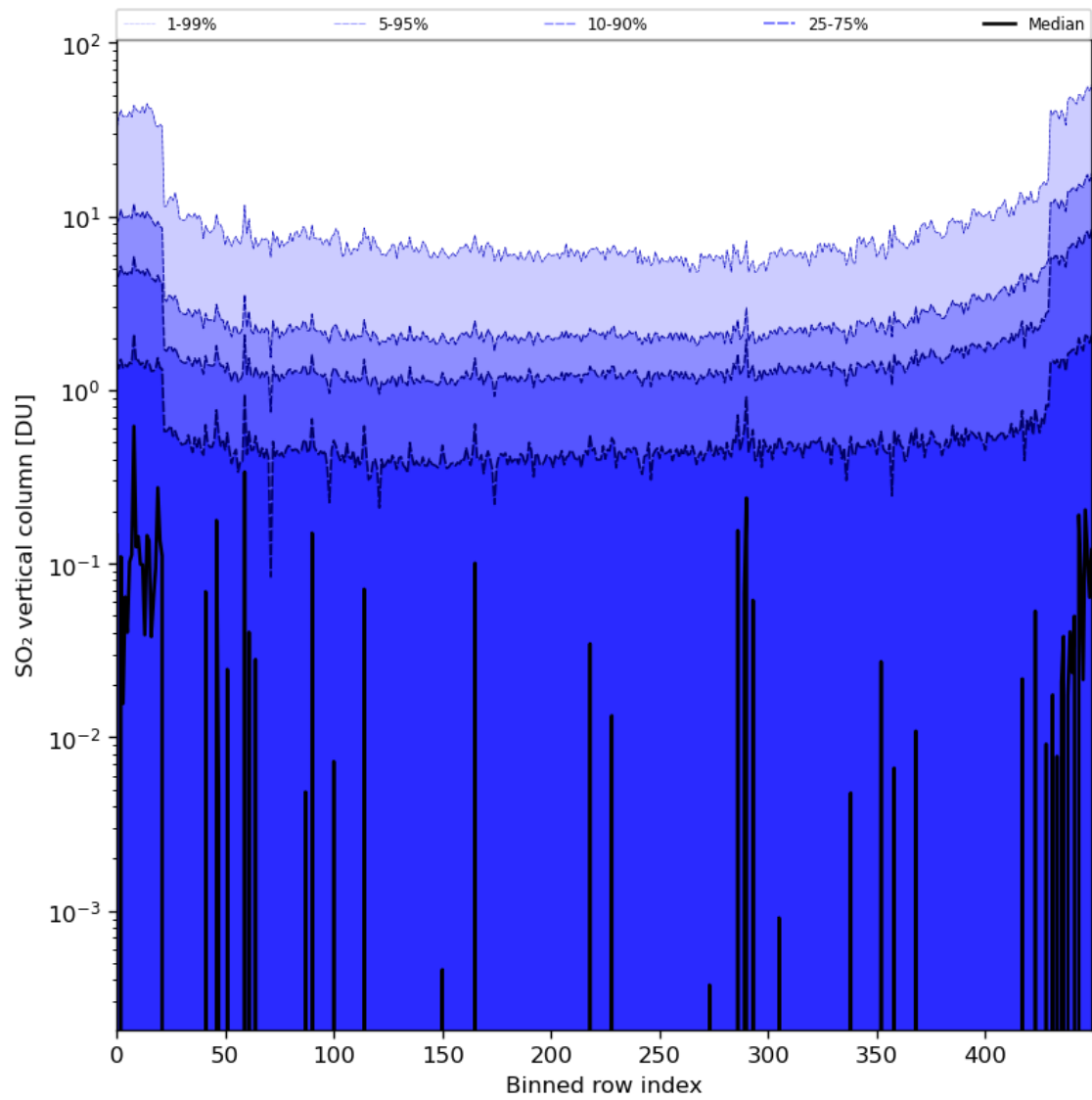
Figure 76: Along track statistics of “SO 2 vertical column” for 2024-03-28 to 2024-03-30
