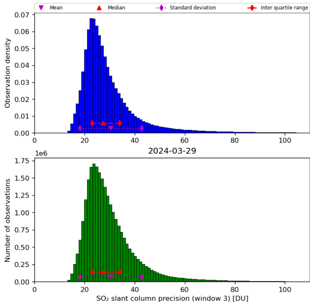
Figure 65: Histogram of “SO 2 slant column precision (window 3)” for 2024-03-28 to 2024-03-30
