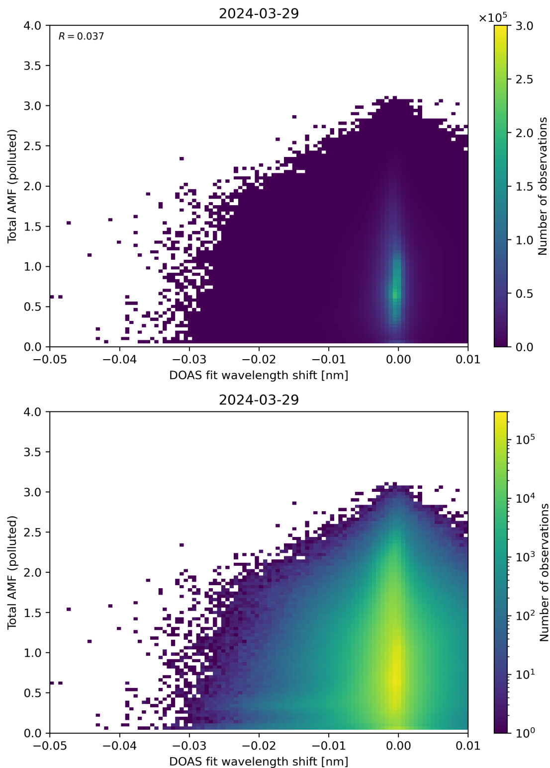
Figure 130: Scatter density plot of “DOAS fit wavelength shift” against “Total AMF (polluted)” for 2024-03-28 to 2024-03-30.
