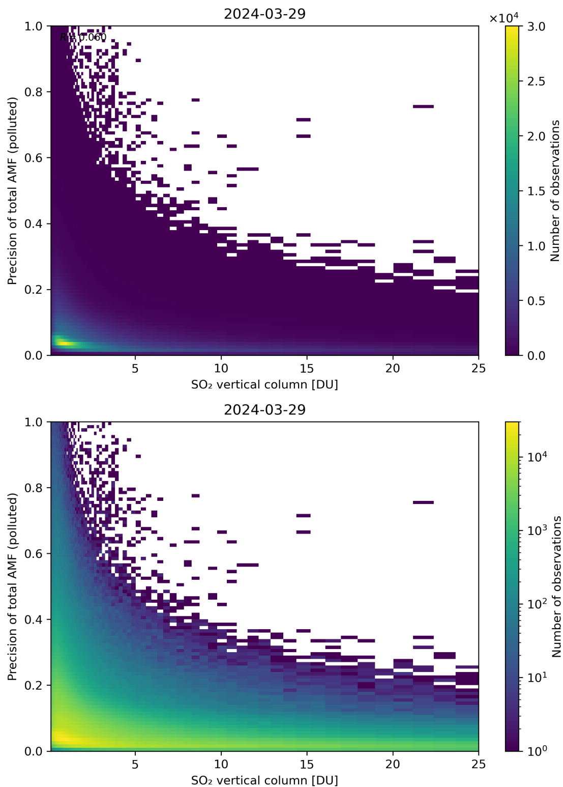
Figure 306: Scatter density plot of “SO 2 vertical column” against “Precision of total AMF (polluted)” for 2024-03-28 to 2024-03-30.
