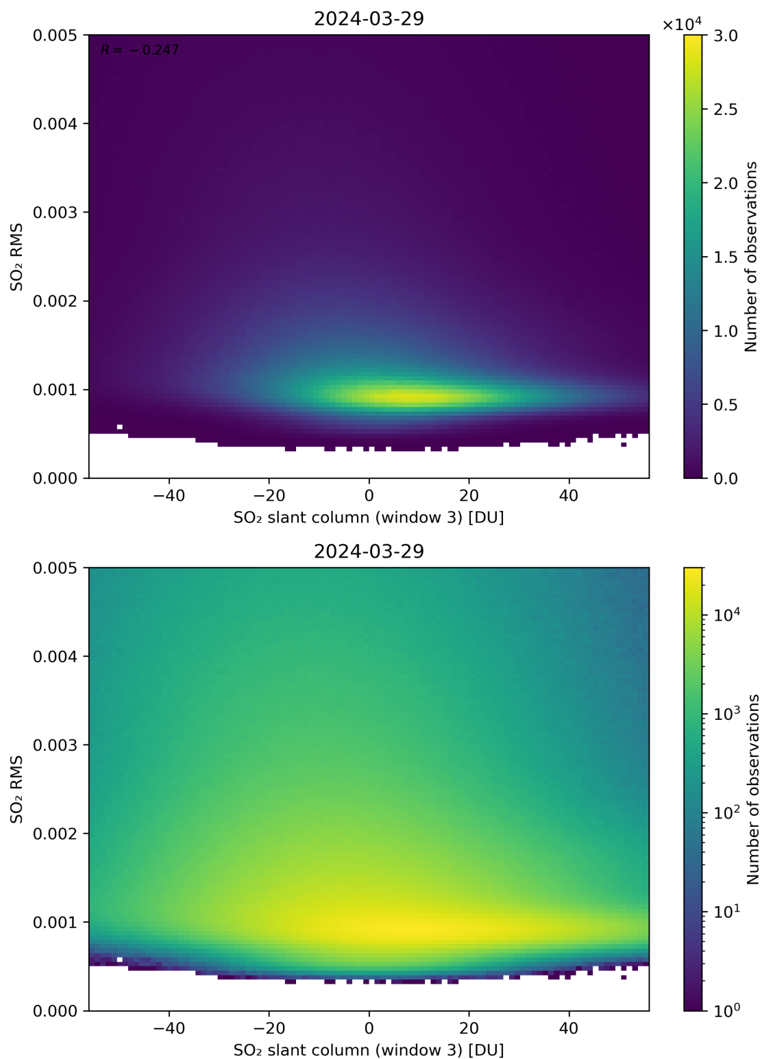
Figure 256: Scatter density plot of “SO 2 slant column (window 3)” against “SO 2 RMS” for 2024-03-28 to 2024-03-30.
