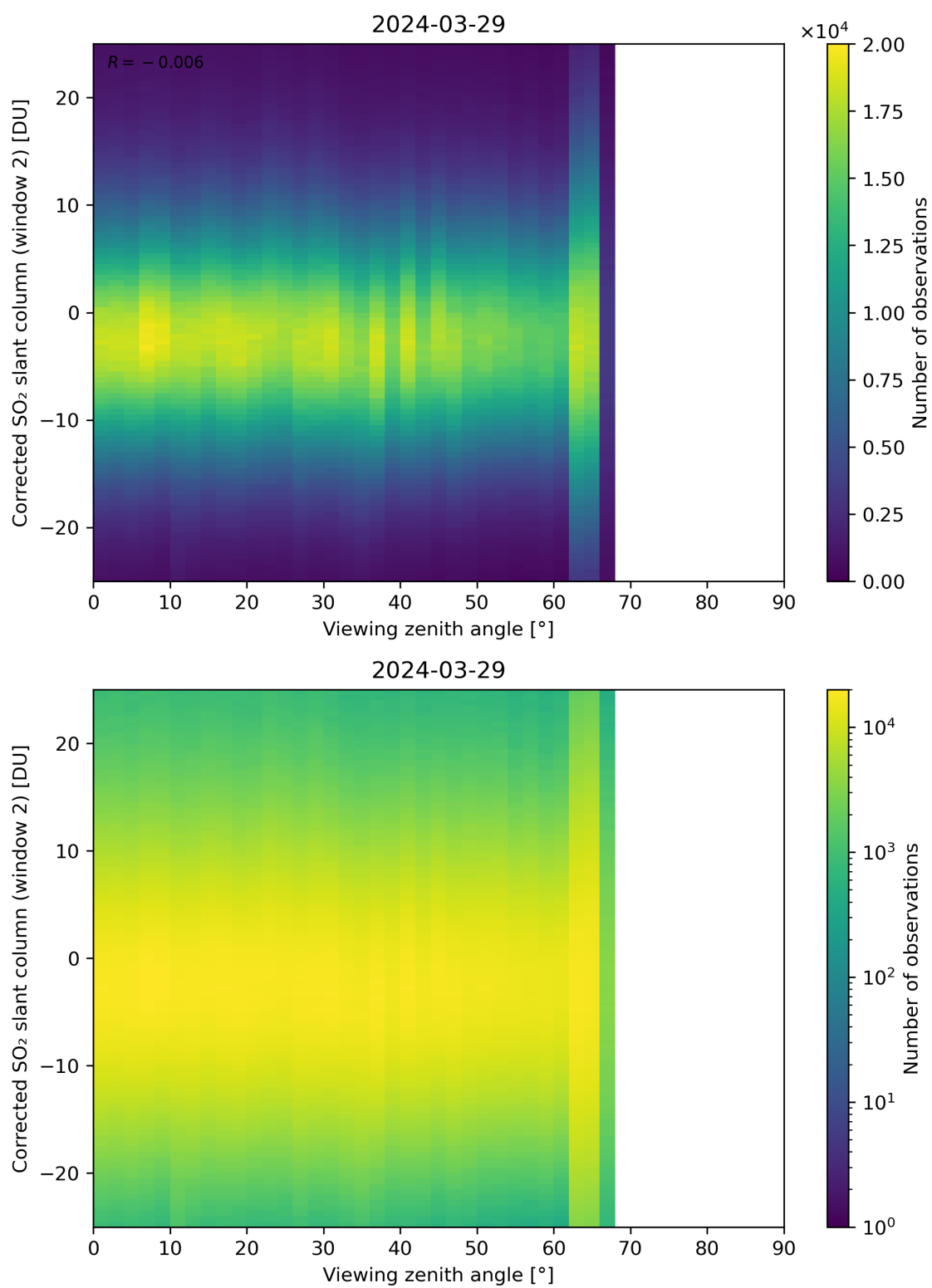
Figure 318: Scatter density plot of “Viewing zenith angle” against “Corrected SO 2 slant column (window 2)” for 2024-03-28 to 2024-03-30.
