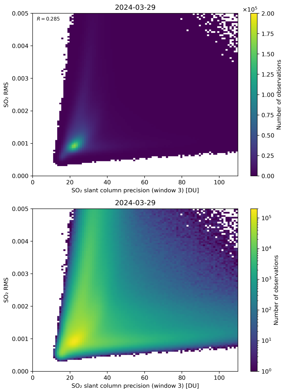
Figure 260: Scatter density plot of “SO 2 slant column precision (window 3)” against “SO 2 RMS” for 2024-03-28 to 2024-03-30.
