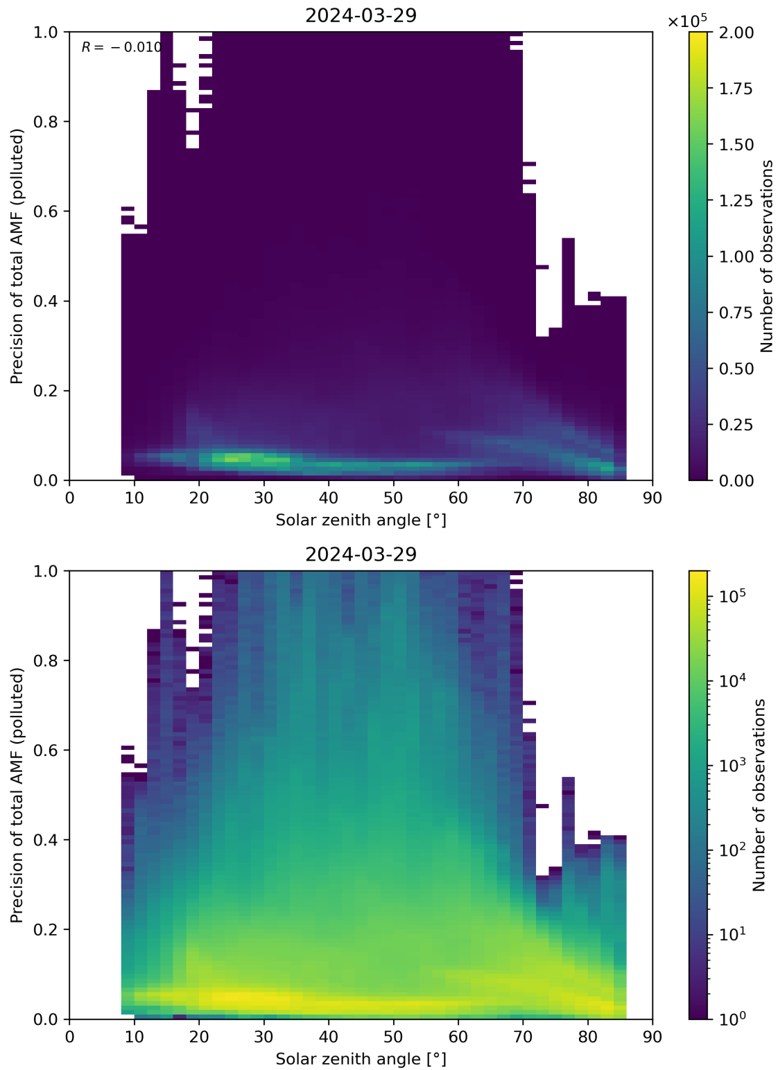
Figure 175: Scatter density plot of “Solar zenith angle” against “Precision of total AMF (polluted)” for 2024-03-28 to 2024-03-30.
