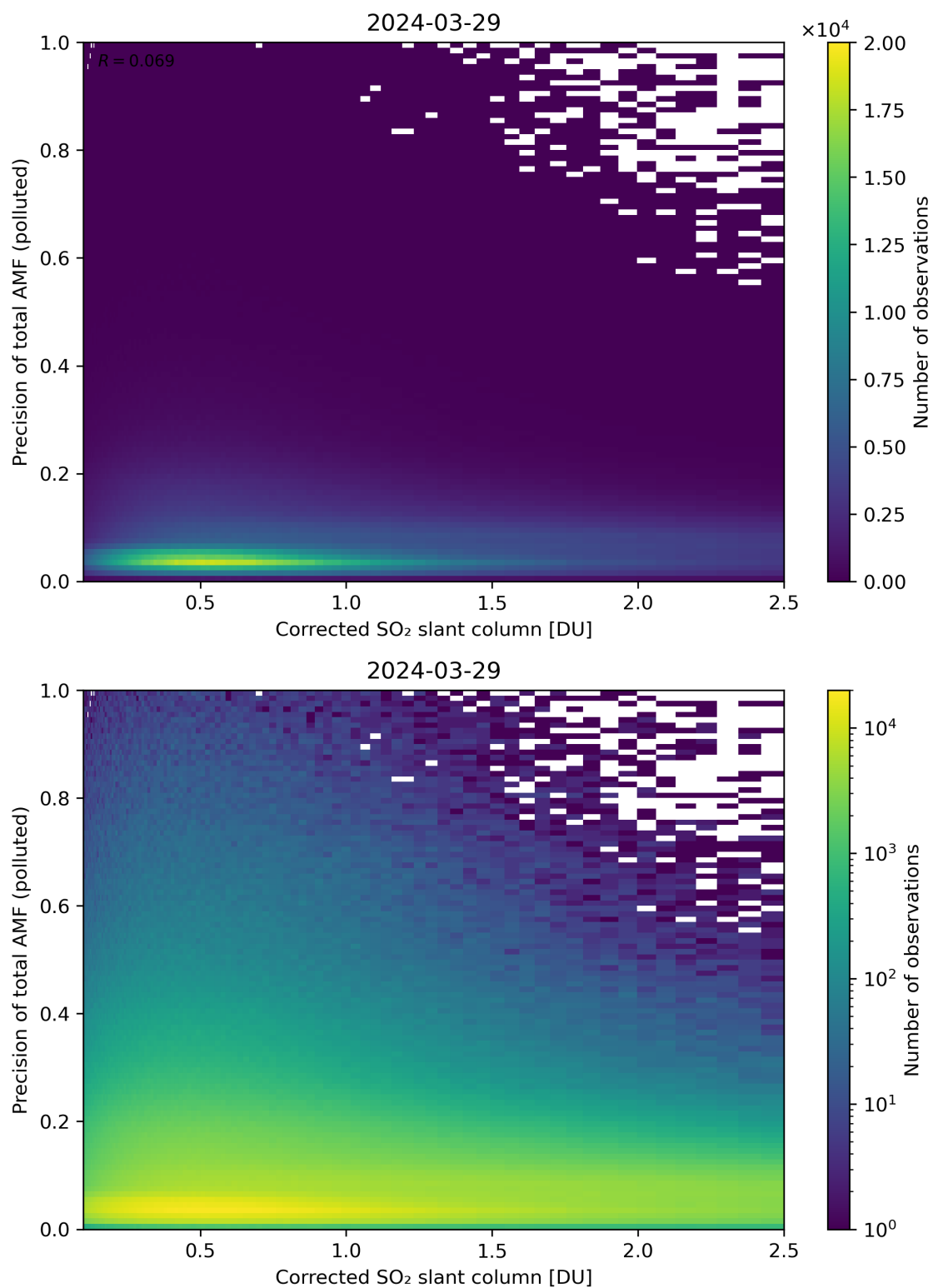
Figure 193: Scatter density plot of “Corrected SO 2 slant column” against “Precision of total AMF (polluted)” for 2024-03-28 to 2024-03-30.
