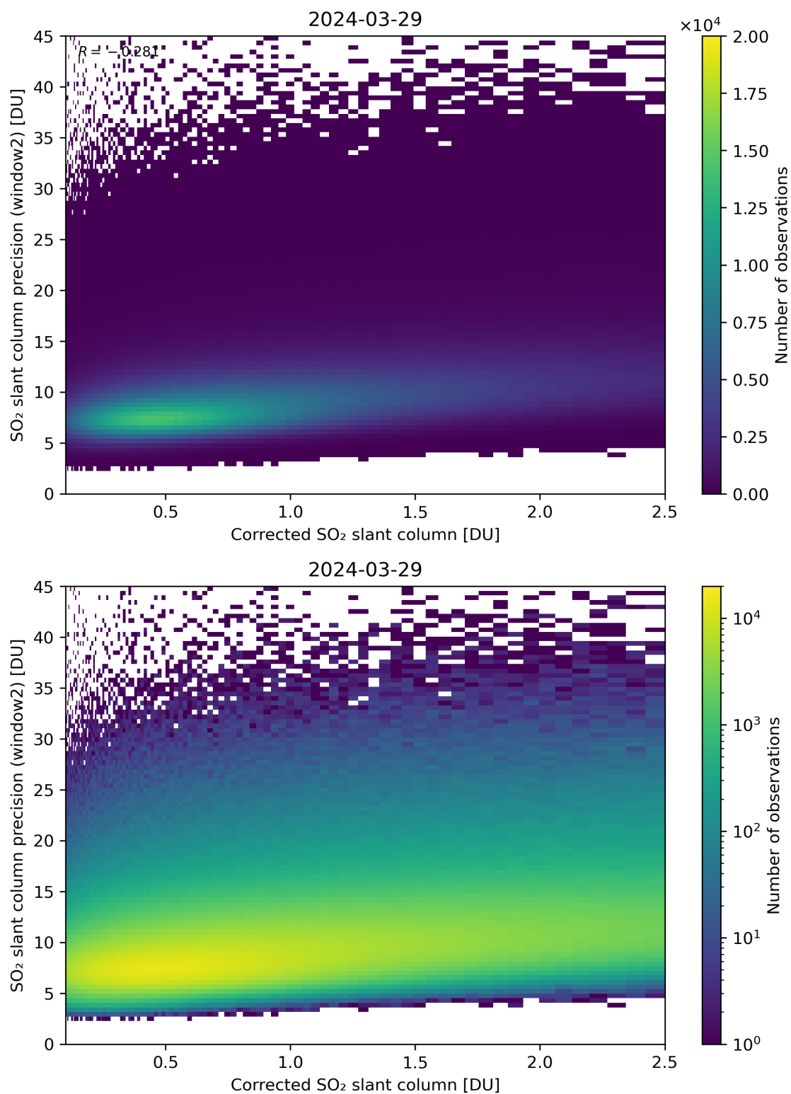
Figure 189: Scatter density plot of “Corrected SO 2 slant column” against “SO 2 slant column precision (window2)” for 2024-03-28 to 2024-03-30.
