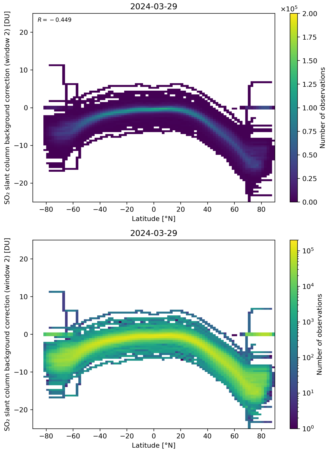
Figure 140: Scatter density plot of “Latitude” against “SO 2 slant column background correction (window 2)” for 2024-03-28 to 2024-03-30.
