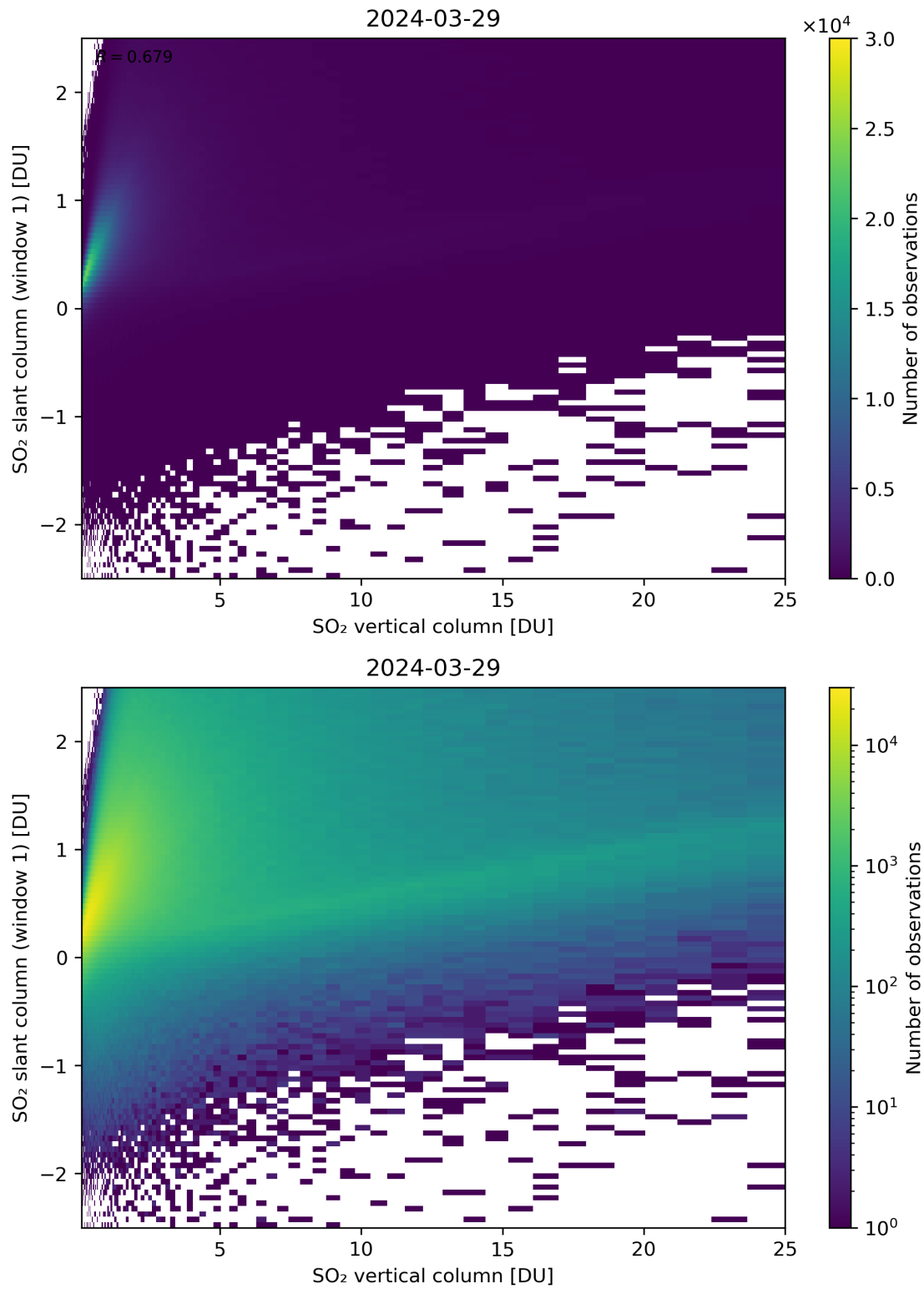
Figure 300: Scatter density plot of “SO 2 vertical column” against “SO 2 slant column (window 1)” for 2024-03-28 to 2024-03-30.
