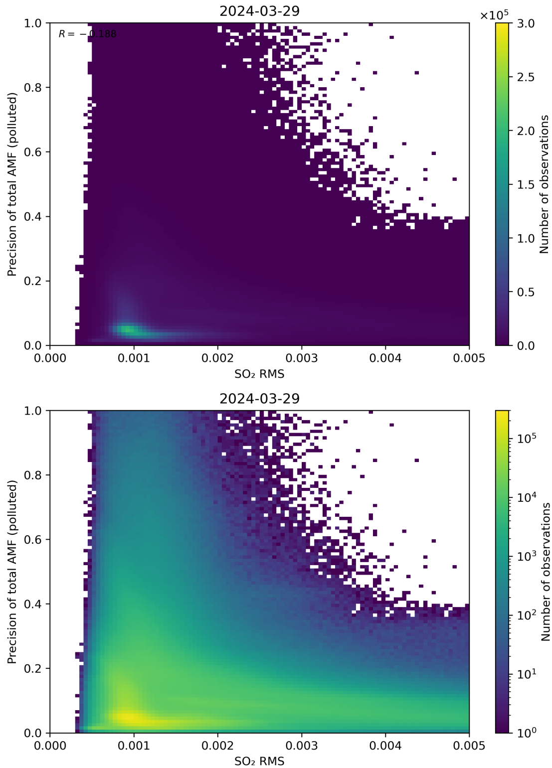
Figure 138: Scatter density plot of “SO 2 RMS” against “Precision of total AMF (polluted)” for 2024-03-28 to 2024-03-30.
