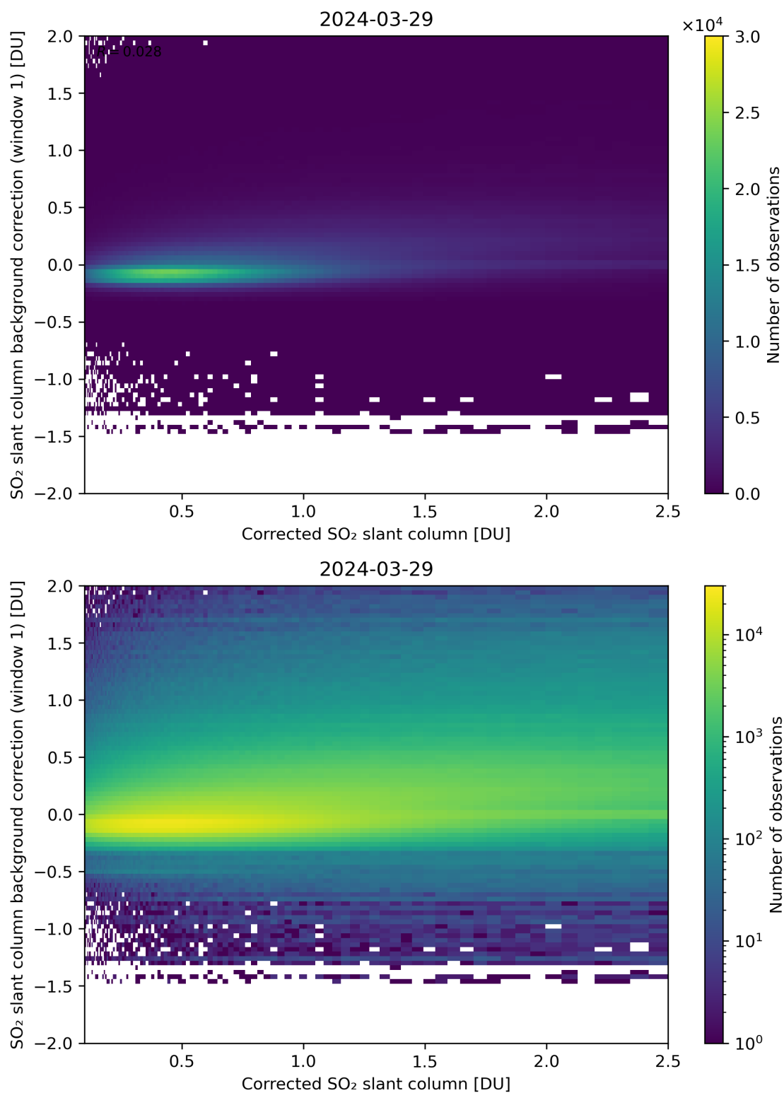
Figure 178: Scatter density plot of “Corrected SO 2 slant column” against “SO 2 slant column background correction (window 1)” for 2024-03-28 to 2024-03-30.
