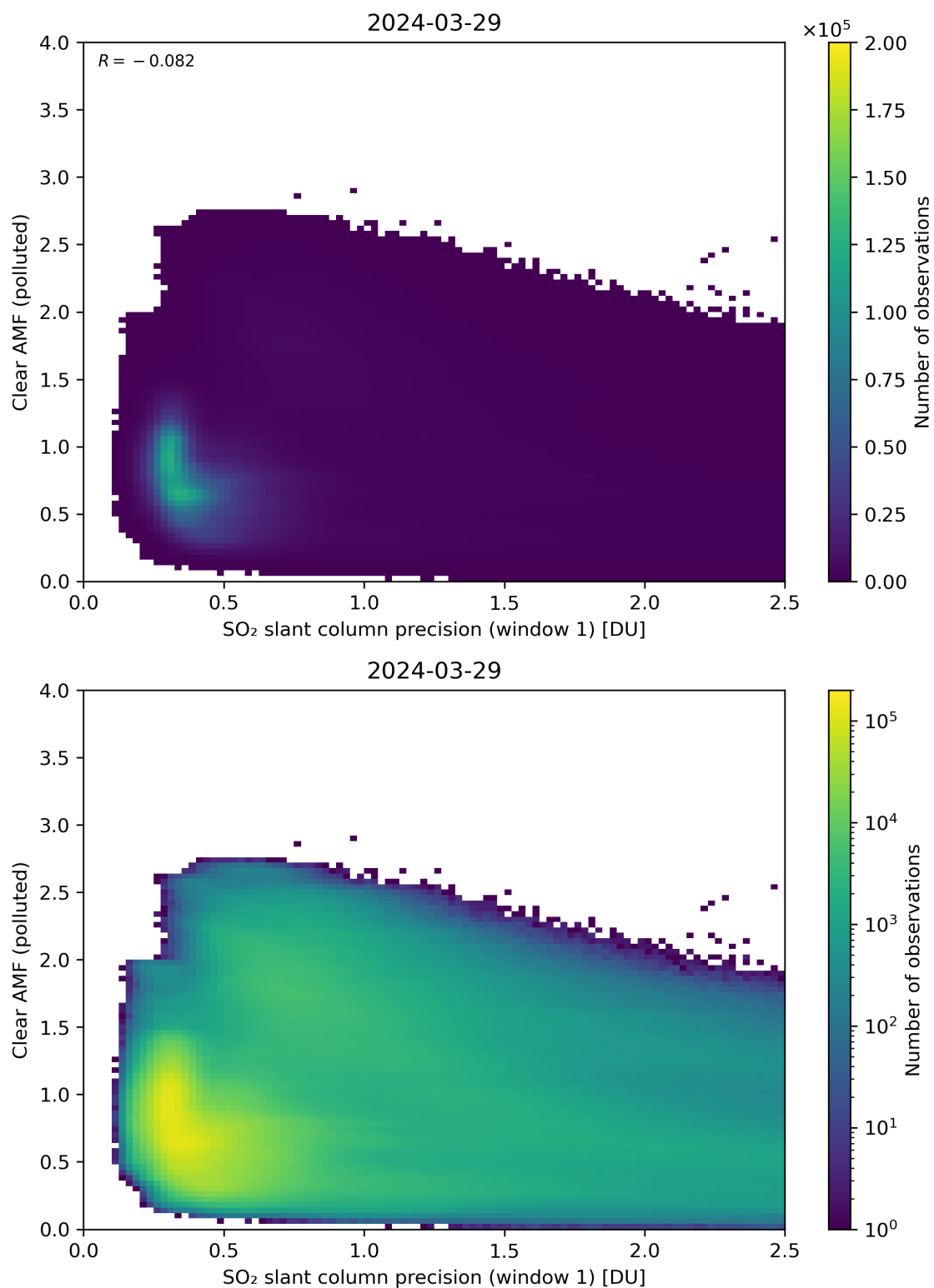
Figure 224: Scatter density plot of “SO 2 slant column precision (window 1)” against “Clear AMF (polluted)” for 2024-03-28 to 2024-03-30.
