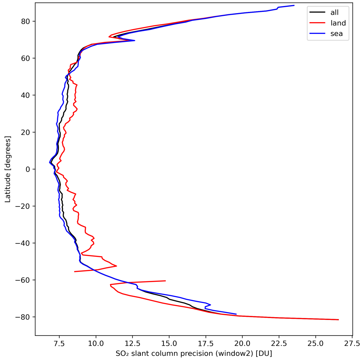
Figure 38: Zonal average of “SO 2 slant column precision (window2)” for 2024-03-28 to 2024-03-30.
