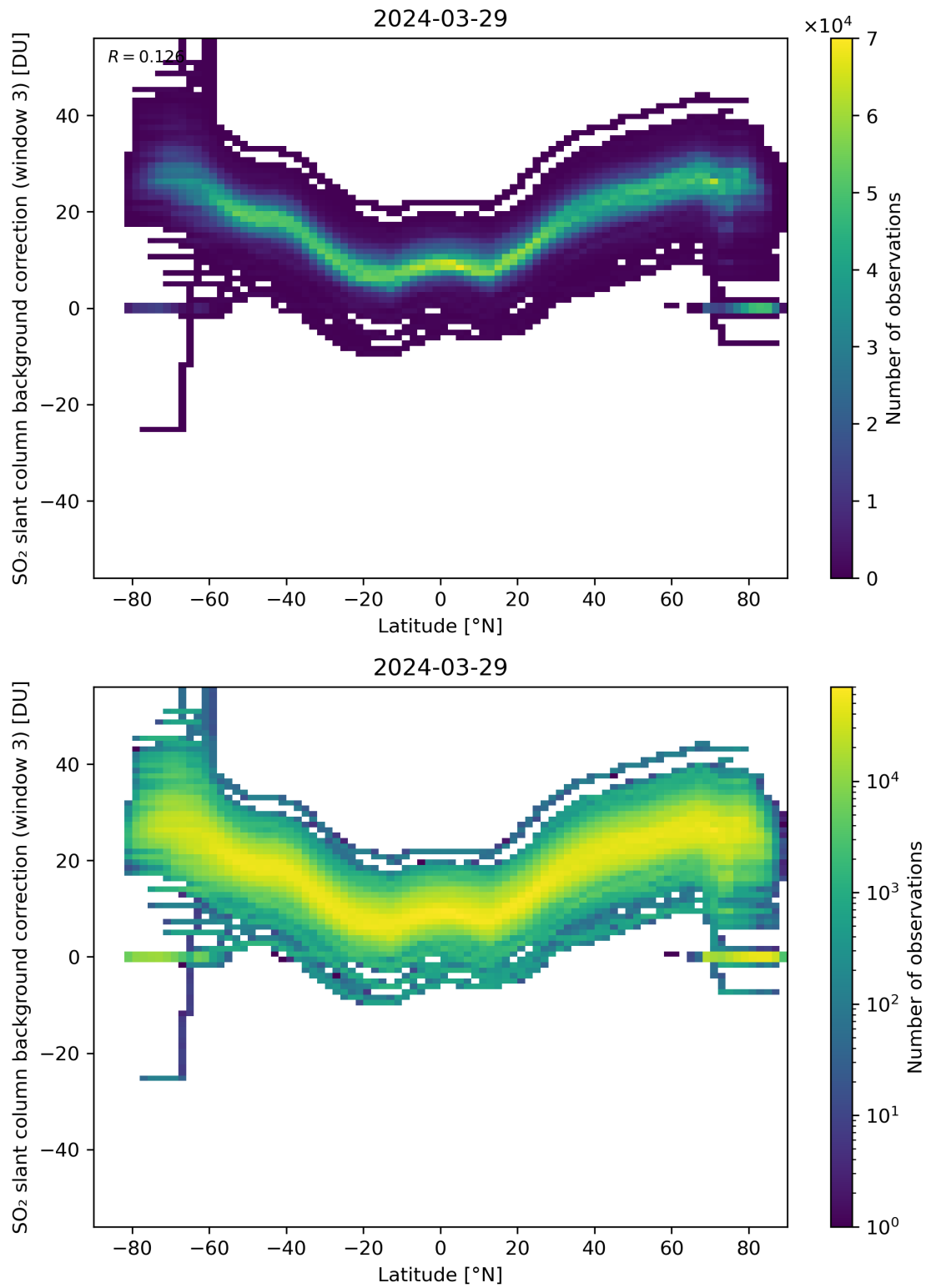
Figure 141: Scatter density plot of “Latitude” against “SO 2 slant column background correction (window 3)” for 2024-03-28 to 2024-03-30.
