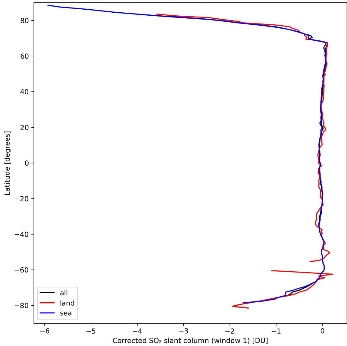
Figure 35: Zonal average of “Corrected SO 2 slant column (window 1)” for 2024-03-28 to 2024-03-30.
