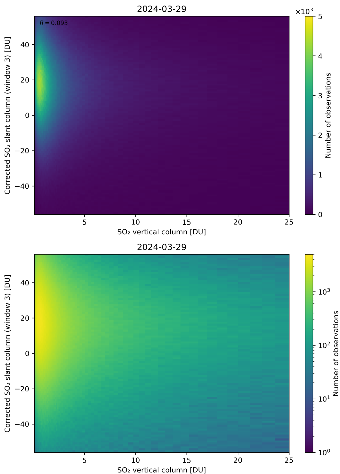
Figure 299: Scatter density plot of “SO 2 vertical column” against “Corrected SO 2 slant column (window 3)” for 2024-03-28 to 2024-03-30.
