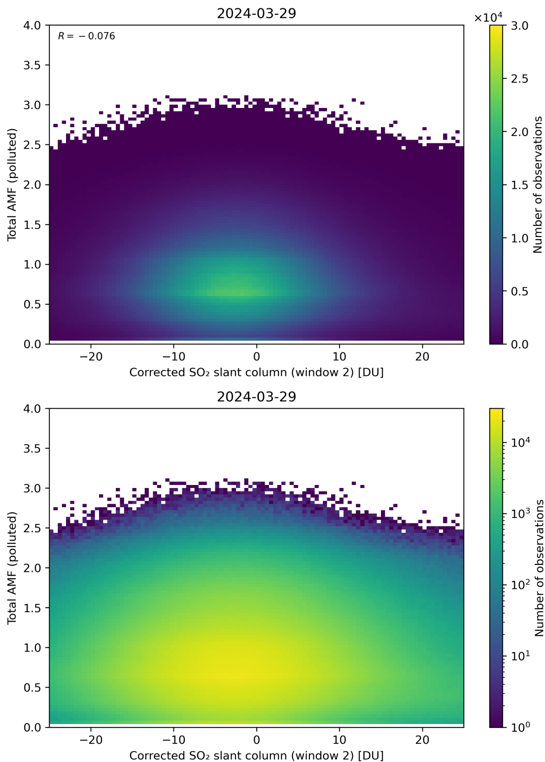
Figure 203: Scatter density plot of “Corrected SO 2 slant column (window 2)” against “Total AMF (polluted)” for 2024-03-28 to 2024-03-30.
