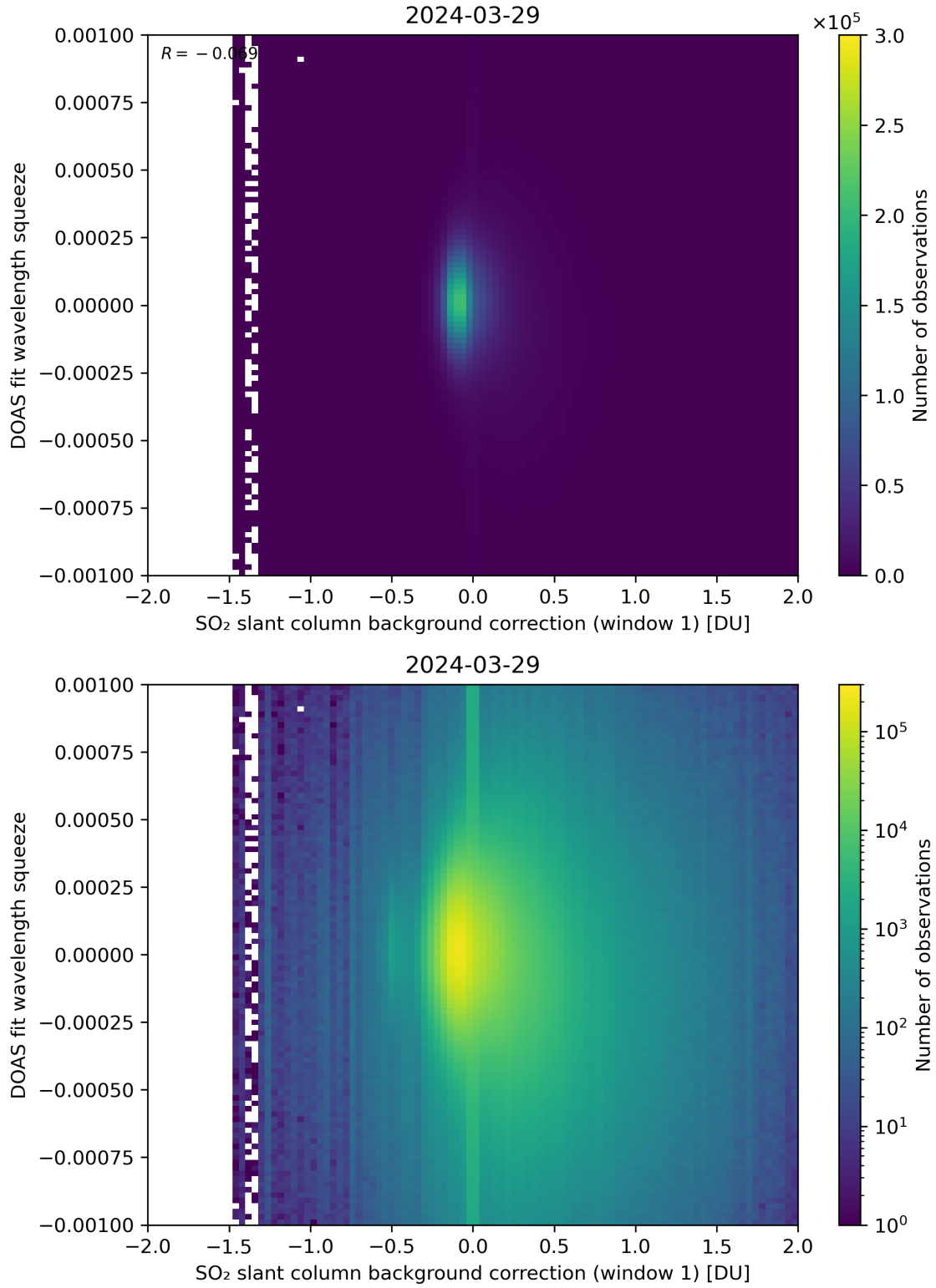
Figure 101: Scatter density plot of “SO 2 slant column background correction (window 1)” against “DOAS fit wavelength squeeze” for 2024-03-28 to 2024-03-30.
