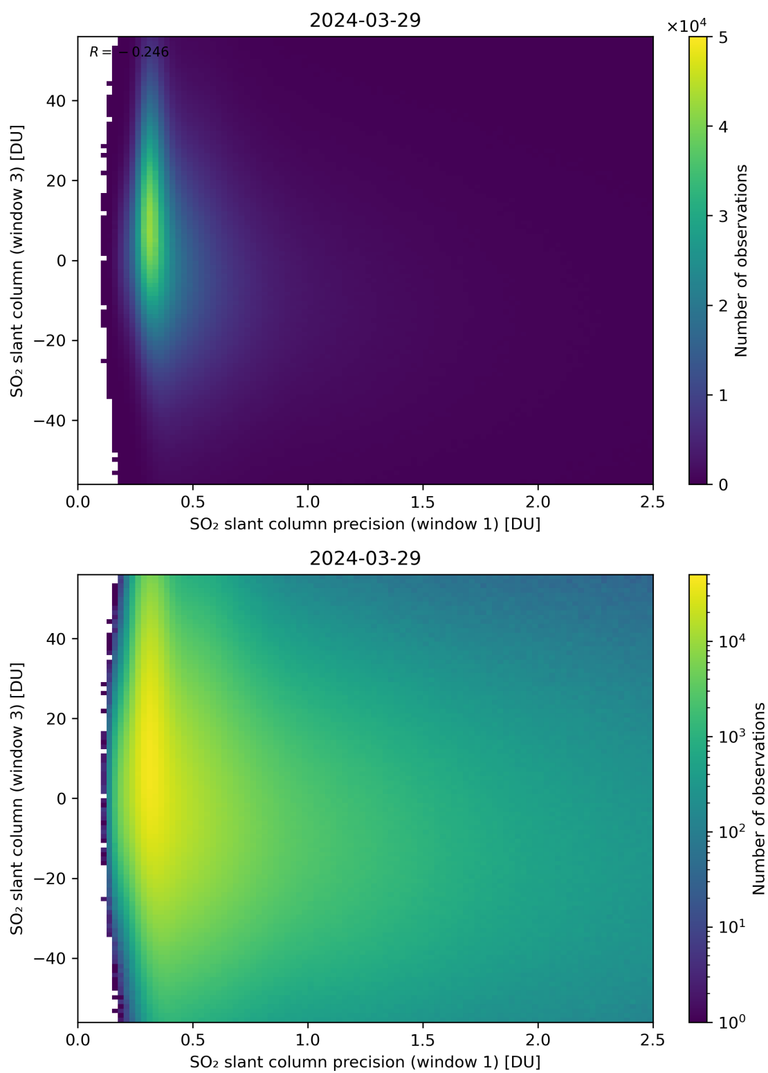
Figure 228: Scatter density plot of “SO 2 slant column precision (window 1)” against “SO 2 slant column (window 3)” for 2024-03-28 to 2024-03-30.
