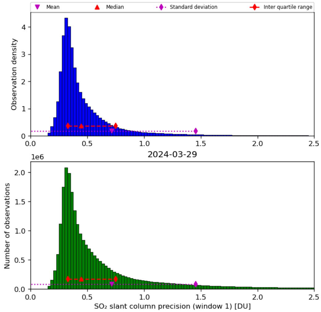
Figure 57: Histogram of “SO 2 slant column precision (window 1)” for 2024-03-28 to 2024-03-30
