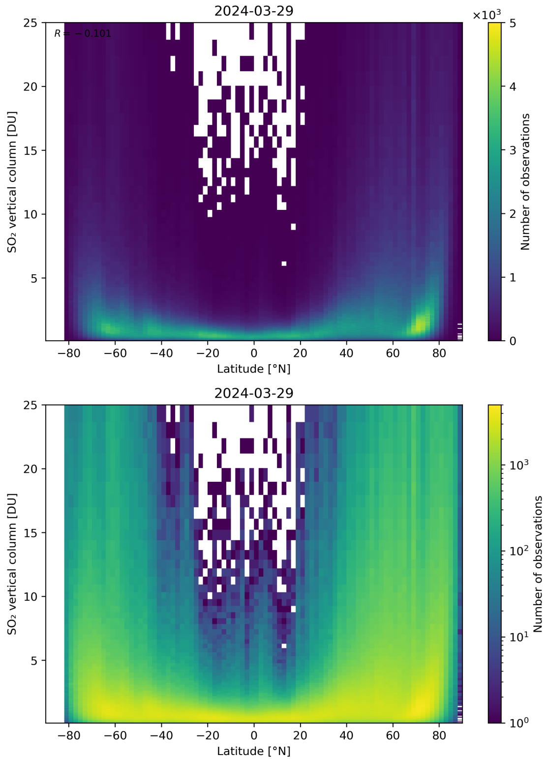
Figure 156: Scatter density plot of “Latitude” against “SO 2 vertical column” for 2024-03-28 to 2024-03-30.
