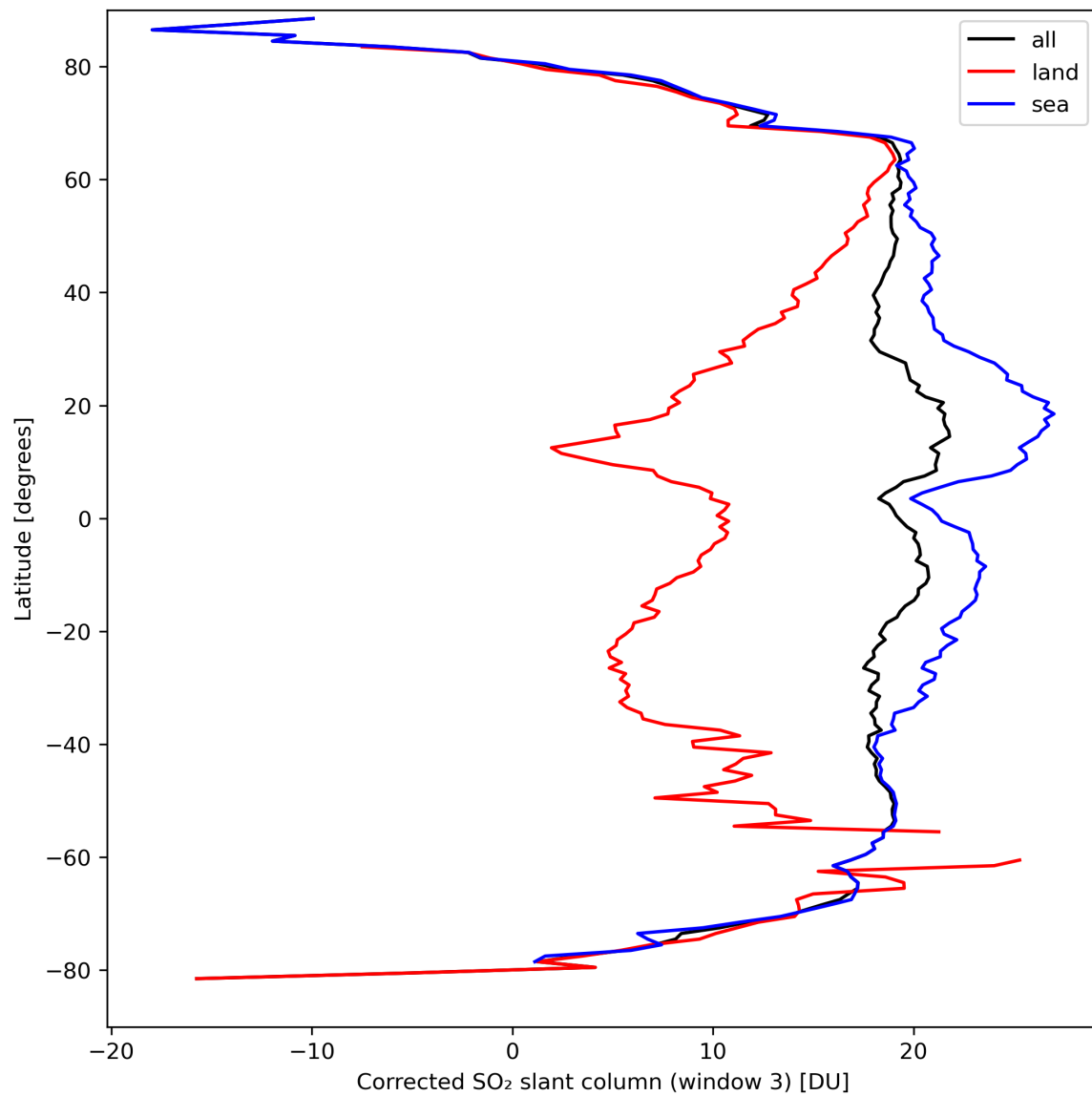
Figure 43: Zonal average of “Corrected SO 2 slant column (window 3)” for 2024-03-28 to 2024-03-30.
