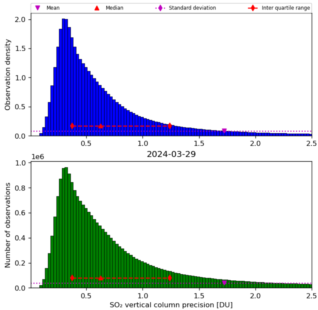
Figure 54: Histogram of “SO 2 vertical column precision” for 2024-03-28 to 2024-03-30
