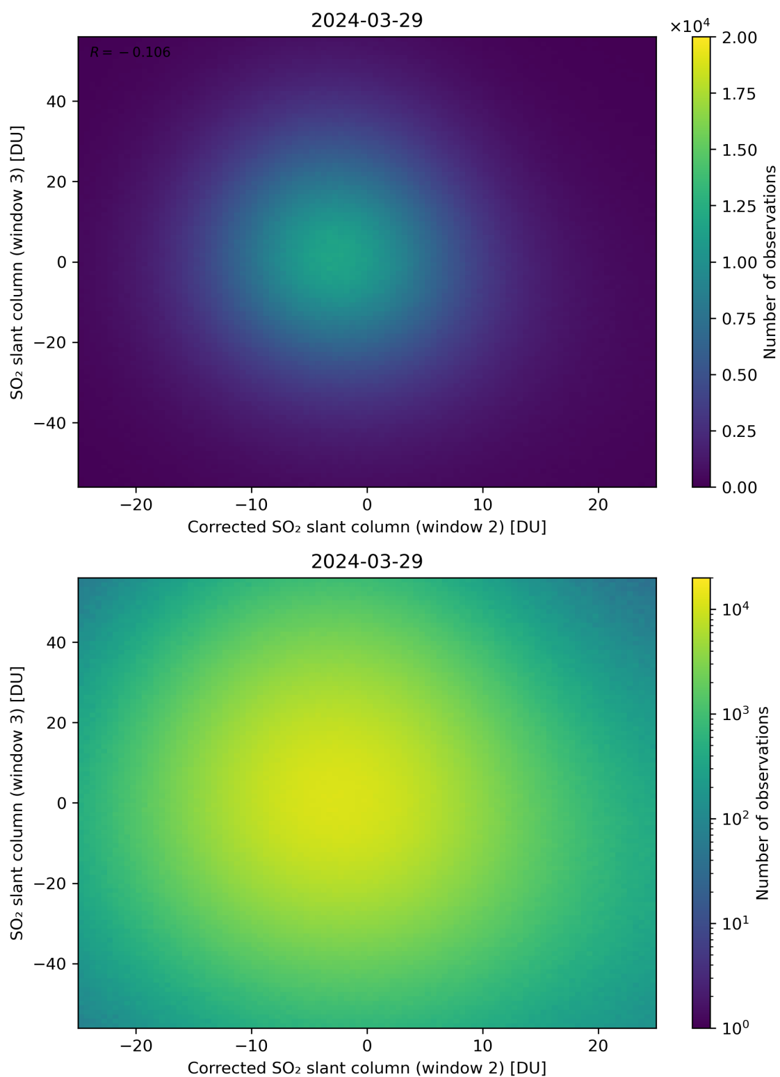
Figure 201: Scatter density plot of “Corrected SO 2 slant column (window 2)” against “SO 2 slant column (window 3)” for 2024-03-28 to 2024-03-30.
