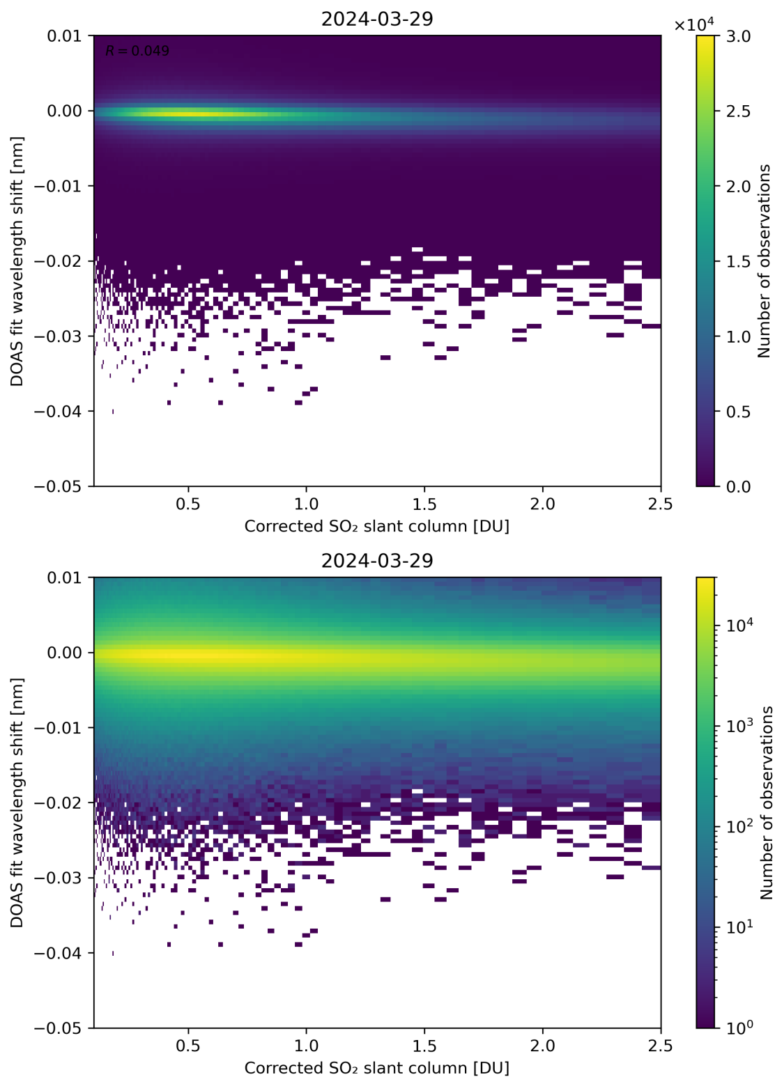
Figure 181: Scatter density plot of “Corrected SO 2 slant column” against “DOAS fit wavelength shift” for 2024-03-28 to 2024-03-30.
