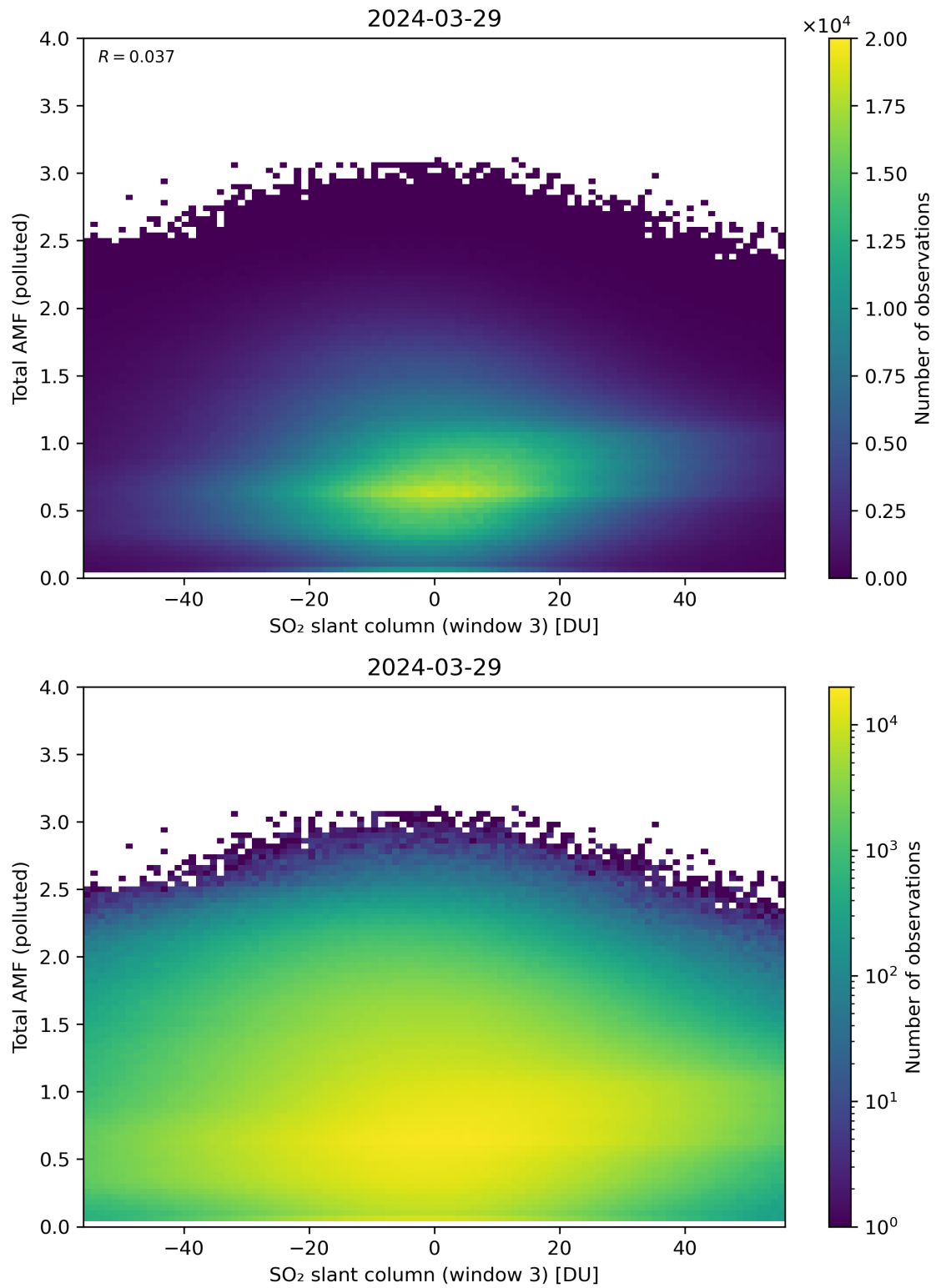
Figure 268: Scatter density plot of “SO 2 slant column (window 3)” against “Total AMF (polluted)” for 2024-03-28 to 2024-03-30.
