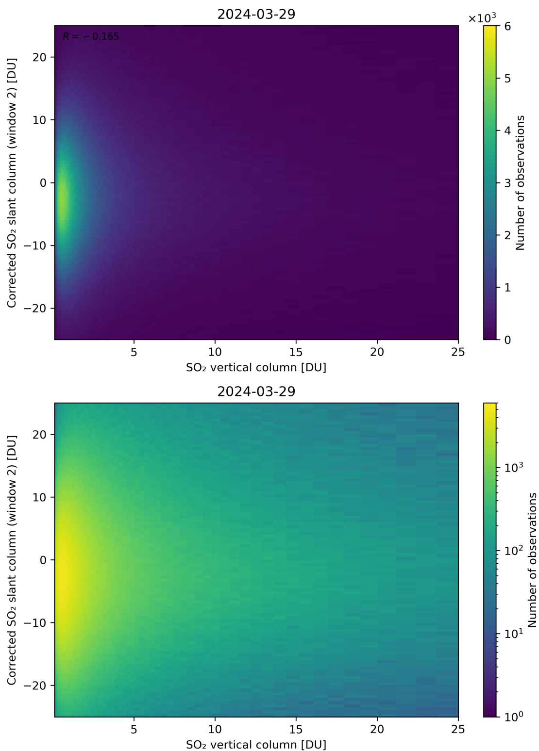
Figure 298: Scatter density plot of “SO 2 vertical column” against “Corrected SO 2 slant column (window 2)” for 2024-03-28 to 2024-03-30.
