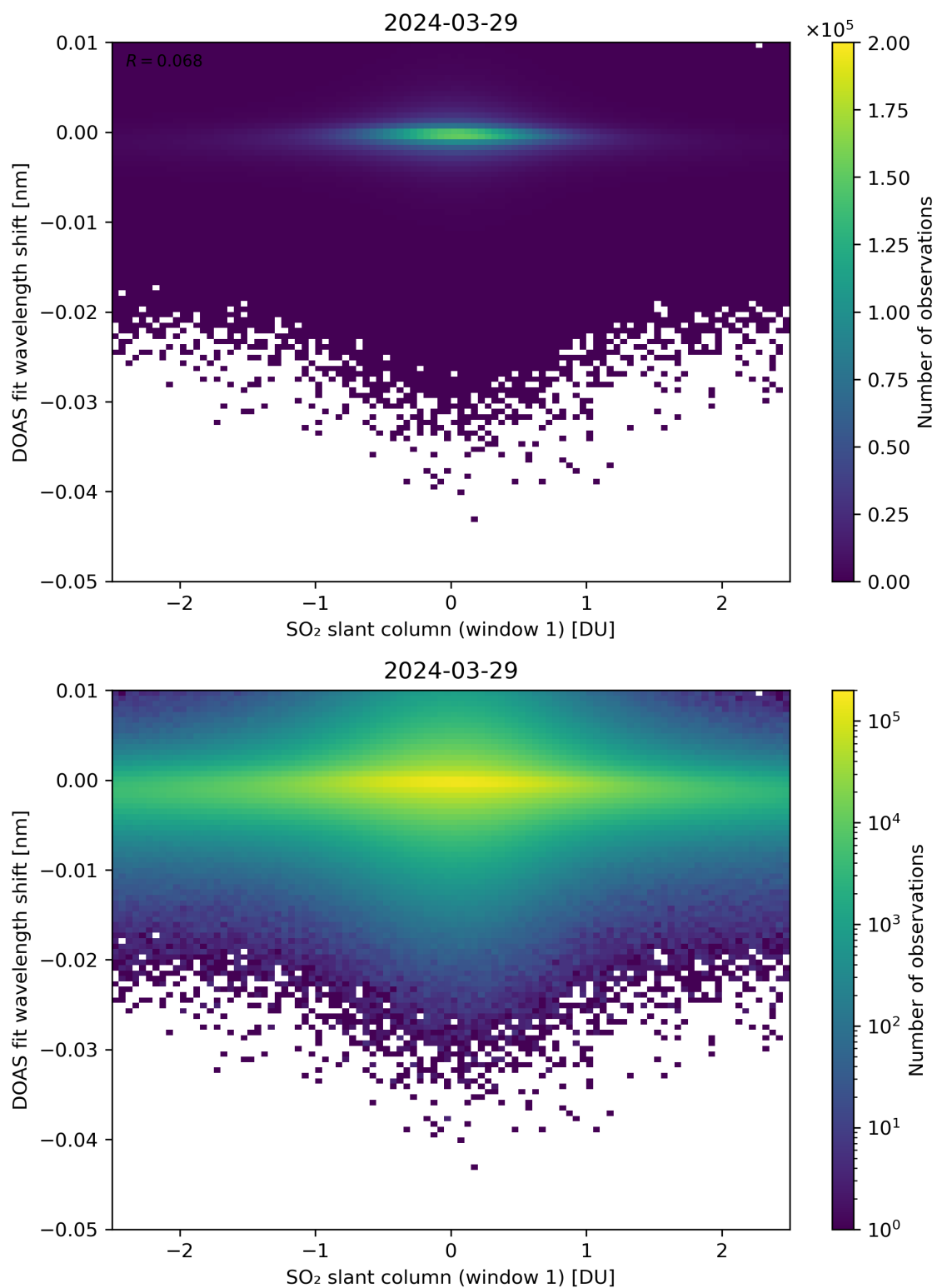
Figure 215: Scatter density plot of “SO 2 slant column (window 1)” against “DOAS fit wavelength shift” for 2024-03-28 to 2024-03-30.
