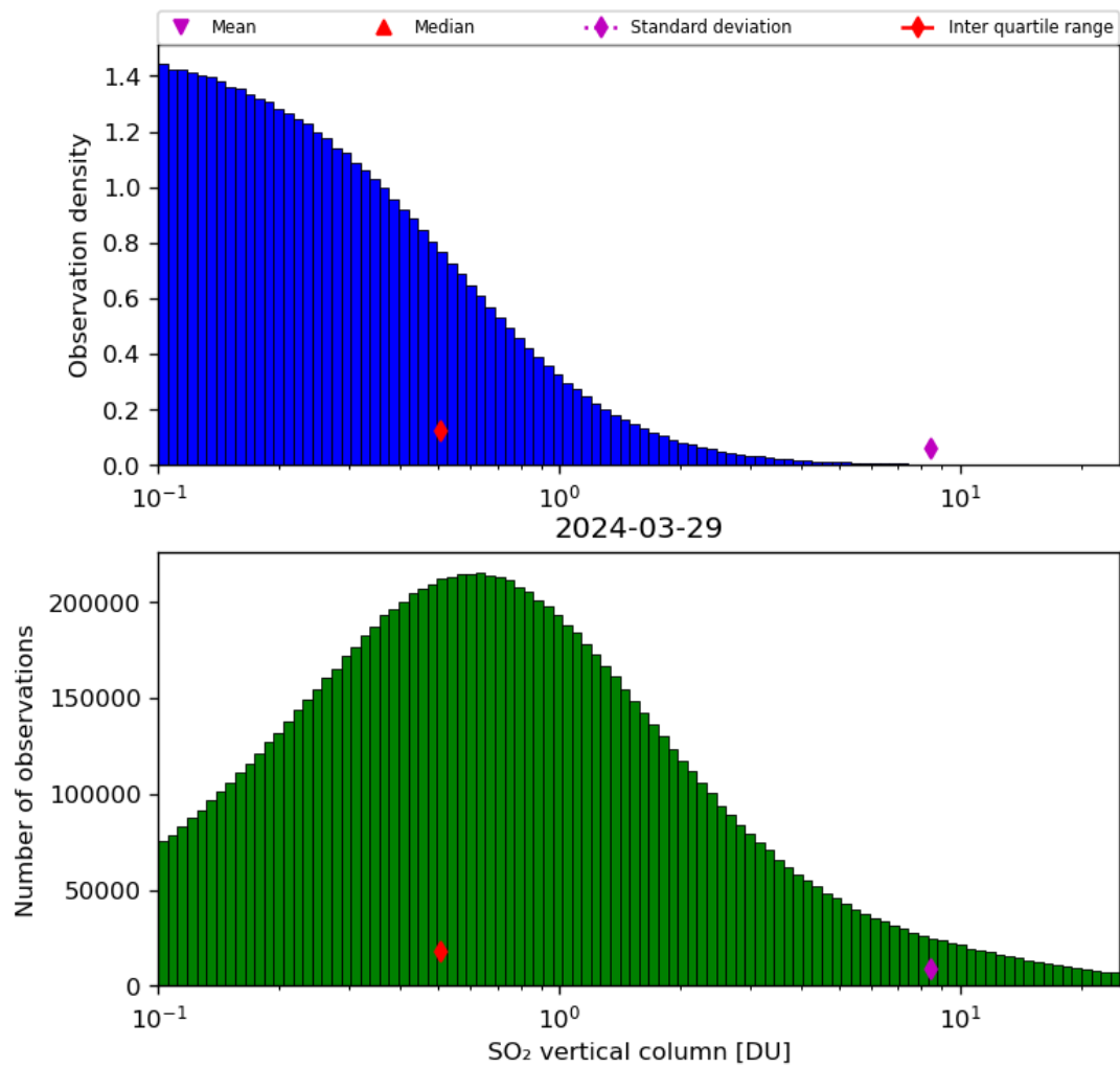
Figure 53: Histogram of “SO 2 vertical column” for 2024-03-28 to 2024-03-30
