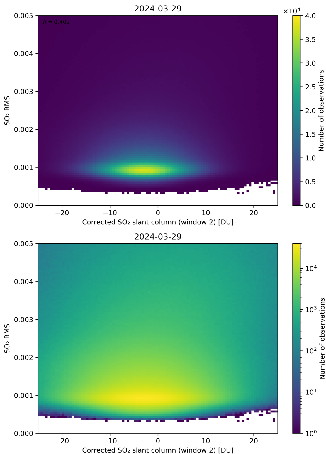
Figure 198: Scatter density plot of “Corrected SO 2 slant column (window 2)” against “SO 2 RMS” for 2024-03-28 to 2024-03-30.
