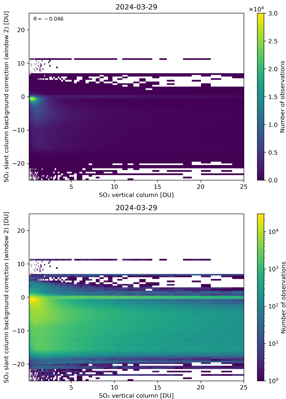
Figure 274: Scatter density plot of “SO 2 vertical column” against “SO 2 slant column background correction (window 2)” for 2024-03-28 to 2024-03-30.
