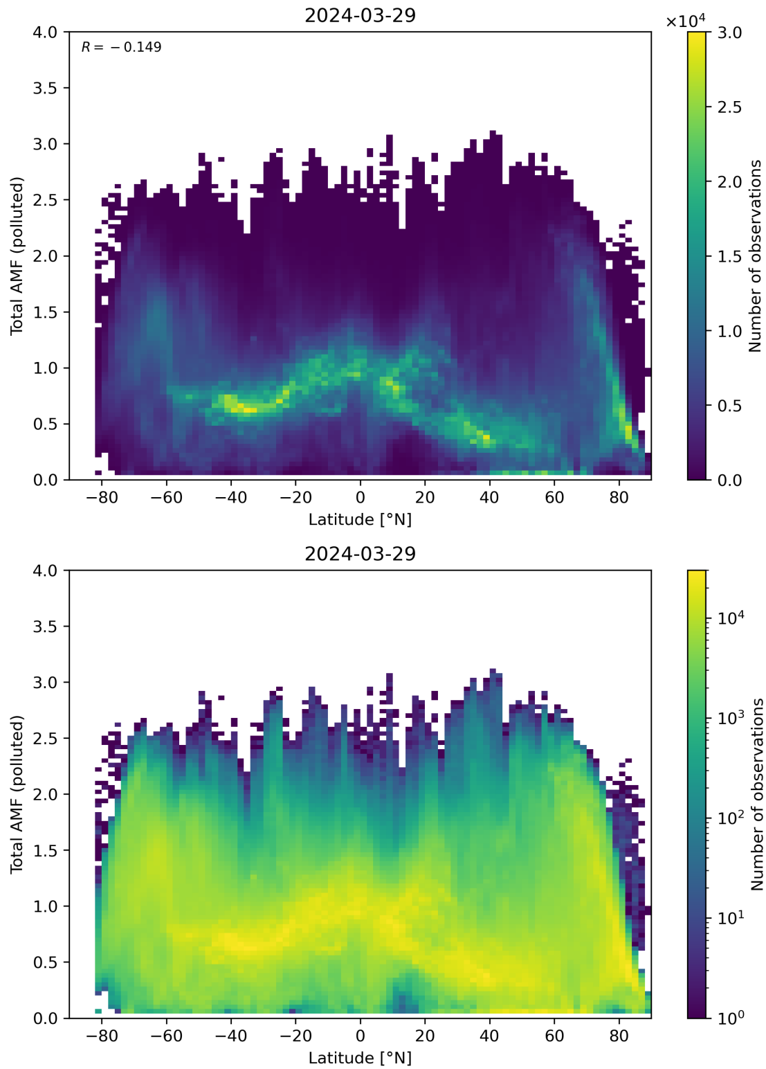
Figure 154: Scatter density plot of “Latitude” against “Total AMF (polluted)” for 2024-03-28 to 2024-03-30.
