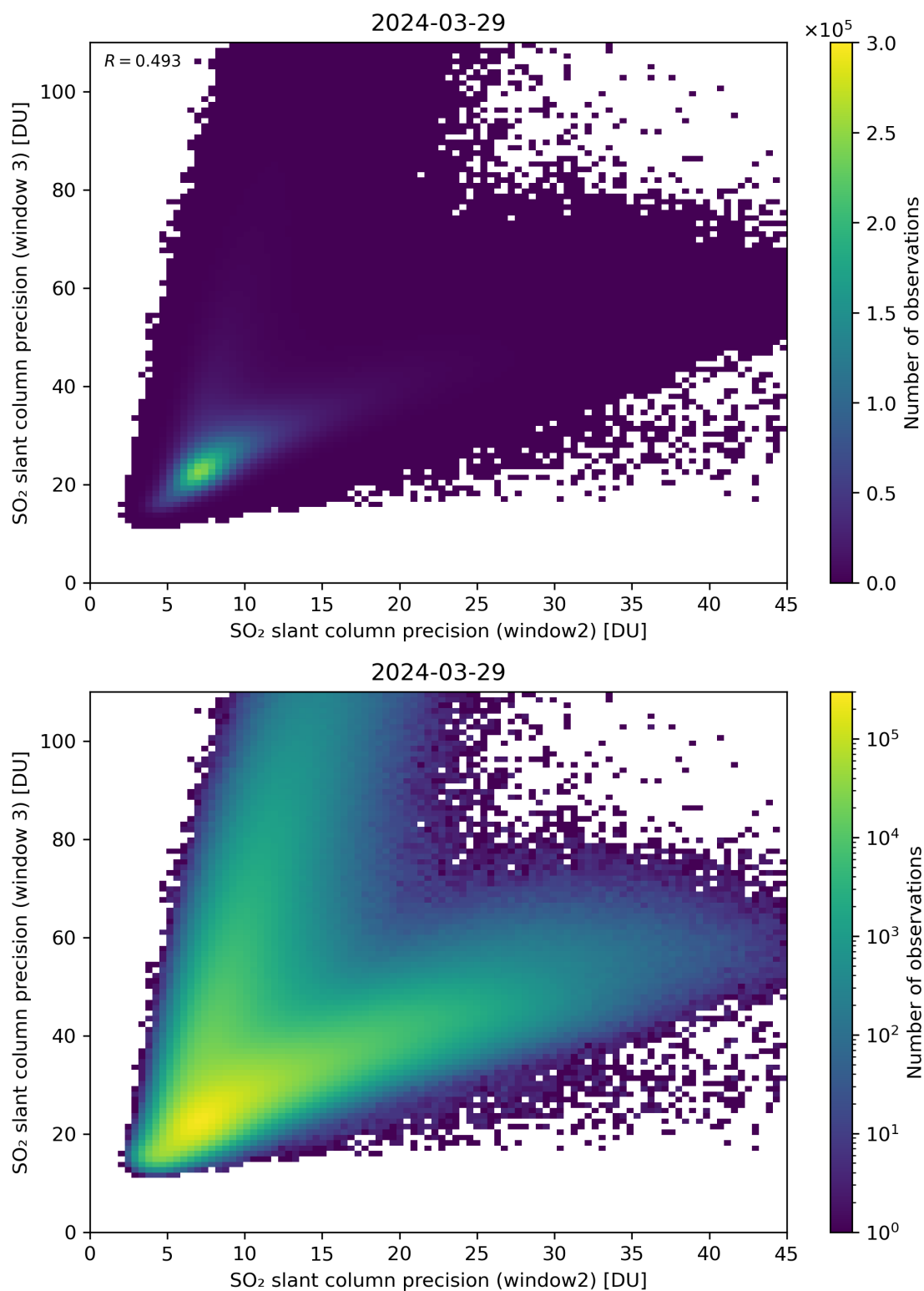
Figure 250: Scatter density plot of “SO 2 slant column precision (window2)” against “SO 2 slant column precision (window 3)” for 2024-03-28 to 2024-03-30.
