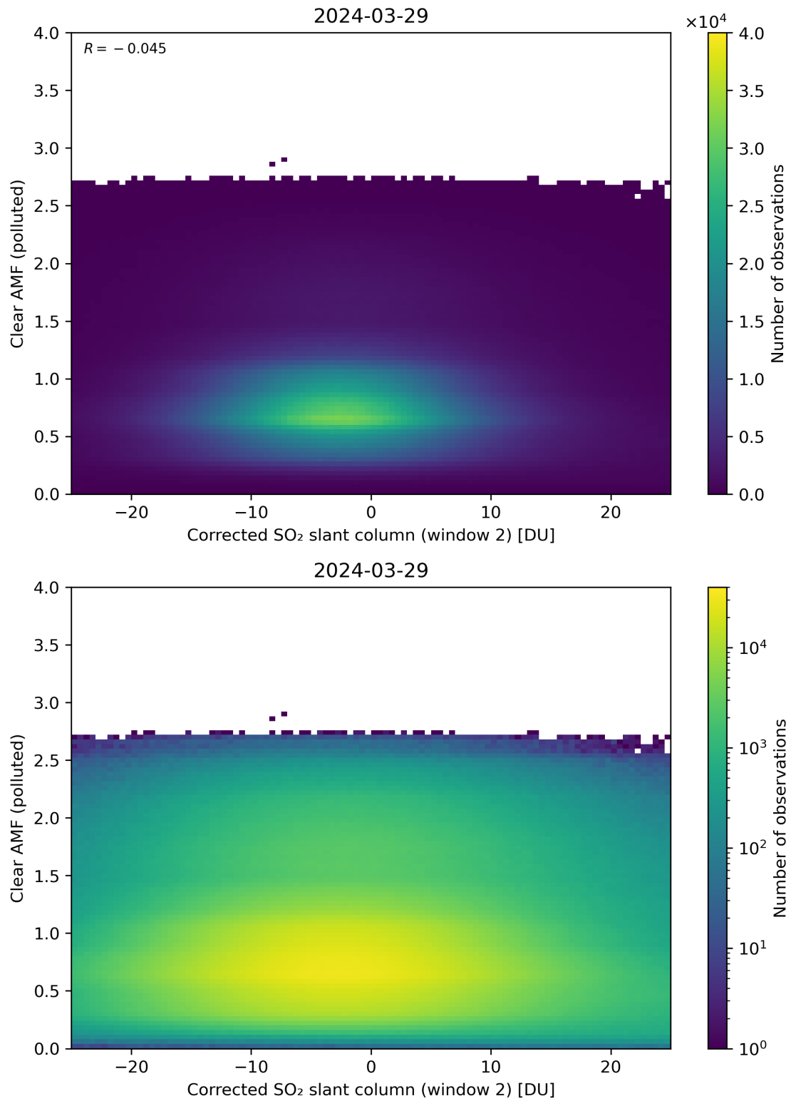
Figure 199: Scatter density plot of “Corrected SO 2 slant column (window 2)” against “Clear AMF (polluted)” for 2024-03-28 to 2024-03-30.
