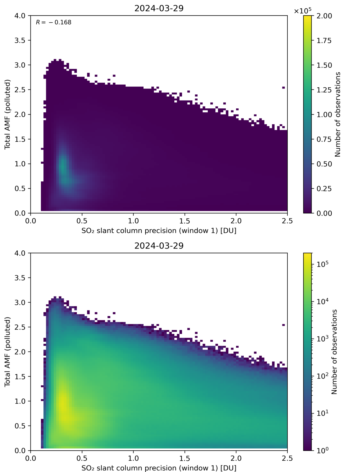
Figure 230: Scatter density plot of “SO 2 slant column precision (window 1)” against “Total AMF (polluted)” for 2024-03-28 to 2024-03-30.
