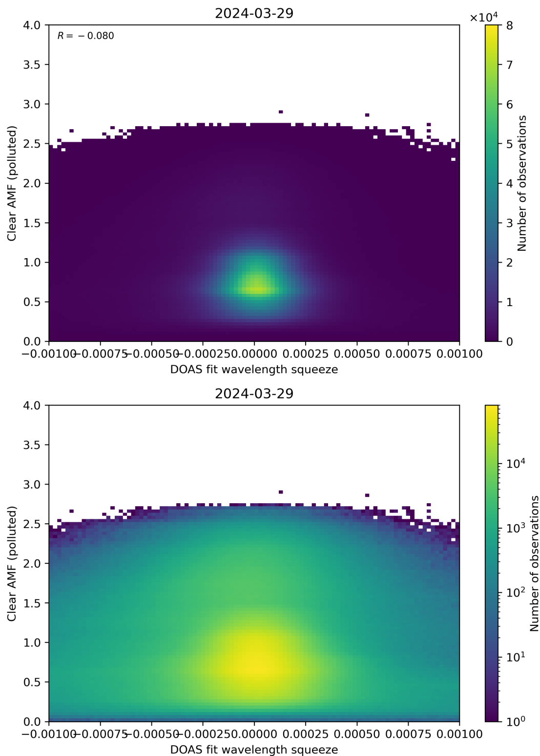
Figure 133: Scatter density plot of “DOAS fit wavelength squeeze” against “Clear AMF (polluted)” for 2024-03-28 to 2024-03-30.
