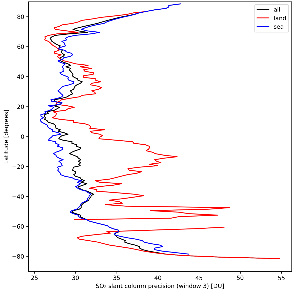
Figure 42: Zonal average of “SO 2 slant column precision (window 3)” for 2024-03-28 to 2024-03-30.
