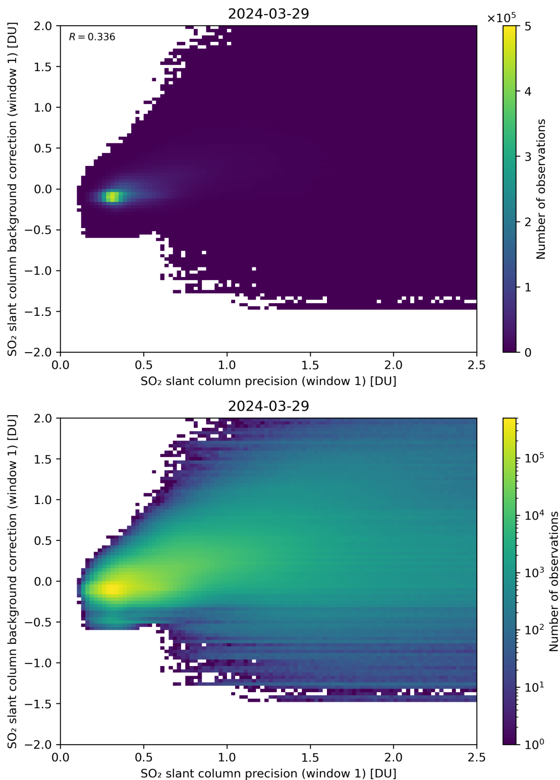
Figure 218: Scatter density plot of “SO 2 slant column precision (window 1)” against “SO 2 slant column background correction (window 1)” for 2024-03-28 to 2024-03-30.
