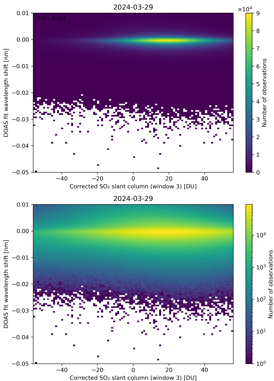
Figure 206: Scatter density plot of “Corrected SO 2 slant column (window 3)” against “DOAS fit wavelength shift” for 2024-03-28 to 2024-03-30.
