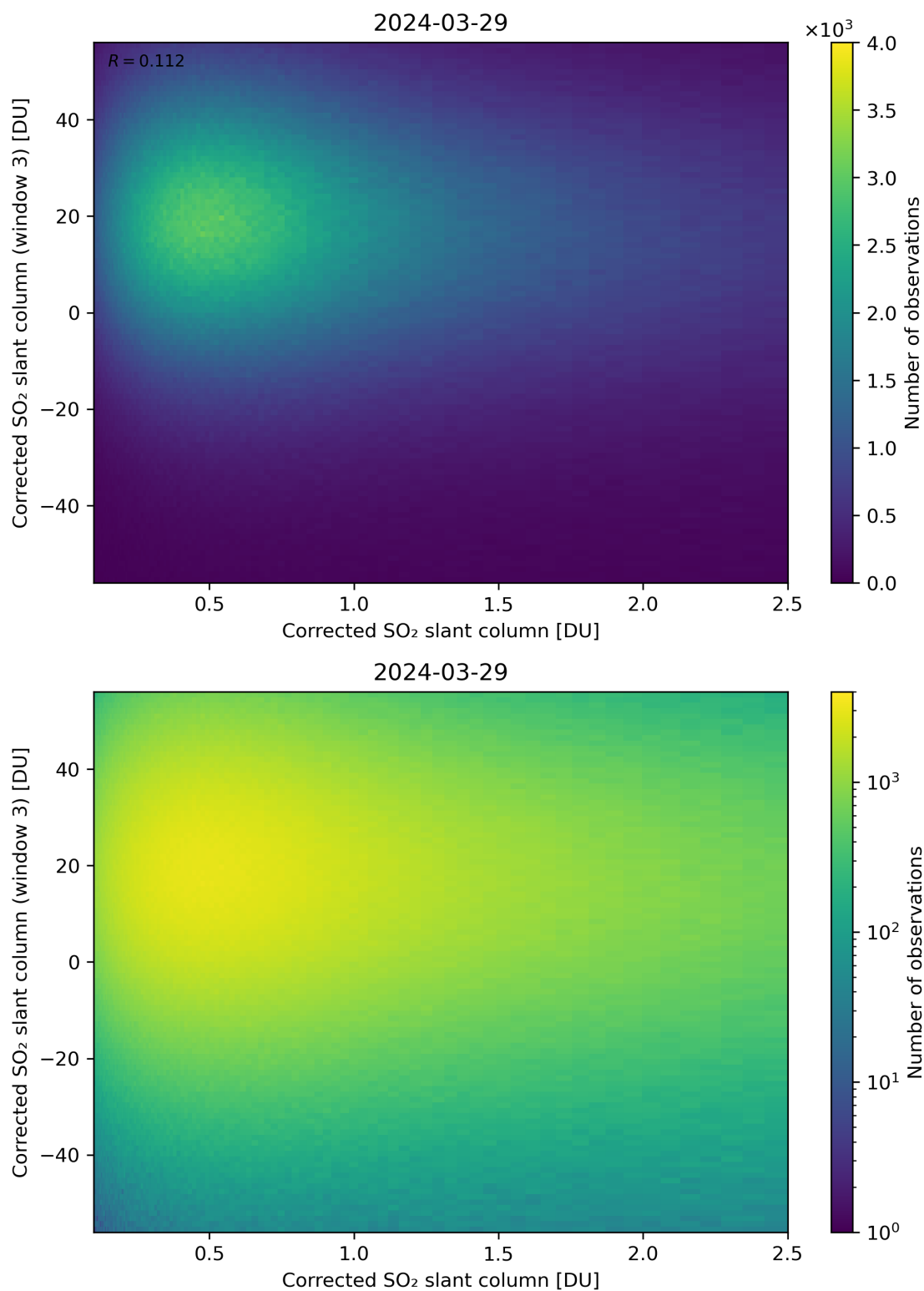
Figure 186: Scatter density plot of “Corrected SO 2 slant column” against “Corrected SO 2 slant column (window 3)” for 2024-03-28 to 2024-03-30.
