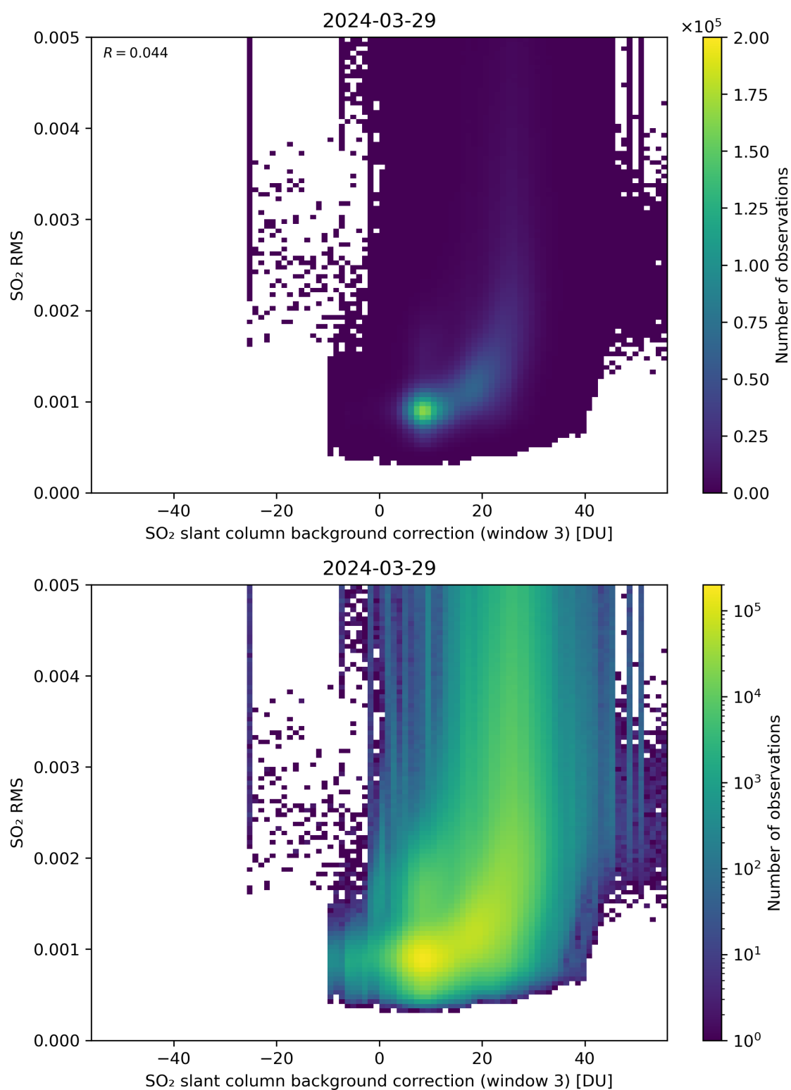
Figure 123: Scatter density plot of “SO 2 slant column background correction (window 3)” against “SO 2 RMS” for 2024-03-28 to 2024-03-30.
