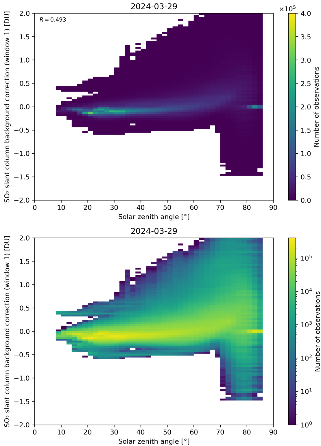
Figure 158: Scatter density plot of “Solar zenith angle” against “SO 2 slant column background correction (window 1)” for 2024-03-28 to 2024-03-30.
