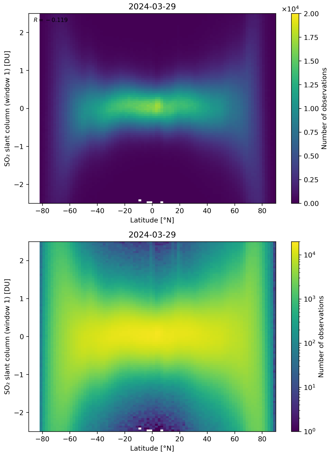
Figure 149: Scatter density plot of “Latitude” against “SO 2 slant column (window 1)” for 2024-03-28 to 2024-03-30.
