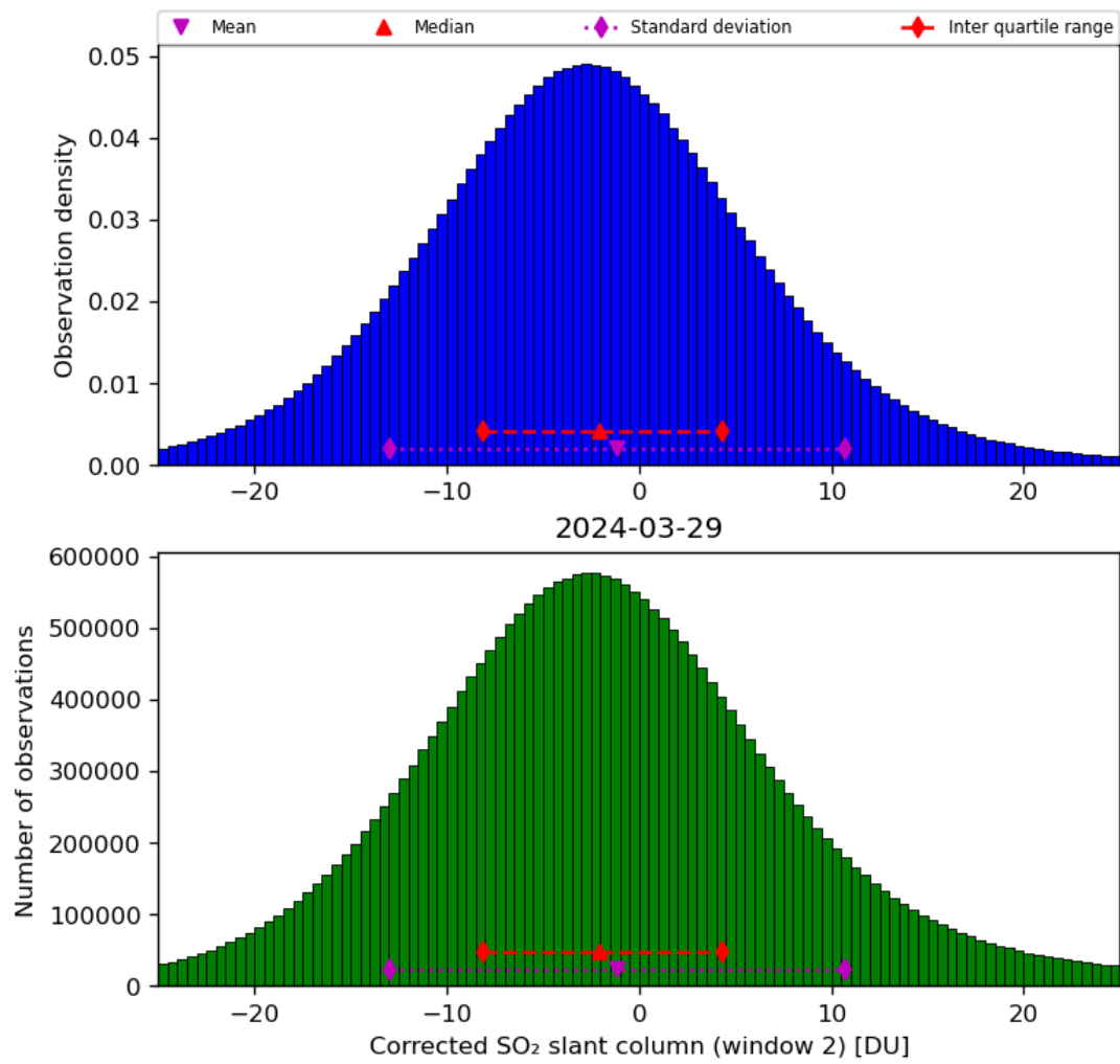
Figure 62: Histogram of “Corrected SO 2 slant column (window 2)” for 2024-03-28 to 2024-03-30
