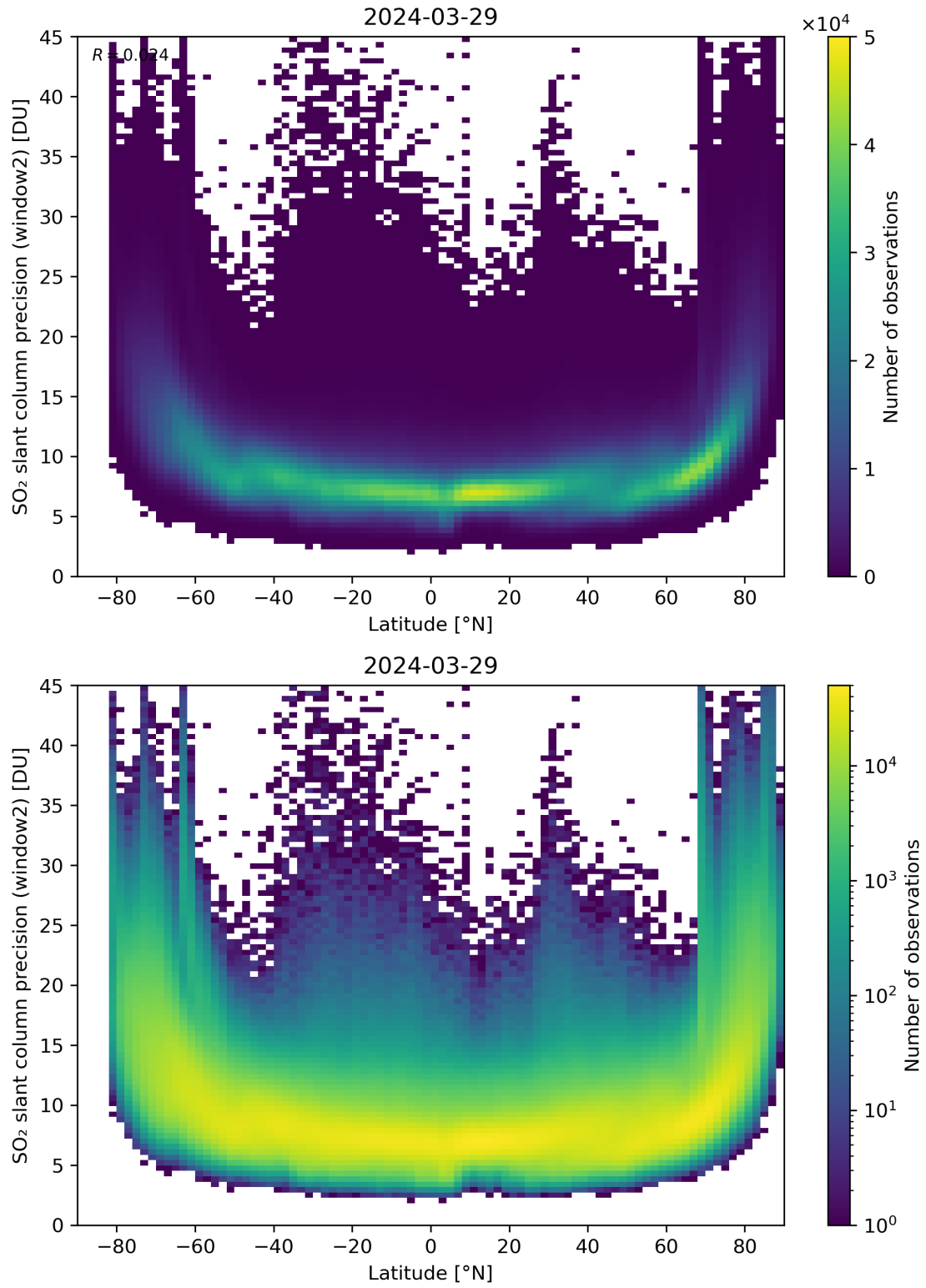
Figure 151: Scatter density plot of “Latitude” against “SO 2 slant column precision (window2)” for 2024-03-28 to 2024-03-30.
