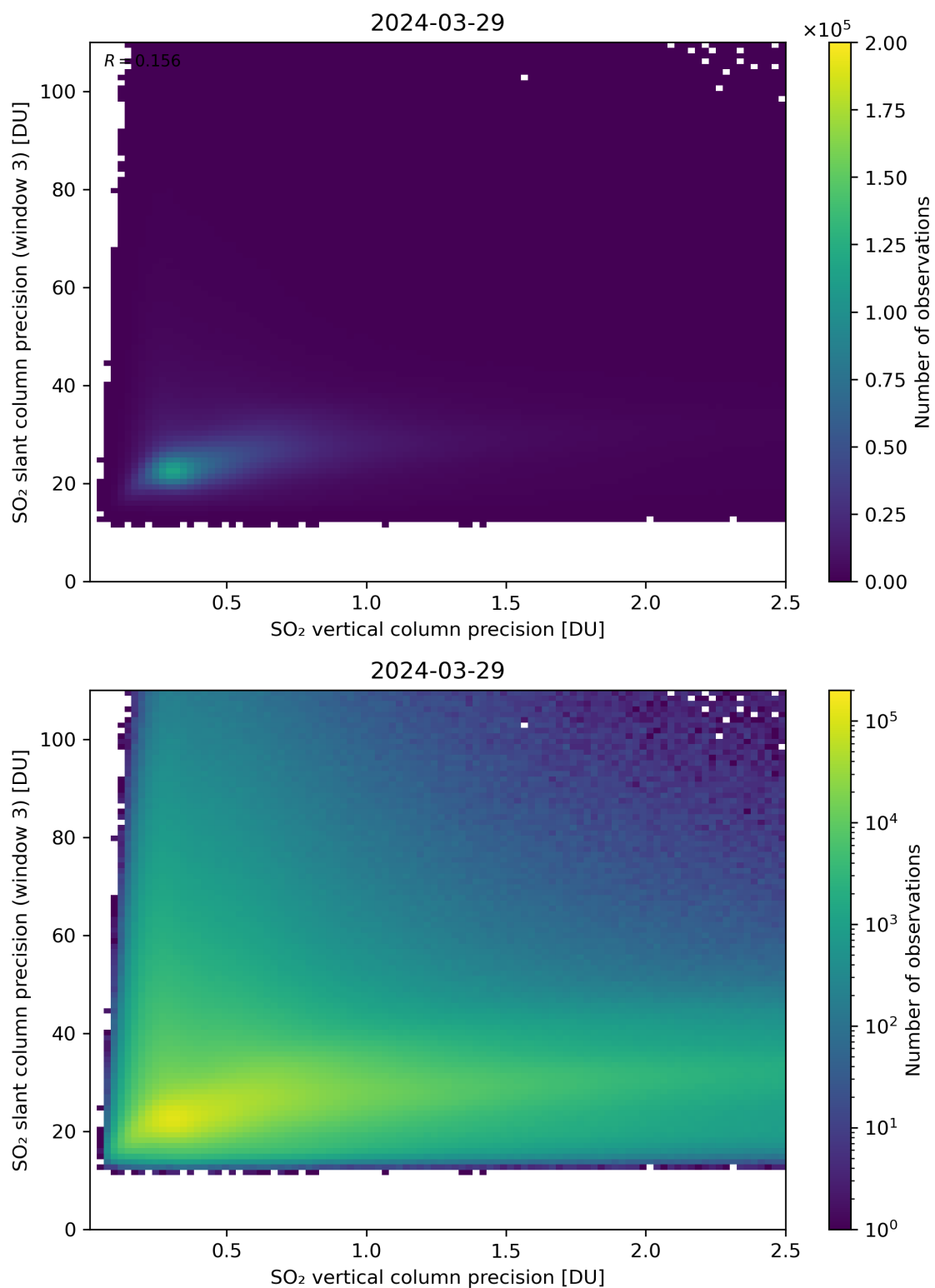
Figure 293: Scatter density plot of “SO 2 vertical column precision” against “SO 2 slant column precision (window 3)” for 2024-03-28 to 2024-03-30.
