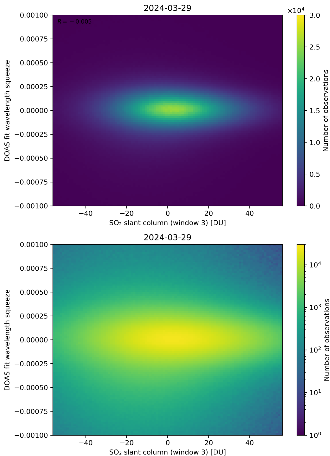
Figure 255: Scatter density plot of “SO 2 slant column (window 3)” against “DOAS fit wavelength squeeze” for 2024-03-28 to 2024-03-30.
