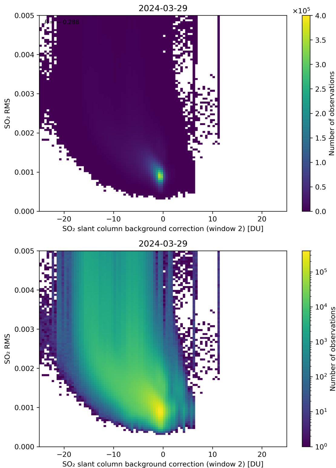
Figure 114: Scatter density plot of “SO 2 slant column background correction (window 2)” against “SO 2 RMS” for 2024-03-28 to 2024-03-30.
