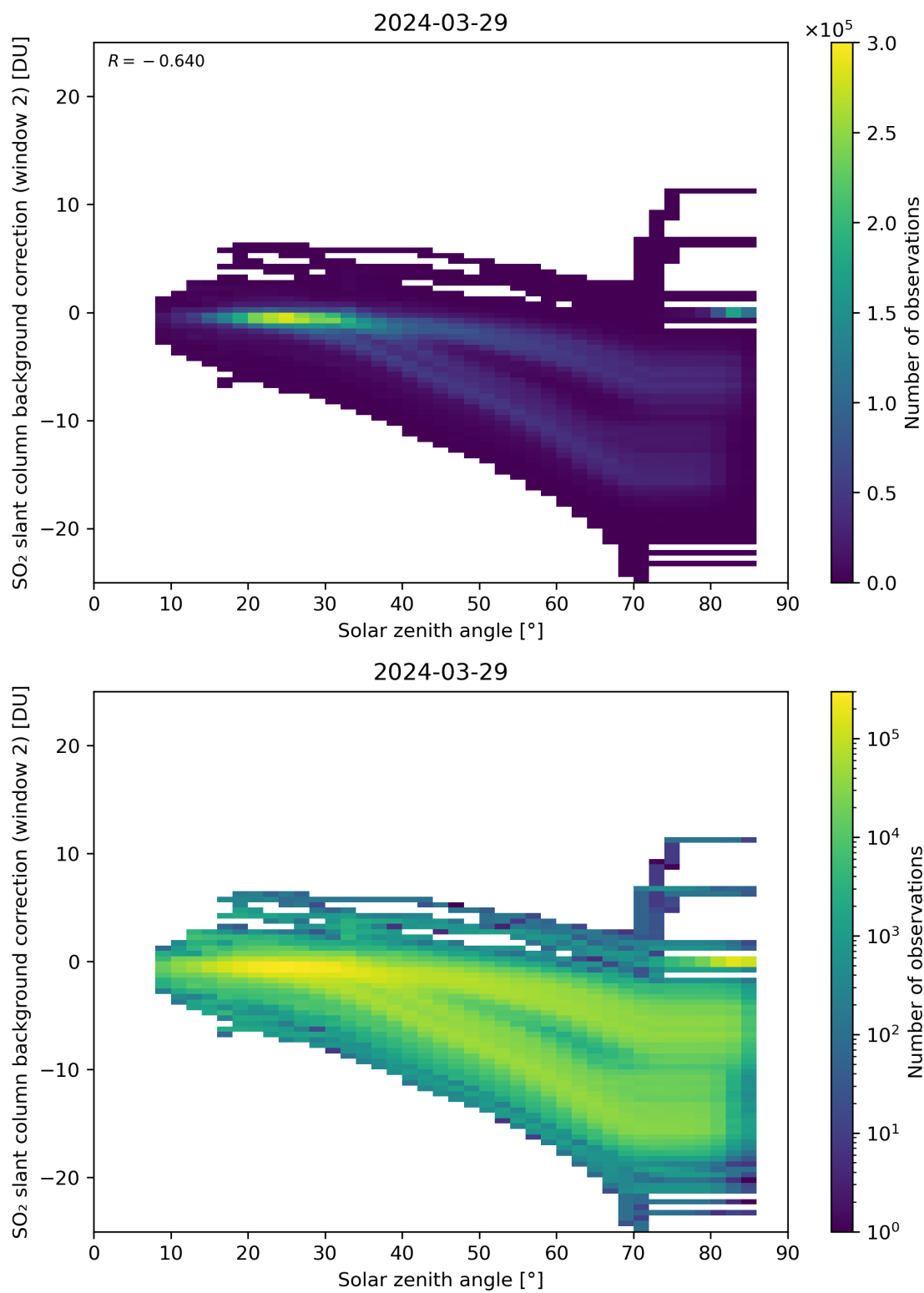
Figure 159: Scatter density plot of “Solar zenith angle” against “SO 2 slant column background correction (window 2)” for 2024-03-28 to 2024-03-30.
