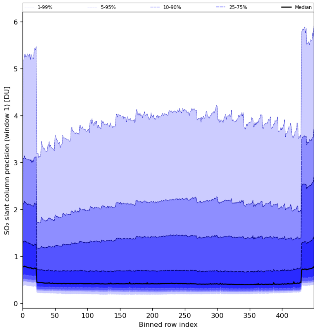
Figure 80: Along track statistics of “SO 2 slant column precision (window 1)” for 2024-03-28 to 2024-03-30
