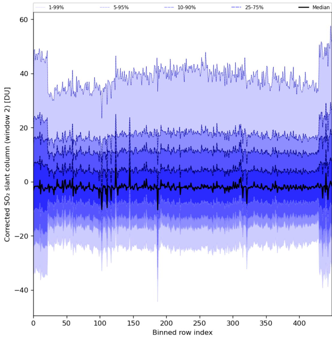
Figure 85: Along track statistics of “Corrected SO 2 slant column (window 2)” for 2024-03-28 to 2024-03-30
