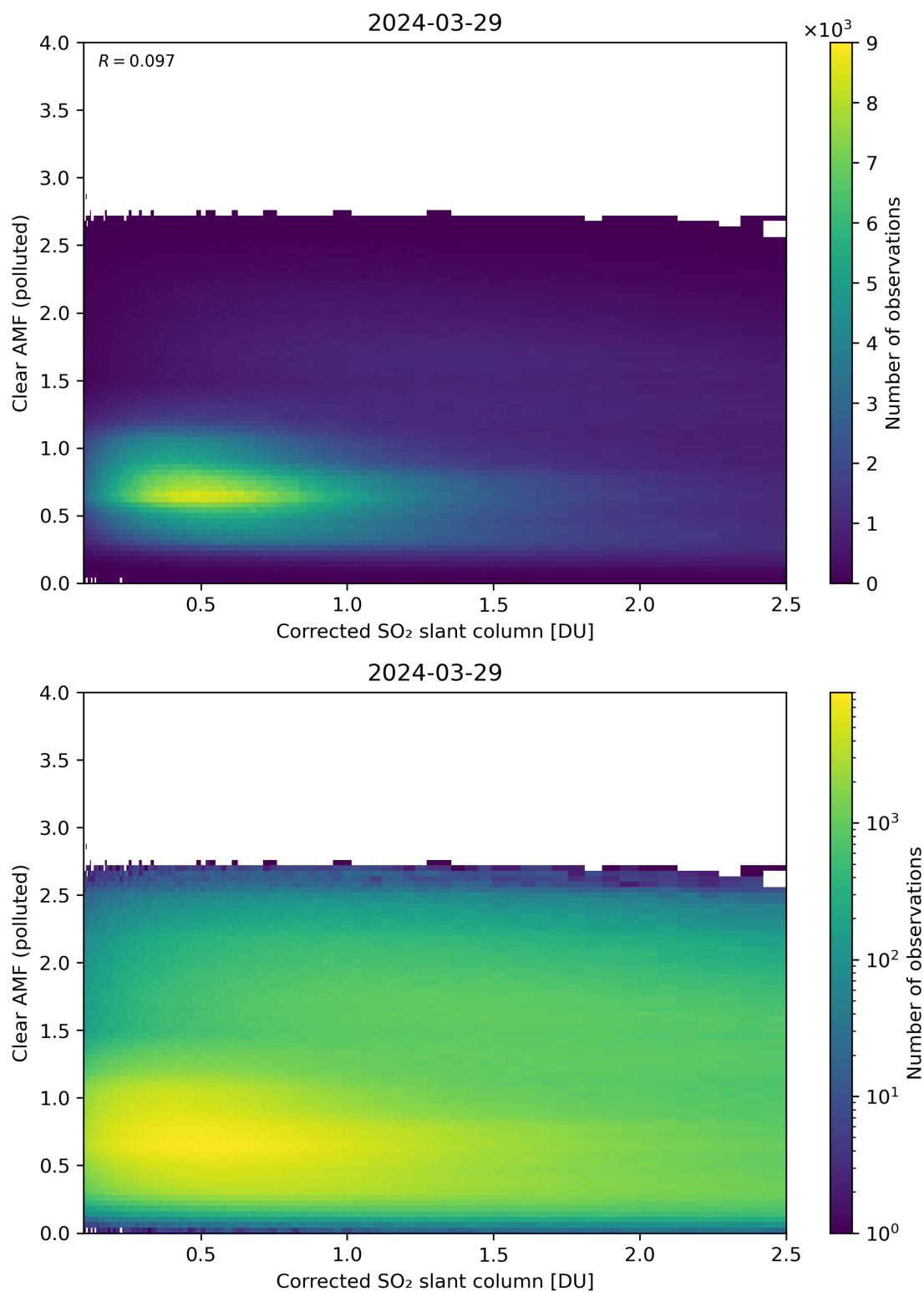
Figure 184: Scatter density plot of “Corrected SO 2 slant column” against “Clear AMF (polluted)” for 2024-03-28 to 2024-03-30.
