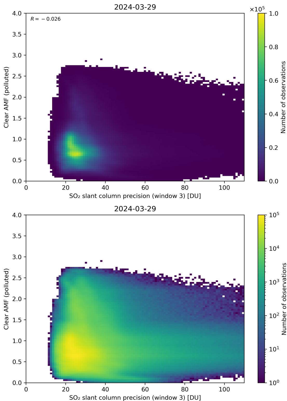
Figure 261: Scatter density plot of “SO 2 slant column precision (window 3)” against “Clear AMF (polluted)” for 2024-03-28 to 2024-03-30.
