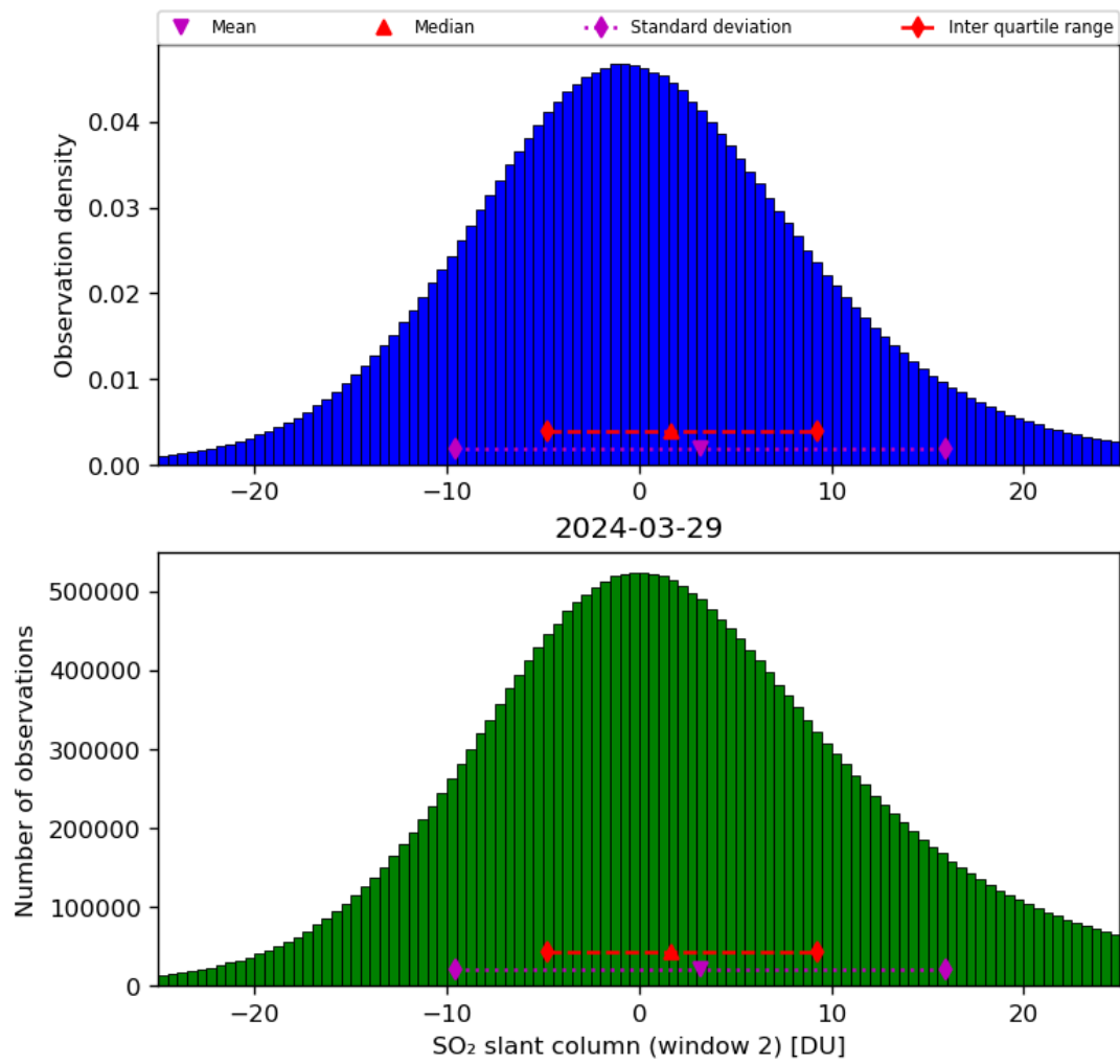
Figure 60: Histogram of “SO 2 slant column (window 2)” for 2024-03-28 to 2024-03-30
