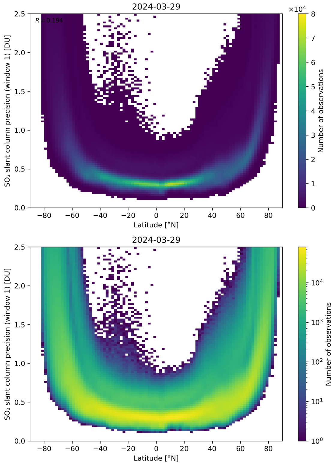
Figure 150: Scatter density plot of “Latitude” against “SO 2 slant column precision (window 1)” for 2024-03-28 to 2024-03-30.
