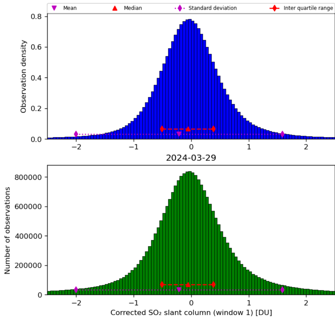
Figure 58: Histogram of “Corrected SO 2 slant column (window 1)” for 2024-03-28 to 2024-03-30
