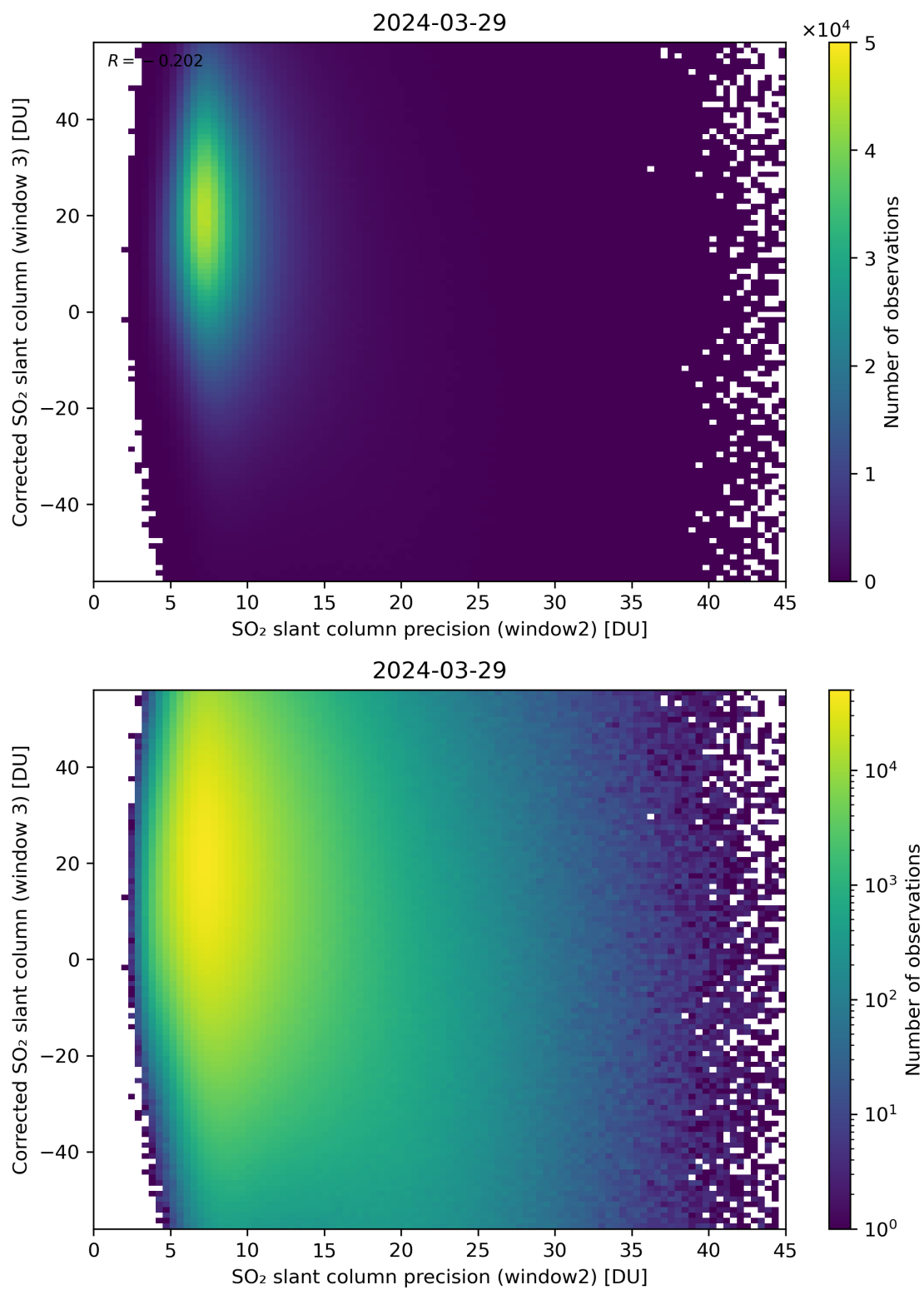
Figure 248: Scatter density plot of “SO 2 slant column precision (window2)” against “Corrected SO 2 slant column (window 3)” for 2024-03-28 to 2024-03-30.
