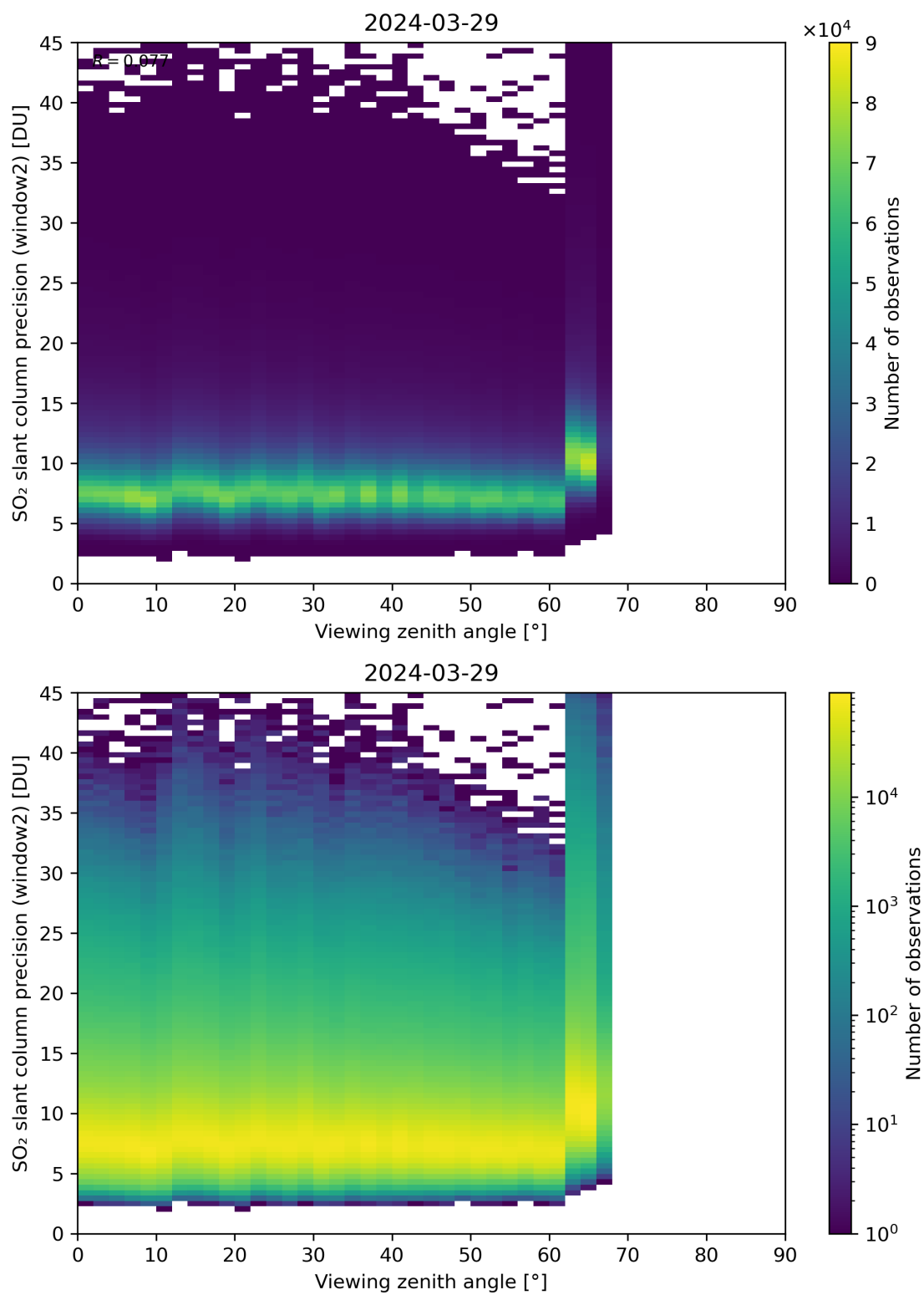
Figure 322: Scatter density plot of “Viewing zenith angle” against “SO 2 slant column precision (window2)” for 2024-03-28 to 2024-03-30.
