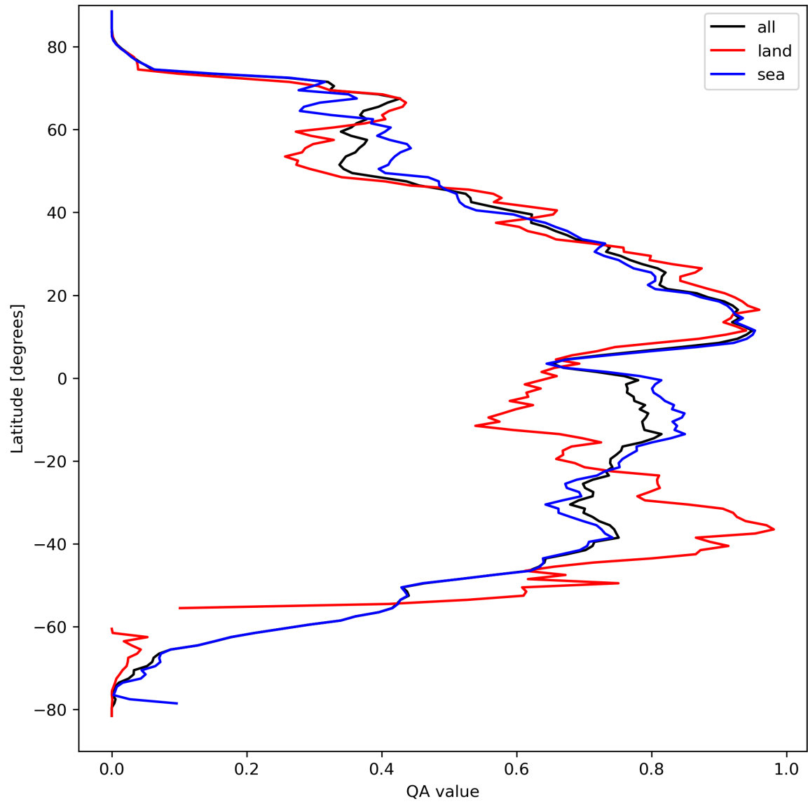
Figure 29: Zonal average of “QA value” for 2024-03-28 to 2024-03-30.
