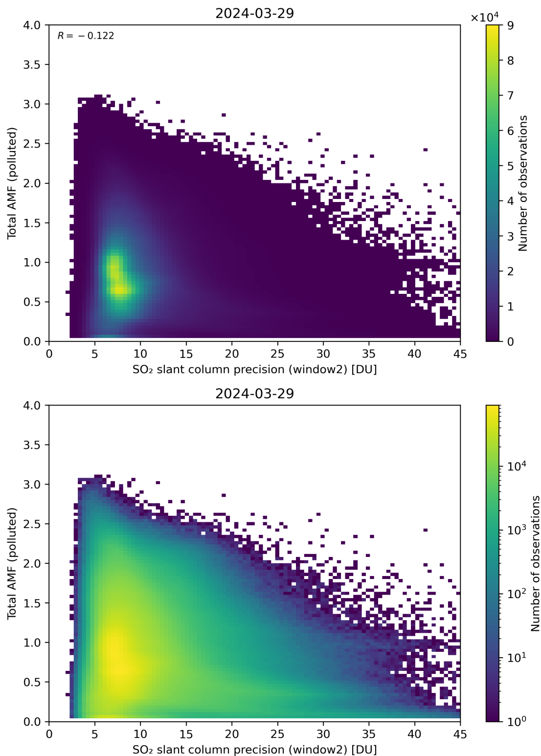
Figure 251: Scatter density plot of “SO 2 slant column precision (window2)” against “Total AMF (polluted)” for 2024-03-28 to 2024-03-30.
