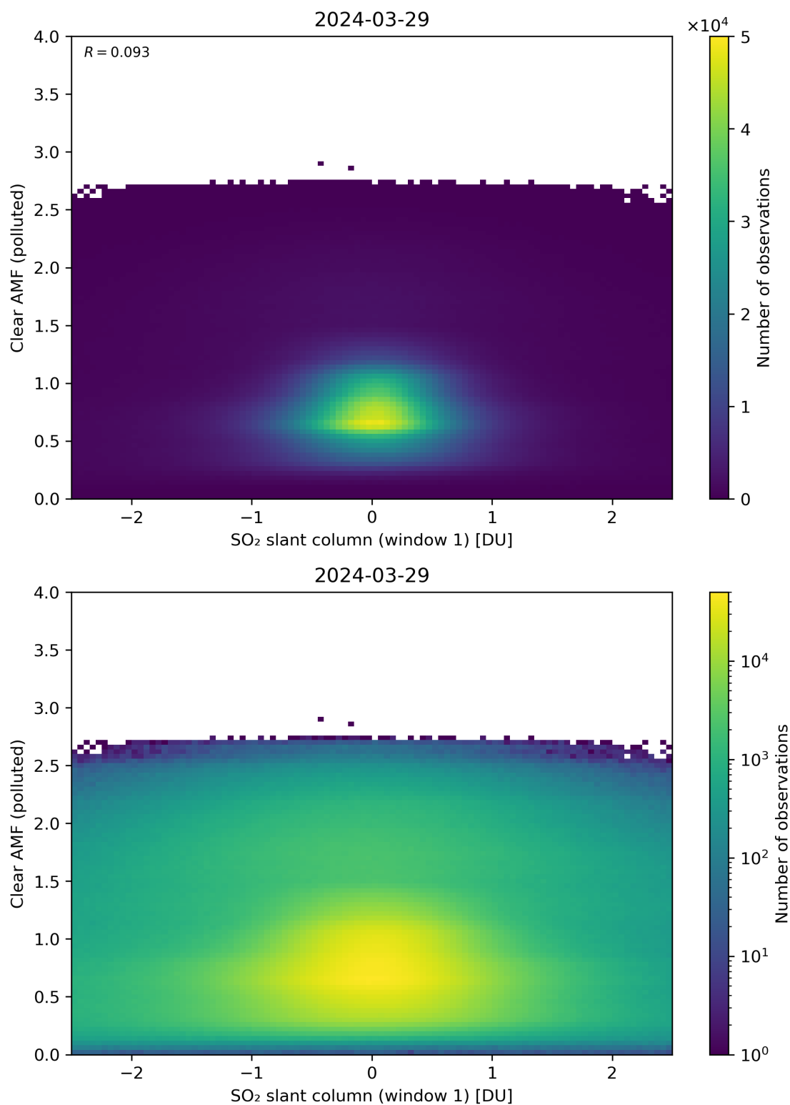
Figure 232: Scatter density plot of “SO 2 slant column (window 1)” against “Clear AMF (polluted)” for 2024-03-28 to 2024-03-30.
