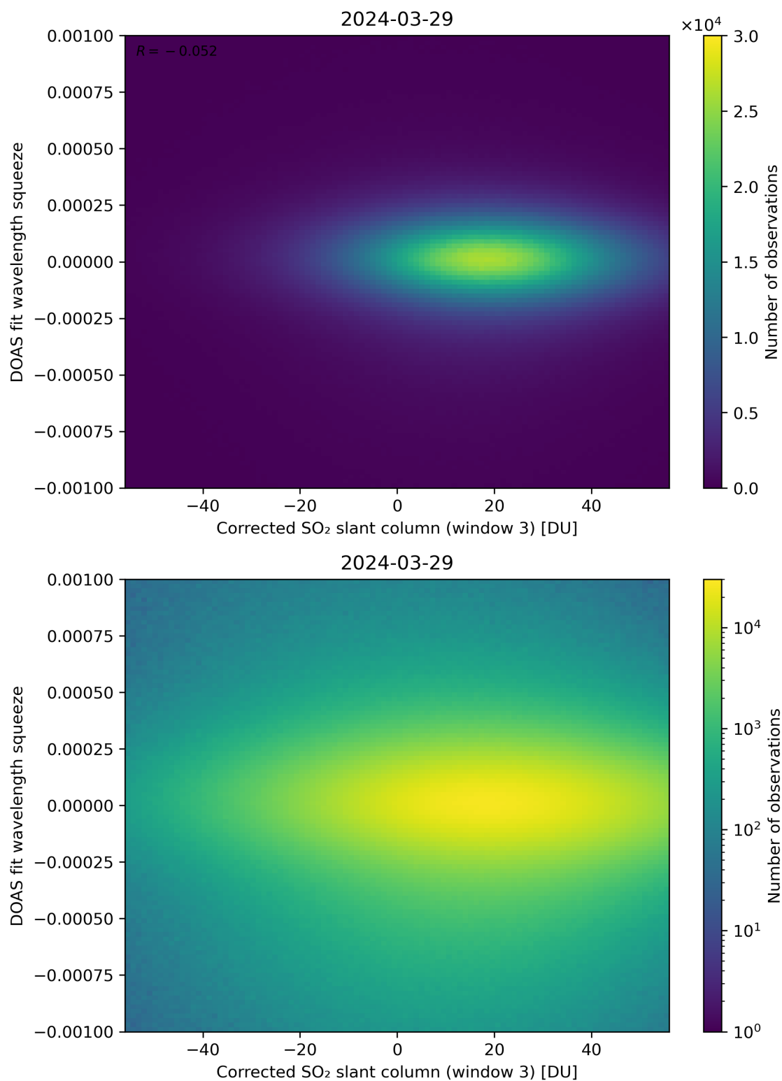
Figure 207: Scatter density plot of “Corrected SO 2 slant column (window 3)” against “DOAS fit wavelength squeeze” for 2024-03-28 to 2024-03-30.
