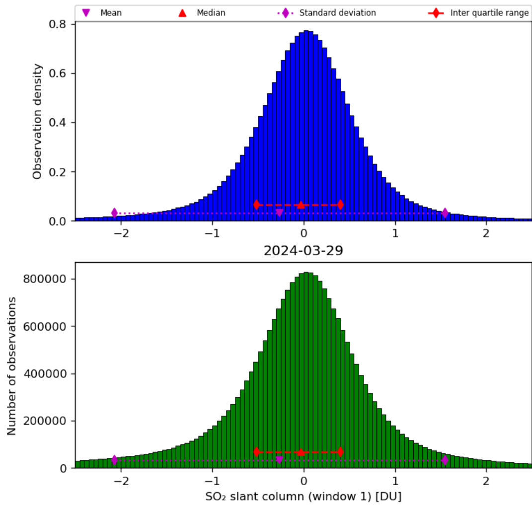
Figure 56: Histogram of “SO 2 slant column (window 1)” for 2024-03-28 to 2024-03-30
