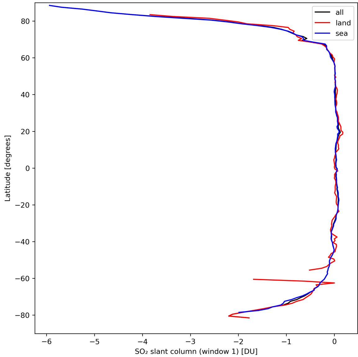
Figure 33: Zonal average of “SO 2 slant column (window 1)” for 2024-03-28 to 2024-03-30.
