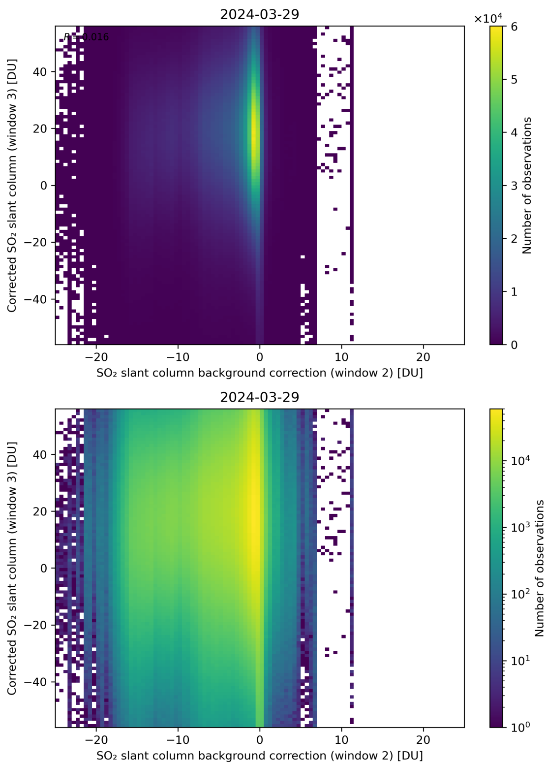
Figure 116: Scatter density plot of “SO 2 slant column background correction (window 2)” against “Corrected SO 2 slant column (window 3)” for 2024-03-28 to 2024-03-30.
