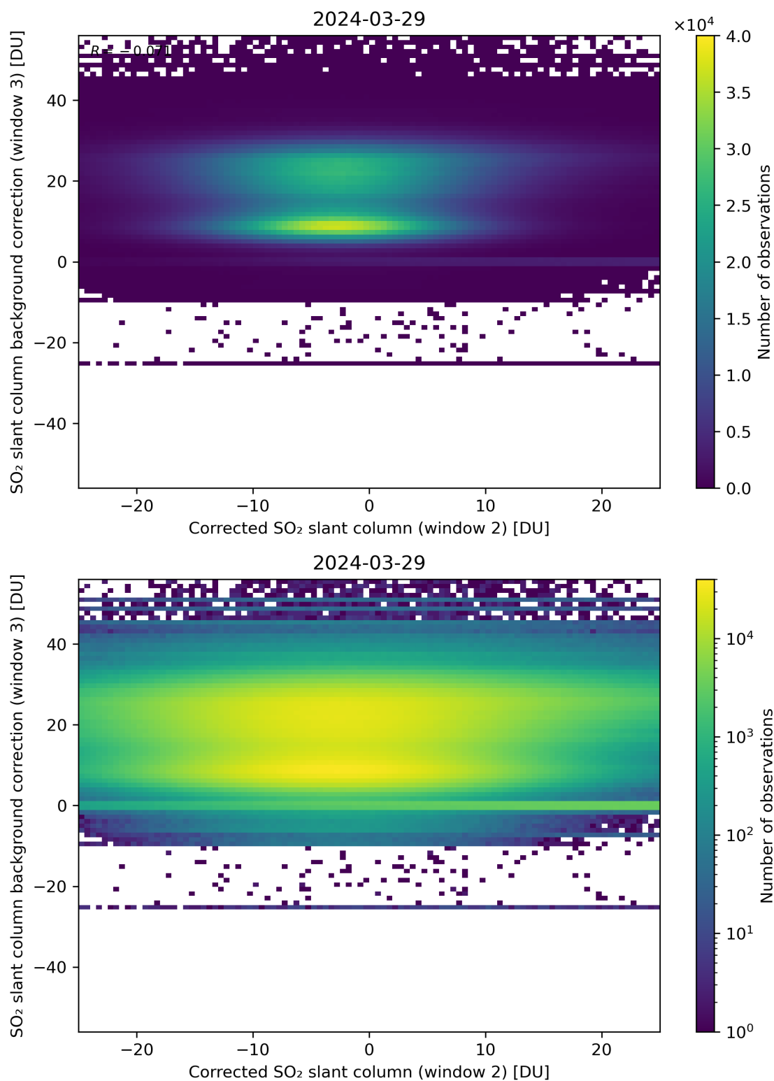
Figure 195: Scatter density plot of “Corrected SO 2 slant column (window 2)” against “SO 2 slant column background correction (window 3)” for 2024-03-28 to 2024-03-30.
