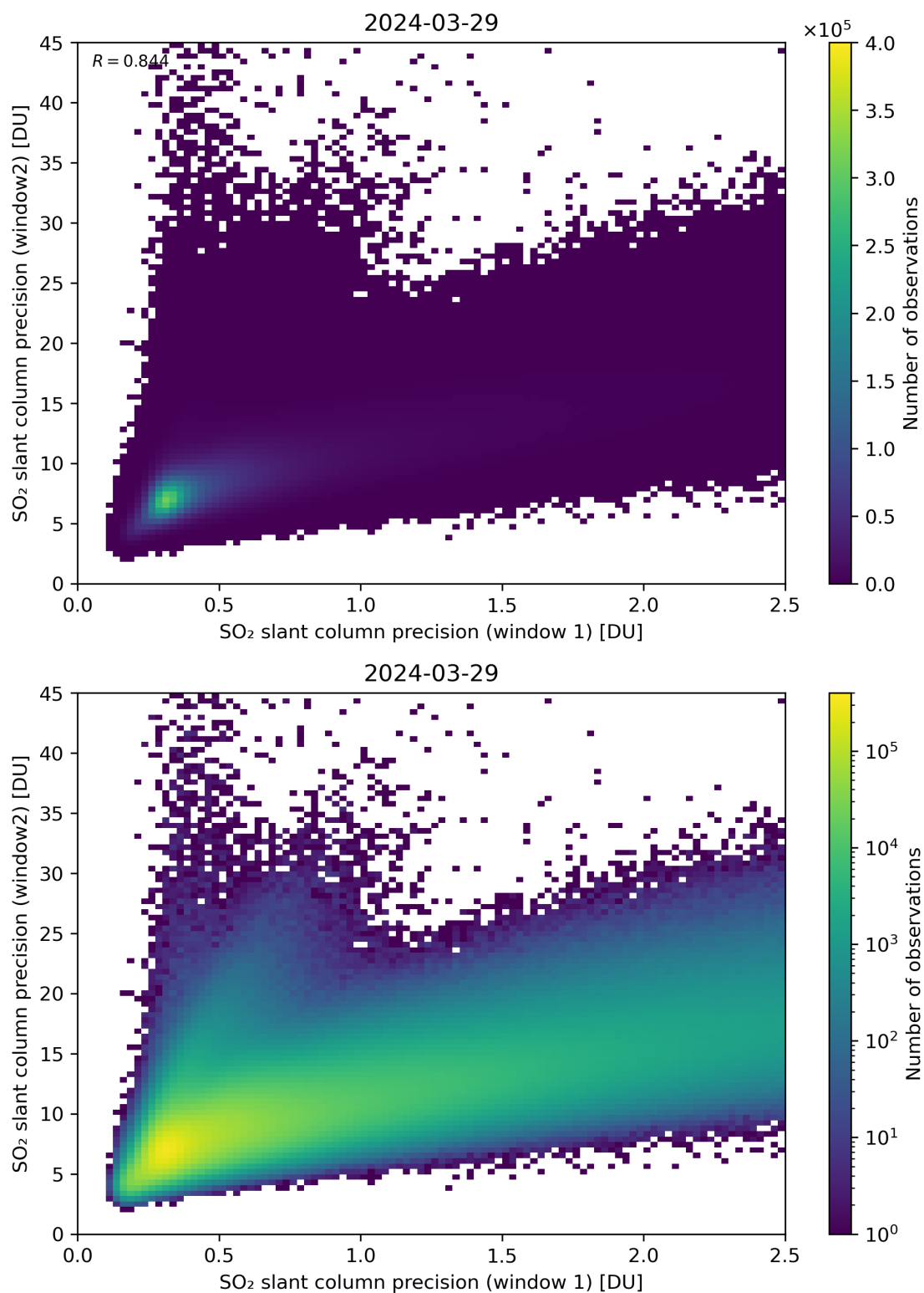
Figure 227: Scatter density plot of “SO 2 slant column precision (window 1)” against “SO 2 slant column precision (window 2)” for 2024-03-28 to 2024-03-30.
