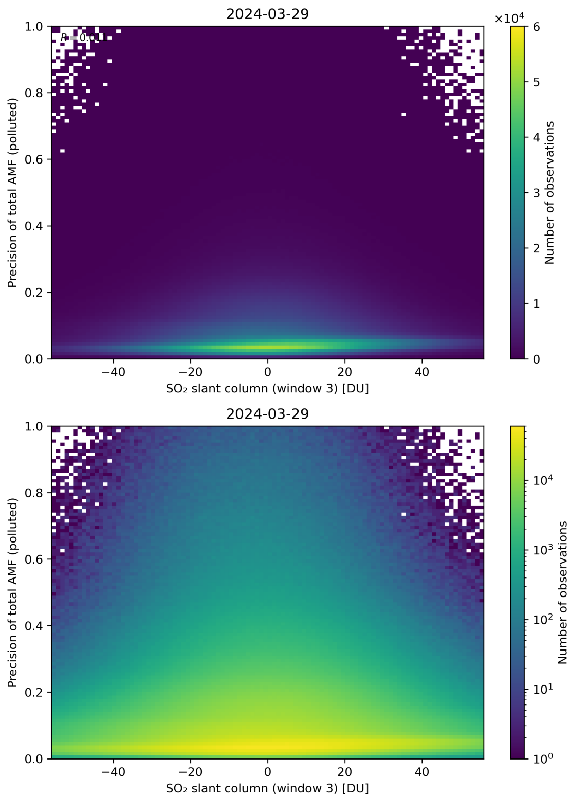
Figure 269: Scatter density plot of “SO 2 slant column (window 3)” against “Precision of total AMF (polluted)” for 2024-03-28 to 2024-03-30.
