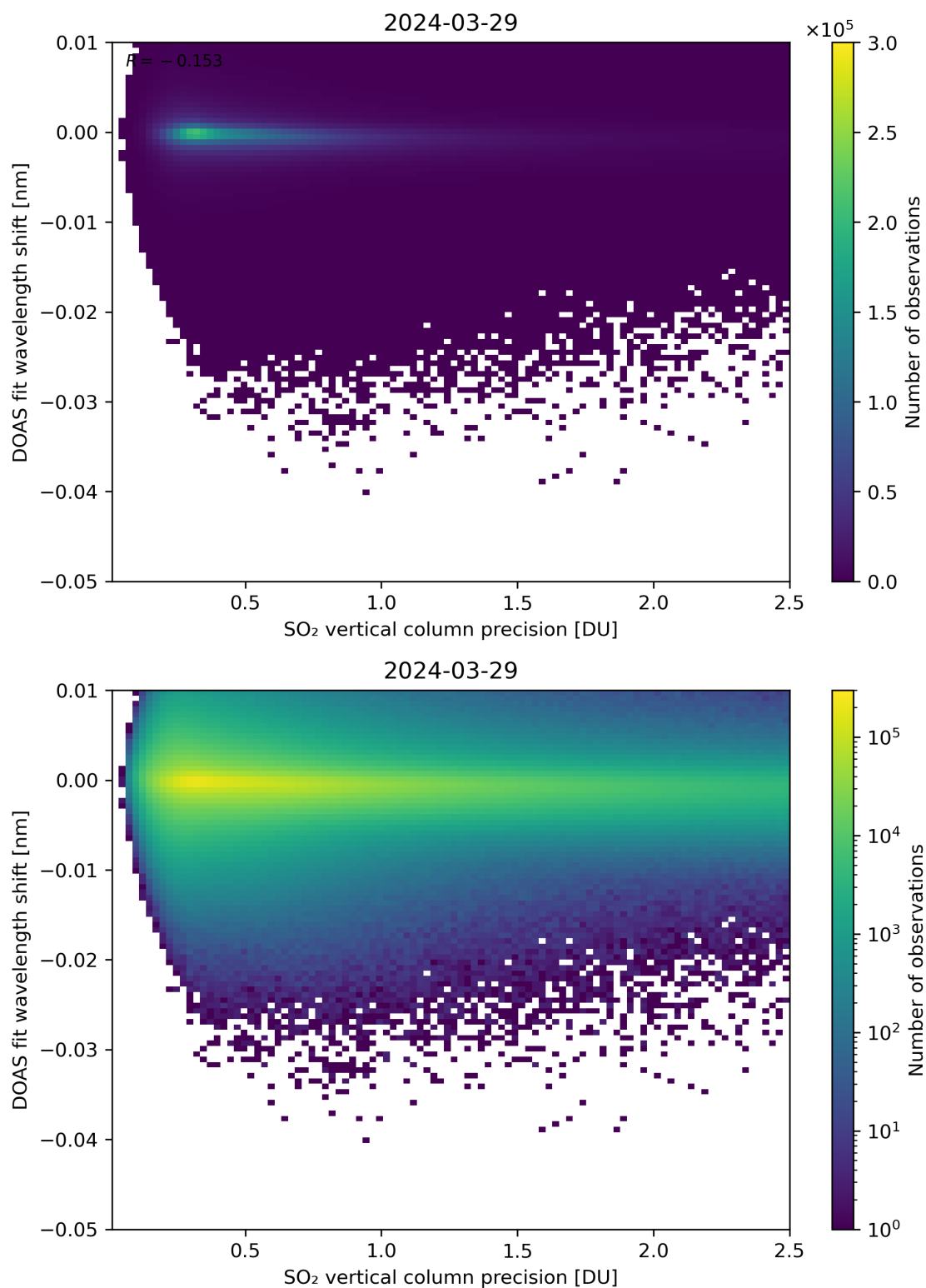
Figure 282: Scatter density plot of “SO 2 vertical column precision” against “DOAS fit wavelength shift” for 2024-03-28 to 2024-03-30.
