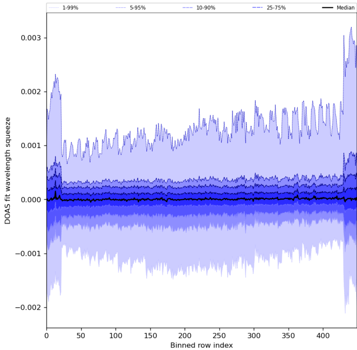
Figure 92: Along track statistics of “DOAS fit wavelength squeeze” for 2024-03-28 to 2024-03-30
