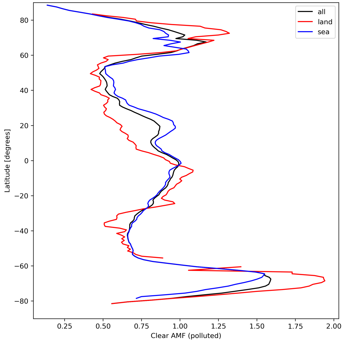
Figure 50: Zonal average of “Clear AMF (polluted)” for 2024-03-28 to 2024-03-30.
