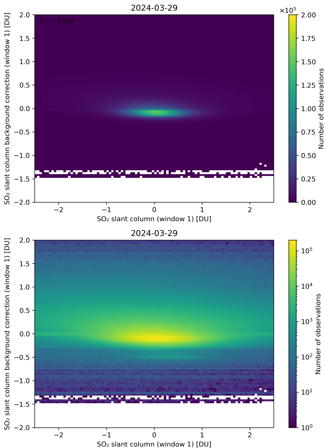
Figure 212: Scatter density plot of “SO 2 slant column (window 1)” against “SO 2 slant column background correction (window 1)” for 2024-03-28 to 2024-03-30.
