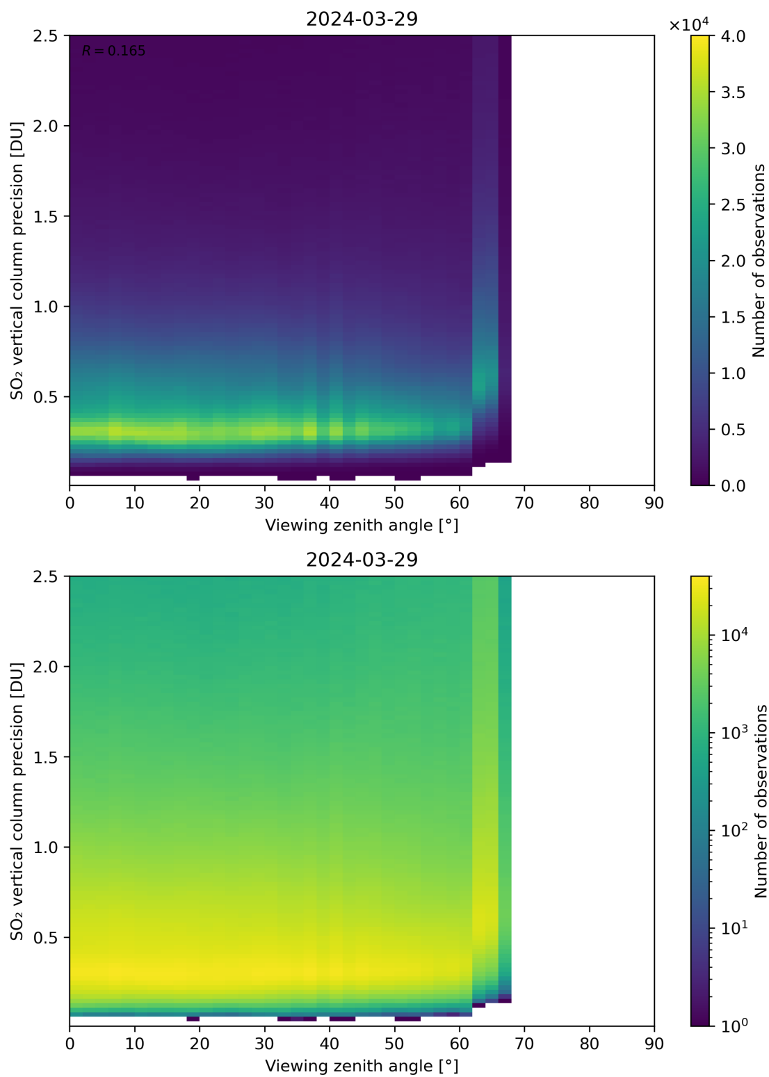
Figure 328: Scatter density plot of “Viewing zenith angle” against “SO 2 vertical column precision” for 2024-03-28 to 2024-03-30.
