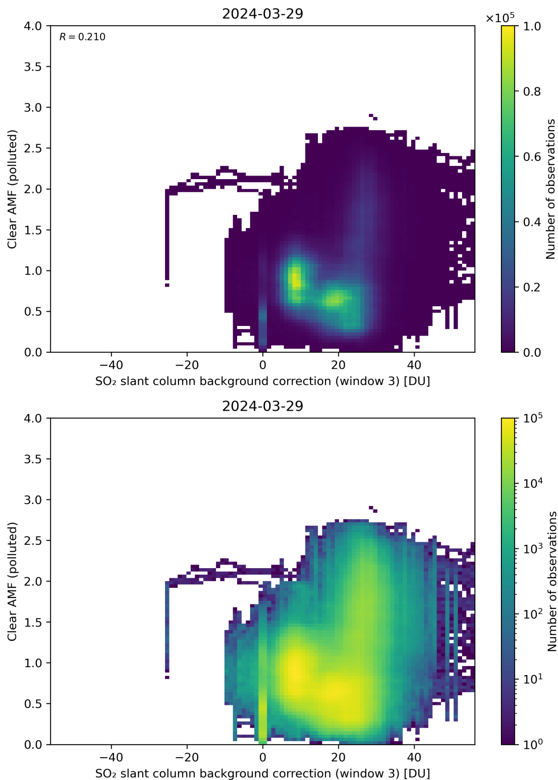
Figure 124: Scatter density plot of “SO 2 slant column background correction (window 3)” against “Clear AMF (polluted)” for 2024-03-28 to 2024-03-30.
