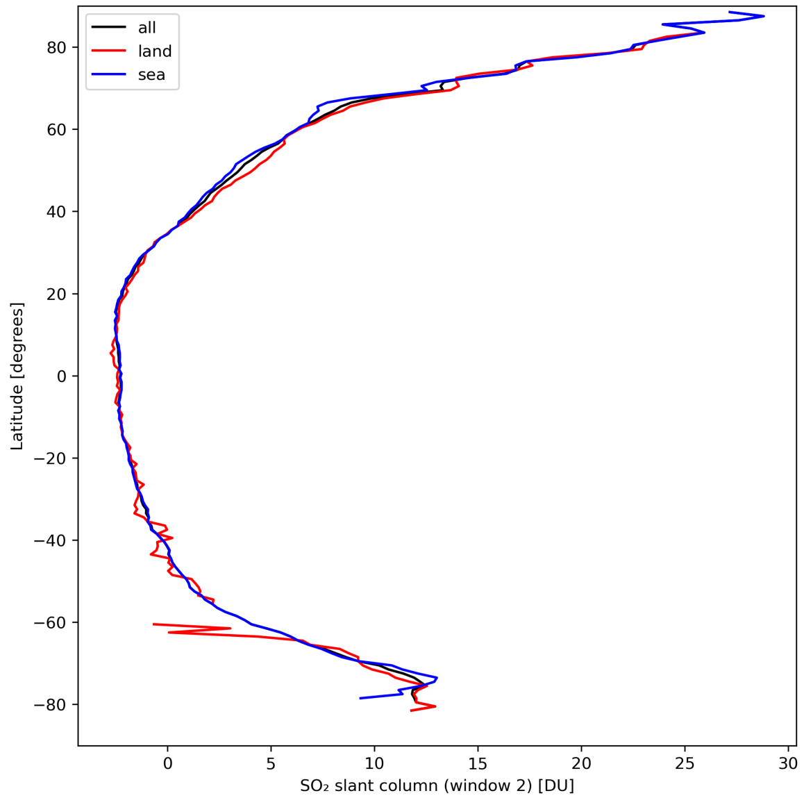
Figure 37: Zonal average of “SO 2 slant column (window 2)” for 2024-03-28 to 2024-03-30.
