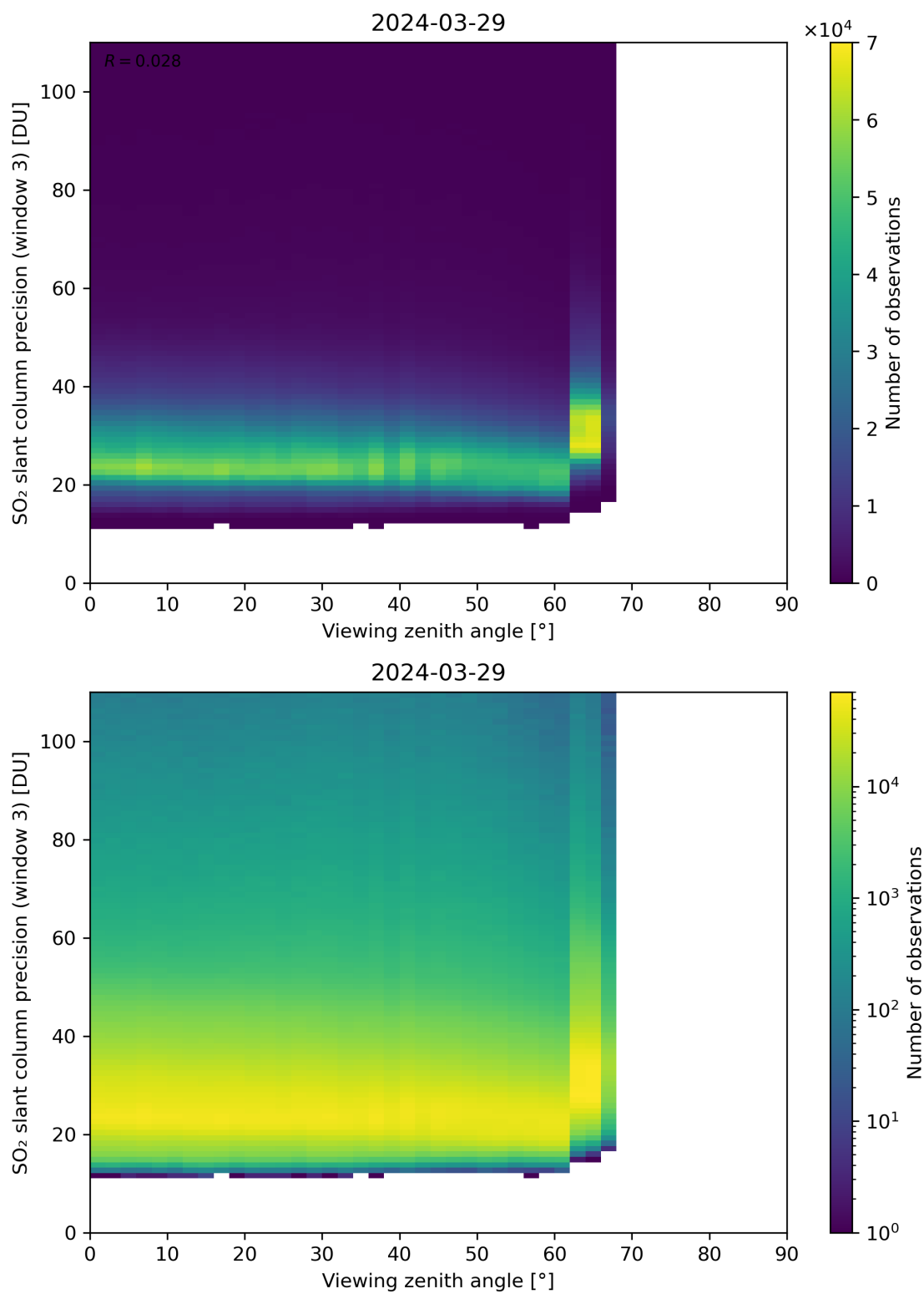
Figure 324: Scatter density plot of “Viewing zenith angle” against “SO 2 slant column precision (window 3)” for 2024-03-28 to 2024-03-30.
