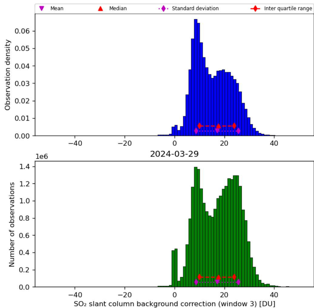
Figure 67: Histogram of “SO 2 slant column background correction (window 3)” for 2024-03-28 to 2024-03-30
