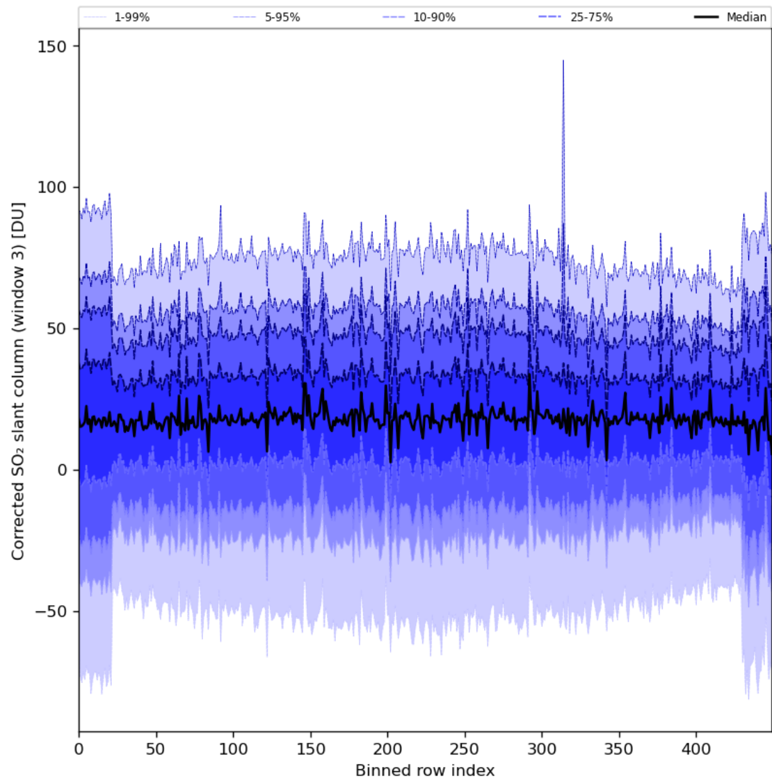
Figure 89: Along track statistics of “Corrected SO 2 slant column (window 3)” for 2024-03-28 to 2024-03-30
