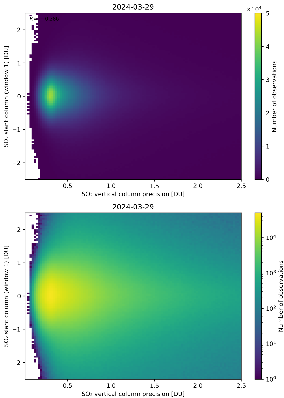
Figure 289: Scatter density plot of “SO 2 vertical column precision” against “SO 2 slant column (window 1)” for 2024-03-28 to 2024-03-30.
