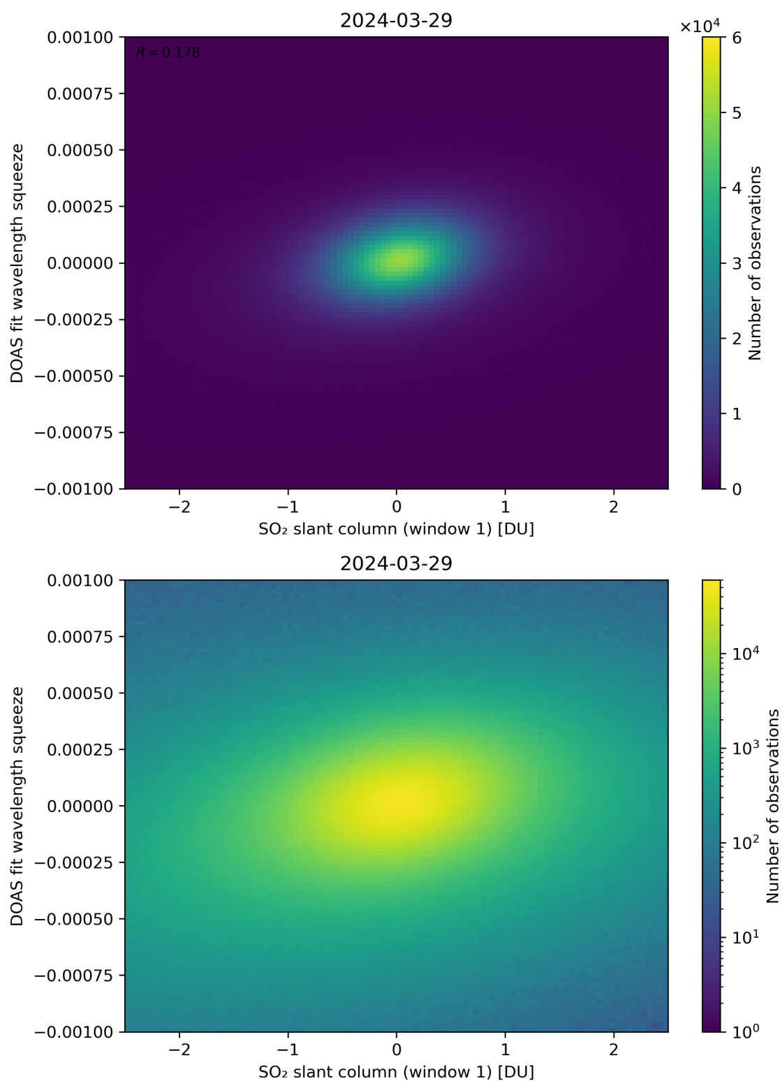
Figure 216: Scatter density plot of “SO 2 slant column (window 1)” against “DOAS fit wavelength squeeze” for 2024-03-28 to 2024-03-30.
