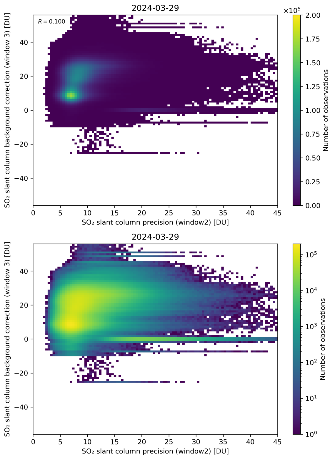
Figure 242: Scatter density plot of “SO 2 slant column precision (window2)” against “SO 2 slant column background correction (window 3)” for 2024-03-28 to 2024-03-30.
