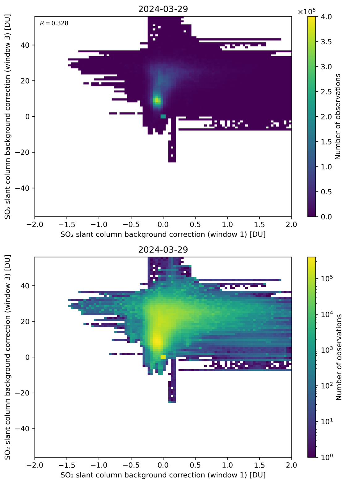
Figure 99: Scatter density plot of “SO 2 slant column background correction (window 1)” against “SO 2 slant column background correction (window 3)” for 2024-03-28 to 2024-03-30.
