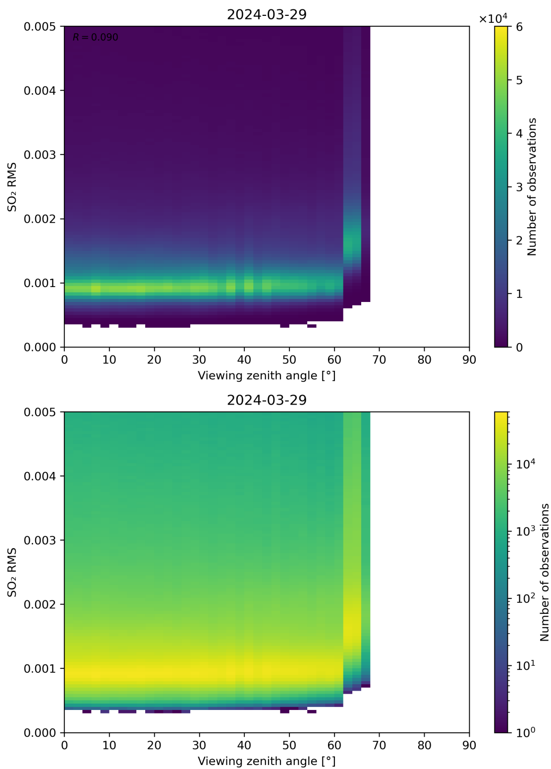
Figure 313: Scatter density plot of “Viewing zenith angle” against “SO 2 RMS” for 2024-03-28 to 2024-03-30.
