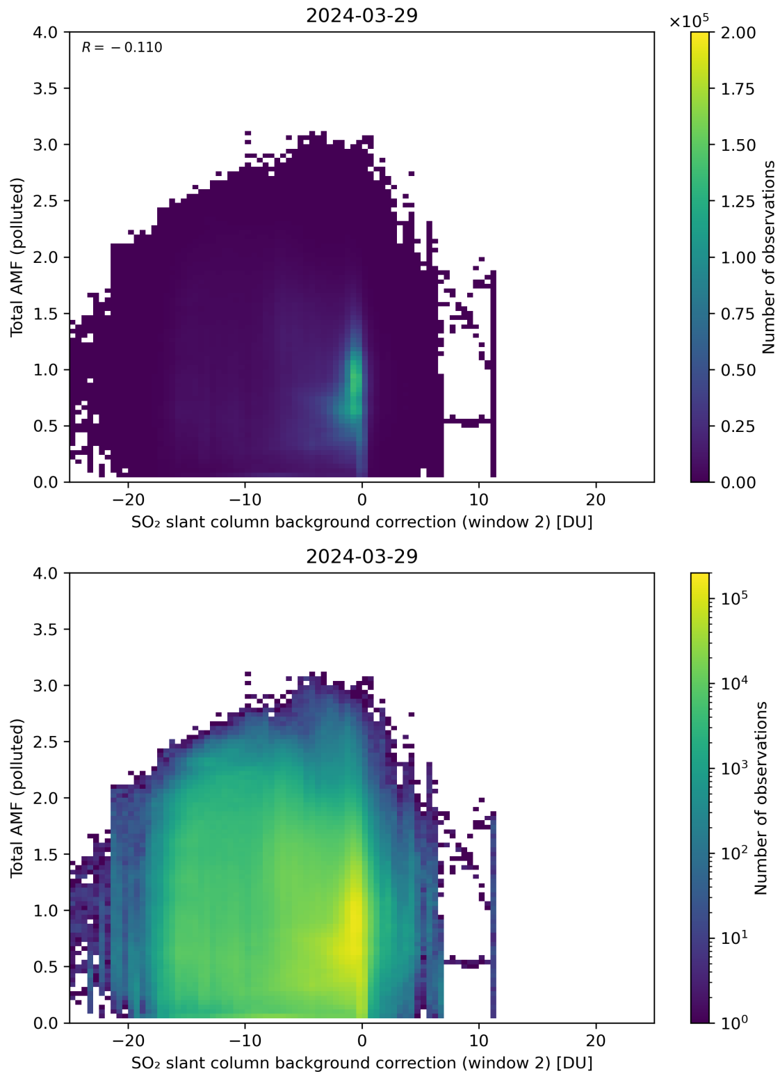
Figure 119: Scatter density plot of “SO 2 slant column background correction (window 2)” against “Total AMF (polluted)” for 2024-03-28 to 2024-03-30.
