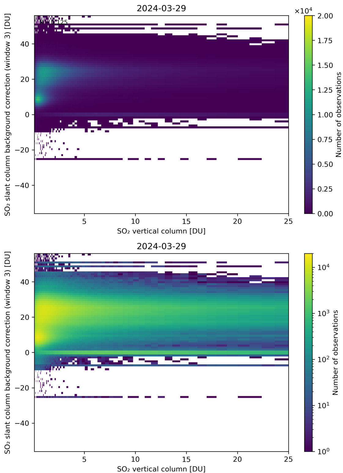
Figure 275: Scatter density plot of “SO 2 vertical column” against “SO 2 slant column background correction (window 3)” for 2024-03-28 to 2024-03-30.
