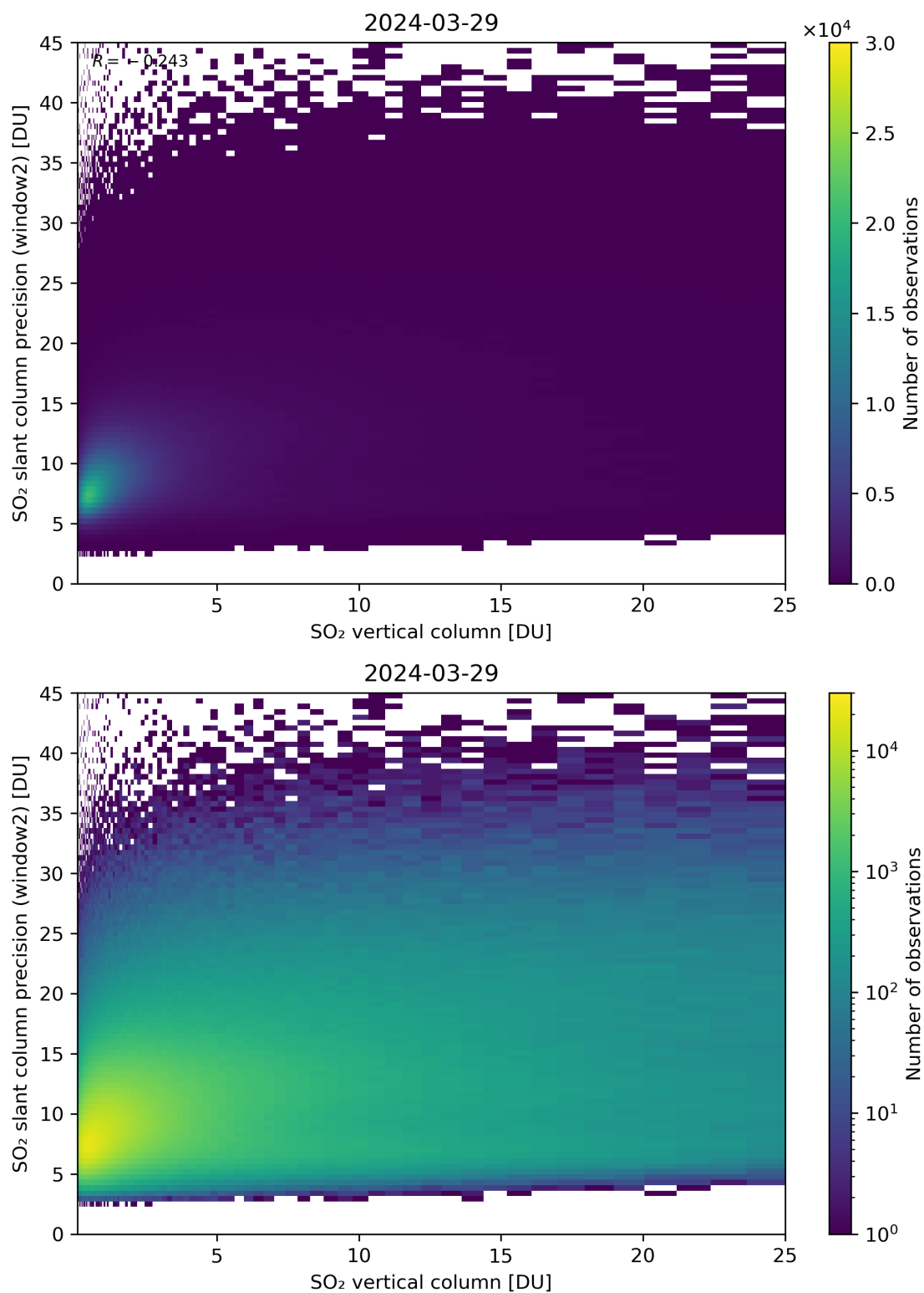
Figure 302: Scatter density plot of “SO 2 vertical column” against “SO 2 slant column precision (window2)” for 2024-03-28 to 2024-03-30.
