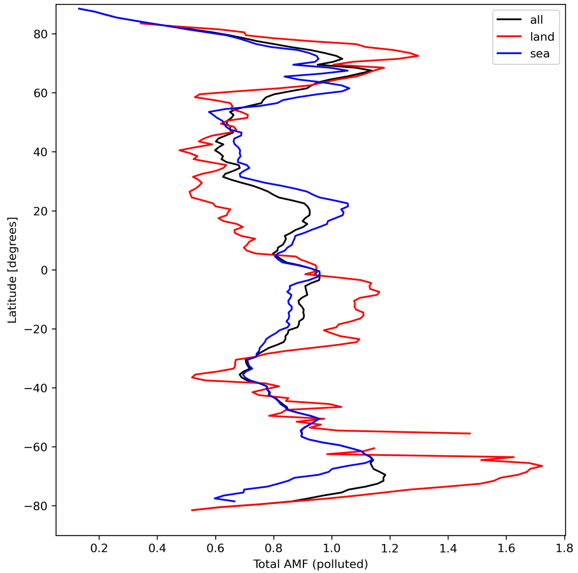
Figure 48: Zonal average of “Total AMF (polluted)” for 2024-03-28 to 2024-03-30.
