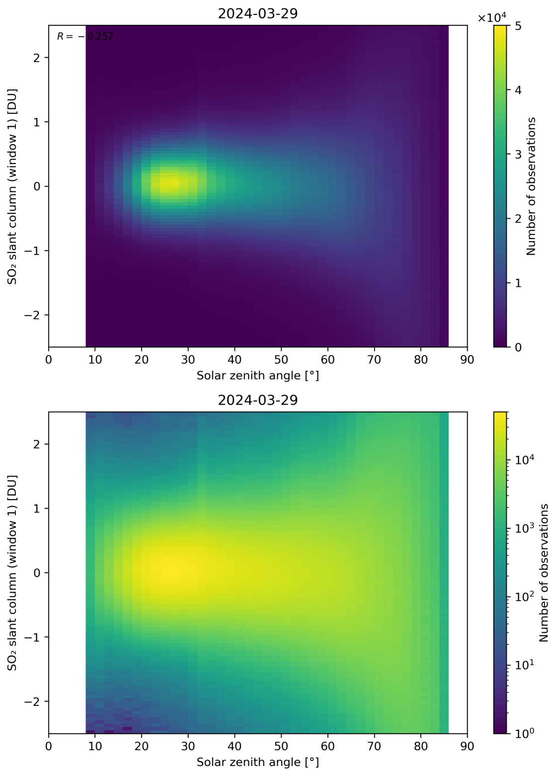
Figure 169: Scatter density plot of “Solar zenith angle” against “SO 2 slant column (window 1)” for 2024-03-28 to 2024-03-30.
