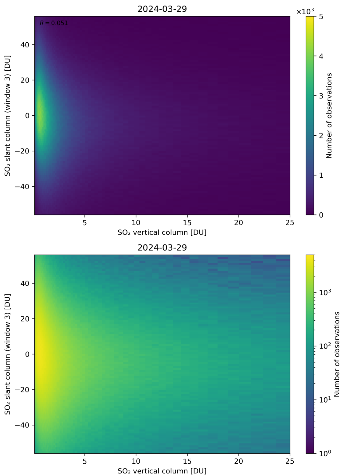
Figure 303: Scatter density plot of “SO 2 vertical column” against “SO 2 slant column (window 3)” for 2024-03-28 to 2024-03-30.
