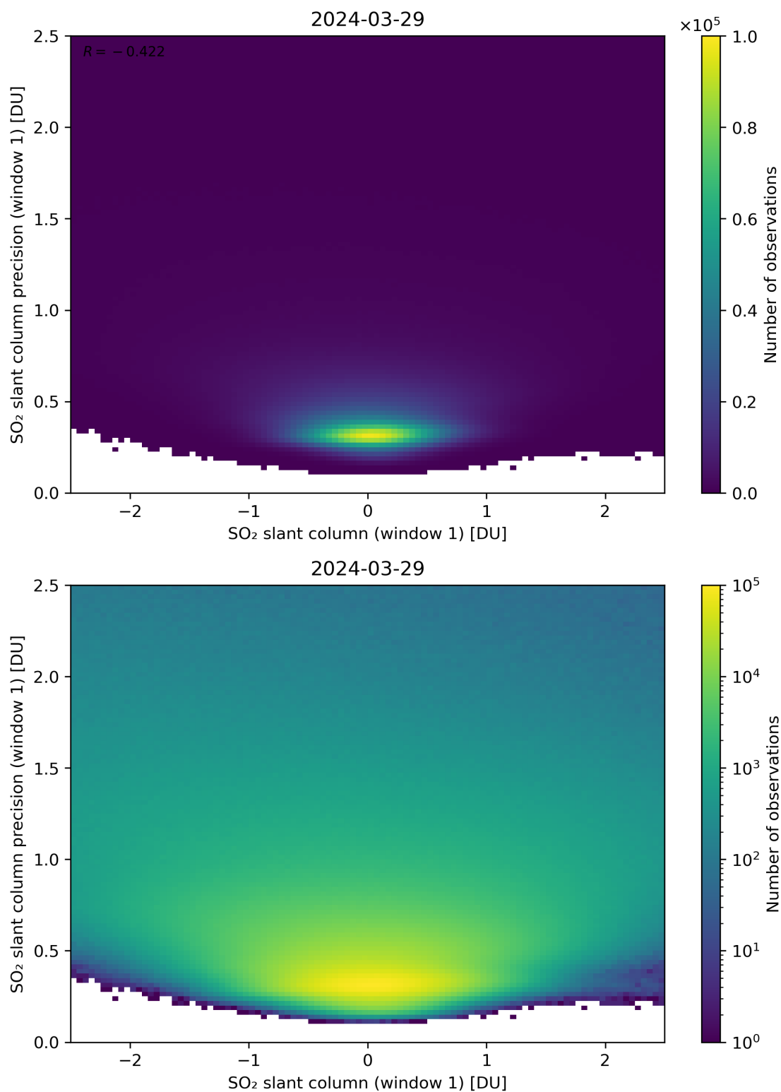
Figure 235: Scatter density plot of “SO 2 slant column (window 1)” against “SO 2 slant column precision (window 1)” for 2024-03-28 to 2024-03-30.
