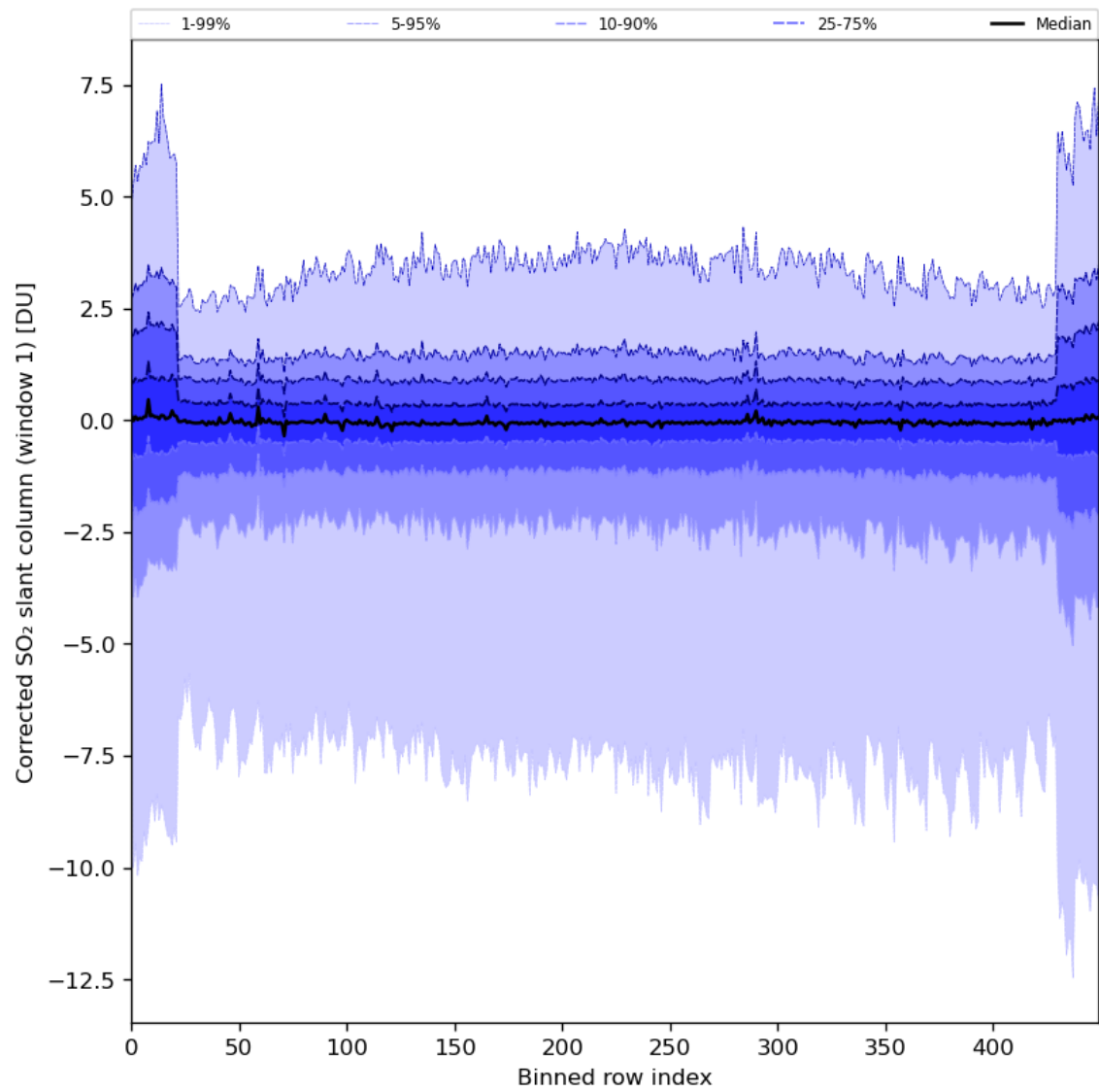
Figure 81: Along track statistics of “Corrected SO 2 slant column (window 1)” for 2024-03-28 to 2024-03-30
