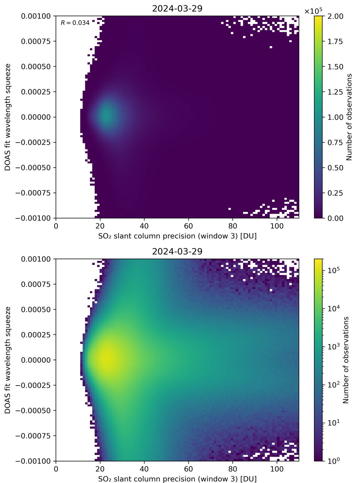
Figure 259: Scatter density plot of “SO 2 slant column precision (window 3)” against “DOAS fit wavelength squeeze” for 2024-03-28 to 2024-03-30.
