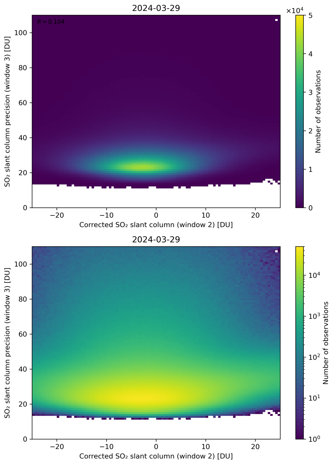
Figure 202: Scatter density plot of “Corrected SO 2 slant column (window 2)” against “SO 2 slant column precision (window 3)” for 2024-03-28 to 2024-03-30.
