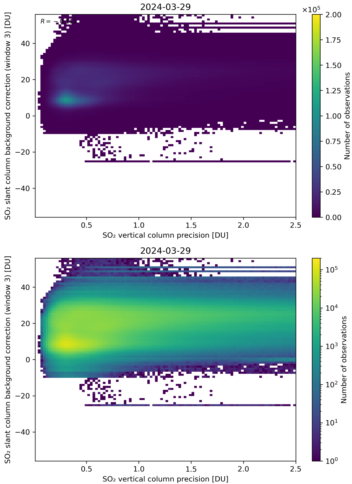
Figure 281: Scatter density plot of “SO 2 vertical column precision” against “SO 2 slant column background correction (window 3)” for 2024-03-28 to 2024-03-30.
