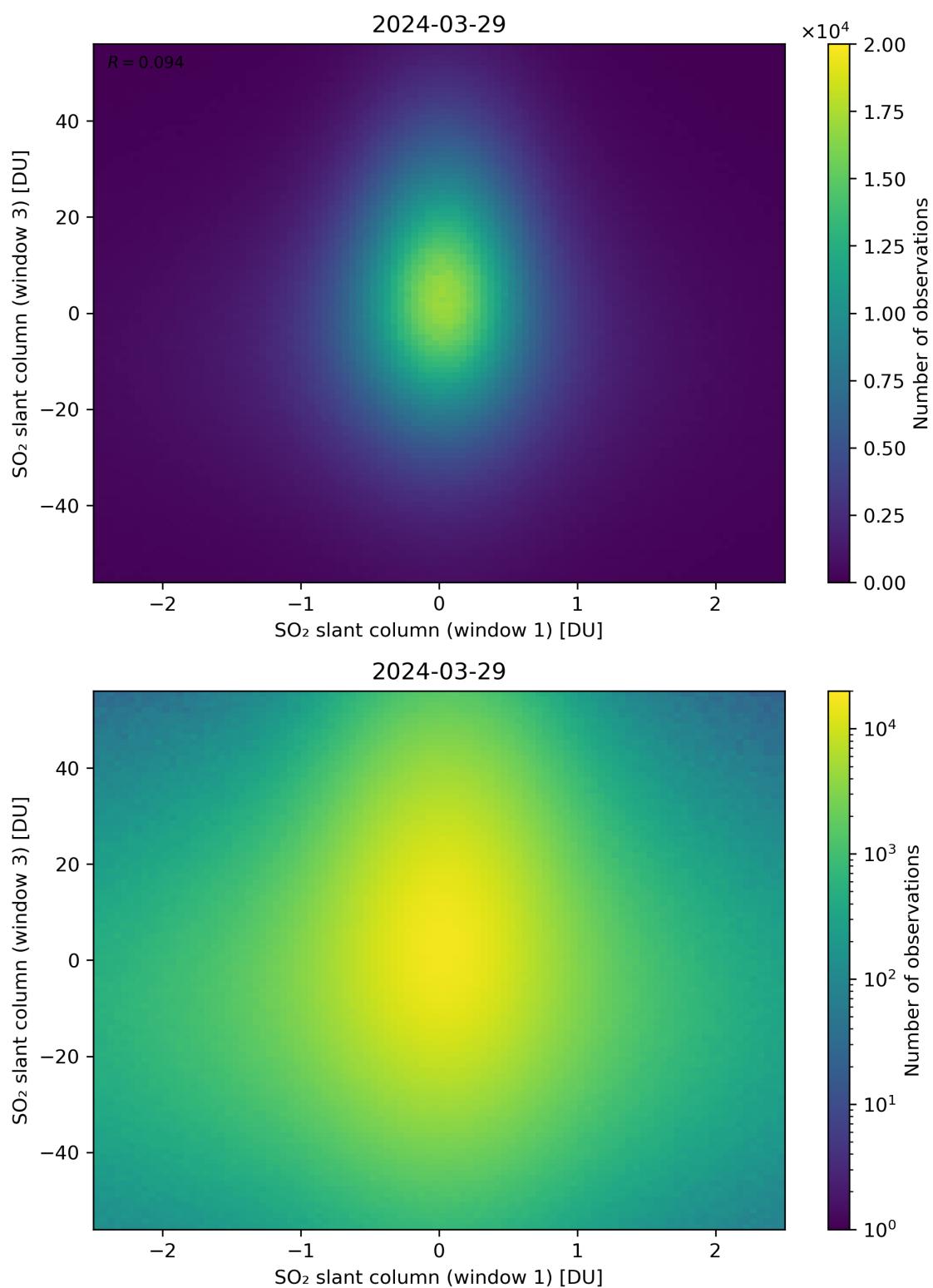
Figure 237: Scatter density plot of “SO 2 slant column (window 1)” against “SO 2 slant column (window 3)” for 2024-03-28 to 2024-03-30.
