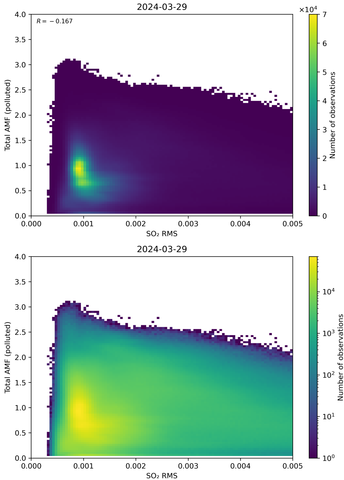
Figure 137: Scatter density plot of “SO 2 RMS” against “Total AMF (polluted)” for 2024-03-28 to 2024-03-30.
