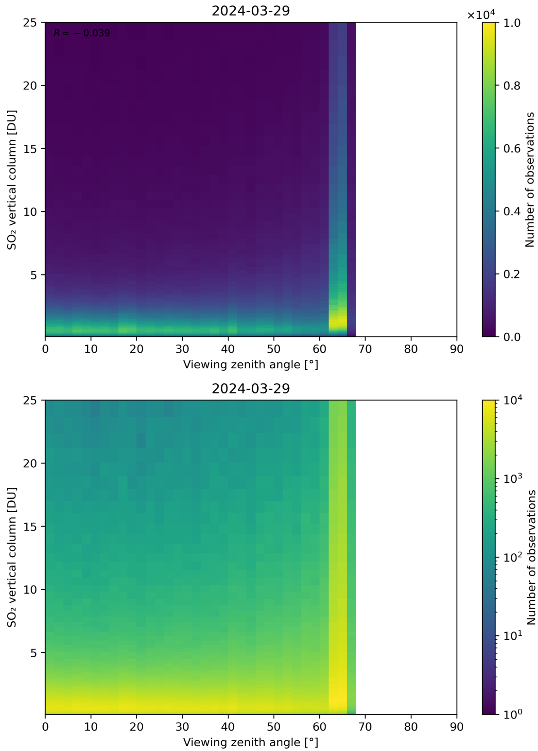
Figure 327: Scatter density plot of “Viewing zenith angle” against “SO 2 vertical column” for 2024-03-28 to 2024-03-30.
