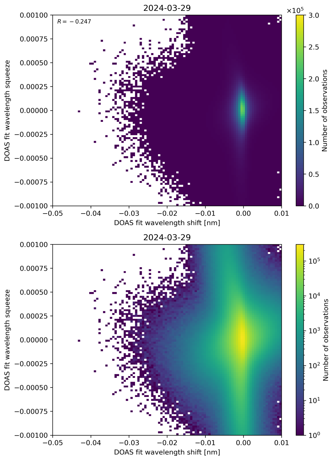
Figure 127: Scatter density plot of “DOAS fit wavelength shift” against “DOAS fit wavelength squeeze” for 2024-03-28 to 2024-03-30.
