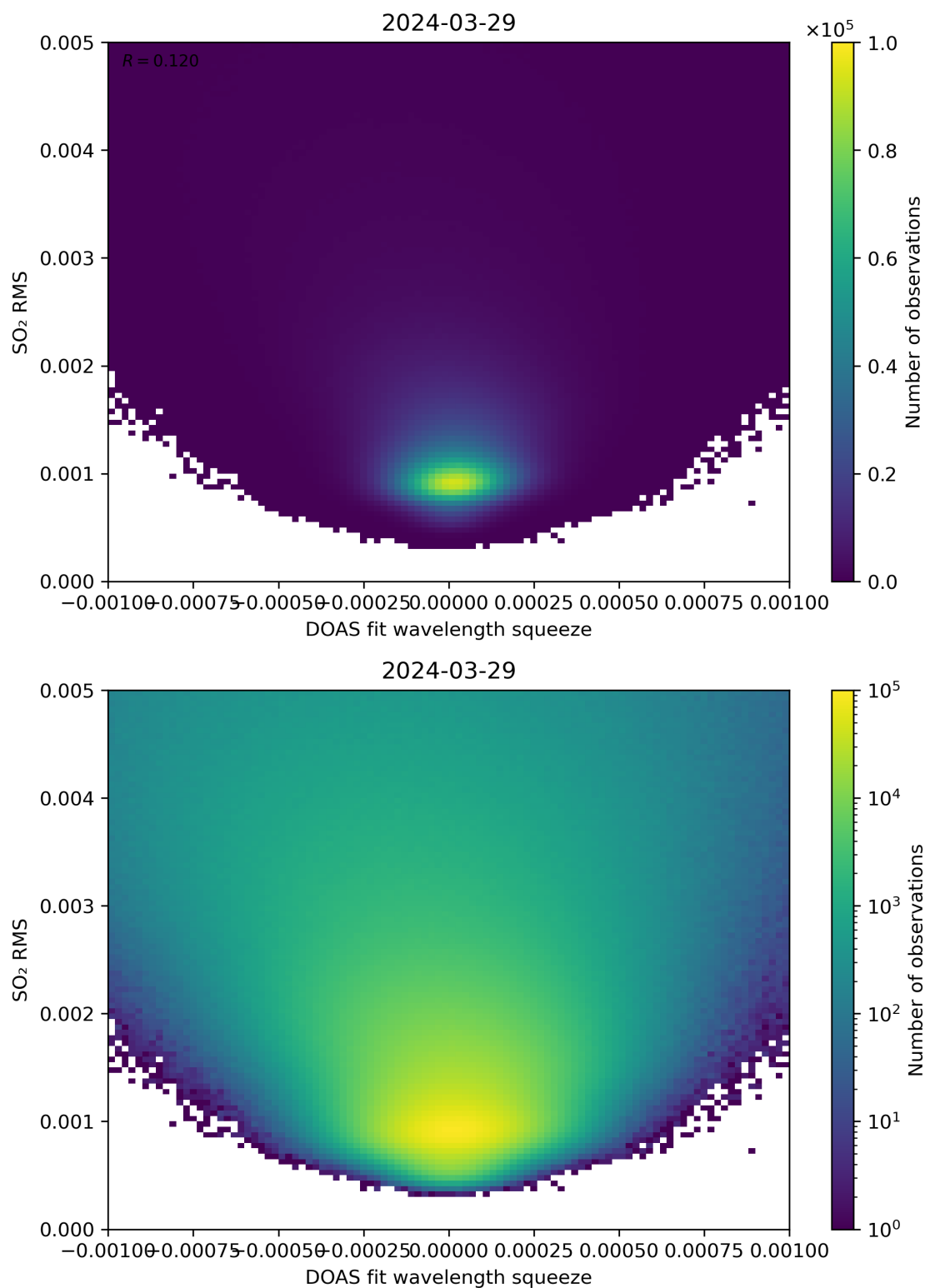
Figure 132: Scatter density plot of “DOAS fit wavelength squeeze” against “SO 2 RMS” for 2024-03-28 to 2024-03-30.
