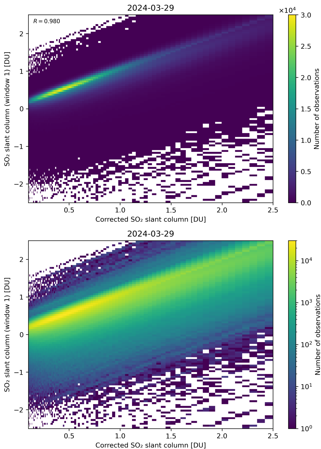
Figure 187: Scatter density plot of “Corrected SO 2 slant column” against “SO 2 slant column (window 1)” for 2024-03-28 to 2024-03-30.
