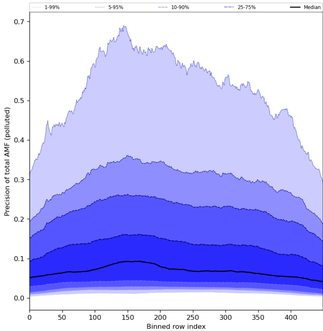
Figure 95: Along track statistics of “Precision of total AMF (polluted)” for 2024-03-28 to 2024-03-30
