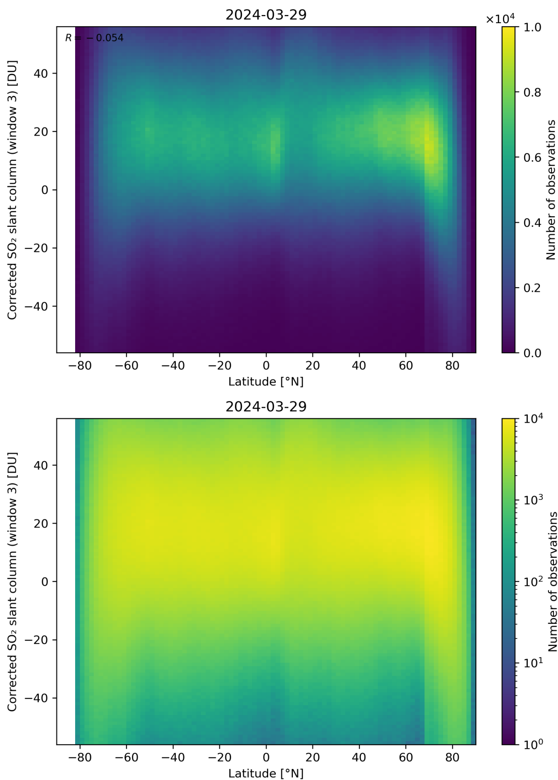
Figure 148: Scatter density plot of “Latitude” against “Corrected SO 2 slant column (window 3)” for 2024-03-28 to 2024-03-30.
