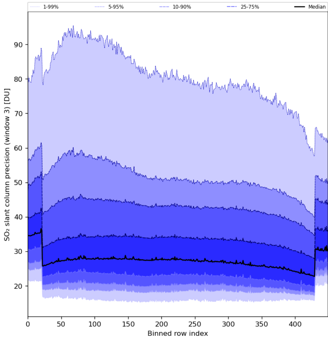
Figure 88: Along track statistics of “SO 2 slant column precision (window 3)” for 2024-03-28 to 2024-03-30
