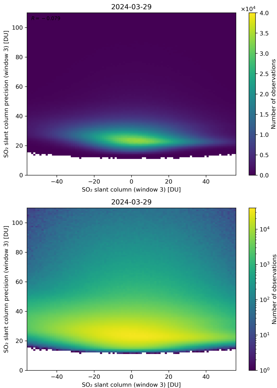
Figure 267: Scatter density plot of “SO 2 slant column (window 3)” against “SO 2 slant column precision (window 3)” for 2024-03-28 to 2024-03-30.
