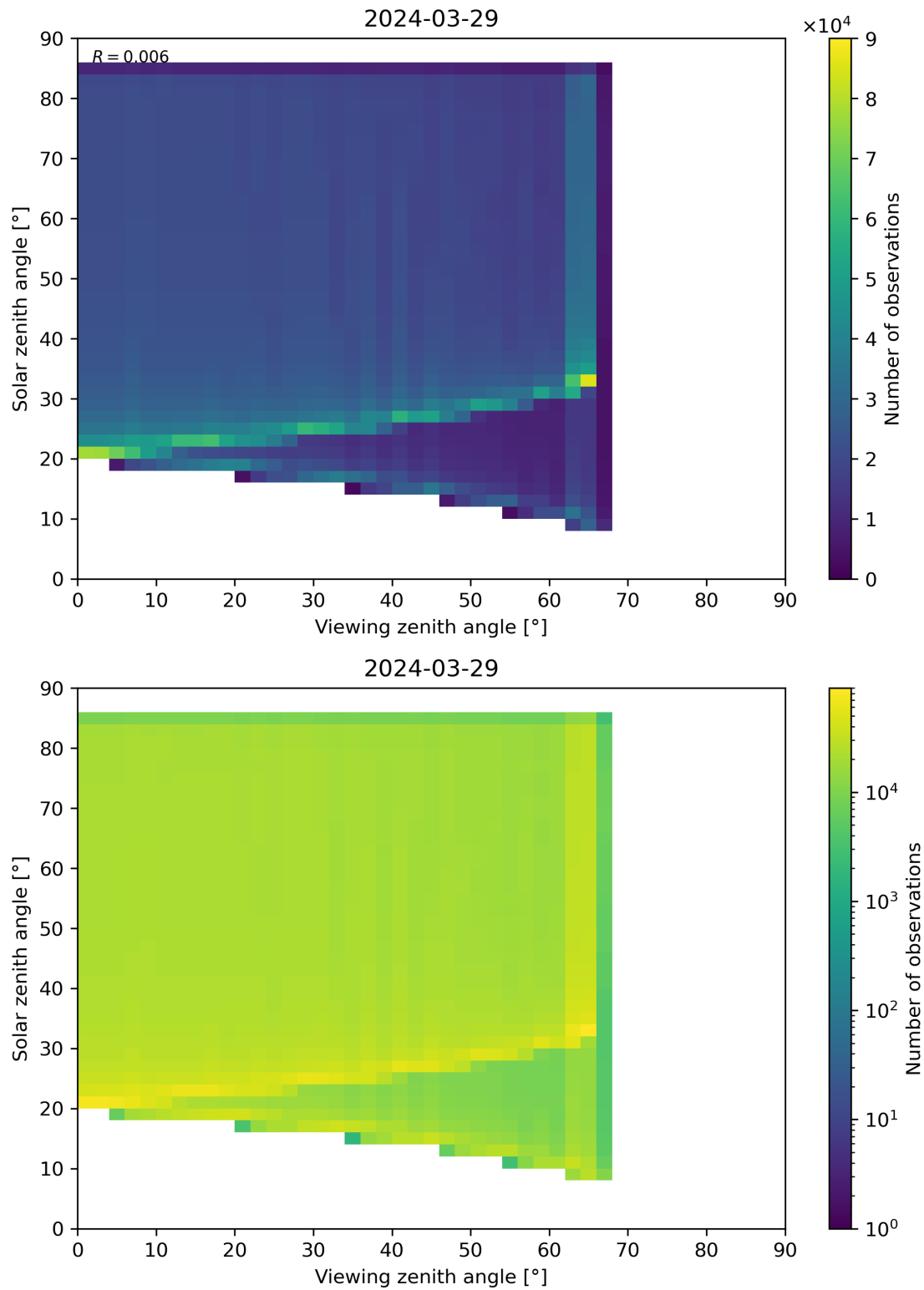
Figure 315: Scatter density plot of “Viewing zenith angle” against “Solar zenith angle” for 2024-03-28 to 2024-03-30.
