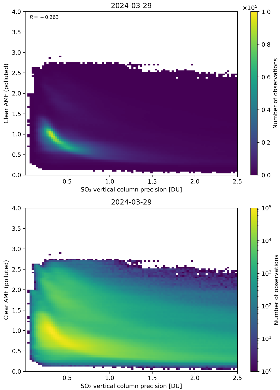
Figure 285: Scatter density plot of “SO 2 vertical column precision” against “Clear AMF (polluted)” for 2024-03-28 to 2024-03-30.
