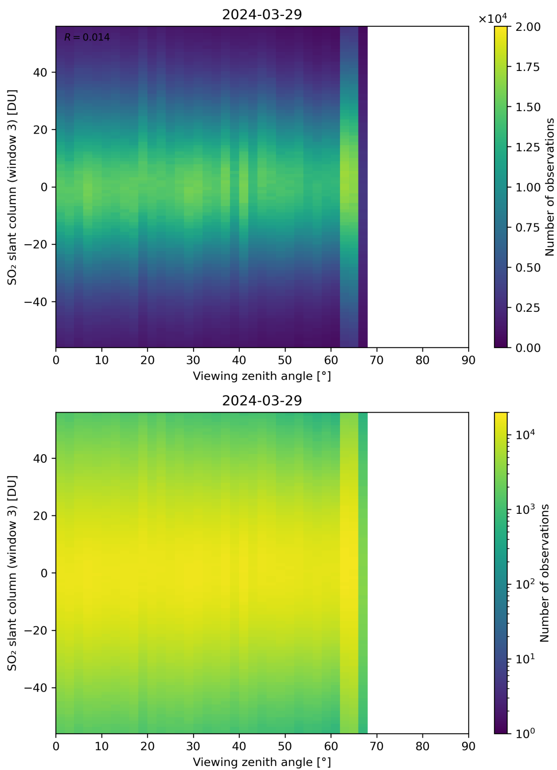
Figure 323: Scatter density plot of “Viewing zenith angle” against “SO 2 slant column (window 3)” for 2024-03-28 to 2024-03-30.
