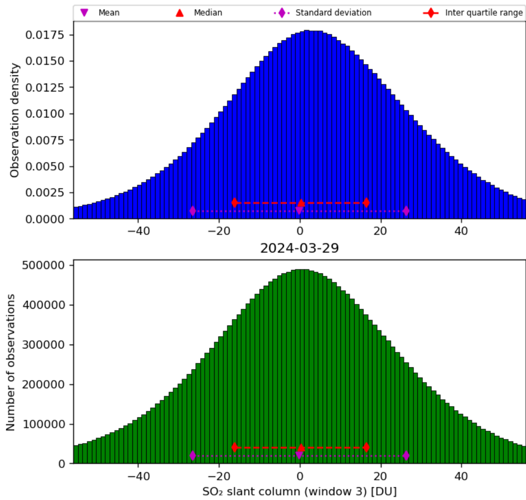
Figure 64: Histogram of “SO 2 slant column (window 3)” for 2024-03-28 to 2024-03-30
