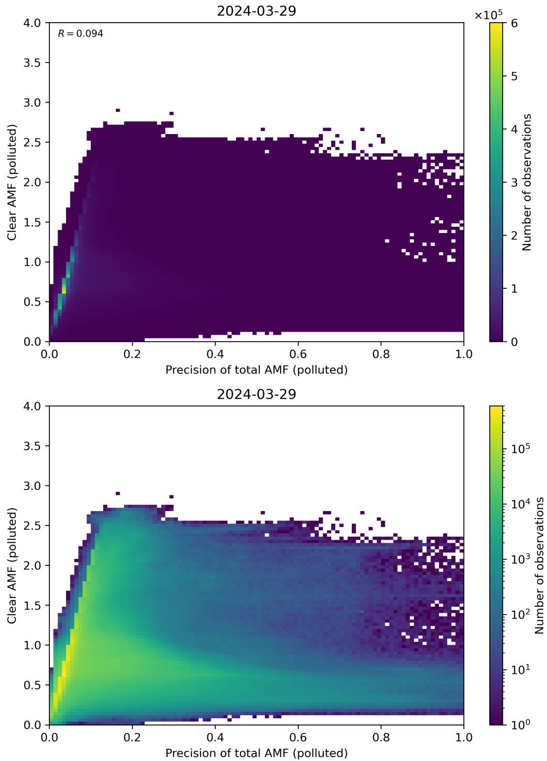
Figure 270: Scatter density plot of “Precision of total AMF (polluted)” against “Clear AMF (polluted)” for 2024-03-28 to 2024-03-30.
