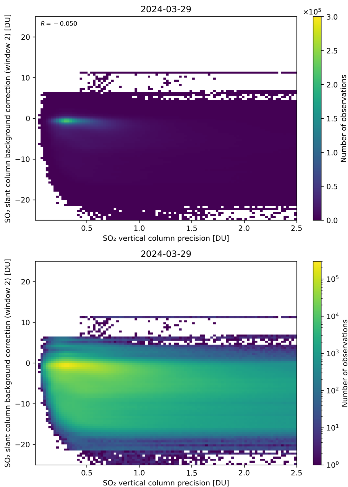
Figure 280: Scatter density plot of “SO 2 vertical column precision” against “SO 2 slant column background correction (window 2)” for 2024-03-28 to 2024-03-30.
