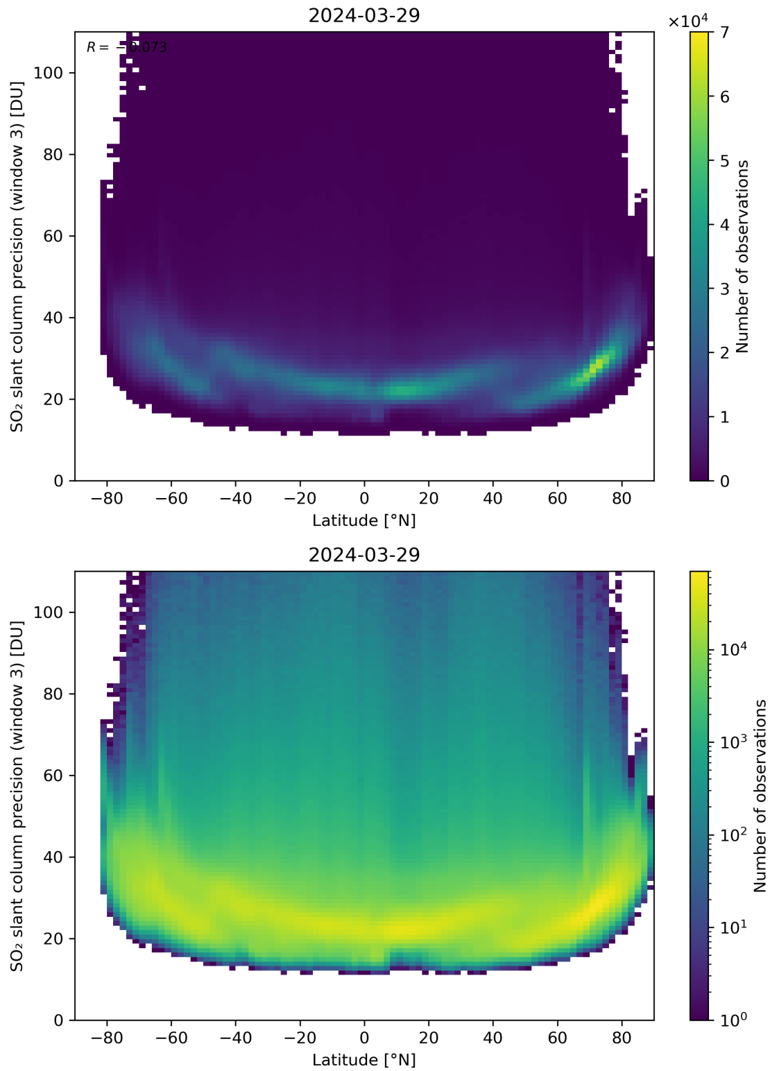
Figure 153: Scatter density plot of “Latitude” against “SO 2 slant column precision (window 3)” for 2024-03-28 to 2024-03-30.
