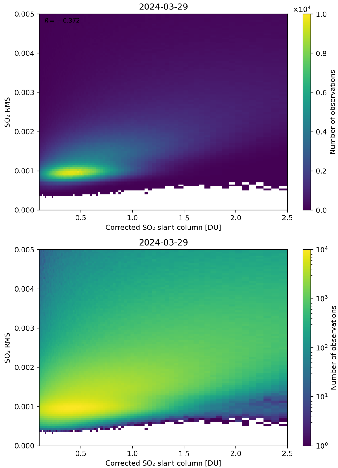
Figure 183: Scatter density plot of “Corrected SO 2 slant column” against “SO 2 RMS” for 2024-03-28 to 2024-03-30.
