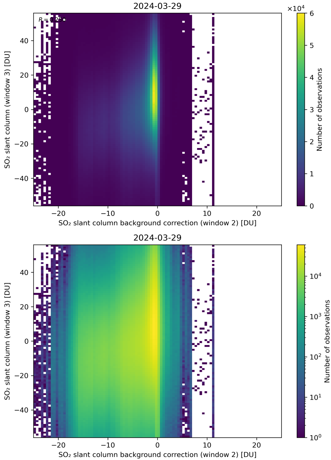
Figure 117: Scatter density plot of “SO 2 slant column background correction (window 2)” against “SO 2 slant column (window 3)” for 2024-03-28 to 2024-03-30.
