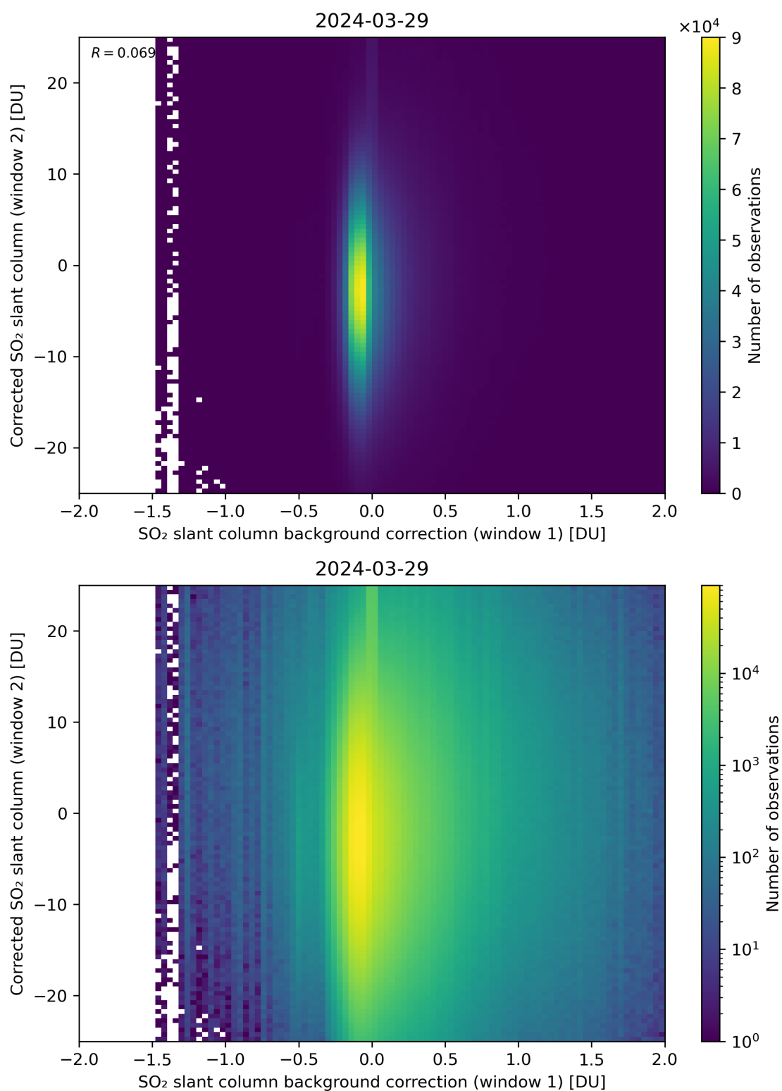
Figure 104: Scatter density plot of “SO 2 slant column background correction (window 1)” against “Corrected SO 2 slant column (window 2)” for 2024-03-28 to 2024-03-30.
