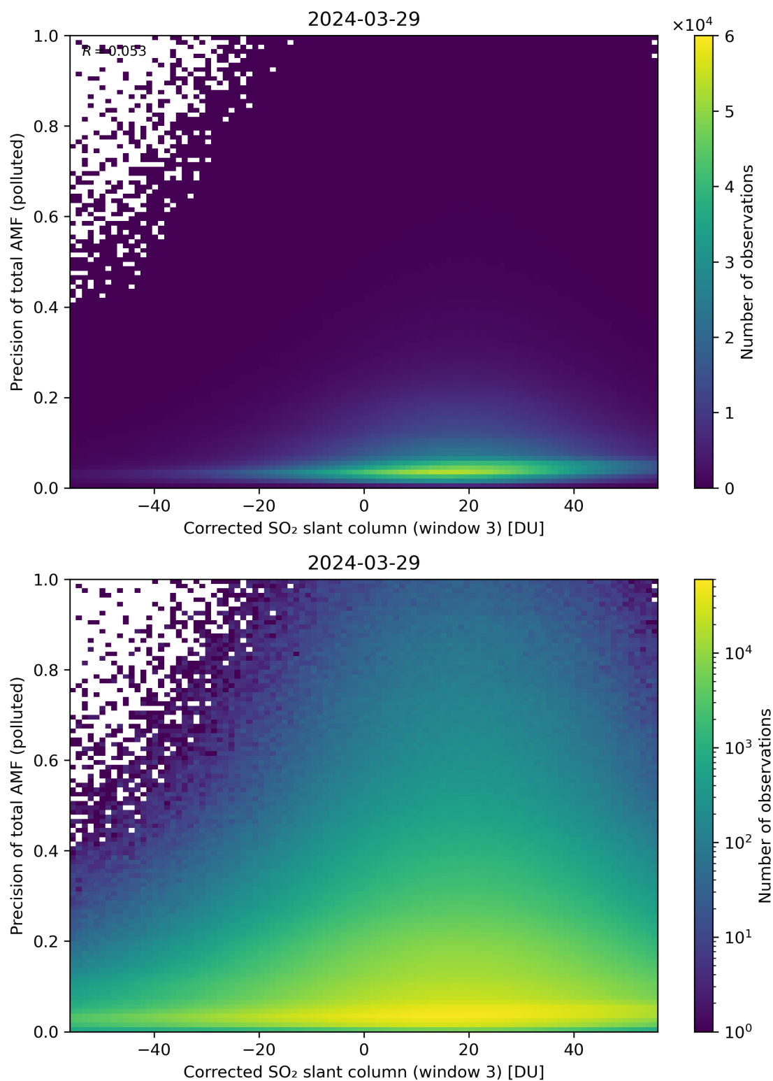
Figure 211: Scatter density plot of “Corrected SO 2 slant column (window 3)” against “Precision of total AMF (polluted)” for 2024-03-28 to 2024-03-30.
