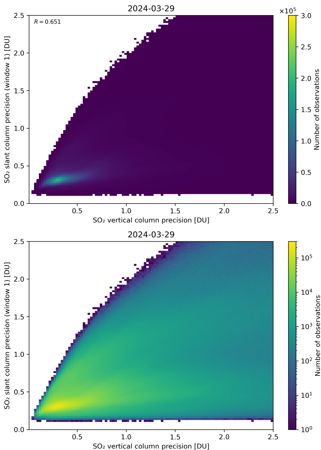
Figure 290: Scatter density plot of “SO 2 vertical column precision” against “SO 2 slant column precision (window 1)” for 2024-03-28 to 2024-03-30.
