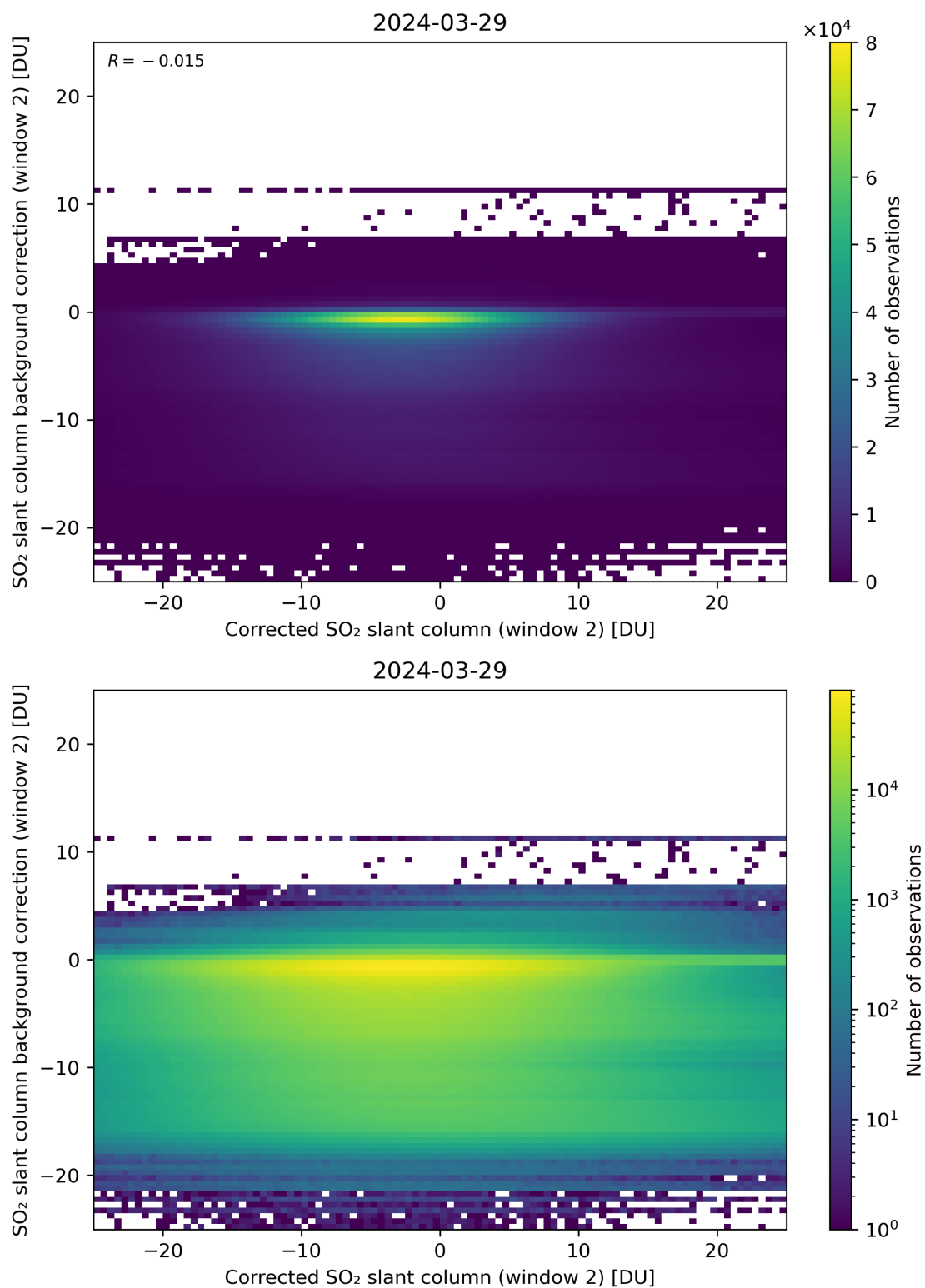
Figure 194: Scatter density plot of “Corrected SO 2 slant column (window 2)” against “SO 2 slant column background correction (window 2)” for 2024-03-28 to 2024-03-30.
