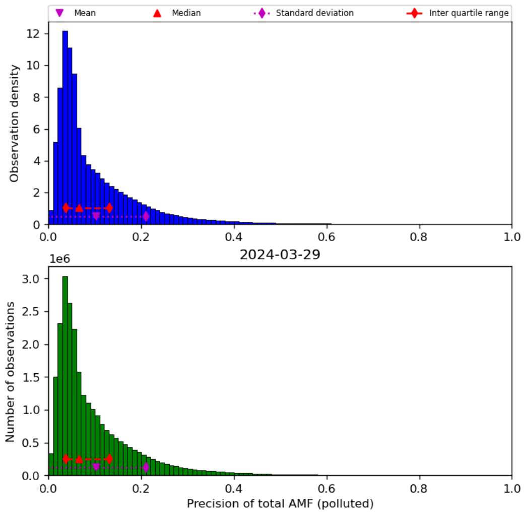
Figure 72: Histogram of “Precision of total AMF (polluted)” for 2024-03-28 to 2024-03-30
