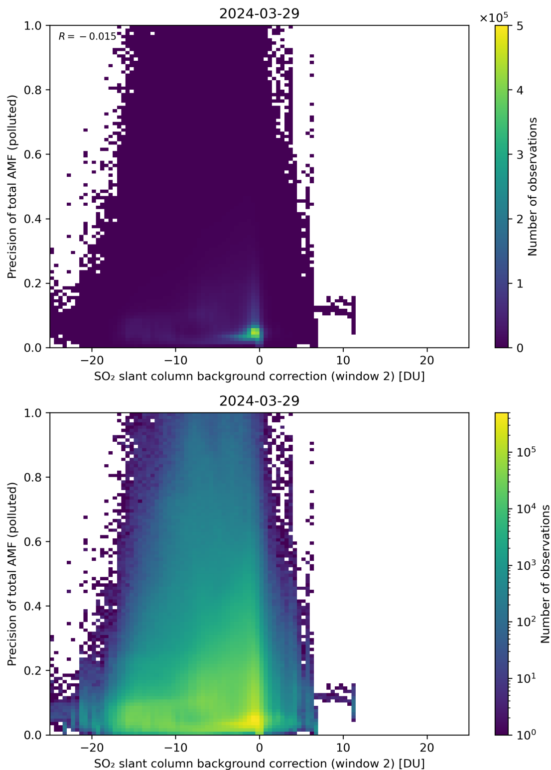
Figure 120: Scatter density plot of “SO 2 slant column background correction (window 2)” against “Precision of total AMF (polluted)” for 2024-03-28 to 2024-03-30.
