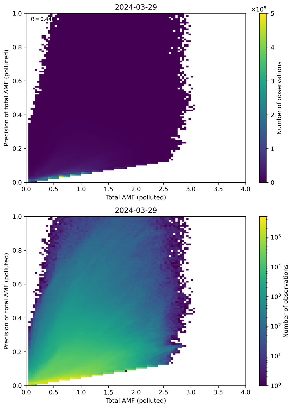
Figure 272: Scatter density plot of “Total AMF (polluted)” against “Precision of total AMF (polluted)” for 2024-03-28 to 2024-03-30.
