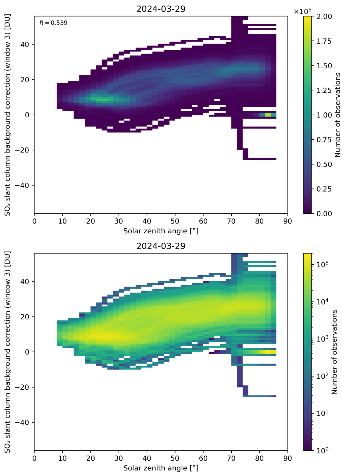
Figure 160: Scatter density plot of “Solar zenith angle” against “SO 2 slant column background correction (window 3)” for 2024-03-28 to 2024-03-30.
