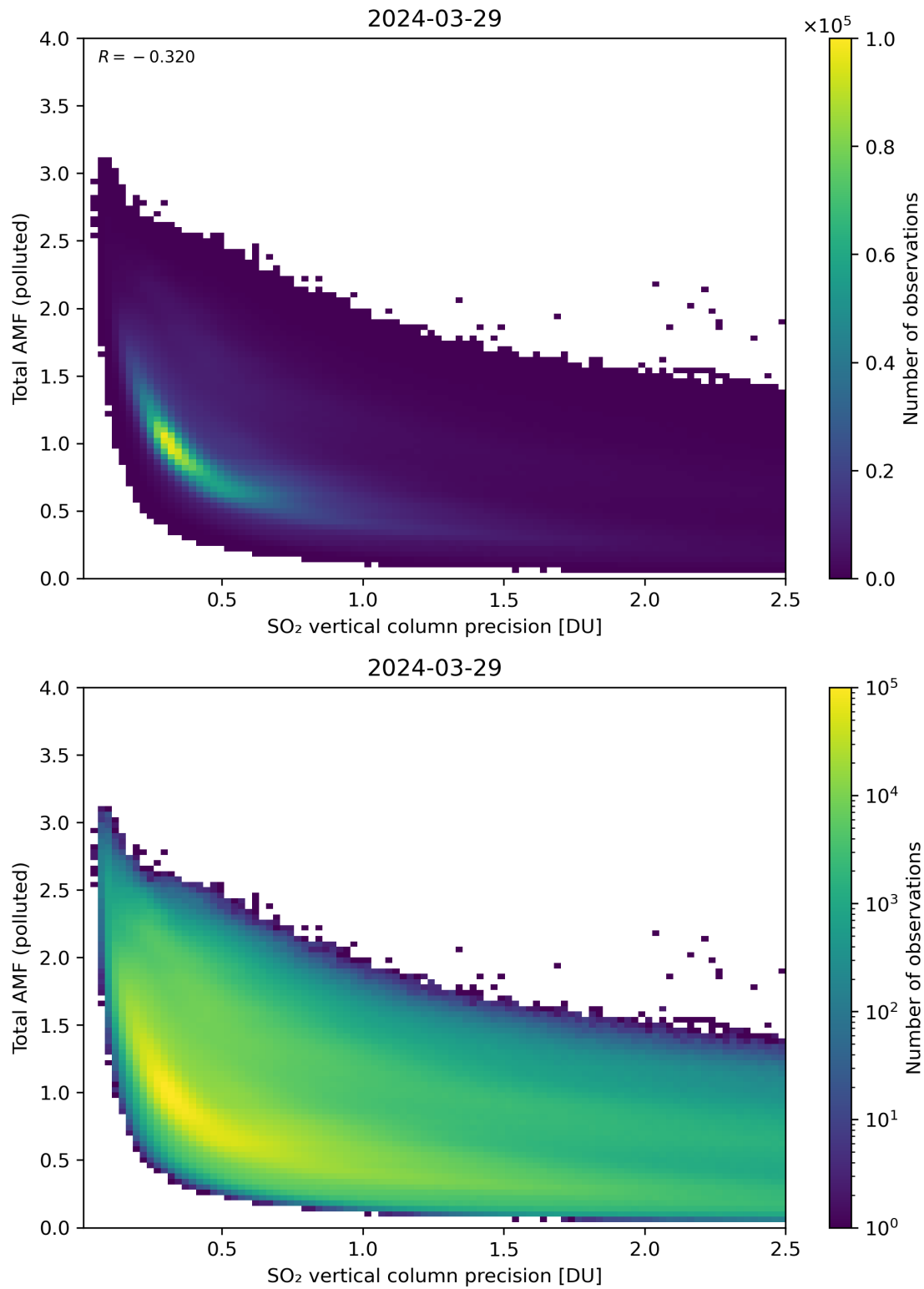
Figure 294: Scatter density plot of “SO 2 vertical column precision” against “Total AMF (polluted)” for 2024-03-28 to 2024-03-30.
