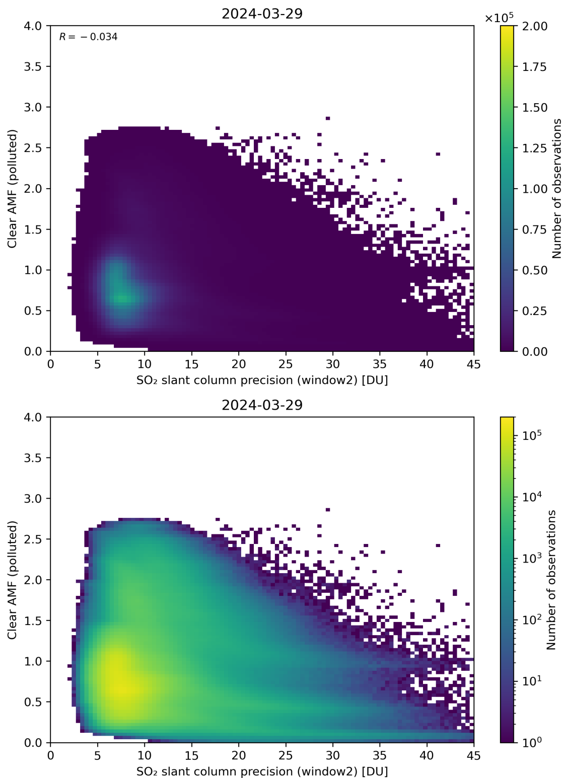
Figure 246: Scatter density plot of “SO 2 slant column precision (window2)” against “Clear AMF (polluted)” for 2024-03-28 to 2024-03-30.
