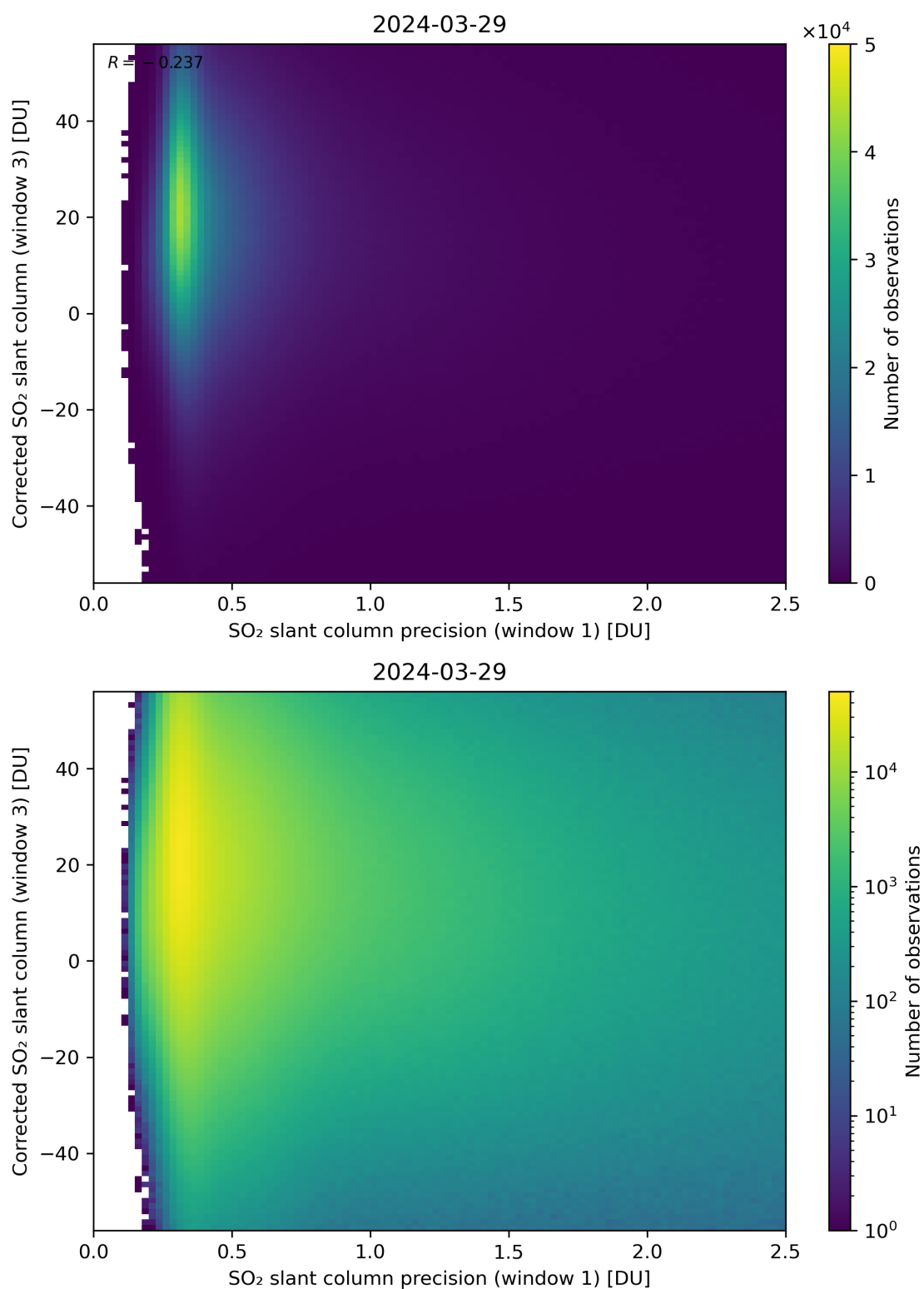
Figure 226: Scatter density plot of “SO 2 slant column precision (window 1)” against “Corrected SO 2 slant column (window 3)” for 2024-03-28 to 2024-03-30.
