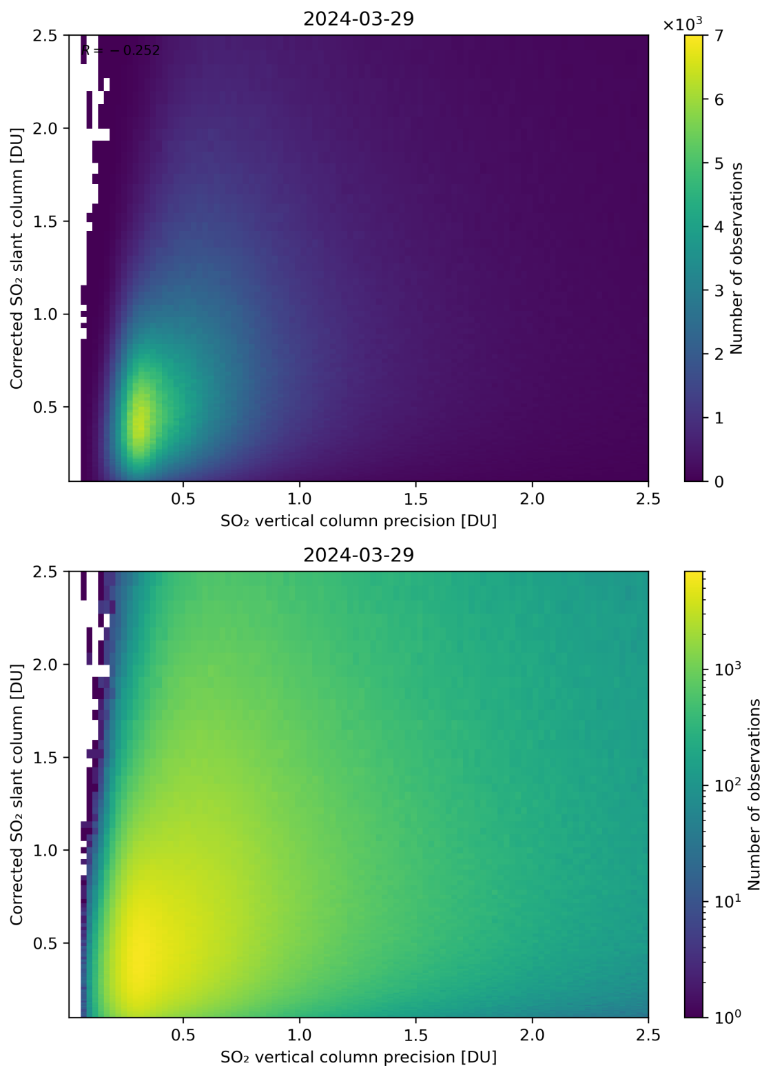
Figure 286: Scatter density plot of “SO 2 vertical column precision” against “Corrected SO 2 slant column” for 2024-03-28 to 2024-03-30.
