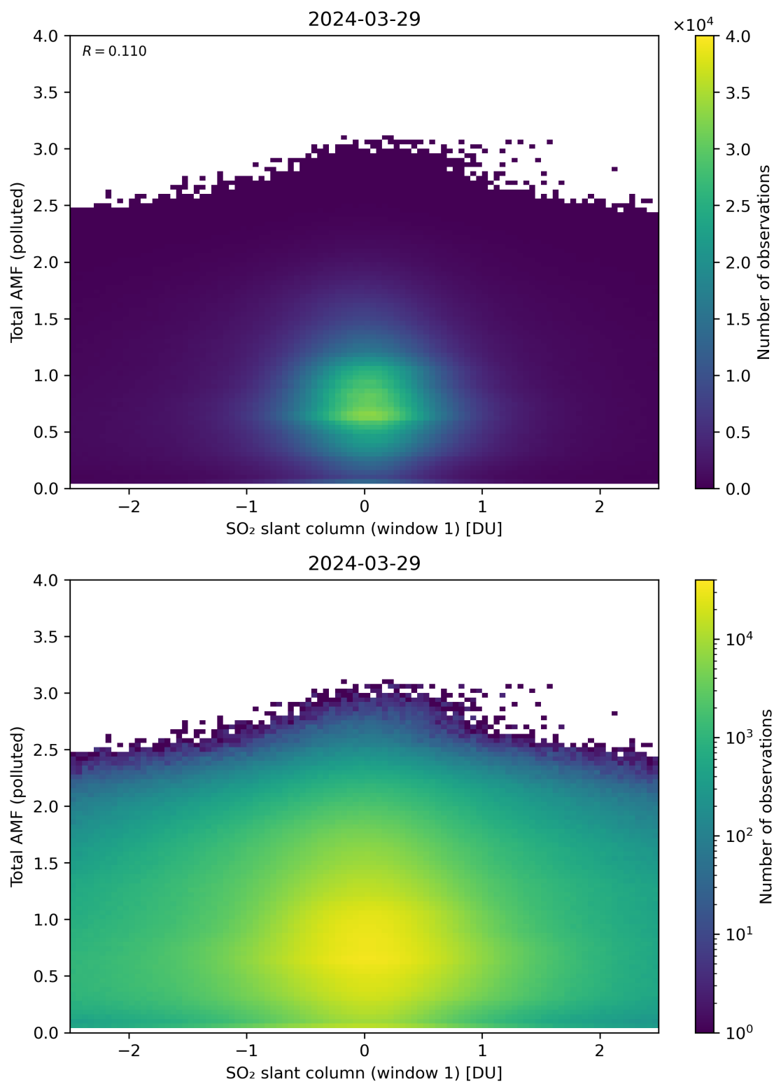
Figure 239: Scatter density plot of “SO 2 slant column (window 1)” against “Total AMF (polluted)” for 2024-03-28 to 2024-03-30.
