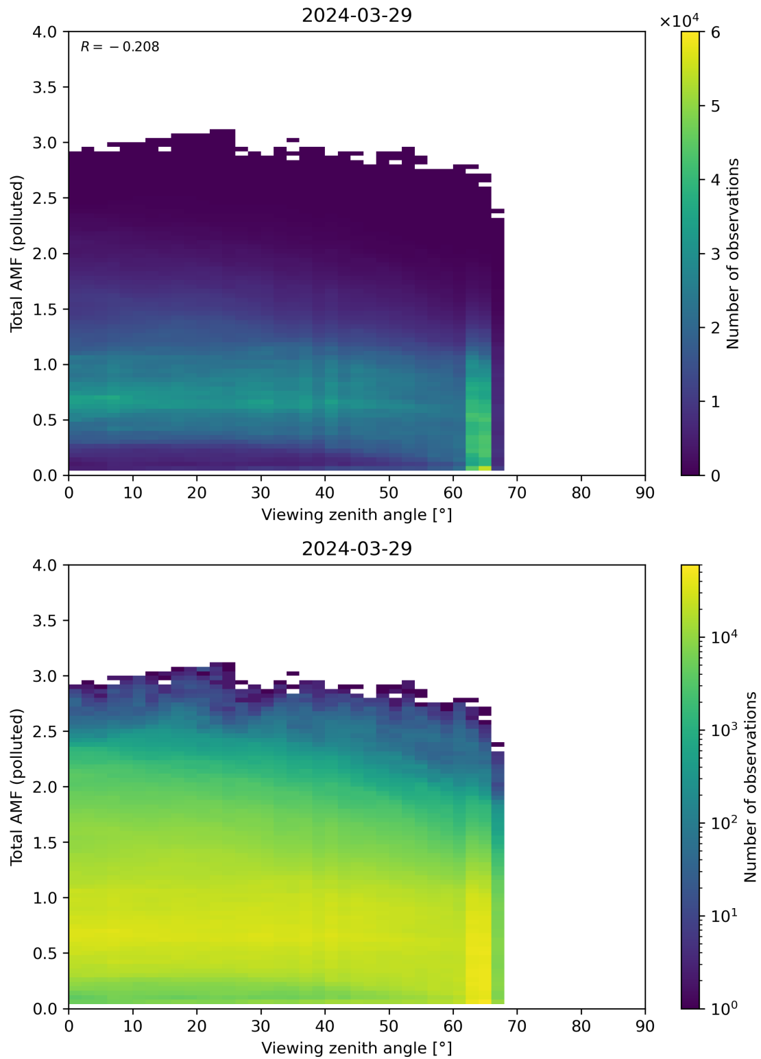
Figure 325: Scatter density plot of “Viewing zenith angle” against “Total AMF (polluted)” for 2024-03-28 to 2024-03-30.
