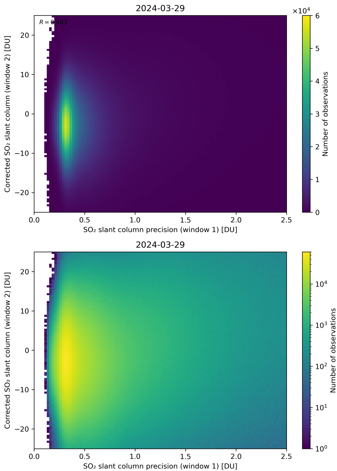
Figure 225: Scatter density plot of “SO 2 slant column precision (window 1)” against “Corrected SO 2 slant column (window 2)” for 2024-03-28 to 2024-03-30.
