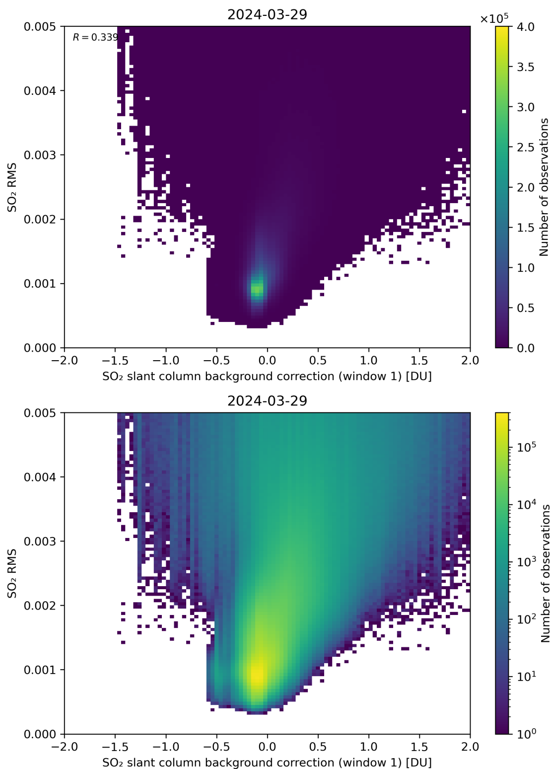
Figure 102: Scatter density plot of “SO 2 slant column background correction (window 1)” against “SO 2 RMS” for 2024-03-28 to 2024-03-30.
