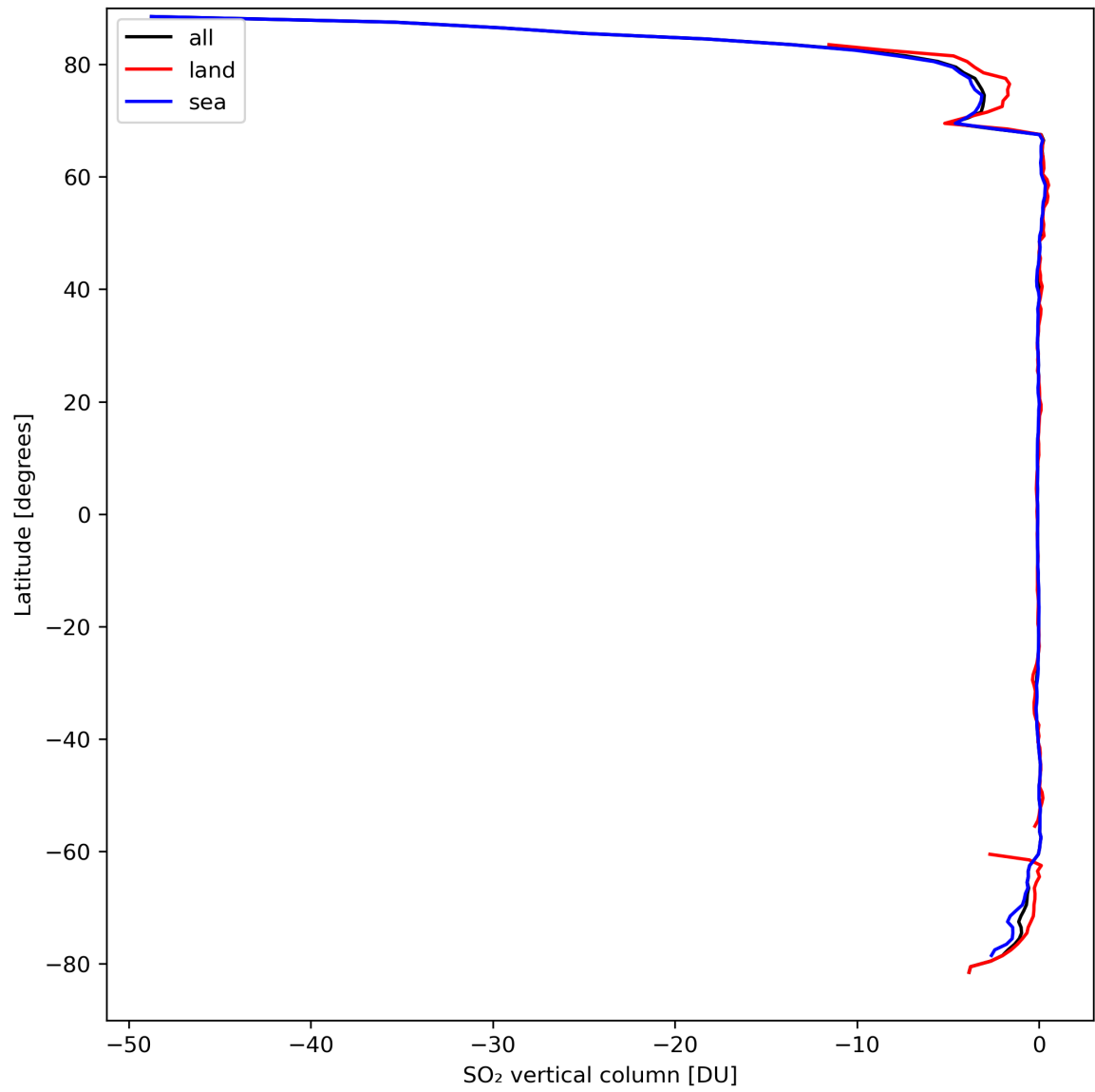
Figure 30: Zonal average of “SO 2 vertical column” for 2024-03-28 to 2024-03-30.
