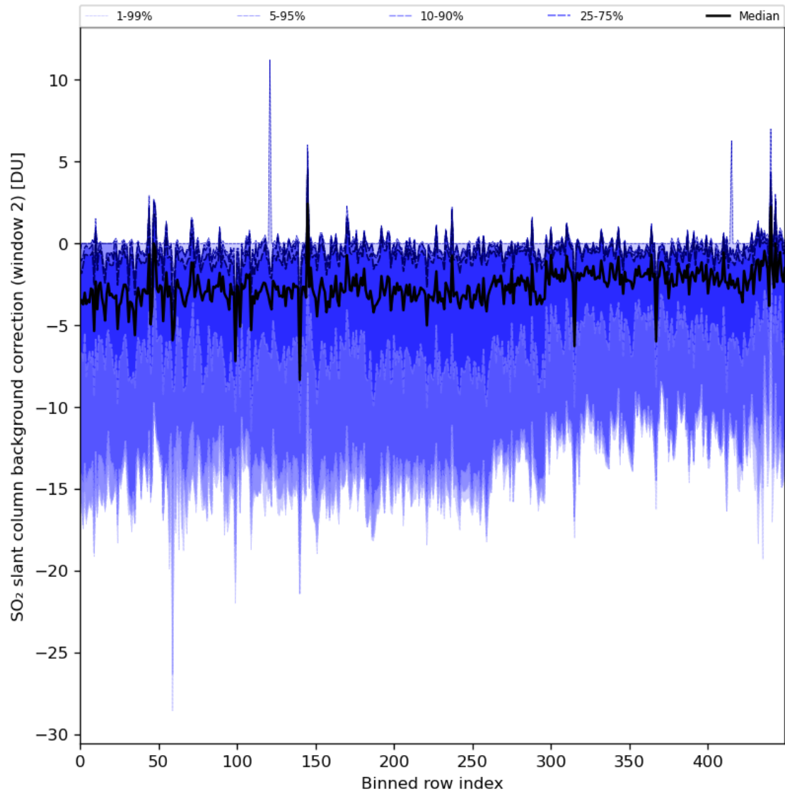
Figure 86: Along track statistics of “SO 2 slant column background correction (window 2)” for 2024-03-28 to 2024-03-30
