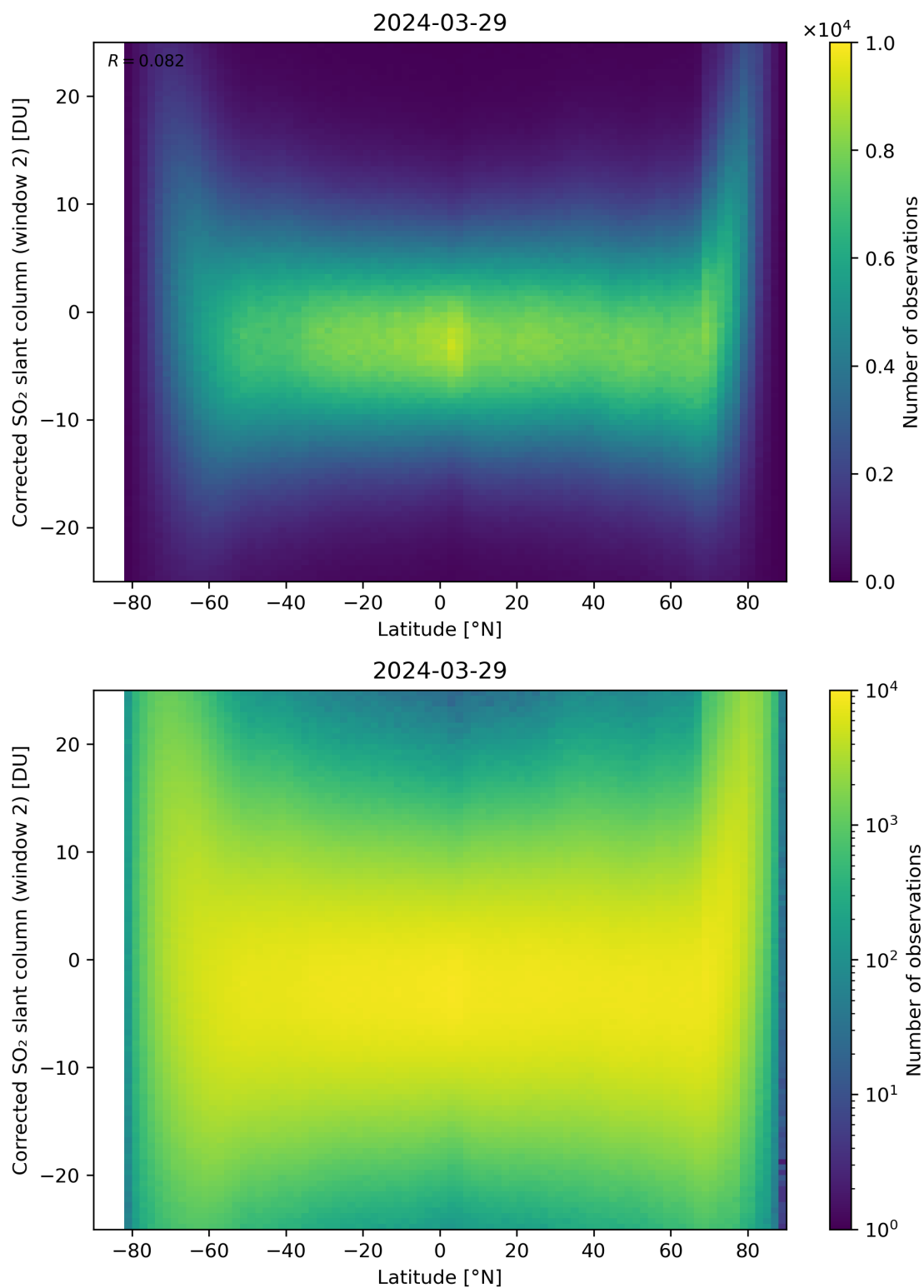
Figure 147: Scatter density plot of “Latitude” against “Corrected SO 2 slant column (window 2)” for 2024-03-28 to 2024-03-30.
