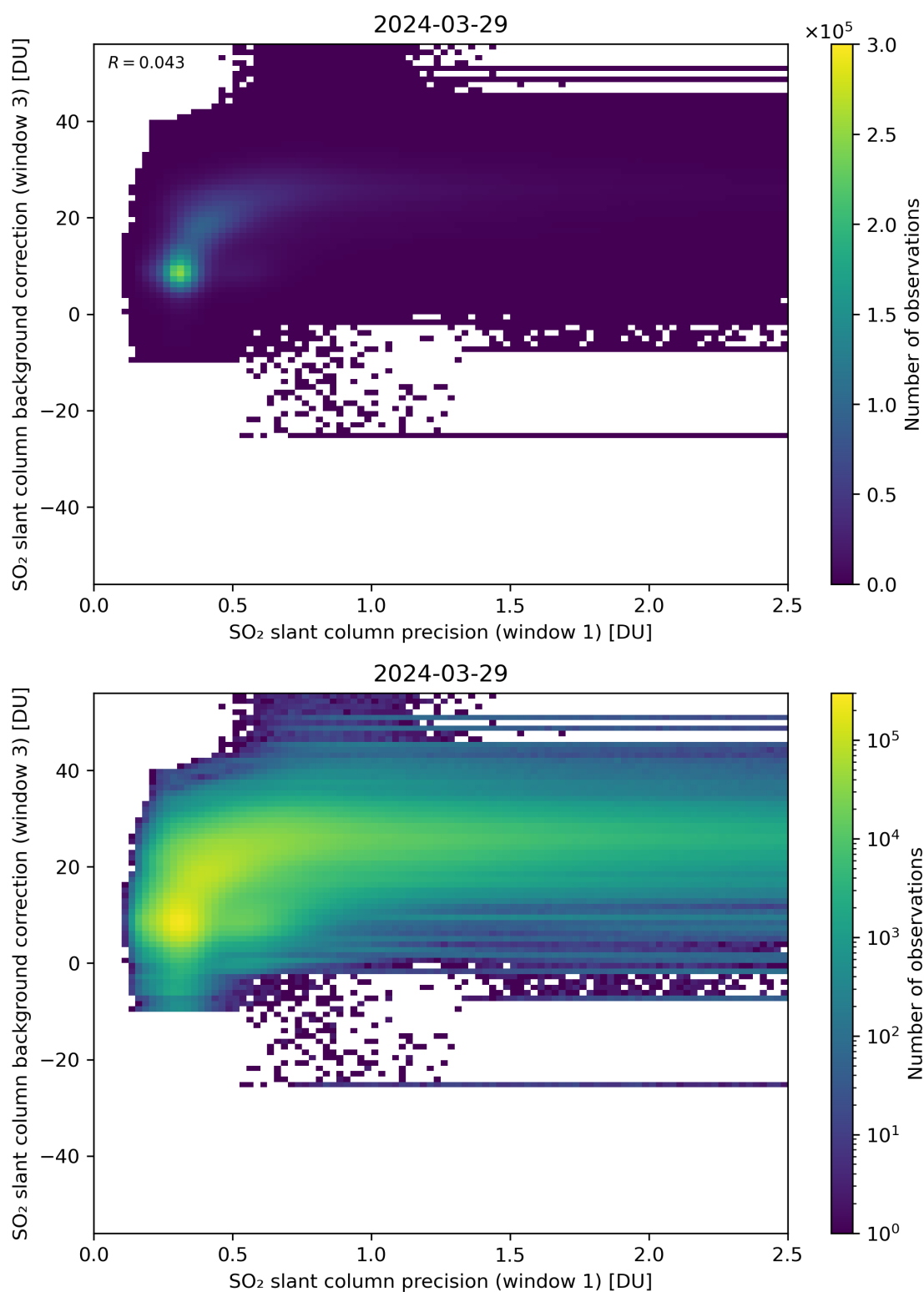
Figure 220: Scatter density plot of “SO 2 slant column precision (window 1)” against “SO 2 slant column background correction (window 3)” for 2024-03-28 to 2024-03-30.
