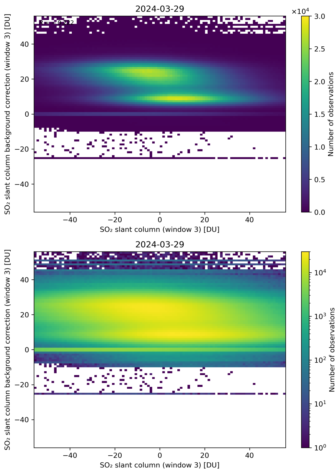
Figure 253: Scatter density plot of “SO 2 slant column (window 3)” against “SO 2 slant column background correction (window 3)” for 2024-03-28 to 2024-03-30.
