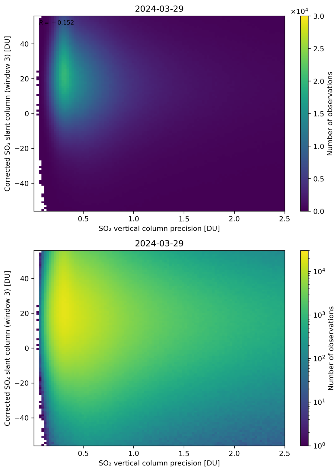
Figure 288: Scatter density plot of “SO 2 vertical column precision” against “Corrected SO 2 slant column (window 3)” for 2024-03-28 to 2024-03-30.
