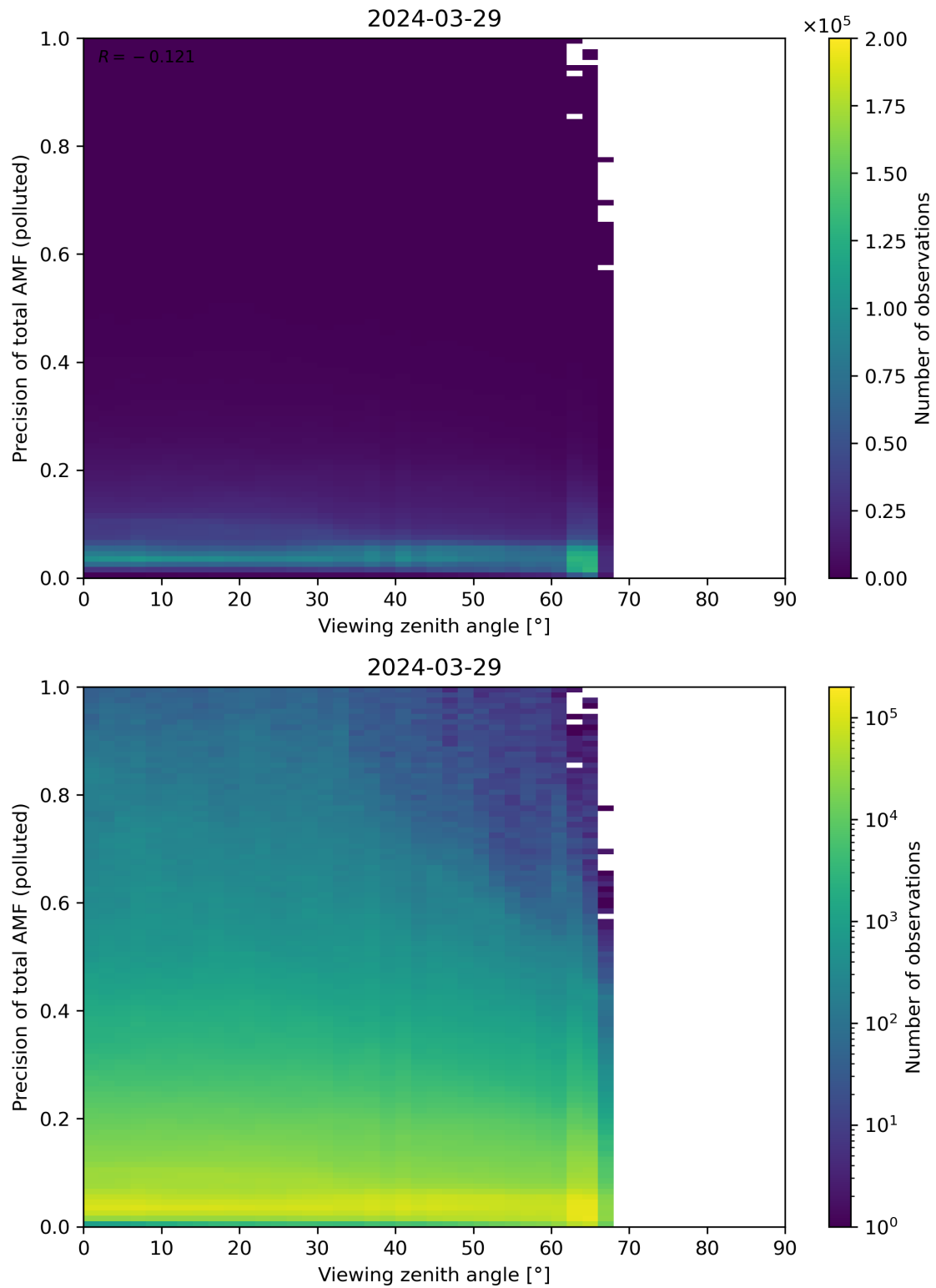
Figure 326: Scatter density plot of “Viewing zenith angle” against “Precision of total AMF (polluted)” for 2024-03-28 to 2024-03-30.
