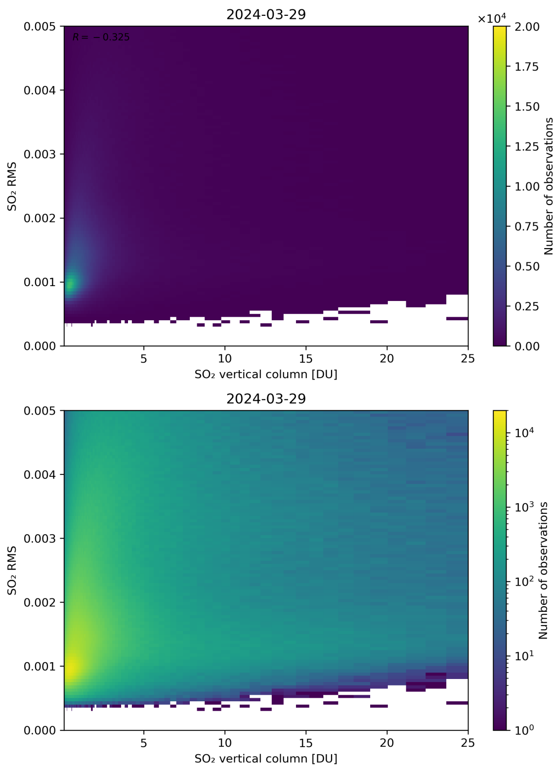
Figure 278: Scatter density plot of “SO 2 vertical column” against “SO 2 RMS” for 2024-03-28 to 2024-03-30.
