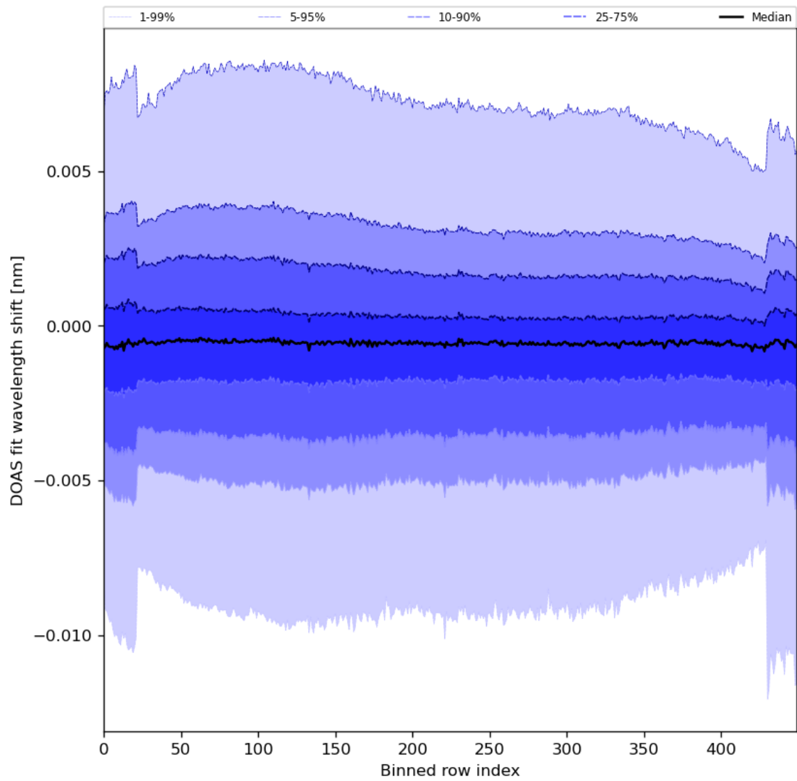
Figure 91: Along track statistics of “DOAS fit wavelength shift” for 2024-03-28 to 2024-03-30
