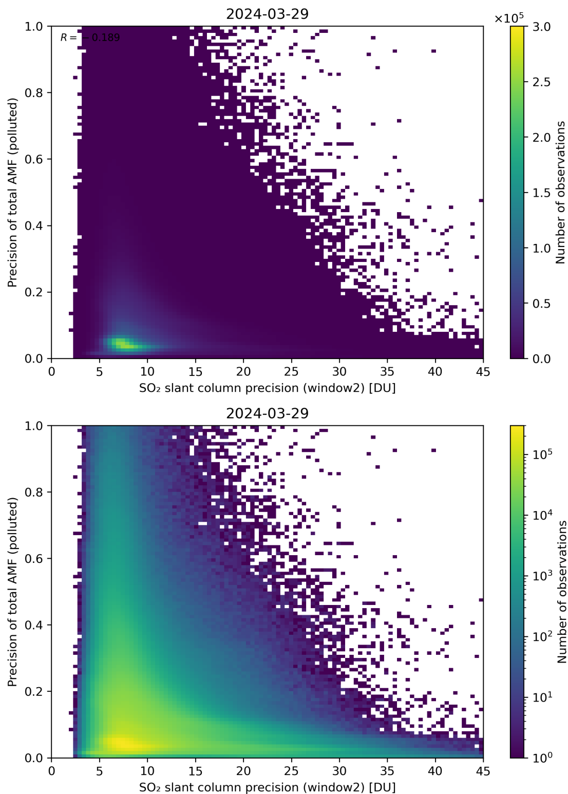
Figure 252: Scatter density plot of “SO 2 slant column precision (window2)” against “Precision of total AMF (polluted)” for 2024-03-28 to 2024-03-30.
