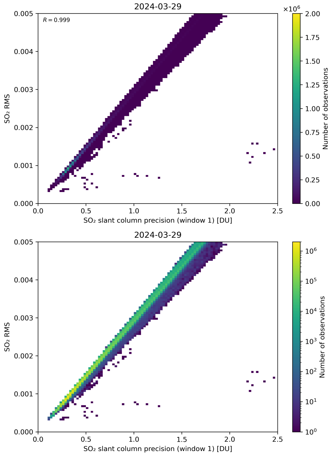
Figure 223: Scatter density plot of “SO 2 slant column precision (window 1)” against “SO 2 RMS” for 2024-03-28 to 2024-03-30.
