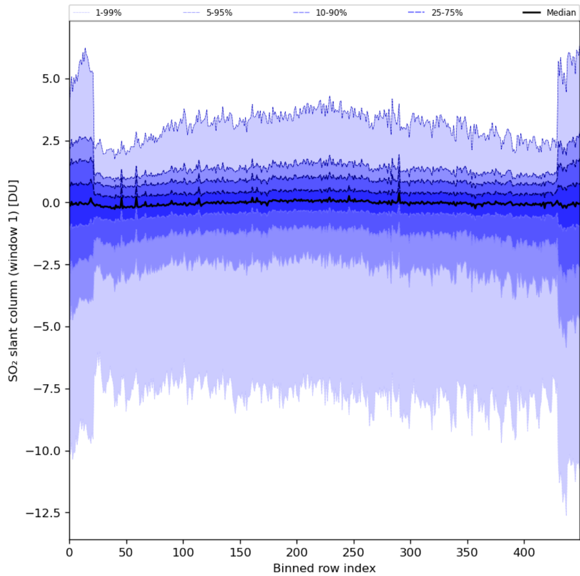
Figure 79: Along track statistics of “SO 2 slant column (window 1)” for 2024-03-28 to 2024-03-30
