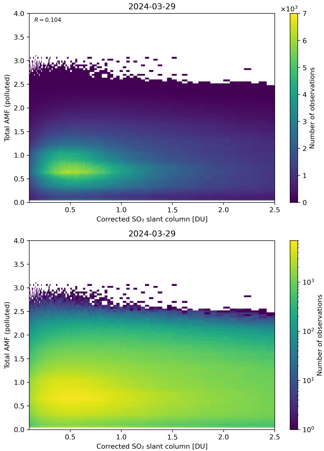
Figure 192: Scatter density plot of “Corrected SO 2 slant column” against “Total AMF (polluted)” for 2024-03-28 to 2024-03-30.
