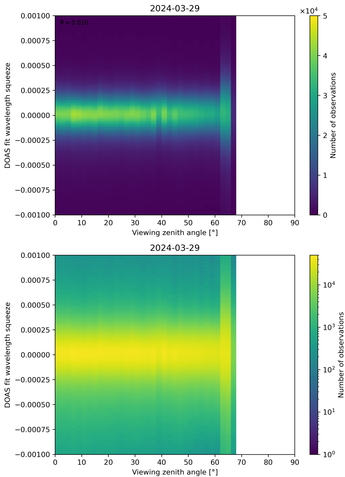
Figure 312: Scatter density plot of “Viewing zenith angle” against “DOAS fit wavelength squeeze” for 2024-03-28 to 2024-03-30.
