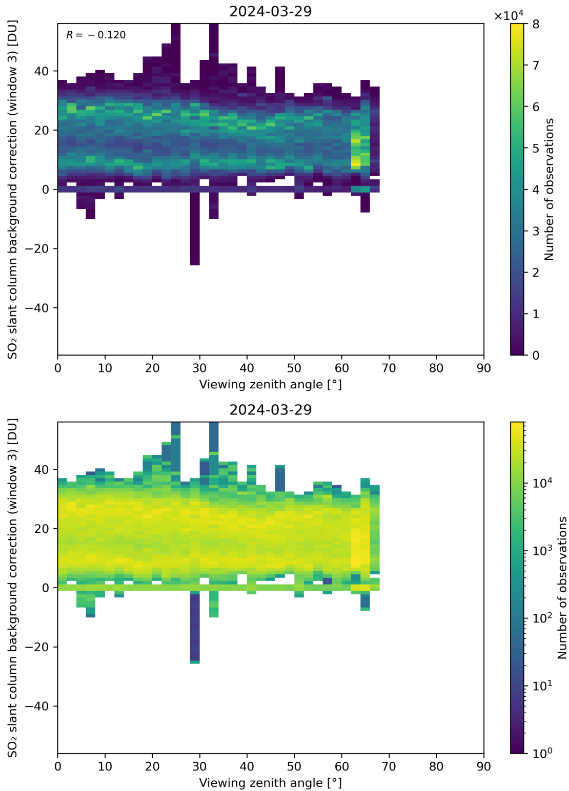
Figure 310: Scatter density plot of “Viewing zenith angle” against “SO 2 slant column background correction (window 3)” for 2024-03-28 to 2024-03-30.
