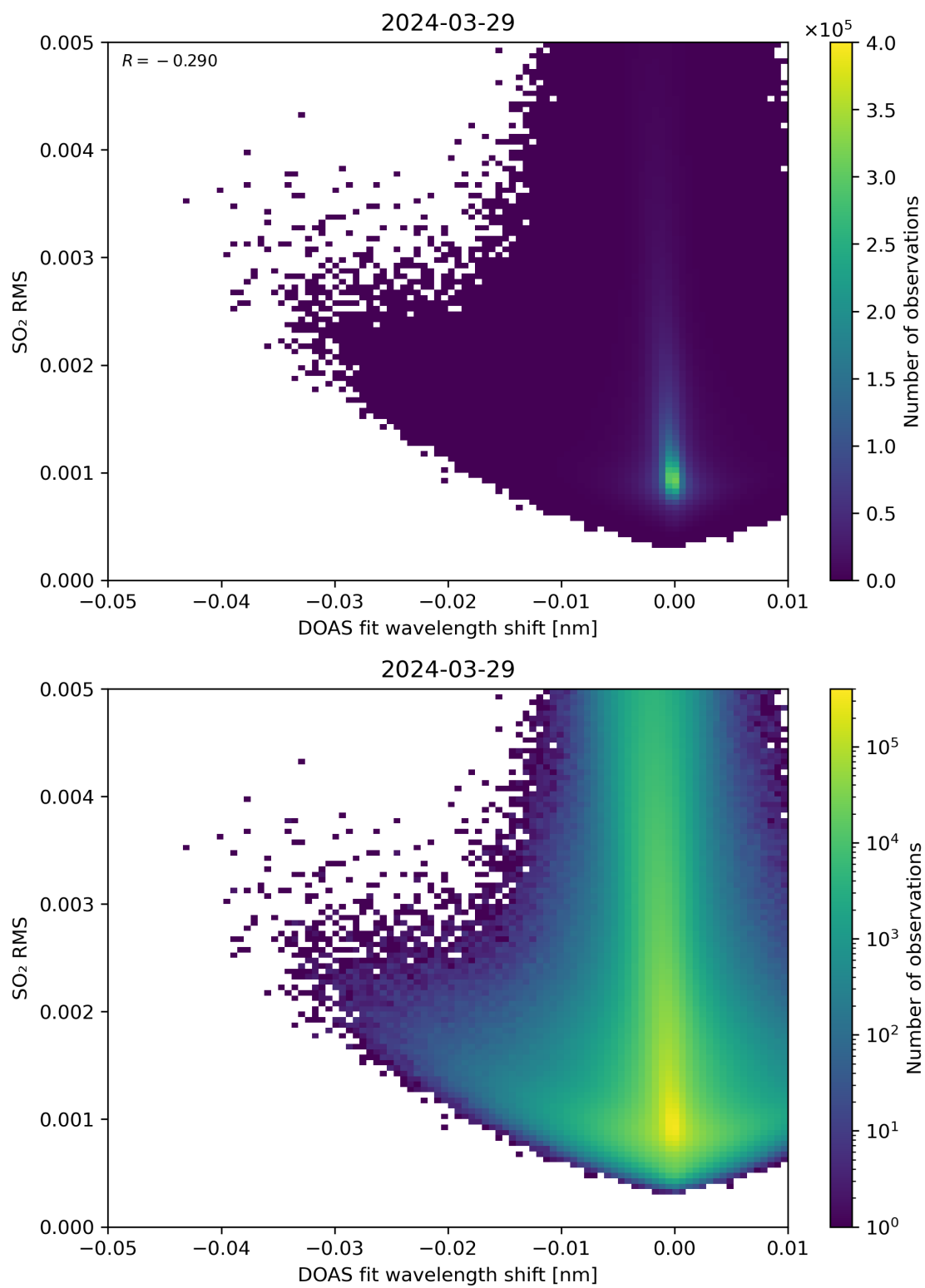
Figure 128: Scatter density plot of “DOAS fit wavelength shift” against “SO 2 RMS” for 2024-03-28 to 2024-03-30.
