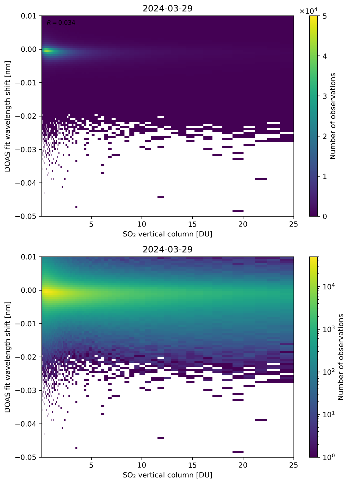
Figure 276: Scatter density plot of “SO 2 vertical column” against “DOAS fit wavelength shift” for 2024-03-28 to 2024-03-30.
