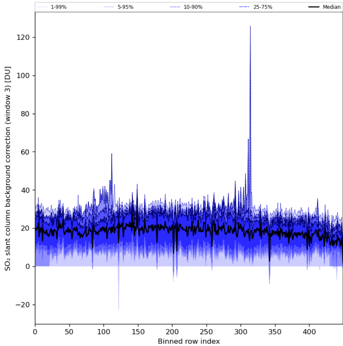
Figure 90: Along track statistics of “SO 2 slant column background correction (window 3)” for 2024-03-28 to 2024-03-30
