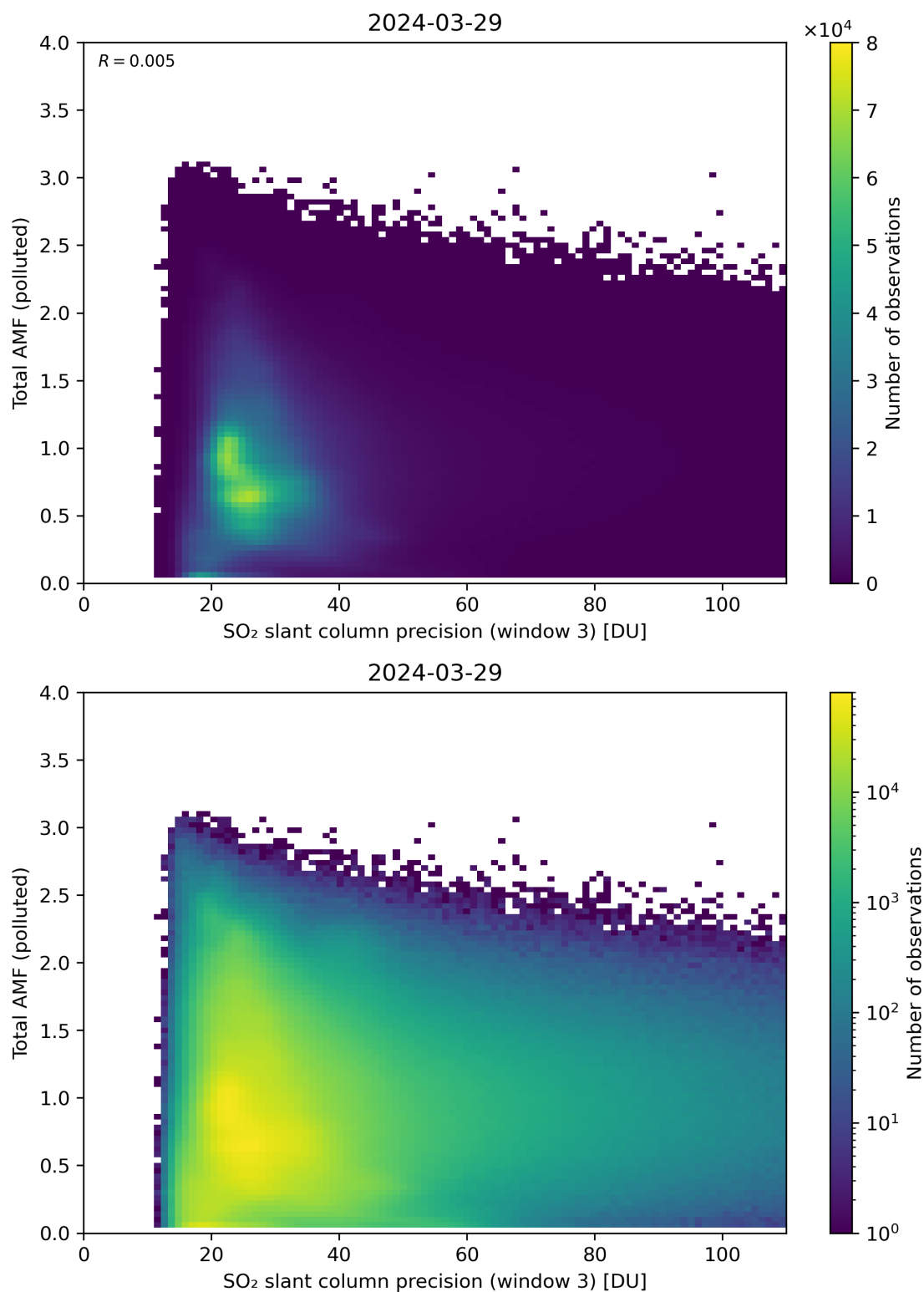
Figure 263: Scatter density plot of “SO 2 slant column precision (window 3)” against “Total AMF (polluted)” for 2024-03-28 to 2024-03-30.
