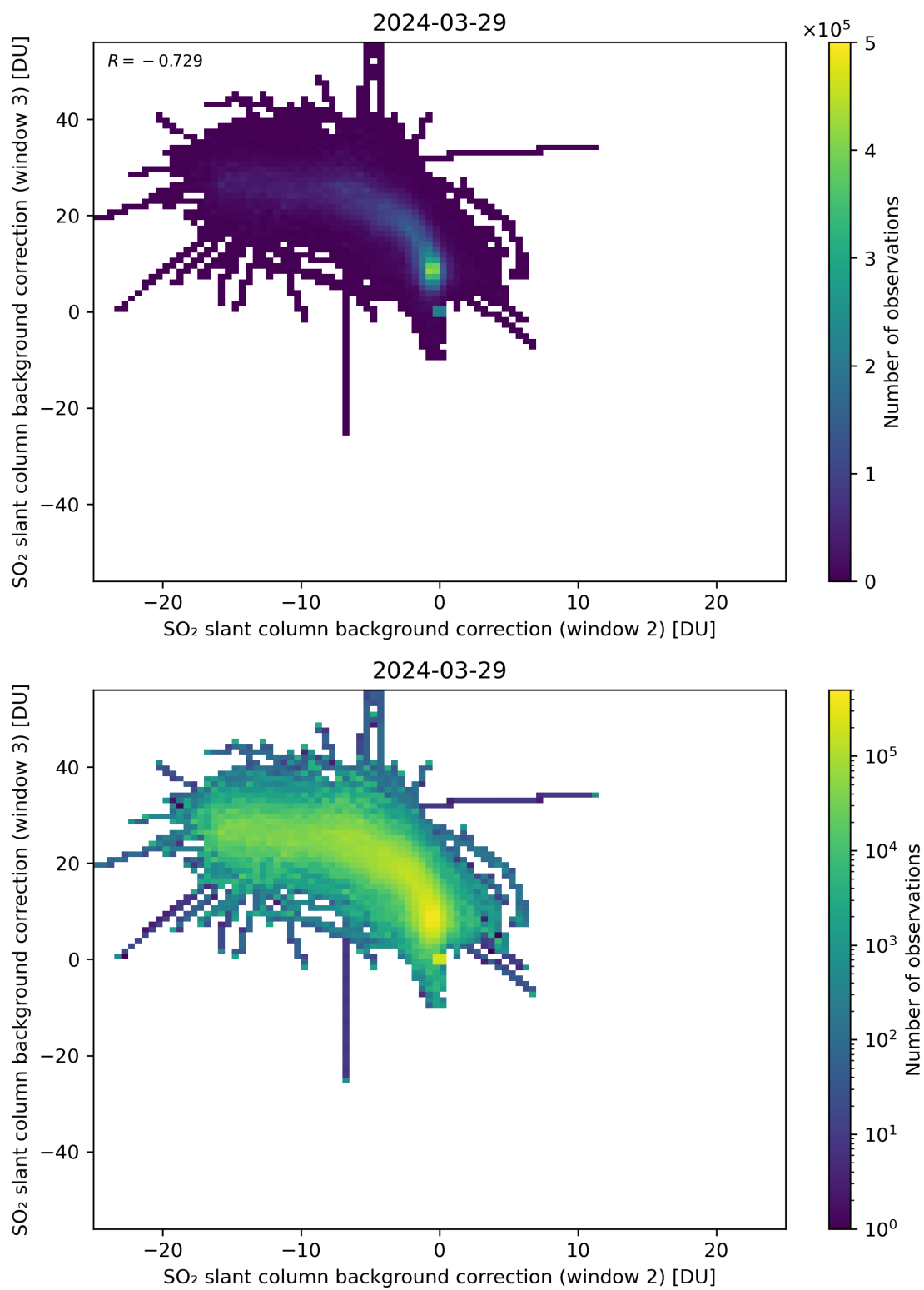
Figure 111: Scatter density plot of “SO 2 slant column background correction (window 2)” against “SO 2 slant column background correction (window 3)” for 2024-03-28 to 2024-03-30.
