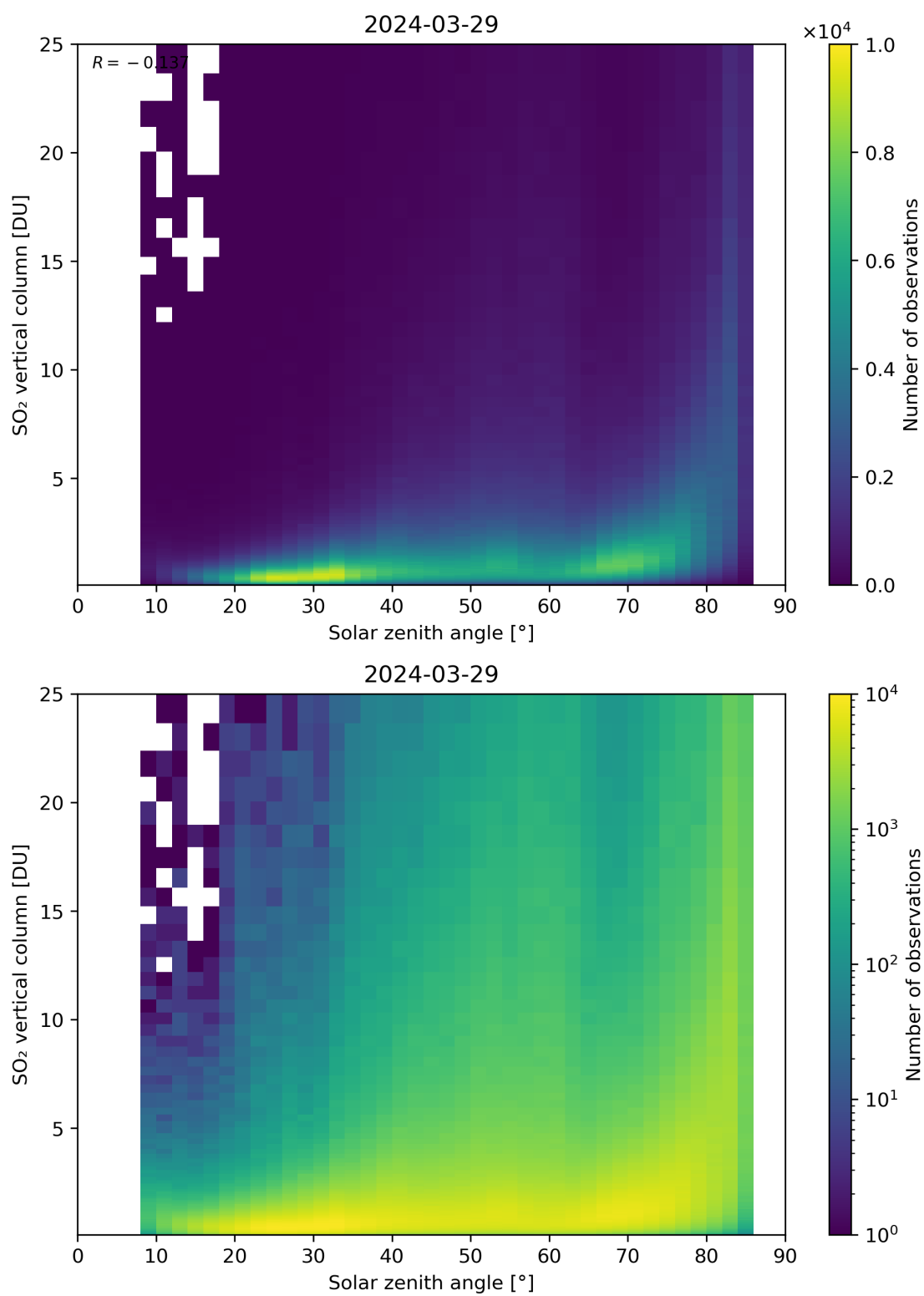
Figure 176: Scatter density plot of “Solar zenith angle” against “SO 2 vertical column” for 2024-03-28 to 2024-03-30.
