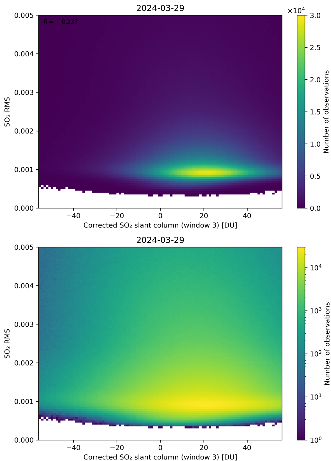
Figure 208: Scatter density plot of “Corrected SO 2 slant column (window 3)” against “SO 2 RMS” for 2024-03-28 to 2024-03-30.
