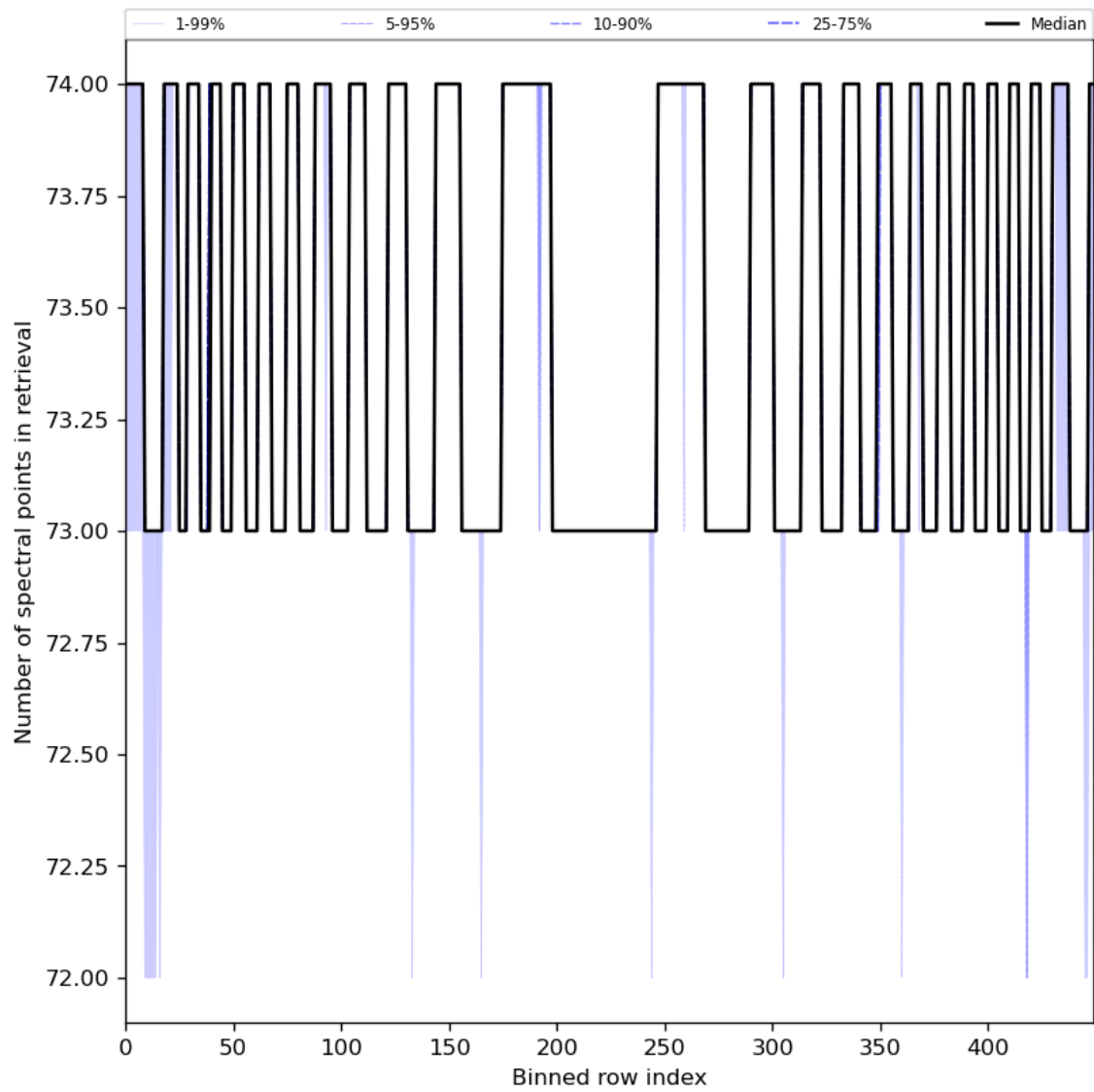
Figure 97: Along track statistics of “Number of spectral points in retrieval” for 2024-03-28 to 2024-03-30
