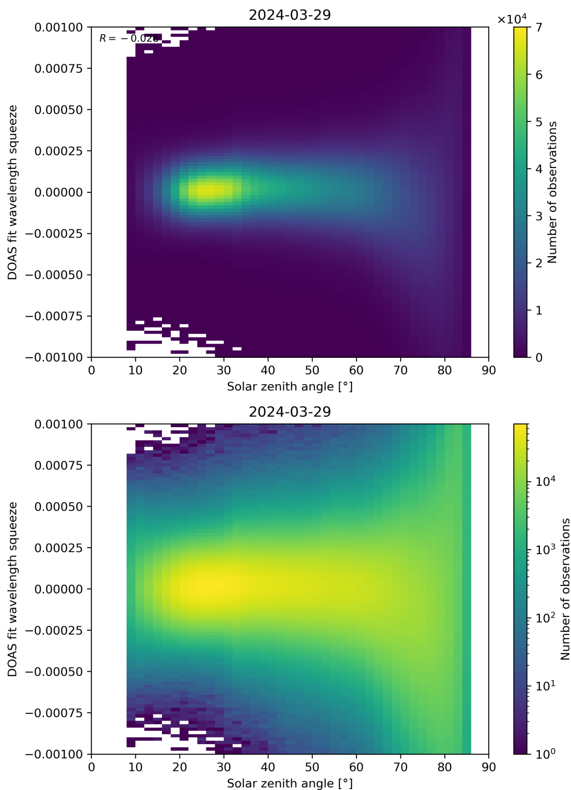
Figure 162: Scatter density plot of “Solar zenith angle” against “DOAS fit wavelength squeeze” for 2024-03-28 to 2024-03-30.
