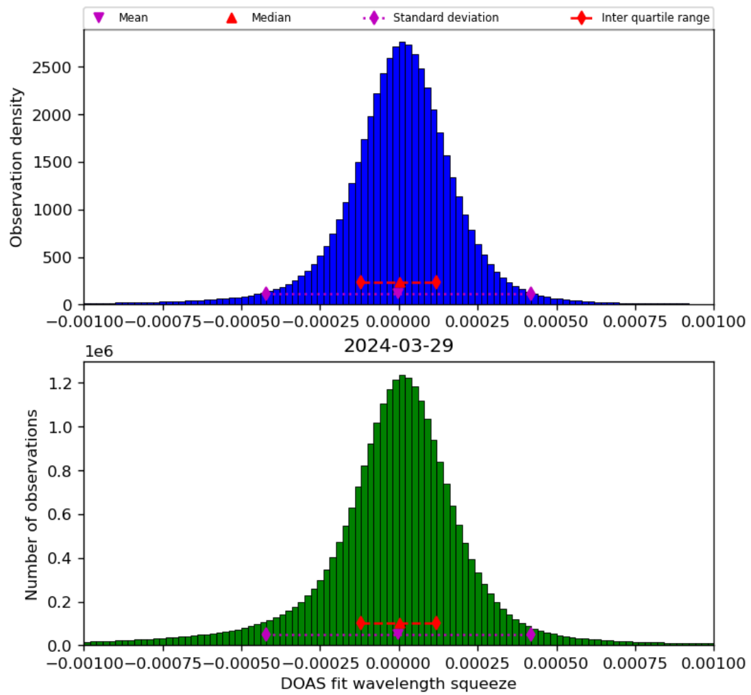
Figure 69: Histogram of “DOAS fit wavelength squeeze” for 2024-03-28 to 2024-03-30
