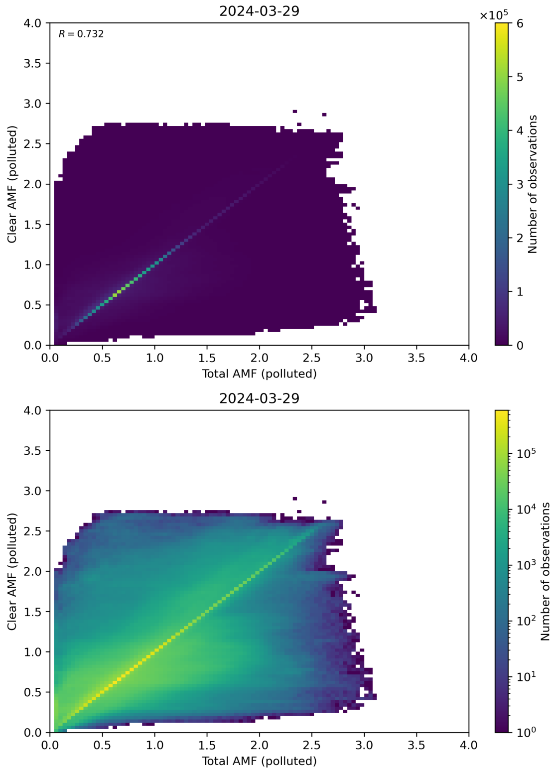
Figure 271: Scatter density plot of “Total AMF (polluted)” against “Clear AMF (polluted)” for 2024-03-28 to 2024-03-30.
