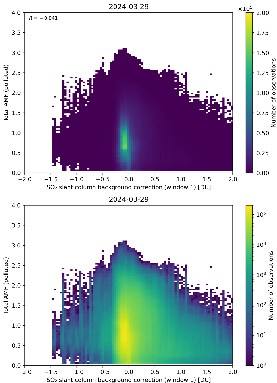
Figure 109: Scatter density plot of “SO 2 slant column background correction (window 1)” against “Total AMF (polluted)” for 2024-03-28 to 2024-03-30.
