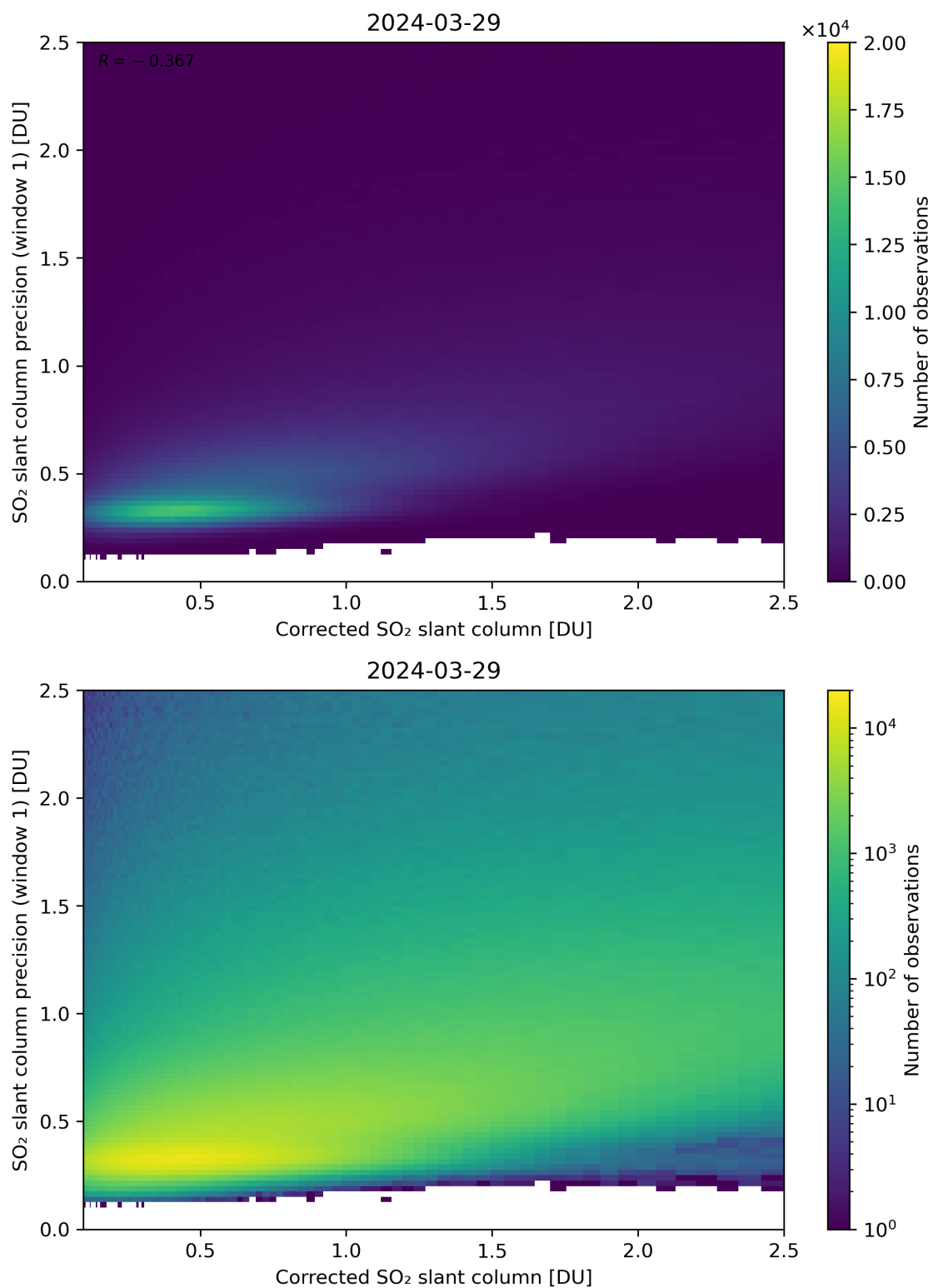
Figure 188: Scatter density plot of “Corrected SO 2 slant column” against “SO 2 slant column precision (window 1)” for 2024-03-28 to 2024-03-30.
