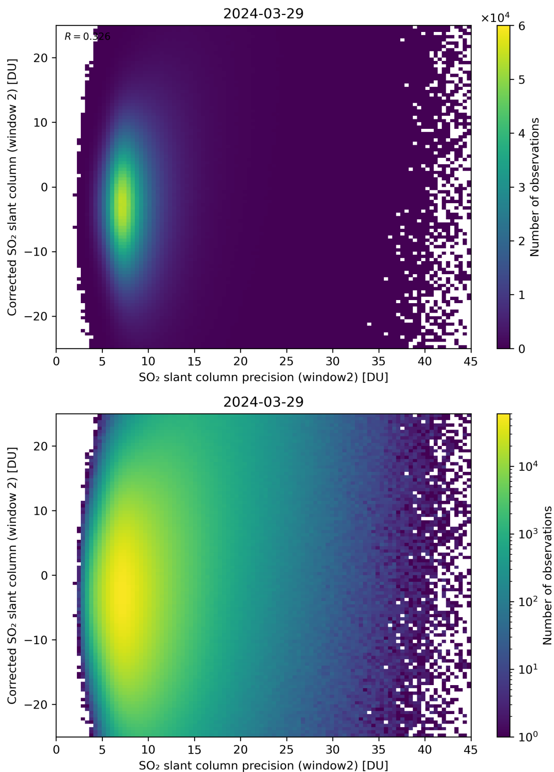
Figure 247: Scatter density plot of “SO 2 slant column precision (window2)” against “Corrected SO 2 slant column (window 2)” for 2024-03-28 to 2024-03-30.
