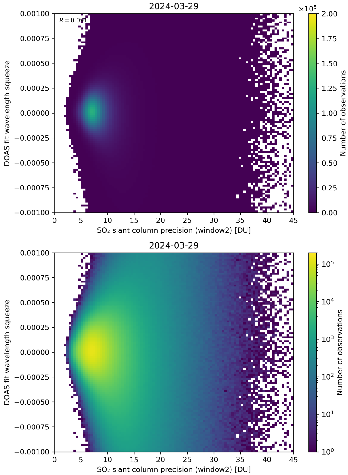
Figure 244: Scatter density plot of “SO 2 slant column precision (window2)” against “DOAS fit wavelength squeeze” for 2024-03-28 to 2024-03-30.
