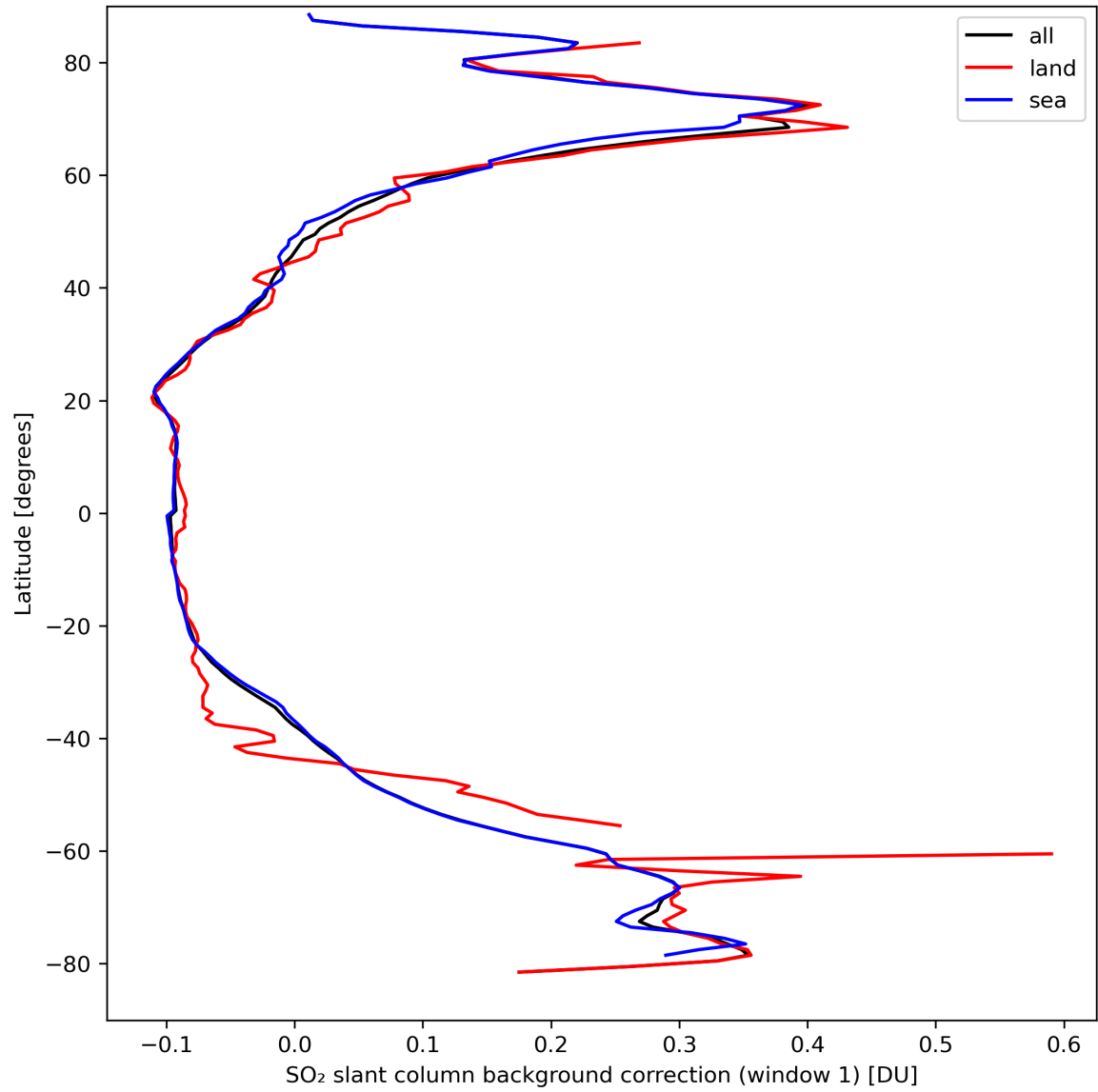
Figure 36: Zonal average of “SO 2 slant column background correction (window 1)” for 2024-03-28 to 2024-03-30.
