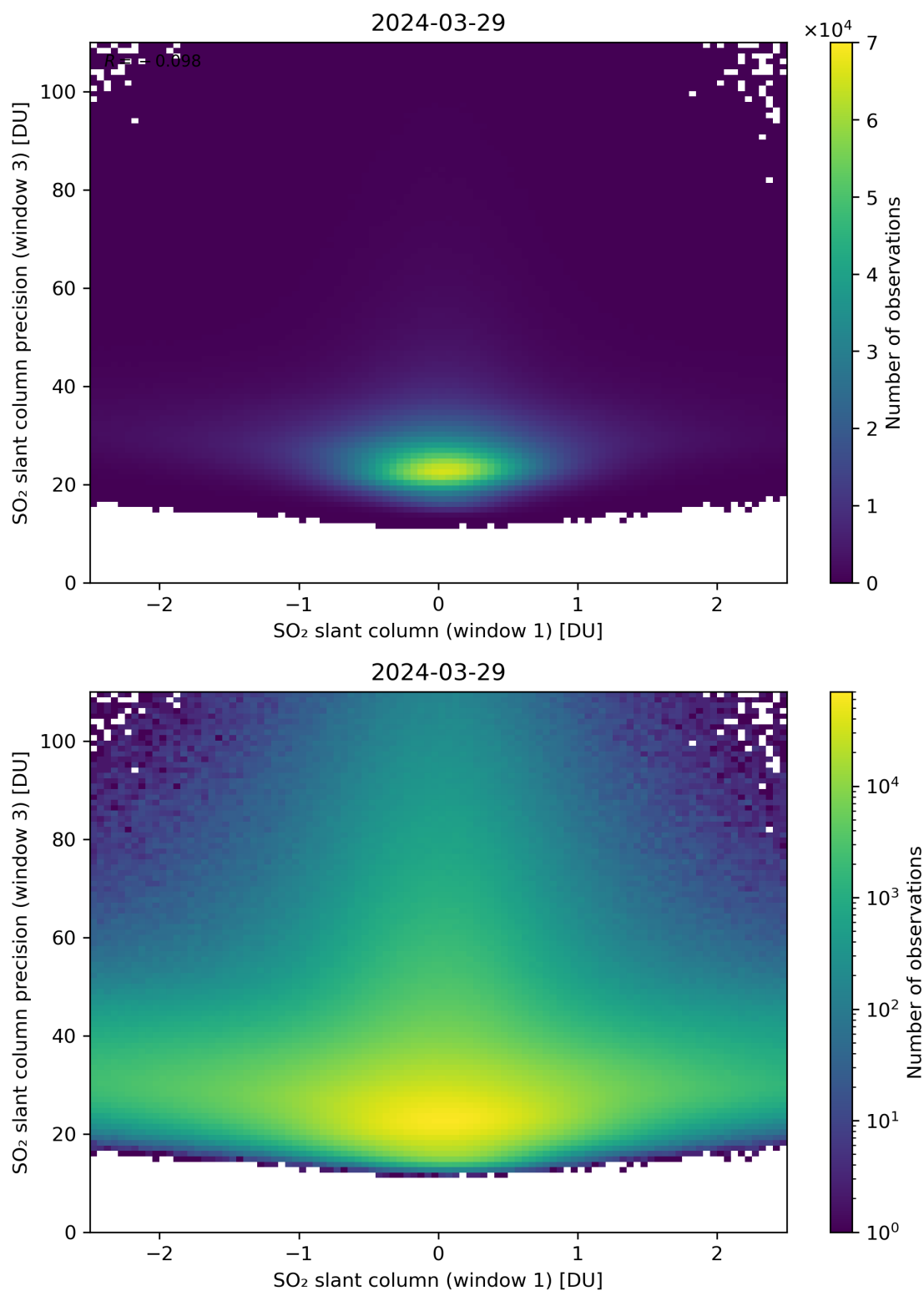
Figure 238: Scatter density plot of “SO 2 slant column (window 1)” against “SO 2 slant column precision (window 3)” for 2024-03-28 to 2024-03-30.
