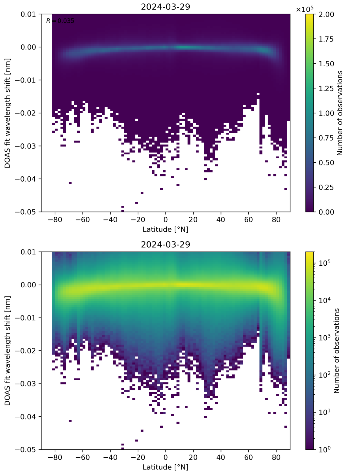
Figure 142: Scatter density plot of “Latitude” against “DOAS fit wavelength shift” for 2024-03-28 to 2024-03-30.
