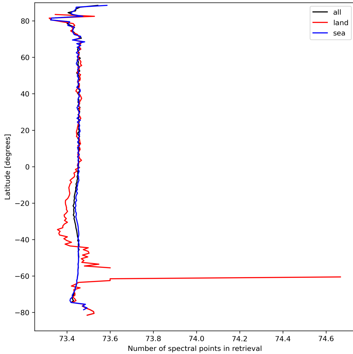
Figure 51: Zonal average of “Number of spectral points in retrieval” for 2024-03-28 to 2024-03-30.
