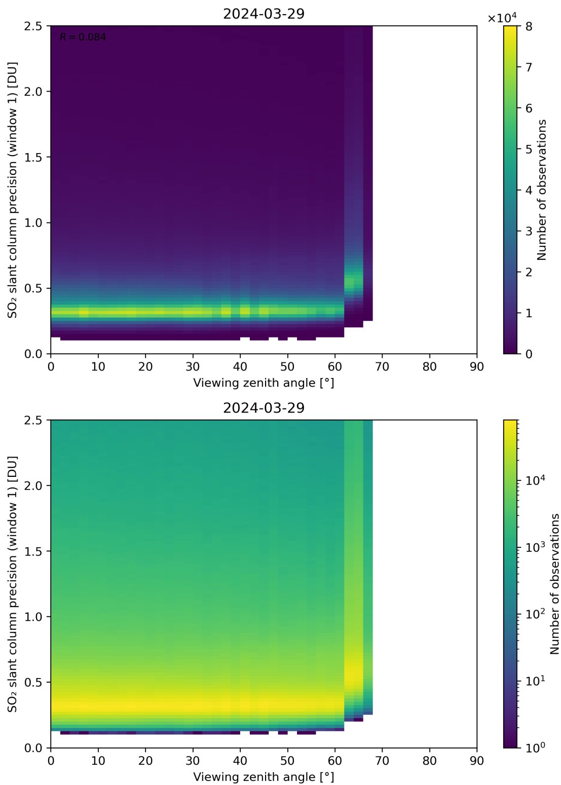
Figure 321: Scatter density plot of “Viewing zenith angle” against “SO 2 slant column precision (window 1)” for 2024-03-28 to 2024-03-30.
