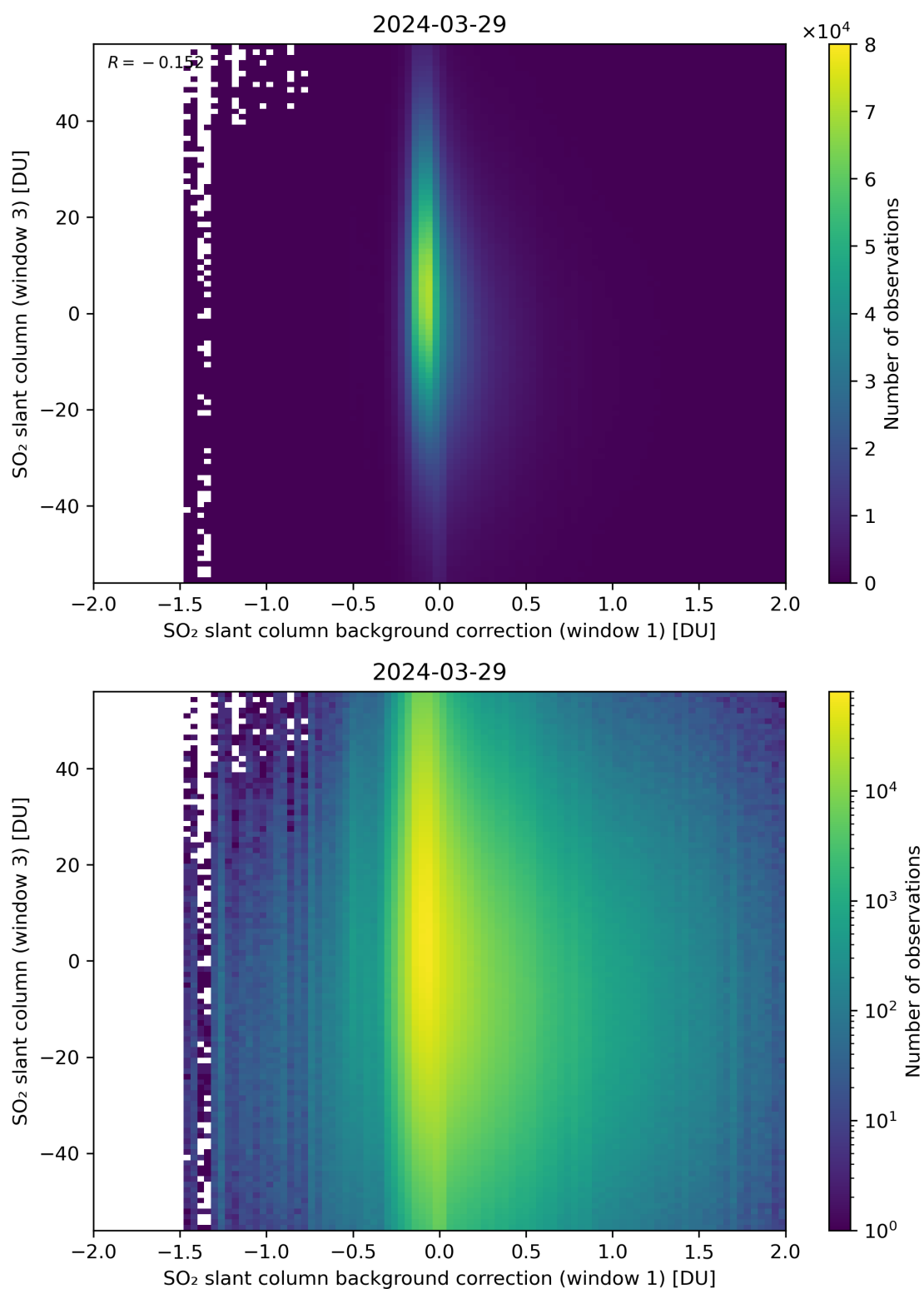
Figure 107: Scatter density plot of “SO 2 slant column background correction (window 1)” against “SO 2 slant column (window 3)” for 2024-03-28 to 2024-03-30.
