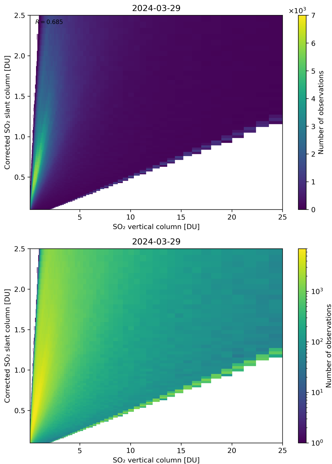
Figure 297: Scatter density plot of “SO 2 vertical column” against “Corrected SO 2 slant column” for 2024-03-28 to 2024-03-30.
