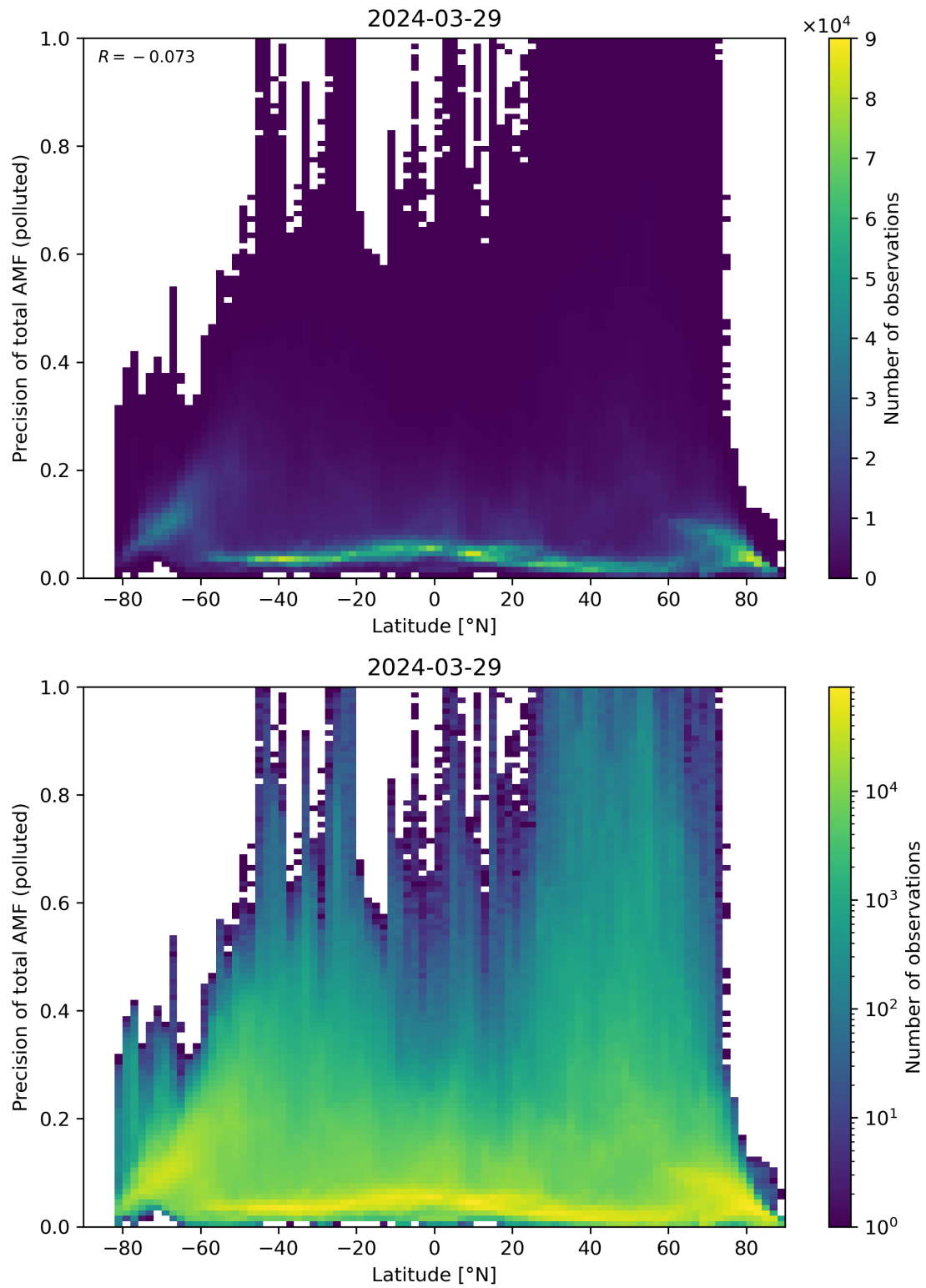
Figure 155: Scatter density plot of “Latitude” against “Precision of total AMF (polluted)” for 2024-03-28 to 2024-03-30.
