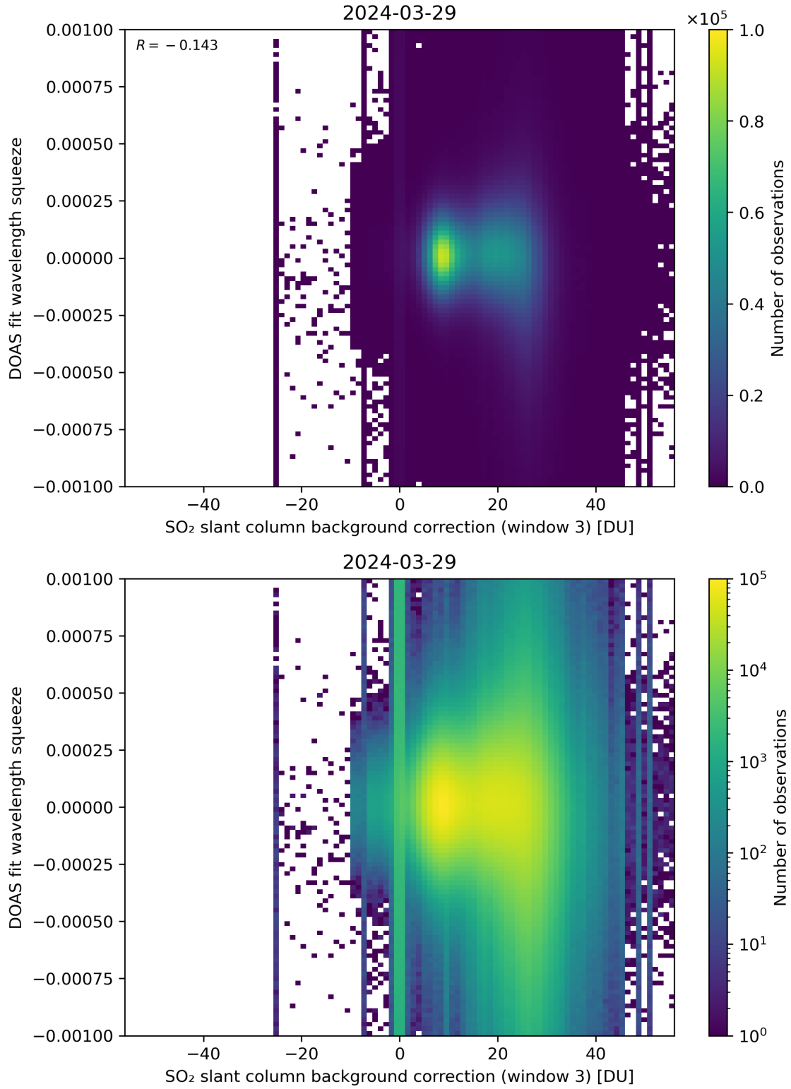
Figure 122: Scatter density plot of “SO 2 slant column background correction (window 3)” against “DOAS fit wavelength squeeze” for 2024-03-28 to 2024-03-30.
