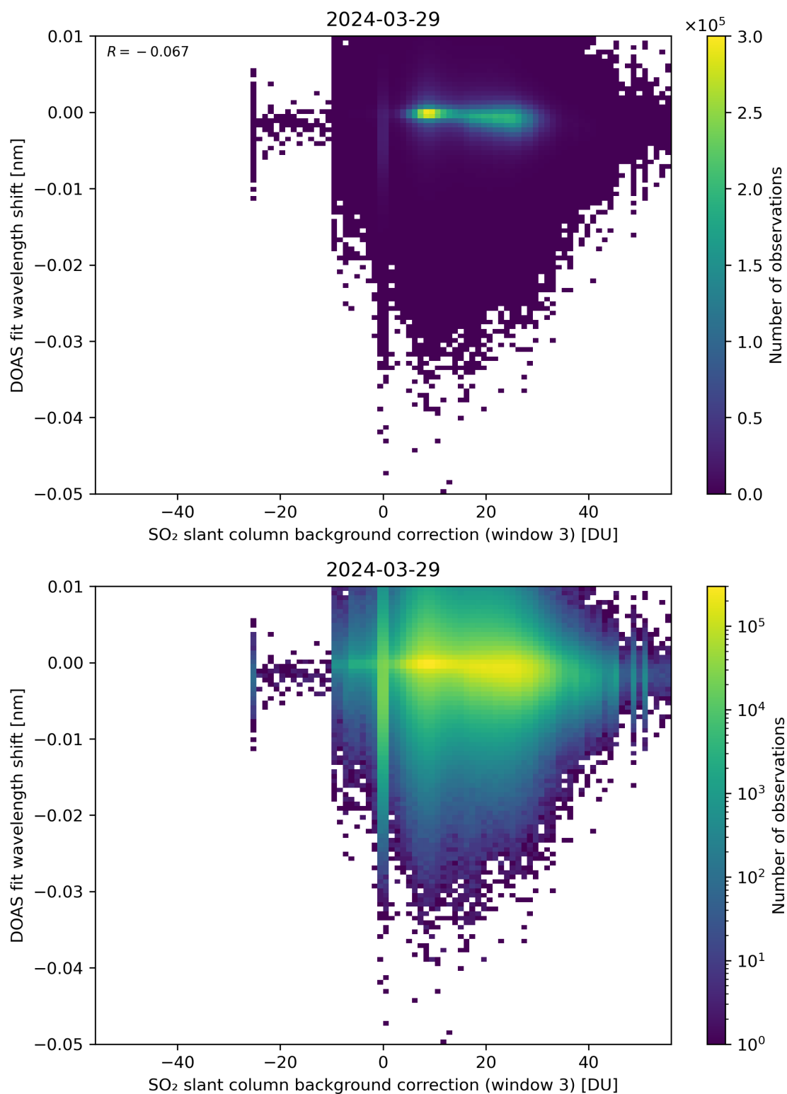
Figure 121: Scatter density plot of “SO 2 slant column background correction (window 3)” against “DOAS fit wavelength shift” for 2024-03-28 to 2024-03-30.
