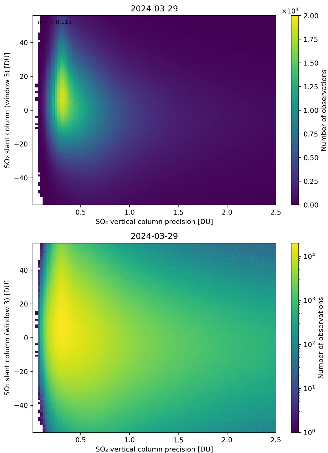
Figure 292: Scatter density plot of “SO 2 vertical column precision” against “SO 2 slant column (window 3)” for 2024-03-28 to 2024-03-30.
