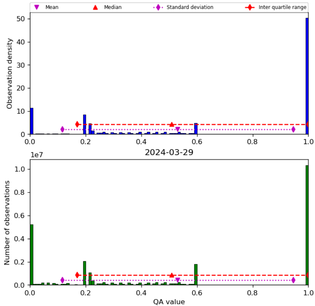
Figure 52: Histogram of “QA value” for 2024-03-28 to 2024-03-30
