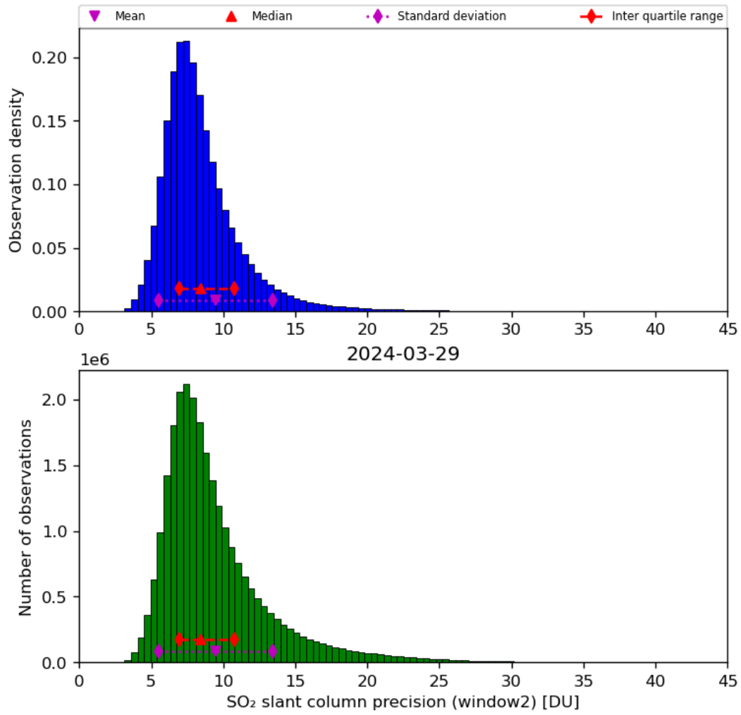
Figure 61: Histogram of “SO 2 slant column precision (window2)” for 2024-03-28 to 2024-03-30
