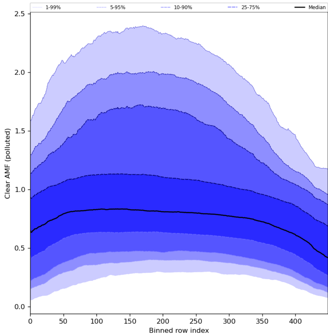
Figure 96: Along track statistics of “Clear AMF (polluted)” for 2024-03-28 to 2024-03-30
