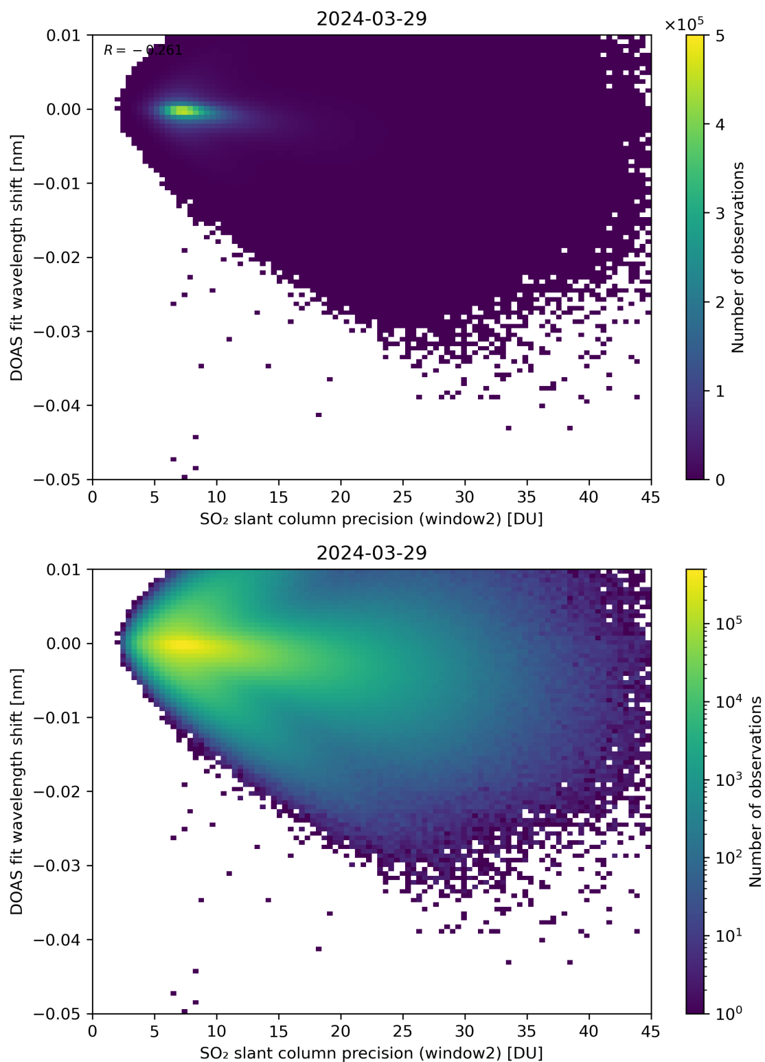
Figure 243: Scatter density plot of “SO 2 slant column precision (window2)” against “DOAS fit wavelength shift” for 2024-03-28 to 2024-03-30.
