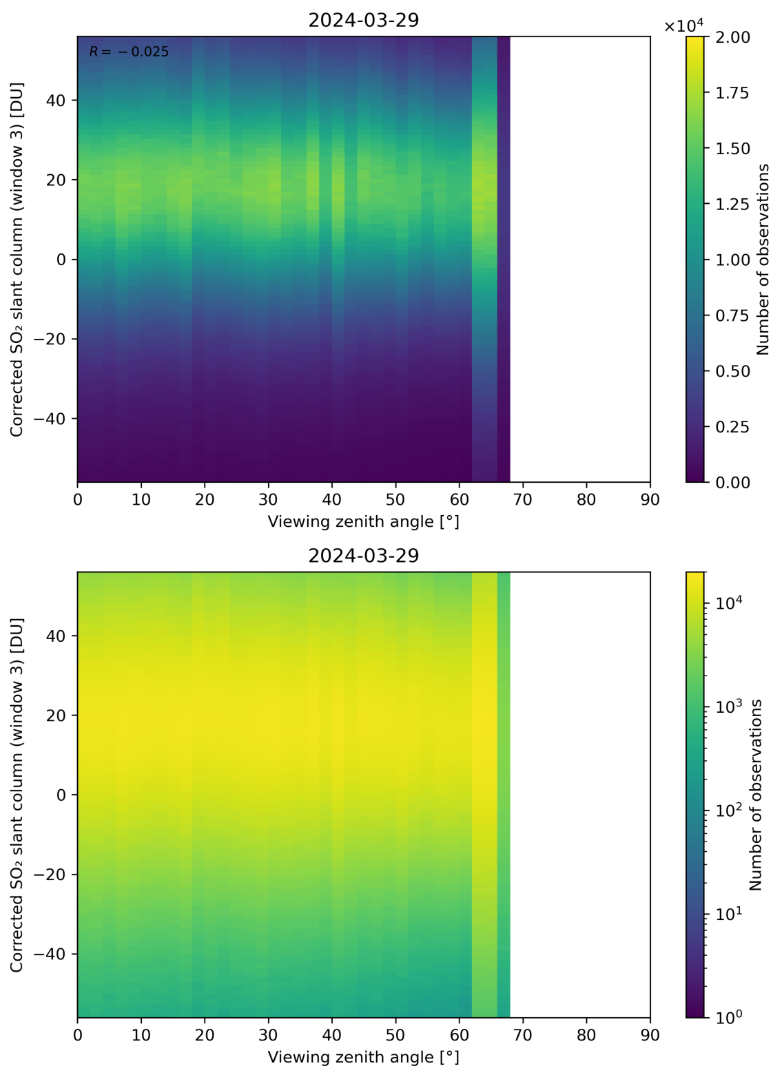
Figure 319: Scatter density plot of “Viewing zenith angle” against “Corrected SO 2 slant column (window 3)” for 2024-03-28 to 2024-03-30.
