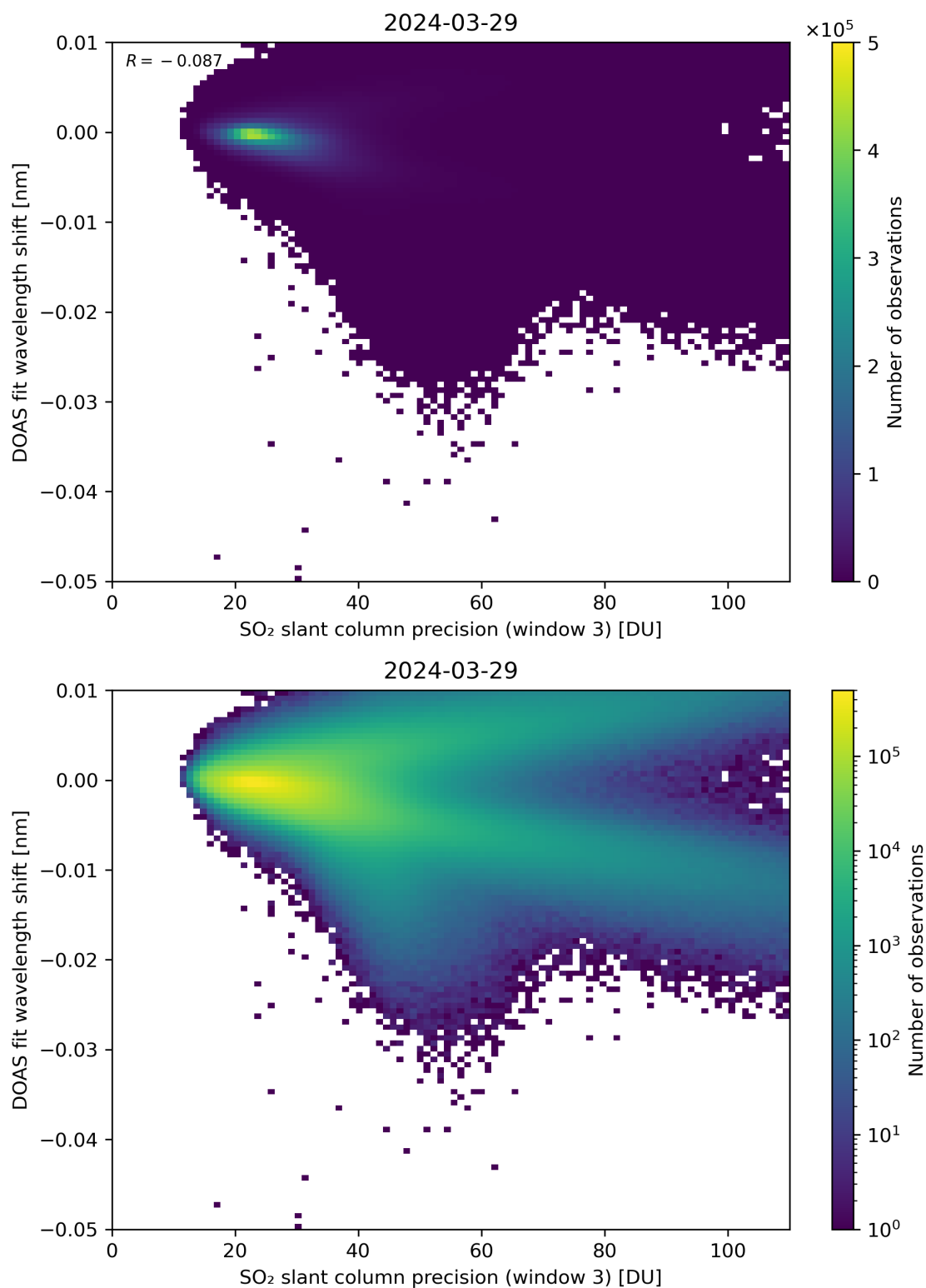
Figure 258: Scatter density plot of “SO 2 slant column precision (window 3)” against “DOAS fit wavelength shift” for 2024-03-28 to 2024-03-30.
