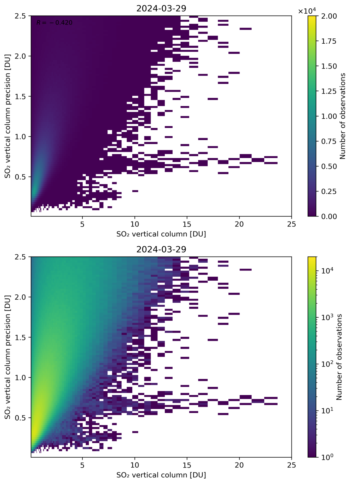
Figure 307: Scatter density plot of “SO 2 vertical column” against “SO 2 vertical column precision” for 2024-03-28 to 2024-03-30.
