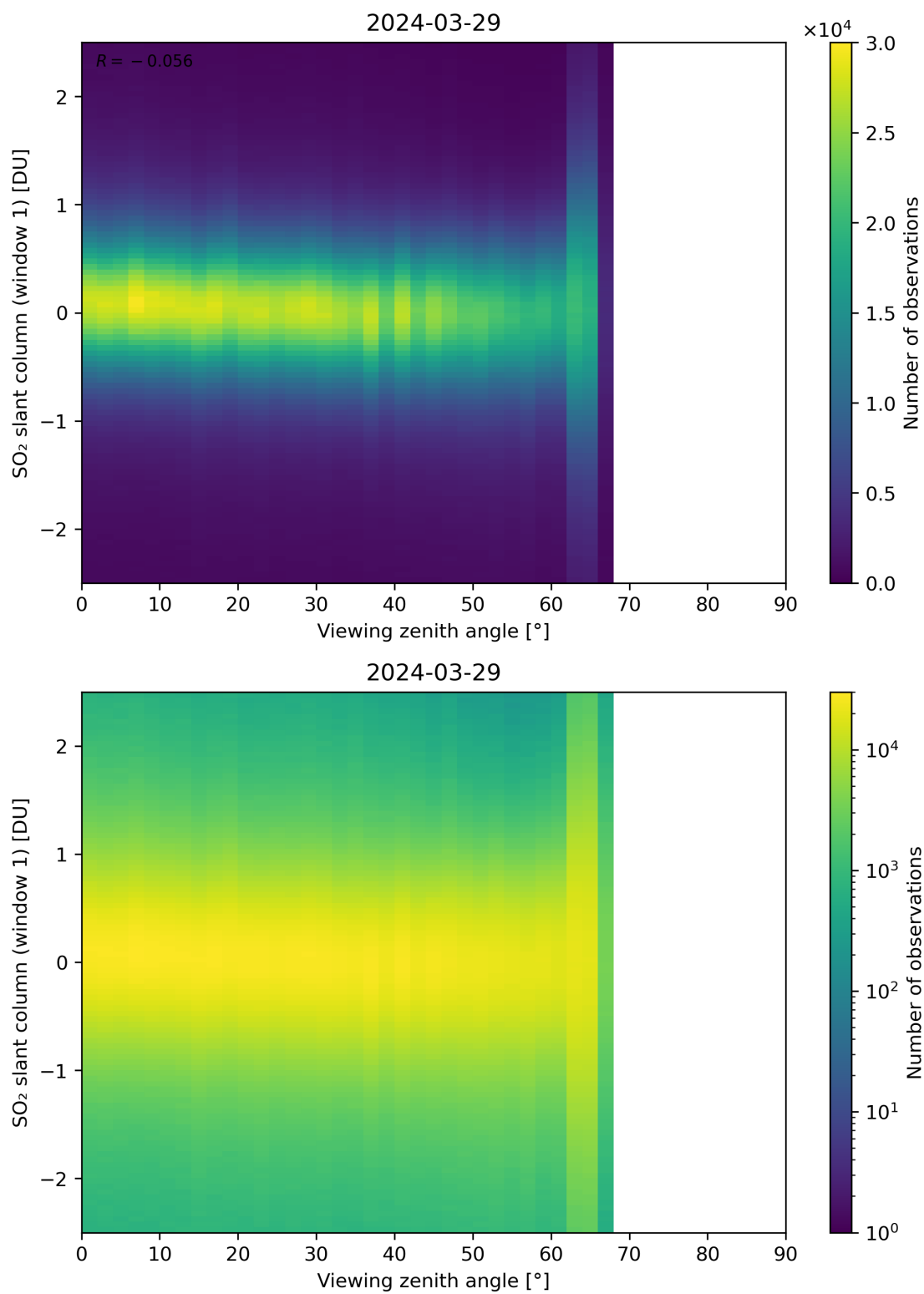
Figure 320: Scatter density plot of “Viewing zenith angle” against “SO 2 slant column (window 1)” for 2024-03-28 to 2024-03-30.
