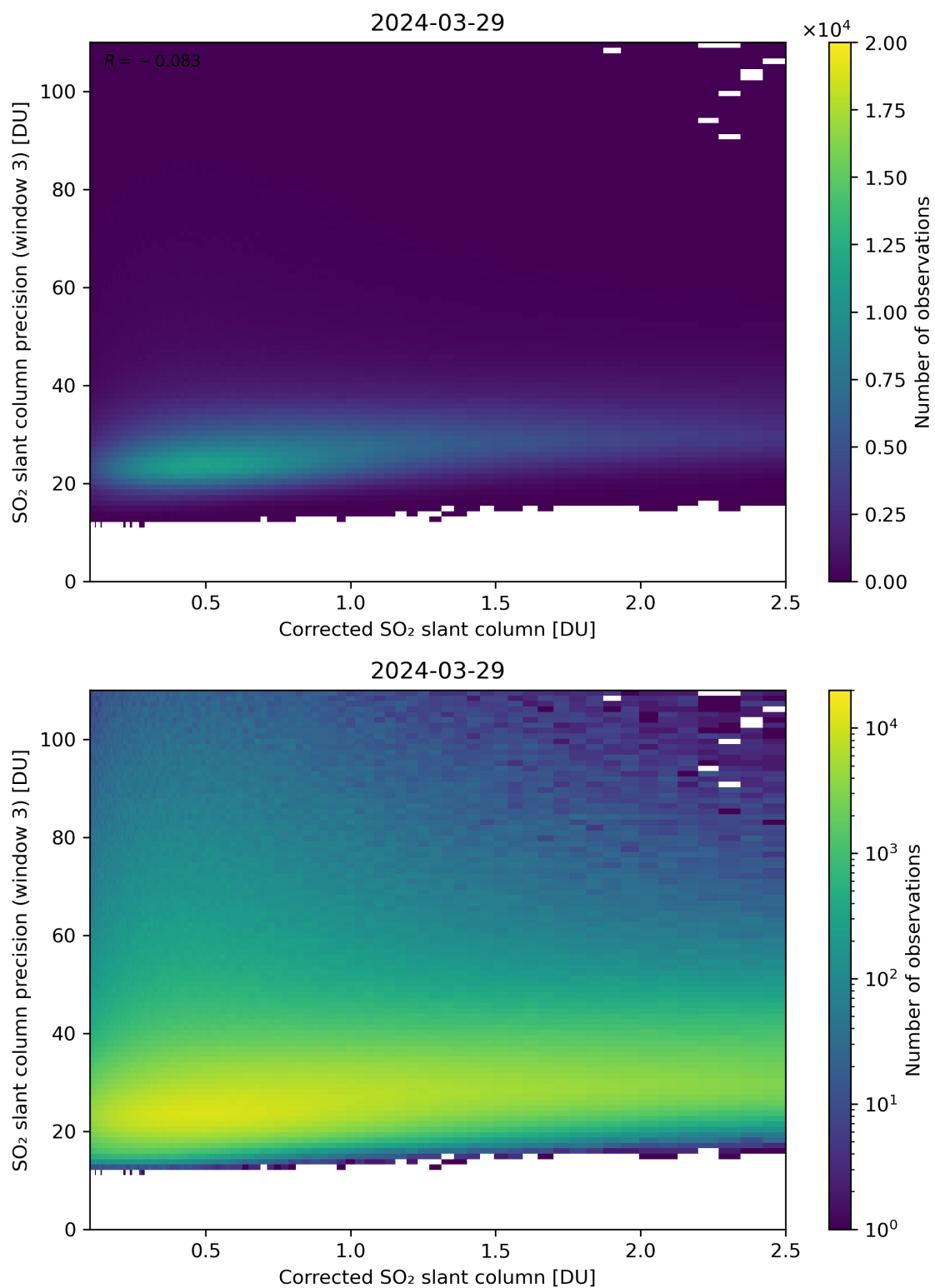
Figure 191: Scatter density plot of “Corrected SO 2 slant column” against “SO 2 slant column precision (window 3)” for 2024-03-28 to 2024-03-30.
