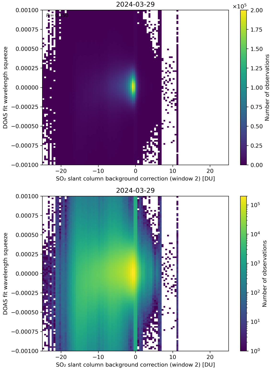
Figure 113: Scatter density plot of “SO 2 slant column background correction (window 2)” against “DOAS fit wavelength squeeze” for 2024-03-28 to 2024-03-30.
