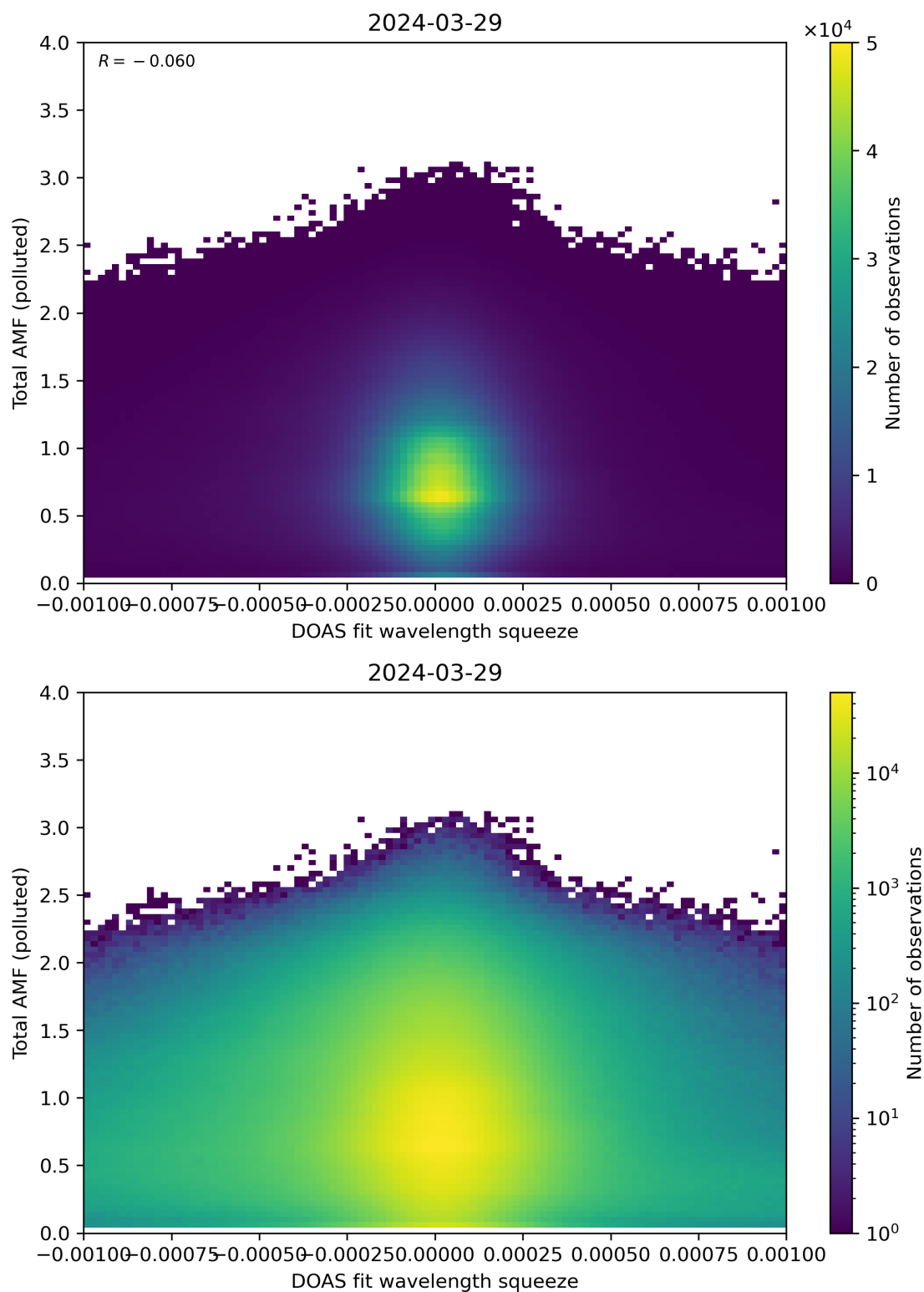
Figure 134: Scatter density plot of “DOAS fit wavelength squeeze” against “Total AMF (polluted)” for 2024-03-28 to 2024-03-30.
