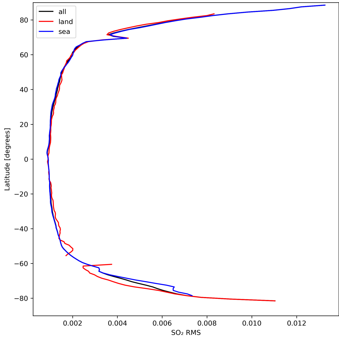
Figure 47: Zonal average of “SO 2 RMS” for 2024-03-28 to 2024-03-30.
