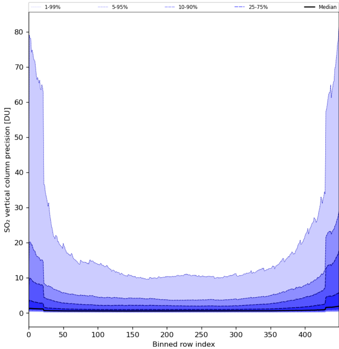
Figure 77: Along track statistics of “SO 2 vertical column precision” for 2024-03-28 to 2024-03-30
