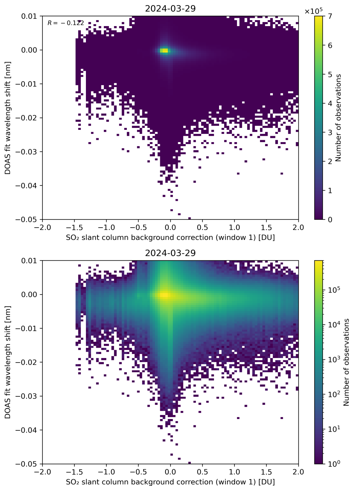
Figure 100: Scatter density plot of “SO 2 slant column background correction (window 1)” against “DOAS fit wavelength shift” for 2024-03-28 to 2024-03-30.
