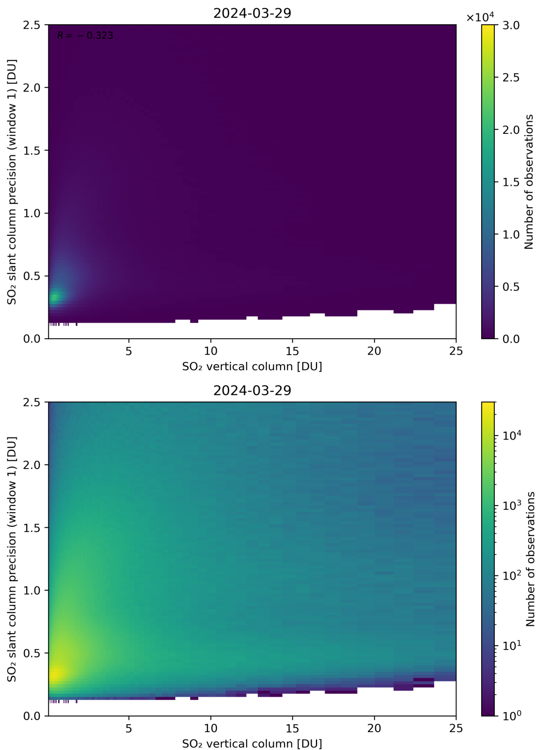
Figure 301: Scatter density plot of “SO 2 vertical column” against “SO 2 slant column precision (window 1)” for 2024-03-28 to 2024-03-30.
