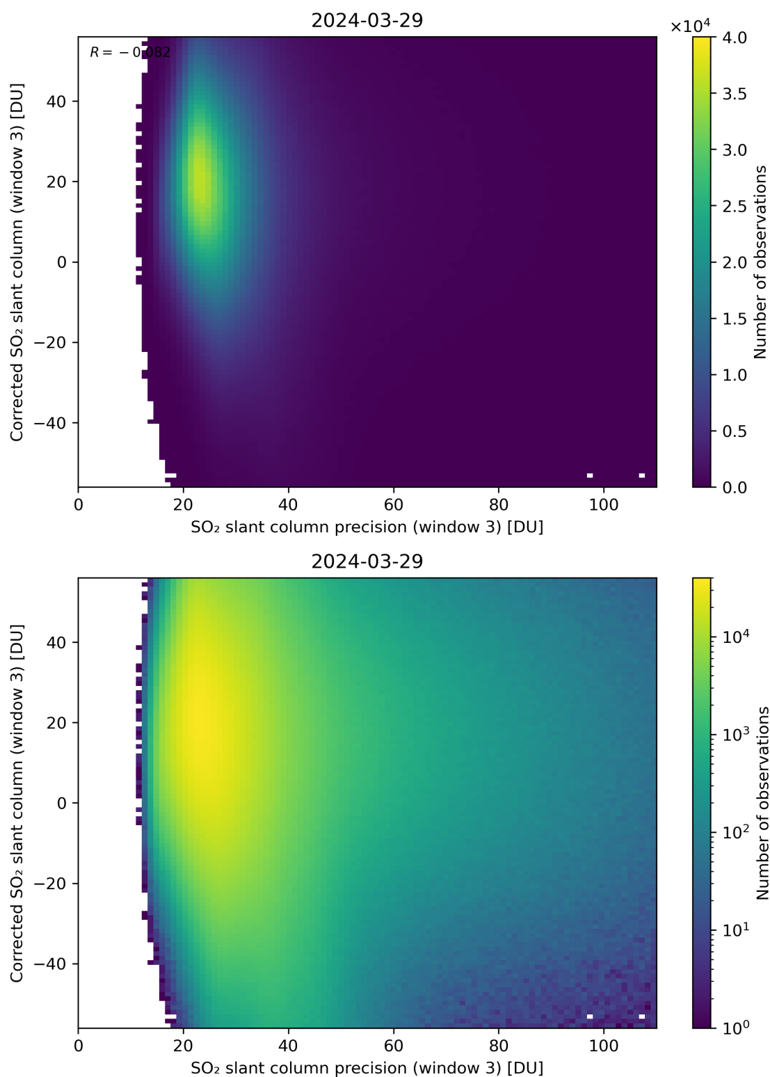
Figure 262: Scatter density plot of “SO 2 slant column precision (window 3)” against “Corrected SO 2 slant column (window 3)” for 2024-03-28 to 2024-03-30.
