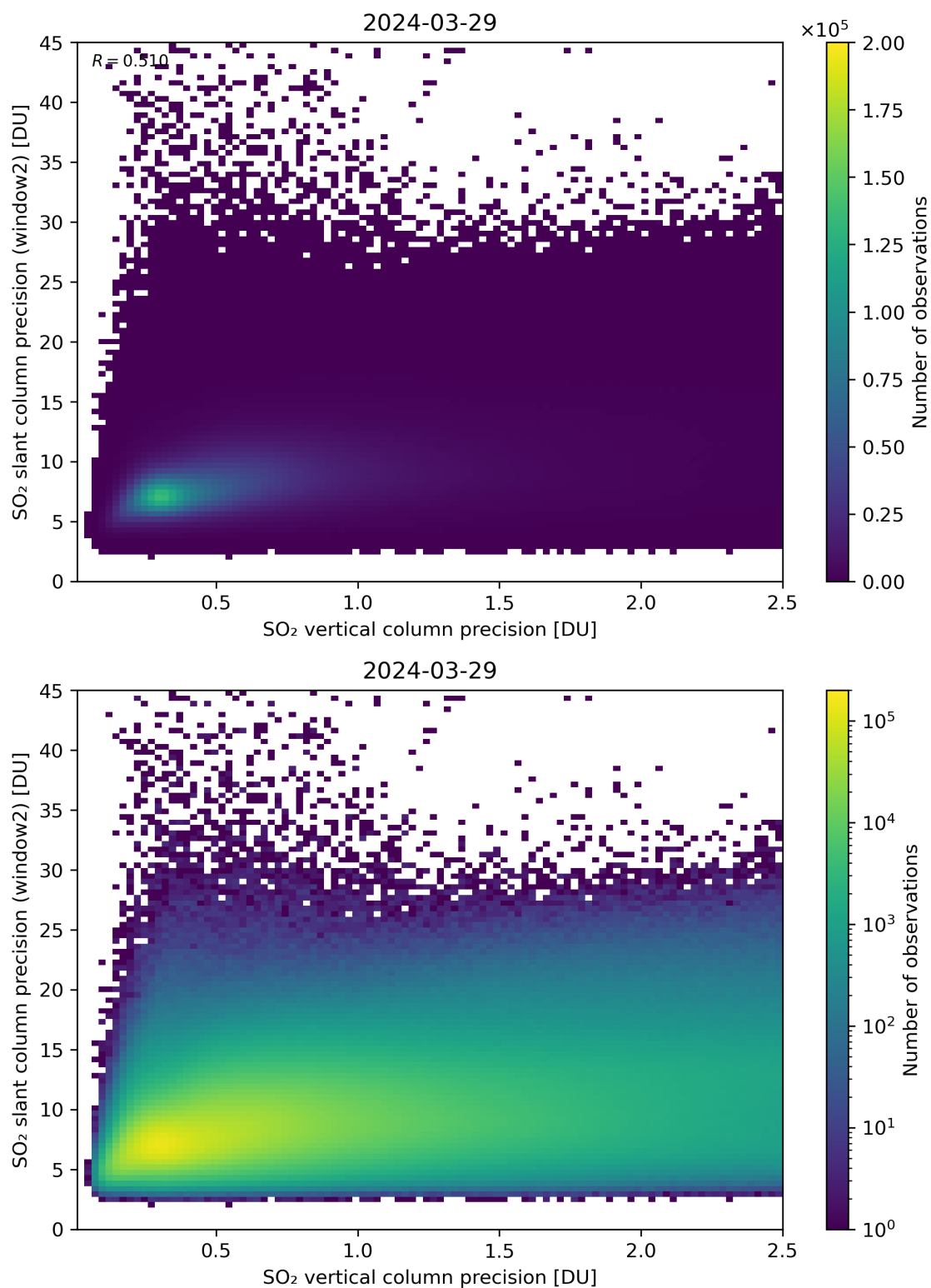
Figure 291: Scatter density plot of “SO 2 vertical column precision” against “SO 2 slant column precision (window2)” for 2024-03-28 to 2024-03-30.
