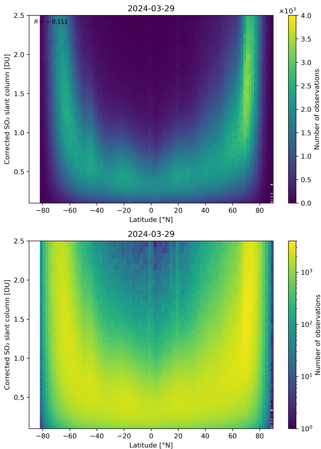
Figure 146: Scatter density plot of “Latitude” against “Corrected SO 2 slant column” for 2024-03-28 to 2024-03-30.
