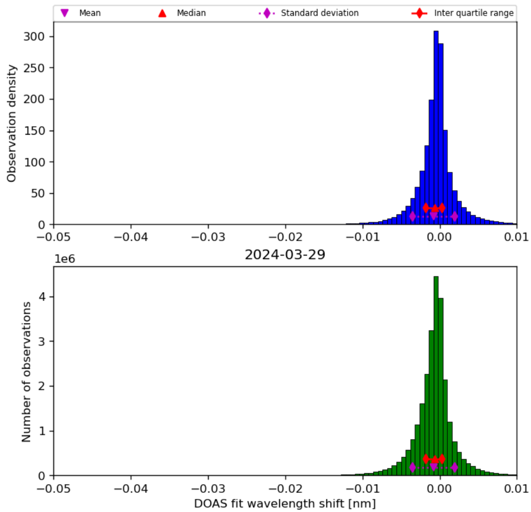
Figure 68: Histogram of “DOAS fit wavelength shift” for 2024-03-28 to 2024-03-30
