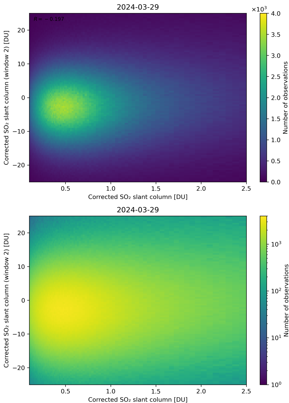
Figure 185: Scatter density plot of “Corrected SO 2 slant column” against “Corrected SO 2 slant column (window 2)” for 2024-03-28 to 2024-03-30.
