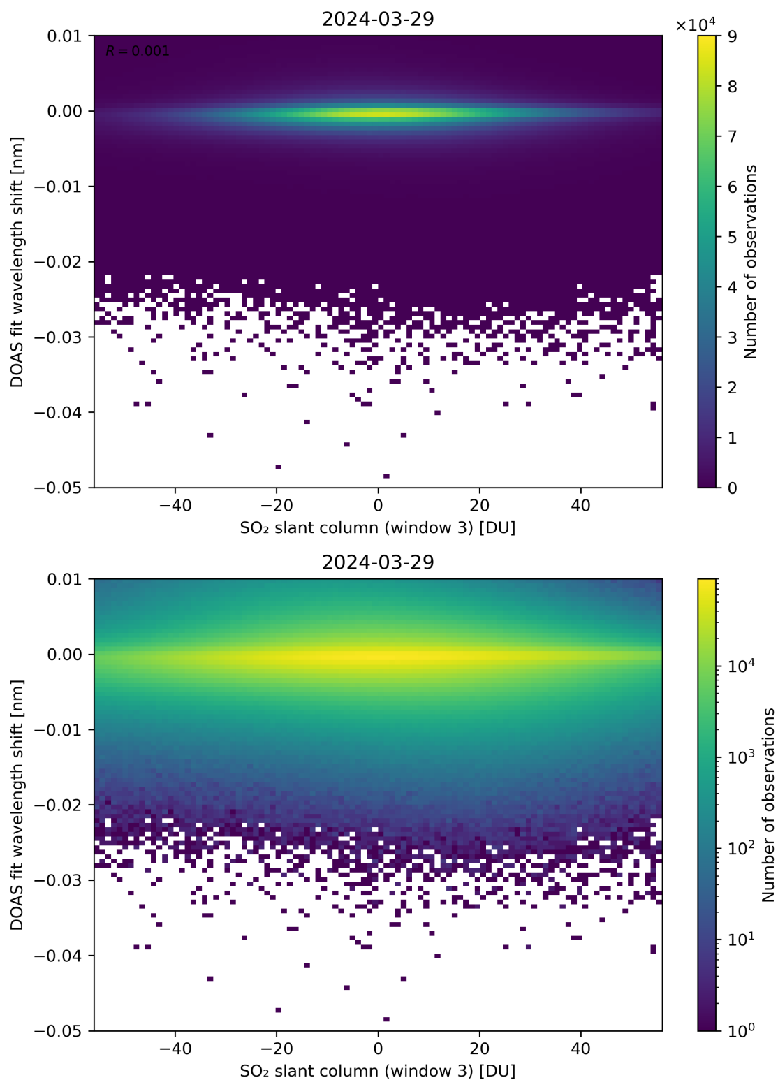
Figure 254: Scatter density plot of “SO 2 slant column (window 3)” against “DOAS fit wavelength shift” for 2024-03-28 to 2024-03-30.
