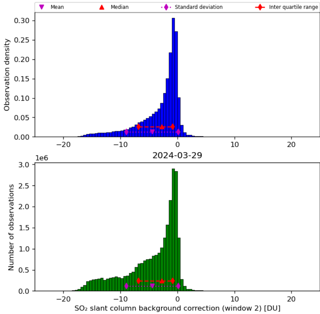
Figure 63: Histogram of “SO 2 slant column background correction (window 2)” for 2024-03-28 to 2024-03-30
