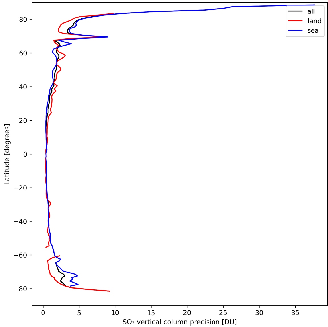
Figure 31: Zonal average of “SO 2 vertical column precision” for 2024-03-28 to 2024-03-30.
