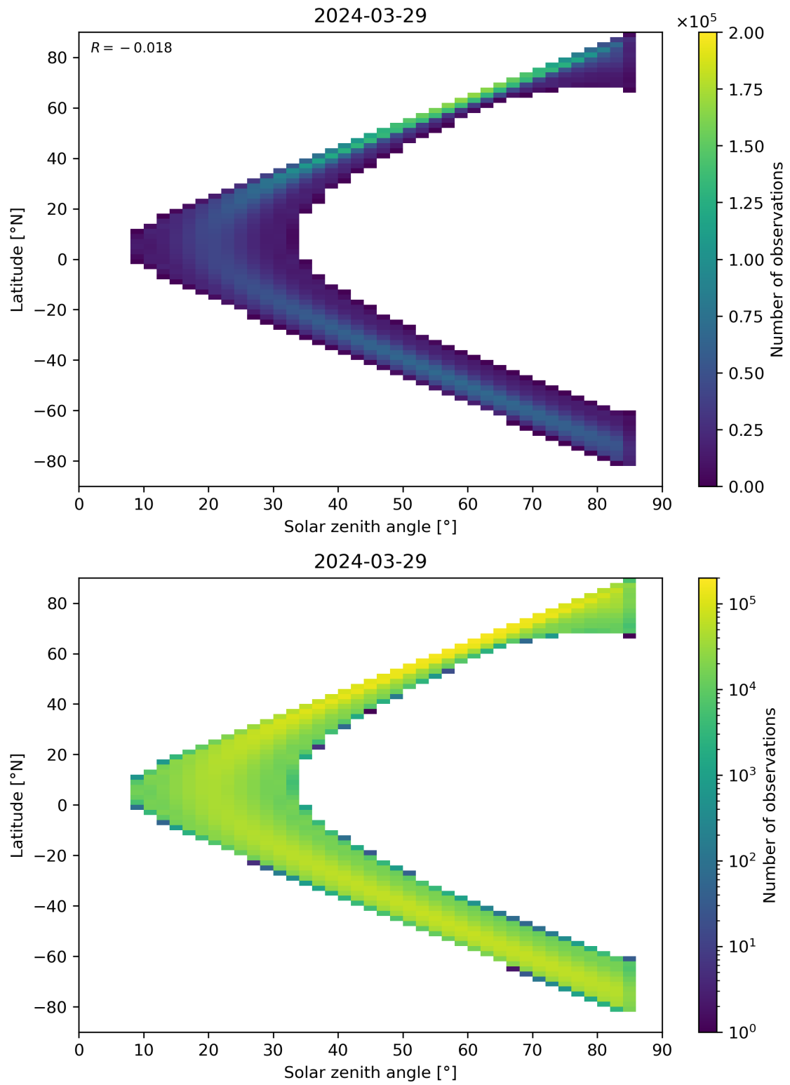
Figure 164: Scatter density plot of “Solar zenith angle” against “Latitude” for 2024-03-28 to 2024-03-30.
