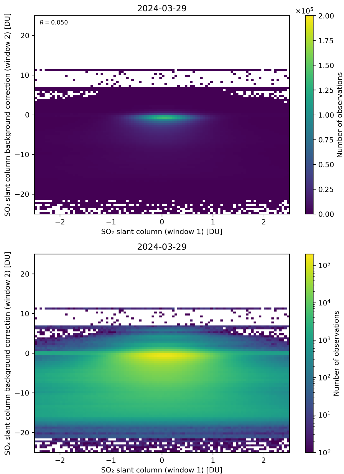
Figure 213: Scatter density plot of “SO 2 slant column (window 1)” against “SO 2 slant column background correction (window 2)” for 2024-03-28 to 2024-03-30.
