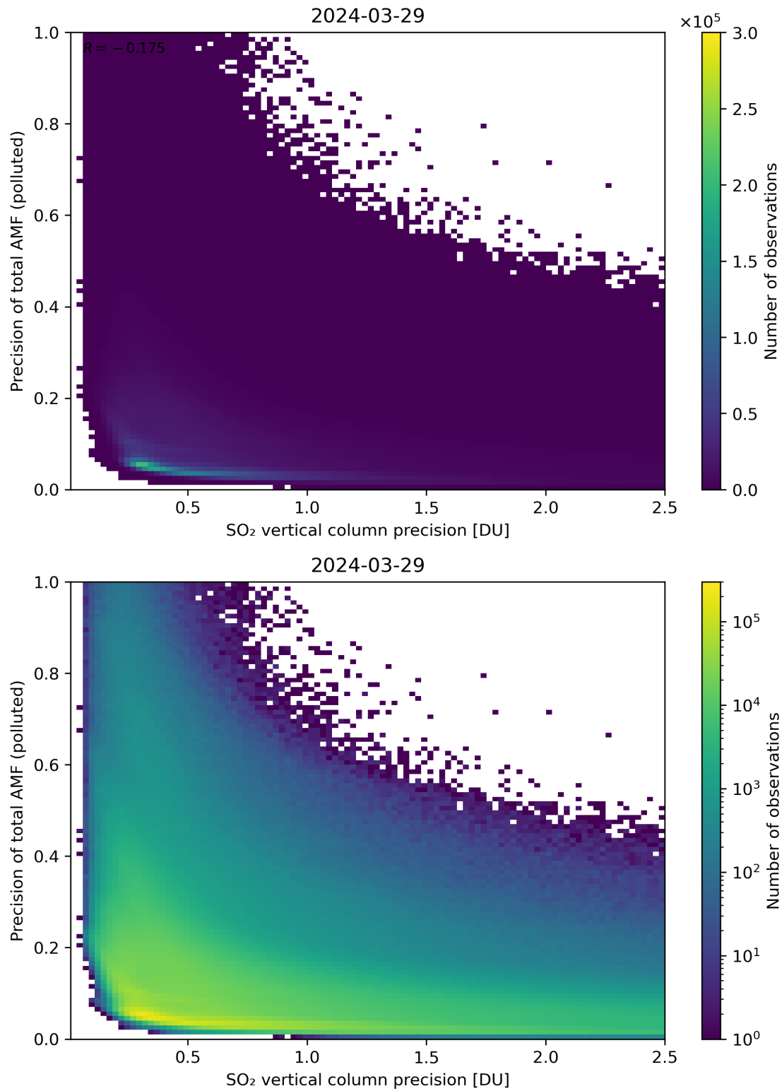
Figure 295: Scatter density plot of “SO 2 vertical column precision” against “Precision of total AMF (polluted)” for 2024-03-28 to 2024-03-30.
