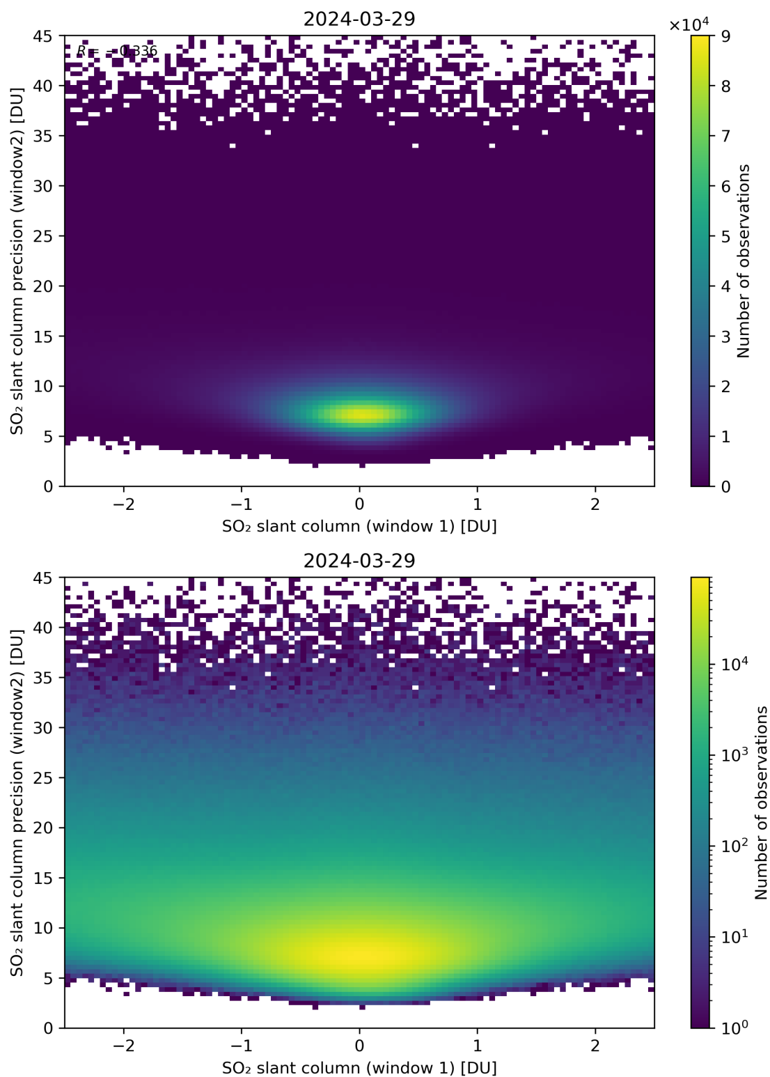
Figure 236: Scatter density plot of “SO 2 slant column (window 1)” against “SO 2 slant column precision (window2)” for 2024-03-28 to 2024-03-30.
