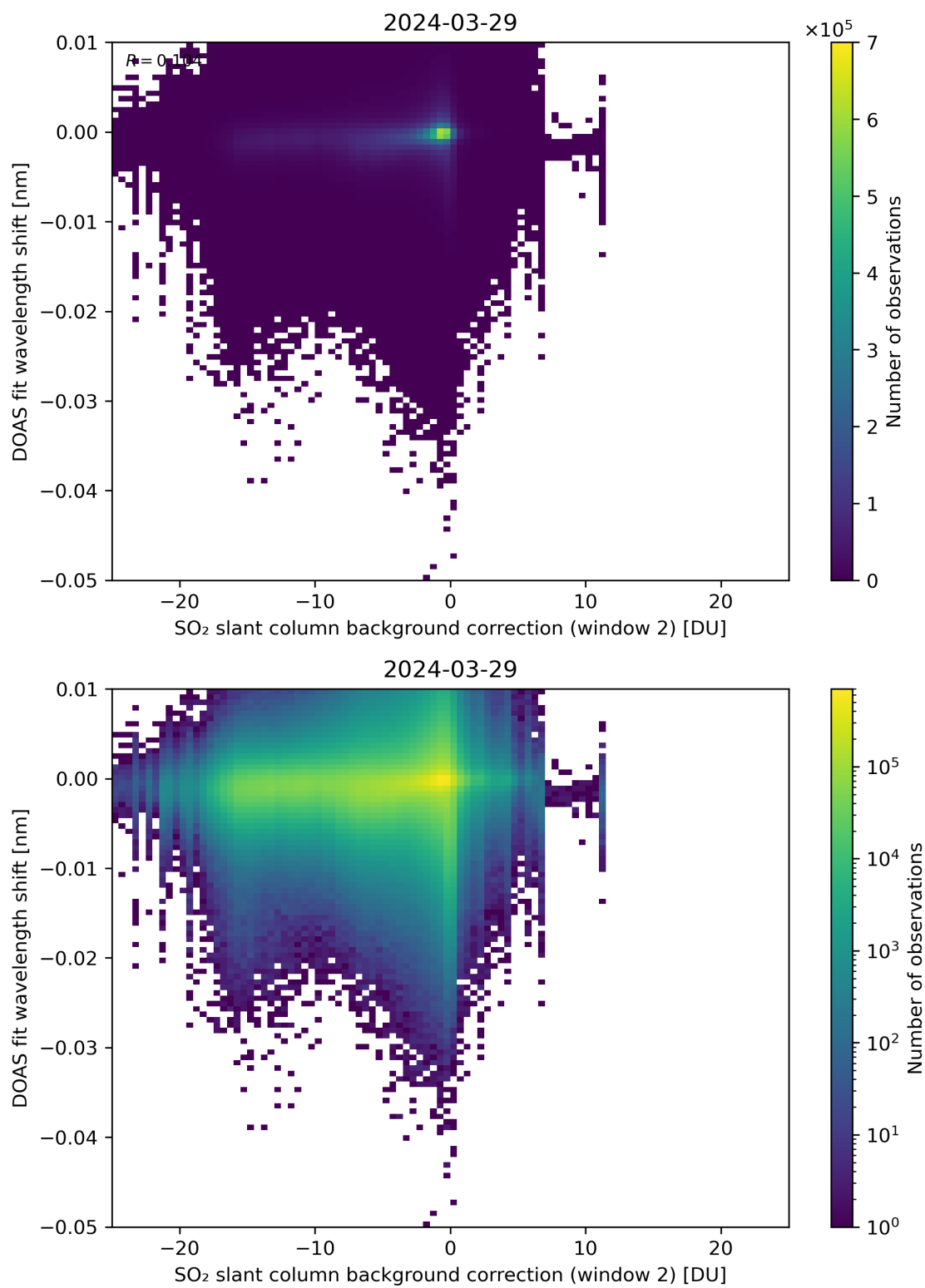
Figure 112: Scatter density plot of “SO 2 slant column background correction (window 2)” against “DOAS fit wavelength shift” for 2024-03-28 to 2024-03-30.
