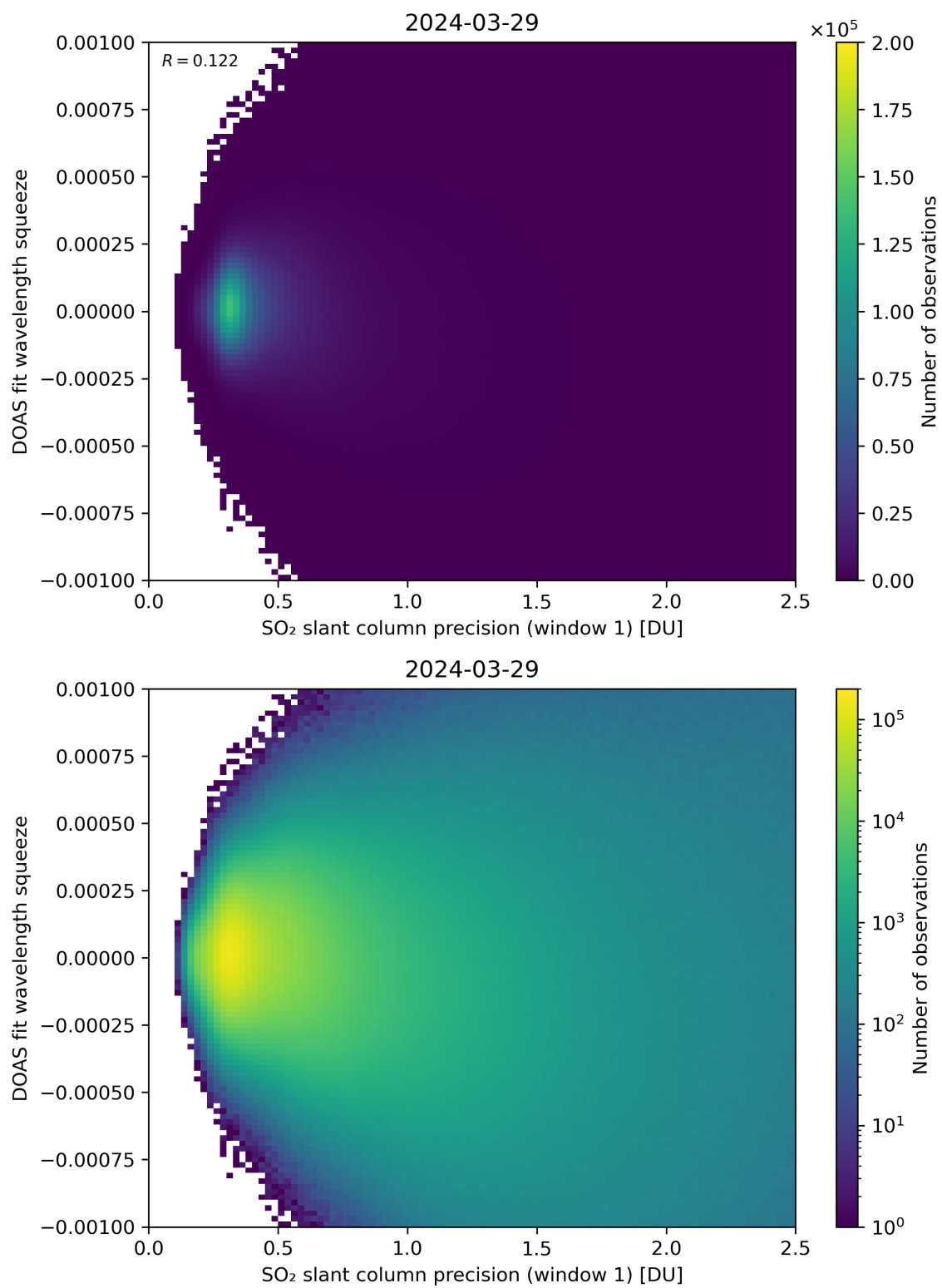
Figure 222: Scatter density plot of “SO 2 slant column precision (window 1)” against “DOAS fit wavelength squeeze” for 2024-03-28 to 2024-03-30.
