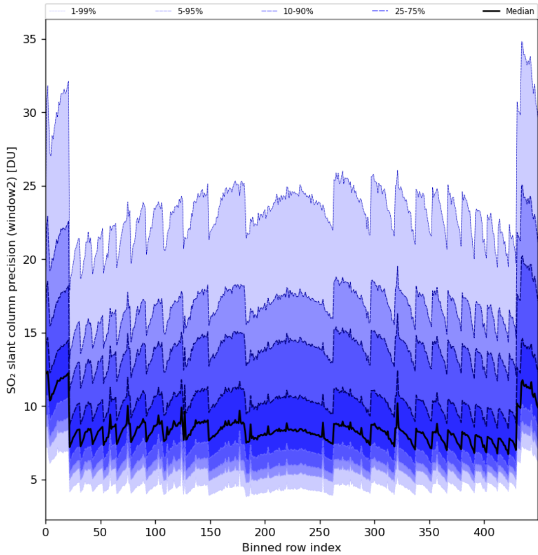
Figure 84: Along track statistics of “SO 2 slant column precision (window2)” for 2024-03-28 to 2024-03-30
