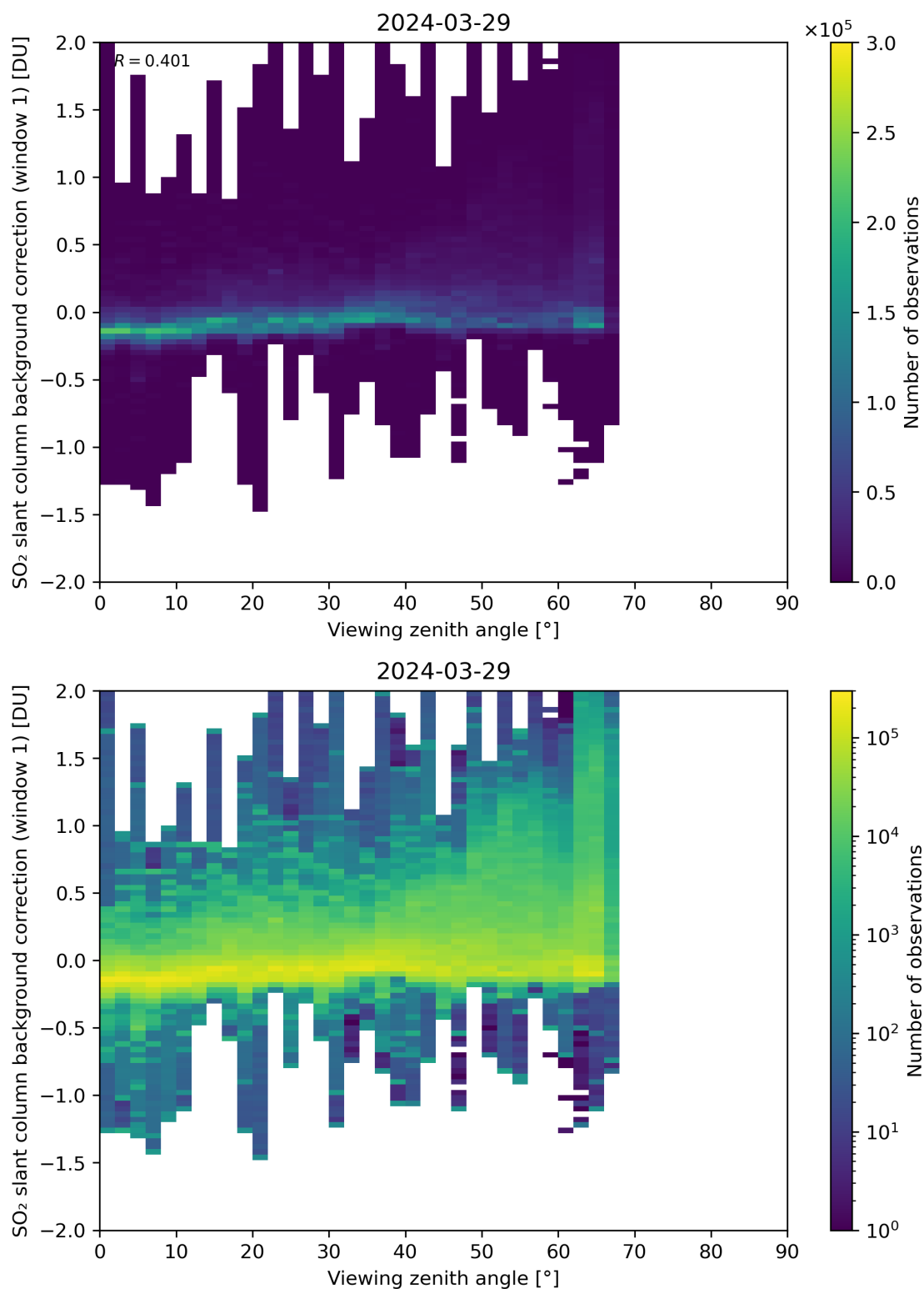
Figure 308: Scatter density plot of “Viewing zenith angle” against “SO 2 slant column background correction (window 1)” for 2024-03-28 to 2024-03-30.
