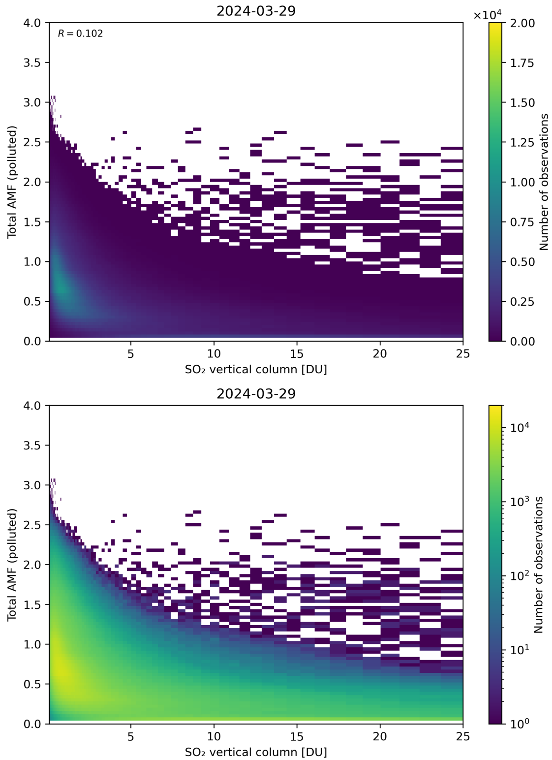
Figure 305: Scatter density plot of “SO 2 vertical column” against “Total AMF (polluted)” for 2024-03-28 to 2024-03-30.
