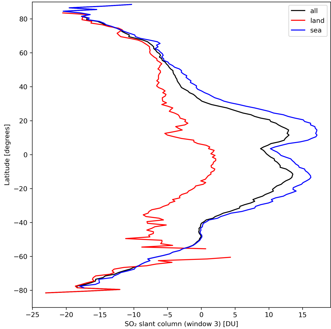
Figure 41: Zonal average of “SO 2 slant column (window 3)” for 2024-03-28 to 2024-03-30.
