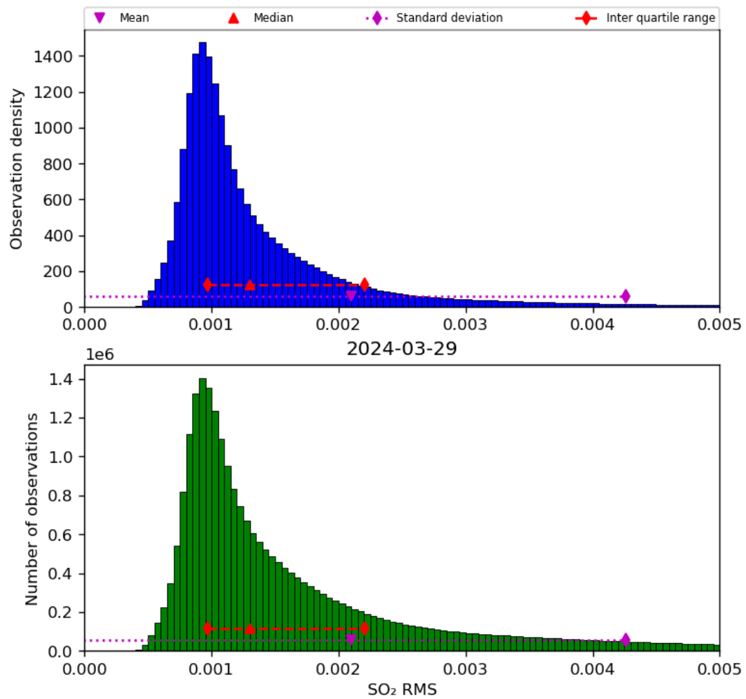
Figure 70: Histogram of “SO 2 RMS” for 2024-03-28 to 2024-03-30
