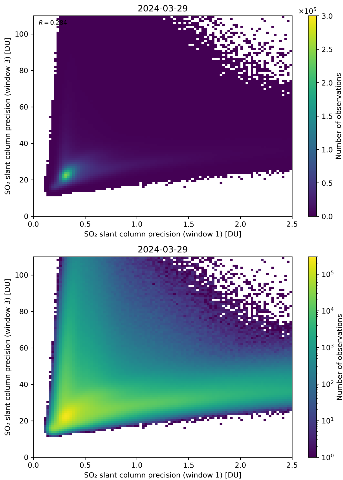
Figure 229: Scatter density plot of “SO 2 slant column precision (window 1)” against “SO 2 slant column precision (window 3)” for 2024-03-28 to 2024-03-30.
