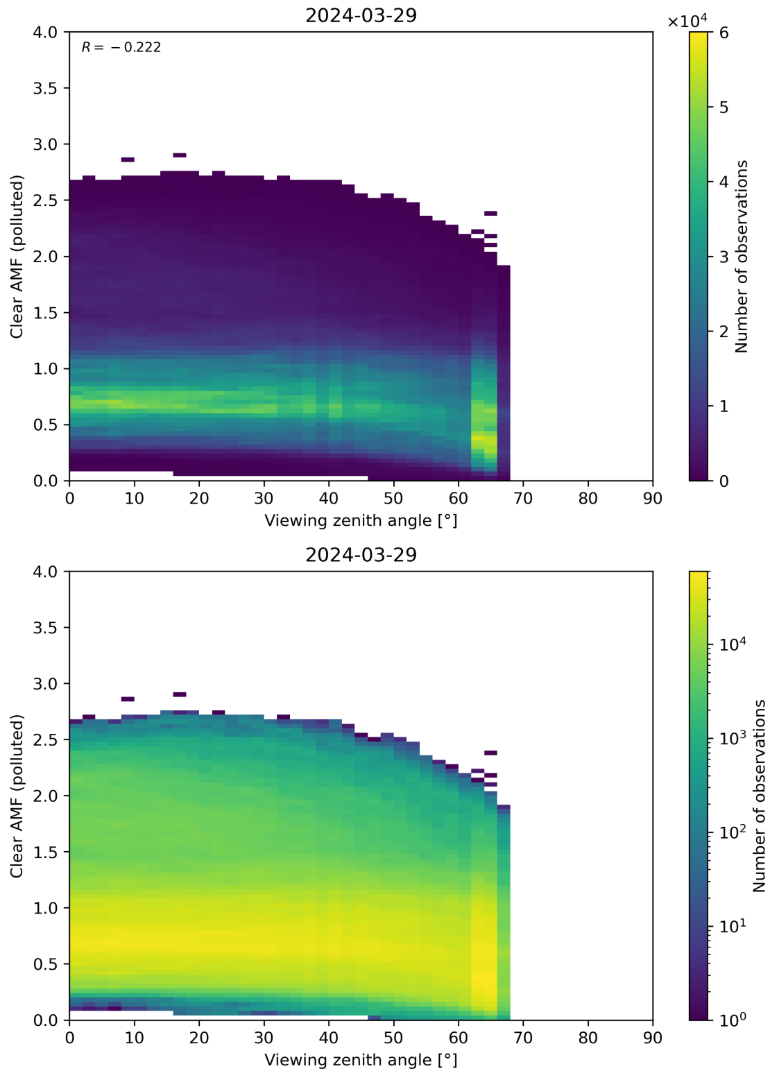
Figure 316: Scatter density plot of “Viewing zenith angle” against “Clear AMF (polluted)” for 2024-03-28 to 2024-03-30.
