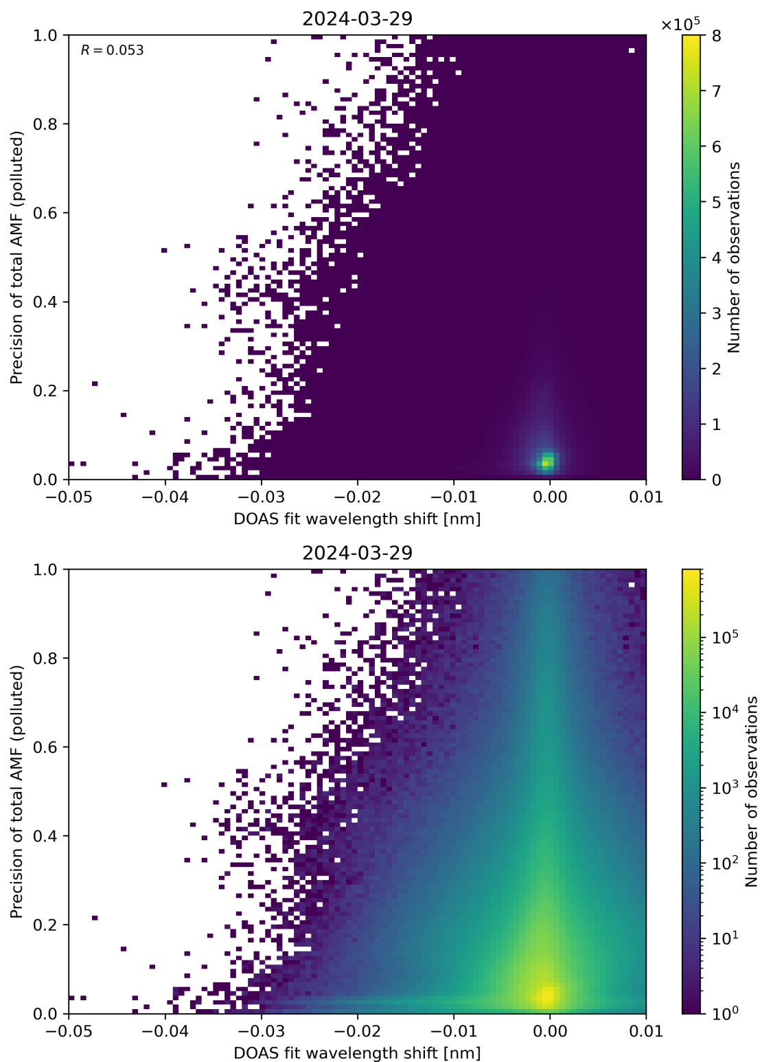
Figure 131: Scatter density plot of “DOAS fit wavelength shift” against “Precision of total AMF (polluted)” for 2024-03-28 to 2024-03-30.
