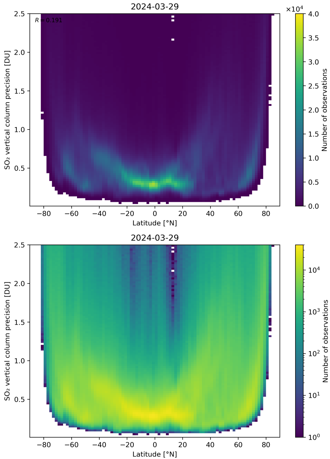
Figure 157: Scatter density plot of “Latitude” against “SO 2 vertical column precision” for 2024-03-28 to 2024-03-30.
