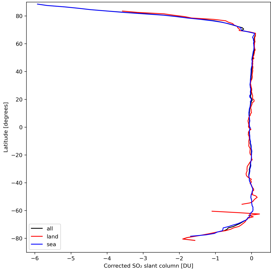
Figure 32: Zonal average of “Corrected SO 2 slant column” for 2024-03-28 to 2024-03-30.
