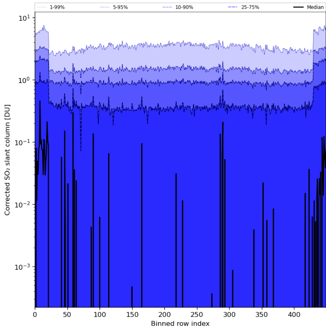
Figure 78: Along track statistics of “Corrected SO 2 slant column” for 2024-03-28 to 2024-03-30
