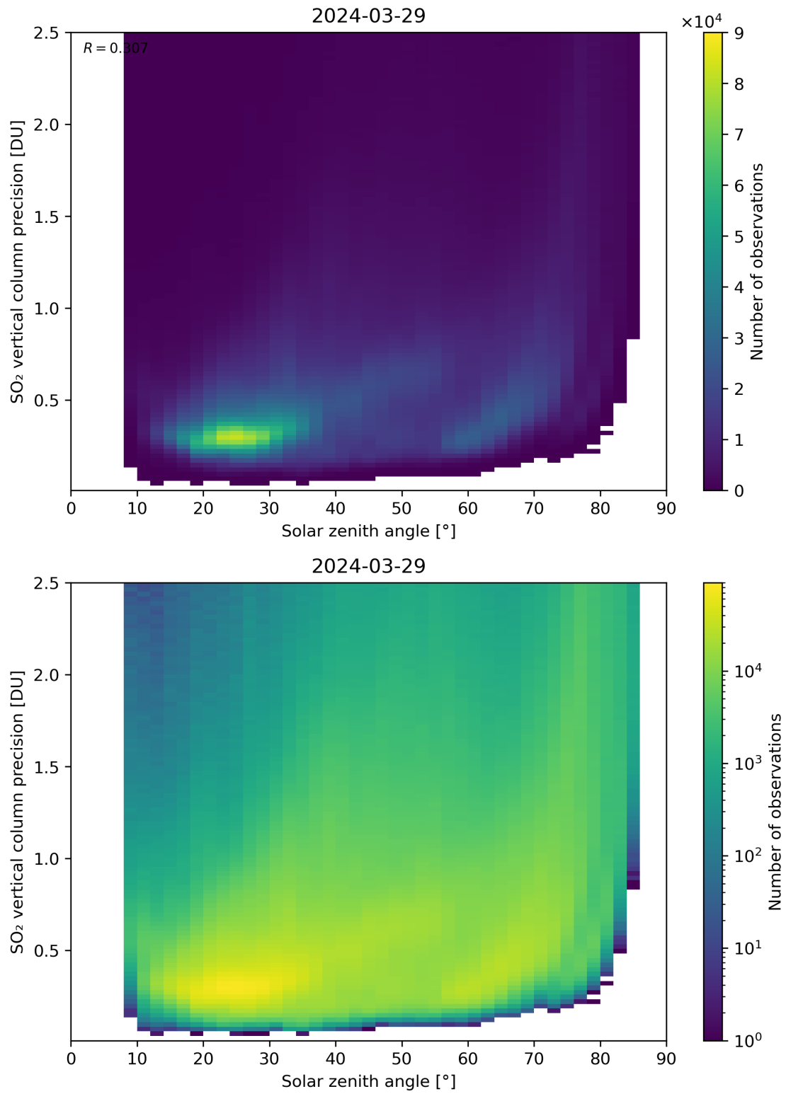
Figure 177: Scatter density plot of “Solar zenith angle” against “SO 2 vertical column precision” for 2024-03-28 to 2024-03-30.
