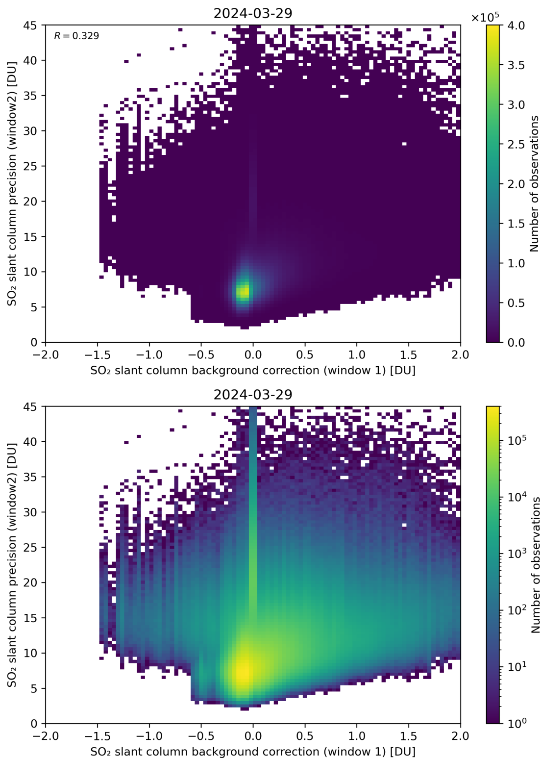
Figure 106: Scatter density plot of “SO 2 slant column background correction (window 1)” against “SO 2 slant column precision (window2)” for 2024-03-28 to 2024-03-30.
