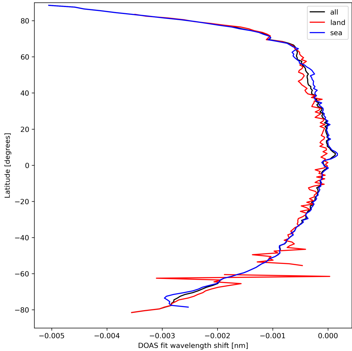
Figure 45: Zonal average of “DOAS fit wavelength shift” for 2024-03-28 to 2024-03-30.
