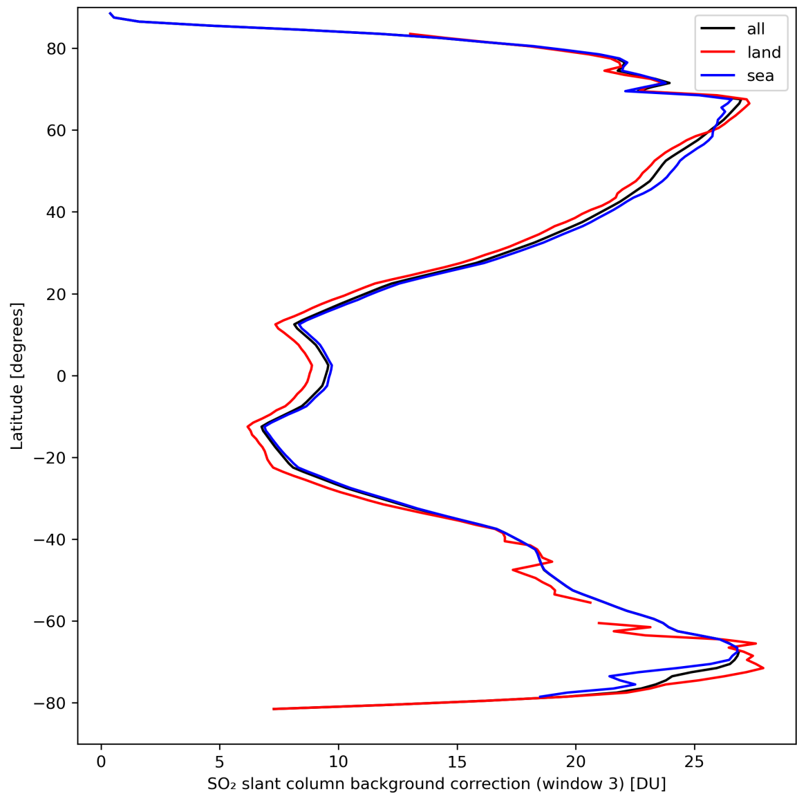
Figure 44: Zonal average of “SO 2 slant column background correction (window 3)” for 2024-03-28 to 2024-03-30.
