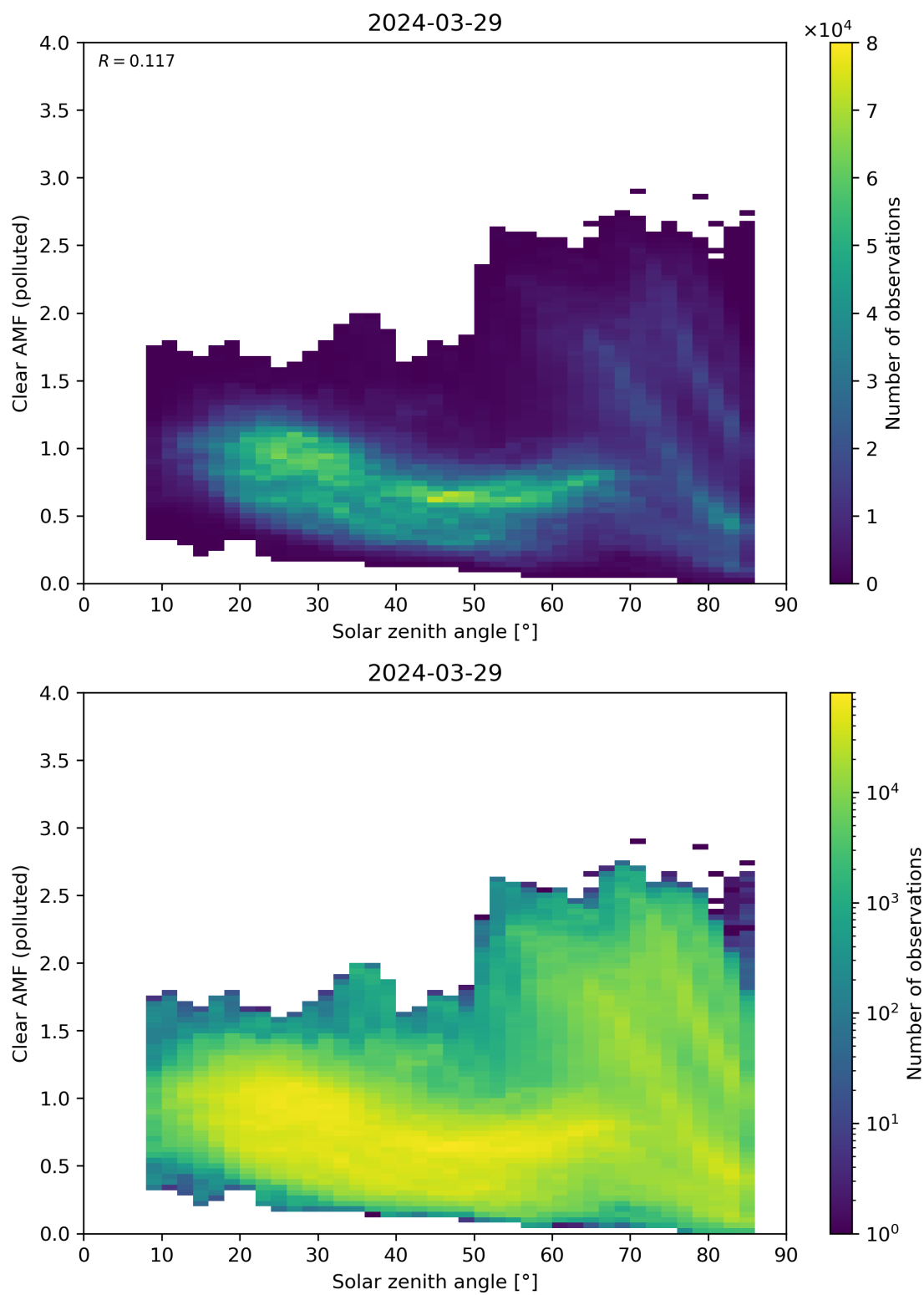
Figure 165: Scatter density plot of “Solar zenith angle” against “Clear AMF (polluted)” for 2024-03-28 to 2024-03-30.
