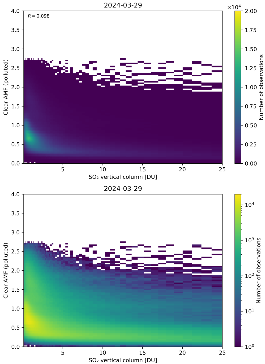
Figure 296: Scatter density plot of “SO 2 vertical column” against “Clear AMF (polluted)” for 2024-03-28 to 2024-03-30.
