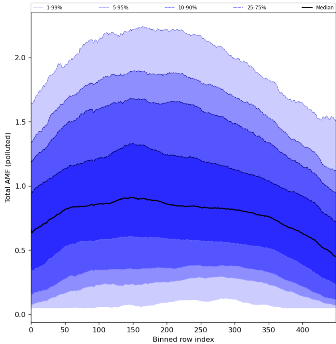
Figure 94: Along track statistics of “Total AMF (polluted)” for 2024-03-28 to 2024-03-30
