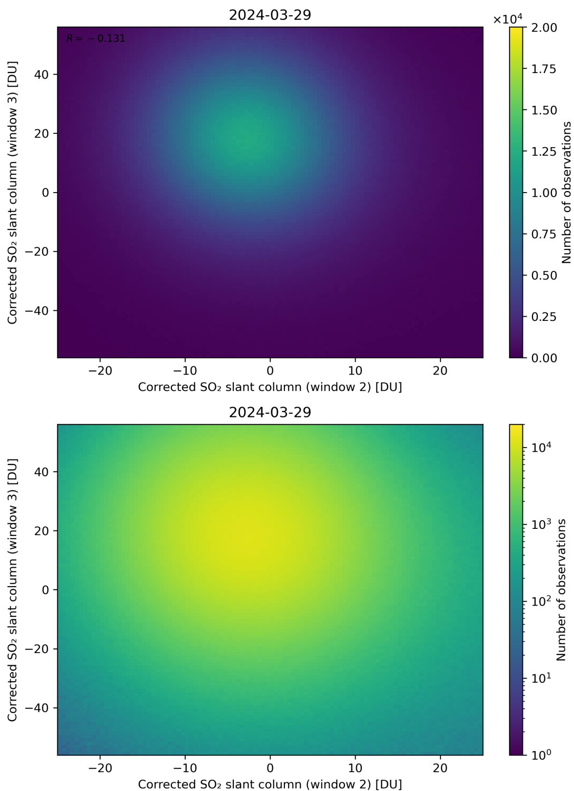
Figure 200: Scatter density plot of “Corrected SO 2 slant column (window 2)” against “Corrected SO 2 slant column (window 3)” for 2024-03-28 to 2024-03-30.
