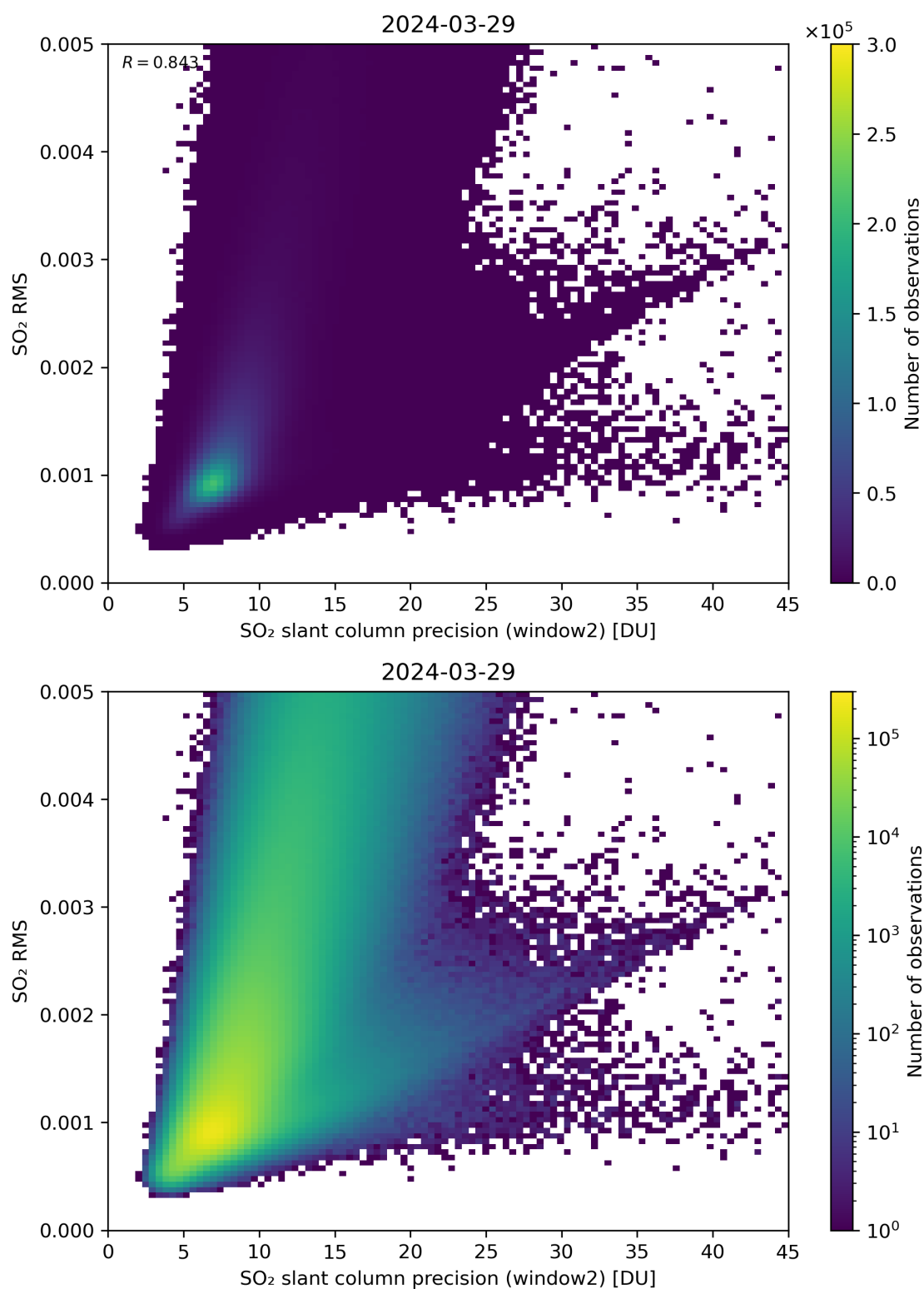
Figure 245: Scatter density plot of “SO 2 slant column precision (window2)” against “SO 2 RMS” for 2024-03-28 to 2024-03-30.
