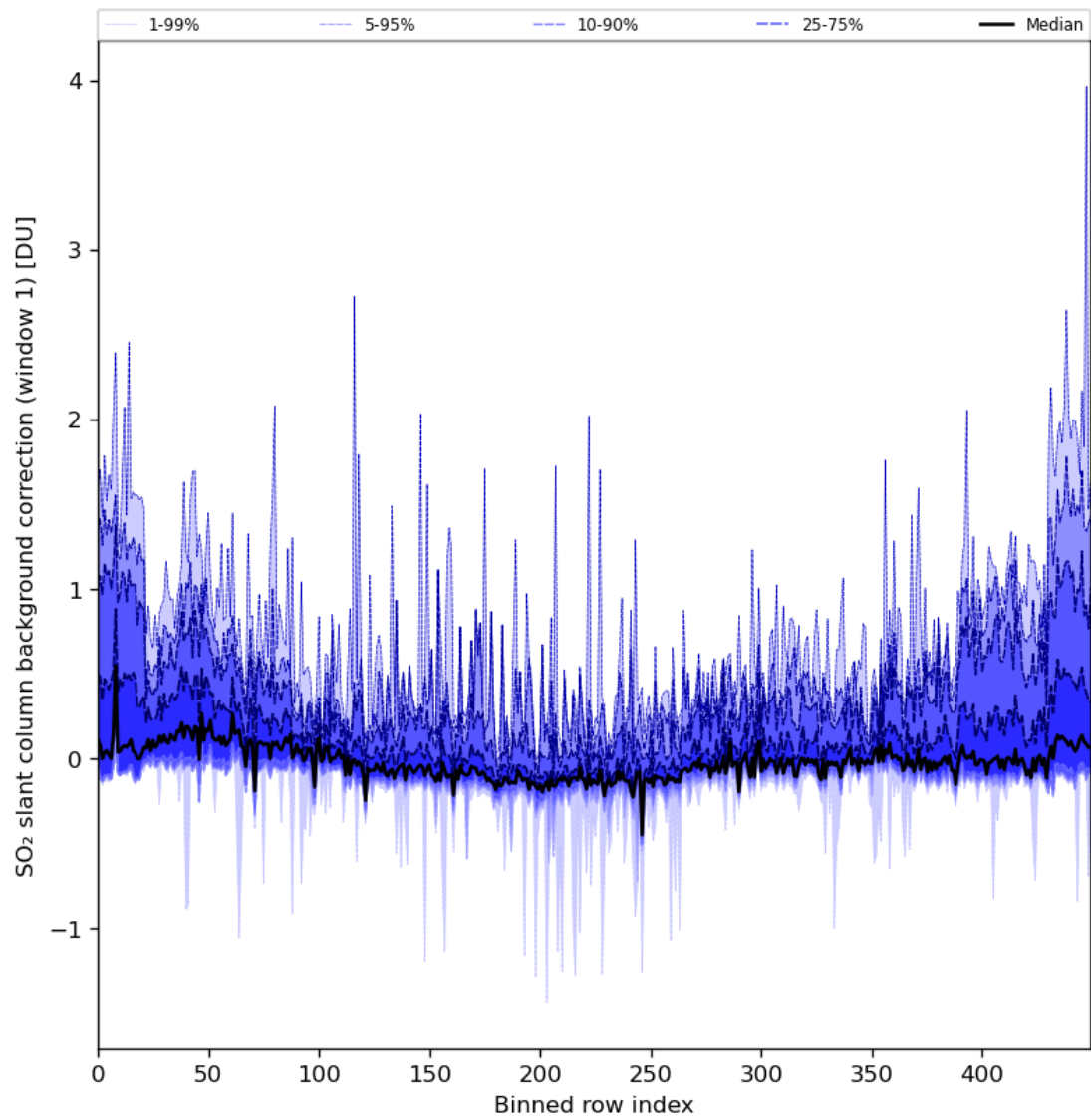
Figure 82: Along track statistics of “SO 2 slant column background correction (window 1)” for 2024-03-28 to 2024-03-30
