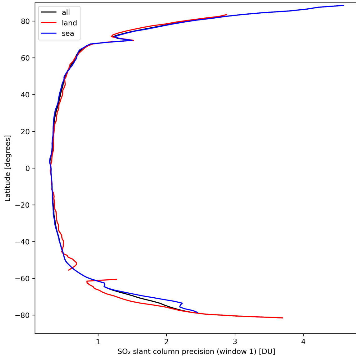
Figure 34: Zonal average of “SO 2 slant column precision (window 1)” for 2024-03-28 to 2024-03-30.
