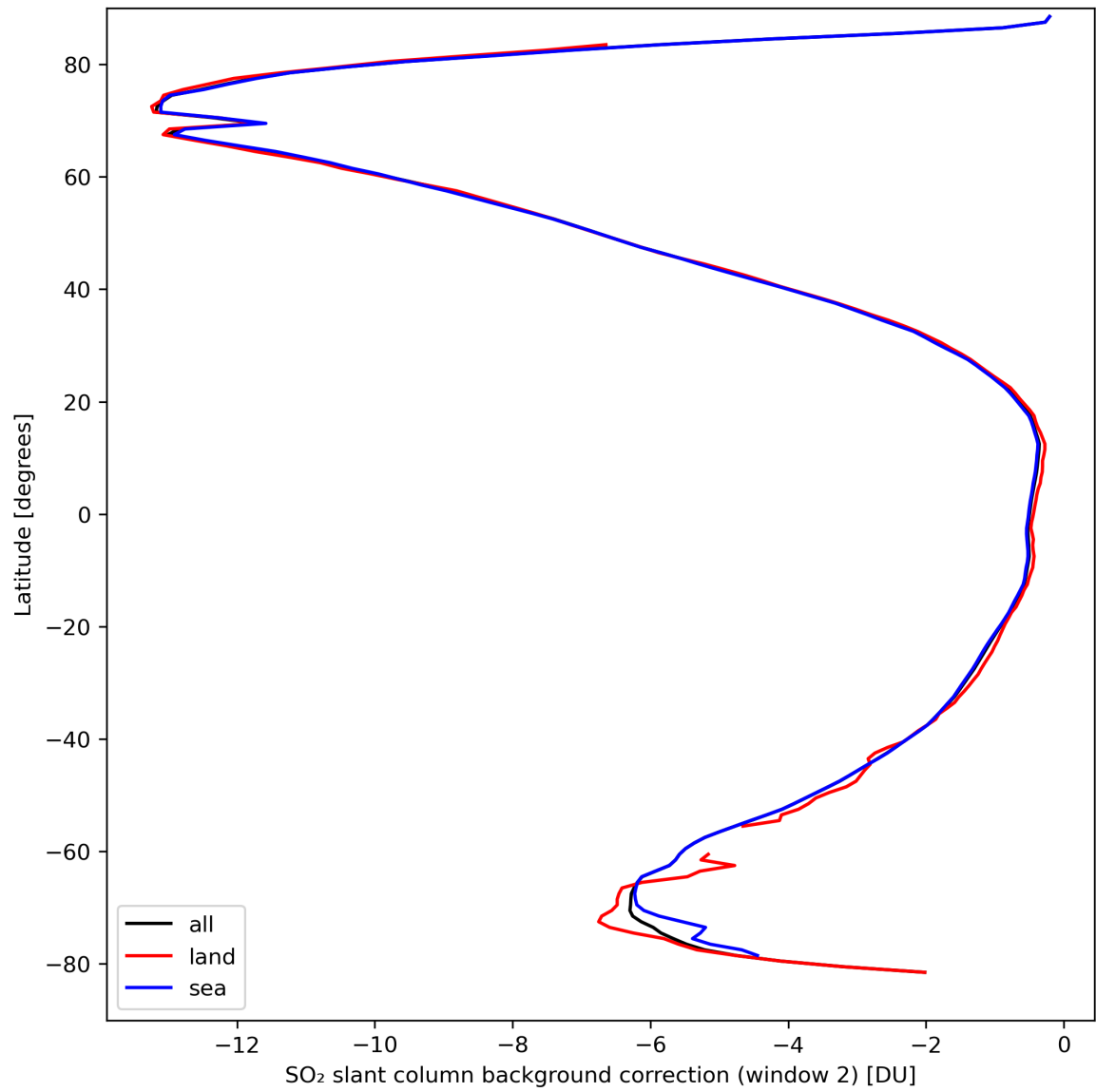
Figure 40: Zonal average of “SO 2 slant column background correction (window 2)” for 2024-03-28 to 2024-03-30.
