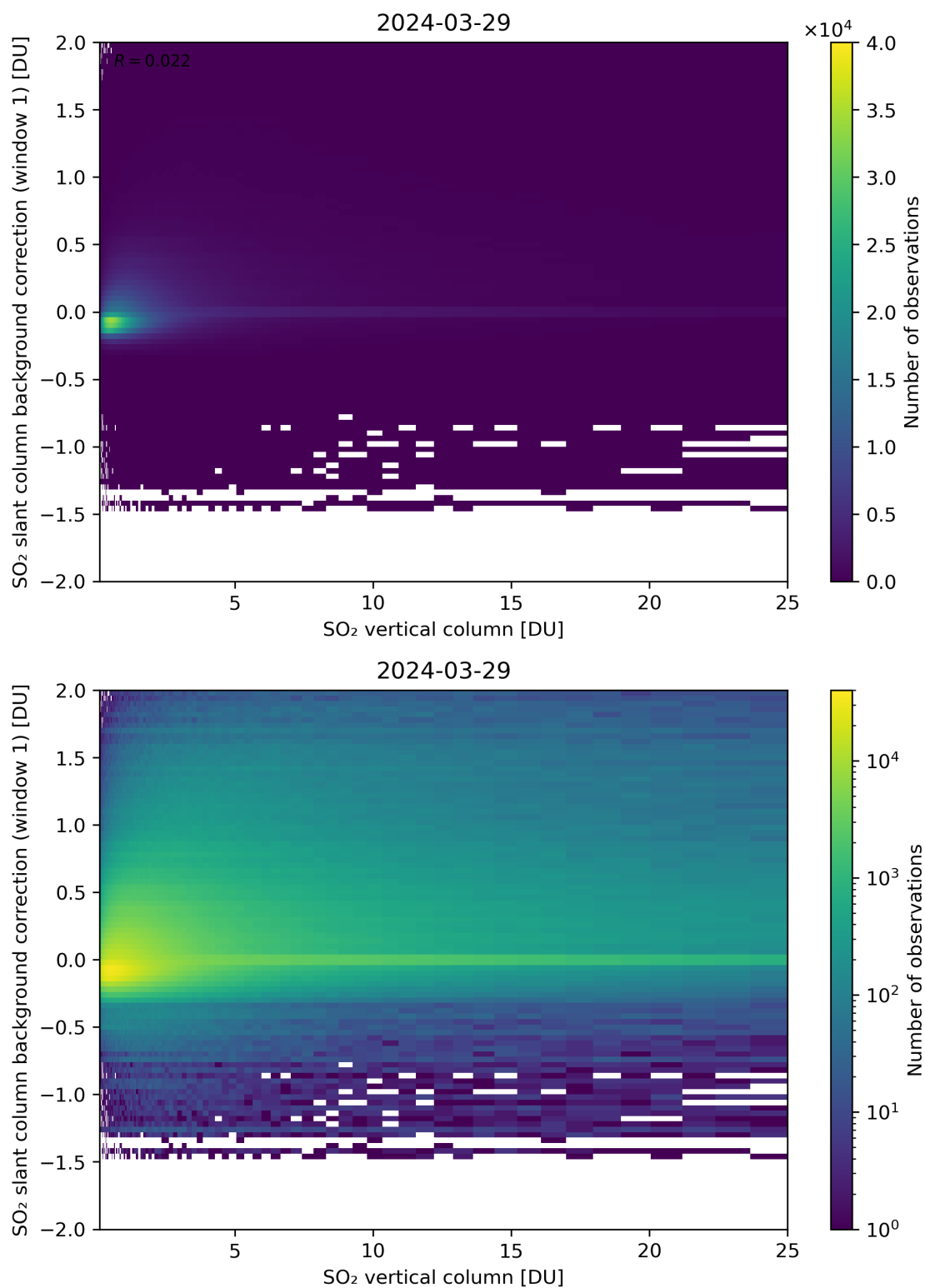
Figure 273: Scatter density plot of “SO 2 vertical column” against “SO 2 slant column background correction (window 1)” for 2024-03-28 to 2024-03-30.
