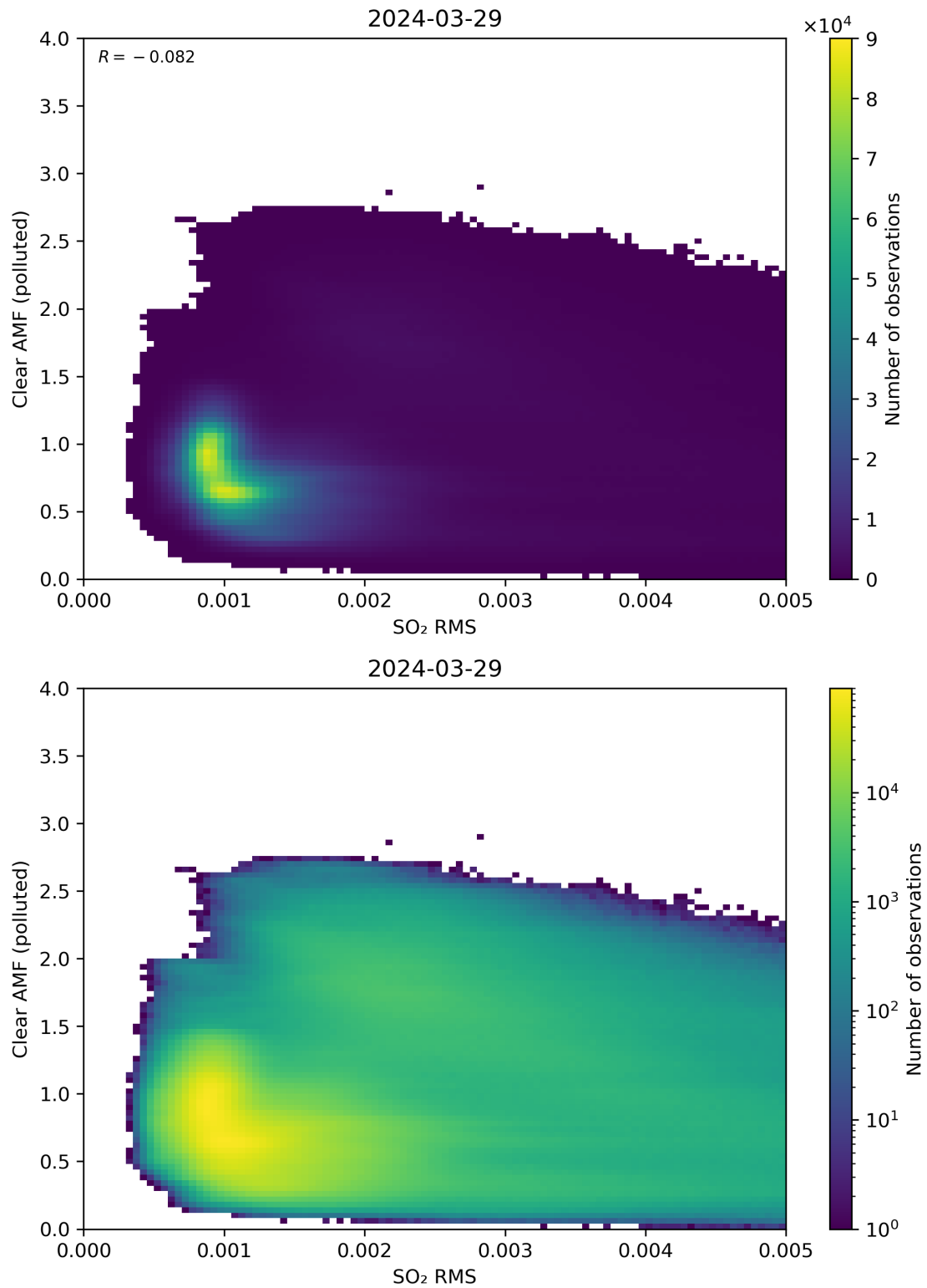
Figure 136: Scatter density plot of “SO 2 RMS” against “Clear AMF (polluted)” for 2024-03-28 to 2024-03-30.
