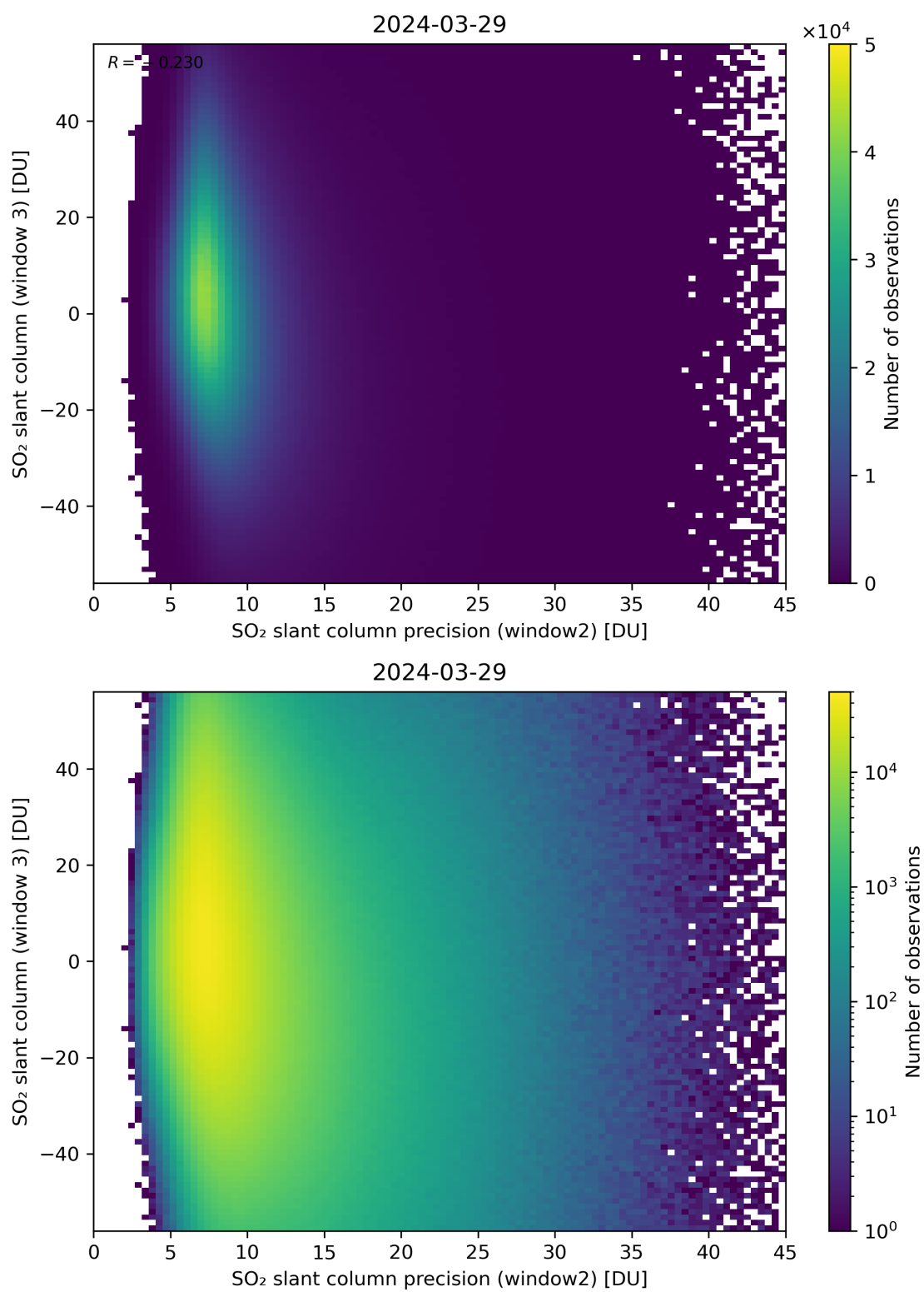
Figure 249: Scatter density plot of “SO 2 slant column precision (window2)” against “SO 2 slant column (window 3)” for 2024-03-28 to 2024-03-30.
