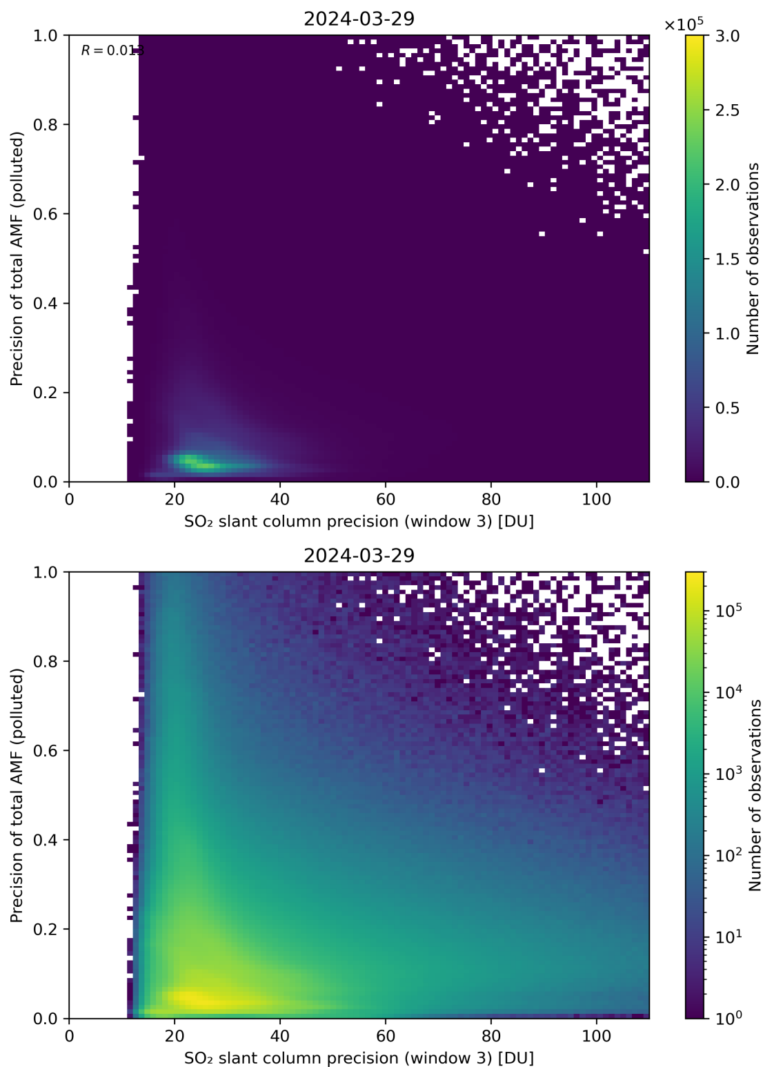
Figure 264: Scatter density plot of “SO 2 slant column precision (window 3)” against “Precision of total AMF (polluted)” for 2024-03-28 to 2024-03-30.
