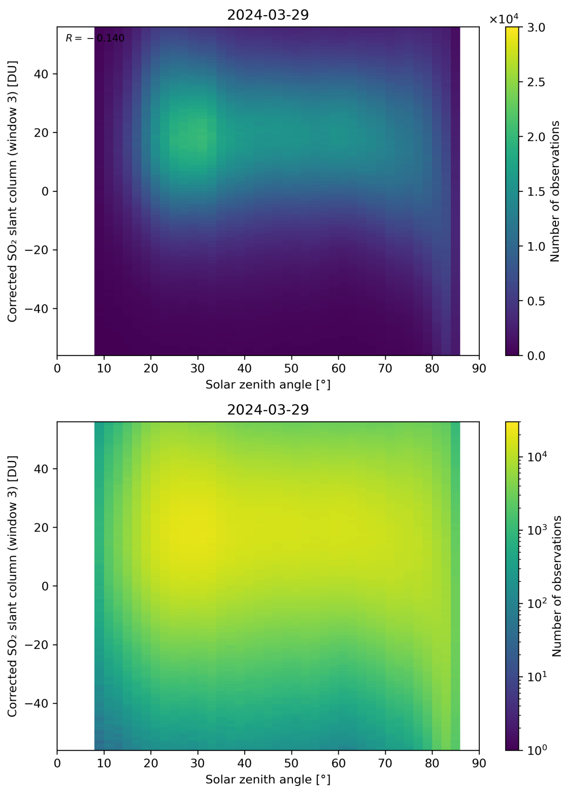
Figure 168: Scatter density plot of “Solar zenith angle” against “Corrected SO 2 slant column (window 3)” for 2024-03-28 to 2024-03-30.
