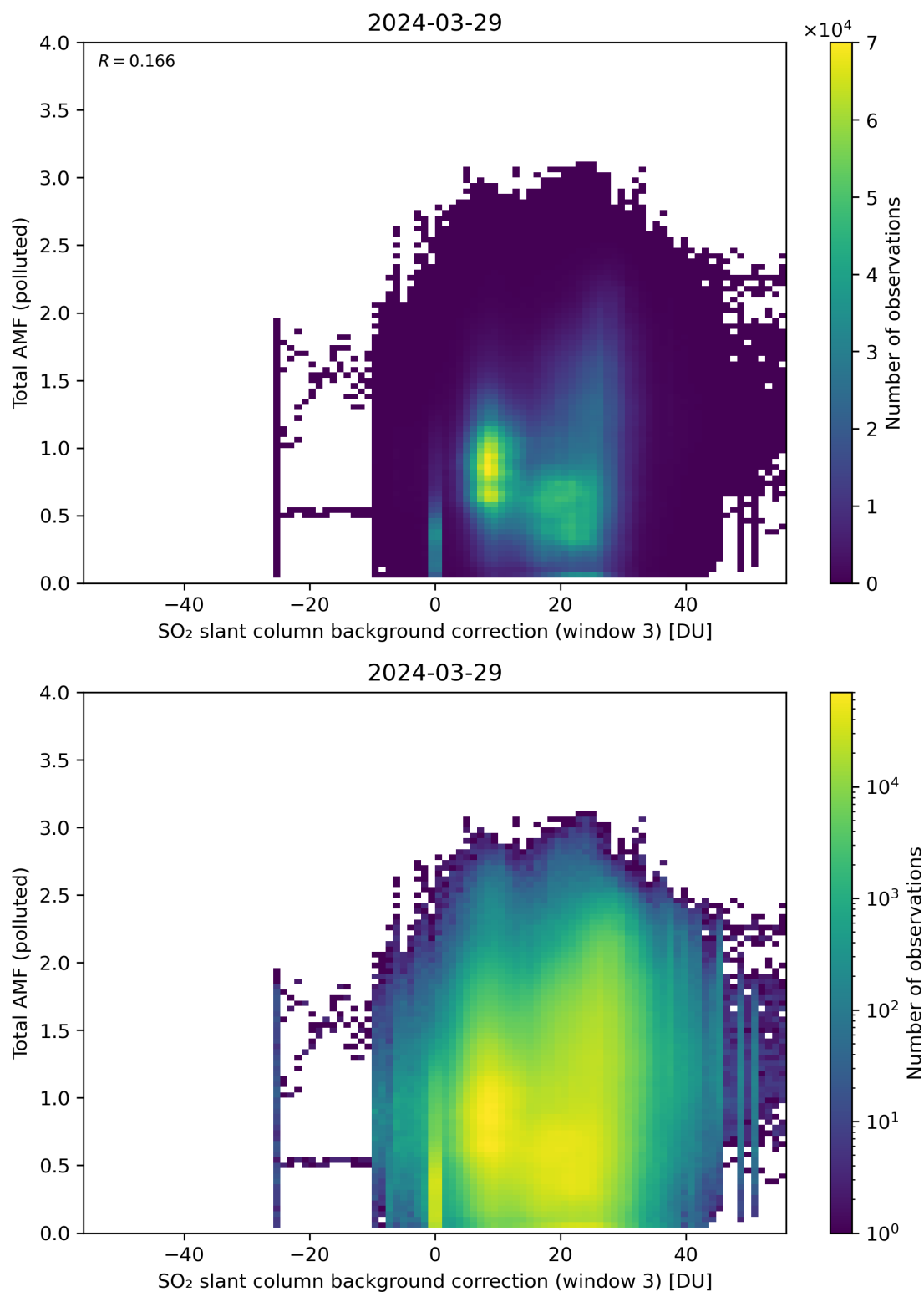
Figure 125: Scatter density plot of “SO 2 slant column background correction (window 3)” against “Total AMF (polluted)” for 2024-03-28 to 2024-03-30.
