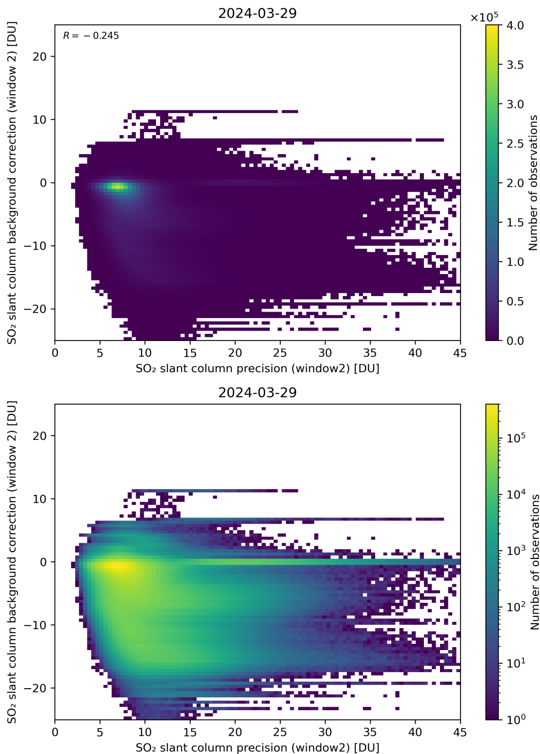
Figure 241: Scatter density plot of “SO 2 slant column precision (window2)” against “SO 2 slant column background correction (window 2)” for 2024-03-28 to 2024-03-30.
