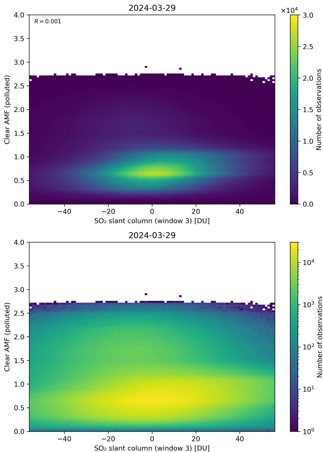
Figure 265: Scatter density plot of “SO 2 slant column (window 3)” against “Clear AMF (polluted)” for 2024-03-28 to 2024-03-30.
