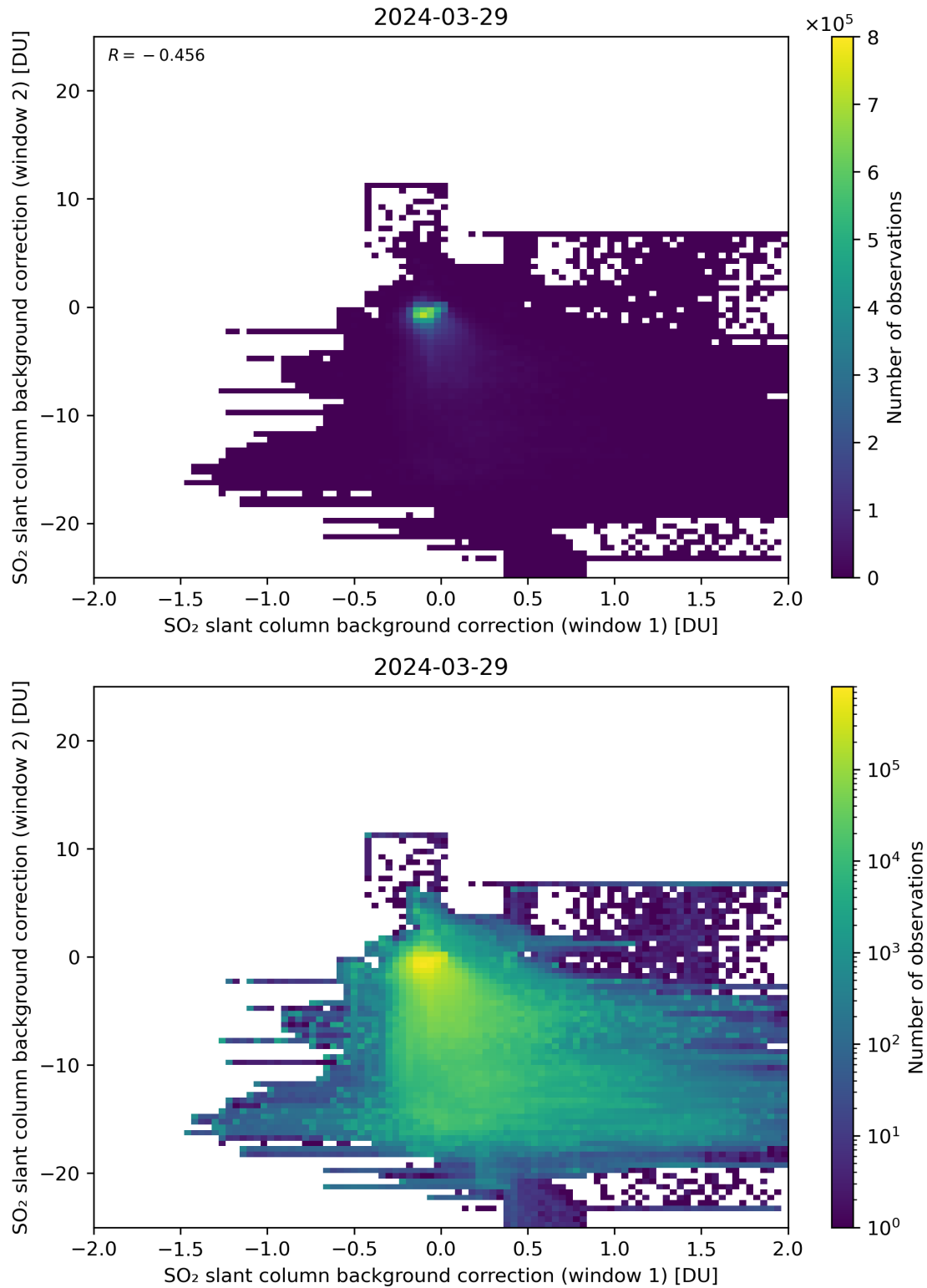
Figure 98: Scatter density plot of “SO 2 slant column background correction (window 1)” against “SO 2 slant column background correction (window 2)” for 2024-03-28 to 2024-03-30.
