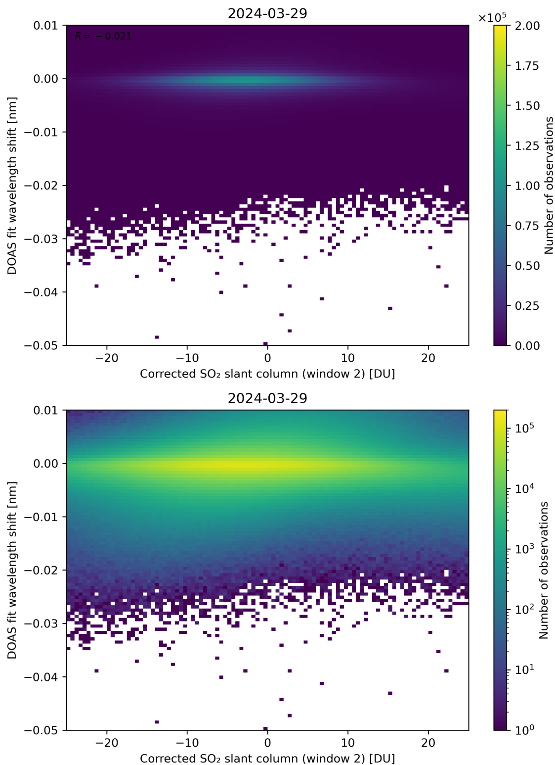
Figure 196: Scatter density plot of “Corrected SO 2 slant column (window 2)” against “DOAS fit wavelength shift” for 2024-03-28 to 2024-03-30.
