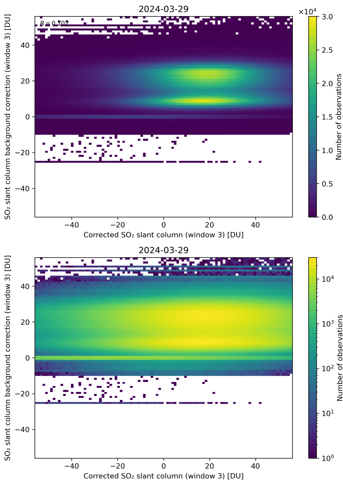
Figure 205: Scatter density plot of “Corrected SO 2 slant column (window 3)” against “SO 2 slant column background correction (window 3)” for 2024-03-28 to 2024-03-30.
