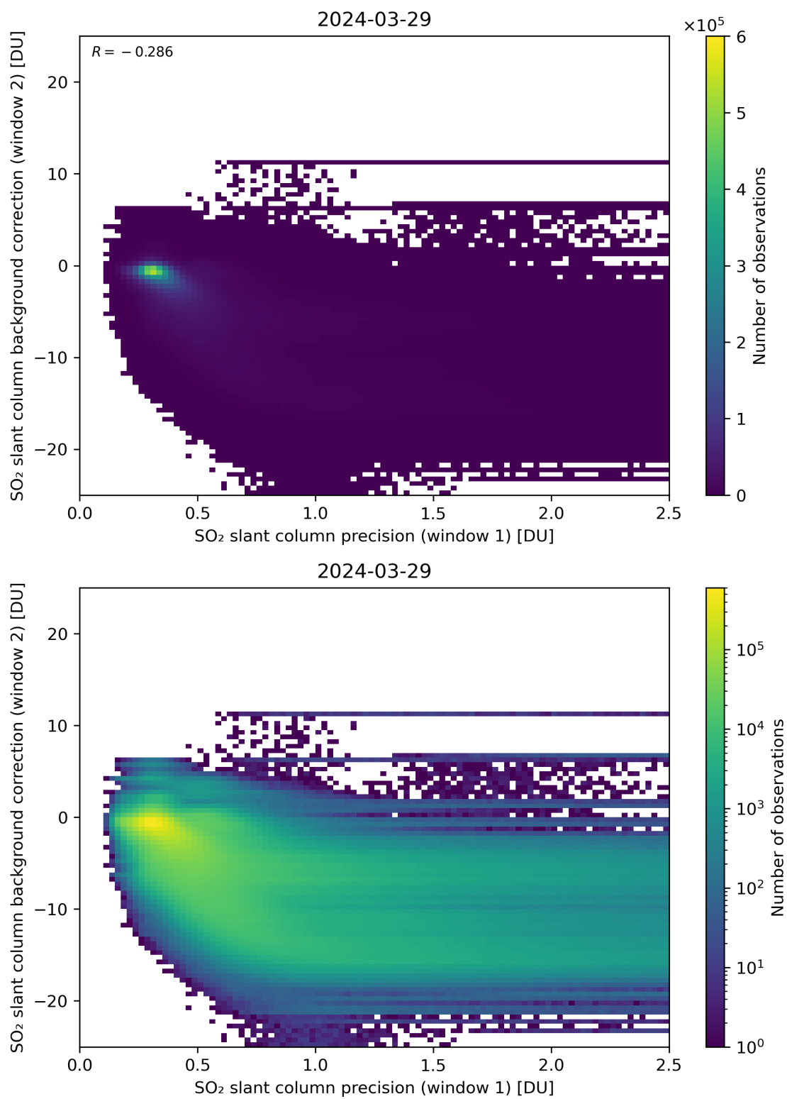
Figure 219: Scatter density plot of “SO 2 slant column precision (window 1)” against “SO 2 slant column background correction (window 2)” for 2024-03-28 to 2024-03-30.
