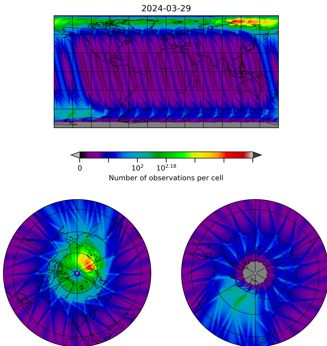
Figure 28: Map of the number of observations for 2024-03-28 to 2024-03-30
