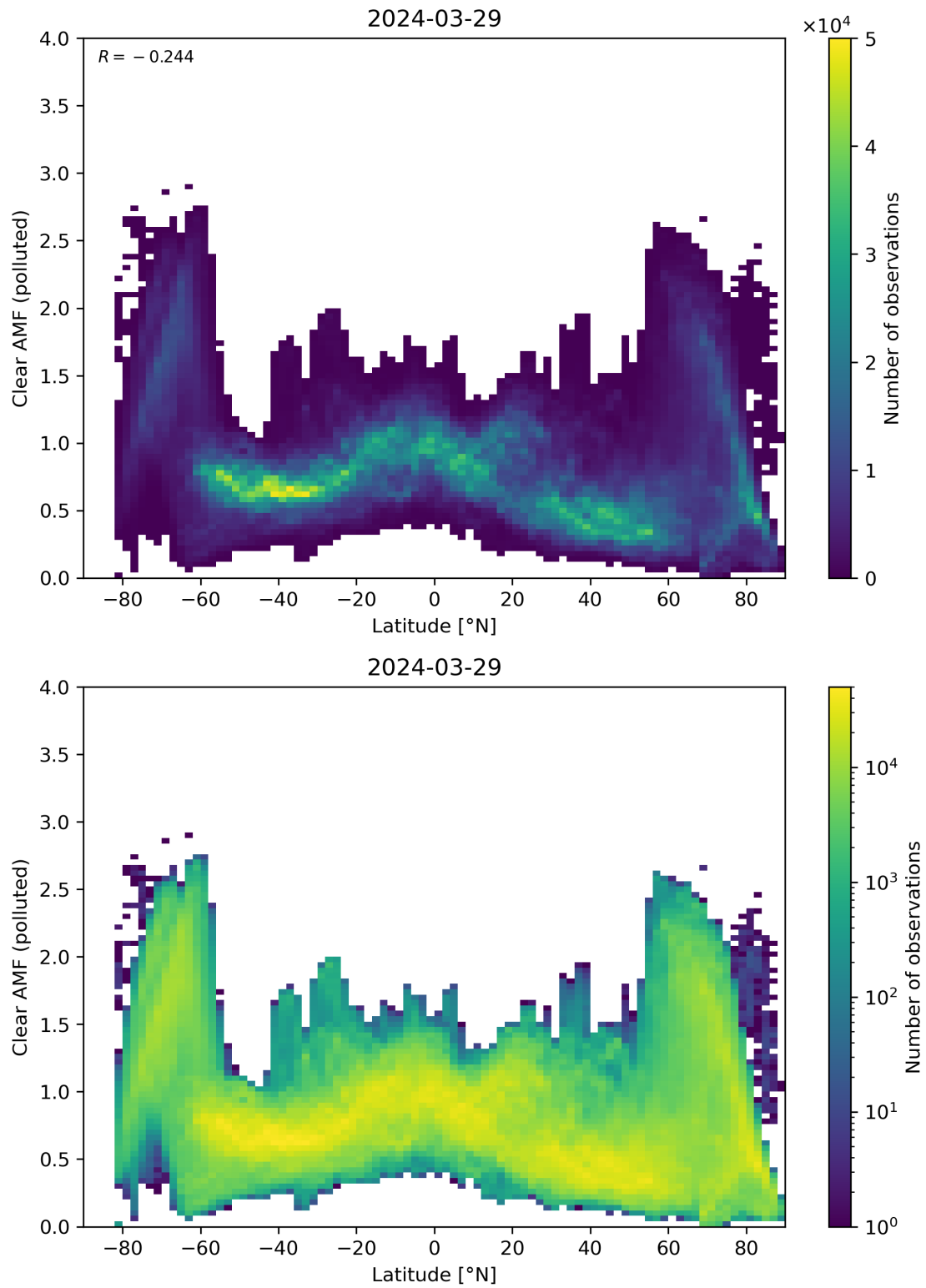
Figure 145: Scatter density plot of “Latitude” against “Clear AMF (polluted)” for 2024-03-28 to 2024-03-30.
