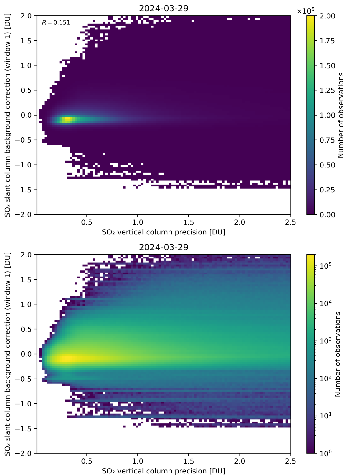
Figure 279: Scatter density plot of “SO 2 vertical column precision” against “SO 2 slant column background correction (window 1)” for 2024-03-28 to 2024-03-30.
