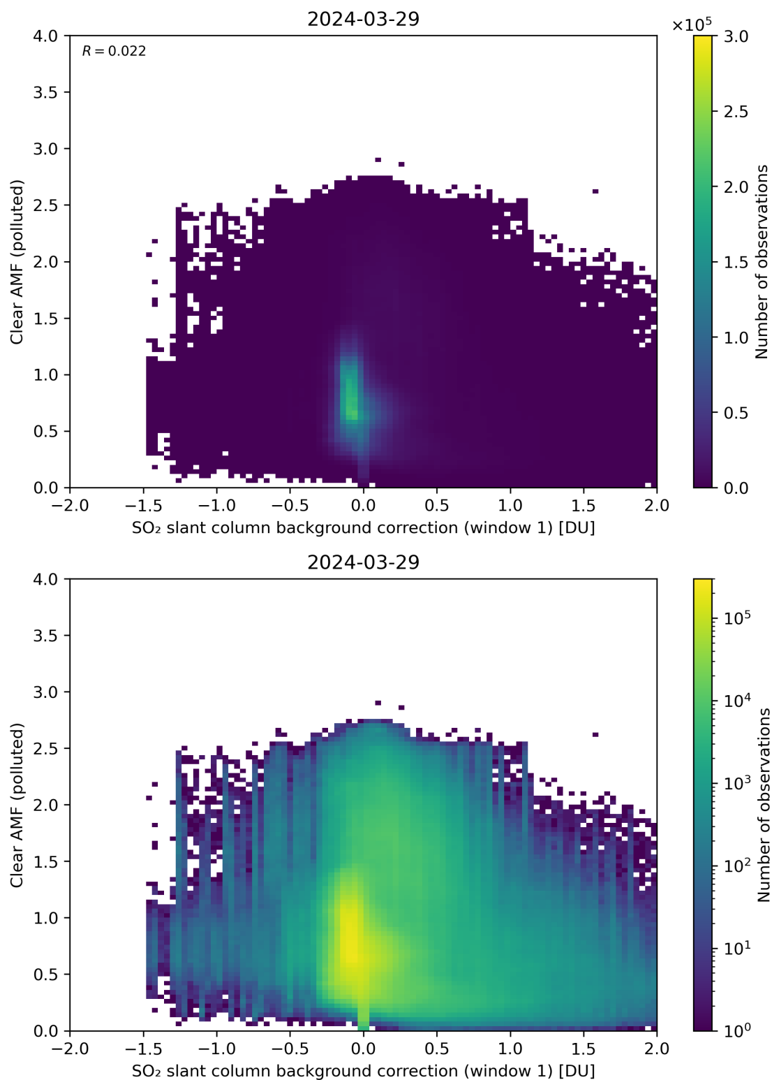
Figure 103: Scatter density plot of “SO 2 slant column background correction (window 1)” against “Clear AMF (polluted)” for 2024-03-28 to 2024-03-30.
