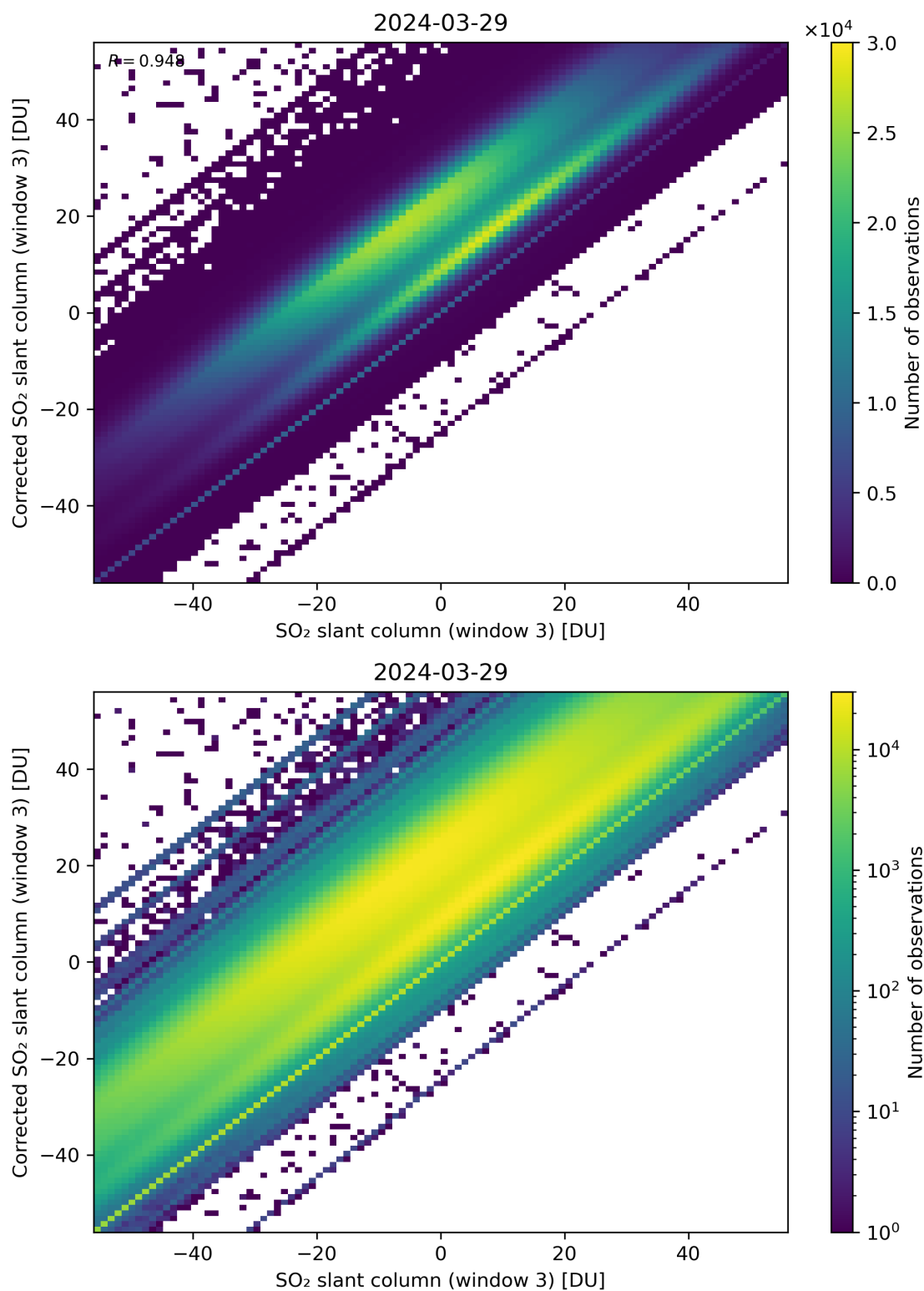
Figure 266: Scatter density plot of “SO 2 slant column (window 3)” against “Corrected SO 2 slant column (window 3)” for 2024-03-28 to 2024-03-30.
