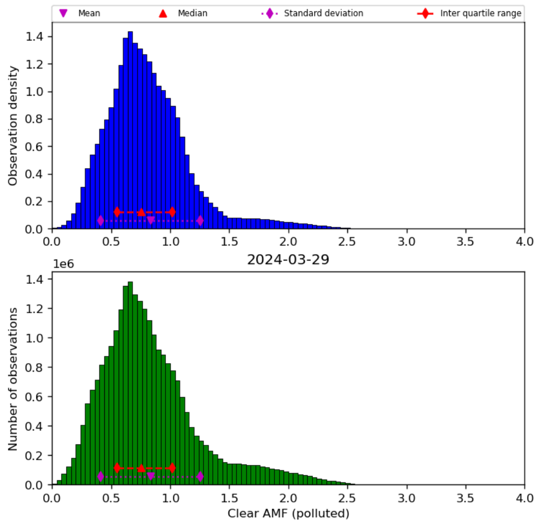
Figure 73: Histogram of “Clear AMF (polluted)” for 2024-03-28 to 2024-03-30
