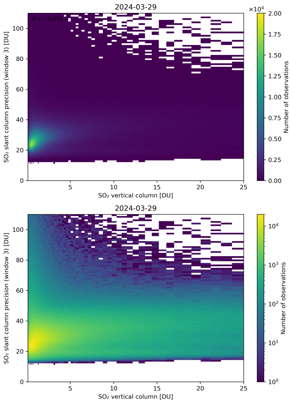
Figure 304: Scatter density plot of “SO 2 vertical column” against “SO 2 slant column precision (window 3)” for 2024-03-28 to 2024-03-30.
