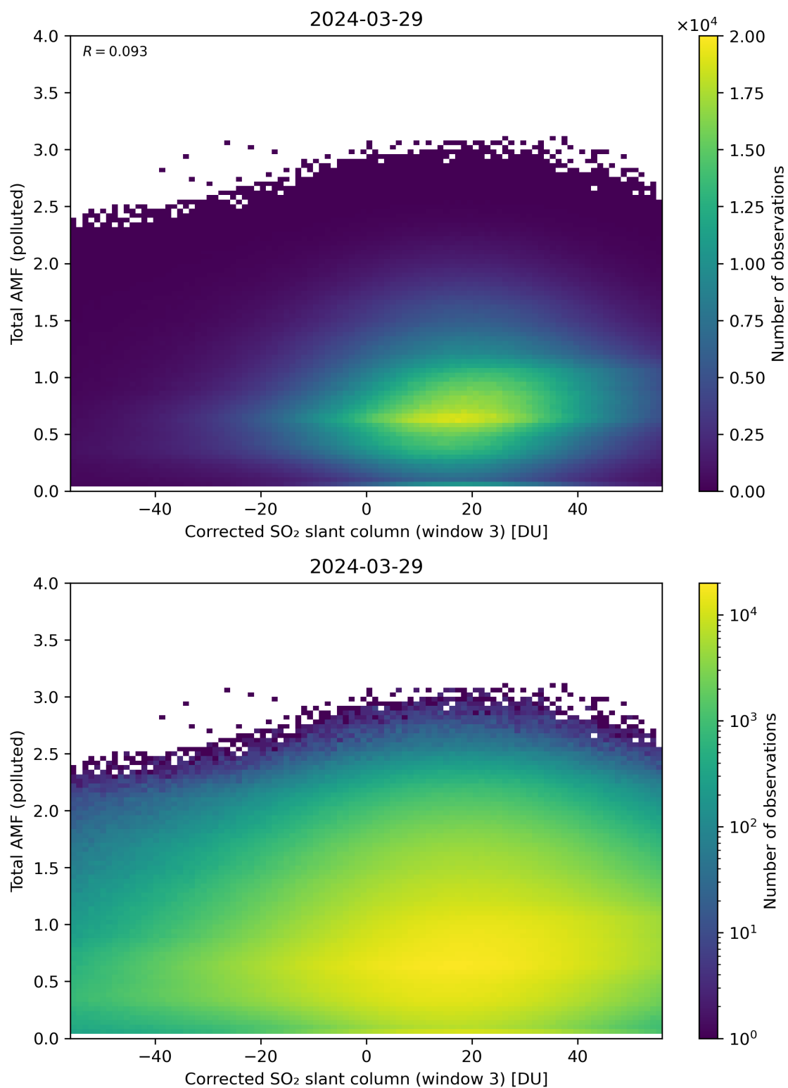
Figure 210: Scatter density plot of “Corrected SO 2 slant column (window 3)” against “Total AMF (polluted)” for 2024-03-28 to 2024-03-30.
