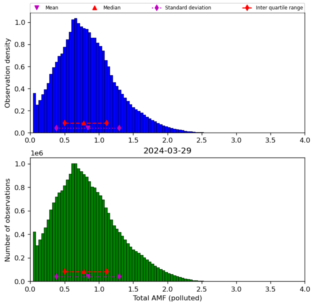
Figure 71: Histogram of “Total AMF (polluted)” for 2024-03-28 to 2024-03-30
