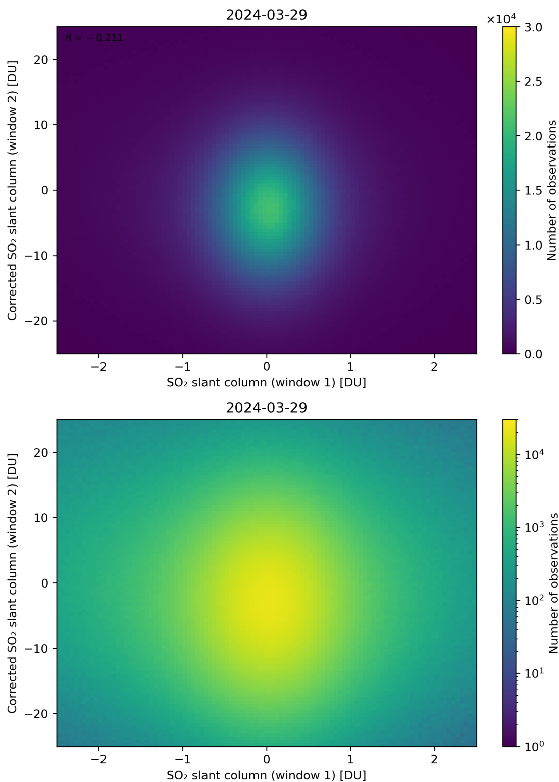
Figure 233: Scatter density plot of “SO 2 slant column (window 1)” against “Corrected SO 2 slant column (window 2)” for 2024-03-28 to 2024-03-30.
