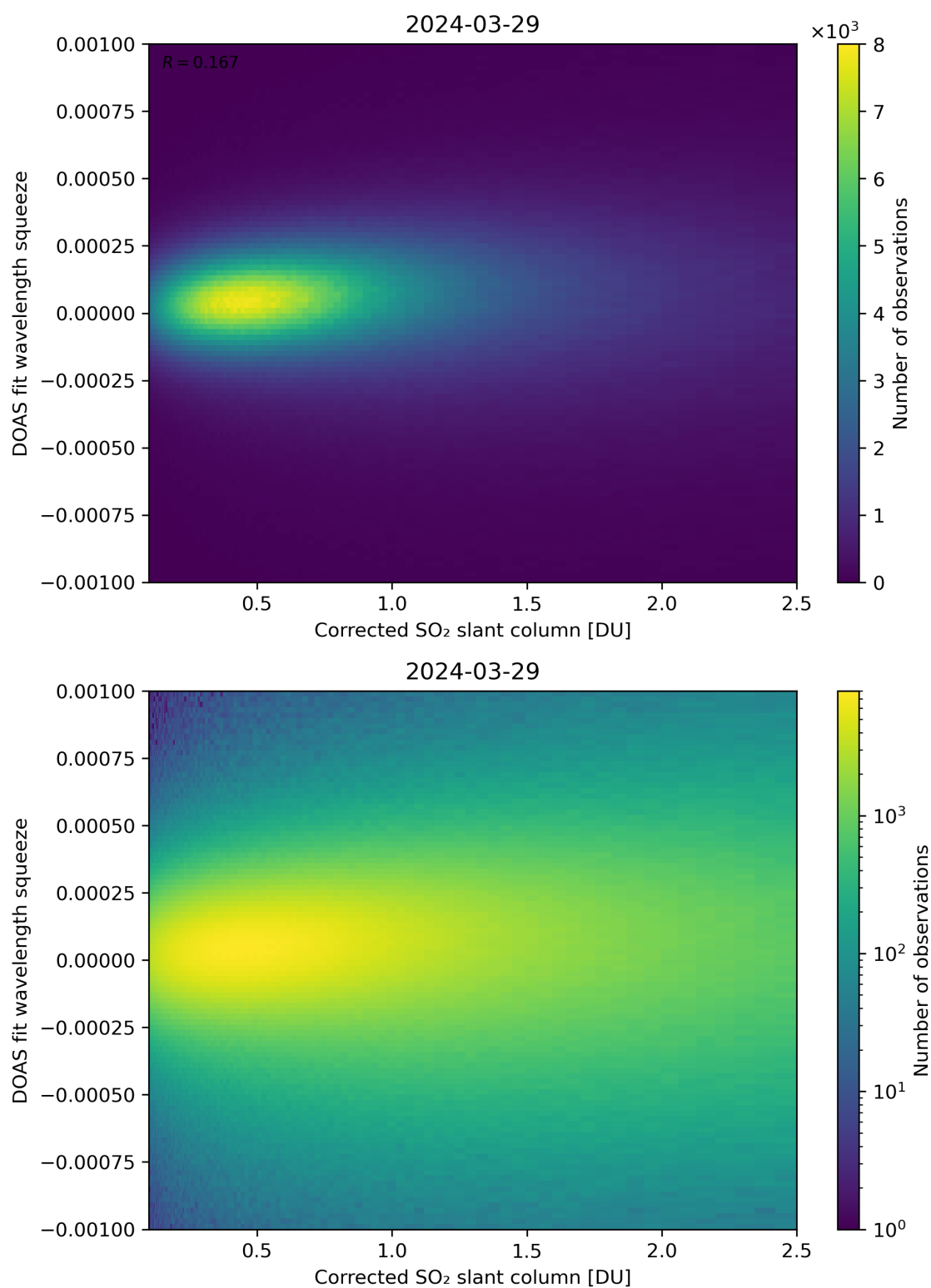
Figure 182: Scatter density plot of “Corrected SO 2 slant column” against “DOAS fit wavelength squeeze” for 2024-03-28 to 2024-03-30.
