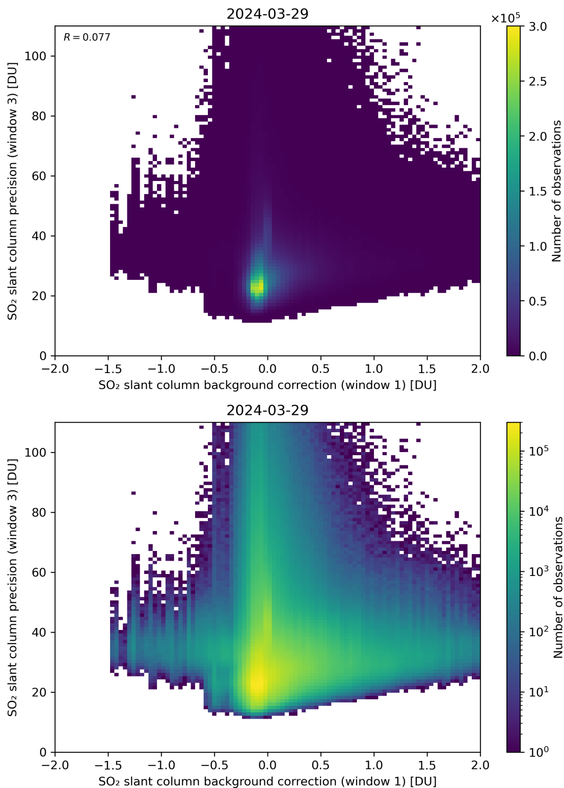
Figure 108: Scatter density plot of “SO 2 slant column background correction (window 1)” against “SO 2 slant column precision (window 3)” for 2024-03-28 to 2024-03-30.
