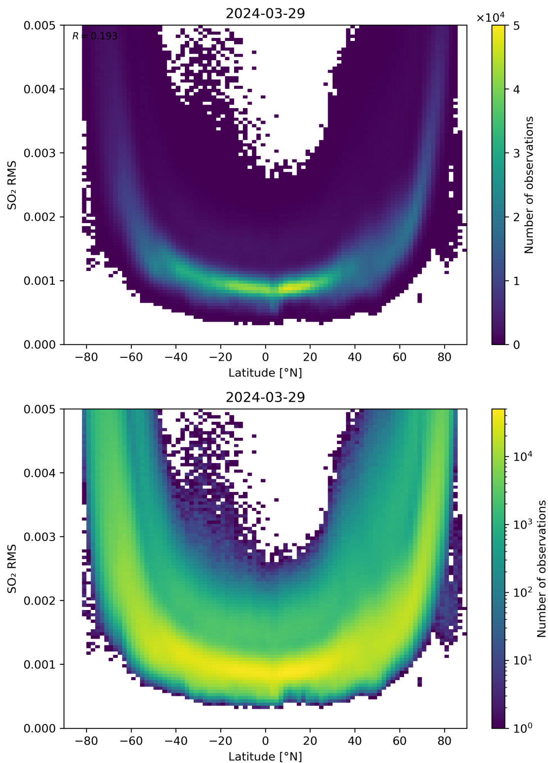
Figure 144: Scatter density plot of “Latitude” against “SO 2 RMS” for 2024-03-28 to 2024-03-30.
