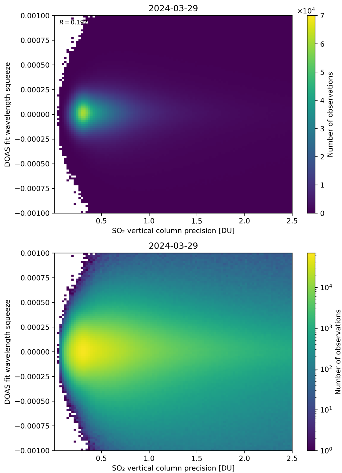
Figure 283: Scatter density plot of “SO 2 vertical column precision” against “DOAS fit wavelength squeeze” for 2024-03-28 to 2024-03-30.
