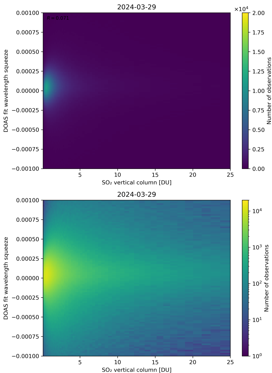
Figure 277: Scatter density plot of “SO 2 vertical column” against “DOAS fit wavelength squeeze” for 2024-03-28 to 2024-03-30.
