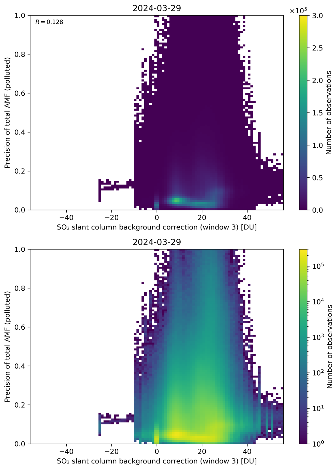
Figure 126: Scatter density plot of “SO 2 slant column background correction (window 3)” against “Precision of total AMF (polluted)” for 2024-03-28 to 2024-03-30.
