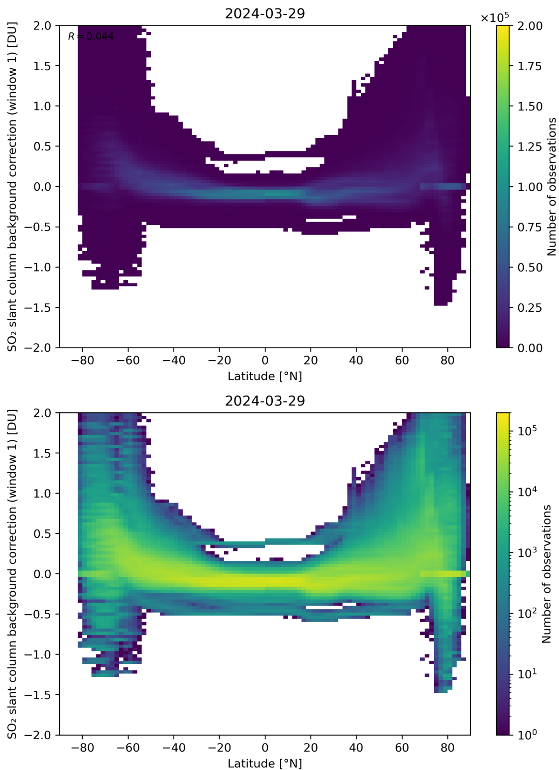
Figure 139: Scatter density plot of “Latitude” against “SO 2 slant column background correction (window 1)” for 2024-03-28 to 2024-03-30.
