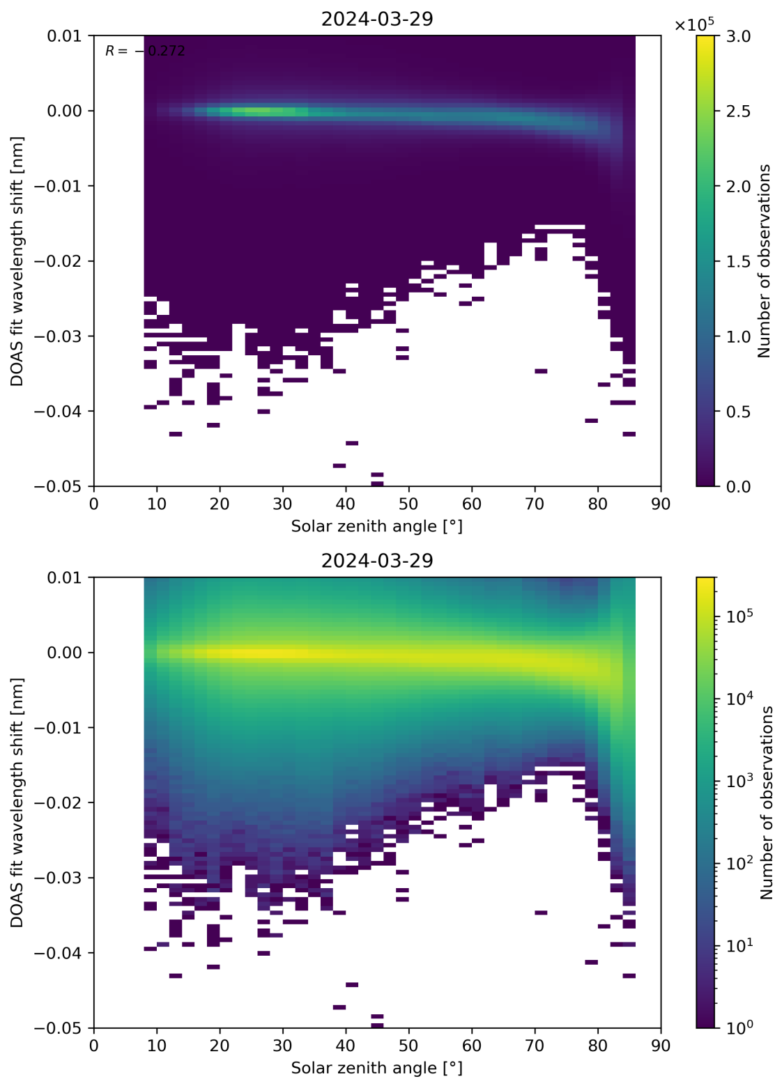
Figure 161: Scatter density plot of “Solar zenith angle” against “DOAS fit wavelength shift” for 2024-03-28 to 2024-03-30.
