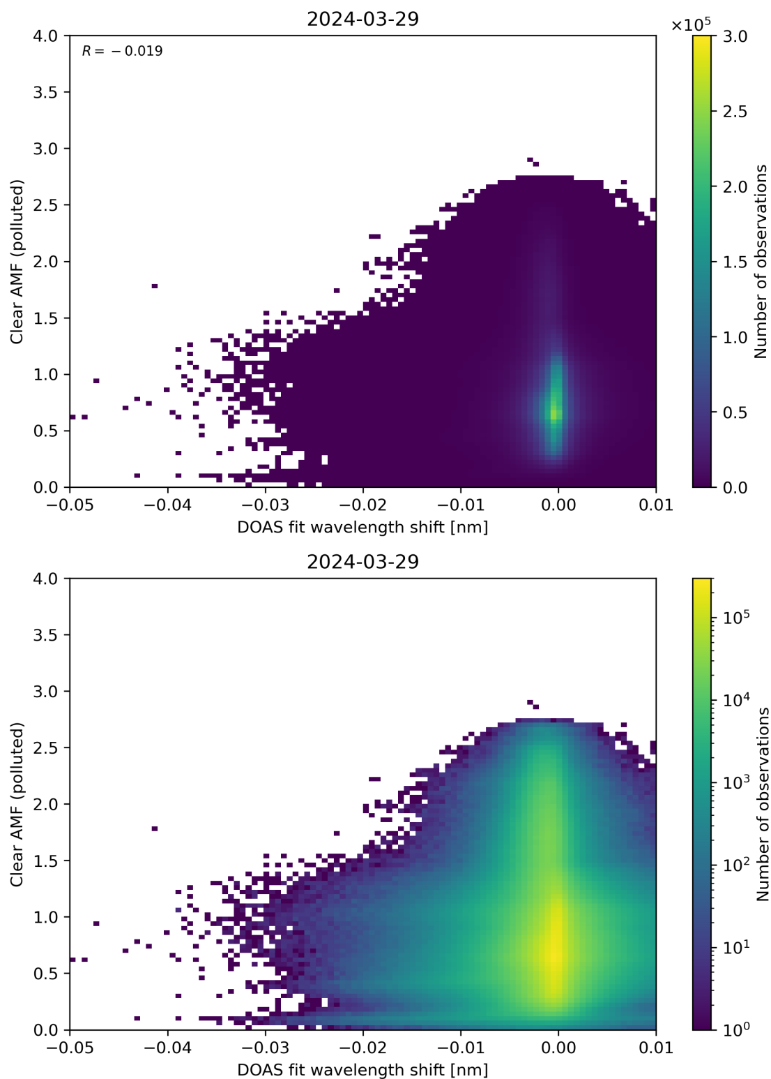
Figure 129: Scatter density plot of “DOAS fit wavelength shift” against “Clear AMF (polluted)” for 2024-03-28 to 2024-03-30.
