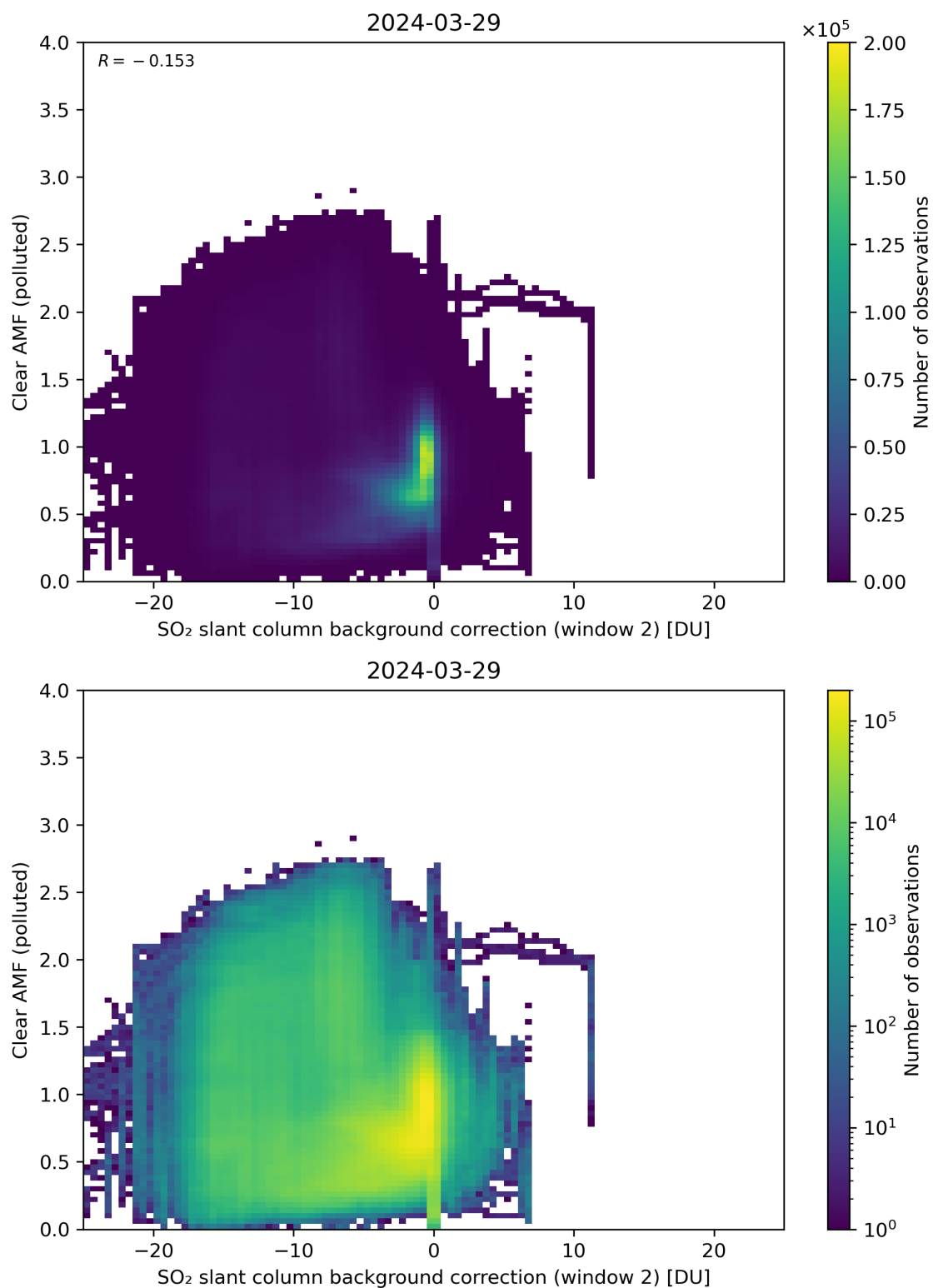
Figure 115: Scatter density plot of “SO 2 slant column background correction (window 2)” against “Clear AMF (polluted)” for 2024-03-28 to 2024-03-30.
