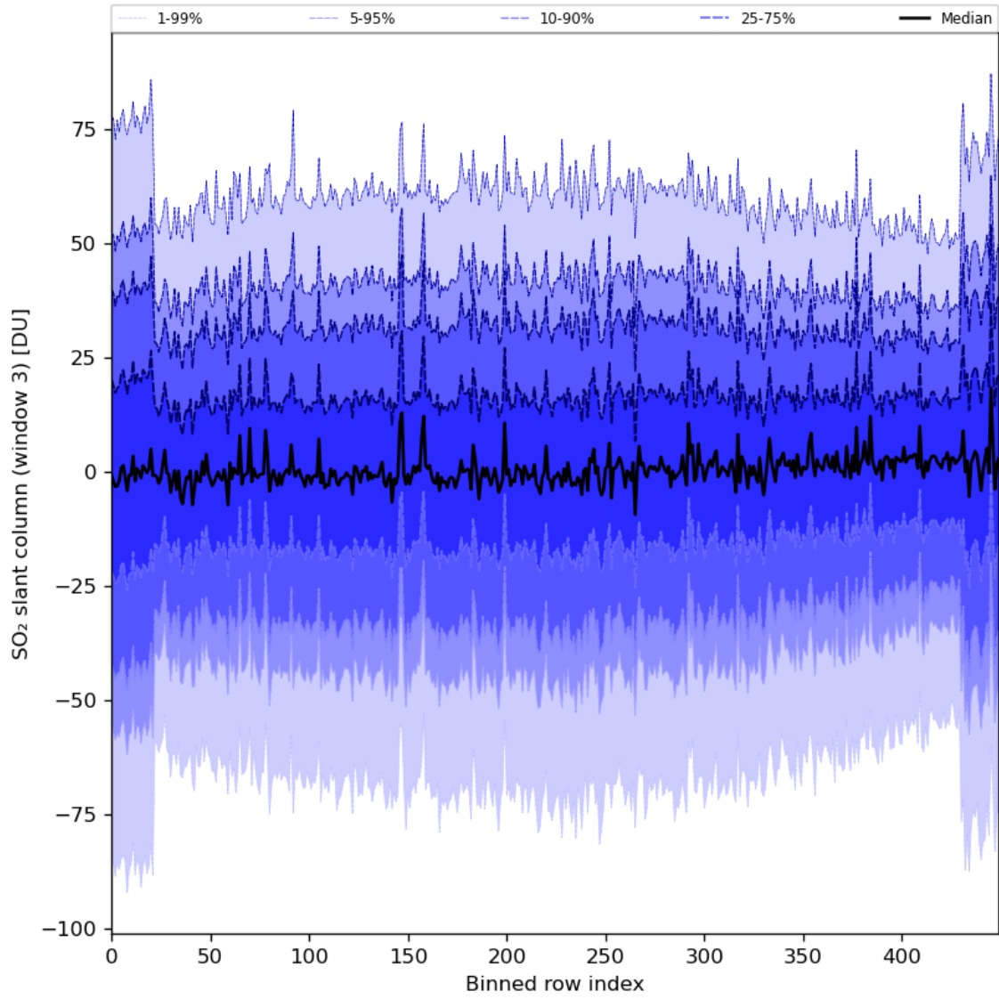
Figure 87: Along track statistics of “SO 2 slant column (window 3)” for 2024-03-28 to 2024-03-30
