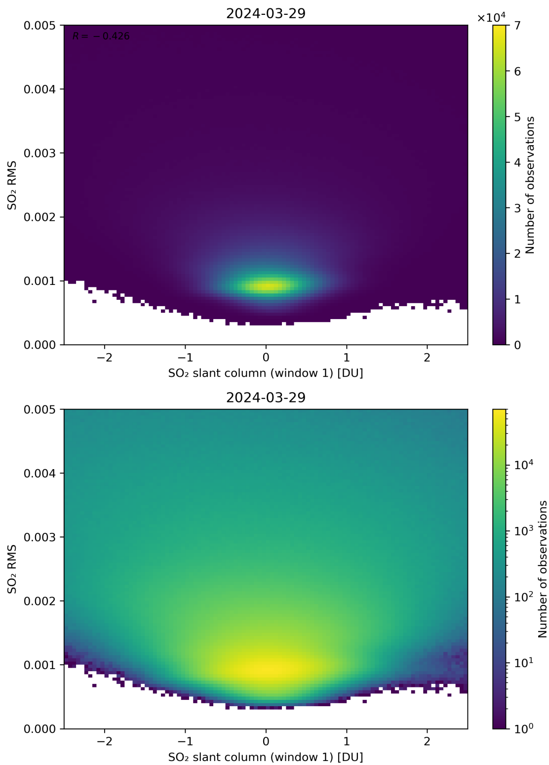
Figure 217: Scatter density plot of “SO 2 slant column (window 1)” against “SO 2 RMS” for 2024-03-28 to 2024-03-30.
