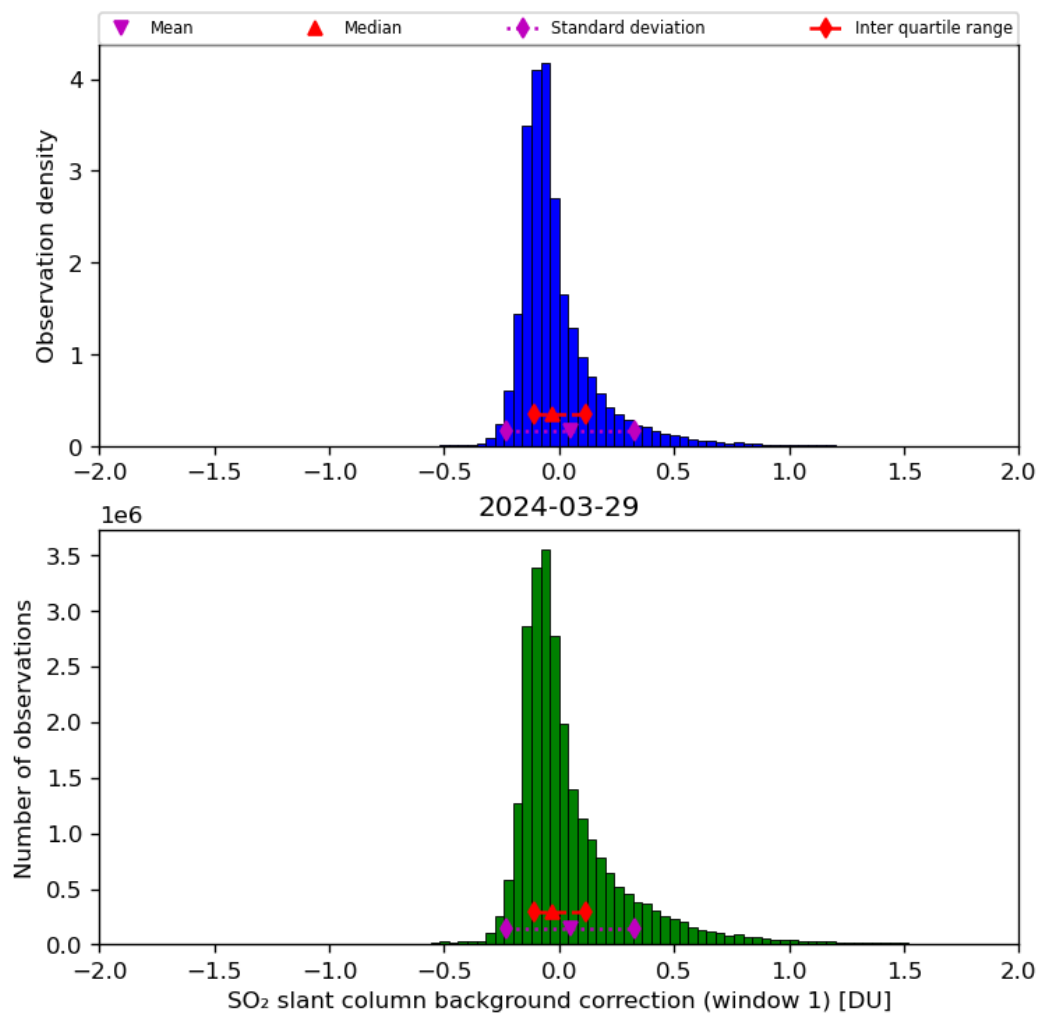
Figure 59: Histogram of “SO 2 slant column background correction (window 1)” for 2024-03-28 to 2024-03-30
