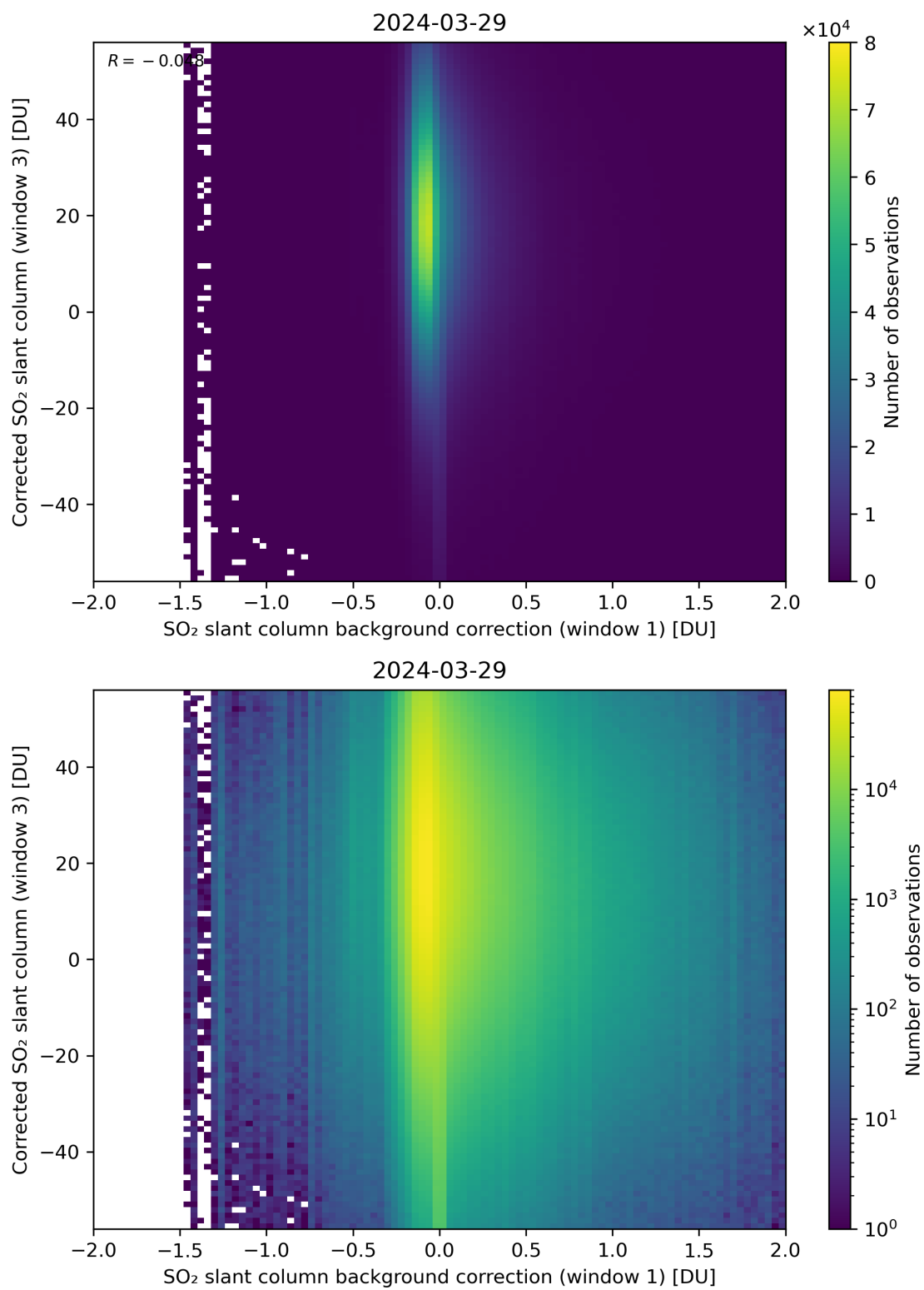
Figure 105: Scatter density plot of “SO 2 slant column background correction (window 1)” against “Corrected SO 2 slant column (window 3)” for 2024-03-28 to 2024-03-30.
