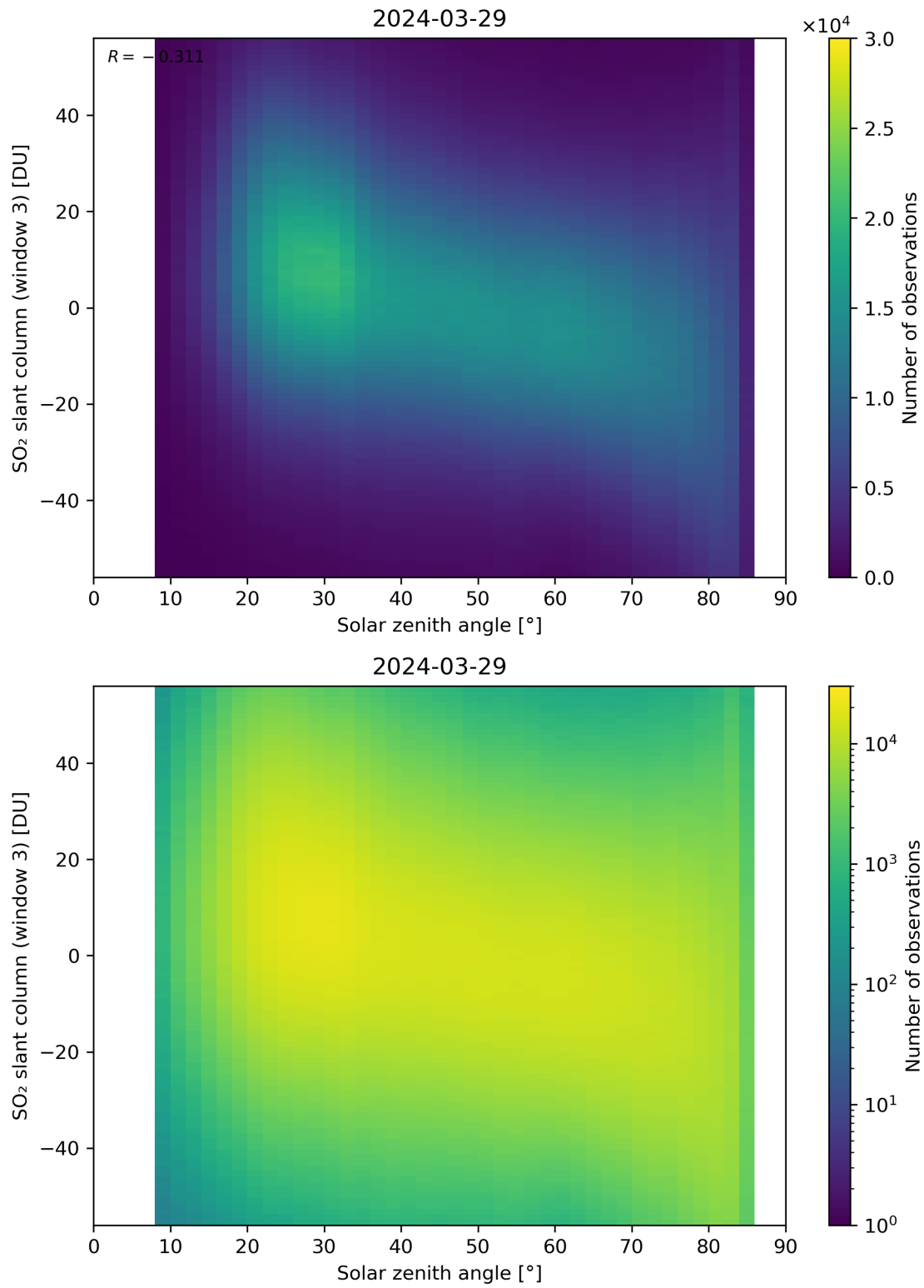
Figure 172: Scatter density plot of “Solar zenith angle” against “SO 2 slant column (window 3)” for 2024-03-28 to 2024-03-30.
