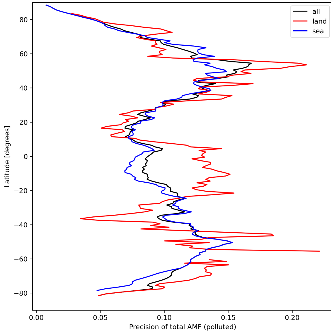
Figure 49: Zonal average of “Precision of total AMF (polluted)” for 2024-03-28 to 2024-03-30.
