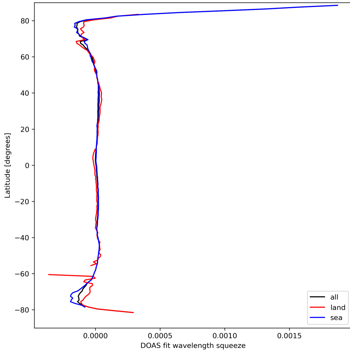
Figure 46: Zonal average of “DOAS fit wavelength squeeze” for 2024-03-28 to 2024-03-30.
