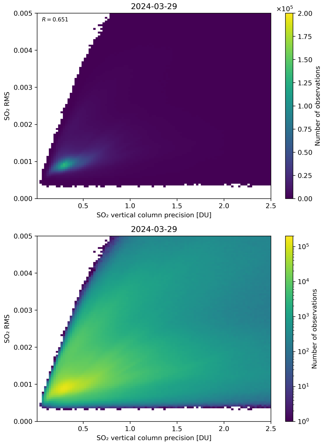
Figure 284: Scatter density plot of “SO 2 vertical column precision” against “SO 2 RMS” for 2024-03-28 to 2024-03-30.
