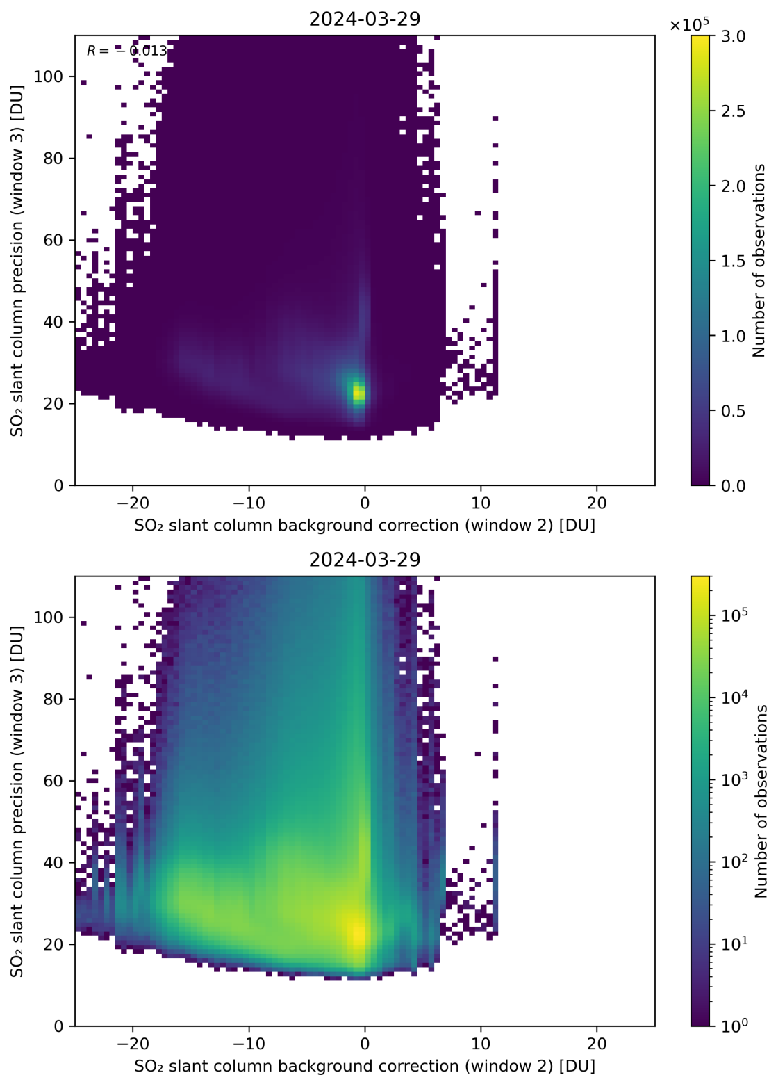
Figure 118: Scatter density plot of “SO 2 slant column background correction (window 2)” against “SO 2 slant column precision (window 3)” for 2024-03-28 to 2024-03-30.
