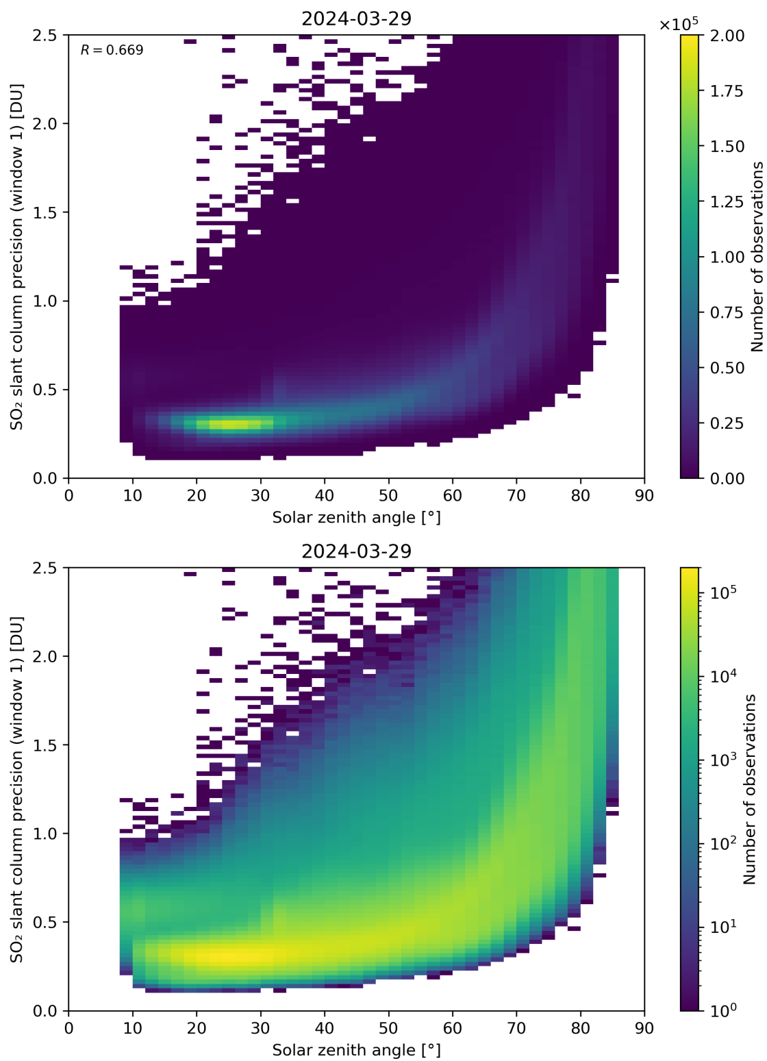
Figure 170: Scatter density plot of “Solar zenith angle” against “SO 2 slant column precision (window 1)” for 2024-03-28 to 2024-03-30.
