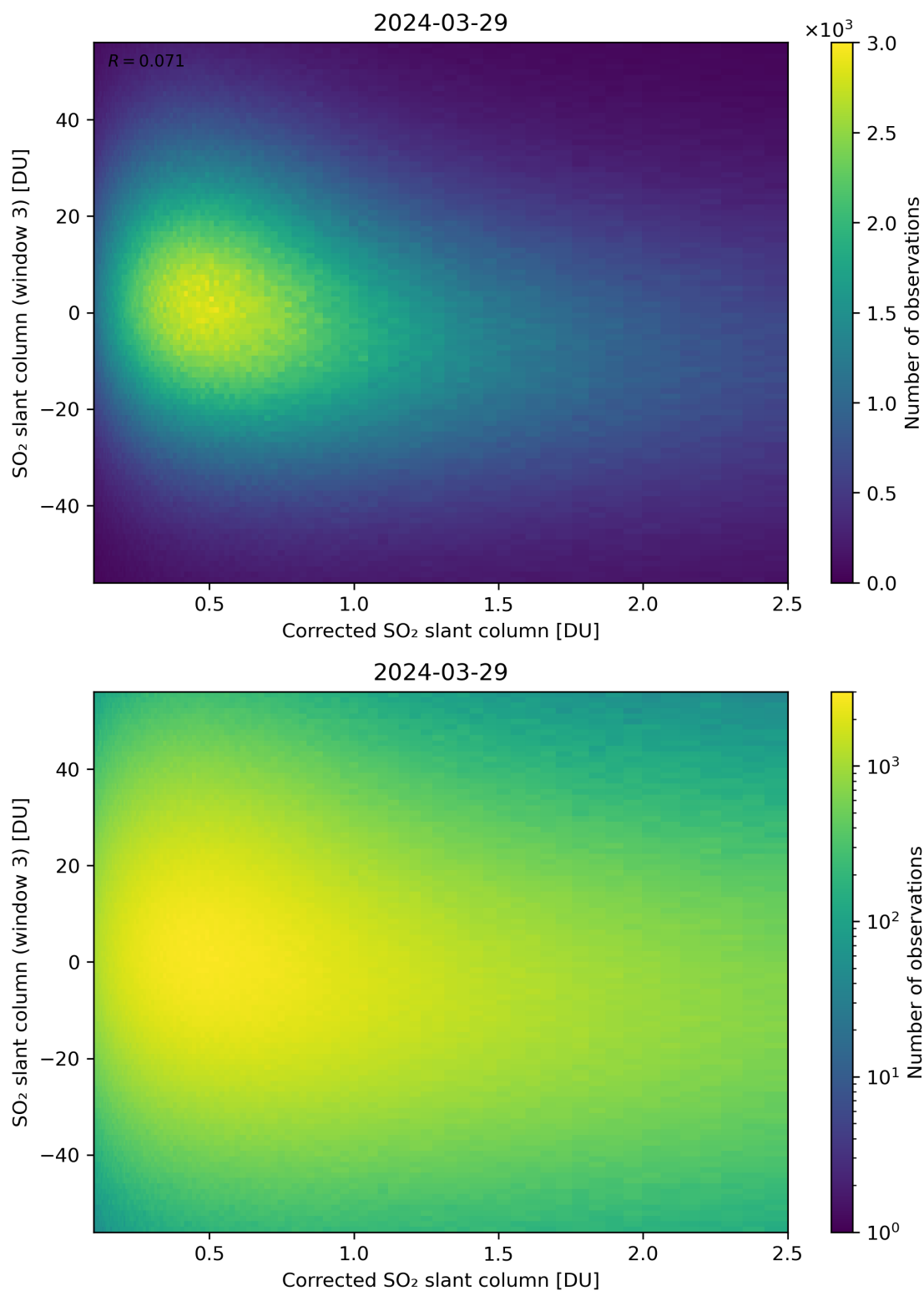
Figure 190: Scatter density plot of “Corrected SO 2 slant column” against “SO 2 slant column (window 3)” for 2024-03-28 to 2024-03-30.
