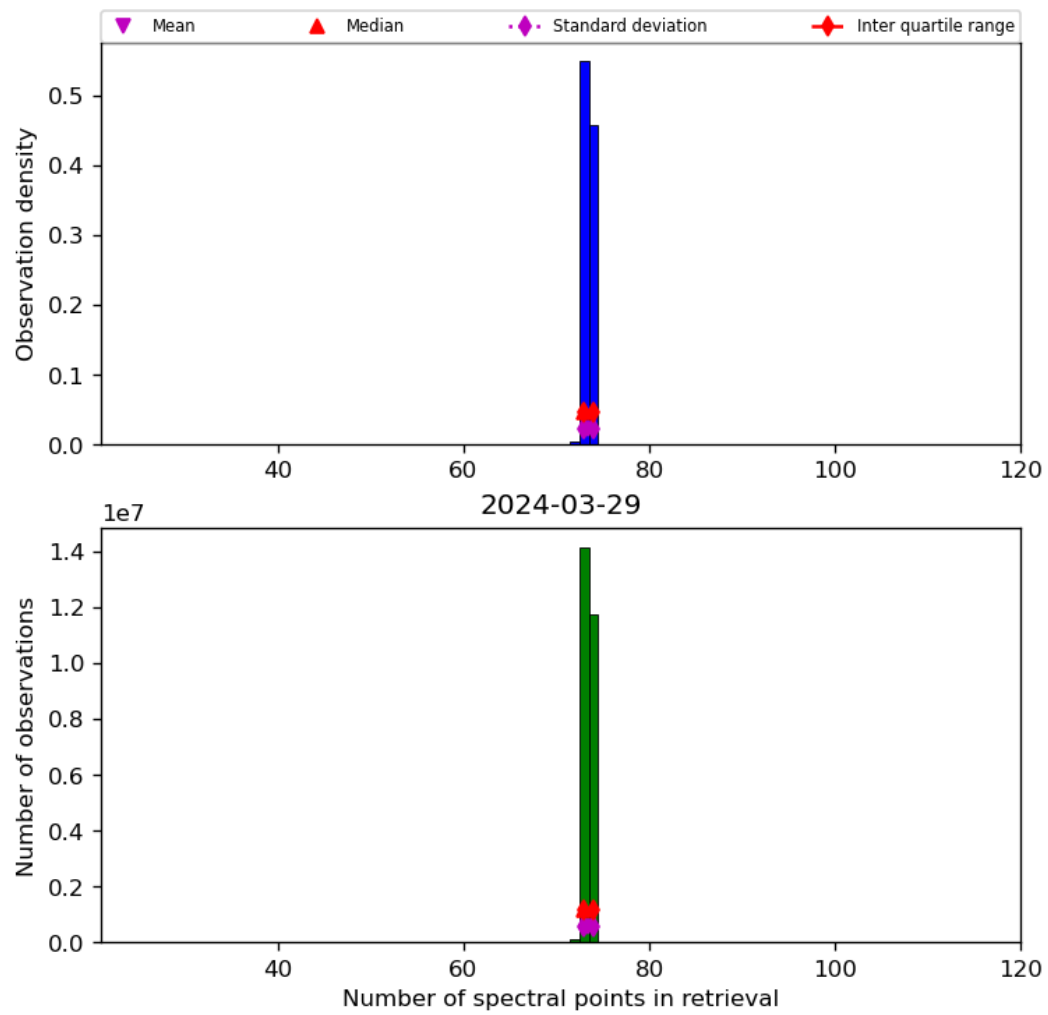
Figure 74: Histogram of “Number of spectral points in retrieval” for 2024-03-28 to 2024-03-30
