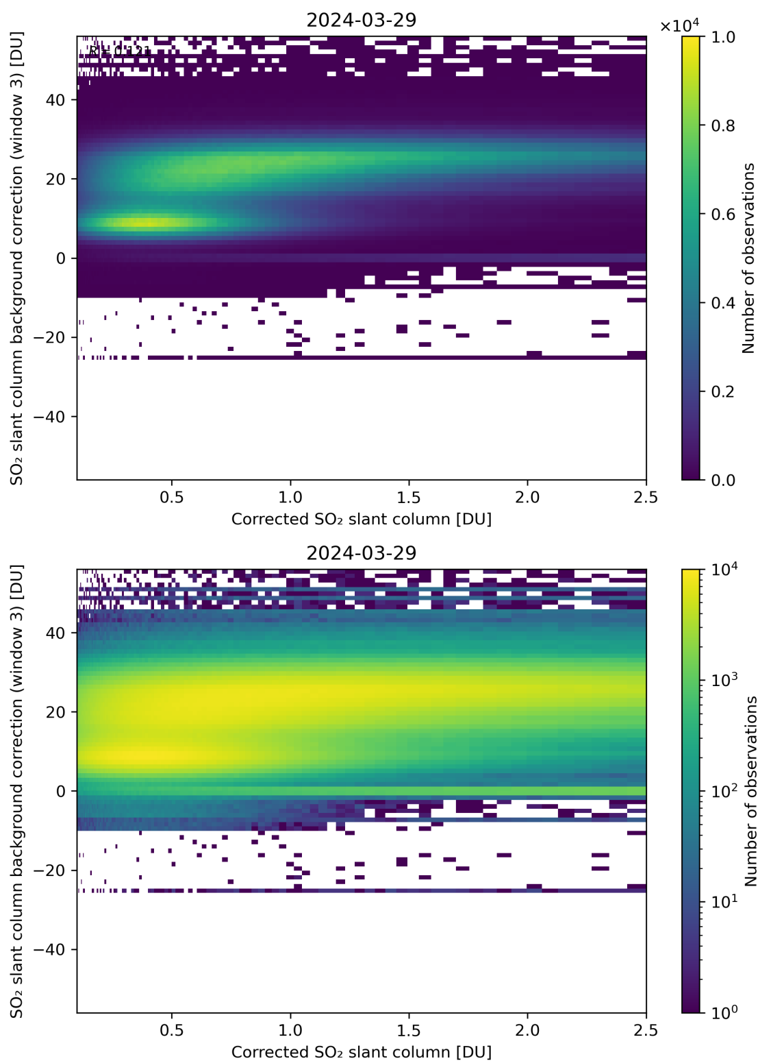
Figure 180: Scatter density plot of “Corrected SO 2 slant column” against “SO 2 slant column background correction (window 3)” for 2024-03-28 to 2024-03-30.
