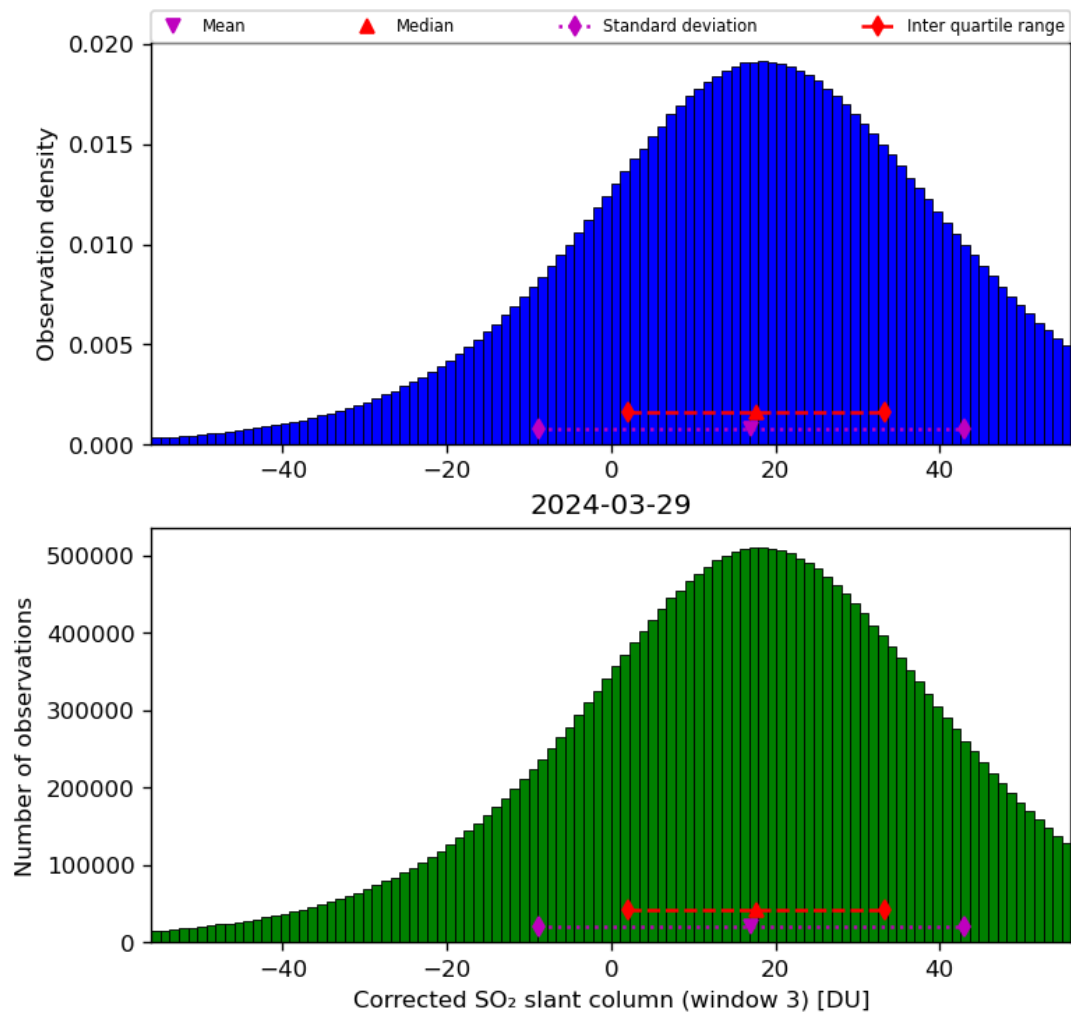
Figure 66: Histogram of “Corrected SO 2 slant column (window 3)” for 2024-03-28 to 2024-03-30
