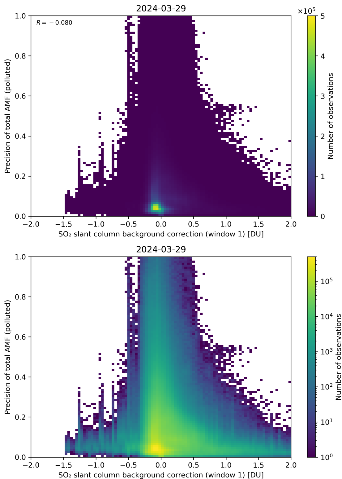
Figure 110: Scatter density plot of “SO 2 slant column background correction (window 1)” against “Precision of total AMF (polluted)” for 2024-03-28 to 2024-03-30.
