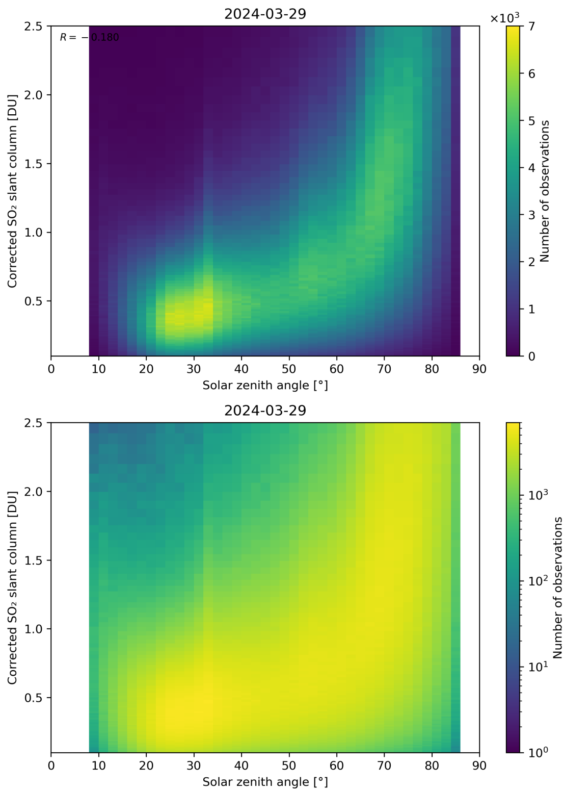
Figure 166: Scatter density plot of “Solar zenith angle” against “Corrected SO 2 slant column” for 2024-03-28 to 2024-03-30.
