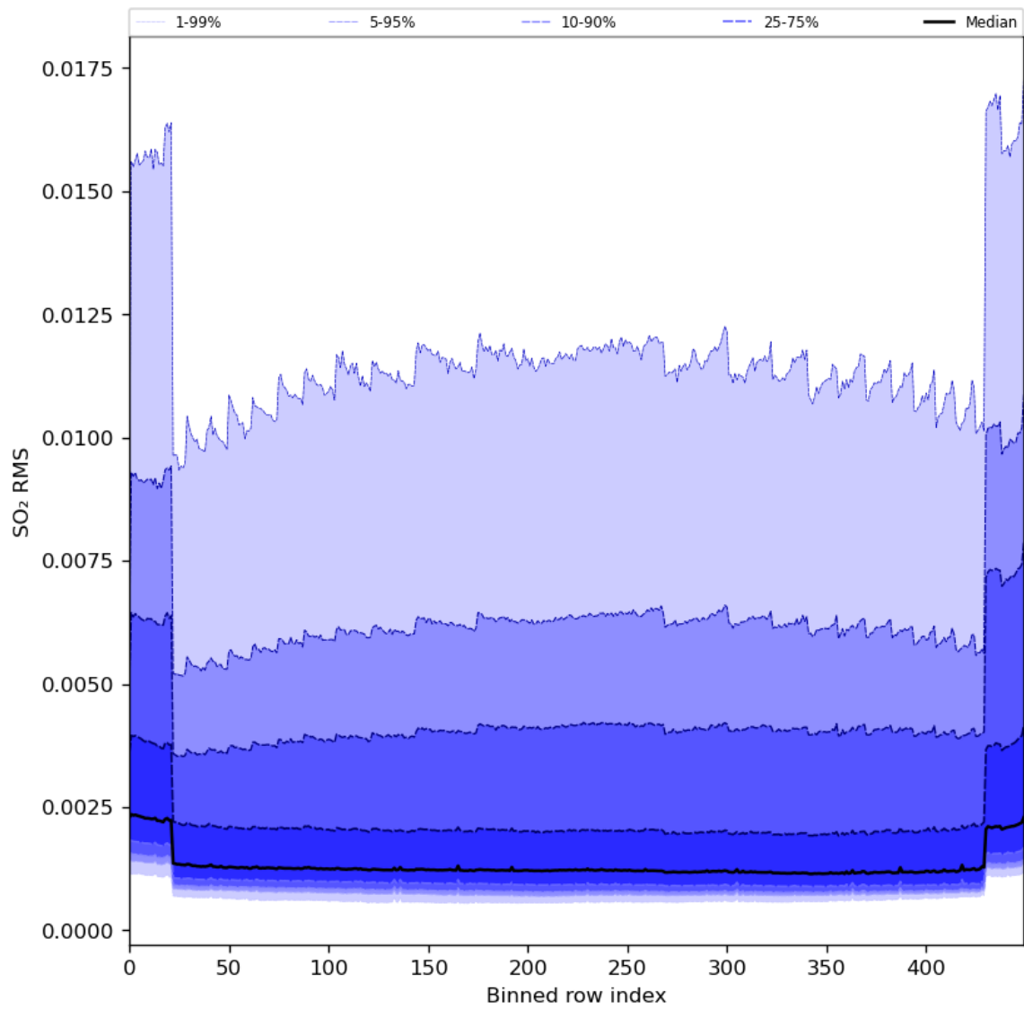
Figure 93: Along track statistics of “SO 2 RMS” for 2024-03-28 to 2024-03-30
