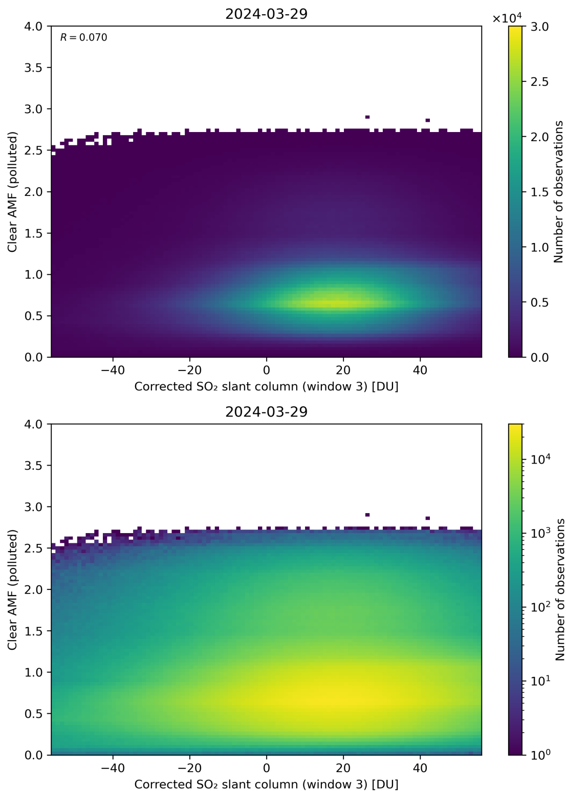
Figure 209: Scatter density plot of “Corrected SO 2 slant column (window 3)” against “Clear AMF (polluted)” for 2024-03-28 to 2024-03-30.
