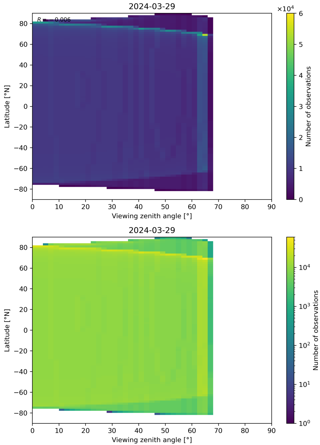
Figure 314: Scatter density plot of “Viewing zenith angle” against “Latitude” for 2024-03-28 to 2024-03-30.
