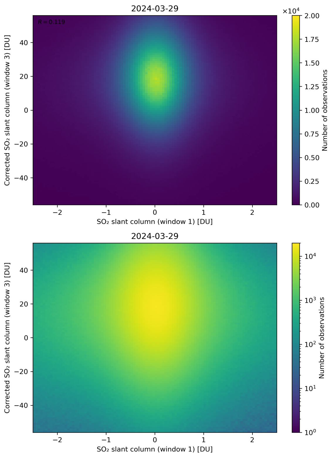
Figure 234: Scatter density plot of “SO 2 slant column (window 1)” against “Corrected SO 2 slant column (window 3)” for 2024-03-28 to 2024-03-30.
