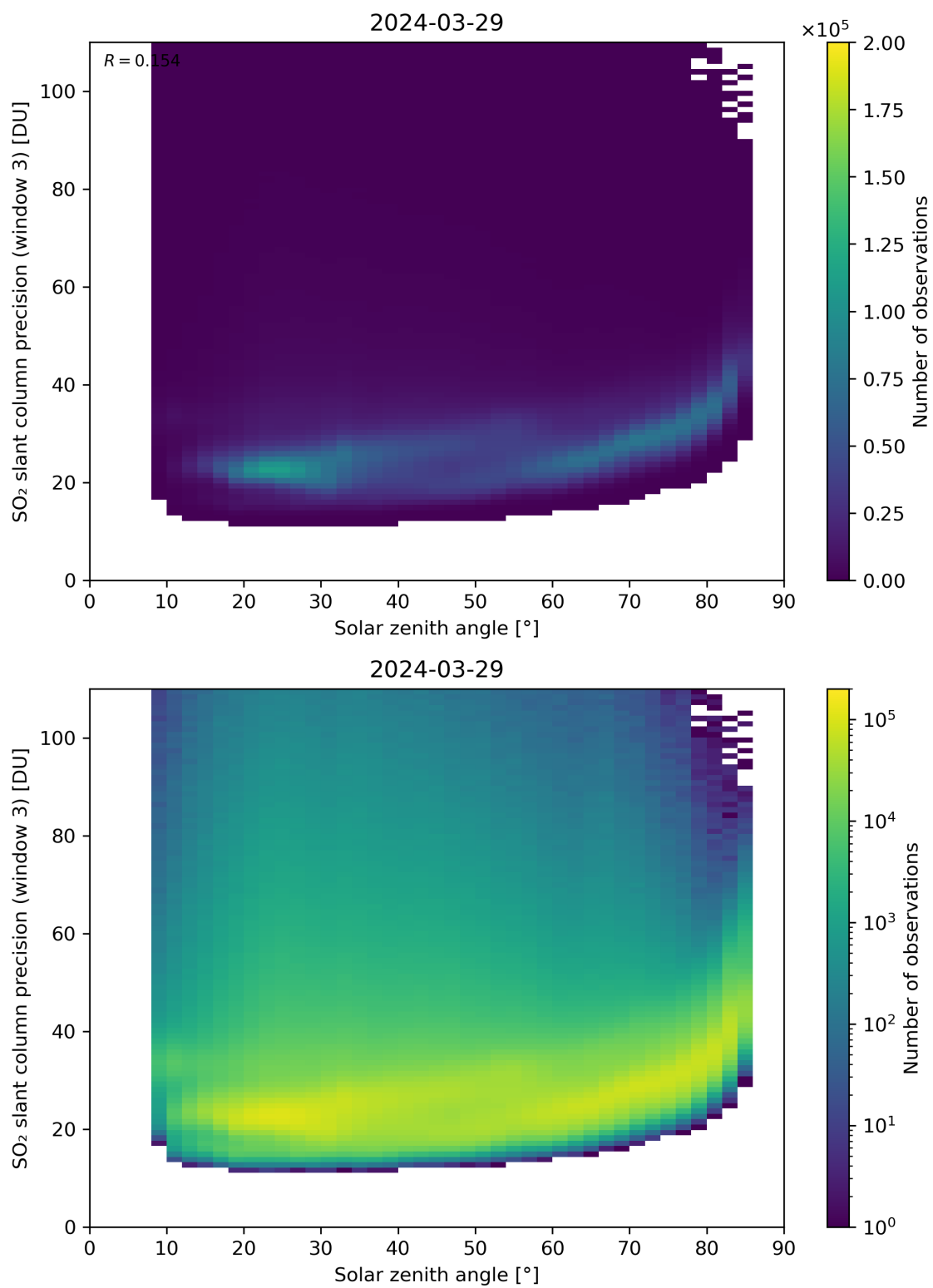
Figure 173: Scatter density plot of “Solar zenith angle” against “SO 2 slant column precision (window 3)” for 2024-03-28 to 2024-03-30.
