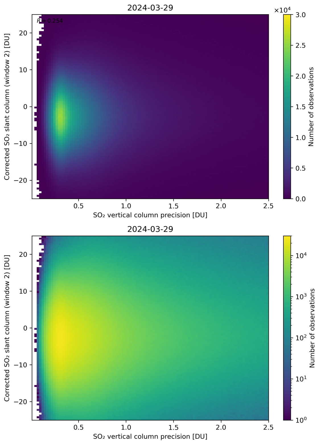
Figure 287: Scatter density plot of “SO 2 vertical column precision” against “Corrected SO 2 slant column (window 2)” for 2024-03-28 to 2024-03-30.
