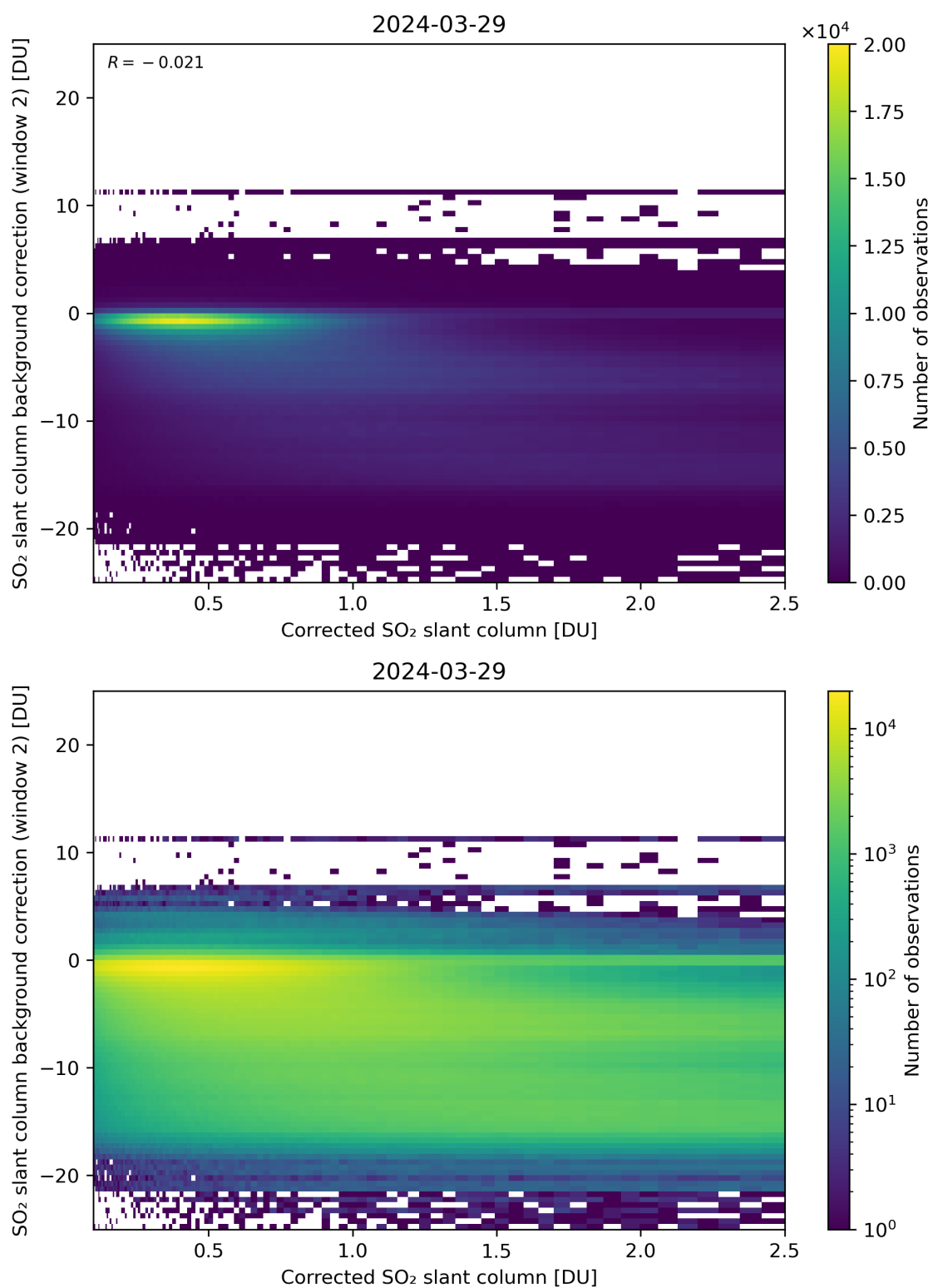
Figure 179: Scatter density plot of “Corrected SO 2 slant column” against “SO 2 slant column background correction (window 2)” for 2024-03-28 to 2024-03-30.
