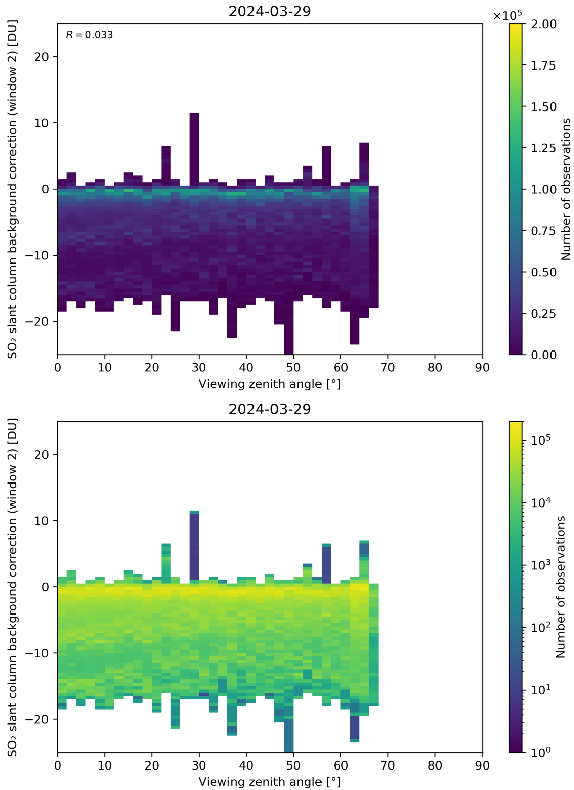
Figure 309: Scatter density plot of “Viewing zenith angle” against “SO 2 slant column background correction (window 2)” for 2024-03-28 to 2024-03-30.
