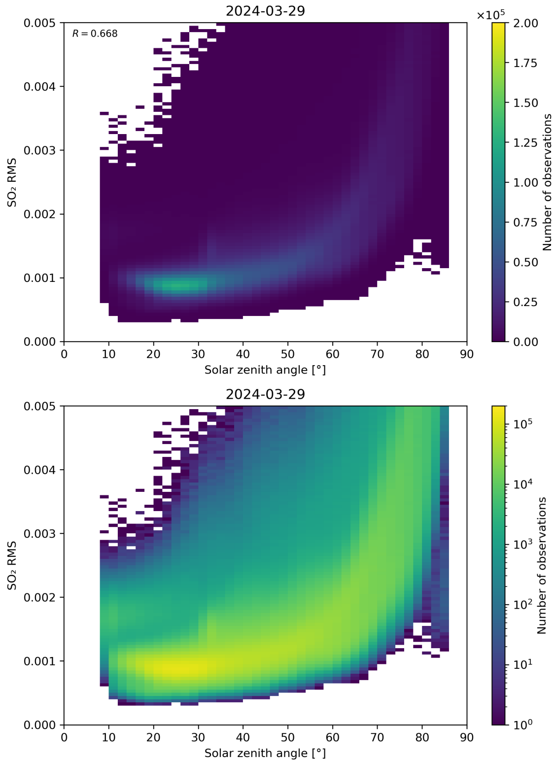
Figure 163: Scatter density plot of “Solar zenith angle” against “SO 2 RMS” for 2024-03-28 to 2024-03-30.
