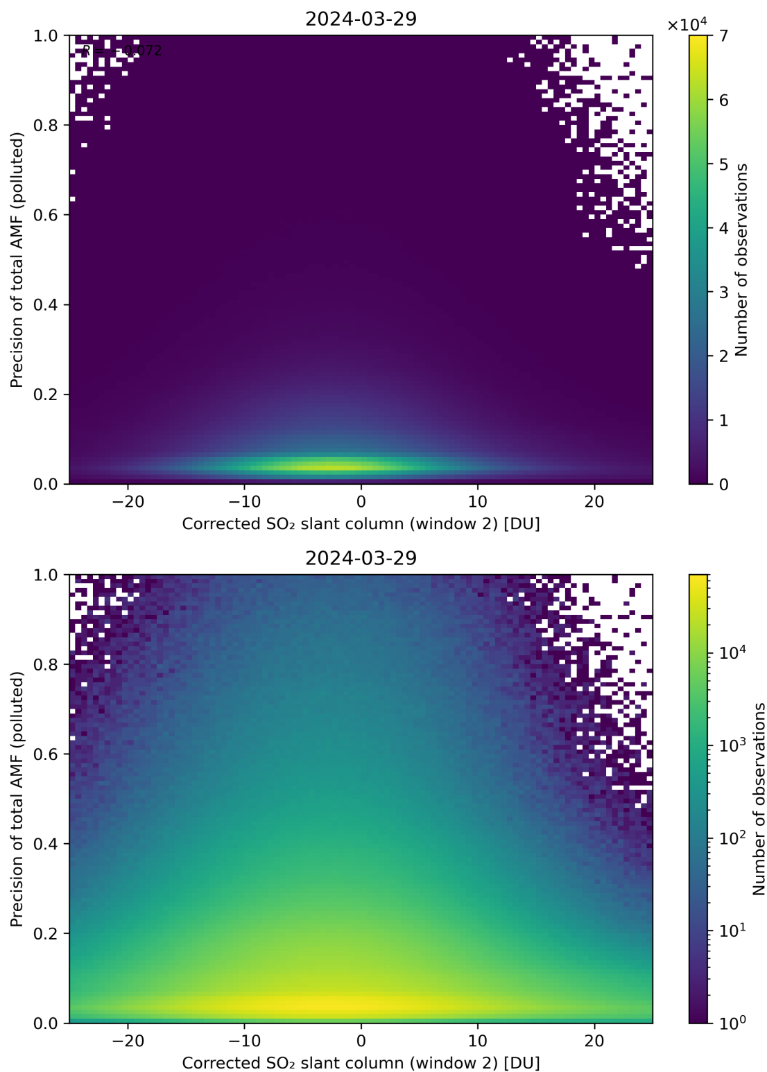
Figure 204: Scatter density plot of “Corrected SO 2 slant column (window 2)” against “Precision of total AMF (polluted)” for 2024-03-28 to 2024-03-30.
