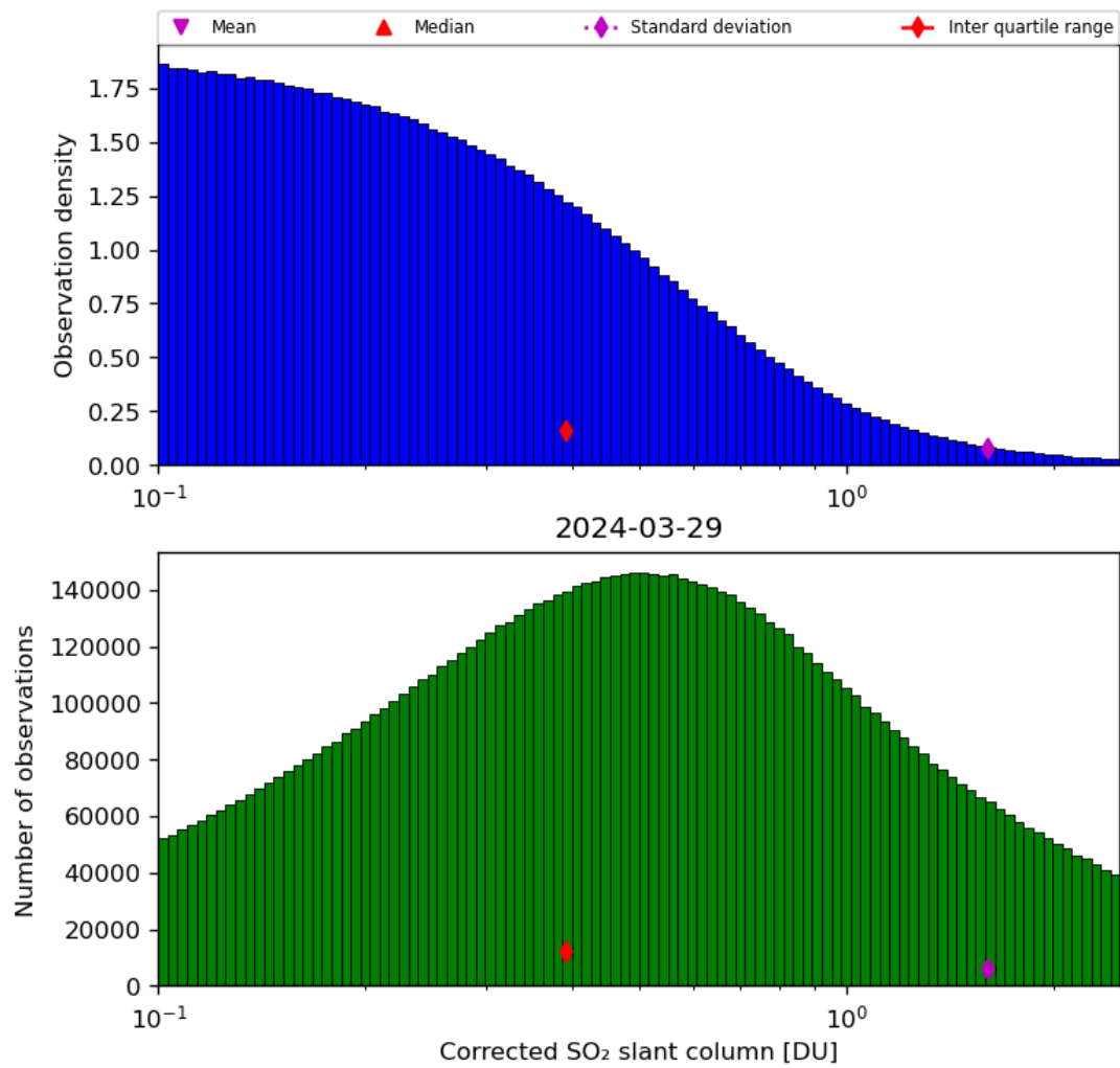
Figure 55: Histogram of “Corrected SO 2 slant column” for 2024-03-28 to 2024-03-30
