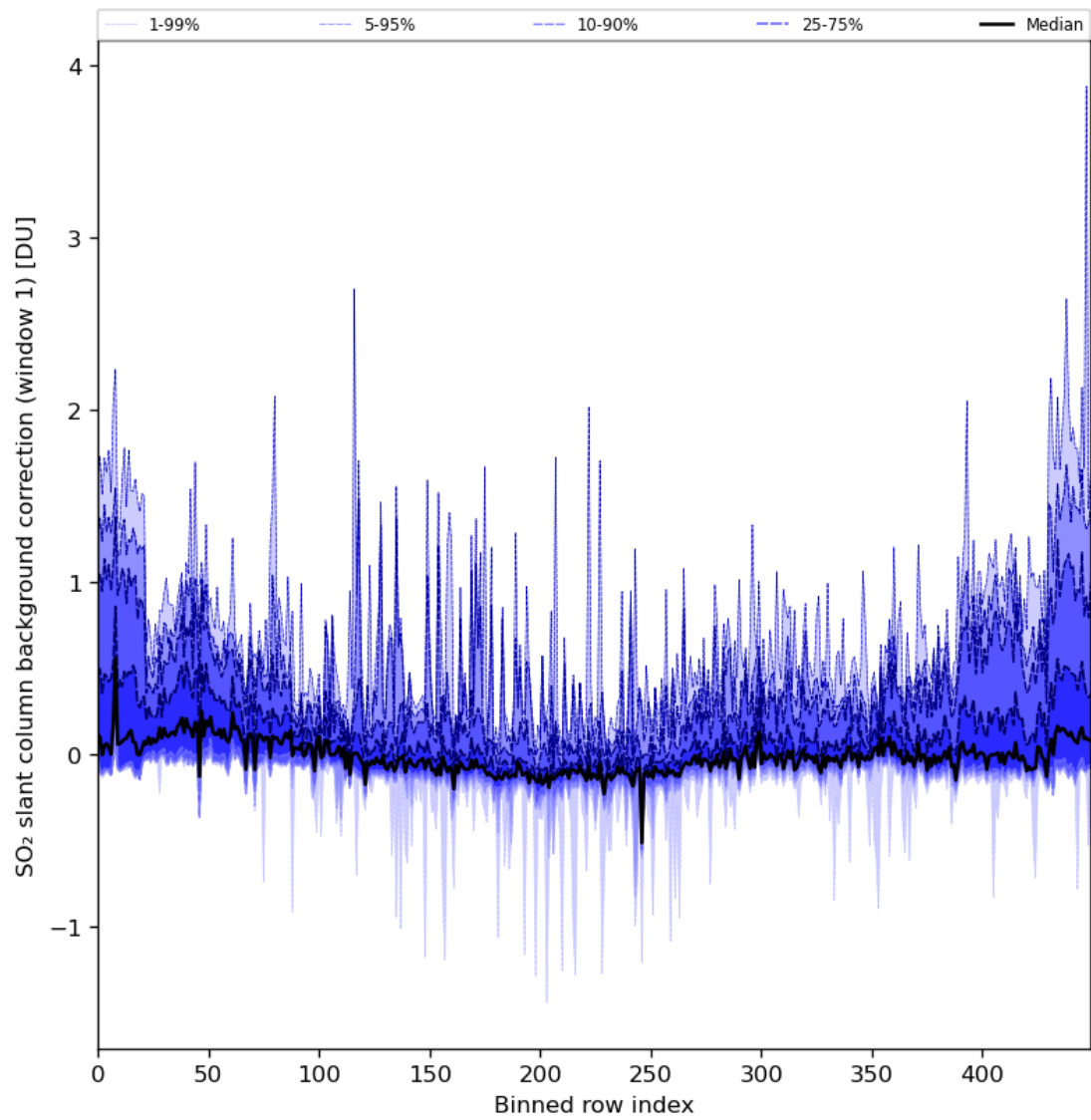
Figure 82: Along track statistics of “SO 2 slant column background correction (window 1)” for 2024-03-30 to 2024-03-31
