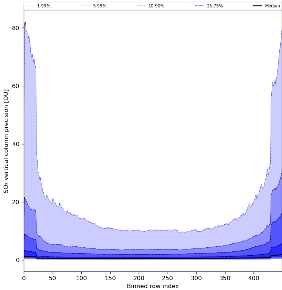
Figure 77: Along track statistics of “SO 2 vertical column precision” for 2024-03-30 to 2024-03-31
