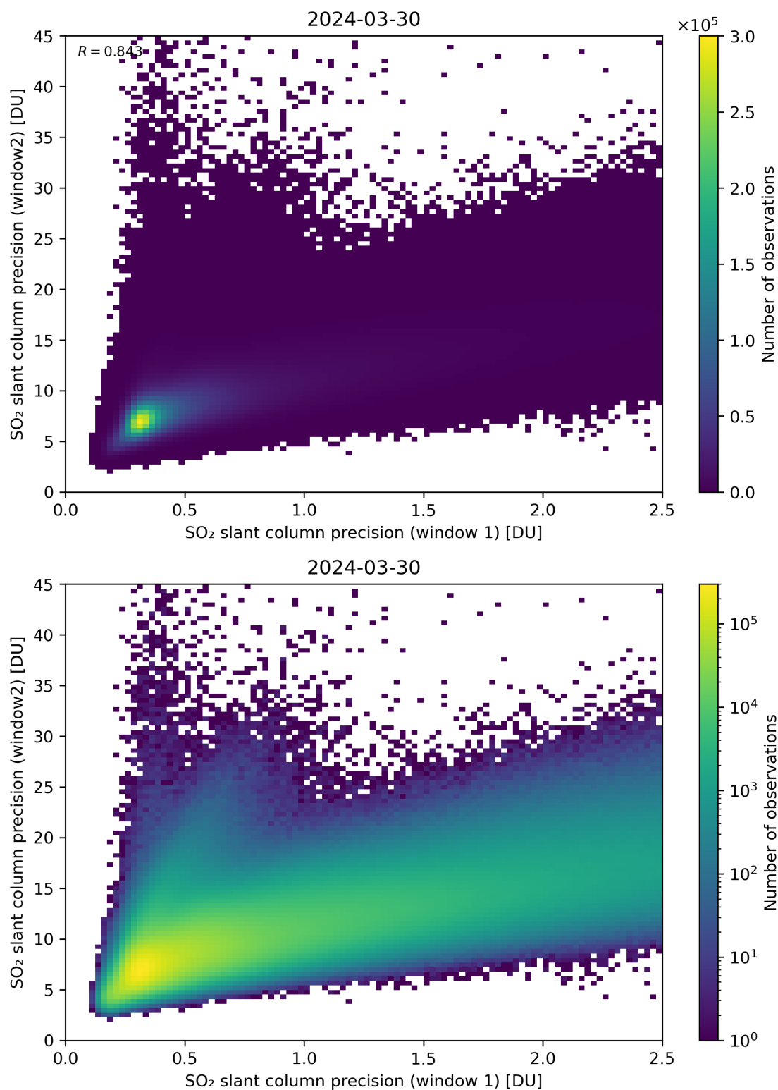
Figure 227: Scatter density plot of “SO 2 slant column precision (window 1)” against “SO 2 slant column precision (window2)” for 2024-03-30 to 2024-03-31.
