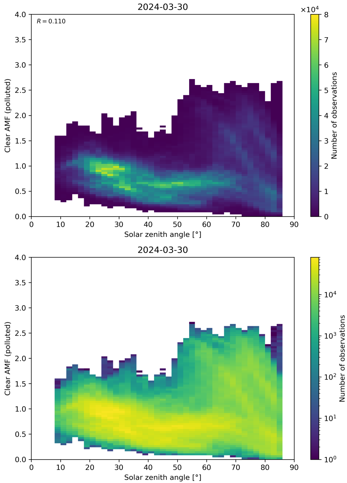
Figure 165: Scatter density plot of “Solar zenith angle” against “Clear AMF (polluted)” for 2024-03-30 to 2024-03-31.
