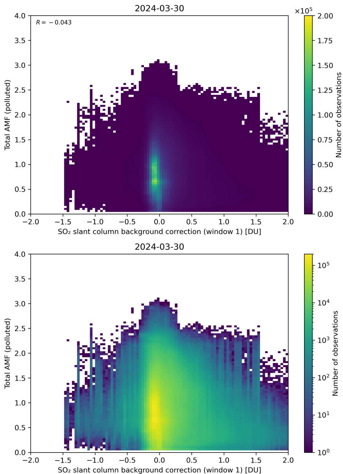
Figure 109: Scatter density plot of “SO 2 slant column background correction (window 1)” against “Total AMF (polluted)” for 2024-03-30 to 2024-03-31.
