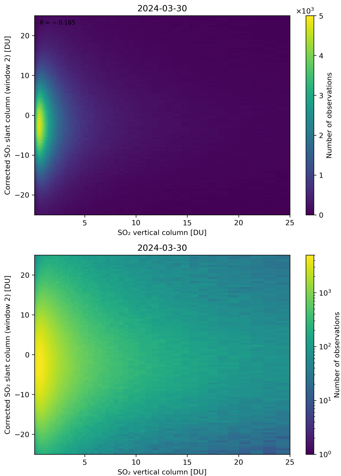
Figure 298: Scatter density plot of “SO 2 vertical column” against “Corrected SO 2 slant column (window 2)” for 2024-03-30 to 2024-03-31.
