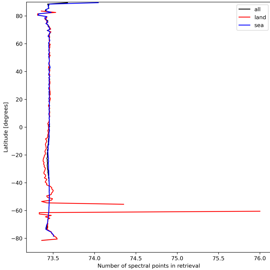
Figure 51: Zonal average of “Number of spectral points in retrieval” for 2024-03-30 to 2024-03-31.
