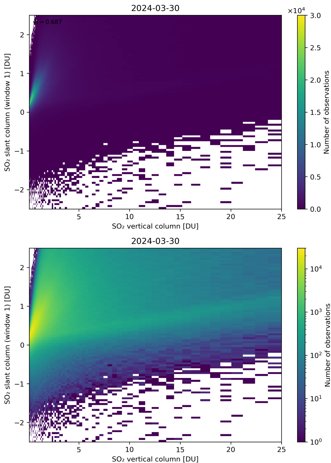
Figure 300: Scatter density plot of “SO 2 vertical column” against “SO 2 slant column (window 1)” for 2024-03-30 to 2024-03-31.
