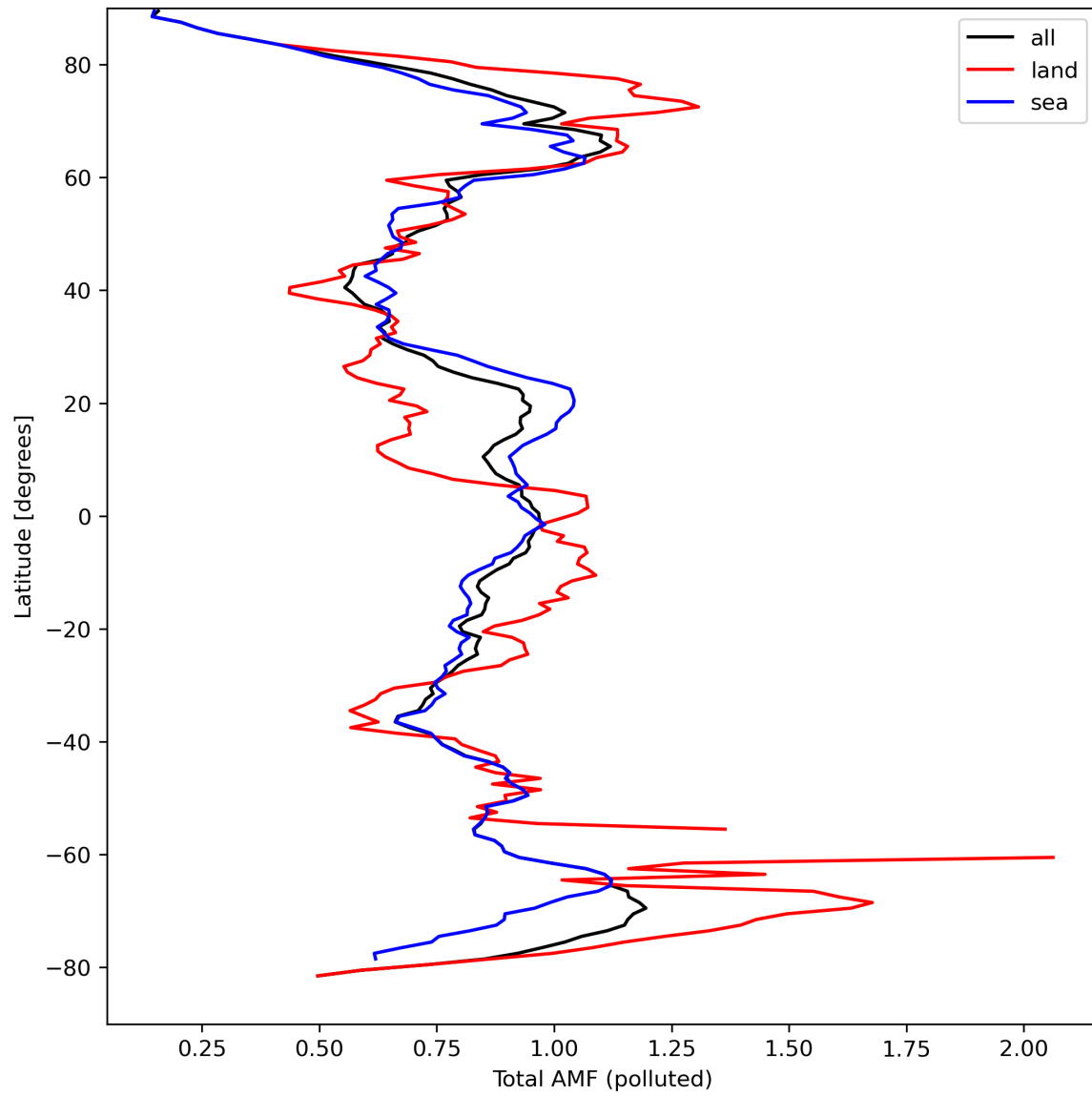
Figure 48: Zonal average of “Total AMF (polluted)” for 2024-03-30 to 2024-03-31.
