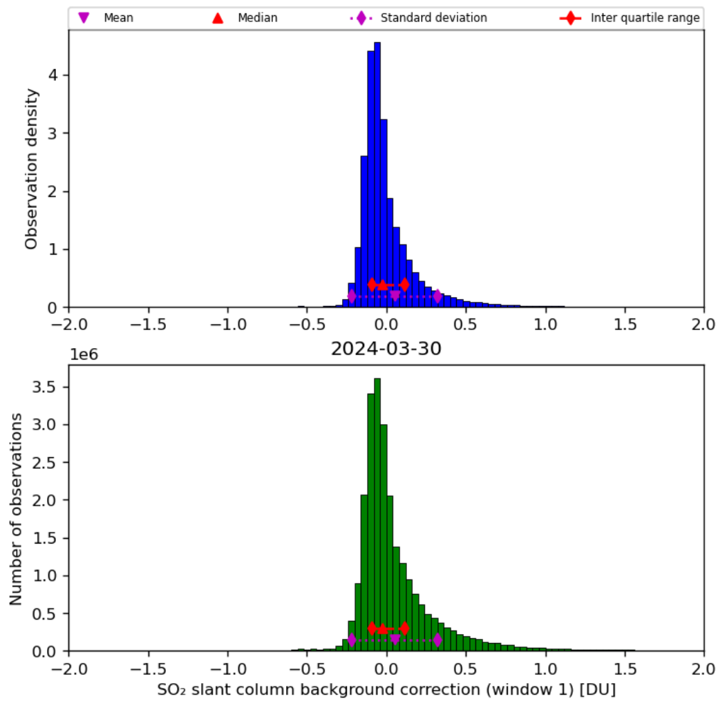
Figure 59: Histogram of “SO 2 slant column background correction (window 1)” for 2024-03-30 to 2024-03-31
