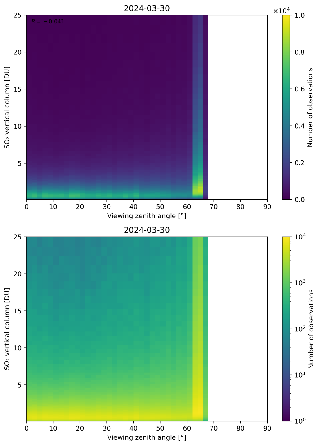
Figure 327: Scatter density plot of “Viewing zenith angle” against “SO 2 vertical column” for 2024-03-30 to 2024-03-31.
