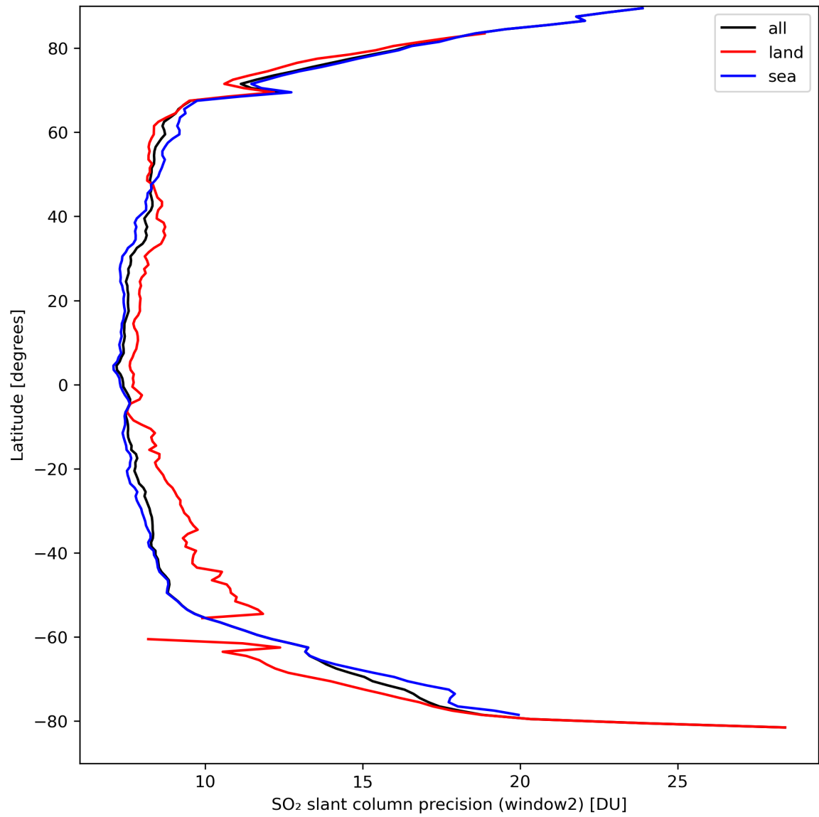
Figure 38: Zonal average of “SO 2 slant column precision (window2)” for 2024-03-30 to 2024-03-31.
