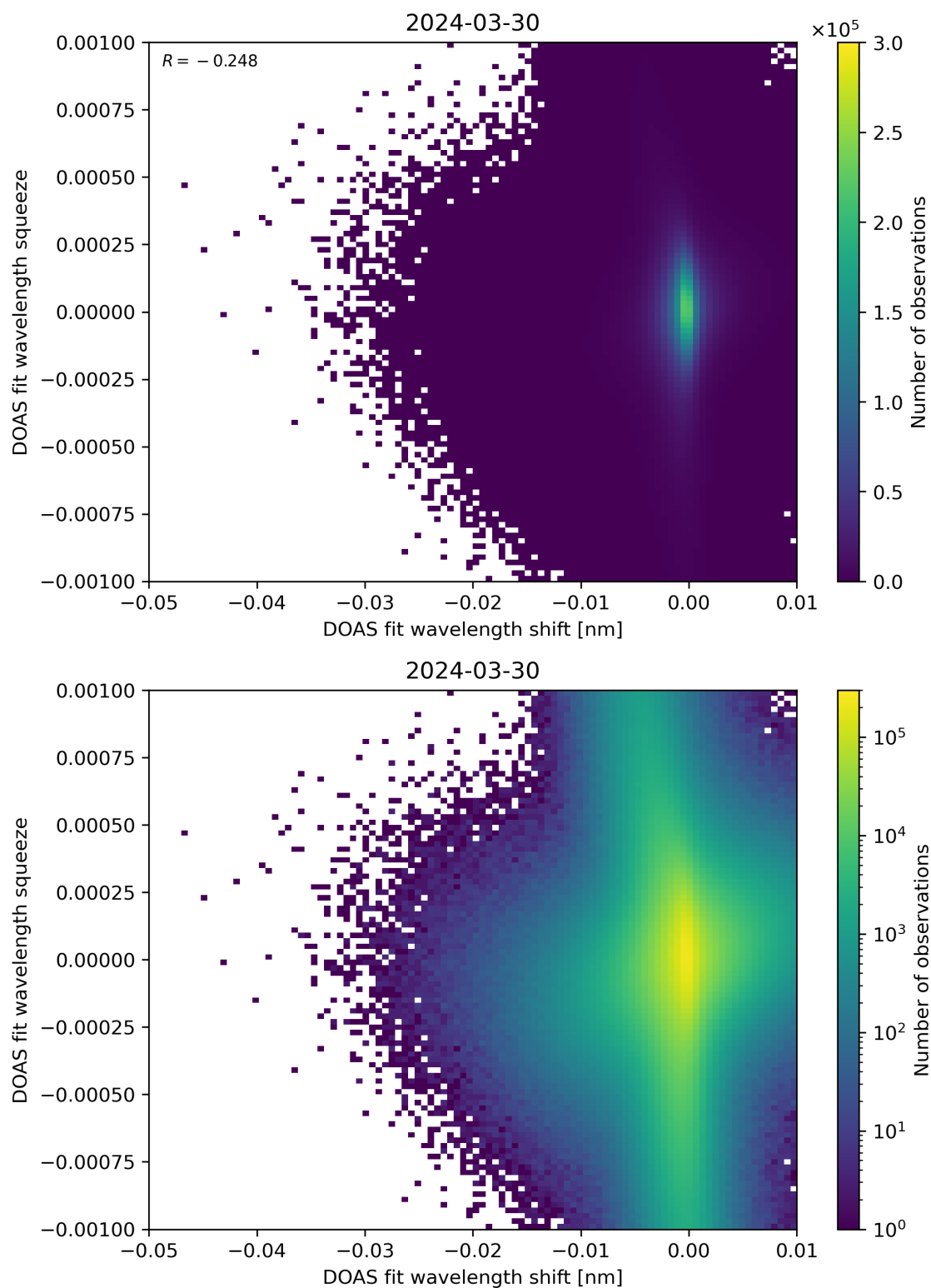
Figure 127: Scatter density plot of “DOAS fit wavelength shift” against “DOAS fit wavelength squeeze” for 2024-03-30 to 2024-03-31.
