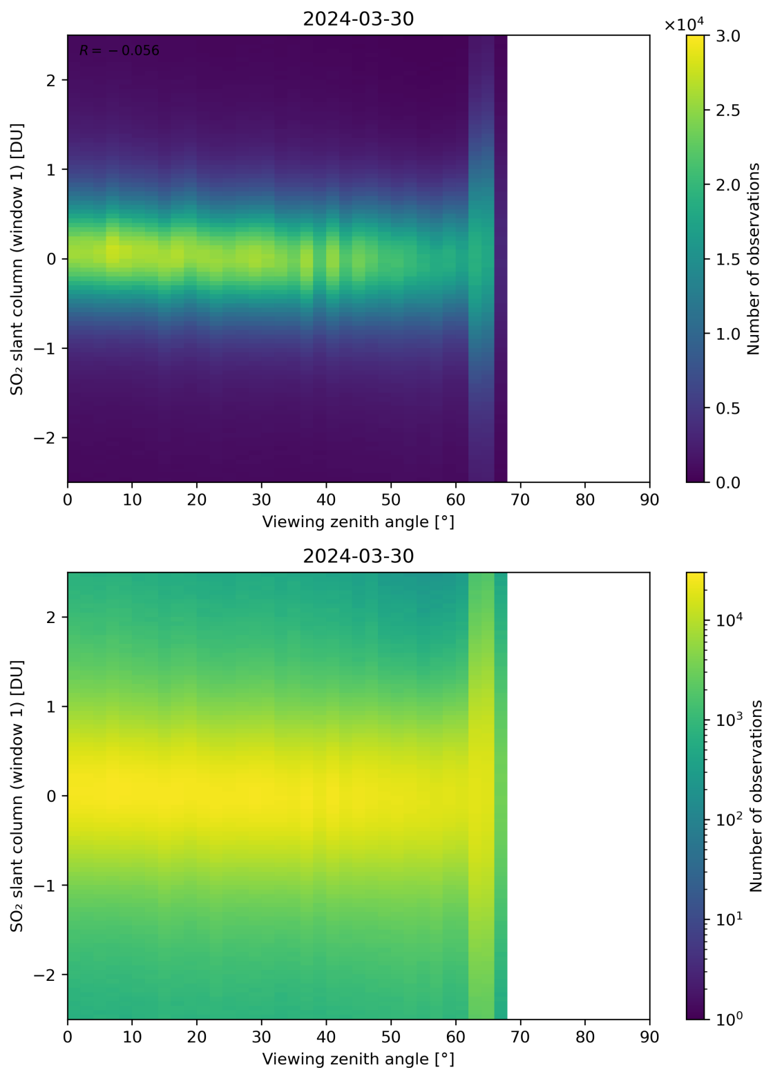
Figure 320: Scatter density plot of “Viewing zenith angle” against “SO 2 slant column (window 1)” for 2024-03-30 to 2024-03-31.
