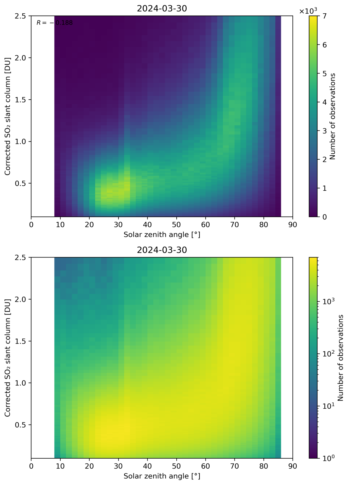
Figure 166: Scatter density plot of “Solar zenith angle” against “Corrected SO 2 slant column” for 2024-03-30 to 2024-03-31.
