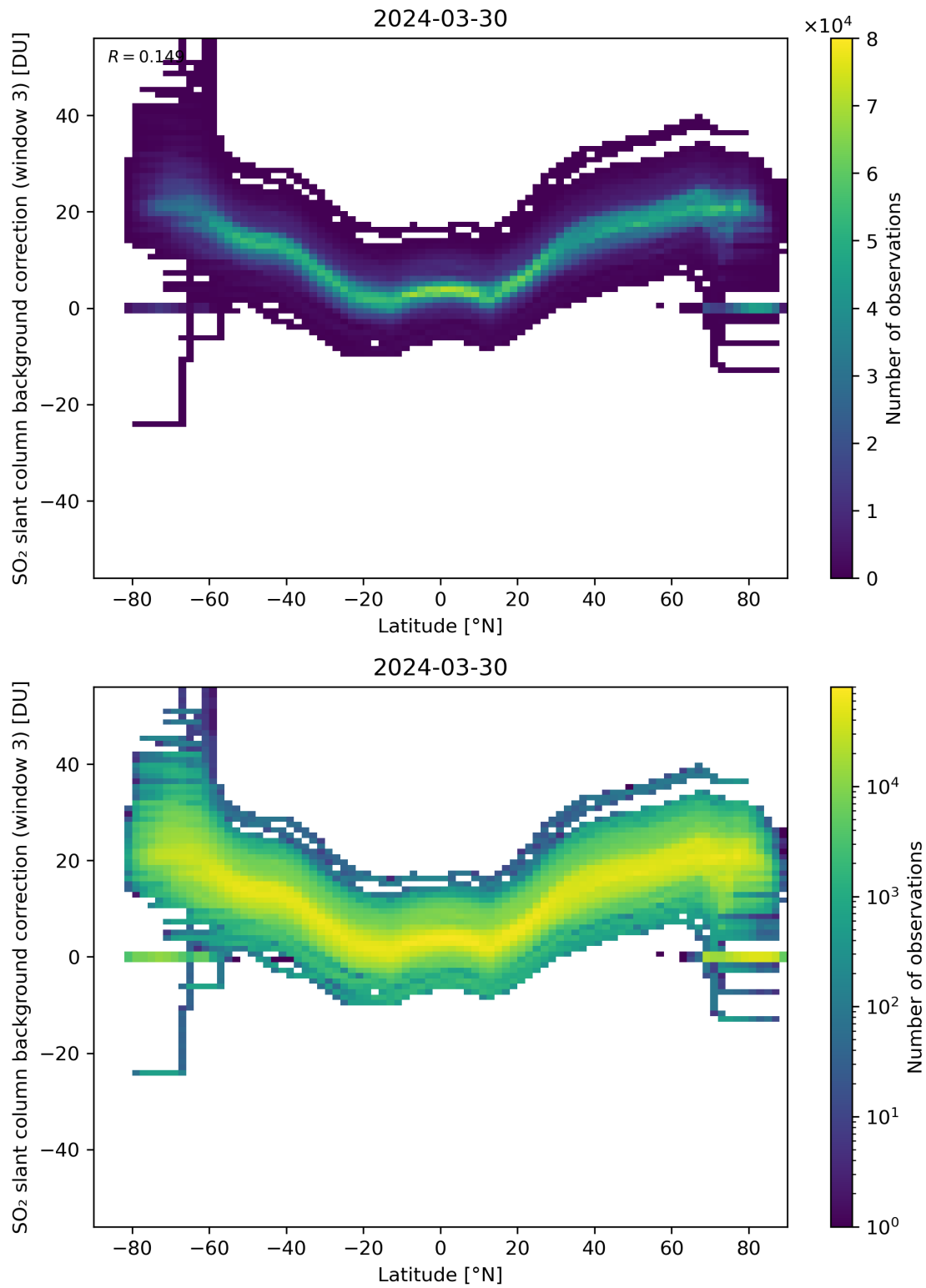
Figure 141: Scatter density plot of “Latitude” against “SO 2 slant column background correction (window 3)” for 2024-03-30 to 2024-03-31.
