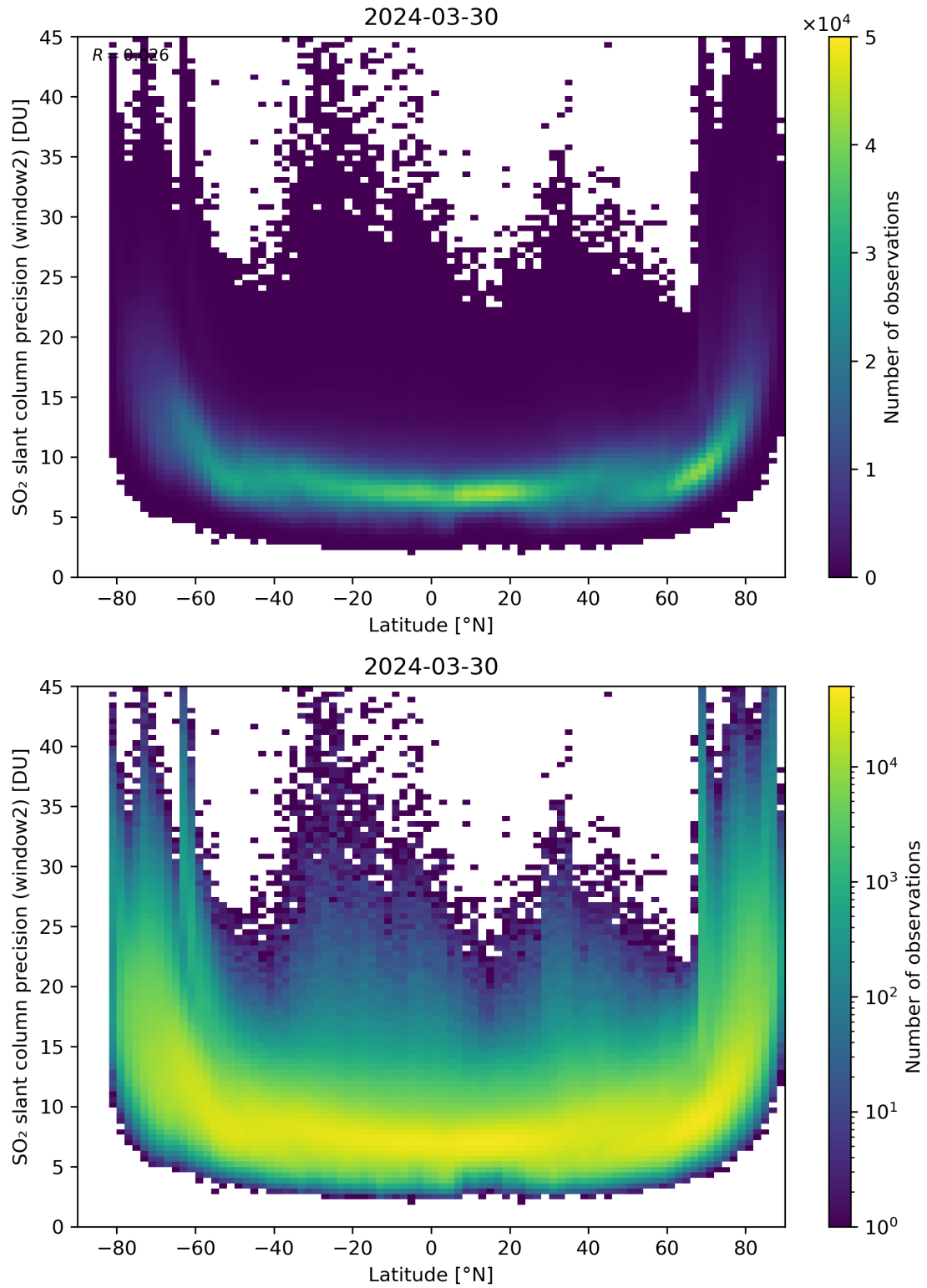
Figure 151: Scatter density plot of “Latitude” against “SO 2 slant column precision (window2)” for 2024-03-30 to 2024-03-31.
