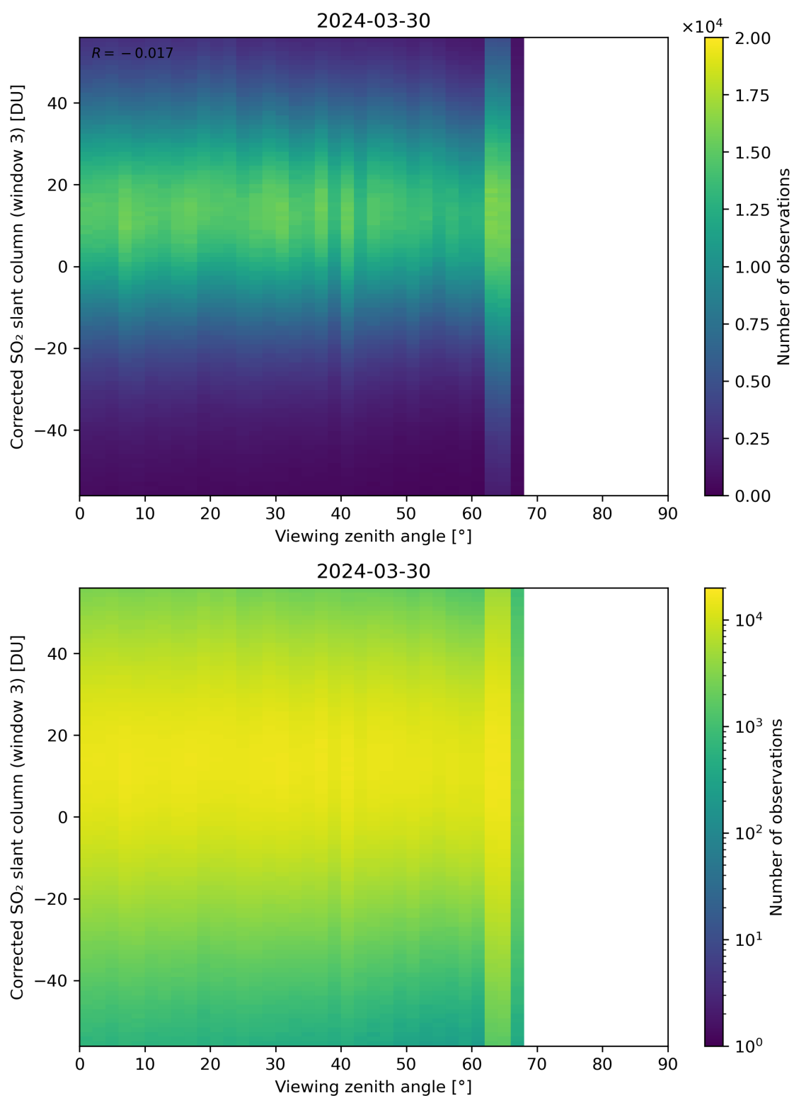
Figure 319: Scatter density plot of “Viewing zenith angle” against “Corrected SO 2 slant column (window 3)” for 2024-03-30 to 2024-03-31.
