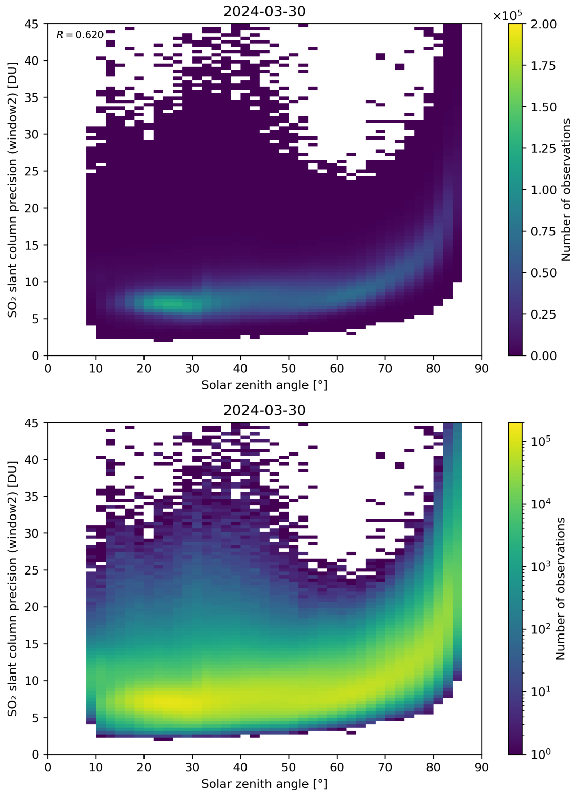
Figure 171: Scatter density plot of “Solar zenith angle” against “SO 2 slant column precision (window2)” for 2024-03-30 to 2024-03-31.
