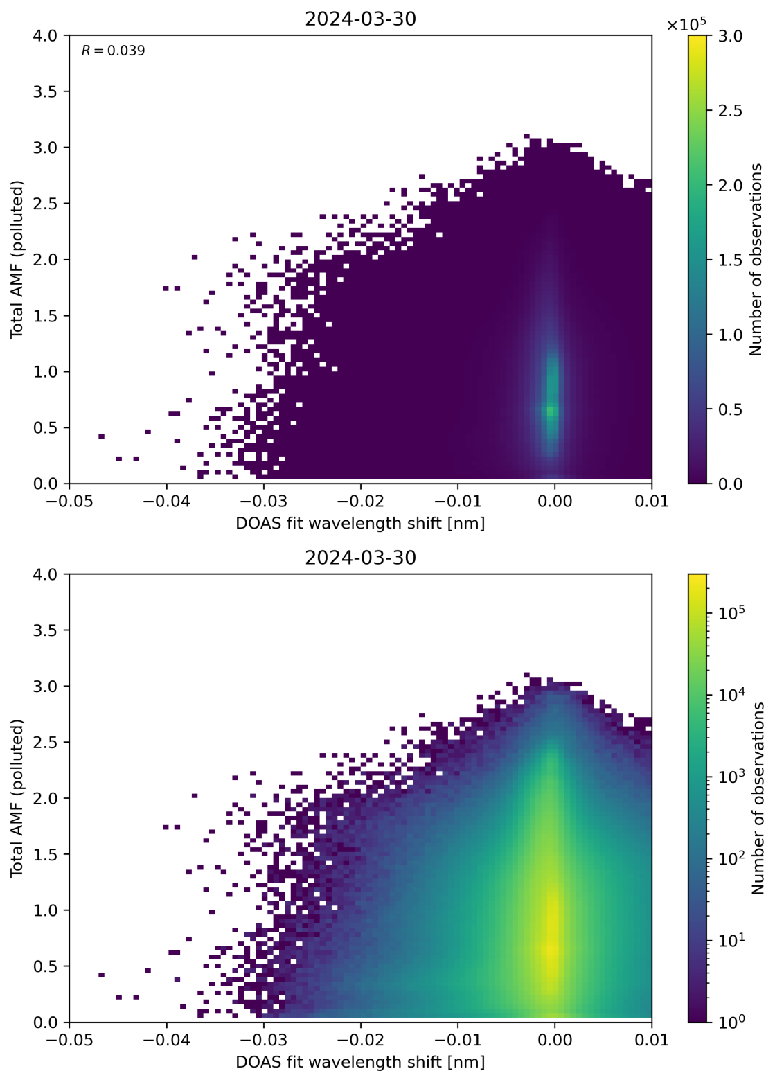
Figure 130: Scatter density plot of “DOAS fit wavelength shift” against “Total AMF (polluted)” for 2024-03-30 to 2024-03-31.
