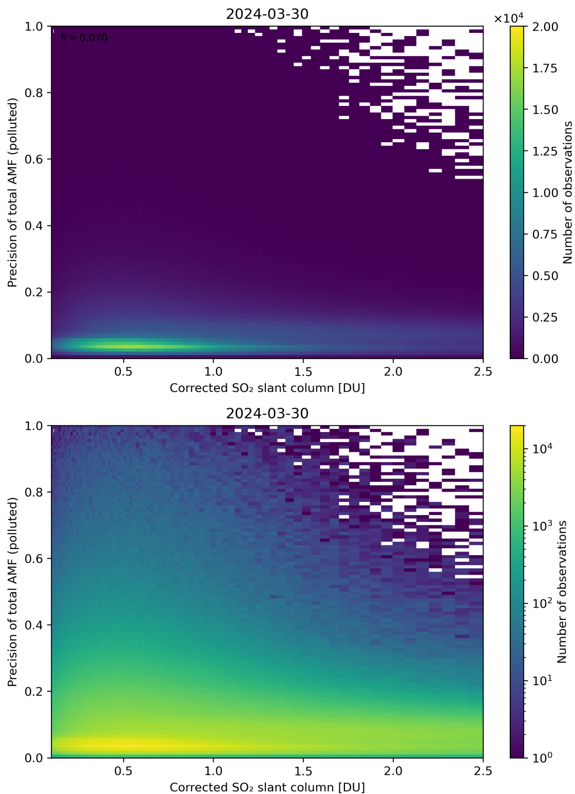
Figure 193: Scatter density plot of “Corrected SO 2 slant column” against “Precision of total AMF (polluted)” for 2024-03-30 to 2024-03-31.
