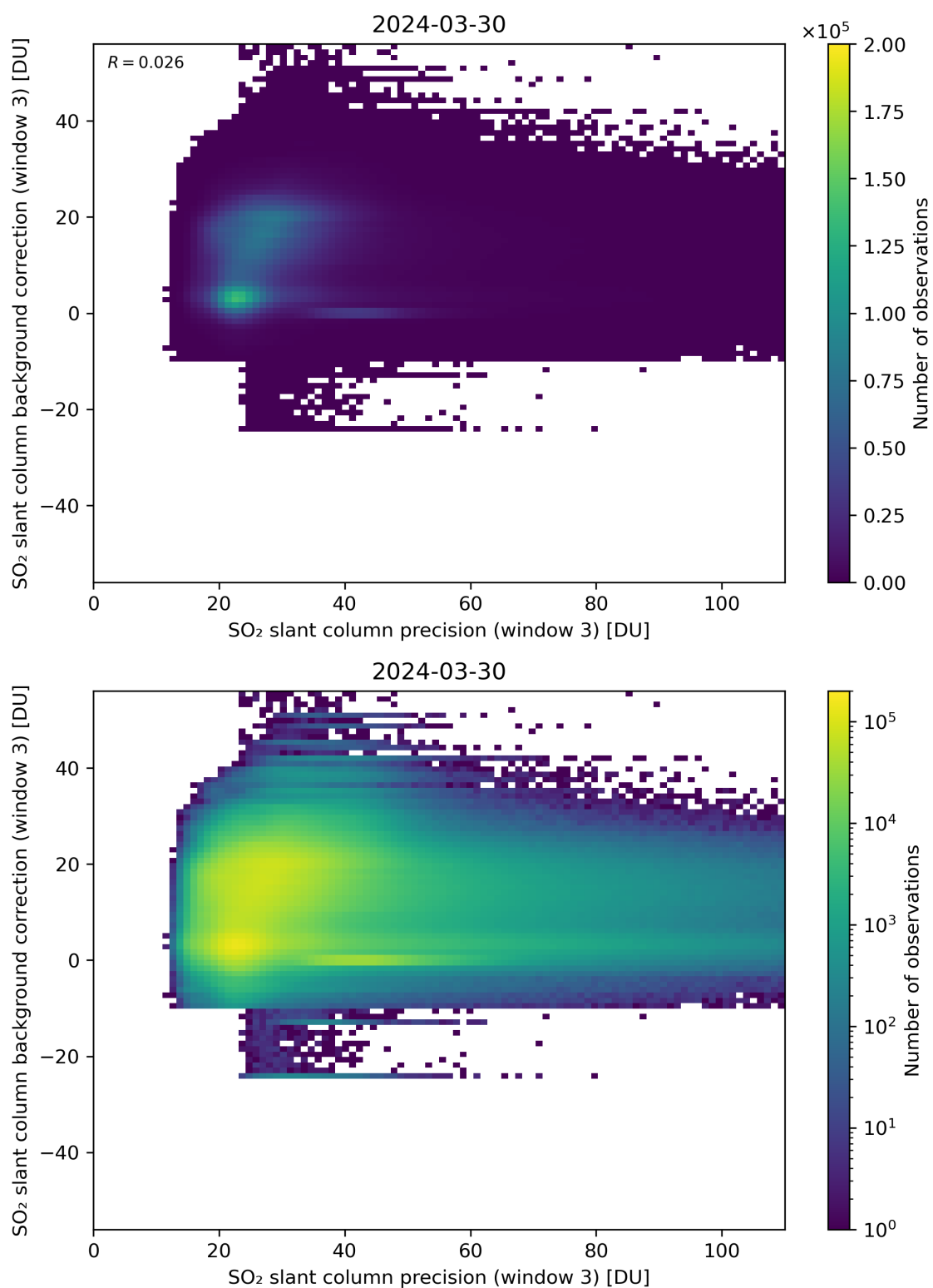
Figure 257: Scatter density plot of “SO 2 slant column precision (window 3)” against “SO 2 slant column background correction (window 3)” for 2024-03-30 to 2024-03-31.
