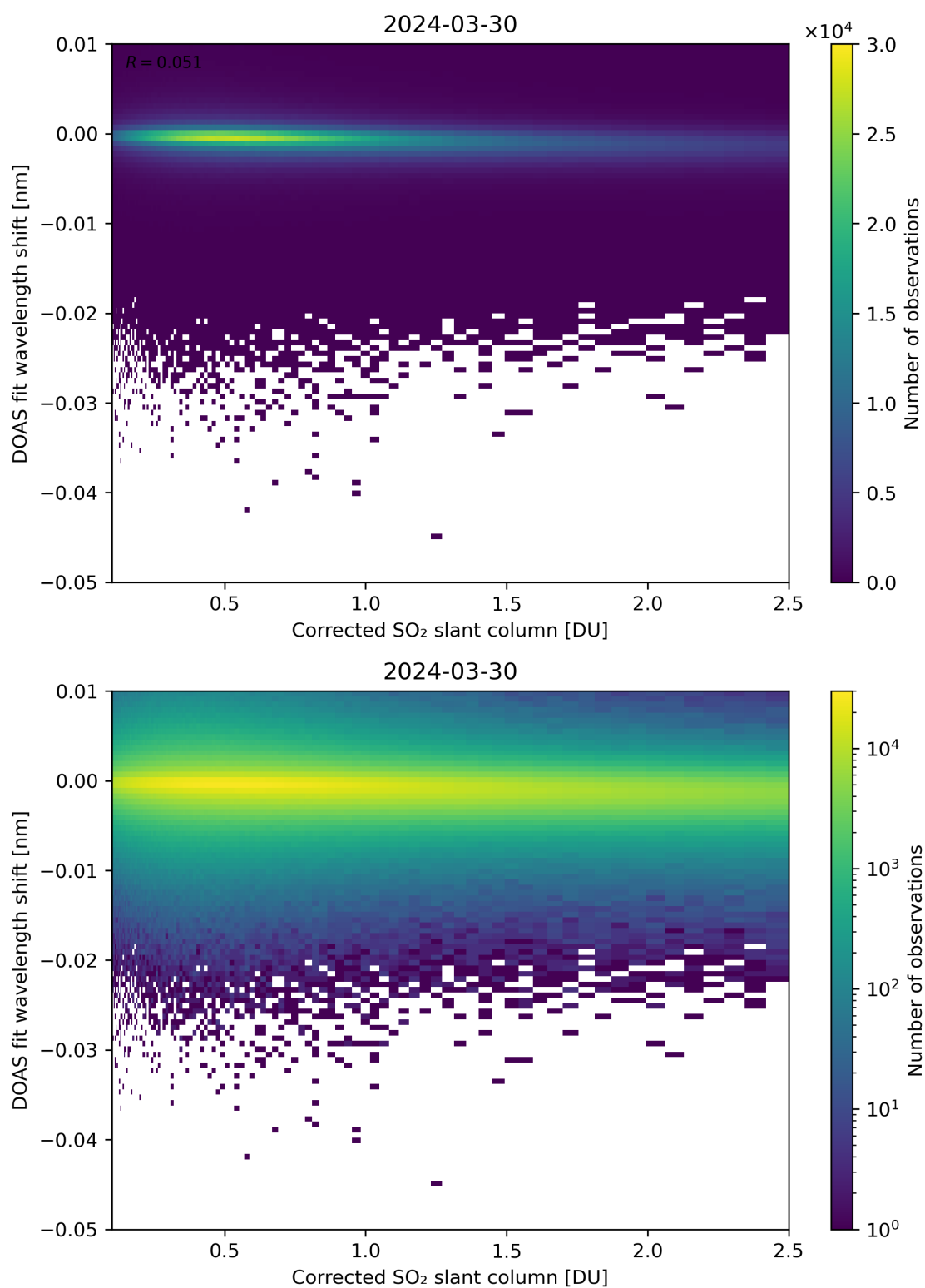
Figure 181: Scatter density plot of “Corrected SO 2 slant column” against “DOAS fit wavelength shift” for 2024-03-30 to 2024-03-31.
