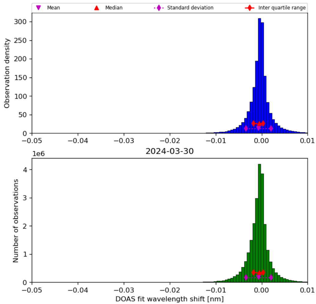
Figure 68: Histogram of “DOAS fit wavelength shift” for 2024-03-30 to 2024-03-31
