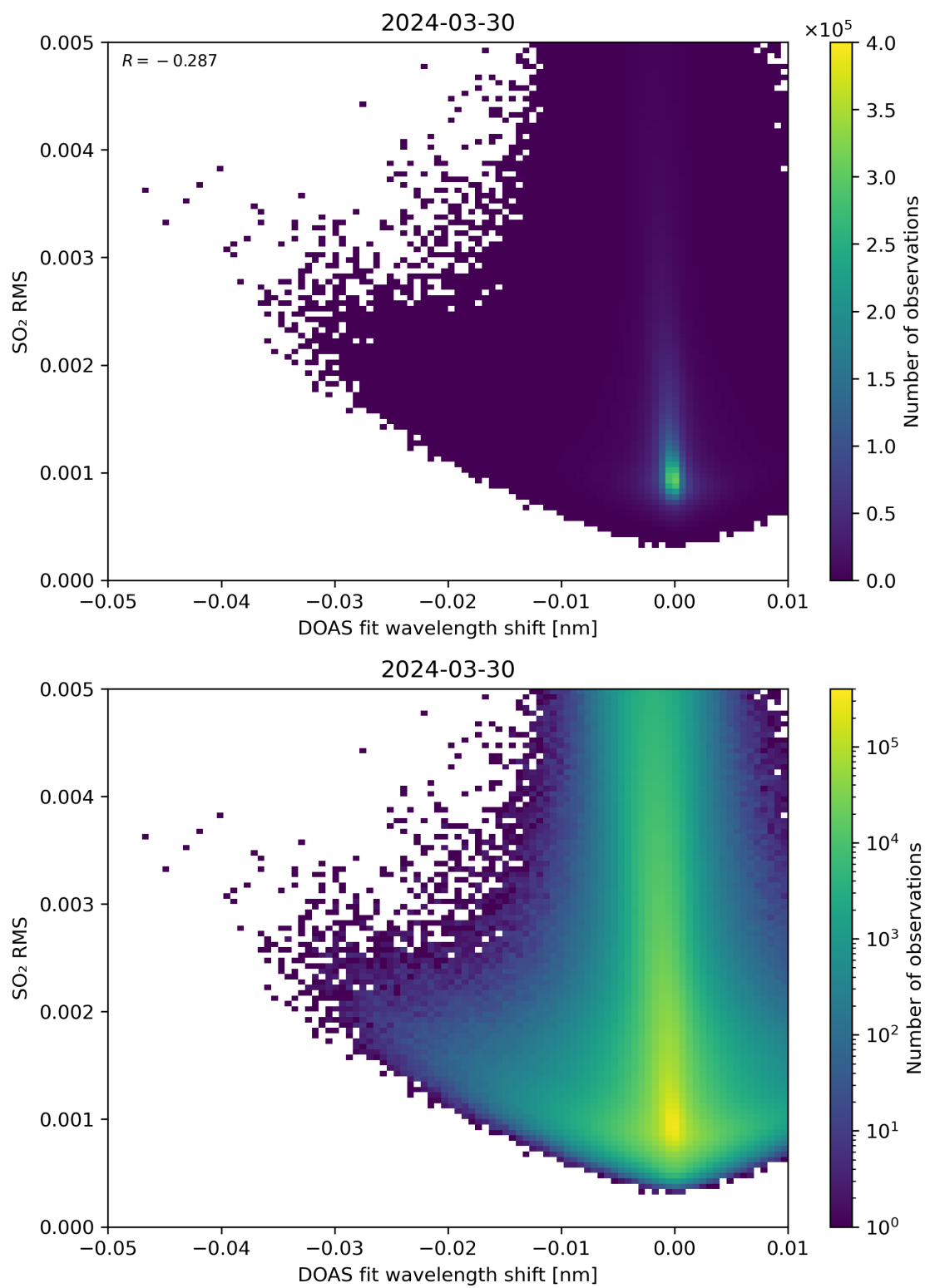
Figure 128: Scatter density plot of “DOAS fit wavelength shift” against “SO 2 RMS” for 2024-03-30 to 2024-03-31.
