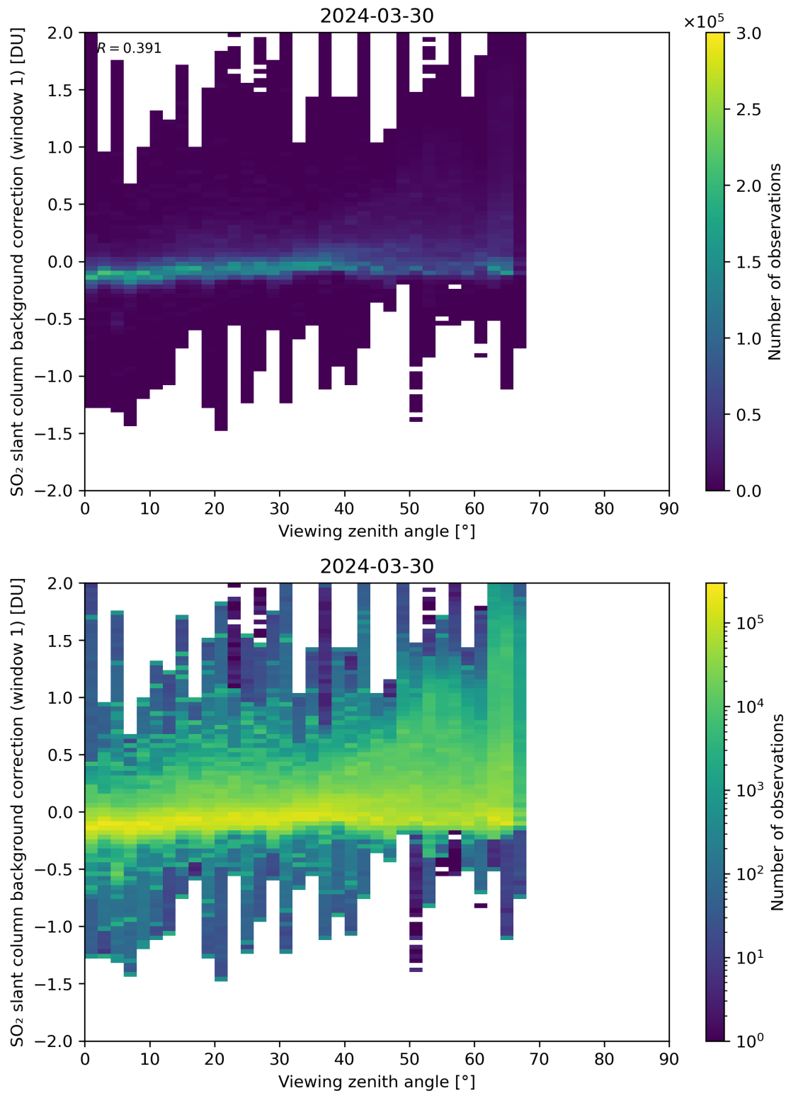
Figure 308: Scatter density plot of “Viewing zenith angle” against “SO 2 slant column background correction (window 1)” for 2024-03-30 to 2024-03-31.
