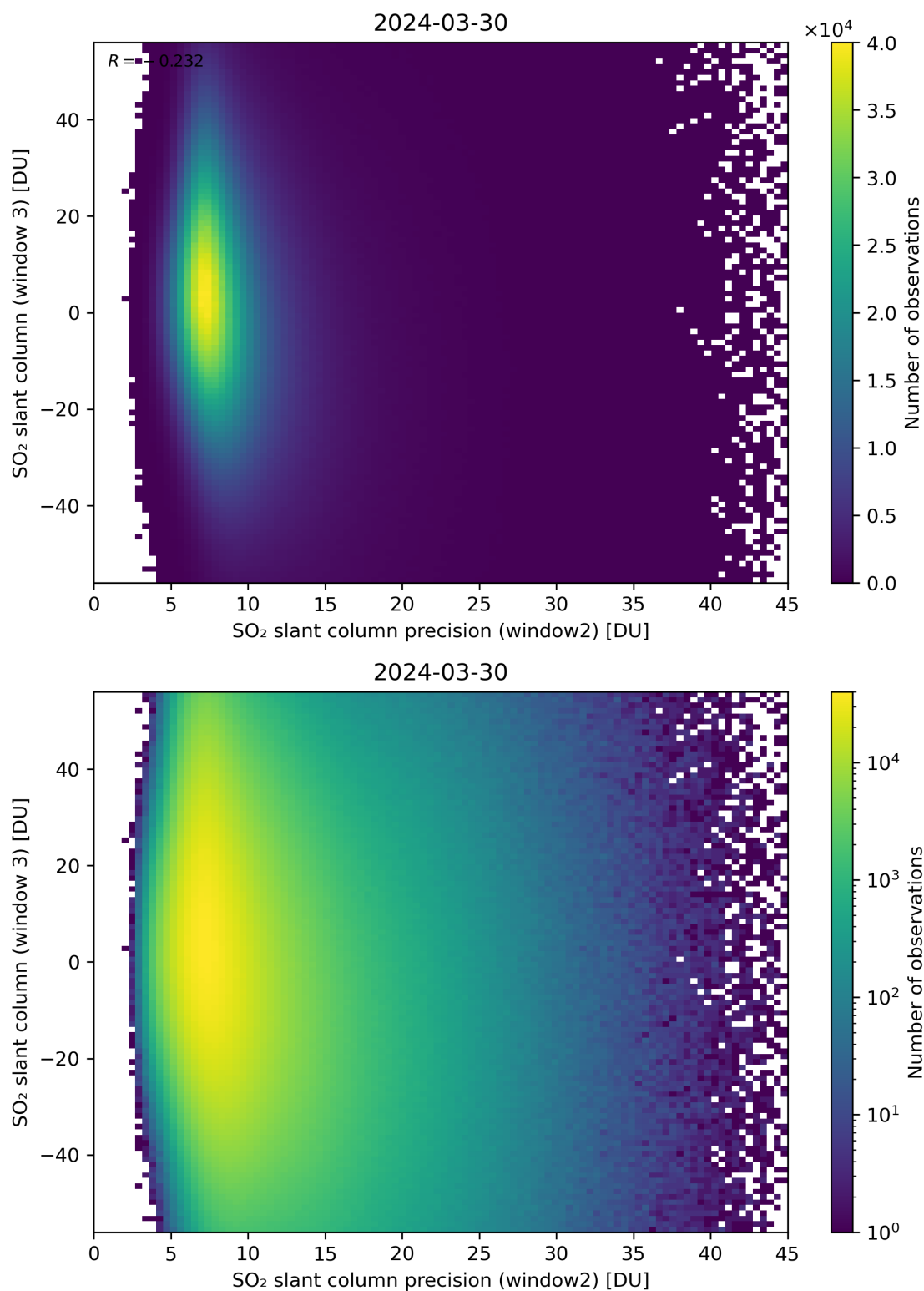
Figure 249: Scatter density plot of “SO 2 slant column precision (window2)” against “SO 2 slant column (window 3)” for 2024-03-30 to 2024-03-31.
