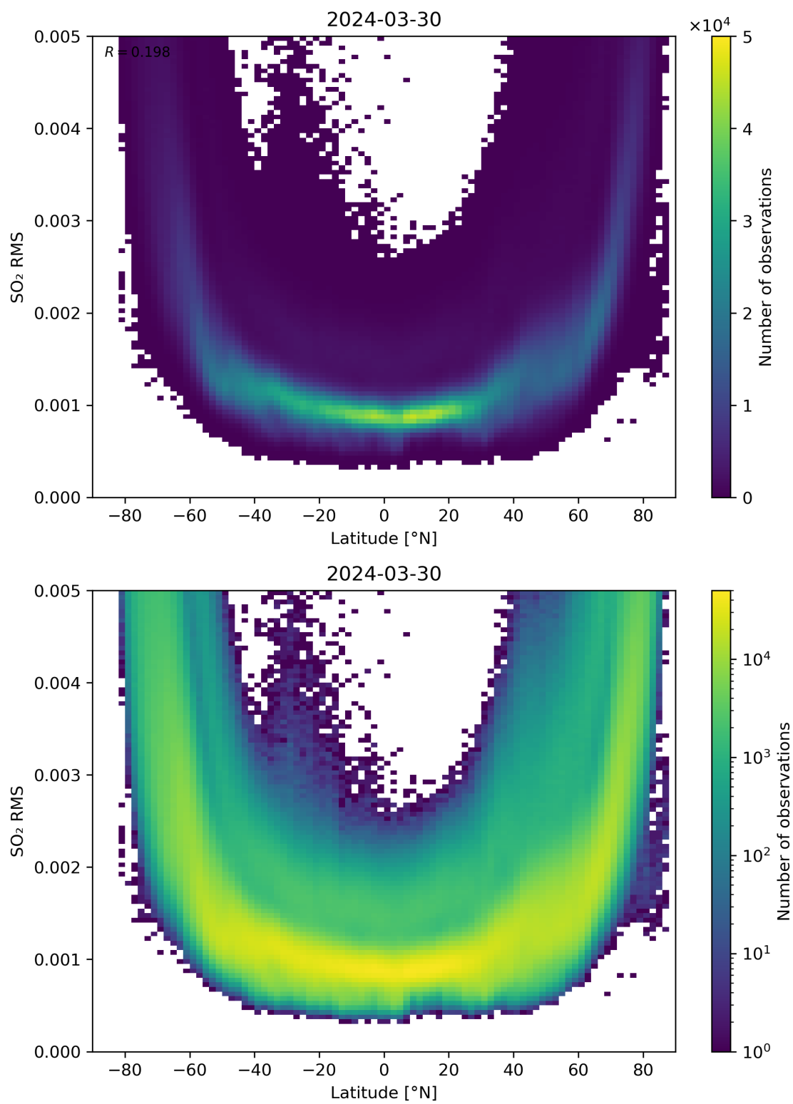
Figure 144: Scatter density plot of “Latitude” against “SO 2 RMS” for 2024-03-30 to 2024-03-31.
