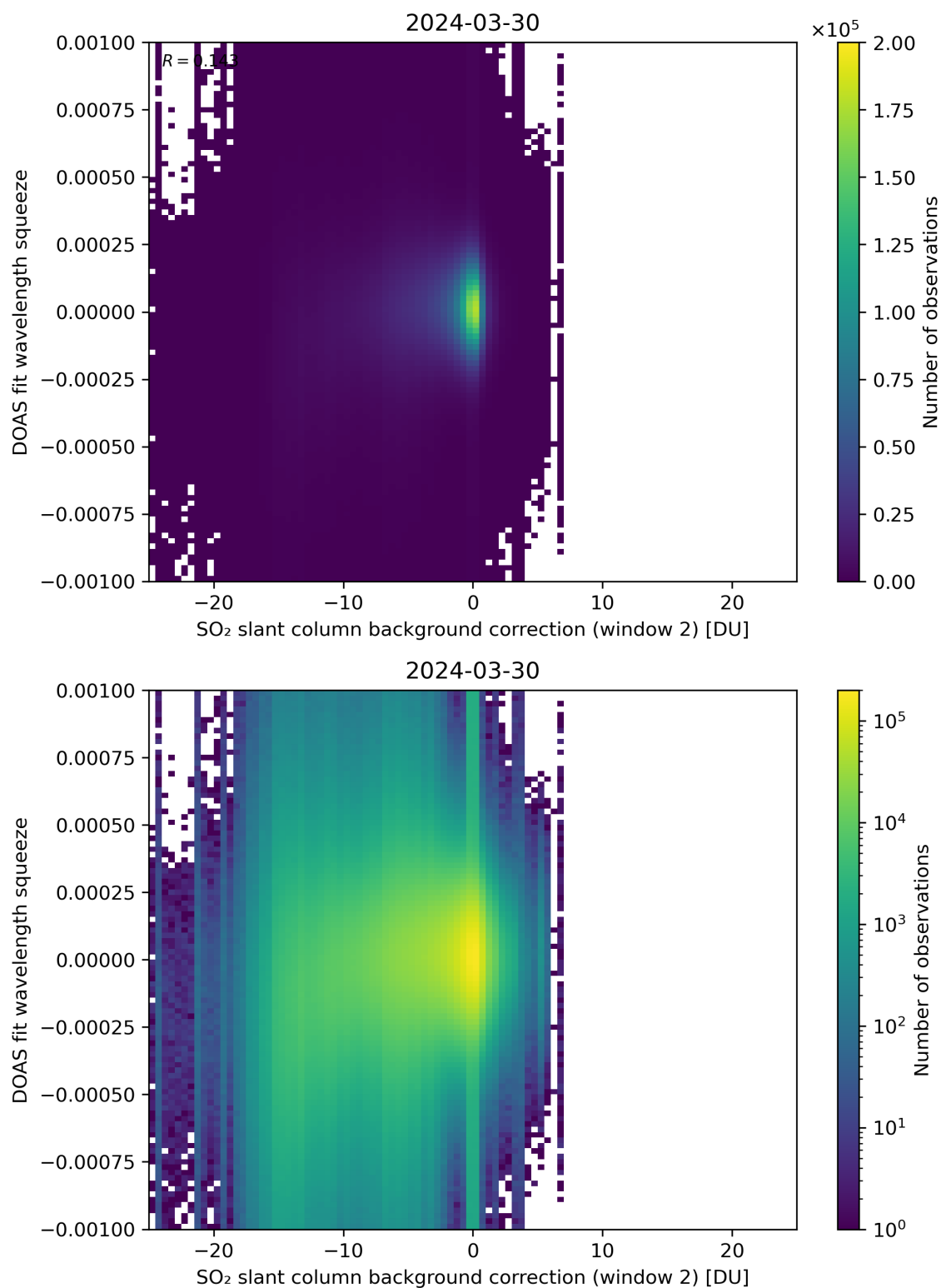
Figure 113: Scatter density plot of “SO 2 slant column background correction (window 2)” against “DOAS fit wavelength squeeze” for 2024-03-30 to 2024-03-31.
