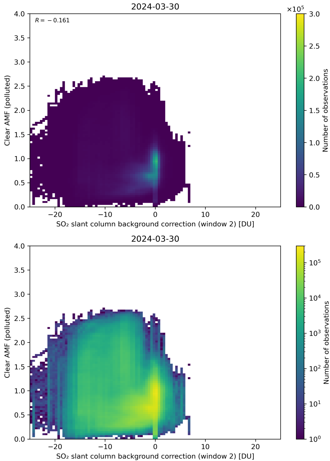
Figure 115: Scatter density plot of “SO 2 slant column background correction (window 2)” against “Clear AMF (polluted)” for 2024-03-30 to 2024-03-31.
