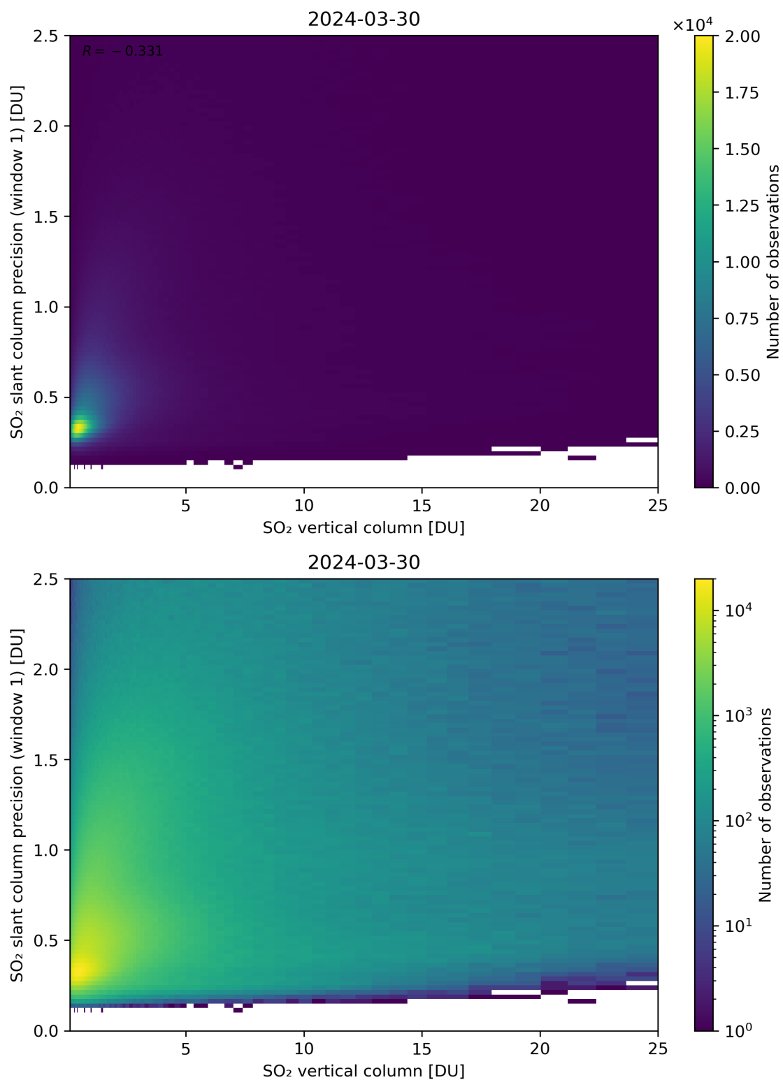
Figure 301: Scatter density plot of “SO 2 vertical column” against “SO 2 slant column precision (window 1)” for 2024-03-30 to 2024-03-31.
