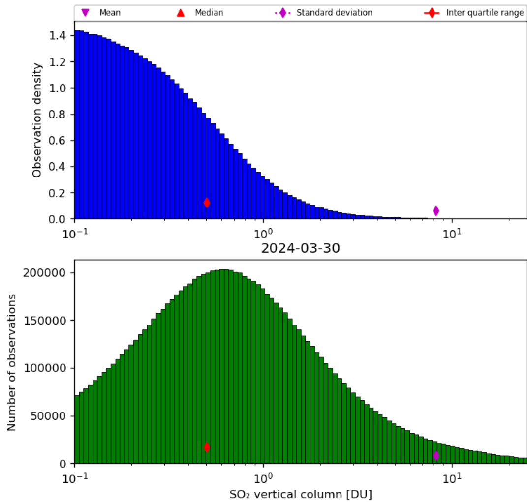
Figure 53: Histogram of “SO 2 vertical column” for 2024-03-30 to 2024-03-31
