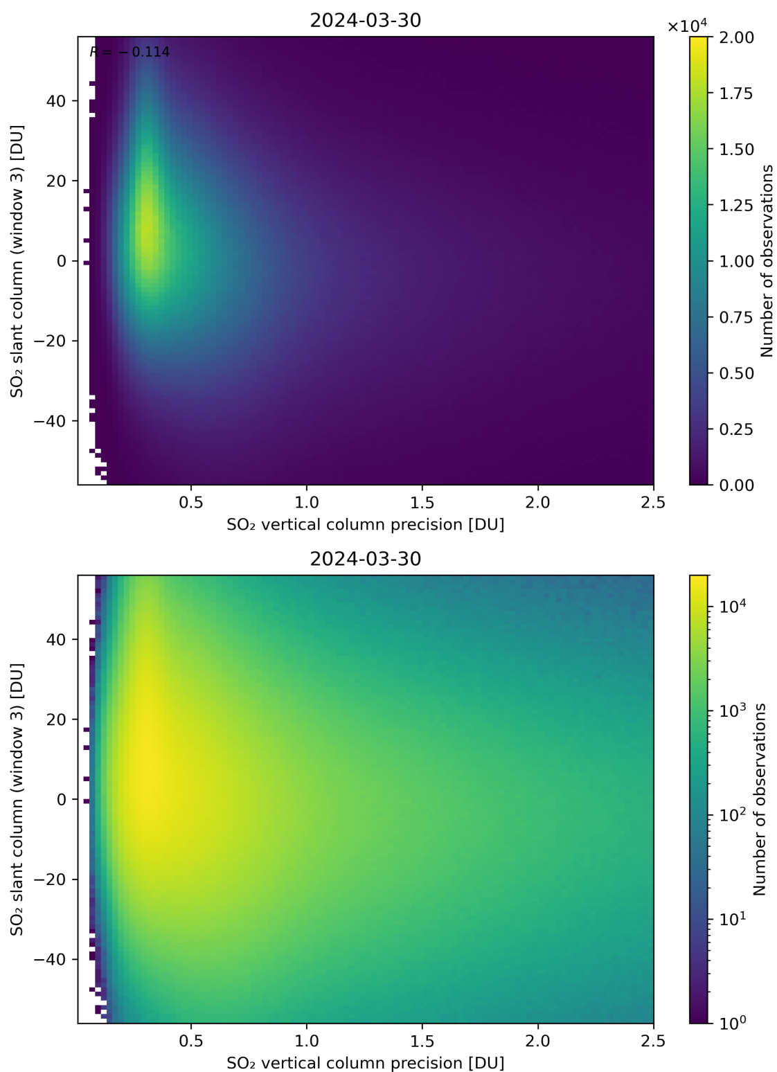
Figure 292: Scatter density plot of “SO 2 vertical column precision” against “SO 2 slant column (window 3)” for 2024-03-30 to 2024-03-31.
