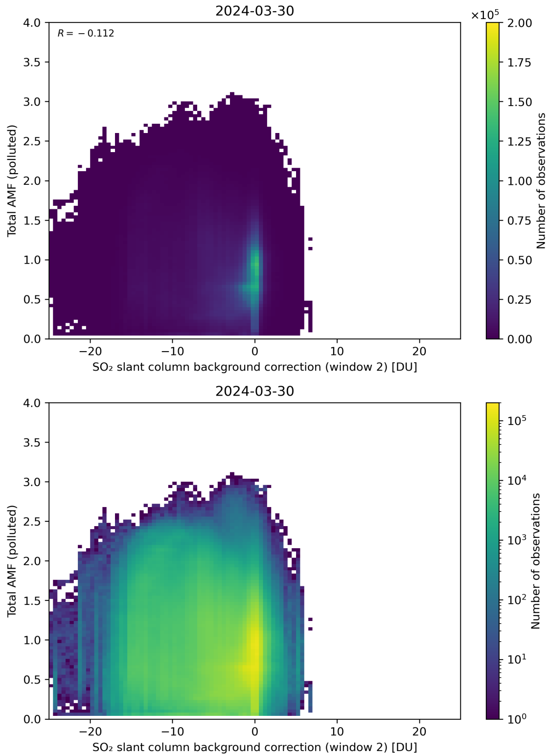
Figure 119: Scatter density plot of “SO 2 slant column background correction (window 2)” against “Total AMF (polluted)” for 2024-03-30 to 2024-03-31.
