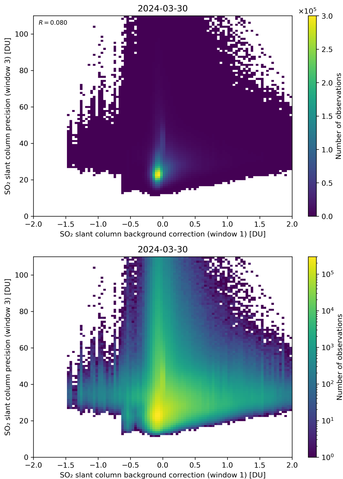
Figure 108: Scatter density plot of “SO 2 slant column background correction (window 1)” against “SO 2 slant column precision (window 3)” for 2024-03-30 to 2024-03-31.
