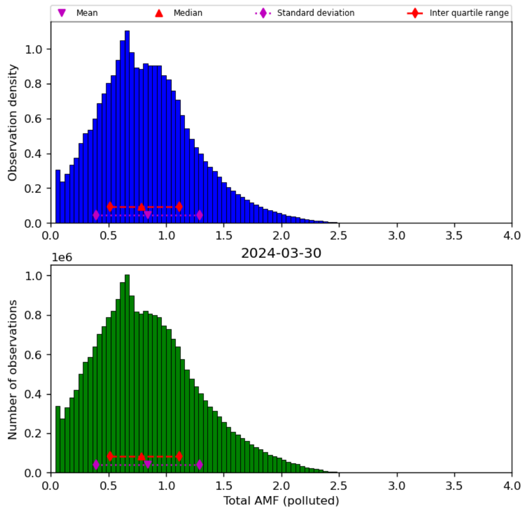
Figure 71: Histogram of “Total AMF (polluted)” for 2024-03-30 to 2024-03-31
