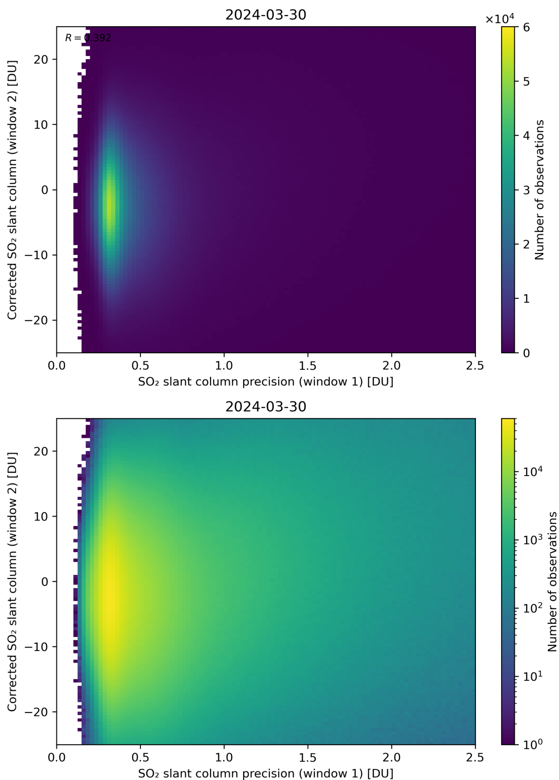
Figure 225: Scatter density plot of “SO 2 slant column precision (window 1)” against “Corrected SO 2 slant column (window 2)” for 2024-03-30 to 2024-03-31.
