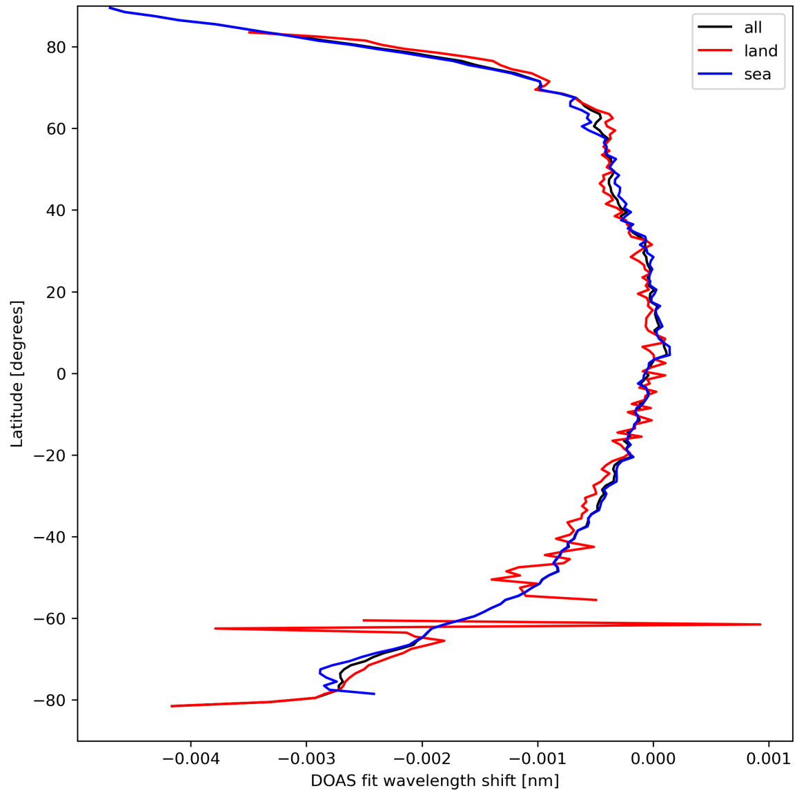
Figure 45: Zonal average of “DOAS fit wavelength shift” for 2024-03-30 to 2024-03-31.
