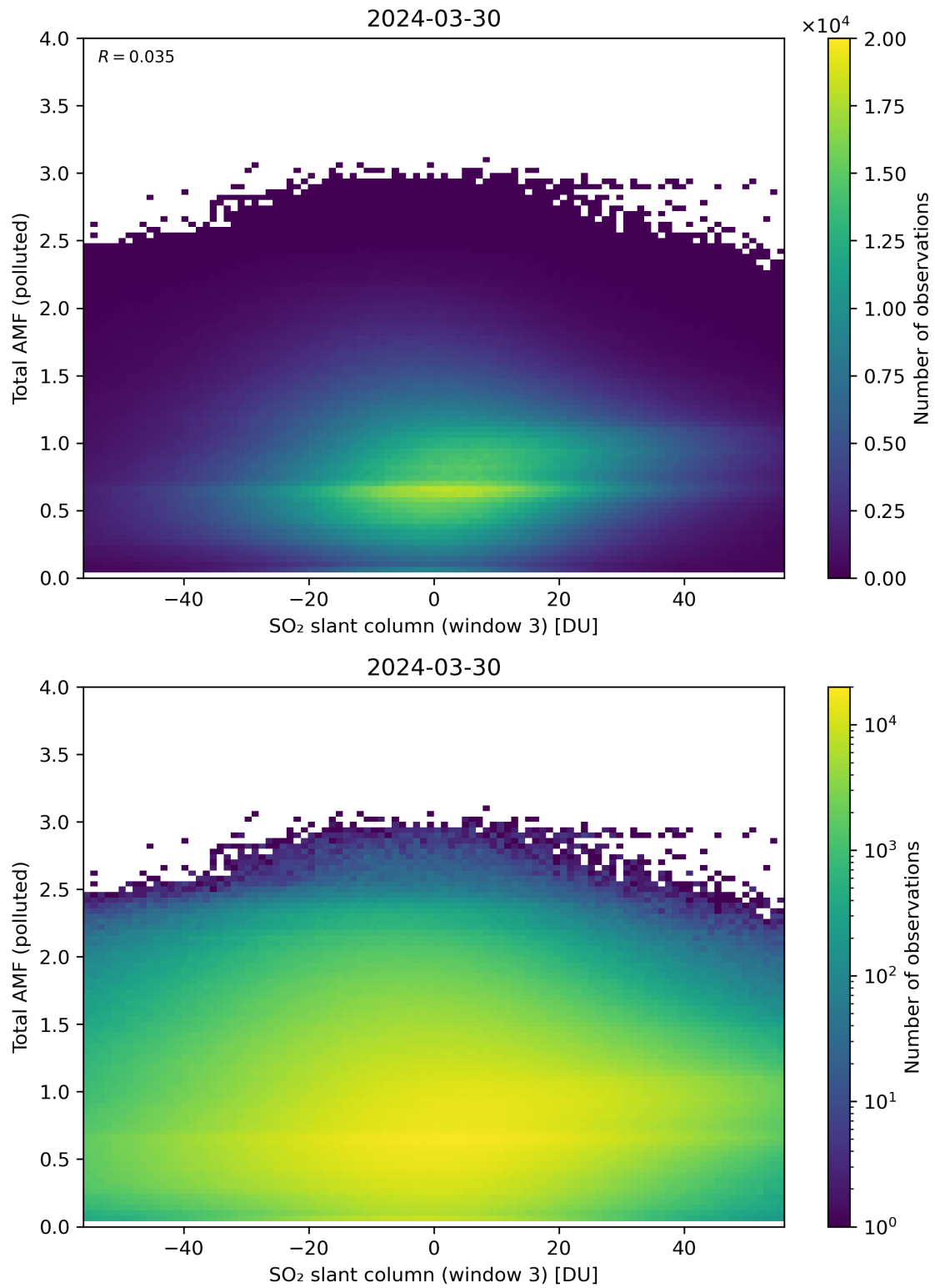
Figure 268: Scatter density plot of “SO 2 slant column (window 3)” against “Total AMF (polluted)” for 2024-03-30 to 2024-03-31.
