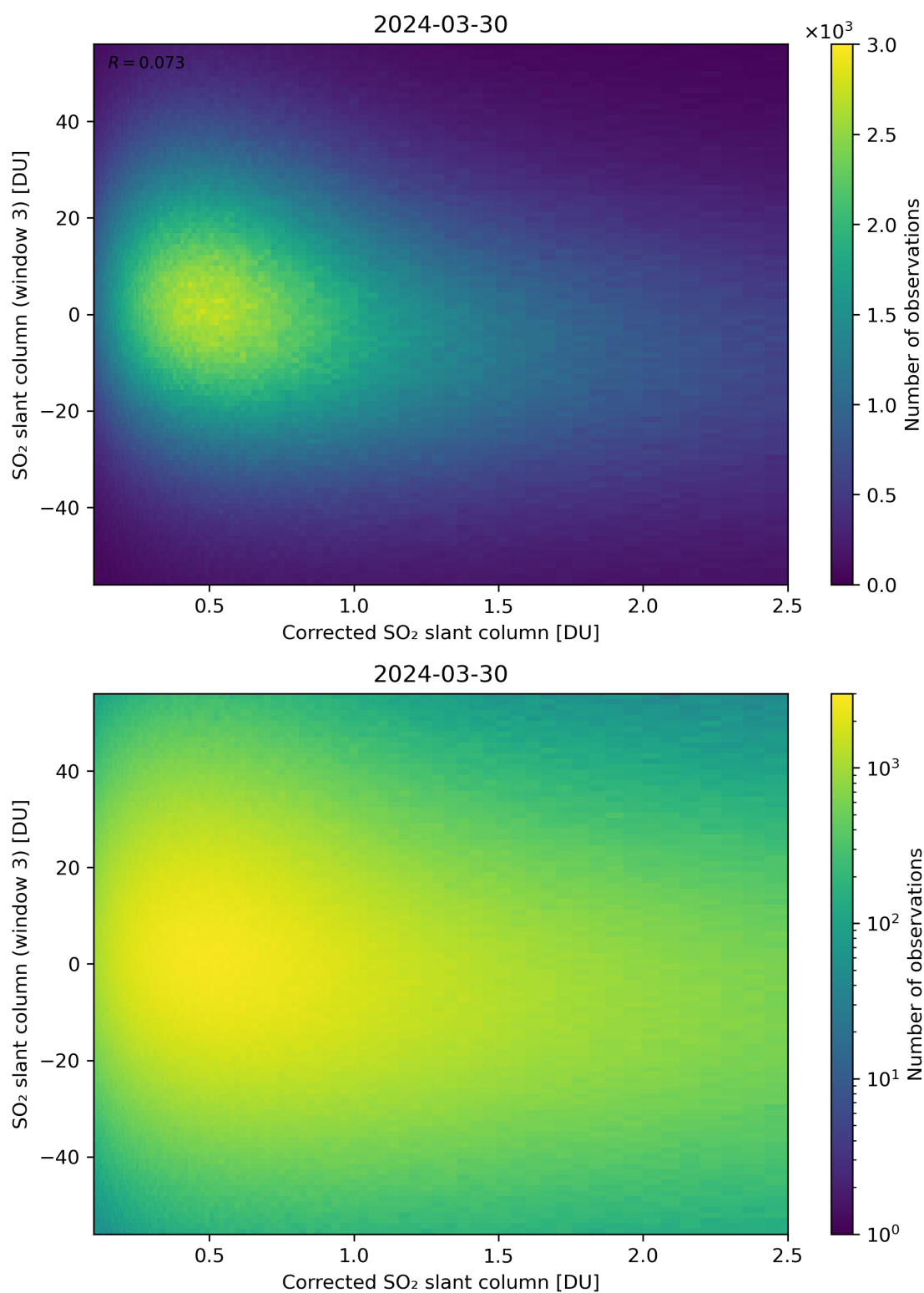
Figure 190: Scatter density plot of “Corrected SO 2 slant column” against “SO 2 slant column (window 3)” for 2024-03-30 to 2024-03-31.
