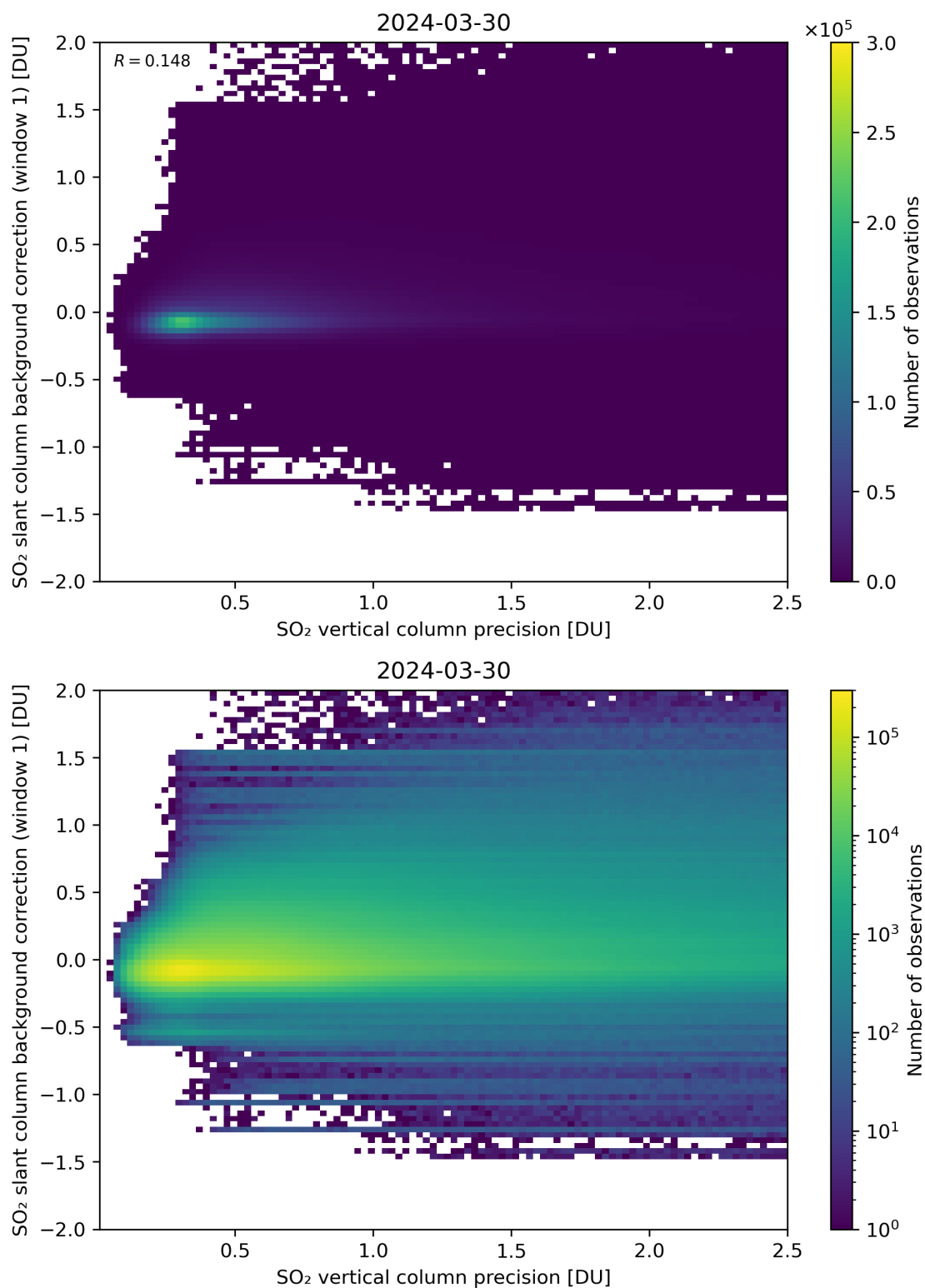
Figure 279: Scatter density plot of “SO 2 vertical column precision” against “SO 2 slant column background correction (window 1)” for 2024-03-30 to 2024-03-31.
