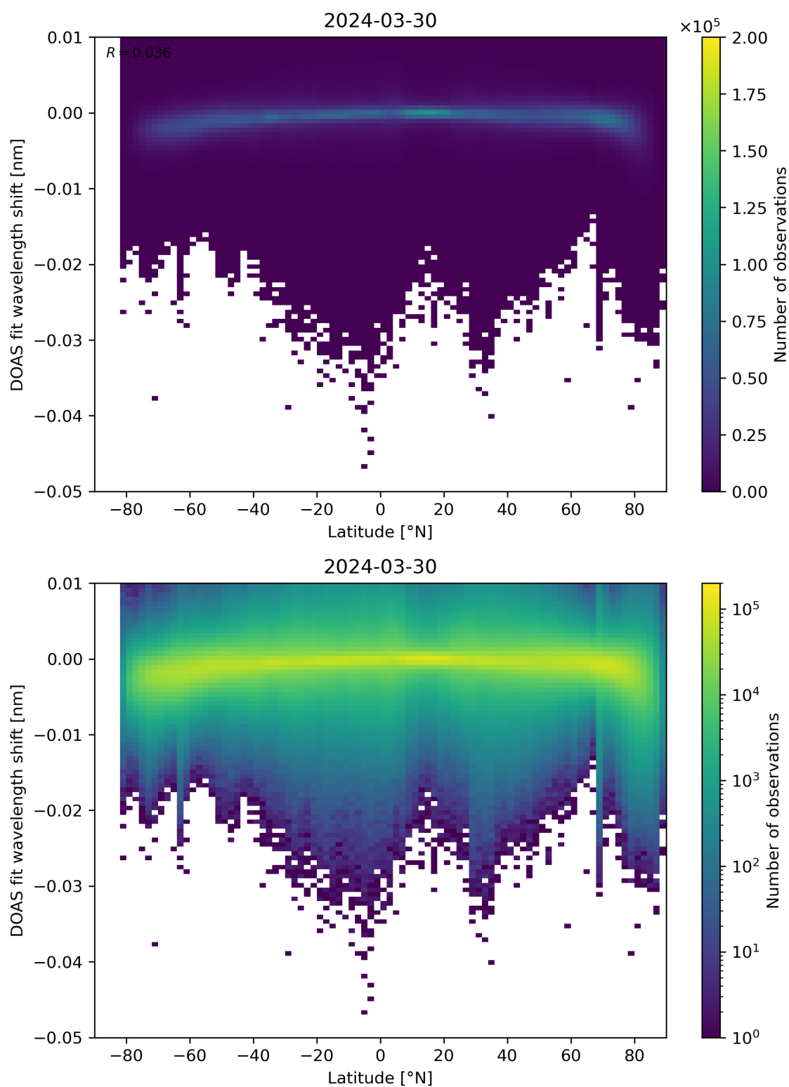
Figure 142: Scatter density plot of “Latitude” against “DOAS fit wavelength shift” for 2024-03-30 to 2024-03-31.
