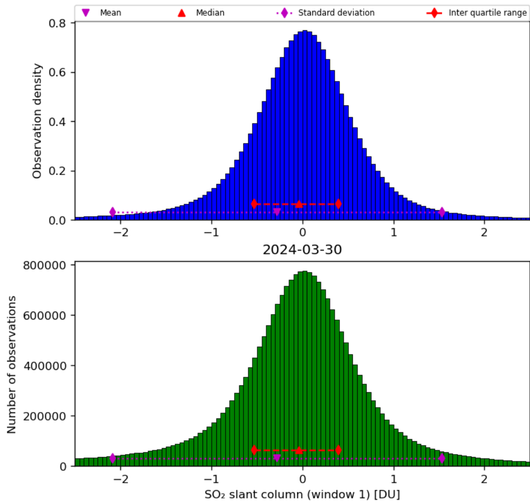
Figure 56: Histogram of “SO 2 slant column (window 1)” for 2024-03-30 to 2024-03-31
