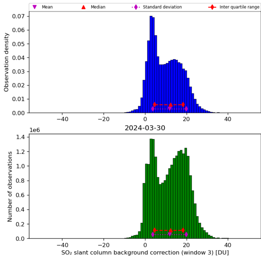
Figure 67: Histogram of “SO 2 slant column background correction (window 3)” for 2024-03-30 to 2024-03-31
