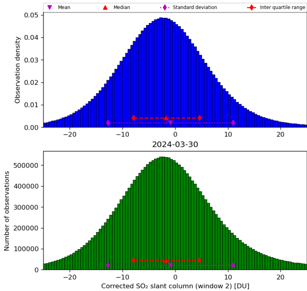
Figure 62: Histogram of “Corrected SO 2 slant column (window 2)” for 2024-03-30 to 2024-03-31
