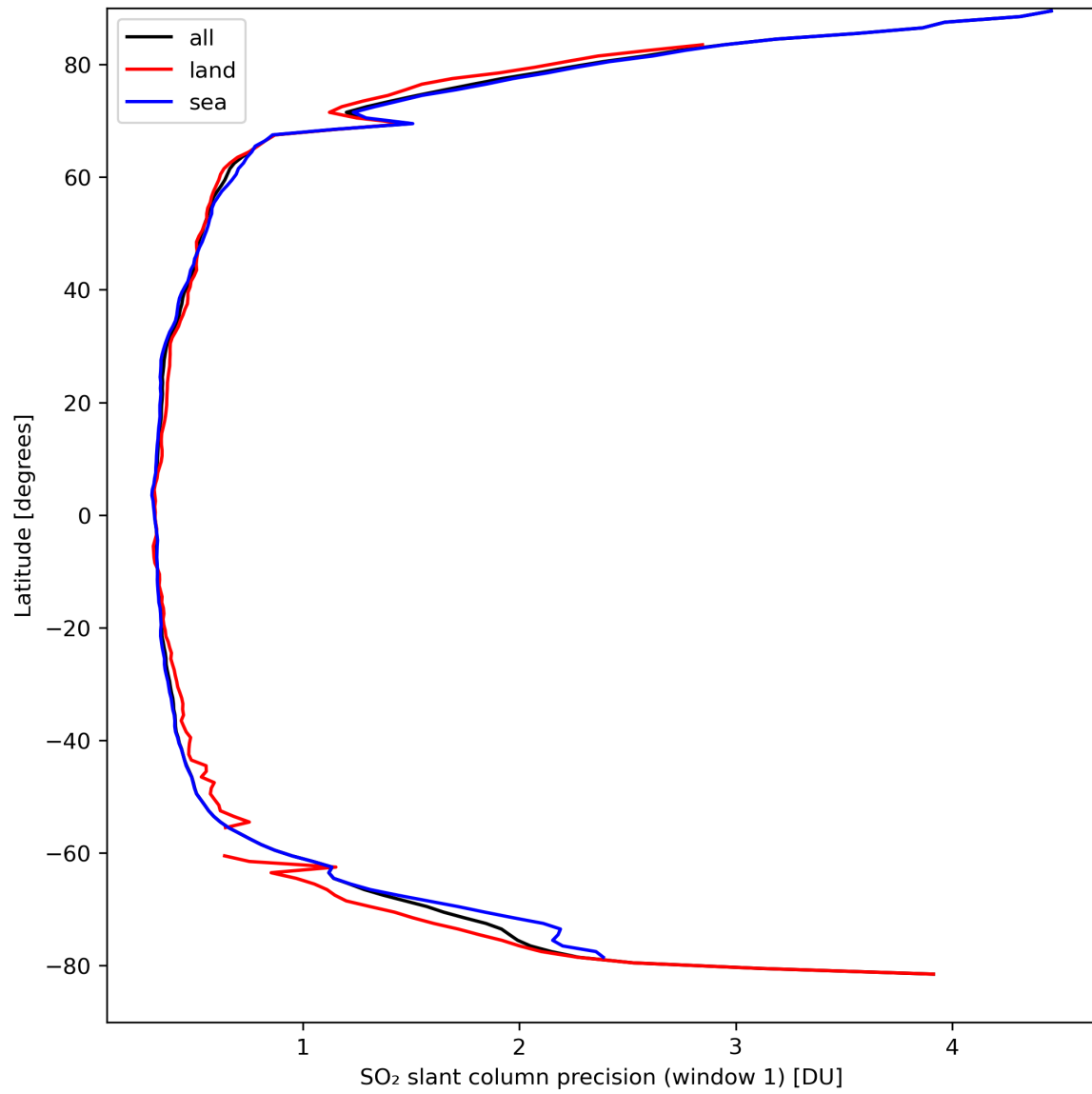
Figure 34: Zonal average of “SO 2 slant column precision (window 1)” for 2024-03-30 to 2024-03-31.
