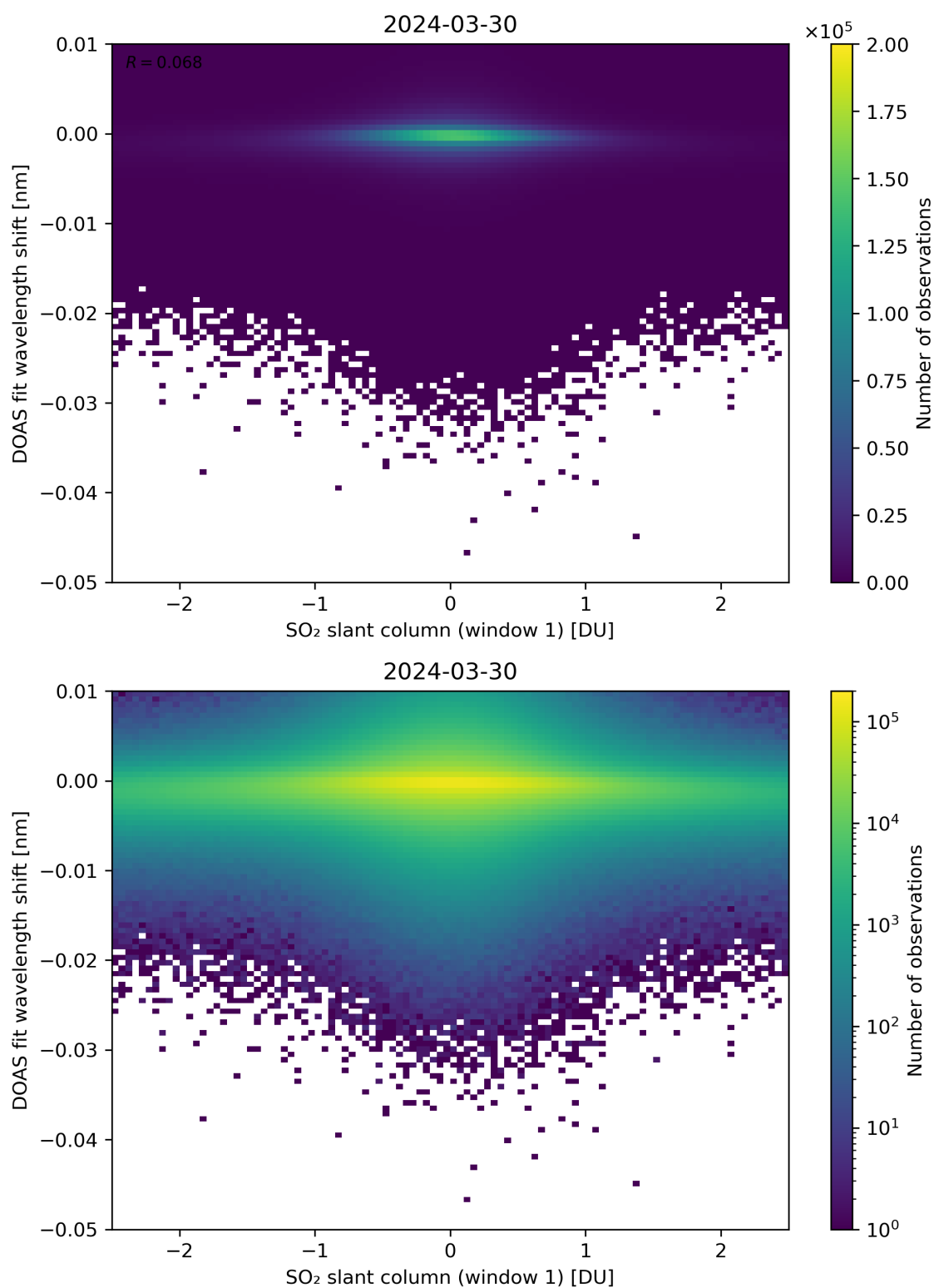
Figure 215: Scatter density plot of “SO 2 slant column (window 1)” against “DOAS fit wavelength shift” for 2024-03-30 to 2024-03-31.
