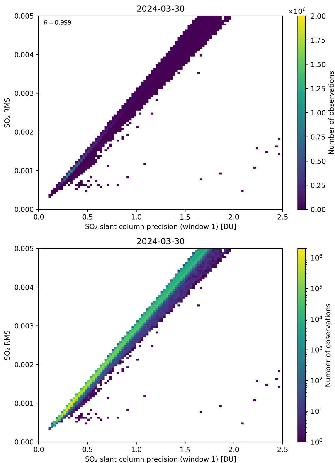
Figure 223: Scatter density plot of “SO 2 slant column precision (window 1)” against “SO 2 RMS” for 2024-03-30 to 2024-03-31.
