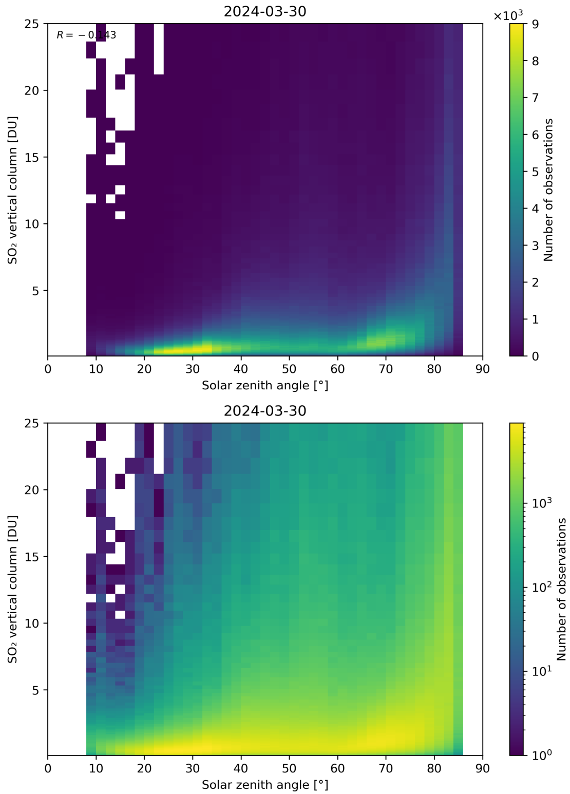
Figure 176: Scatter density plot of “Solar zenith angle” against “SO 2 vertical column” for 2024-03-30 to 2024-03-31.
