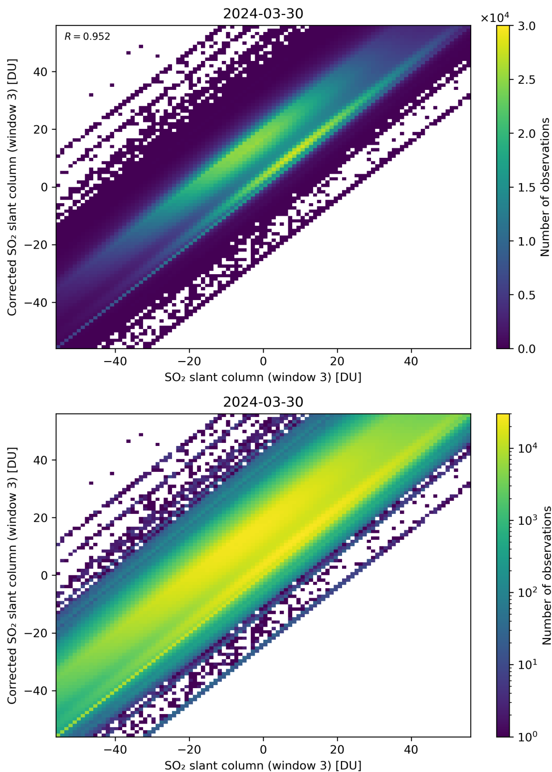
Figure 266: Scatter density plot of “SO 2 slant column (window 3)” against “Corrected SO 2 slant column (window 3)” for 2024-03-30 to 2024-03-31.
