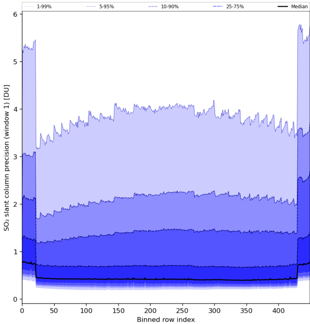
Figure 80: Along track statistics of “SO 2 slant column precision (window 1)” for 2024-03-30 to 2024-03-31
