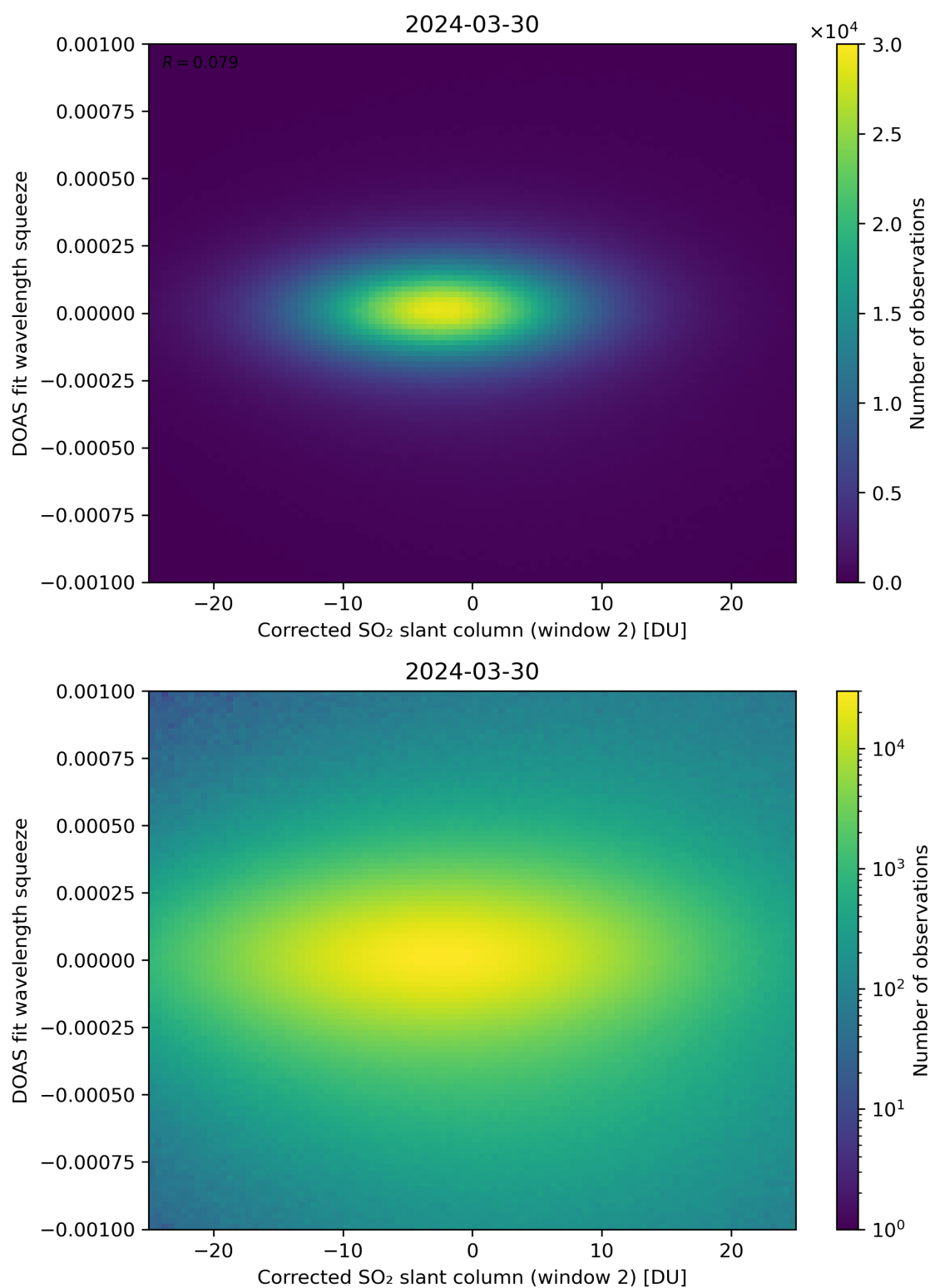
Figure 197: Scatter density plot of “Corrected SO 2 slant column (window 2)” against “DOAS fit wavelength squeeze” for 2024-03-30 to 2024-03-31.
