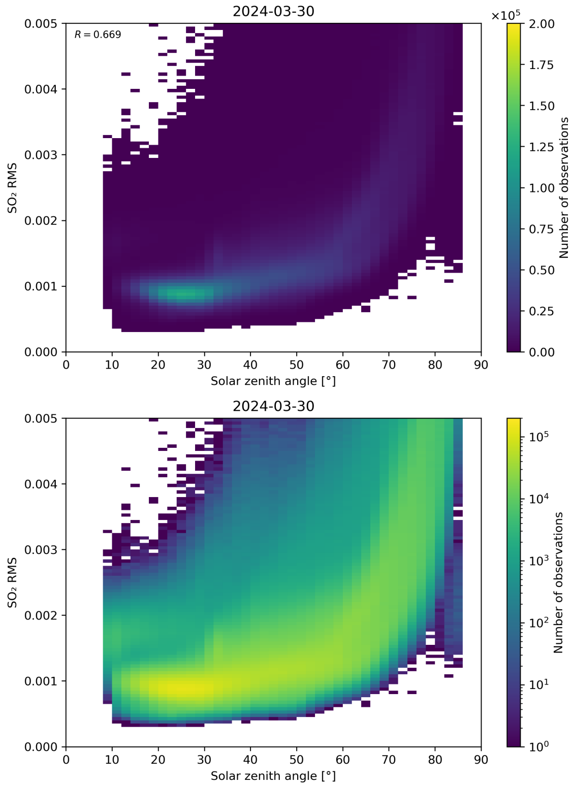
Figure 163: Scatter density plot of “Solar zenith angle” against “SO 2 RMS” for 2024-03-30 to 2024-03-31.
