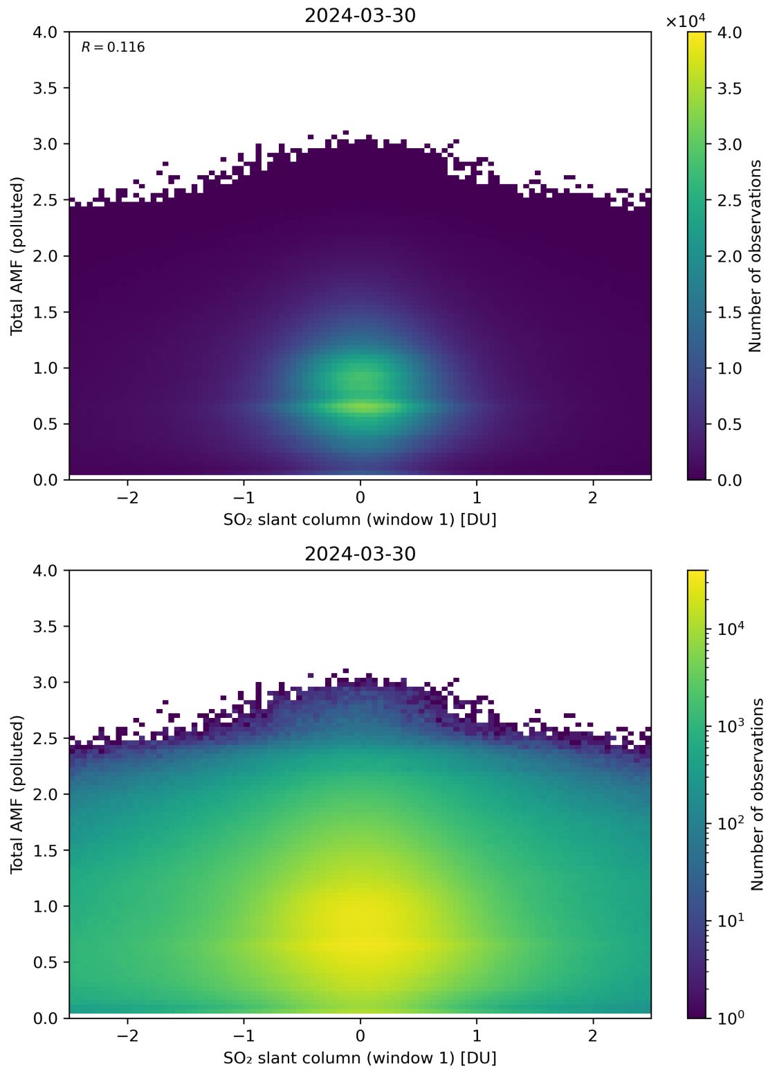
Figure 239: Scatter density plot of “SO 2 slant column (window 1)” against “Total AMF (polluted)” for 2024-03-30 to 2024-03-31.
