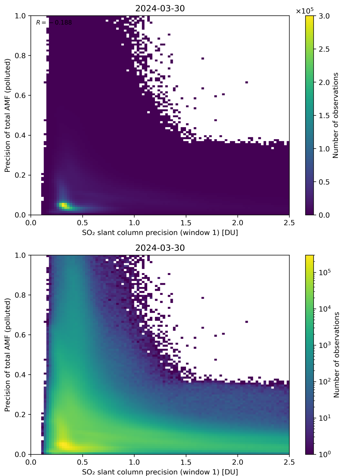
Figure 231: Scatter density plot of “SO 2 slant column precision (window 1)” against “Precision of total AMF (polluted)” for 2024-03-30 to 2024-03-31.
