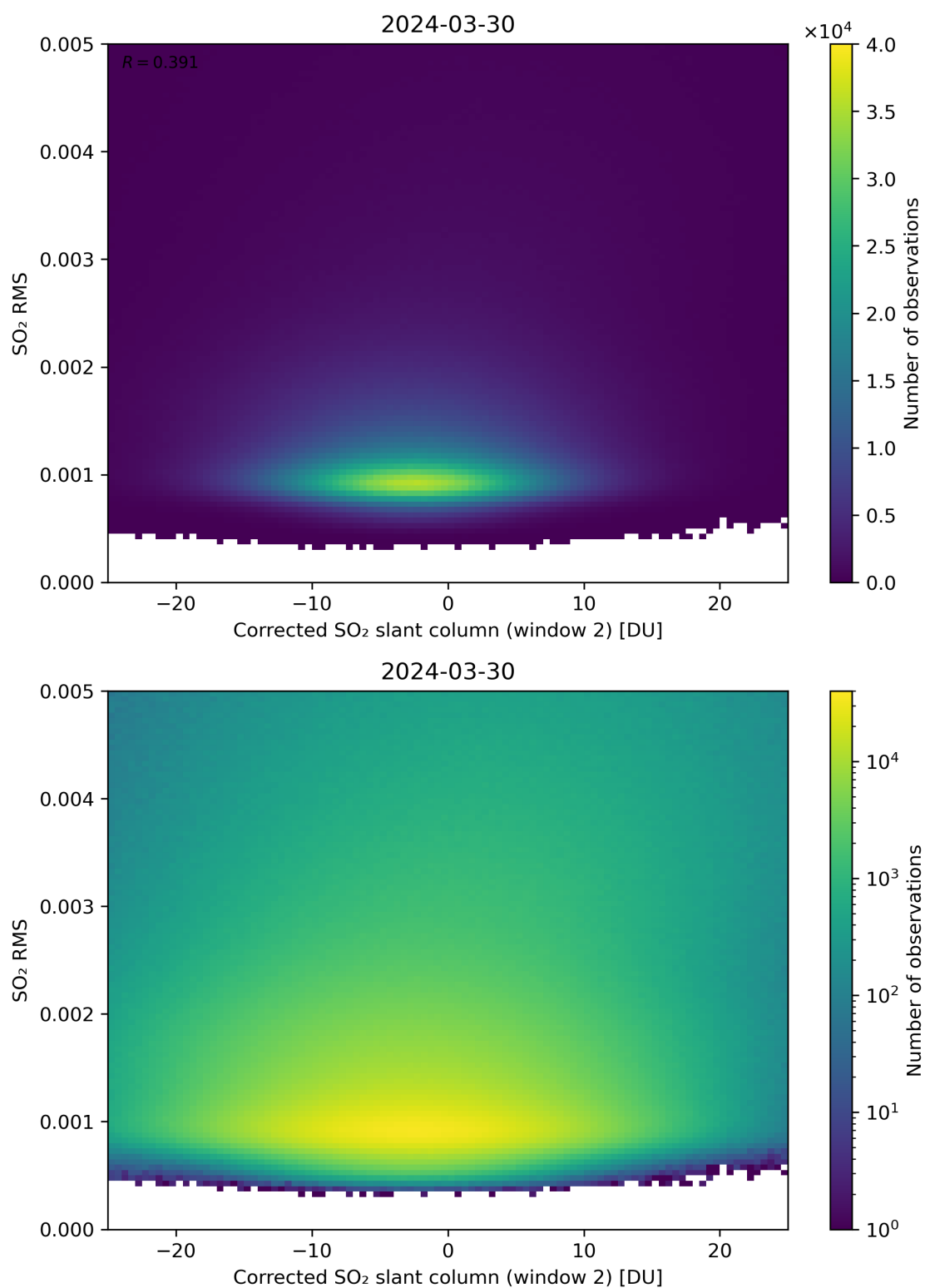
Figure 198: Scatter density plot of “Corrected SO 2 slant column (window 2)” against “SO 2 RMS” for 2024-03-30 to 2024-03-31.
