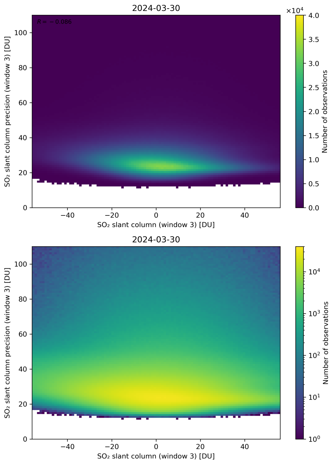
Figure 267: Scatter density plot of “SO 2 slant column (window 3)” against “SO 2 slant column precision (window 3)” for 2024-03-30 to 2024-03-31.
