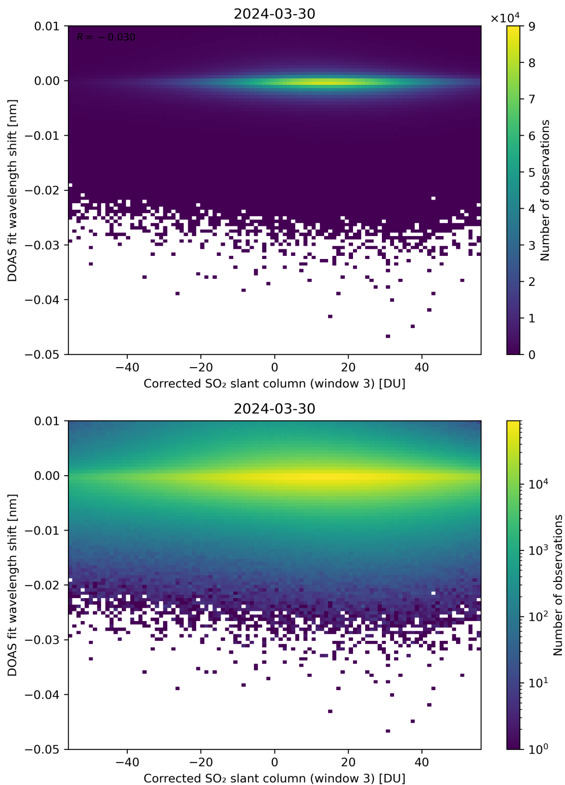
Figure 206: Scatter density plot of “Corrected SO 2 slant column (window 3)” against “DOAS fit wavelength shift” for 2024-03-30 to 2024-03-31.
