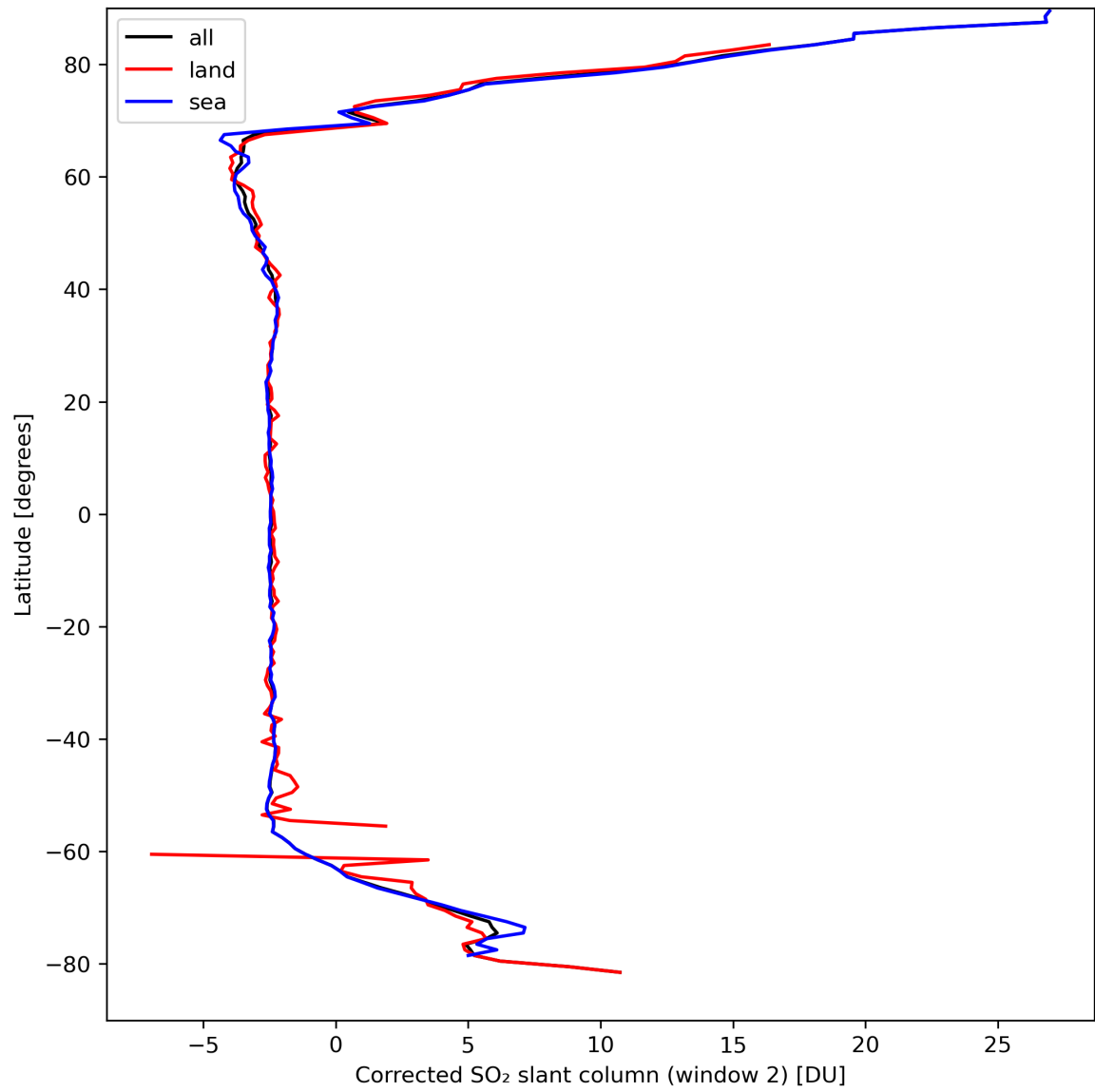
Figure 39: Zonal average of “Corrected SO 2 slant column (window 2)” for 2024-03-30 to 2024-03-31.
