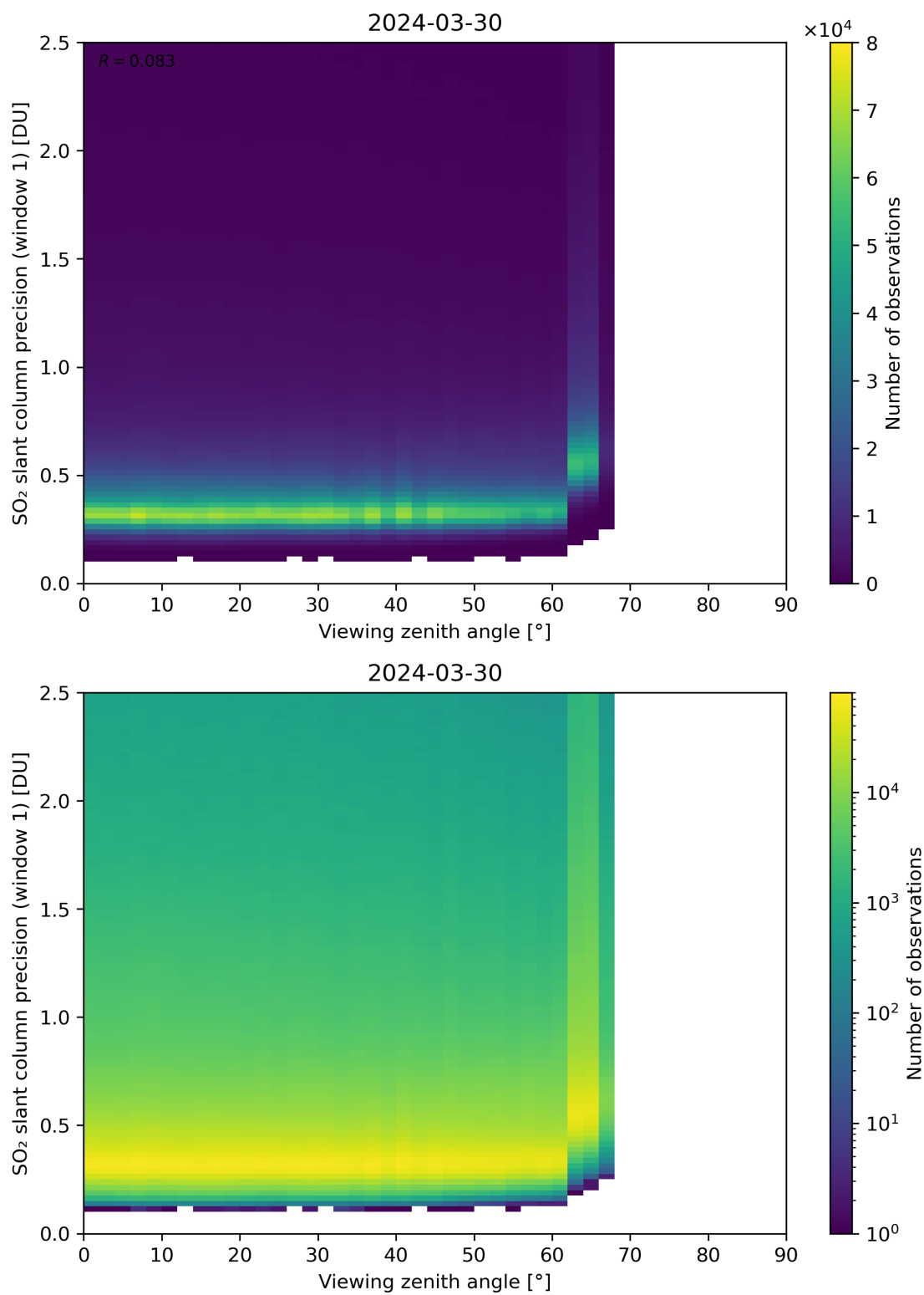
Figure 321: Scatter density plot of “Viewing zenith angle” against “SO 2 slant column precision (window 1)” for 2024-03-30 to 2024-03-31.
