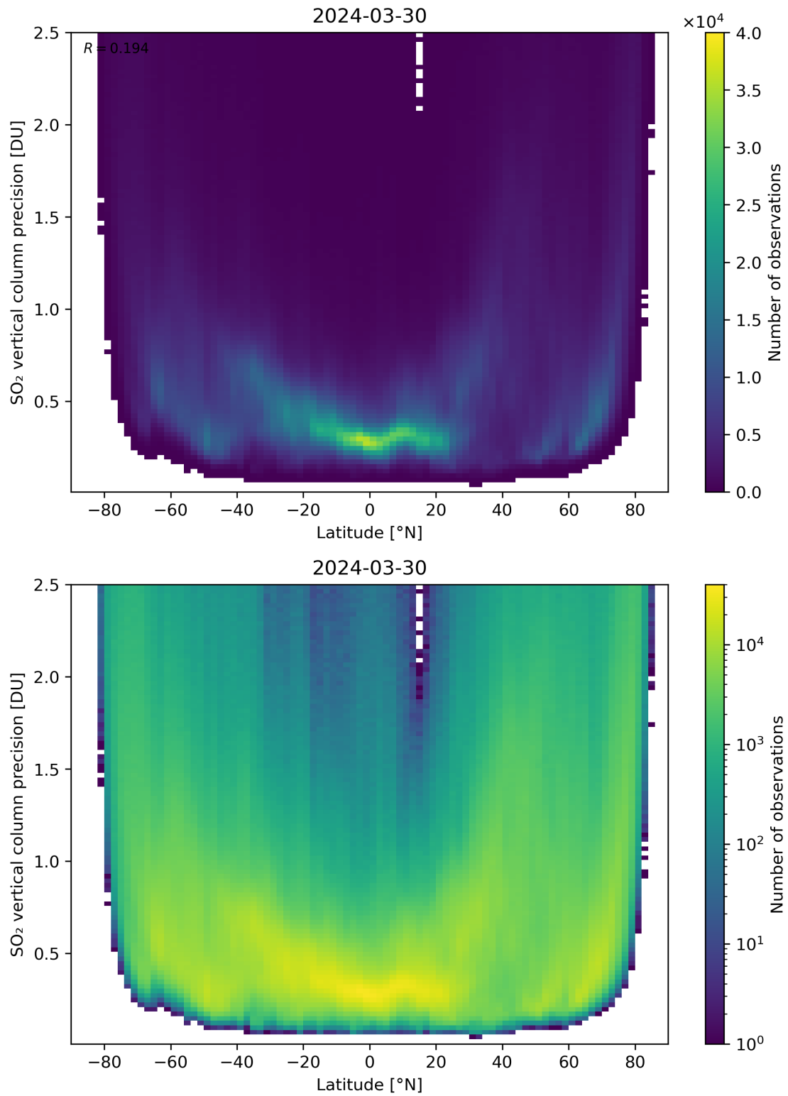
Figure 157: Scatter density plot of “Latitude” against “SO 2 vertical column precision” for 2024-03-30 to 2024-03-31.
