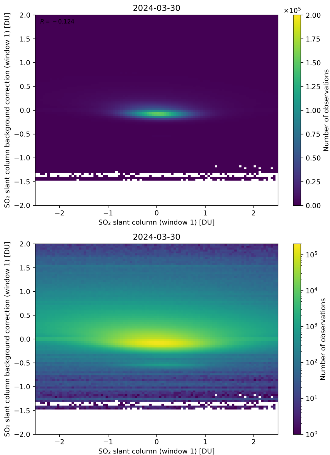
Figure 212: Scatter density plot of “SO 2 slant column (window 1)” against “SO 2 slant column background correction (window 1)” for 2024-03-30 to 2024-03-31.
