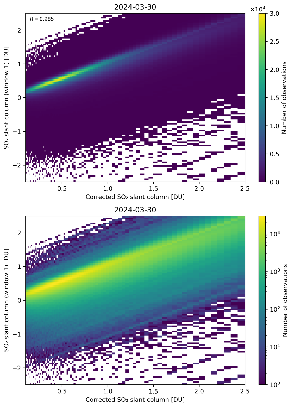
Figure 187: Scatter density plot of “Corrected SO 2 slant column” against “SO 2 slant column (window 1)” for 2024-03-30 to 2024-03-31.
