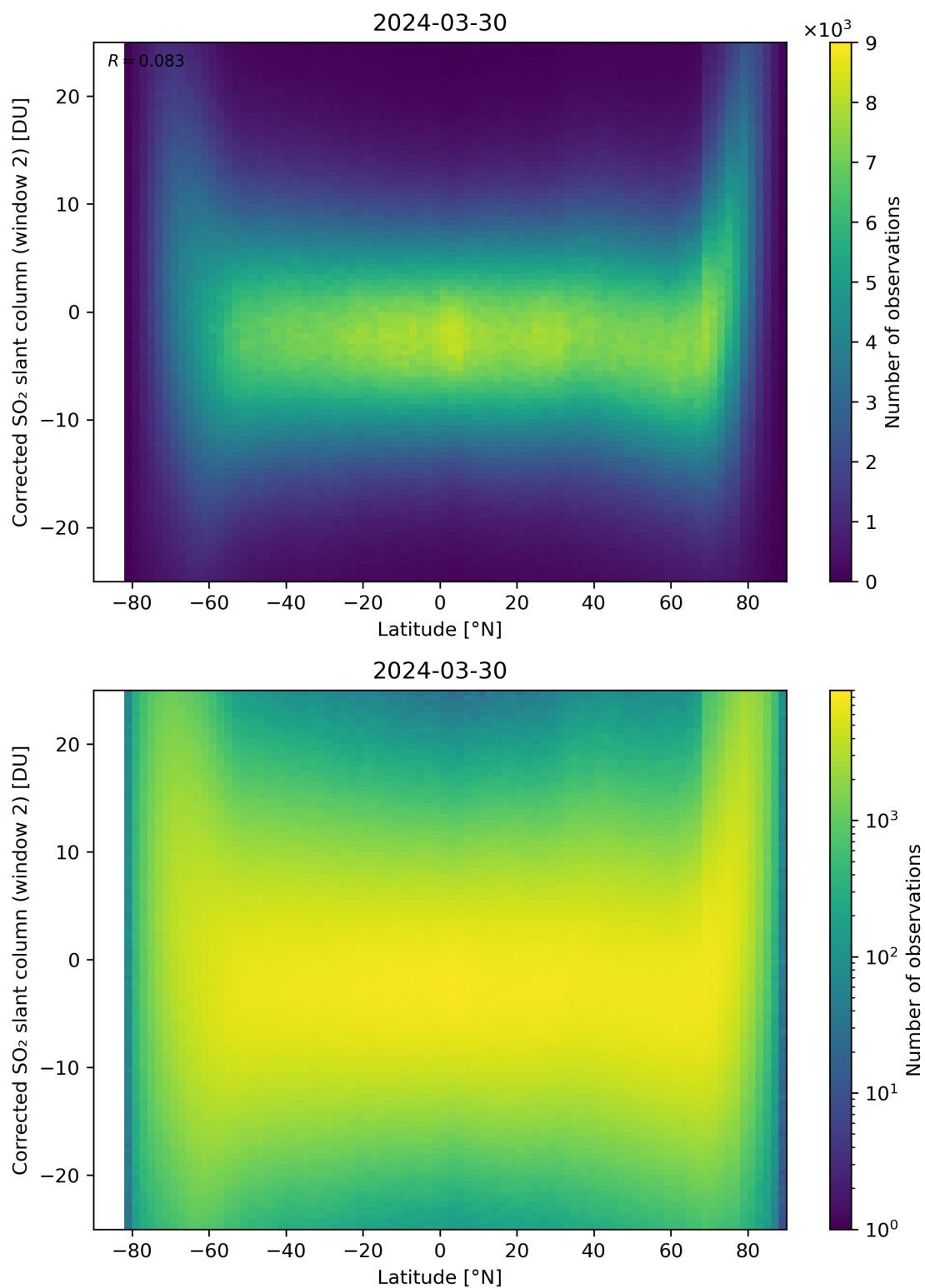
Figure 147: Scatter density plot of “Latitude” against “Corrected SO 2 slant column (window 2)” for 2024-03-30 to 2024-03-31.
