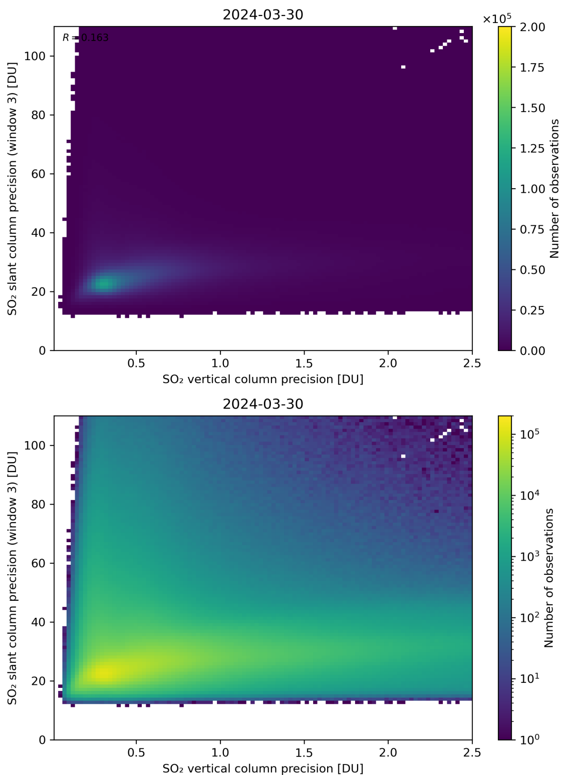
Figure 293: Scatter density plot of “SO 2 vertical column precision” against “SO 2 slant column precision (window 3)” for 2024-03-30 to 2024-03-31.
