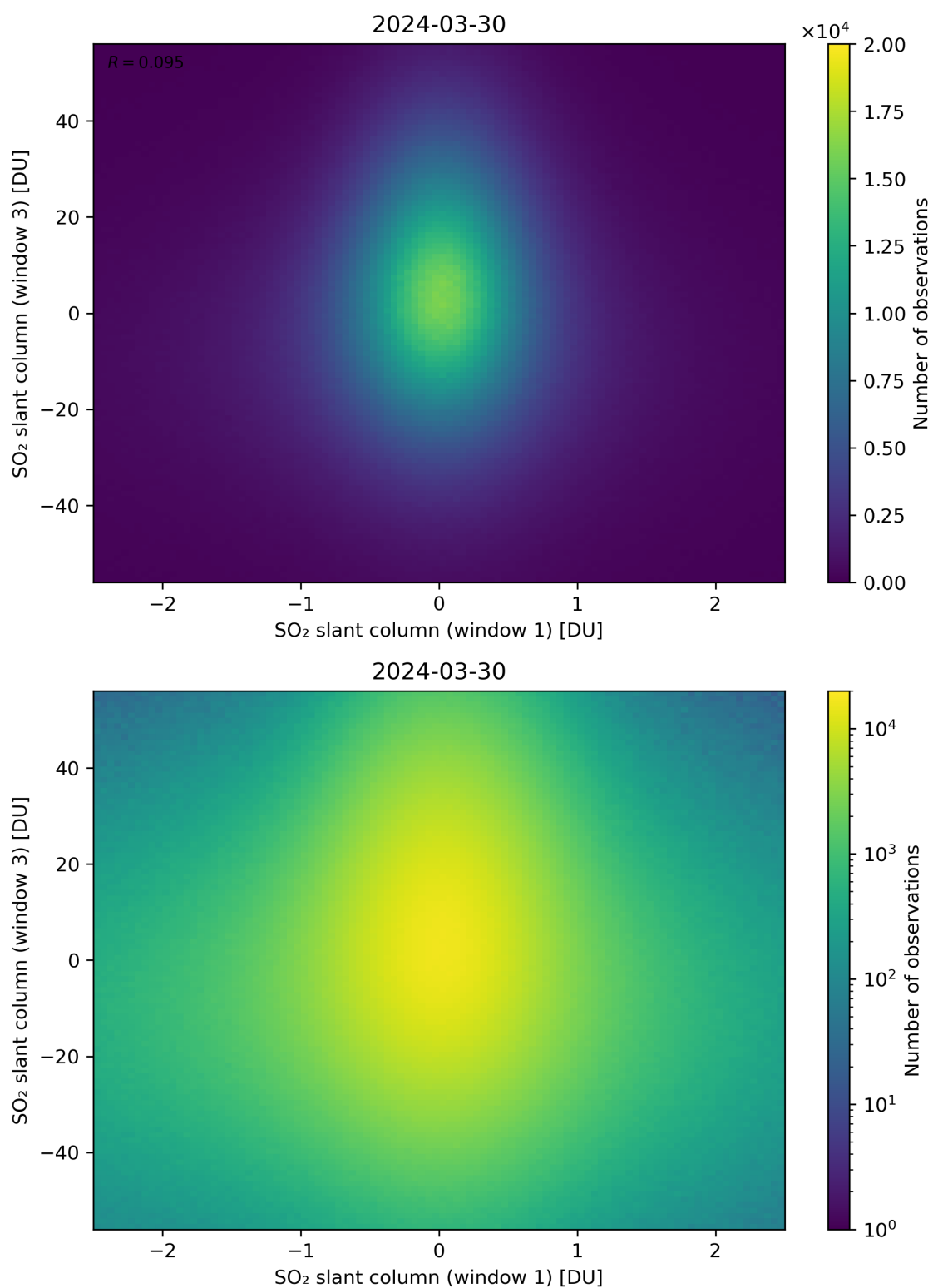
Figure 237: Scatter density plot of “SO 2 slant column (window 1)” against “SO 2 slant column (window 3)” for 2024-03-30 to 2024-03-31.
