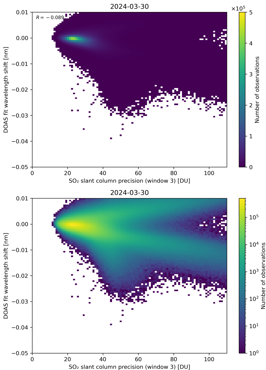
Figure 258: Scatter density plot of “SO 2 slant column precision (window 3)” against “DOAS fit wavelength shift” for 2024-03-30 to 2024-03-31.
