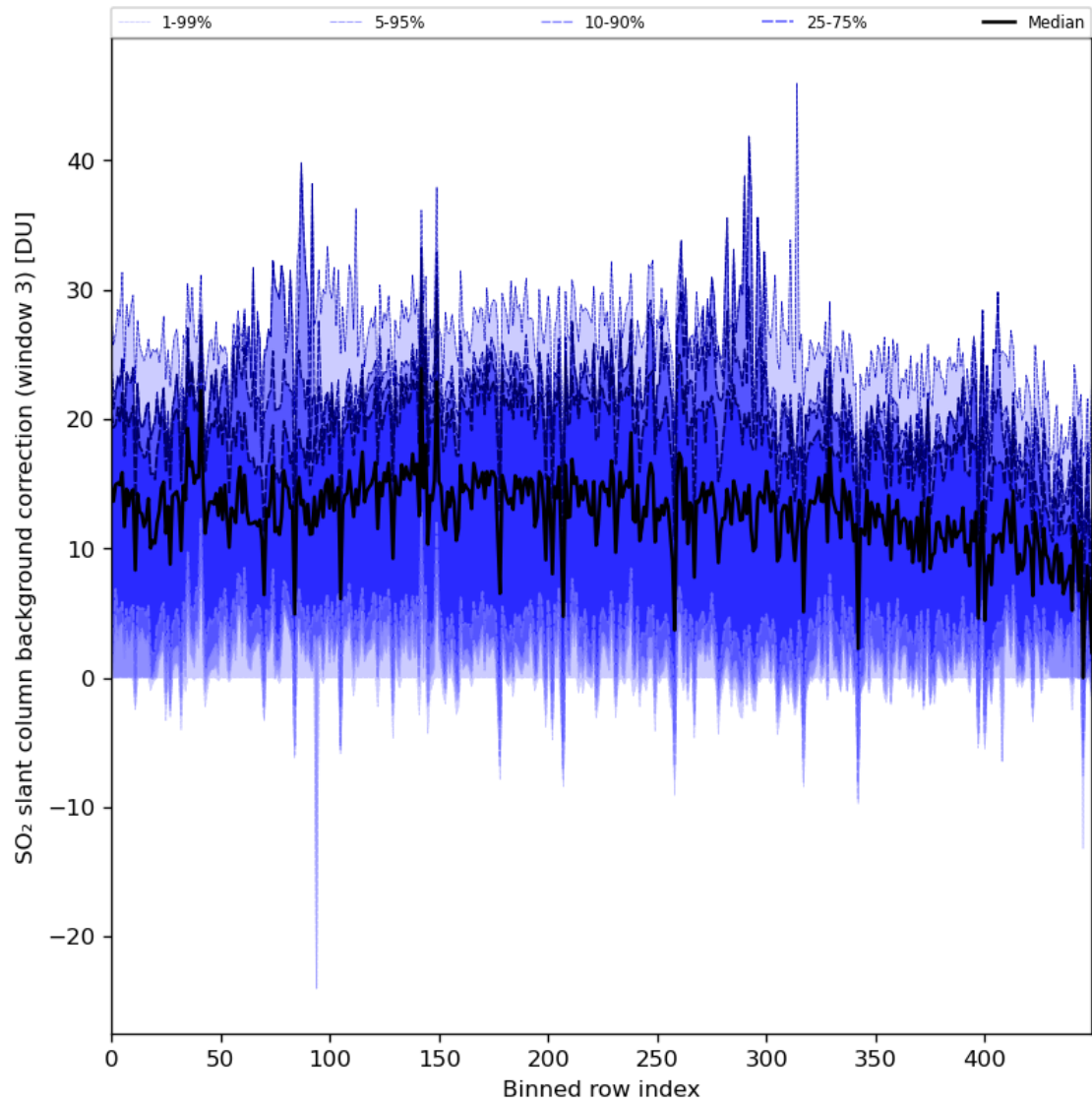
Figure 90: Along track statistics of “SO 2 slant column background correction (window 3)” for 2024-03-30 to 2024-03-31
