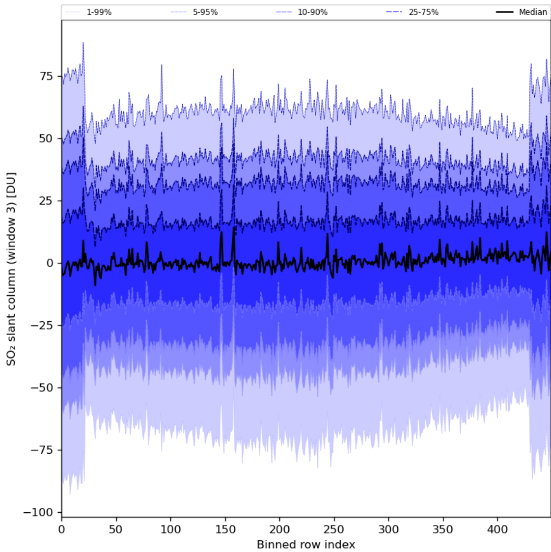
Figure 87: Along track statistics of “SO 2 slant column (window 3)” for 2024-03-30 to 2024-03-31
