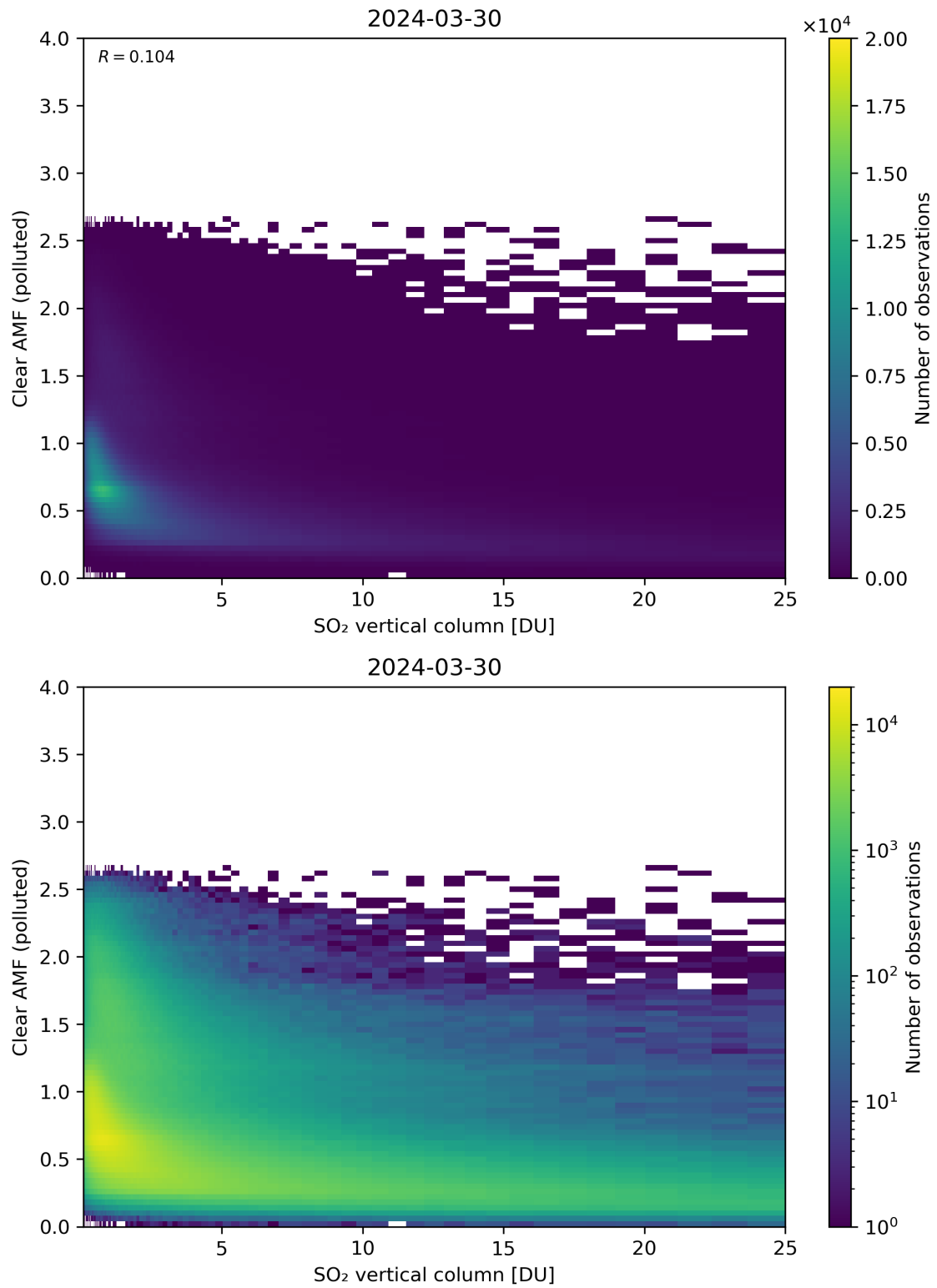
Figure 296: Scatter density plot of “SO 2 vertical column” against “Clear AMF (polluted)” for 2024-03-30 to 2024-03-31.
