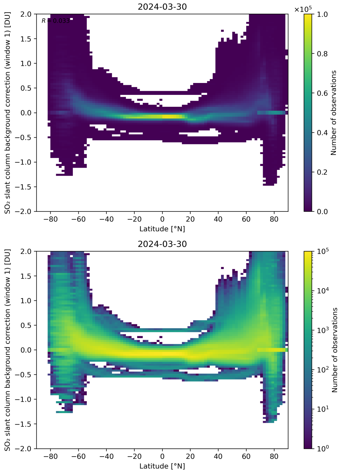
Figure 139: Scatter density plot of “Latitude” against “SO 2 slant column background correction (window 1)” for 2024-03-30 to 2024-03-31.
