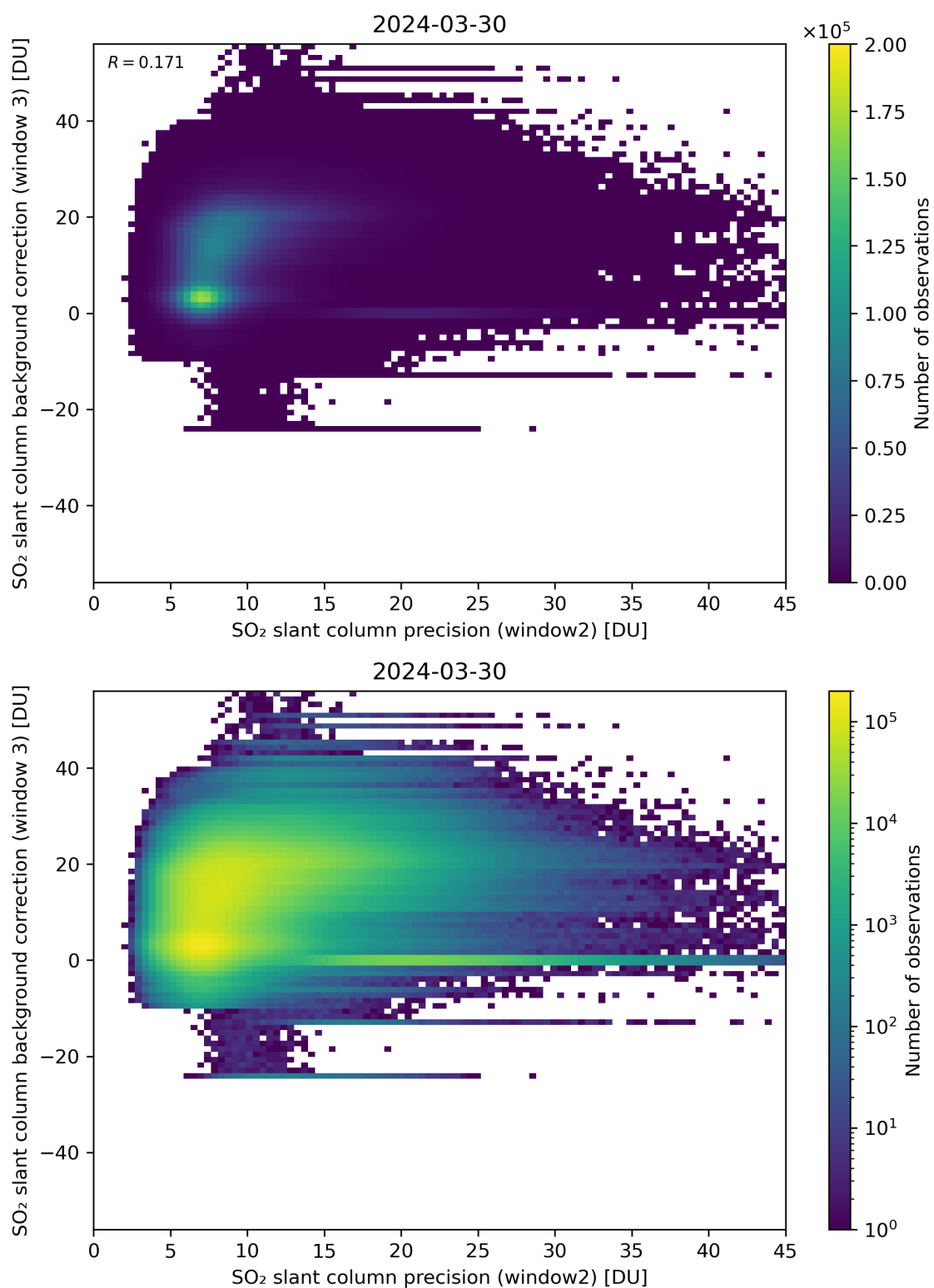
Figure 242: Scatter density plot of “SO 2 slant column precision (window2)” against “SO 2 slant column background correction (window 3)” for 2024-03-30 to 2024-03-31.
