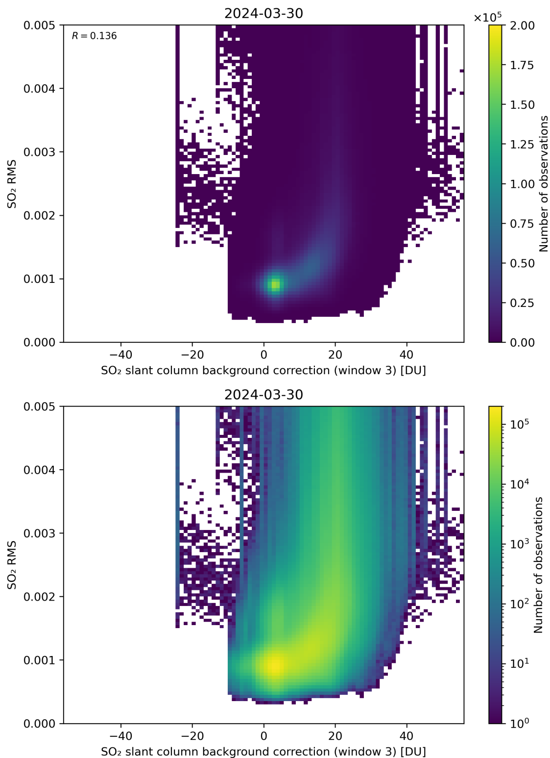
Figure 123: Scatter density plot of “SO 2 slant column background correction (window 3)” against “SO 2 RMS” for 2024-03-30 to 2024-03-31.
