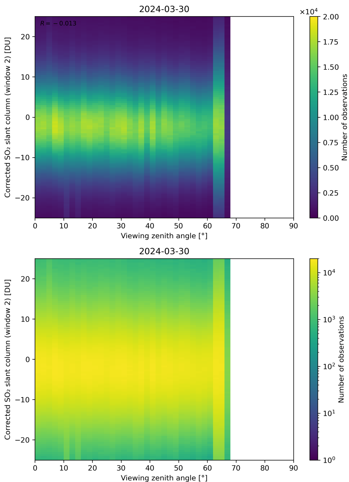
Figure 318: Scatter density plot of “Viewing zenith angle” against “Corrected SO 2 slant column (window 2)” for 2024-03-30 to 2024-03-31.
