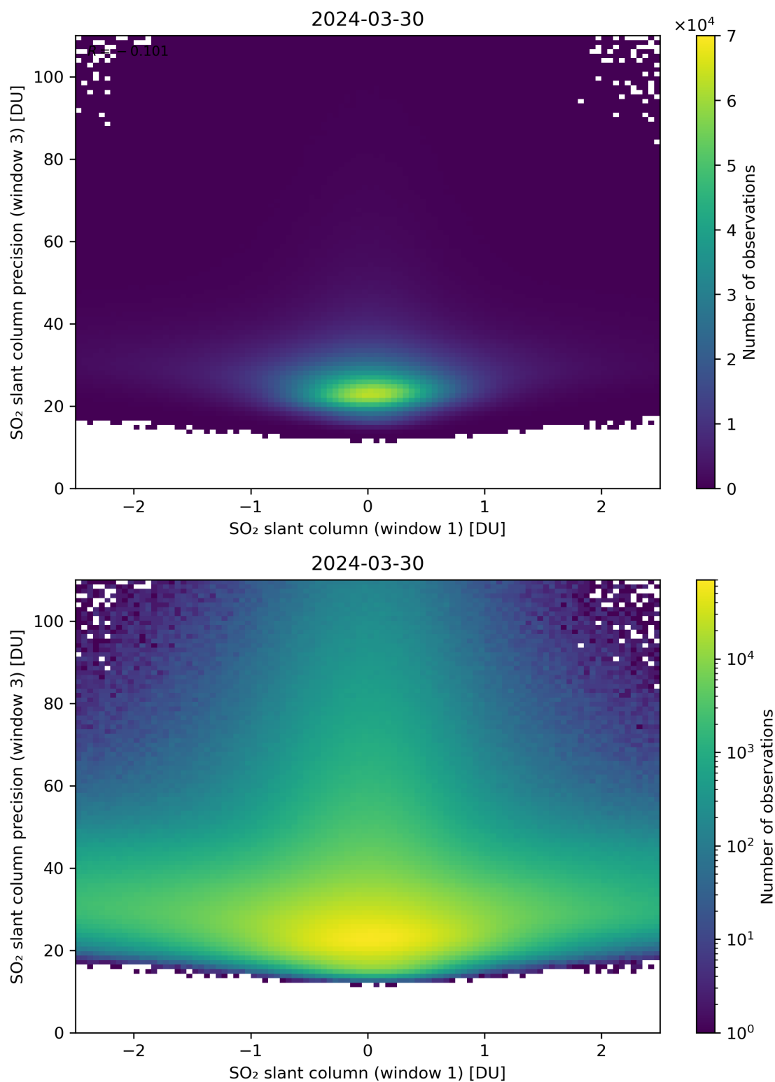
Figure 238: Scatter density plot of “SO 2 slant column (window 1)” against “SO 2 slant column precision (window 3)” for 2024-03-30 to 2024-03-31.
