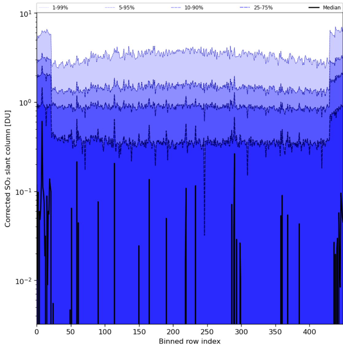
Figure 78: Along track statistics of “Corrected SO 2 slant column” for 2024-03-30 to 2024-03-31
