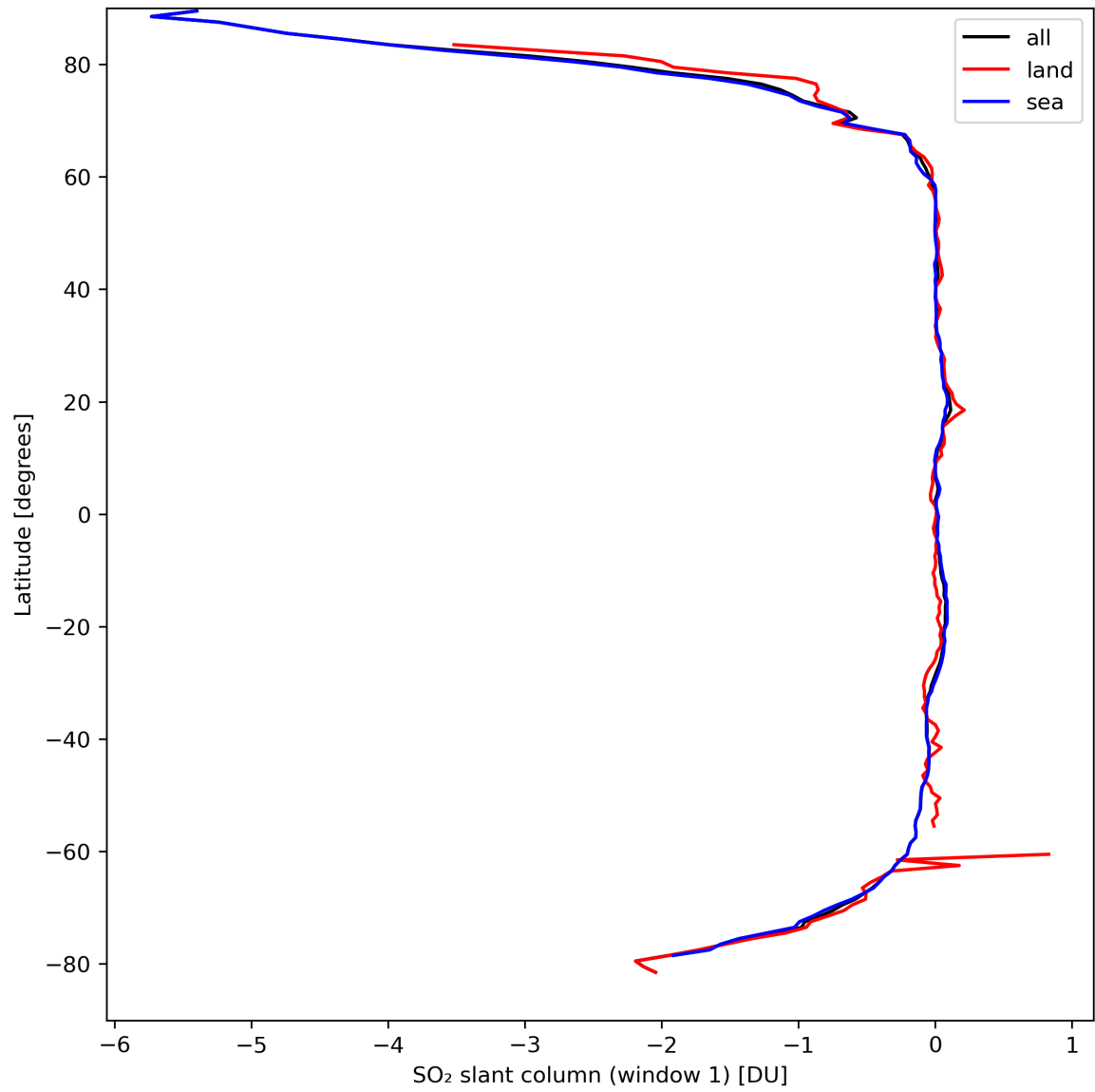
Figure 33: Zonal average of “SO 2 slant column (window 1)” for 2024-03-30 to 2024-03-31.
