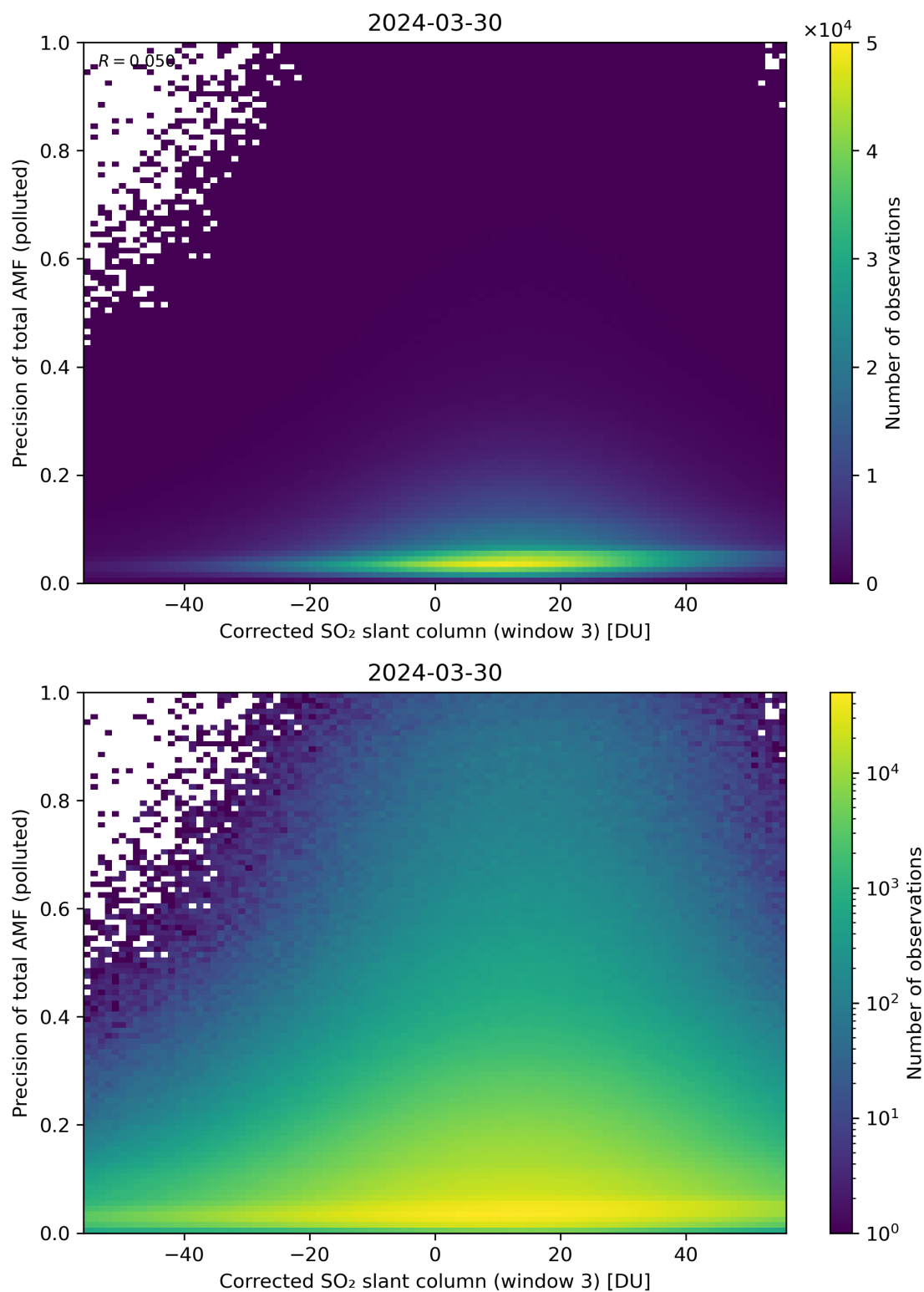
Figure 211: Scatter density plot of “Corrected SO 2 slant column (window 3)” against “Precision of total AMF (polluted)” for 2024-03-30 to 2024-03-31.
