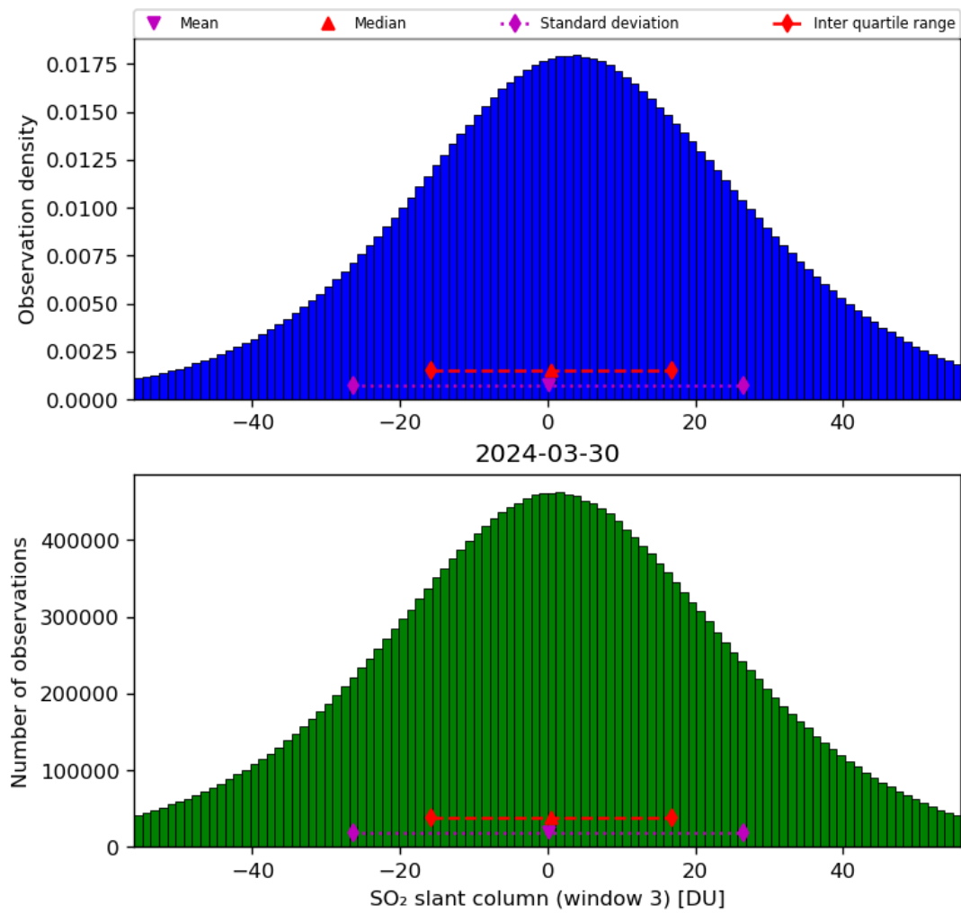
Figure 64: Histogram of “SO 2 slant column (window 3)” for 2024-03-30 to 2024-03-31
