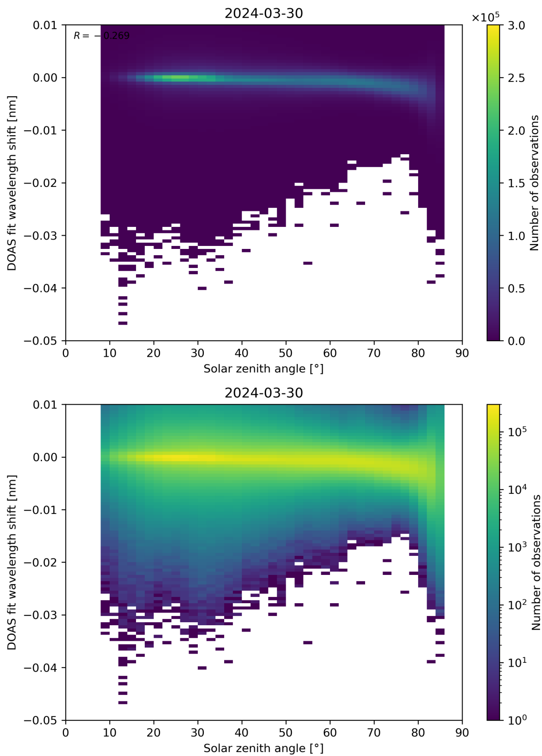
Figure 161: Scatter density plot of “Solar zenith angle” against “DOAS fit wavelength shift” for 2024-03-30 to 2024-03-31.
