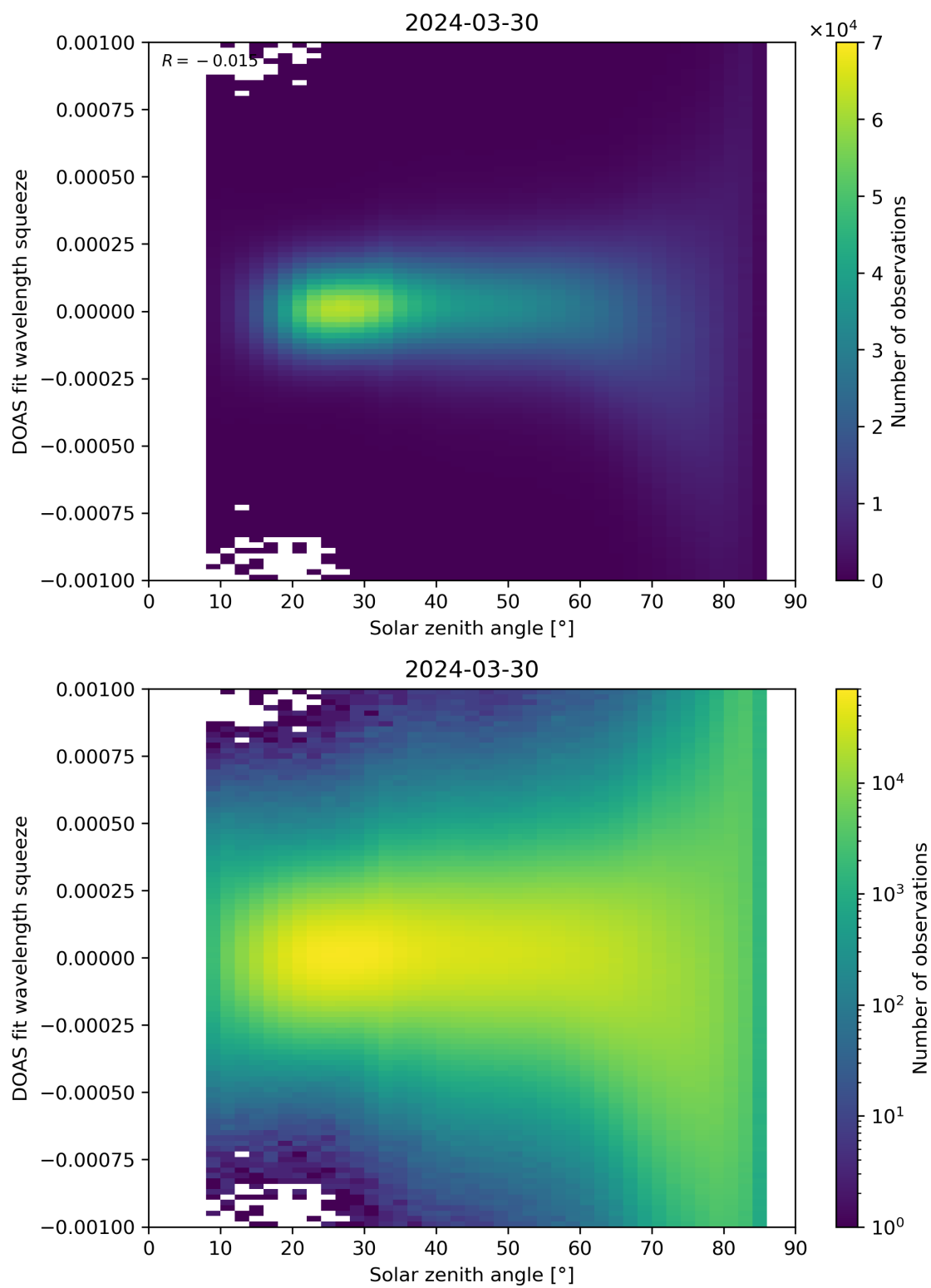
Figure 162: Scatter density plot of “Solar zenith angle” against “DOAS fit wavelength squeeze” for 2024-03-30 to 2024-03-31.
