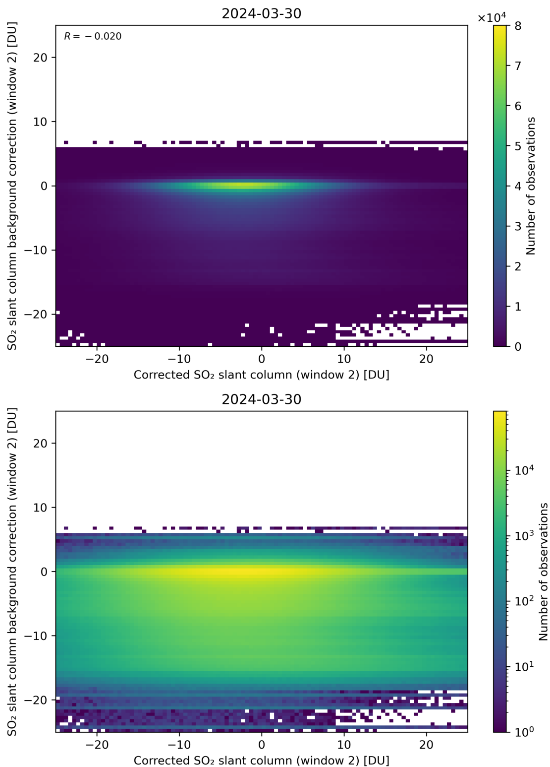
Figure 194: Scatter density plot of “Corrected SO 2 slant column (window 2)” against “SO 2 slant column background correction (window 2)” for 2024-03-30 to 2024-03-31.
