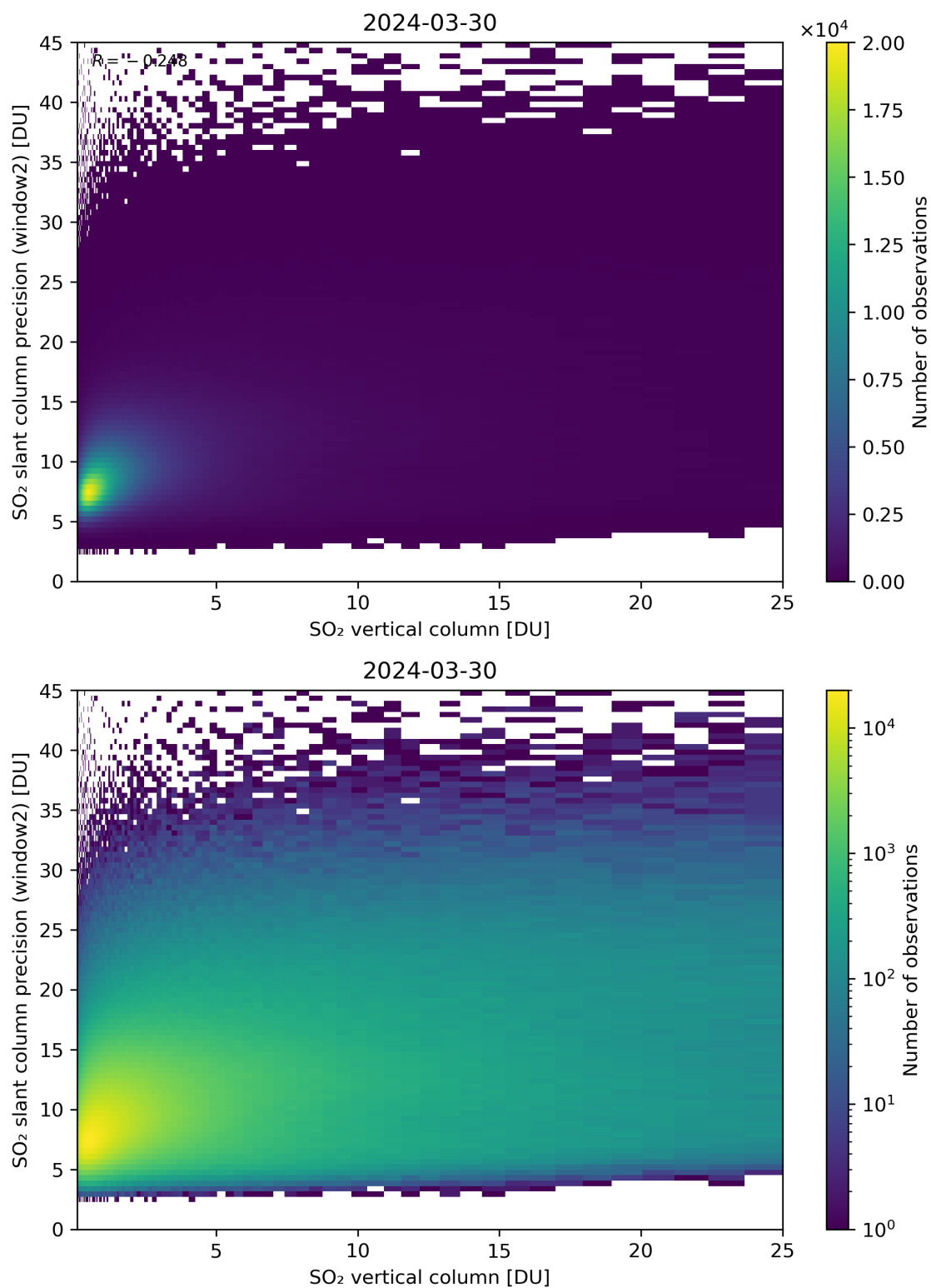
Figure 302: Scatter density plot of “SO 2 vertical column” against “SO 2 slant column precision (window2)” for 2024-03-30 to 2024-03-31.
