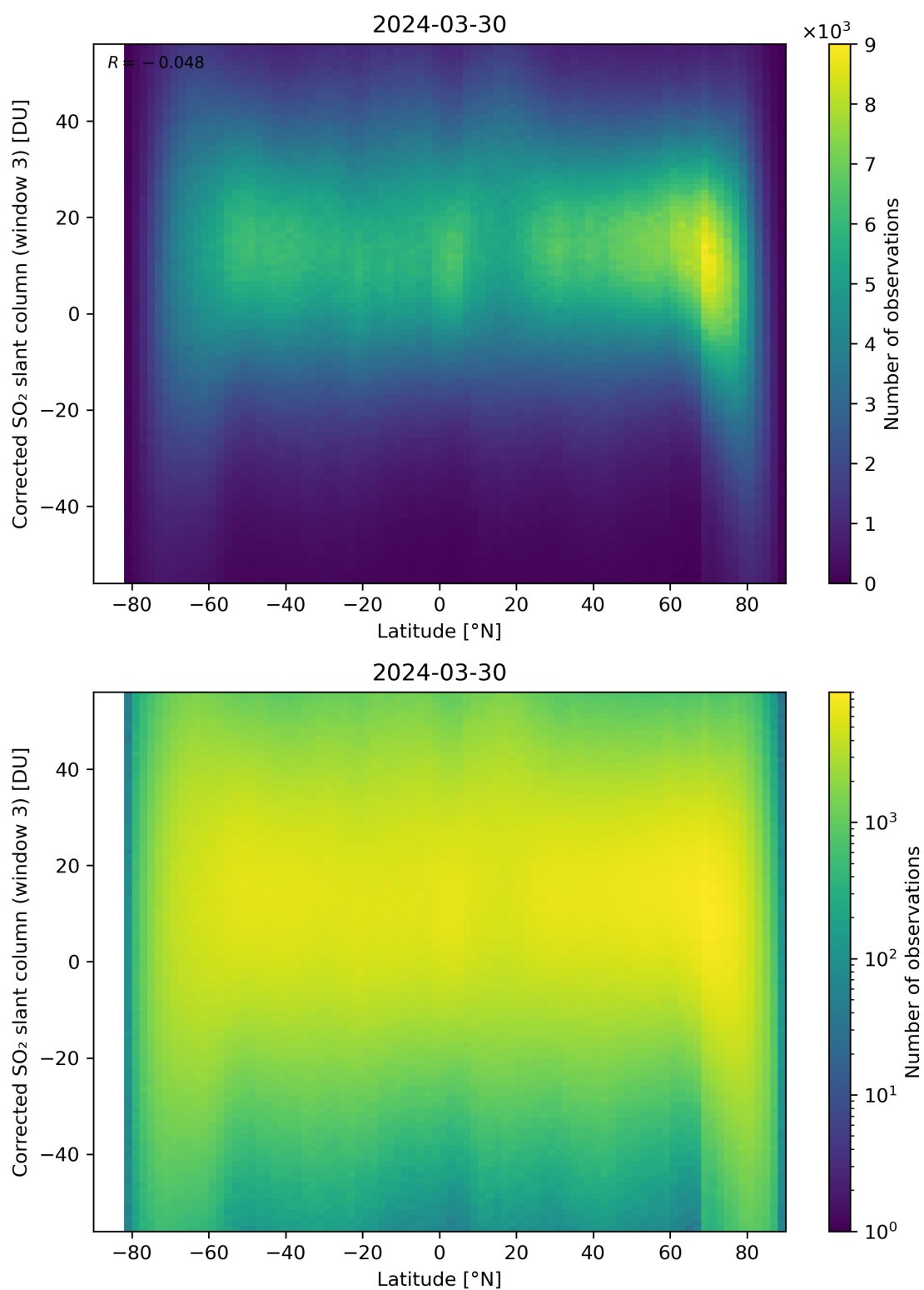
Figure 148: Scatter density plot of “Latitude” against “Corrected SO 2 slant column (window 3)” for 2024-03-30 to 2024-03-31.
