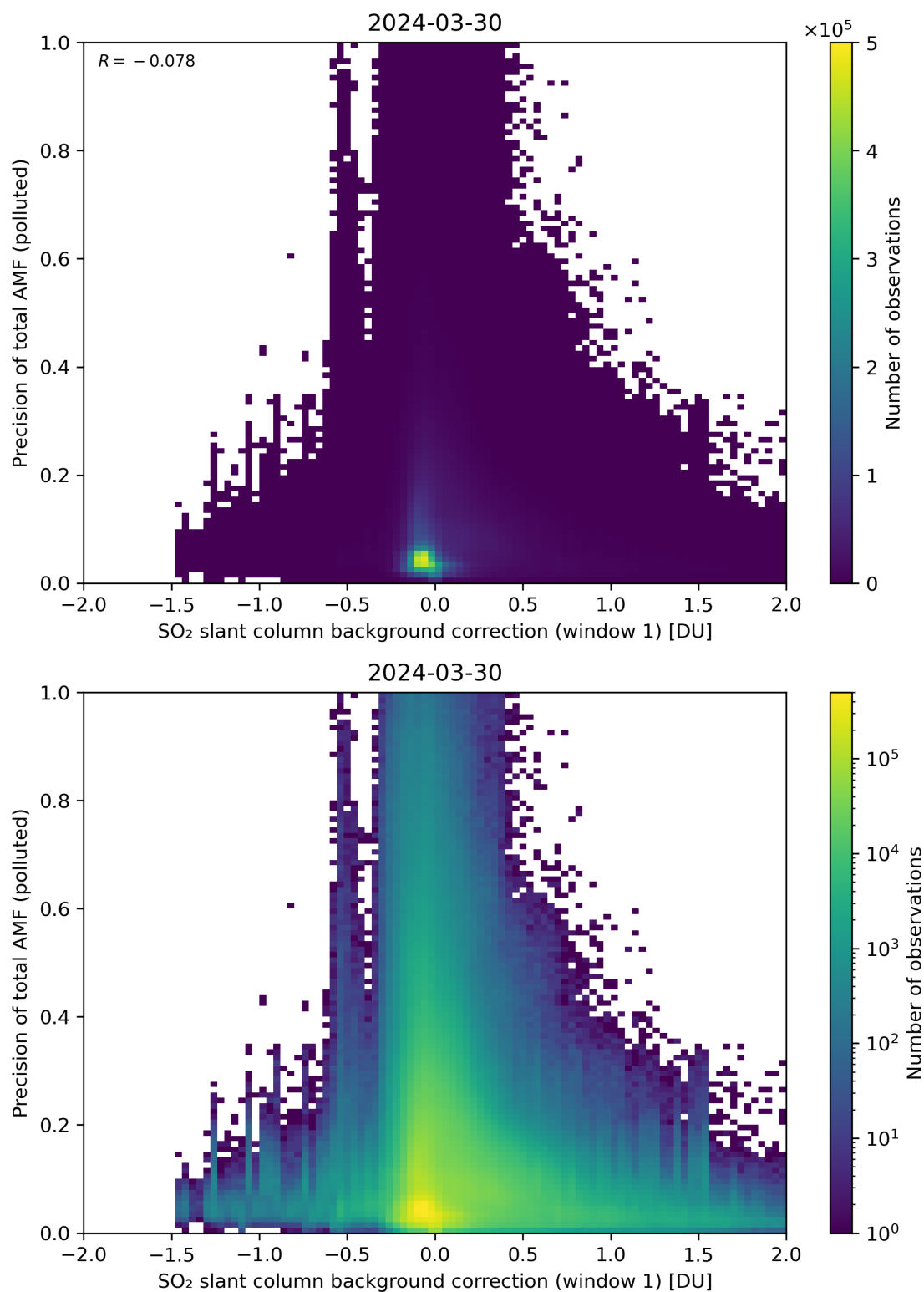
Figure 110: Scatter density plot of “SO 2 slant column background correction (window 1)” against “Precision of total AMF (polluted)” for 2024-03-30 to 2024-03-31.
