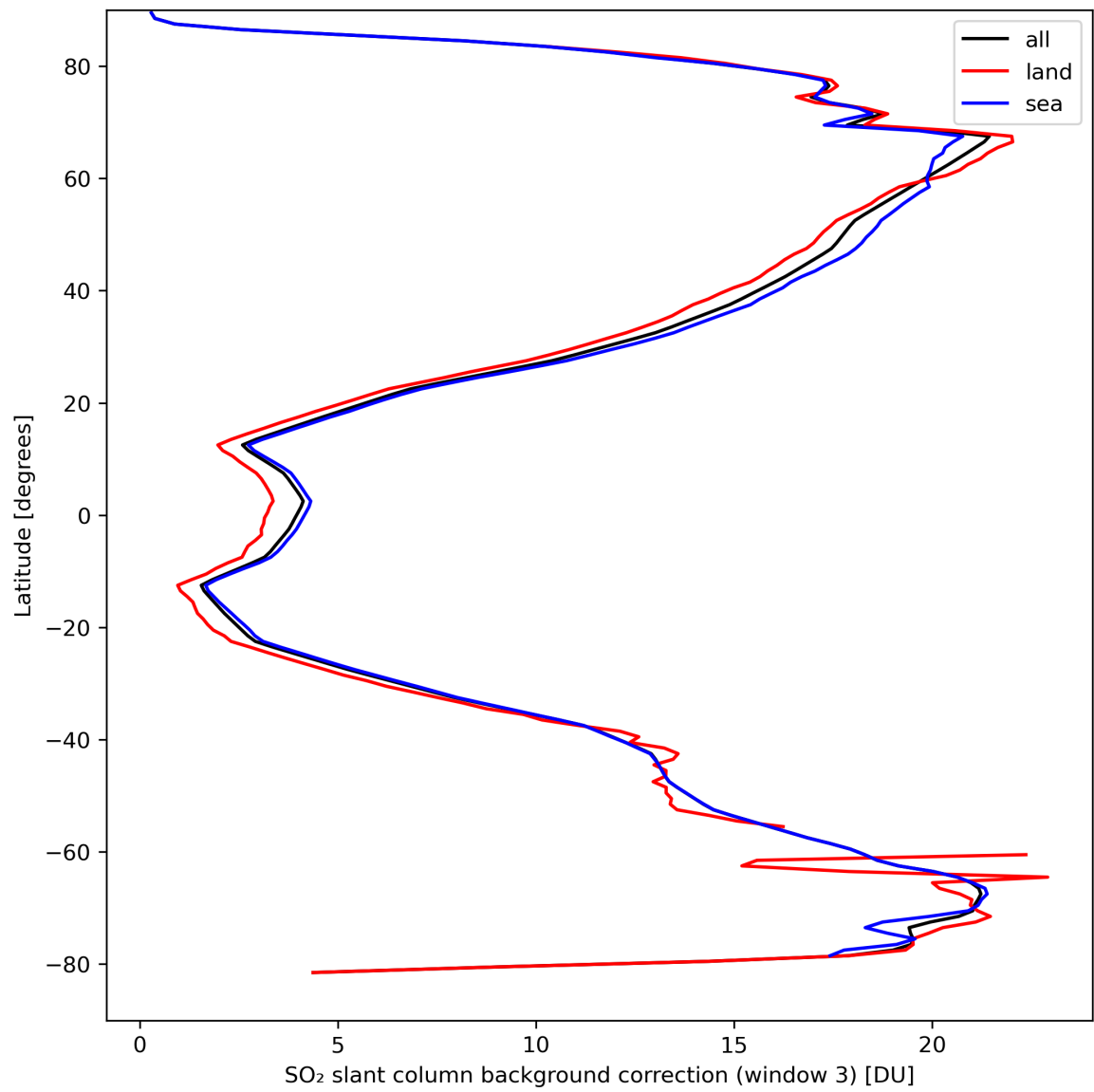
Figure 44: Zonal average of "SO 2 slant column background correction (window 3)" for 2024-03-30 to 2024-03-31.
