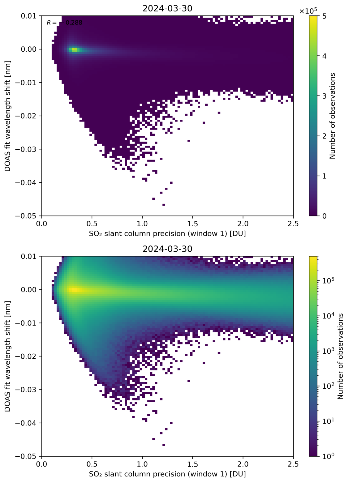
Figure 221: Scatter density plot of “SO 2 slant column precision (window 1)” against “DOAS fit wavelength shift” for 2024-03-30 to 2024-03-31.
