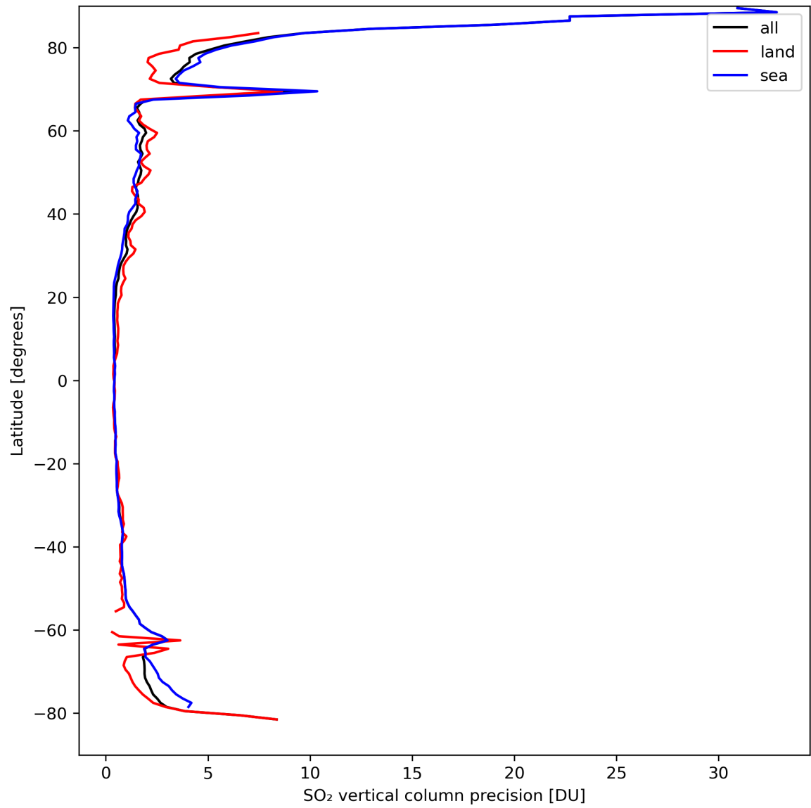
Figure 31: Zonal average of “SO 2 vertical column precision” for 2024-03-30 to 2024-03-31.
