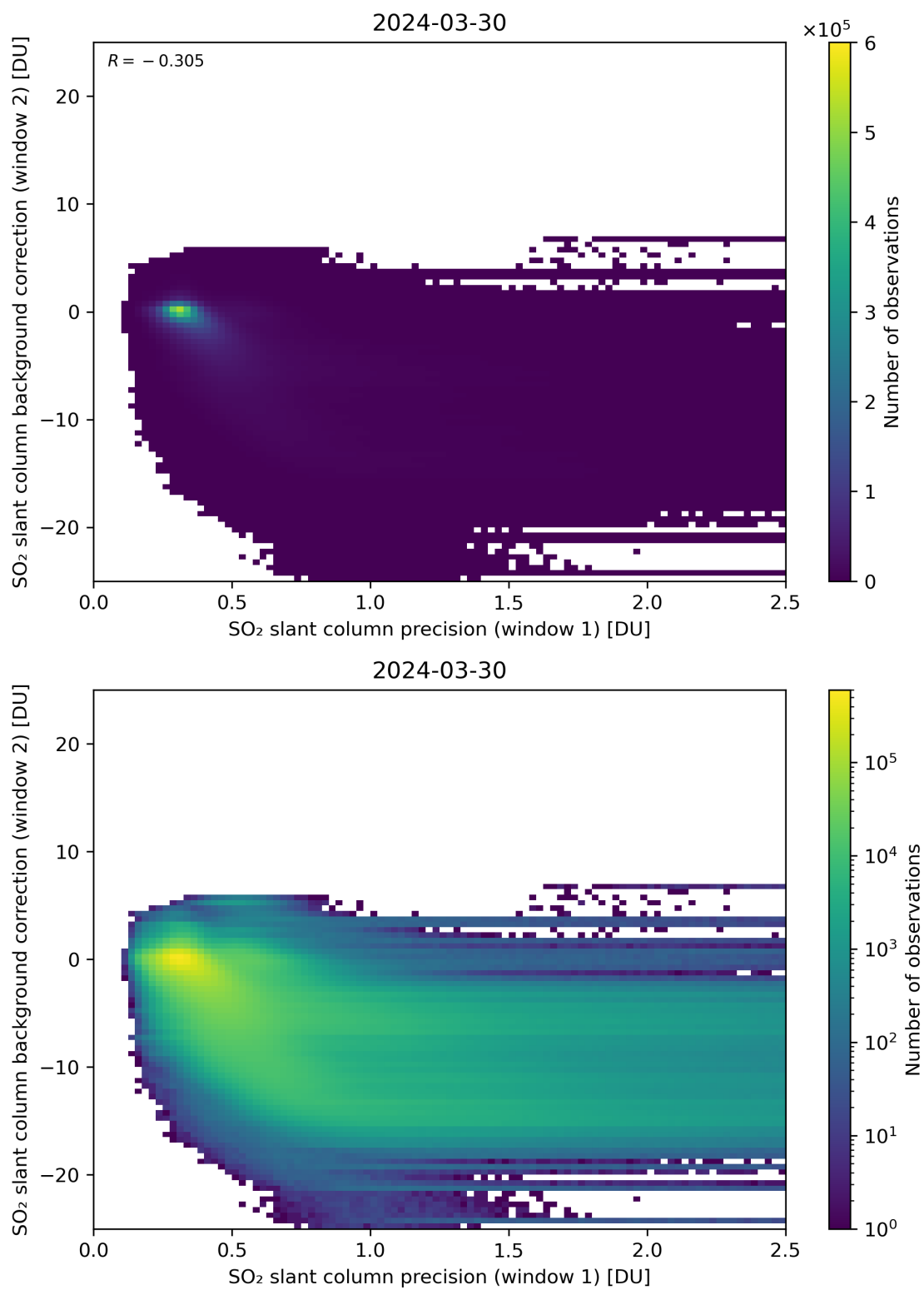
Figure 219: Scatter density plot of “SO 2 slant column precision (window 1)” against “SO 2 slant column background correction (window 2)” for 2024-03-30 to 2024-03-31.
