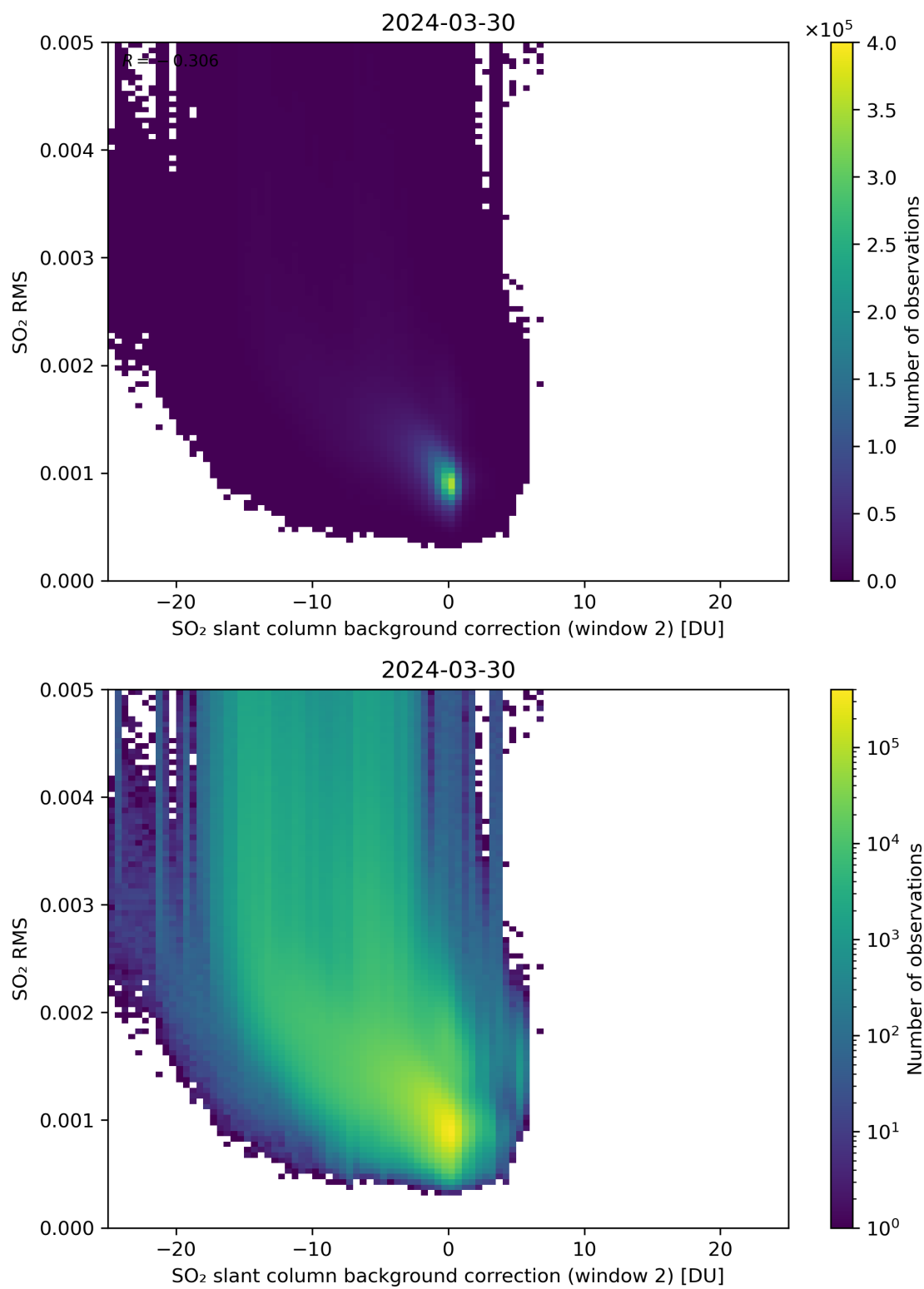
Figure 114: Scatter density plot of “SO 2 slant column background correction (window 2)” against “SO 2 RMS” for 2024-03-30 to 2024-03-31.
