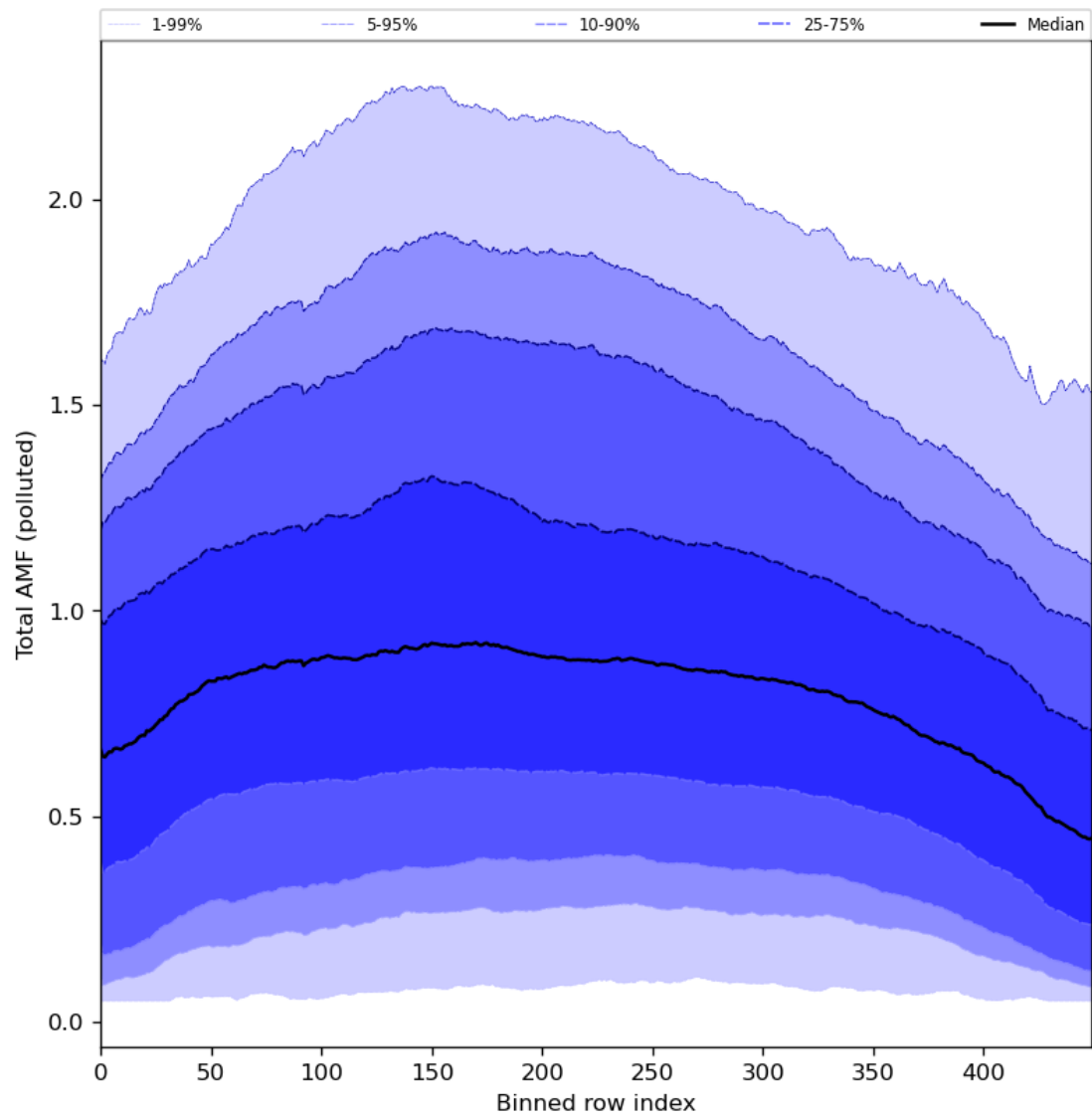
Figure 94: Along track statistics of “Total AMF (polluted)” for 2024-03-30 to 2024-03-31
