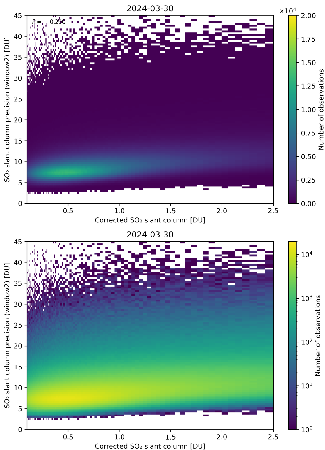
Figure 189: Scatter density plot of “Corrected SO 2 slant column” against “SO 2 slant column precision (window2)” for 2024-03-30 to 2024-03-31.
