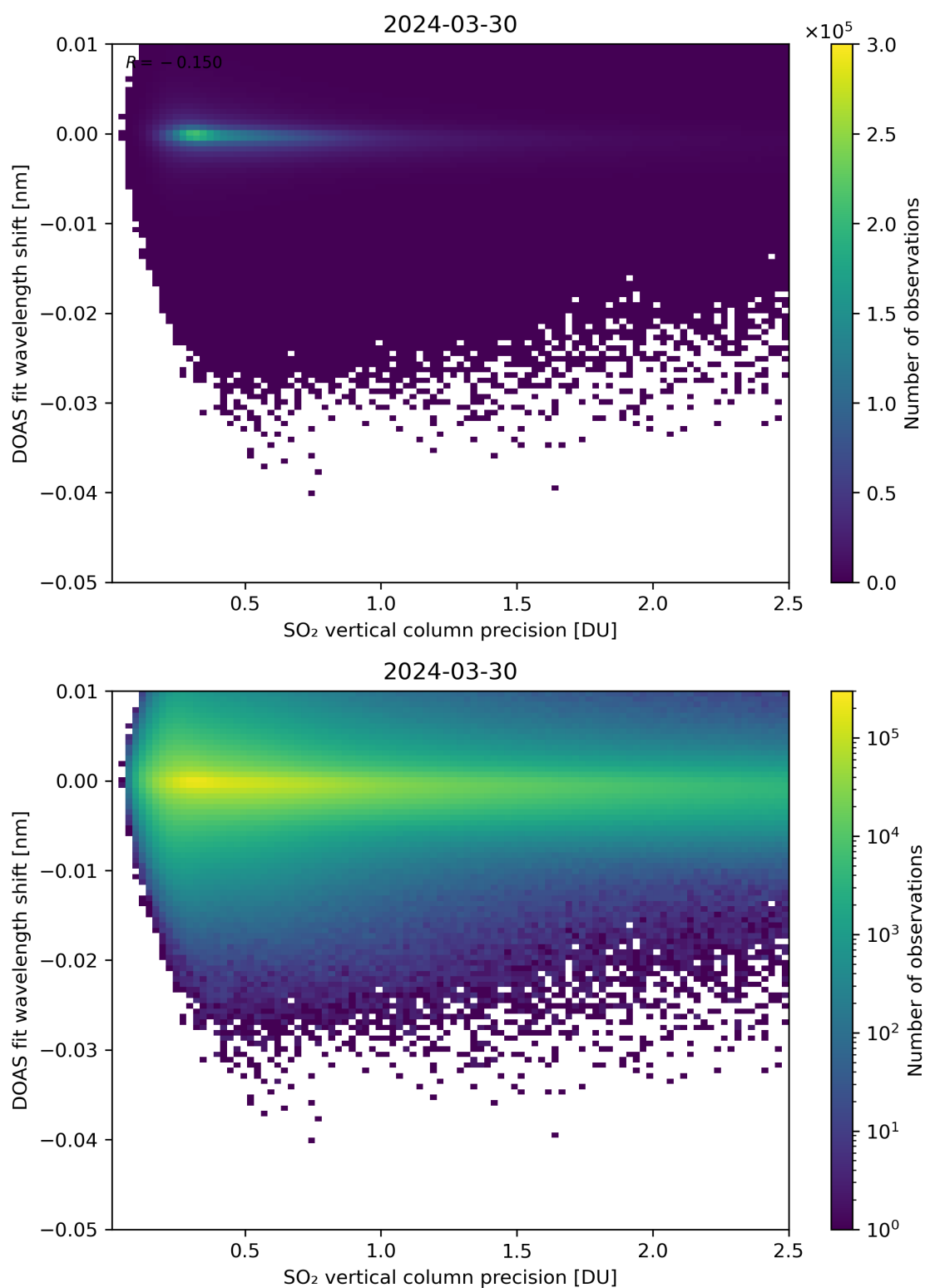
Figure 282: Scatter density plot of “SO 2 vertical column precision” against “DOAS fit wavelength shift” for 2024-03-30 to 2024-03-31.
