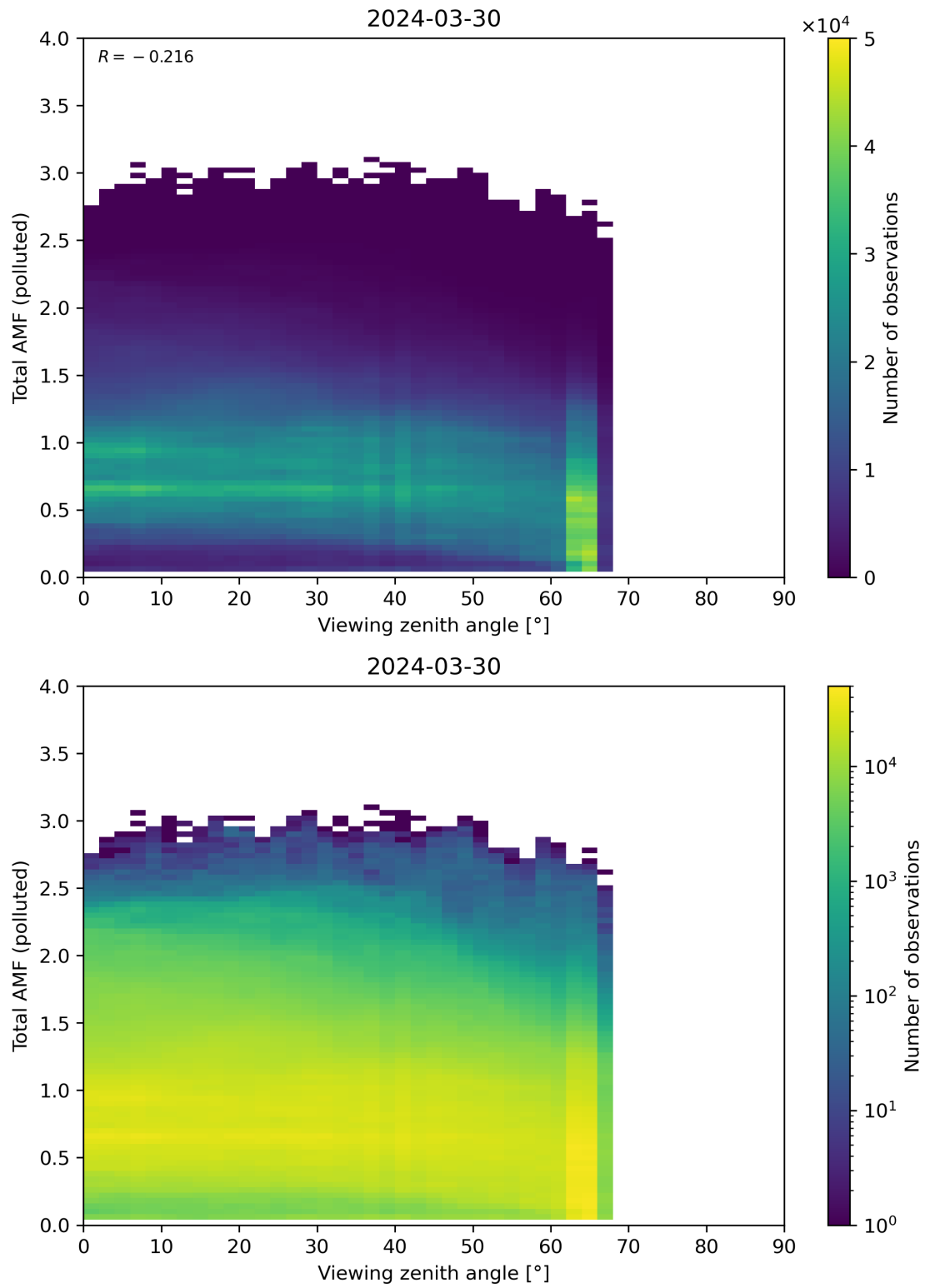
Figure 325: Scatter density plot of “Viewing zenith angle” against “Total AMF (polluted)” for 2024-03-30 to 2024-03-31.
