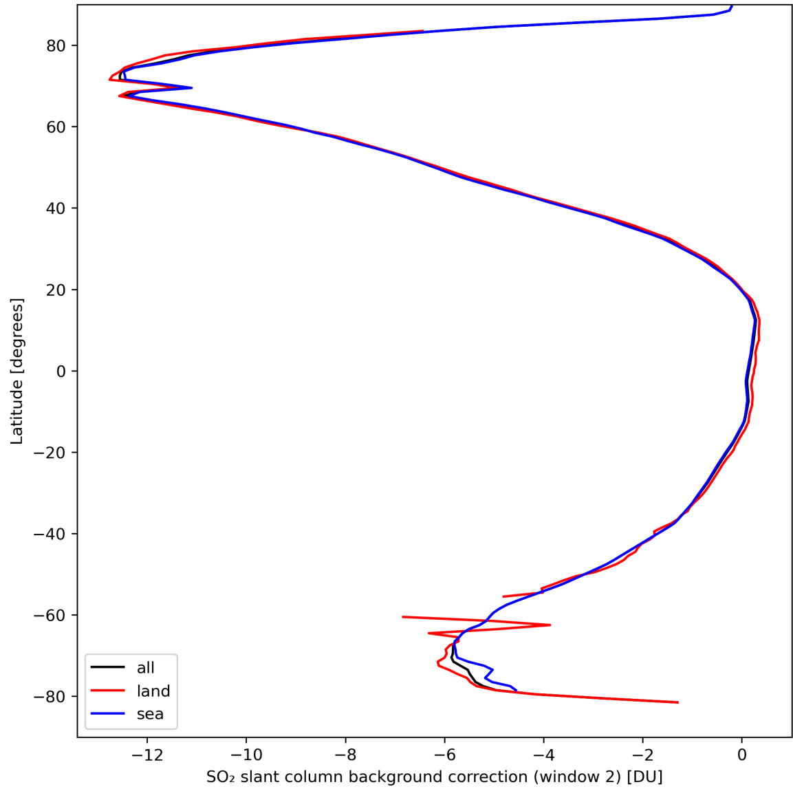
Figure 40: Zonal average of “SO 2 slant column background correction (window 2)” for 2024-03-30 to 2024-03-31.
