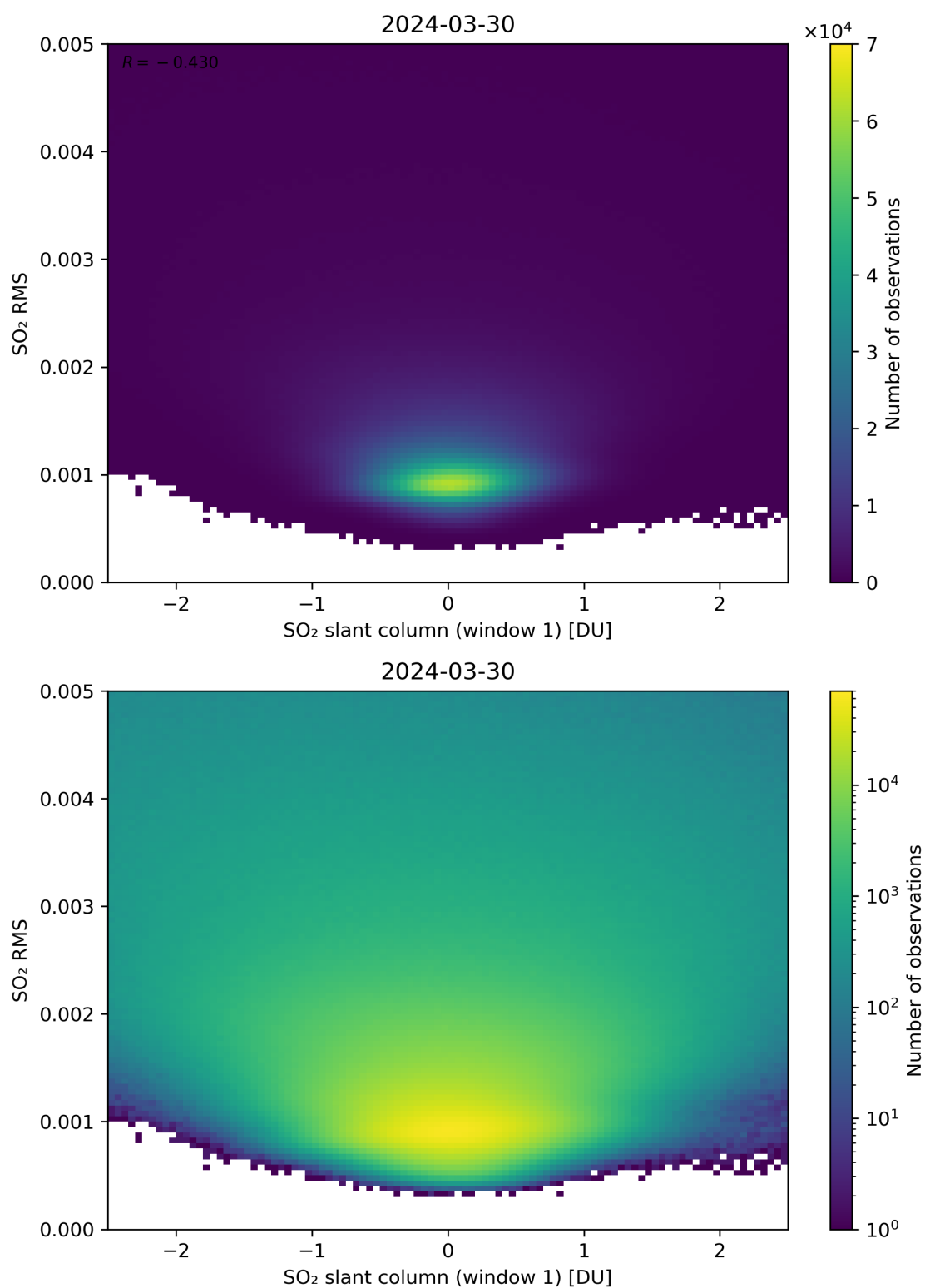
Figure 217: Scatter density plot of “SO 2 slant column (window 1)” against “SO 2 RMS” for 2024-03-30 to 2024-03-31.
