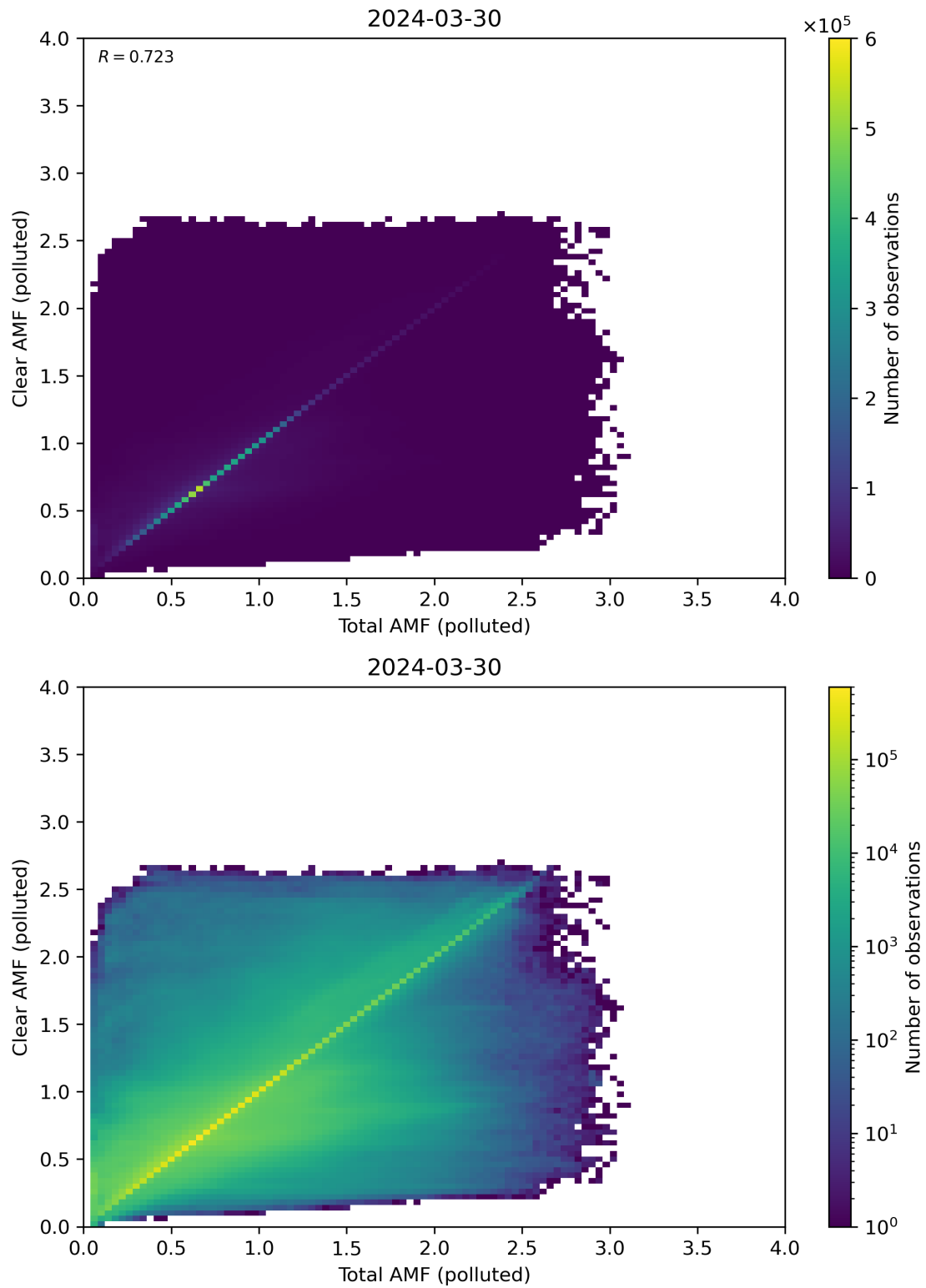
Figure 271: Scatter density plot of “Total AMF (polluted)” against “Clear AMF (polluted)” for 2024-03-30 to 2024-03-31.
