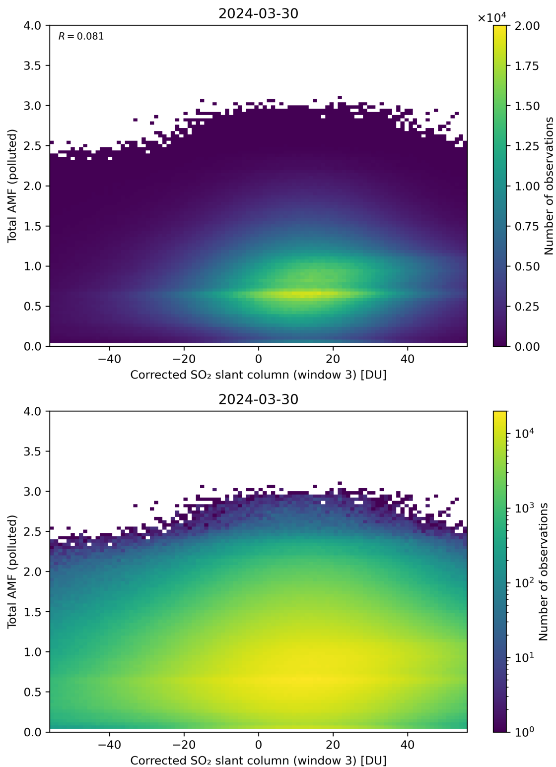
Figure 210: Scatter density plot of “Corrected SO 2 slant column (window 3)” against “Total AMF (polluted)” for 2024-03-30 to 2024-03-31.
