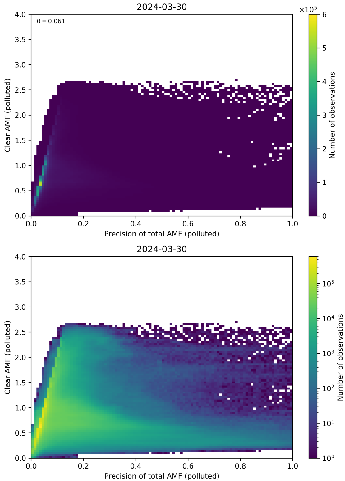
Figure 270: Scatter density plot of “Precision of total AMF (polluted)” against “Clear AMF (polluted)” for 2024-03-30 to 2024-03-31.
