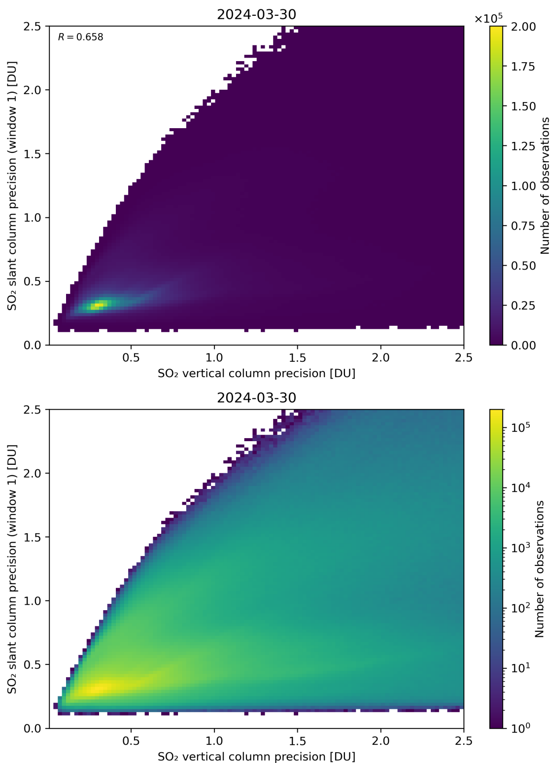
Figure 290: Scatter density plot of “SO 2 vertical column precision” against “SO 2 slant column precision (window 1)” for 2024-03-30 to 2024-03-31.
