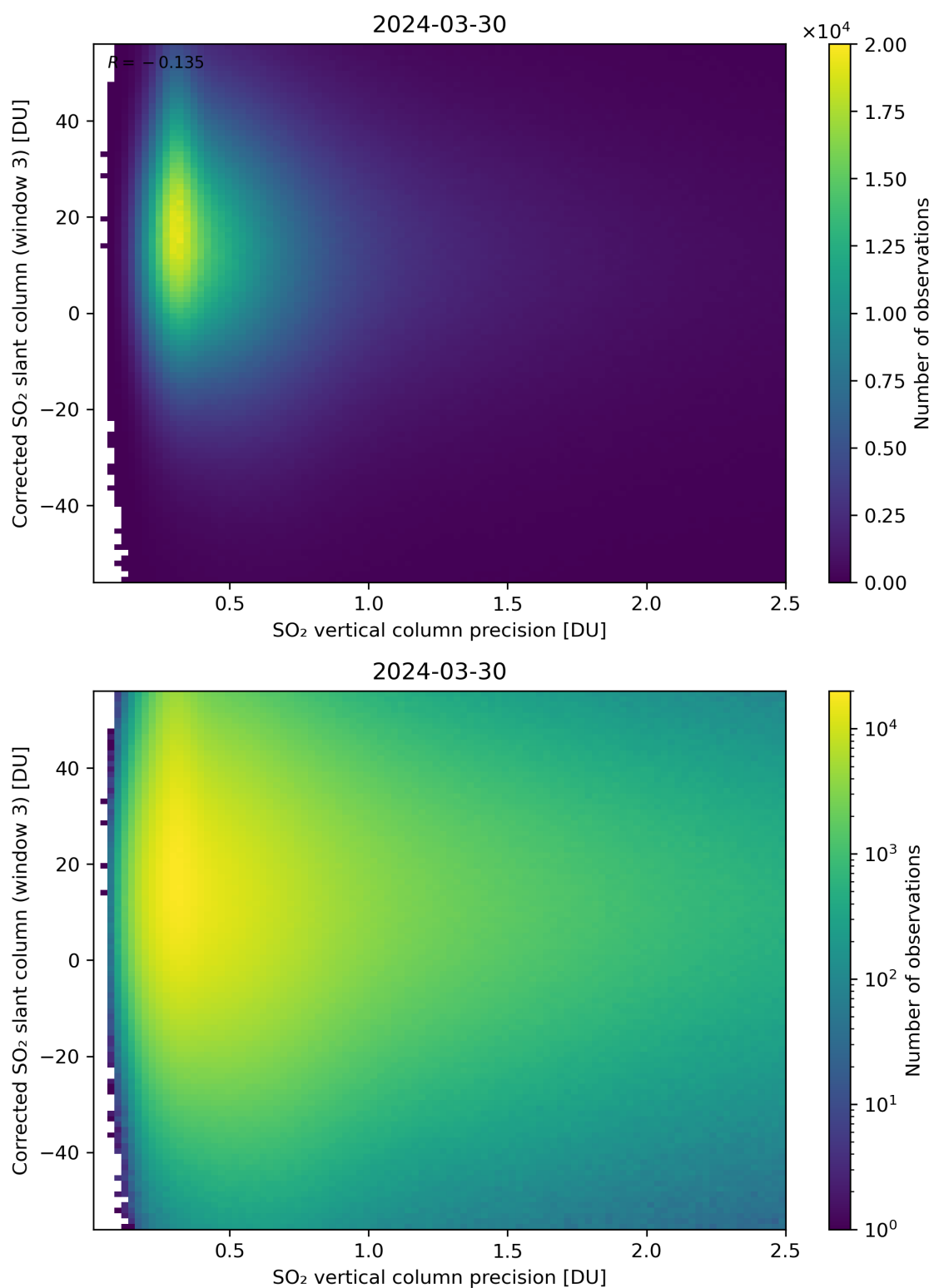
Figure 288: Scatter density plot of “SO 2 vertical column precision” against “Corrected SO 2 slant column (window 3)” for 2024-03-30 to 2024-03-31.
