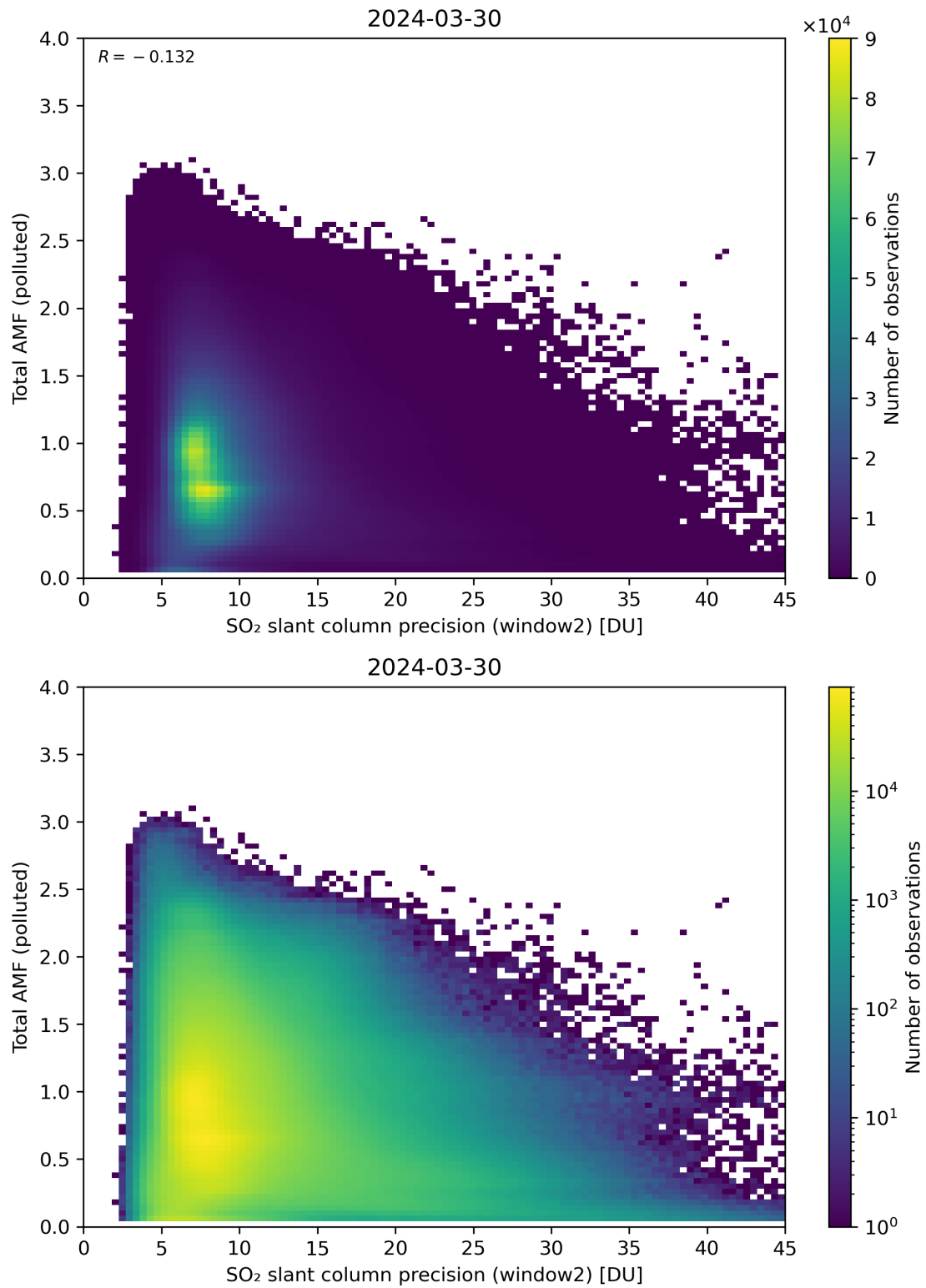
Figure 251: Scatter density plot of “SO 2 slant column precision (window2)” against “Total AMF (polluted)” for 2024-03-30 to 2024-03-31.
