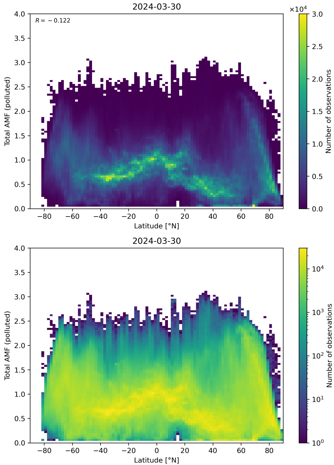
Figure 154: Scatter density plot of “Latitude” against “Total AMF (polluted)” for 2024-03-30 to 2024-03-31.
