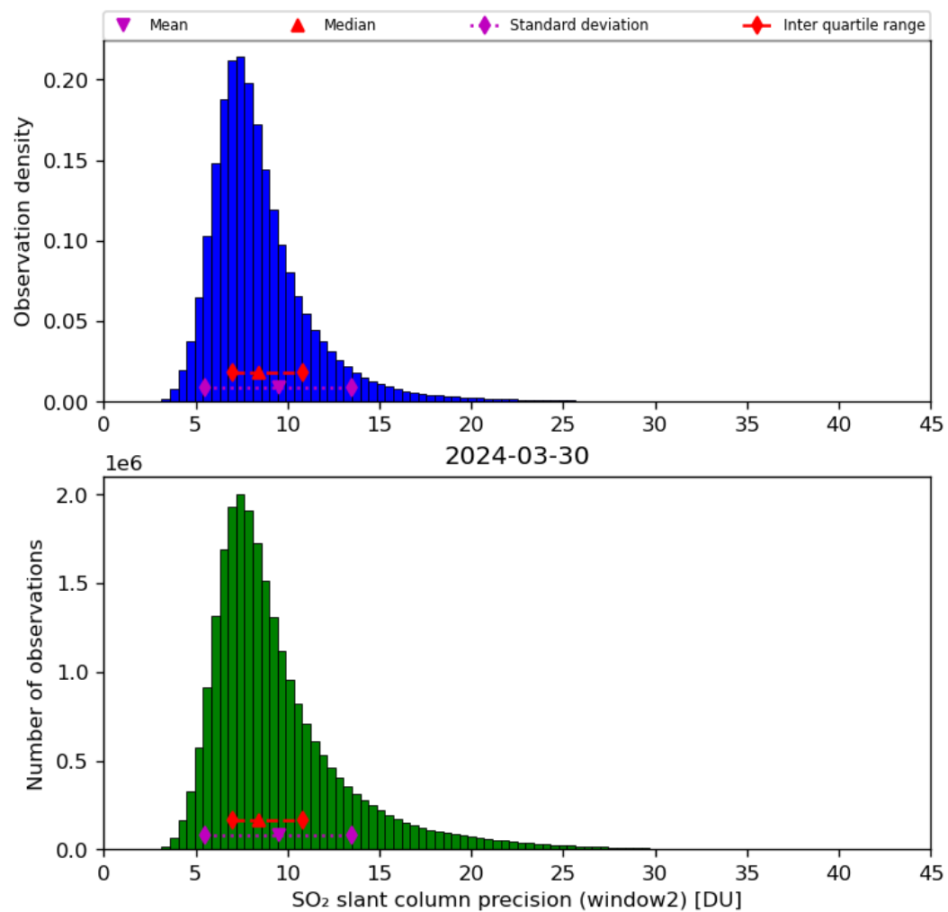
Figure 61: Histogram of “SO 2 slant column precision (window2)” for 2024-03-30 to 2024-03-31
