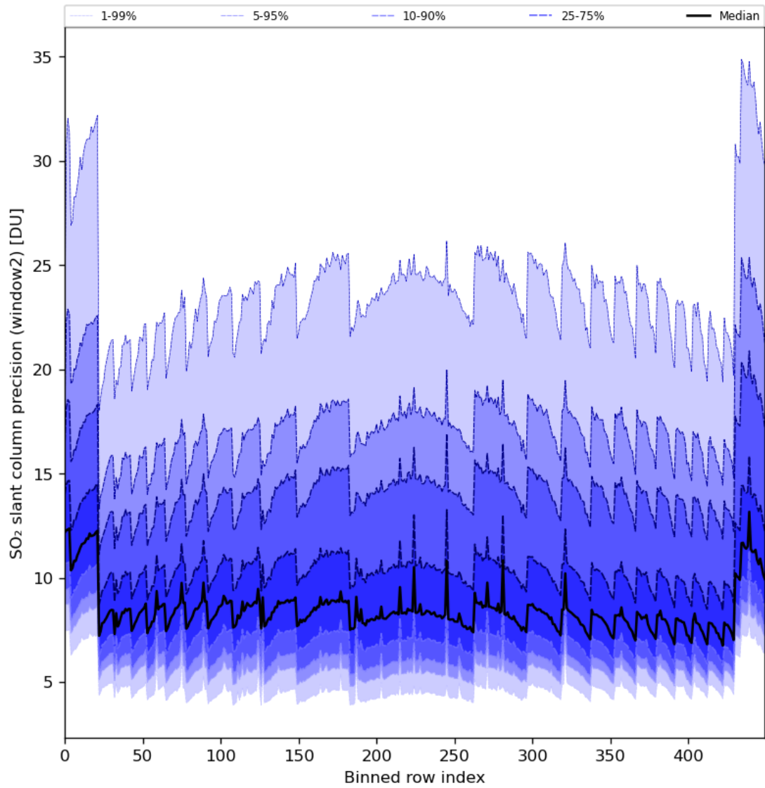
Figure 84: Along track statistics of “SO 2 slant column precision (window2)” for 2024-03-30 to 2024-03-31
