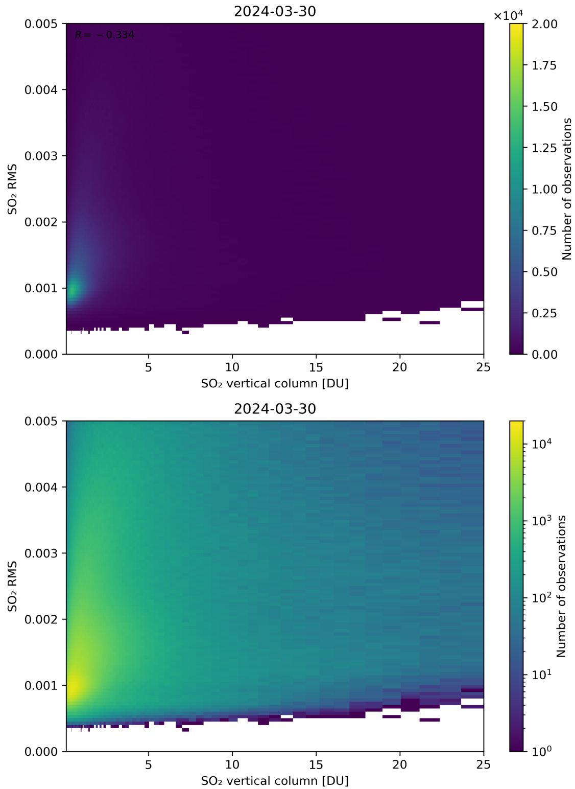
Figure 278: Scatter density plot of “SO 2 vertical column” against “SO 2 RMS” for 2024-03-30 to 2024-03-31.
