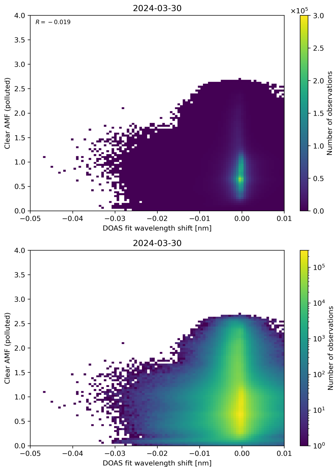
Figure 129: Scatter density plot of “DOAS fit wavelength shift” against “Clear AMF (polluted)” for 2024-03-30 to 2024-03-31.
