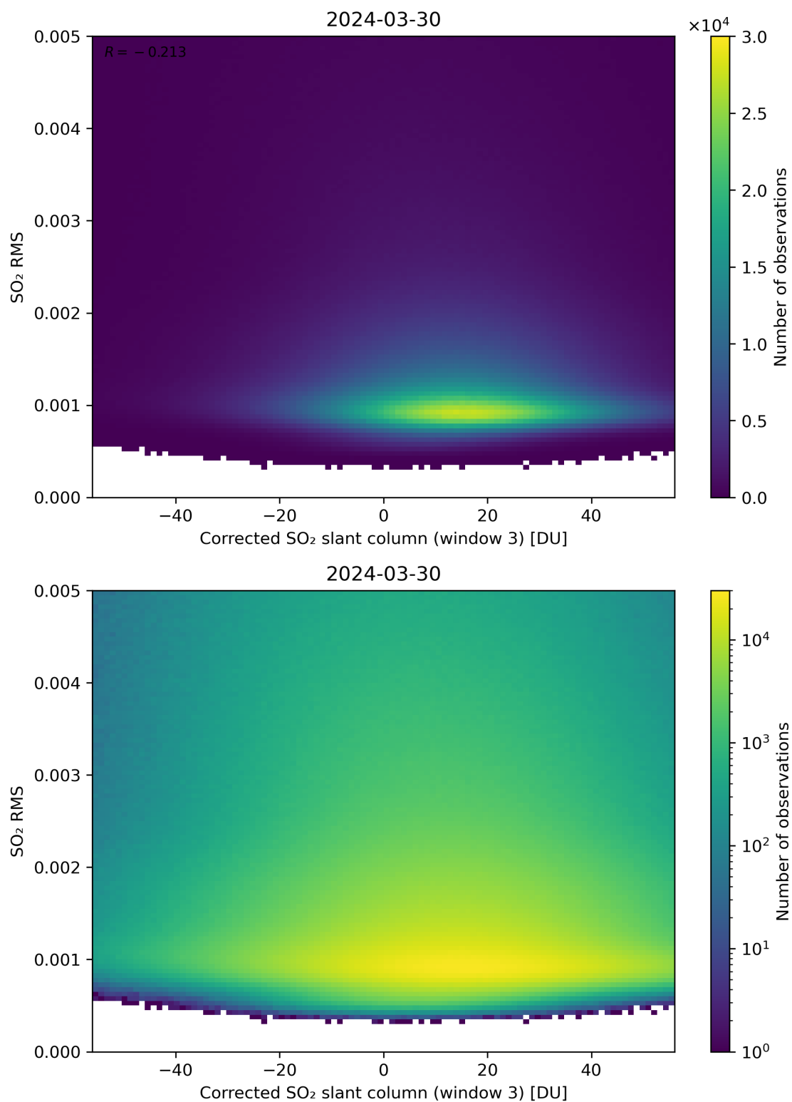
Figure 208: Scatter density plot of “Corrected SO 2 slant column (window 3)” against “SO 2 RMS” for 2024-03-30 to 2024-03-31.
