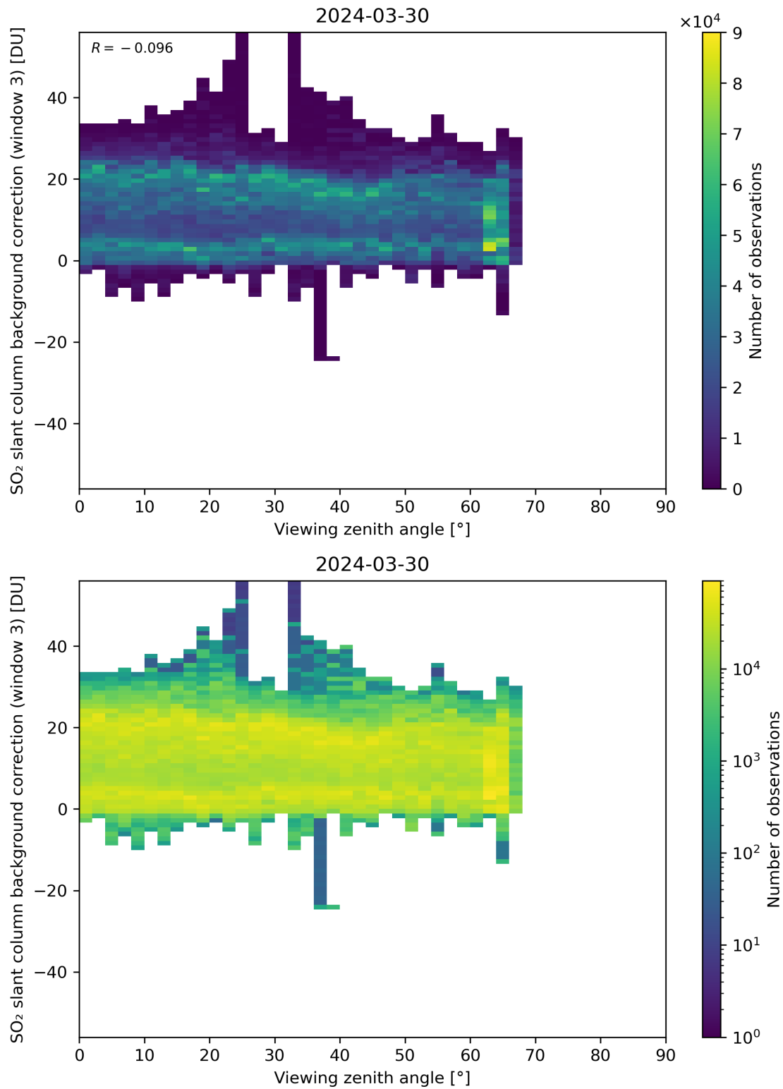
Figure 310: Scatter density plot of “Viewing zenith angle” against “SO 2 slant column background correction (window 3)” for 2024-03-30 to 2024-03-31.
