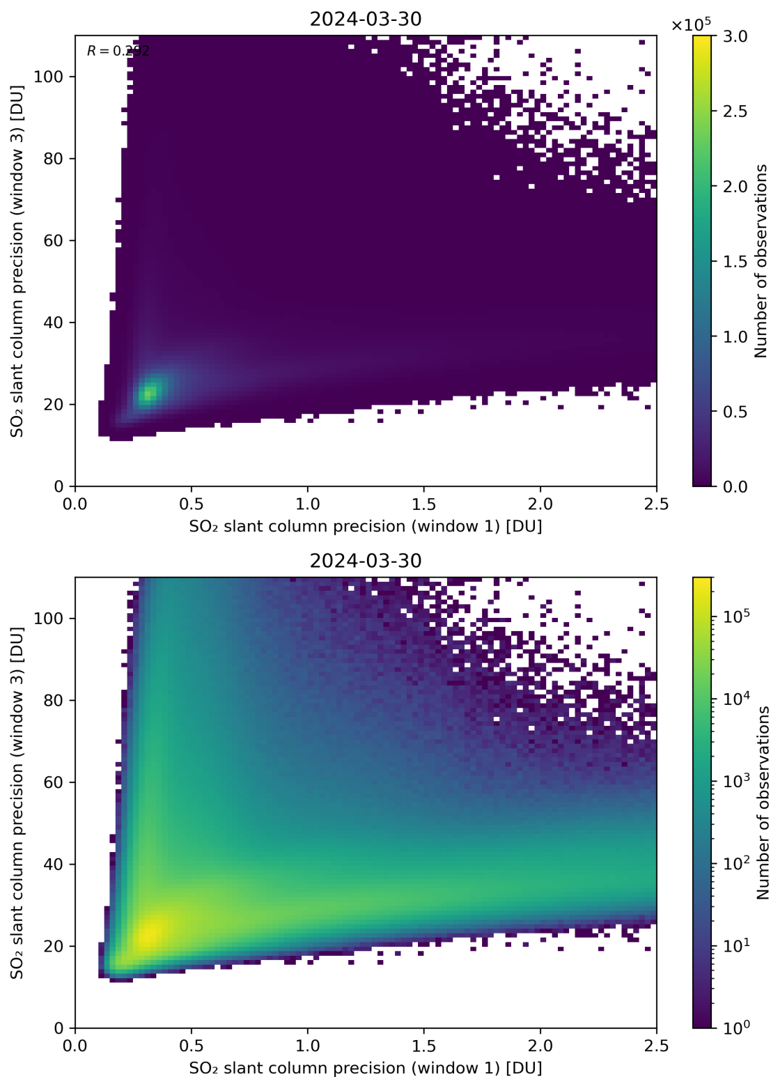
Figure 229: Scatter density plot of “SO 2 slant column precision (window 1)” against “SO 2 slant column precision (window 3)” for 2024-03-30 to 2024-03-31.
