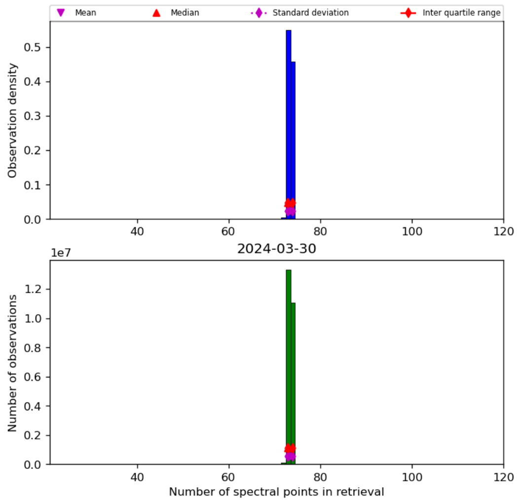
Figure 74: Histogram of “Number of spectral points in retrieval” for 2024-03-30 to 2024-03-31
