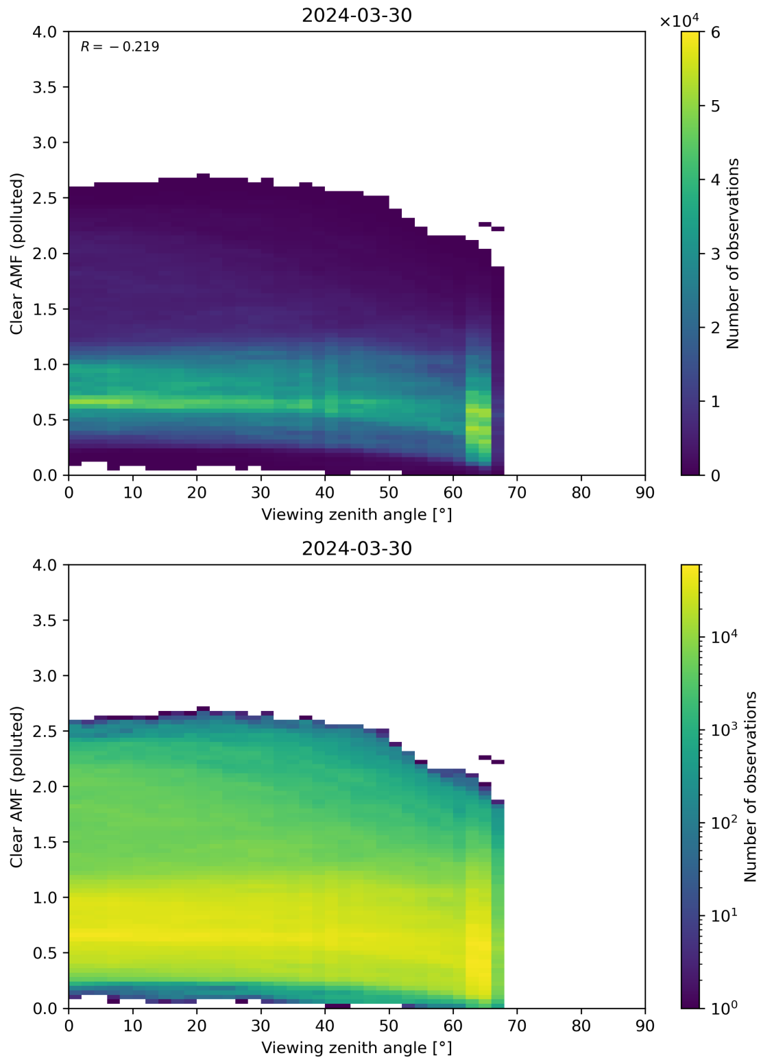
Figure 316: Scatter density plot of “Viewing zenith angle” against “Clear AMF (polluted)” for 2024-03-30 to 2024-03-31.
