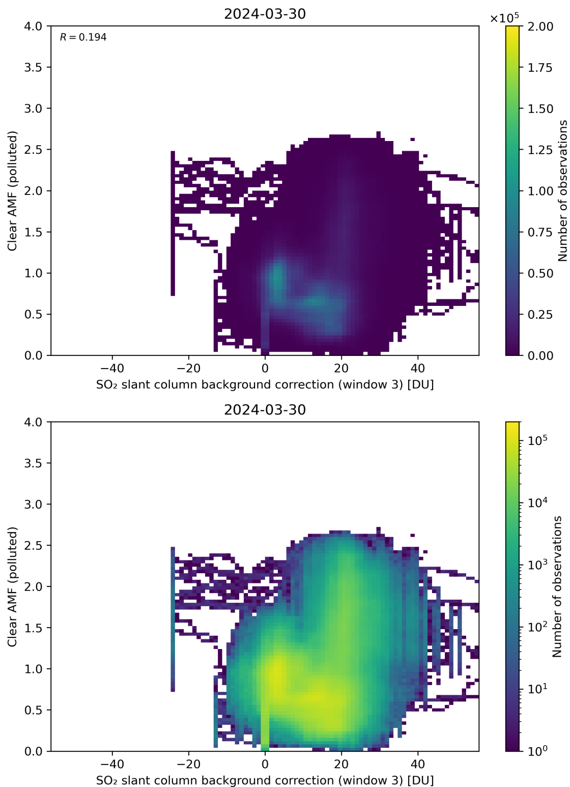
Figure 124: Scatter density plot of “SO 2 slant column background correction (window 3)” against “Clear AMF (polluted)” for 2024-03-30 to 2024-03-31.
