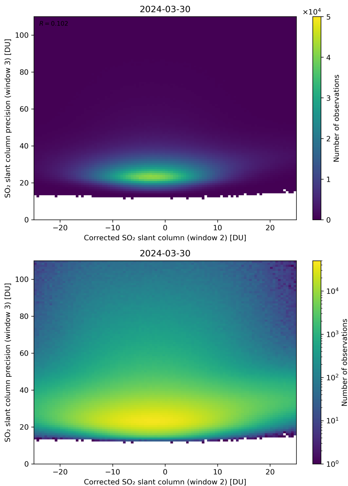
Figure 202: Scatter density plot of “Corrected SO 2 slant column (window 2)” against “SO 2 slant column precision (window 3)” for 2024-03-30 to 2024-03-31.
