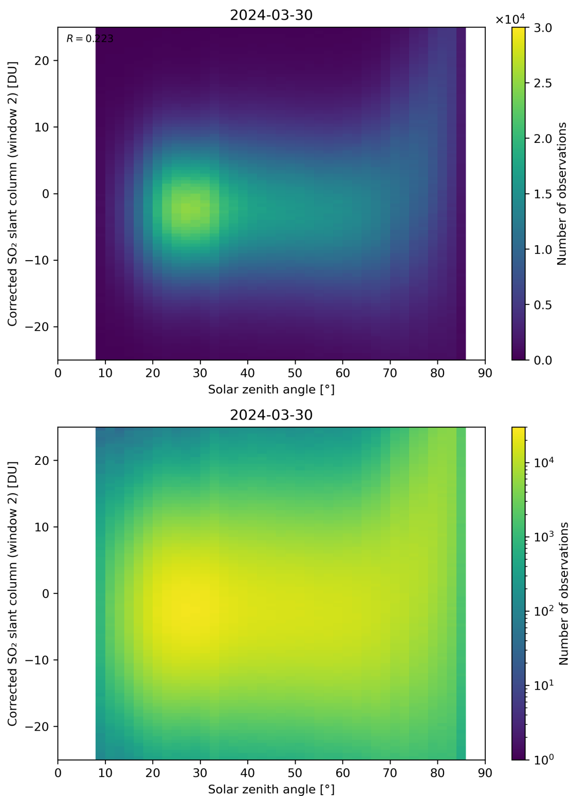
Figure 167: Scatter density plot of “Solar zenith angle” against “Corrected SO 2 slant column (window 2)” for 2024-03-30 to 2024-03-31.
