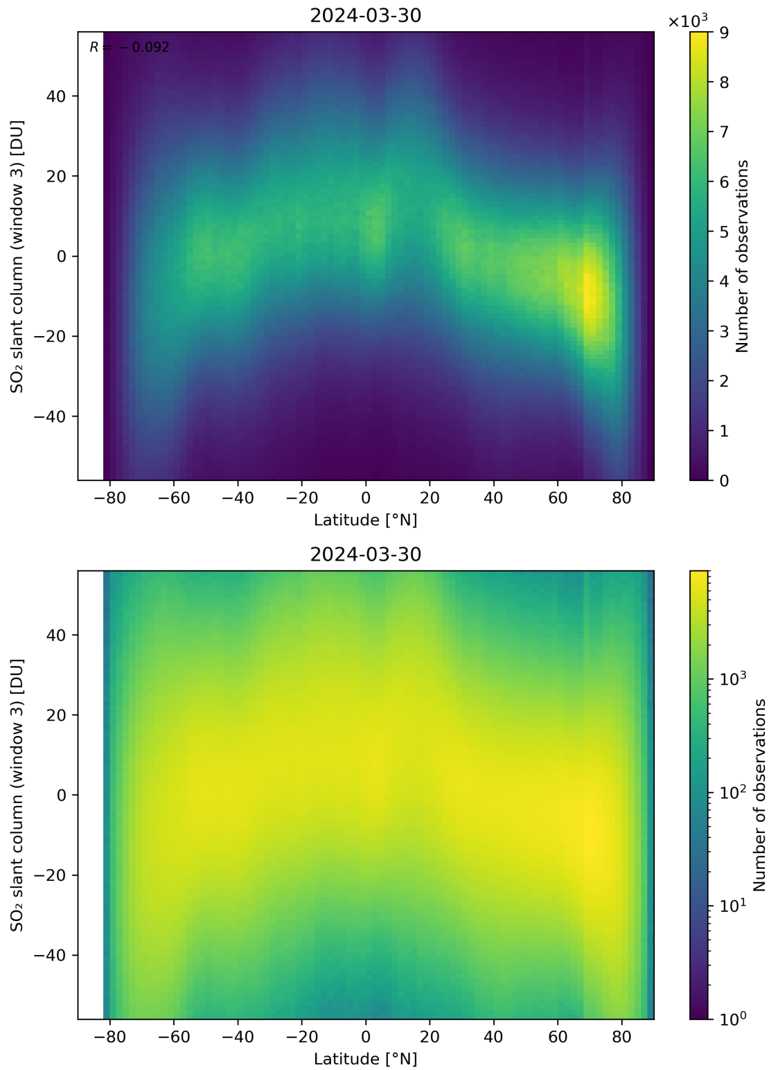
Figure 152: Scatter density plot of “Latitude” against “SO 2 slant column (window 3)” for 2024-03-30 to 2024-03-31.
