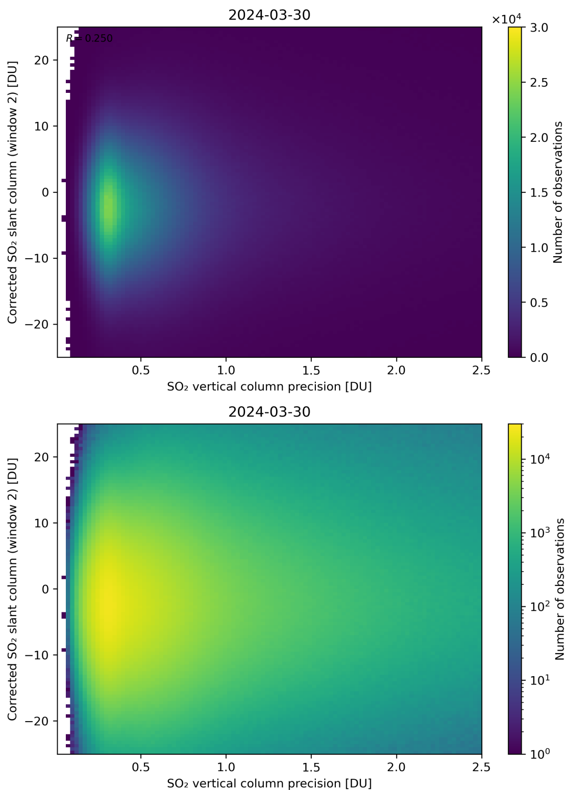
Figure 287: Scatter density plot of “SO 2 vertical column precision” against “Corrected SO 2 slant column (window 2)” for 2024-03-30 to 2024-03-31.
