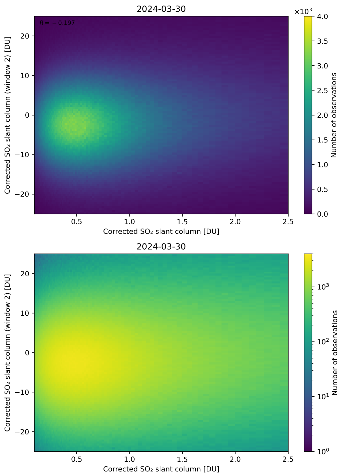
Figure 185: Scatter density plot of “Corrected SO 2 slant column” against “Corrected SO 2 slant column (window 2)” for 2024-03-30 to 2024-03-31.
