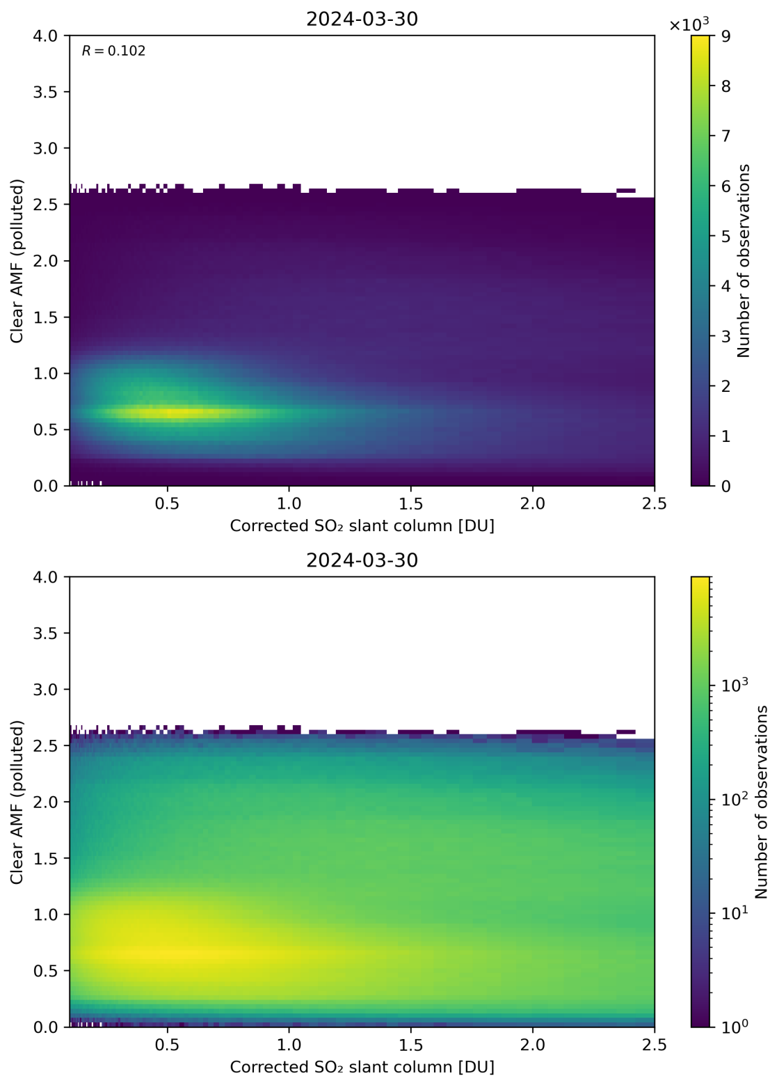
Figure 184: Scatter density plot of “Corrected SO 2 slant column” against “Clear AMF (polluted)” for 2024-03-30 to 2024-03-31.
