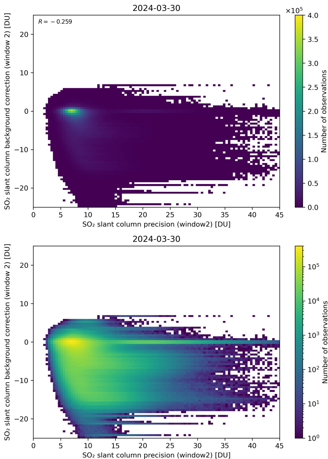
Figure 241: Scatter density plot of “SO 2 slant column precision (window2)” against “SO 2 slant column background correction (window 2)” for 2024-03-30 to 2024-03-31.
