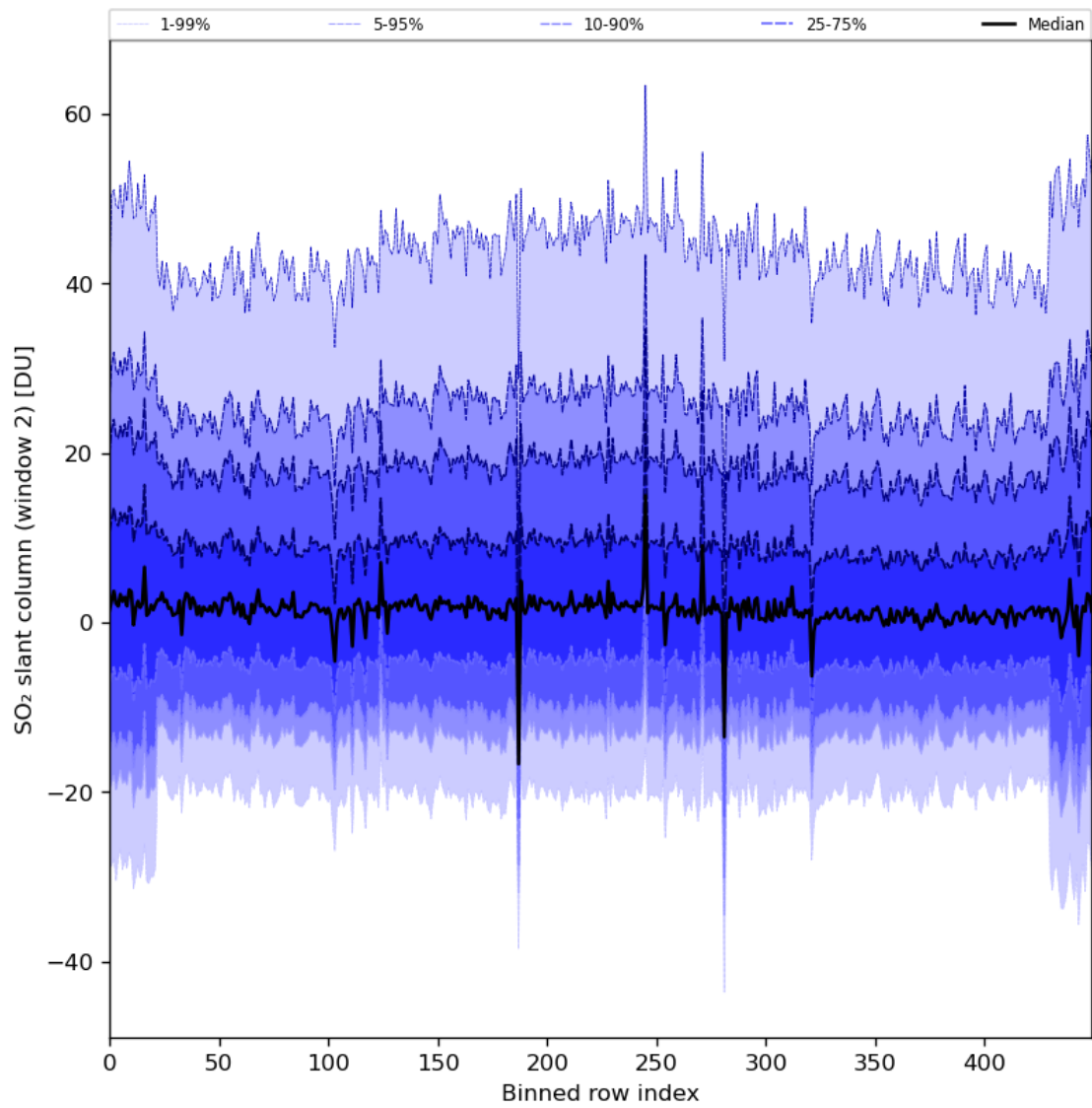
Figure 83: Along track statistics of “SO 2 slant column (window 2)” for 2024-03-30 to 2024-03-31
