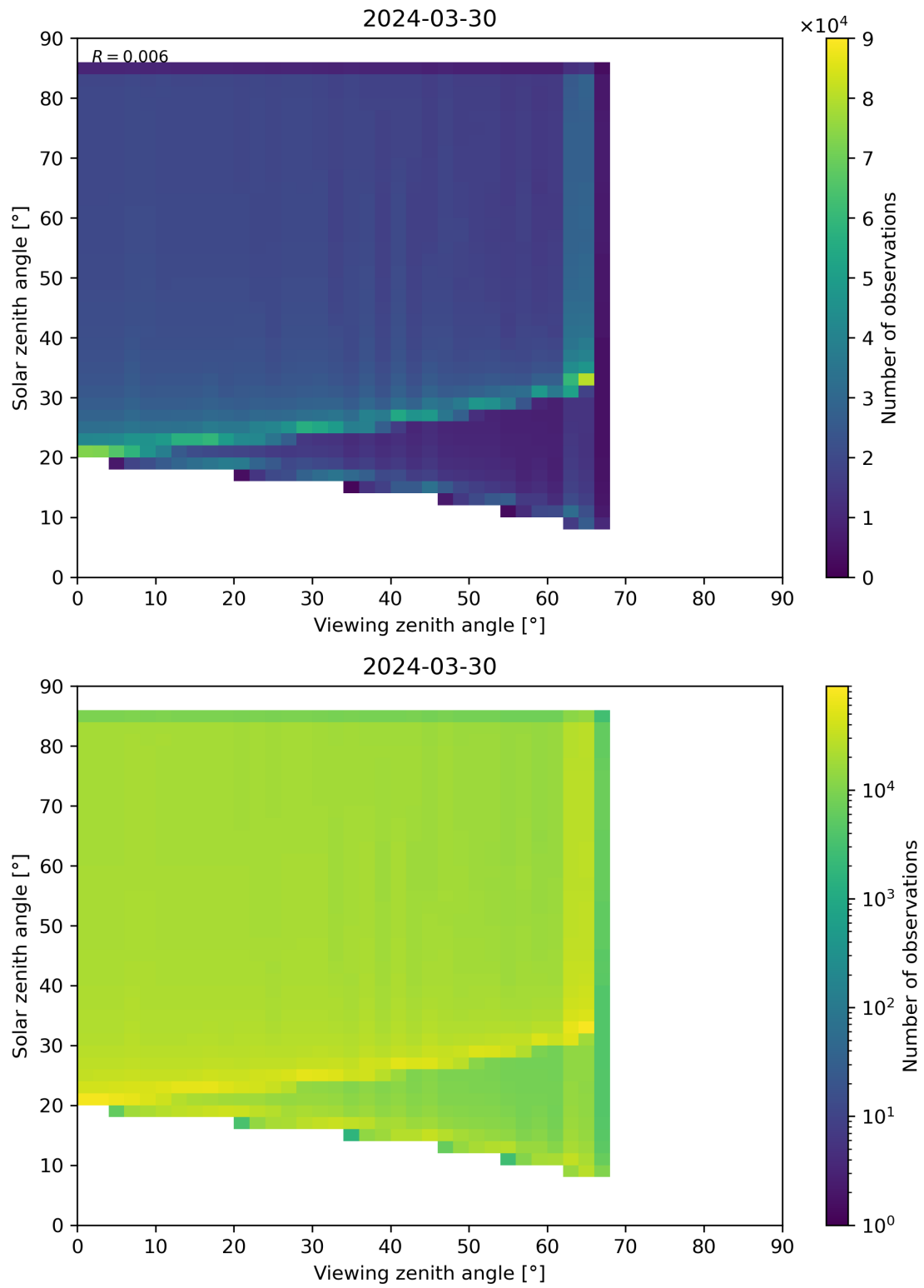
Figure 315: Scatter density plot of “Viewing zenith angle” against “Solar zenith angle” for 2024-03-30 to 2024-03-31.
