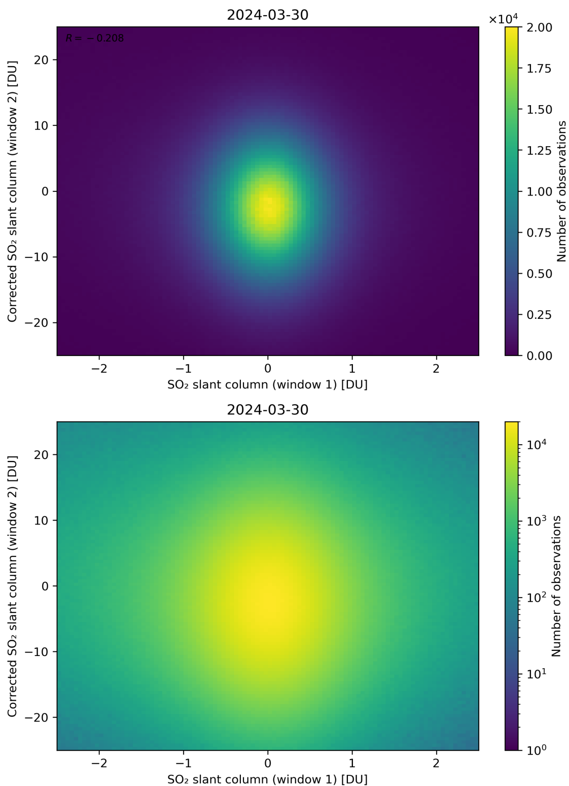
Figure 233: Scatter density plot of “SO 2 slant column (window 1)” against “Corrected SO 2 slant column (window 2)” for 2024-03-30 to 2024-03-31.
