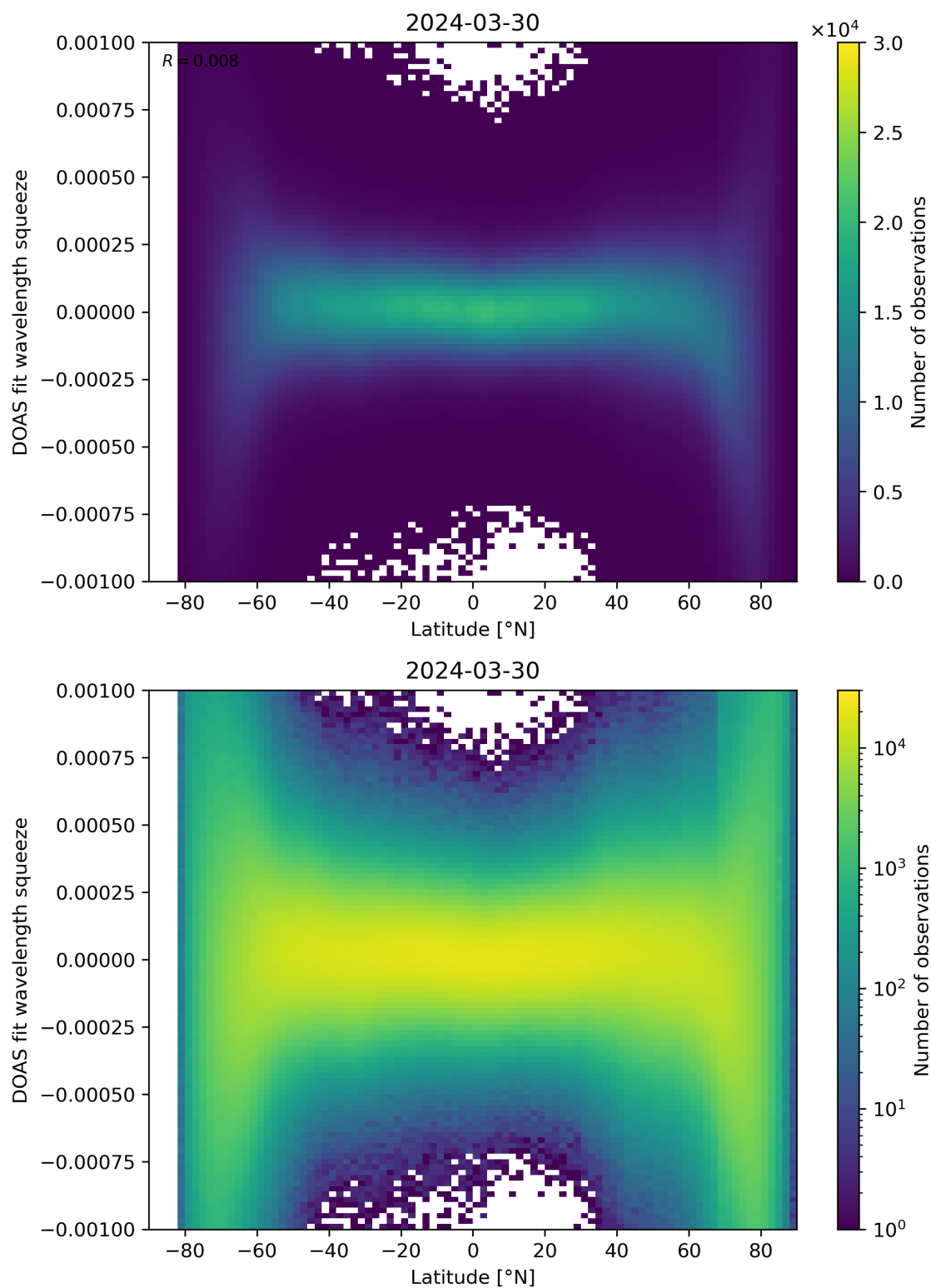
Figure 143: Scatter density plot of “Latitude” against “DOAS fit wavelength squeeze” for 2024-03-30 to 2024-03-31.
