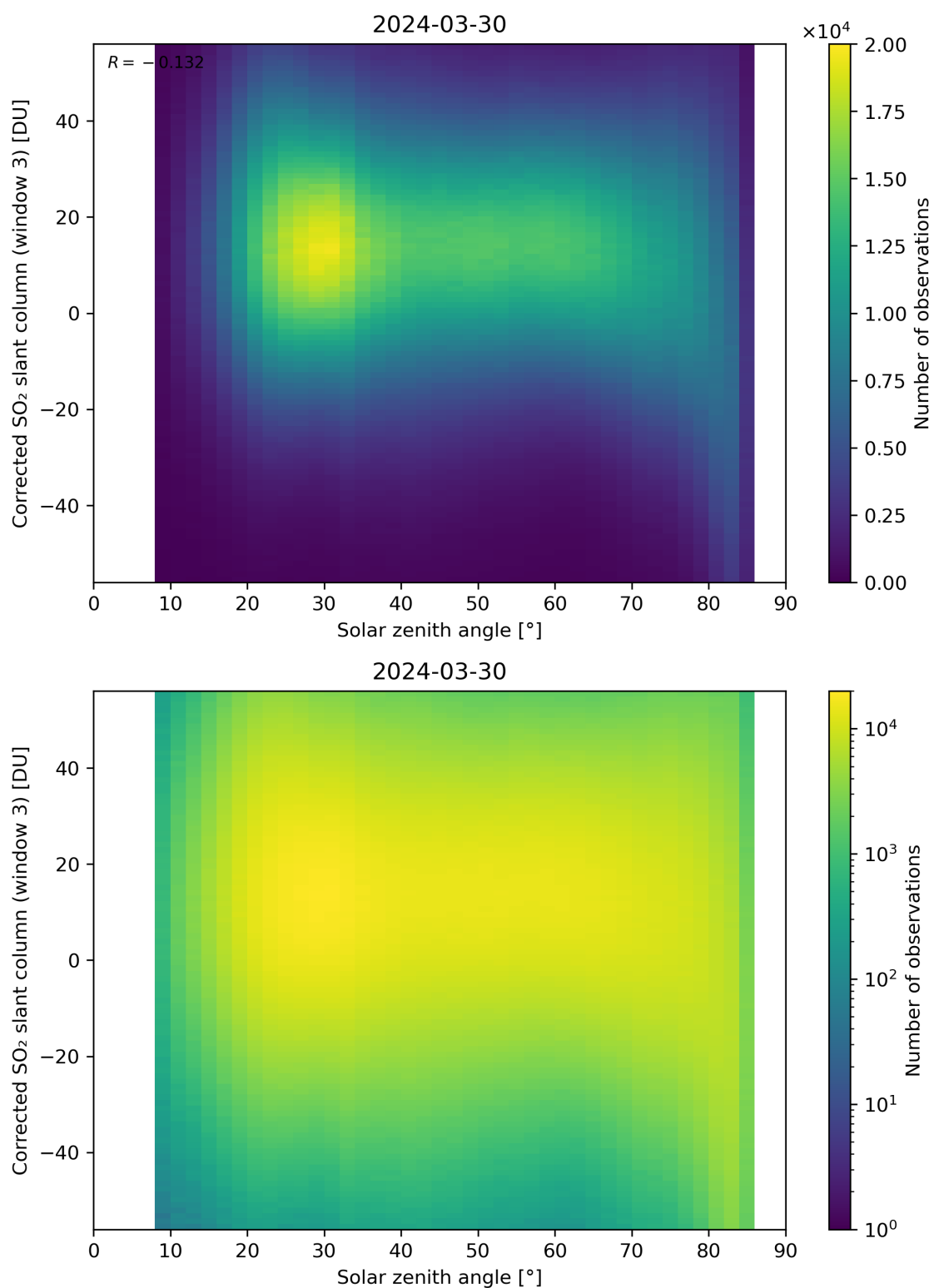
Figure 168: Scatter density plot of “Solar zenith angle” against “Corrected SO 2 slant column (window 3)” for 2024-03-30 to 2024-03-31.
