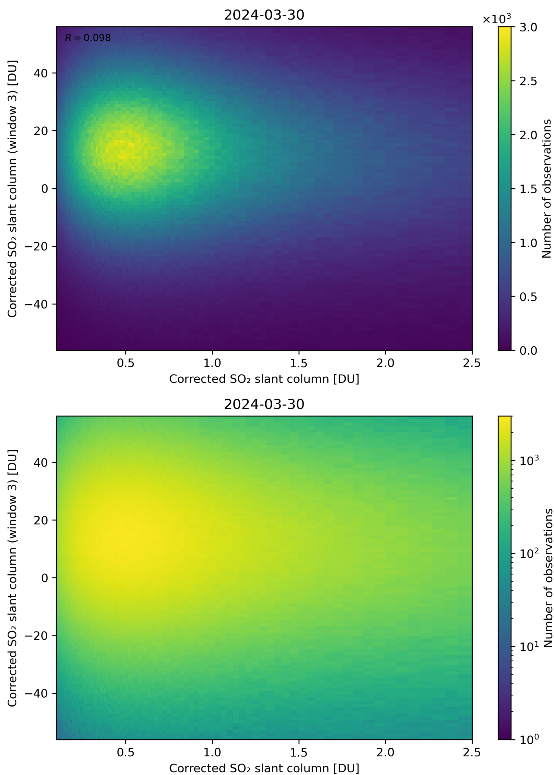
Figure 186: Scatter density plot of “Corrected SO 2 slant column” against “Corrected SO 2 slant column (window 3)” for 2024-03-30 to 2024-03-31.
