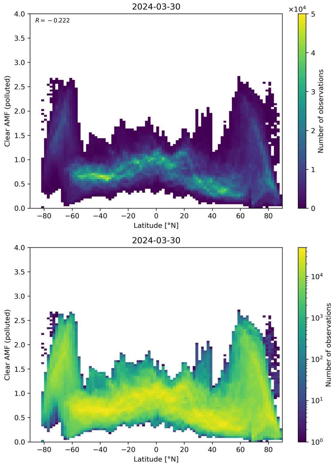
Figure 145: Scatter density plot of “Latitude” against “Clear AMF (polluted)” for 2024-03-30 to 2024-03-31.
