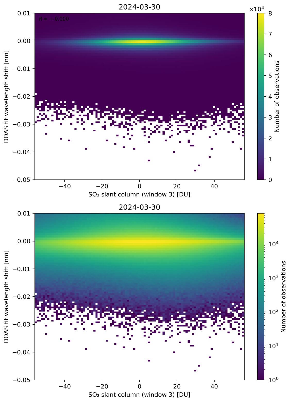
Figure 254: Scatter density plot of “SO 2 slant column (window 3)” against “DOAS fit wavelength shift” for 2024-03-30 to 2024-03-31.
