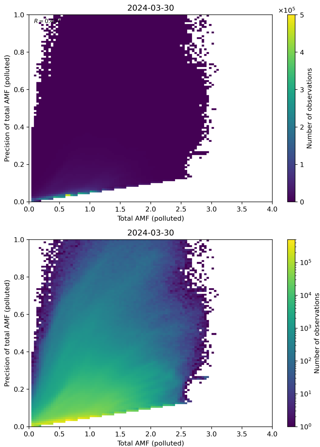
Figure 272: Scatter density plot of “Total AMF (polluted)” against “Precision of total AMF (polluted)” for 2024-03-30 to 2024-03-31.
