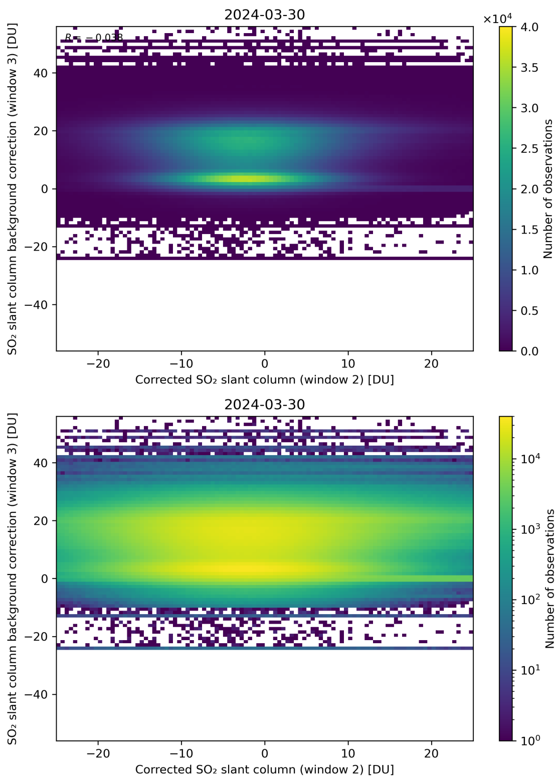
Figure 195: Scatter density plot of “Corrected SO 2 slant column (window 2)” against “SO 2 slant column background correction (window 3)” for 2024-03-30 to 2024-03-31.
