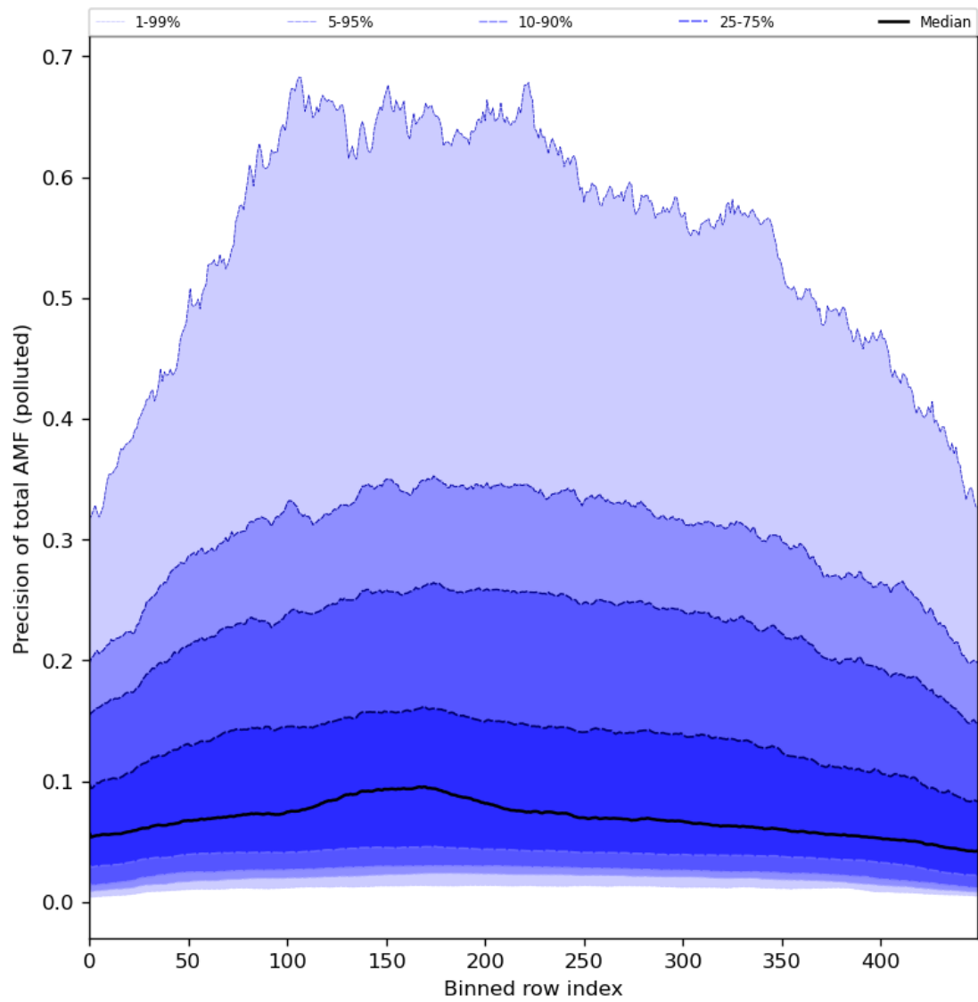
Figure 95: Along track statistics of “Precision of total AMF (polluted)” for 2024-03-30 to 2024-03-31
