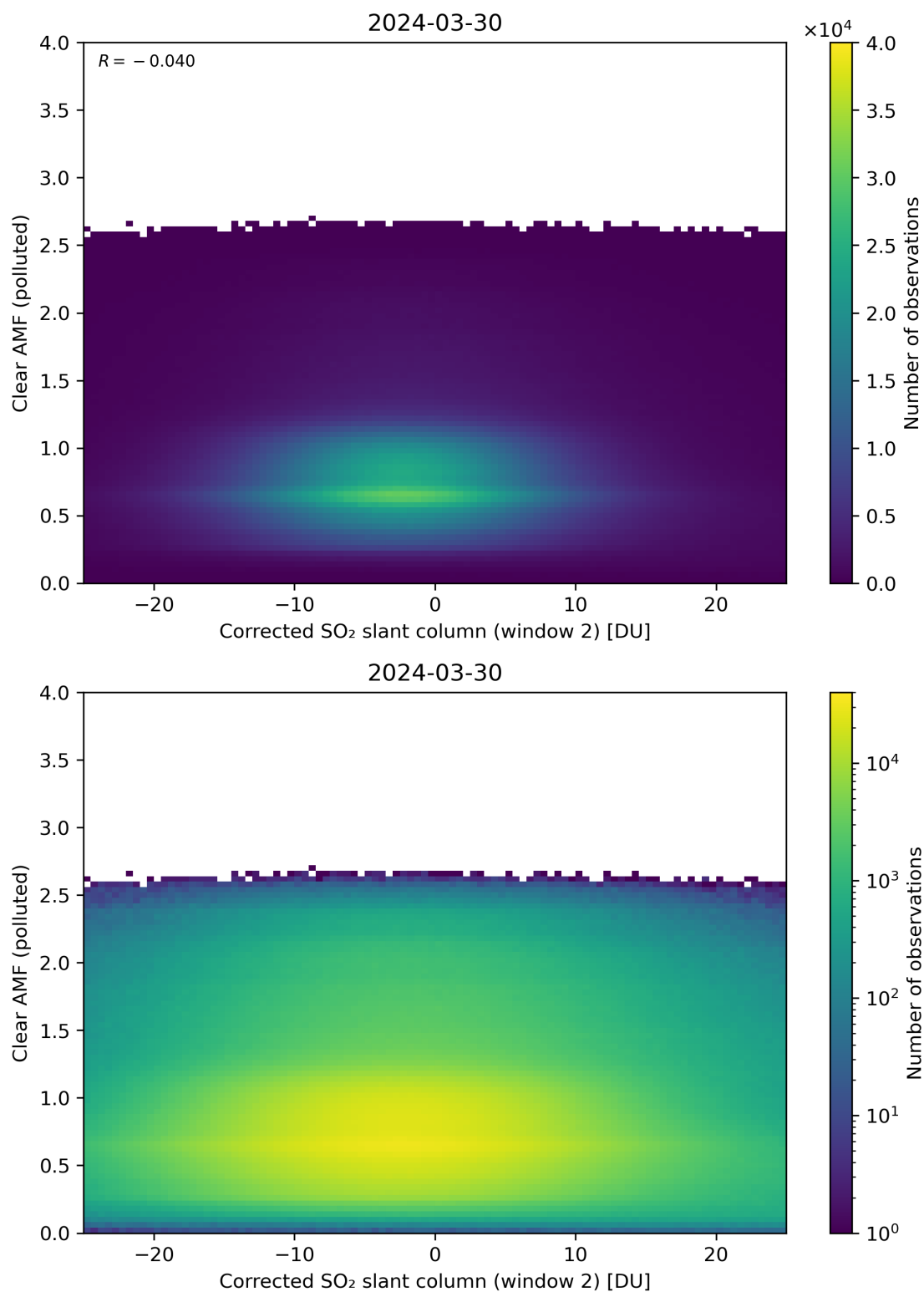
Figure 199: Scatter density plot of “Corrected SO 2 slant column (window 2)” against “Clear AMF (polluted)” for 2024-03-30 to 2024-03-31.
