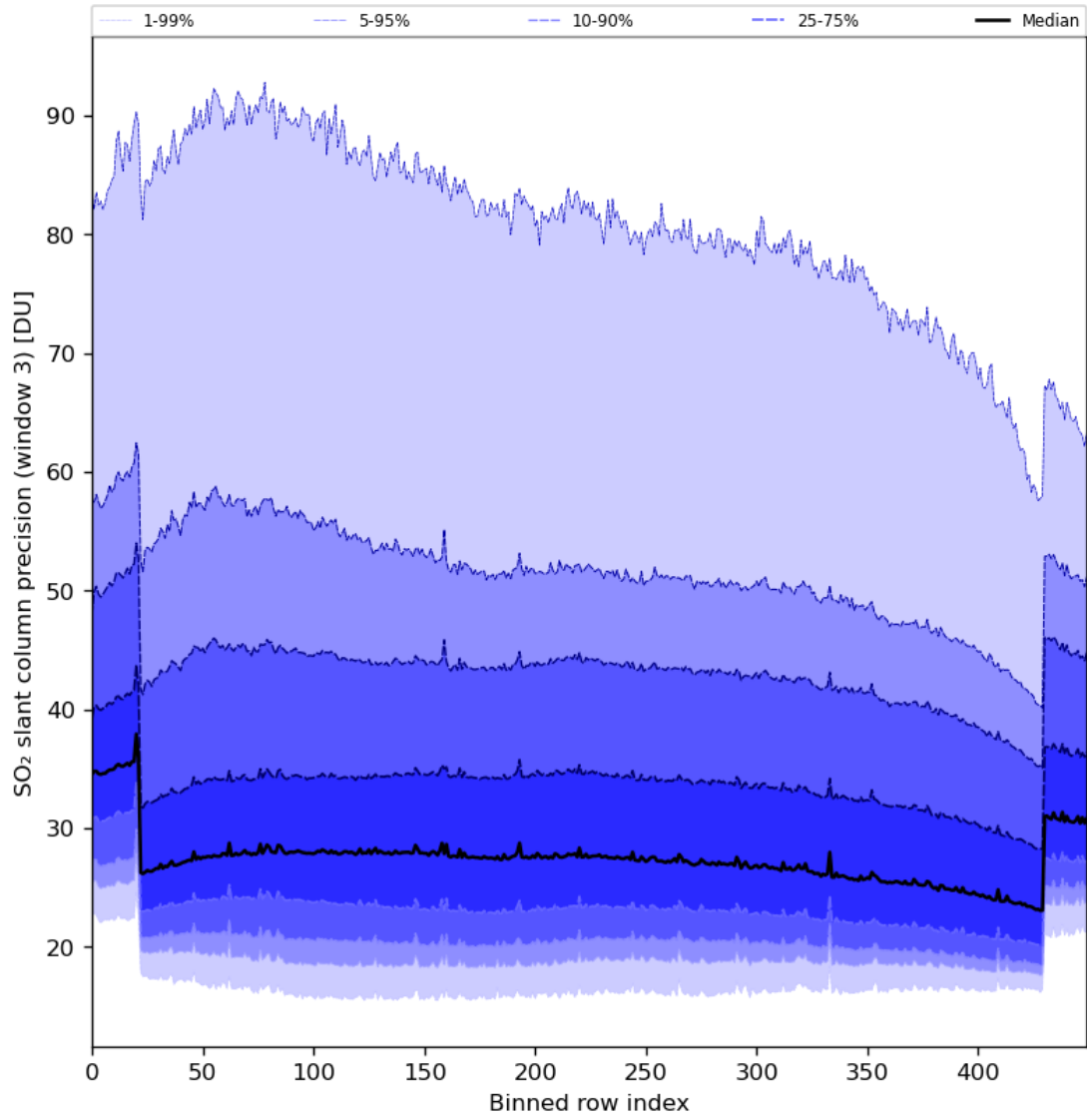
Figure 88: Along track statistics of “SO 2 slant column precision (window 3)” for 2024-03-30 to 2024-03-31
