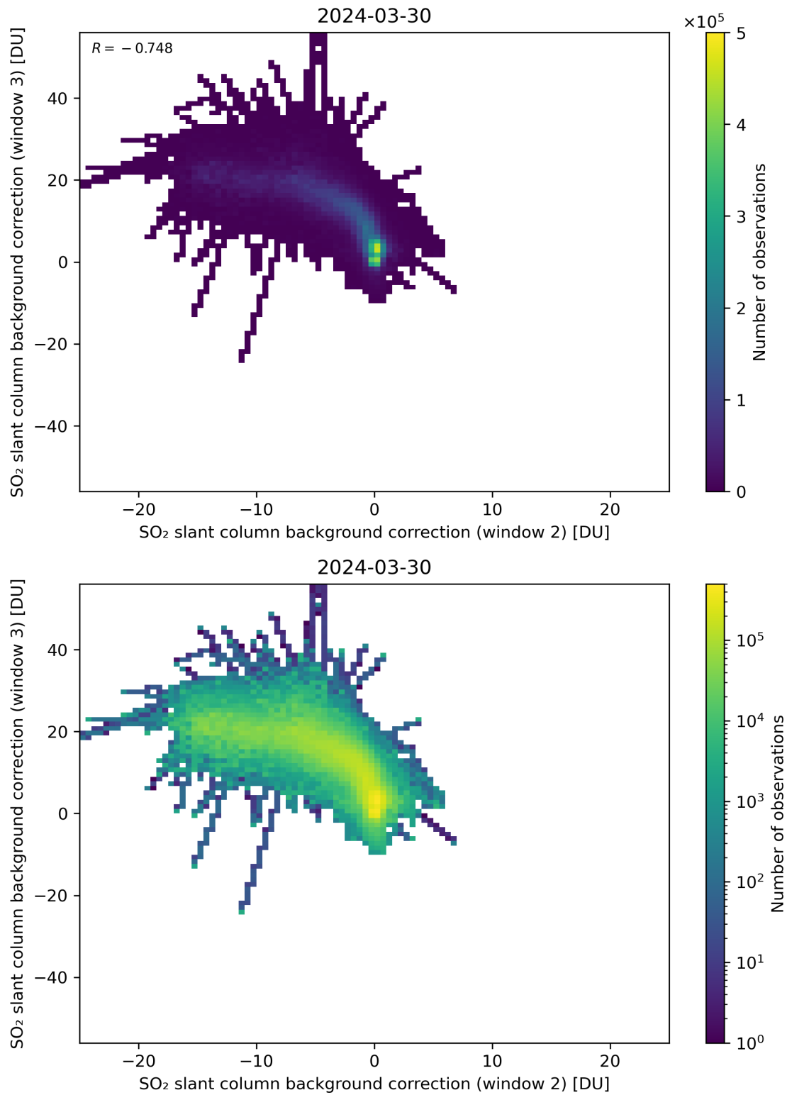
Figure 111: Scatter density plot of “SO 2 slant column background correction (window 2)” against “SO 2 slant column background correction (window 3)” for 2024-03-30 to 2024-03-31.
