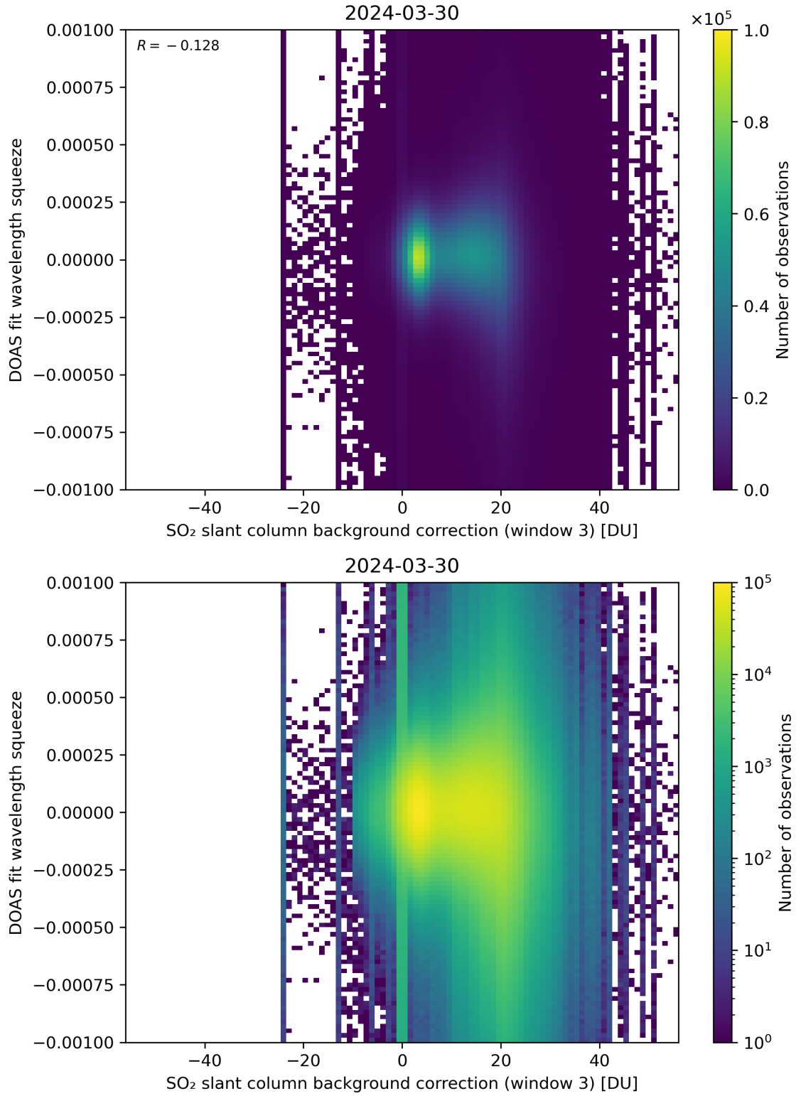
Figure 122: Scatter density plot of “SO 2 slant column background correction (window 3)” against “DOAS fit wavelength squeeze” for 2024-03-30 to 2024-03-31.
