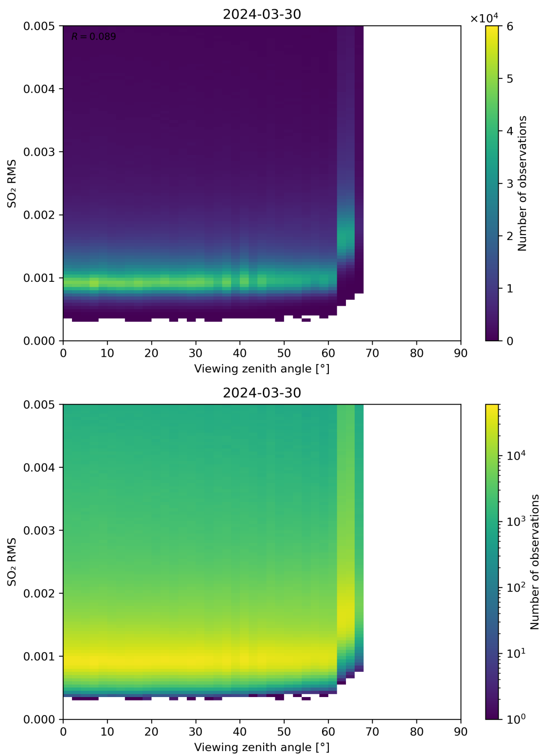
Figure 313: Scatter density plot of “Viewing zenith angle” against “SO 2 RMS” for 2024-03-30 to 2024-03-31.
