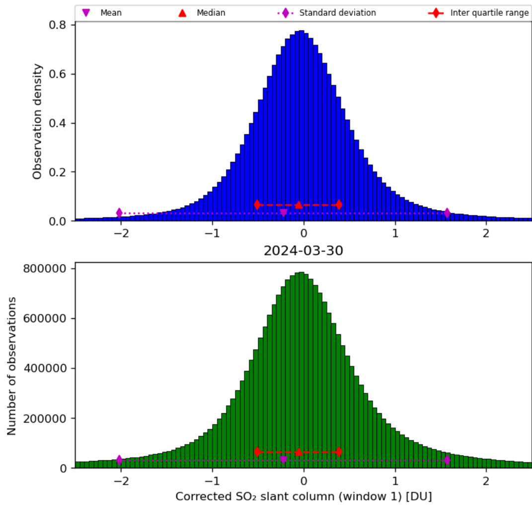
Figure 58: Histogram of “Corrected SO 2 slant column (window 1)” for 2024-03-30 to 2024-03-31
