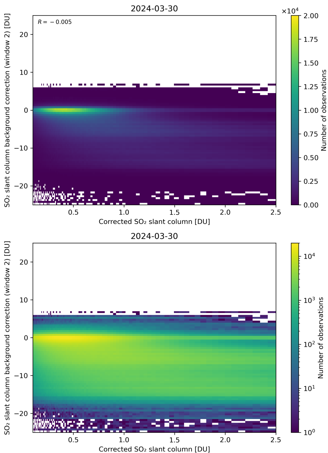
Figure 179: Scatter density plot of “Corrected SO 2 slant column” against “SO 2 slant column background correction (window 2)” for 2024-03-30 to 2024-03-31.
