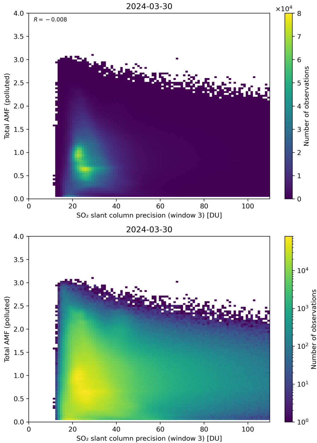
Figure 263: Scatter density plot of “SO 2 slant column precision (window 3)” against “Total AMF (polluted)” for 2024-03-30 to 2024-03-31.
