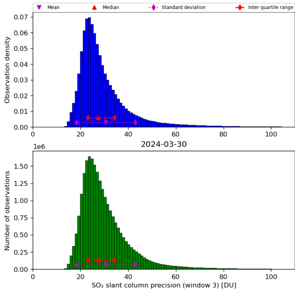
Figure 65: Histogram of “SO 2 slant column precision (window 3)” for 2024-03-30 to 2024-03-31
