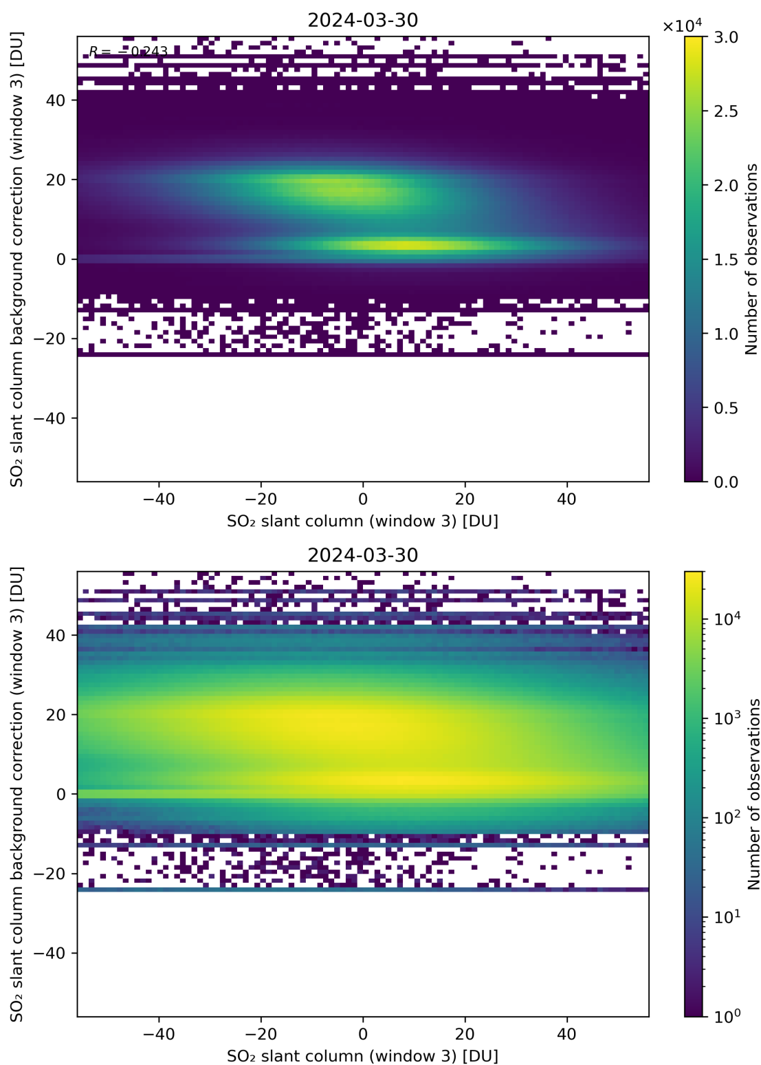
Figure 253: Scatter density plot of “SO 2 slant column (window 3)” against “SO 2 slant column background correction (window 3)” for 2024-03-30 to 2024-03-31.
