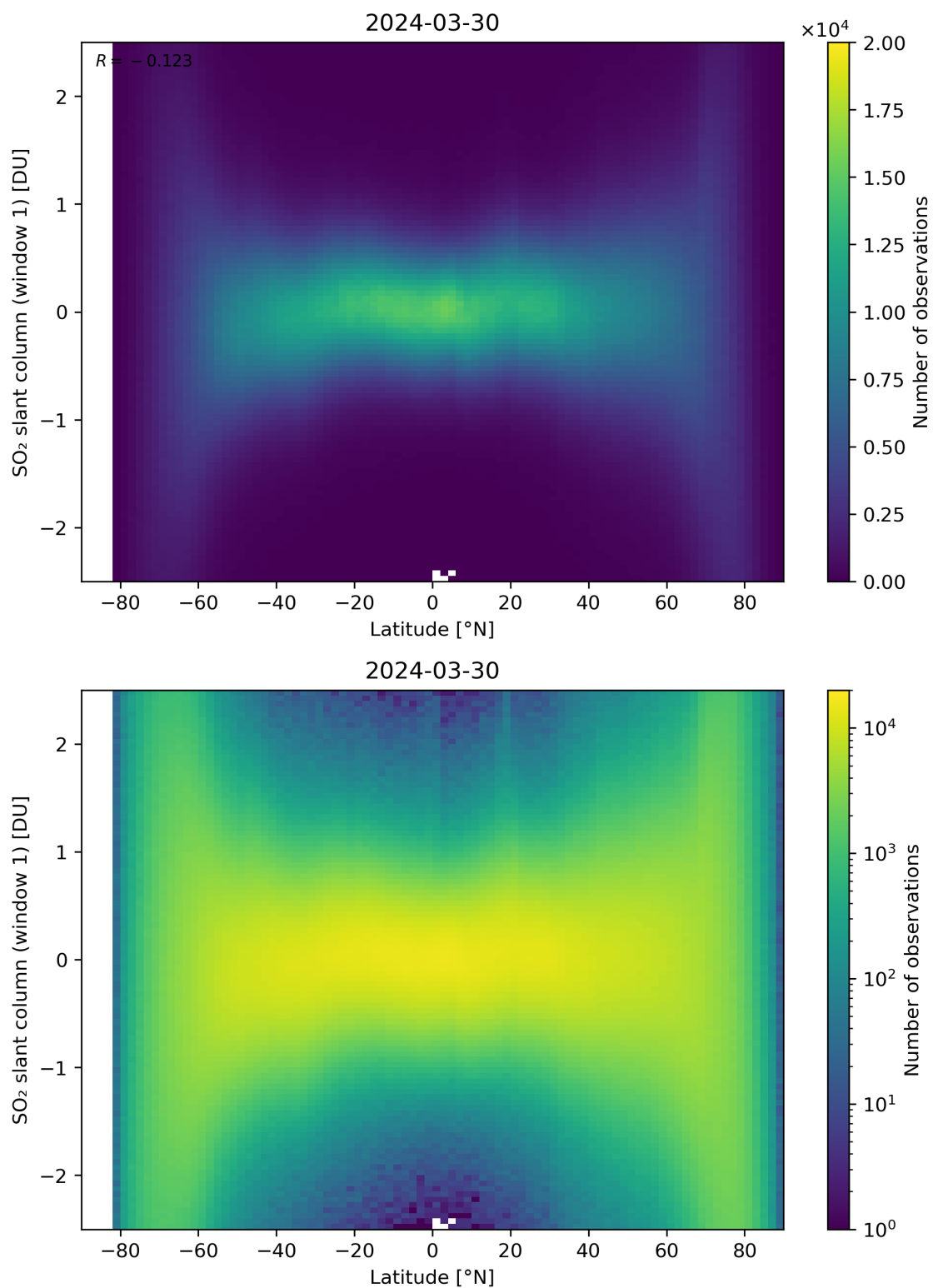
Figure 149: Scatter density plot of “Latitude” against “SO 2 slant column (window 1)” for 2024-03-30 to 2024-03-31.
