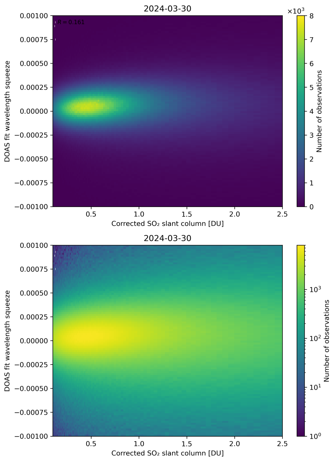
Figure 182: Scatter density plot of “Corrected SO 2 slant column” against “DOAS fit wavelength squeeze” for 2024-03-30 to 2024-03-31.
