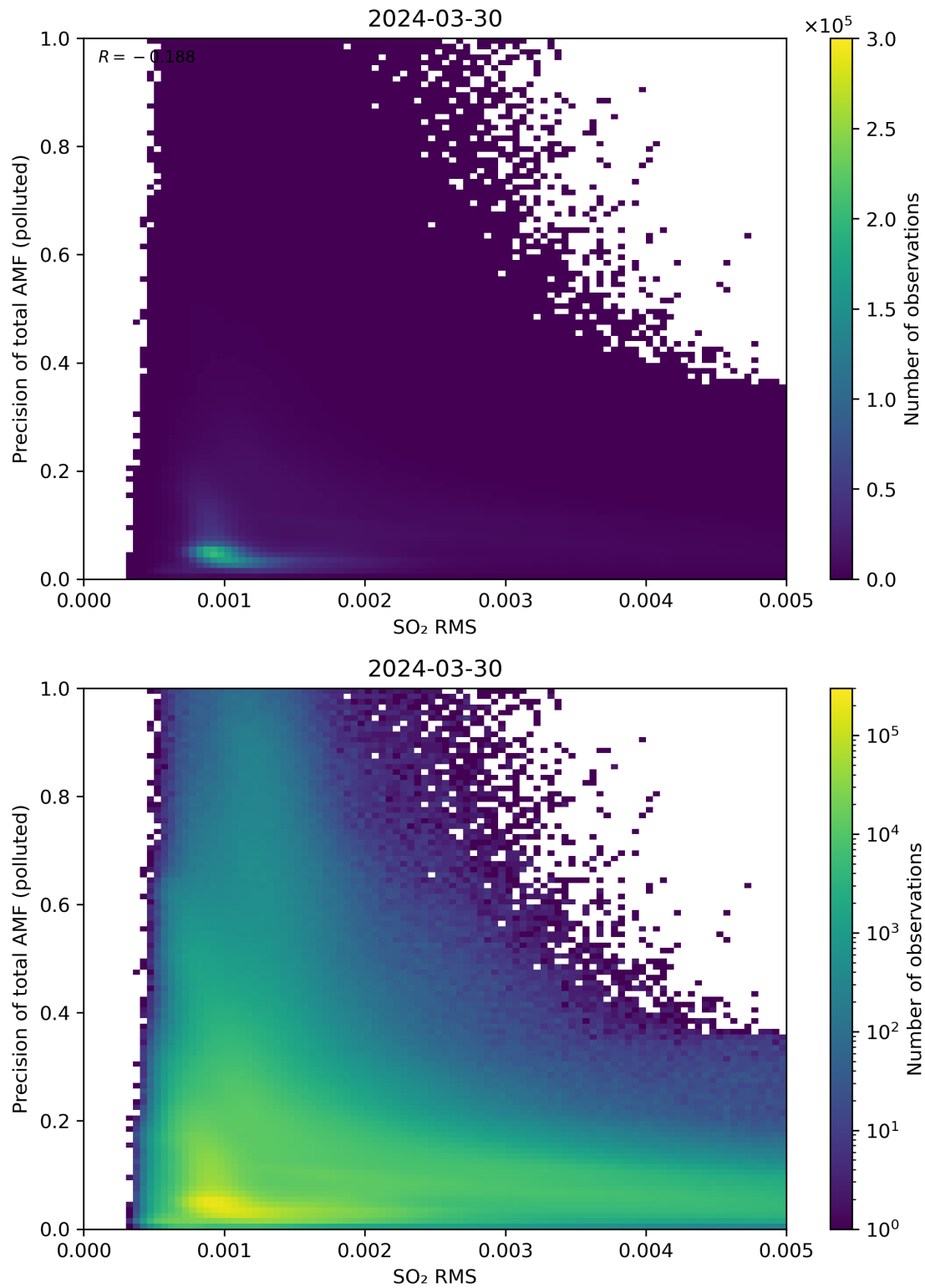
Figure 138: Scatter density plot of “SO 2 RMS” against “Precision of total AMF (polluted)” for 2024-03-30 to 2024-03-31.
