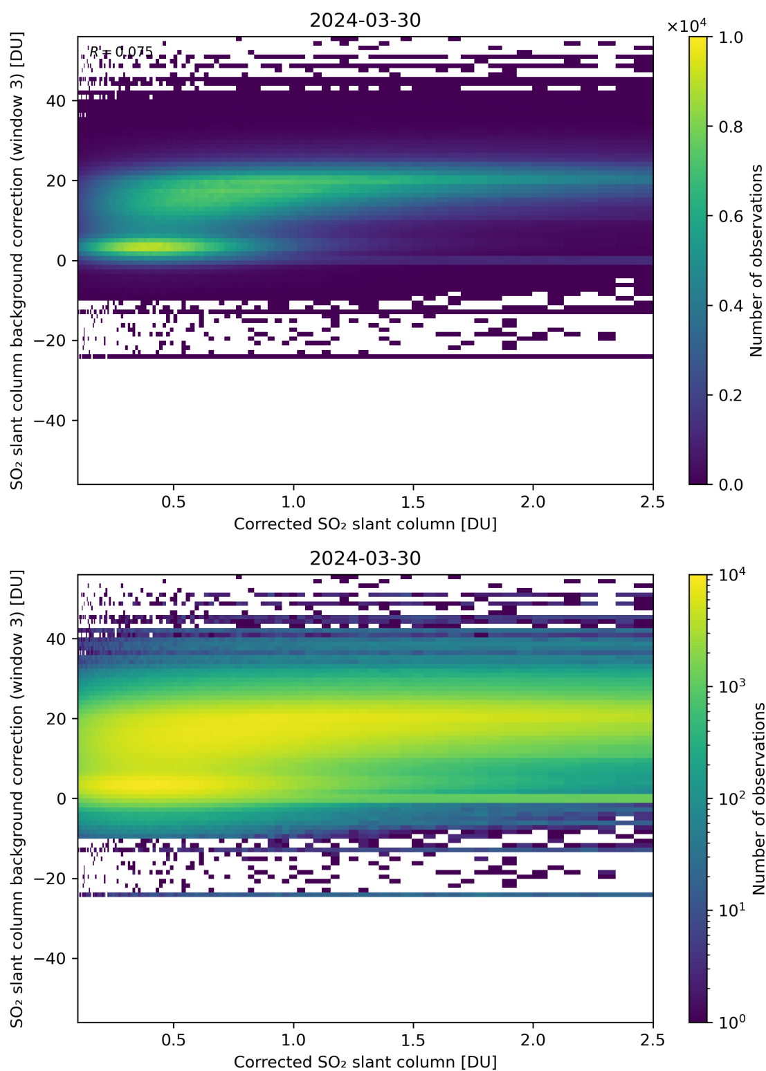
Figure 180: Scatter density plot of “Corrected SO 2 slant column” against “SO 2 slant column background correction (window 3)” for 2024-03-30 to 2024-03-31.
