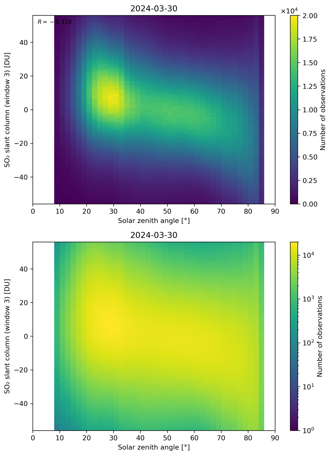
Figure 172: Scatter density plot of “Solar zenith angle” against “SO 2 slant column (window 3)” for 2024-03-30 to 2024-03-31.
