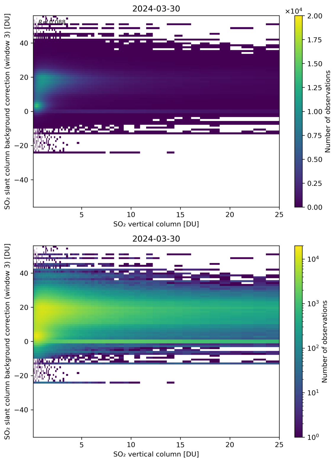
Figure 275: Scatter density plot of “SO 2 vertical column” against “SO 2 slant column background correction (window 3)” for 2024-03-30 to 2024-03-31.
