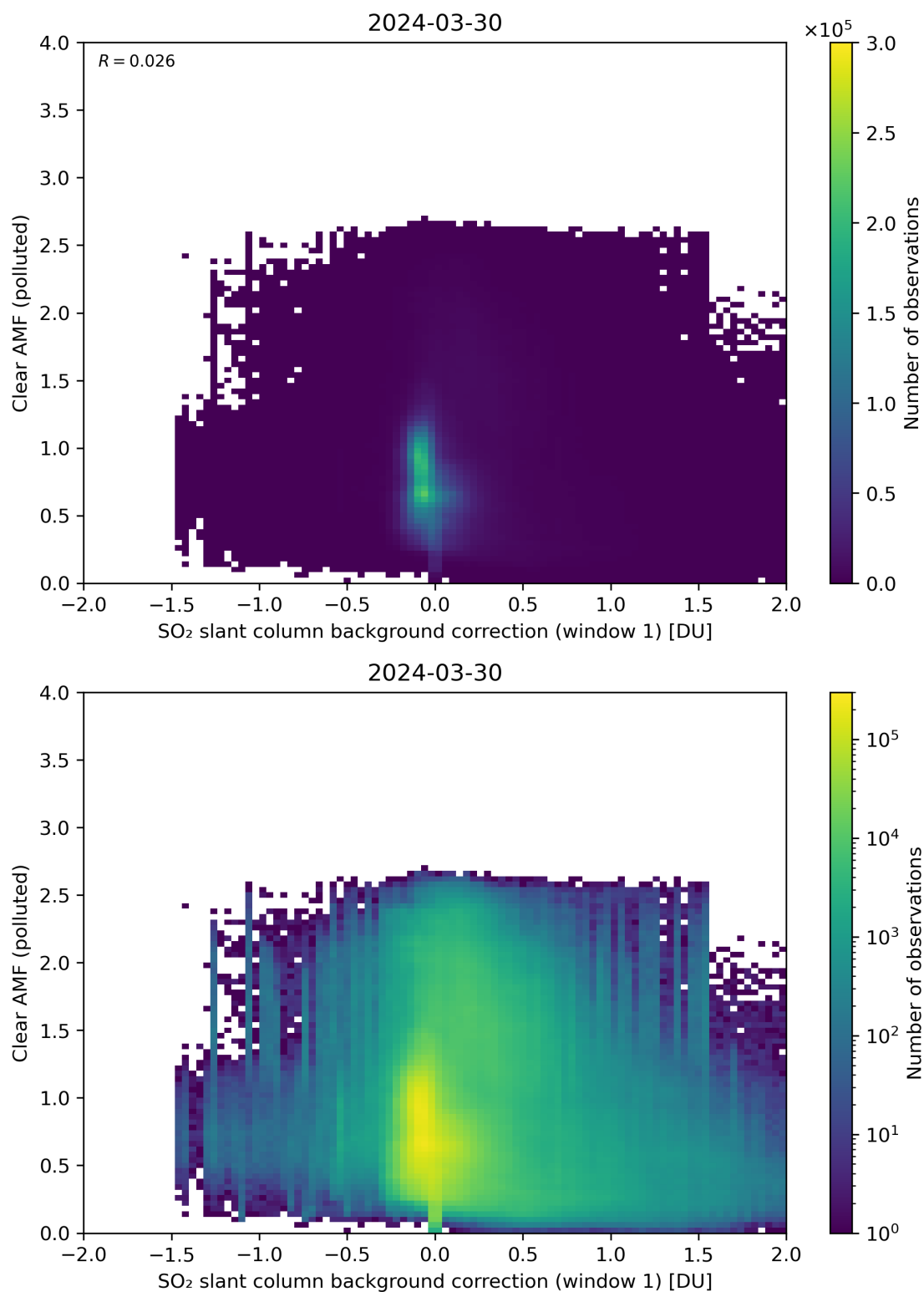
Figure 103: Scatter density plot of “SO 2 slant column background correction (window 1)” against “Clear AMF (polluted)” for 2024-03-30 to 2024-03-31.
