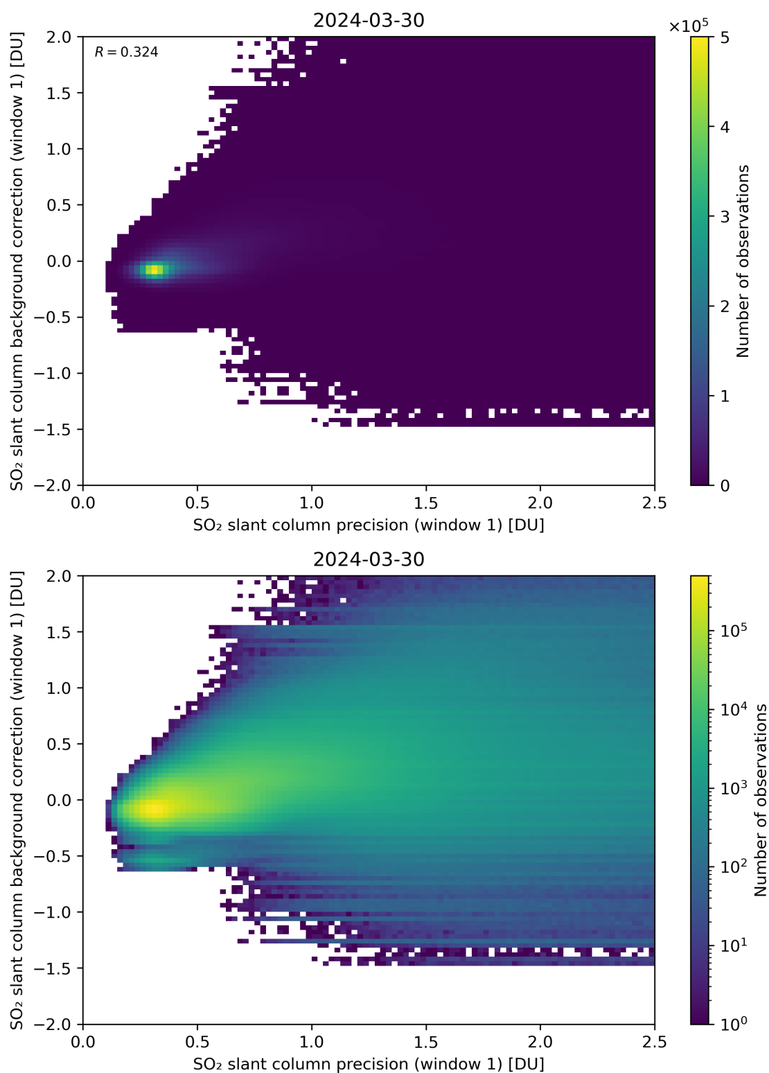
Figure 218: Scatter density plot of “SO 2 slant column precision (window 1)” against “SO 2 slant column background correction (window 1)” for 2024-03-30 to 2024-03-31.
