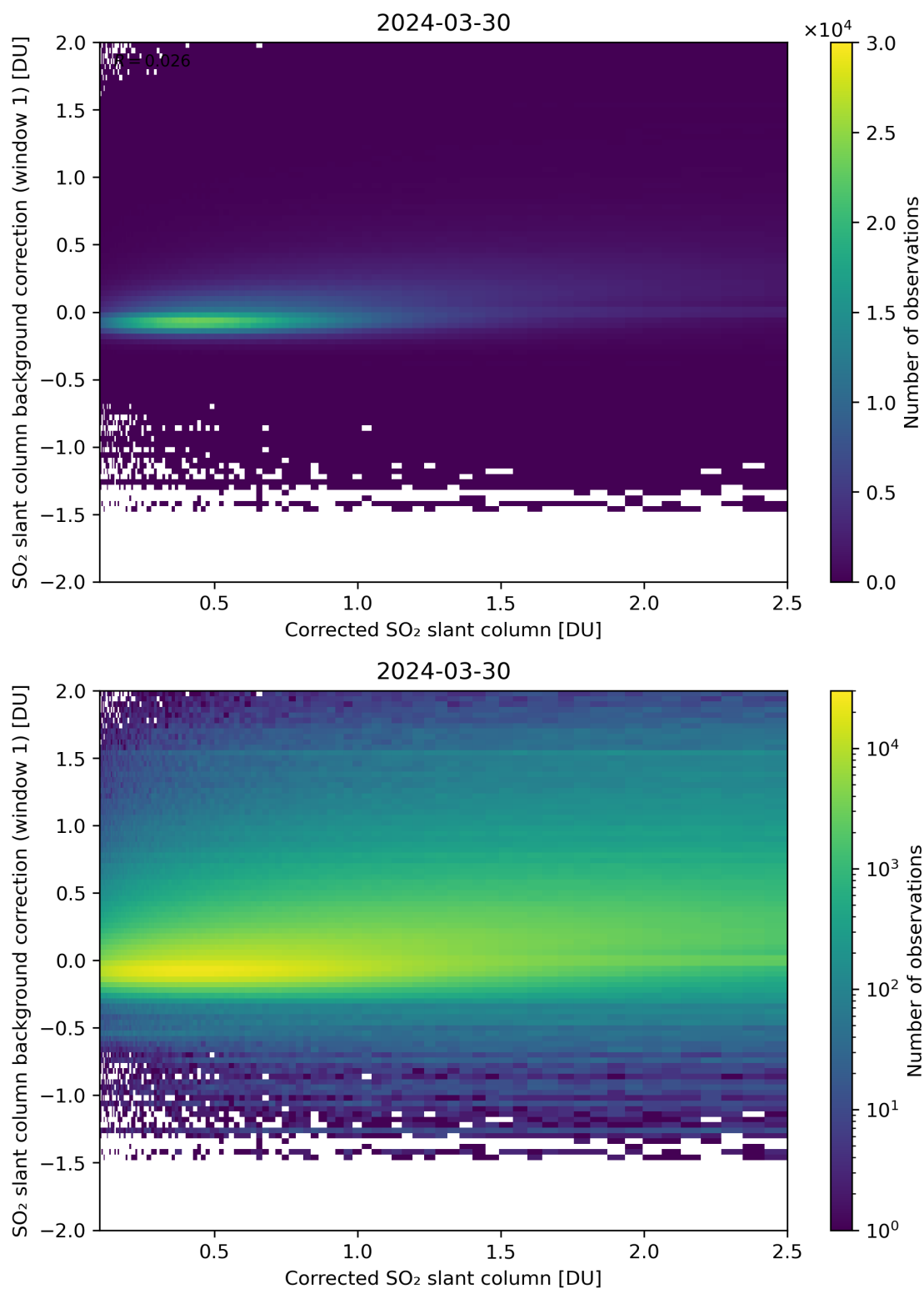
Figure 178: Scatter density plot of “Corrected SO 2 slant column” against “SO 2 slant column background correction (window 1)” for 2024-03-30 to 2024-03-31.
