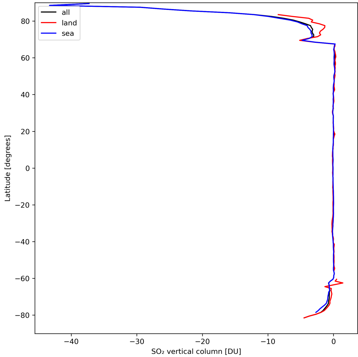
Figure 30: Zonal average of “SO 2 vertical column” for 2024-03-30 to 2024-03-31.
