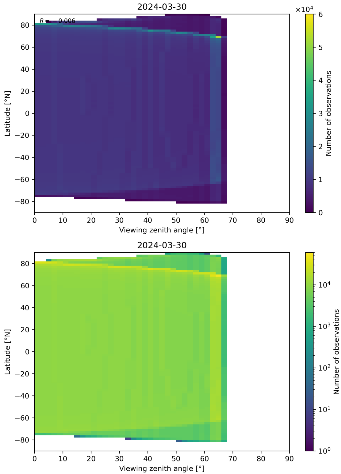
Figure 314: Scatter density plot of “Viewing zenith angle” against “Latitude” for 2024-03-30 to 2024-03-31.
