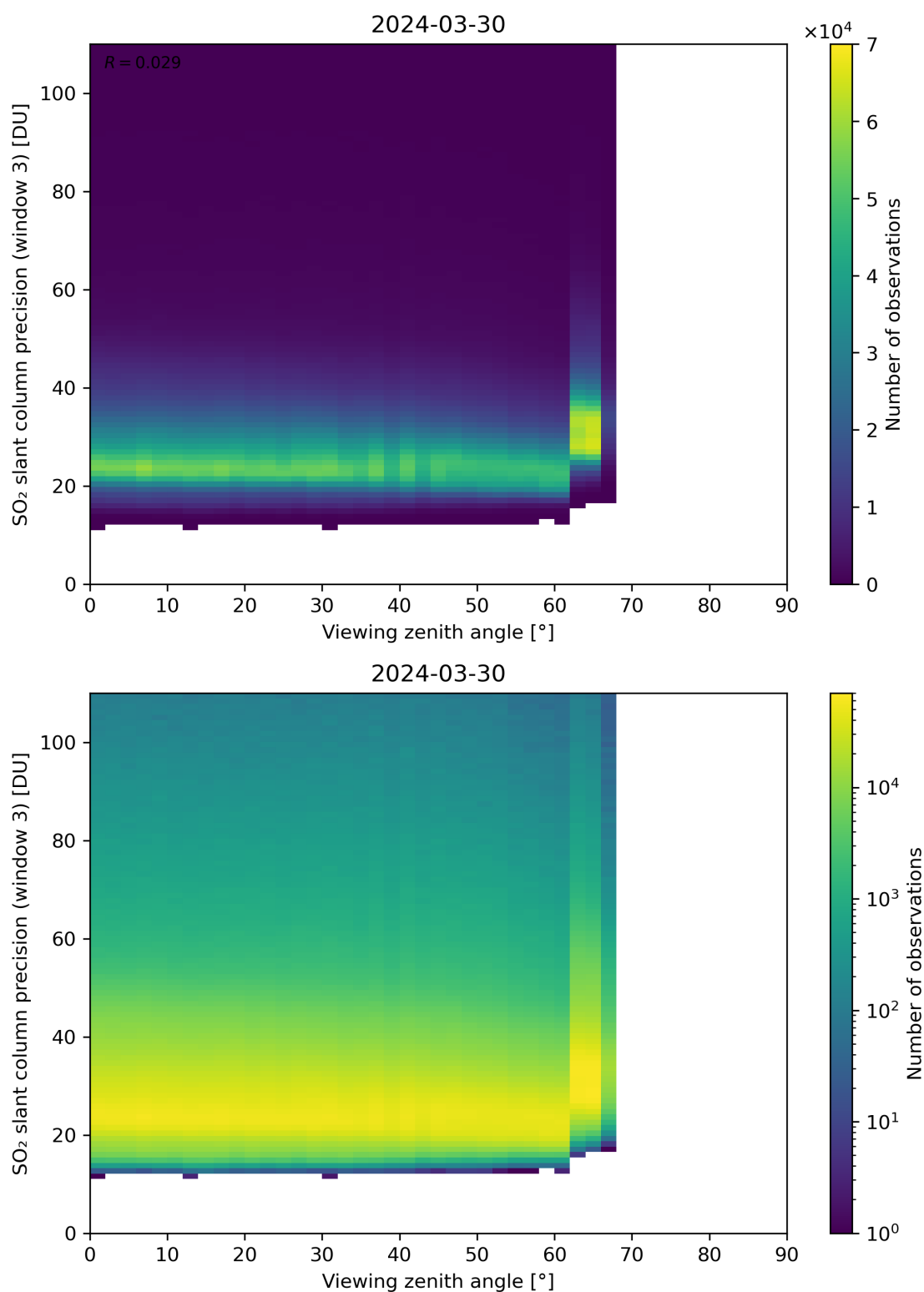
Figure 324: Scatter density plot of “Viewing zenith angle” against “SO 2 slant column precision (window 3)” for 2024-03-30 to 2024-03-31.
