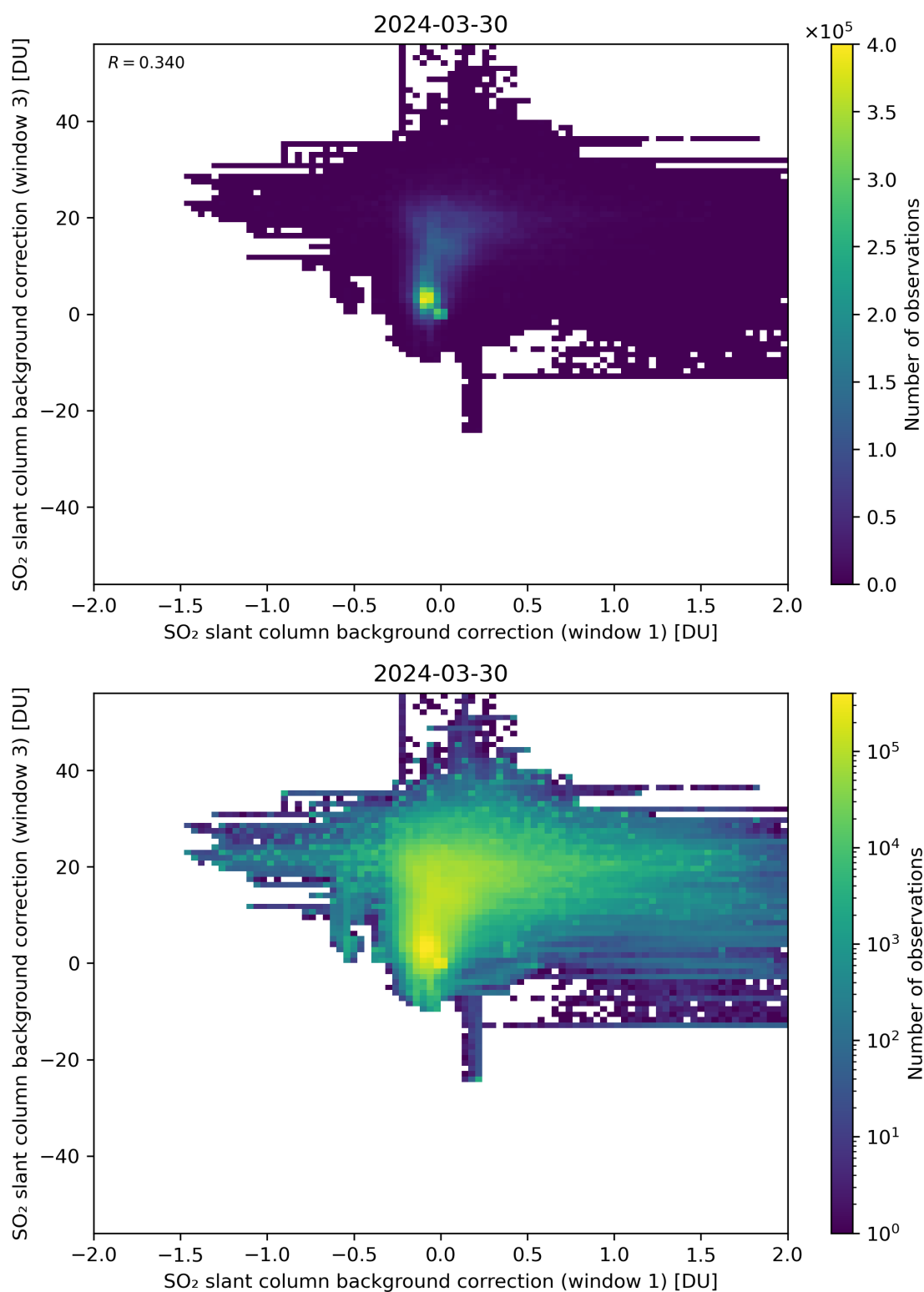
Figure 99: Scatter density plot of “SO 2 slant column background correction (window 1)” against “SO 2 slant column background correction (window 3)” for 2024-03-30 to 2024-03-31.
