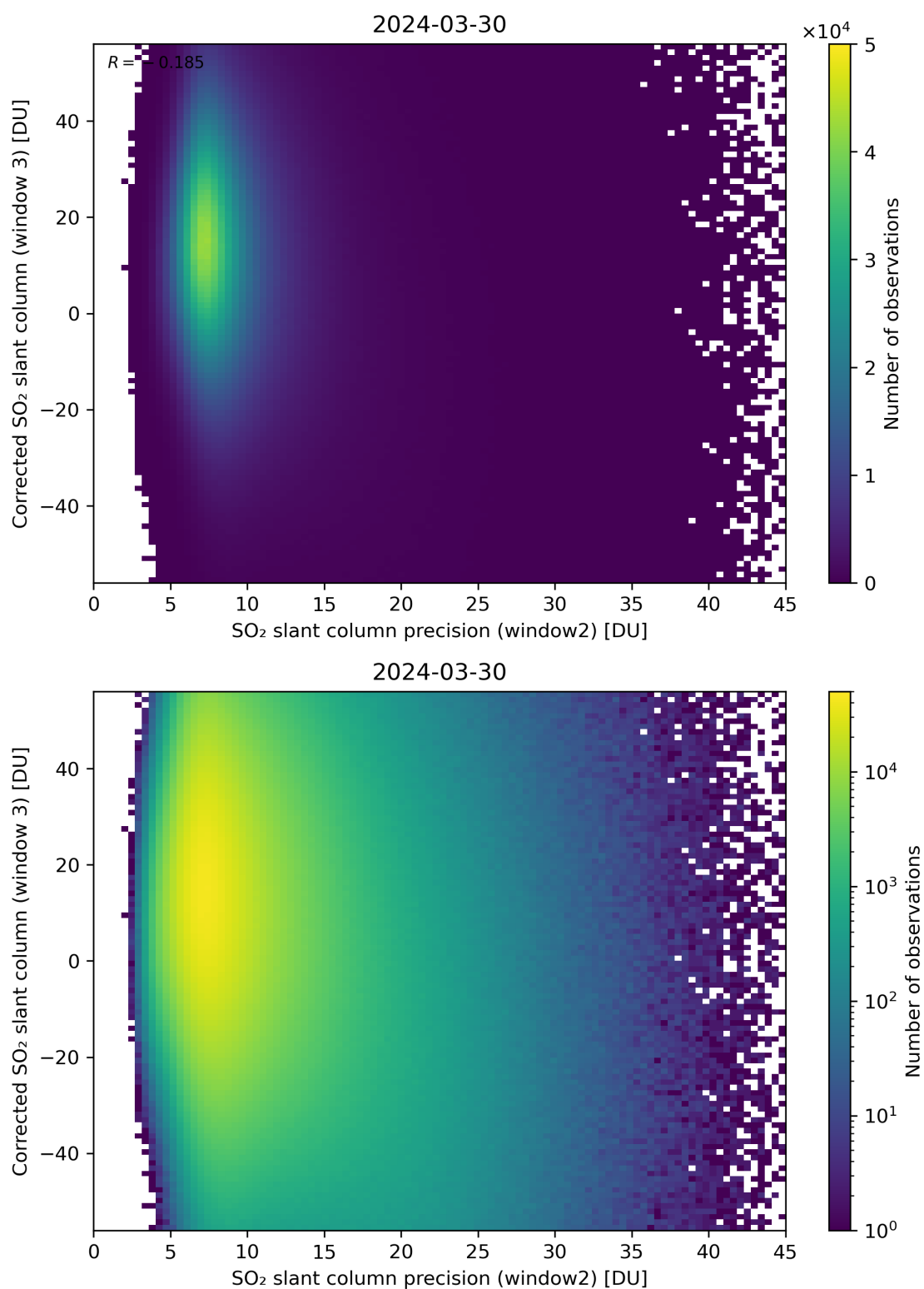
Figure 248: Scatter density plot of “SO 2 slant column precision (window2)” against “Corrected SO 2 slant column (window 3)” for 2024-03-30 to 2024-03-31.
