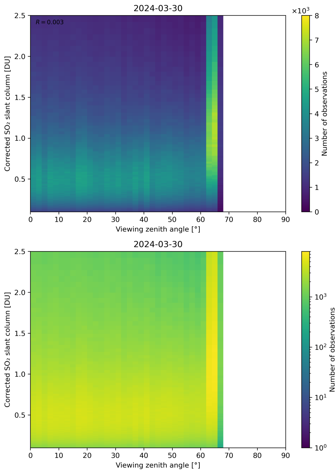
Figure 317: Scatter density plot of “Viewing zenith angle” against “Corrected SO 2 slant column” for 2024-03-30 to 2024-03-31.
