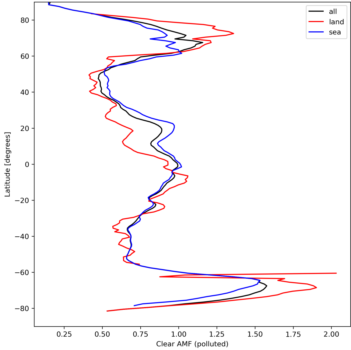
Figure 50: Zonal average of “Clear AMF (polluted)” for 2024-03-30 to 2024-03-31.
