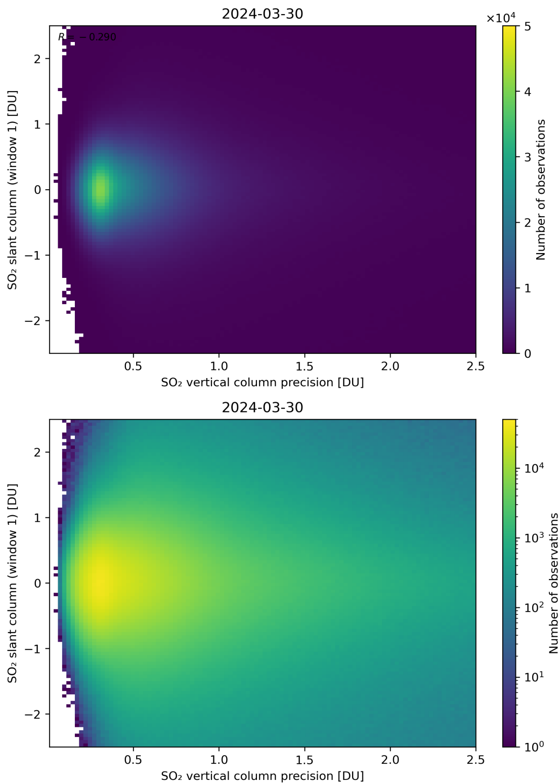
Figure 289: Scatter density plot of “SO 2 vertical column precision” against “SO 2 slant column (window 1)” for 2024-03-30 to 2024-03-31.
