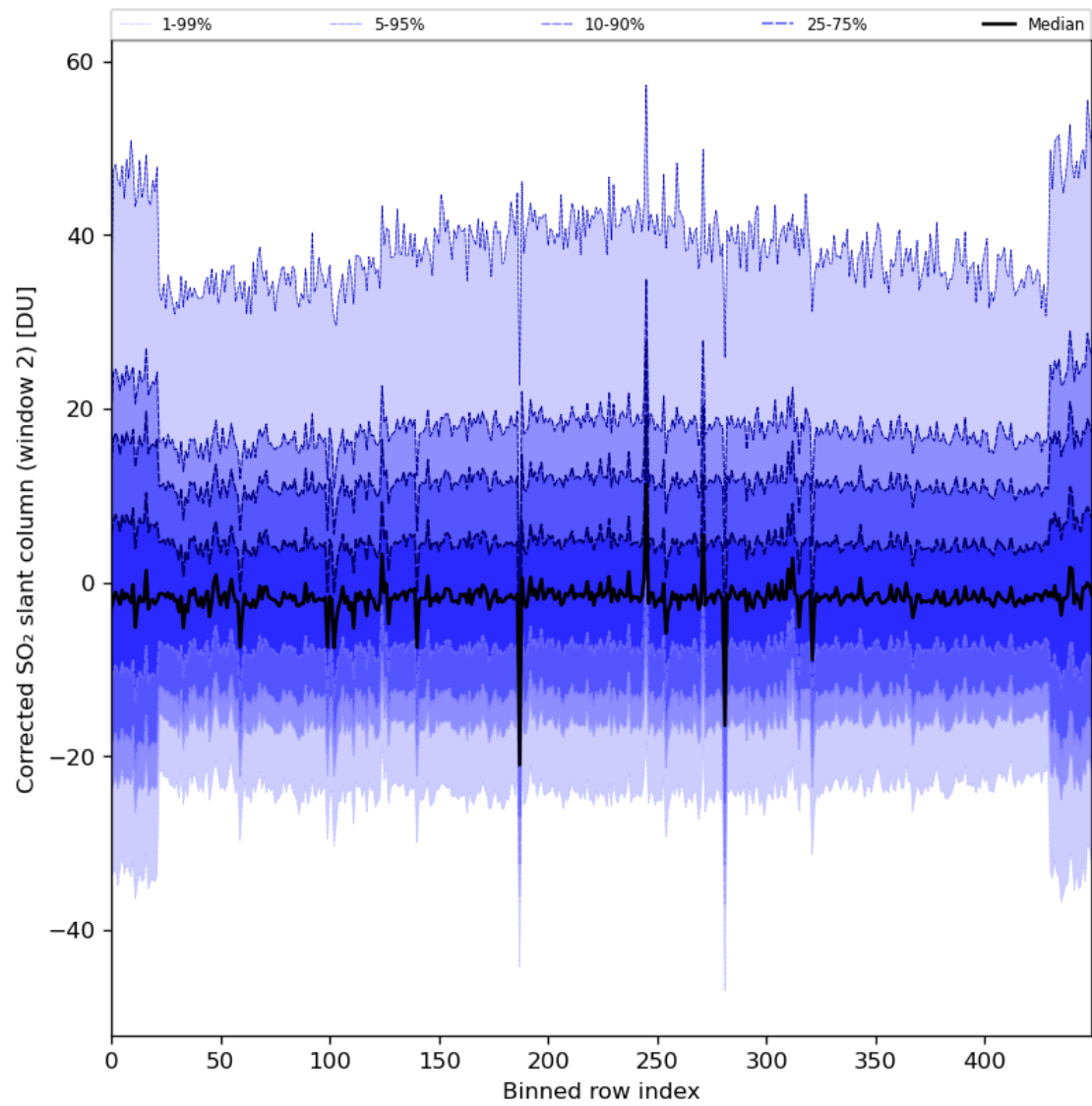
Figure 85: Along track statistics of “Corrected SO 2 slant column (window 2)” for 2024-03-30 to 2024-03-31
