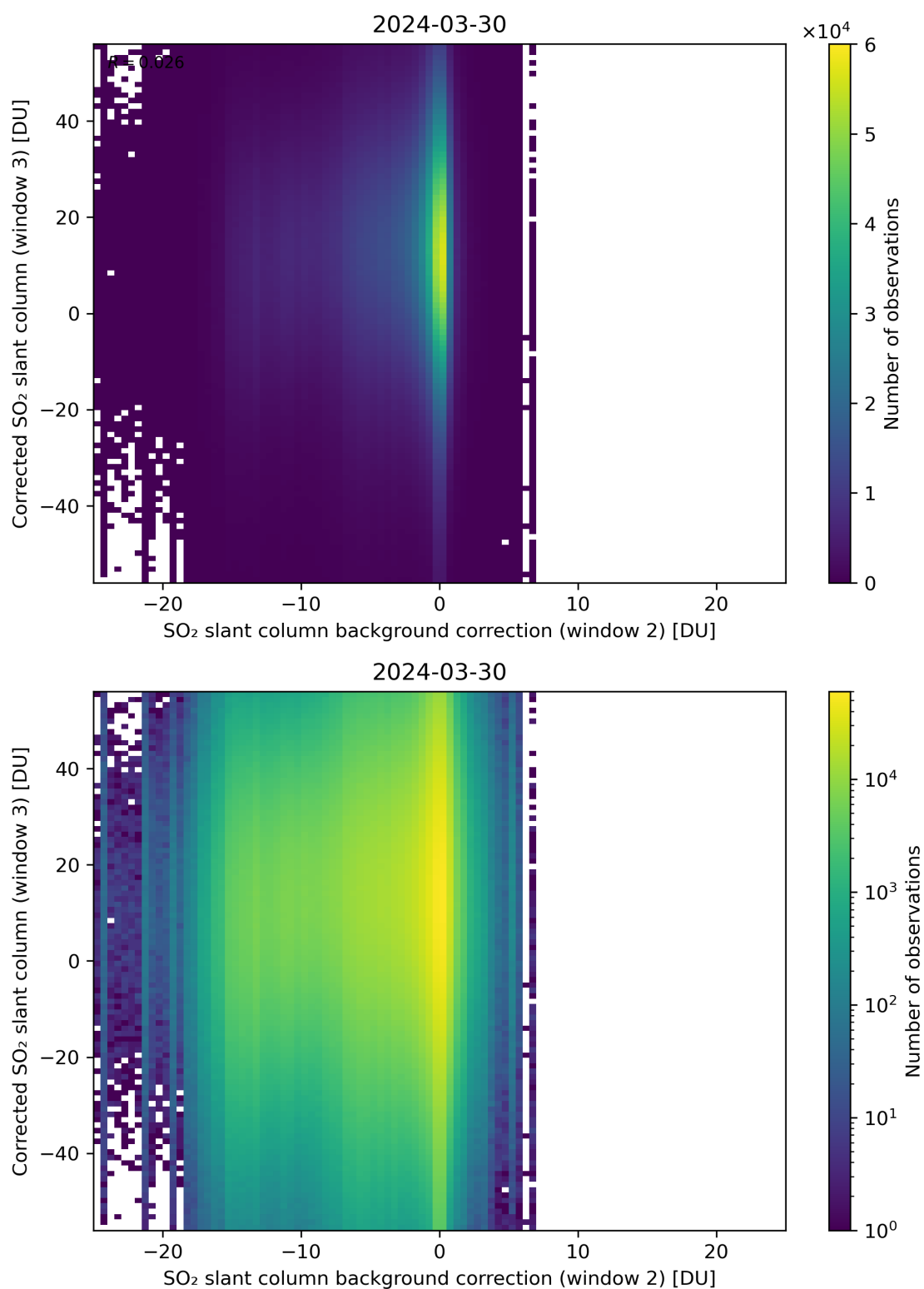
Figure 116: Scatter density plot of “SO 2 slant column background correction (window 2)” against “Corrected SO 2 slant column (window 3)” for 2024-03-30 to 2024-03-31.
