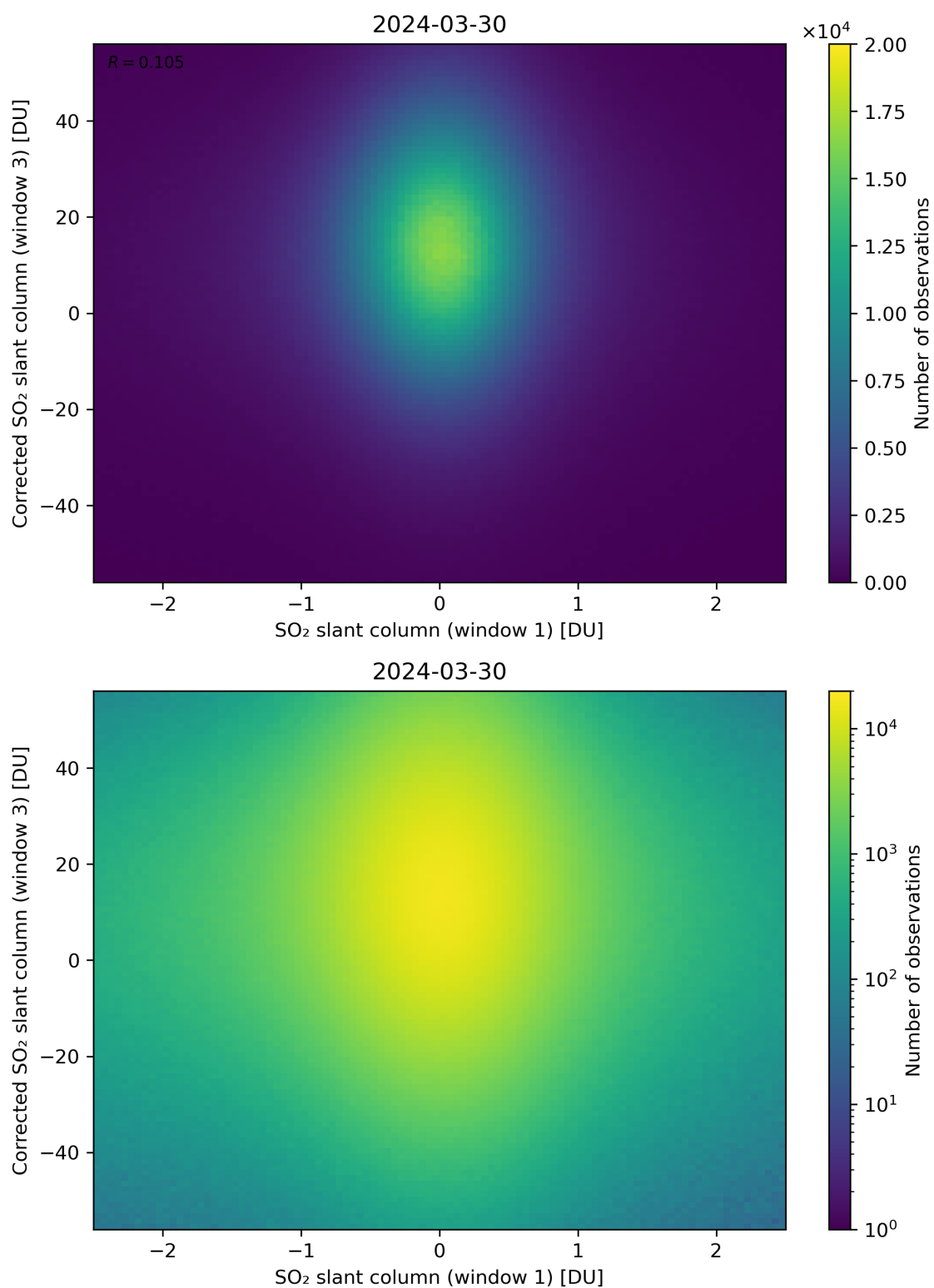
Figure 234: Scatter density plot of “SO 2 slant column (window 1)” against “Corrected SO 2 slant column (window 3)” for 2024-03-30 to 2024-03-31.
