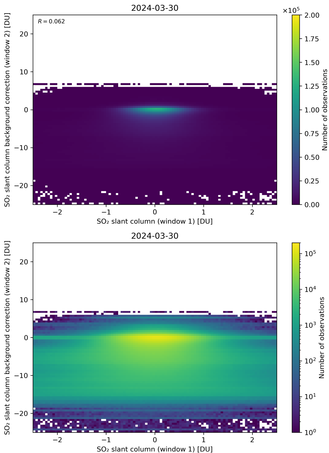
Figure 213: Scatter density plot of “SO 2 slant column (window 1)” against “SO 2 slant column background correction (window 2)” for 2024-03-30 to 2024-03-31.
