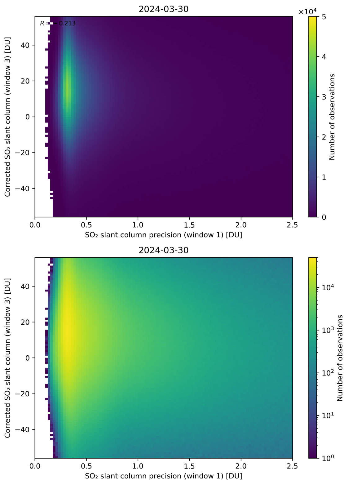
Figure 226: Scatter density plot of “SO 2 slant column precision (window 1)” against “Corrected SO 2 slant column (window 3)” for 2024-03-30 to 2024-03-31.
