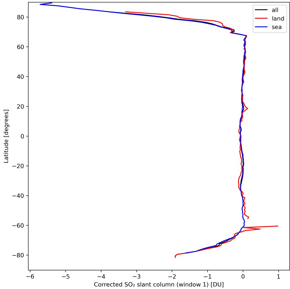
Figure 35: Zonal average of “Corrected SO 2 slant column (window 1)” for 2024-03-30 to 2024-03-31.
