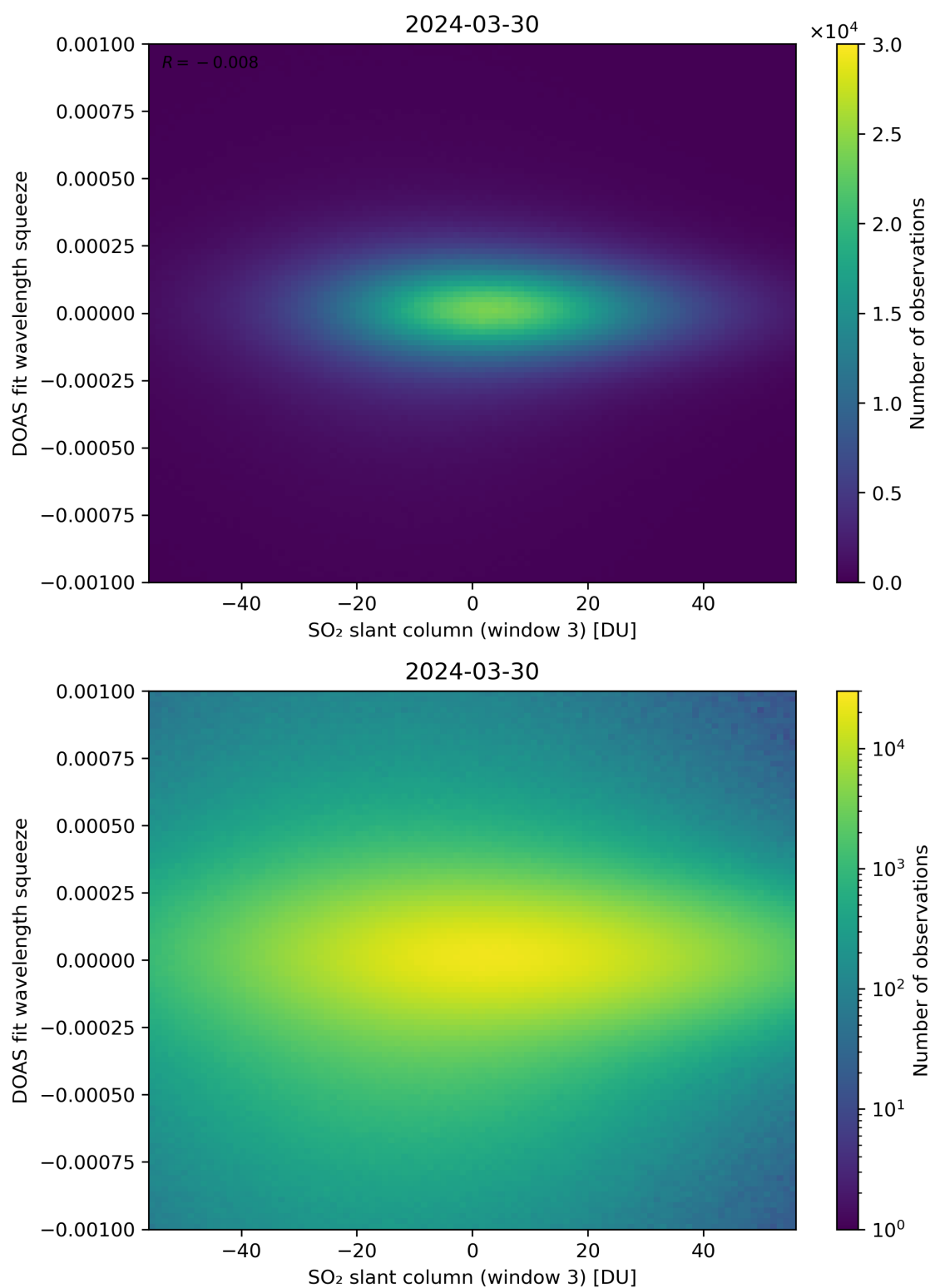
Figure 255: Scatter density plot of “SO 2 slant column (window 3)” against “DOAS fit wavelength squeeze” for 2024-03-30 to 2024-03-31.
