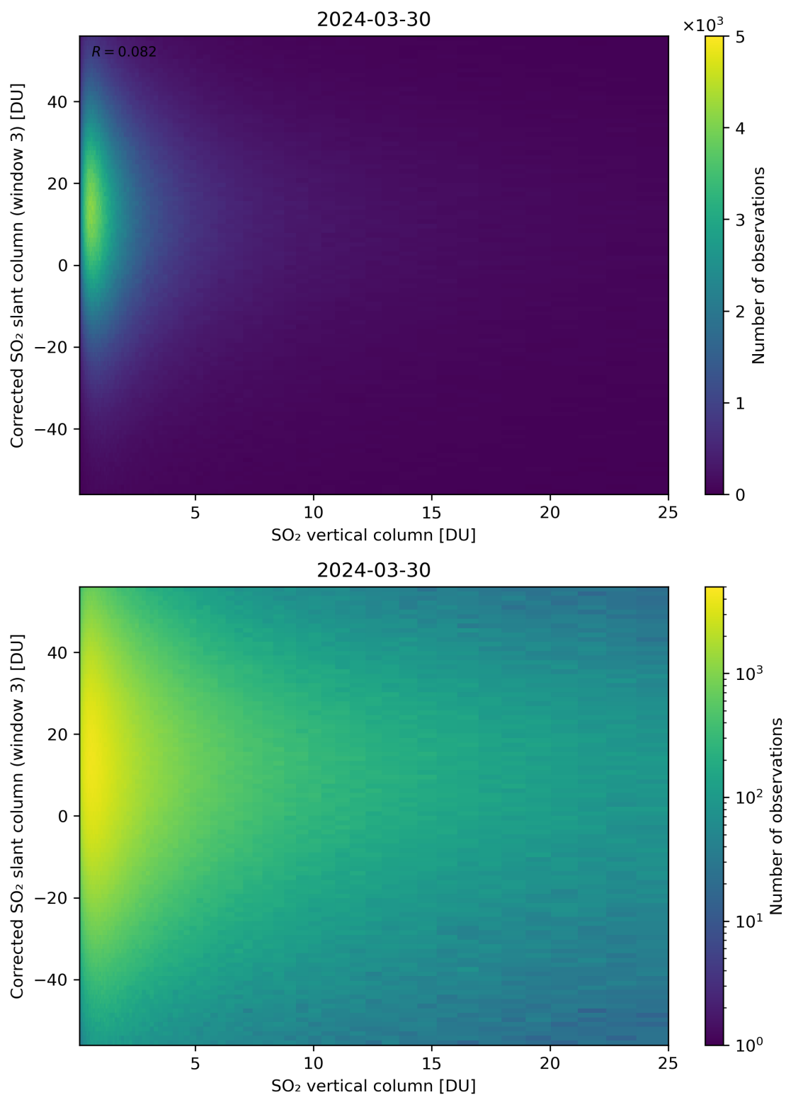
Figure 299: Scatter density plot of “SO 2 vertical column” against “Corrected SO 2 slant column (window 3)” for 2024-03-30 to 2024-03-31.
