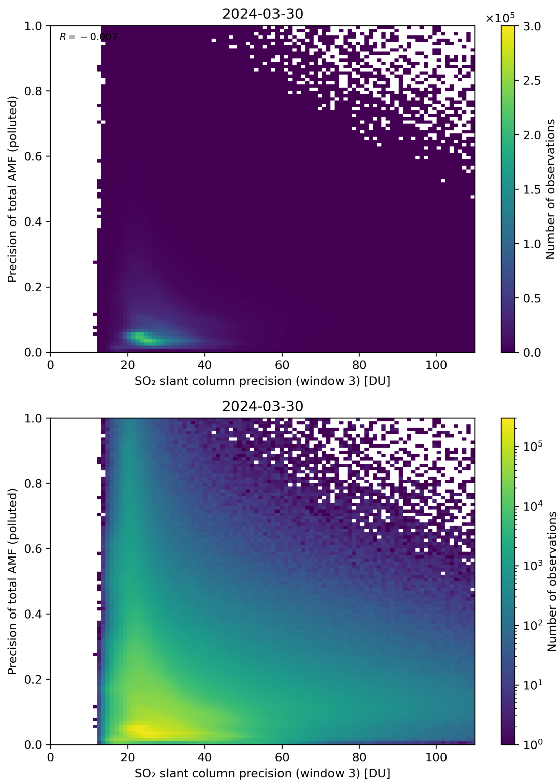
Figure 264: Scatter density plot of “SO 2 slant column precision (window 3)” against “Precision of total AMF (polluted)” for 2024-03-30 to 2024-03-31.
