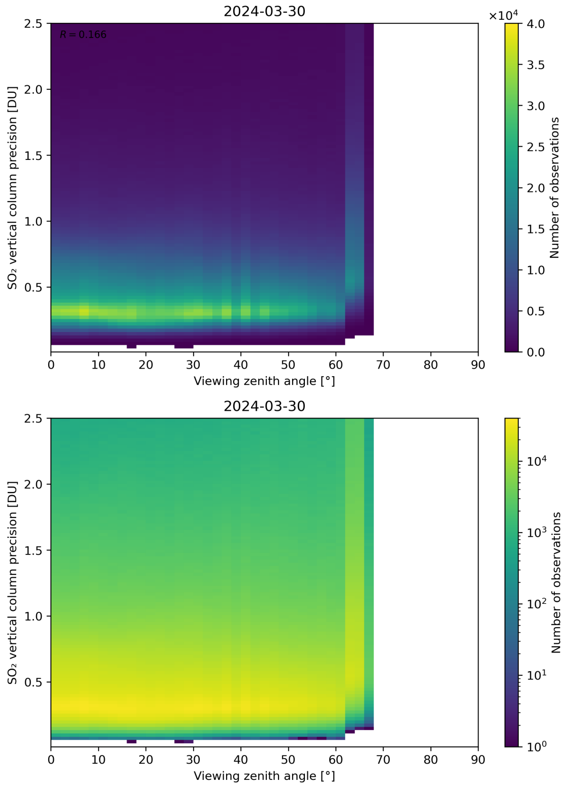
Figure 328: Scatter density plot of “Viewing zenith angle” against “SO 2 vertical column precision” for 2024-03-30 to 2024-03-31.
