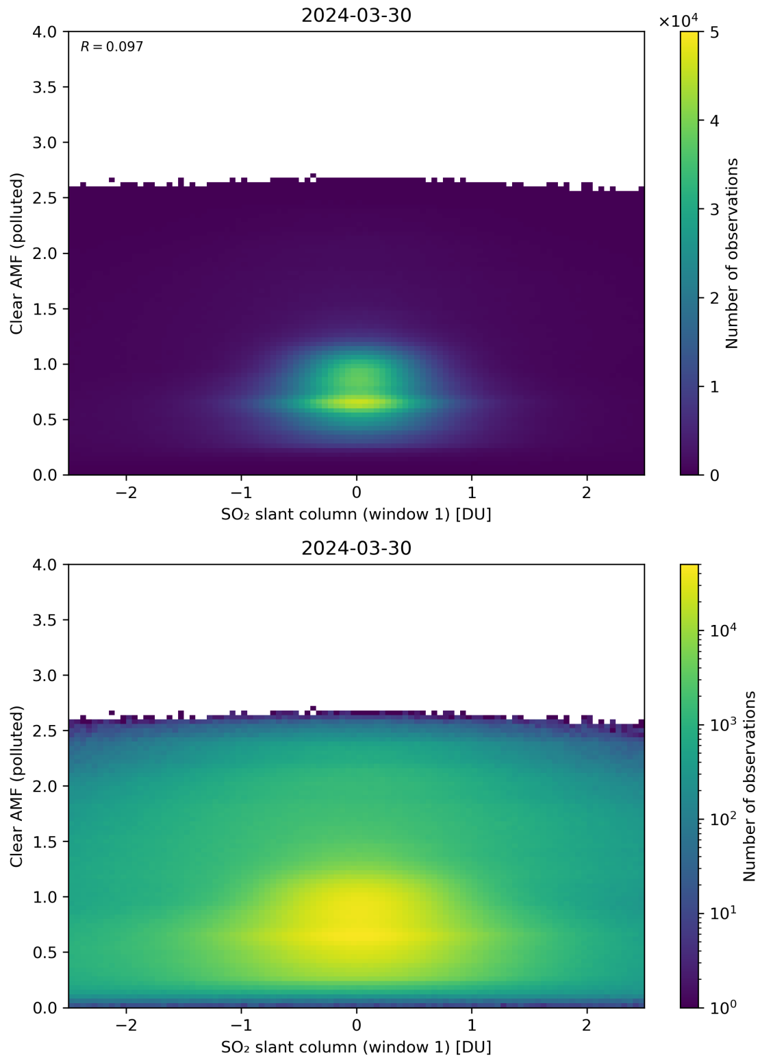
Figure 232: Scatter density plot of “SO 2 slant column (window 1)” against “Clear AMF (polluted)” for 2024-03-30 to 2024-03-31.
