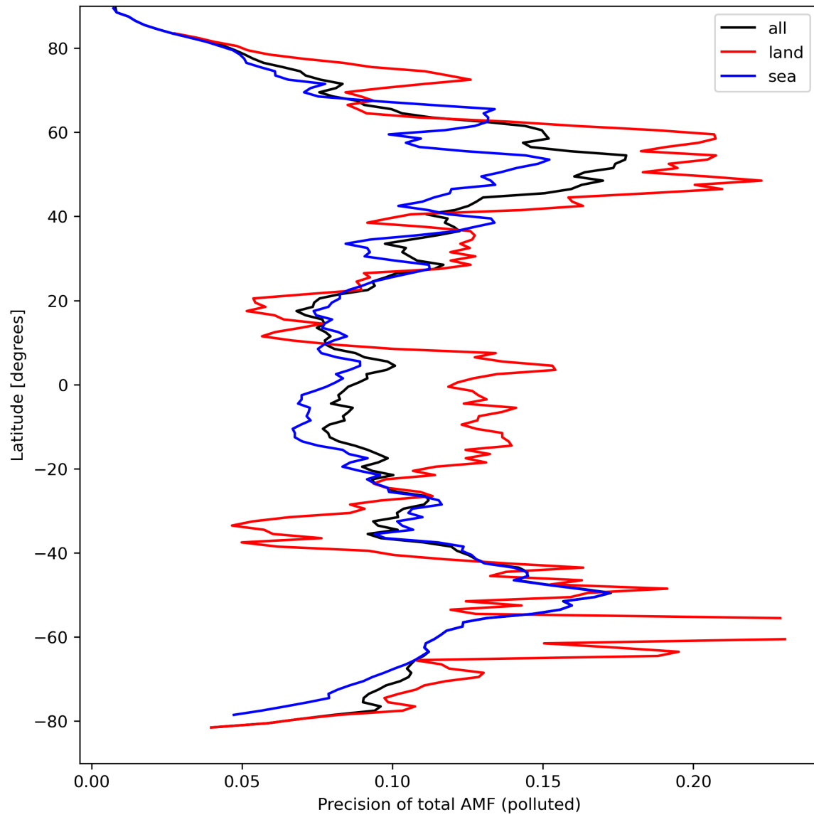
Figure 49: Zonal average of “Precision of total AMF (polluted)” for 2024-03-30 to 2024-03-31.
