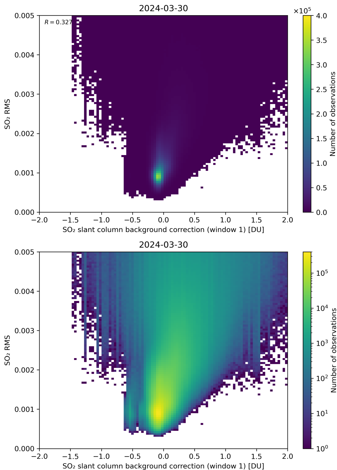
Figure 102: Scatter density plot of “SO 2 slant column background correction (window 1)” against “SO 2 RMS” for 2024-03-30 to 2024-03-31.
