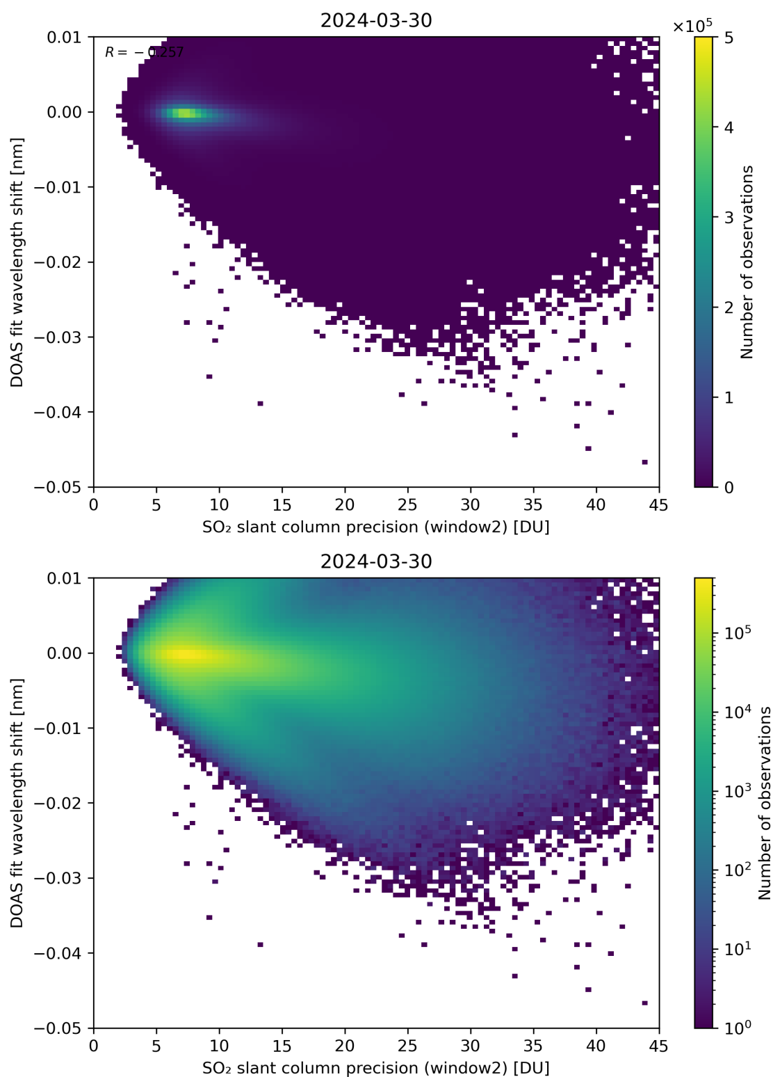
Figure 243: Scatter density plot of “SO 2 slant column precision (window2)” against “DOAS fit wavelength shift” for 2024-03-30 to 2024-03-31.
