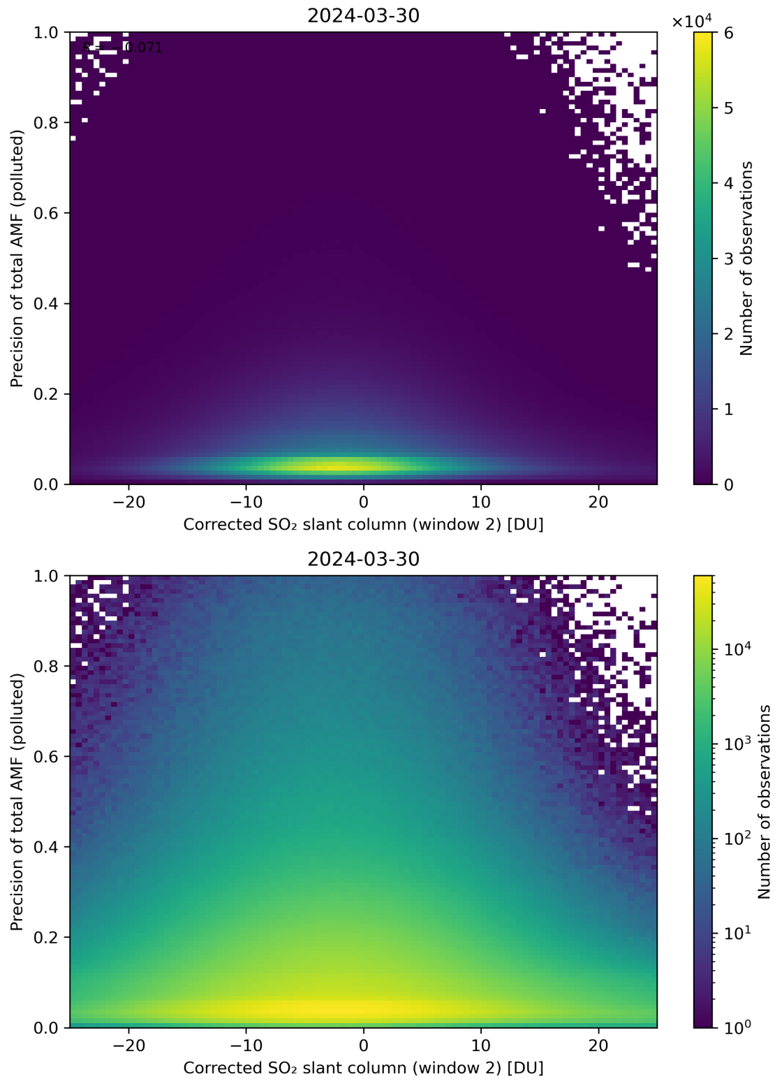
Figure 204: Scatter density plot of “Corrected SO 2 slant column (window 2)” against “Precision of total AMF (polluted)” for 2024-03-30 to 2024-03-31.
