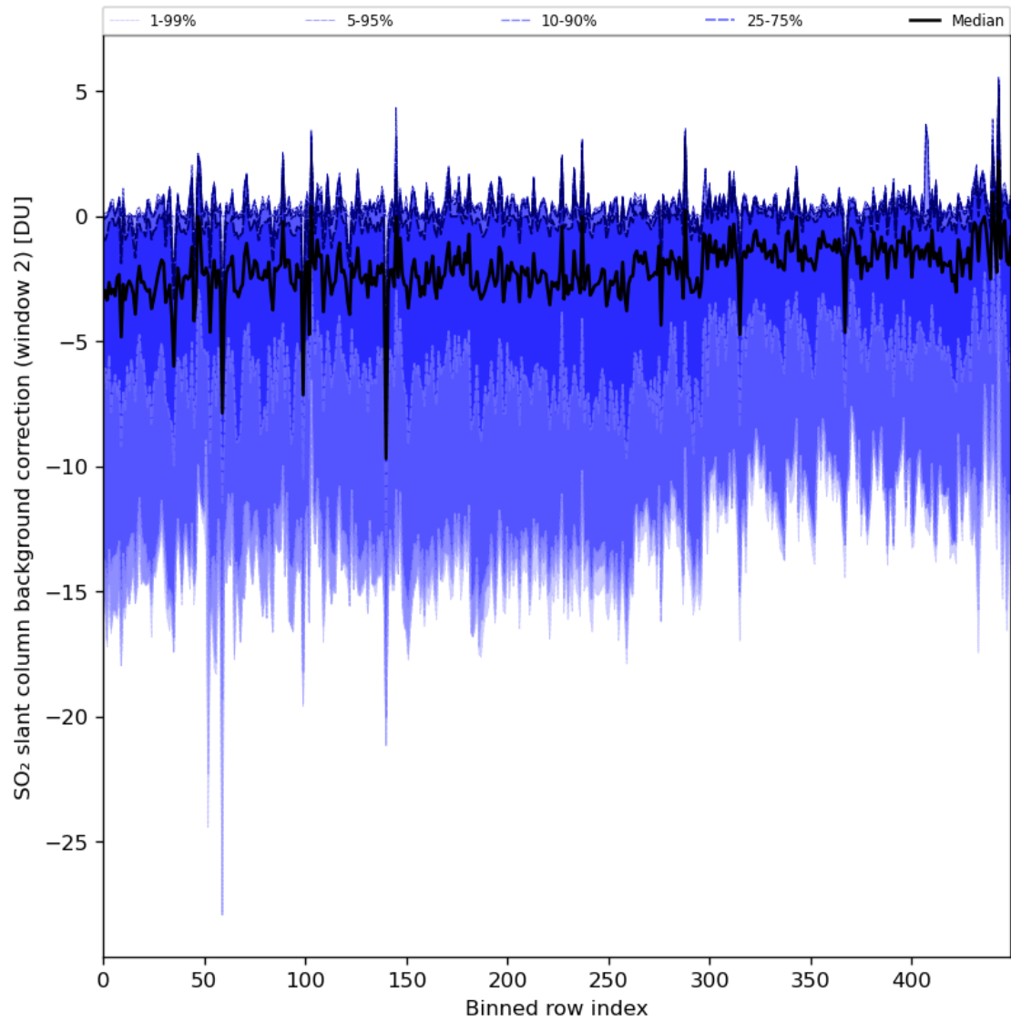
Figure 86: Along track statistics of “SO 2 slant column background correction (window 2)” for 2024-03-30 to 2024-03-31
