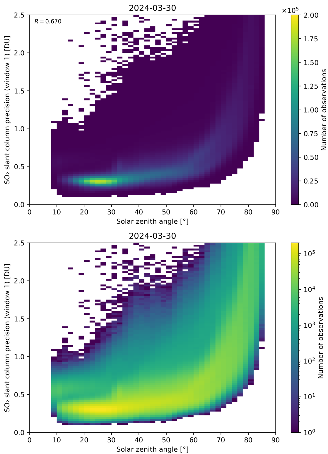
Figure 170: Scatter density plot of “Solar zenith angle” against “SO 2 slant column precision (window 1)” for 2024-03-30 to 2024-03-31.
