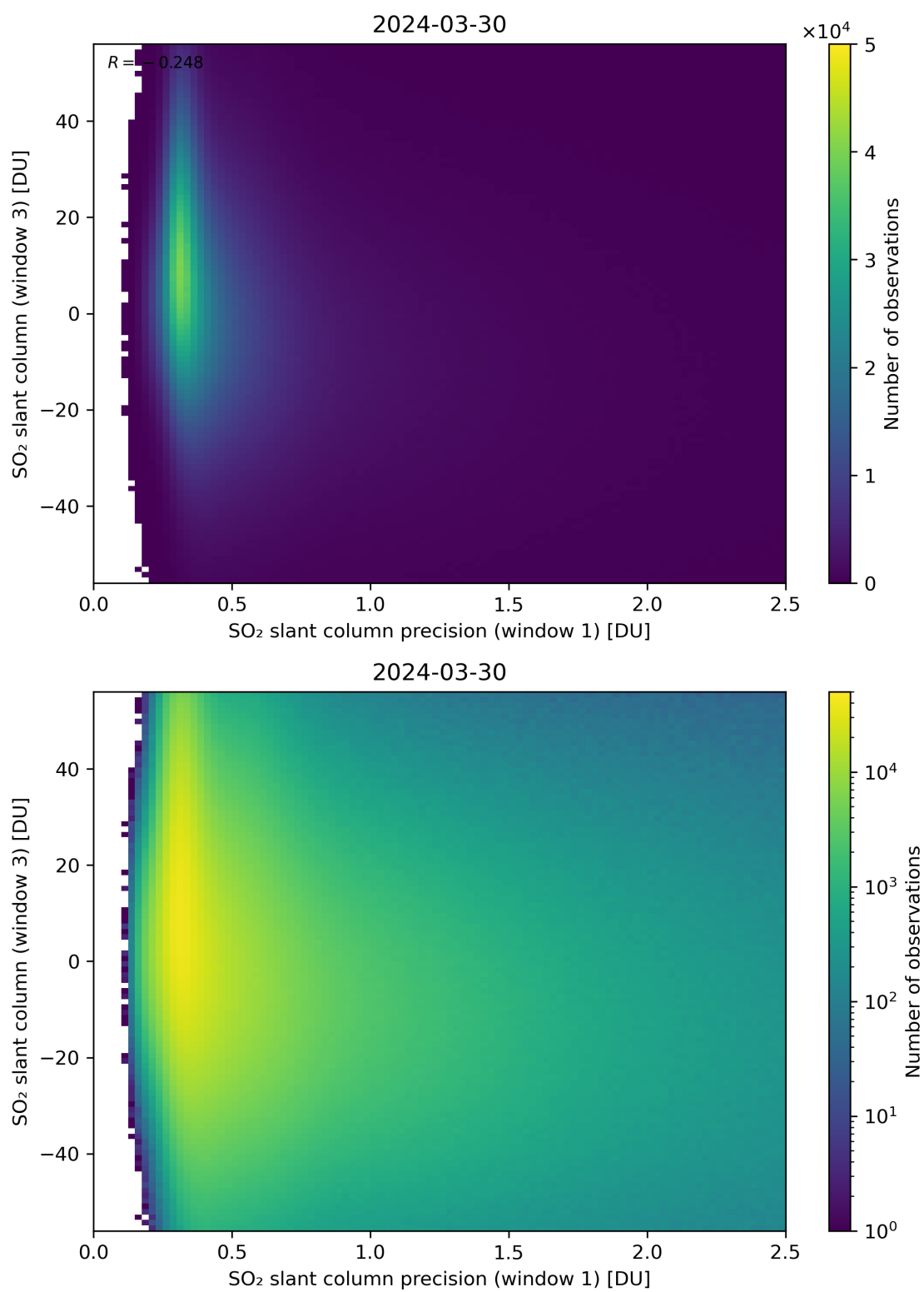
Figure 228: Scatter density plot of “SO 2 slant column precision (window 1)” against “SO 2 slant column (window 3)” for 2024-03-30 to 2024-03-31.
