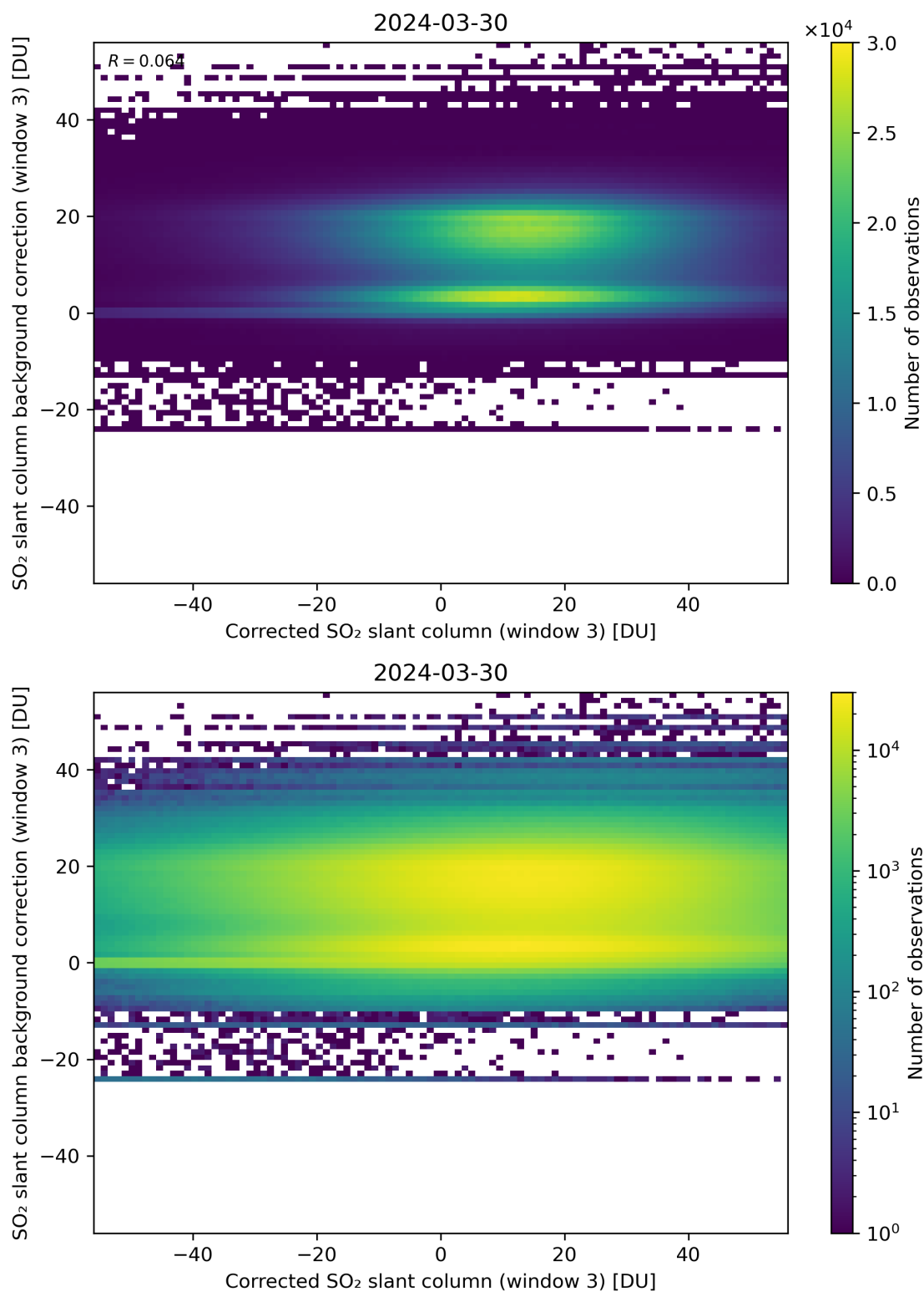
Figure 205: Scatter density plot of “Corrected SO 2 slant column (window 3)” against “SO 2 slant column background correction (window 3)” for 2024-03-30 to 2024-03-31.
