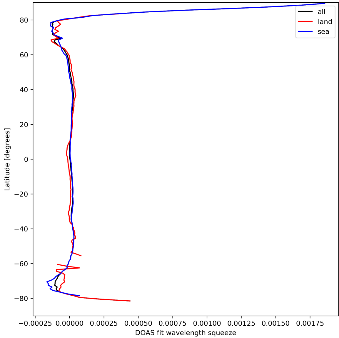
Figure 46: Zonal average of “DOAS fit wavelength squeeze” for 2024-03-30 to 2024-03-31.
