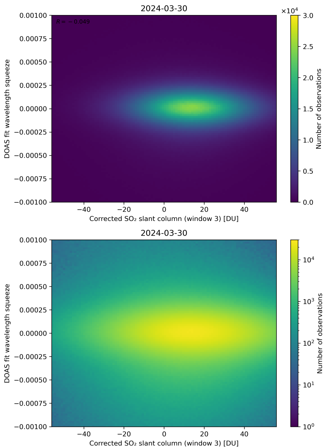
Figure 207: Scatter density plot of “Corrected SO 2 slant column (window 3)” against “DOAS fit wavelength squeeze” for 2024-03-30 to 2024-03-31.
