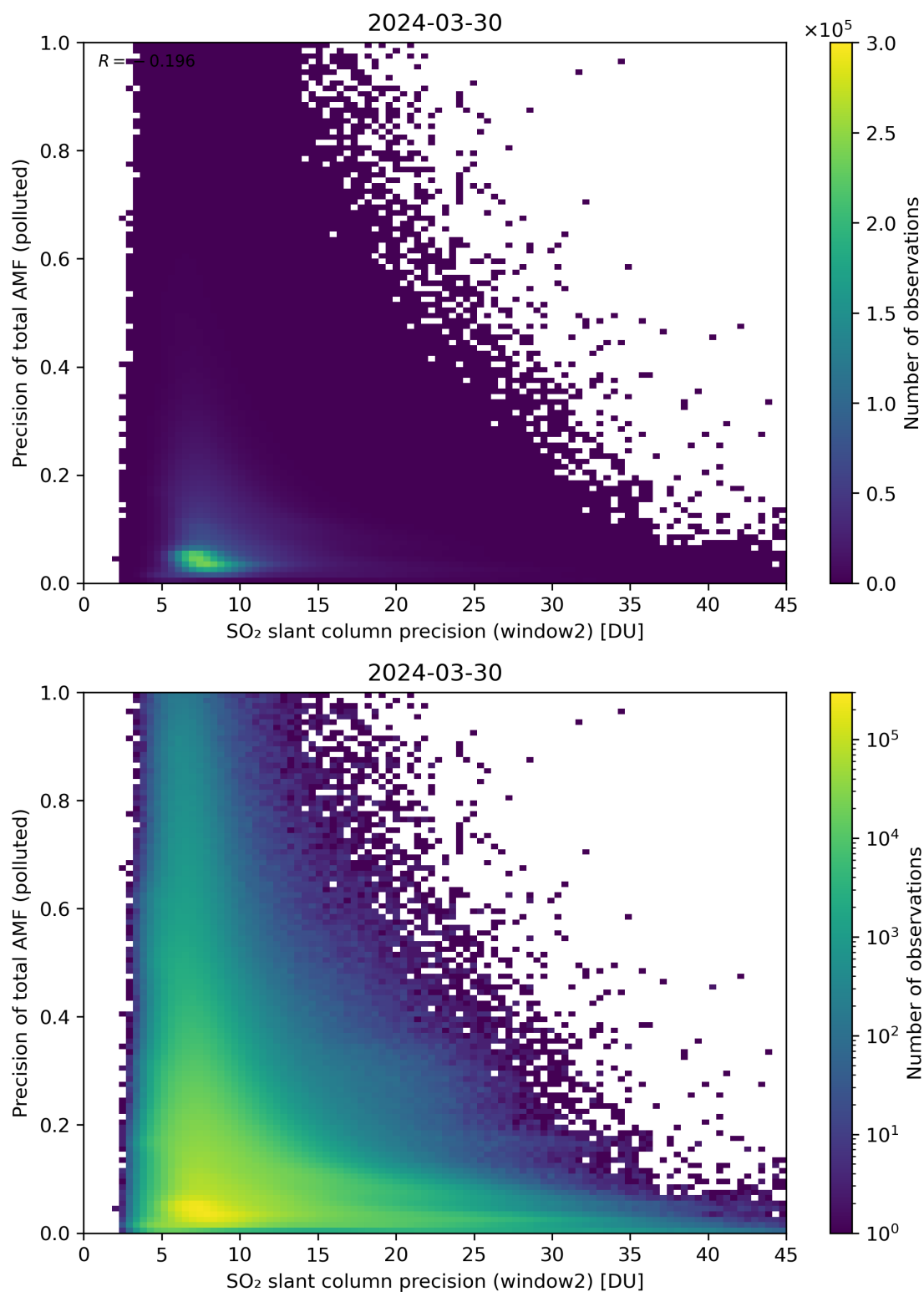
Figure 252: Scatter density plot of “SO 2 slant column precision (window2)” against “Precision of total AMF (polluted)” for 2024-03-30 to 2024-03-31.
