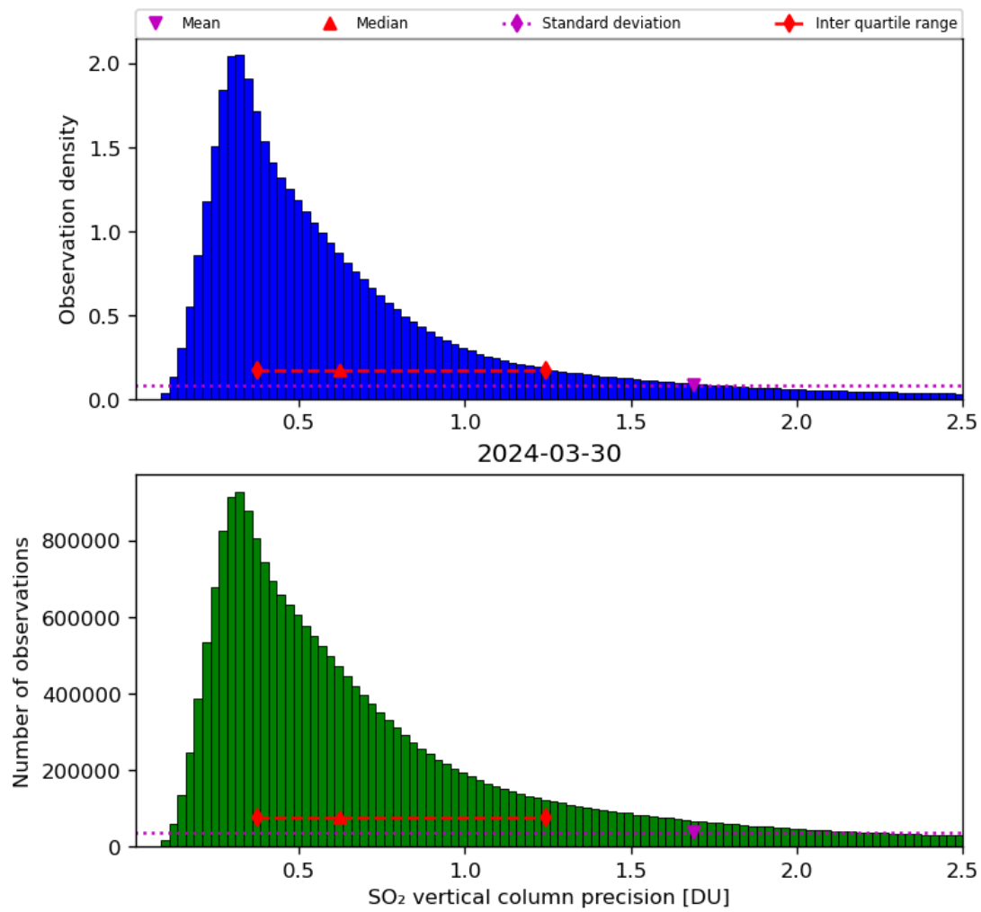
Figure 54: Histogram of “SO 2 vertical column precision” for 2024-03-30 to 2024-03-31
