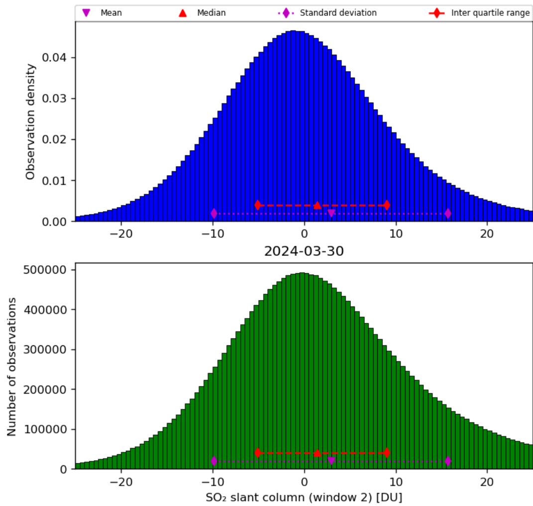
Figure 60: Histogram of “SO 2 slant column (window 2)” for 2024-03-30 to 2024-03-31
