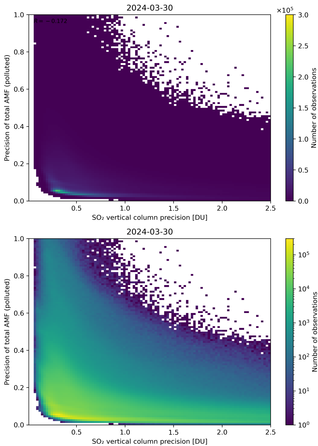
Figure 295: Scatter density plot of “SO 2 vertical column precision” against “Precision of total AMF (polluted)” for 2024-03-30 to 2024-03-31.
