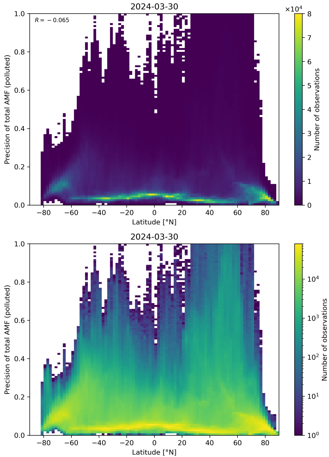
Figure 155: Scatter density plot of “Latitude” against “Precision of total AMF (polluted)” for 2024-03-30 to 2024-03-31.
