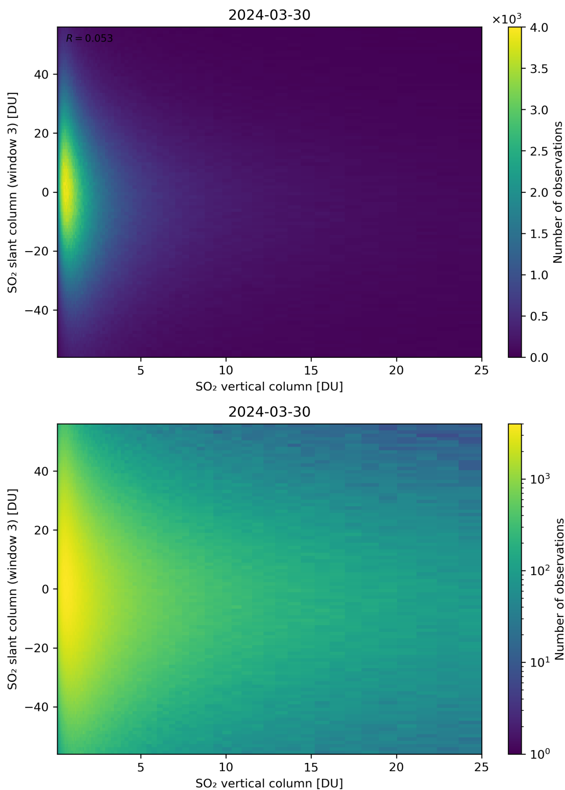
Figure 303: Scatter density plot of “SO 2 vertical column” against “SO 2 slant column (window 3)” for 2024-03-30 to 2024-03-31.
