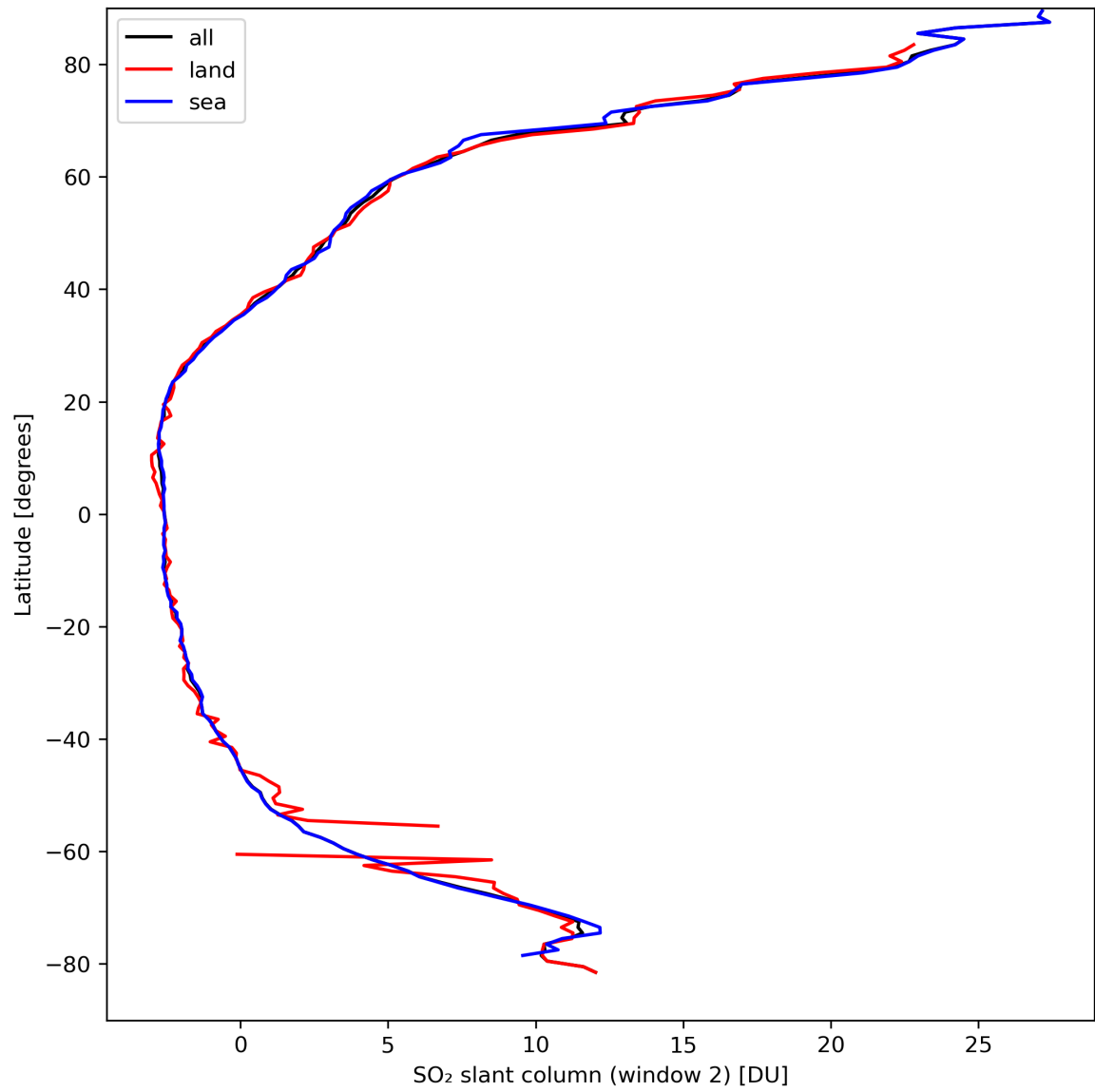
Figure 37: Zonal average of “SO 2 slant column (window 2)” for 2024-03-30 to 2024-03-31.
