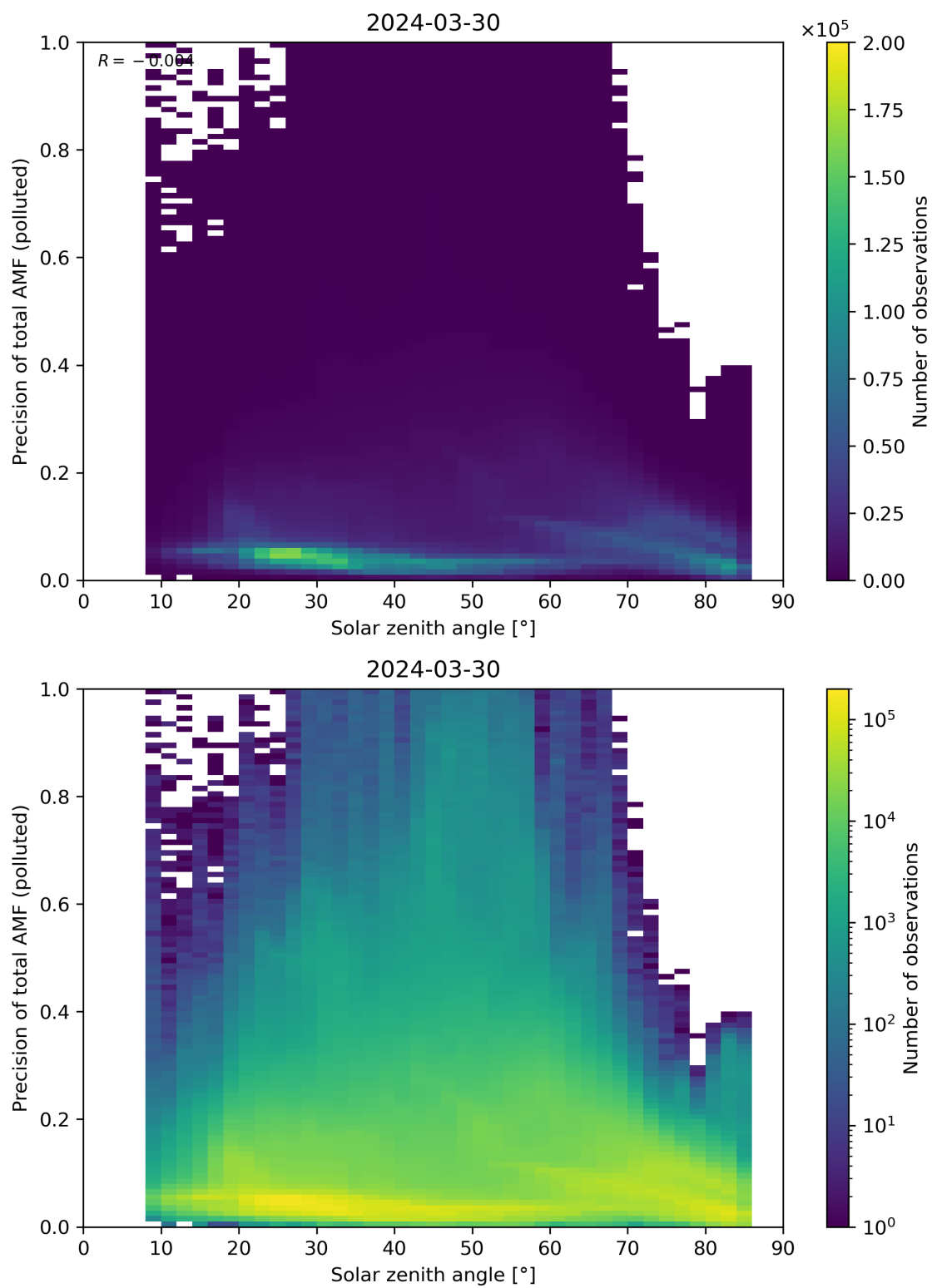
Figure 175: Scatter density plot of “Solar zenith angle” against “Precision of total AMF (polluted)” for 2024-03-30 to 2024-03-31.
