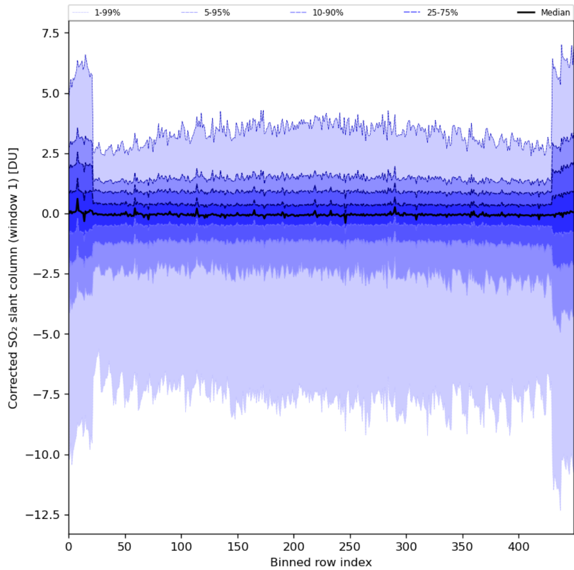
Figure 81: Along track statistics of “Corrected SO 2 slant column (window 1)” for 2024-03-30 to 2024-03-31
