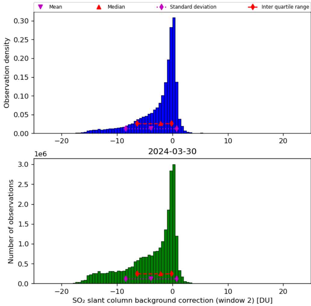
Figure 63: Histogram of “SO 2 slant column background correction (window 2)” for 2024-03-30 to 2024-03-31
