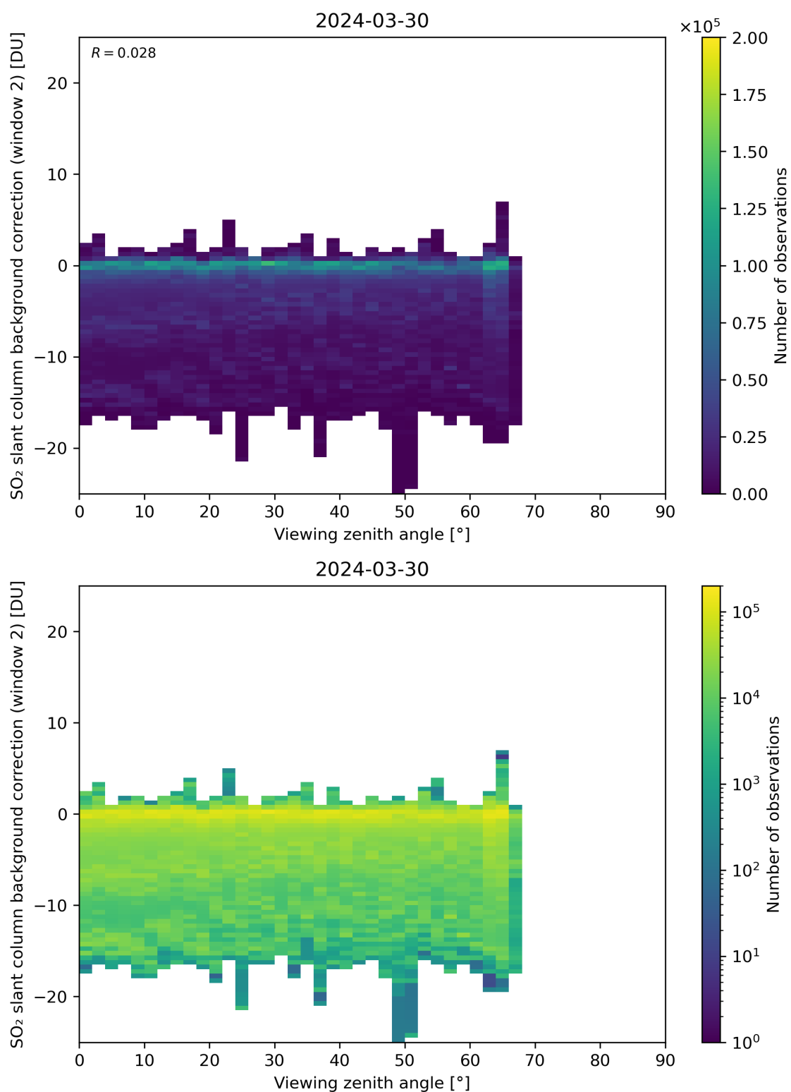
Figure 309: Scatter density plot of “Viewing zenith angle” against “SO 2 slant column background correction (window 2)” for 2024-03-30 to 2024-03-31.
