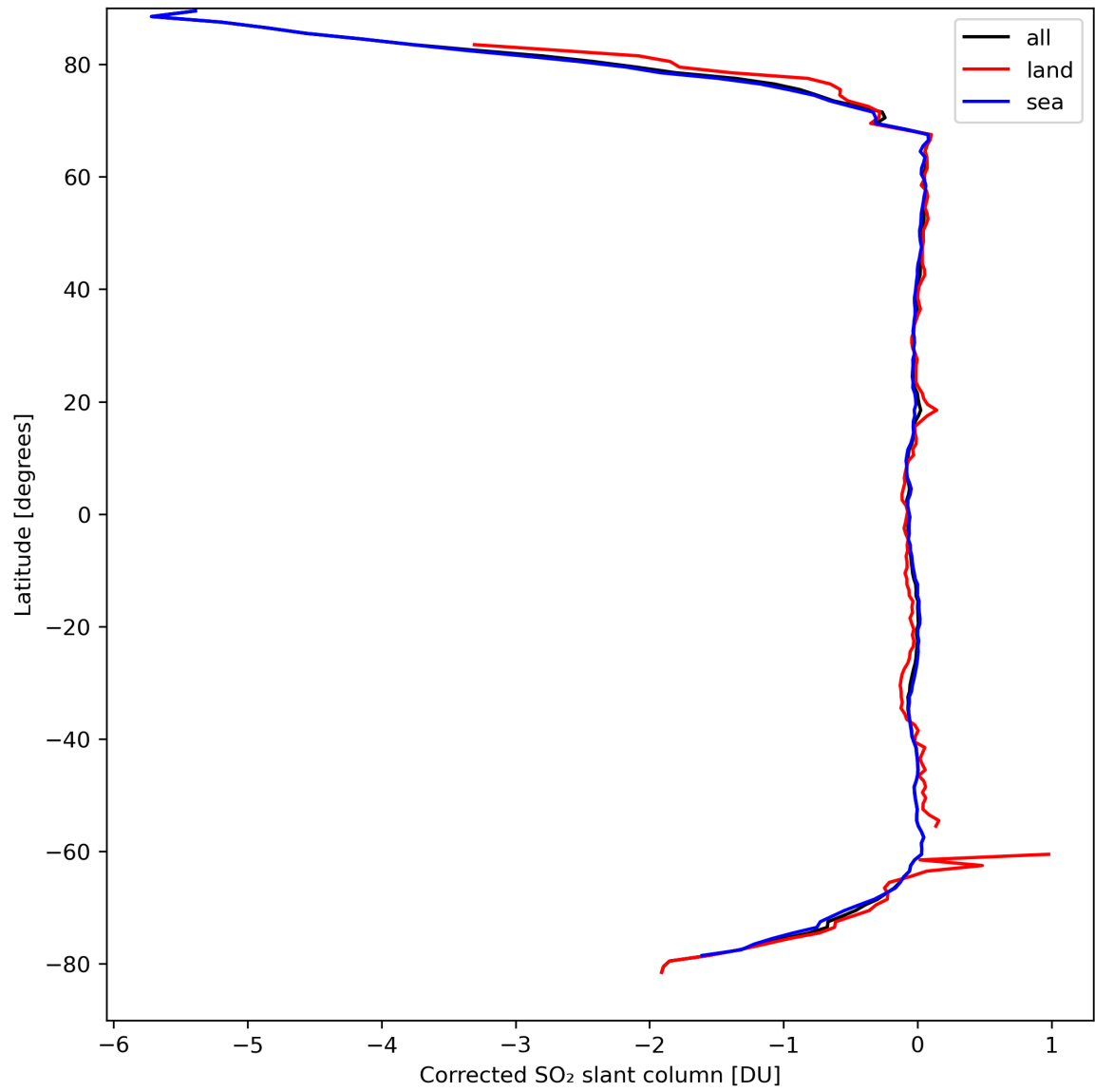
Figure 32: Zonal average of “Corrected SO 2 slant column” for 2024-03-30 to 2024-03-31.
