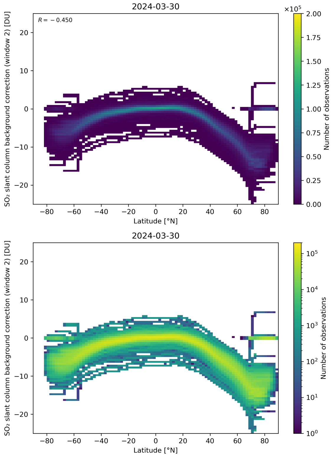
Figure 140: Scatter density plot of “Latitude” against “SO 2 slant column background correction (window 2)” for 2024-03-30 to 2024-03-31.
