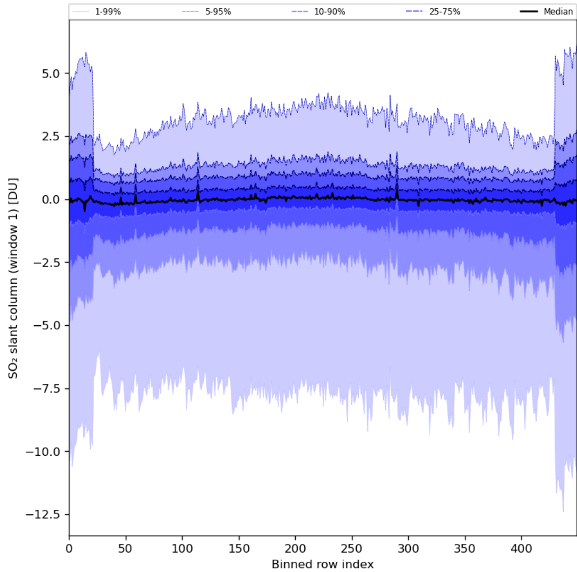
Figure 79: Along track statistics of “SO 2 slant column (window 1)” for 2024-03-30 to 2024-03-31
