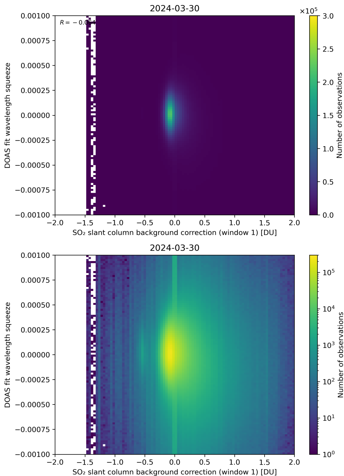
Figure 101: Scatter density plot of “SO 2 slant column background correction (window 1)” against “DOAS fit wavelength squeeze” for 2024-03-30 to 2024-03-31.
