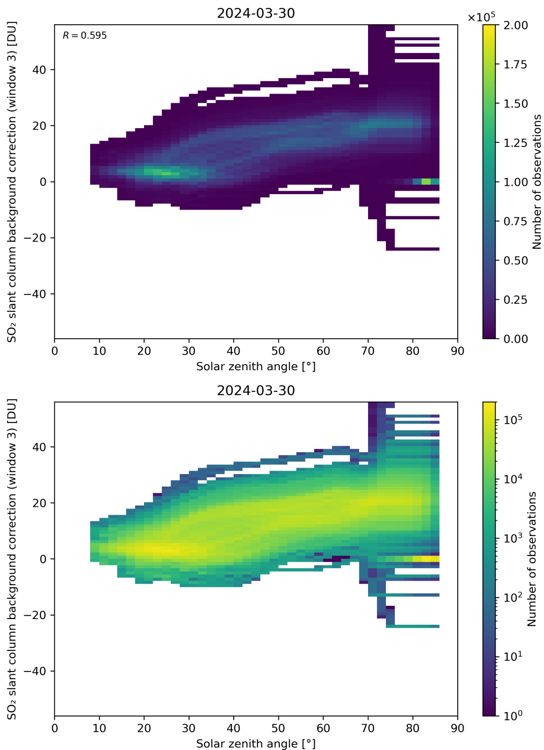
Figure 160: Scatter density plot of “Solar zenith angle” against “SO 2 slant column background correction (window 3)” for 2024-03-30 to 2024-03-31.
