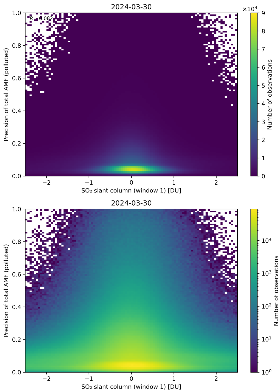
Figure 240: Scatter density plot of “SO 2 slant column (window 1)” against “Precision of total AMF (polluted)” for 2024-03-30 to 2024-03-31.
