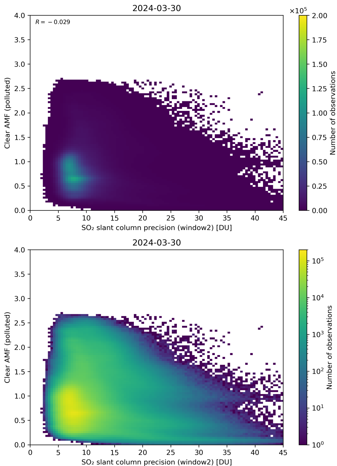
Figure 246: Scatter density plot of “SO 2 slant column precision (window2)” against “Clear AMF (polluted)” for 2024-03-30 to 2024-03-31.
