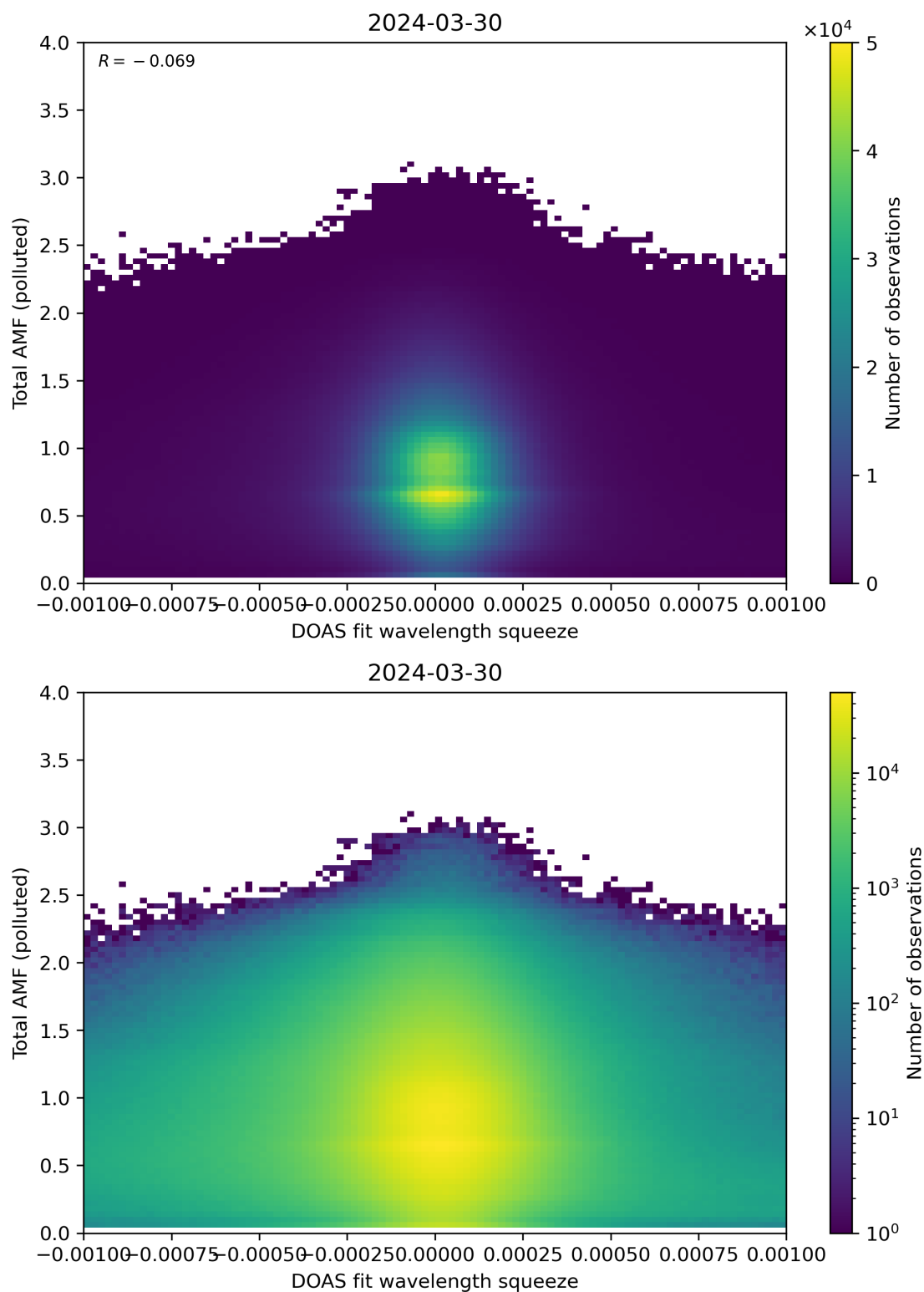
Figure 134: Scatter density plot of “DOAS fit wavelength squeeze” against “Total AMF (polluted)” for 2024-03-30 to 2024-03-31.
