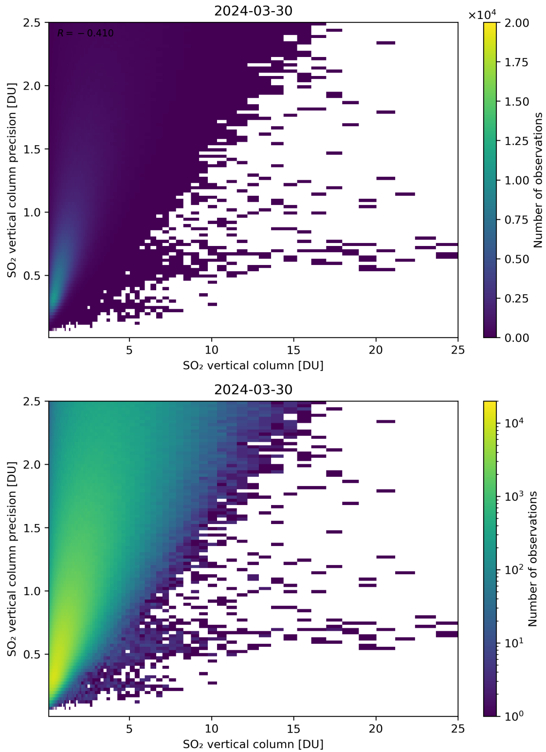
Figure 307: Scatter density plot of “SO 2 vertical column” against “SO 2 vertical column precision” for 2024-03-30 to 2024-03-31.
