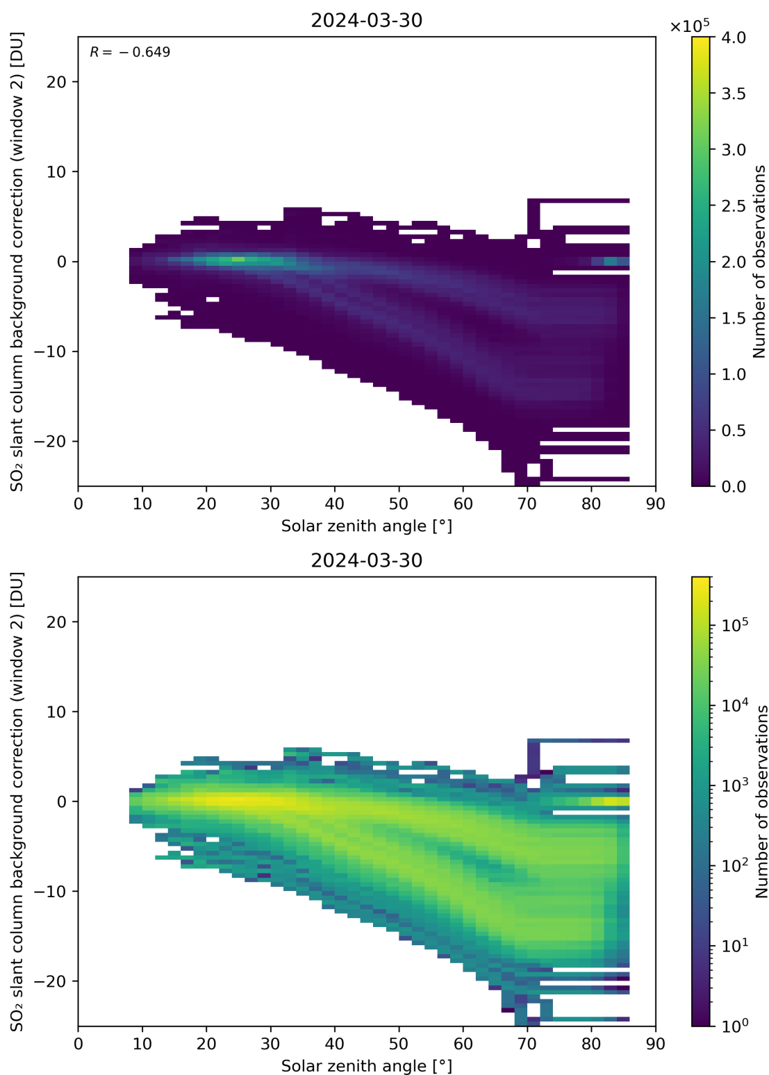
Figure 159: Scatter density plot of “Solar zenith angle” against “SO 2 slant column background correction (window 2)” for 2024-03-30 to 2024-03-31.
