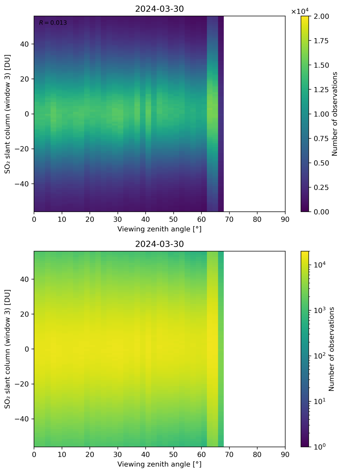
Figure 323: Scatter density plot of “Viewing zenith angle” against “SO 2 slant column (window 3)” for 2024-03-30 to 2024-03-31.
