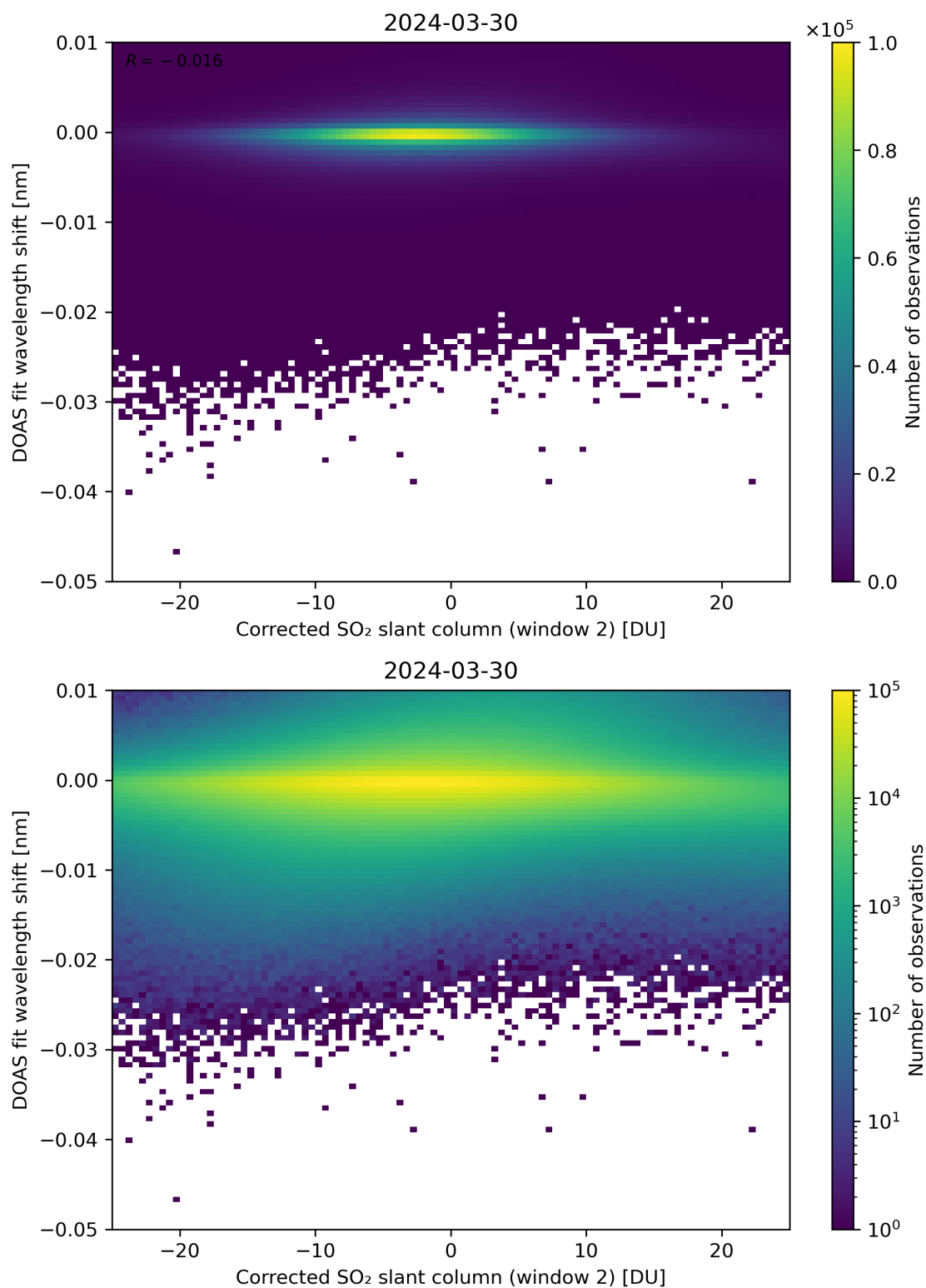
Figure 196: Scatter density plot of “Corrected SO 2 slant column (window 2)” against “DOAS fit wavelength shift” for 2024-03-30 to 2024-03-31.
