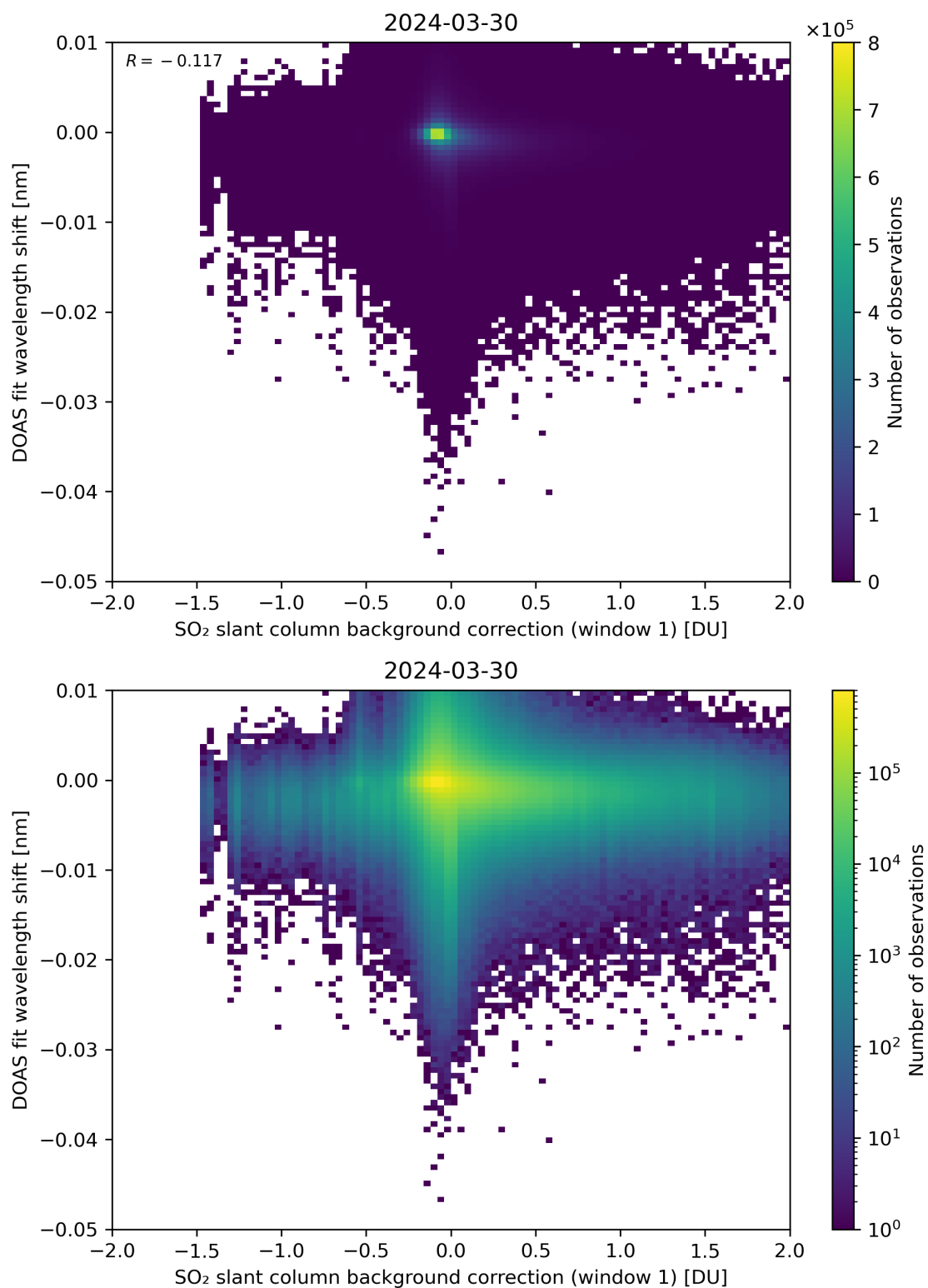
Figure 100: Scatter density plot of “SO 2 slant column background correction (window 1)” against “DOAS fit wavelength shift” for 2024-03-30 to 2024-03-31.
