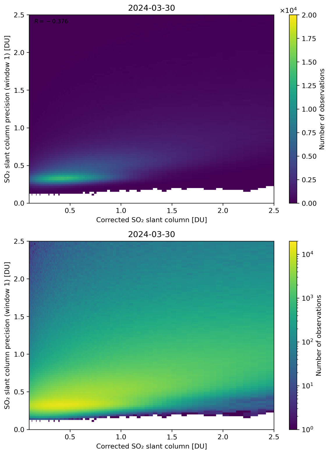
Figure 188: Scatter density plot of “Corrected SO 2 slant column” against “SO 2 slant column precision (window 1)” for 2024-03-30 to 2024-03-31.
