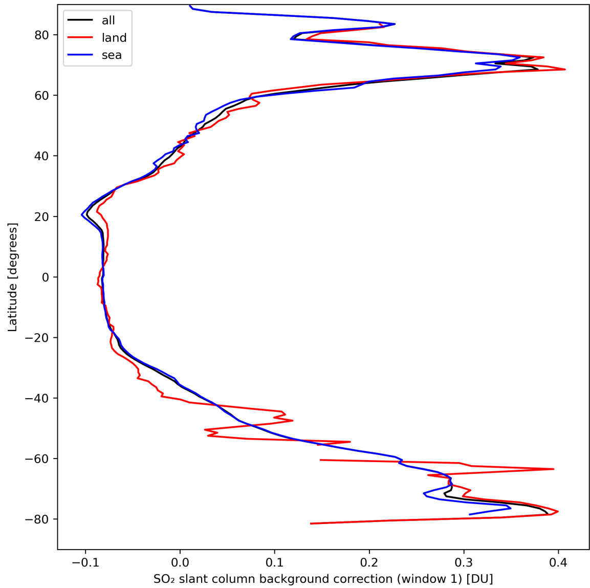
Figure 36: Zonal average of “SO 2 slant column background correction (window 1)” for 2024-03-30 to 2024-03-31.
