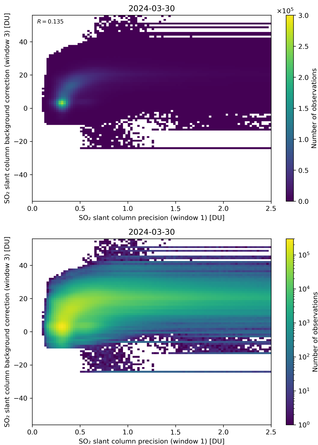
Figure 220: Scatter density plot of “SO 2 slant column precision (window 1)” against “SO 2 slant column background correction (window 3)” for 2024-03-30 to 2024-03-31.
