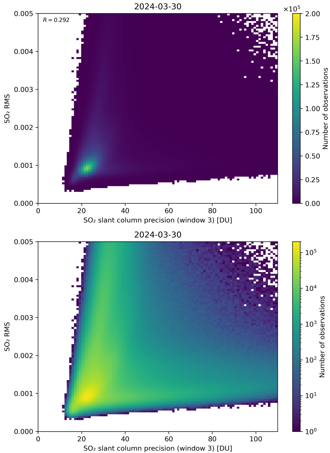
Figure 260: Scatter density plot of “SO 2 slant column precision (window 3)” against “SO 2 RMS” for 2024-03-30 to 2024-03-31.
