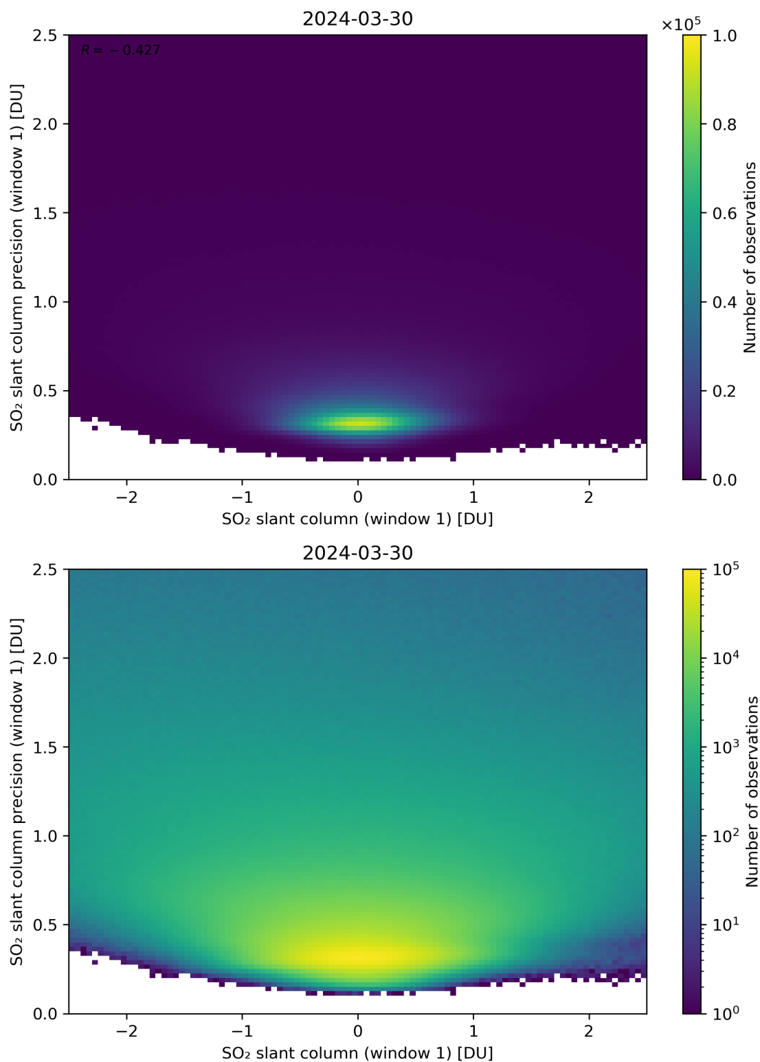
Figure 235: Scatter density plot of “SO 2 slant column (window 1)” against “SO 2 slant column precision (window 1)” for 2024-03-30 to 2024-03-31.
