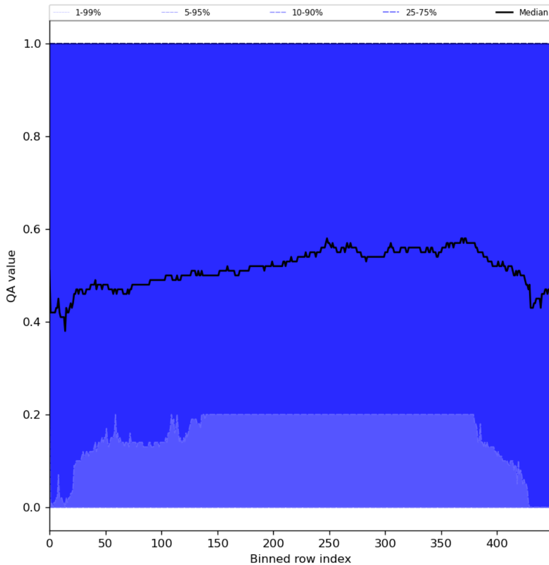
Figure 75: Along track statistics of “QA value” for 2024-03-30 to 2024-03-31
