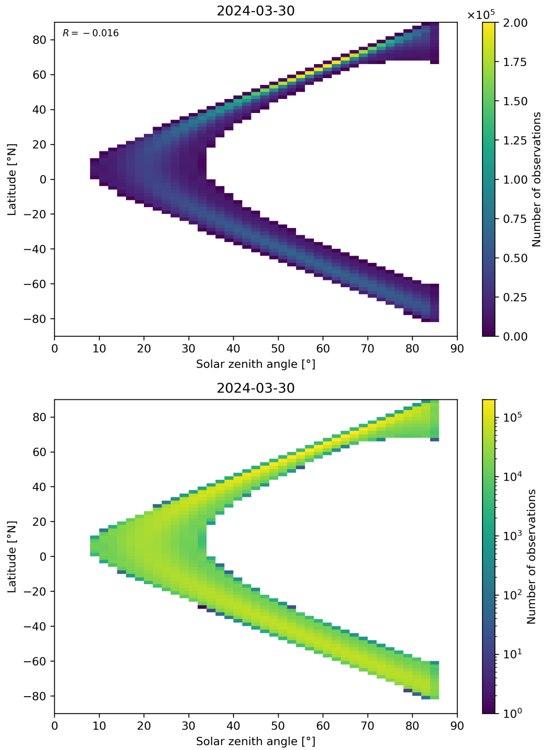
Figure 164: Scatter density plot of “Solar zenith angle” against “Latitude” for 2024-03-30 to 2024-03-31.
