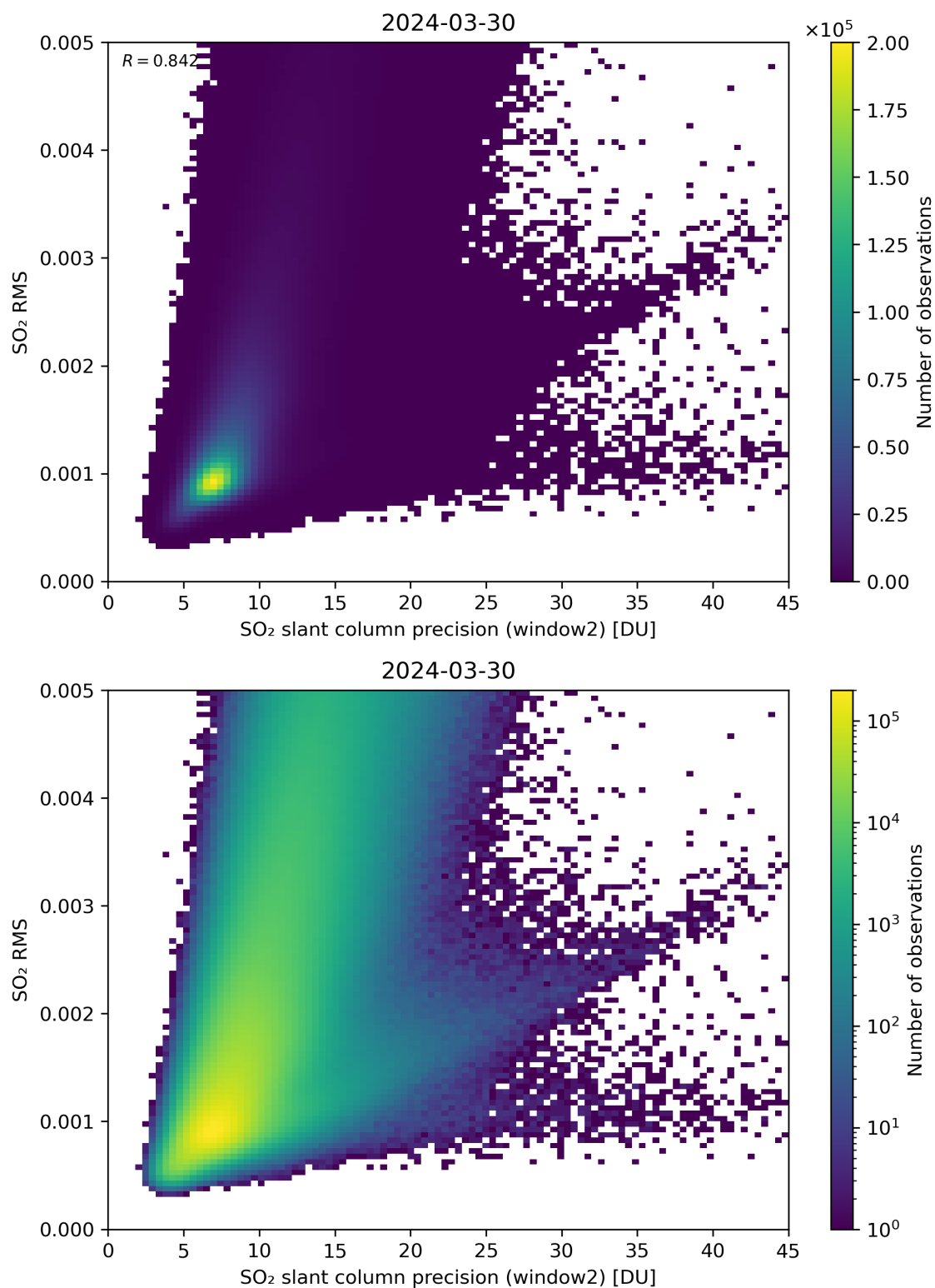
Figure 245: Scatter density plot of “SO 2 slant column precision (window2)” against “SO 2 RMS” for 2024-03-30 to 2024-03-31.
