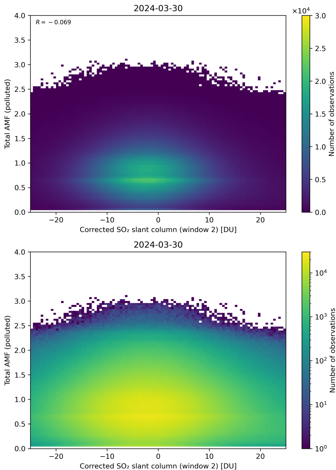
Figure 203: Scatter density plot of “Corrected SO 2 slant column (window 2)” against “Total AMF (polluted)” for 2024-03-30 to 2024-03-31.
