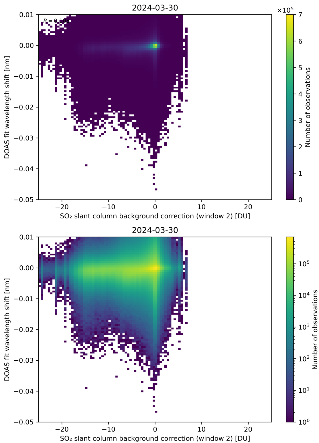
Figure 112: Scatter density plot of “SO 2 slant column background correction (window 2)” against “DOAS fit wavelength shift” for 2024-03-30 to 2024-03-31.
