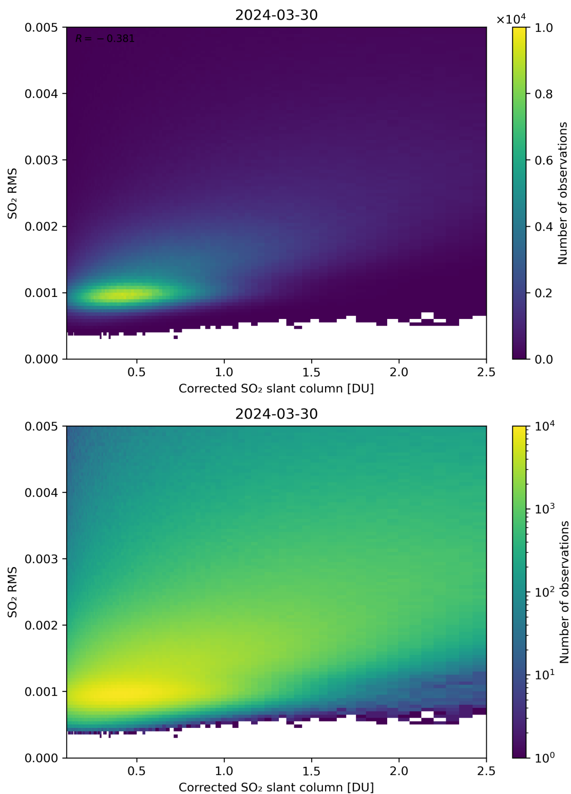
Figure 183: Scatter density plot of “Corrected SO 2 slant column” against “SO 2 RMS” for 2024-03-30 to 2024-03-31.
