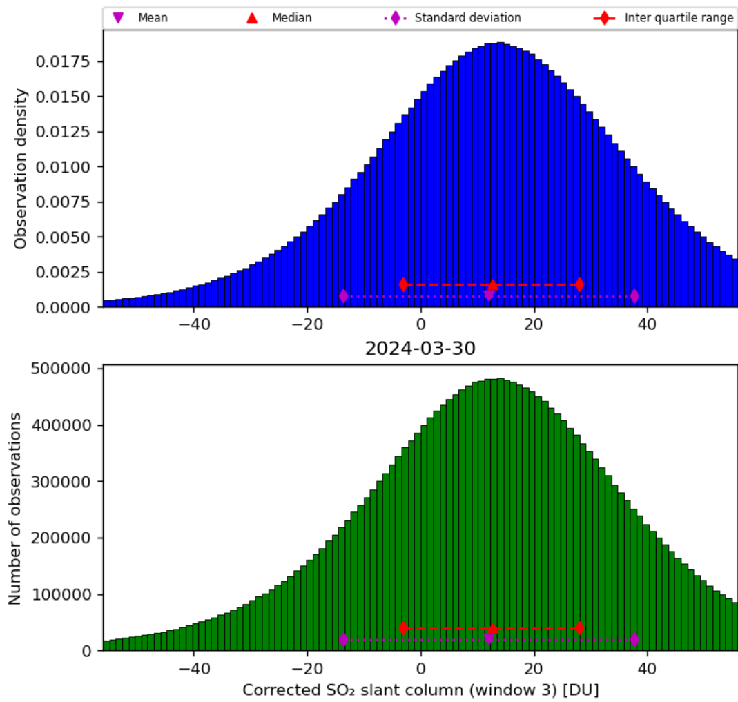
Figure 66: Histogram of “Corrected SO 2 slant column (window 3)” for 2024-03-30 to 2024-03-31
