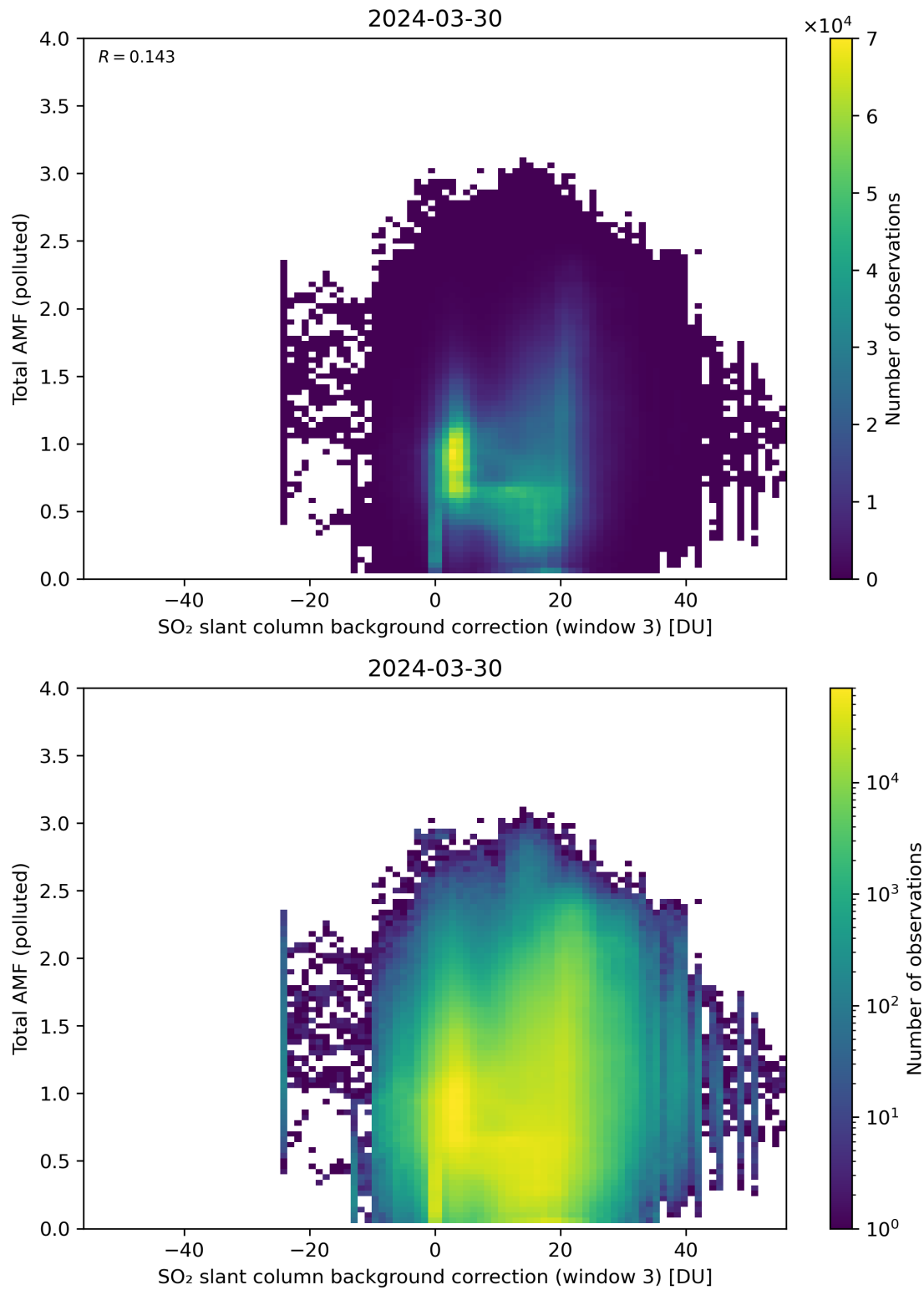
Figure 125: Scatter density plot of “SO 2 slant column background correction (window 3)” against “Total AMF (polluted)” for 2024-03-30 to 2024-03-31.
