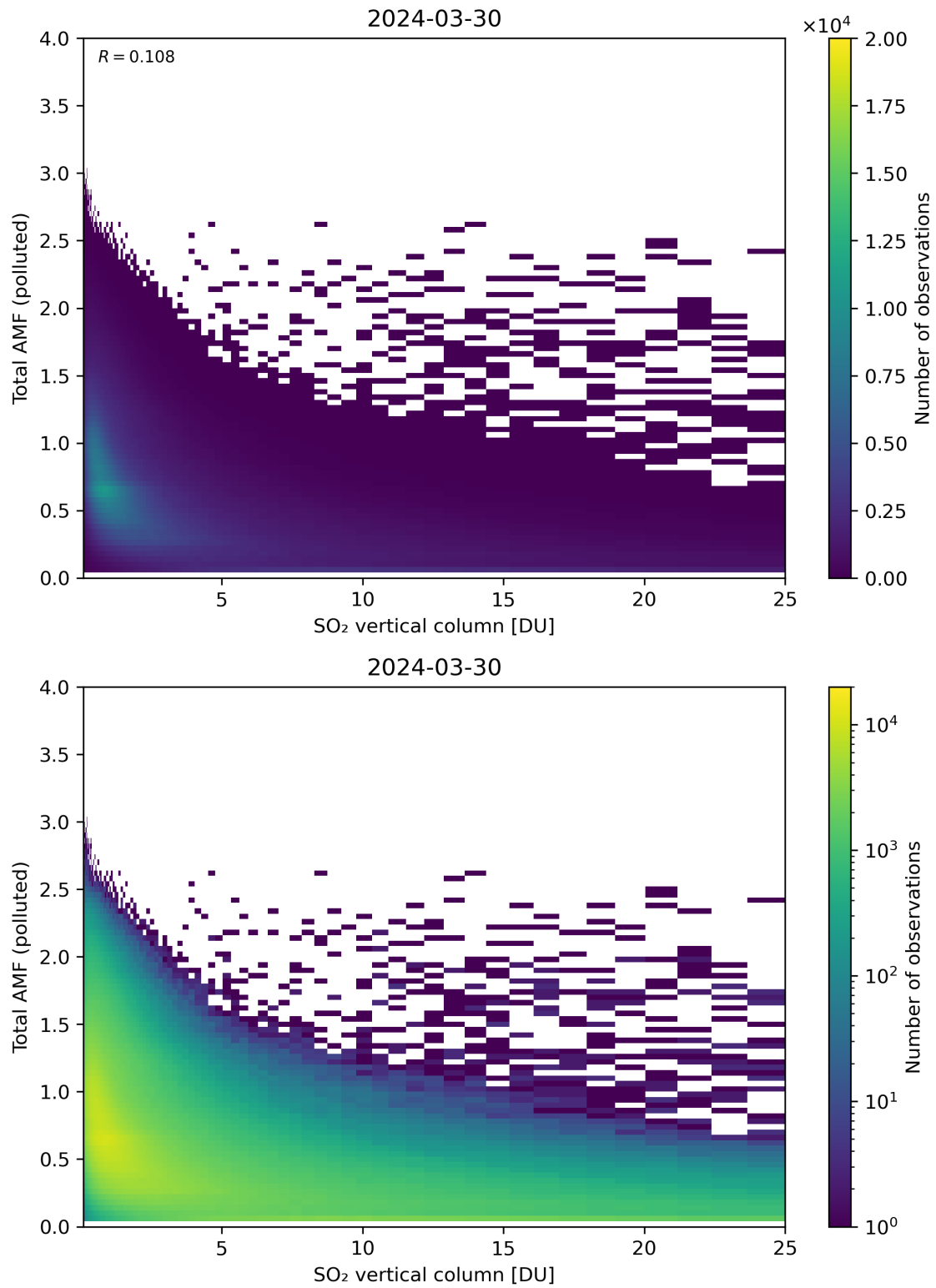
Figure 305: Scatter density plot of “SO 2 vertical column” against “Total AMF (polluted)” for 2024-03-30 to 2024-03-31.
