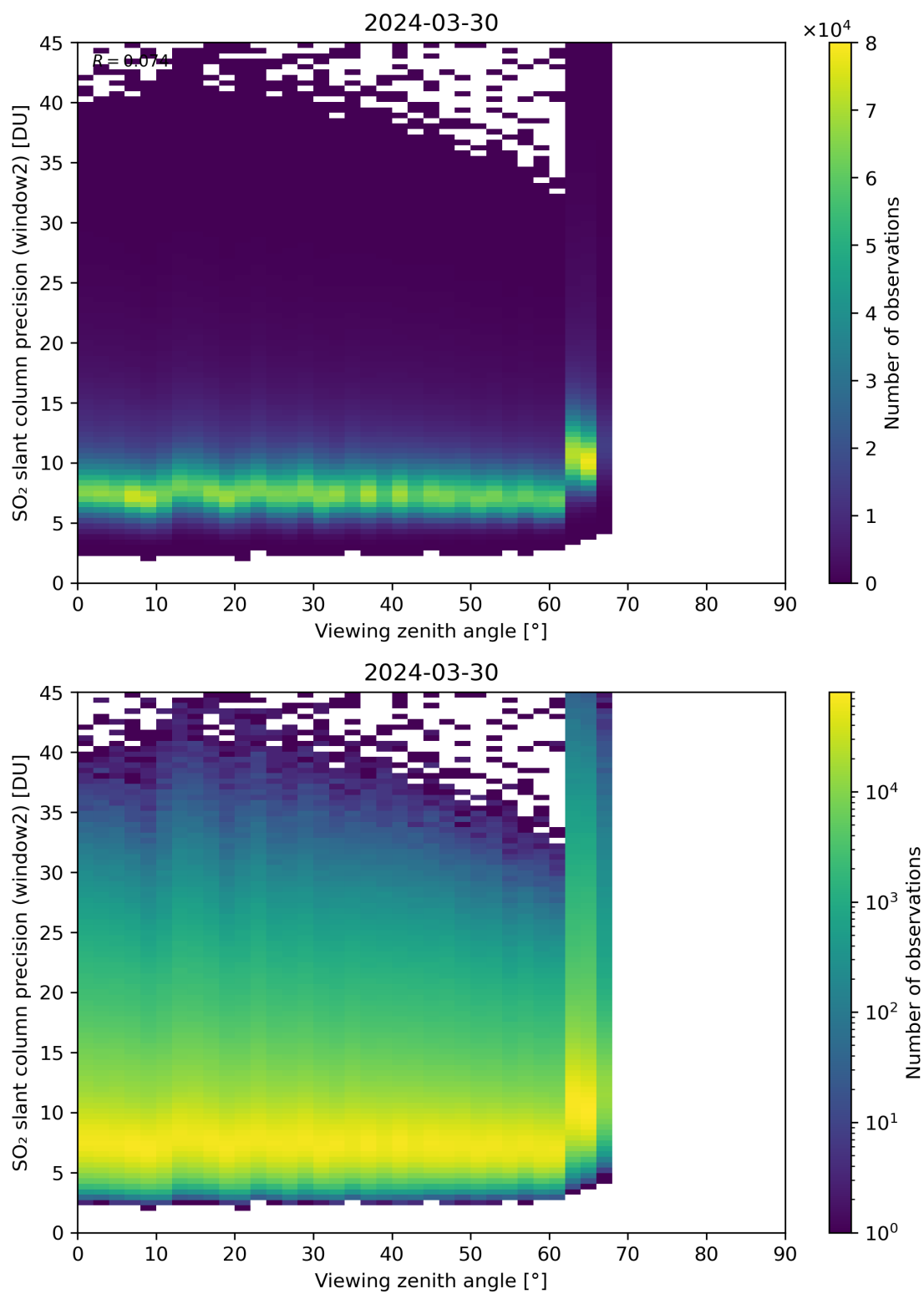
Figure 322: Scatter density plot of “Viewing zenith angle” against “SO 2 slant column precision (window2)” for 2024-03-30 to 2024-03-31.
