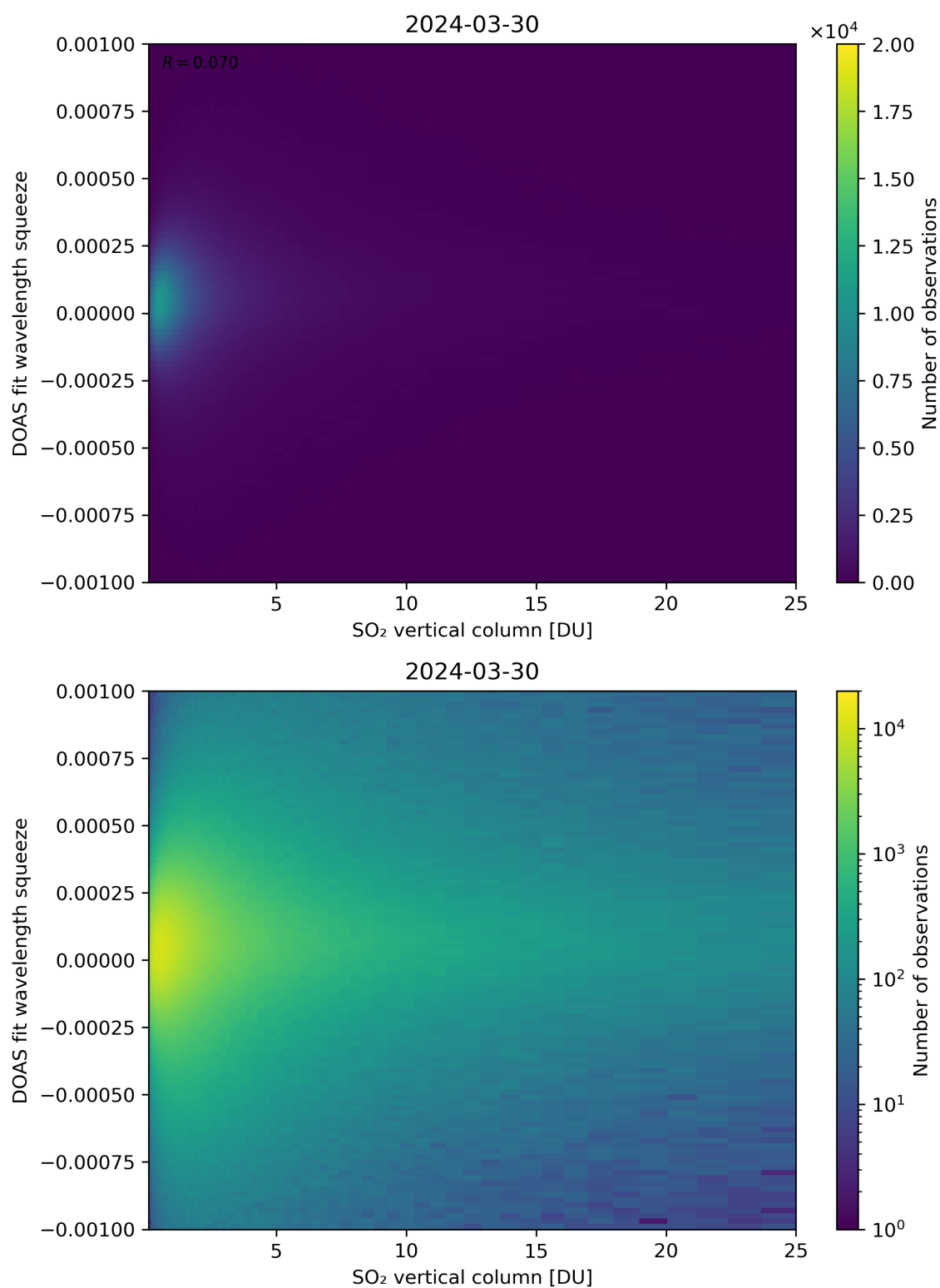
Figure 277: Scatter density plot of “SO 2 vertical column” against “DOAS fit wavelength squeeze” for 2024-03-30 to 2024-03-31.
