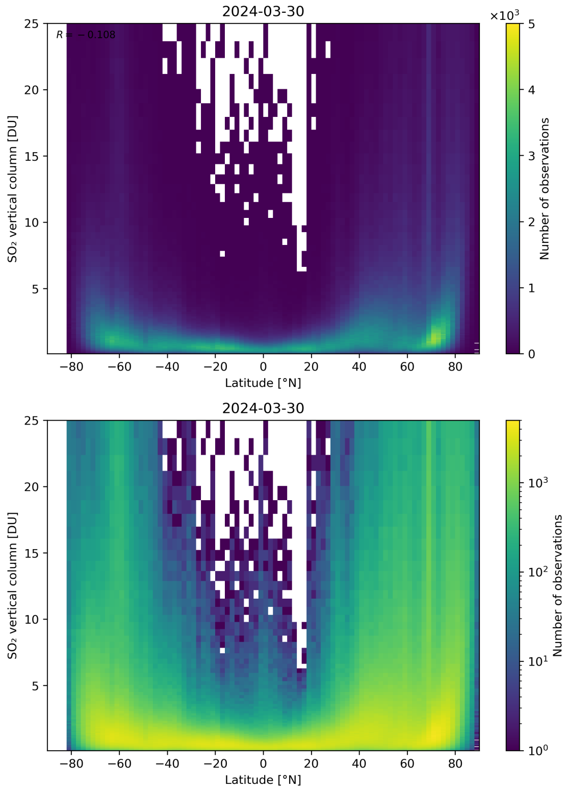
Figure 156: Scatter density plot of “Latitude” against “SO 2 vertical column” for 2024-03-30 to 2024-03-31.
