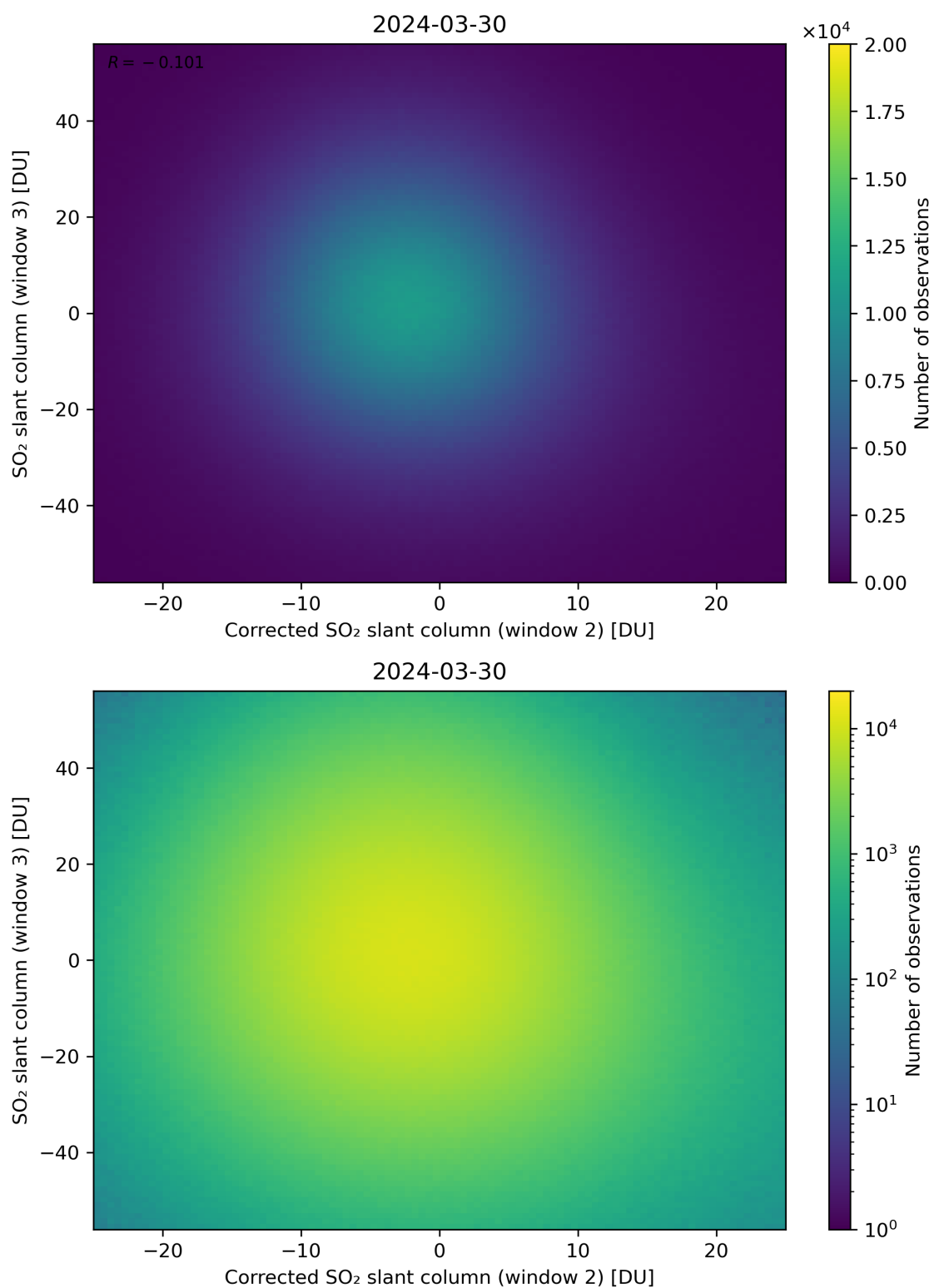
Figure 201: Scatter density plot of “Corrected SO 2 slant column (window 2)” against “SO 2 slant column (window 3)” for 2024-03-30 to 2024-03-31.
