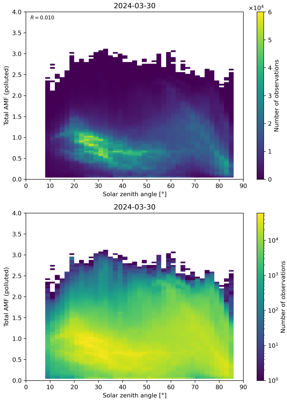
Figure 174: Scatter density plot of “Solar zenith angle” against “Total AMF (polluted)” for 2024-03-30 to 2024-03-31.
