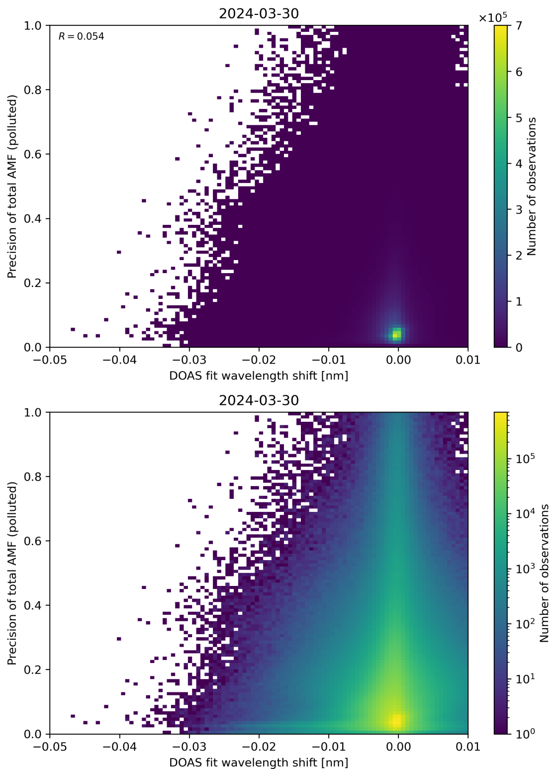
Figure 131: Scatter density plot of “DOAS fit wavelength shift” against “Precision of total AMF (polluted)” for 2024-03-30 to 2024-03-31.
