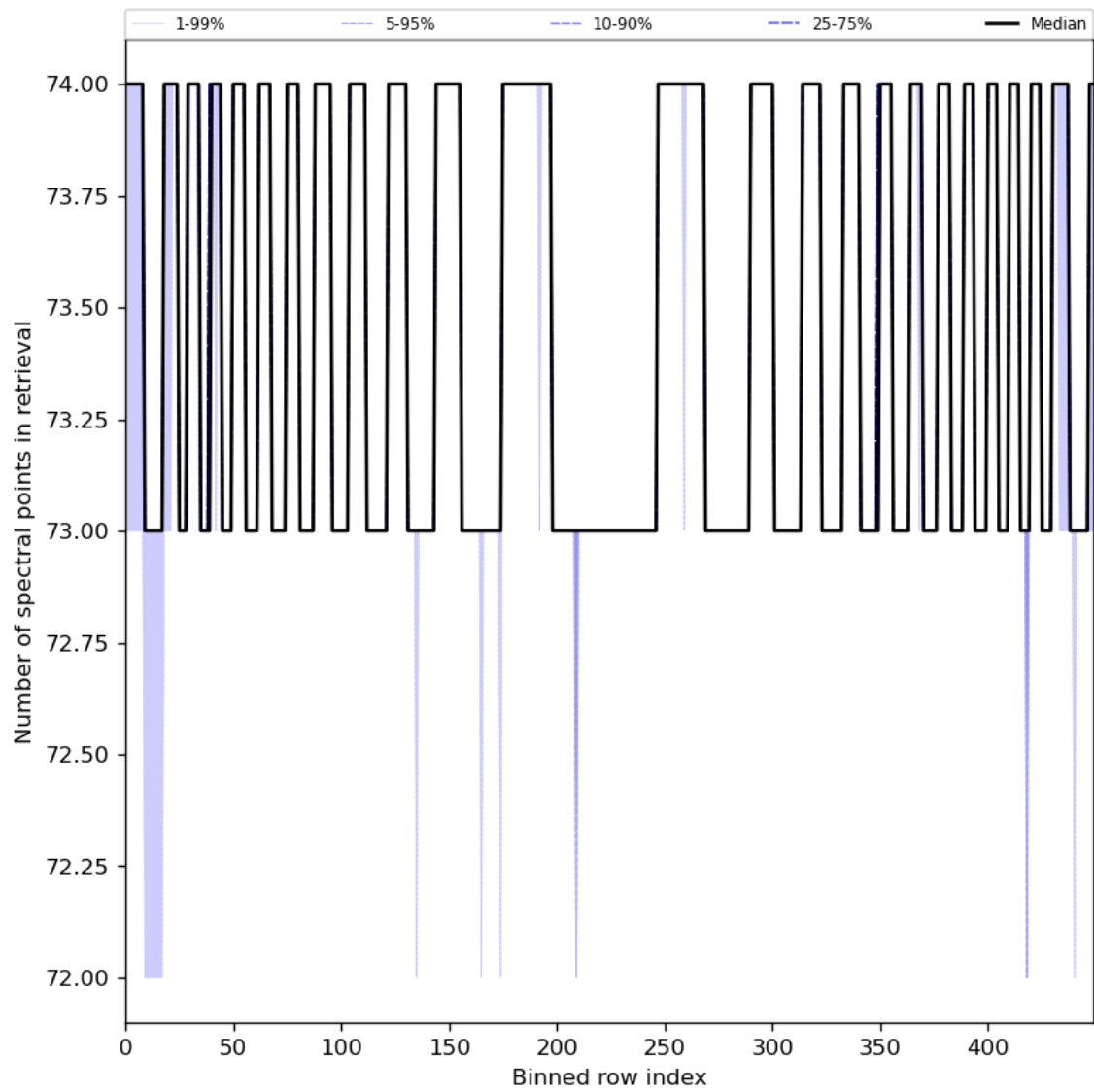
Figure 97: Along track statistics of “Number of spectral points in retrieval” for 2024-03-30 to 2024-03-31
