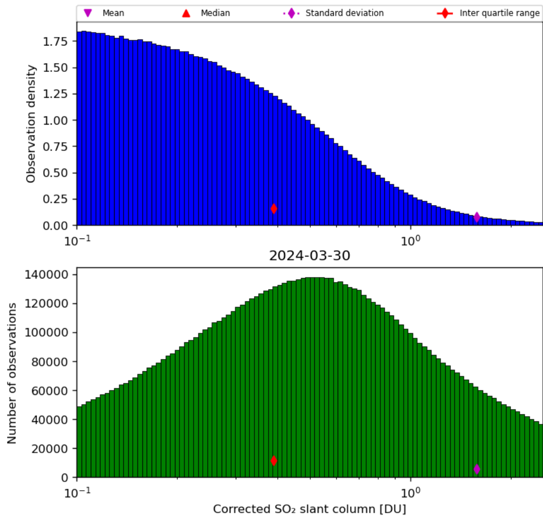
Figure 55: Histogram of “Corrected SO 2 slant column” for 2024-03-30 to 2024-03-31
