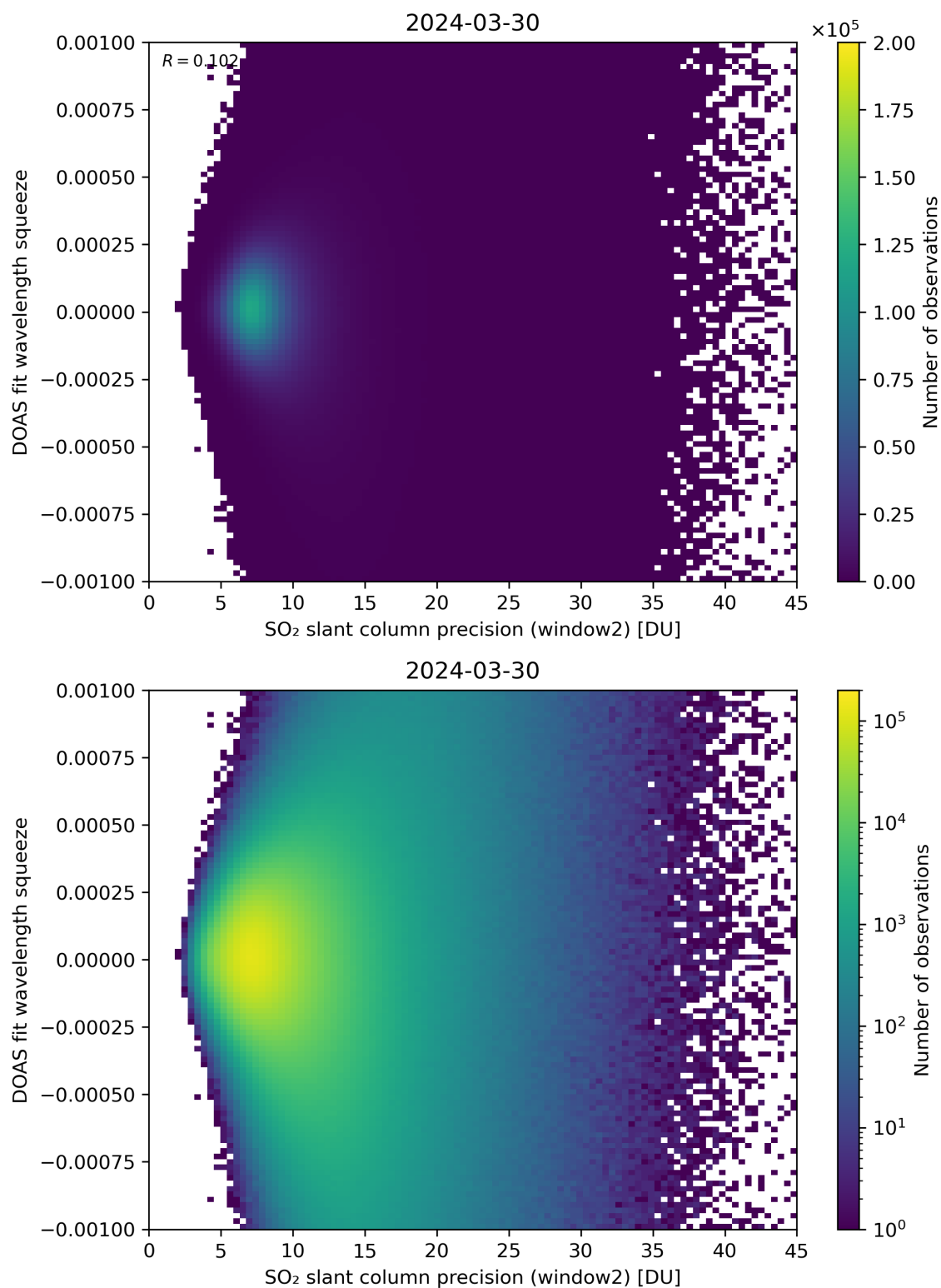
Figure 244: Scatter density plot of “SO 2 slant column precision (window2)” against “DOAS fit wavelength squeeze” for 2024-03-30 to 2024-03-31.
