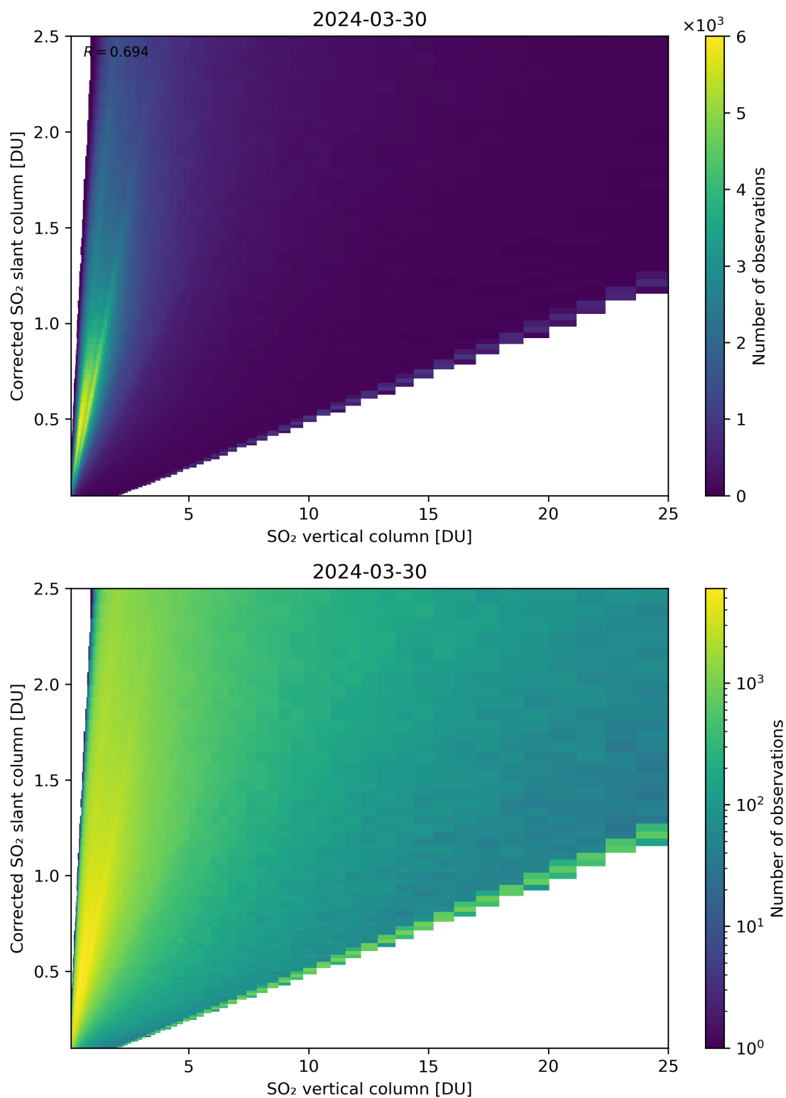
Figure 297: Scatter density plot of “SO 2 vertical column” against “Corrected SO 2 slant column” for 2024-03-30 to 2024-03-31.
