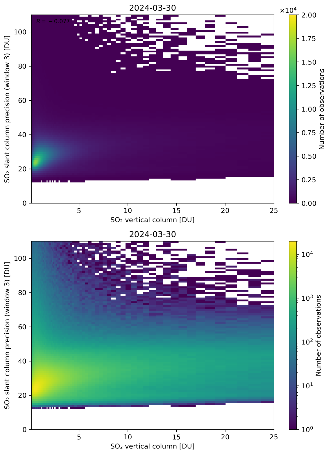
Figure 304: Scatter density plot of “SO 2 vertical column” against “SO 2 slant column precision (window 3)” for 2024-03-30 to 2024-03-31.
