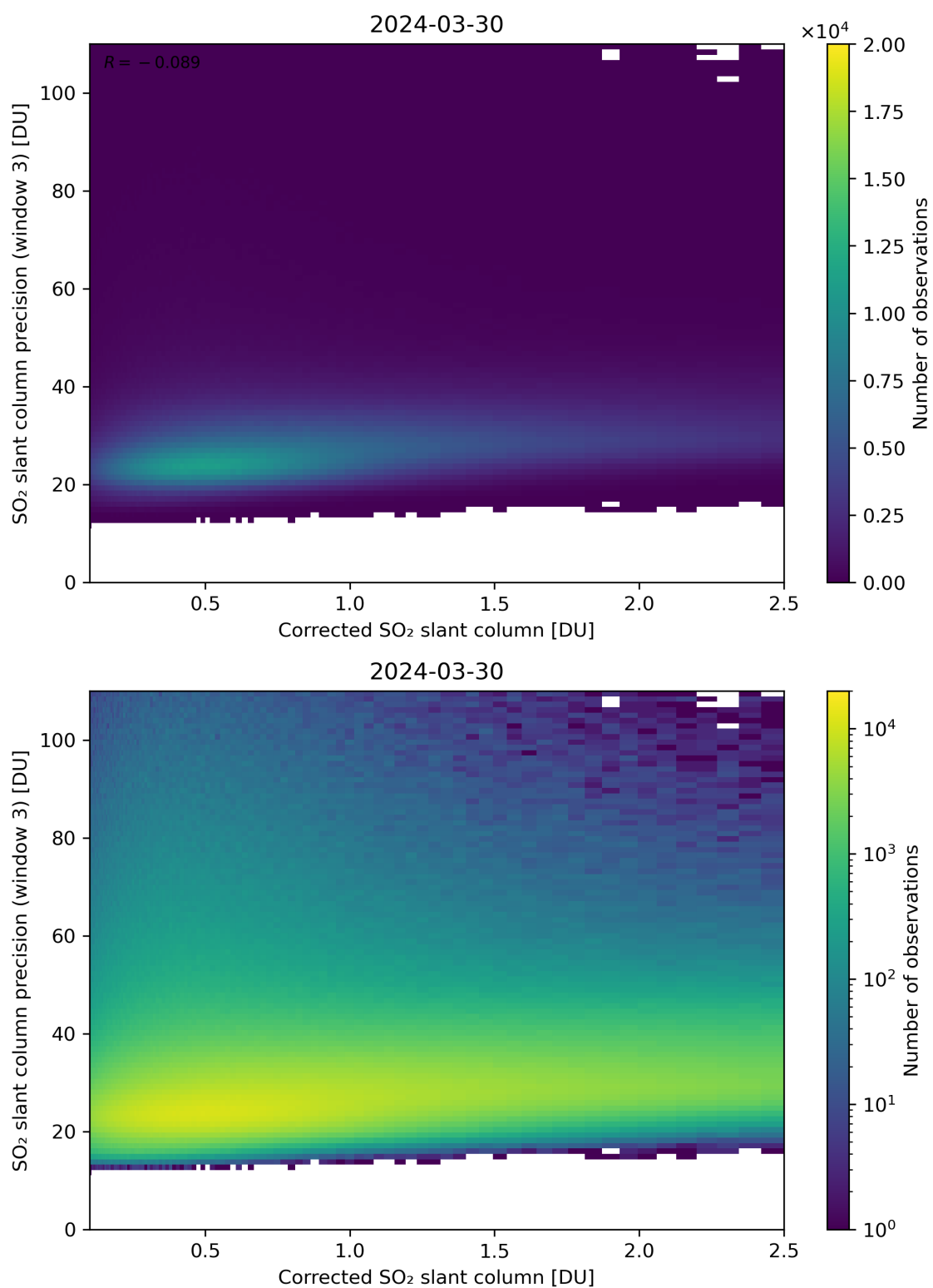
Figure 191: Scatter density plot of “Corrected SO 2 slant column” against “SO 2 slant column precision (window 3)” for 2024-03-30 to 2024-03-31.
