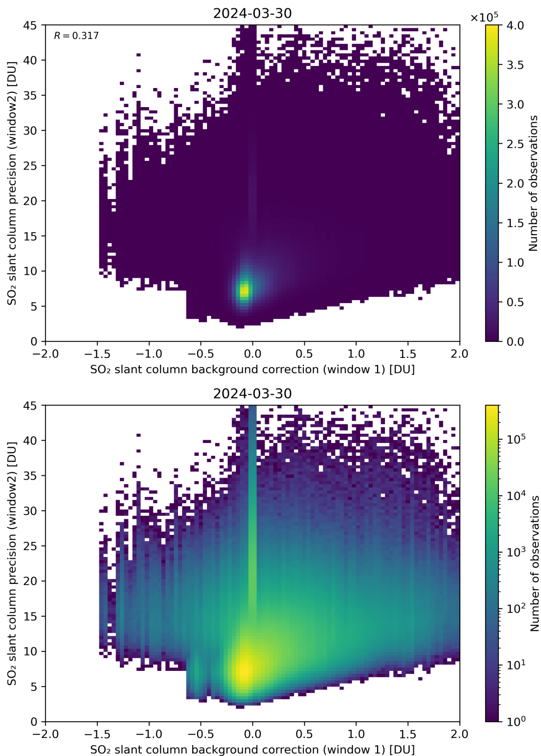
Figure 106: Scatter density plot of “SO 2 slant column background correction (window 1)” against “SO 2 slant column precision (window2)” for 2024-03-30 to 2024-03-31.
