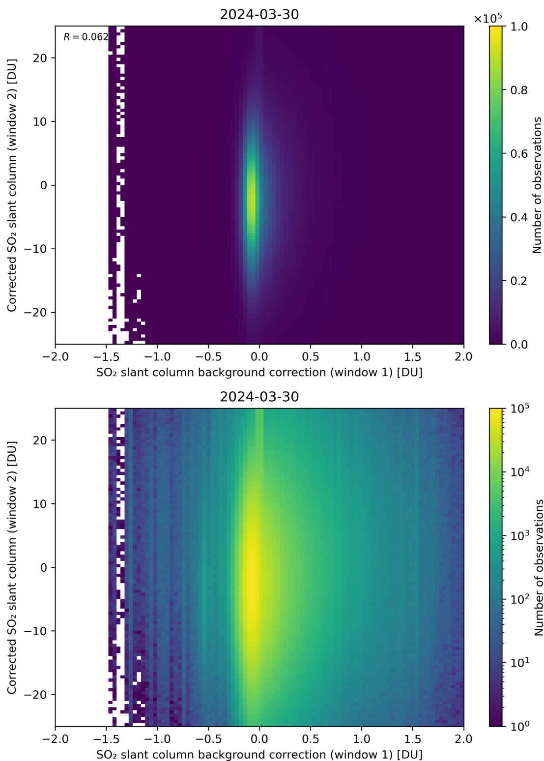
Figure 104: Scatter density plot of “SO 2 slant column background correction (window 1)” against “Corrected SO 2 slant column (window 2)” for 2024-03-30 to 2024-03-31.
