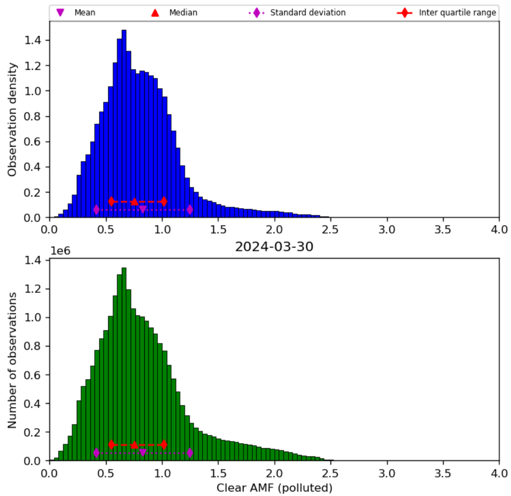
Figure 73: Histogram of “Clear AMF (polluted)” for 2024-03-30 to 2024-03-31
