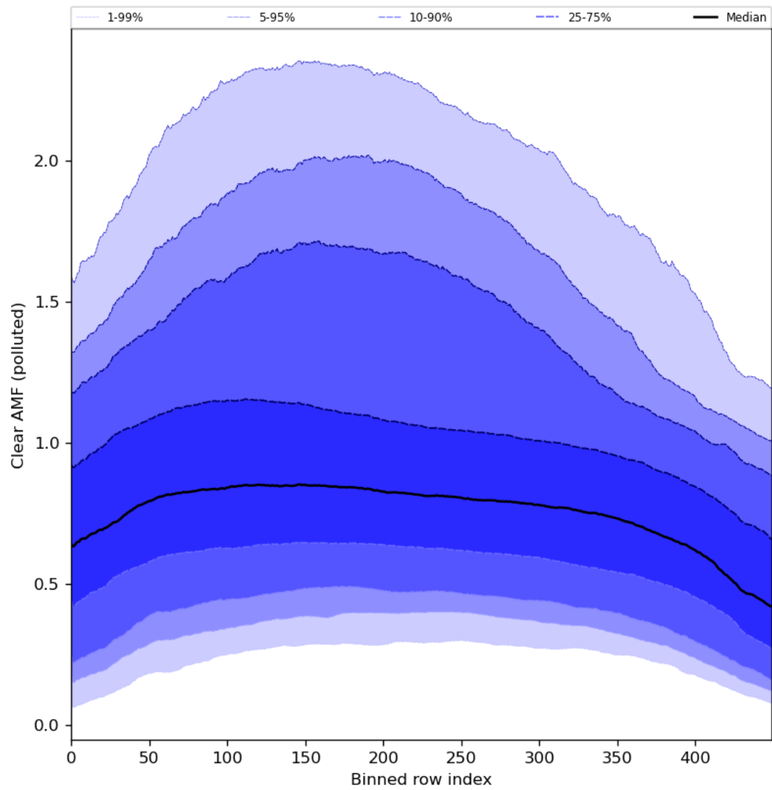
Figure 96: Along track statistics of “Clear AMF (polluted)” for 2024-03-30 to 2024-03-31
