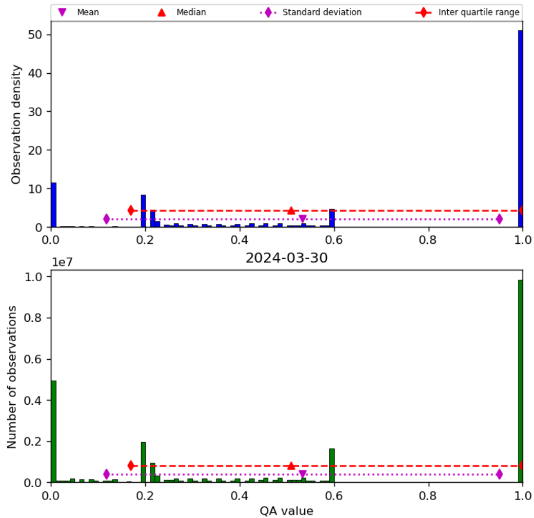
Figure 52: Histogram of “QA value” for 2024-03-30 to 2024-03-31
