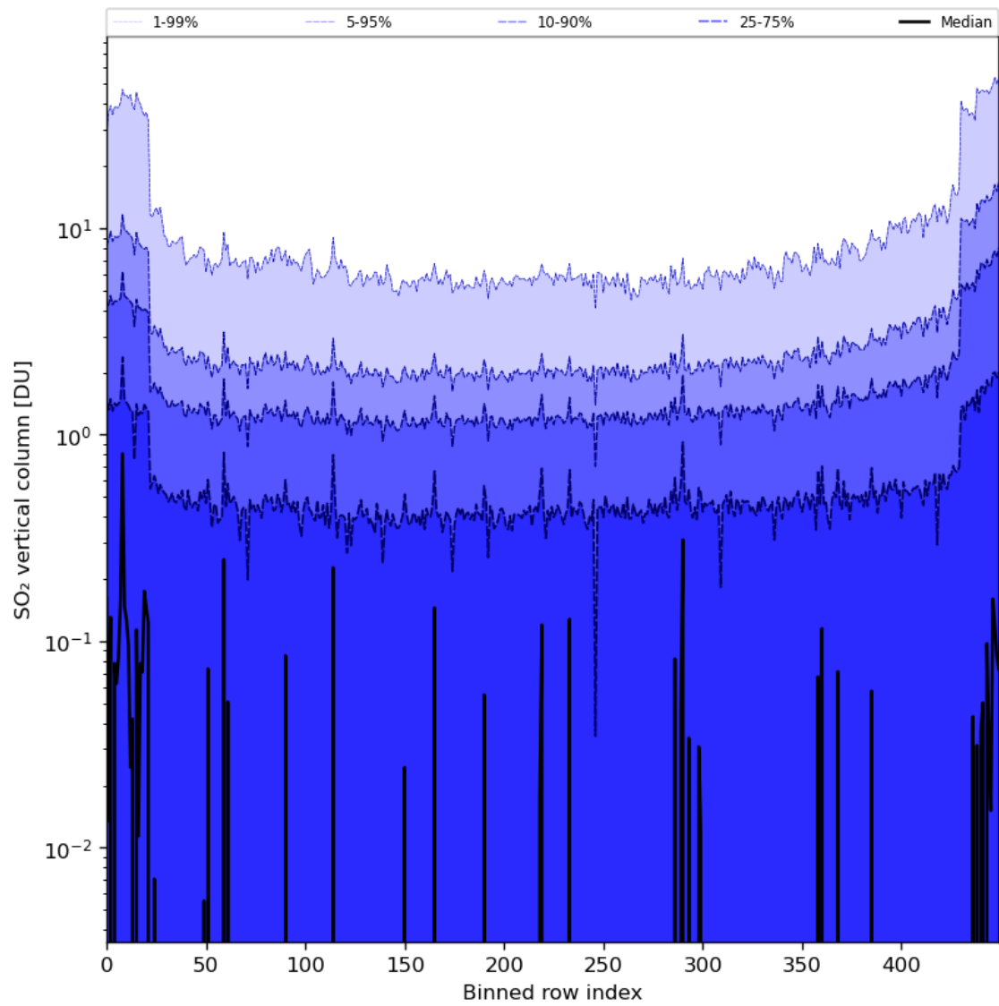
Figure 76: Along track statistics of “SO 2 vertical column” for 2024-03-30 to 2024-03-31
