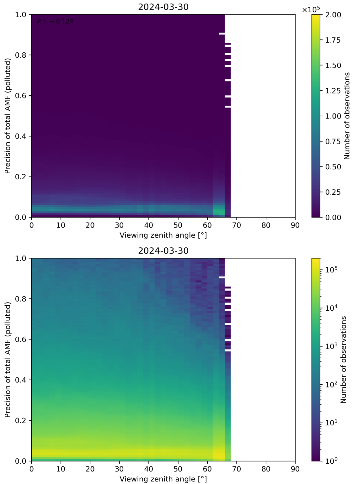
Figure 326: Scatter density plot of “Viewing zenith angle” against “Precision of total AMF (polluted)” for 2024-03-30 to 2024-03-31.
