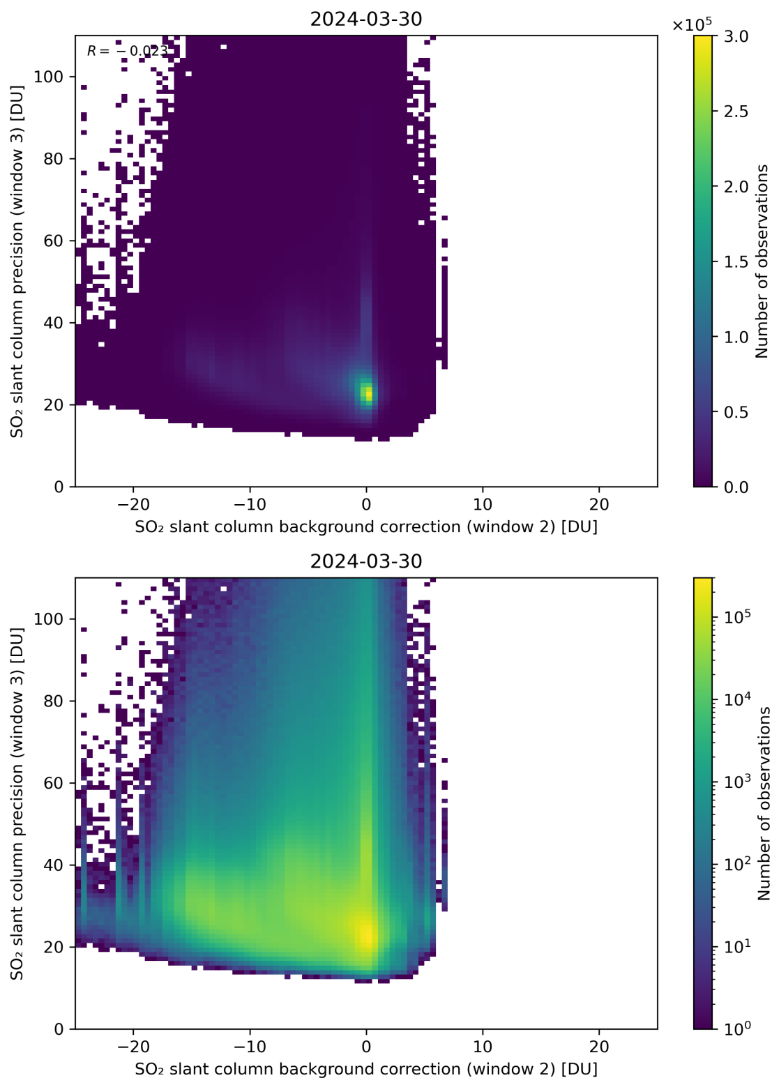
Figure 118: Scatter density plot of “SO 2 slant column background correction (window 2)” against “SO 2 slant column precision (window 3)” for 2024-03-30 to 2024-03-31.
