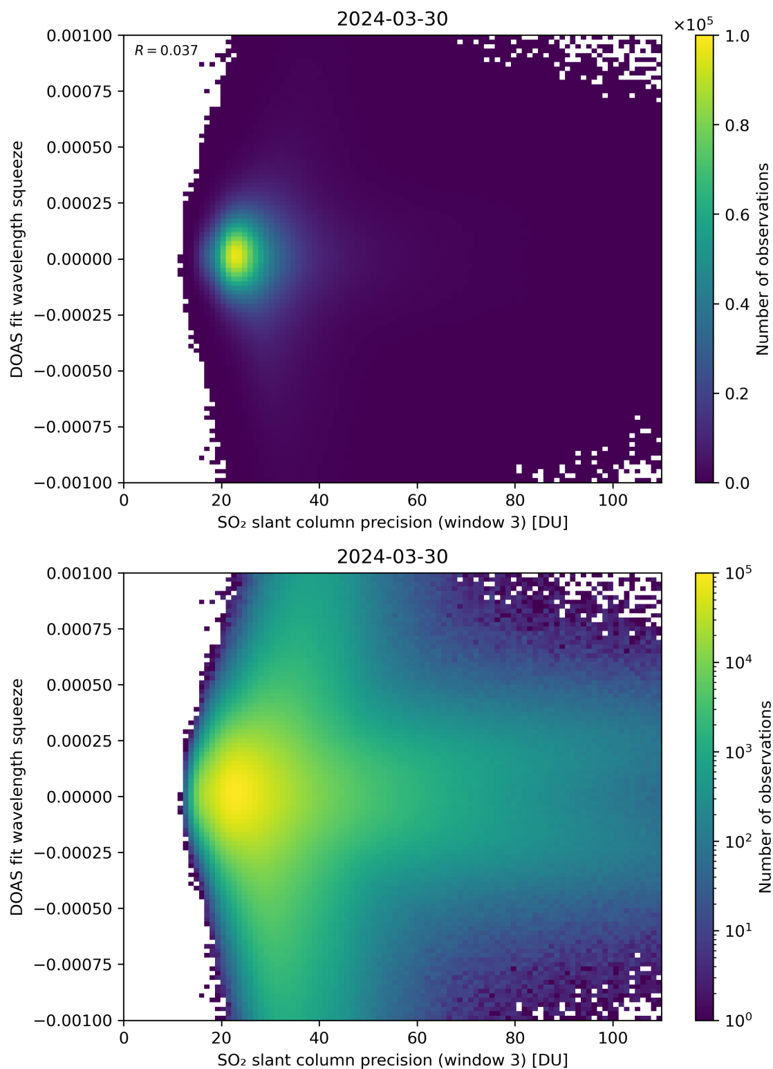
Figure 259: Scatter density plot of “SO 2 slant column precision (window 3)” against “DOAS fit wavelength squeeze” for 2024-03-30 to 2024-03-31.
