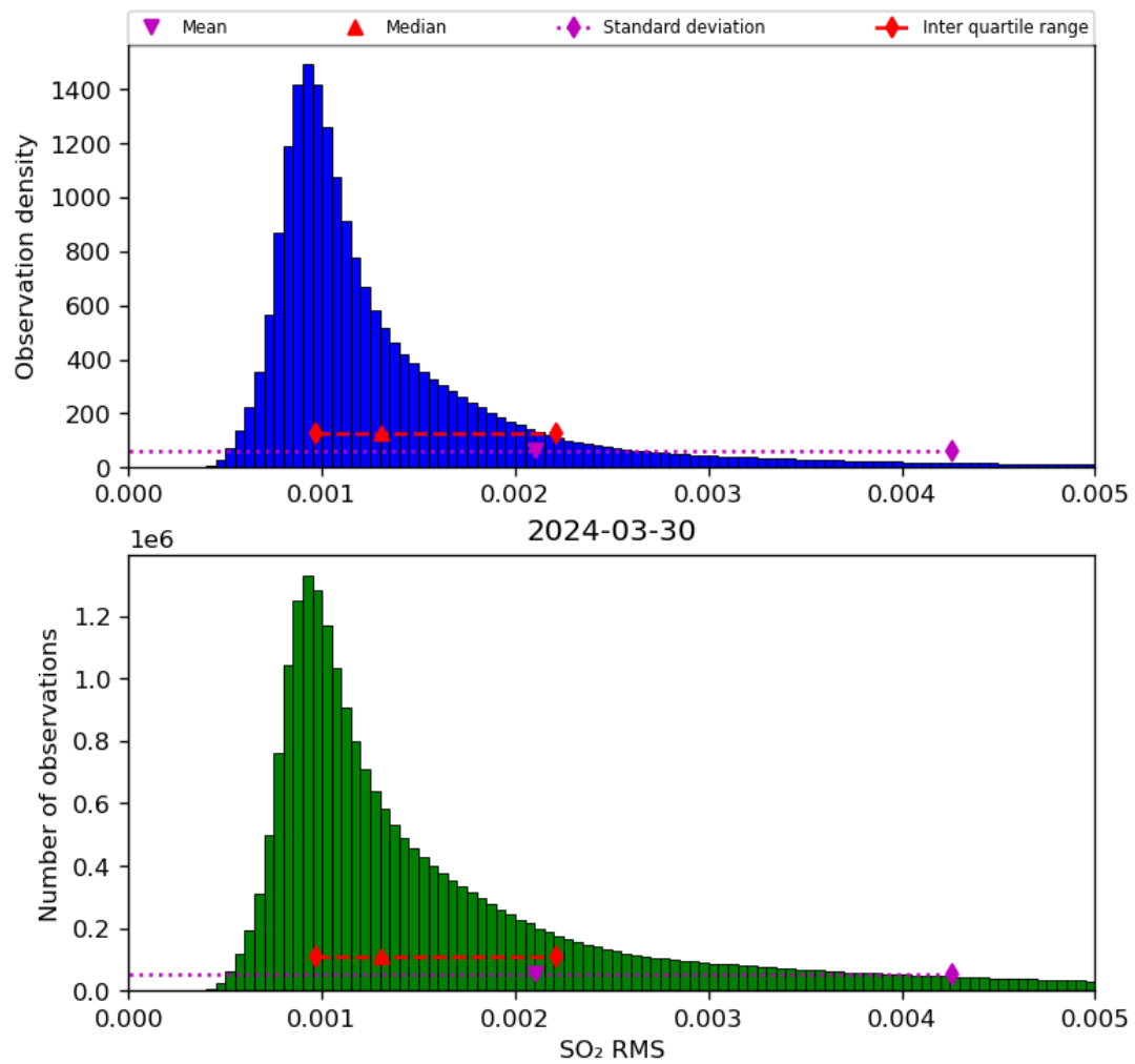
Figure 70: Histogram of “SO 2 RMS” for 2024-03-30 to 2024-03-31
