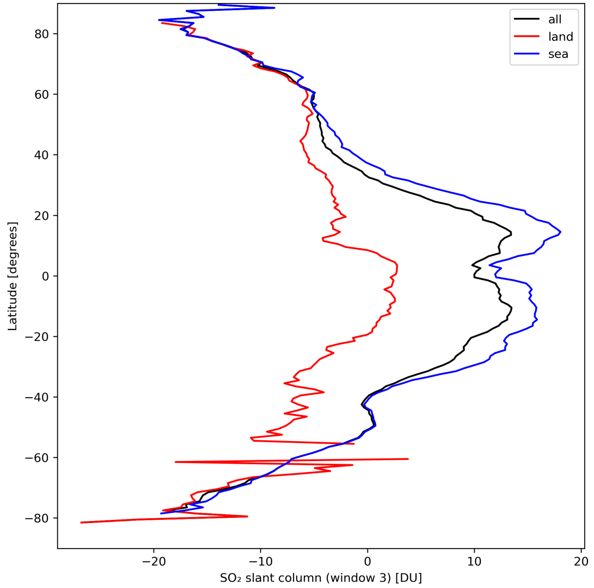
Figure 41: Zonal average of “SO 2 slant column (window 3)” for 2024-03-30 to 2024-03-31.
