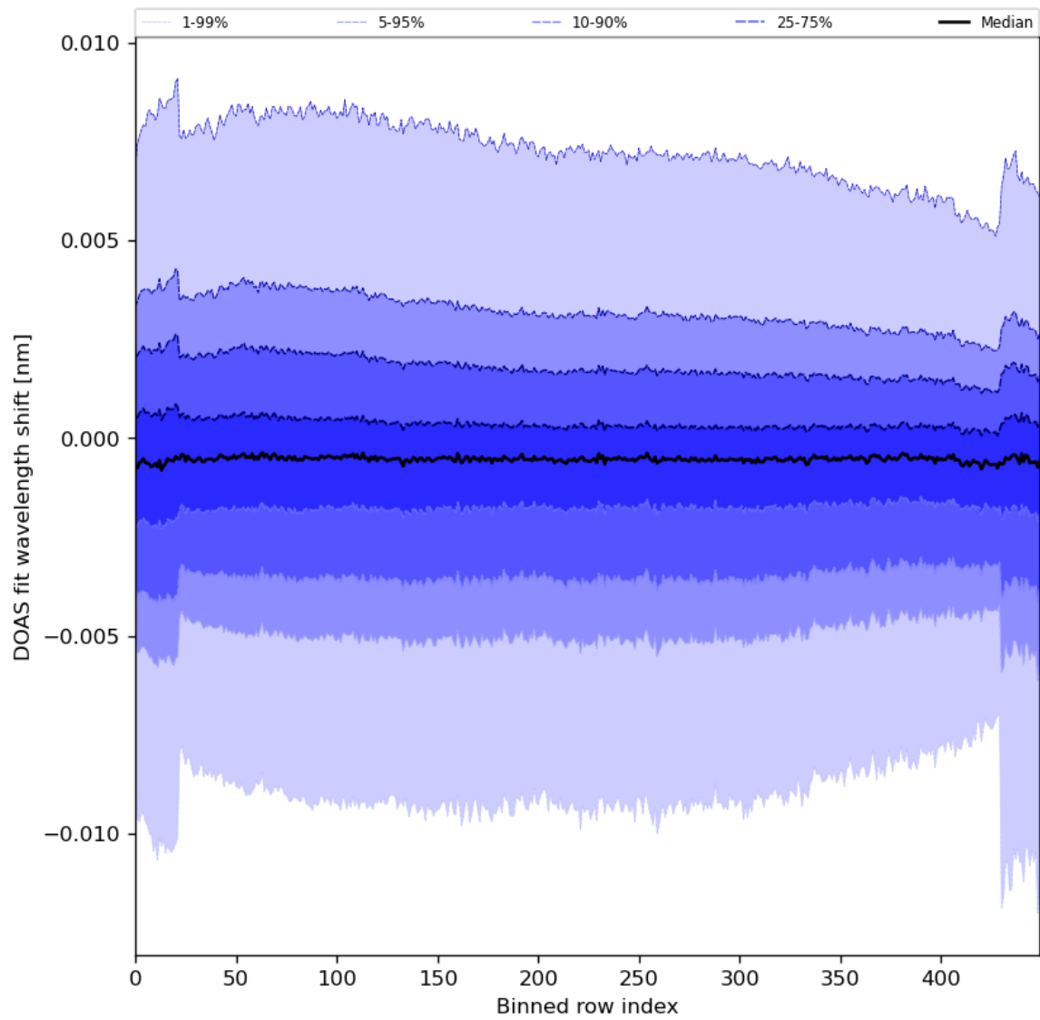
Figure 91: Along track statistics of “DOAS fit wavelength shift” for 2024-03-30 to 2024-03-31
