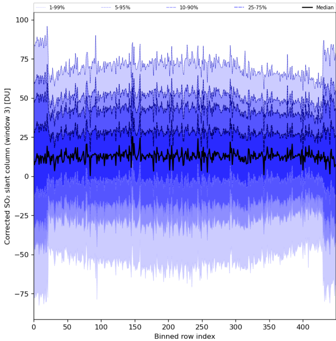
Figure 89: Along track statistics of “Corrected SO 2 slant column (window 3)” for 2024-03-30 to 2024-03-31
