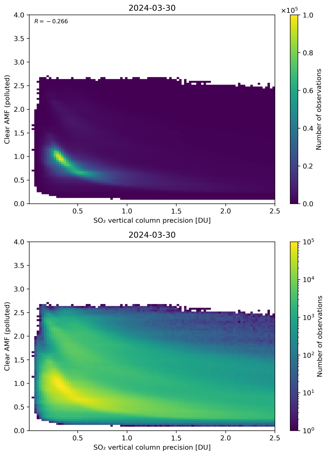
Figure 285: Scatter density plot of “SO 2 vertical column precision” against “Clear AMF (polluted)” for 2024-03-30 to 2024-03-31.
