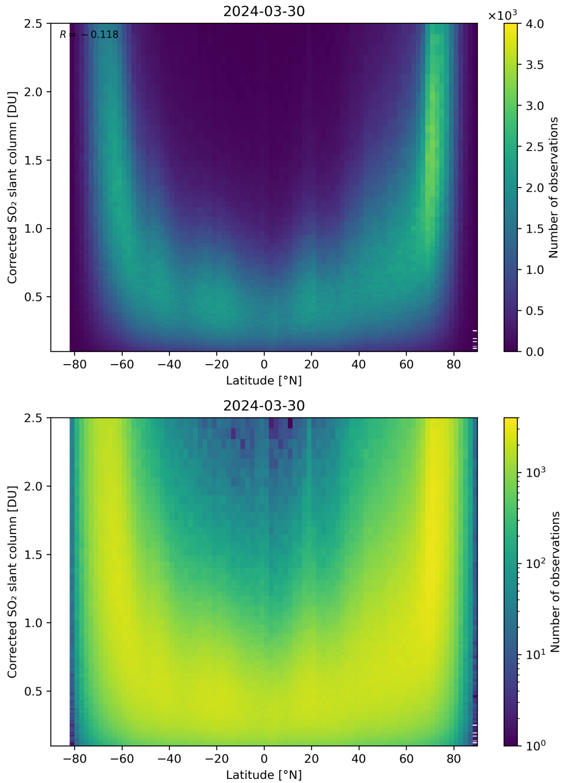
Figure 146: Scatter density plot of “Latitude” against “Corrected SO 2 slant column” for 2024-03-30 to 2024-03-31.
