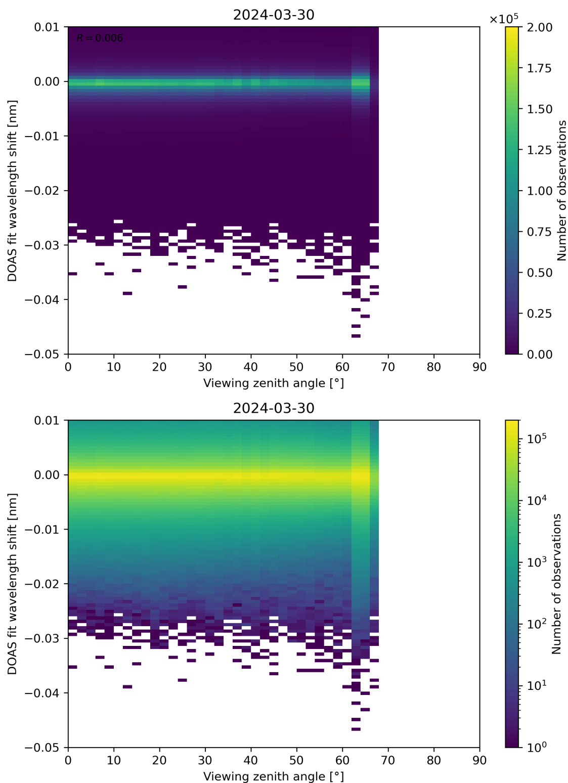
Figure 311: Scatter density plot of “Viewing zenith angle” against “DOAS fit wavelength shift” for 2024-03-30 to 2024-03-31.
