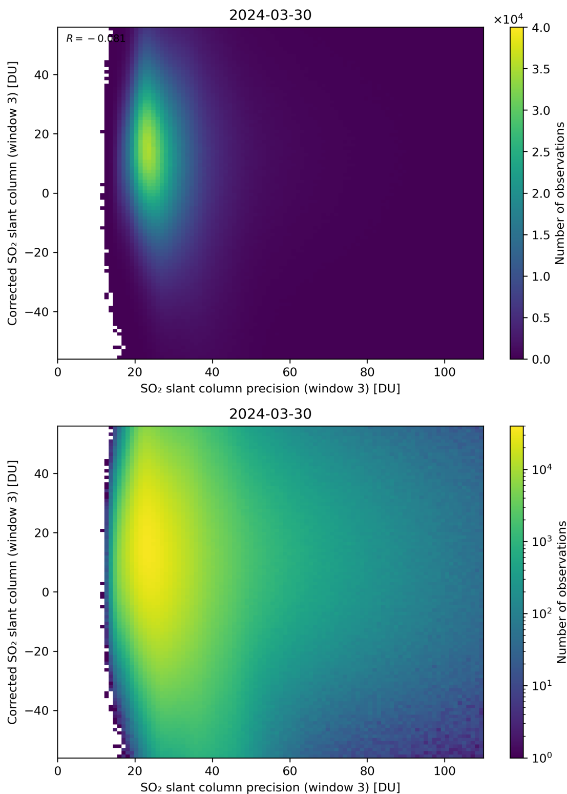
Figure 262: Scatter density plot of “SO 2 slant column precision (window 3)” against “Corrected SO 2 slant column (window 3)” for 2024-03-30 to 2024-03-31.
