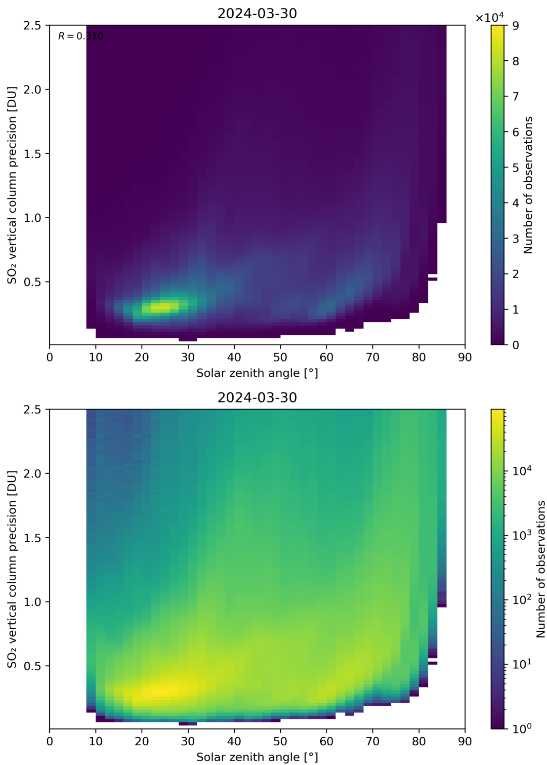
Figure 177: Scatter density plot of “Solar zenith angle” against “SO 2 vertical column precision” for 2024-03-30 to 2024-03-31.
