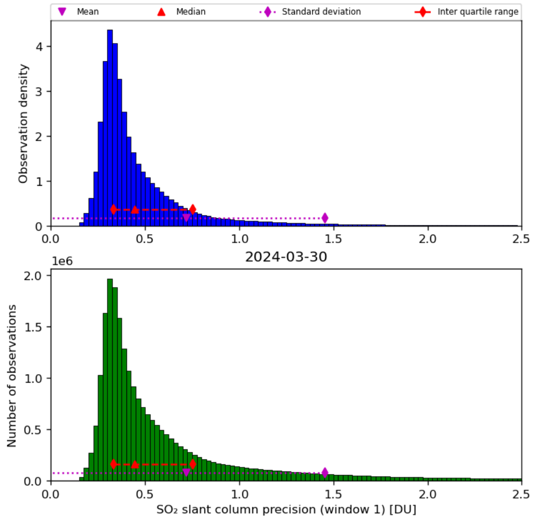
Figure 57: Histogram of “SO 2 slant column precision (window 1)” for 2024-03-30 to 2024-03-31
