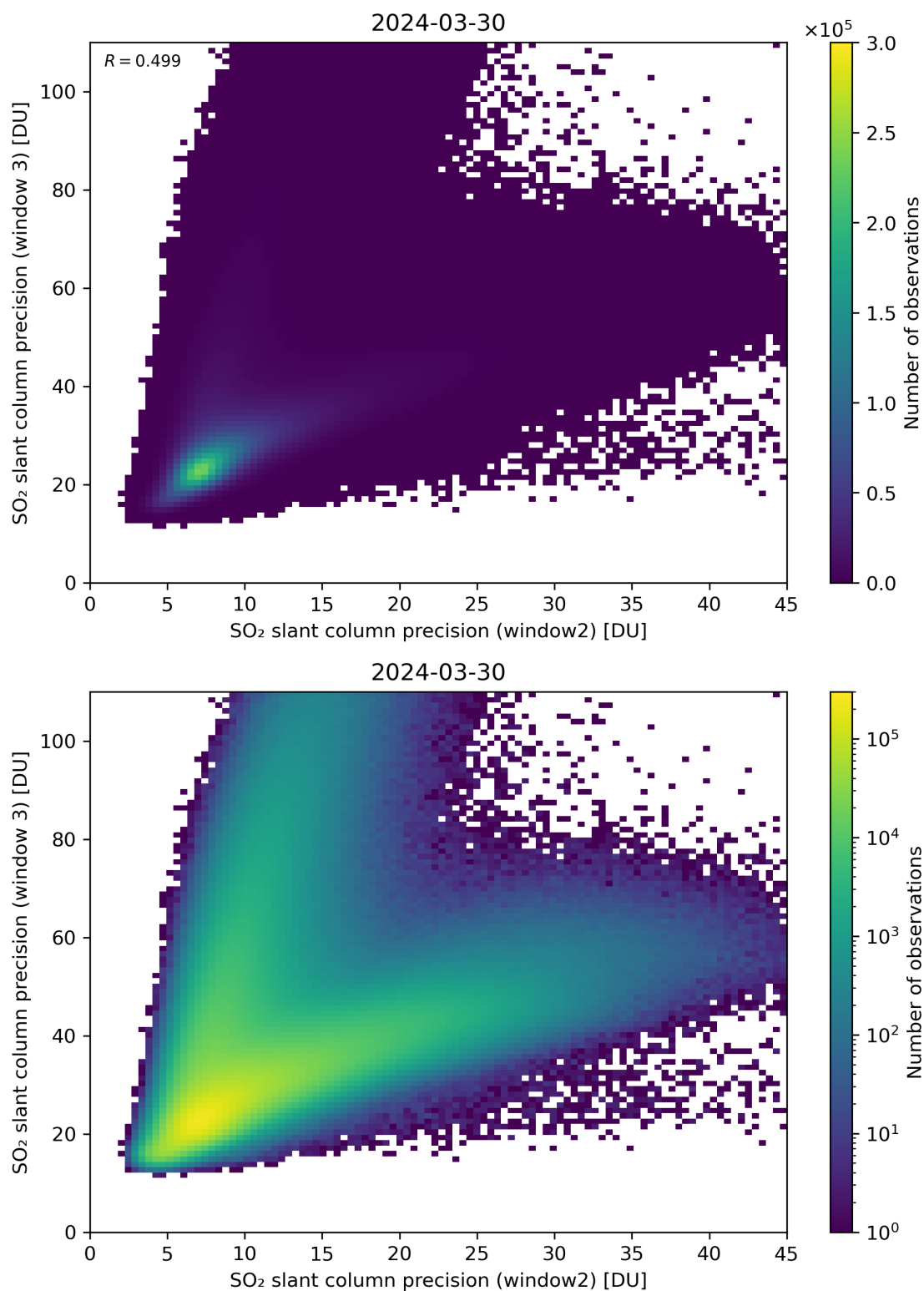
Figure 250: Scatter density plot of “SO 2 slant column precision (window2)” against “SO 2 slant column precision (window 3)” for 2024-03-30 to 2024-03-31.
