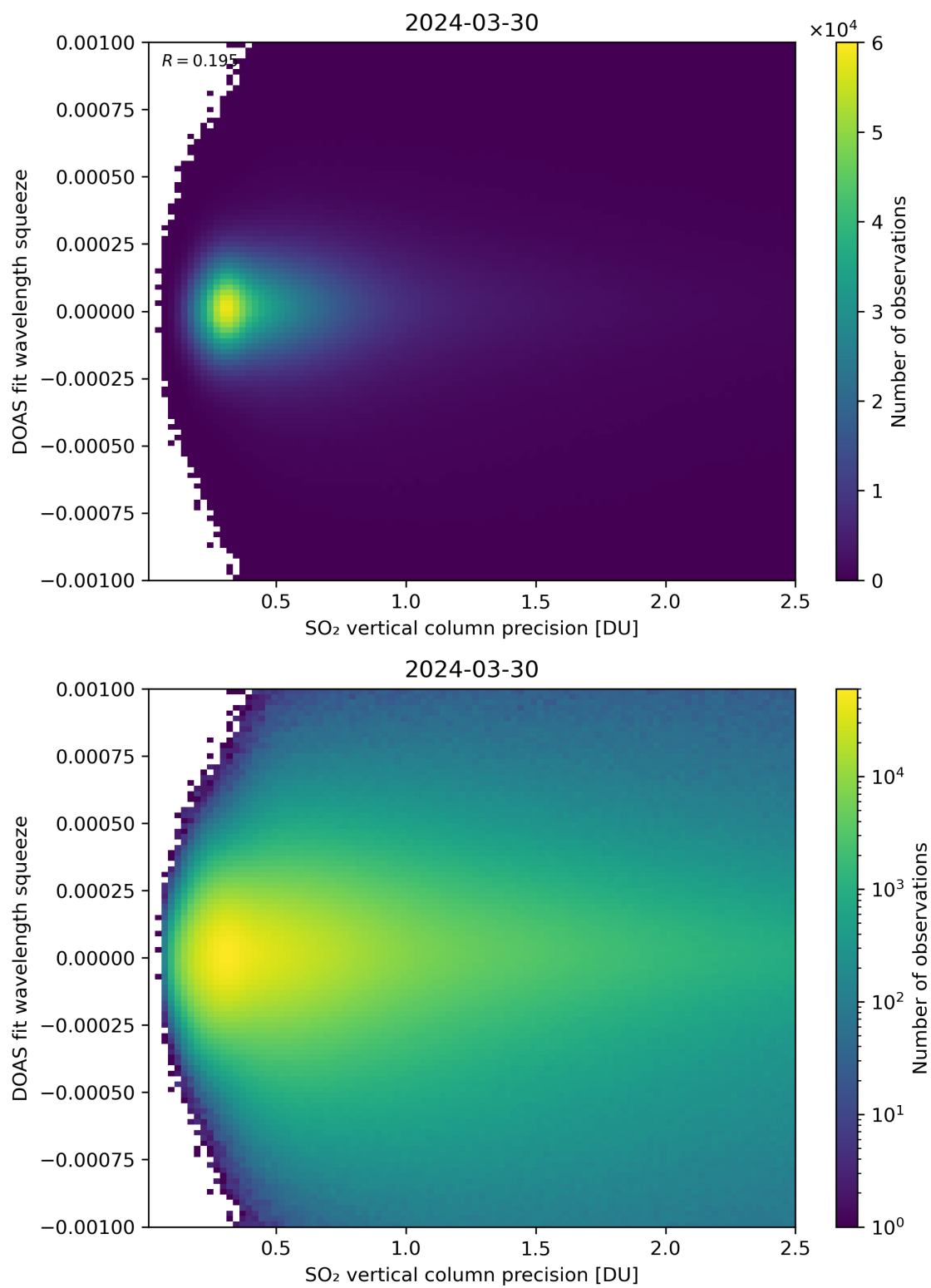
Figure 283: Scatter density plot of “SO 2 vertical column precision” against “DOAS fit wavelength squeeze” for 2024-03-30 to 2024-03-31.
