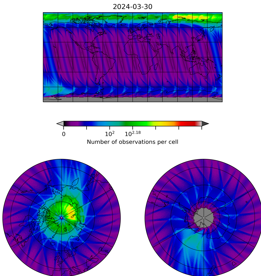
Figure 28: Map of the number of observations for 2024-03-30 to 2024-03-31
