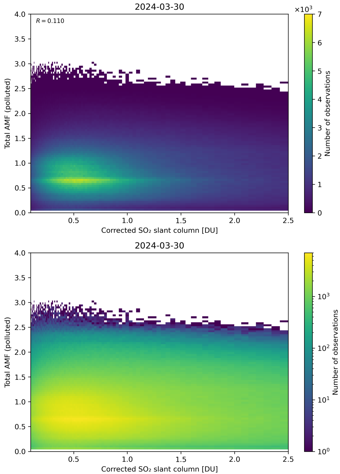
Figure 192: Scatter density plot of “Corrected SO 2 slant column” against “Total AMF (polluted)” for 2024-03-30 to 2024-03-31.
