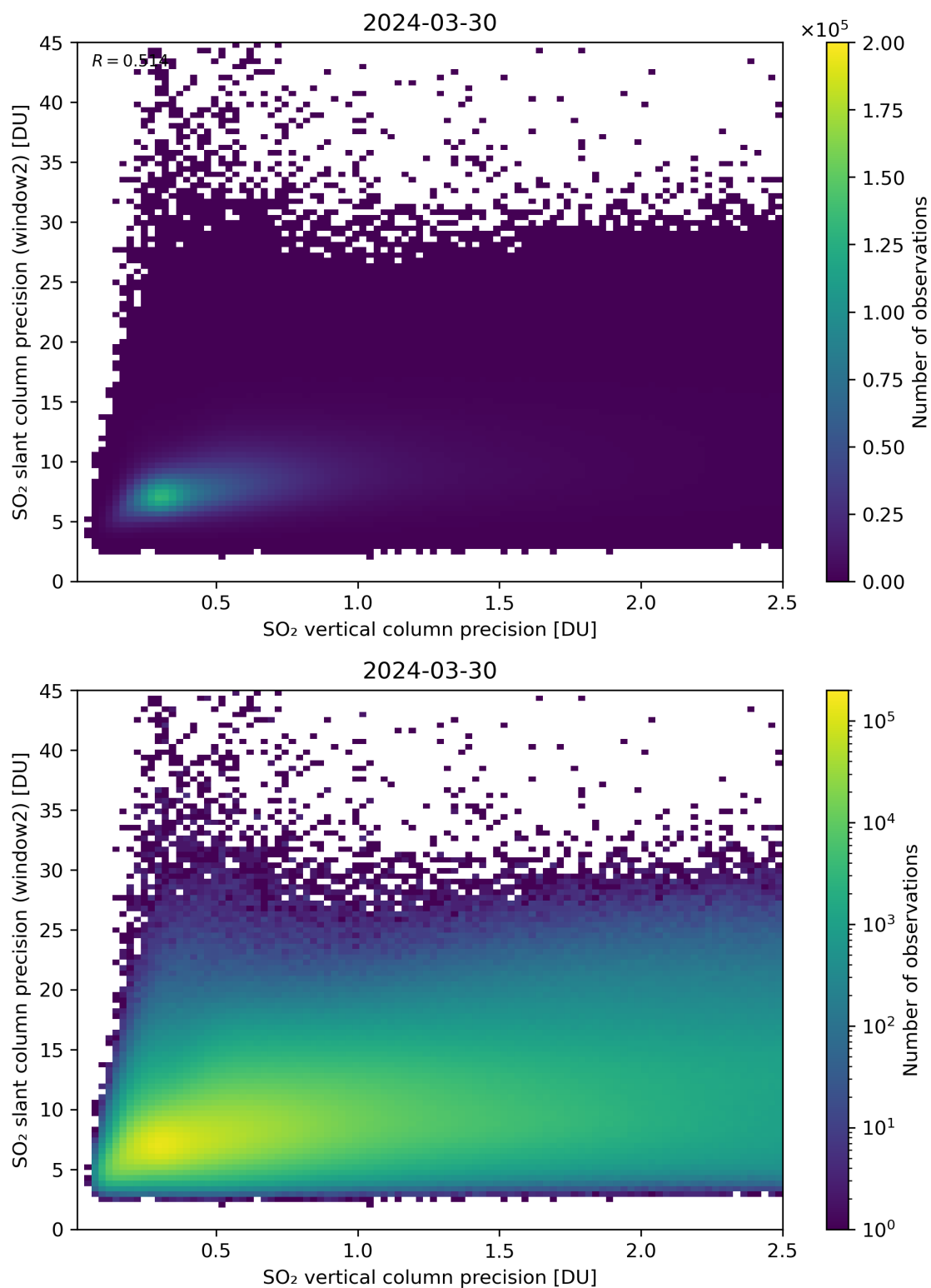
Figure 291: Scatter density plot of “SO 2 vertical column precision” against “SO 2 slant column precision (window2)” for 2024-03-30 to 2024-03-31.
