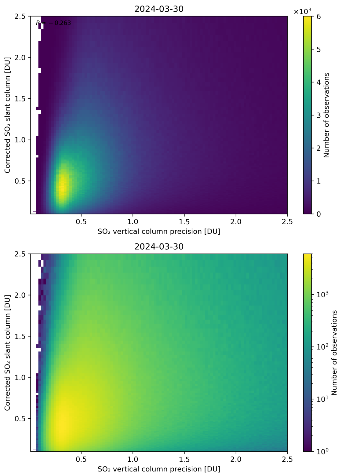
Figure 286: Scatter density plot of “SO 2 vertical column precision” against “Corrected SO 2 slant column” for 2024-03-30 to 2024-03-31.
