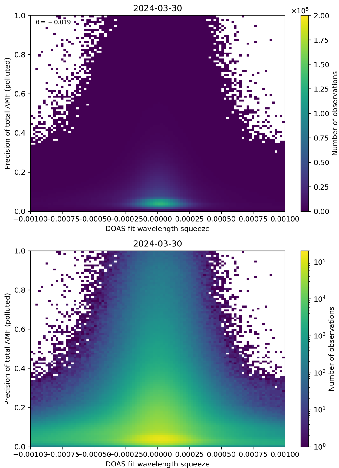
Figure 135: Scatter density plot of “DOAS fit wavelength squeeze” against “Precision of total AMF (polluted)” for 2024-03-30 to 2024-03-31.
