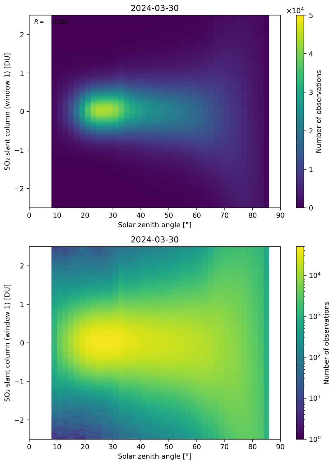
Figure 169: Scatter density plot of “Solar zenith angle” against “SO 2 slant column (window 1)” for 2024-03-30 to 2024-03-31.
