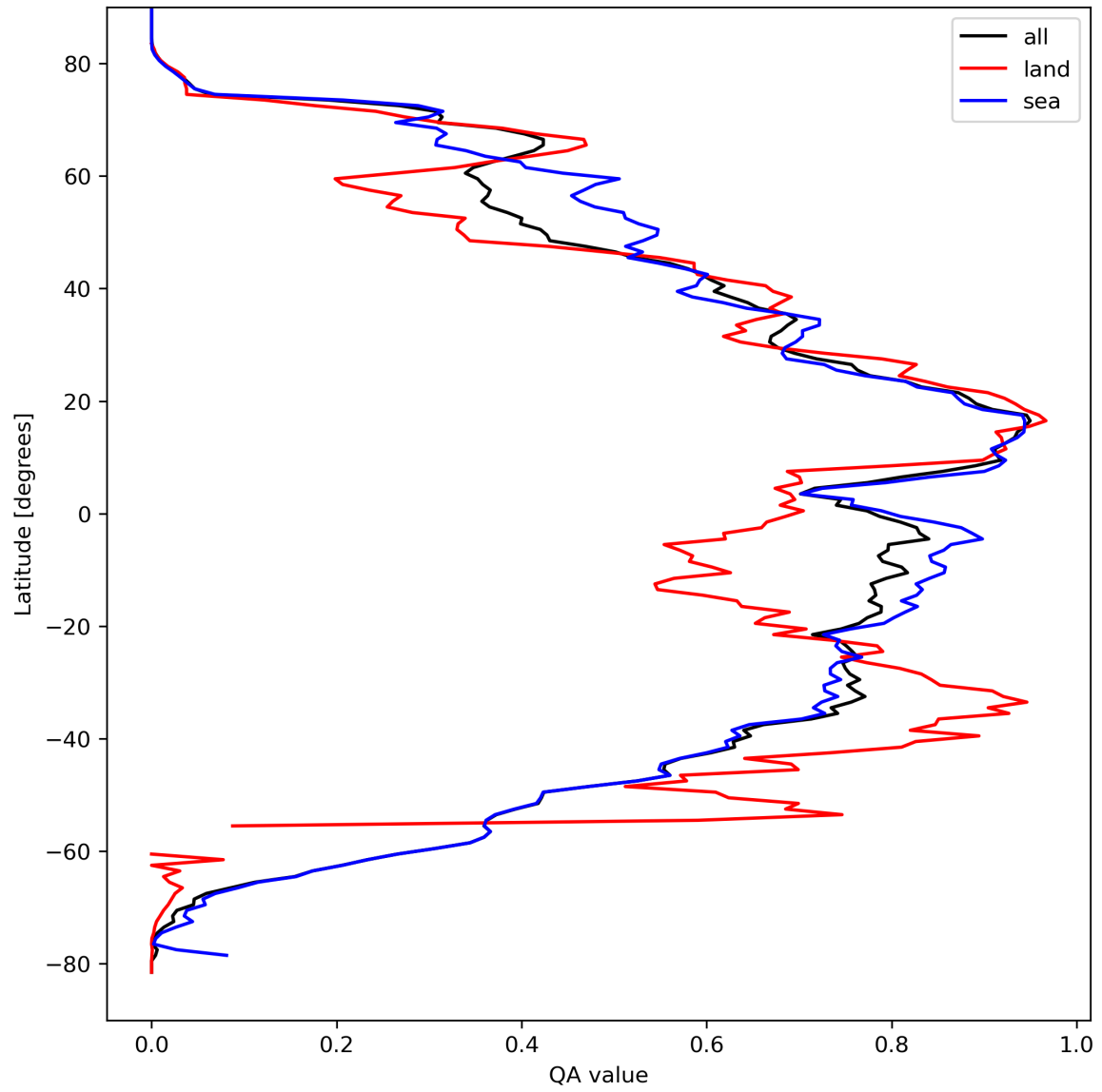
Figure 29: Zonal average of “QA value” for 2024-03-30 to 2024-03-31.
