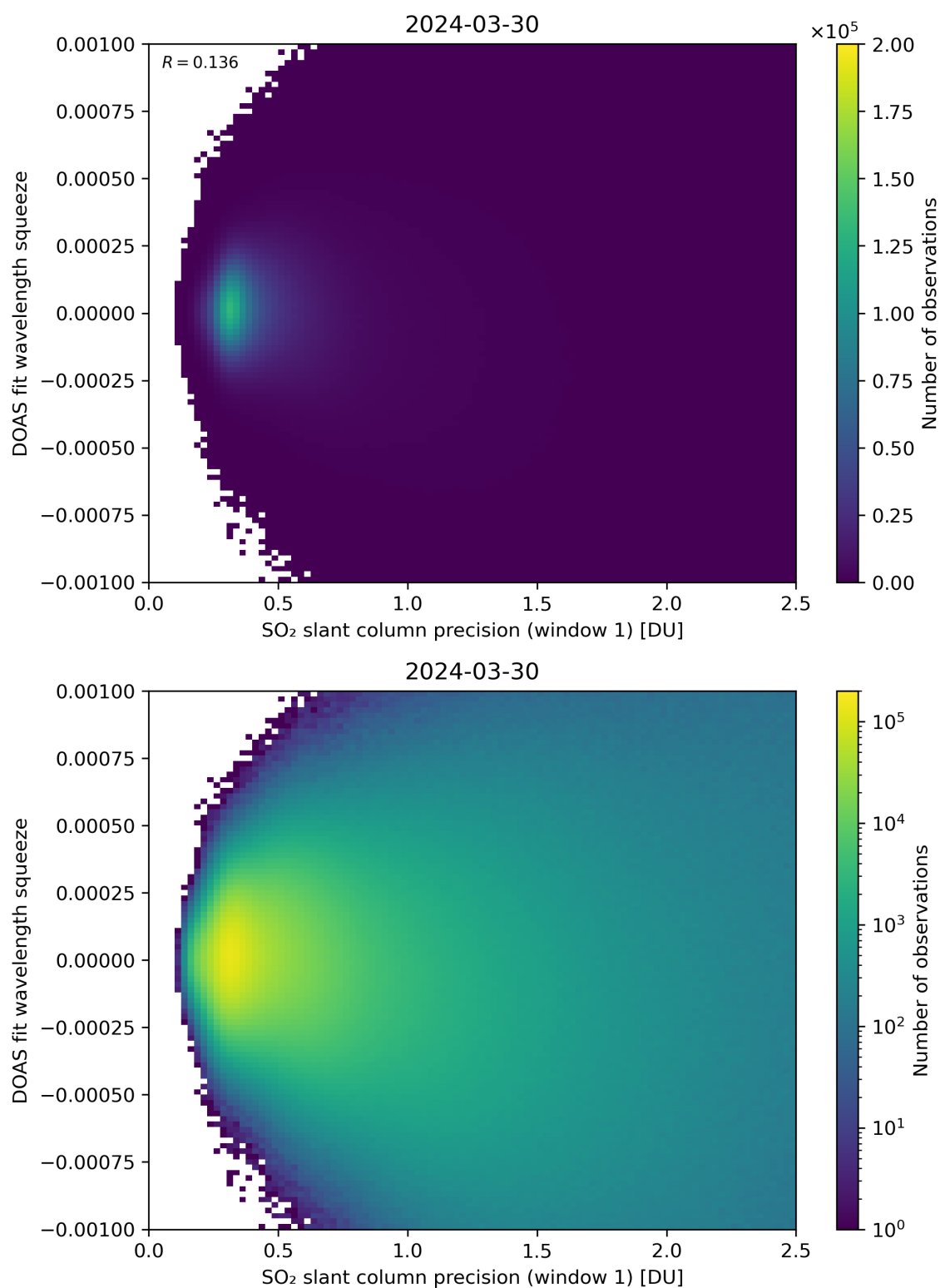
Figure 222: Scatter density plot of “SO 2 slant column precision (window 1)” against “DOAS fit wavelength squeeze” for 2024-03-30 to 2024-03-31.
