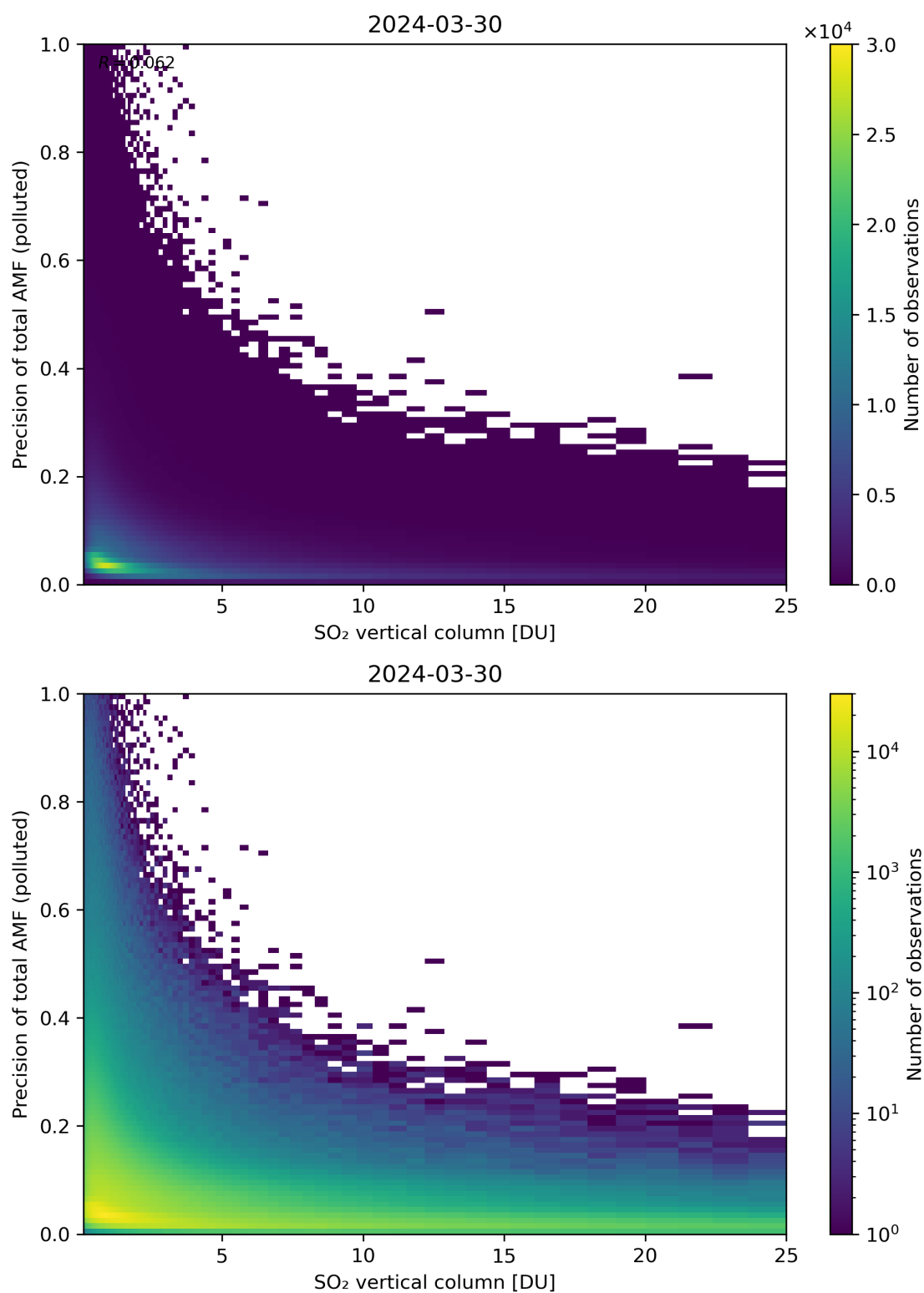
Figure 306: Scatter density plot of “SO 2 vertical column” against “Precision of total AMF (polluted)” for 2024-03-30 to 2024-03-31.
