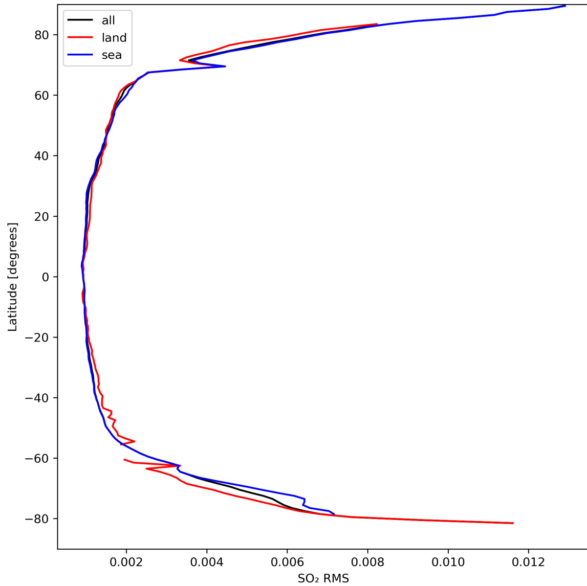
Figure 47: Zonal average of “SO 2 RMS” for 2024-03-30 to 2024-03-31.
