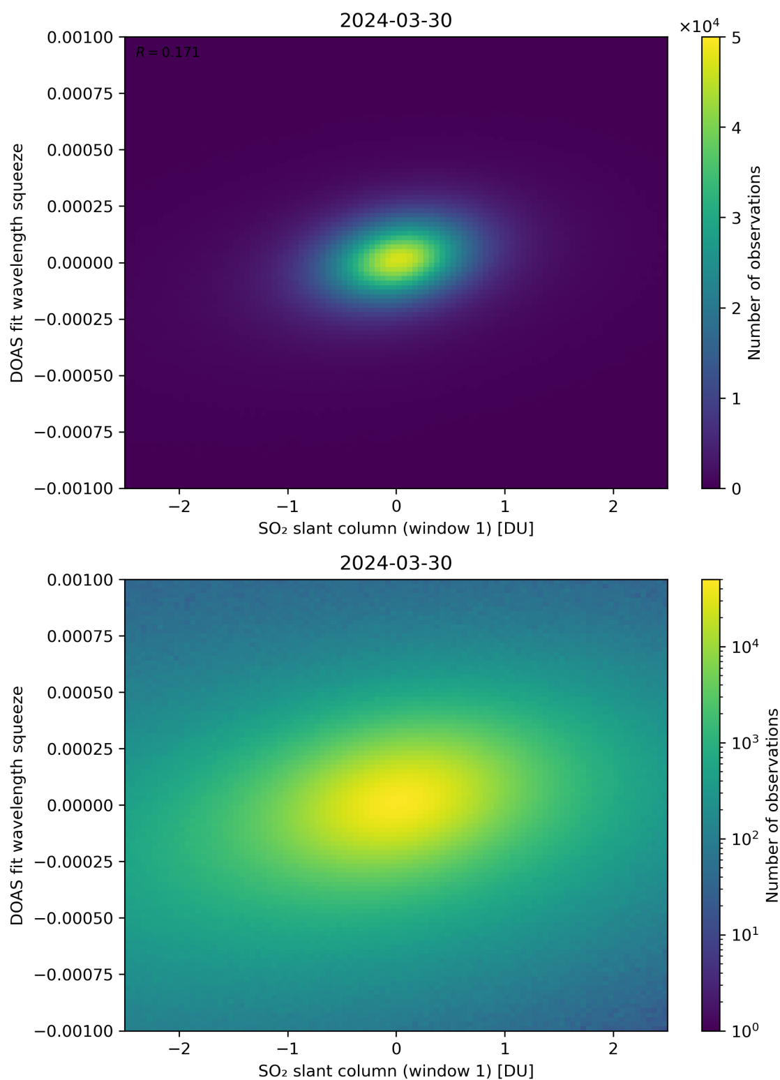
Figure 216: Scatter density plot of “SO 2 slant column (window 1)” against “DOAS fit wavelength squeeze” for 2024-03-30 to 2024-03-31.
