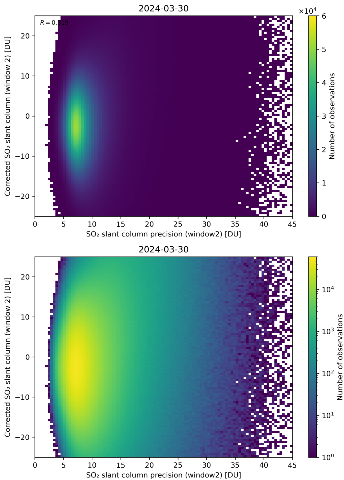
Figure 247: Scatter density plot of “SO 2 slant column precision (window2)” against “Corrected SO 2 slant column (window 2)” for 2024-03-30 to 2024-03-31.
