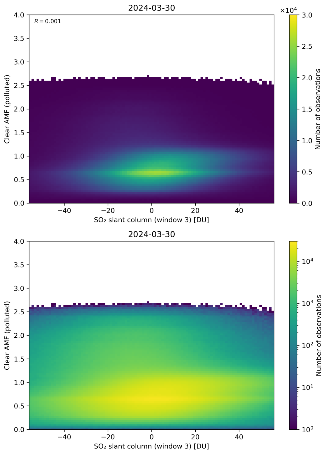
Figure 265: Scatter density plot of “SO 2 slant column (window 3)” against “Clear AMF (polluted)” for 2024-03-30 to 2024-03-31.
