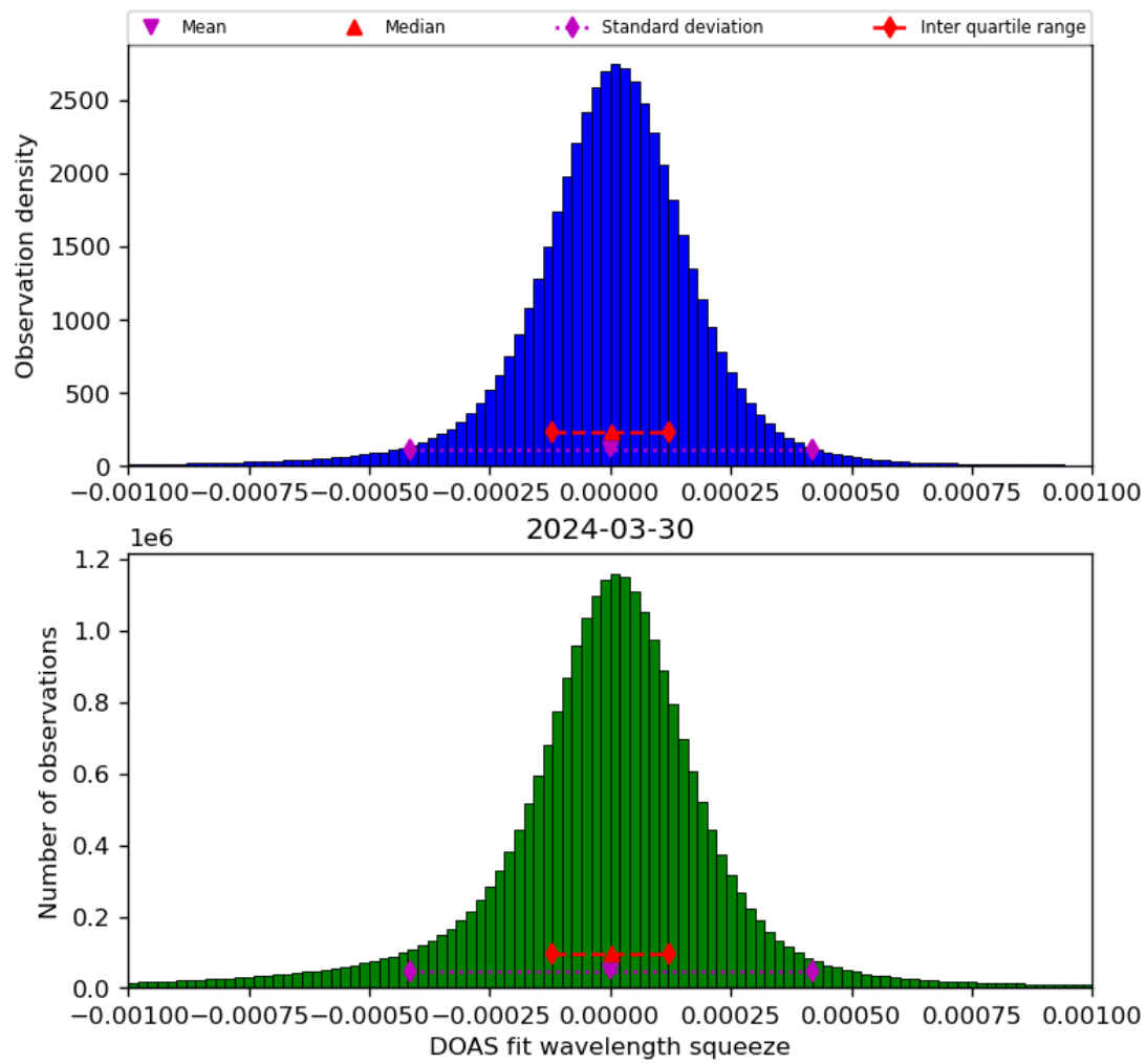
Figure 69: Histogram of “DOAS fit wavelength squeeze” for 2024-03-30 to 2024-03-31
