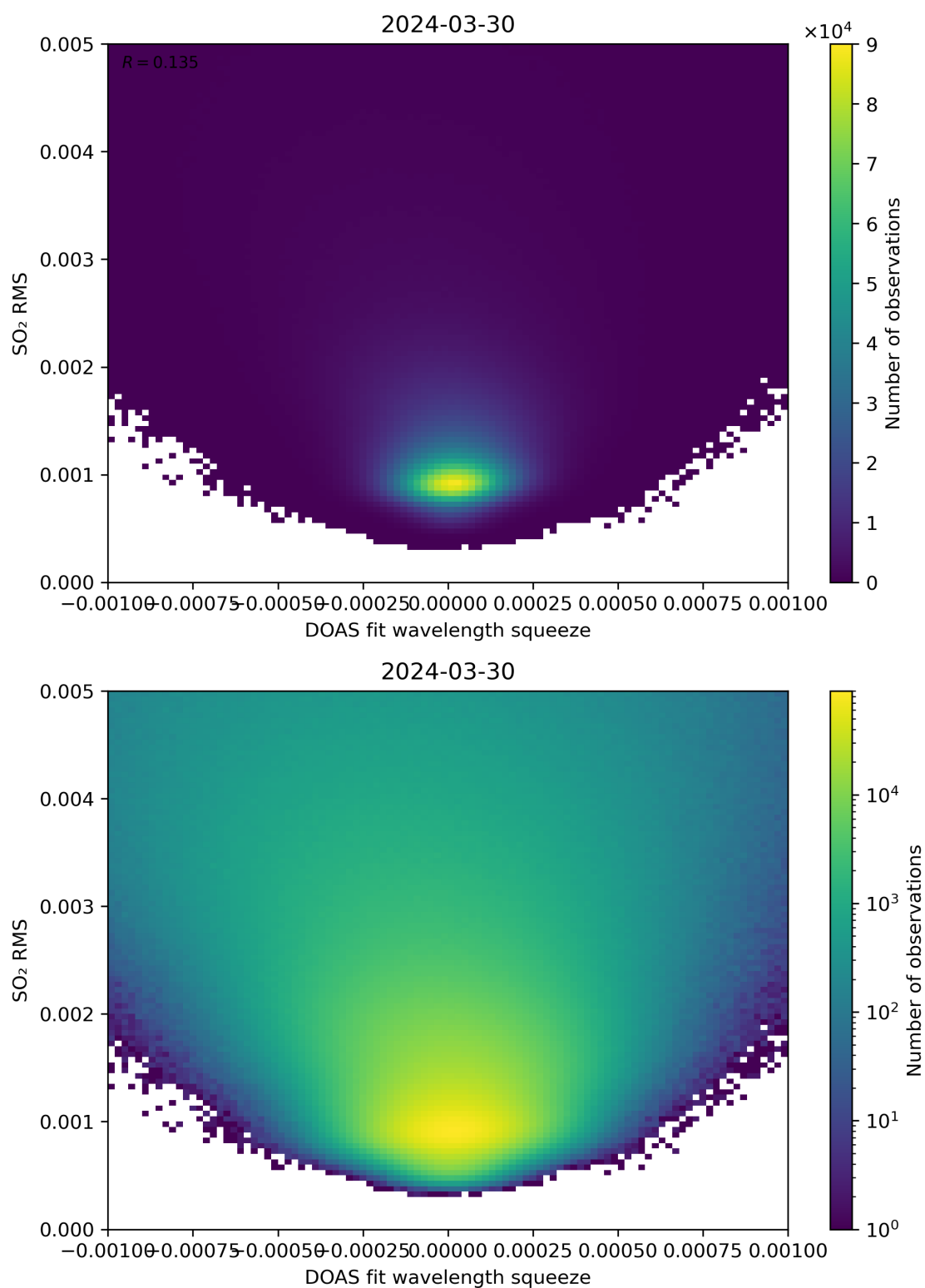
Figure 132: Scatter density plot of “DOAS fit wavelength squeeze” against “SO 2 RMS” for 2024-03-30 to 2024-03-31.
