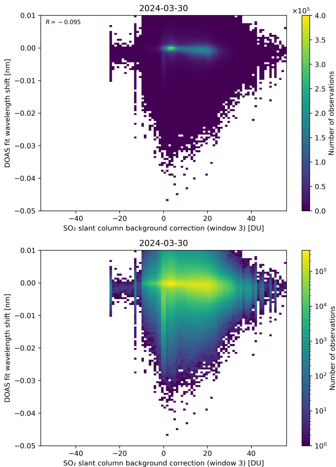
Figure 121: Scatter density plot of “SO 2 slant column background correction (window 3)” against “DOAS fit wavelength shift” for 2024-03-30 to 2024-03-31.
