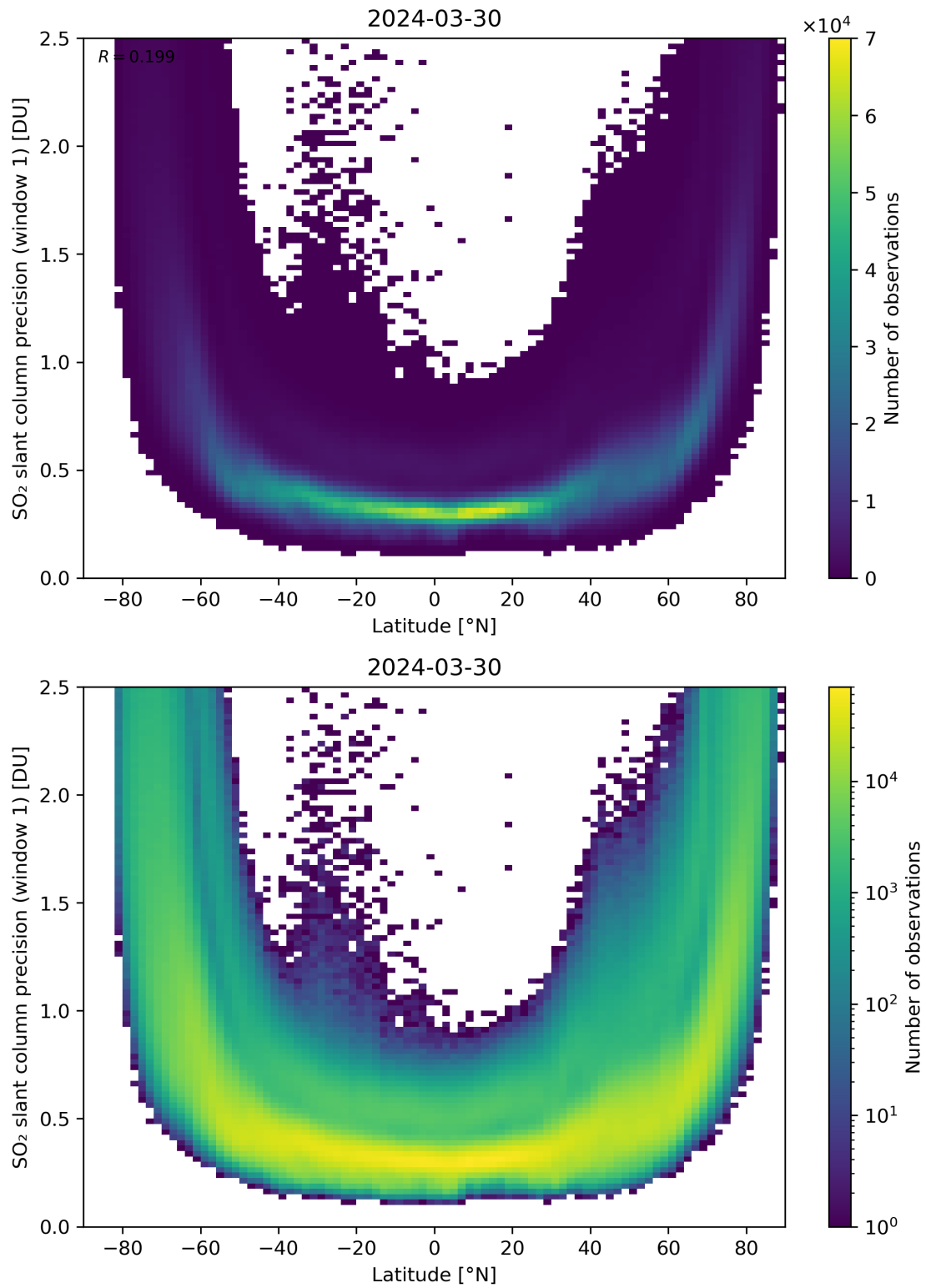
Figure 150: Scatter density plot of “Latitude” against “SO 2 slant column precision (window 1)” for 2024-03-30 to 2024-03-31.
