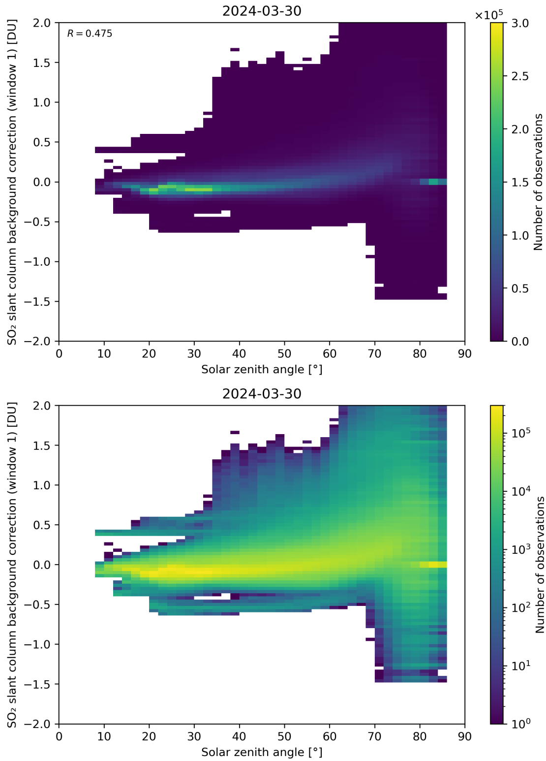
Figure 158: Scatter density plot of “Solar zenith angle” against “SO 2 slant column background correction (window 1)” for 2024-03-30 to 2024-03-31.
