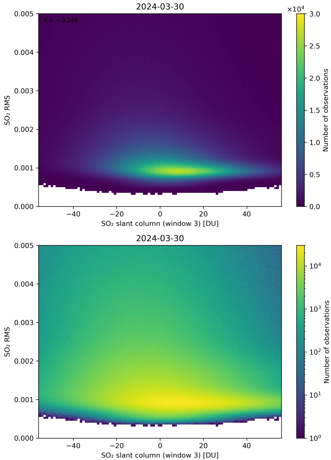
Figure 256: Scatter density plot of “SO 2 slant column (window 3)” against “SO 2 RMS” for 2024-03-30 to 2024-03-31.
