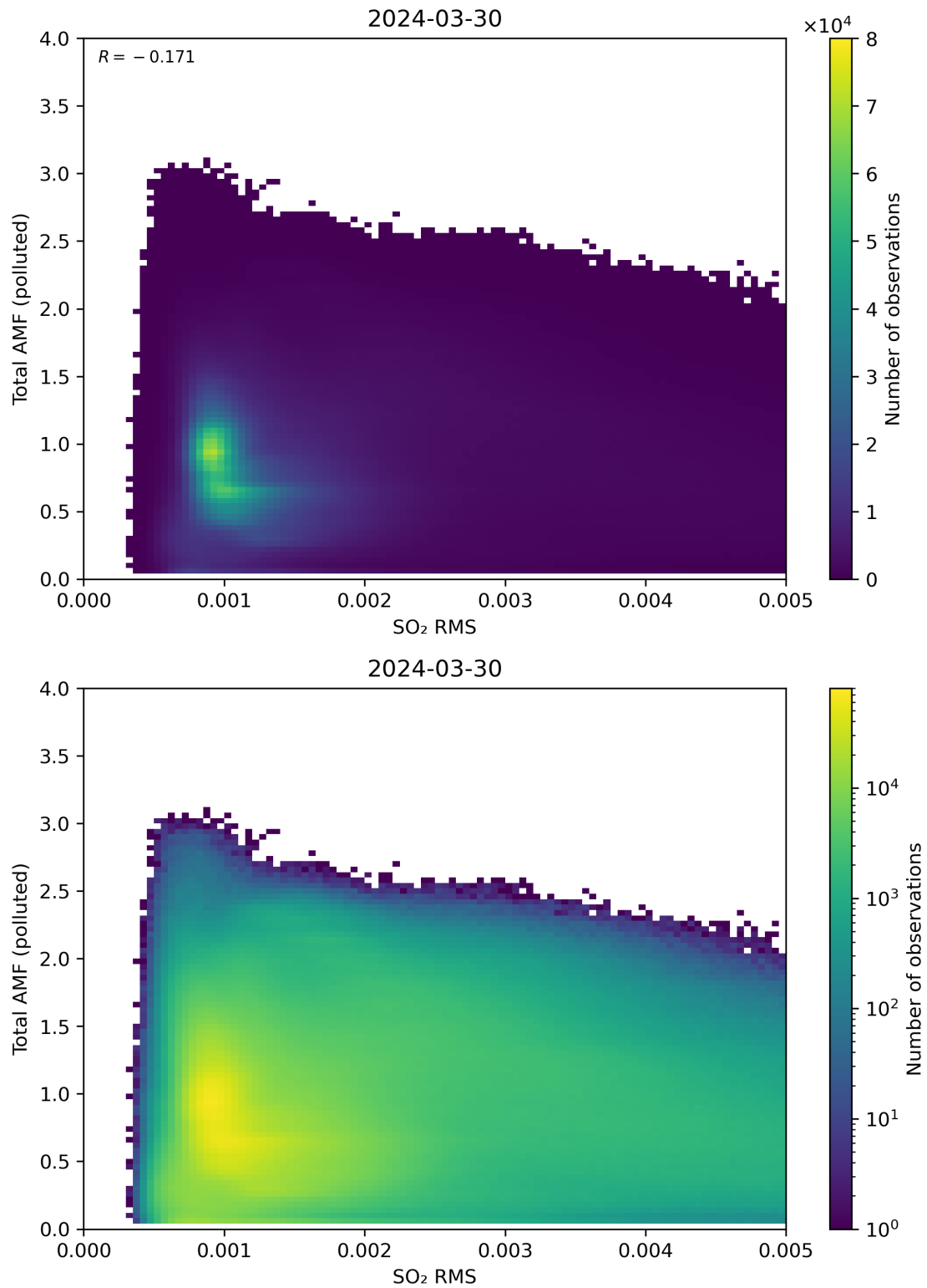
Figure 137: Scatter density plot of “SO 2 RMS” against “Total AMF (polluted)” for 2024-03-30 to 2024-03-31.
