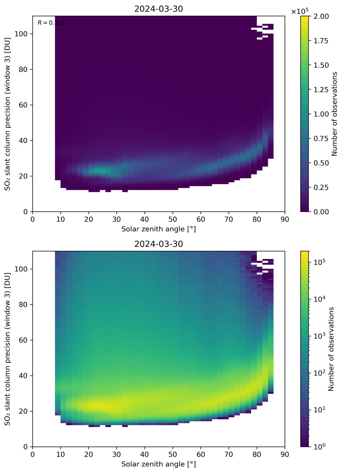
Figure 173: Scatter density plot of “Solar zenith angle” against “SO 2 slant column precision (window 3)” for 2024-03-30 to 2024-03-31.
