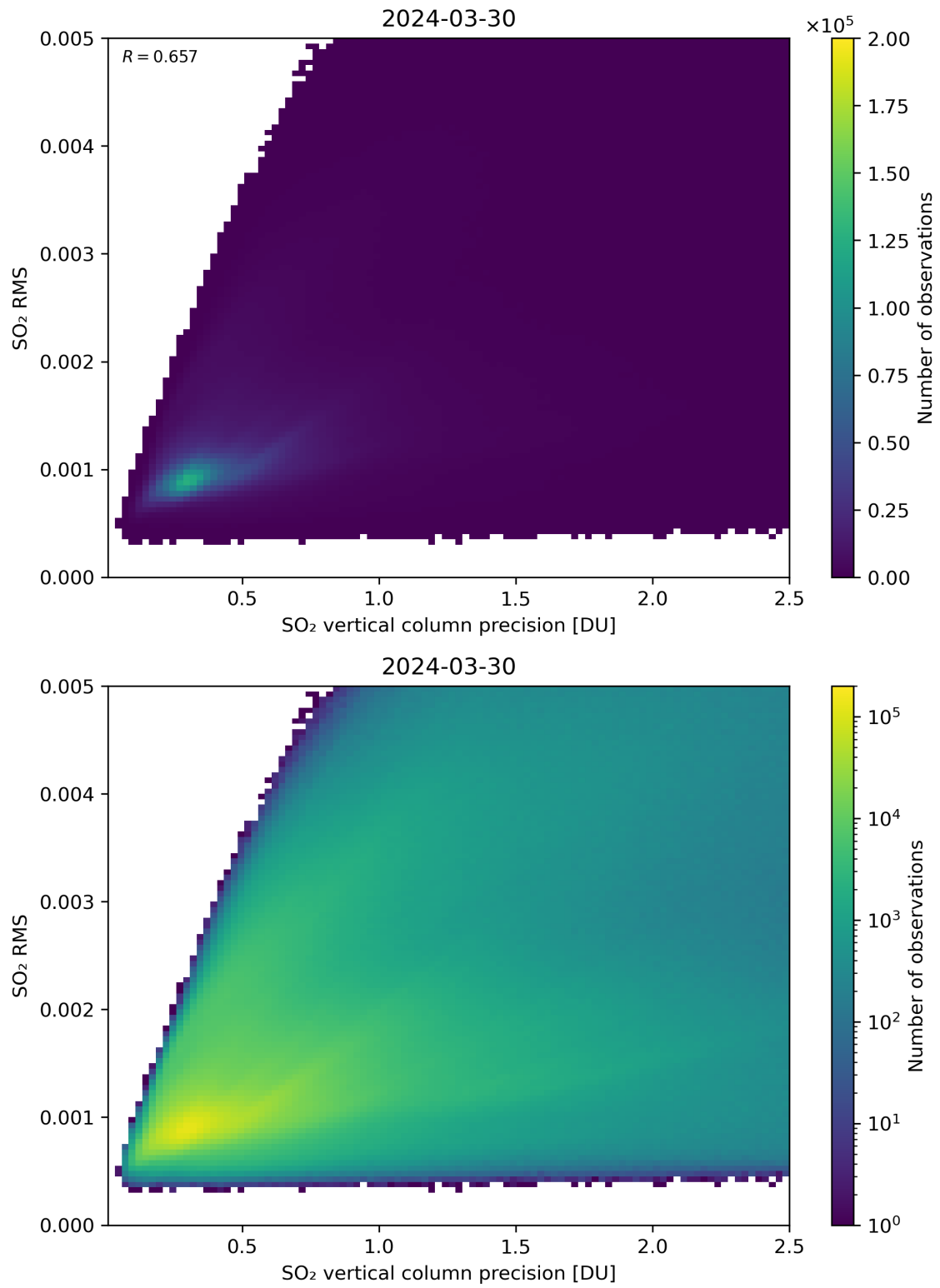
Figure 284: Scatter density plot of “SO 2 vertical column precision” against “SO 2 RMS” for 2024-03-30 to 2024-03-31.
