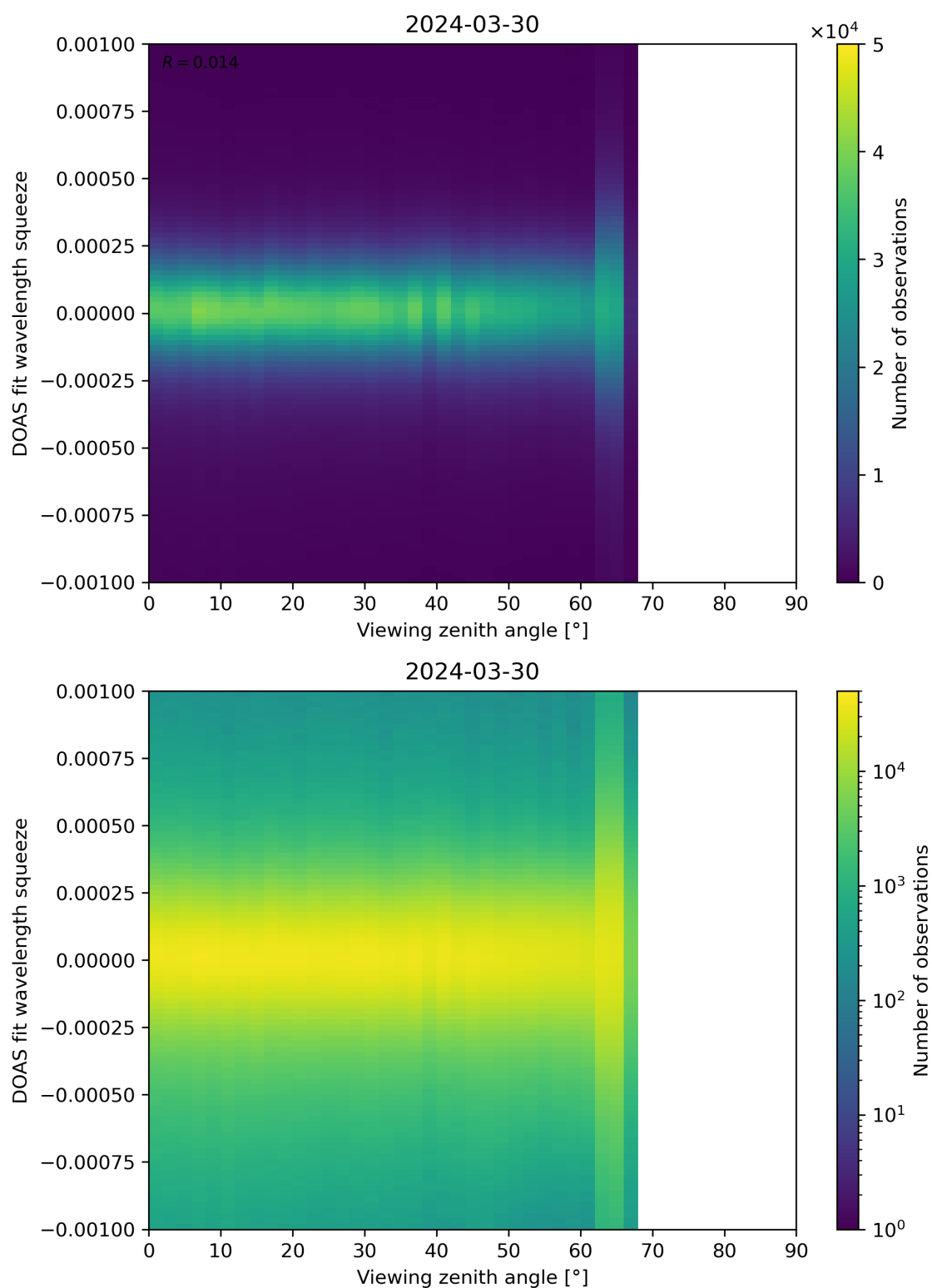
Figure 312: Scatter density plot of “Viewing zenith angle” against “DOAS fit wavelength squeeze” for 2024-03-30 to 2024-03-31.
