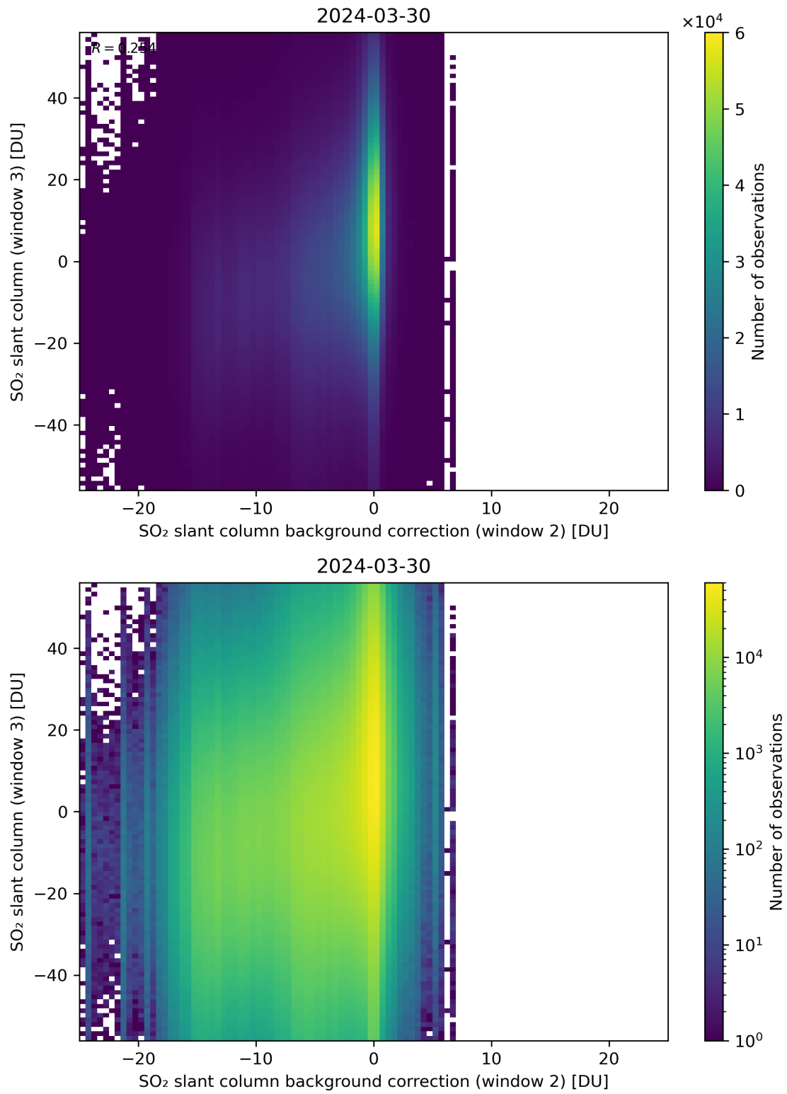
Figure 117: Scatter density plot of “SO 2 slant column background correction (window 2)” against “SO 2 slant column (window 3)” for 2024-03-30 to 2024-03-31.
