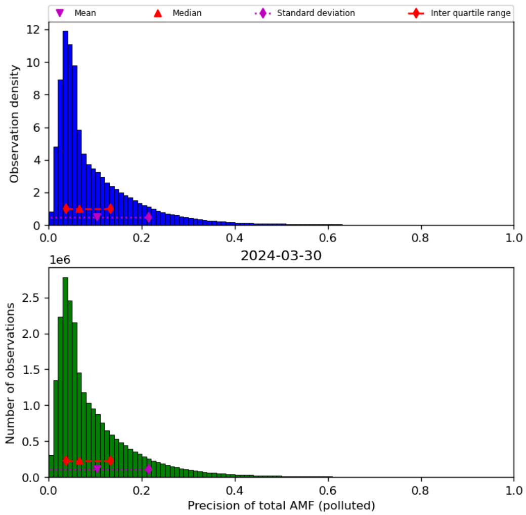
Figure 72: Histogram of “Precision of total AMF (polluted)” for 2024-03-30 to 2024-03-31
