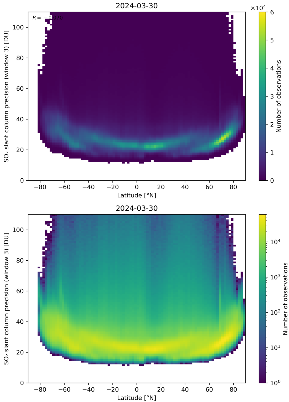
Figure 153: Scatter density plot of “Latitude” against “SO 2 slant column precision (window 3)” for 2024-03-30 to 2024-03-31.
