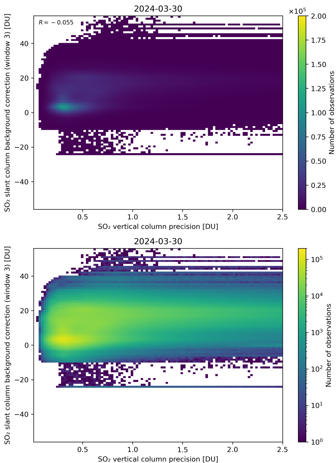
Figure 281: Scatter density plot of “SO 2 vertical column precision” against “SO 2 slant column background correction (window 3)” for 2024-03-30 to 2024-03-31.
