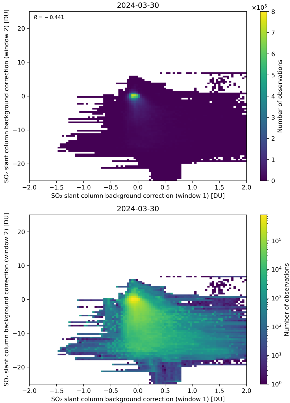
Figure 98: Scatter density plot of “SO 2 slant column background correction (window 1)” against “SO 2 slant column background correction (window 2)” for 2024-03-30 to 2024-03-31.
