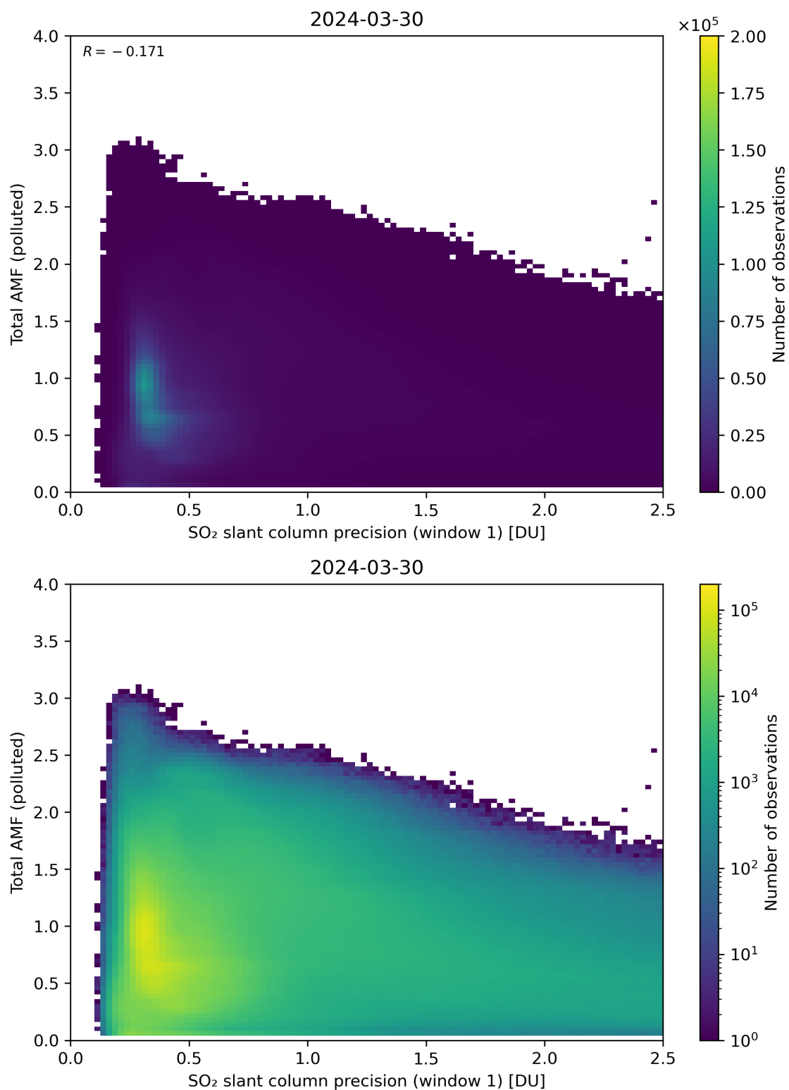
Figure 230: Scatter density plot of “SO 2 slant column precision (window 1)” against “Total AMF (polluted)” for 2024-03-30 to 2024-03-31.
