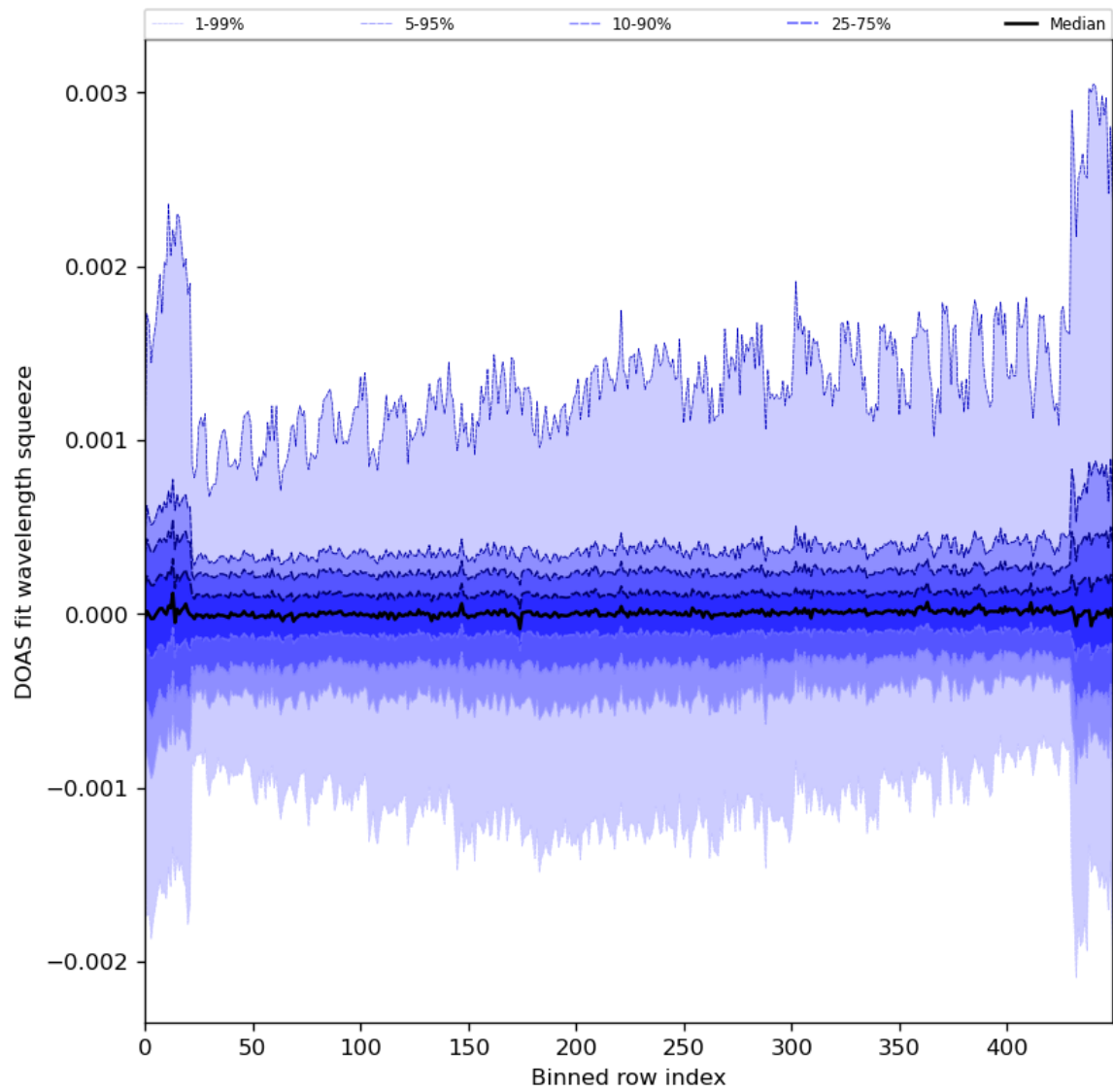
Figure 92: Along track statistics of “DOAS fit wavelength squeeze” for 2024-03-30 to 2024-03-31
