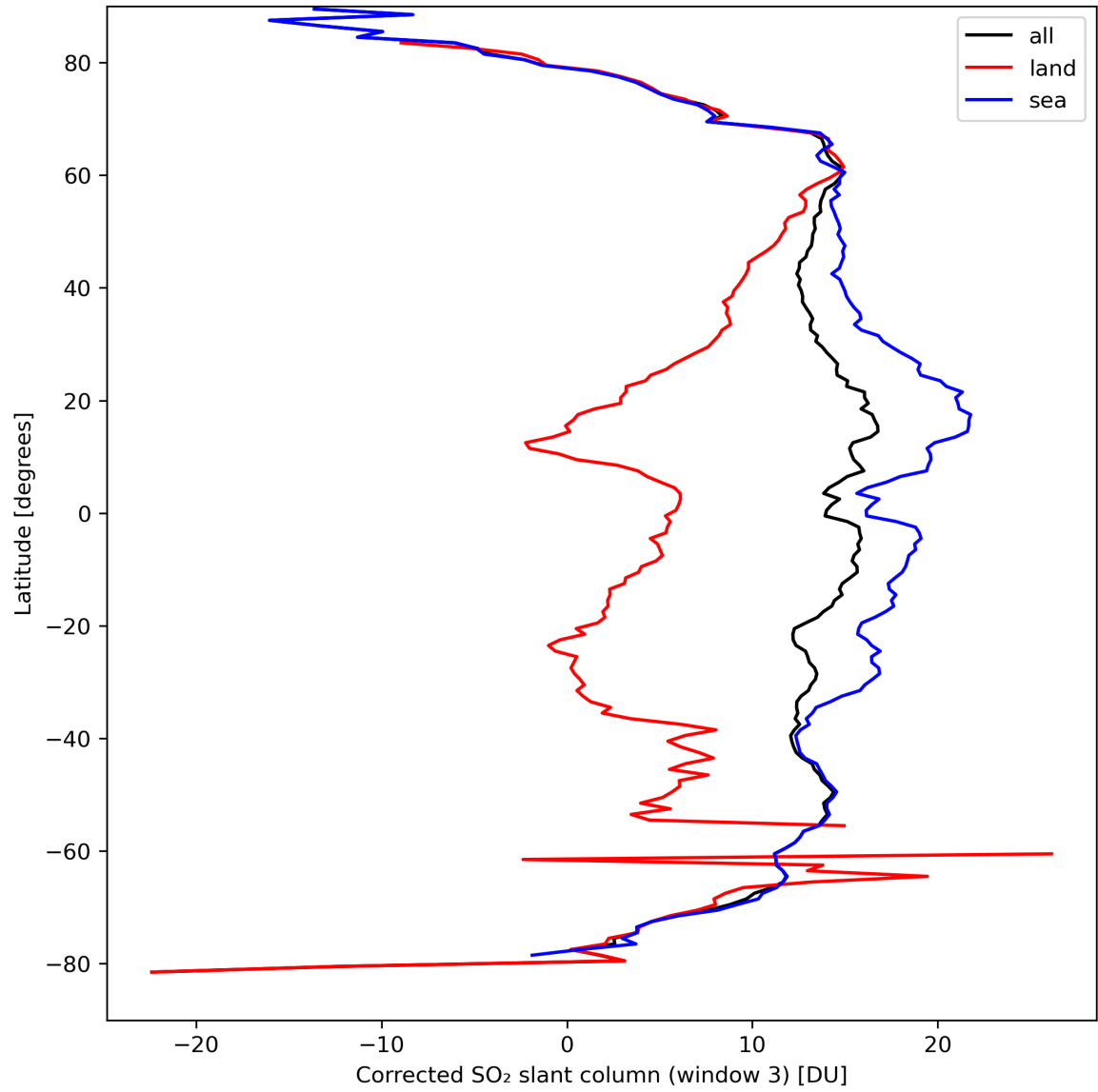
Figure 43: Zonal average of “Corrected SO 2 slant column (window 3)” for 2024-03-30 to 2024-03-31.
