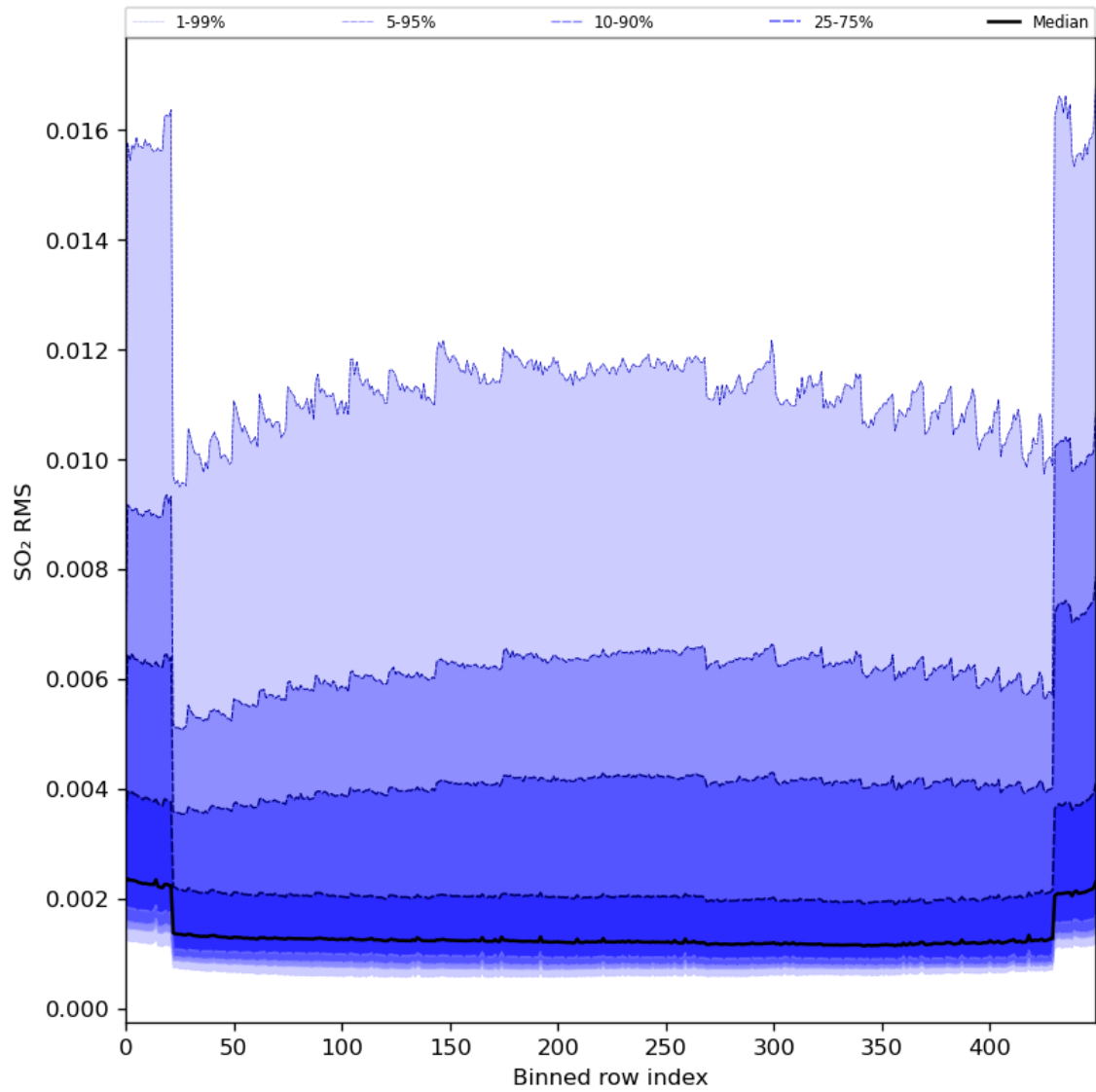
Figure 93: Along track statistics of “SO 2 RMS” for 2024-03-30 to 2024-03-31
