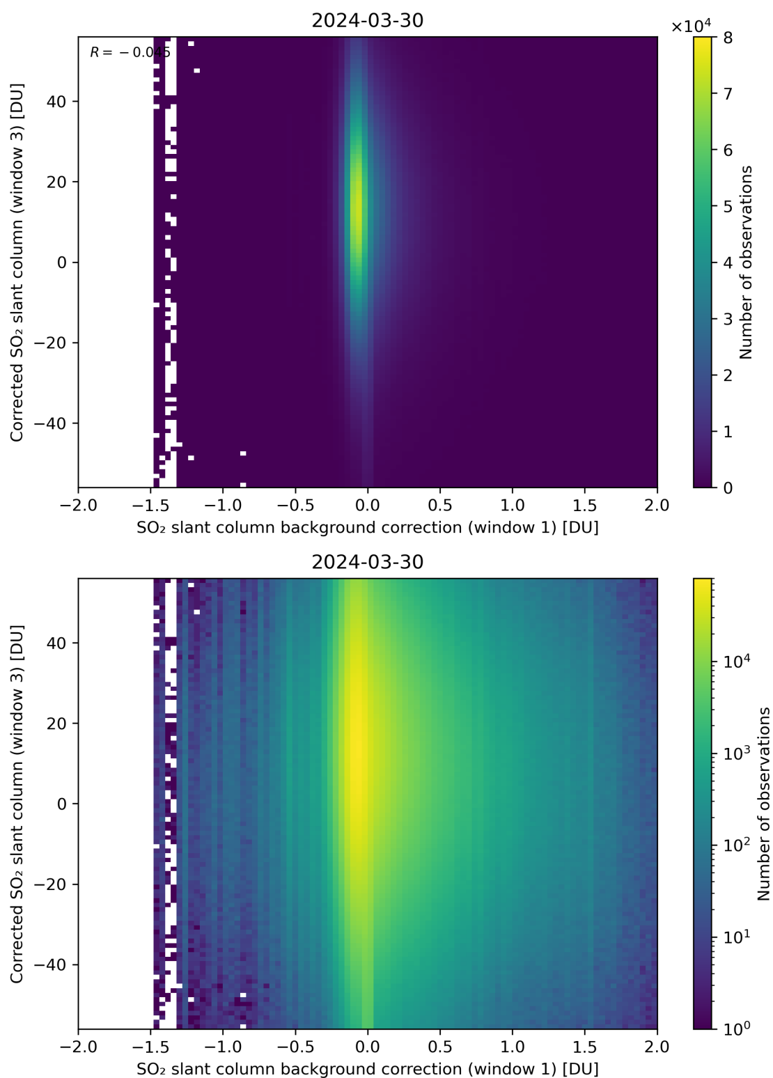
Figure 105: Scatter density plot of “SO 2 slant column background correction (window 1)” against “Corrected SO 2 slant column (window 3)” for 2024-03-30 to 2024-03-31.
