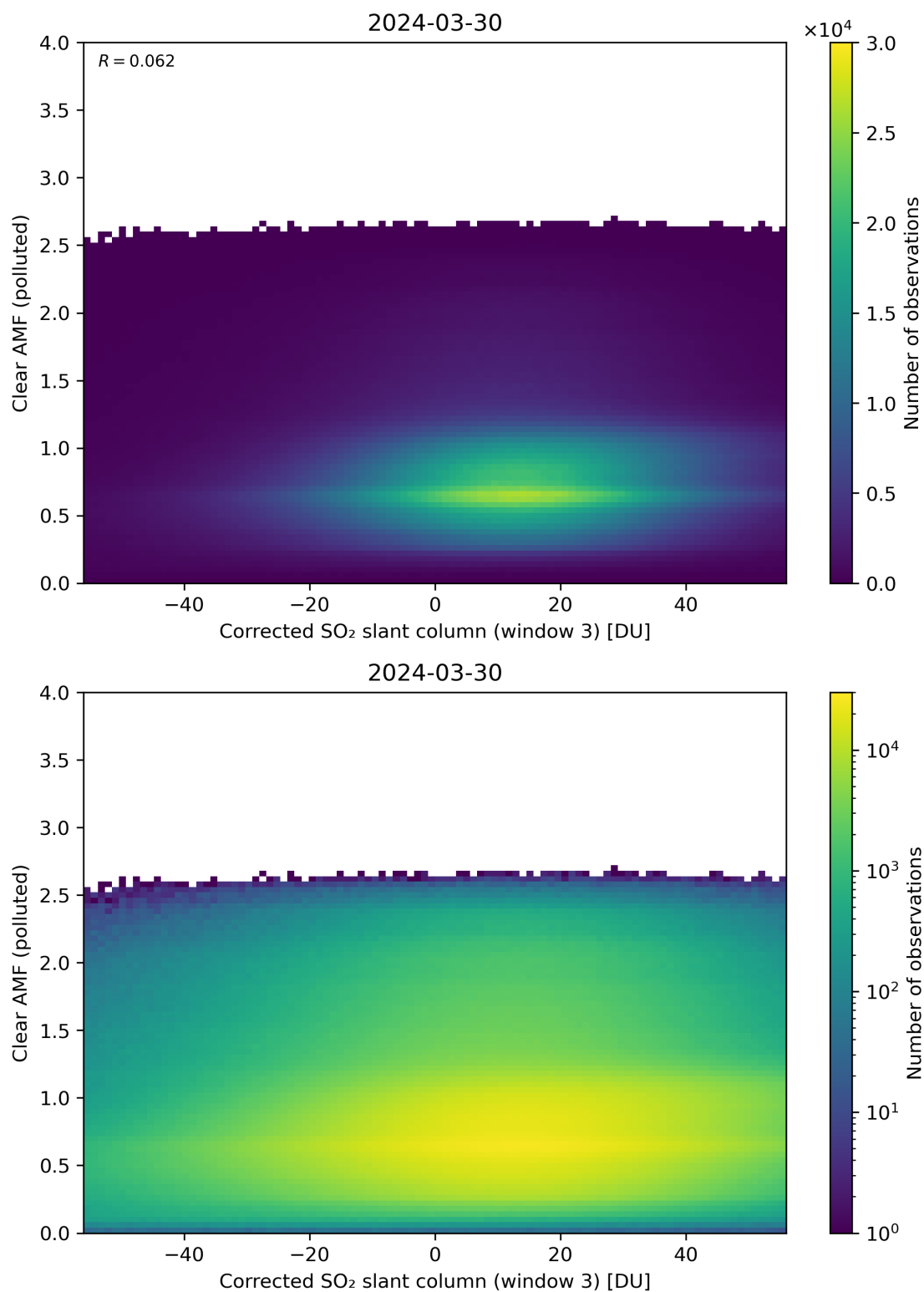
Figure 209: Scatter density plot of “Corrected SO 2 slant column (window 3)” against “Clear AMF (polluted)” for 2024-03-30 to 2024-03-31.
