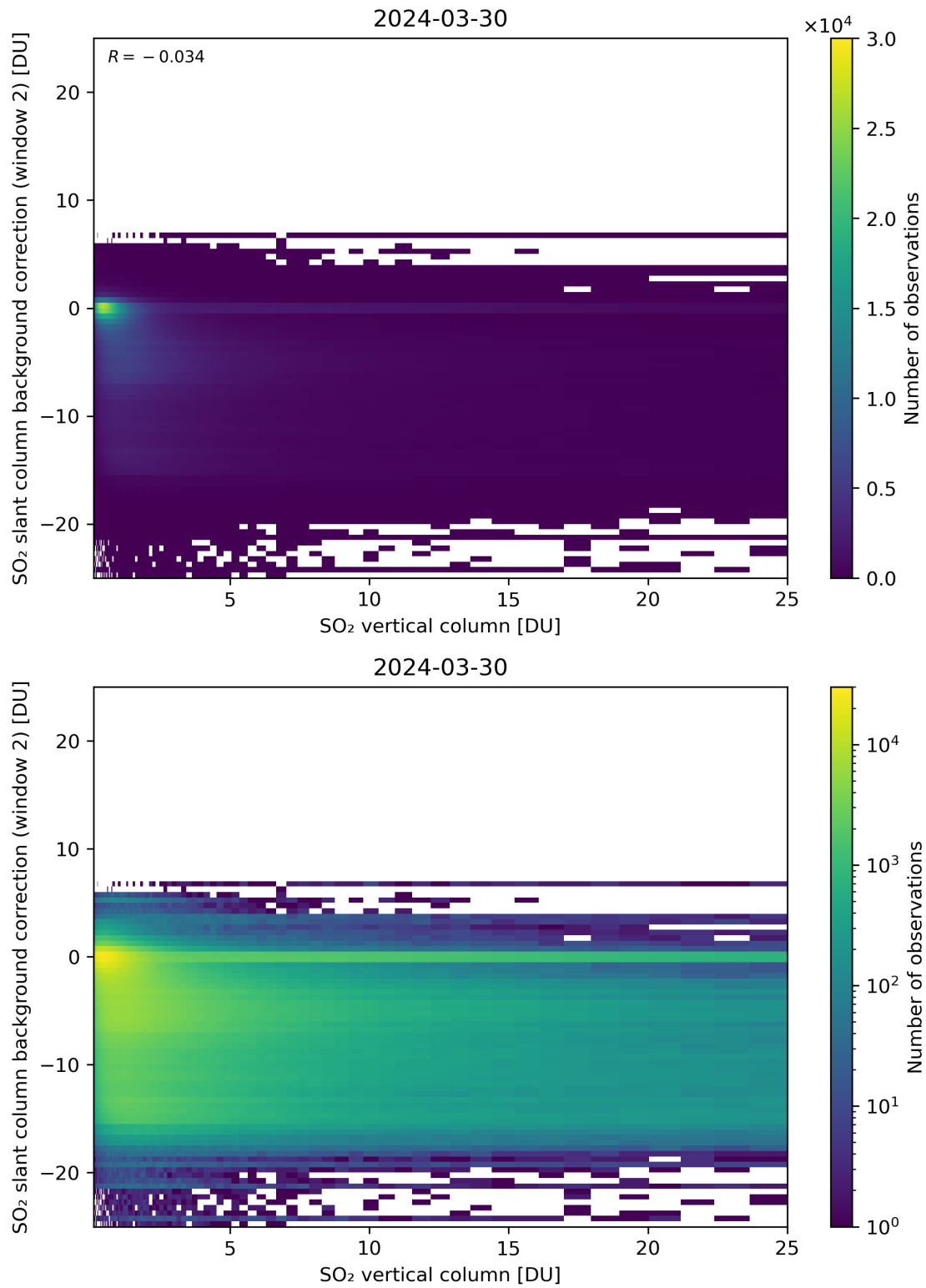
Figure 274: Scatter density plot of “SO 2 vertical column” against “SO 2 slant column background correction (window 2)” for 2024-03-30 to 2024-03-31.
