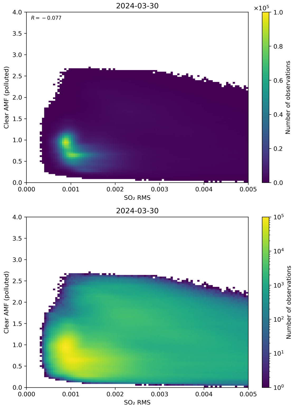
Figure 136: Scatter density plot of “SO 2 RMS” against “Clear AMF (polluted)” for 2024-03-30 to 2024-03-31.
