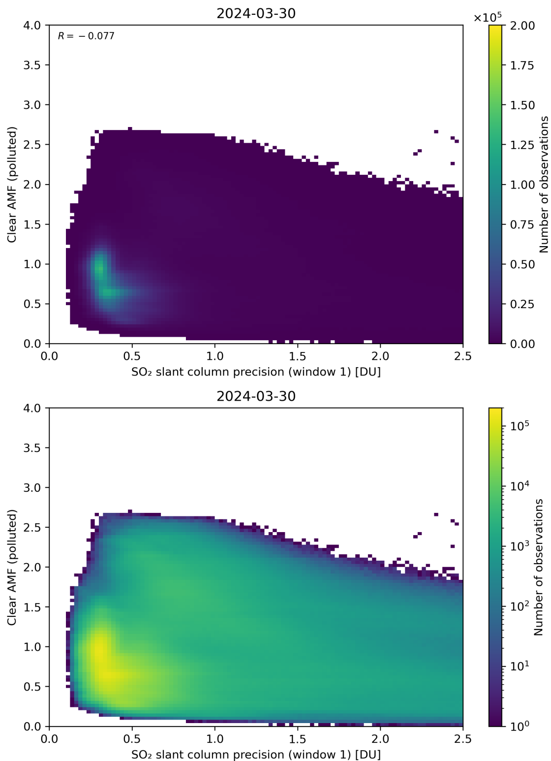
Figure 224: Scatter density plot of “SO 2 slant column precision (window 1)” against “Clear AMF (polluted)” for 2024-03-30 to 2024-03-31.
