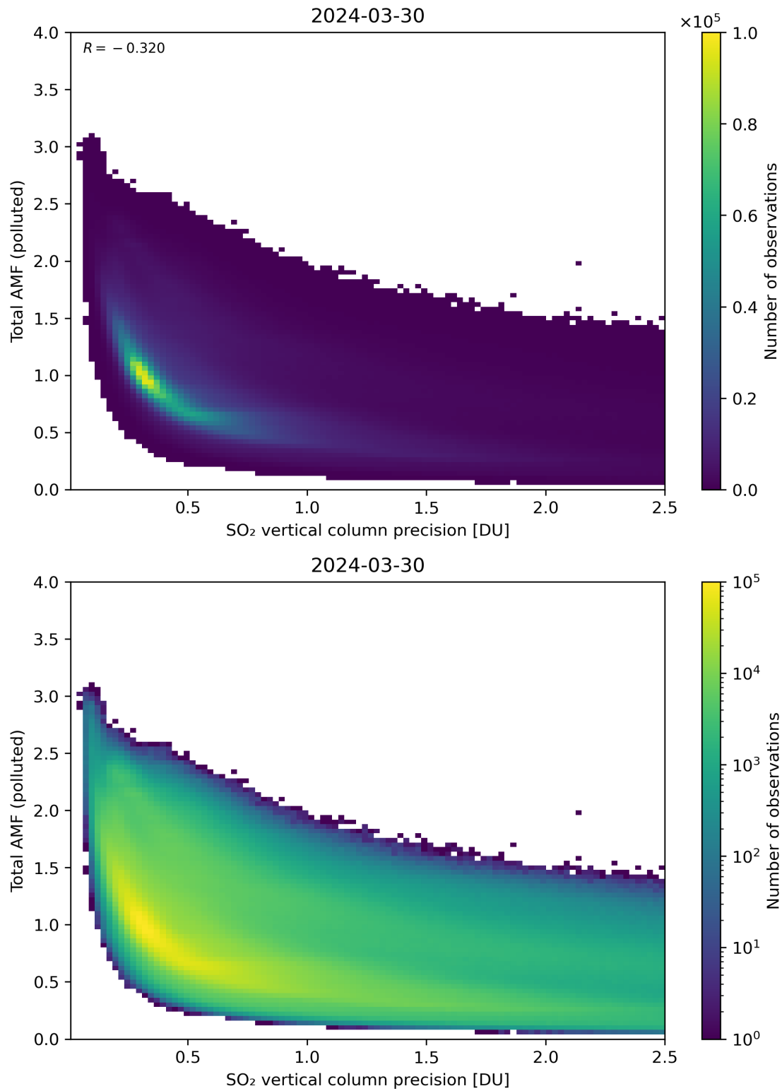
Figure 294: Scatter density plot of “SO 2 vertical column precision” against “Total AMF (polluted)” for 2024-03-30 to 2024-03-31.
