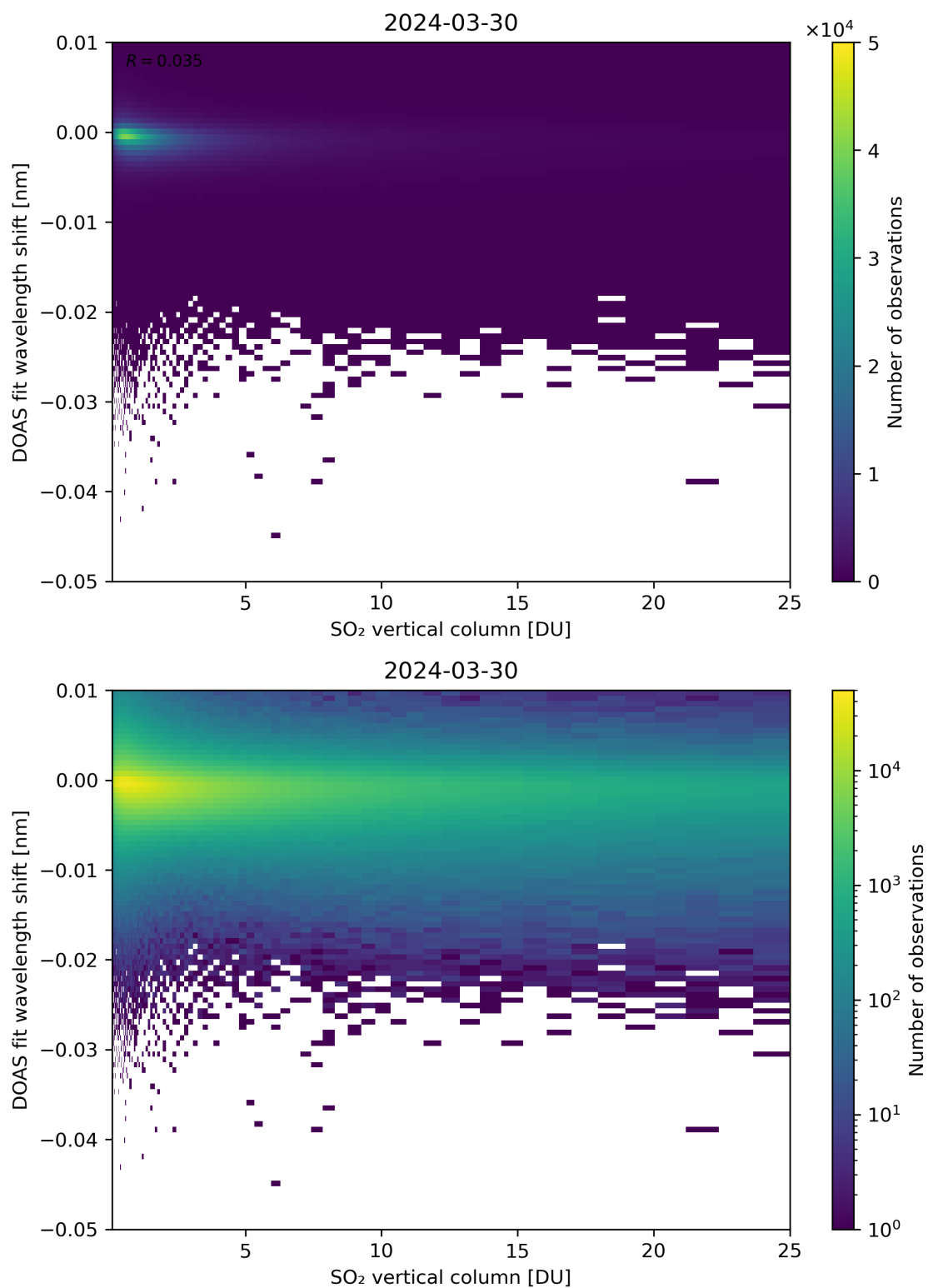
Figure 276: Scatter density plot of “SO 2 vertical column” against “DOAS fit wavelength shift” for 2024-03-30 to 2024-03-31.
