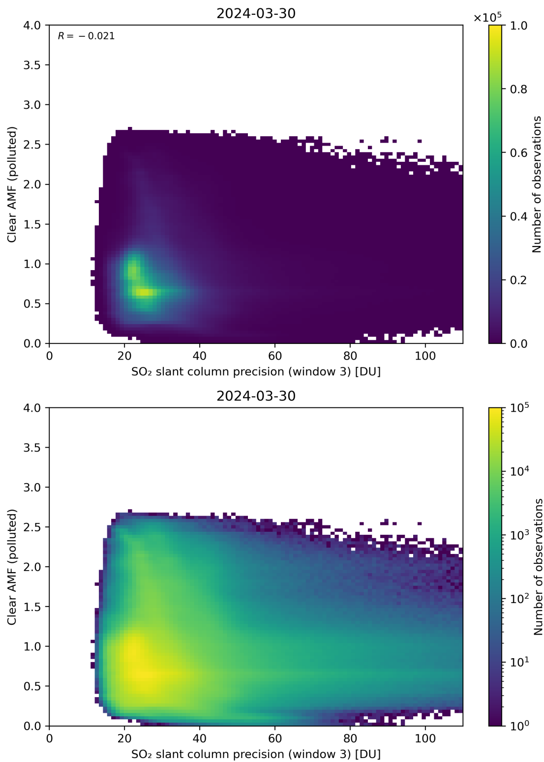
Figure 261: Scatter density plot of “SO 2 slant column precision (window 3)” against “Clear AMF (polluted)” for 2024-03-30 to 2024-03-31.
