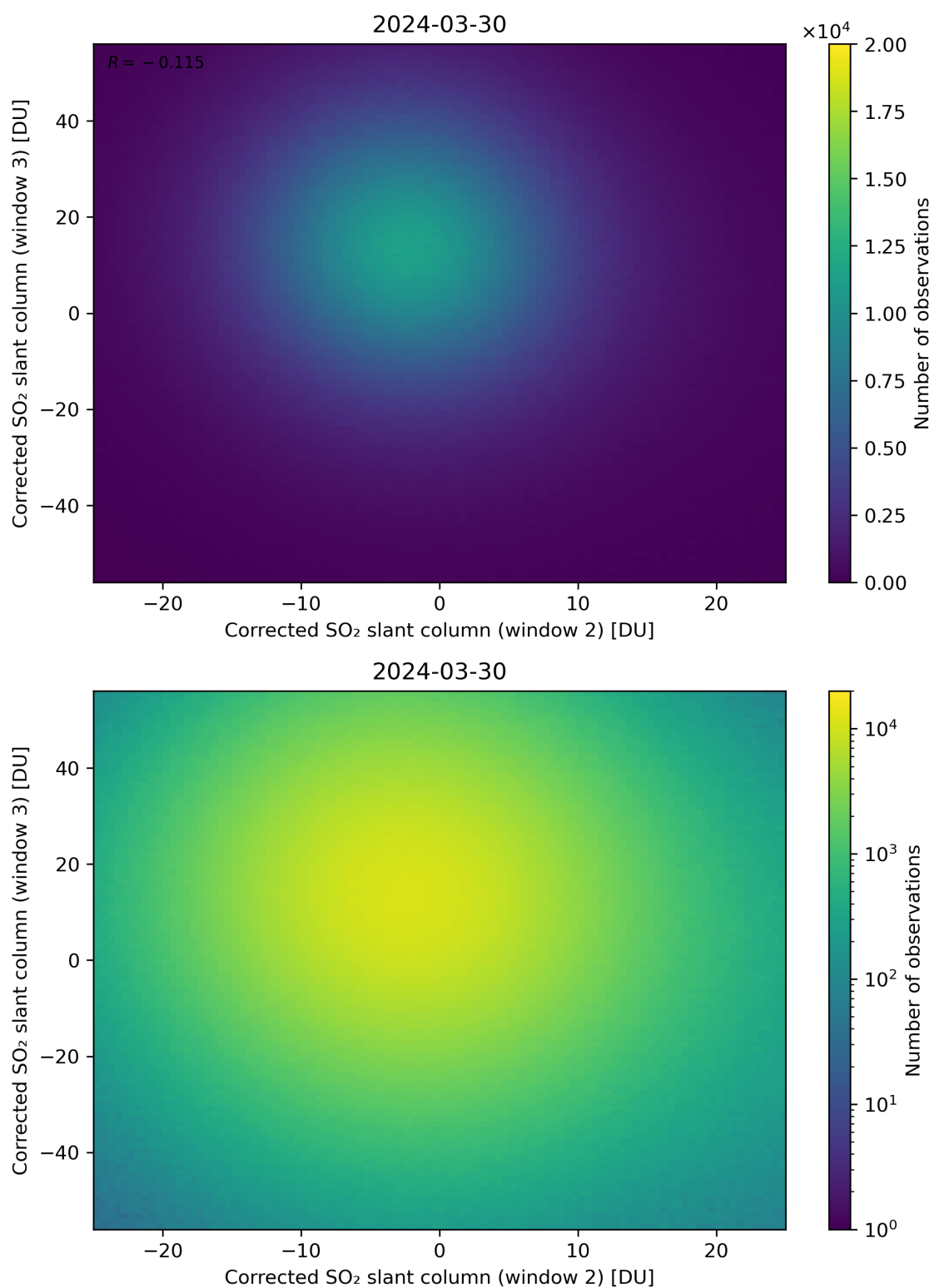
Figure 200: Scatter density plot of “Corrected SO 2 slant column (window 2)” against “Corrected SO 2 slant column (window 3)” for 2024-03-30 to 2024-03-31.
