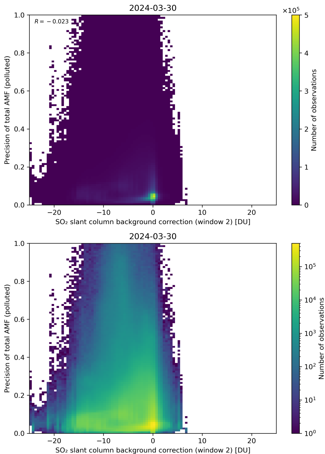
Figure 120: Scatter density plot of “SO 2 slant column background correction (window 2)” against “Precision of total AMF (polluted)” for 2024-03-30 to 2024-03-31.
