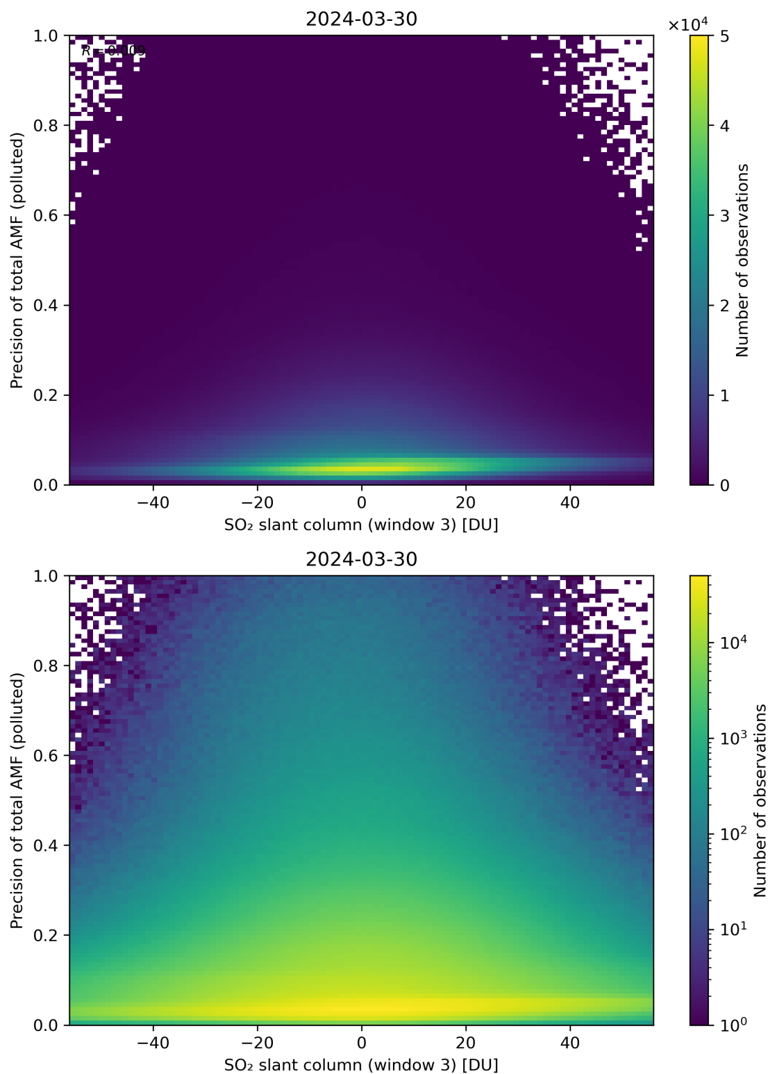
Figure 269: Scatter density plot of “SO 2 slant column (window 3)” against “Precision of total AMF (polluted)” for 2024-03-30 to 2024-03-31.
