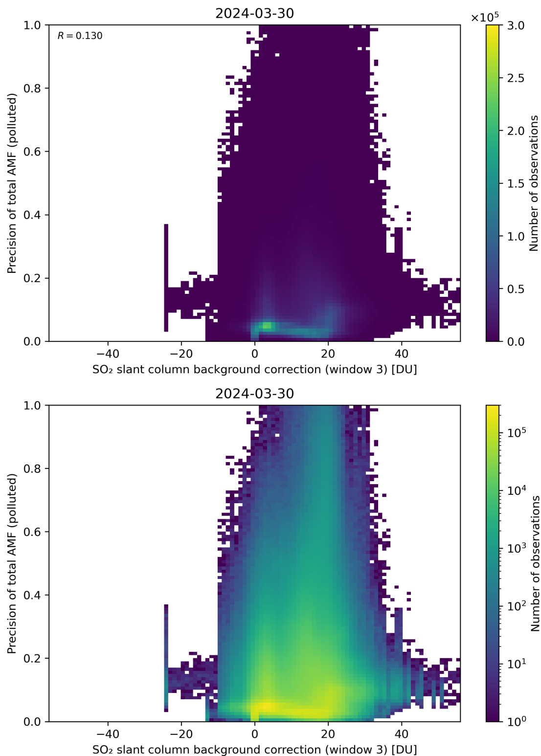
Figure 126: Scatter density plot of “SO 2 slant column background correction (window 3)” against “Precision of total AMF (polluted)” for 2024-03-30 to 2024-03-31.
