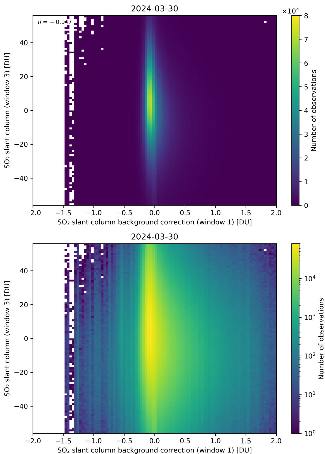
Figure 107: Scatter density plot of “SO 2 slant column background correction (window 1)” against “SO 2 slant column (window 3)” for 2024-03-30 to 2024-03-31.
