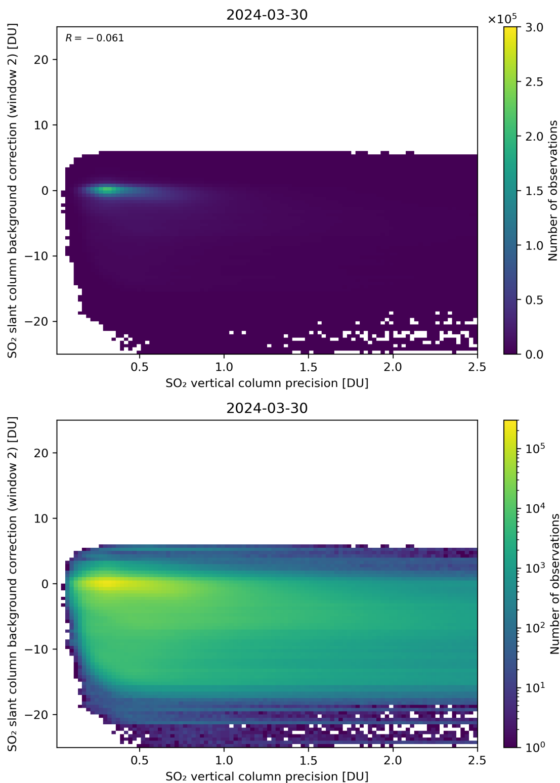
Figure 280: Scatter density plot of “SO 2 vertical column precision” against “SO 2 slant column background correction (window 2)” for 2024-03-30 to 2024-03-31.
