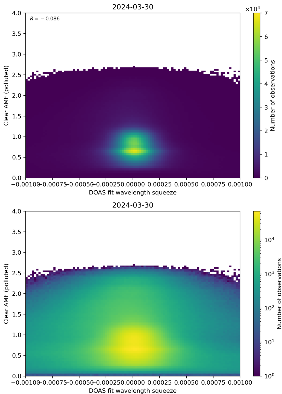
Figure 133: Scatter density plot of “DOAS fit wavelength squeeze” against “Clear AMF (polluted)” for 2024-03-30 to 2024-03-31.
