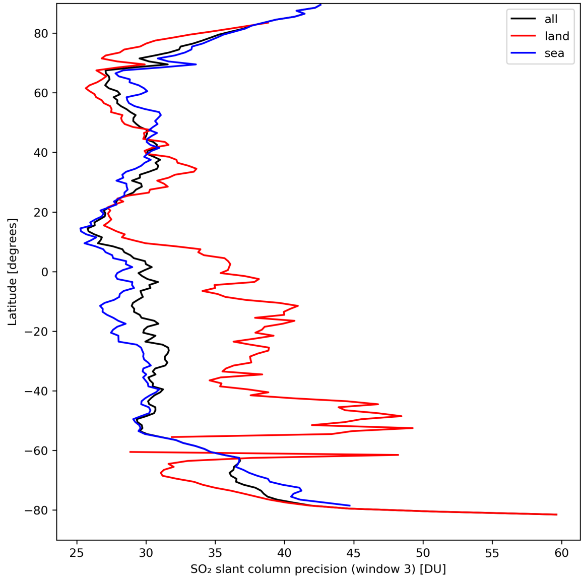
Figure 42: Zonal average of “SO 2 slant column precision (window 3)” for 2024-03-30 to 2024-03-31.
