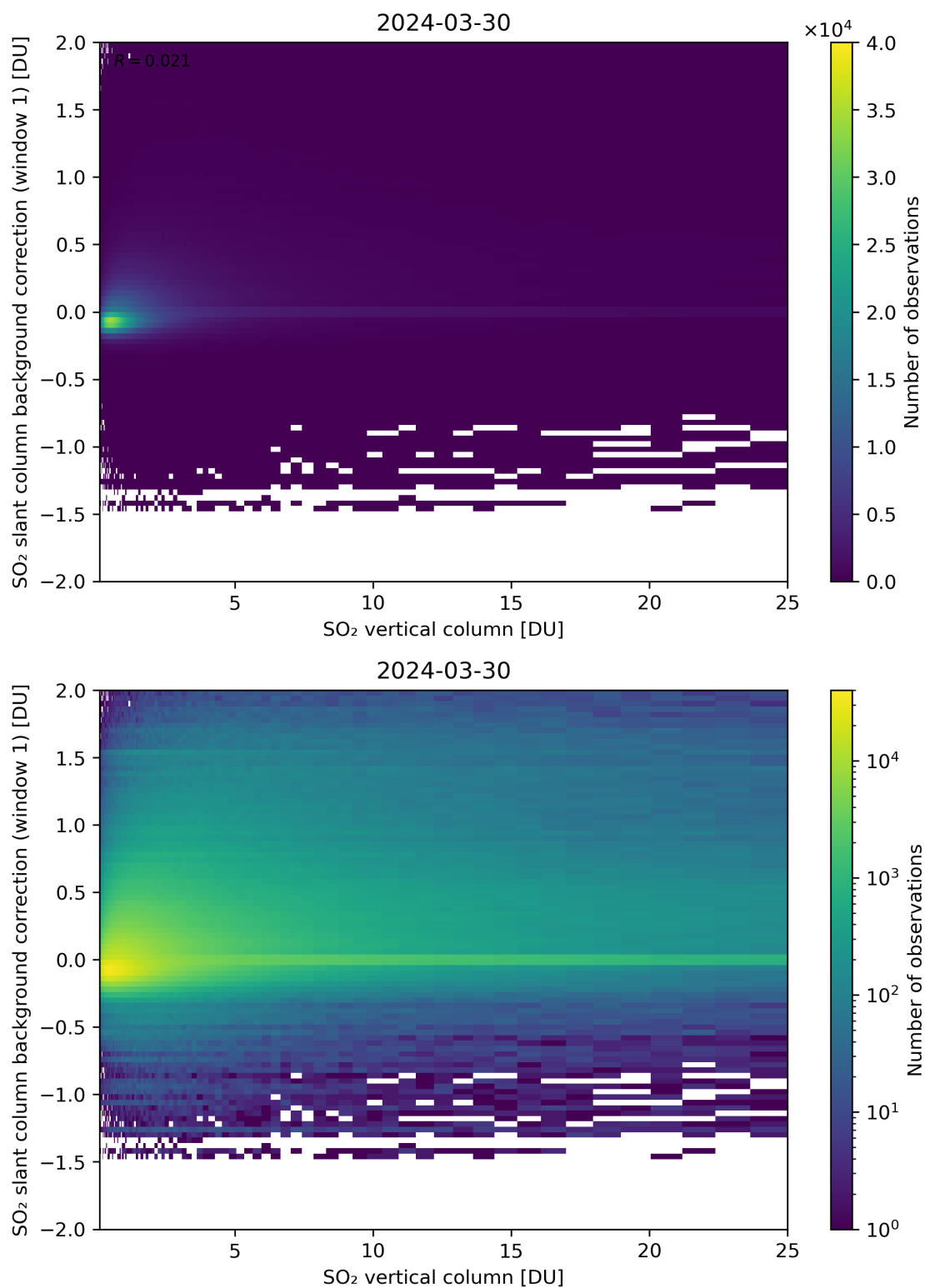
Figure 273: Scatter density plot of “SO 2 vertical column” against “SO 2 slant column background correction (window 1)” for 2024-03-30 to 2024-03-31.
