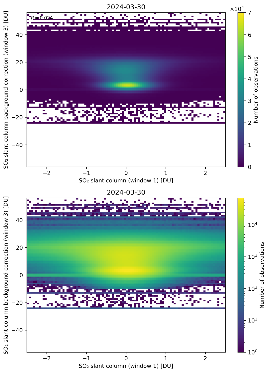
Figure 214: Scatter density plot of “SO 2 slant column (window 1)” against “SO 2 slant column background correction (window 3)” for 2024-03-30 to 2024-03-31.
