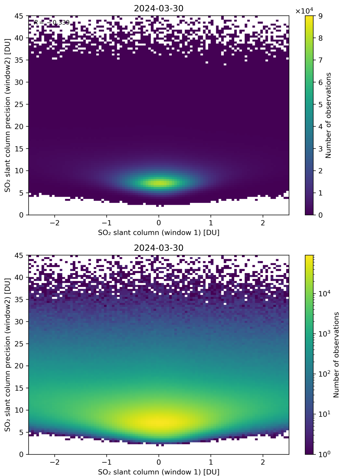
Figure 236: Scatter density plot of “SO 2 slant column (window 1)” against “SO 2 slant column precision (window2)” for 2024-03-30 to 2024-03-31.
