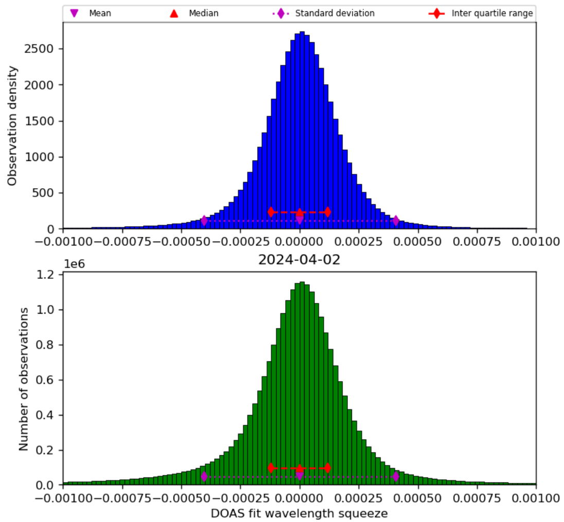
Figure 69: Histogram of “DOAS fit wavelength squeeze” for 2024-04-01 to 2024-04-03
