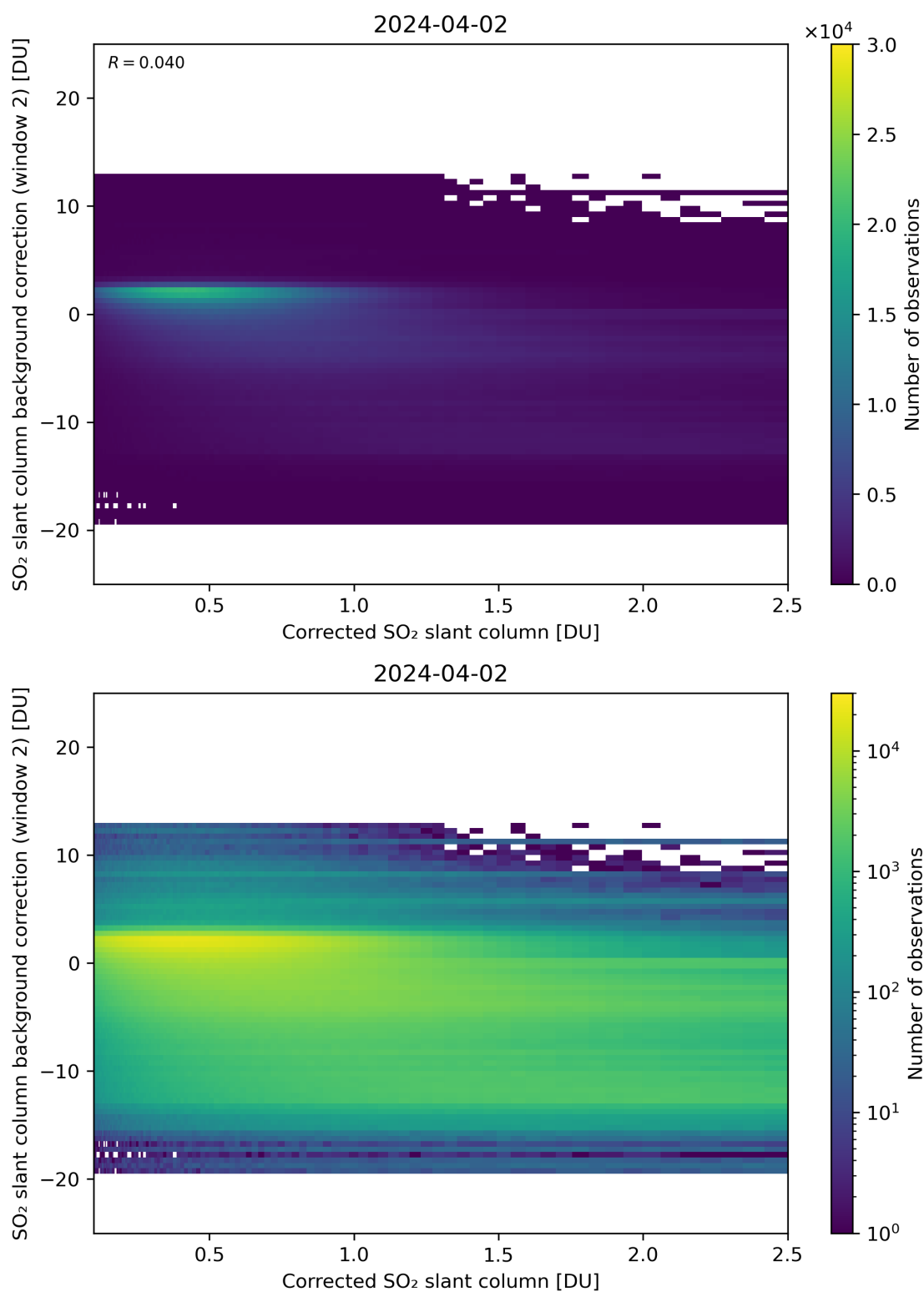
Figure 179: Scatter density plot of “Corrected SO 2 slant column” against “SO 2 slant column background correction (window 2)” for 2024-04-01 to 2024-04-03.
