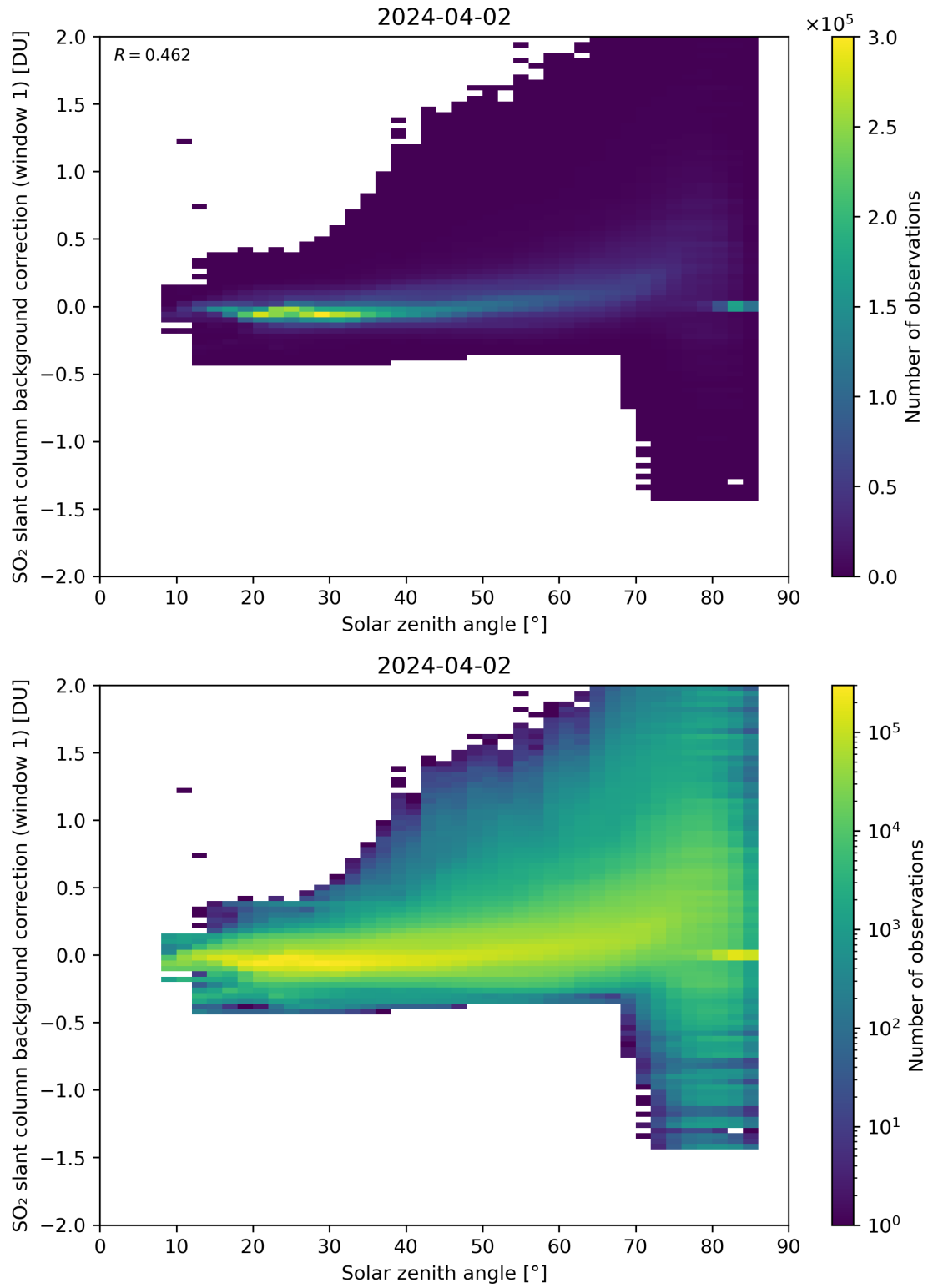
Figure 158: Scatter density plot of “Solar zenith angle” against “SO 2 slant column background correction (window 1)” for 2024-04-01 to 2024-04-03.
