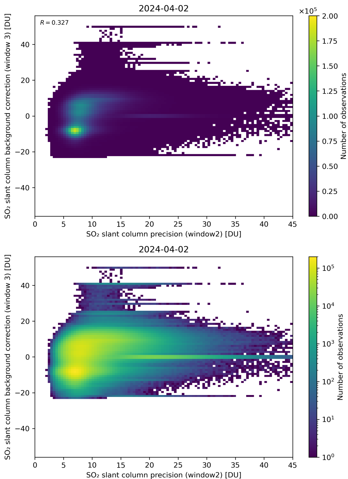
Figure 242: Scatter density plot of “SO 2 slant column precision (window2)” against “SO 2 slant column background correction (window 3)” for 2024-04-01 to 2024-04-03.
