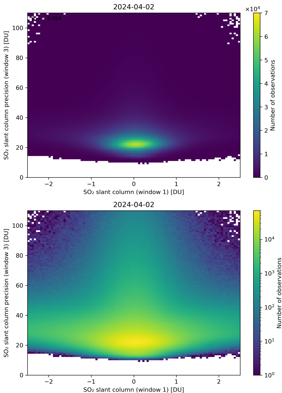
Figure 238: Scatter density plot of “SO 2 slant column (window 1)” against “SO 2 slant column precision (window 3)” for 2024-04-01 to 2024-04-03.
