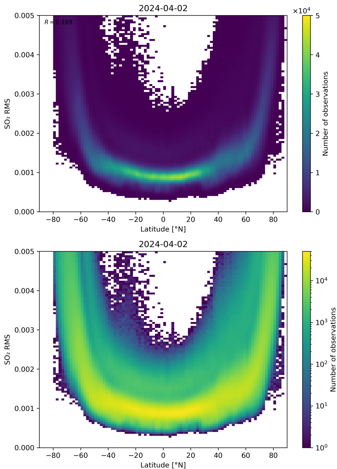
Figure 144: Scatter density plot of “Latitude” against “SO 2 RMS” for 2024-04-01 to 2024-04-03.
