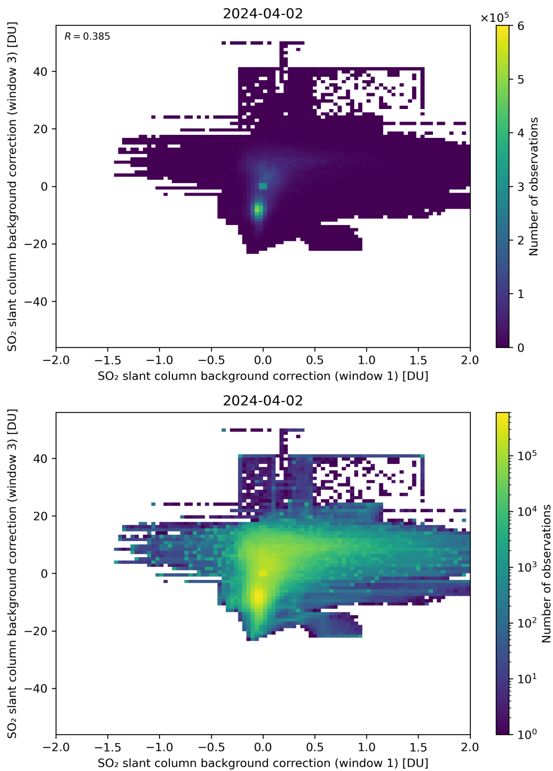
Figure 99: Scatter density plot of “SO 2 slant column background correction (window 1)” against “SO 2 slant column background correction (window 3)” for 2024-04-01 to 2024-04-03.
