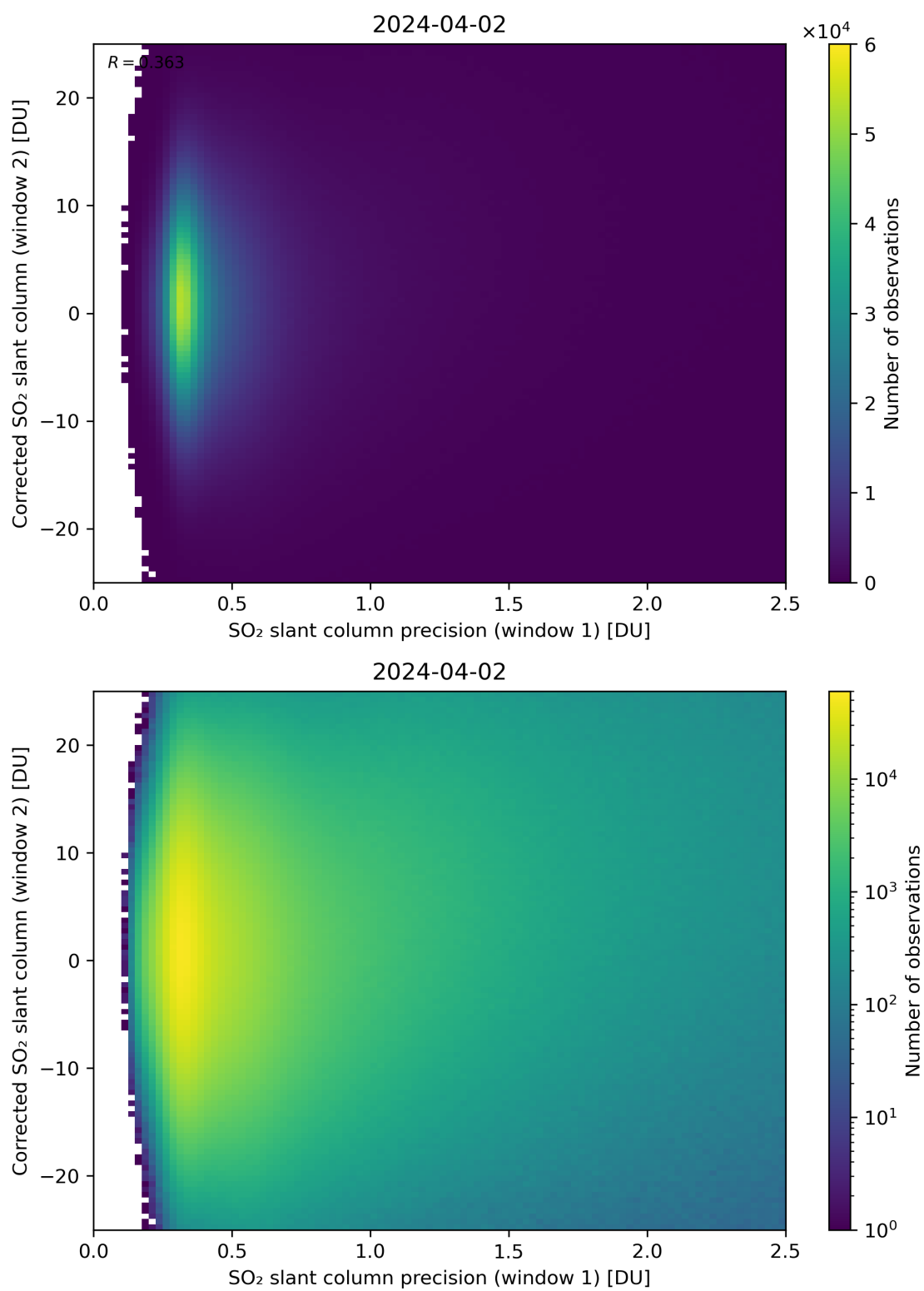
Figure 225: Scatter density plot of “SO 2 slant column precision (window 1)” against “Corrected SO 2 slant column (window 2)” for 2024-04-01 to 2024-04-03.
