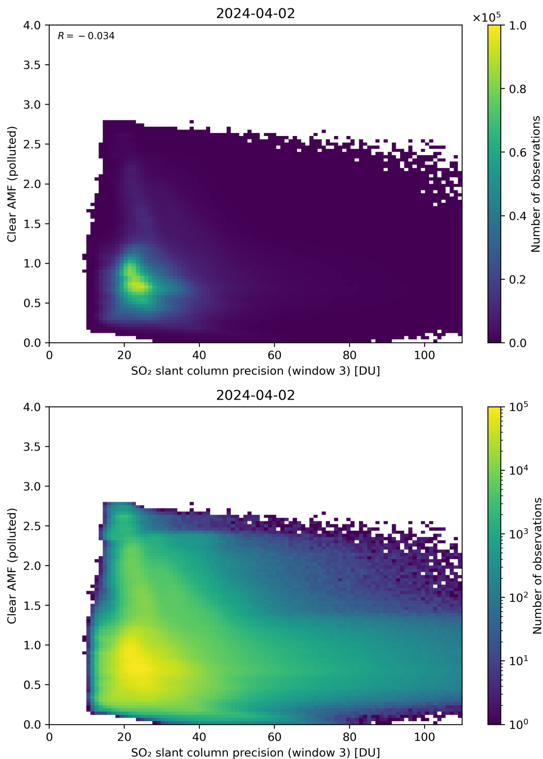
Figure 261: Scatter density plot of “SO 2 slant column precision (window 3)” against “Clear AMF (polluted)” for 2024-04-01 to 2024-04-03.
