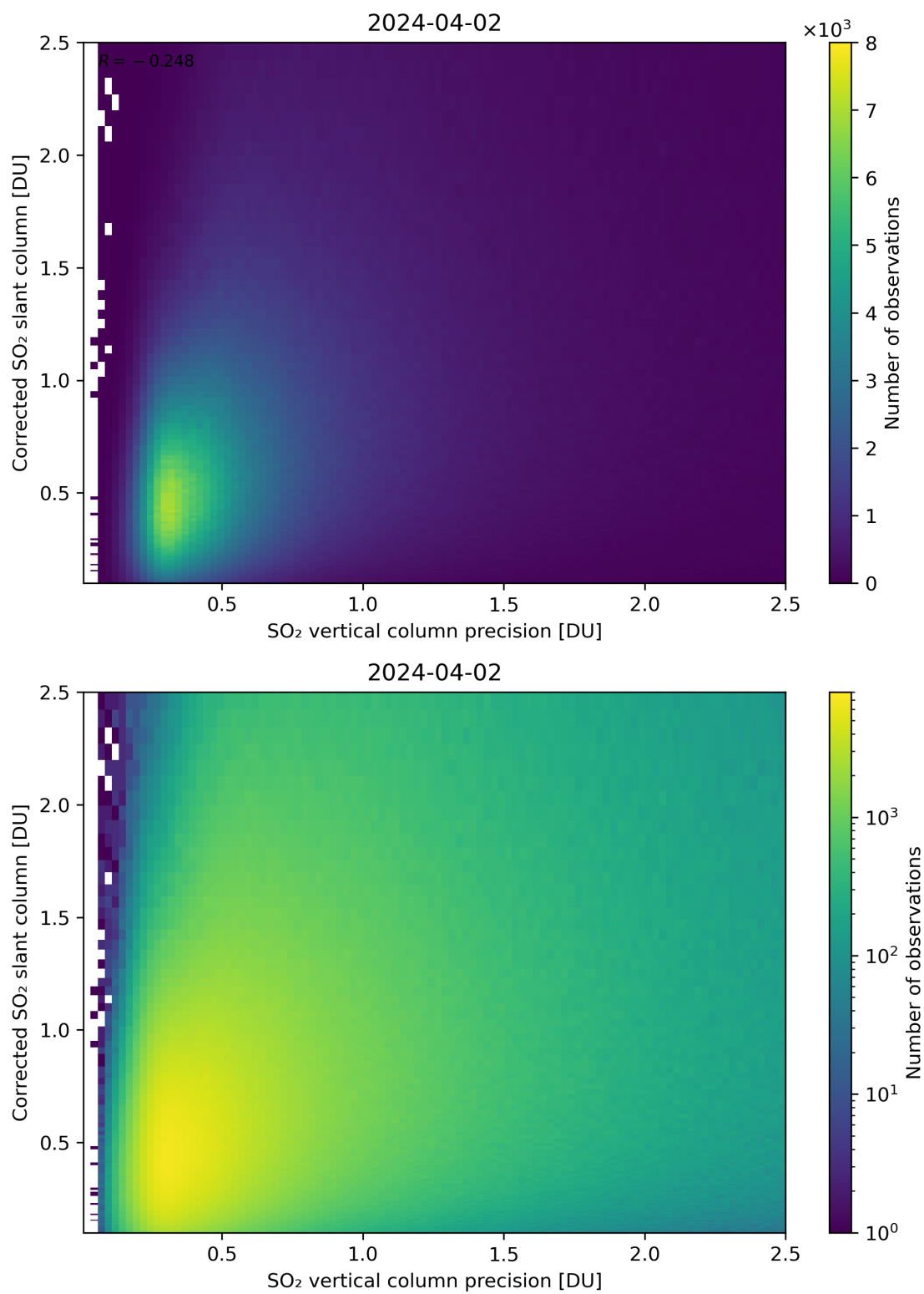
Figure 286: Scatter density plot of “SO 2 vertical column precision” against “Corrected SO 2 slant column” for 2024-04-01 to 2024-04-03.
