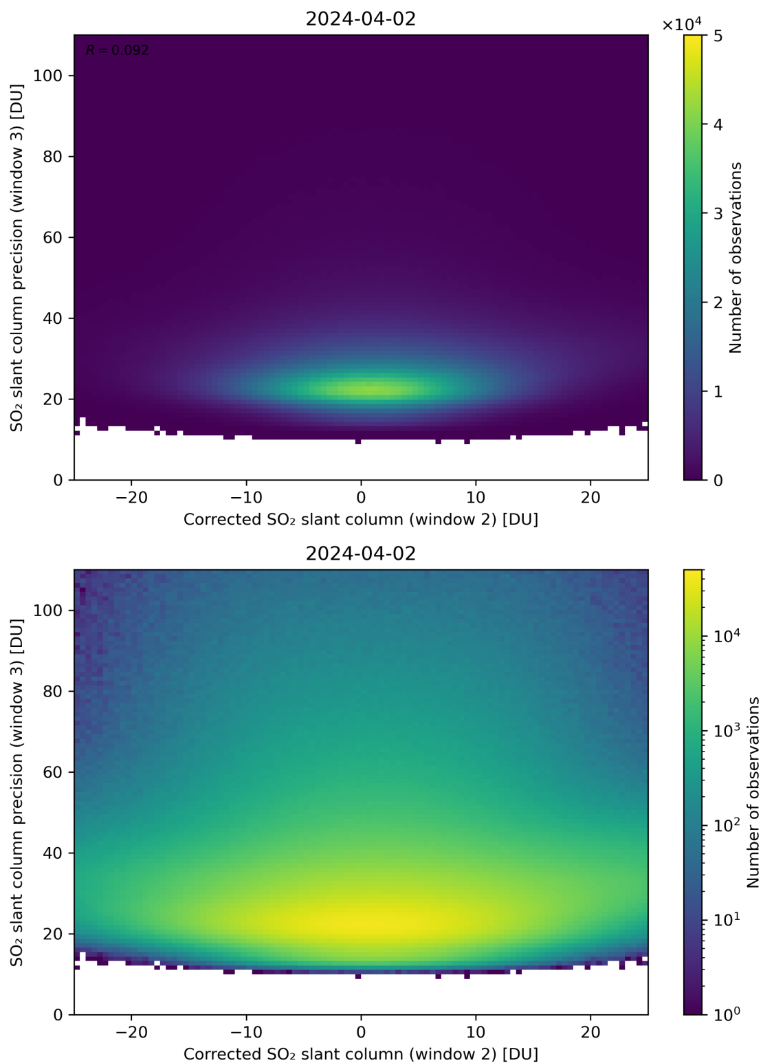
Figure 202: Scatter density plot of “Corrected SO 2 slant column (window 2)” against “SO 2 slant column precision (window 3)” for 2024-04-01 to 2024-04-03.
