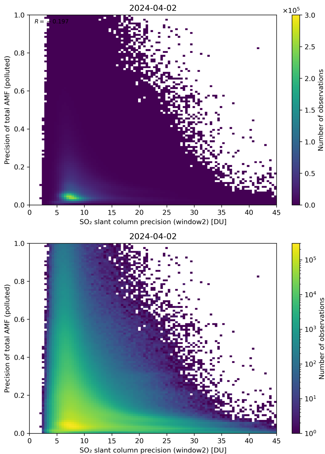
Figure 252: Scatter density plot of “SO 2 slant column precision (window2)” against “Precision of total AMF (polluted)” for 2024-04-01 to 2024-04-03.
