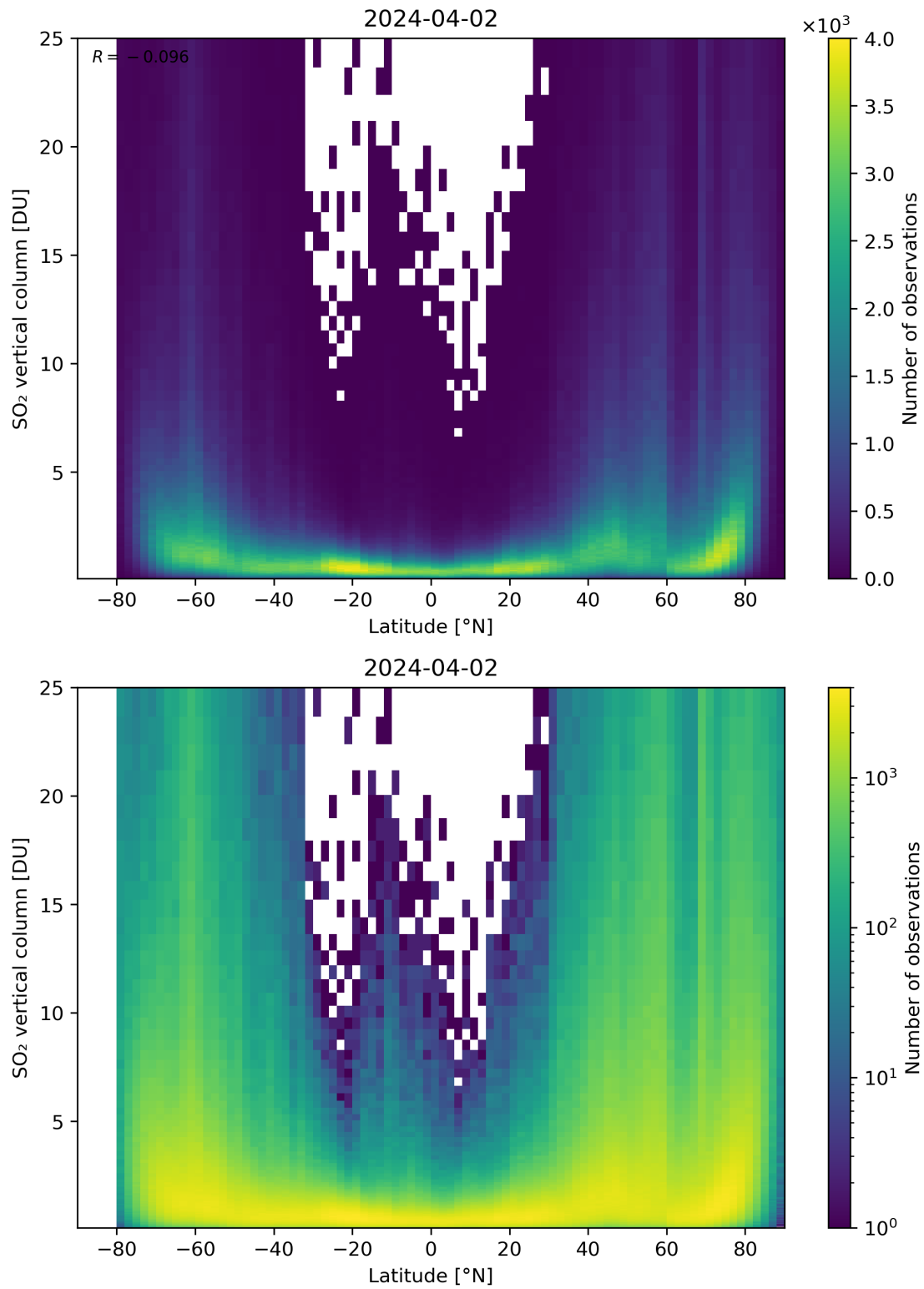
Figure 156: Scatter density plot of “Latitude” against “SO 2 vertical column” for 2024-04-01 to 2024-04-03.
