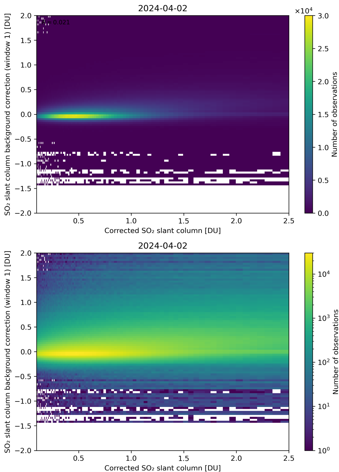
Figure 178: Scatter density plot of "Corrected SO 2 slant column" against "SO 2 slant column background correction (window 1)" for 2024-04-01 to 2024-04-03.
