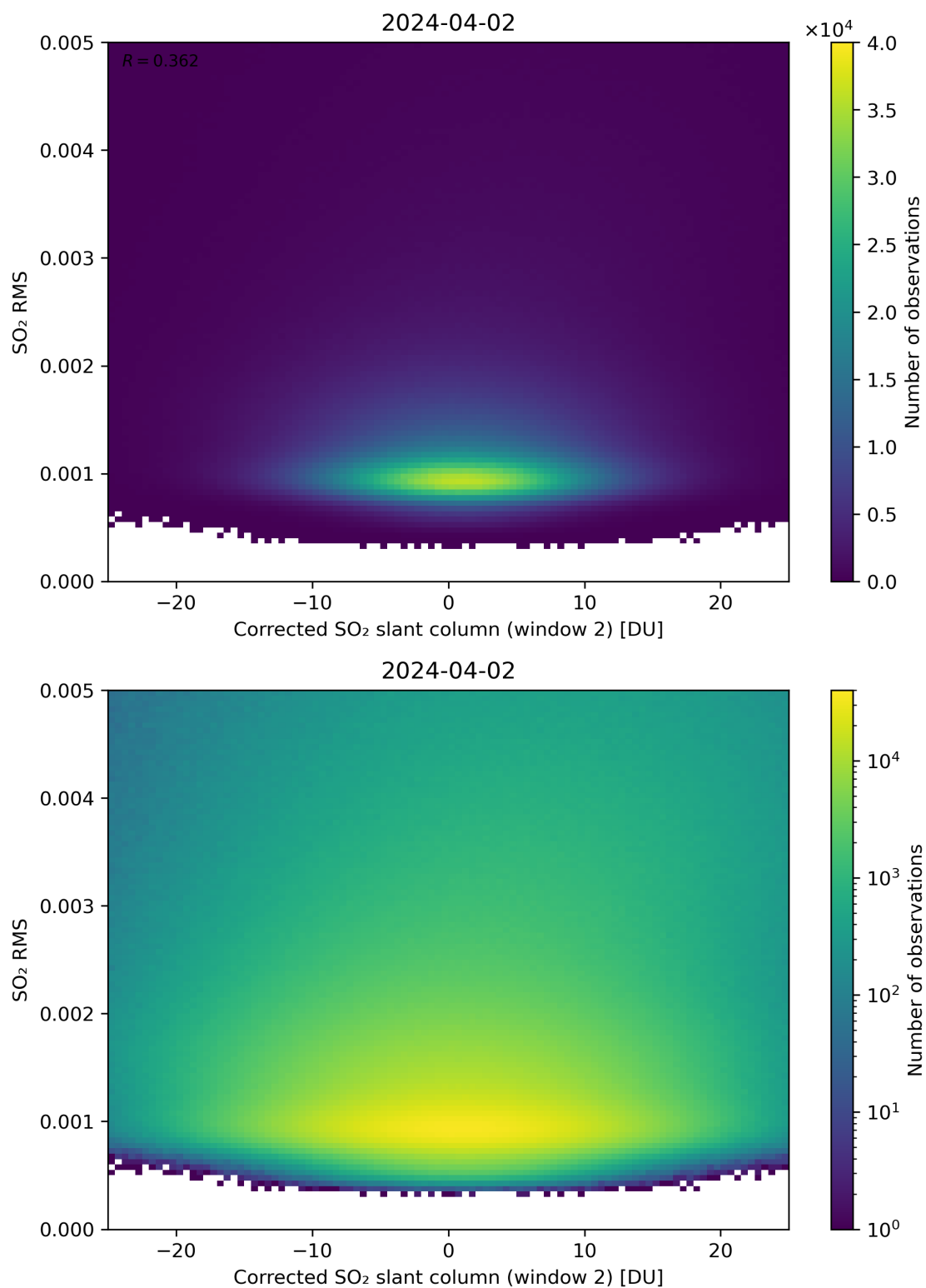
Figure 198: Scatter density plot of “Corrected SO 2 slant column (window 2)” against “SO 2 RMS” for 2024-04-01 to 2024-04-03.
