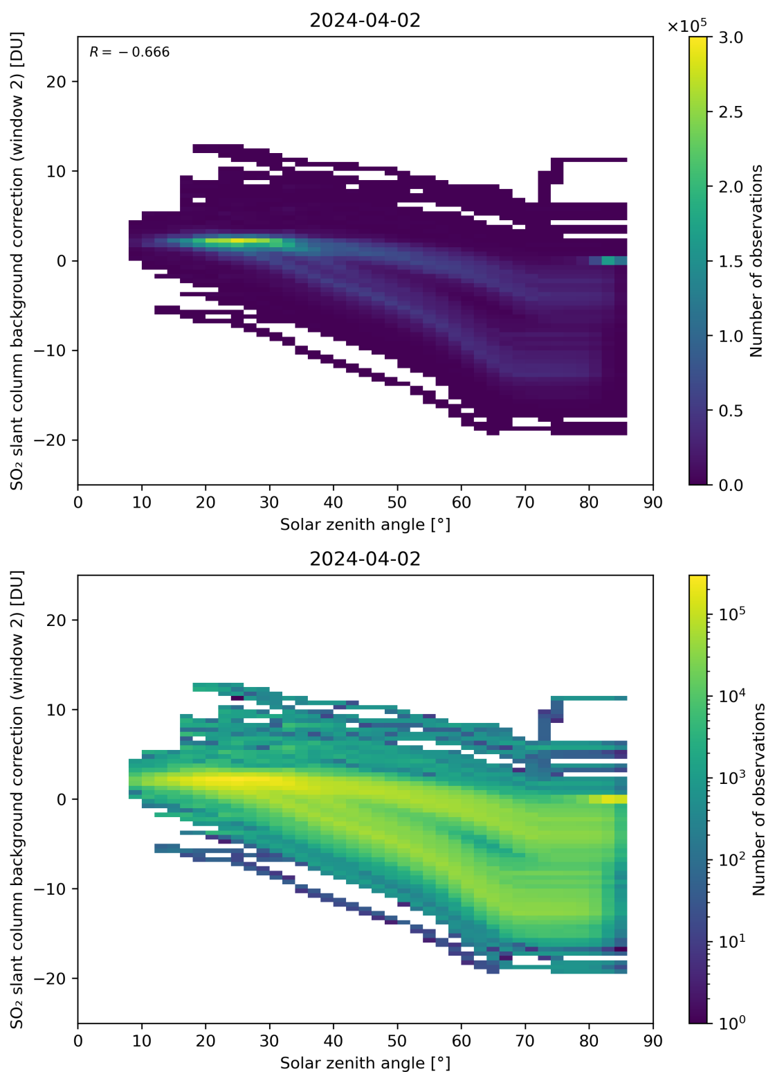
Figure 159: Scatter density plot of “Solar zenith angle” against “SO 2 slant column background correction (window 2)” for 2024-04-01 to 2024-04-03.
