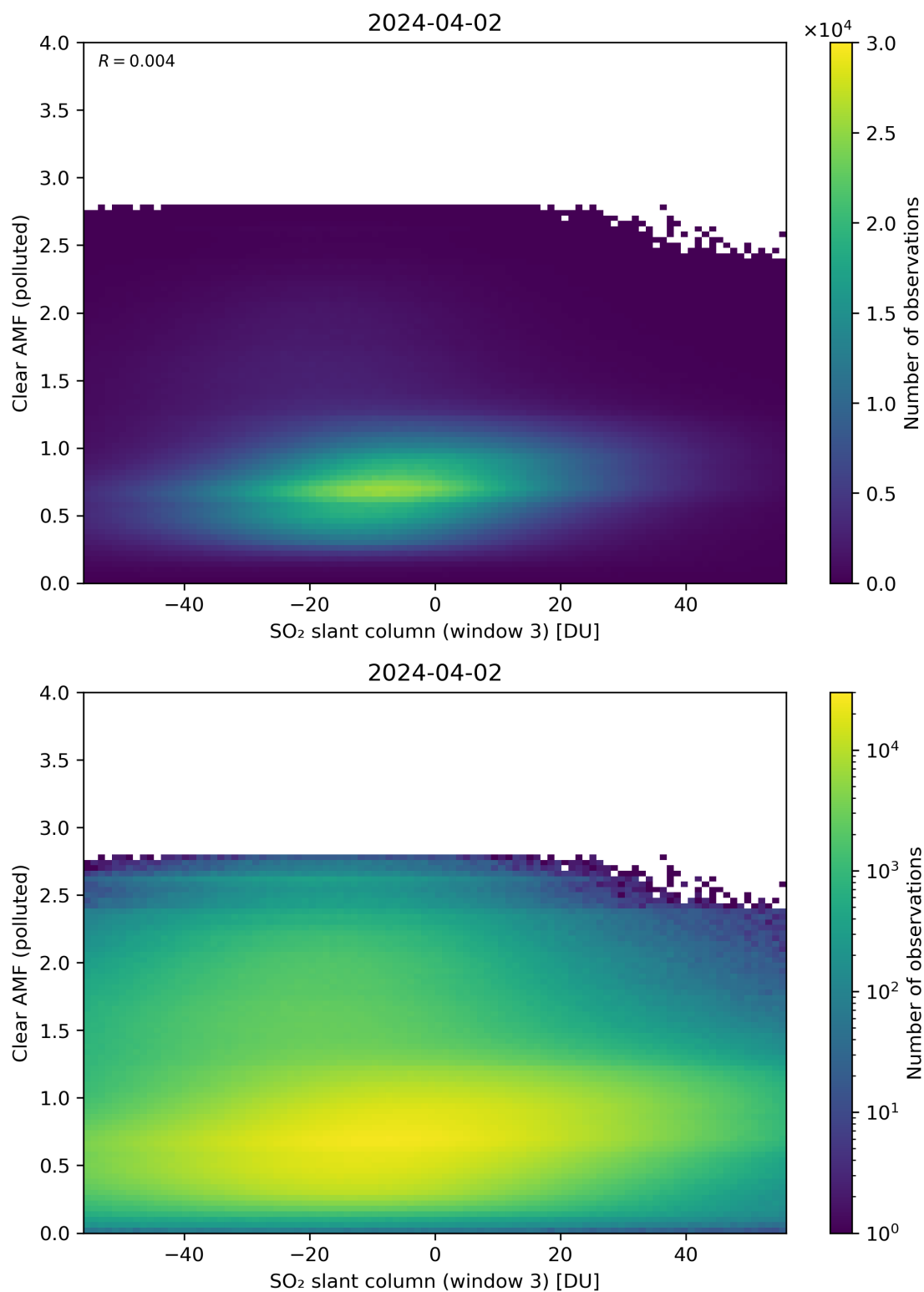
Figure 265: Scatter density plot of “SO 2 slant column (window 3)” against “Clear AMF (polluted)” for 2024-04-01 to 2024-04-03.
