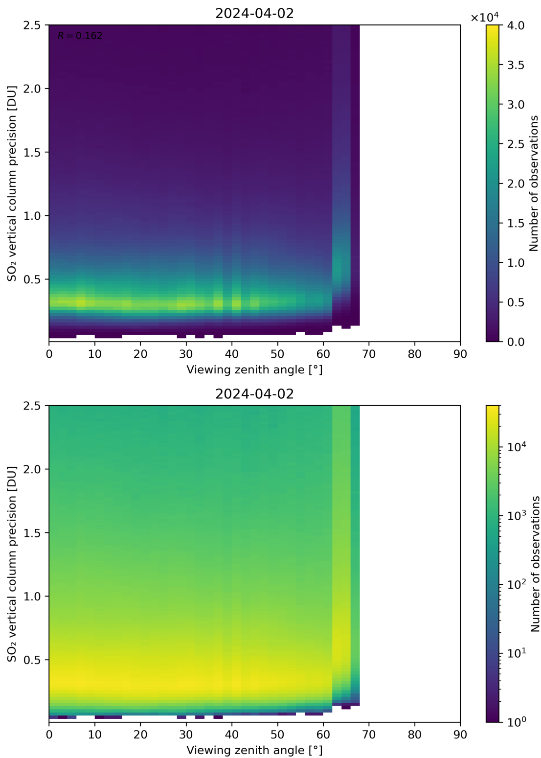
Figure 328: Scatter density plot of “Viewing zenith angle” against “SO 2 vertical column precision” for 2024-04-01 to 2024-04-03.
