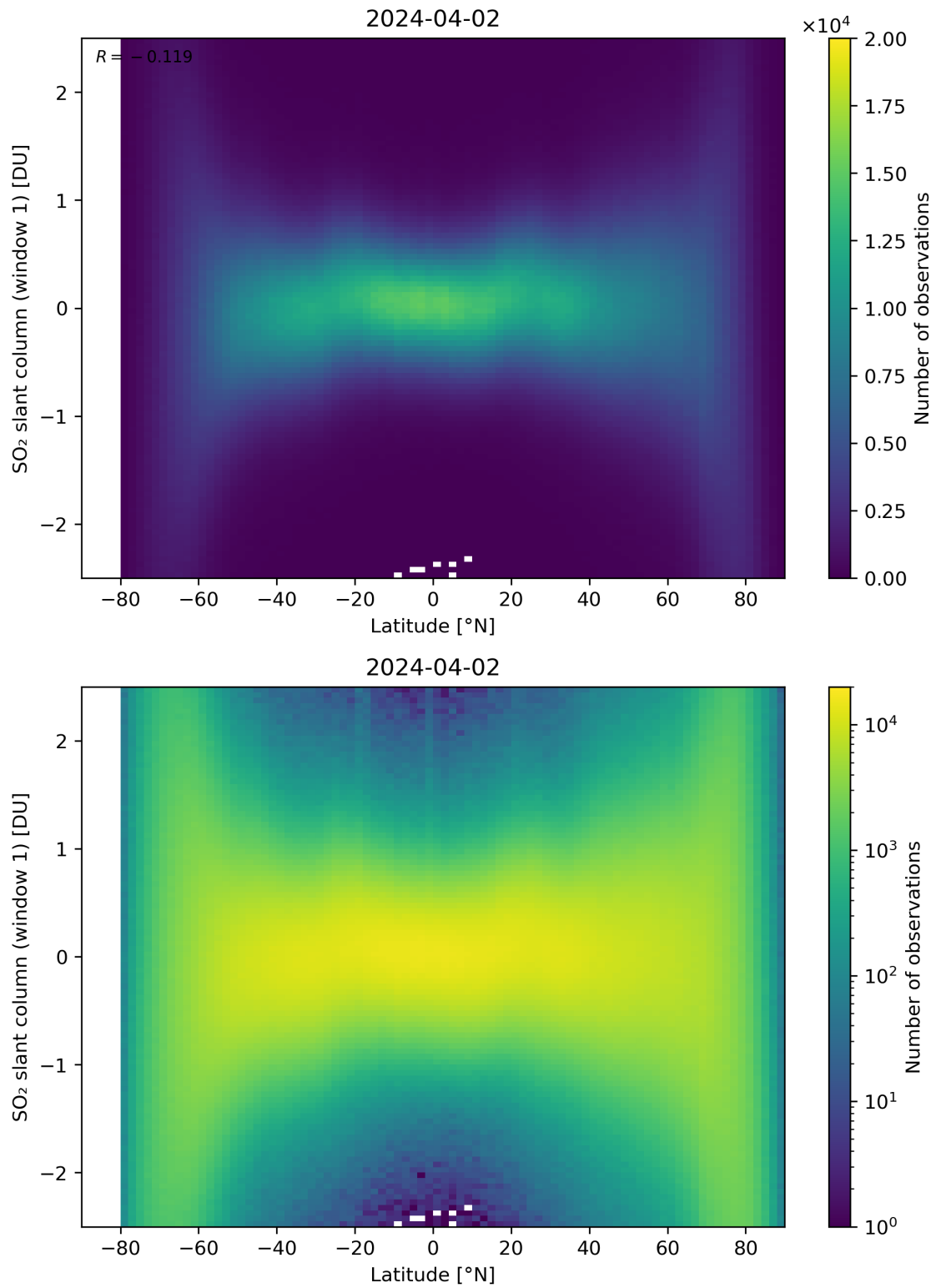
Figure 149: Scatter density plot of “Latitude” against “SO 2 slant column (window 1)” for 2024-04-01 to 2024-04-03.
