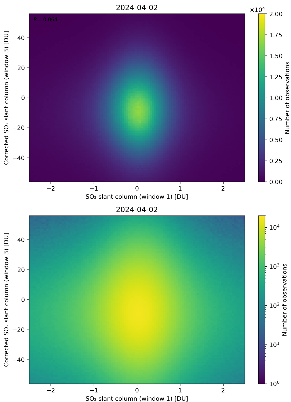
Figure 234: Scatter density plot of “SO 2 slant column (window 1)” against “Corrected SO 2 slant column (window 3)” for 2024-04-01 to 2024-04-03.
