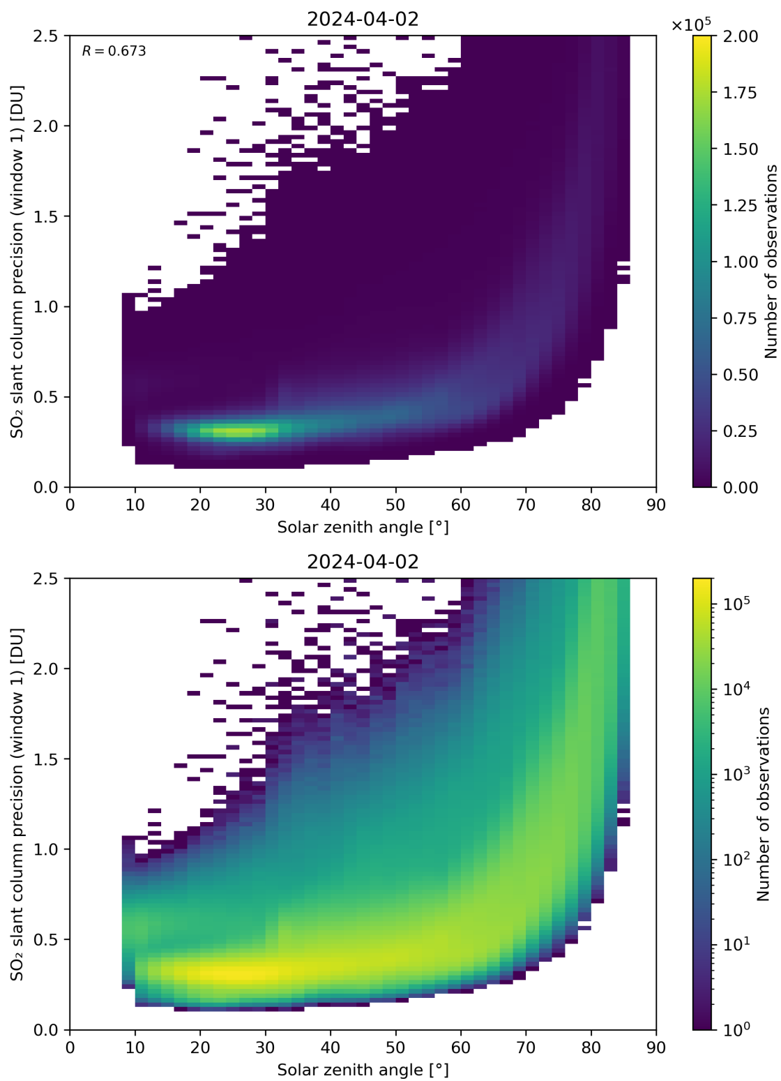
Figure 170: Scatter density plot of “Solar zenith angle” against “SO 2 slant column precision (window 1)” for 2024-04-01 to 2024-04-03.
