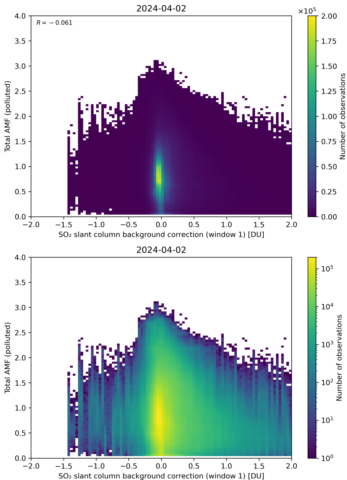
Figure 109: Scatter density plot of “SO 2 slant column background correction (window 1)” against “Total AMF (polluted)” for 2024-04-01 to 2024-04-03.
