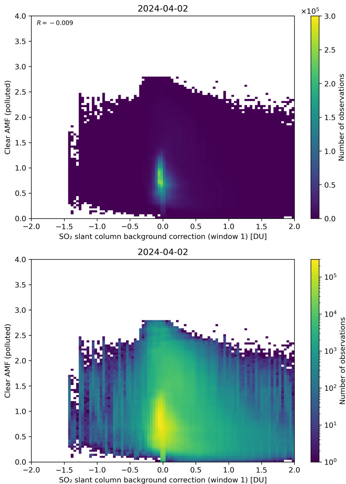
Figure 103: Scatter density plot of “SO 2 slant column background correction (window 1)” against “Clear AMF (polluted)” for 2024-04-01 to 2024-04-03.
