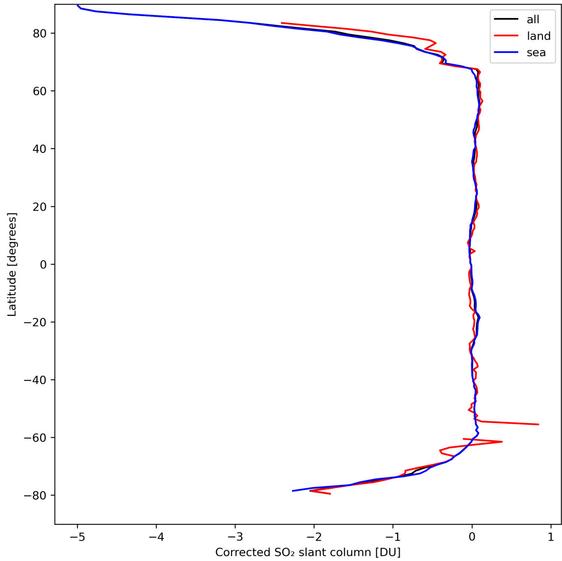
Figure 32: Zonal average of “Corrected SO 2 slant column” for 2024-04-01 to 2024-04-03.
