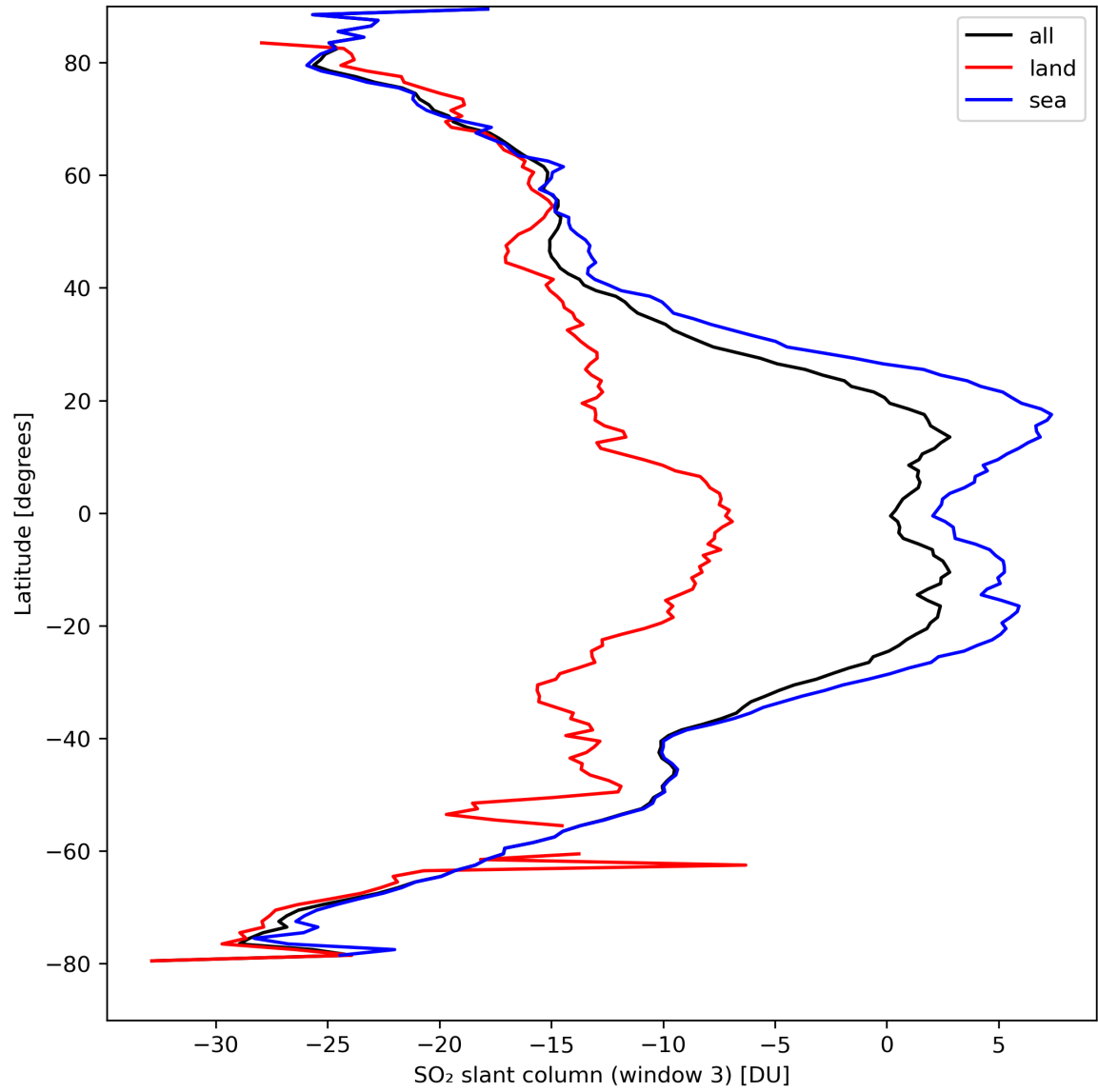
Figure 41: Zonal average of “SO 2 slant column (window 3)” for 2024-04-01 to 2024-04-03.
