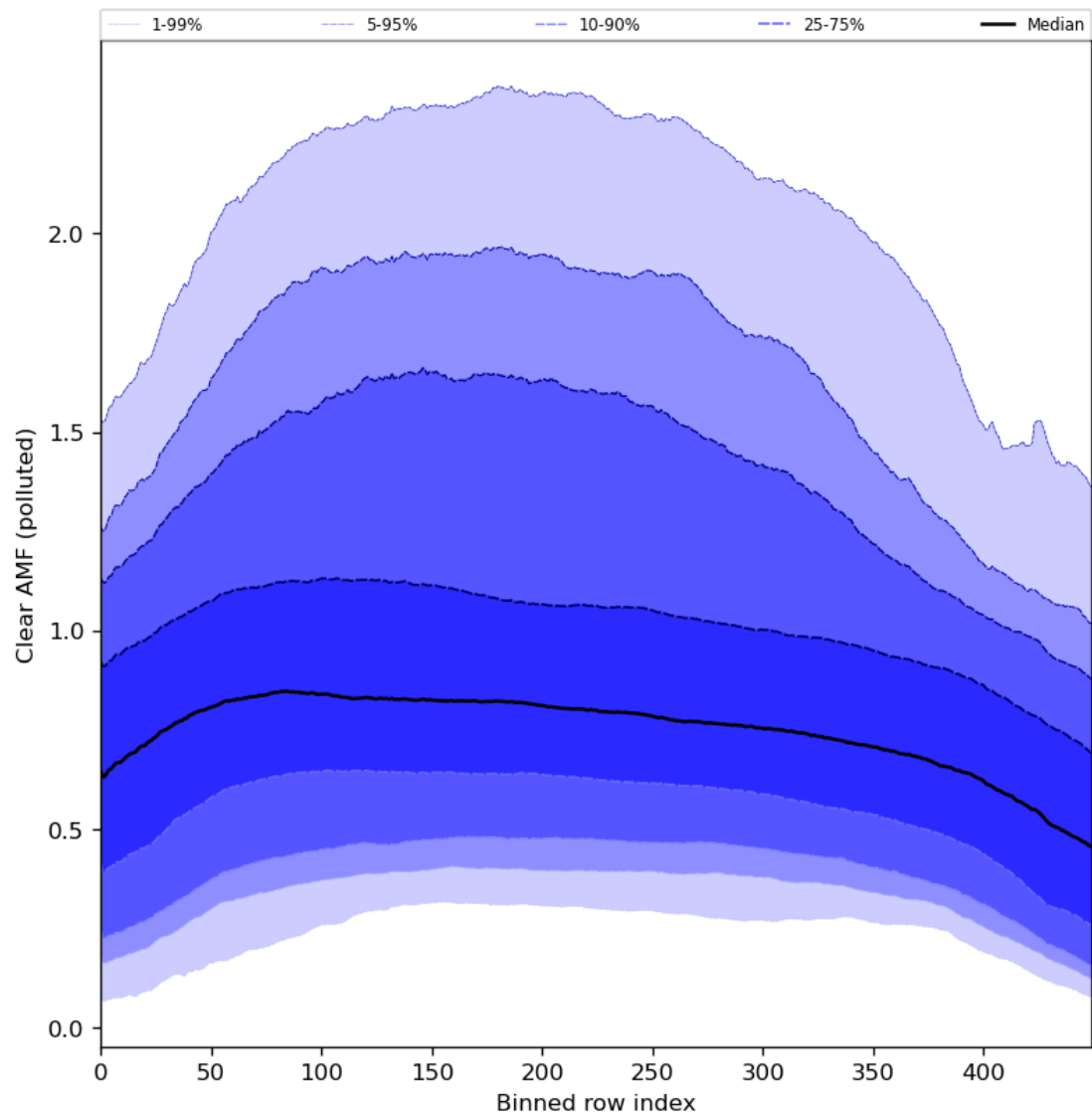
Figure 96: Along track statistics of “Clear AMF (polluted)” for 2024-04-01 to 2024-04-03
