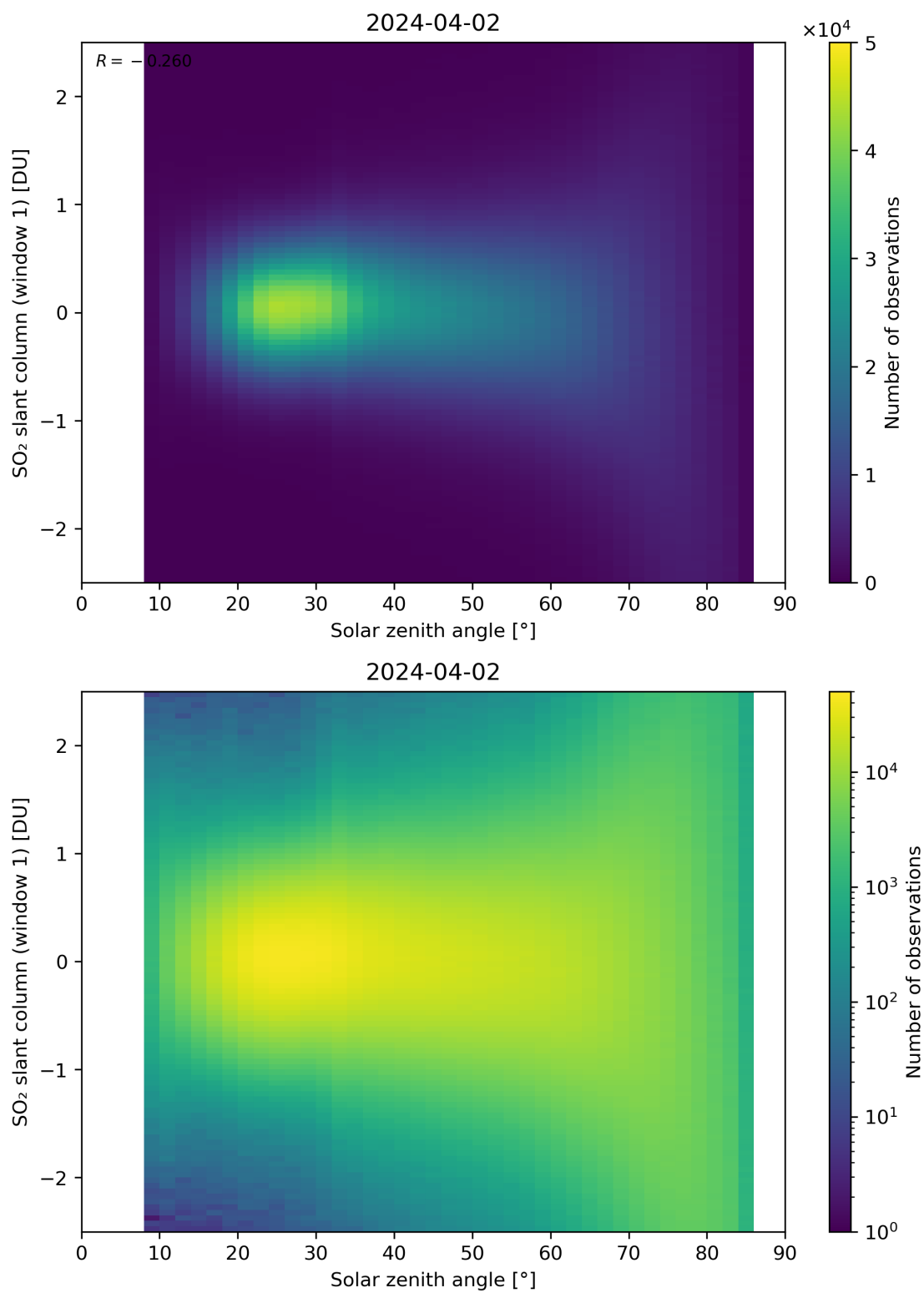
Figure 169: Scatter density plot of “Solar zenith angle” against “SO 2 slant column (window 1)” for 2024-04-01 to 2024-04-03.
