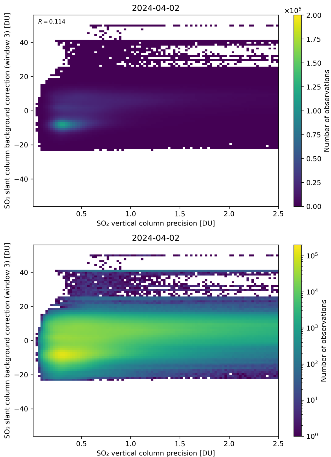
Figure 281: Scatter density plot of “SO 2 vertical column precision” against “SO 2 slant column background correction (window 3)” for 2024-04-01 to 2024-04-03.
