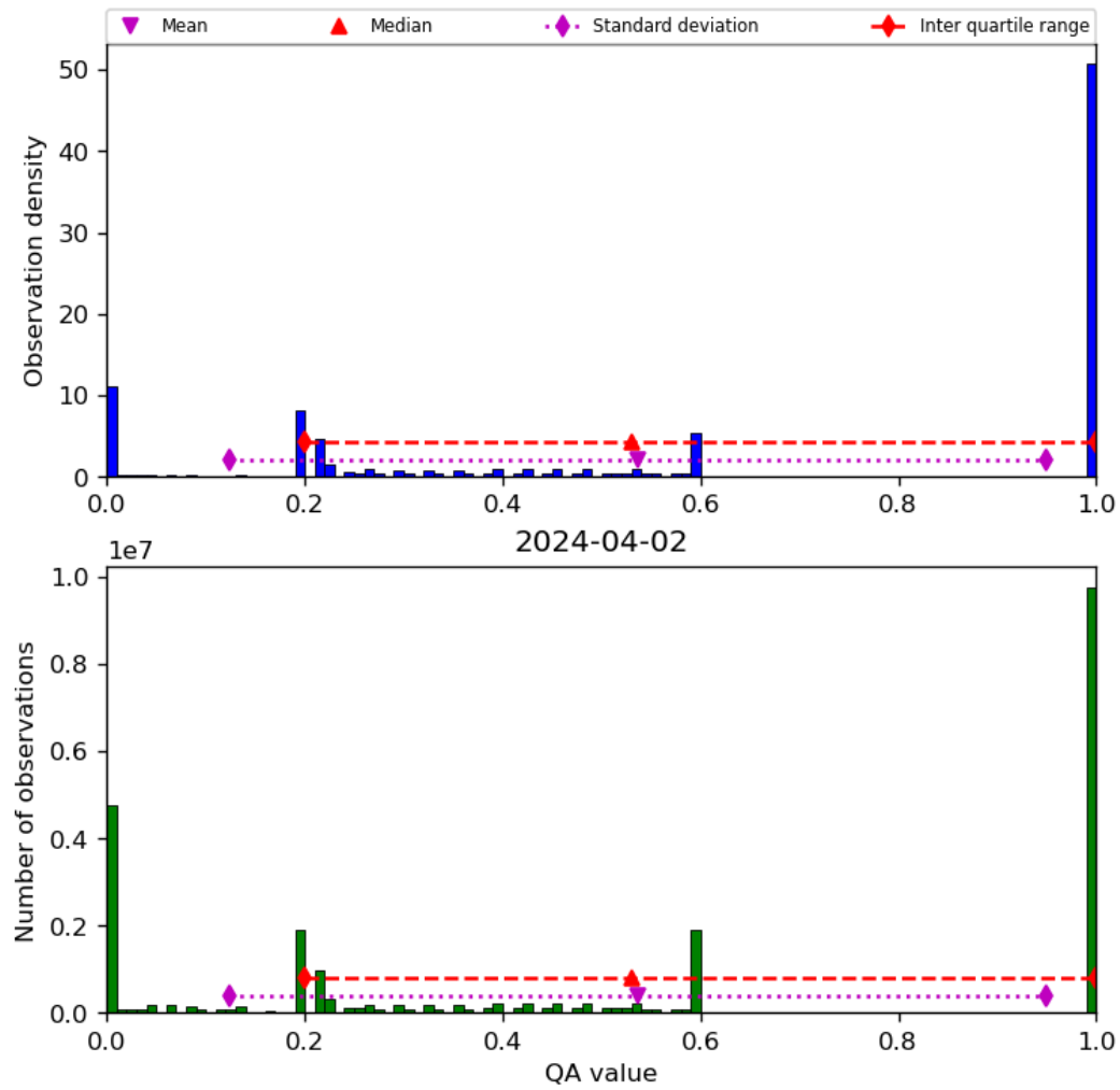
Figure 52: Histogram of “QA value” for 2024-04-01 to 2024-04-03
