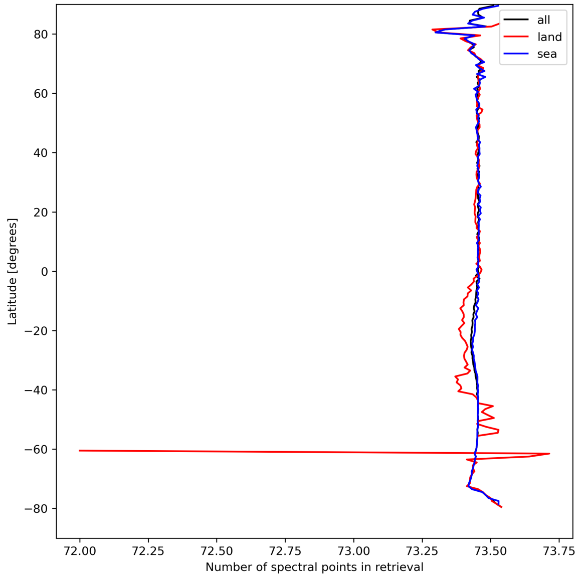
Figure 51: Zonal average of “Number of spectral points in retrieval” for 2024-04-01 to 2024-04-03.
