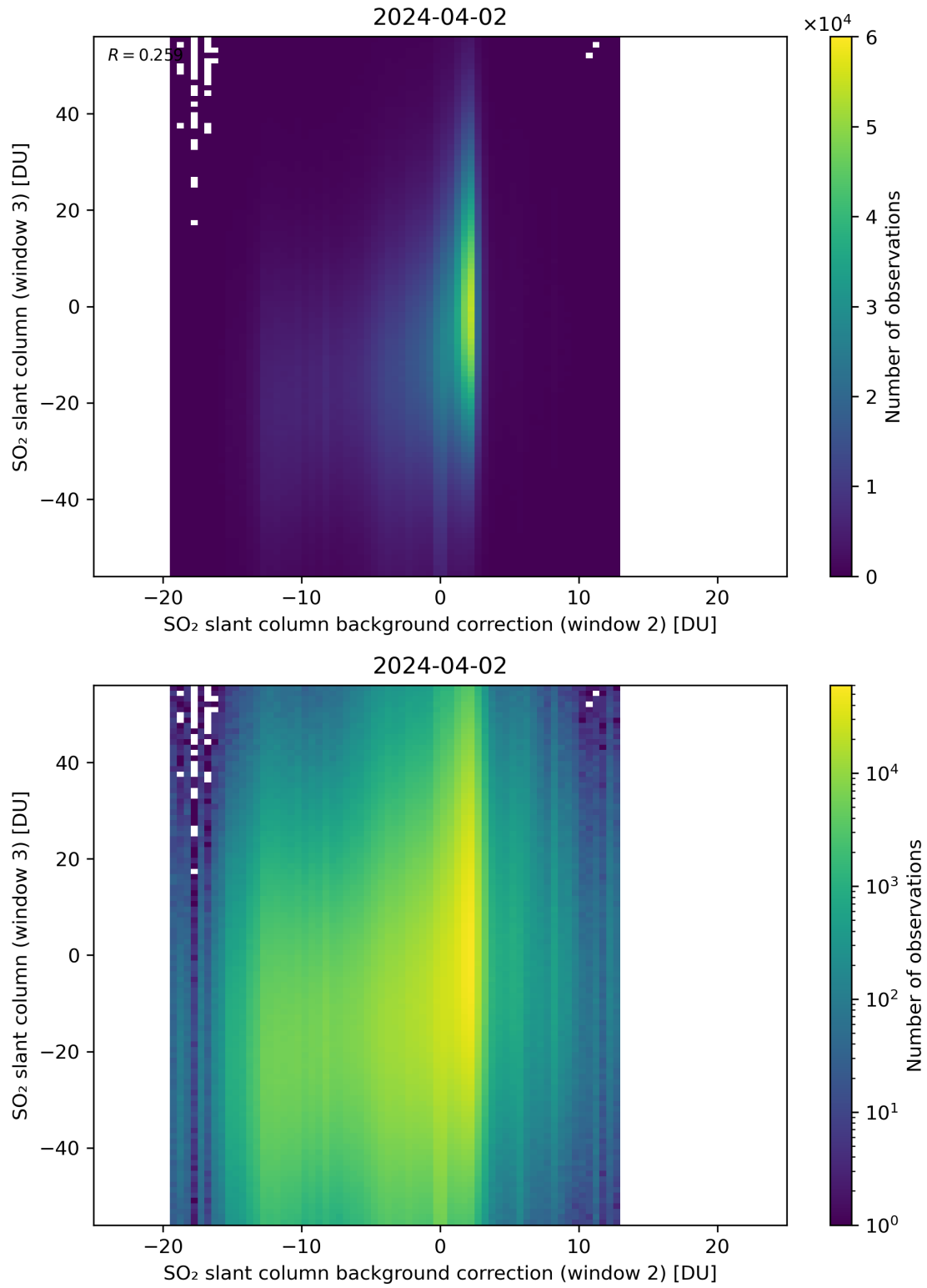
Figure 117: Scatter density plot of “SO 2 slant column background correction (window 2)” against “SO 2 slant column (window 3)” for 2024-04-01 to 2024-04-03.
