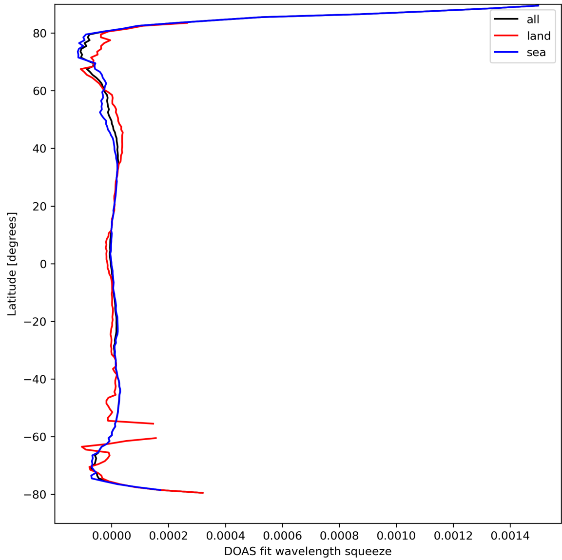
Figure 46: Zonal average of “DOAS fit wavelength squeeze” for 2024-04-01 to 2024-04-03.
