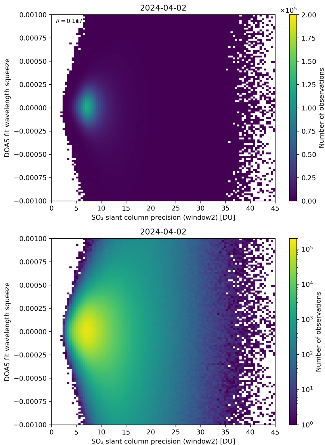
Figure 244: Scatter density plot of “SO 2 slant column precision (window2)” against “DOAS fit wavelength squeeze” for 2024-04-01 to 2024-04-03.
