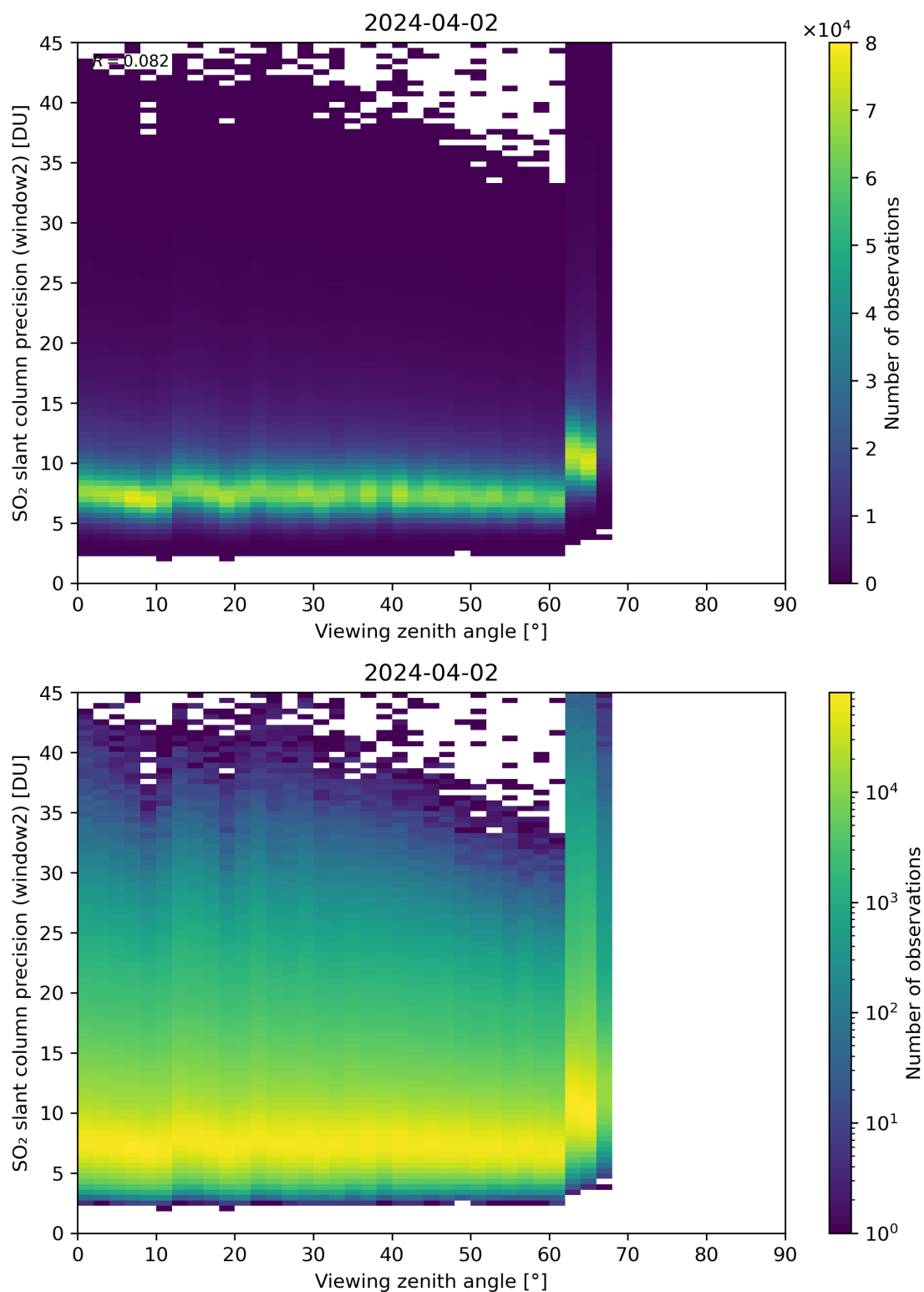
Figure 322: Scatter density plot of “Viewing zenith angle” against “SO 2 slant column precision (window2)” for 2024-04-01 to 2024-04-03.
