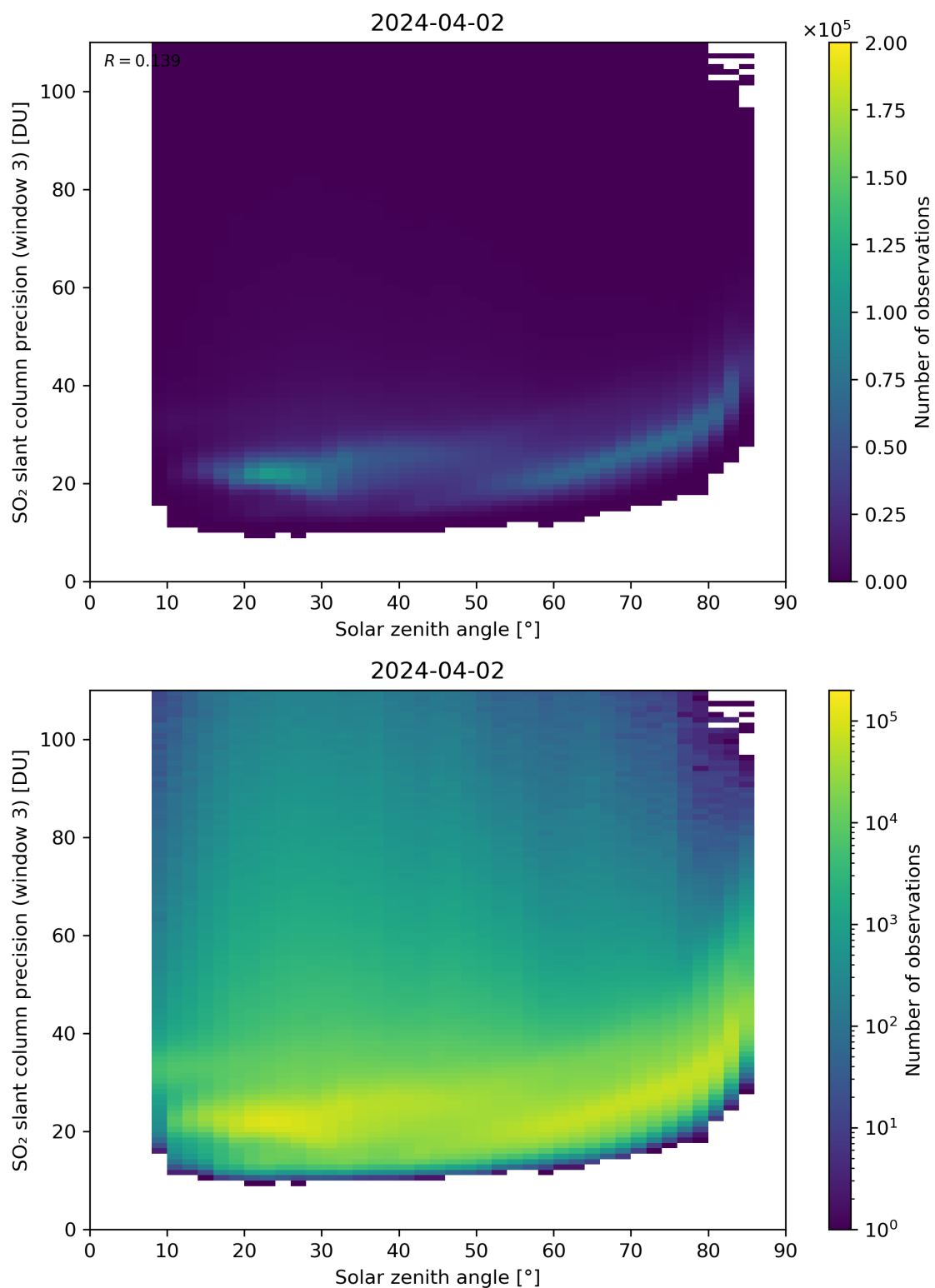
Figure 173: Scatter density plot of “Solar zenith angle” against “SO 2 slant column precision (window 3)” for 2024-04-01 to 2024-04-03.
