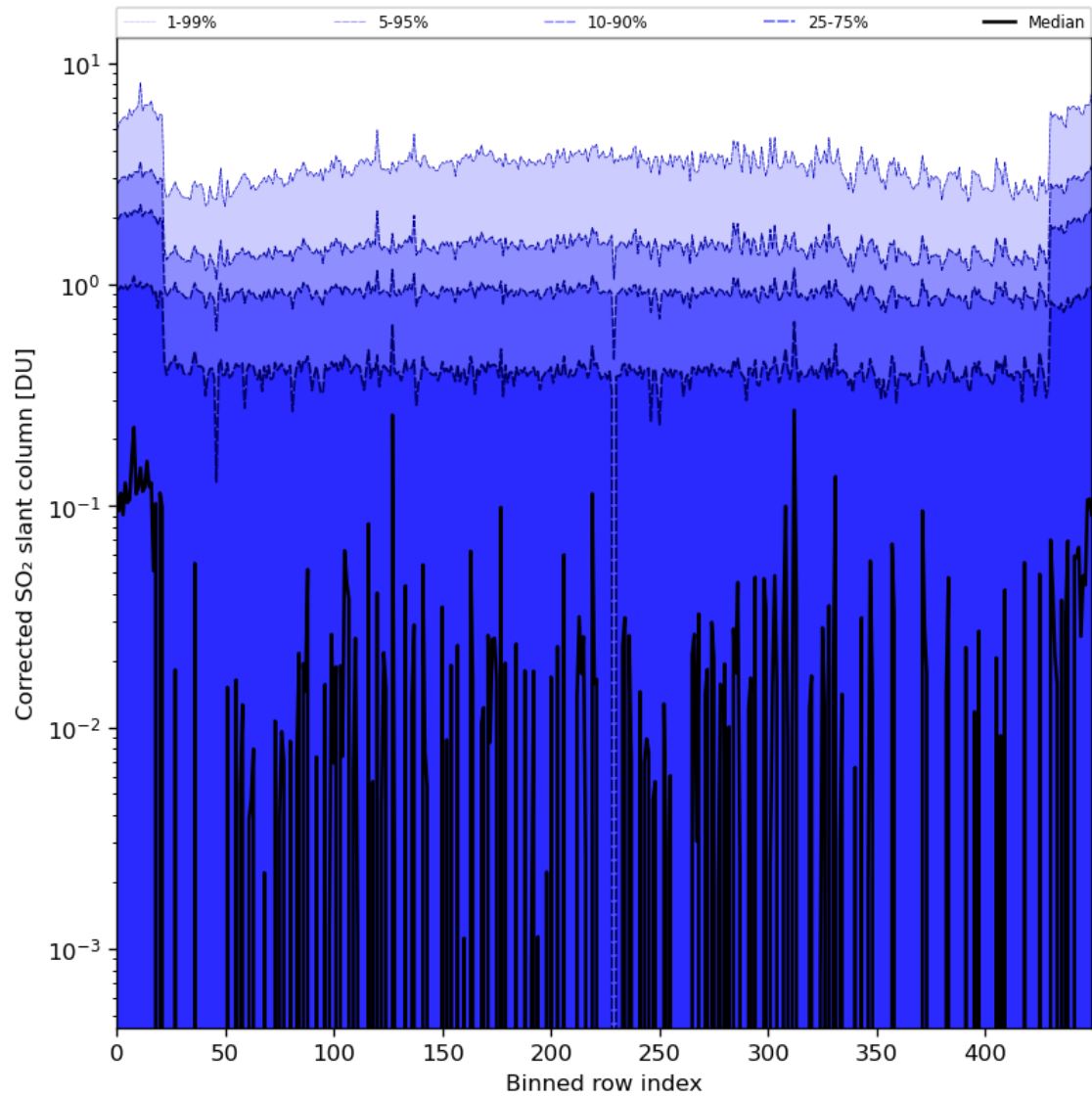
Figure 78: Along track statistics of “Corrected SO 2 slant column” for 2024-04-01 to 2024-04-03
