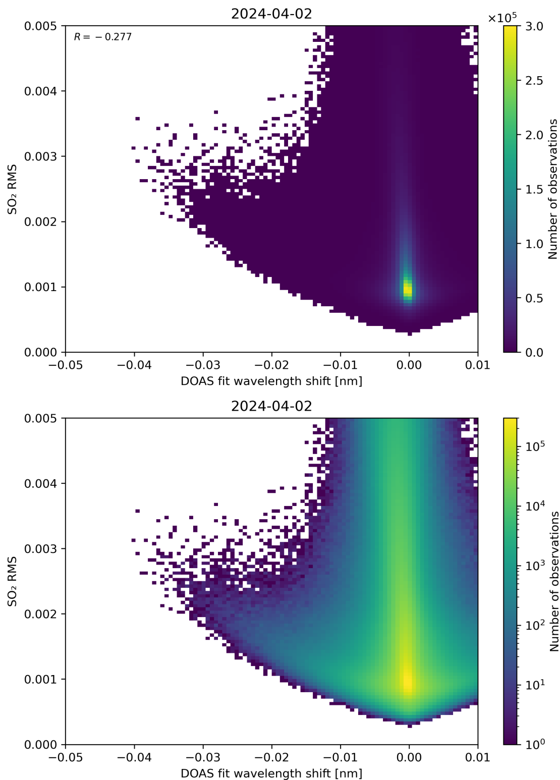
Figure 128: Scatter density plot of “DOAS fit wavelength shift” against “SO 2 RMS” for 2024-04-01 to 2024-04-03.
