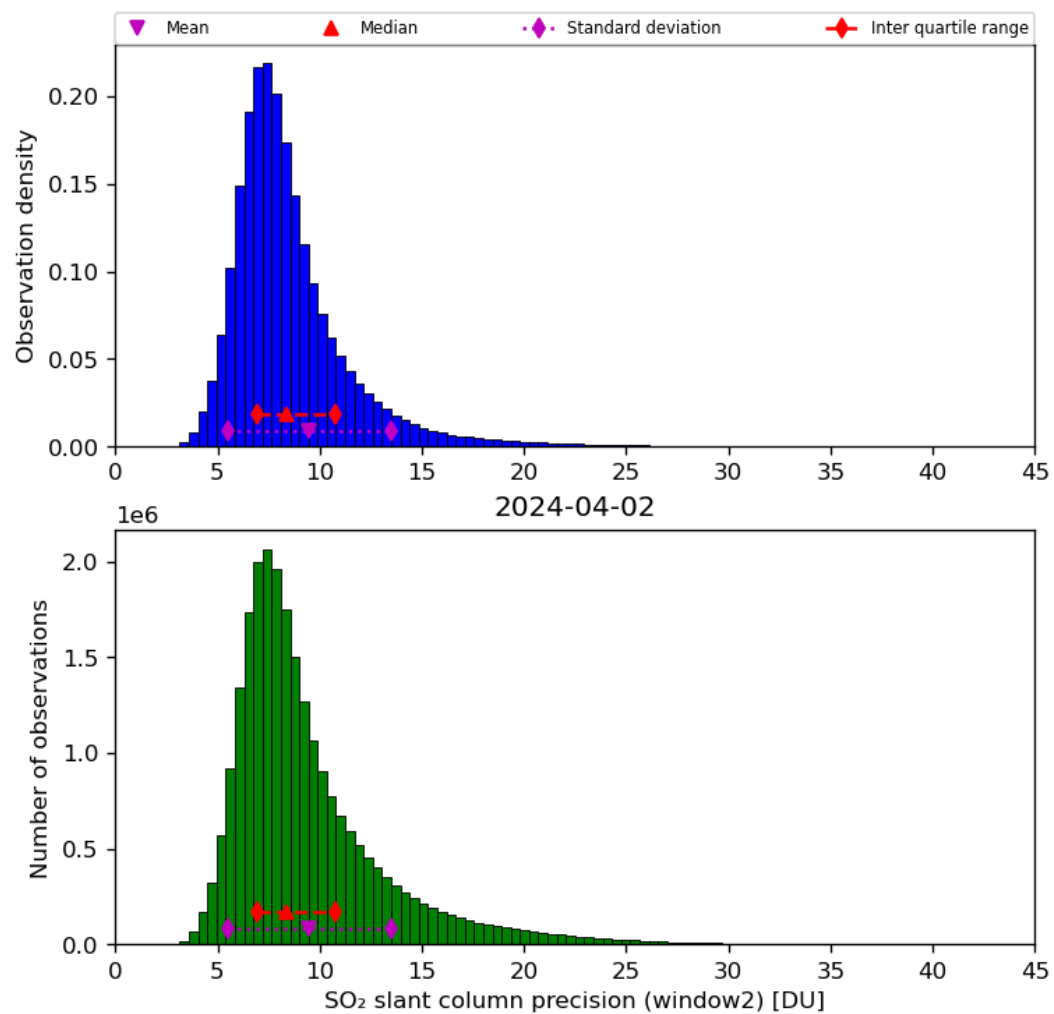
Figure 61: Histogram of “SO 2 slant column precision (window2)” for 2024-04-01 to 2024-04-03
