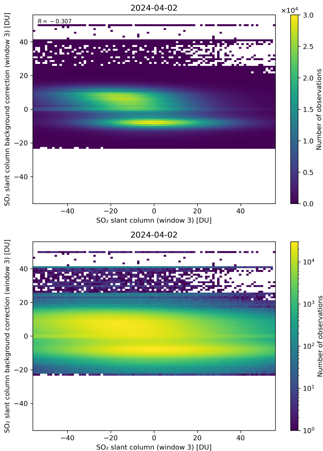
Figure 253: Scatter density plot of “SO 2 slant column (window 3)” against “SO 2 slant column background correction (window 3)” for 2024-04-01 to 2024-04-03.
