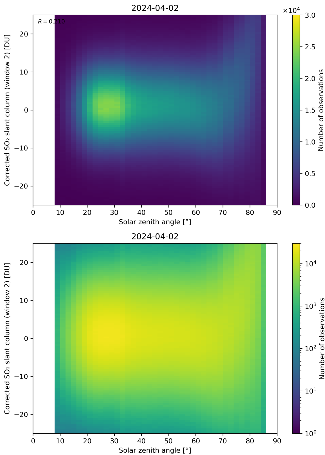
Figure 167: Scatter density plot of “Solar zenith angle” against “Corrected SO 2 slant column (window 2)” for 2024-04-01 to 2024-04-03.
