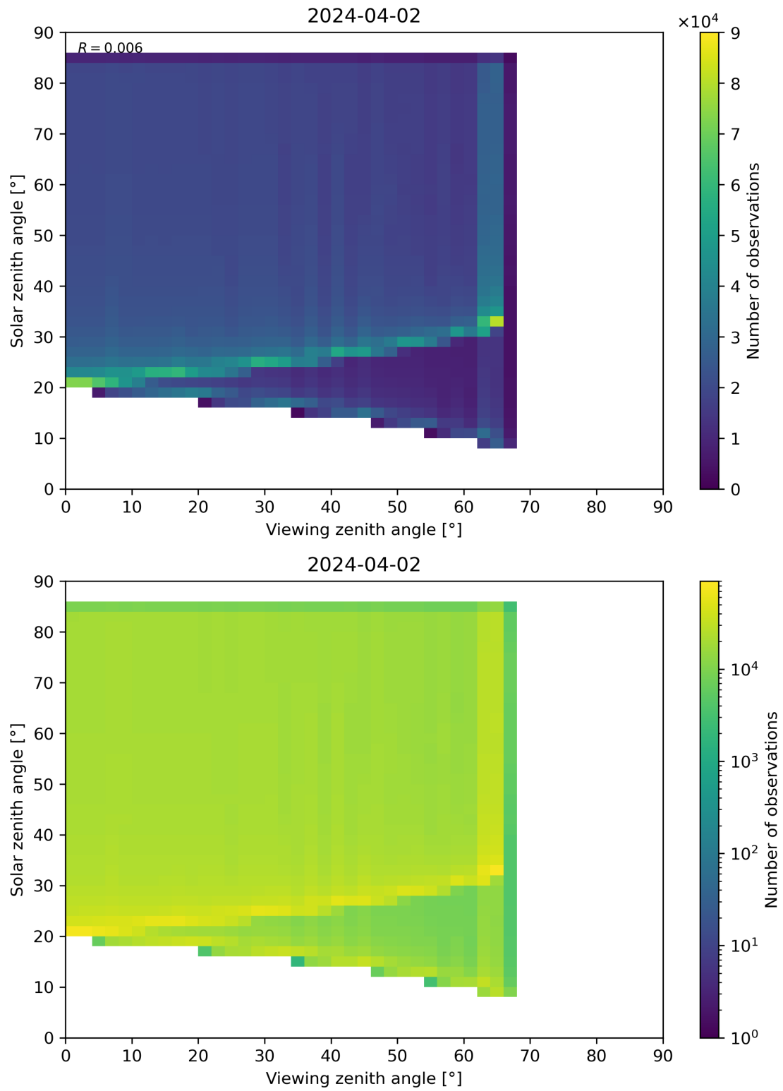
Figure 315: Scatter density plot of “Viewing zenith angle” against “Solar zenith angle” for 2024-04-01 to 2024-04-03.
