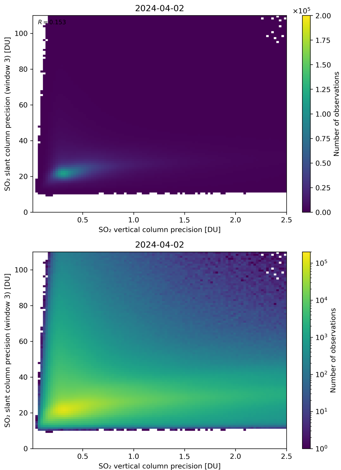
Figure 293: Scatter density plot of “SO 2 vertical column precision” against “SO 2 slant column precision (window 3)” for 2024-04-01 to 2024-04-03.
