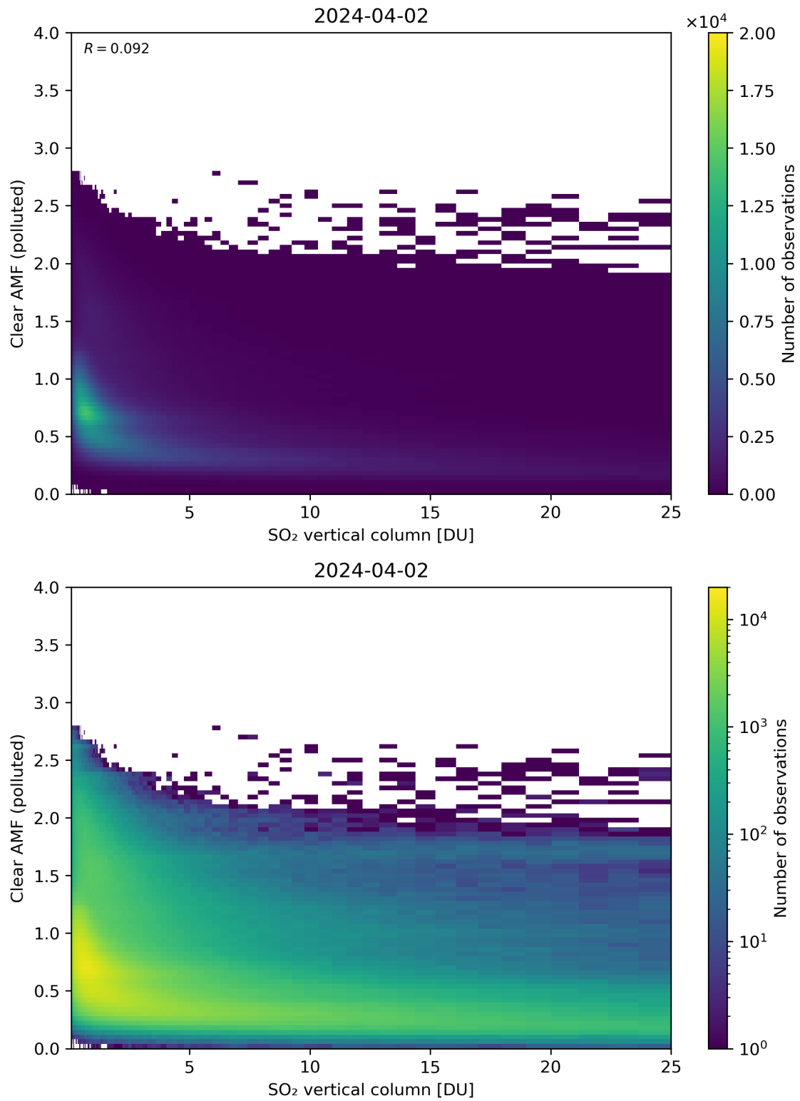
Figure 296: Scatter density plot of “SO 2 vertical column” against “Clear AMF (polluted)” for 2024-04-01 to 2024-04-03.
