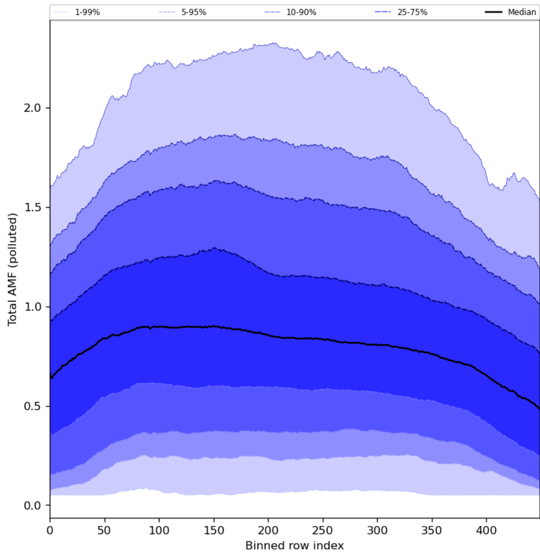
Figure 94: Along track statistics of “Total AMF (polluted)” for 2024-04-01 to 2024-04-03
