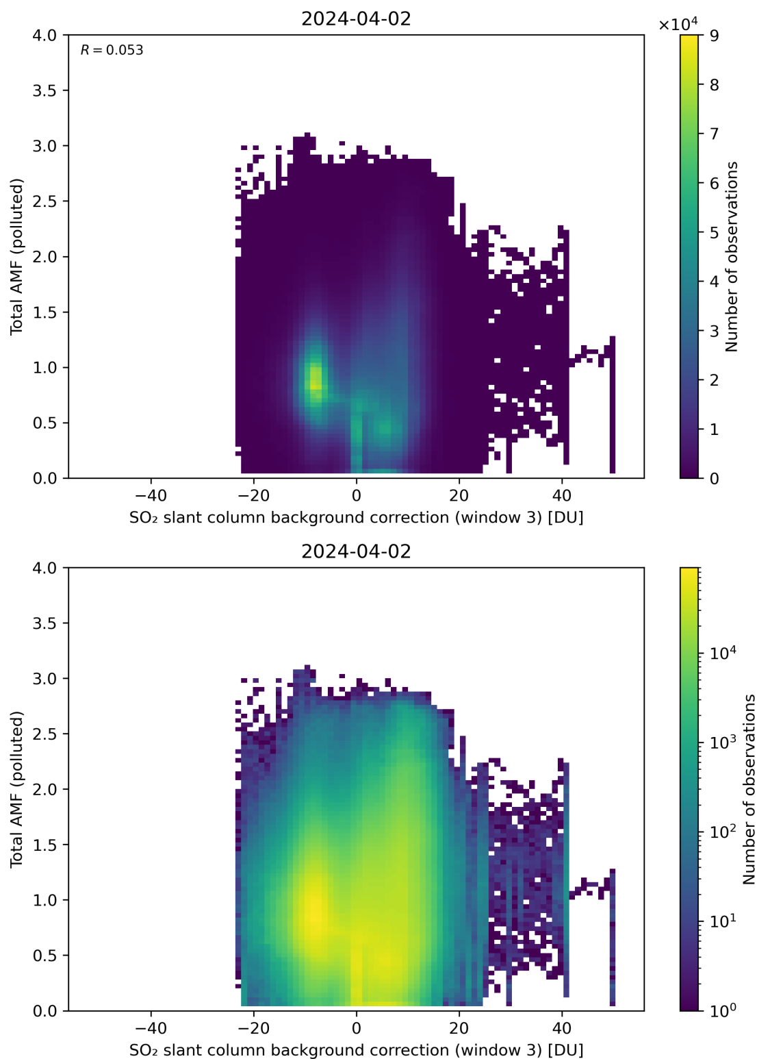
Figure 125: Scatter density plot of “SO 2 slant column background correction (window 3)” against “Total AMF (polluted)” for 2024-04-01 to 2024-04-03.
