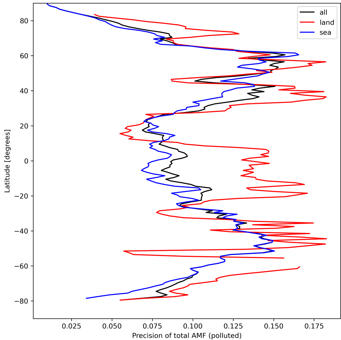
Figure 49: Zonal average of “Precision of total AMF (polluted)” for 2024-04-01 to 2024-04-03.
