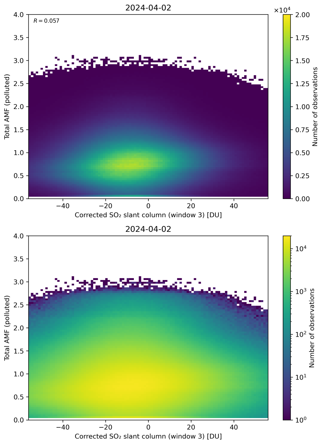
Figure 210: Scatter density plot of “Corrected SO 2 slant column (window 3)” against “Total AMF (polluted)” for 2024-04-01 to 2024-04-03.
