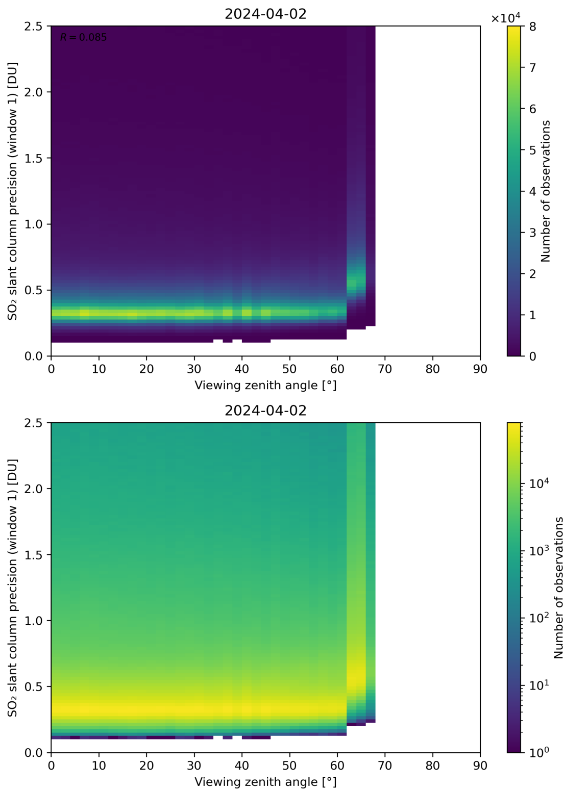
Figure 321: Scatter density plot of “Viewing zenith angle” against “SO 2 slant column precision (window 1)” for 2024-04-01 to 2024-04-03.
