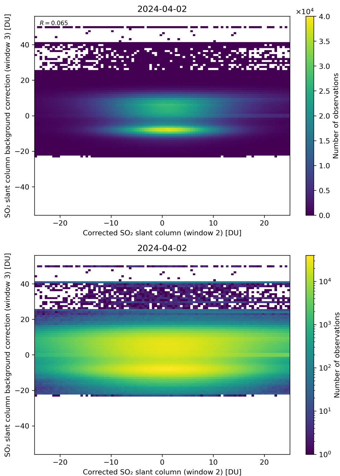
Figure 195: Scatter density plot of “Corrected SO 2 slant column (window 2)” against “SO 2 slant column background correction (window 3)” for 2024-04-01 to 2024-04-03.
