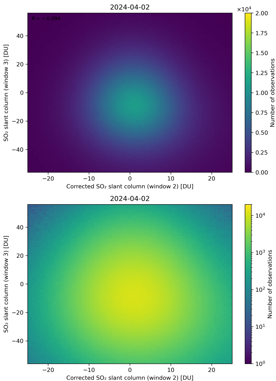
Figure 201: Scatter density plot of “Corrected SO 2 slant column (window 2)” against “SO 2 slant column (window 3)” for 2024-04-01 to 2024-04-03.
