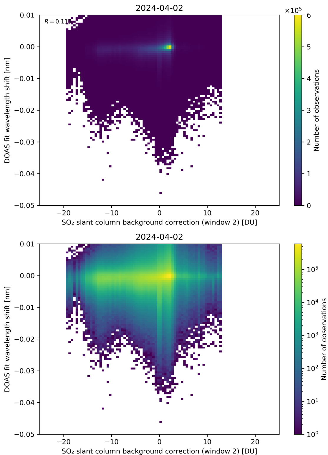
Figure 112: Scatter density plot of “SO 2 slant column background correction (window 2)” against “DOAS fit wavelength shift” for 2024-04-01 to 2024-04-03.
