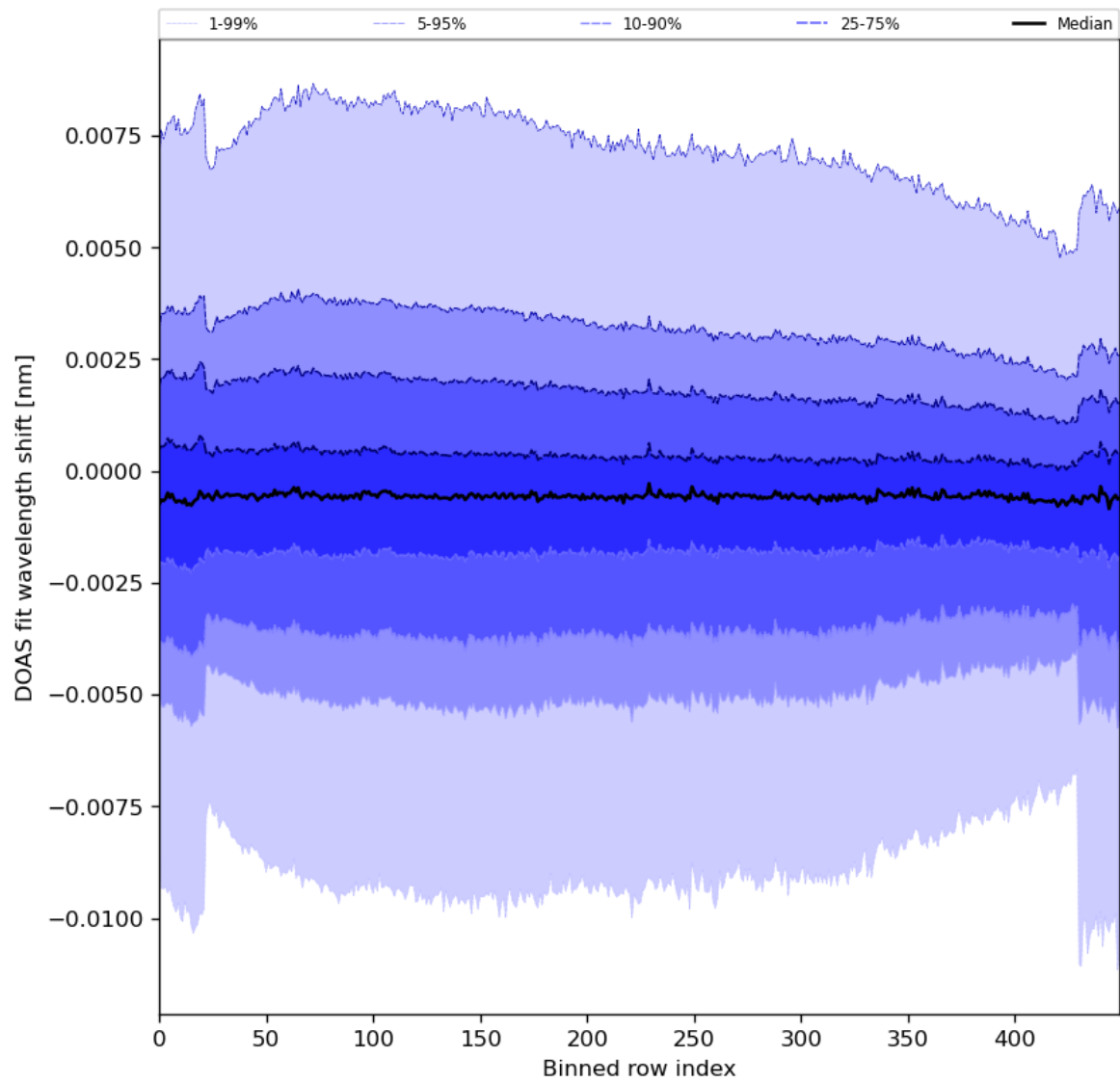
Figure 91: Along track statistics of “DOAS fit wavelength shift” for 2024-04-01 to 2024-04-03
