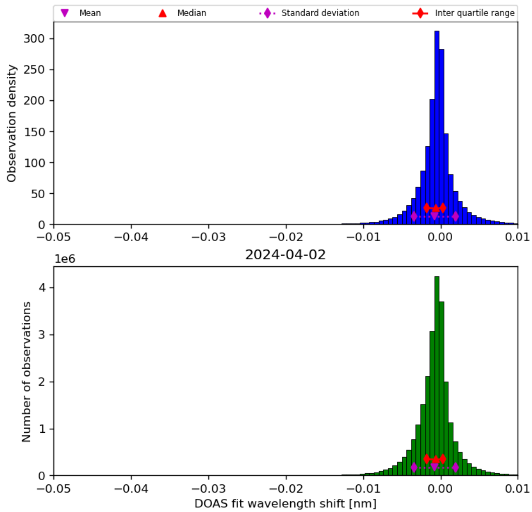
Figure 68: Histogram of “DOAS fit wavelength shift” for 2024-04-01 to 2024-04-03
