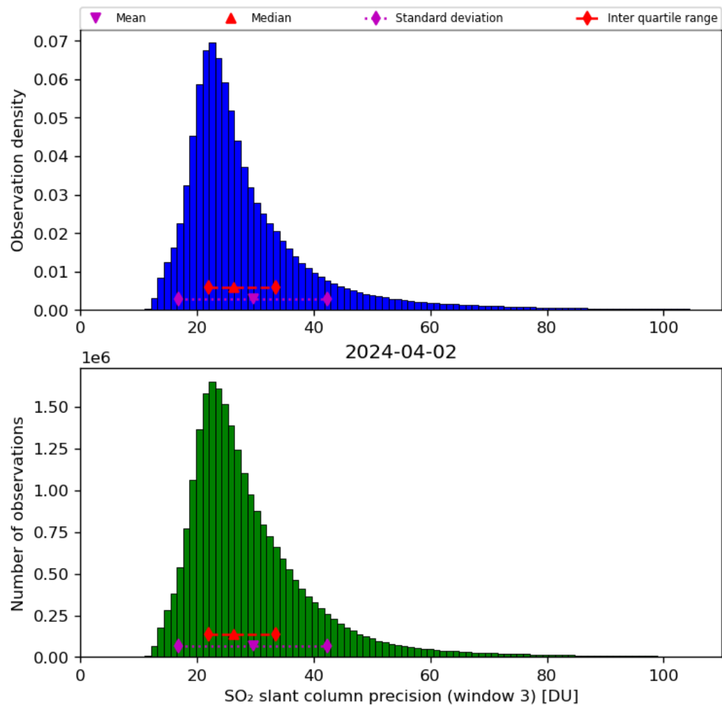
Figure 65: Histogram of “SO 2 slant column precision (window 3)” for 2024-04-01 to 2024-04-03
