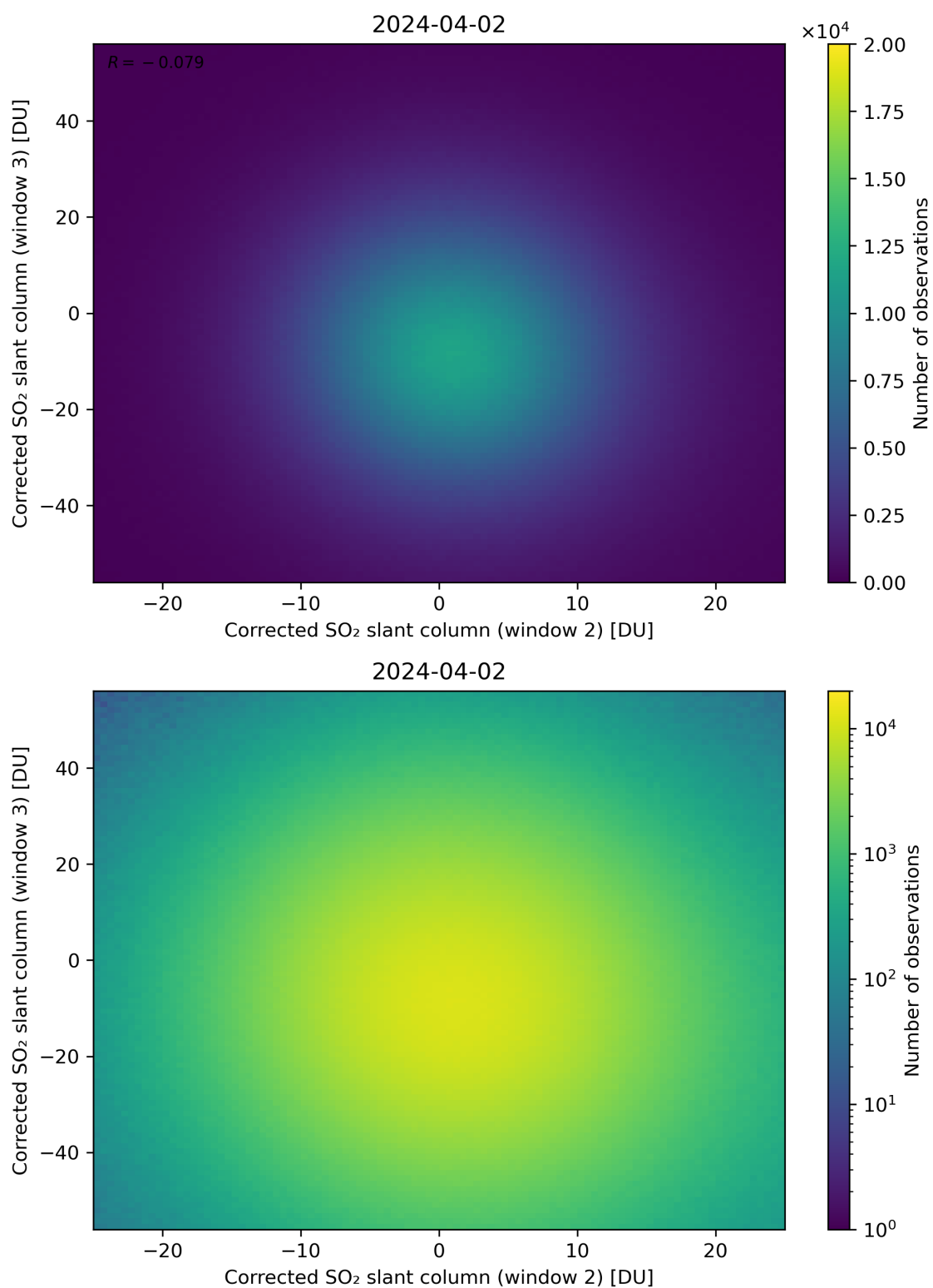
Figure 200: Scatter density plot of “Corrected SO 2 slant column (window 2)” against “Corrected SO 2 slant column (window 3)” for 2024-04-01 to 2024-04-03.
