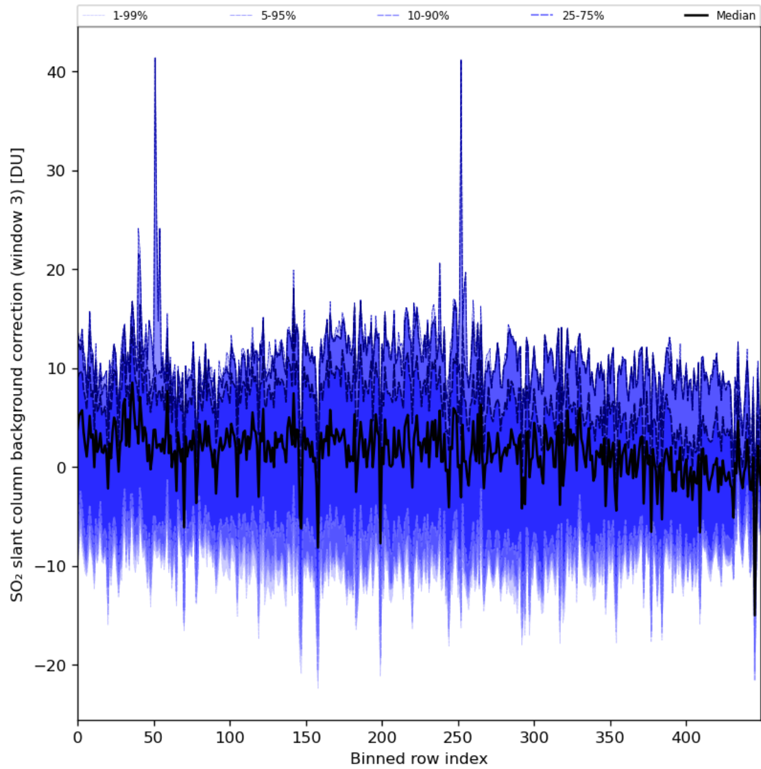
Figure 90: Along track statistics of “SO 2 slant column background correction (window 3)” for 2024-04-01 to 2024-04-03
