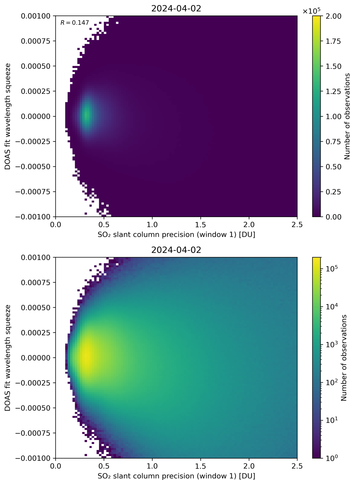
Figure 222: Scatter density plot of “SO 2 slant column precision (window 1)” against “DOAS fit wavelength squeeze” for 2024-04-01 to 2024-04-03.
