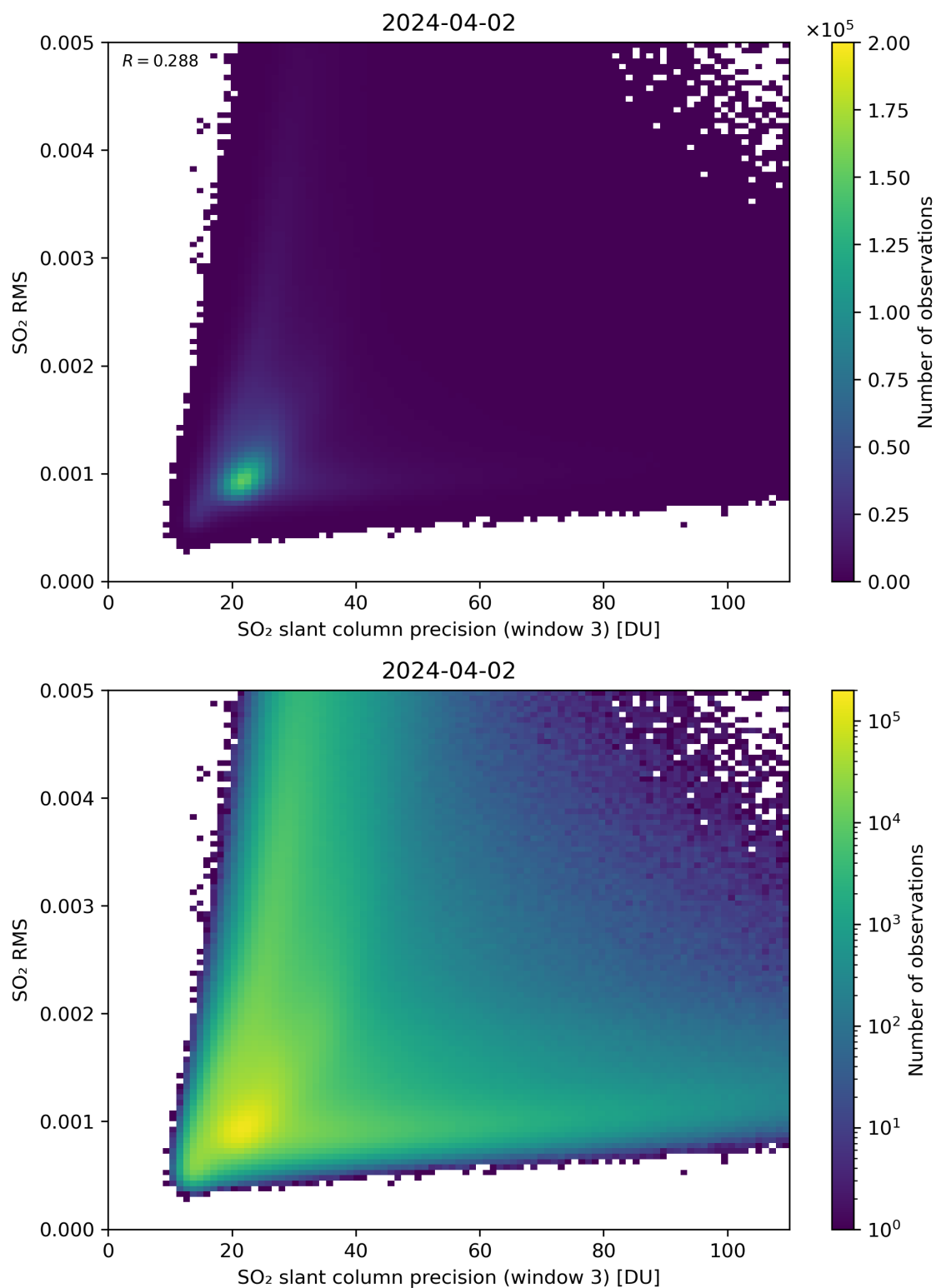
Figure 260: Scatter density plot of “SO 2 slant column precision (window 3)” against “SO 2 RMS” for 2024-04-01 to 2024-04-03.
