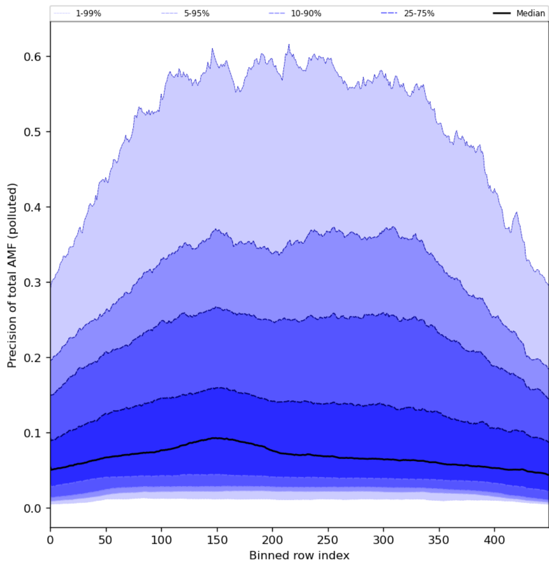
Figure 95: Along track statistics of “Precision of total AMF (polluted)” for 2024-04-01 to 2024-04-03
