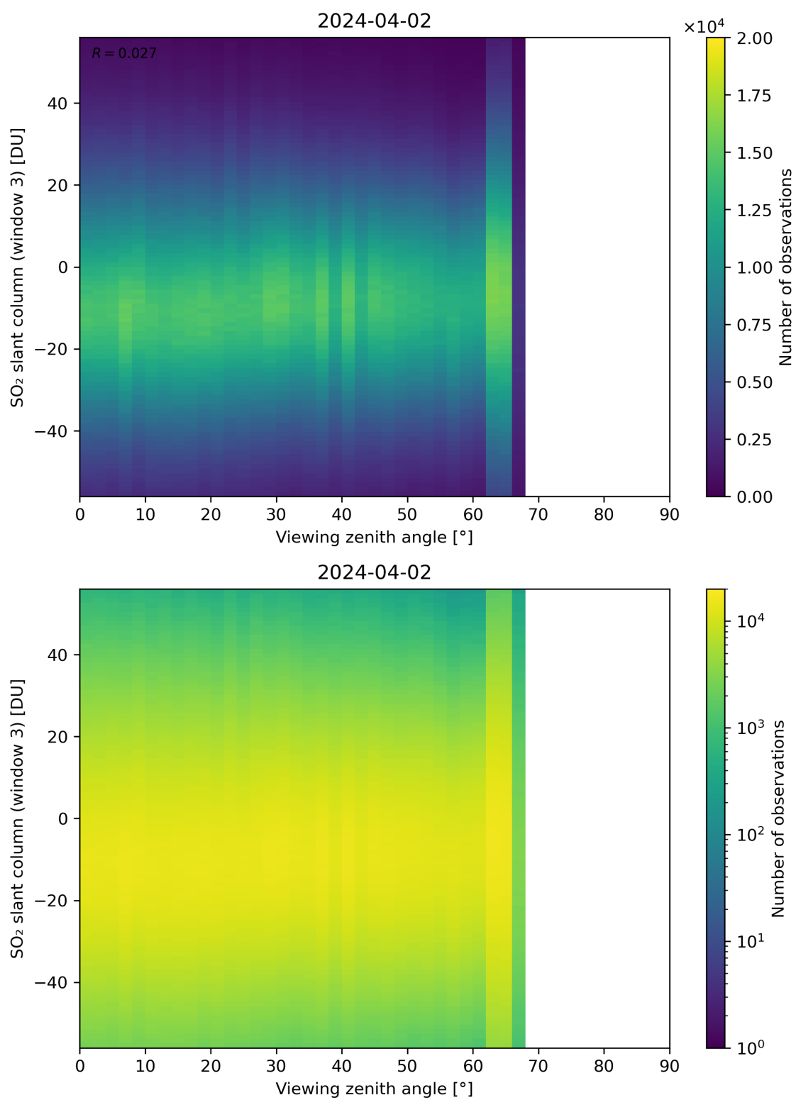
Figure 323: Scatter density plot of “Viewing zenith angle” against “SO 2 slant column (window 3)” for 2024-04-01 to 2024-04-03.
