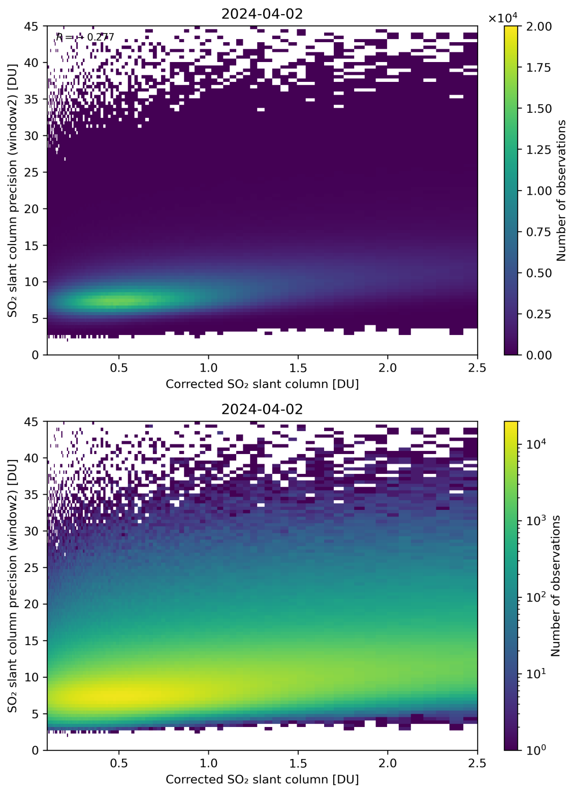
Figure 189: Scatter density plot of “Corrected SO 2 slant column” against “SO 2 slant column precision (window2)” for 2024-04-01 to 2024-04-03.
