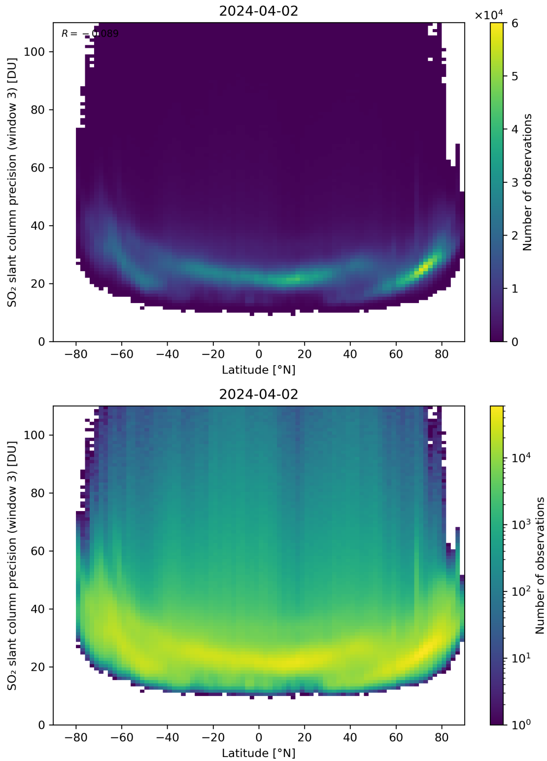
Figure 153: Scatter density plot of “Latitude” against “SO 2 slant column precision (window 3)” for 2024-04-01 to 2024-04-03.
