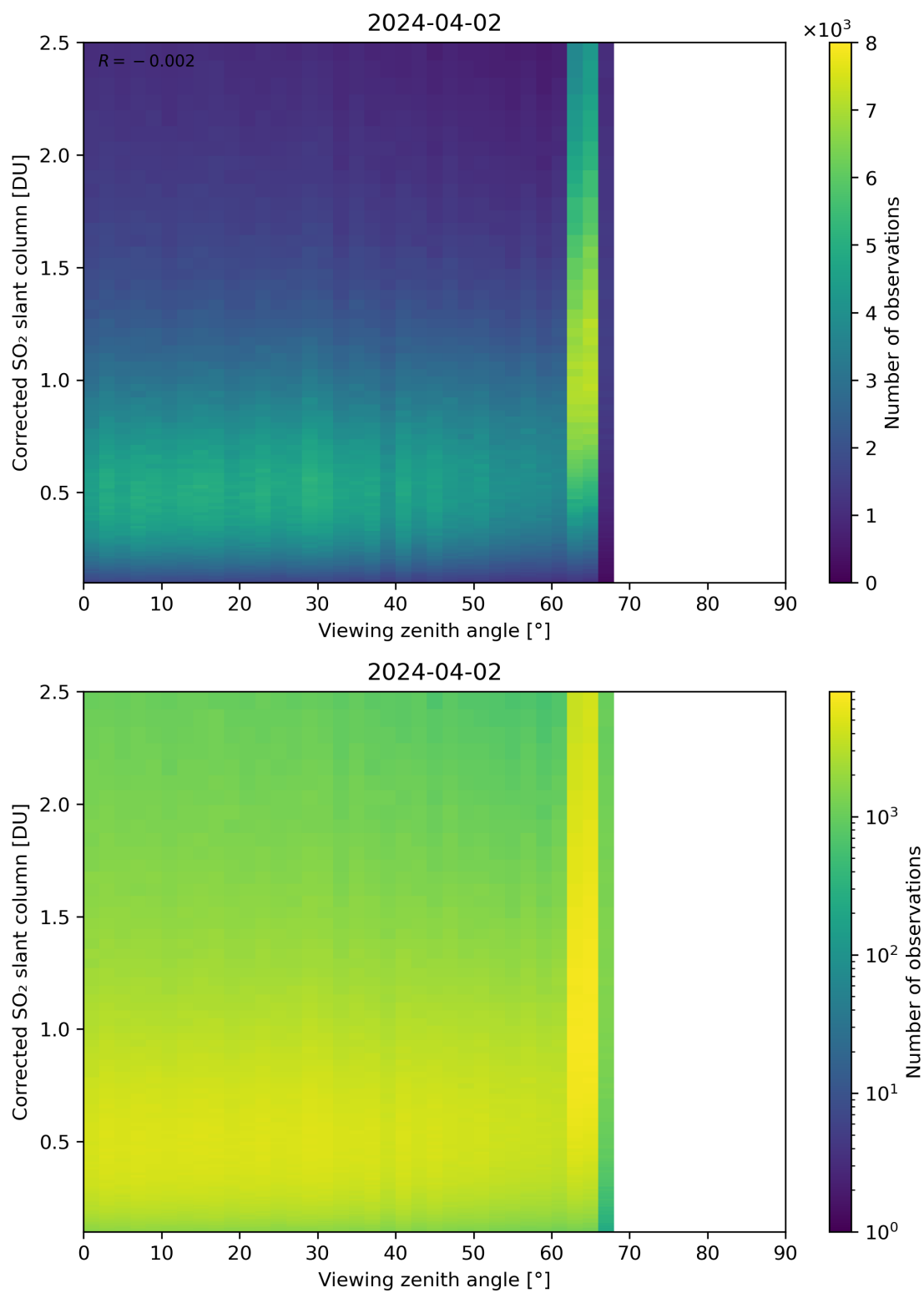
Figure 317: Scatter density plot of “Viewing zenith angle” against “Corrected SO 2 slant column” for 2024-04-01 to 2024-04-03.
