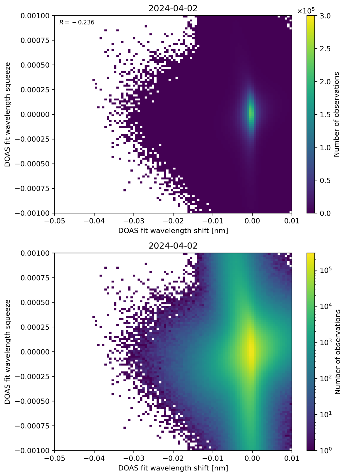
Figure 127: Scatter density plot of “DOAS fit wavelength shift” against “DOAS fit wavelength squeeze” for 2024-04-01 to 2024-04-03.
