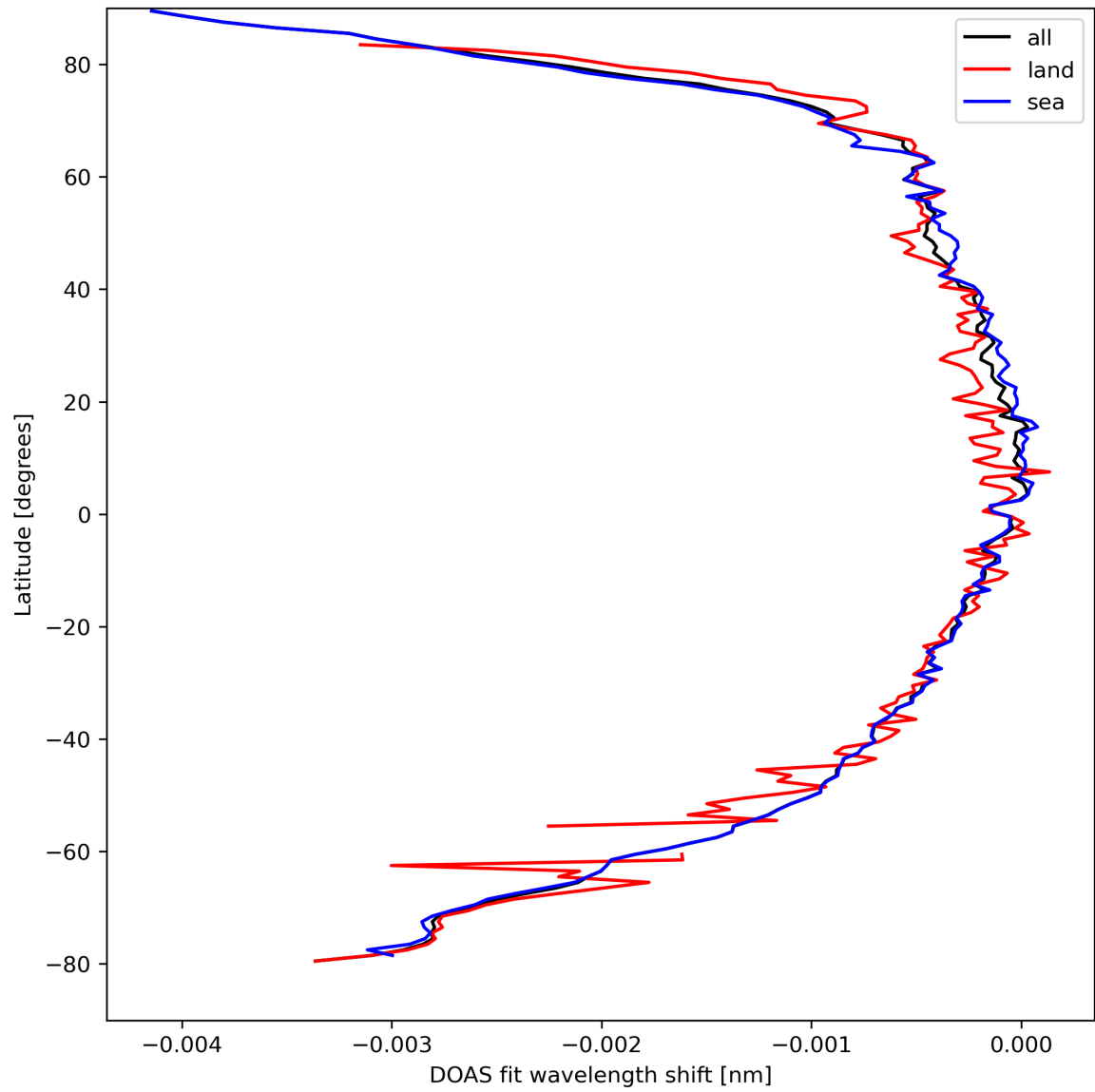
Figure 45: Zonal average of “DOAS fit wavelength shift” for 2024-04-01 to 2024-04-03.
