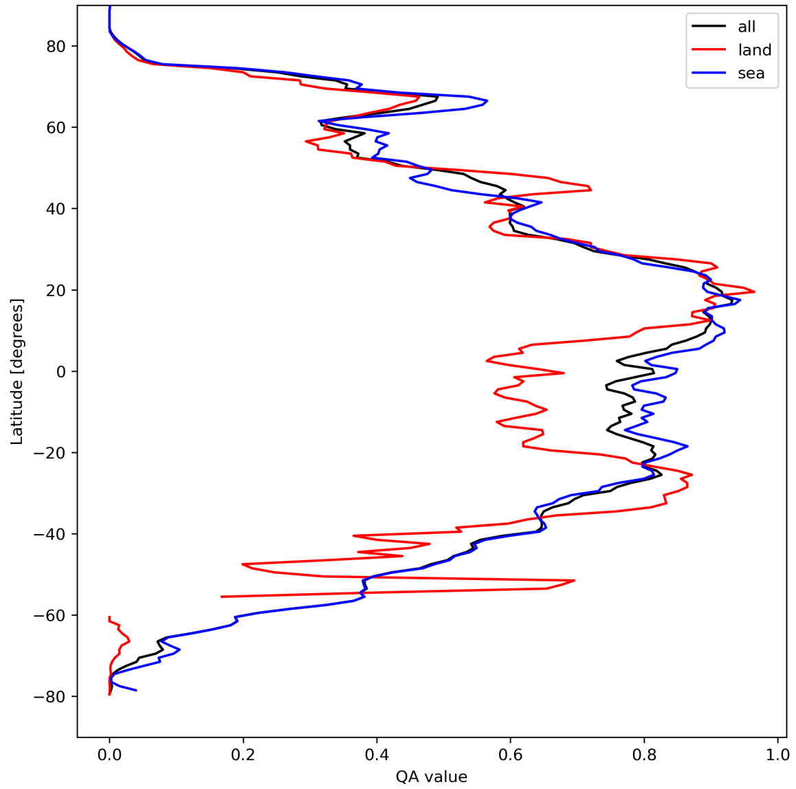
Figure 29: Zonal average of “QA value” for 2024-04-01 to 2024-04-03.
