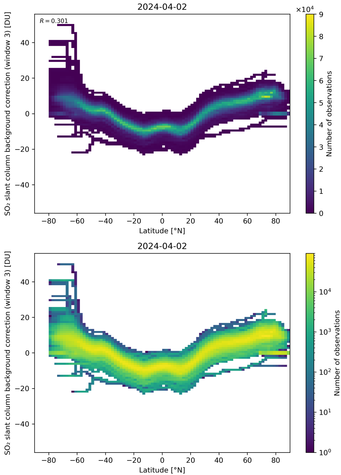
Figure 141: Scatter density plot of “Latitude” against “SO 2 slant column background correction (window 3)” for 2024-04-01 to 2024-04-03.
