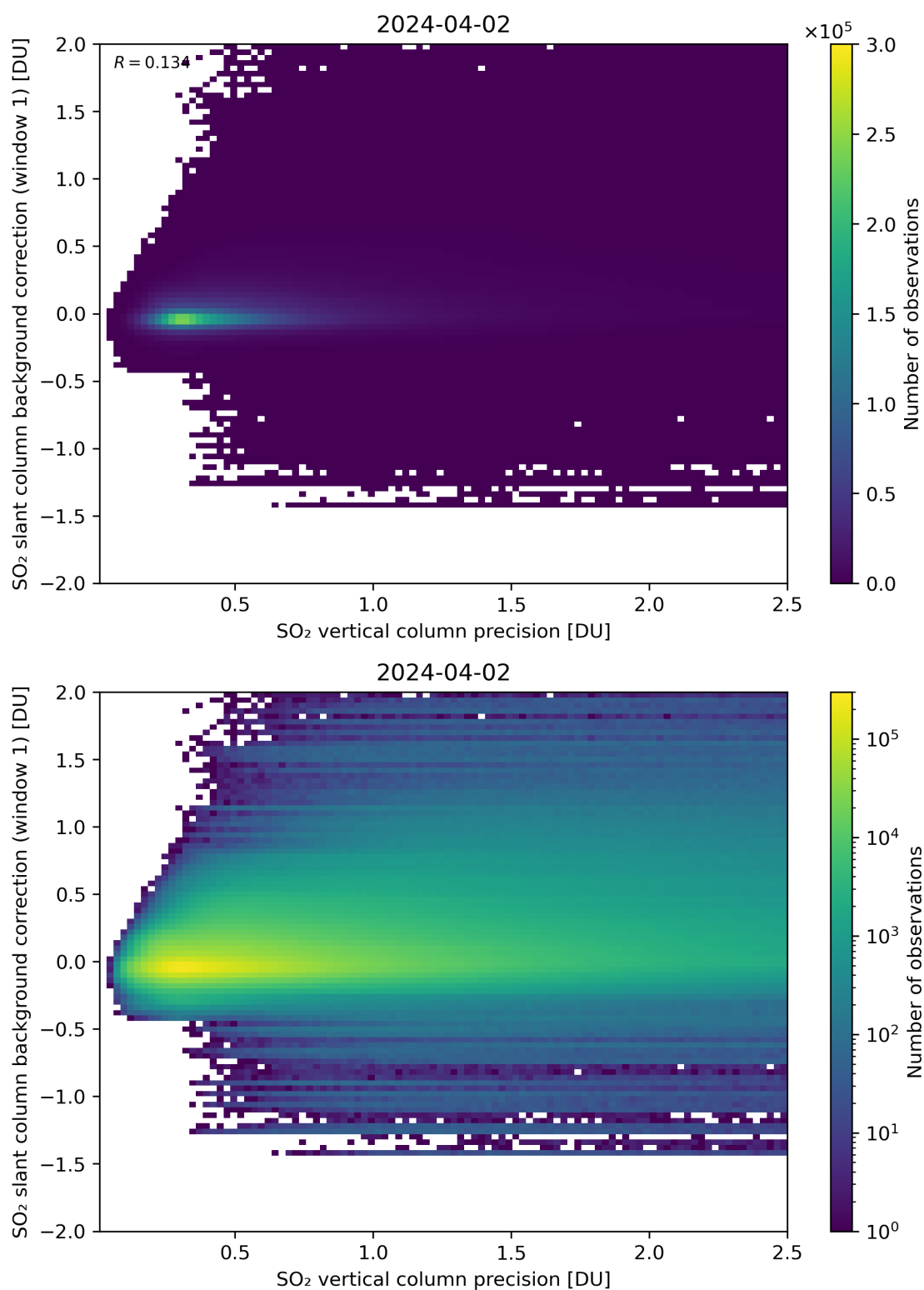
Figure 279: Scatter density plot of “SO 2 vertical column precision” against “SO 2 slant column background correction (window 1)” for 2024-04-01 to 2024-04-03.
