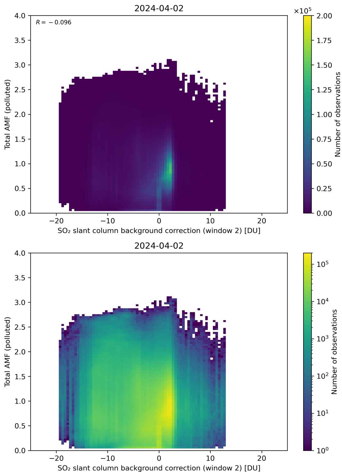
Figure 119: Scatter density plot of “SO 2 slant column background correction (window 2)” against “Total AMF (polluted)” for 2024-04-01 to 2024-04-03.
