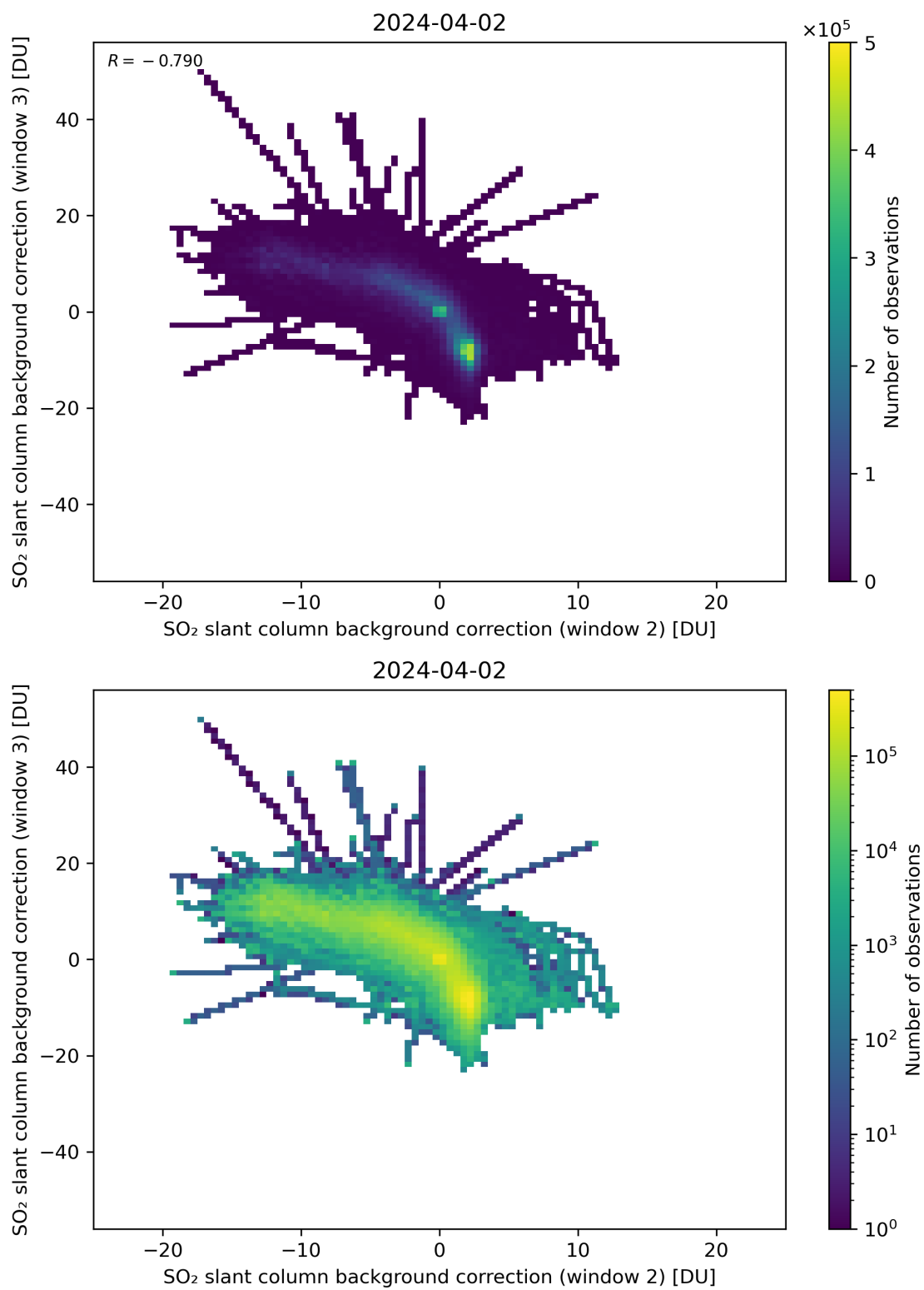
Figure 111: Scatter density plot of “SO 2 slant column background correction (window 2)” against “SO 2 slant column background correction (window 3)” for 2024-04-01 to 2024-04-03.
