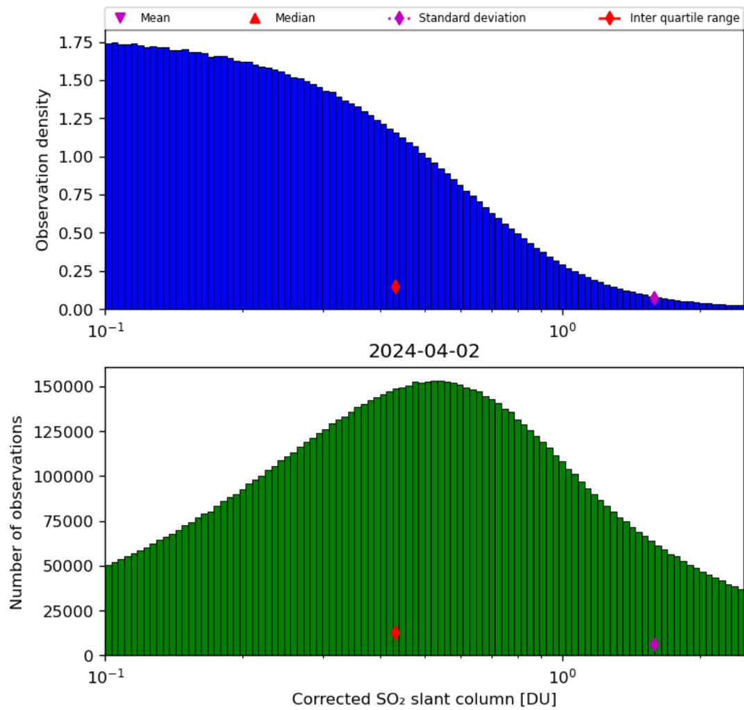
Figure 55: Histogram of “Corrected SO 2 slant column” for 2024-04-01 to 2024-04-03
