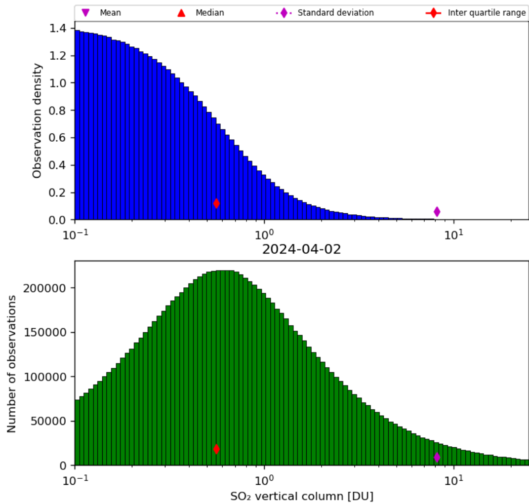
Figure 53: Histogram of “SO 2 vertical column” for 2024-04-01 to 2024-04-03
