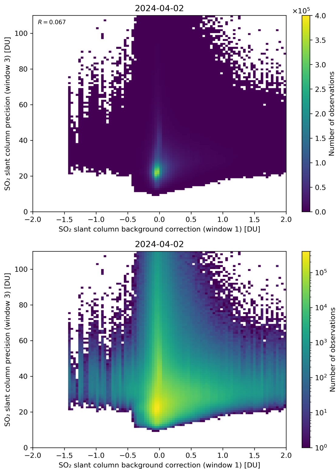
Figure 108: Scatter density plot of “SO 2 slant column background correction (window 1)” against “SO 2 slant column precision (window 3)” for 2024-04-01 to 2024-04-03.
