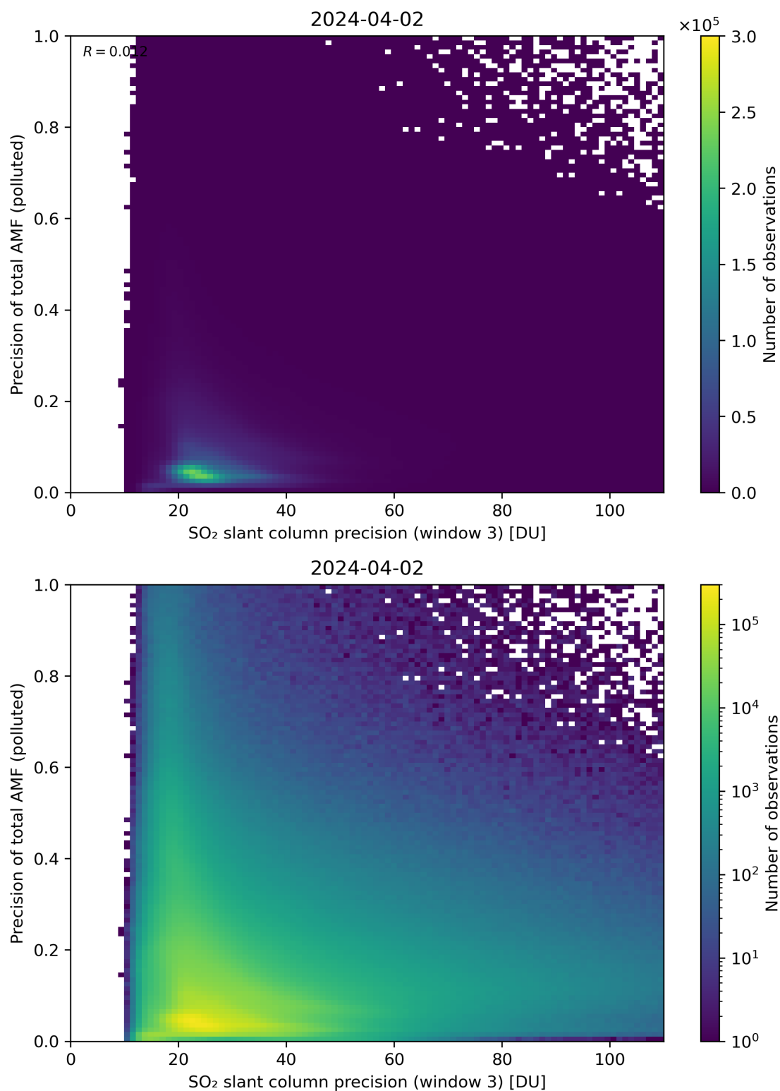
Figure 264: Scatter density plot of “SO 2 slant column precision (window 3)” against “Precision of total AMF (polluted)” for 2024-04-01 to 2024-04-03.
