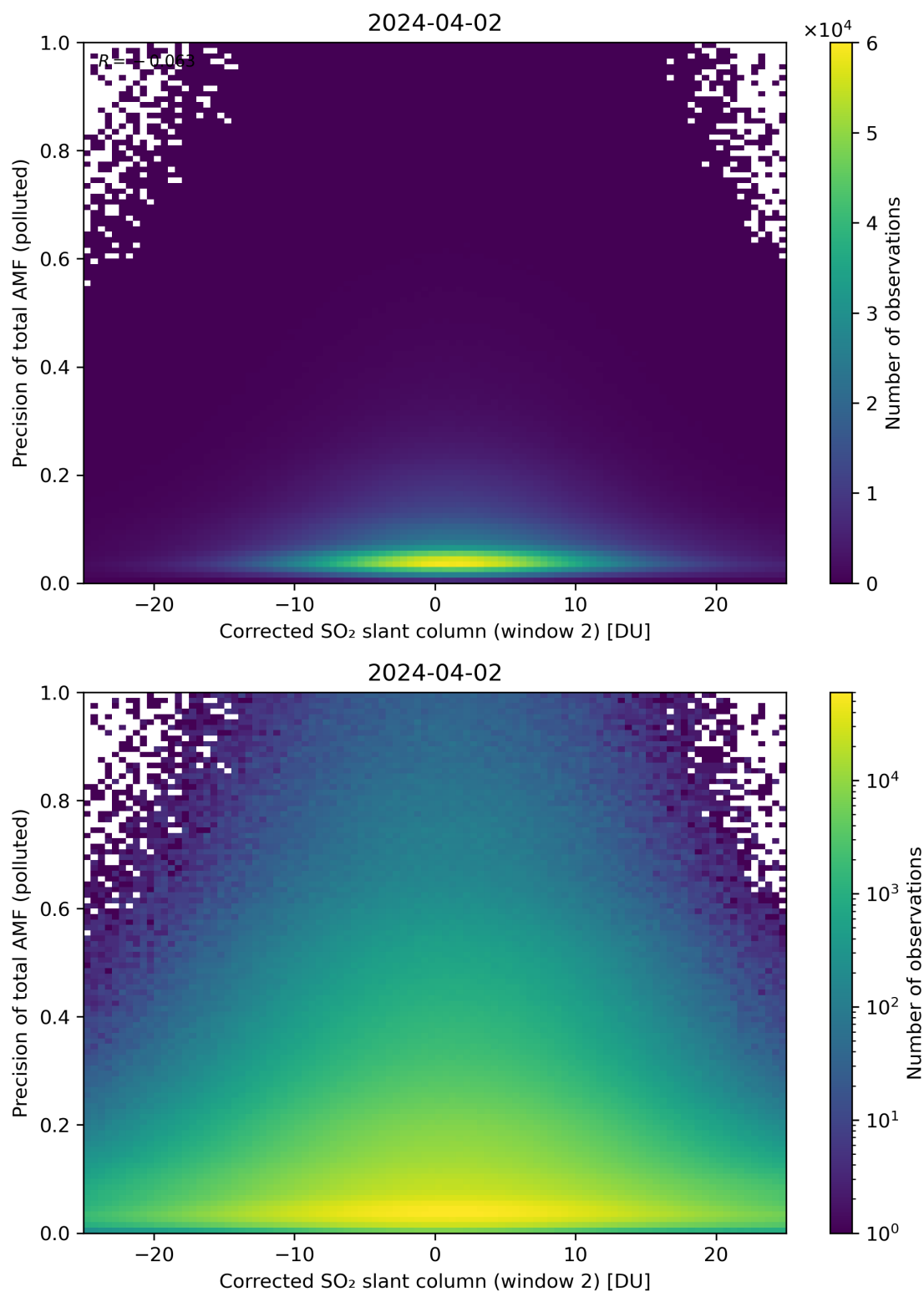
Figure 204: Scatter density plot of “Corrected SO 2 slant column (window 2)” against “Precision of total AMF (polluted)” for 2024-04-01 to 2024-04-03.
