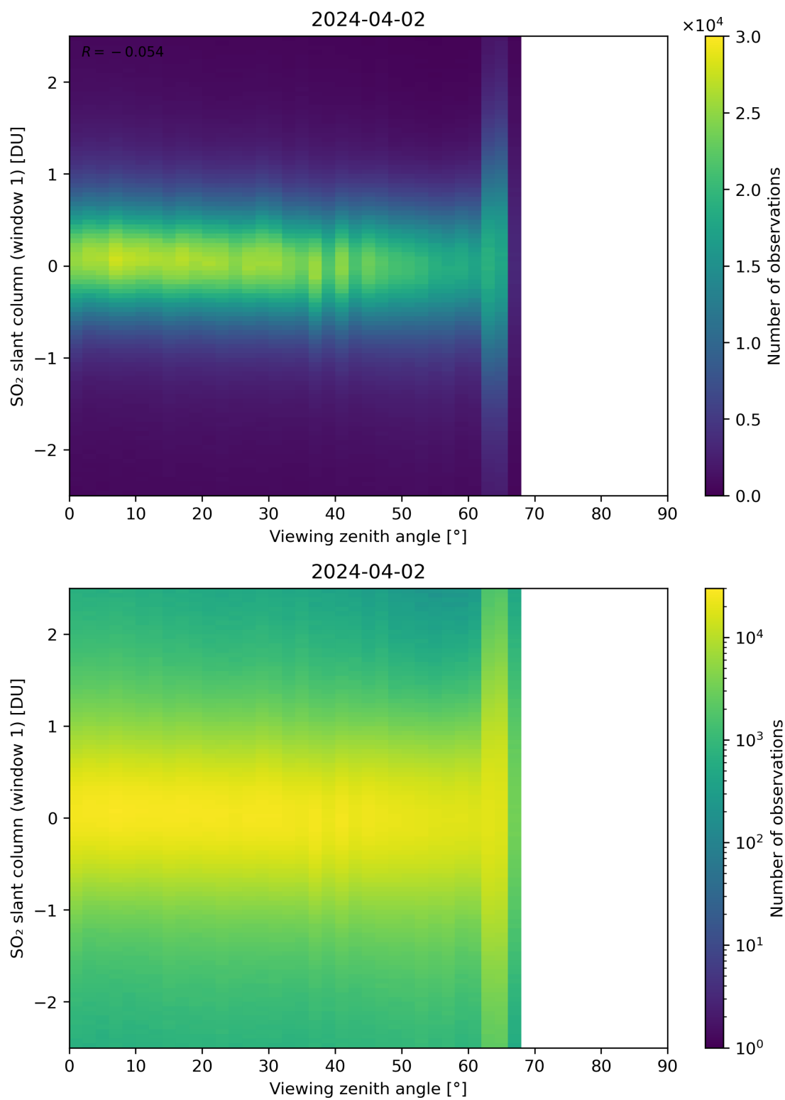
Figure 320: Scatter density plot of “Viewing zenith angle” against “SO 2 slant column (window 1)” for 2024-04-01 to 2024-04-03.
