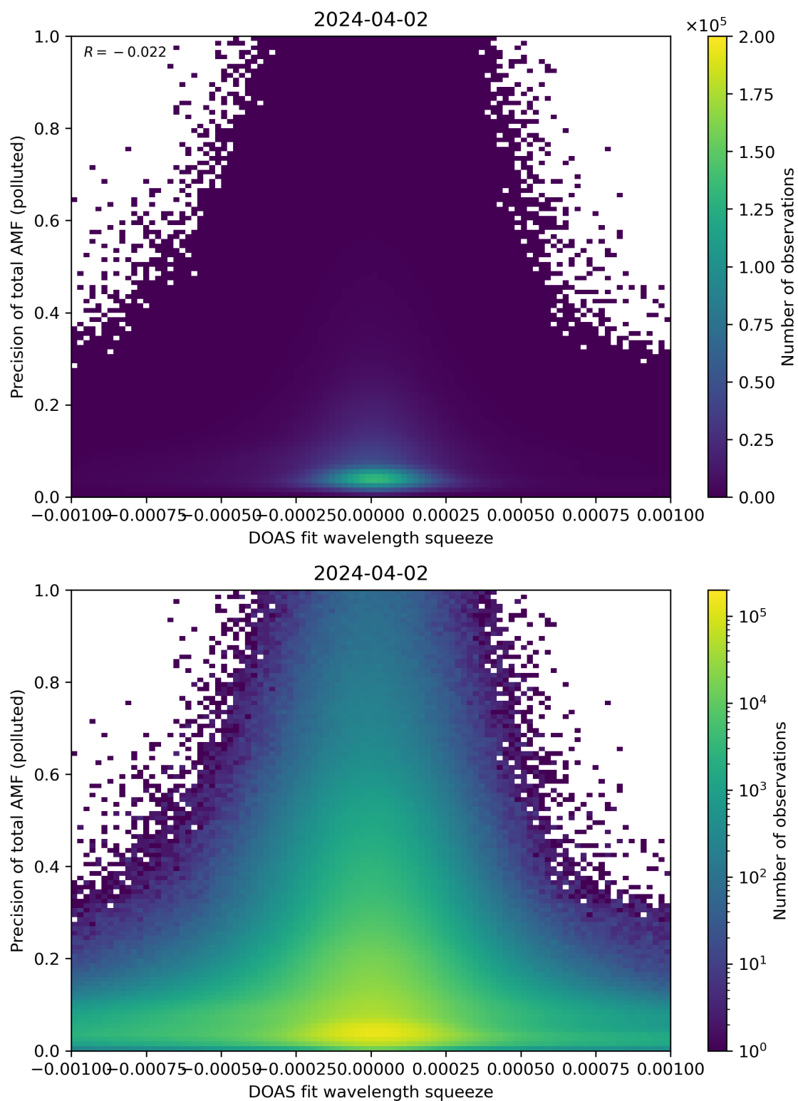
Figure 135: Scatter density plot of “DOAS fit wavelength squeeze” against “Precision of total AMF (polluted)” for 2024-04-01 to 2024-04-03.
