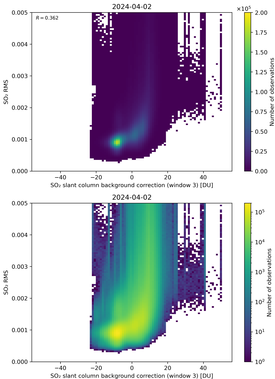
Figure 123: Scatter density plot of “SO 2 slant column background correction (window 3)” against “SO 2 RMS” for 2024-04-01 to 2024-04-03.
