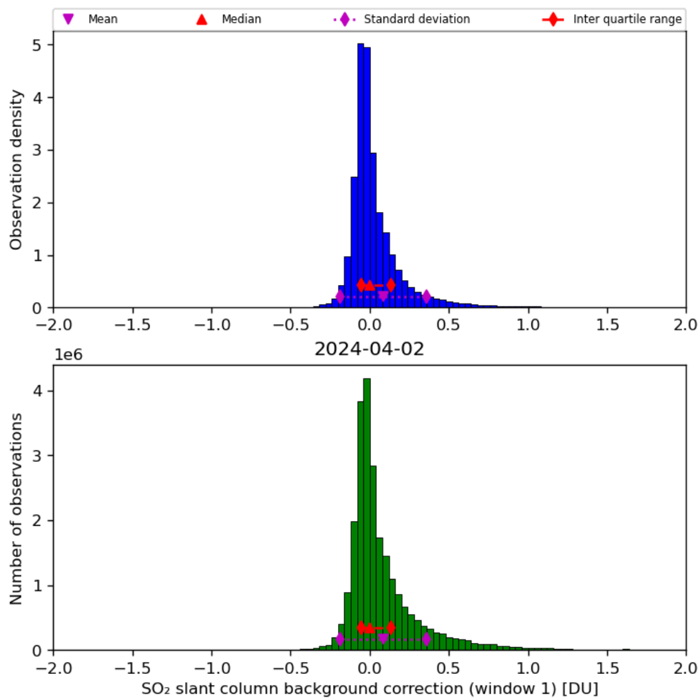
Figure 59: Histogram of “SO 2 slant column background correction (window 1)” for 2024-04-01 to 2024-04-03
