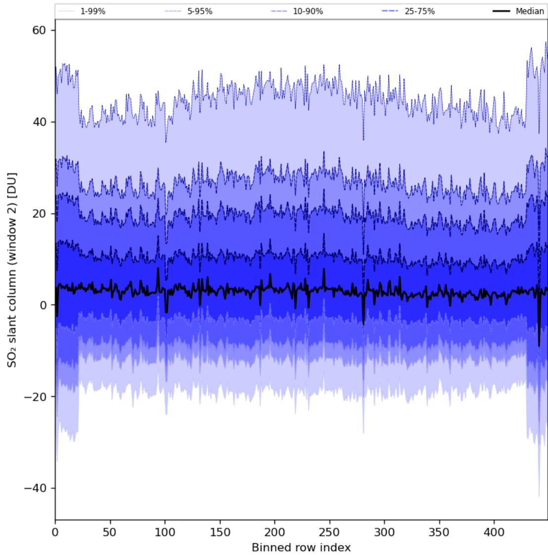
Figure 83: Along track statistics of “SO 2 slant column (window 2)” for 2024-04-01 to 2024-04-03
