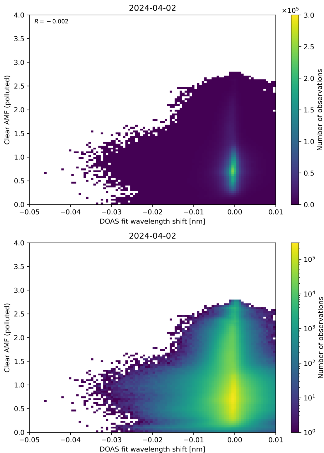
Figure 129: Scatter density plot of “DOAS fit wavelength shift” against “Clear AMF (polluted)” for 2024-04-01 to 2024-04-03.
