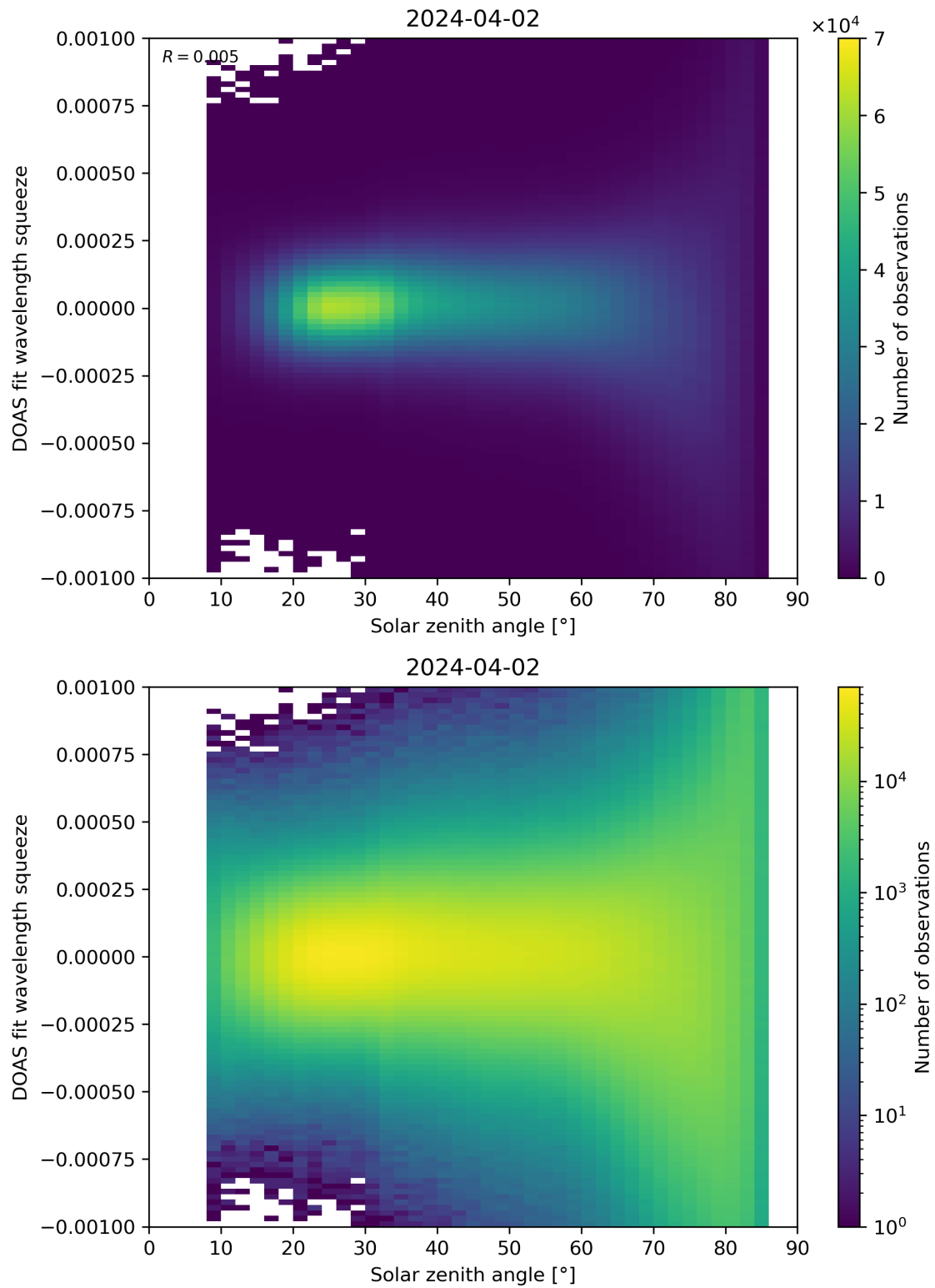
Figure 162: Scatter density plot of “Solar zenith angle” against “DOAS fit wavelength squeeze” for 2024-04-01 to 2024-04-03.
