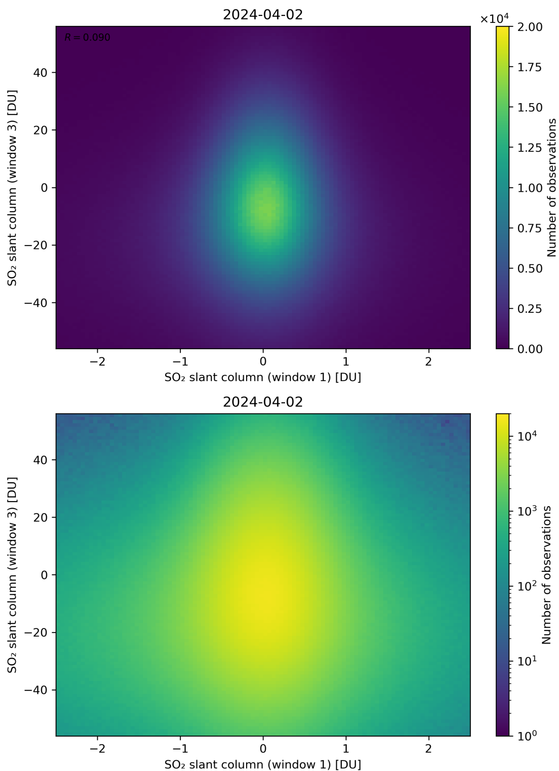
Figure 237: Scatter density plot of “SO 2 slant column (window 1)” against “SO 2 slant column (window 3)” for 2024-04-01 to 2024-04-03.
