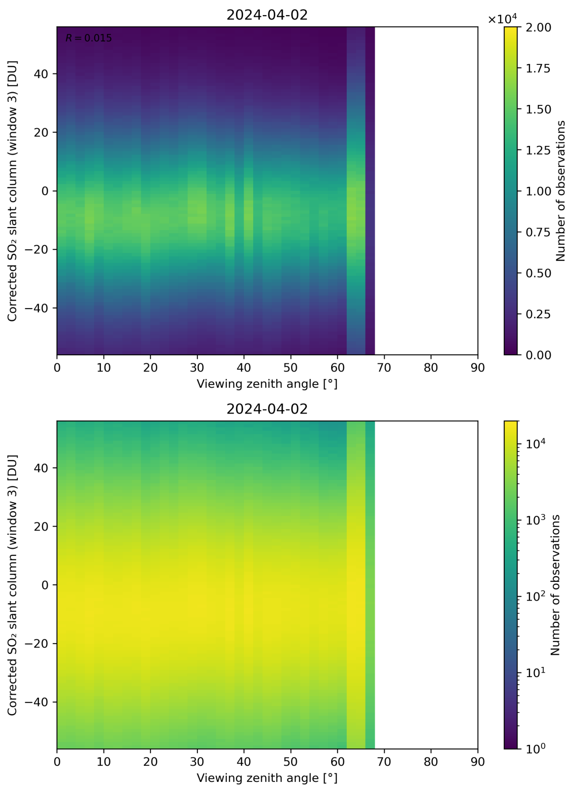
Figure 319: Scatter density plot of “Viewing zenith angle” against “Corrected SO 2 slant column (window 3)” for 2024-04-01 to 2024-04-03.
