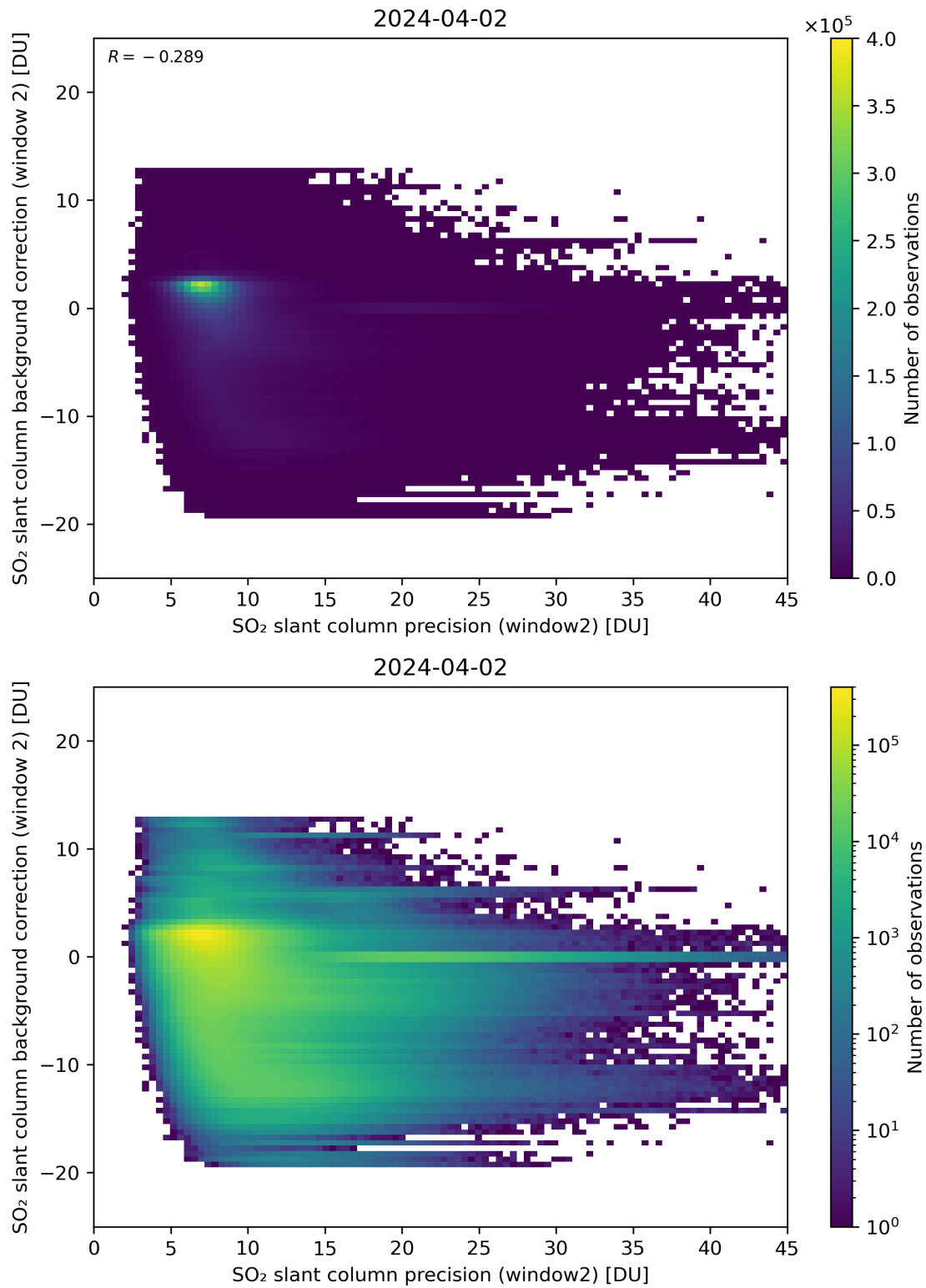
Figure 241: Scatter density plot of “SO 2 slant column precision (window2)” against “SO 2 slant column background correction (window 2)” for 2024-04-01 to 2024-04-03.
