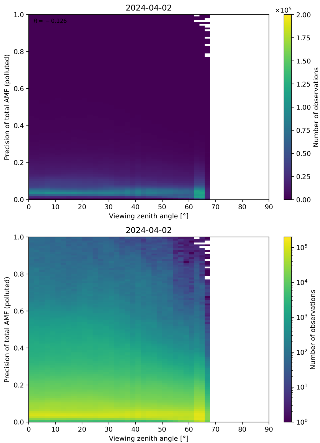
Figure 326: Scatter density plot of “Viewing zenith angle” against “Precision of total AMF (polluted)” for 2024-04-01 to 2024-04-03.
