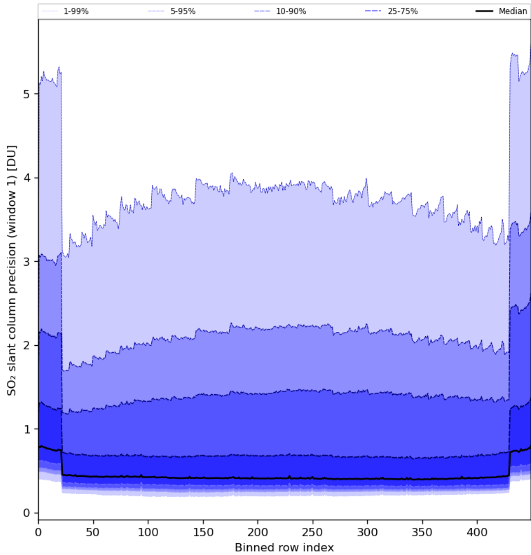
Figure 80: Along track statistics of “SO 2 slant column precision (window 1)” for 2024-04-01 to 2024-04-03
