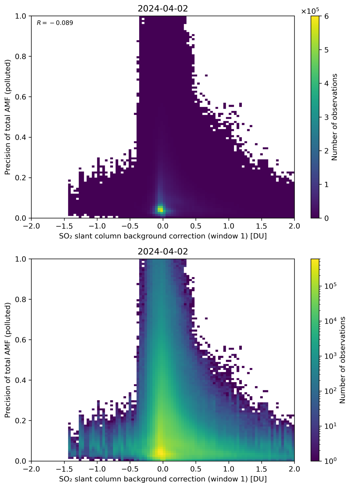
Figure 110: Scatter density plot of “SO 2 slant column background correction (window 1)” against “Precision of total AMF (polluted)” for 2024-04-01 to 2024-04-03.
