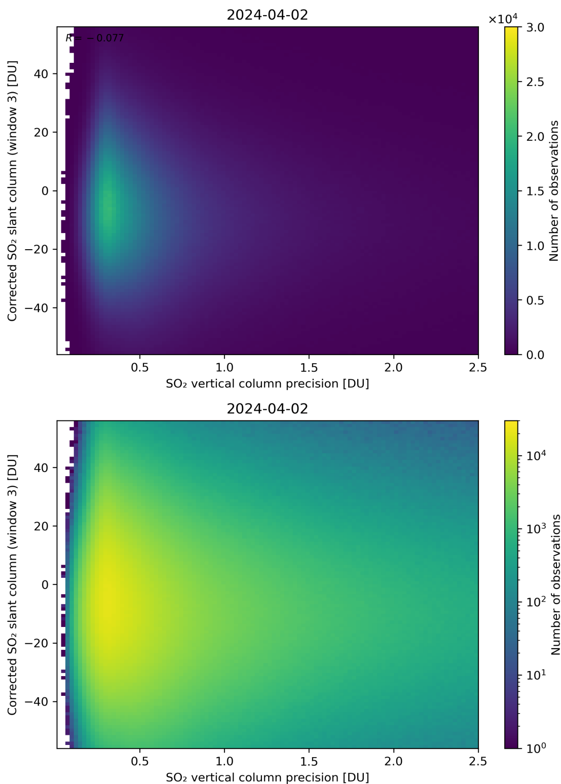
Figure 288: Scatter density plot of “SO 2 vertical column precision” against “Corrected SO 2 slant column (window 3)” for 2024-04-01 to 2024-04-03.
