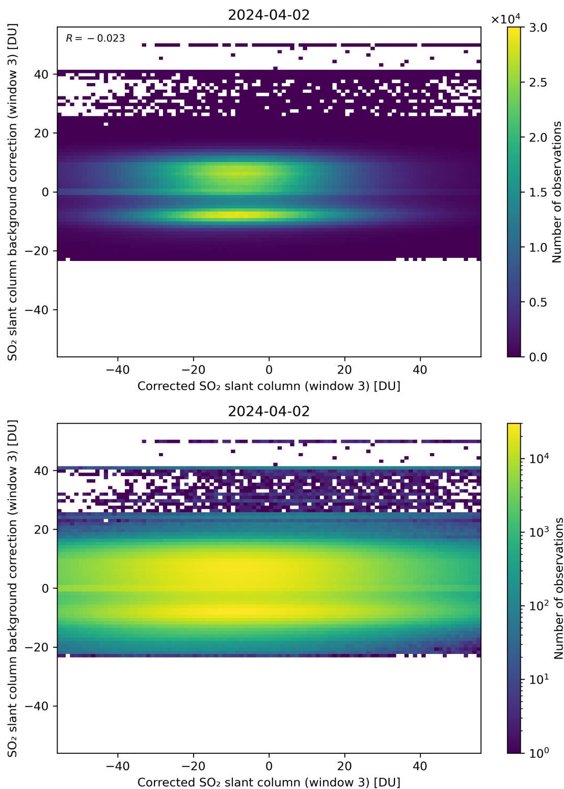
Figure 205: Scatter density plot of “Corrected SO 2 slant column (window 3)” against “SO 2 slant column background correction (window 3)” for 2024-04-01 to 2024-04-03.
