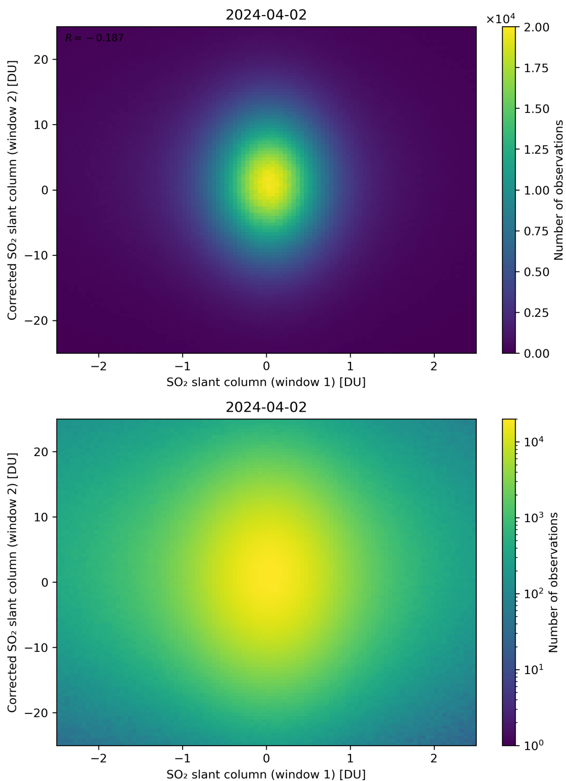
Figure 233: Scatter density plot of “SO 2 slant column (window 1)” against “Corrected SO 2 slant column (window 2)” for 2024-04-01 to 2024-04-03.
