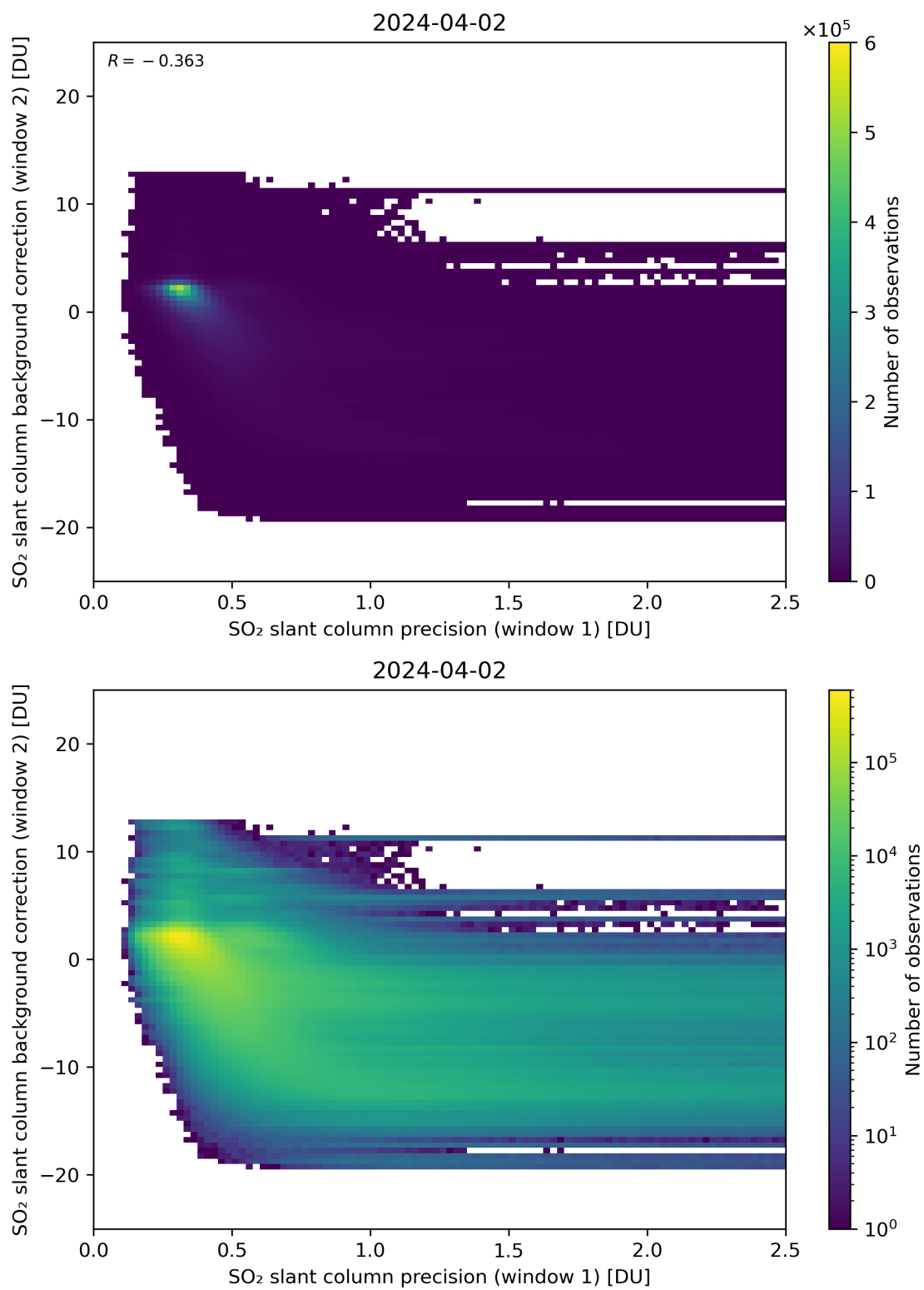
Figure 219: Scatter density plot of “SO 2 slant column precision (window 1)” against “SO 2 slant column background correction (window 2)” for 2024-04-01 to 2024-04-03.
