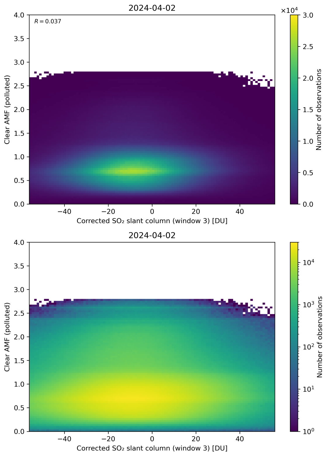
Figure 209: Scatter density plot of “Corrected SO 2 slant column (window 3)” against “Clear AMF (polluted)” for 2024-04-01 to 2024-04-03.
