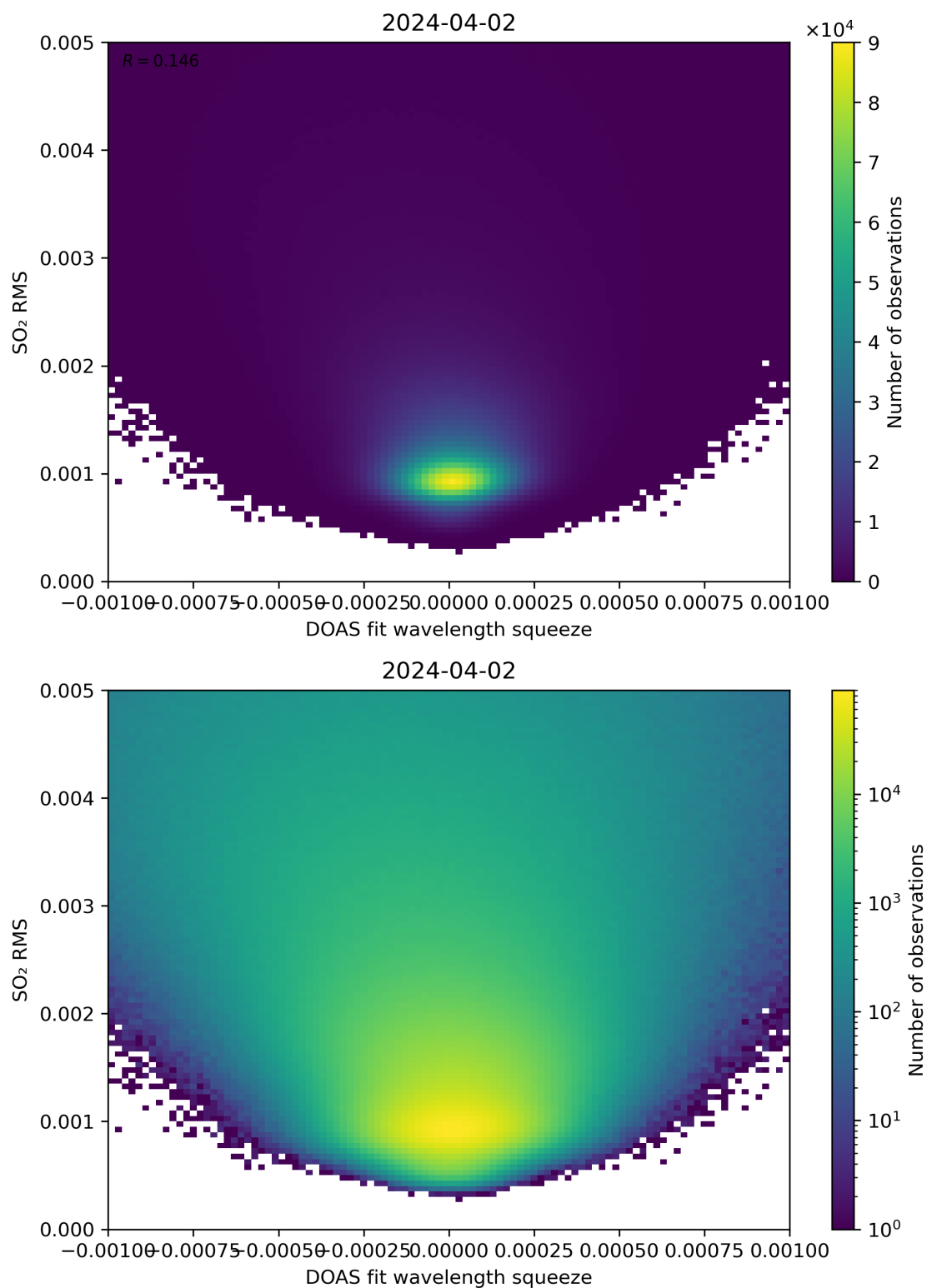
Figure 132: Scatter density plot of “DOAS fit wavelength squeeze” against “SO 2 RMS” for 2024-04-01 to 2024-04-03.
