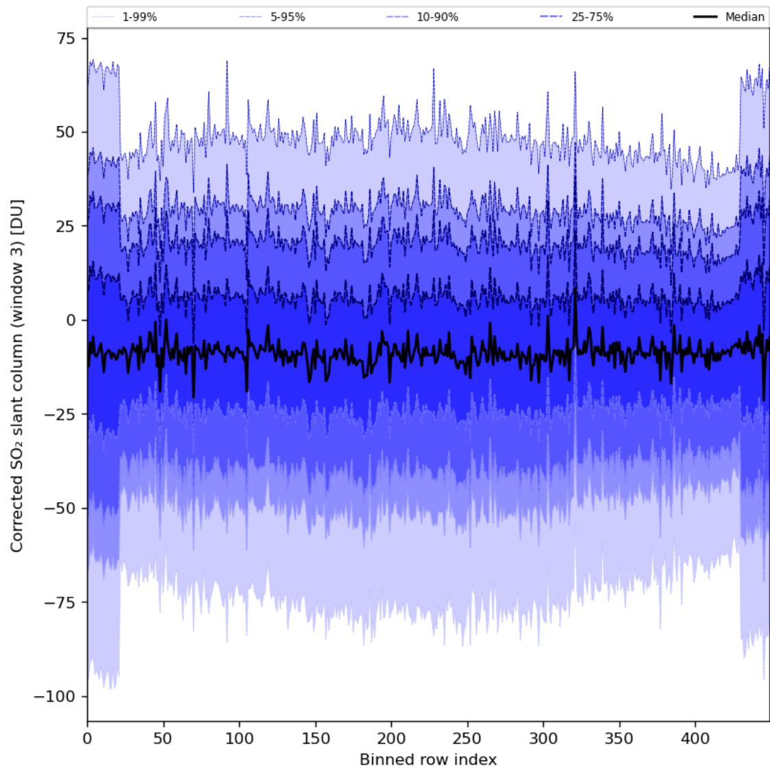
Figure 89: Along track statistics of “Corrected SO 2 slant column (window 3)” for 2024-04-01 to 2024-04-03
