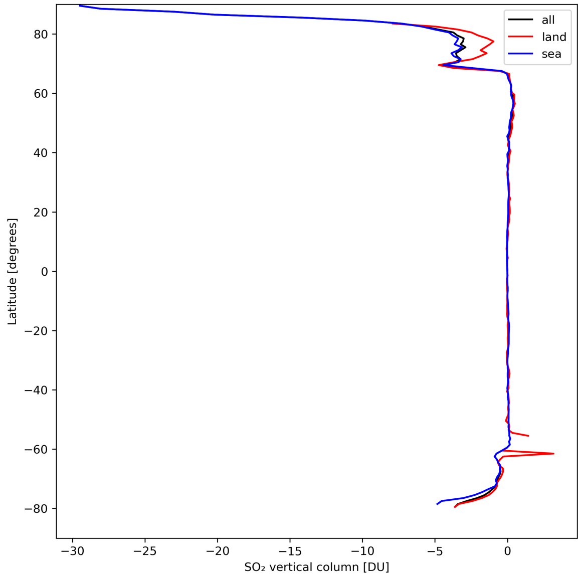
Figure 30: Zonal average of “SO 2 vertical column” for 2024-04-01 to 2024-04-03.
