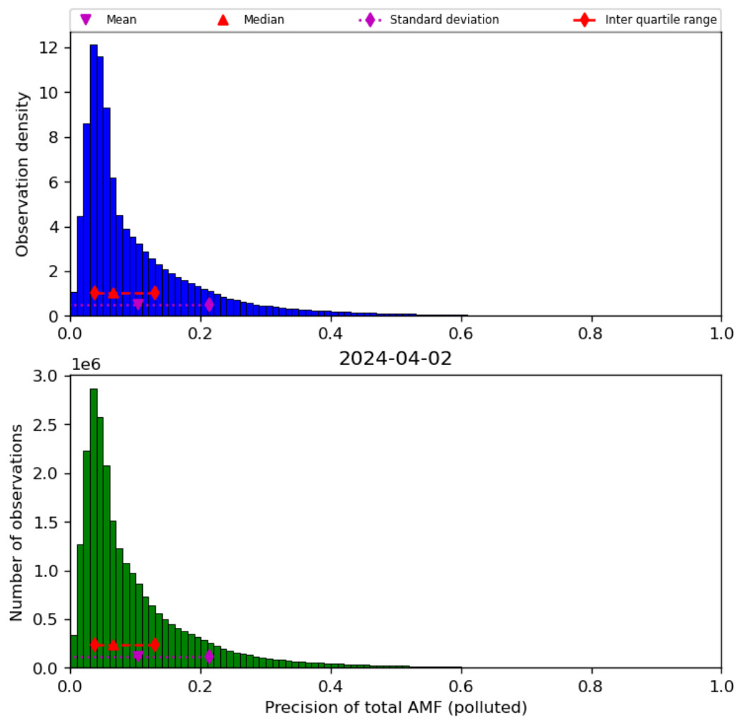
Figure 72: Histogram of “Precision of total AMF (polluted)” for 2024-04-01 to 2024-04-03
