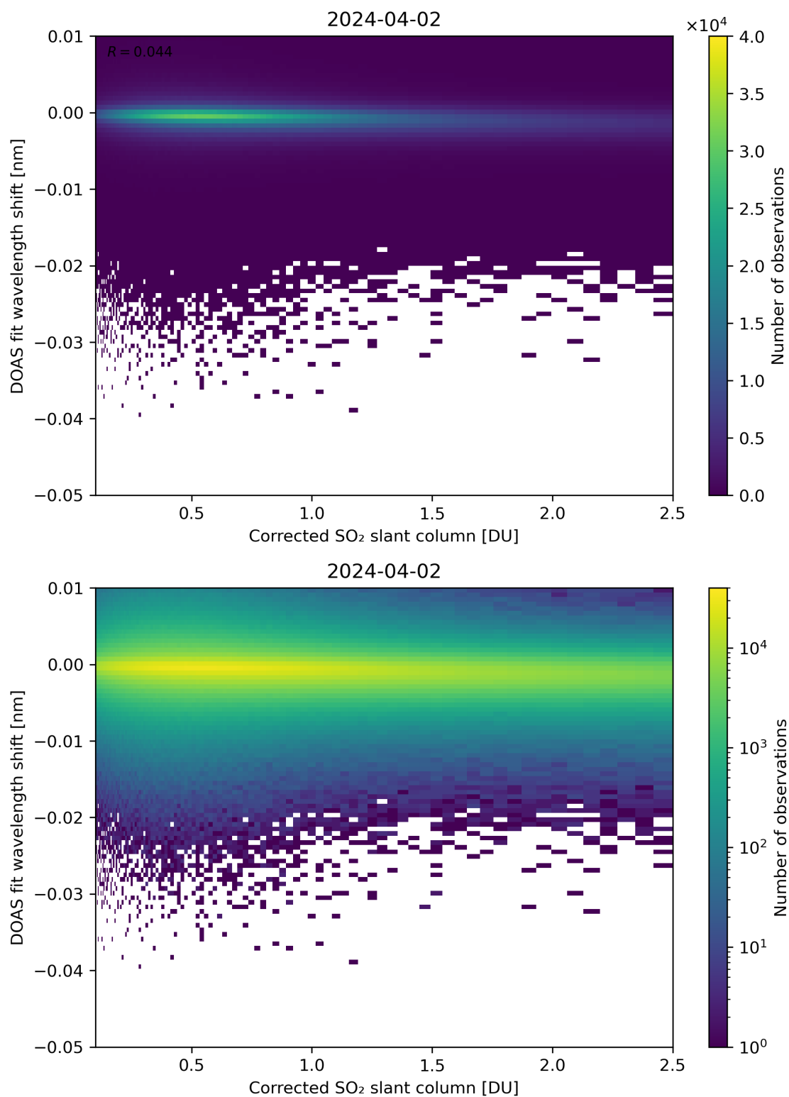
Figure 181: Scatter density plot of “Corrected SO 2 slant column” against “DOAS fit wavelength shift” for 2024-04-01 to 2024-04-03.
