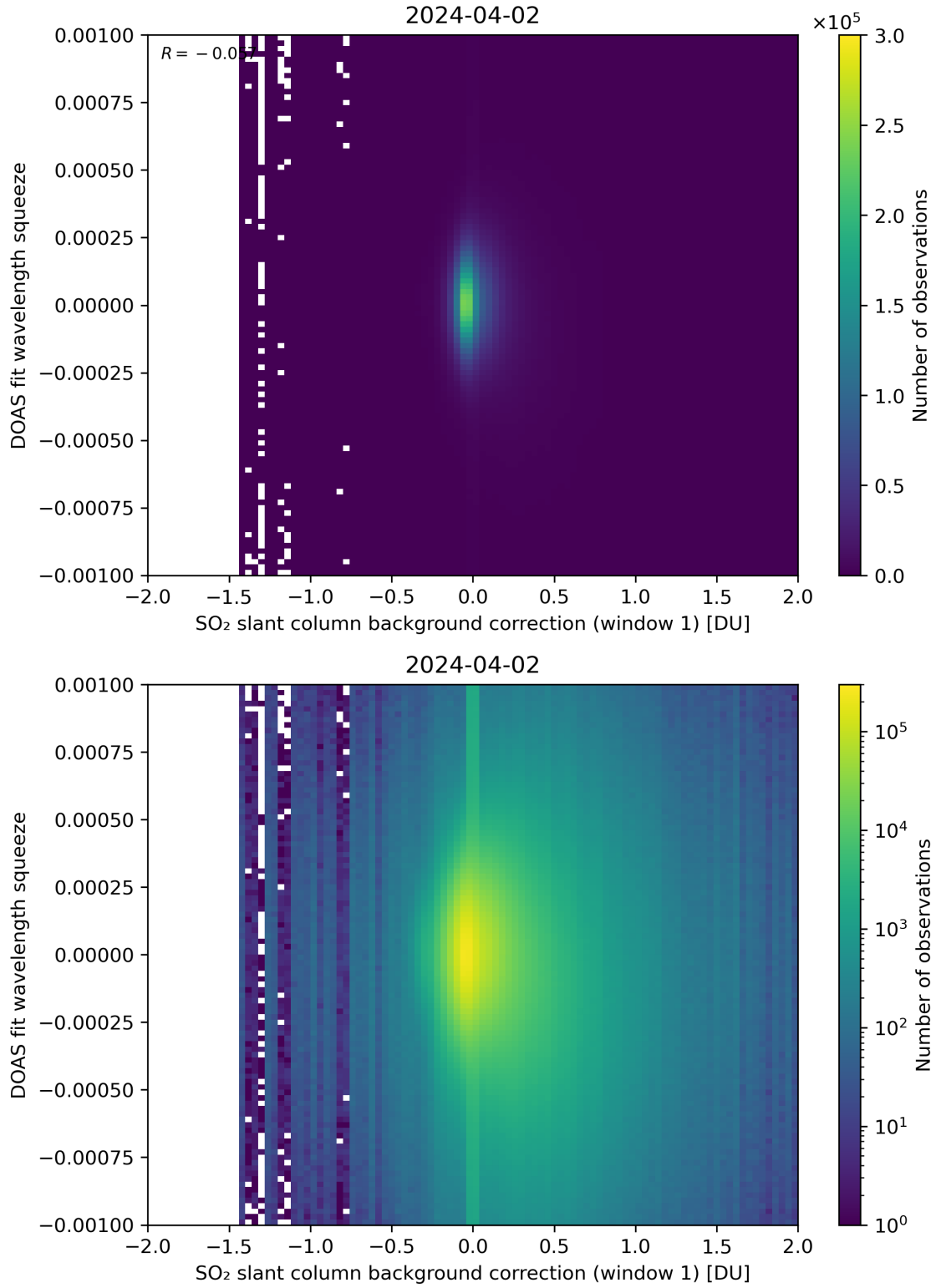
Figure 101: Scatter density plot of “SO 2 slant column background correction (window 1)” against “DOAS fit wavelength squeeze” for 2024-04-01 to 2024-04-03.
