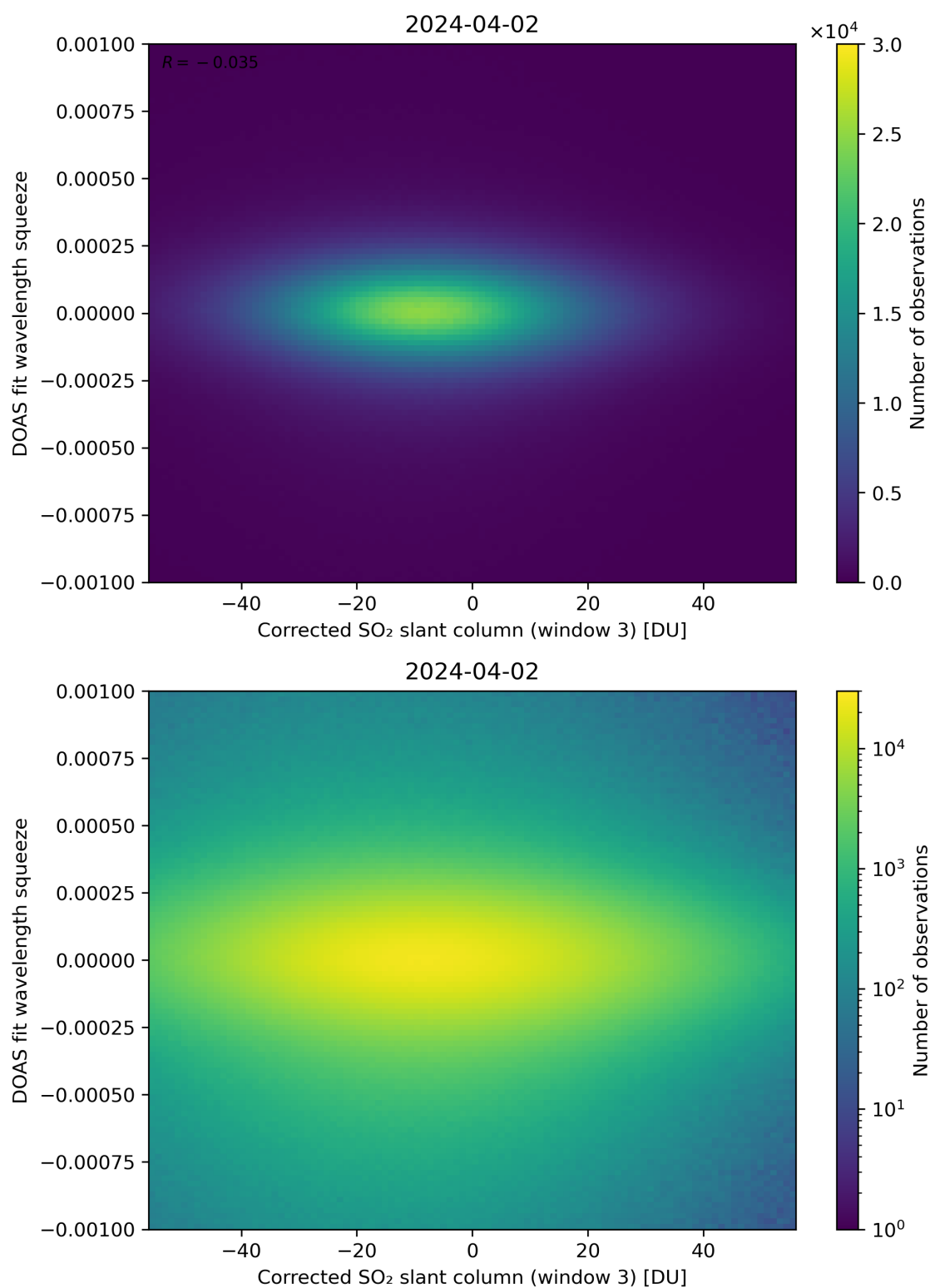
Figure 207: Scatter density plot of “Corrected SO 2 slant column (window 3)” against “DOAS fit wavelength squeeze” for 2024-04-01 to 2024-04-03.
