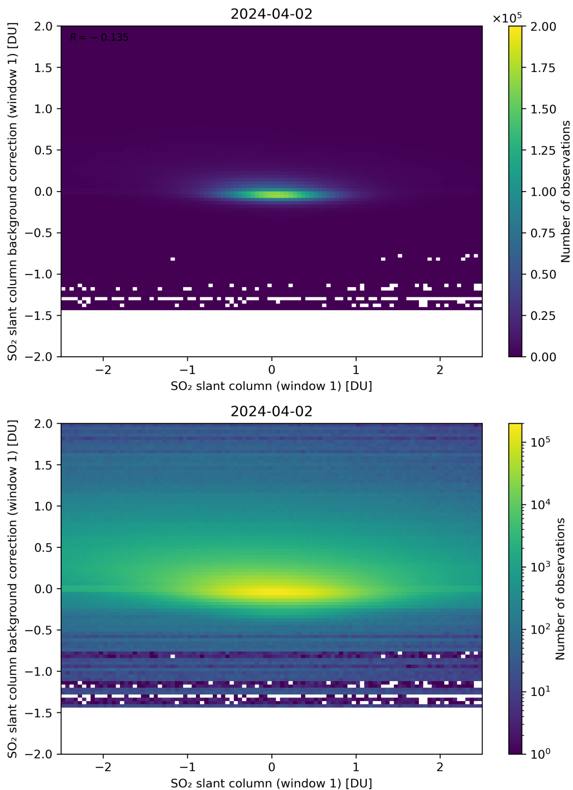
Figure 212: Scatter density plot of “SO 2 slant column (window 1)” against “SO 2 slant column background correction (window 1)” for 2024-04-01 to 2024-04-03.
