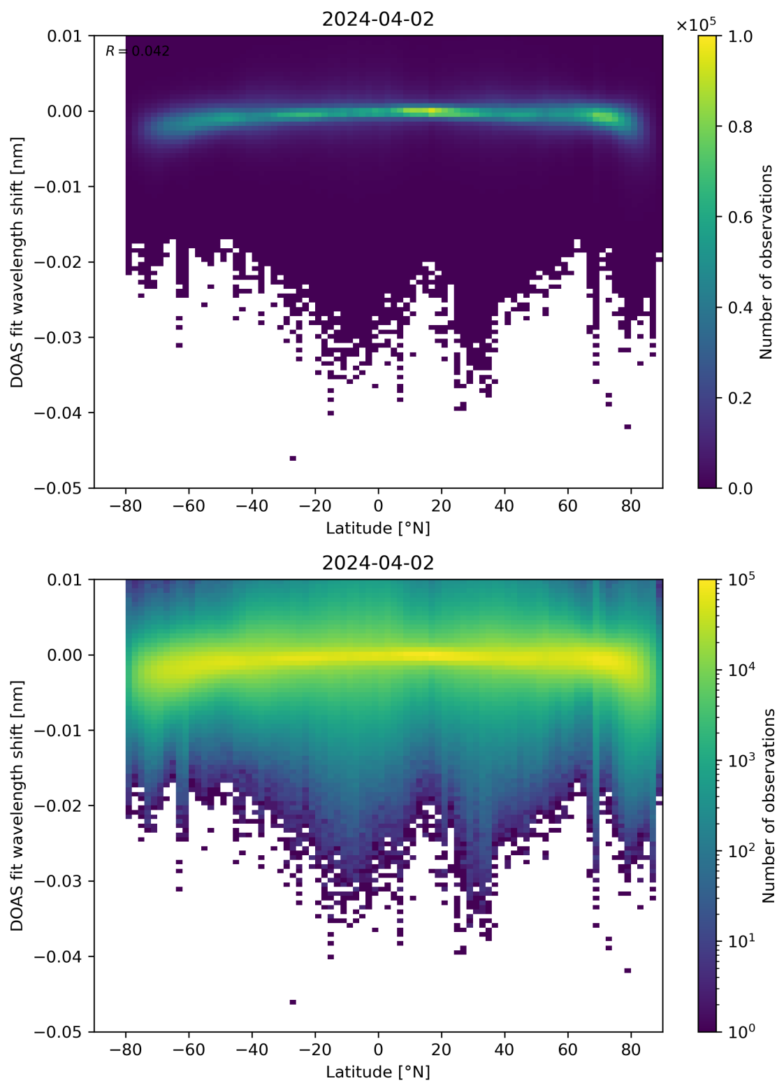
Figure 142: Scatter density plot of “Latitude” against “DOAS fit wavelength shift” for 2024-04-01 to 2024-04-03.
