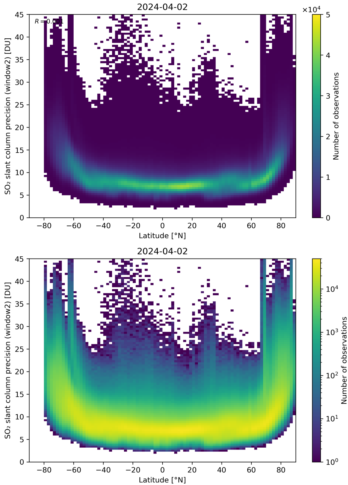
Figure 151: Scatter density plot of “Latitude” against “SO 2 slant column precision (window2)” for 2024-04-01 to 2024-04-03.
