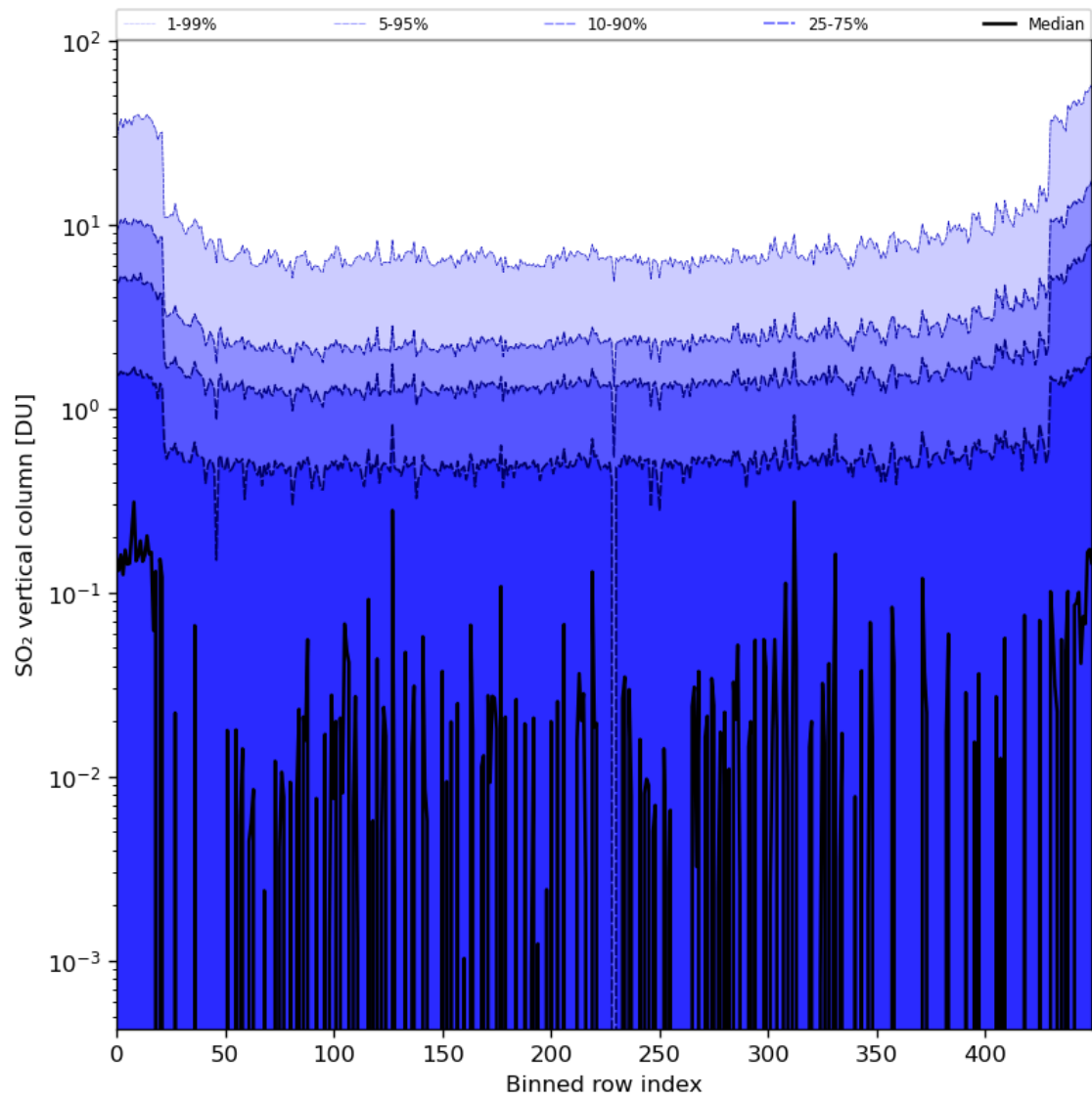
Figure 76: Along track statistics of “SO 2 vertical column” for 2024-04-01 to 2024-04-03
