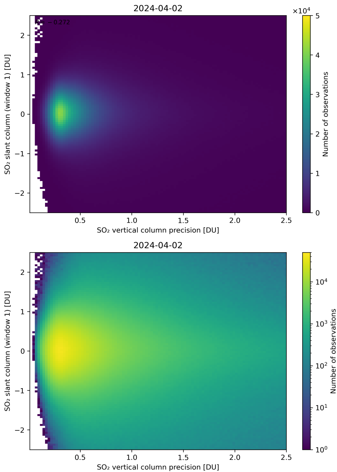
Figure 289: Scatter density plot of “SO 2 vertical column precision” against “SO 2 slant column (window 1)” for 2024-04-01 to 2024-04-03.
