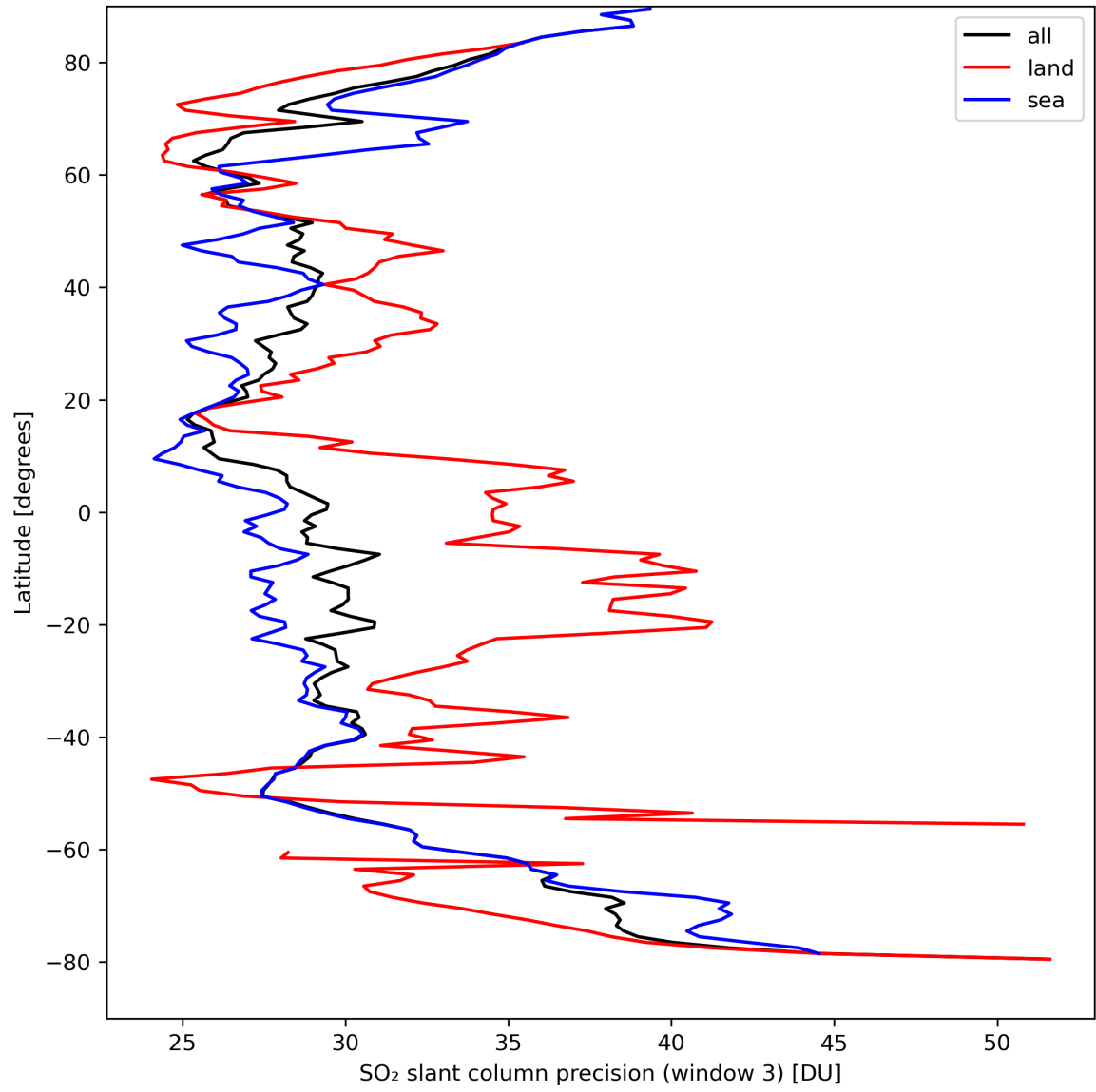
Figure 42: Zonal average of "SO 2 slant column precision (window 3)" for 2024-04-01 to 2024-04-03.
