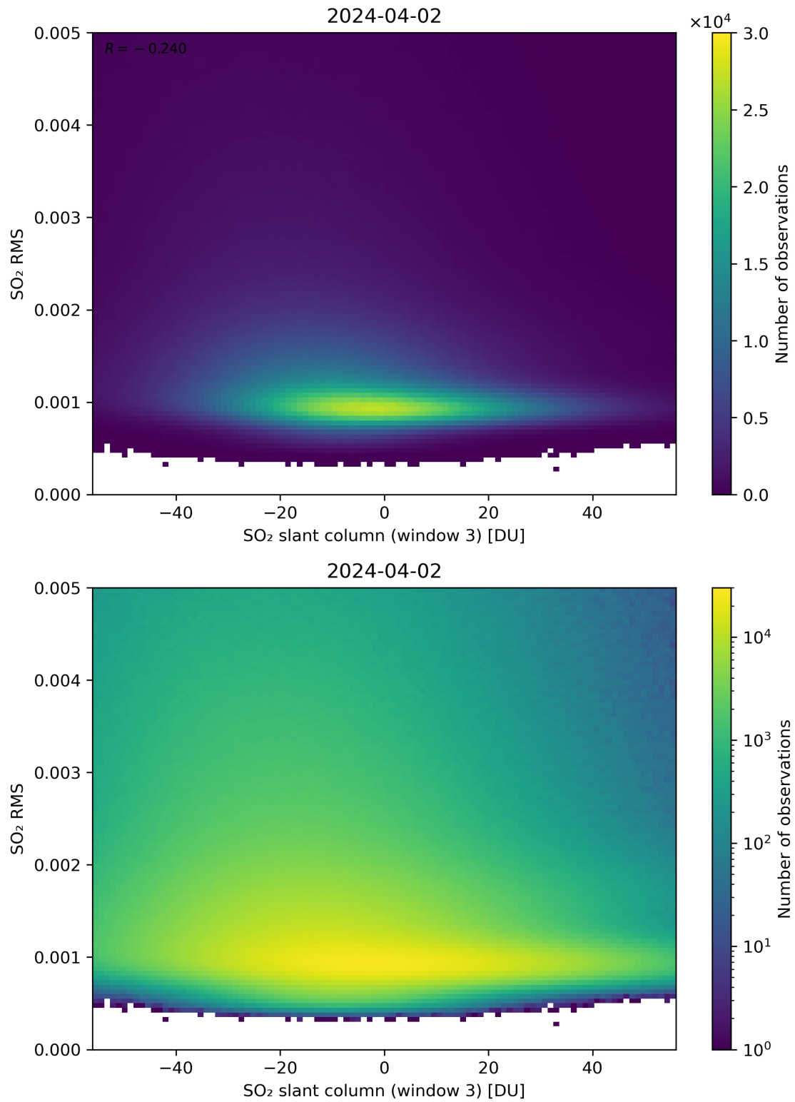
Figure 256: Scatter density plot of “SO 2 slant column (window 3)” against “SO 2 RMS” for 2024-04-01 to 2024-04-03.
