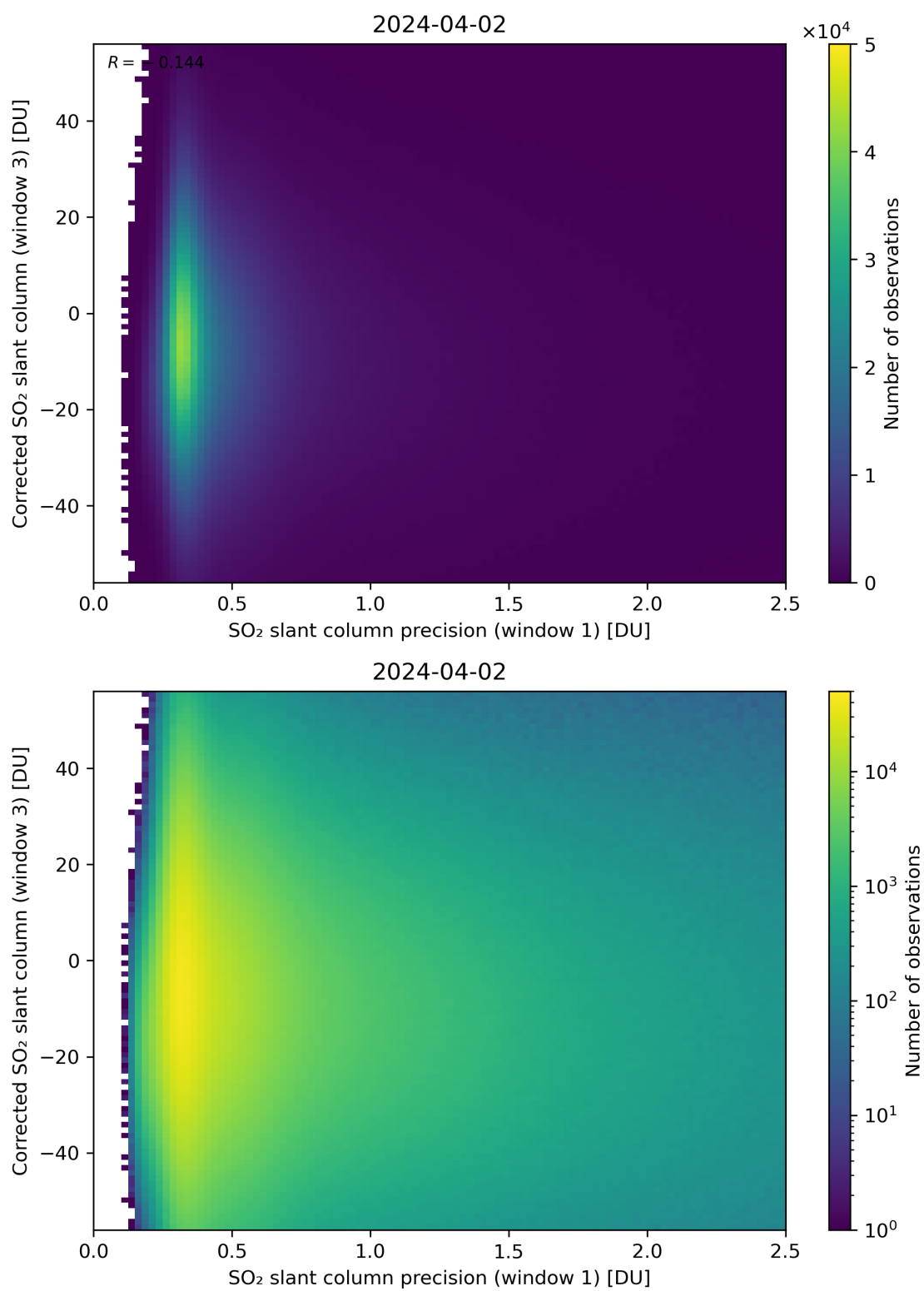
Figure 226: Scatter density plot of “SO 2 slant column precision (window 1)” against “Corrected SO 2 slant column (window 3)” for 2024-04-01 to 2024-04-03.
