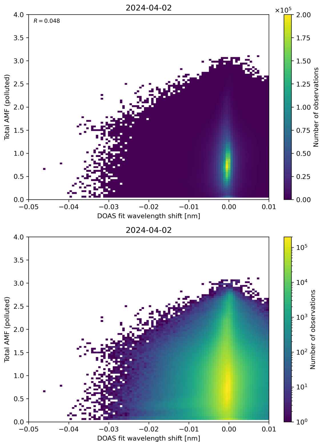
Figure 130: Scatter density plot of “DOAS fit wavelength shift” against “Total AMF (polluted)” for 2024-04-01 to 2024-04-03.
