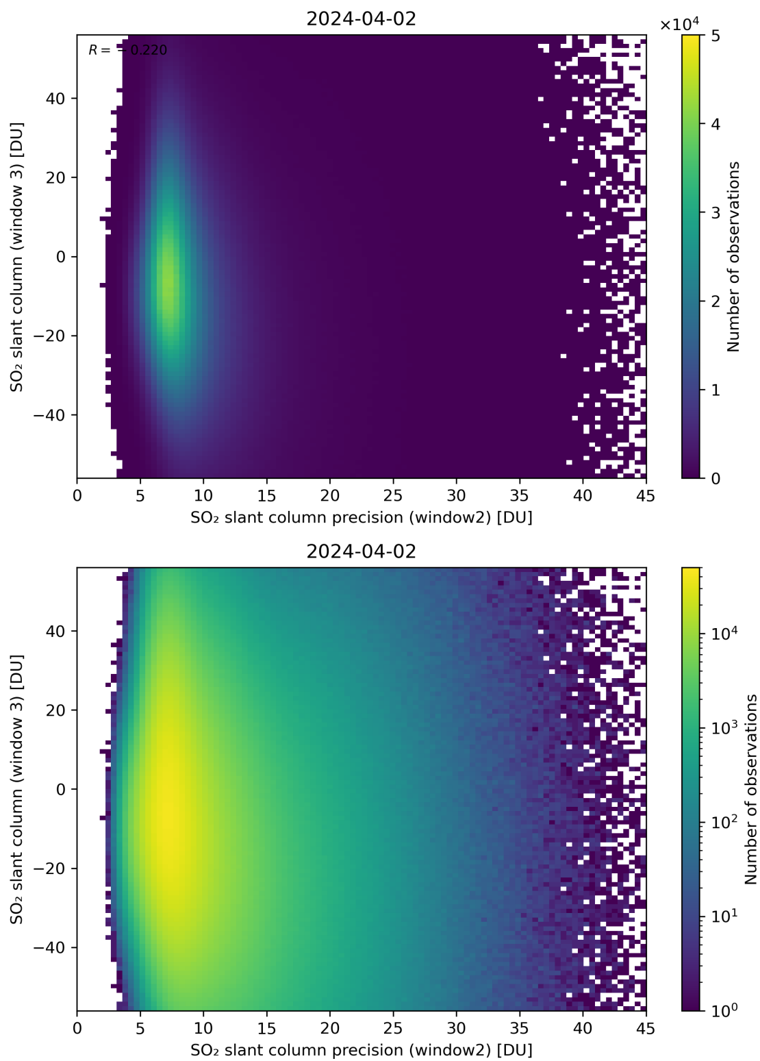
Figure 249: Scatter density plot of “SO 2 slant column precision (window2)” against “SO 2 slant column (window 3)” for 2024-04-01 to 2024-04-03.
