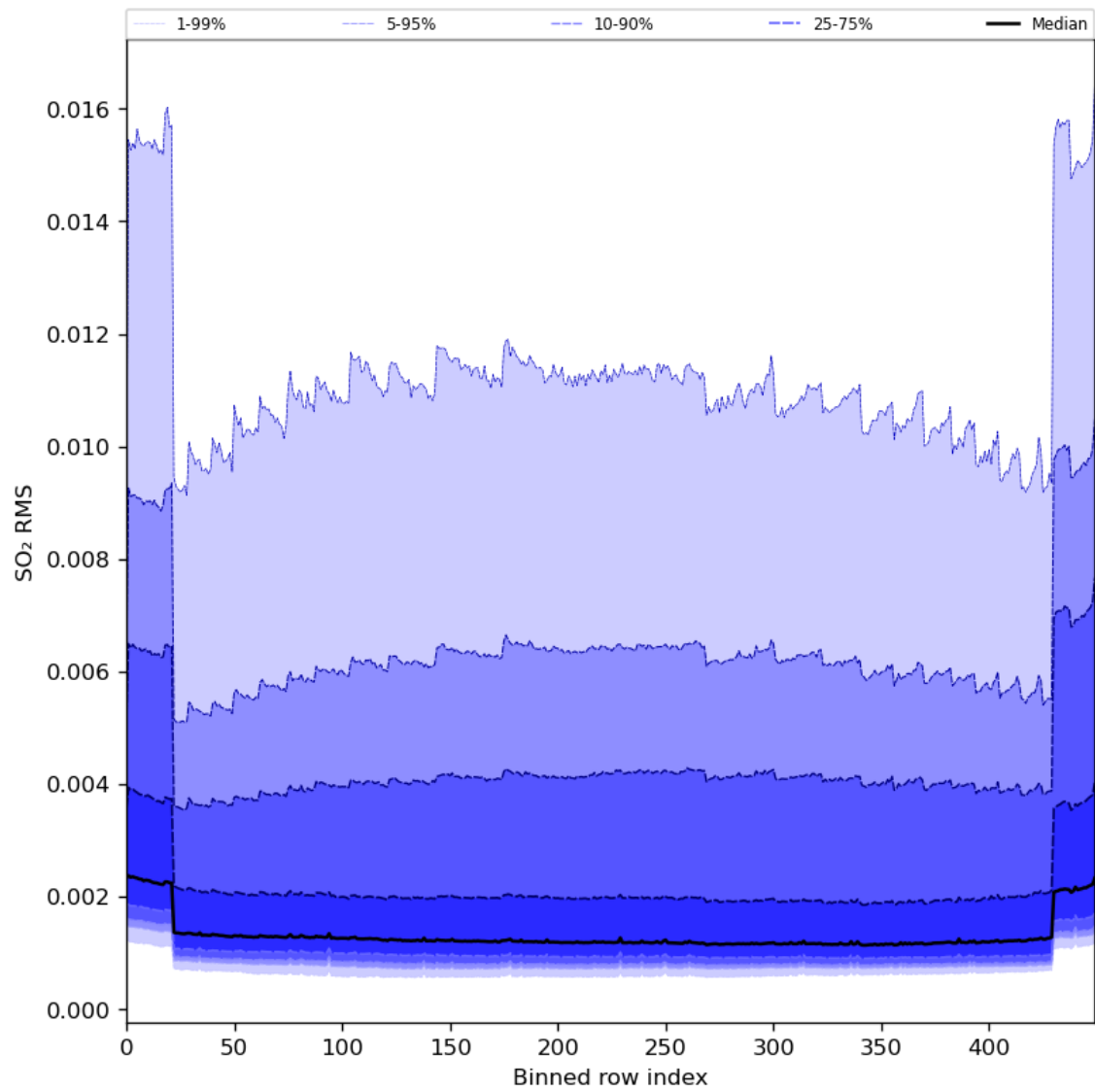
Figure 93: Along track statistics of “SO 2 RMS” for 2024-04-01 to 2024-04-03
