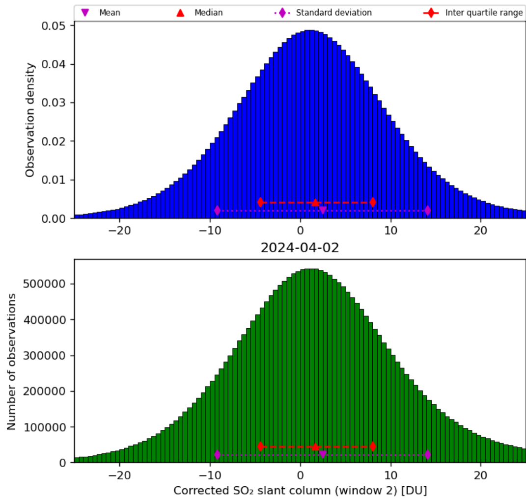
Figure 62: Histogram of “Corrected SO 2 slant column (window 2)” for 2024-04-01 to 2024-04-03
