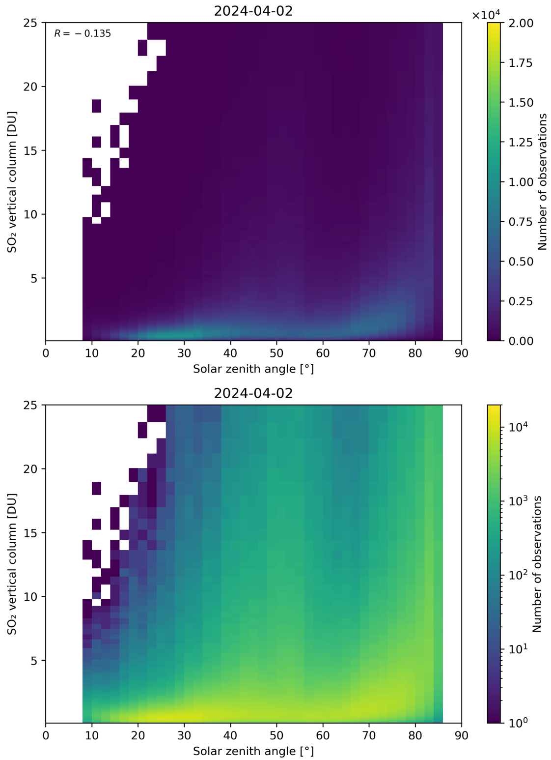
Figure 176: Scatter density plot of “Solar zenith angle” against “SO 2 vertical column” for 2024-04-01 to 2024-04-03.
