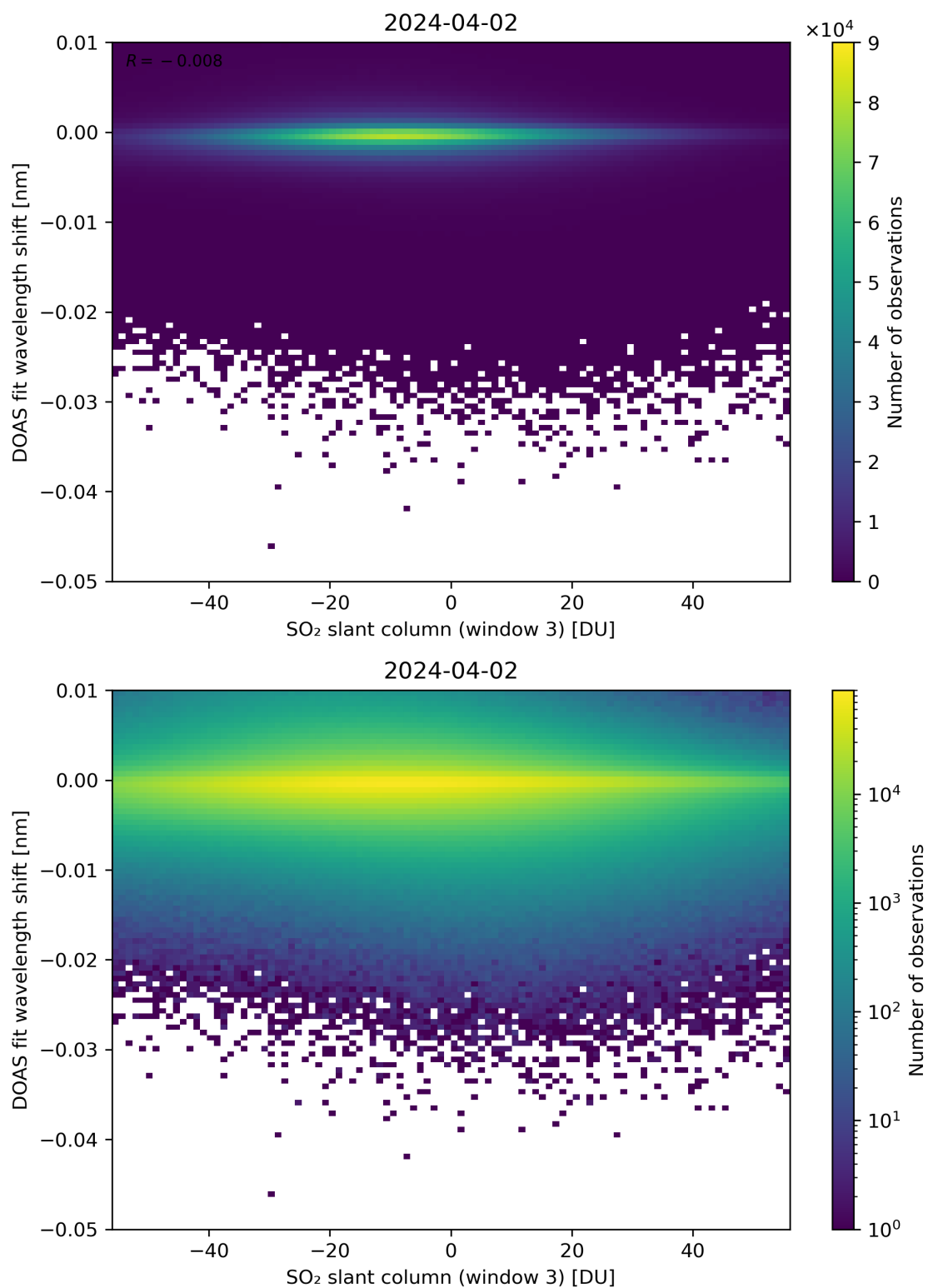
Figure 254: Scatter density plot of “SO 2 slant column (window 3)” against “DOAS fit wavelength shift” for 2024-04-01 to 2024-04-03.
