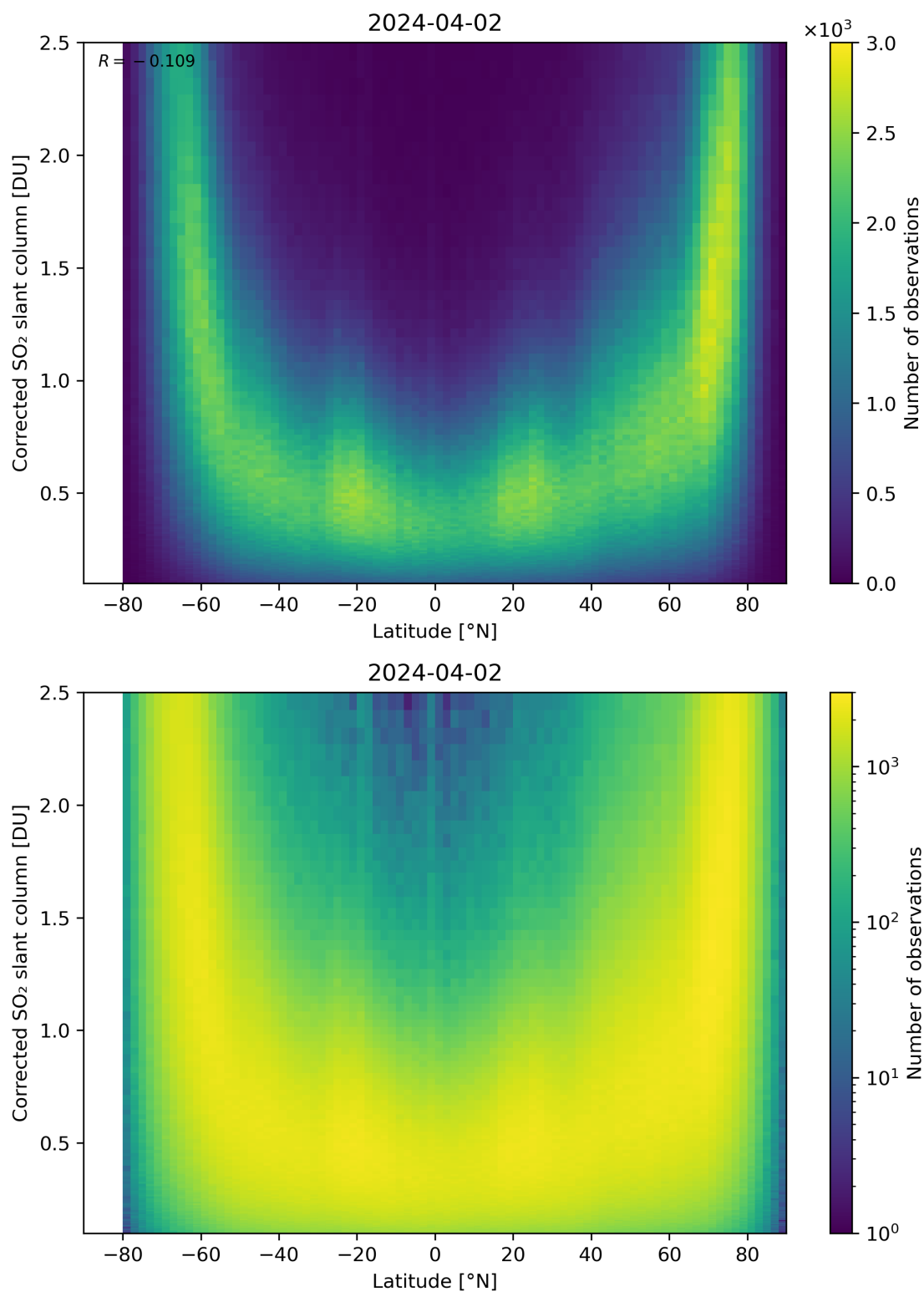
Figure 146: Scatter density plot of “Latitude” against “Corrected SO 2 slant column” for 2024-04-01 to 2024-04-03.
