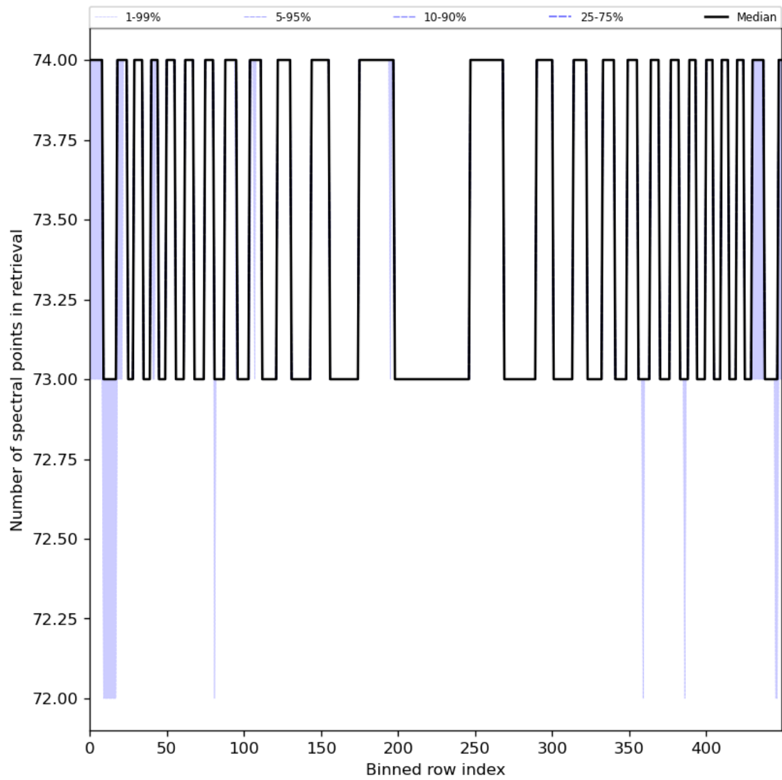
Figure 97: Along track statistics of “Number of spectral points in retrieval” for 2024-04-01 to 2024-04-03
