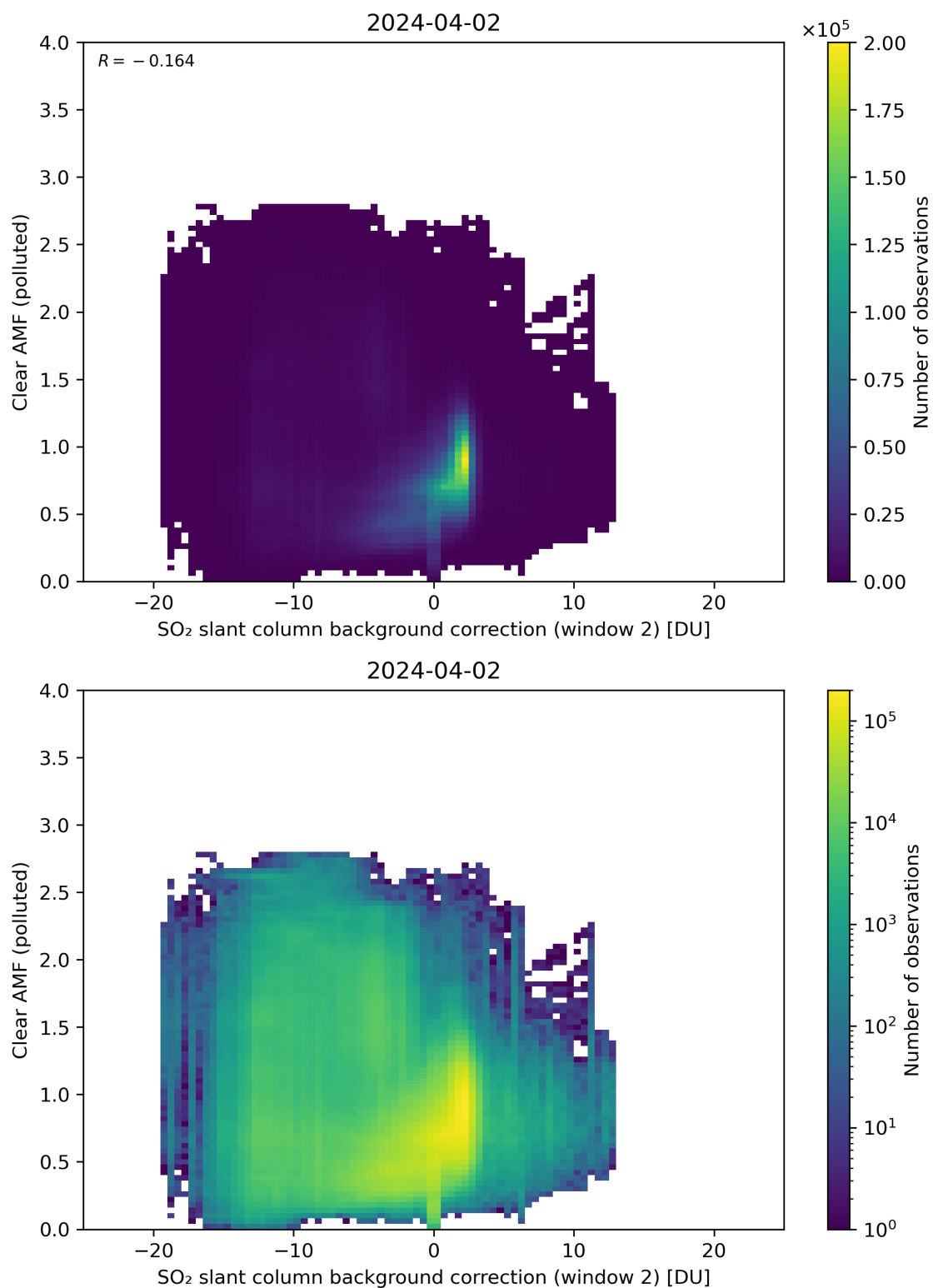
Figure 115: Scatter density plot of “SO 2 slant column background correction (window 2)” against “Clear AMF (polluted)” for 2024-04-01 to 2024-04-03.
