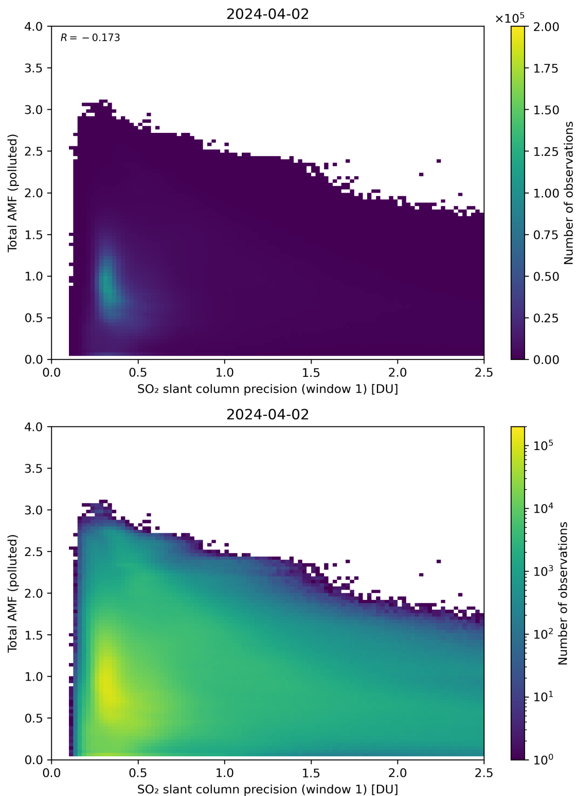
Figure 230: Scatter density plot of “SO 2 slant column precision (window 1)” against “Total AMF (polluted)” for 2024-04-01 to 2024-04-03.
