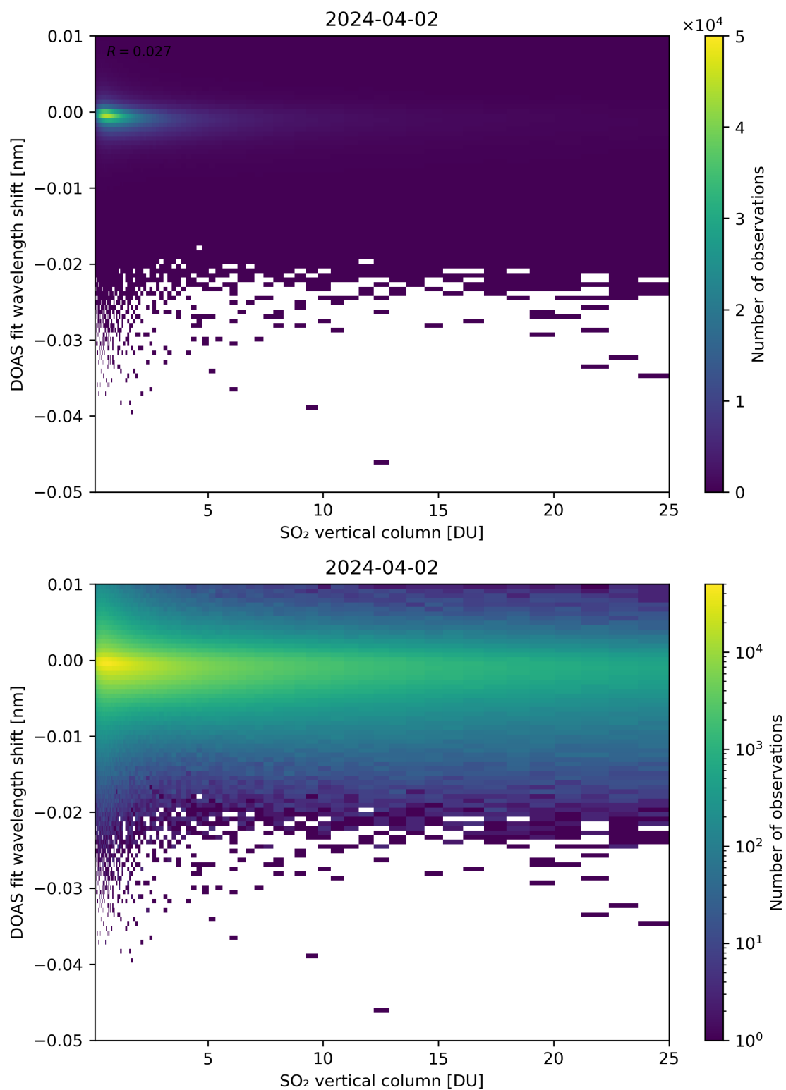
Figure 276: Scatter density plot of “SO 2 vertical column” against “DOAS fit wavelength shift” for 2024-04-01 to 2024-04-03.
