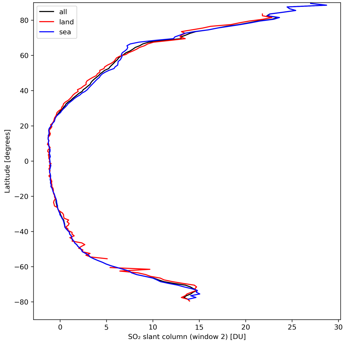
Figure 37: Zonal average of “SO 2 slant column (window 2)” for 2024-04-01 to 2024-04-03.
