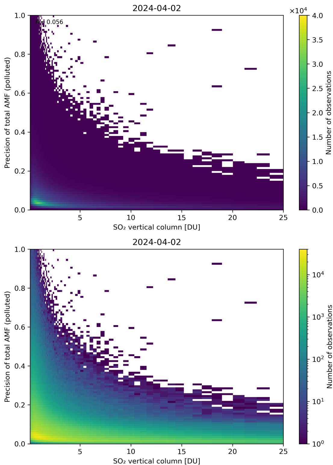
Figure 306: Scatter density plot of “SO 2 vertical column” against “Precision of total AMF (polluted)” for 2024-04-01 to 2024-04-03.
