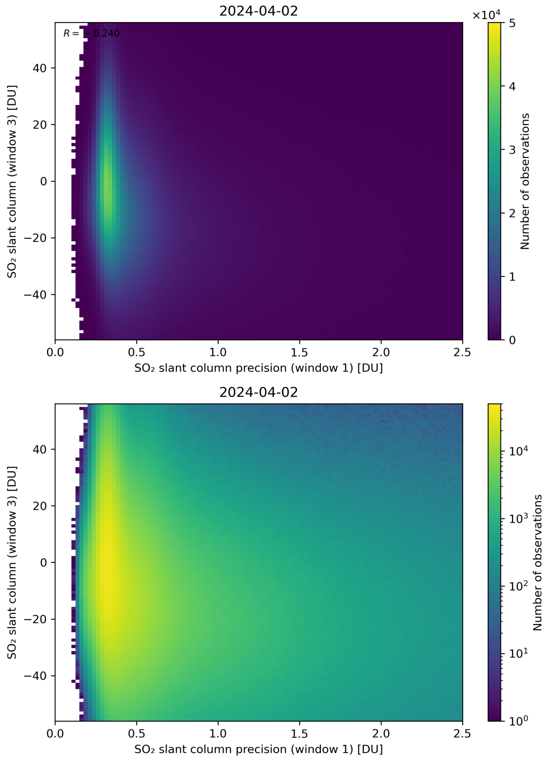
Figure 228: Scatter density plot of “SO 2 slant column precision (window 1)” against “SO 2 slant column (window 3)” for 2024-04-01 to 2024-04-03.
