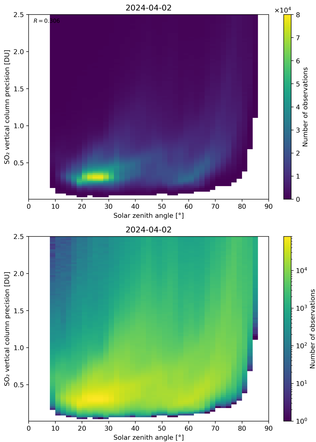
Figure 177: Scatter density plot of “Solar zenith angle” against “SO 2 vertical column precision” for 2024-04-01 to 2024-04-03.
