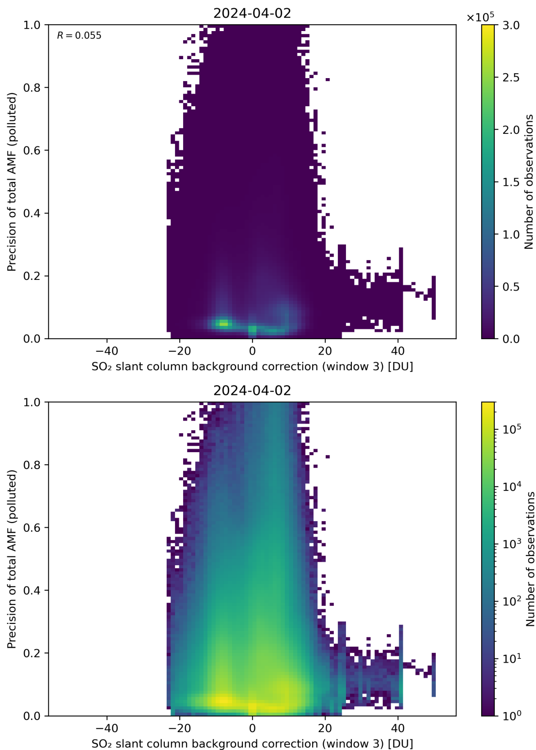
Figure 126: Scatter density plot of “SO 2 slant column background correction (window 3)” against “Precision of total AMF (polluted)” for 2024-04-01 to 2024-04-03.
