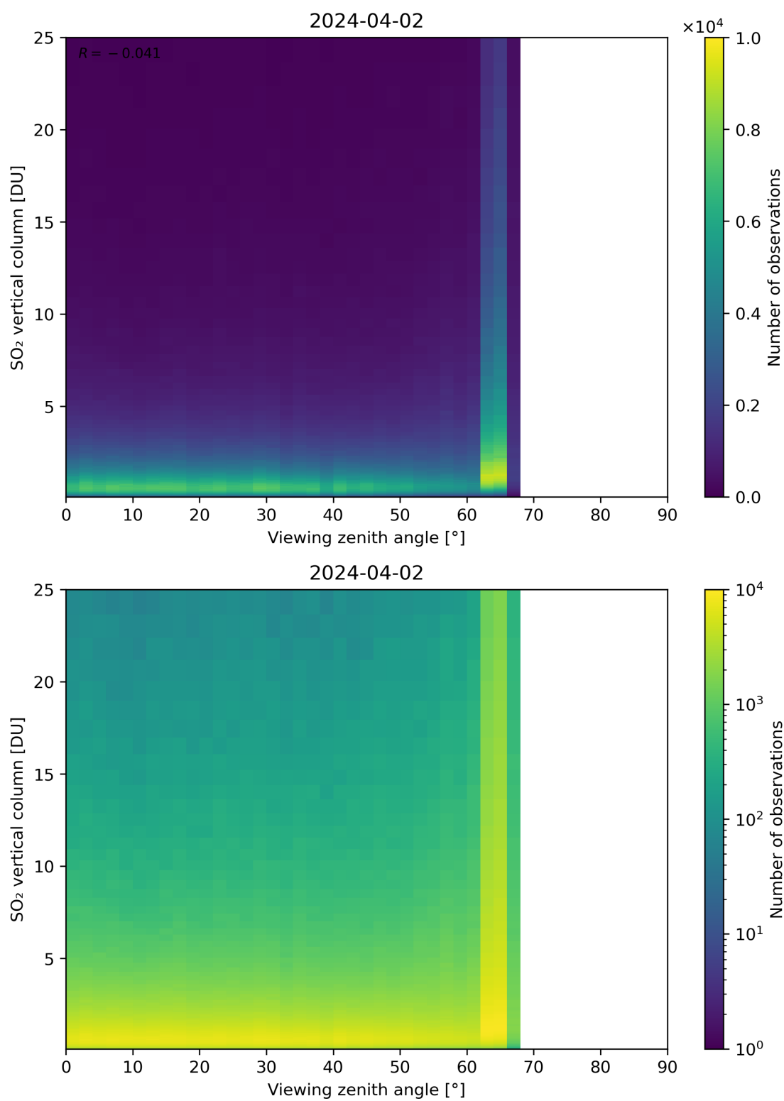
Figure 327: Scatter density plot of “Viewing zenith angle” against “SO 2 vertical column” for 2024-04-01 to 2024-04-03.
