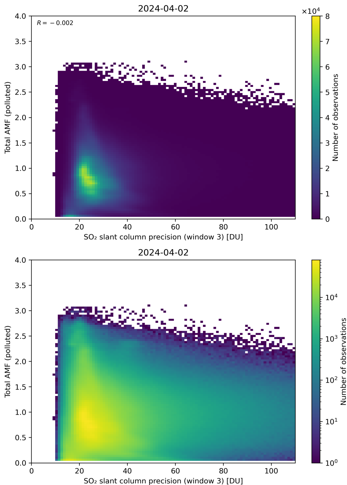
Figure 263: Scatter density plot of “SO 2 slant column precision (window 3)” against “Total AMF (polluted)” for 2024-04-01 to 2024-04-03.
