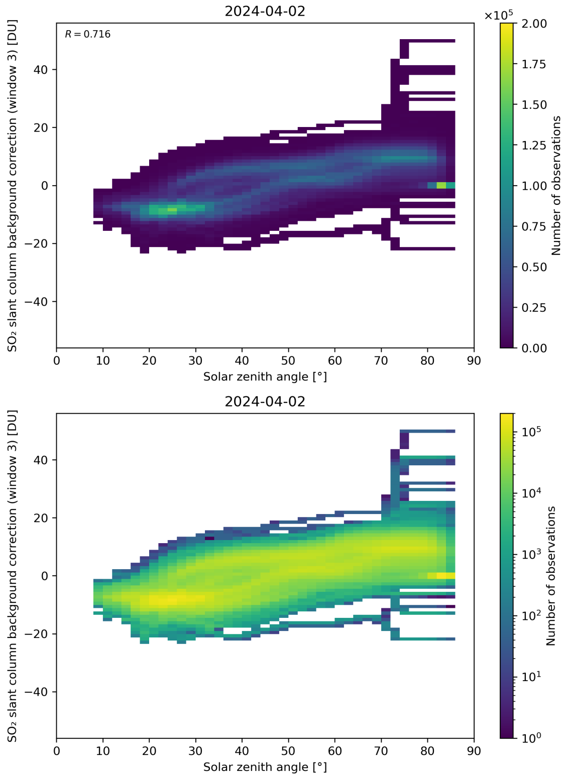
Figure 160: Scatter density plot of “Solar zenith angle” against “SO 2 slant column background correction (window 3)” for 2024-04-01 to 2024-04-03.
