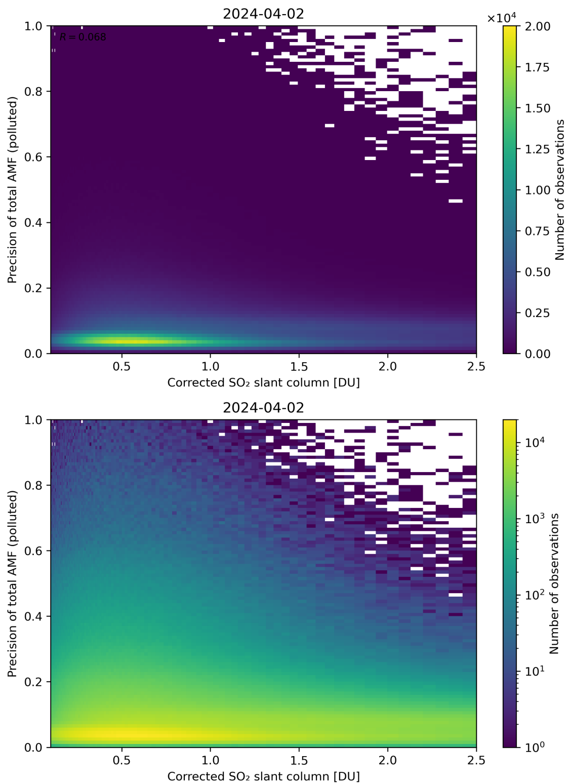
Figure 193: Scatter density plot of “Corrected SO 2 slant column” against “Precision of total AMF (polluted)” for 2024-04-01 to 2024-04-03.
