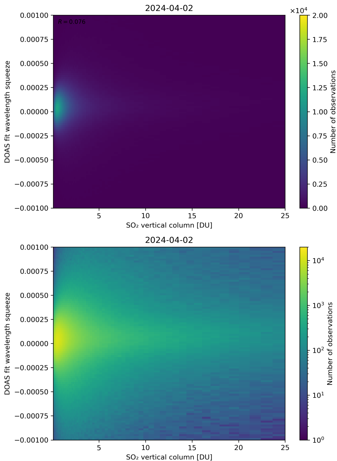
Figure 277: Scatter density plot of “SO 2 vertical column” against “DOAS fit wavelength squeeze” for 2024-04-01 to 2024-04-03.
