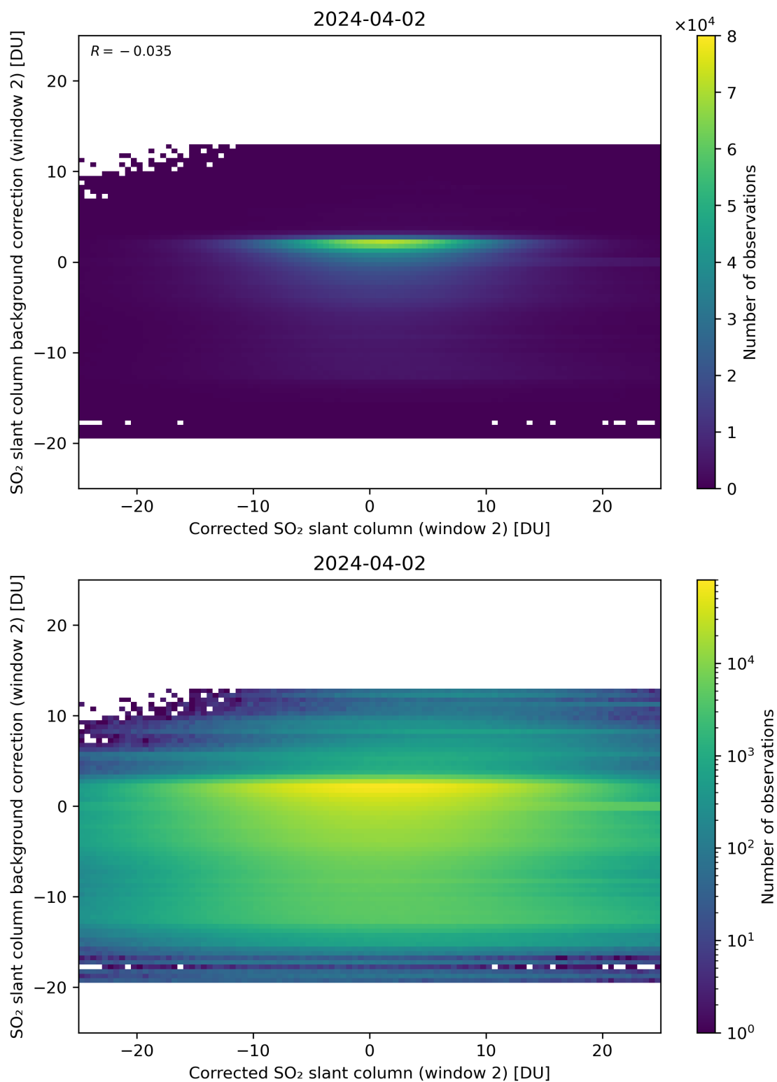
Figure 194: Scatter density plot of “Corrected SO 2 slant column (window 2)” against “SO 2 slant column background correction (window 2)” for 2024-04-01 to 2024-04-03.
