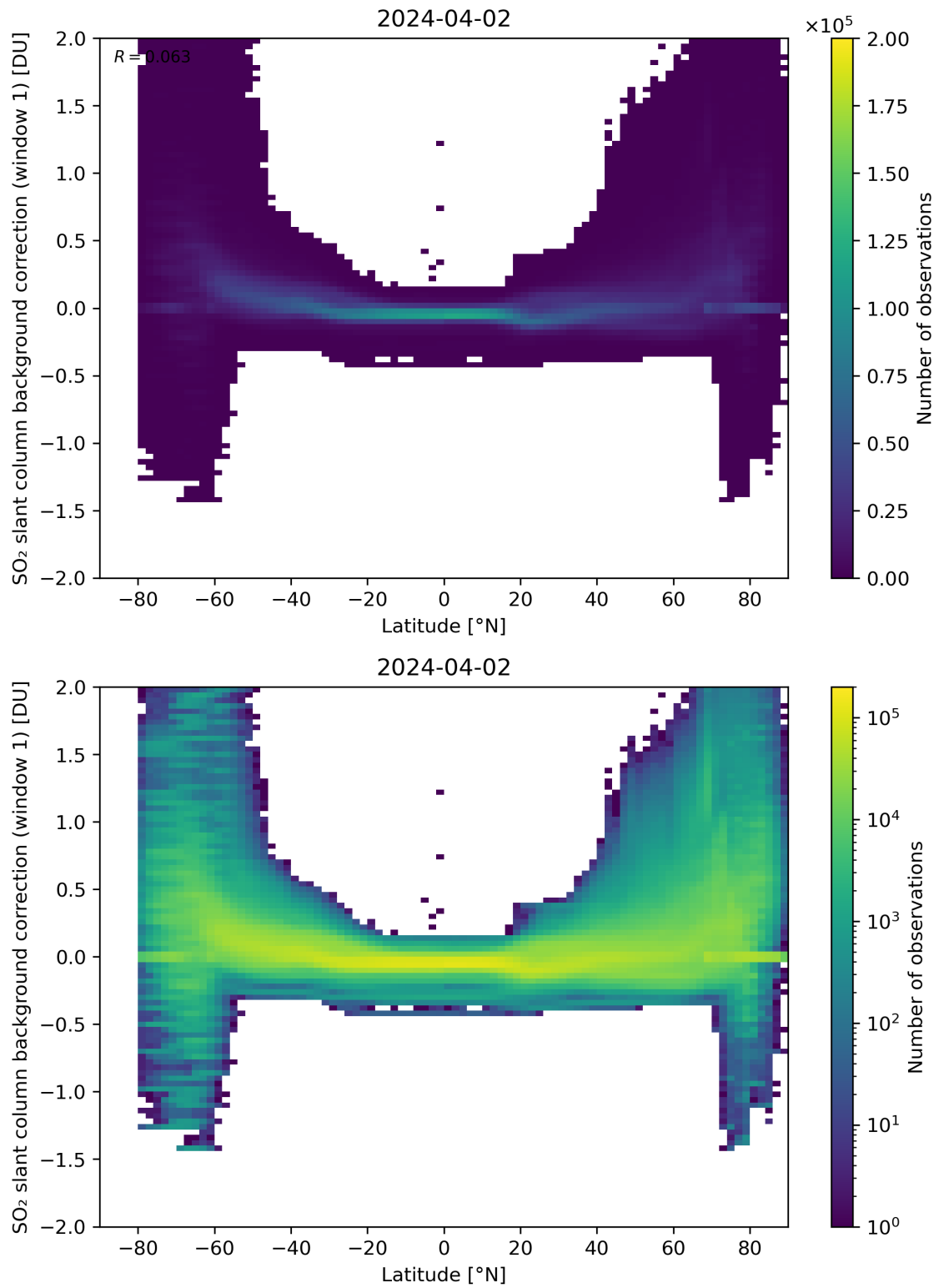
Figure 139: Scatter density plot of “Latitude” against “SO 2 slant column background correction (window 1)” for 2024-04-01 to 2024-04-03.
