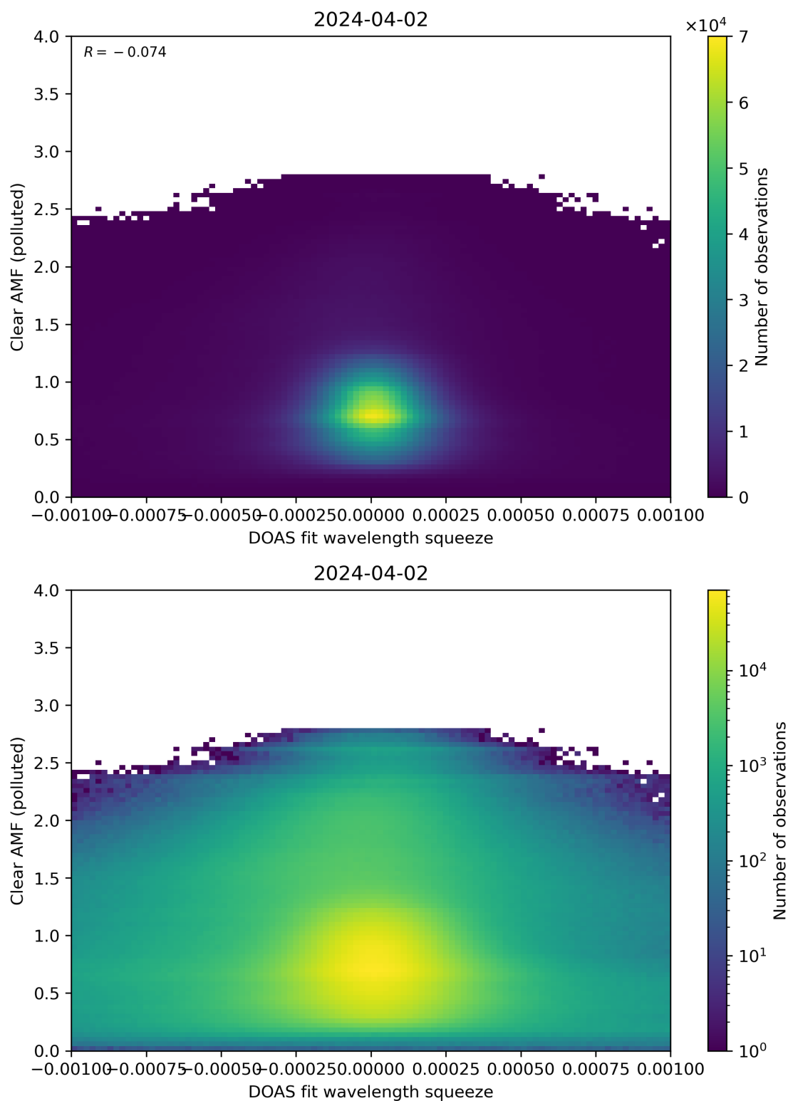
Figure 133: Scatter density plot of “DOAS fit wavelength squeeze” against “Clear AMF (polluted)” for 2024-04-01 to 2024-04-03.
