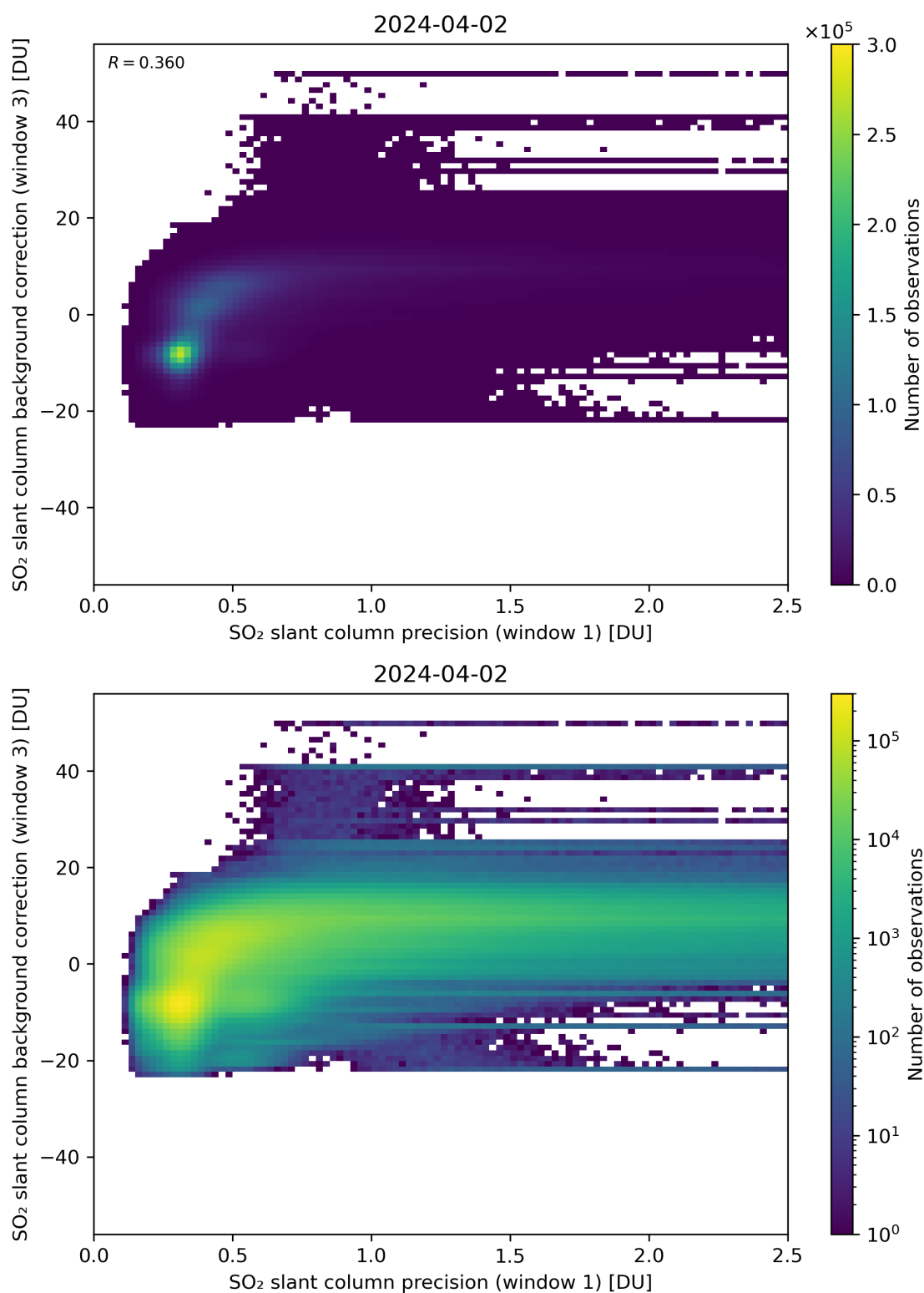
Figure 220: Scatter density plot of “SO 2 slant column precision (window 1)” against “SO 2 slant column background correction (window 3)” for 2024-04-01 to 2024-04-03.
