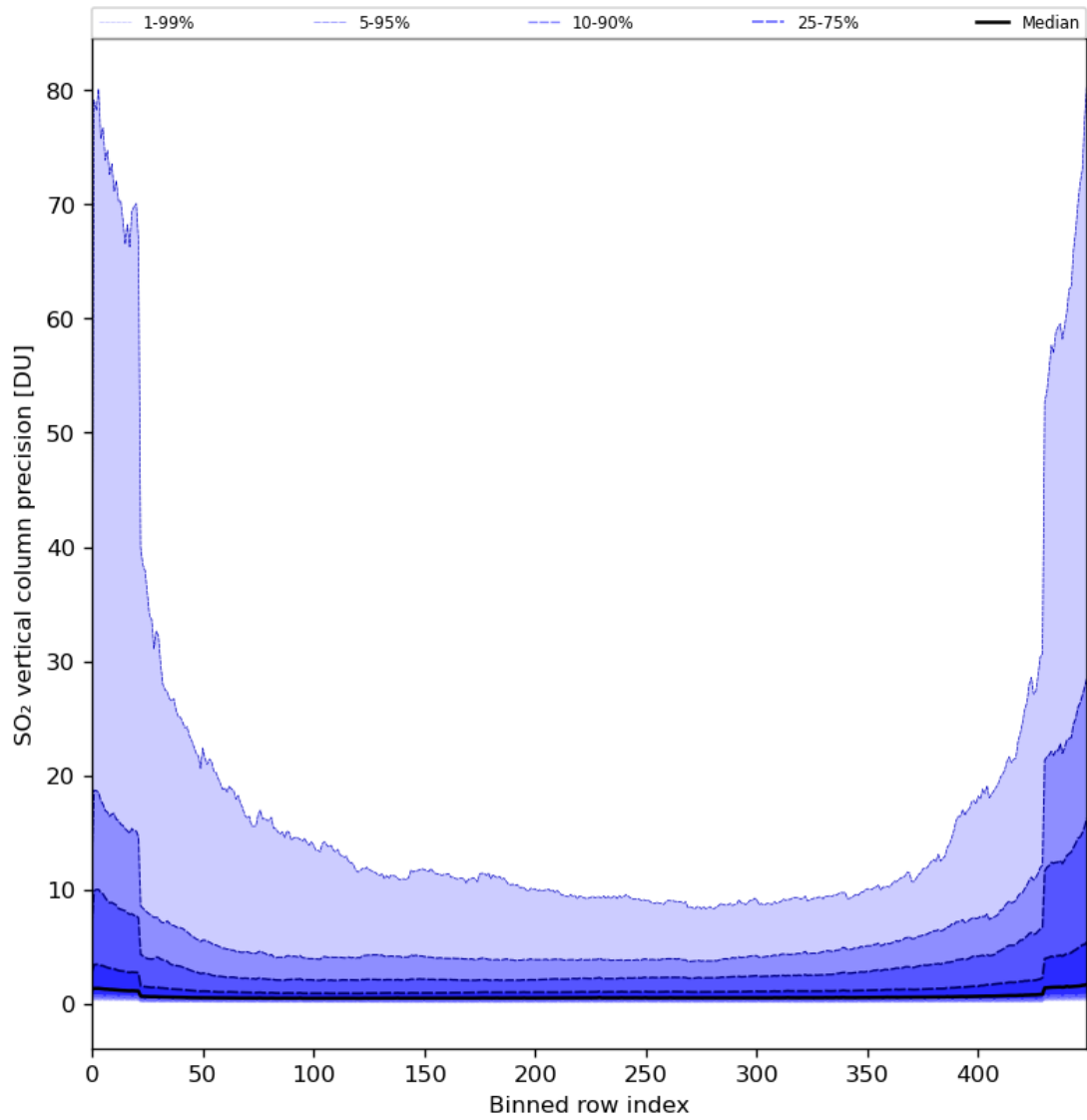
Figure 77: Along track statistics of “SO 2 vertical column precision” for 2024-04-01 to 2024-04-03
