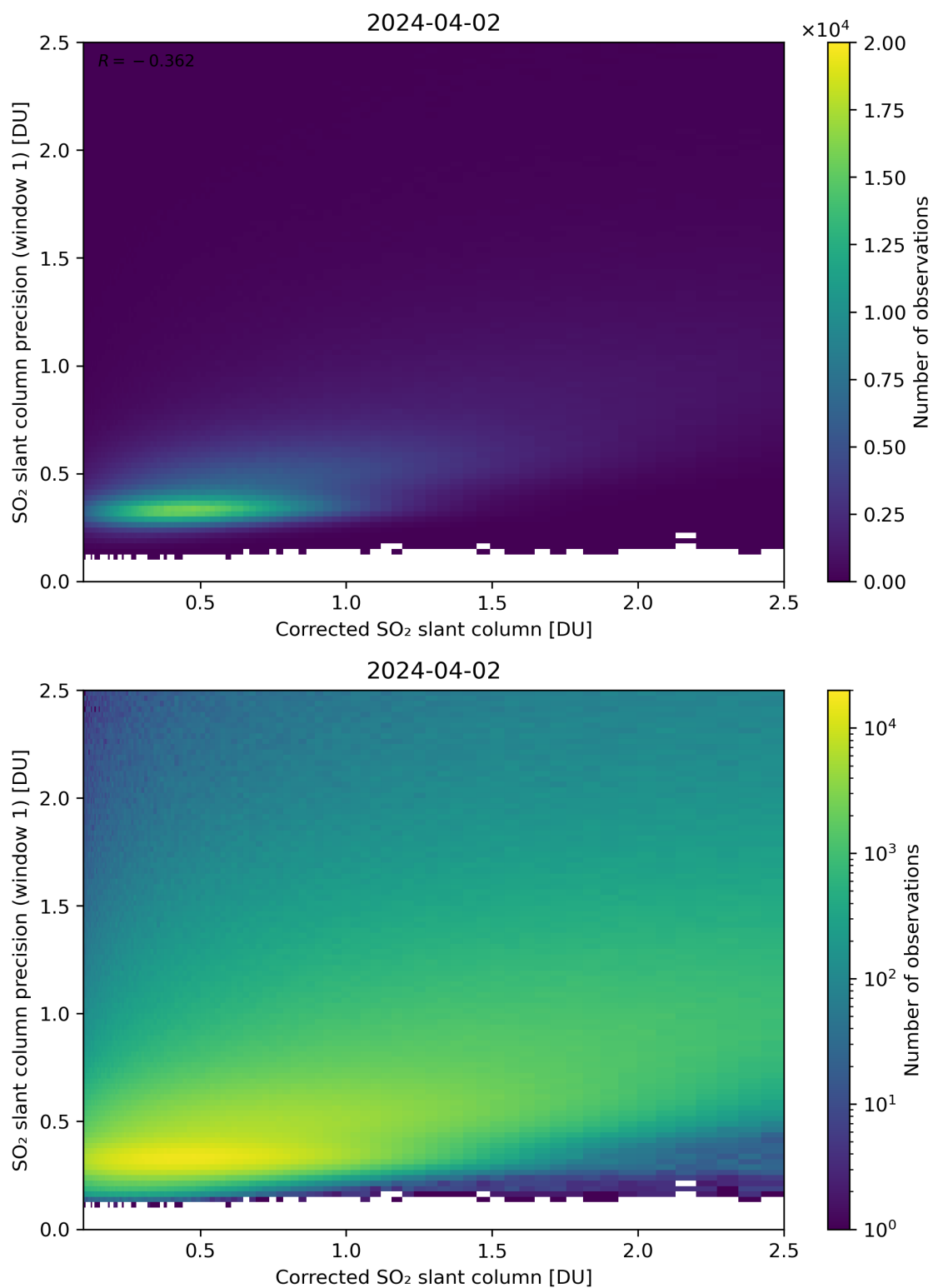
Figure 188: Scatter density plot of “Corrected SO 2 slant column” against “SO 2 slant column precision (window 1)” for 2024-04-01 to 2024-04-03.
