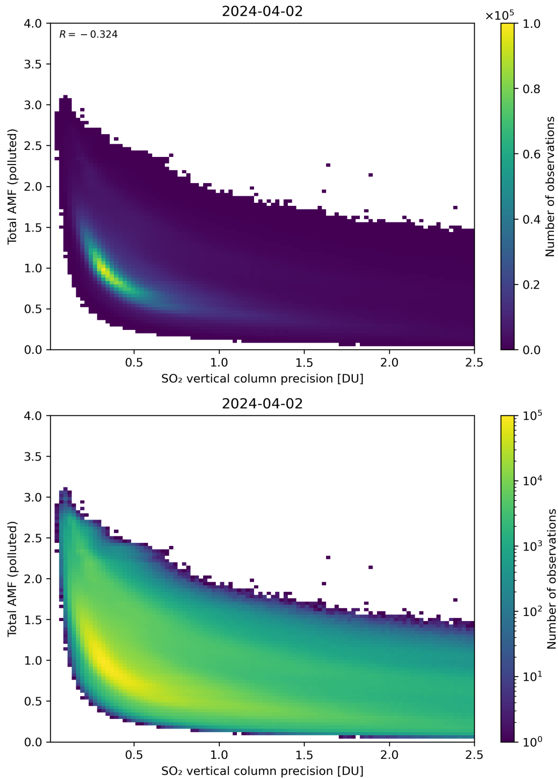
Figure 294: Scatter density plot of “SO 2 vertical column precision” against “Total AMF (polluted)” for 2024-04-01 to 2024-04-03.
