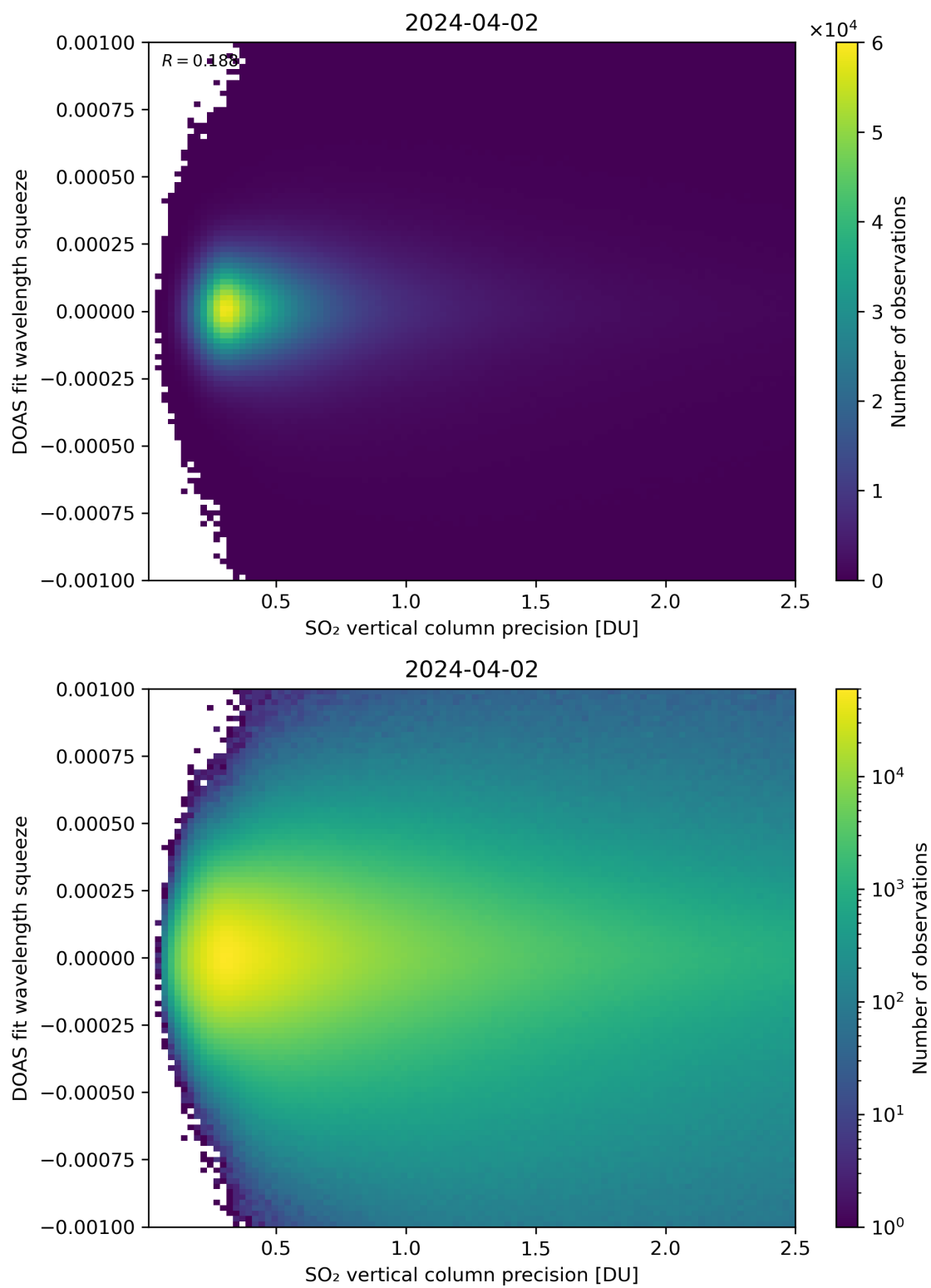
Figure 283: Scatter density plot of “SO 2 vertical column precision” against “DOAS fit wavelength squeeze” for 2024-04-01 to 2024-04-03.
