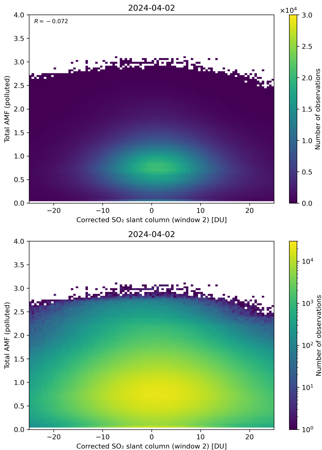
Figure 203: Scatter density plot of “Corrected SO 2 slant column (window 2)” against “Total AMF (polluted)” for 2024-04-01 to 2024-04-03.
