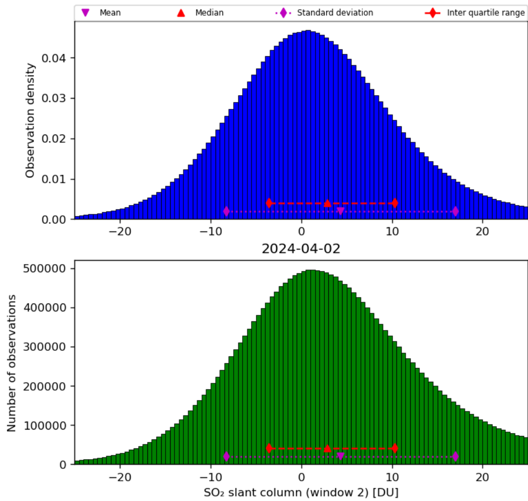
Figure 60: Histogram of “SO 2 slant column (window 2)” for 2024-04-01 to 2024-04-03
