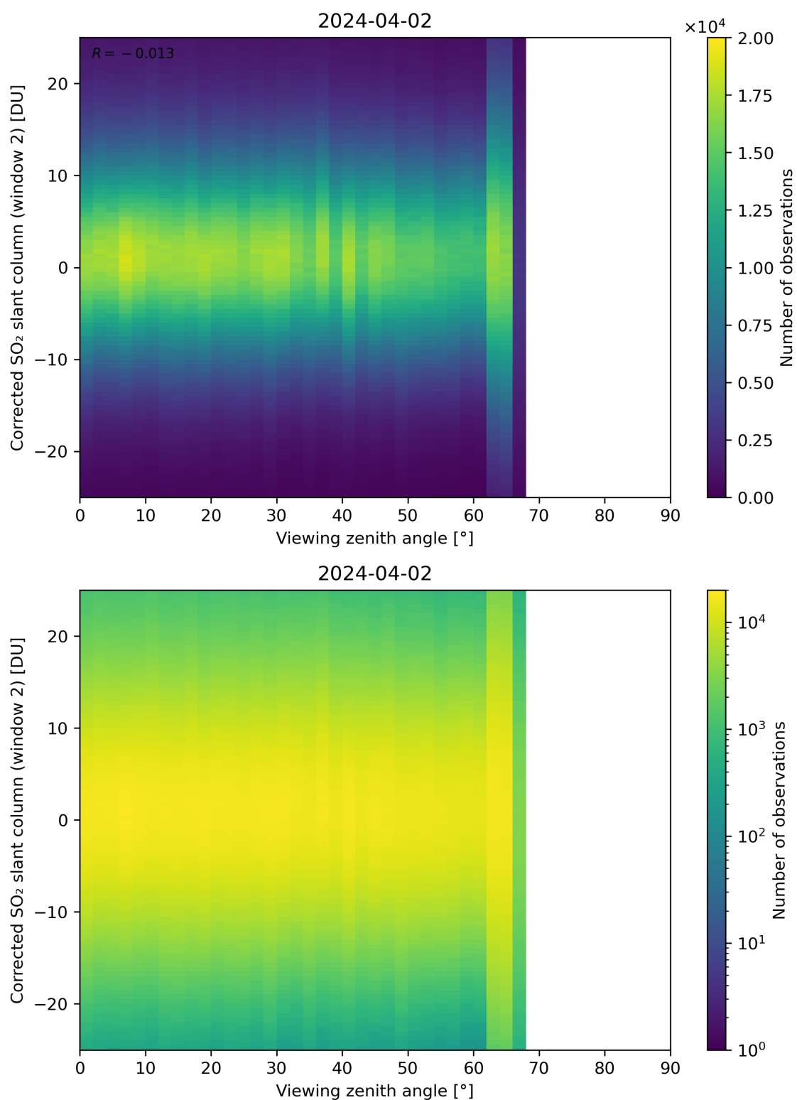
Figure 318: Scatter density plot of “Viewing zenith angle” against “Corrected SO 2 slant column (window 2)” for 2024-04-01 to 2024-04-03.
