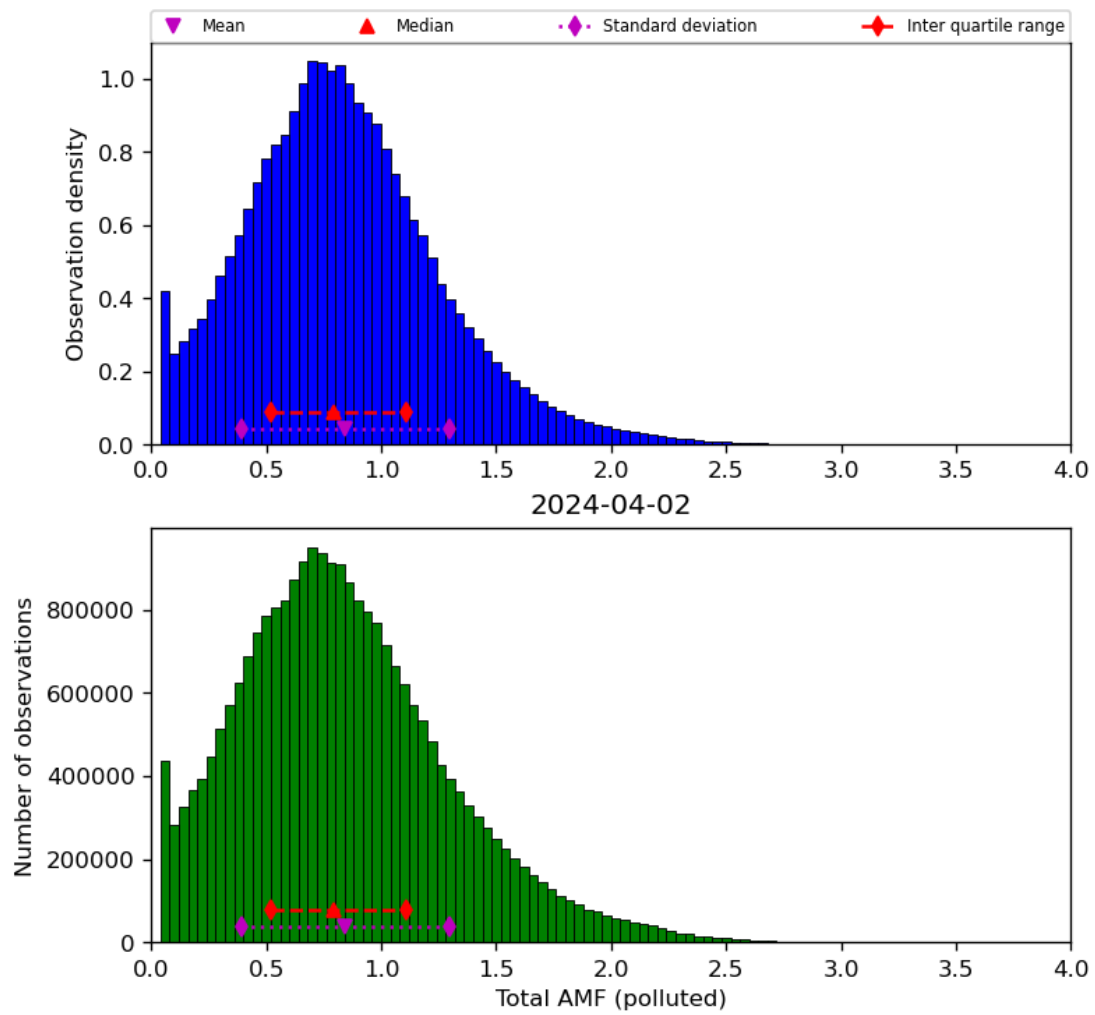
Figure 71: Histogram of “Total AMF (polluted)” for 2024-04-01 to 2024-04-03
