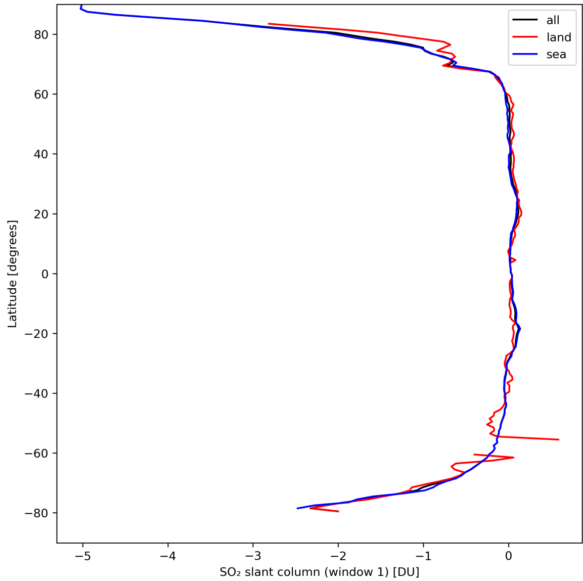
Figure 33: Zonal average of “SO 2 slant column (window 1)” for 2024-04-01 to 2024-04-03.
