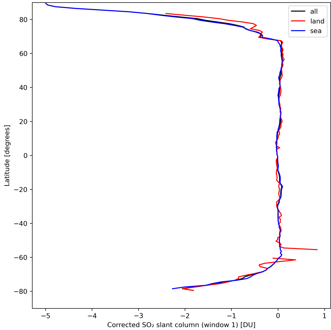
Figure 35: Zonal average of “Corrected SO 2 slant column (window 1)” for 2024-04-01 to 2024-04-03.
