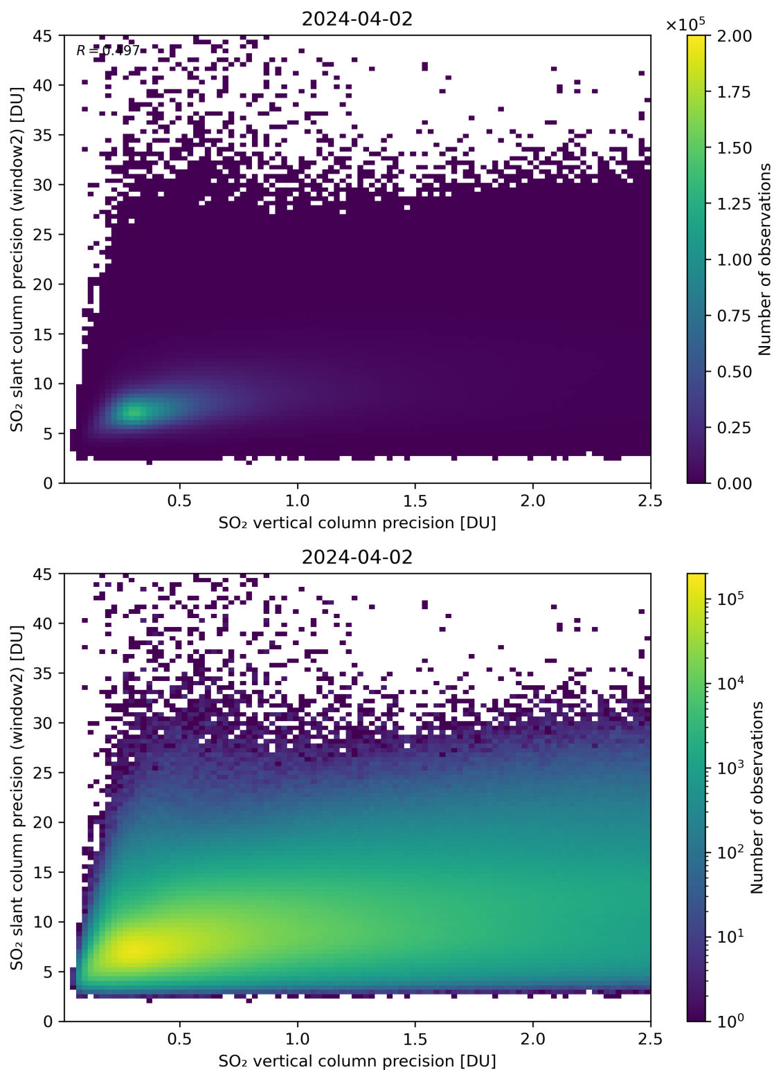
Figure 291: Scatter density plot of “SO 2 vertical column precision” against “SO 2 slant column precision (window2)” for 2024-04-01 to 2024-04-03.
