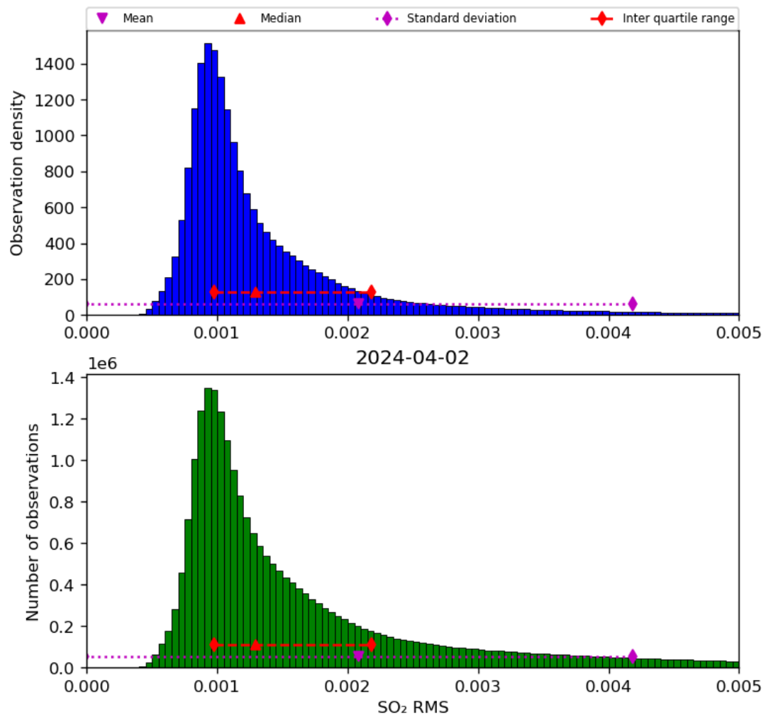
Figure 70: Histogram of “SO 2 RMS” for 2024-04-01 to 2024-04-03
