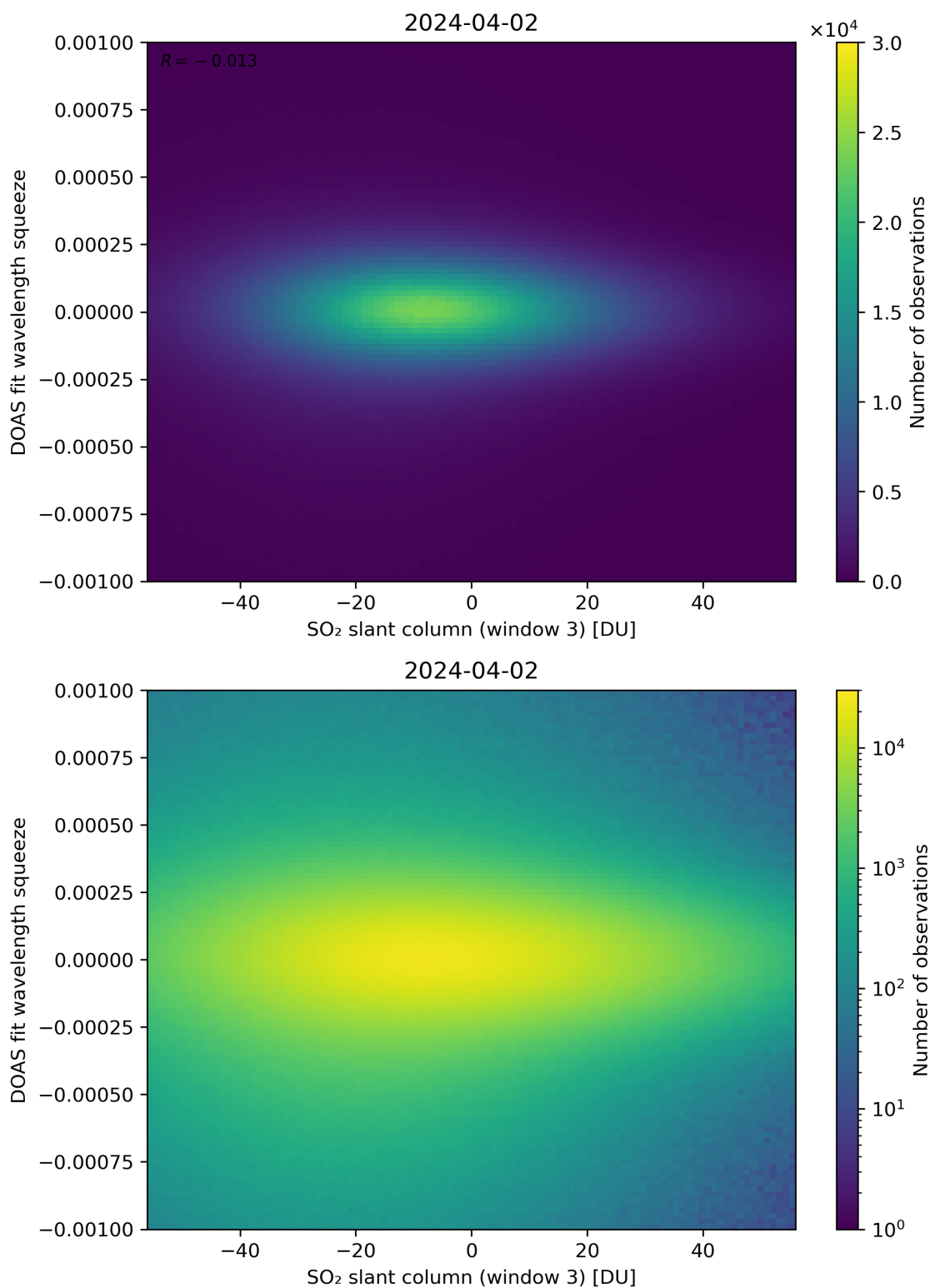
Figure 255: Scatter density plot of “SO 2 slant column (window 3)” against “DOAS fit wavelength squeeze” for 2024-04-01 to 2024-04-03.
