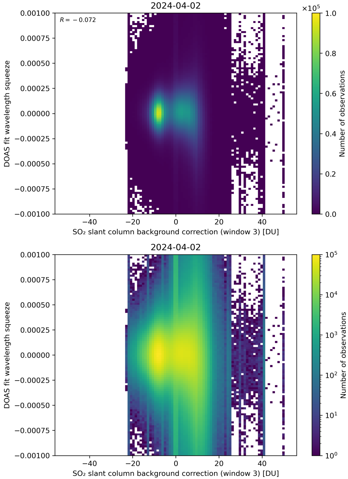
Figure 122: Scatter density plot of “SO 2 slant column background correction (window 3)” against “DOAS fit wavelength squeeze” for 2024-04-01 to 2024-04-03.
