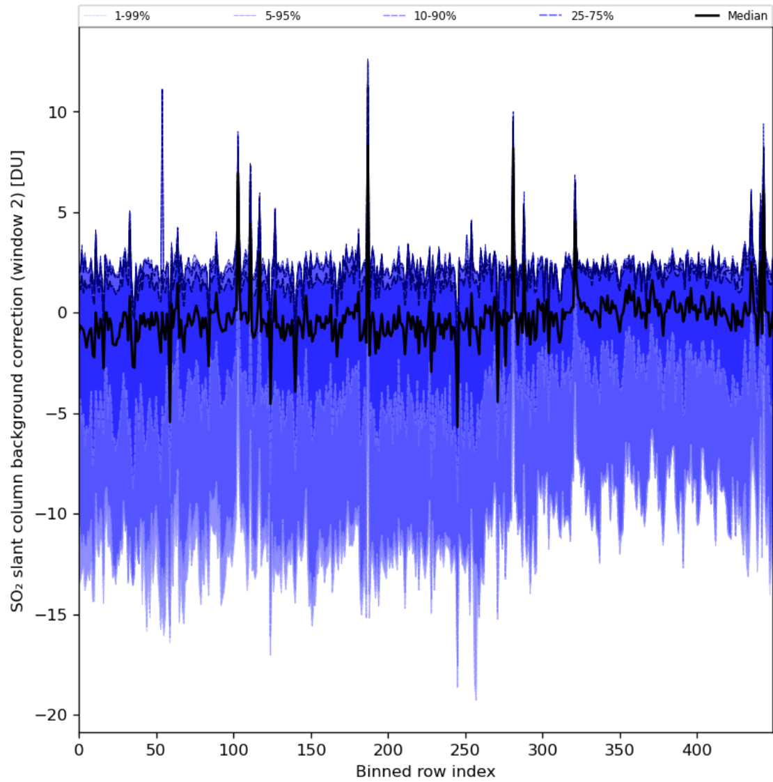
Figure 86: Along track statistics of “SO 2 slant column background correction (window 2)” for 2024-04-01 to 2024-04-03
