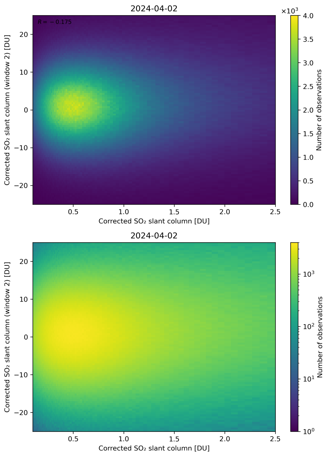
Figure 185: Scatter density plot of “Corrected SO 2 slant column” against “Corrected SO 2 slant column (window 2)” for 2024-04-01 to 2024-04-03.
