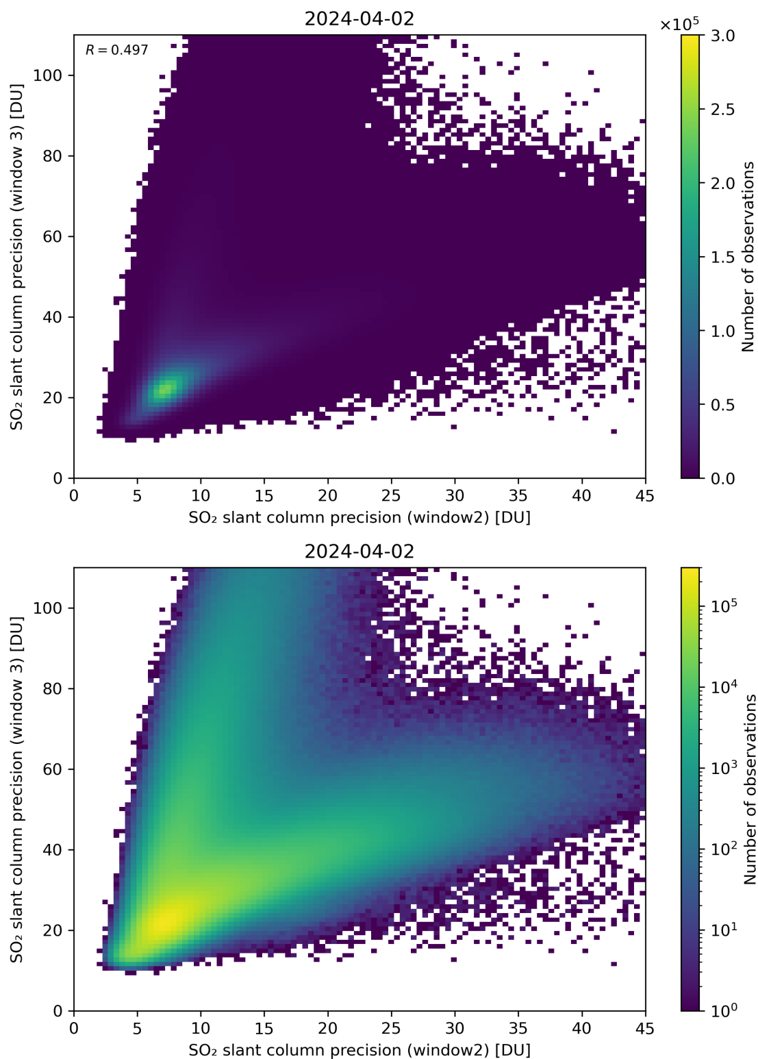
Figure 250: Scatter density plot of “SO 2 slant column precision (window2)” against “SO 2 slant column precision (window 3)” for 2024-04-01 to 2024-04-03.
