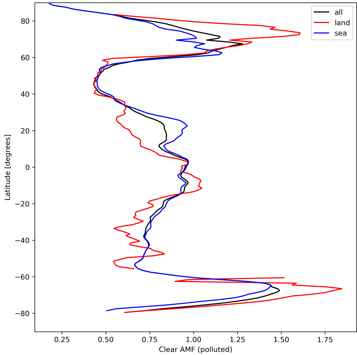
Figure 50: Zonal average of “Clear AMF (polluted)” for 2024-04-01 to 2024-04-03.
