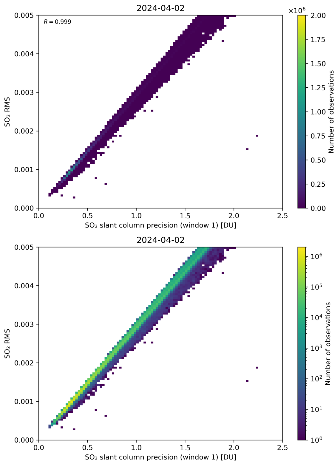
Figure 223: Scatter density plot of “SO 2 slant column precision (window 1)” against “SO 2 RMS” for 2024-04-01 to 2024-04-03.
