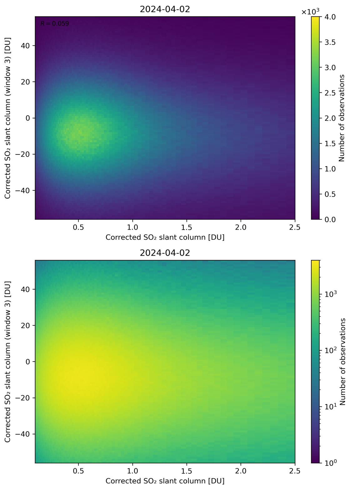
Figure 186: Scatter density plot of “Corrected SO 2 slant column” against “Corrected SO 2 slant column (window 3)” for 2024-04-01 to 2024-04-03.
