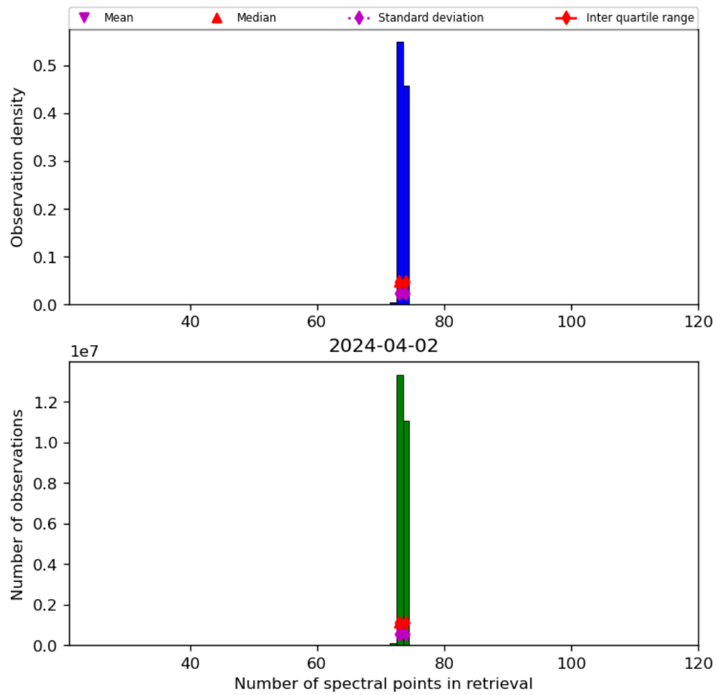
Figure 74: Histogram of “Number of spectral points in retrieval” for 2024-04-01 to 2024-04-03
