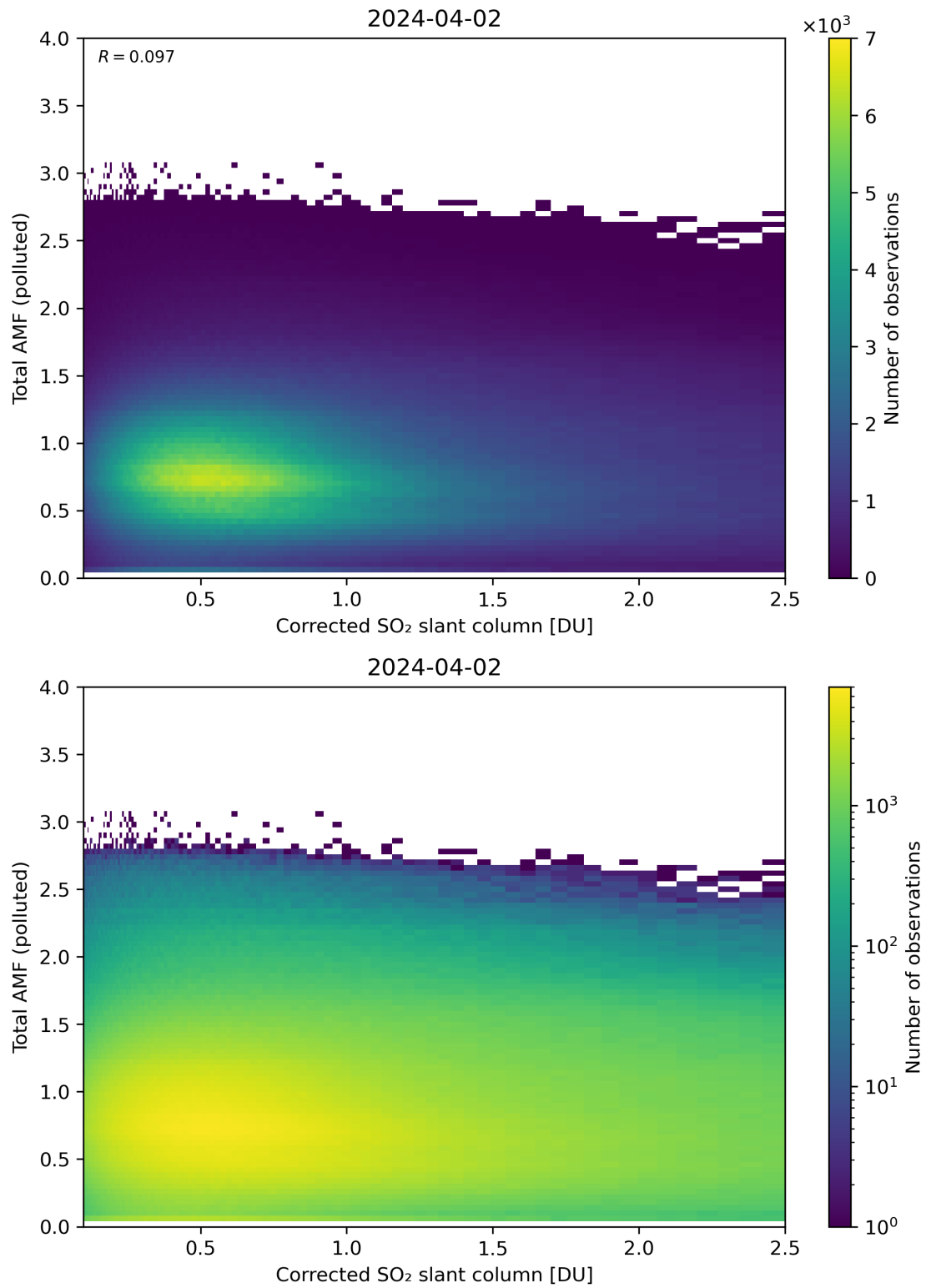
Figure 192: Scatter density plot of “Corrected SO 2 slant column” against “Total AMF (polluted)” for 2024-04-01 to 2024-04-03.
