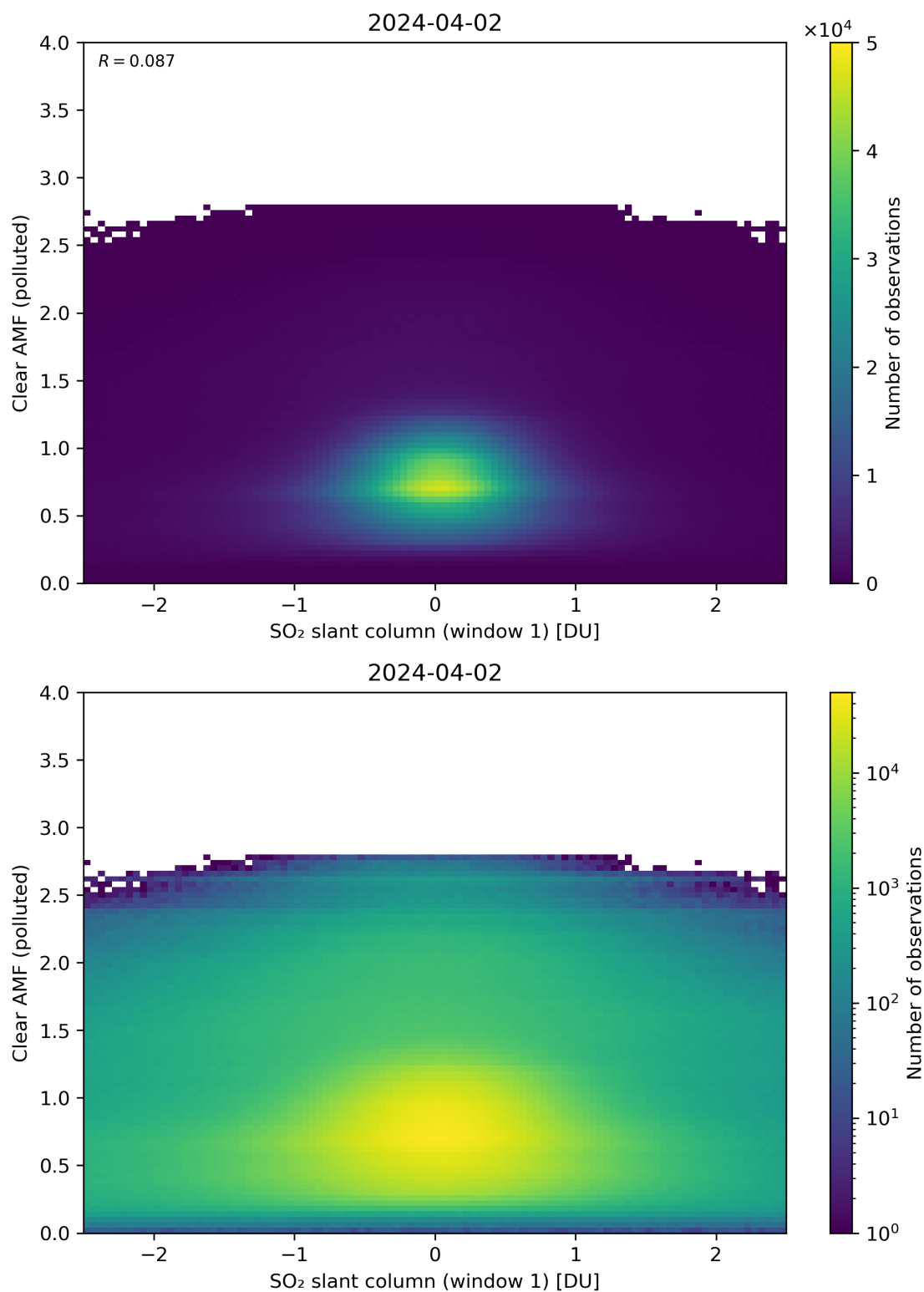
Figure 232: Scatter density plot of “SO 2 slant column (window 1)” against “Clear AMF (polluted)” for 2024-04-01 to 2024-04-03.
