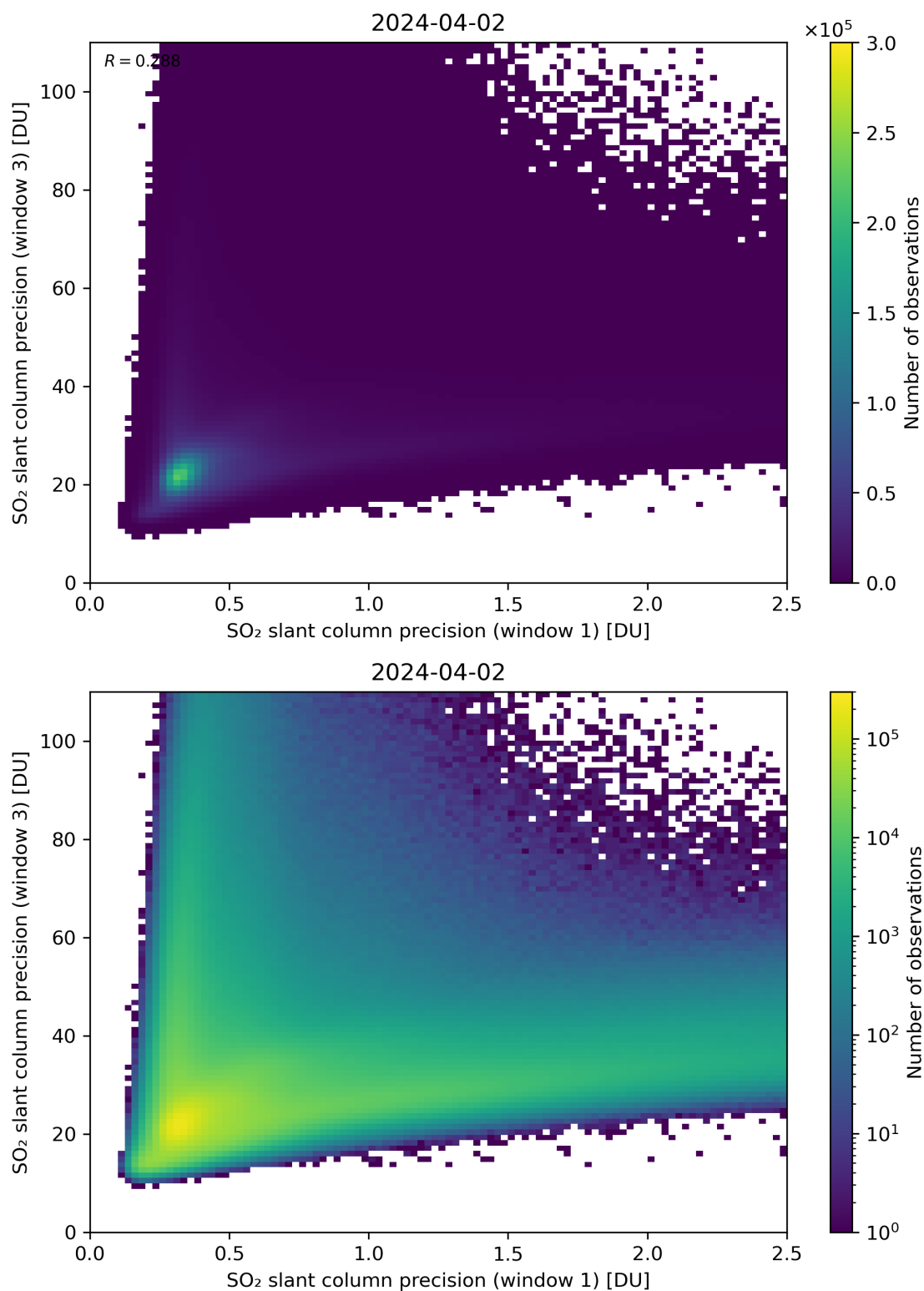
Figure 229: Scatter density plot of “SO 2 slant column precision (window 1)” against “SO 2 slant column precision (window 3)” for 2024-04-01 to 2024-04-03.
