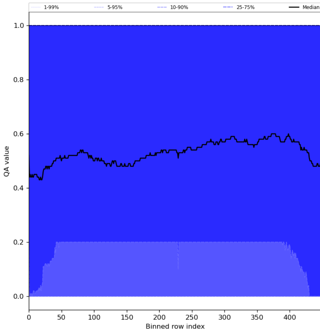
Figure 75: Along track statistics of “QA value” for 2024-04-01 to 2024-04-03
