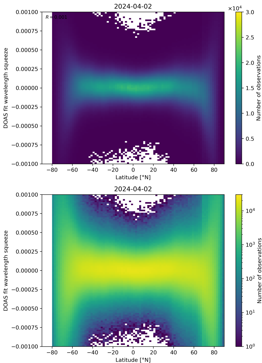
Figure 143: Scatter density plot of “Latitude” against “DOAS fit wavelength squeeze” for 2024-04-01 to 2024-04-03.
