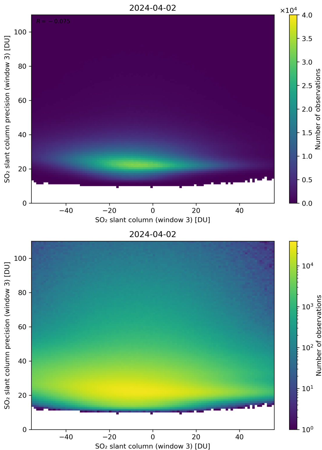
Figure 267: Scatter density plot of “SO 2 slant column (window 3)” against “SO 2 slant column precision (window 3)” for 2024-04-01 to 2024-04-03.
