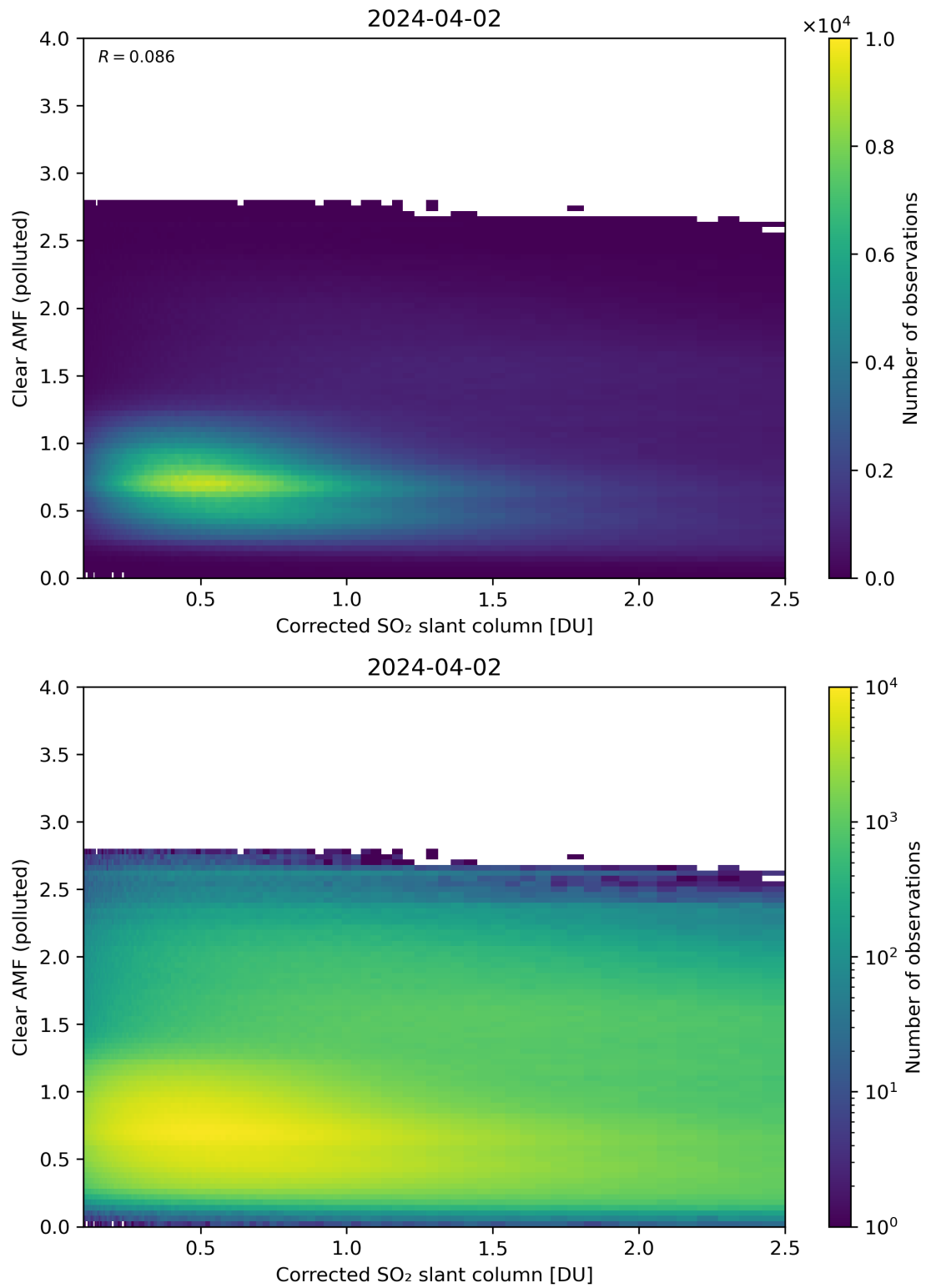
Figure 184: Scatter density plot of “Corrected SO 2 slant column” against “Clear AMF (polluted)” for 2024-04-01 to 2024-04-03.
