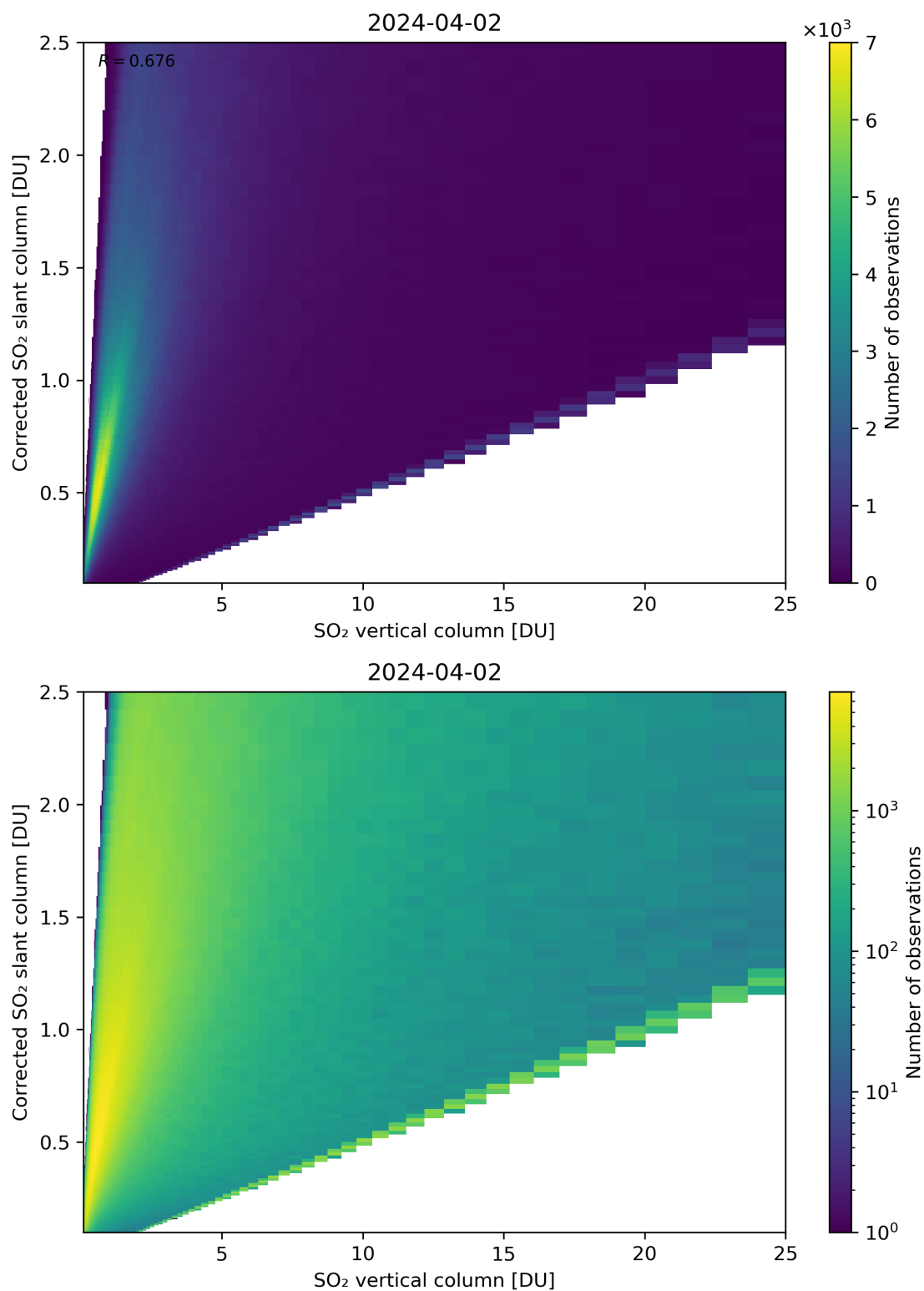
Figure 297: Scatter density plot of “SO 2 vertical column” against “Corrected SO 2 slant column” for 2024-04-01 to 2024-04-03.
