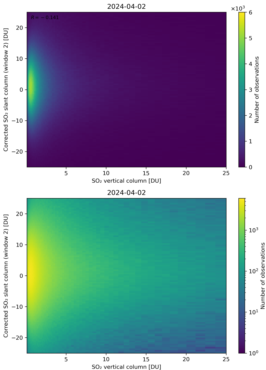
Figure 298: Scatter density plot of “SO 2 vertical column” against “Corrected SO 2 slant column (window 2)” for 2024-04-01 to 2024-04-03.
