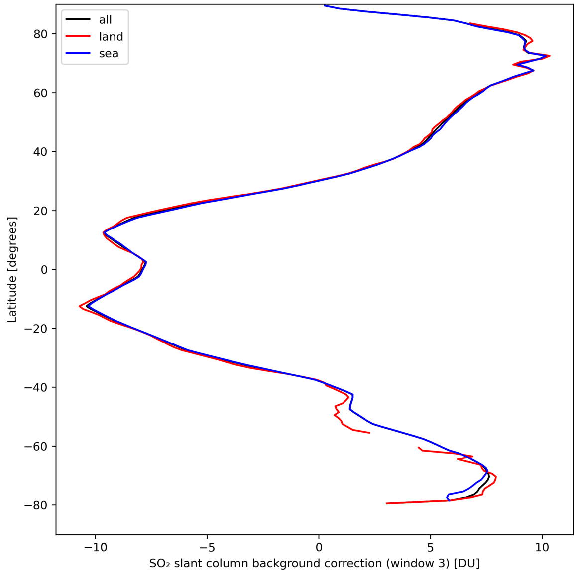
Figure 44: Zonal average of “SO 2 slant column background correction (window 3)” for 2024-04-01 to 2024-04-03.
