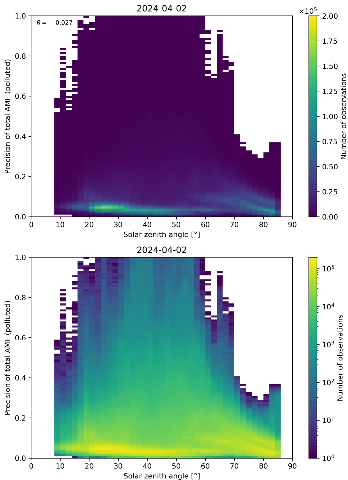
Figure 175: Scatter density plot of “Solar zenith angle” against “Precision of total AMF (polluted)” for 2024-04-01 to 2024-04-03.
