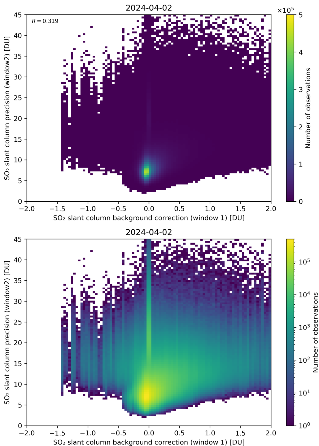
Figure 106: Scatter density plot of “SO 2 slant column background correction (window 1)” against “SO 2 slant column precision (window2)” for 2024-04-01 to 2024-04-03.
