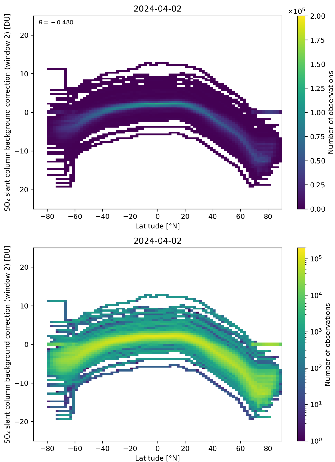
Figure 140: Scatter density plot of “Latitude” against “SO 2 slant column background correction (window 2)” for 2024-04-01 to 2024-04-03.
