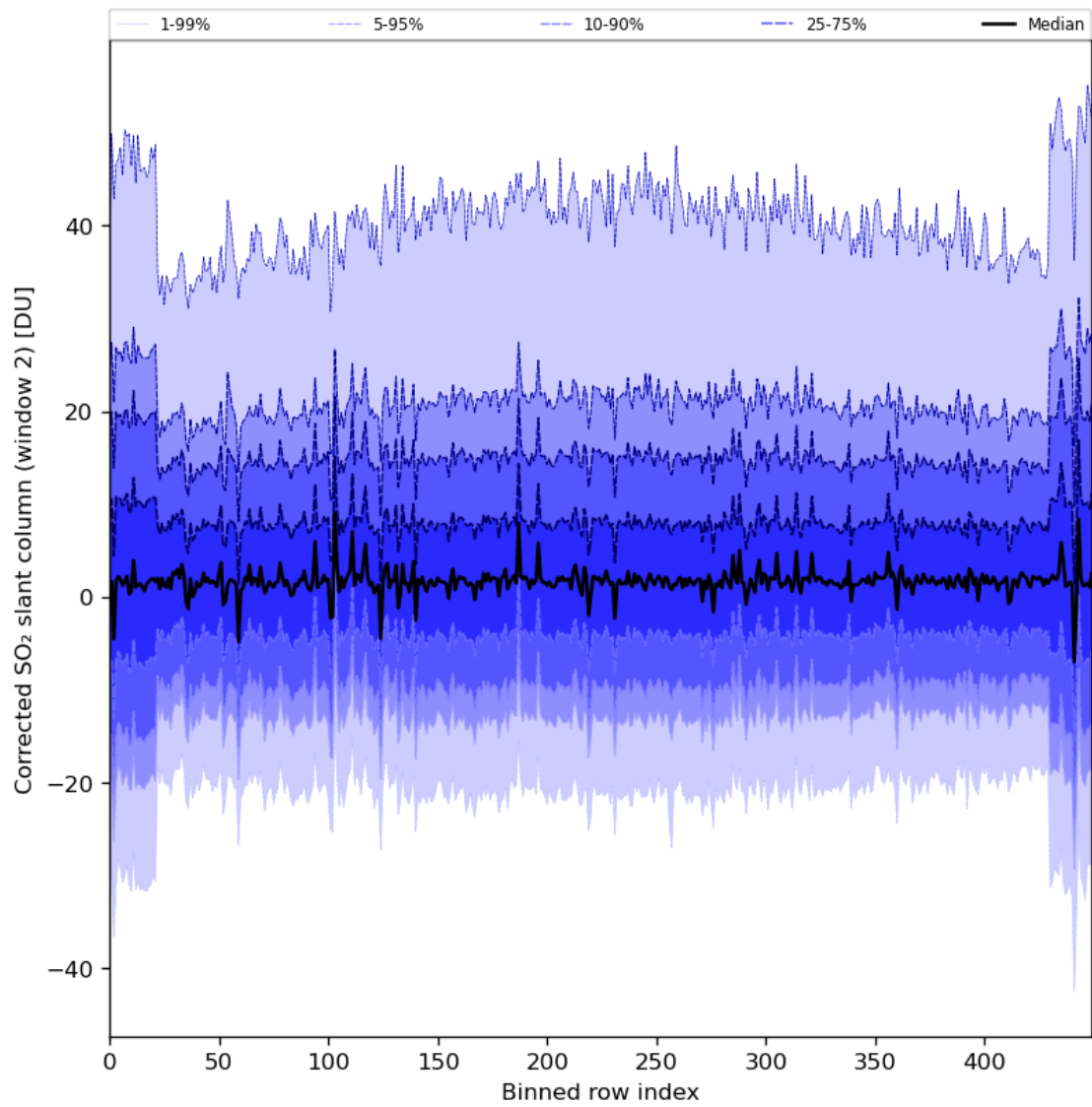
Figure 85: Along track statistics of “Corrected SO 2 slant column (window 2)” for 2024-04-01 to 2024-04-03
