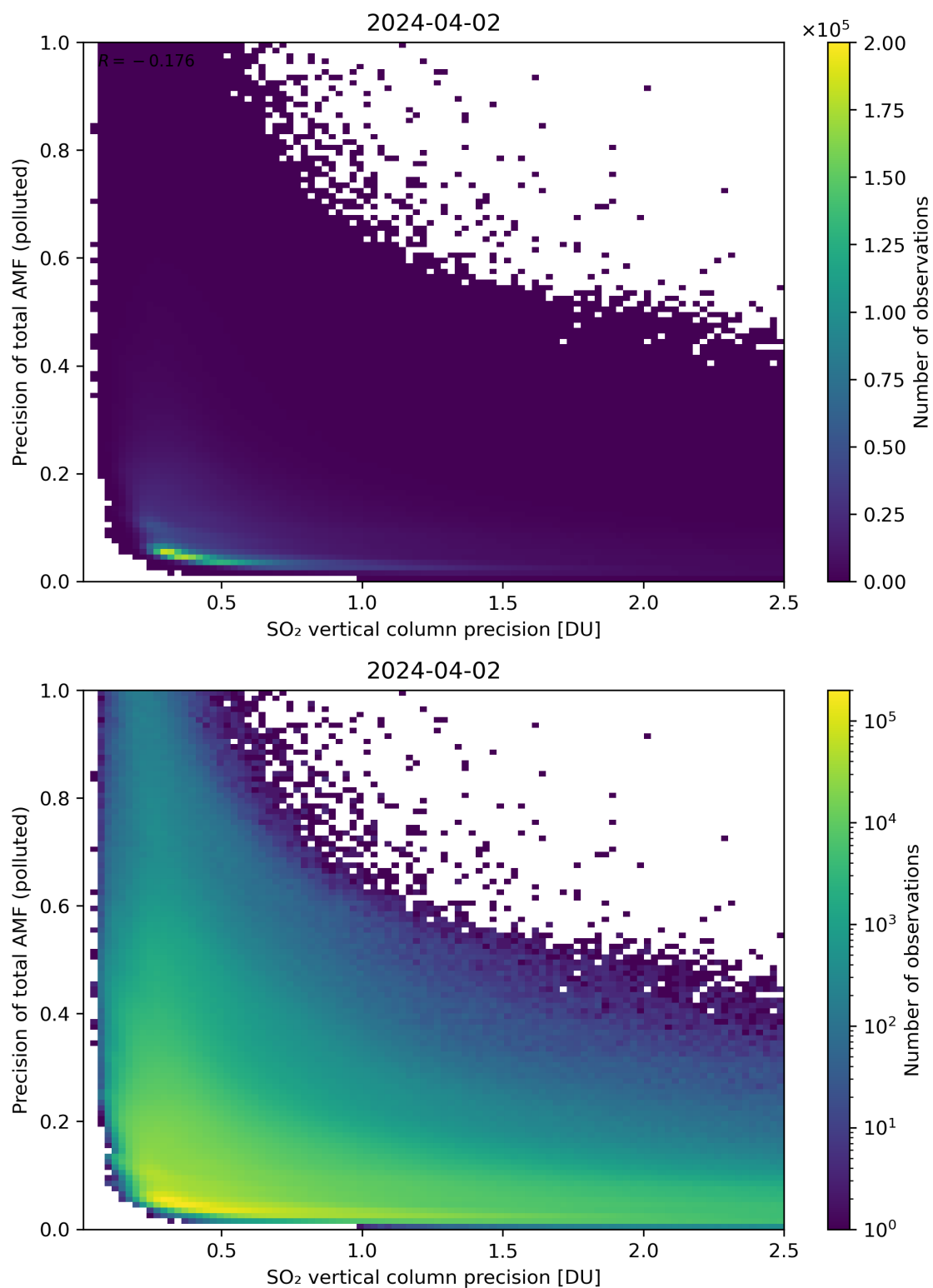
Figure 295: Scatter density plot of “SO 2 vertical column precision” against “Precision of total AMF (polluted)” for 2024-04-01 to 2024-04-03.
