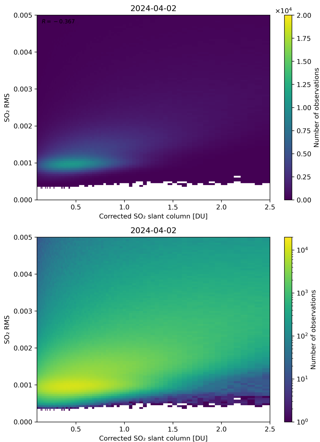
Figure 183: Scatter density plot of “Corrected SO 2 slant column” against “SO 2 RMS” for 2024-04-01 to 2024-04-03.
