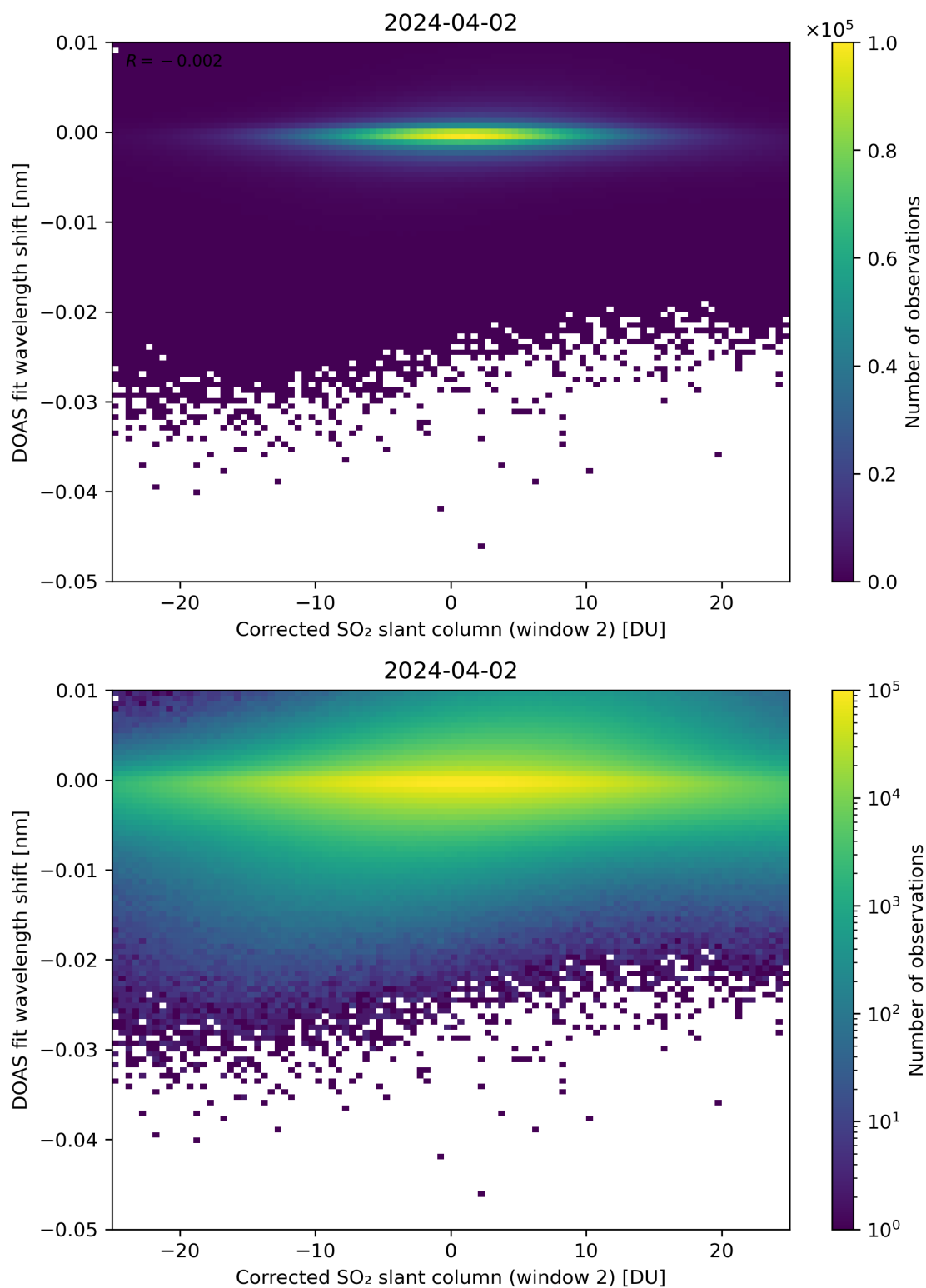
Figure 196: Scatter density plot of “Corrected SO 2 slant column (window 2)” against “DOAS fit wavelength shift” for 2024-04-01 to 2024-04-03.
