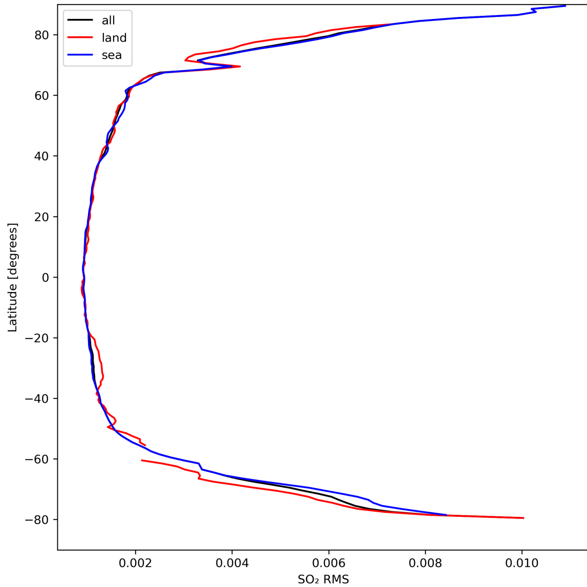
Figure 47: Zonal average of “SO 2 RMS” for 2024-04-01 to 2024-04-03.
