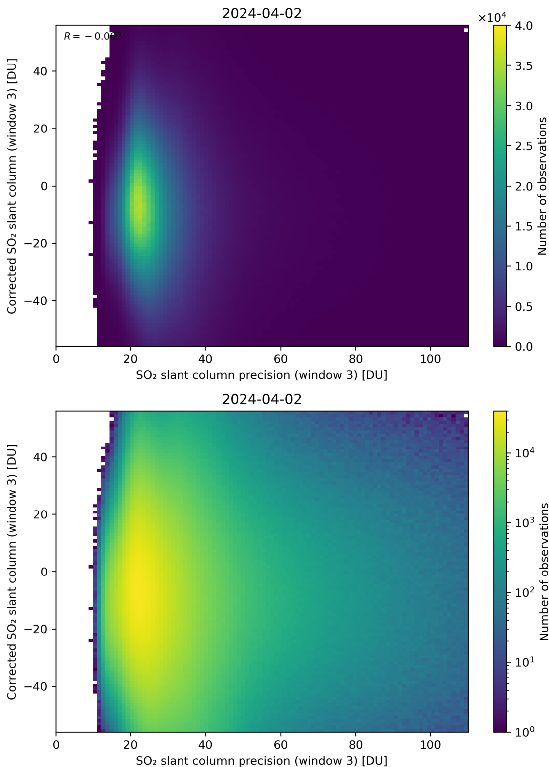
Figure 262: Scatter density plot of “SO 2 slant column precision (window 3)” against “Corrected SO 2 slant column (window 3)” for 2024-04-01 to 2024-04-03.
