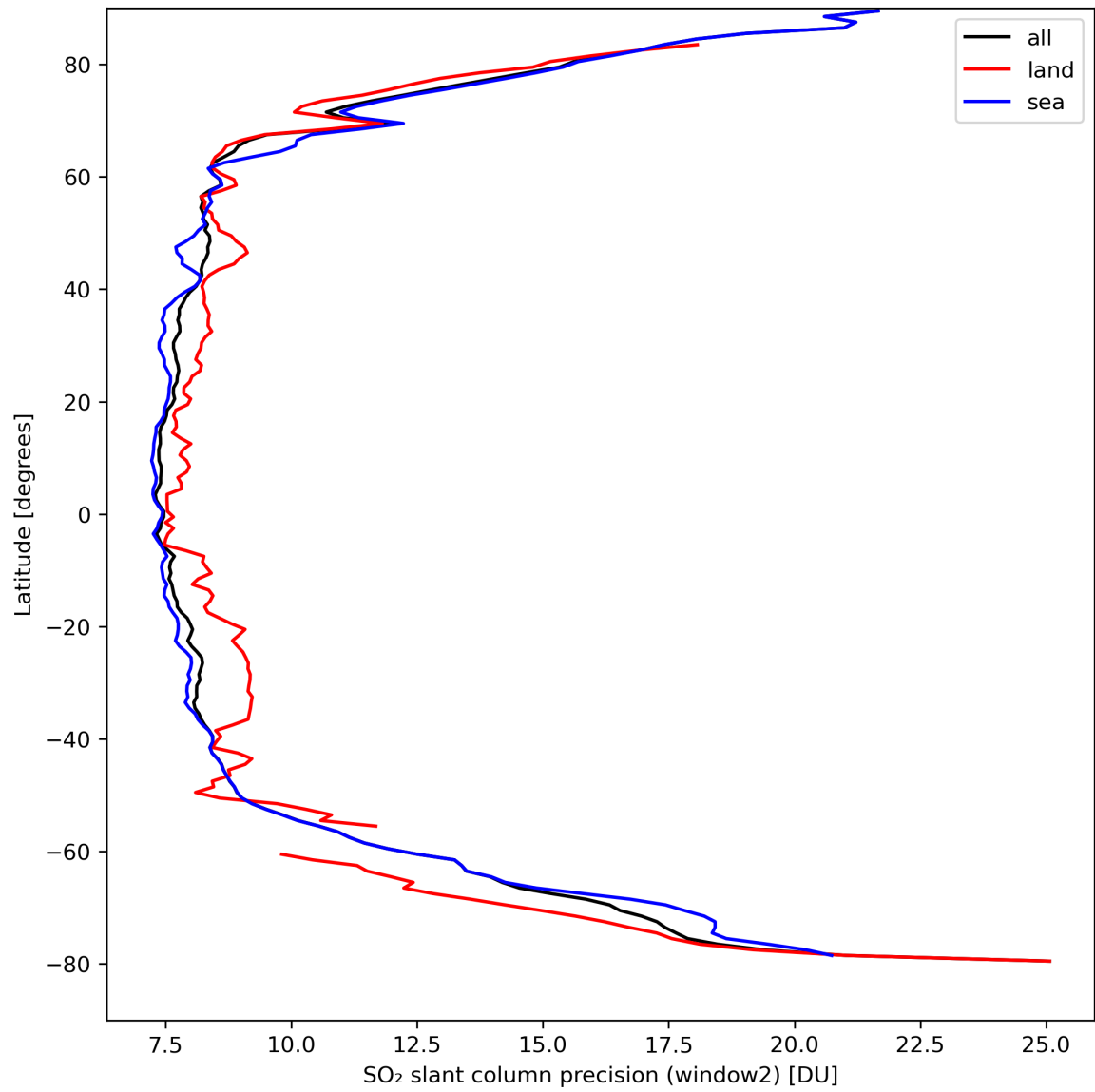
Figure 38: Zonal average of “SO 2 slant column precision (window2)” for 2024-04-01 to 2024-04-03.
