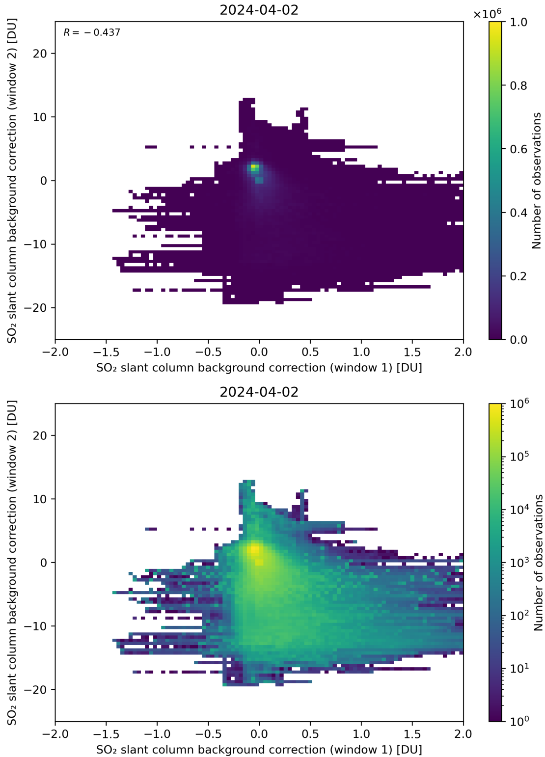
Figure 98: Scatter density plot of “SO 2 slant column background correction (window 1)” against “SO 2 slant column background correction (window 2)” for 2024-04-01 to 2024-04-03.
