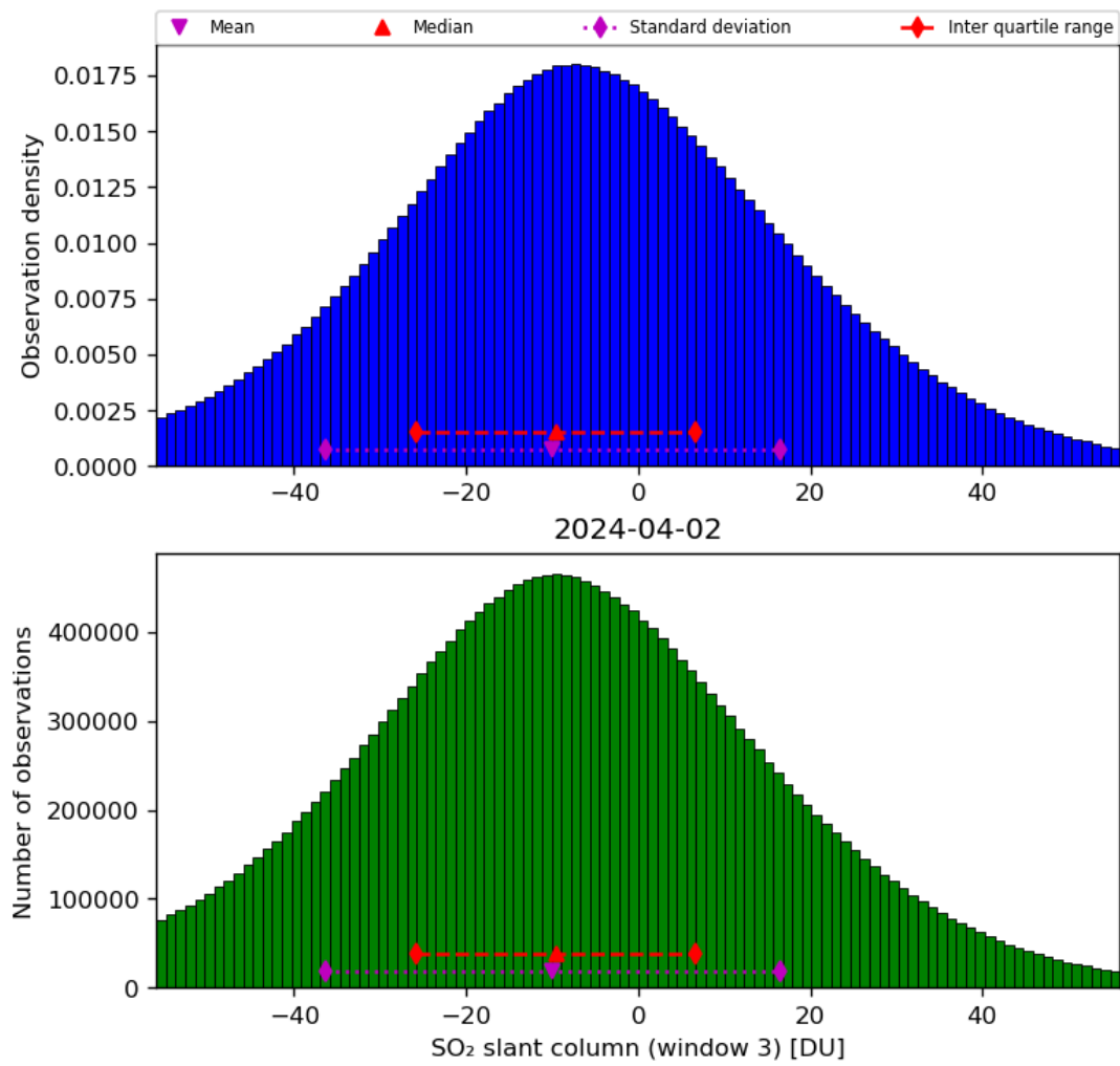
Figure 64: Histogram of “SO 2 slant column (window 3)” for 2024-04-01 to 2024-04-03
