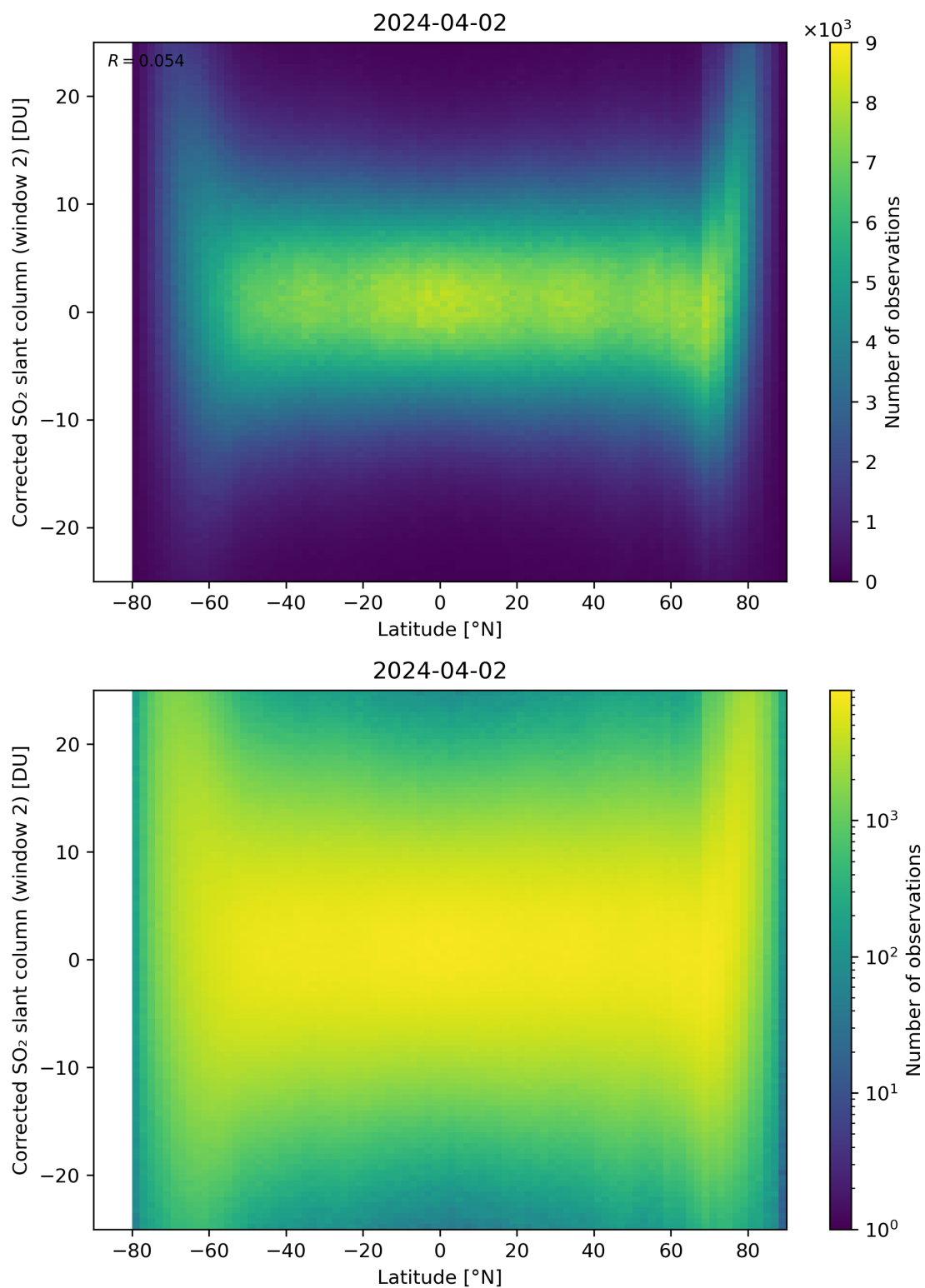
Figure 147: Scatter density plot of “Latitude” against “Corrected SO 2 slant column (window 2)” for 2024-04-01 to 2024-04-03.
