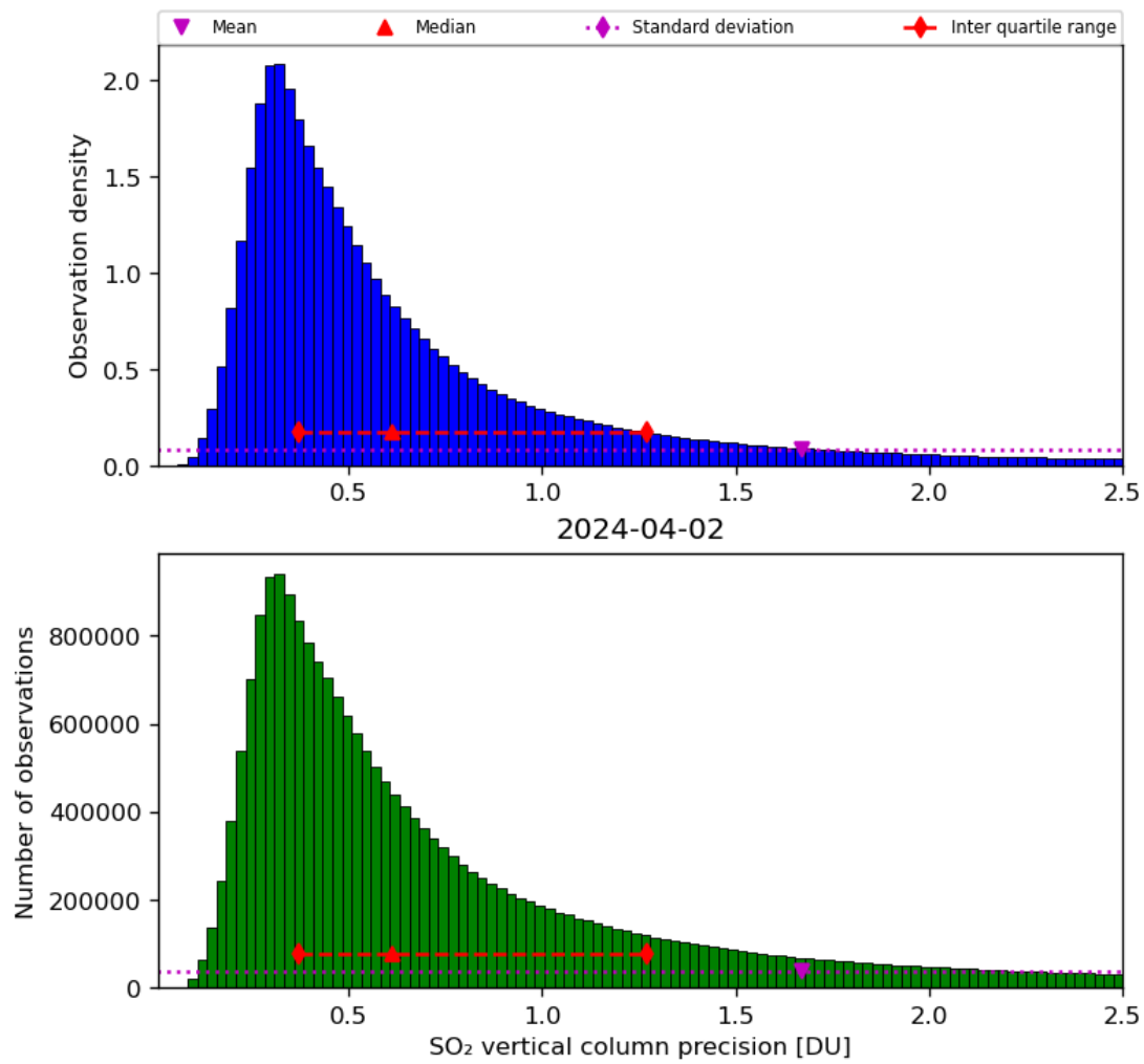
Figure 54: Histogram of “SO 2 vertical column precision” for 2024-04-01 to 2024-04-03
