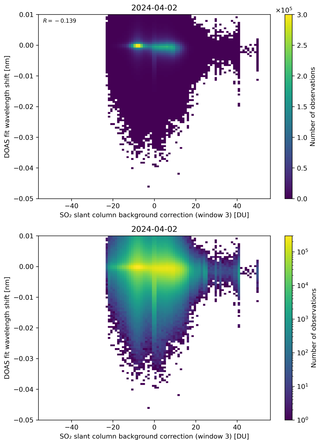
Figure 121: Scatter density plot of “SO 2 slant column background correction (window 3)” against “DOAS fit wavelength shift” for 2024-04-01 to 2024-04-03.
