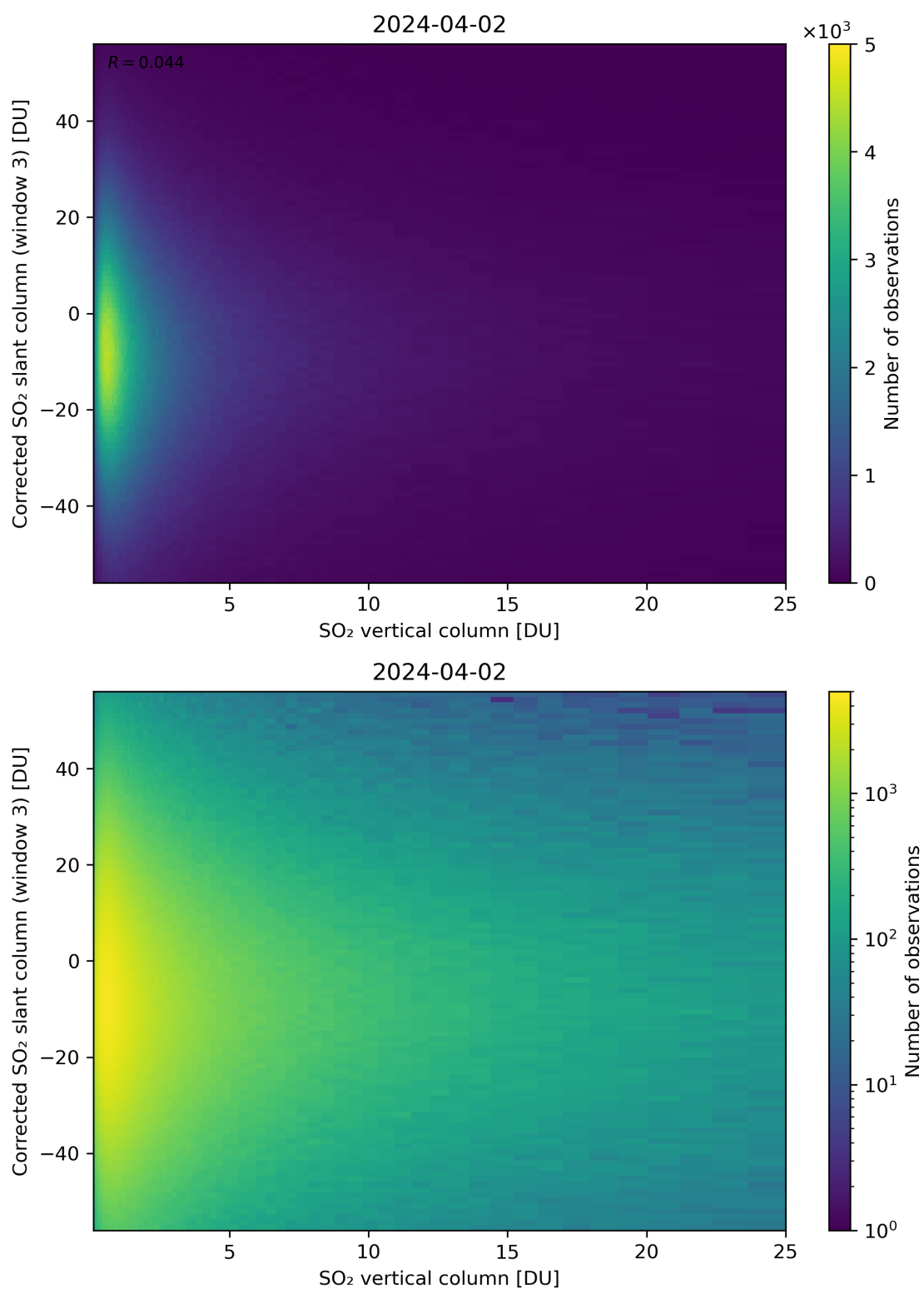
Figure 299: Scatter density plot of “SO 2 vertical column” against “Corrected SO 2 slant column (window 3)” for 2024-04-01 to 2024-04-03.
