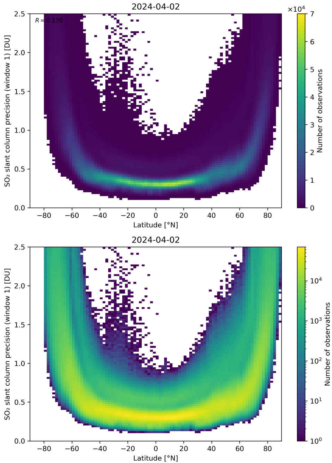
Figure 150: Scatter density plot of “Latitude” against “SO 2 slant column precision (window 1)” for 2024-04-01 to 2024-04-03.
