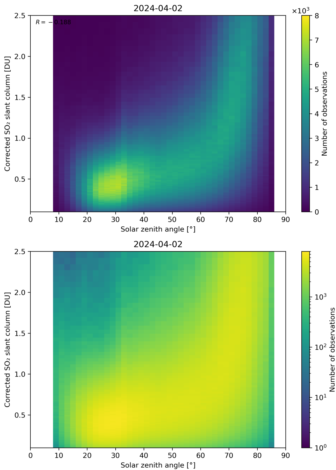
Figure 166: Scatter density plot of “Solar zenith angle” against “Corrected SO 2 slant column” for 2024-04-01 to 2024-04-03.
