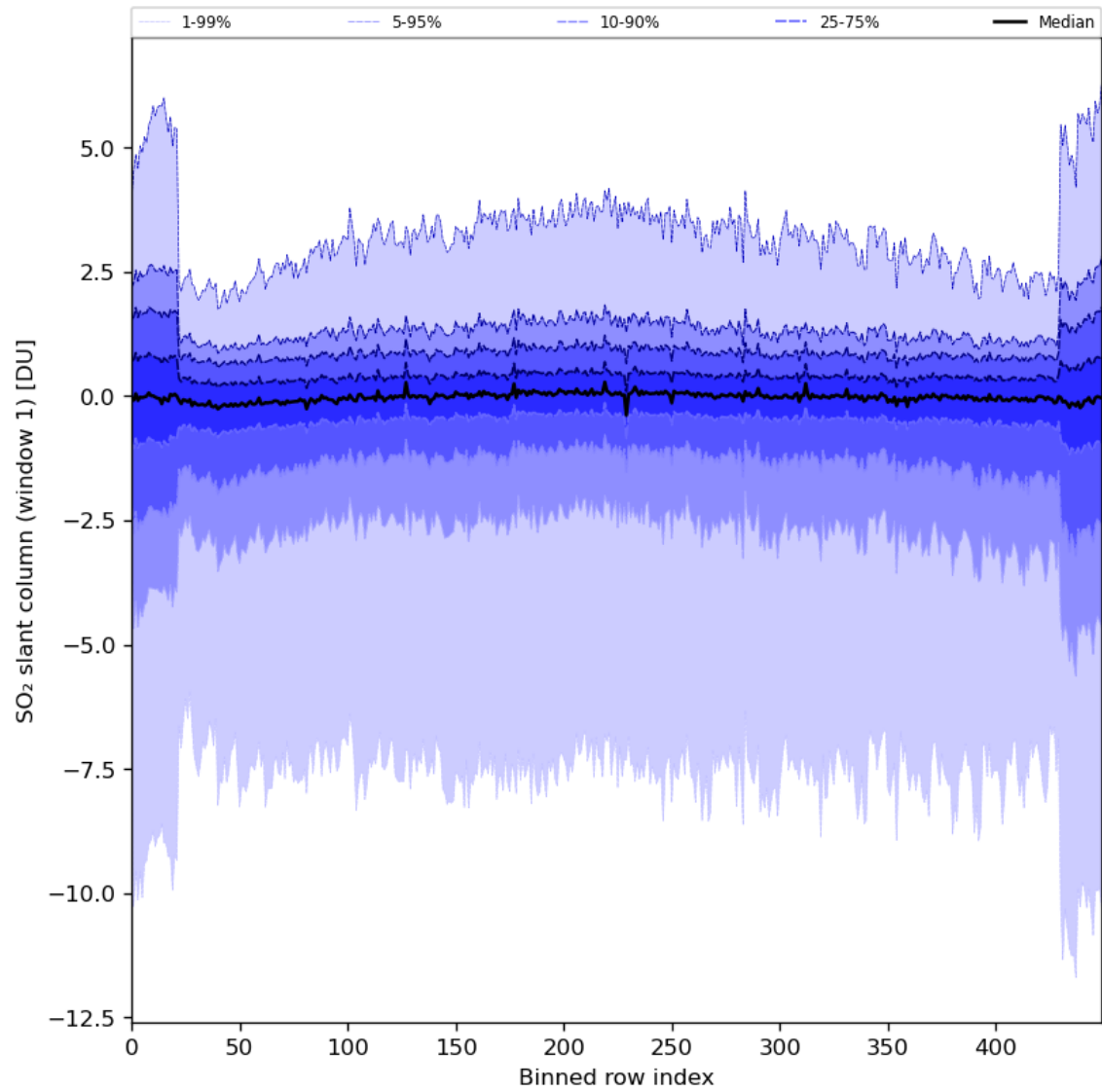
Figure 79: Along track statistics of “SO 2 slant column (window 1)” for 2024-04-01 to 2024-04-03
