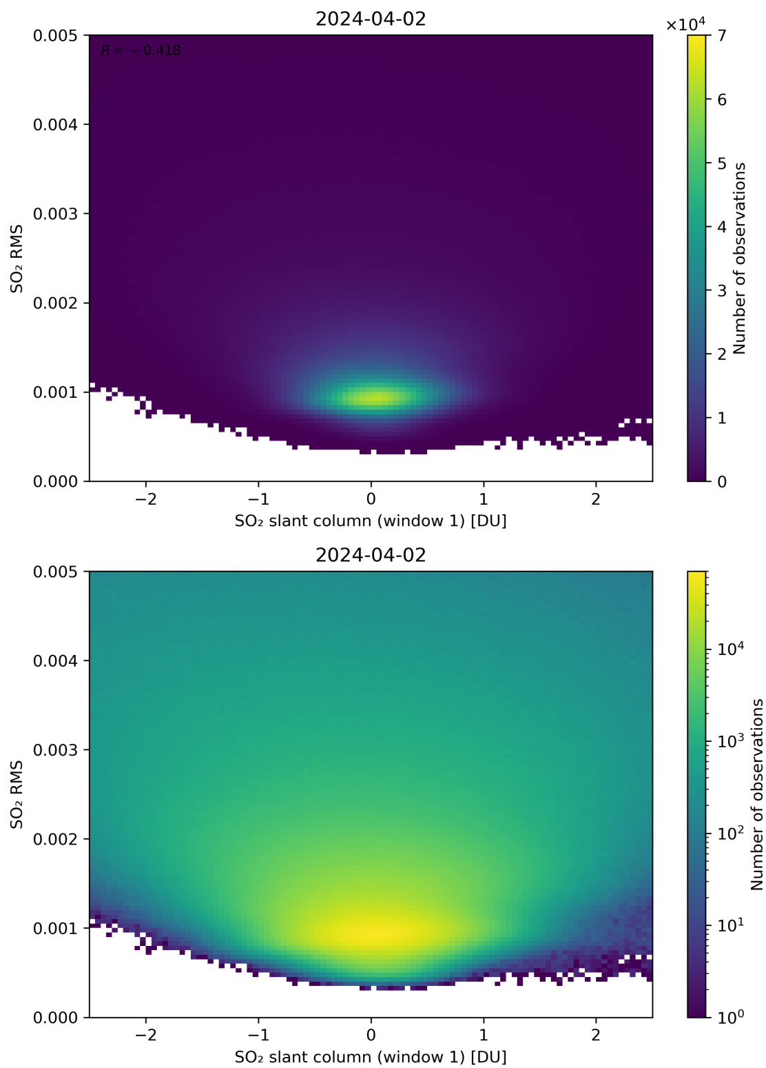
Figure 217: Scatter density plot of “SO 2 slant column (window 1)” against “SO 2 RMS” for 2024-04-01 to 2024-04-03.
