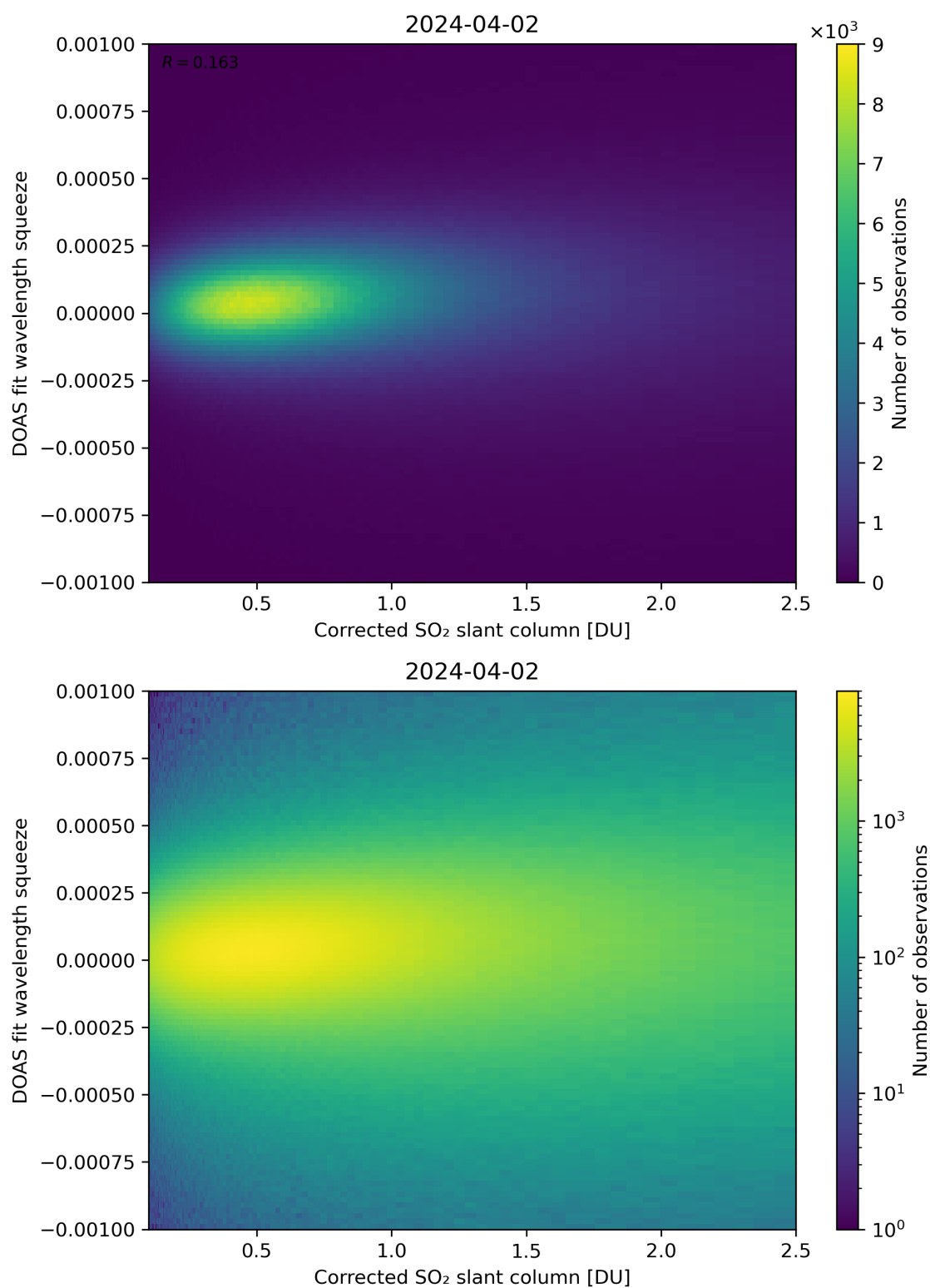
Figure 182: Scatter density plot of “Corrected SO 2 slant column” against “DOAS fit wavelength squeeze” for 2024-04-01 to 2024-04-03.
