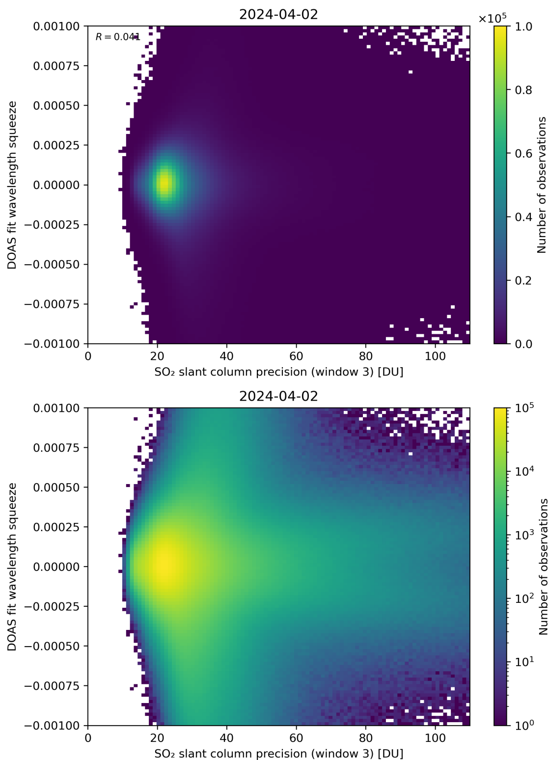
Figure 259: Scatter density plot of “SO 2 slant column precision (window 3)” against “DOAS fit wavelength squeeze” for 2024-04-01 to 2024-04-03.
