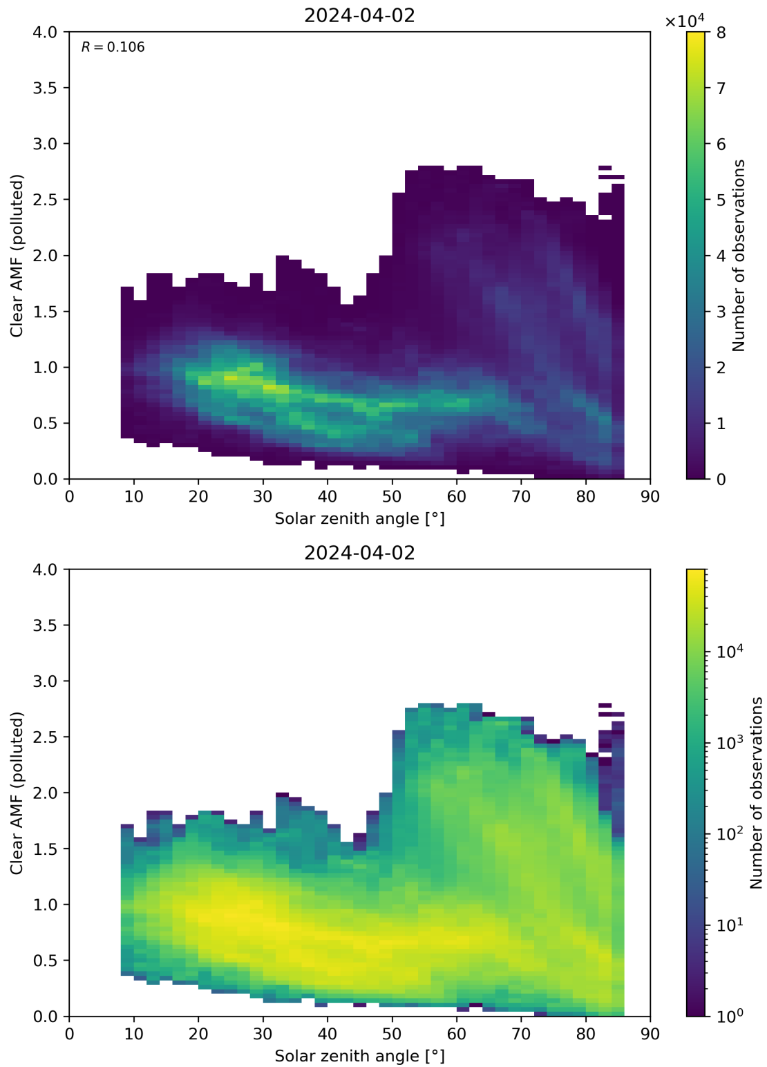
Figure 165: Scatter density plot of “Solar zenith angle” against “Clear AMF (polluted)” for 2024-04-01 to 2024-04-03.
