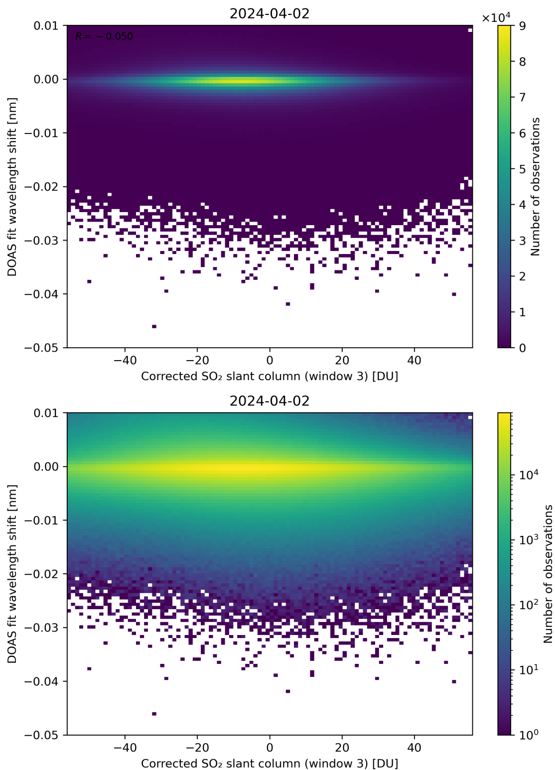
Figure 206: Scatter density plot of “Corrected SO 2 slant column (window 3)” against “DOAS fit wavelength shift” for 2024-04-01 to 2024-04-03.
