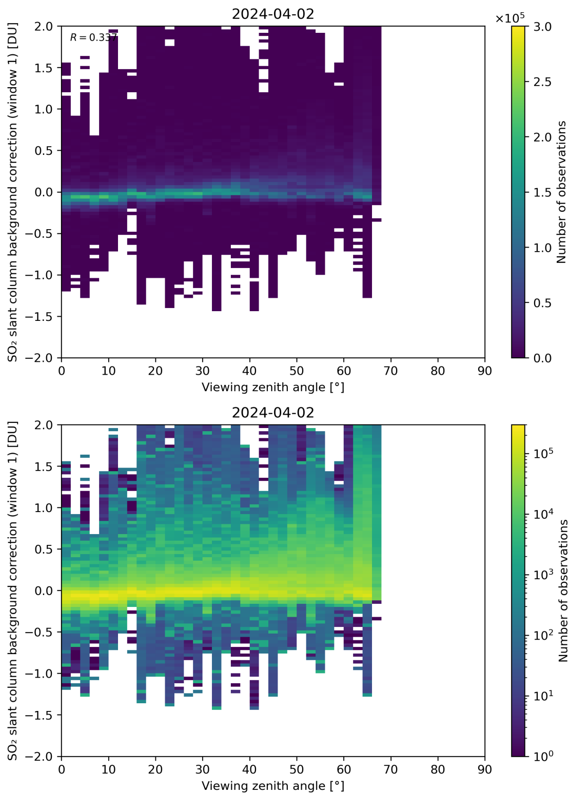
Figure 308: Scatter density plot of “Viewing zenith angle” against “SO 2 slant column background correction (window 1)” for 2024-04-01 to 2024-04-03.
