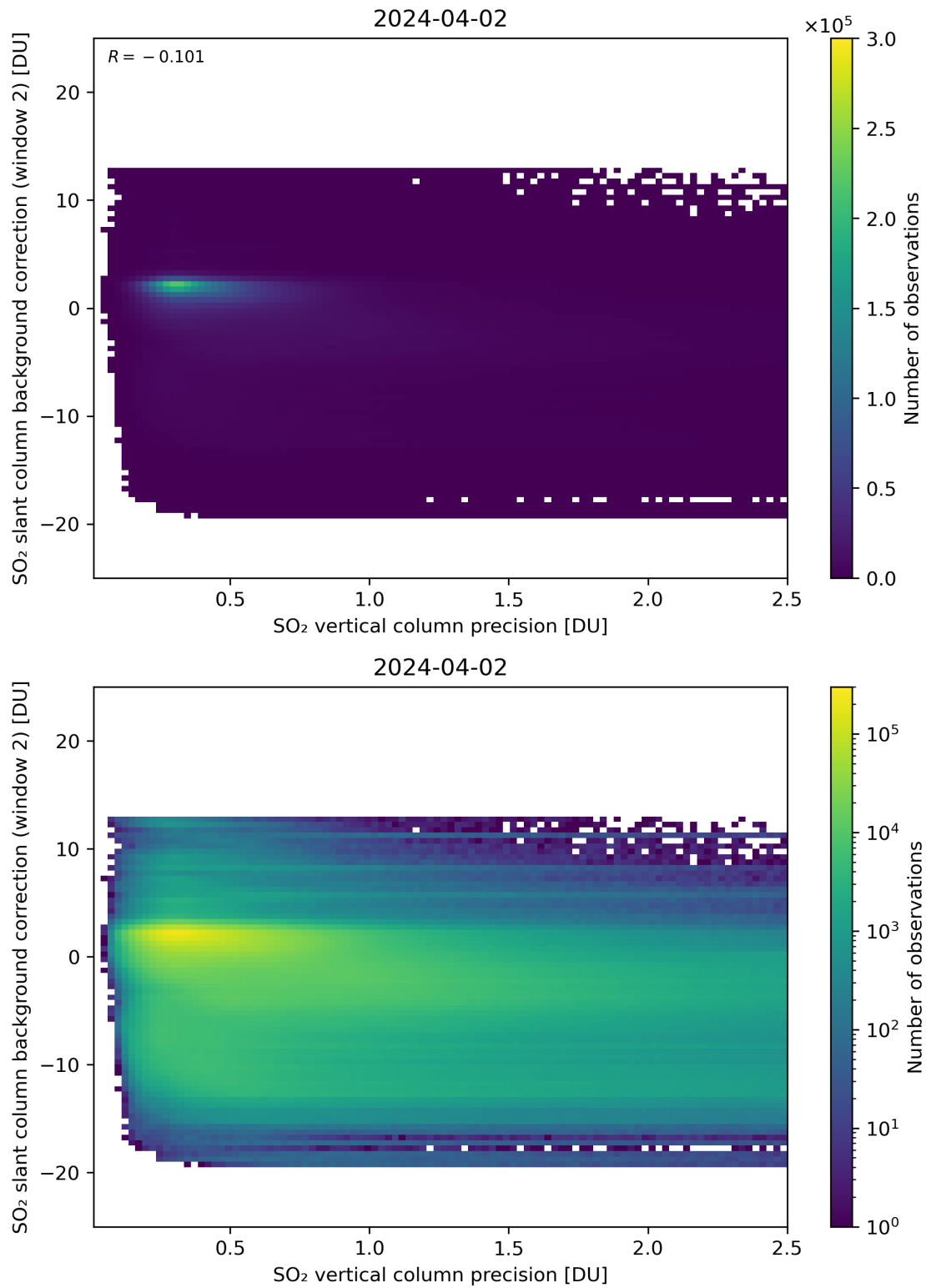
Figure 280: Scatter density plot of “SO 2 vertical column precision” against “SO 2 slant column background correction (window 2)” for 2024-04-01 to 2024-04-03.
