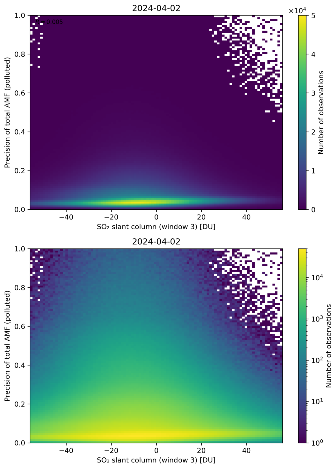
Figure 269: Scatter density plot of “SO 2 slant column (window 3)” against “Precision of total AMF (polluted)” for 2024-04-01 to 2024-04-03.
