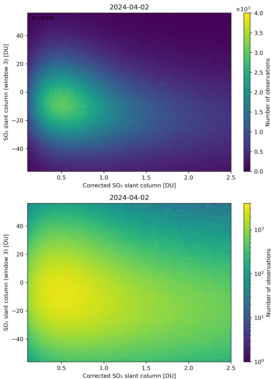
Figure 190: Scatter density plot of “Corrected SO 2 slant column” against “SO 2 slant column (window 3)” for 2024-04-01 to 2024-04-03.
