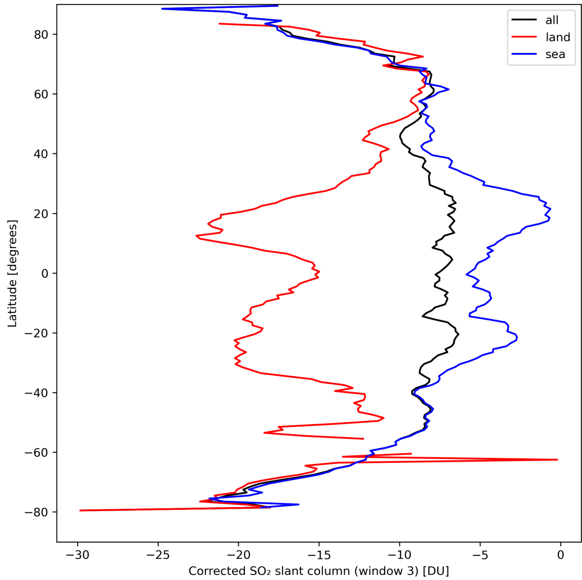
Figure 43: Zonal average of “Corrected SO 2 slant column (window 3)” for 2024-04-01 to 2024-04-03.
