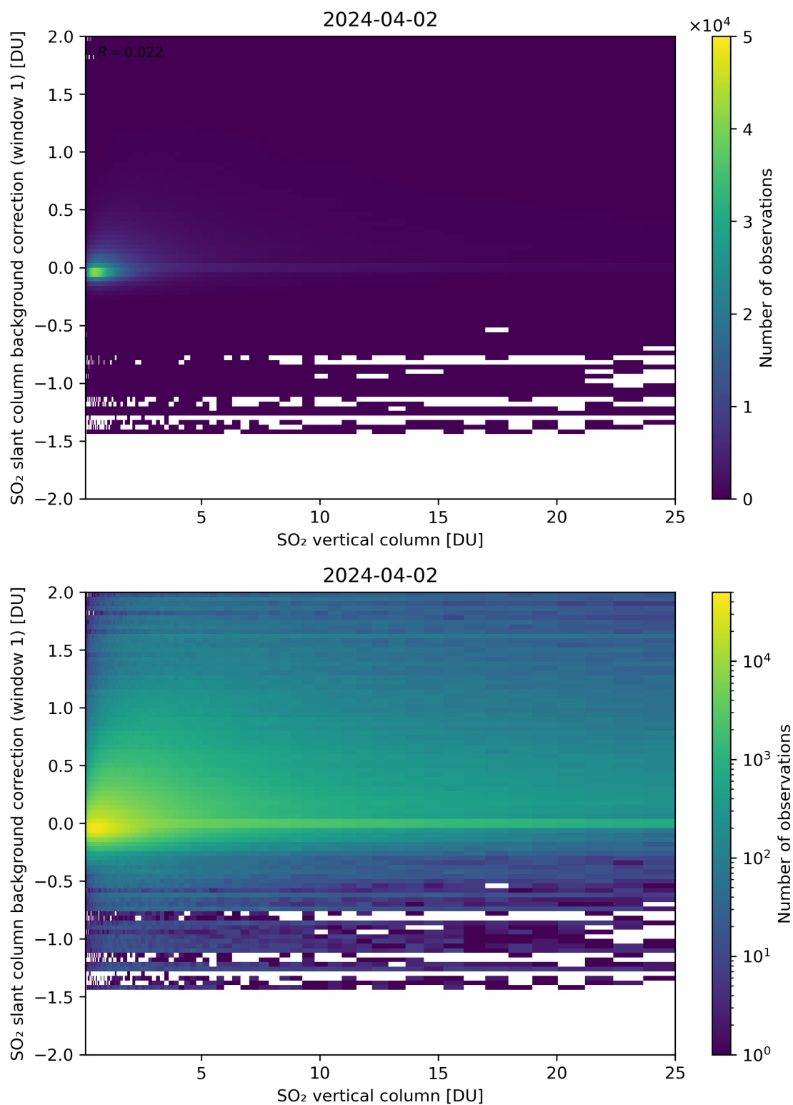
Figure 273: Scatter density plot of “SO 2 vertical column” against “SO 2 slant column background correction (window 1)” for 2024-04-01 to 2024-04-03.
