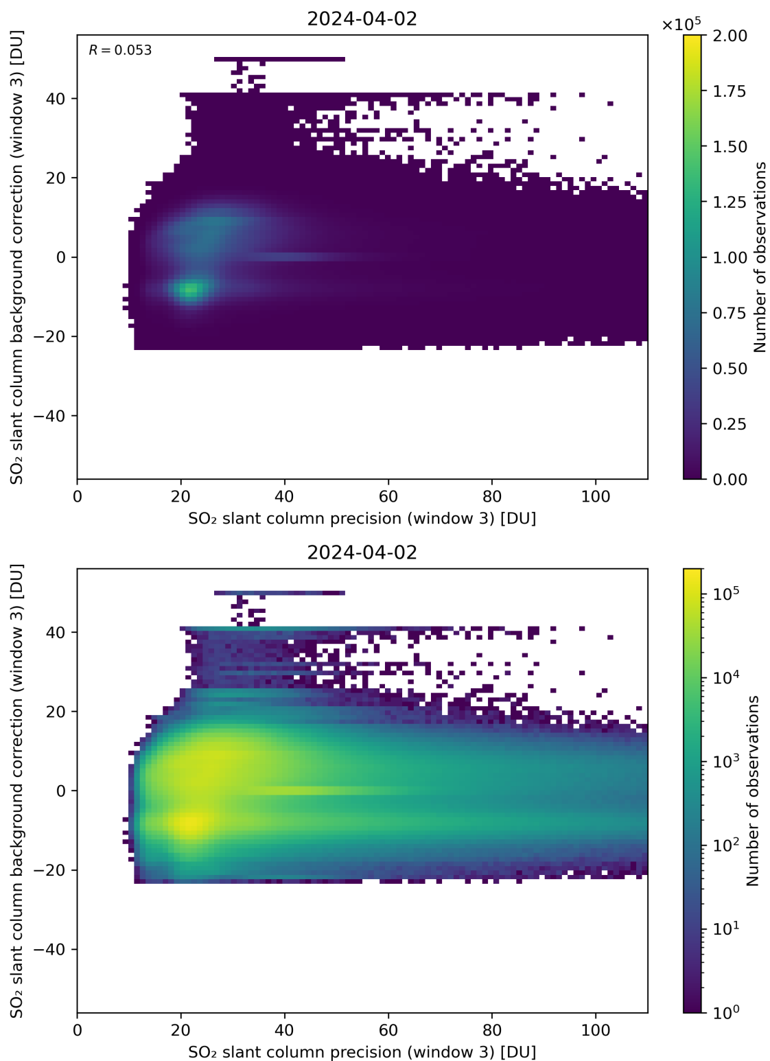
Figure 257: Scatter density plot of “SO 2 slant column precision (window 3)” against “SO 2 slant column background correction (window 3)” for 2024-04-01 to 2024-04-03.
