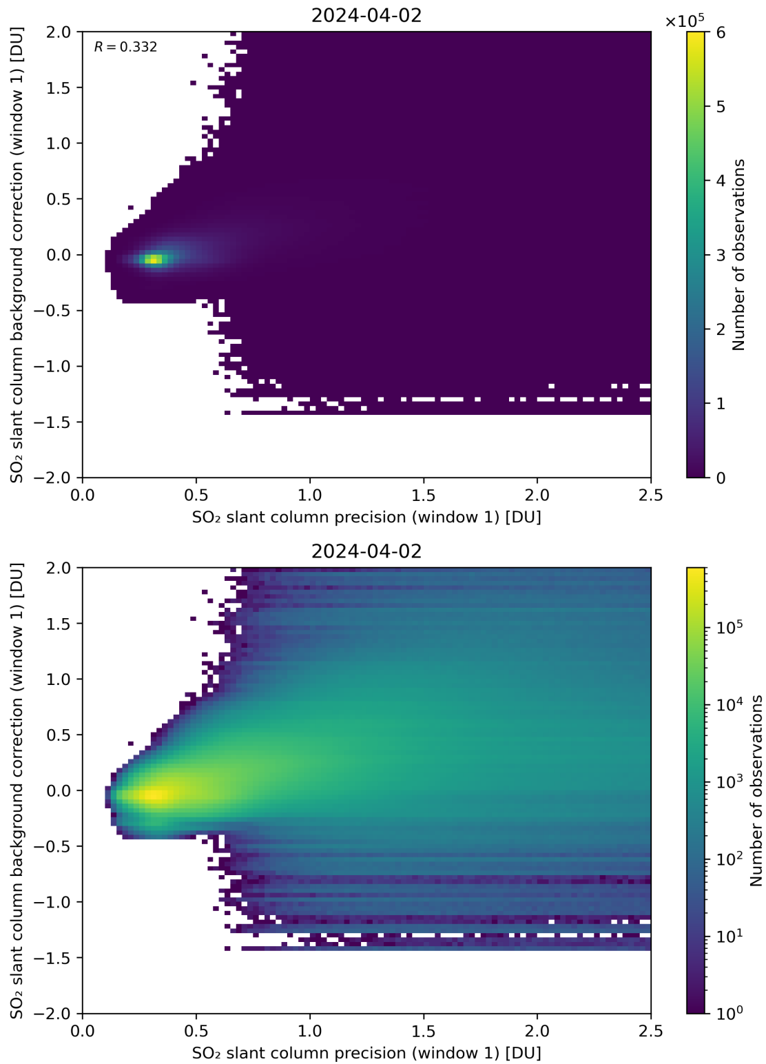
Figure 218: Scatter density plot of “SO 2 slant column precision (window 1)” against “SO 2 slant column background correction (window 1)” for 2024-04-01 to 2024-04-03.
