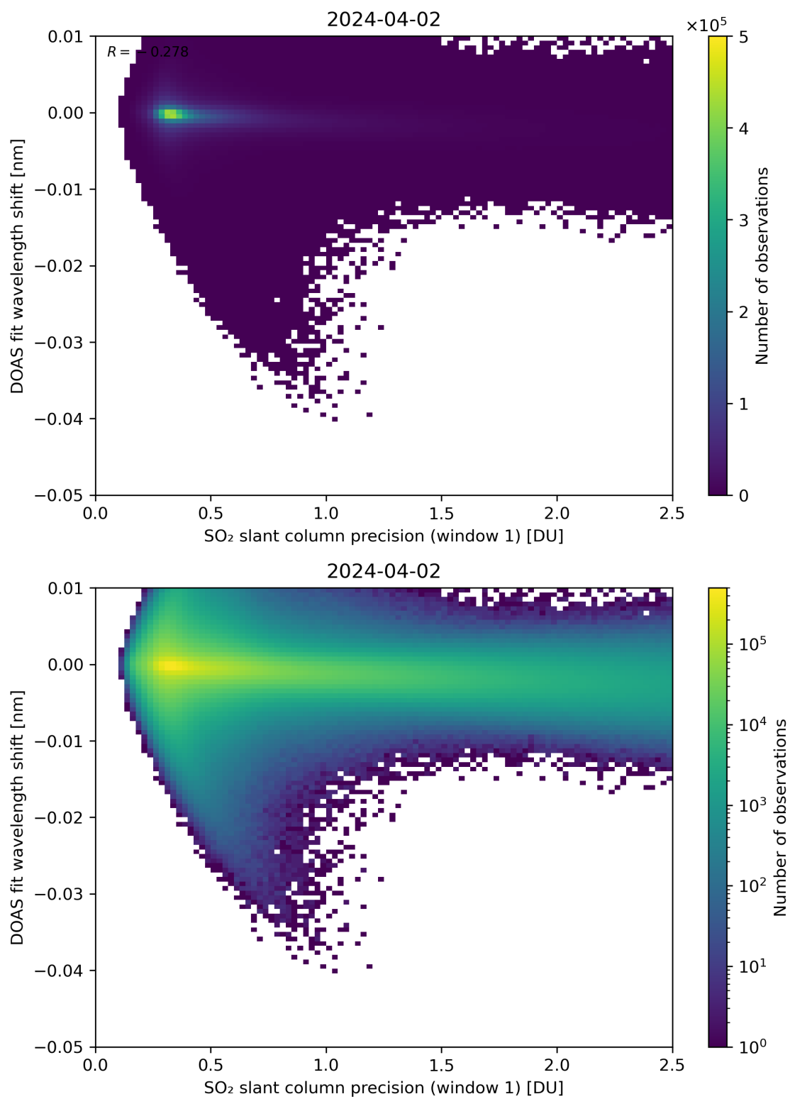
Figure 221: Scatter density plot of “SO 2 slant column precision (window 1)” against “DOAS fit wavelength shift” for 2024-04-01 to 2024-04-03.
