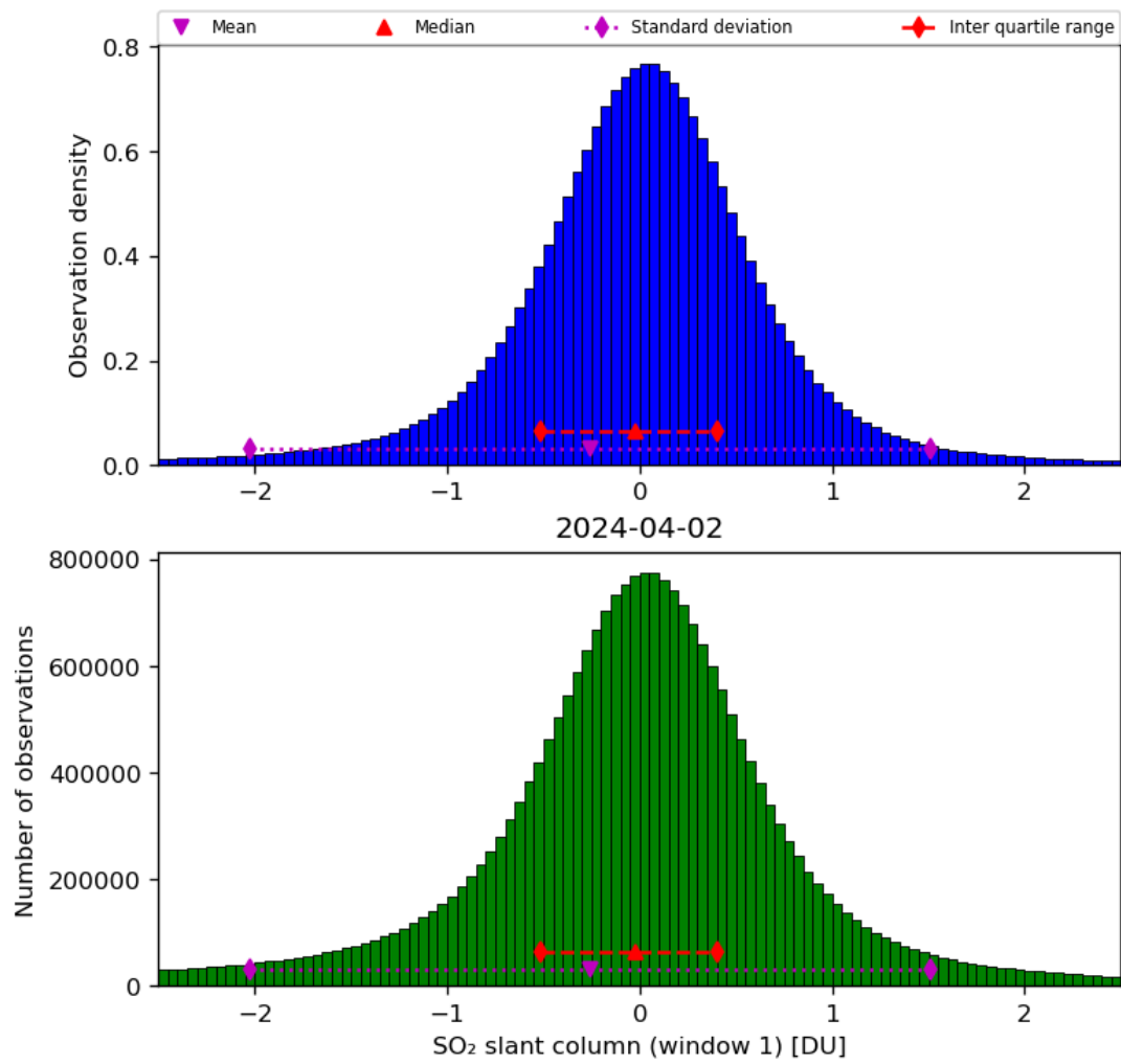
Figure 56: Histogram of “SO 2 slant column (window 1)” for 2024-04-01 to 2024-04-03
