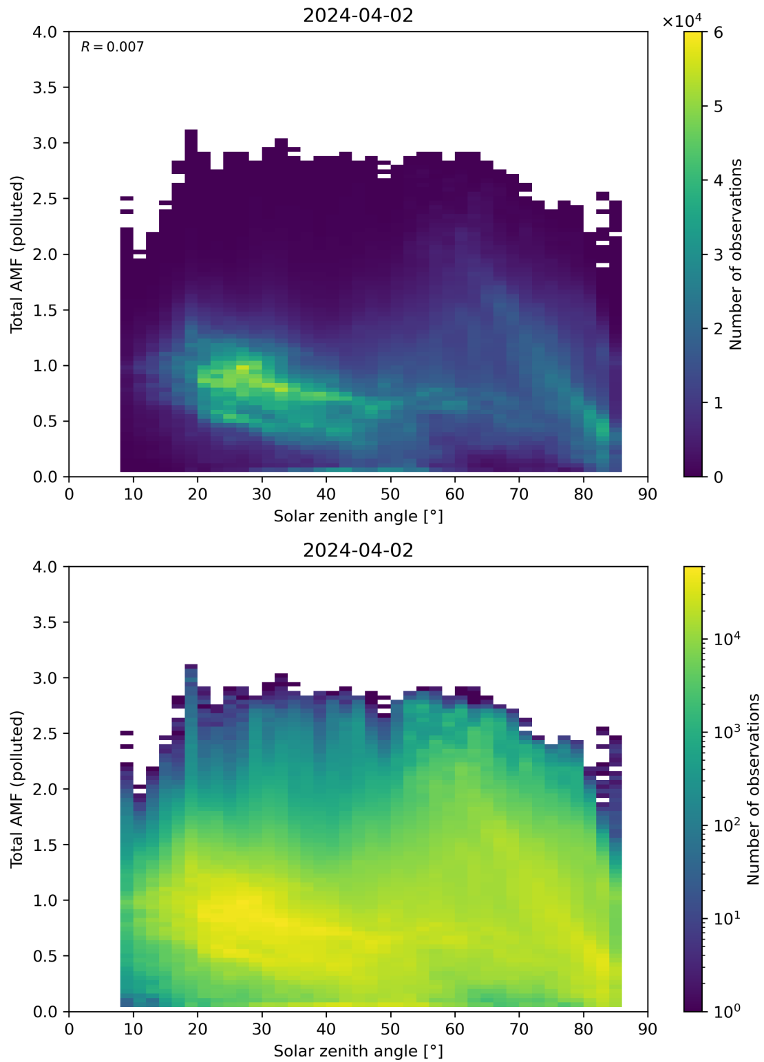
Figure 174: Scatter density plot of “Solar zenith angle” against “Total AMF (polluted)” for 2024-04-01 to 2024-04-03.
