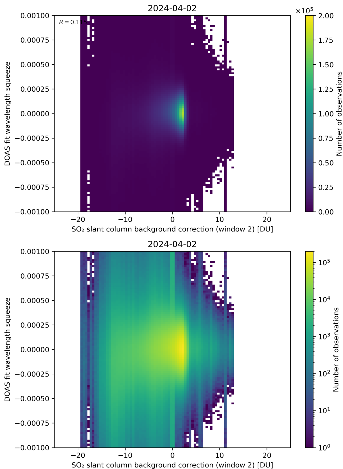
Figure 113: Scatter density plot of “SO 2 slant column background correction (window 2)” against “DOAS fit wavelength squeeze” for 2024-04-01 to 2024-04-03.
