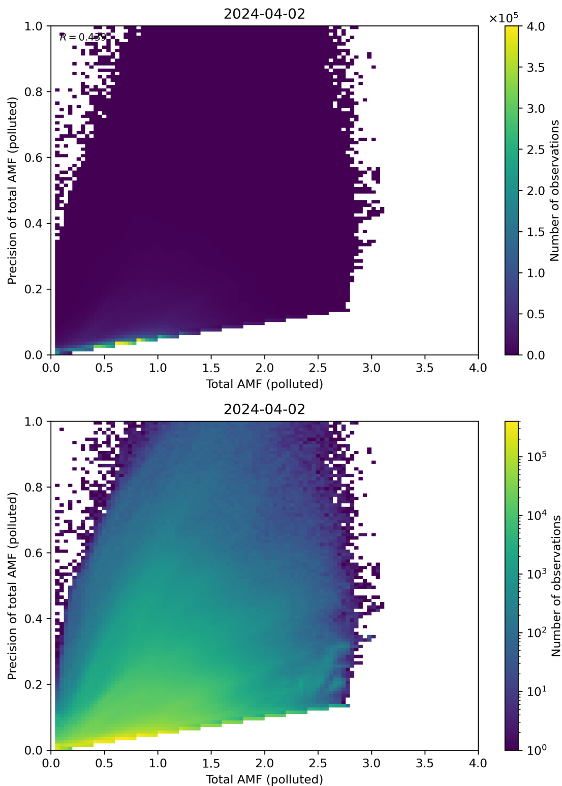
Figure 272: Scatter density plot of “Total AMF (polluted)” against “Precision of total AMF (polluted)” for 2024-04-01 to 2024-04-03.
