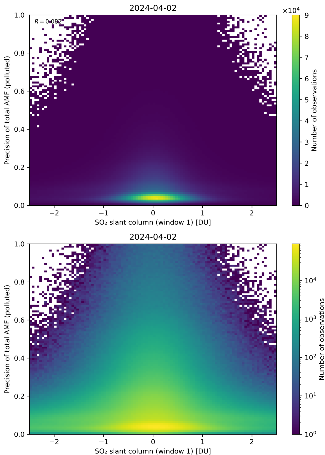
Figure 240: Scatter density plot of “SO 2 slant column (window 1)” against “Precision of total AMF (polluted)” for 2024-04-01 to 2024-04-03.
