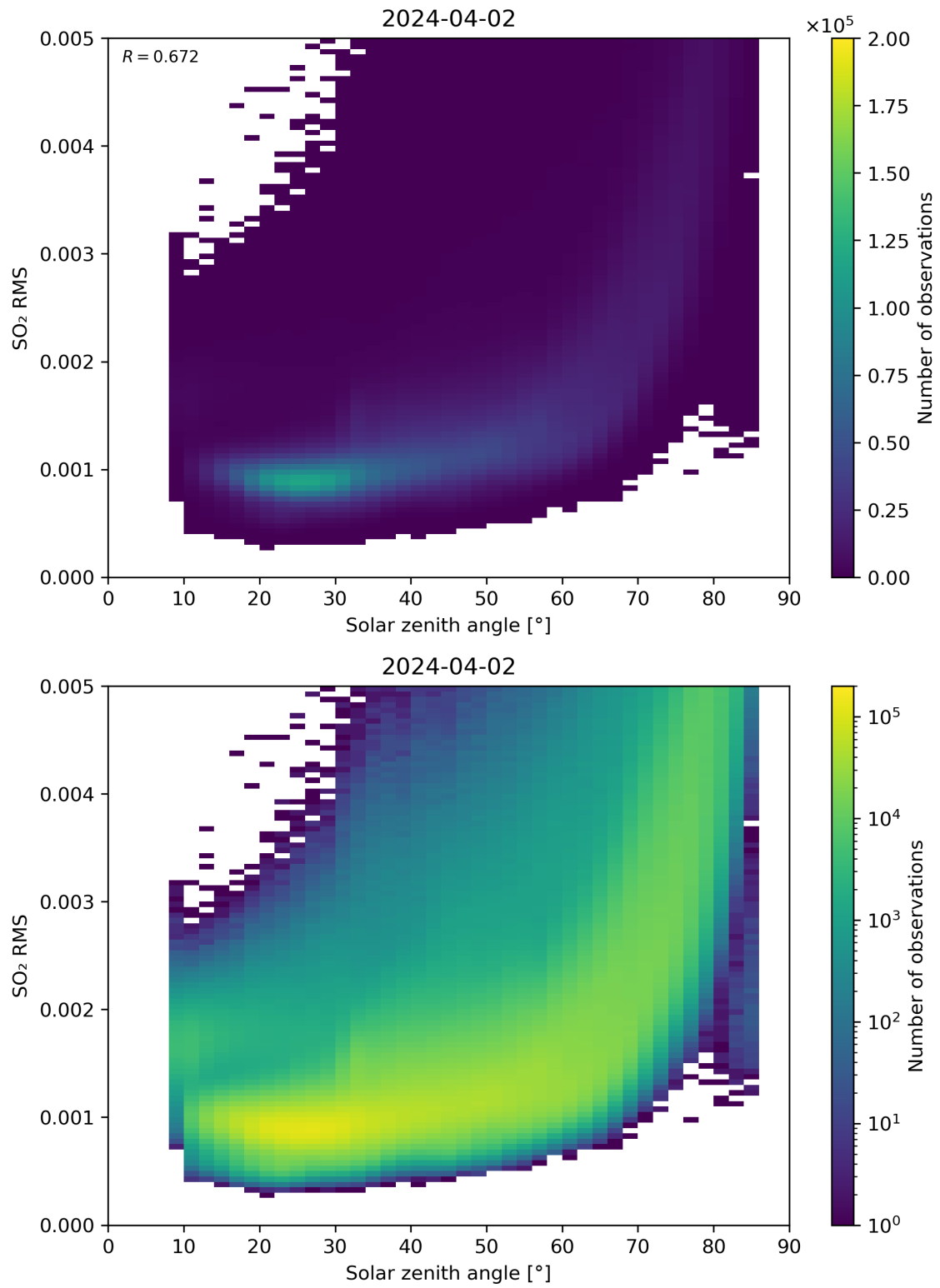
Figure 163: Scatter density plot of “Solar zenith angle” against “SO 2 RMS” for 2024-04-01 to 2024-04-03.
