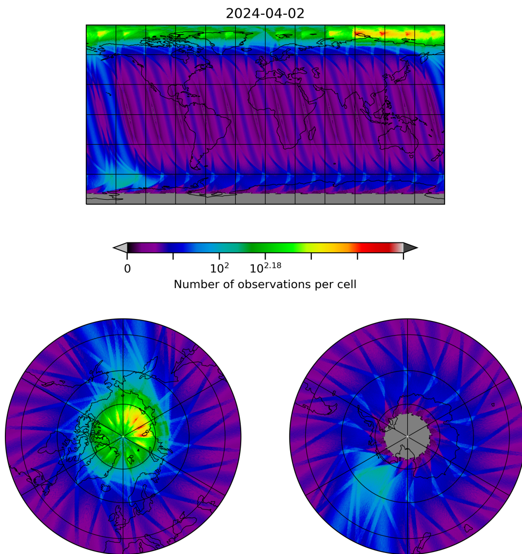
Figure 28: Map of the number of observations for 2024-04-01 to 2024-04-03
