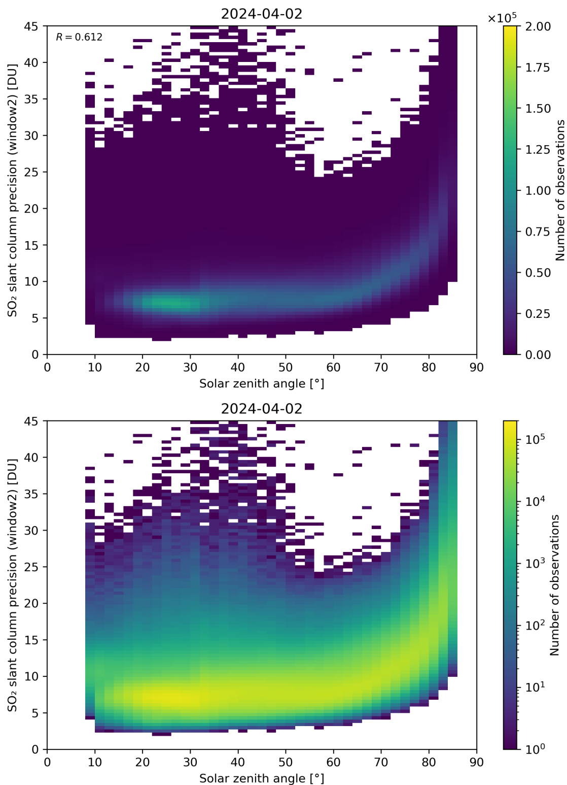
Figure 171: Scatter density plot of “Solar zenith angle” against “SO 2 slant column precision (window2)” for 2024-04-01 to 2024-04-03.
