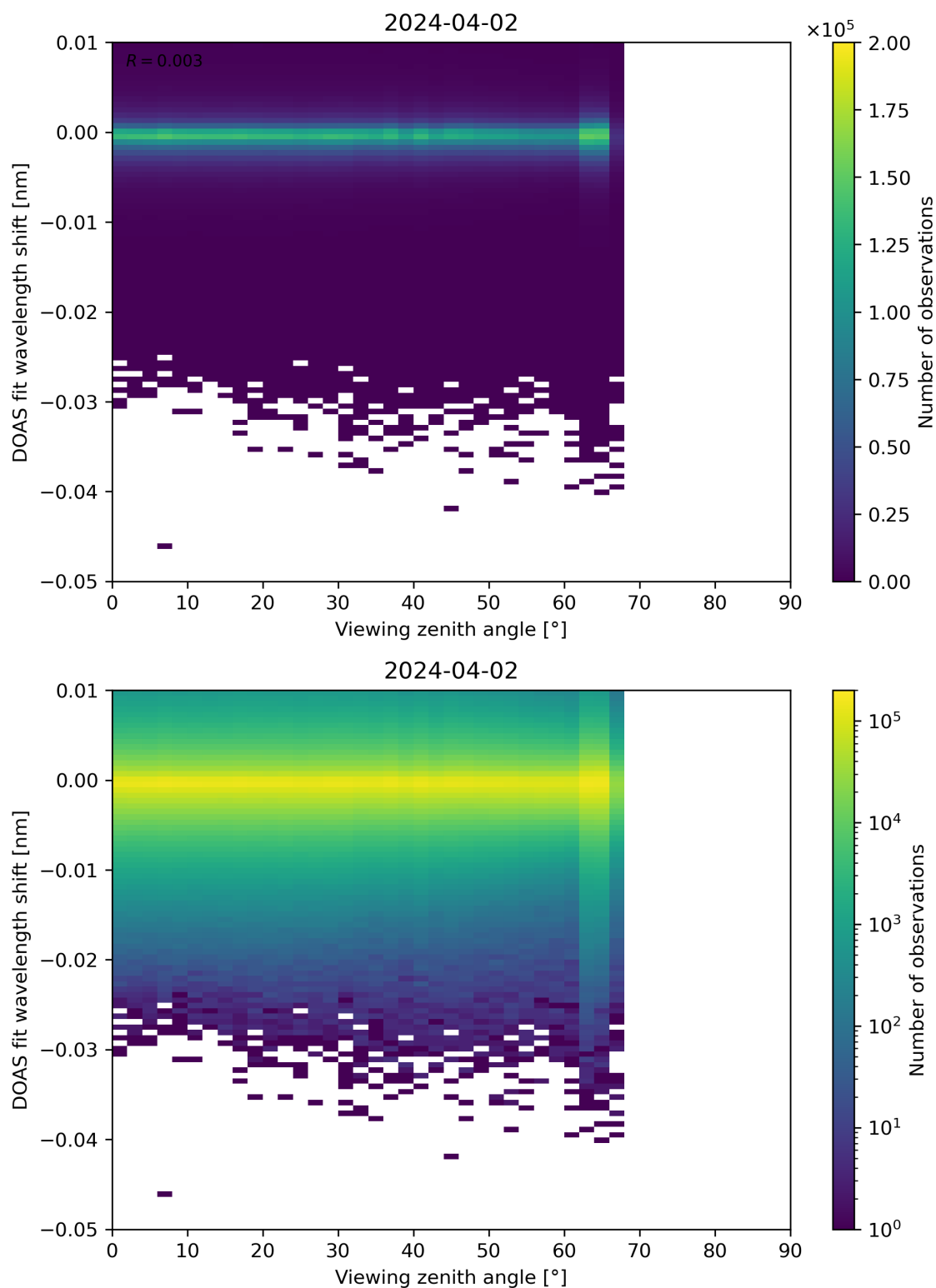
Figure 311: Scatter density plot of “Viewing zenith angle” against “DOAS fit wavelength shift” for 2024-04-01 to 2024-04-03.
