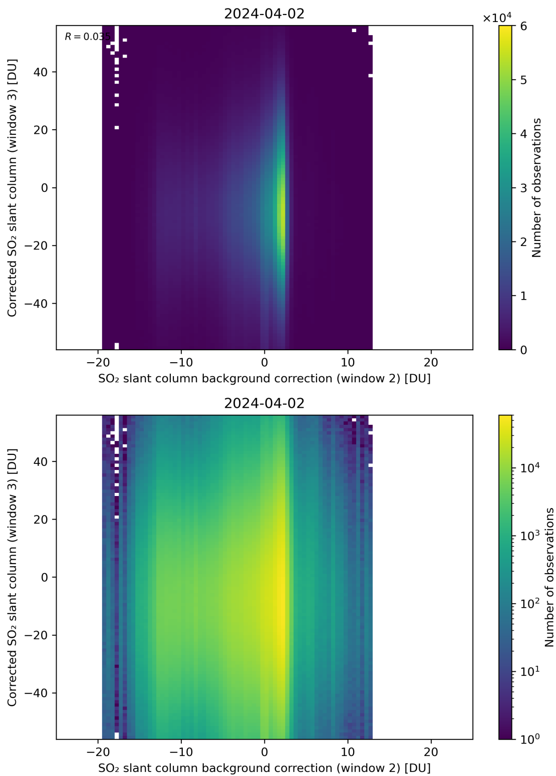
Figure 116: Scatter density plot of “SO 2 slant column background correction (window 2)” against “Corrected SO 2 slant column (window 3)” for 2024-04-01 to 2024-04-03.
