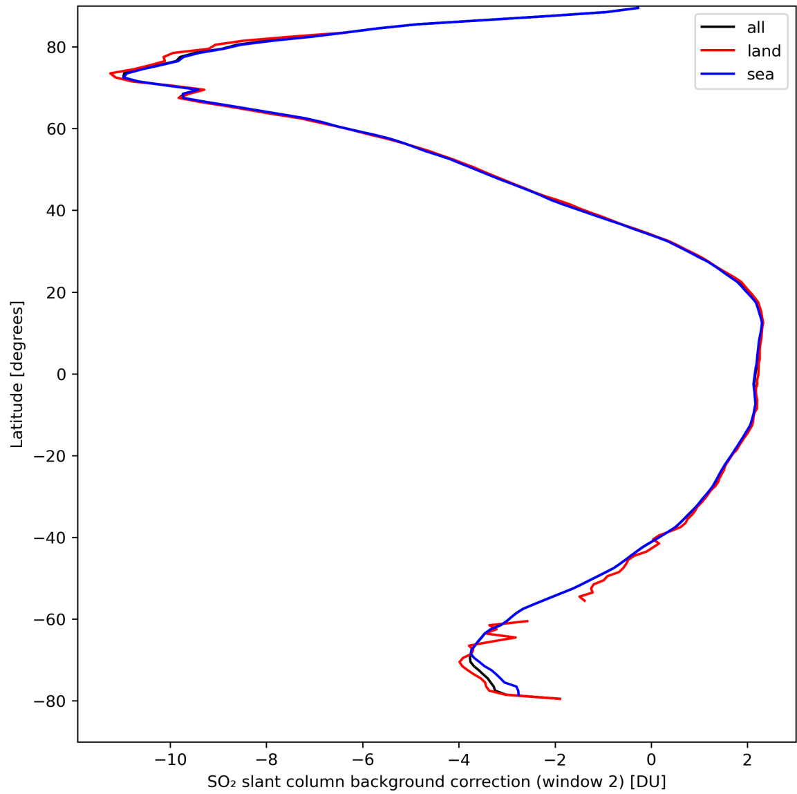
Figure 40: Zonal average of “SO 2 slant column background correction (window 2)” for 2024-04-01 to 2024-04-03.
