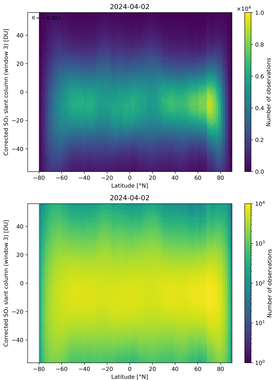
Figure 148: Scatter density plot of “Latitude” against “Corrected SO 2 slant column (window 3)” for 2024-04-01 to 2024-04-03.
