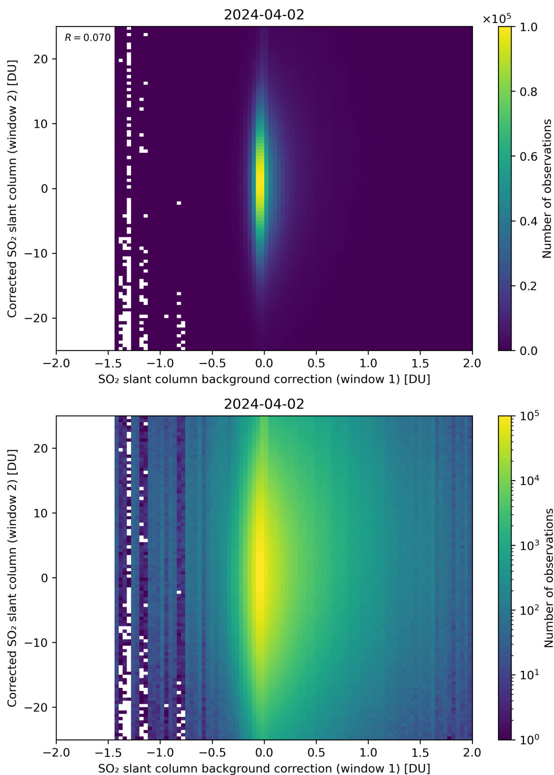
Figure 104: Scatter density plot of “SO 2 slant column background correction (window 1)” against “Corrected SO 2 slant column (window 2)” for 2024-04-01 to 2024-04-03.
