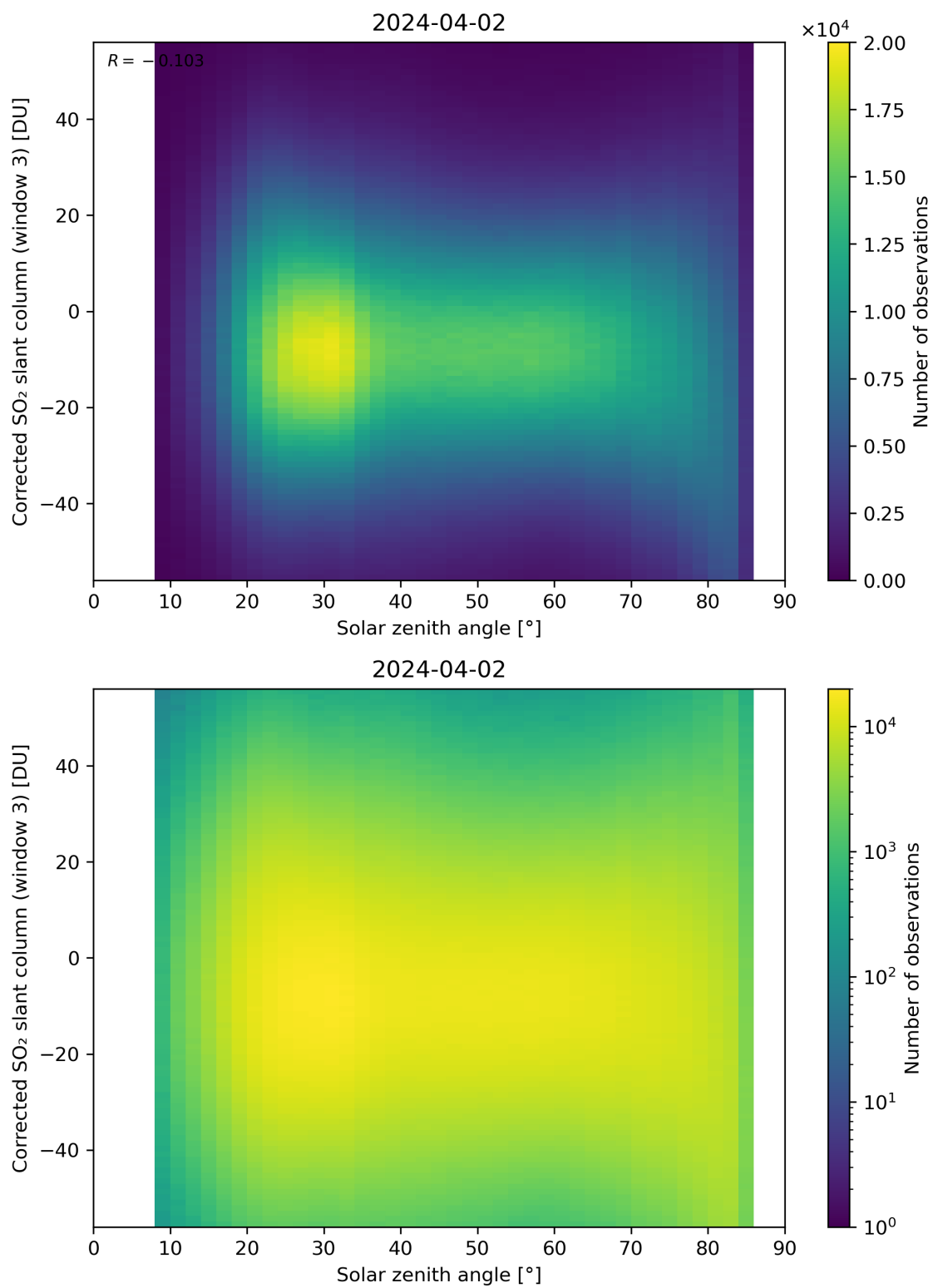
Figure 168: Scatter density plot of “Solar zenith angle” against “Corrected SO 2 slant column (window 3)” for 2024-04-01 to 2024-04-03.
