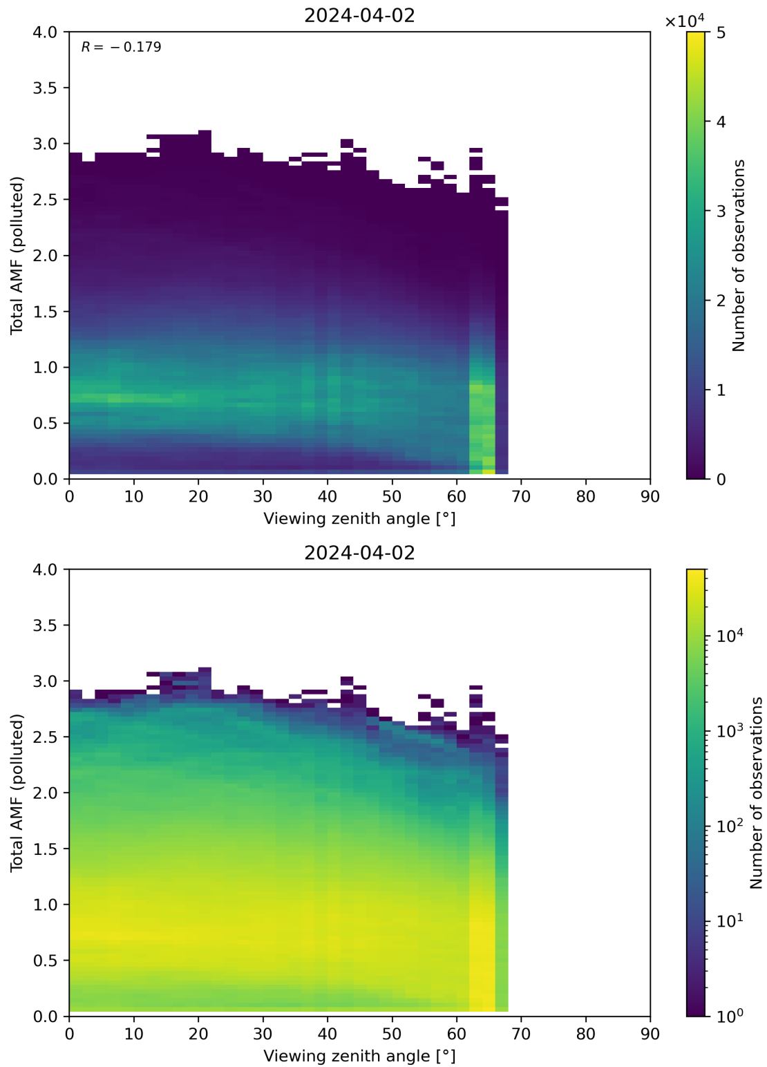
Figure 325: Scatter density plot of “Viewing zenith angle” against “Total AMF (polluted)” for 2024-04-01 to 2024-04-03.
