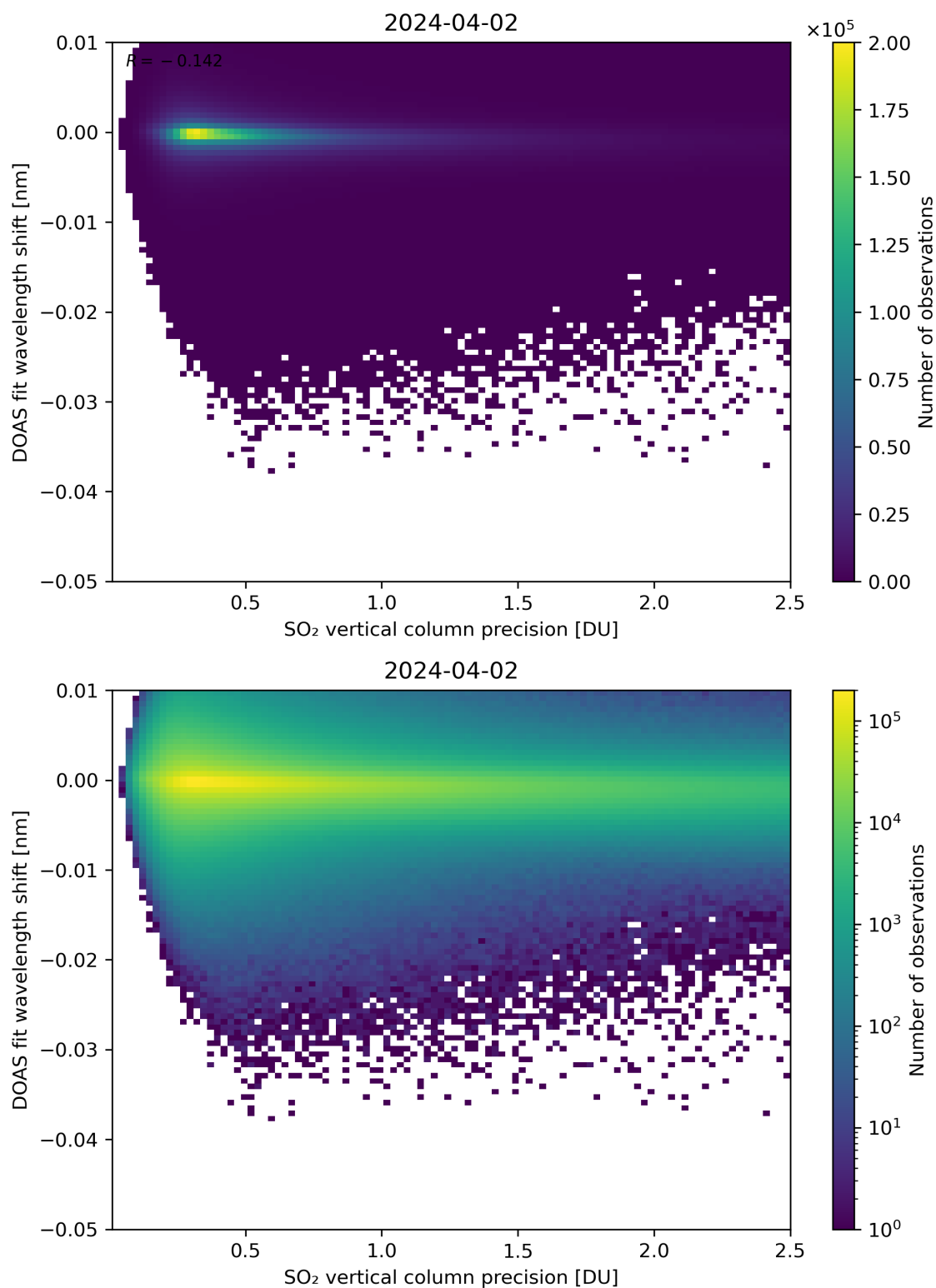
Figure 282: Scatter density plot of “SO 2 vertical column precision” against “DOAS fit wavelength shift” for 2024-04-01 to 2024-04-03.
