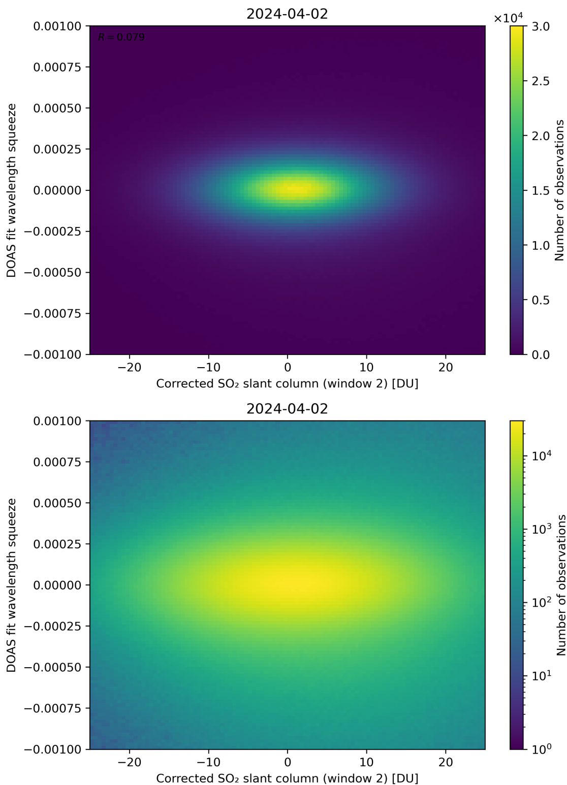
Figure 197: Scatter density plot of “Corrected SO 2 slant column (window 2)” against “DOAS fit wavelength squeeze” for 2024-04-01 to 2024-04-03.
