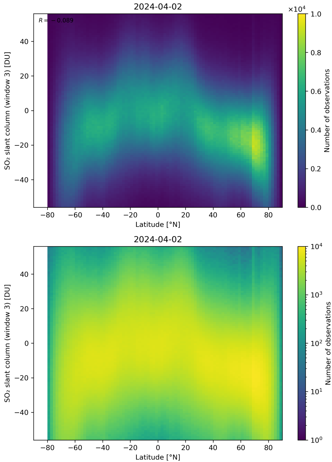
Figure 152: Scatter density plot of “Latitude” against “SO 2 slant column (window 3)” for 2024-04-01 to 2024-04-03.
