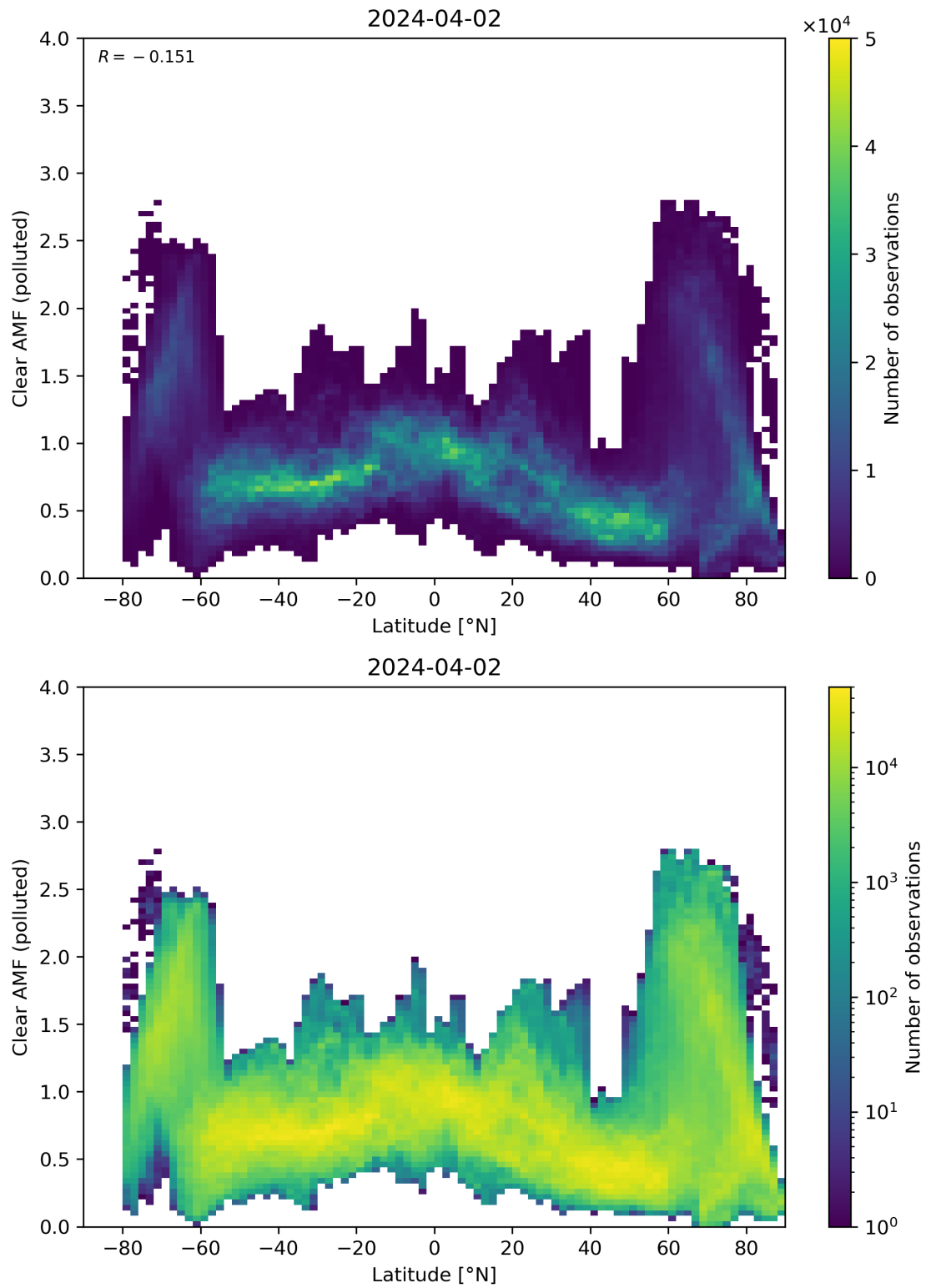
Figure 145: Scatter density plot of “Latitude” against “Clear AMF (polluted)” for 2024-04-01 to 2024-04-03.
