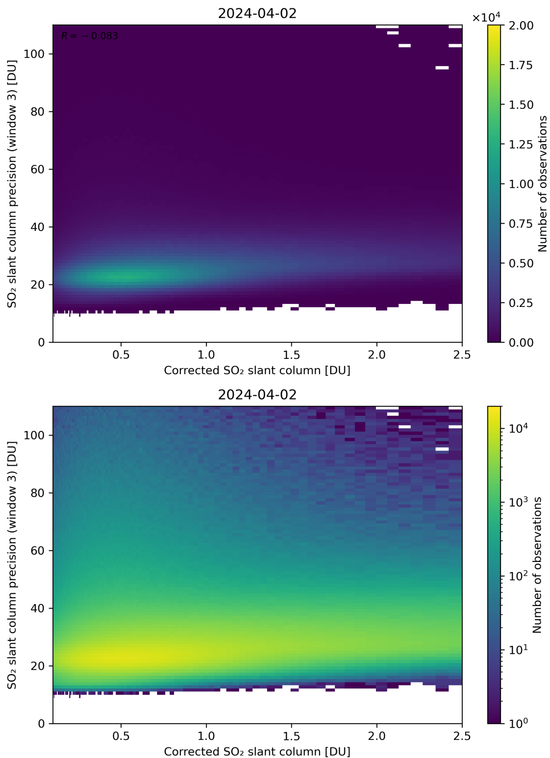
Figure 191: Scatter density plot of “Corrected SO 2 slant column” against “SO 2 slant column precision (window 3)” for 2024-04-01 to 2024-04-03.
