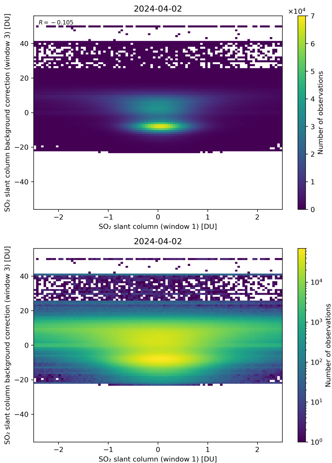
Figure 214: Scatter density plot of “SO 2 slant column (window 1)” against “SO 2 slant column background correction (window 3)” for 2024-04-01 to 2024-04-03.
