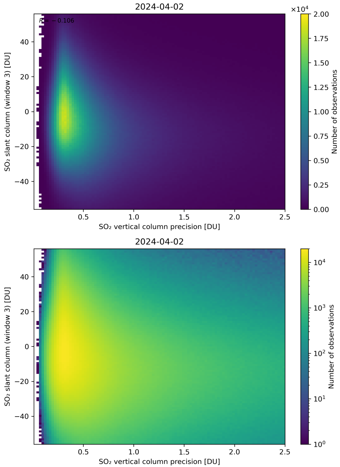
Figure 292: Scatter density plot of “SO 2 vertical column precision” against “SO 2 slant column (window 3)” for 2024-04-01 to 2024-04-03.
