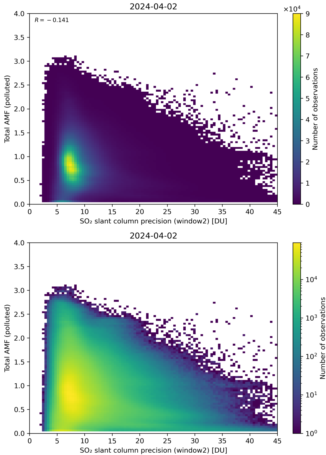
Figure 251: Scatter density plot of “SO 2 slant column precision (window2)” against “Total AMF (polluted)” for 2024-04-01 to 2024-04-03.
