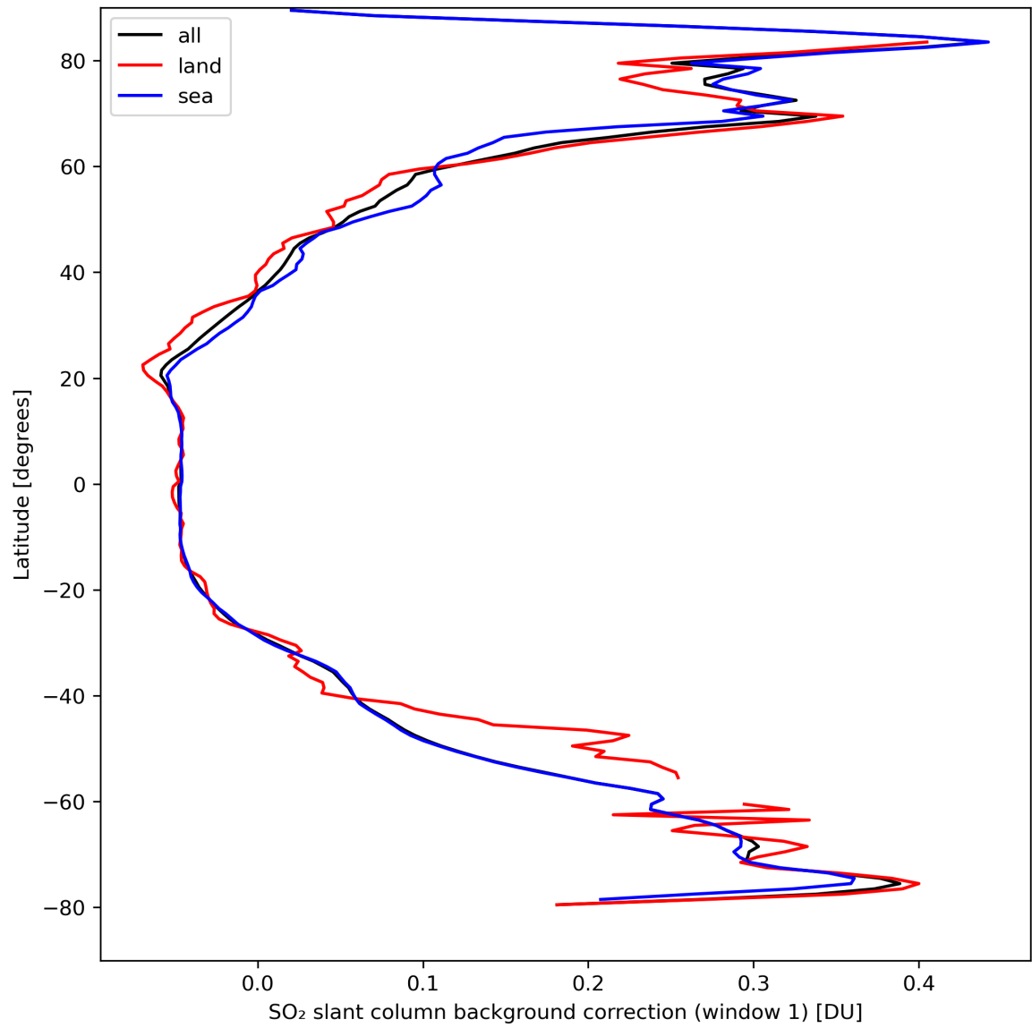
Figure 36: Zonal average of “SO 2 slant column background correction (window 1)” for 2024-04-01 to 2024-04-03.
