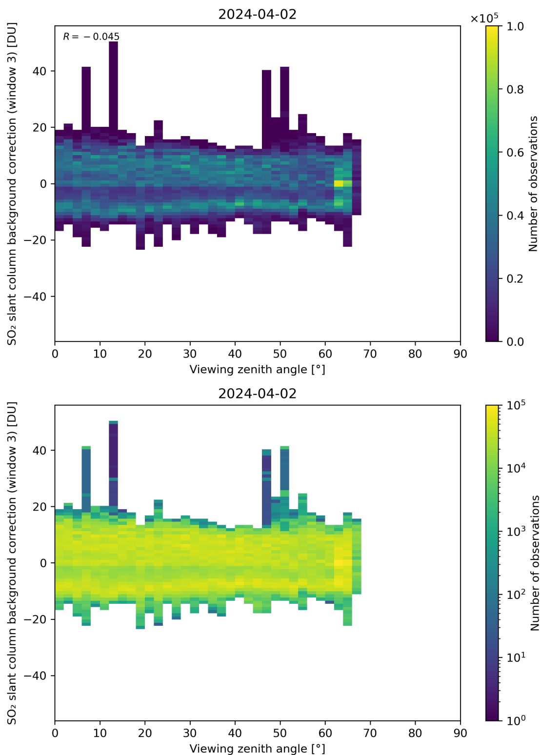
Figure 310: Scatter density plot of “Viewing zenith angle” against “SO 2 slant column background correction (window 3)” for 2024-04-01 to 2024-04-03.
