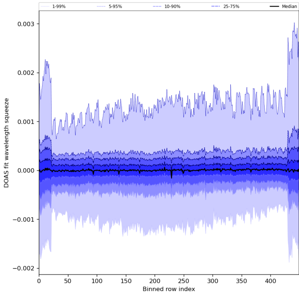
Figure 92: Along track statistics of “DOAS fit wavelength squeeze” for 2024-04-01 to 2024-04-03
