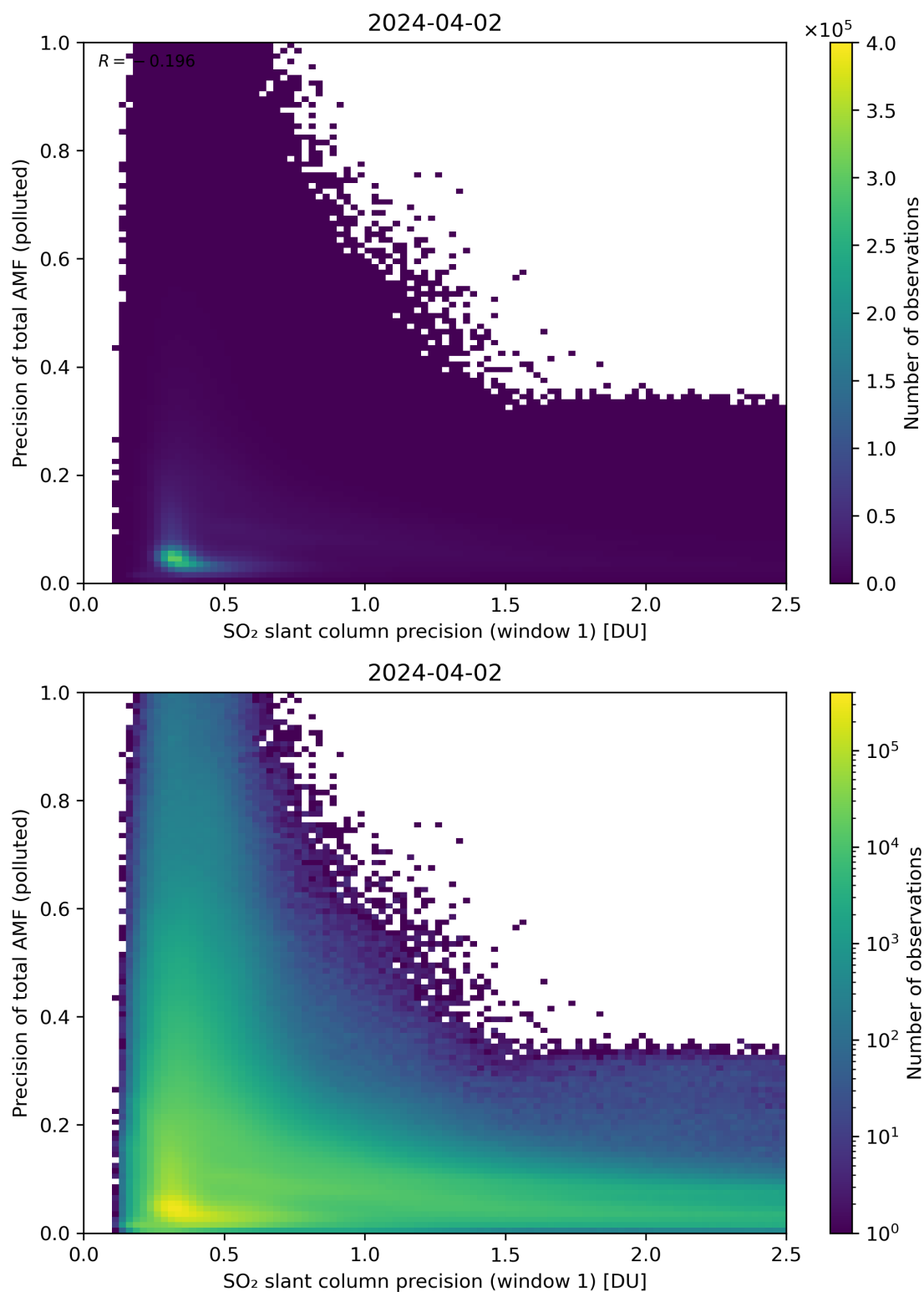
Figure 231: Scatter density plot of “SO 2 slant column precision (window 1)” against “Precision of total AMF (polluted)” for 2024-04-01 to 2024-04-03.
