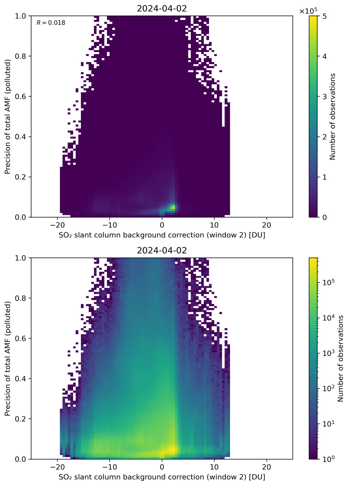
Figure 120: Scatter density plot of “SO 2 slant column background correction (window 2)” against “Precision of total AMF (polluted)” for 2024-04-01 to 2024-04-03.
