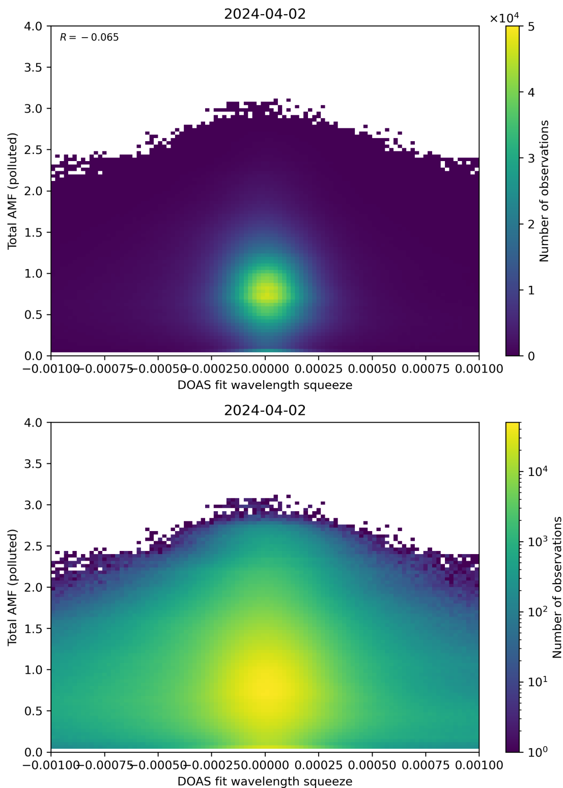
Figure 134: Scatter density plot of “DOAS fit wavelength squeeze” against “Total AMF (polluted)” for 2024-04-01 to 2024-04-03.
