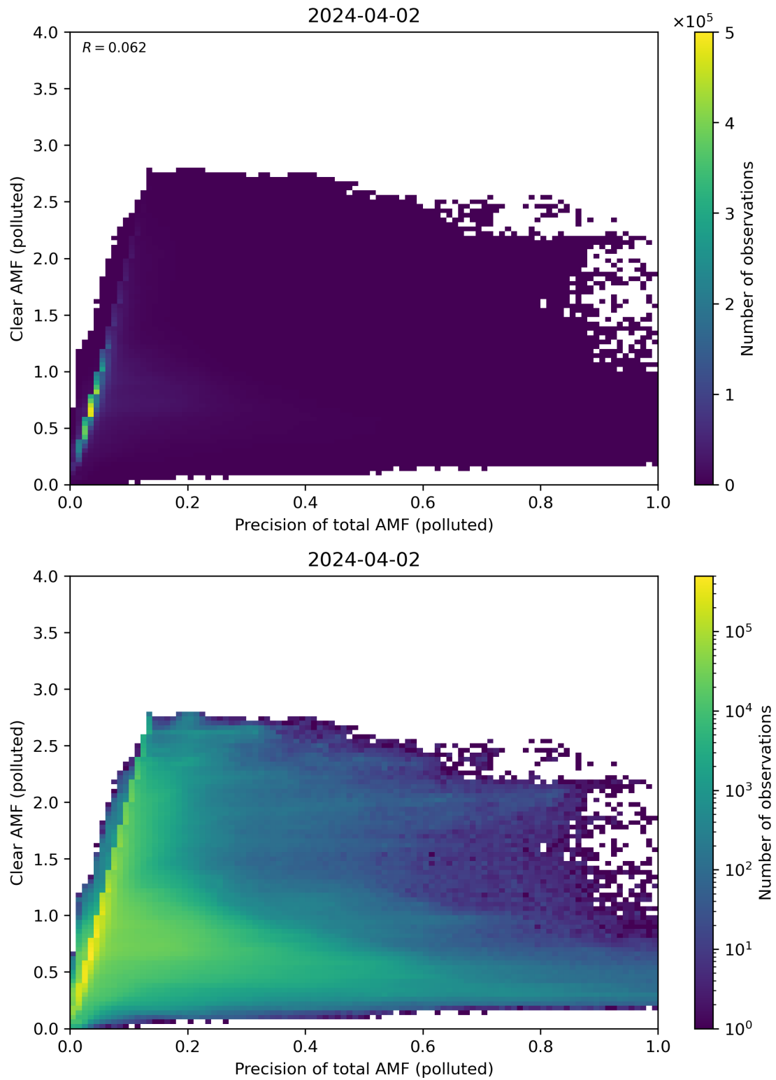
Figure 270: Scatter density plot of “Precision of total AMF (polluted)” against “Clear AMF (polluted)” for 2024-04-01 to 2024-04-03.
