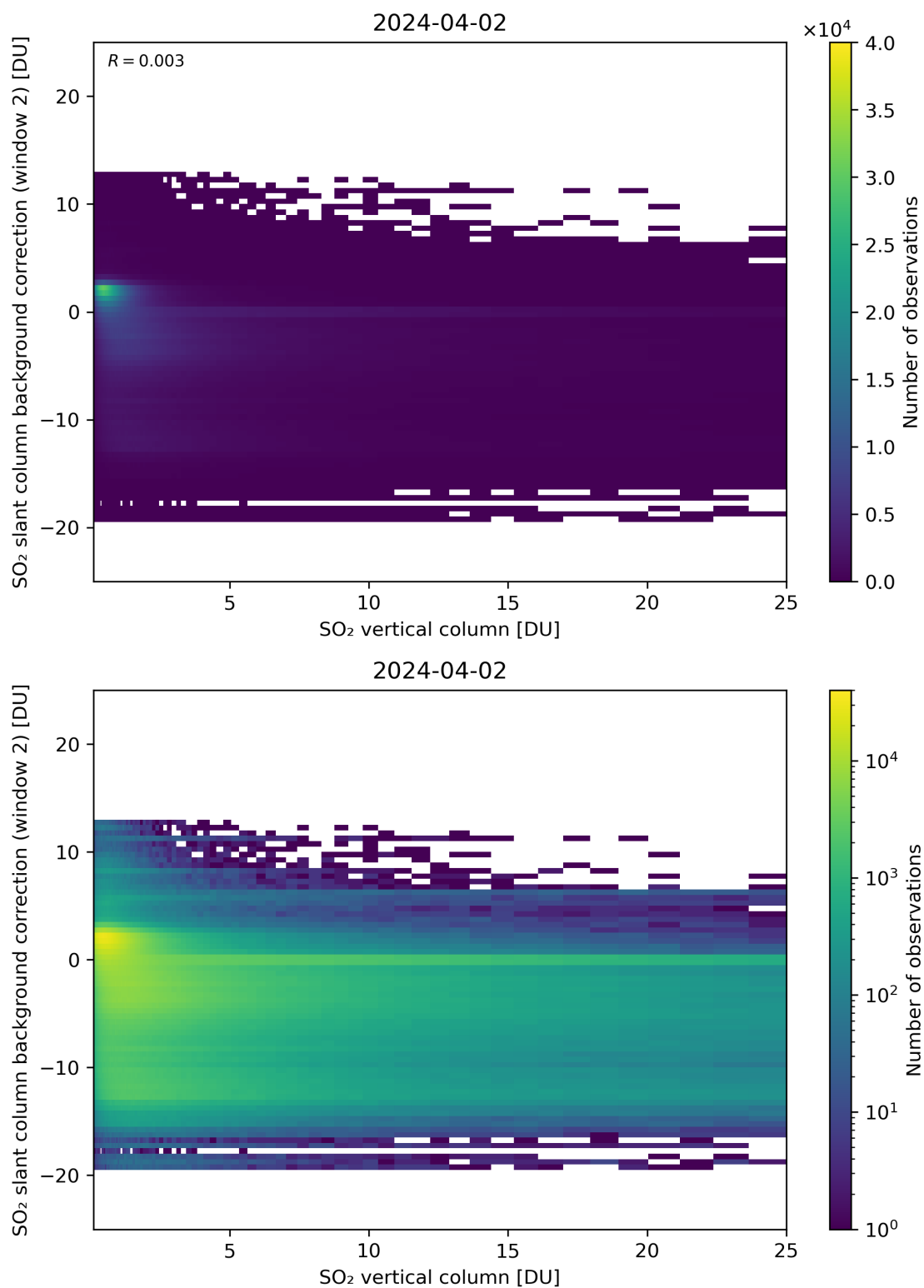
Figure 274: Scatter density plot of “SO 2 vertical column” against “SO 2 slant column background correction (window 2)” for 2024-04-01 to 2024-04-03.
