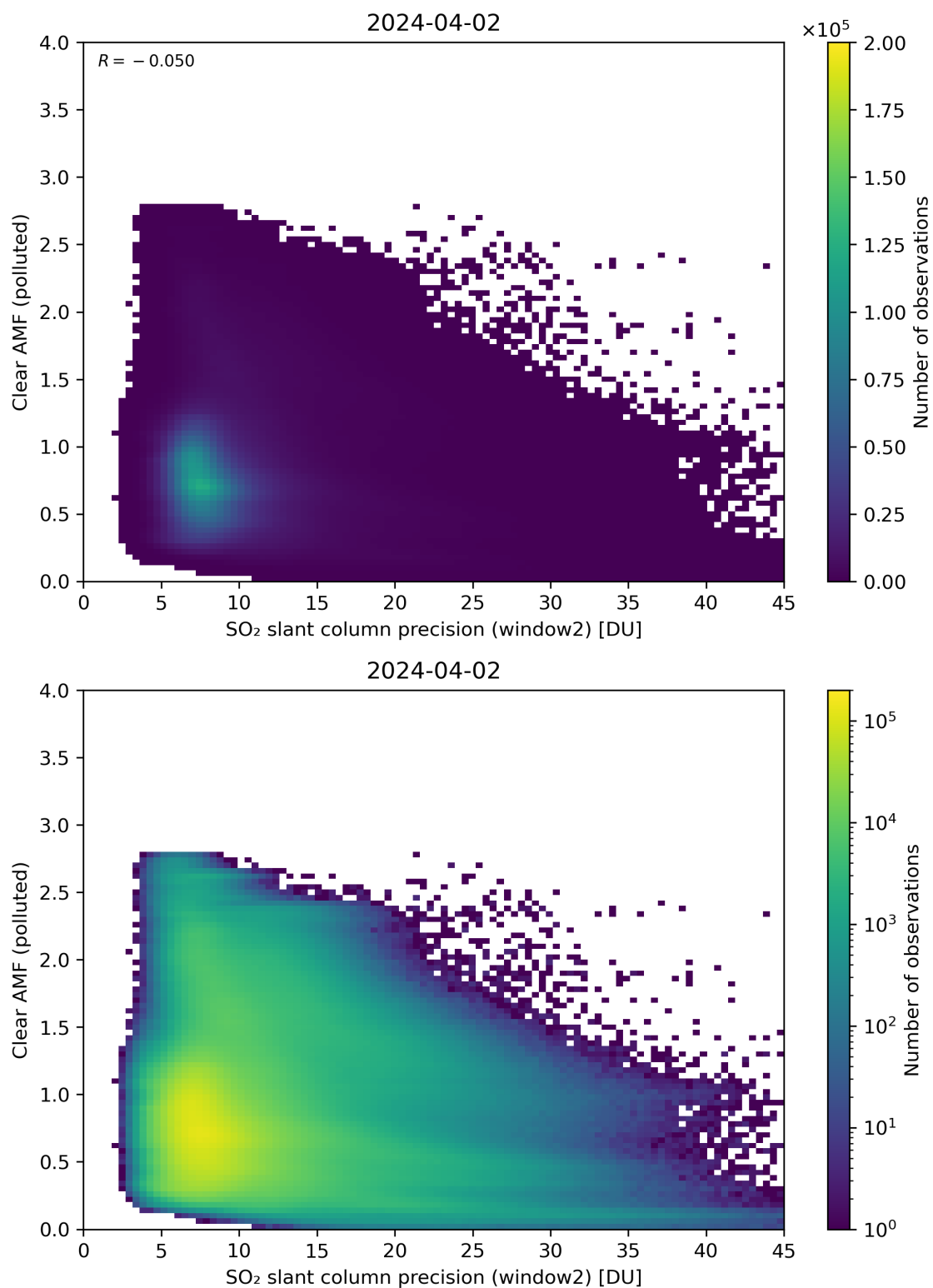
Figure 246: Scatter density plot of “SO 2 slant column precision (window2)” against “Clear AMF (polluted)” for 2024-04-01 to 2024-04-03.
