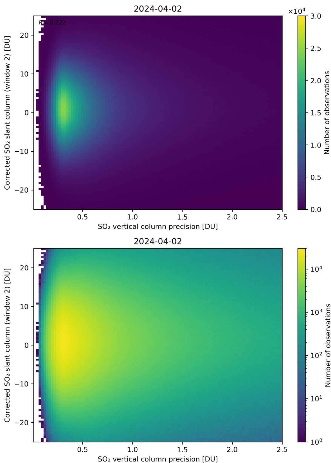
Figure 287: Scatter density plot of “SO 2 vertical column precision” against “Corrected SO 2 slant column (window 2)” for 2024-04-01 to 2024-04-03.
