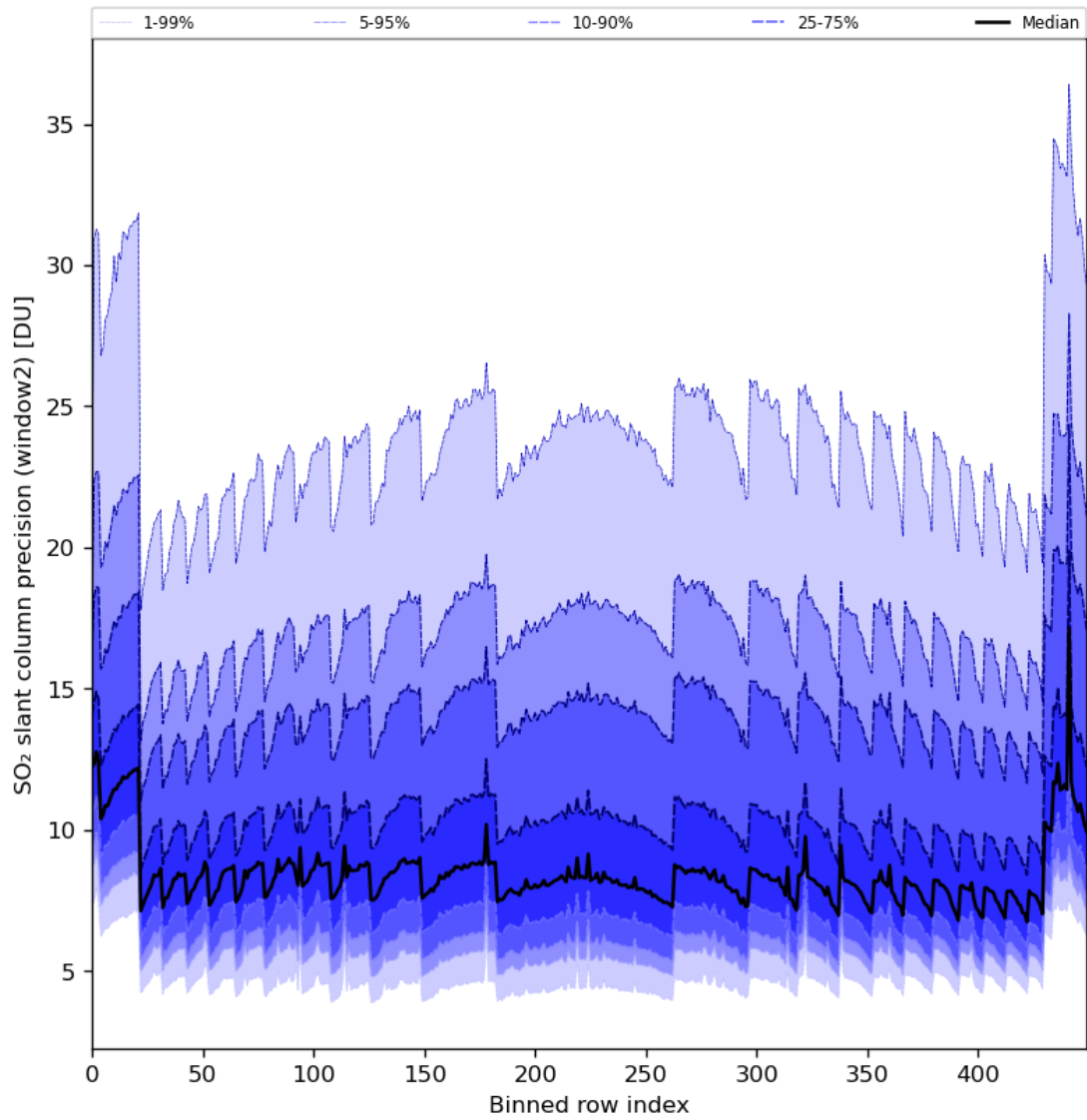
Figure 84: Along track statistics of “SO 2 slant column precision (window2)” for 2024-04-01 to 2024-04-03
