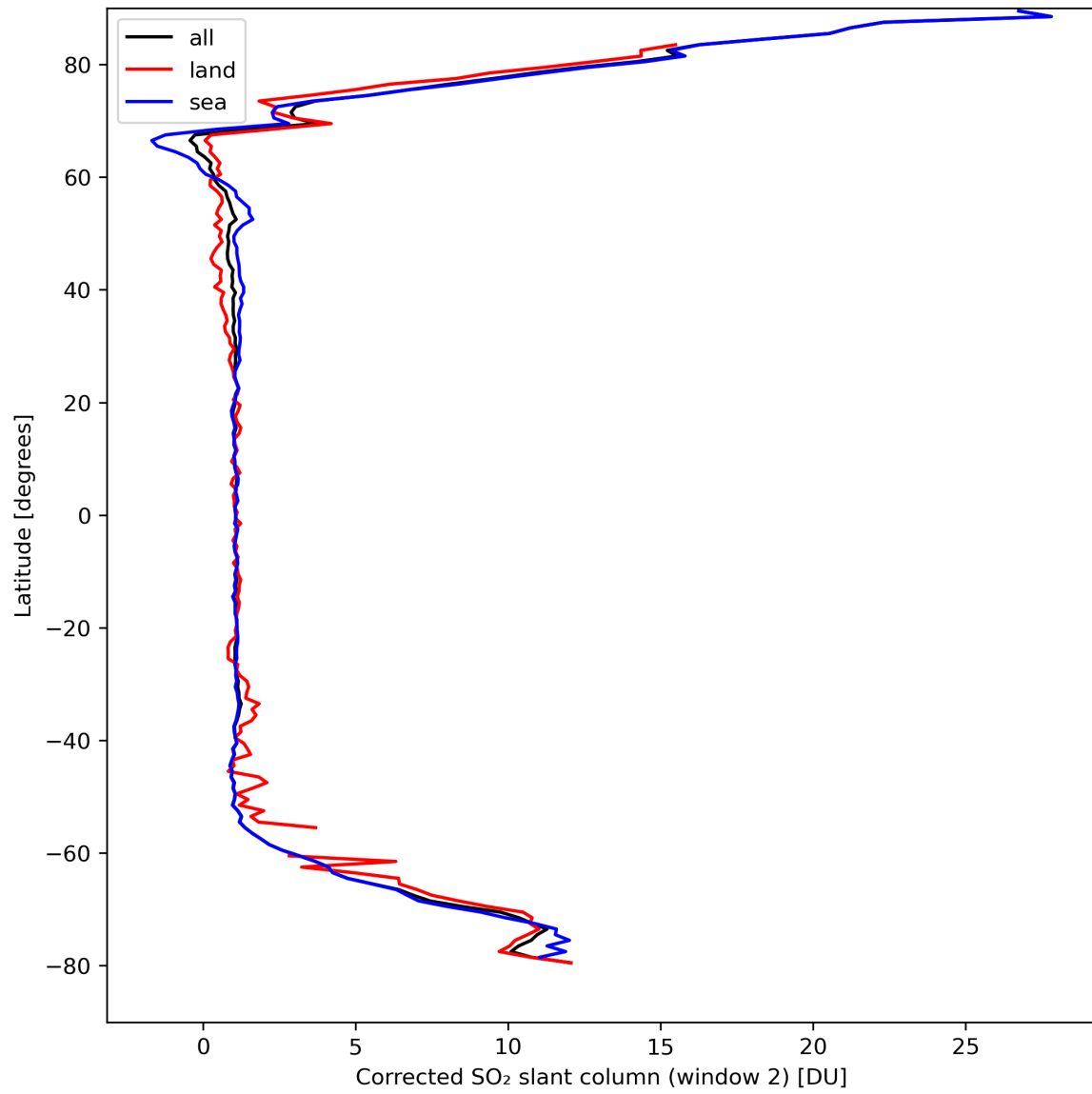
Figure 39: Zonal average of “Corrected SO 2 slant column (window 2)” for 2024-04-01 to 2024-04-03.
