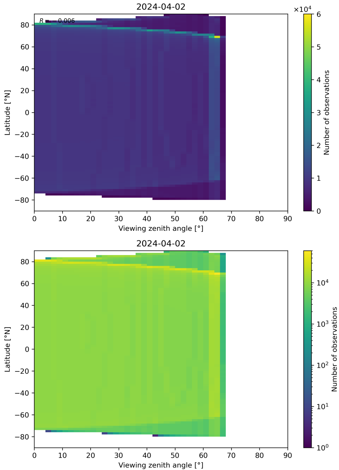
Figure 314: Scatter density plot of “Viewing zenith angle” against “Latitude” for 2024-04-01 to 2024-04-03.
