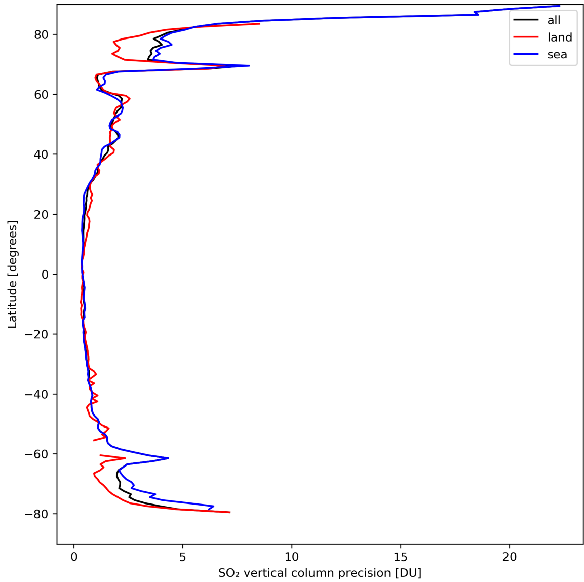
Figure 31: Zonal average of “SO 2 vertical column precision” for 2024-04-01 to 2024-04-03.
