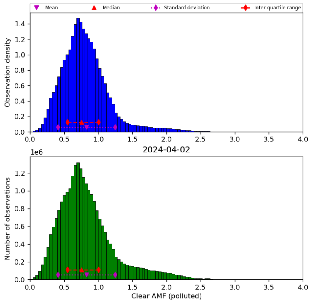
Figure 73: Histogram of “Clear AMF (polluted)” for 2024-04-01 to 2024-04-03
