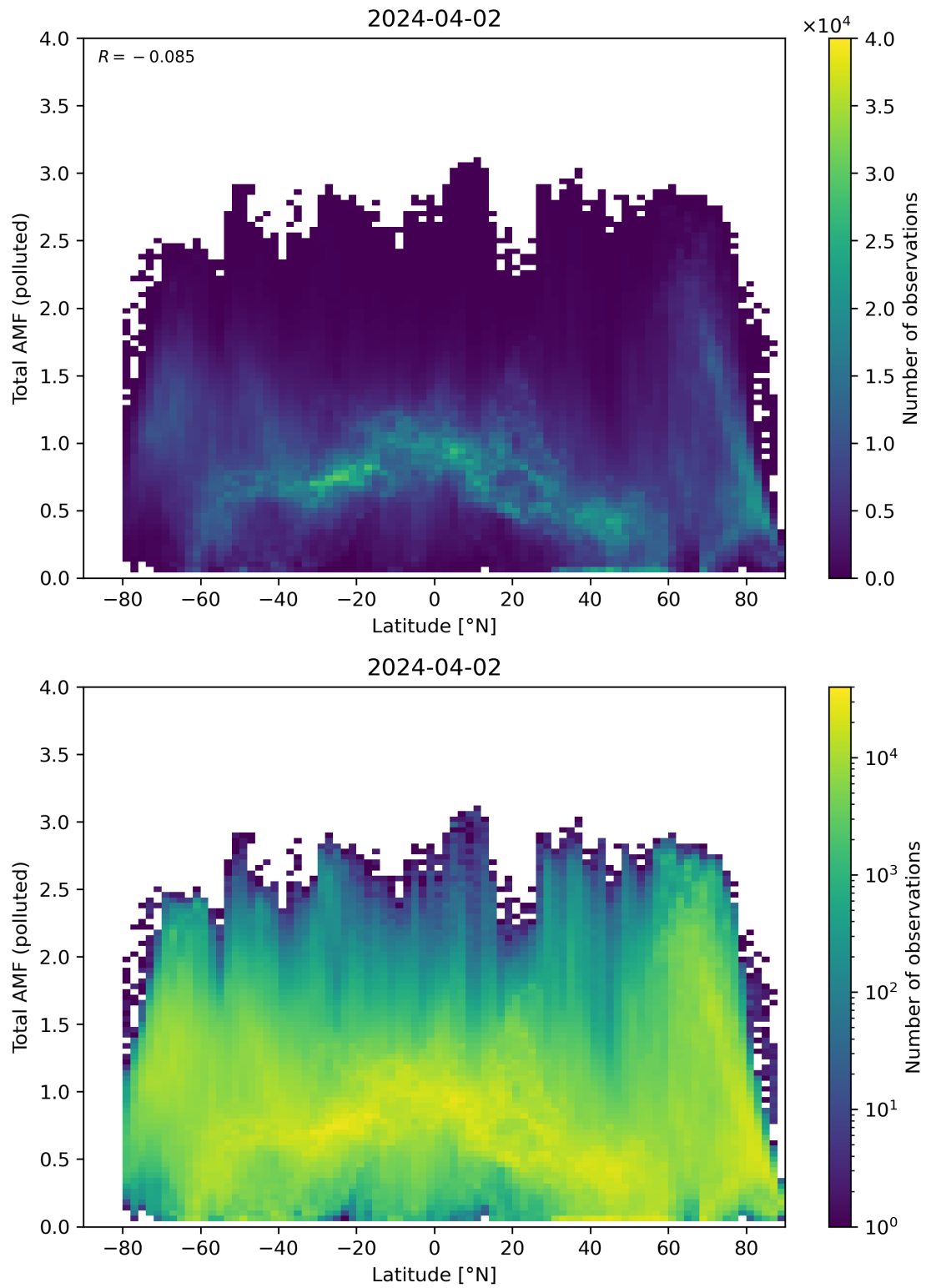
Figure 154: Scatter density plot of “Latitude” against “Total AMF (polluted)” for 2024-04-01 to 2024-04-03.
