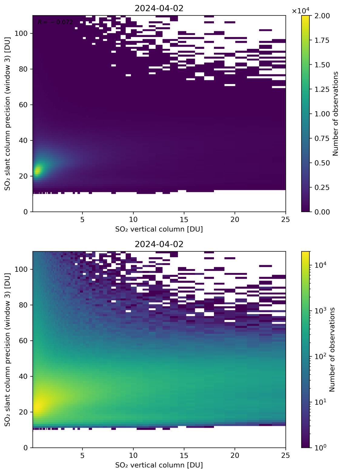
Figure 304: Scatter density plot of “SO 2 vertical column” against “SO 2 slant column precision (window 3)” for 2024-04-01 to 2024-04-03.
