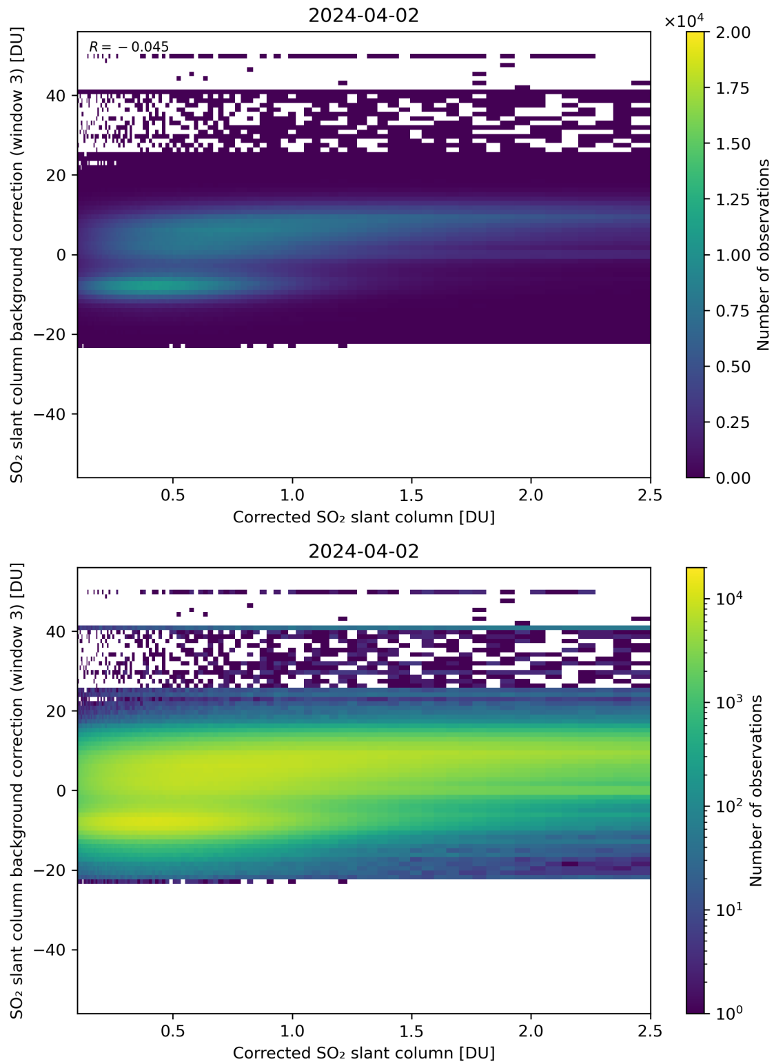
Figure 180: Scatter density plot of “Corrected SO 2 slant column” against “SO 2 slant column background correction (window 3)” for 2024-04-01 to 2024-04-03.
