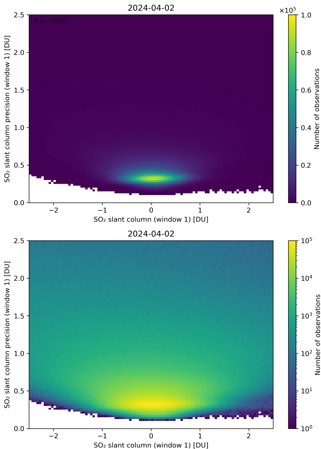
Figure 235: Scatter density plot of “SO 2 slant column (window 1)” against “SO 2 slant column precision (window 1)” for 2024-04-01 to 2024-04-03.
