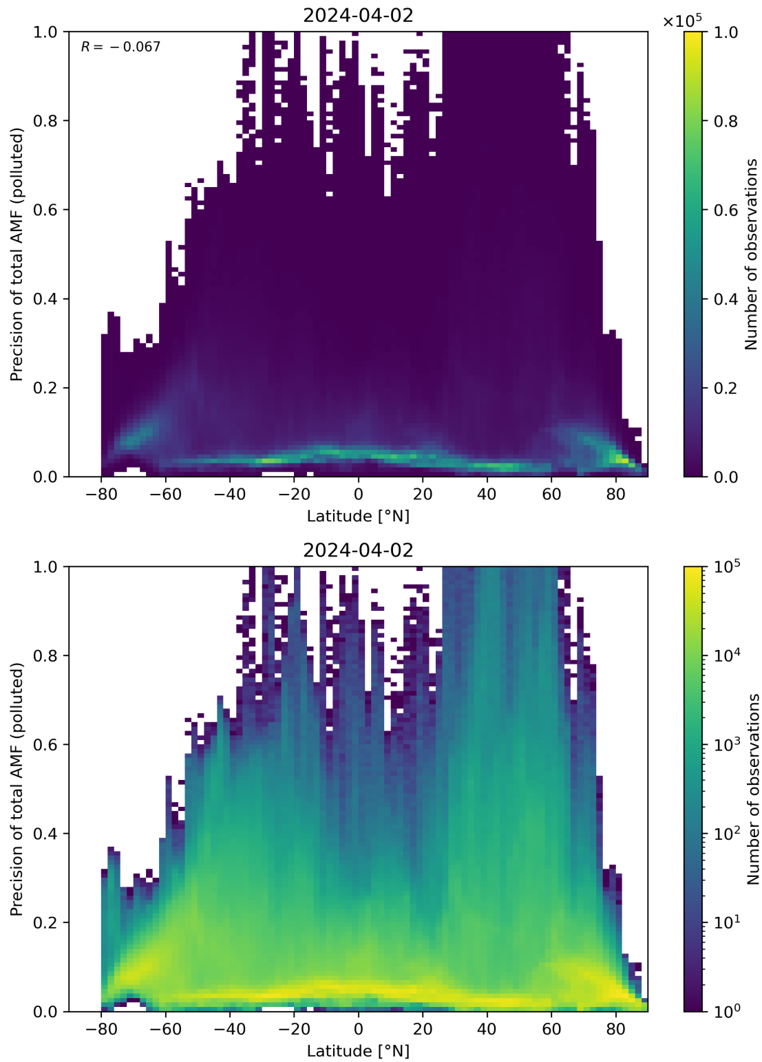
Figure 155: Scatter density plot of “Latitude” against “Precision of total AMF (polluted)” for 2024-04-01 to 2024-04-03.
