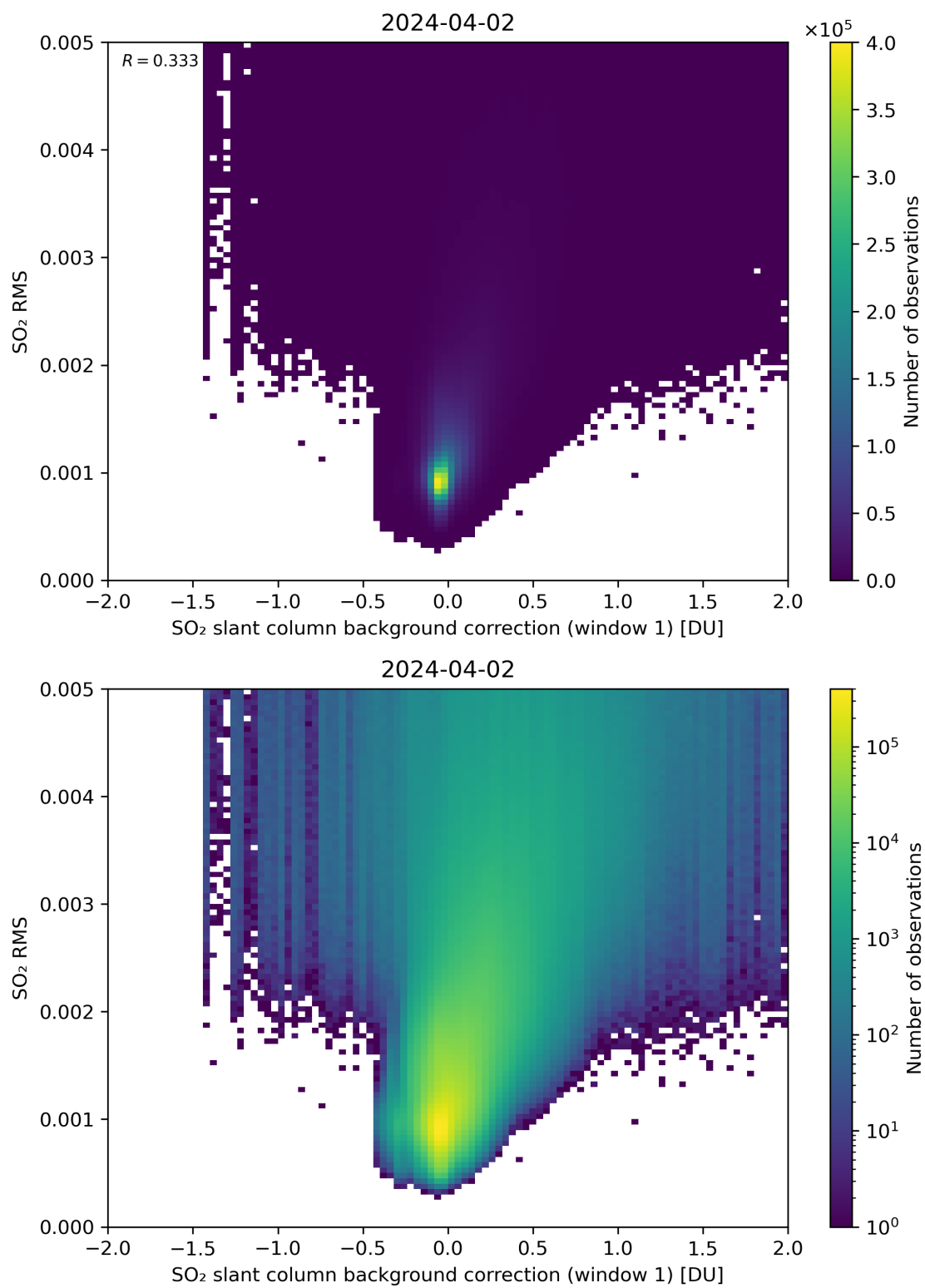
Figure 102: Scatter density plot of “SO 2 slant column background correction (window 1)” against “SO 2 RMS” for 2024-04-01 to 2024-04-03.
