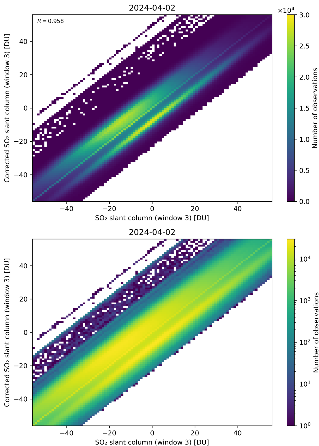
Figure 266: Scatter density plot of “SO 2 slant column (window 3)” against “Corrected SO 2 slant column (window 3)” for 2024-04-01 to 2024-04-03.
