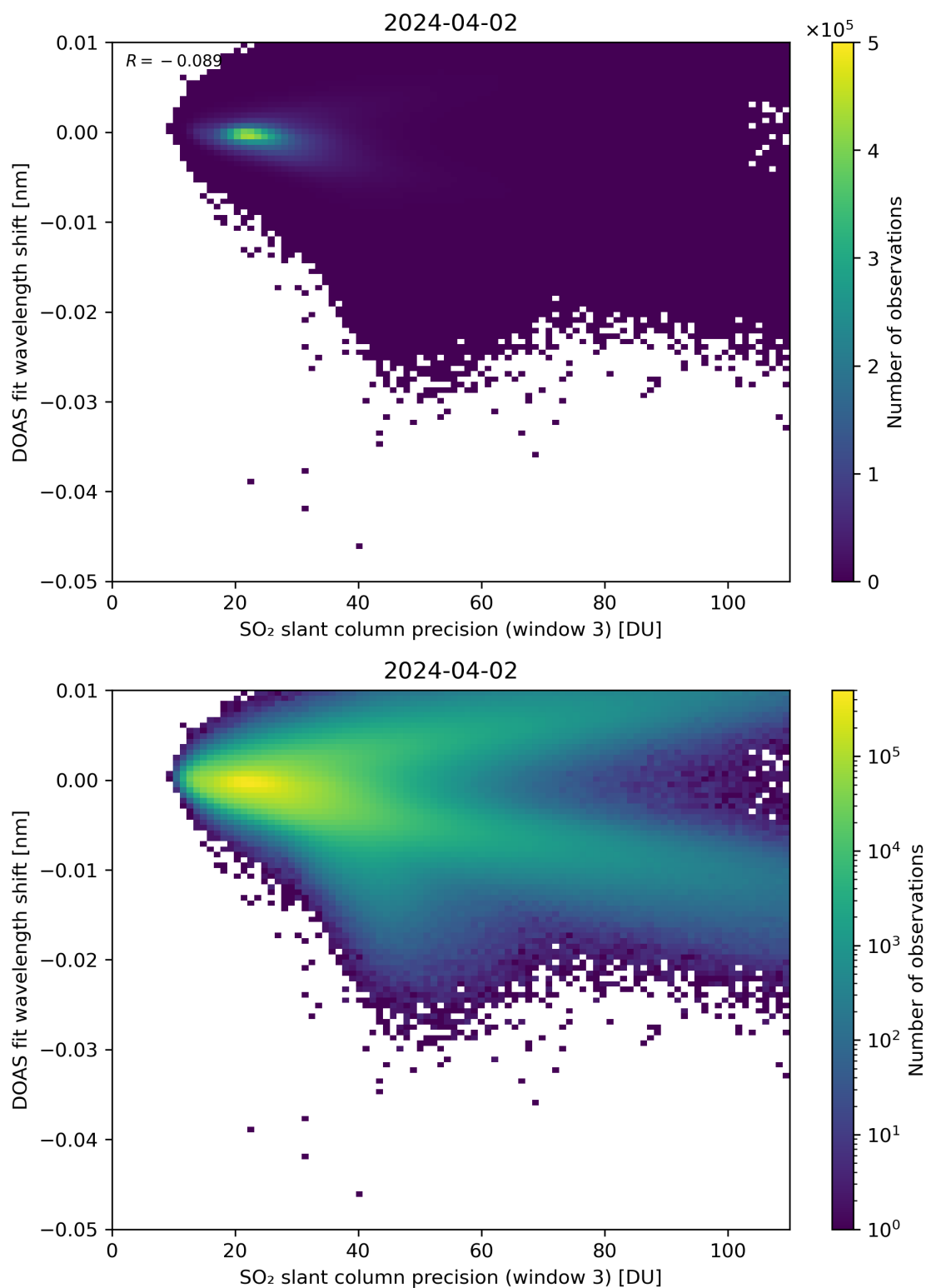
Figure 258: Scatter density plot of “SO 2 slant column precision (window 3)” against “DOAS fit wavelength shift” for 2024-04-01 to 2024-04-03.
