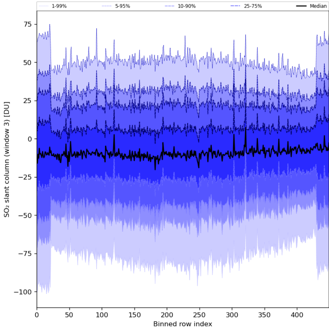
Figure 87: Along track statistics of “SO 2 slant column (window 3)” for 2024-04-01 to 2024-04-03
