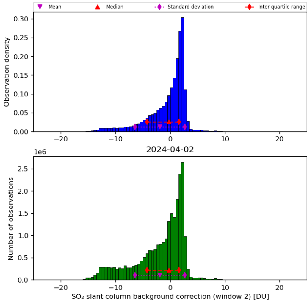
Figure 63: Histogram of “SO 2 slant column background correction (window 2)” for 2024-04-01 to 2024-04-03
