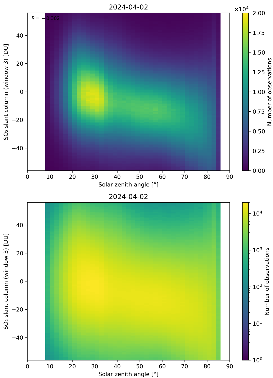
Figure 172: Scatter density plot of “Solar zenith angle” against “SO 2 slant column (window 3)” for 2024-04-01 to 2024-04-03.
