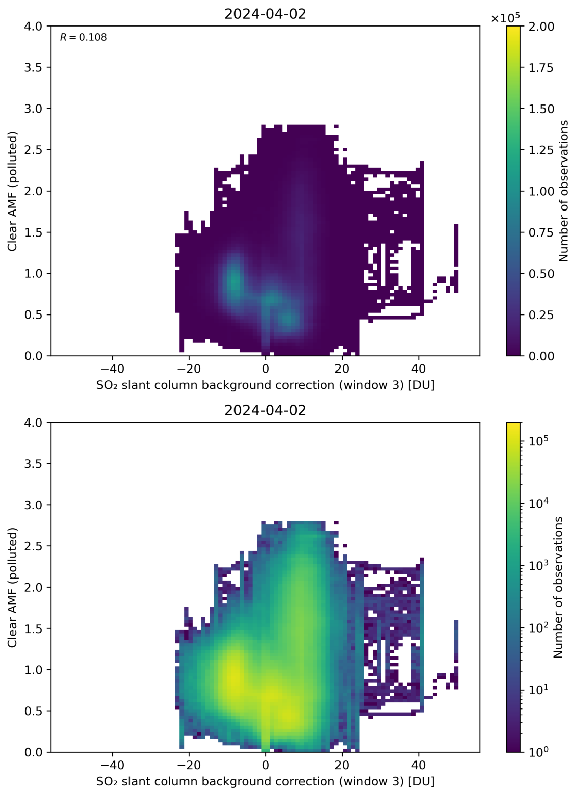
Figure 124: Scatter density plot of “SO 2 slant column background correction (window 3)” against “Clear AMF (polluted)” for 2024-04-01 to 2024-04-03.
