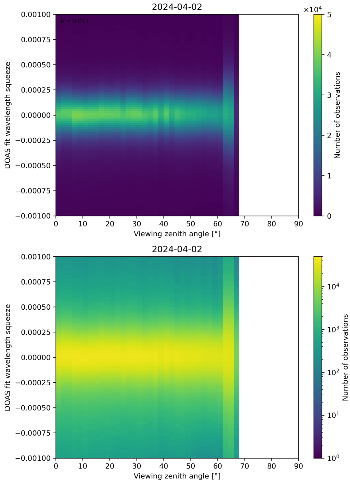
Figure 312: Scatter density plot of “Viewing zenith angle” against “DOAS fit wavelength squeeze” for 2024-04-01 to 2024-04-03.
