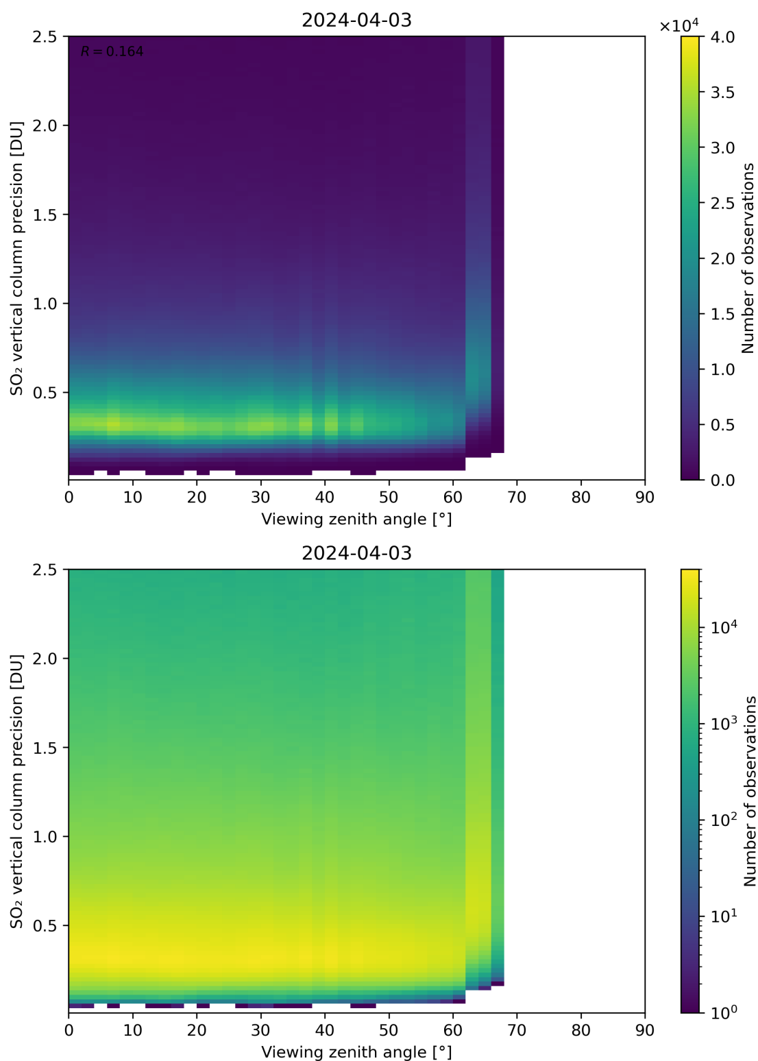
Figure 328: Scatter density plot of “Viewing zenith angle” against “SO 2 vertical column precision” for 2024-04-02 to 2024-04-04.
