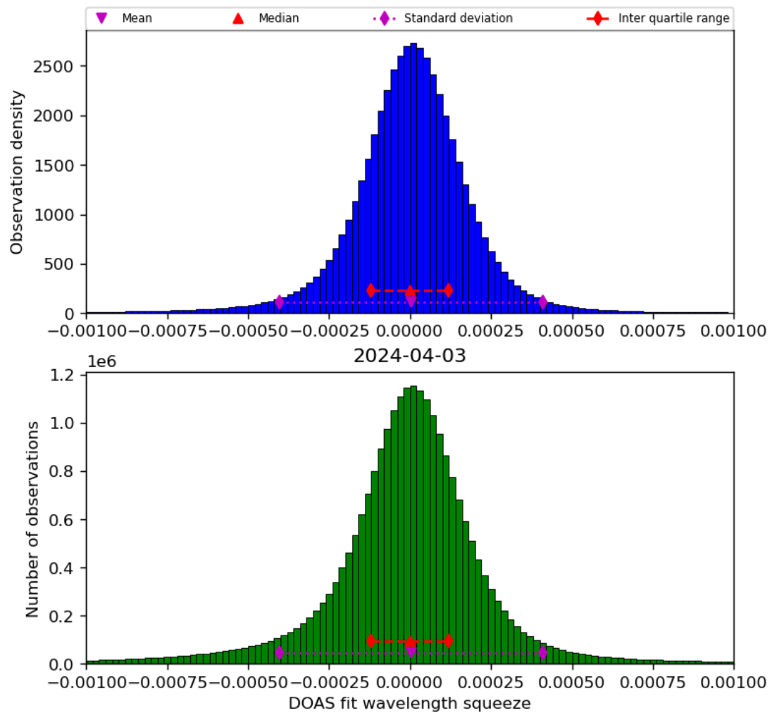
Figure 69: Histogram of “DOAS fit wavelength squeeze” for 2024-04-02 to 2024-04-04
