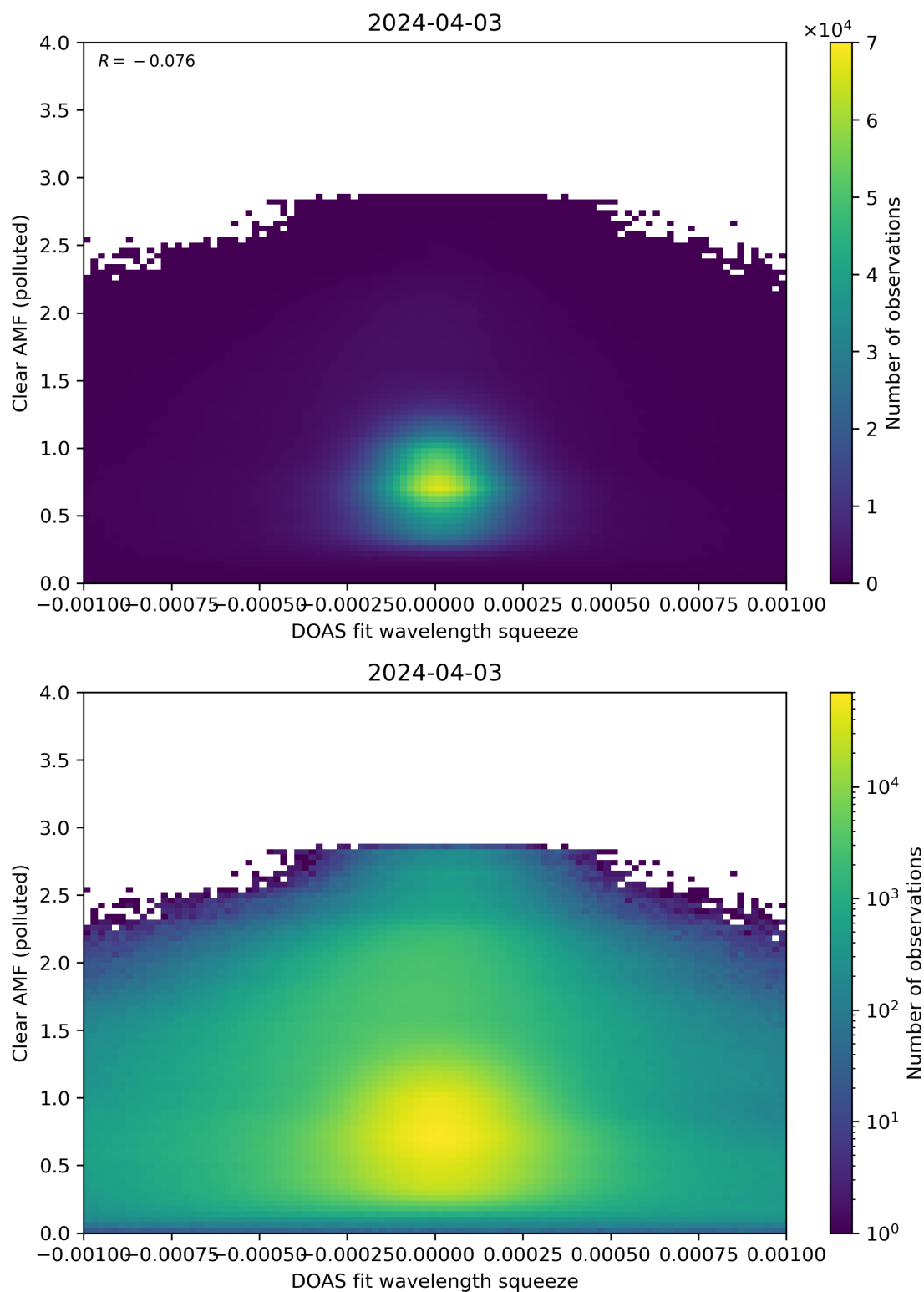
Figure 133: Scatter density plot of “DOAS fit wavelength squeeze” against “Clear AMF (polluted)” for 2024-04-02 to 2024-04-04.
