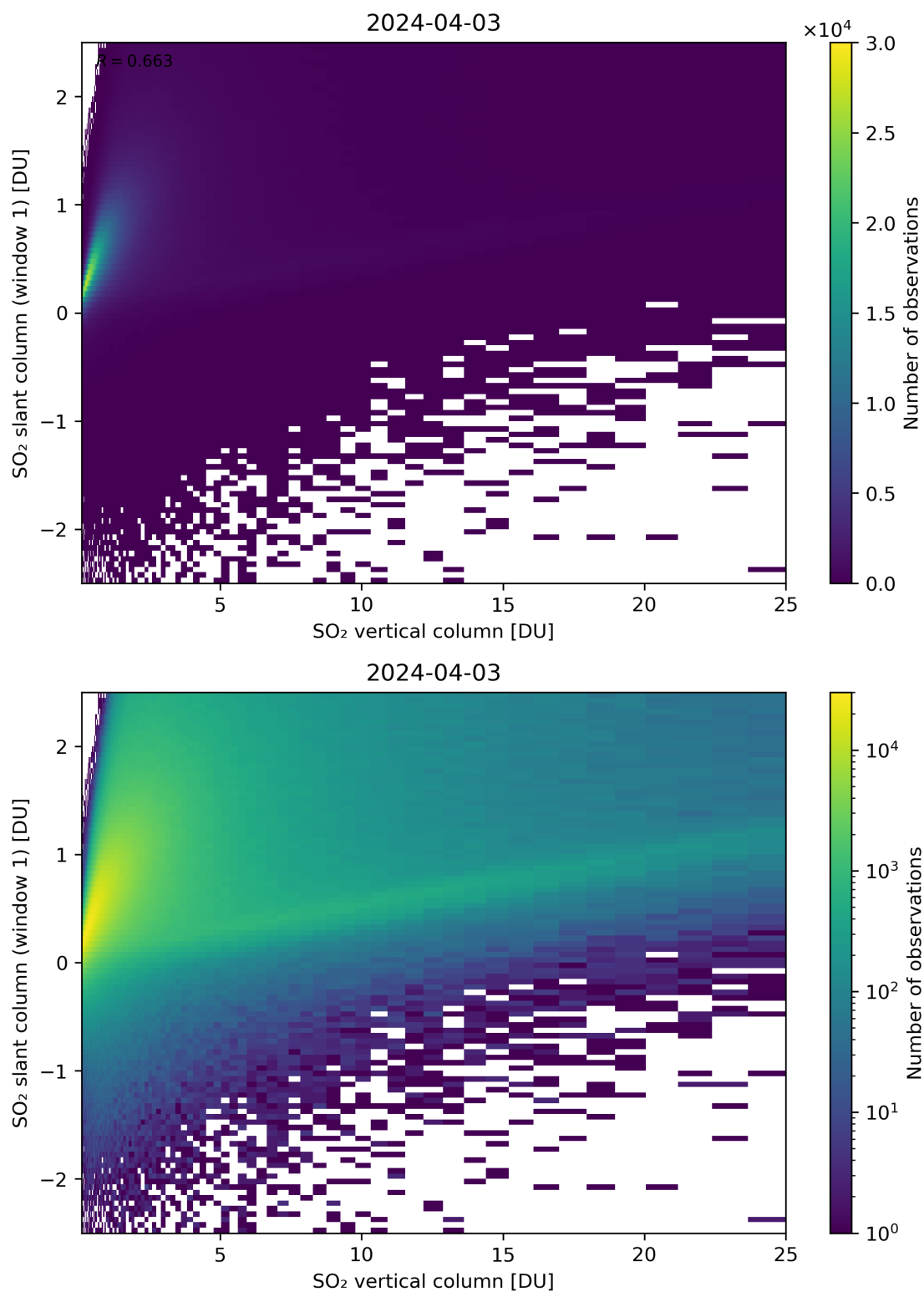
Figure 300: Scatter density plot of “SO 2 vertical column” against “SO 2 slant column (window 1)” for 2024-04-02 to 2024-04-04.
