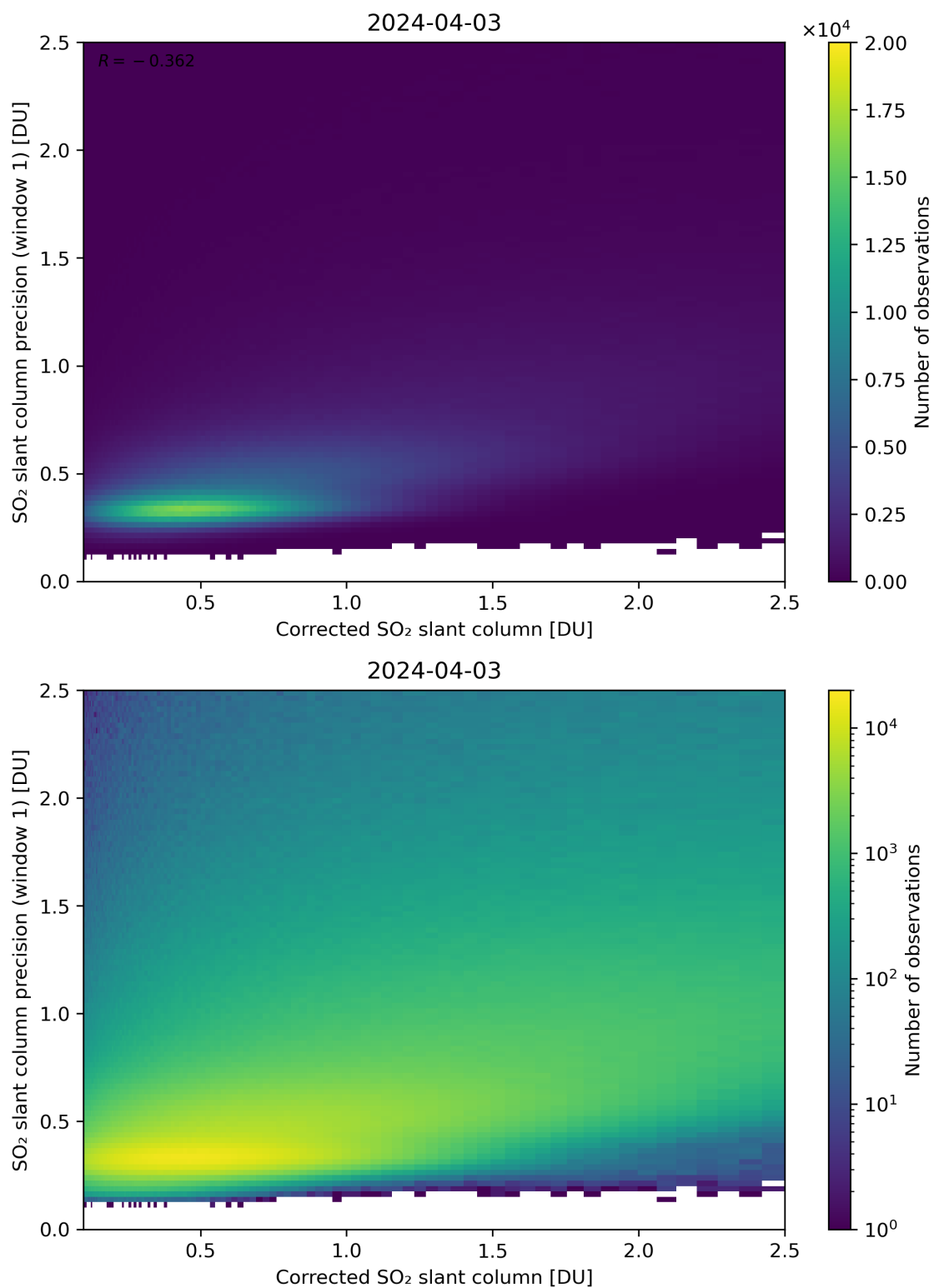
Figure 188: Scatter density plot of “Corrected SO 2 slant column” against “SO 2 slant column precision (window 1)” for 2024-04-02 to 2024-04-04.
