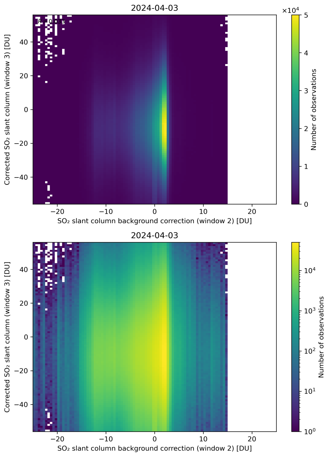
Figure 116: Scatter density plot of “SO 2 slant column background correction (window 2)” against “Corrected SO 2 slant column (window 3)” for 2024-04-02 to 2024-04-04.
