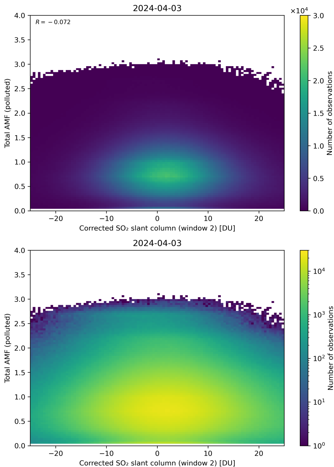
Figure 203: Scatter density plot of “Corrected SO 2 slant column (window 2)” against “Total AMF (polluted)” for 2024-04-02 to 2024-04-04.
