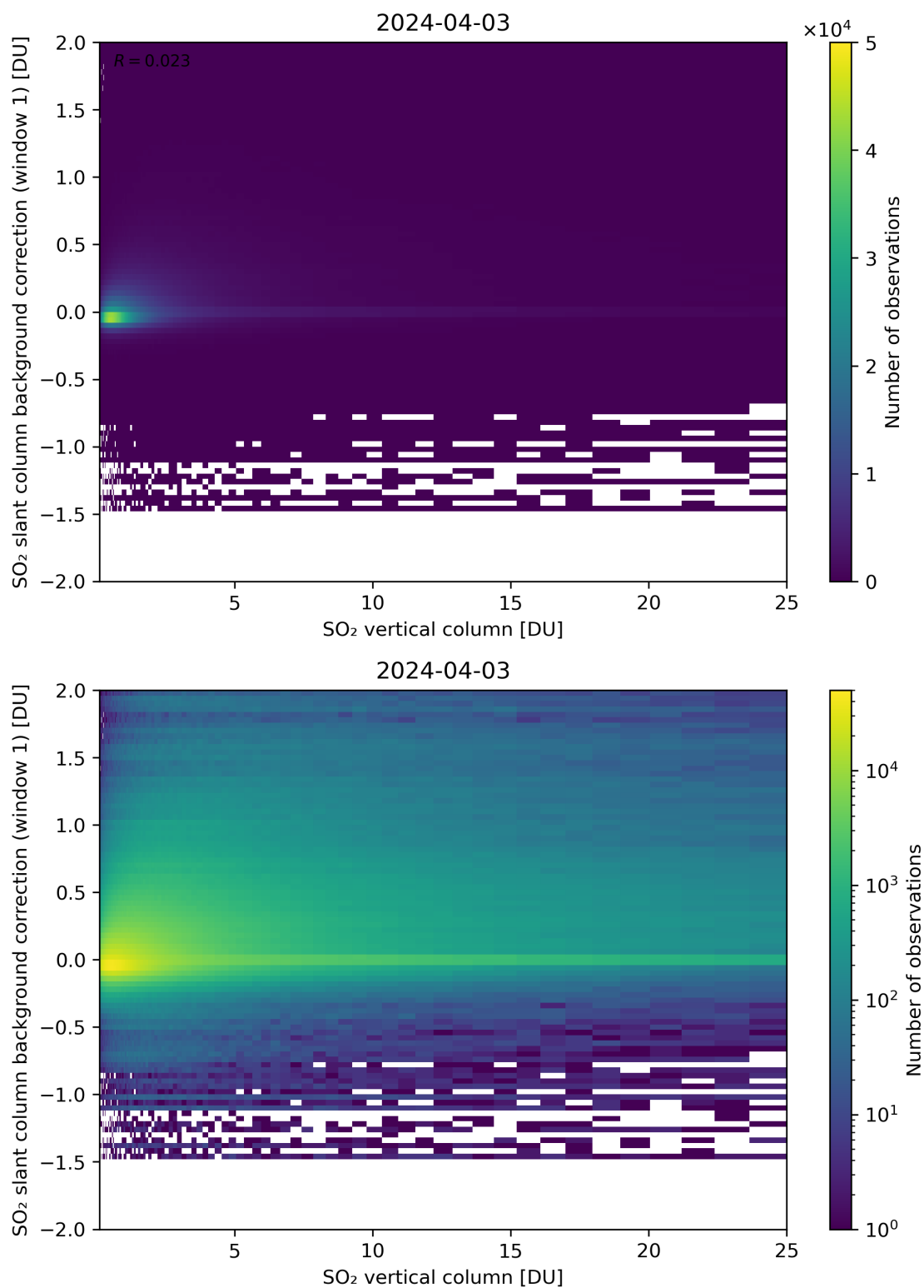
Figure 273: Scatter density plot of “SO 2 vertical column” against “SO 2 slant column background correction (window 1)” for 2024-04-02 to 2024-04-04.
