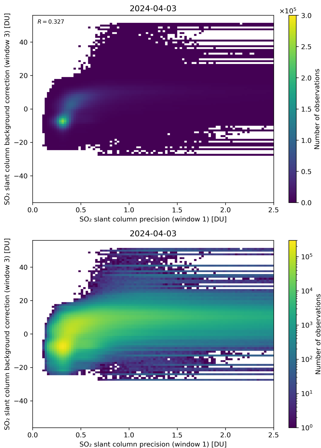
Figure 220: Scatter density plot of “SO 2 slant column precision (window 1)” against “SO 2 slant column background correction (window 3)” for 2024-04-02 to 2024-04-04.
