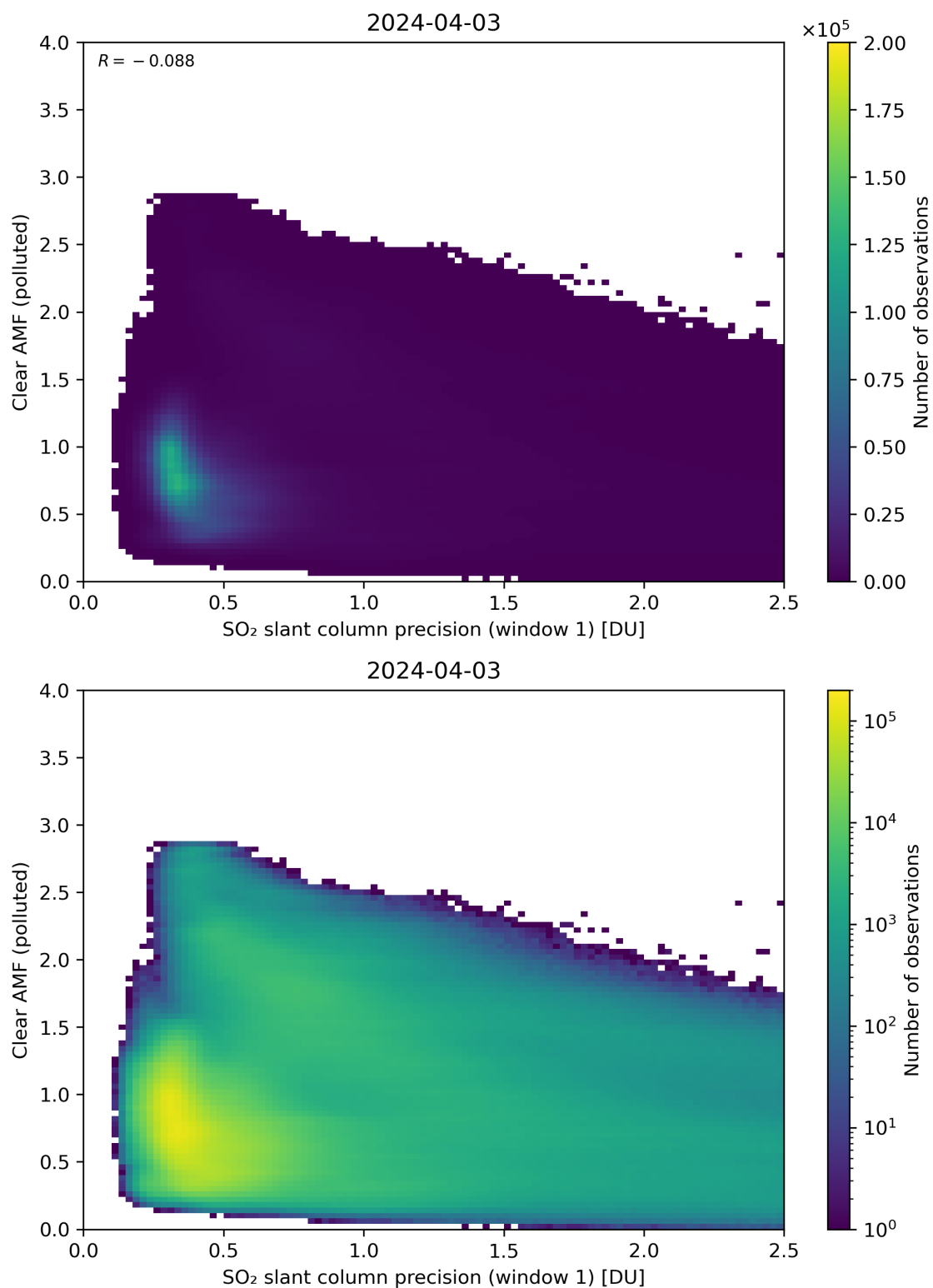
Figure 224: Scatter density plot of “SO 2 slant column precision (window 1)” against “Clear AMF (polluted)” for 2024-04-02 to 2024-04-04.
