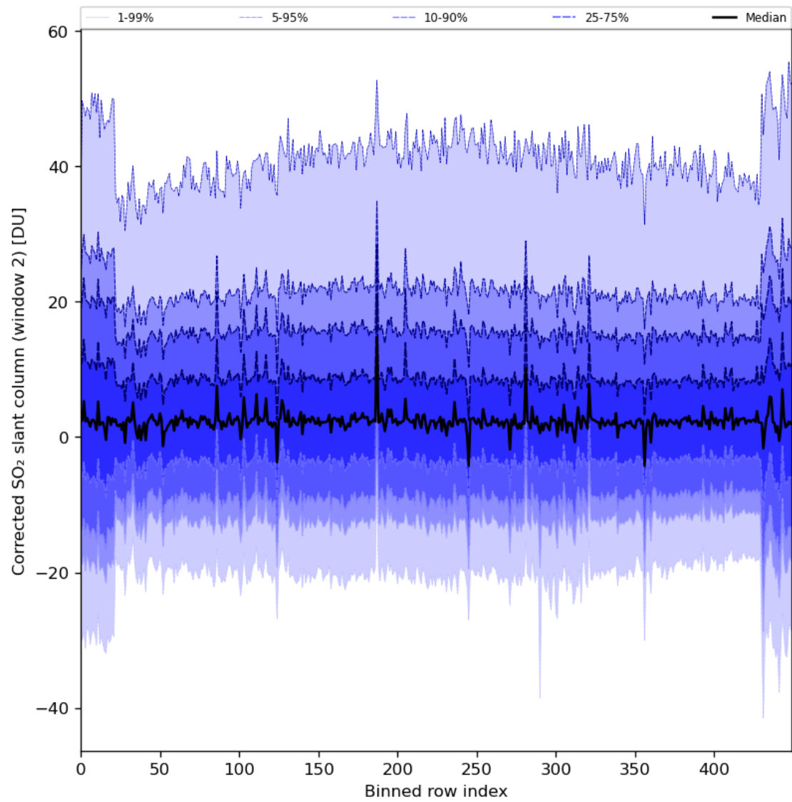
Figure 85: Along track statistics of “Corrected SO 2 slant column (window 2)” for 2024-04-02 to 2024-04-04
