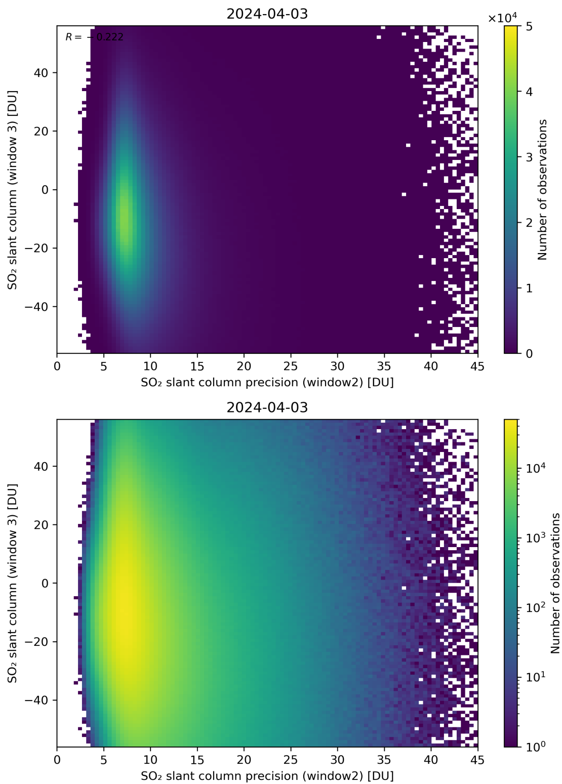
Figure 249: Scatter density plot of “SO 2 slant column precision (window2)” against “SO 2 slant column (window 3)” for 2024-04-02 to 2024-04-04.
