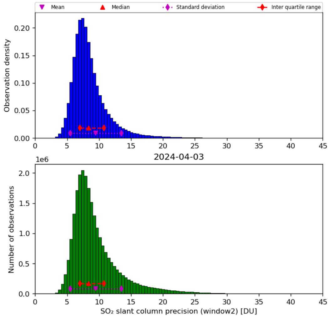
Figure 61: Histogram of “SO 2 slant column precision (window2)” for 2024-04-02 to 2024-04-04
