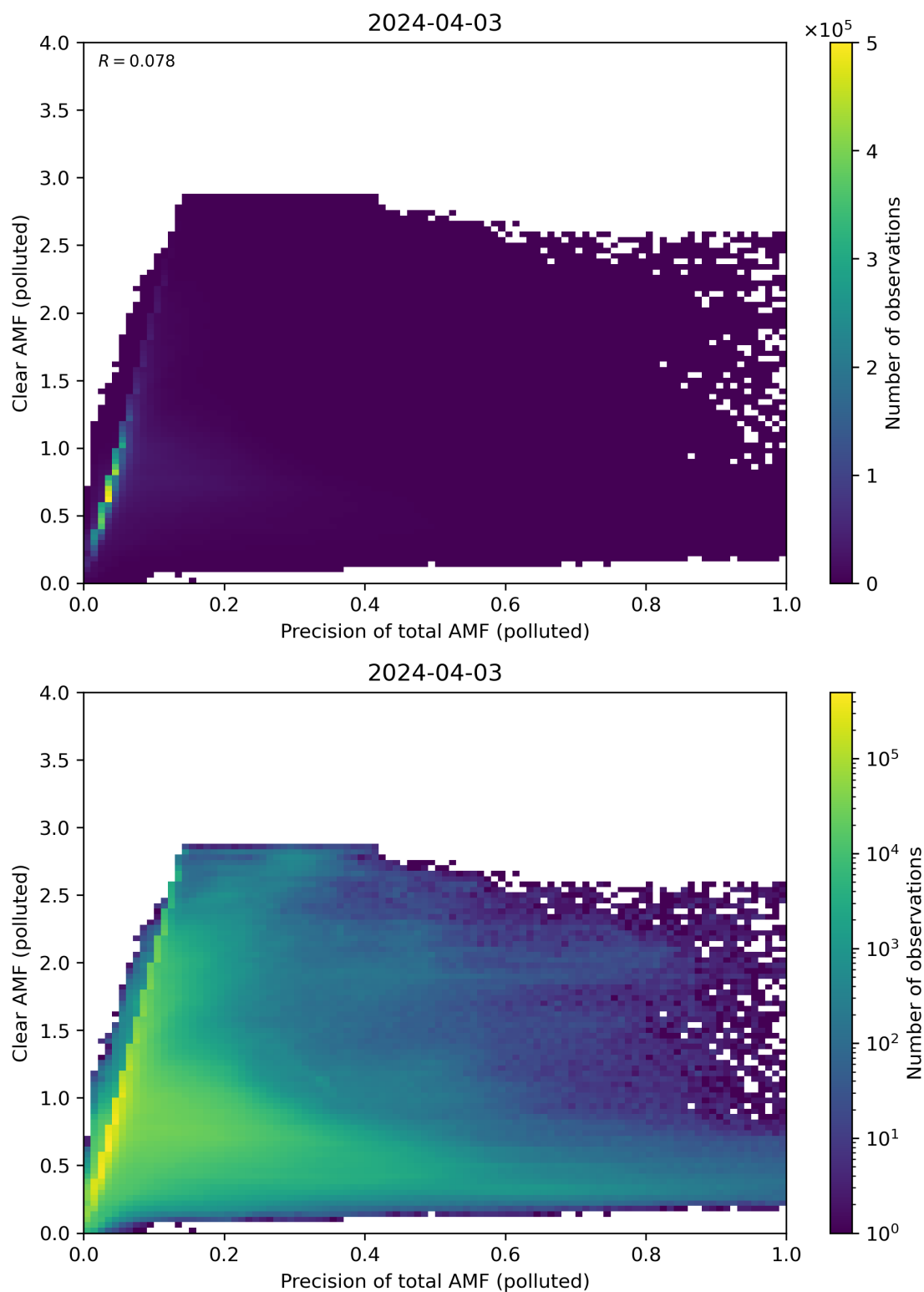
Figure 270: Scatter density plot of “Precision of total AMF (polluted)” against “Clear AMF (polluted)” for 2024-04-02 to 2024-04-04.
