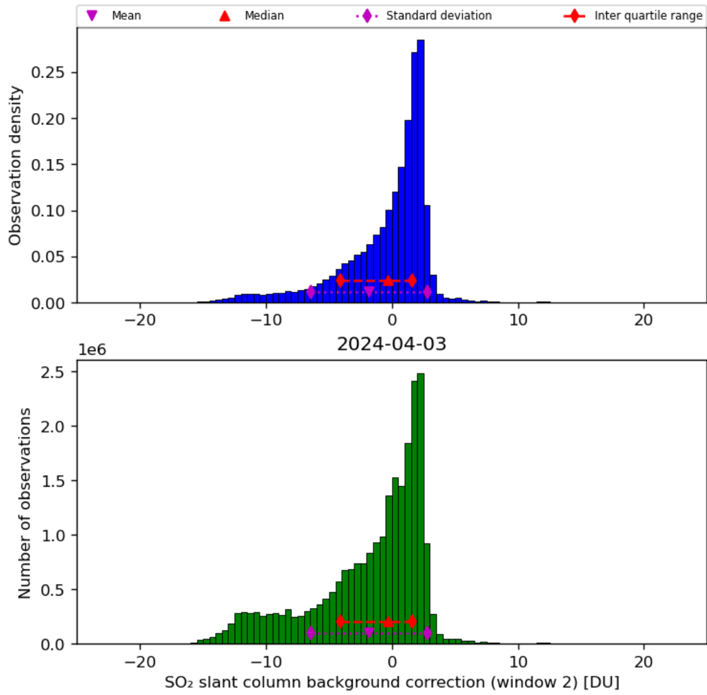
Figure 63: Histogram of “SO 2 slant column background correction (window 2)” for 2024-04-02 to 2024-04-04
