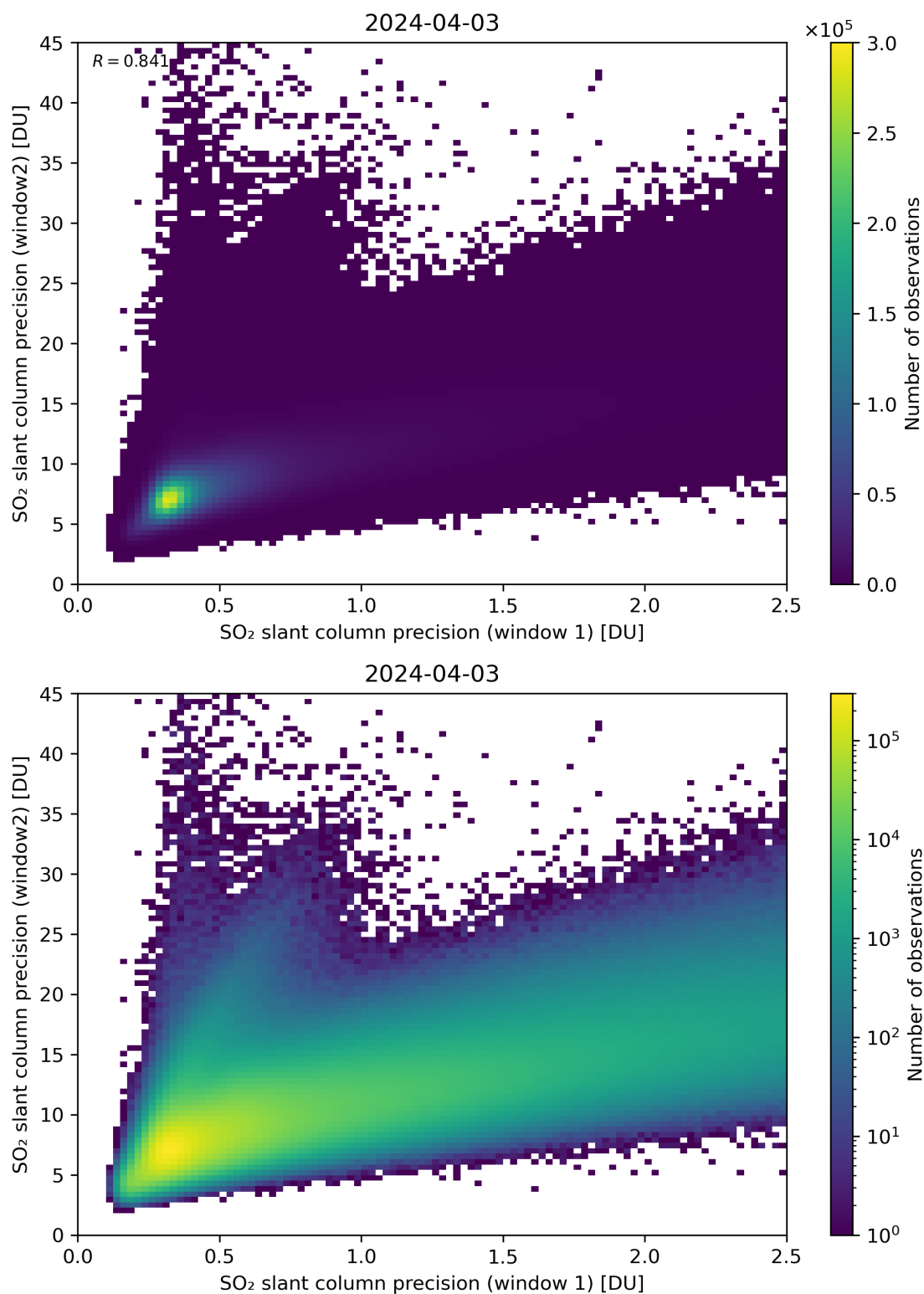
Figure 227: Scatter density plot of “SO 2 slant column precision (window 1)” against “SO 2 slant column precision (window 2)” for 2024-04-02 to 2024-04-04.
