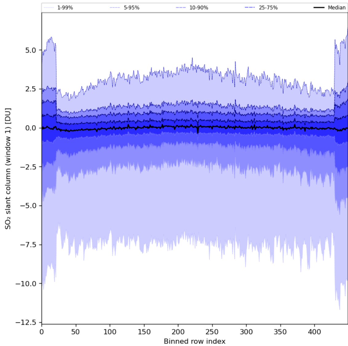
Figure 79: Along track statistics of “SO 2 slant column (window 1)” for 2024-04-02 to 2024-04-04
