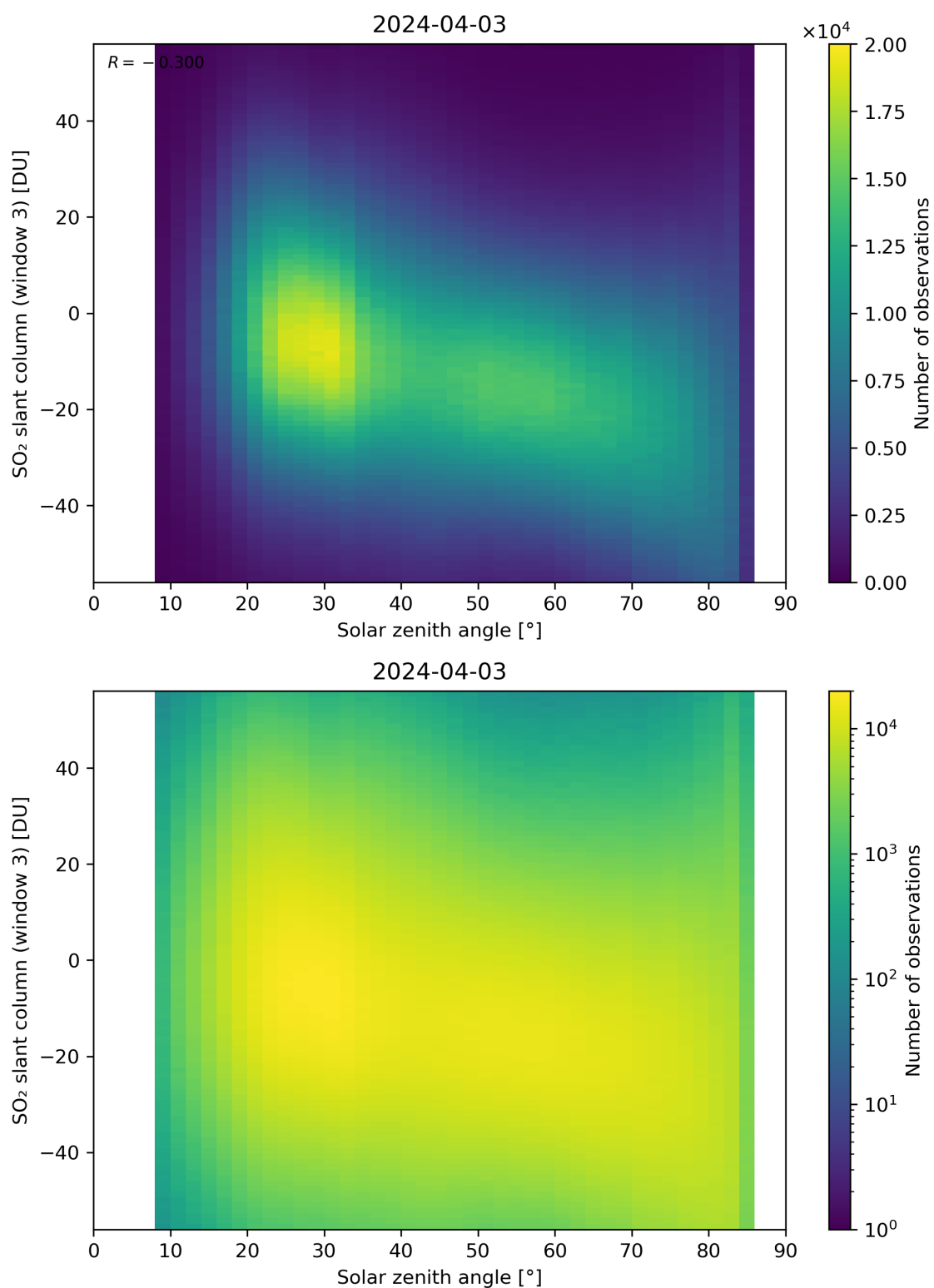
Figure 172: Scatter density plot of “Solar zenith angle” against “SO 2 slant column (window 3)” for 2024-04-02 to 2024-04-04.
