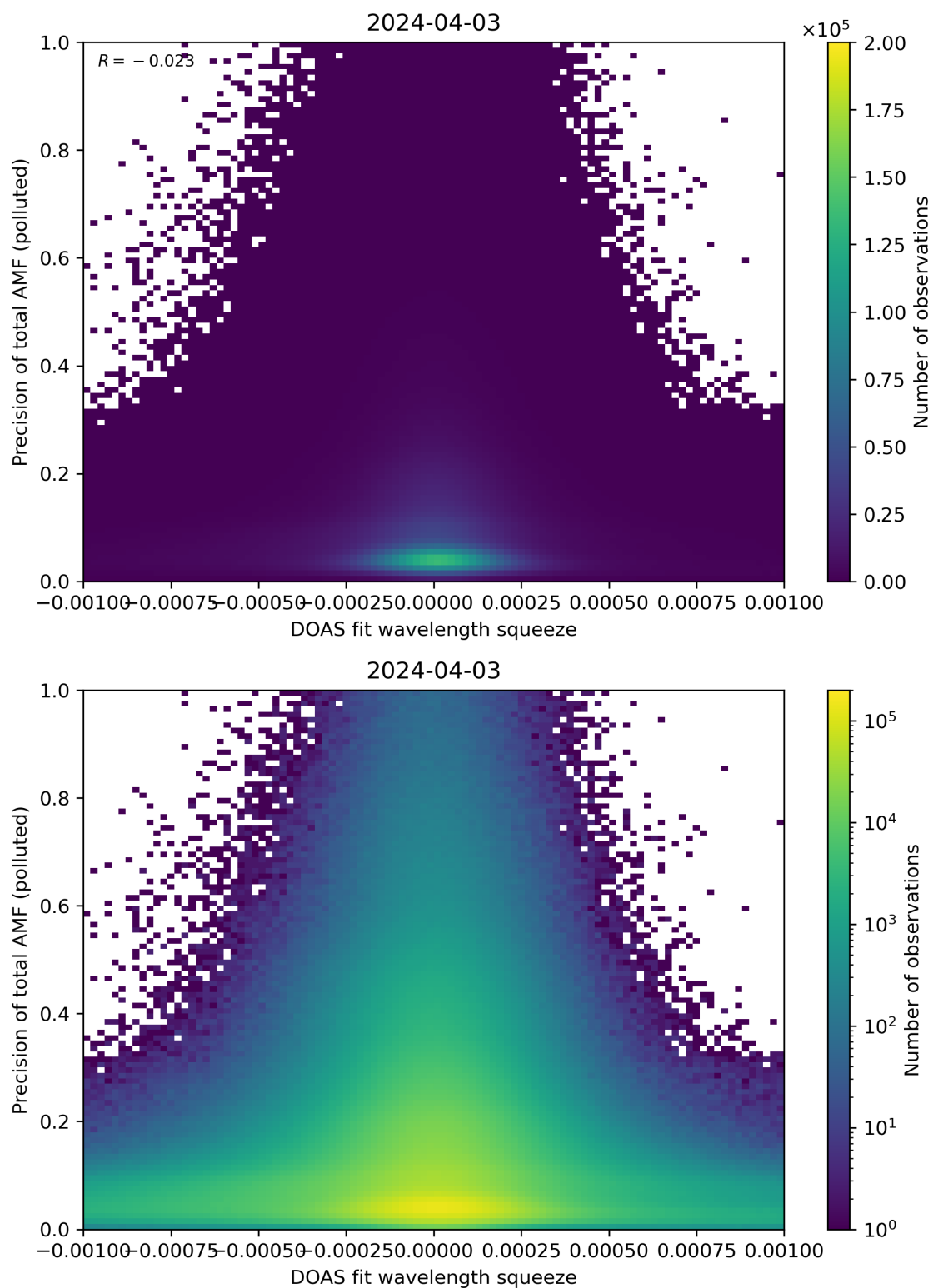
Figure 135: Scatter density plot of “DOAS fit wavelength squeeze” against “Precision of total AMF (polluted)” for 2024-04-02 to 2024-04-04.
