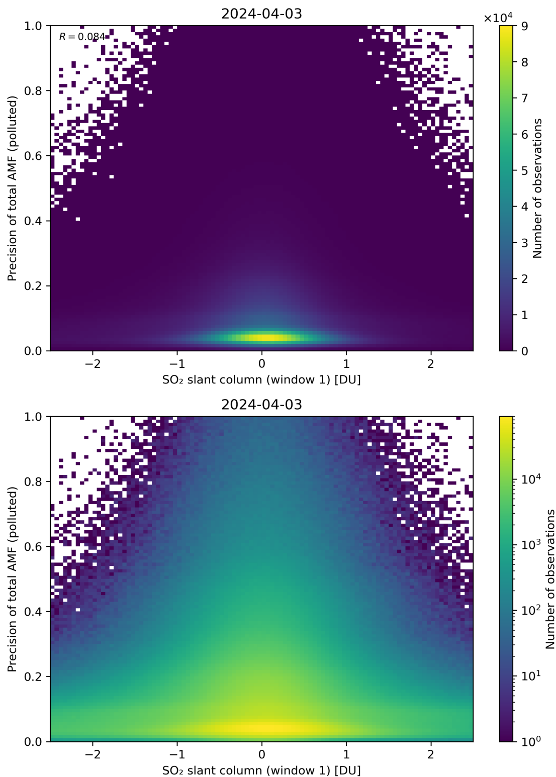
Figure 240: Scatter density plot of “SO 2 slant column (window 1)” against “Precision of total AMF (polluted)” for 2024-04-02 to 2024-04-04.
