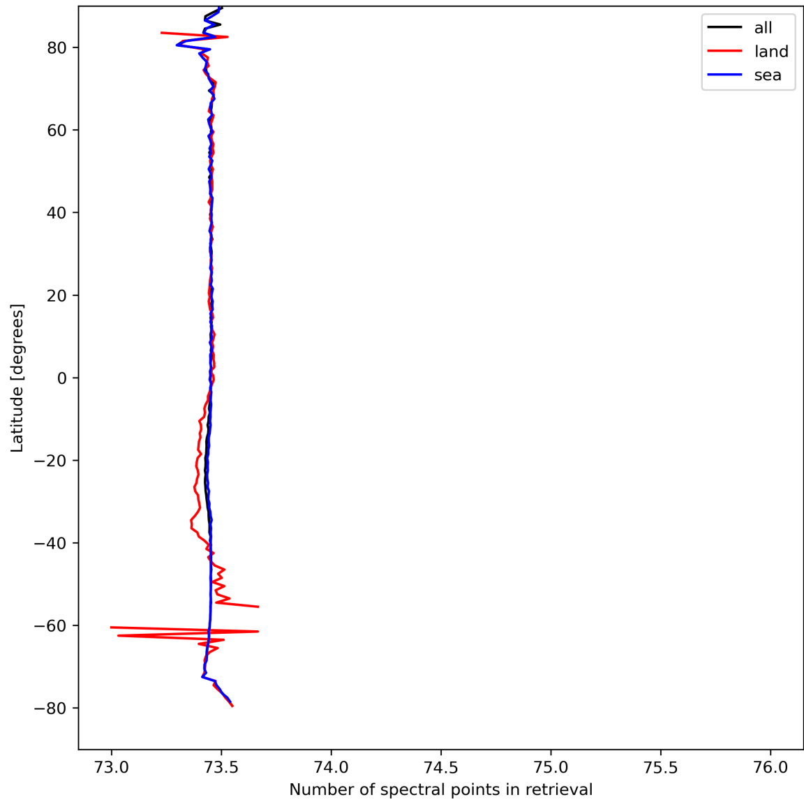
Figure 51: Zonal average of “Number of spectral points in retrieval” for 2024-04-02 to 2024-04-04.
