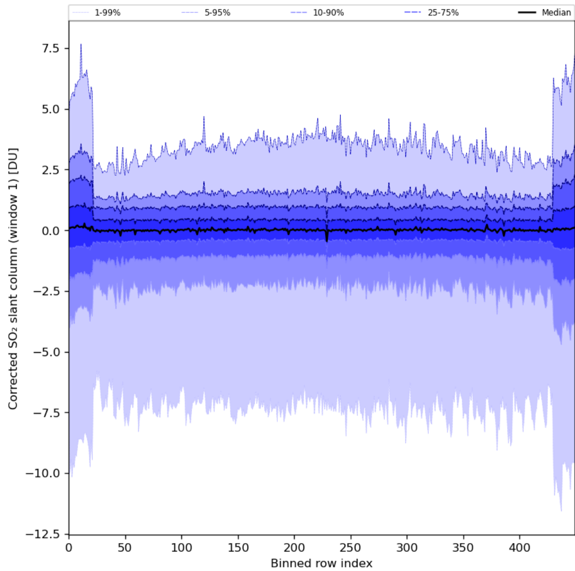
Figure 81: Along track statistics of “Corrected SO 2 slant column (window 1)” for 2024-04-02 to 2024-04-04
