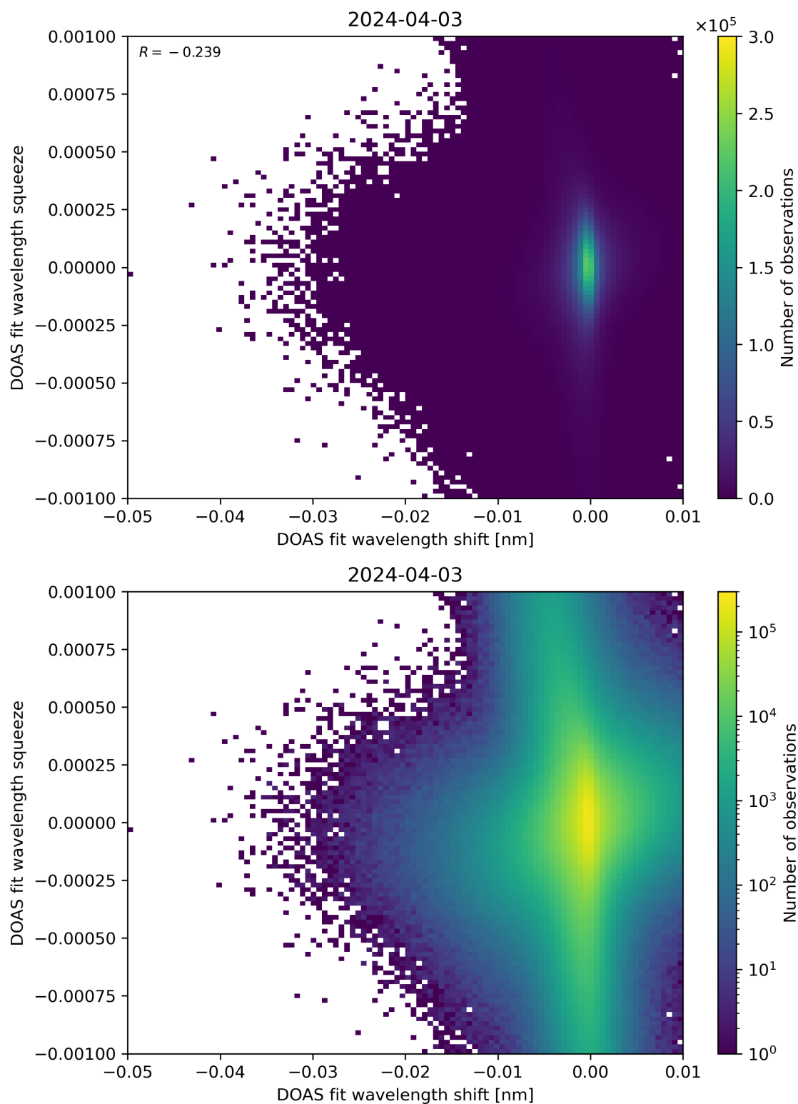
Figure 127: Scatter density plot of “DOAS fit wavelength shift” against “DOAS fit wavelength squeeze” for 2024-04-02 to 2024-04-04.
