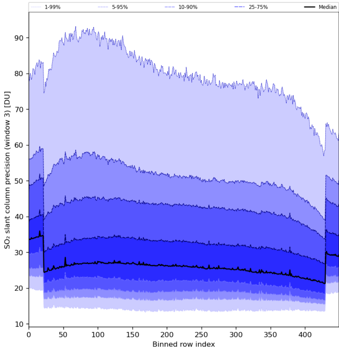
Figure 88: Along track statistics of “SO 2 slant column precision (window 3)” for 2024-04-02 to 2024-04-04
