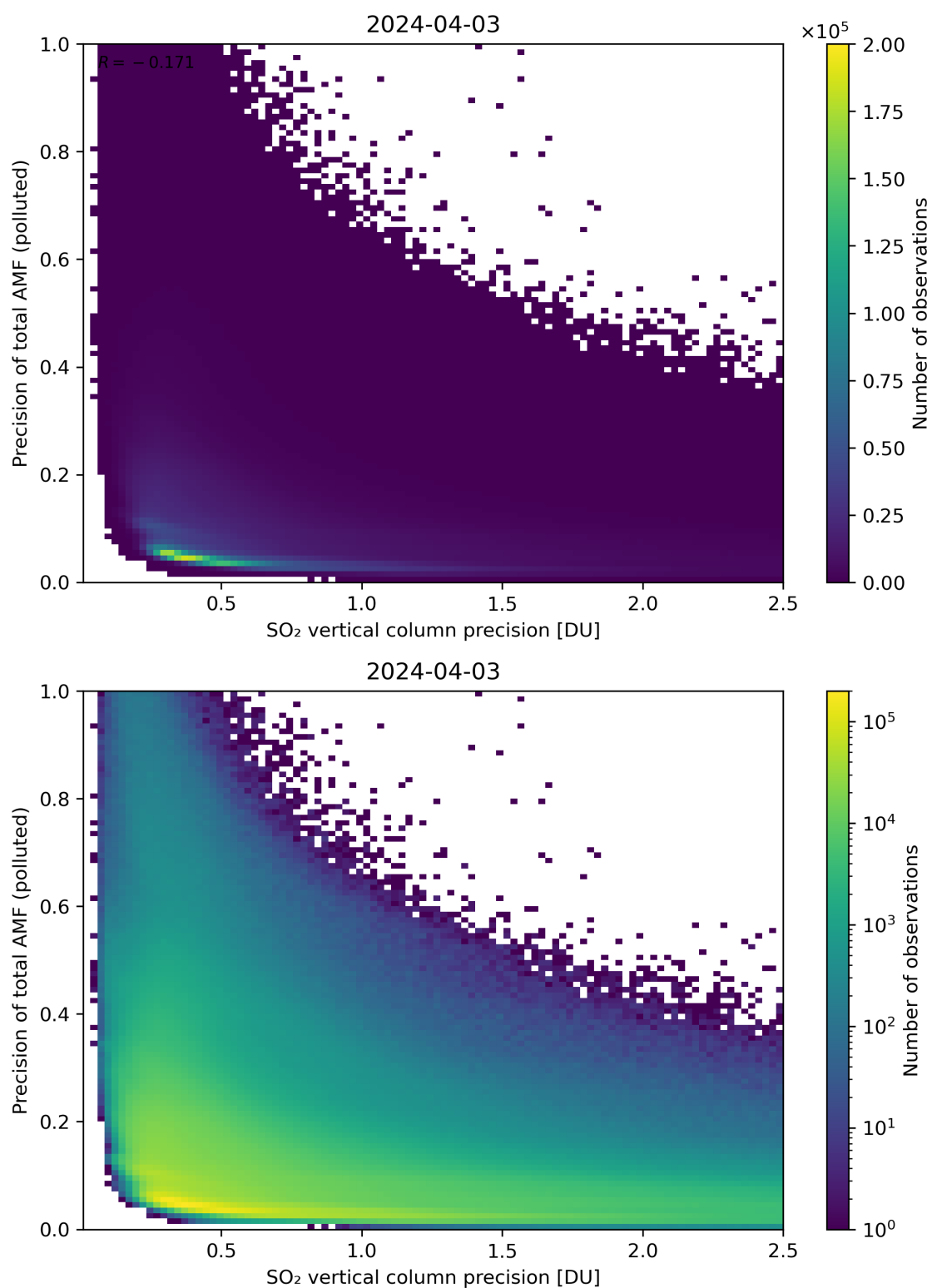
Figure 295: Scatter density plot of “SO 2 vertical column precision” against “Precision of total AMF (polluted)” for 2024-04-02 to 2024-04-04.
