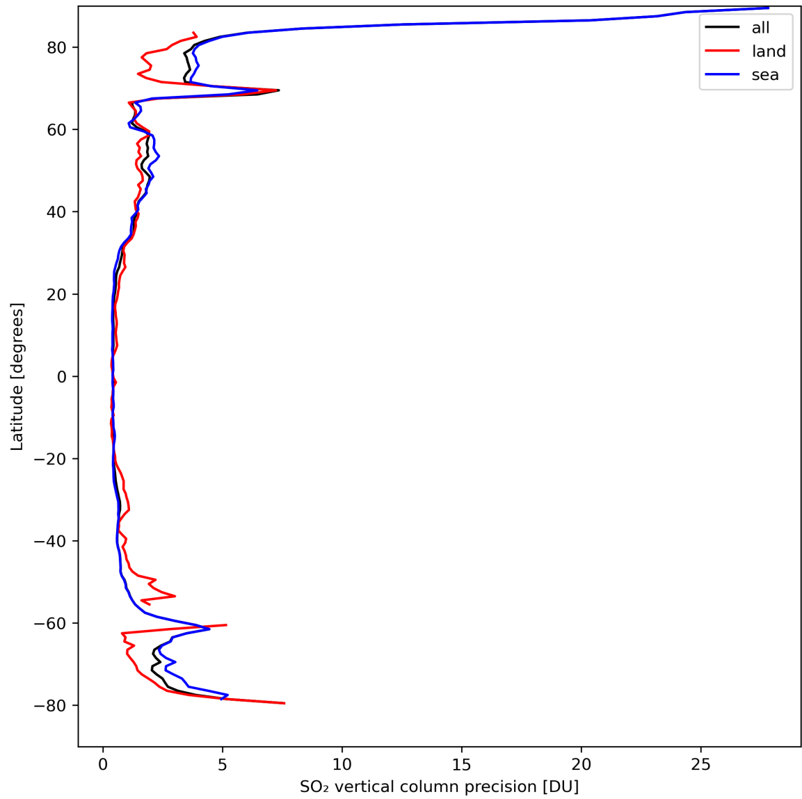
Figure 31: Zonal average of “SO 2 vertical column precision” for 2024-04-02 to 2024-04-04.
