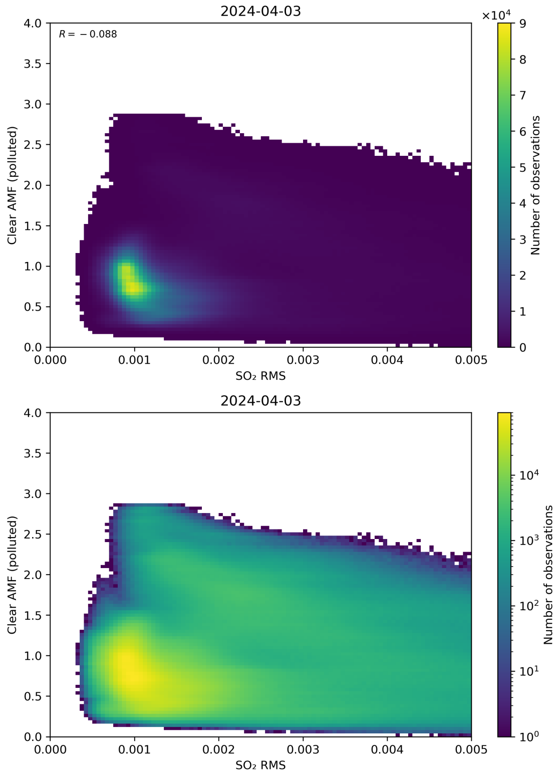
Figure 136: Scatter density plot of “SO 2 RMS” against “Clear AMF (polluted)” for 2024-04-02 to 2024-04-04.
