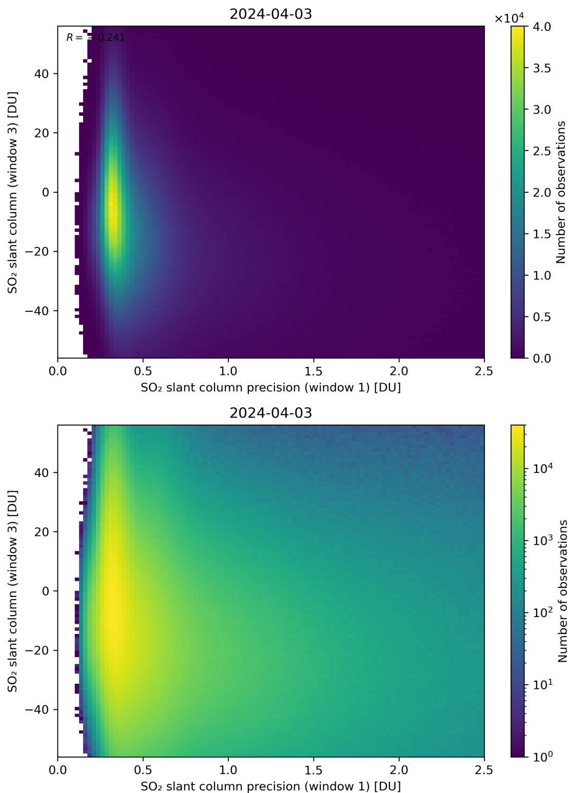
Figure 228: Scatter density plot of “SO 2 slant column precision (window 1)” against “SO 2 slant column (window 3)” for 2024-04-02 to 2024-04-04.
