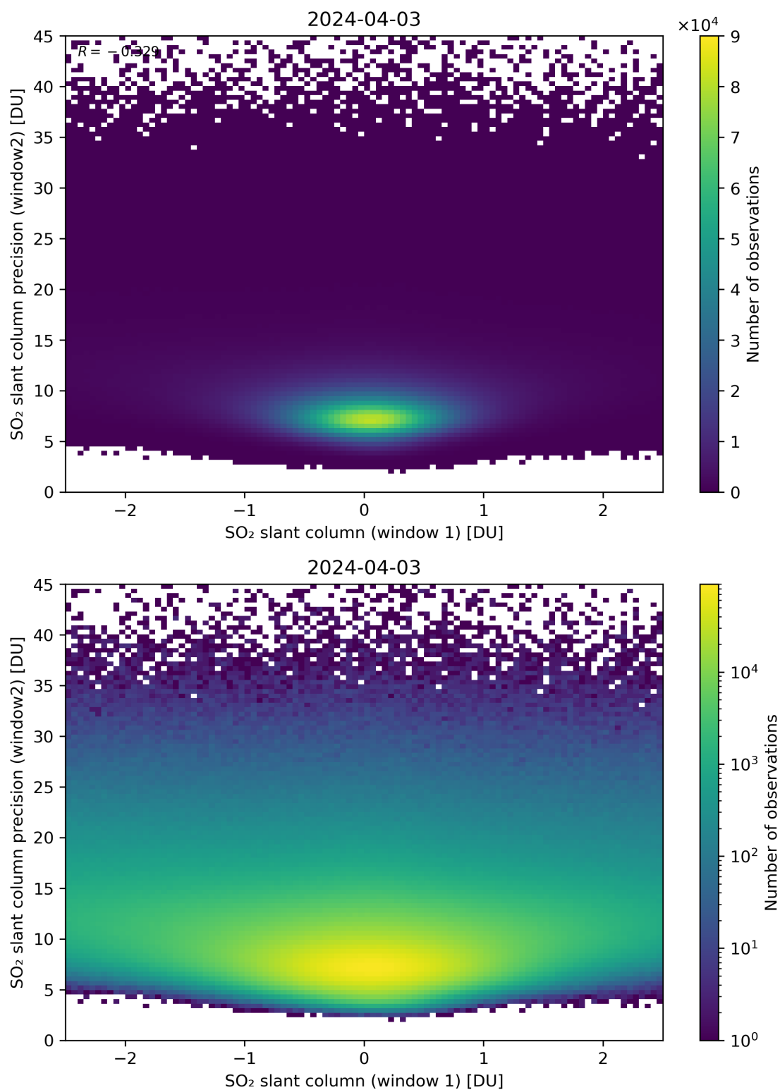
Figure 236: Scatter density plot of “SO 2 slant column (window 1)” against “SO 2 slant column precision (window2)” for 2024-04-02 to 2024-04-04.
