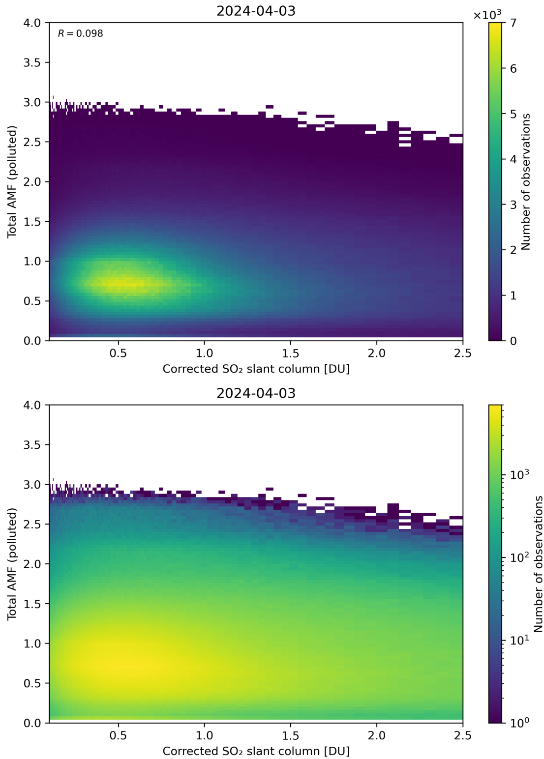
Figure 192: Scatter density plot of “Corrected SO 2 slant column” against “Total AMF (polluted)” for 2024-04-02 to 2024-04-04.
