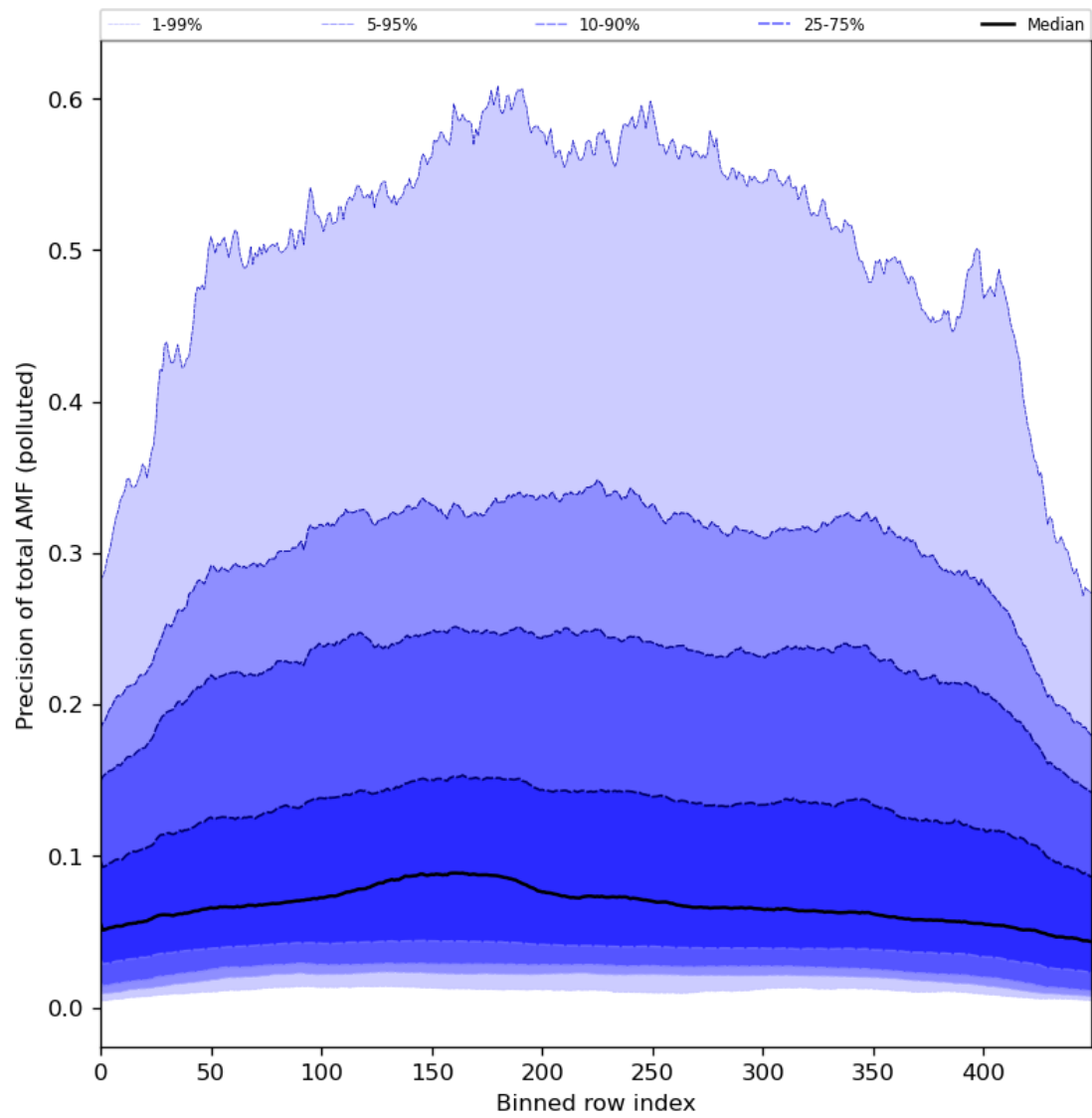
Figure 95: Along track statistics of “Precision of total AMF (polluted)” for 2024-04-02 to 2024-04-04
