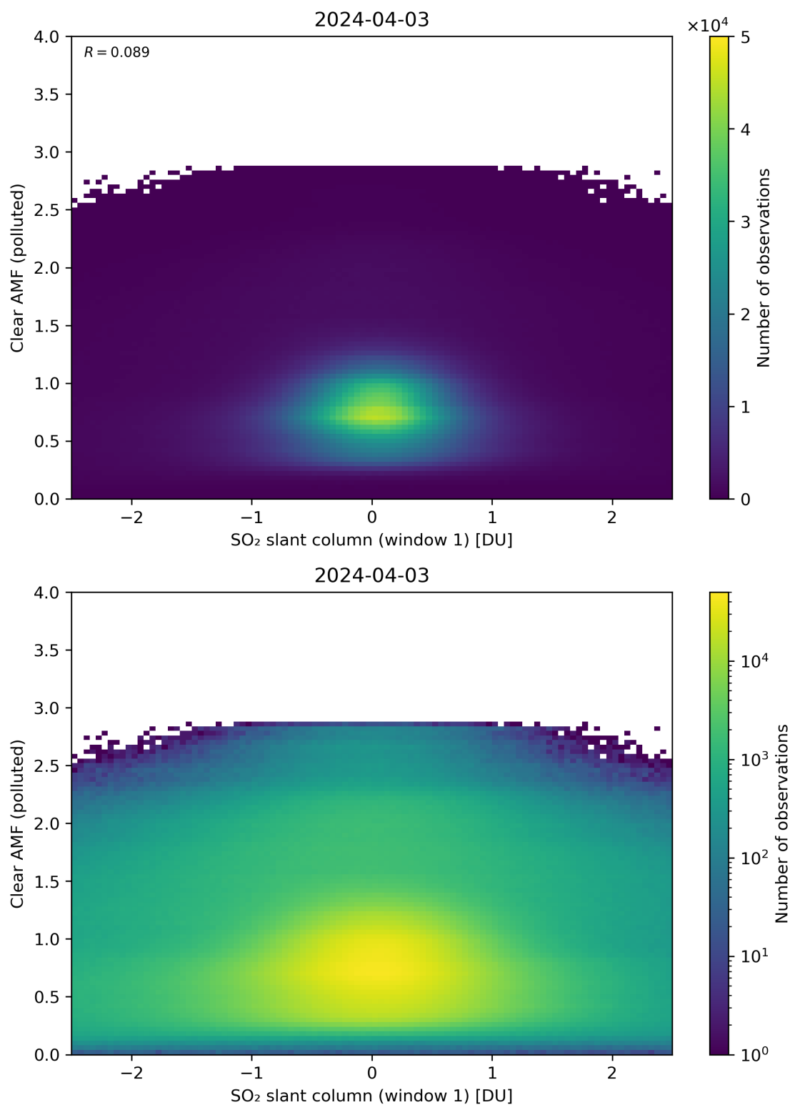
Figure 232: Scatter density plot of “SO 2 slant column (window 1)” against “Clear AMF (polluted)” for 2024-04-02 to 2024-04-04.
