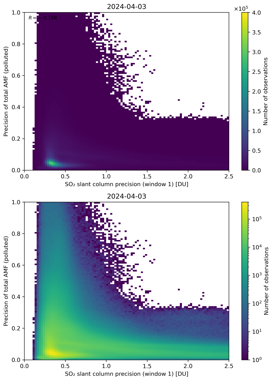
Figure 231: Scatter density plot of “SO 2 slant column precision (window 1)” against “Precision of total AMF (polluted)” for 2024-04-02 to 2024-04-04.
