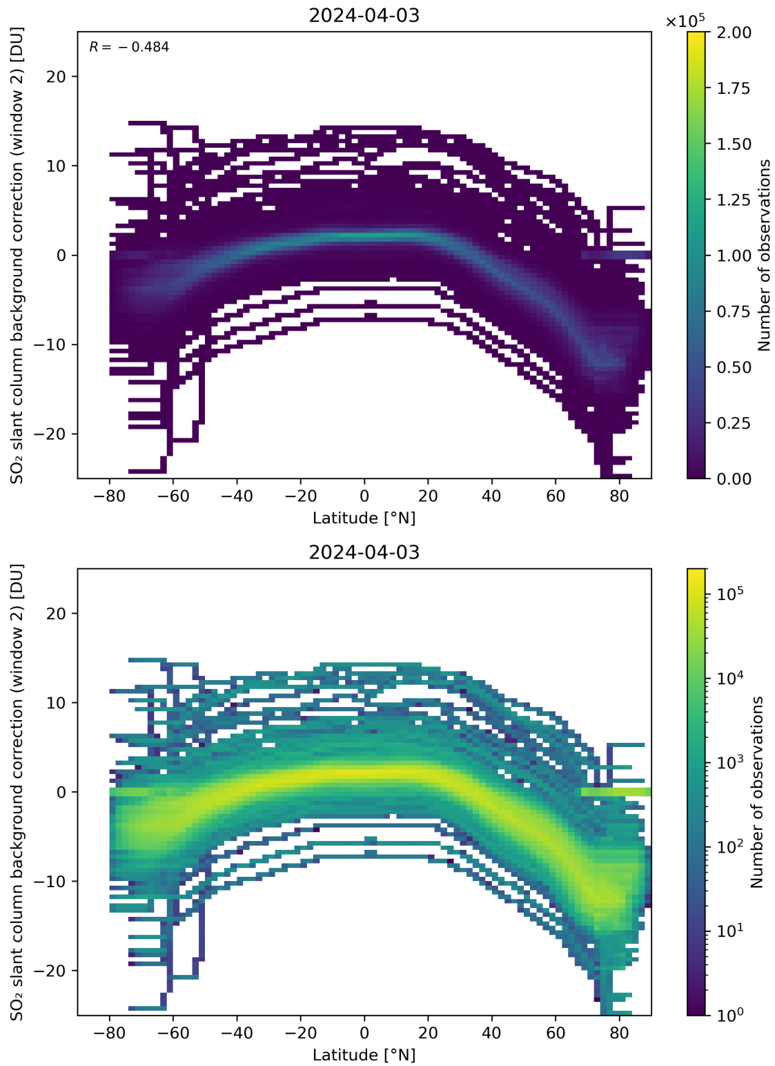
Figure 140: Scatter density plot of “Latitude” against “SO 2 slant column background correction (window 2)” for 2024-04-02 to 2024-04-04.
