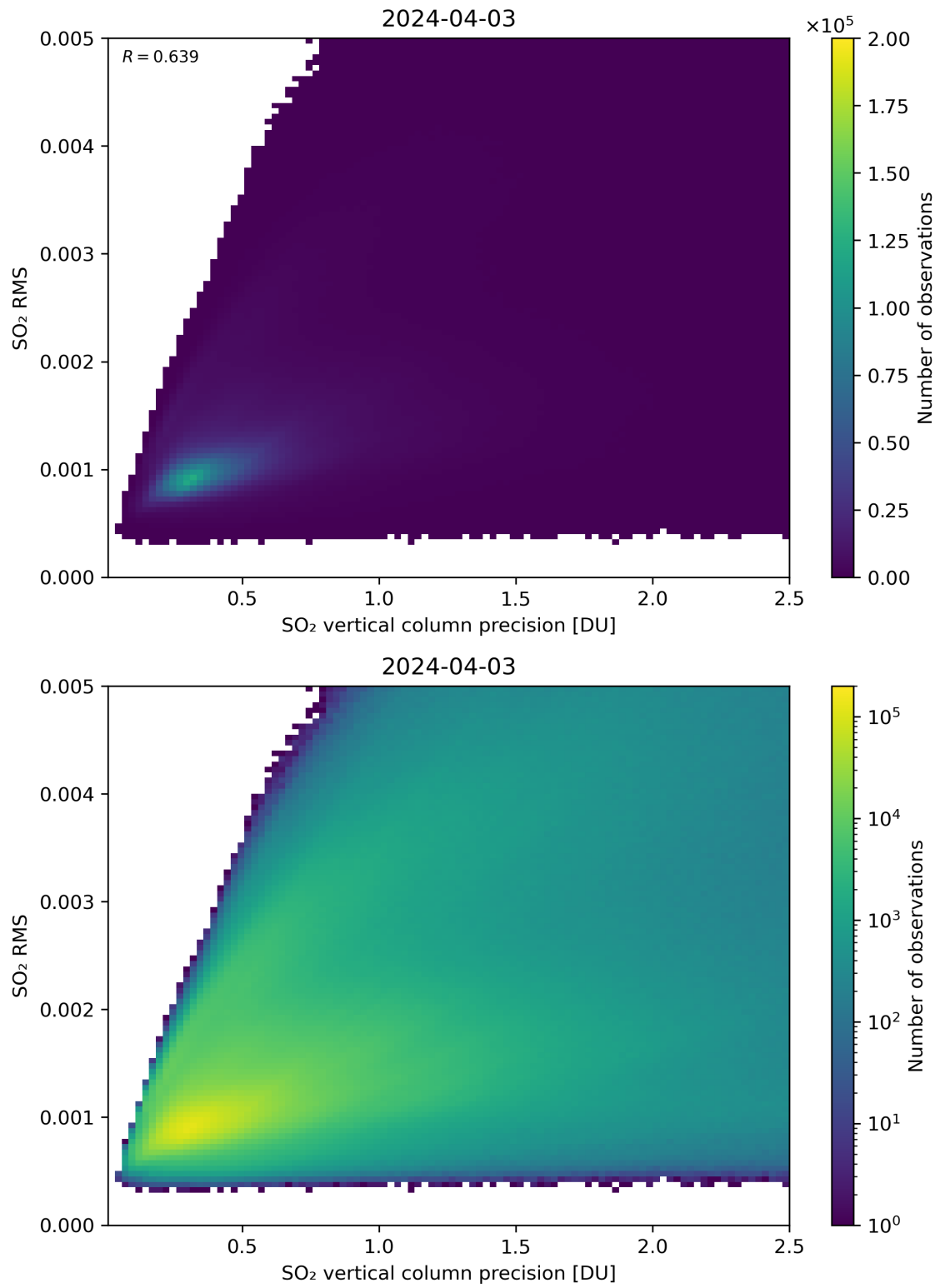
Figure 284: Scatter density plot of “SO 2 vertical column precision” against “SO 2 RMS” for 2024-04-02 to 2024-04-04.
