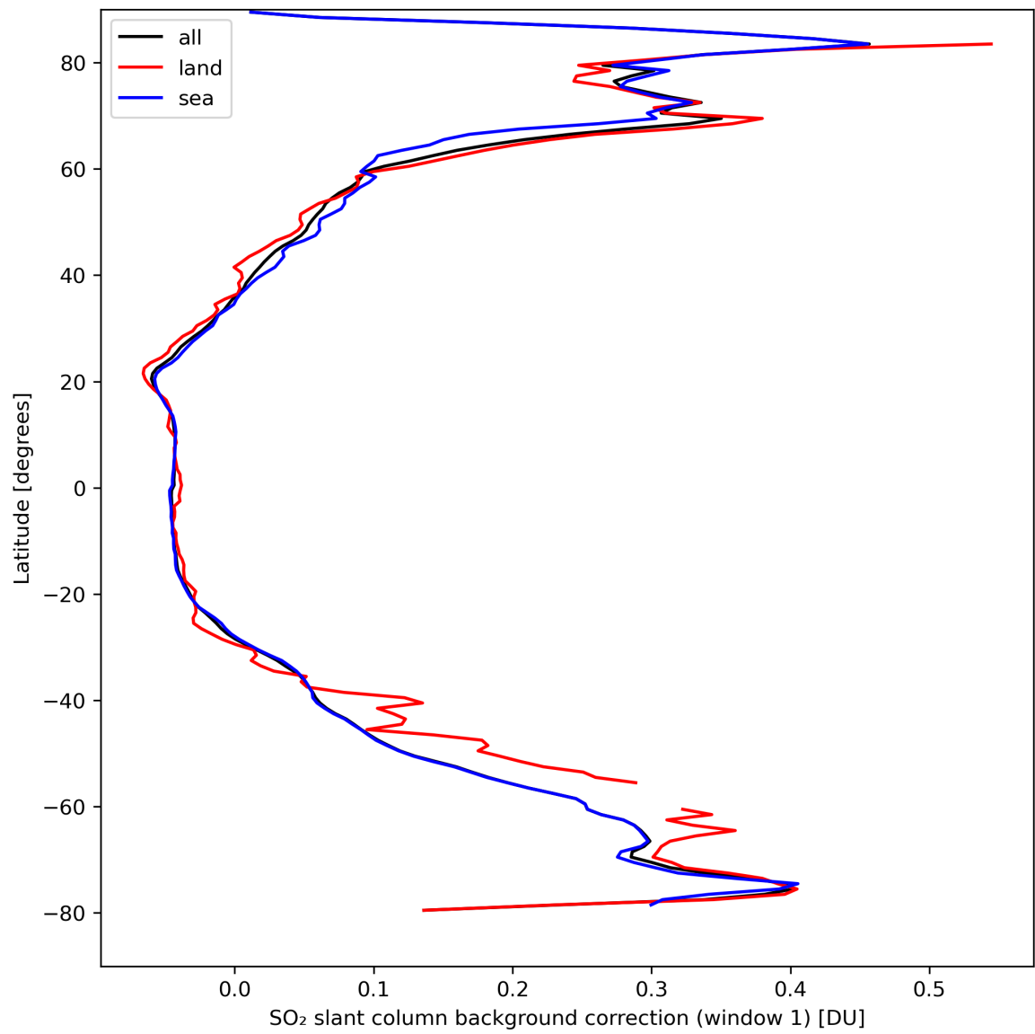
Figure 36: Zonal average of “SO 2 slant column background correction (window 1)” for 2024-04-02 to 2024-04-04.
