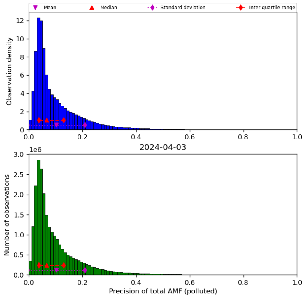
Figure 72: Histogram of “Precision of total AMF (polluted)” for 2024-04-02 to 2024-04-04
