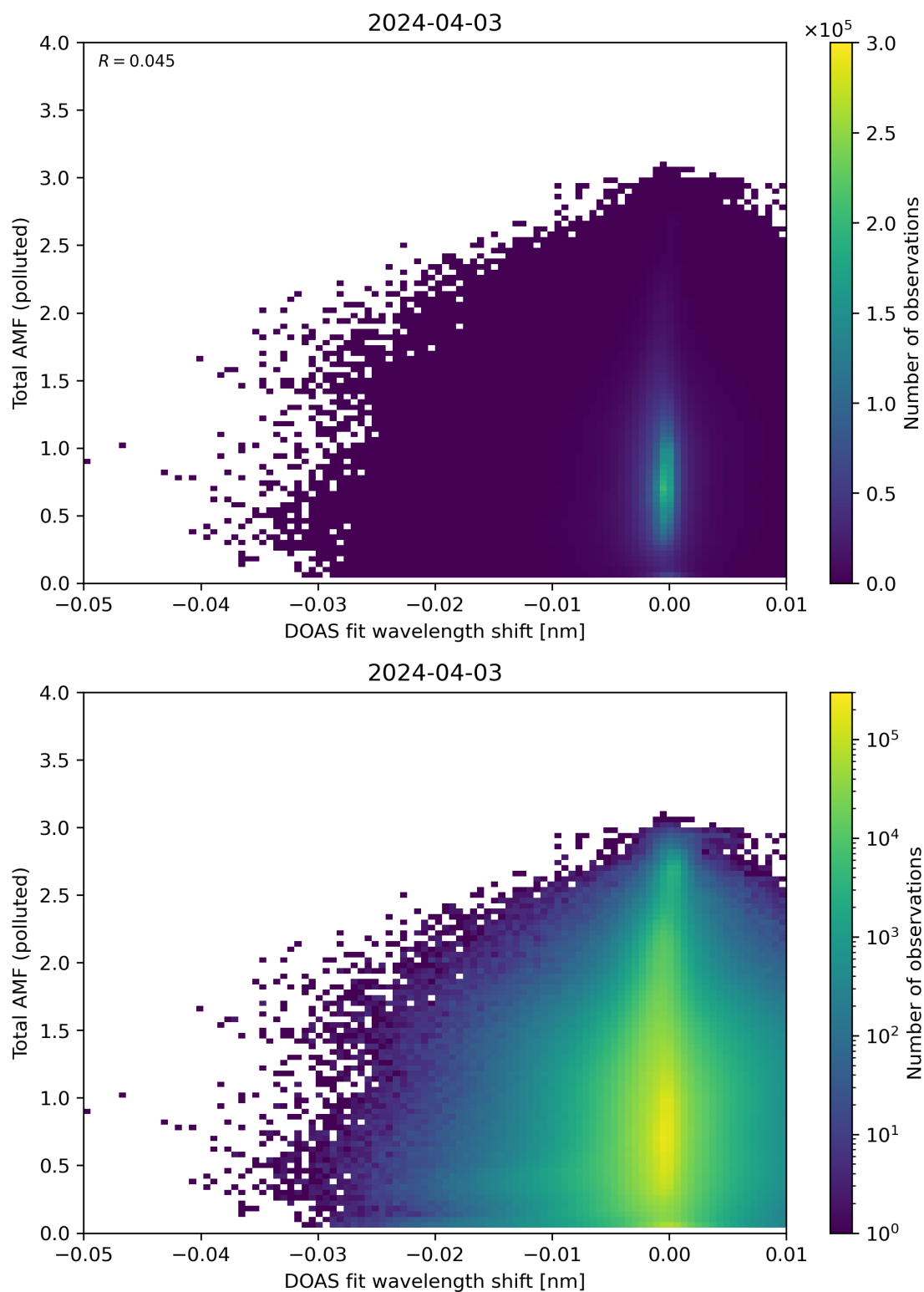
Figure 130: Scatter density plot of “DOAS fit wavelength shift” against “Total AMF (polluted)” for 2024-04-02 to 2024-04-04.
