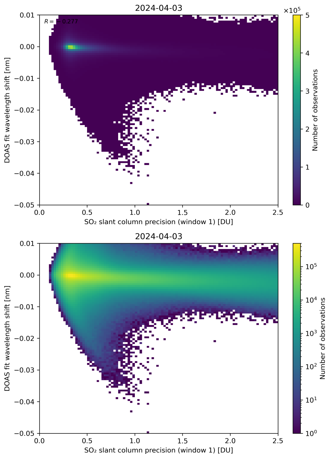
Figure 221: Scatter density plot of “SO 2 slant column precision (window 1)” against “DOAS fit wavelength shift” for 2024-04-02 to 2024-04-04.
