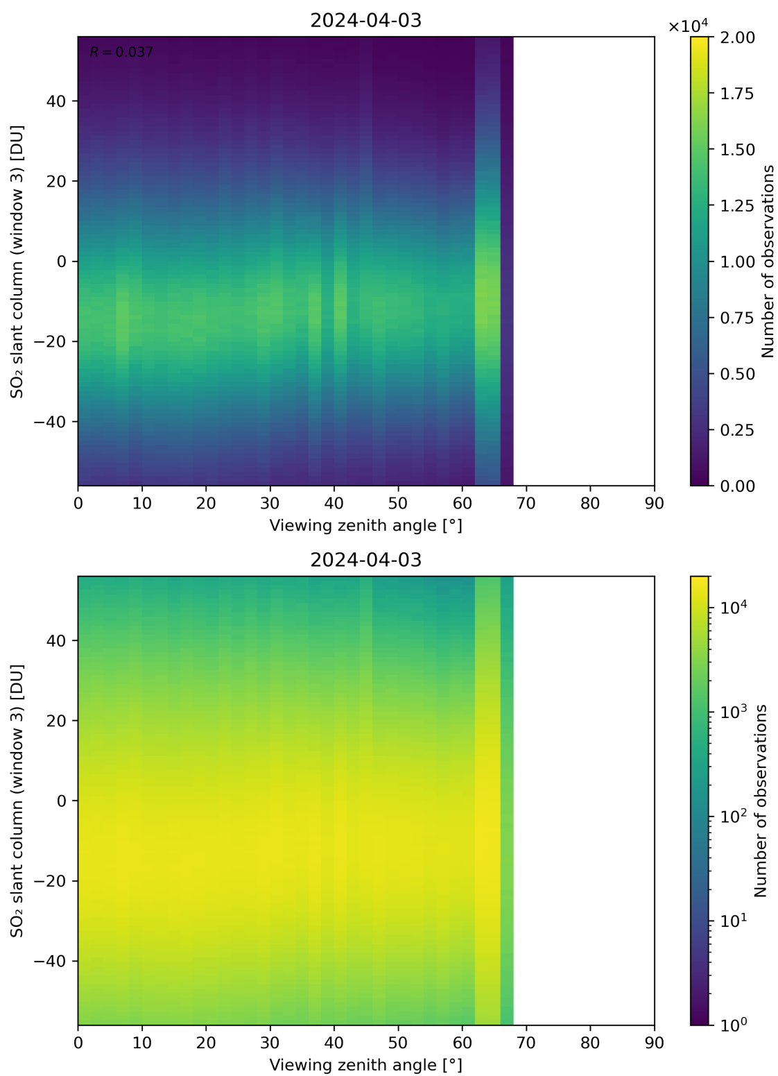
Figure 323: Scatter density plot of “Viewing zenith angle” against “SO 2 slant column (window 3)” for 2024-04-02 to 2024-04-04.
