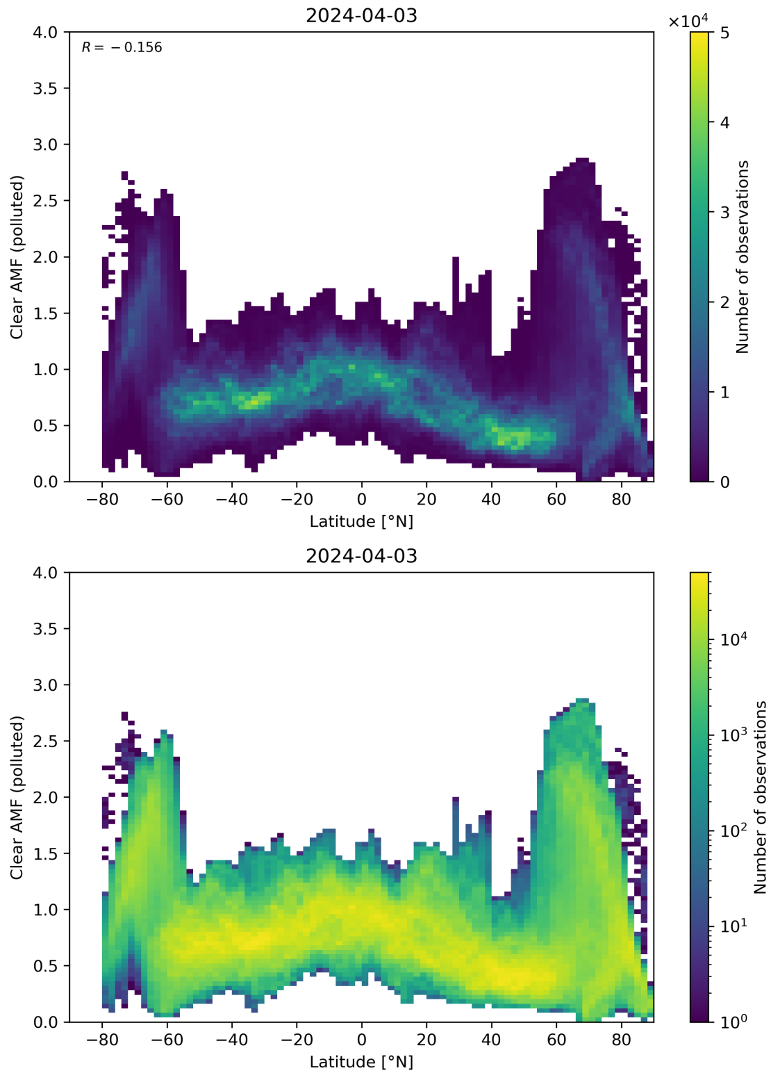
Figure 145: Scatter density plot of “Latitude” against “Clear AMF (polluted)” for 2024-04-02 to 2024-04-04.
