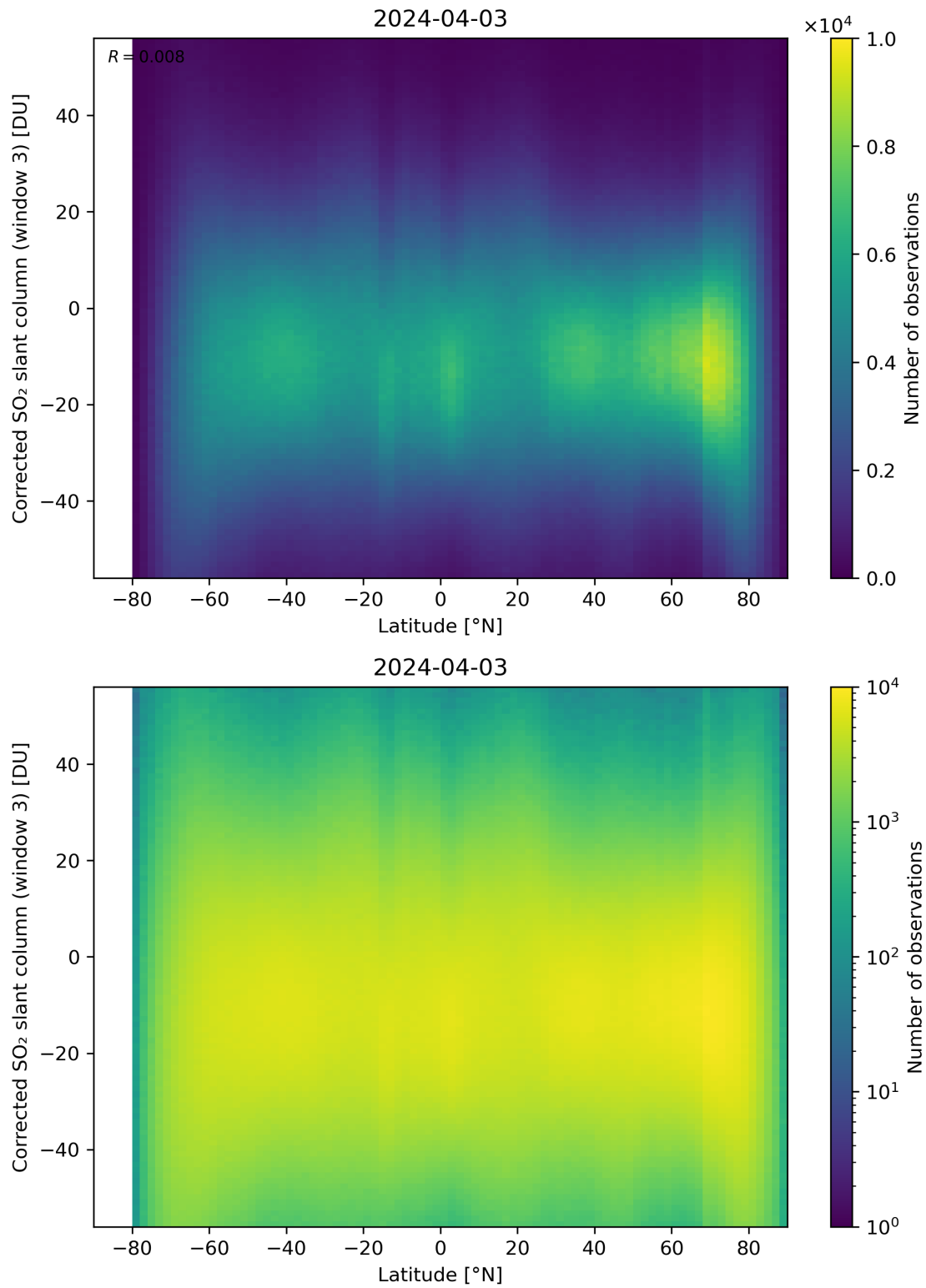
Figure 148: Scatter density plot of “Latitude” against “Corrected SO 2 slant column (window 3)” for 2024-04-02 to 2024-04-04.
