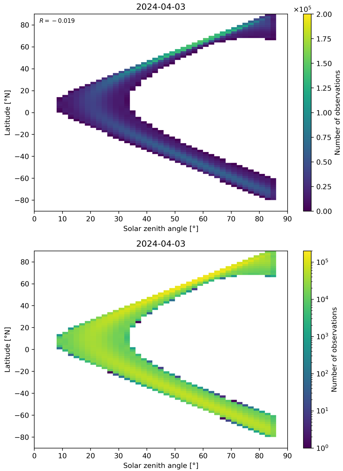
Figure 164: Scatter density plot of “Solar zenith angle” against “Latitude” for 2024-04-02 to 2024-04-04.
