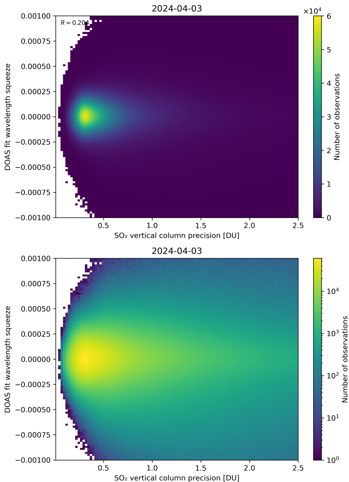
Figure 283: Scatter density plot of “SO 2 vertical column precision” against “DOAS fit wavelength squeeze” for 2024-04-02 to 2024-04-04.
