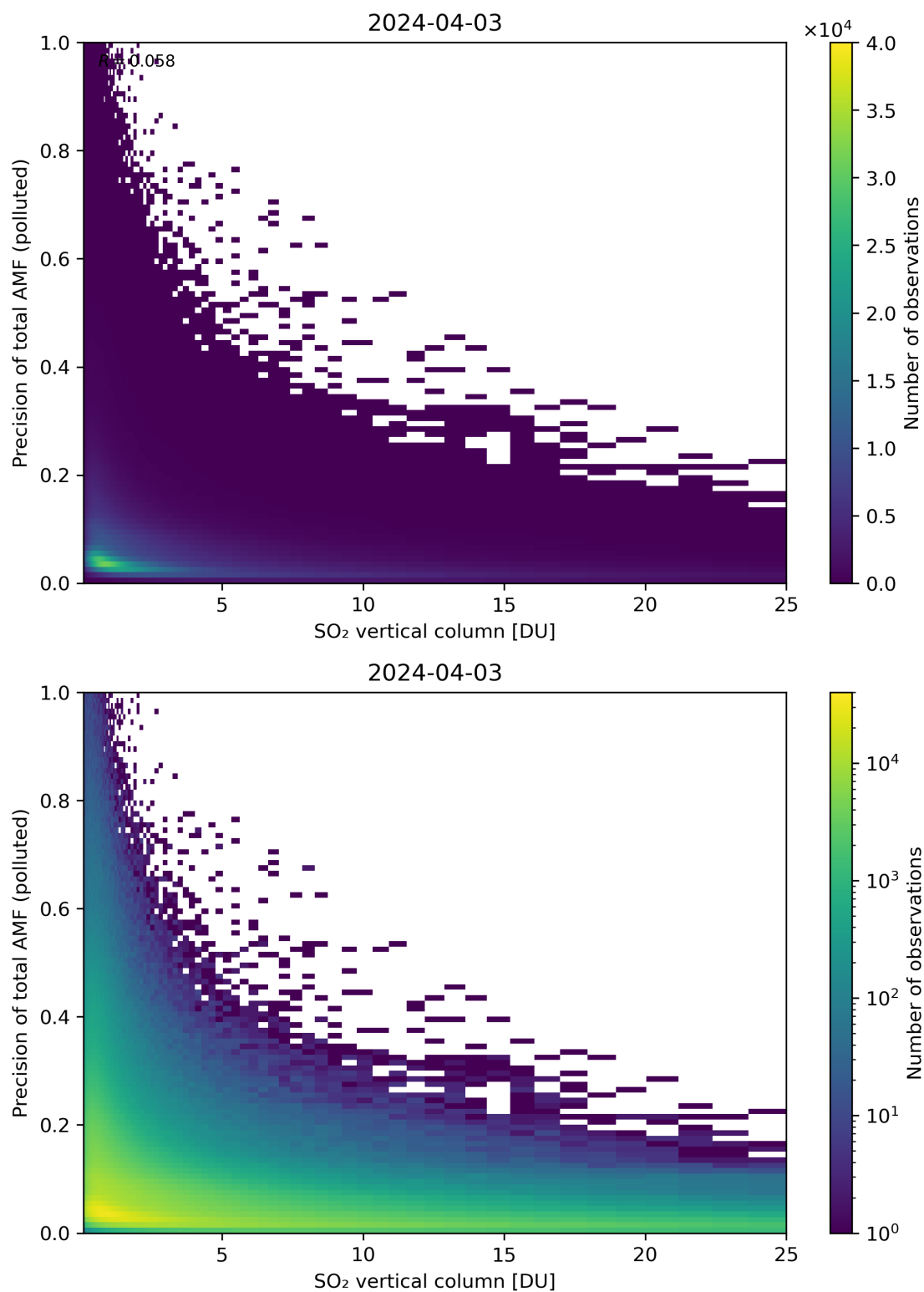
Figure 306: Scatter density plot of “SO 2 vertical column” against “Precision of total AMF (polluted)” for 2024-04-02 to 2024-04-04.
