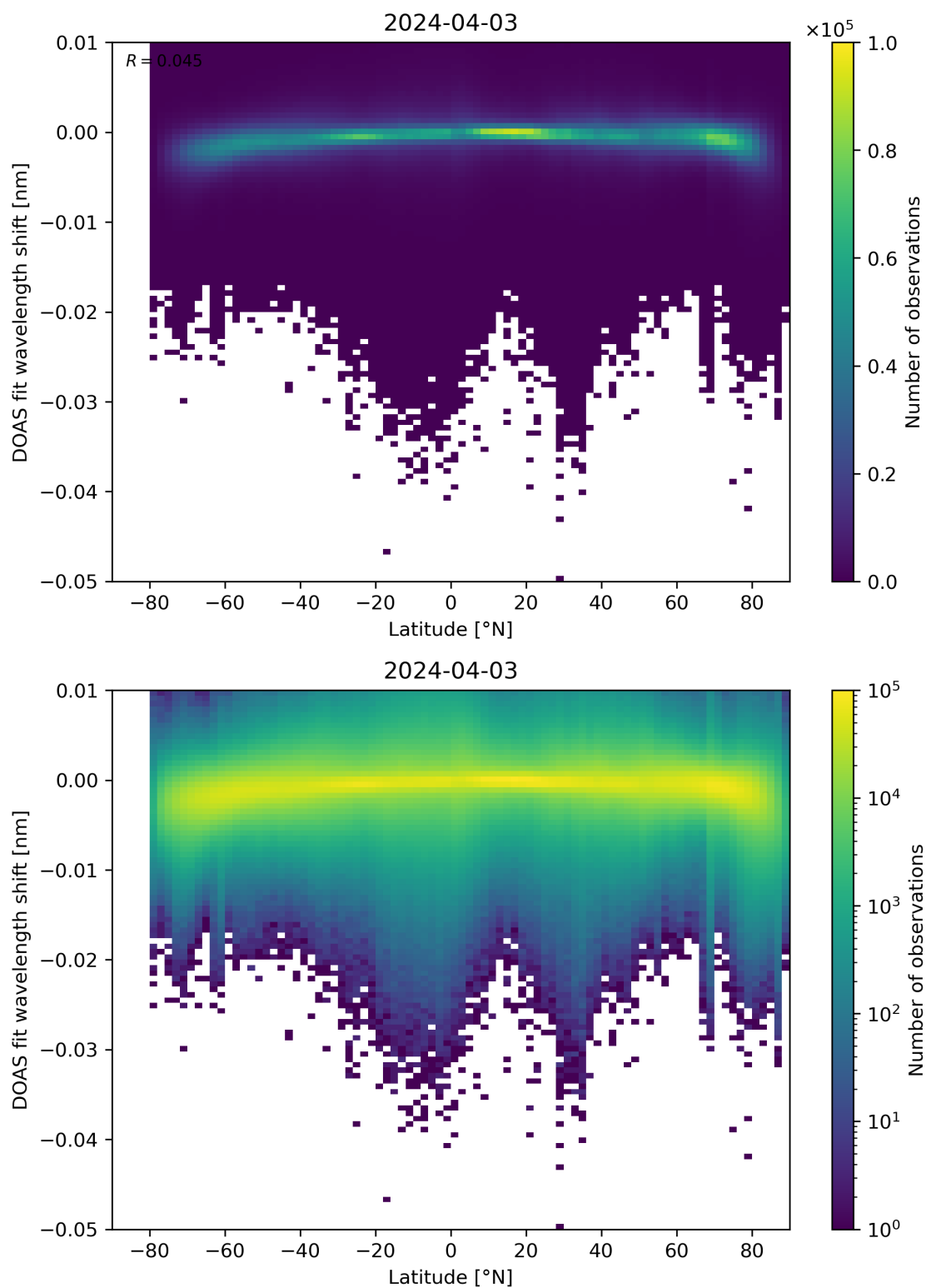
Figure 142: Scatter density plot of “Latitude” against “DOAS fit wavelength shift” for 2024-04-02 to 2024-04-04.
