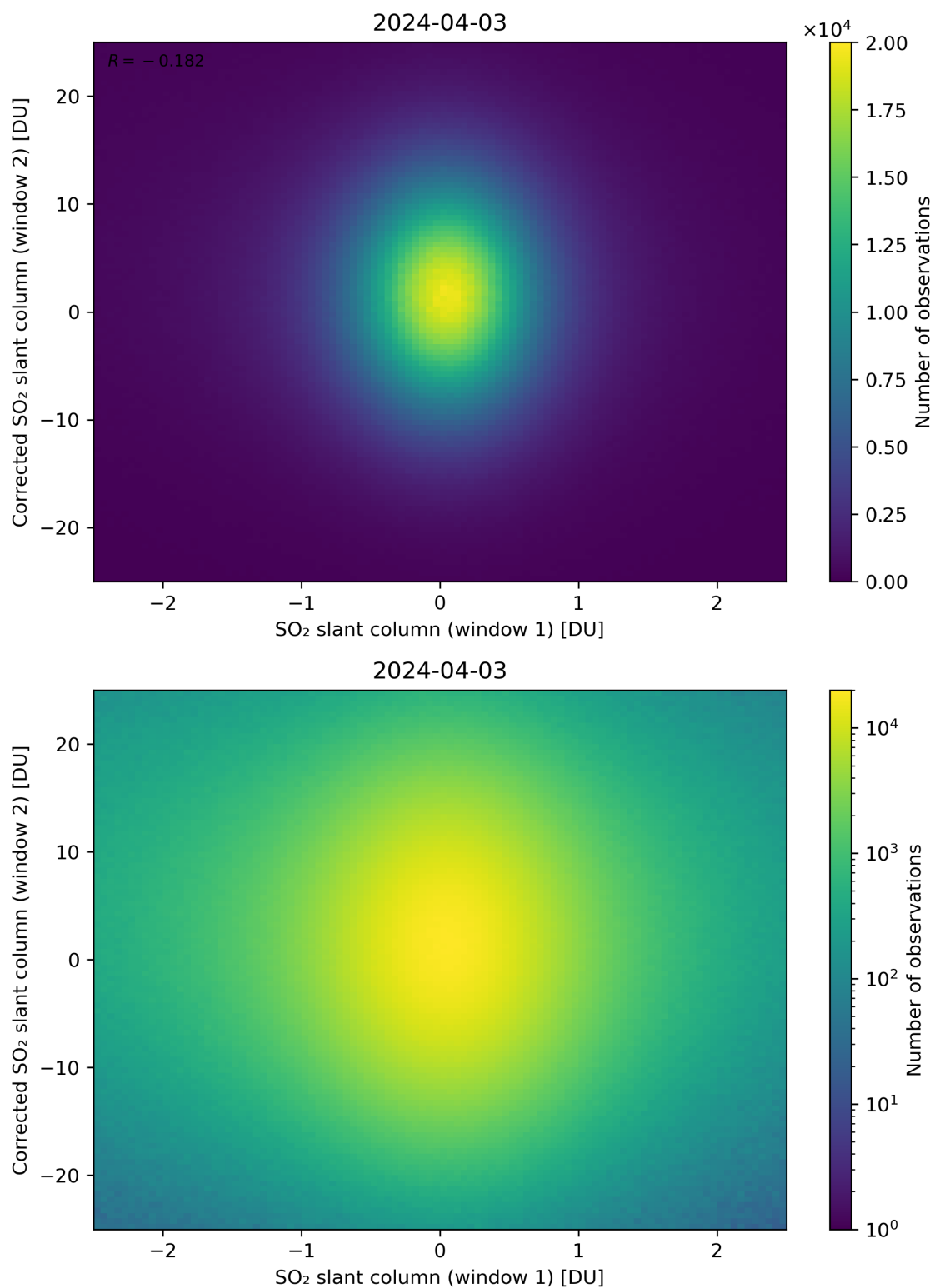
Figure 233: Scatter density plot of “SO 2 slant column (window 1)” against “Corrected SO 2 slant column (window 2)” for 2024-04-02 to 2024-04-04.
