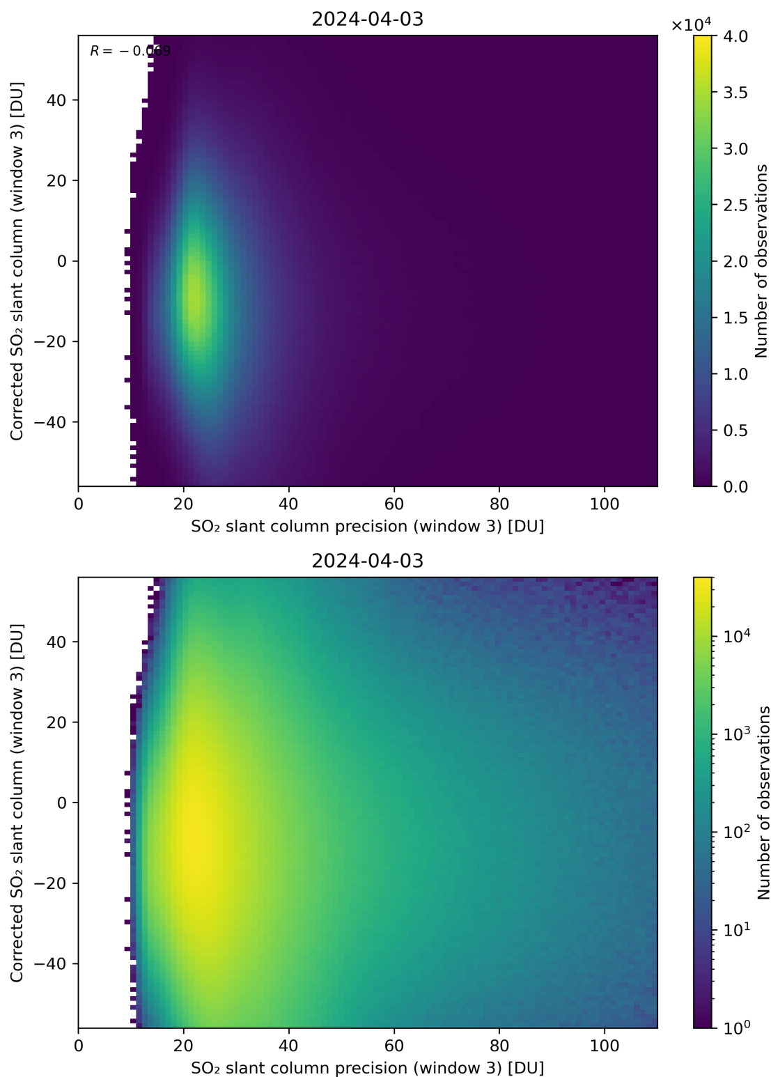
Figure 262: Scatter density plot of “SO 2 slant column precision (window 3)” against “Corrected SO 2 slant column (window 3)” for 2024-04-02 to 2024-04-04.
