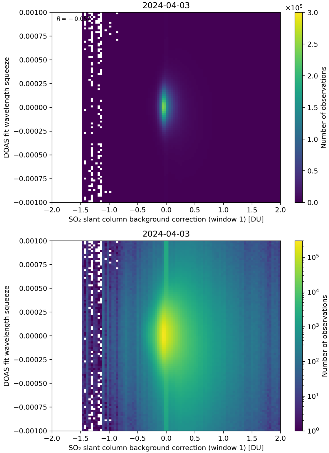
Figure 101: Scatter density plot of “SO 2 slant column background correction (window 1)” against “DOAS fit wavelength squeeze” for 2024-04-02 to 2024-04-04.
