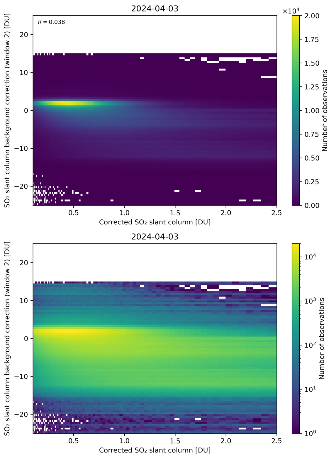
Figure 179: Scatter density plot of “Corrected SO 2 slant column” against “SO 2 slant column background correction (window 2)” for 2024-04-02 to 2024-04-04.
