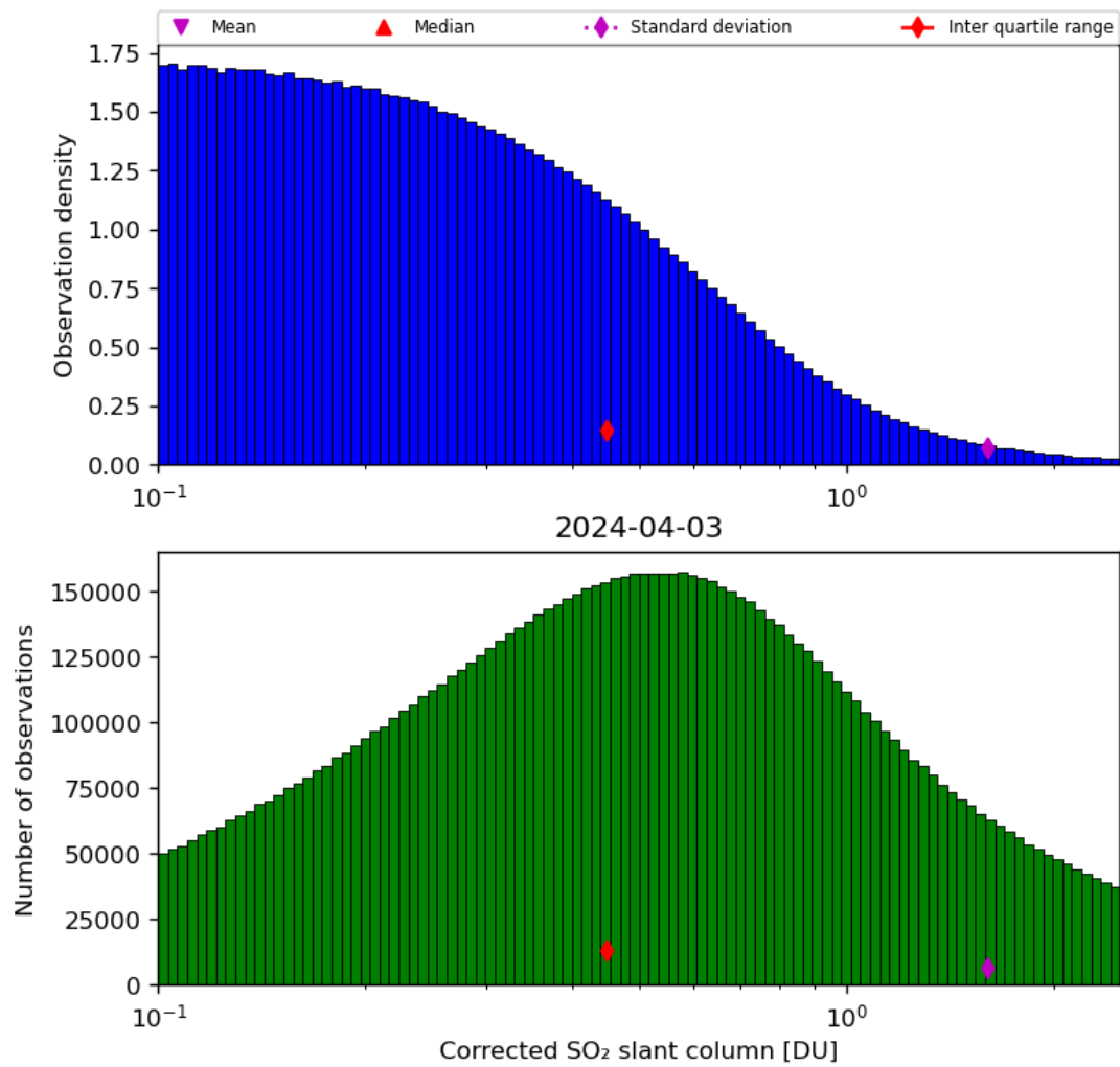
Figure 55: Histogram of “Corrected SO 2 slant column” for 2024-04-02 to 2024-04-04
