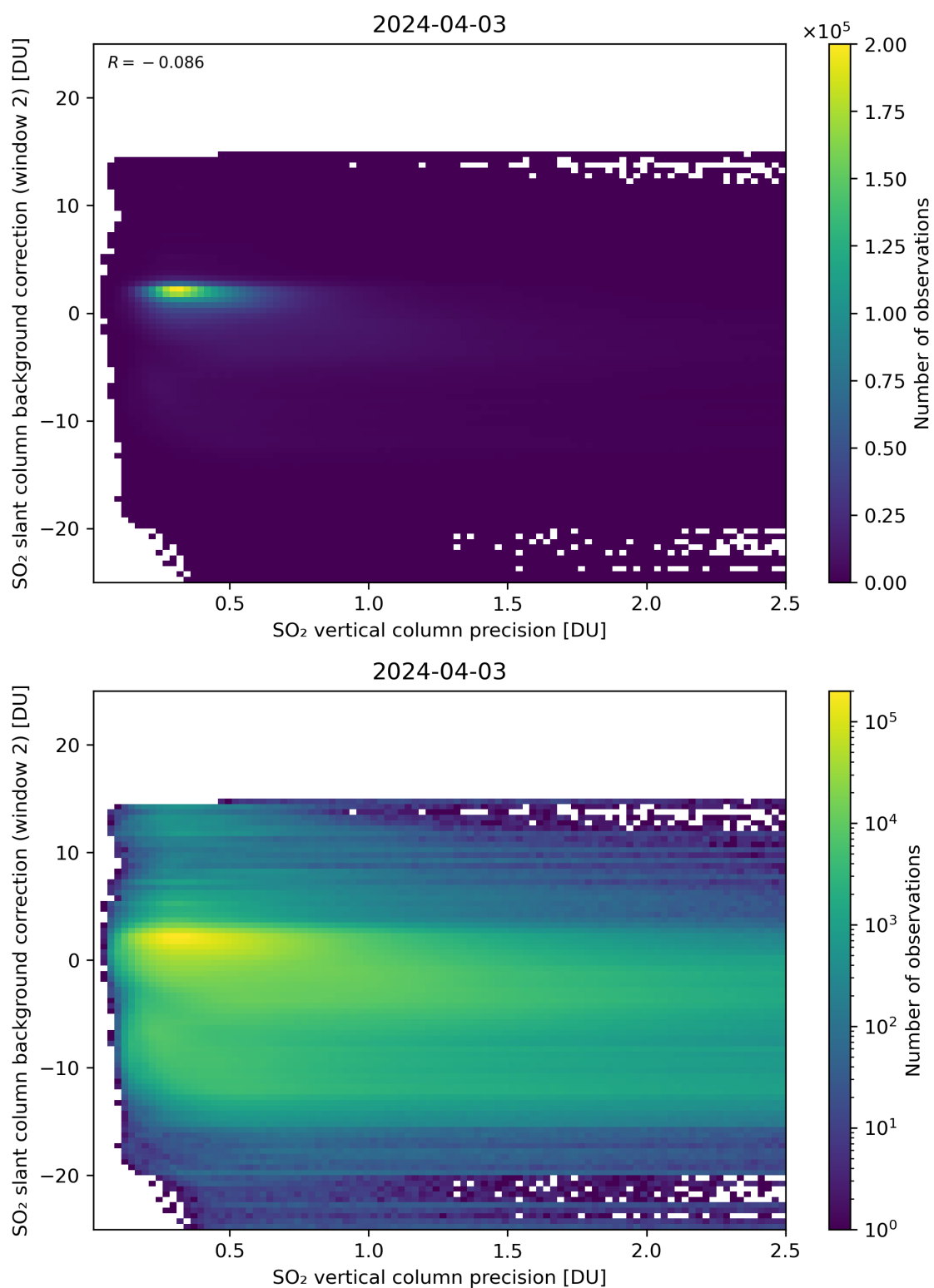
Figure 280: Scatter density plot of “SO 2 vertical column precision” against “SO 2 slant column background correction (window 2)” for 2024-04-02 to 2024-04-04.
