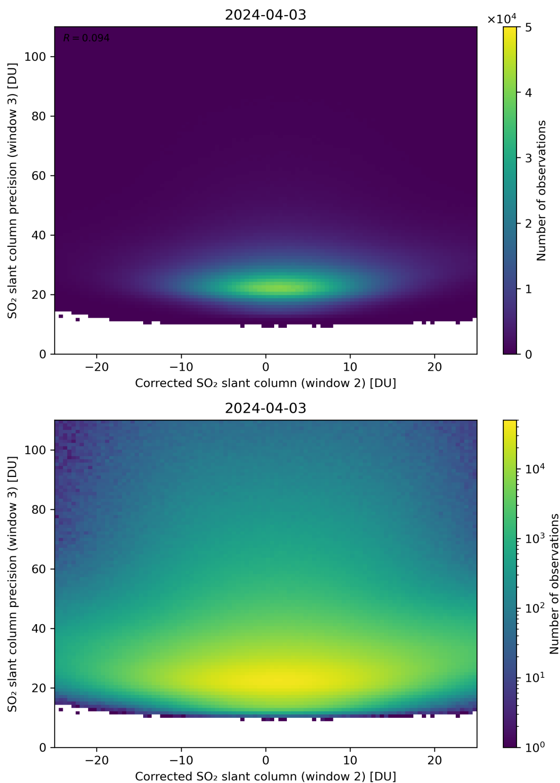
Figure 202: Scatter density plot of “Corrected SO 2 slant column (window 2)” against “SO 2 slant column precision (window 3)” for 2024-04-02 to 2024-04-04.
