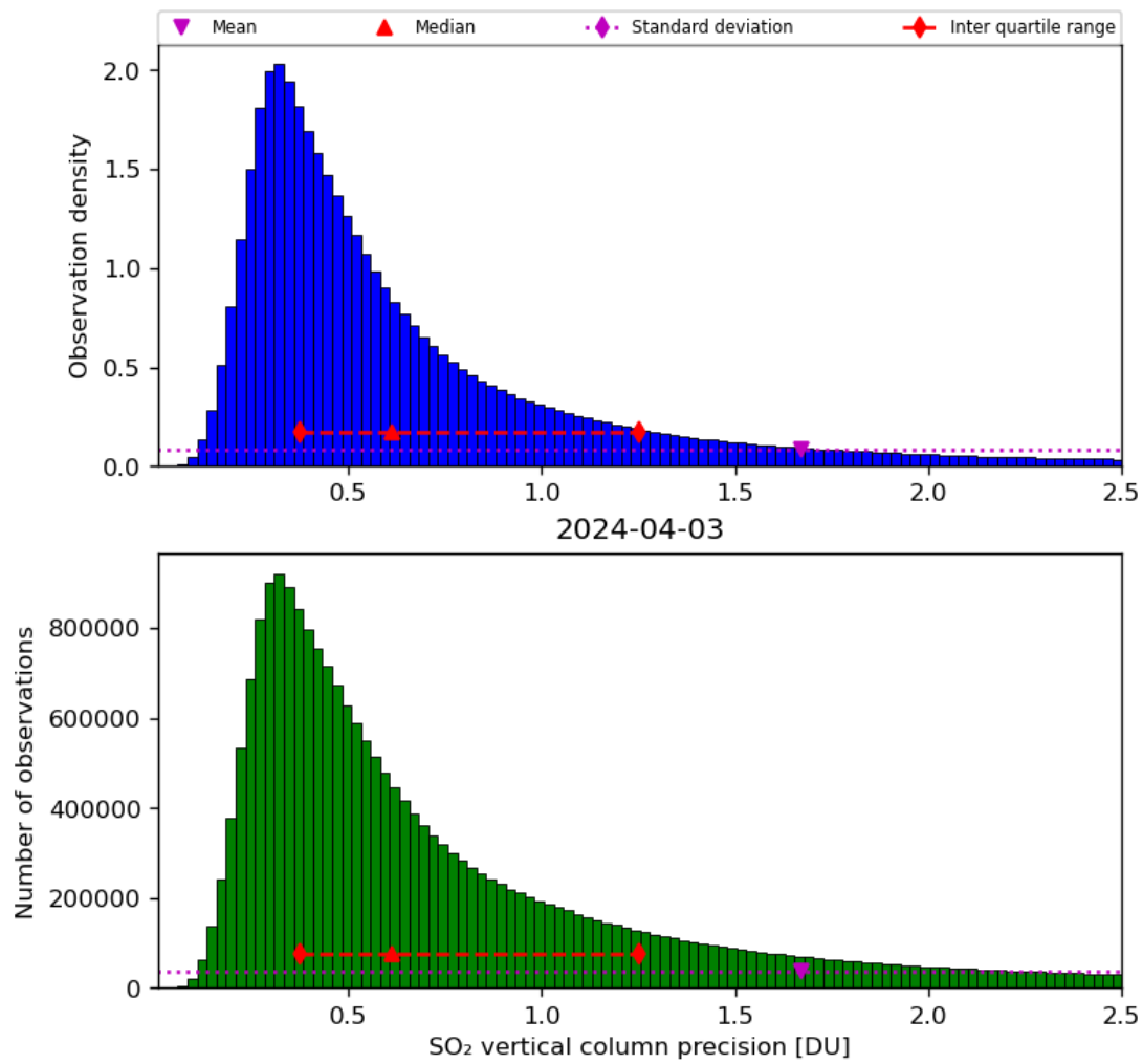
Figure 54: Histogram of “SO 2 vertical column precision” for 2024-04-02 to 2024-04-04
