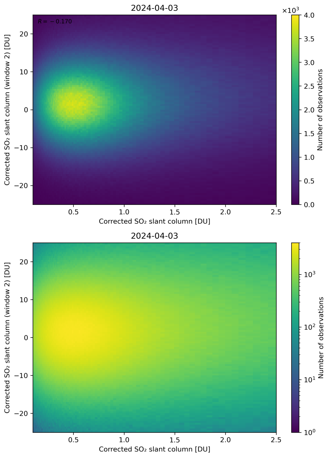
Figure 185: Scatter density plot of “Corrected SO 2 slant column” against “Corrected SO 2 slant column (window 2)” for 2024-04-02 to 2024-04-04.
