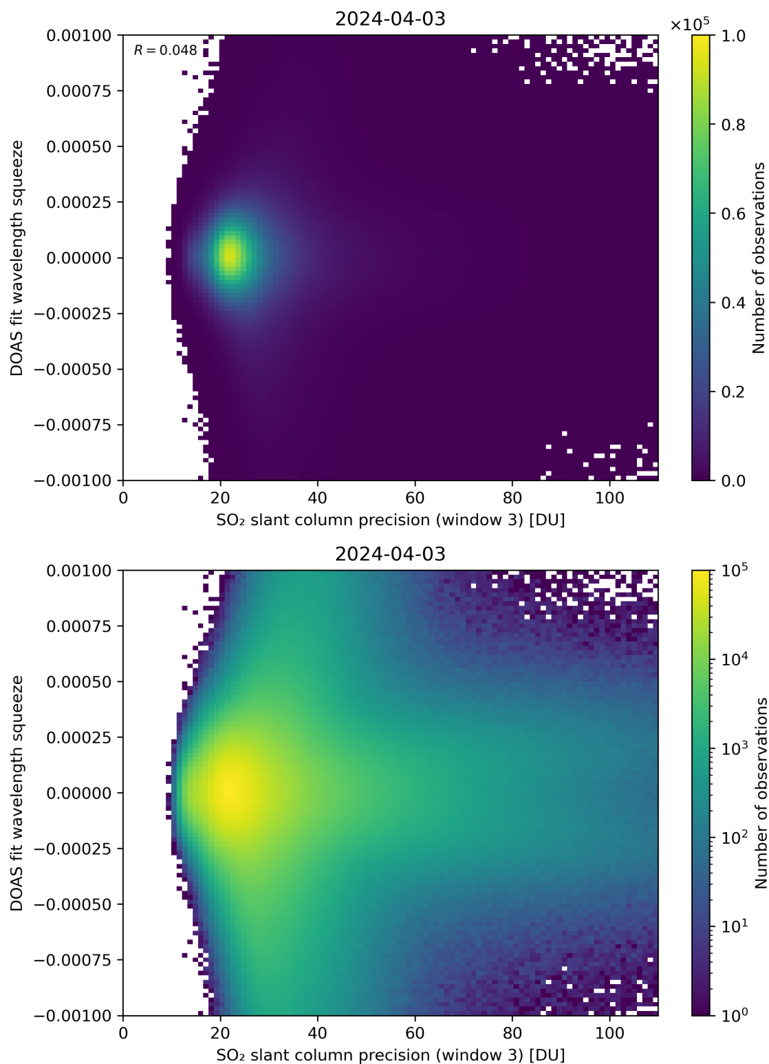
Figure 259: Scatter density plot of “SO 2 slant column precision (window 3)” against “DOAS fit wavelength squeeze” for 2024-04-02 to 2024-04-04.
