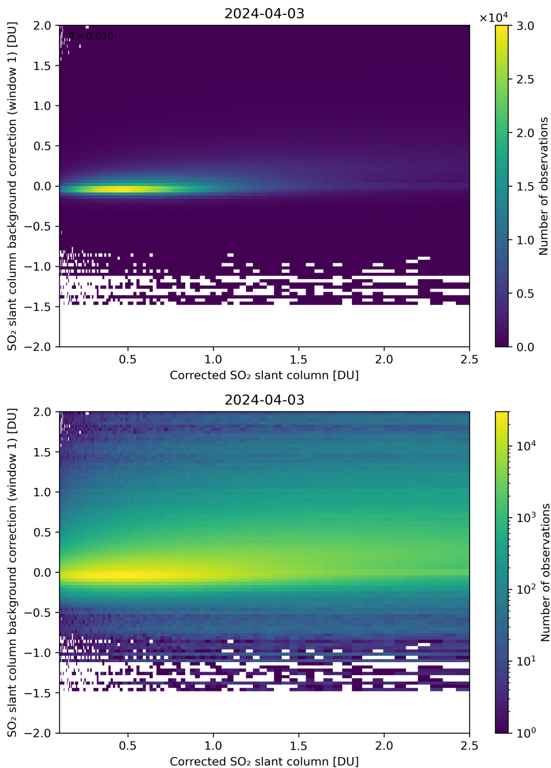
Figure 178: Scatter density plot of “Corrected SO 2 slant column” against “SO 2 slant column background correction (window 1)” for 2024-04-02 to 2024-04-04.
