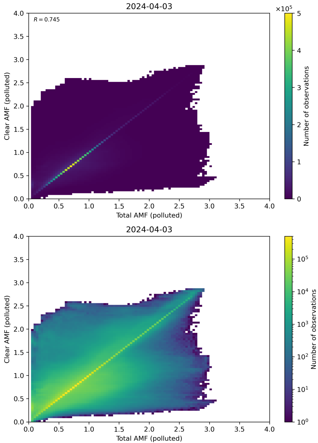
Figure 271: Scatter density plot of “Total AMF (polluted)” against “Clear AMF (polluted)” for 2024-04-02 to 2024-04-04.
