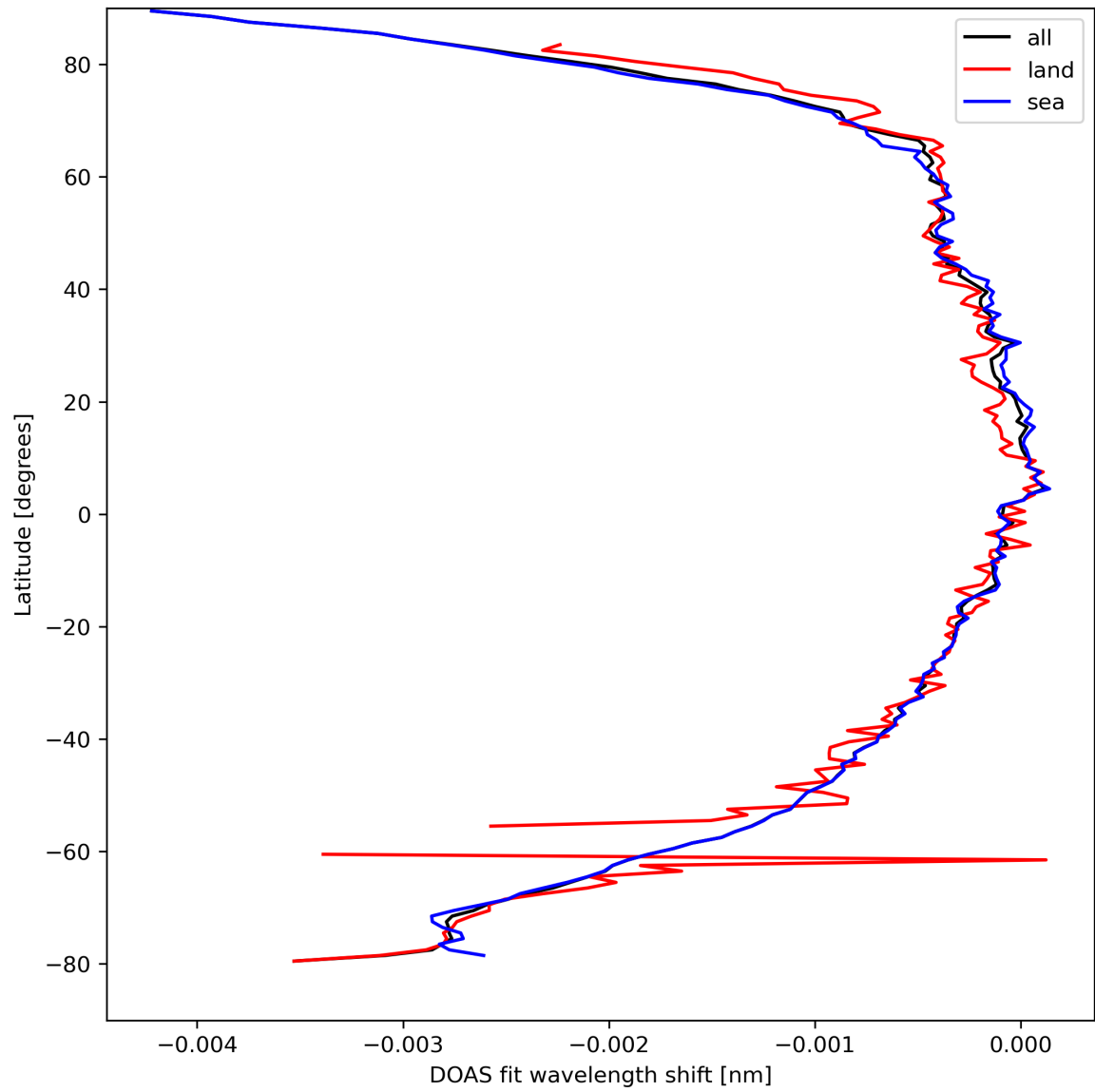
Figure 45: Zonal average of “DOAS fit wavelength shift” for 2024-04-02 to 2024-04-04.
