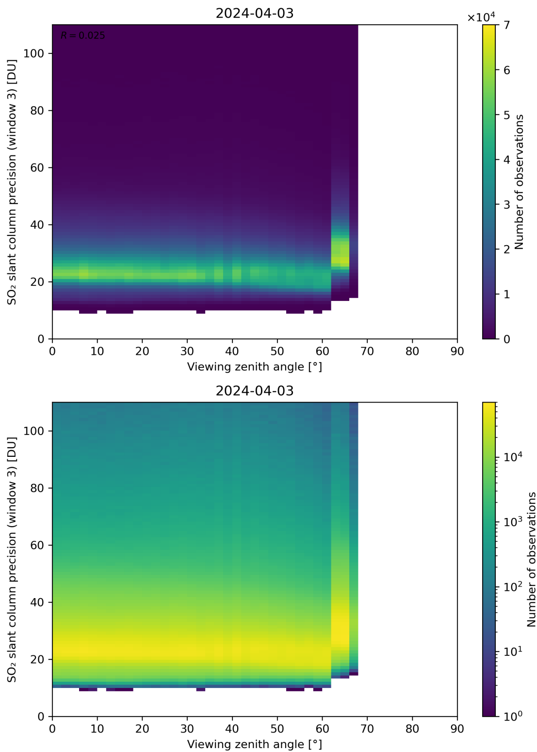
Figure 324: Scatter density plot of “Viewing zenith angle” against “SO 2 slant column precision (window 3)” for 2024-04-02 to 2024-04-04.
