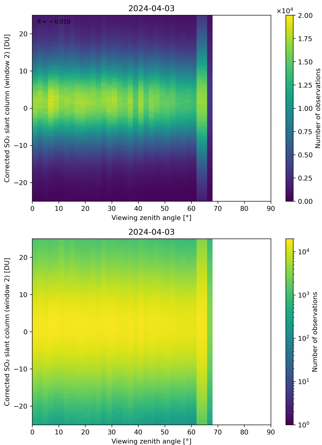
Figure 318: Scatter density plot of “Viewing zenith angle” against “Corrected SO 2 slant column (window 2)” for 2024-04-02 to 2024-04-04.
