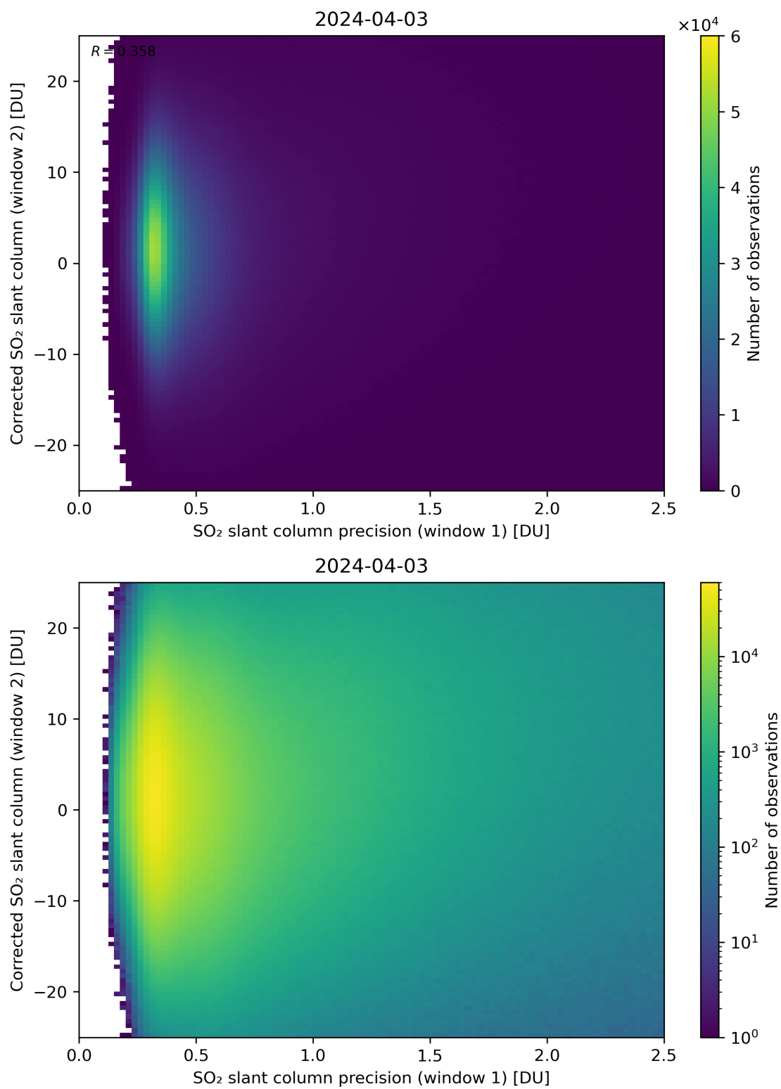
Figure 225: Scatter density plot of “SO 2 slant column precision (window 1)” against “Corrected SO 2 slant column (window 2)” for 2024-04-02 to 2024-04-04.
