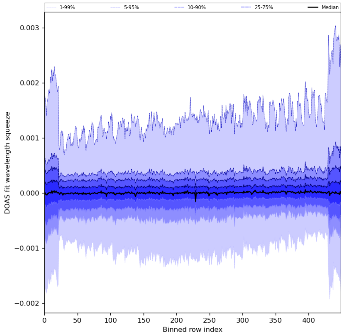
Figure 92: Along track statistics of “DOAS fit wavelength squeeze” for 2024-04-02 to 2024-04-04
