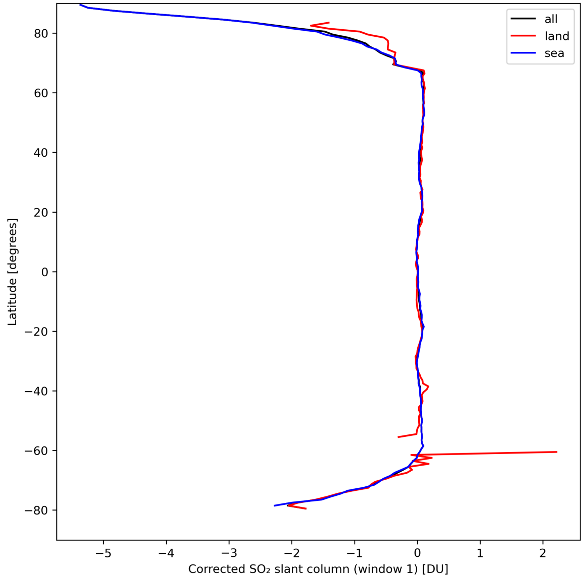
Figure 35: Zonal average of “Corrected SO 2 slant column (window 1)” for 2024-04-02 to 2024-04-04.
