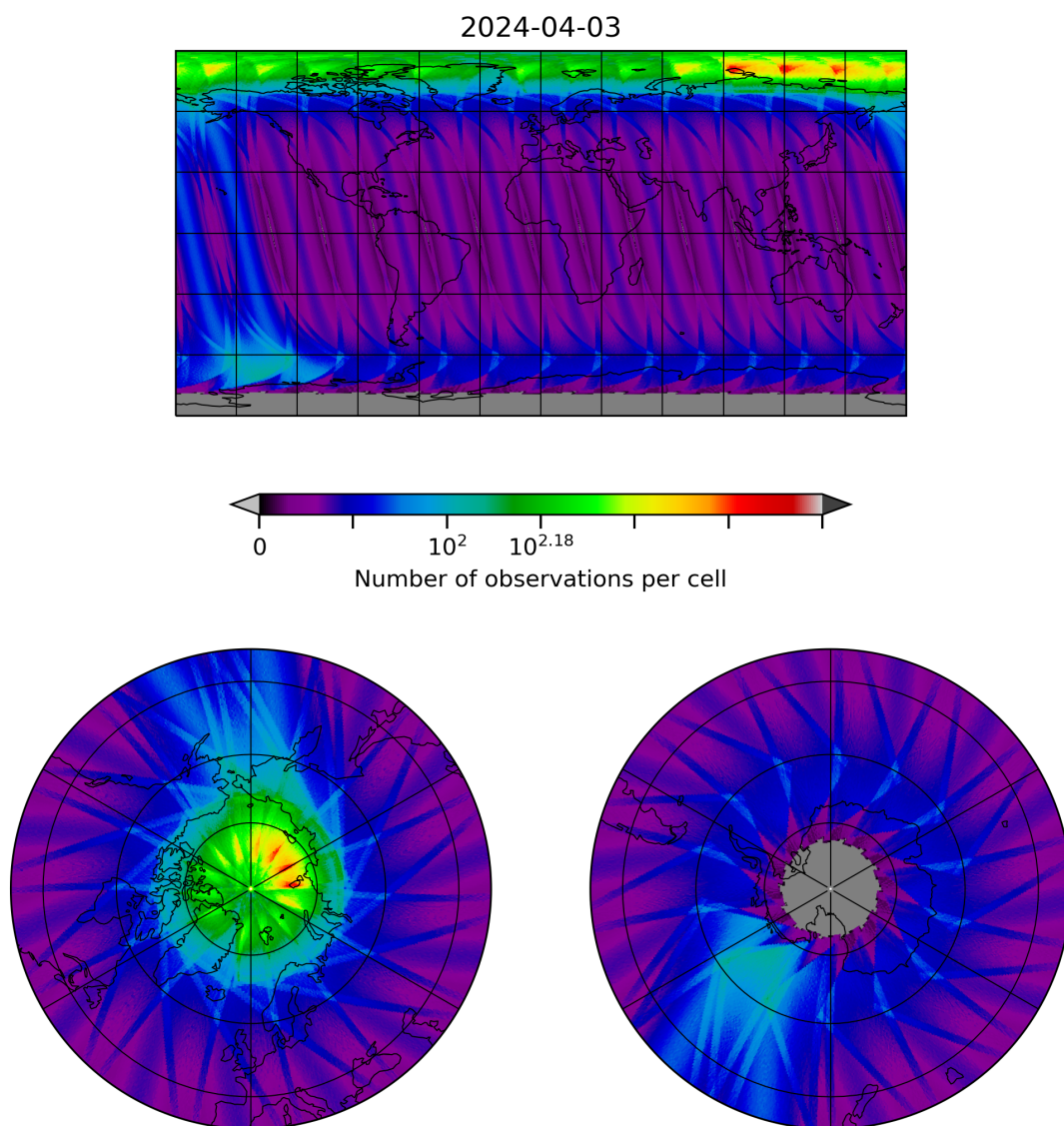
Figure 28: Map of the number of observations for 2024-04-02 to 2024-04-04
