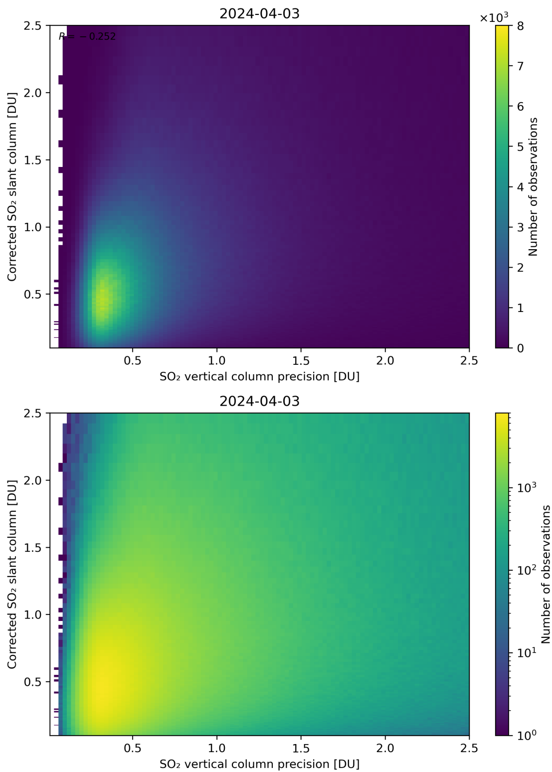
Figure 286: Scatter density plot of “SO 2 vertical column precision” against “Corrected SO 2 slant column” for 2024-04-02 to 2024-04-04.
