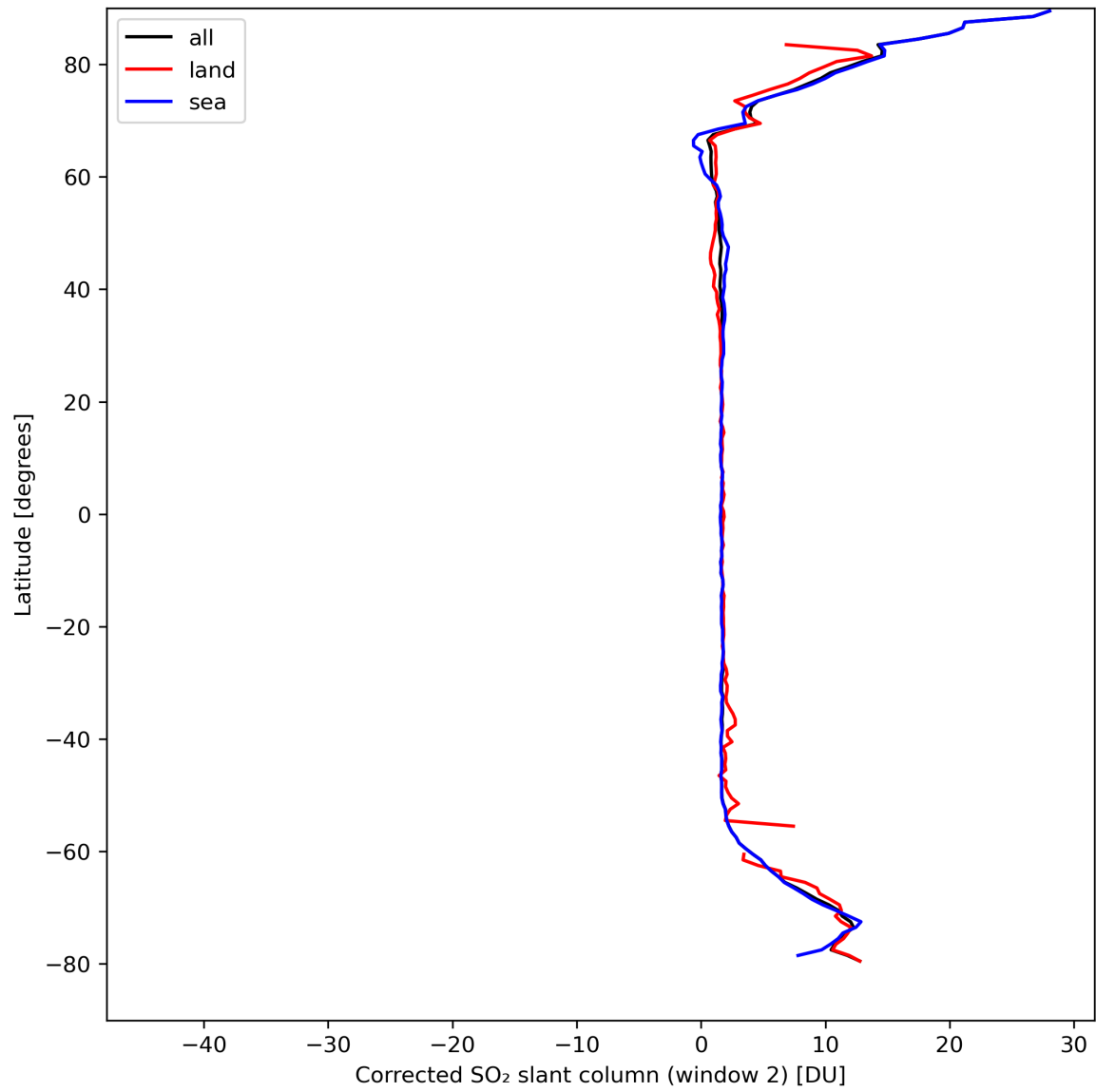
Figure 39: Zonal average of “Corrected SO 2 slant column (window 2)” for 2024-04-02 to 2024-04-04.
