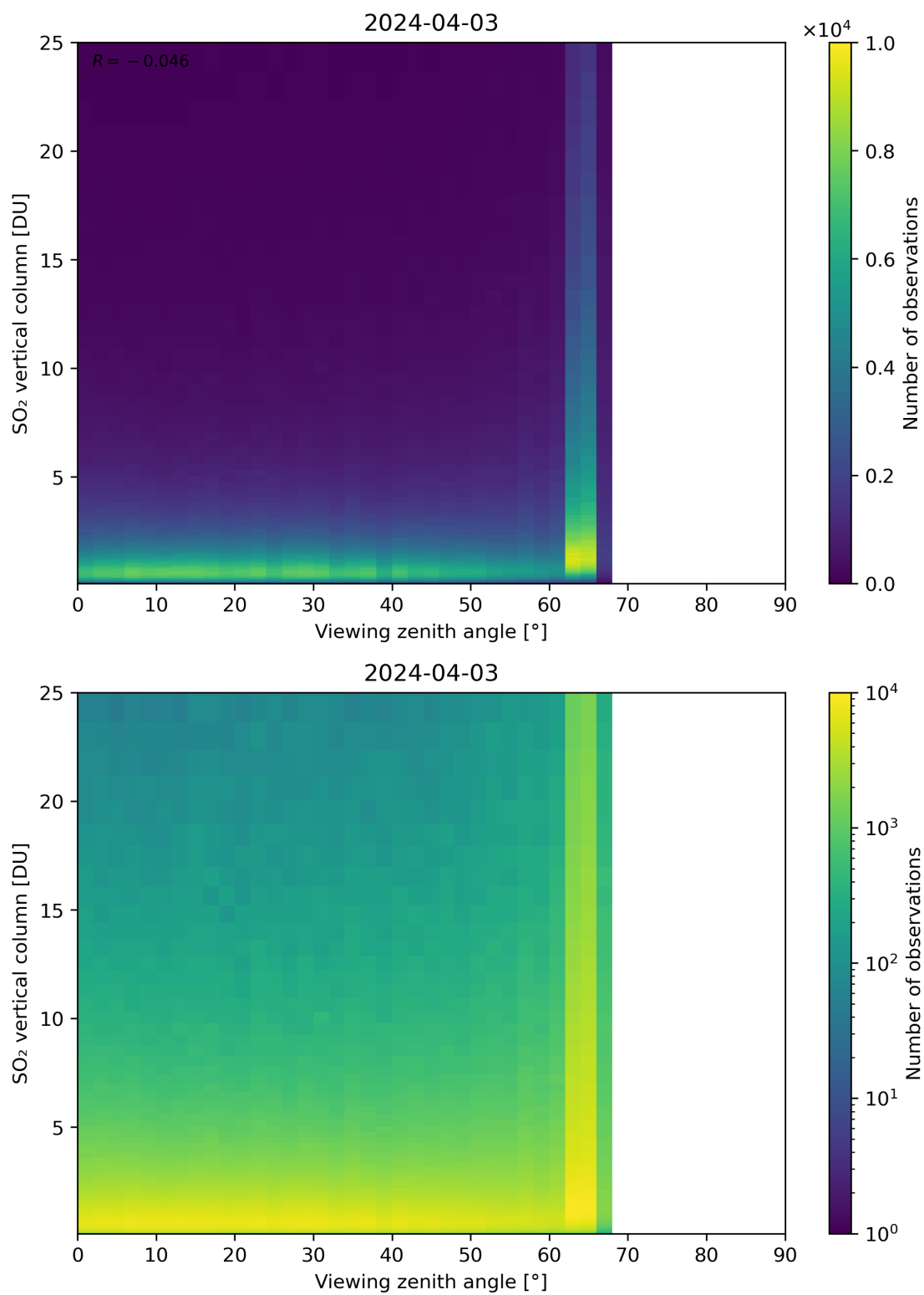
Figure 327: Scatter density plot of “Viewing zenith angle” against “SO 2 vertical column” for 2024-04-02 to 2024-04-04.
