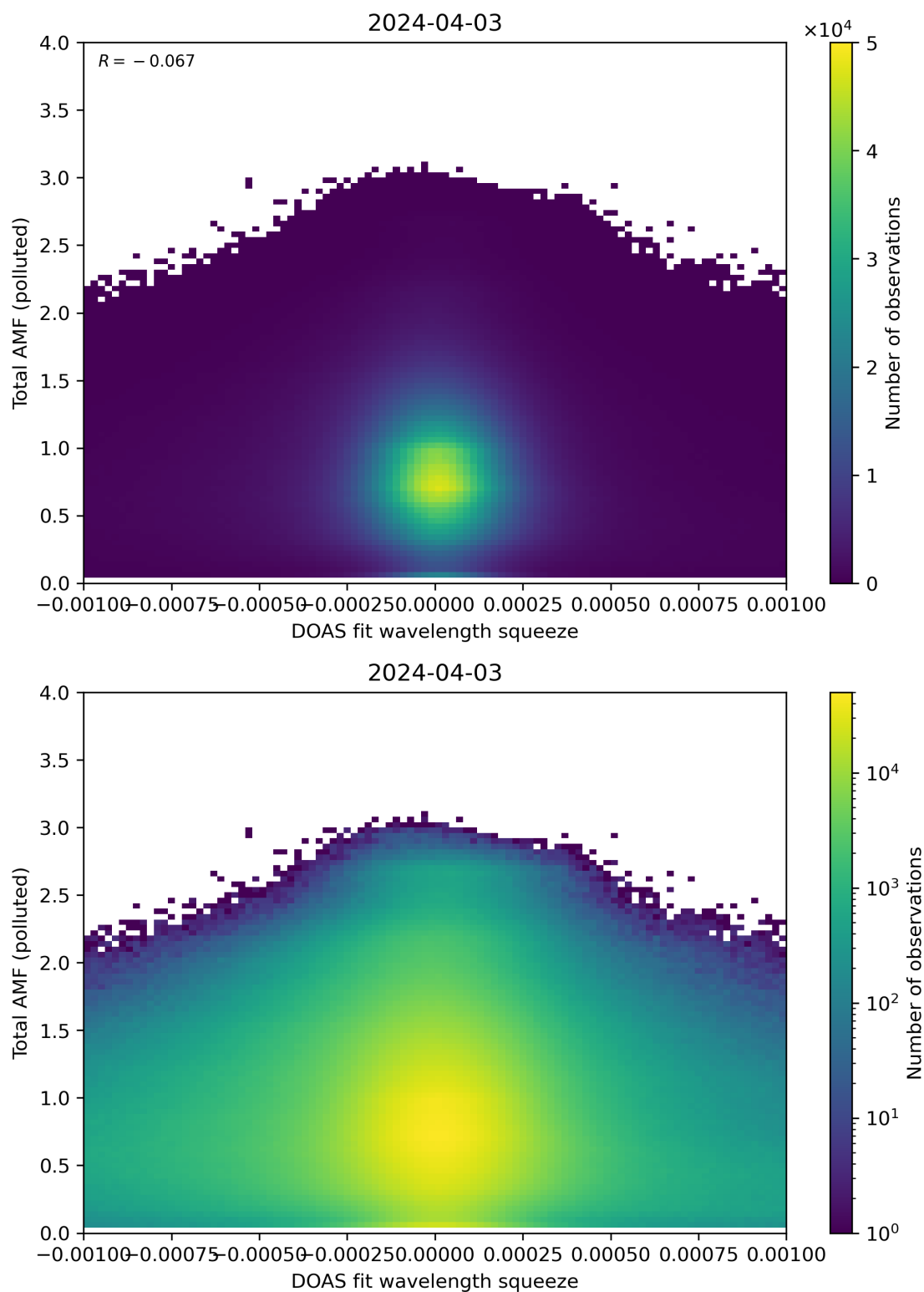
Figure 134: Scatter density plot of “DOAS fit wavelength squeeze” against “Total AMF (polluted)” for 2024-04-02 to 2024-04-04.
