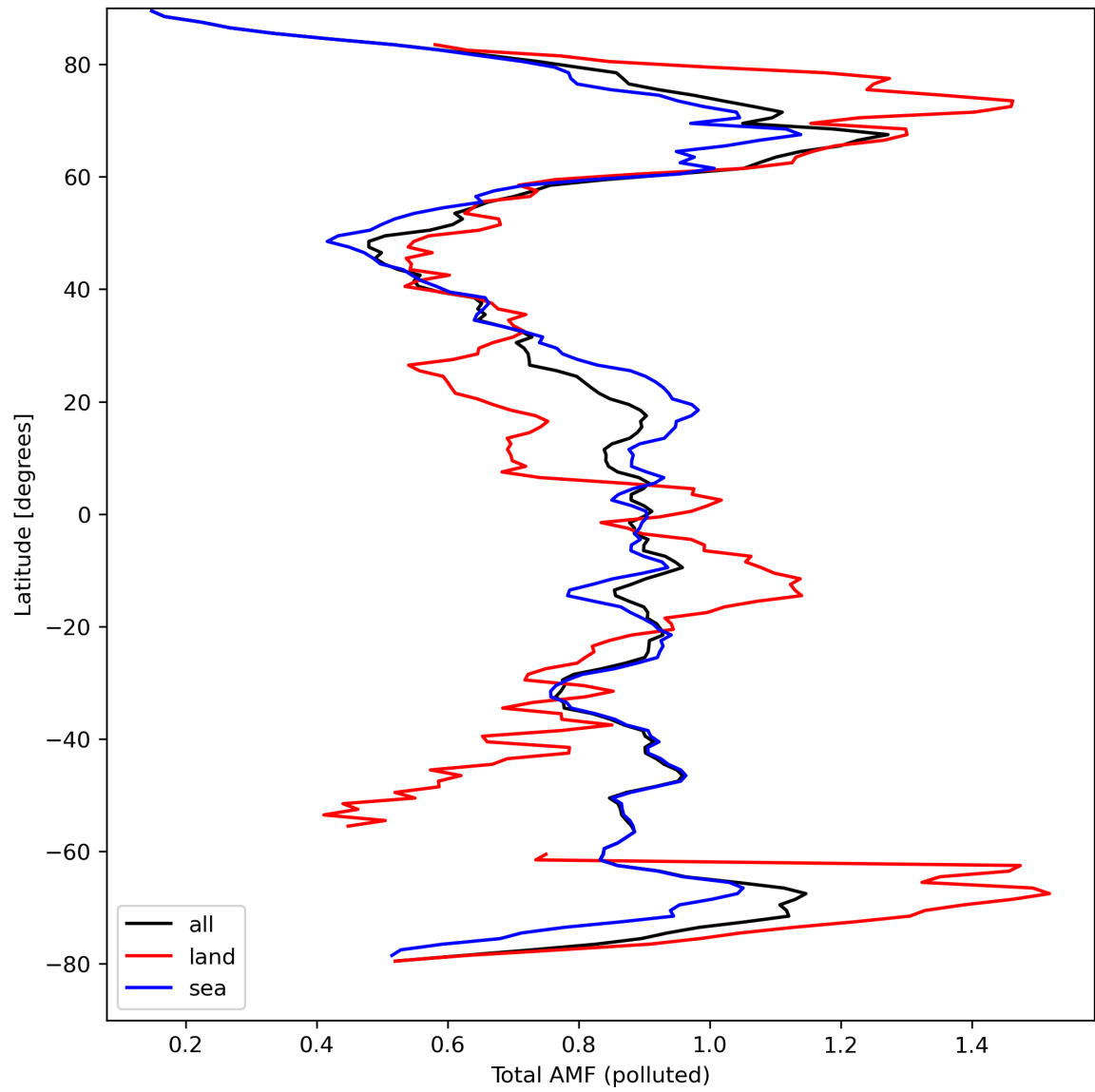
Figure 48: Zonal average of “Total AMF (polluted)” for 2024-04-02 to 2024-04-04.
