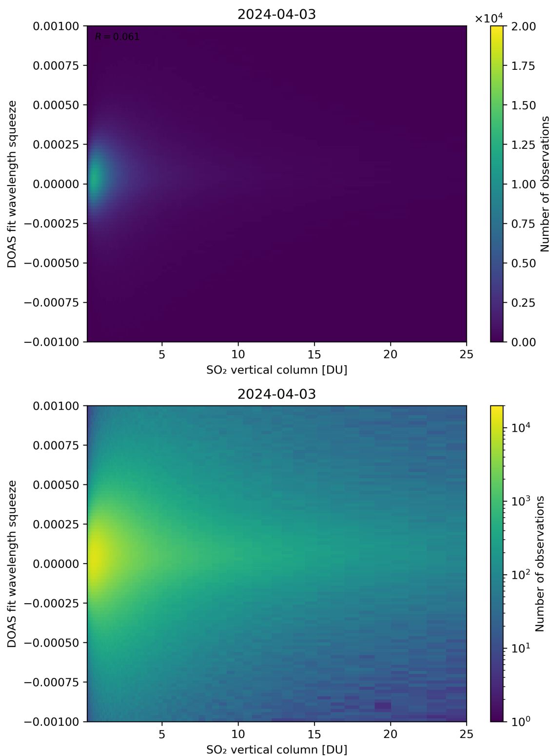
Figure 277: Scatter density plot of “SO 2 vertical column” against “DOAS fit wavelength squeeze” for 2024-04-02 to 2024-04-04.
