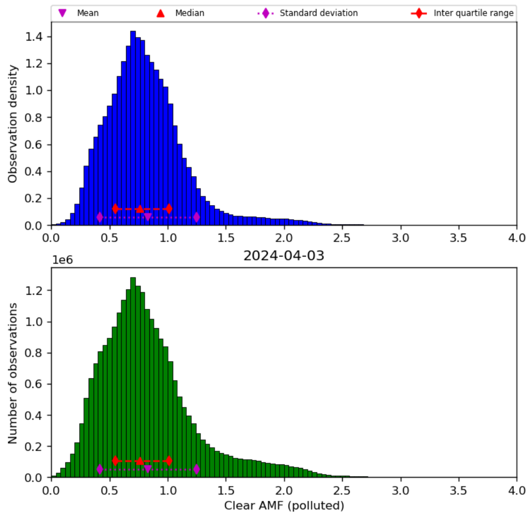
Figure 73: Histogram of “Clear AMF (polluted)” for 2024-04-02 to 2024-04-04
