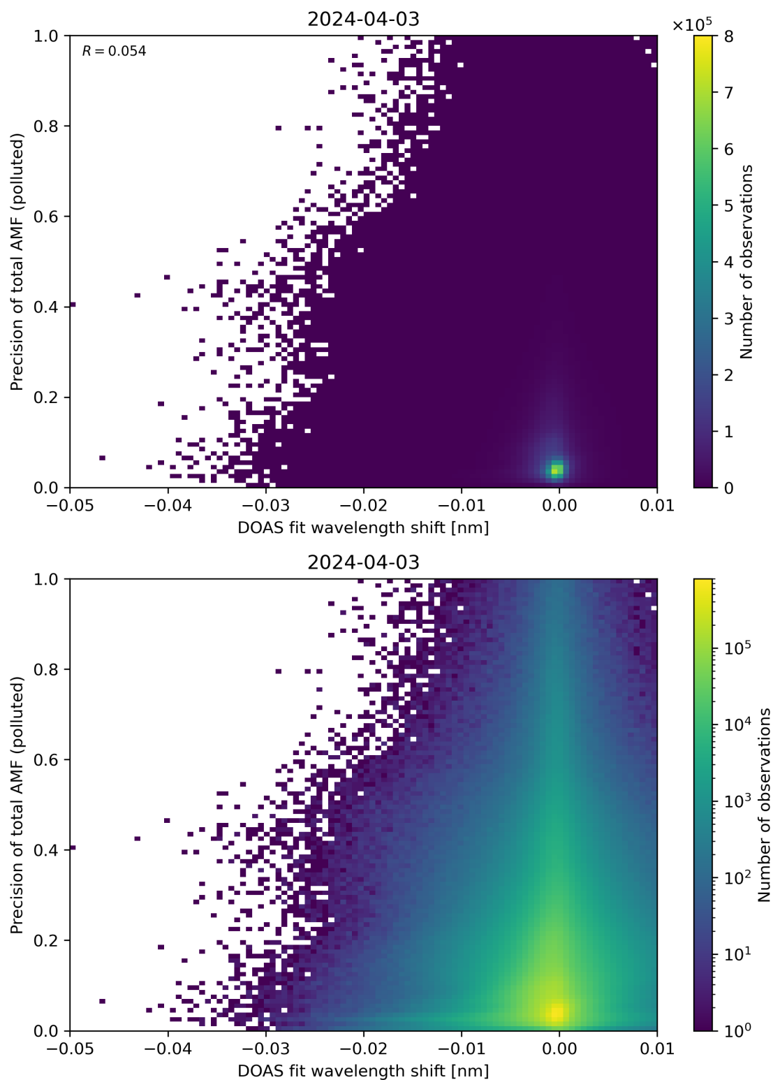
Figure 131: Scatter density plot of “DOAS fit wavelength shift” against “Precision of total AMF (polluted)” for 2024-04-02 to 2024-04-04.
