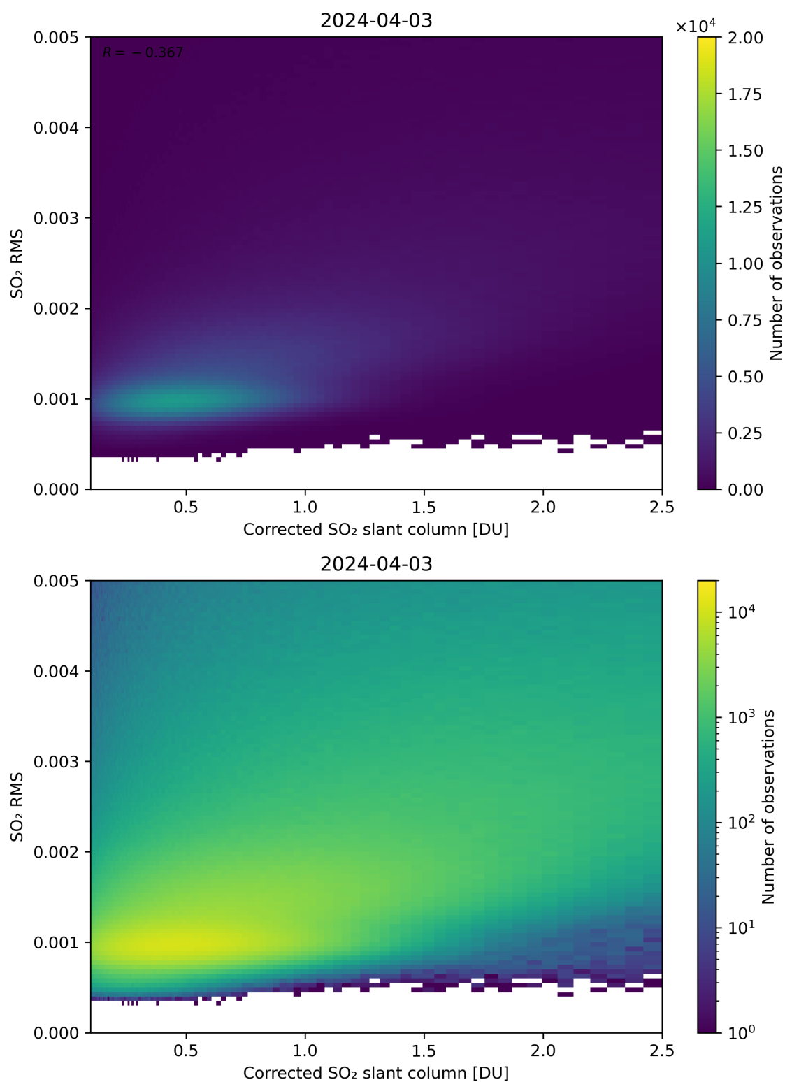
Figure 183: Scatter density plot of “Corrected SO 2 slant column” against “SO 2 RMS” for 2024-04-02 to 2024-04-04.
