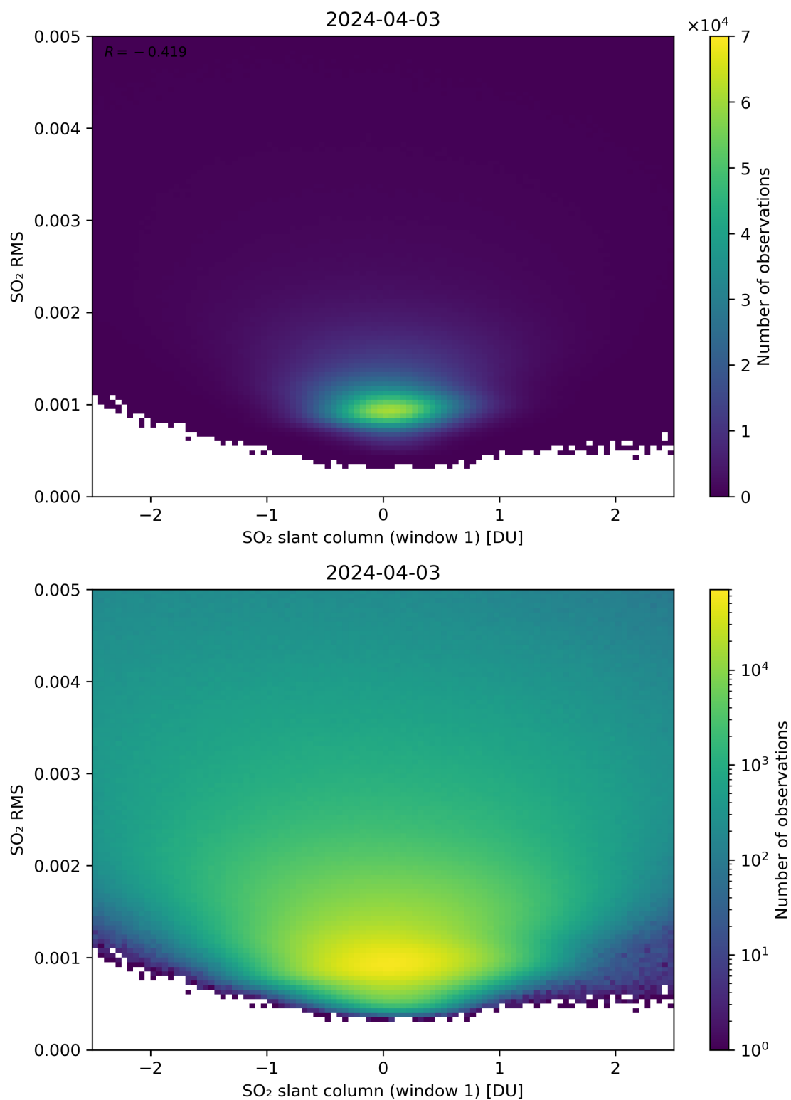
Figure 217: Scatter density plot of “SO 2 slant column (window 1)” against “SO 2 RMS” for 2024-04-02 to 2024-04-04.
