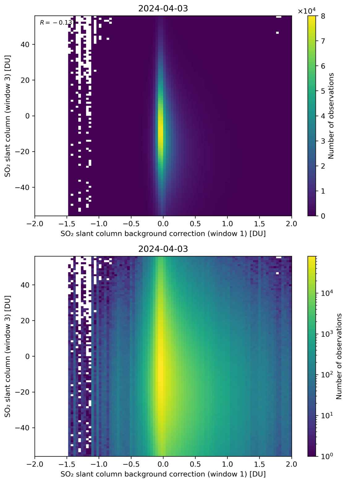
Figure 107: Scatter density plot of “SO 2 slant column background correction (window 1)” against “SO 2 slant column (window 3)” for 2024-04-02 to 2024-04-04.
