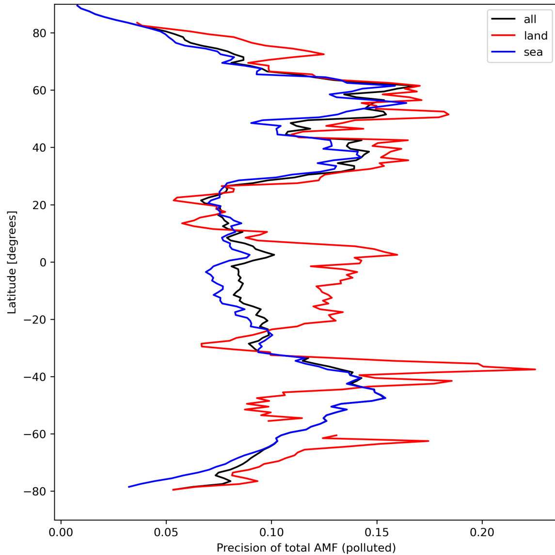
Figure 49: Zonal average of “Precision of total AMF (polluted)” for 2024-04-02 to 2024-04-04.
