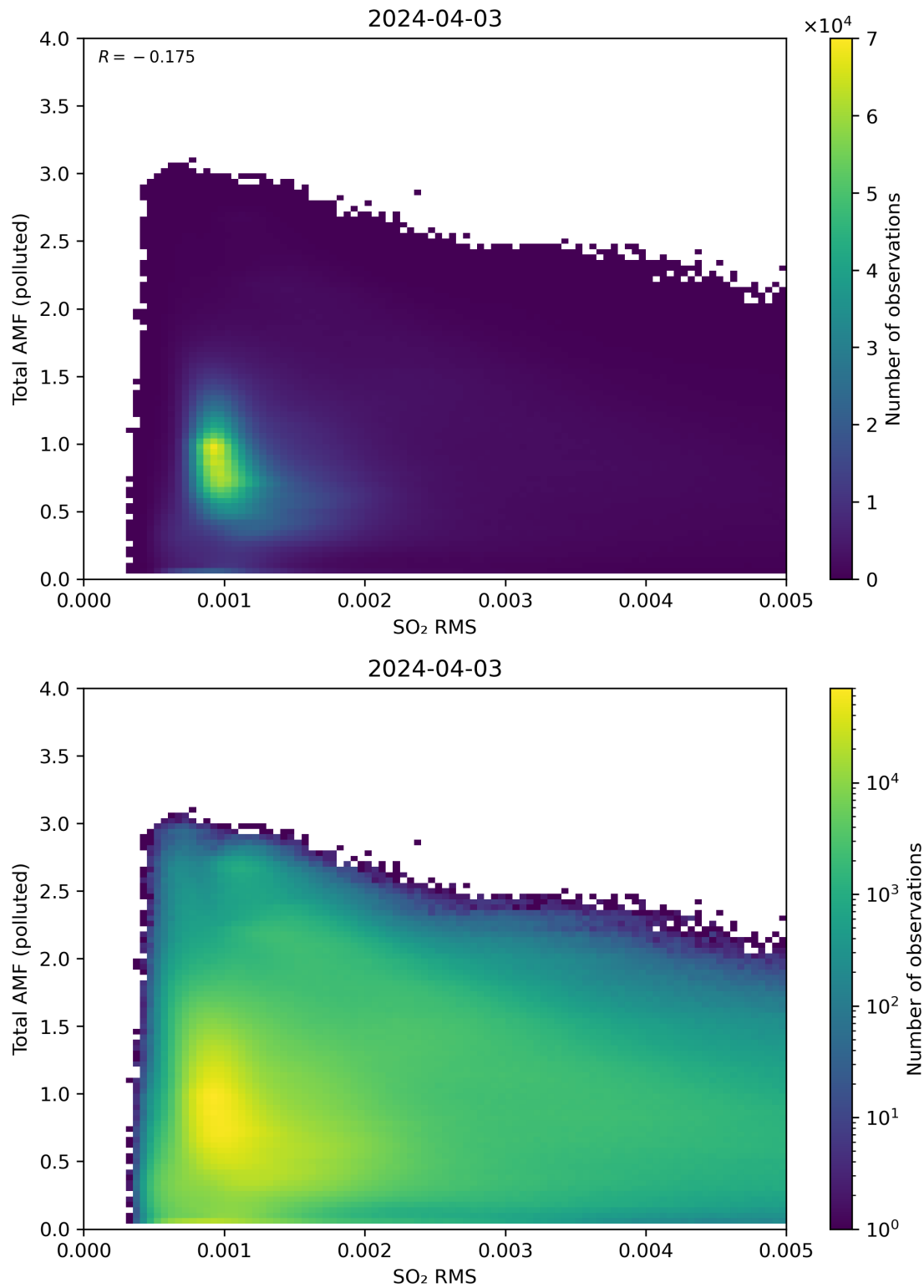
Figure 137: Scatter density plot of “SO 2 RMS” against “Total AMF (polluted)” for 2024-04-02 to 2024-04-04.
