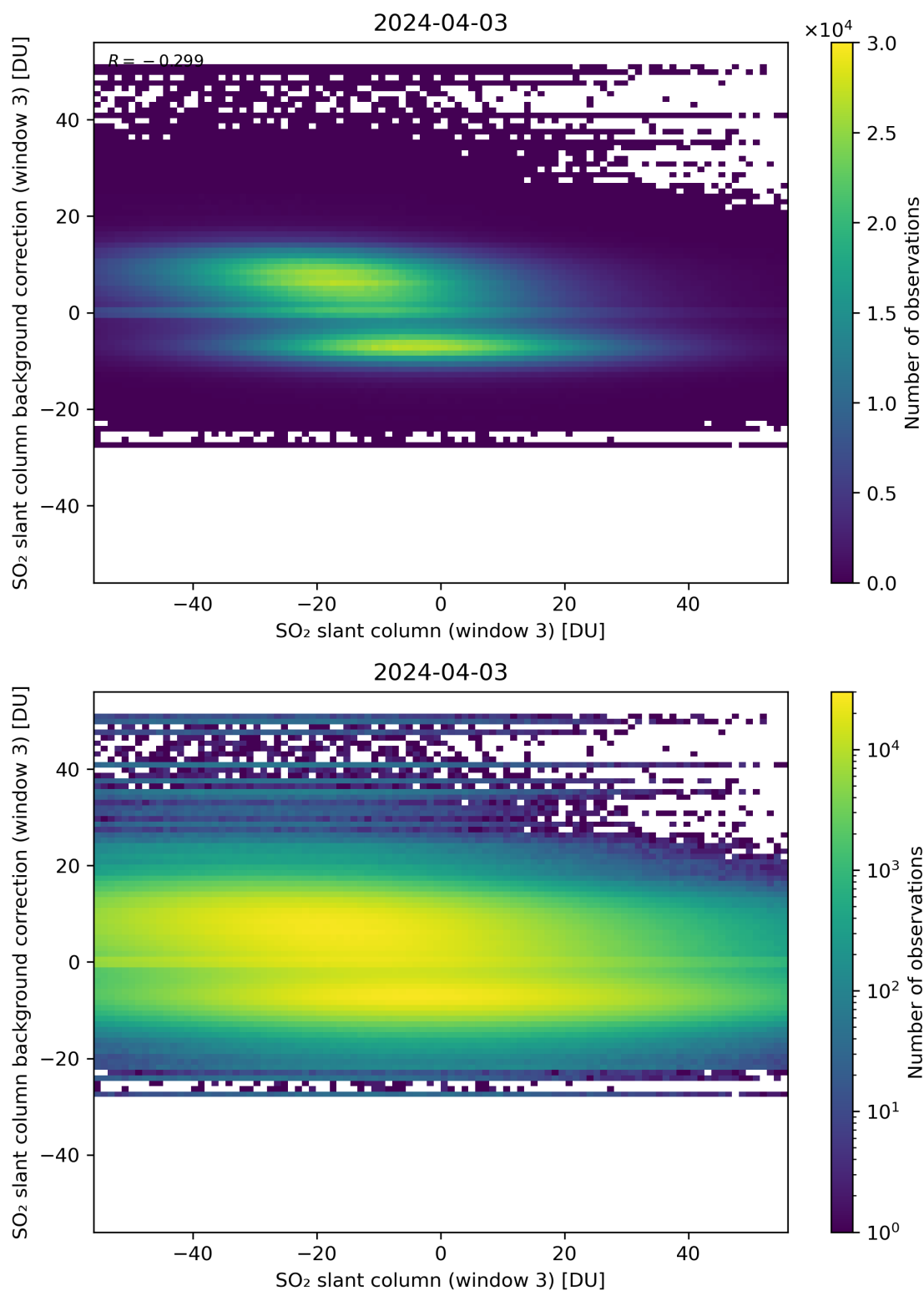
Figure 253: Scatter density plot of “SO 2 slant column (window 3)” against “SO 2 slant column background correction (window 3)” for 2024-04-02 to 2024-04-04.
