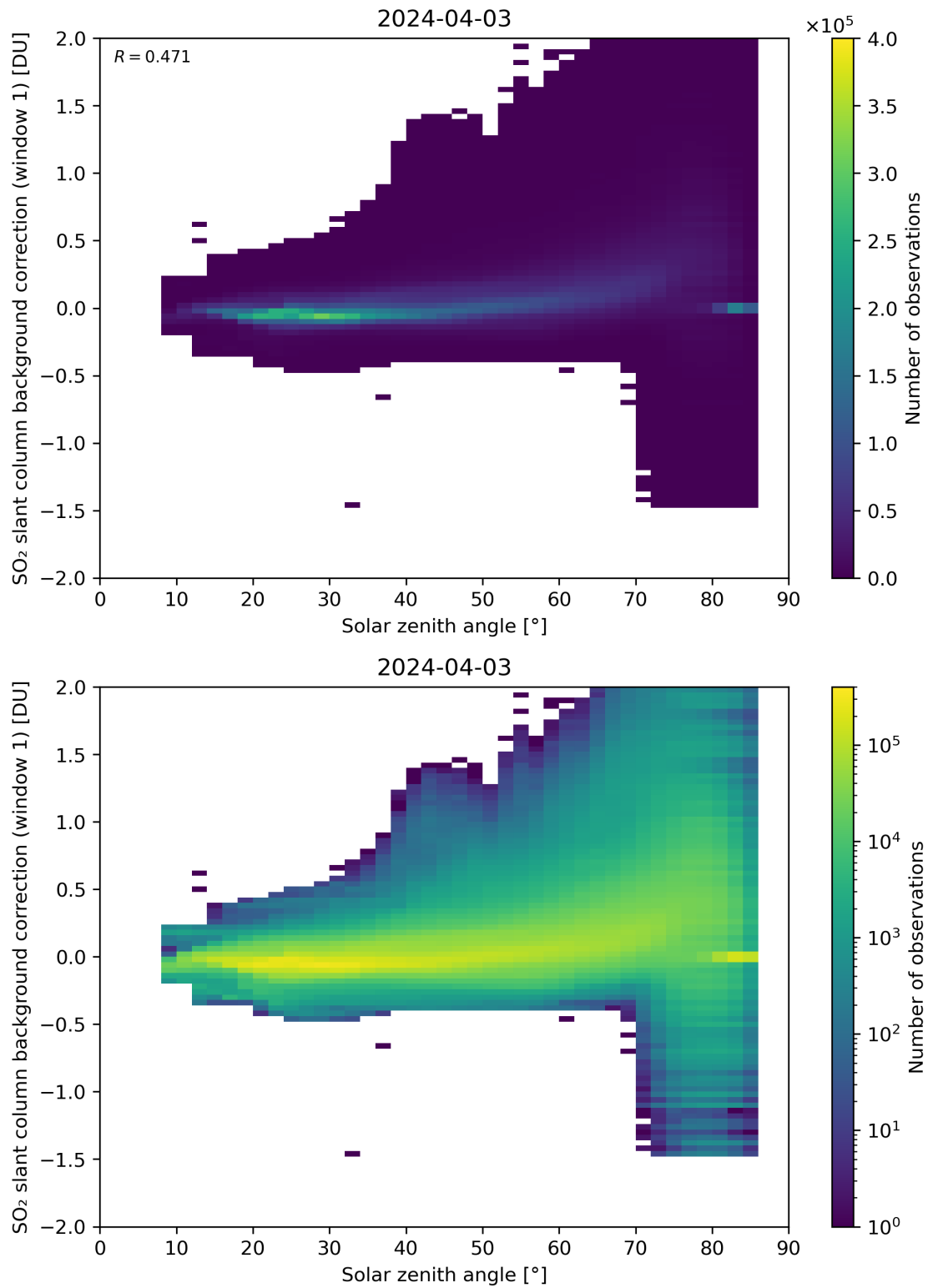
Figure 158: Scatter density plot of “Solar zenith angle” against “SO 2 slant column background correction (window 1)” for 2024-04-02 to 2024-04-04.
