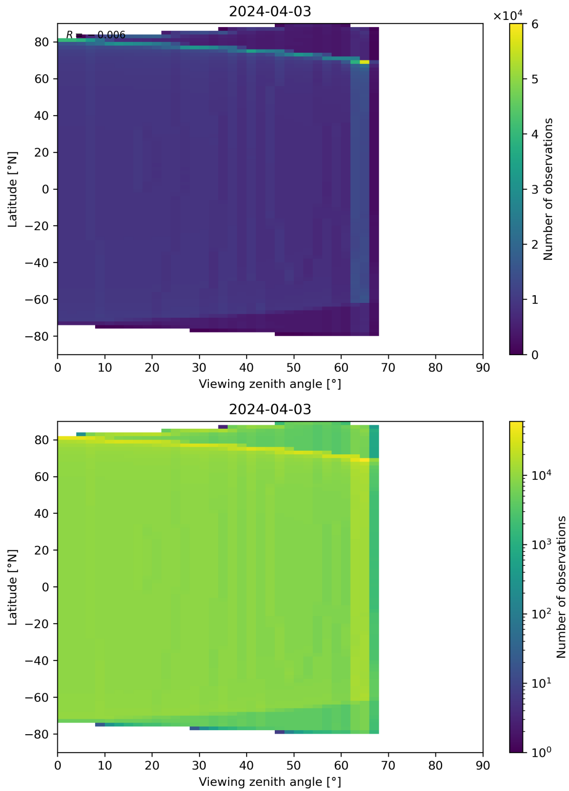
Figure 314: Scatter density plot of “Viewing zenith angle” against “Latitude” for 2024-04-02 to 2024-04-04.
