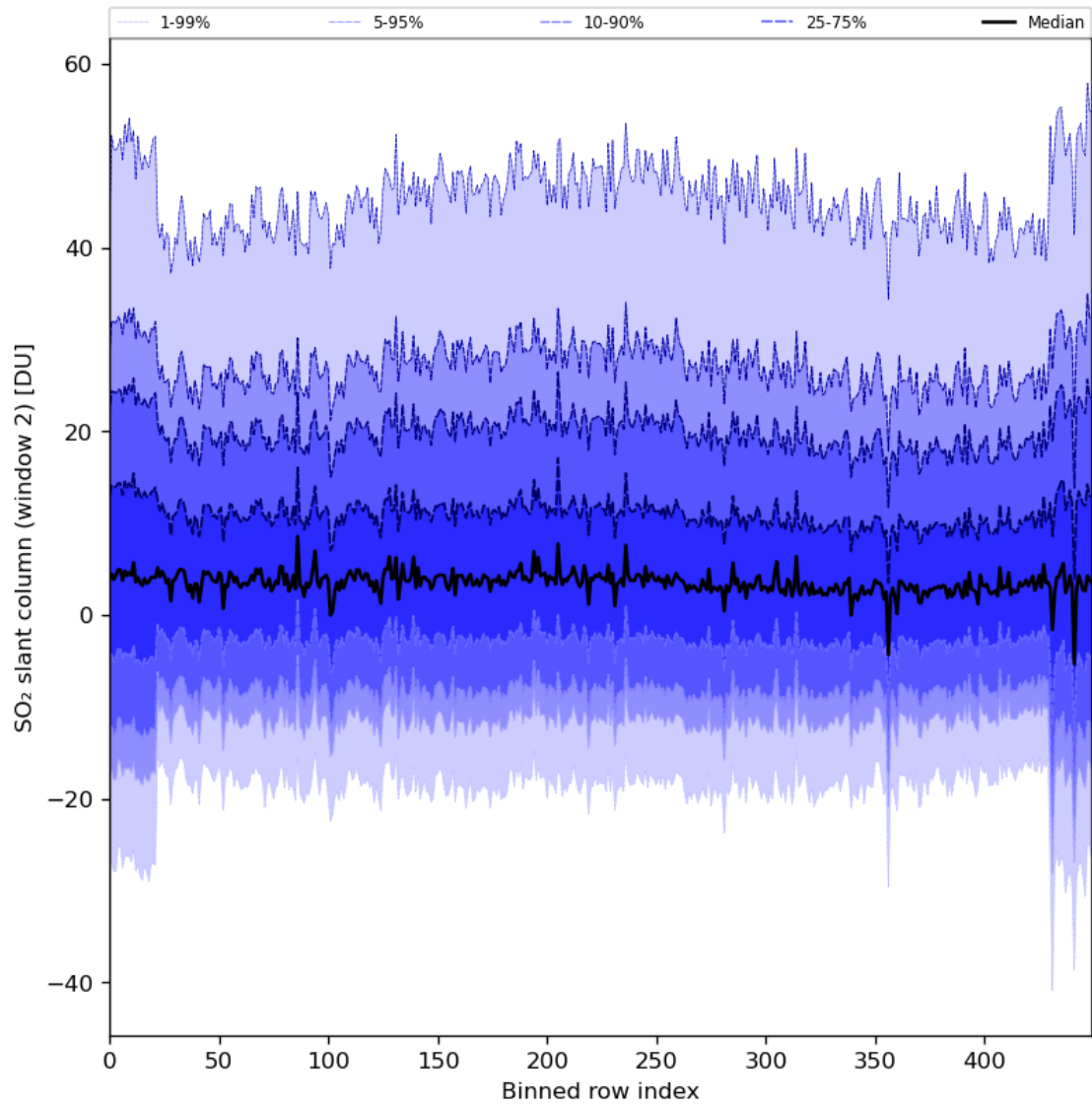
Figure 83: Along track statistics of “SO 2 slant column (window 2)” for 2024-04-02 to 2024-04-04
