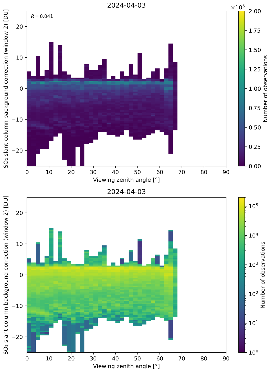
Figure 309: Scatter density plot of “Viewing zenith angle” against “SO 2 slant column background correction (window 2)” for 2024-04-02 to 2024-04-04.
