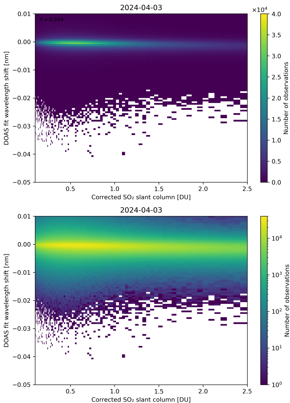
Figure 181: Scatter density plot of “Corrected SO 2 slant column” against “DOAS fit wavelength shift” for 2024-04-02 to 2024-04-04.
