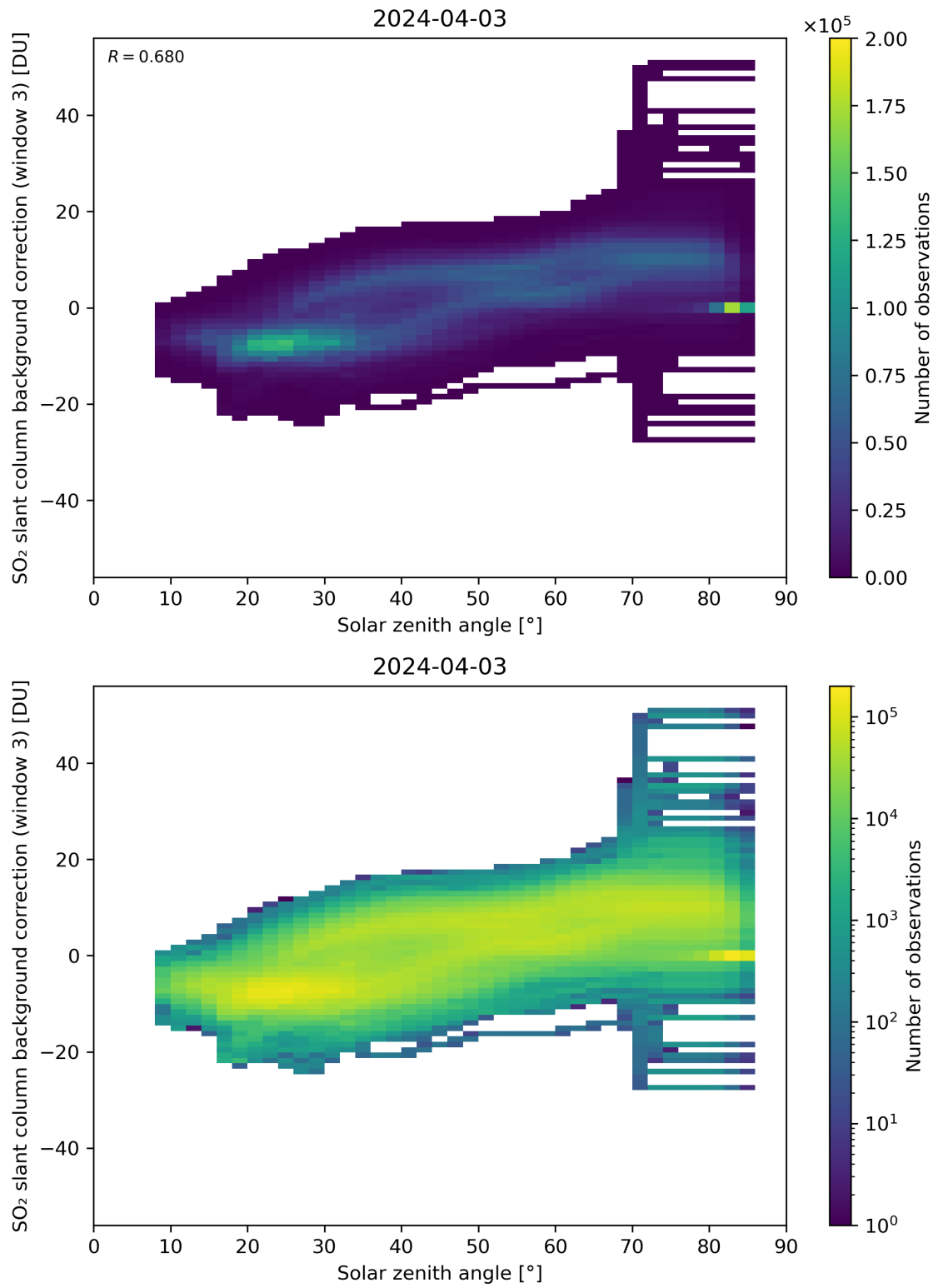
Figure 160: Scatter density plot of “Solar zenith angle” against “SO 2 slant column background correction (window 3)” for 2024-04-02 to 2024-04-04.
