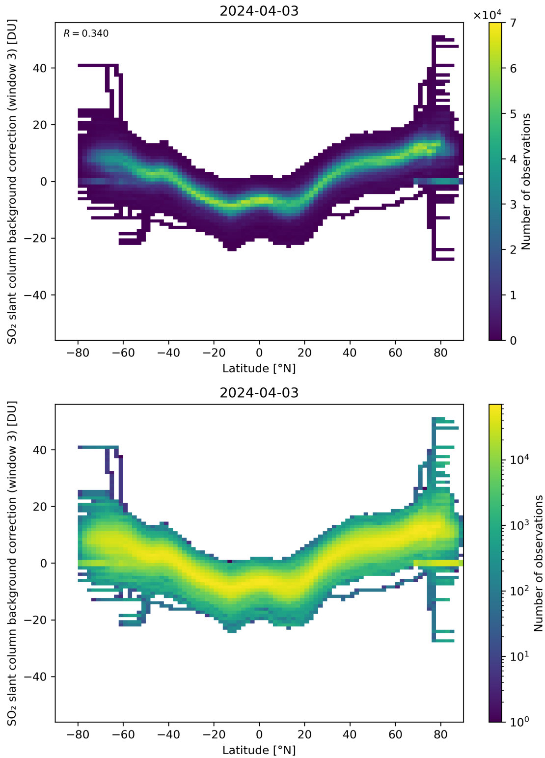
Figure 141: Scatter density plot of “Latitude” against “SO 2 slant column background correction (window 3)” for 2024-04-02 to 2024-04-04.
