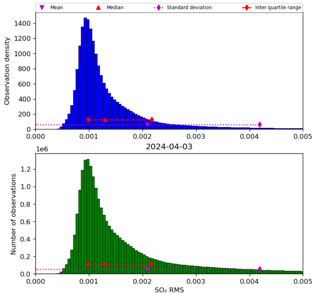
Figure 70: Histogram of “SO 2 RMS” for 2024-04-02 to 2024-04-04
