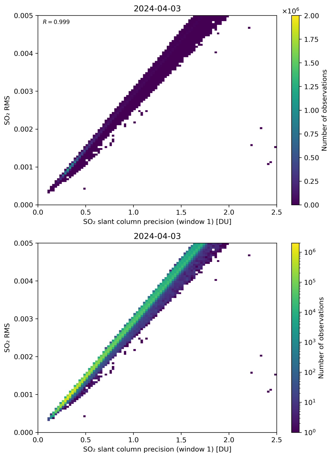
Figure 223: Scatter density plot of “SO 2 slant column precision (window 1)” against “SO 2 RMS” for 2024-04-02 to 2024-04-04.
