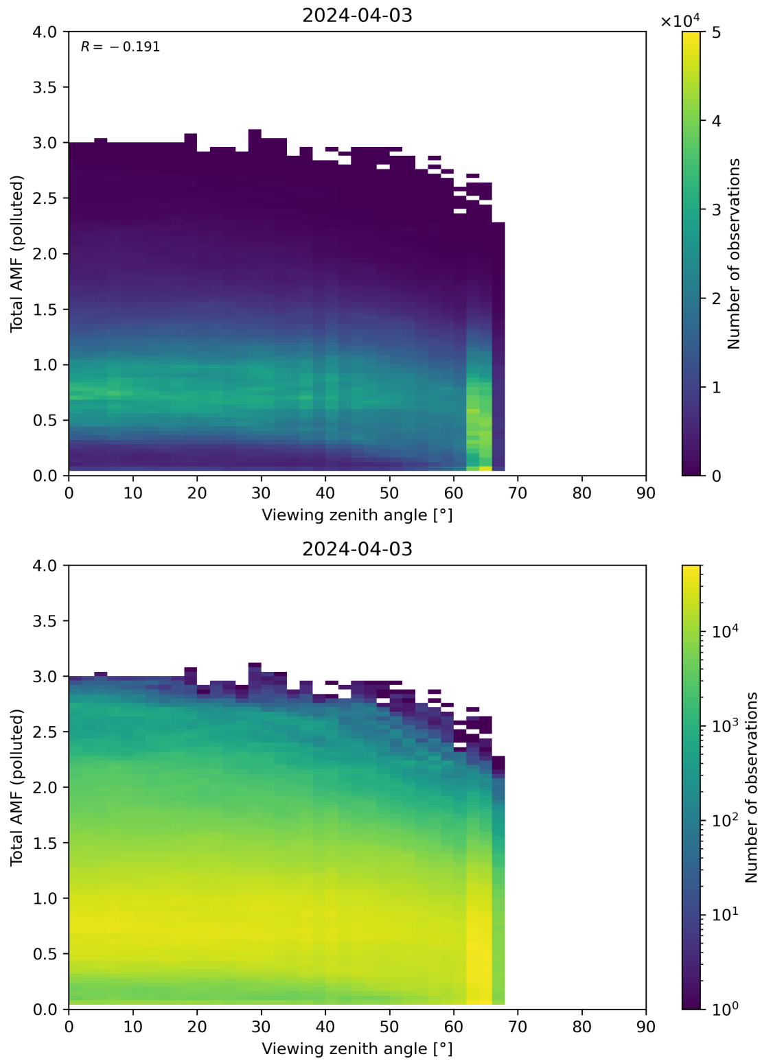
Figure 325: Scatter density plot of “Viewing zenith angle” against “Total AMF (polluted)” for 2024-04-02 to 2024-04-04.
