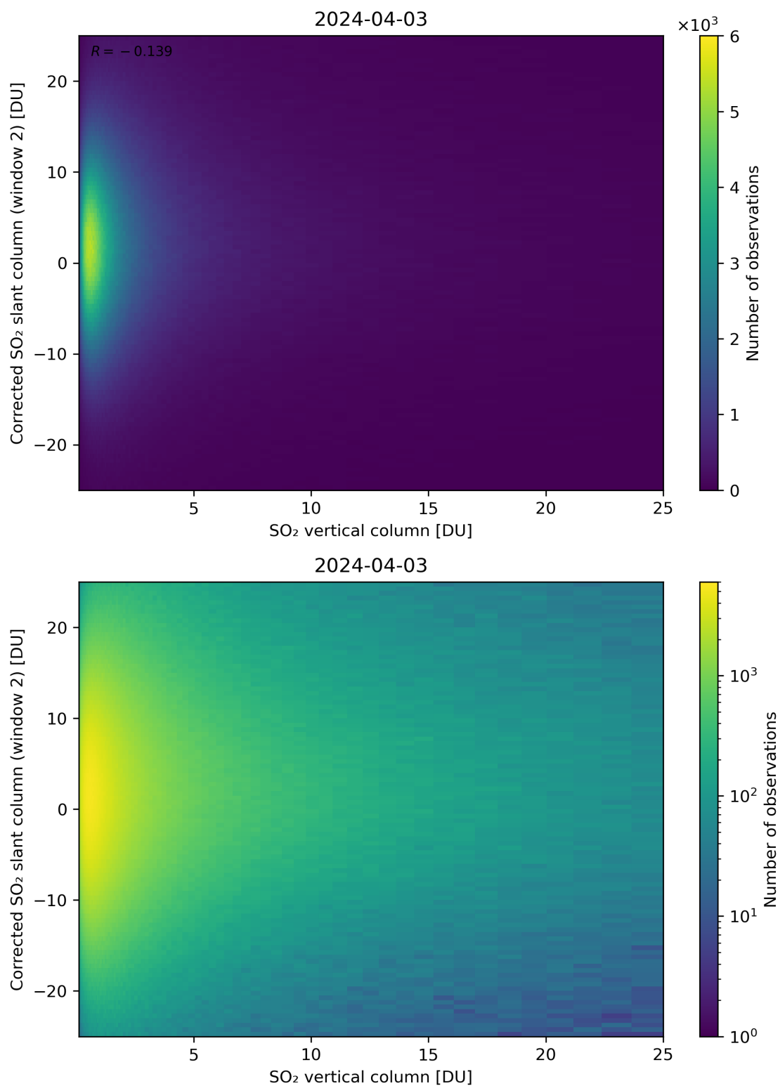
Figure 298: Scatter density plot of “SO 2 vertical column” against “Corrected SO 2 slant column (window 2)” for 2024-04-02 to 2024-04-04.
