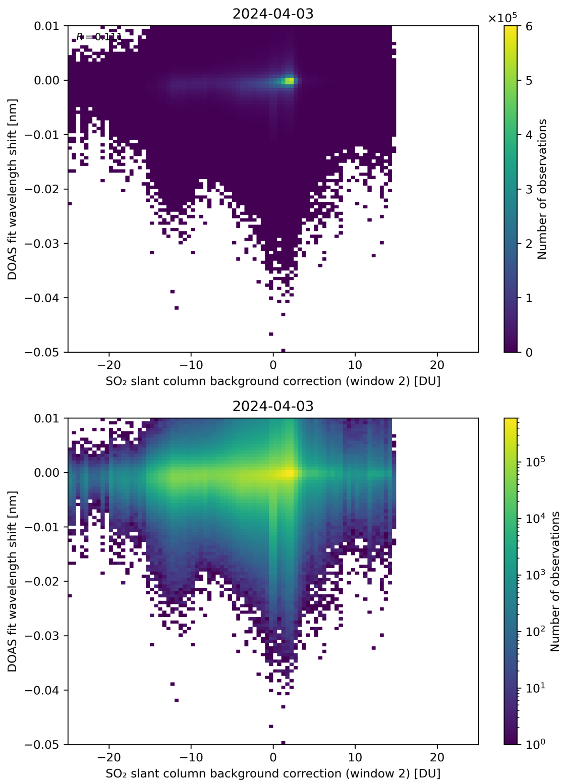
Figure 112: Scatter density plot of “SO 2 slant column background correction (window 2)” against “DOAS fit wavelength shift” for 2024-04-02 to 2024-04-04.
