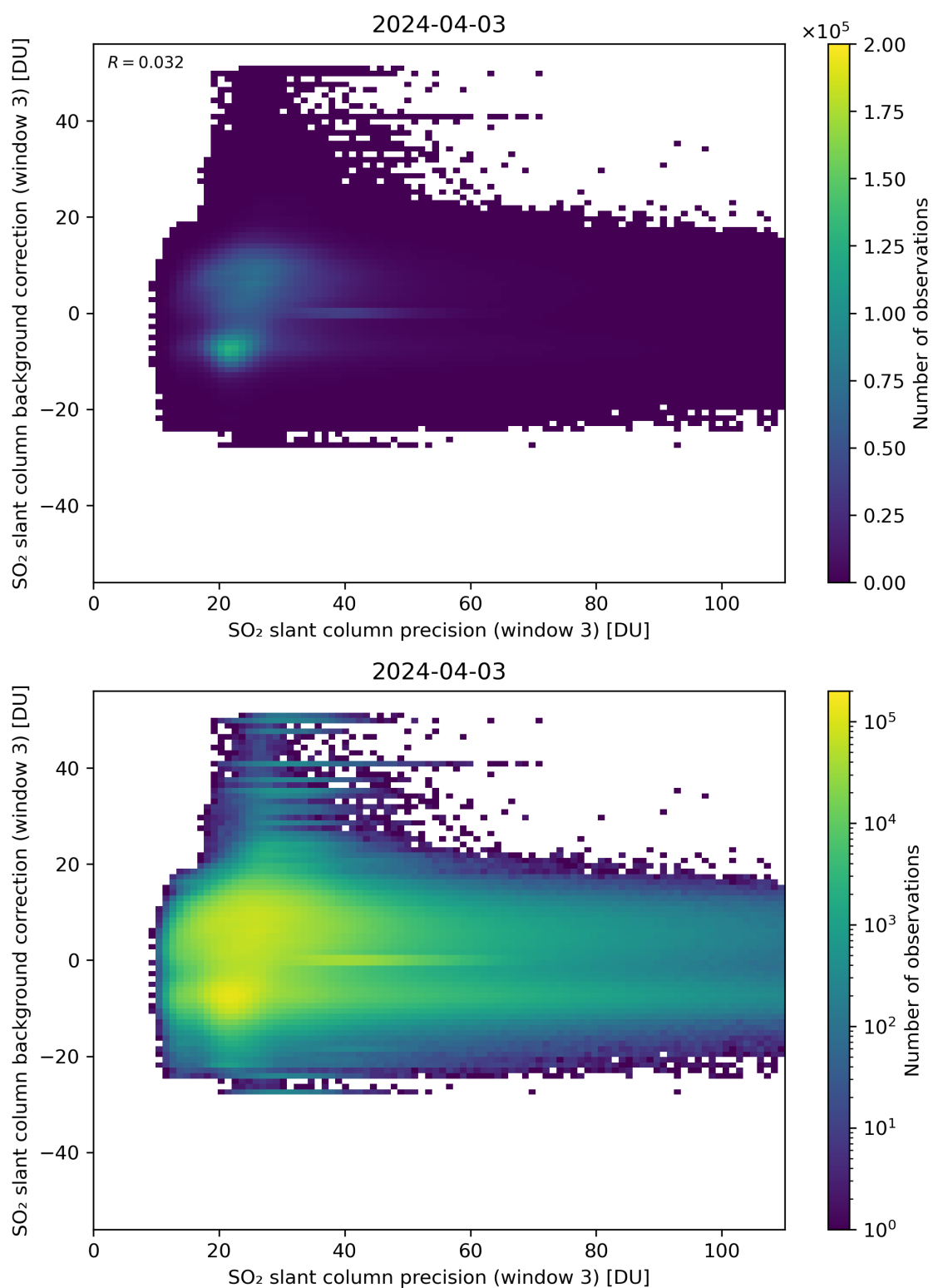
Figure 257: Scatter density plot of “SO 2 slant column precision (window 3)” against “SO 2 slant column background correction (window 3)” for 2024-04-02 to 2024-04-04.
