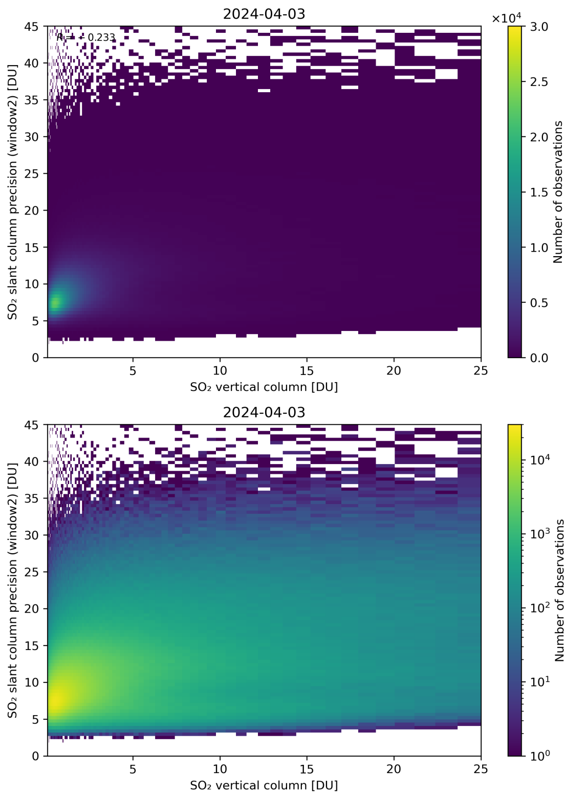
Figure 302: Scatter density plot of “SO 2 vertical column” against “SO 2 slant column precision (window2)” for 2024-04-02 to 2024-04-04.
