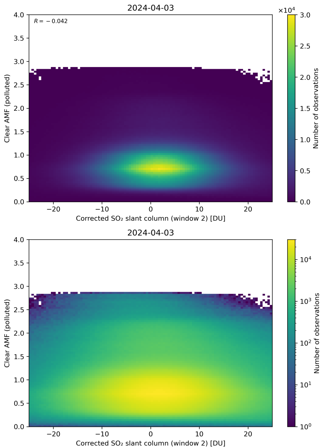
Figure 199: Scatter density plot of “Corrected SO 2 slant column (window 2)” against “Clear AMF (polluted)” for 2024-04-02 to 2024-04-04.
