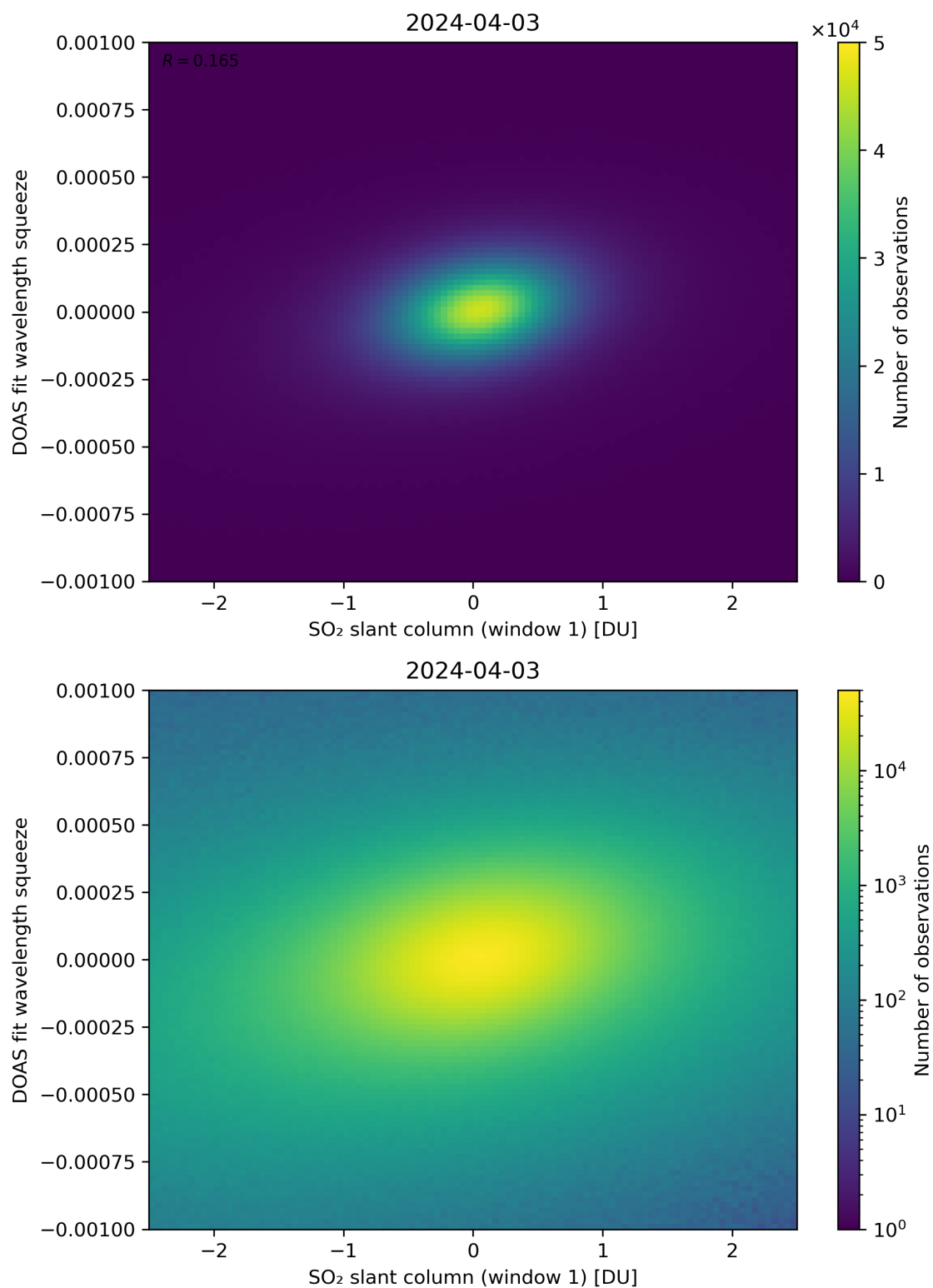
Figure 216: Scatter density plot of “SO 2 slant column (window 1)” against “DOAS fit wavelength squeeze” for 2024-04-02 to 2024-04-04.
