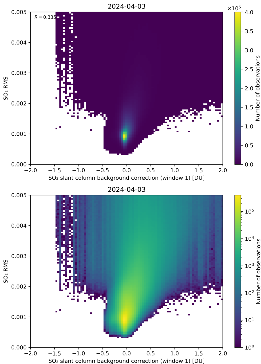
Figure 102: Scatter density plot of “SO 2 slant column background correction (window 1)” against “SO 2 RMS” for 2024-04-02 to 2024-04-04.
