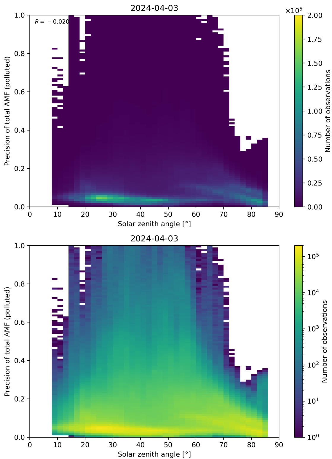
Figure 175: Scatter density plot of “Solar zenith angle” against “Precision of total AMF (polluted)” for 2024-04-02 to 2024-04-04.
