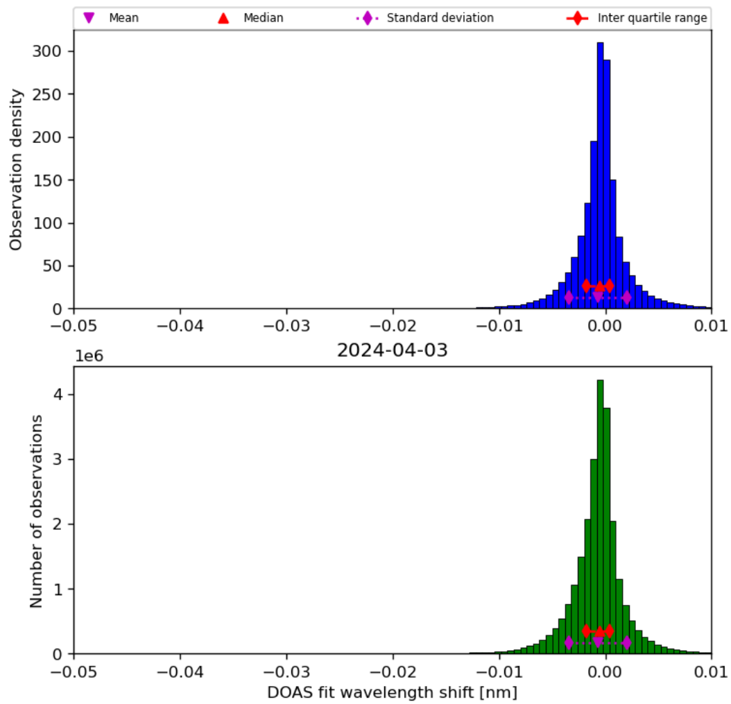
Figure 68: Histogram of “DOAS fit wavelength shift” for 2024-04-02 to 2024-04-04
