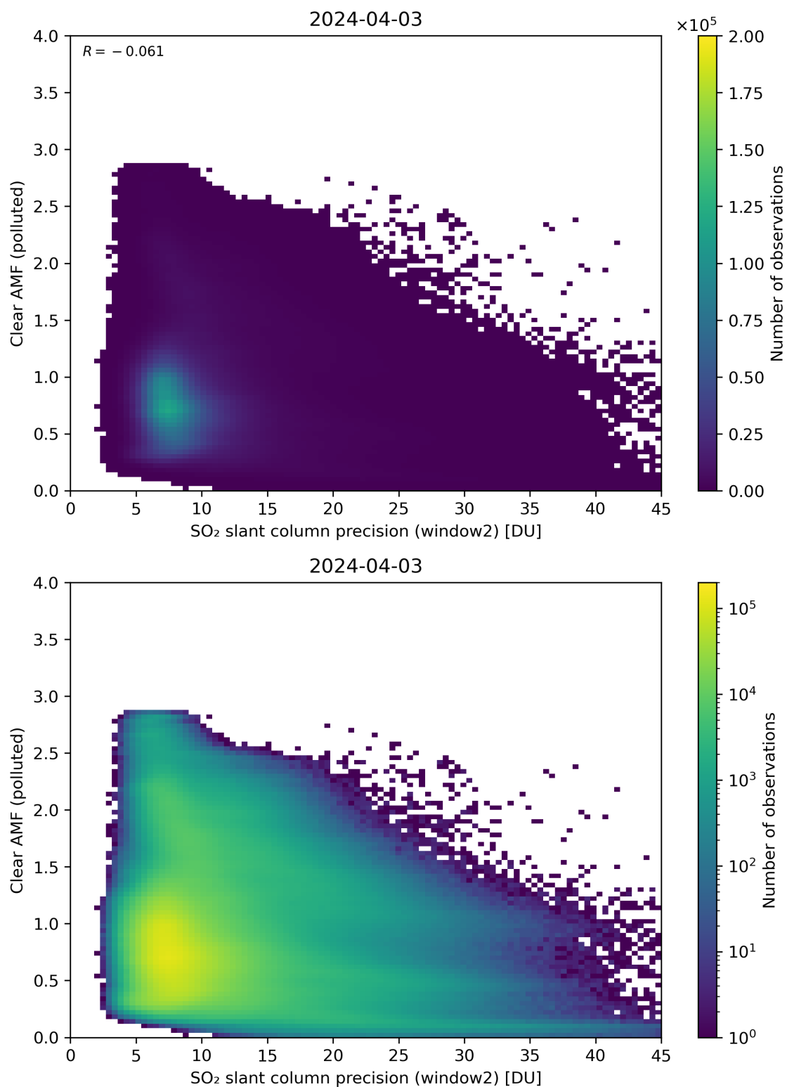
Figure 246: Scatter density plot of “SO 2 slant column precision (window2)” against “Clear AMF (polluted)” for 2024-04-02 to 2024-04-04.
