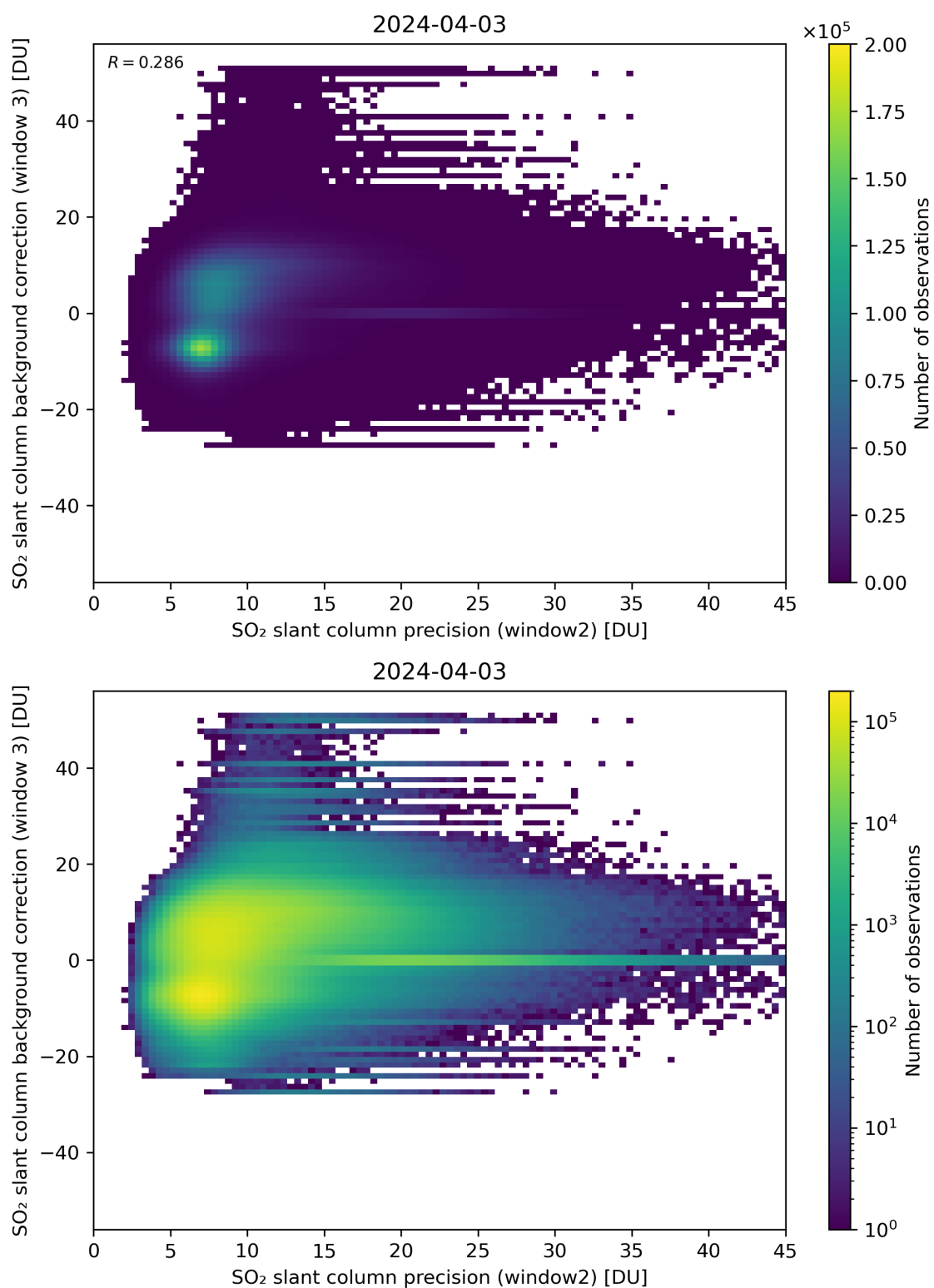
Figure 242: Scatter density plot of “SO 2 slant column precision (window2)” against “SO 2 slant column background correction (window 3)” for 2024-04-02 to 2024-04-04.
