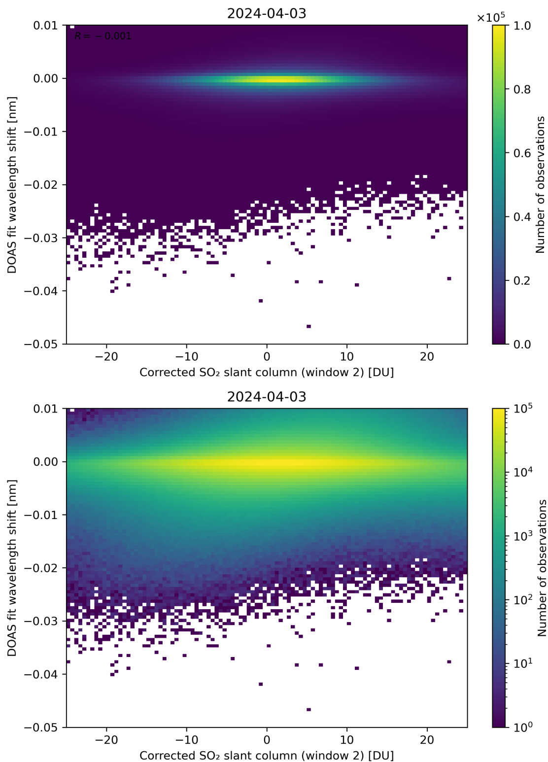
Figure 196: Scatter density plot of “Corrected SO 2 slant column (window 2)” against “DOAS fit wavelength shift” for 2024-04-02 to 2024-04-04.
