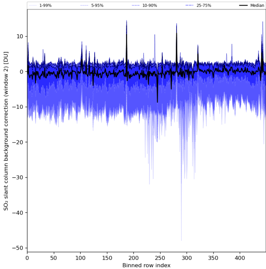
Figure 86: Along track statistics of “SO 2 slant column background correction (window 2)” for 2024-04-02 to 2024-04-04
