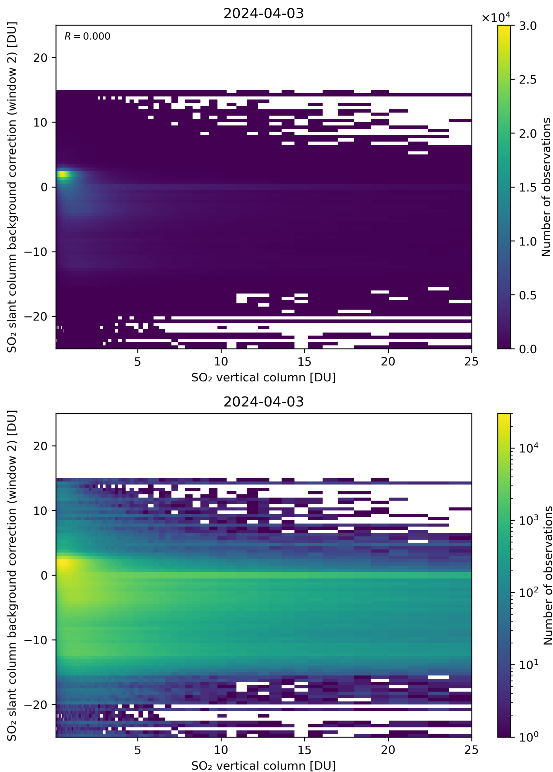
Figure 274: Scatter density plot of “SO 2 vertical column” against “SO 2 slant column background correction (window 2)” for 2024-04-02 to 2024-04-04.
