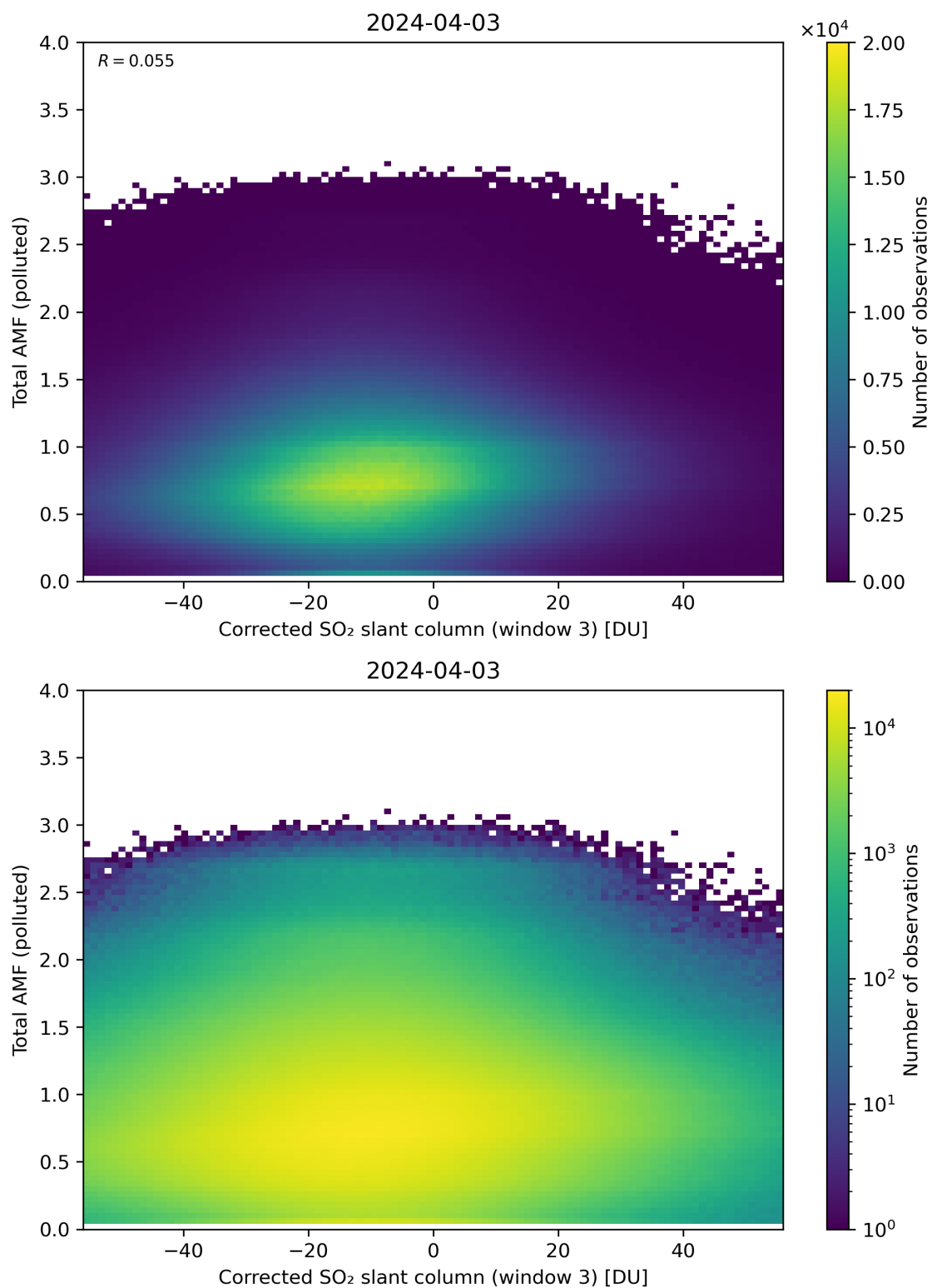
Figure 210: Scatter density plot of “Corrected SO 2 slant column (window 3)” against “Total AMF (polluted)” for 2024-04-02 to 2024-04-04.
