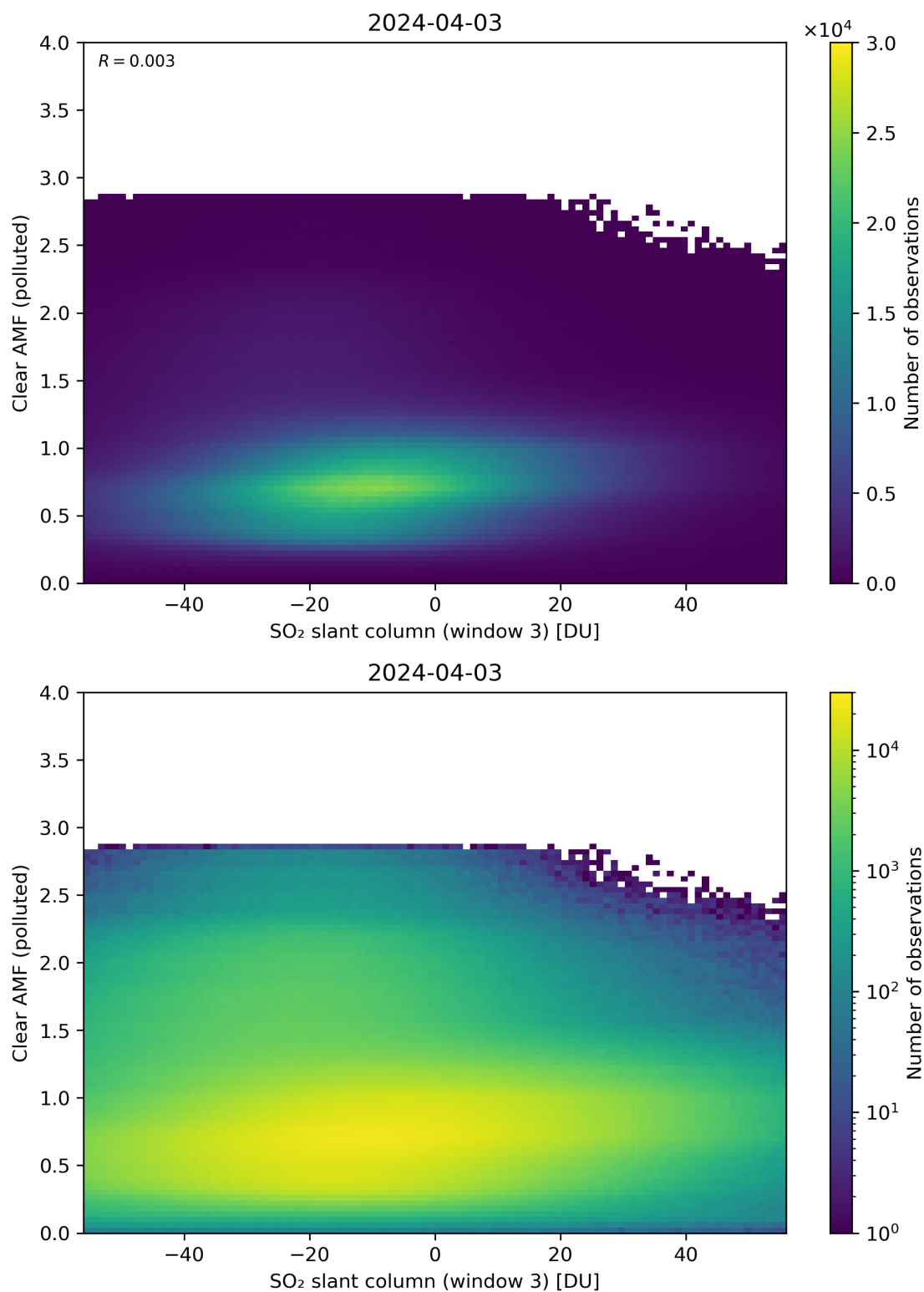
Figure 265: Scatter density plot of “SO 2 slant column (window 3)” against “Clear AMF (polluted)” for 2024-04-02 to 2024-04-04.
