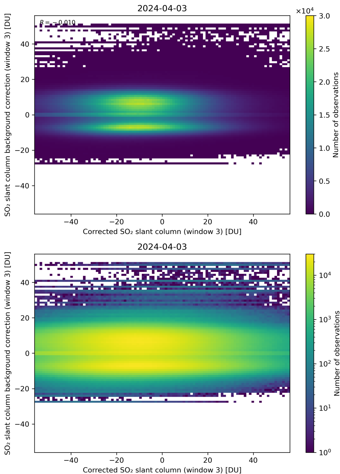
Figure 205: Scatter density plot of “Corrected SO 2 slant column (window 3)” against “SO 2 slant column background correction (window 3)” for 2024-04-02 to 2024-04-04.
