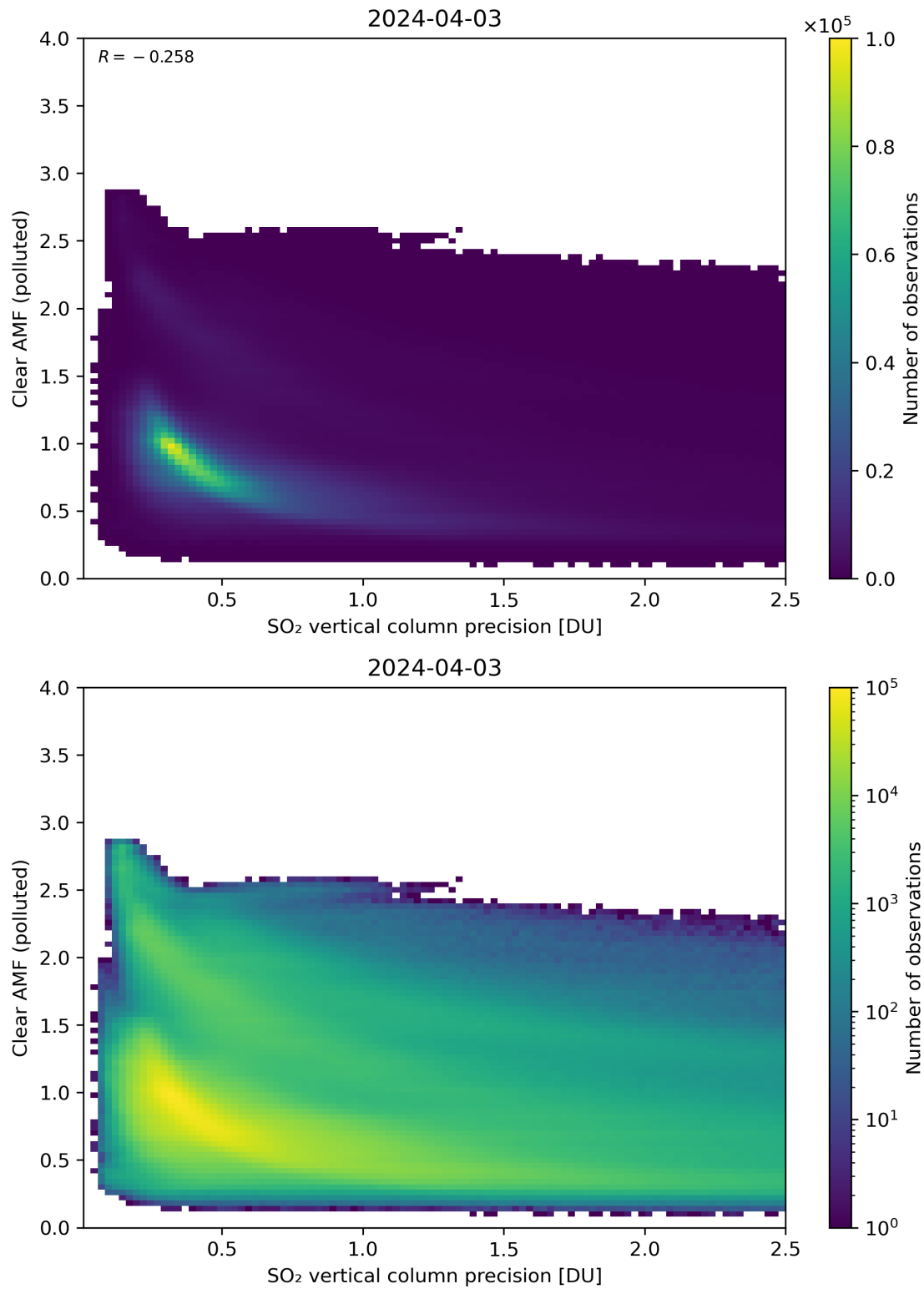
Figure 285: Scatter density plot of “SO 2 vertical column precision” against “Clear AMF (polluted)” for 2024-04-02 to 2024-04-04.
