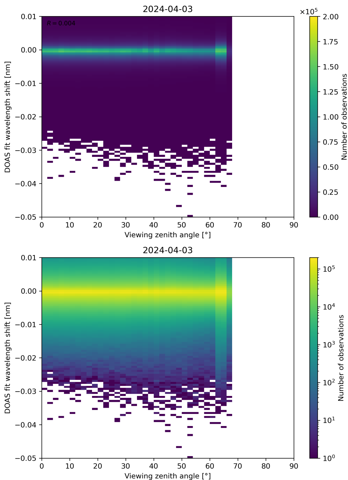
Figure 311: Scatter density plot of “Viewing zenith angle” against “DOAS fit wavelength shift” for 2024-04-02 to 2024-04-04.
