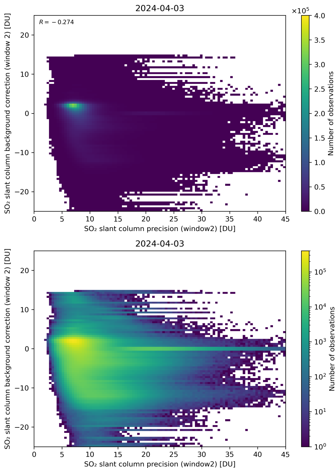
Figure 241: Scatter density plot of “SO 2 slant column precision (window2)” against “SO 2 slant column background correction (window 2)” for 2024-04-02 to 2024-04-04.
