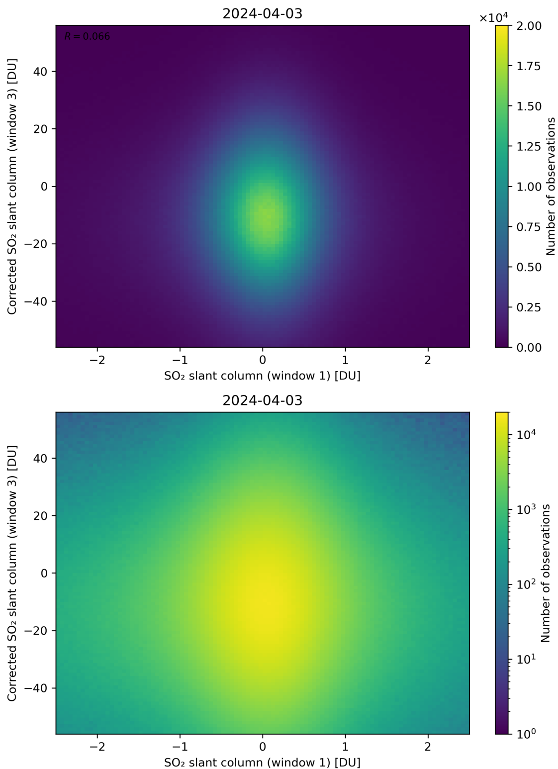
Figure 234: Scatter density plot of “SO 2 slant column (window 1)” against “Corrected SO 2 slant column (window 3)” for 2024-04-02 to 2024-04-04.
