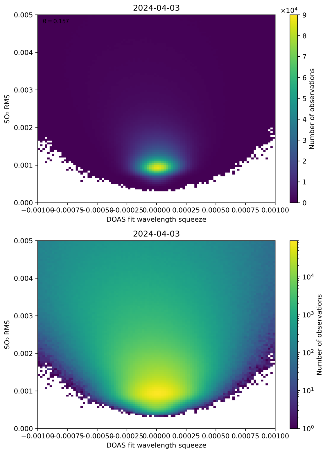
Figure 132: Scatter density plot of “DOAS fit wavelength squeeze” against “SO 2 RMS” for 2024-04-02 to 2024-04-04.
