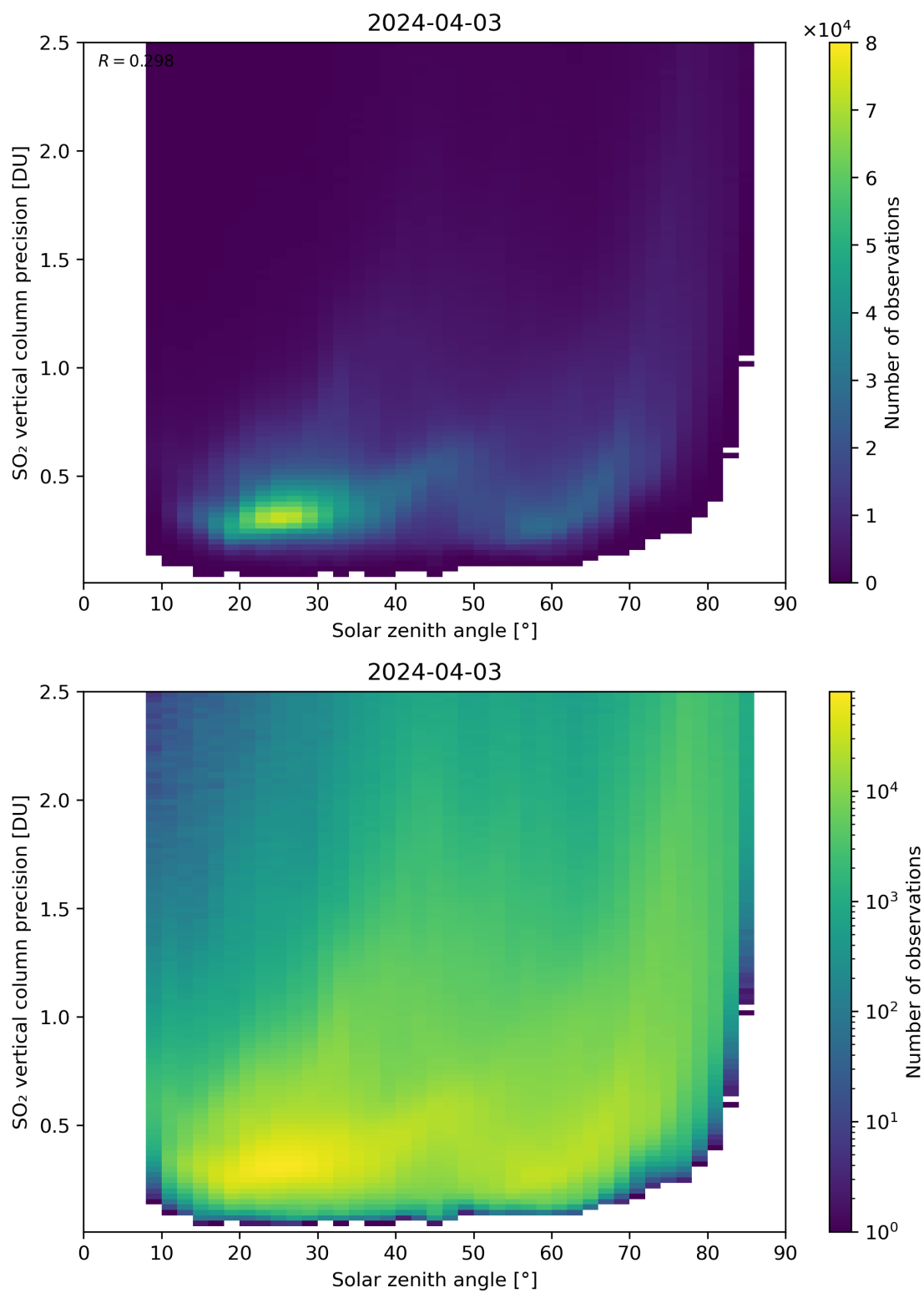
Figure 177: Scatter density plot of “Solar zenith angle” against “SO 2 vertical column precision” for 2024-04-02 to 2024-04-04.
