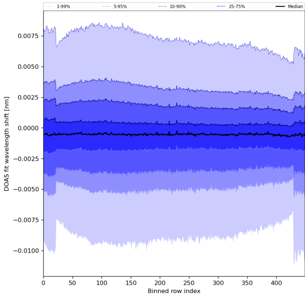
Figure 91: Along track statistics of “DOAS fit wavelength shift” for 2024-04-02 to 2024-04-04
