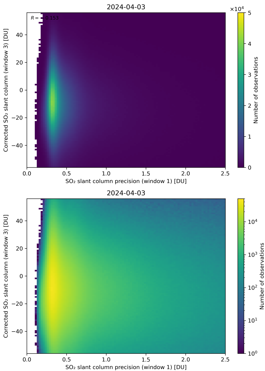
Figure 226: Scatter density plot of “SO 2 slant column precision (window 1)” against “Corrected SO 2 slant column (window 3)” for 2024-04-02 to 2024-04-04.
