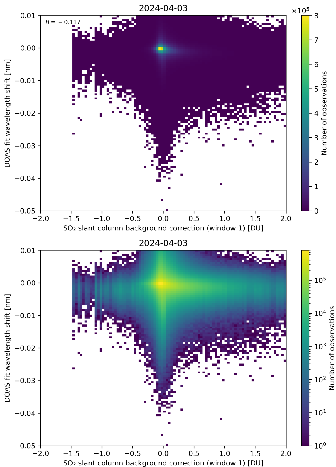
Figure 100: Scatter density plot of “SO 2 slant column background correction (window 1)” against “DOAS fit wavelength shift” for 2024-04-02 to 2024-04-04.
