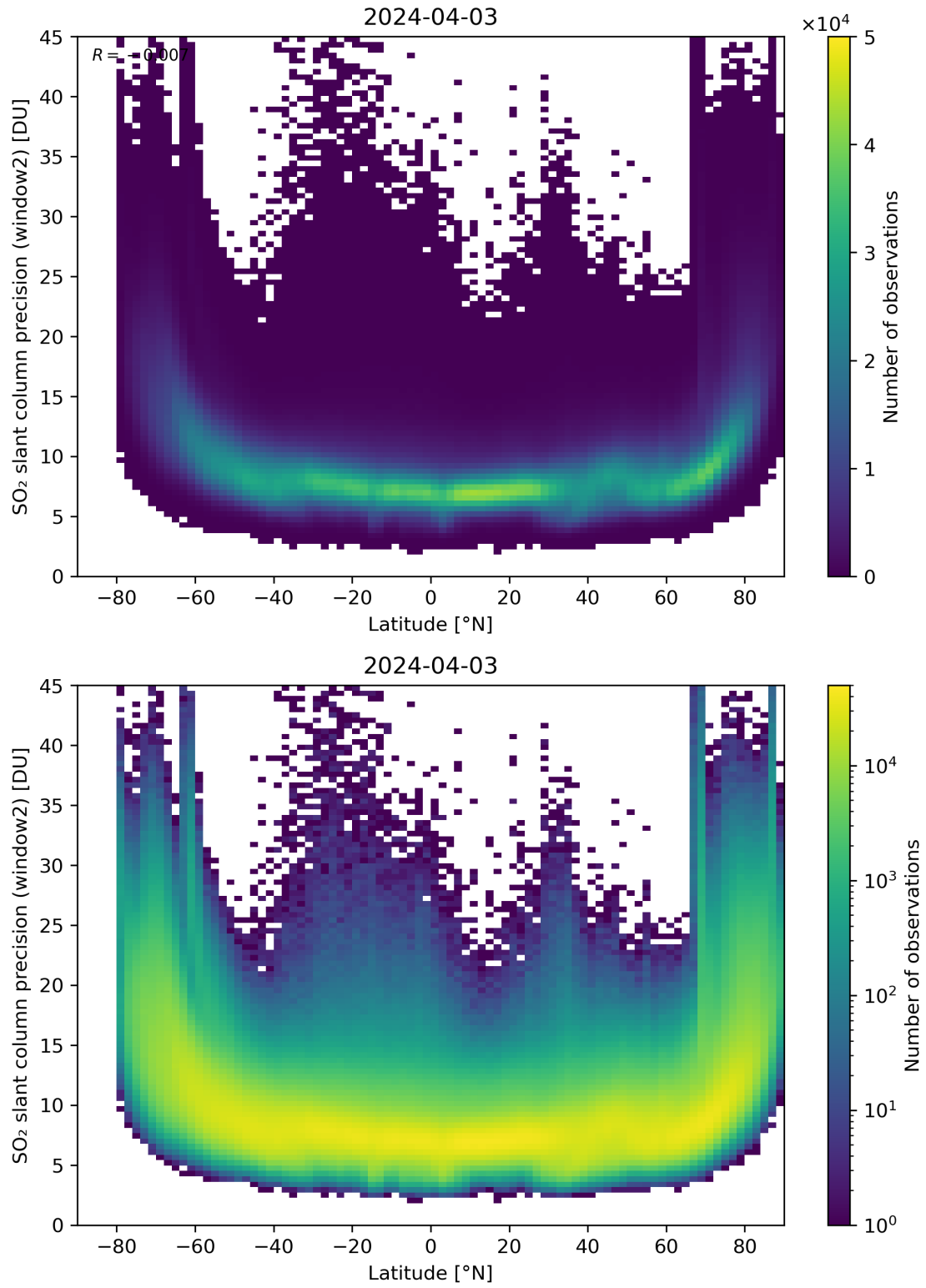
Figure 151: Scatter density plot of “Latitude” against “SO 2 slant column precision (window2)” for 2024-04-02 to 2024-04-04.
