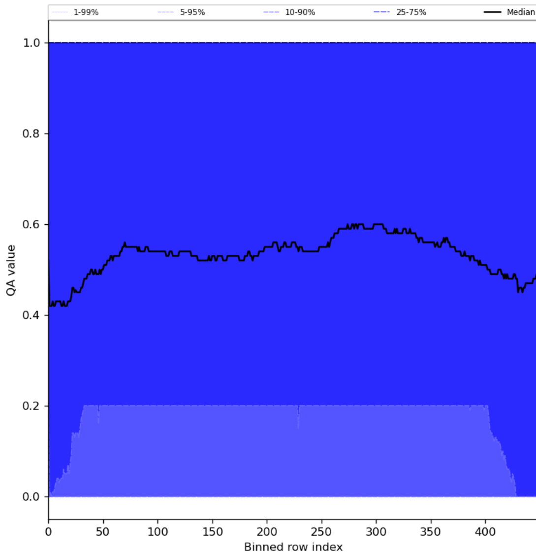
Figure 75: Along track statistics of “QA value” for 2024-04-02 to 2024-04-04
