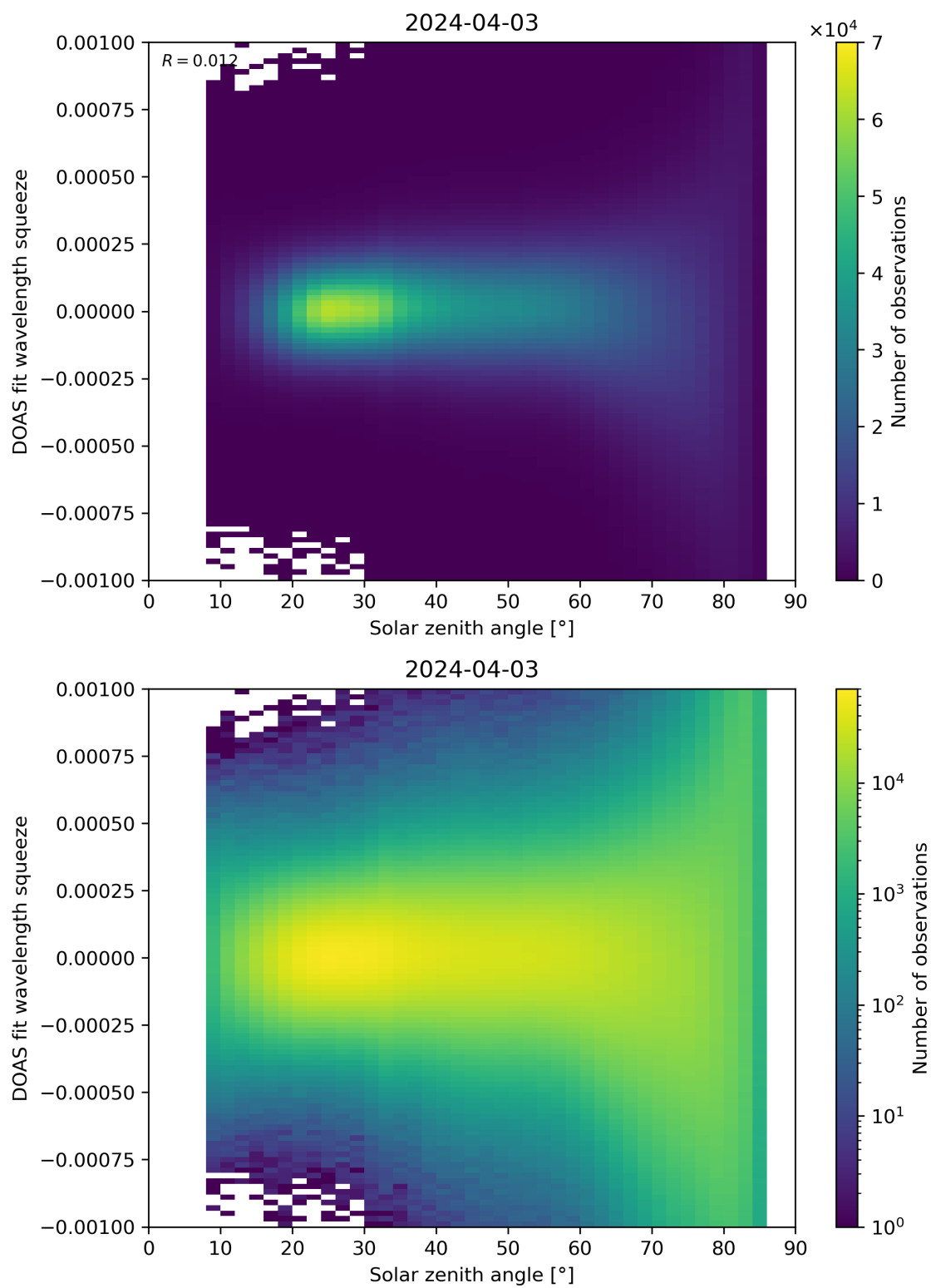
Figure 162: Scatter density plot of “Solar zenith angle” against “DOAS fit wavelength squeeze” for 2024-04-02 to 2024-04-04.
