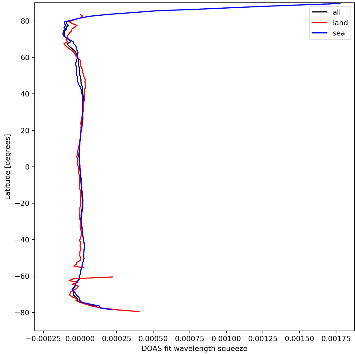
Figure 46: Zonal average of “DOAS fit wavelength squeeze” for 2024-04-02 to 2024-04-04.
