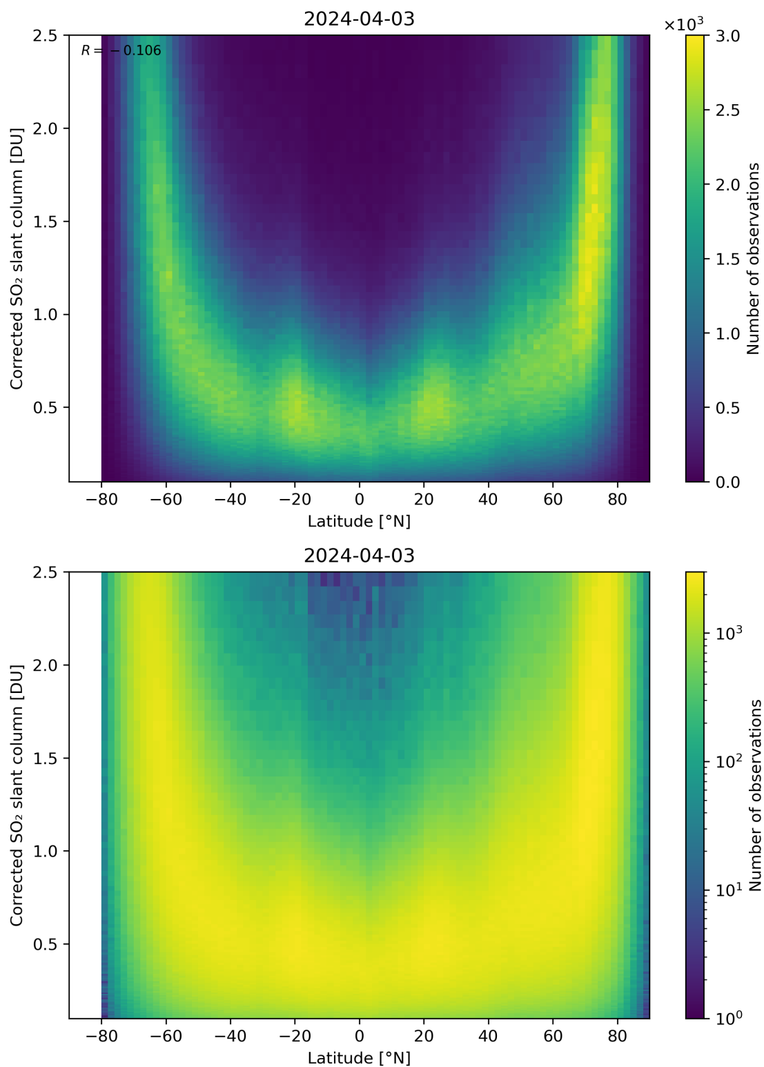
Figure 146: Scatter density plot of “Latitude” against “Corrected SO 2 slant column” for 2024-04-02 to 2024-04-04.
