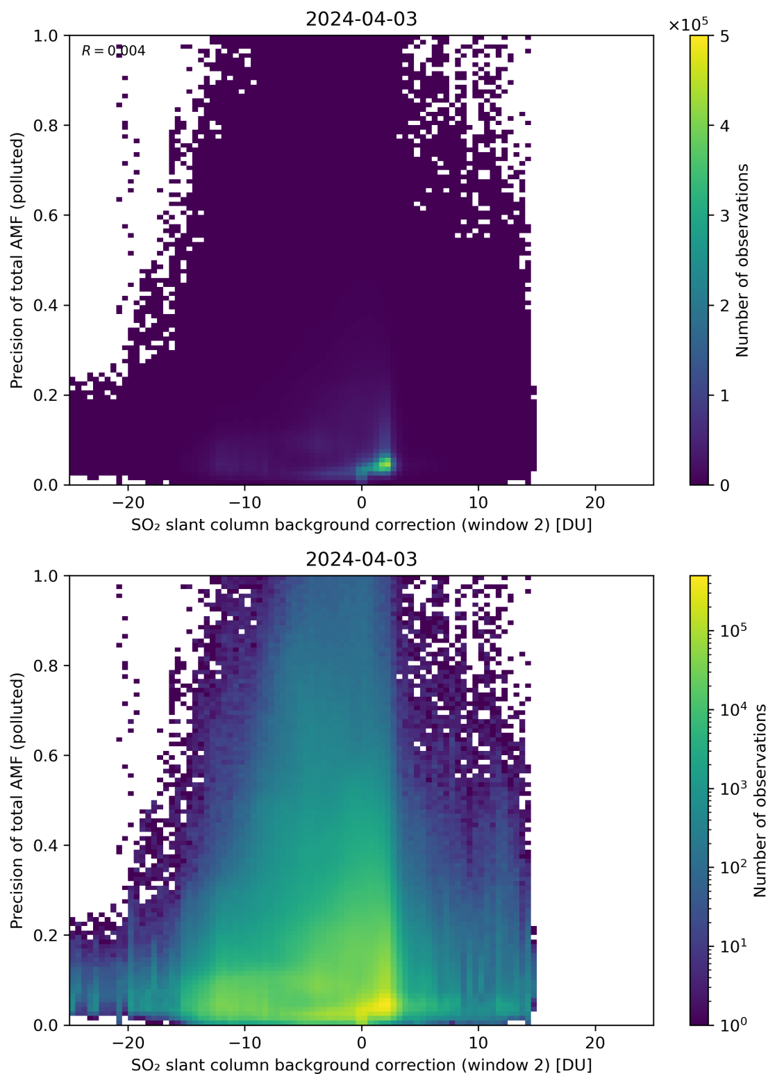
Figure 120: Scatter density plot of “SO 2 slant column background correction (window 2)” against “Precision of total AMF (polluted)” for 2024-04-02 to 2024-04-04.
