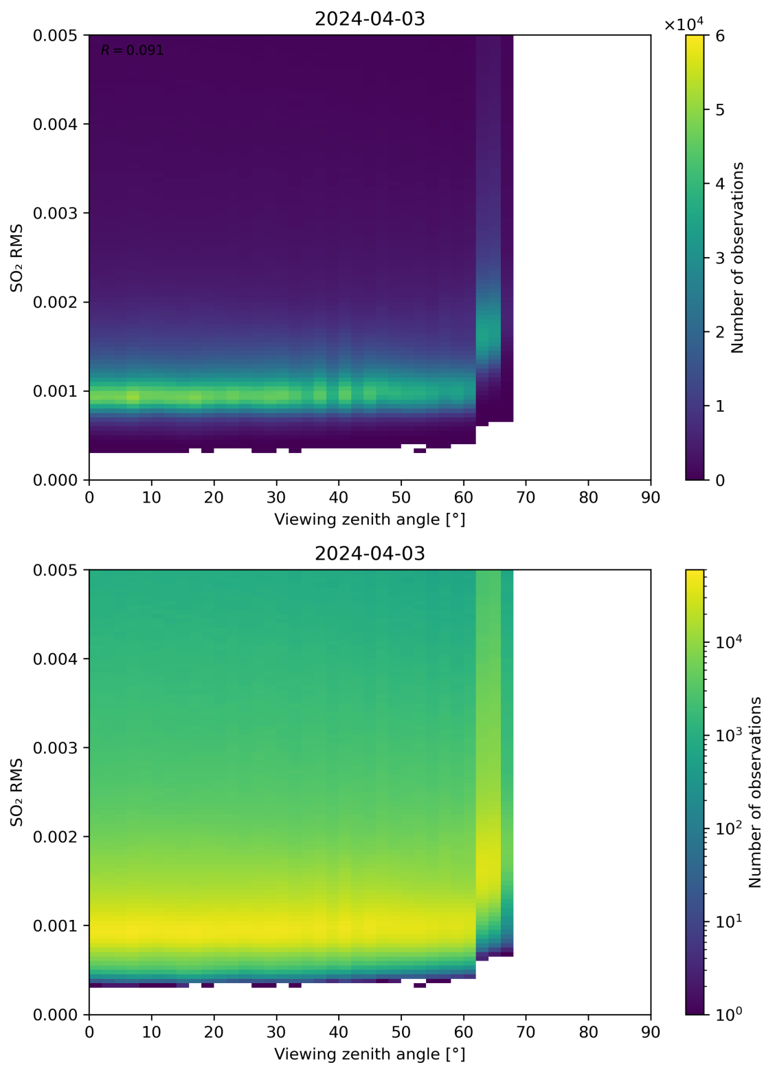
Figure 313: Scatter density plot of “Viewing zenith angle” against “SO 2 RMS” for 2024-04-02 to 2024-04-04.
