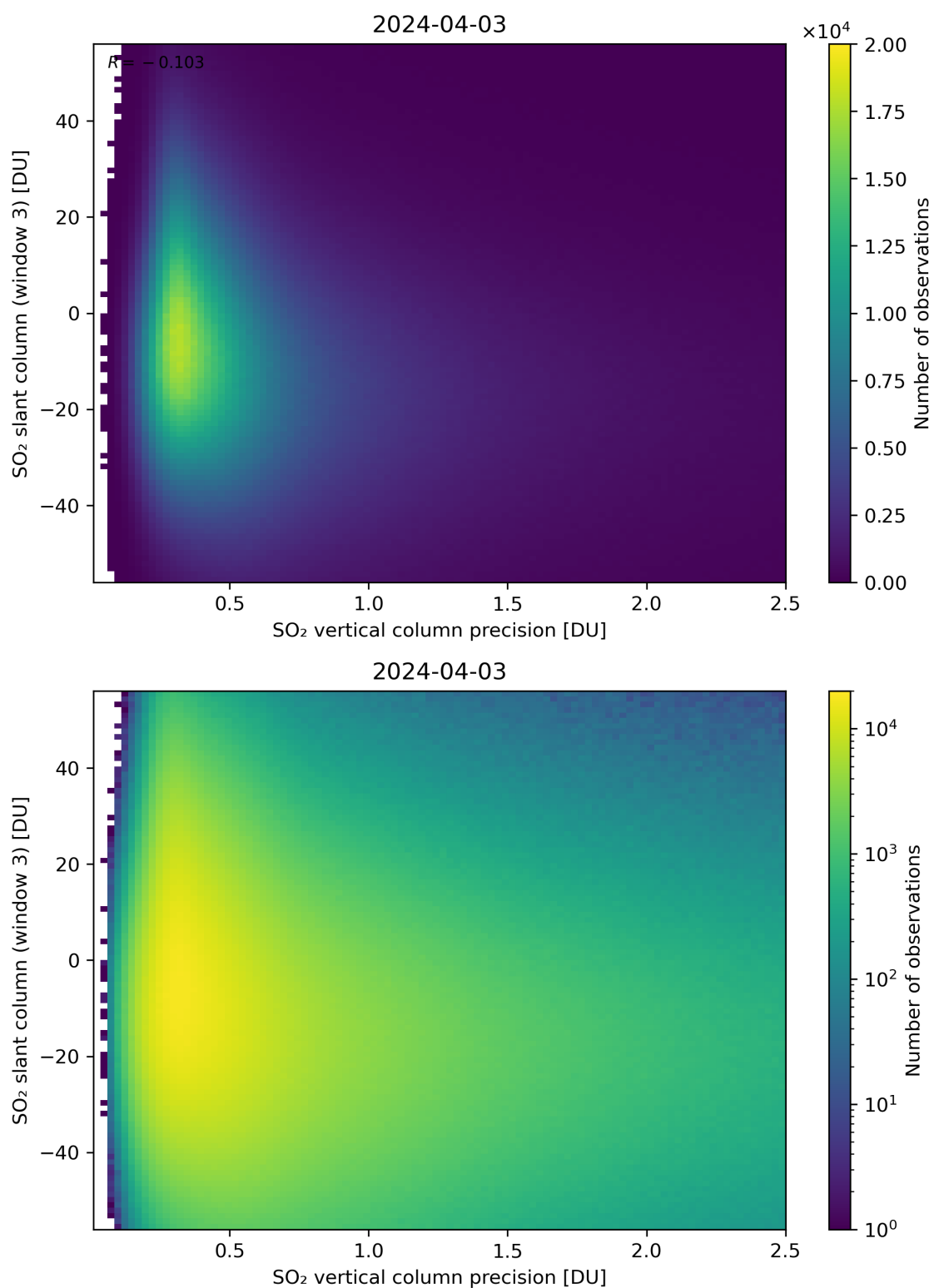
Figure 292: Scatter density plot of “SO 2 vertical column precision” against “SO 2 slant column (window 3)” for 2024-04-02 to 2024-04-04.
