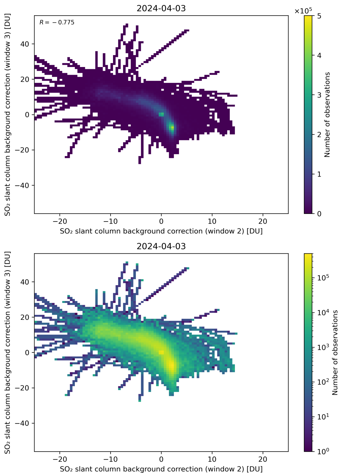
Figure 111: Scatter density plot of “SO 2 slant column background correction (window 2)” against “SO 2 slant column background correction (window 3)” for 2024-04-02 to 2024-04-04.
