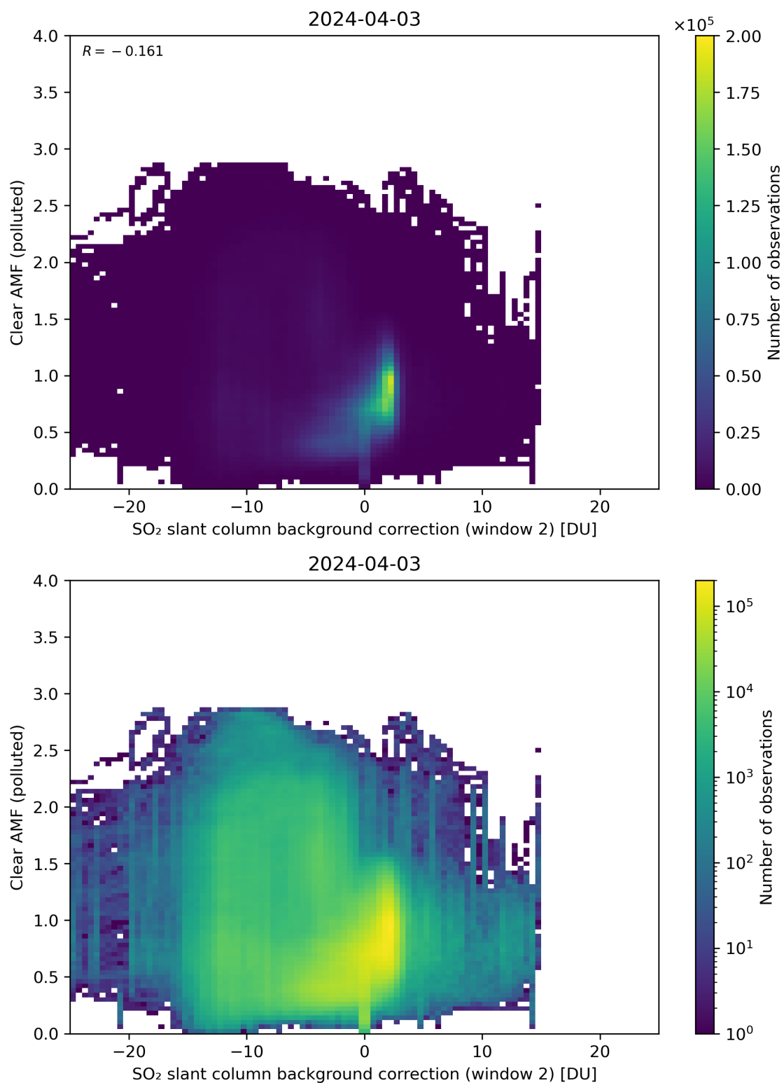
Figure 115: Scatter density plot of “SO 2 slant column background correction (window 2)” against “Clear AMF (polluted)” for 2024-04-02 to 2024-04-04.
