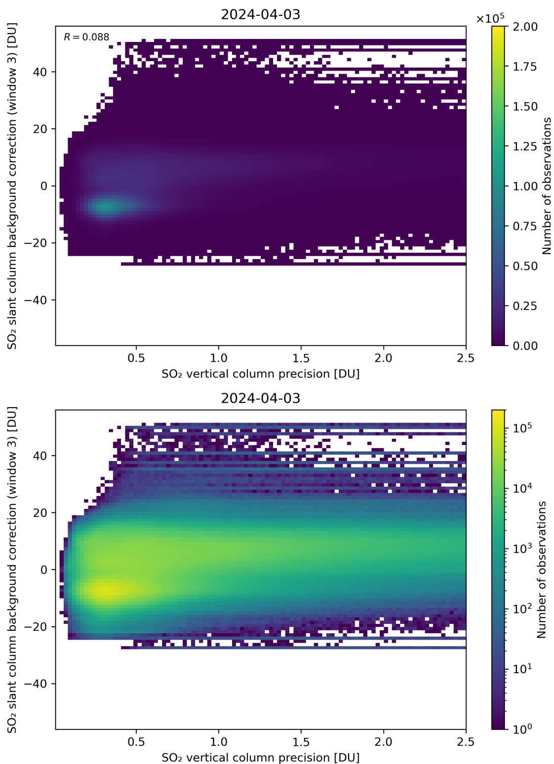
Figure 281: Scatter density plot of “SO 2 vertical column precision” against “SO 2 slant column background correction (window 3)” for 2024-04-02 to 2024-04-04.
