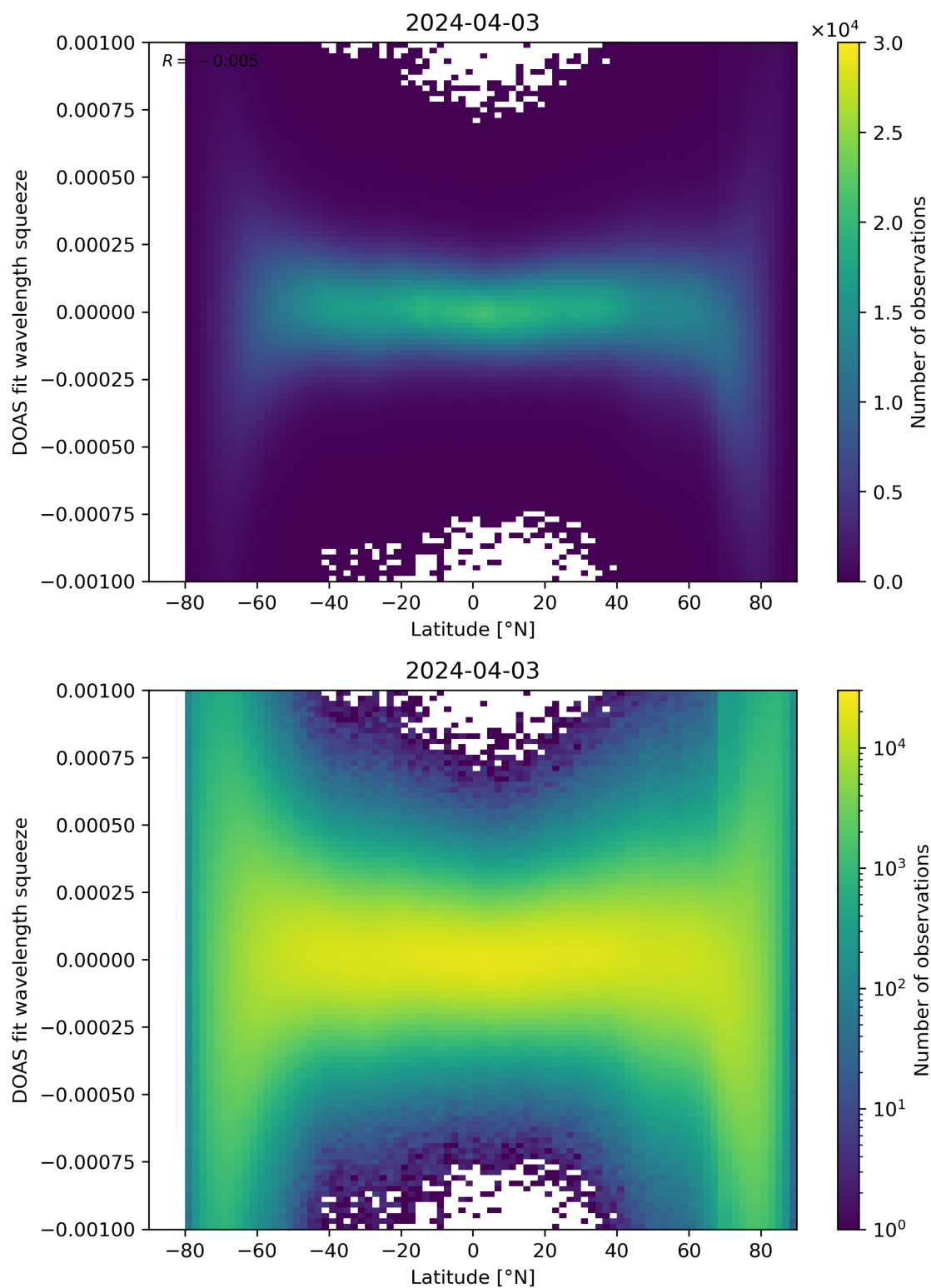
Figure 143: Scatter density plot of “Latitude” against “DOAS fit wavelength squeeze” for 2024-04-02 to 2024-04-04.
