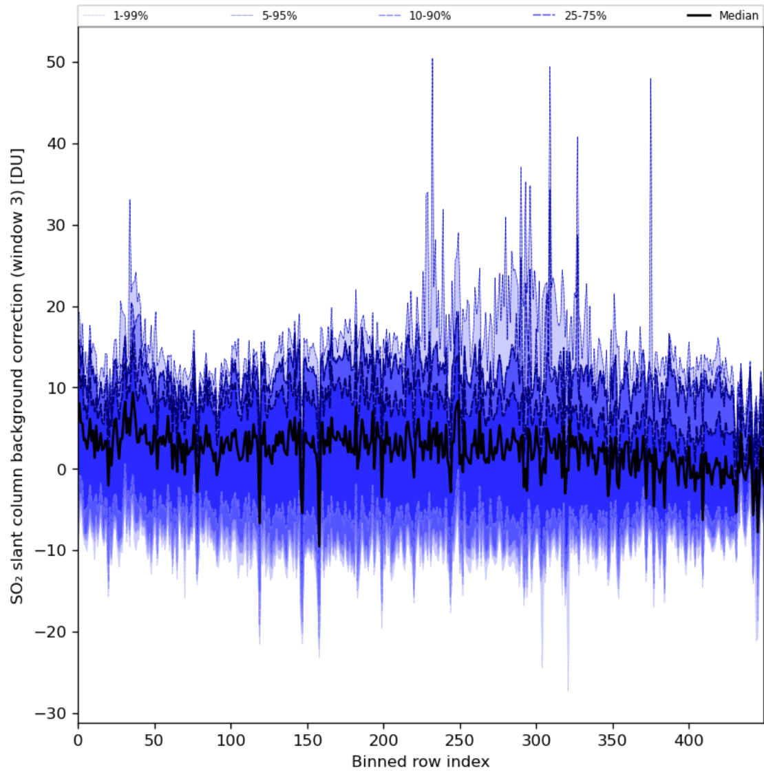
Figure 90: Along track statistics of “SO 2 slant column background correction (window 3)” for 2024-04-02 to 2024-04-04
