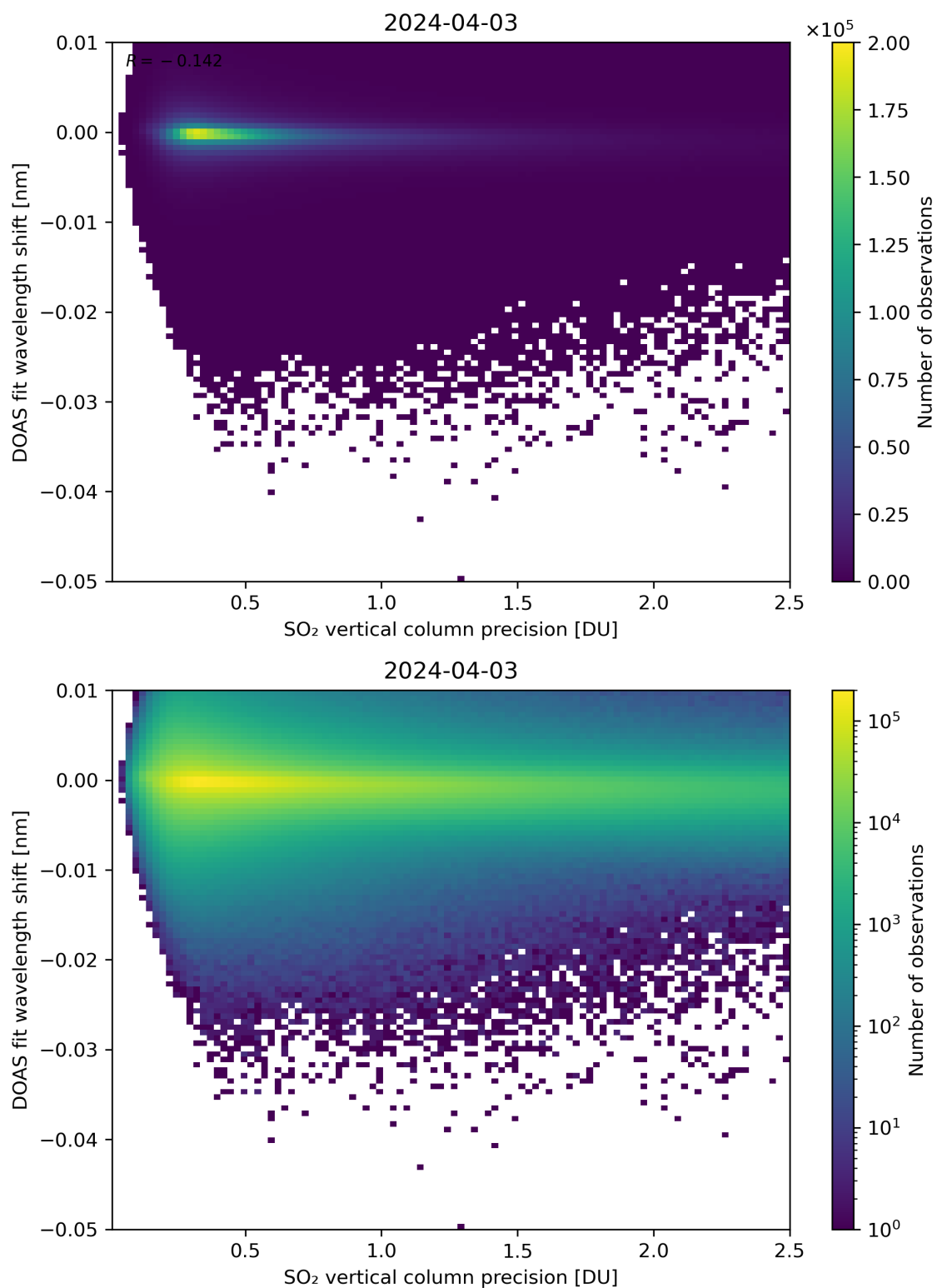
Figure 282: Scatter density plot of “SO 2 vertical column precision” against “DOAS fit wavelength shift” for 2024-04-02 to 2024-04-04.
