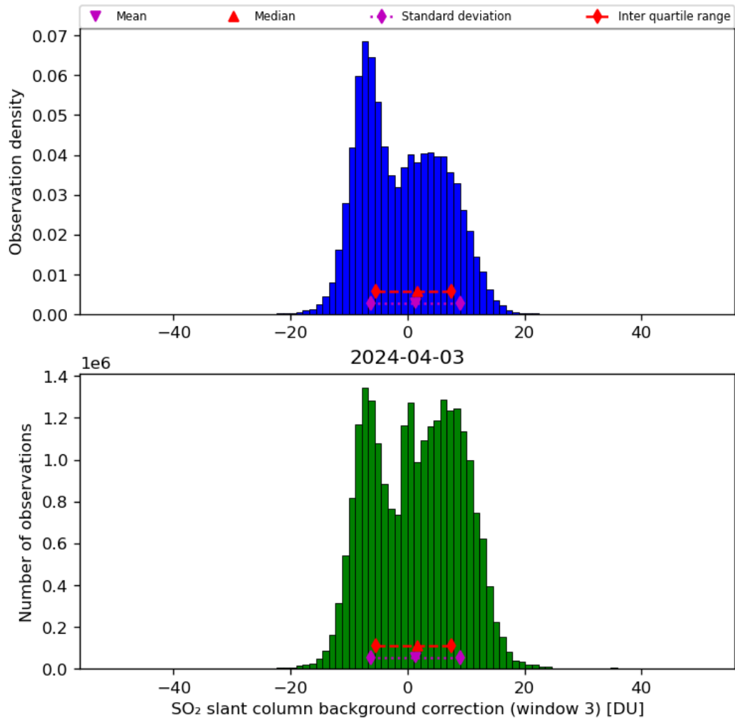
Figure 67: Histogram of “SO 2 slant column background correction (window 3)” for 2024-04-02 to 2024-04-04
