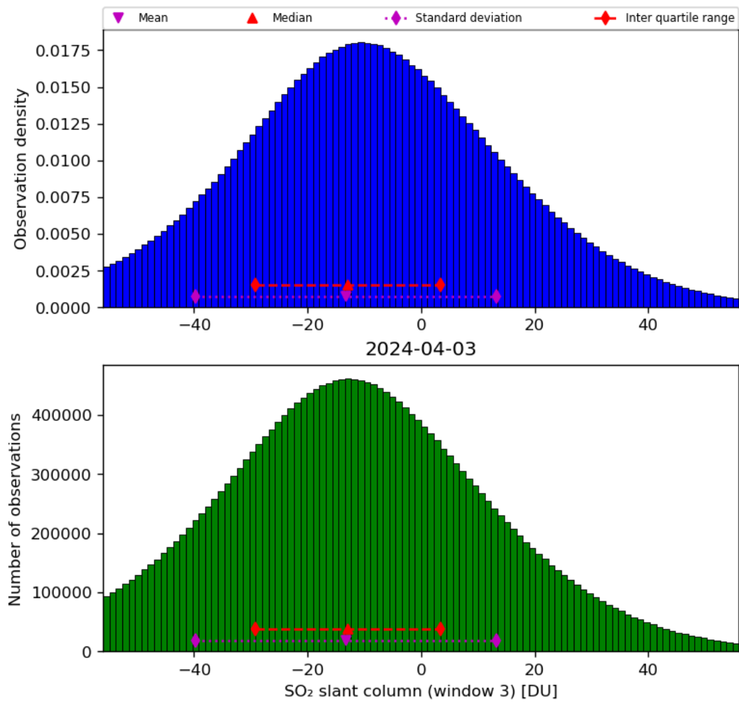
Figure 64: Histogram of “SO 2 slant column (window 3)” for 2024-04-02 to 2024-04-04
