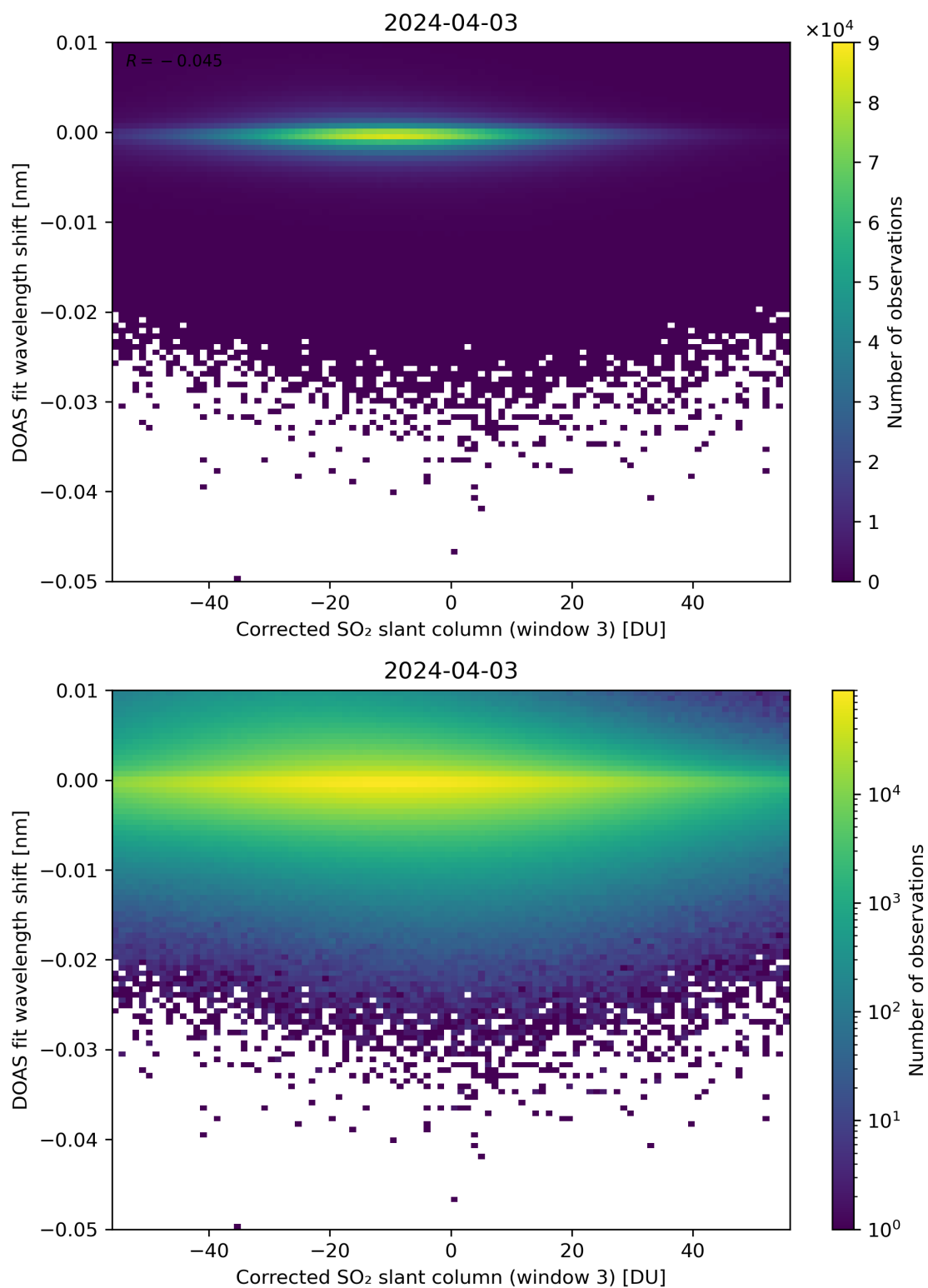
Figure 206: Scatter density plot of “Corrected SO 2 slant column (window 3)” against “DOAS fit wavelength shift” for 2024-04-02 to 2024-04-04.
