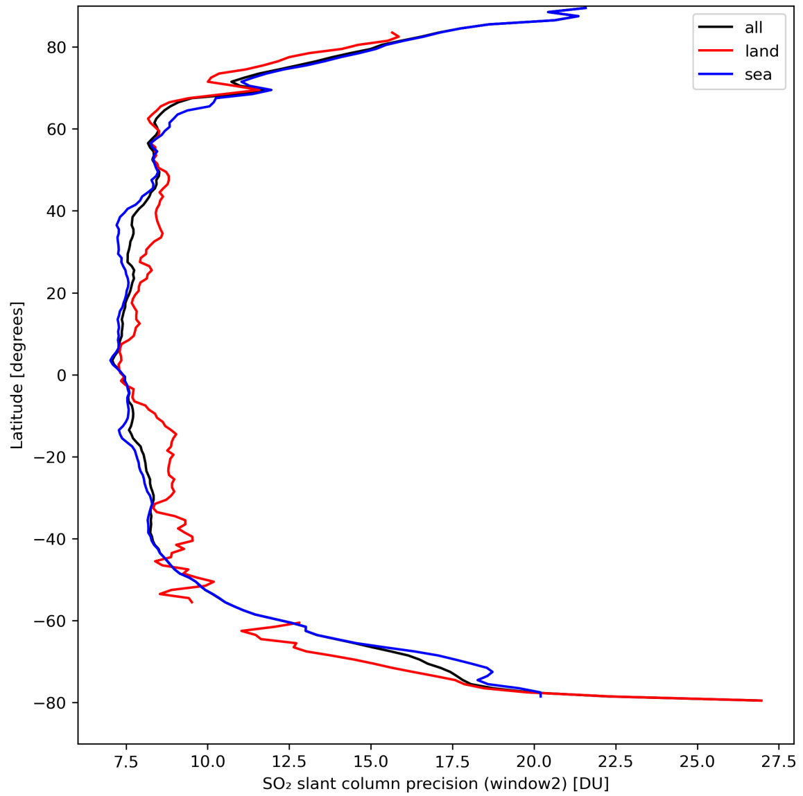
Figure 38: Zonal average of “SO 2 slant column precision (window2)” for 2024-04-02 to 2024-04-04.
