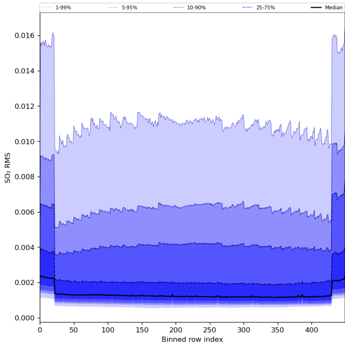
Figure 93: Along track statistics of “SO 2 RMS” for 2024-04-02 to 2024-04-04
