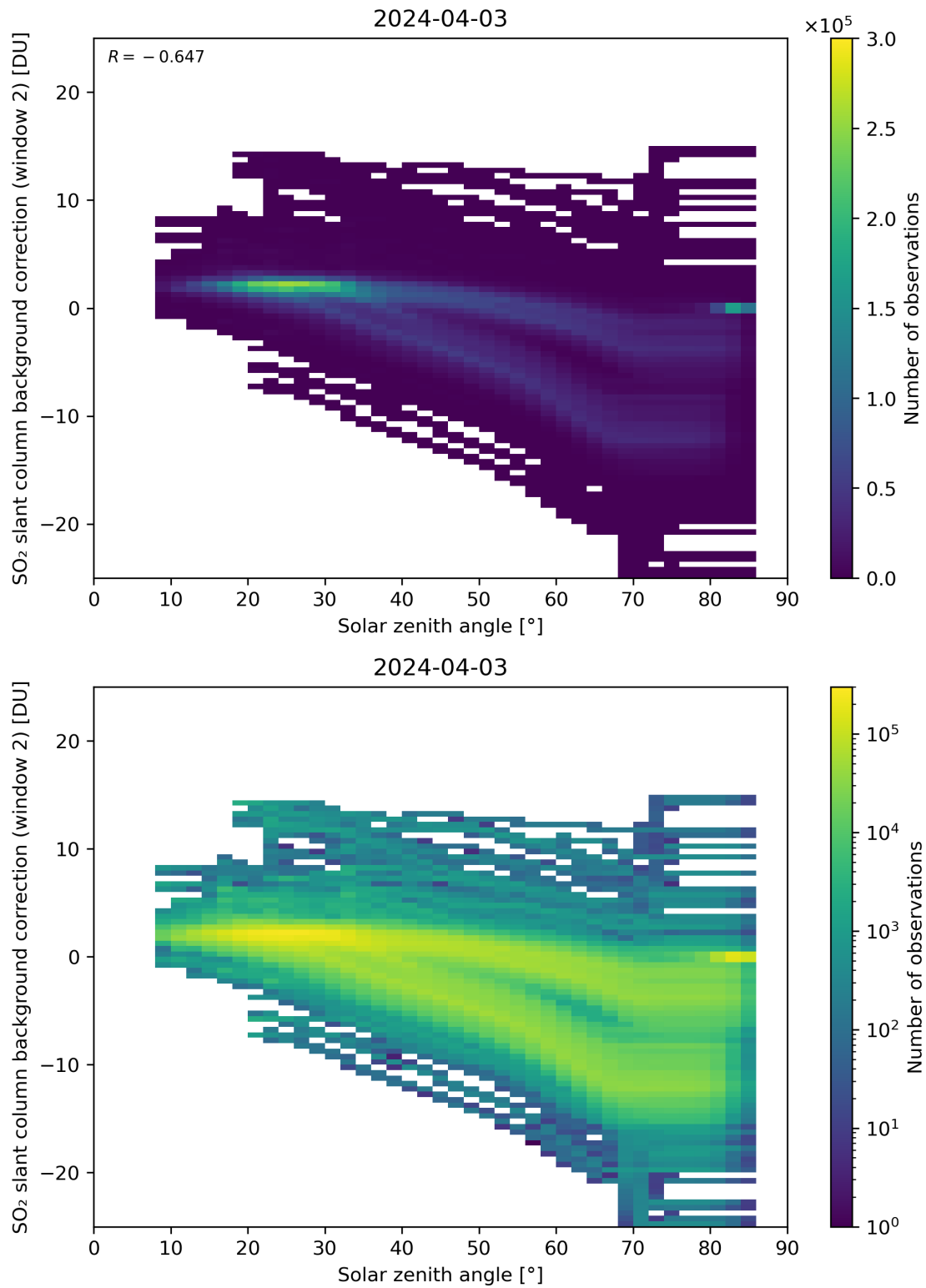
Figure 159: Scatter density plot of “Solar zenith angle” against “SO 2 slant column background correction (window 2)” for 2024-04-02 to 2024-04-04.
