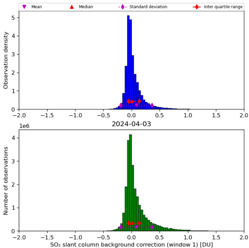
Figure 59: Histogram of “SO 2 slant column background correction (window 1)” for 2024-04-02 to 2024-04-04
