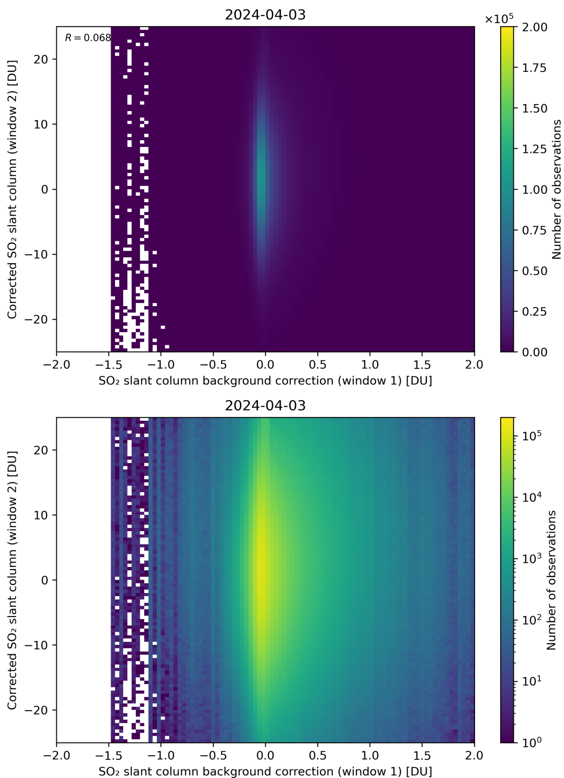
Figure 104: Scatter density plot of “SO 2 slant column background correction (window 1)” against “Corrected SO 2 slant column (window 2)” for 2024-04-02 to 2024-04-04.
