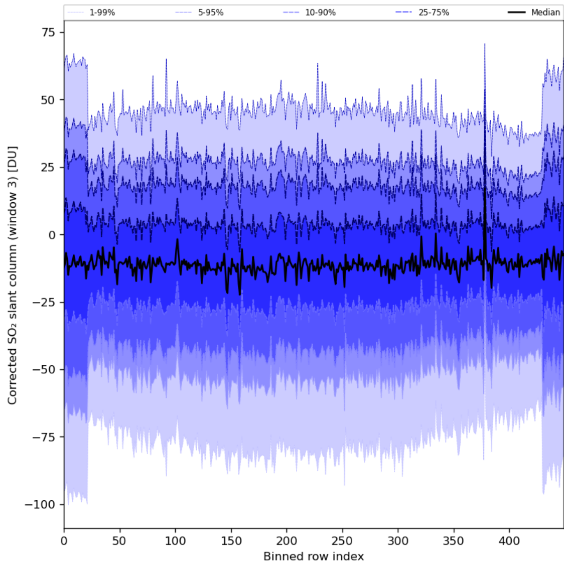
Figure 89: Along track statistics of “Corrected SO 2 slant column (window 3)” for 2024-04-02 to 2024-04-04
