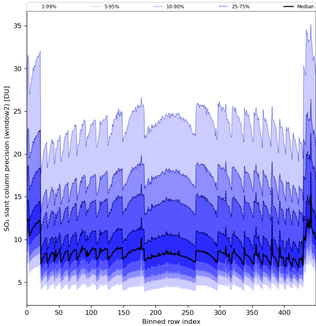
Figure 84: Along track statistics of “SO 2 slant column precision (window2)” for 2024-04-02 to 2024-04-04
