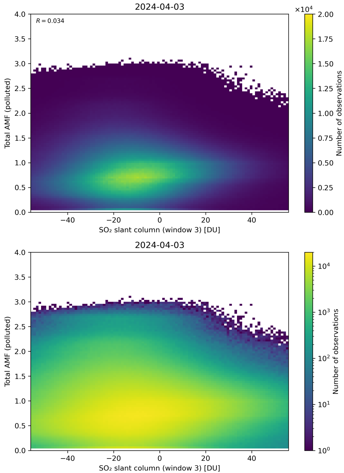
Figure 268: Scatter density plot of “SO 2 slant column (window 3)” against “Total AMF (polluted)” for 2024-04-02 to 2024-04-04.
