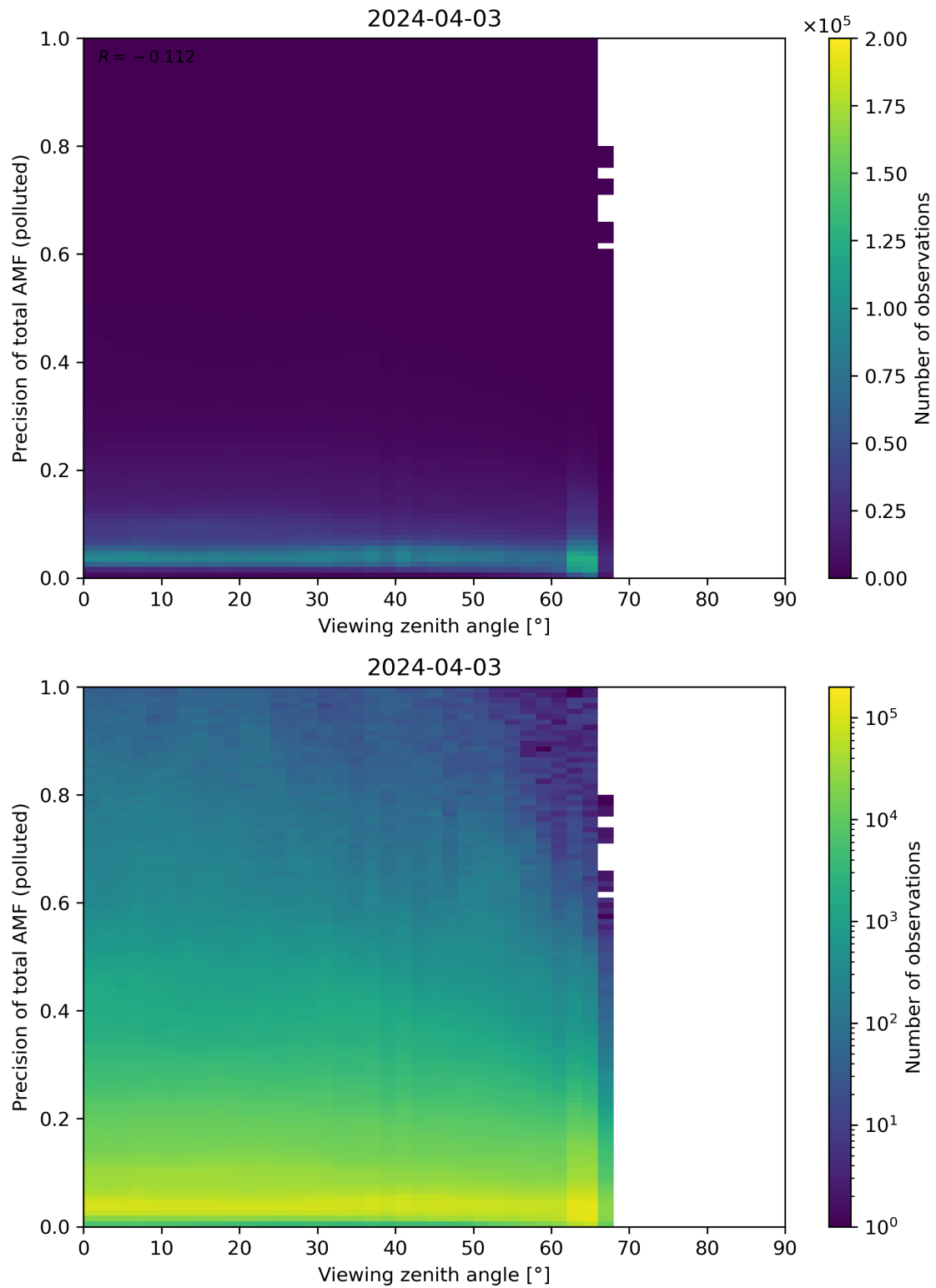
Figure 326: Scatter density plot of “Viewing zenith angle” against “Precision of total AMF (polluted)” for 2024-04-02 to 2024-04-04.
