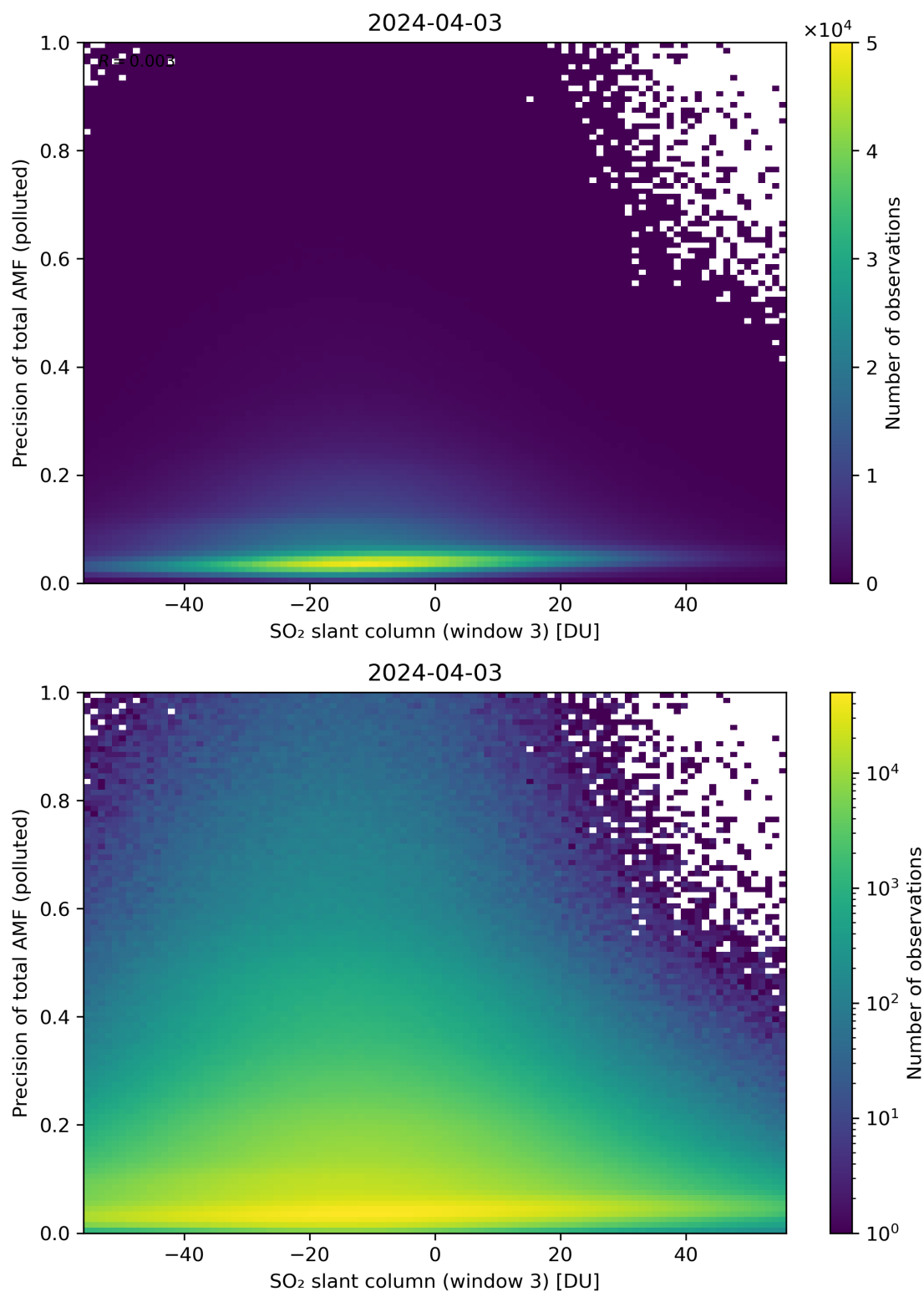
Figure 269: Scatter density plot of “SO 2 slant column (window 3)” against “Precision of total AMF (polluted)” for 2024-04-02 to 2024-04-04.
