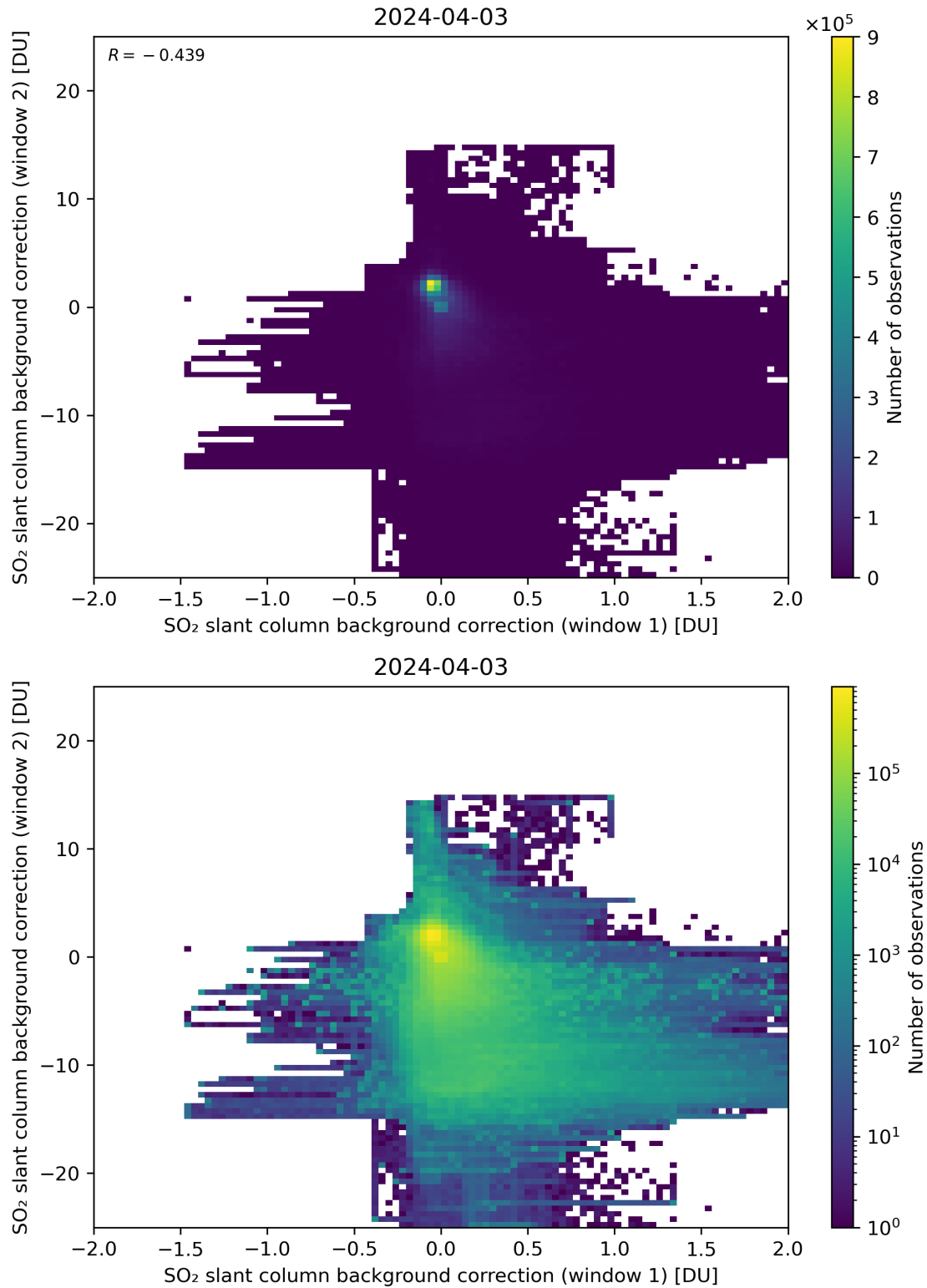
Figure 98: Scatter density plot of “SO 2 slant column background correction (window 1)” against “SO 2 slant column background correction (window 2)” for 2024-04-02 to 2024-04-04.
