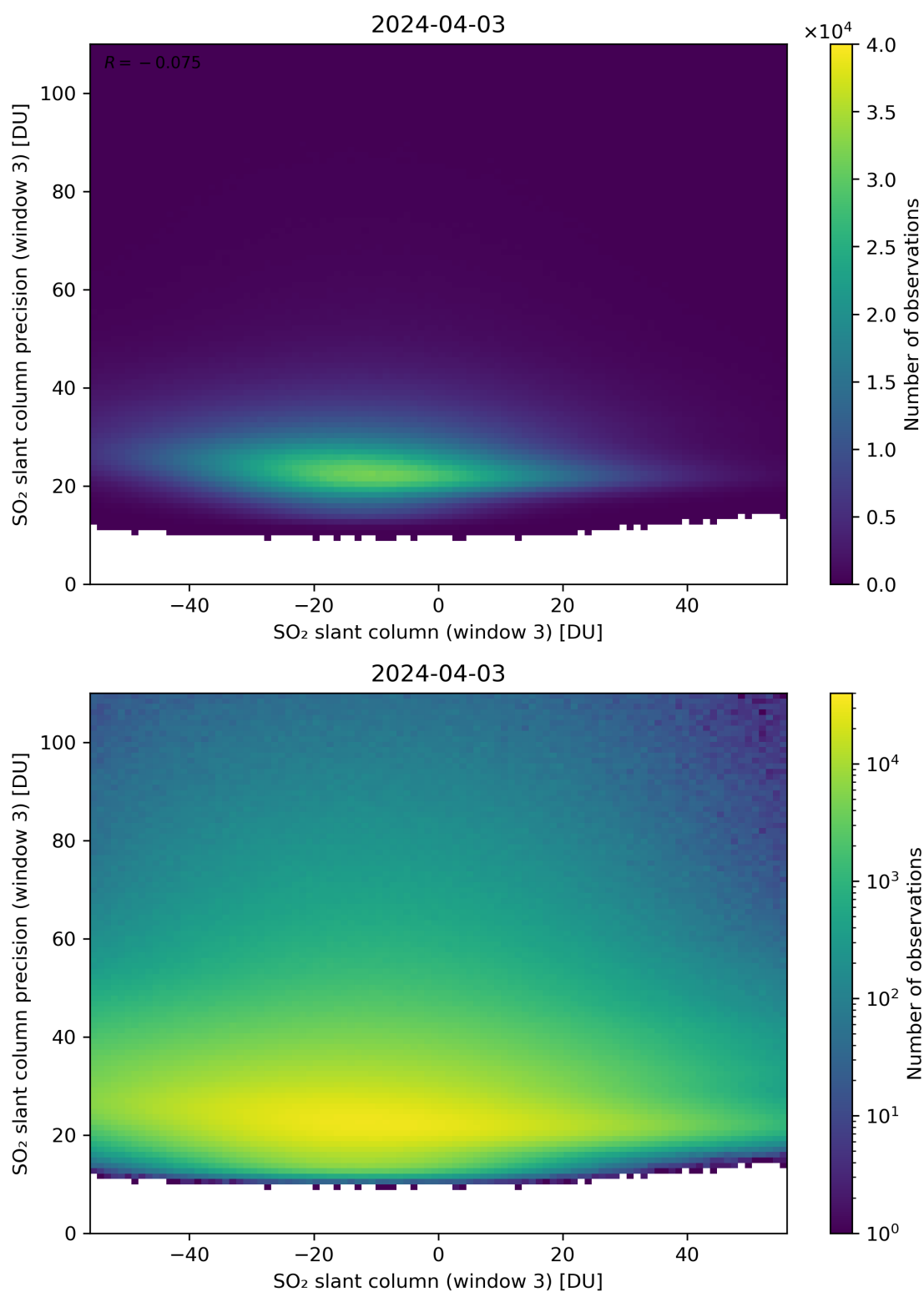
Figure 267: Scatter density plot of “SO 2 slant column (window 3)” against “SO 2 slant column precision (window 3)” for 2024-04-02 to 2024-04-04.
