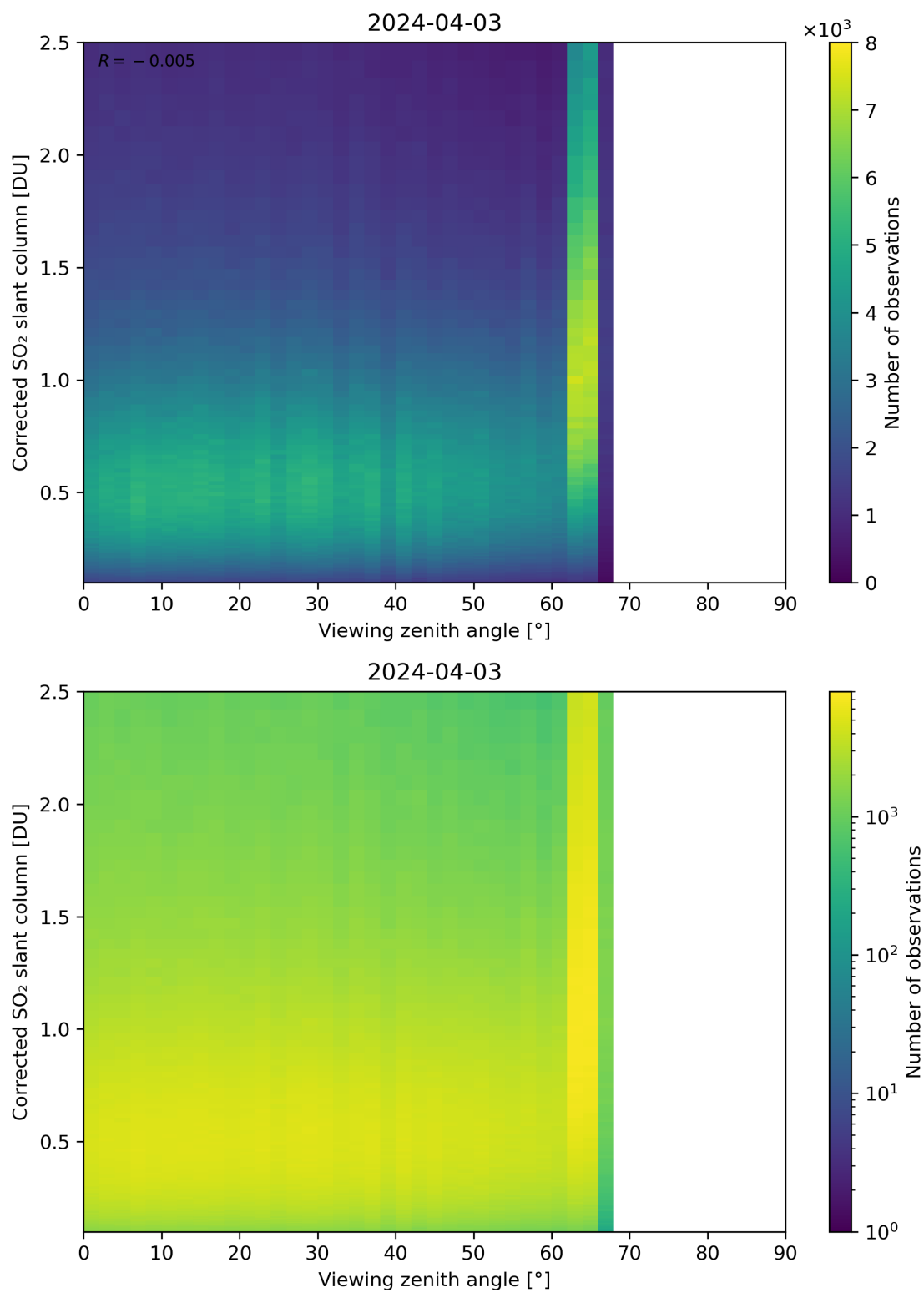
Figure 317: Scatter density plot of “Viewing zenith angle” against “Corrected SO 2 slant column” for 2024-04-02 to 2024-04-04.
