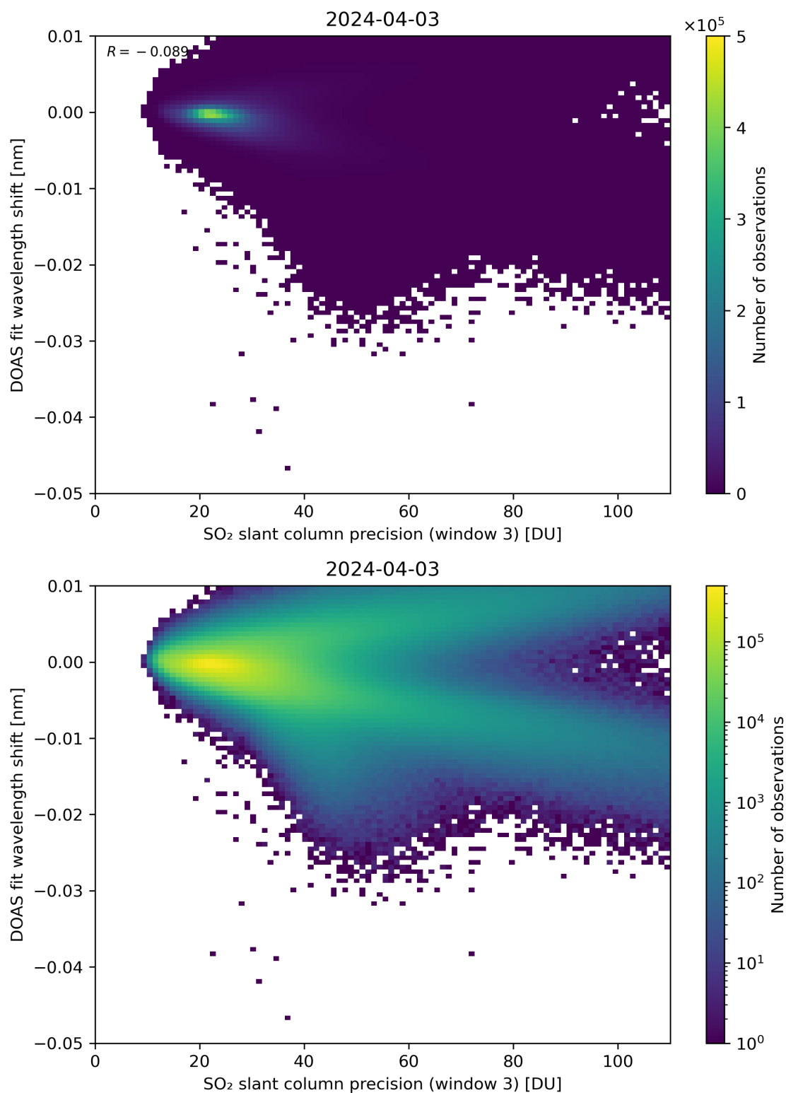
Figure 258: Scatter density plot of “SO 2 slant column precision (window 3)” against “DOAS fit wavelength shift” for 2024-04-02 to 2024-04-04.
