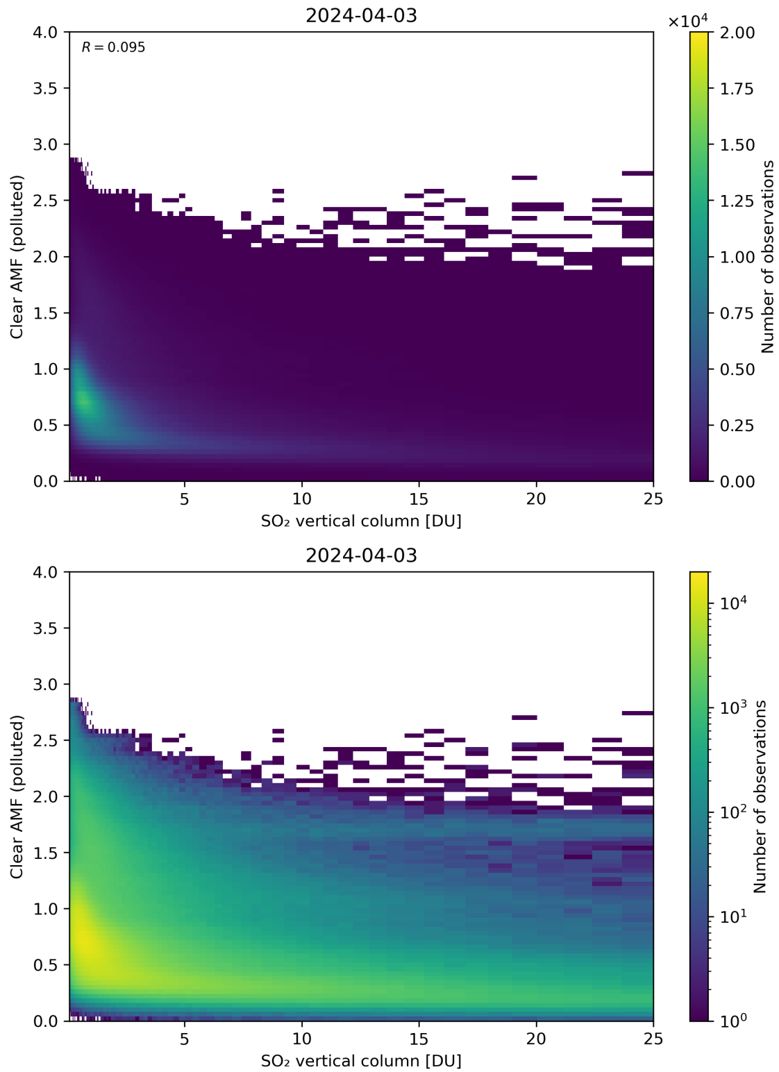
Figure 296: Scatter density plot of “SO 2 vertical column” against “Clear AMF (polluted)” for 2024-04-02 to 2024-04-04.
