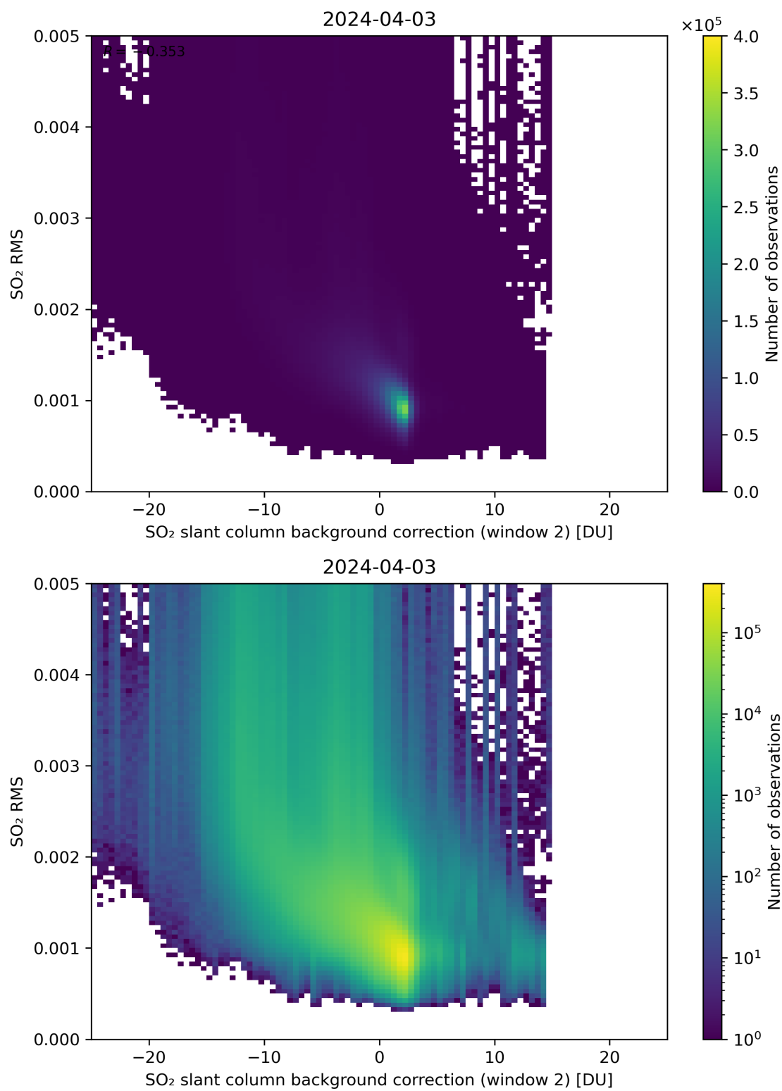
Figure 114: Scatter density plot of “SO 2 slant column background correction (window 2)” against “SO 2 RMS” for 2024-04-02 to 2024-04-04.
