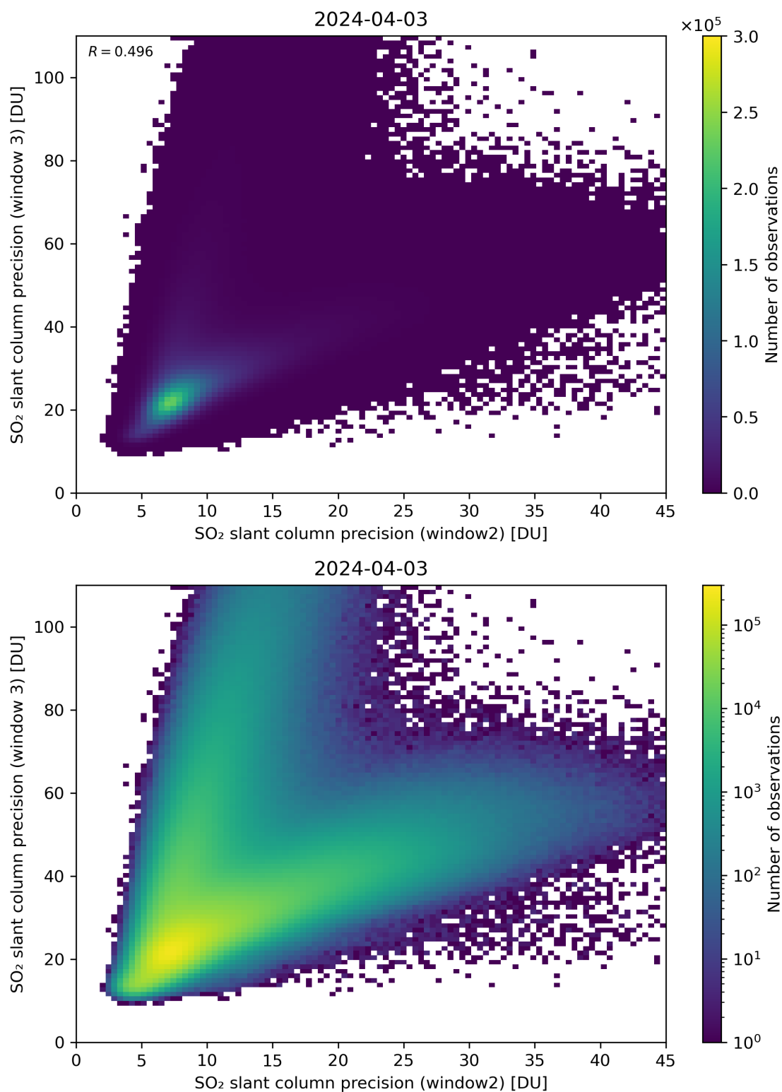
Figure 250: Scatter density plot of “SO 2 slant column precision (window2)” against “SO 2 slant column precision (window 3)” for 2024-04-02 to 2024-04-04.
