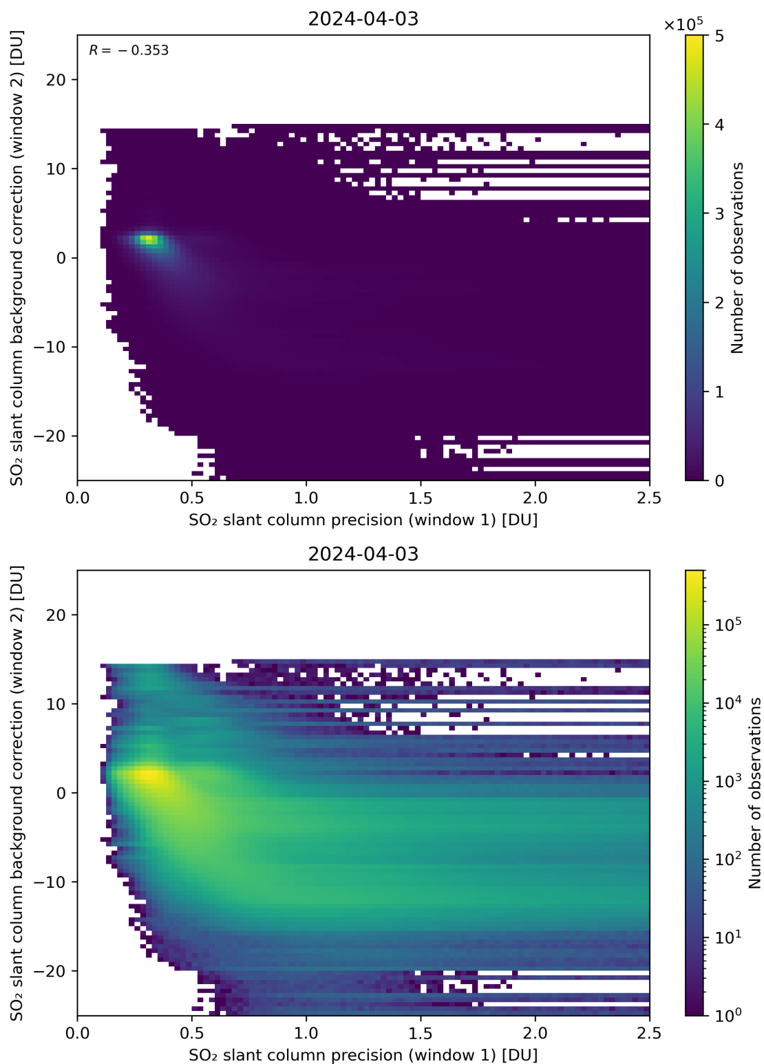
Figure 219: Scatter density plot of “SO 2 slant column precision (window 1)” against “SO 2 slant column background correction (window 2)” for 2024-04-02 to 2024-04-04.
