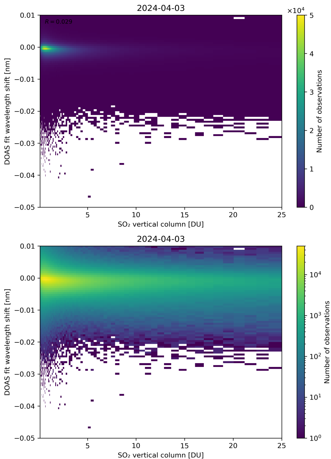
Figure 276: Scatter density plot of “SO 2 vertical column” against “DOAS fit wavelength shift” for 2024-04-02 to 2024-04-04.
