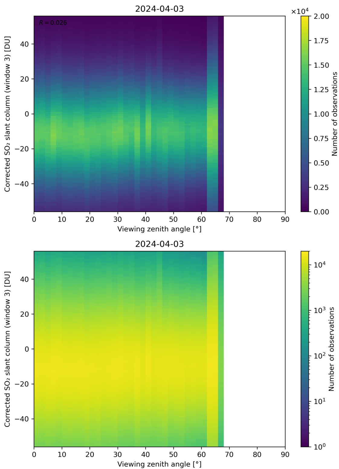
Figure 319: Scatter density plot of “Viewing zenith angle” against “Corrected SO 2 slant column (window 3)” for 2024-04-02 to 2024-04-04.
