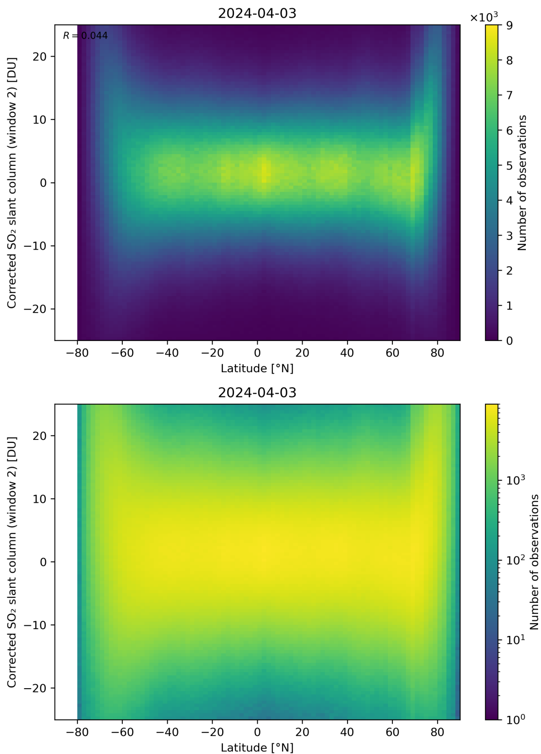
Figure 147: Scatter density plot of “Latitude” against “Corrected SO 2 slant column (window 2)” for 2024-04-02 to 2024-04-04.
