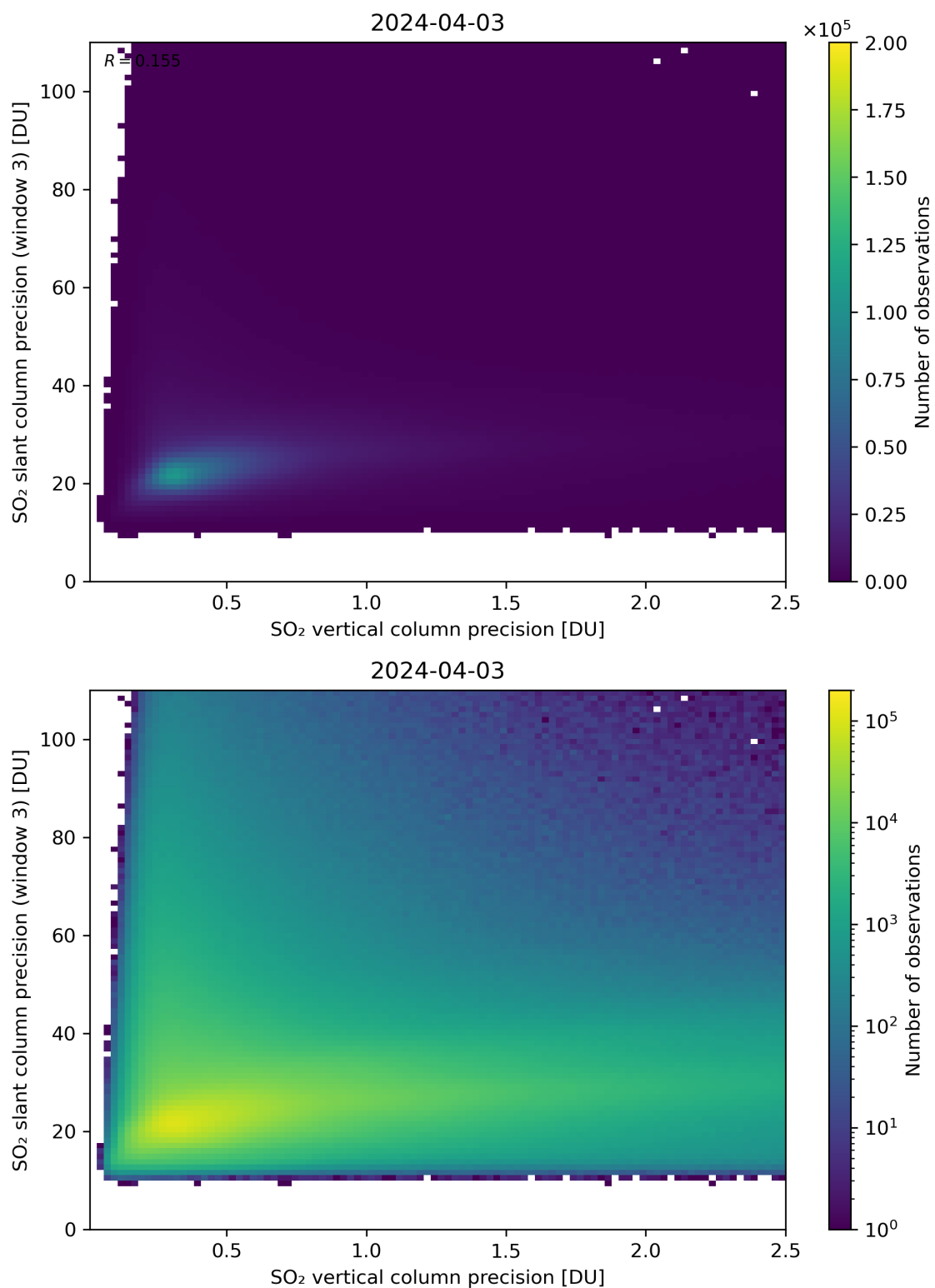
Figure 293: Scatter density plot of “SO 2 vertical column precision” against “SO 2 slant column precision (window 3)” for 2024-04-02 to 2024-04-04.
