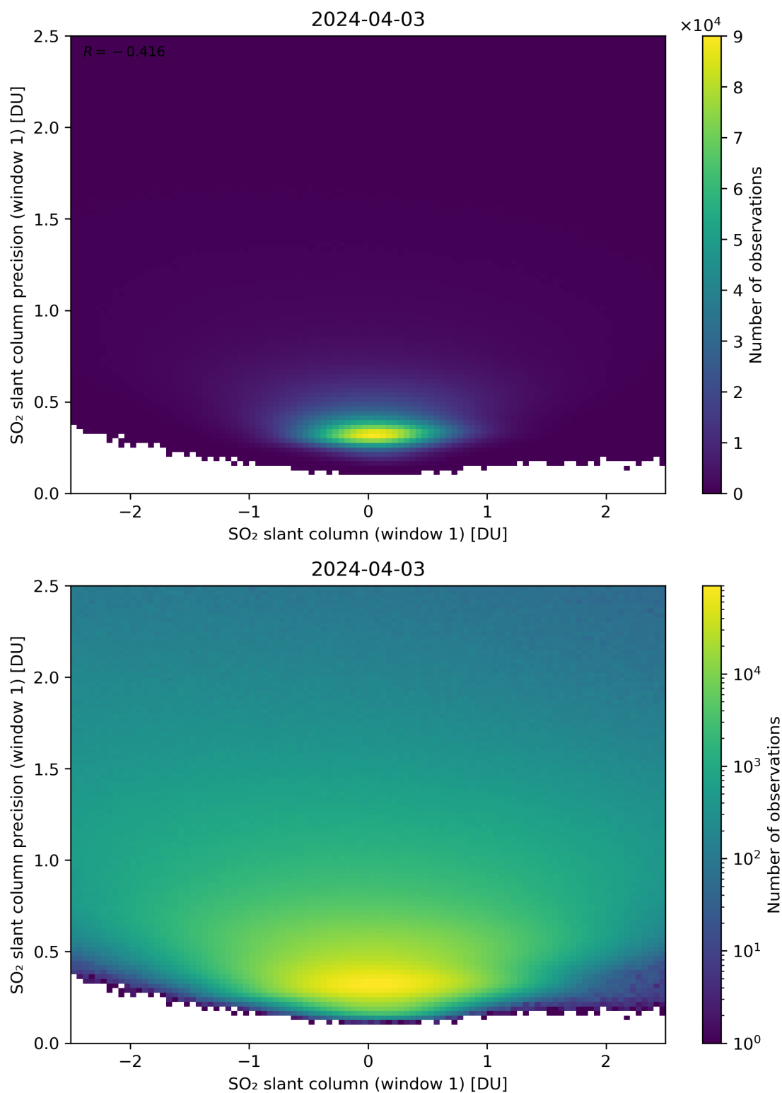
Figure 235: Scatter density plot of “SO 2 slant column (window 1)” against “SO 2 slant column precision (window 1)” for 2024-04-02 to 2024-04-04.
