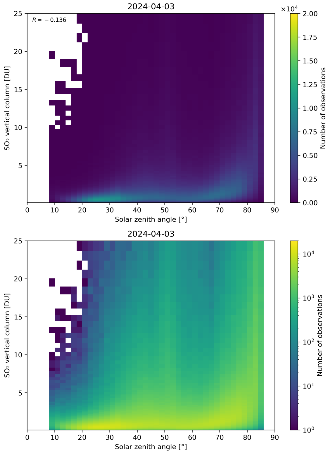
Figure 176: Scatter density plot of “Solar zenith angle” against “SO 2 vertical column” for 2024-04-02 to 2024-04-04.
