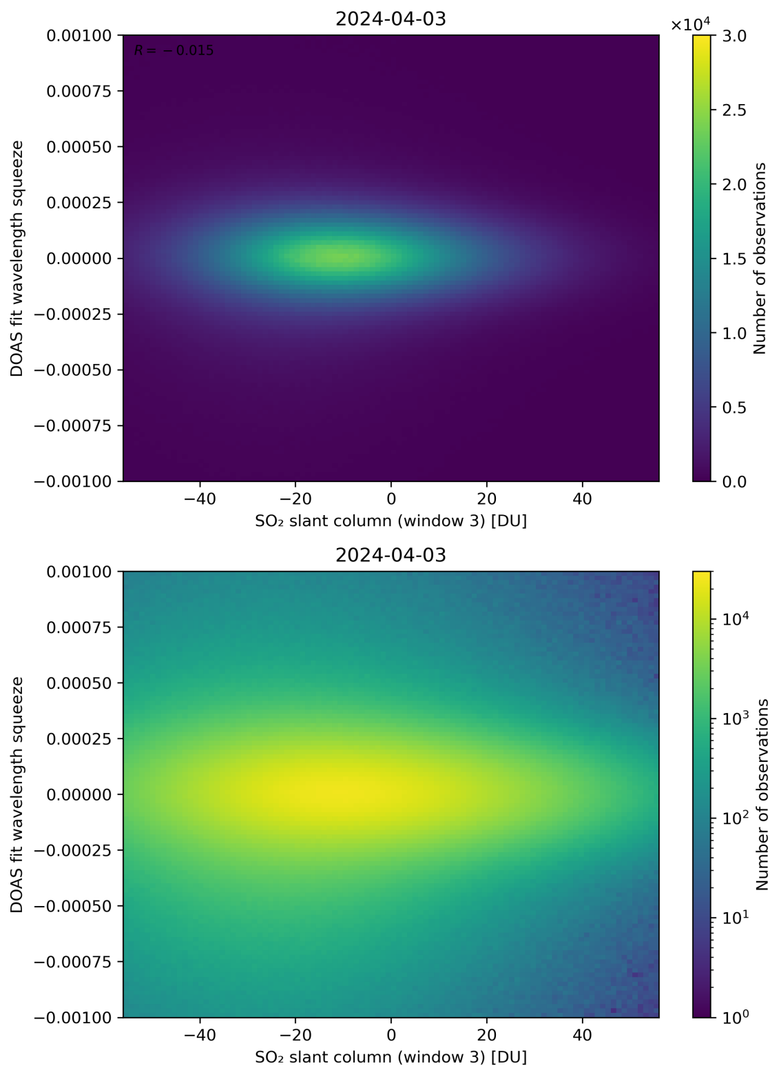
Figure 255: Scatter density plot of “SO 2 slant column (window 3)” against “DOAS fit wavelength squeeze” for 2024-04-02 to 2024-04-04.
