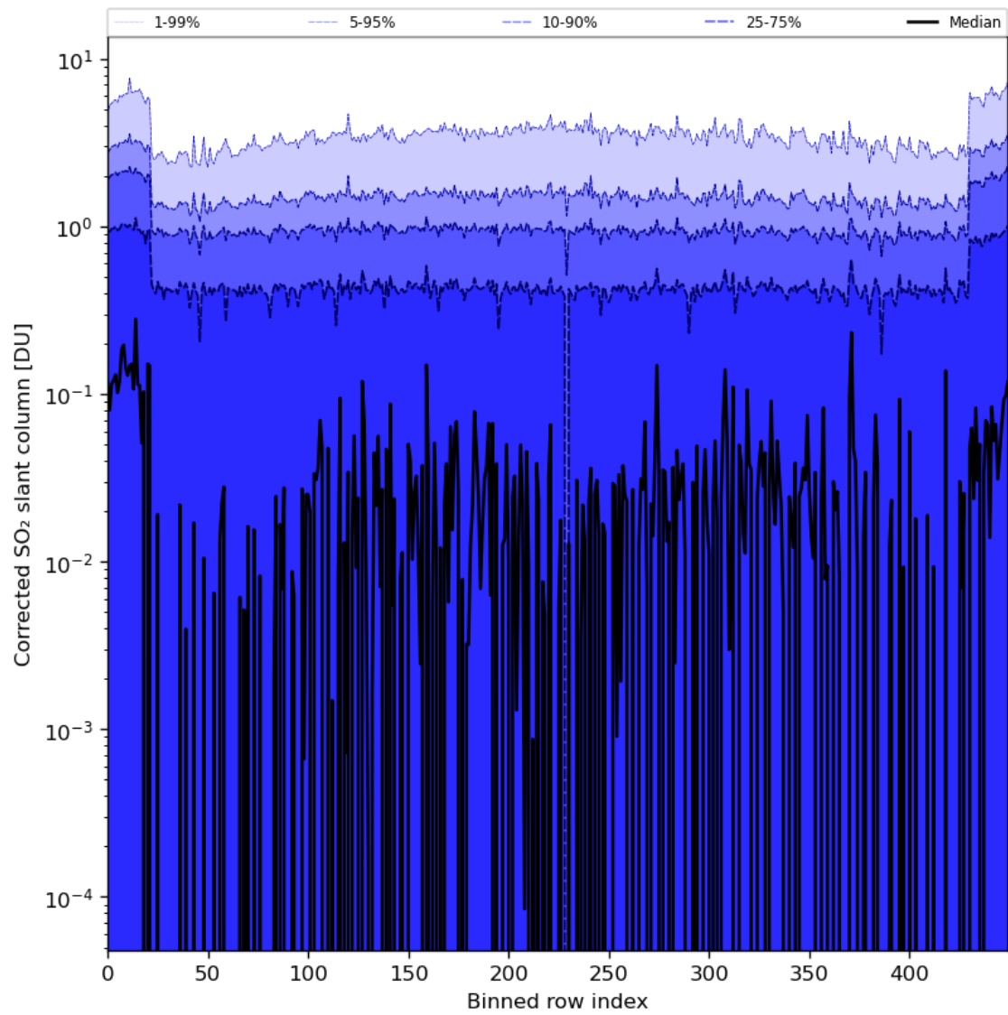
Figure 78: Along track statistics of “Corrected SO 2 slant column” for 2024-04-02 to 2024-04-04
