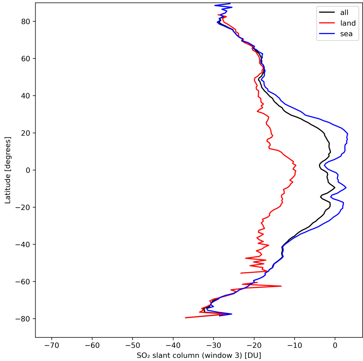
Figure 41: Zonal average of “SO 2 slant column (window 3)” for 2024-04-02 to 2024-04-04.
