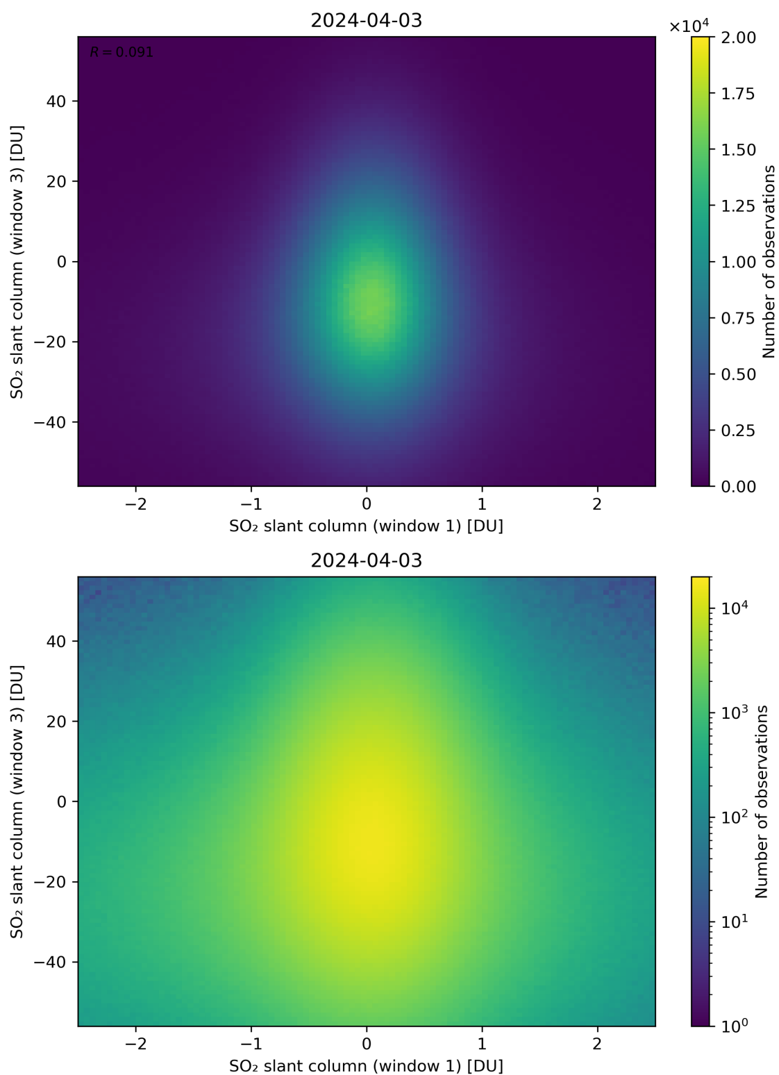
Figure 237: Scatter density plot of “SO 2 slant column (window 1)” against “SO 2 slant column (window 3)” for 2024-04-02 to 2024-04-04.
