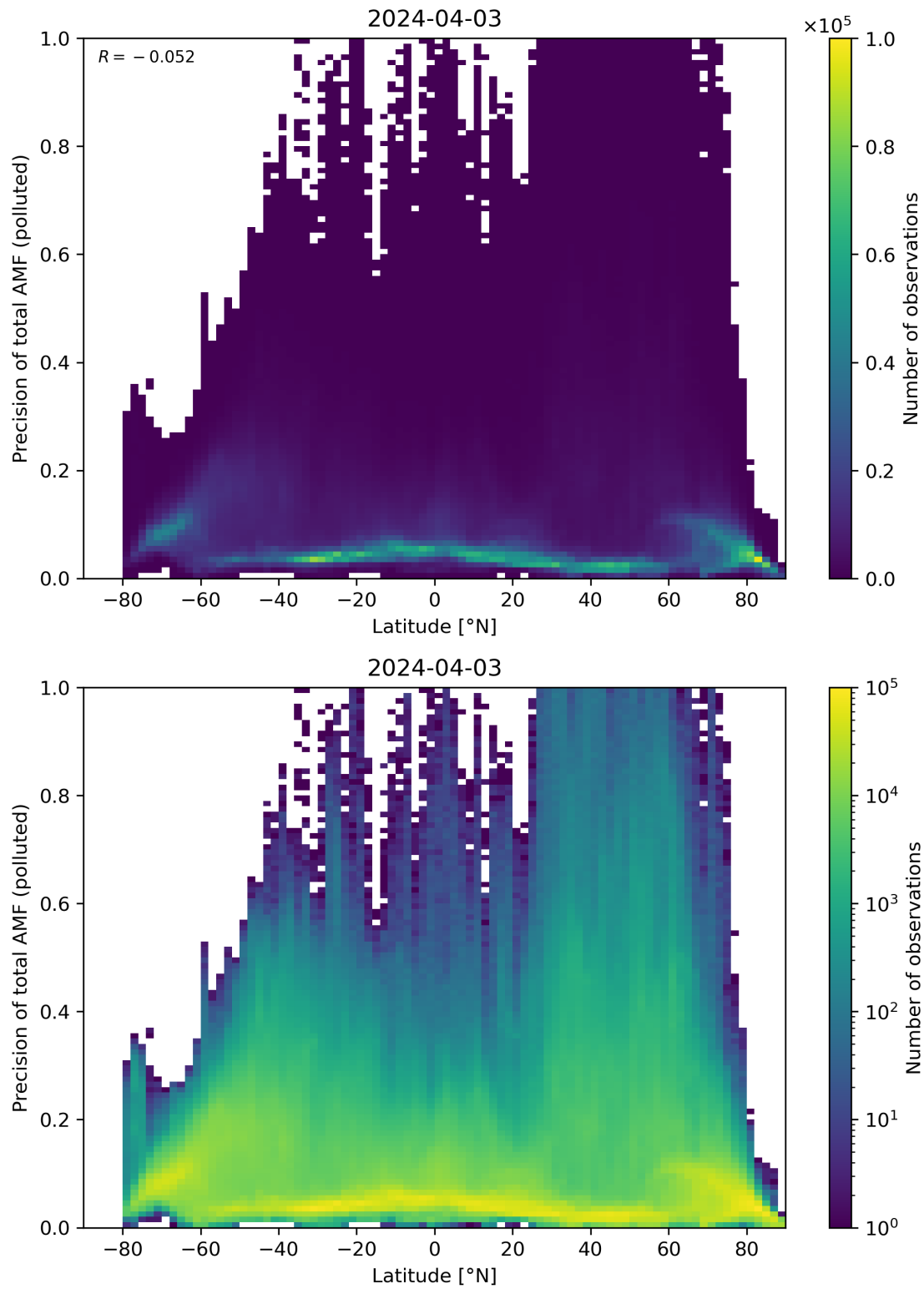
Figure 155: Scatter density plot of “Latitude” against “Precision of total AMF (polluted)” for 2024-04-02 to 2024-04-04.
