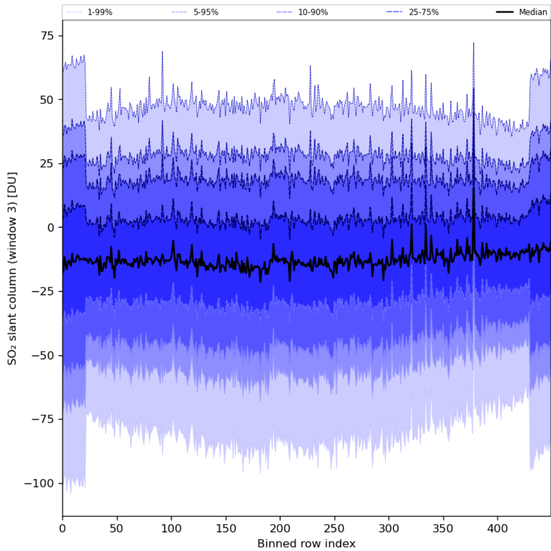
Figure 87: Along track statistics of “SO 2 slant column (window 3)” for 2024-04-02 to 2024-04-04
