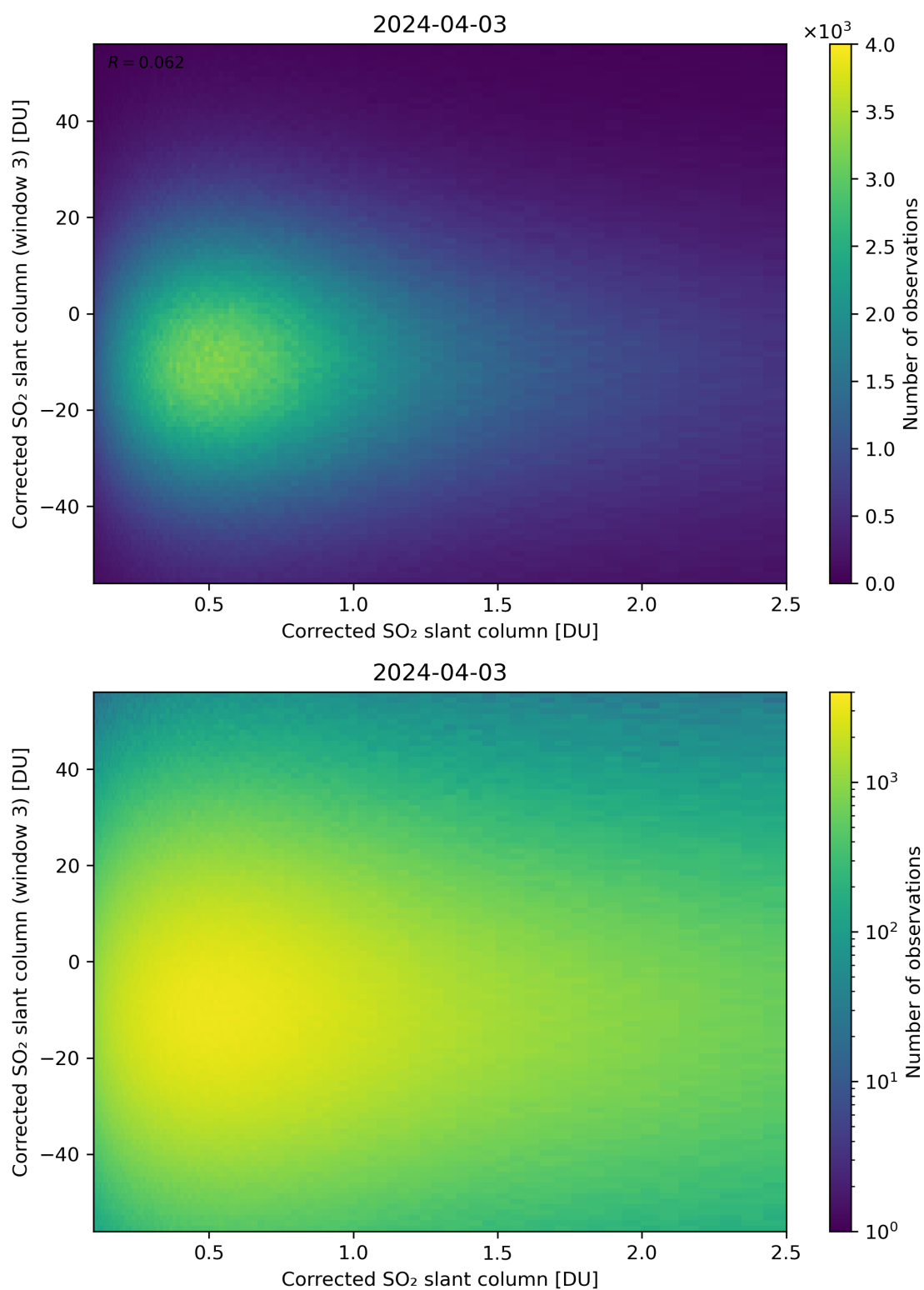
Figure 186: Scatter density plot of “Corrected SO 2 slant column” against “Corrected SO 2 slant column (window 3)” for 2024-04-02 to 2024-04-04.
