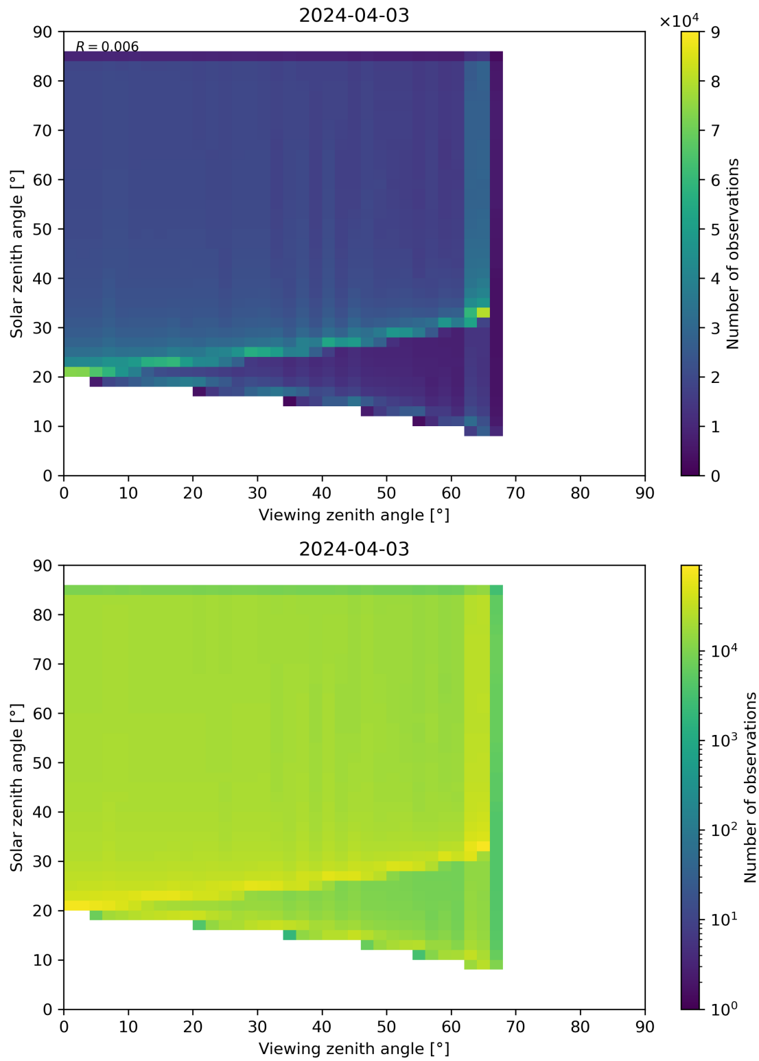
Figure 315: Scatter density plot of “Viewing zenith angle” against “Solar zenith angle” for 2024-04-02 to 2024-04-04.
