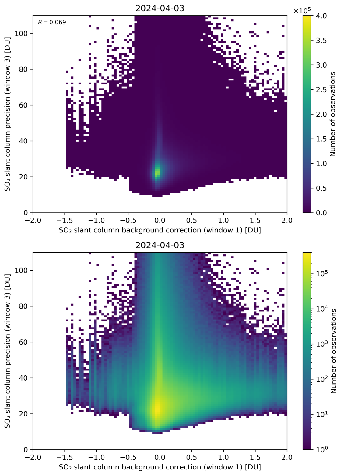
Figure 108: Scatter density plot of “SO 2 slant column background correction (window 1)” against “SO 2 slant column precision (window 3)” for 2024-04-02 to 2024-04-04.
