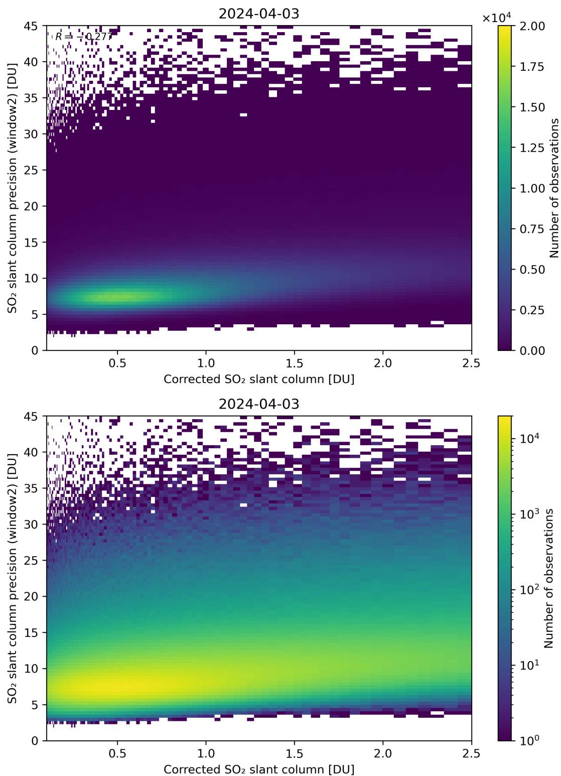
Figure 189: Scatter density plot of “Corrected SO 2 slant column” against “SO 2 slant column precision (window2)” for 2024-04-02 to 2024-04-04.
