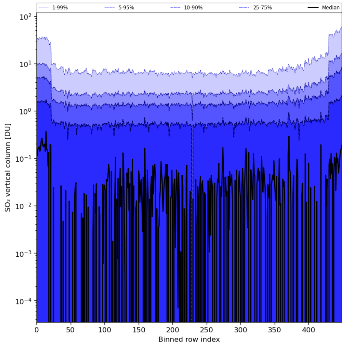
Figure 76: Along track statistics of “SO 2 vertical column” for 2024-04-02 to 2024-04-04
