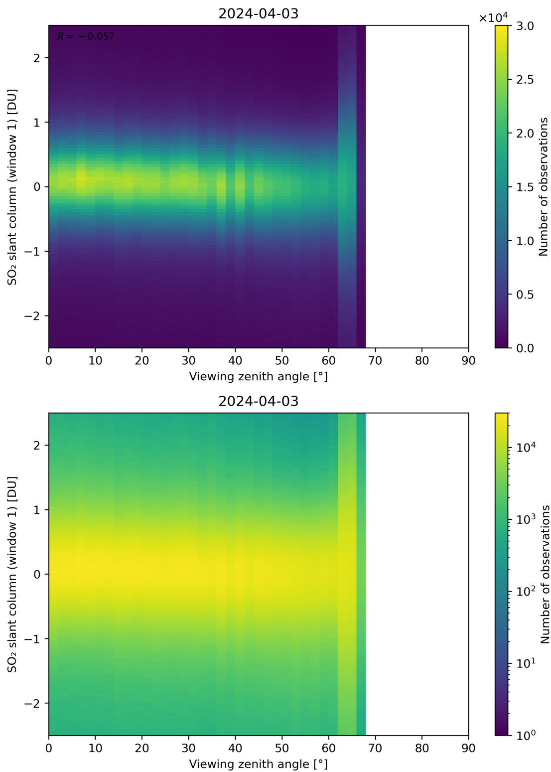
Figure 320: Scatter density plot of “Viewing zenith angle” against “SO 2 slant column (window 1)” for 2024-04-02 to 2024-04-04.
