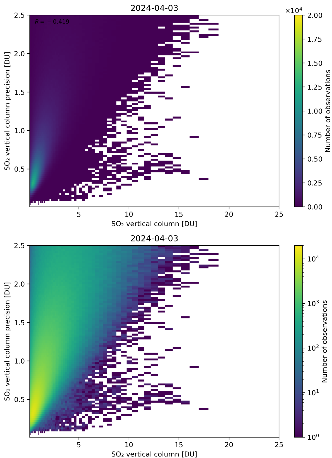
Figure 307: Scatter density plot of “SO 2 vertical column” against “SO 2 vertical column precision” for 2024-04-02 to 2024-04-04.
