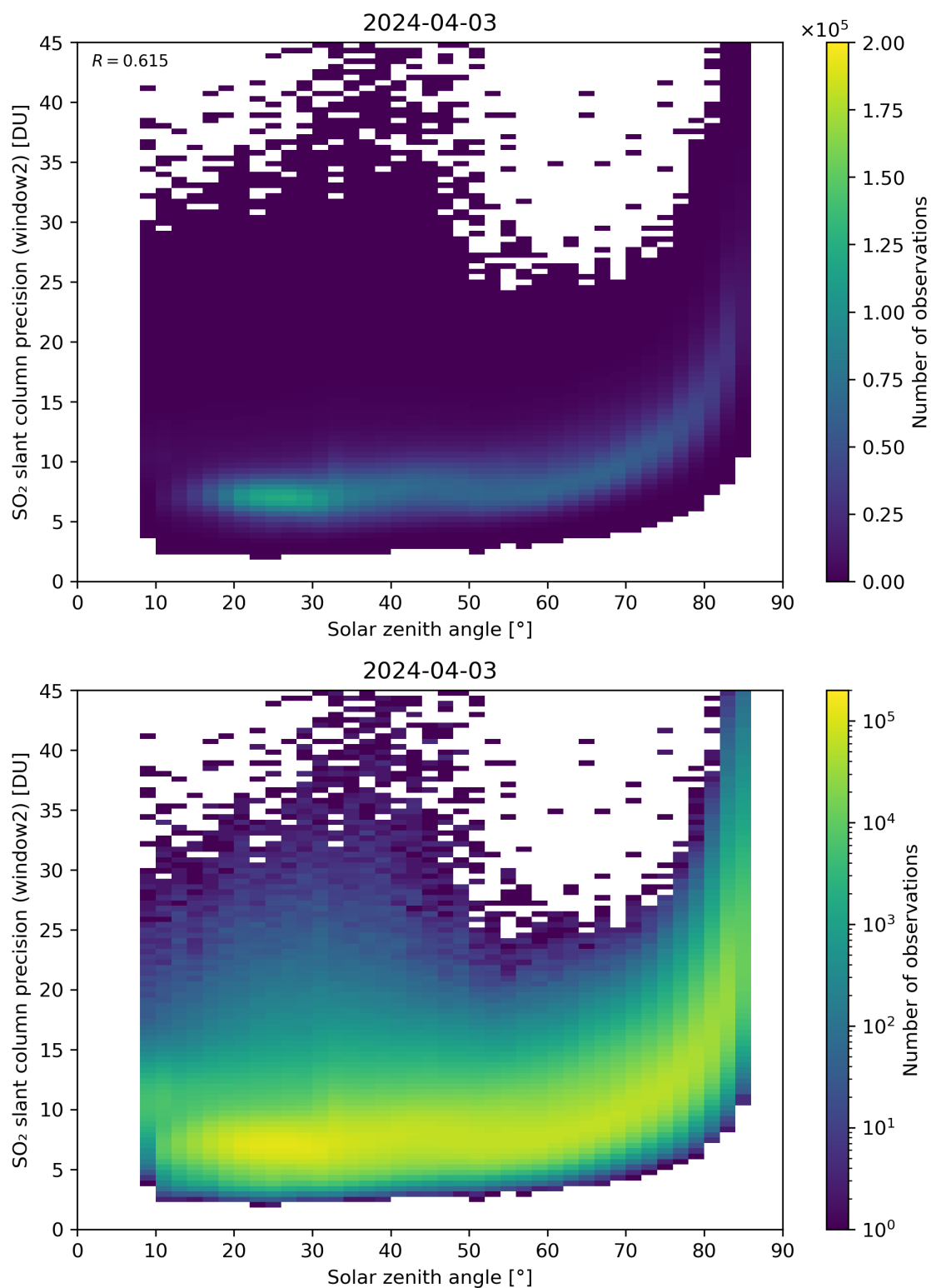
Figure 171: Scatter density plot of “Solar zenith angle” against “SO 2 slant column precision (window2)” for 2024-04-02 to 2024-04-04.
