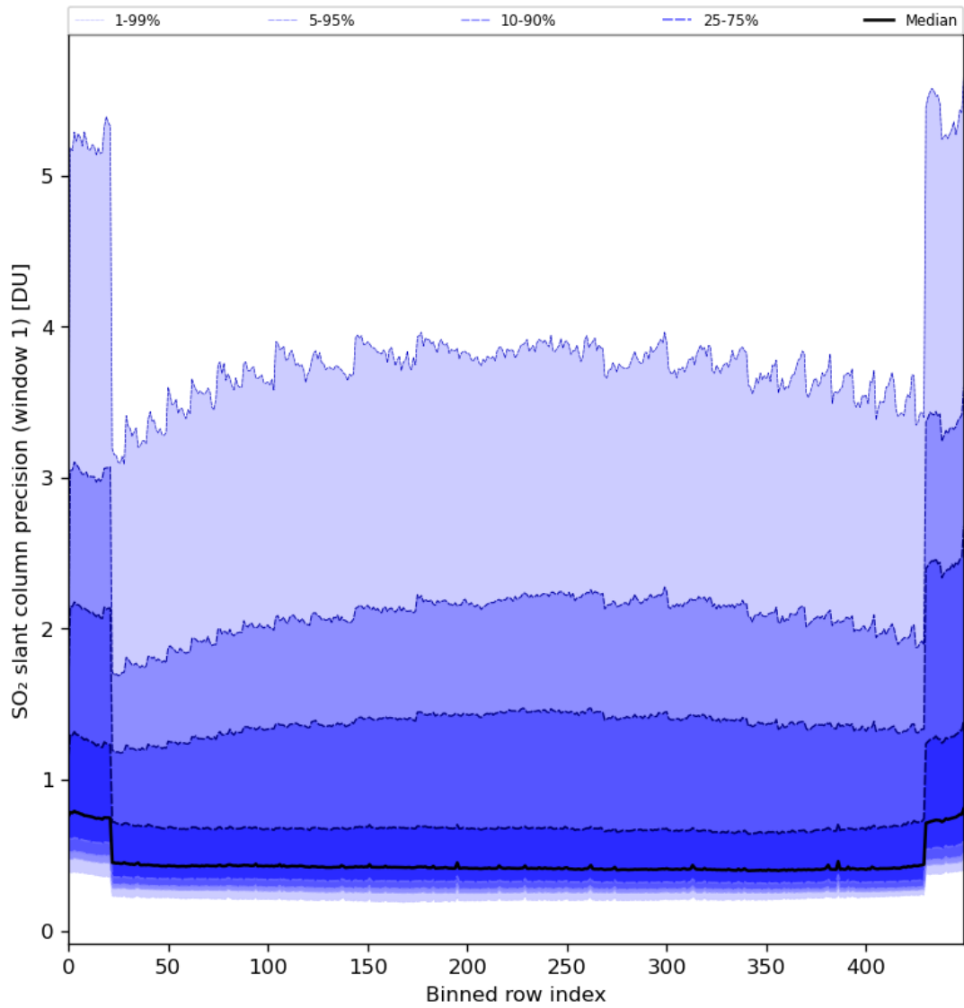
Figure 80: Along track statistics of “SO 2 slant column precision (window 1)” for 2024-04-02 to 2024-04-04
