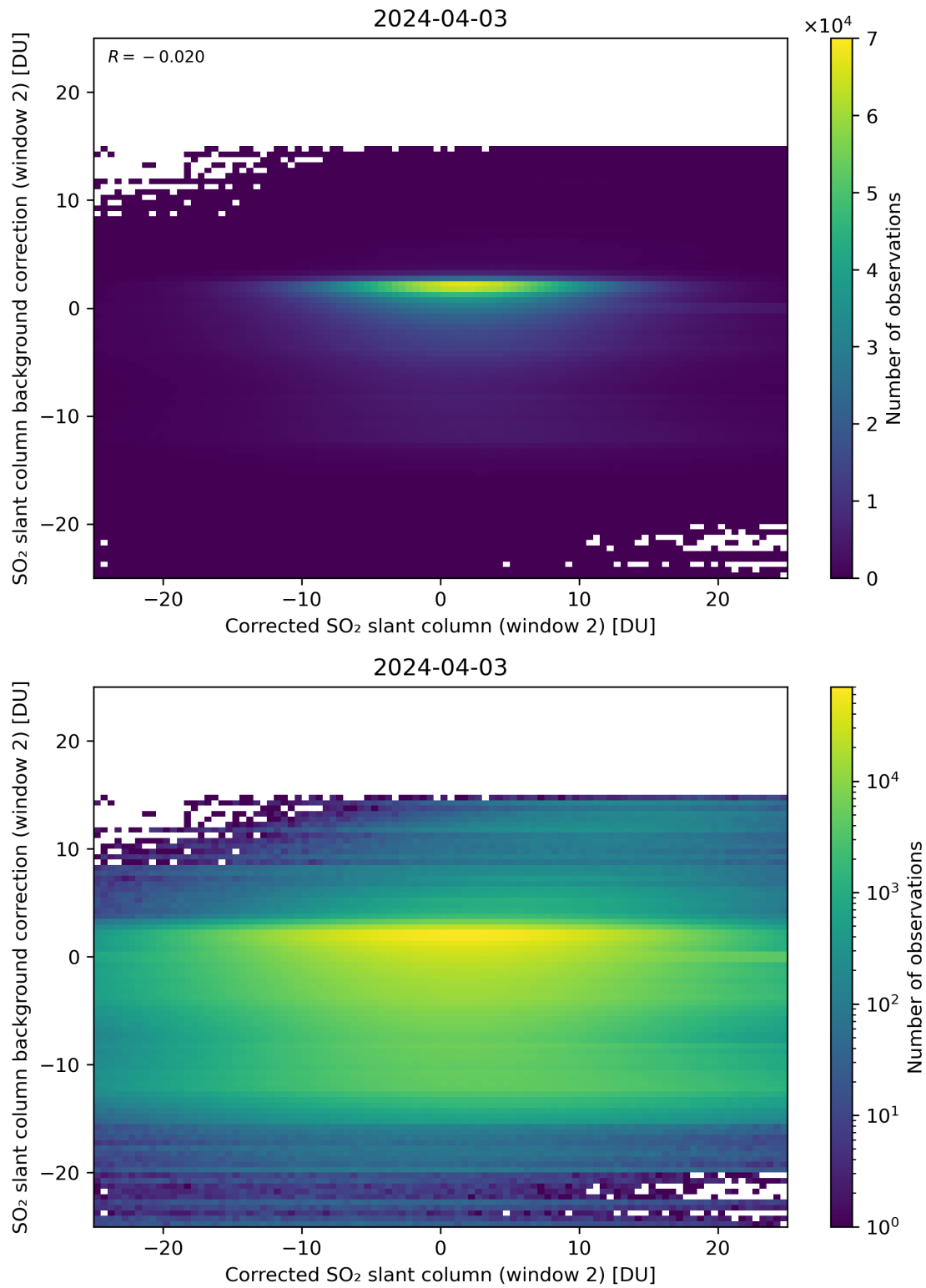
Figure 194: Scatter density plot of “Corrected SO 2 slant column (window 2)” against “SO 2 slant column background correction (window 2)” for 2024-04-02 to 2024-04-04.
