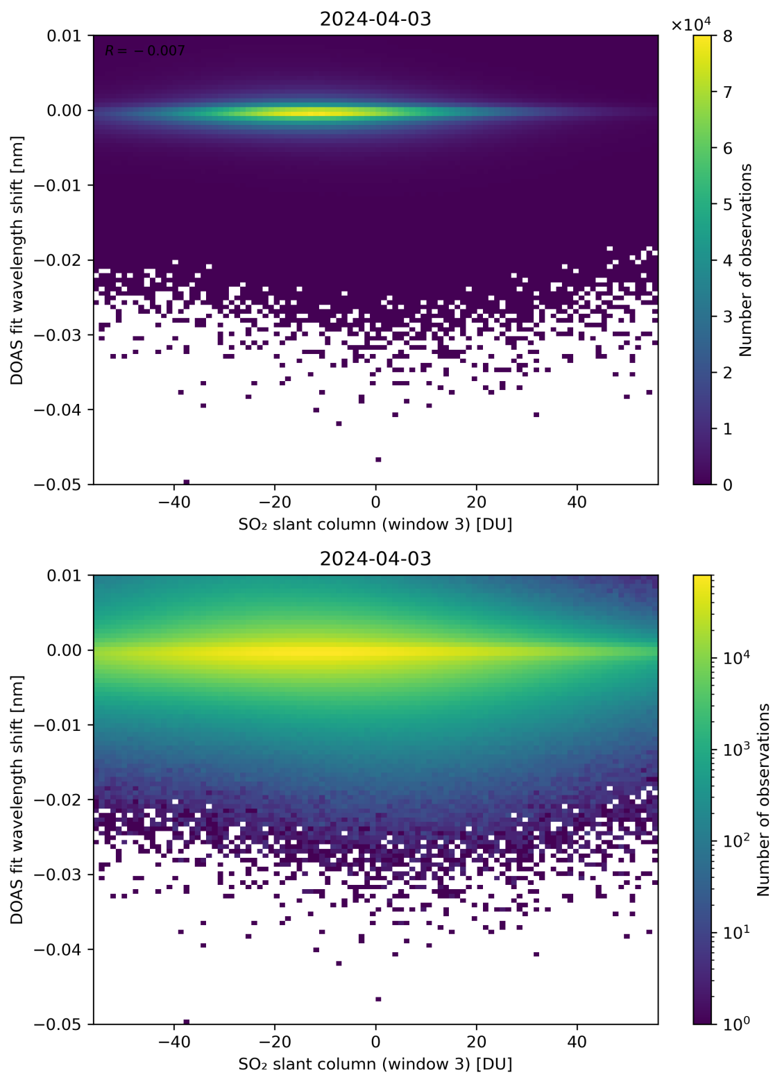
Figure 254: Scatter density plot of “SO 2 slant column (window 3)” against “DOAS fit wavelength shift” for 2024-04-02 to 2024-04-04.
