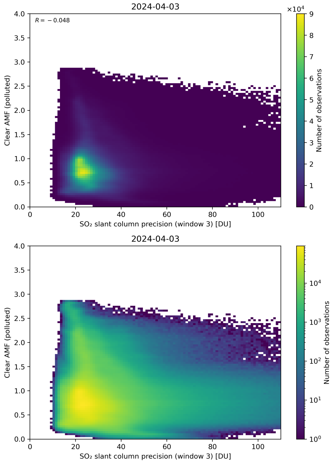
Figure 261: Scatter density plot of “SO 2 slant column precision (window 3)” against “Clear AMF (polluted)” for 2024-04-02 to 2024-04-04.
