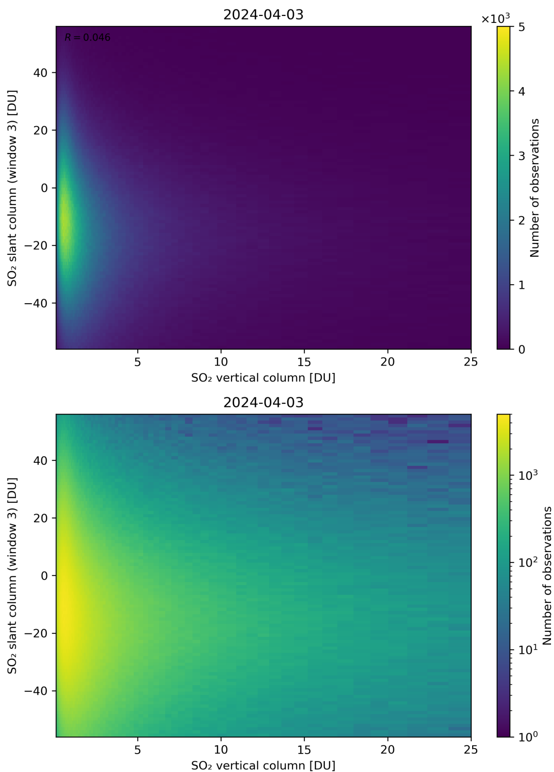
Figure 303: Scatter density plot of “SO 2 vertical column” against “SO 2 slant column (window 3)” for 2024-04-02 to 2024-04-04.
