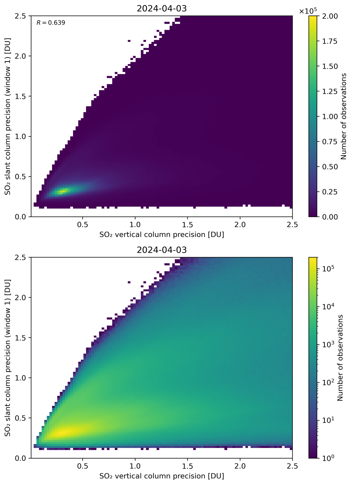
Figure 290: Scatter density plot of “SO 2 vertical column precision” against “SO 2 slant column precision (window 1)” for 2024-04-02 to 2024-04-04.
