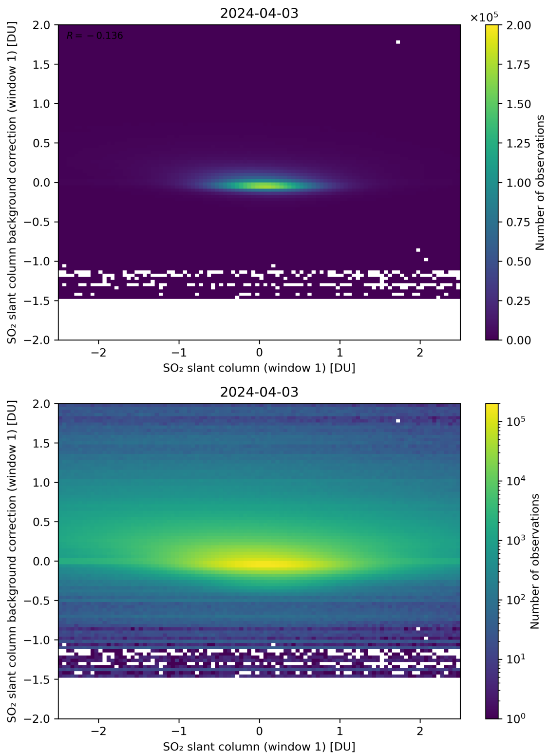
Figure 212: Scatter density plot of “SO 2 slant column (window 1)” against “SO 2 slant column background correction (window 1)” for 2024-04-02 to 2024-04-04.
