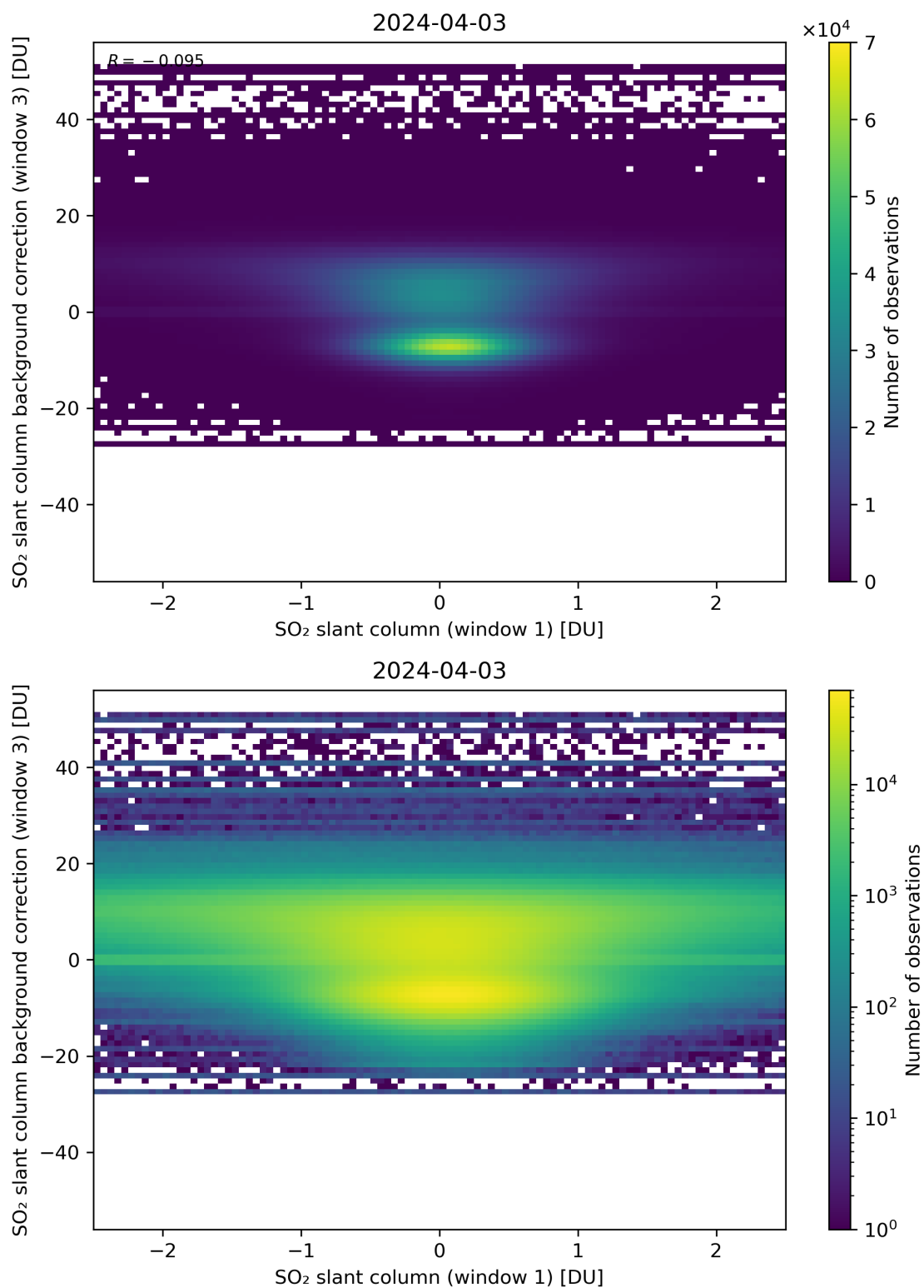
Figure 214: Scatter density plot of “SO 2 slant column (window 1)” against “SO 2 slant column background correction (window 3)” for 2024-04-02 to 2024-04-04.
