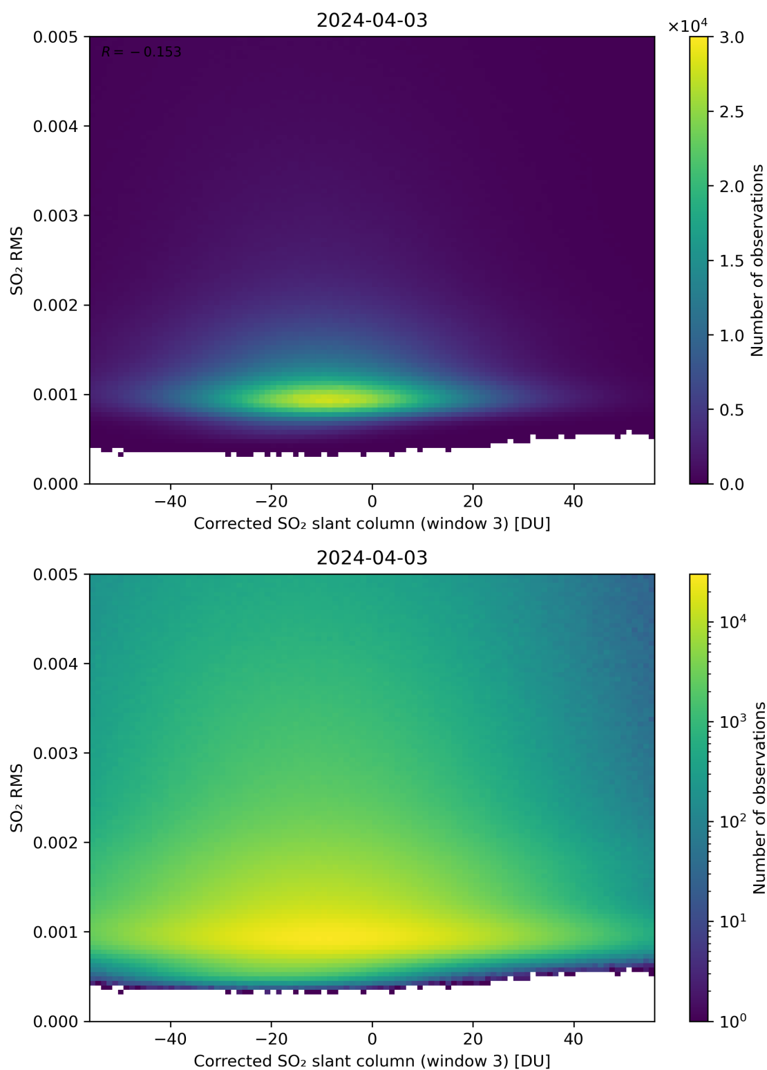
Figure 208: Scatter density plot of “Corrected SO 2 slant column (window 3)” against “SO 2 RMS” for 2024-04-02 to 2024-04-04.
