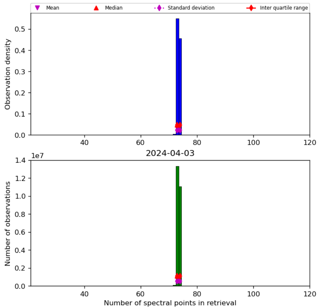
Figure 74: Histogram of “Number of spectral points in retrieval” for 2024-04-02 to 2024-04-04
