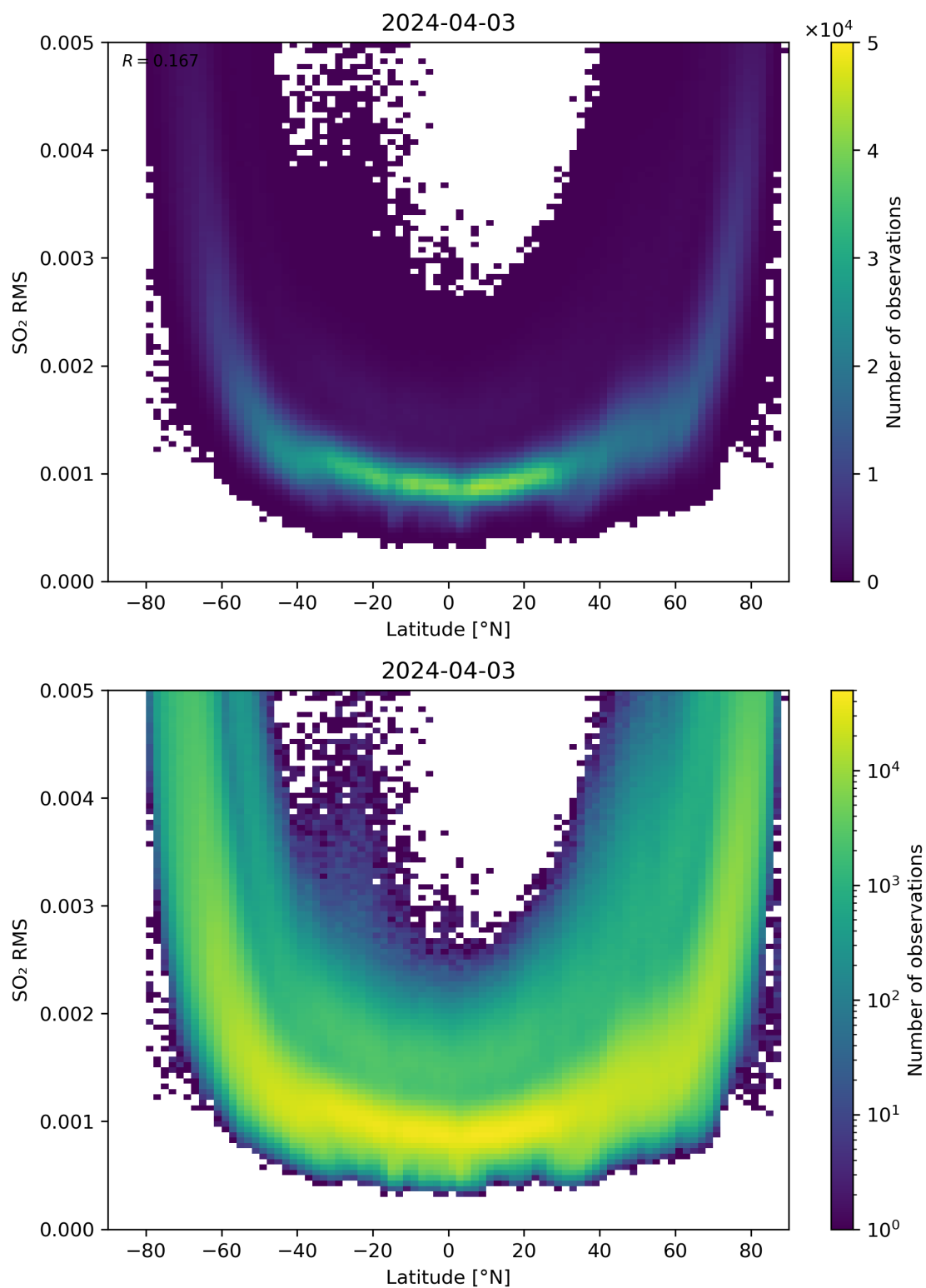
Figure 144: Scatter density plot of “Latitude” against “SO 2 RMS” for 2024-04-02 to 2024-04-04.
