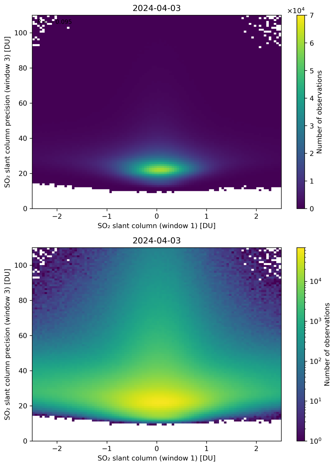
Figure 238: Scatter density plot of “SO 2 slant column (window 1)” against “SO 2 slant column precision (window 3)” for 2024-04-02 to 2024-04-04.
