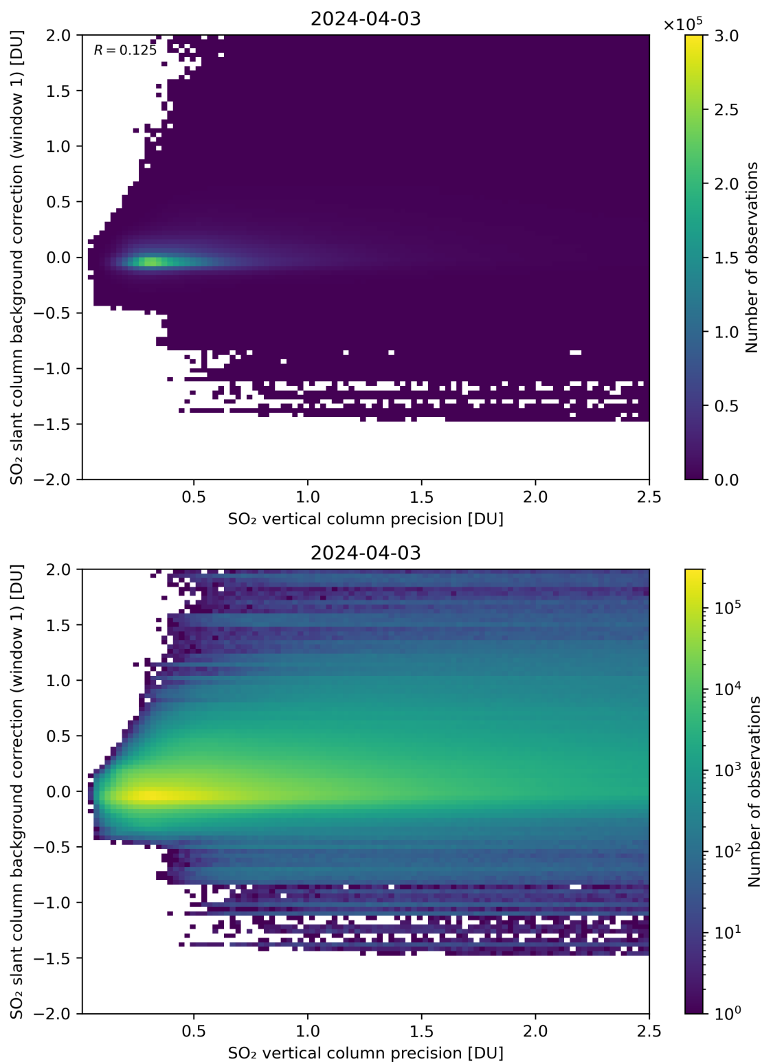
Figure 279: Scatter density plot of “SO 2 vertical column precision” against “SO 2 slant column background correction (window 1)” for 2024-04-02 to 2024-04-04.
