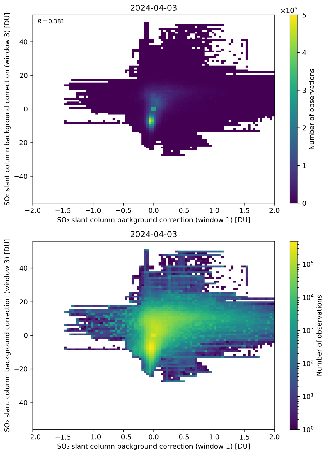
Figure 99: Scatter density plot of “SO 2 slant column background correction (window 1)” against “SO 2 slant column background correction (window 3)” for 2024-04-02 to 2024-04-04.
