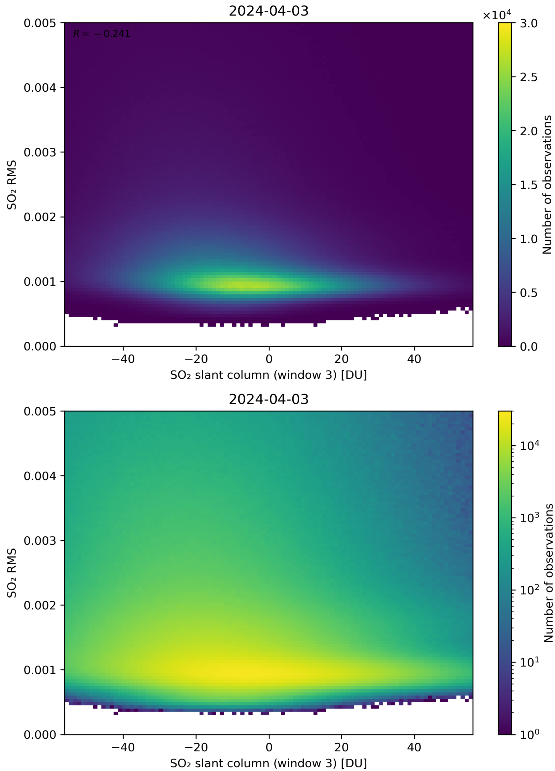
Figure 256: Scatter density plot of “SO 2 slant column (window 3)” against “SO 2 RMS” for 2024-04-02 to 2024-04-04.
