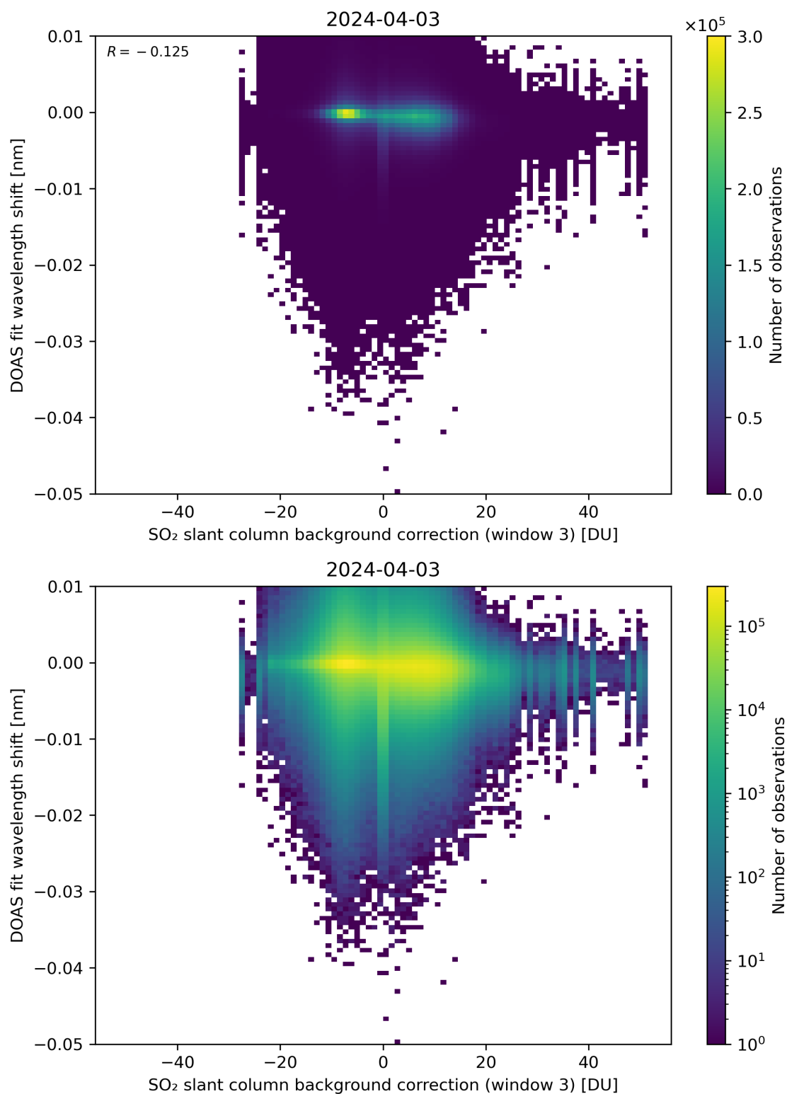
Figure 121: Scatter density plot of “SO 2 slant column background correction (window 3)” against “DOAS fit wavelength shift” for 2024-04-02 to 2024-04-04.
