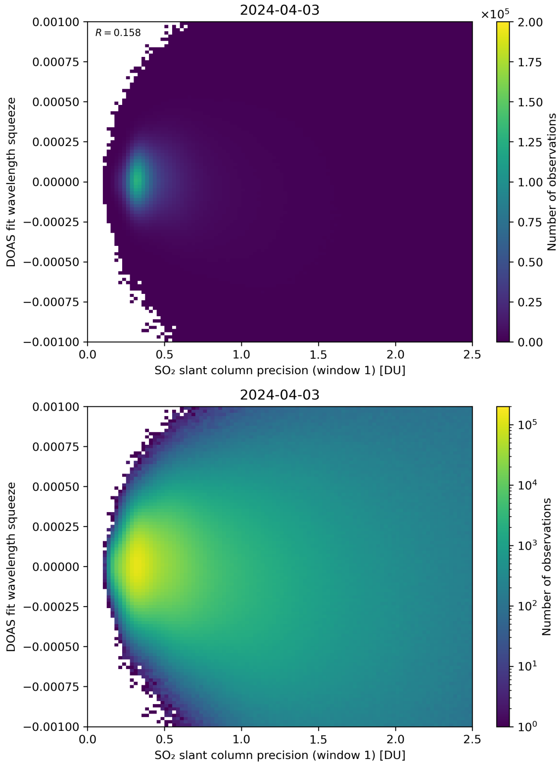
Figure 222: Scatter density plot of “SO 2 slant column precision (window 1)” against “DOAS fit wavelength squeeze” for 2024-04-02 to 2024-04-04.
