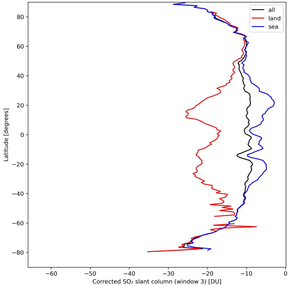
Figure 43: Zonal average of “Corrected SO 2 slant column (window 3)” for 2024-04-02 to 2024-04-04.
