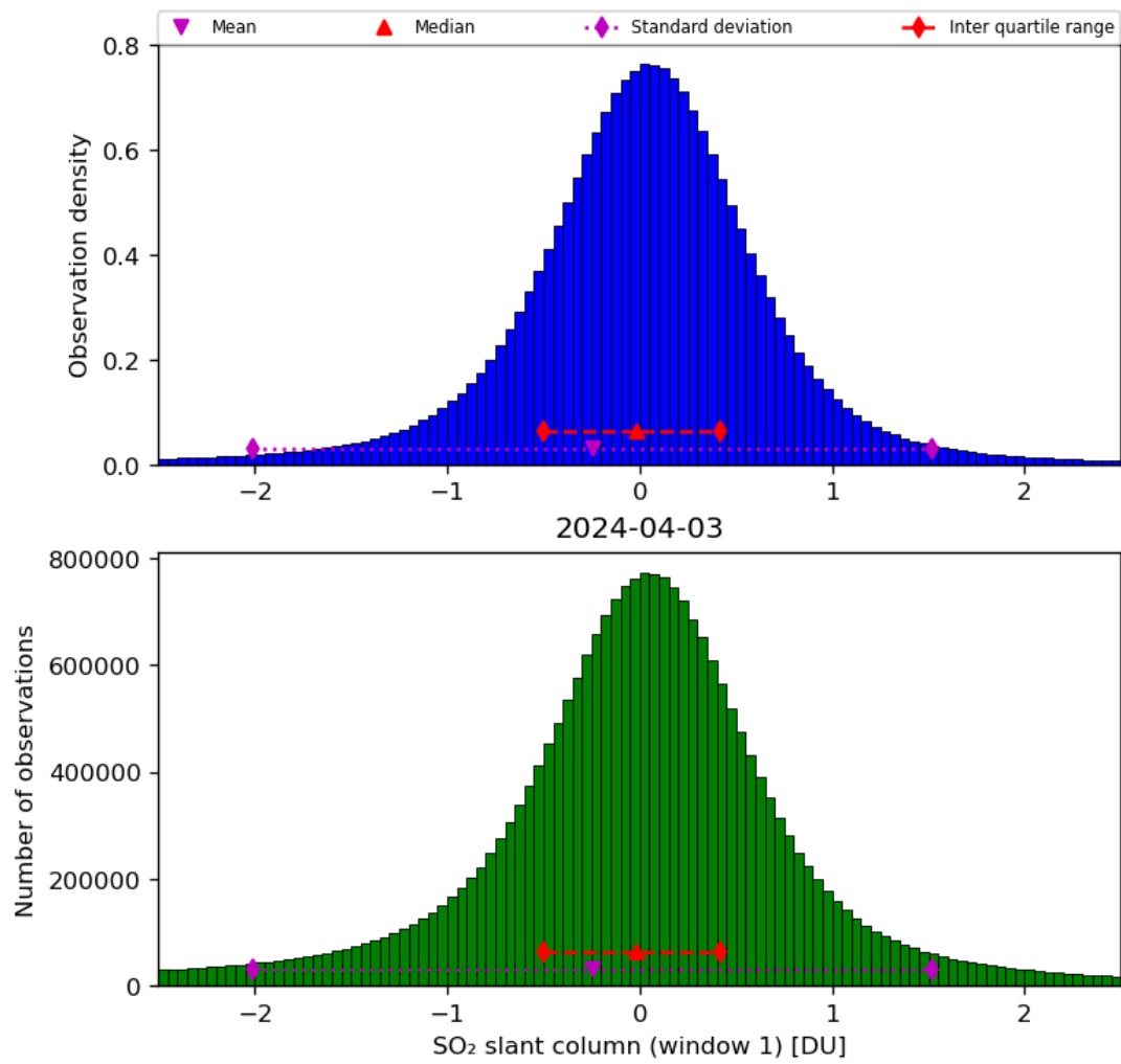
Figure 56: Histogram of “SO 2 slant column (window 1)” for 2024-04-02 to 2024-04-04
