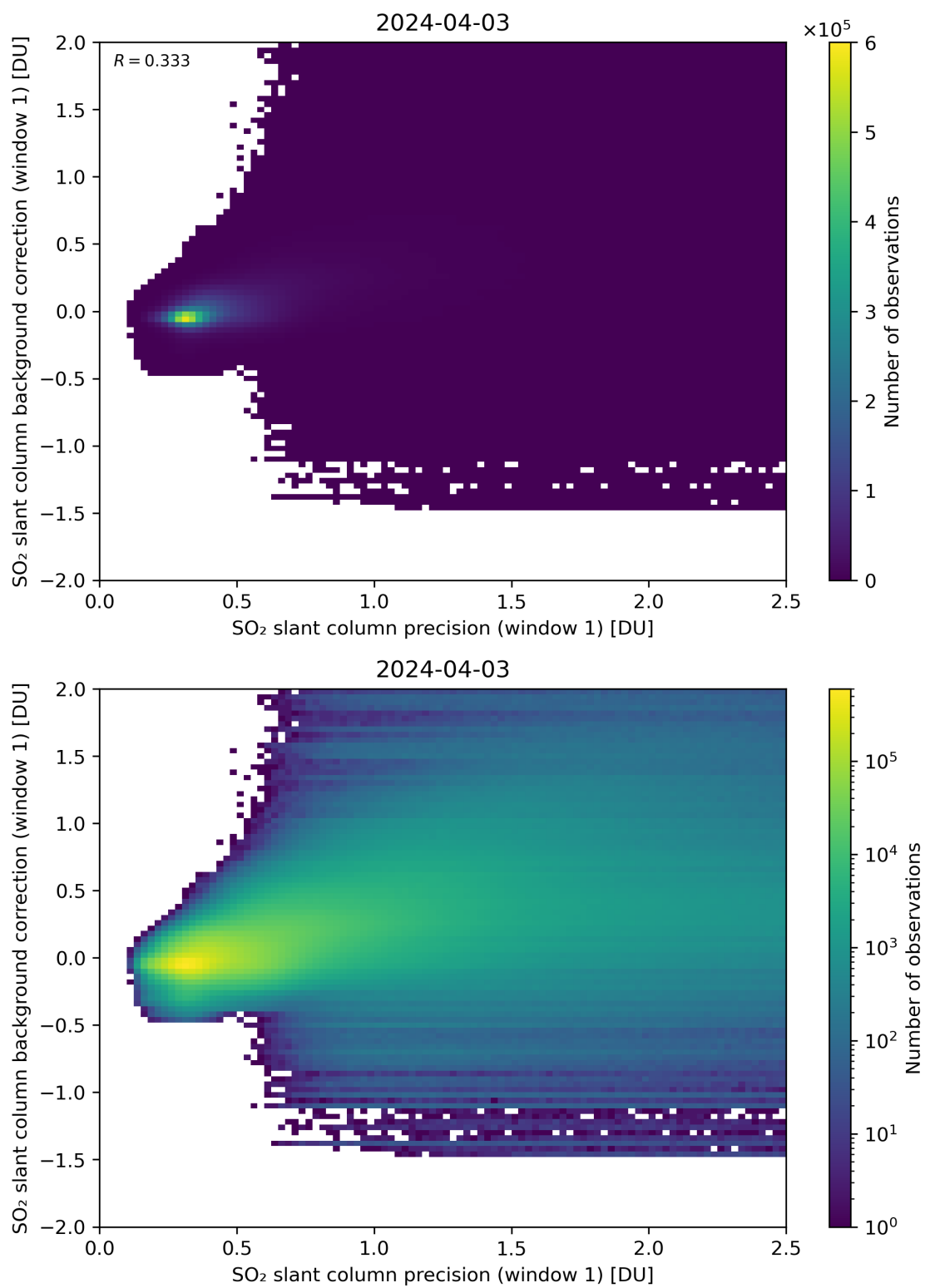
Figure 218: Scatter density plot of “SO 2 slant column precision (window 1)” against “SO 2 slant column background correction (window 1)” for 2024-04-02 to 2024-04-04.
