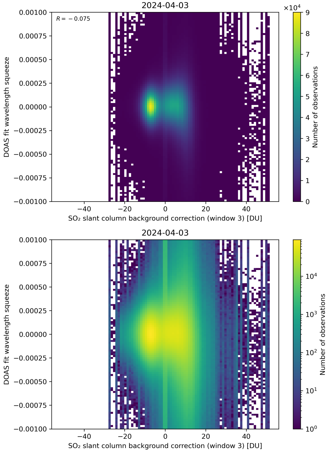
Figure 122: Scatter density plot of “SO 2 slant column background correction (window 3)” against “DOAS fit wavelength squeeze” for 2024-04-02 to 2024-04-04.
