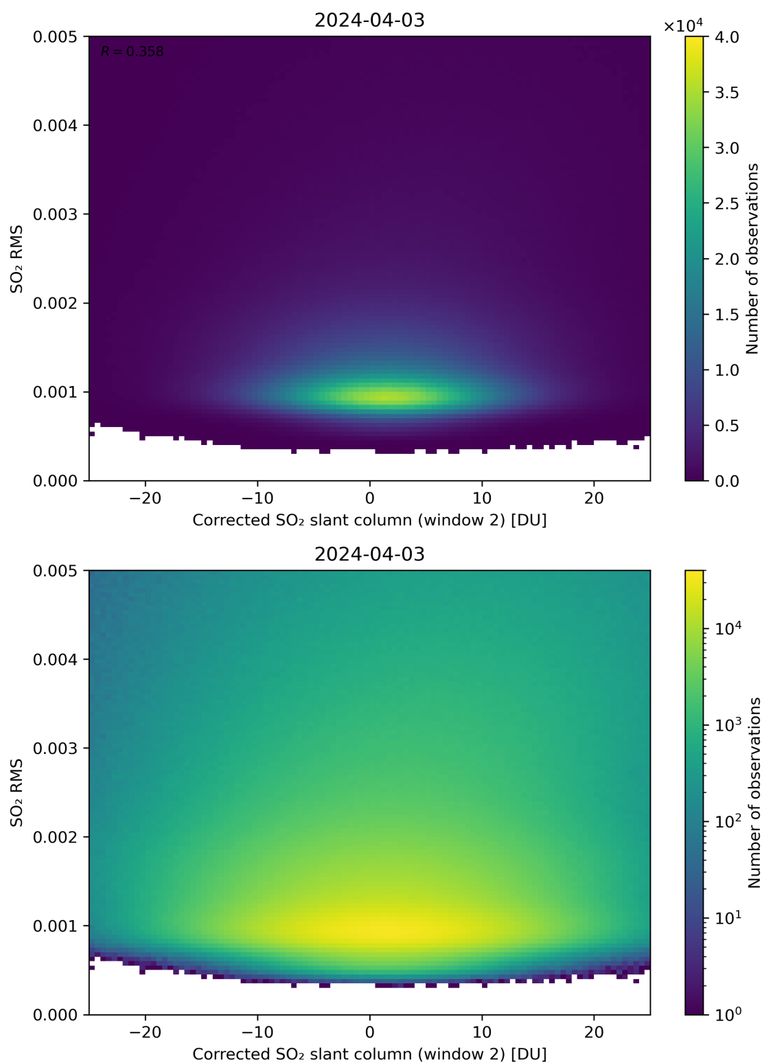
Figure 198: Scatter density plot of “Corrected SO 2 slant column (window 2)” against “SO 2 RMS” for 2024-04-02 to 2024-04-04.
