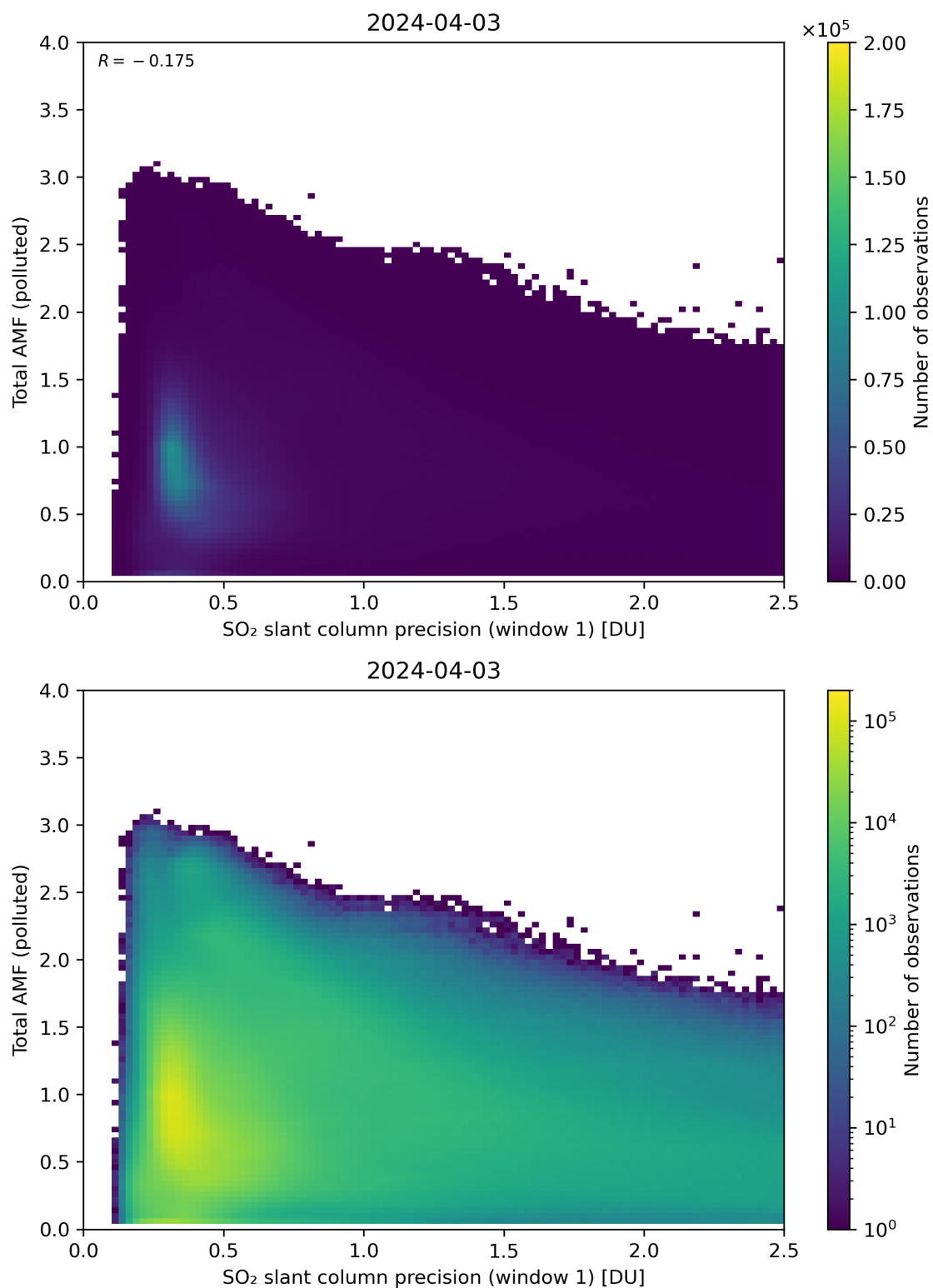
Figure 230: Scatter density plot of “SO 2 slant column precision (window 1)” against “Total AMF (polluted)” for 2024-04-02 to 2024-04-04.
