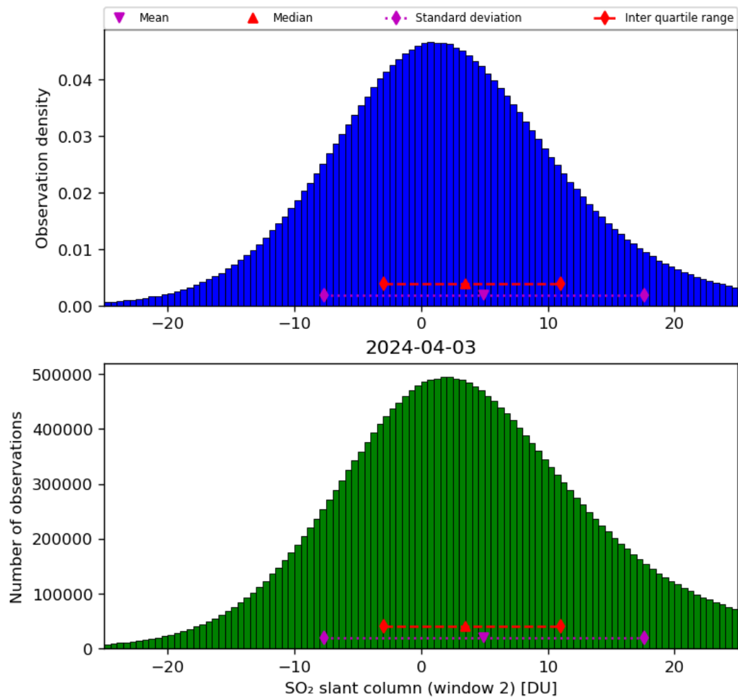
Figure 60: Histogram of “SO 2 slant column (window 2)” for 2024-04-02 to 2024-04-04
