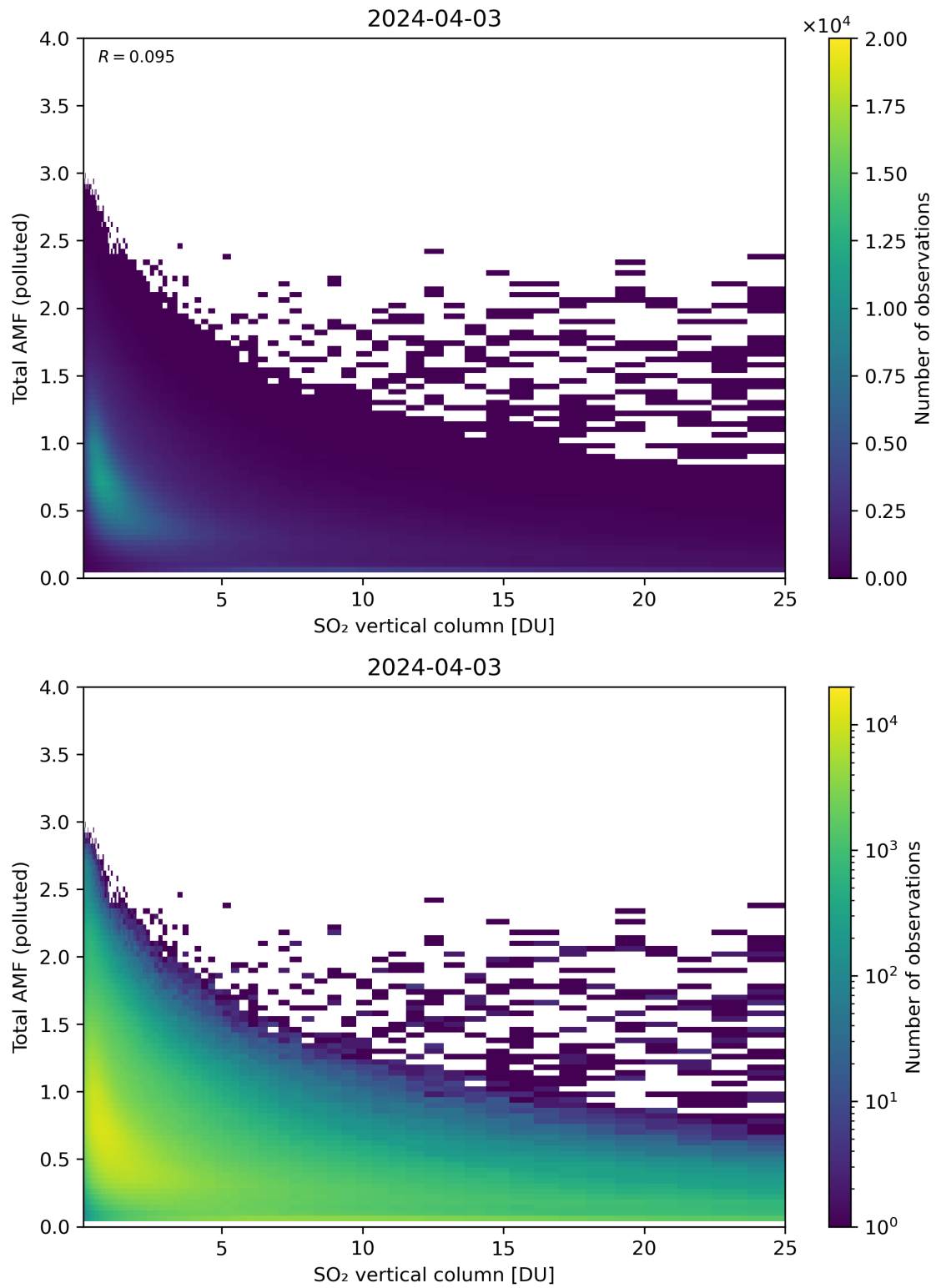
Figure 305: Scatter density plot of “SO 2 vertical column” against “Total AMF (polluted)” for 2024-04-02 to 2024-04-04.
