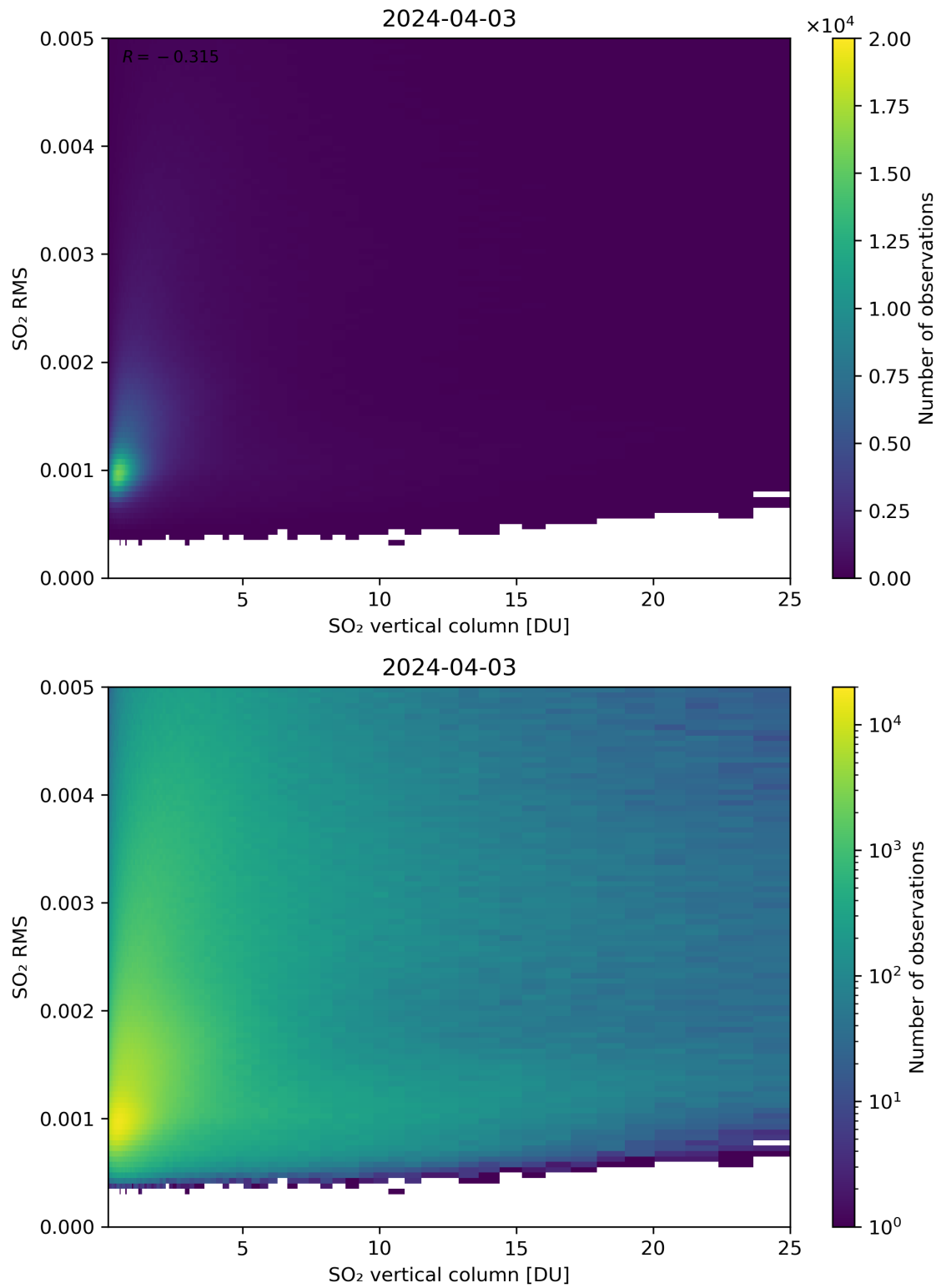
Figure 278: Scatter density plot of “SO 2 vertical column” against “SO 2 RMS” for 2024-04-02 to 2024-04-04.
