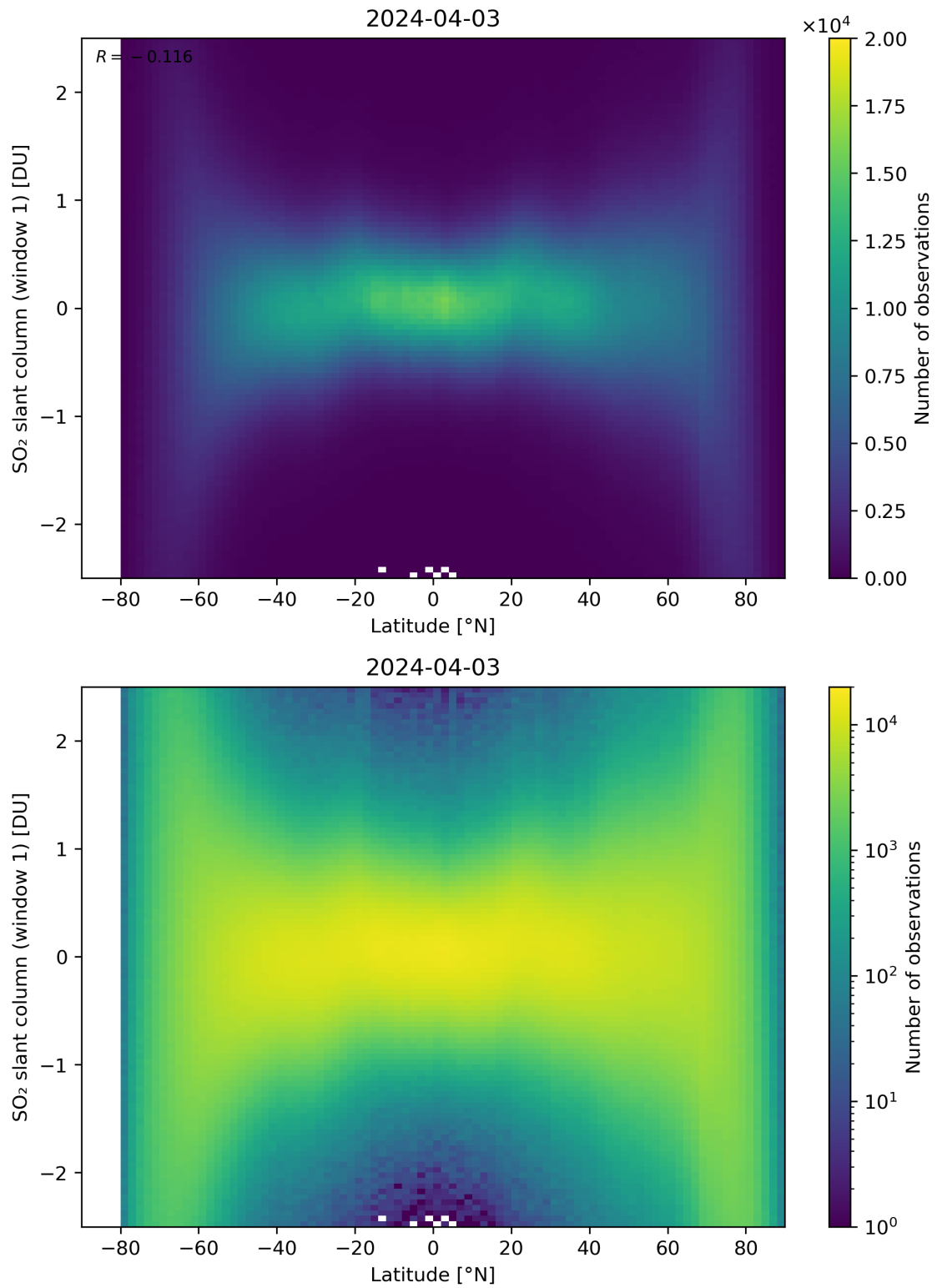
Figure 149: Scatter density plot of “Latitude” against “SO 2 slant column (window 1)” for 2024-04-02 to 2024-04-04.
