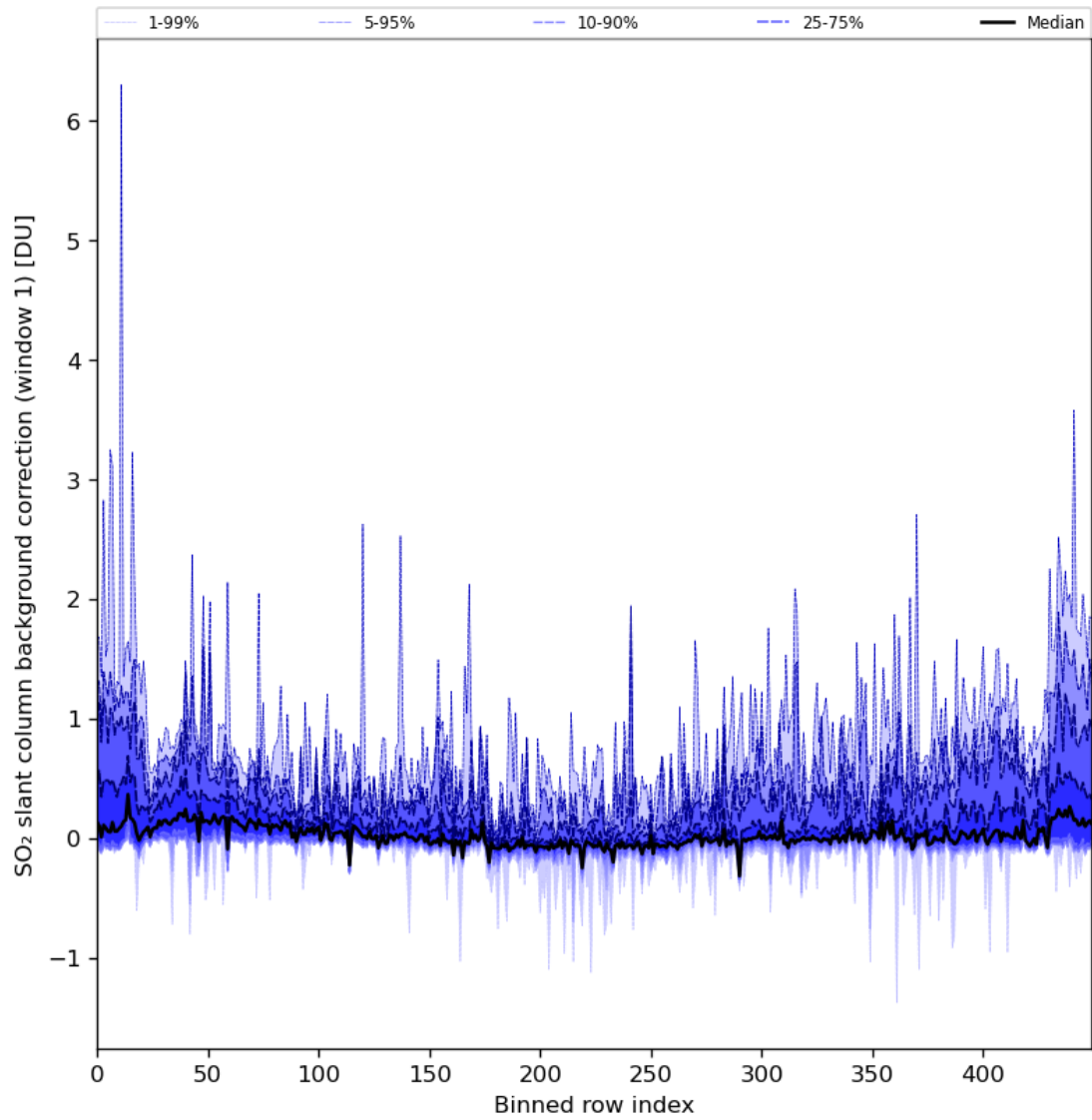
Figure 82: Along track statistics of “SO 2 slant column background correction (window 1)” for 2024-04-02 to 2024-04-04
