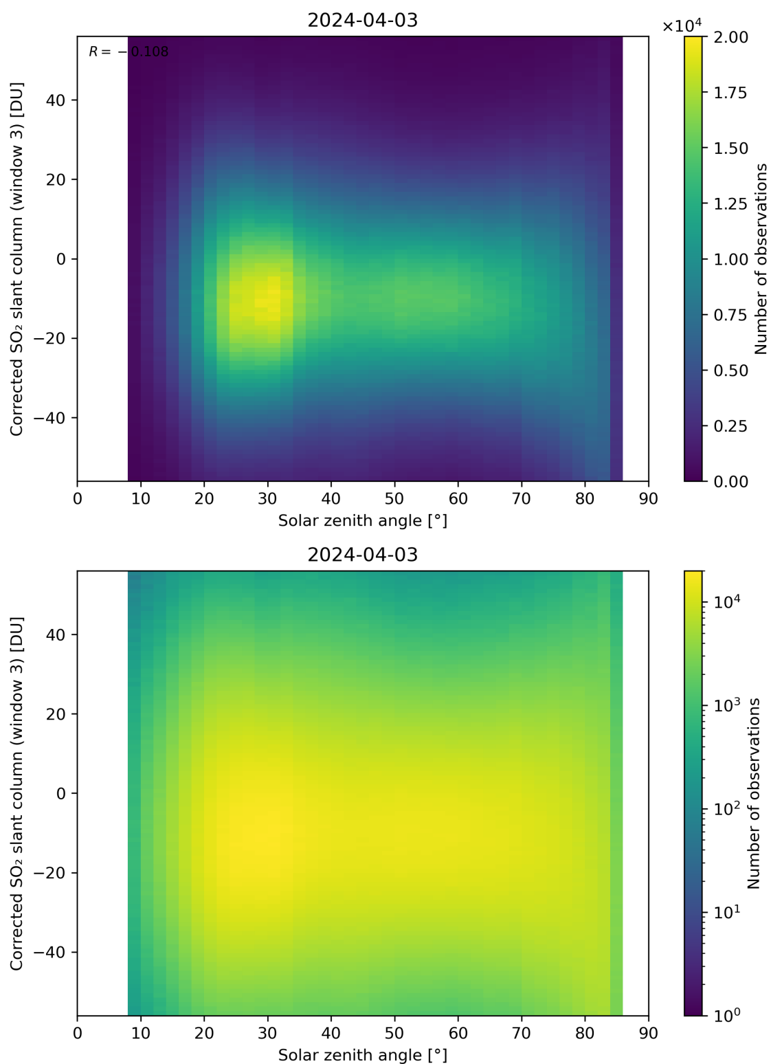
Figure 168: Scatter density plot of “Solar zenith angle” against “Corrected SO 2 slant column (window 3)” for 2024-04-02 to 2024-04-04.
