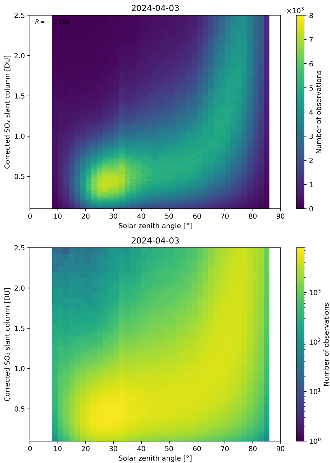
Figure 166: Scatter density plot of “Solar zenith angle” against “Corrected SO 2 slant column” for 2024-04-02 to 2024-04-04.
