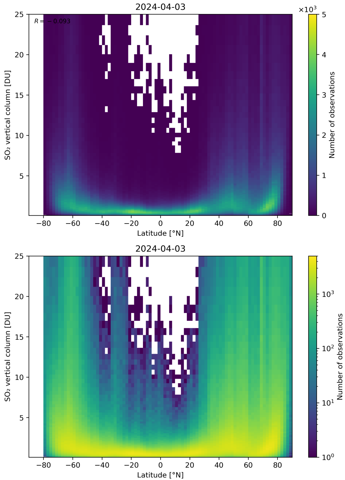
Figure 156: Scatter density plot of “Latitude” against “SO 2 vertical column” for 2024-04-02 to 2024-04-04.
