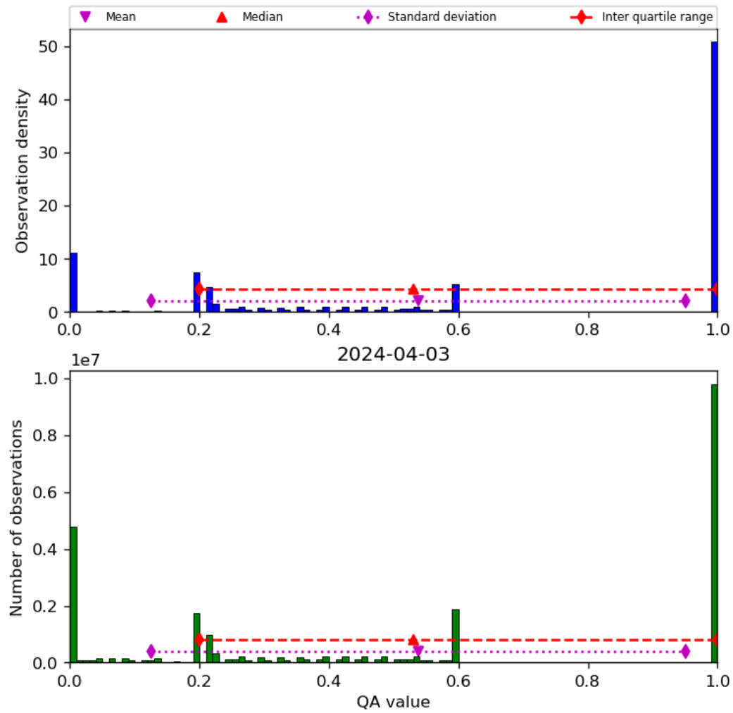
Figure 52: Histogram of “QA value” for 2024-04-02 to 2024-04-04
