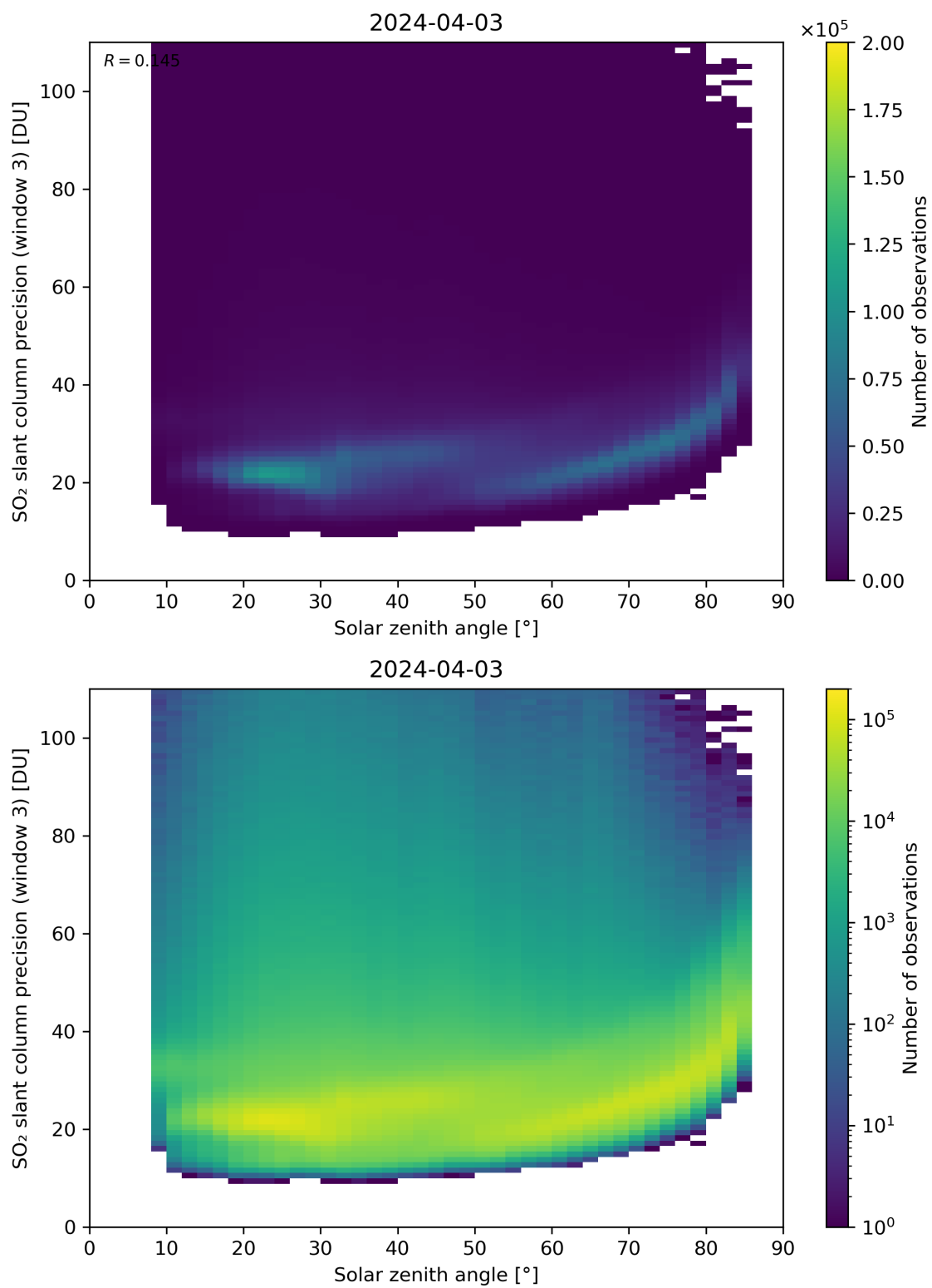
Figure 173: Scatter density plot of “Solar zenith angle” against “SO 2 slant column precision (window 3)” for 2024-04-02 to 2024-04-04.
