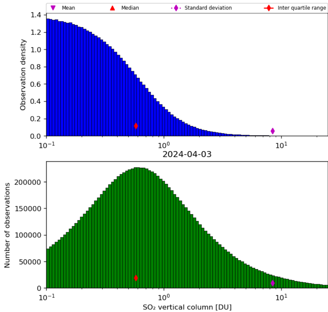
Figure 53: Histogram of “SO 2 vertical column” for 2024-04-02 to 2024-04-04
