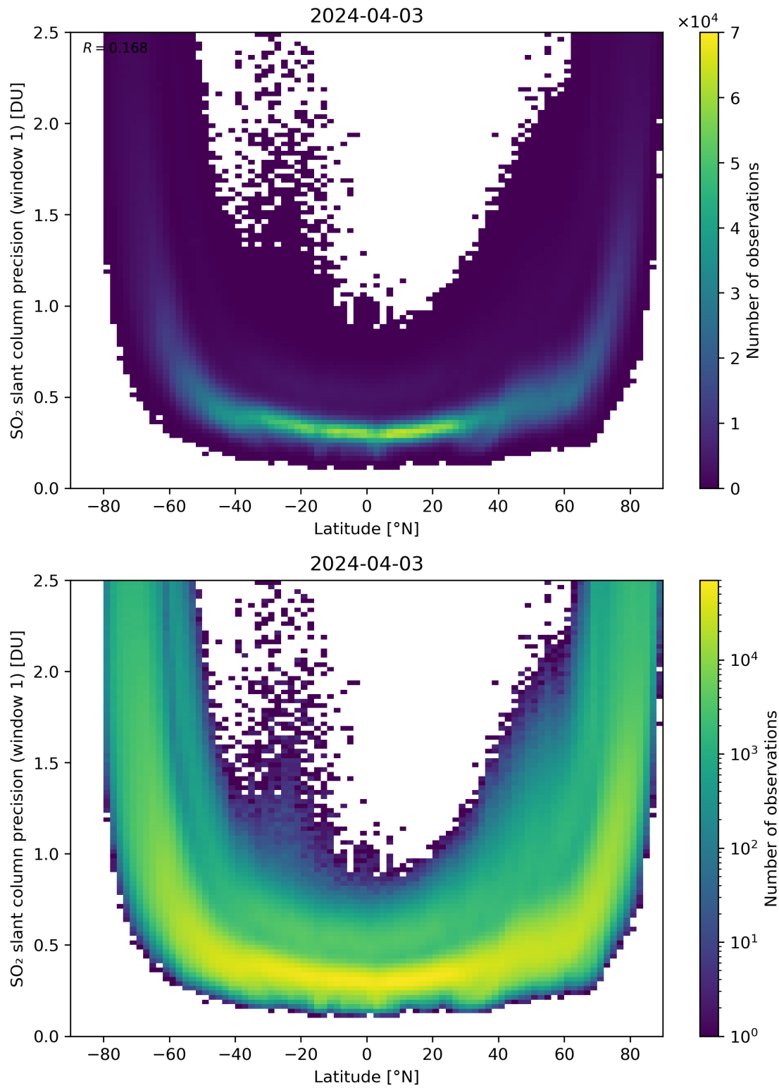
Figure 150: Scatter density plot of “Latitude” against “SO 2 slant column precision (window 1)” for 2024-04-02 to 2024-04-04.
