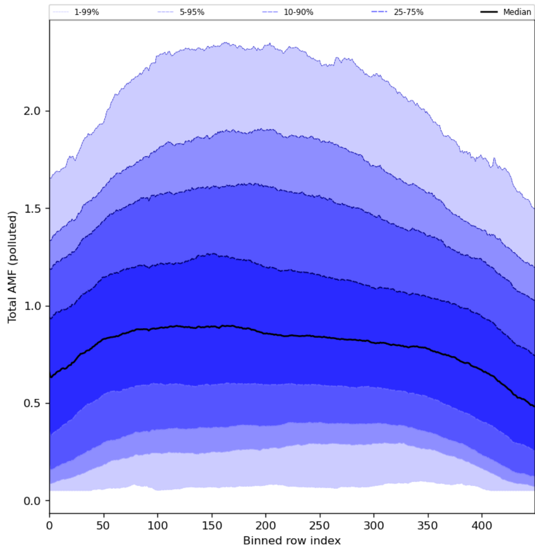
Figure 94: Along track statistics of “Total AMF (polluted)” for 2024-04-02 to 2024-04-04
