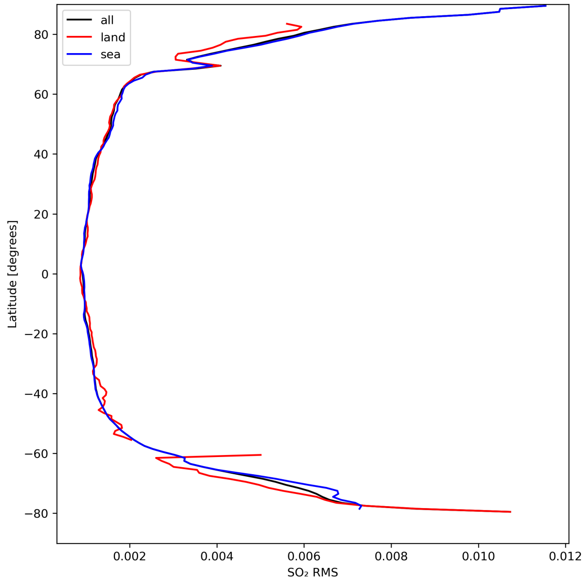
Figure 47: Zonal average of “SO 2 RMS” for 2024-04-02 to 2024-04-04.
