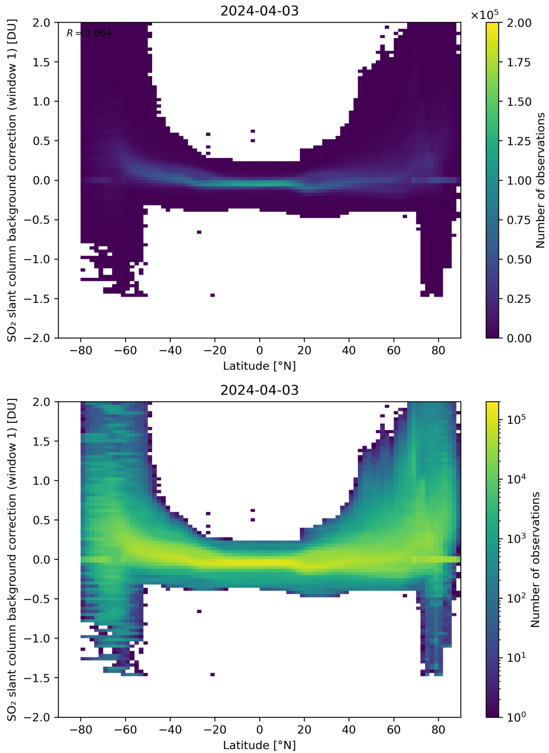
Figure 139: Scatter density plot of “Latitude” against “SO 2 slant column background correction (window 1)” for 2024-04-02 to 2024-04-04.
