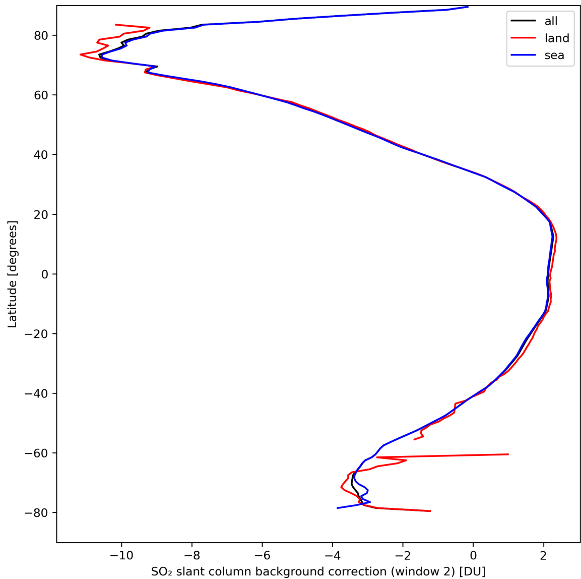
Figure 40: Zonal average of “SO 2 slant column background correction (window 2)” for 2024-04-02 to 2024-04-04.
