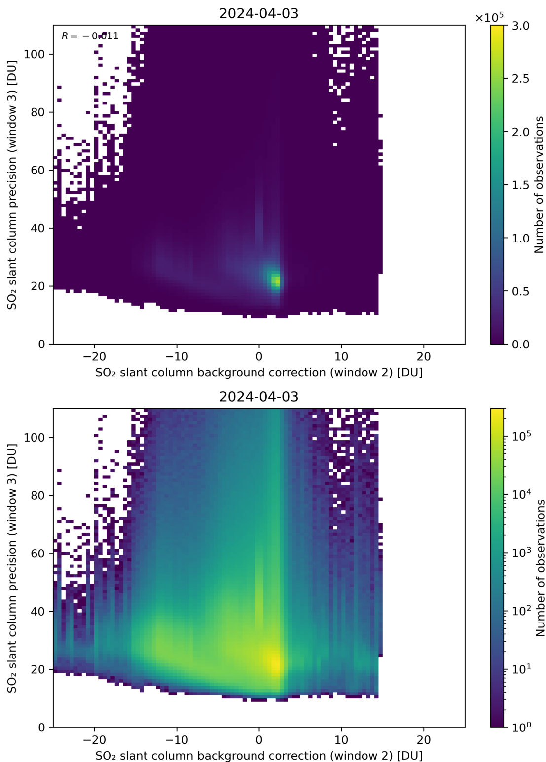
Figure 118: Scatter density plot of “SO 2 slant column background correction (window 2)” against “SO 2 slant column precision (window 3)” for 2024-04-02 to 2024-04-04.
