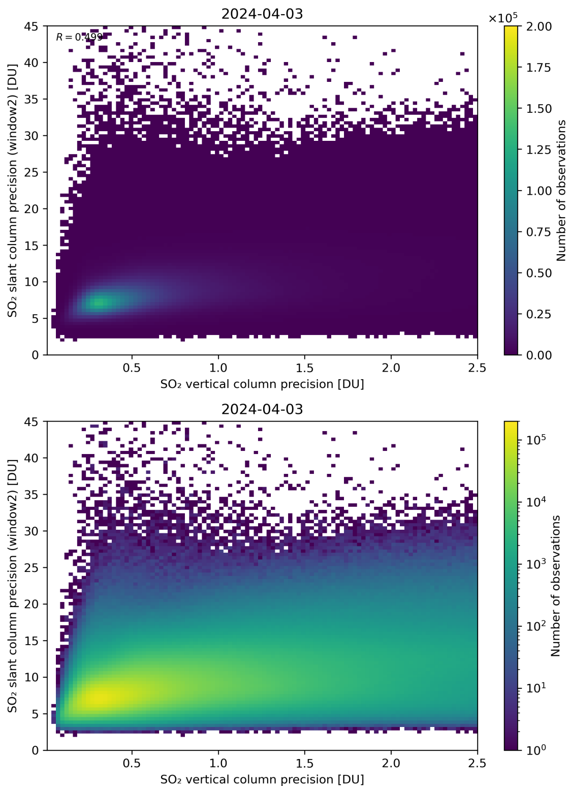
Figure 291: Scatter density plot of “SO 2 vertical column precision” against “SO 2 slant column precision (window2)” for 2024-04-02 to 2024-04-04.
