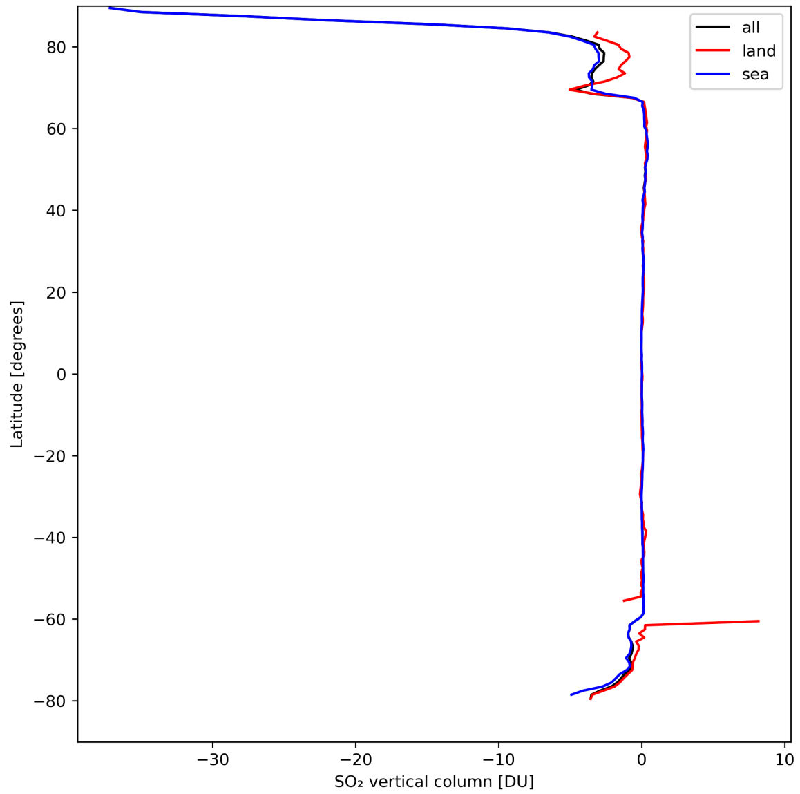
Figure 30: Zonal average of “SO 2 vertical column” for 2024-04-02 to 2024-04-04.
