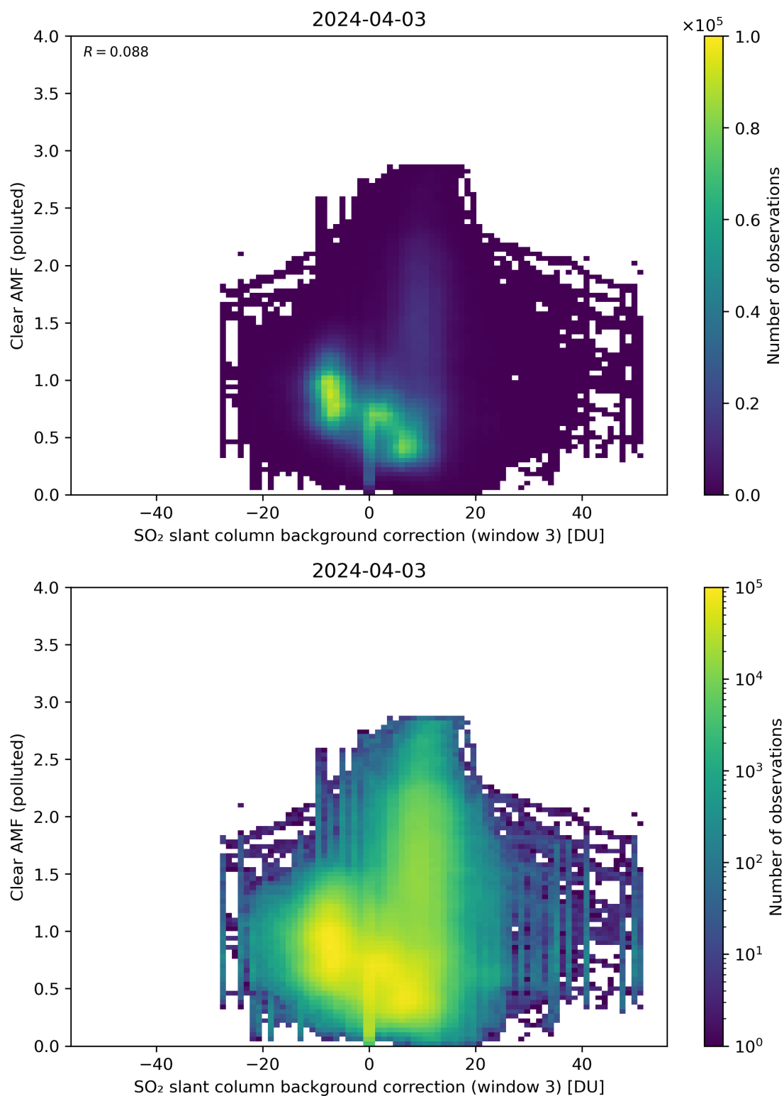
Figure 124: Scatter density plot of “SO 2 slant column background correction (window 3)” against “Clear AMF (polluted)” for 2024-04-02 to 2024-04-04.
