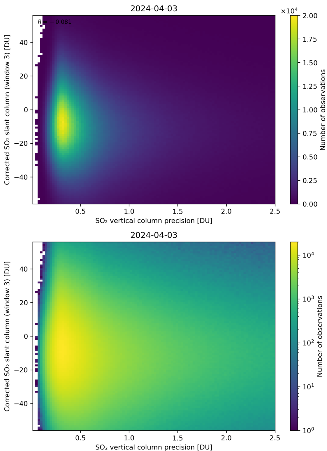
Figure 288: Scatter density plot of “SO 2 vertical column precision” against “Corrected SO 2 slant column (window 3)” for 2024-04-02 to 2024-04-04.
