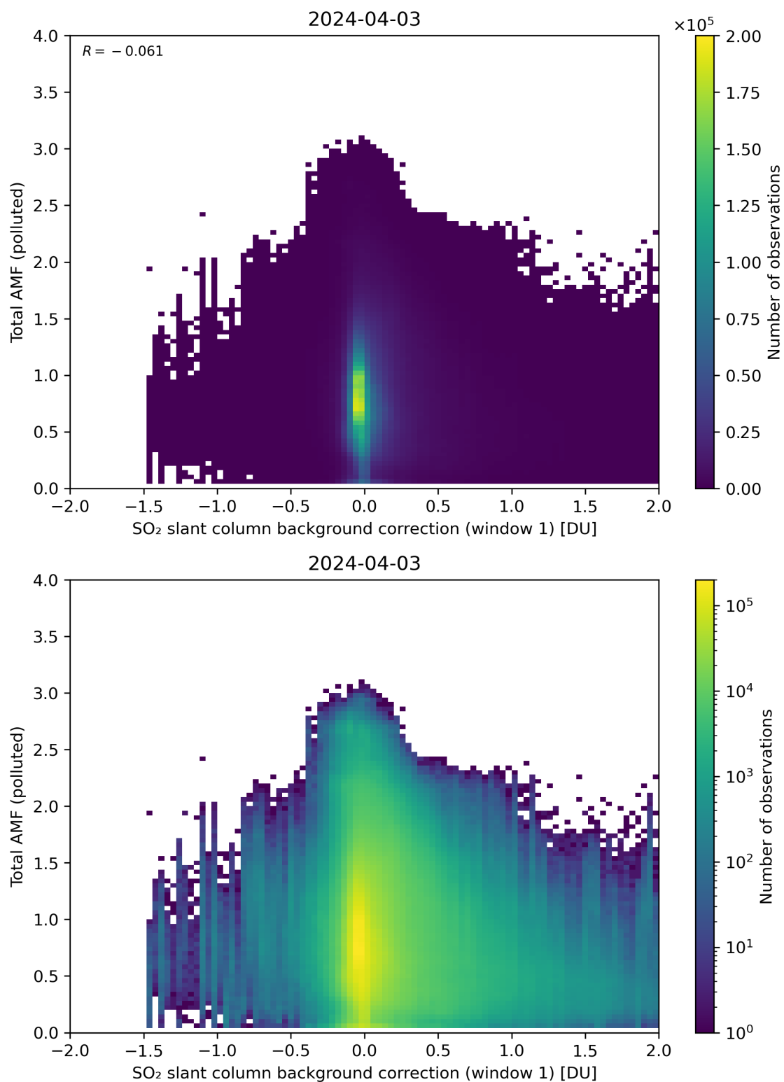
Figure 109: Scatter density plot of “SO 2 slant column background correction (window 1)” against “Total AMF (polluted)” for 2024-04-02 to 2024-04-04.
