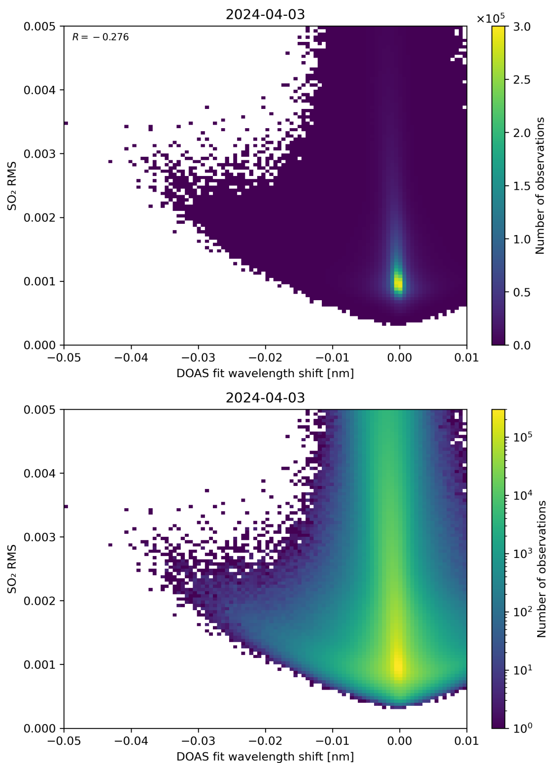
Figure 128: Scatter density plot of “DOAS fit wavelength shift” against “SO 2 RMS” for 2024-04-02 to 2024-04-04.
