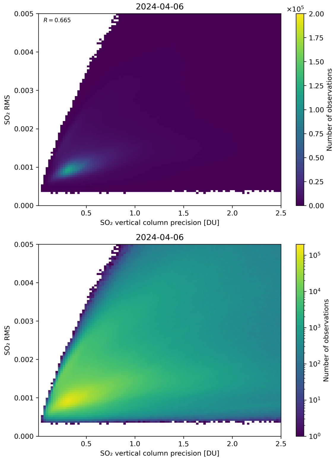
Figure 284: Scatter density plot of “SO 2 vertical column precision” against “SO 2 RMS” for 2024-04-05 to 2024-04-07.
