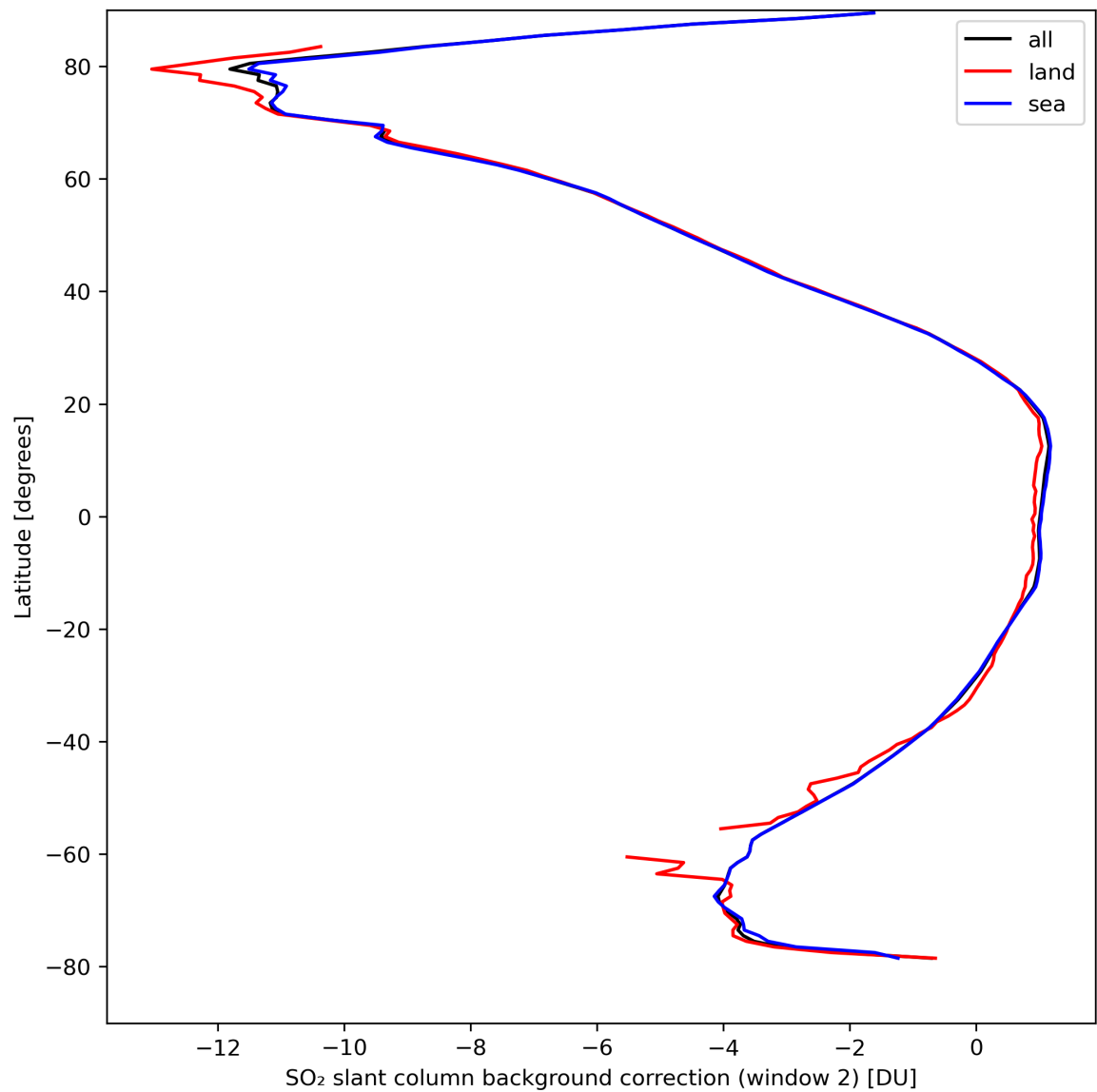
Figure 40: Zonal average of “SO 2 slant column background correction (window 2)” for 2024-04-05 to 2024-04-07.
