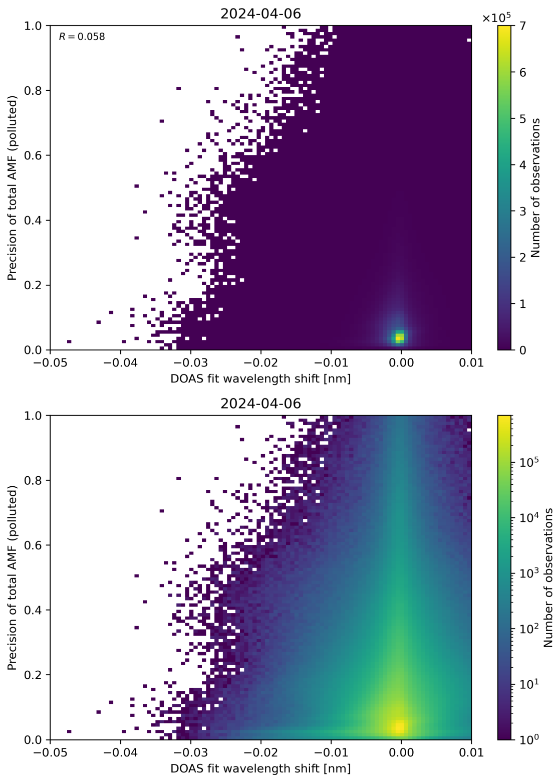
Figure 131: Scatter density plot of “DOAS fit wavelength shift” against “Precision of total AMF (polluted)” for 2024-04-05 to 2024-04-07.
