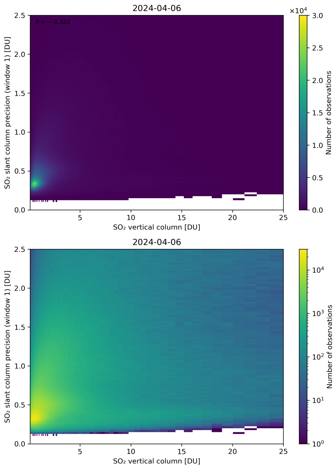
Figure 301: Scatter density plot of “SO 2 vertical column” against “SO 2 slant column precision (window 1)” for 2024-04-05 to 2024-04-07.
