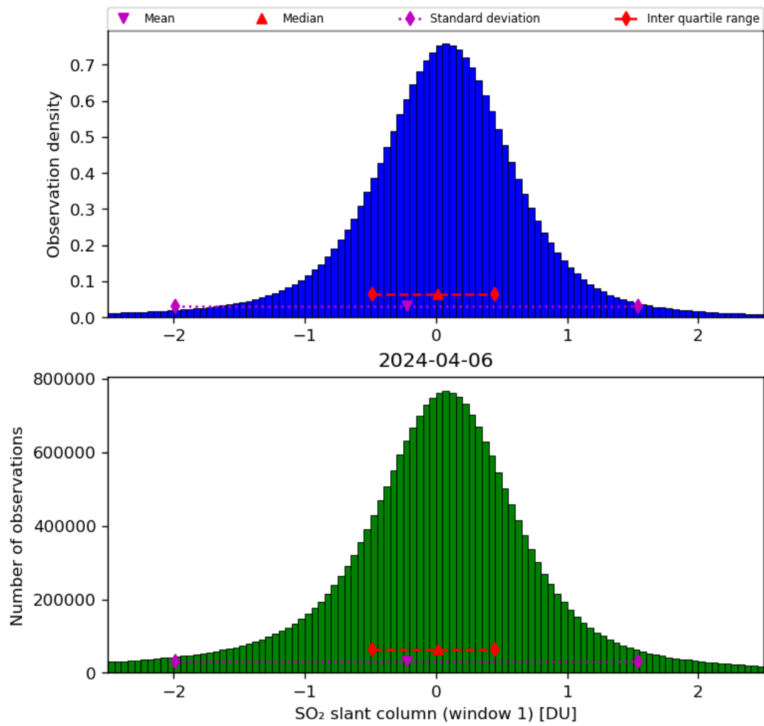
Figure 56: Histogram of “SO 2 slant column (window 1)” for 2024-04-05 to 2024-04-07
