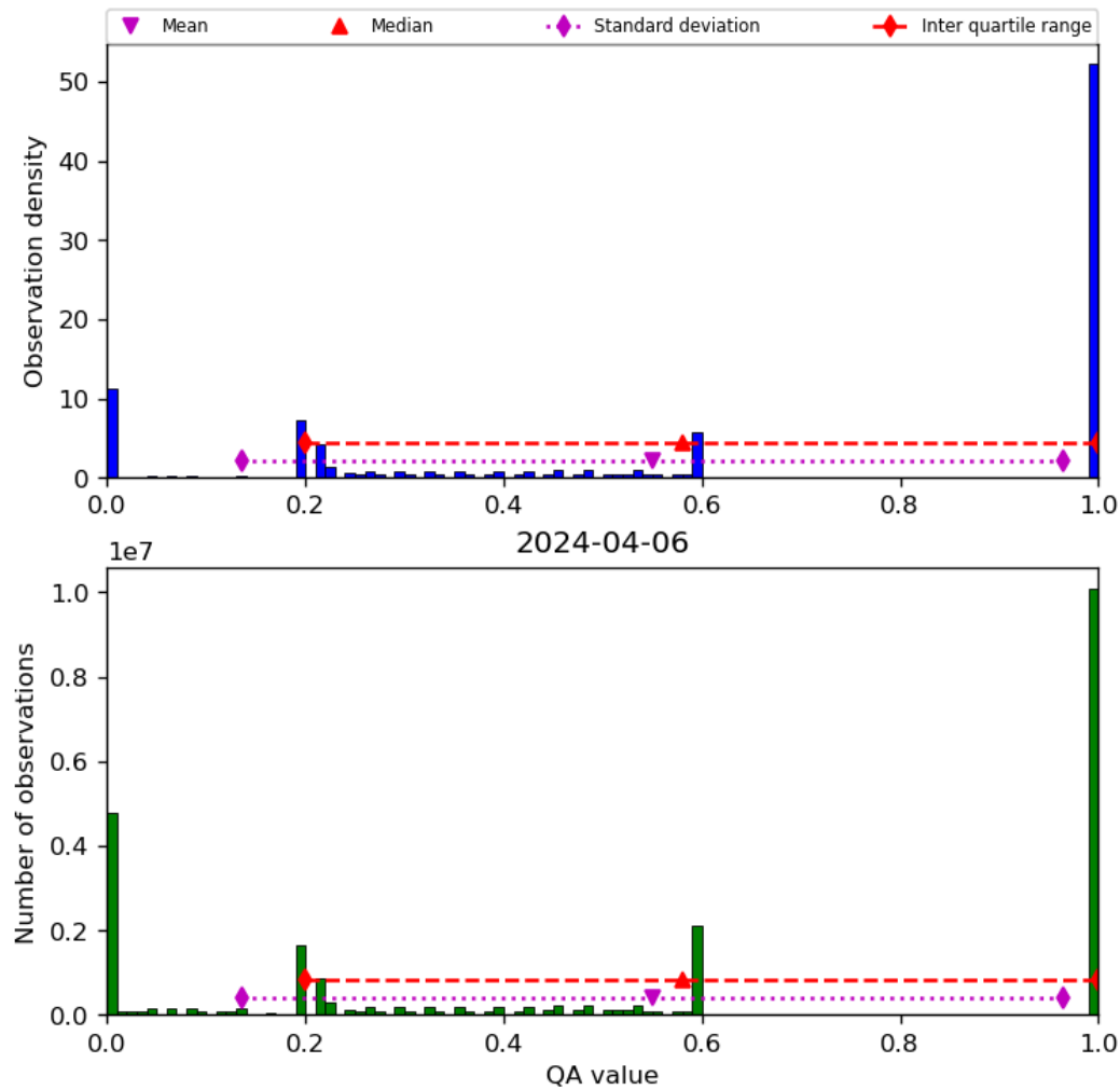
Figure 52: Histogram of “QA value” for 2024-04-05 to 2024-04-07
