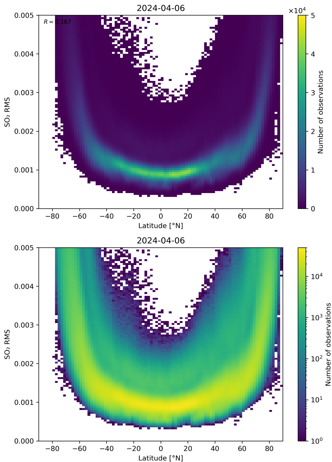
Figure 144: Scatter density plot of “Latitude” against “SO 2 RMS” for 2024-04-05 to 2024-04-07.
