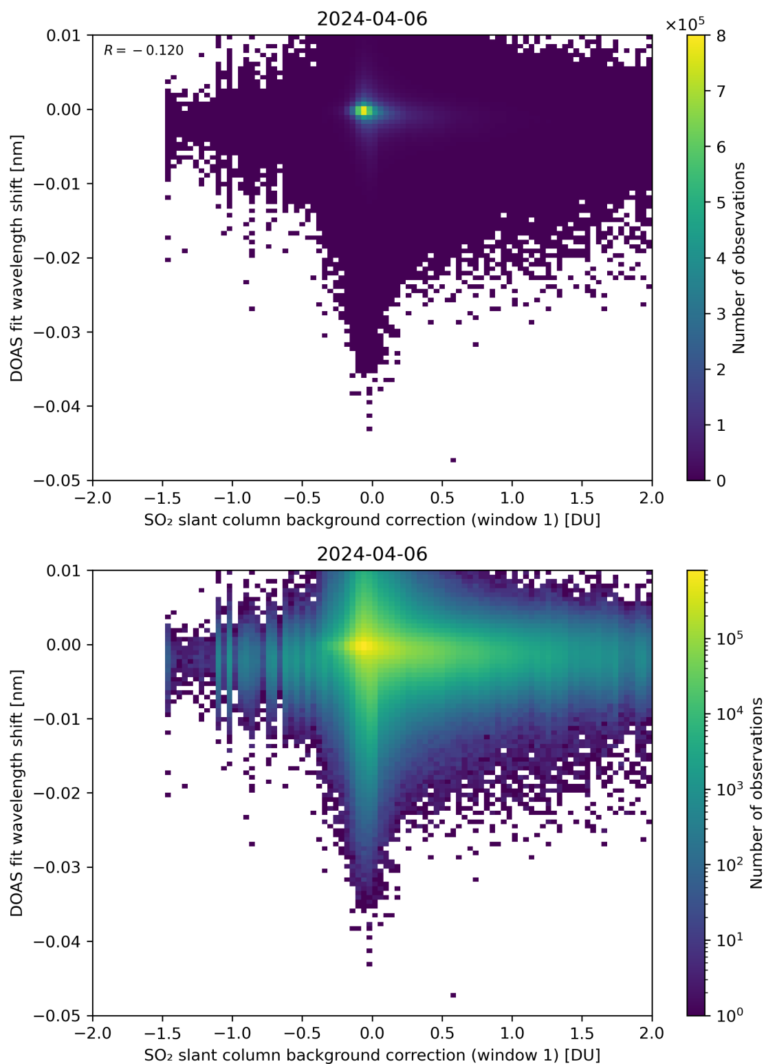
Figure 100: Scatter density plot of “SO 2 slant column background correction (window 1)” against “DOAS fit wavelength shift” for 2024-04-05 to 2024-04-07.
