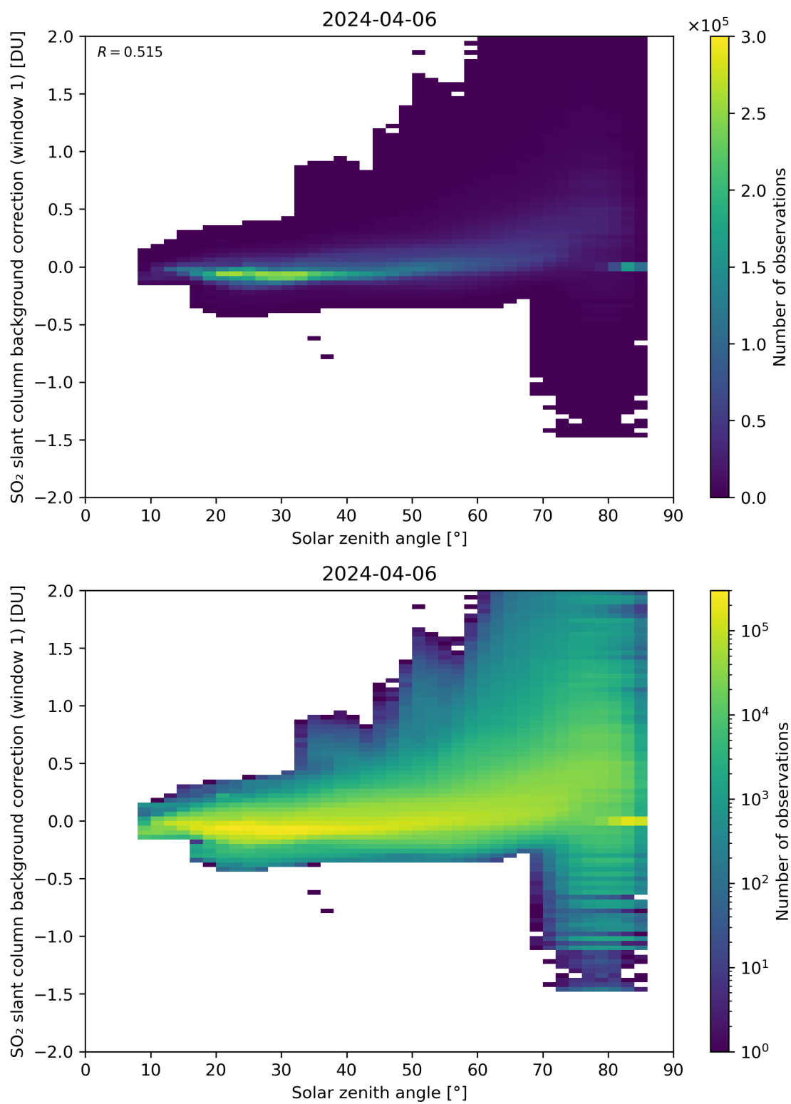
Figure 158: Scatter density plot of “Solar zenith angle” against “SO 2 slant column background correction (window 1)” for 2024-04-05 to 2024-04-07.
