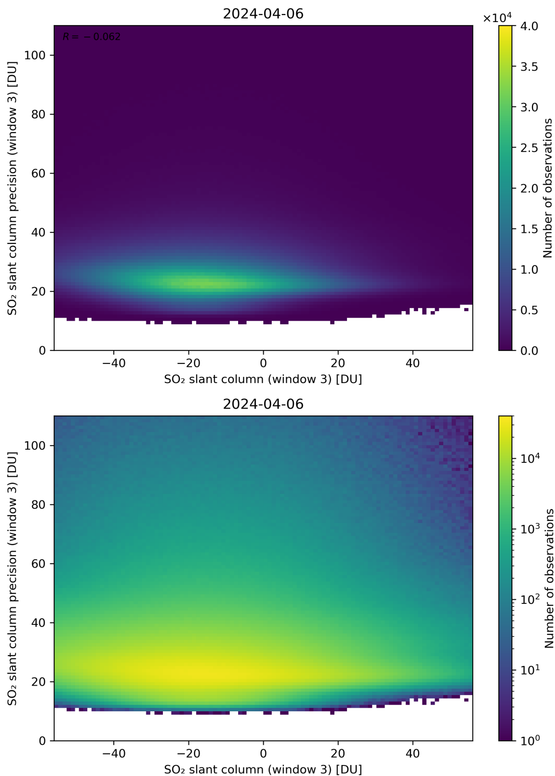
Figure 267: Scatter density plot of “SO 2 slant column (window 3)” against “SO 2 slant column precision (window 3)” for 2024-04-05 to 2024-04-07.
