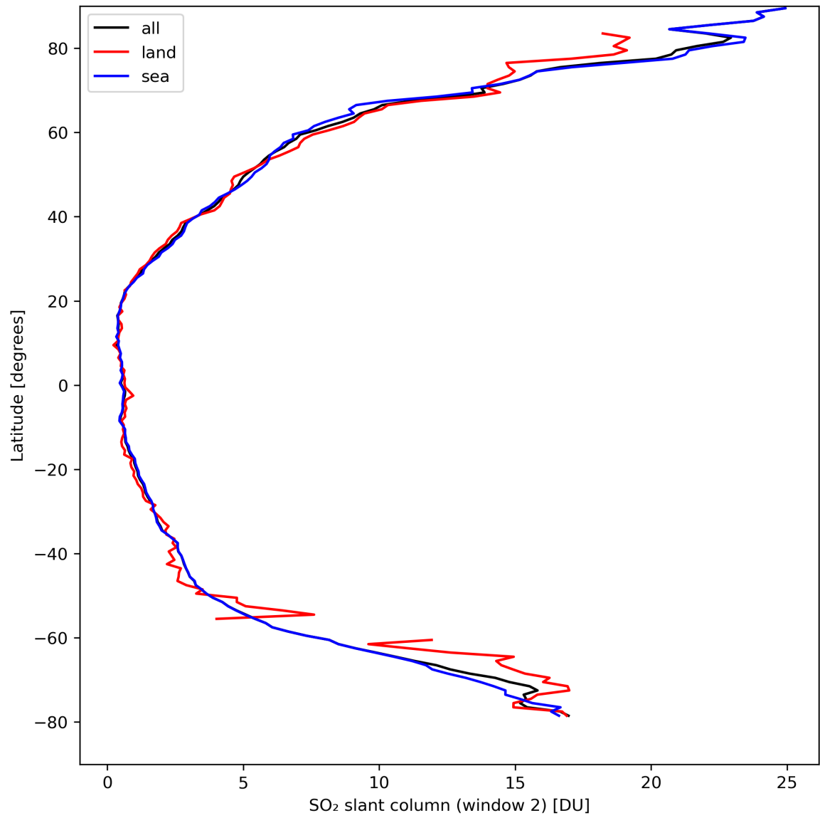
Figure 37: Zonal average of “SO 2 slant column (window 2)” for 2024-04-05 to 2024-04-07.
