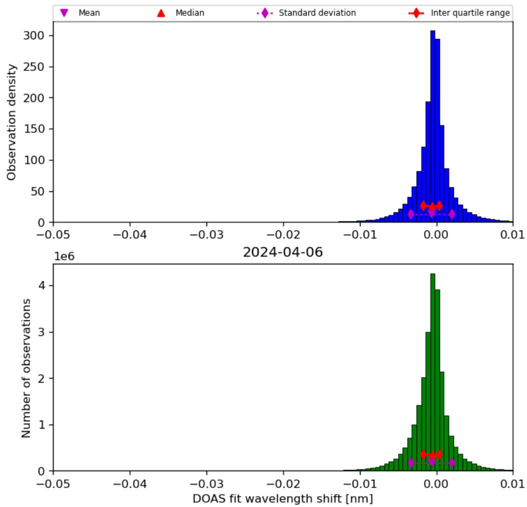
Figure 68: Histogram of “DOAS fit wavelength shift” for 2024-04-05 to 2024-04-07
