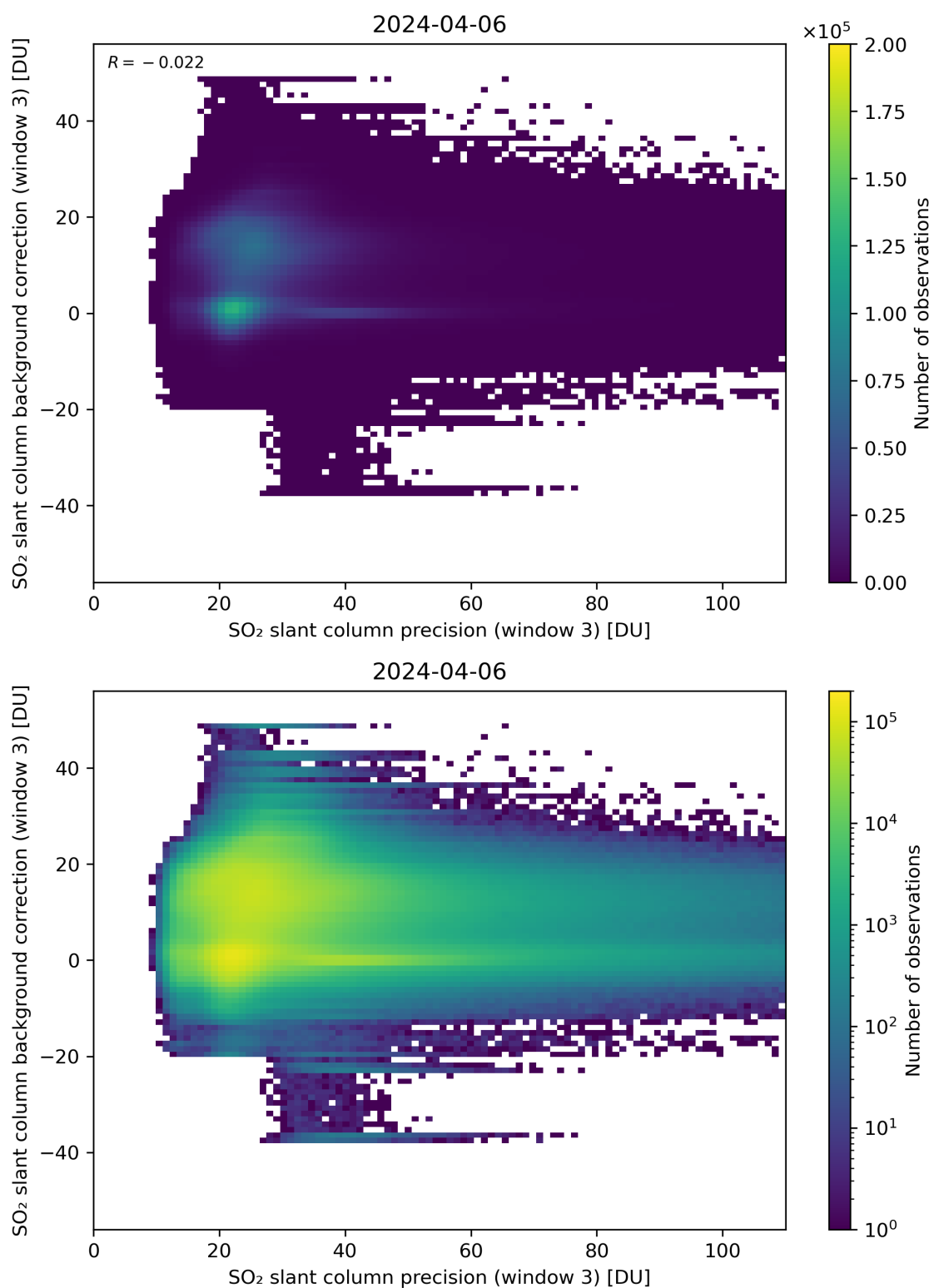
Figure 257: Scatter density plot of “SO 2 slant column precision (window 3)” against “SO 2 slant column background correction (window 3)” for 2024-04-05 to 2024-04-07.
