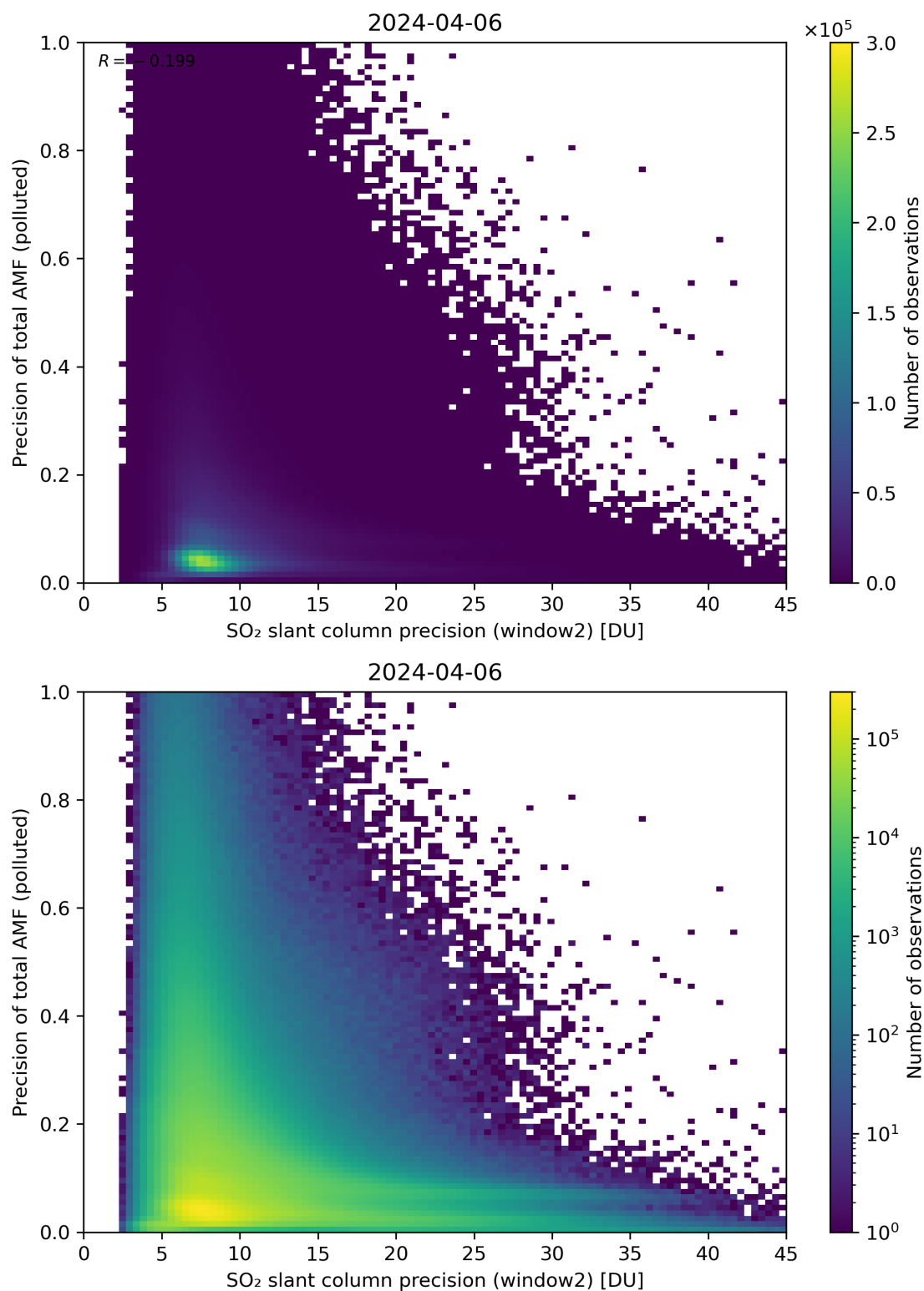
Figure 252: Scatter density plot of “SO 2 slant column precision (window2)” against “Precision of total AMF (polluted)” for 2024-04-05 to 2024-04-07.
