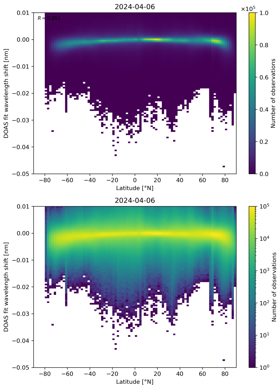
Figure 142: Scatter density plot of “Latitude” against “DOAS fit wavelength shift” for 2024-04-05 to 2024-04-07.
