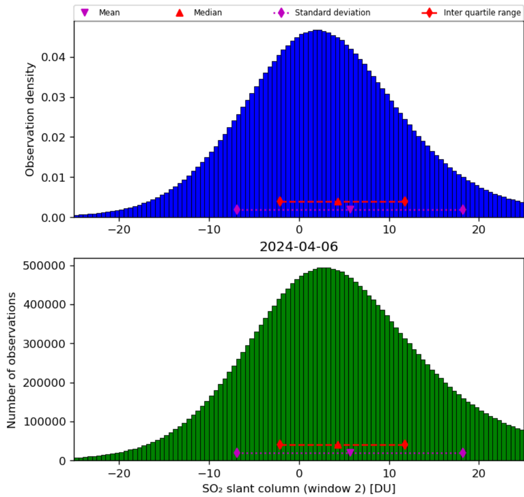
Figure 60: Histogram of “SO 2 slant column (window 2)” for 2024-04-05 to 2024-04-07
