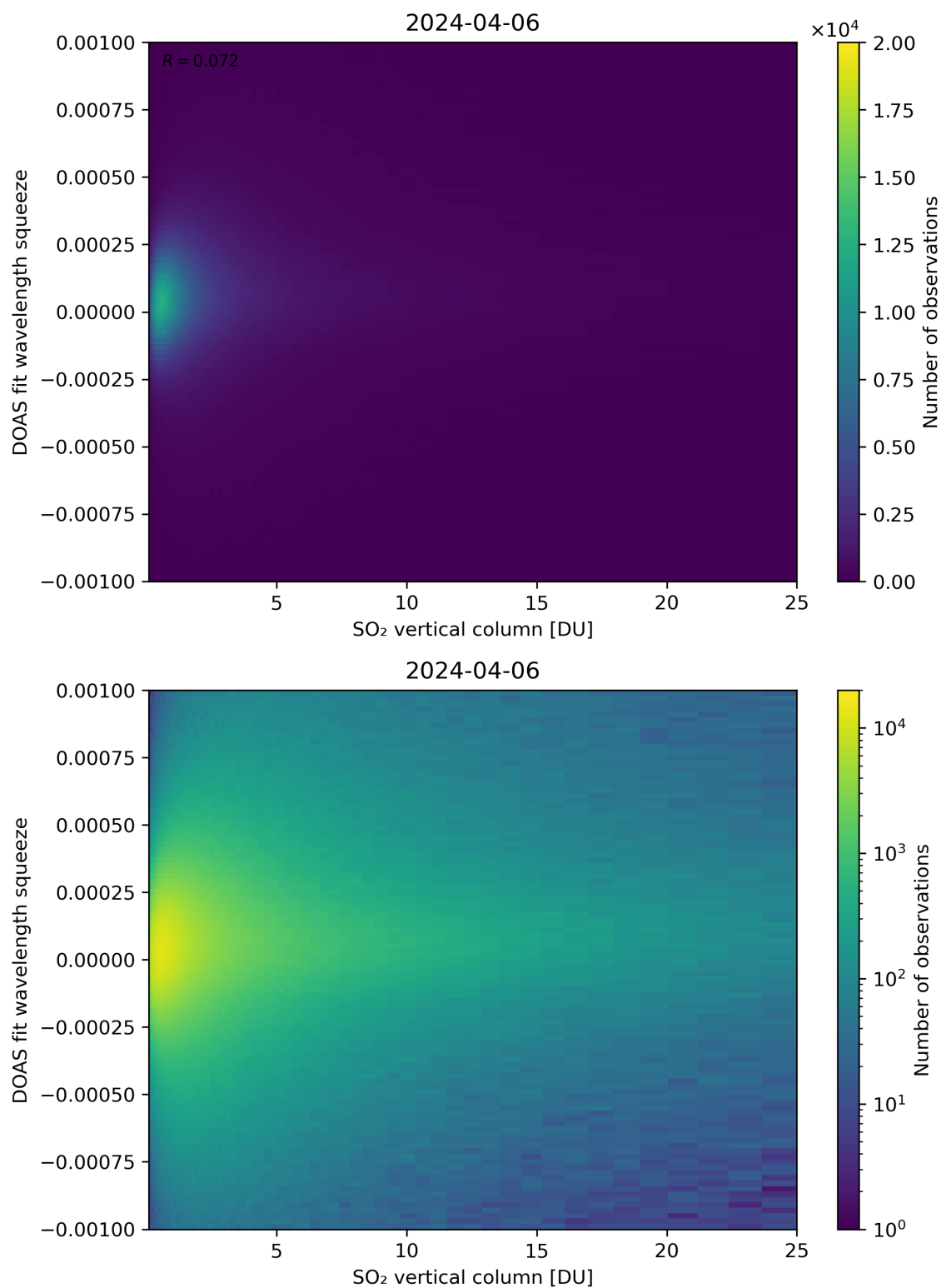
Figure 277: Scatter density plot of “SO 2 vertical column” against “DOAS fit wavelength squeeze” for 2024-04-05 to 2024-04-07.
