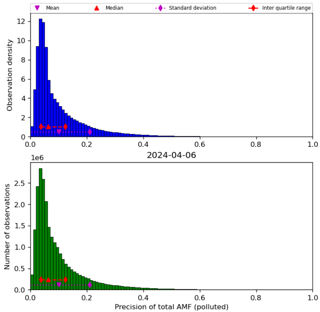
Figure 72: Histogram of “Precision of total AMF (polluted)” for 2024-04-05 to 2024-04-07
