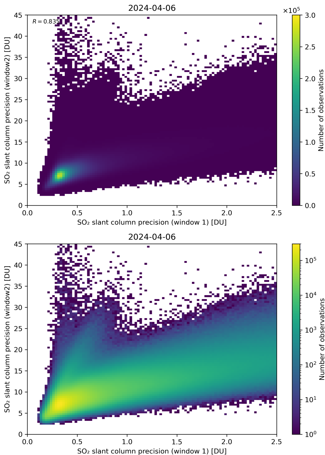
Figure 227: Scatter density plot of “SO 2 slant column precision (window 1)” against “SO 2 slant column precision (window2)” for 2024-04-05 to 2024-04-07.
