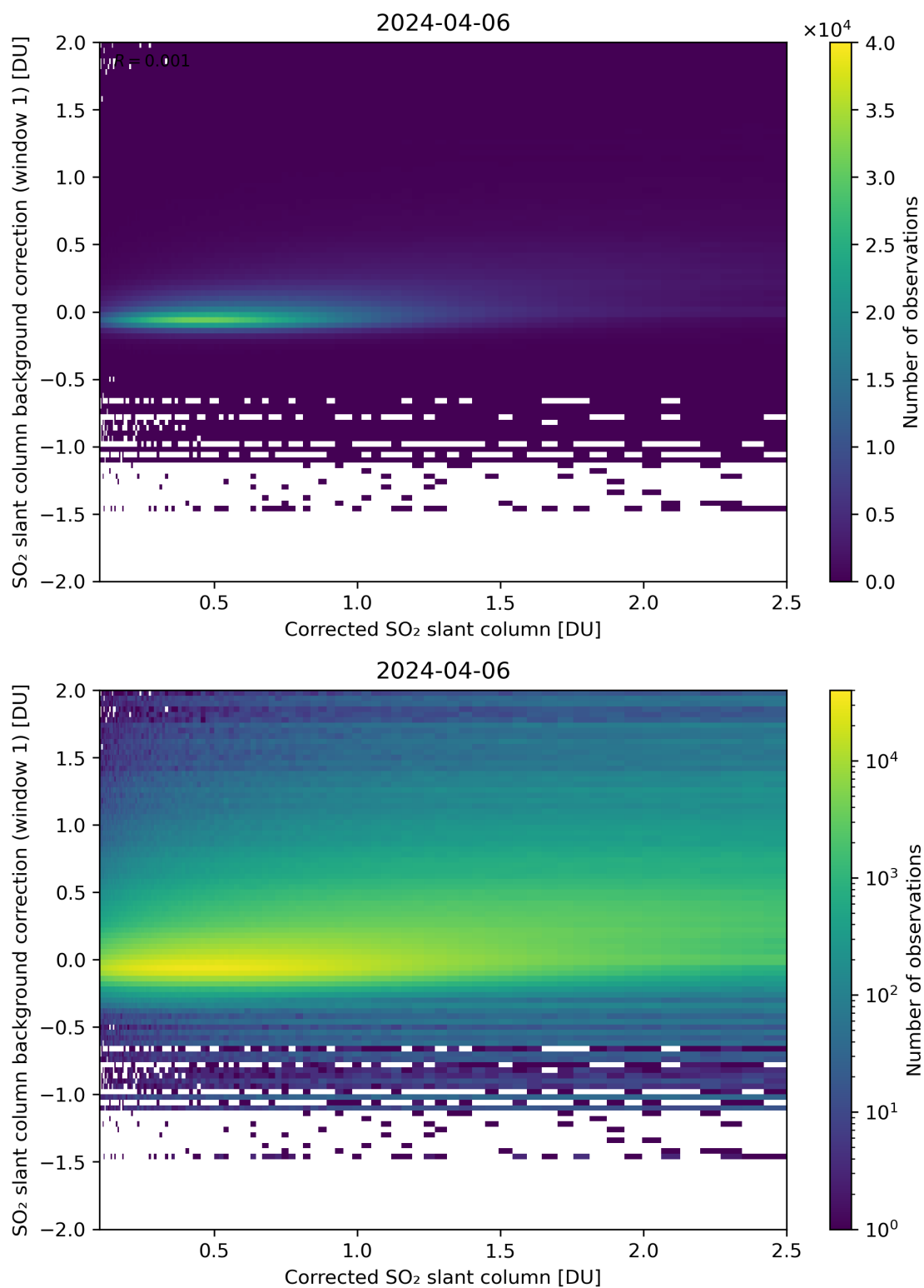
Figure 178: Scatter density plot of “Corrected SO 2 slant column” against “SO 2 slant column background correction (window 1)” for 2024-04-05 to 2024-04-07.
