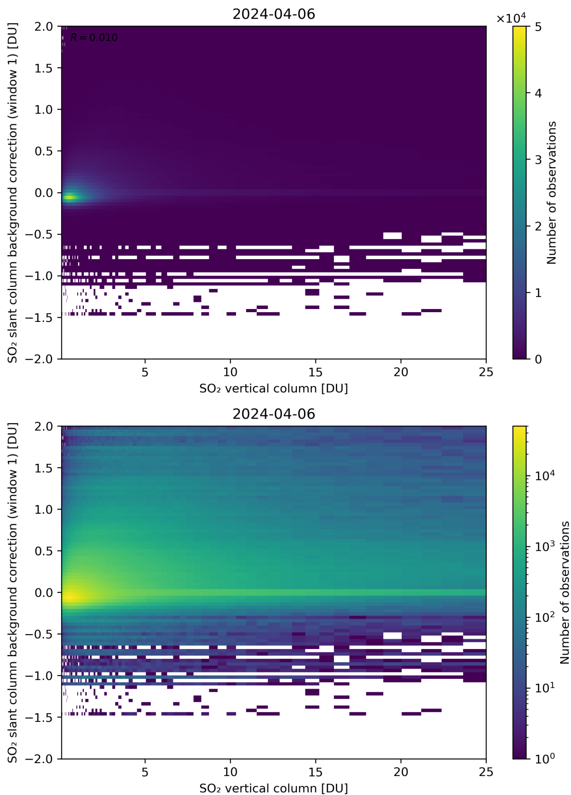
Figure 273: Scatter density plot of “SO 2 vertical column” against “SO 2 slant column background correction (window 1)” for 2024-04-05 to 2024-04-07.
