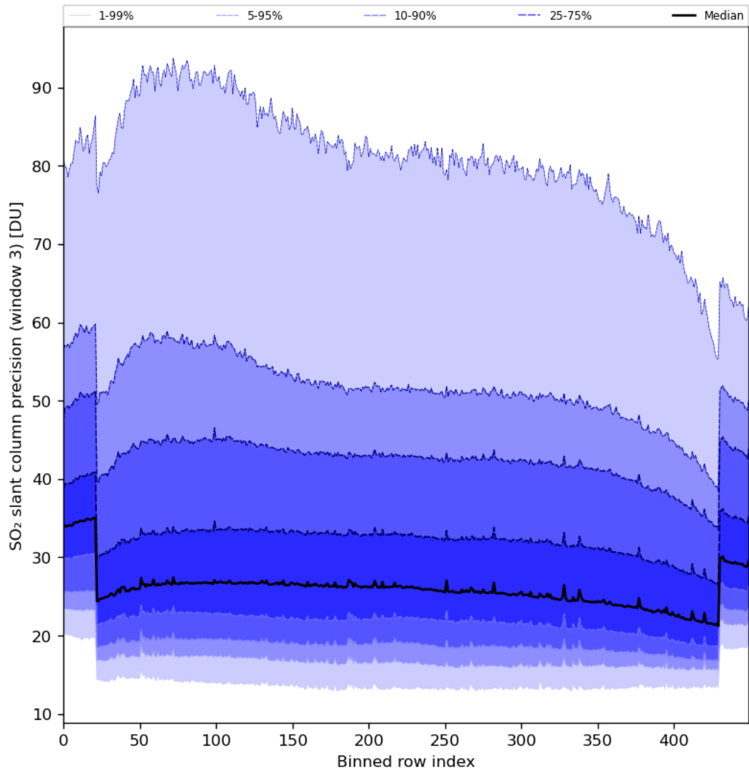
Figure 88: Along track statistics of “SO 2 slant column precision (window 3)” for 2024-04-05 to 2024-04-07
