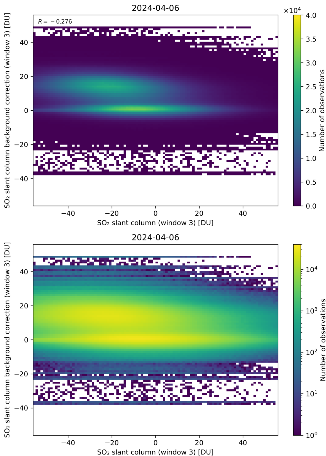
Figure 253: Scatter density plot of “SO 2 slant column (window 3)” against “SO 2 slant column background correction (window 3)” for 2024-04-05 to 2024-04-07.
