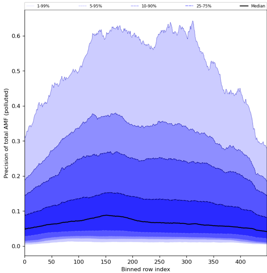
Figure 95: Along track statistics of “Precision of total AMF (polluted)” for 2024-04-05 to 2024-04-07
