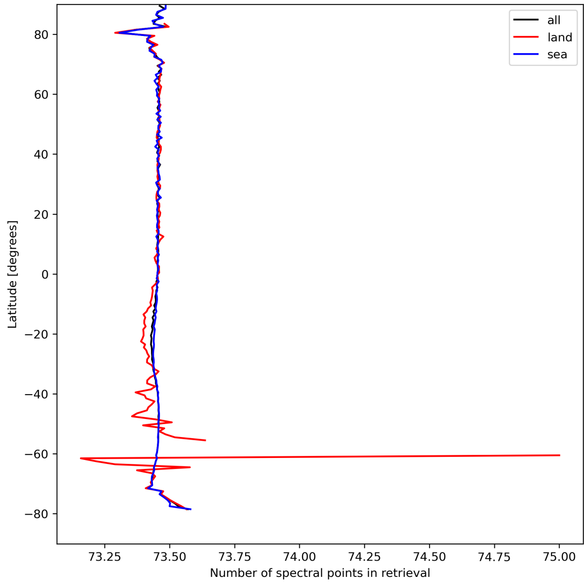
Figure 51: Zonal average of “Number of spectral points in retrieval” for 2024-04-05 to 2024-04-07.
