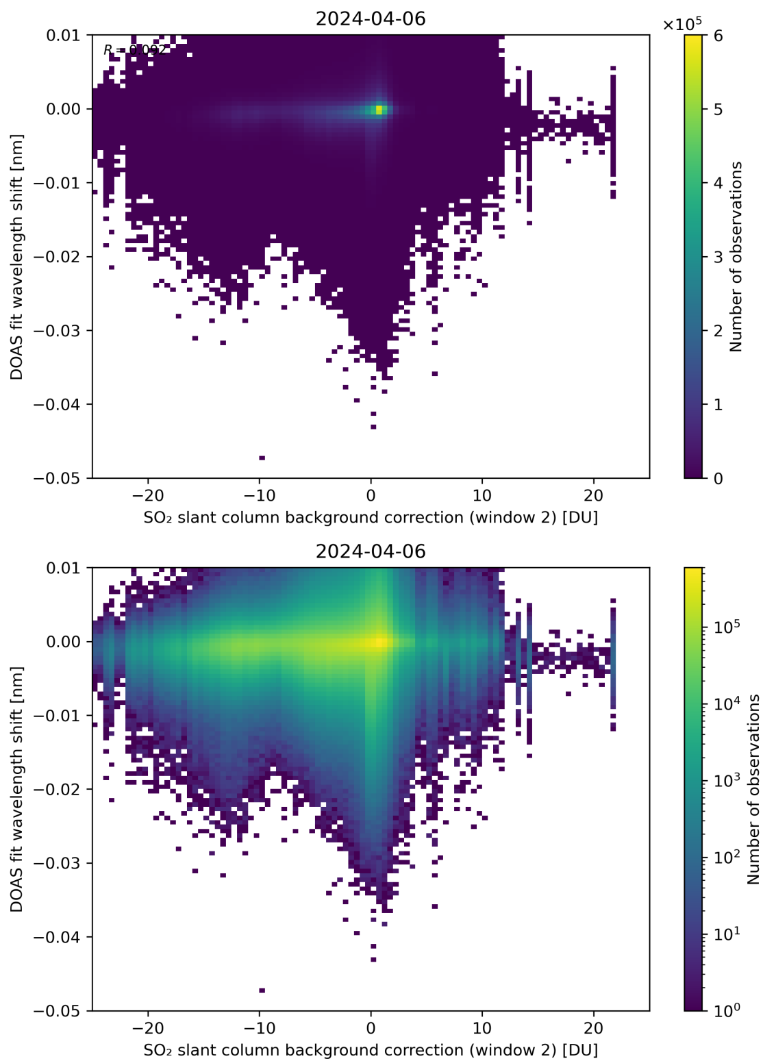
Figure 112: Scatter density plot of “SO 2 slant column background correction (window 2)” against “DOAS fit wavelength shift” for 2024-04-05 to 2024-04-07.
