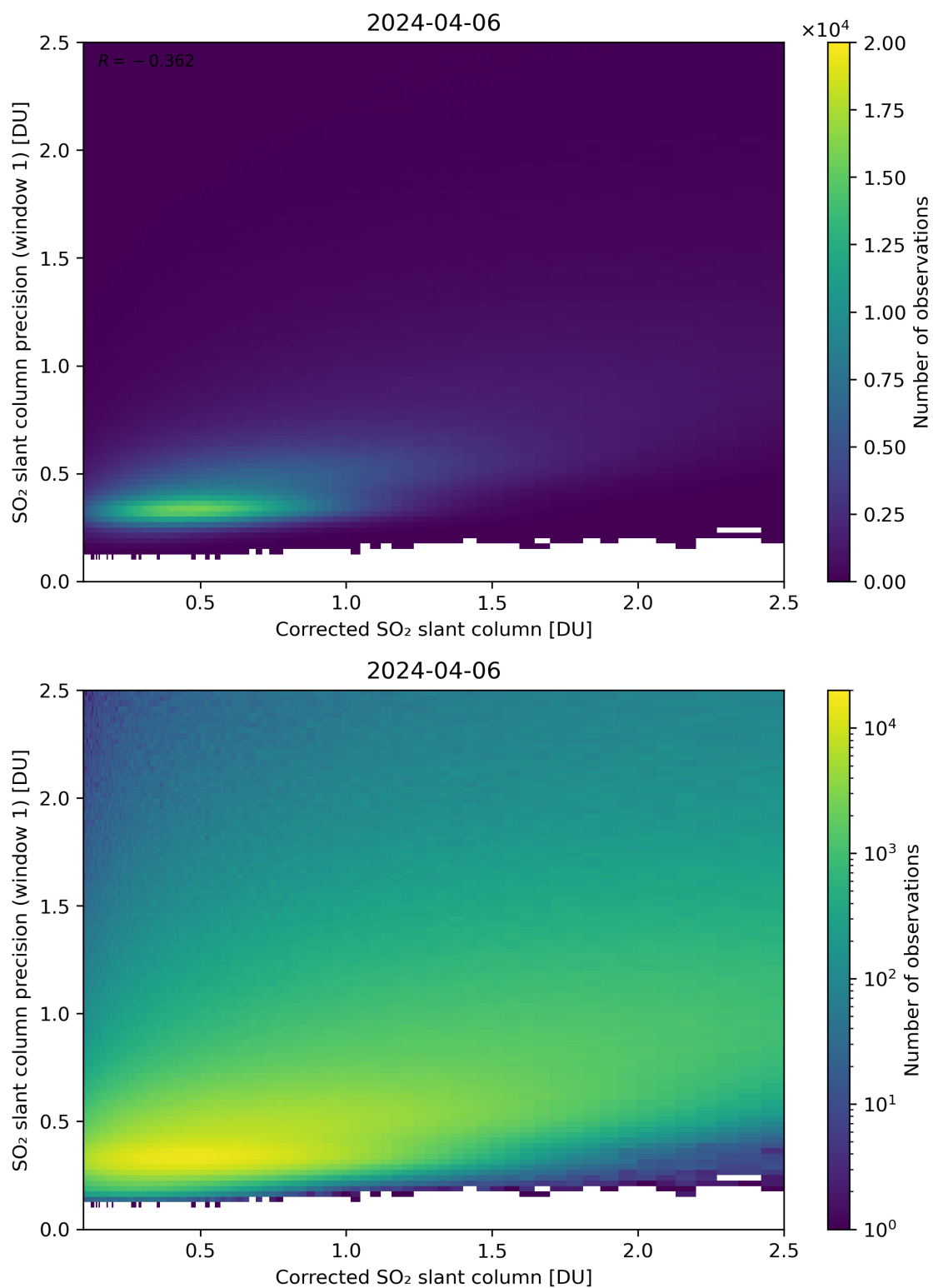
Figure 188: Scatter density plot of “Corrected SO 2 slant column” against “SO 2 slant column precision (window 1)” for 2024-04-05 to 2024-04-07.
