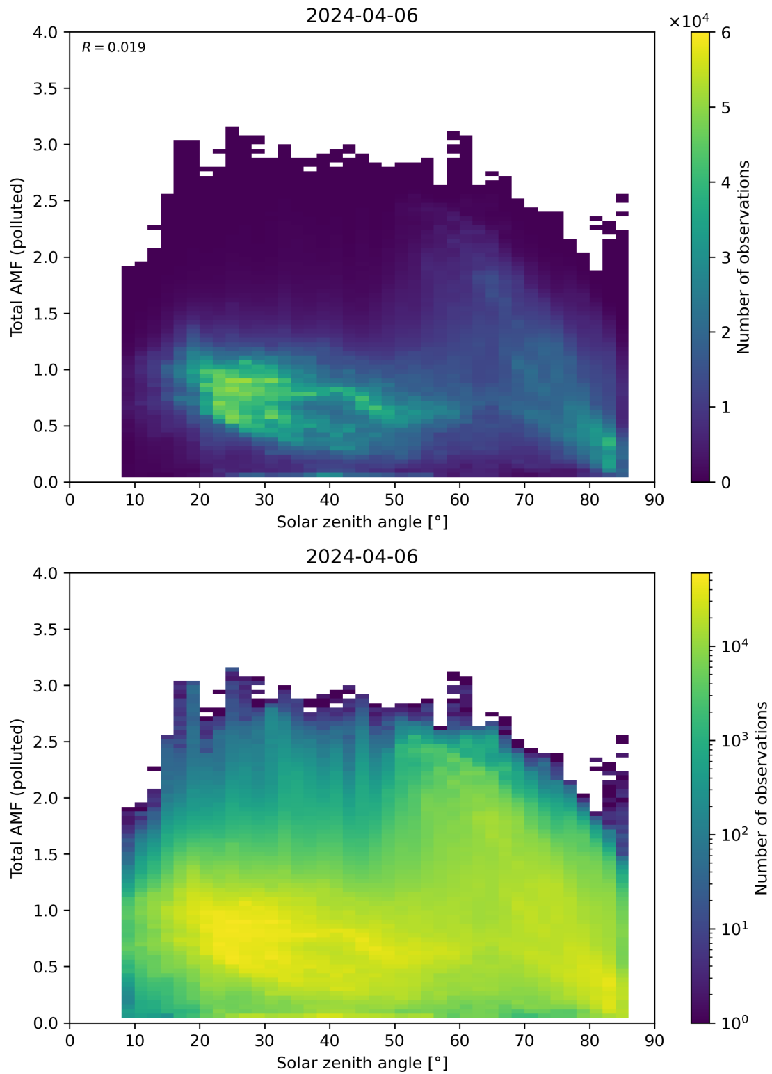
Figure 174: Scatter density plot of “Solar zenith angle” against “Total AMF (polluted)” for 2024-04-05 to 2024-04-07.
