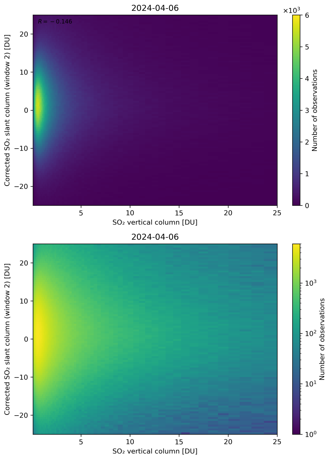
Figure 298: Scatter density plot of “SO 2 vertical column” against “Corrected SO 2 slant column (window 2)” for 2024-04-05 to 2024-04-07.
