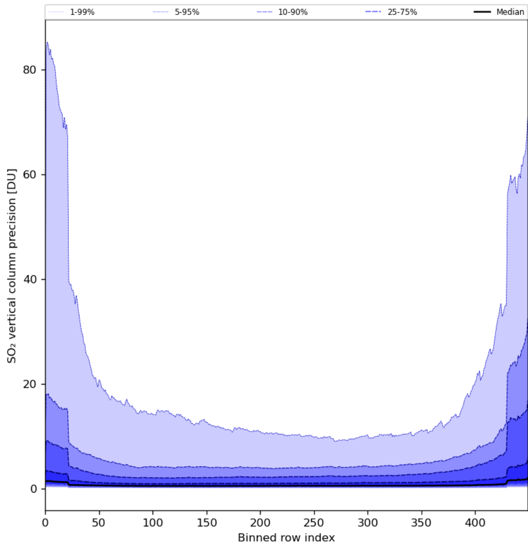
Figure 77: Along track statistics of “SO 2 vertical column precision” for 2024-04-05 to 2024-04-07
