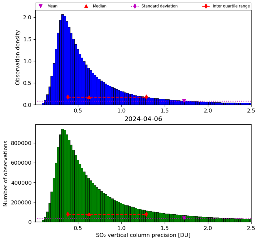
Figure 54: Histogram of “SO 2 vertical column precision” for 2024-04-05 to 2024-04-07
