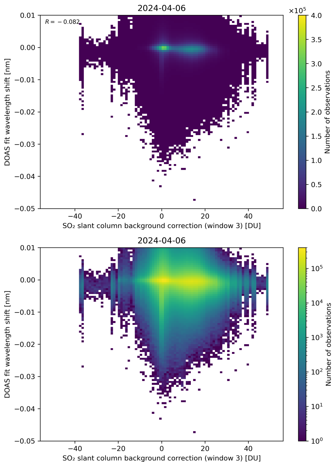
Figure 121: Scatter density plot of “SO 2 slant column background correction (window 3)” against “DOAS fit wavelength shift” for 2024-04-05 to 2024-04-07.
