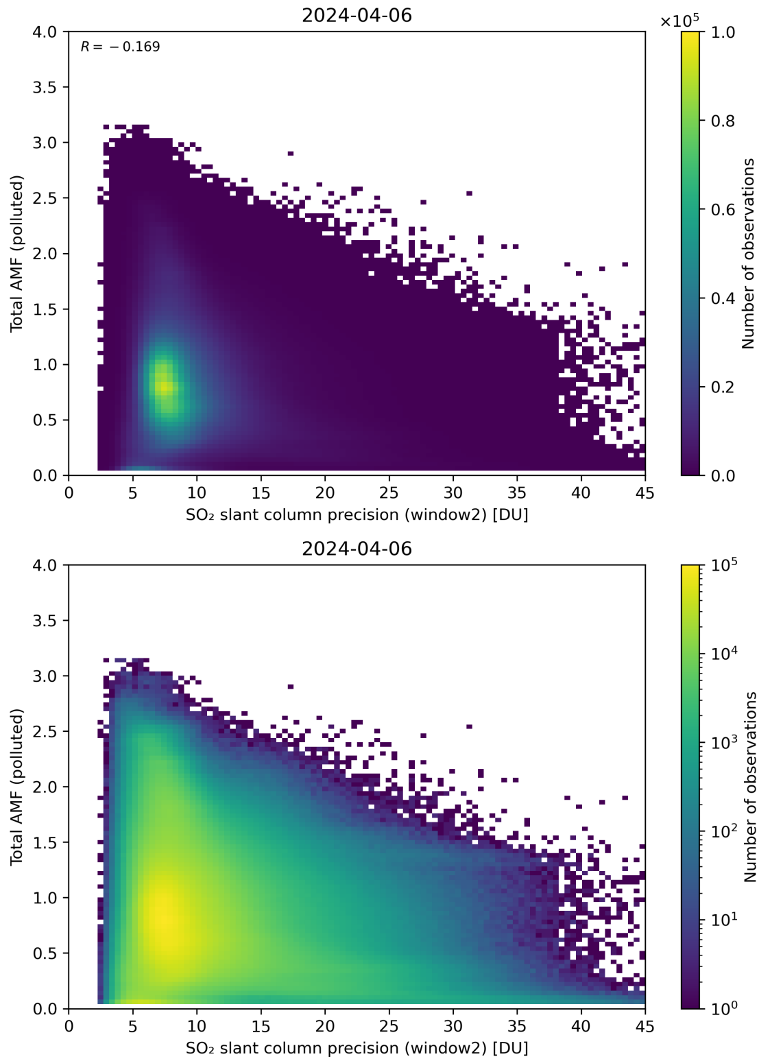
Figure 251: Scatter density plot of “SO 2 slant column precision (window2)” against “Total AMF (polluted)” for 2024-04-05 to 2024-04-07.
