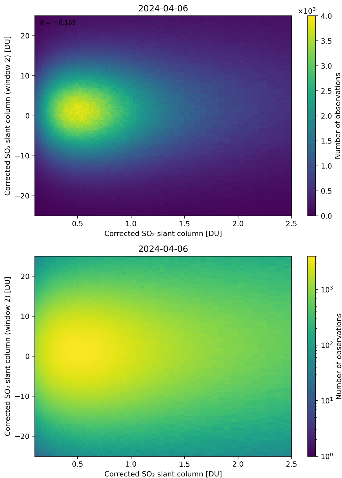
Figure 185: Scatter density plot of “Corrected SO 2 slant column” against “Corrected SO 2 slant column (window 2)” for 2024-04-05 to 2024-04-07.
