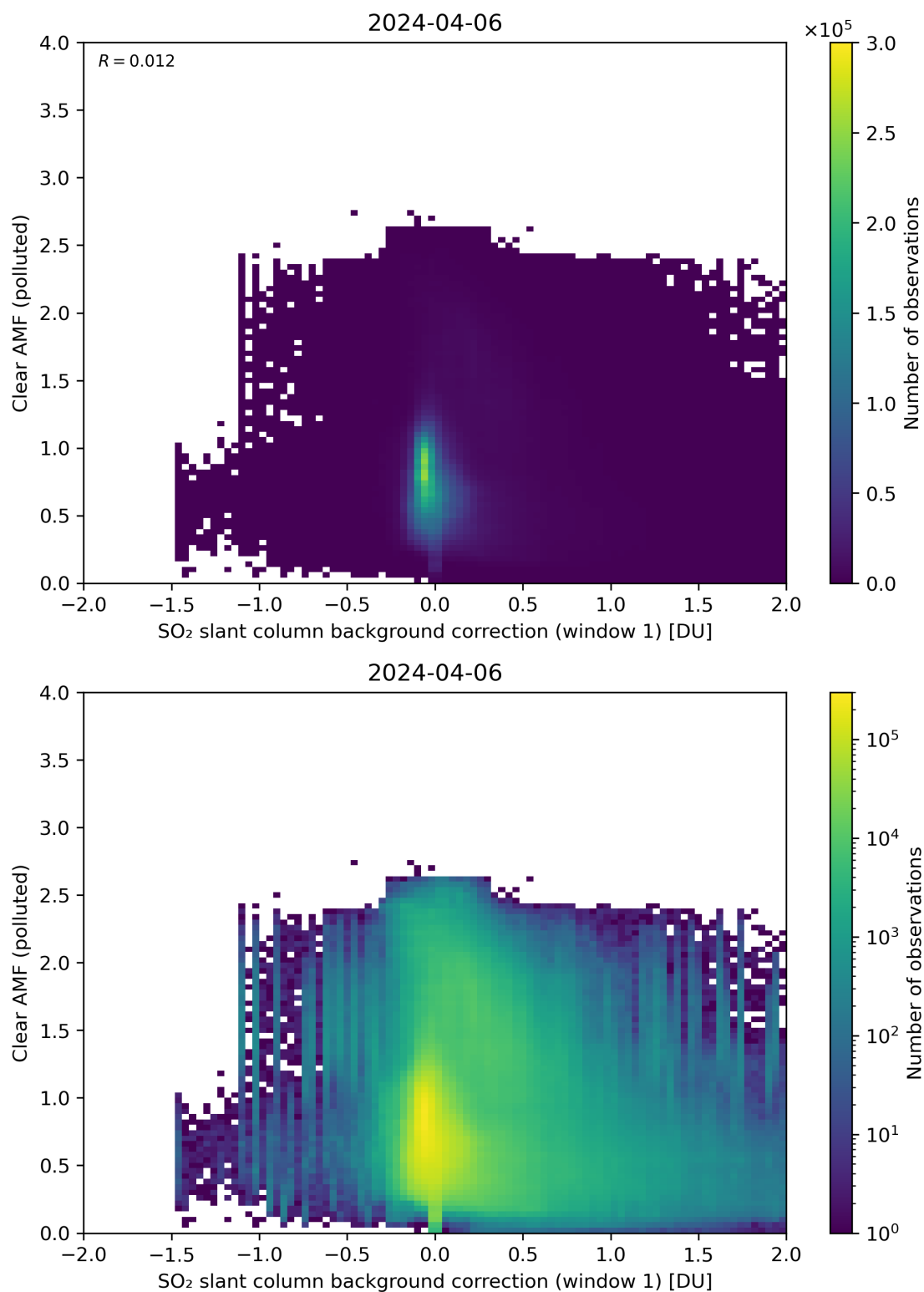
Figure 103: Scatter density plot of “SO 2 slant column background correction (window 1)” against “Clear AMF (polluted)” for 2024-04-05 to 2024-04-07.
