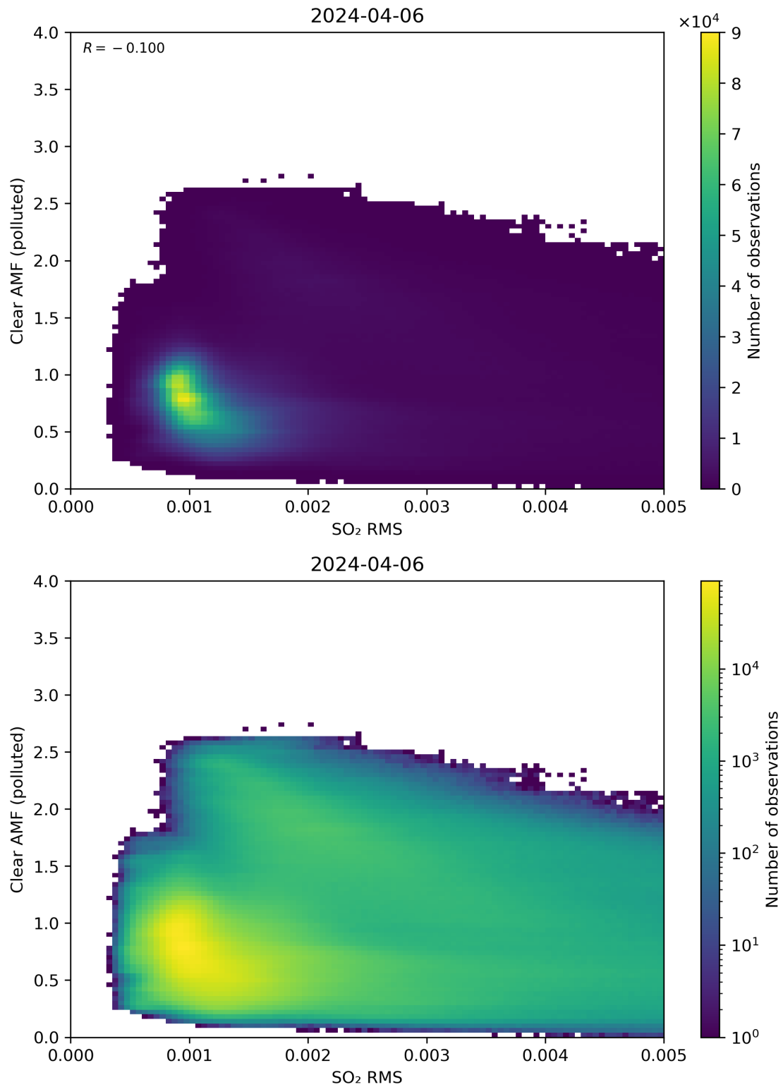
Figure 136: Scatter density plot of “SO 2 RMS” against “Clear AMF (polluted)” for 2024-04-05 to 2024-04-07.
