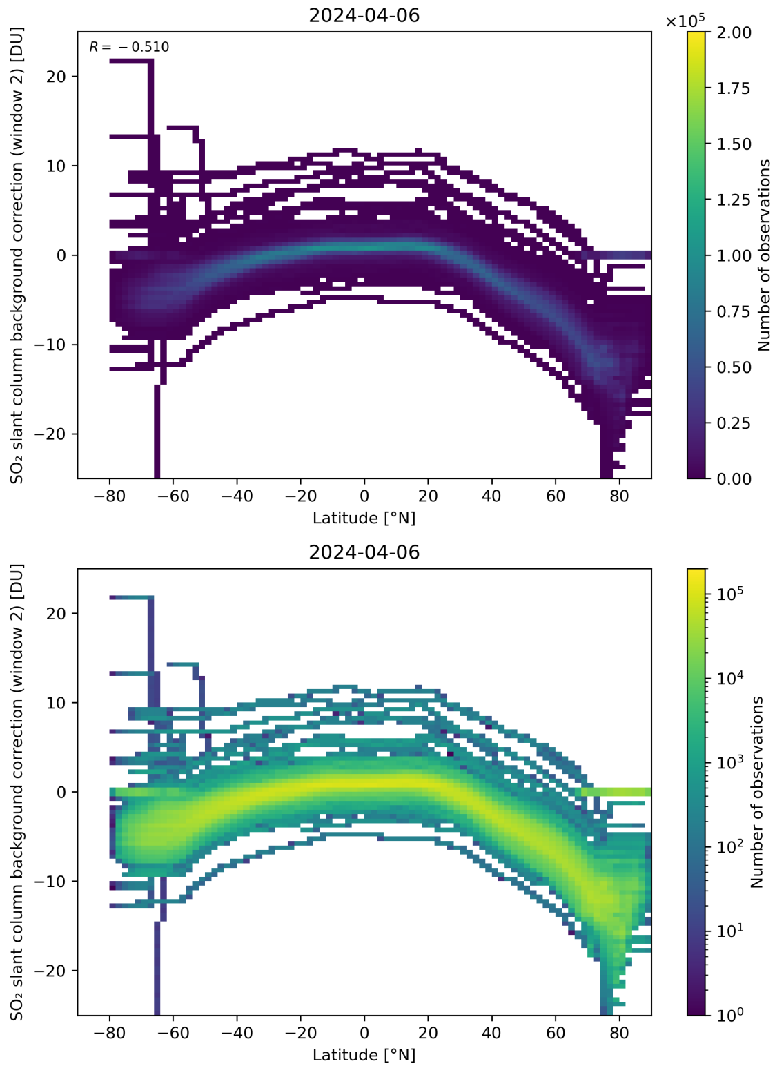
Figure 140: Scatter density plot of “Latitude” against “SO 2 slant column background correction (window 2)” for 2024-04-05 to 2024-04-07.
