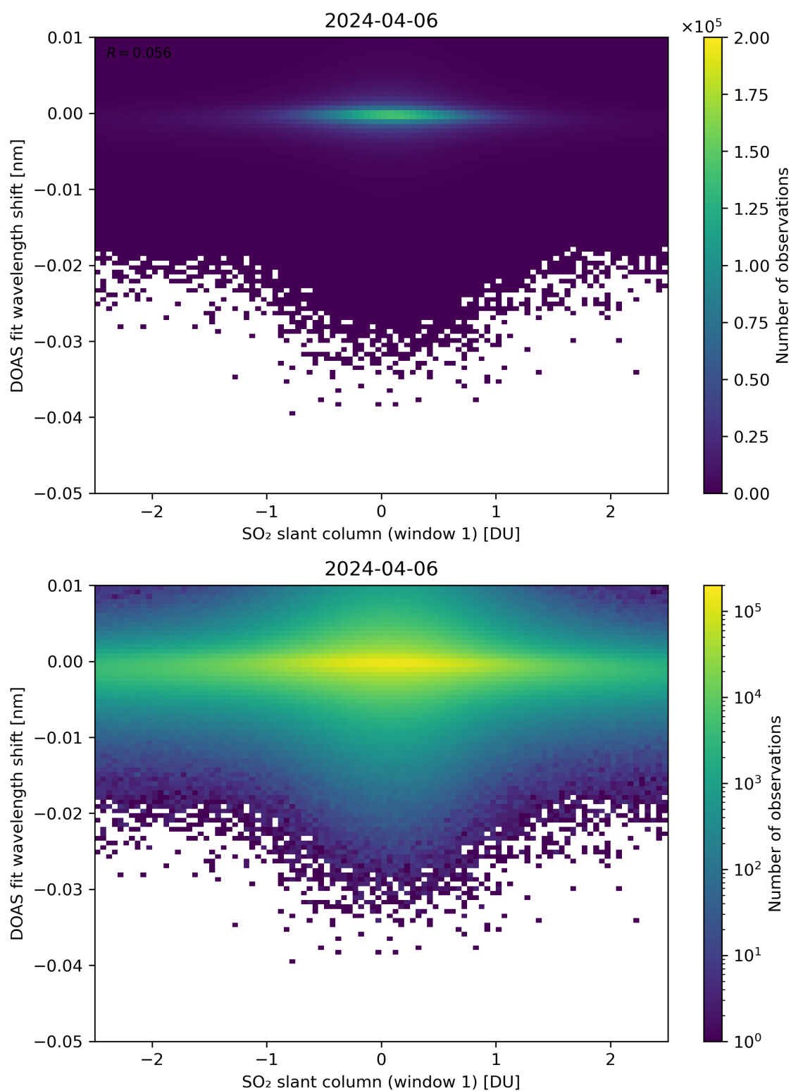
Figure 215: Scatter density plot of “SO 2 slant column (window 1)” against “DOAS fit wavelength shift” for 2024-04-05 to 2024-04-07.
