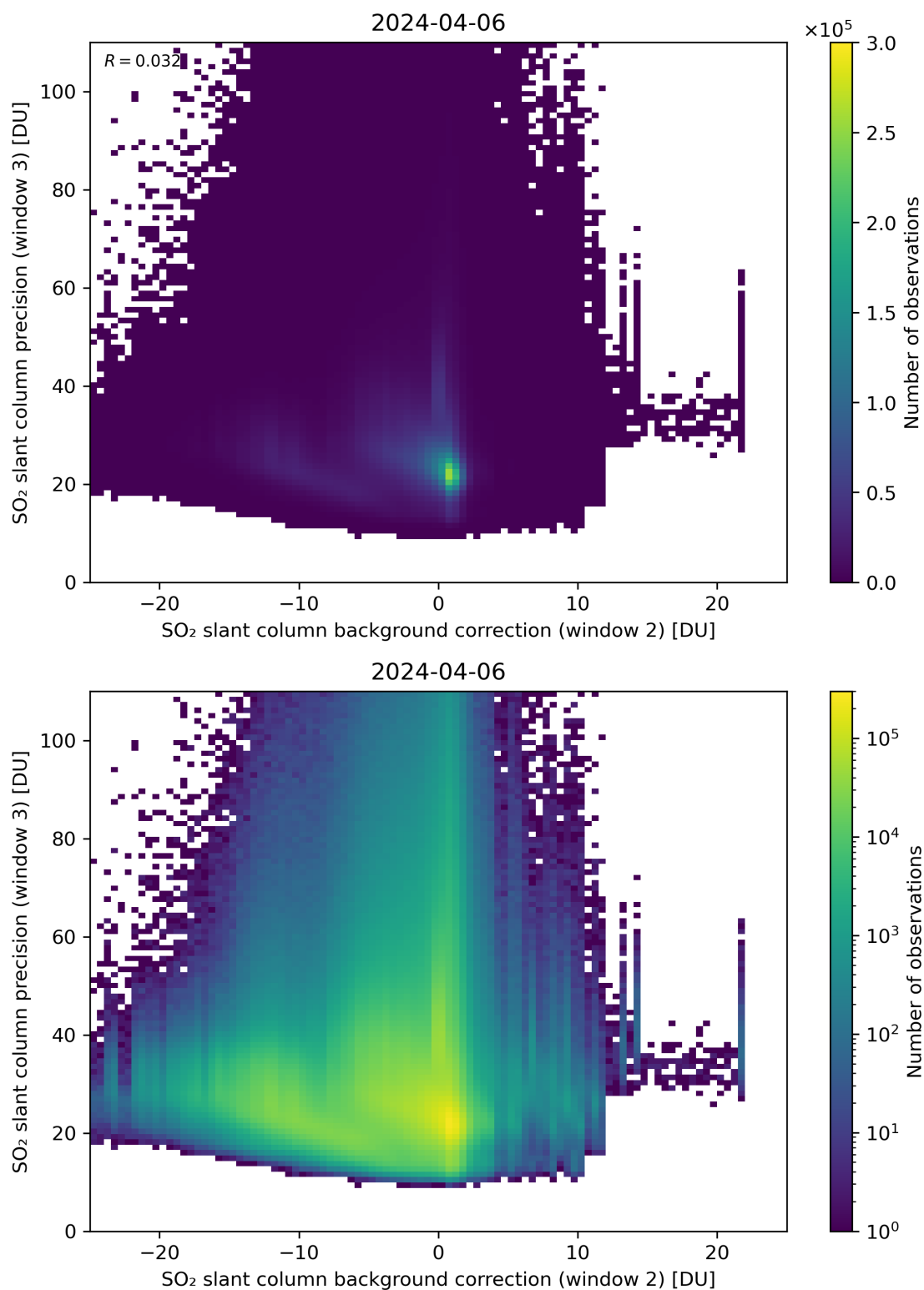
Figure 118: Scatter density plot of “SO 2 slant column background correction (window 2)” against “SO 2 slant column precision (window 3)” for 2024-04-05 to 2024-04-07.
