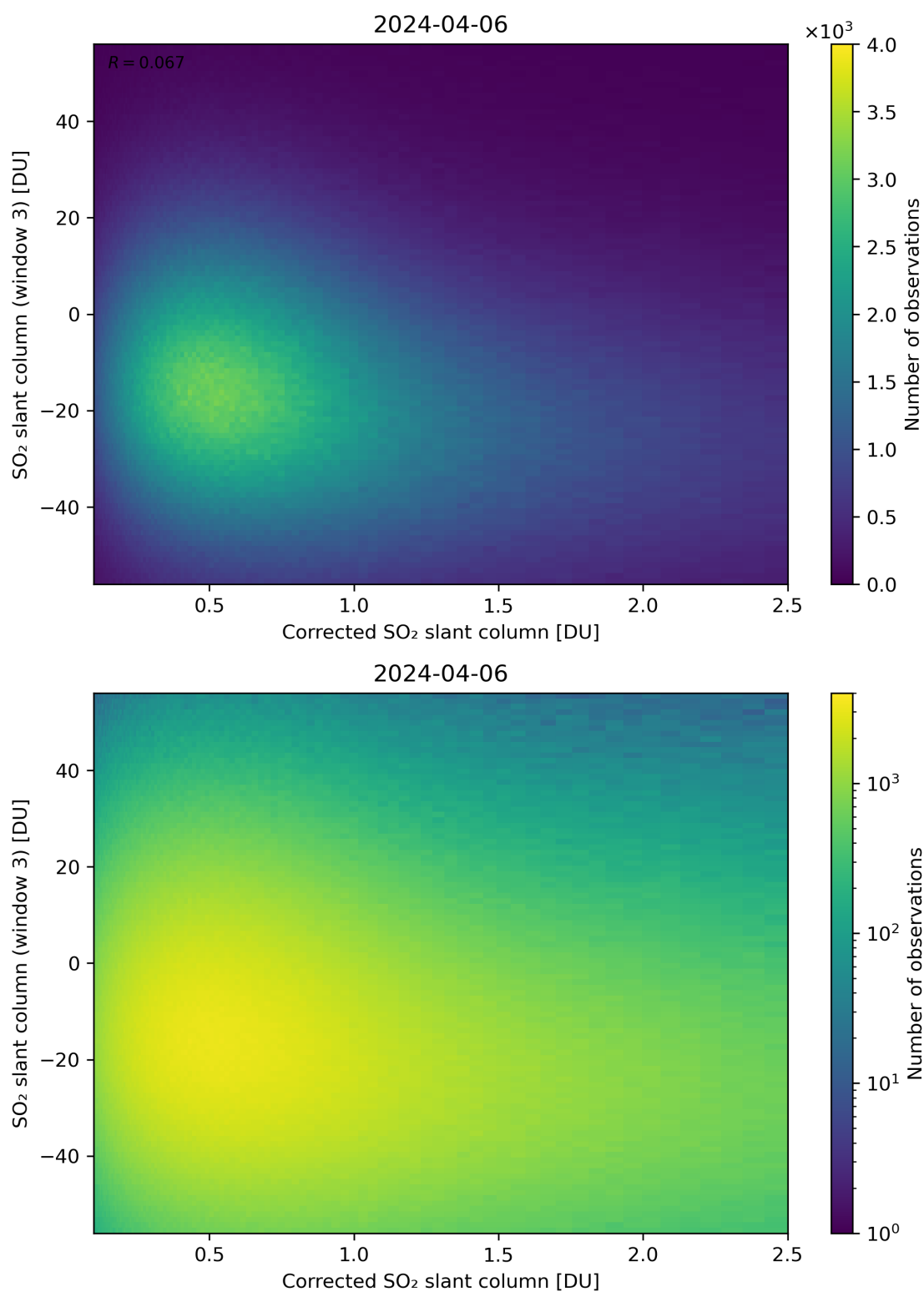
Figure 190: Scatter density plot of “Corrected SO 2 slant column” against “SO 2 slant column (window 3)” for 2024-04-05 to 2024-04-07.
