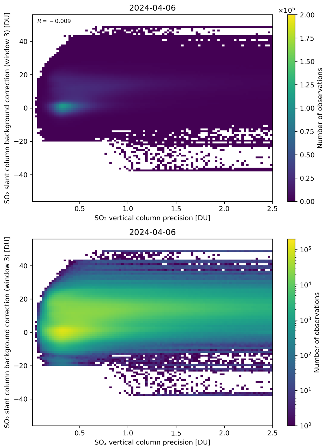
Figure 281: Scatter density plot of “SO 2 vertical column precision” against “SO 2 slant column background correction (window 3)” for 2024-04-05 to 2024-04-07.
