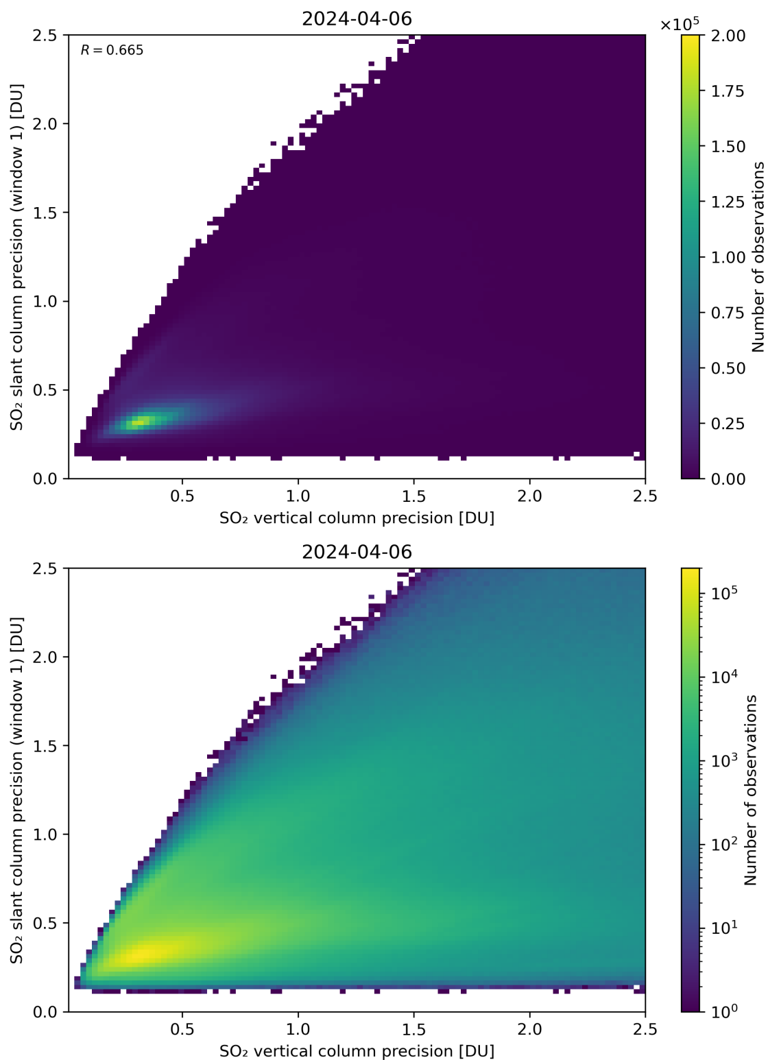
Figure 290: Scatter density plot of “SO 2 vertical column precision” against “SO 2 slant column precision (window 1)” for 2024-04-05 to 2024-04-07.
