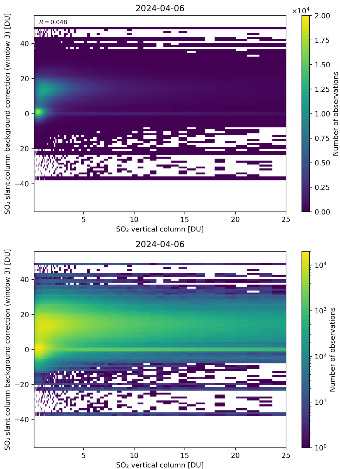
Figure 275: Scatter density plot of “SO 2 vertical column” against “SO 2 slant column background correction (window 3)” for 2024-04-05 to 2024-04-07.
