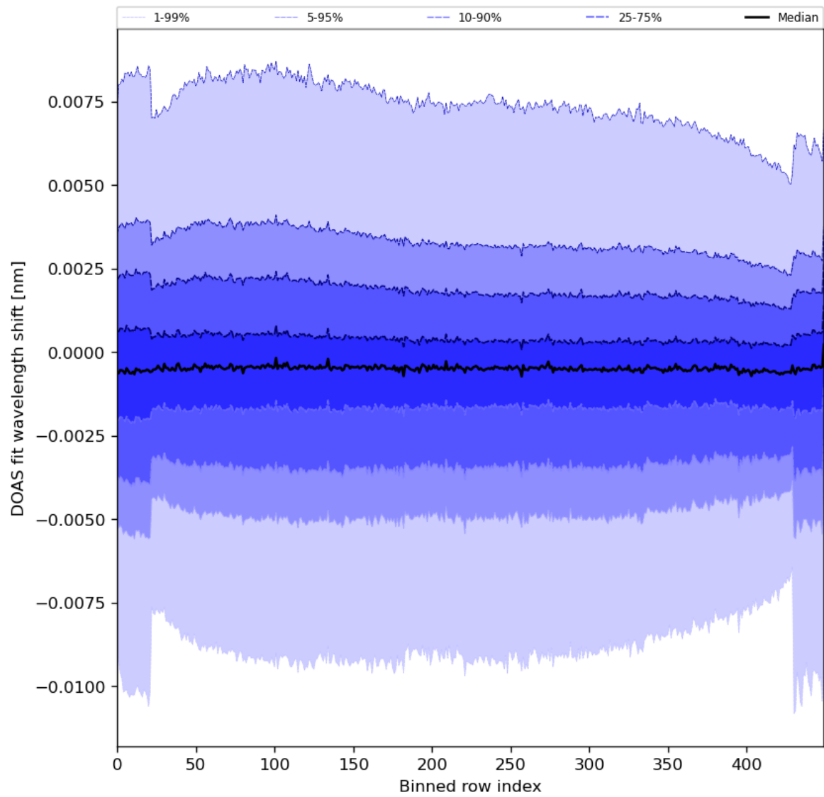
Figure 91: Along track statistics of “DOAS fit wavelength shift” for 2024-04-05 to 2024-04-07
