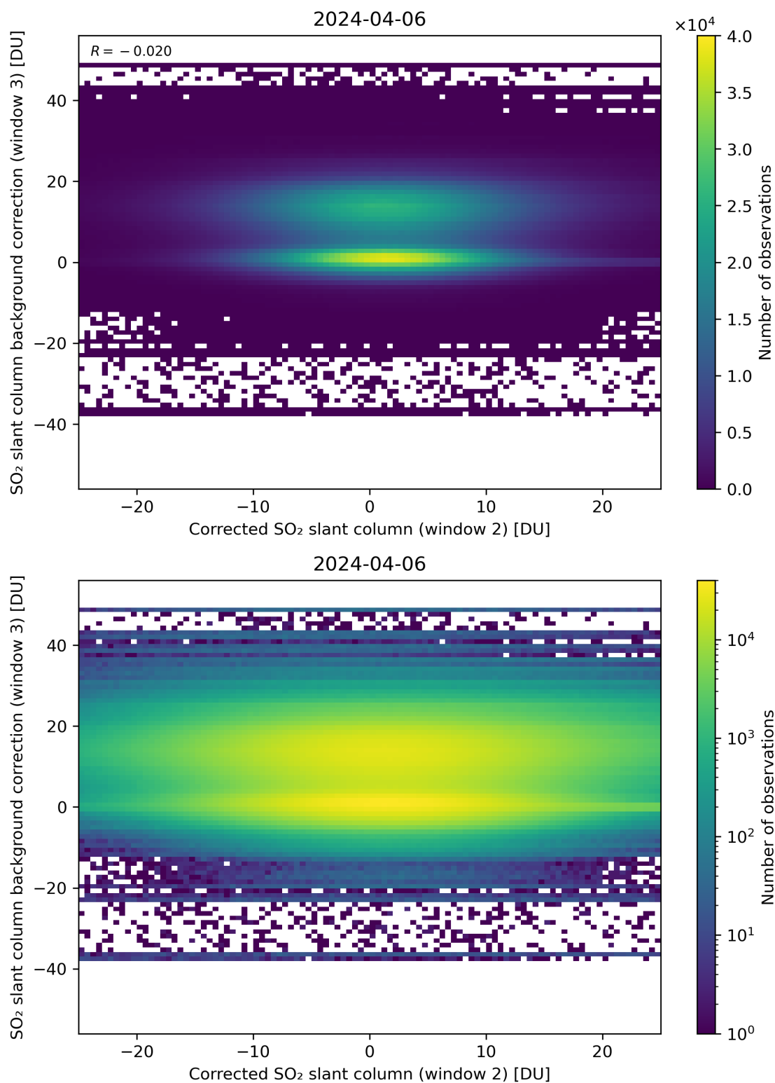
Figure 195: Scatter density plot of “Corrected SO 2 slant column (window 2)” against “SO 2 slant column background correction (window 3)” for 2024-04-05 to 2024-04-07.
