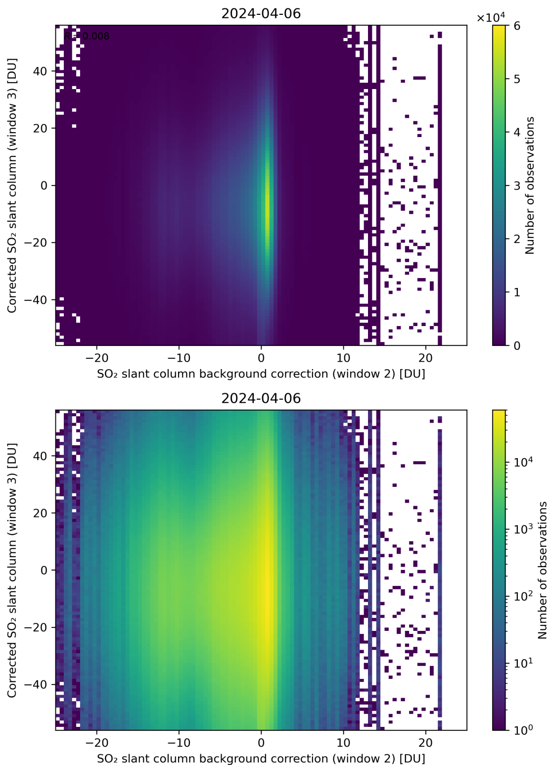
Figure 116: Scatter density plot of “SO 2 slant column background correction (window 2)” against “Corrected SO 2 slant column (window 3)” for 2024-04-05 to 2024-04-07.
