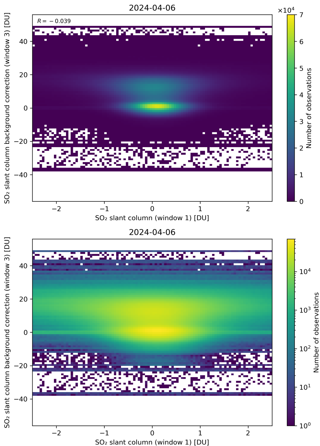
Figure 214: Scatter density plot of “SO 2 slant column (window 1)” against “SO 2 slant column background correction (window 3)” for 2024-04-05 to 2024-04-07.
