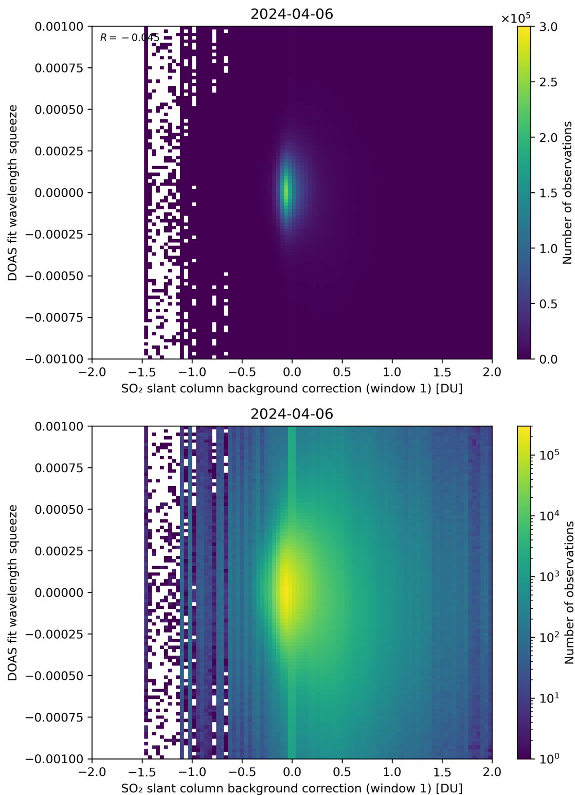
Figure 101: Scatter density plot of “SO 2 slant column background correction (window 1)” against “DOAS fit wavelength squeeze” for 2024-04-05 to 2024-04-07.
