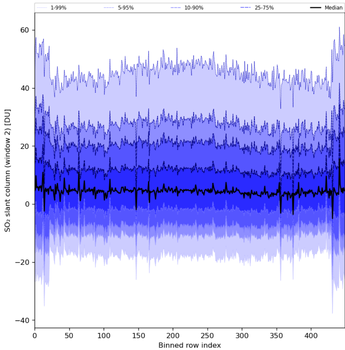
Figure 83: Along track statistics of “SO 2 slant column (window 2)” for 2024-04-05 to 2024-04-07
