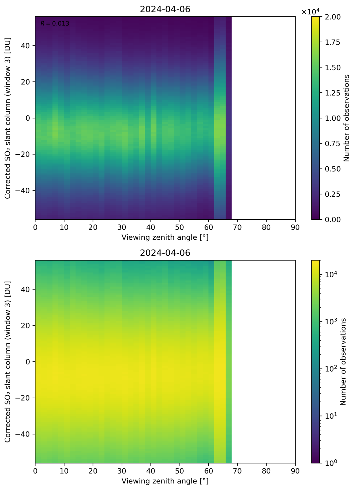
Figure 319: Scatter density plot of “Viewing zenith angle” against “Corrected SO 2 slant column (window 3)” for 2024-04-05 to 2024-04-07.
