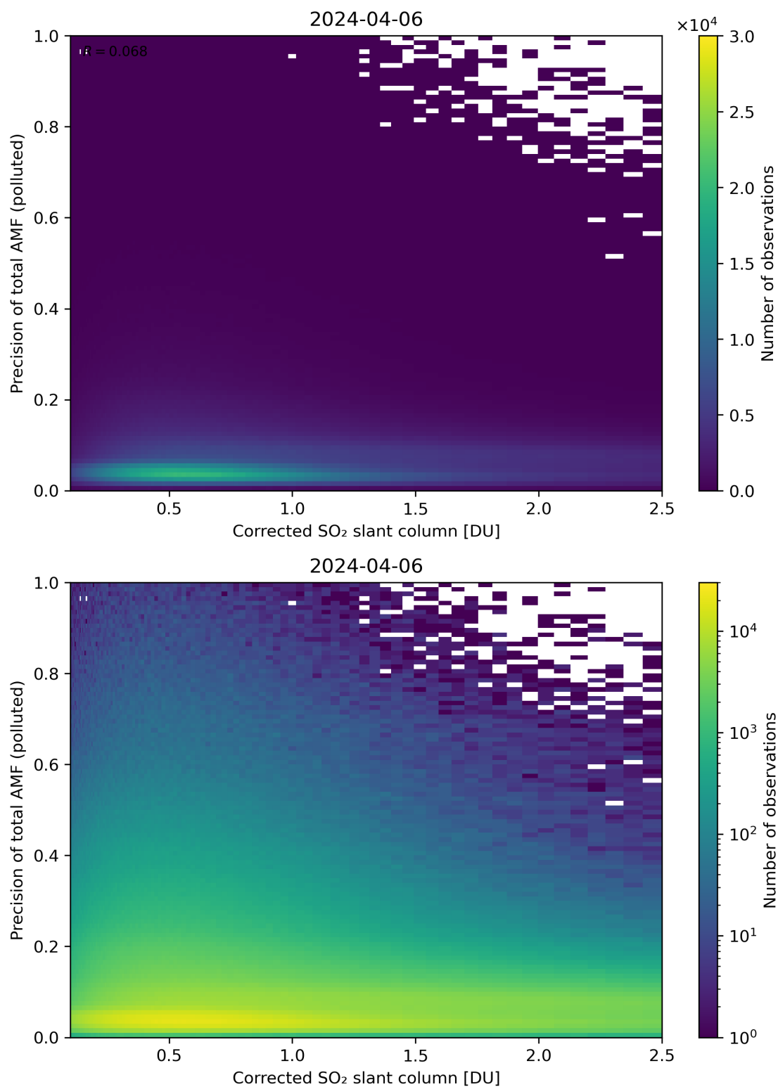
Figure 193: Scatter density plot of “Corrected SO 2 slant column” against “Precision of total AMF (polluted)” for 2024-04-05 to 2024-04-07.
