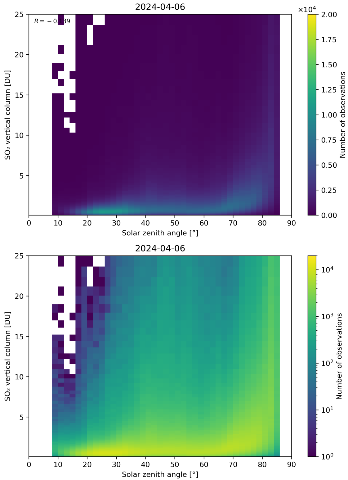
Figure 176: Scatter density plot of “Solar zenith angle” against “SO 2 vertical column” for 2024-04-05 to 2024-04-07.
