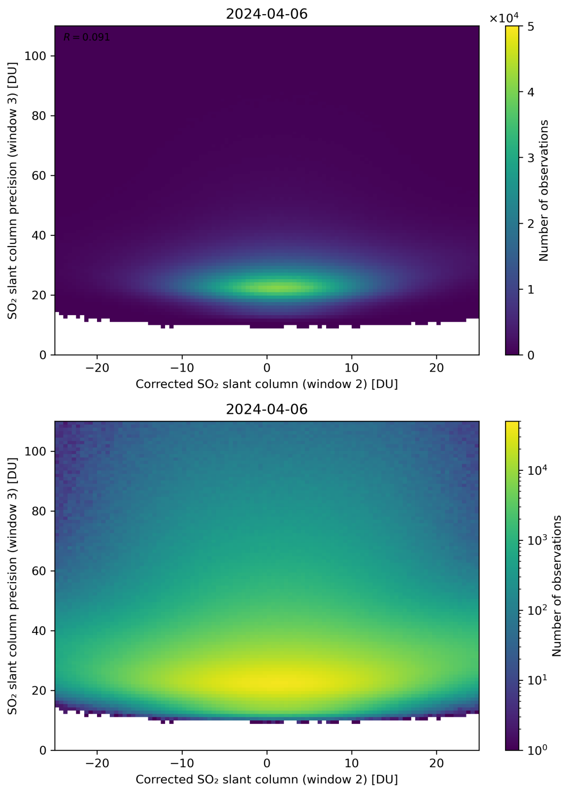
Figure 202: Scatter density plot of “Corrected SO 2 slant column (window 2)” against “SO 2 slant column precision (window 3)” for 2024-04-05 to 2024-04-07.
