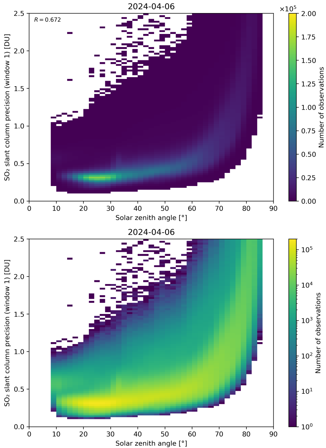
Figure 170: Scatter density plot of “Solar zenith angle” against “SO 2 slant column precision (window 1)” for 2024-04-05 to 2024-04-07.
