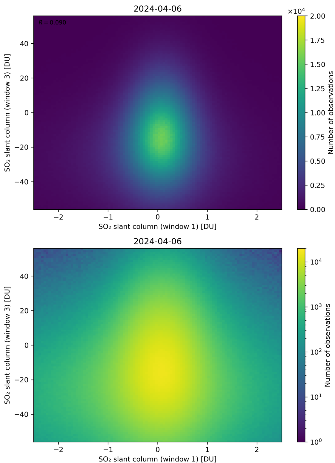
Figure 237: Scatter density plot of “SO 2 slant column (window 1)” against “SO 2 slant column (window 3)” for 2024-04-05 to 2024-04-07.
