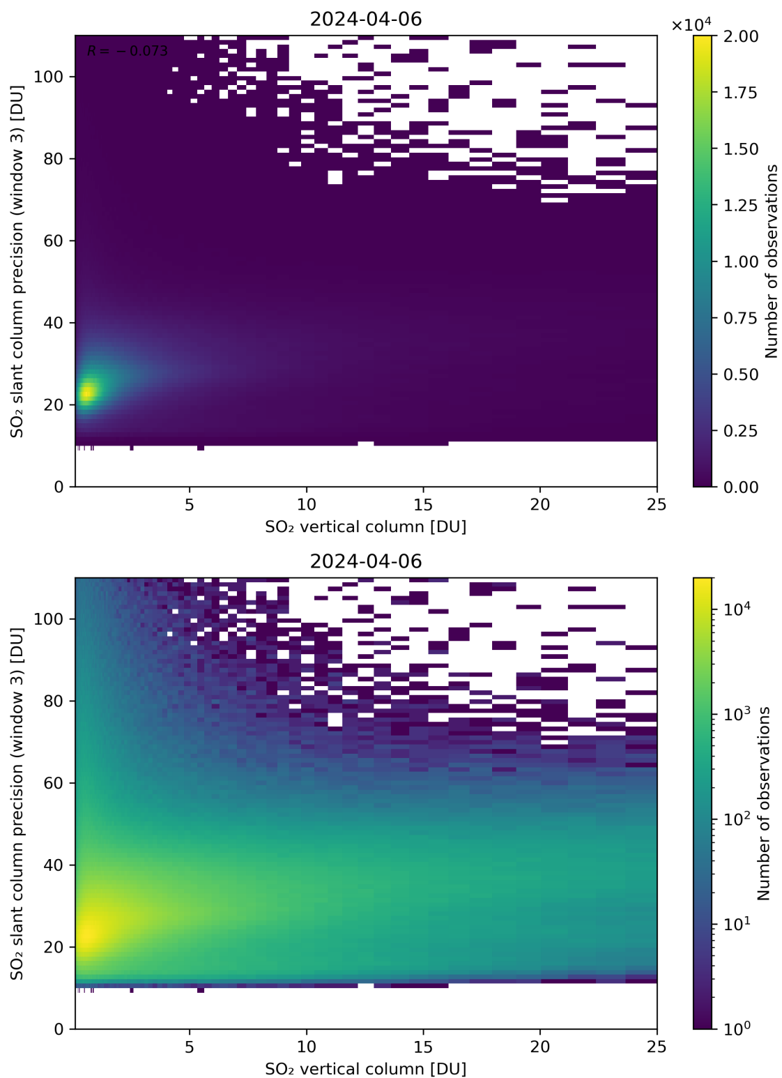
Figure 304: Scatter density plot of “SO 2 vertical column” against “SO 2 slant column precision (window 3)” for 2024-04-05 to 2024-04-07.
