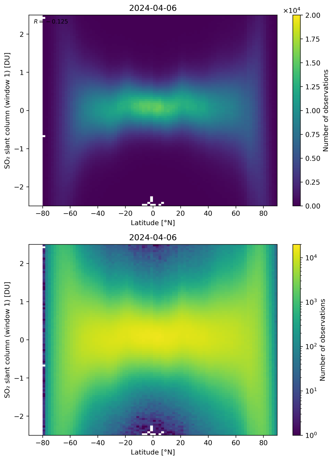
Figure 149: Scatter density plot of “Latitude” against “SO 2 slant column (window 1)” for 2024-04-05 to 2024-04-07.
