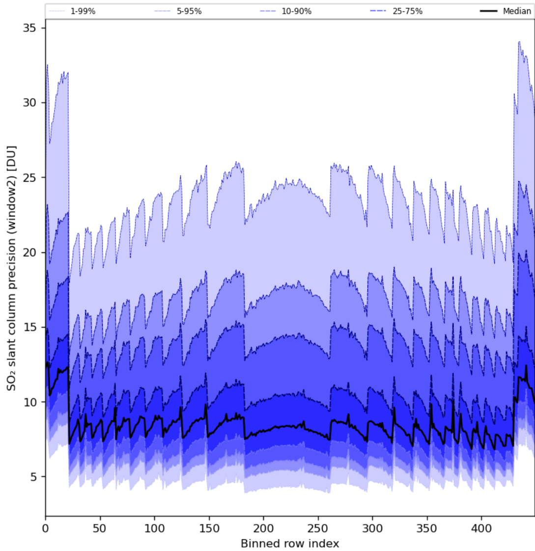
Figure 84: Along track statistics of “SO 2 slant column precision (window2)” for 2024-04-05 to 2024-04-07
