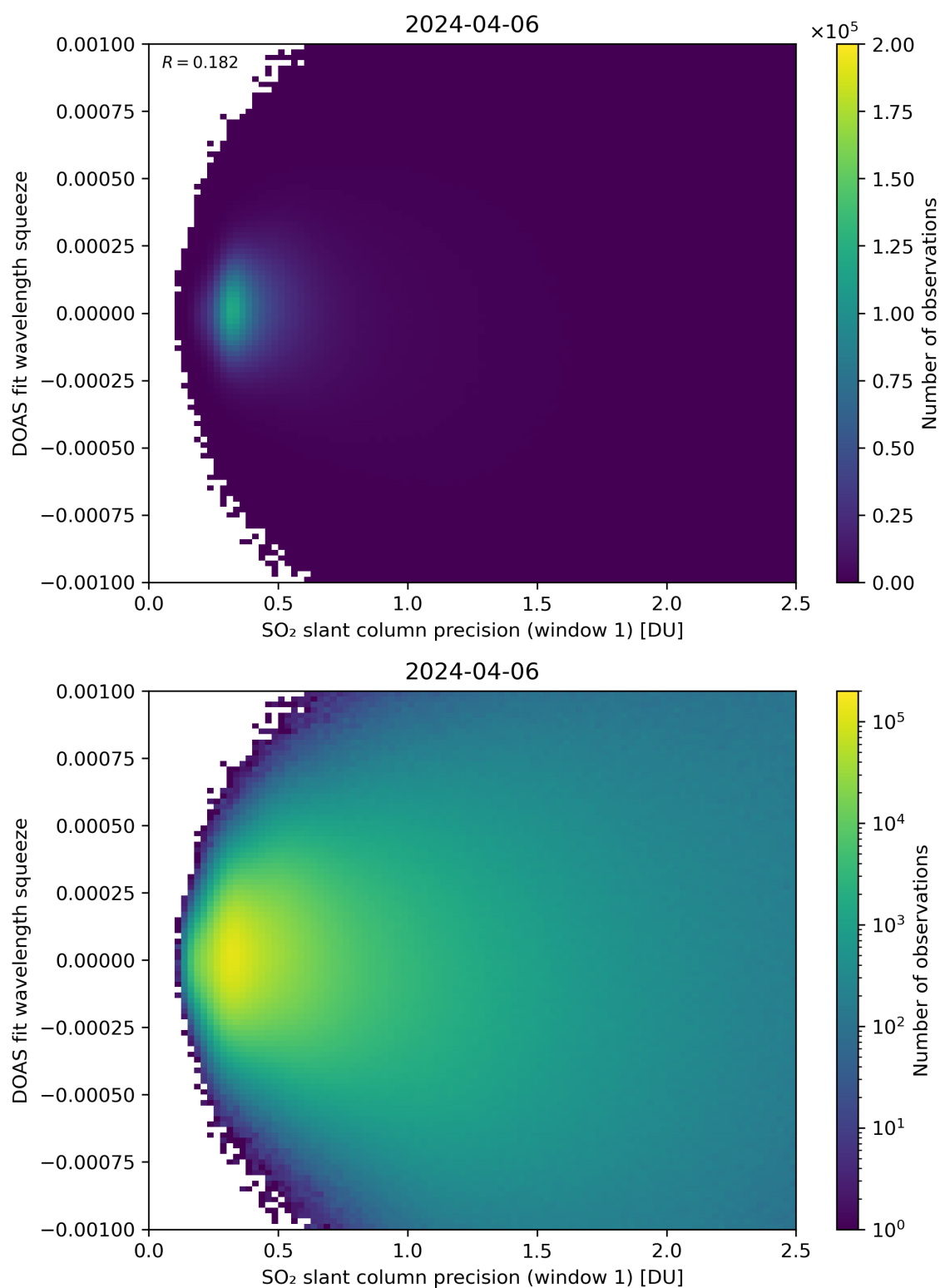
Figure 222: Scatter density plot of “SO 2 slant column precision (window 1)” against “DOAS fit wavelength squeeze” for 2024-04-05 to 2024-04-07.
