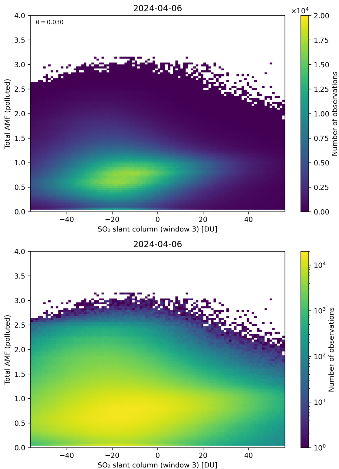
Figure 268: Scatter density plot of “SO 2 slant column (window 3)” against “Total AMF (polluted)” for 2024-04-05 to 2024-04-07.
