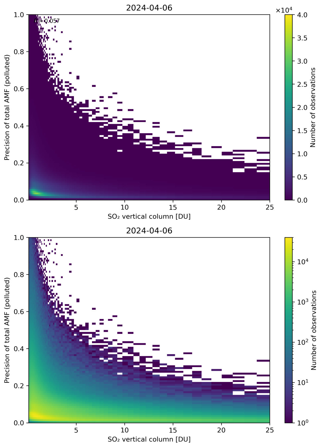
Figure 306: Scatter density plot of “SO 2 vertical column” against “Precision of total AMF (polluted)” for 2024-04-05 to 2024-04-07.
