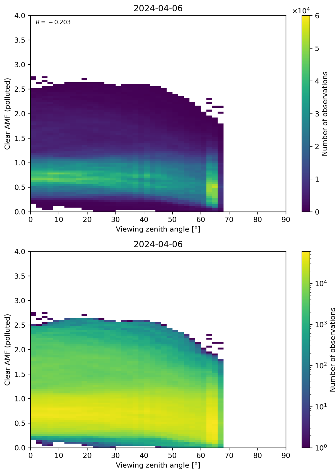
Figure 316: Scatter density plot of “Viewing zenith angle” against “Clear AMF (polluted)” for 2024-04-05 to 2024-04-07.
