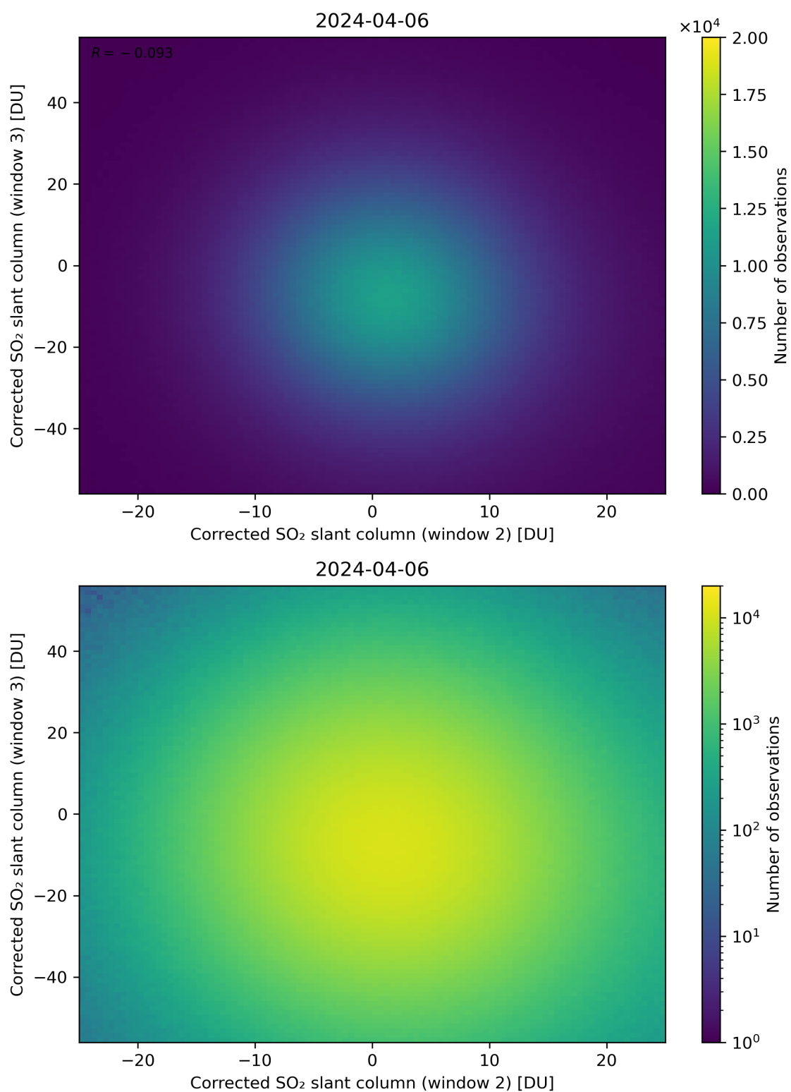
Figure 200: Scatter density plot of “Corrected SO 2 slant column (window 2)” against “Corrected SO 2 slant column (window 3)” for 2024-04-05 to 2024-04-07.
