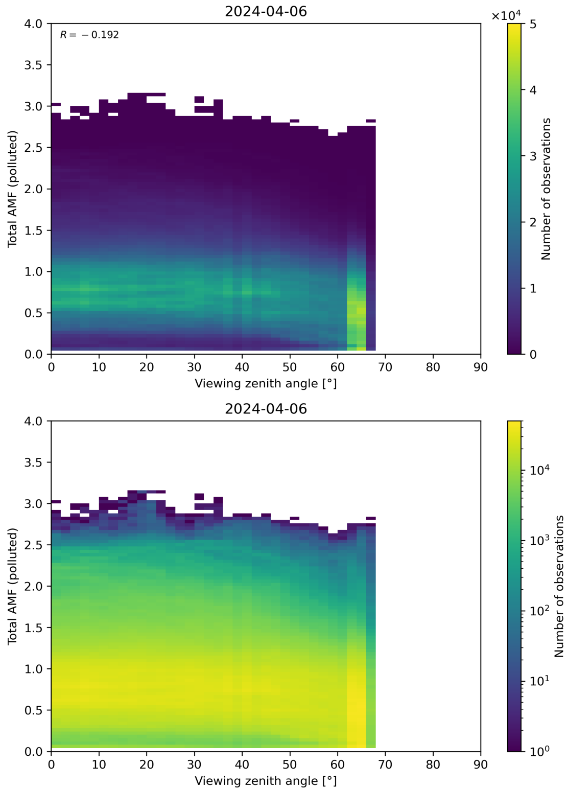
Figure 325: Scatter density plot of “Viewing zenith angle” against “Total AMF (polluted)” for 2024-04-05 to 2024-04-07.
