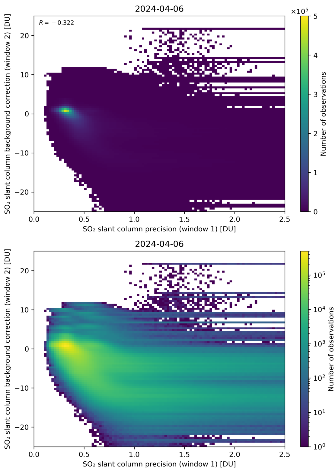
Figure 219: Scatter density plot of “SO 2 slant column precision (window 1)” against “SO 2 slant column background correction (window 2)” for 2024-04-05 to 2024-04-07.
