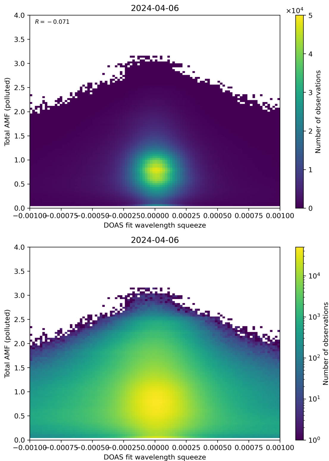
Figure 134: Scatter density plot of “DOAS fit wavelength squeeze” against “Total AMF (polluted)” for 2024-04-05 to 2024-04-07.
