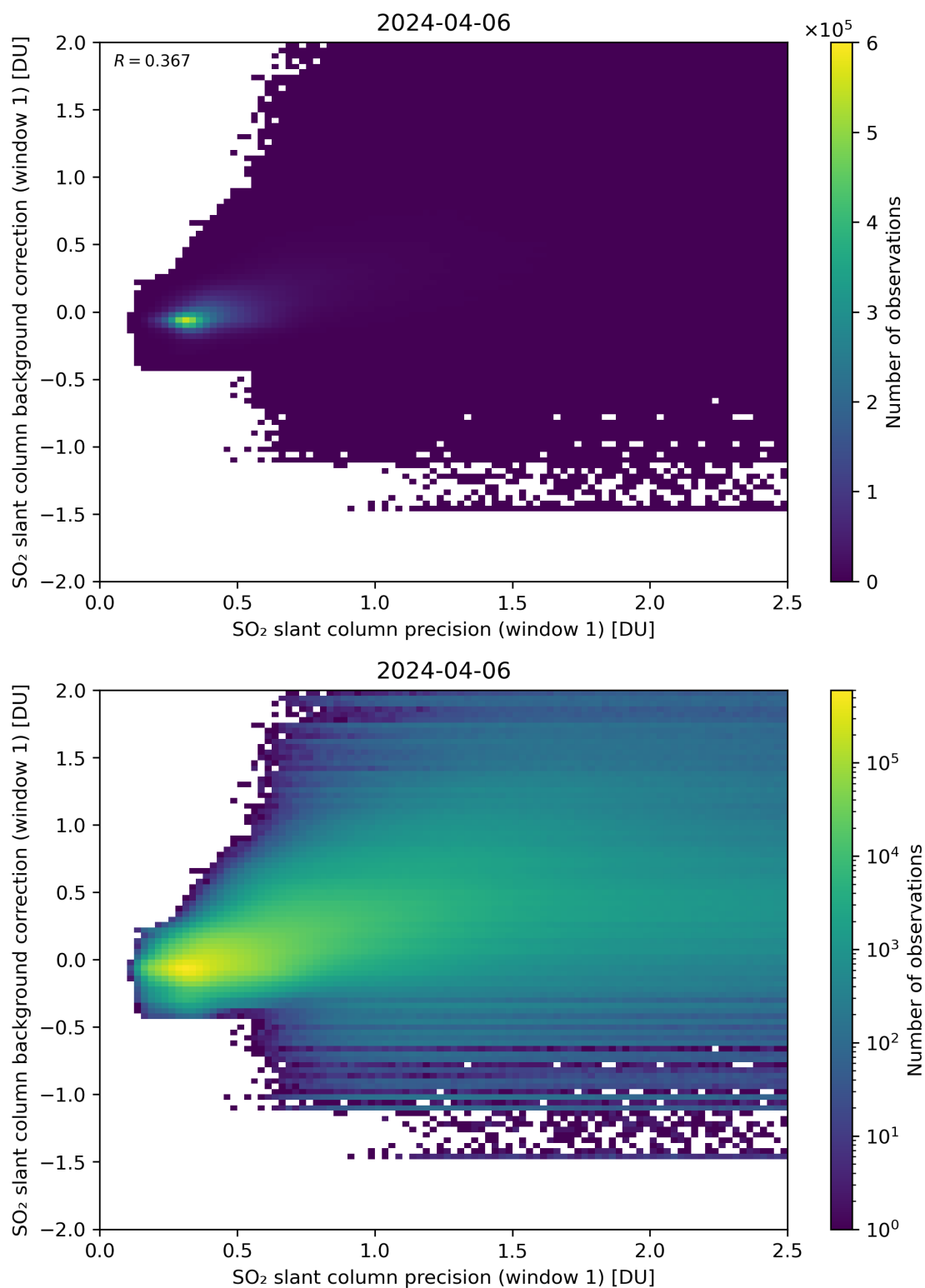
Figure 218: Scatter density plot of “SO 2 slant column precision (window 1)” against “SO 2 slant column background correction (window 1)” for 2024-04-05 to 2024-04-07.
