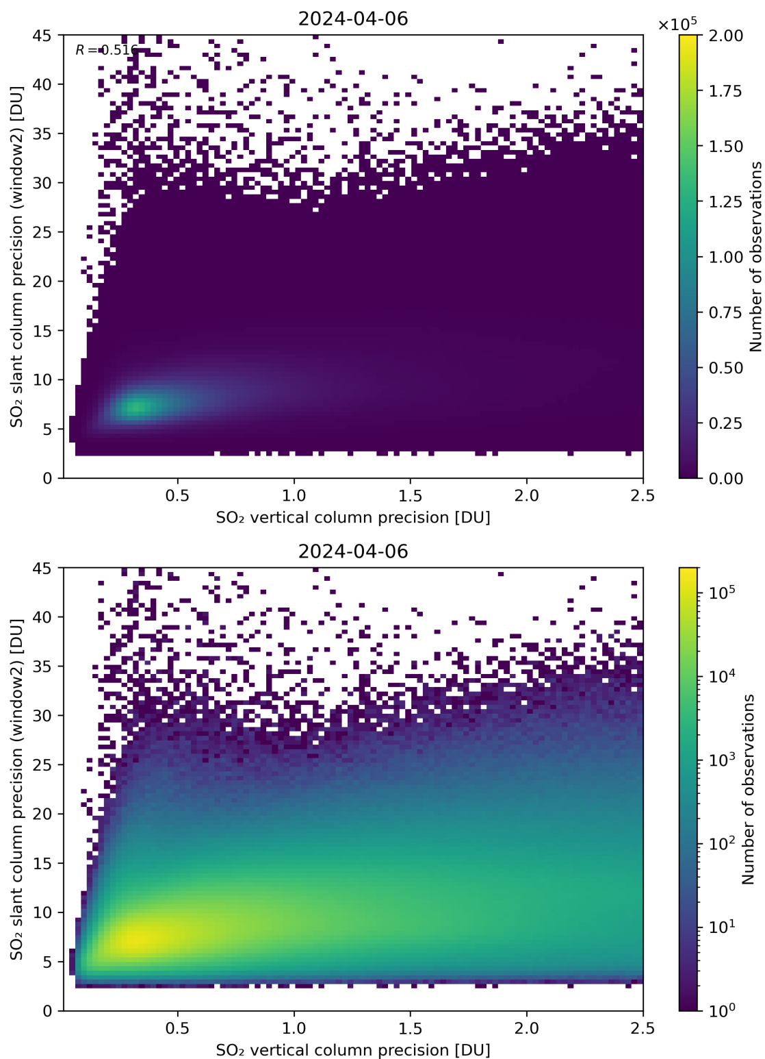
Figure 291: Scatter density plot of “SO 2 vertical column precision” against “SO 2 slant column precision (window2)” for 2024-04-05 to 2024-04-07.
