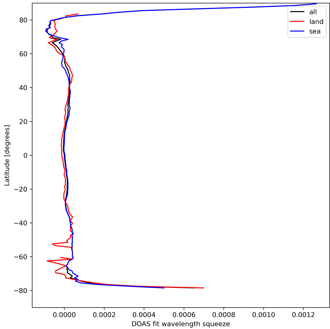
Figure 46: Zonal average of “DOAS fit wavelength squeeze” for 2024-04-05 to 2024-04-07.
