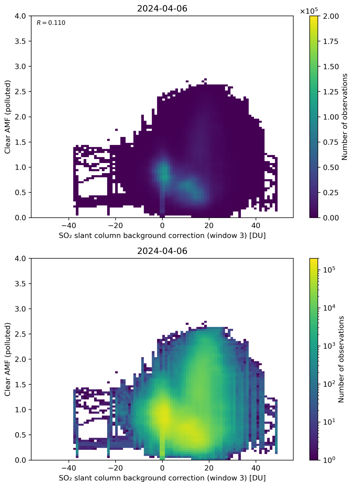
Figure 124: Scatter density plot of “SO 2 slant column background correction (window 3)” against “Clear AMF (polluted)” for 2024-04-05 to 2024-04-07.
