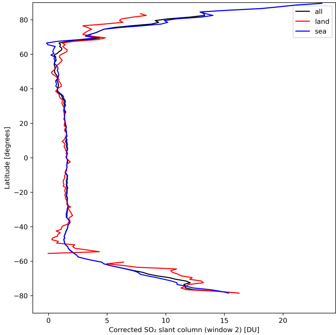
Figure 39: Zonal average of “Corrected SO 2 slant column (window 2)” for 2024-04-05 to 2024-04-07.
