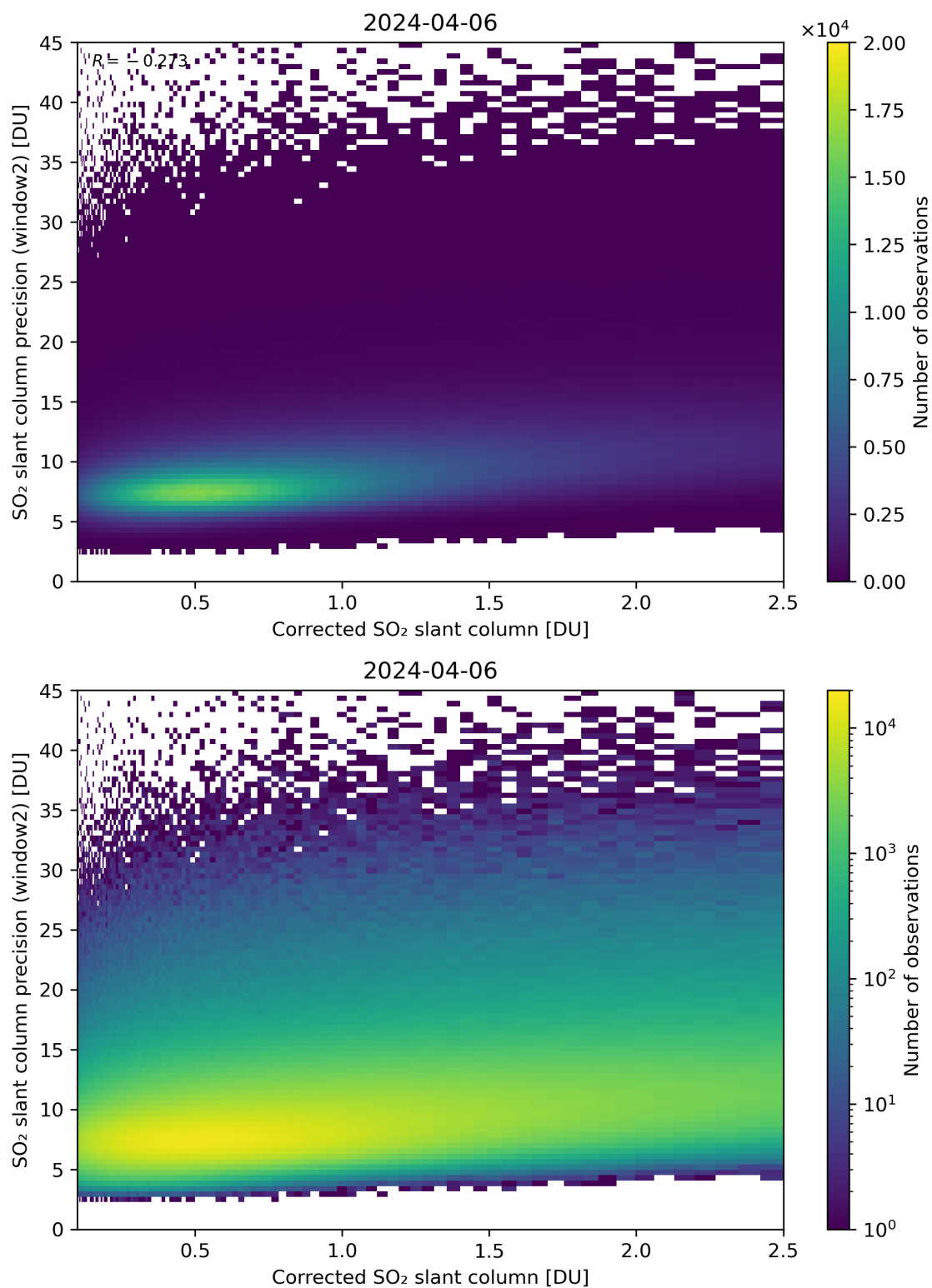
Figure 189: Scatter density plot of “Corrected SO 2 slant column” against “SO 2 slant column precision (window2)” for 2024-04-05 to 2024-04-07.
