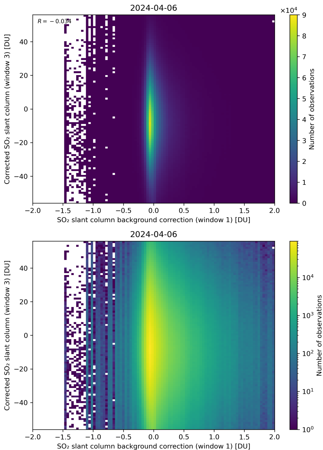
Figure 105: Scatter density plot of “SO 2 slant column background correction (window 1)” against “Corrected SO 2 slant column (window 3)” for 2024-04-05 to 2024-04-07.
