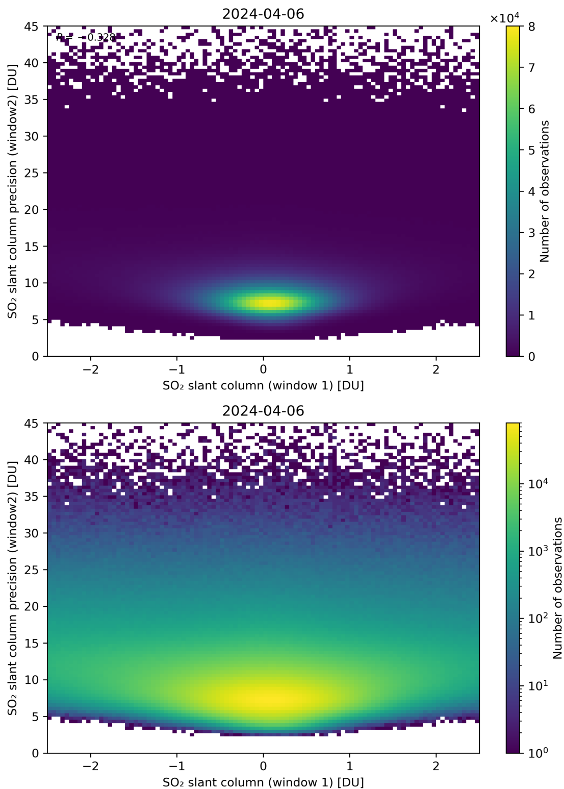
Figure 236: Scatter density plot of “SO 2 slant column (window 1)” against “SO 2 slant column precision (window2)” for 2024-04-05 to 2024-04-07.
