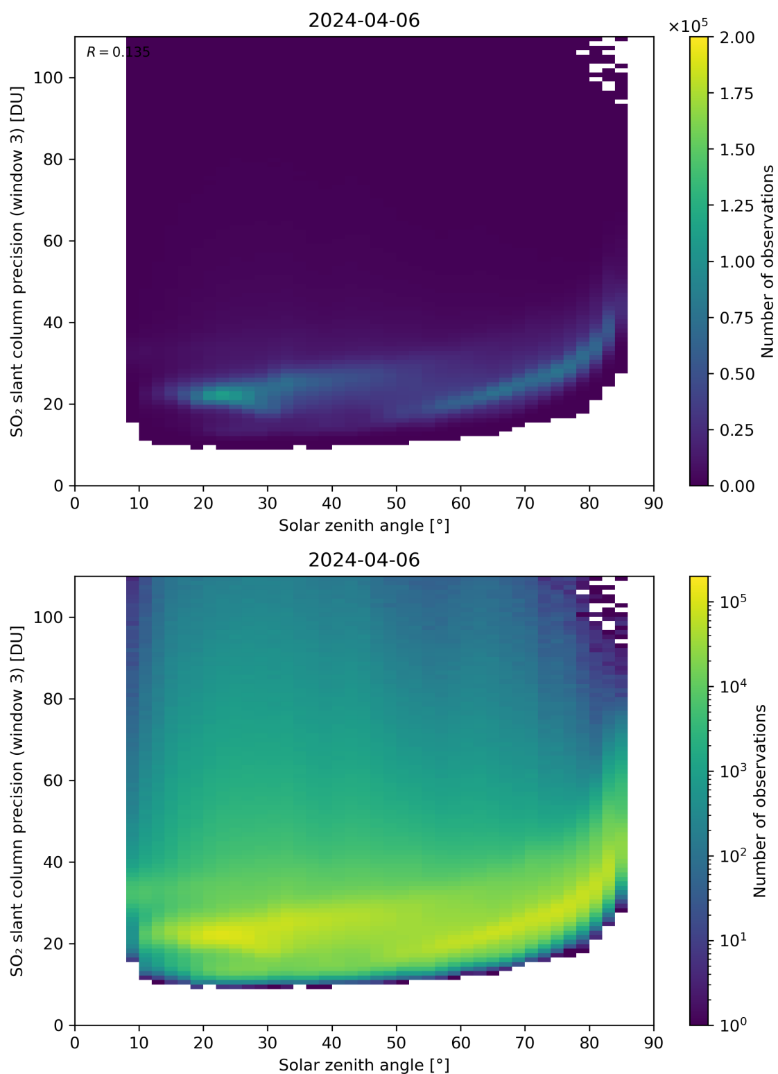
Figure 173: Scatter density plot of “Solar zenith angle” against “SO 2 slant column precision (window 3)” for 2024-04-05 to 2024-04-07.
