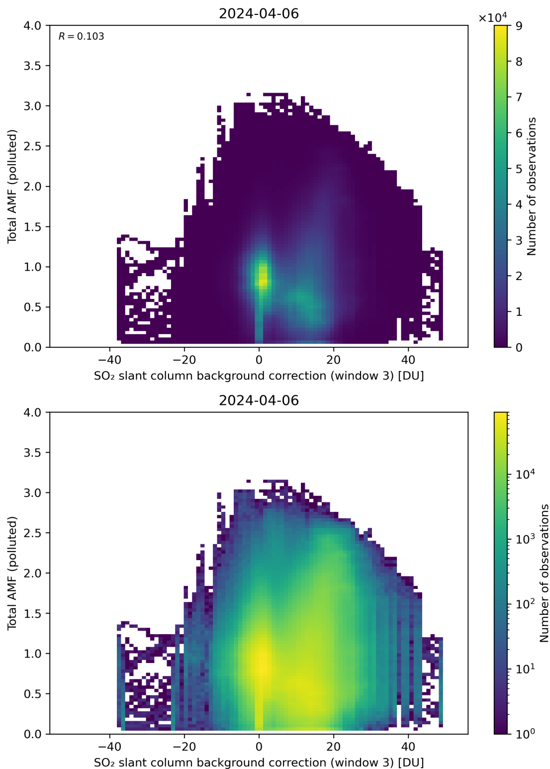
Figure 125: Scatter density plot of “SO 2 slant column background correction (window 3)” against “Total AMF (polluted)” for 2024-04-05 to 2024-04-07.
