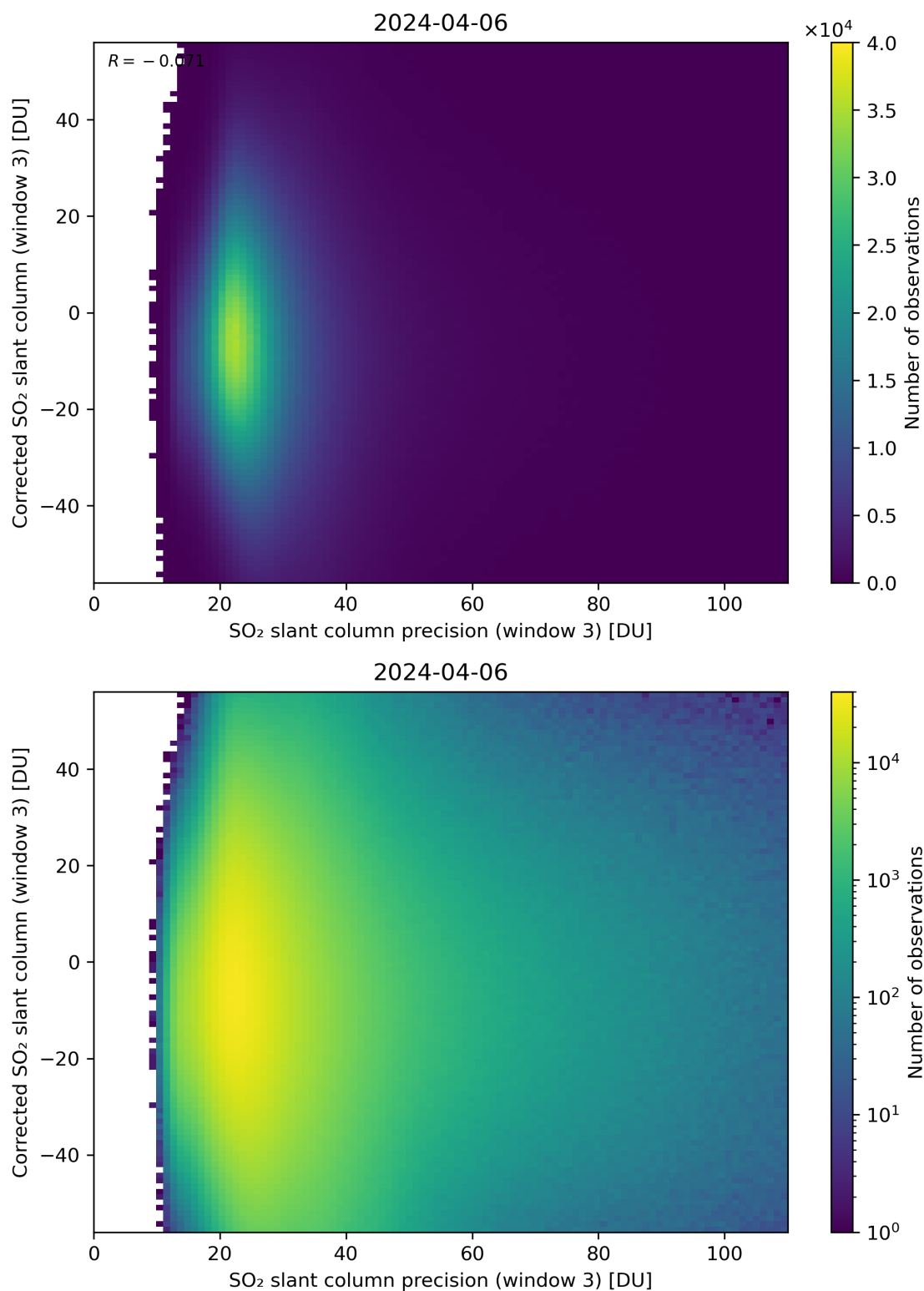
Figure 262: Scatter density plot of “SO 2 slant column precision (window 3)” against “Corrected SO 2 slant column (window 3)” for 2024-04-05 to 2024-04-07.
