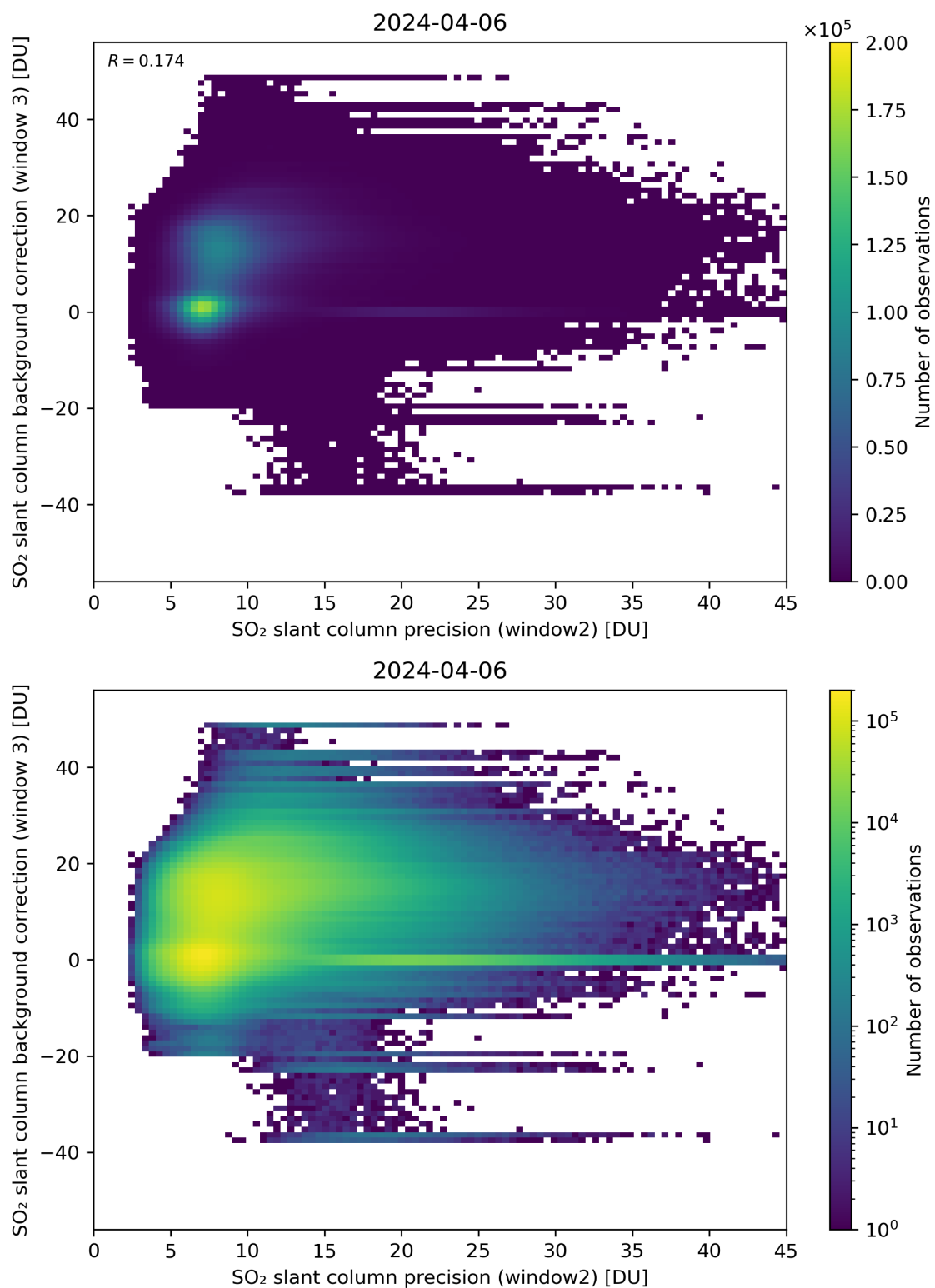
Figure 242: Scatter density plot of “SO 2 slant column precision (window2)” against “SO 2 slant column background correction (window 3)” for 2024-04-05 to 2024-04-07.
