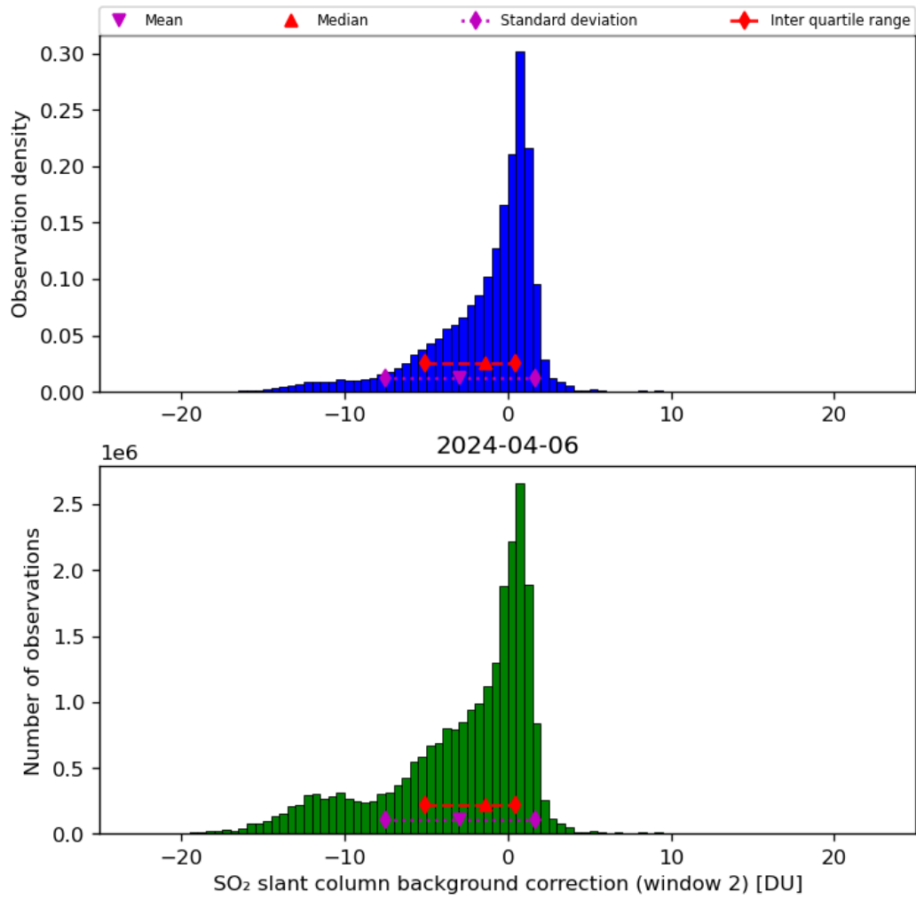
Figure 63: Histogram of “SO 2 slant column background correction (window 2)” for 2024-04-05 to 2024-04-07
