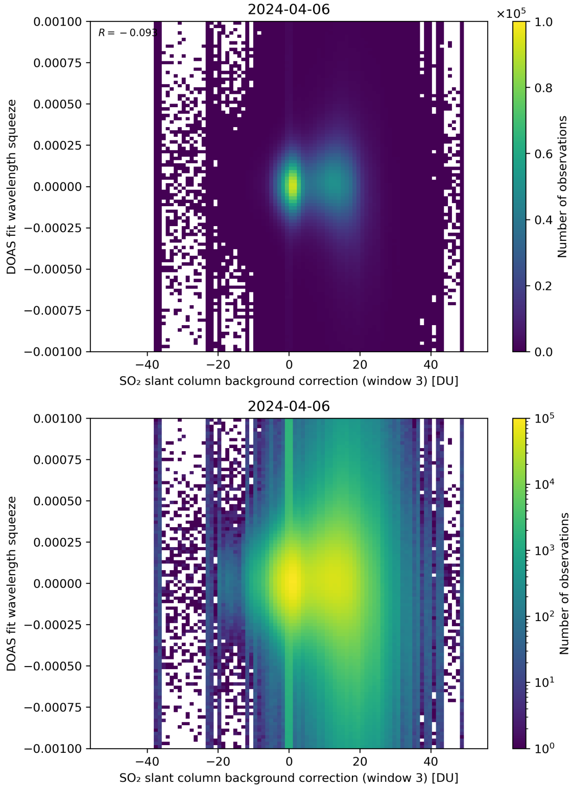
Figure 122: Scatter density plot of “SO 2 slant column background correction (window 3)” against “DOAS fit wavelength squeeze” for 2024-04-05 to 2024-04-07.
