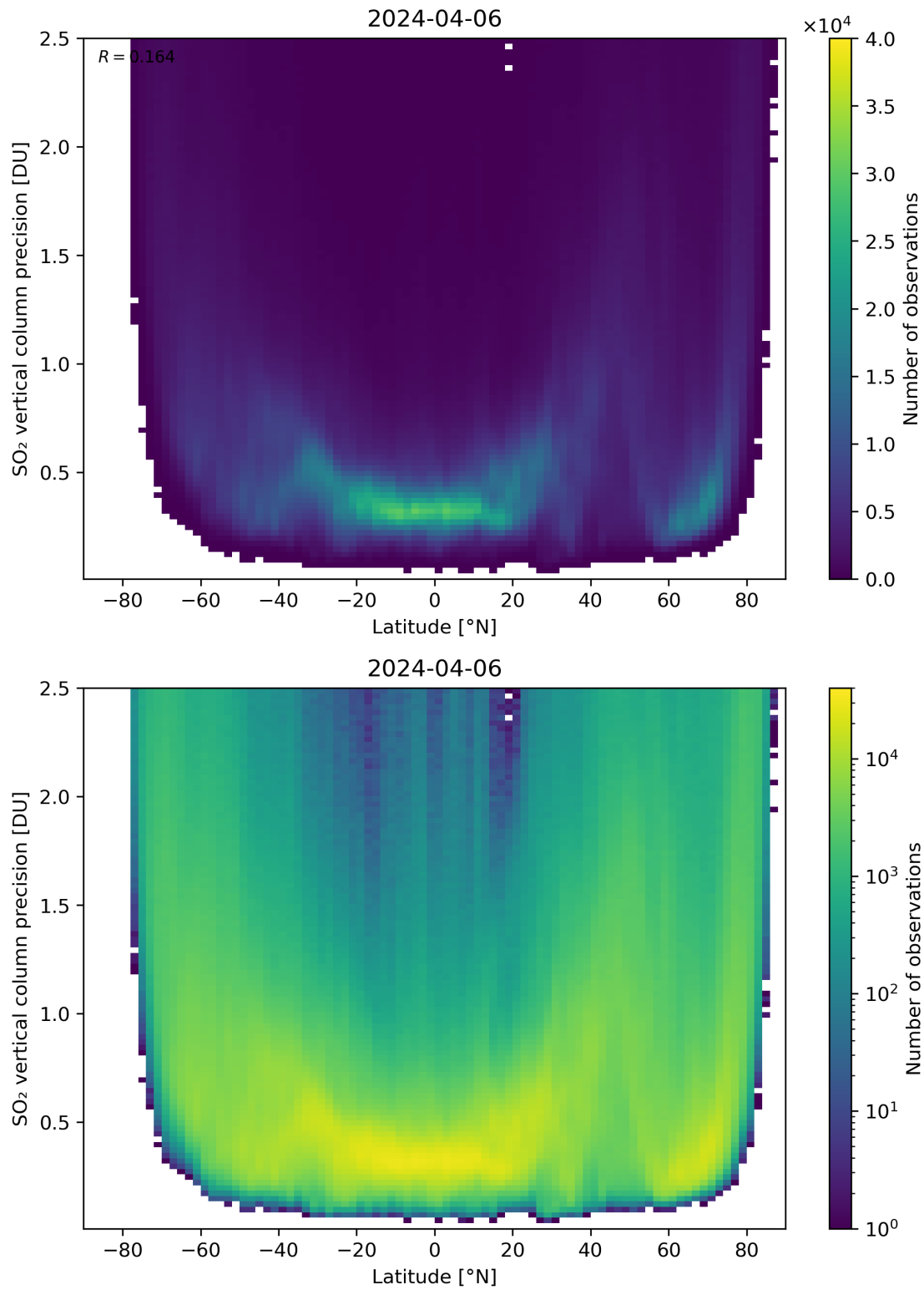
Figure 157: Scatter density plot of “Latitude” against “SO 2 vertical column precision” for 2024-04-05 to 2024-04-07.
