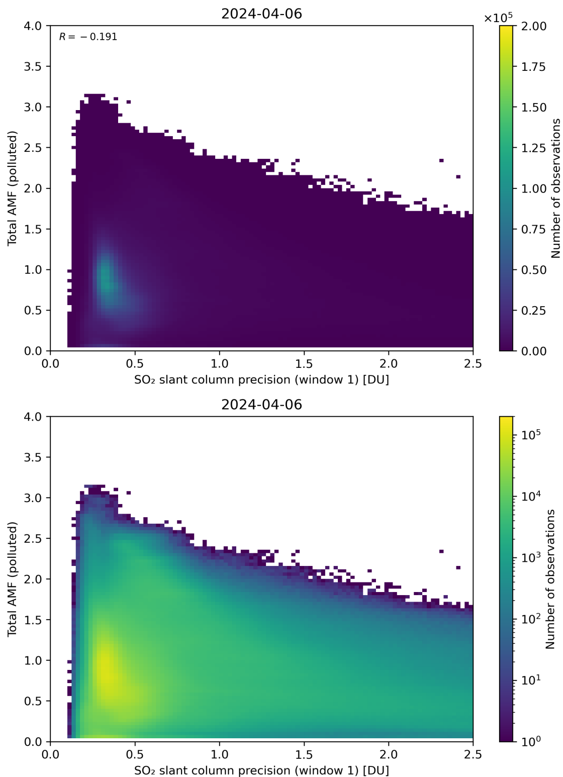
Figure 230: Scatter density plot of “SO 2 slant column precision (window 1)” against “Total AMF (polluted)” for 2024-04-05 to 2024-04-07.
