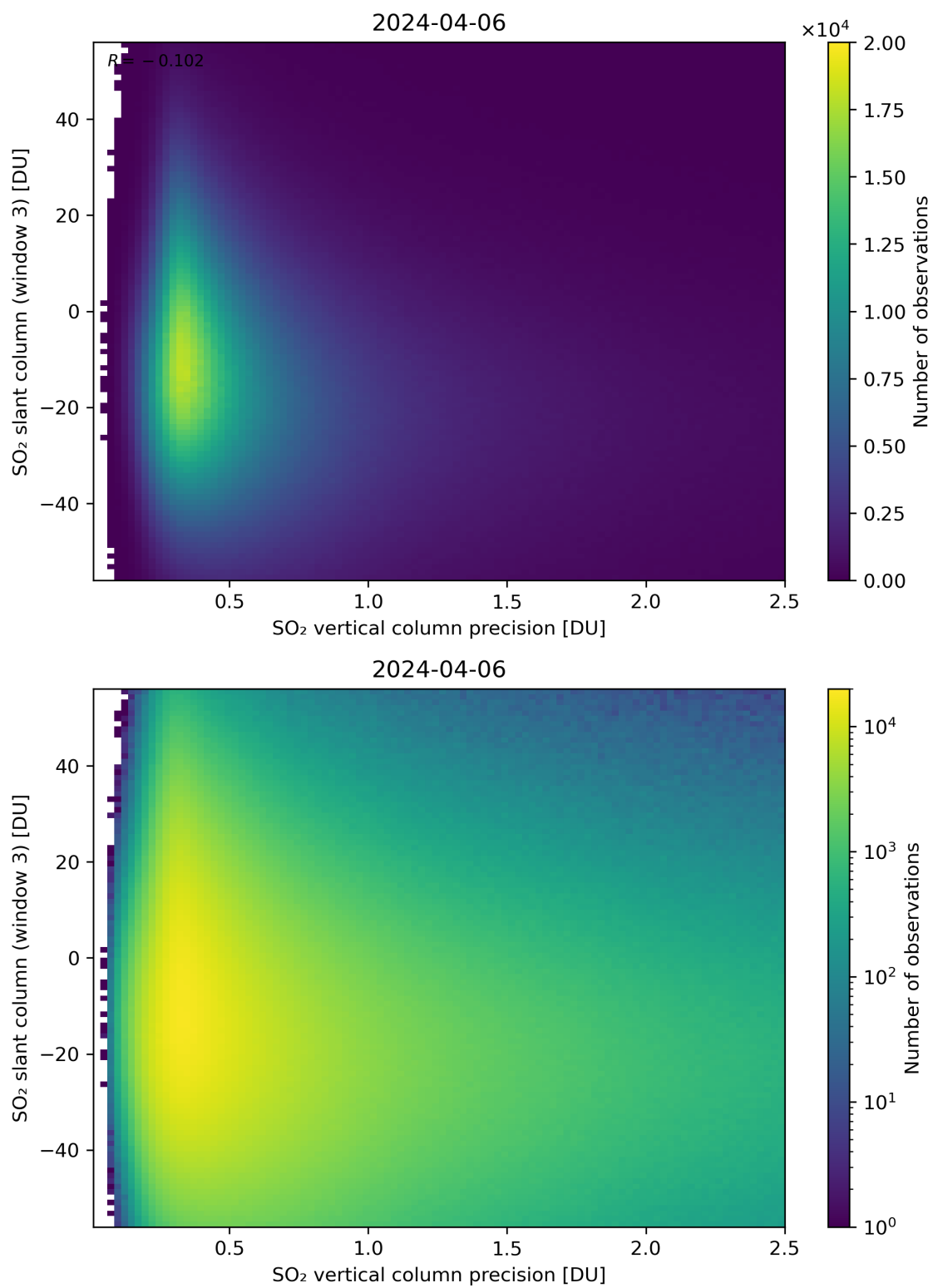
Figure 292: Scatter density plot of “SO 2 vertical column precision” against “SO 2 slant column (window 3)” for 2024-04-05 to 2024-04-07.
