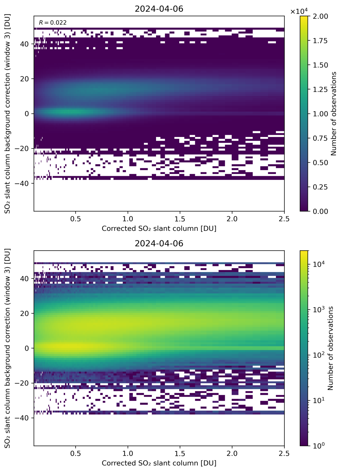
Figure 180: Scatter density plot of “Corrected SO 2 slant column” against “SO 2 slant column background correction (window 3)” for 2024-04-05 to 2024-04-07.
