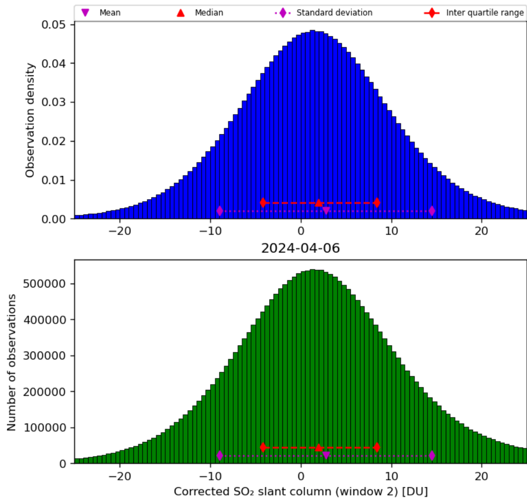
Figure 62: Histogram of “Corrected SO 2 slant column (window 2)” for 2024-04-05 to 2024-04-07
