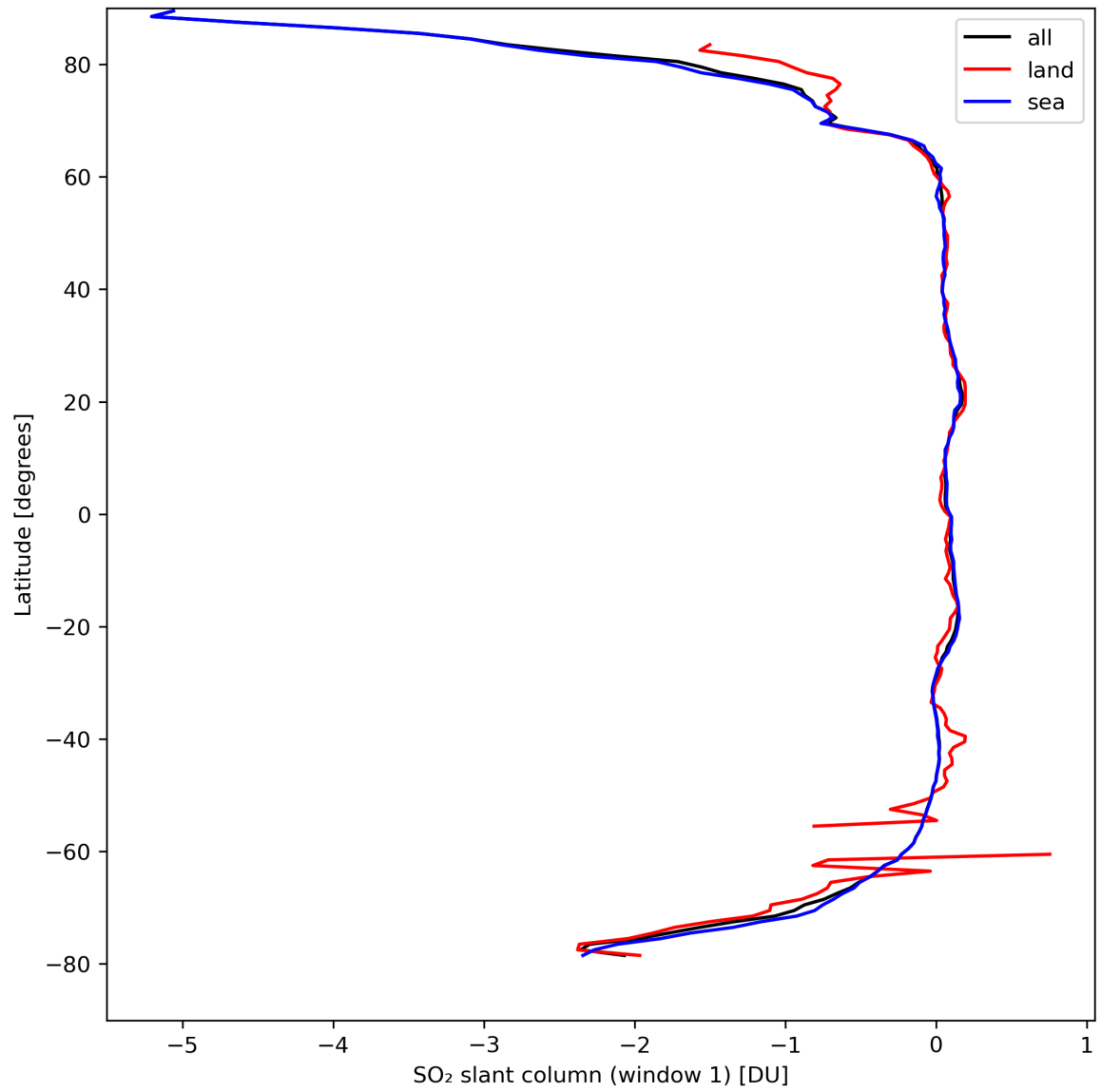
Figure 33: Zonal average of “SO 2 slant column (window 1)” for 2024-04-05 to 2024-04-07.
