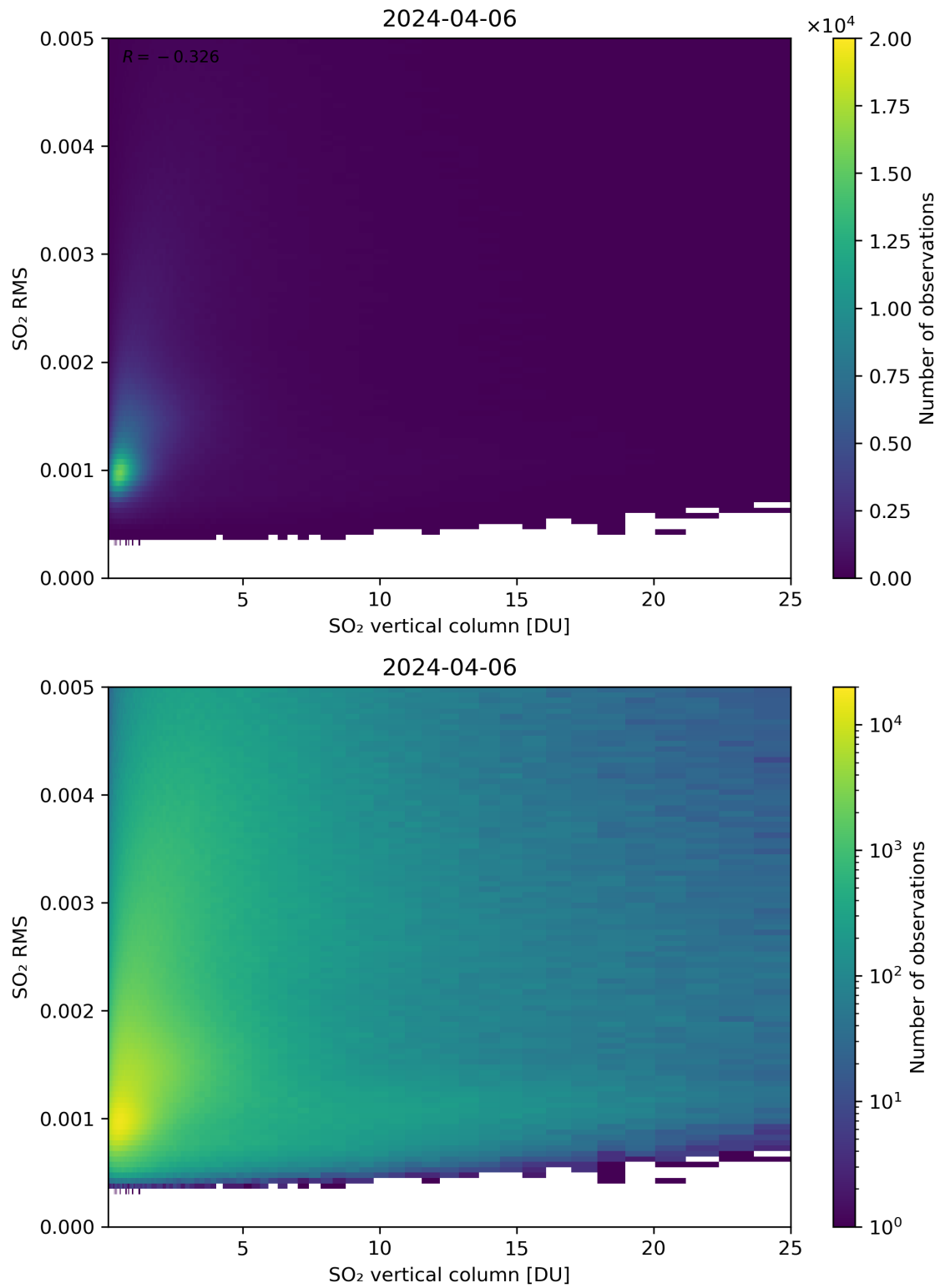
Figure 278: Scatter density plot of “SO 2 vertical column” against “SO 2 RMS” for 2024-04-05 to 2024-04-07.
