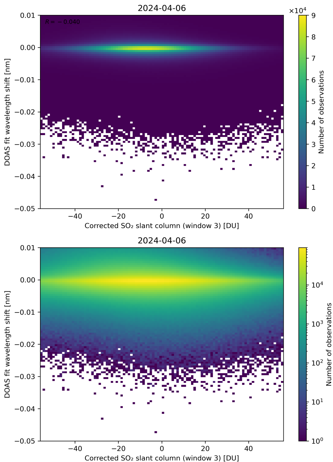
Figure 206: Scatter density plot of “Corrected SO 2 slant column (window 3)” against “DOAS fit wavelength shift” for 2024-04-05 to 2024-04-07.
