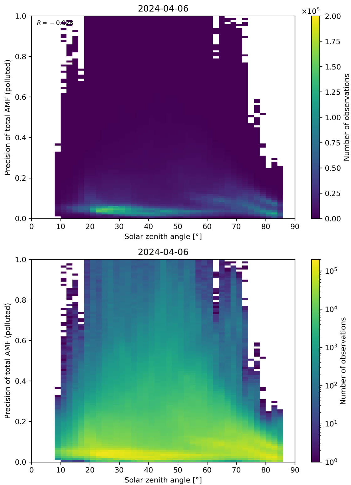
Figure 175: Scatter density plot of “Solar zenith angle” against “Precision of total AMF (polluted)” for 2024-04-05 to 2024-04-07.
