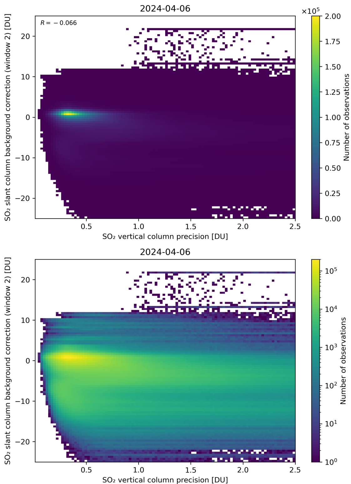
Figure 280: Scatter density plot of “SO 2 vertical column precision” against “SO 2 slant column background correction (window 2)” for 2024-04-05 to 2024-04-07.
