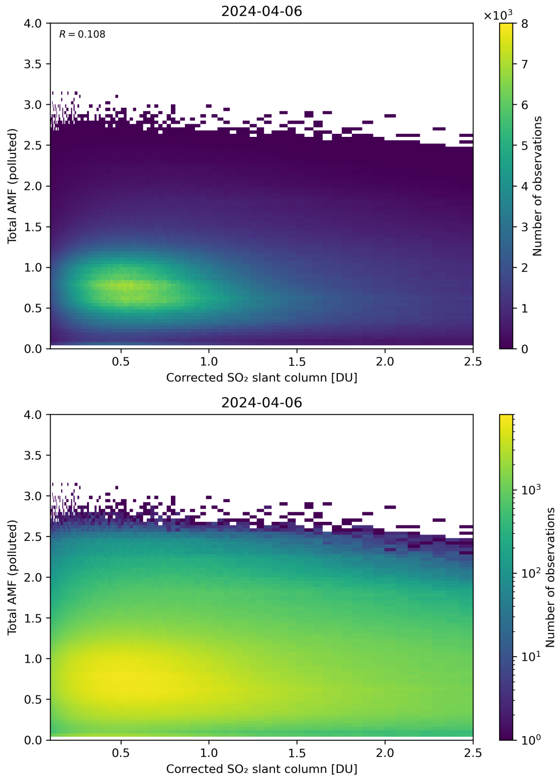
Figure 192: Scatter density plot of “Corrected SO 2 slant column” against “Total AMF (polluted)” for 2024-04-05 to 2024-04-07.
