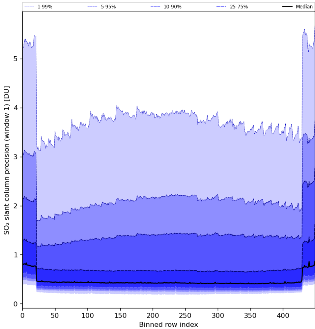
Figure 80: Along track statistics of “SO 2 slant column precision (window 1)” for 2024-04-05 to 2024-04-07
