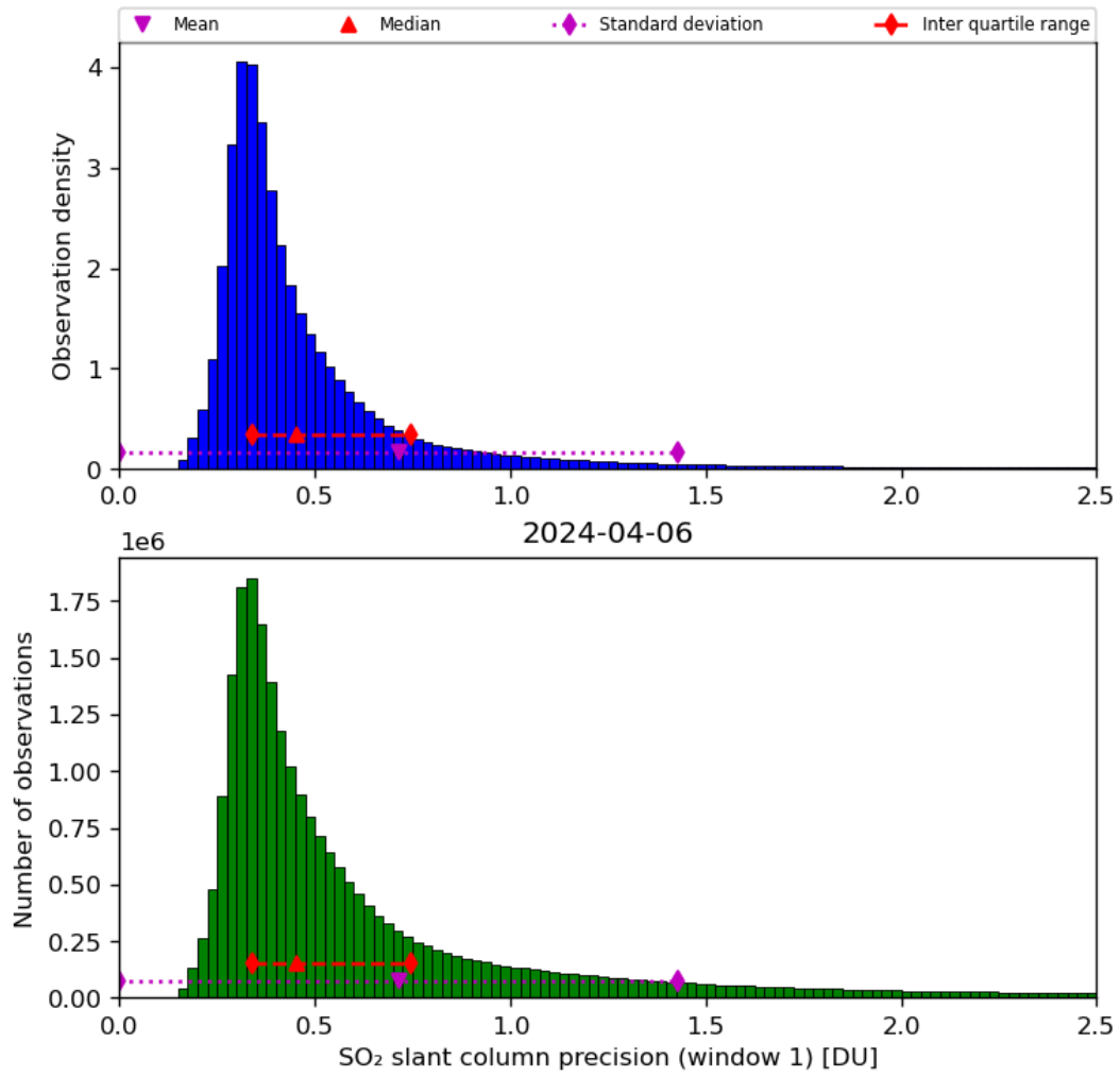
Figure 57: Histogram of “SO 2 slant column precision (window 1)” for 2024-04-05 to 2024-04-07
