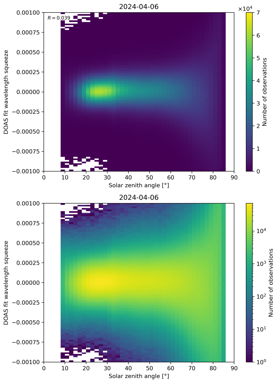
Figure 162: Scatter density plot of “Solar zenith angle” against “DOAS fit wavelength squeeze” for 2024-04-05 to 2024-04-07.
