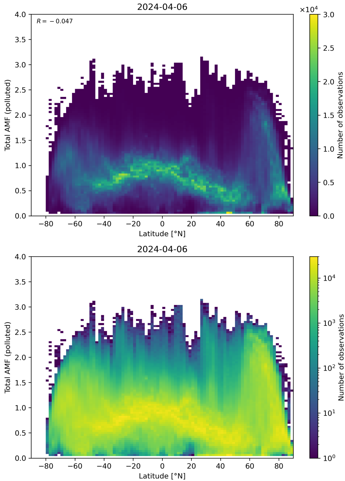
Figure 154: Scatter density plot of “Latitude” against “Total AMF (polluted)” for 2024-04-05 to 2024-04-07.
