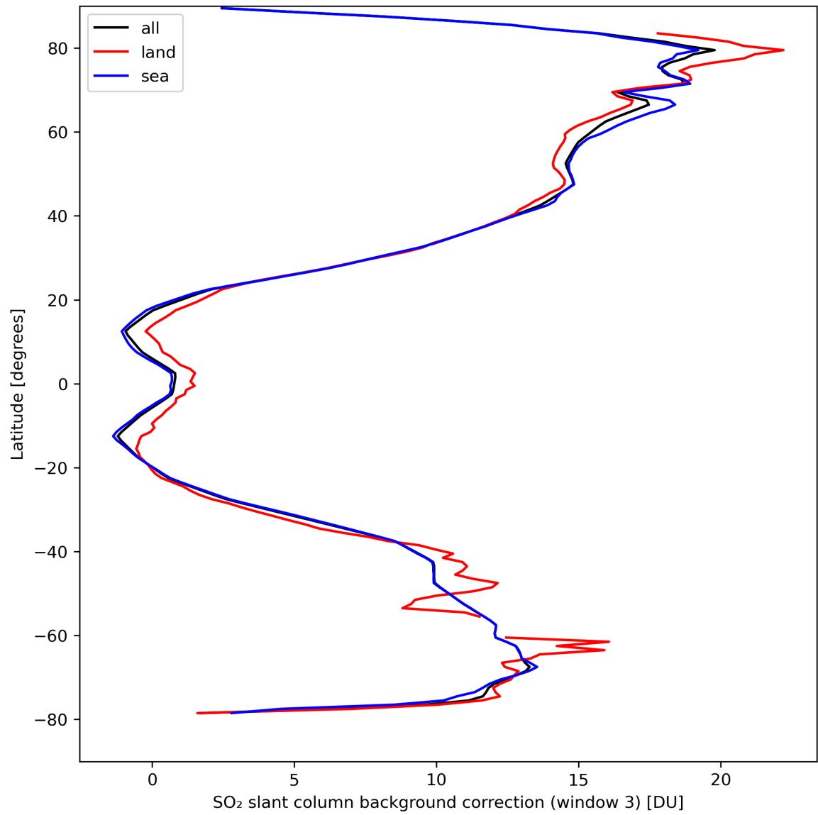
Figure 44: Zonal average of “SO 2 slant column background correction (window 3)” for 2024-04-05 to 2024-04-07.
