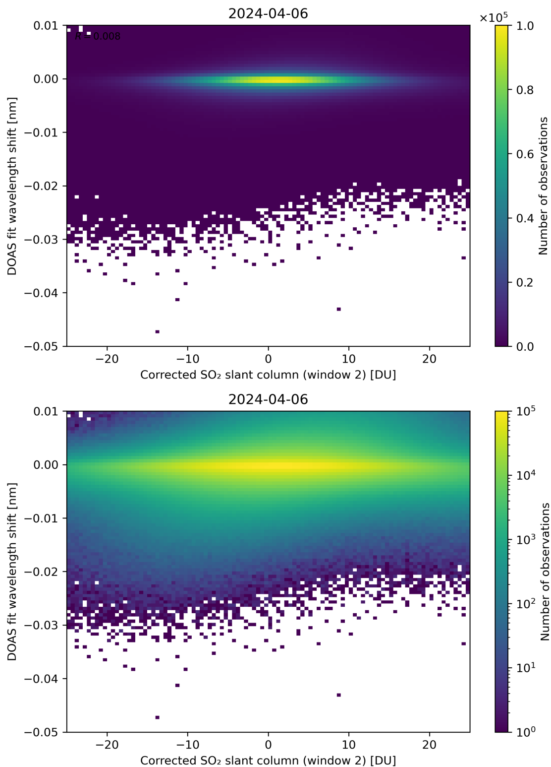
Figure 196: Scatter density plot of “Corrected SO 2 slant column (window 2)” against “DOAS fit wavelength shift” for 2024-04-05 to 2024-04-07.
