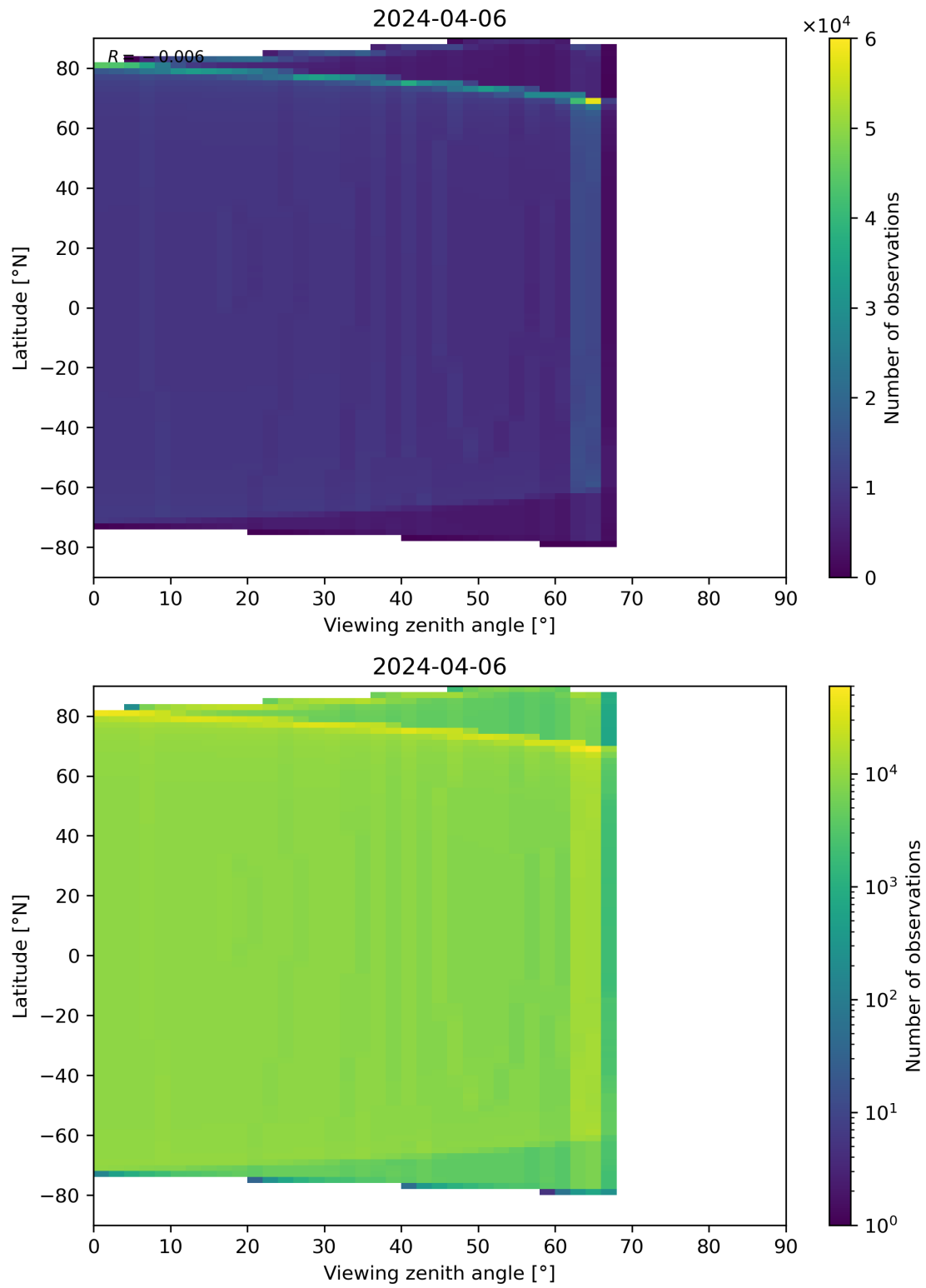
Figure 314: Scatter density plot of “Viewing zenith angle” against “Latitude” for 2024-04-05 to 2024-04-07.
