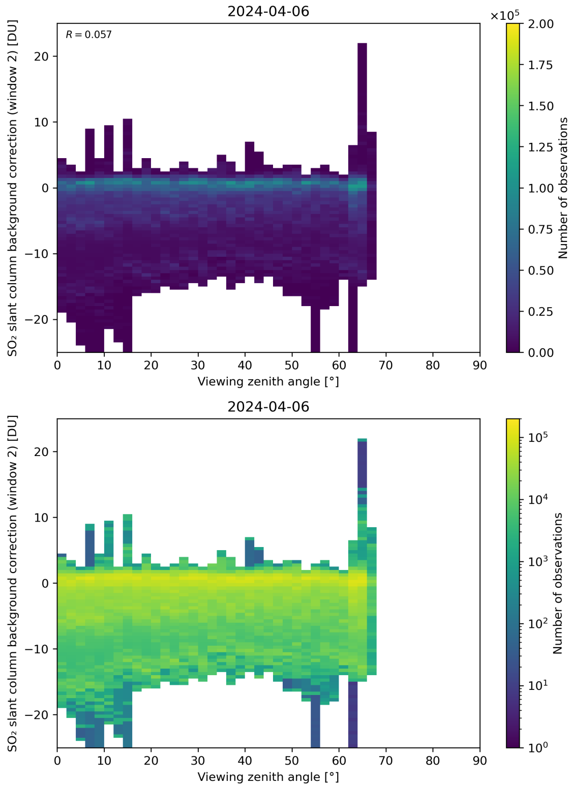
Figure 309: Scatter density plot of “Viewing zenith angle” against “SO 2 slant column background correction (window 2)” for 2024-04-05 to 2024-04-07.
