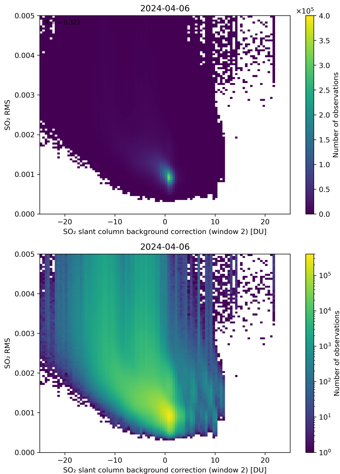
Figure 114: Scatter density plot of “SO 2 slant column background correction (window 2)” against “SO 2 RMS” for 2024-04-05 to 2024-04-07.
