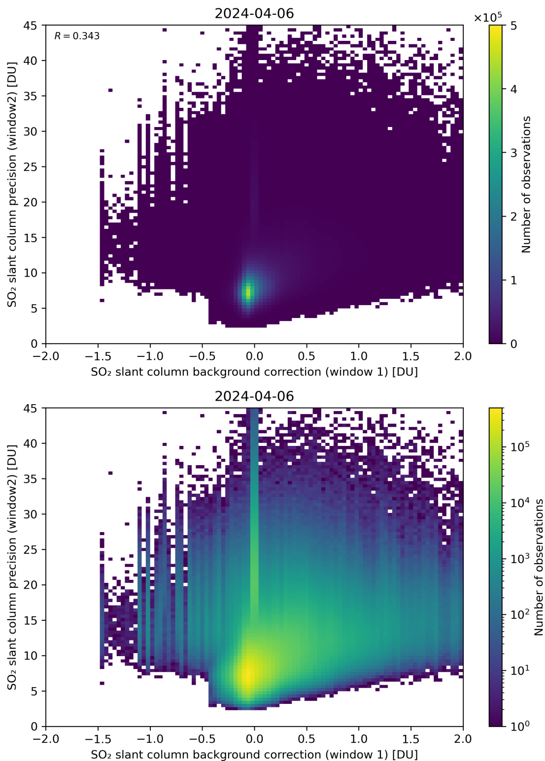
Figure 106: Scatter density plot of “SO 2 slant column background correction (window 1)” against “SO 2 slant column precision (window2)” for 2024-04-05 to 2024-04-07.
