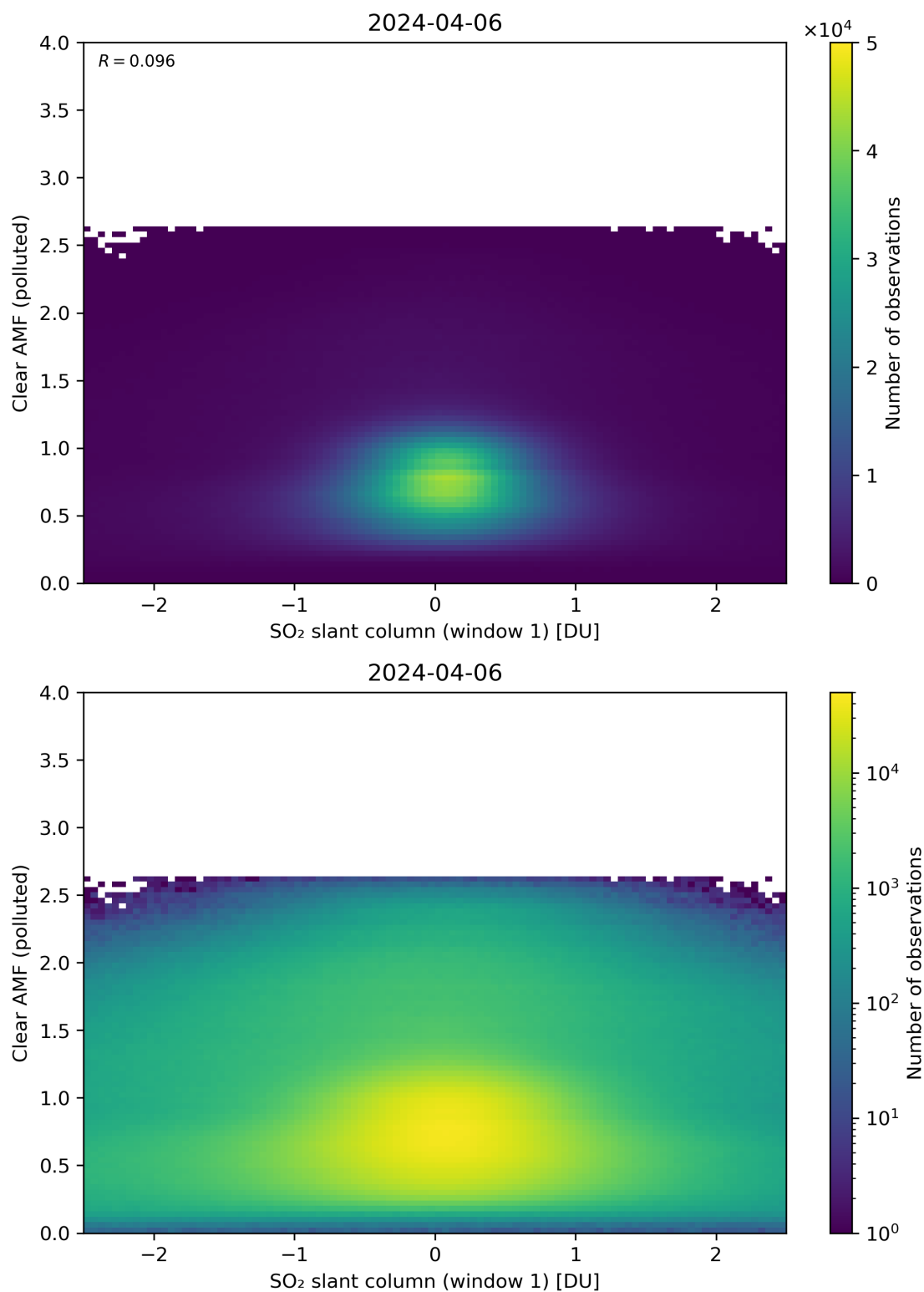
Figure 232: Scatter density plot of “SO 2 slant column (window 1)” against “Clear AMF (polluted)” for 2024-04-05 to 2024-04-07.
