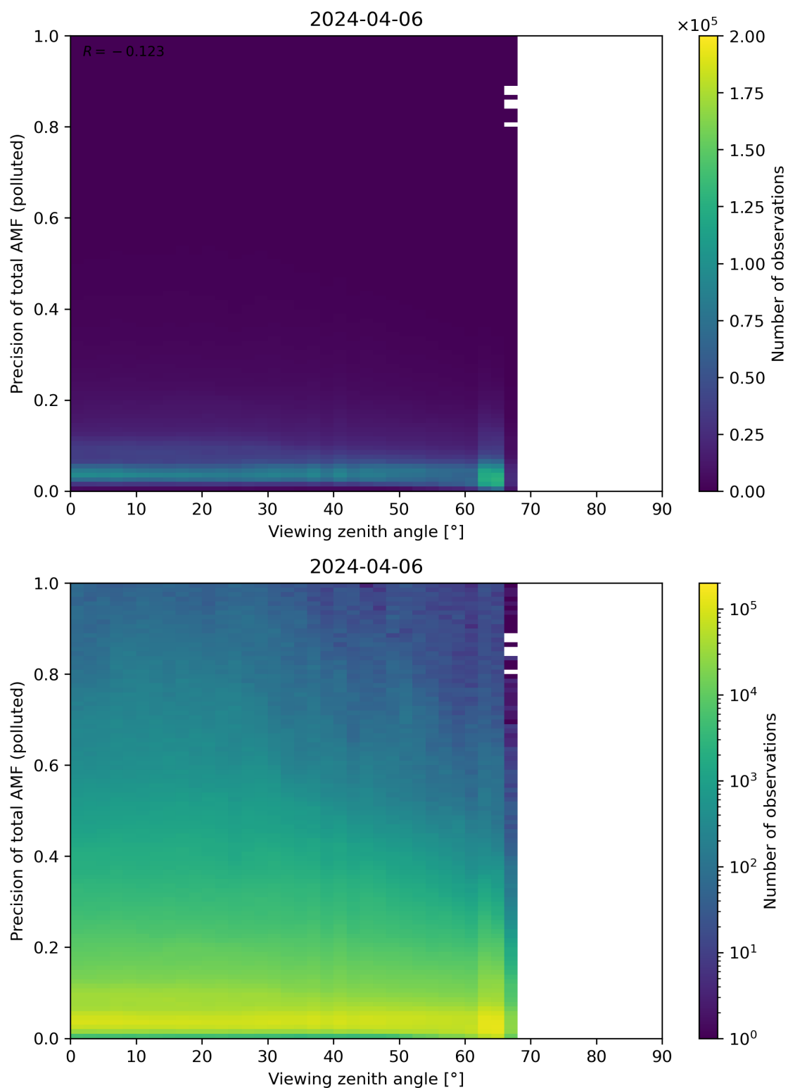
Figure 326: Scatter density plot of “Viewing zenith angle” against “Precision of total AMF (polluted)” for 2024-04-05 to 2024-04-07.
