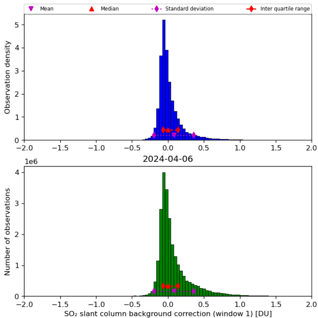
Figure 59: Histogram of “SO 2 slant column background correction (window 1)” for 2024-04-05 to 2024-04-07
