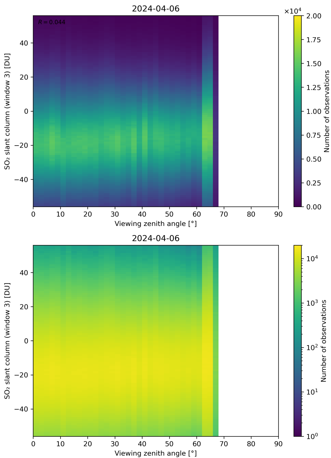
Figure 323: Scatter density plot of “Viewing zenith angle” against “SO 2 slant column (window 3)” for 2024-04-05 to 2024-04-07.
