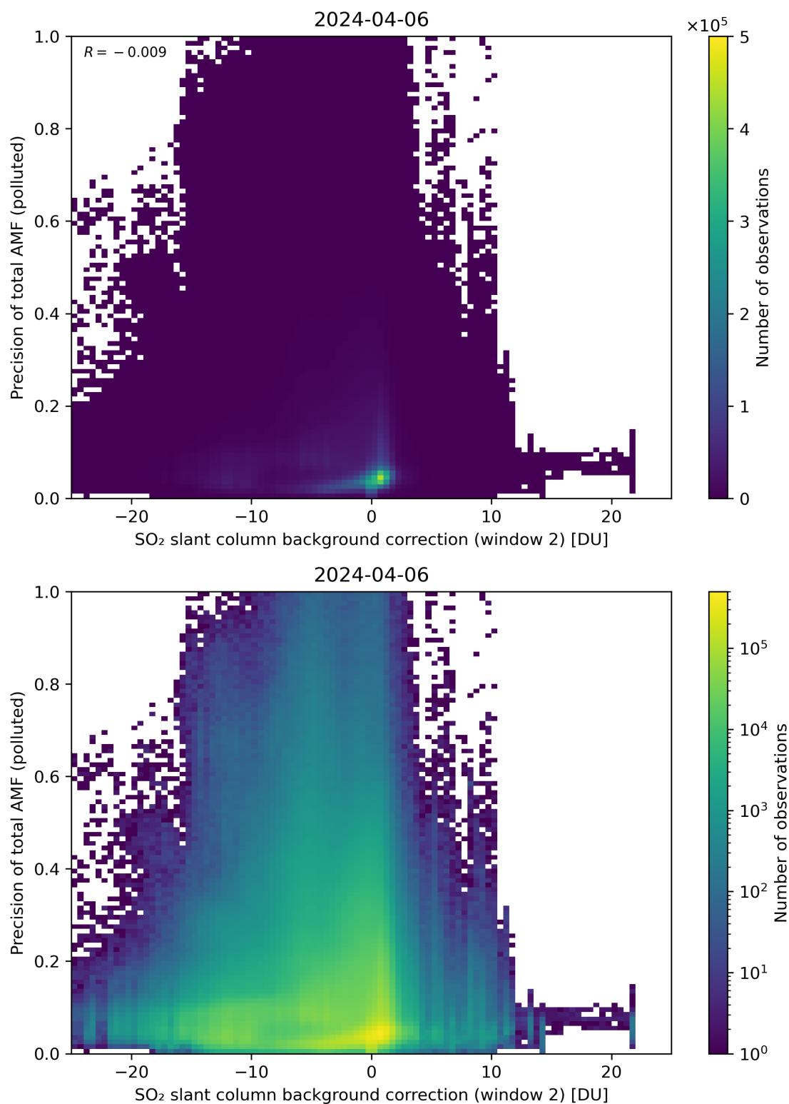
Figure 120: Scatter density plot of “SO 2 slant column background correction (window 2)” against “Precision of total AMF (polluted)” for 2024-04-05 to 2024-04-07.
