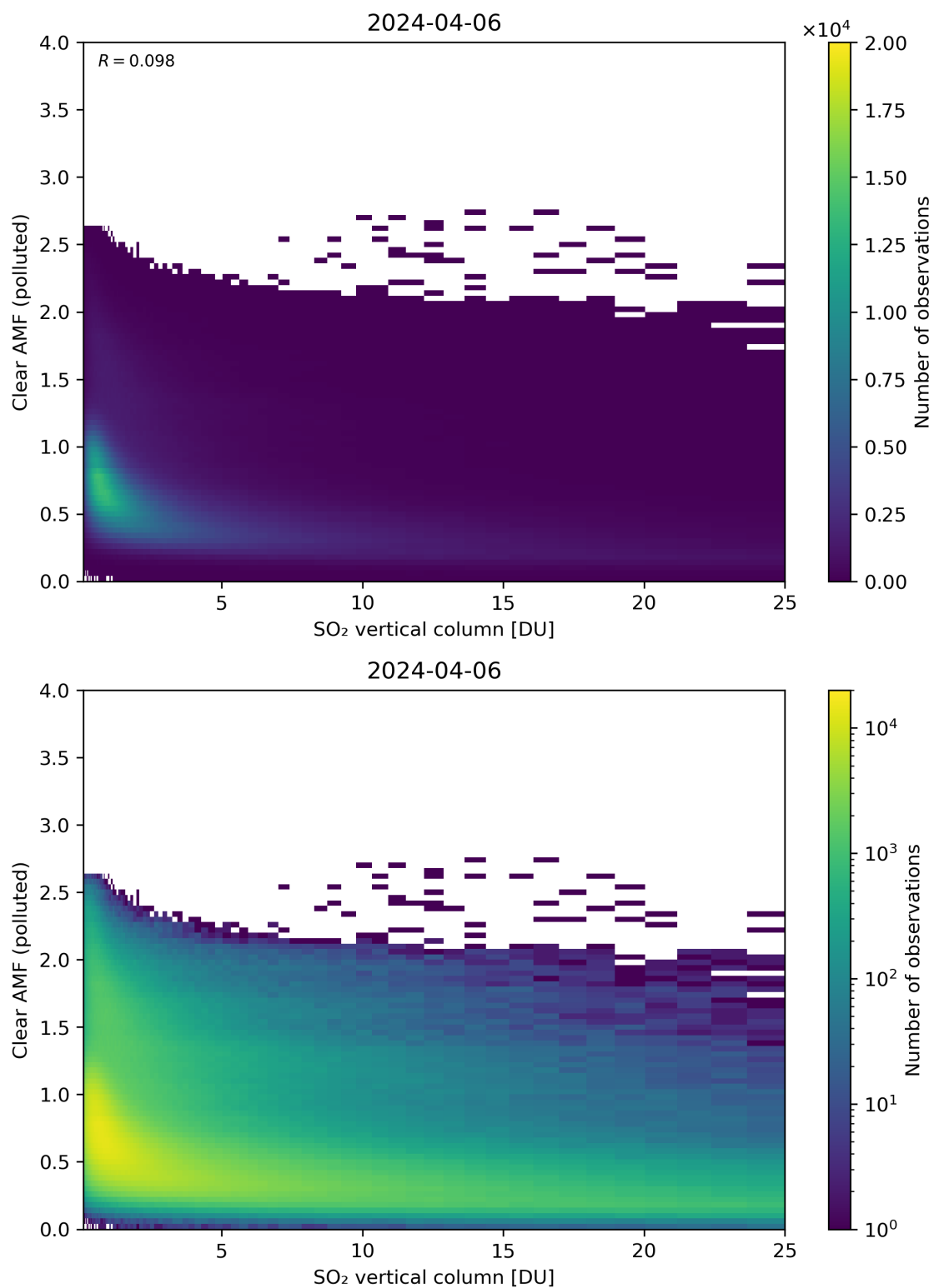
Figure 296: Scatter density plot of “SO 2 vertical column” against “Clear AMF (polluted)” for 2024-04-05 to 2024-04-07.
