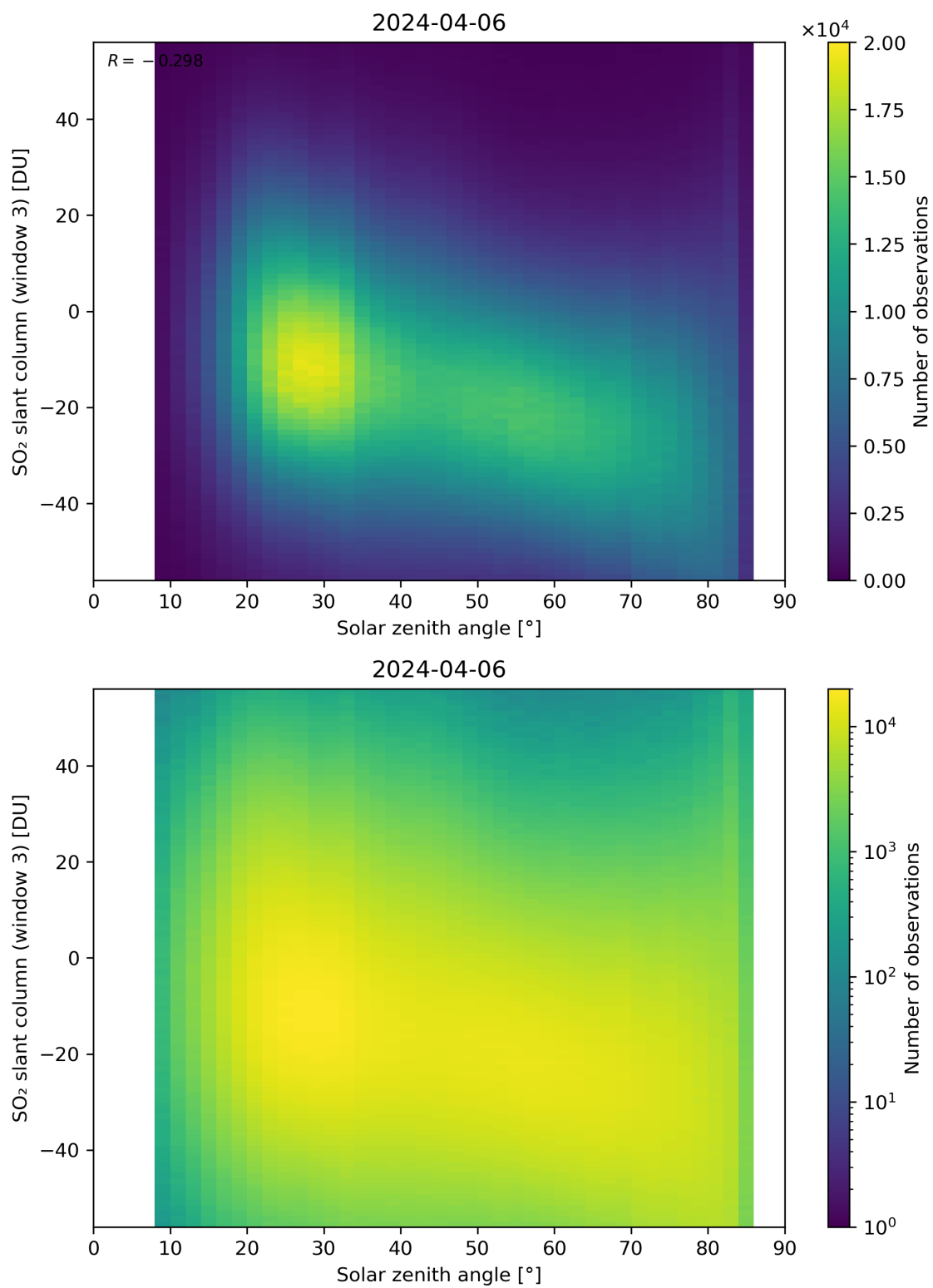
Figure 172: Scatter density plot of “Solar zenith angle” against “SO 2 slant column (window 3)” for 2024-04-05 to 2024-04-07.
