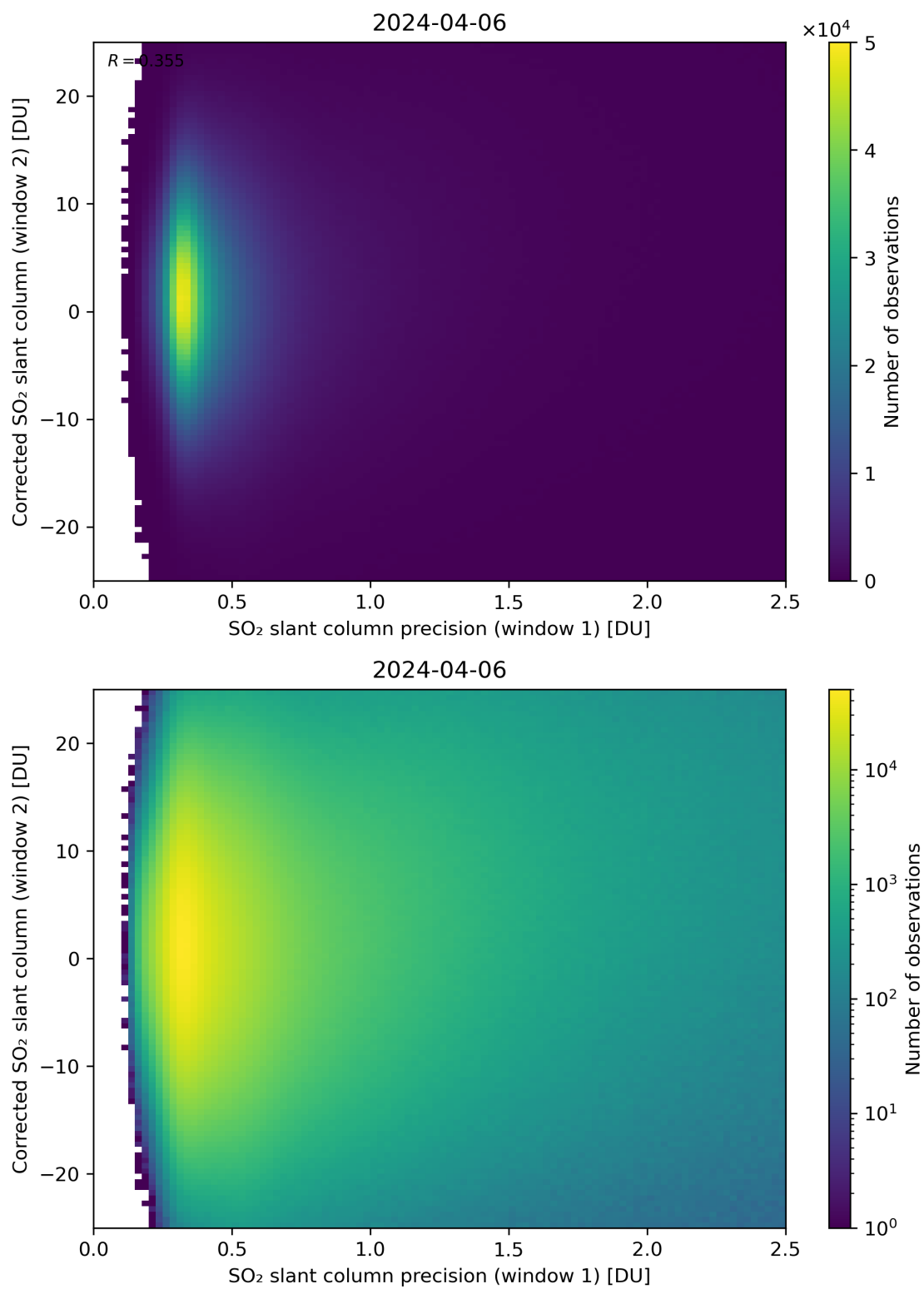
Figure 225: Scatter density plot of “SO 2 slant column precision (window 1)” against “Corrected SO 2 slant column (window 2)” for 2024-04-05 to 2024-04-07.
