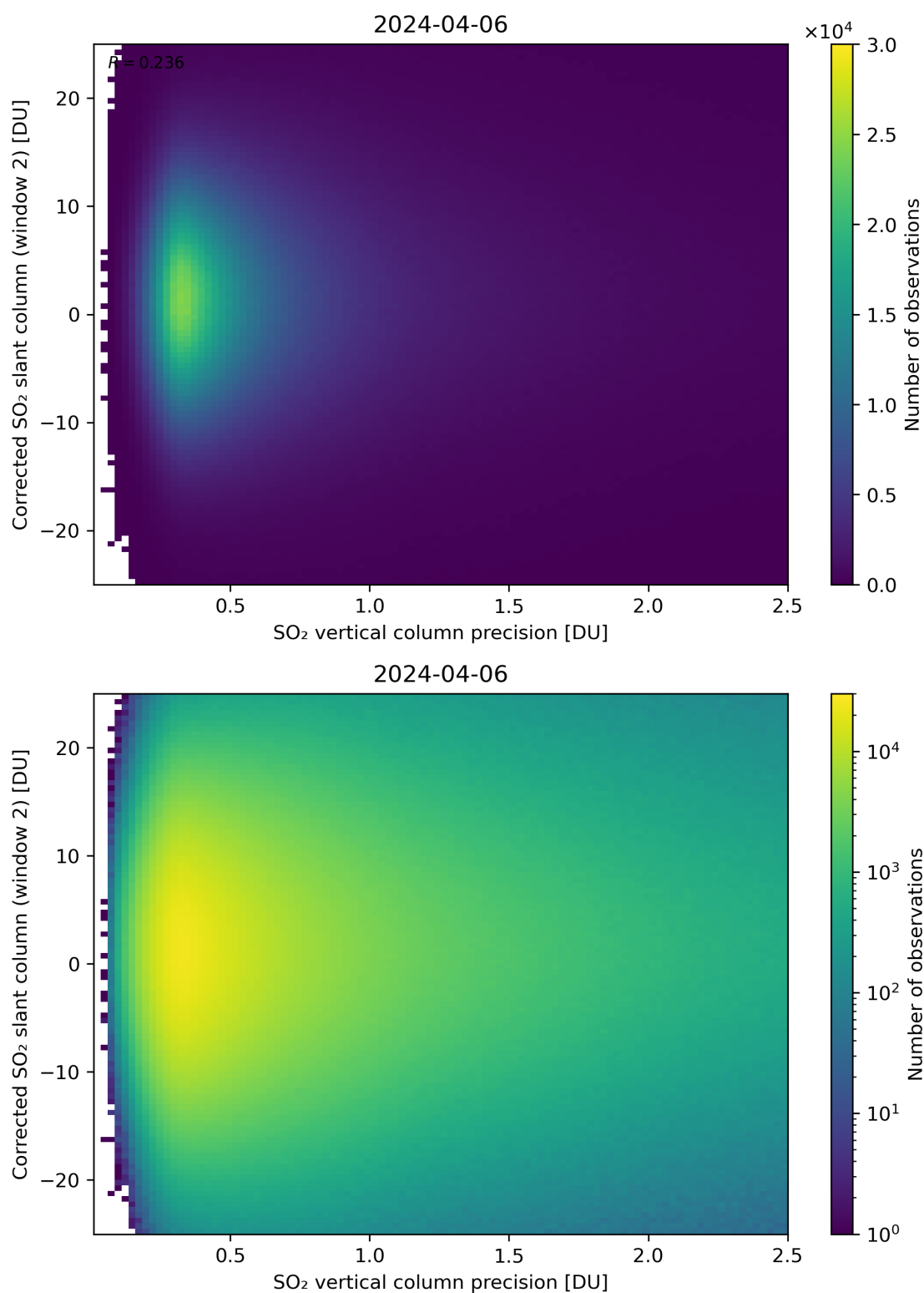
Figure 287: Scatter density plot of “SO 2 vertical column precision” against “Corrected SO 2 slant column (window 2)” for 2024-04-05 to 2024-04-07.
