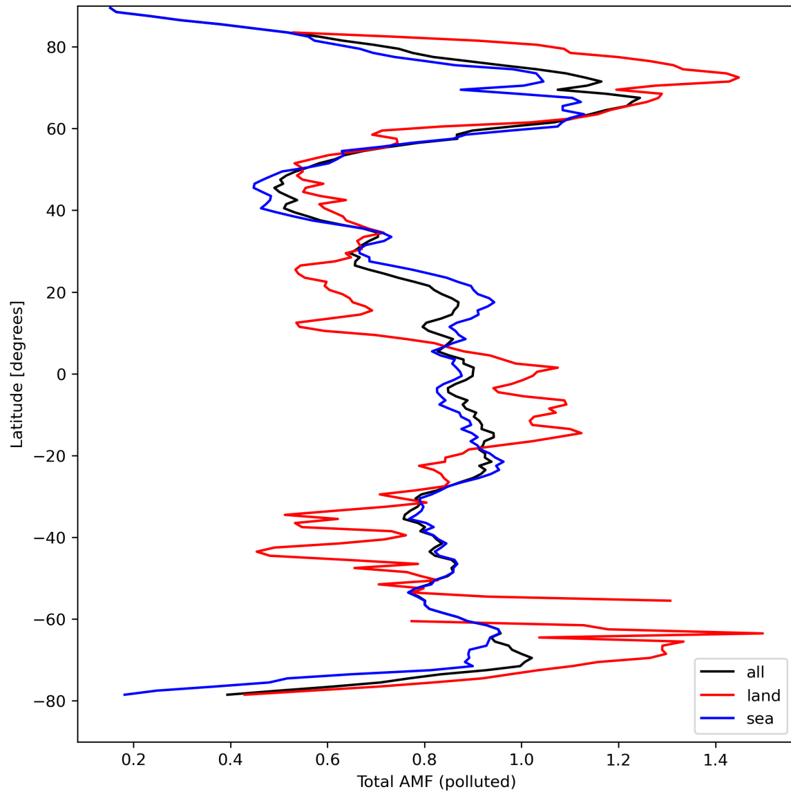
Figure 48: Zonal average of “Total AMF (polluted)” for 2024-04-05 to 2024-04-07.
