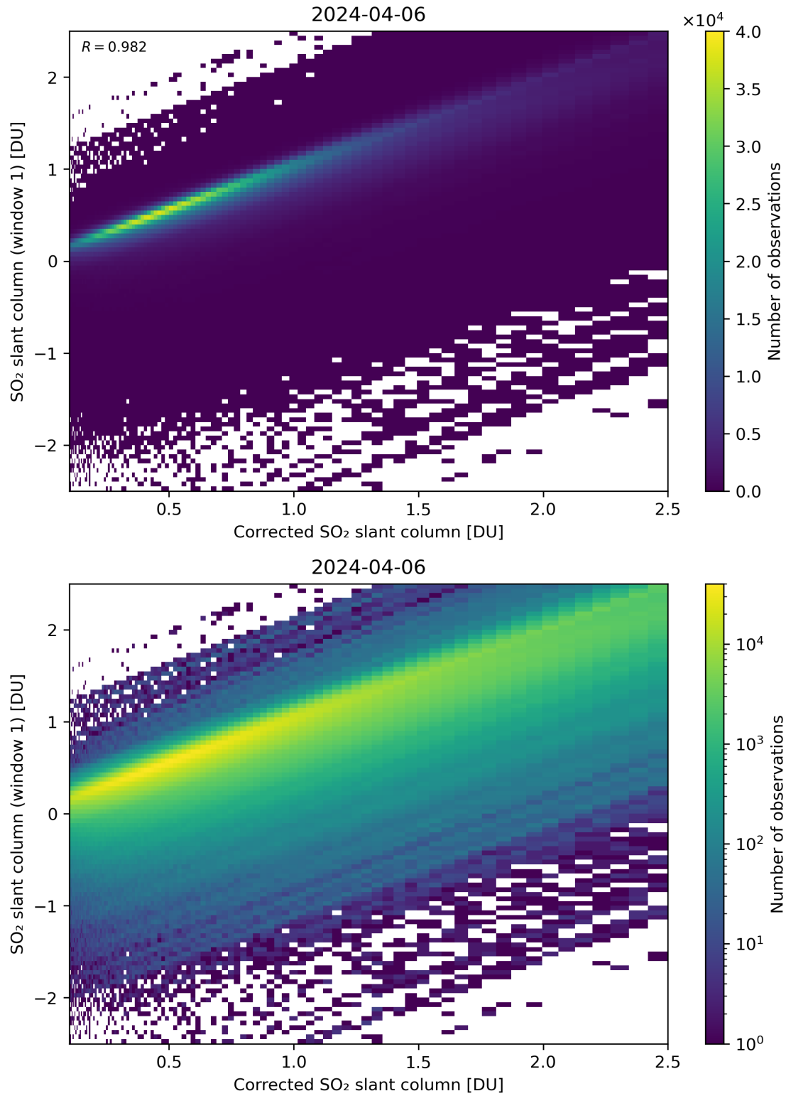
Figure 187: Scatter density plot of “Corrected SO 2 slant column” against “SO 2 slant column (window 1)” for 2024-04-05 to 2024-04-07.
