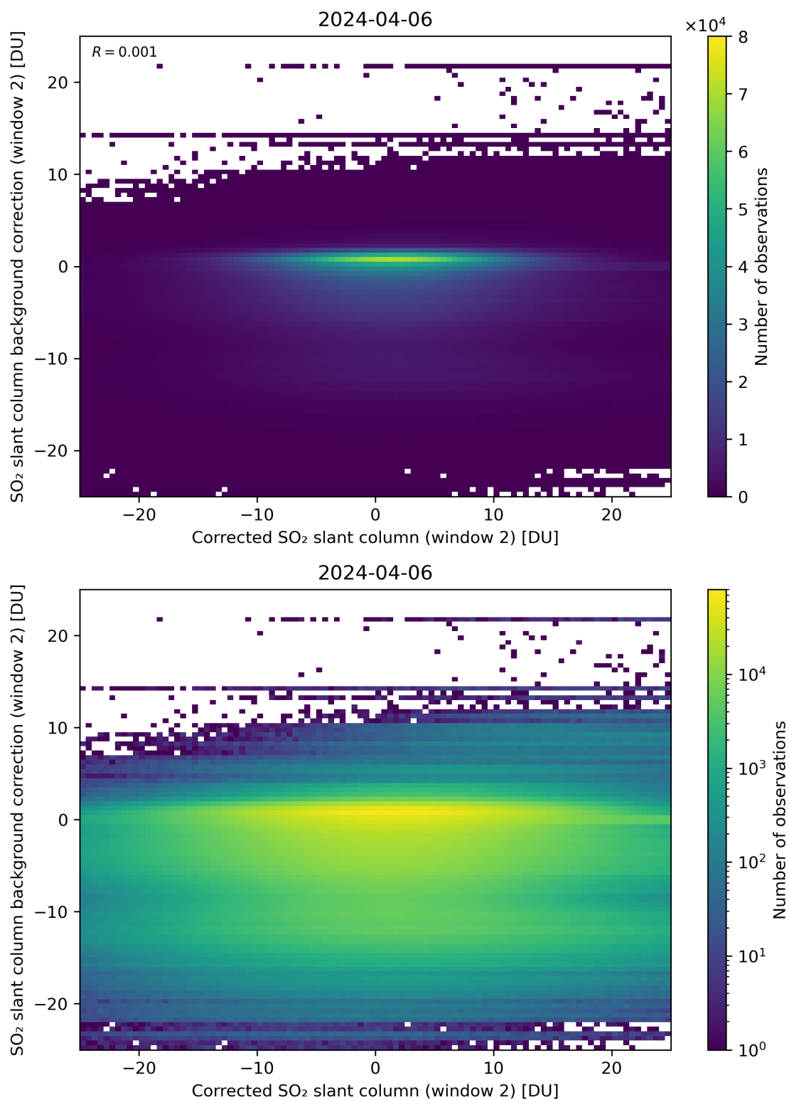
Figure 194: Scatter density plot of “Corrected SO 2 slant column (window 2)” against “SO 2 slant column background correction (window 2)” for 2024-04-05 to 2024-04-07.
