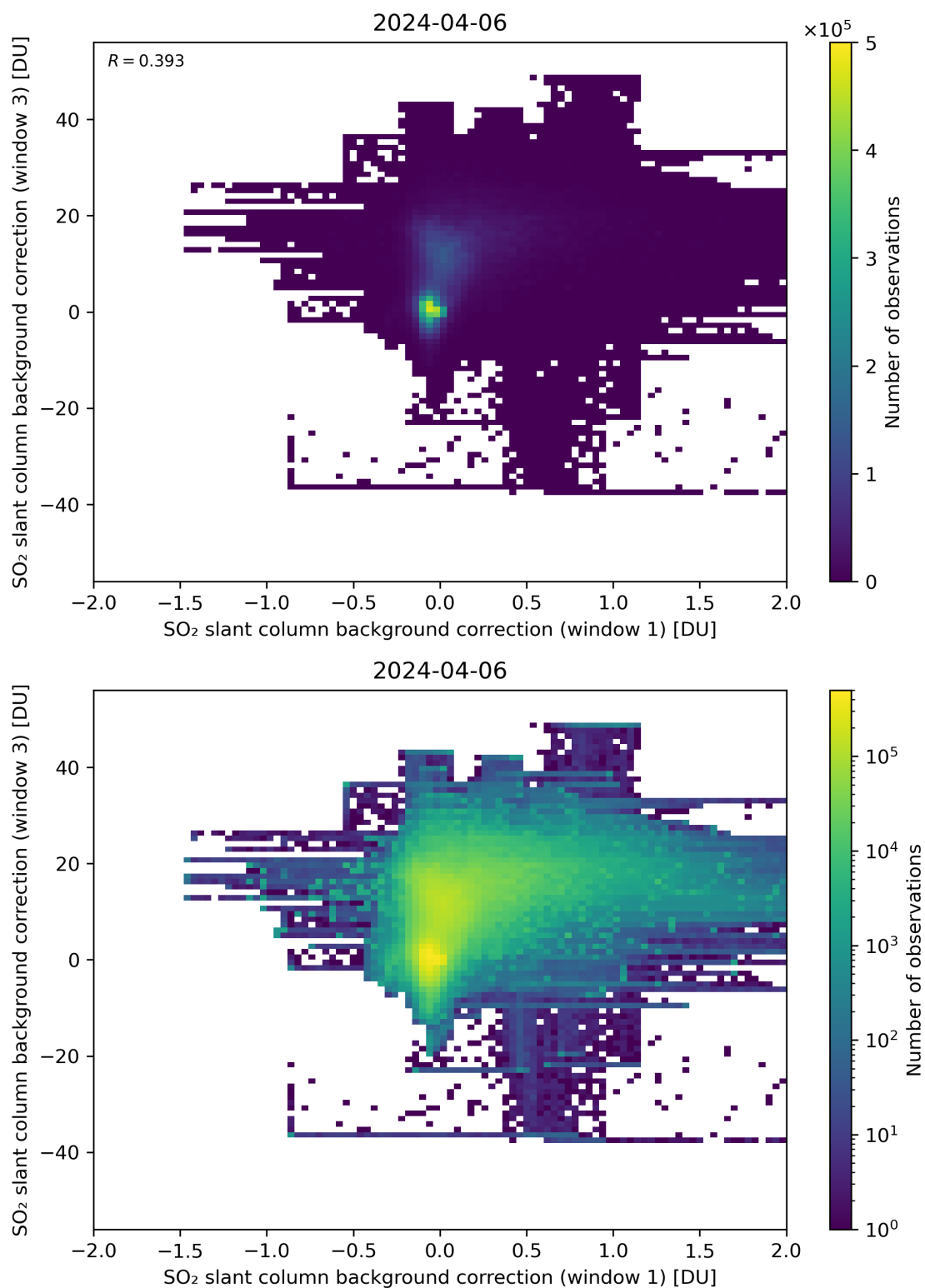
Figure 99: Scatter density plot of “SO 2 slant column background correction (window 1)” against “SO 2 slant column background correction (window 3)” for 2024-04-05 to 2024-04-07.
