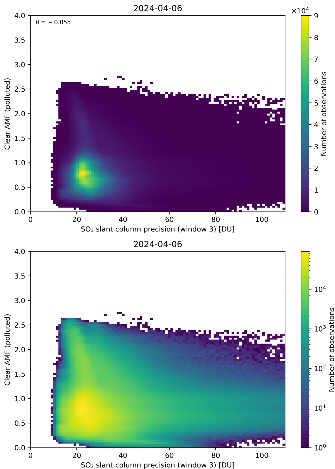
Figure 261: Scatter density plot of “SO 2 slant column precision (window 3)” against “Clear AMF (polluted)” for 2024-04-05 to 2024-04-07.
