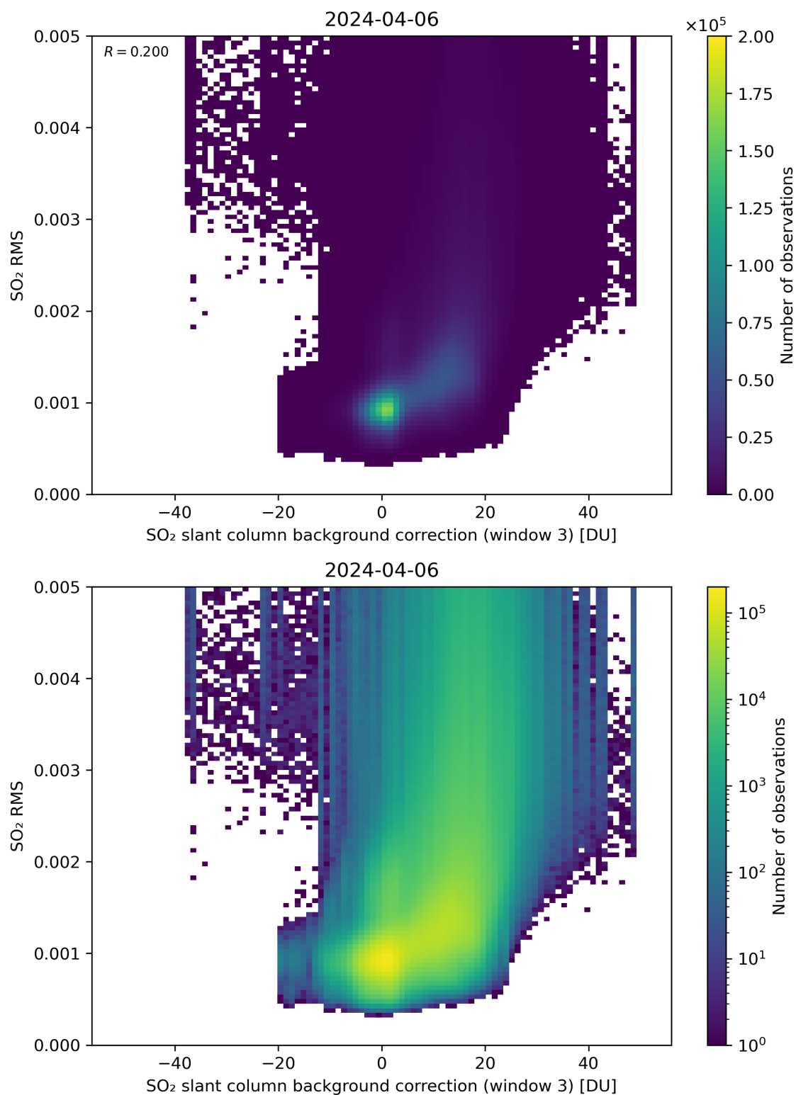
Figure 123: Scatter density plot of “SO 2 slant column background correction (window 3)” against “SO 2 RMS” for 2024-04-05 to 2024-04-07.
