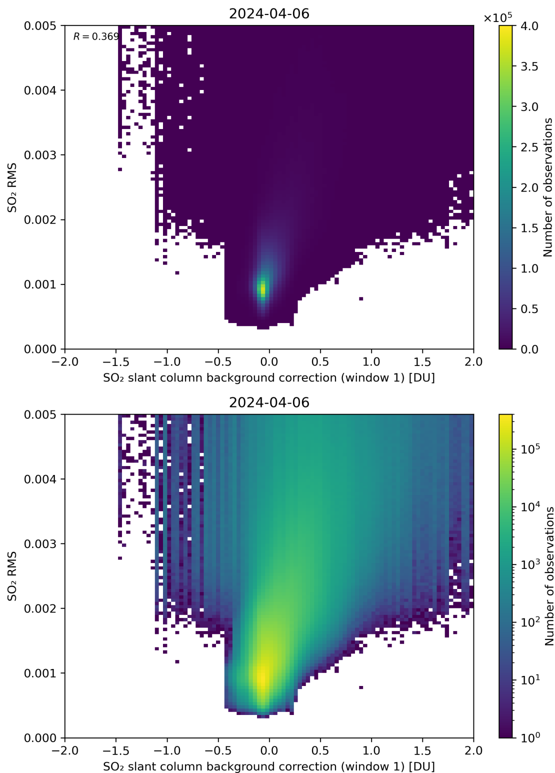
Figure 102: Scatter density plot of “SO 2 slant column background correction (window 1)” against “SO 2 RMS” for 2024-04-05 to 2024-04-07.
