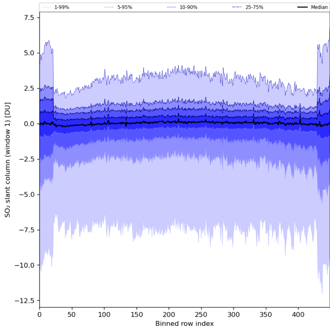
Figure 79: Along track statistics of “SO 2 slant column (window 1)” for 2024-04-05 to 2024-04-07
