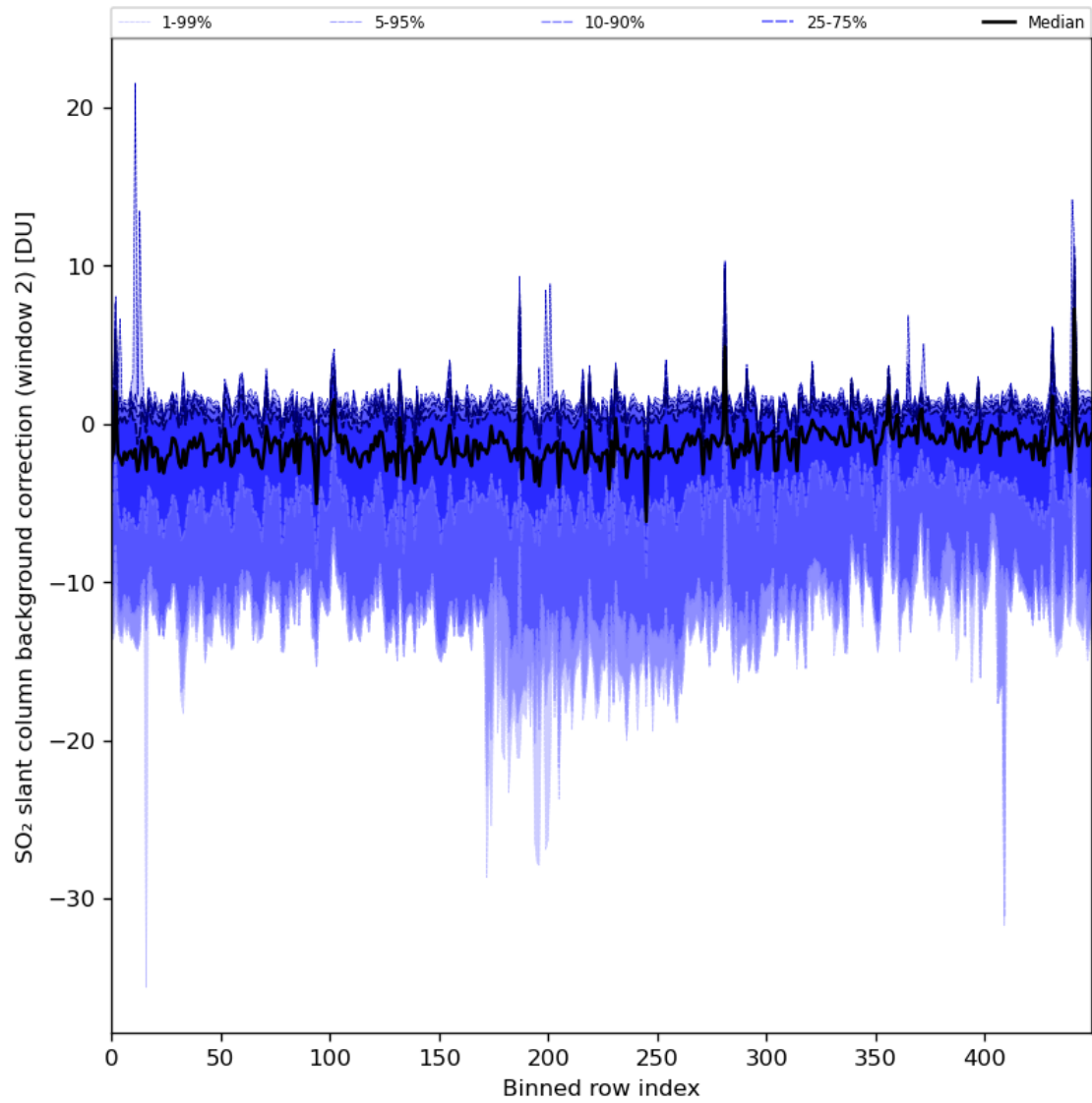
Figure 86: Along track statistics of “SO 2 slant column background correction (window 2)” for 2024-04-05 to 2024-04-07
