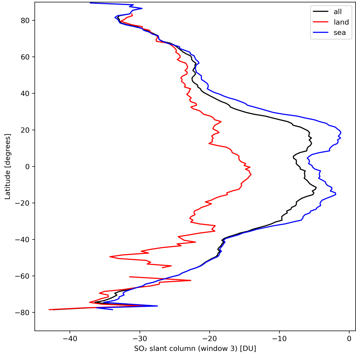
Figure 41: Zonal average of “SO 2 slant column (window 3)” for 2024-04-05 to 2024-04-07.
