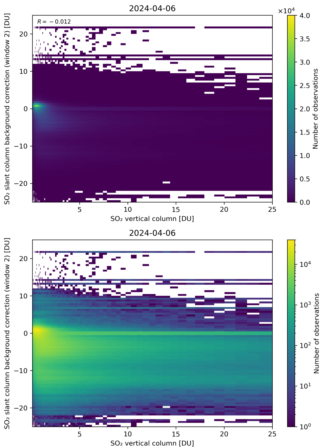
Figure 274: Scatter density plot of “SO 2 vertical column” against “SO 2 slant column background correction (window 2)” for 2024-04-05 to 2024-04-07.
