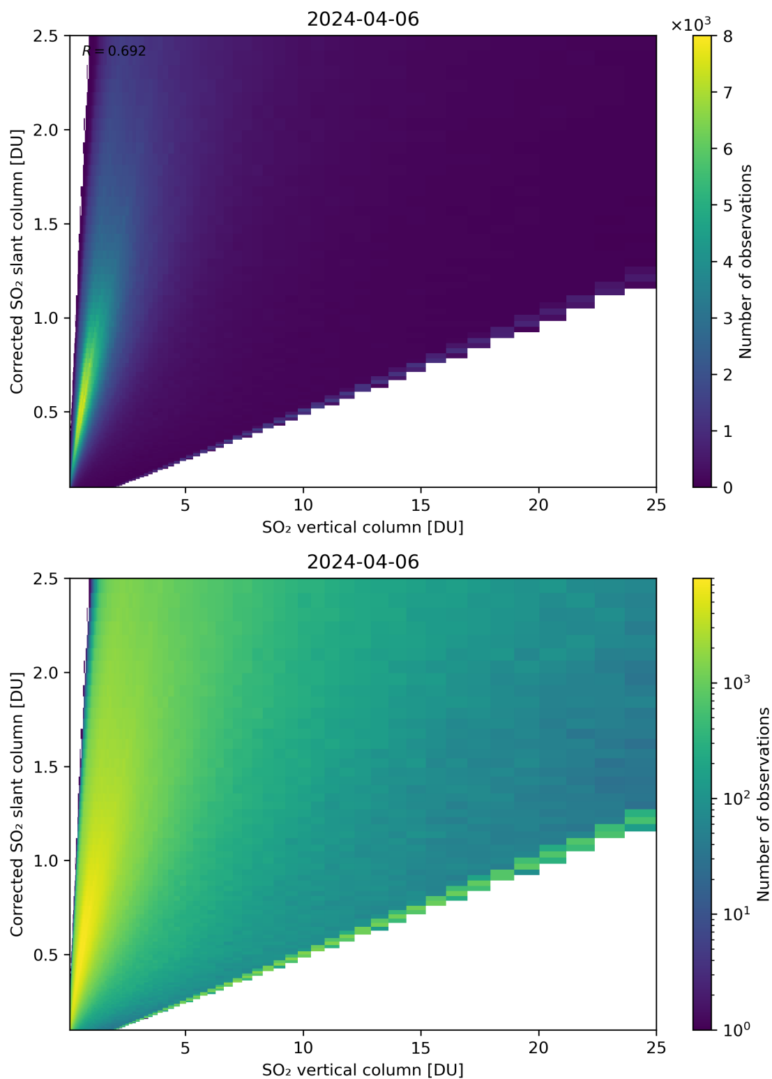
Figure 297: Scatter density plot of “SO 2 vertical column” against “Corrected SO 2 slant column” for 2024-04-05 to 2024-04-07.
