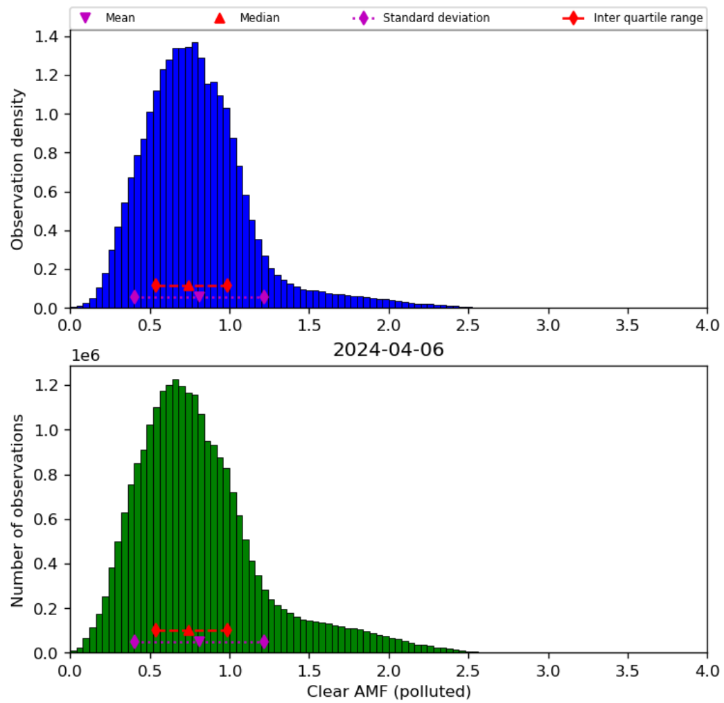
Figure 73: Histogram of “Clear AMF (polluted)” for 2024-04-05 to 2024-04-07
