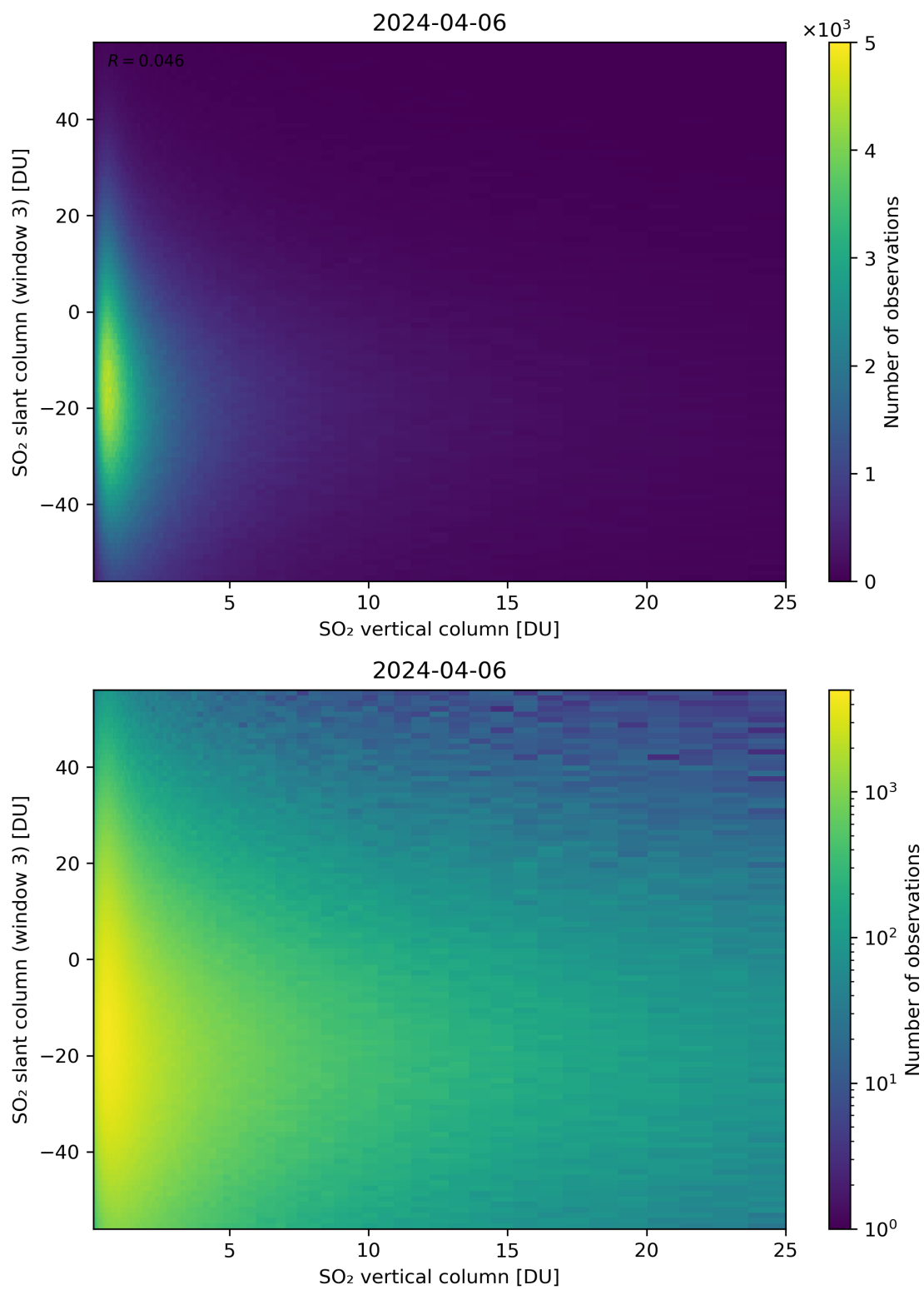
Figure 303: Scatter density plot of “SO 2 vertical column” against “SO 2 slant column (window 3)” for 2024-04-05 to 2024-04-07.
