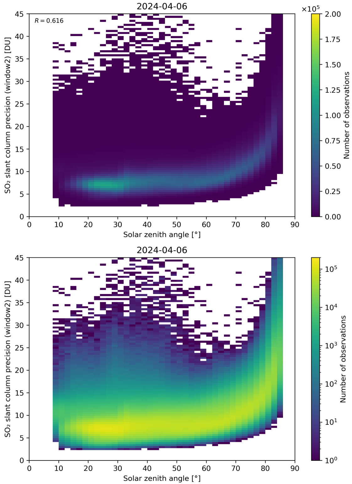
Figure 171: Scatter density plot of “Solar zenith angle” against “SO 2 slant column precision (window2)” for 2024-04-05 to 2024-04-07.
