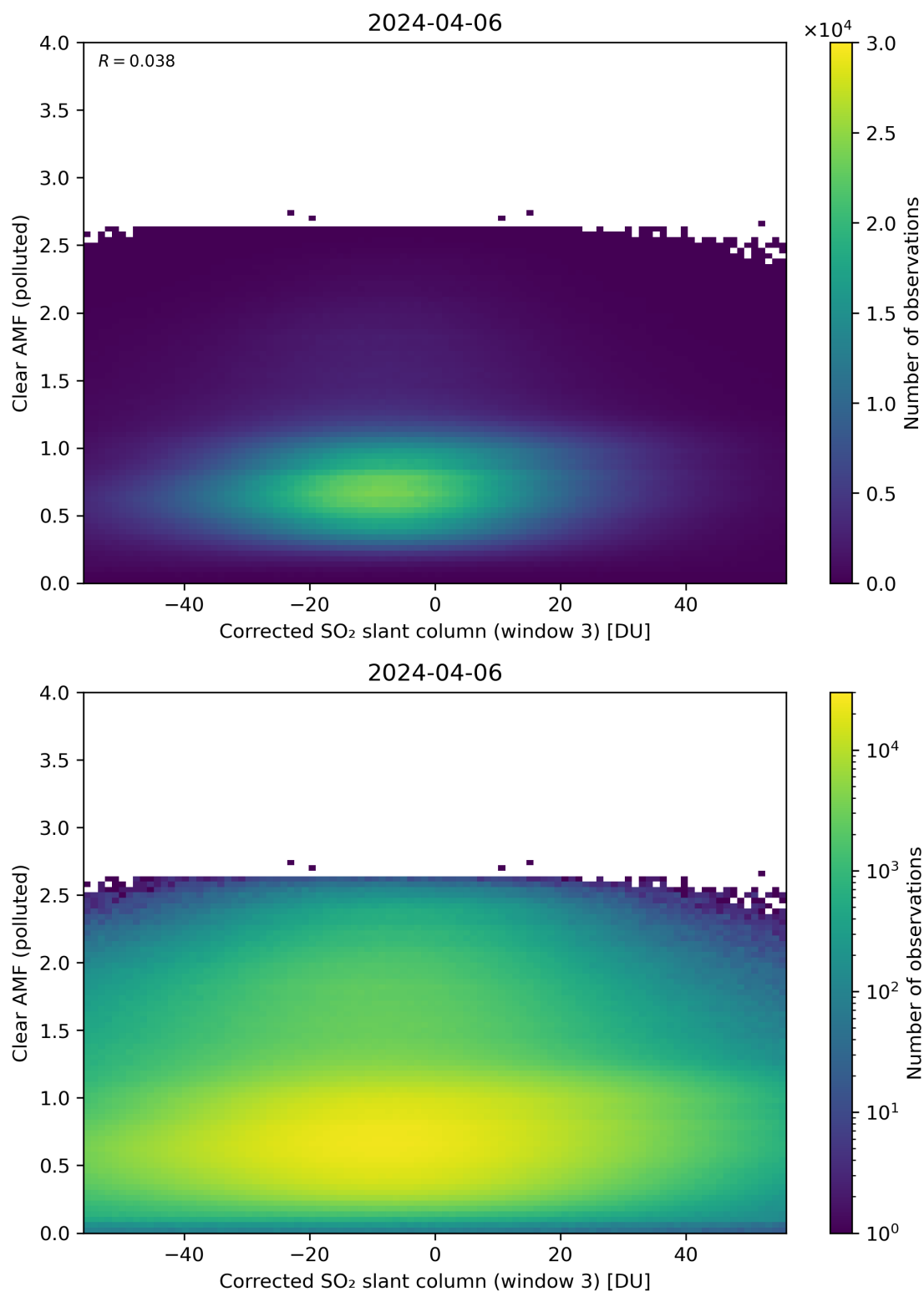
Figure 209: Scatter density plot of “Corrected SO 2 slant column (window 3)” against “Clear AMF (polluted)” for 2024-04-05 to 2024-04-07.
