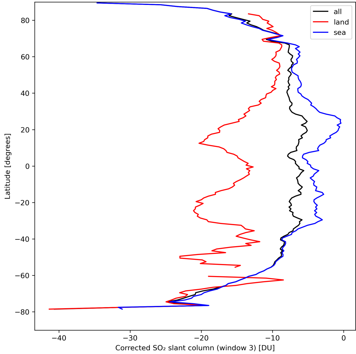
Figure 43: Zonal average of “Corrected SO 2 slant column (window 3)” for 2024-04-05 to 2024-04-07.
