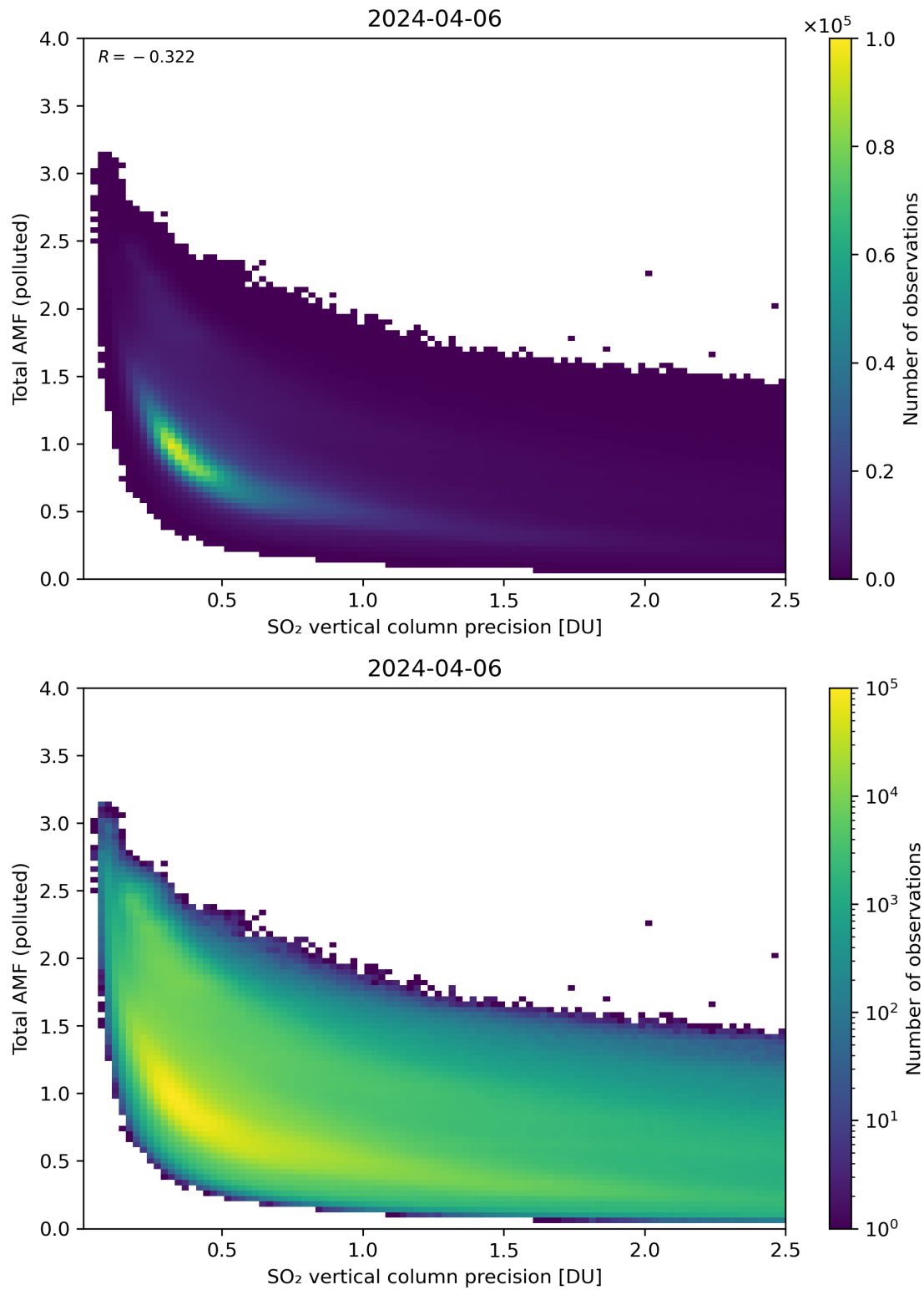
Figure 294: Scatter density plot of “SO 2 vertical column precision” against “Total AMF (polluted)” for 2024-04-05 to 2024-04-07.
