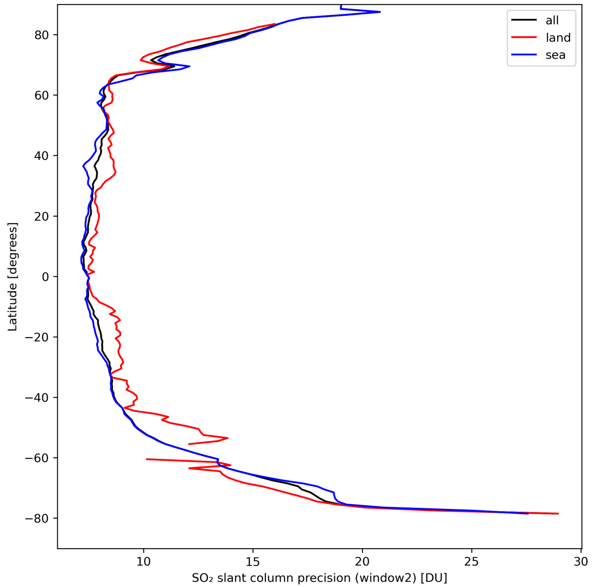
Figure 38: Zonal average of “SO 2 slant column precision (window2)” for 2024-04-05 to 2024-04-07.
