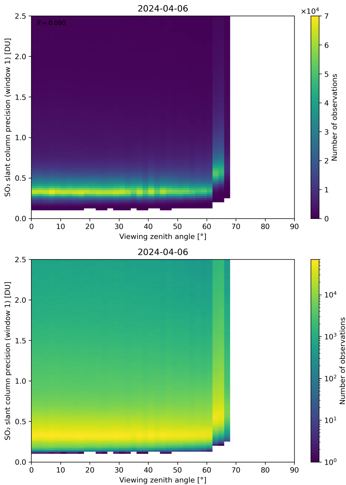
Figure 321: Scatter density plot of “Viewing zenith angle” against “SO 2 slant column precision (window 1)” for 2024-04-05 to 2024-04-07.
