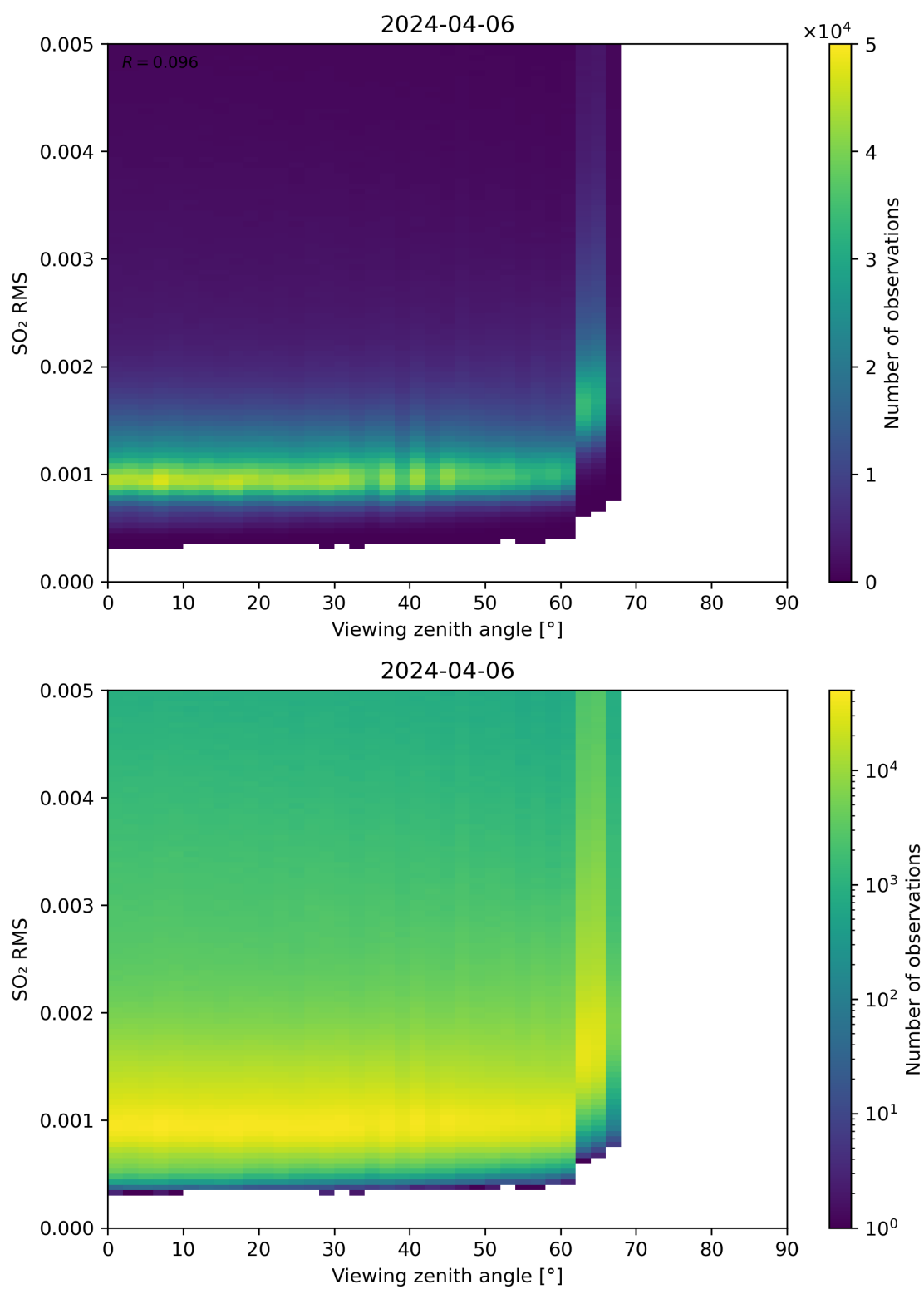
Figure 313: Scatter density plot of “Viewing zenith angle” against “SO 2 RMS” for 2024-04-05 to 2024-04-07.
