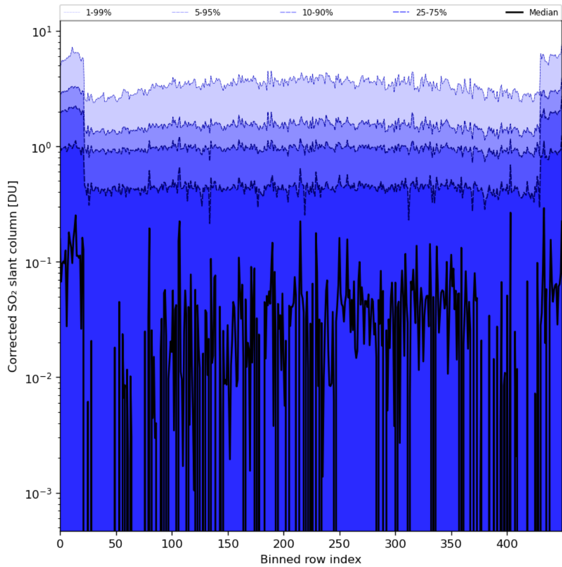
Figure 78: Along track statistics of “Corrected SO 2 slant column” for 2024-04-05 to 2024-04-07
