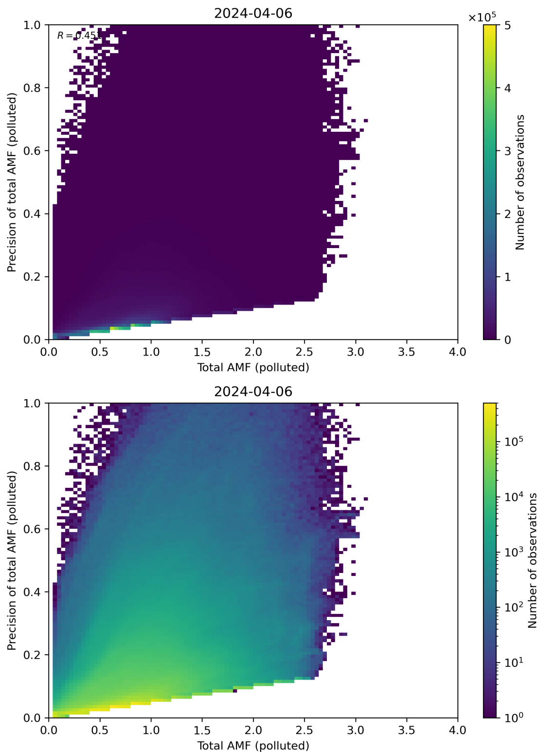
Figure 272: Scatter density plot of “Total AMF (polluted)” against “Precision of total AMF (polluted)” for 2024-04-05 to 2024-04-07.
