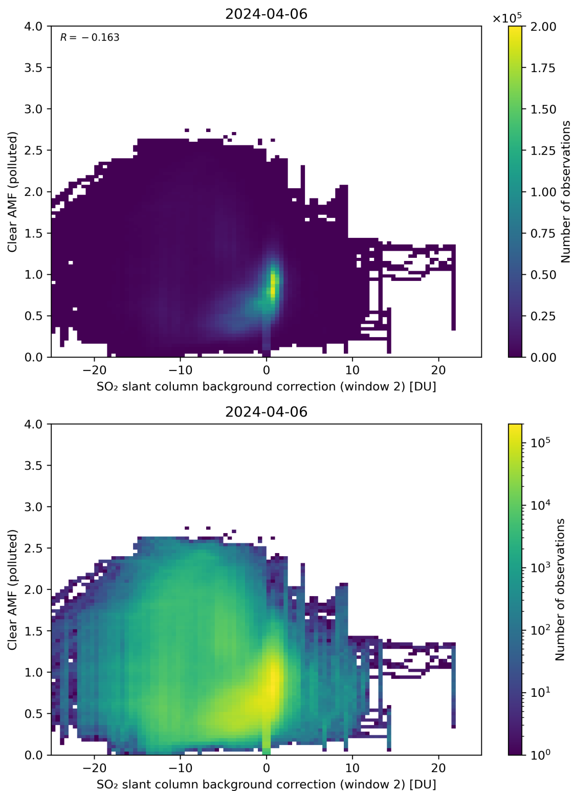
Figure 115: Scatter density plot of “SO 2 slant column background correction (window 2)” against “Clear AMF (polluted)” for 2024-04-05 to 2024-04-07.
