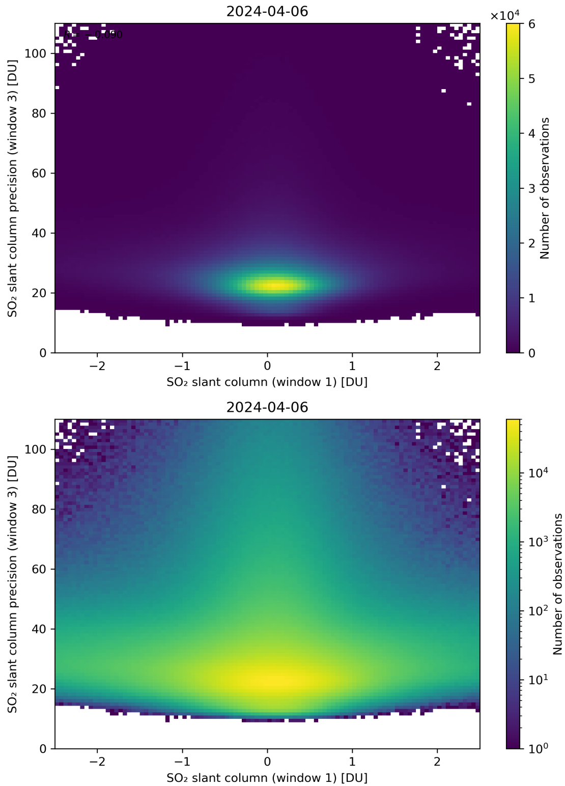
Figure 238: Scatter density plot of “SO 2 slant column (window 1)” against “SO 2 slant column precision (window 3)” for 2024-04-05 to 2024-04-07.
