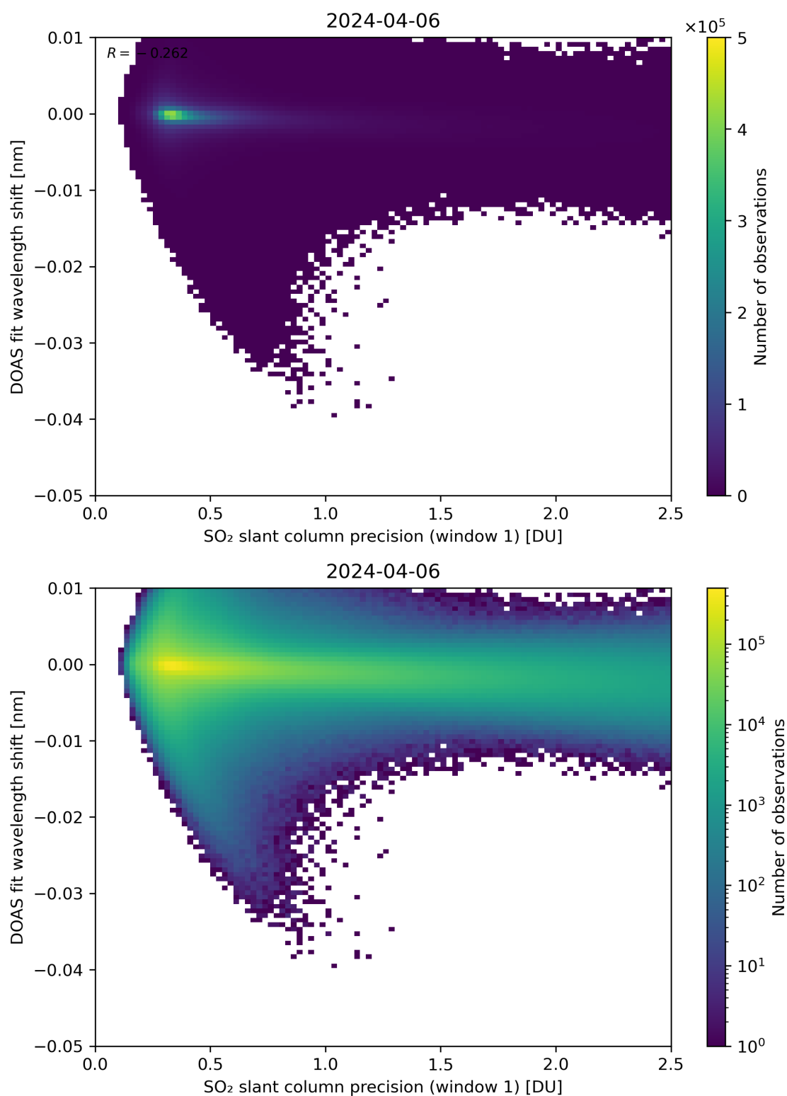
Figure 221: Scatter density plot of “SO 2 slant column precision (window 1)” against “DOAS fit wavelength shift” for 2024-04-05 to 2024-04-07.
