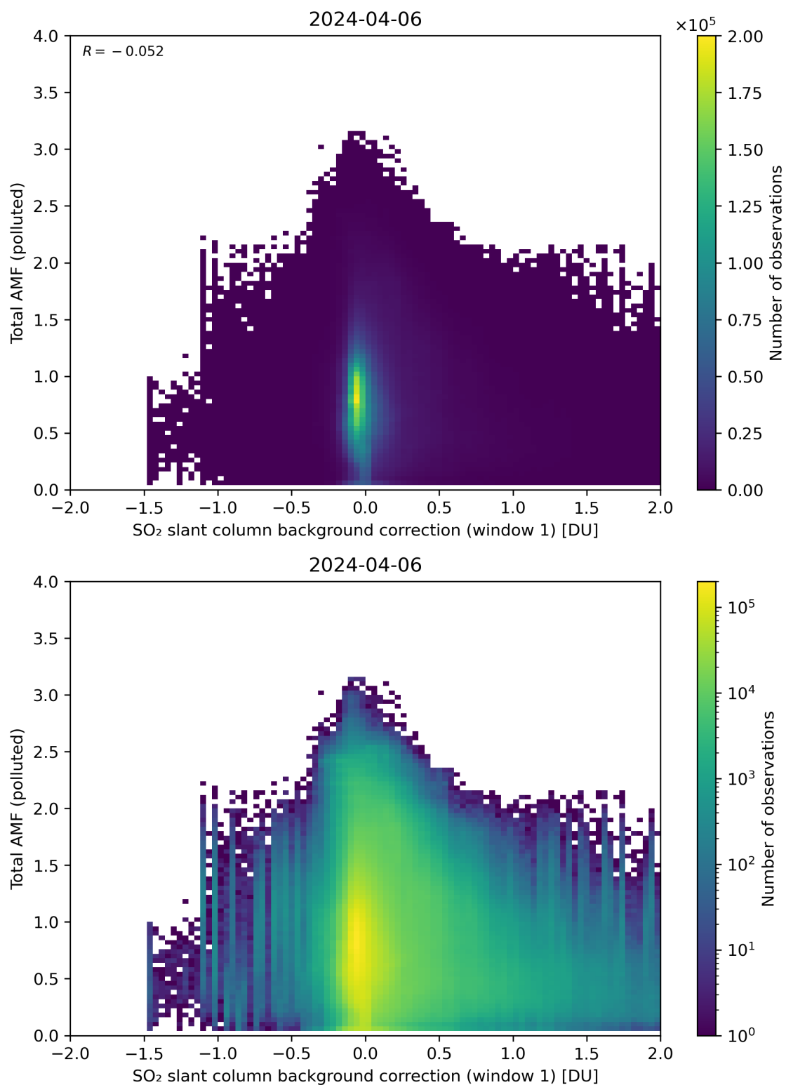
Figure 109: Scatter density plot of “SO 2 slant column background correction (window 1)” against “Total AMF (polluted)” for 2024-04-05 to 2024-04-07.
