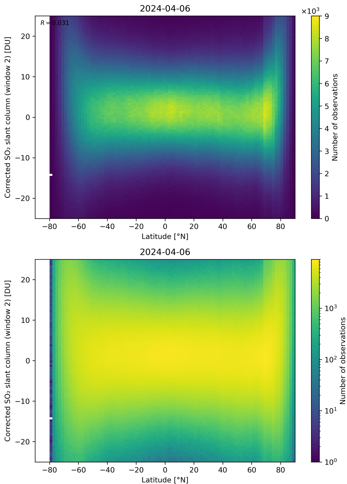
Figure 147: Scatter density plot of “Latitude” against “Corrected SO 2 slant column (window 2)” for 2024-04-05 to 2024-04-07.
