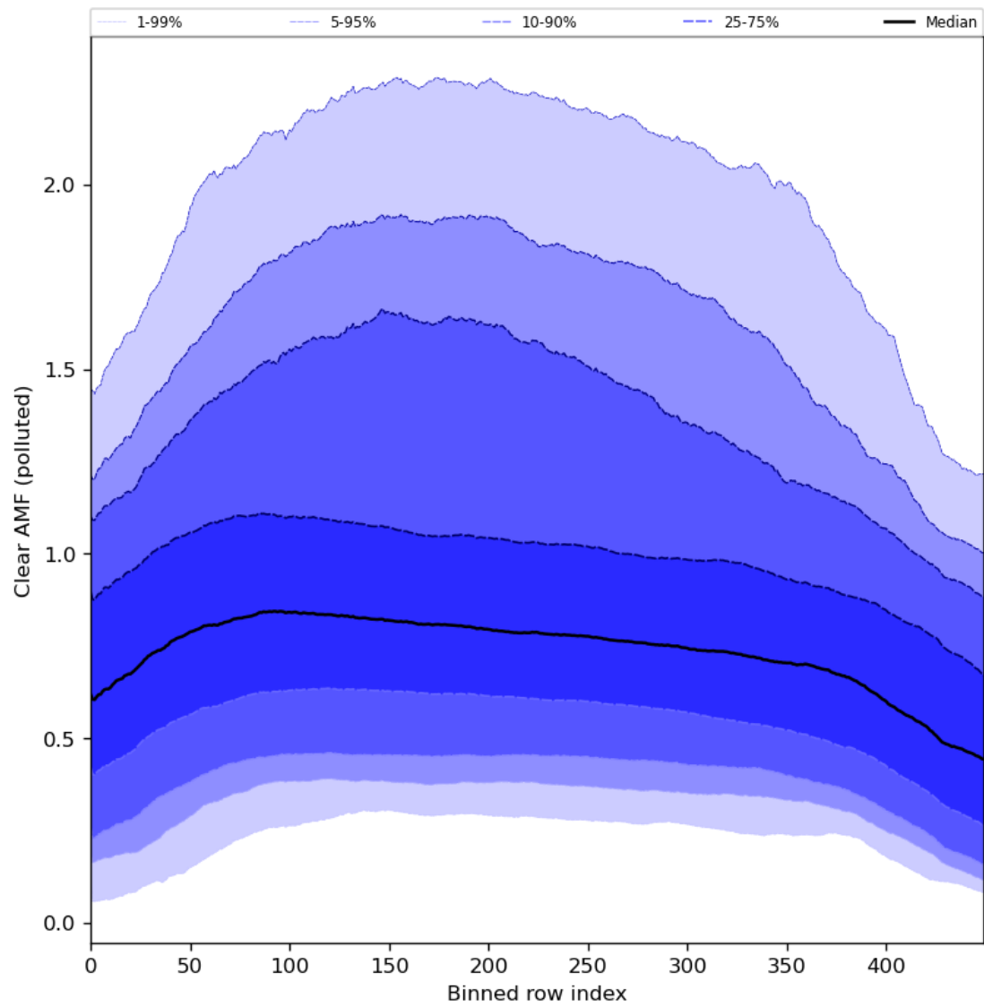
Figure 96: Along track statistics of “Clear AMF (polluted)” for 2024-04-05 to 2024-04-07
