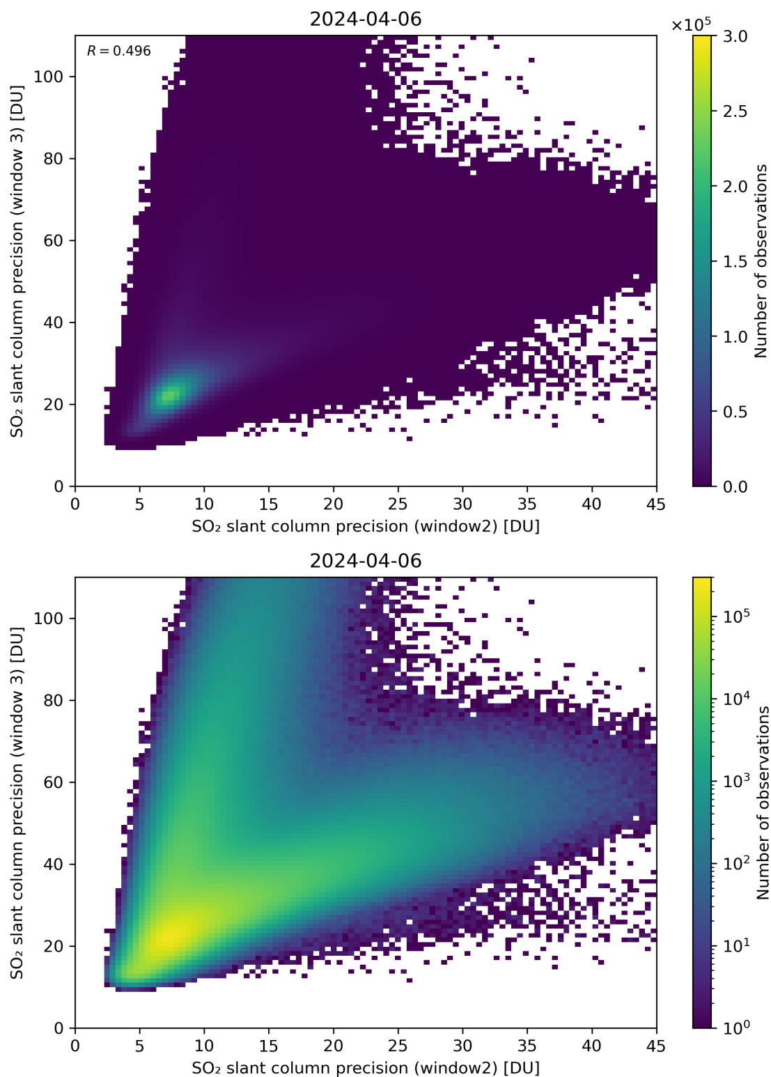
Figure 250: Scatter density plot of “SO 2 slant column precision (window2)” against “SO 2 slant column precision (window 3)” for 2024-04-05 to 2024-04-07.
