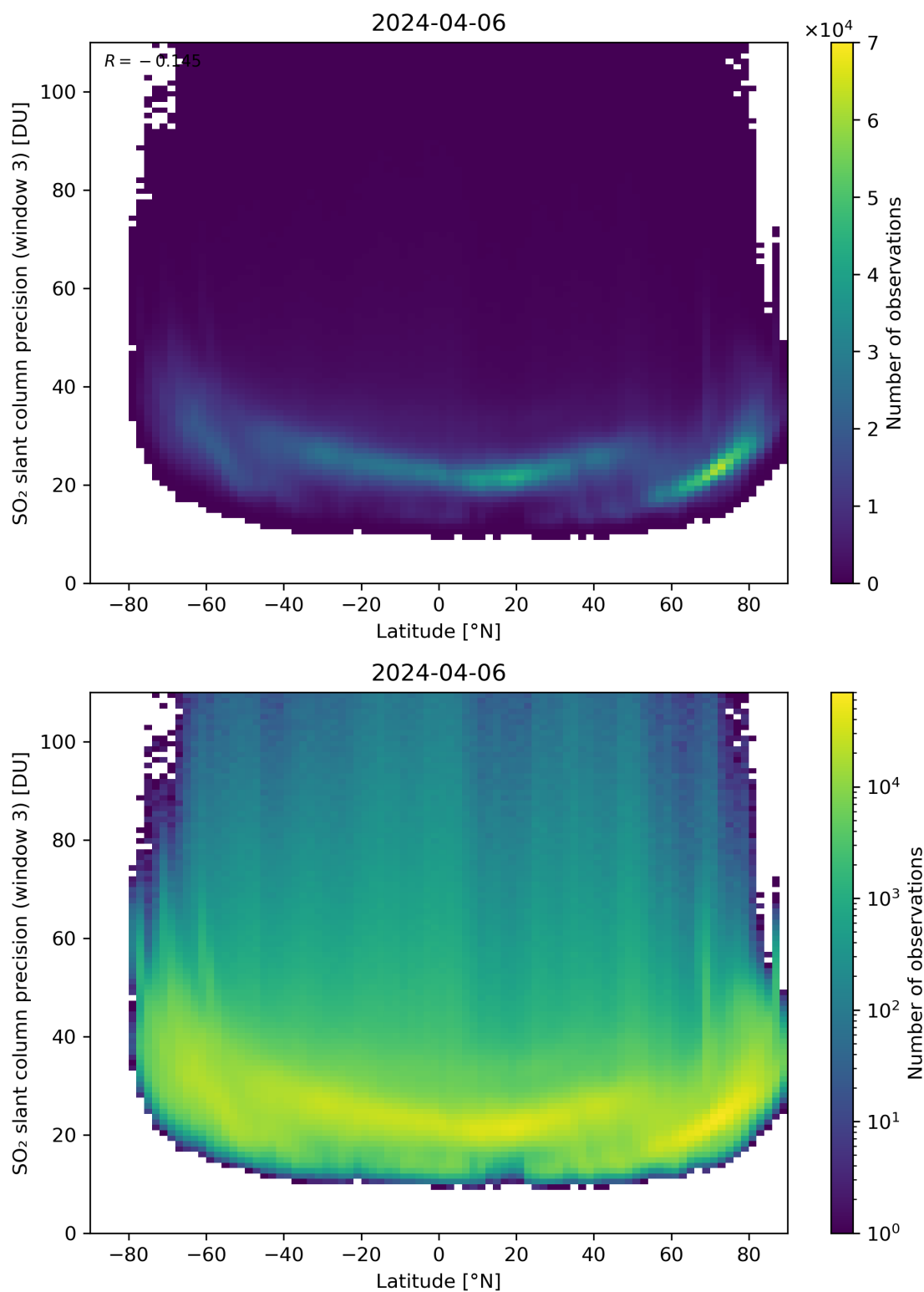
Figure 153: Scatter density plot of “Latitude” against “SO 2 slant column precision (window 3)” for 2024-04-05 to 2024-04-07.
