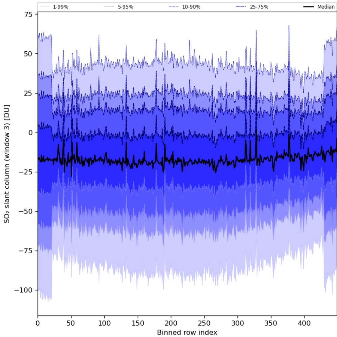
Figure 87: Along track statistics of “SO 2 slant column (window 3)” for 2024-04-05 to 2024-04-07
