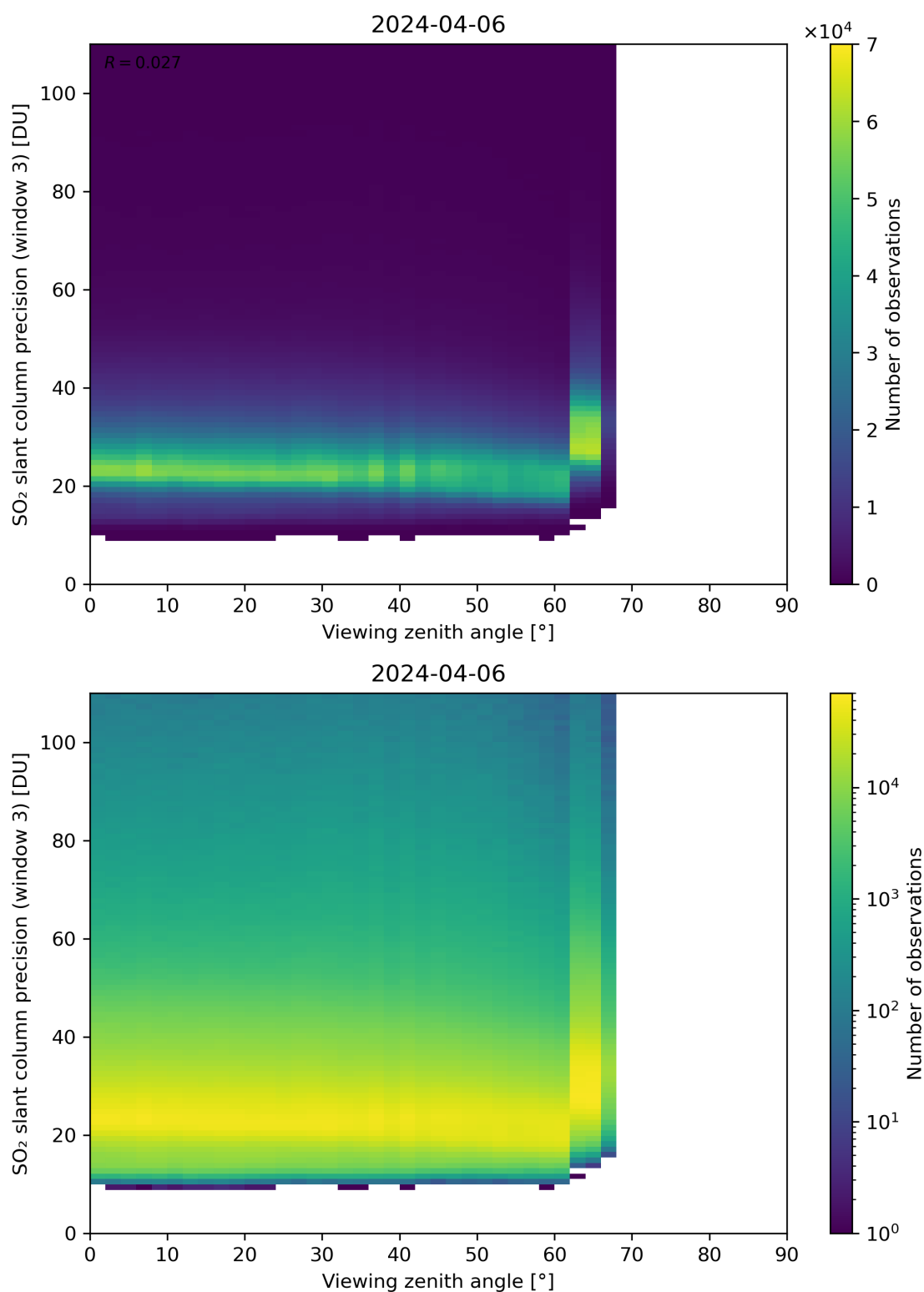
Figure 324: Scatter density plot of “Viewing zenith angle” against “SO 2 slant column precision (window 3)” for 2024-04-05 to 2024-04-07.
