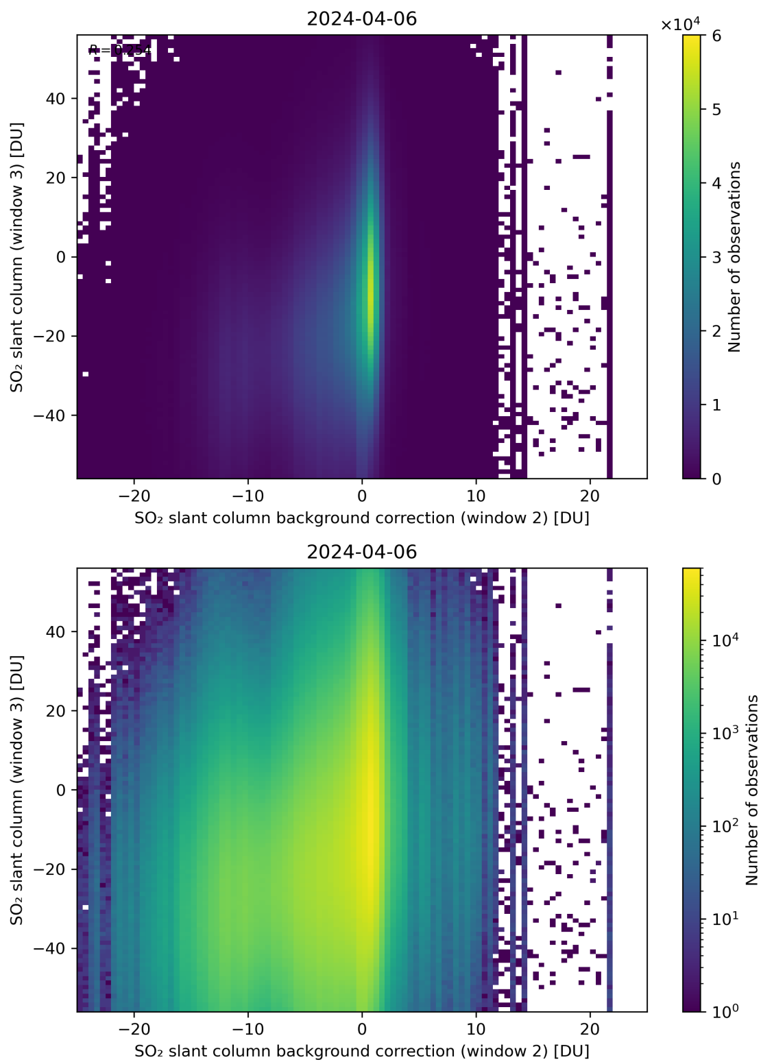
Figure 117: Scatter density plot of “SO 2 slant column background correction (window 2)” against “SO 2 slant column (window 3)” for 2024-04-05 to 2024-04-07.
