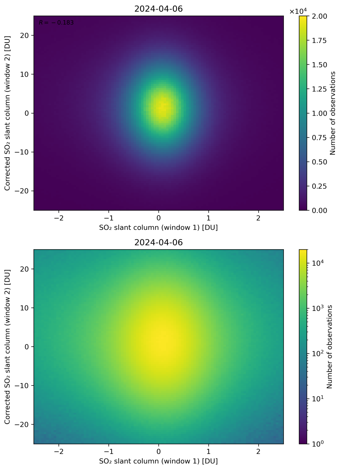
Figure 233: Scatter density plot of “SO 2 slant column (window 1)” against “Corrected SO 2 slant column (window 2)” for 2024-04-05 to 2024-04-07.
