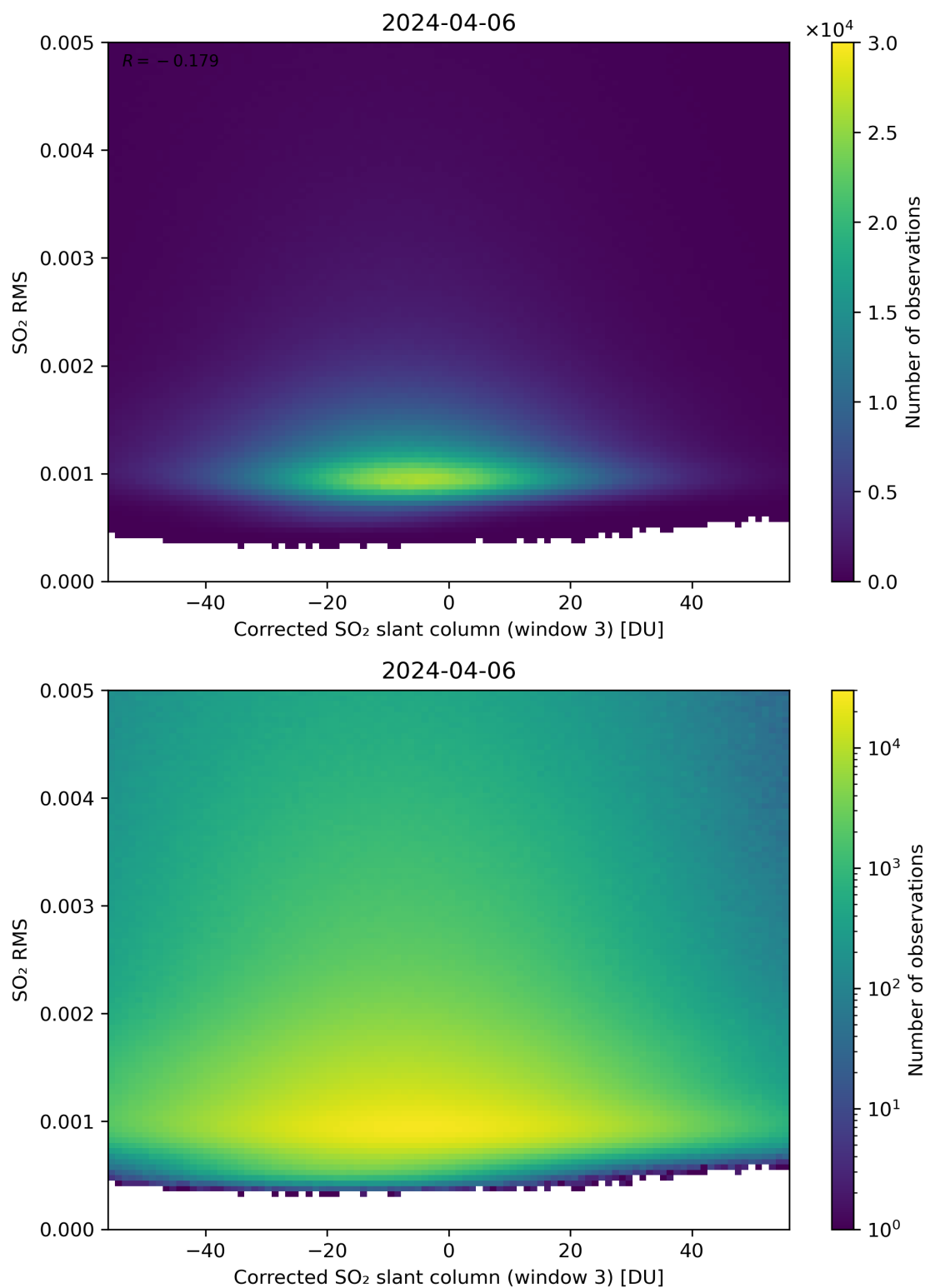
Figure 208: Scatter density plot of “Corrected SO 2 slant column (window 3)” against “SO 2 RMS” for 2024-04-05 to 2024-04-07.
