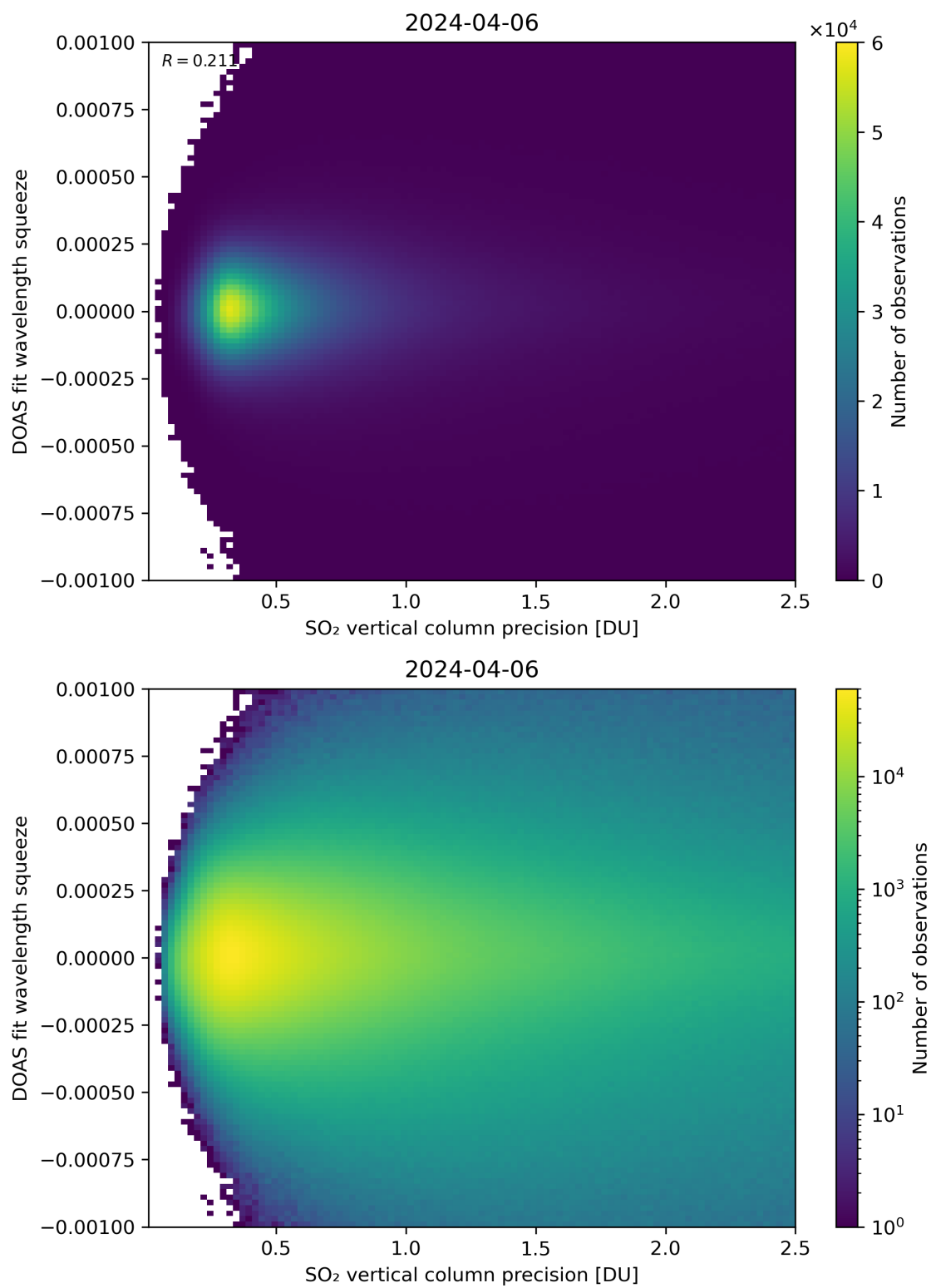
Figure 283: Scatter density plot of “SO 2 vertical column precision” against “DOAS fit wavelength squeeze” for 2024-04-05 to 2024-04-07.
