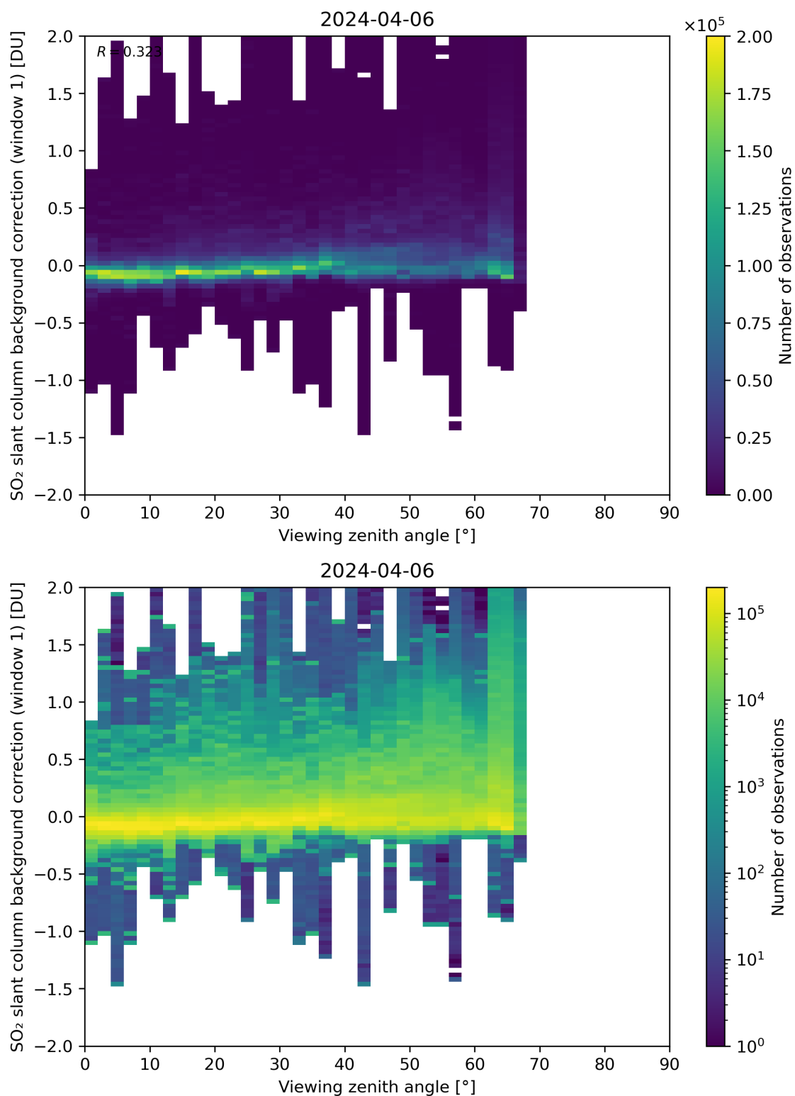
Figure 308: Scatter density plot of “Viewing zenith angle” against “SO 2 slant column background correction (window 1)” for 2024-04-05 to 2024-04-07.
