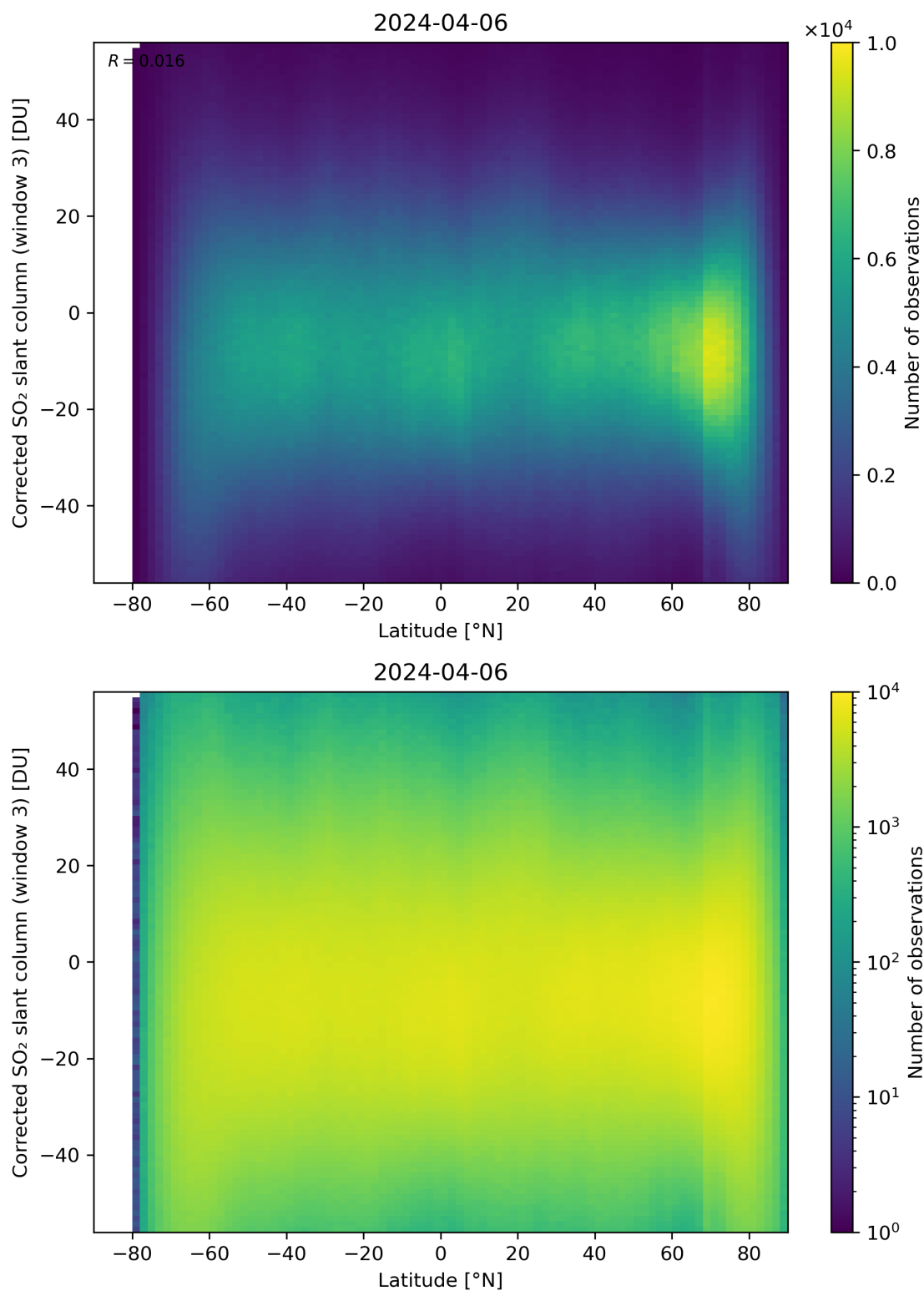
Figure 148: Scatter density plot of “Latitude” against “Corrected SO 2 slant column (window 3)” for 2024-04-05 to 2024-04-07.
