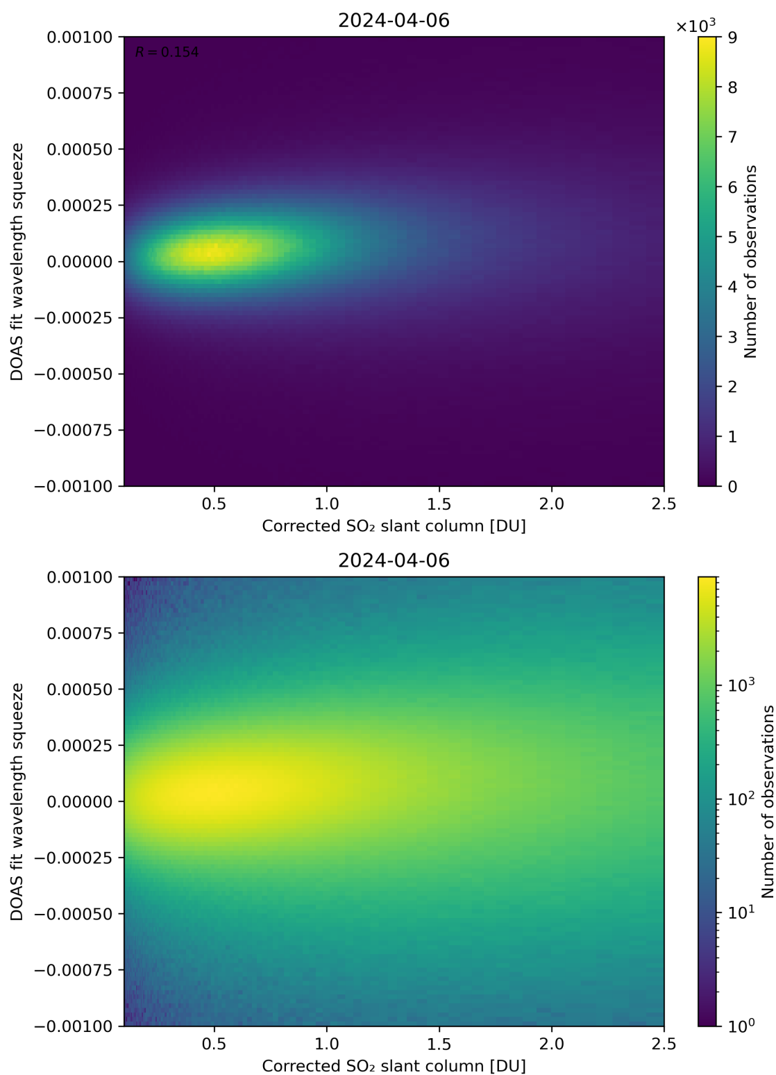
Figure 182: Scatter density plot of “Corrected SO 2 slant column” against “DOAS fit wavelength squeeze” for 2024-04-05 to 2024-04-07.
