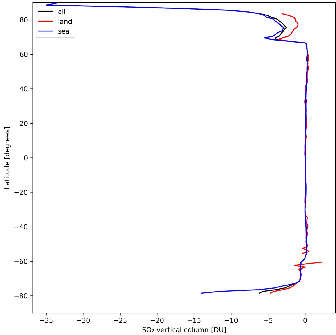
Figure 30: Zonal average of “SO 2 vertical column” for 2024-04-05 to 2024-04-07.
