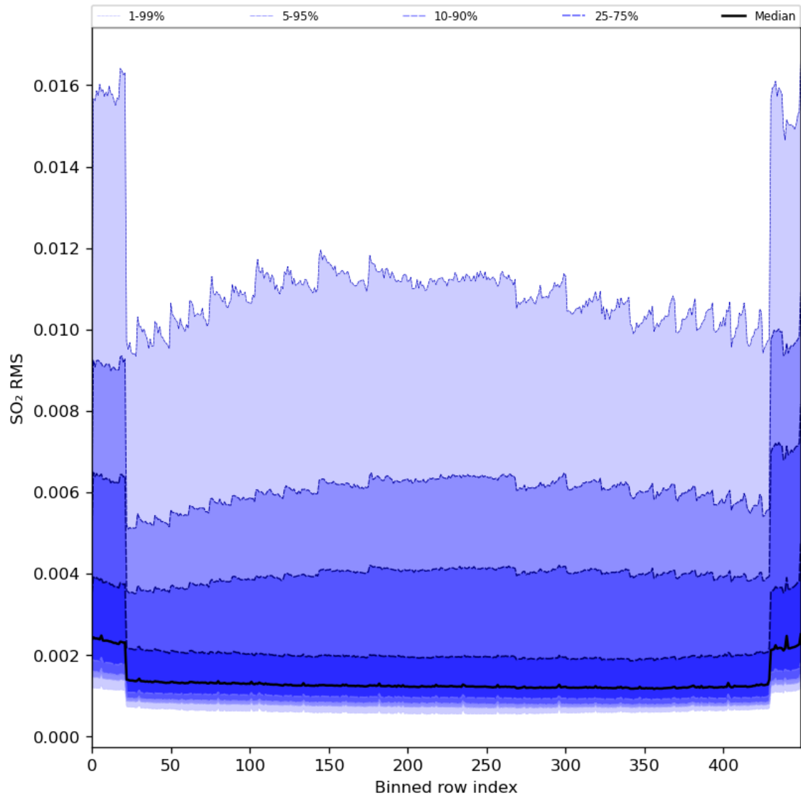
Figure 93: Along track statistics of “SO 2 RMS” for 2024-04-05 to 2024-04-07
