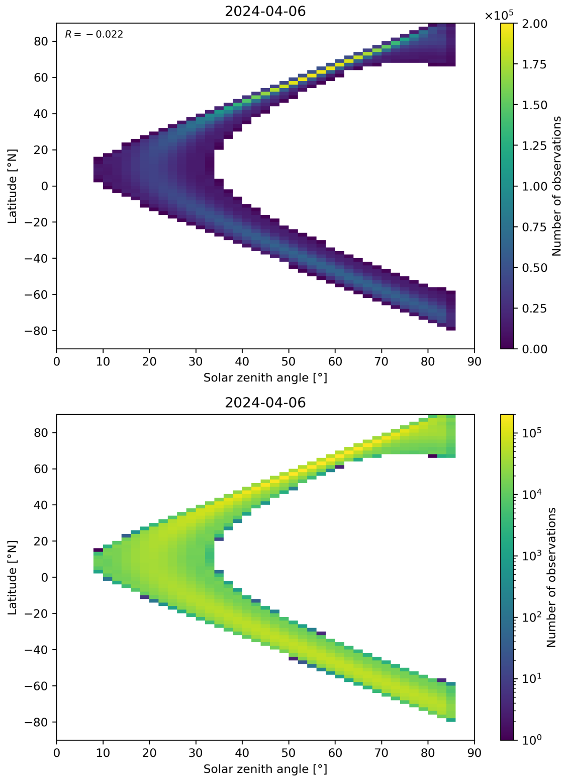
Figure 164: Scatter density plot of “Solar zenith angle” against “Latitude” for 2024-04-05 to 2024-04-07.
