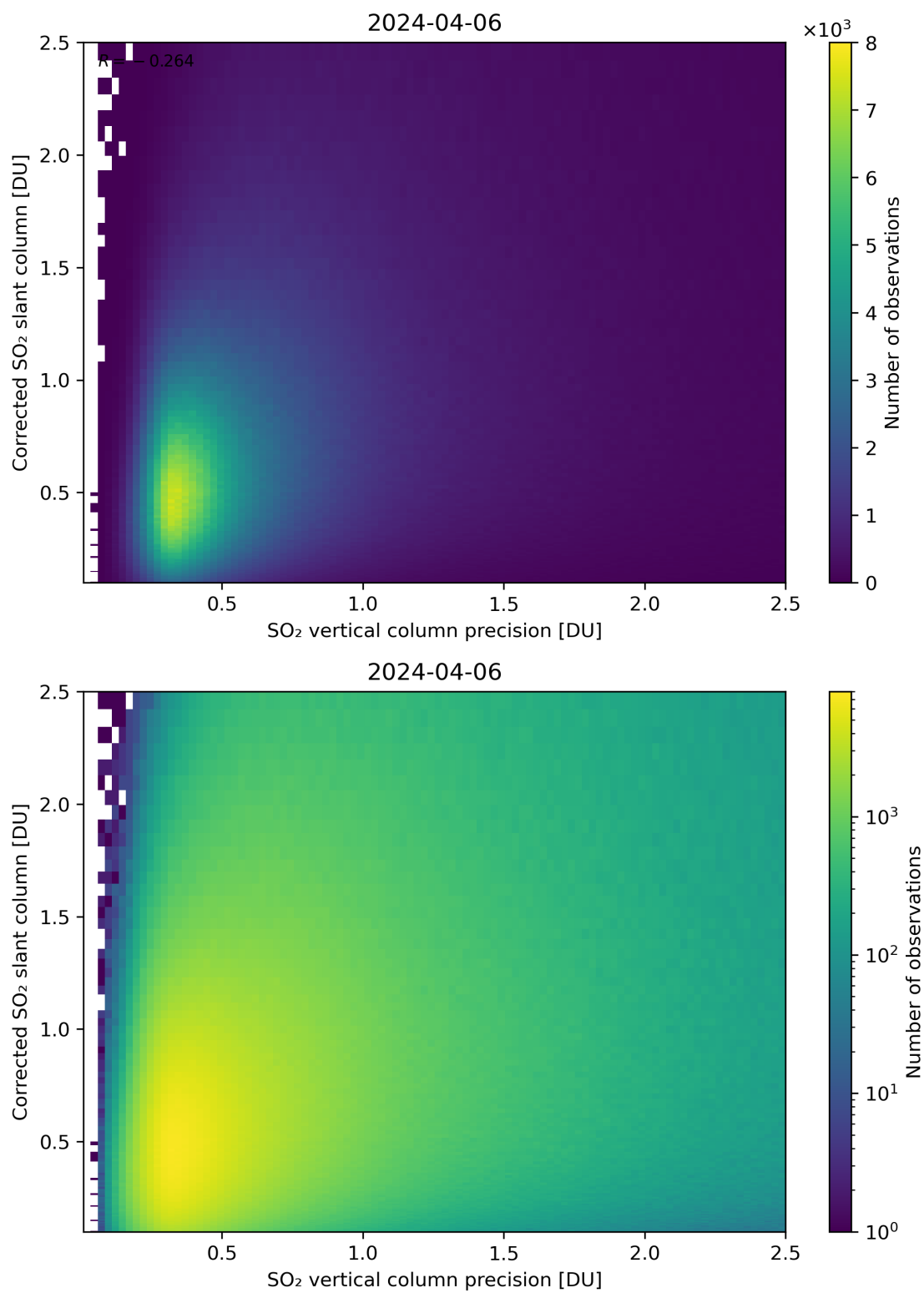
Figure 286: Scatter density plot of “SO 2 vertical column precision” against “Corrected SO 2 slant column” for 2024-04-05 to 2024-04-07.
