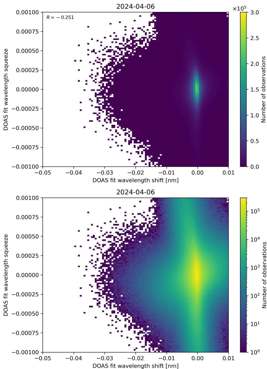
Figure 127: Scatter density plot of “DOAS fit wavelength shift” against “DOAS fit wavelength squeeze” for 2024-04-05 to 2024-04-07.
