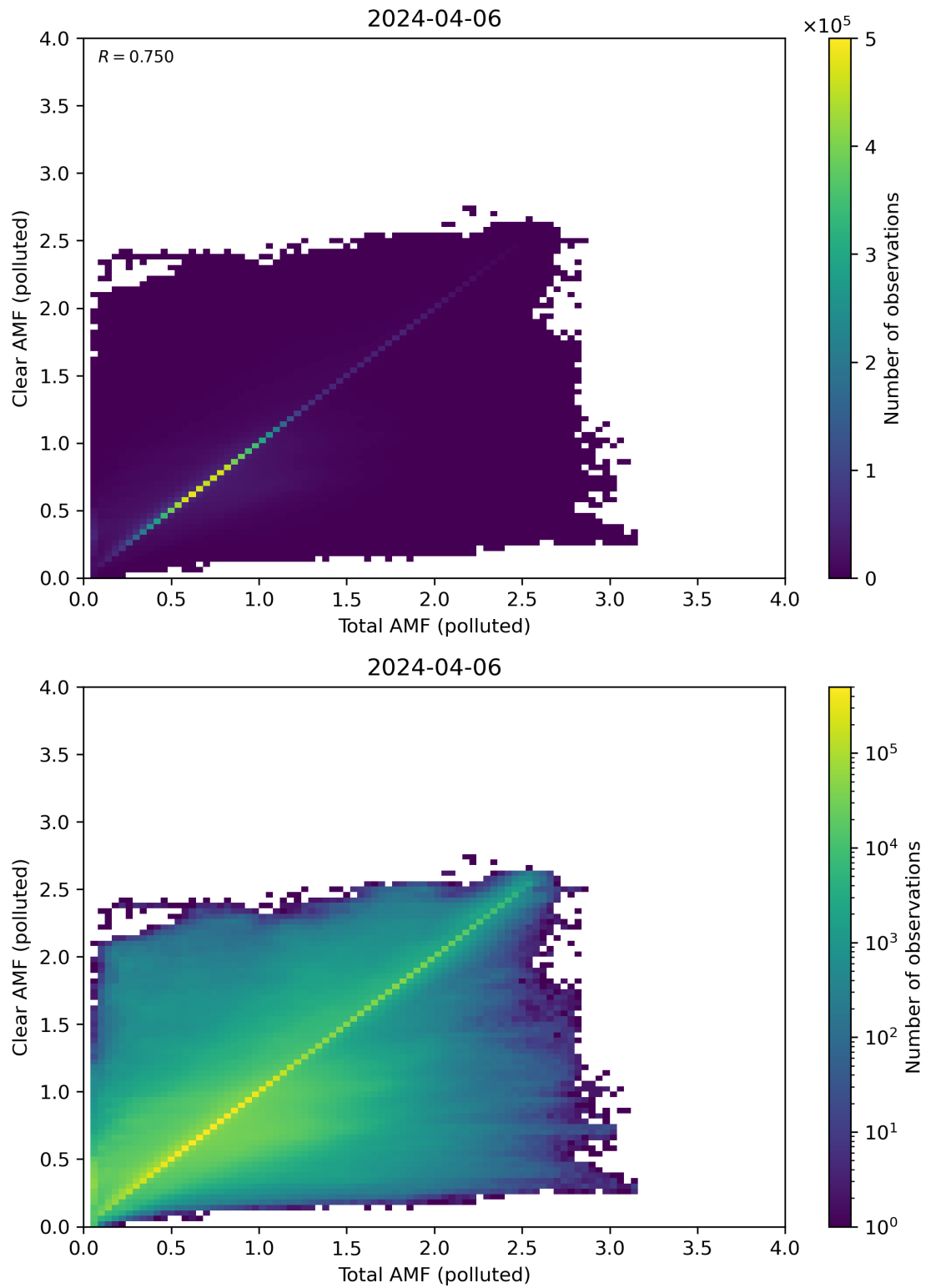
Figure 271: Scatter density plot of “Total AMF (polluted)” against “Clear AMF (polluted)” for 2024-04-05 to 2024-04-07.
