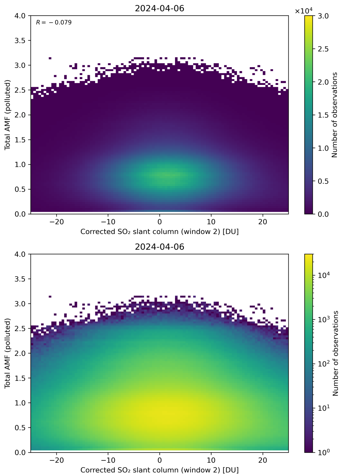
Figure 203: Scatter density plot of “Corrected SO 2 slant column (window 2)” against “Total AMF (polluted)” for 2024-04-05 to 2024-04-07.
