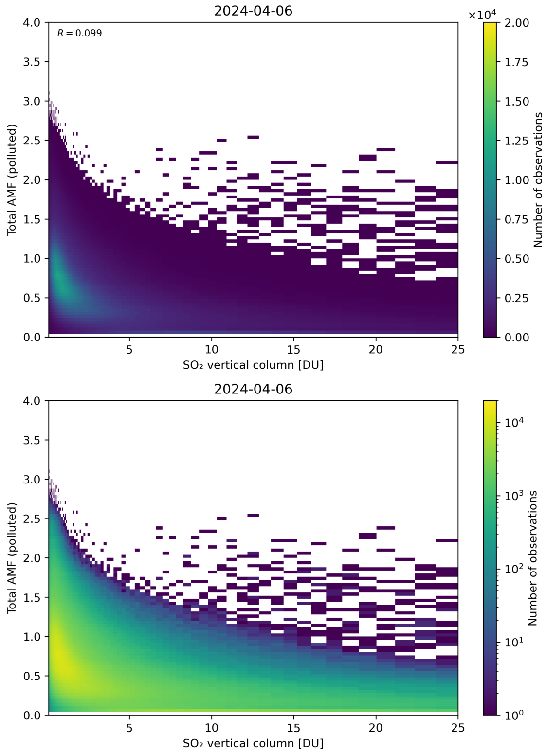
Figure 305: Scatter density plot of “SO 2 vertical column” against “Total AMF (polluted)” for 2024-04-05 to 2024-04-07.
