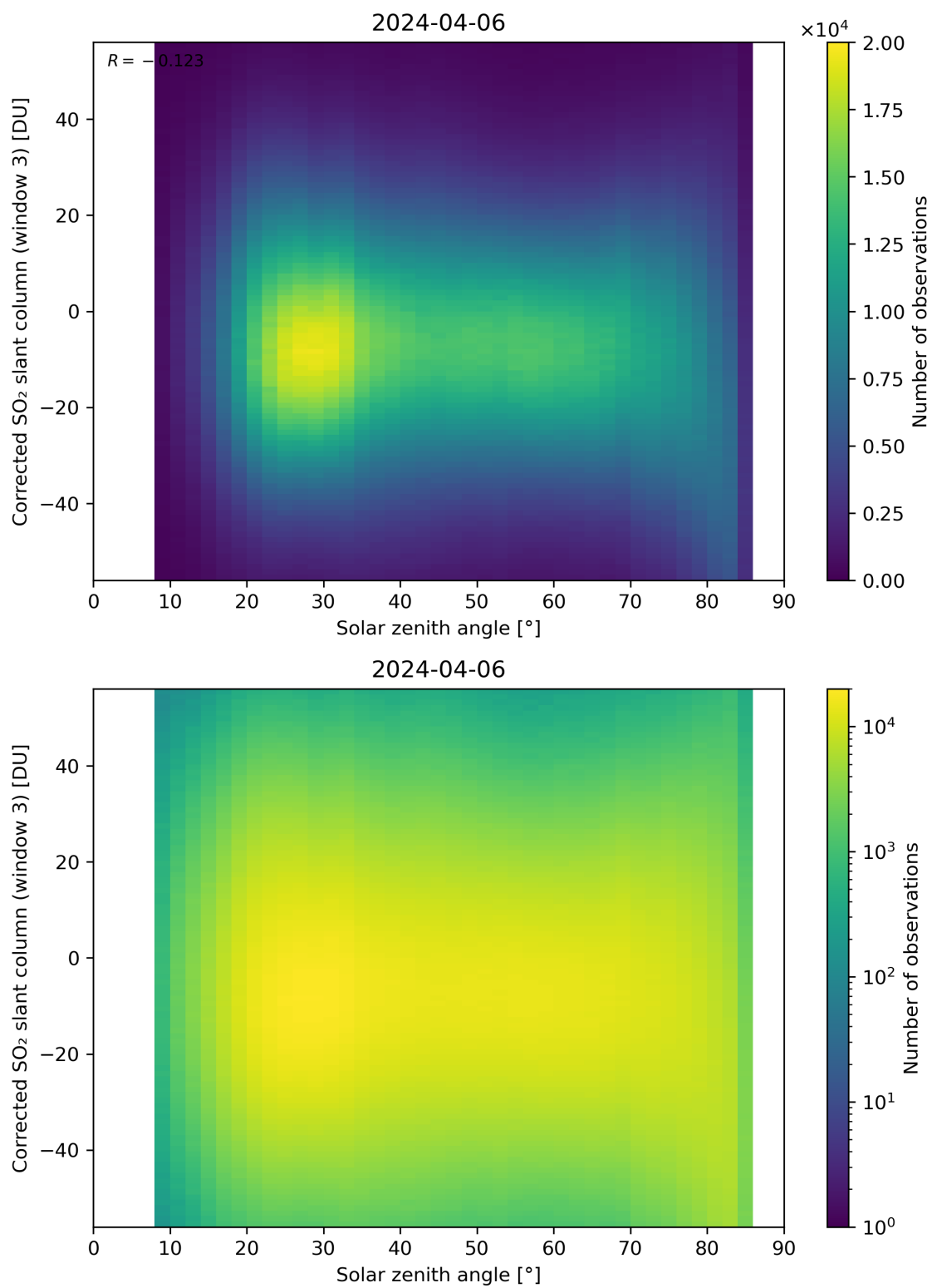
Figure 168: Scatter density plot of “Solar zenith angle” against “Corrected SO 2 slant column (window 3)” for 2024-04-05 to 2024-04-07.
