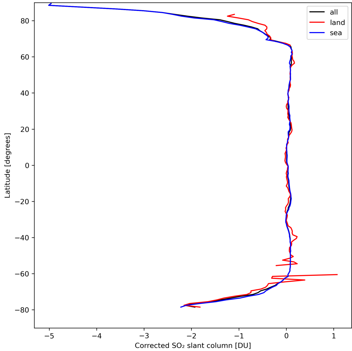
Figure 32: Zonal average of “Corrected SO 2 slant column” for 2024-04-05 to 2024-04-07.
