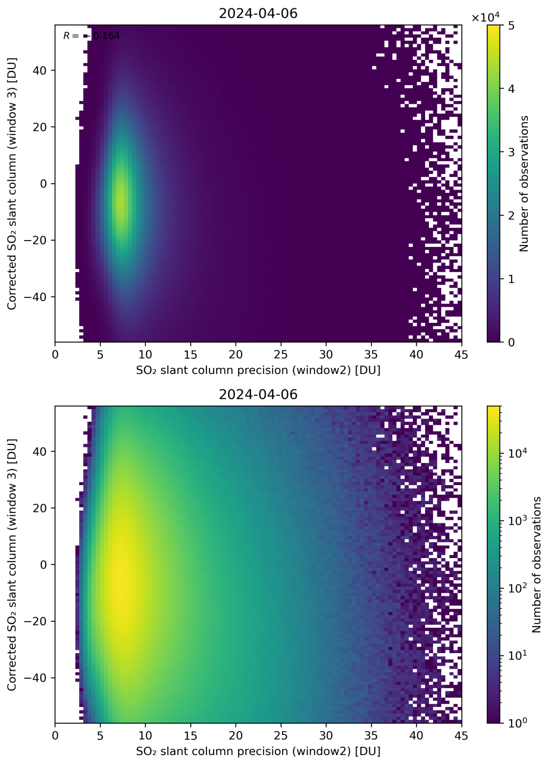
Figure 248: Scatter density plot of “SO 2 slant column precision (window2)” against “Corrected SO 2 slant column (window 3)” for 2024-04-05 to 2024-04-07.
