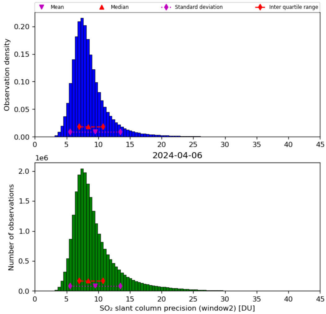
Figure 61: Histogram of “SO 2 slant column precision (window2)” for 2024-04-05 to 2024-04-07
