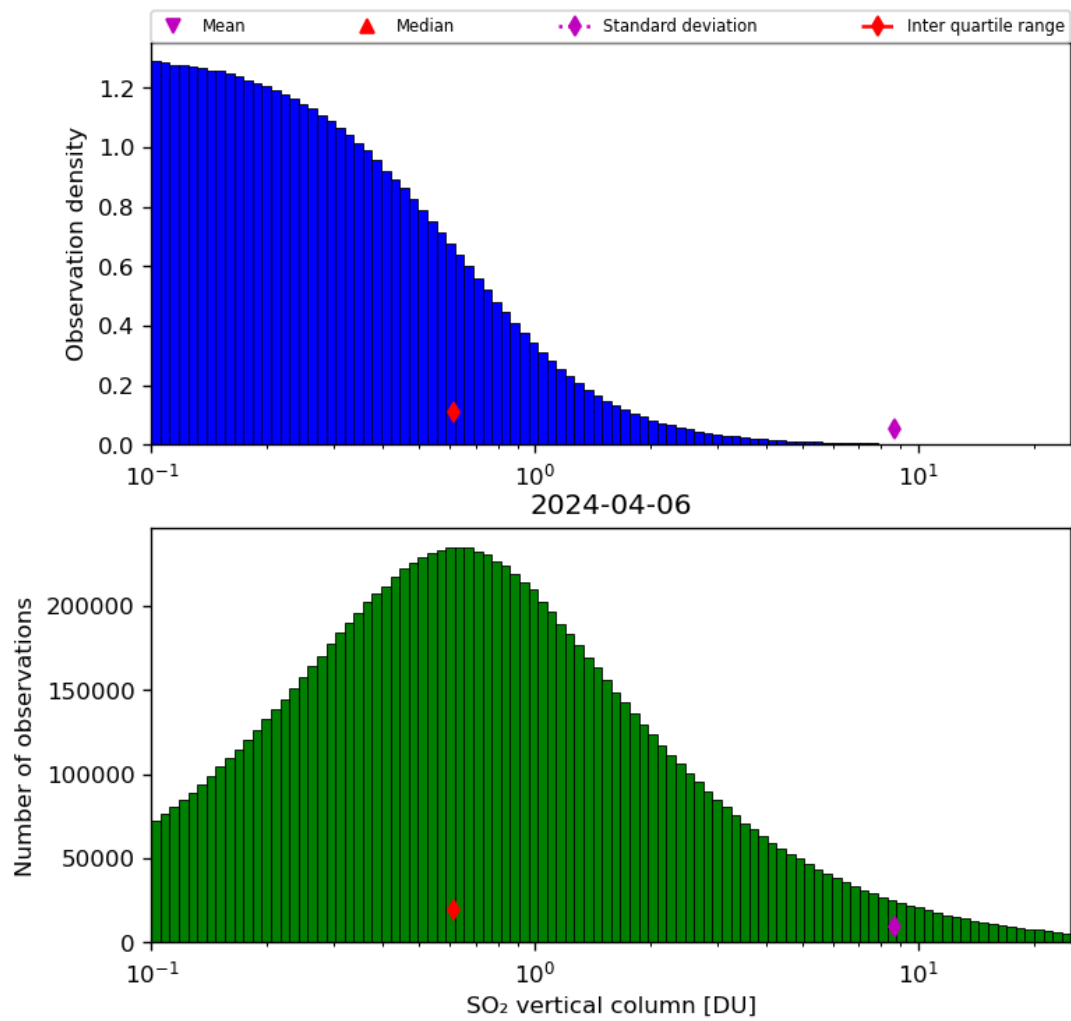
Figure 53: Histogram of “SO 2 vertical column” for 2024-04-05 to 2024-04-07
