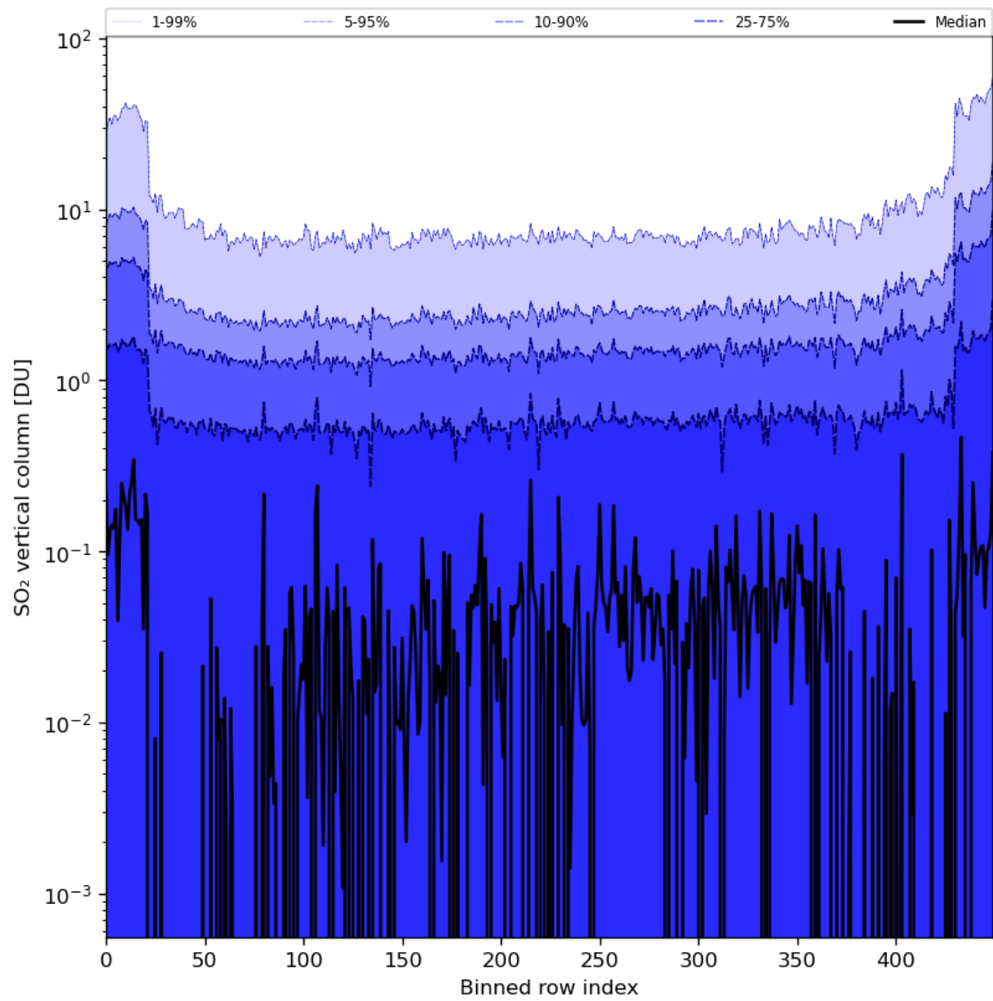
Figure 76: Along track statistics of “SO 2 vertical column” for 2024-04-05 to 2024-04-07
