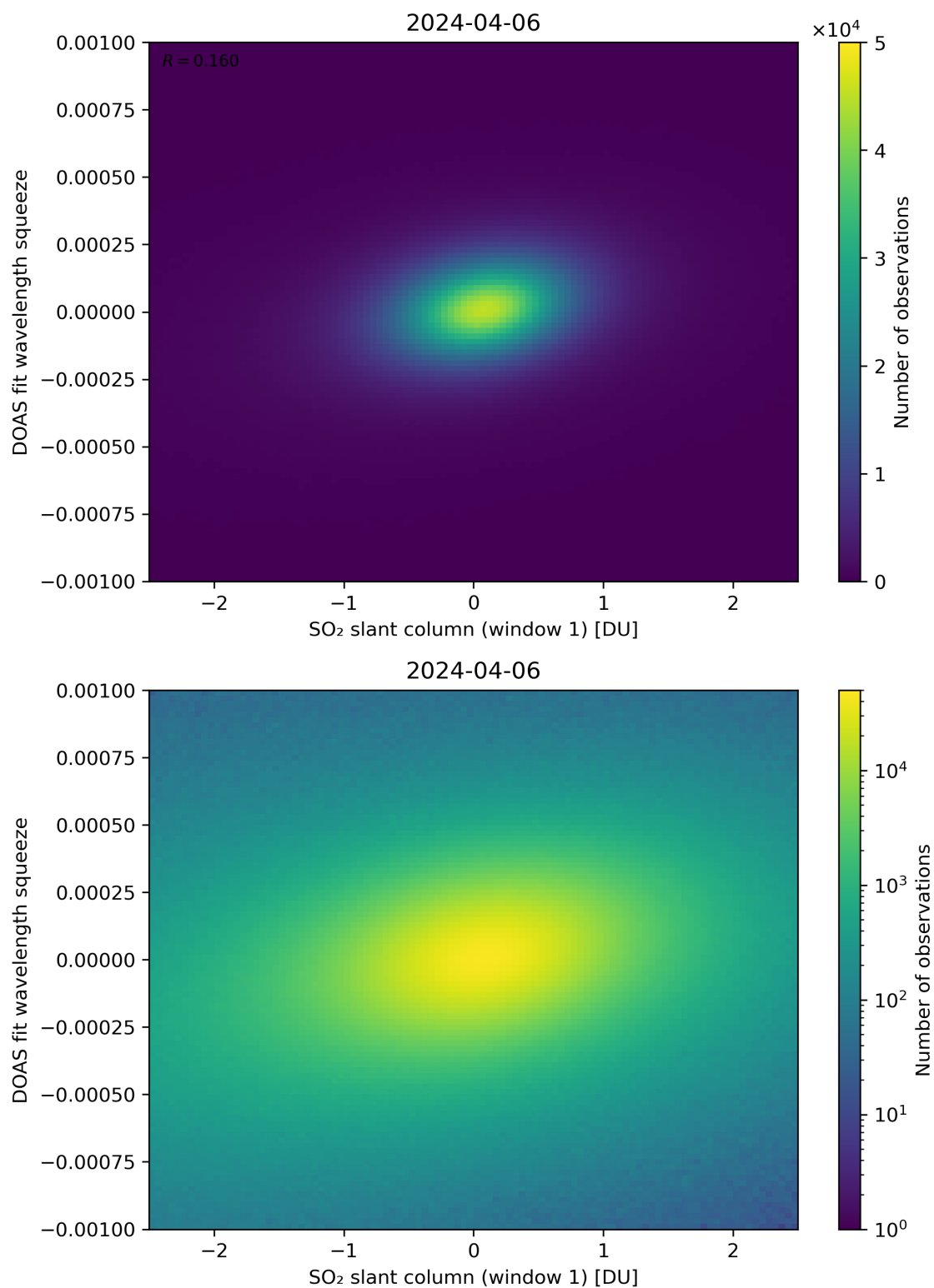
Figure 216: Scatter density plot of “SO 2 slant column (window 1)” against “DOAS fit wavelength squeeze” for 2024-04-05 to 2024-04-07.
