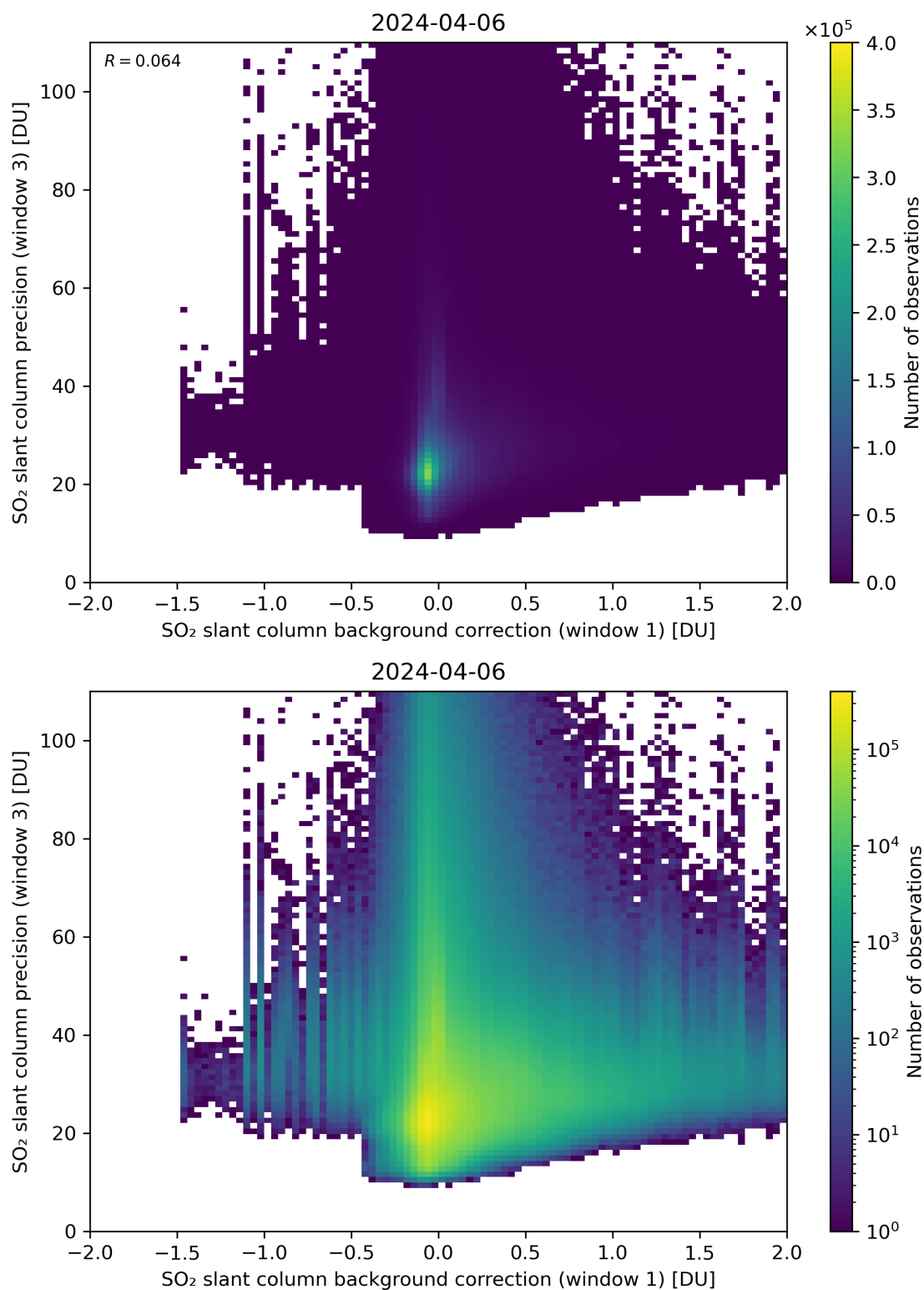
Figure 108: Scatter density plot of “SO 2 slant column background correction (window 1)” against “SO 2 slant column precision (window 3)” for 2024-04-05 to 2024-04-07.
