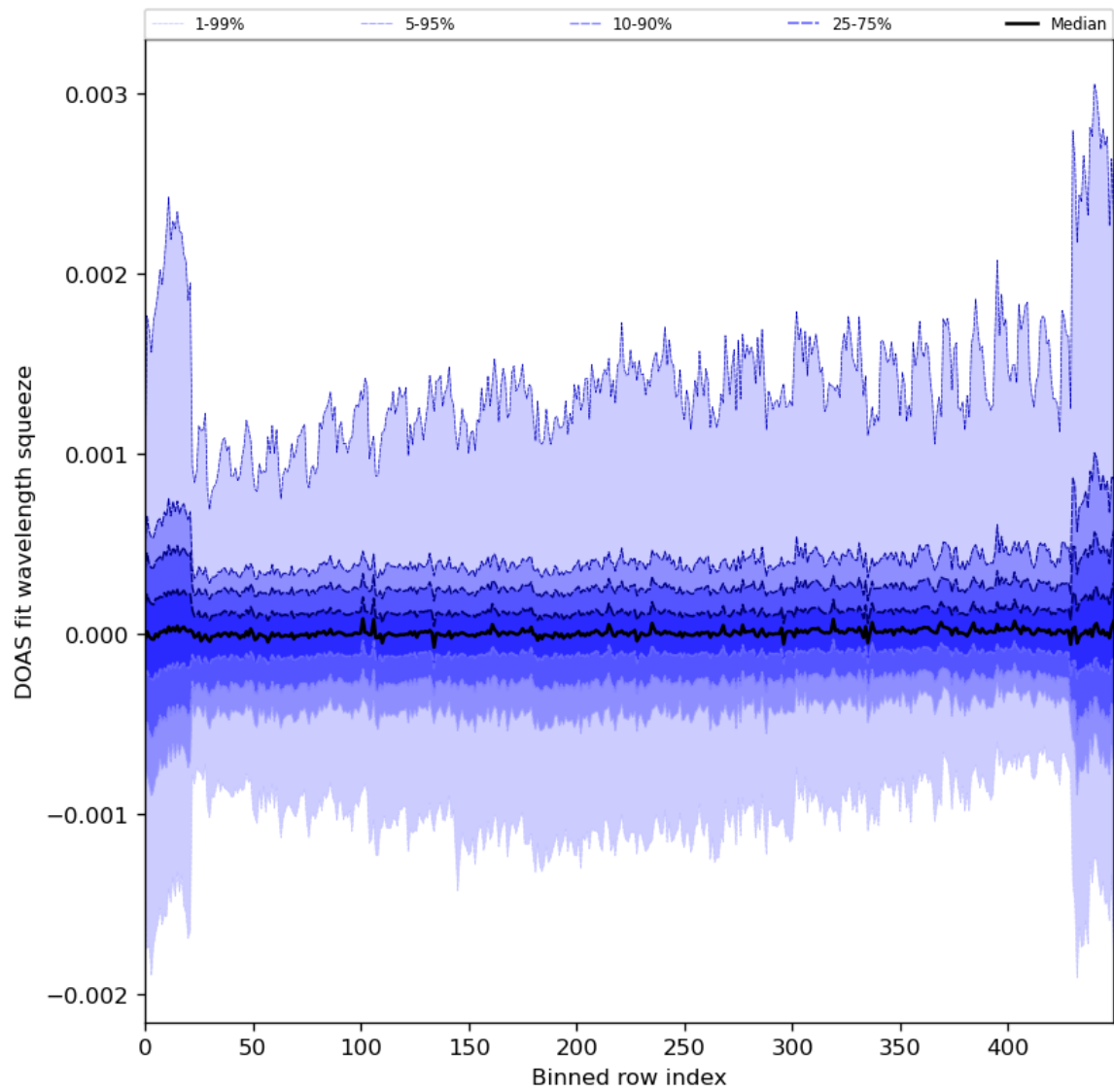
Figure 92: Along track statistics of “DOAS fit wavelength squeeze” for 2024-04-05 to 2024-04-07
