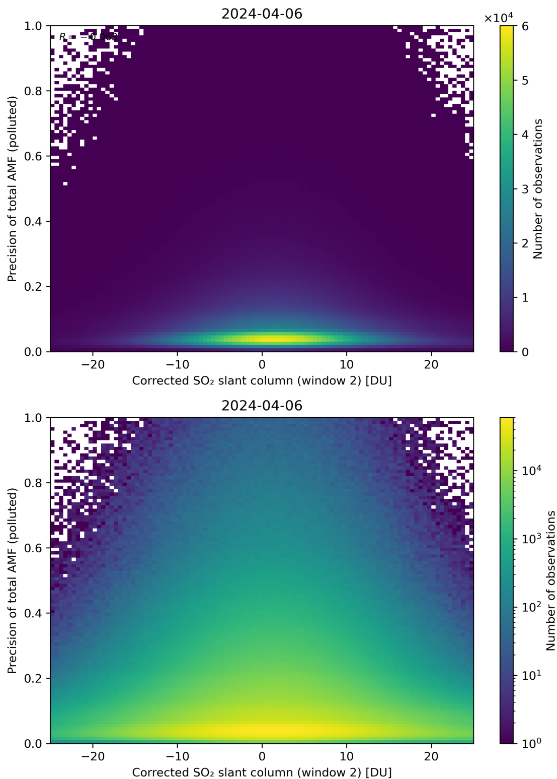
Figure 204: Scatter density plot of “Corrected SO 2 slant column (window 2)” against “Precision of total AMF (polluted)” for 2024-04-05 to 2024-04-07.
