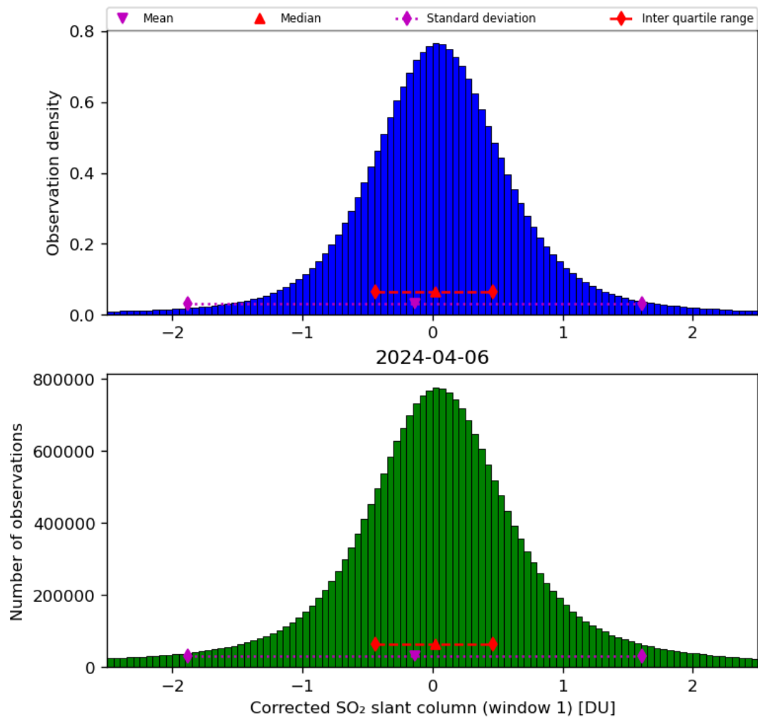
Figure 58: Histogram of “Corrected SO 2 slant column (window 1)” for 2024-04-05 to 2024-04-07
