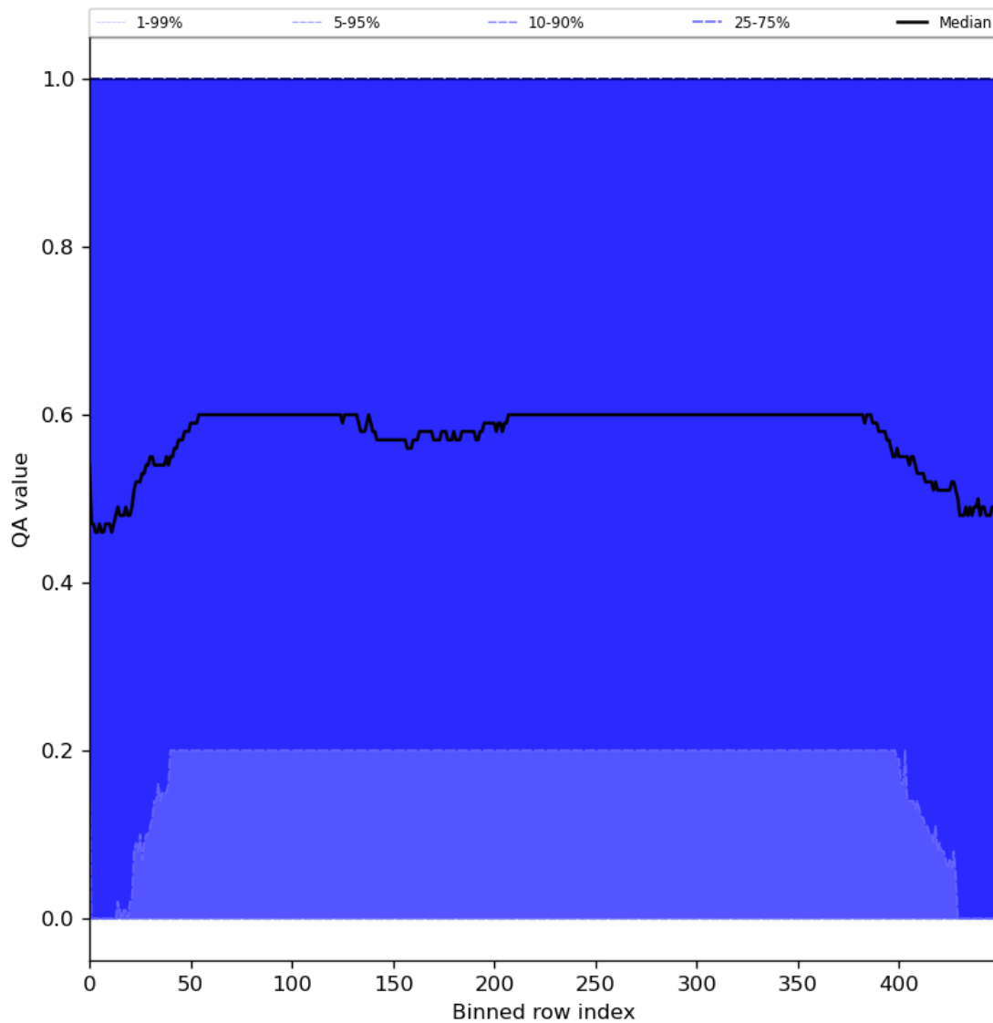
Figure 75: Along track statistics of “QA value” for 2024-04-05 to 2024-04-07
