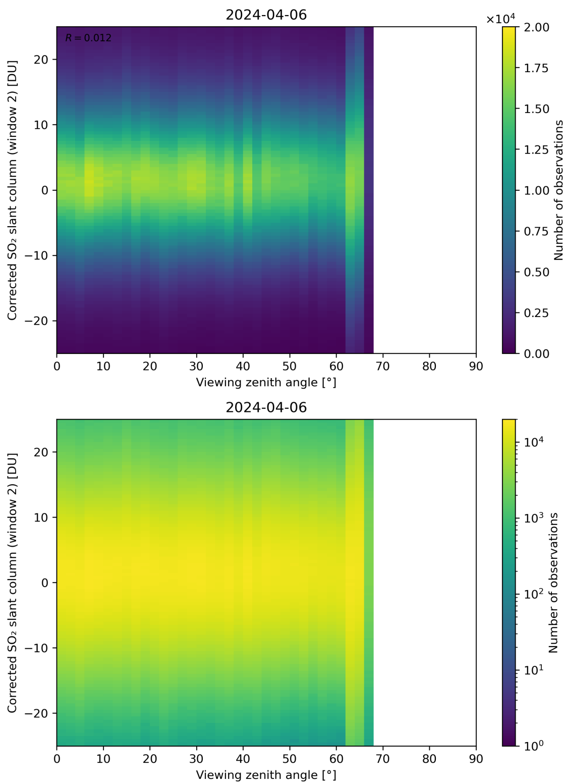
Figure 318: Scatter density plot of “Viewing zenith angle” against “Corrected SO 2 slant column (window 2)” for 2024-04-05 to 2024-04-07.
