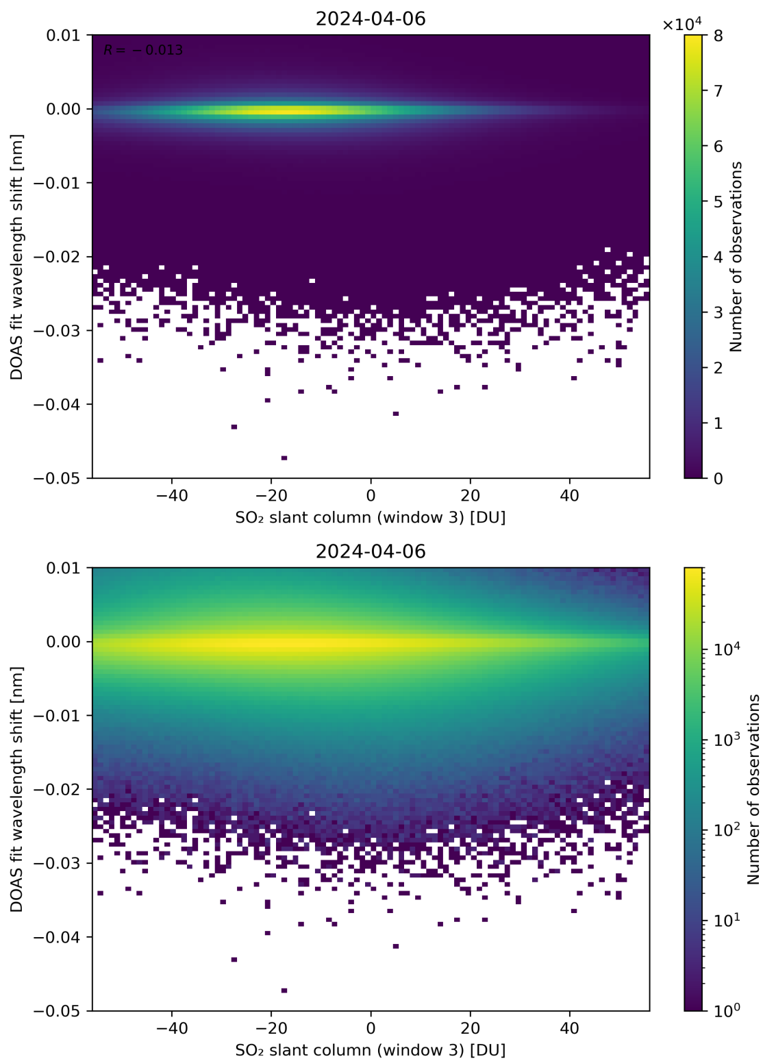
Figure 254: Scatter density plot of “SO 2 slant column (window 3)” against “DOAS fit wavelength shift” for 2024-04-05 to 2024-04-07.
