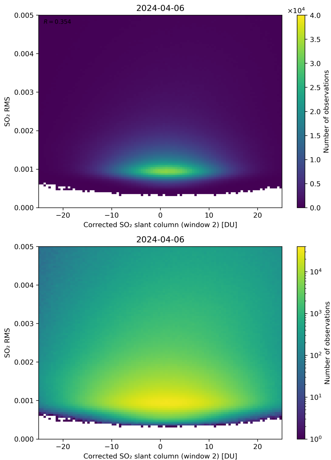
Figure 198: Scatter density plot of “Corrected SO 2 slant column (window 2)” against “SO 2 RMS” for 2024-04-05 to 2024-04-07.
