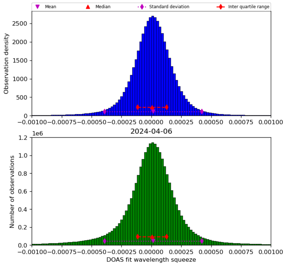
Figure 69: Histogram of “DOAS fit wavelength squeeze” for 2024-04-05 to 2024-04-07
