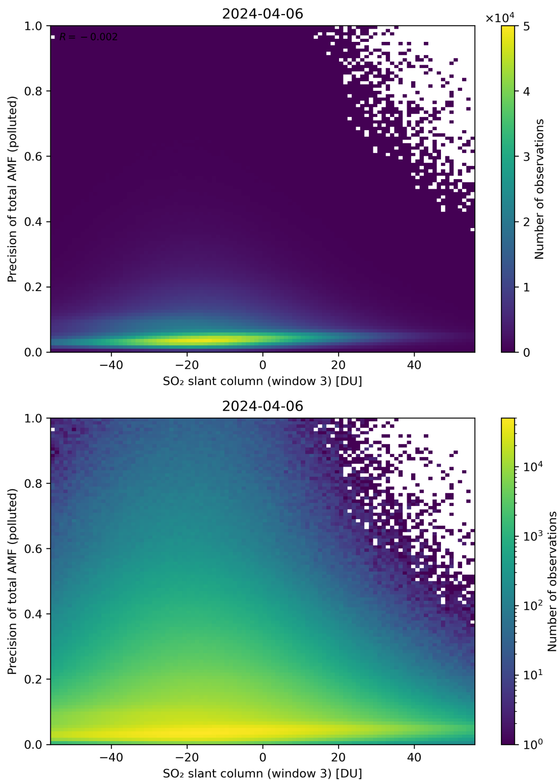
Figure 269: Scatter density plot of “SO 2 slant column (window 3)” against “Precision of total AMF (polluted)” for 2024-04-05 to 2024-04-07.
