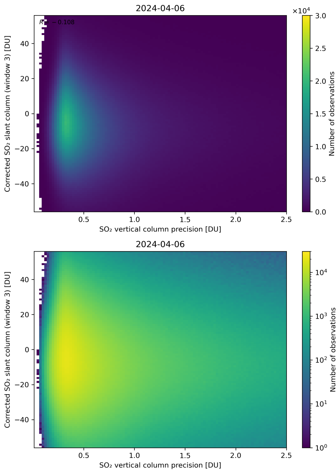
Figure 288: Scatter density plot of “SO 2 vertical column precision” against “Corrected SO 2 slant column (window 3)” for 2024-04-05 to 2024-04-07.
