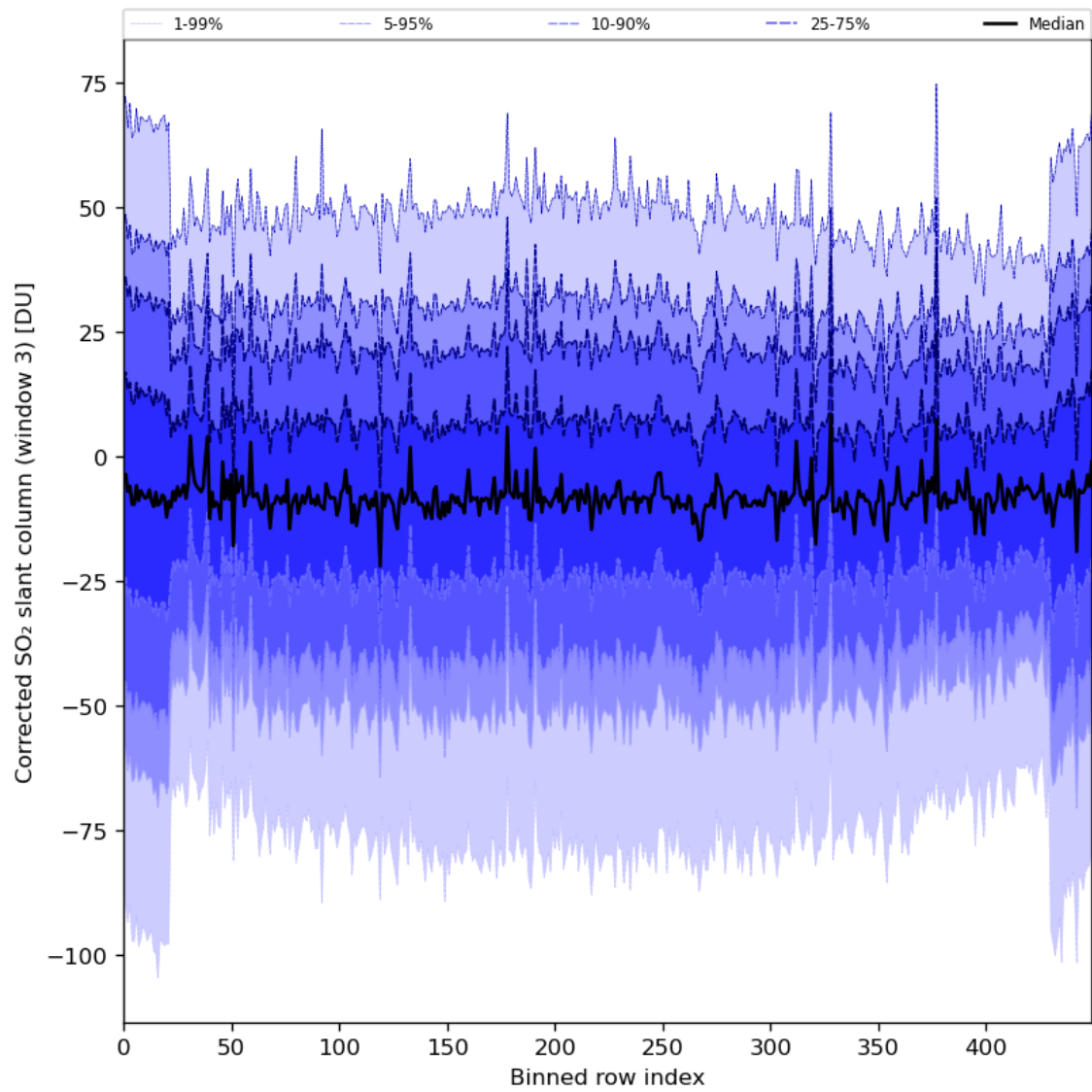
Figure 89: Along track statistics of “Corrected SO 2 slant column (window 3)” for 2024-04-05 to 2024-04-07
