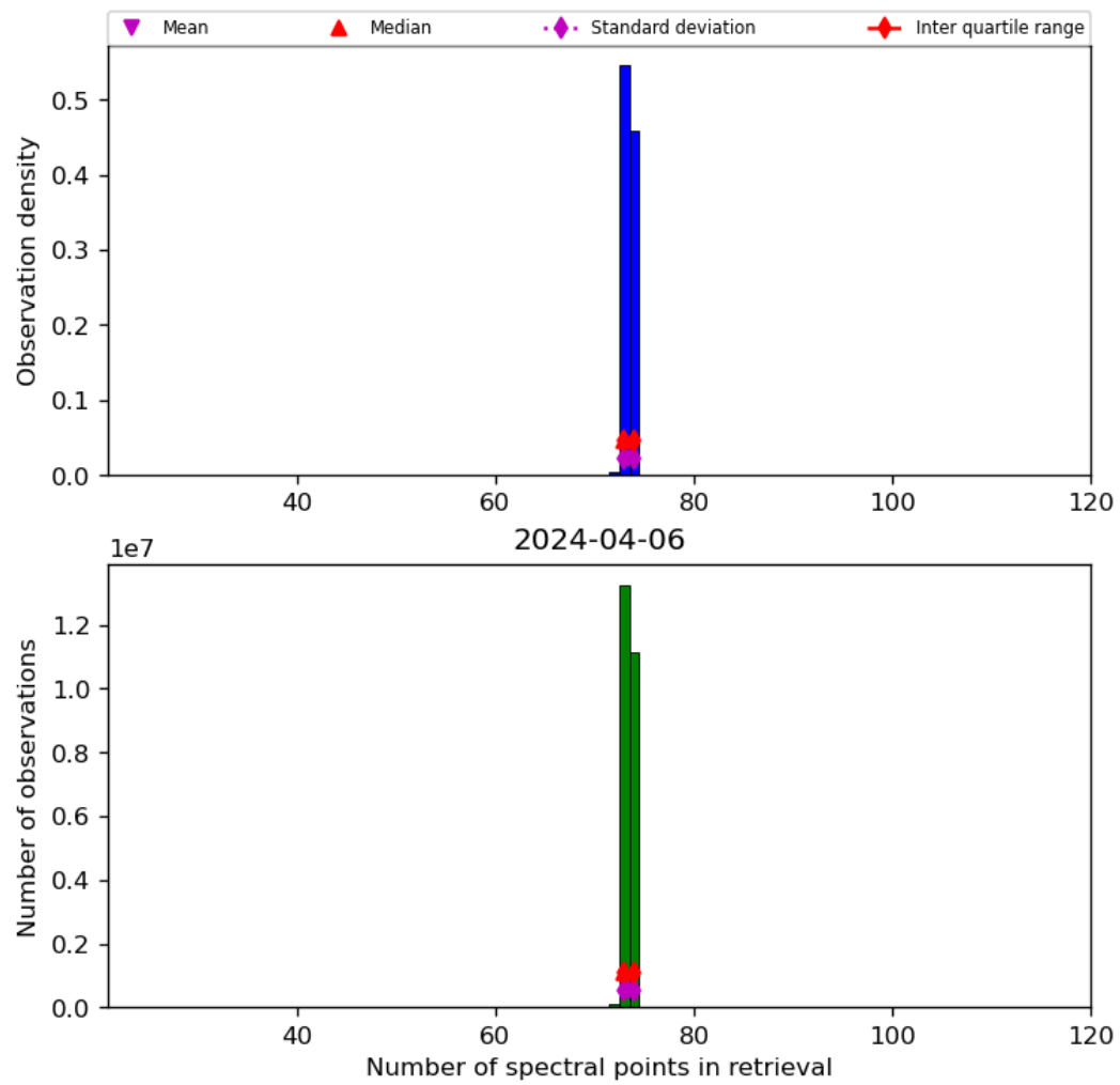
Figure 74: Histogram of “Number of spectral points in retrieval” for 2024-04-05 to 2024-04-07
