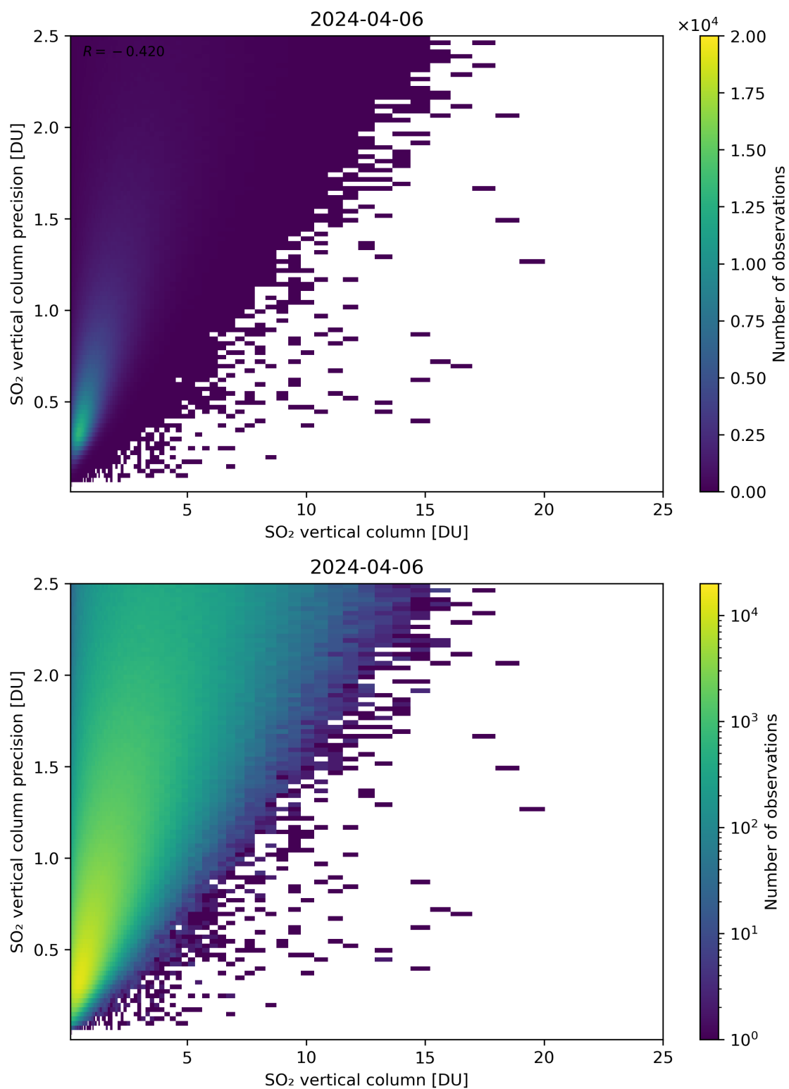
Figure 307: Scatter density plot of “SO 2 vertical column” against “SO 2 vertical column precision” for 2024-04-05 to 2024-04-07.
