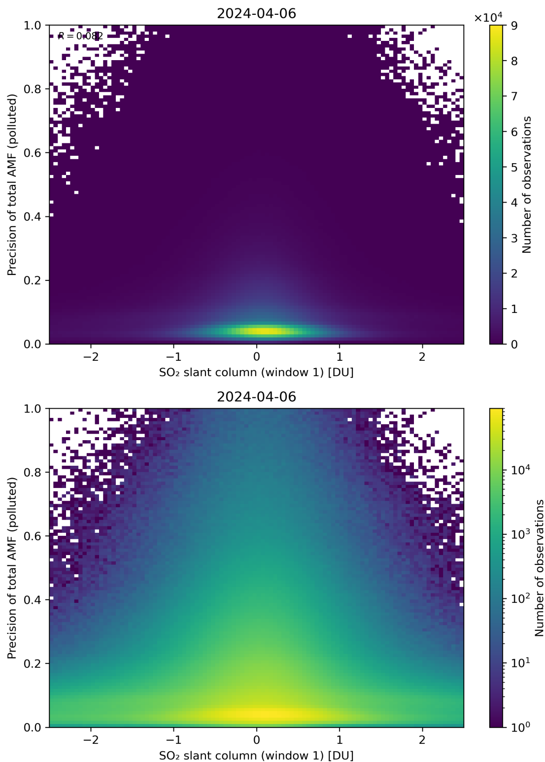
Figure 240: Scatter density plot of “SO 2 slant column (window 1)” against “Precision of total AMF (polluted)” for 2024-04-05 to 2024-04-07.
