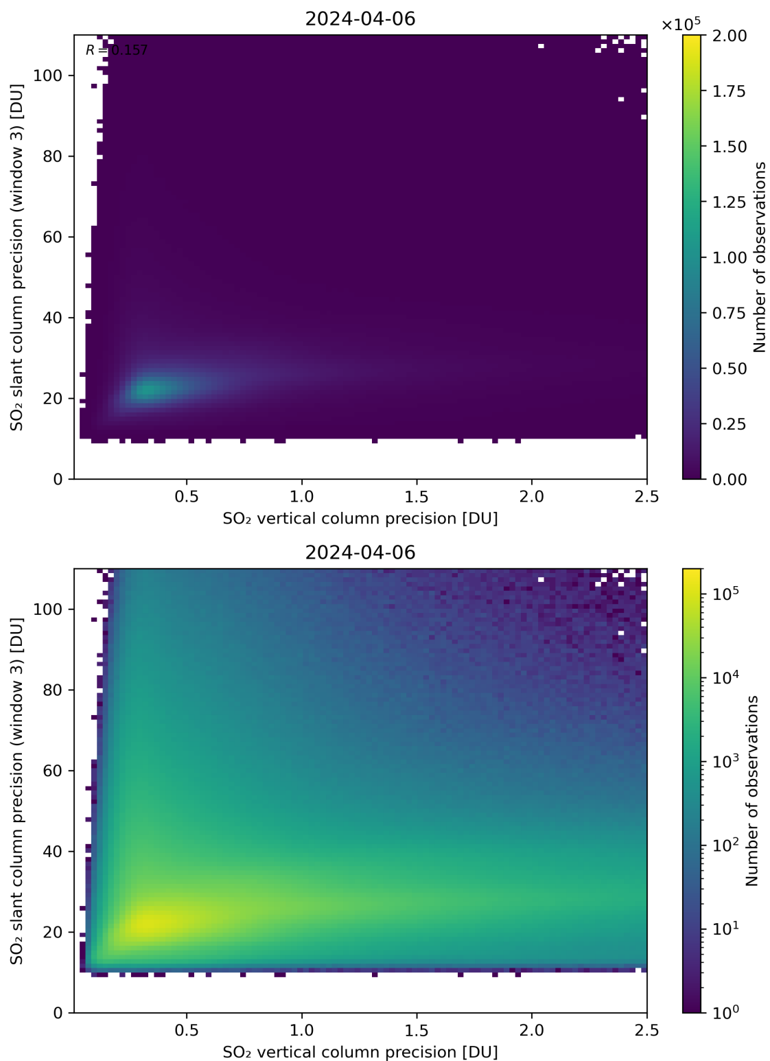
Figure 293: Scatter density plot of “SO 2 vertical column precision” against “SO 2 slant column precision (window 3)” for 2024-04-05 to 2024-04-07.
