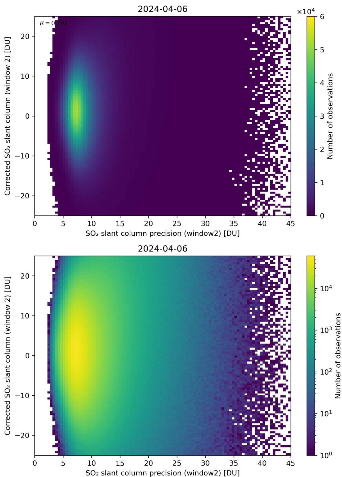
Figure 247: Scatter density plot of “SO 2 slant column precision (window2)” against “Corrected SO 2 slant column (window 2)” for 2024-04-05 to 2024-04-07.
