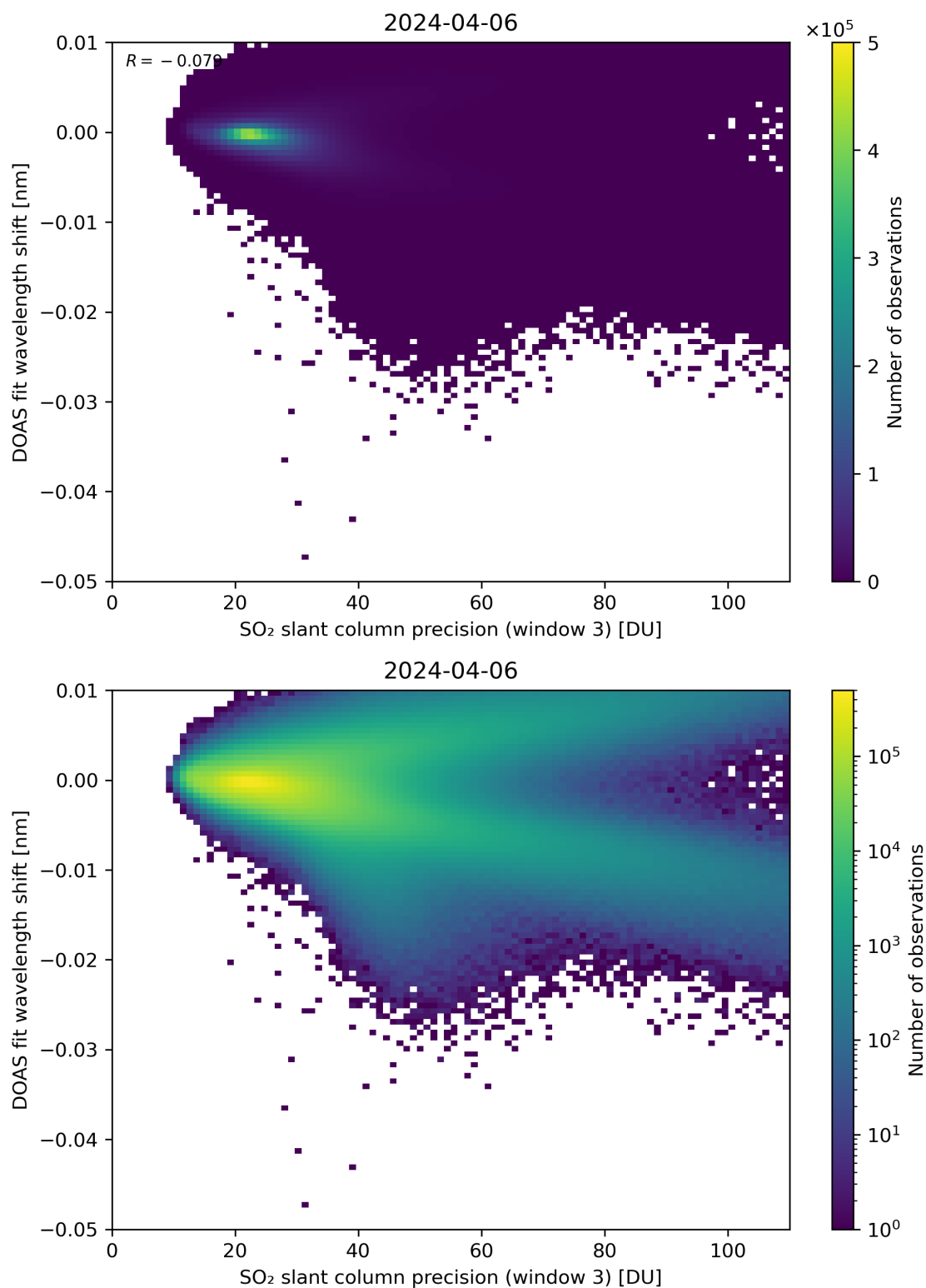
Figure 258: Scatter density plot of “SO 2 slant column precision (window 3)” against “DOAS fit wavelength shift” for 2024-04-05 to 2024-04-07.
