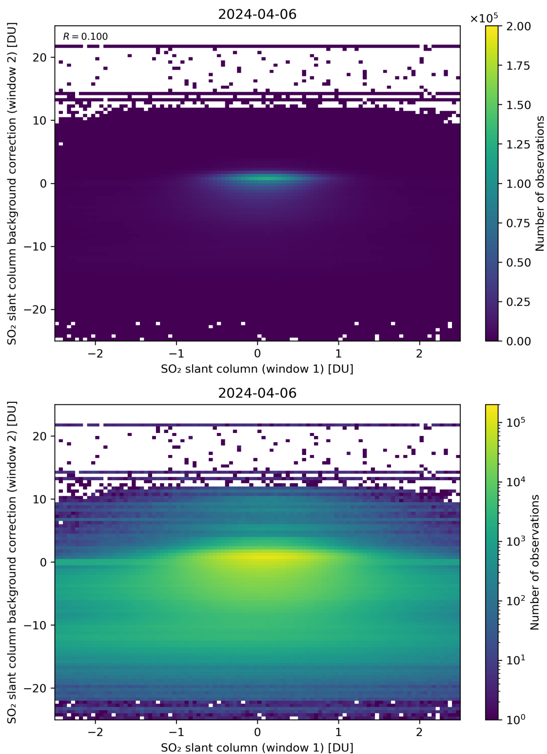
Figure 213: Scatter density plot of “SO 2 slant column (window 1)” against “SO 2 slant column background correction (window 2)” for 2024-04-05 to 2024-04-07.
