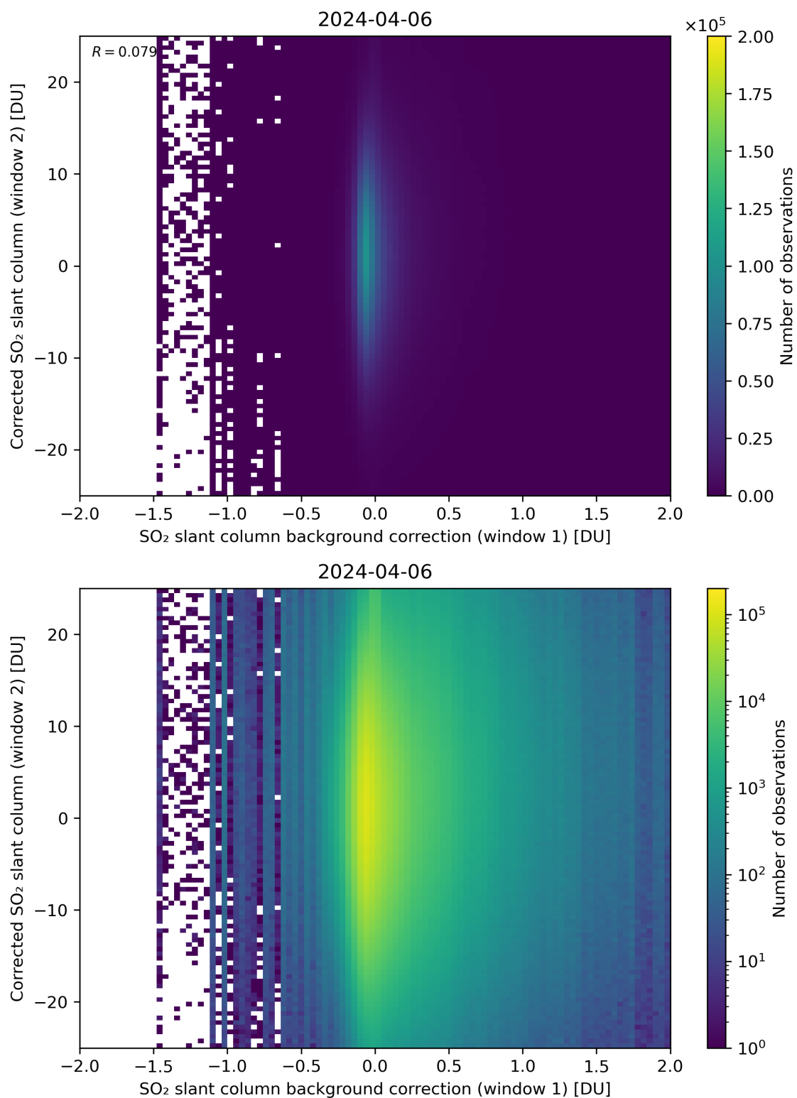
Figure 104: Scatter density plot of “SO 2 slant column background correction (window 1)” against “Corrected SO 2 slant column (window 2)” for 2024-04-05 to 2024-04-07.
