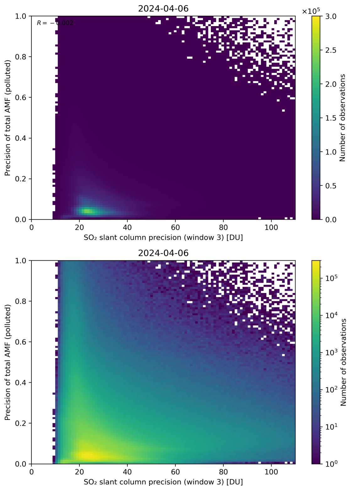
Figure 264: Scatter density plot of “SO 2 slant column precision (window 3)” against “Precision of total AMF (polluted)” for 2024-04-05 to 2024-04-07.
