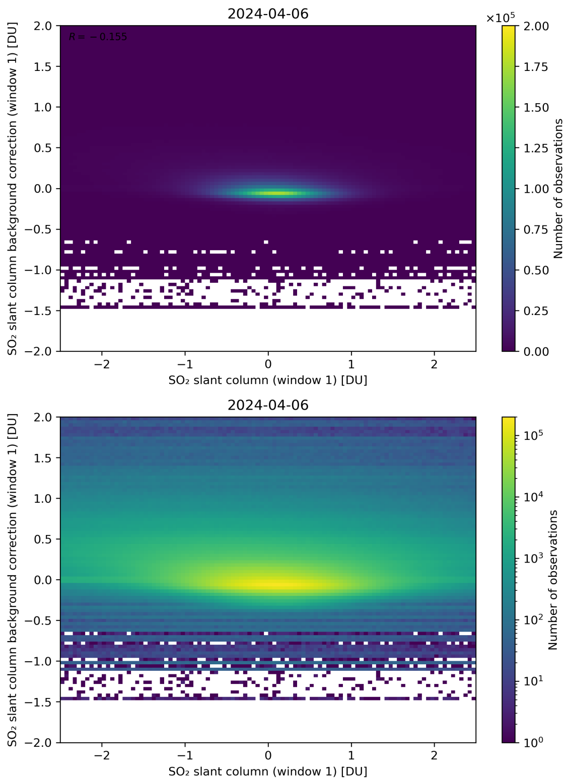
Figure 212: Scatter density plot of “SO 2 slant column (window 1)” against “SO 2 slant column background correction (window 1)” for 2024-04-05 to 2024-04-07.
