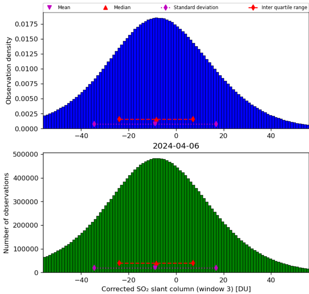
Figure 66: Histogram of “Corrected SO 2 slant column (window 3)” for 2024-04-05 to 2024-04-07
