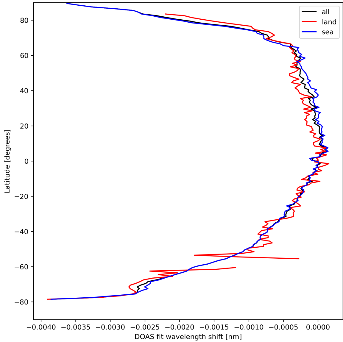
Figure 45: Zonal average of “DOAS fit wavelength shift” for 2024-04-05 to 2024-04-07.
