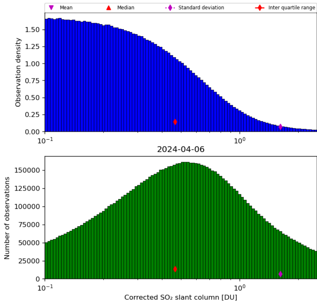
Figure 55: Histogram of “Corrected SO 2 slant column” for 2024-04-05 to 2024-04-07
