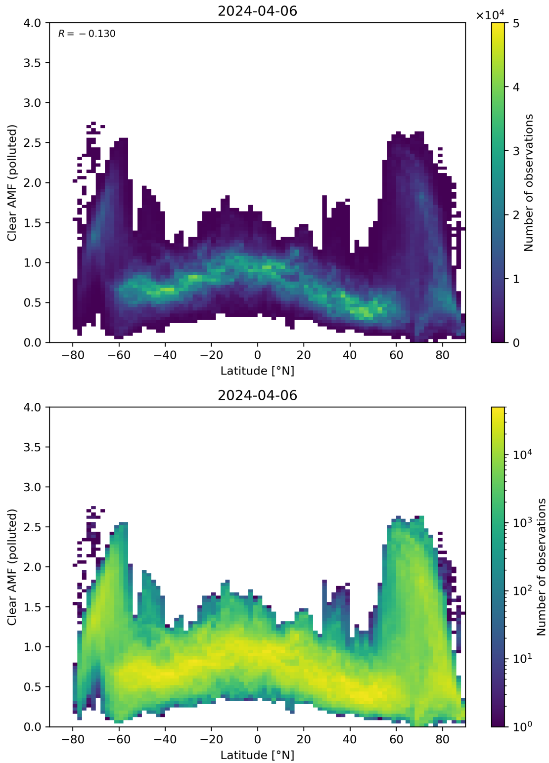
Figure 145: Scatter density plot of “Latitude” against “Clear AMF (polluted)” for 2024-04-05 to 2024-04-07.
