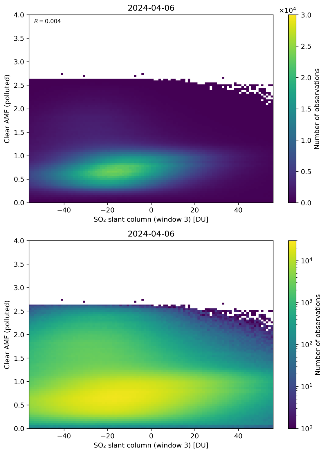
Figure 265: Scatter density plot of “SO 2 slant column (window 3)” against “Clear AMF (polluted)” for 2024-04-05 to 2024-04-07.
