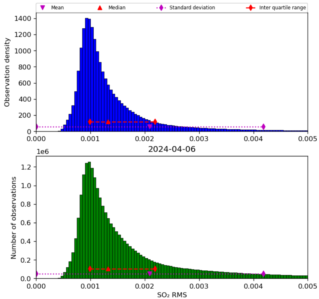
Figure 70: Histogram of “SO 2 RMS” for 2024-04-05 to 2024-04-07
