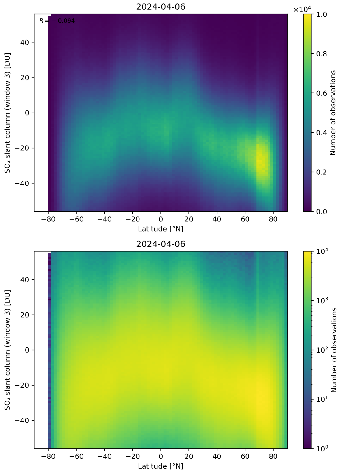
Figure 152: Scatter density plot of “Latitude” against “SO 2 slant column (window 3)” for 2024-04-05 to 2024-04-07.
