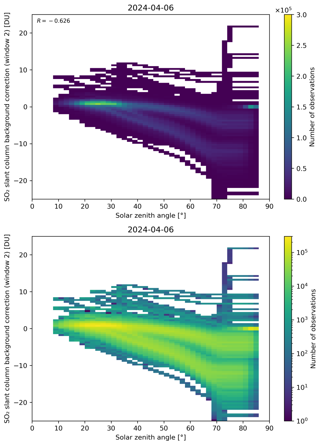
Figure 159: Scatter density plot of “Solar zenith angle” against “SO 2 slant column background correction (window 2)” for 2024-04-05 to 2024-04-07.
