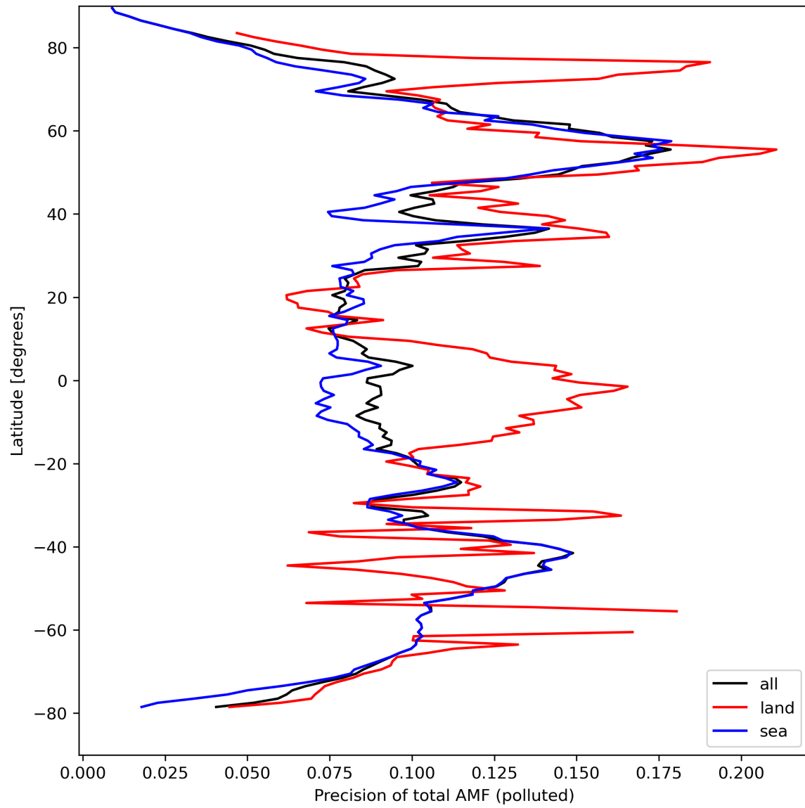
Figure 49: Zonal average of “Precision of total AMF (polluted)” for 2024-04-05 to 2024-04-07.
