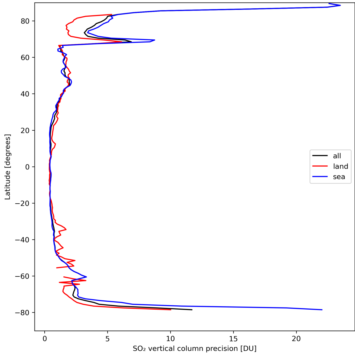
Figure 31: Zonal average of “SO 2 vertical column precision” for 2024-04-05 to 2024-04-07.
