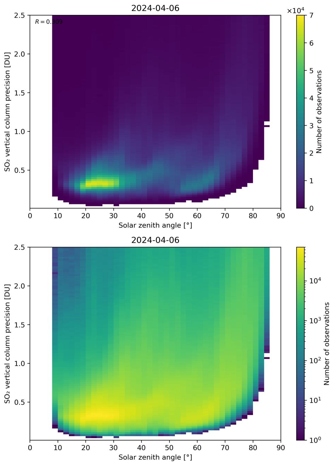
Figure 177: Scatter density plot of “Solar zenith angle” against “SO 2 vertical column precision” for 2024-04-05 to 2024-04-07.
