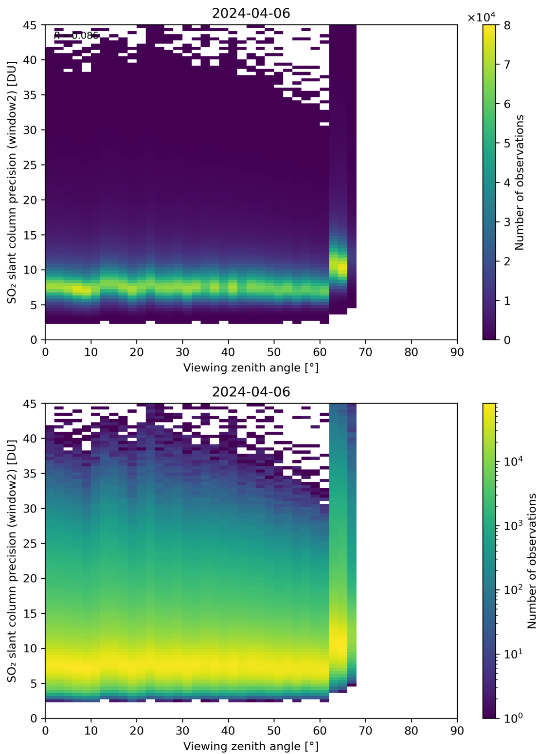
Figure 322: Scatter density plot of “Viewing zenith angle” against “SO 2 slant column precision (window2)” for 2024-04-05 to 2024-04-07.
