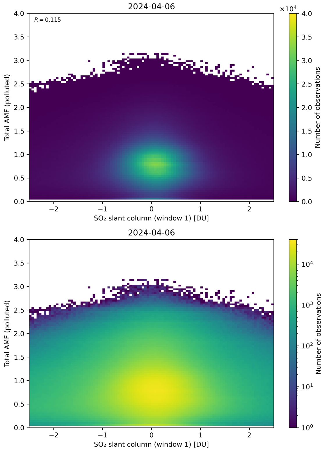
Figure 239: Scatter density plot of “SO 2 slant column (window 1)” against “Total AMF (polluted)” for 2024-04-05 to 2024-04-07.
