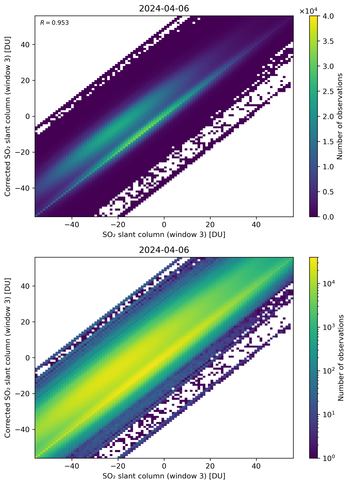
Figure 266: Scatter density plot of “SO 2 slant column (window 3)” against “Corrected SO 2 slant column (window 3)” for 2024-04-05 to 2024-04-07.
