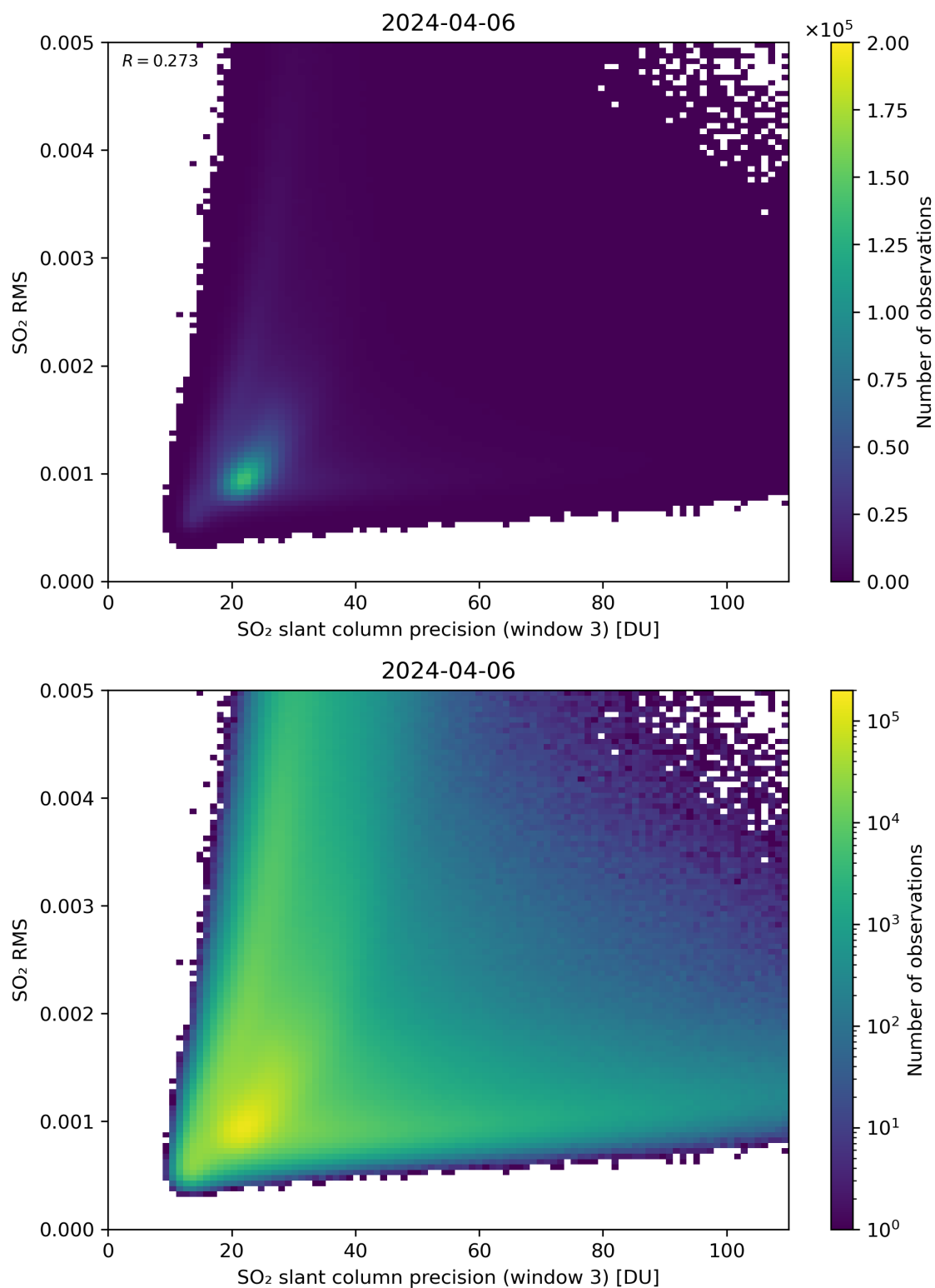
Figure 260: Scatter density plot of “SO 2 slant column precision (window 3)” against “SO 2 RMS” for 2024-04-05 to 2024-04-07.
