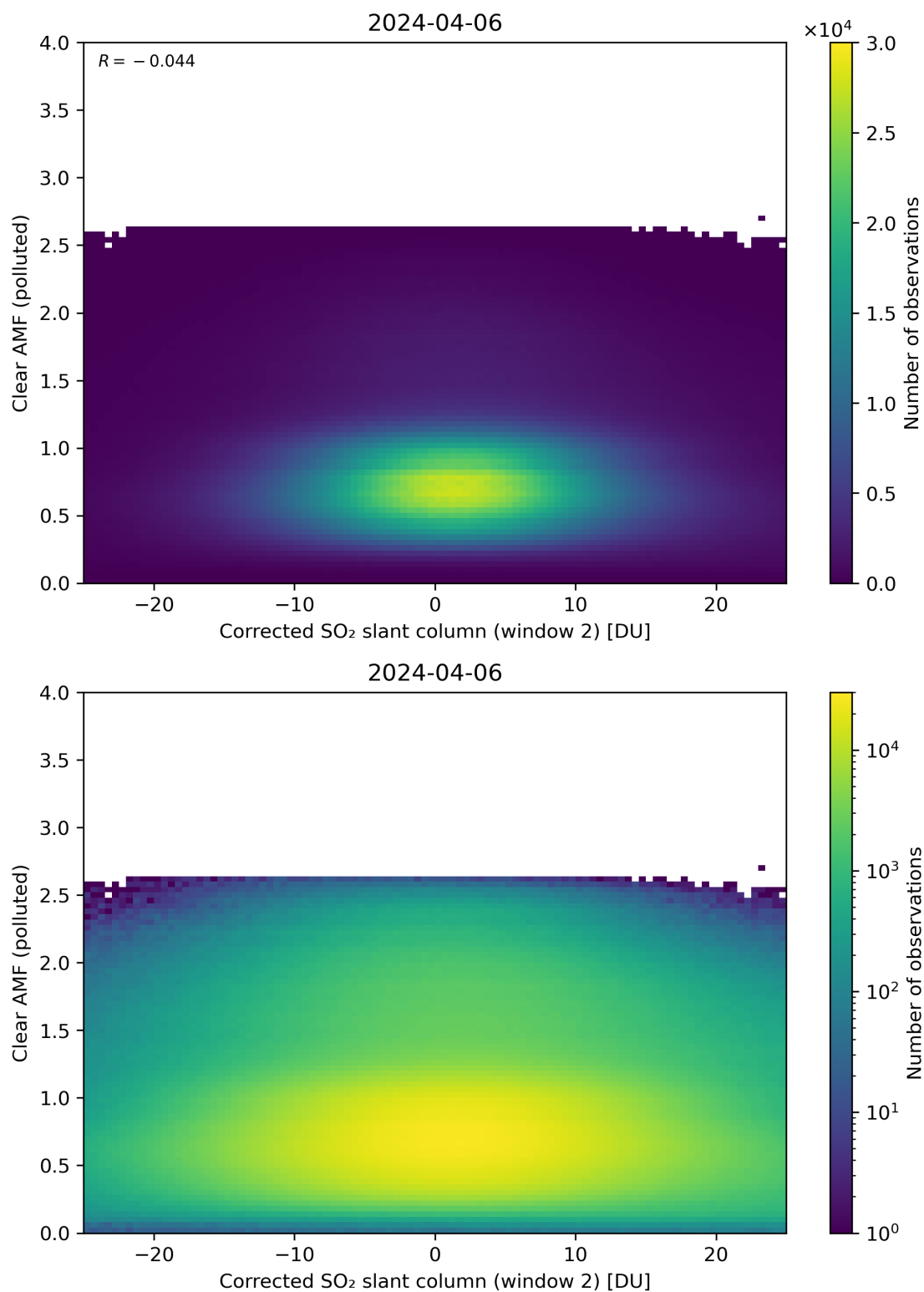
Figure 199: Scatter density plot of “Corrected SO 2 slant column (window 2)” against “Clear AMF (polluted)” for 2024-04-05 to 2024-04-07.
