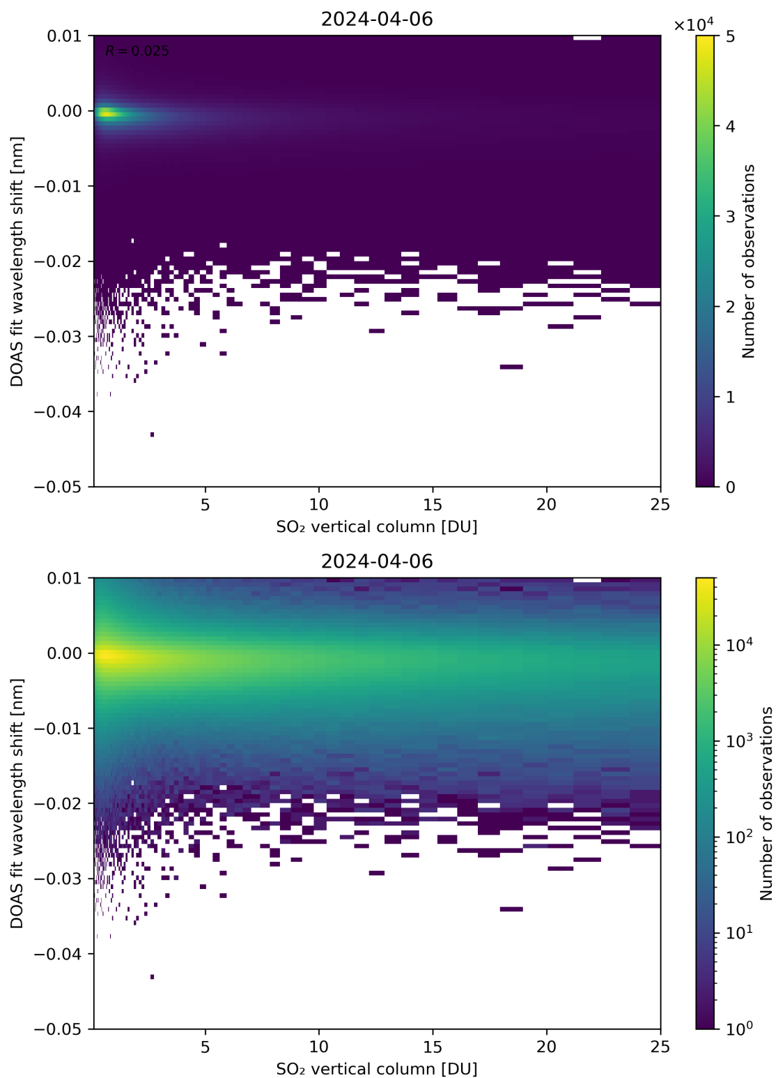
Figure 276: Scatter density plot of “SO 2 vertical column” against “DOAS fit wavelength shift” for 2024-04-05 to 2024-04-07.
