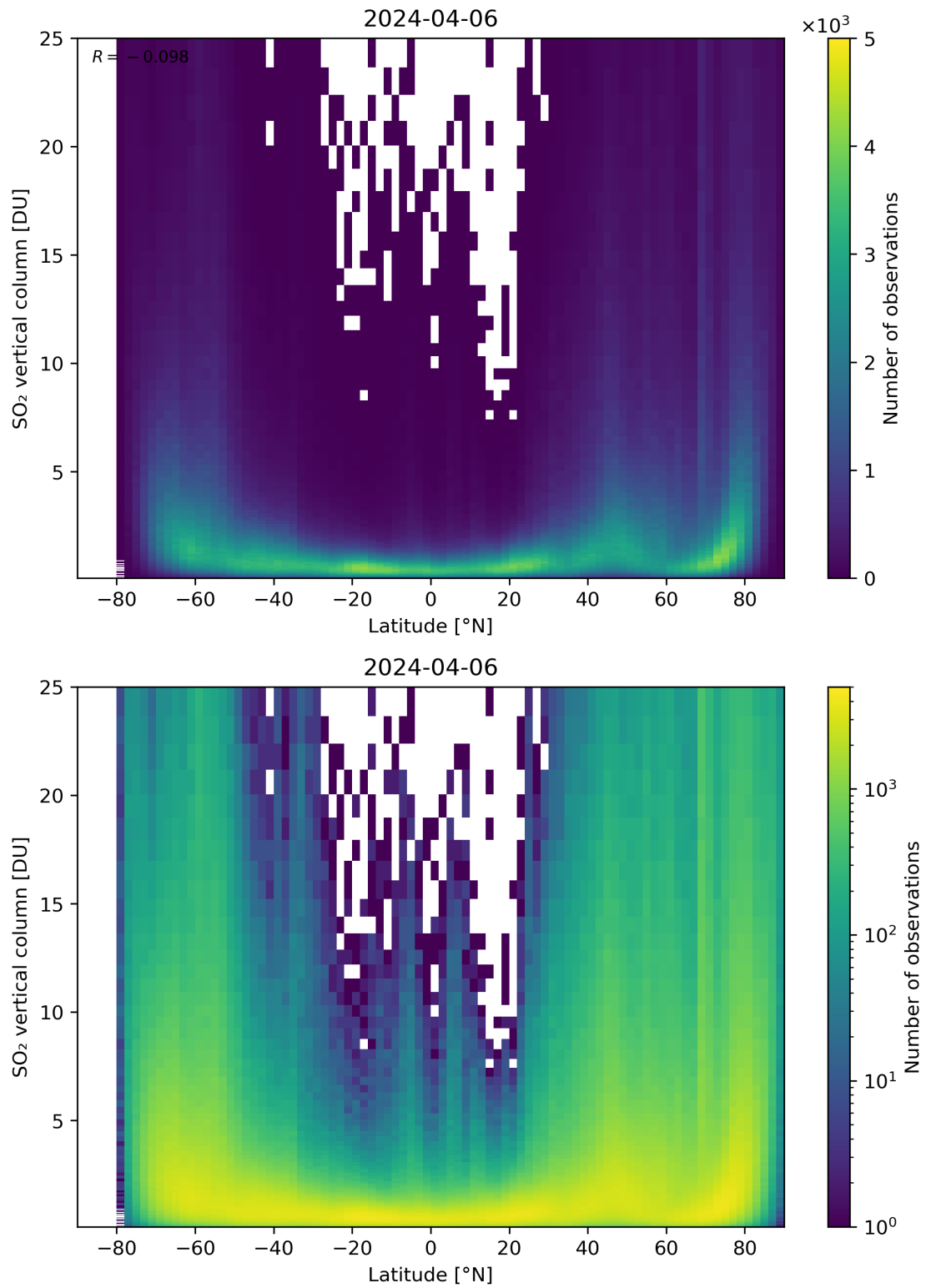
Figure 156: Scatter density plot of “Latitude” against “SO 2 vertical column” for 2024-04-05 to 2024-04-07.
