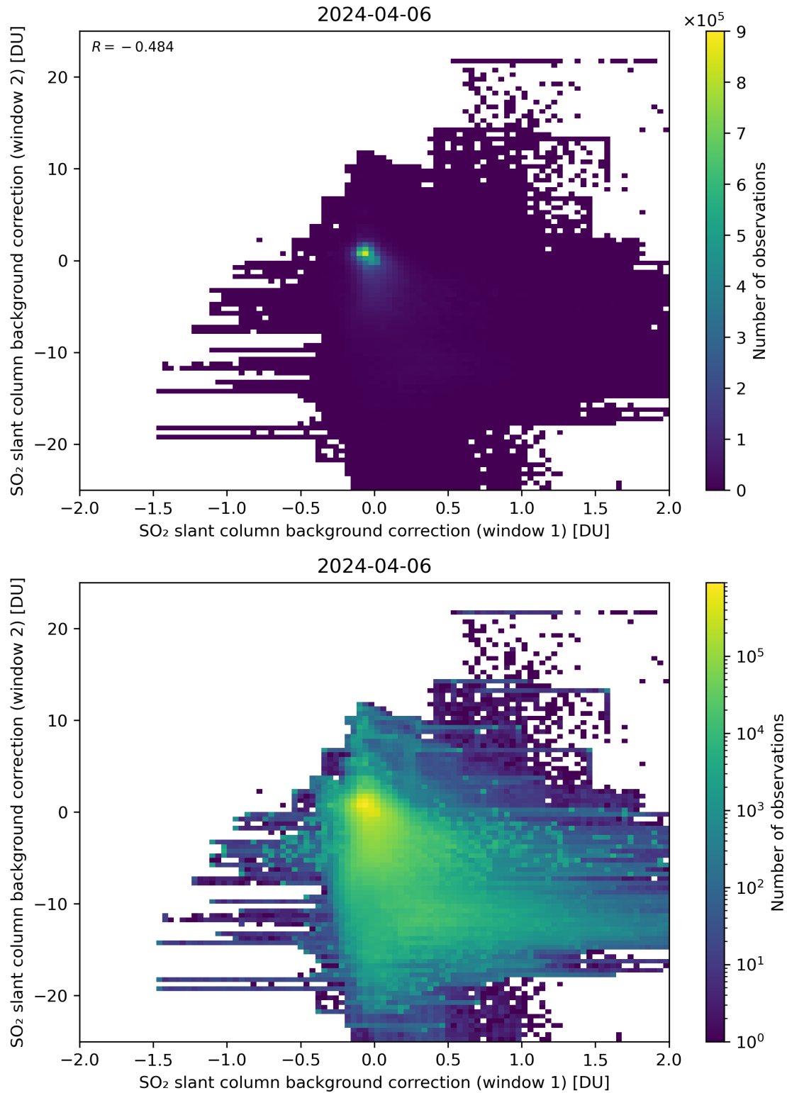
Figure 98: Scatter density plot of “SO 2 slant column background correction (window 1)” against “SO 2 slant column background correction (window 2)” for 2024-04-05 to 2024-04-07.
