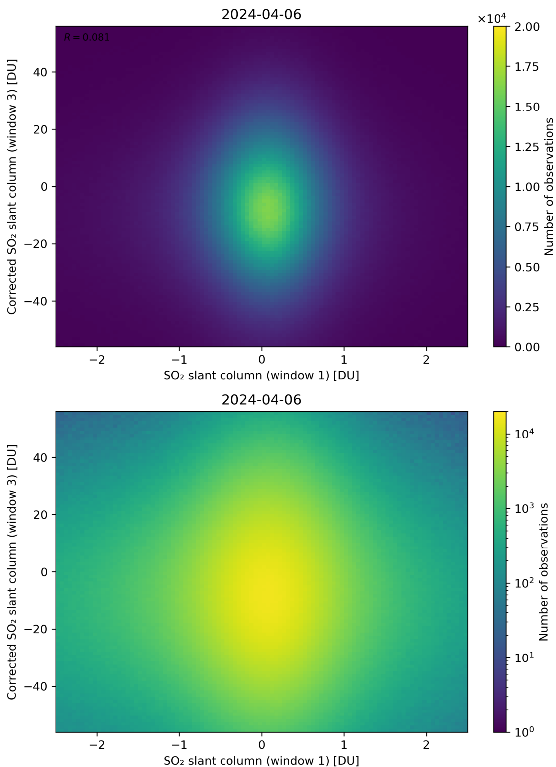
Figure 234: Scatter density plot of “SO 2 slant column (window 1)” against “Corrected SO 2 slant column (window 3)” for 2024-04-05 to 2024-04-07.
