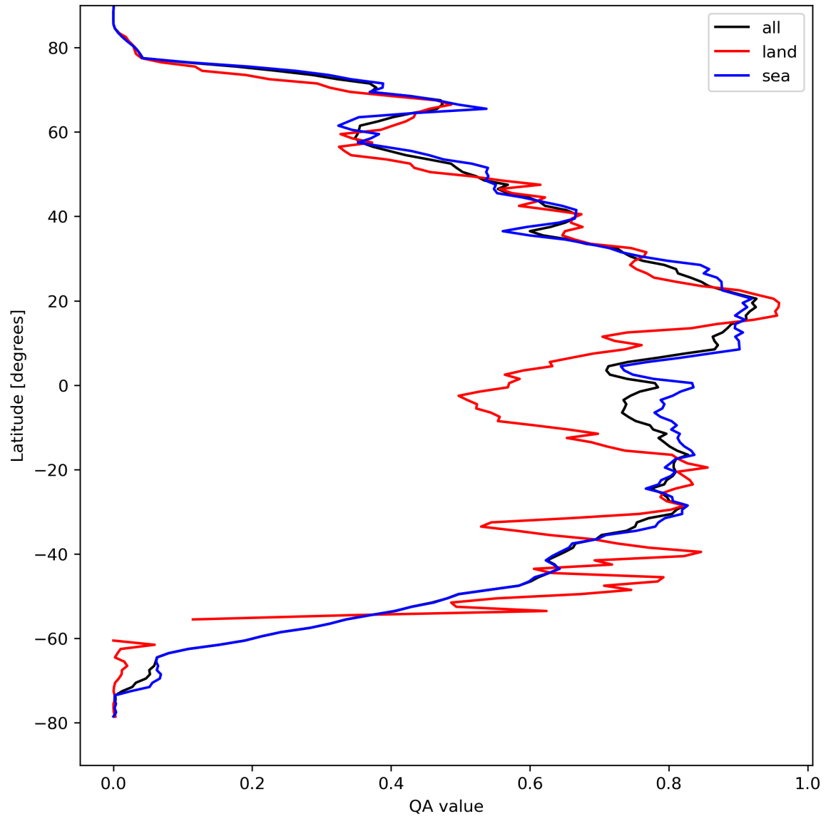
Figure 29: Zonal average of “QA value” for 2024-04-05 to 2024-04-07.
