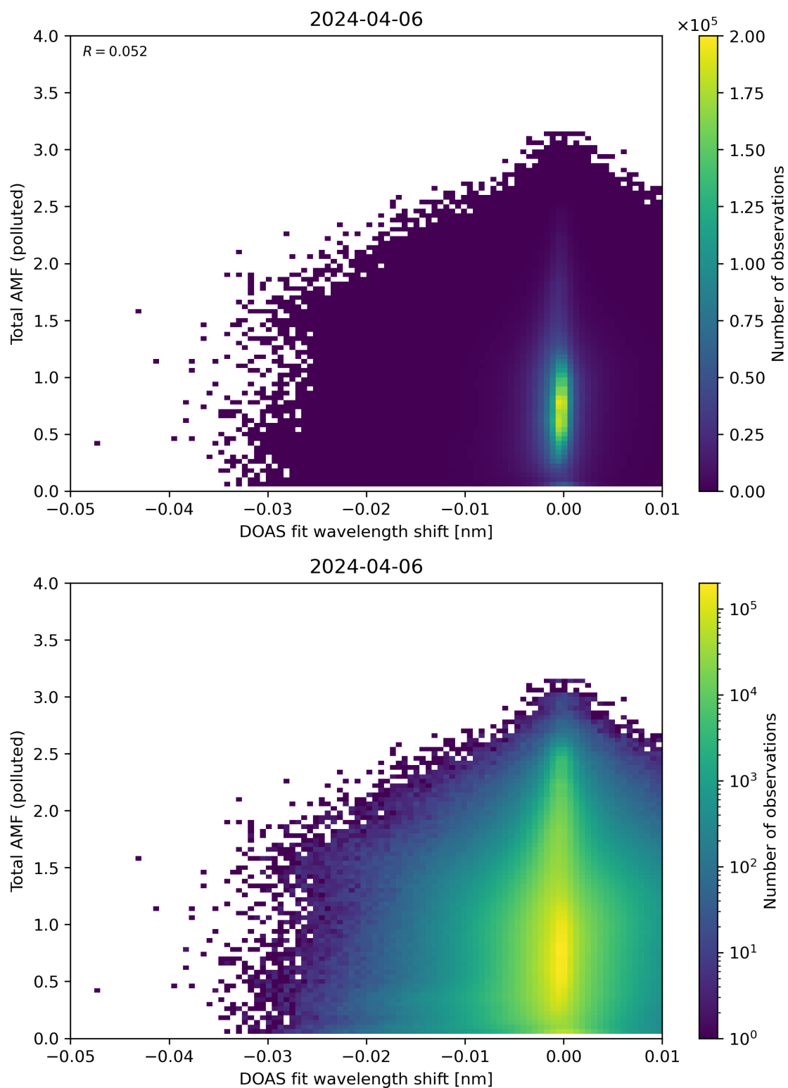
Figure 130: Scatter density plot of “DOAS fit wavelength shift” against “Total AMF (polluted)” for 2024-04-05 to 2024-04-07.
