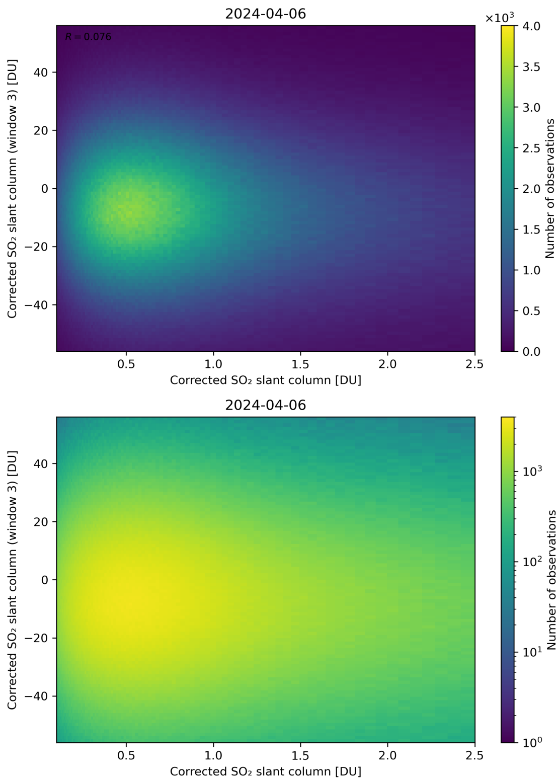
Figure 186: Scatter density plot of “Corrected SO 2 slant column” against “Corrected SO 2 slant column (window 3)” for 2024-04-05 to 2024-04-07.
