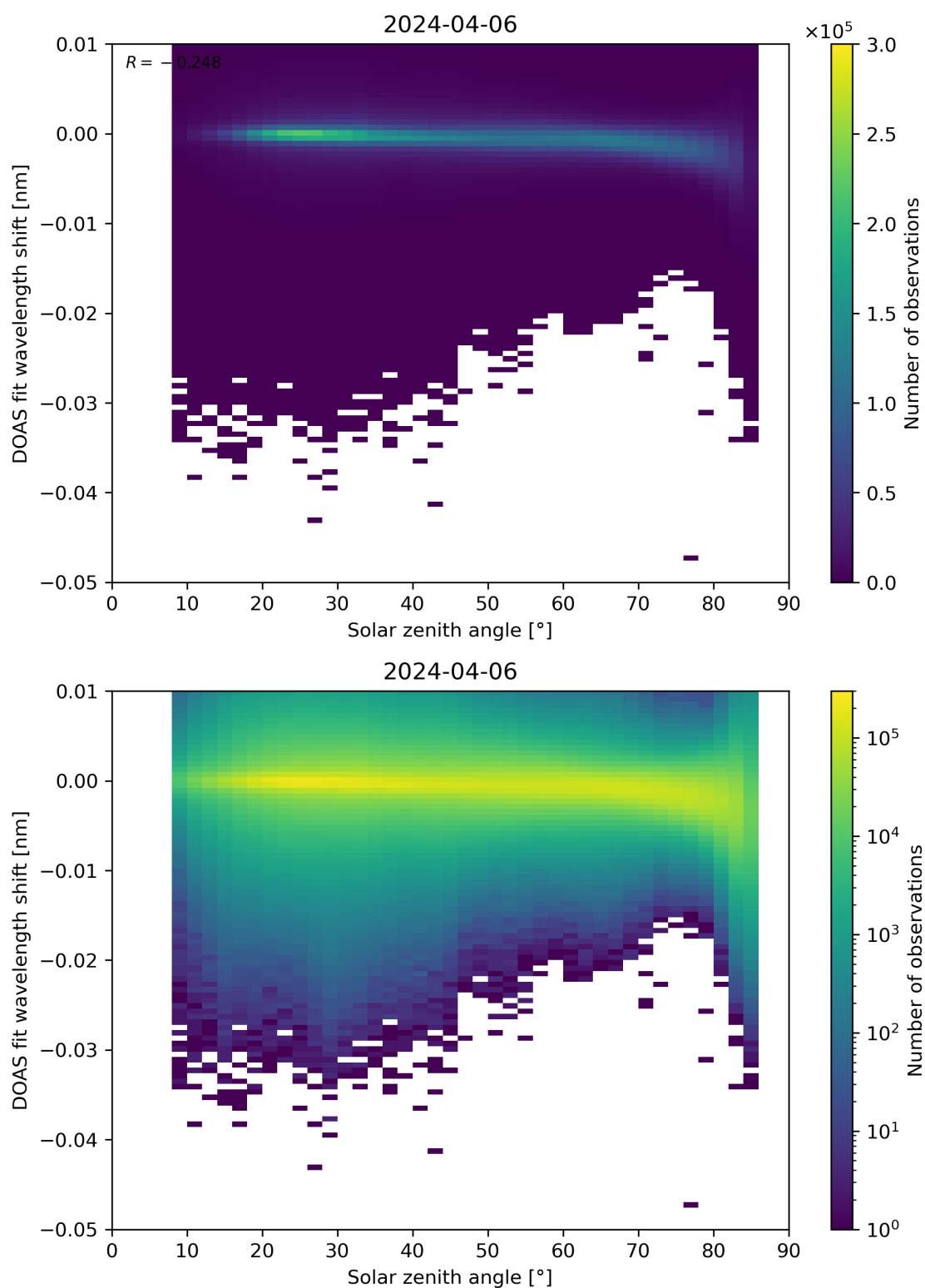
Figure 161: Scatter density plot of “Solar zenith angle” against “DOAS fit wavelength shift” for 2024-04-05 to 2024-04-07.
