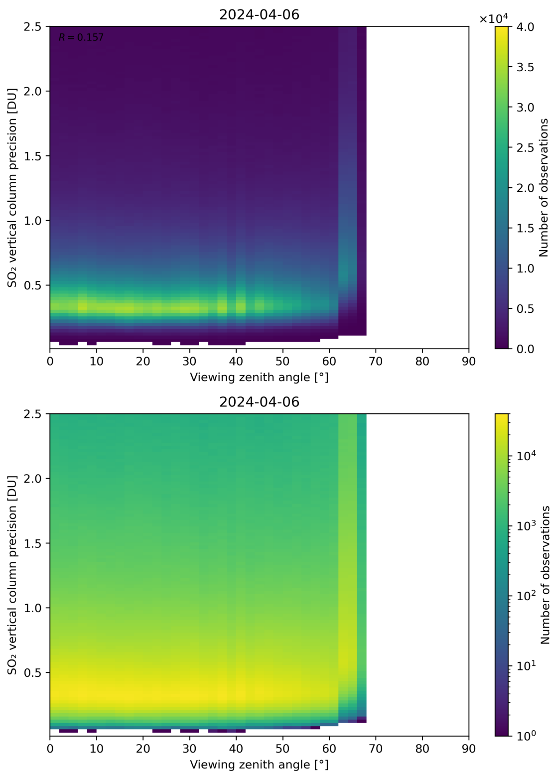
Figure 328: Scatter density plot of “Viewing zenith angle” against “SO 2 vertical column precision” for 2024-04-05 to 2024-04-07.
