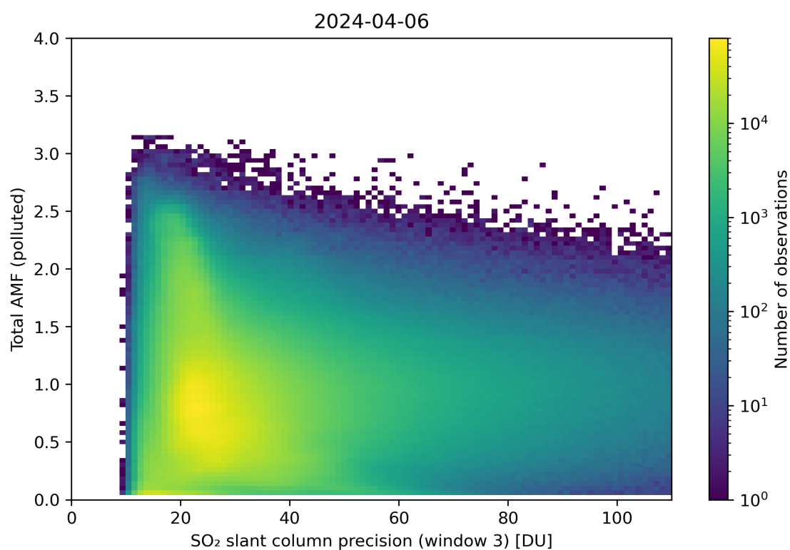
Figure 263: Scatter density plot of “SO 2 slant column precision (window 3)” against “Total AMF (polluted)” for 2024-04-05 to 2024-04-07.
