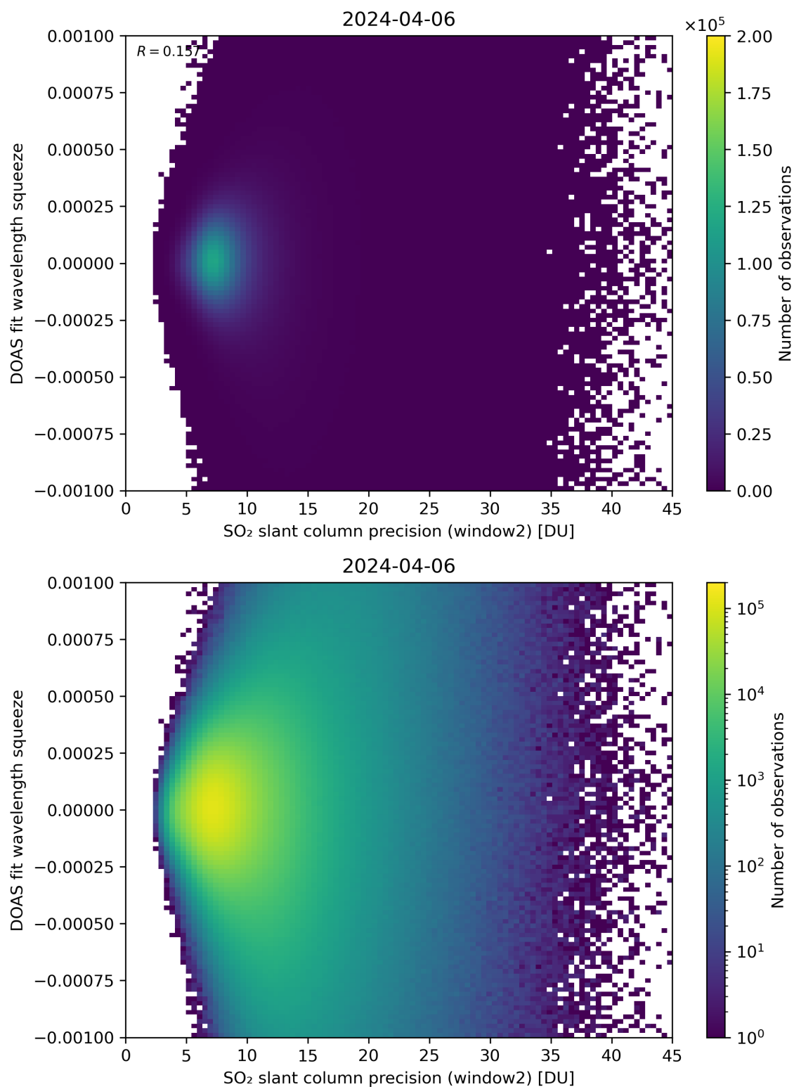
Figure 244: Scatter density plot of “SO 2 slant column precision (window2)” against “DOAS fit wavelength squeeze” for 2024-04-05 to 2024-04-07.
