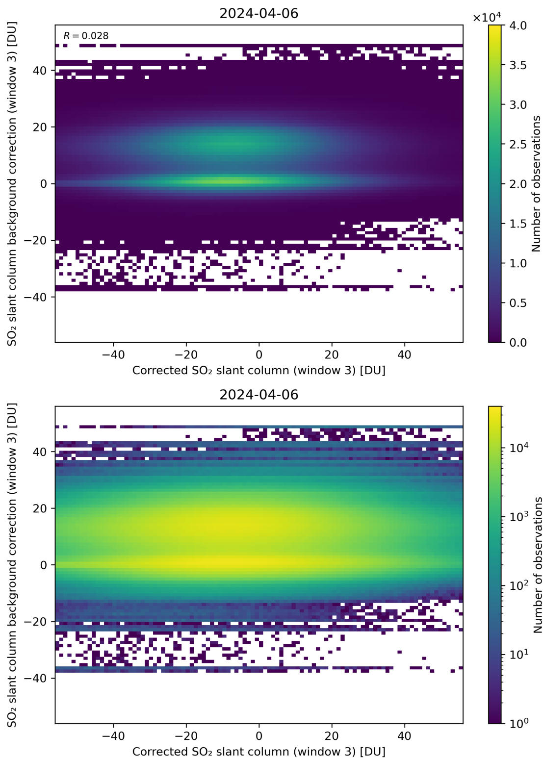
Figure 205: Scatter density plot of “Corrected SO 2 slant column (window 3)” against “SO 2 slant column background correction (window 3)” for 2024-04-05 to 2024-04-07.
