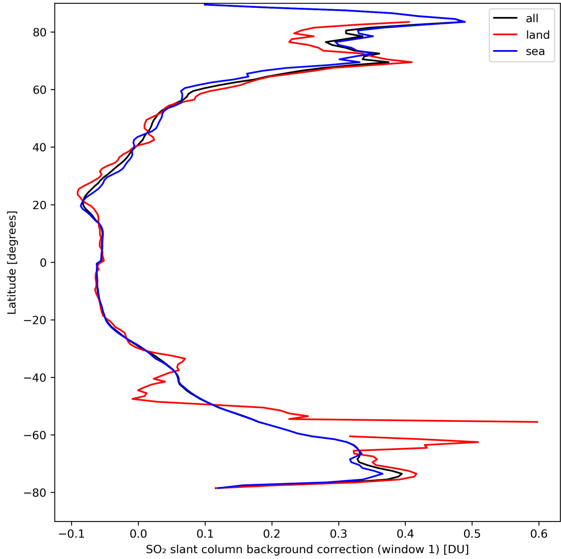
Figure 36: Zonal average of “SO 2 slant column background correction (window 1)” for 2024-04-05 to 2024-04-07.
