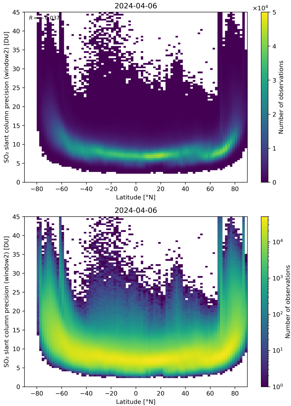
Figure 151: Scatter density plot of “Latitude” against “SO 2 slant column precision (window2)” for 2024-04-05 to 2024-04-07.
