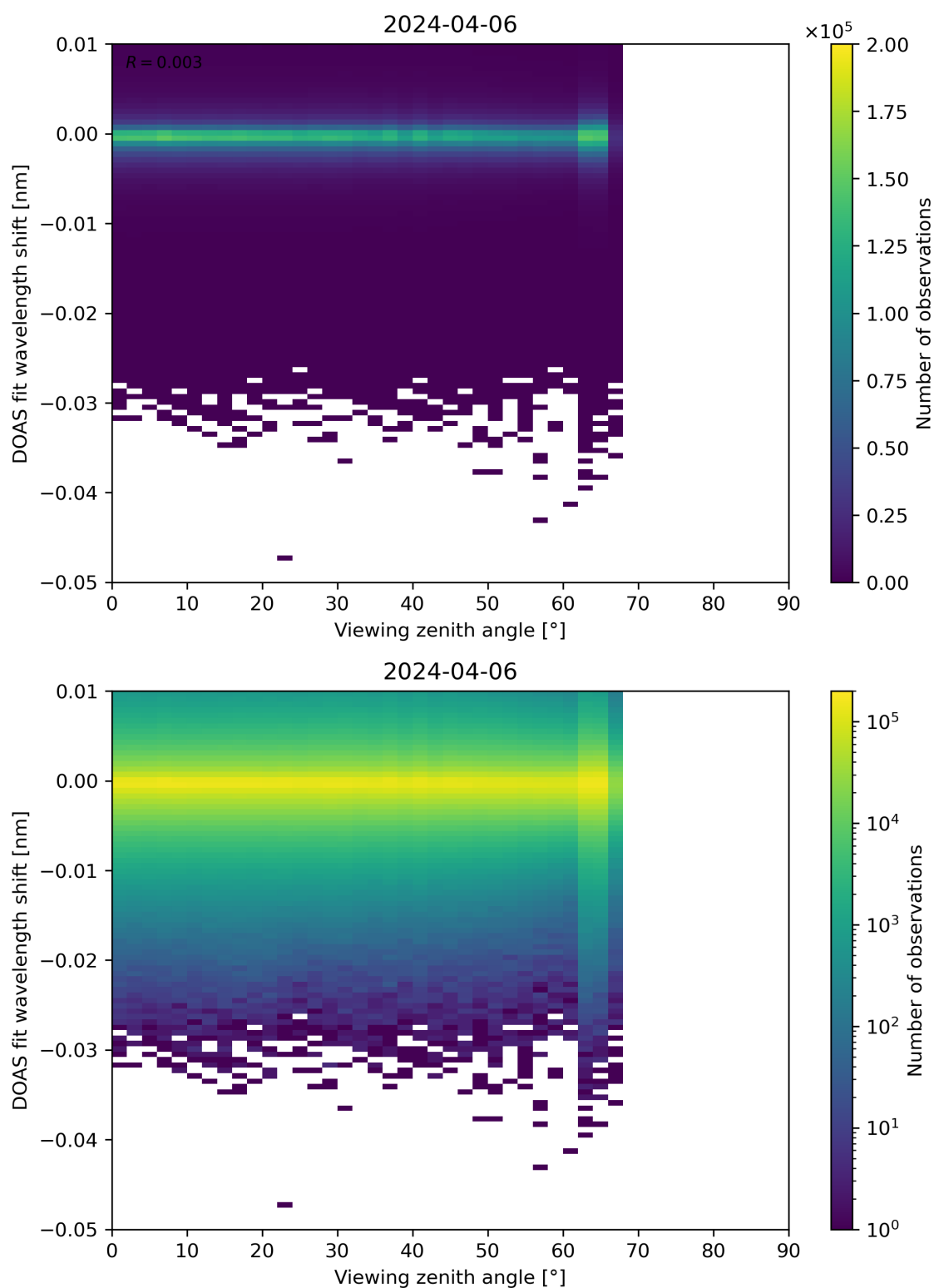
Figure 311: Scatter density plot of “Viewing zenith angle” against “DOAS fit wavelength shift” for 2024-04-05 to 2024-04-07.
