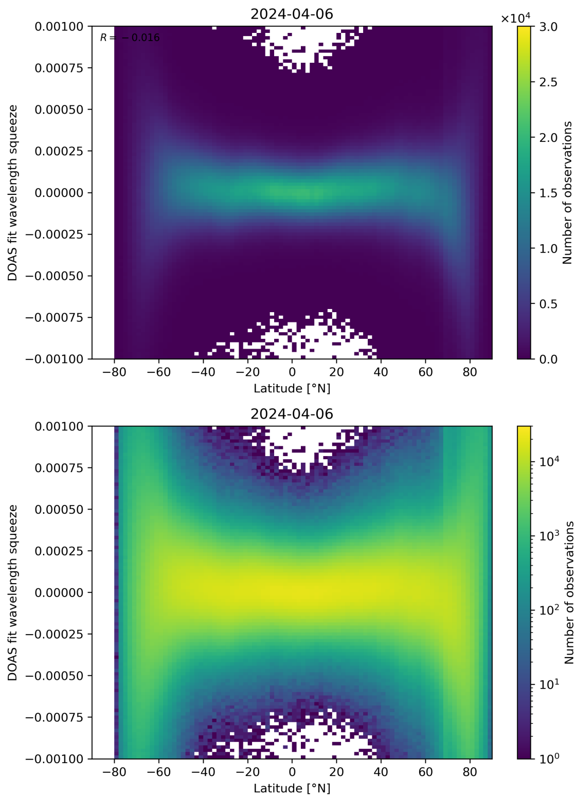
Figure 143: Scatter density plot of “Latitude” against “DOAS fit wavelength squeeze” for 2024-04-05 to 2024-04-07.
