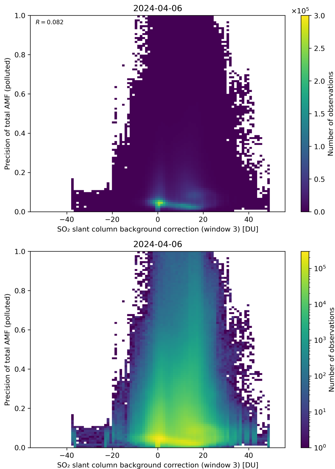
Figure 126: Scatter density plot of “SO 2 slant column background correction (window 3)” against “Precision of total AMF (polluted)” for 2024-04-05 to 2024-04-07.
