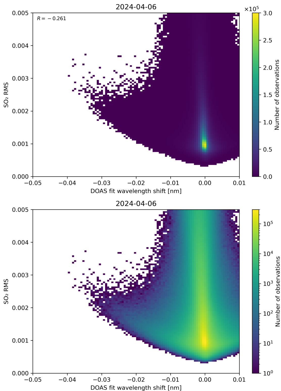
Figure 128: Scatter density plot of “DOAS fit wavelength shift” against “SO 2 RMS” for 2024-04-05 to 2024-04-07.
