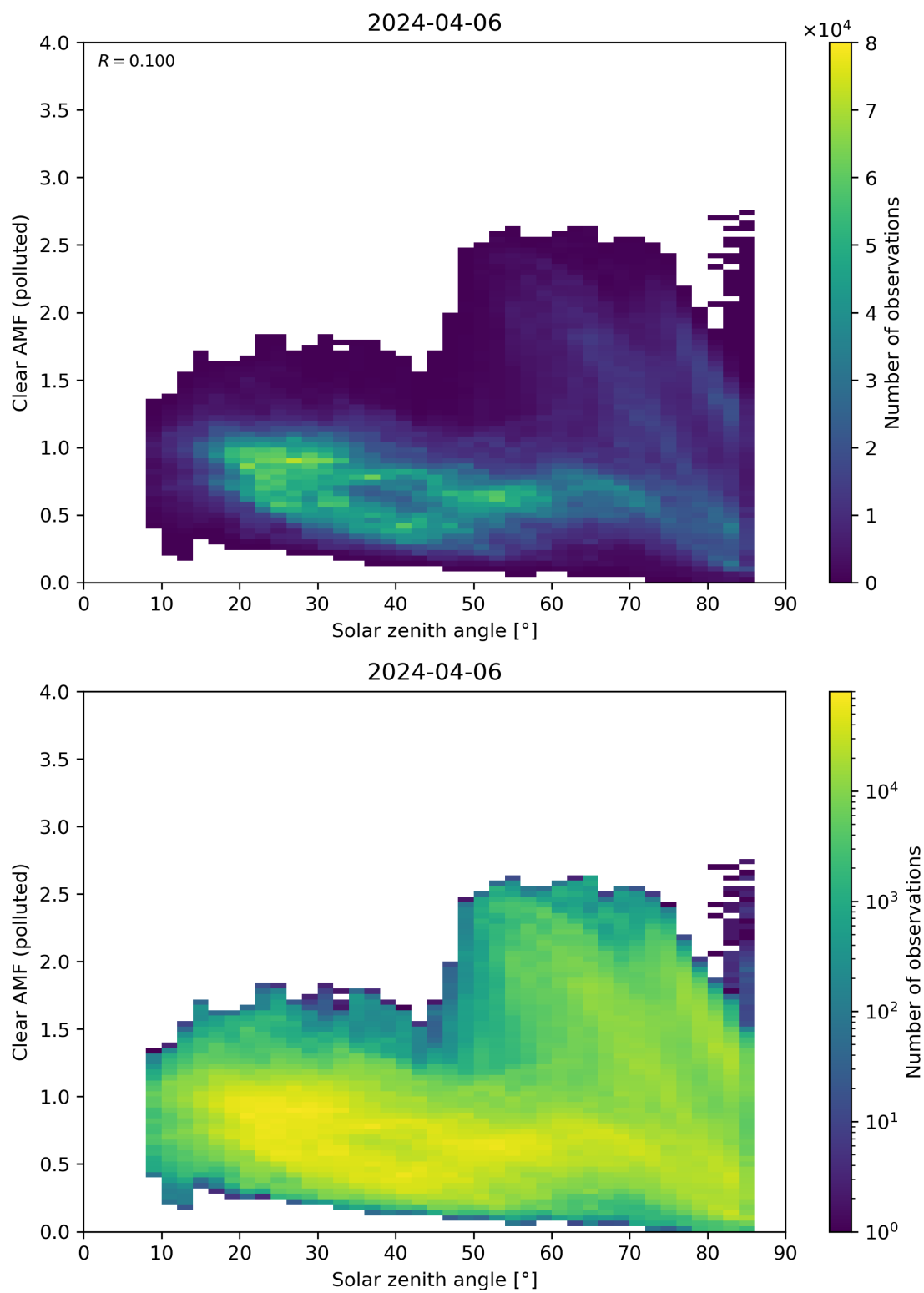
Figure 165: Scatter density plot of “Solar zenith angle” against “Clear AMF (polluted)” for 2024-04-05 to 2024-04-07.
