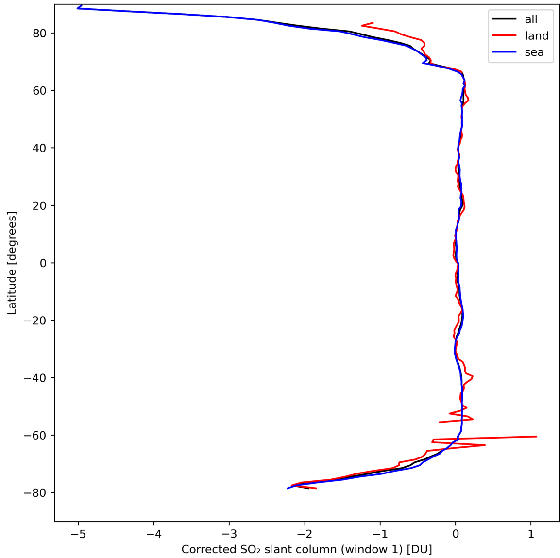
Figure 35: Zonal average of “Corrected SO 2 slant column (window 1)” for 2024-04-05 to 2024-04-07.
