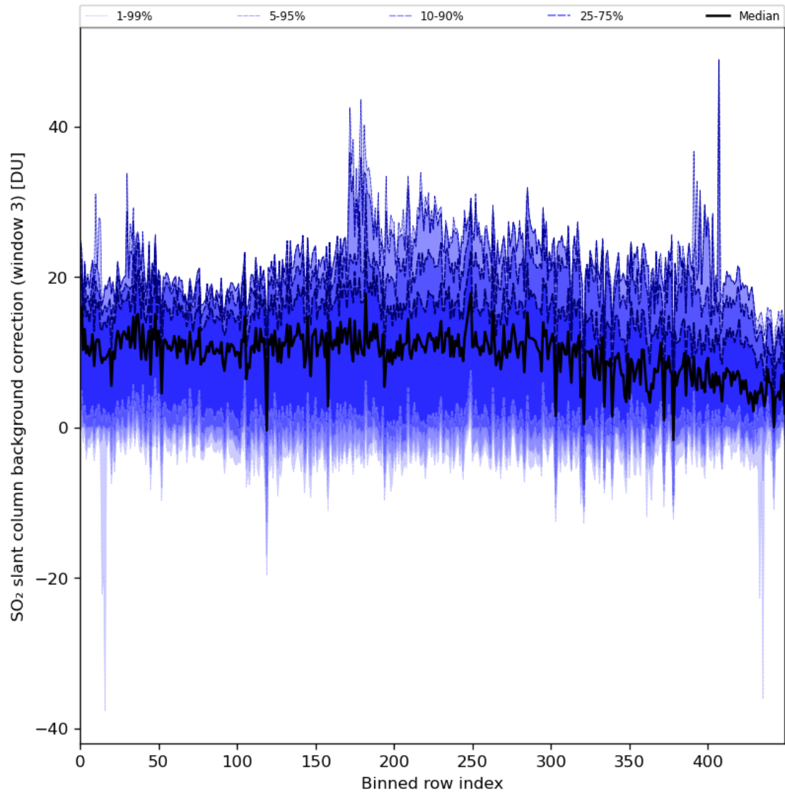
Figure 90: Along track statistics of “SO 2 slant column background correction (window 3)” for 2024-04-05 to 2024-04-07
