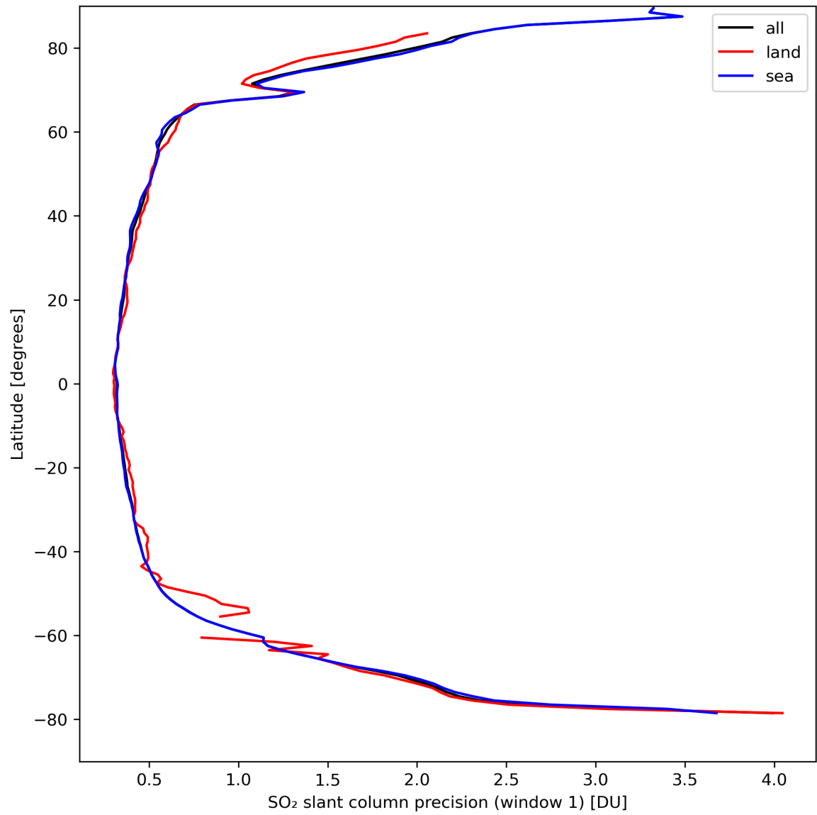
Figure 34: Zonal average of “SO 2 slant column precision (window 1)” for 2024-04-05 to 2024-04-07.
