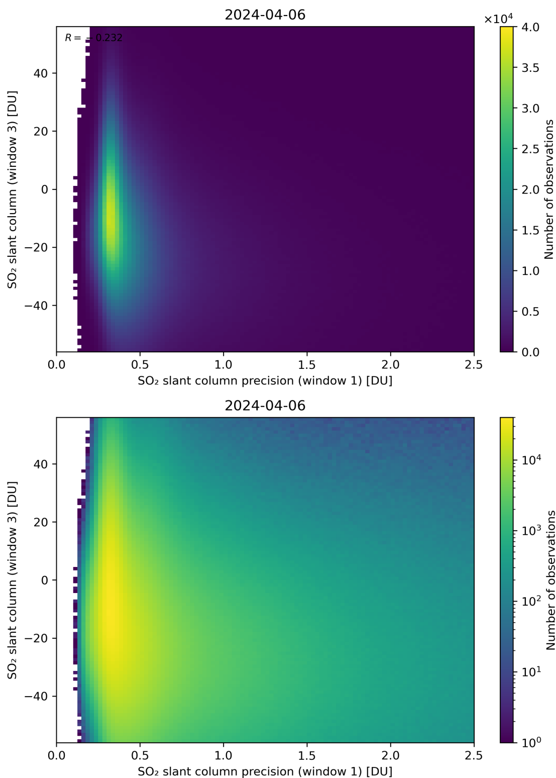
Figure 228: Scatter density plot of “SO 2 slant column precision (window 1)” against “SO 2 slant column (window 3)” for 2024-04-05 to 2024-04-07.
