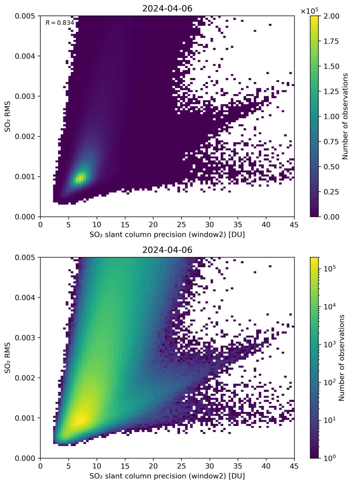
Figure 245: Scatter density plot of “SO 2 slant column precision (window2)” against “SO 2 RMS” for 2024-04-05 to 2024-04-07.
