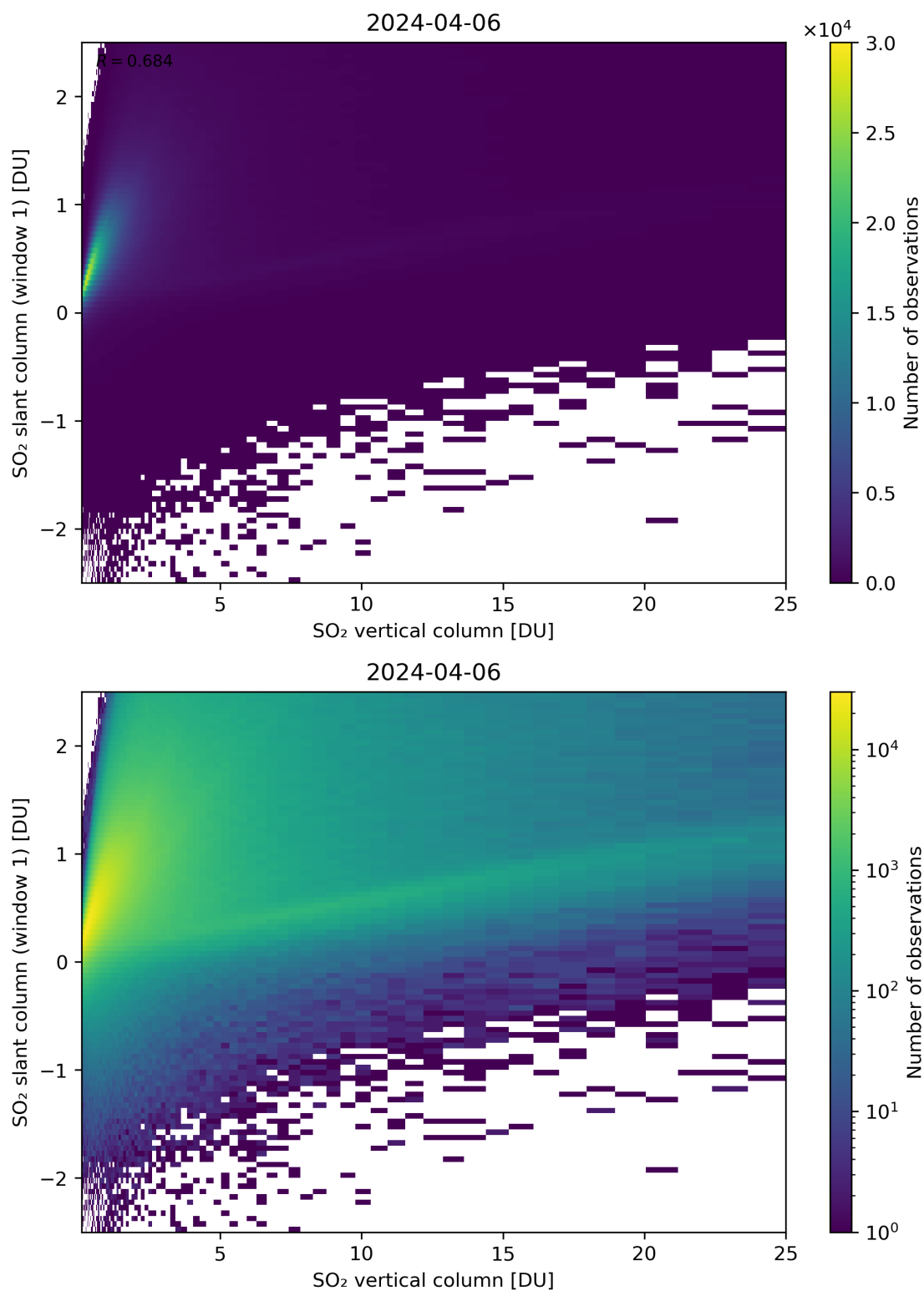
Figure 300: Scatter density plot of “SO 2 vertical column” against “SO 2 slant column (window 1)” for 2024-04-05 to 2024-04-07.
