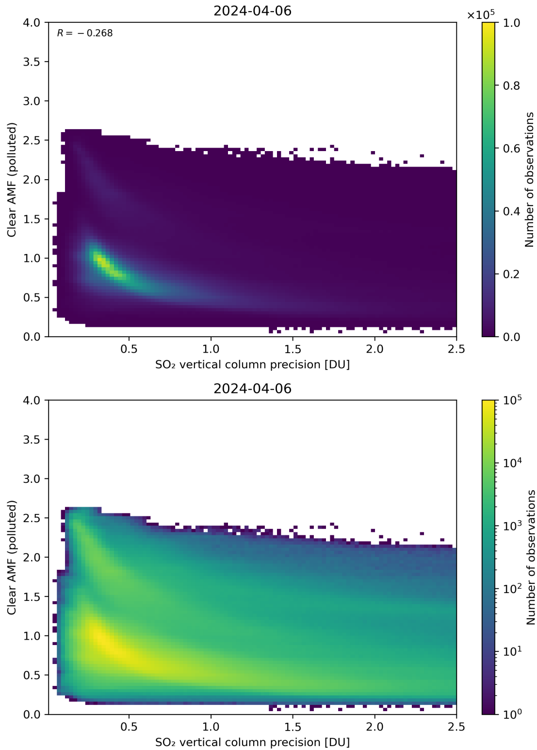
Figure 285: Scatter density plot of “SO 2 vertical column precision” against “Clear AMF (polluted)” for 2024-04-05 to 2024-04-07.
