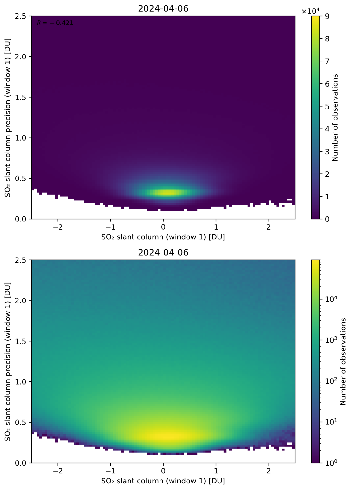
Figure 235: Scatter density plot of “SO 2 slant column (window 1)” against “SO 2 slant column precision (window 1)” for 2024-04-05 to 2024-04-07.
