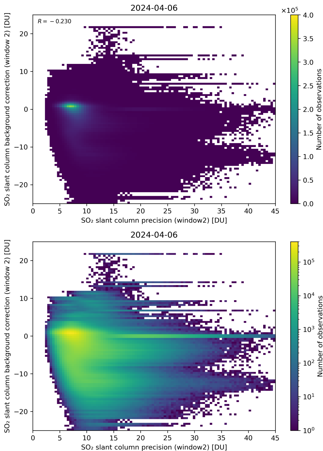
Figure 241: Scatter density plot of “SO 2 slant column precision (window2)” against “SO 2 slant column background correction (window 2)” for 2024-04-05 to 2024-04-07.
