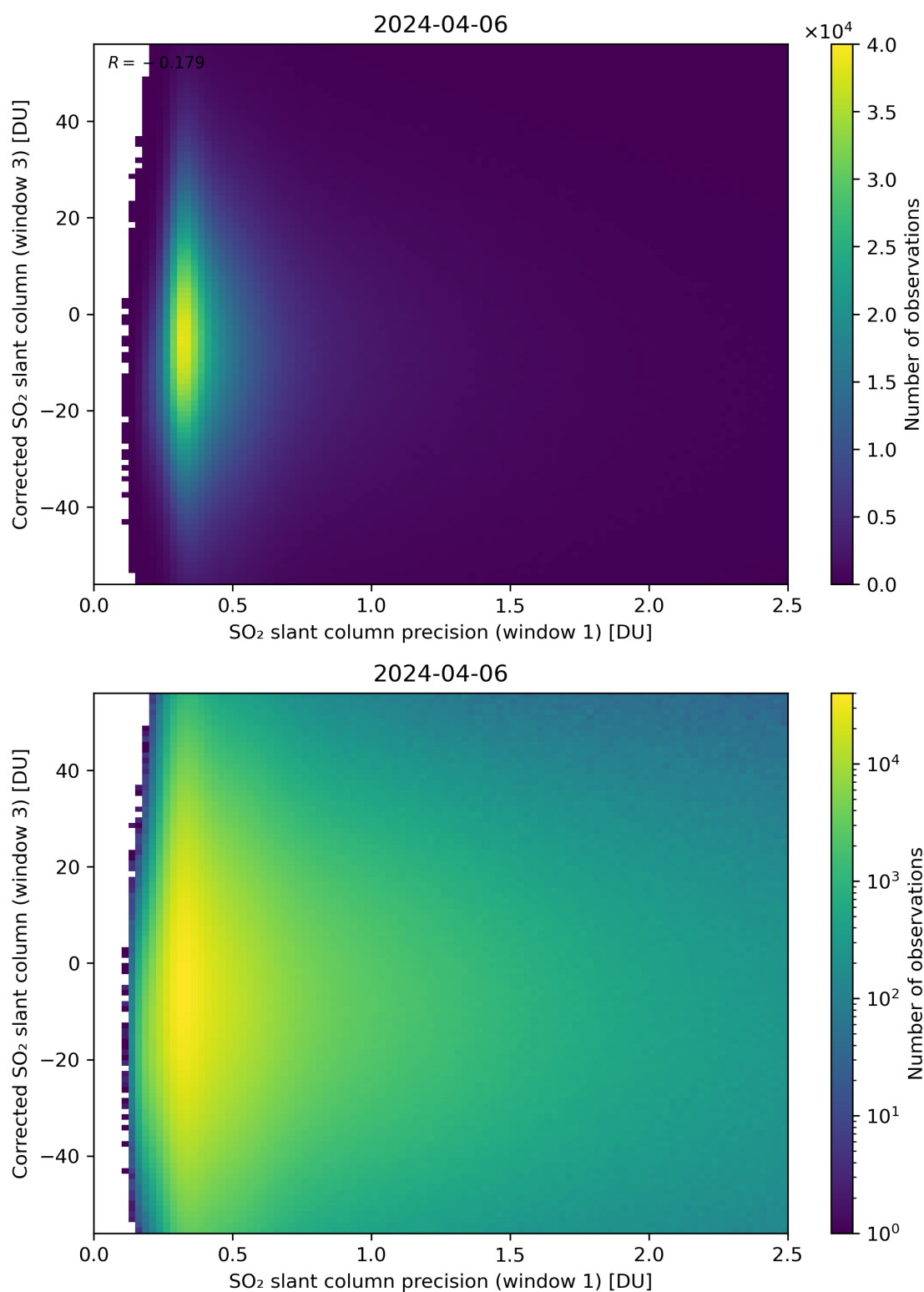
Figure 226: Scatter density plot of “SO 2 slant column precision (window 1)” against “Corrected SO 2 slant column (window 3)” for 2024-04-05 to 2024-04-07.
