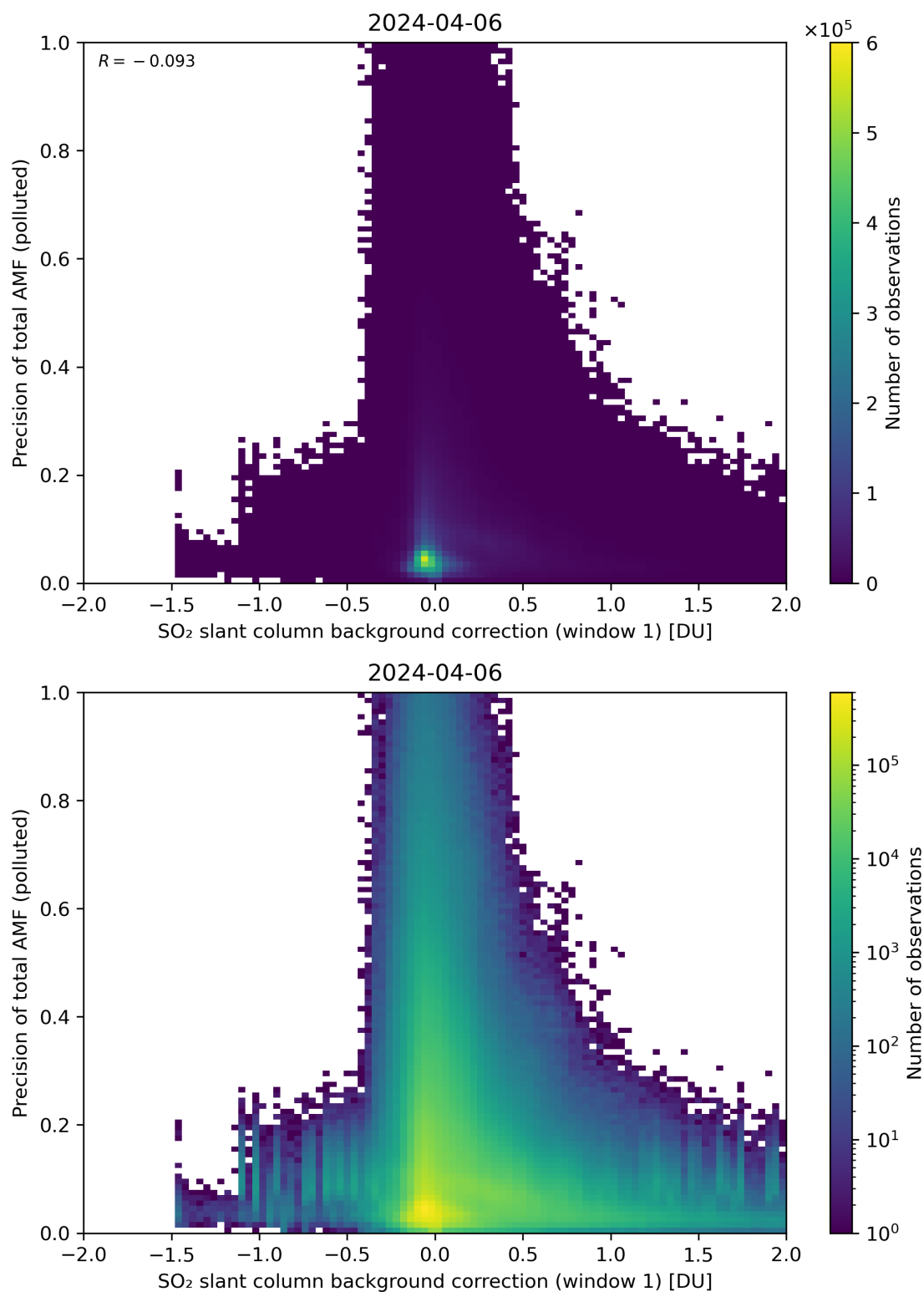
Figure 110: Scatter density plot of “SO 2 slant column background correction (window 1)” against “Precision of total AMF (polluted)” for 2024-04-05 to 2024-04-07.
