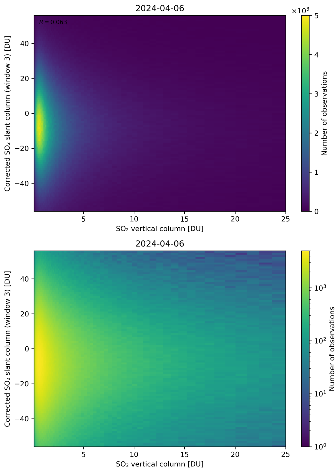
Figure 299: Scatter density plot of “SO 2 vertical column” against “Corrected SO 2 slant column (window 3)” for 2024-04-05 to 2024-04-07.
