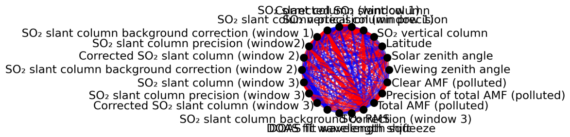
Figure 1: Map of correlation graph for 2024-04-05 to 2024-04-07.
