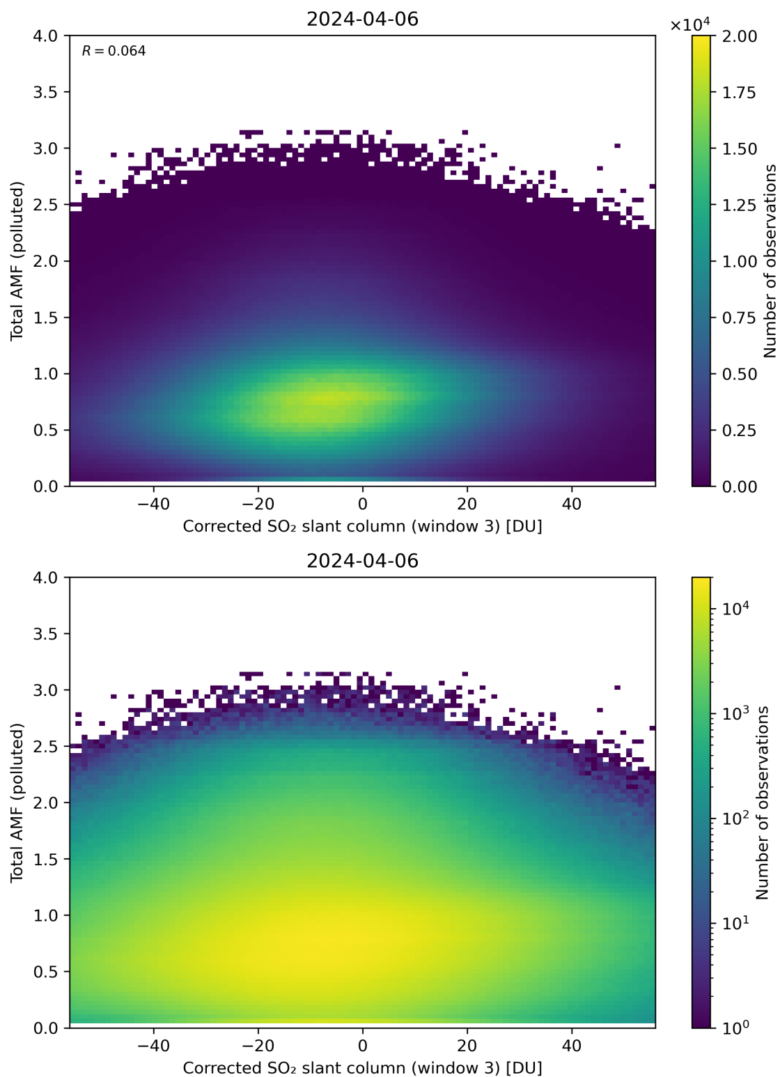
Figure 210: Scatter density plot of “Corrected SO 2 slant column (window 3)” against “Total AMF (polluted)” for 2024-04-05 to 2024-04-07.
