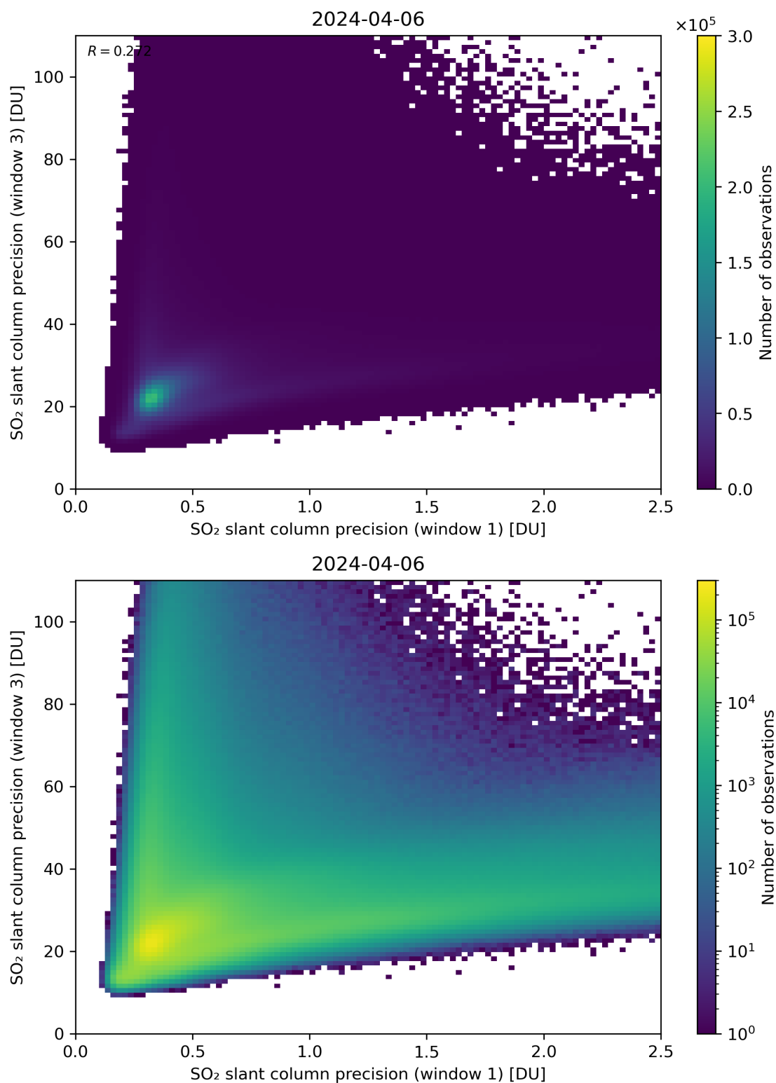
Figure 229: Scatter density plot of “SO 2 slant column precision (window 1)” against “SO 2 slant column precision (window 3)” for 2024-04-05 to 2024-04-07.
