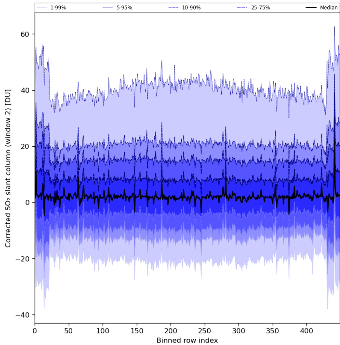
Figure 85: Along track statistics of “Corrected SO 2 slant column (window 2)” for 2024-04-05 to 2024-04-07
