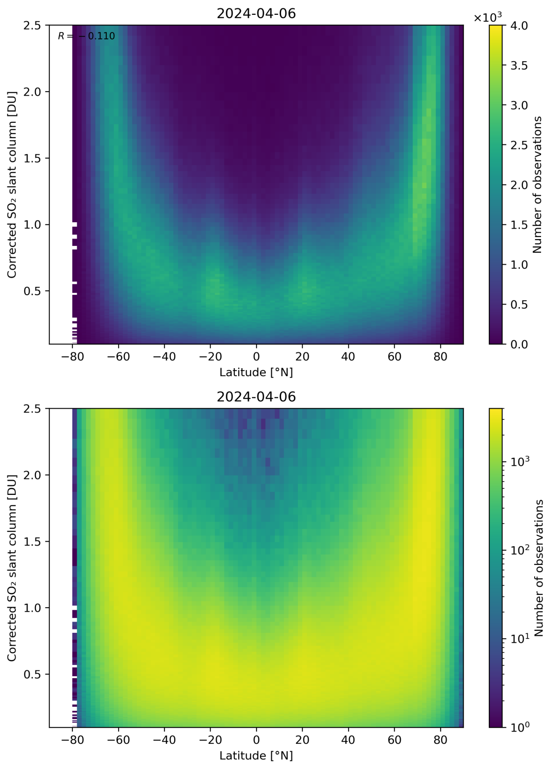
Figure 146: Scatter density plot of “Latitude” against “Corrected SO 2 slant column” for 2024-04-05 to 2024-04-07.
