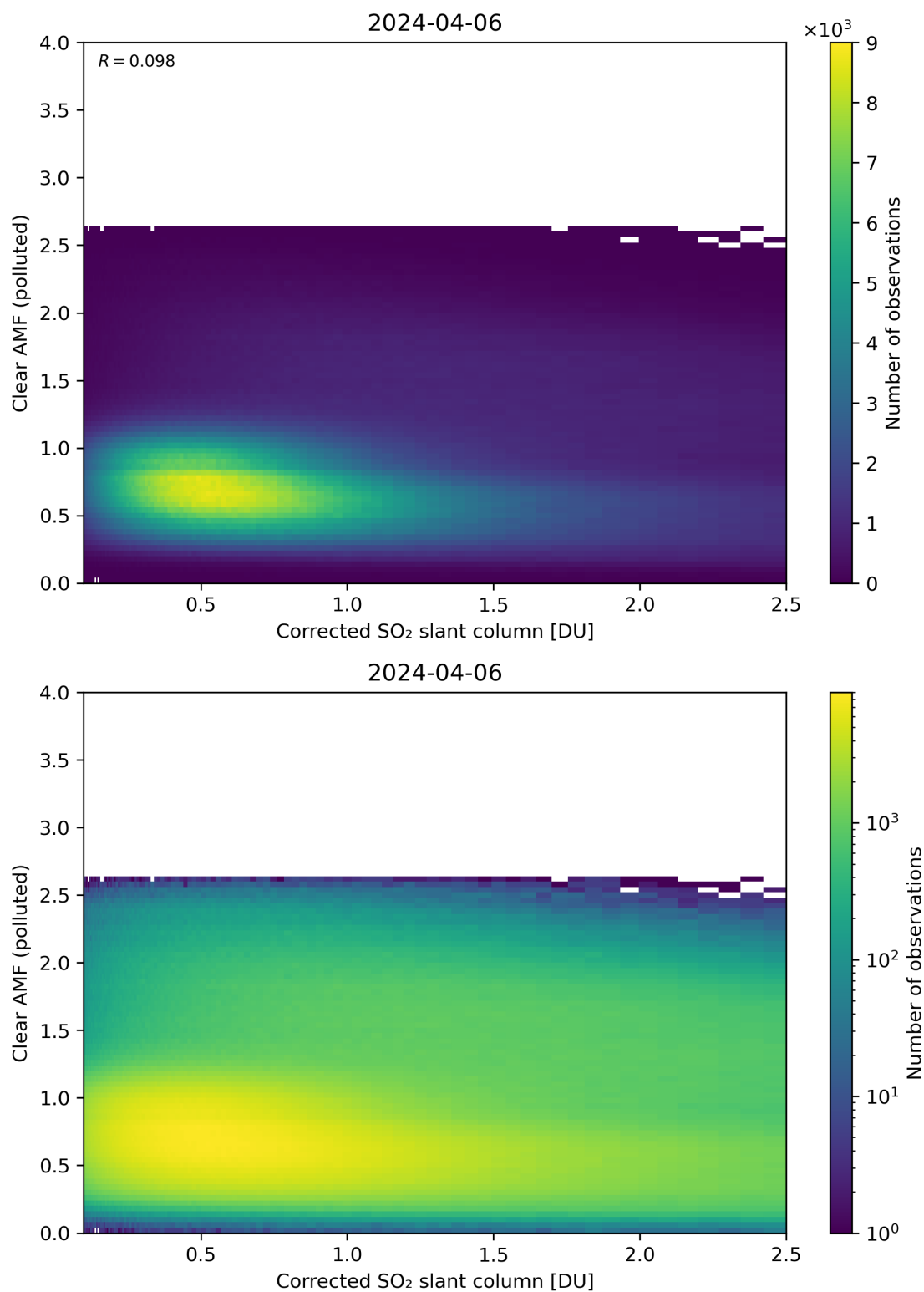
Figure 184: Scatter density plot of “Corrected SO 2 slant column” against “Clear AMF (polluted)” for 2024-04-05 to 2024-04-07.
