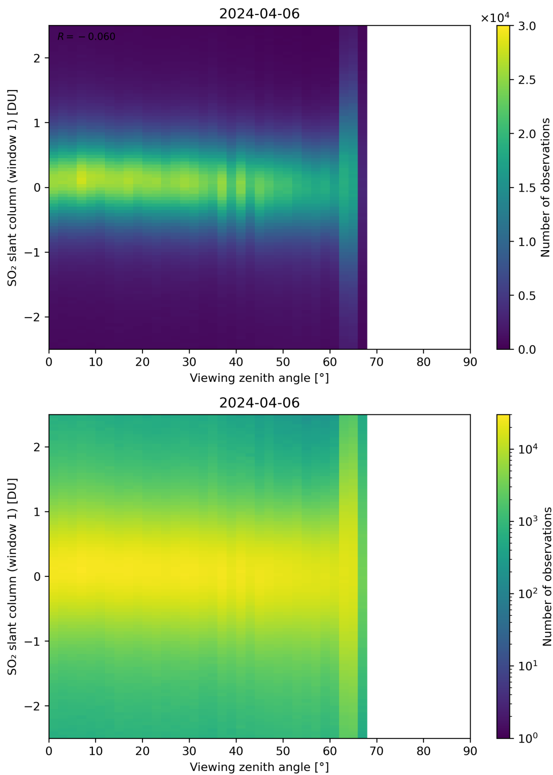
Figure 320: Scatter density plot of “Viewing zenith angle” against “SO 2 slant column (window 1)” for 2024-04-05 to 2024-04-07.
