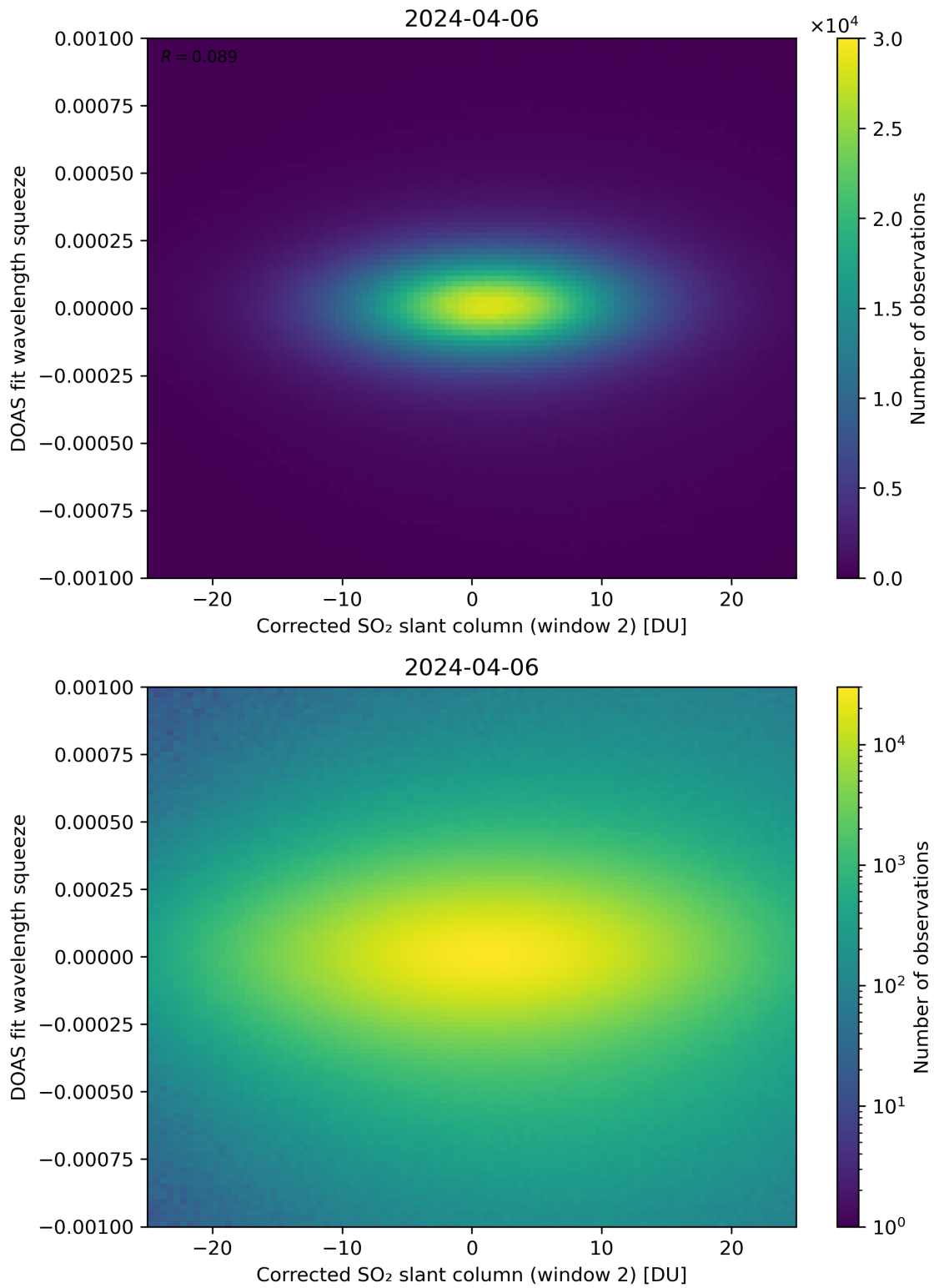
Figure 197: Scatter density plot of “Corrected SO 2 slant column (window 2)” against “DOAS fit wavelength squeeze” for 2024-04-05 to 2024-04-07.
