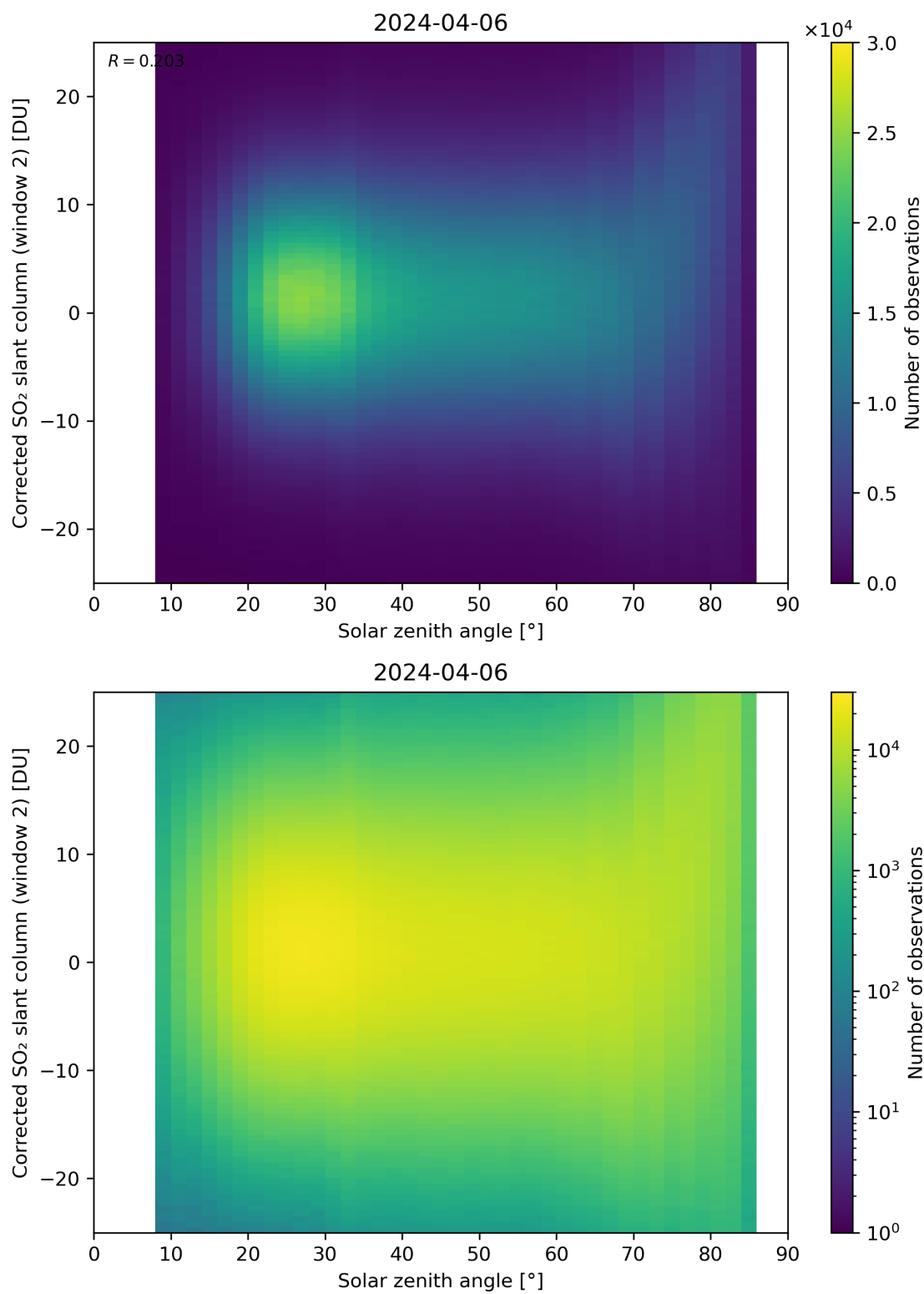
Figure 167: Scatter density plot of “Solar zenith angle” against “Corrected SO 2 slant column (window 2)” for 2024-04-05 to 2024-04-07.
