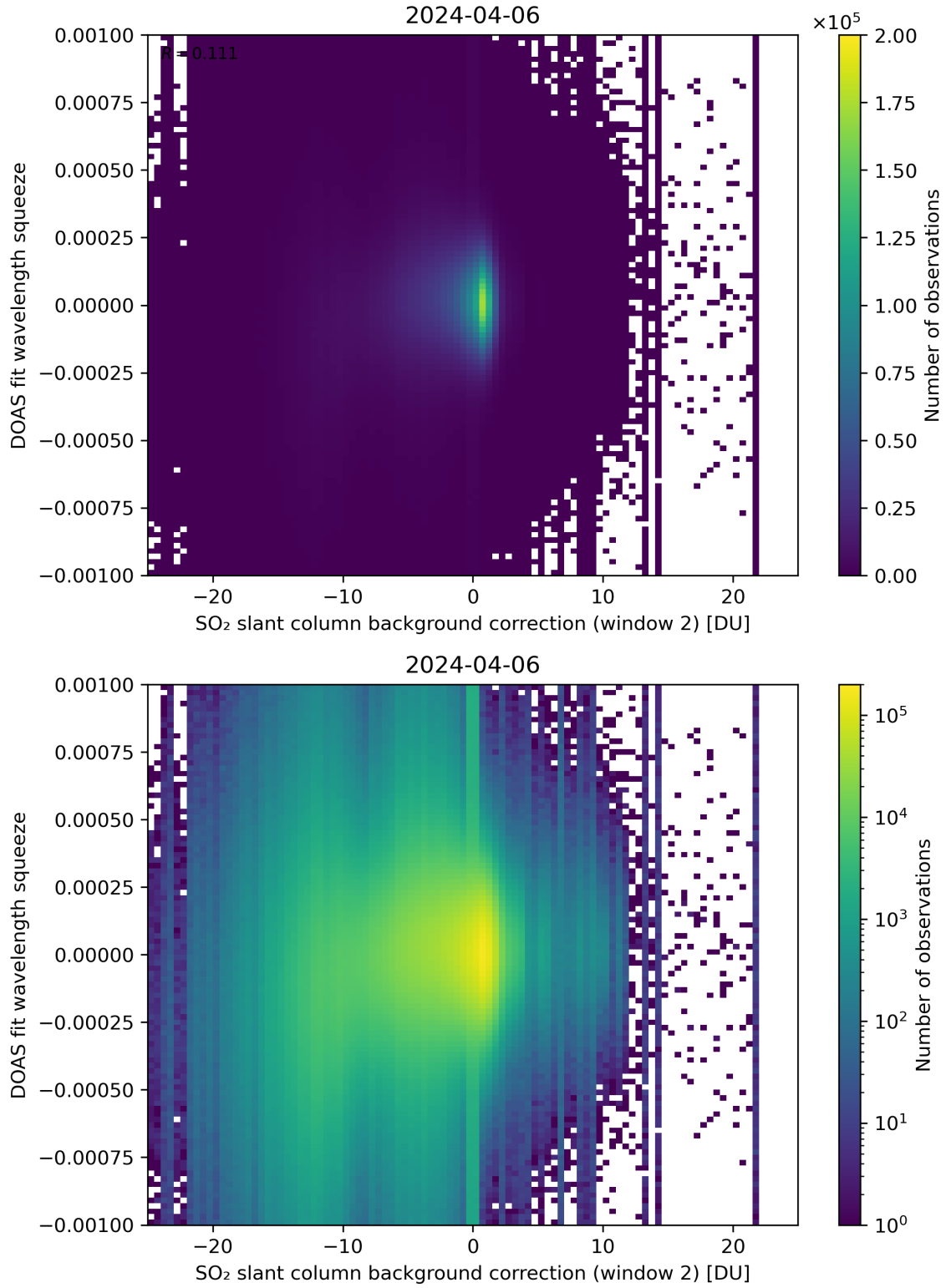
Figure 113: Scatter density plot of “SO 2 slant column background correction (window 2)” against “DOAS fit wavelength squeeze” for 2024-04-05 to 2024-04-07.
