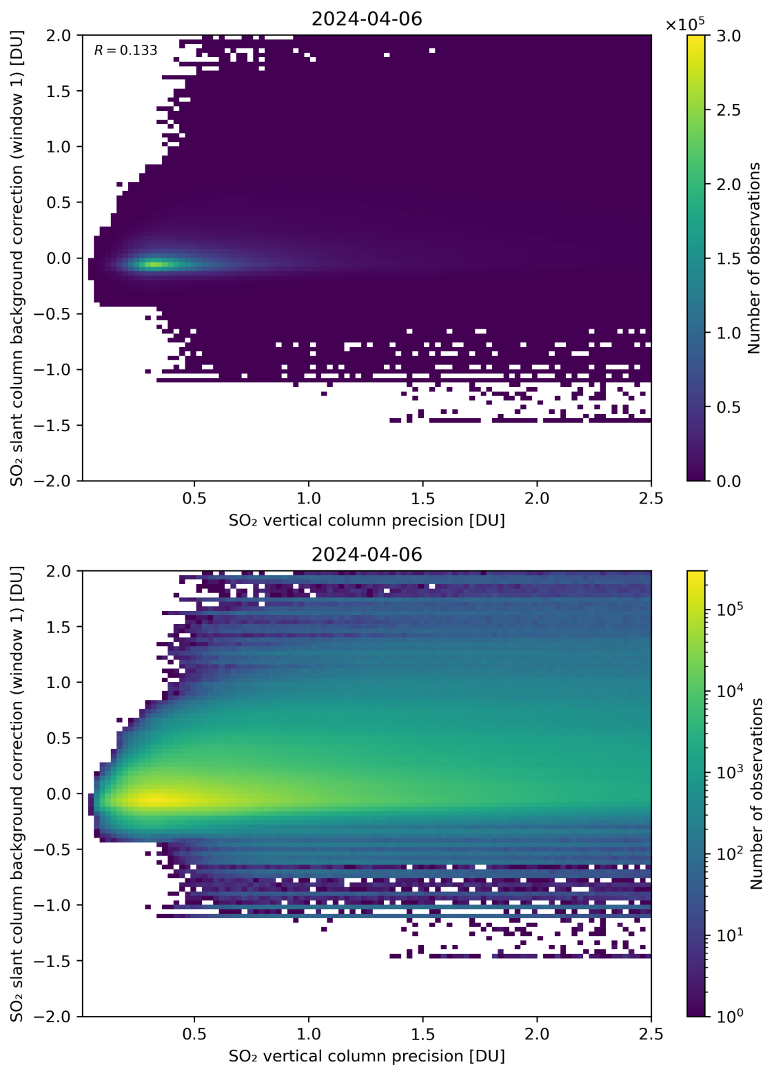
Figure 279: Scatter density plot of “SO 2 vertical column precision” against “SO 2 slant column background correction (window 1)” for 2024-04-05 to 2024-04-07.
