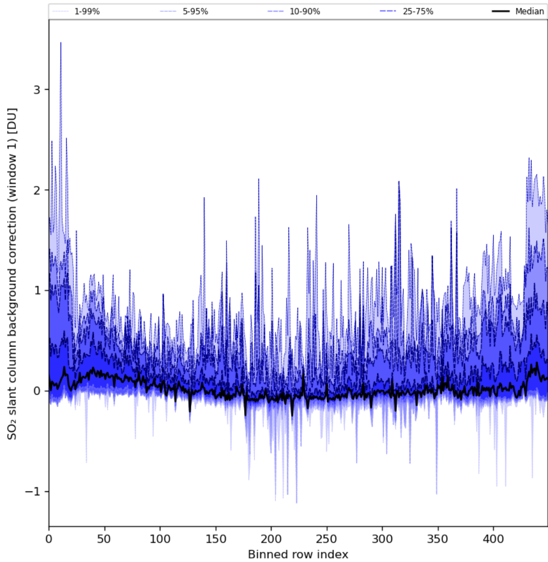
Figure 82: Along track statistics of “SO 2 slant column background correction (window 1)” for 2024-04-05 to 2024-04-07
