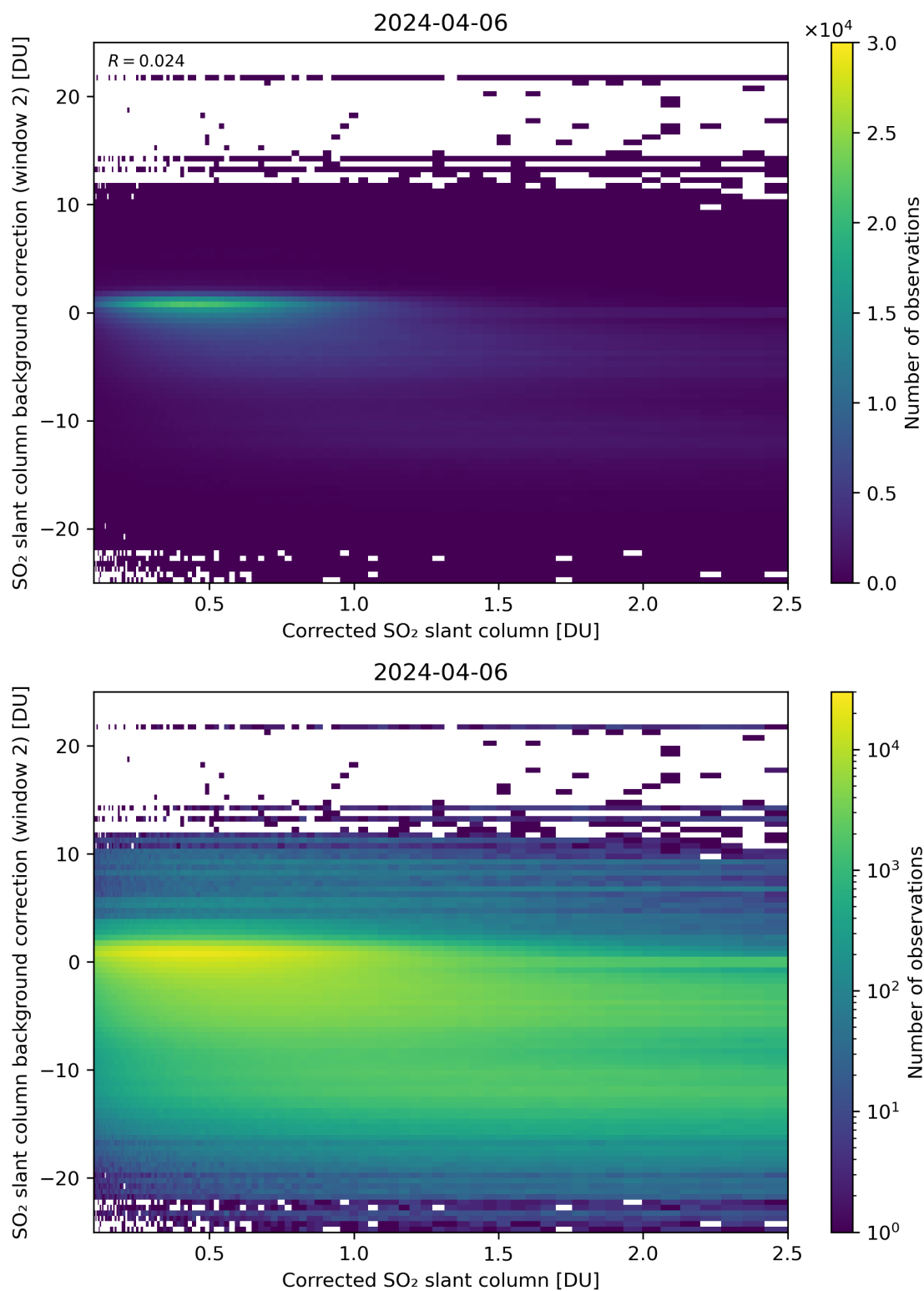
Figure 179: Scatter density plot of “Corrected SO 2 slant column” against “SO 2 slant column background correction (window 2)” for 2024-04-05 to 2024-04-07.
