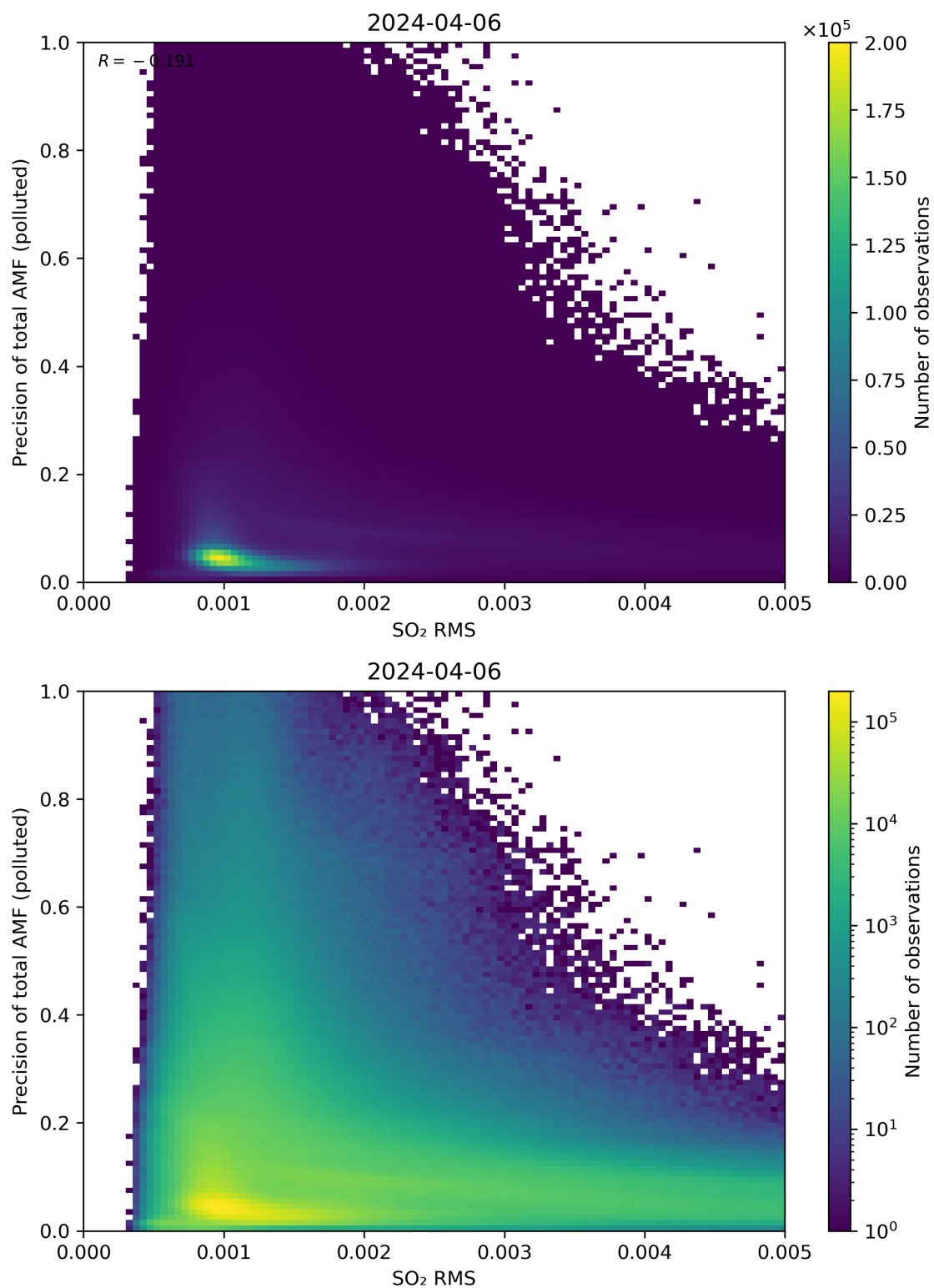
Figure 138: Scatter density plot of “SO 2 RMS” against “Precision of total AMF (polluted)” for 2024-04-05 to 2024-04-07.
