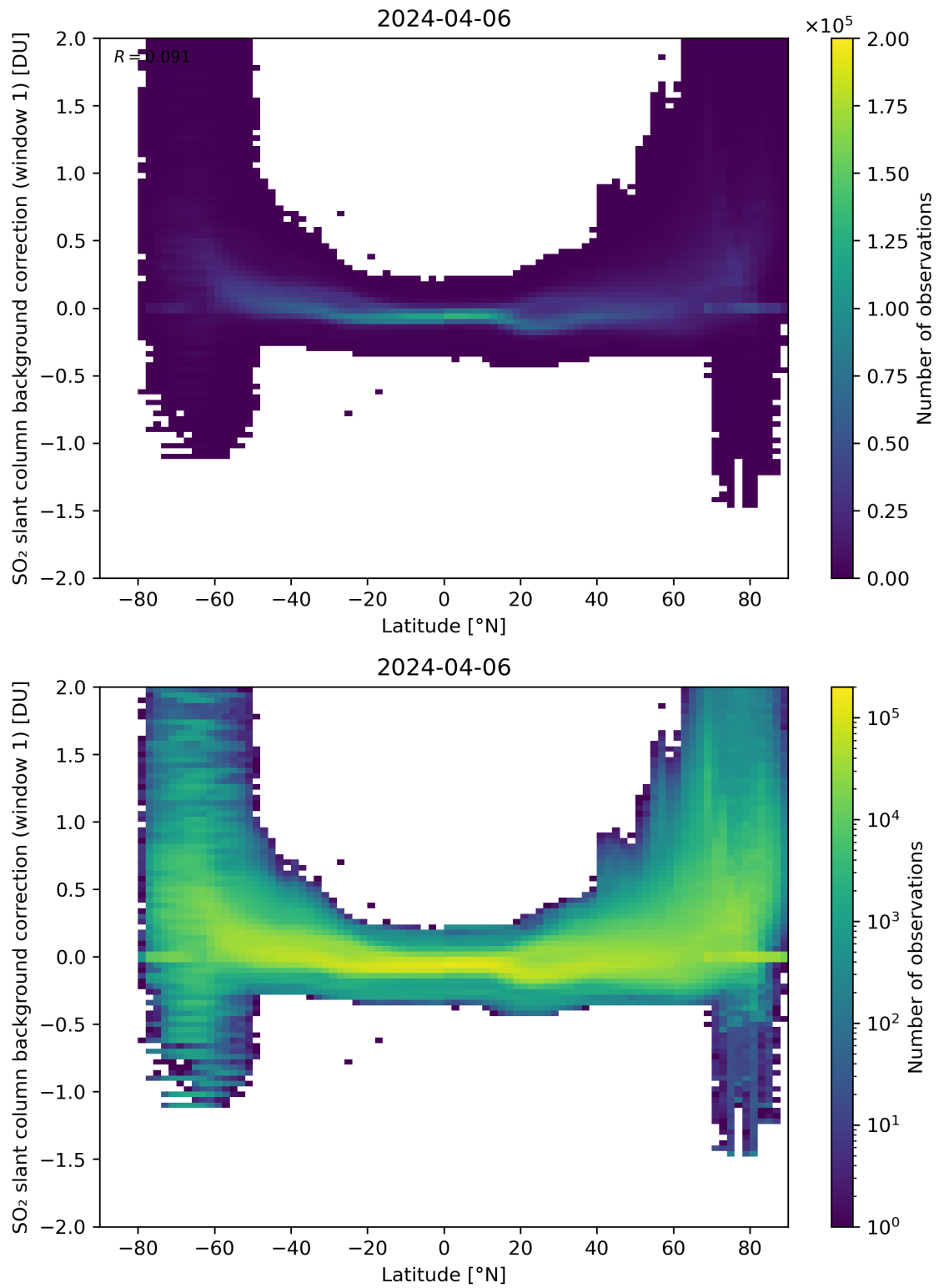
Figure 139: Scatter density plot of “Latitude” against “SO 2 slant column background correction (window 1)” for 2024-04-05 to 2024-04-07.
