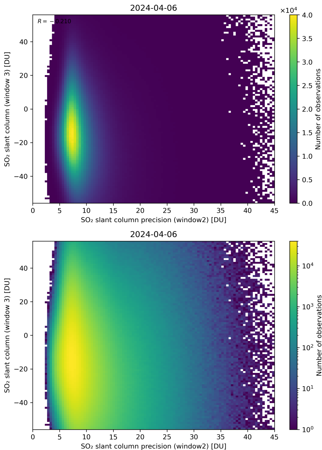
Figure 249: Scatter density plot of “SO 2 slant column precision (window2)” against “SO 2 slant column (window 3)” for 2024-04-05 to 2024-04-07.
