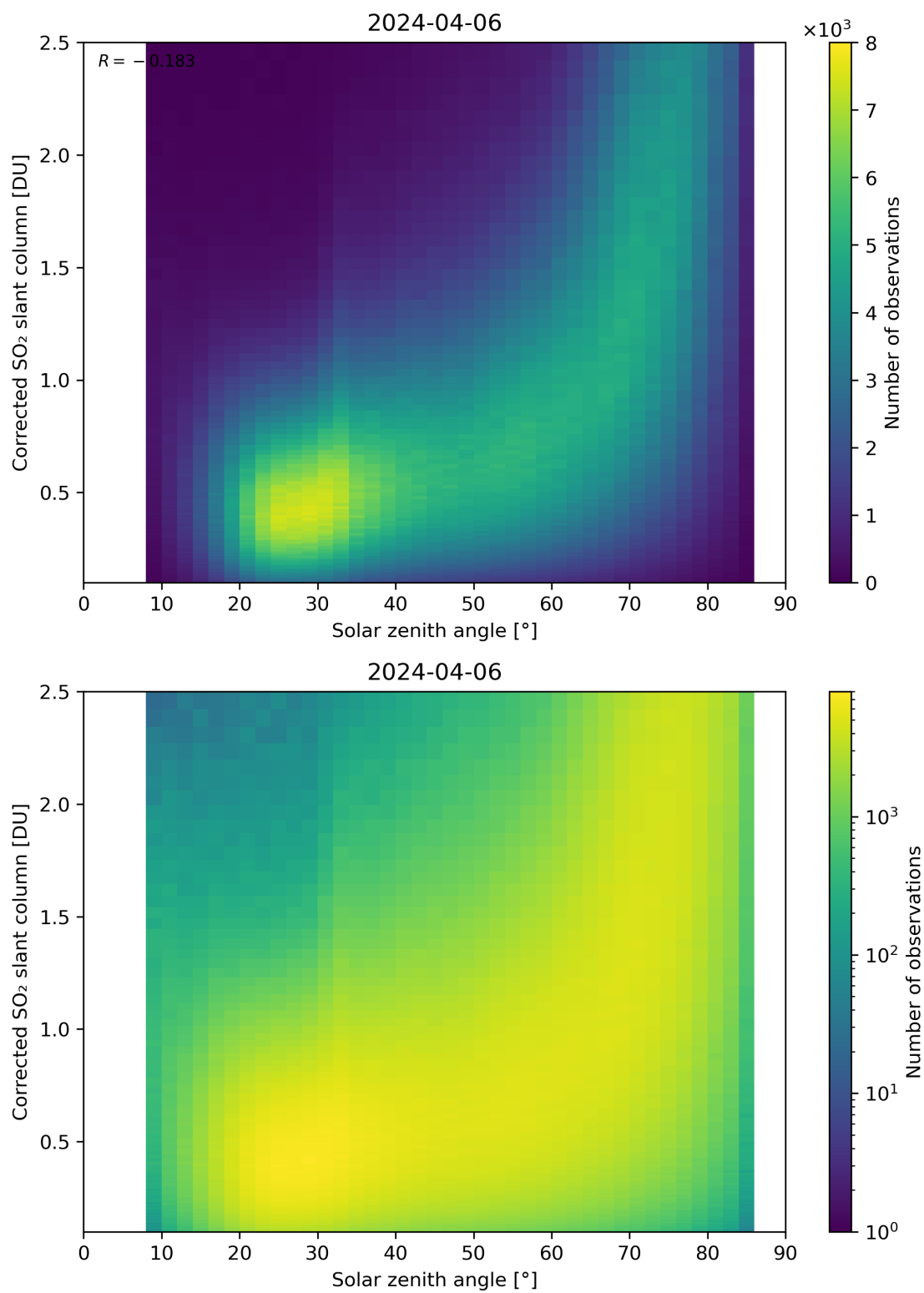
Figure 166: Scatter density plot of “Solar zenith angle” against “Corrected SO 2 slant column” for 2024-04-05 to 2024-04-07.
