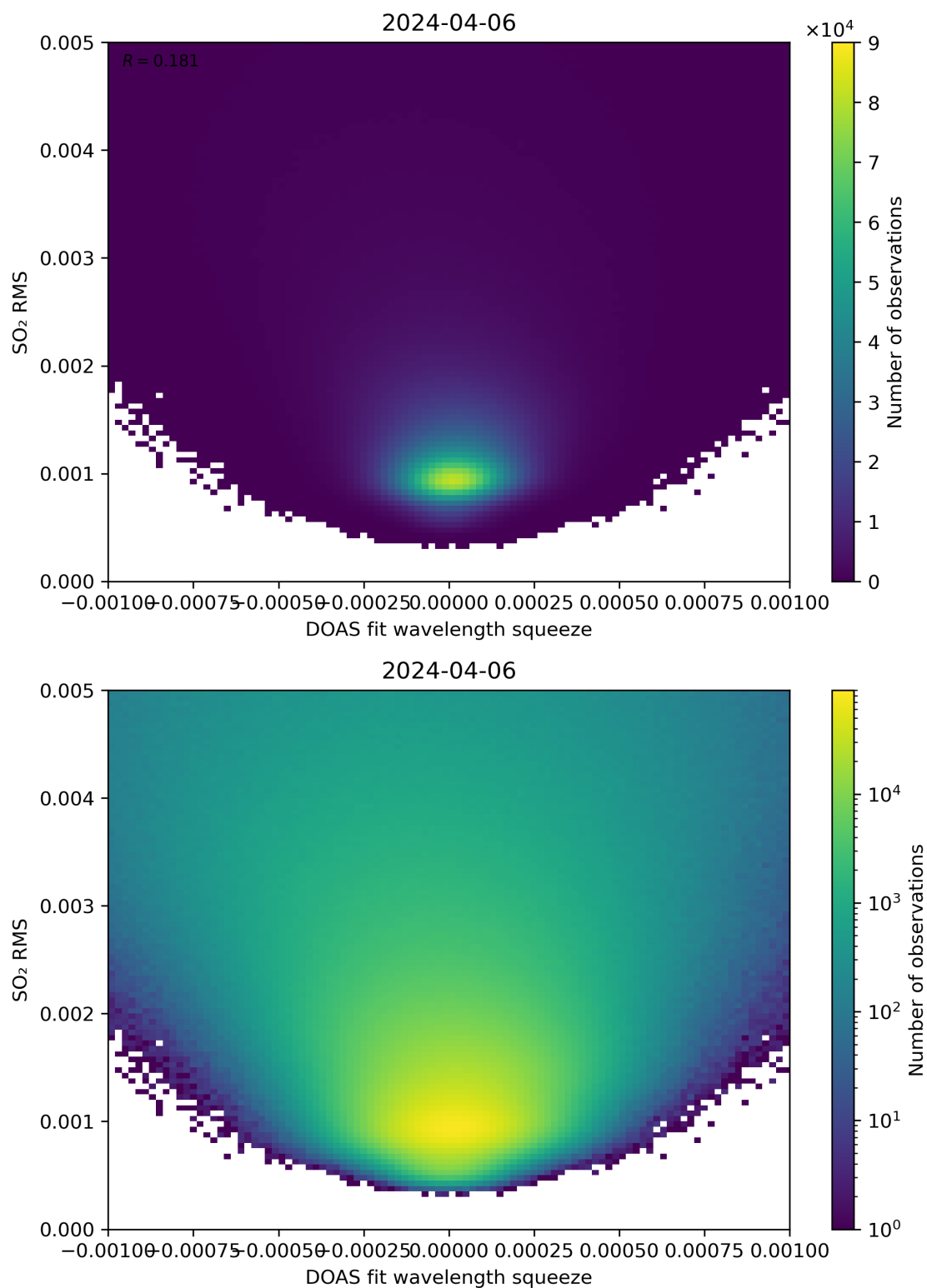
Figure 132: Scatter density plot of “DOAS fit wavelength squeeze” against “SO 2 RMS” for 2024-04-05 to 2024-04-07.
