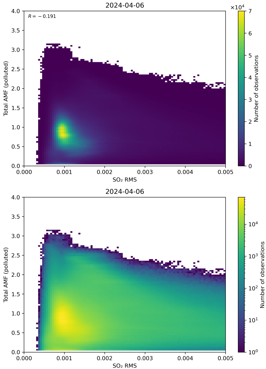
Figure 137: Scatter density plot of “SO 2 RMS” against “Total AMF (polluted)” for 2024-04-05 to 2024-04-07.
