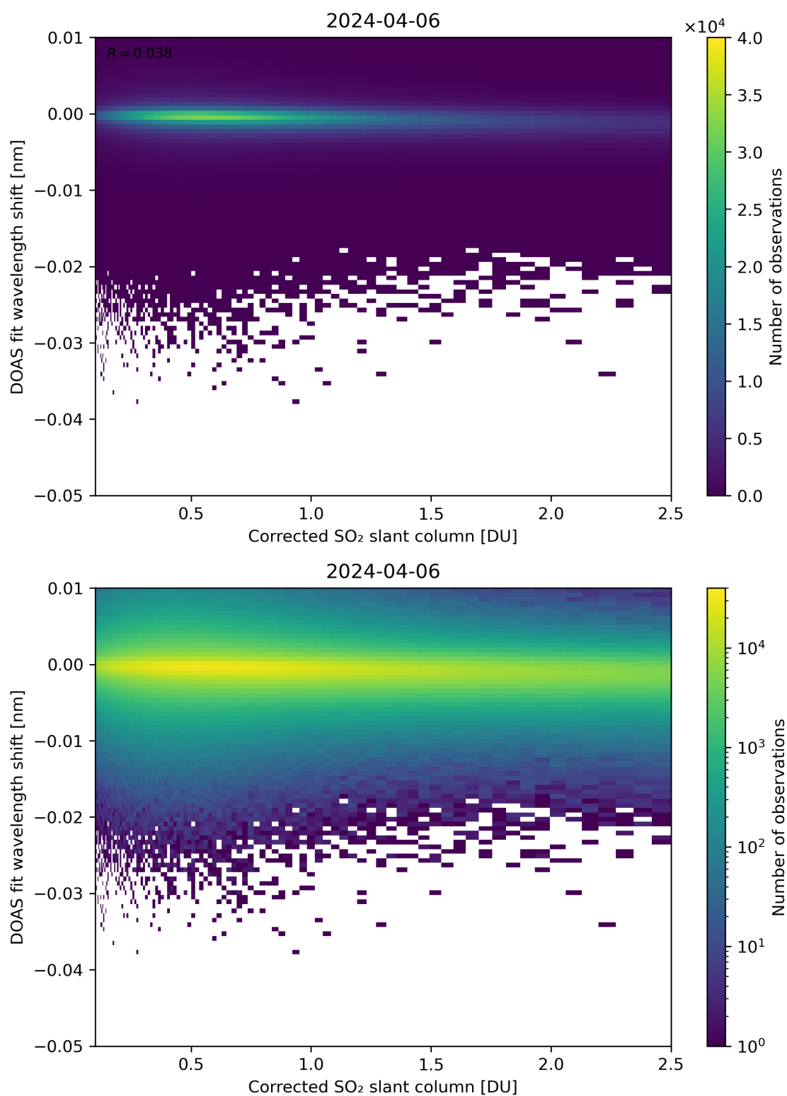
Figure 181: Scatter density plot of “Corrected SO 2 slant column” against “DOAS fit wavelength shift” for 2024-04-05 to 2024-04-07.
