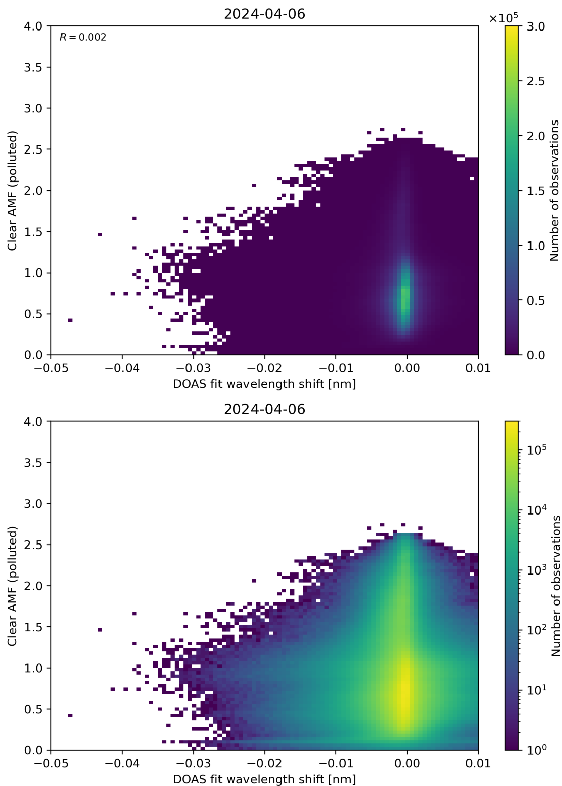
Figure 129: Scatter density plot of “DOAS fit wavelength shift” against “Clear AMF (polluted)” for 2024-04-05 to 2024-04-07.
