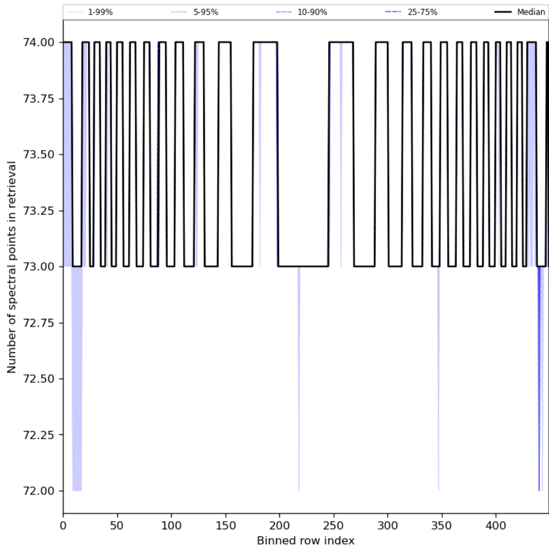
Figure 97: Along track statistics of “Number of spectral points in retrieval” for 2024-04-05 to 2024-04-07
