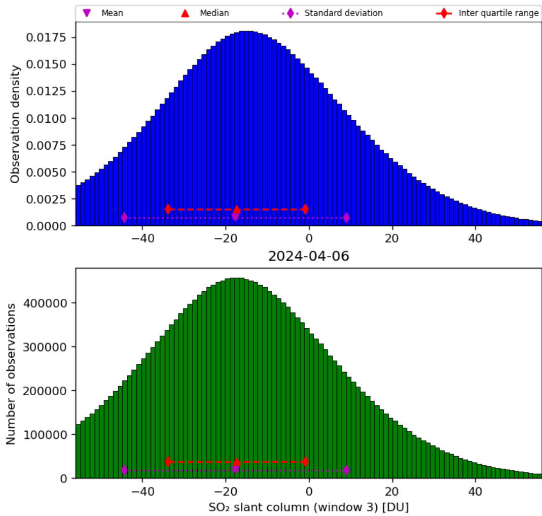
Figure 64: Histogram of “SO 2 slant column (window 3)” for 2024-04-05 to 2024-04-07
