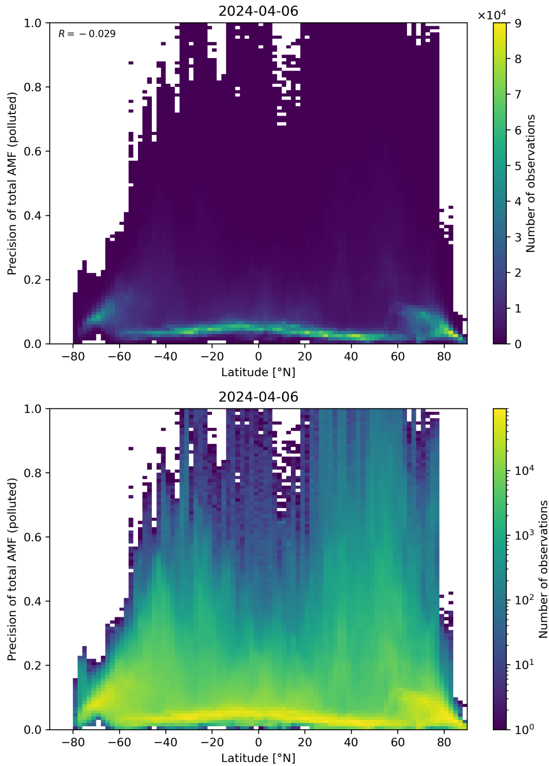
Figure 155: Scatter density plot of “Latitude” against “Precision of total AMF (polluted)” for 2024-04-05 to 2024-04-07.
