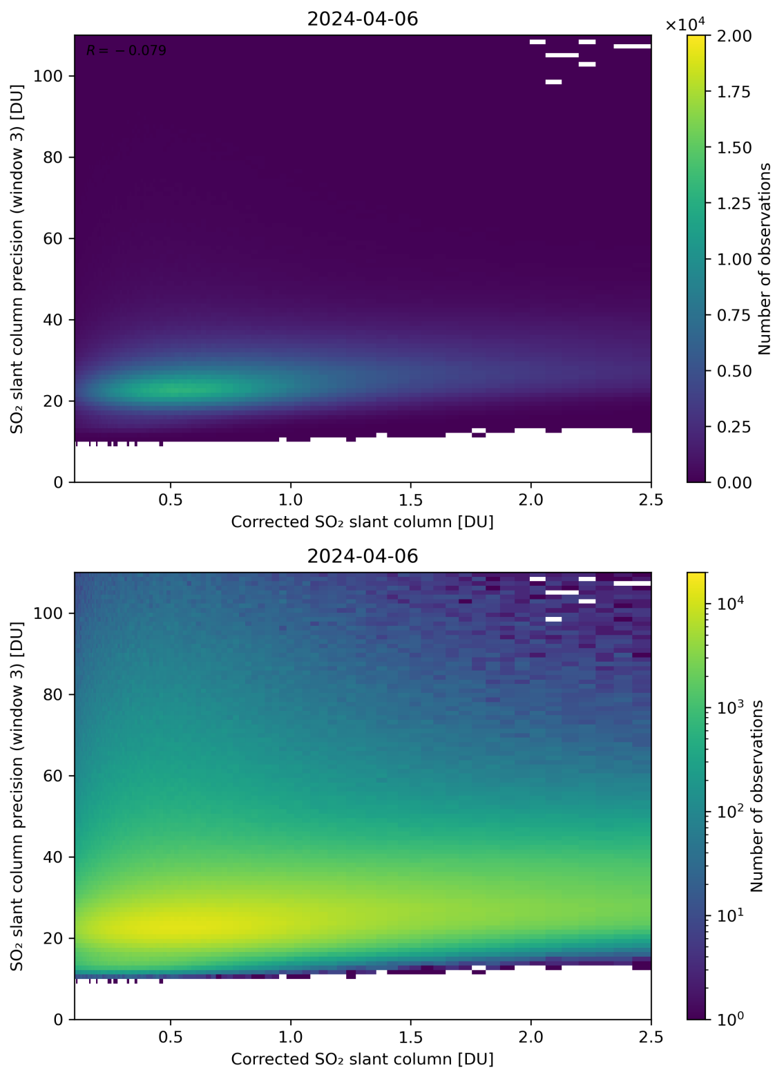
Figure 191: Scatter density plot of “Corrected SO 2 slant column” against “SO 2 slant column precision (window 3)” for 2024-04-05 to 2024-04-07.
