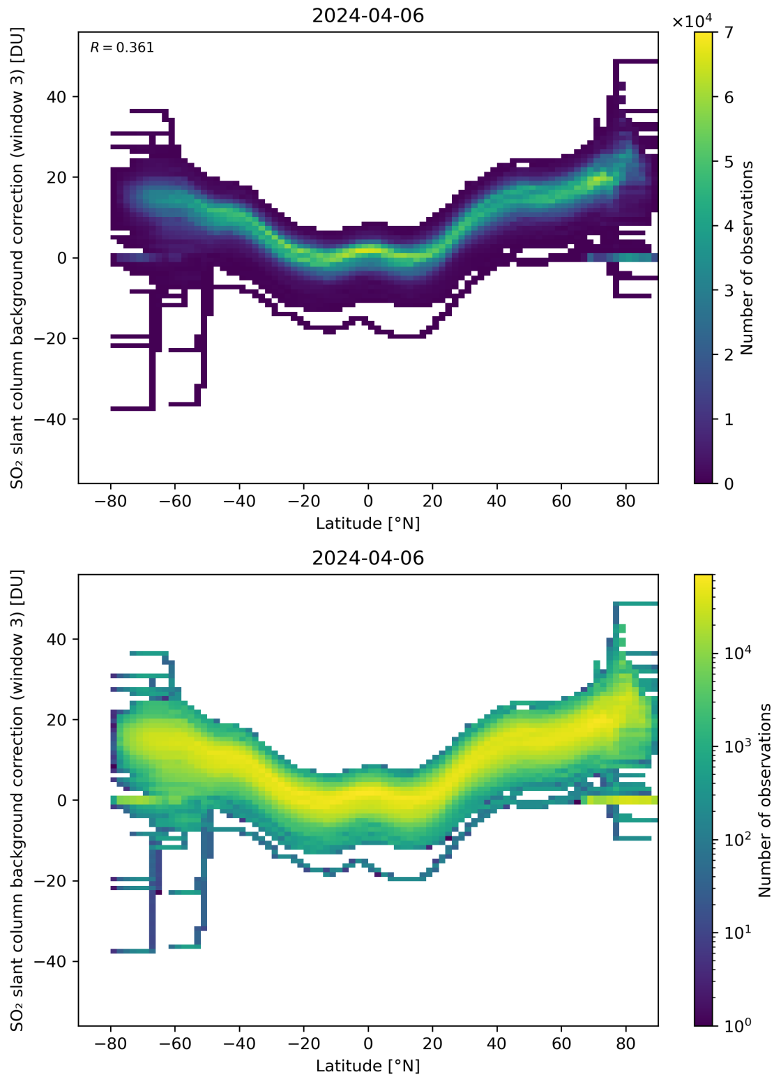
Figure 141: Scatter density plot of “Latitude” against “SO 2 slant column background correction (window 3)” for 2024-04-05 to 2024-04-07.
