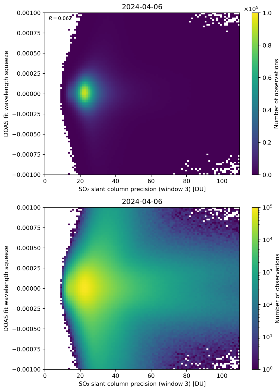
Figure 259: Scatter density plot of “SO 2 slant column precision (window 3)” against “DOAS fit wavelength squeeze” for 2024-04-05 to 2024-04-07.
