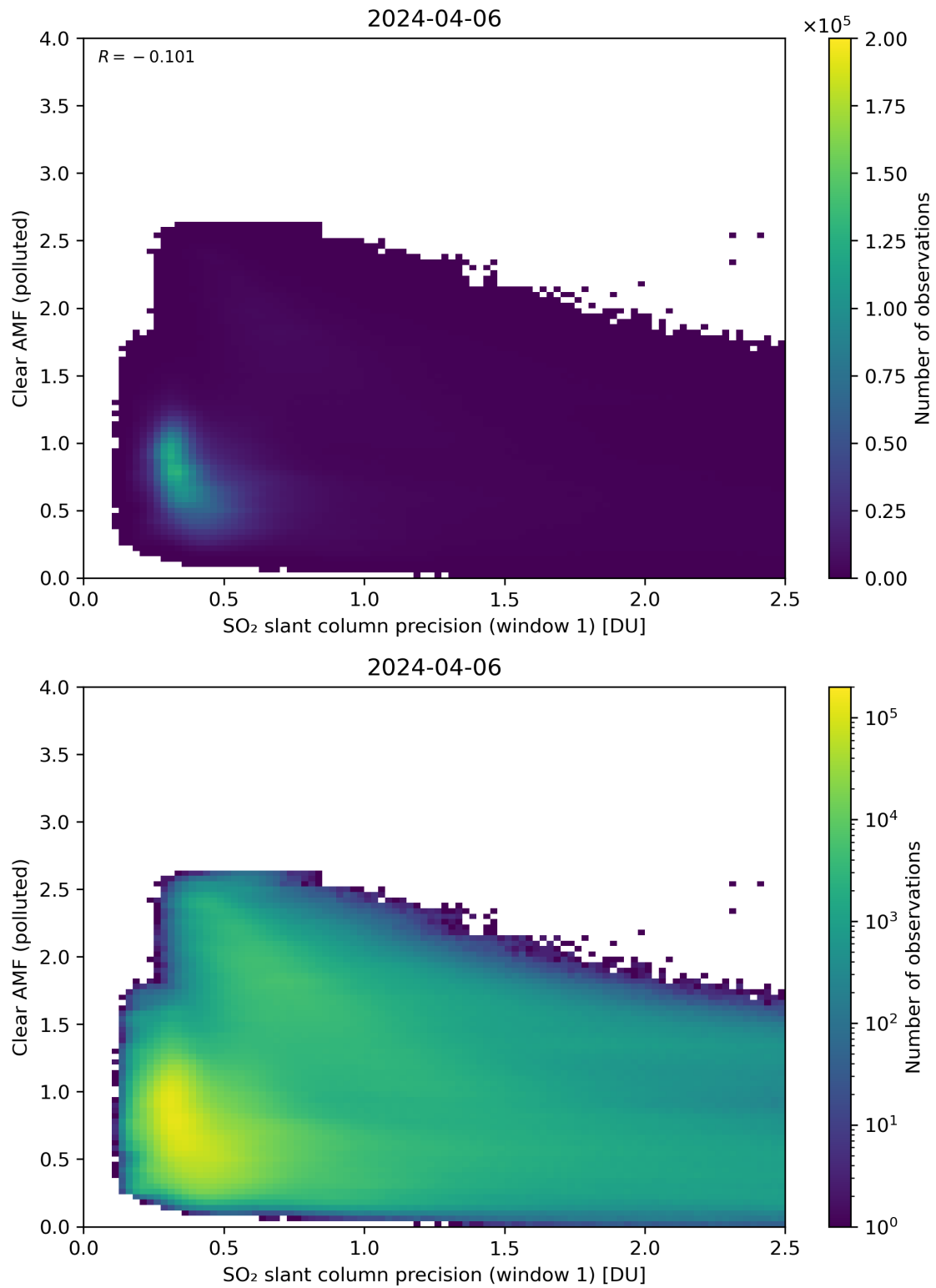
Figure 224: Scatter density plot of “SO 2 slant column precision (window 1)” against “Clear AMF (polluted)” for 2024-04-05 to 2024-04-07.
