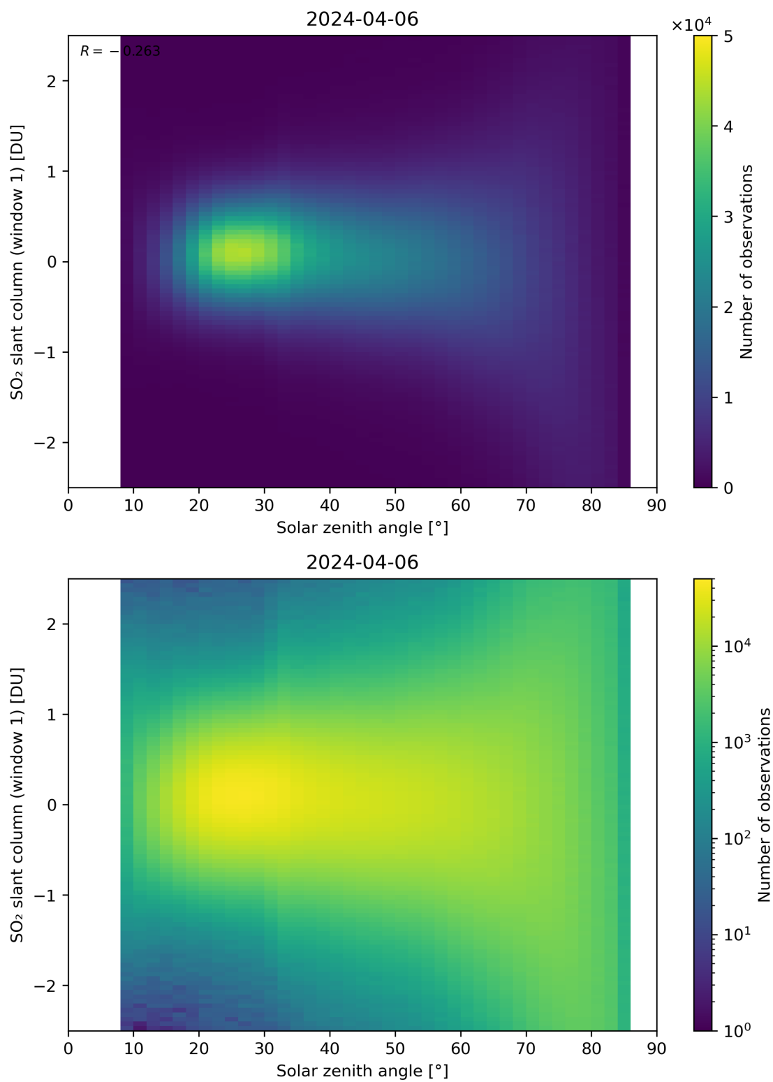
Figure 169: Scatter density plot of “Solar zenith angle” against “SO 2 slant column (window 1)” for 2024-04-05 to 2024-04-07.
