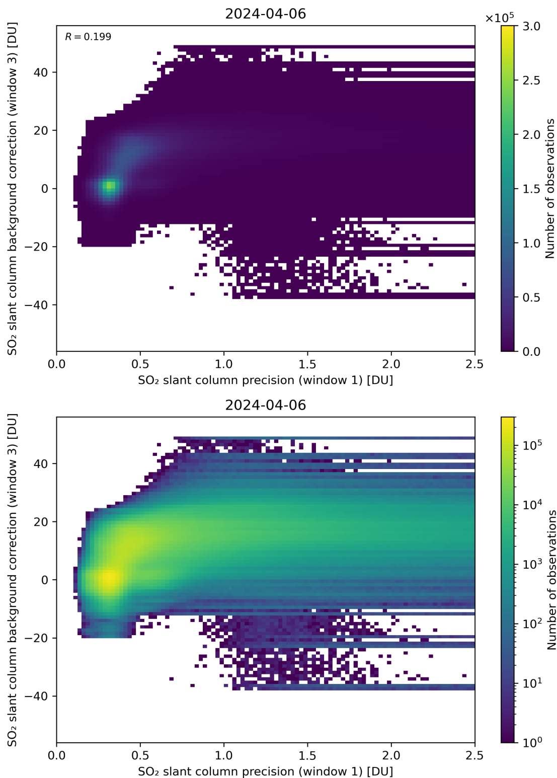
Figure 220: Scatter density plot of “SO 2 slant column precision (window 1)” against “SO 2 slant column background correction (window 3)” for 2024-04-05 to 2024-04-07.
