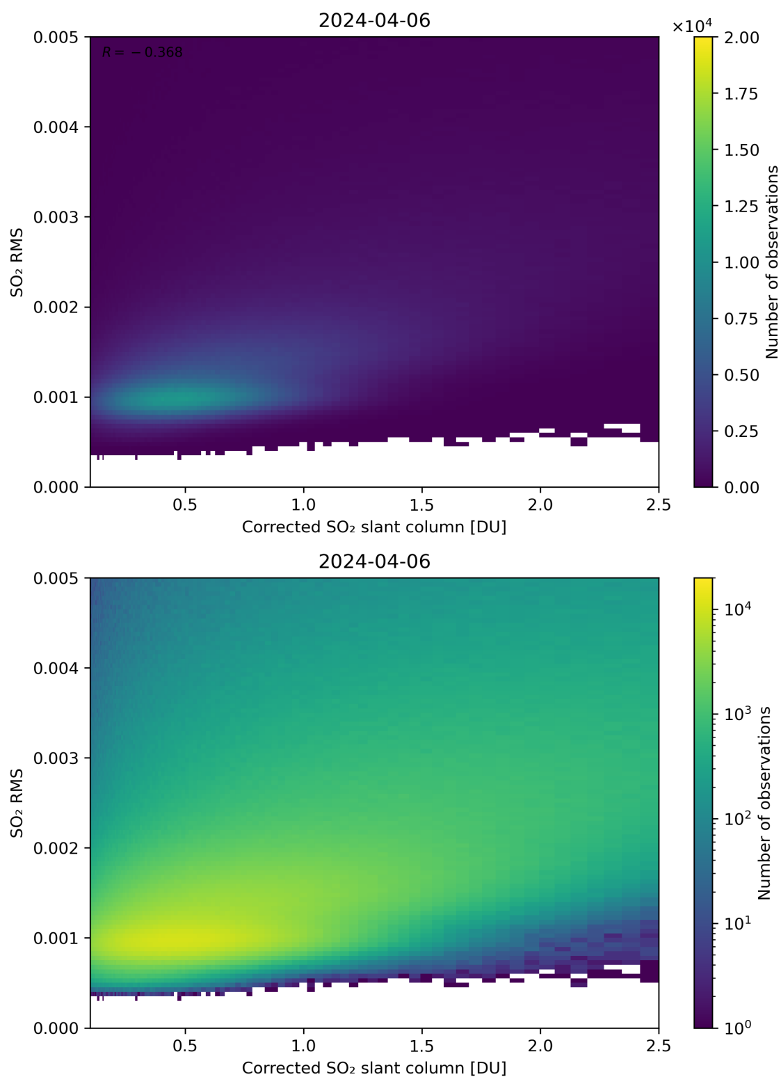
Figure 183: Scatter density plot of “Corrected SO 2 slant column” against “SO 2 RMS” for 2024-04-05 to 2024-04-07.
