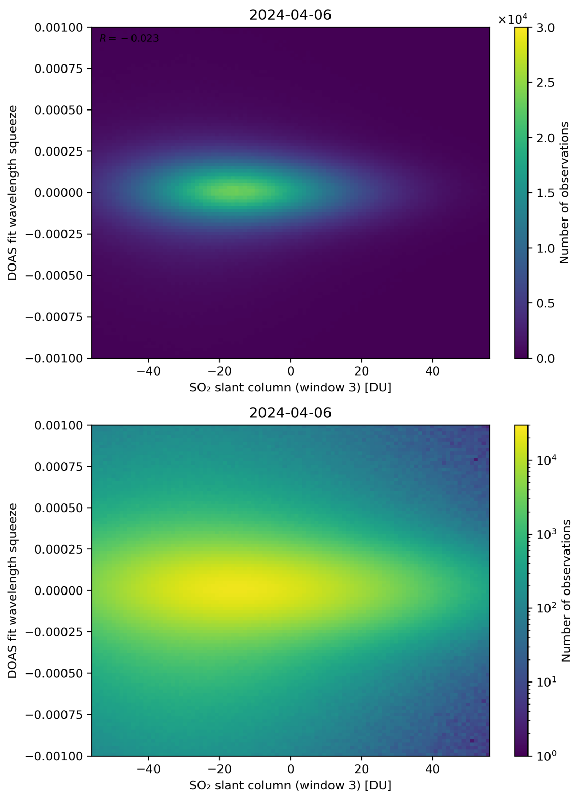
Figure 255: Scatter density plot of “SO 2 slant column (window 3)” against “DOAS fit wavelength squeeze” for 2024-04-05 to 2024-04-07.
