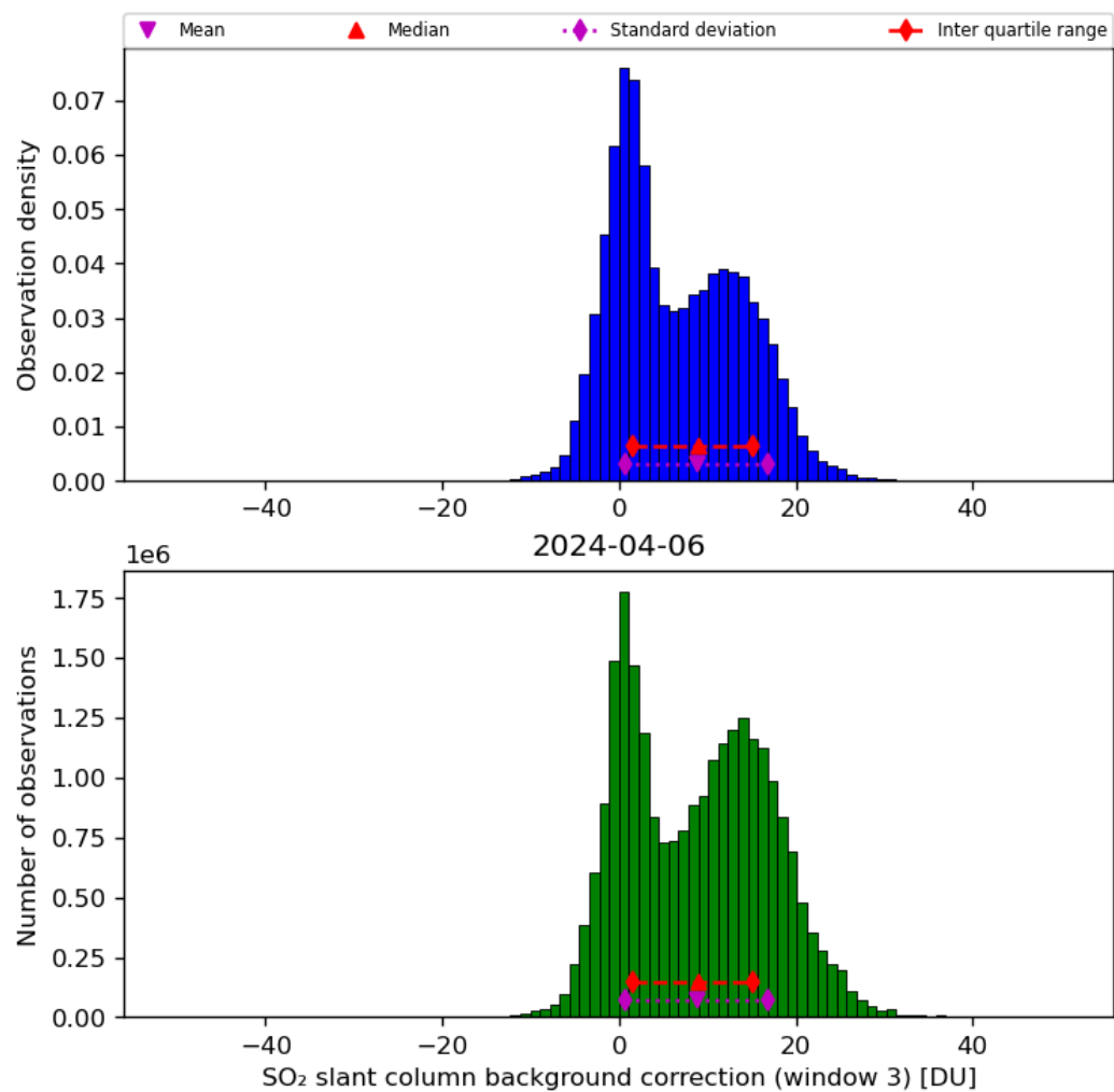
Figure 67: Histogram of “SO 2 slant column background correction (window 3)” for 2024-04-05 to 2024-04-07
