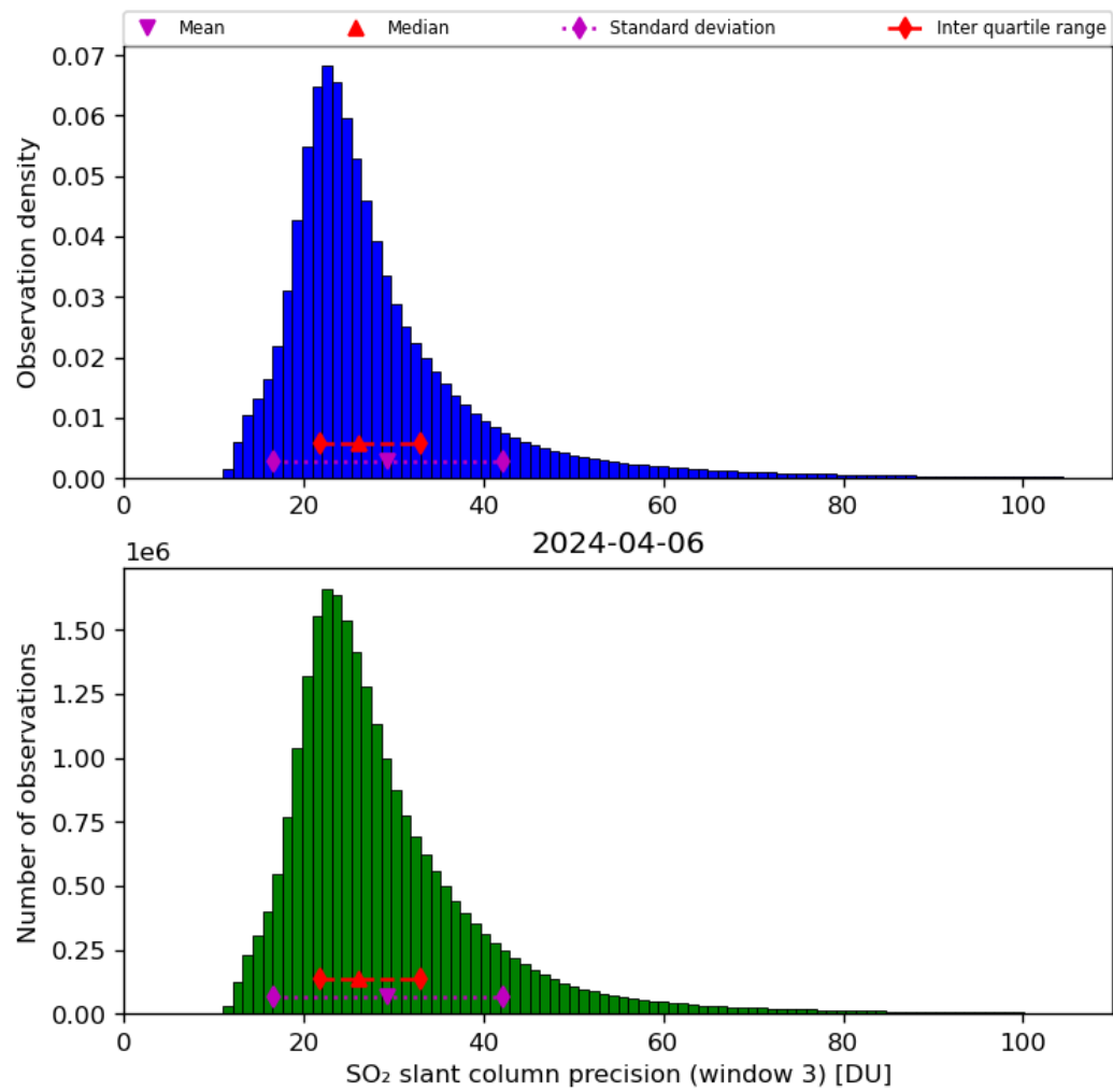
Figure 65: Histogram of “SO 2 slant column precision (window 3)” for 2024-04-05 to 2024-04-07
