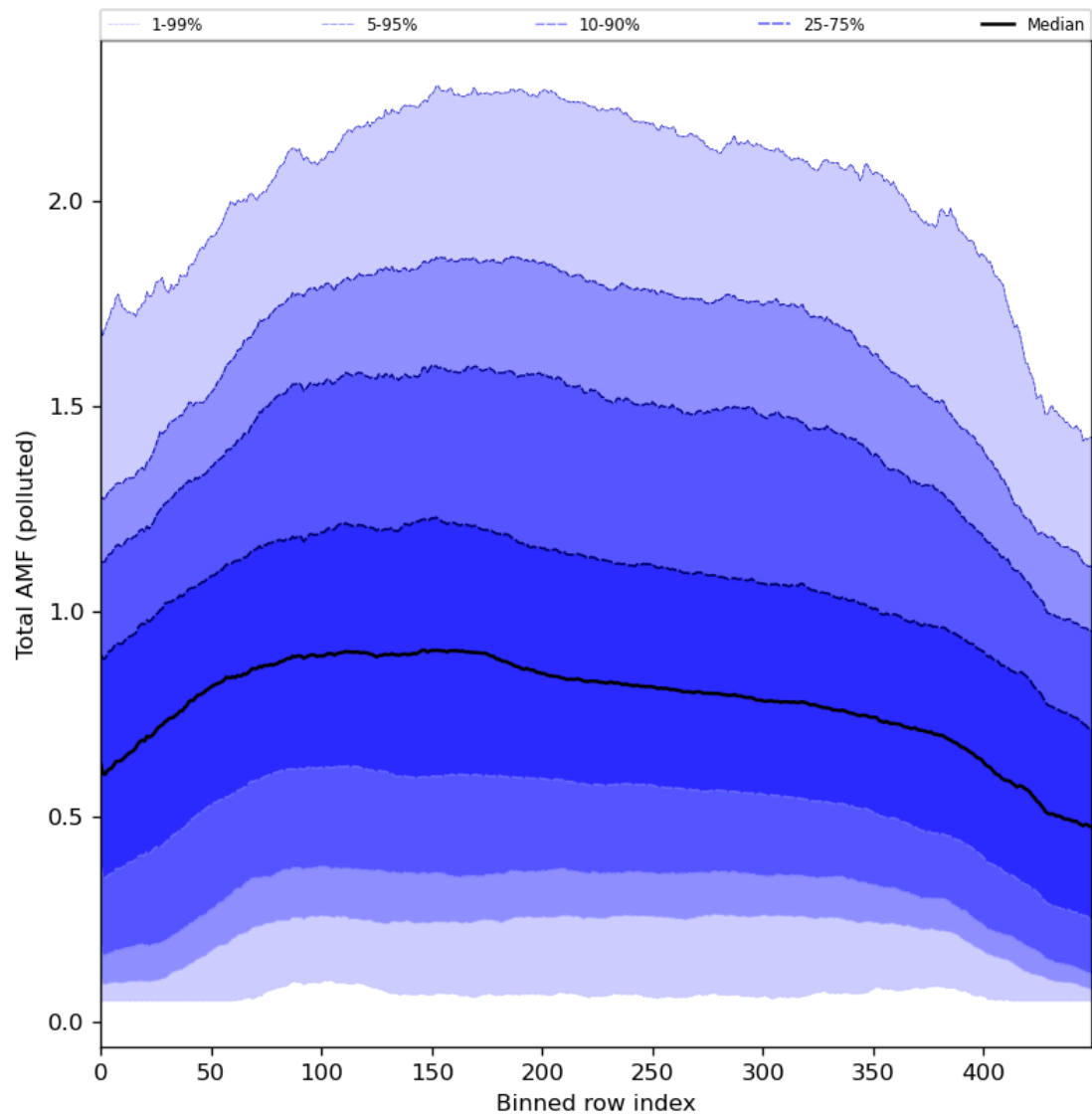
Figure 94: Along track statistics of “Total AMF (polluted)” for 2024-04-05 to 2024-04-07
