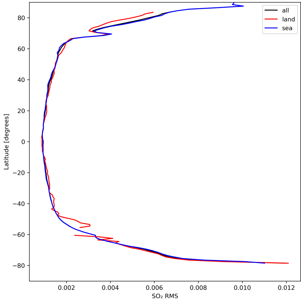
Figure 47: Zonal average of “SO 2 RMS” for 2024-04-05 to 2024-04-07.
