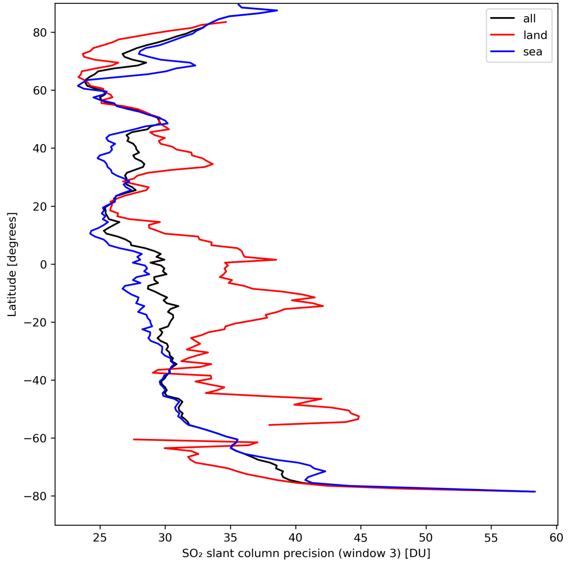
Figure 42: Zonal average of “SO 2 slant column precision (window 3)” for 2024-04-05 to 2024-04-07.
