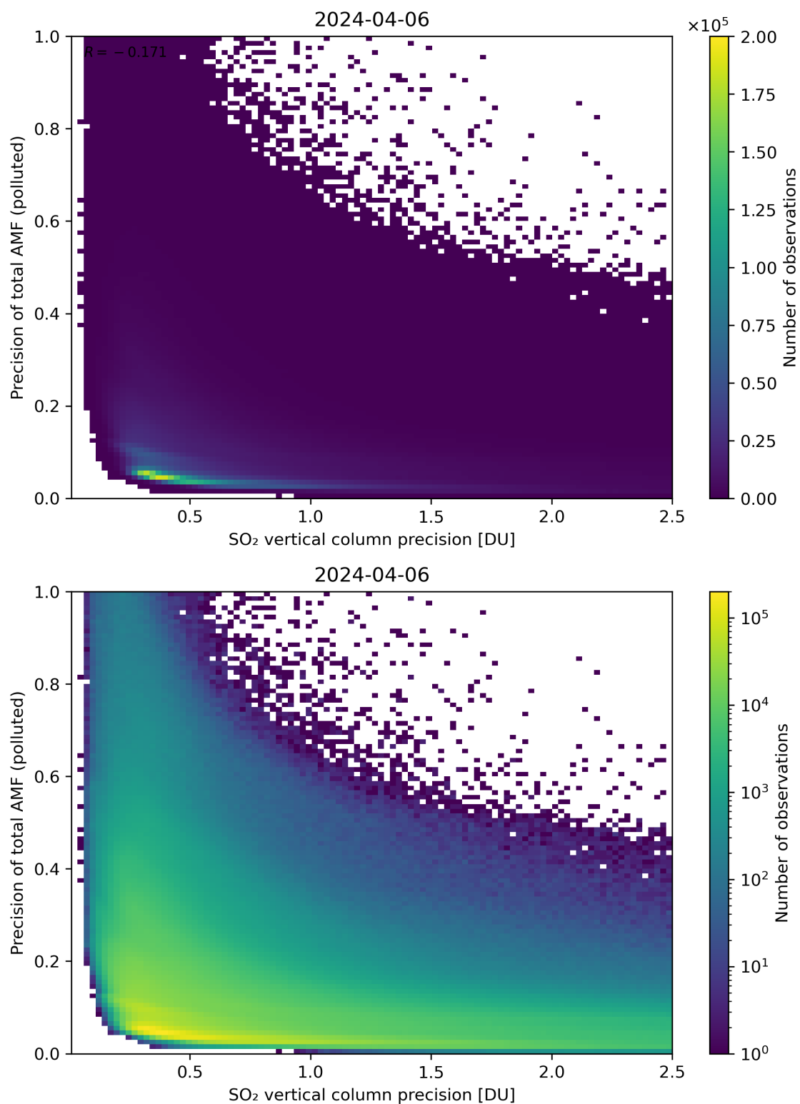
Figure 295: Scatter density plot of “SO 2 vertical column precision” against “Precision of total AMF (polluted)” for 2024-04-05 to 2024-04-07.
