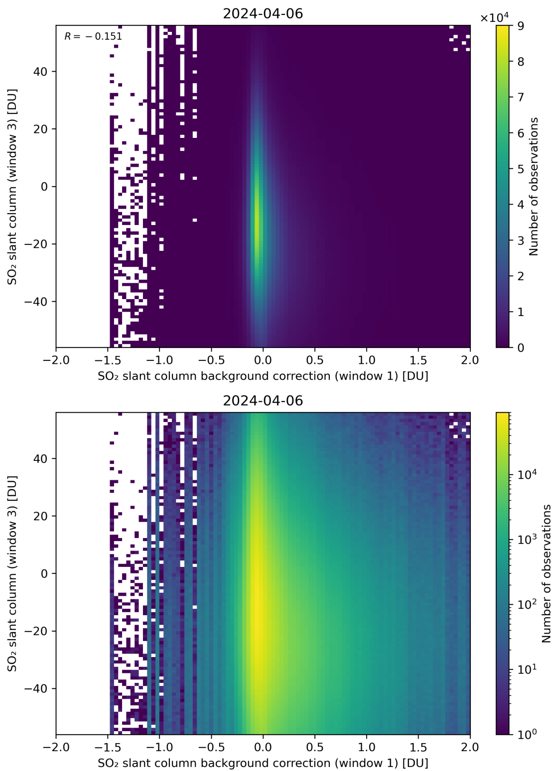
Figure 107: Scatter density plot of “SO 2 slant column background correction (window 1)” against “SO 2 slant column (window 3)” for 2024-04-05 to 2024-04-07.
