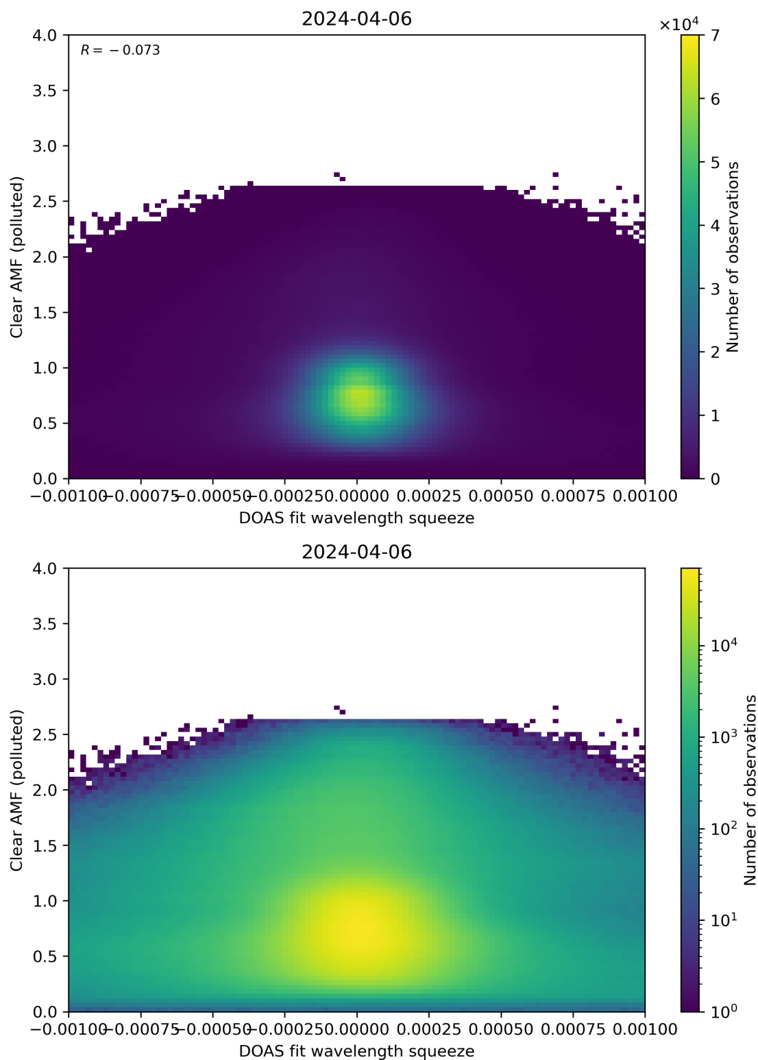
Figure 133: Scatter density plot of “DOAS fit wavelength squeeze” against “Clear AMF (polluted)” for 2024-04-05 to 2024-04-07.
