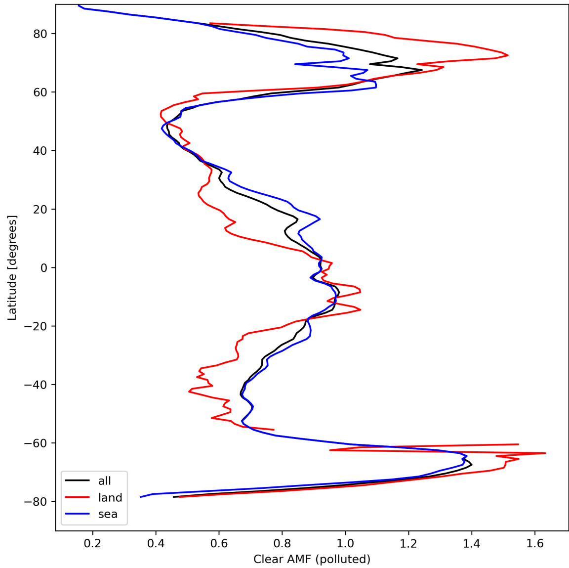
Figure 50: Zonal average of “Clear AMF (polluted)” for 2024-04-05 to 2024-04-07.
