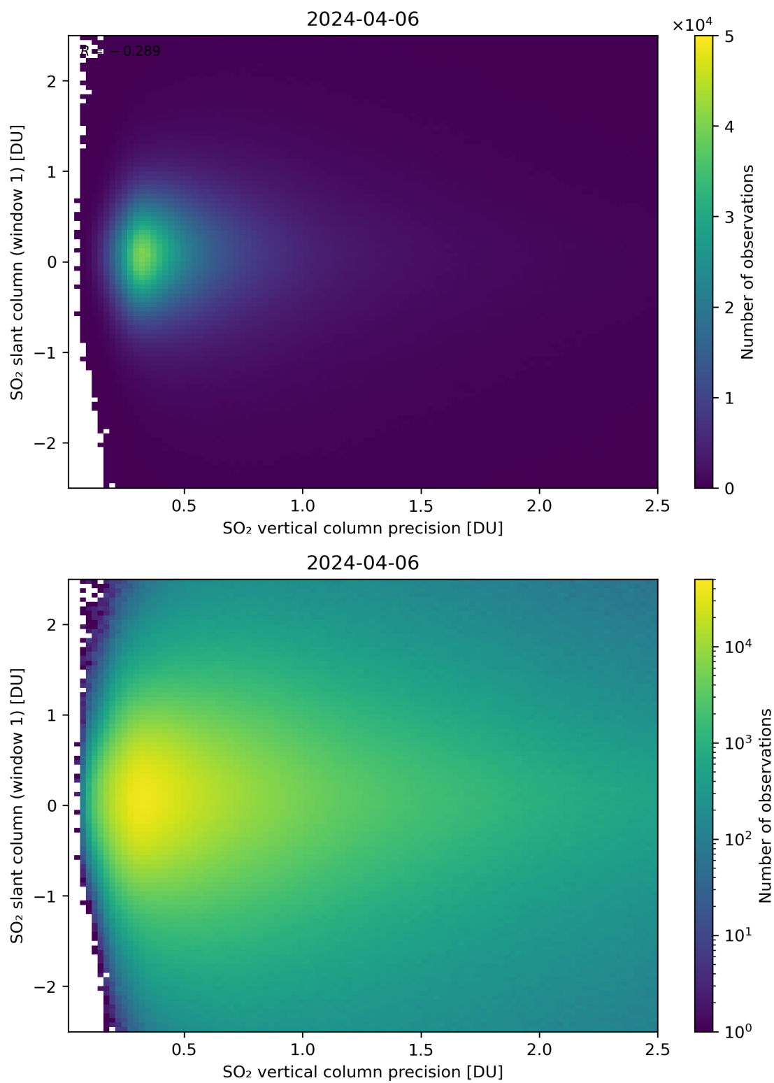
Figure 289: Scatter density plot of “SO 2 vertical column precision” against “SO 2 slant column (window 1)” for 2024-04-05 to 2024-04-07.
