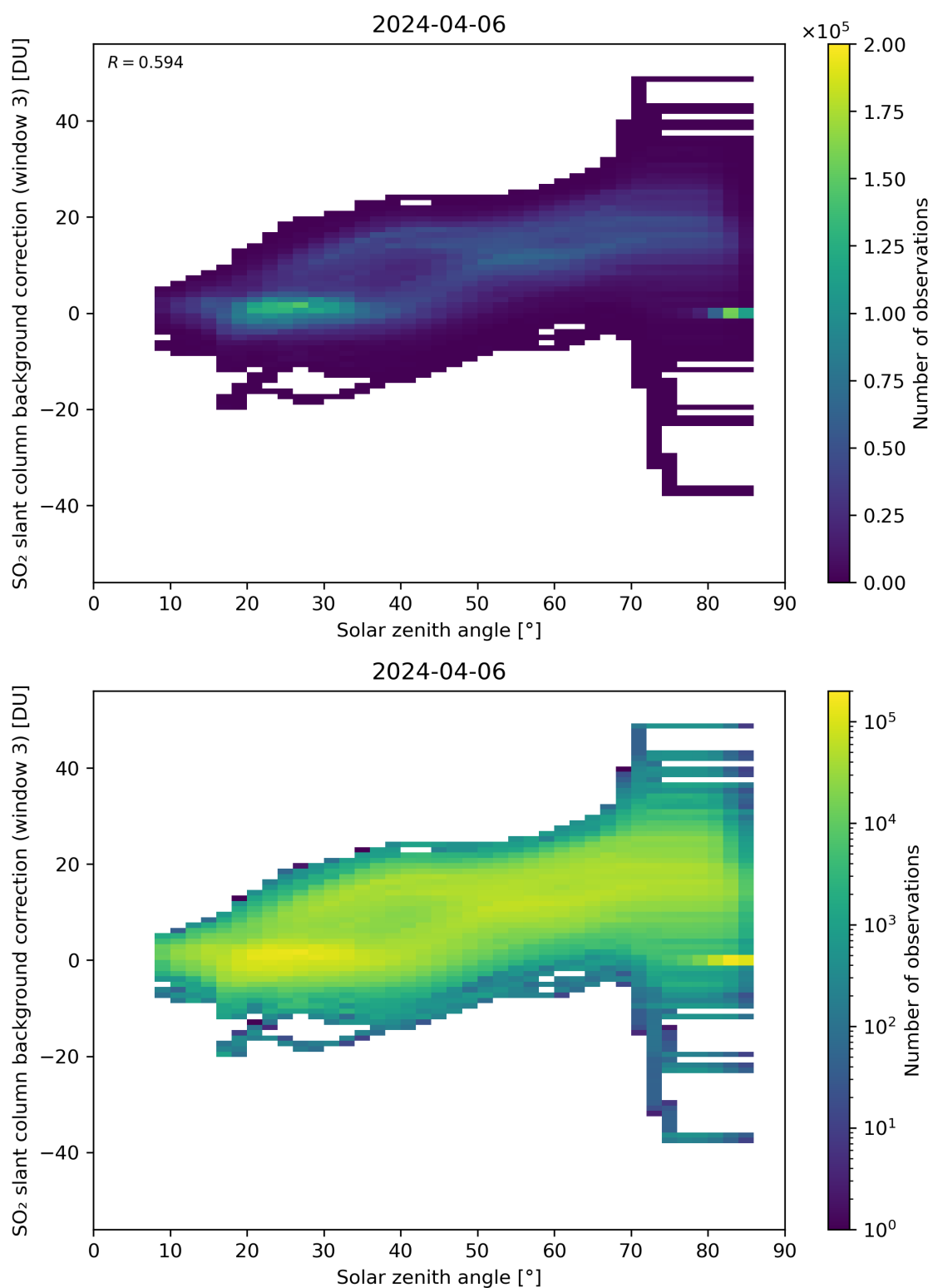
Figure 160: Scatter density plot of “Solar zenith angle” against “SO 2 slant column background correction (window 3)” for 2024-04-05 to 2024-04-07.
