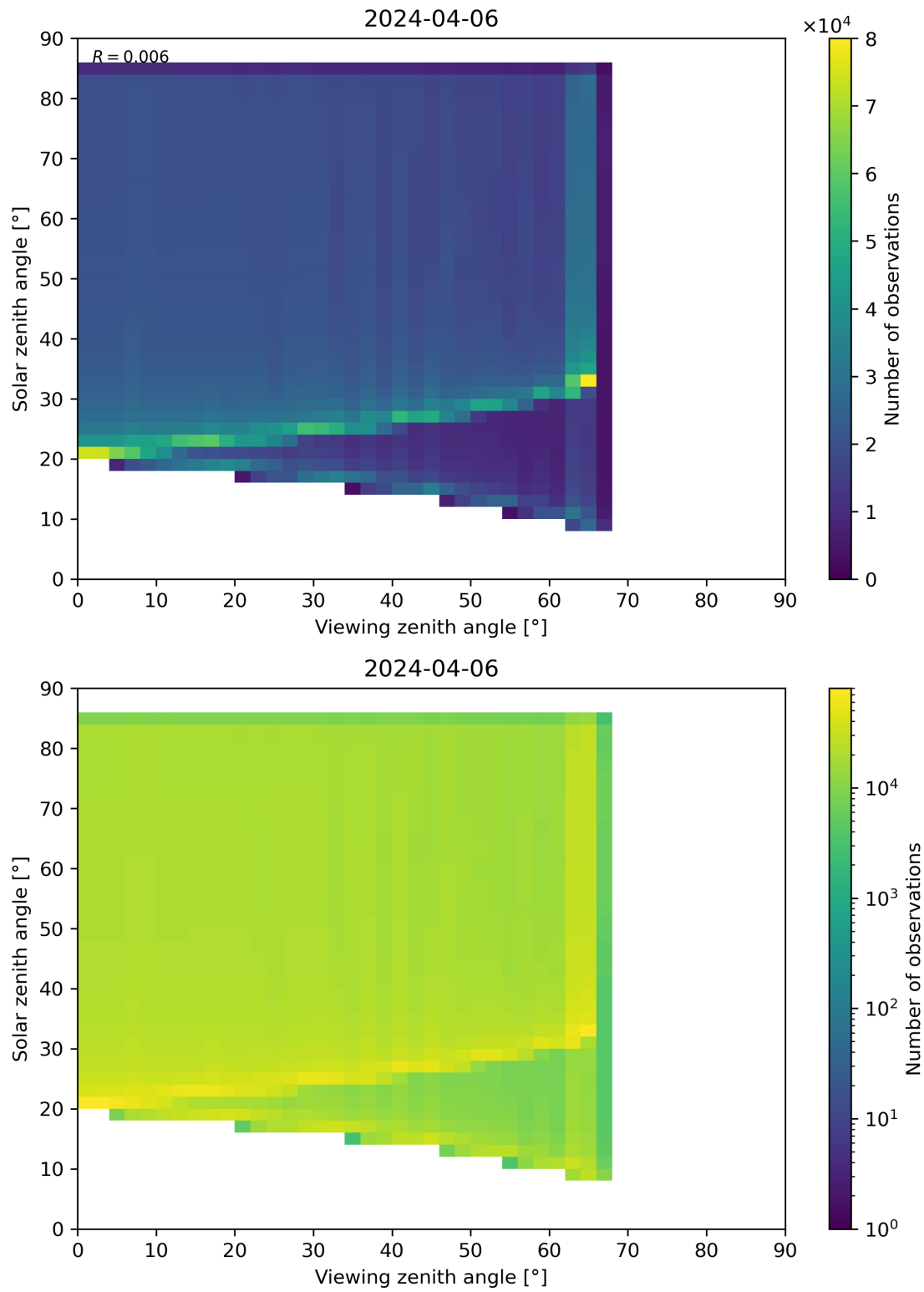
Figure 315: Scatter density plot of “Viewing zenith angle” against “Solar zenith angle” for 2024-04-05 to 2024-04-07.
