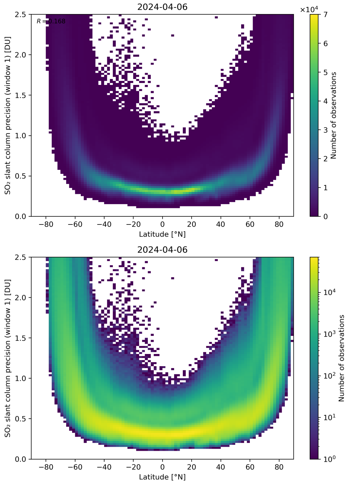
Figure 150: Scatter density plot of “Latitude” against “SO 2 slant column precision (window 1)” for 2024-04-05 to 2024-04-07.
