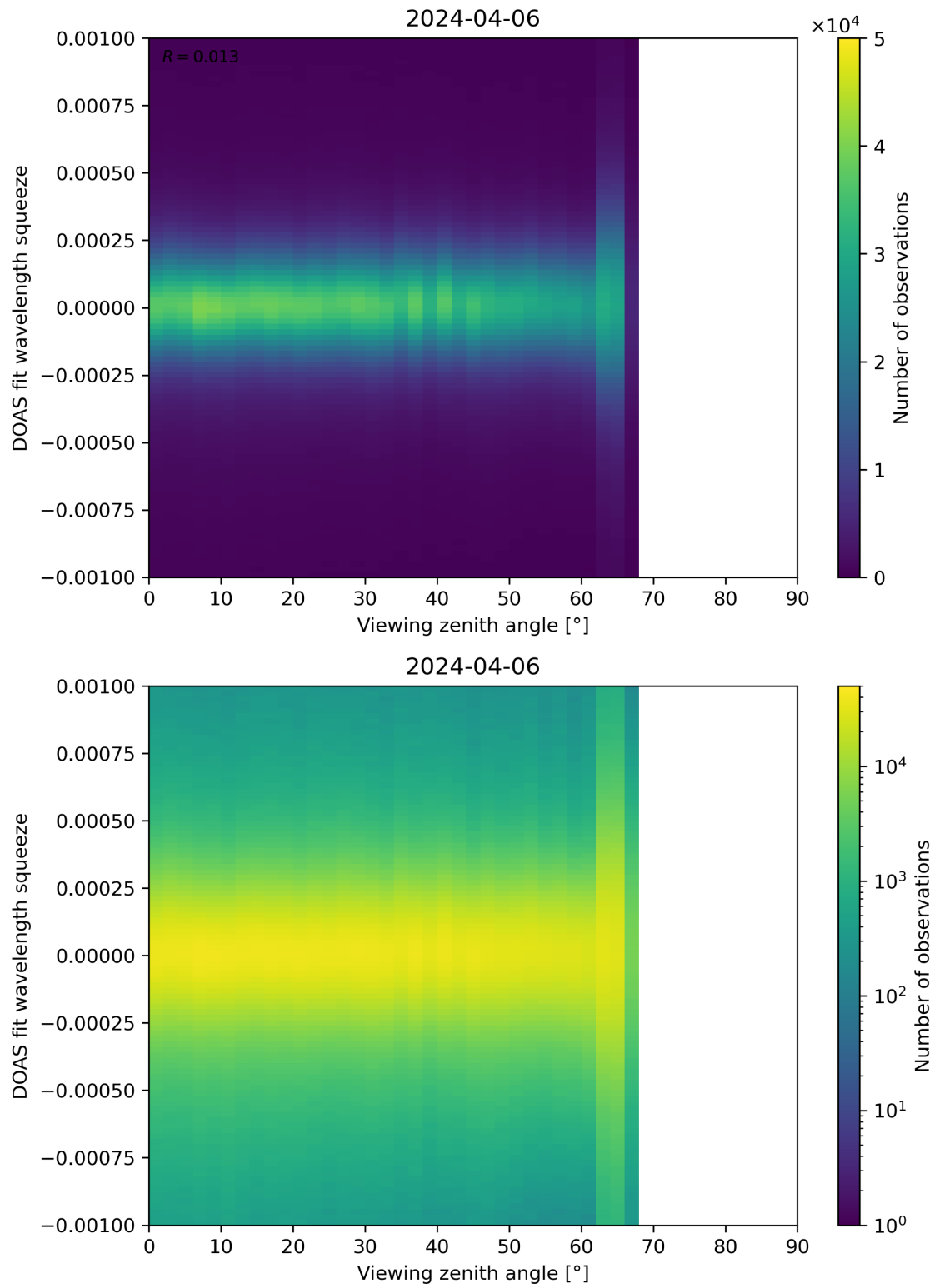
Figure 312: Scatter density plot of “Viewing zenith angle” against “DOAS fit wavelength squeeze” for 2024-04-05 to 2024-04-07.
