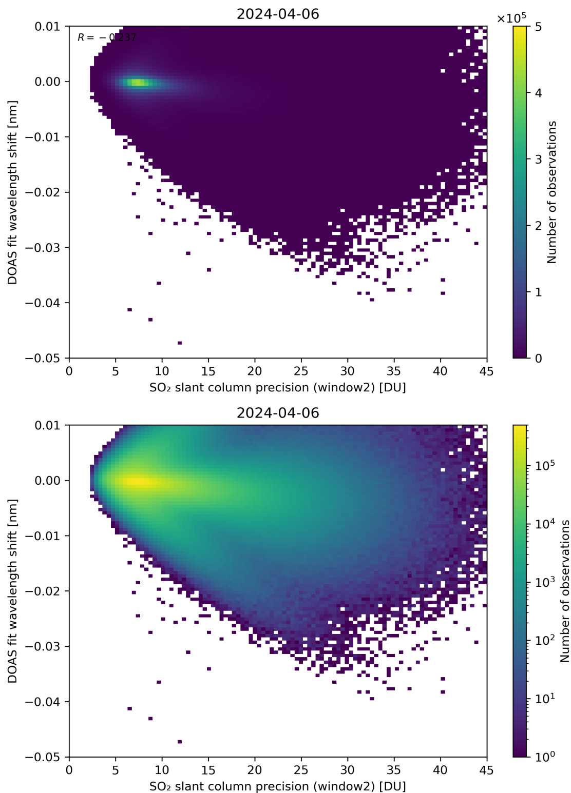
Figure 243: Scatter density plot of “SO 2 slant column precision (window2)” against “DOAS fit wavelength shift” for 2024-04-05 to 2024-04-07.
