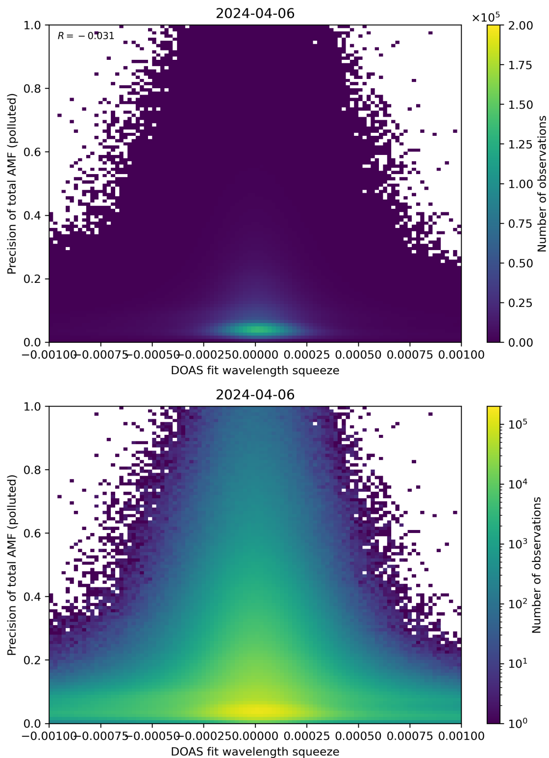
Figure 135: Scatter density plot of “DOAS fit wavelength squeeze” against “Precision of total AMF (polluted)” for 2024-04-05 to 2024-04-07.
