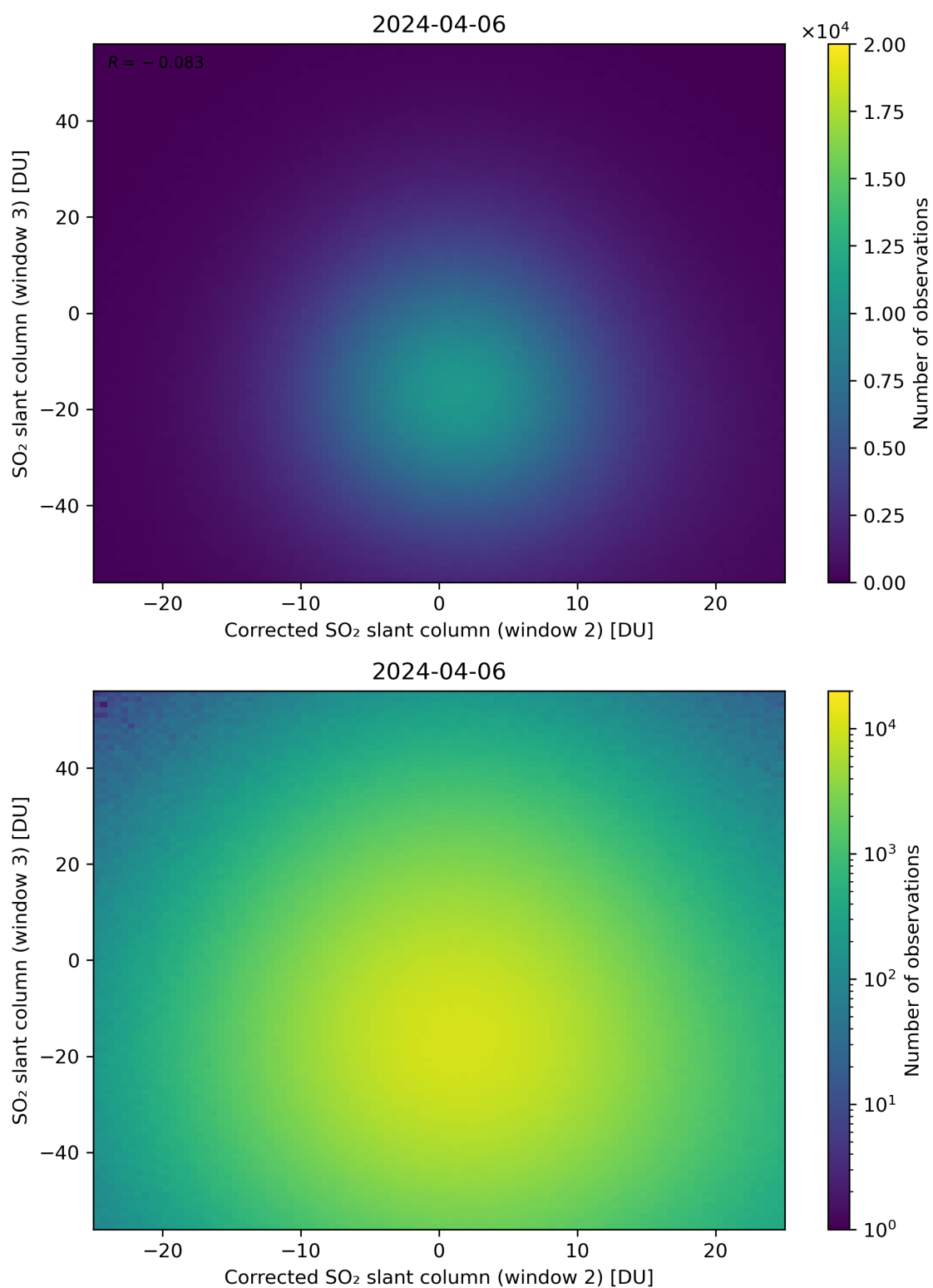
Figure 201: Scatter density plot of “Corrected SO 2 slant column (window 2)” against “SO 2 slant column (window 3)” for 2024-04-05 to 2024-04-07.
