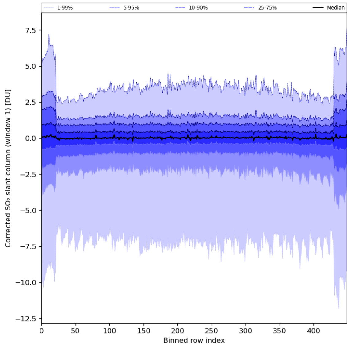
Figure 81: Along track statistics of “Corrected SO 2 slant column (window 1)” for 2024-04-05 to 2024-04-07
