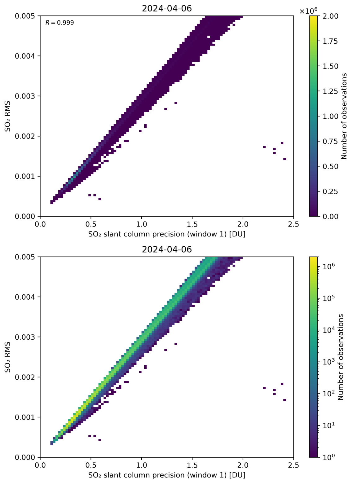
Figure 223: Scatter density plot of “SO 2 slant column precision (window 1)” against “SO 2 RMS” for 2024-04-05 to 2024-04-07.
