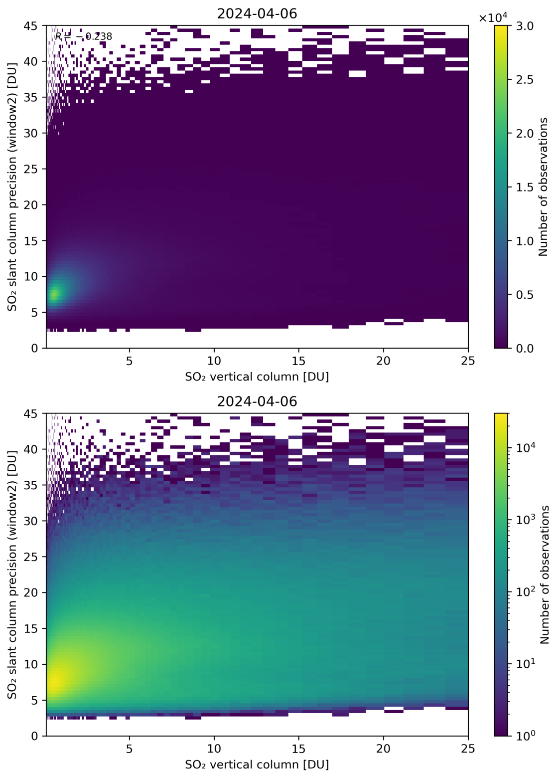
Figure 302: Scatter density plot of “SO 2 vertical column” against “SO 2 slant column precision (window2)” for 2024-04-05 to 2024-04-07.
