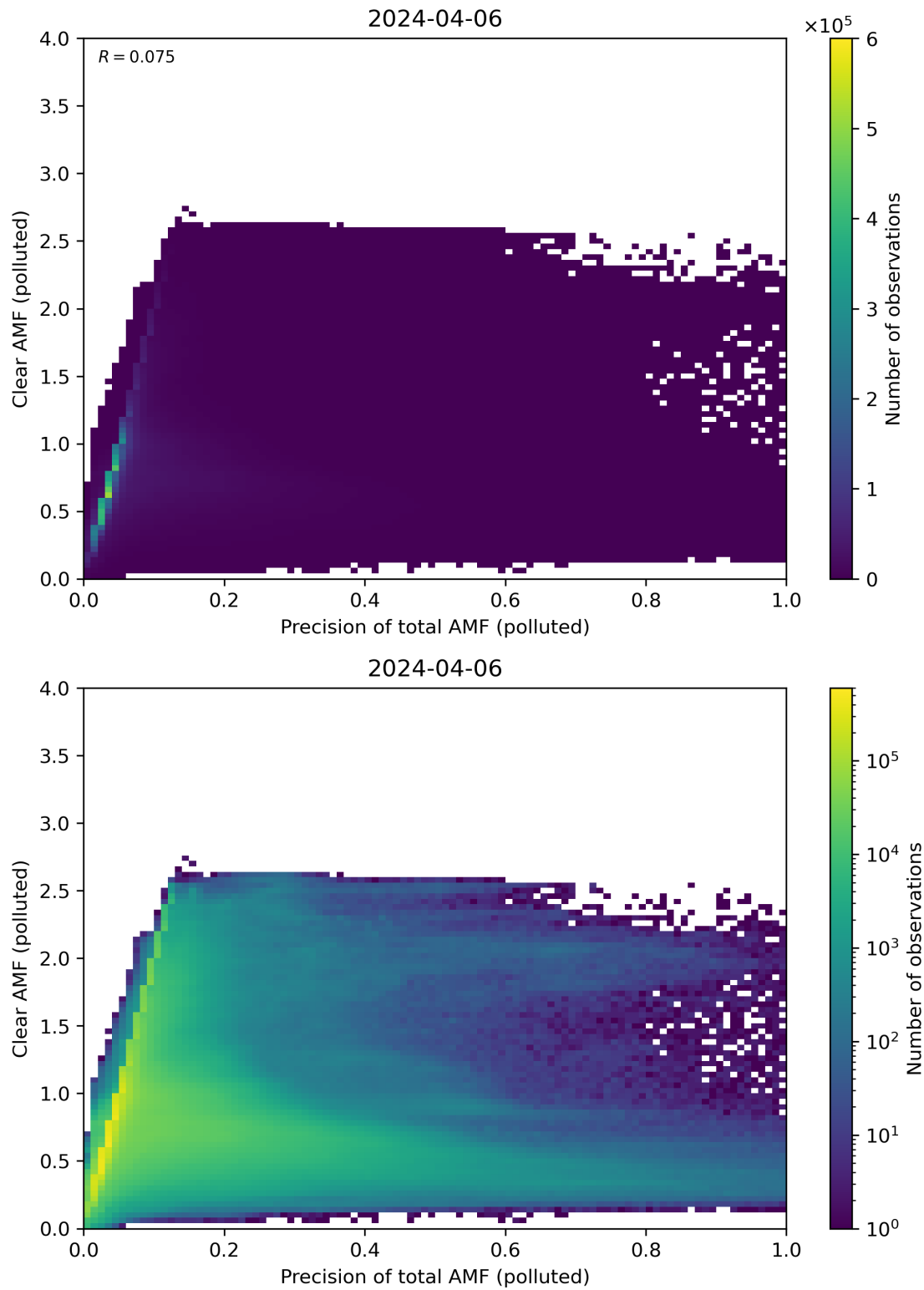
Figure 270: Scatter density plot of “Precision of total AMF (polluted)” against “Clear AMF (polluted)” for 2024-04-05 to 2024-04-07.
