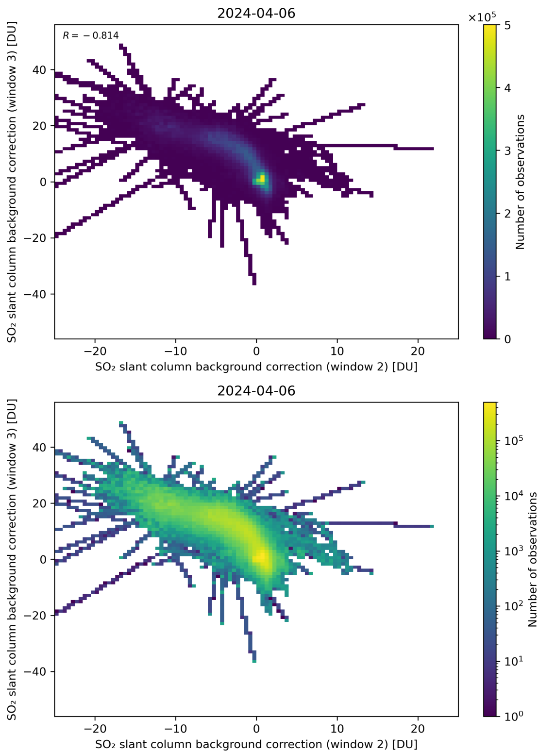
Figure 111: Scatter density plot of “SO 2 slant column background correction (window 2)” against “SO 2 slant column background correction (window 3)” for 2024-04-05 to 2024-04-07.
