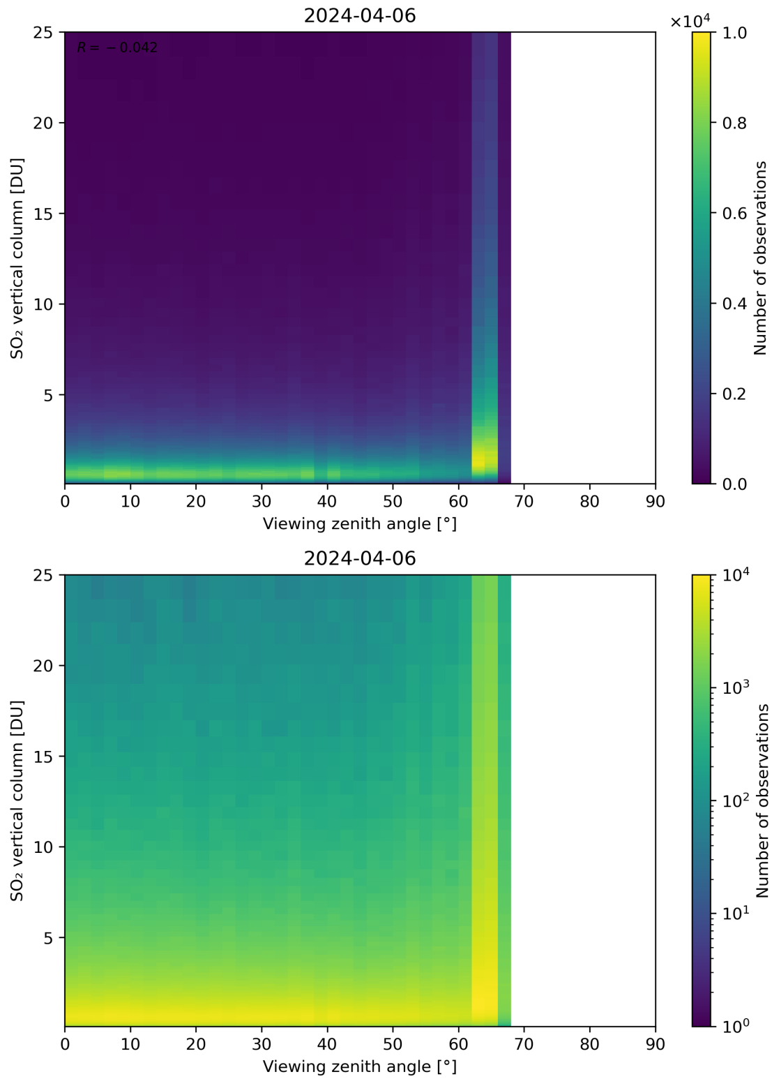
Figure 327: Scatter density plot of “Viewing zenith angle” against “SO 2 vertical column” for 2024-04-05 to 2024-04-07.
