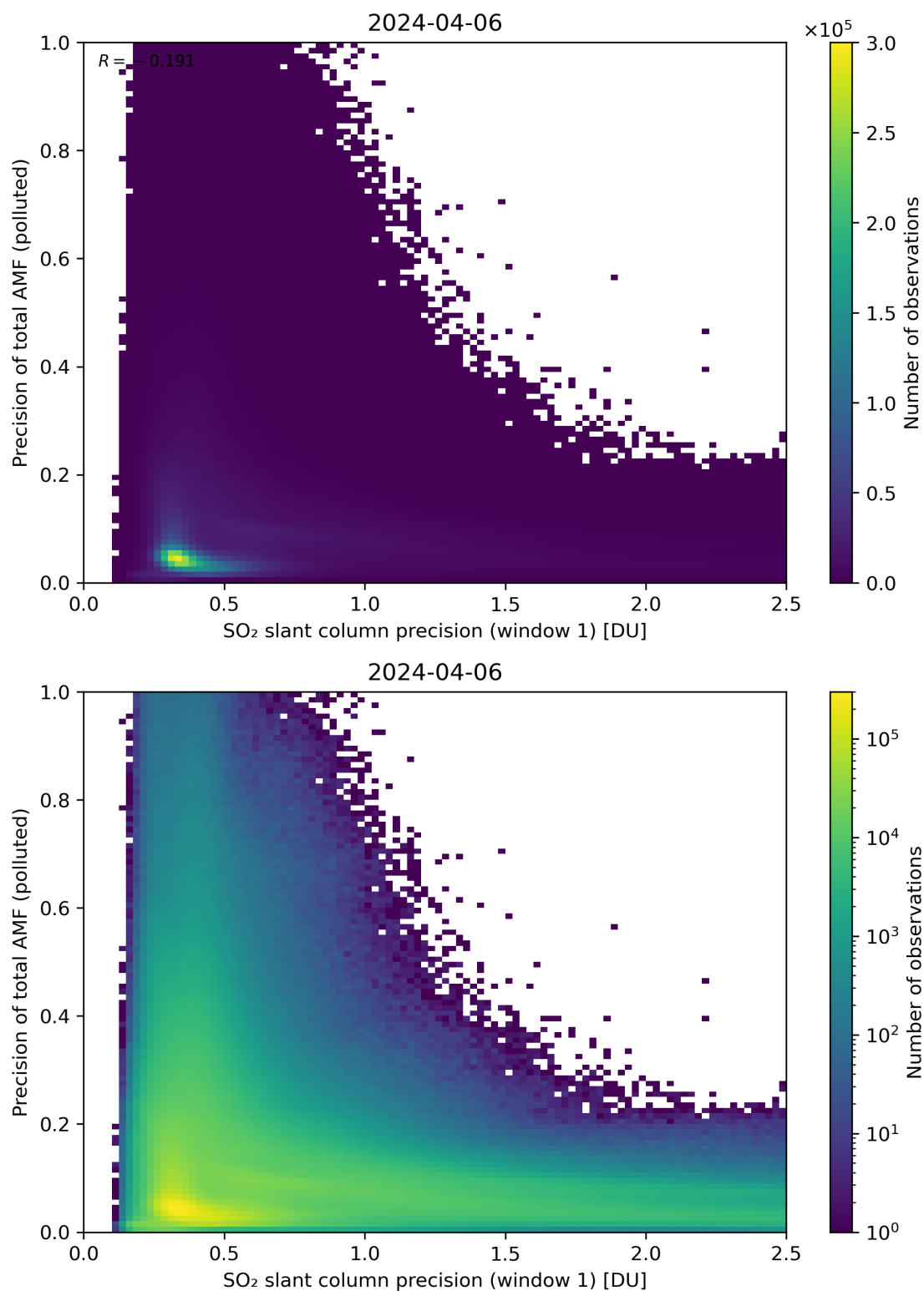
Figure 231: Scatter density plot of “SO 2 slant column precision (window 1)” against “Precision of total AMF (polluted)” for 2024-04-05 to 2024-04-07.
