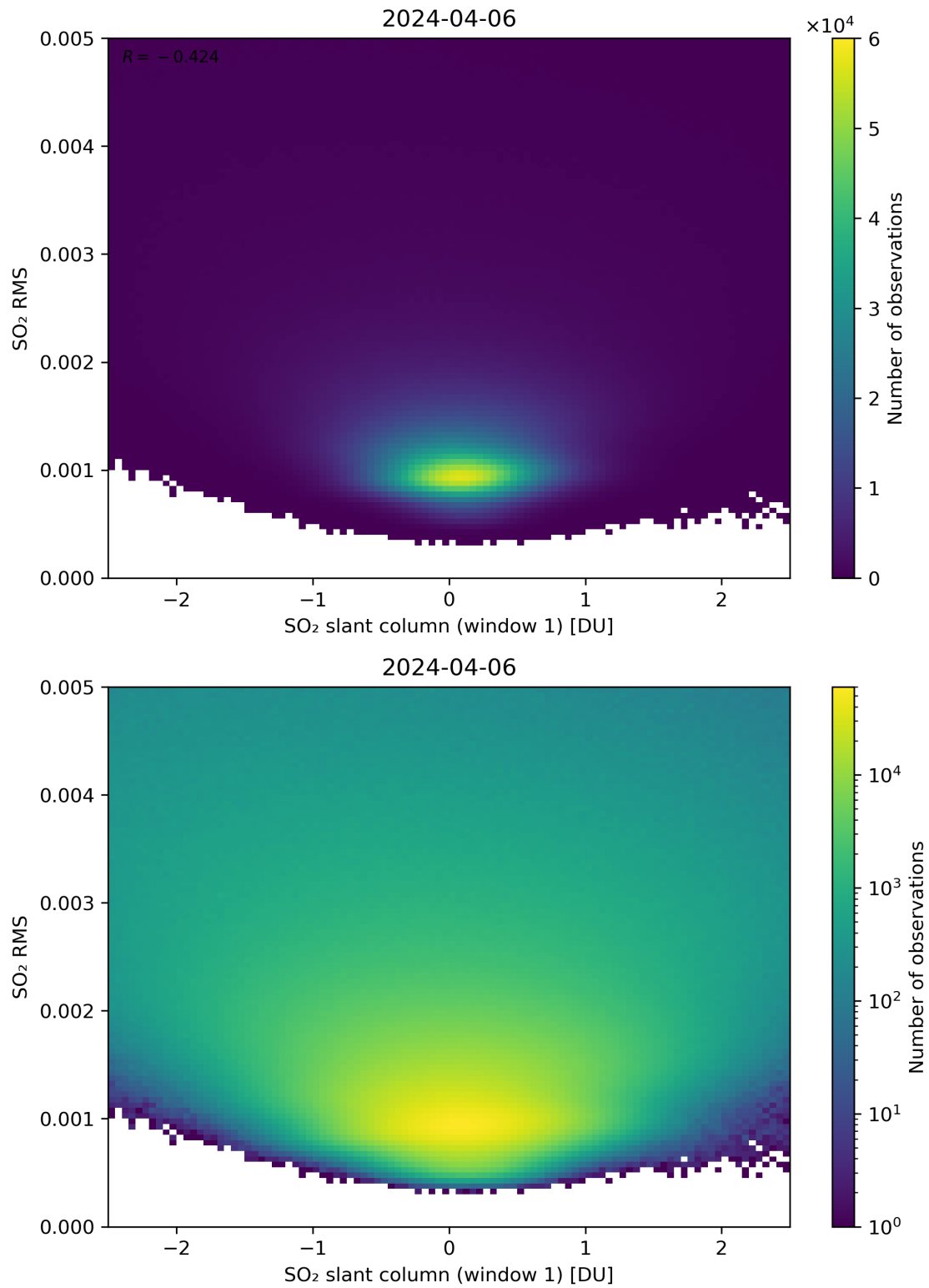
Figure 217: Scatter density plot of “SO 2 slant column (window 1)” against “SO 2 RMS” for 2024-04-05 to 2024-04-07.
