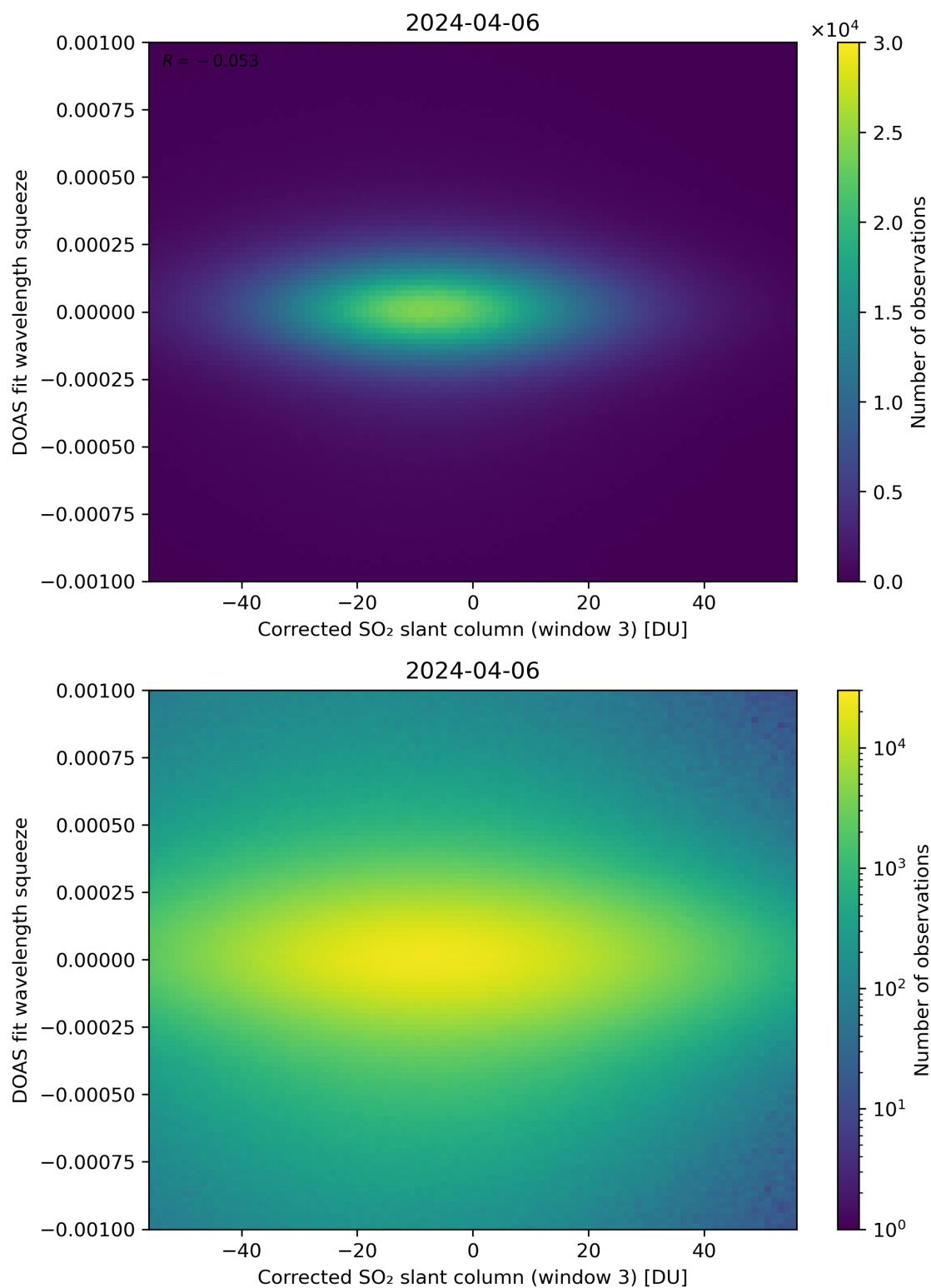
Figure 207: Scatter density plot of “Corrected SO 2 slant column (window 3)” against “DOAS fit wavelength squeeze” for 2024-04-05 to 2024-04-07.
