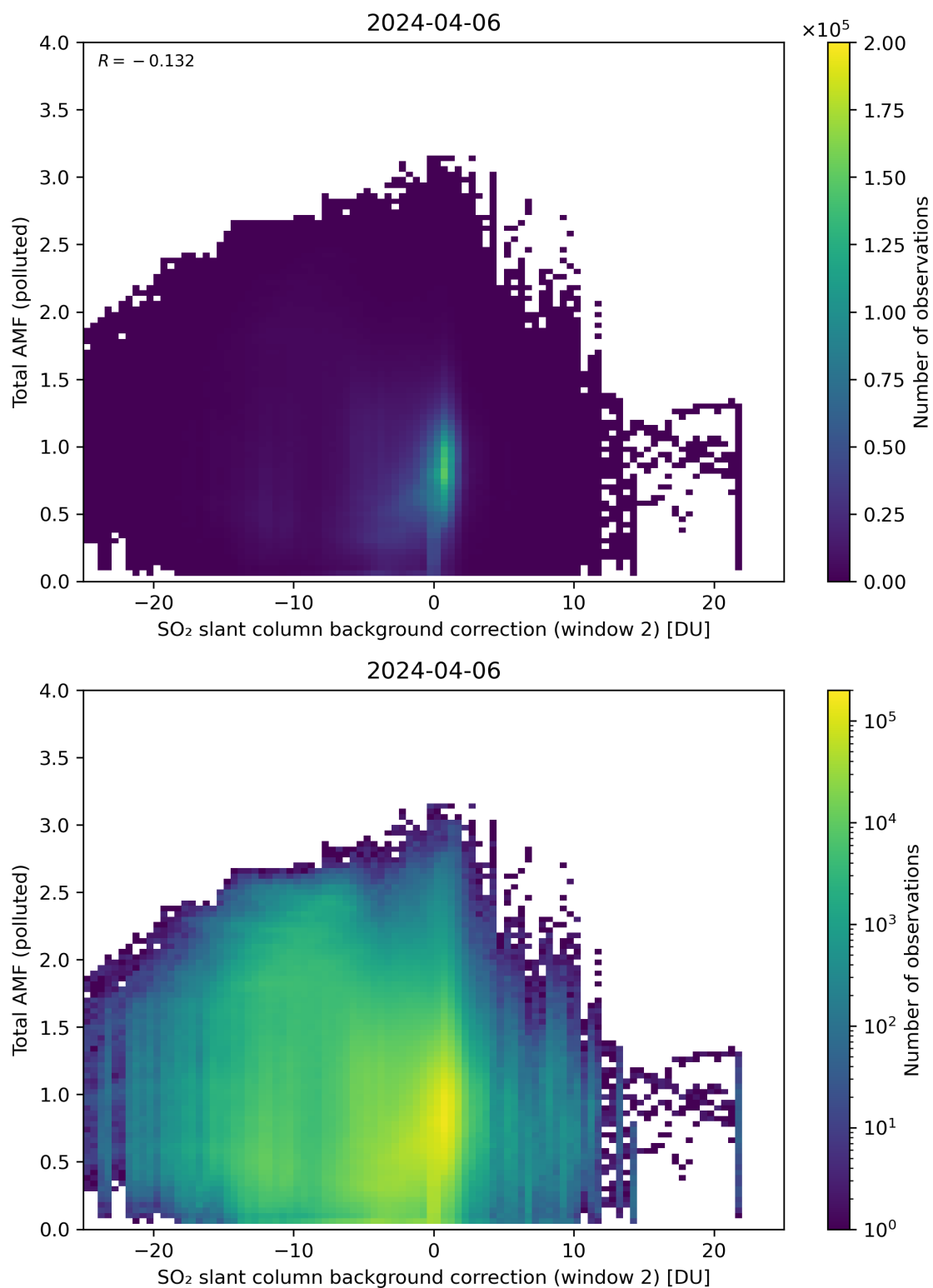
Figure 119: Scatter density plot of “SO 2 slant column background correction (window 2)” against “Total AMF (polluted)” for 2024-04-05 to 2024-04-07.
