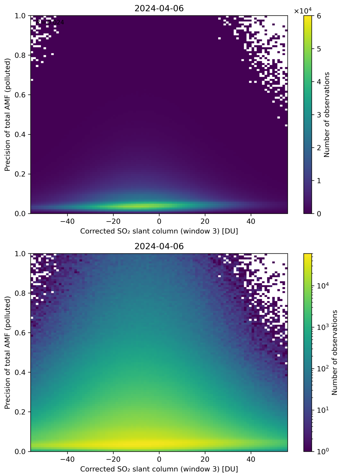
Figure 211: Scatter density plot of “Corrected SO 2 slant column (window 3)” against “Precision of total AMF (polluted)” for 2024-04-05 to 2024-04-07.
