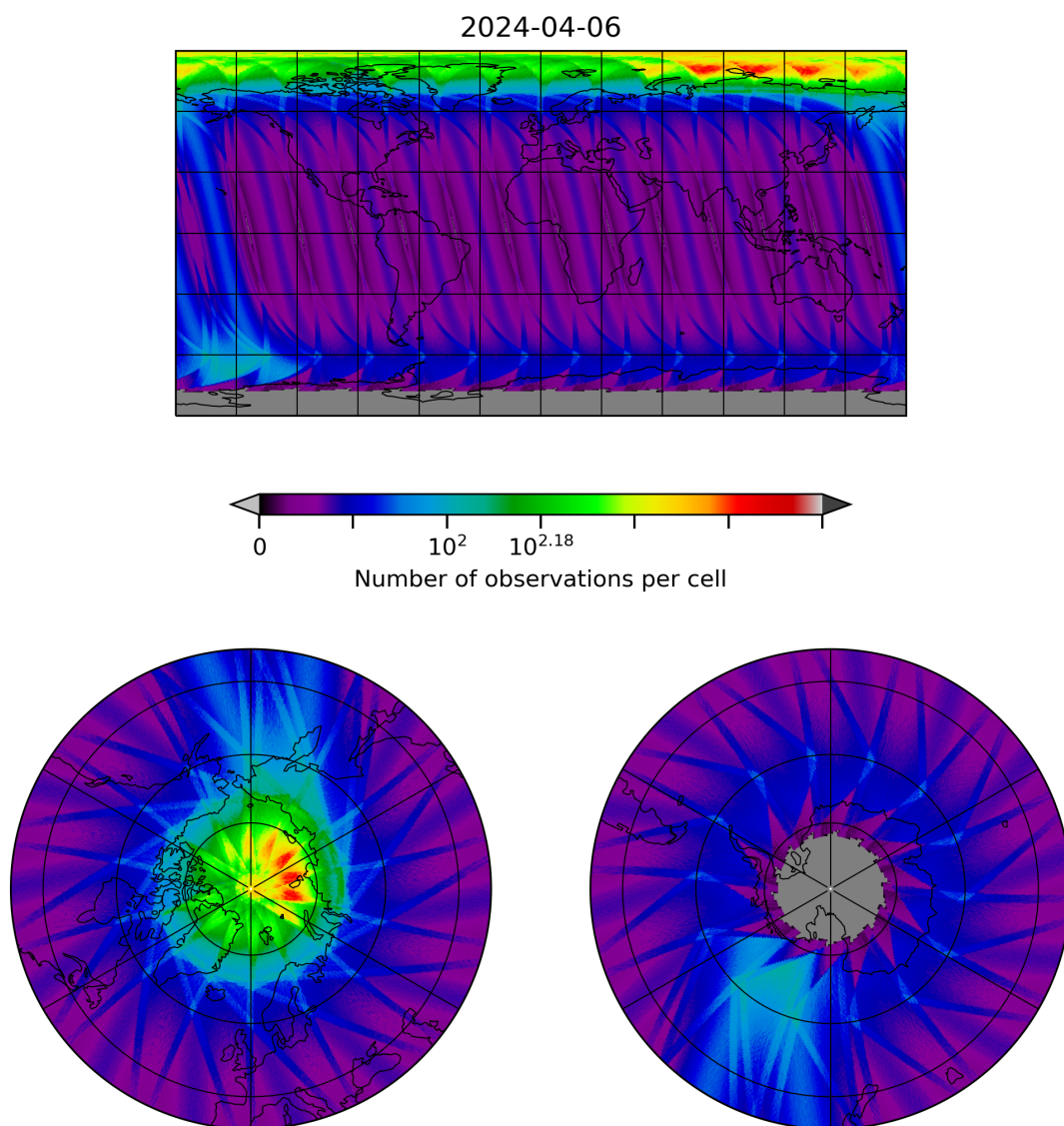
Figure 28: Map of the number of observations for 2024-04-05 to 2024-04-07
