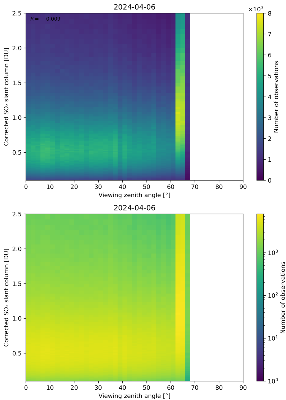
Figure 317: Scatter density plot of “Viewing zenith angle” against “Corrected SO 2 slant column” for 2024-04-05 to 2024-04-07.
