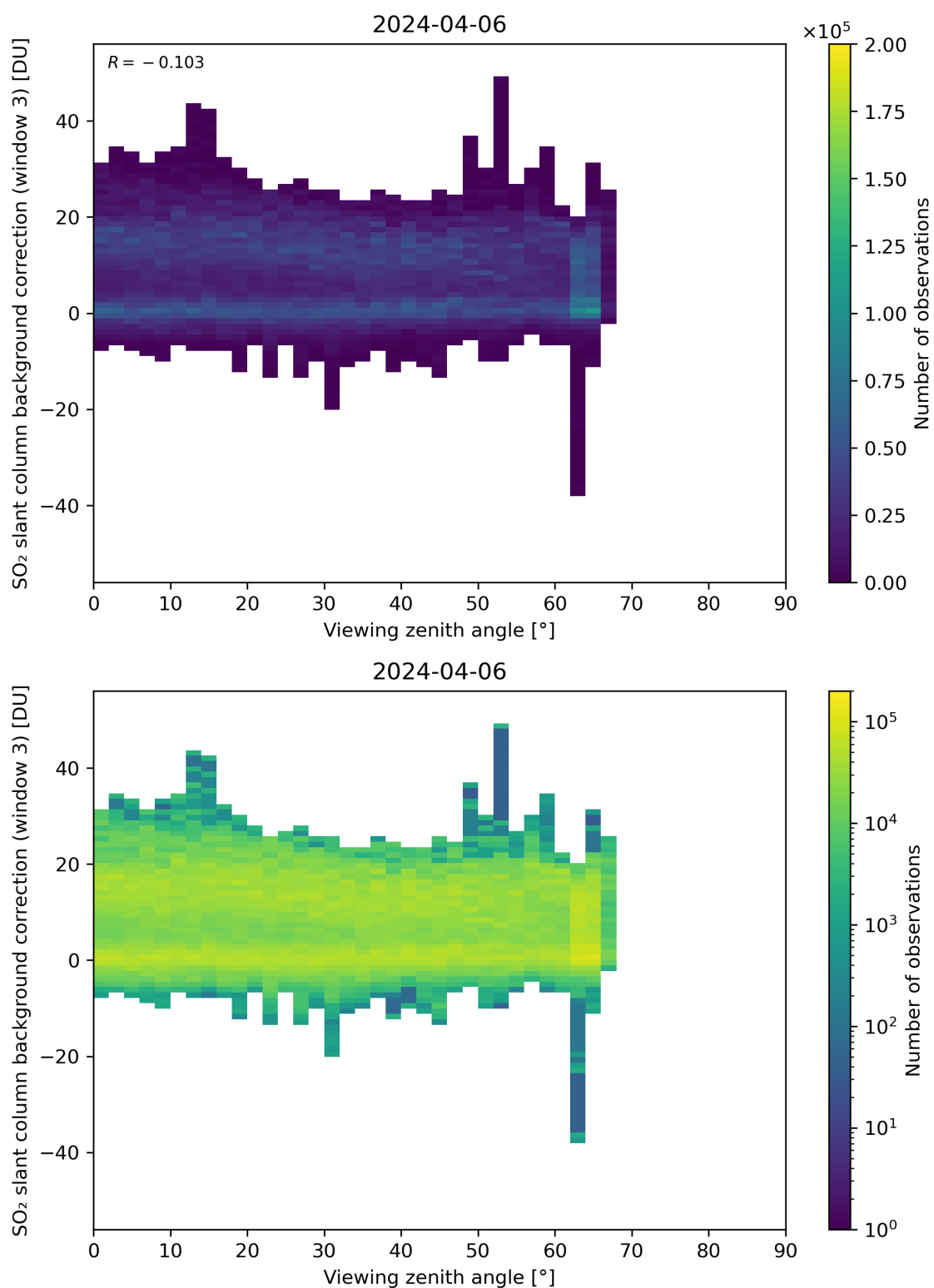
Figure 310: Scatter density plot of “Viewing zenith angle” against “SO 2 slant column background correction (window 3)” for 2024-04-05 to 2024-04-07.
