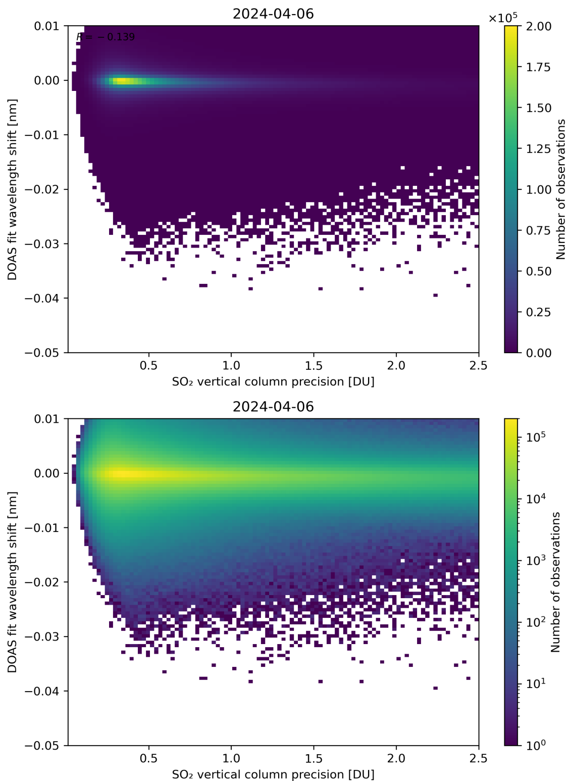
Figure 282: Scatter density plot of “SO 2 vertical column precision” against “DOAS fit wavelength shift” for 2024-04-05 to 2024-04-07.
