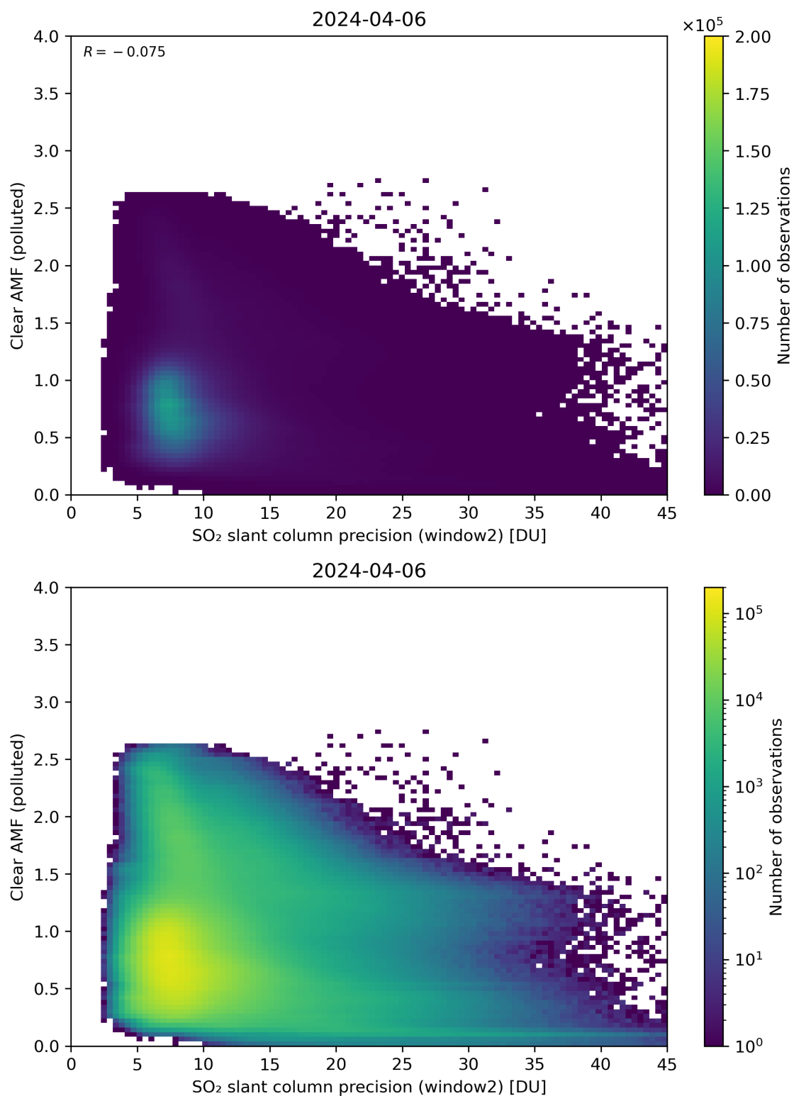
Figure 246: Scatter density plot of “SO 2 slant column precision (window2)” against “Clear AMF (polluted)” for 2024-04-05 to 2024-04-07.
