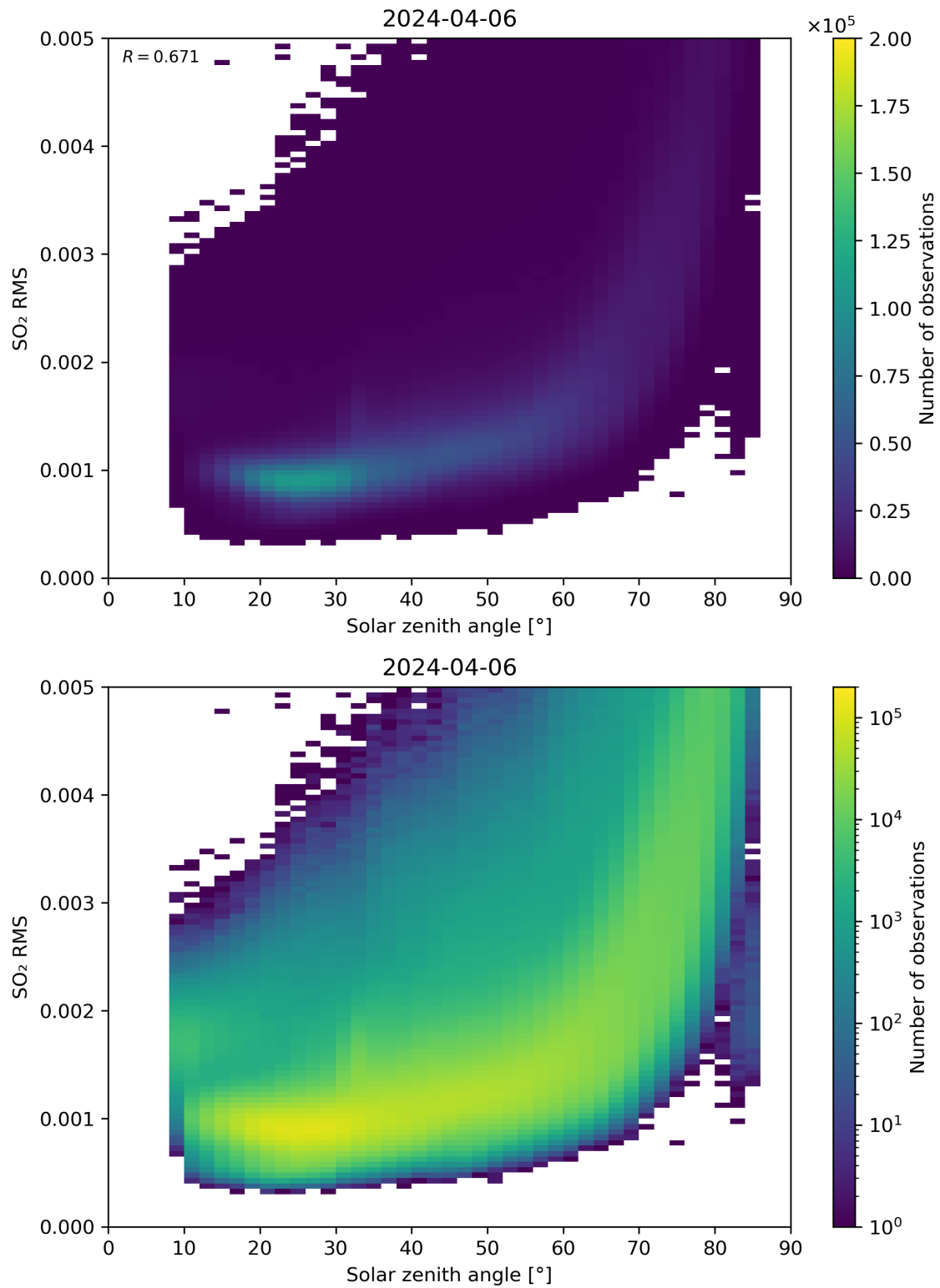
Figure 163: Scatter density plot of “Solar zenith angle” against “SO 2 RMS” for 2024-04-05 to 2024-04-07.
