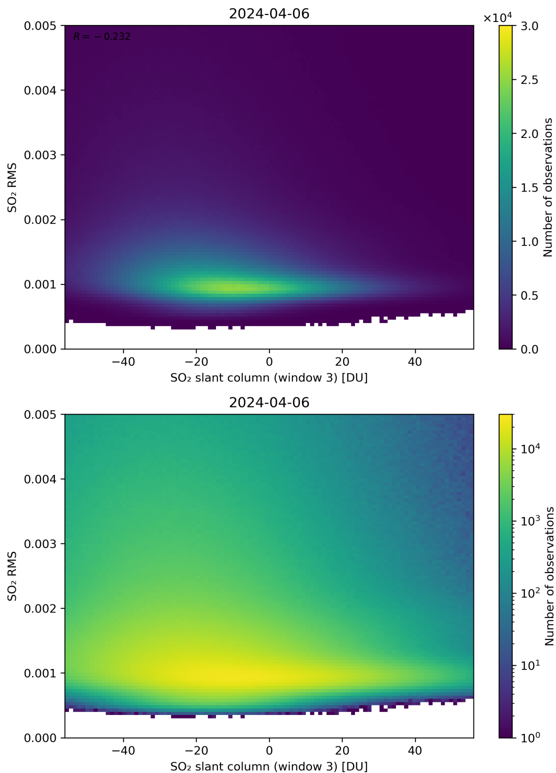
Figure 256: Scatter density plot of “SO 2 slant column (window 3)” against “SO 2 RMS” for 2024-04-05 to 2024-04-07.
