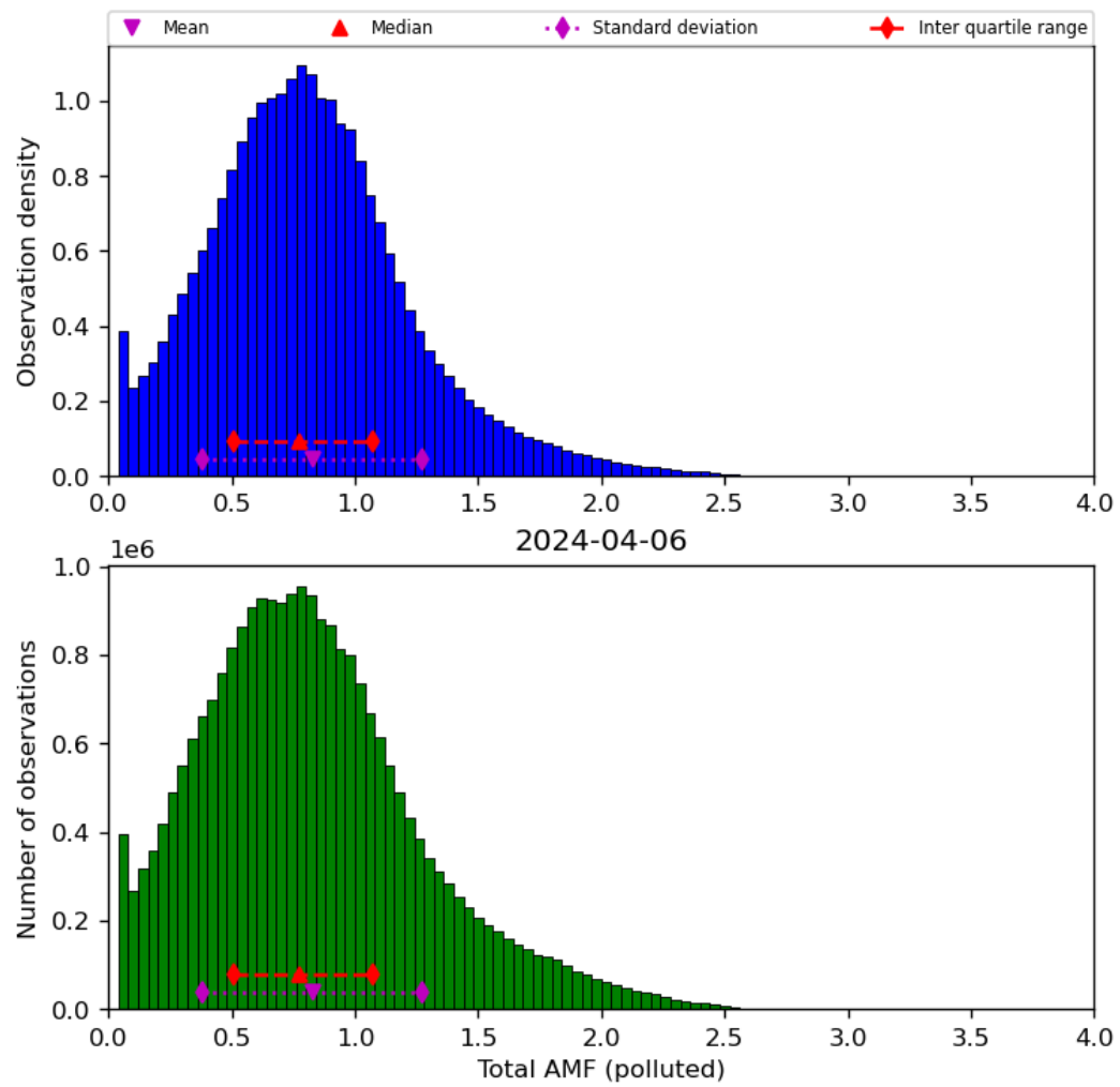
Figure 71: Histogram of “Total AMF (polluted)” for 2024-04-05 to 2024-04-07
