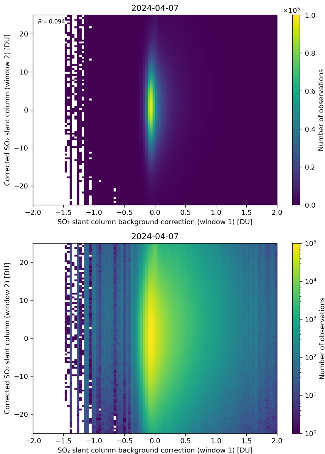
Figure 104: Scatter density plot of “SO 2 slant column background correction (window 1)” against “Corrected SO 2 slant column (window 2)” for 2024-04-06 to 2024-04-08.
