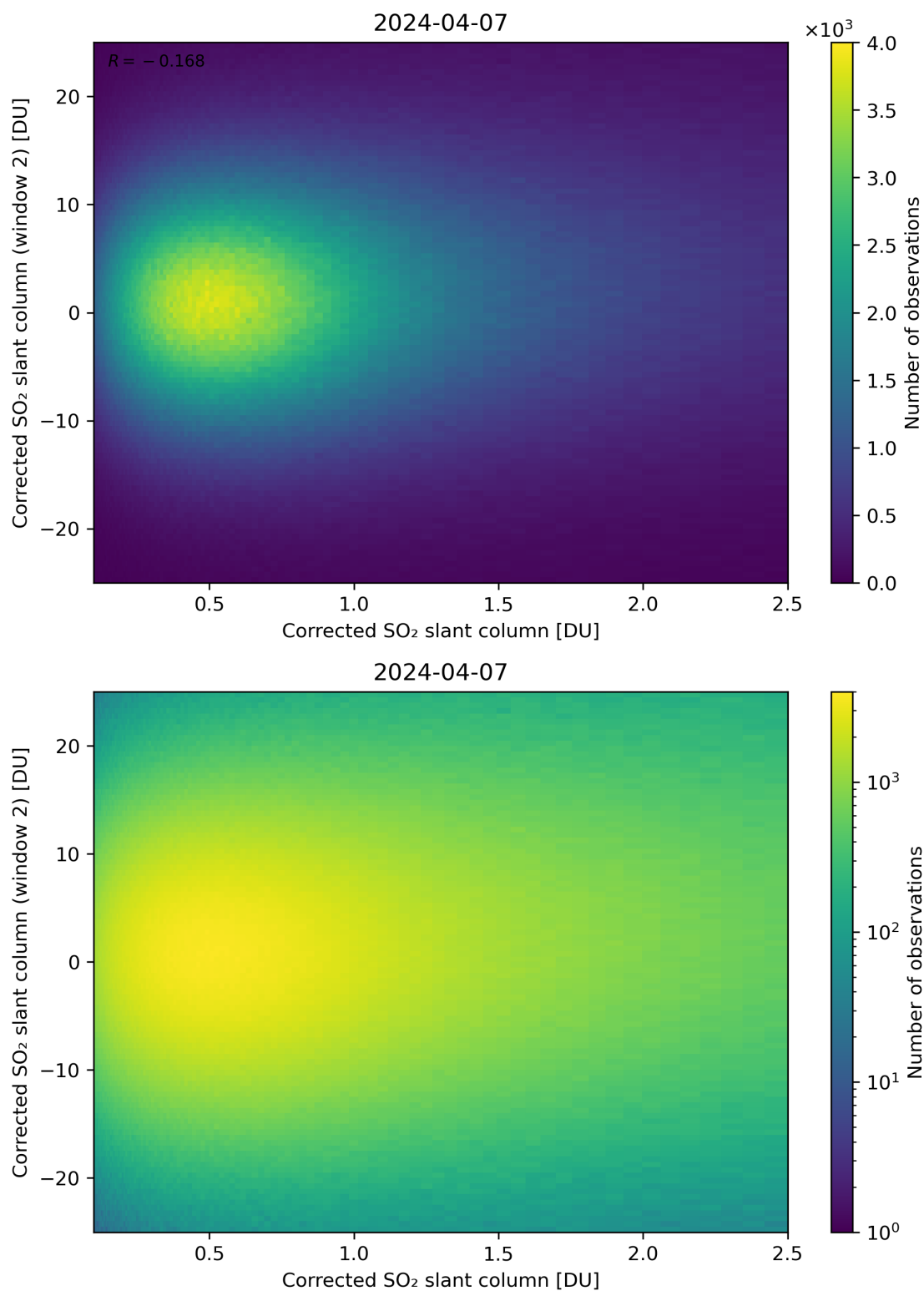
Figure 185: Scatter density plot of “Corrected SO 2 slant column” against “Corrected SO 2 slant column (window 2)” for 2024-04-06 to 2024-04-08.
