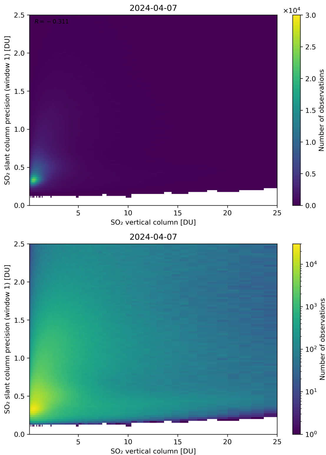
Figure 301: Scatter density plot of “SO 2 vertical column” against “SO 2 slant column precision (window 1)” for 2024-04-06 to 2024-04-08.
