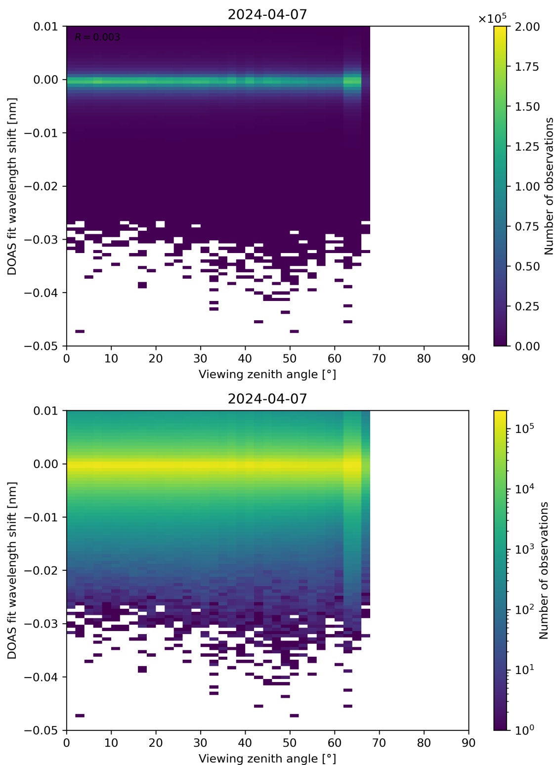
Figure 311: Scatter density plot of “Viewing zenith angle” against “DOAS fit wavelength shift” for 2024-04-06 to 2024-04-08.
