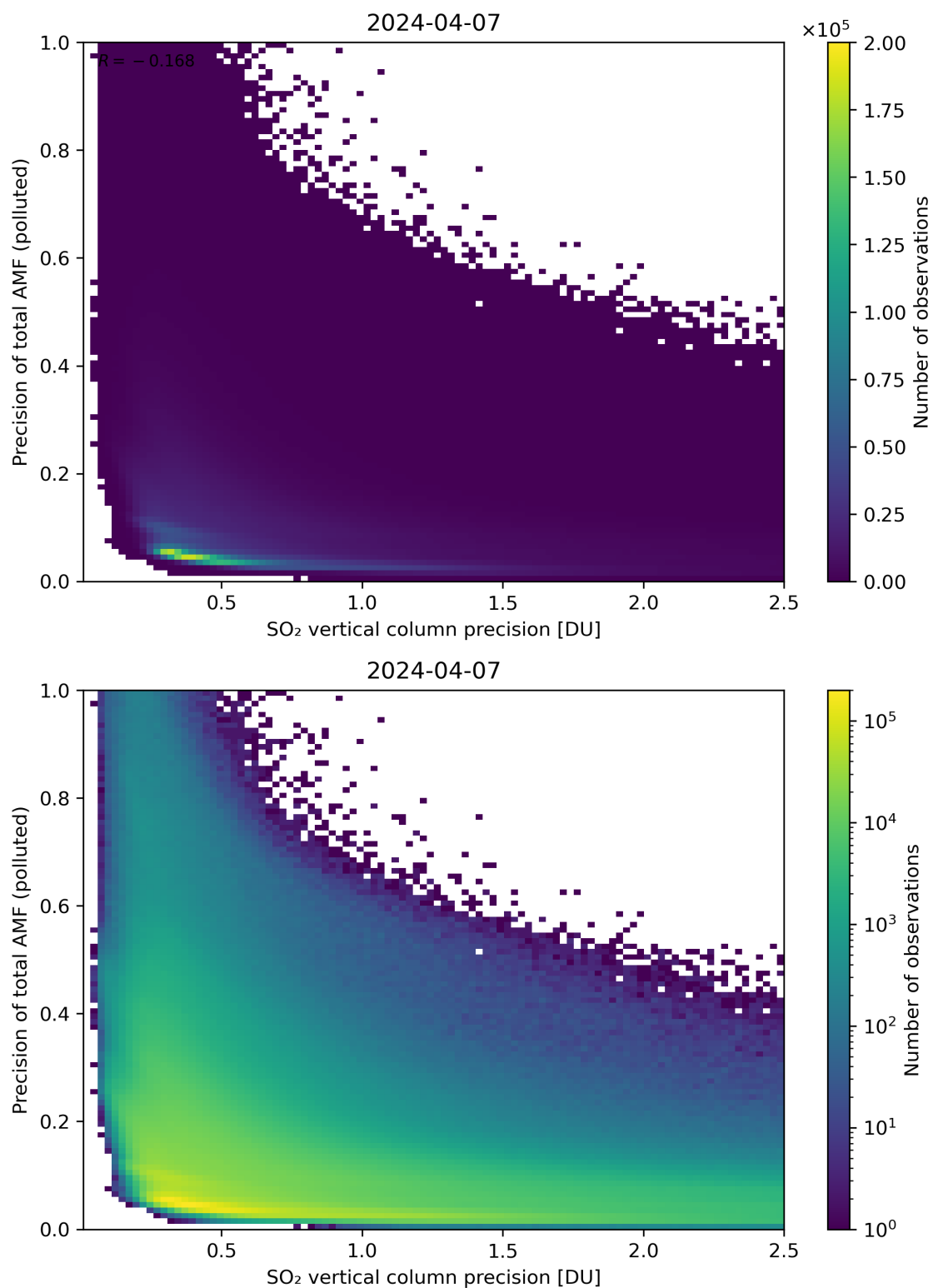
Figure 295: Scatter density plot of “SO 2 vertical column precision” against “Precision of total AMF (polluted)” for 2024-04-06 to 2024-04-08.
