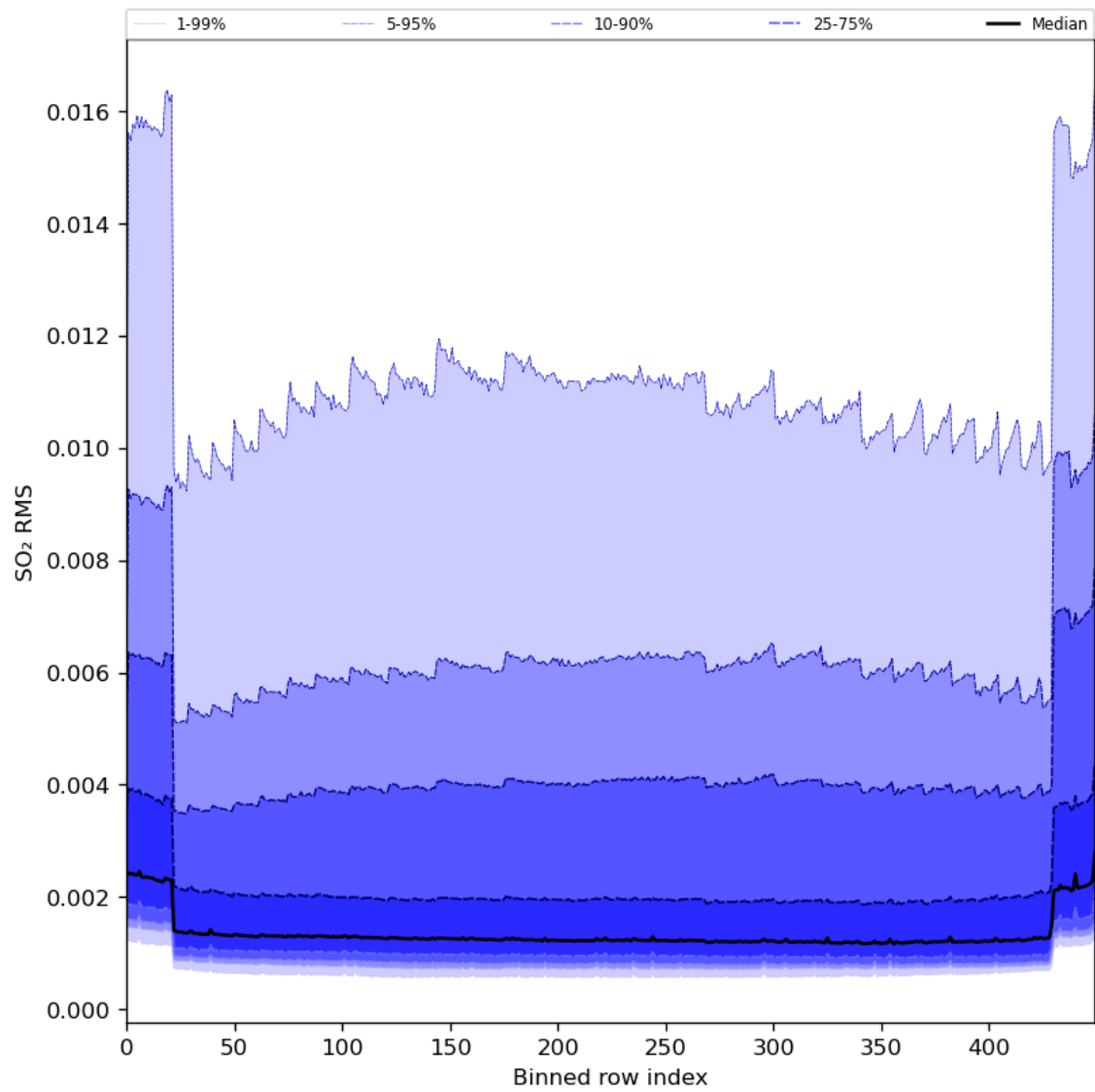
Figure 93: Along track statistics of “SO 2 RMS” for 2024-04-06 to 2024-04-08
