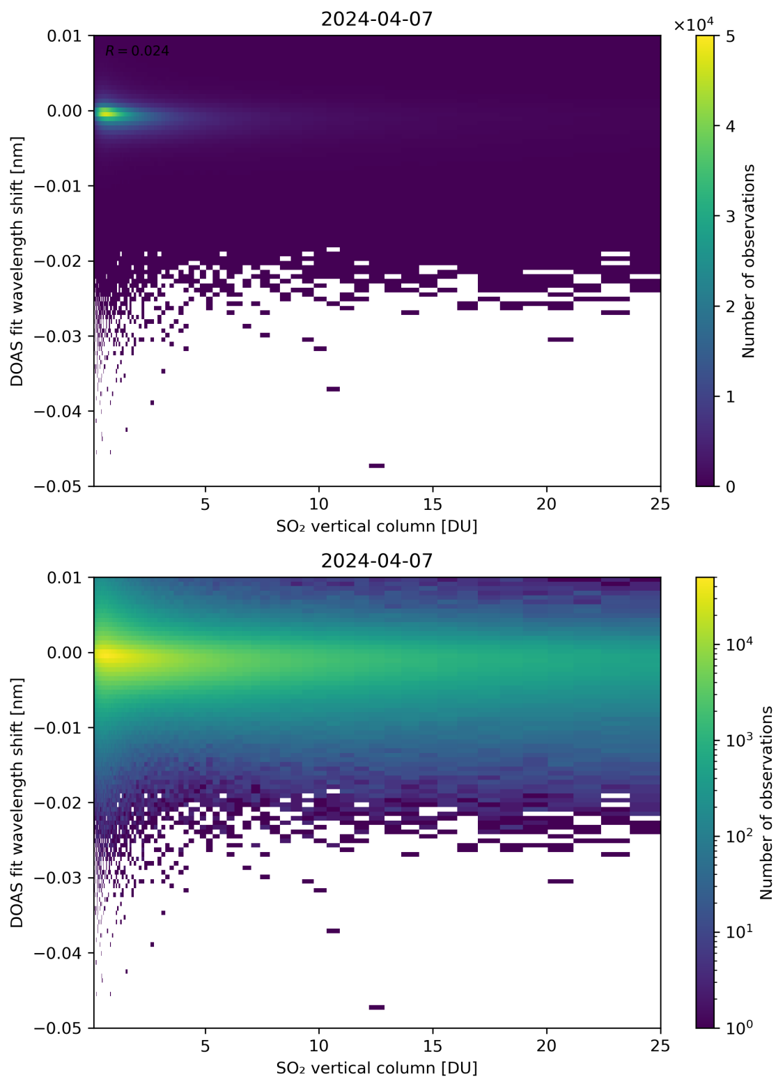
Figure 276: Scatter density plot of “SO 2 vertical column” against “DOAS fit wavelength shift” for 2024-04-06 to 2024-04-08.
