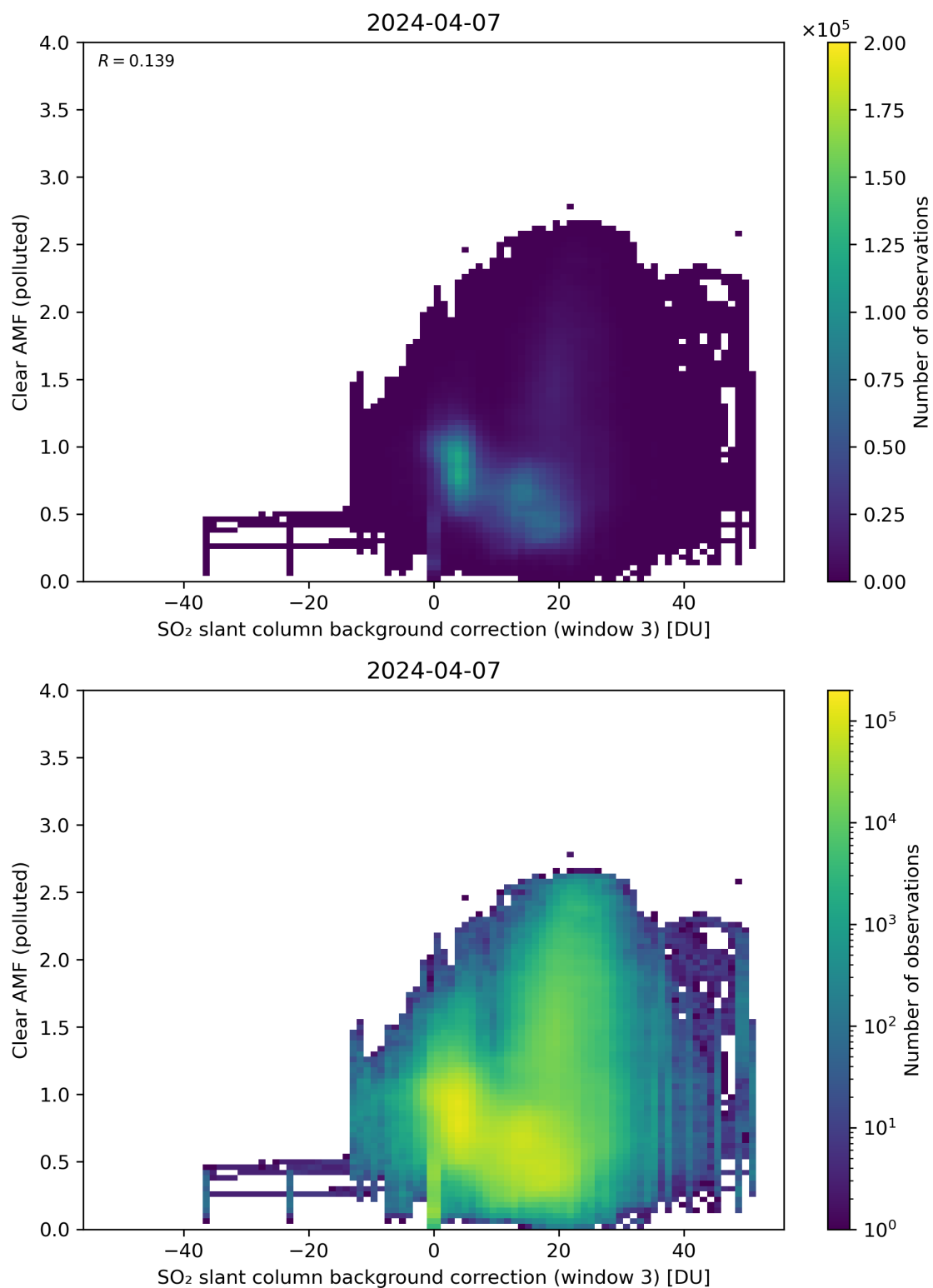
Figure 124: Scatter density plot of “SO 2 slant column background correction (window 3)” against “Clear AMF (polluted)” for 2024-04-06 to 2024-04-08.
