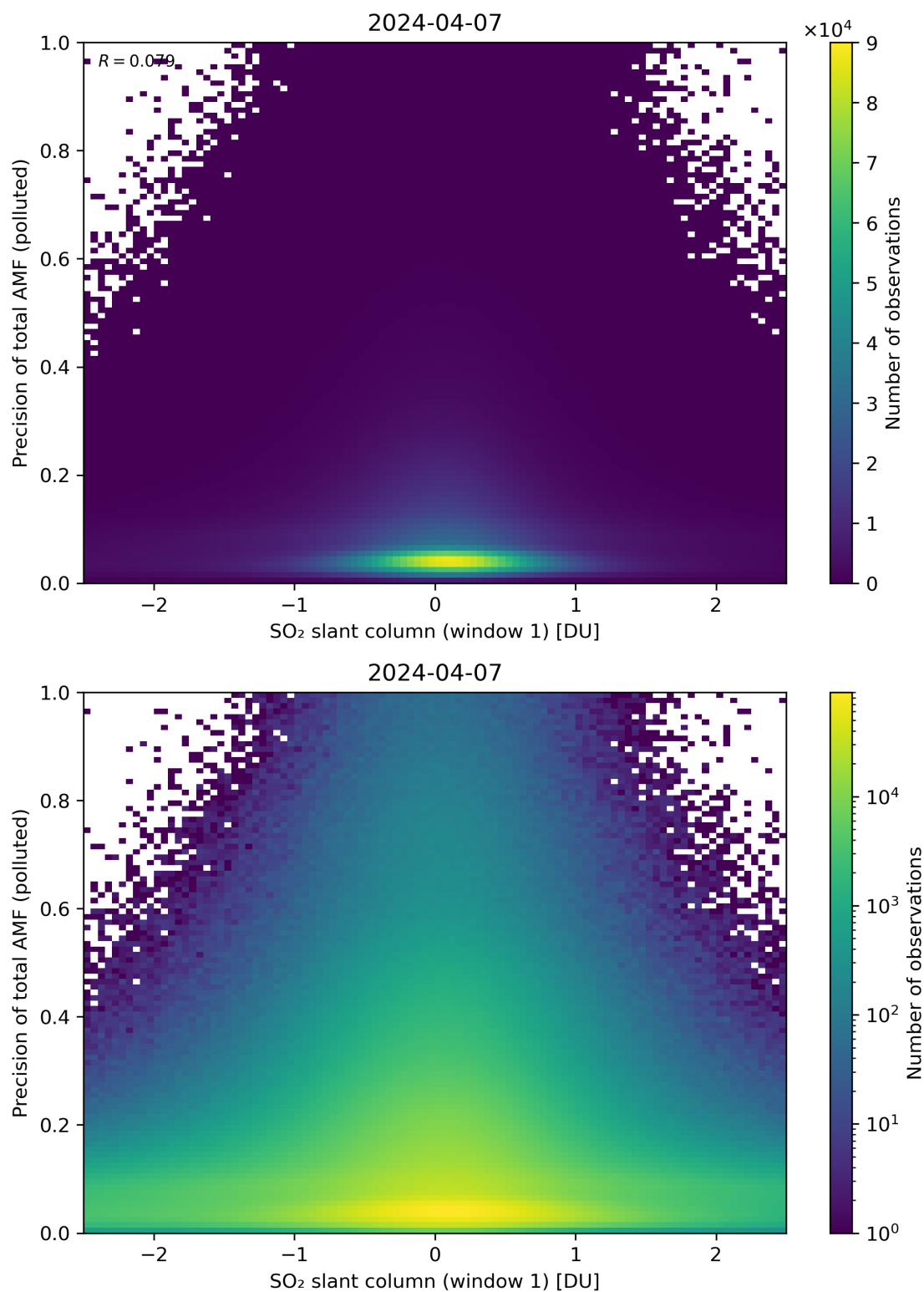
Figure 240: Scatter density plot of “SO 2 slant column (window 1)” against “Precision of total AMF (polluted)” for 2024-04-06 to 2024-04-08.
