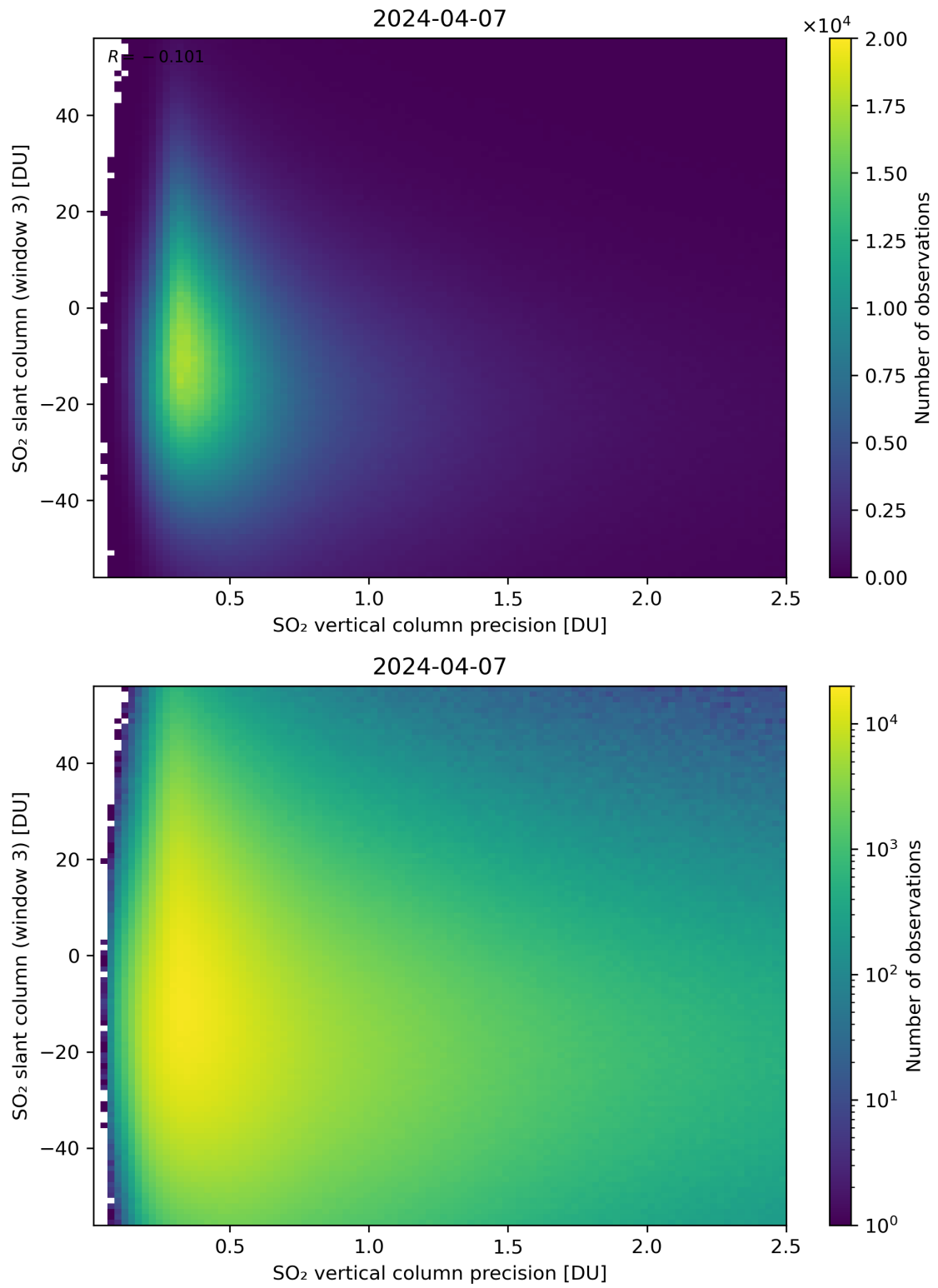
Figure 292: Scatter density plot of “SO 2 vertical column precision” against “SO 2 slant column (window 3)” for 2024-04-06 to 2024-04-08.
