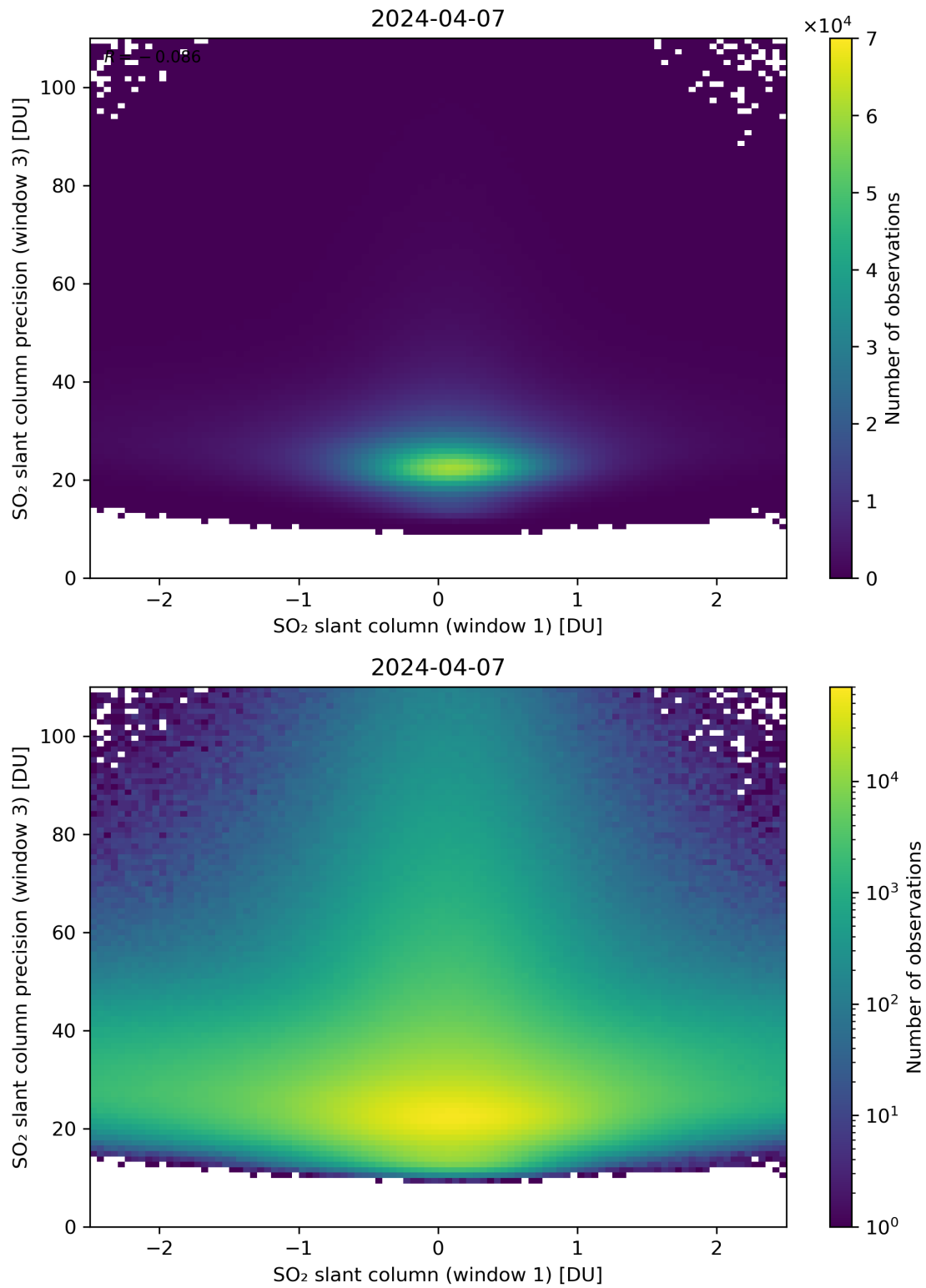
Figure 238: Scatter density plot of “SO 2 slant column (window 1)” against “SO 2 slant column precision (window 3)” for 2024-04-06 to 2024-04-08.
