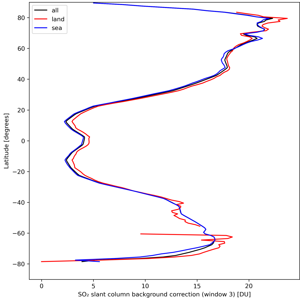
Figure 44: Zonal average of “SO 2 slant column background correction (window 3)” for 2024-04-06 to 2024-04-08.
