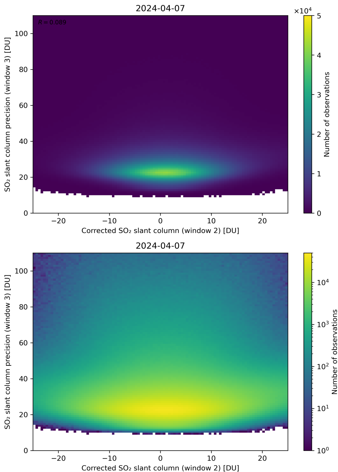
Figure 202: Scatter density plot of “Corrected SO 2 slant column (window 2)” against “SO 2 slant column precision (window 3)” for 2024-04-06 to 2024-04-08.
