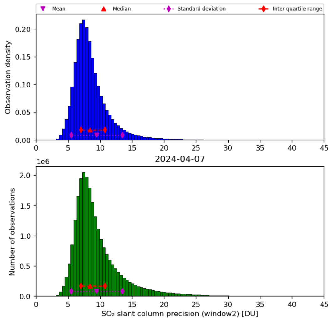
Figure 61: Histogram of “SO 2 slant column precision (window2)” for 2024-04-06 to 2024-04-08
