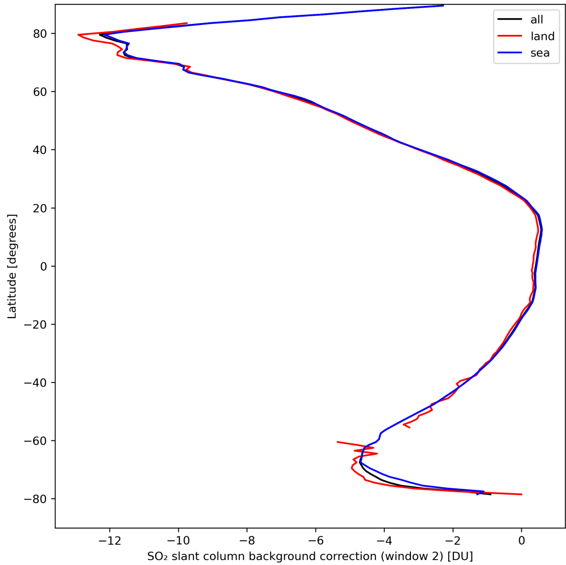
Figure 40: Zonal average of “SO 2 slant column background correction (window 2)” for 2024-04-06 to 2024-04-08.
