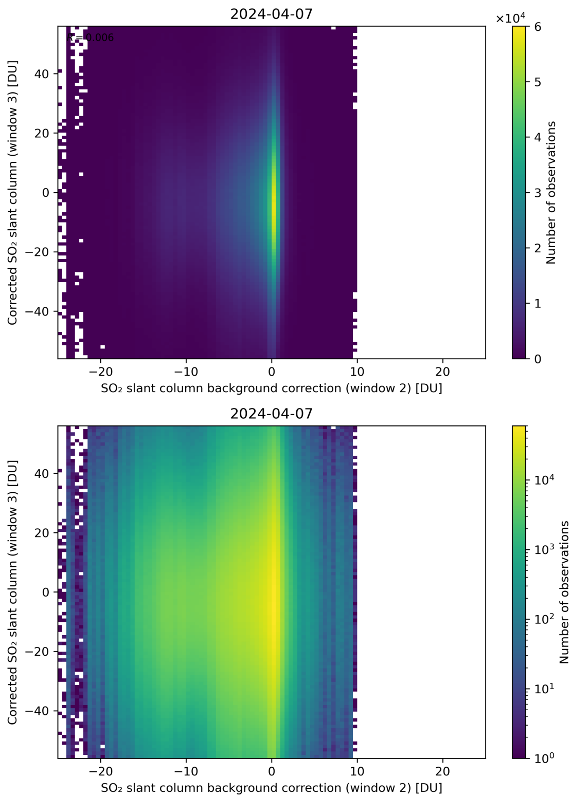
Figure 116: Scatter density plot of “SO 2 slant column background correction (window 2)” against “Corrected SO 2 slant column (window 3)” for 2024-04-06 to 2024-04-08.
