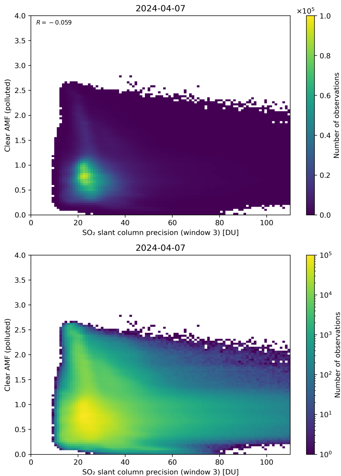
Figure 261: Scatter density plot of “SO 2 slant column precision (window 3)” against “Clear AMF (polluted)” for 2024-04-06 to 2024-04-08.
