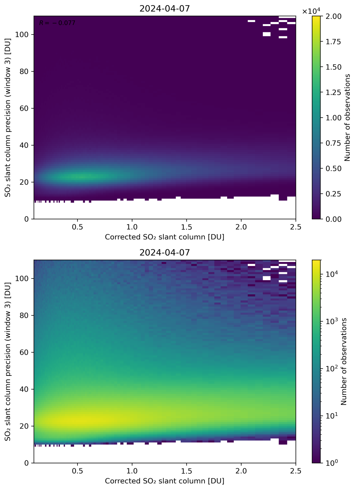
Figure 191: Scatter density plot of “Corrected SO 2 slant column” against “SO 2 slant column precision (window 3)” for 2024-04-06 to 2024-04-08.
