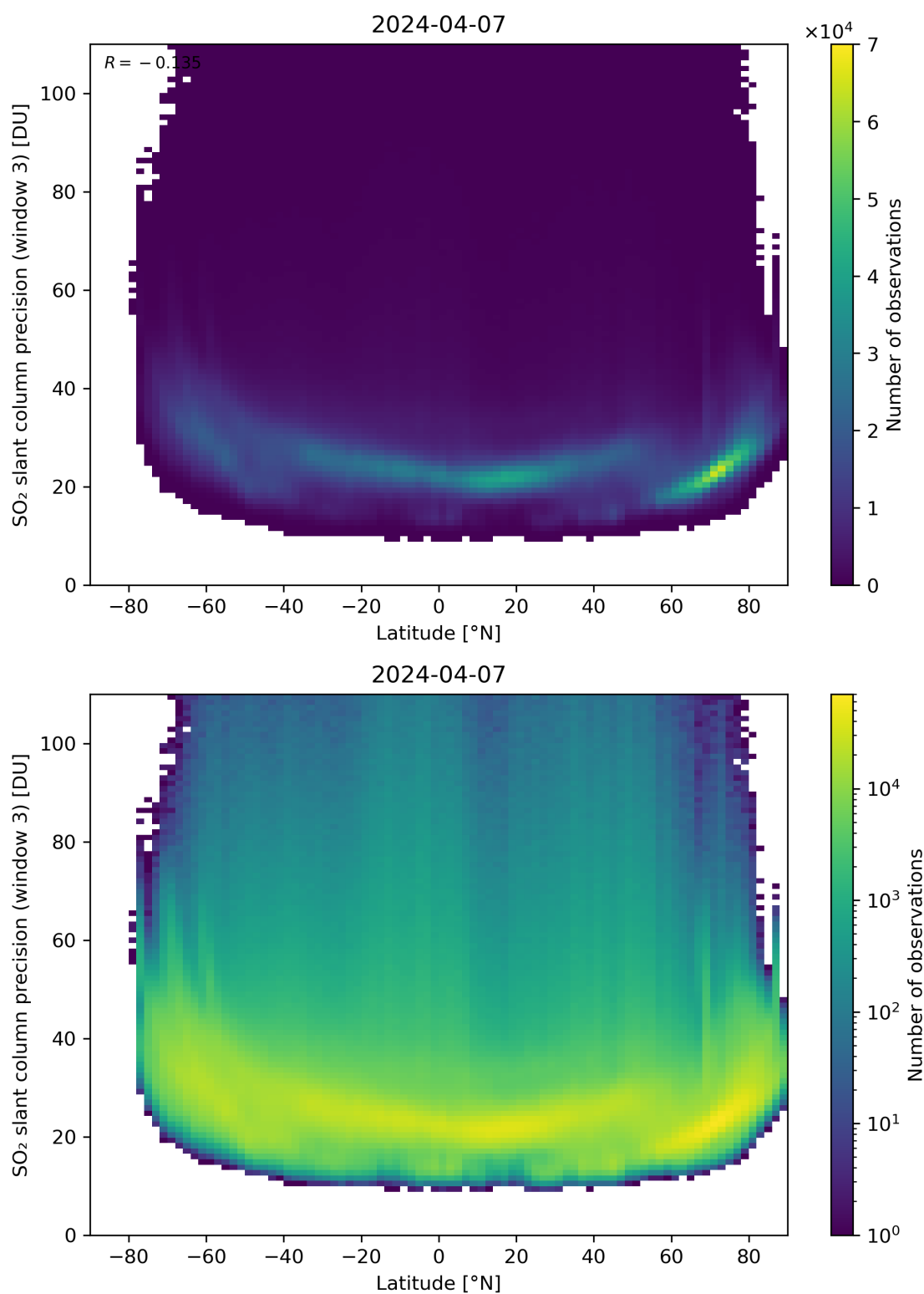
Figure 153: Scatter density plot of “Latitude” against “SO 2 slant column precision (window 3)” for 2024-04-06 to 2024-04-08.
