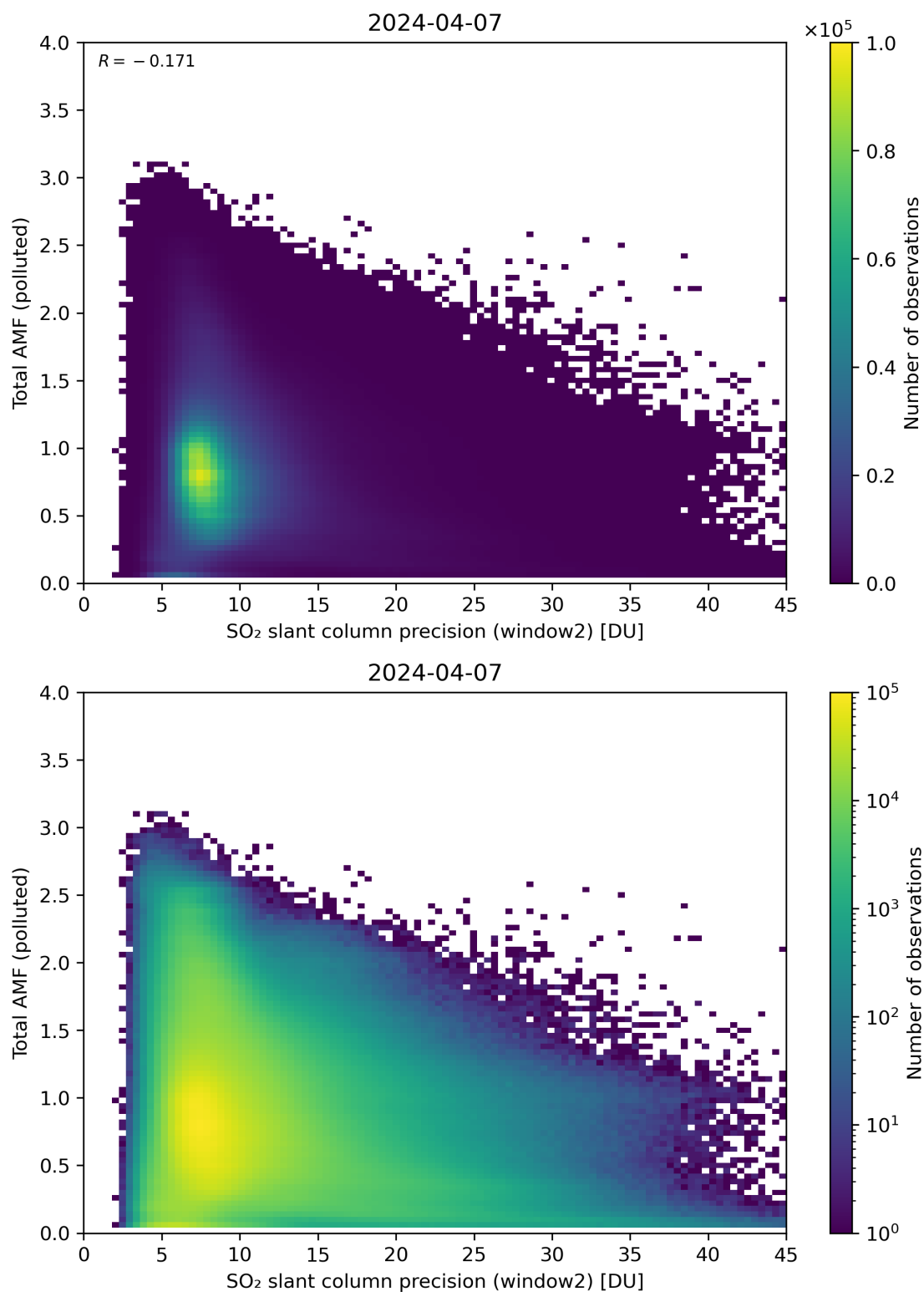
Figure 251: Scatter density plot of “SO 2 slant column precision (window2)” against “Total AMF (polluted)” for 2024-04-06 to 2024-04-08.
