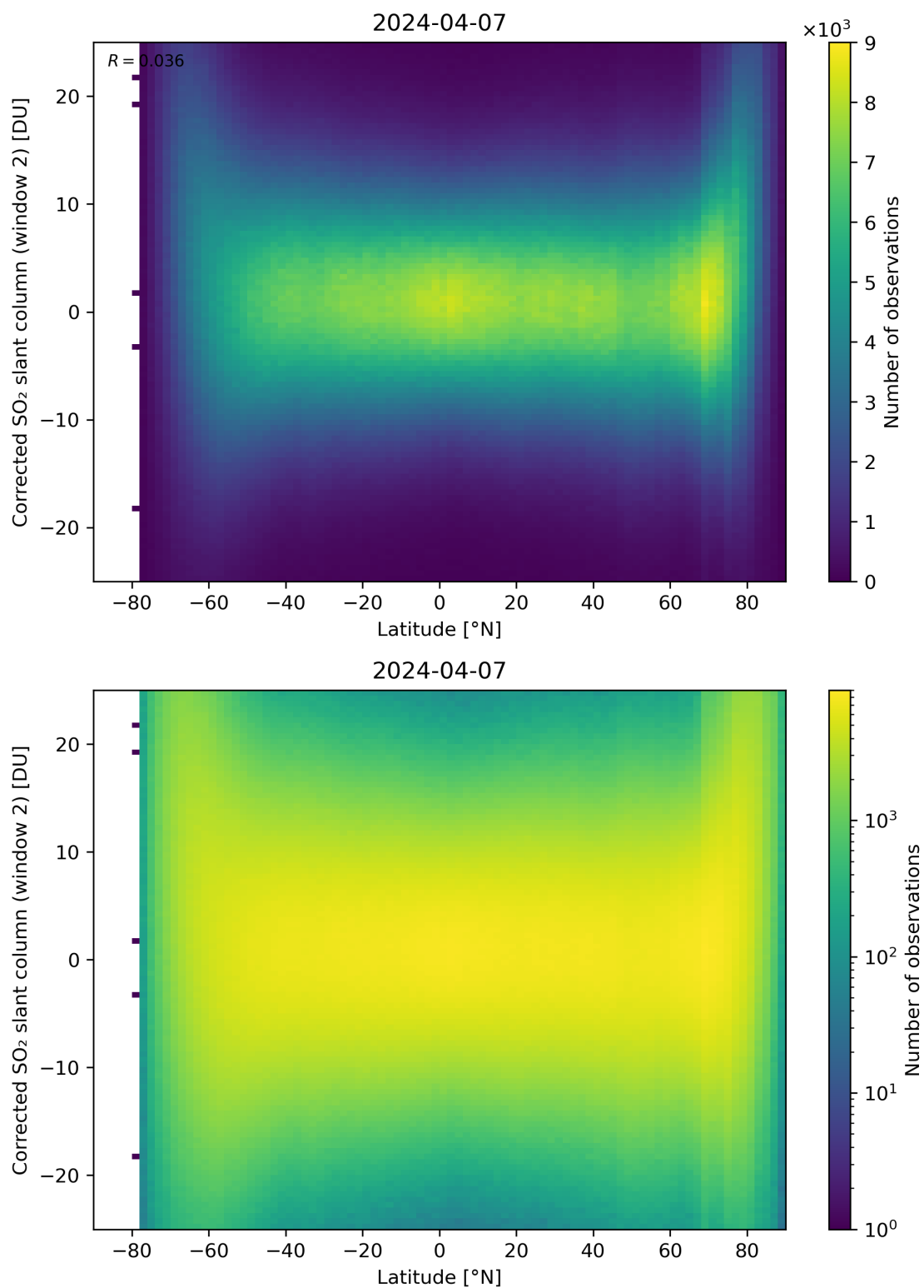
Figure 147: Scatter density plot of “Latitude” against “Corrected SO 2 slant column (window 2)” for 2024-04-06 to 2024-04-08.
