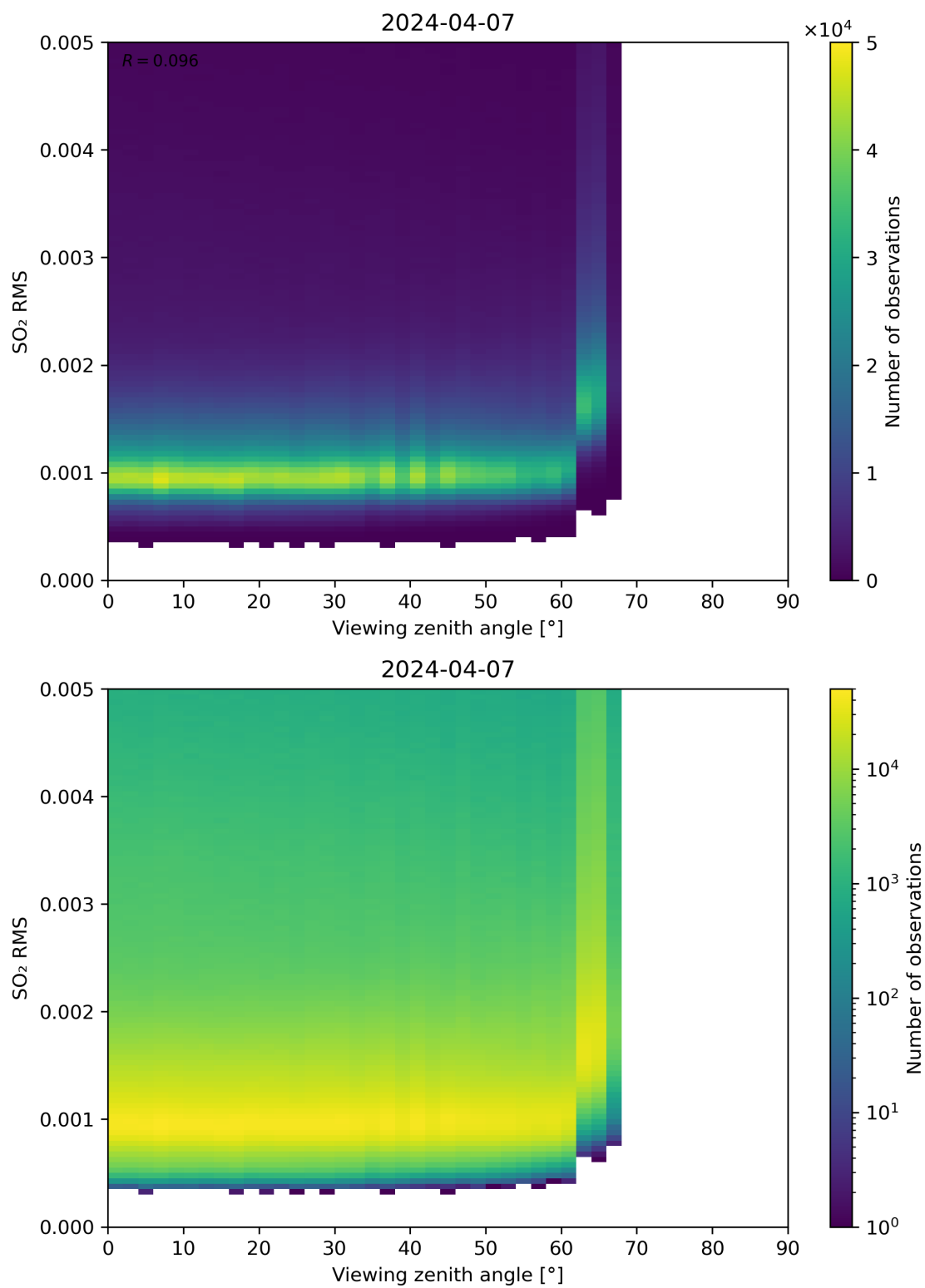
Figure 313: Scatter density plot of “Viewing zenith angle” against “SO 2 RMS” for 2024-04-06 to 2024-04-08.
