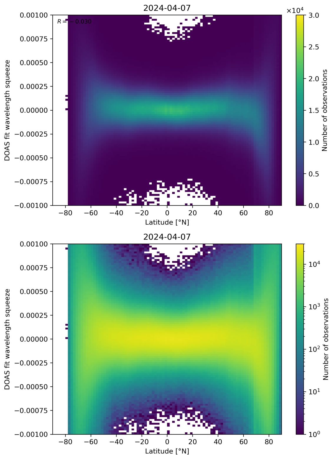
Figure 143: Scatter density plot of “Latitude” against “DOAS fit wavelength squeeze” for 2024-04-06 to 2024-04-08.
