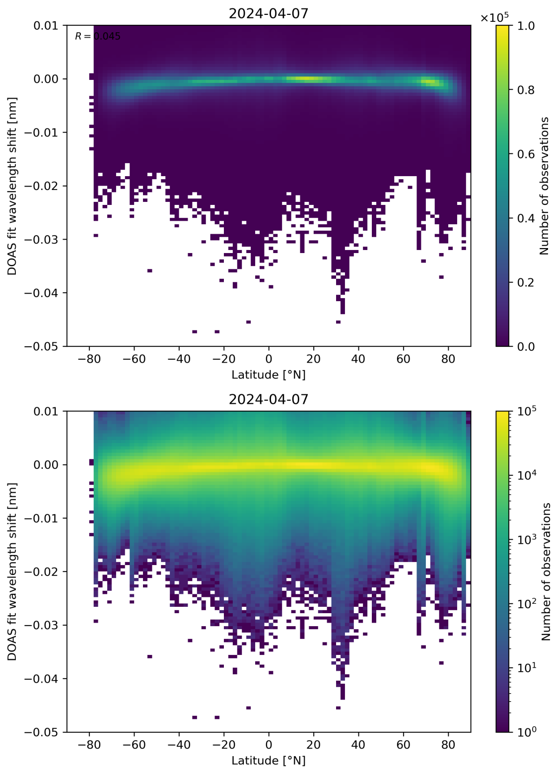
Figure 142: Scatter density plot of “Latitude” against “DOAS fit wavelength shift” for 2024-04-06 to 2024-04-08.
