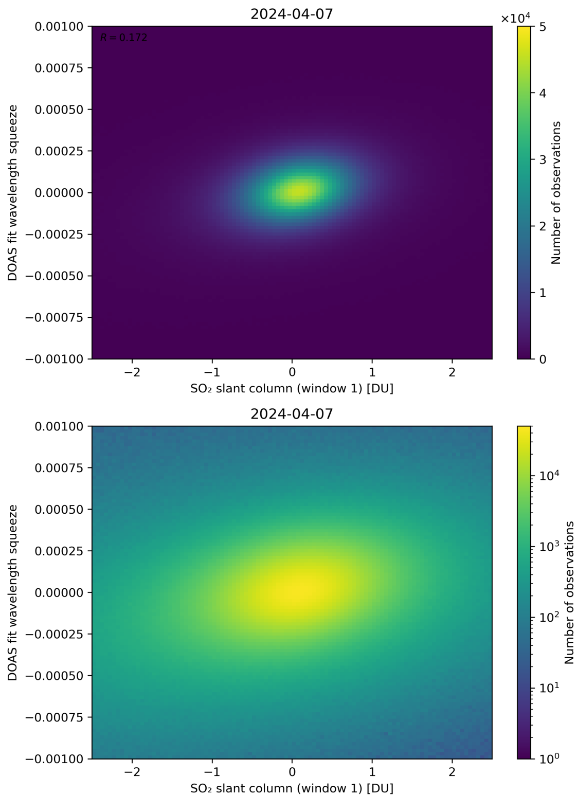
Figure 216: Scatter density plot of “SO 2 slant column (window 1)” against “DOAS fit wavelength squeeze” for 2024-04-06 to 2024-04-08.
