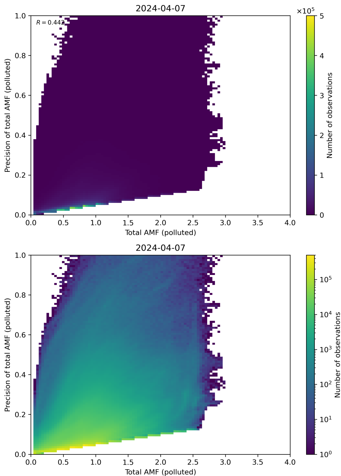
Figure 272: Scatter density plot of “Total AMF (polluted)” against “Precision of total AMF (polluted)” for 2024-04-06 to 2024-04-08.
