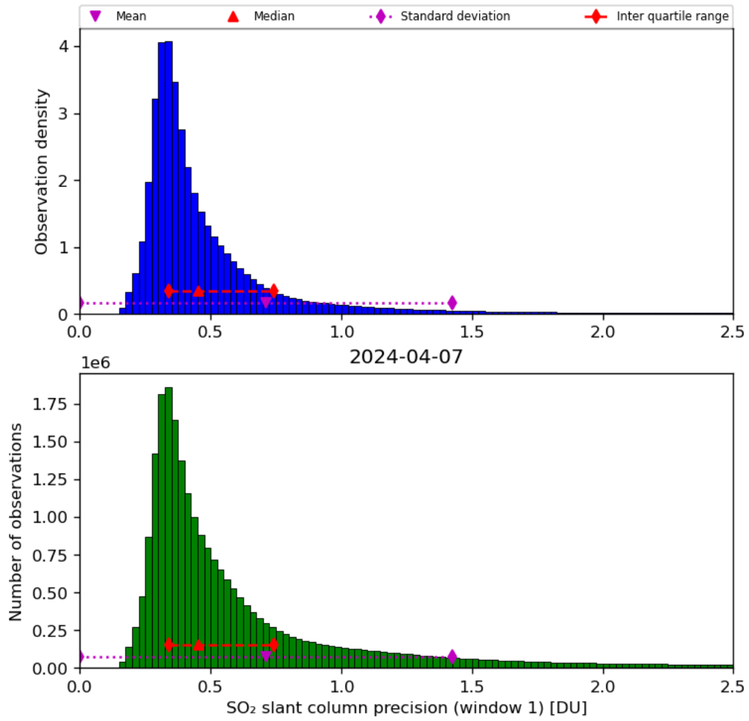
Figure 57: Histogram of “SO 2 slant column precision (window 1)” for 2024-04-06 to 2024-04-08
