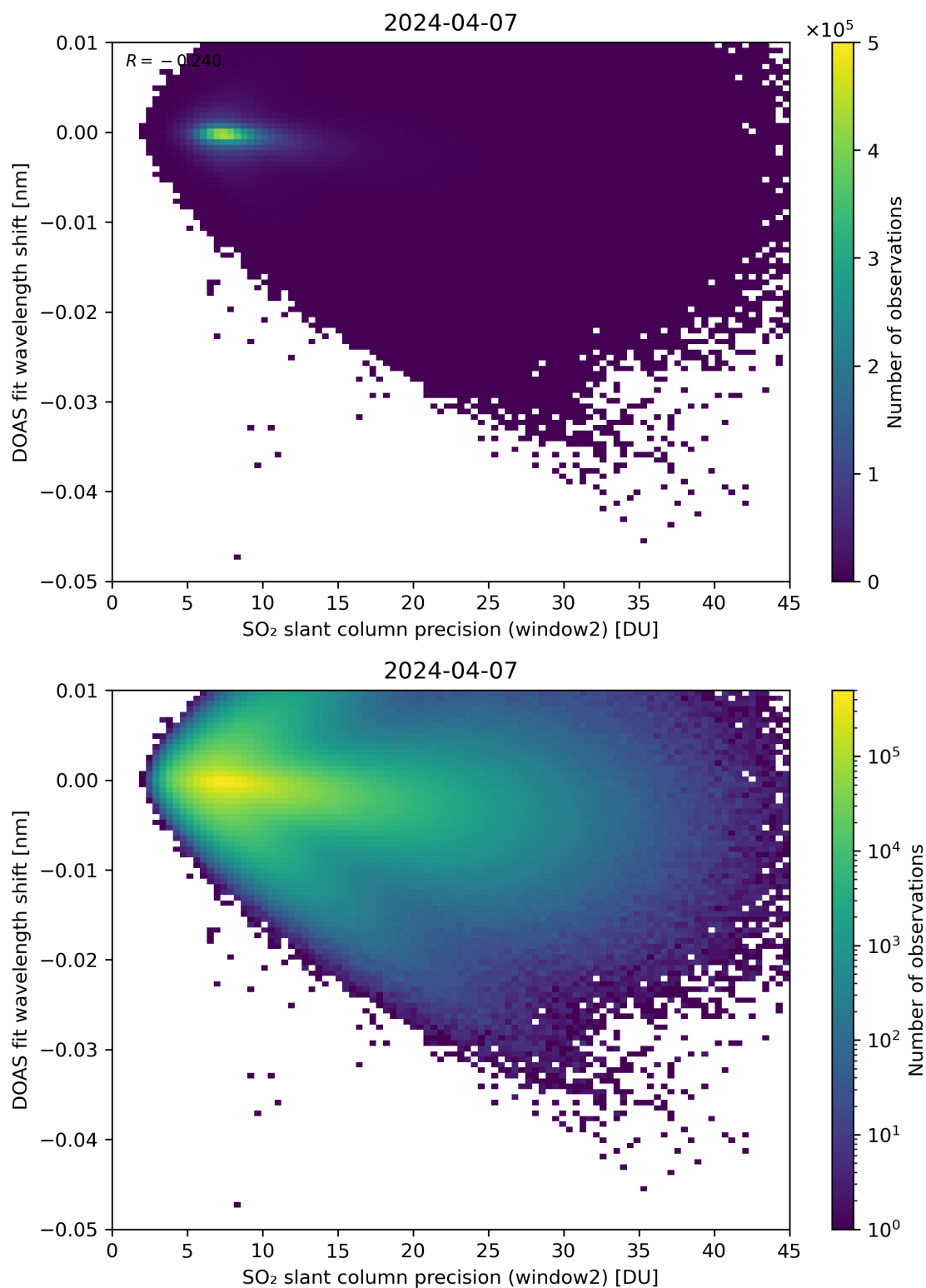
Figure 243: Scatter density plot of “SO 2 slant column precision (window2)” against “DOAS fit wavelength shift” for 2024-04-06 to 2024-04-08.
