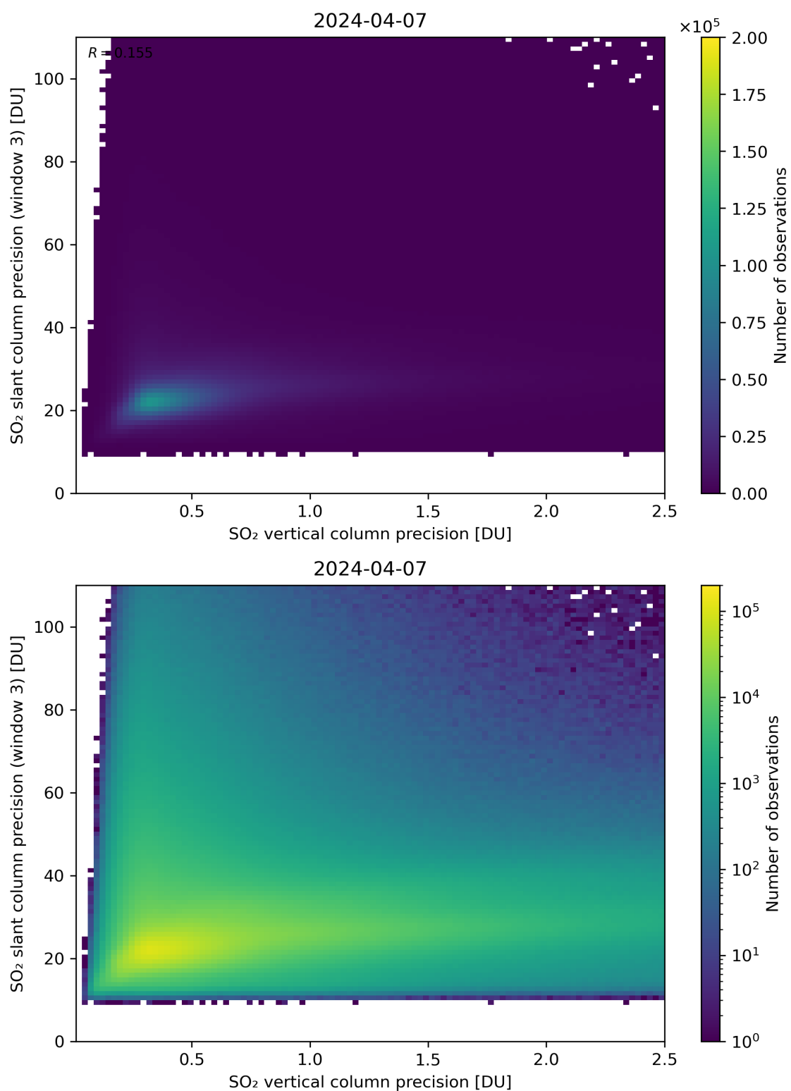
Figure 293: Scatter density plot of “SO 2 vertical column precision” against “SO 2 slant column precision (window 3)” for 2024-04-06 to 2024-04-08.
