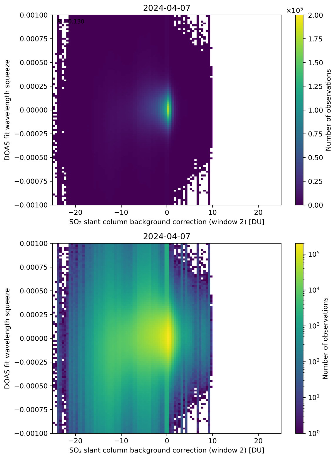
Figure 113: Scatter density plot of “SO 2 slant column background correction (window 2)” against “DOAS fit wavelength squeeze” for 2024-04-06 to 2024-04-08.
