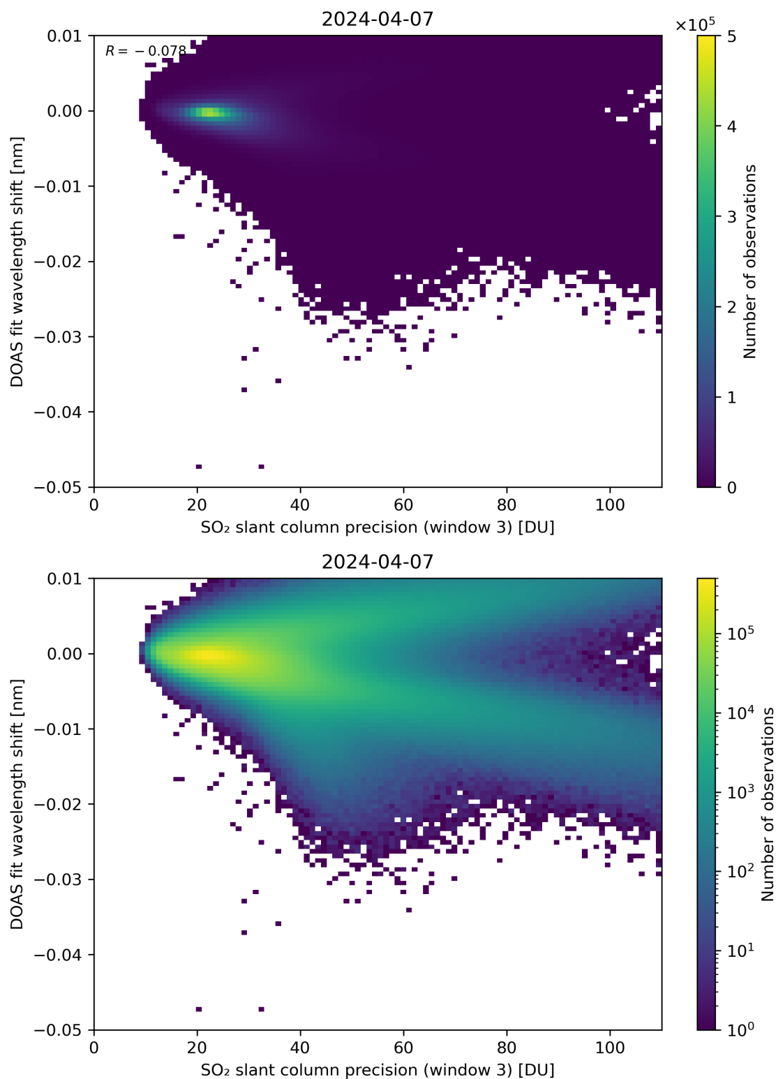
Figure 258: Scatter density plot of “SO 2 slant column precision (window 3)” against “DOAS fit wavelength shift” for 2024-04-06 to 2024-04-08.
