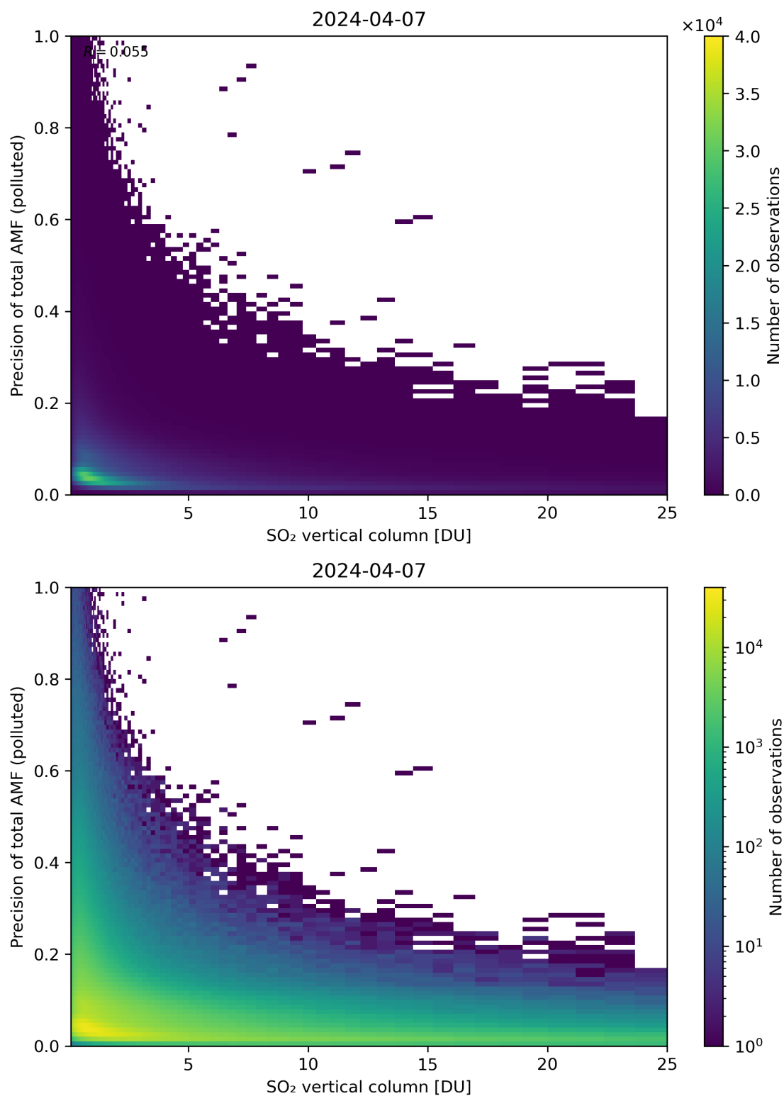
Figure 306: Scatter density plot of “SO 2 vertical column” against “Precision of total AMF (polluted)” for 2024-04-06 to 2024-04-08.
