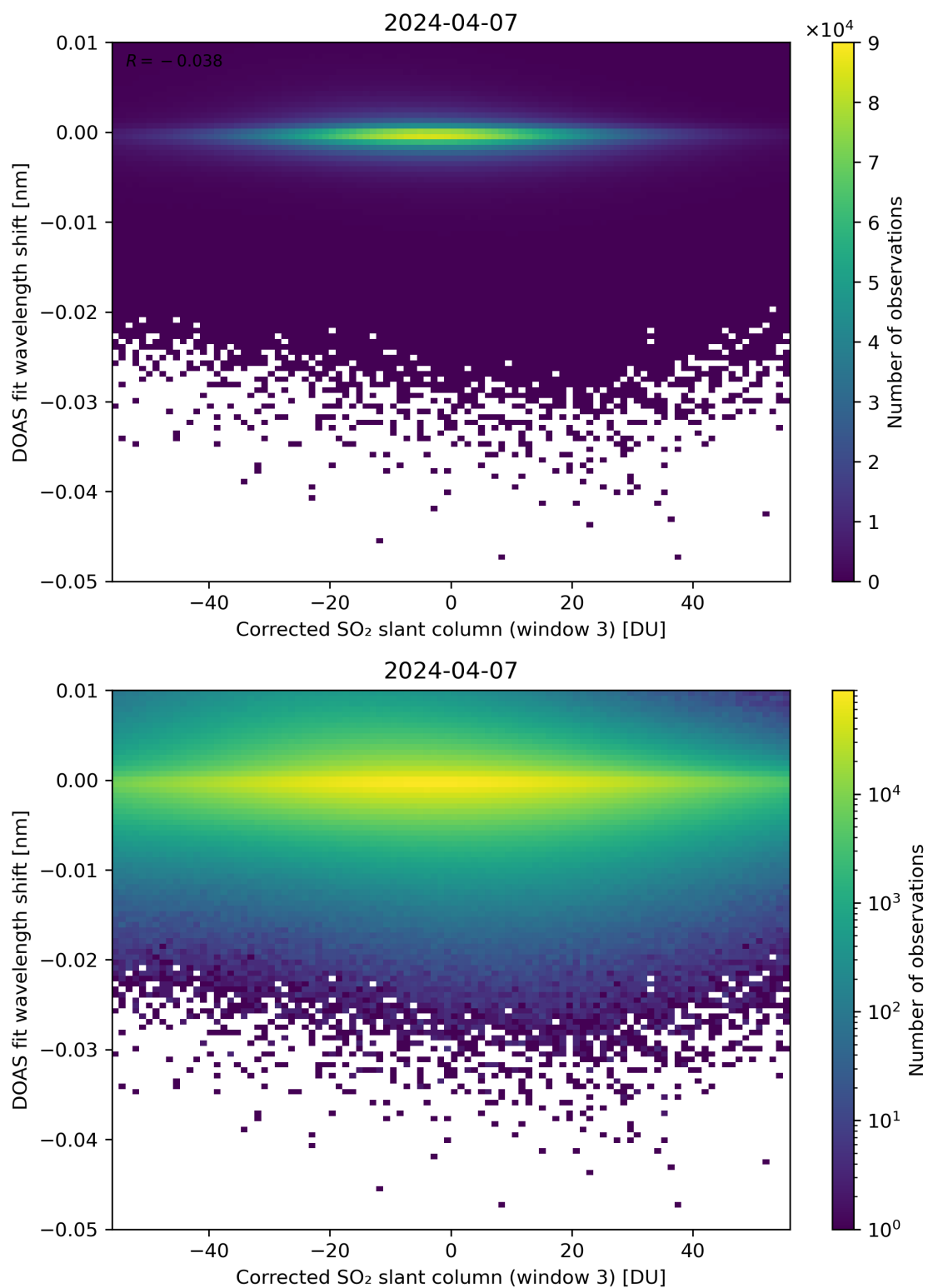
Figure 206: Scatter density plot of “Corrected SO 2 slant column (window 3)” against “DOAS fit wavelength shift” for 2024-04-06 to 2024-04-08.
