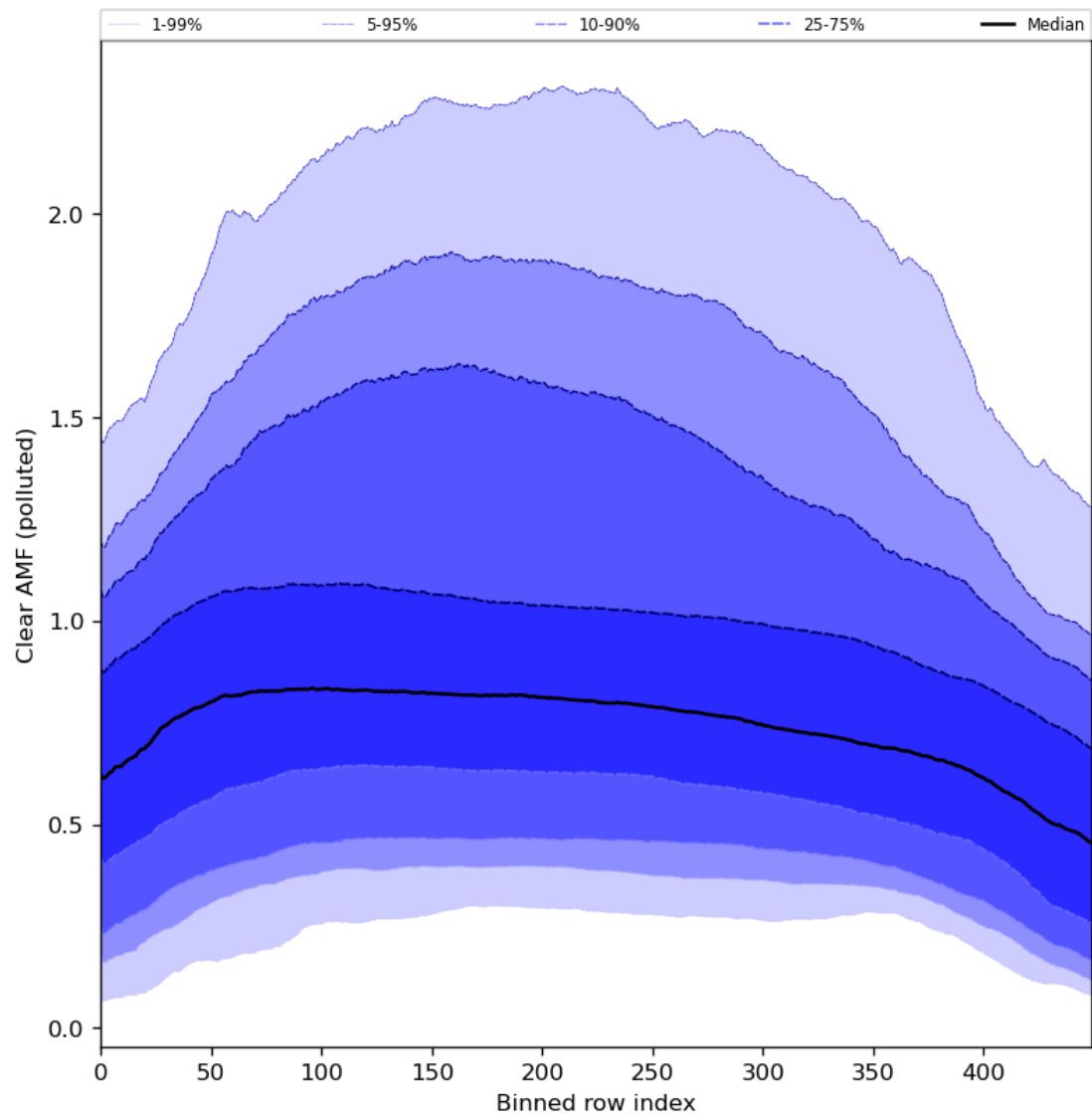
Figure 96: Along track statistics of “Clear AMF (polluted)” for 2024-04-06 to 2024-04-08
