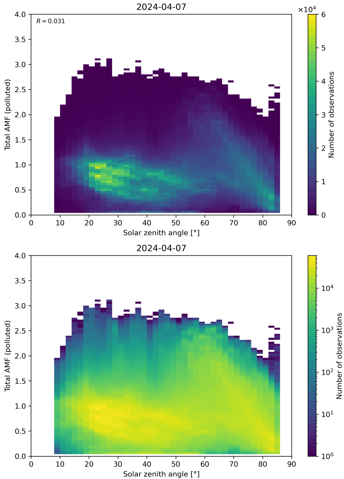
Figure 174: Scatter density plot of “Solar zenith angle” against “Total AMF (polluted)” for 2024-04-06 to 2024-04-08.
