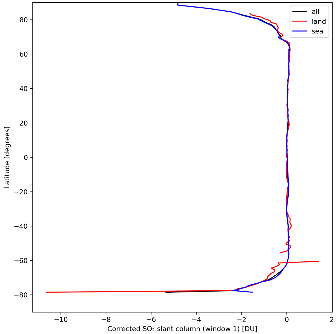
Figure 35: Zonal average of “Corrected SO 2 slant column (window 1)” for 2024-04-06 to 2024-04-08.
