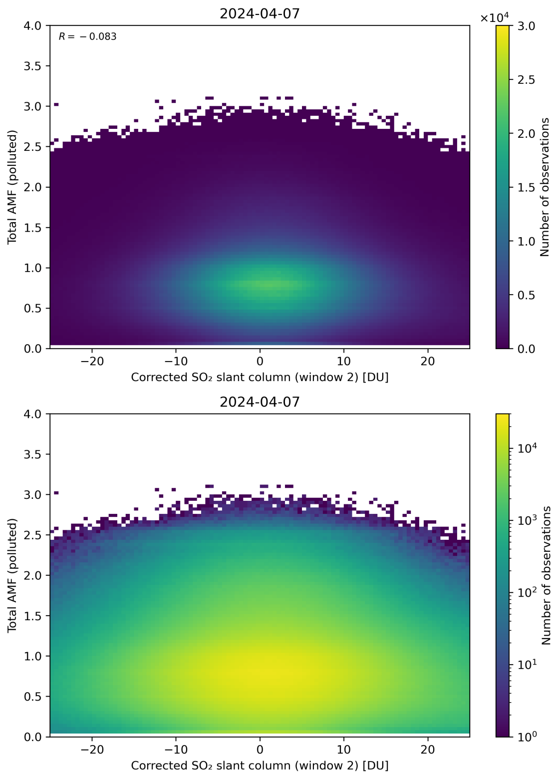
Figure 203: Scatter density plot of “Corrected SO 2 slant column (window 2)” against “Total AMF (polluted)” for 2024-04-06 to 2024-04-08.
