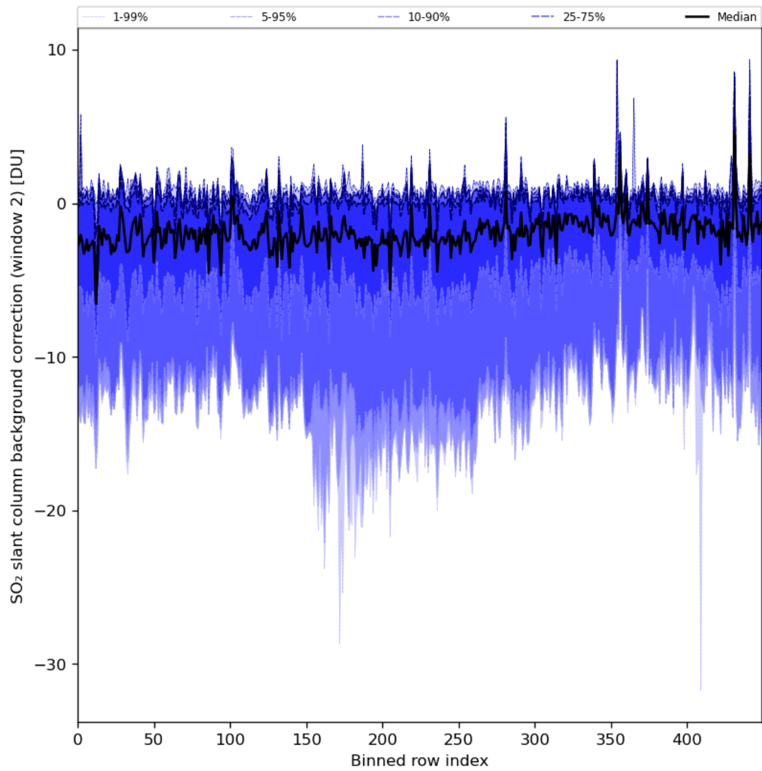
Figure 86: Along track statistics of “SO 2 slant column background correction (window 2)” for 2024-04-06 to 2024-04-08
