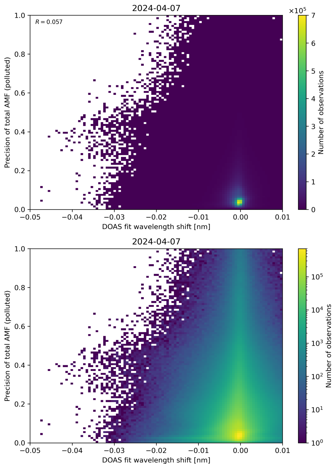
Figure 131: Scatter density plot of “DOAS fit wavelength shift” against “Precision of total AMF (polluted)” for 2024-04-06 to 2024-04-08.
