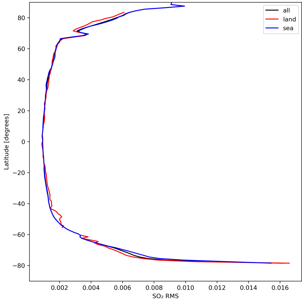
Figure 47: Zonal average of “SO 2 RMS” for 2024-04-06 to 2024-04-08.
