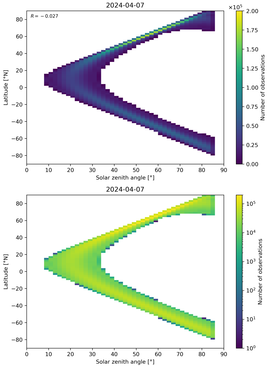
Figure 164: Scatter density plot of “Solar zenith angle” against “Latitude” for 2024-04-06 to 2024-04-08.
