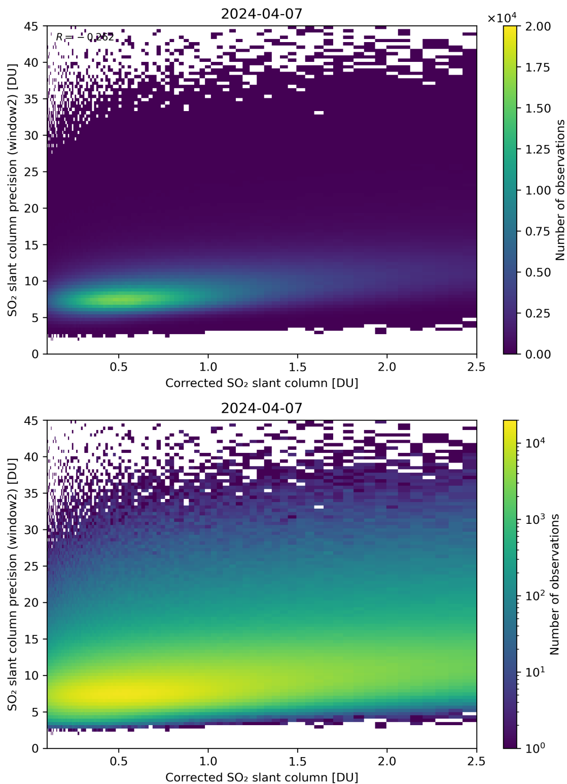
Figure 189: Scatter density plot of “Corrected SO 2 slant column” against “SO 2 slant column precision (window2)” for 2024-04-06 to 2024-04-08.
