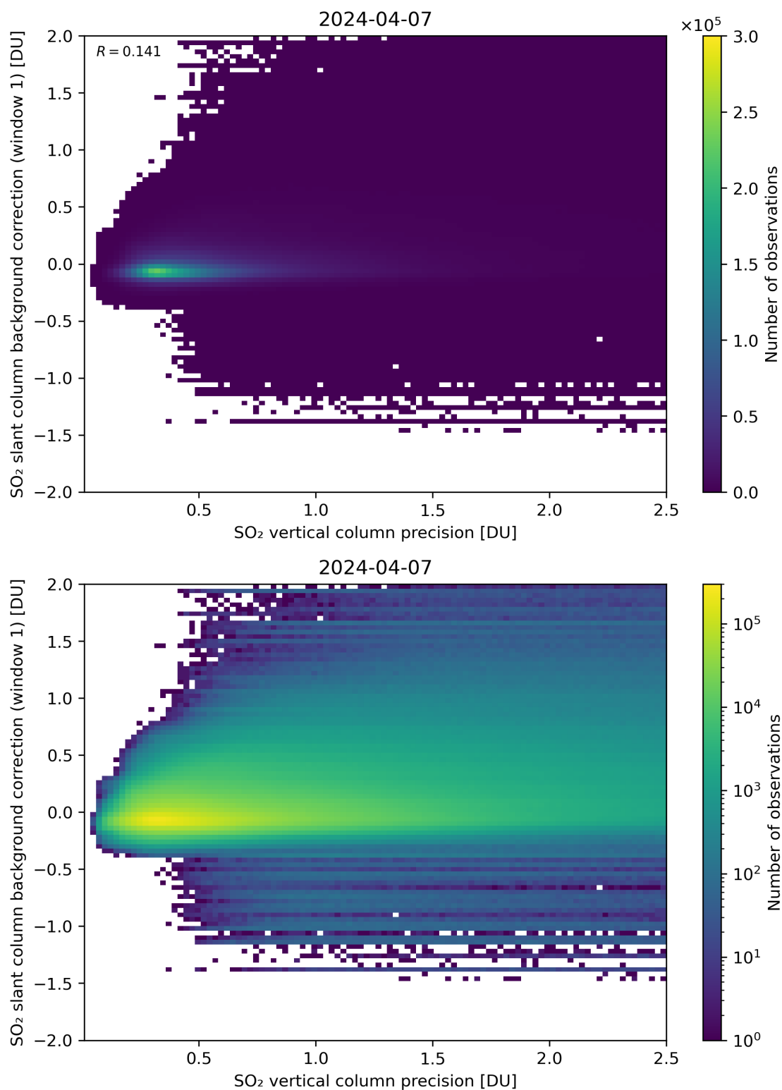
Figure 279: Scatter density plot of “SO 2 vertical column precision” against “SO 2 slant column background correction (window 1)” for 2024-04-06 to 2024-04-08.
