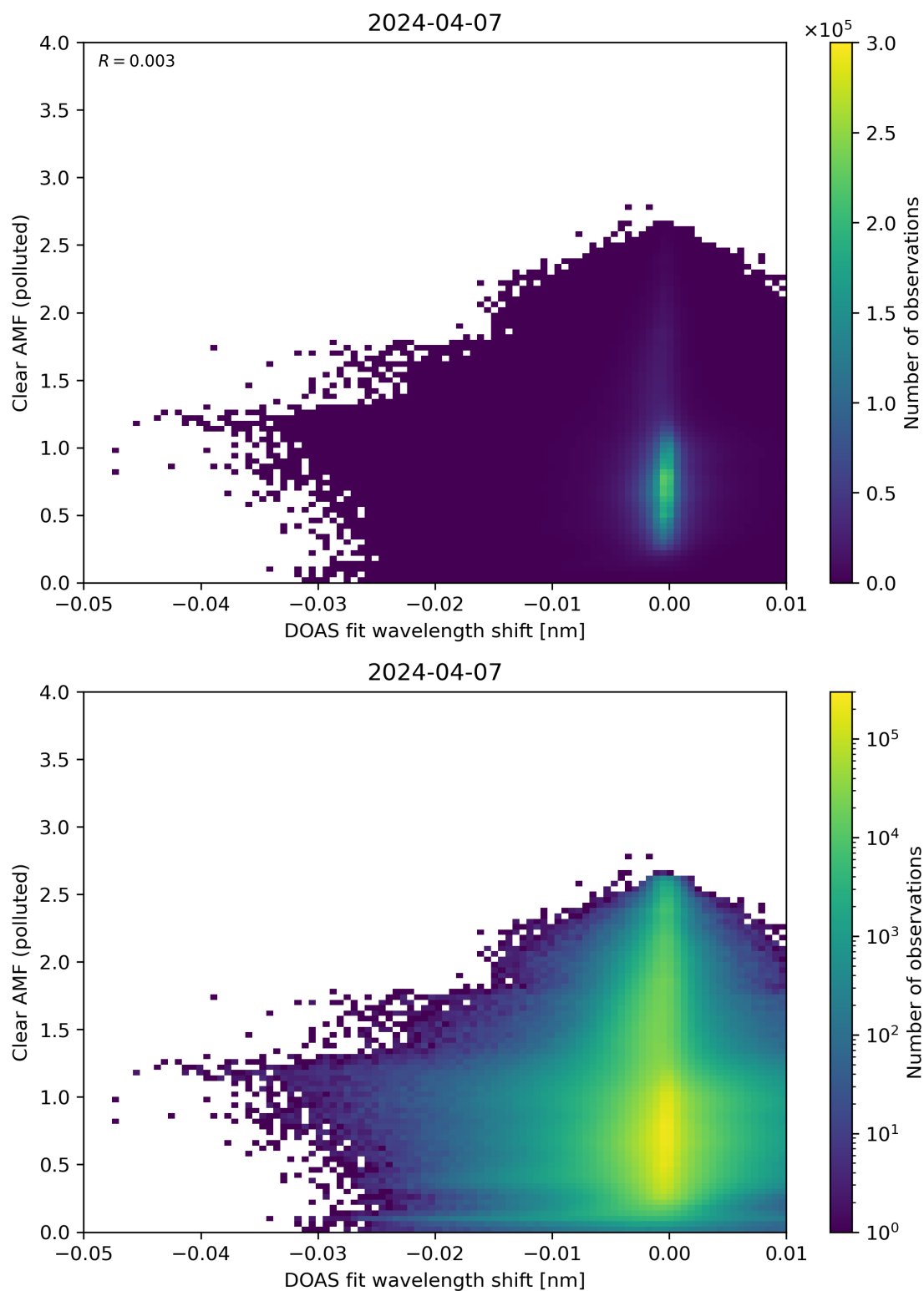
Figure 129: Scatter density plot of “DOAS fit wavelength shift” against “Clear AMF (polluted)” for 2024-04-06 to 2024-04-08.
