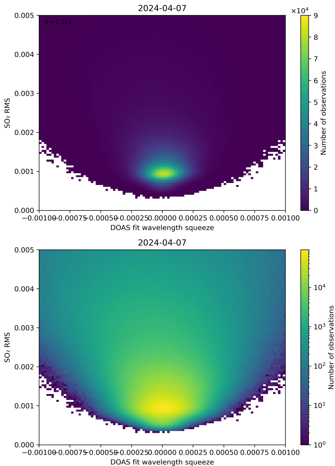
Figure 132: Scatter density plot of “DOAS fit wavelength squeeze” against “SO 2 RMS” for 2024-04-06 to 2024-04-08.
