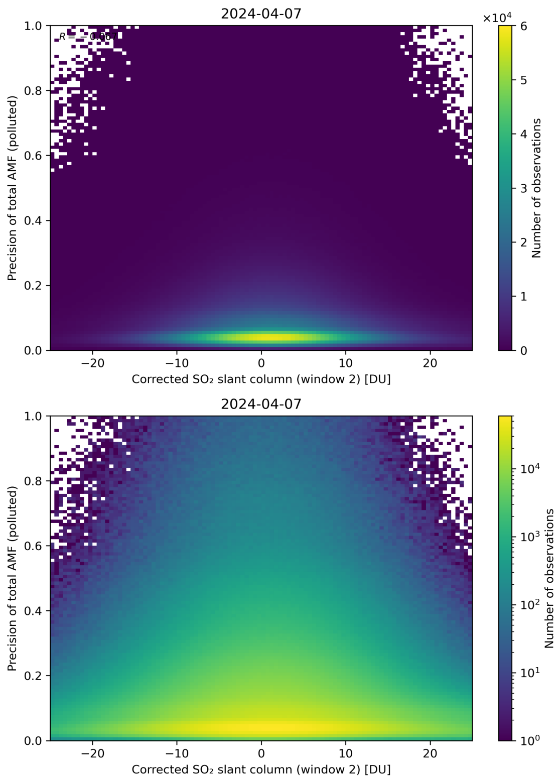
Figure 204: Scatter density plot of “Corrected SO 2 slant column (window 2)” against “Precision of total AMF (polluted)” for 2024-04-06 to 2024-04-08.
