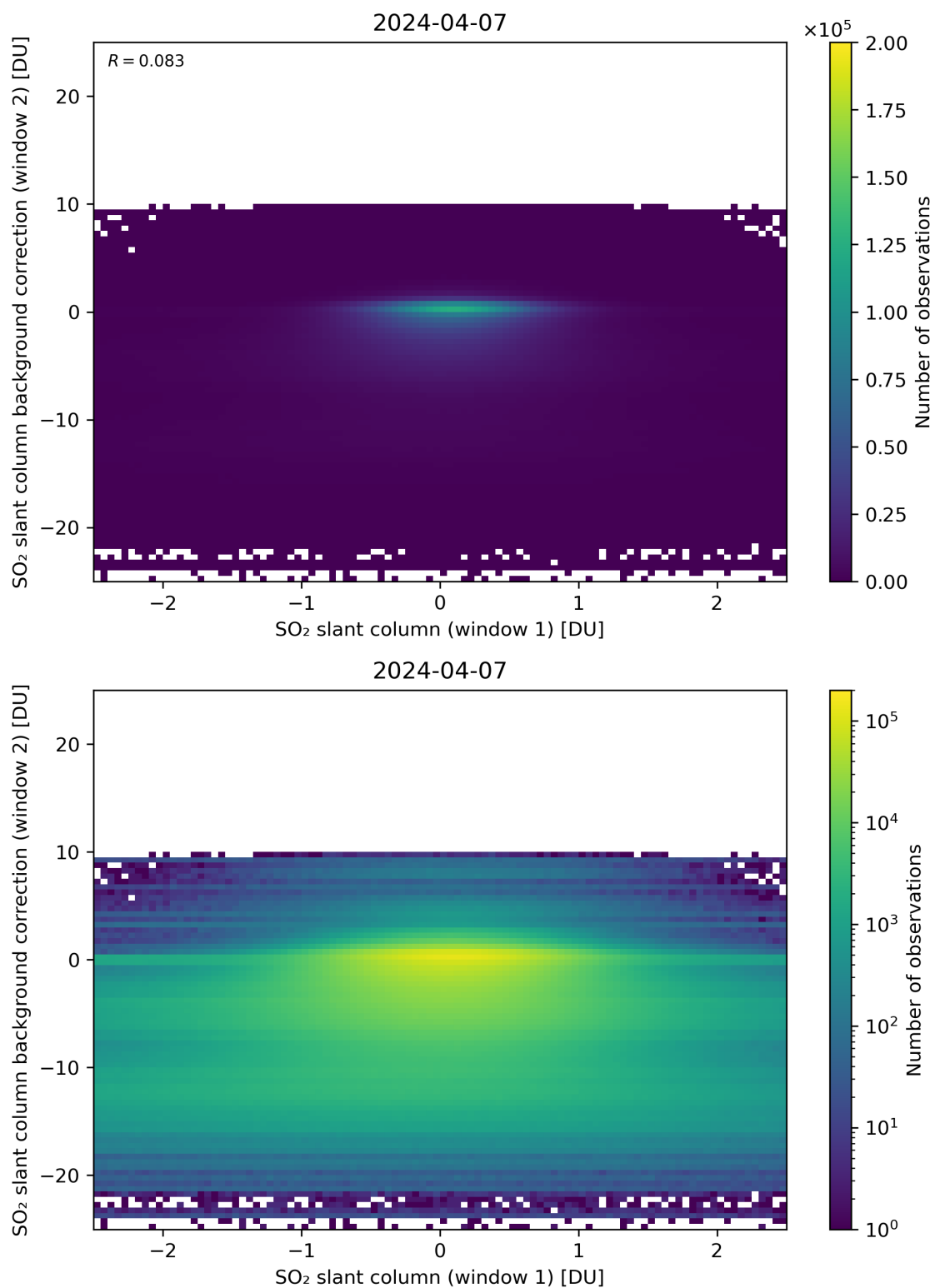
Figure 213: Scatter density plot of “SO 2 slant column (window 1)” against “SO 2 slant column background correction (window 2)” for 2024-04-06 to 2024-04-08.
