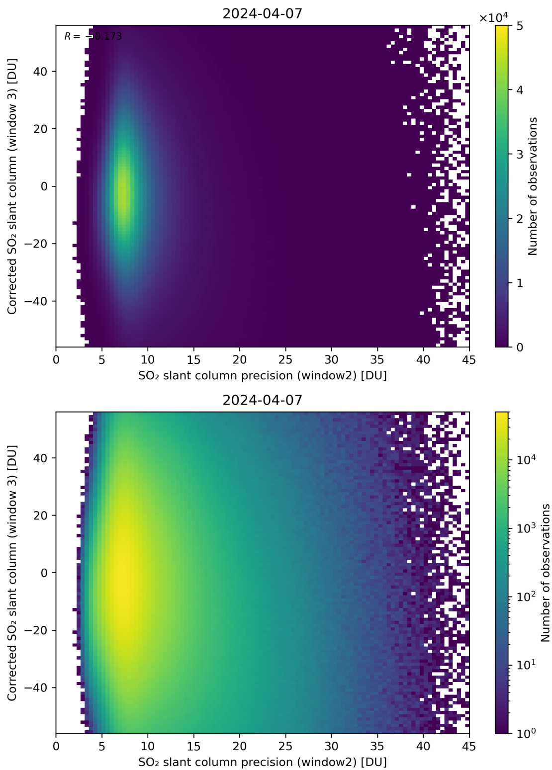
Figure 248: Scatter density plot of “SO 2 slant column precision (window2)” against “Corrected SO 2 slant column (window 3)” for 2024-04-06 to 2024-04-08.
