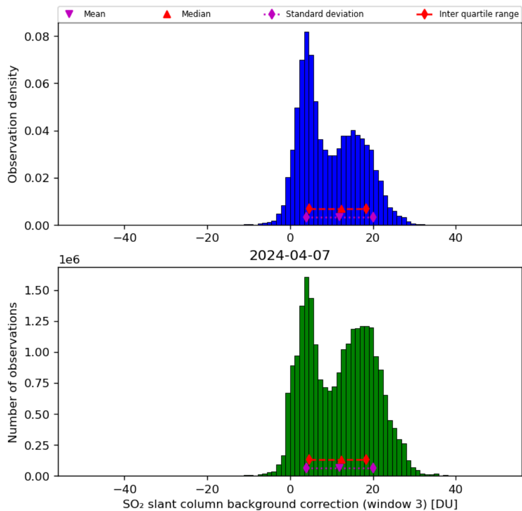
Figure 67: Histogram of “SO 2 slant column background correction (window 3)” for 2024-04-06 to 2024-04-08
