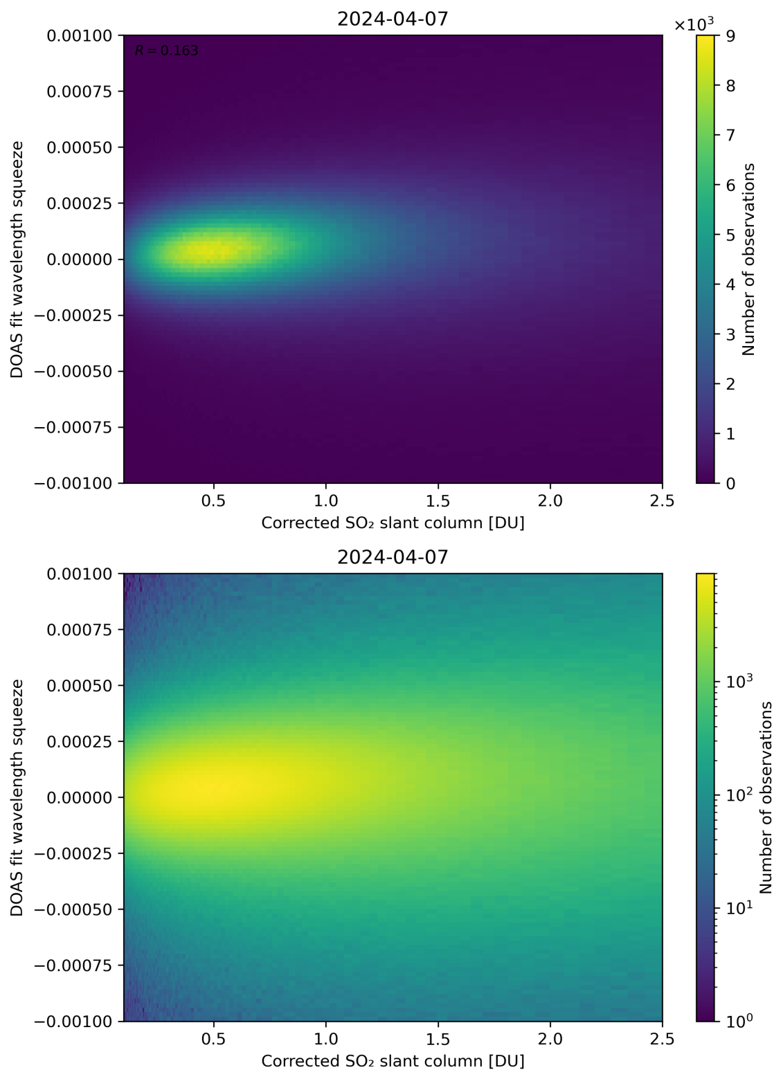
Figure 182: Scatter density plot of “Corrected SO 2 slant column” against “DOAS fit wavelength squeeze” for 2024-04-06 to 2024-04-08.
