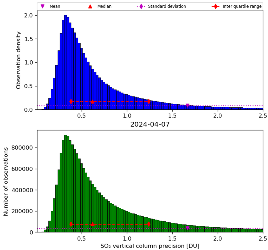
Figure 54: Histogram of “SO 2 vertical column precision” for 2024-04-06 to 2024-04-08
