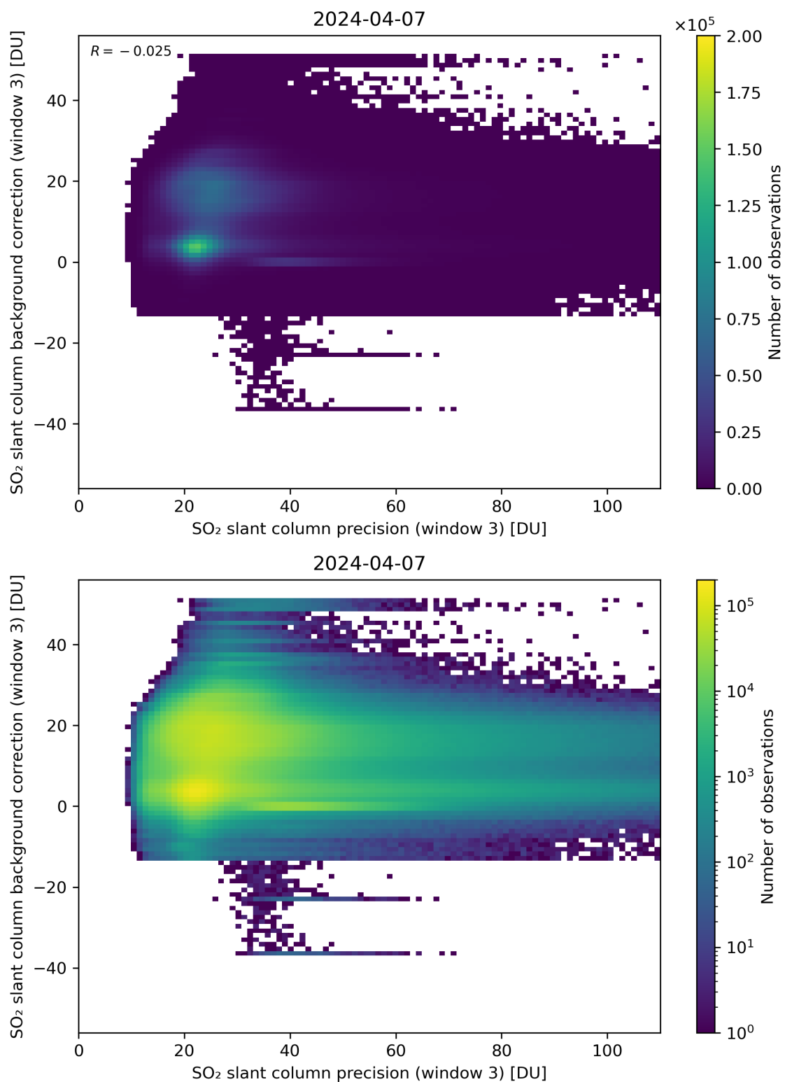
Figure 257: Scatter density plot of “SO 2 slant column precision (window 3)” against “SO 2 slant column background correction (window 3)” for 2024-04-06 to 2024-04-08.
