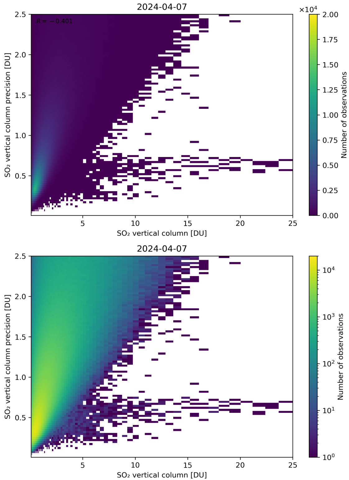
Figure 307: Scatter density plot of “SO 2 vertical column” against “SO 2 vertical column precision” for 2024-04-06 to 2024-04-08.
