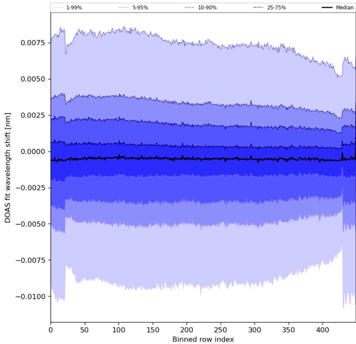
Figure 91: Along track statistics of “DOAS fit wavelength shift” for 2024-04-06 to 2024-04-08
