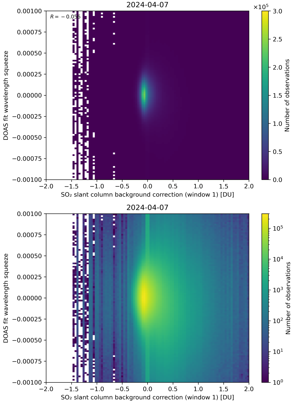
Figure 101: Scatter density plot of “SO 2 slant column background correction (window 1)” against “DOAS fit wavelength squeeze” for 2024-04-06 to 2024-04-08.
