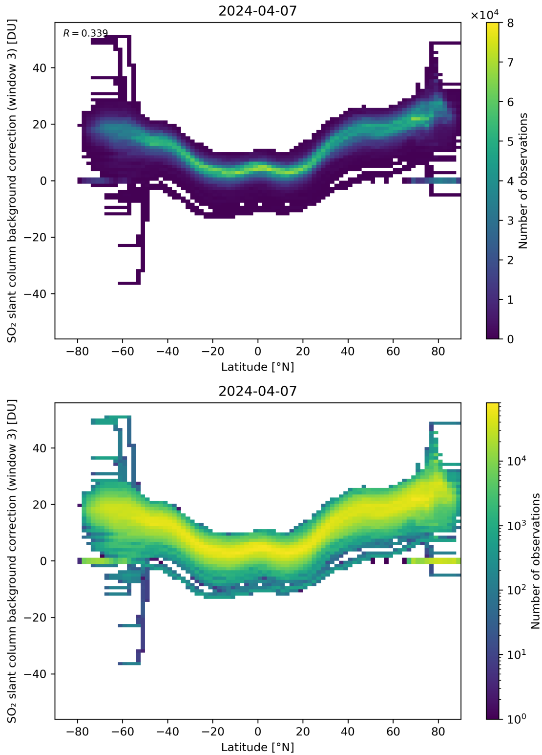
Figure 141: Scatter density plot of “Latitude” against “SO 2 slant column background correction (window 3)” for 2024-04-06 to 2024-04-08.
