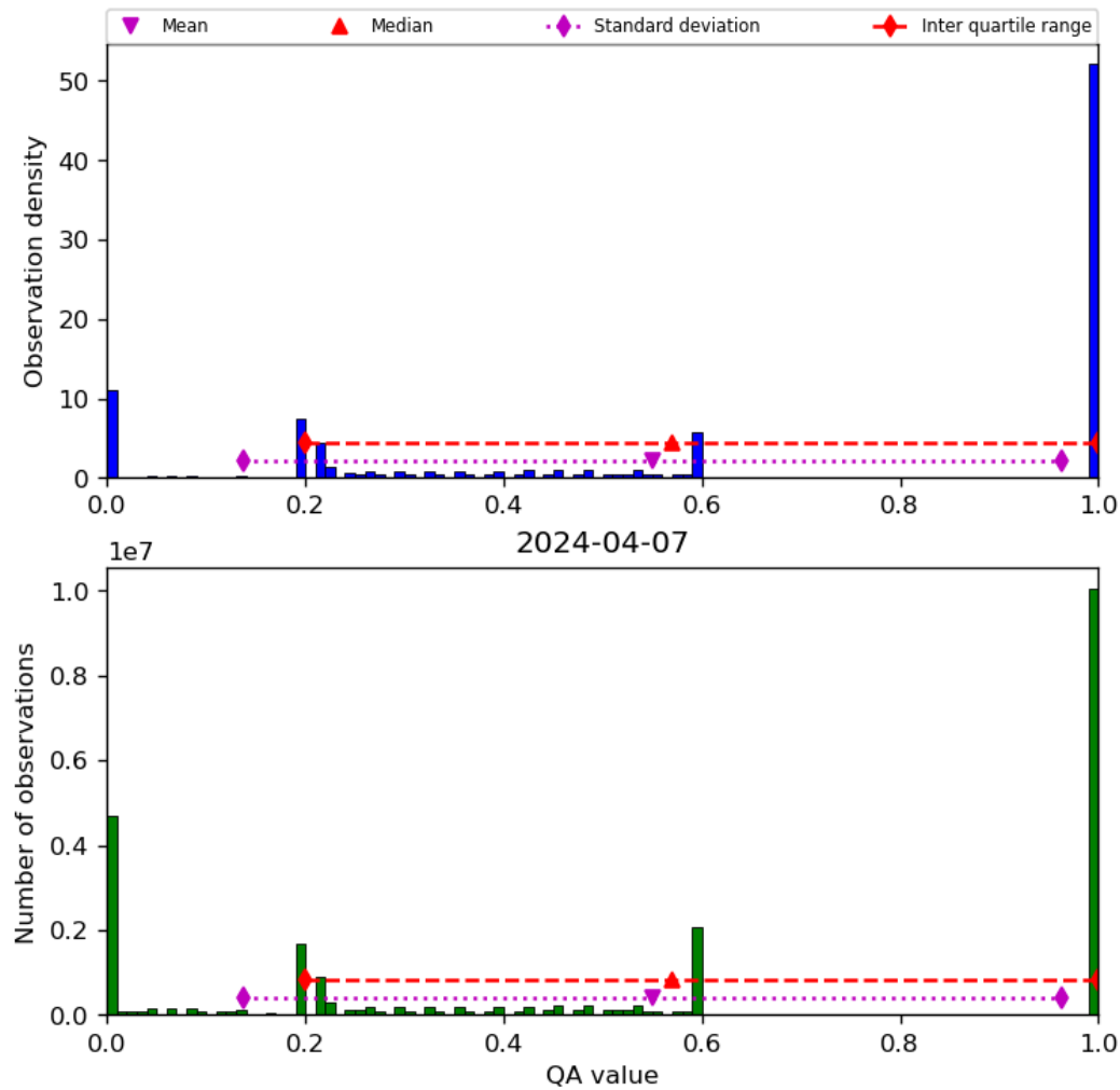
Figure 52: Histogram of “QA value” for 2024-04-06 to 2024-04-08
