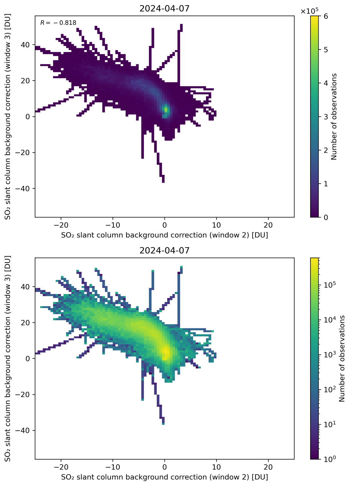
Figure 111: Scatter density plot of “SO 2 slant column background correction (window 2)” against “SO 2 slant column background correction (window 3)” for 2024-04-06 to 2024-04-08.
