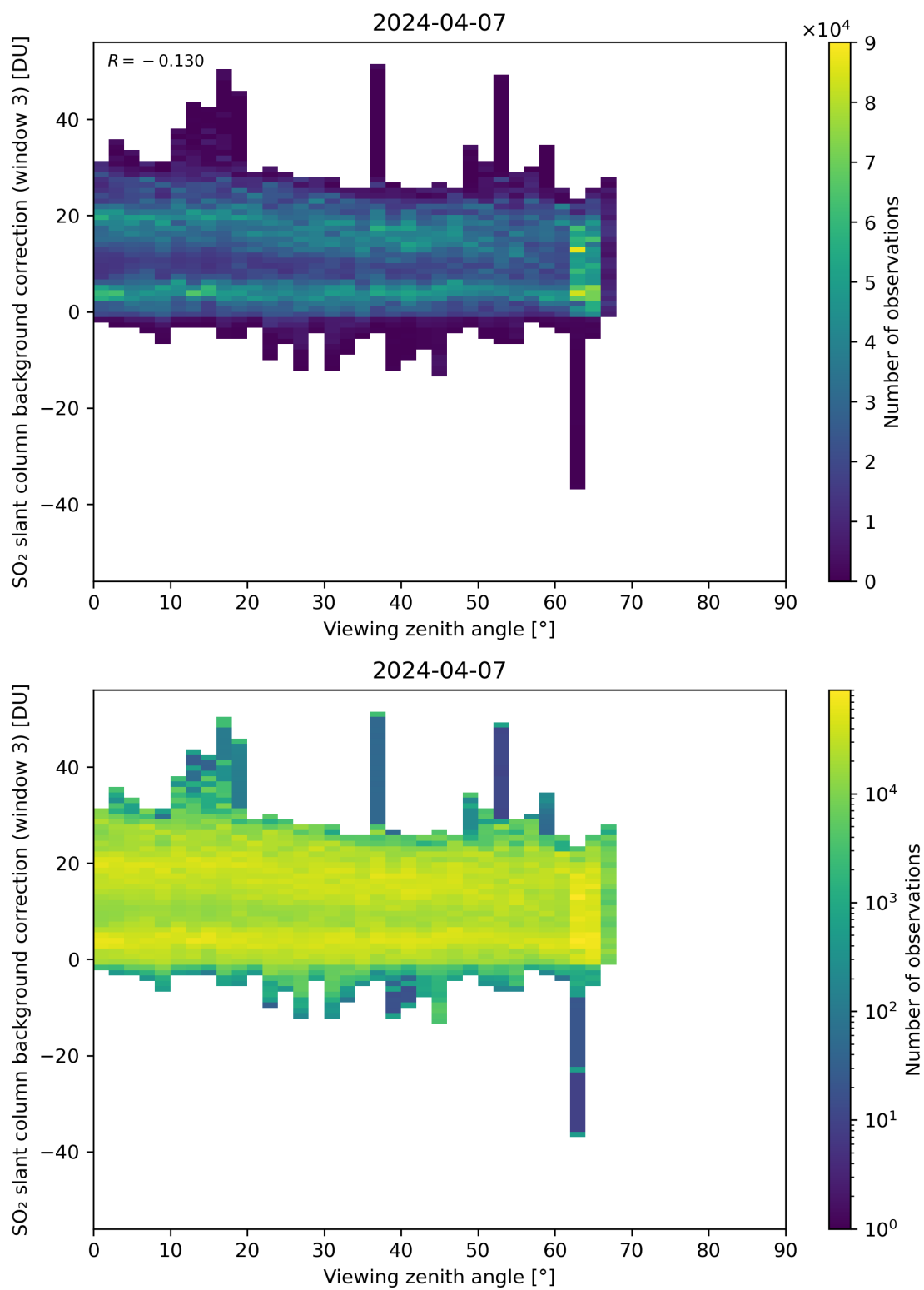
Figure 310: Scatter density plot of “Viewing zenith angle” against “SO 2 slant column background correction (window 3)” for 2024-04-06 to 2024-04-08.
