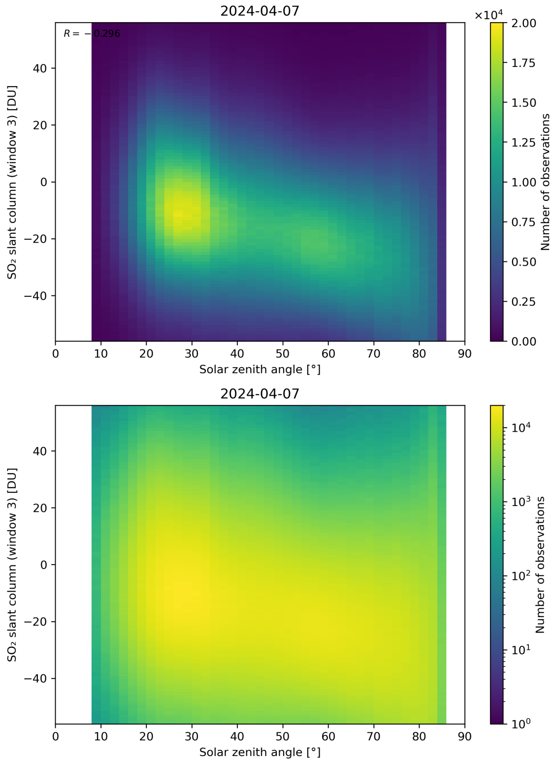
Figure 172: Scatter density plot of “Solar zenith angle” against “SO 2 slant column (window 3)” for 2024-04-06 to 2024-04-08.
