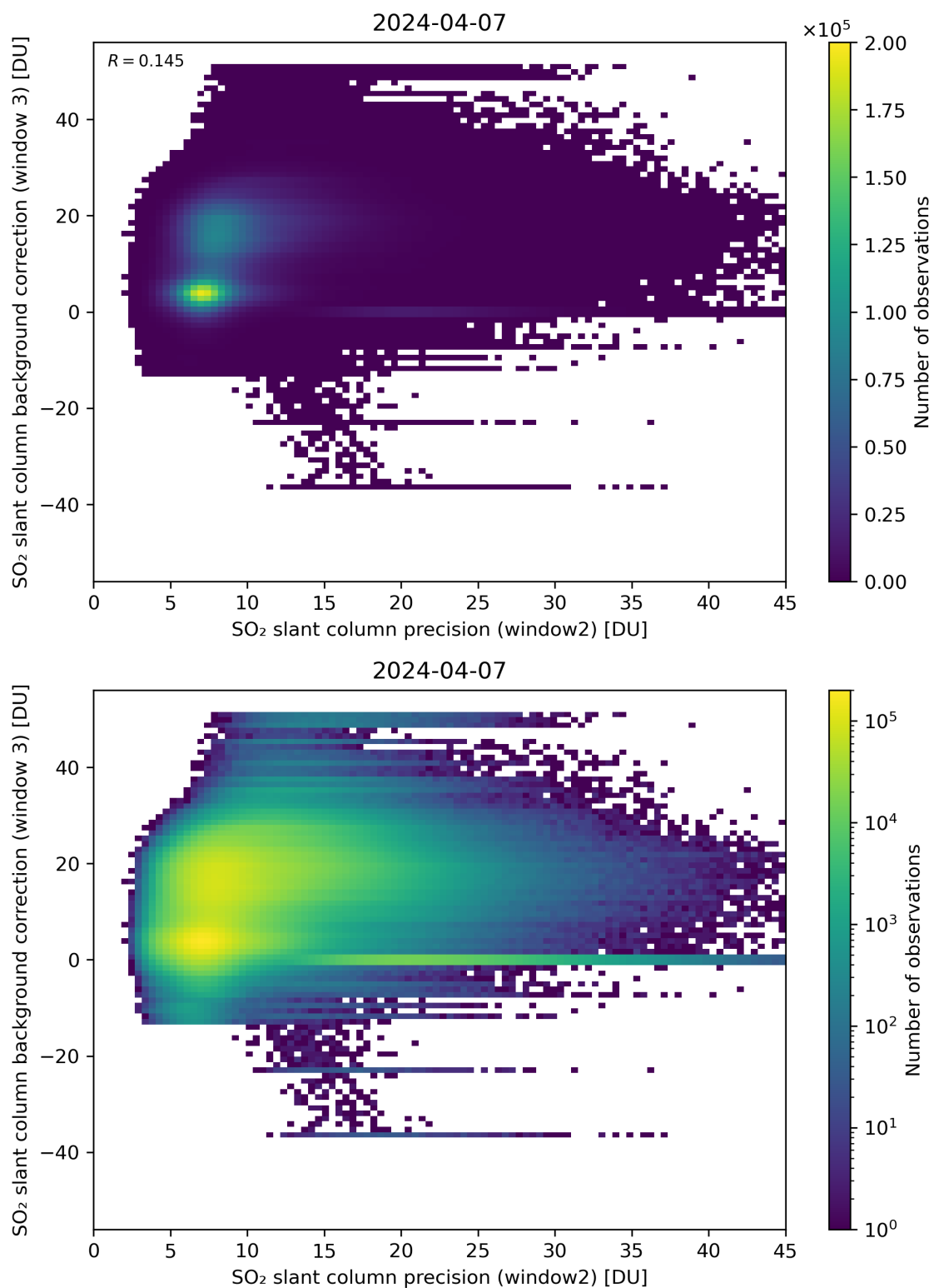
Figure 242: Scatter density plot of “SO 2 slant column precision (window2)” against “SO 2 slant column background correction (window 3)” for 2024-04-06 to 2024-04-08.
