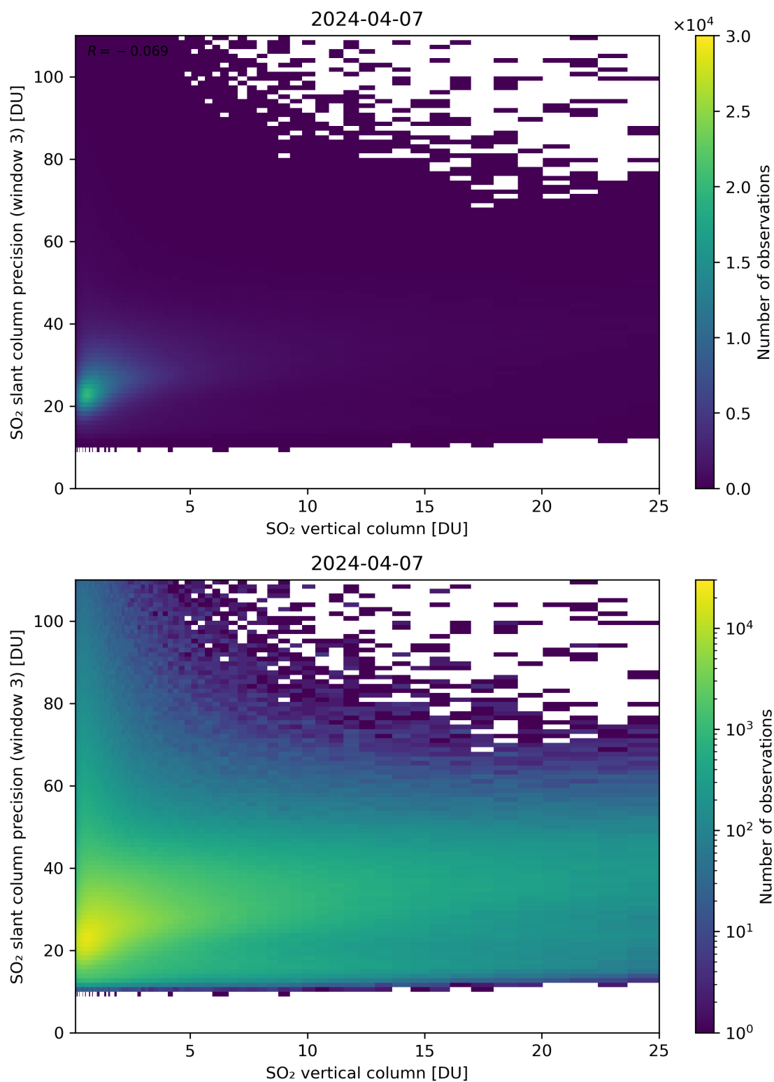
Figure 304: Scatter density plot of “SO 2 vertical column” against “SO 2 slant column precision (window 3)” for 2024-04-06 to 2024-04-08.
