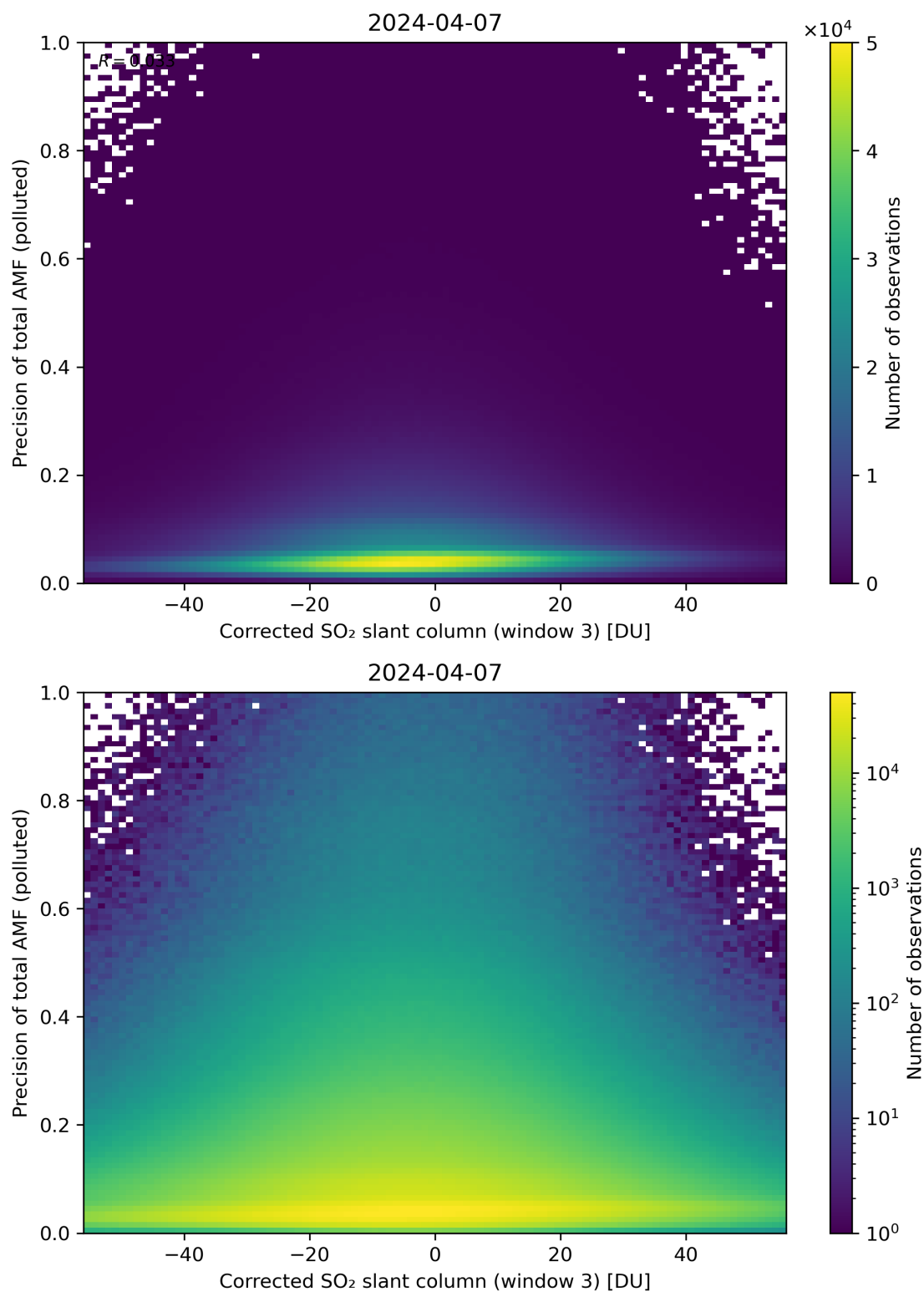
Figure 211: Scatter density plot of “Corrected SO 2 slant column (window 3)” against “Precision of total AMF (polluted)” for 2024-04-06 to 2024-04-08.
