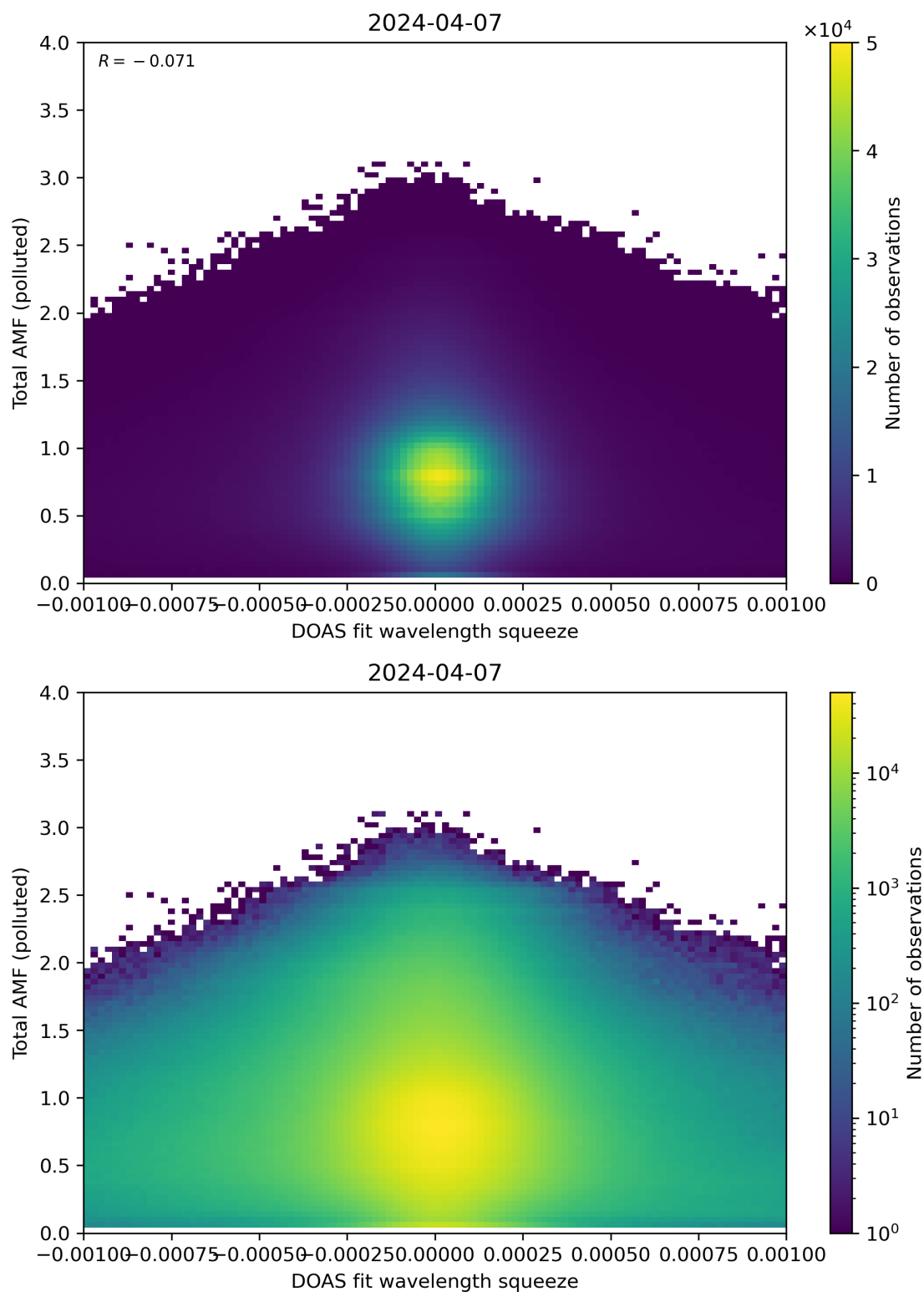
Figure 134: Scatter density plot of “DOAS fit wavelength squeeze” against “Total AMF (polluted)” for 2024-04-06 to 2024-04-08.
