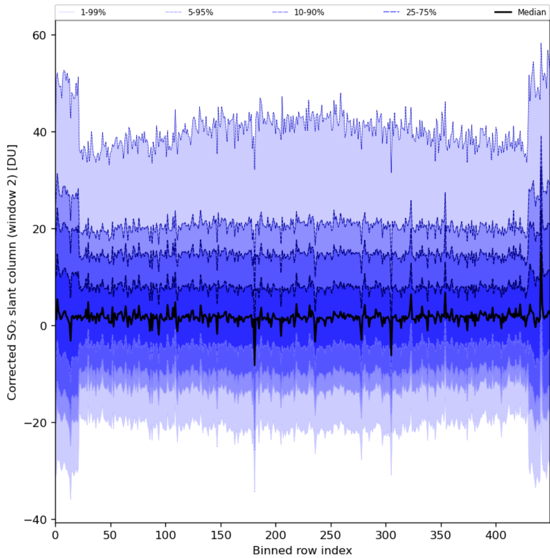
Figure 85: Along track statistics of “Corrected SO 2 slant column (window 2)” for 2024-04-06 to 2024-04-08
