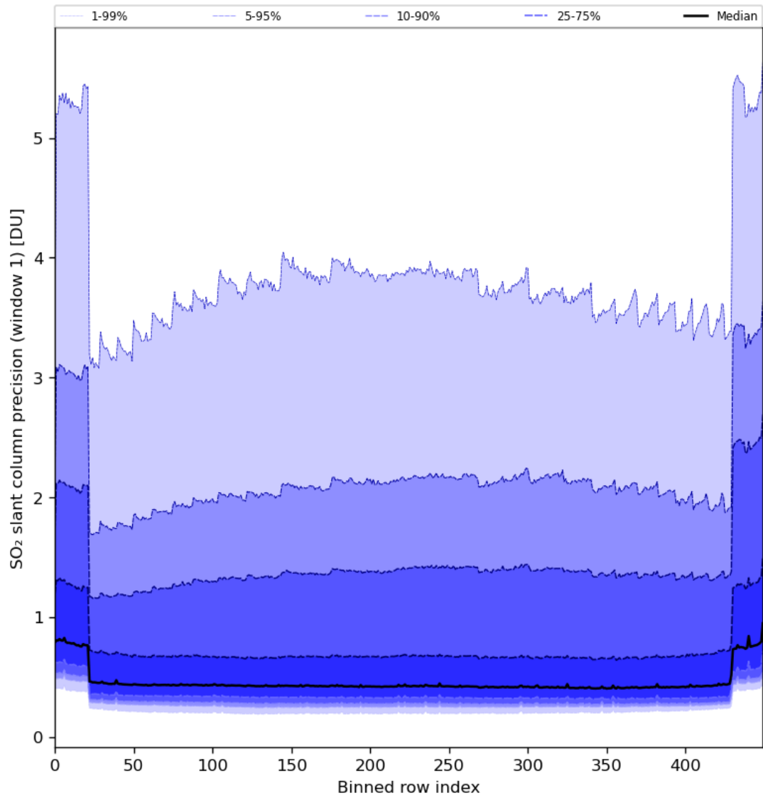
Figure 80: Along track statistics of “SO 2 slant column precision (window 1)” for 2024-04-06 to 2024-04-08
