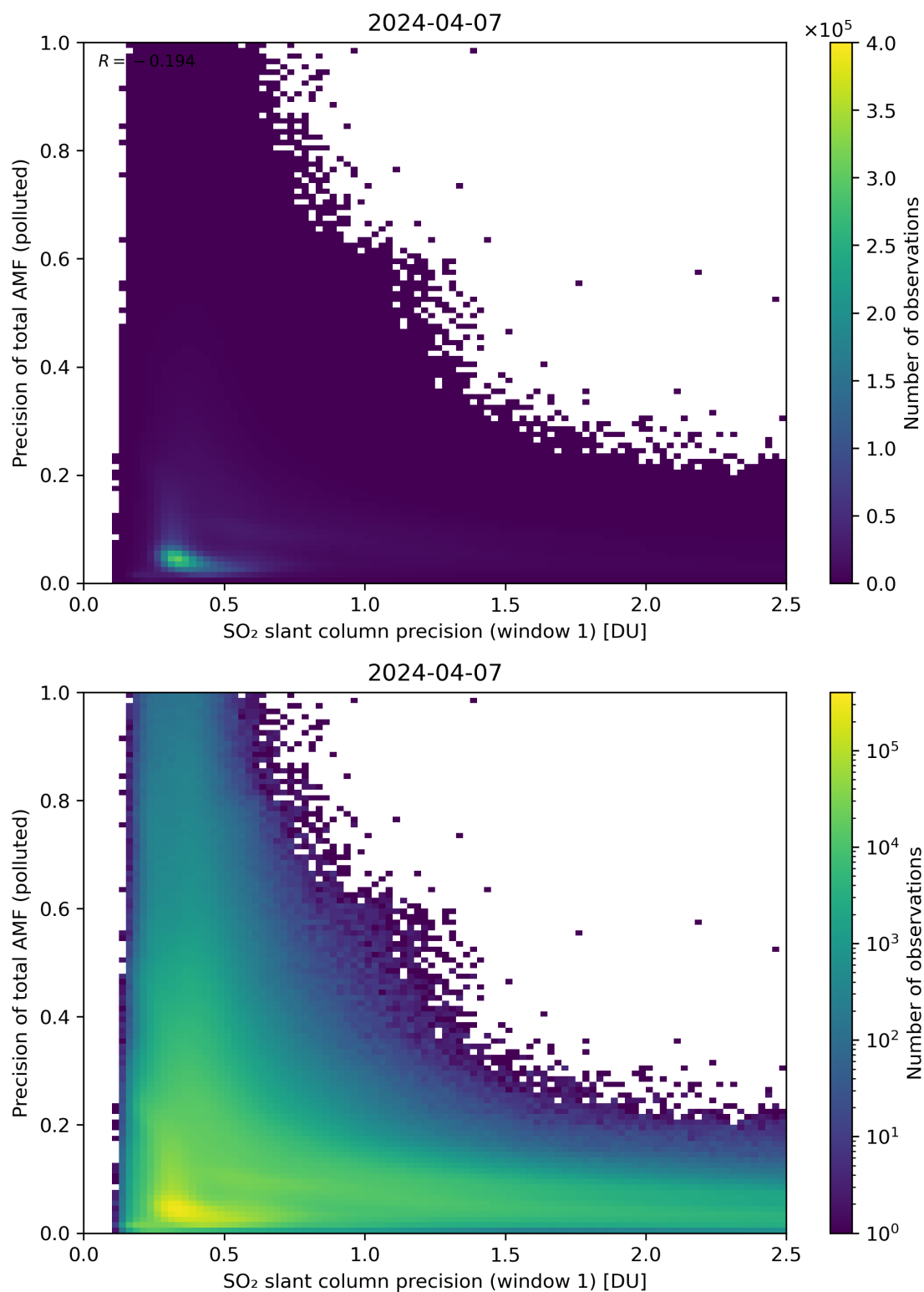
Figure 231: Scatter density plot of “SO 2 slant column precision (window 1)” against “Precision of total AMF (polluted)” for 2024-04-06 to 2024-04-08.
