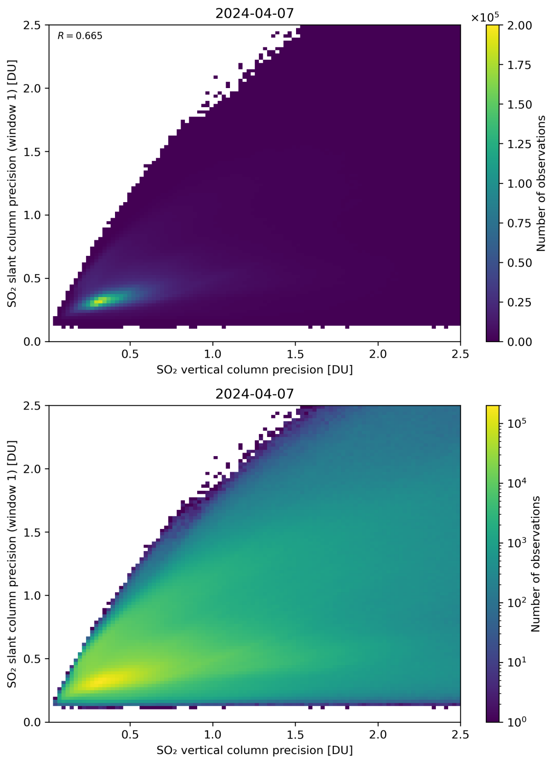
Figure 290: Scatter density plot of “SO 2 vertical column precision” against “SO 2 slant column precision (window 1)” for 2024-04-06 to 2024-04-08.
