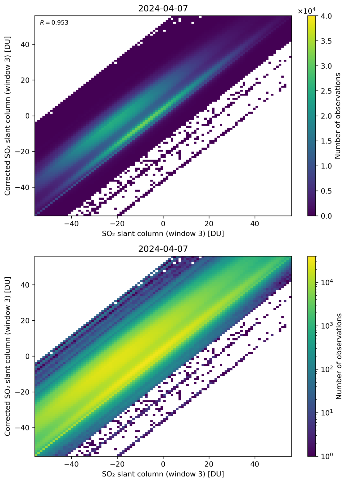
Figure 266: Scatter density plot of “SO 2 slant column (window 3)” against “Corrected SO 2 slant column (window 3)” for 2024-04-06 to 2024-04-08.
