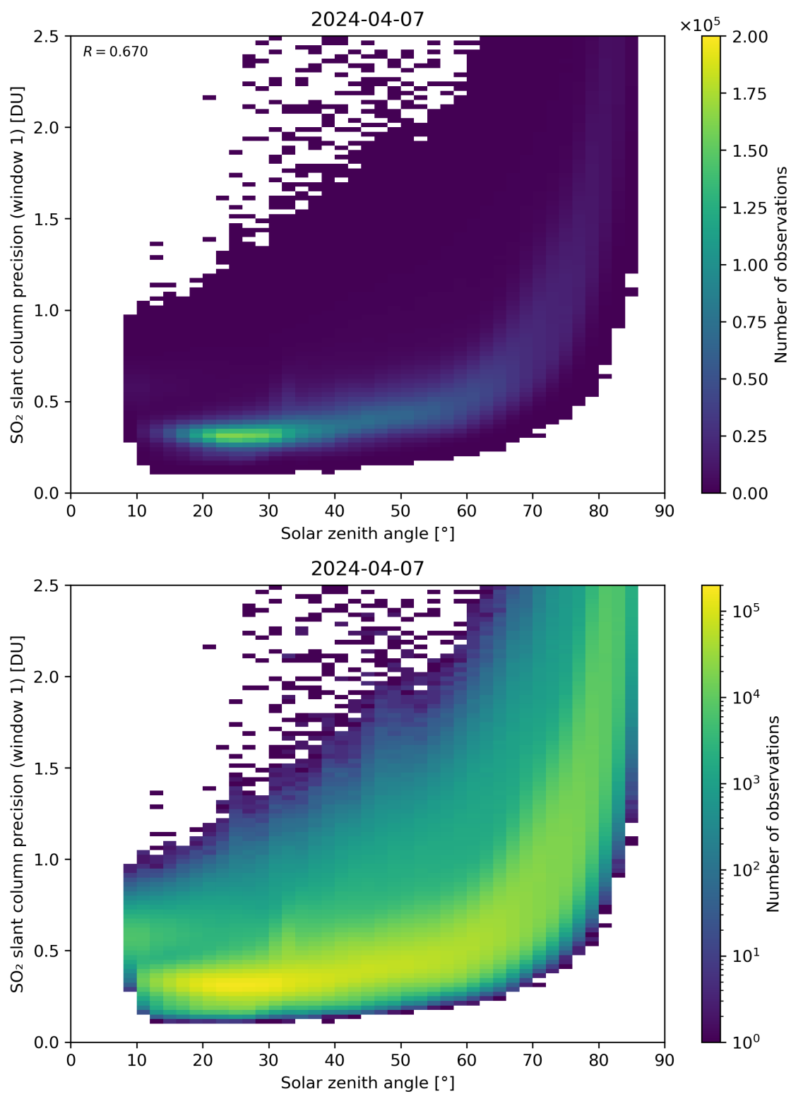
Figure 170: Scatter density plot of “Solar zenith angle” against “SO 2 slant column precision (window 1)” for 2024-04-06 to 2024-04-08.
