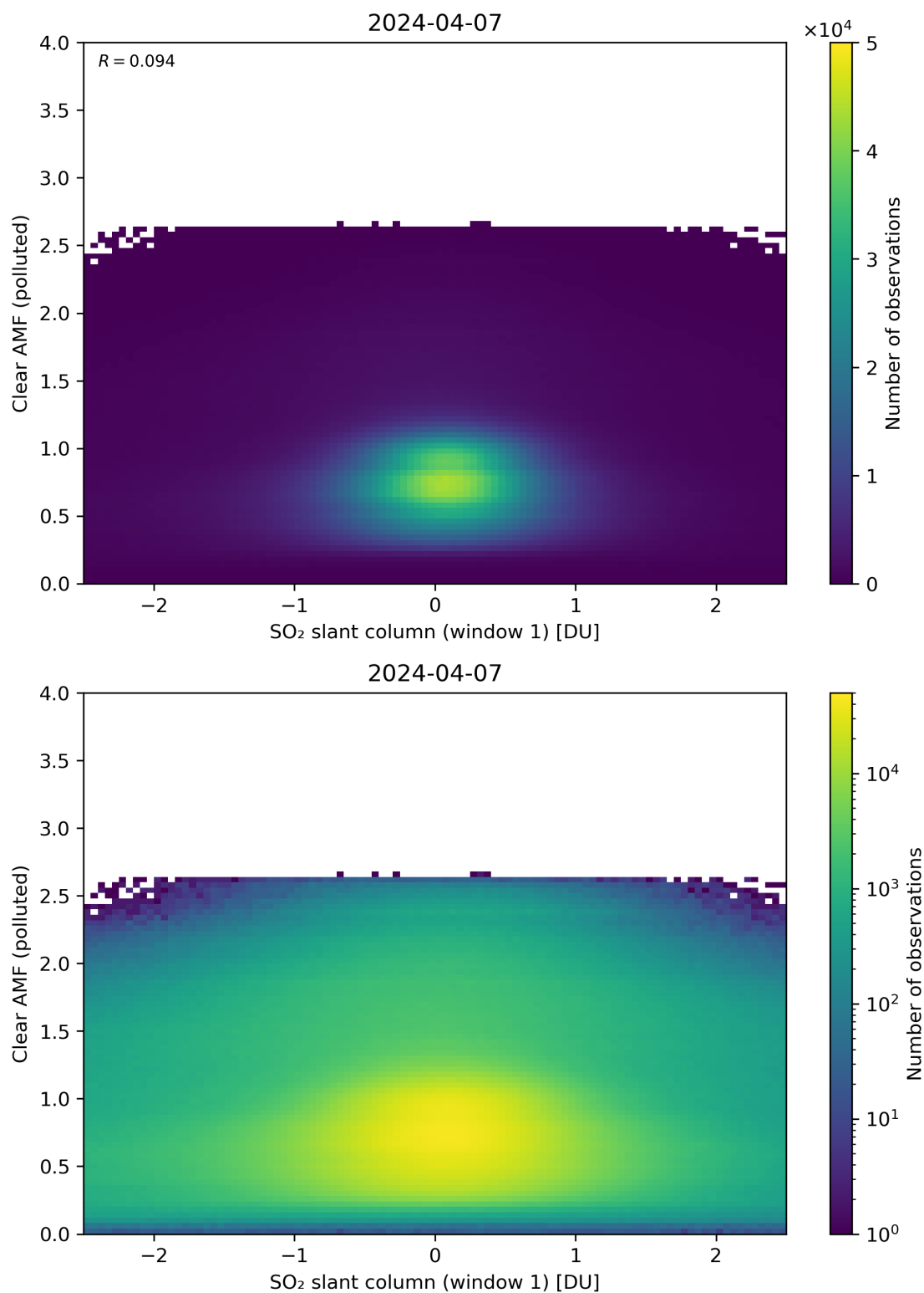
Figure 232: Scatter density plot of “SO 2 slant column (window 1)” against “Clear AMF (polluted)” for 2024-04-06 to 2024-04-08.
