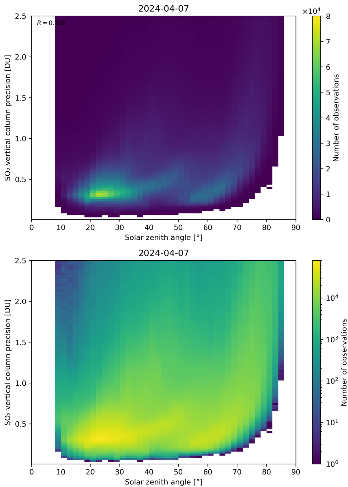
Figure 177: Scatter density plot of “Solar zenith angle” against “SO 2 vertical column precision” for 2024-04-06 to 2024-04-08.
