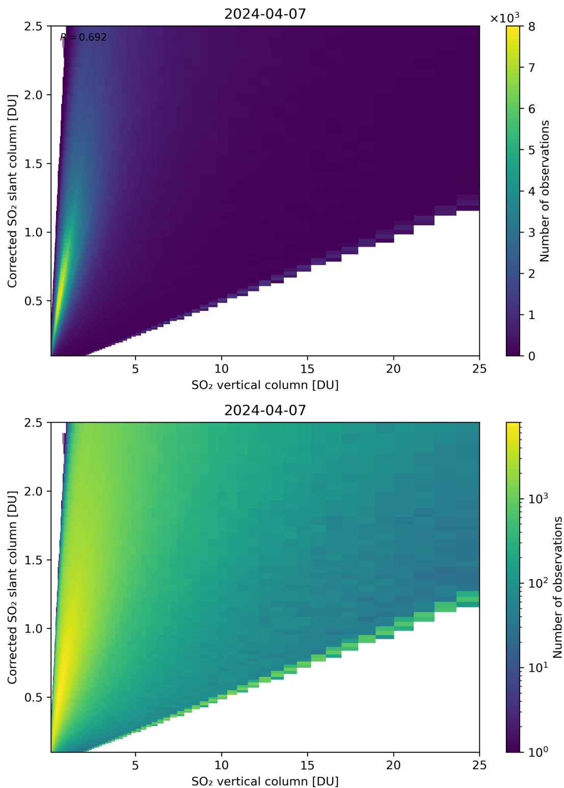
Figure 297: Scatter density plot of “SO 2 vertical column” against “Corrected SO 2 slant column” for 2024-04-06 to 2024-04-08.
