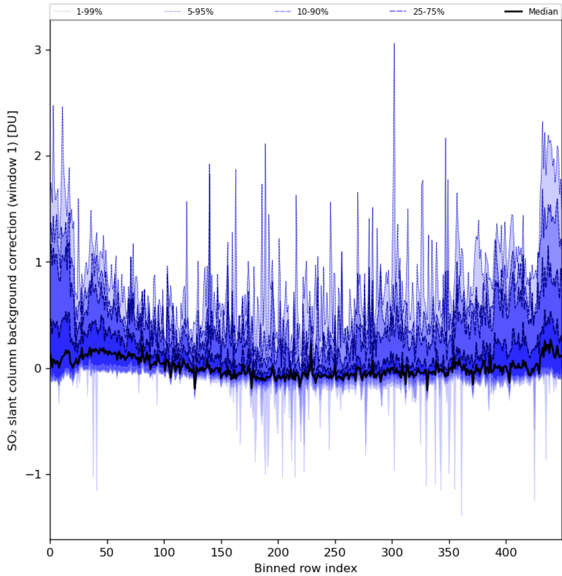
Figure 82: Along track statistics of “SO 2 slant column background correction (window 1)” for 2024-04-06 to 2024-04-08
