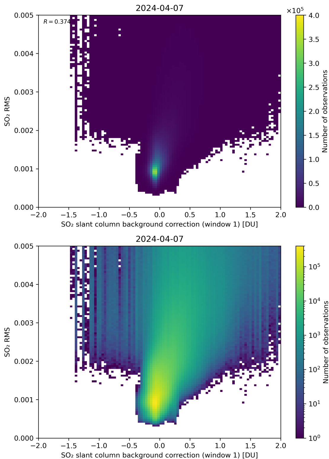
Figure 102: Scatter density plot of “SO 2 slant column background correction (window 1)” against “SO 2 RMS” for 2024-04-06 to 2024-04-08.
