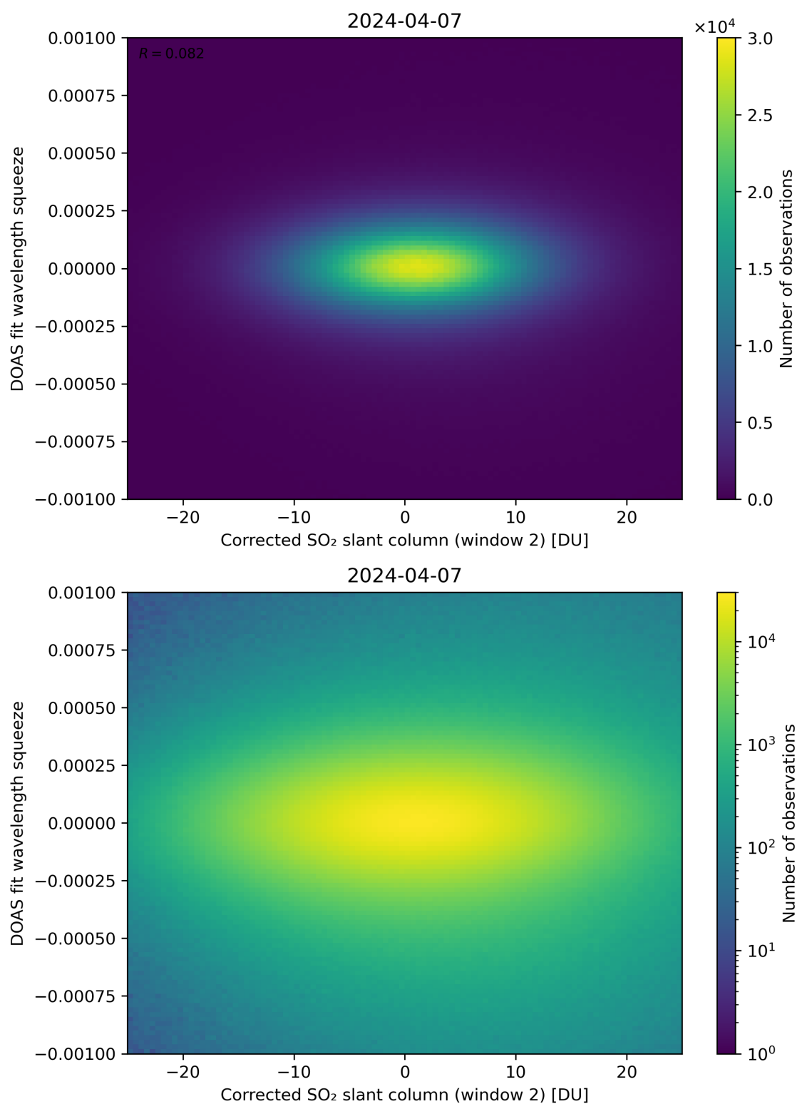
Figure 197: Scatter density plot of “Corrected SO 2 slant column (window 2)” against “DOAS fit wavelength squeeze” for 2024-04-06 to 2024-04-08.
