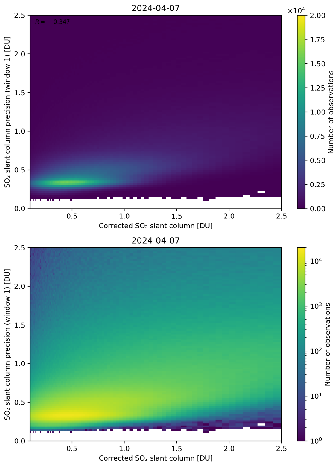
Figure 188: Scatter density plot of “Corrected SO 2 slant column” against “SO 2 slant column precision (window 1)” for 2024-04-06 to 2024-04-08.
