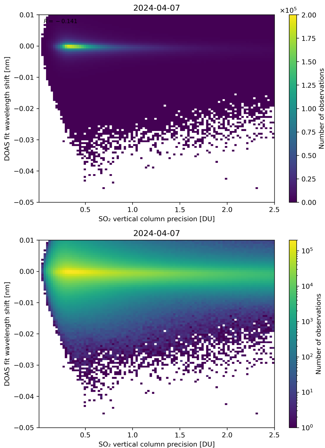
Figure 282: Scatter density plot of “SO 2 vertical column precision” against “DOAS fit wavelength shift” for 2024-04-06 to 2024-04-08.
