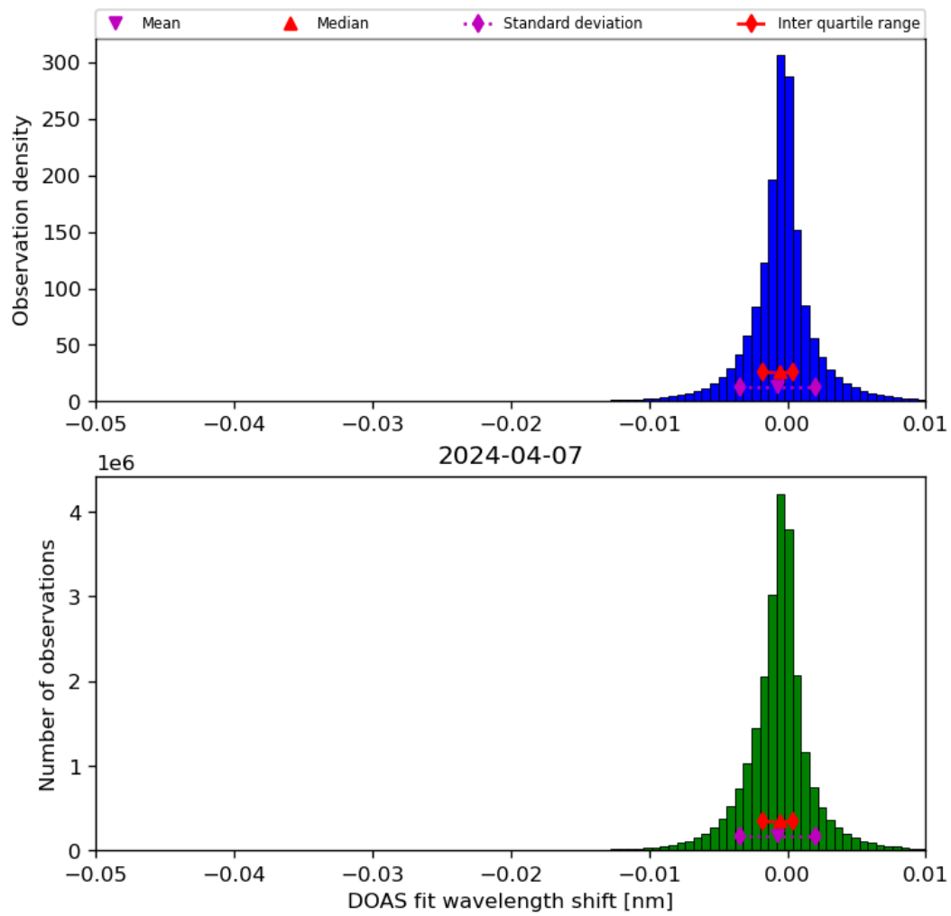
Figure 68: Histogram of “DOAS fit wavelength shift” for 2024-04-06 to 2024-04-08
