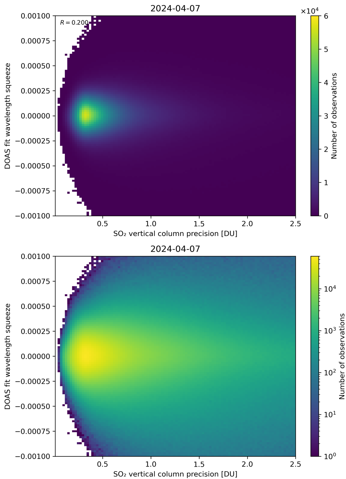
Figure 283: Scatter density plot of “SO 2 vertical column precision” against “DOAS fit wavelength squeeze” for 2024-04-06 to 2024-04-08.
