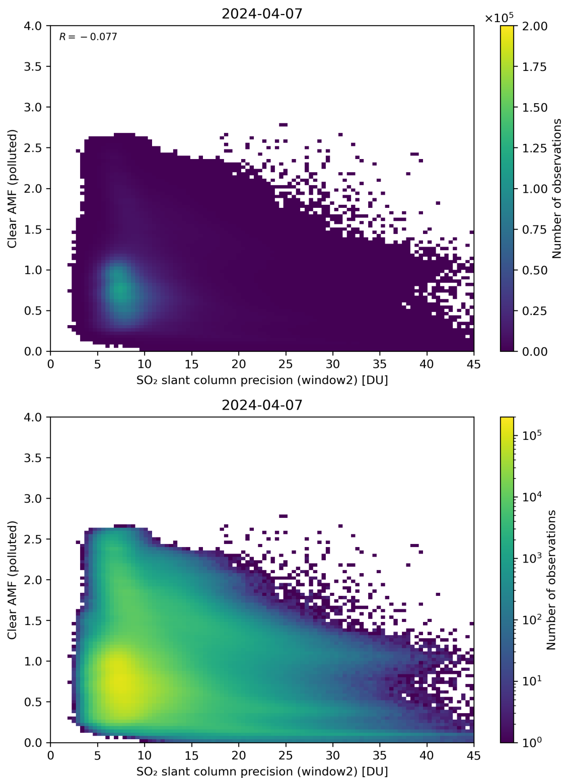
Figure 246: Scatter density plot of “SO 2 slant column precision (window2)” against “Clear AMF (polluted)” for 2024-04-06 to 2024-04-08.
