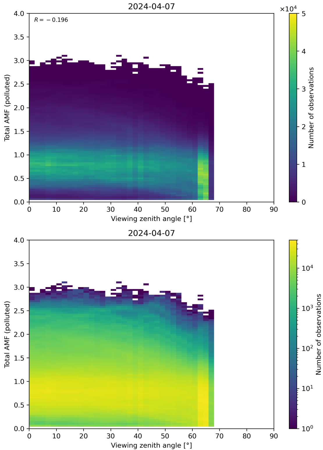
Figure 325: Scatter density plot of “Viewing zenith angle” against “Total AMF (polluted)” for 2024-04-06 to 2024-04-08.
