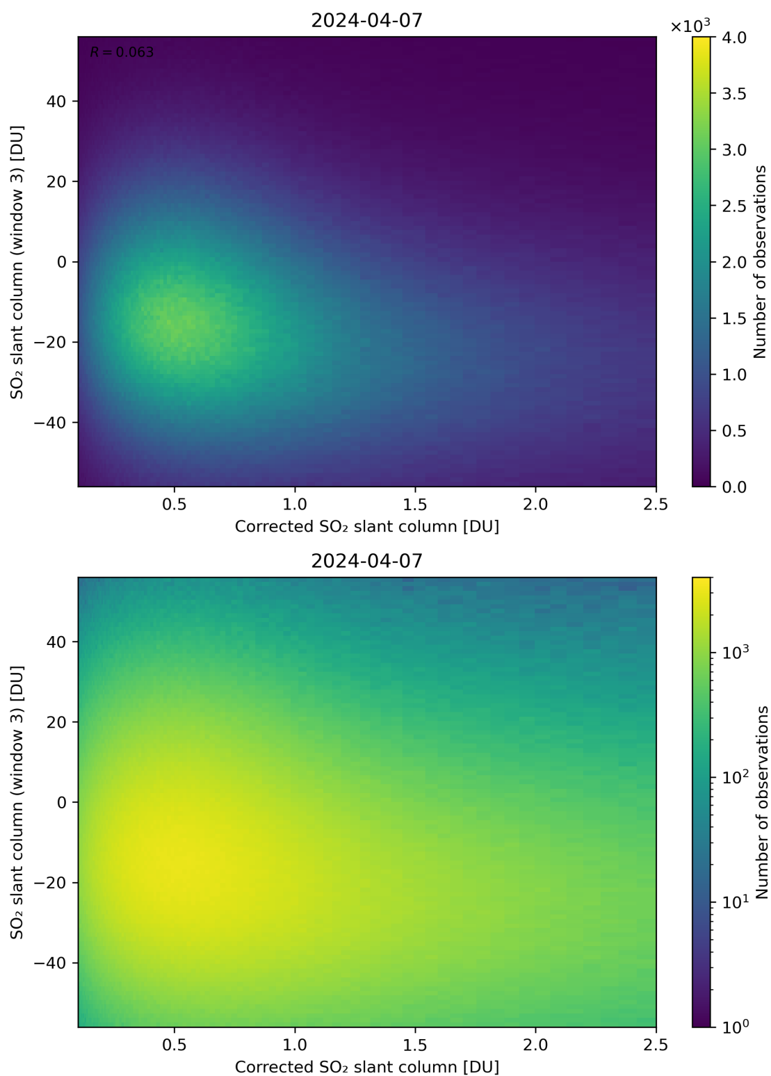
Figure 190: Scatter density plot of “Corrected SO 2 slant column” against “SO 2 slant column (window 3)” for 2024-04-06 to 2024-04-08.
