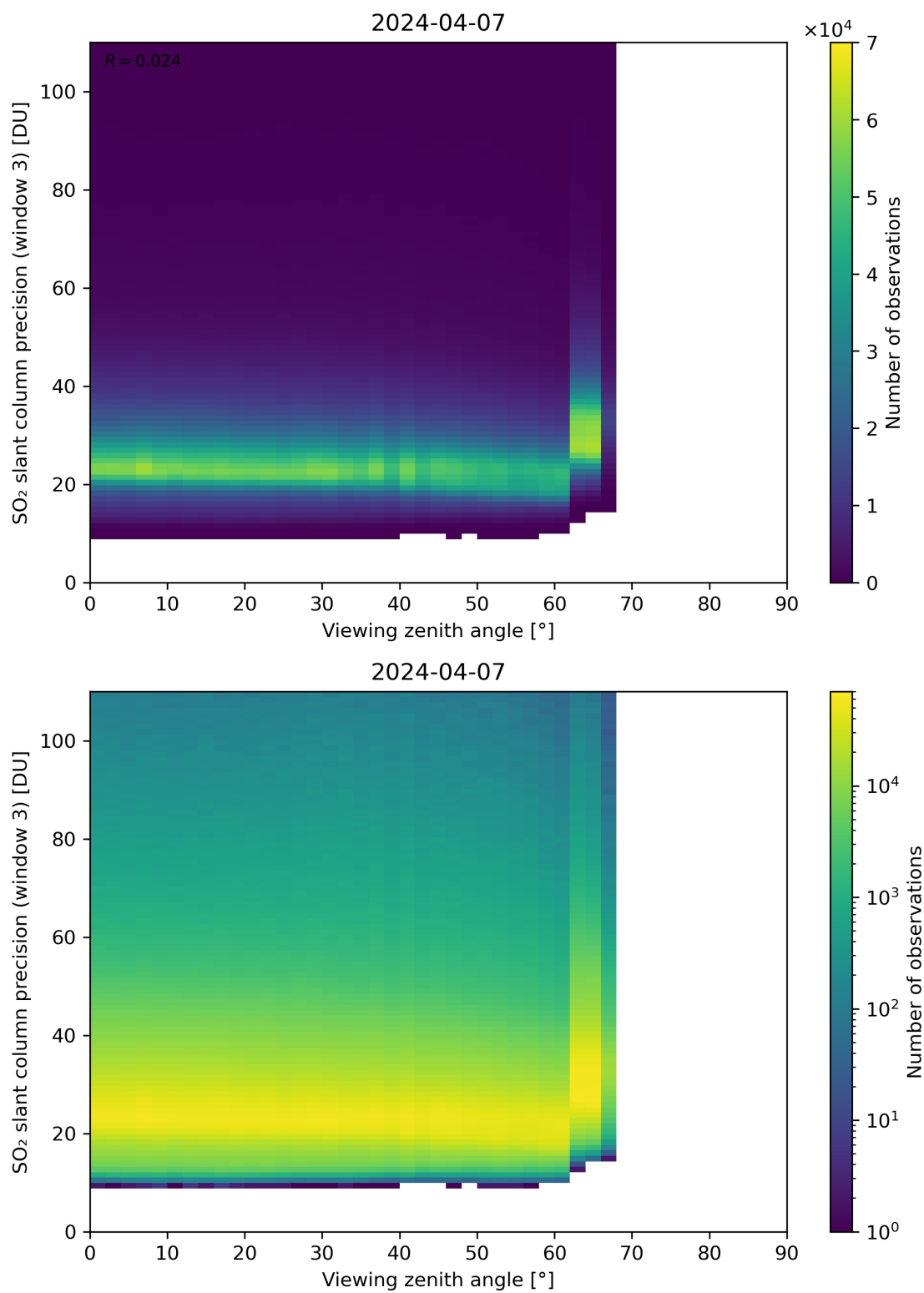
Figure 324: Scatter density plot of “Viewing zenith angle” against “SO 2 slant column precision (window 3)” for 2024-04-06 to 2024-04-08.
