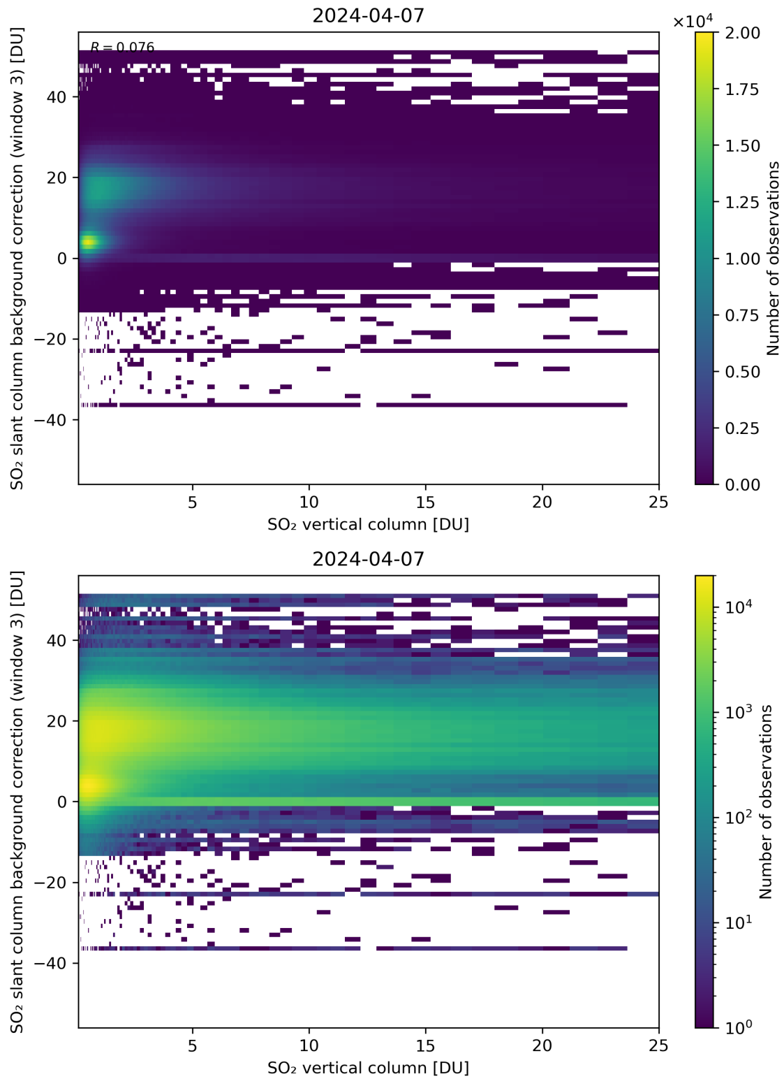
Figure 275: Scatter density plot of “SO 2 vertical column” against “SO 2 slant column background correction (window 3)” for 2024-04-06 to 2024-04-08.
