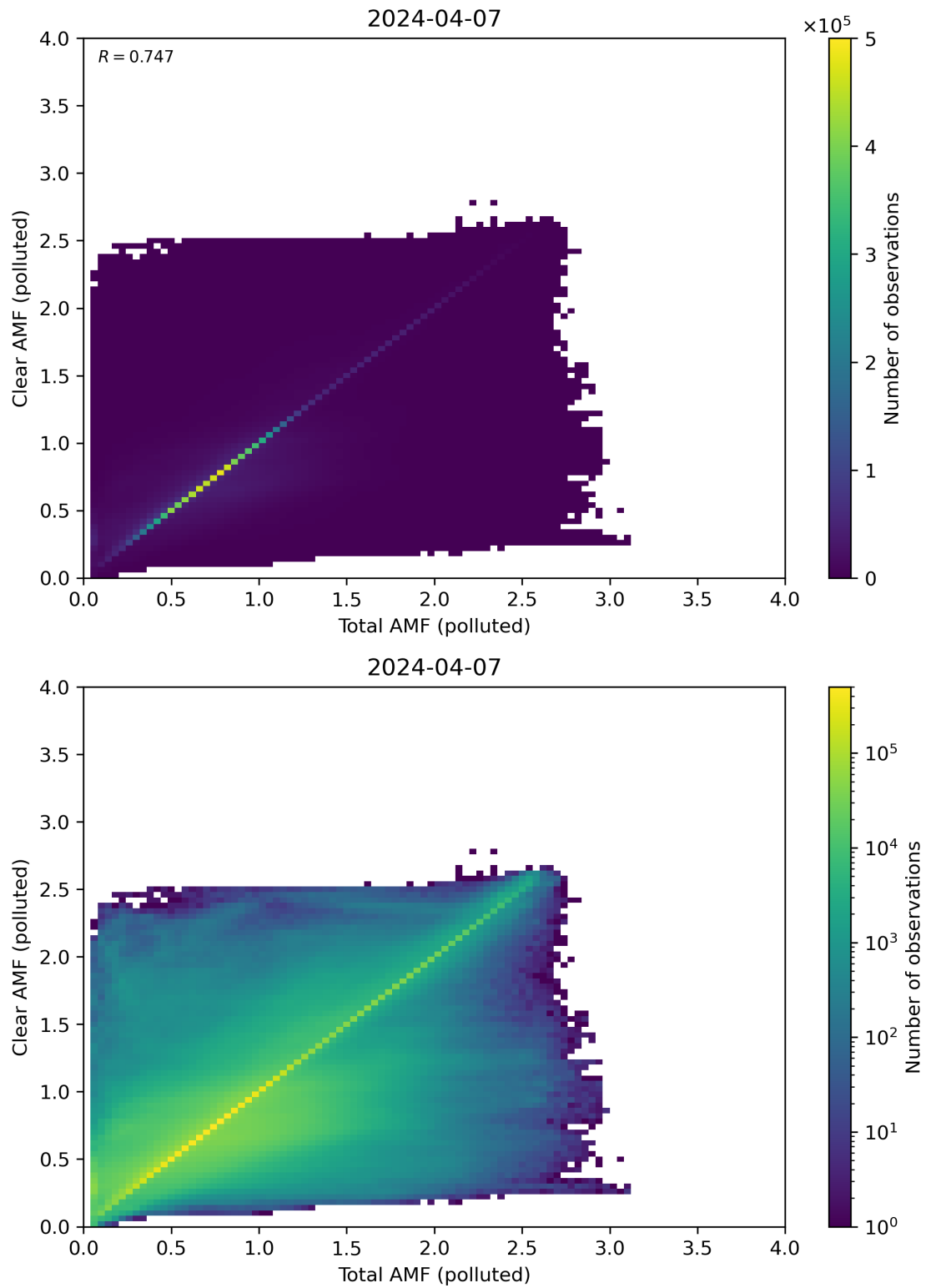
Figure 271: Scatter density plot of “Total AMF (polluted)” against “Clear AMF (polluted)” for 2024-04-06 to 2024-04-08.
