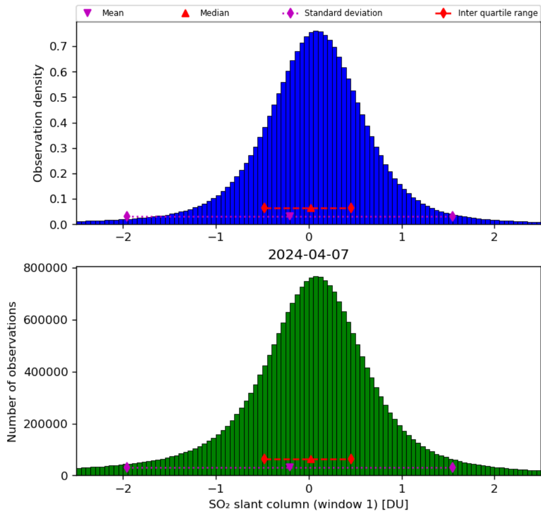
Figure 56: Histogram of “SO 2 slant column (window 1)” for 2024-04-06 to 2024-04-08
