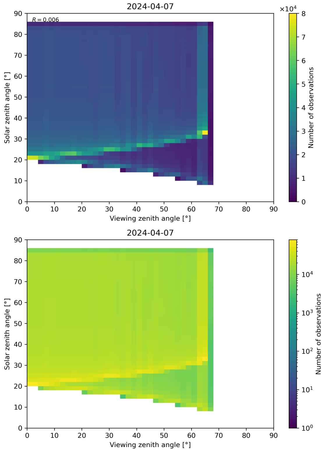
Figure 315: Scatter density plot of “Viewing zenith angle” against “Solar zenith angle” for 2024-04-06 to 2024-04-08.
