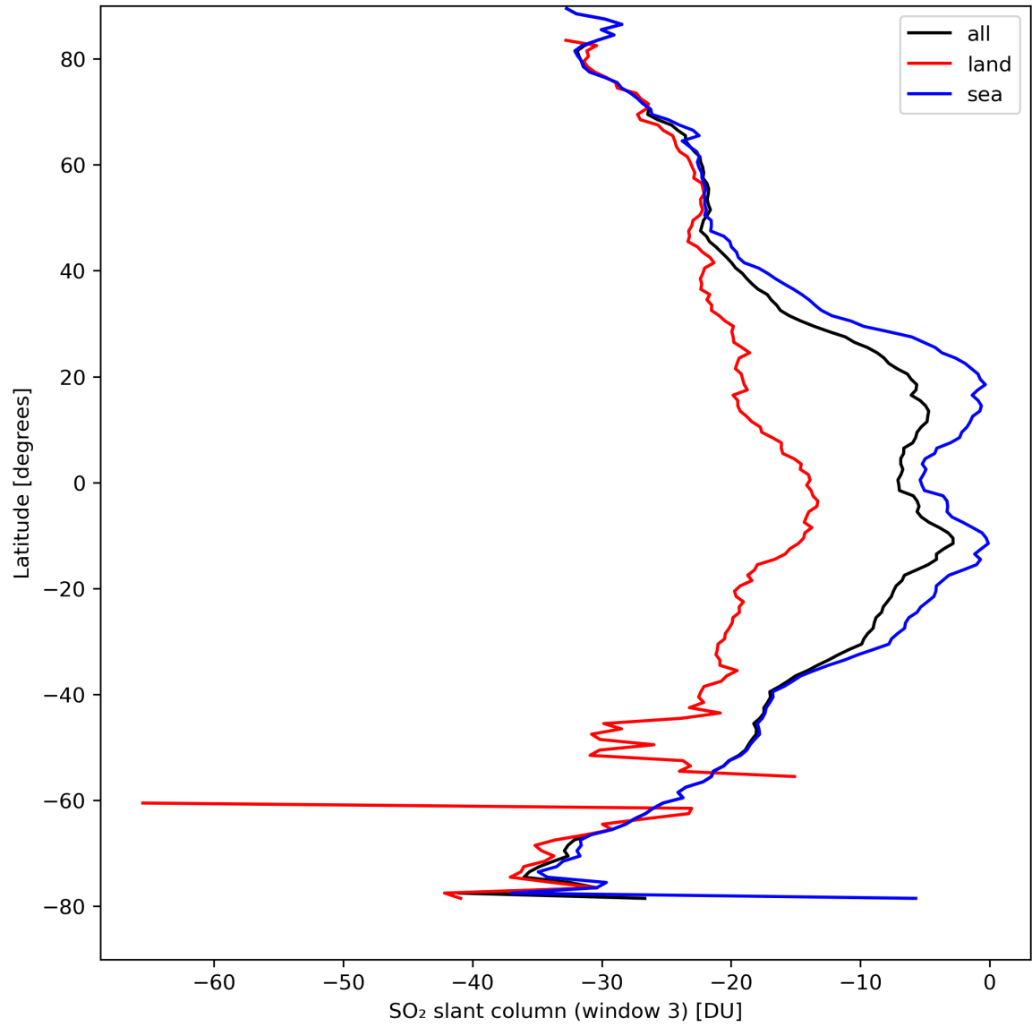
Figure 41: Zonal average of “SO 2 slant column (window 3)” for 2024-04-06 to 2024-04-08.
