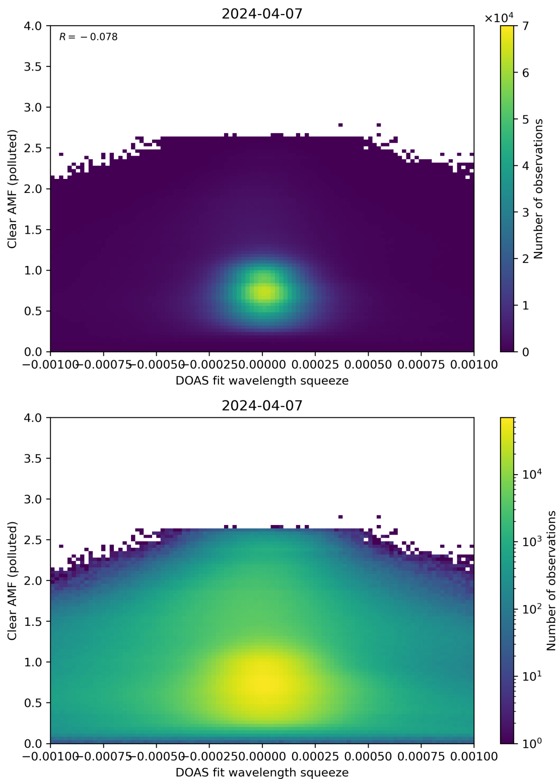
Figure 133: Scatter density plot of “DOAS fit wavelength squeeze” against “Clear AMF (polluted)” for 2024-04-06 to 2024-04-08.
