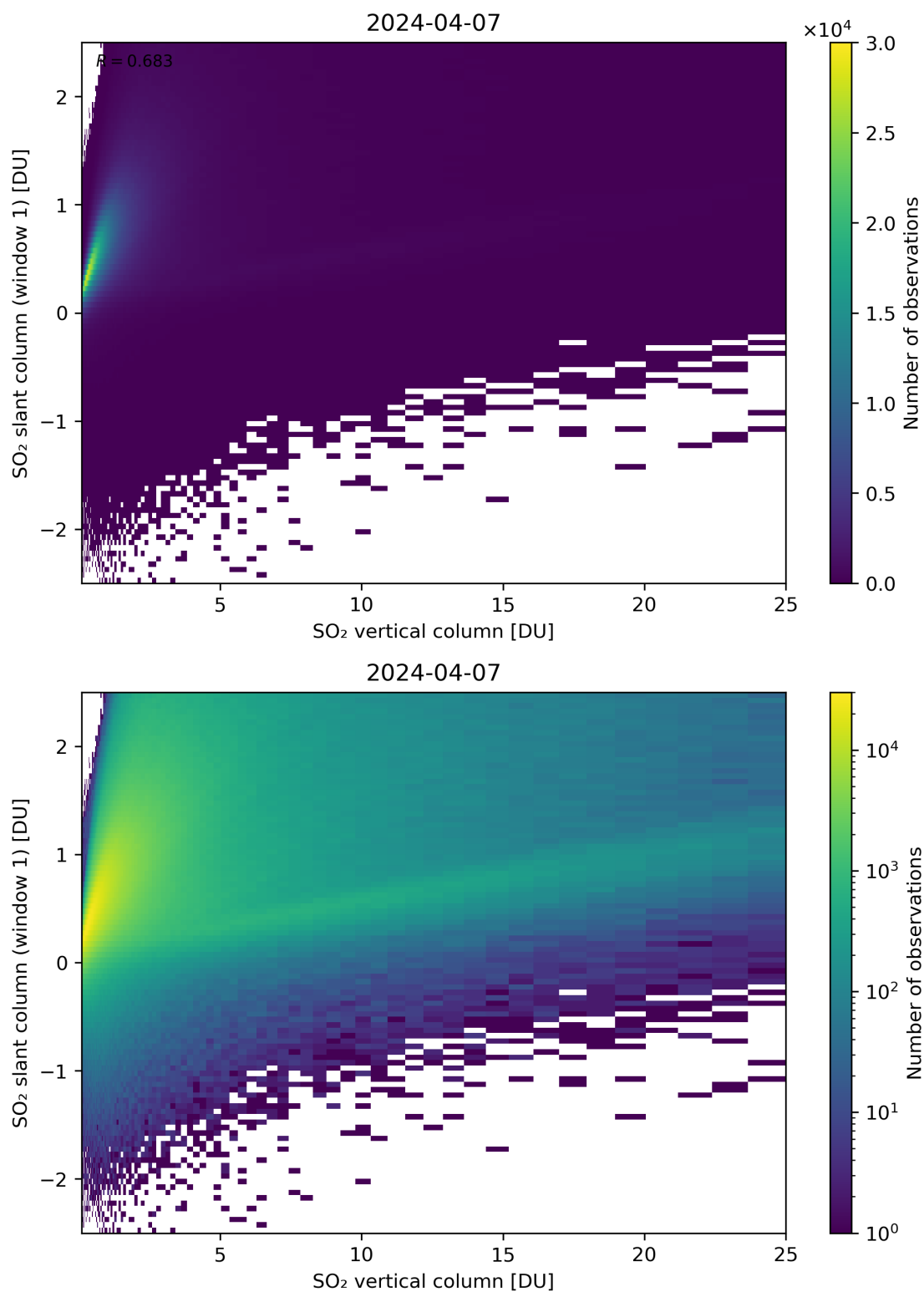
Figure 300: Scatter density plot of “SO 2 vertical column” against “SO 2 slant column (window 1)” for 2024-04-06 to 2024-04-08.
