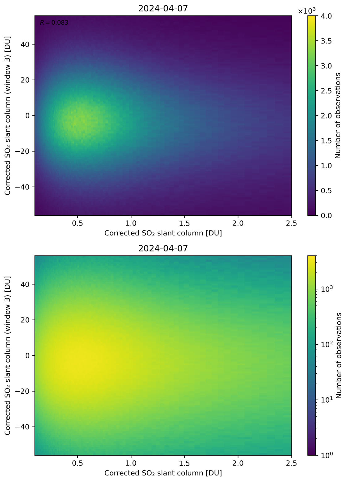
Figure 186: Scatter density plot of “Corrected SO 2 slant column” against “Corrected SO 2 slant column (window 3)” for 2024-04-06 to 2024-04-08.
