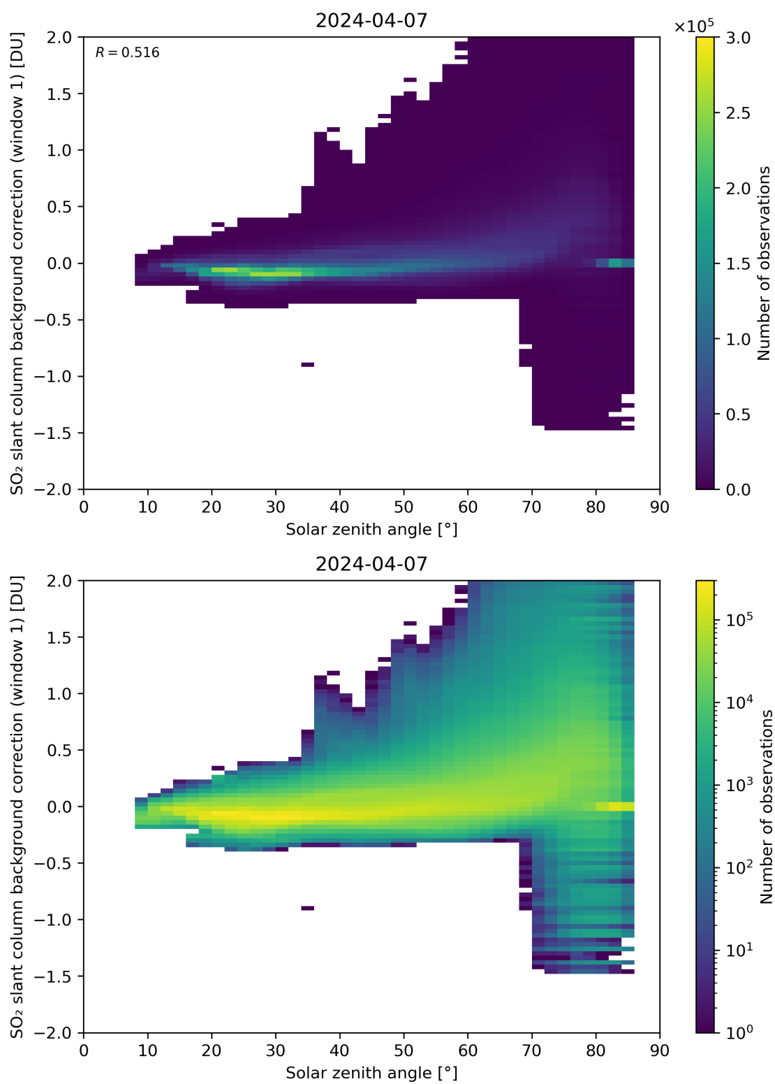
Figure 158: Scatter density plot of “Solar zenith angle” against “SO 2 slant column background correction (window 1)” for 2024-04-06 to 2024-04-08.
