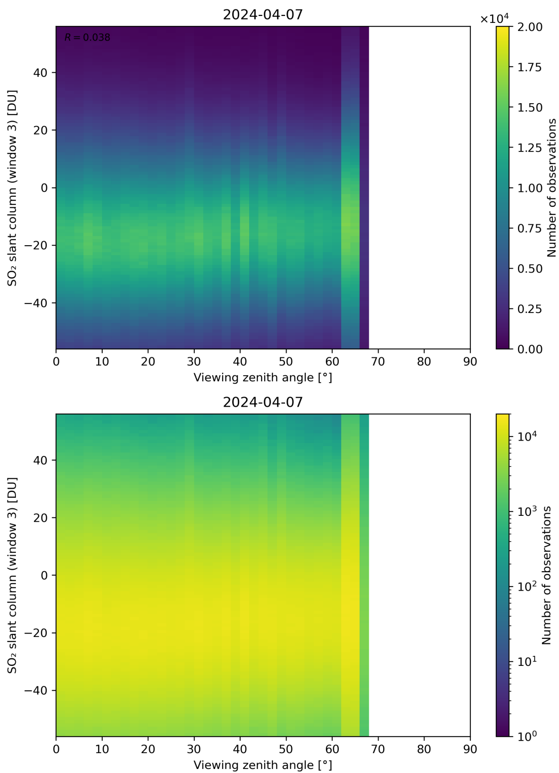
Figure 323: Scatter density plot of “Viewing zenith angle” against “SO 2 slant column (window 3)” for 2024-04-06 to 2024-04-08.
