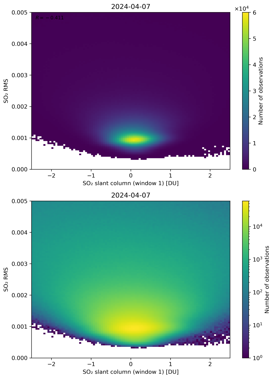
Figure 217: Scatter density plot of “SO 2 slant column (window 1)” against “SO 2 RMS” for 2024-04-06 to 2024-04-08.
