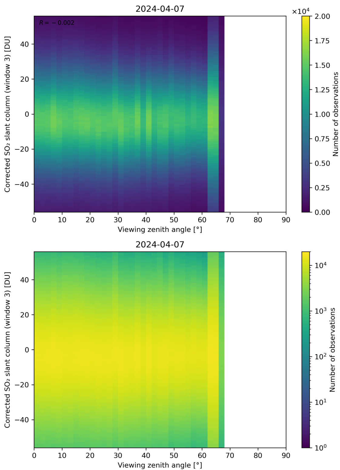
Figure 319: Scatter density plot of “Viewing zenith angle” against “Corrected SO 2 slant column (window 3)” for 2024-04-06 to 2024-04-08.
