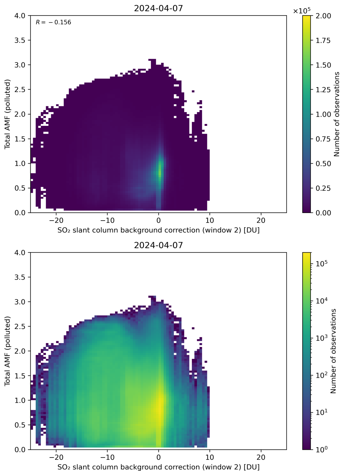
Figure 119: Scatter density plot of “SO 2 slant column background correction (window 2)” against “Total AMF (polluted)” for 2024-04-06 to 2024-04-08.
