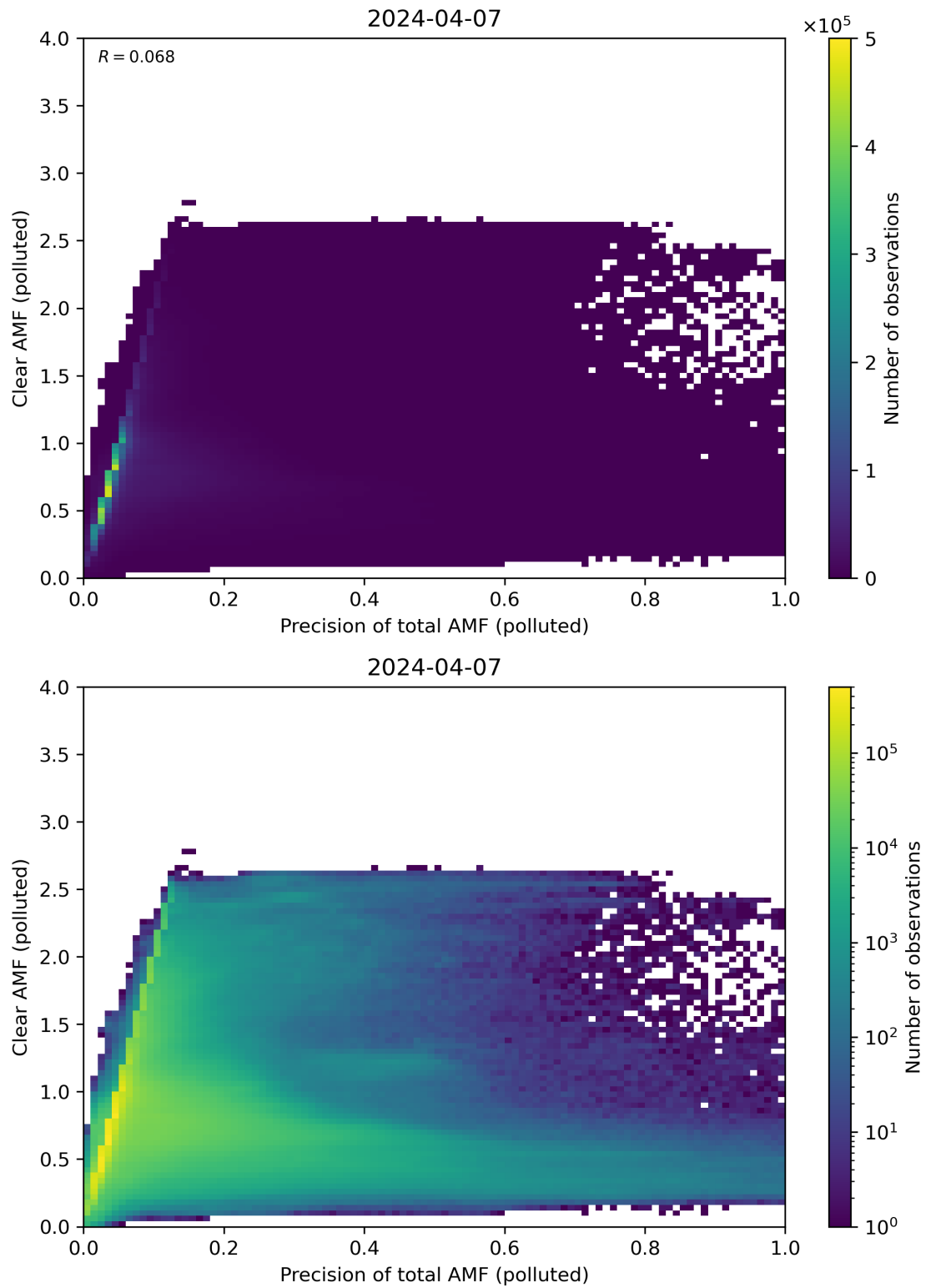
Figure 270: Scatter density plot of “Precision of total AMF (polluted)” against “Clear AMF (polluted)” for 2024-04-06 to 2024-04-08.
