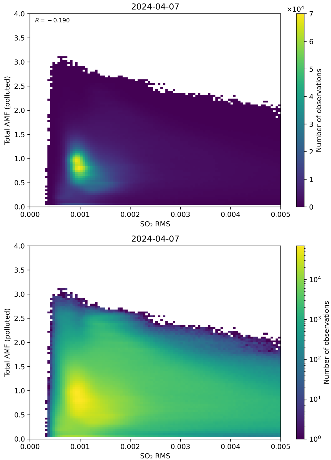
Figure 137: Scatter density plot of “SO 2 RMS” against “Total AMF (polluted)” for 2024-04-06 to 2024-04-08.
