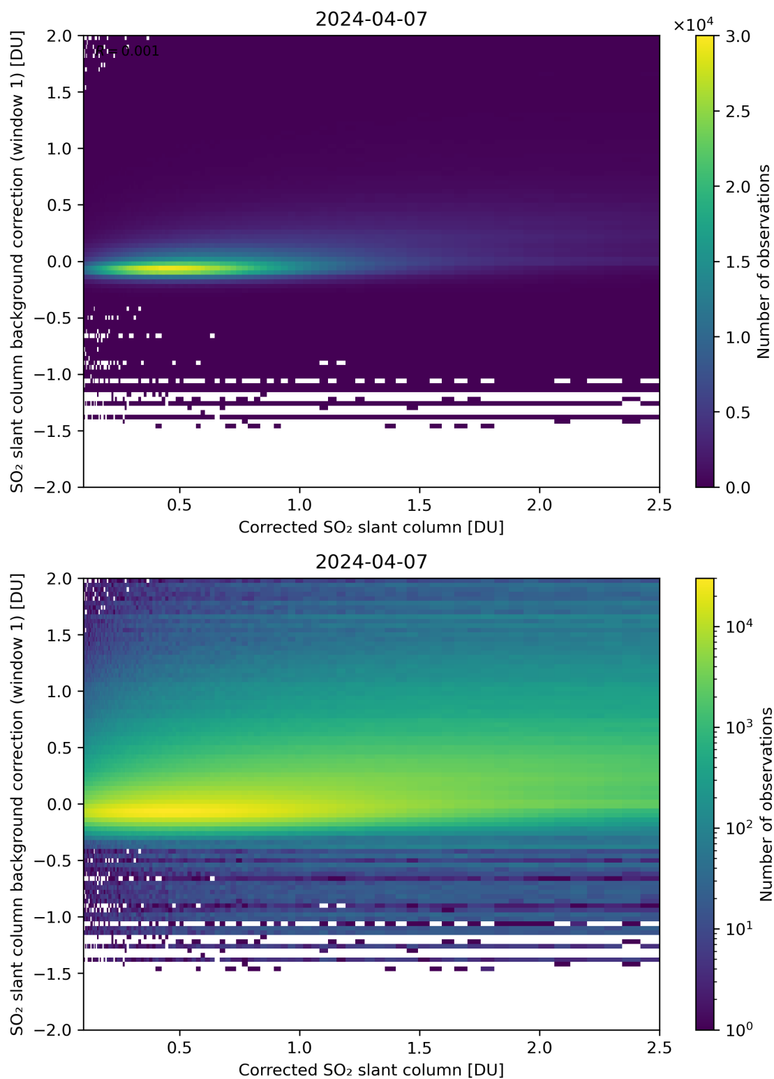
Figure 178: Scatter density plot of “Corrected SO 2 slant column” against “SO 2 slant column background correction (window 1)” for 2024-04-06 to 2024-04-08.
