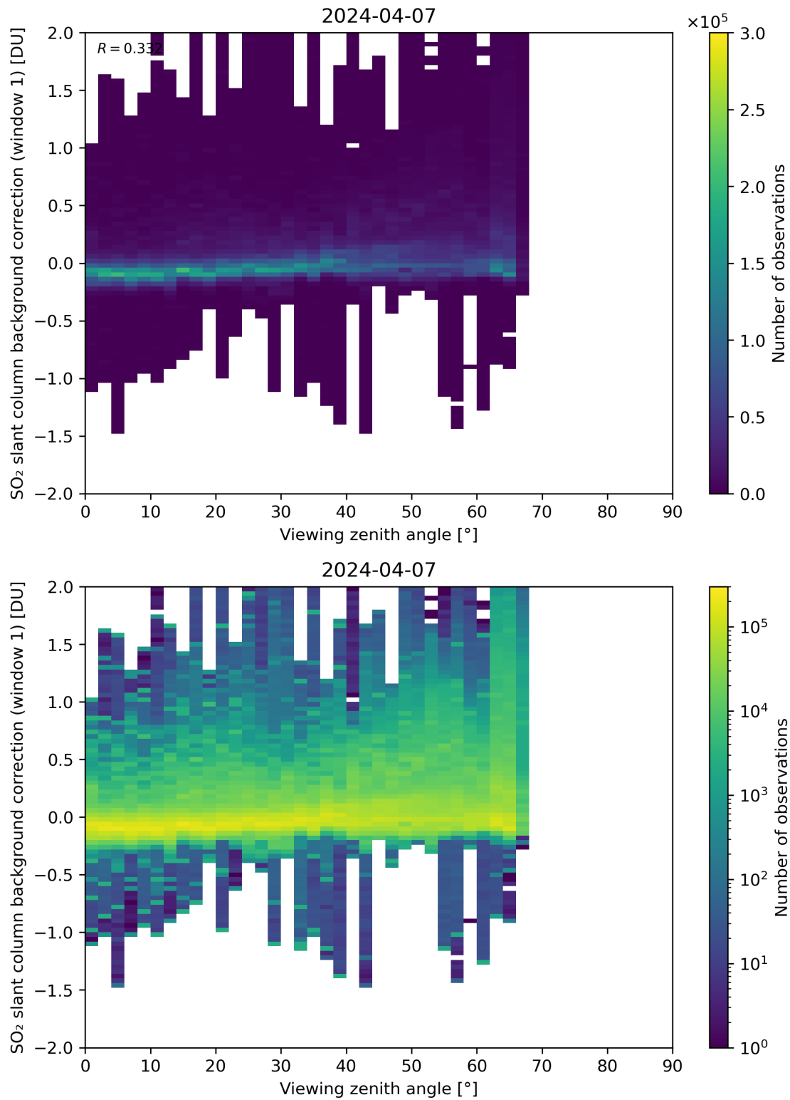
Figure 308: Scatter density plot of “Viewing zenith angle” against “SO 2 slant column background correction (window 1)” for 2024-04-06 to 2024-04-08.
