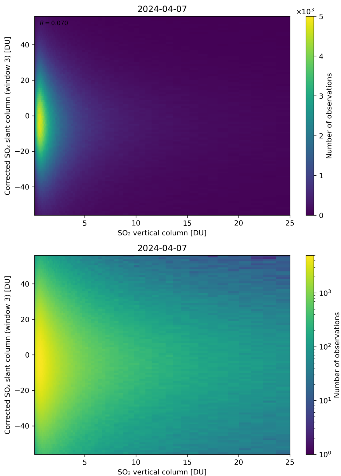
Figure 299: Scatter density plot of “SO 2 vertical column” against “Corrected SO 2 slant column (window 3)” for 2024-04-06 to 2024-04-08.
