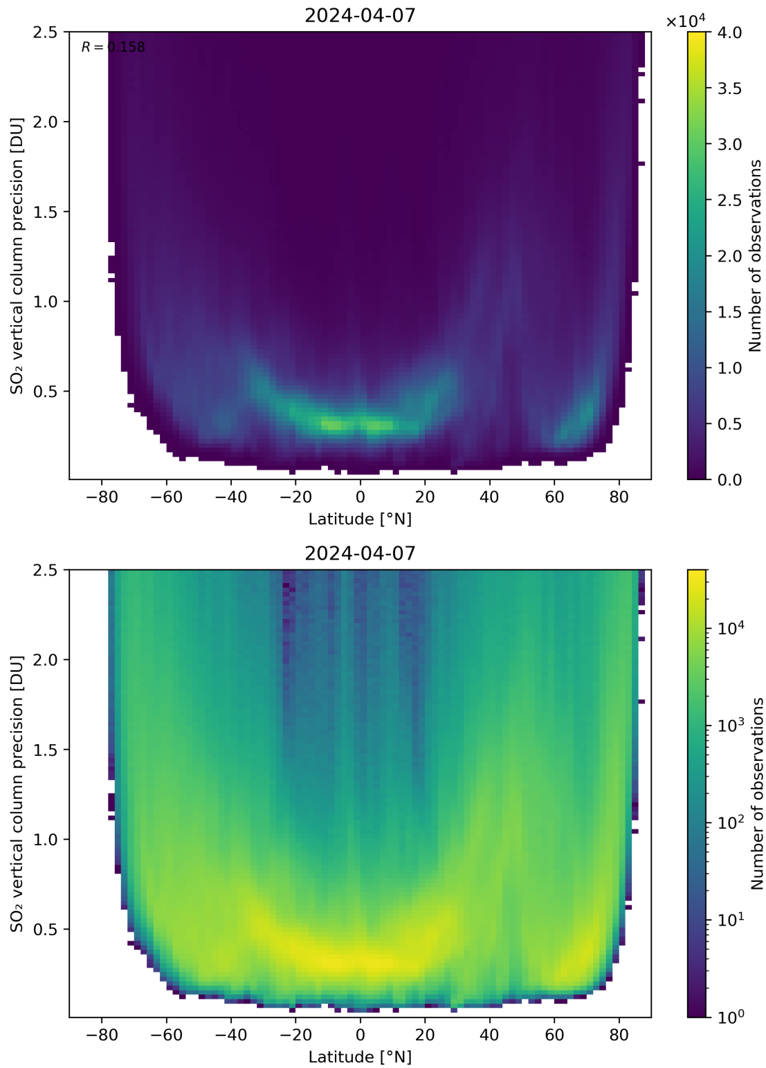
Figure 157: Scatter density plot of “Latitude” against “SO 2 vertical column precision” for 2024-04-06 to 2024-04-08.
