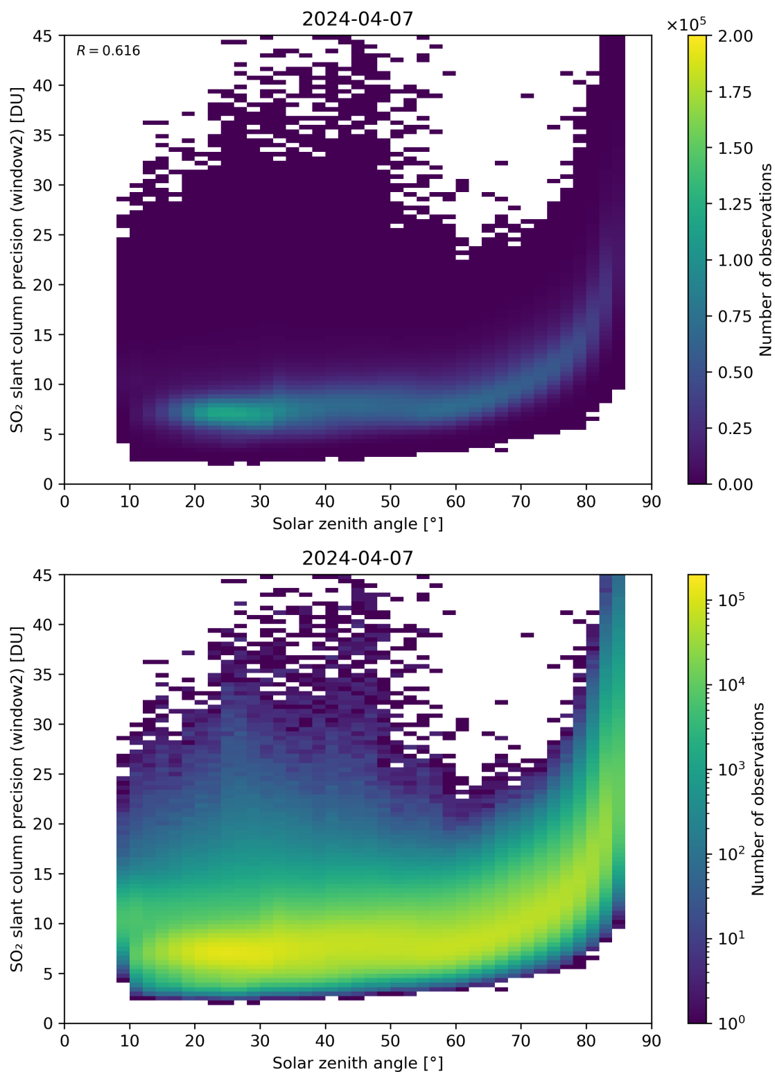
Figure 171: Scatter density plot of “Solar zenith angle” against “SO 2 slant column precision (window2)” for 2024-04-06 to 2024-04-08.
