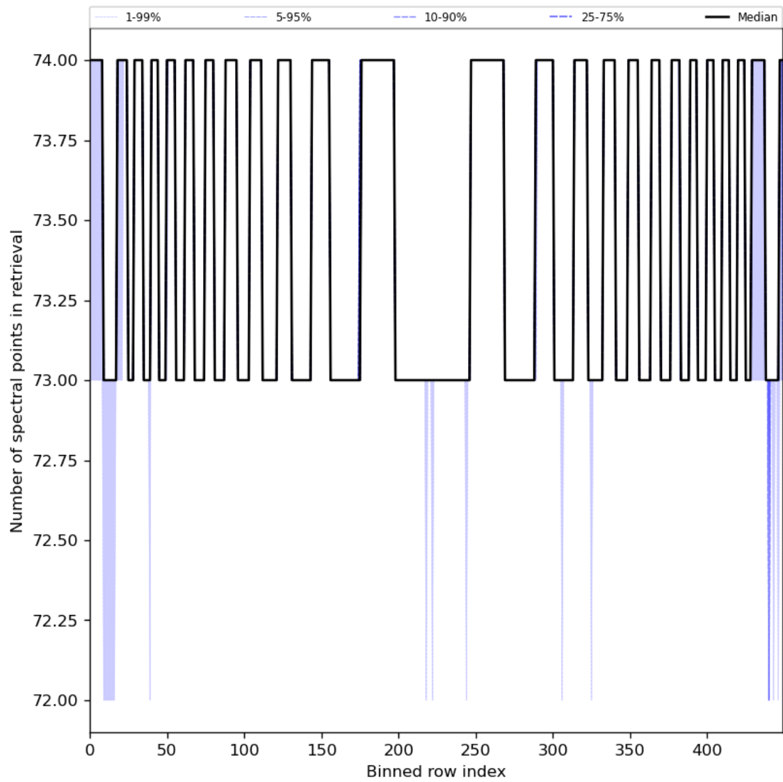
Figure 97: Along track statistics of “Number of spectral points in retrieval” for 2024-04-06 to 2024-04-08
