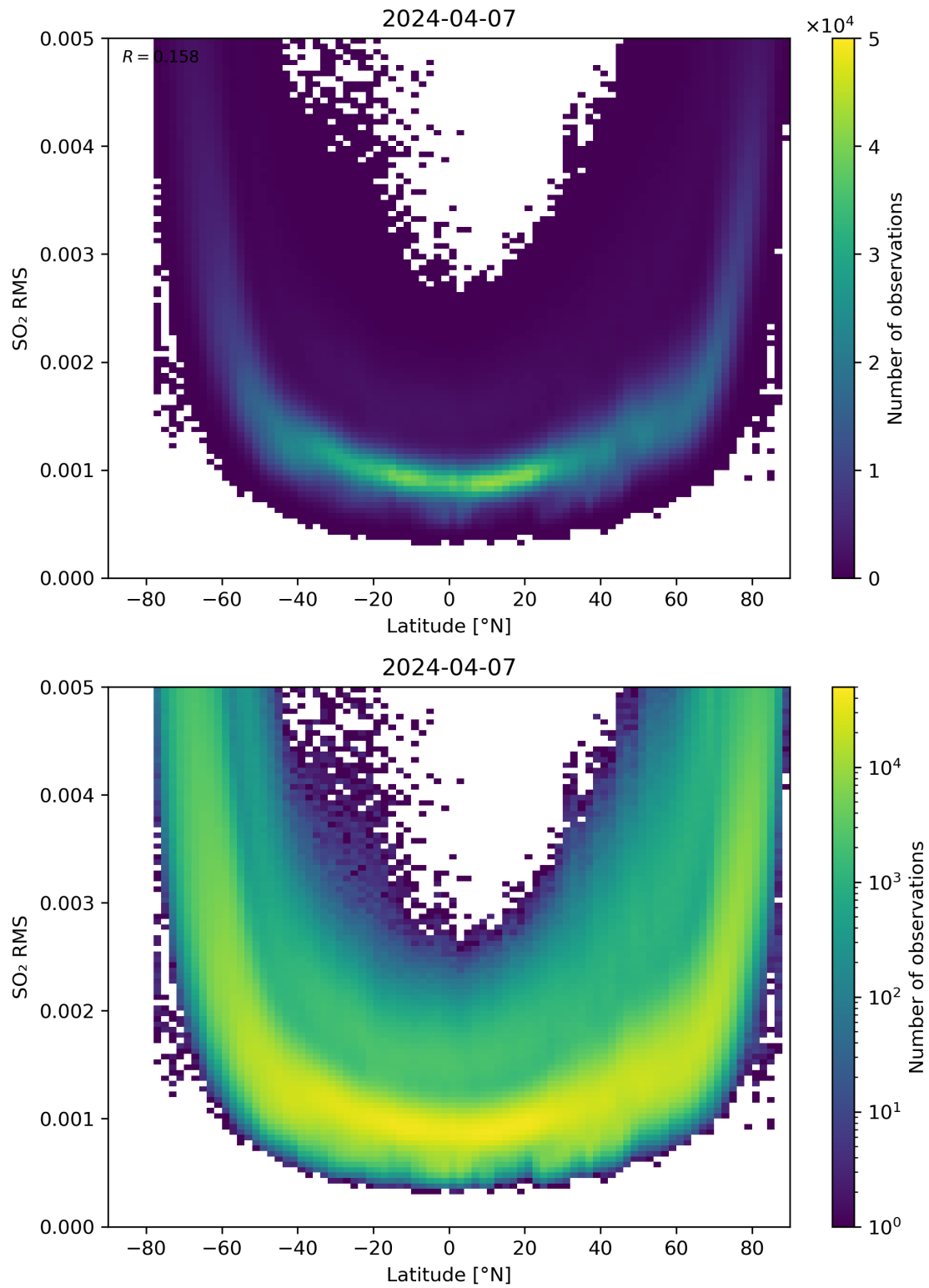
Figure 144: Scatter density plot of “Latitude” against “SO 2 RMS” for 2024-04-06 to 2024-04-08.
