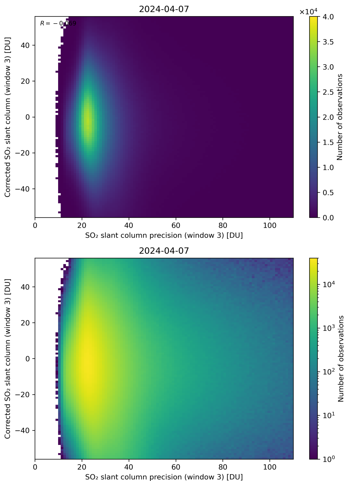
Figure 262: Scatter density plot of “SO 2 slant column precision (window 3)” against “Corrected SO 2 slant column (window 3)” for 2024-04-06 to 2024-04-08.
