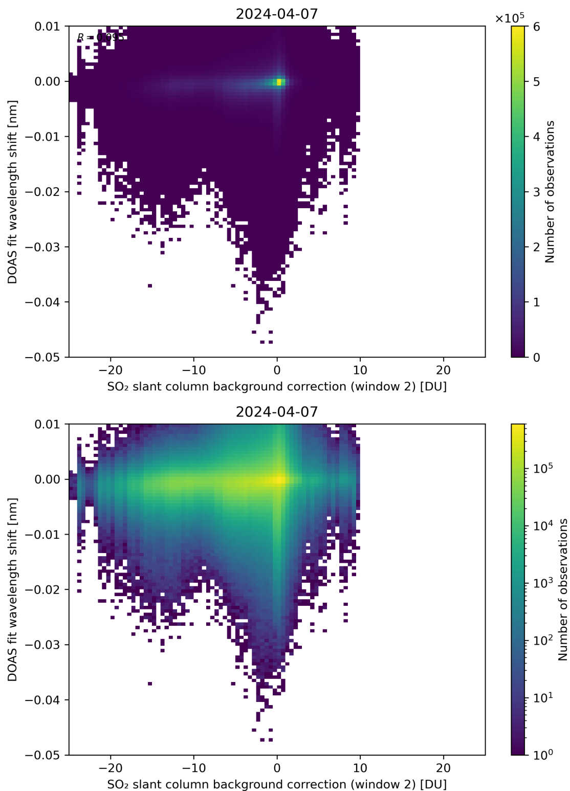
Figure 112: Scatter density plot of “SO 2 slant column background correction (window 2)” against “DOAS fit wavelength shift” for 2024-04-06 to 2024-04-08.
