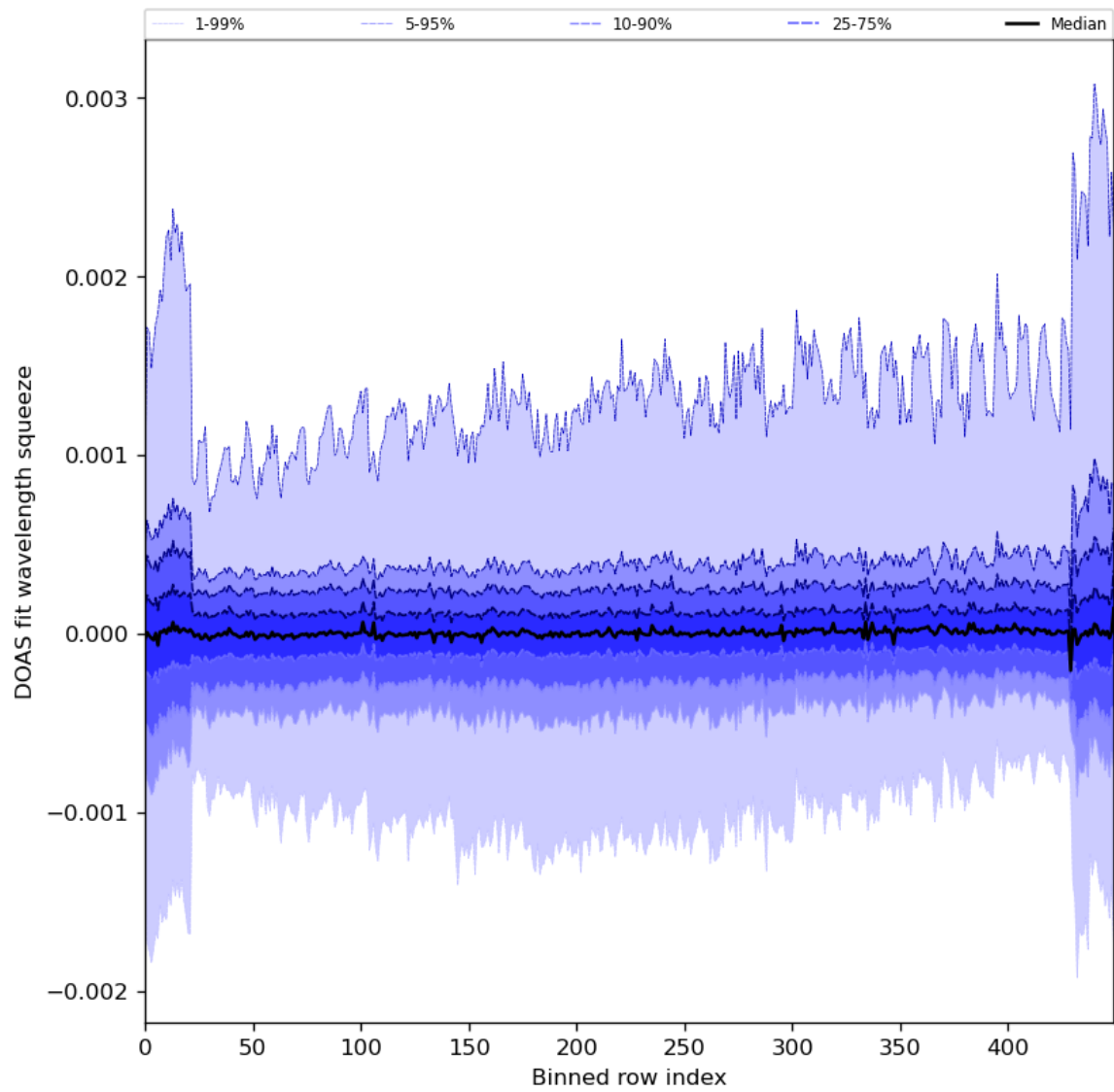
Figure 92: Along track statistics of “DOAS fit wavelength squeeze” for 2024-04-06 to 2024-04-08
