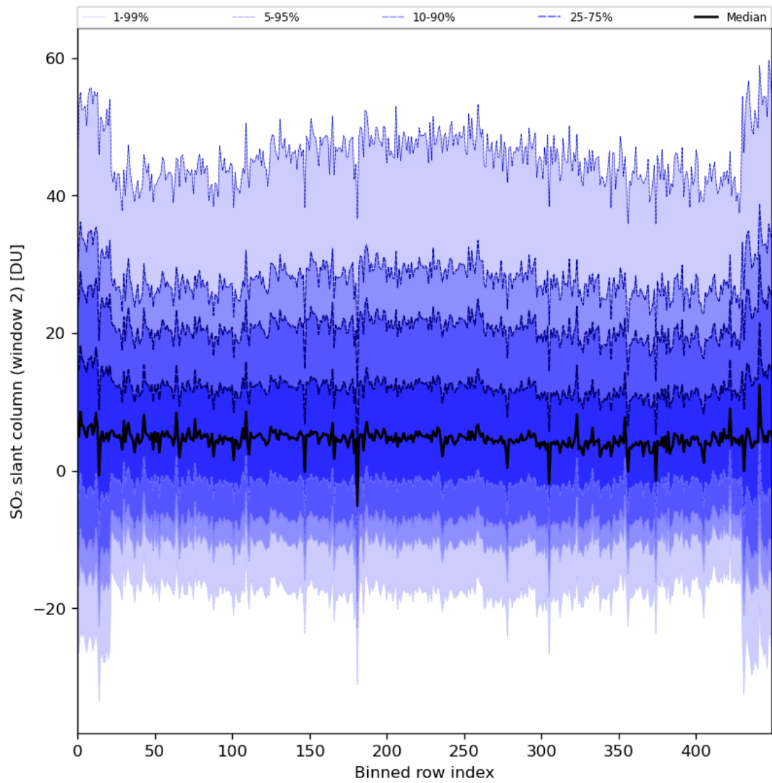
Figure 83: Along track statistics of “SO 2 slant column (window 2)” for 2024-04-06 to 2024-04-08
