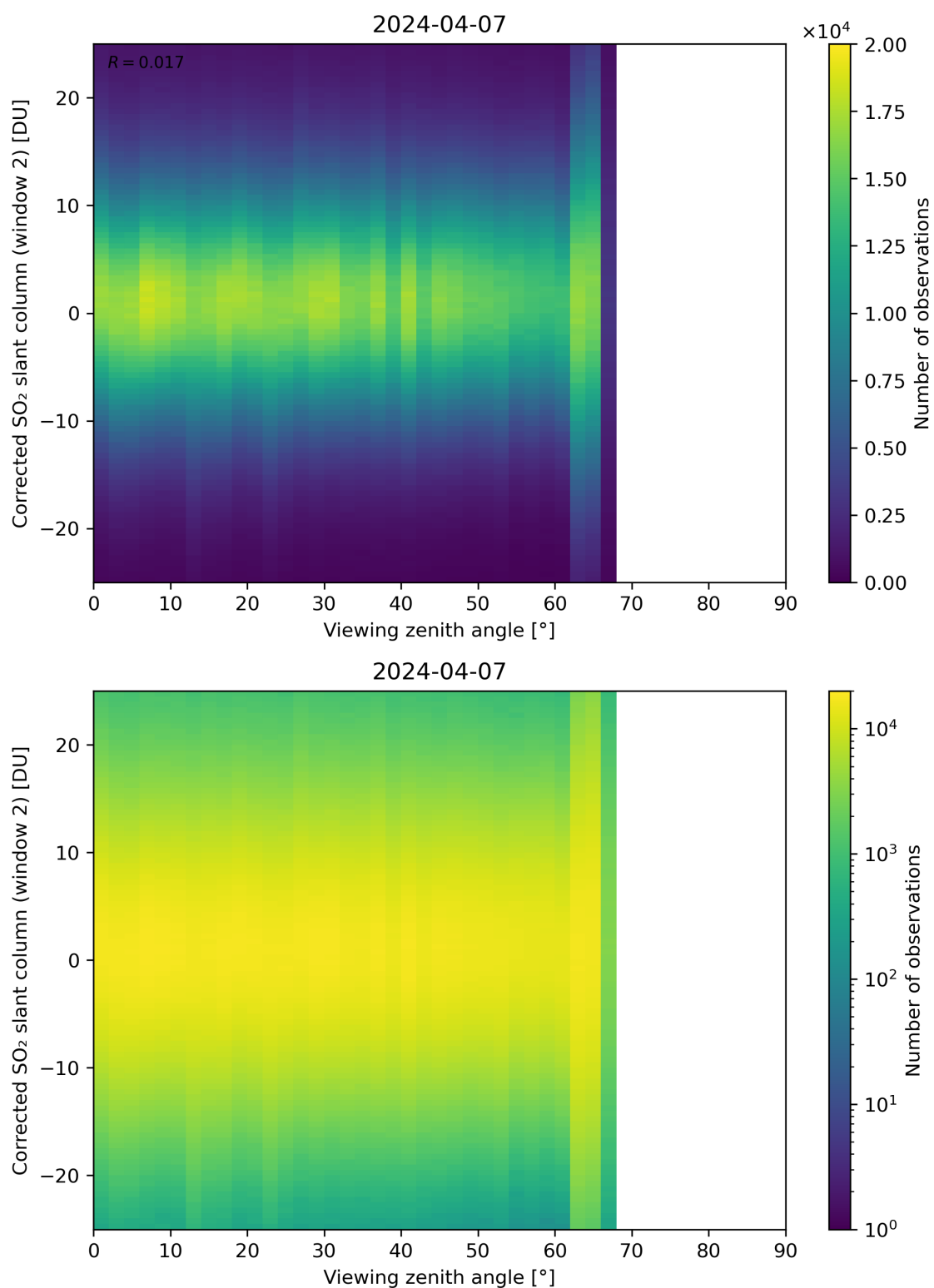
Figure 318: Scatter density plot of “Viewing zenith angle” against “Corrected SO 2 slant column (window 2)” for 2024-04-06 to 2024-04-08.
