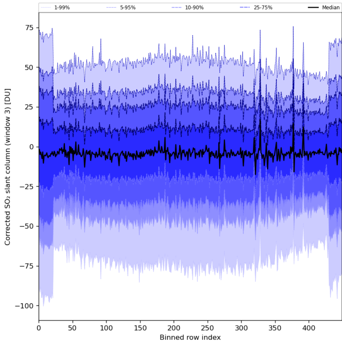
Figure 89: Along track statistics of “Corrected SO 2 slant column (window 3)” for 2024-04-06 to 2024-04-08
