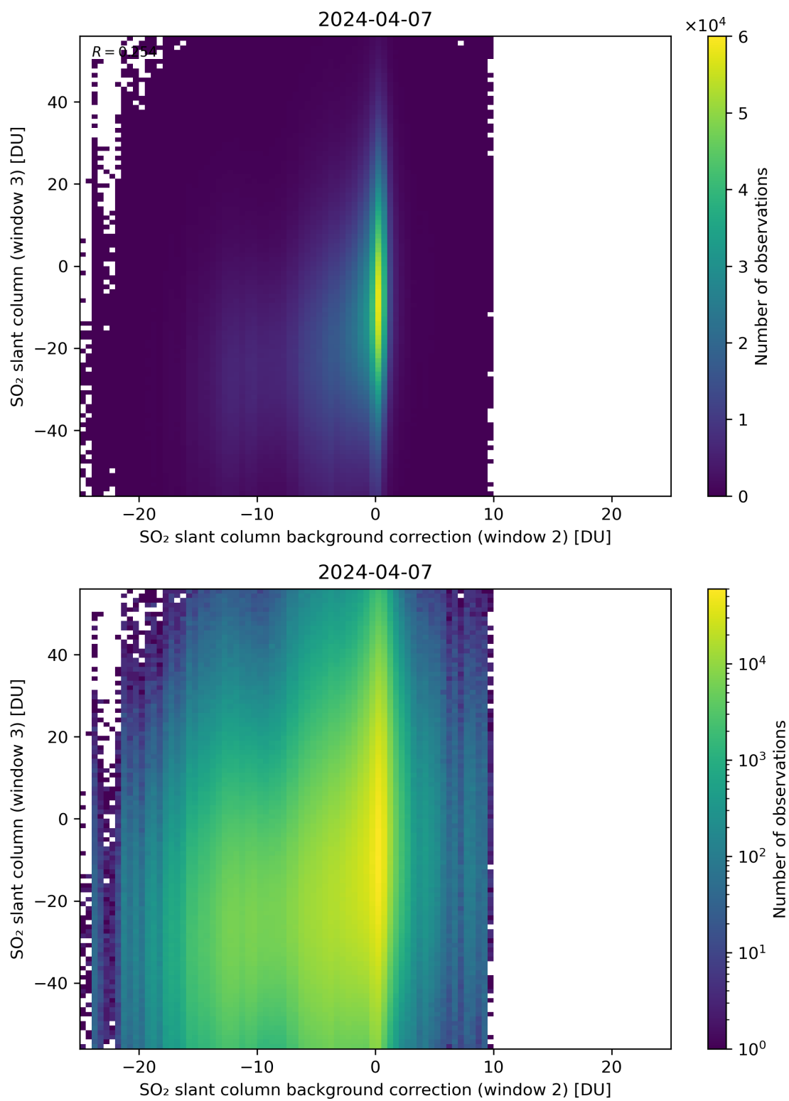
Figure 117: Scatter density plot of “SO 2 slant column background correction (window 2)” against “SO 2 slant column (window 3)” for 2024-04-06 to 2024-04-08.
