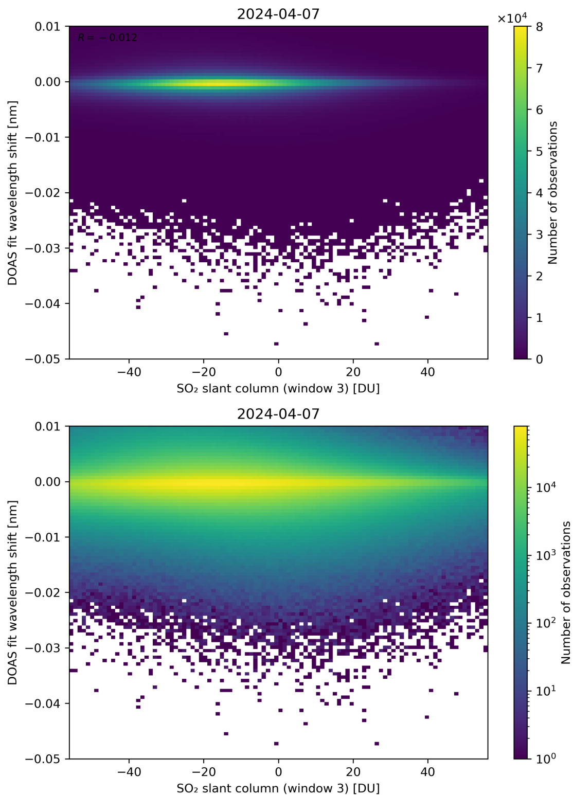
Figure 254: Scatter density plot of “SO 2 slant column (window 3)” against “DOAS fit wavelength shift” for 2024-04-06 to 2024-04-08.
