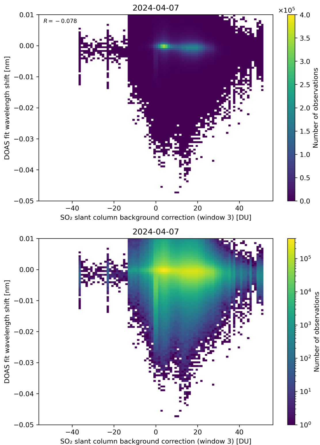
Figure 121: Scatter density plot of “SO 2 slant column background correction (window 3)” against “DOAS fit wavelength shift” for 2024-04-06 to 2024-04-08.
