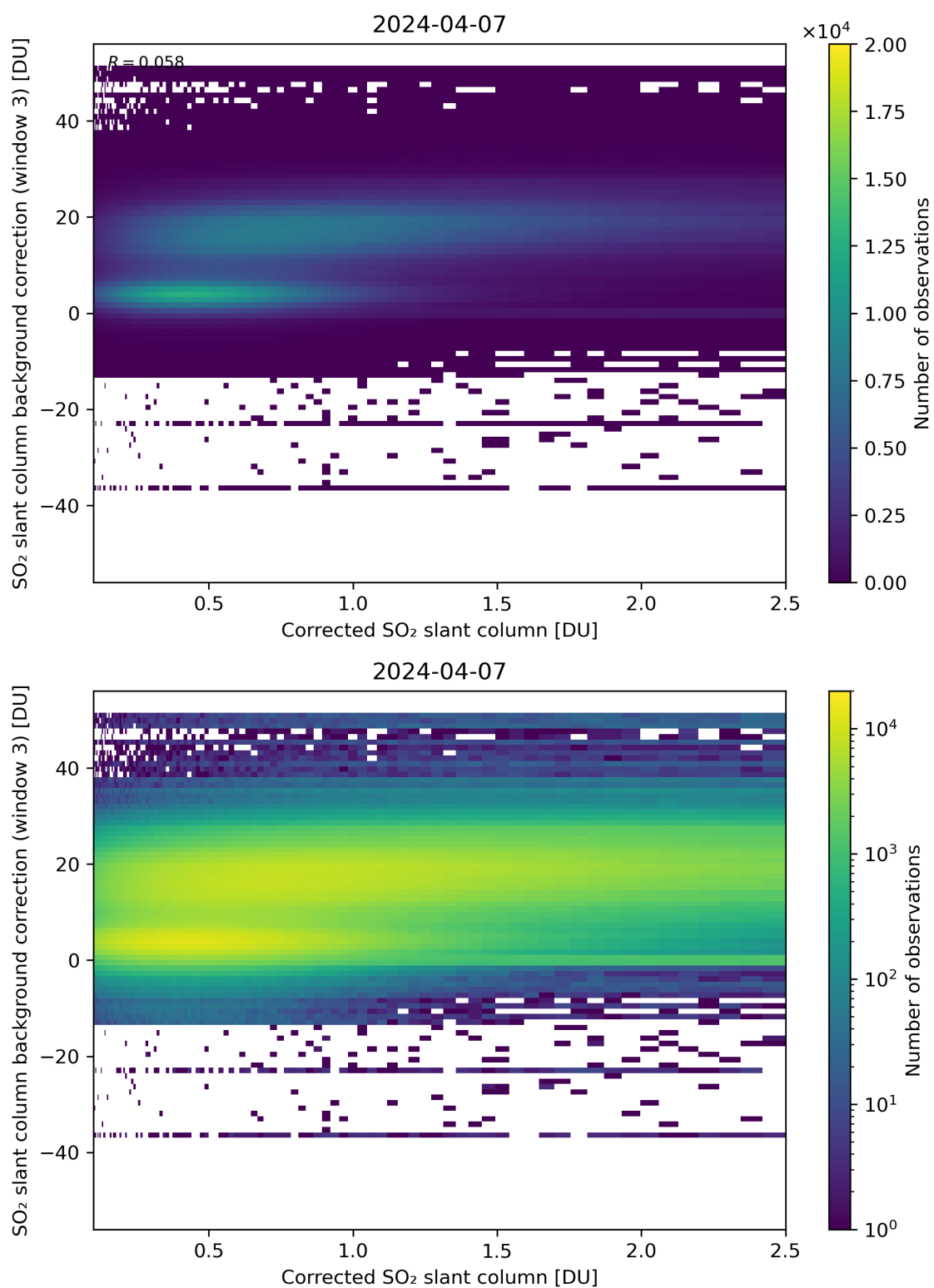
Figure 180: Scatter density plot of “Corrected SO 2 slant column” against “SO 2 slant column background correction (window 3)” for 2024-04-06 to 2024-04-08.
