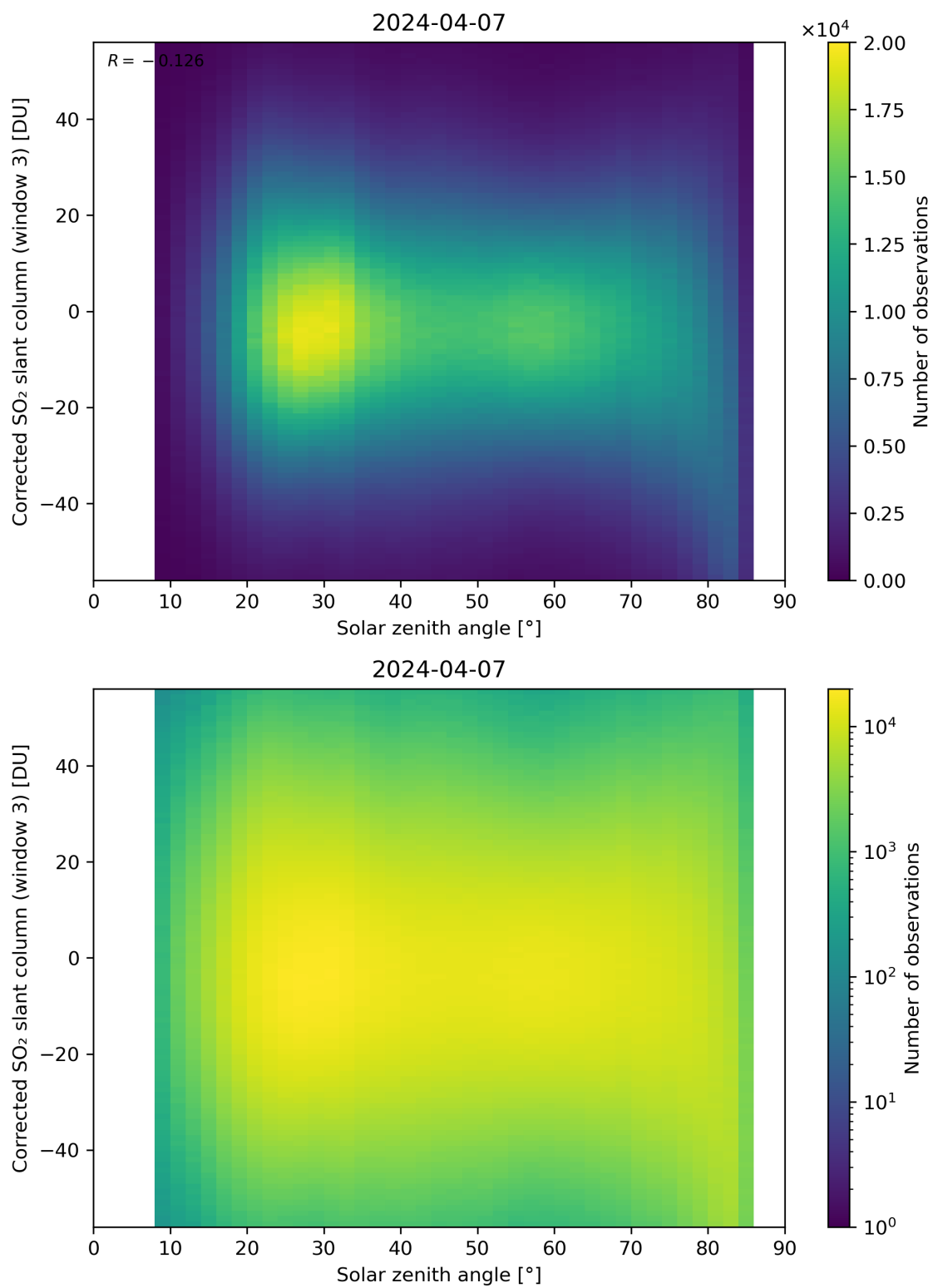
Figure 168: Scatter density plot of “Solar zenith angle” against “Corrected SO 2 slant column (window 3)” for 2024-04-06 to 2024-04-08.
