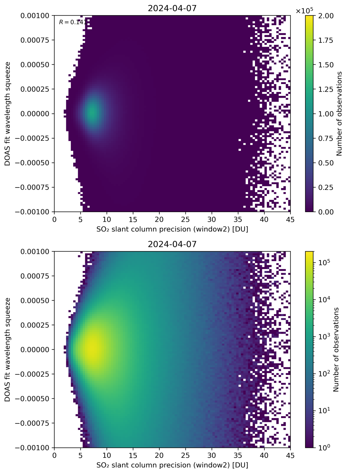
Figure 244: Scatter density plot of “SO 2 slant column precision (window2)” against “DOAS fit wavelength squeeze” for 2024-04-06 to 2024-04-08.
