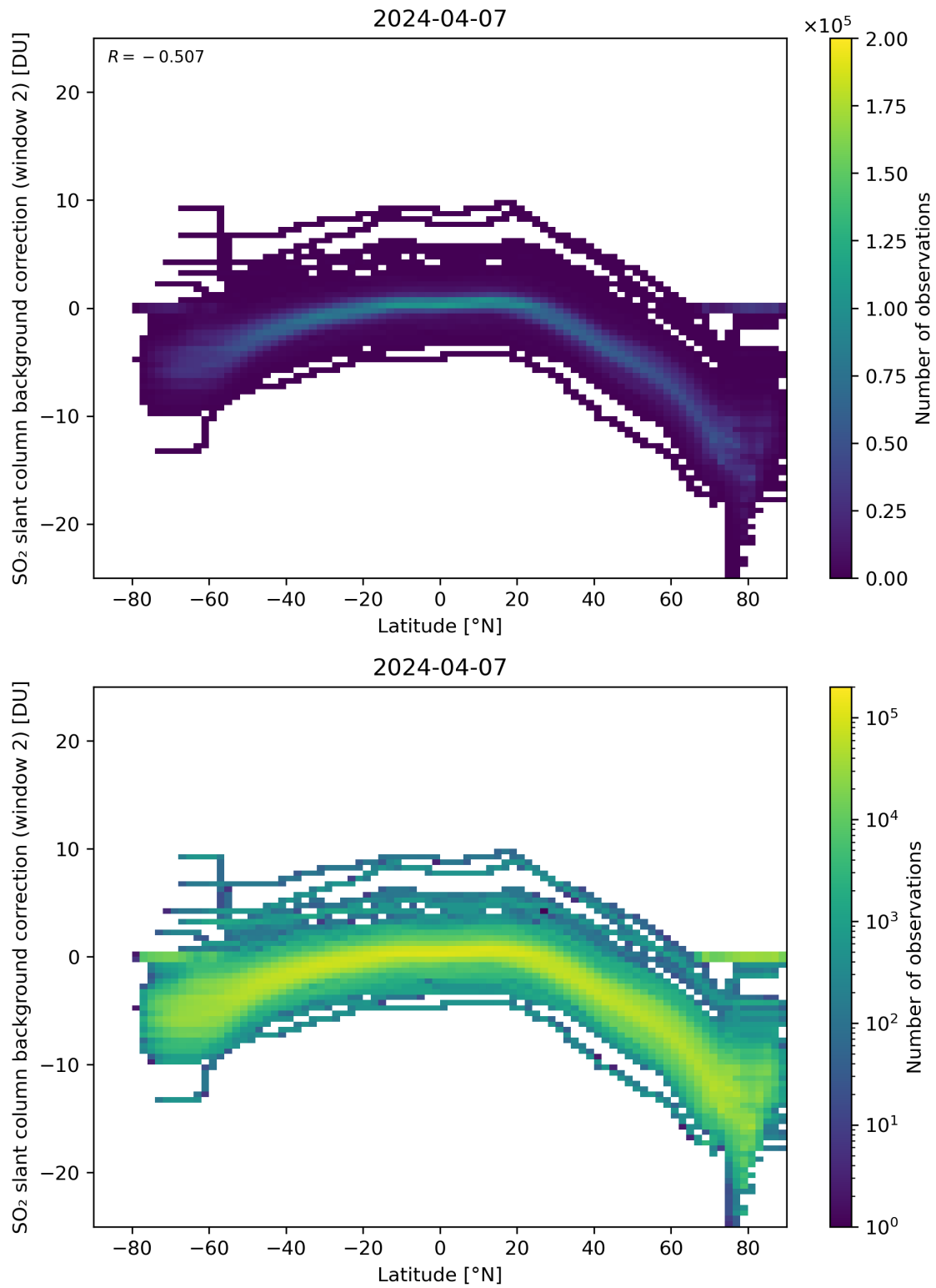
Figure 140: Scatter density plot of “Latitude” against “SO 2 slant column background correction (window 2)” for 2024-04-06 to 2024-04-08.
