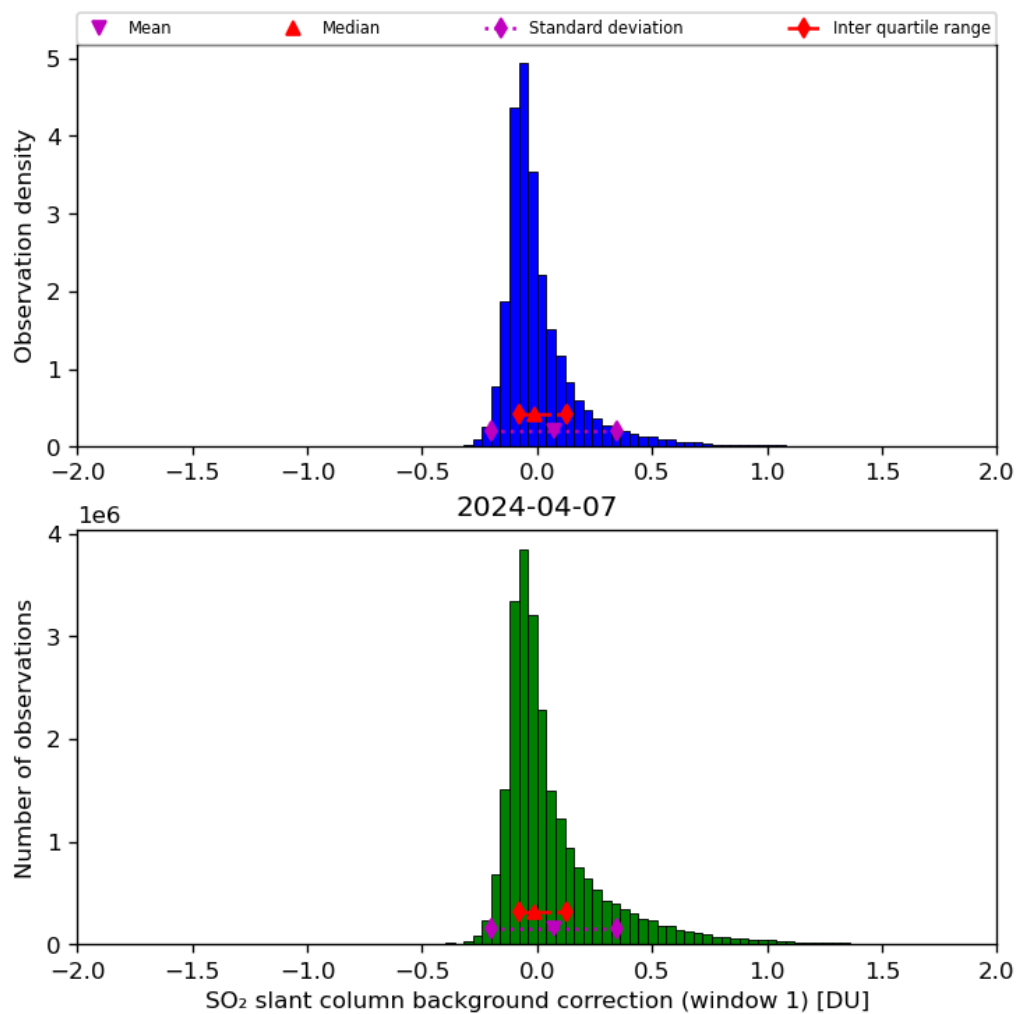
Figure 59: Histogram of “SO 2 slant column background correction (window 1)” for 2024-04-06 to 2024-04-08
