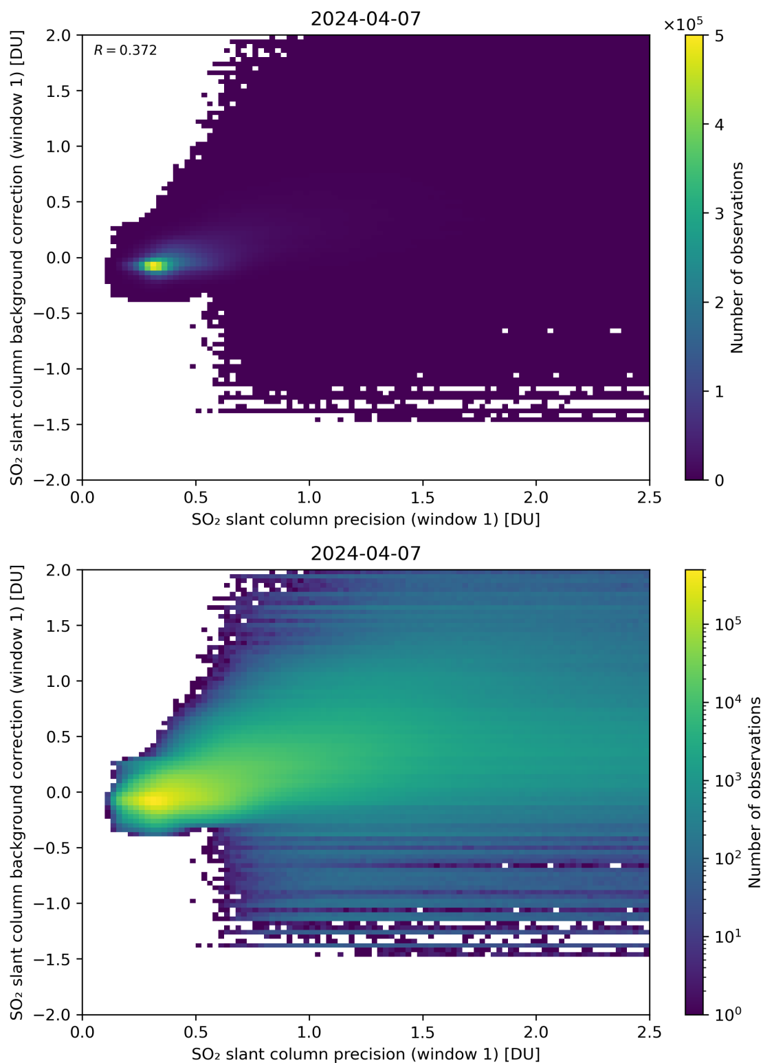
Figure 218: Scatter density plot of “SO 2 slant column precision (window 1)” against “SO 2 slant column background correction (window 1)” for 2024-04-06 to 2024-04-08.
