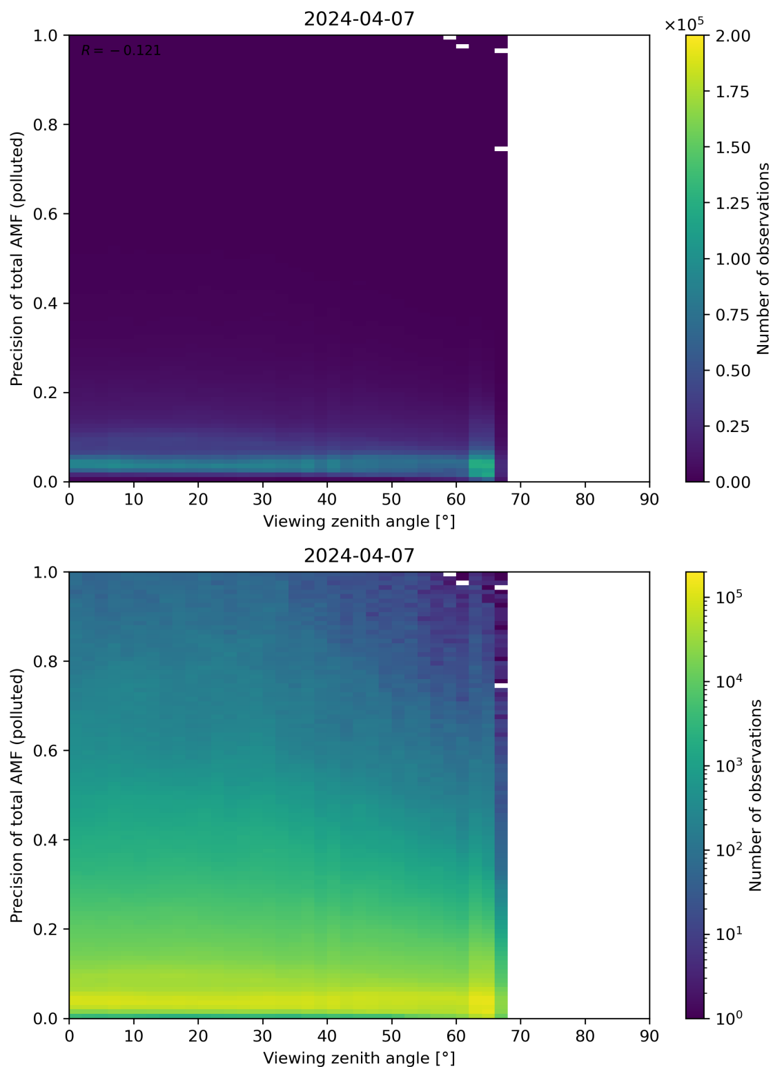
Figure 326: Scatter density plot of “Viewing zenith angle” against “Precision of total AMF (polluted)” for 2024-04-06 to 2024-04-08.
