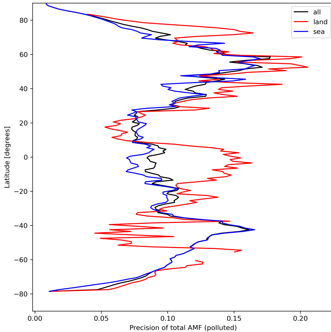
Figure 49: Zonal average of “Precision of total AMF (polluted)” for 2024-04-06 to 2024-04-08.
