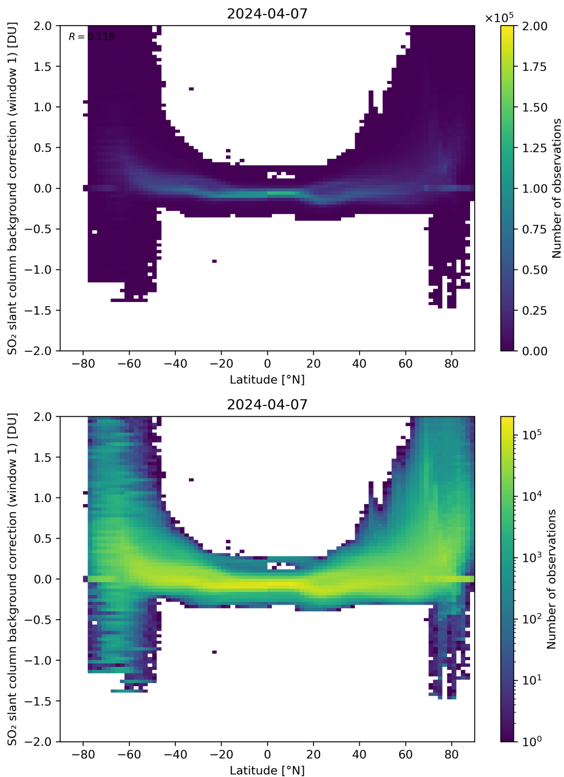
Figure 139: Scatter density plot of “Latitude” against “SO 2 slant column background correction (window 1)” for 2024-04-06 to 2024-04-08.
