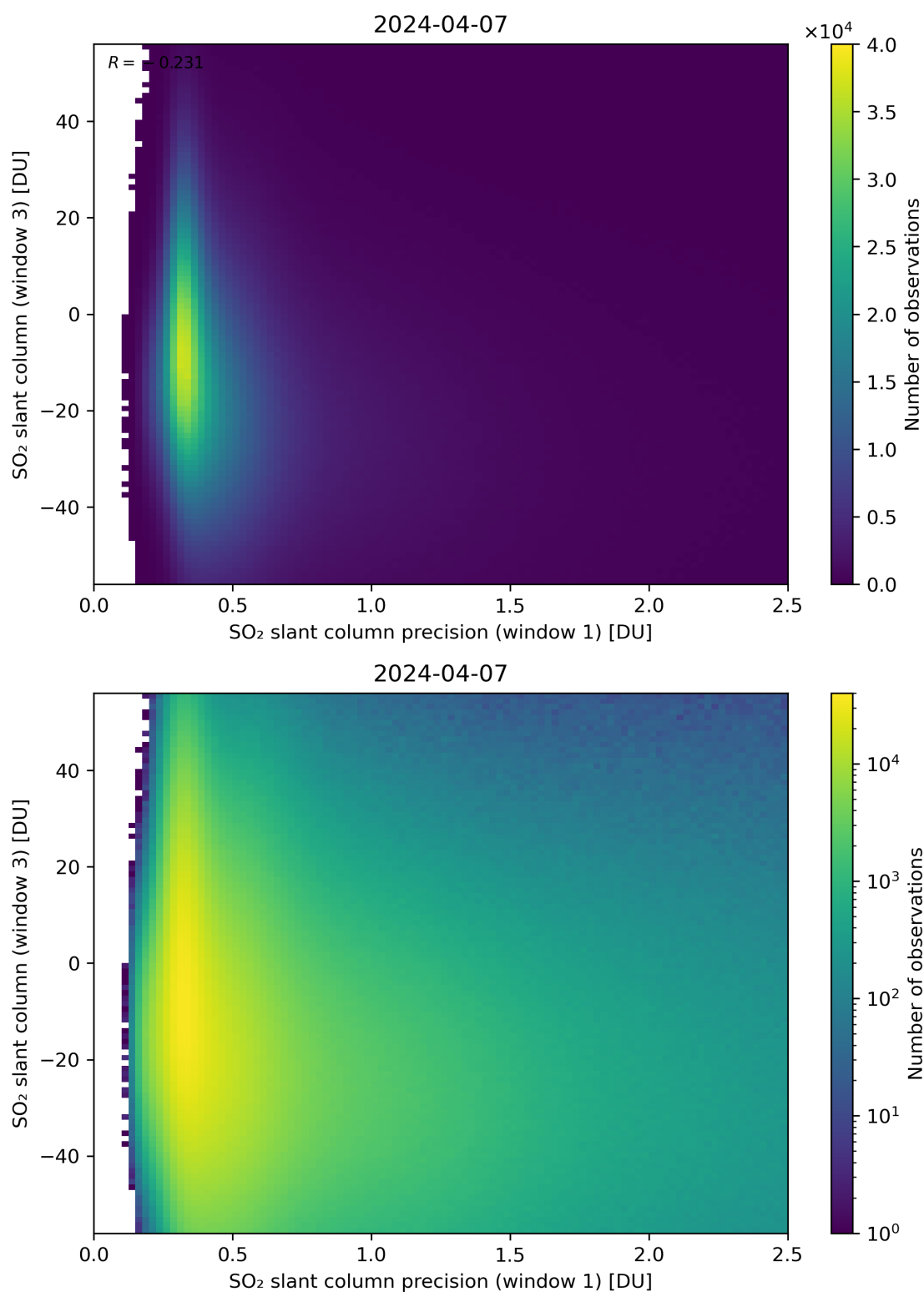
Figure 228: Scatter density plot of “SO 2 slant column precision (window 1)” against “SO 2 slant column (window 3)” for 2024-04-06 to 2024-04-08.
