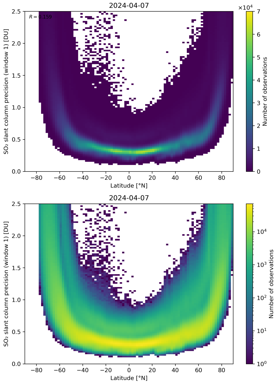
Figure 150: Scatter density plot of “Latitude” against “SO 2 slant column precision (window 1)” for 2024-04-06 to 2024-04-08.
