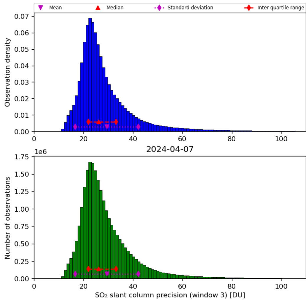
Figure 65: Histogram of “SO 2 slant column precision (window 3)” for 2024-04-06 to 2024-04-08
