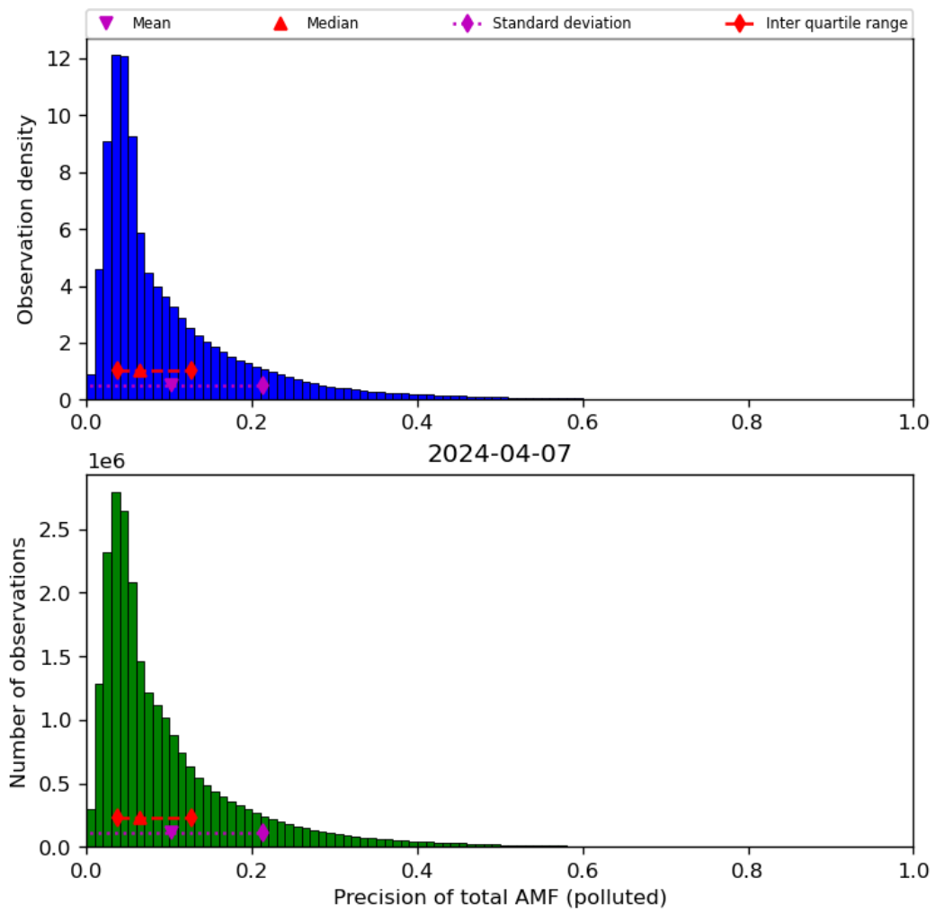
Figure 72: Histogram of “Precision of total AMF (polluted)” for 2024-04-06 to 2024-04-08
