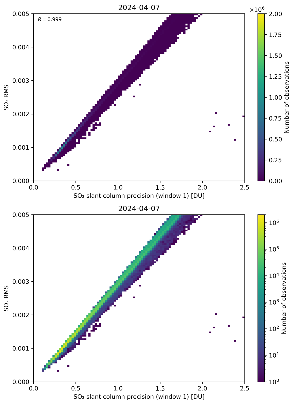
Figure 223: Scatter density plot of “SO 2 slant column precision (window 1)” against “SO 2 RMS” for 2024-04-06 to 2024-04-08.
