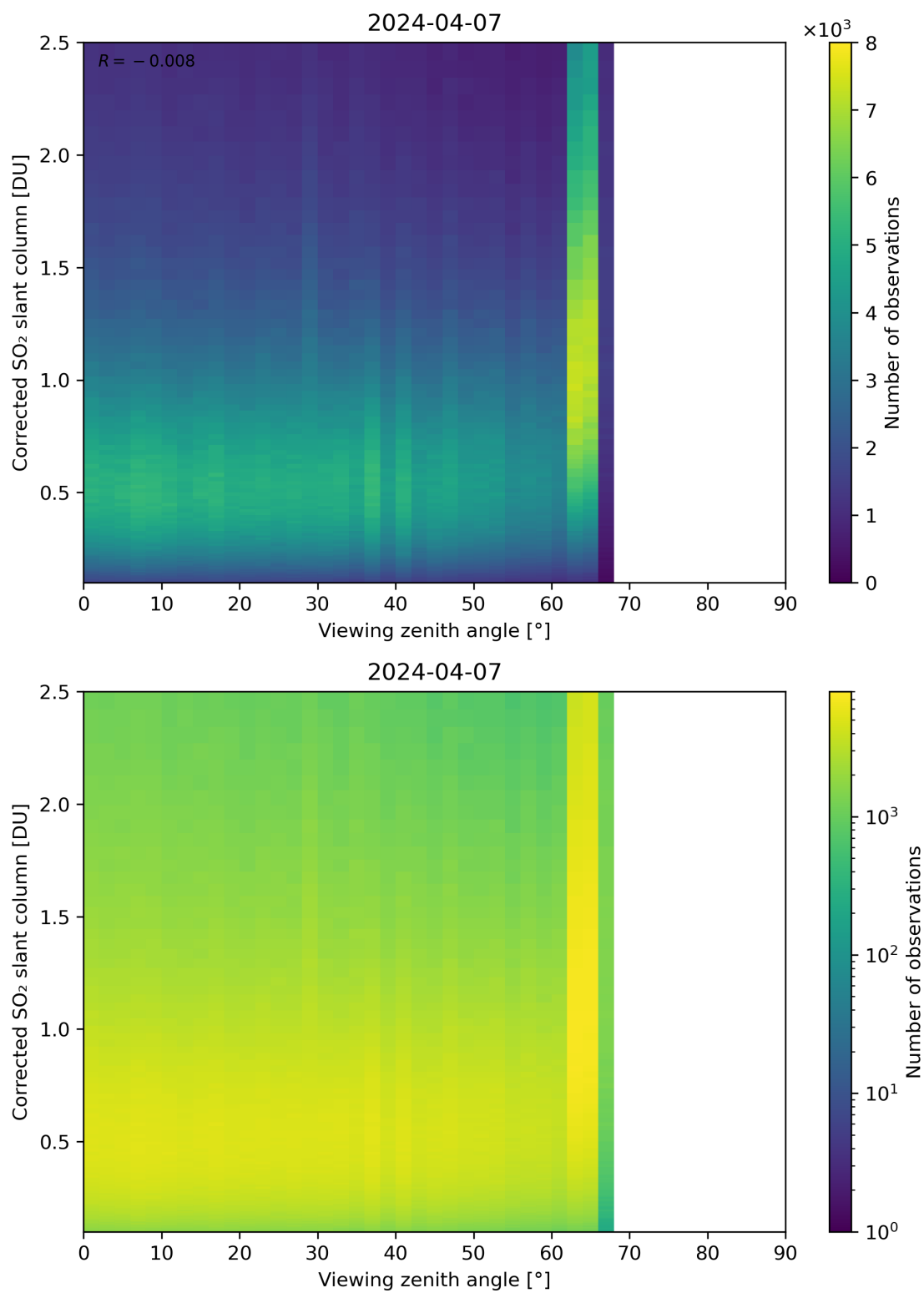
Figure 317: Scatter density plot of “Viewing zenith angle” against “Corrected SO 2 slant column” for 2024-04-06 to 2024-04-08.
