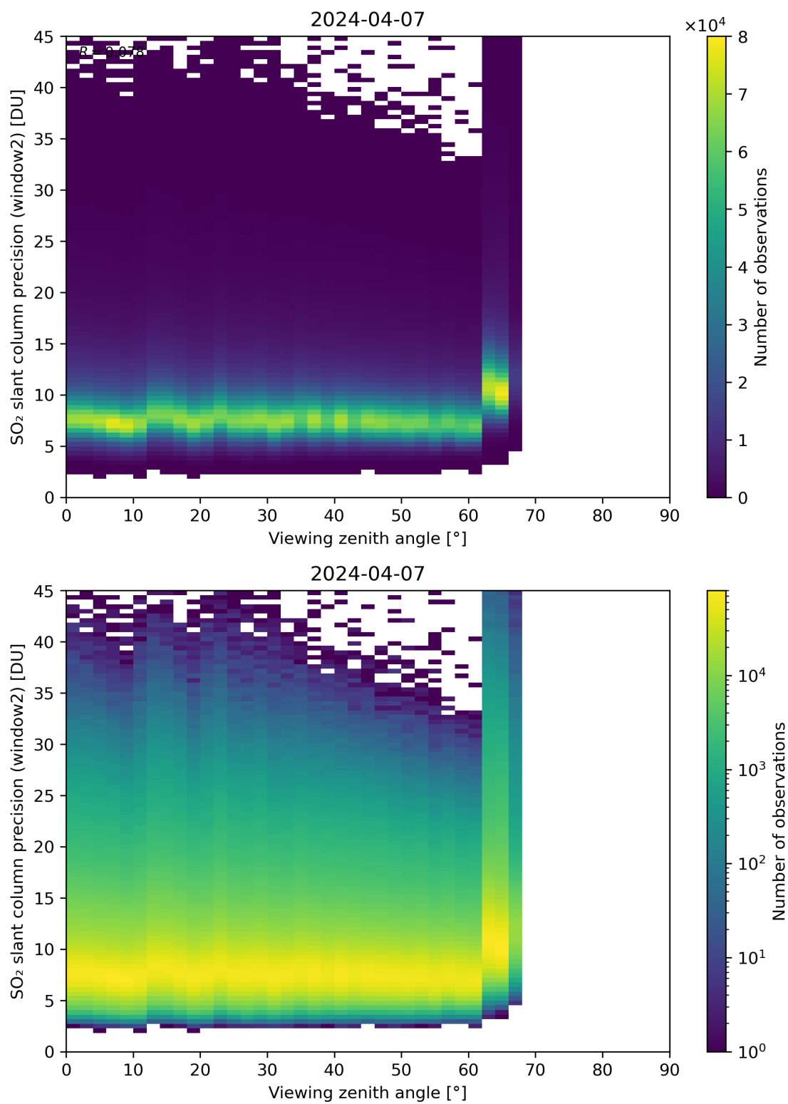
Figure 322: Scatter density plot of “Viewing zenith angle” against “SO 2 slant column precision (window2)” for 2024-04-06 to 2024-04-08.
