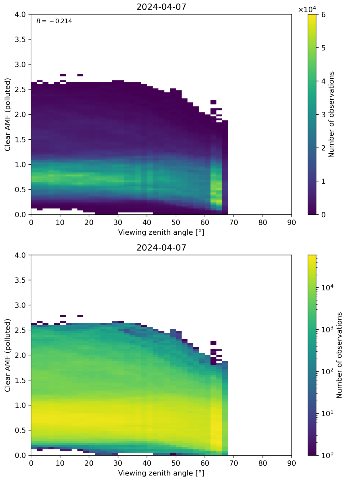
Figure 316: Scatter density plot of “Viewing zenith angle” against “Clear AMF (polluted)” for 2024-04-06 to 2024-04-08.
