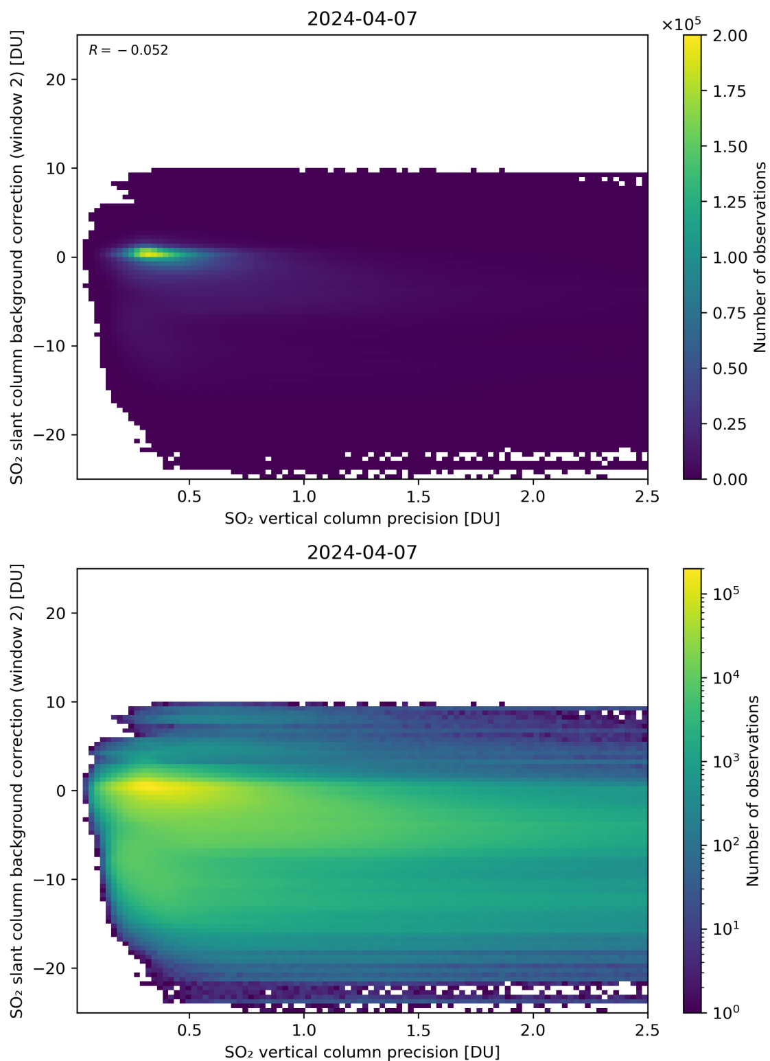
Figure 280: Scatter density plot of “SO 2 vertical column precision” against “SO 2 slant column background correction (window 2)” for 2024-04-06 to 2024-04-08.
