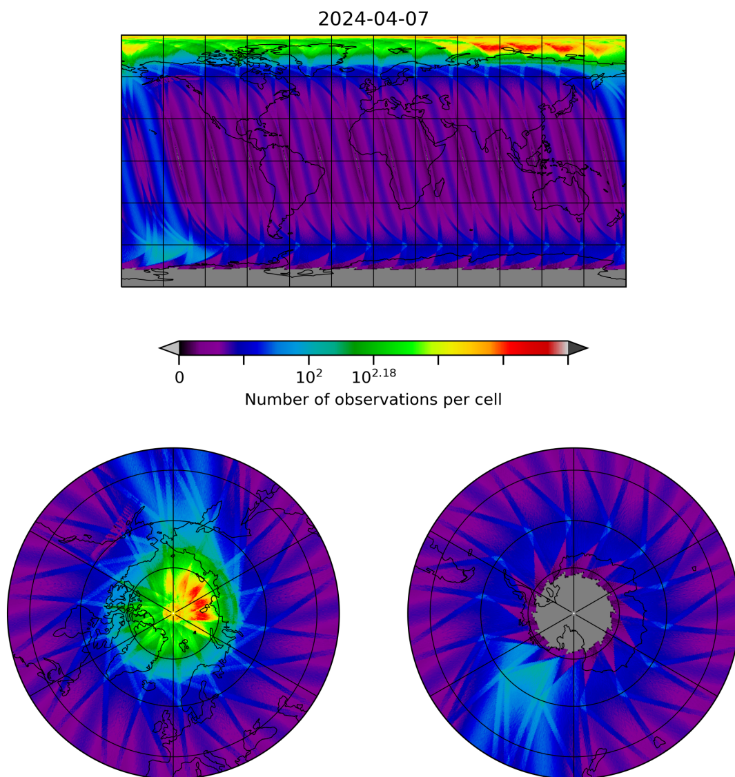
Figure 28: Map of the number of observations for 2024-04-06 to 2024-04-08
