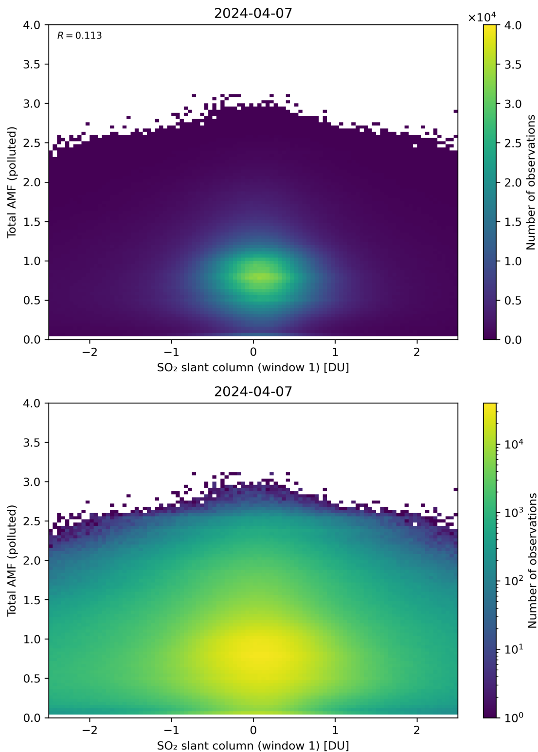
Figure 239: Scatter density plot of “SO 2 slant column (window 1)” against “Total AMF (polluted)” for 2024-04-06 to 2024-04-08.
