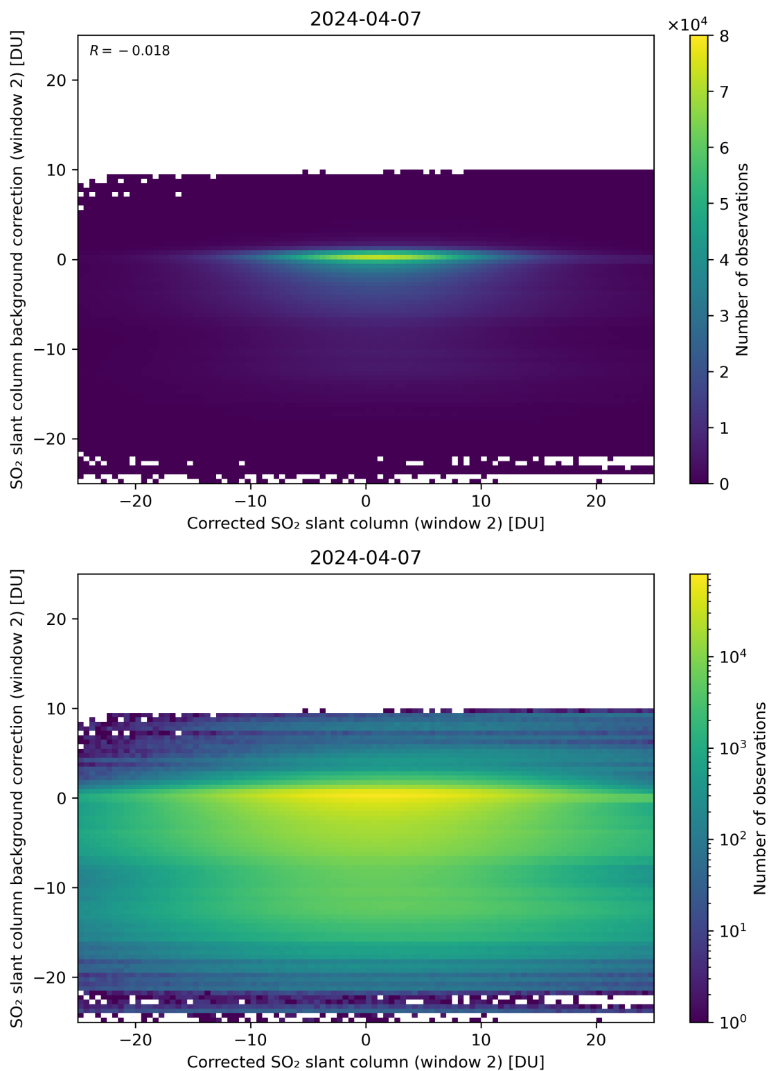
Figure 194: Scatter density plot of “Corrected SO 2 slant column (window 2)” against “SO 2 slant column background correction (window 2)” for 2024-04-06 to 2024-04-08.
