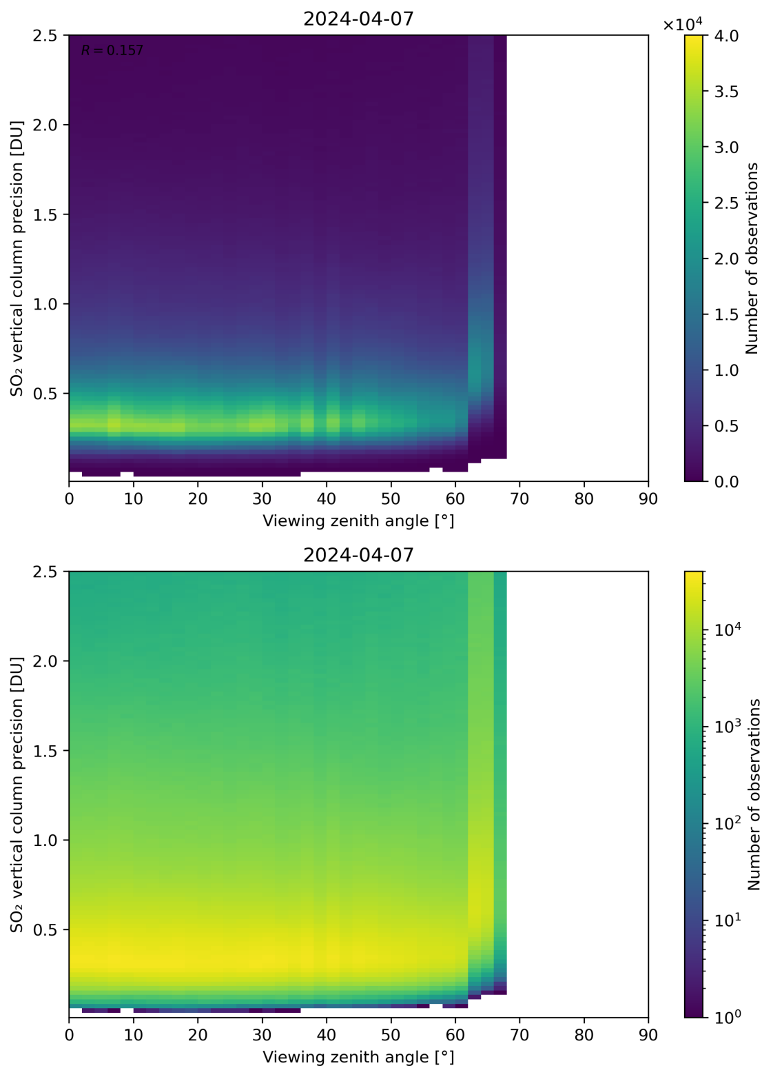
Figure 328: Scatter density plot of “Viewing zenith angle” against “SO 2 vertical column precision” for 2024-04-06 to 2024-04-08.
