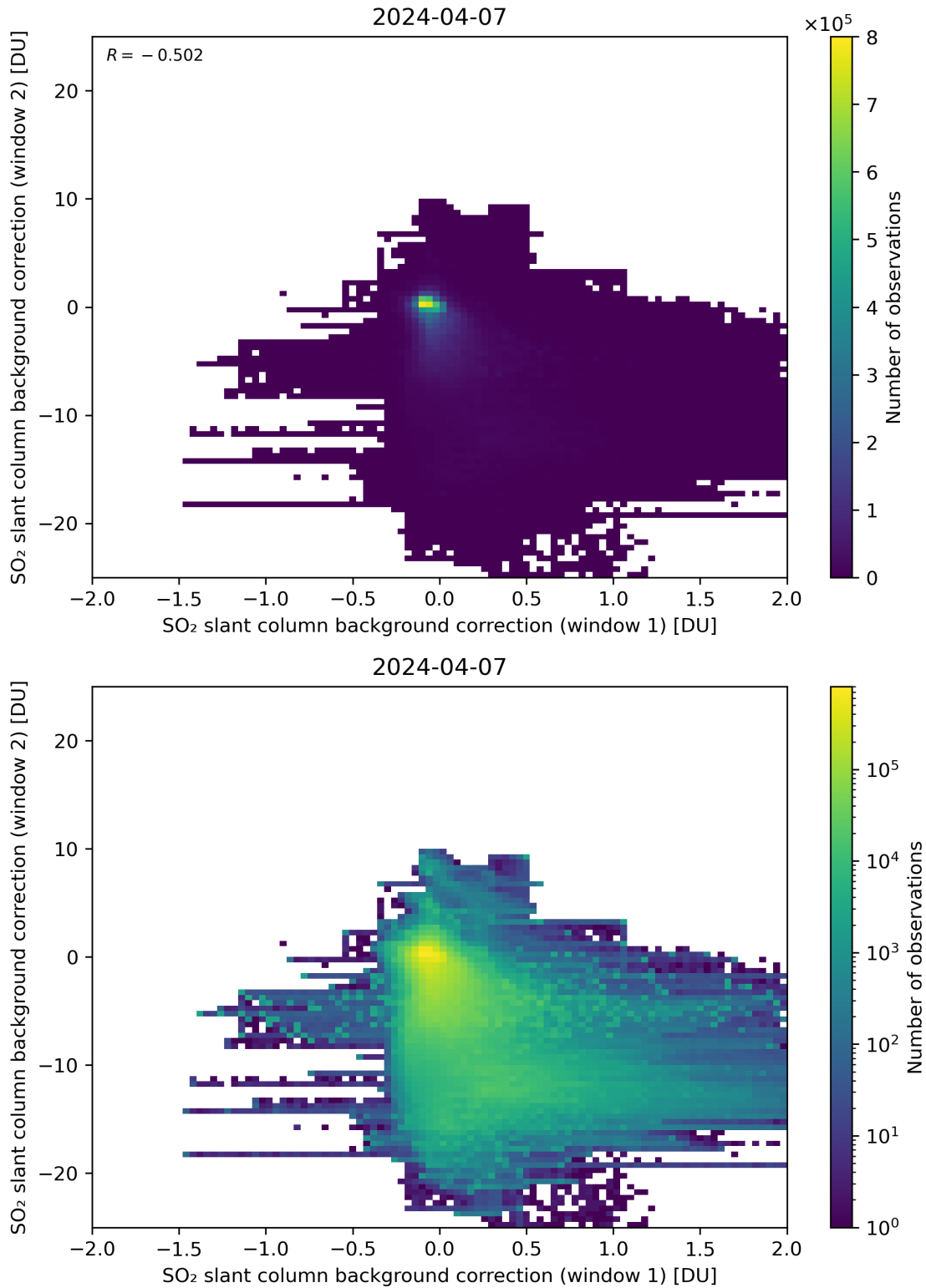
Figure 98: Scatter density plot of “SO 2 slant column background correction (window 1)” against “SO 2 slant column background correction (window 2)” for 2024-04-06 to 2024-04-08.
