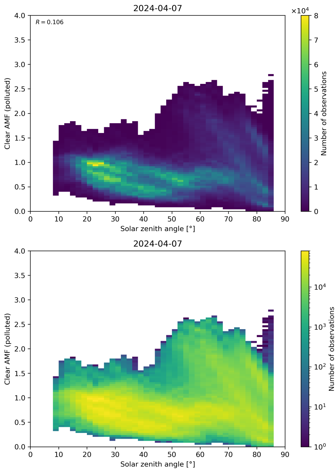
Figure 165: Scatter density plot of “Solar zenith angle” against “Clear AMF (polluted)” for 2024-04-06 to 2024-04-08.
