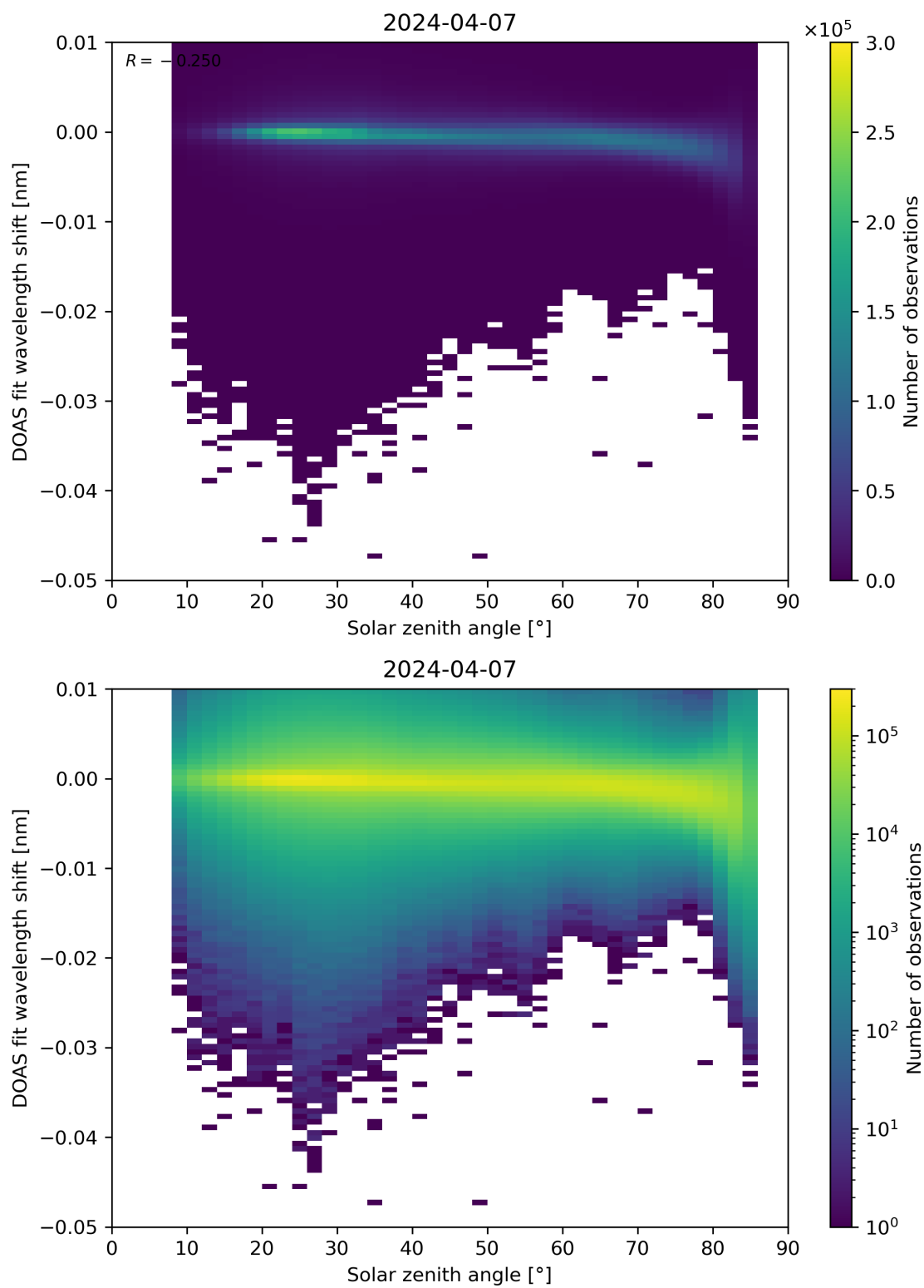
Figure 161: Scatter density plot of “Solar zenith angle” against “DOAS fit wavelength shift” for 2024-04-06 to 2024-04-08.
