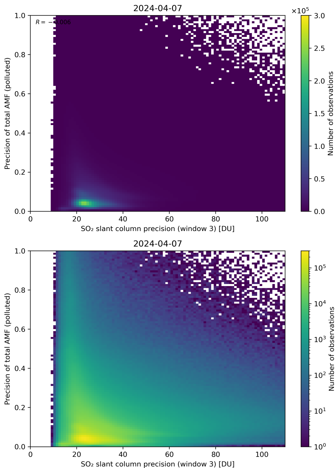
Figure 264: Scatter density plot of “SO 2 slant column precision (window 3)” against “Precision of total AMF (polluted)” for 2024-04-06 to 2024-04-08.
