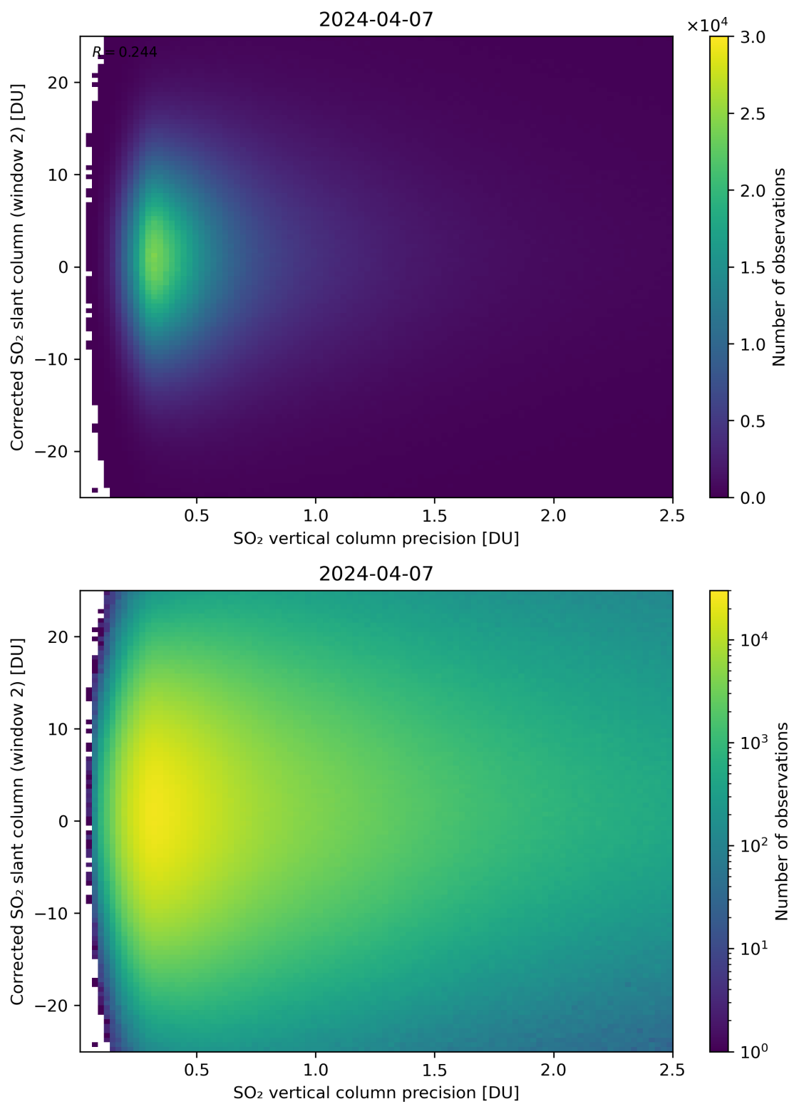
Figure 287: Scatter density plot of “SO 2 vertical column precision” against “Corrected SO 2 slant column (window 2)” for 2024-04-06 to 2024-04-08.
