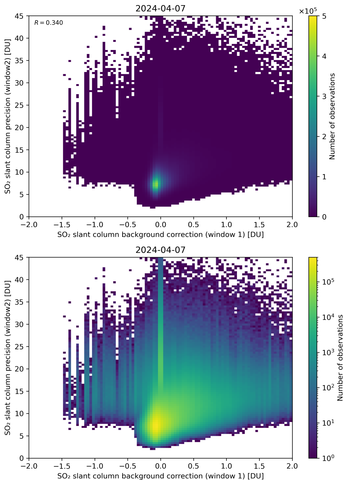
Figure 106: Scatter density plot of “SO 2 slant column background correction (window 1)” against “SO 2 slant column precision (window2)” for 2024-04-06 to 2024-04-08.
