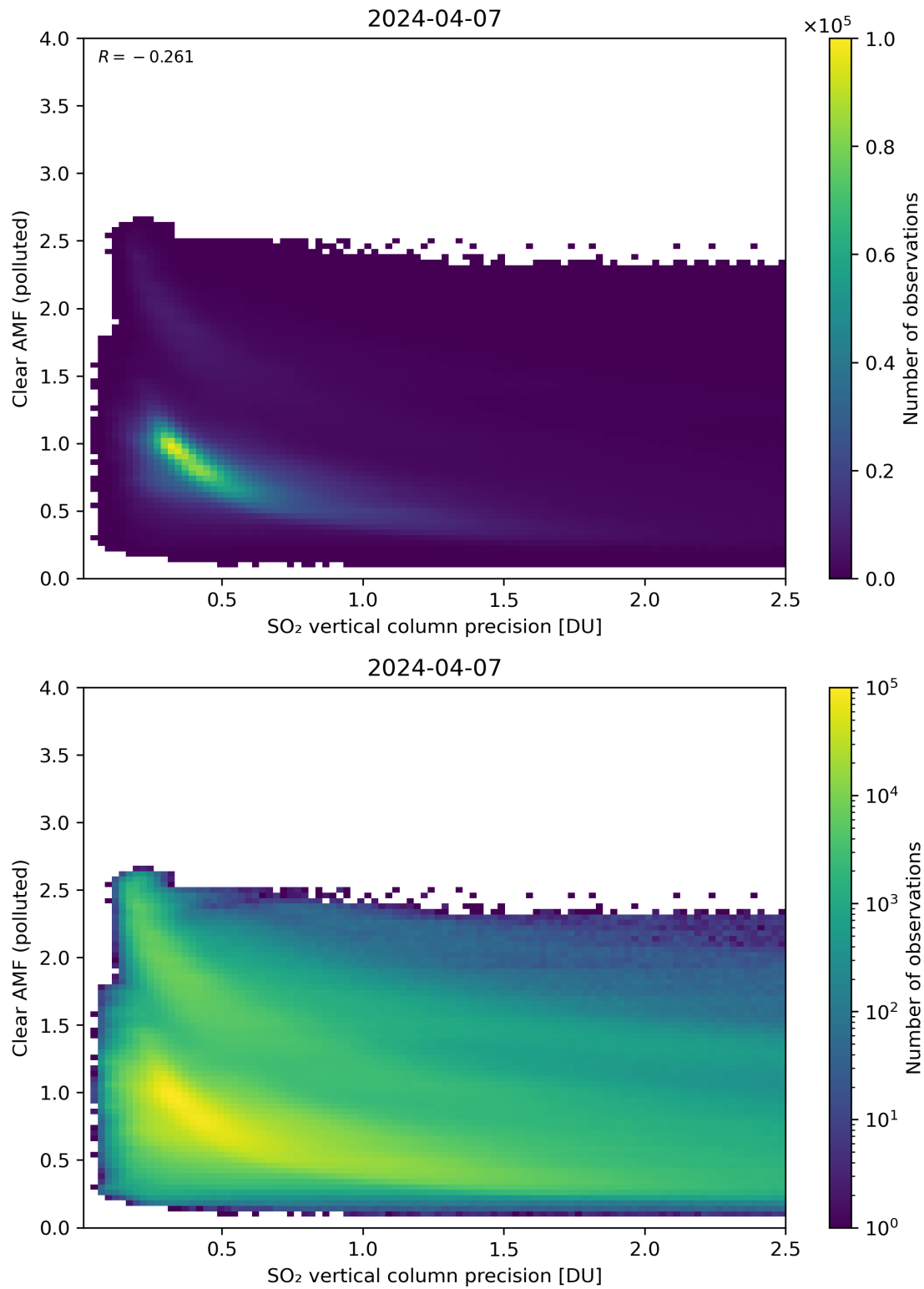
Figure 285: Scatter density plot of “SO 2 vertical column precision” against “Clear AMF (polluted)” for 2024-04-06 to 2024-04-08.
