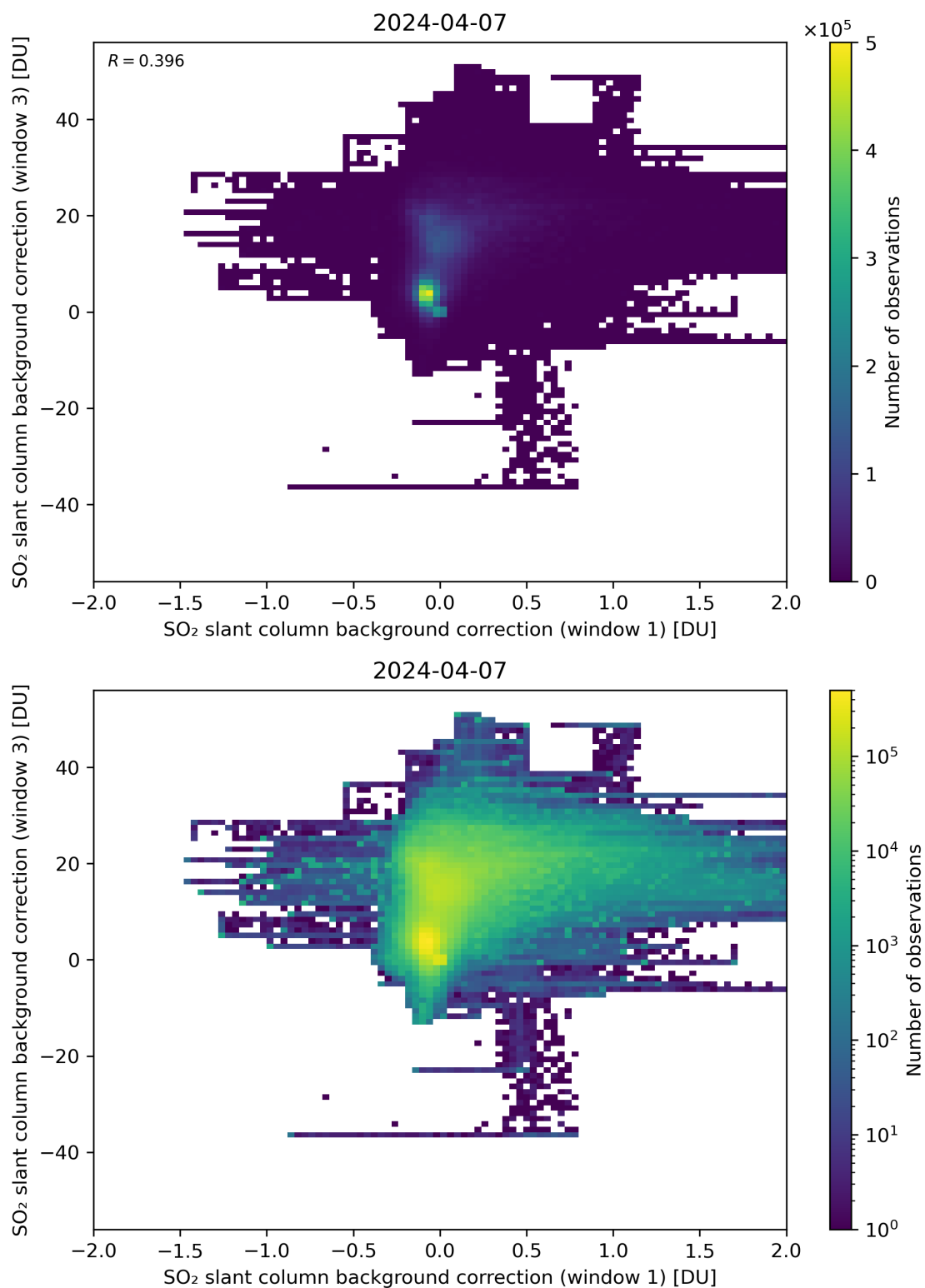
Figure 99: Scatter density plot of “SO 2 slant column background correction (window 1)” against “SO 2 slant column background correction (window 3)” for 2024-04-06 to 2024-04-08.
