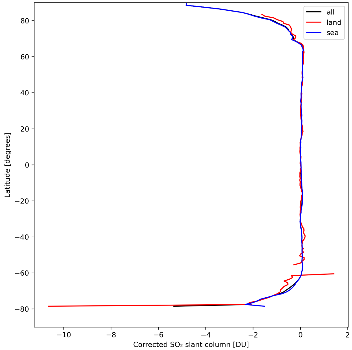
Figure 32: Zonal average of “Corrected SO 2 slant column” for 2024-04-06 to 2024-04-08.
