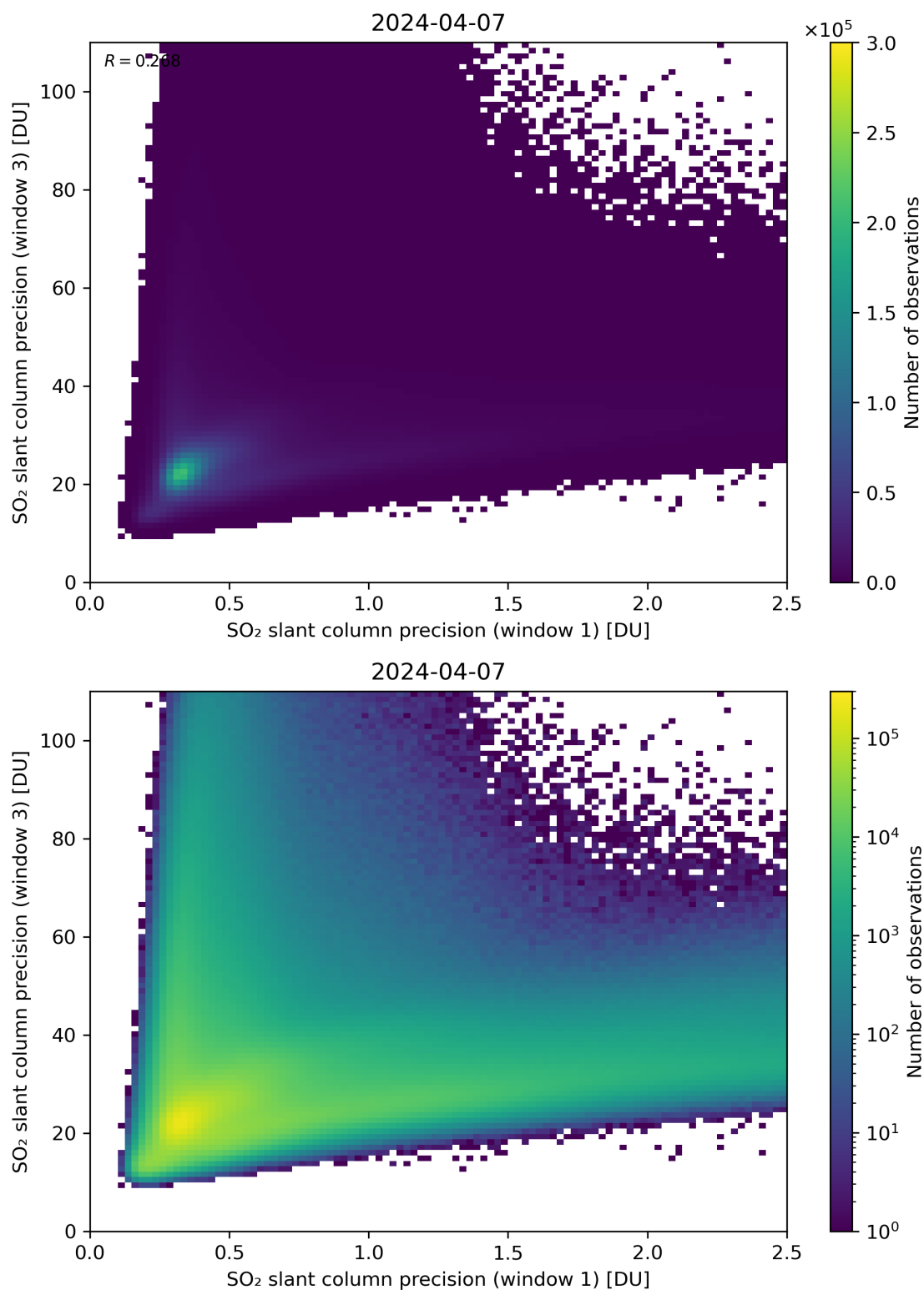
Figure 229: Scatter density plot of “SO 2 slant column precision (window 1)” against “SO 2 slant column precision (window 3)” for 2024-04-06 to 2024-04-08.
