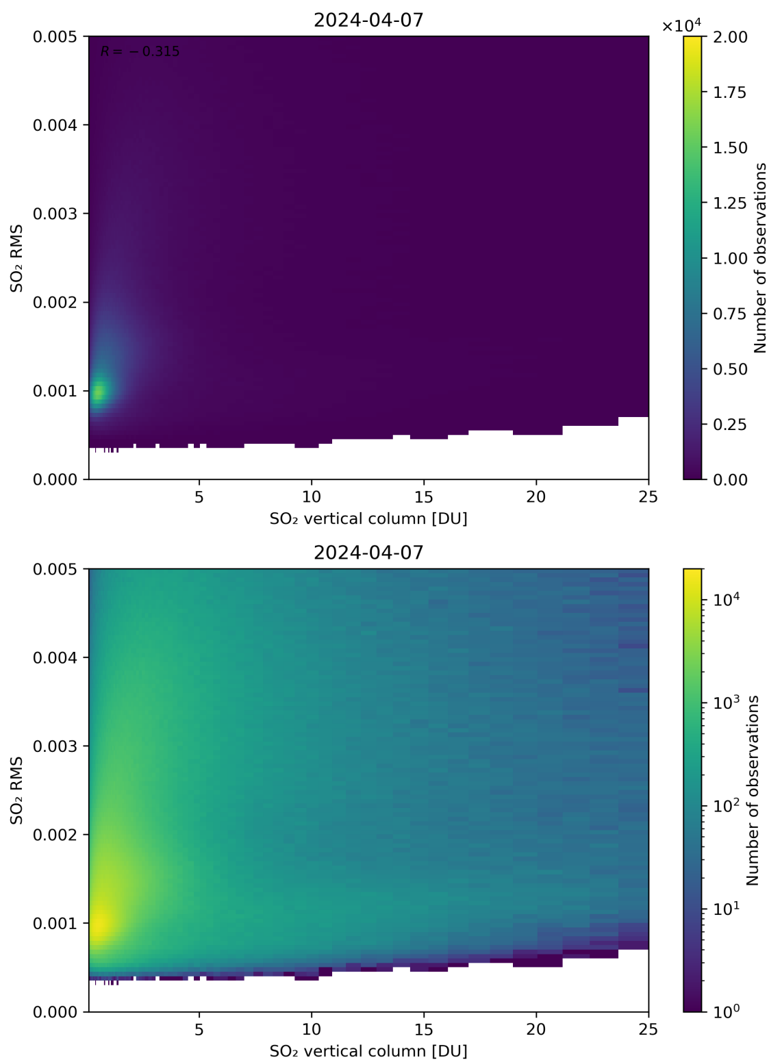
Figure 278: Scatter density plot of “SO 2 vertical column” against “SO 2 RMS” for 2024-04-06 to 2024-04-08.
