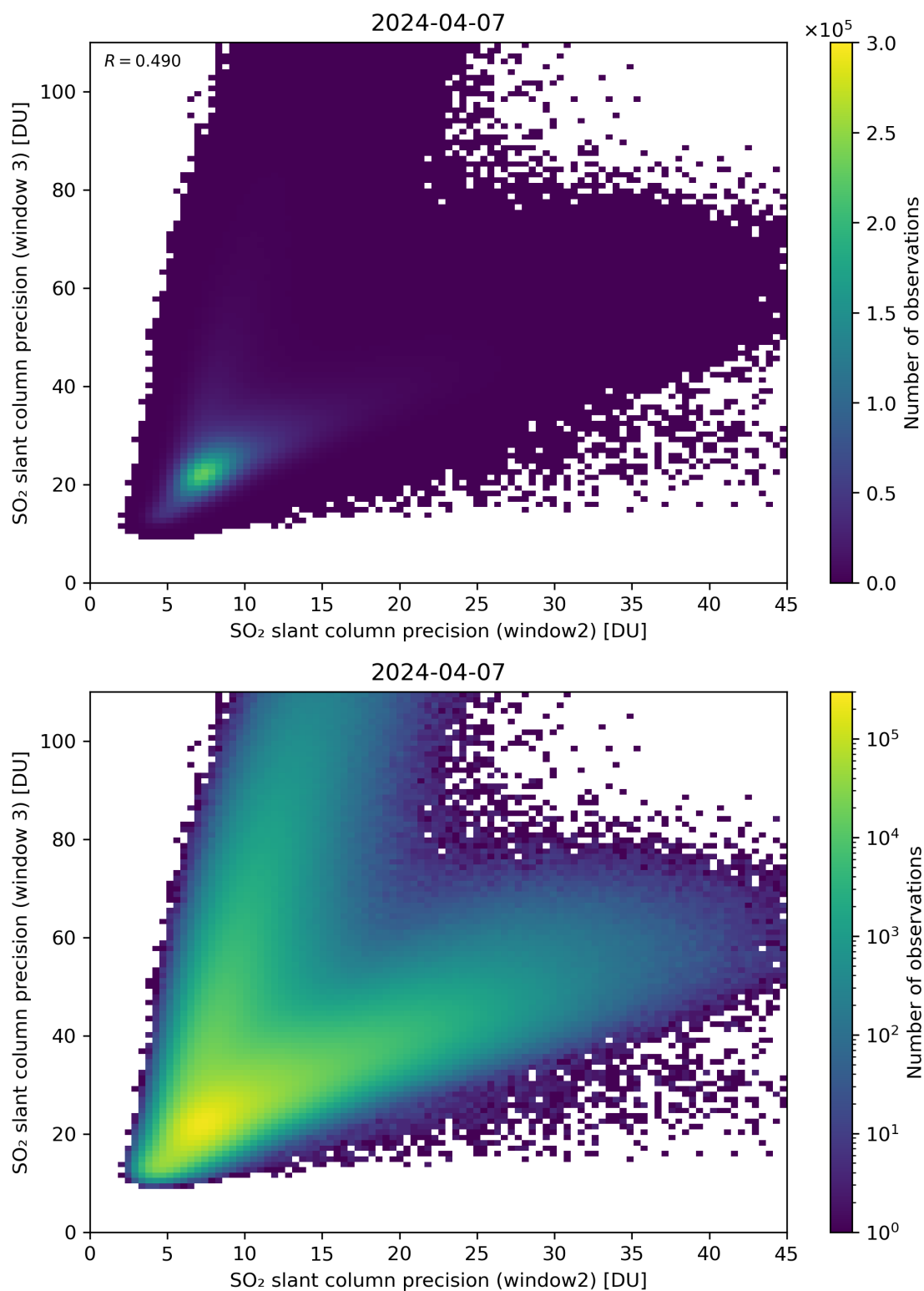
Figure 250: Scatter density plot of “SO 2 slant column precision (window2)” against “SO 2 slant column precision (window 3)” for 2024-04-06 to 2024-04-08.
