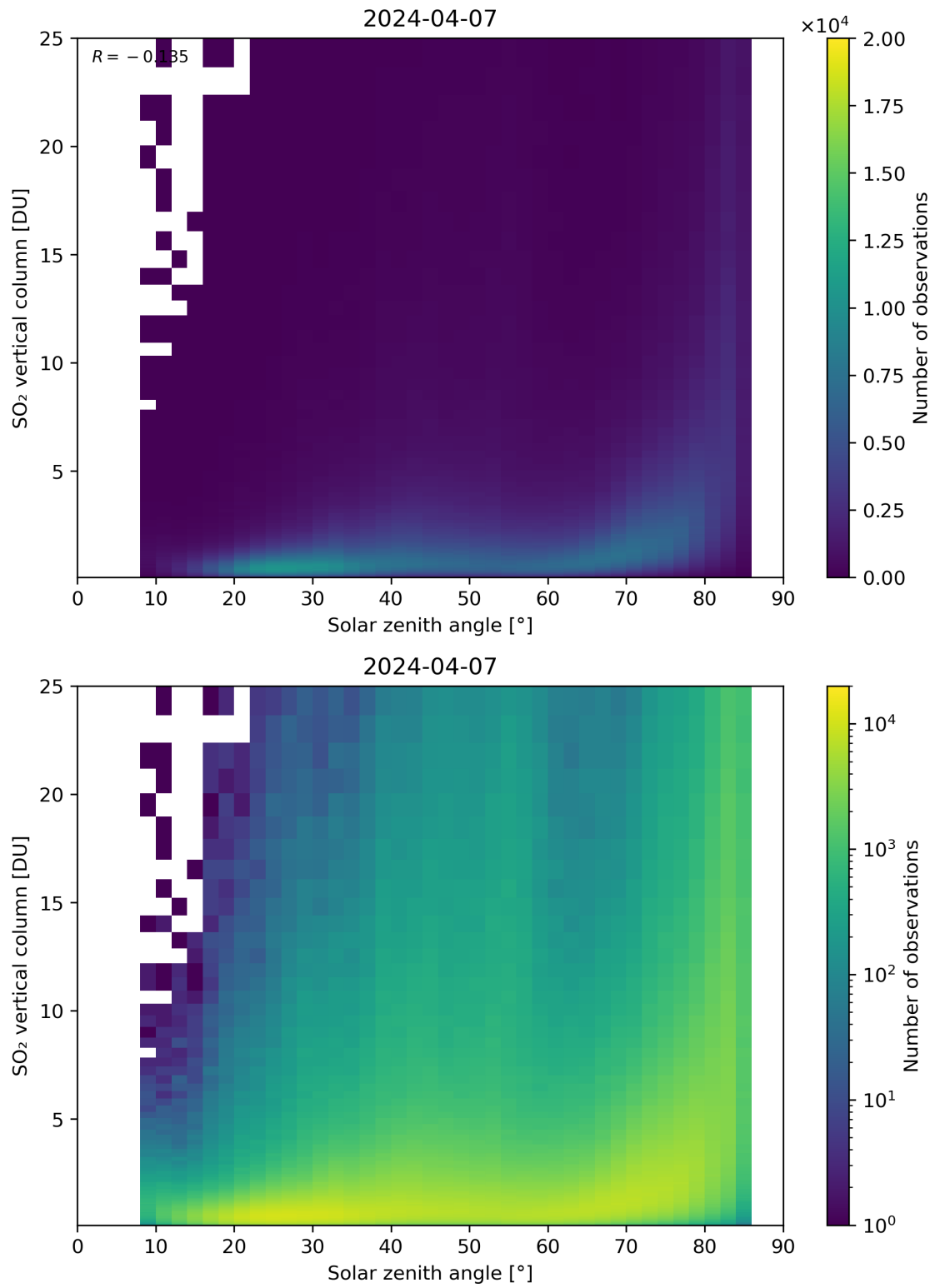
Figure 176: Scatter density plot of “Solar zenith angle” against “SO 2 vertical column” for 2024-04-06 to 2024-04-08.
