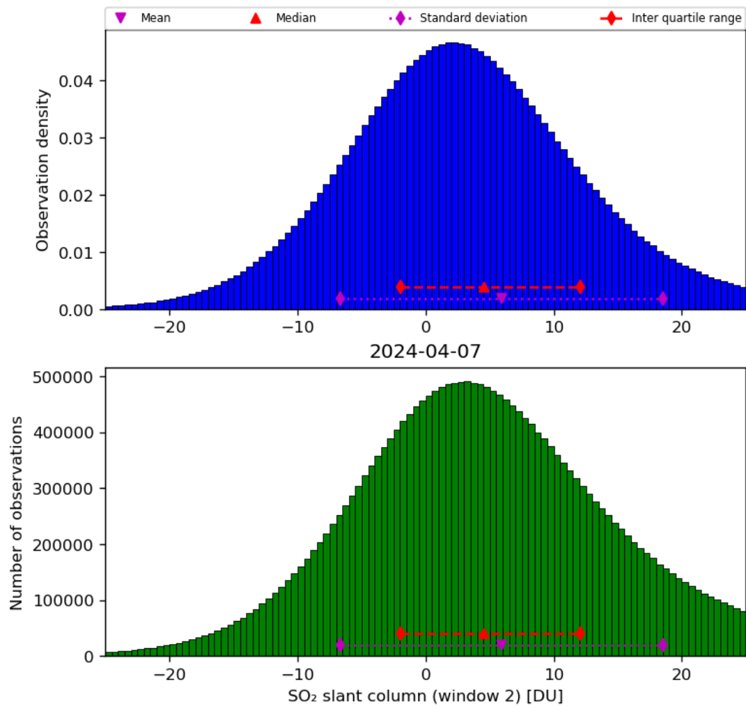
Figure 60: Histogram of “SO 2 slant column (window 2)” for 2024-04-06 to 2024-04-08
