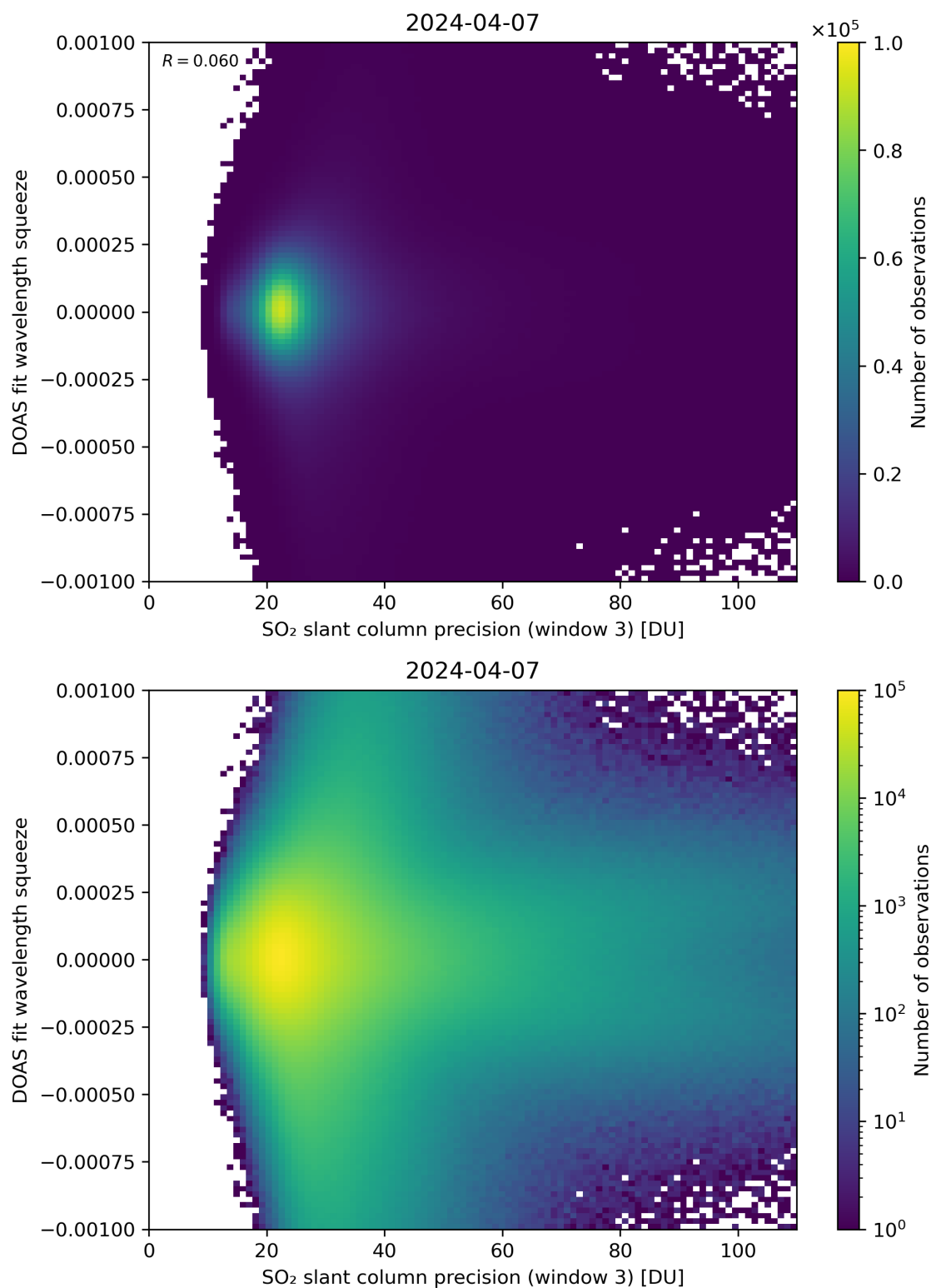
Figure 259: Scatter density plot of “SO 2 slant column precision (window 3)” against “DOAS fit wavelength squeeze” for 2024-04-06 to 2024-04-08.
