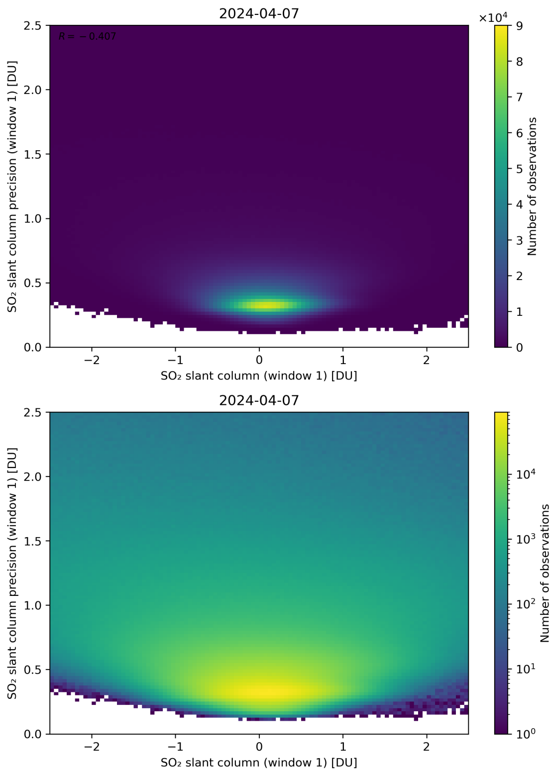
Figure 235: Scatter density plot of “SO 2 slant column (window 1)” against “SO 2 slant column precision (window 1)” for 2024-04-06 to 2024-04-08.
