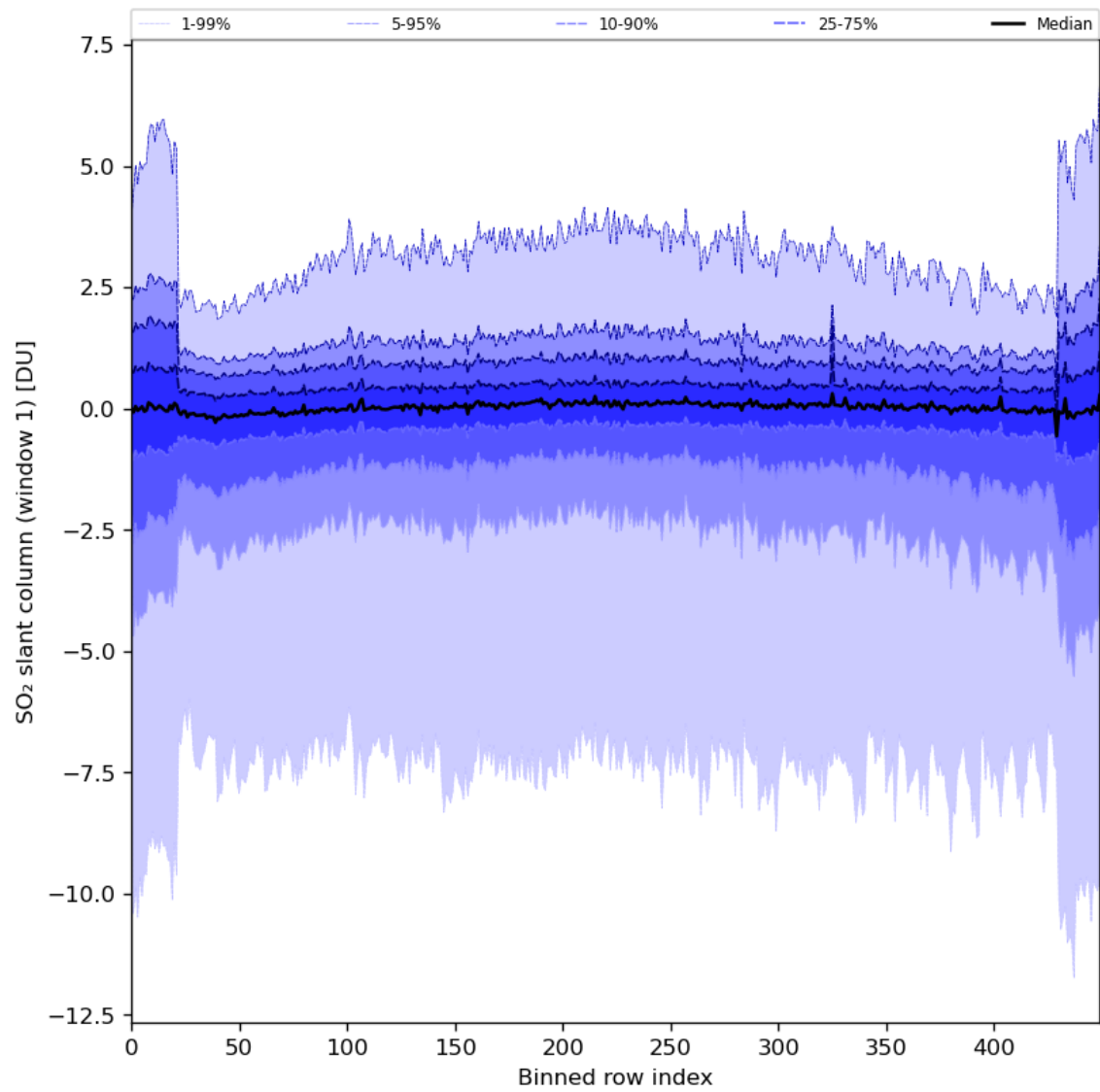
Figure 79: Along track statistics of “SO 2 slant column (window 1)” for 2024-04-06 to 2024-04-08
