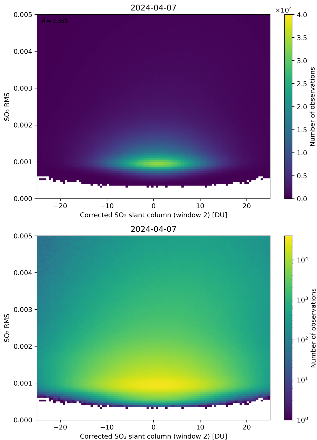
Figure 198: Scatter density plot of “Corrected SO 2 slant column (window 2)” against “SO 2 RMS” for 2024-04-06 to 2024-04-08.
