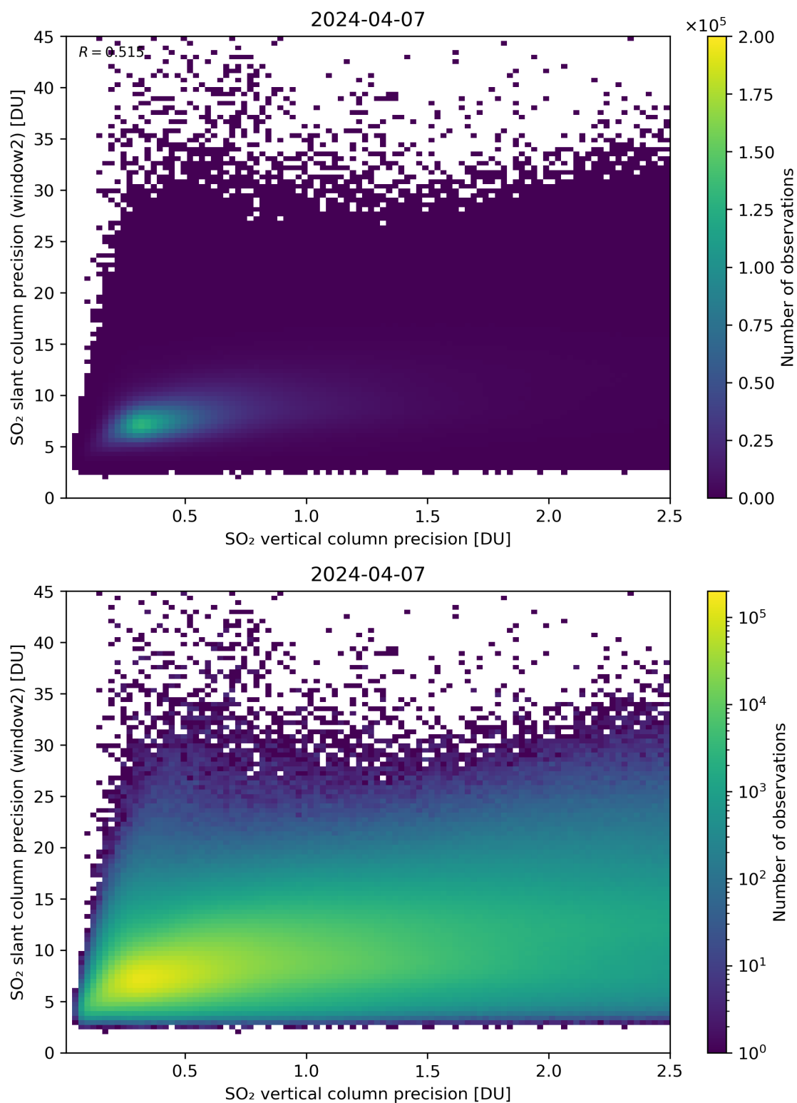
Figure 291: Scatter density plot of “SO 2 vertical column precision” against “SO 2 slant column precision (window2)” for 2024-04-06 to 2024-04-08.
