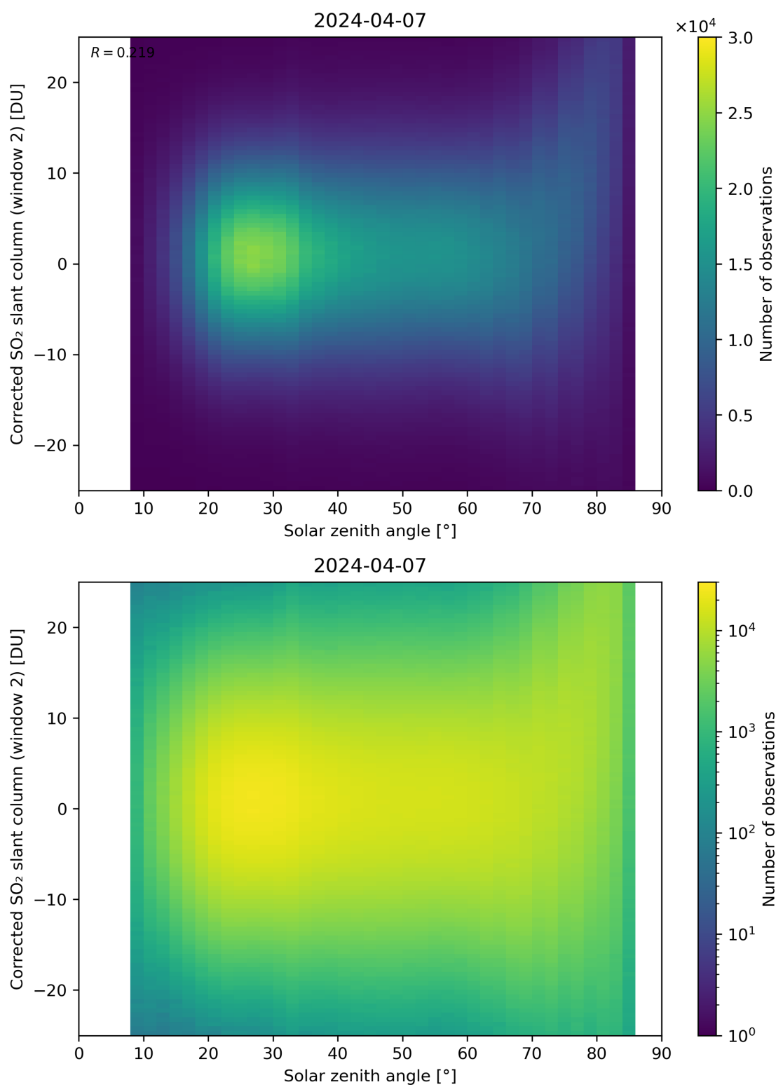
Figure 167: Scatter density plot of “Solar zenith angle” against “Corrected SO 2 slant column (window 2)” for 2024-04-06 to 2024-04-08.
