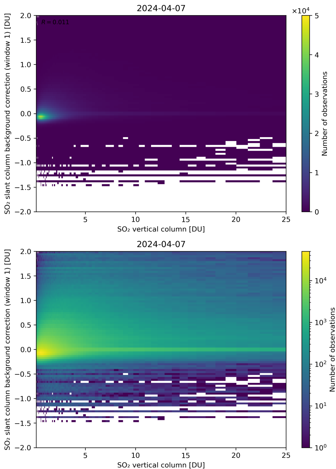
Figure 273: Scatter density plot of “SO 2 vertical column” against “SO 2 slant column background correction (window 1)” for 2024-04-06 to 2024-04-08.
