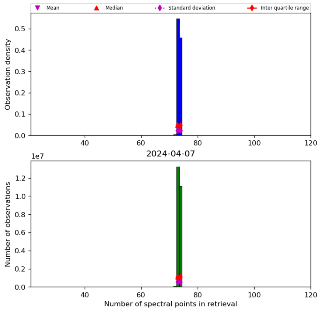
Figure 74: Histogram of “Number of spectral points in retrieval” for 2024-04-06 to 2024-04-08
