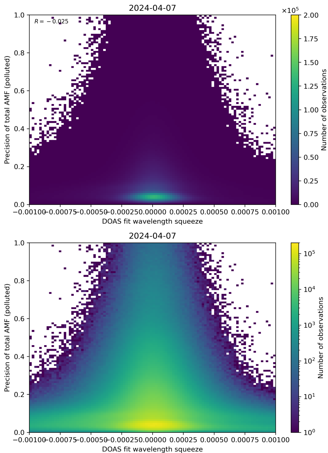
Figure 135: Scatter density plot of “DOAS fit wavelength squeeze” against “Precision of total AMF (polluted)” for 2024-04-06 to 2024-04-08.
