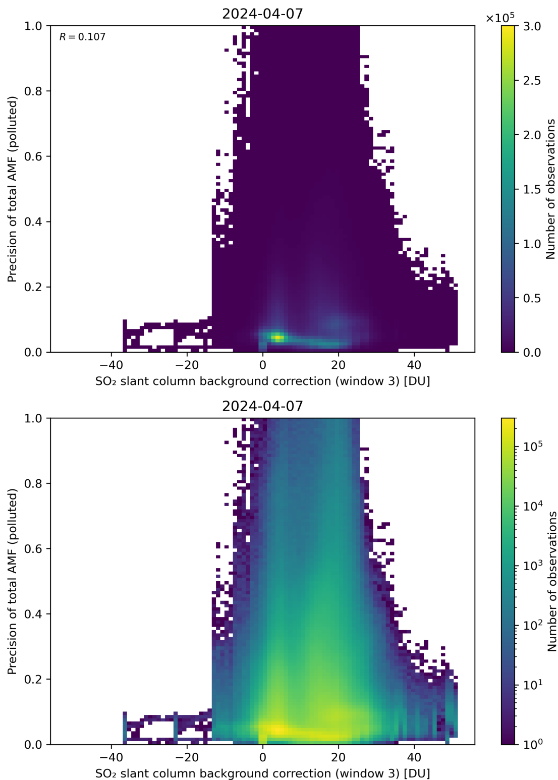
Figure 126: Scatter density plot of “SO 2 slant column background correction (window 3)” against “Precision of total AMF (polluted)” for 2024-04-06 to 2024-04-08.
