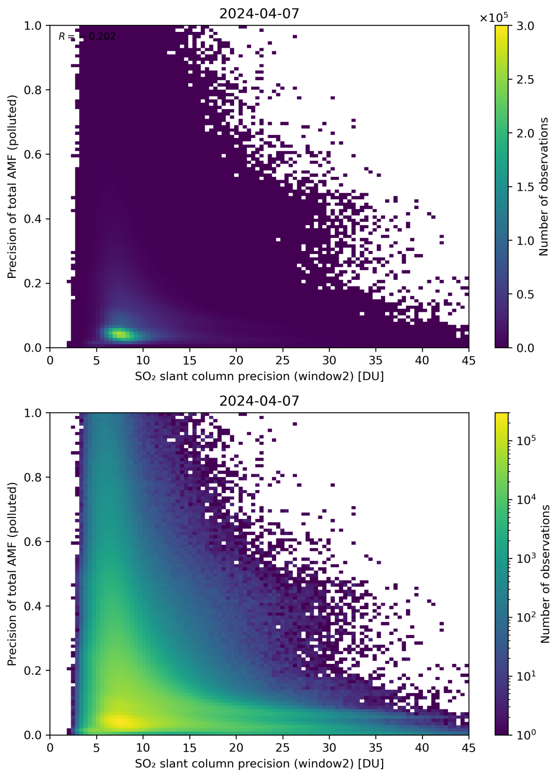
Figure 252: Scatter density plot of “SO 2 slant column precision (window2)” against “Precision of total AMF (polluted)” for 2024-04-06 to 2024-04-08.
