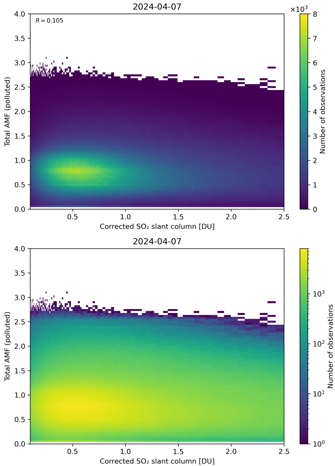
Figure 192: Scatter density plot of “Corrected SO 2 slant column” against “Total AMF (polluted)” for 2024-04-06 to 2024-04-08.
