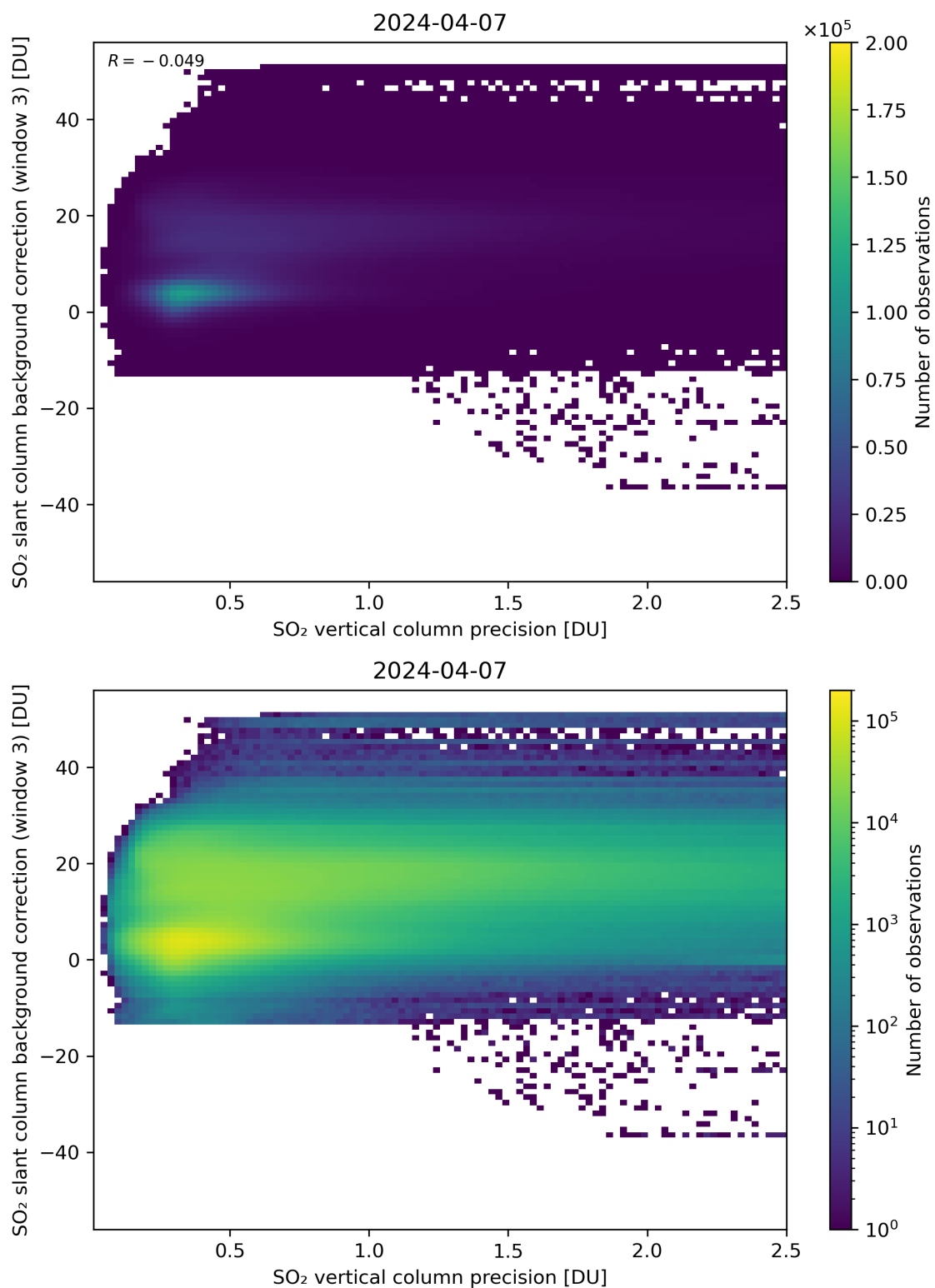
Figure 281: Scatter density plot of “SO 2 vertical column precision” against “SO 2 slant column background correction (window 3)” for 2024-04-06 to 2024-04-08.
