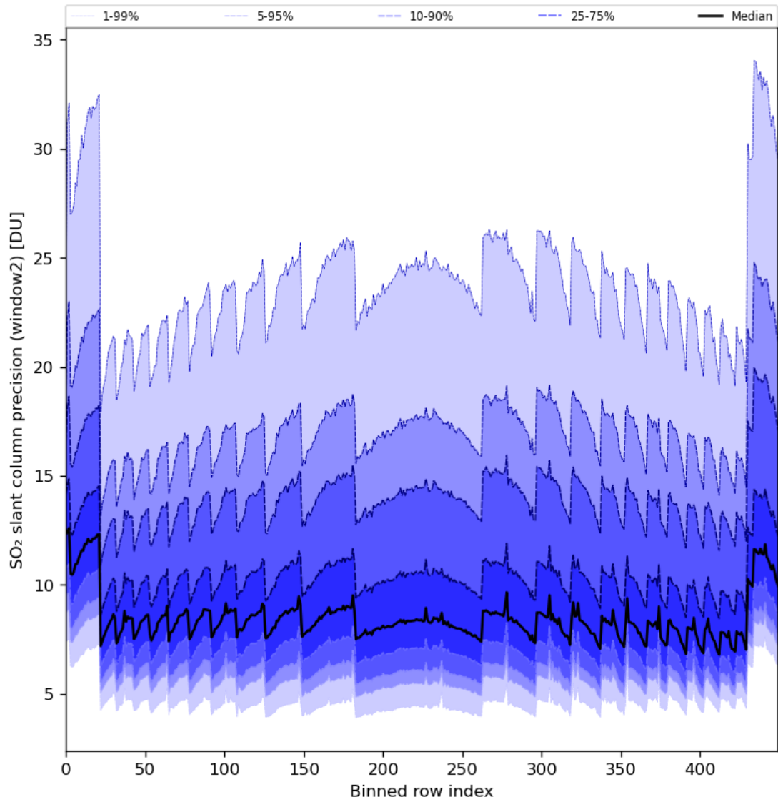
Figure 84: Along track statistics of “SO 2 slant column precision (window2)” for 2024-04-06 to 2024-04-08
