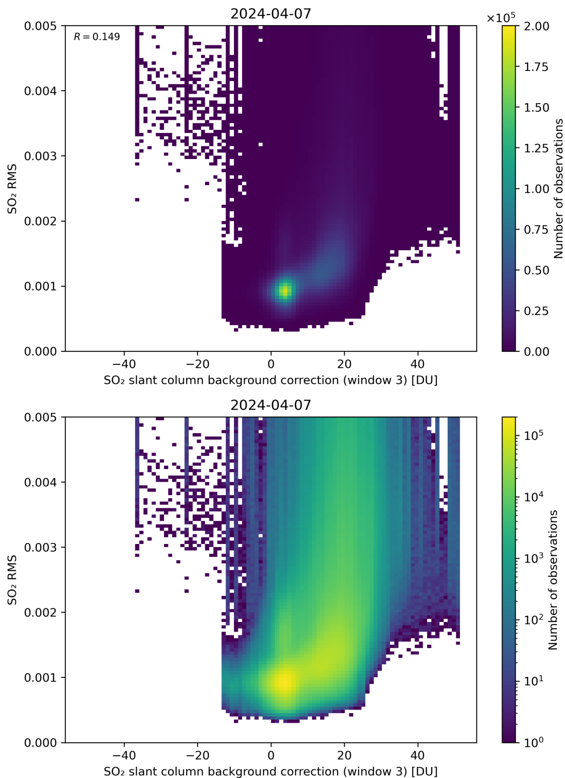
Figure 123: Scatter density plot of “SO 2 slant column background correction (window 3)” against “SO 2 RMS” for 2024-04-06 to 2024-04-08.
