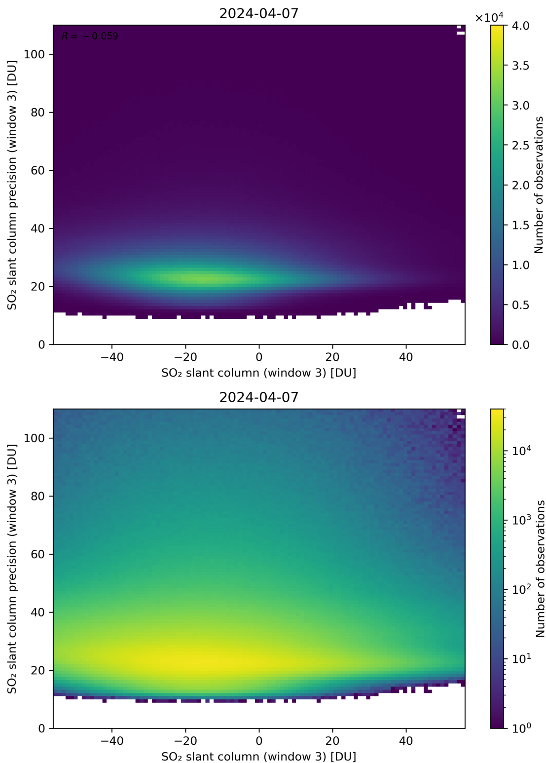
Figure 267: Scatter density plot of “SO 2 slant column (window 3)” against “SO 2 slant column precision (window 3)” for 2024-04-06 to 2024-04-08.
