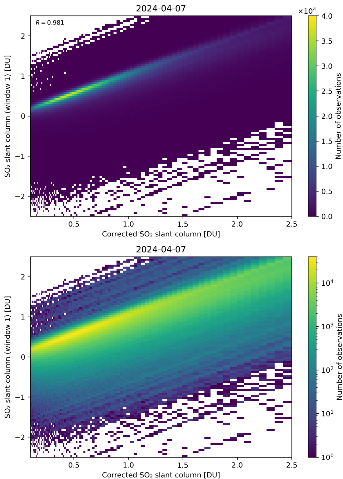
Figure 187: Scatter density plot of “Corrected SO 2 slant column” against “SO 2 slant column (window 1)” for 2024-04-06 to 2024-04-08.
