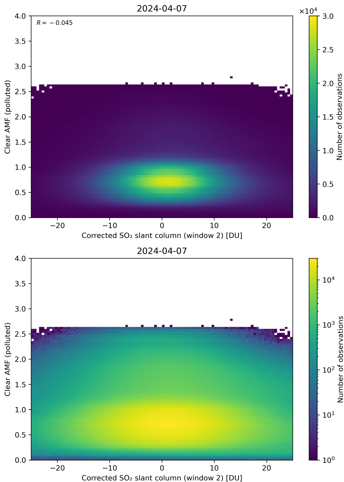
Figure 199: Scatter density plot of “Corrected SO 2 slant column (window 2)” against “Clear AMF (polluted)” for 2024-04-06 to 2024-04-08.
