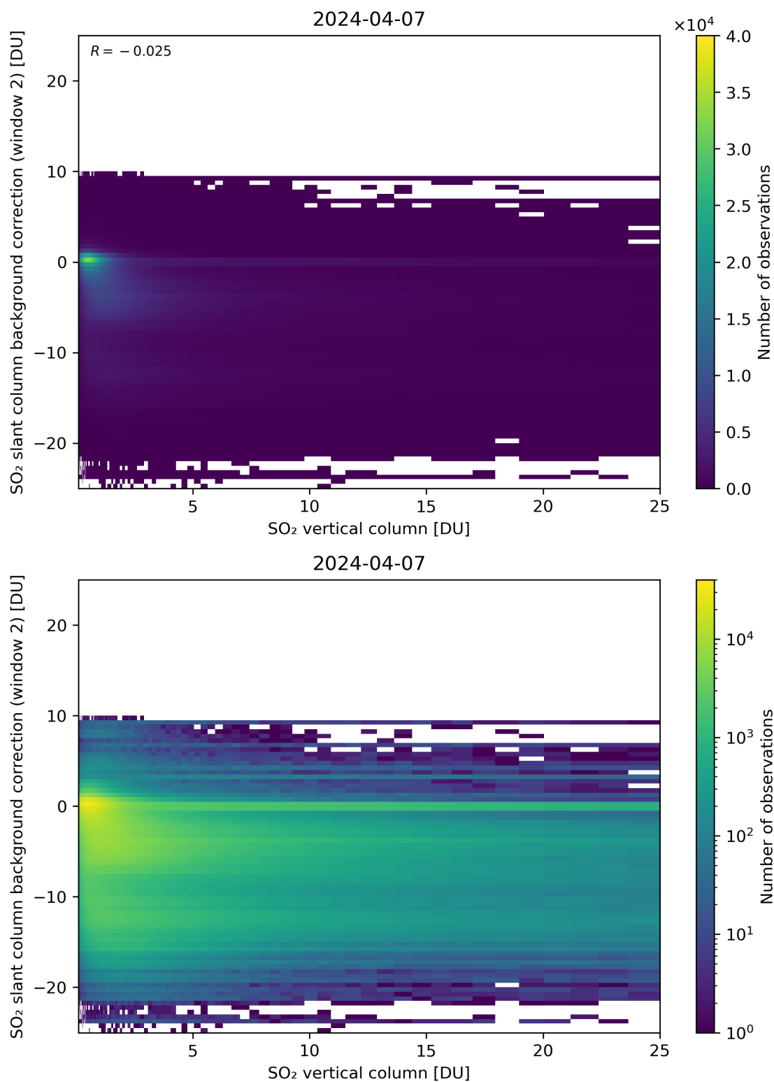
Figure 274: Scatter density plot of “SO 2 vertical column” against “SO 2 slant column background correction (window 2)” for 2024-04-06 to 2024-04-08.
