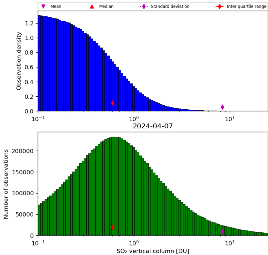
Figure 53: Histogram of “SO 2 vertical column” for 2024-04-06 to 2024-04-08
