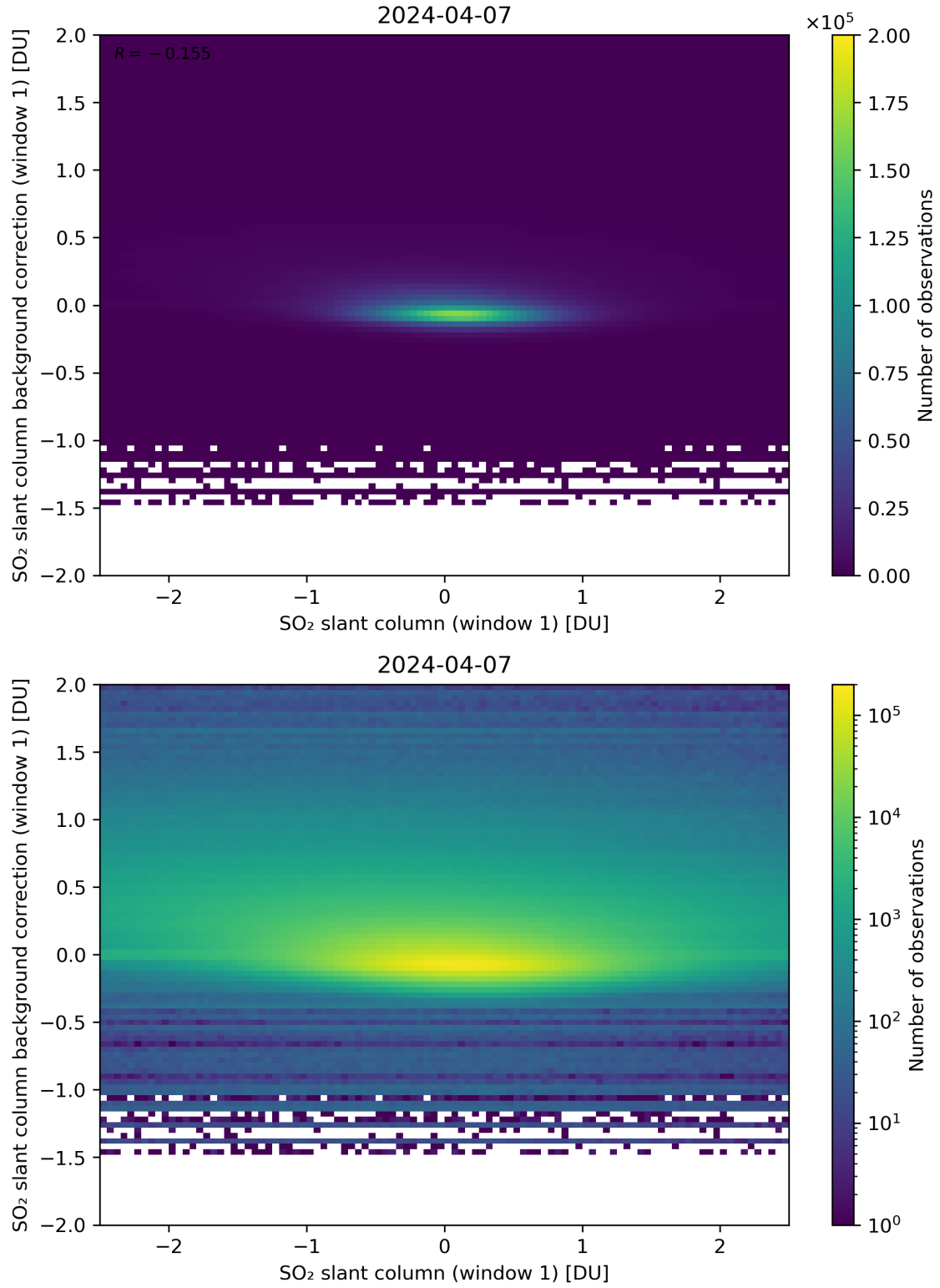
Figure 212: Scatter density plot of “SO 2 slant column (window 1)” against “SO 2 slant column background correction (window 1)” for 2024-04-06 to 2024-04-08.
