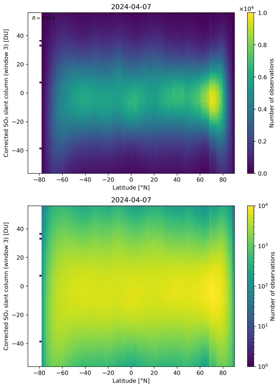
Figure 148: Scatter density plot of “Latitude” against “Corrected SO 2 slant column (window 3)” for 2024-04-06 to 2024-04-08.
