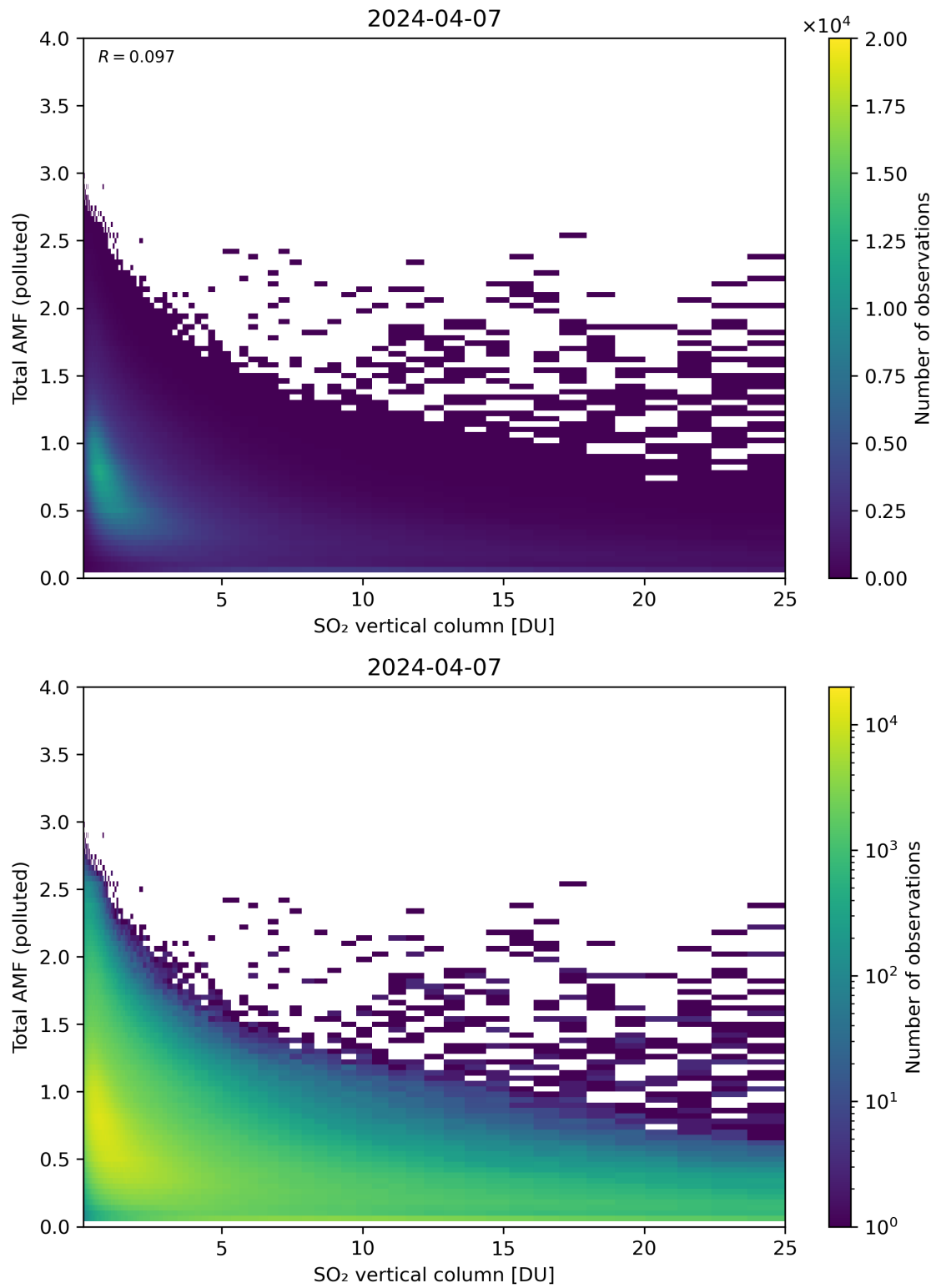
Figure 305: Scatter density plot of “SO 2 vertical column” against “Total AMF (polluted)” for 2024-04-06 to 2024-04-08.
