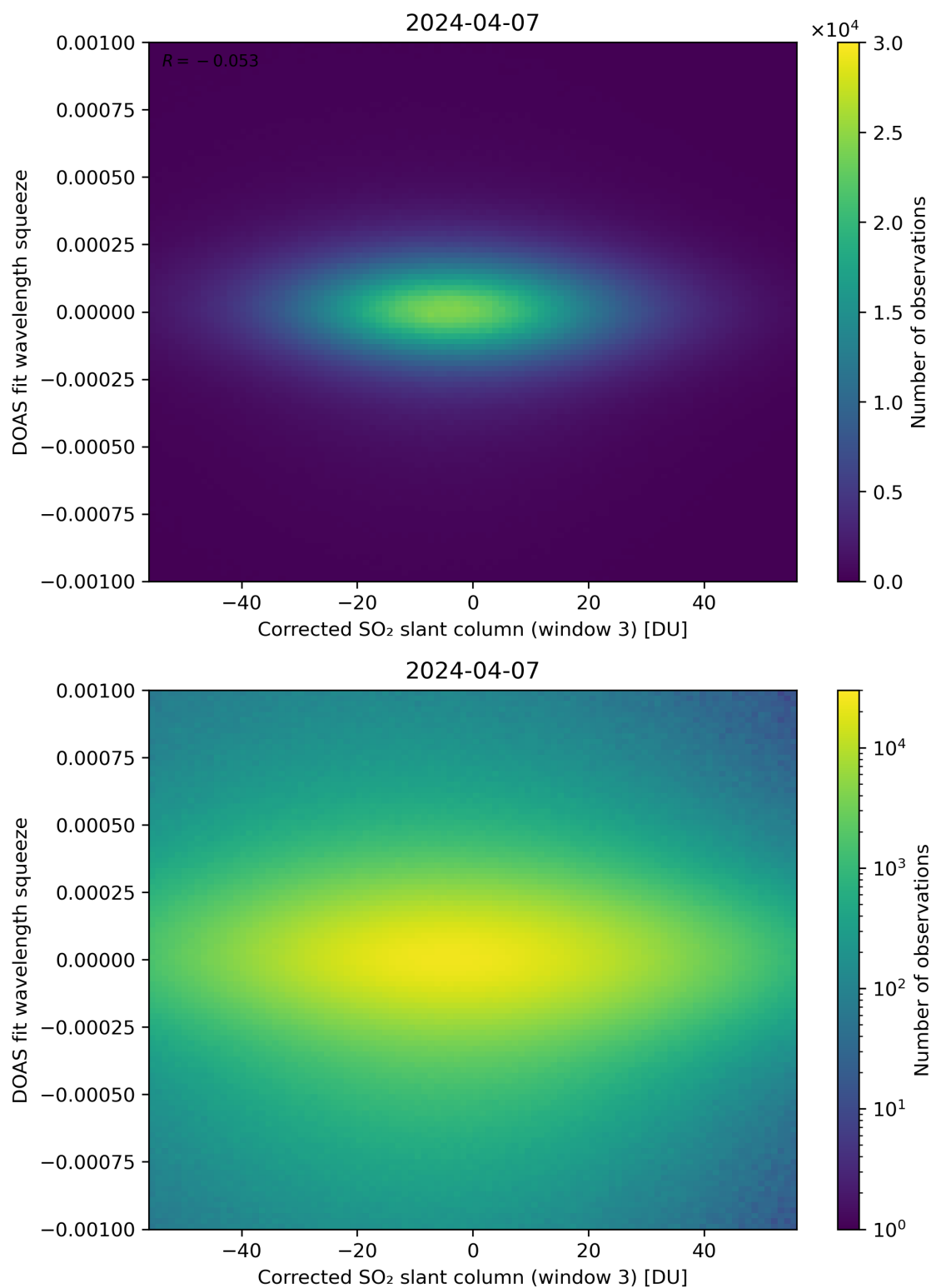
Figure 207: Scatter density plot of “Corrected SO 2 slant column (window 3)” against “DOAS fit wavelength squeeze” for 2024-04-06 to 2024-04-08.
