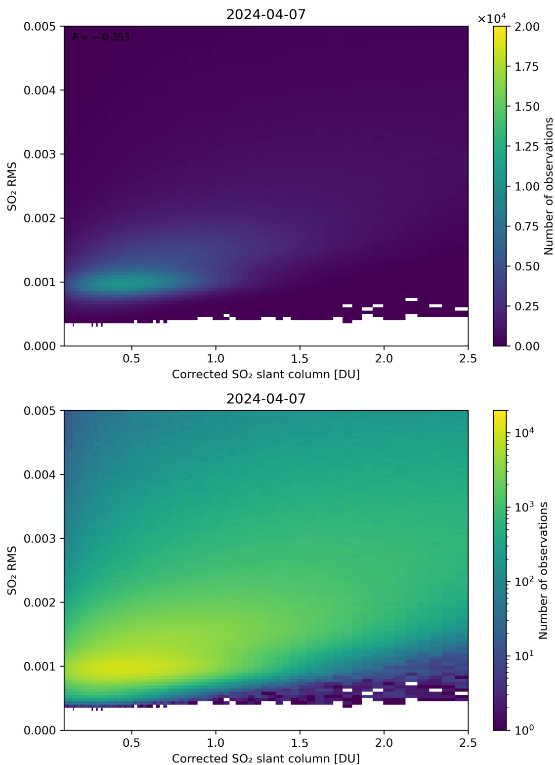
Figure 183: Scatter density plot of “Corrected SO 2 slant column” against “SO 2 RMS” for 2024-04-06 to 2024-04-08.
