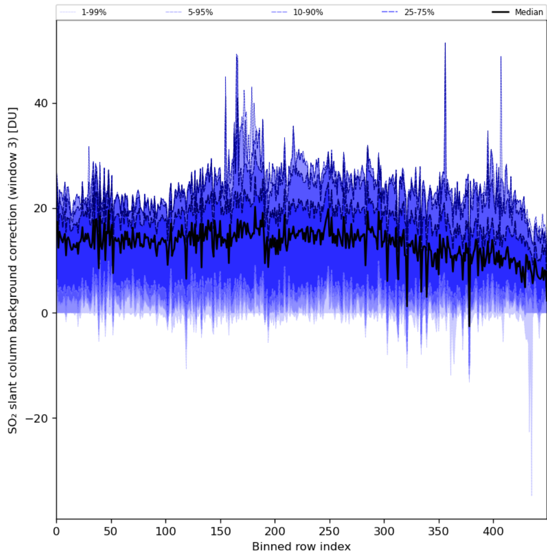
Figure 90: Along track statistics of “SO 2 slant column background correction (window 3)” for 2024-04-06 to 2024-04-08
