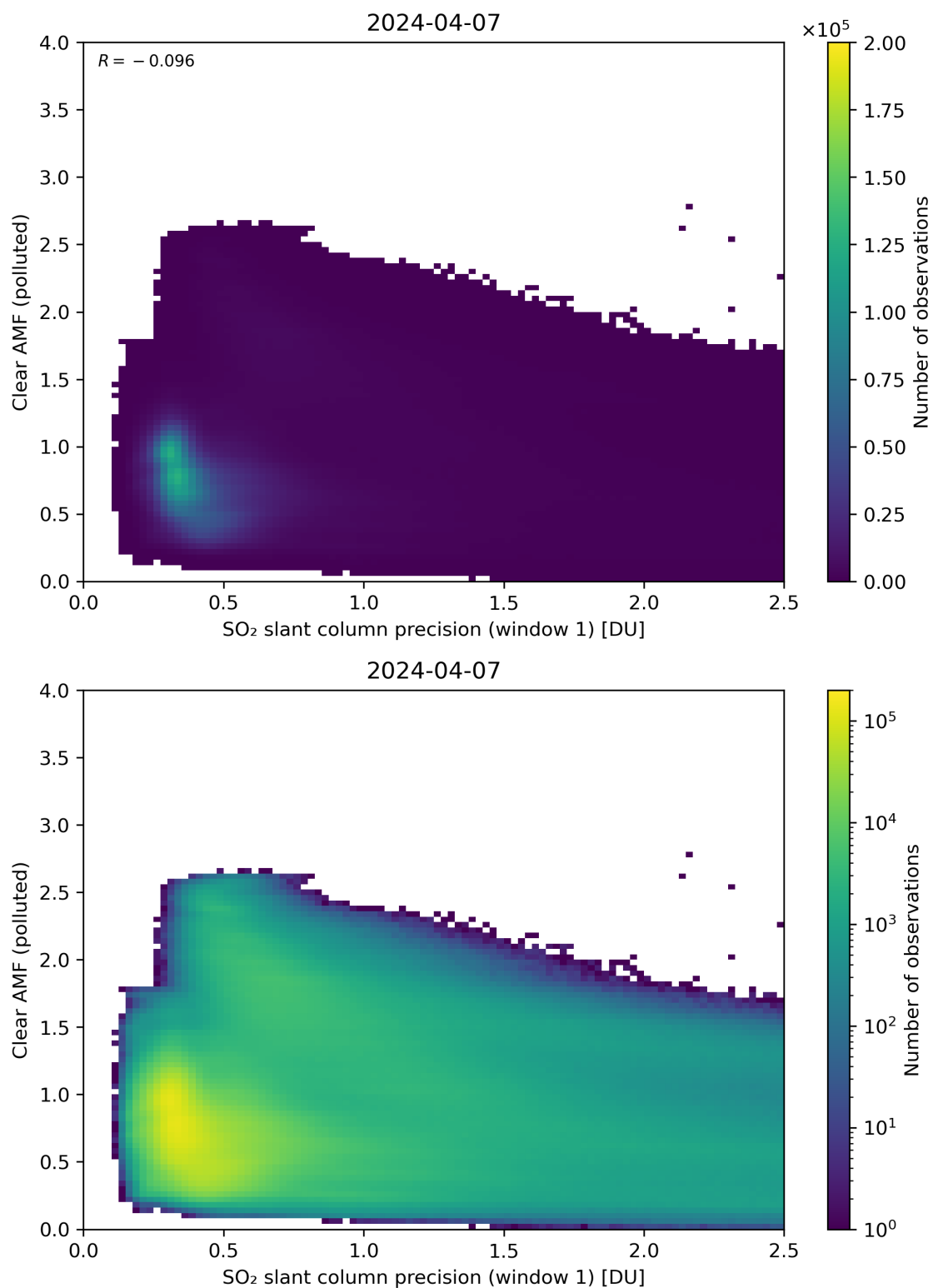
Figure 224: Scatter density plot of “SO 2 slant column precision (window 1)” against “Clear AMF (polluted)” for 2024-04-06 to 2024-04-08.
