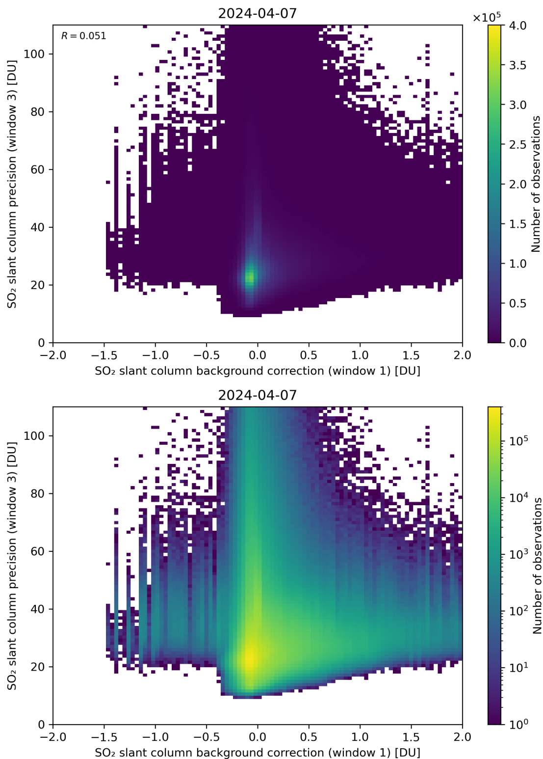
Figure 108: Scatter density plot of “SO 2 slant column background correction (window 1)” against “SO 2 slant column precision (window 3)” for 2024-04-06 to 2024-04-08.
