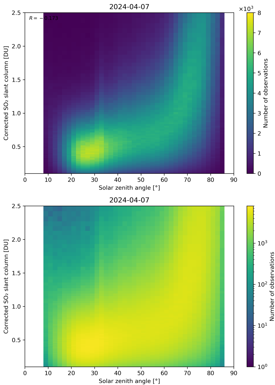
Figure 166: Scatter density plot of “Solar zenith angle” against “Corrected SO 2 slant column” for 2024-04-06 to 2024-04-08.
