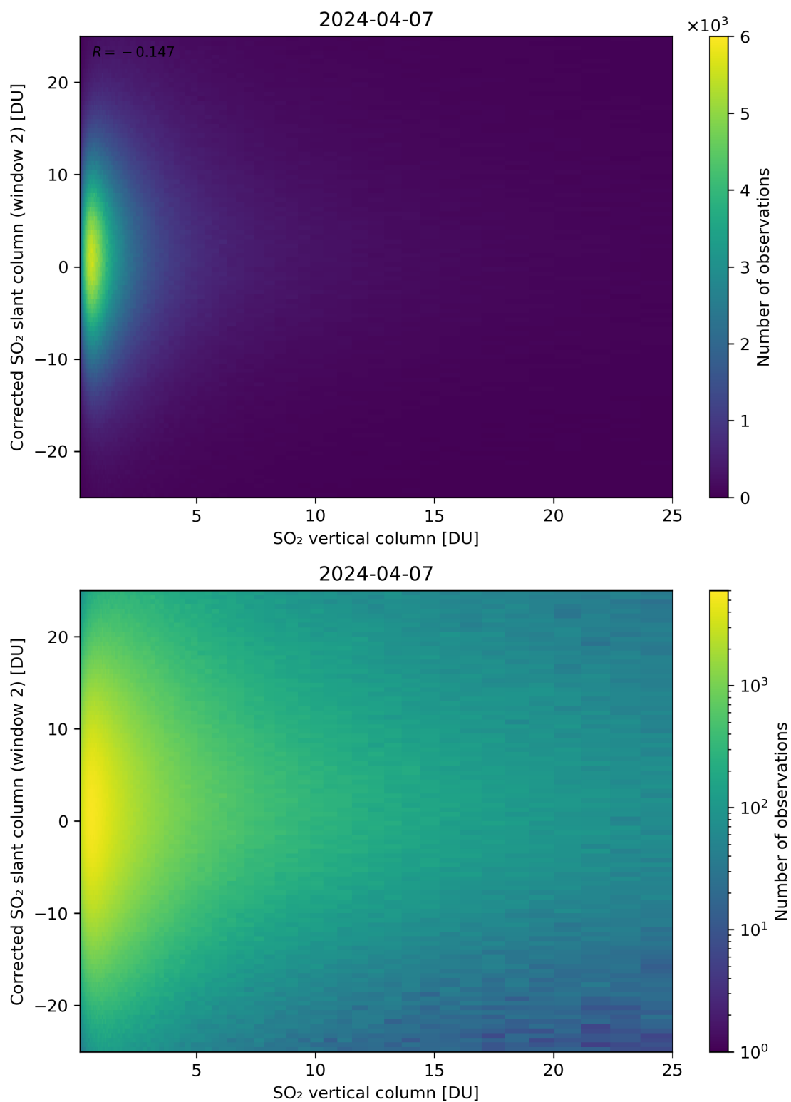
Figure 298: Scatter density plot of “SO 2 vertical column” against “Corrected SO 2 slant column (window 2)” for 2024-04-06 to 2024-04-08.
