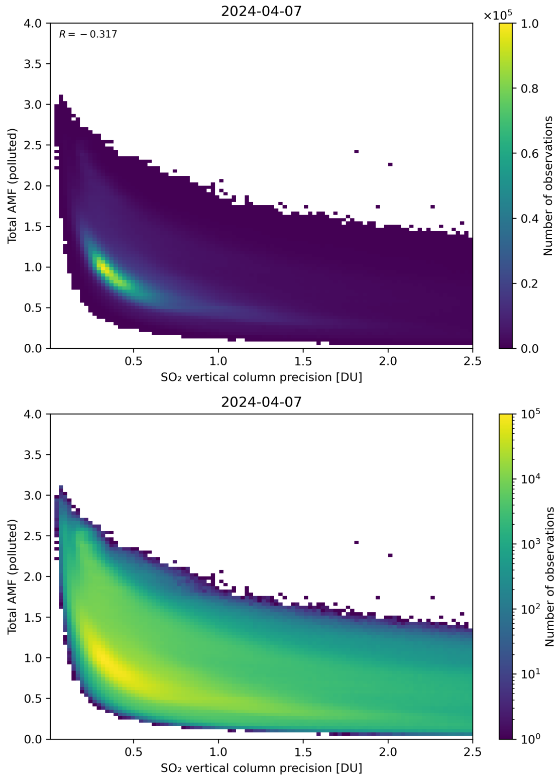
Figure 294: Scatter density plot of “SO 2 vertical column precision” against “Total AMF (polluted)” for 2024-04-06 to 2024-04-08.
