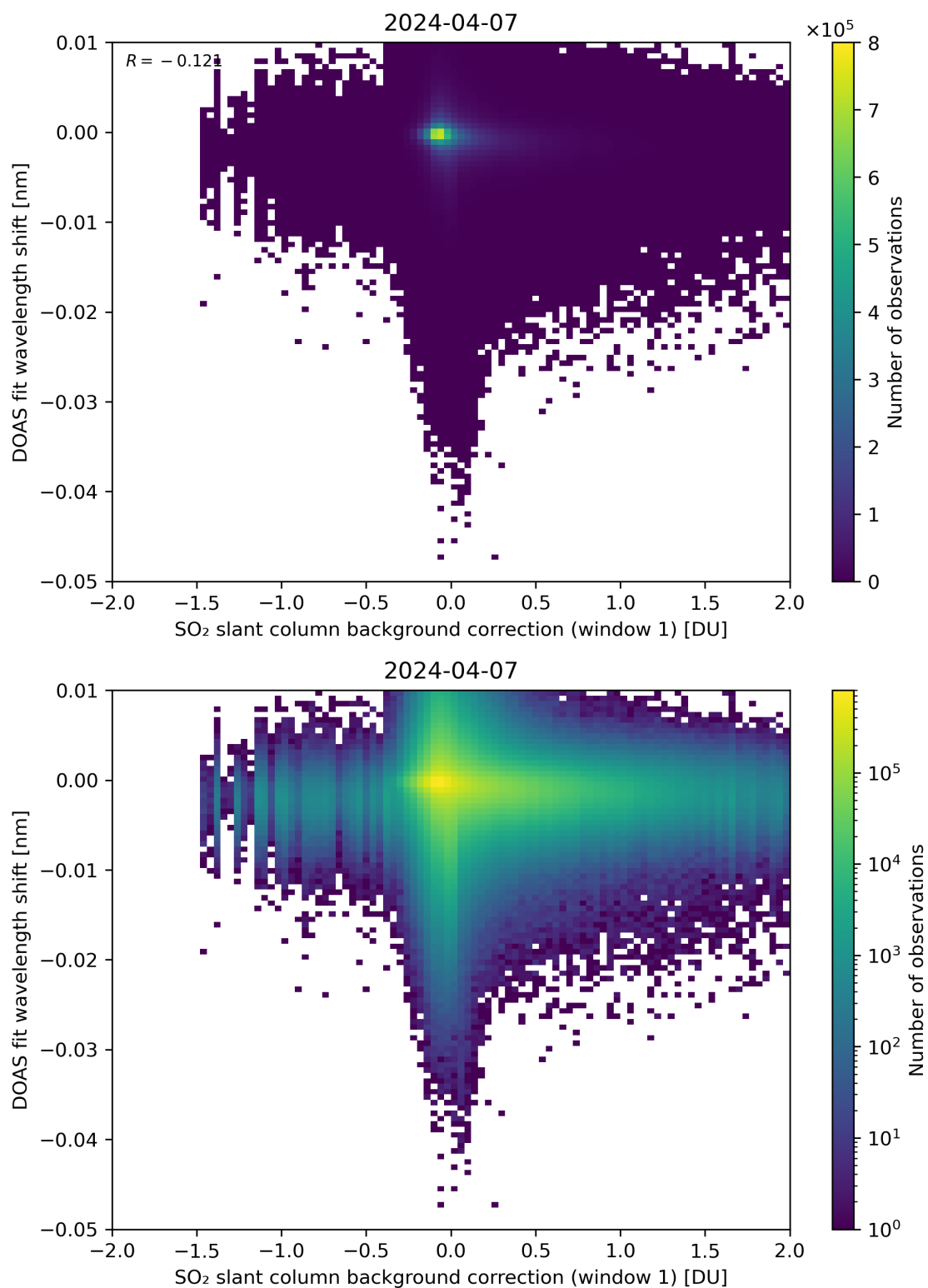
Figure 100: Scatter density plot of “SO 2 slant column background correction (window 1)” against “DOAS fit wavelength shift” for 2024-04-06 to 2024-04-08.
