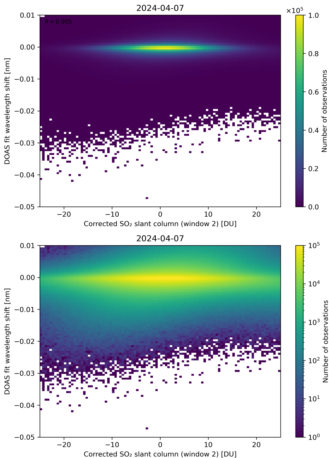
Figure 196: Scatter density plot of “Corrected SO 2 slant column (window 2)” against “DOAS fit wavelength shift” for 2024-04-06 to 2024-04-08.
