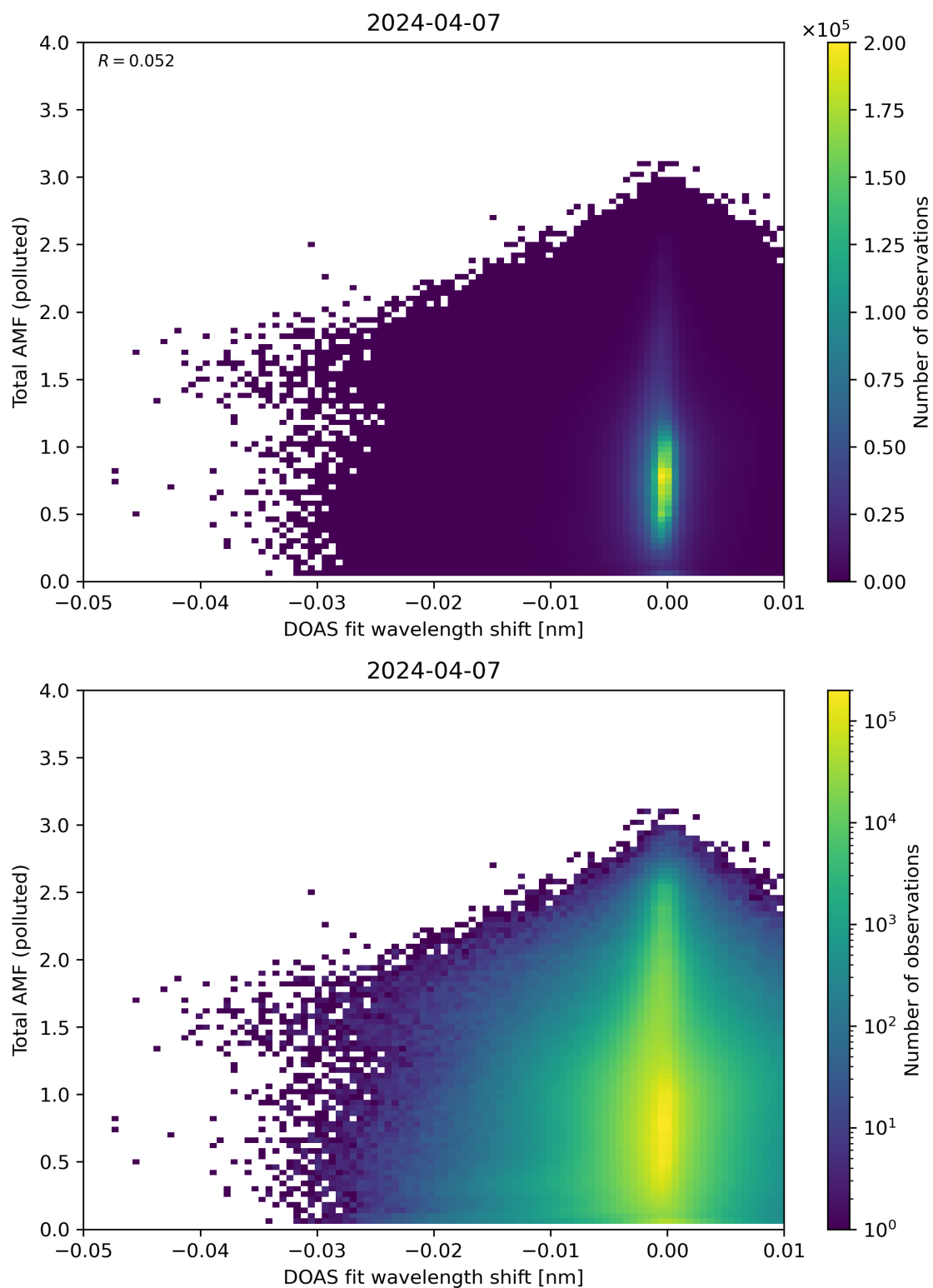
Figure 130: Scatter density plot of “DOAS fit wavelength shift” against “Total AMF (polluted)” for 2024-04-06 to 2024-04-08.
