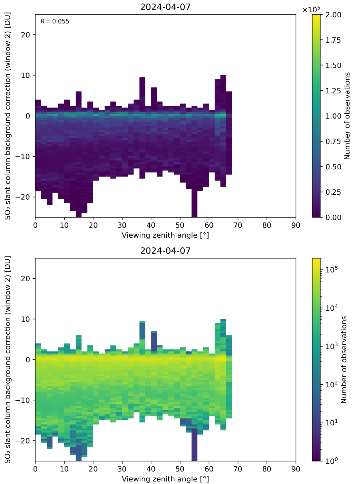
Figure 309: Scatter density plot of “Viewing zenith angle” against “SO 2 slant column background correction (window 2)” for 2024-04-06 to 2024-04-08.
