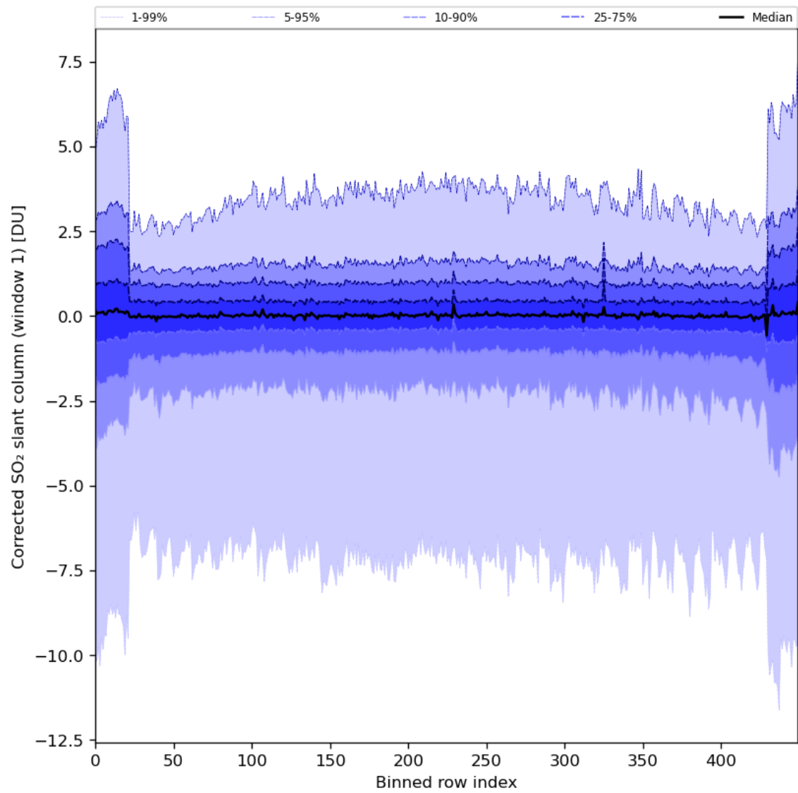
Figure 81: Along track statistics of “Corrected SO 2 slant column (window 1)” for 2024-04-06 to 2024-04-08
