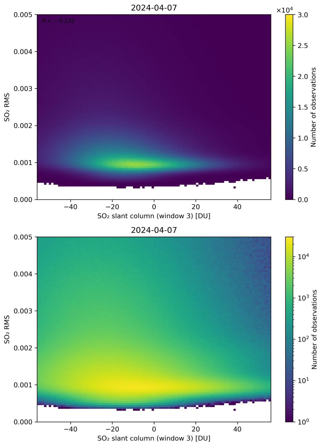
Figure 256: Scatter density plot of “SO 2 slant column (window 3)” against “SO 2 RMS” for 2024-04-06 to 2024-04-08.
