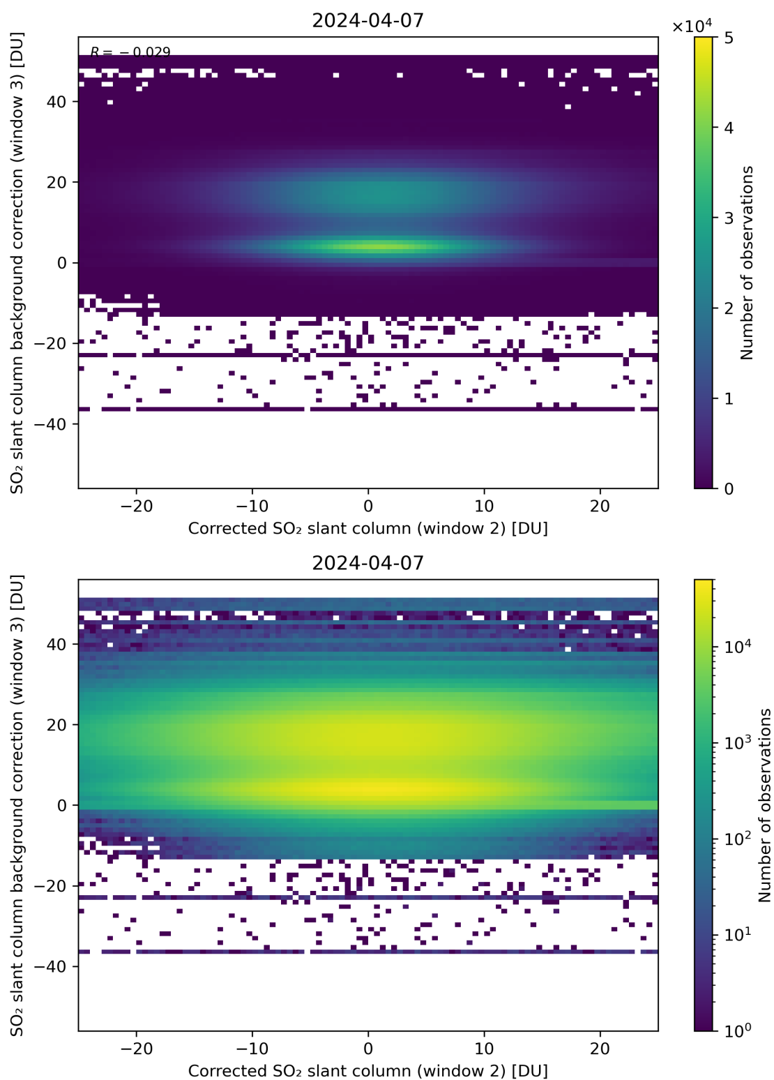
Figure 195: Scatter density plot of “Corrected SO 2 slant column (window 2)” against “SO 2 slant column background correction (window 3)” for 2024-04-06 to 2024-04-08.
