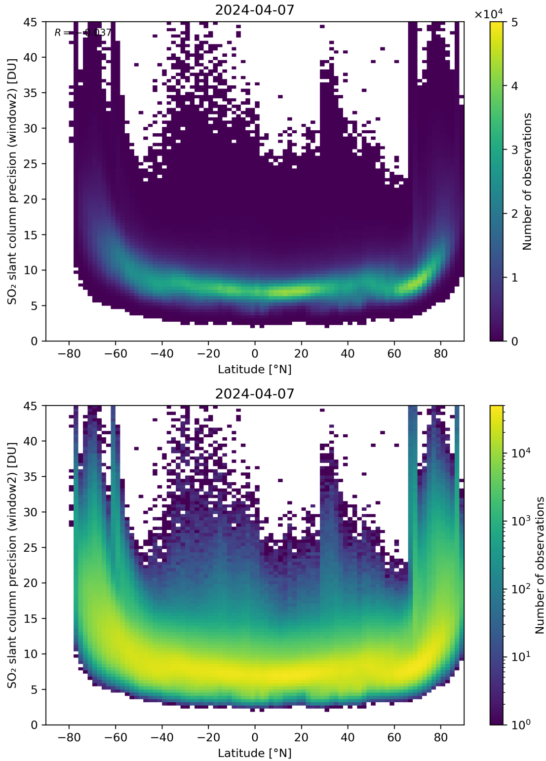
Figure 151: Scatter density plot of “Latitude” against “SO 2 slant column precision (window2)” for 2024-04-06 to 2024-04-08.
