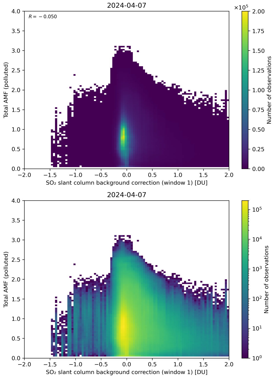
Figure 109: Scatter density plot of “SO 2 slant column background correction (window 1)” against “Total AMF (polluted)” for 2024-04-06 to 2024-04-08.
