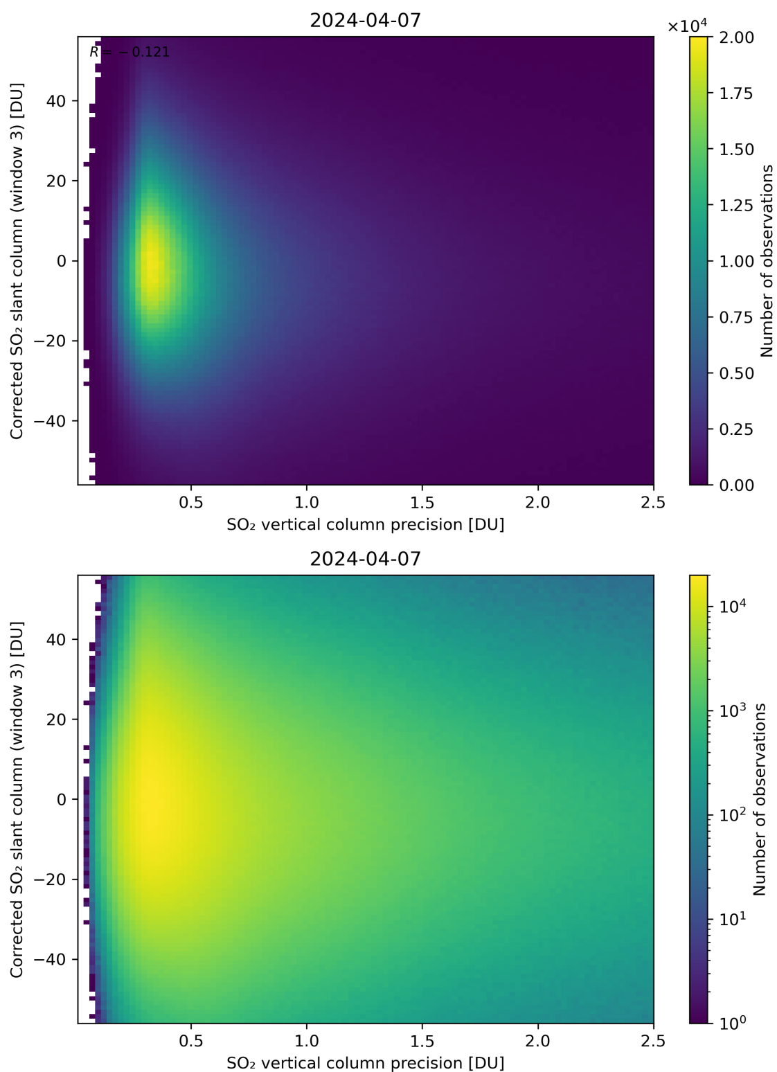
Figure 288: Scatter density plot of “SO 2 vertical column precision” against “Corrected SO 2 slant column (window 3)” for 2024-04-06 to 2024-04-08.
