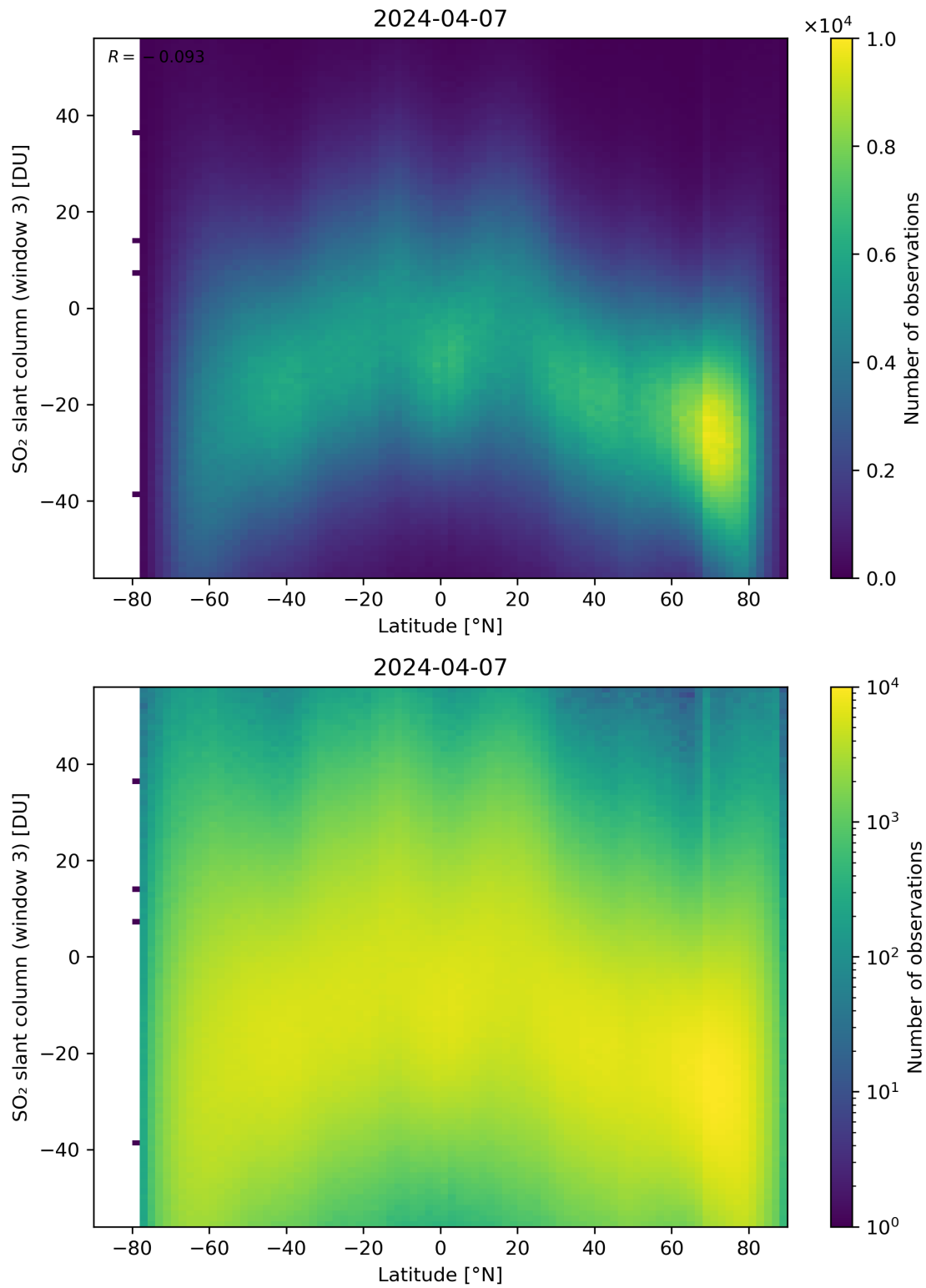
Figure 152: Scatter density plot of “Latitude” against “SO 2 slant column (window 3)” for 2024-04-06 to 2024-04-08.
