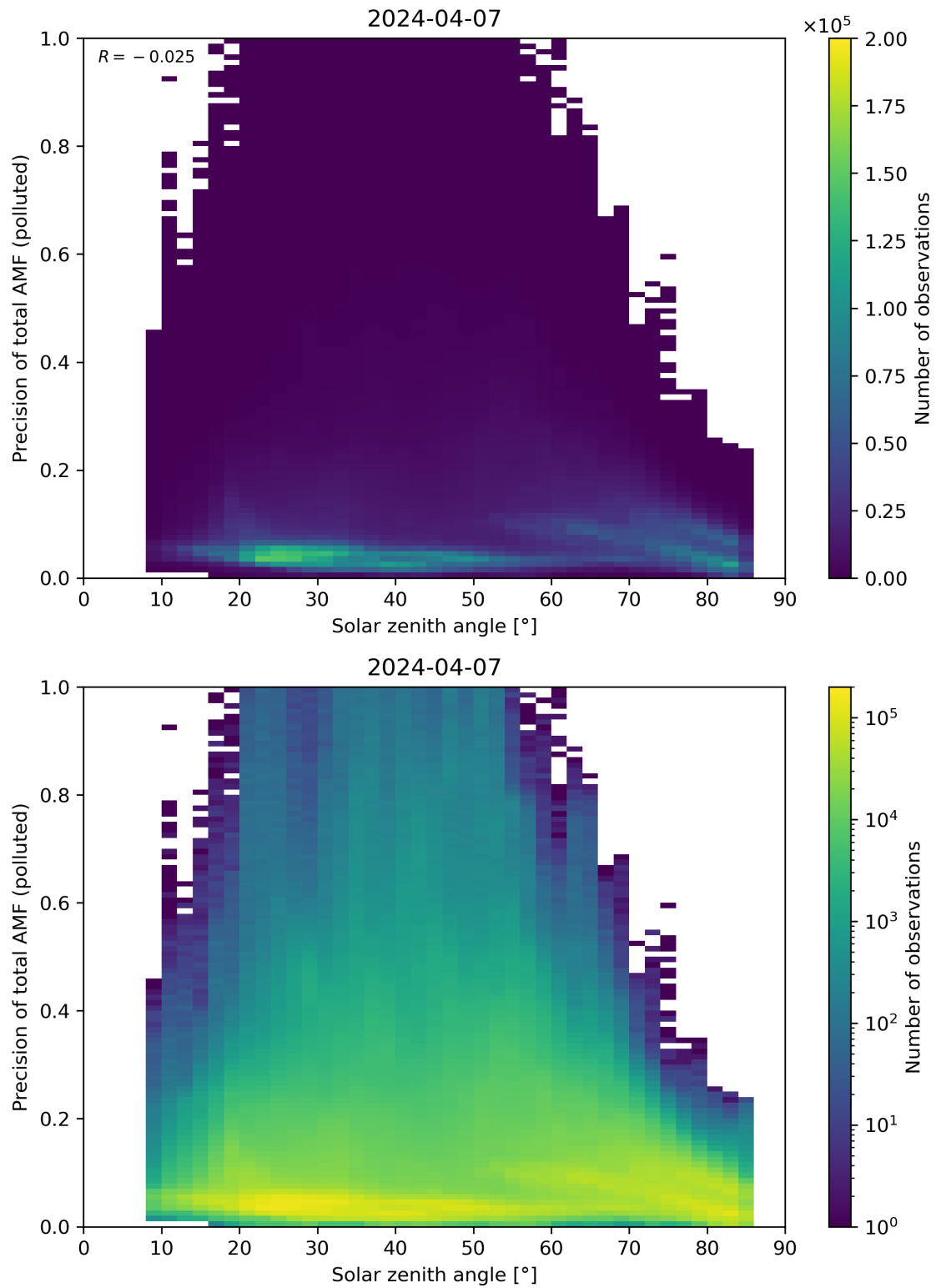
Figure 175: Scatter density plot of “Solar zenith angle” against “Precision of total AMF (polluted)” for 2024-04-06 to 2024-04-08.
