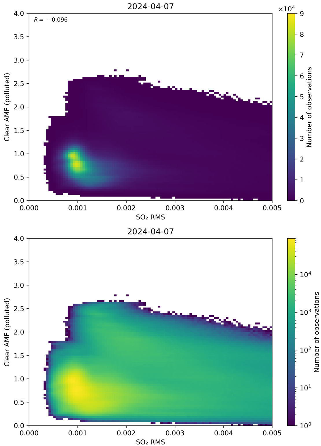
Figure 136: Scatter density plot of “SO 2 RMS” against “Clear AMF (polluted)” for 2024-04-06 to 2024-04-08.
