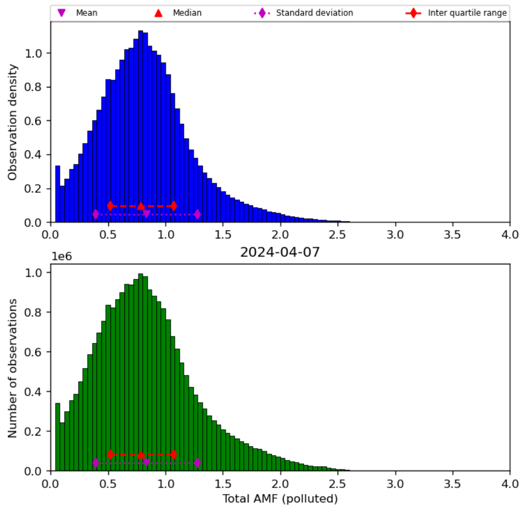
Figure 71: Histogram of “Total AMF (polluted)” for 2024-04-06 to 2024-04-08
