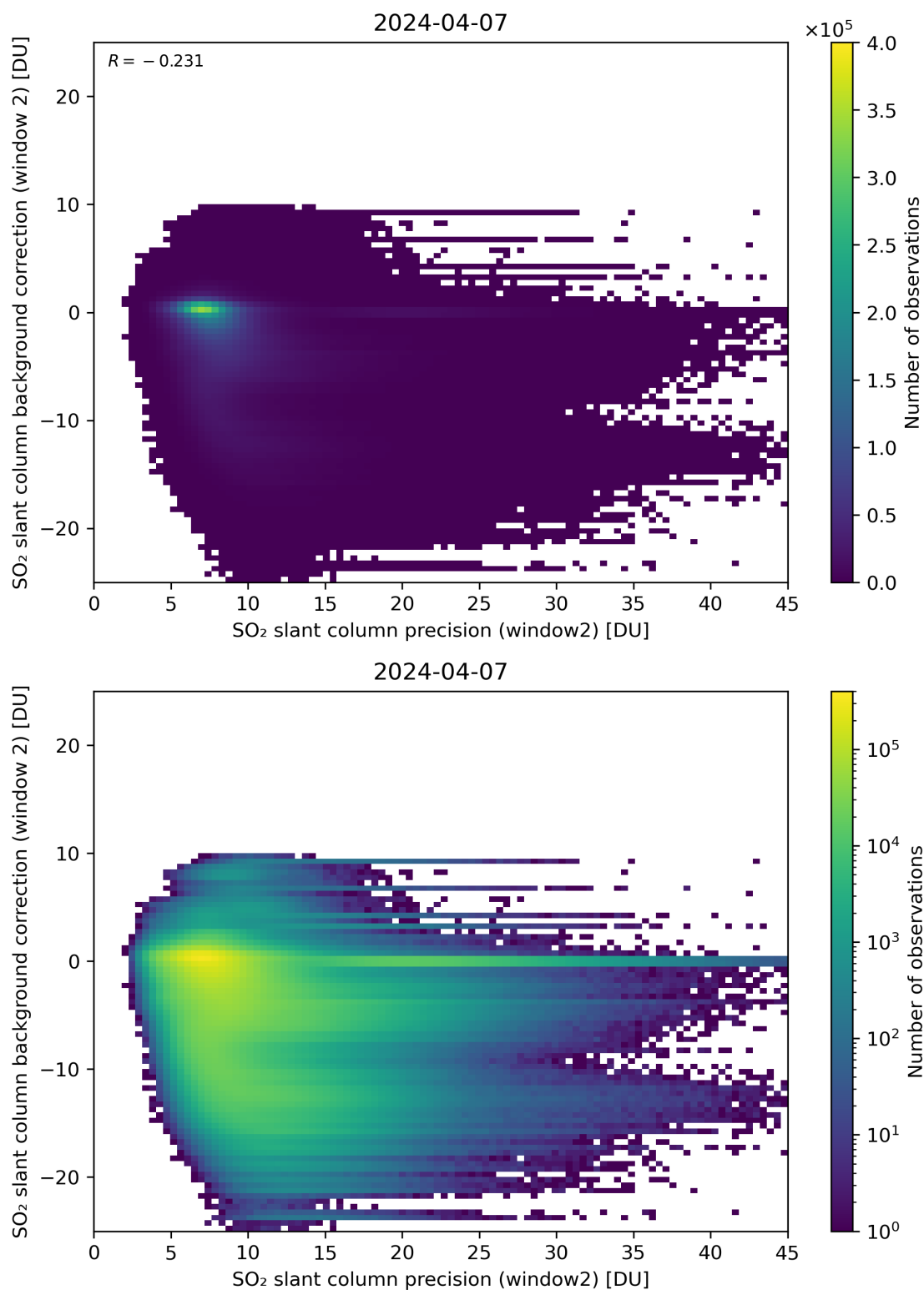
Figure 241: Scatter density plot of “SO 2 slant column precision (window2)” against “SO 2 slant column background correction (window 2)” for 2024-04-06 to 2024-04-08.
