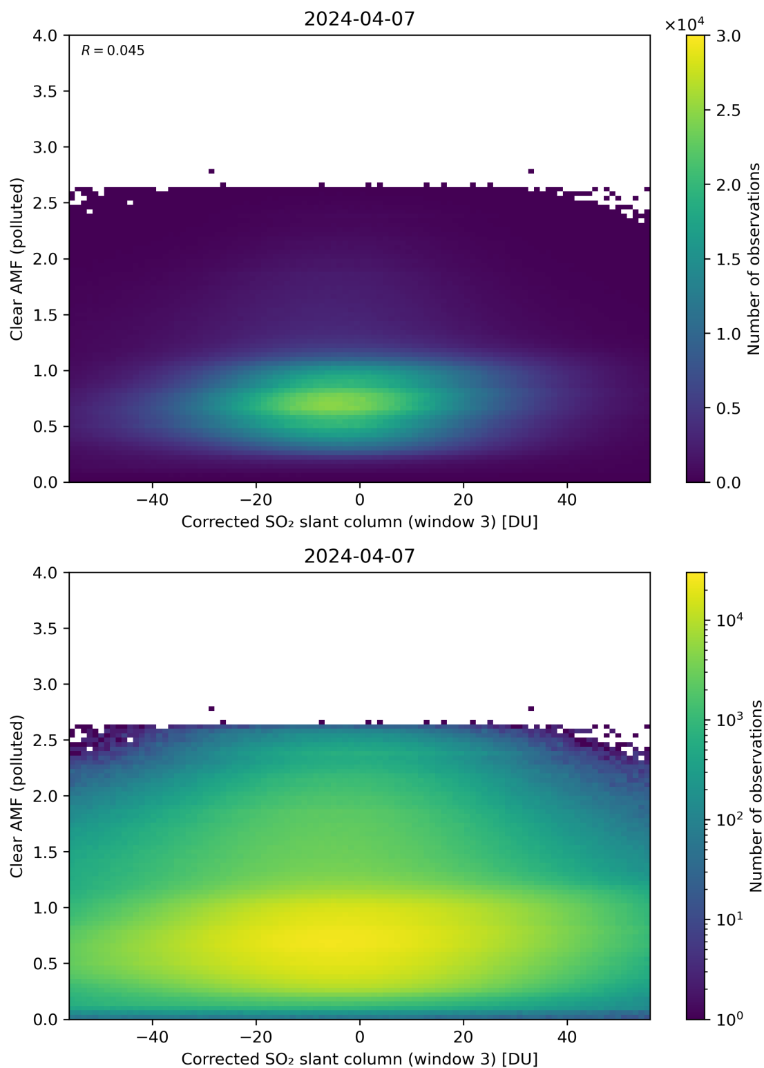
Figure 209: Scatter density plot of “Corrected SO 2 slant column (window 3)” against “Clear AMF (polluted)” for 2024-04-06 to 2024-04-08.
