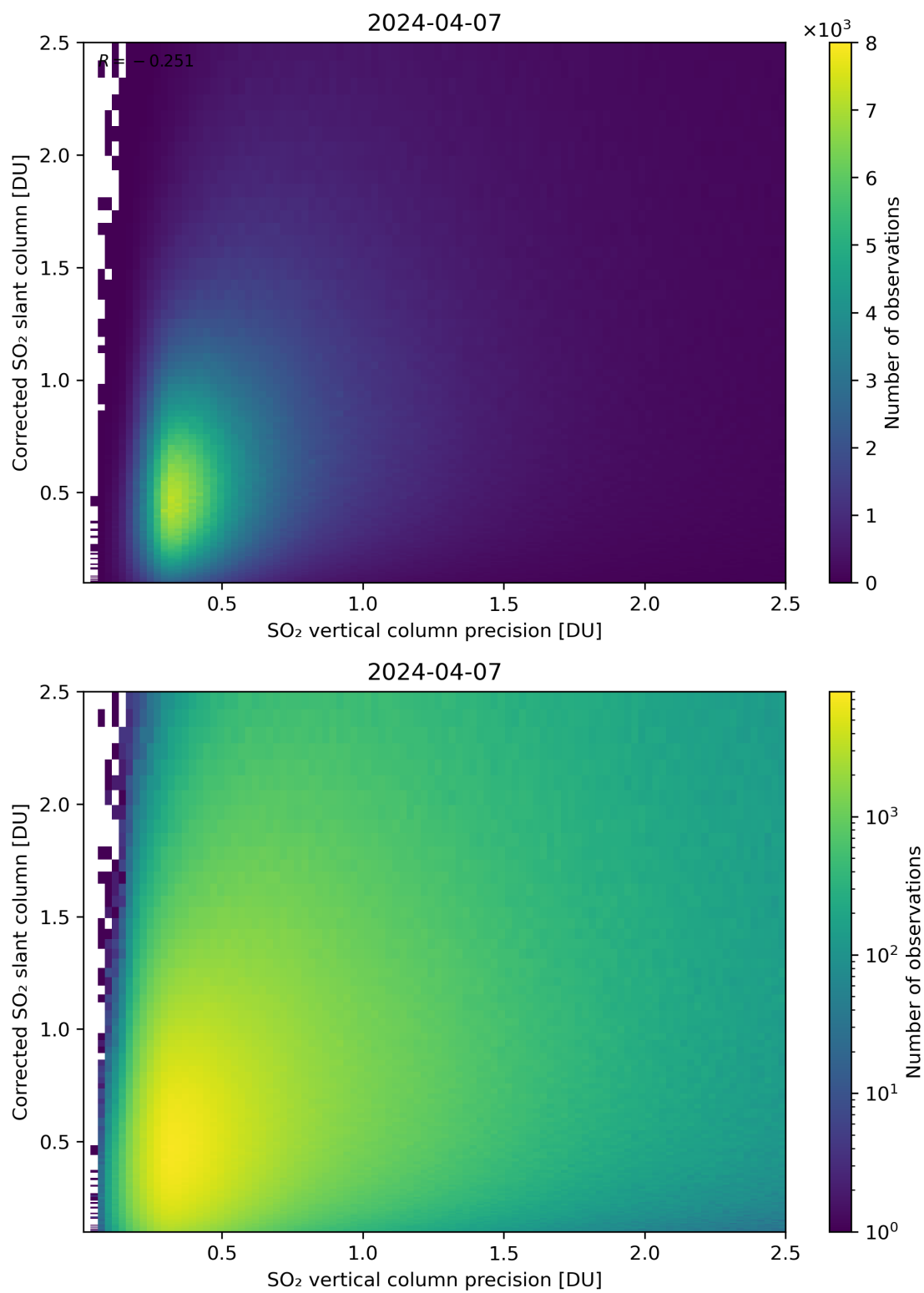
Figure 286: Scatter density plot of “SO 2 vertical column precision” against “Corrected SO 2 slant column” for 2024-04-06 to 2024-04-08.
