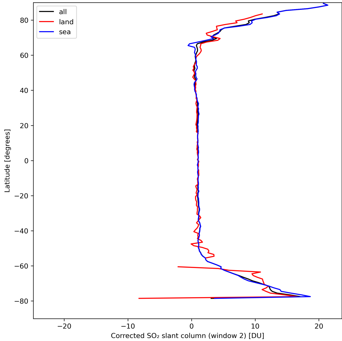
Figure 39: Zonal average of “Corrected SO 2 slant column (window 2)” for 2024-04-06 to 2024-04-08.
