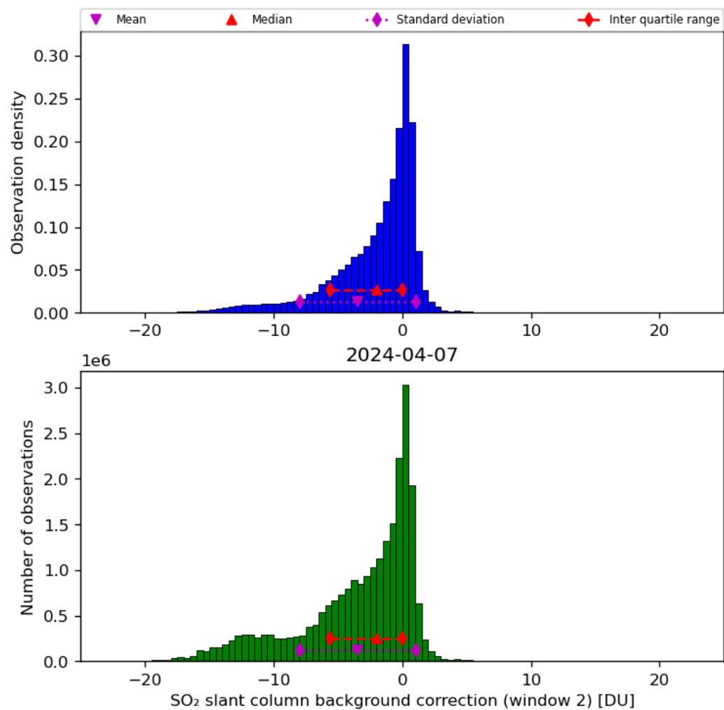
Figure 63: Histogram of “SO 2 slant column background correction (window 2)” for 2024-04-06 to 2024-04-08
