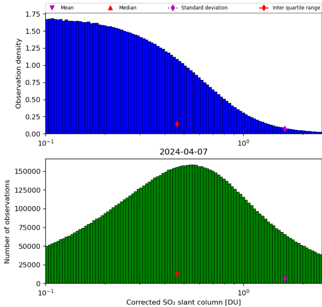
Figure 55: Histogram of “Corrected SO 2 slant column” for 2024-04-06 to 2024-04-08
