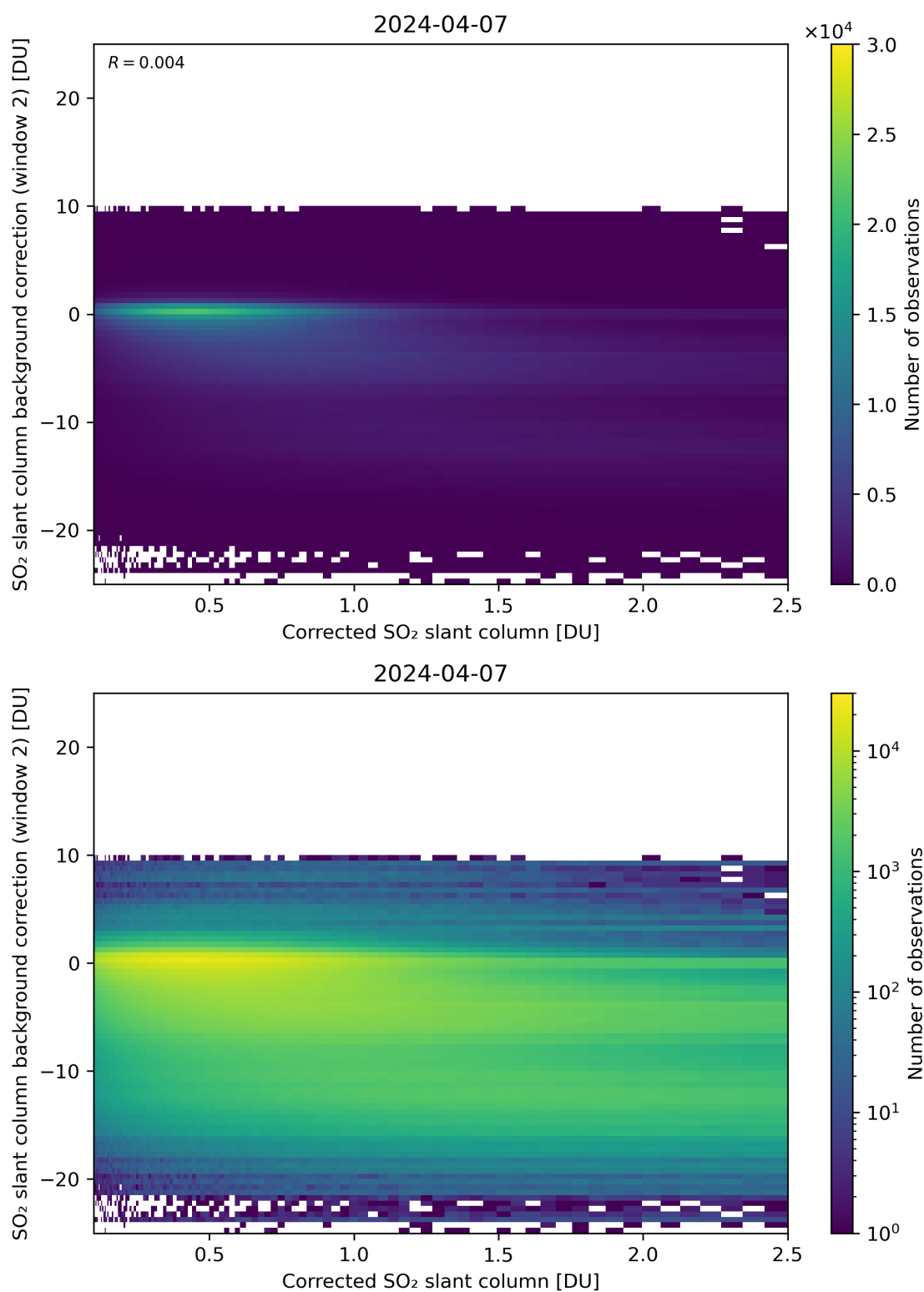
Figure 179: Scatter density plot of “Corrected SO 2 slant column” against “SO 2 slant column background correction (window 2)” for 2024-04-06 to 2024-04-08.
