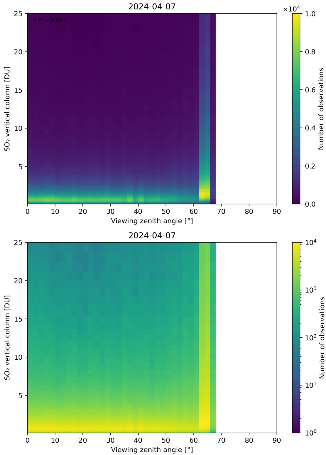
Figure 327: Scatter density plot of “Viewing zenith angle” against “SO 2 vertical column” for 2024-04-06 to 2024-04-08.
