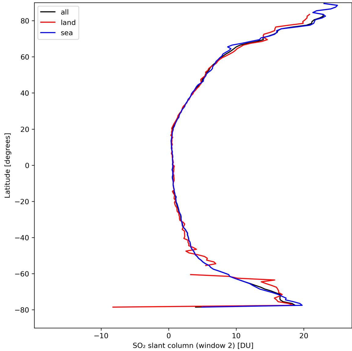
Figure 37: Zonal average of “SO 2 slant column (window 2)” for 2024-04-06 to 2024-04-08.
