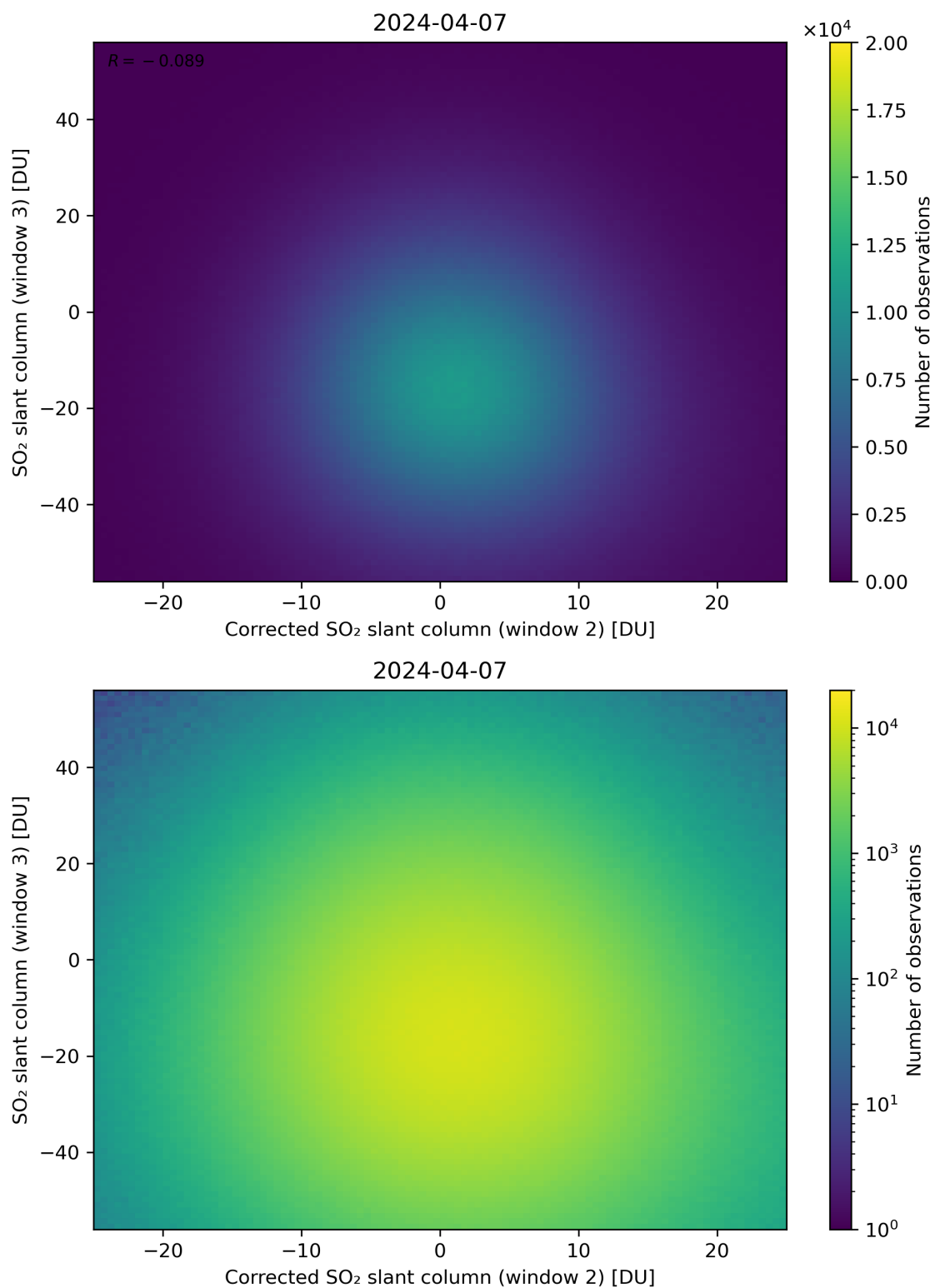
Figure 201: Scatter density plot of “Corrected SO 2 slant column (window 2)” against “SO 2 slant column (window 3)” for 2024-04-06 to 2024-04-08.
