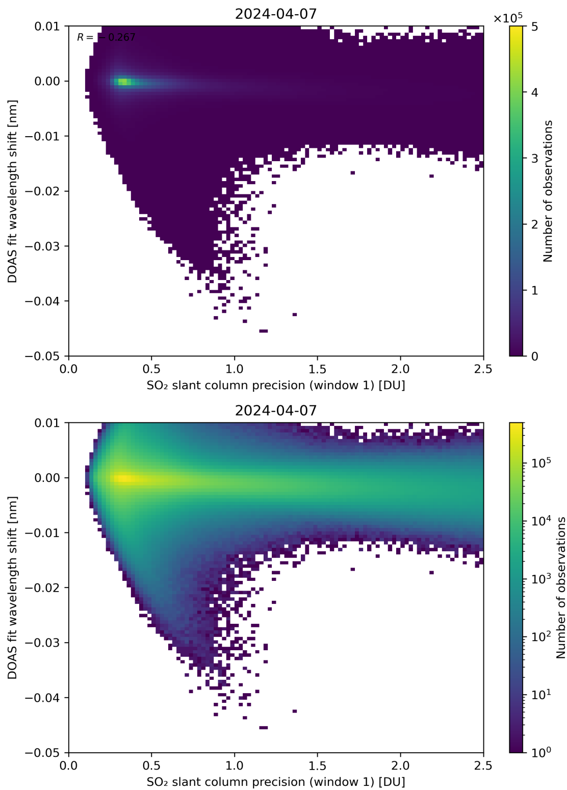
Figure 221: Scatter density plot of “SO 2 slant column precision (window 1)” against “DOAS fit wavelength shift” for 2024-04-06 to 2024-04-08.
