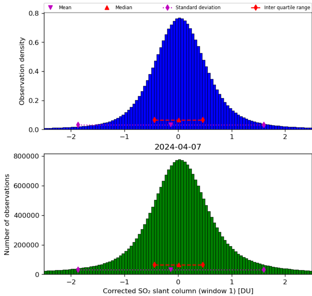
Figure 58: Histogram of “Corrected SO 2 slant column (window 1)” for 2024-04-06 to 2024-04-08
