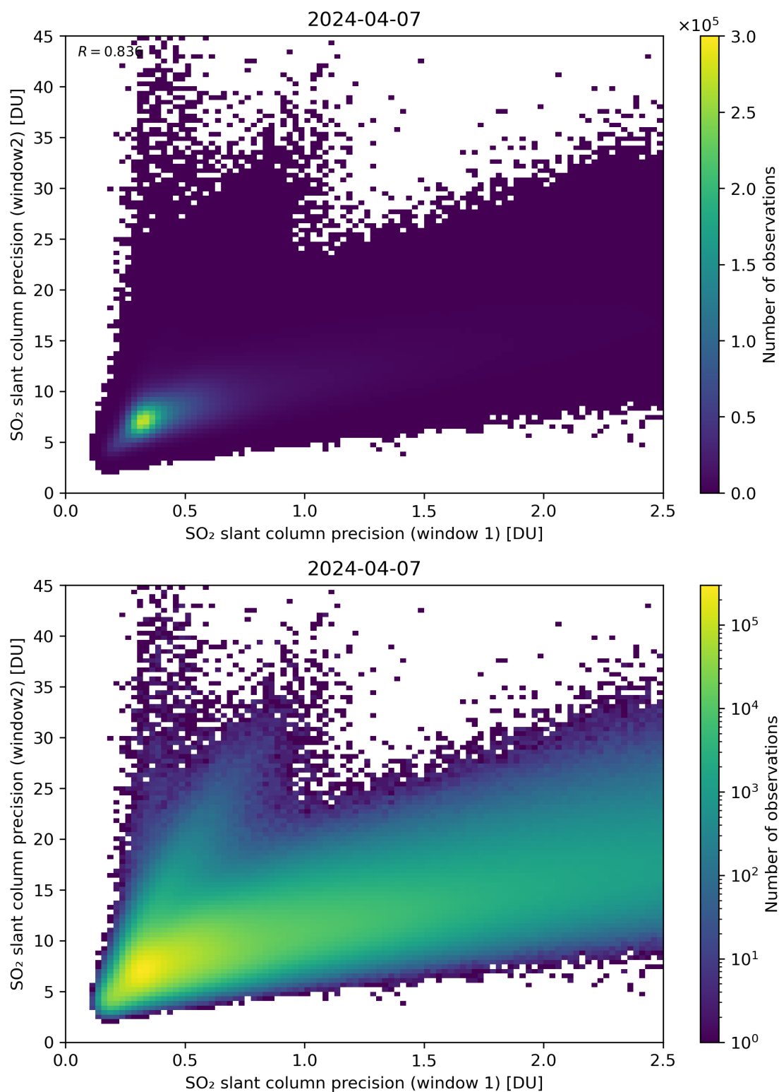
Figure 227: Scatter density plot of “SO 2 slant column precision (window 1)” against “SO 2 slant column precision (window 2)” for 2024-04-06 to 2024-04-08.
