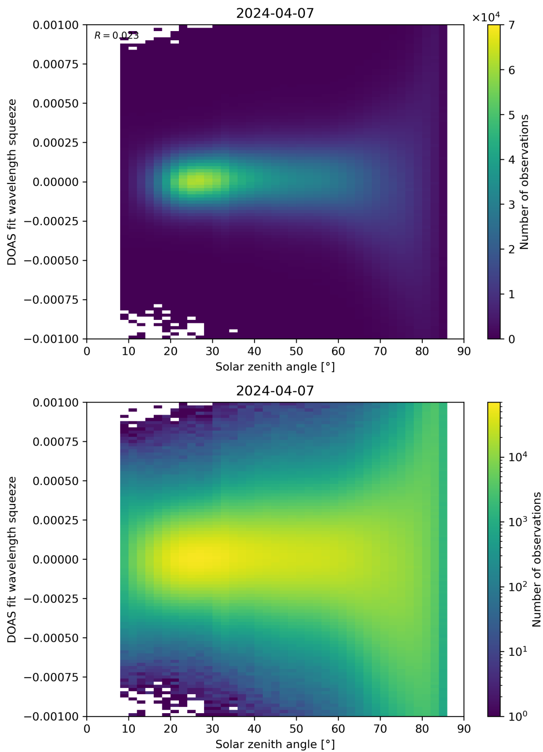
Figure 162: Scatter density plot of “Solar zenith angle” against “DOAS fit wavelength squeeze” for 2024-04-06 to 2024-04-08.
