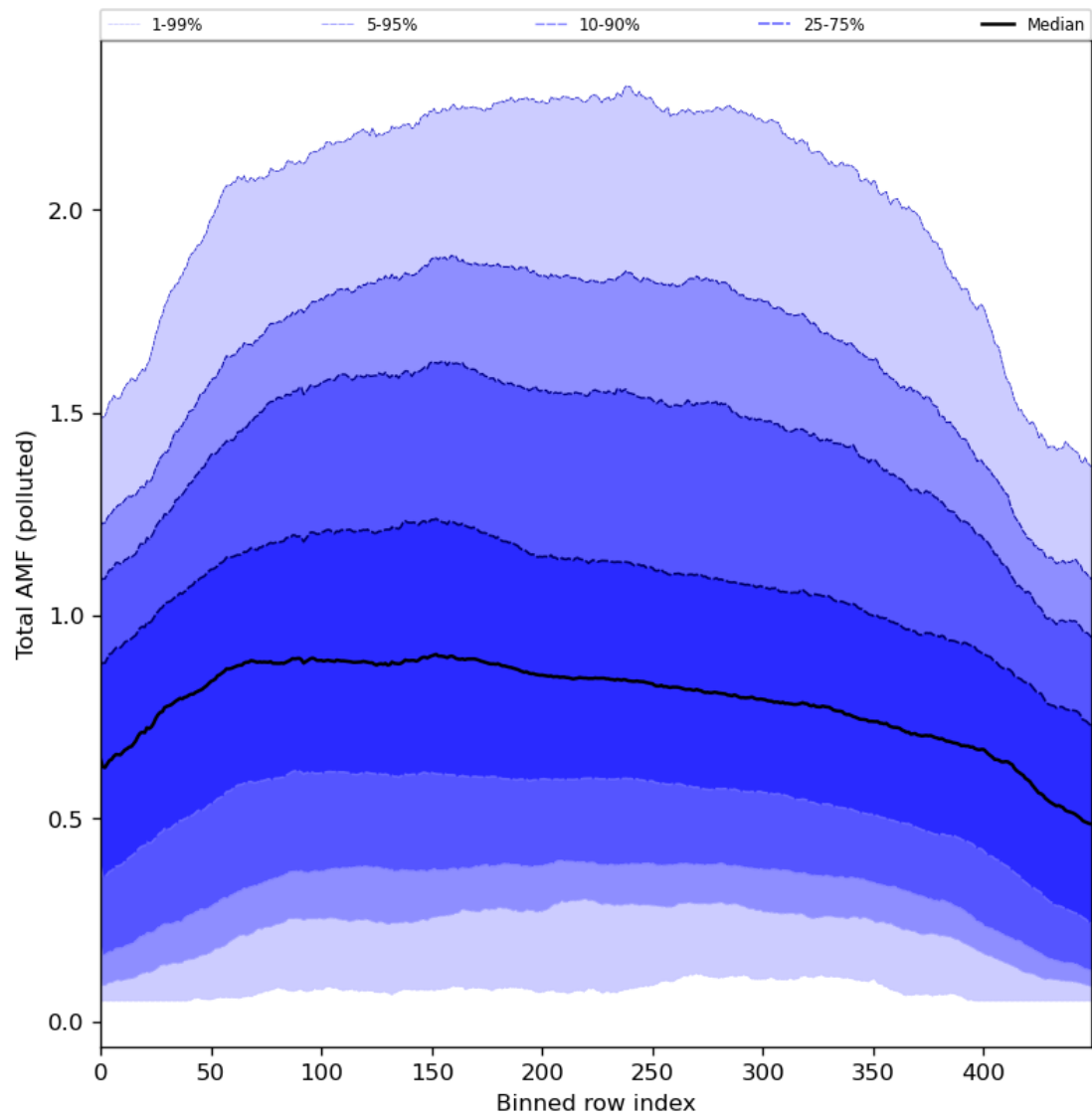
Figure 94: Along track statistics of “Total AMF (polluted)” for 2024-04-06 to 2024-04-08
