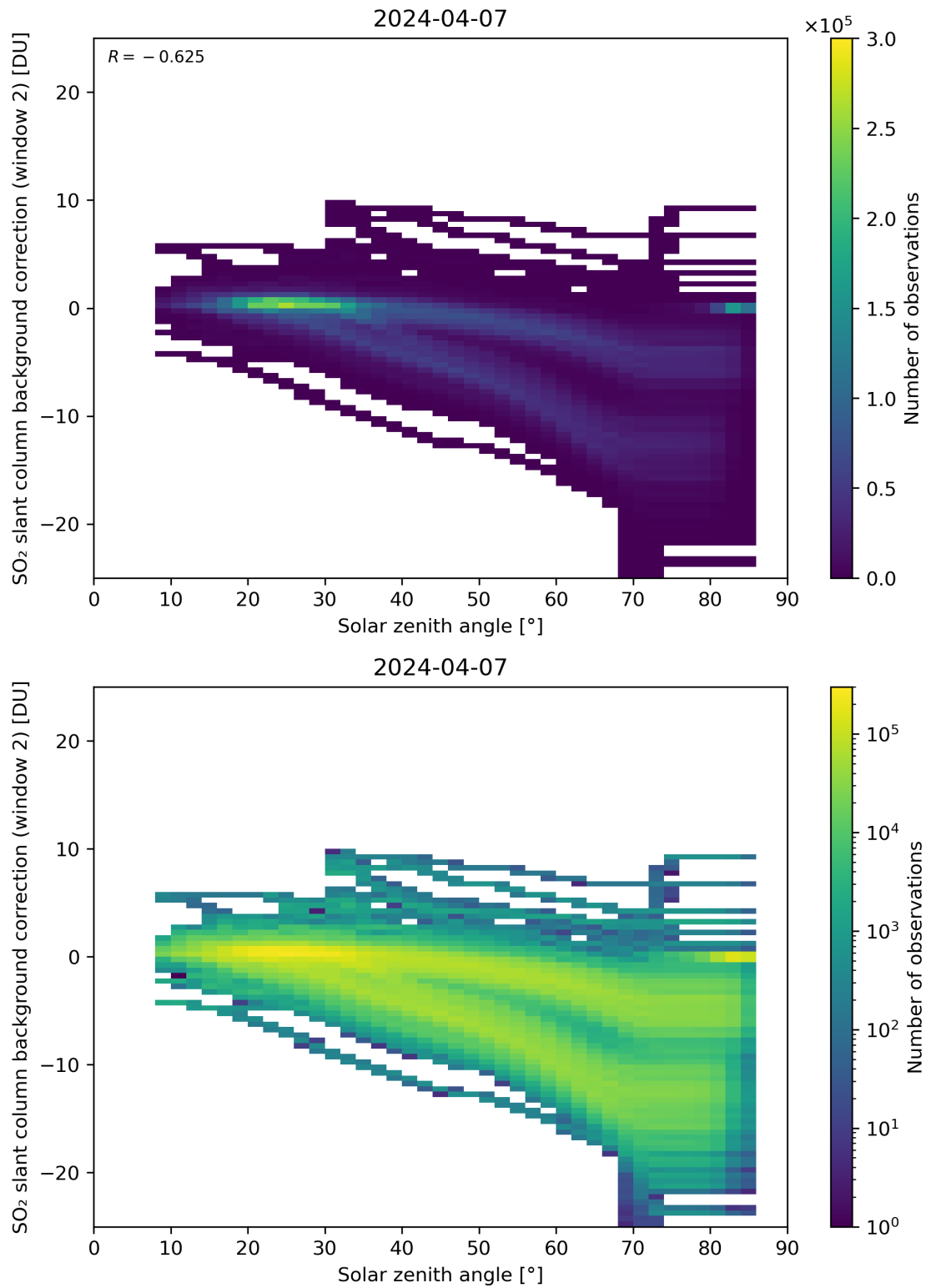
Figure 159: Scatter density plot of “Solar zenith angle” against “SO 2 slant column background correction (window 2)” for 2024-04-06 to 2024-04-08.
