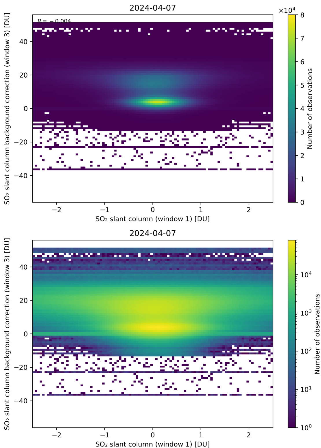
Figure 214: Scatter density plot of “SO 2 slant column (window 1)” against “SO 2 slant column background correction (window 3)” for 2024-04-06 to 2024-04-08.
