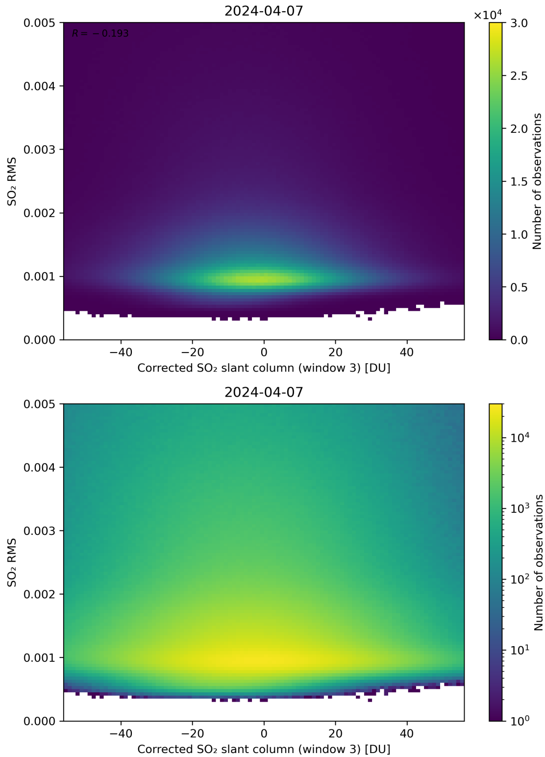
Figure 208: Scatter density plot of “Corrected SO 2 slant column (window 3)” against “SO 2 RMS” for 2024-04-06 to 2024-04-08.
