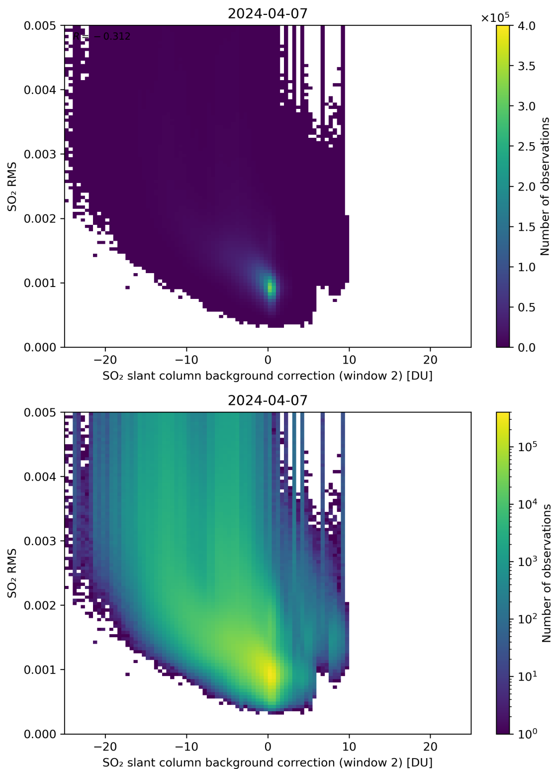
Figure 114: Scatter density plot of “SO 2 slant column background correction (window 2)” against “SO 2 RMS” for 2024-04-06 to 2024-04-08.
