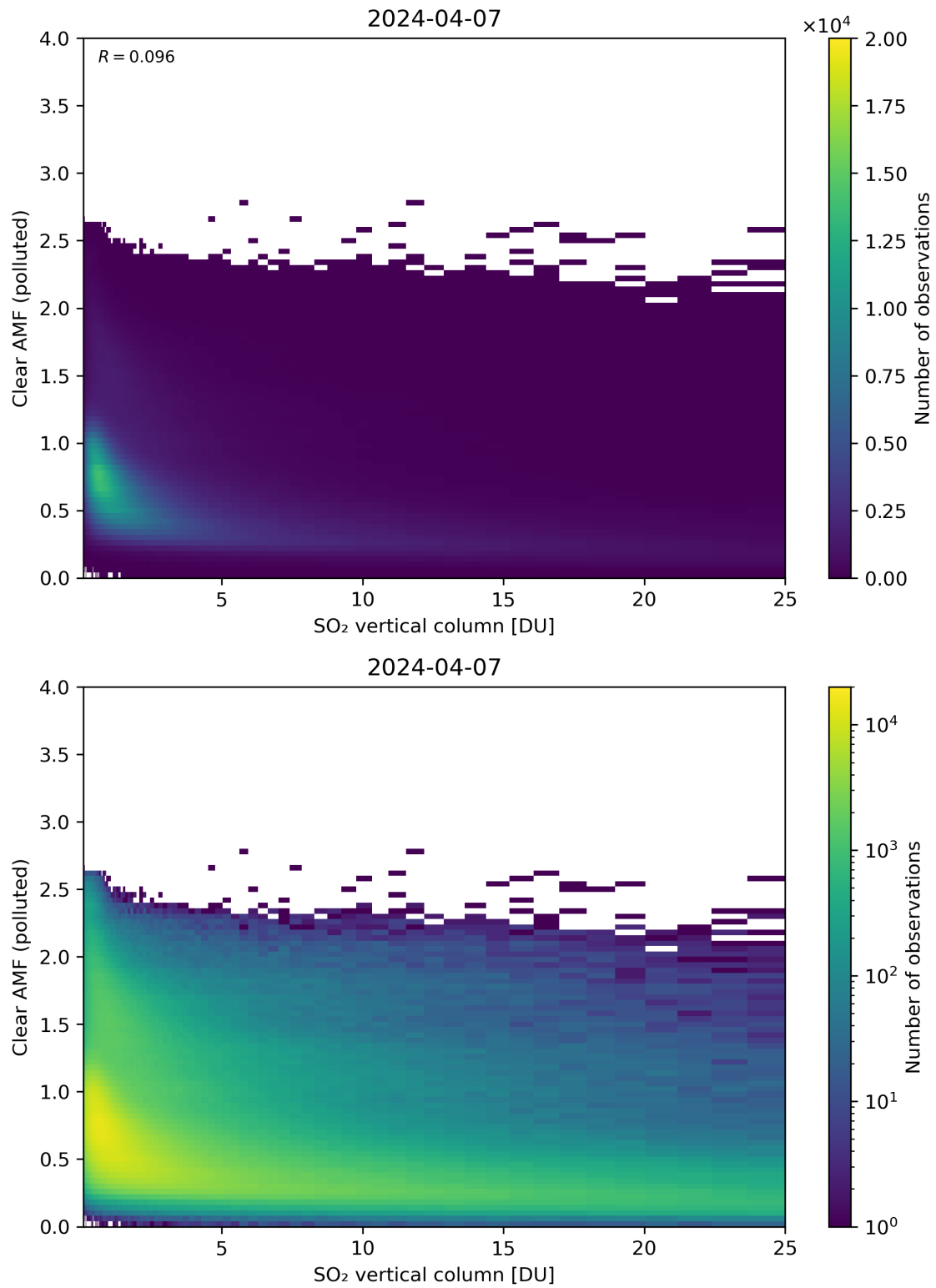
Figure 296: Scatter density plot of “SO 2 vertical column” against “Clear AMF (polluted)” for 2024-04-06 to 2024-04-08.
