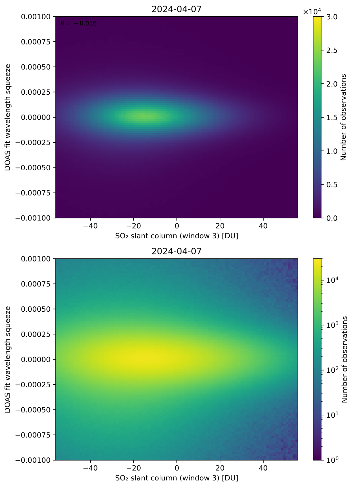
Figure 255: Scatter density plot of “SO 2 slant column (window 3)” against “DOAS fit wavelength squeeze” for 2024-04-06 to 2024-04-08.
