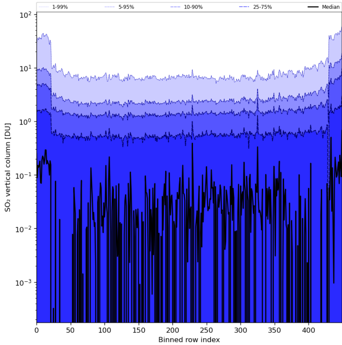
Figure 76: Along track statistics of “SO 2 vertical column” for 2024-04-06 to 2024-04-08
