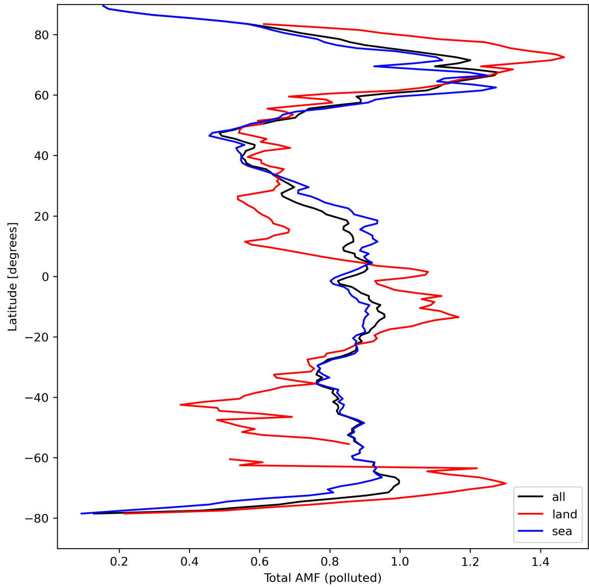
Figure 48: Zonal average of “Total AMF (polluted)” for 2024-04-06 to 2024-04-08.
