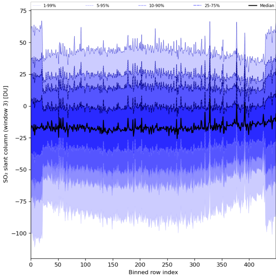
Figure 87: Along track statistics of “SO 2 slant column (window 3)” for 2024-04-06 to 2024-04-08
