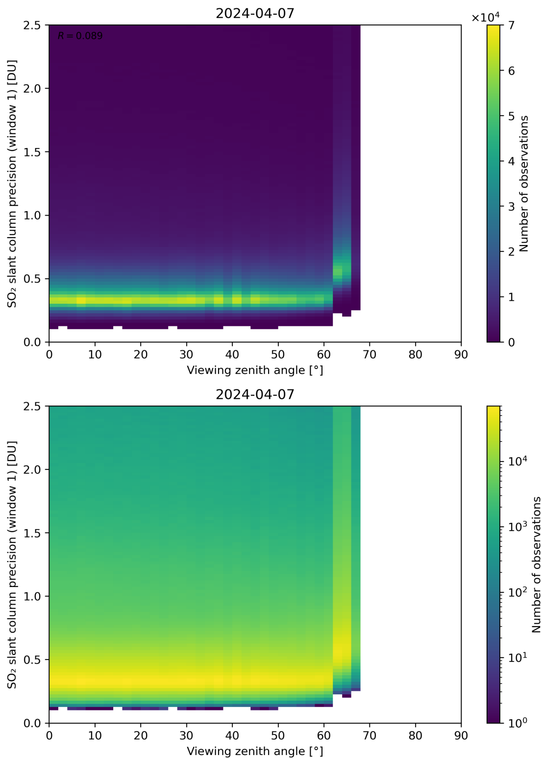
Figure 321: Scatter density plot of “Viewing zenith angle” against “SO 2 slant column precision (window 1)” for 2024-04-06 to 2024-04-08.
