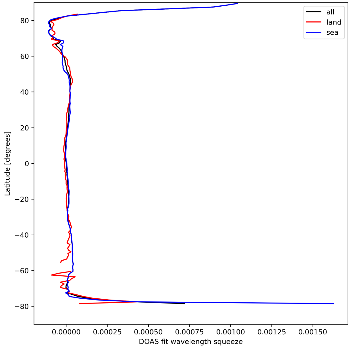
Figure 46: Zonal average of “DOAS fit wavelength squeeze” for 2024-04-06 to 2024-04-08.
