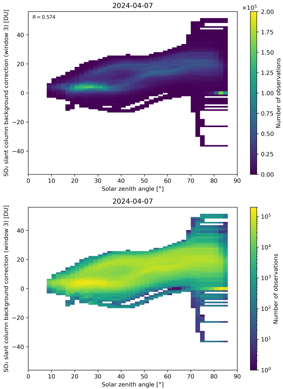
Figure 160: Scatter density plot of “Solar zenith angle” against “SO 2 slant column background correction (window 3)” for 2024-04-06 to 2024-04-08.
