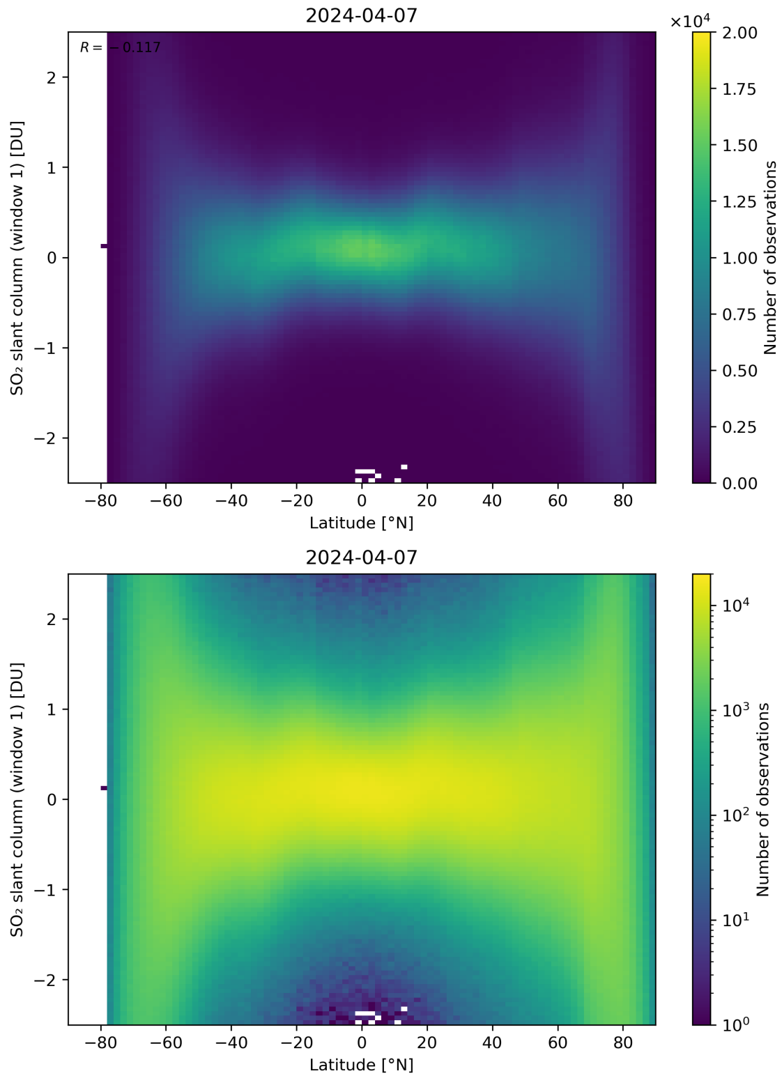
Figure 149: Scatter density plot of “Latitude” against “SO 2 slant column (window 1)” for 2024-04-06 to 2024-04-08.
