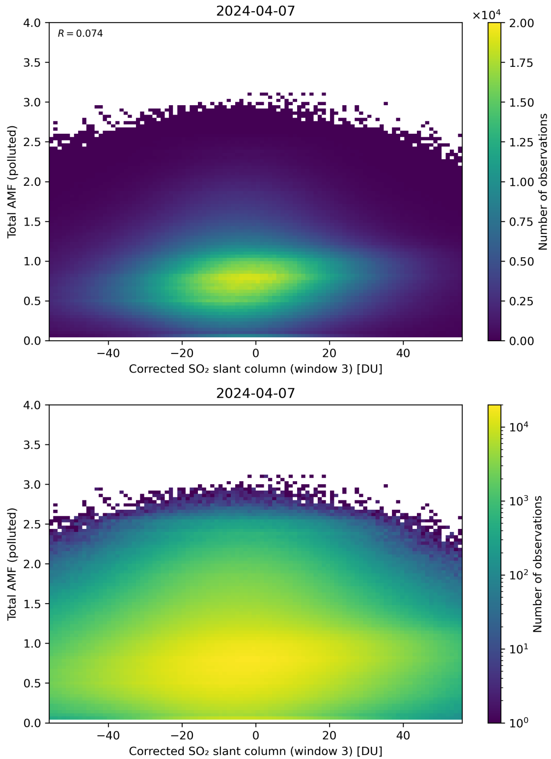
Figure 210: Scatter density plot of “Corrected SO 2 slant column (window 3)” against “Total AMF (polluted)” for 2024-04-06 to 2024-04-08.
