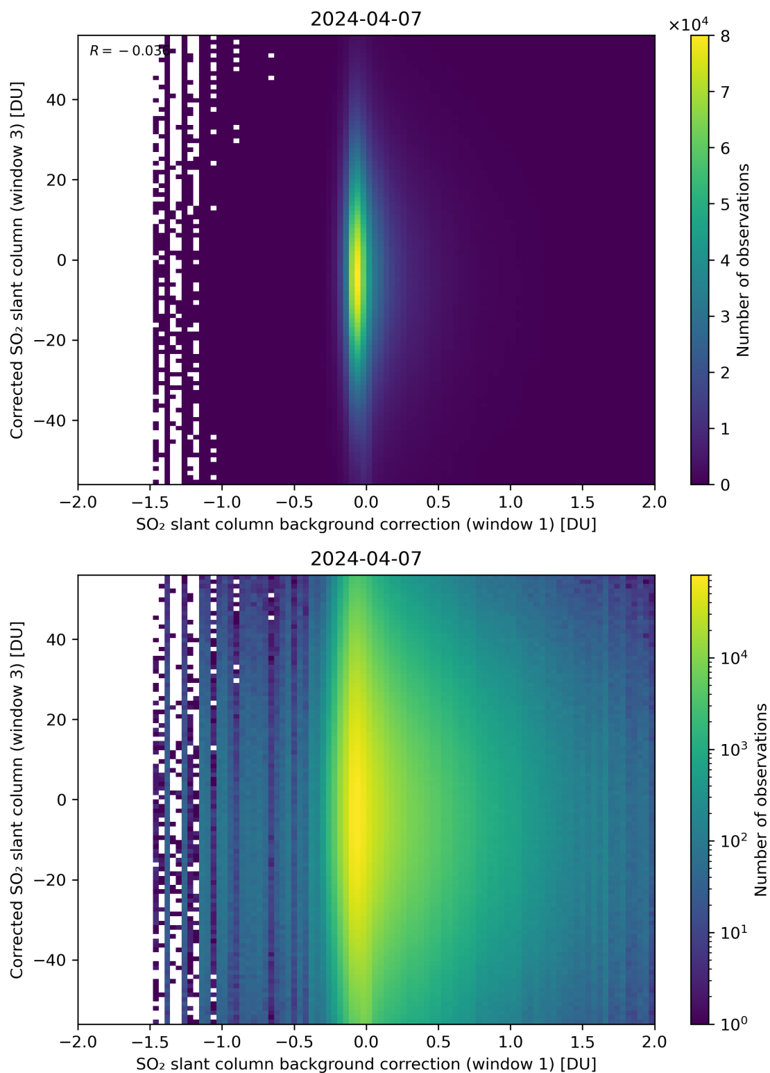
Figure 105: Scatter density plot of “SO 2 slant column background correction (window 1)” against “Corrected SO 2 slant column (window 3)” for 2024-04-06 to 2024-04-08.
