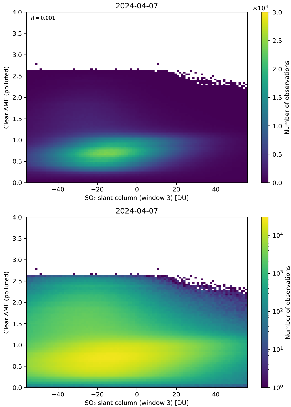
Figure 265: Scatter density plot of “SO 2 slant column (window 3)” against “Clear AMF (polluted)” for 2024-04-06 to 2024-04-08.
