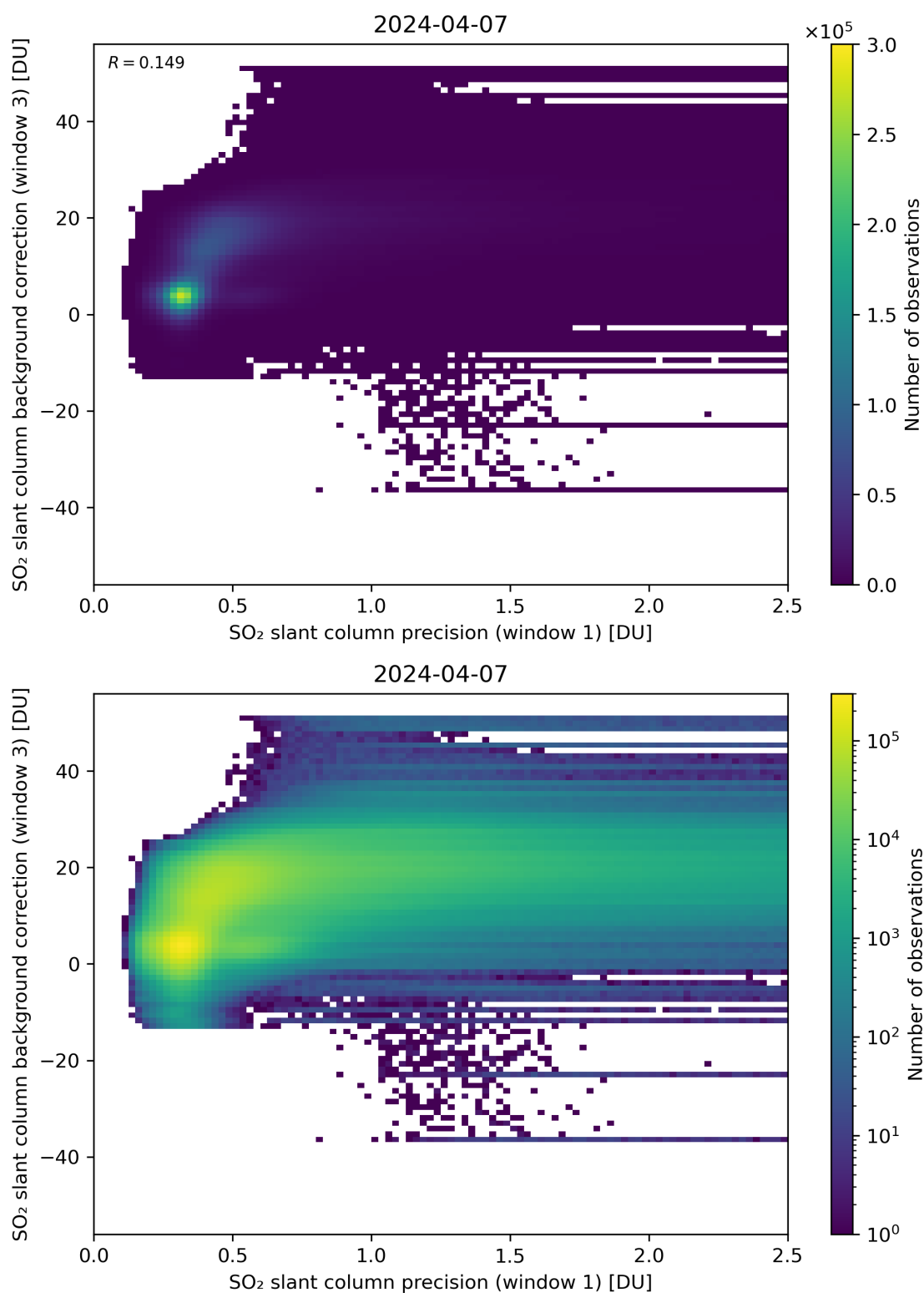
Figure 220: Scatter density plot of “SO 2 slant column precision (window 1)” against “SO 2 slant column background correction (window 3)” for 2024-04-06 to 2024-04-08.
