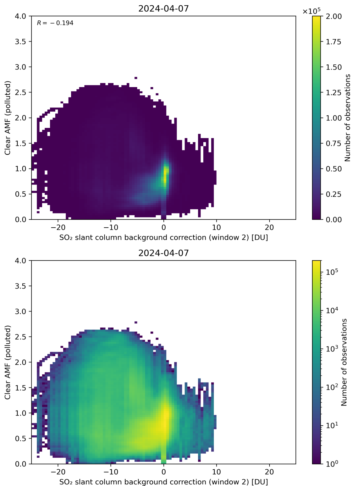
Figure 115: Scatter density plot of “SO 2 slant column background correction (window 2)” against “Clear AMF (polluted)” for 2024-04-06 to 2024-04-08.
