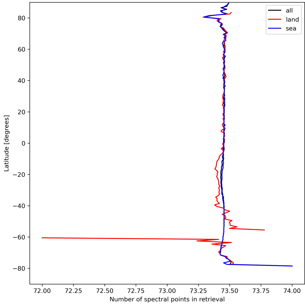
Figure 51: Zonal average of “Number of spectral points in retrieval” for 2024-04-06 to 2024-04-08.
