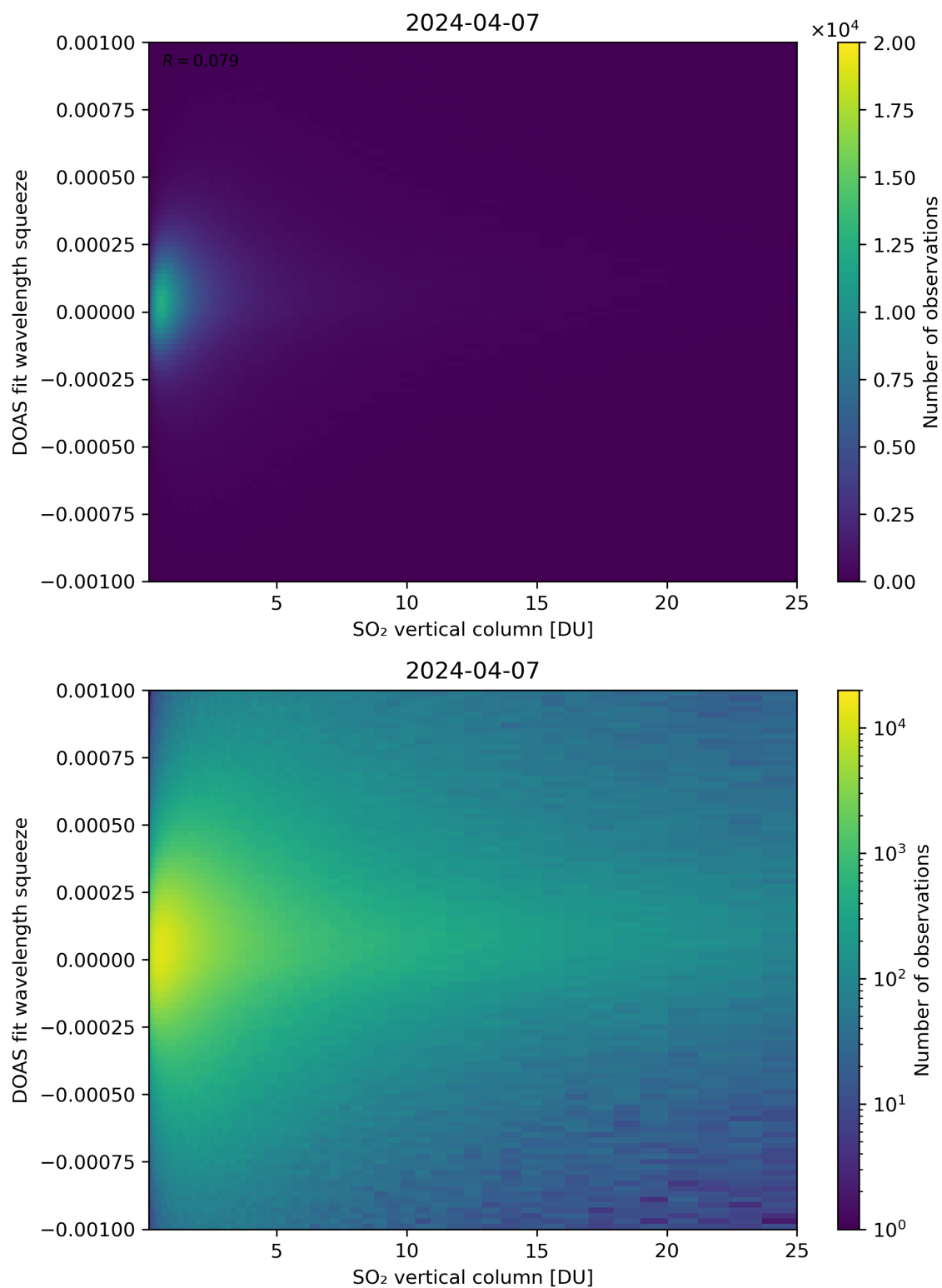
Figure 277: Scatter density plot of “SO 2 vertical column” against “DOAS fit wavelength squeeze” for 2024-04-06 to 2024-04-08.
