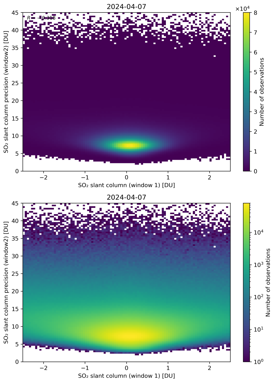
Figure 236: Scatter density plot of “SO 2 slant column (window 1)” against “SO 2 slant column precision (window2)” for 2024-04-06 to 2024-04-08.
