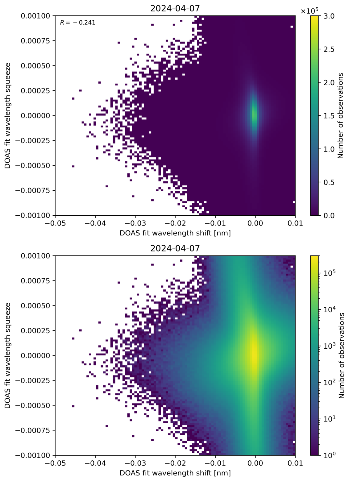
Figure 127: Scatter density plot of “DOAS fit wavelength shift” against “DOAS fit wavelength squeeze” for 2024-04-06 to 2024-04-08.
