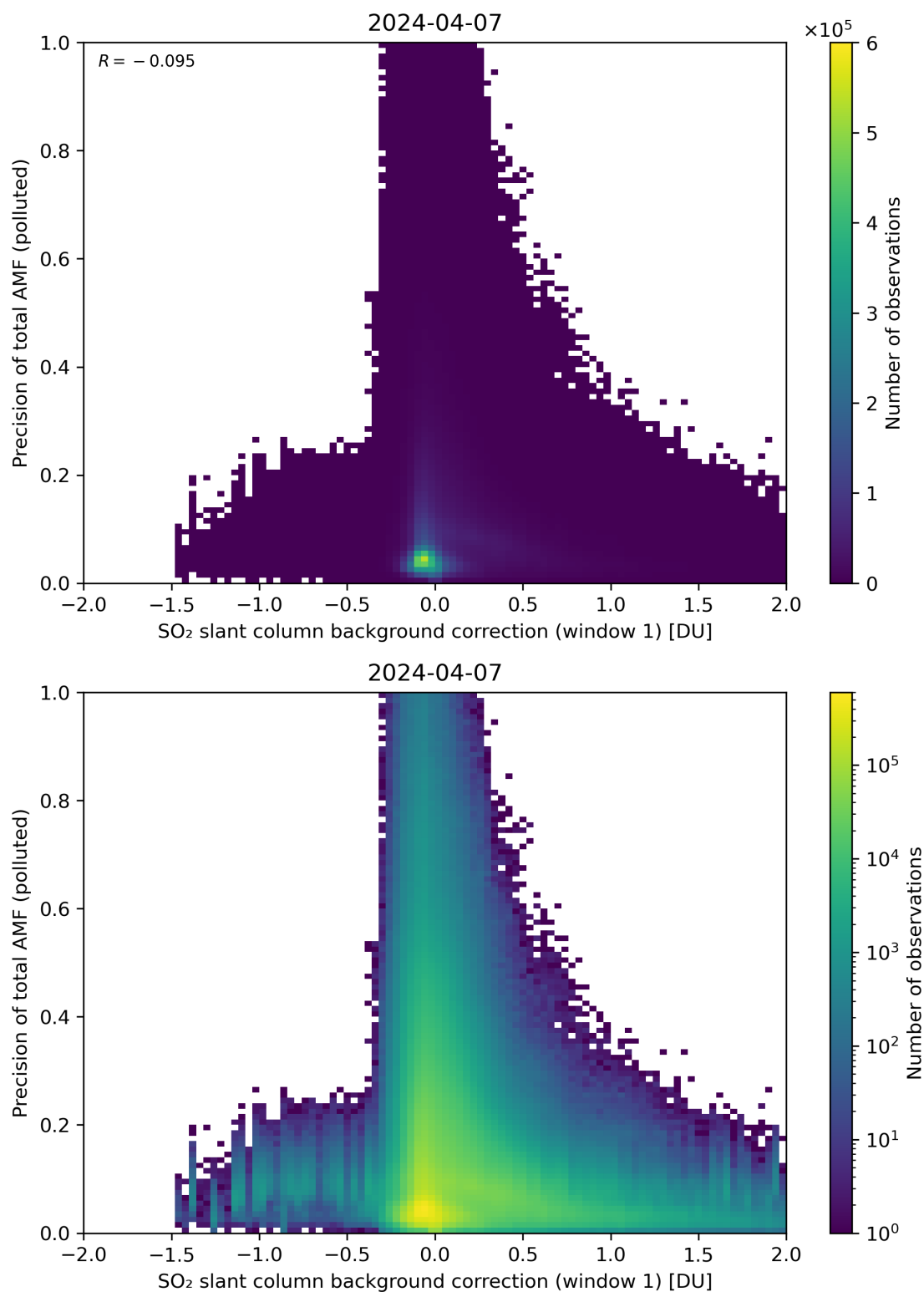
Figure 110: Scatter density plot of “SO 2 slant column background correction (window 1)” against “Precision of total AMF (polluted)” for 2024-04-06 to 2024-04-08.
