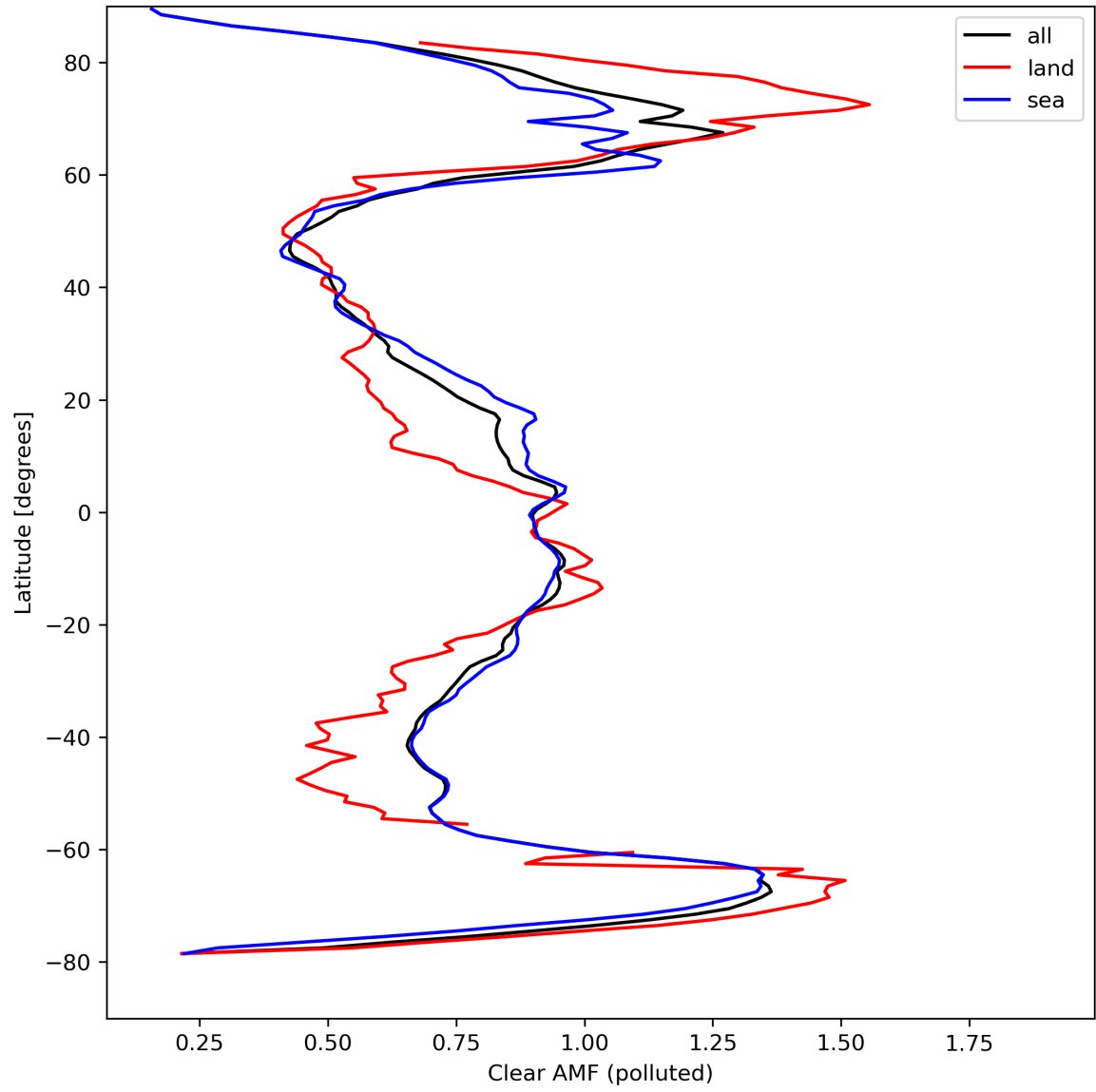
Figure 50: Zonal average of “Clear AMF (polluted)” for 2024-04-06 to 2024-04-08.
