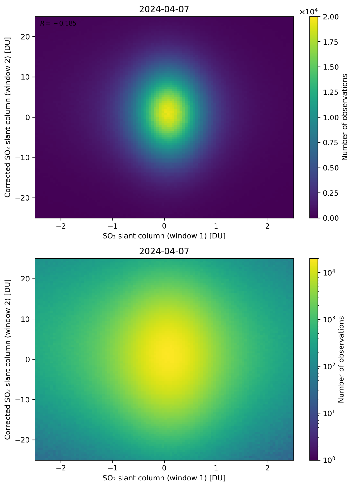
Figure 233: Scatter density plot of “SO 2 slant column (window 1)” against “Corrected SO 2 slant column (window 2)” for 2024-04-06 to 2024-04-08.
