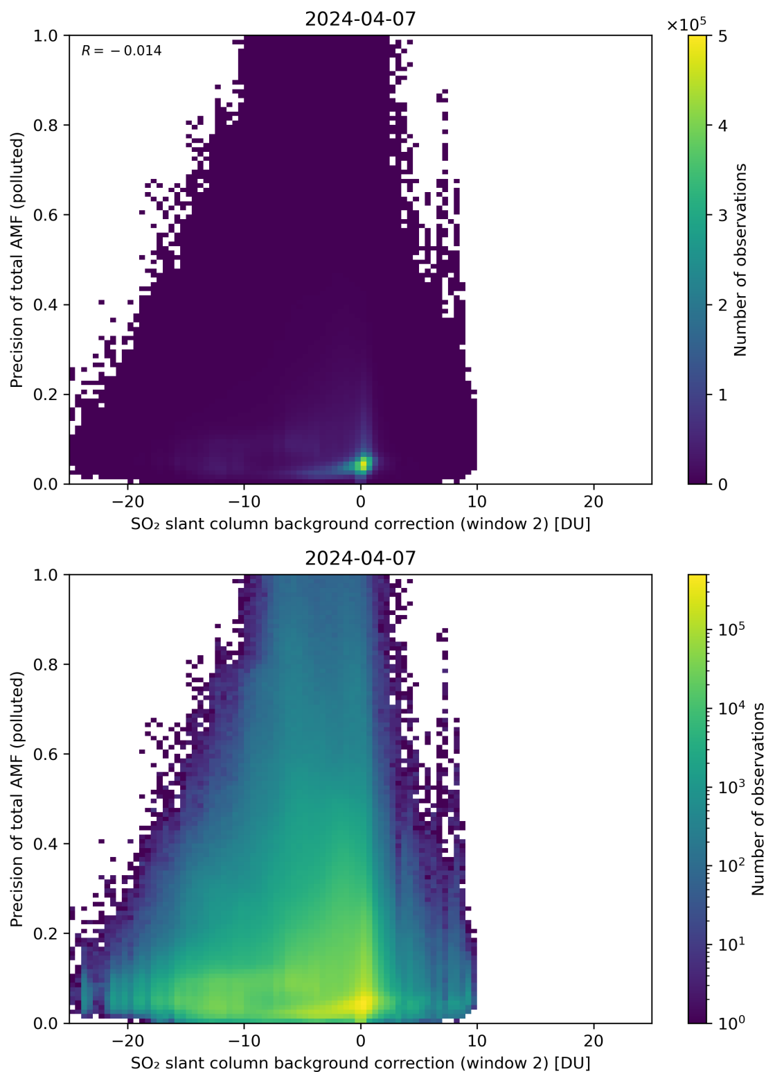
Figure 120: Scatter density plot of “SO 2 slant column background correction (window 2)” against “Precision of total AMF (polluted)” for 2024-04-06 to 2024-04-08.
