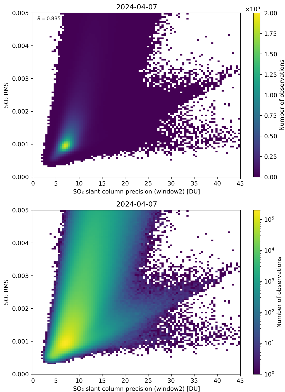
Figure 245: Scatter density plot of “SO 2 slant column precision (window2)” against “SO 2 RMS” for 2024-04-06 to 2024-04-08.
