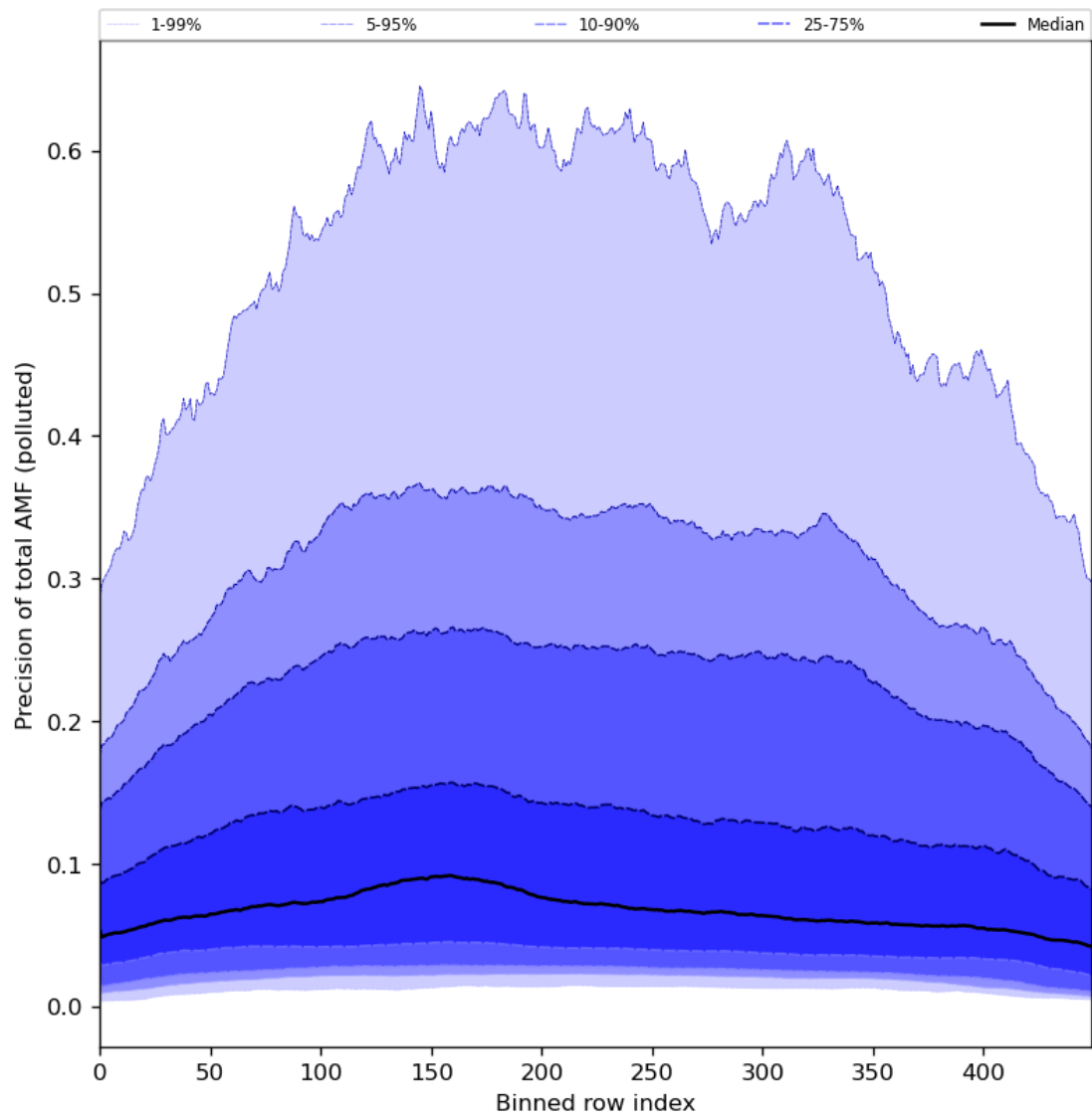
Figure 95: Along track statistics of “Precision of total AMF (polluted)” for 2024-04-06 to 2024-04-08
