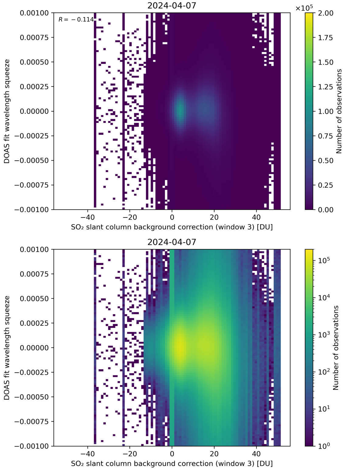
Figure 122: Scatter density plot of “SO 2 slant column background correction (window 3)” against “DOAS fit wavelength squeeze” for 2024-04-06 to 2024-04-08.
