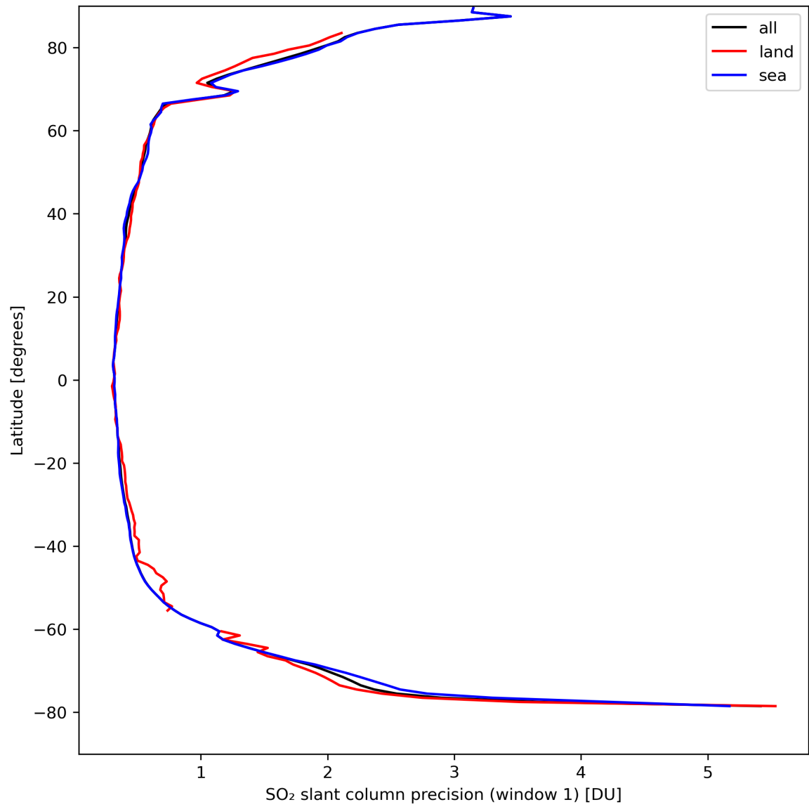
Figure 34: Zonal average of “SO 2 slant column precision (window 1)” for 2024-04-06 to 2024-04-08.
