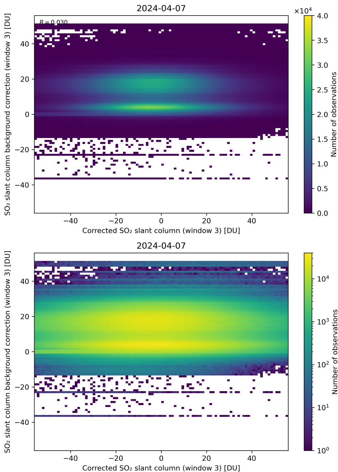
Figure 205: Scatter density plot of “Corrected SO 2 slant column (window 3)” against “SO 2 slant column background correction (window 3)” for 2024-04-06 to 2024-04-08.
