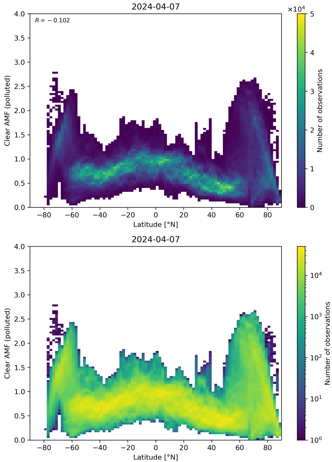
Figure 145: Scatter density plot of “Latitude” against “Clear AMF (polluted)” for 2024-04-06 to 2024-04-08.
