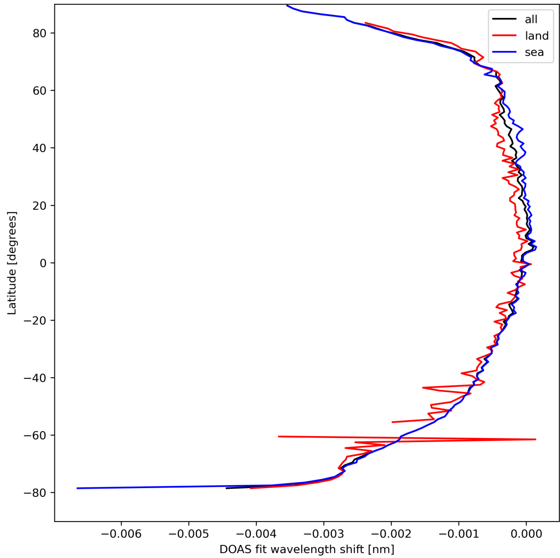
Figure 45: Zonal average of “DOAS fit wavelength shift” for 2024-04-06 to 2024-04-08.
