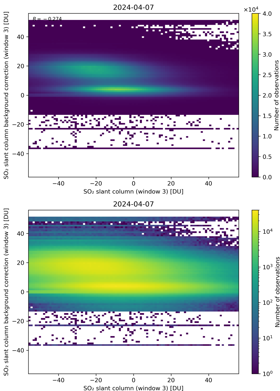
Figure 253: Scatter density plot of “SO 2 slant column (window 3)” against “SO 2 slant column background correction (window 3)” for 2024-04-06 to 2024-04-08.
