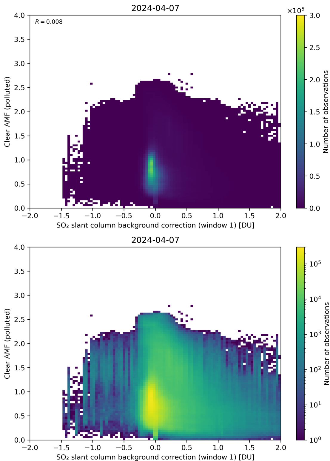
Figure 103: Scatter density plot of “SO 2 slant column background correction (window 1)” against “Clear AMF (polluted)” for 2024-04-06 to 2024-04-08.
