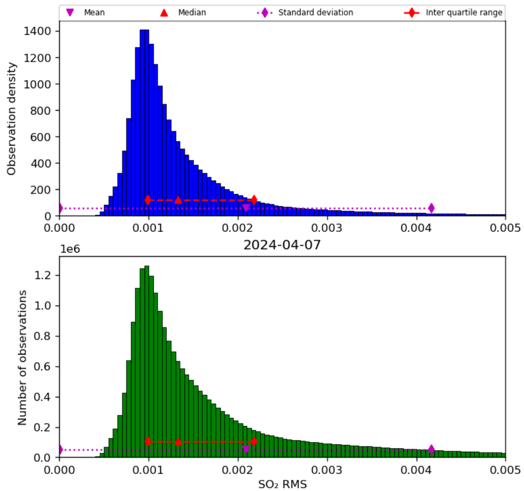
Figure 70: Histogram of “SO 2 RMS” for 2024-04-06 to 2024-04-08
