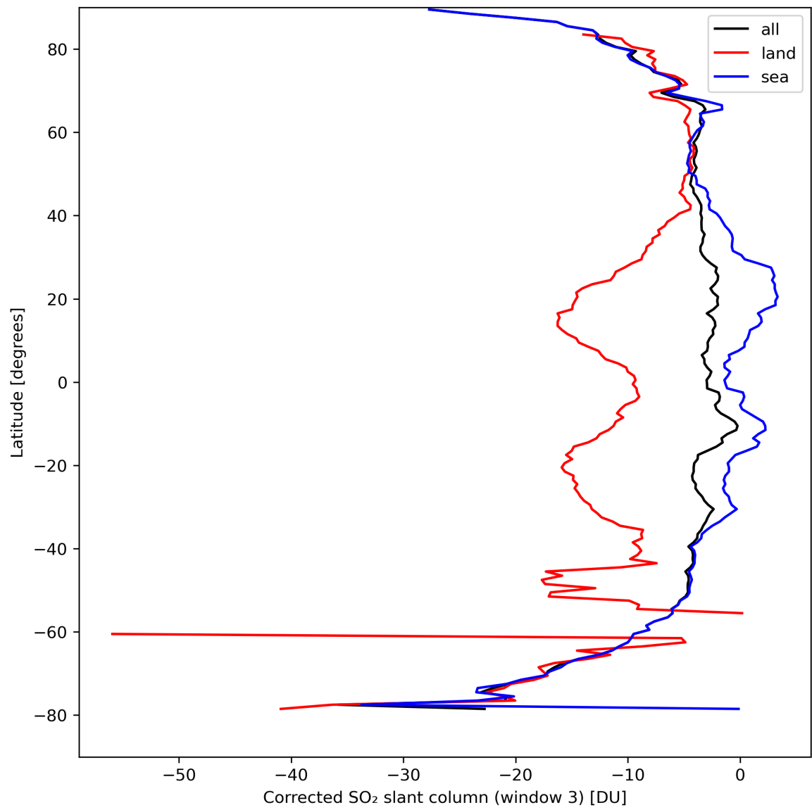
Figure 43: Zonal average of “Corrected SO 2 slant column (window 3)” for 2024-04-06 to 2024-04-08.
