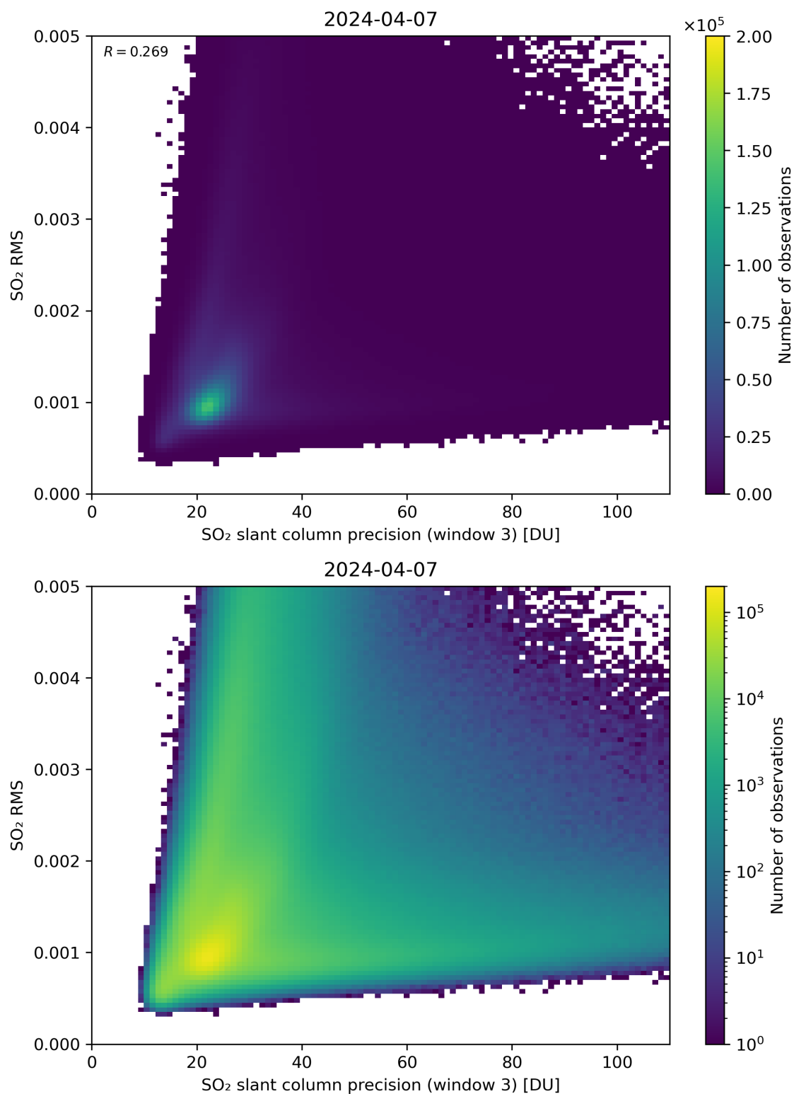
Figure 260: Scatter density plot of “SO 2 slant column precision (window 3)” against “SO 2 RMS” for 2024-04-06 to 2024-04-08.
