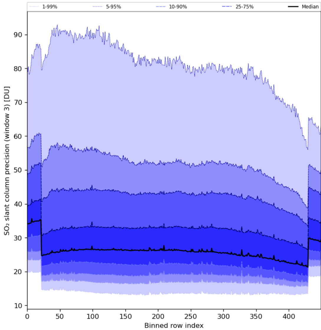
Figure 88: Along track statistics of “SO 2 slant column precision (window 3)” for 2024-04-06 to 2024-04-08
