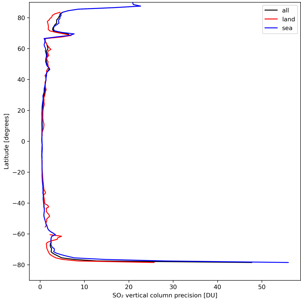
Figure 31: Zonal average of “SO 2 vertical column precision” for 2024-04-06 to 2024-04-08.
