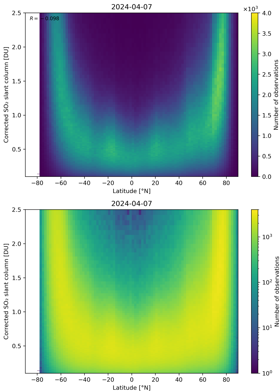
Figure 146: Scatter density plot of “Latitude” against “Corrected SO 2 slant column” for 2024-04-06 to 2024-04-08.
