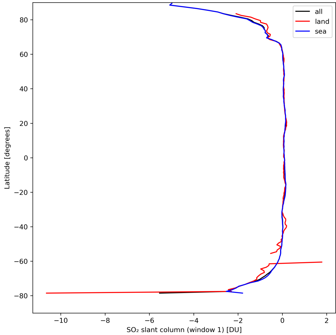
Figure 33: Zonal average of “SO 2 slant column (window 1)” for 2024-04-06 to 2024-04-08.
