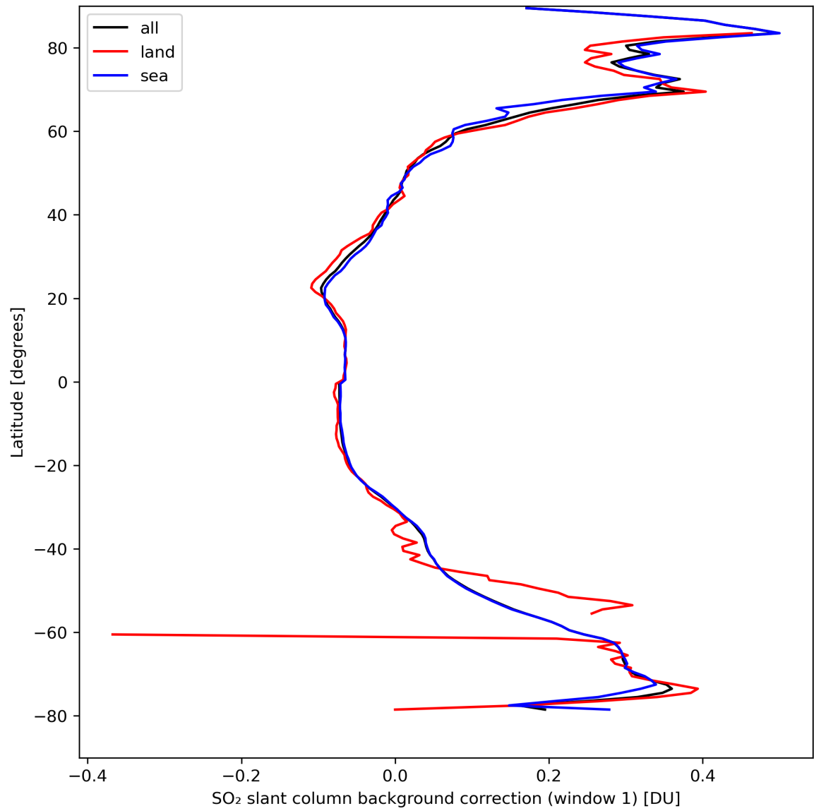
Figure 36: Zonal average of “SO 2 slant column background correction (window 1)” for 2024-04-06 to 2024-04-08.
