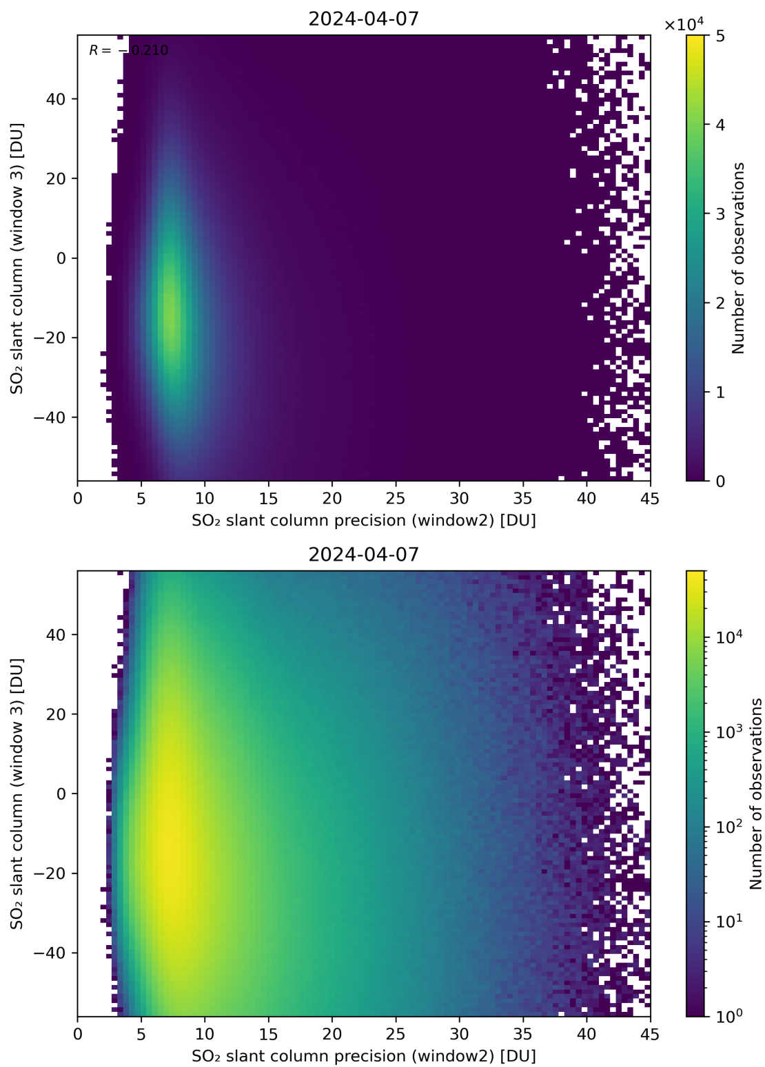
Figure 249: Scatter density plot of “SO 2 slant column precision (window2)” against “SO 2 slant column (window 3)” for 2024-04-06 to 2024-04-08.
