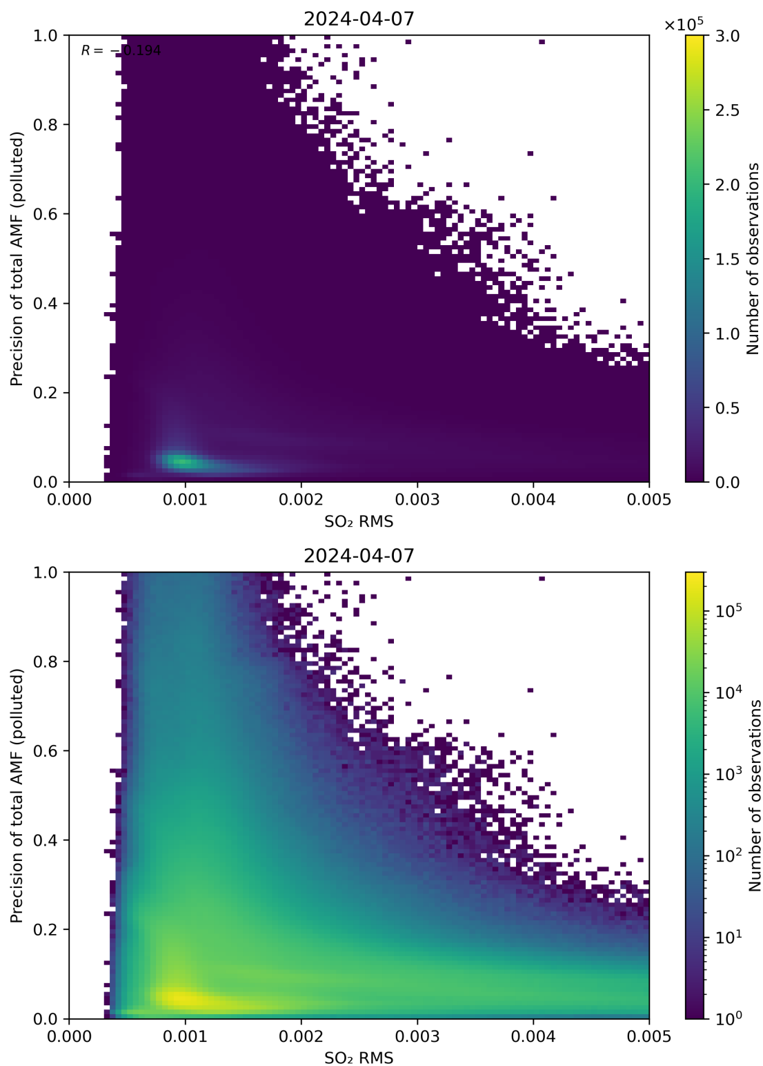
Figure 138: Scatter density plot of “SO 2 RMS” against “Precision of total AMF (polluted)” for 2024-04-06 to 2024-04-08.
