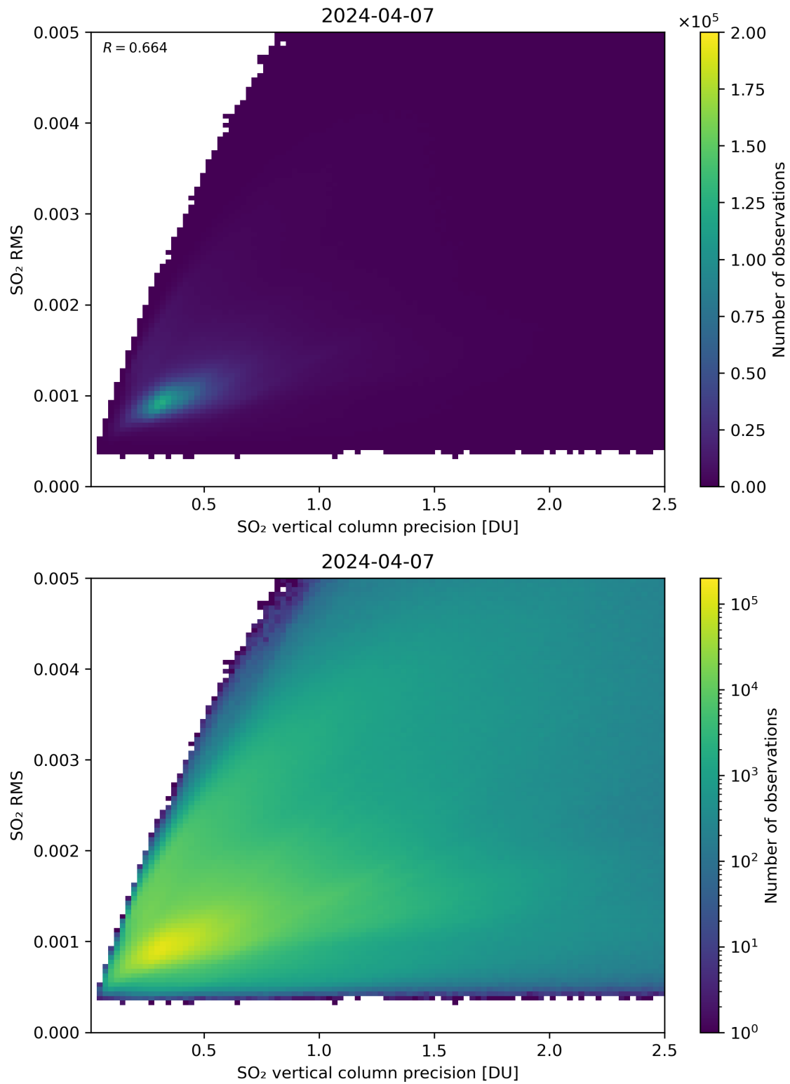
Figure 284: Scatter density plot of “SO 2 vertical column precision” against “SO 2 RMS” for 2024-04-06 to 2024-04-08.
