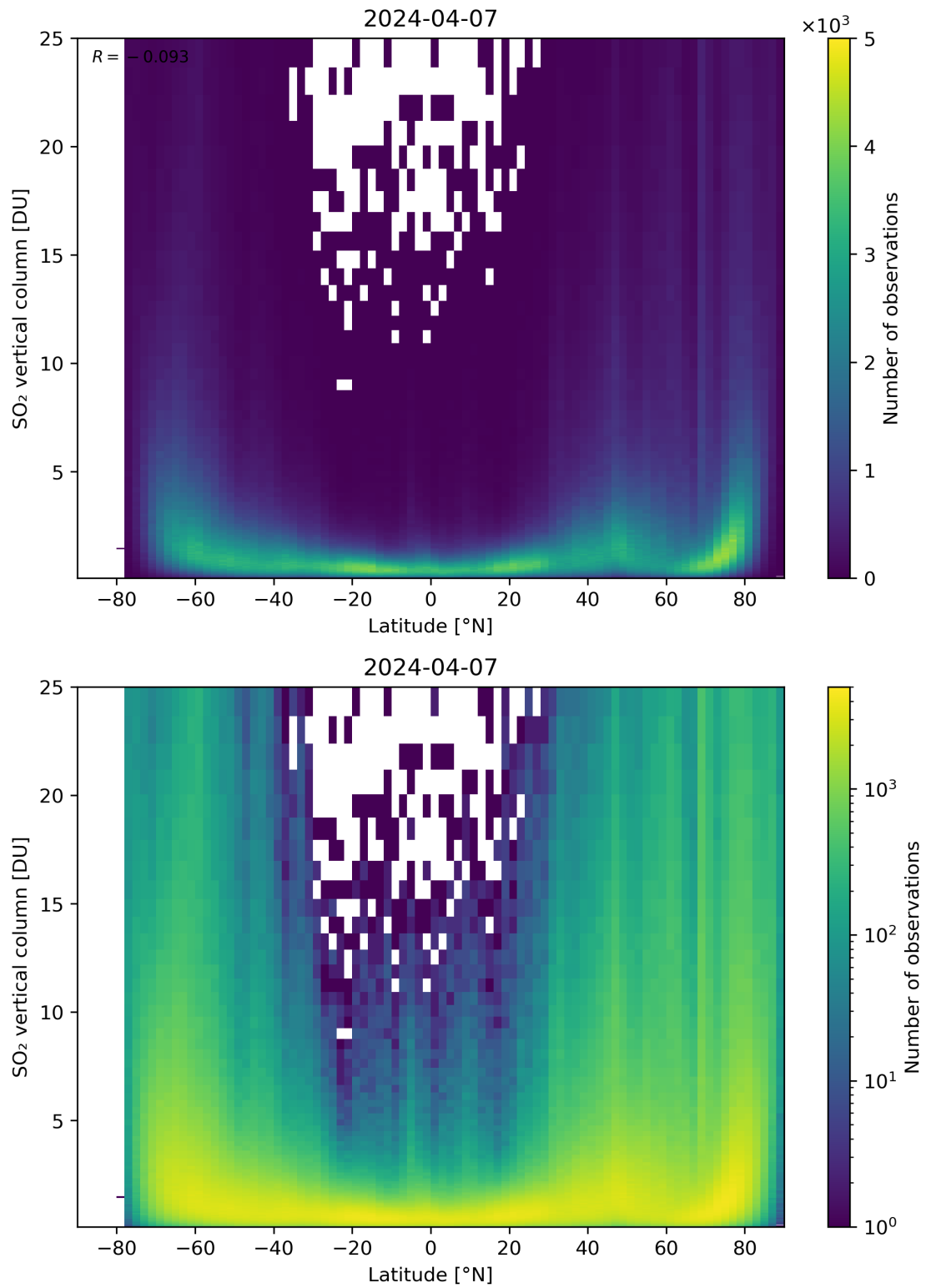
Figure 156: Scatter density plot of “Latitude” against “SO 2 vertical column” for 2024-04-06 to 2024-04-08.
