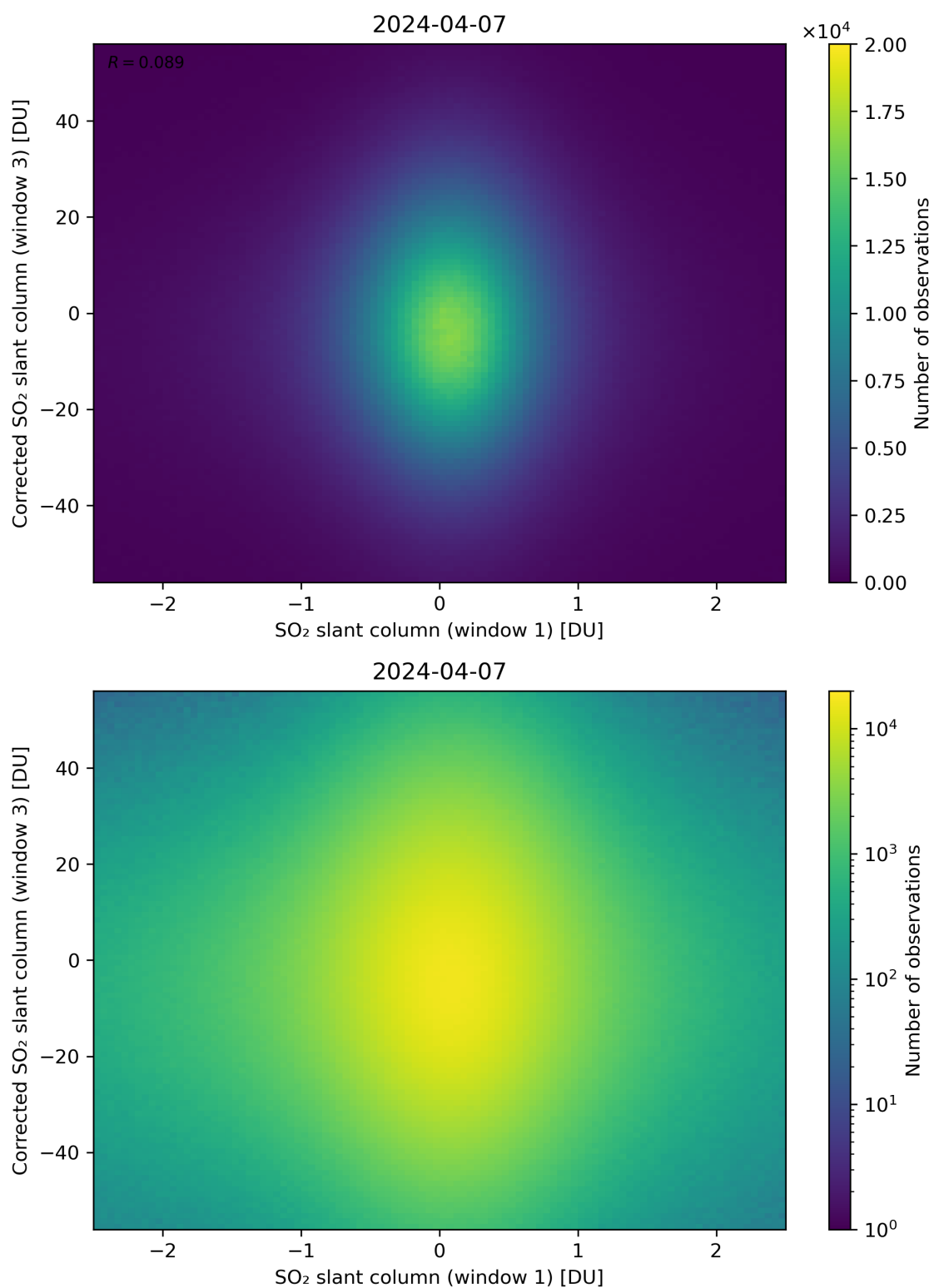
Figure 234: Scatter density plot of “SO 2 slant column (window 1)” against “Corrected SO 2 slant column (window 3)” for 2024-04-06 to 2024-04-08.
