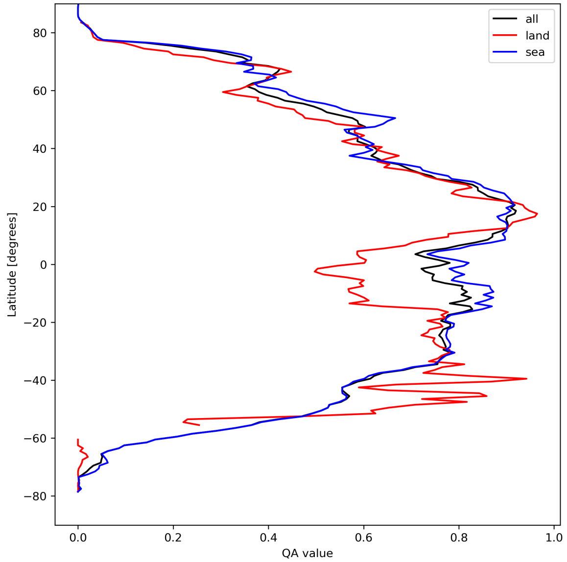
Figure 29: Zonal average of “QA value” for 2024-04-06 to 2024-04-08.
