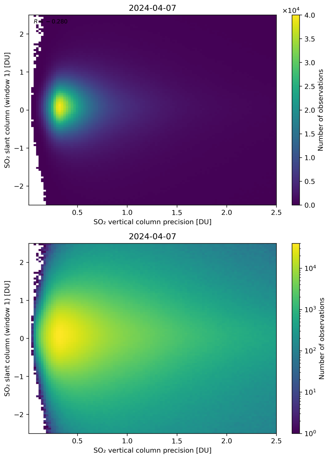
Figure 289: Scatter density plot of “SO 2 vertical column precision” against “SO 2 slant column (window 1)” for 2024-04-06 to 2024-04-08.
