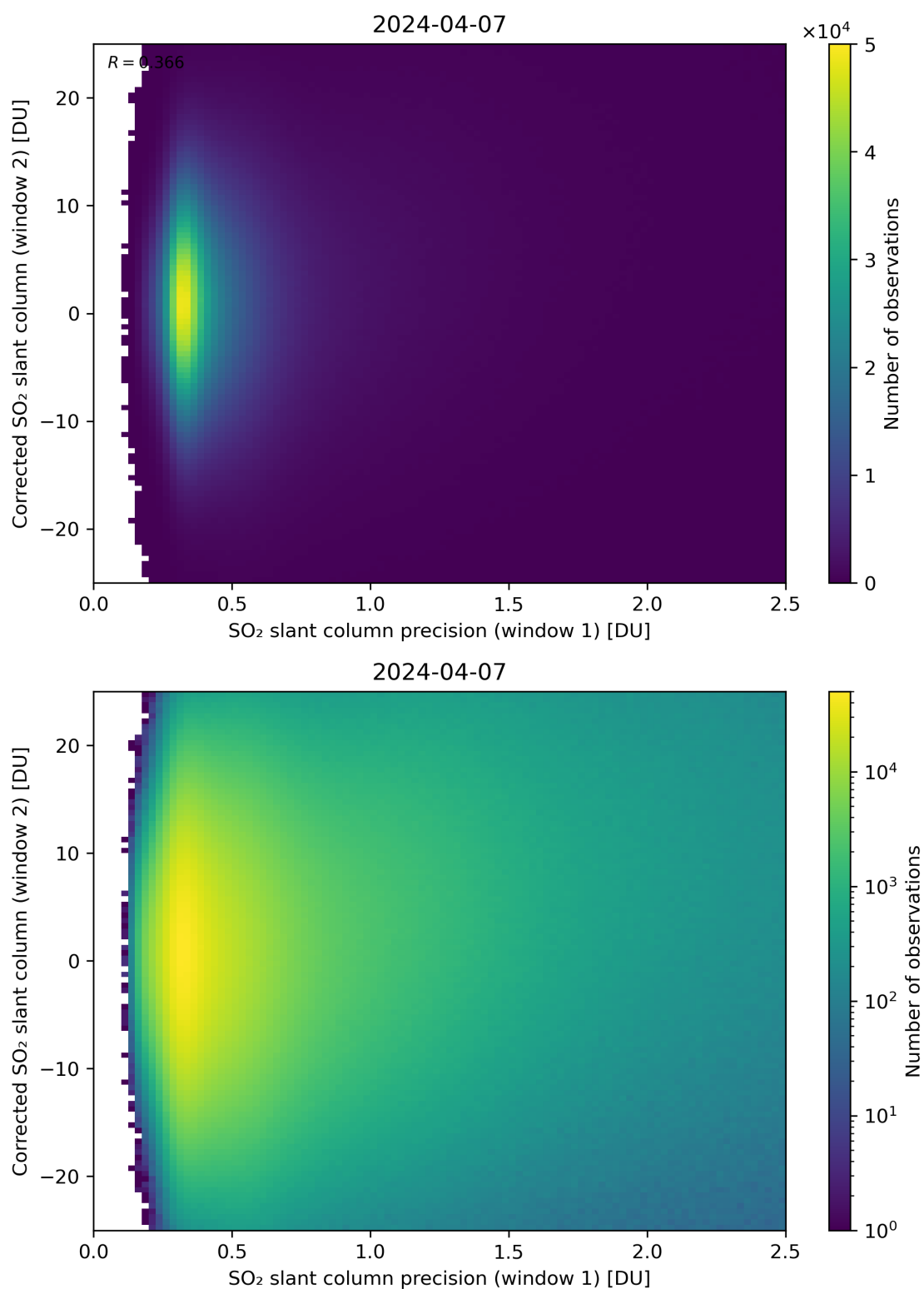
Figure 225: Scatter density plot of “SO 2 slant column precision (window 1)” against “Corrected SO 2 slant column (window 2)” for 2024-04-06 to 2024-04-08.
