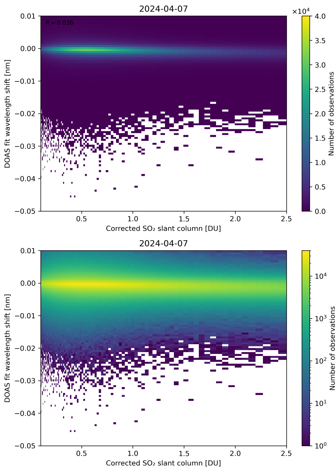
Figure 181: Scatter density plot of “Corrected SO 2 slant column” against “DOAS fit wavelength shift” for 2024-04-06 to 2024-04-08.
