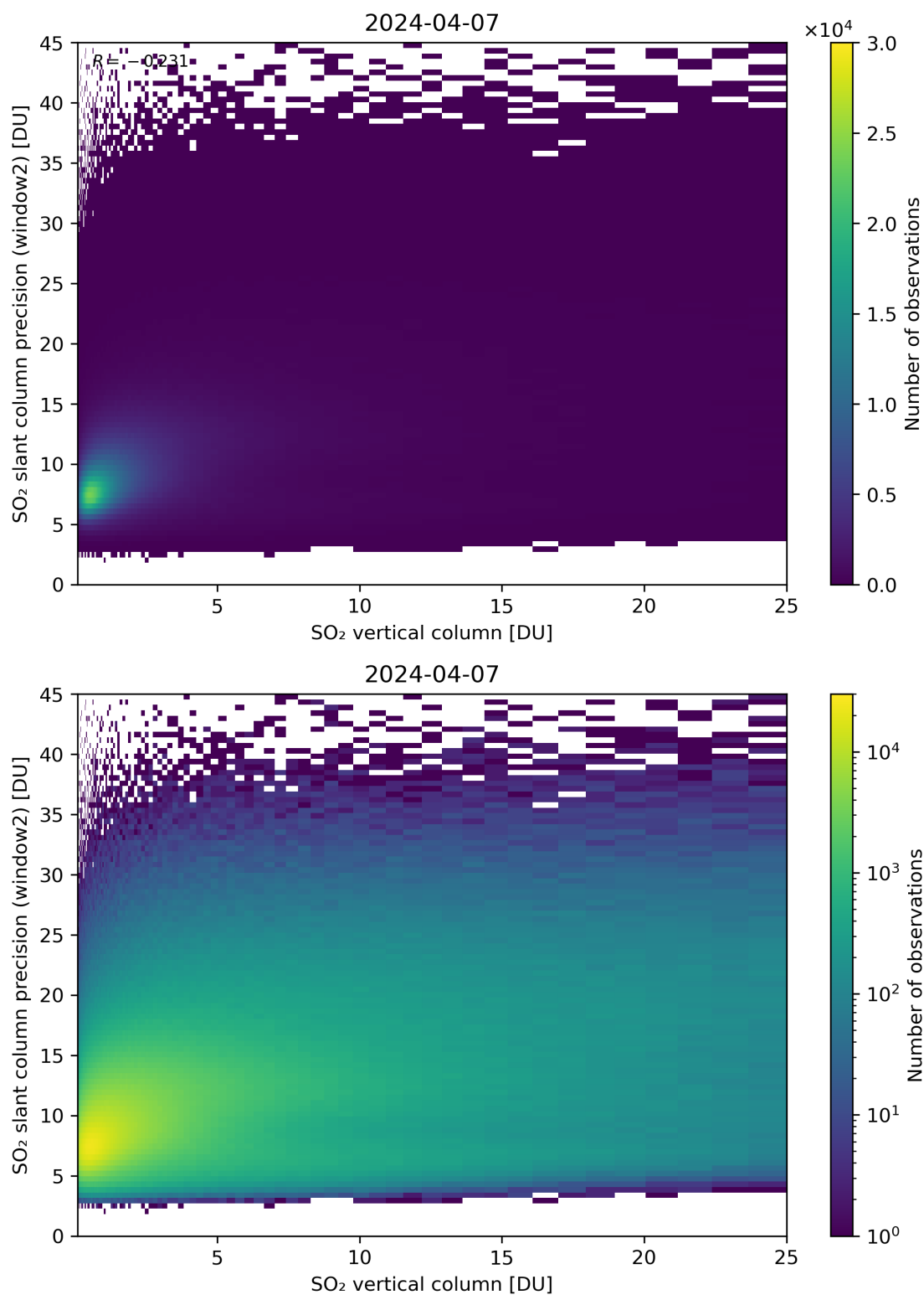
Figure 302: Scatter density plot of “SO 2 vertical column” against “SO 2 slant column precision (window2)” for 2024-04-06 to 2024-04-08.
