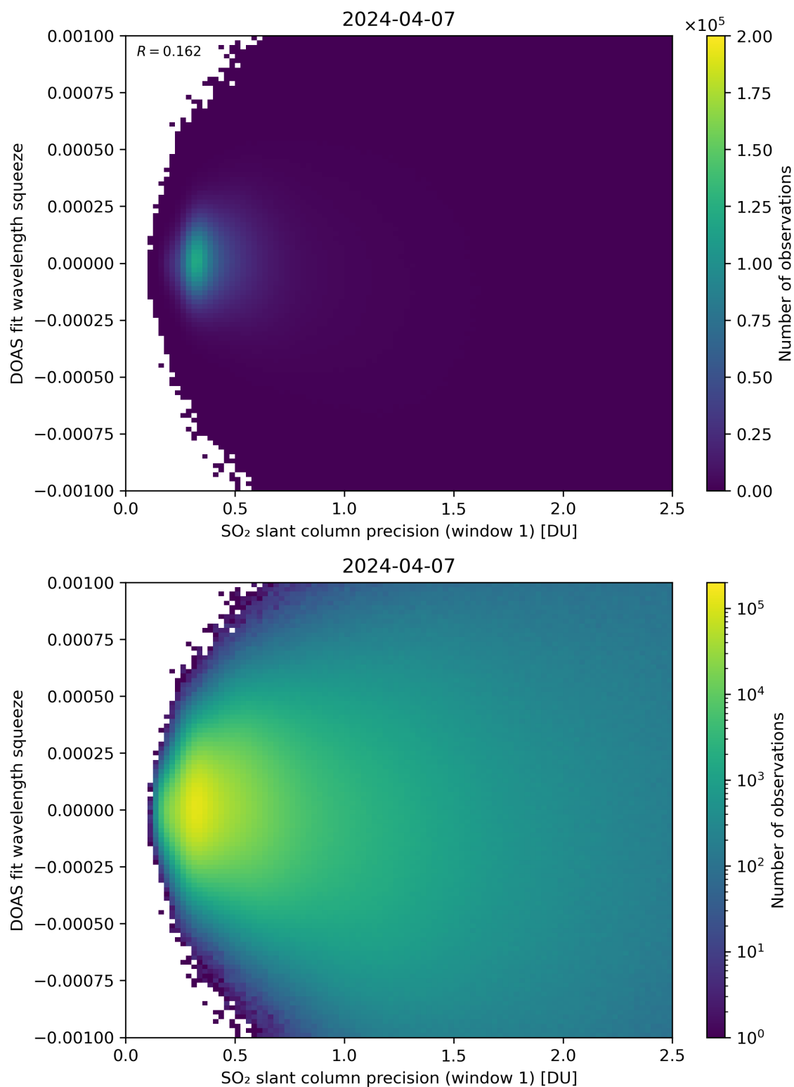
Figure 222: Scatter density plot of “SO 2 slant column precision (window 1)” against “DOAS fit wavelength squeeze” for 2024-04-06 to 2024-04-08.
