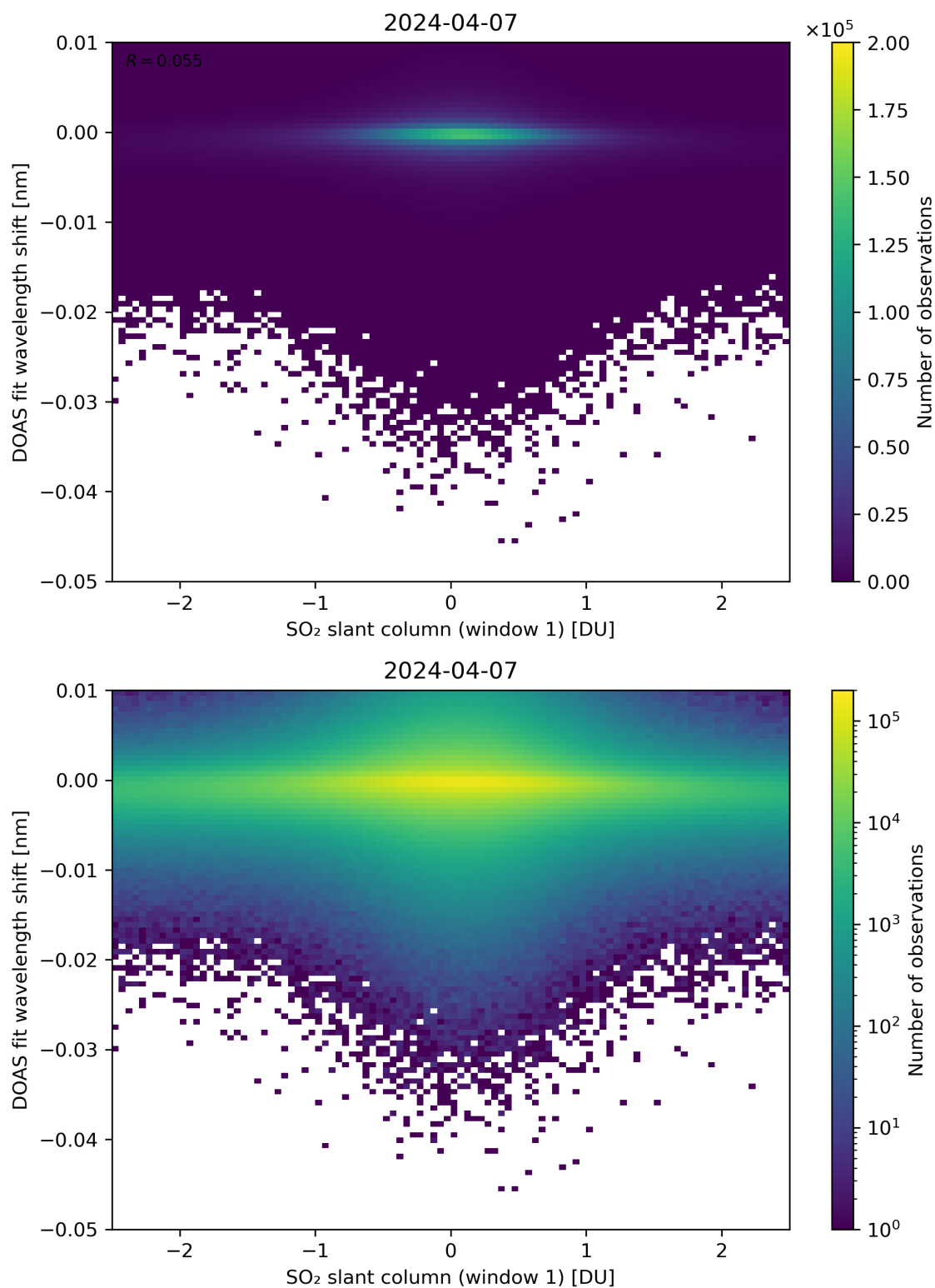
Figure 215: Scatter density plot of “SO 2 slant column (window 1)” against “DOAS fit wavelength shift” for 2024-04-06 to 2024-04-08.
