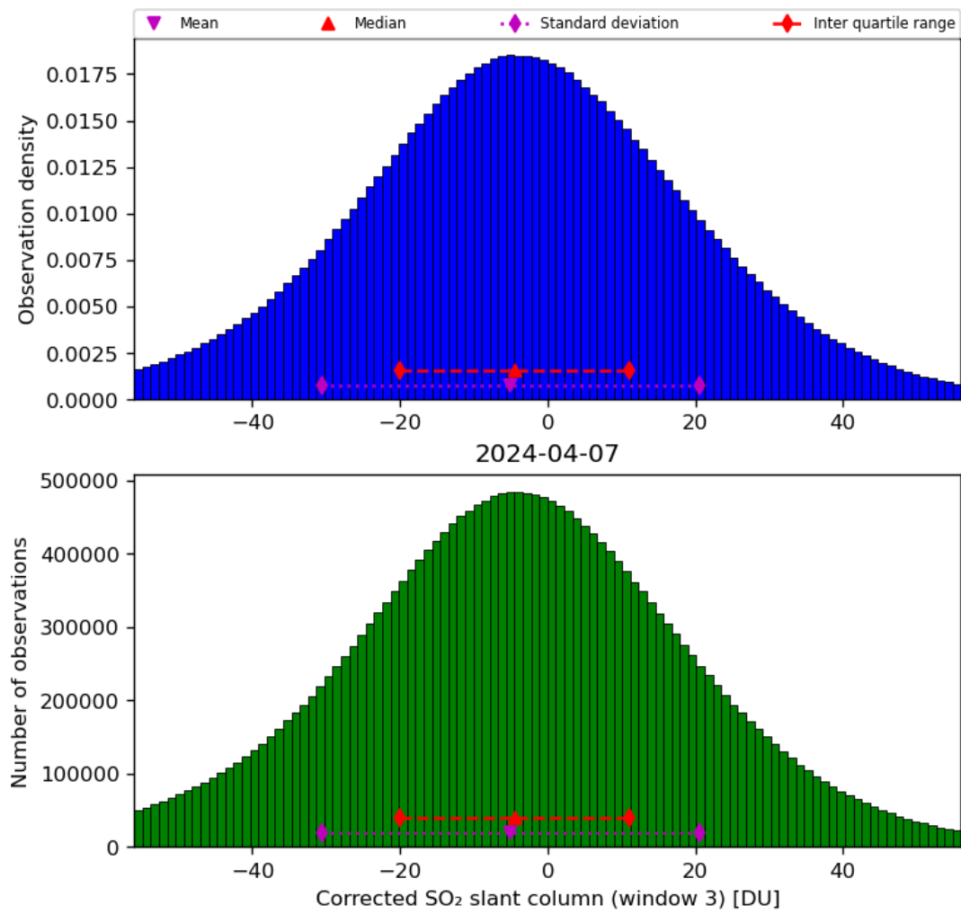
Figure 66: Histogram of “Corrected SO 2 slant column (window 3)” for 2024-04-06 to 2024-04-08
