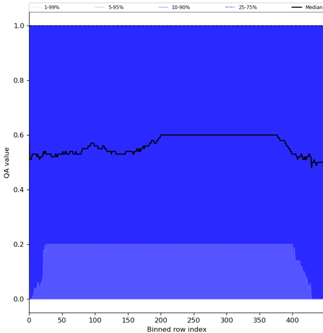
Figure 75: Along track statistics of “QA value” for 2024-04-06 to 2024-04-08
