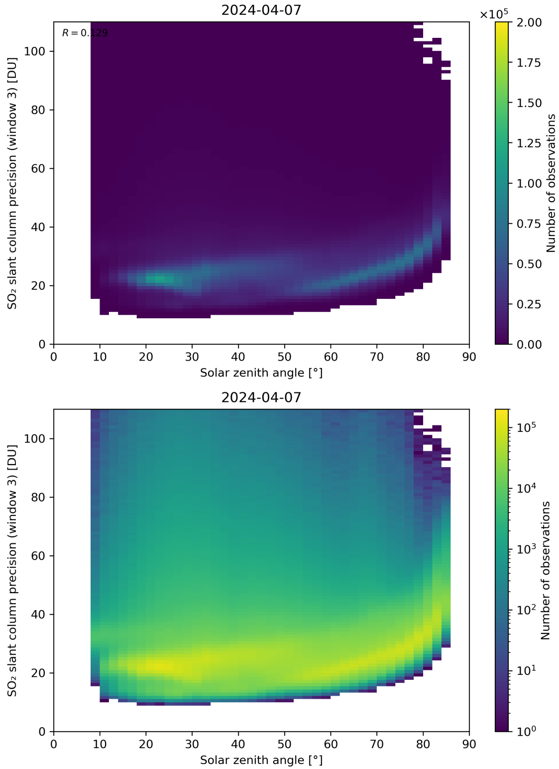
Figure 173: Scatter density plot of “Solar zenith angle” against “SO 2 slant column precision (window 3)” for 2024-04-06 to 2024-04-08.
