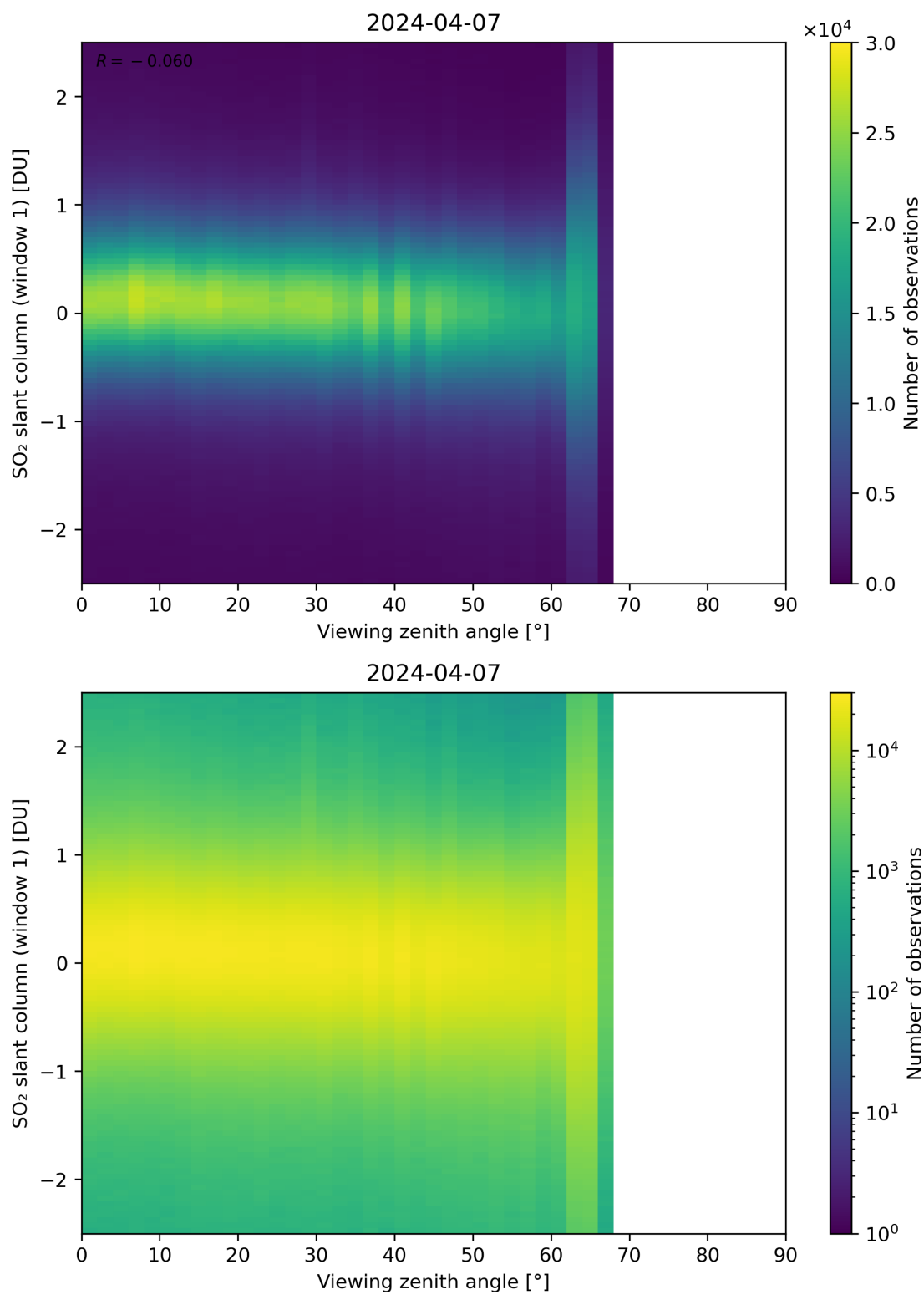
Figure 320: Scatter density plot of “Viewing zenith angle” against “SO 2 slant column (window 1)” for 2024-04-06 to 2024-04-08.
