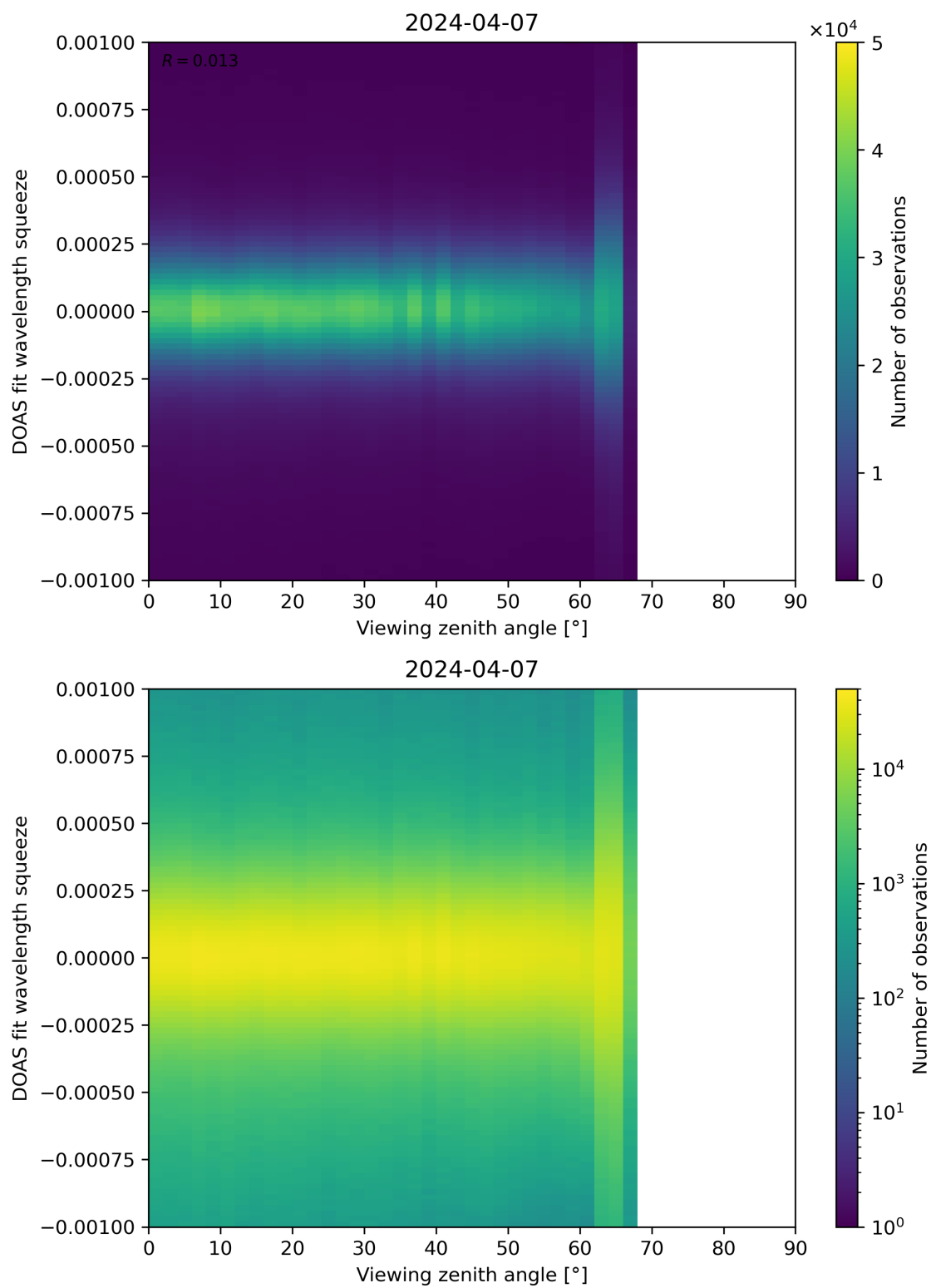
Figure 312: Scatter density plot of “Viewing zenith angle” against “DOAS fit wavelength squeeze” for 2024-04-06 to 2024-04-08.
