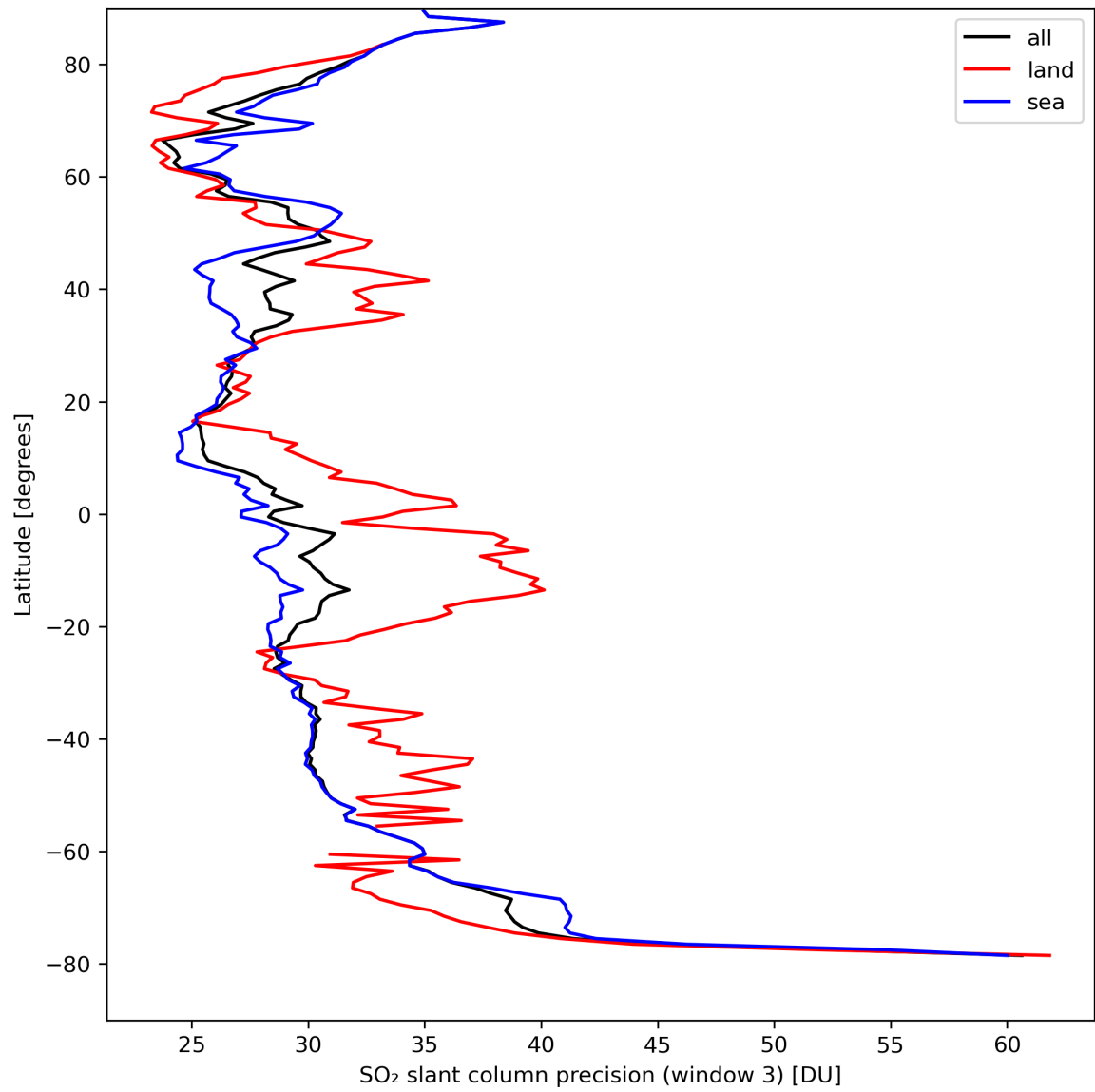
Figure 42: Zonal average of “SO 2 slant column precision (window 3)” for 2024-04-06 to 2024-04-08.
