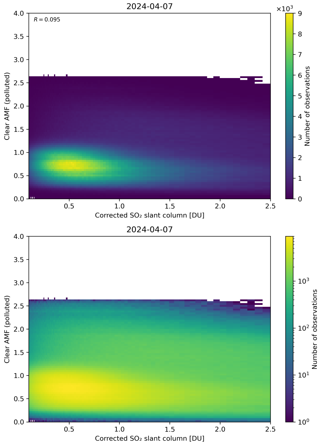
Figure 184: Scatter density plot of “Corrected SO 2 slant column” against “Clear AMF (polluted)” for 2024-04-06 to 2024-04-08.
