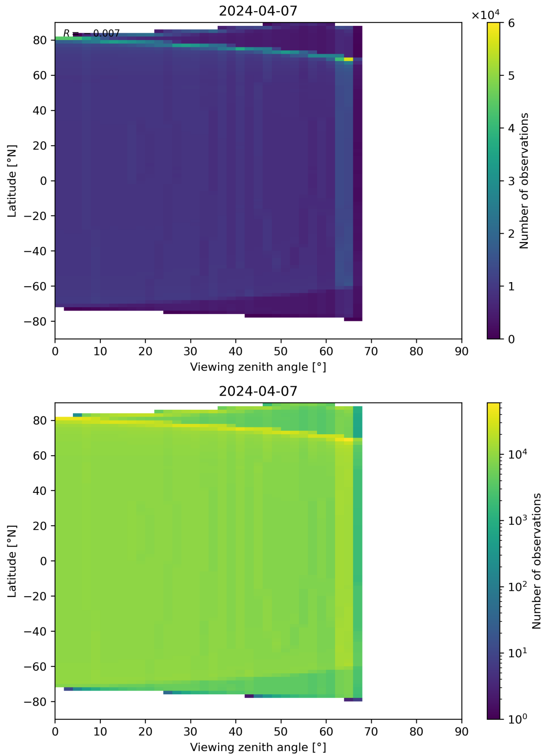
Figure 314: Scatter density plot of “Viewing zenith angle” against “Latitude” for 2024-04-06 to 2024-04-08.
