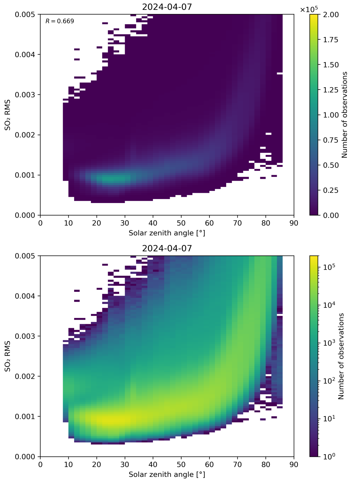
Figure 163: Scatter density plot of “Solar zenith angle” against “SO 2 RMS” for 2024-04-06 to 2024-04-08.
