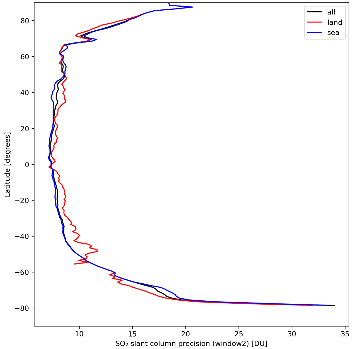
Figure 38: Zonal average of “SO 2 slant column precision (window2)” for 2024-04-06 to 2024-04-08.
