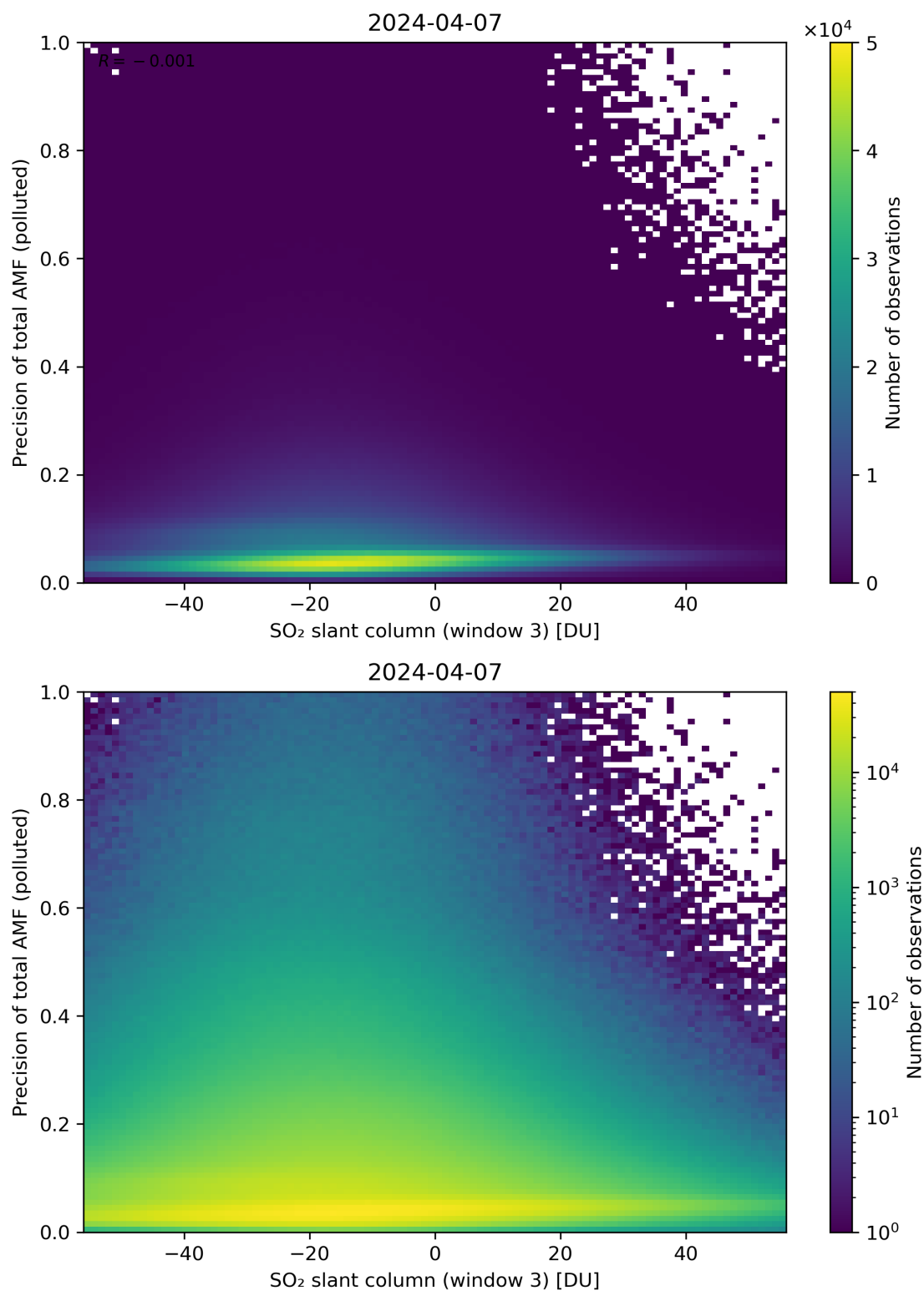
Figure 269: Scatter density plot of “SO 2 slant column (window 3)” against “Precision of total AMF (polluted)” for 2024-04-06 to 2024-04-08.
