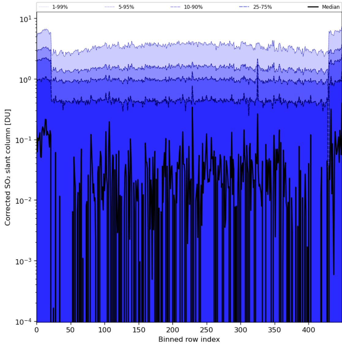
Figure 78: Along track statistics of “Corrected SO 2 slant column” for 2024-04-06 to 2024-04-08
