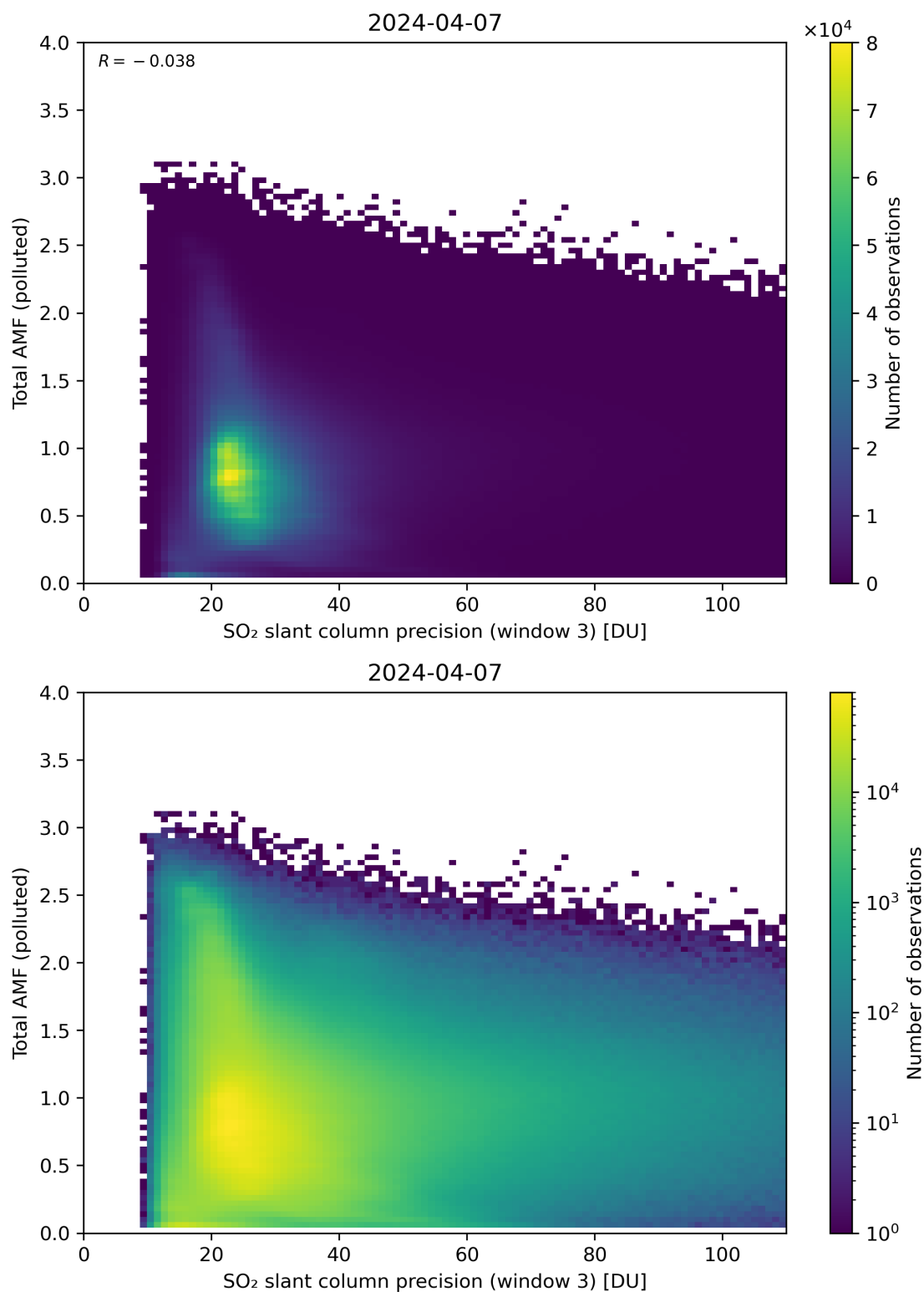
Figure 263: Scatter density plot of “SO 2 slant column precision (window 3)” against “Total AMF (polluted)” for 2024-04-06 to 2024-04-08.
