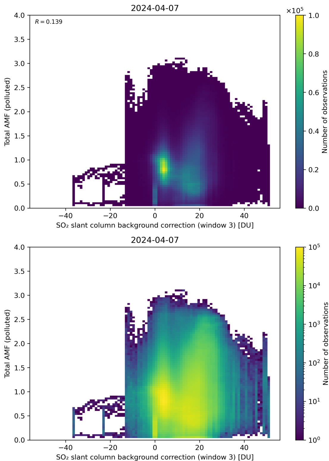
Figure 125: Scatter density plot of “SO 2 slant column background correction (window 3)” against “Total AMF (polluted)” for 2024-04-06 to 2024-04-08.
