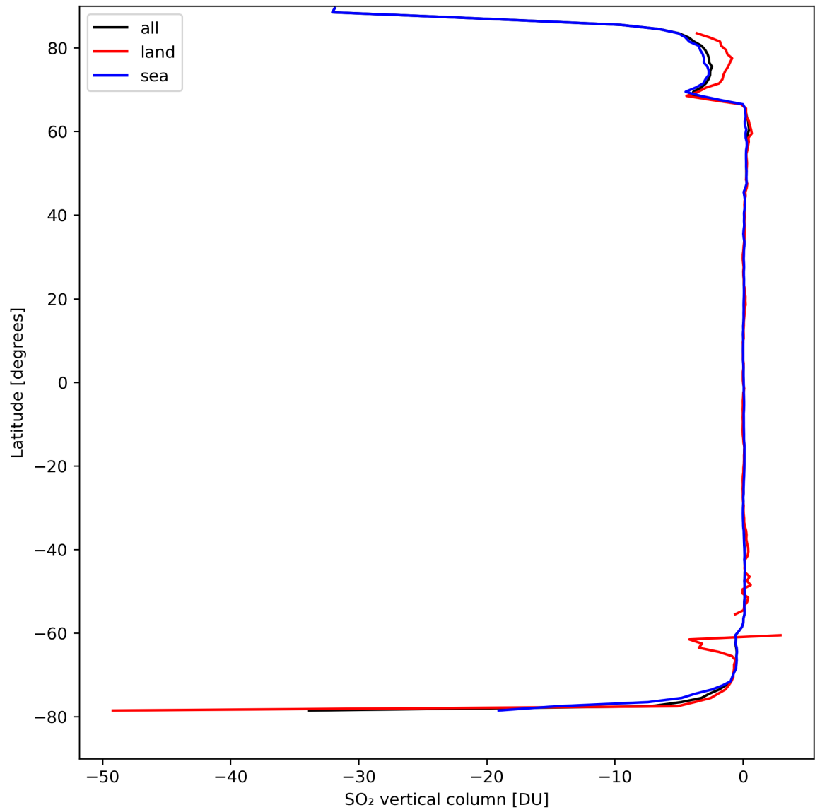
Figure 30: Zonal average of “SO 2 vertical column” for 2024-04-06 to 2024-04-08.
