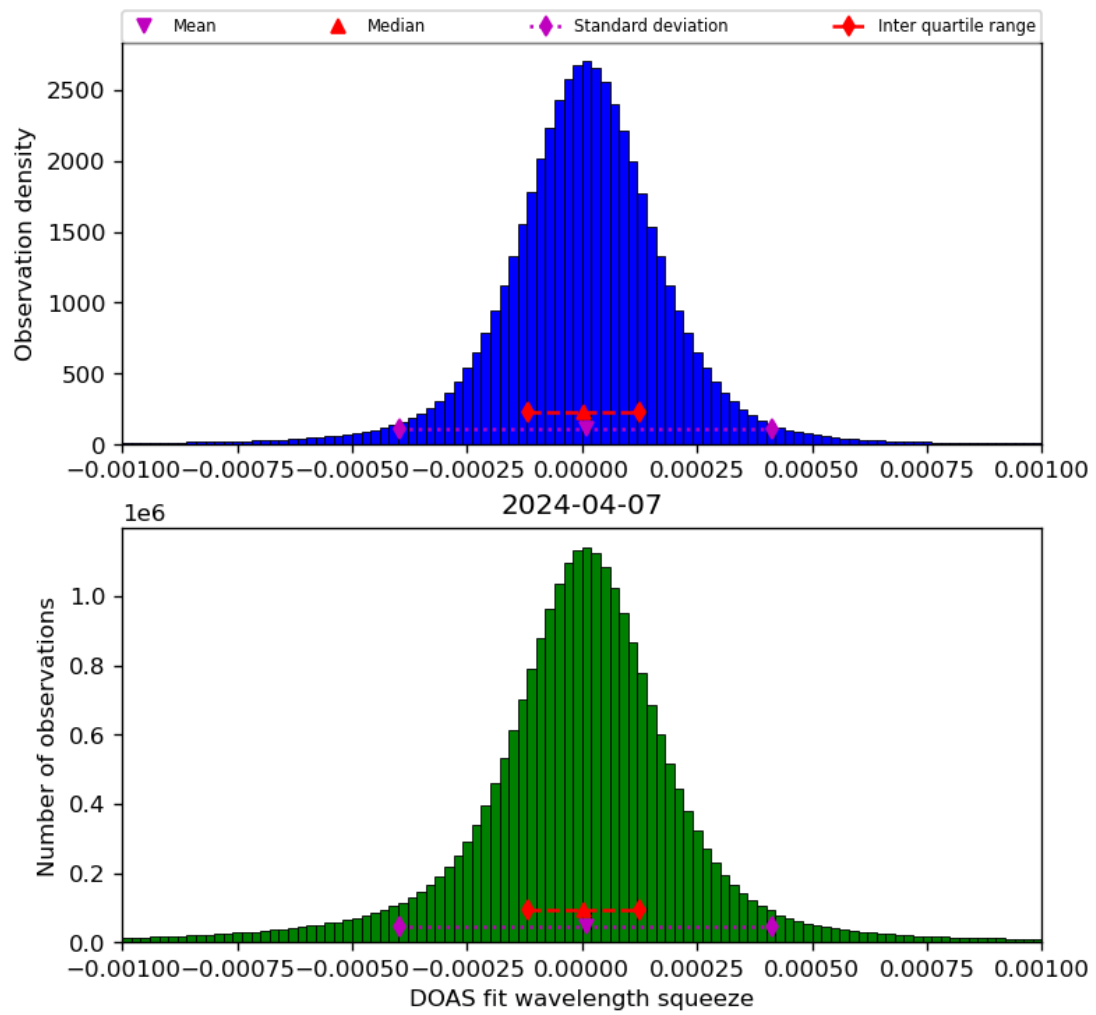
Figure 69: Histogram of “DOAS fit wavelength squeeze” for 2024-04-06 to 2024-04-08
