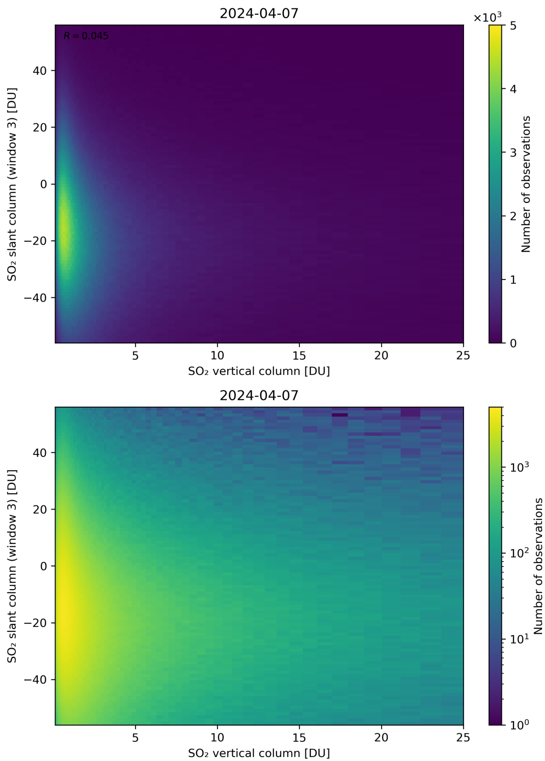
Figure 303: Scatter density plot of “SO 2 vertical column” against “SO 2 slant column (window 3)” for 2024-04-06 to 2024-04-08.
