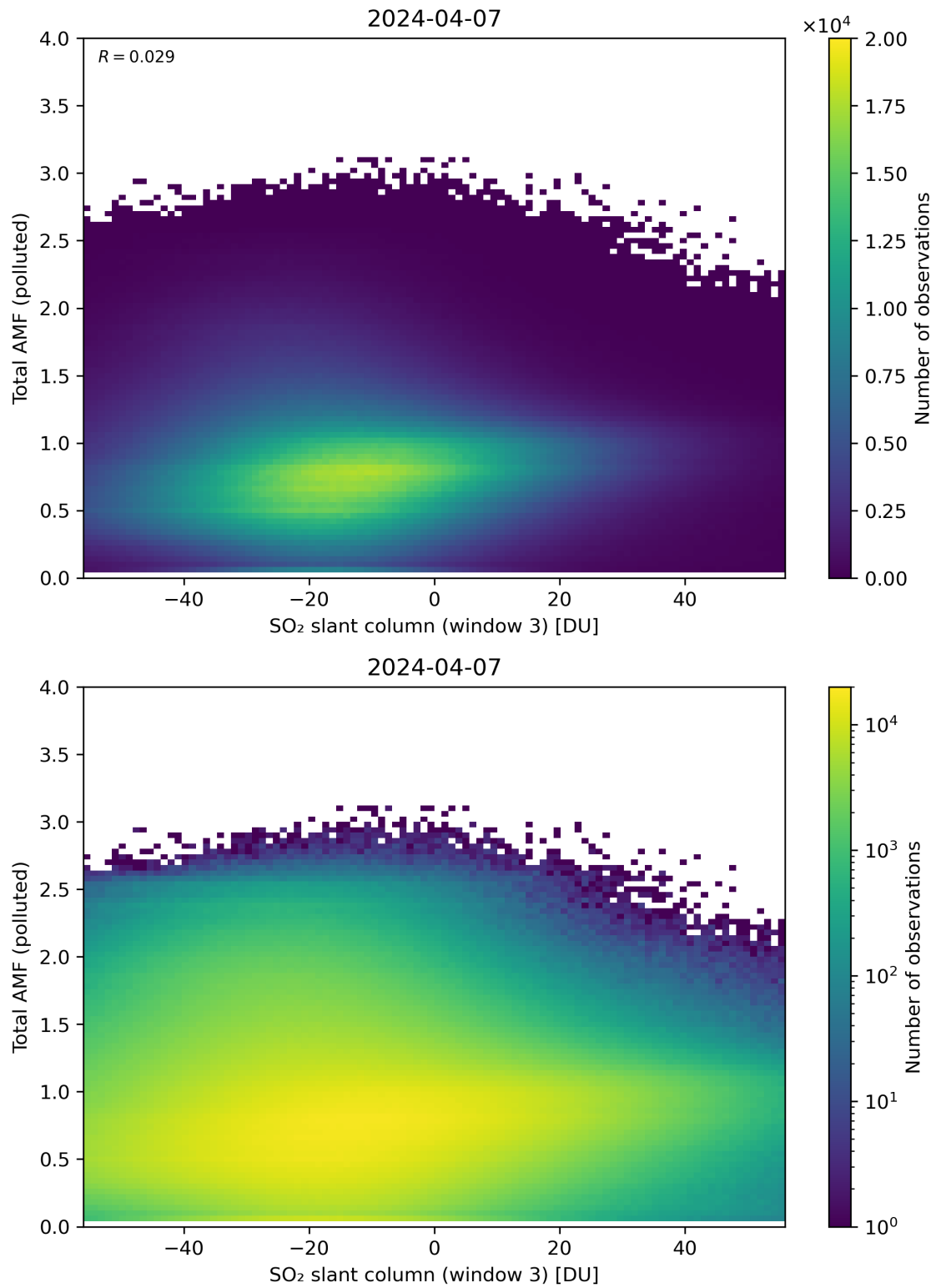
Figure 268: Scatter density plot of “SO 2 slant column (window 3)” against “Total AMF (polluted)” for 2024-04-06 to 2024-04-08.
