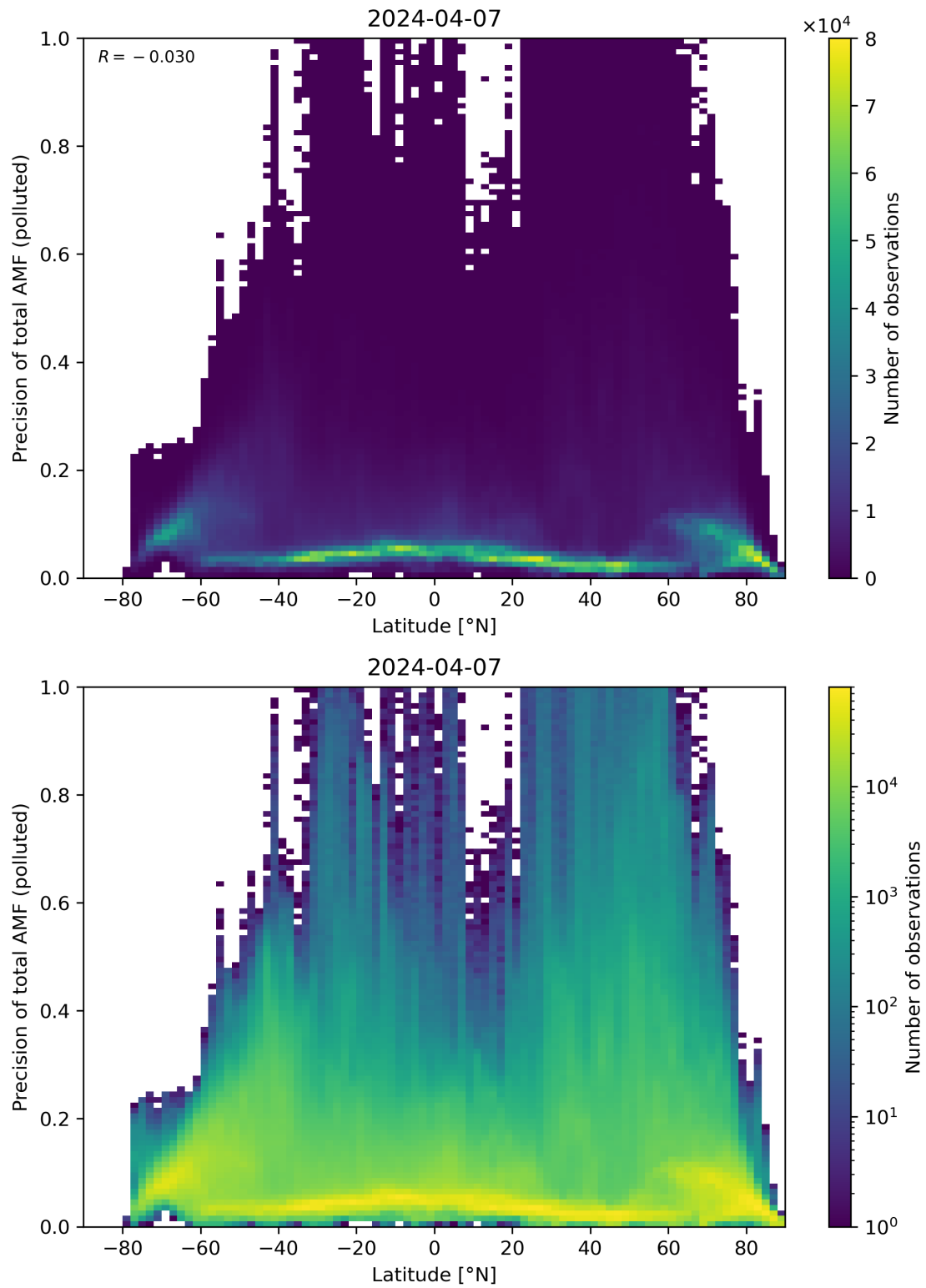
Figure 155: Scatter density plot of “Latitude” against “Precision of total AMF (polluted)” for 2024-04-06 to 2024-04-08.
