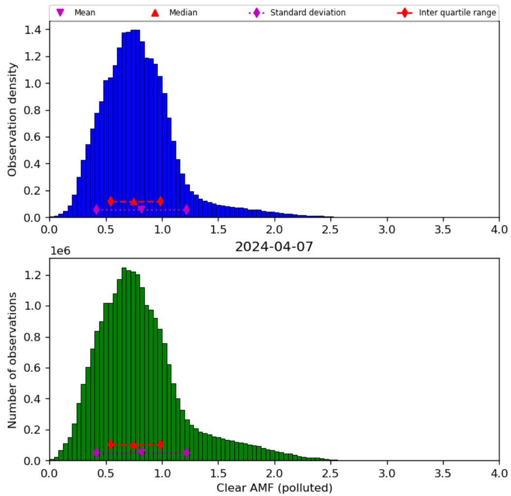
Figure 73: Histogram of “Clear AMF (polluted)” for 2024-04-06 to 2024-04-08
