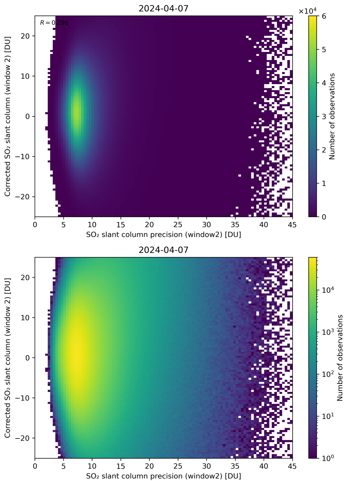
Figure 247: Scatter density plot of “SO 2 slant column precision (window2)” against “Corrected SO 2 slant column (window 2)” for 2024-04-06 to 2024-04-08.
