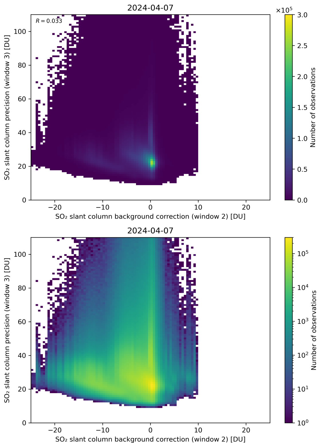
Figure 118: Scatter density plot of “SO 2 slant column background correction (window 2)” against “SO 2 slant column precision (window 3)” for 2024-04-06 to 2024-04-08.
