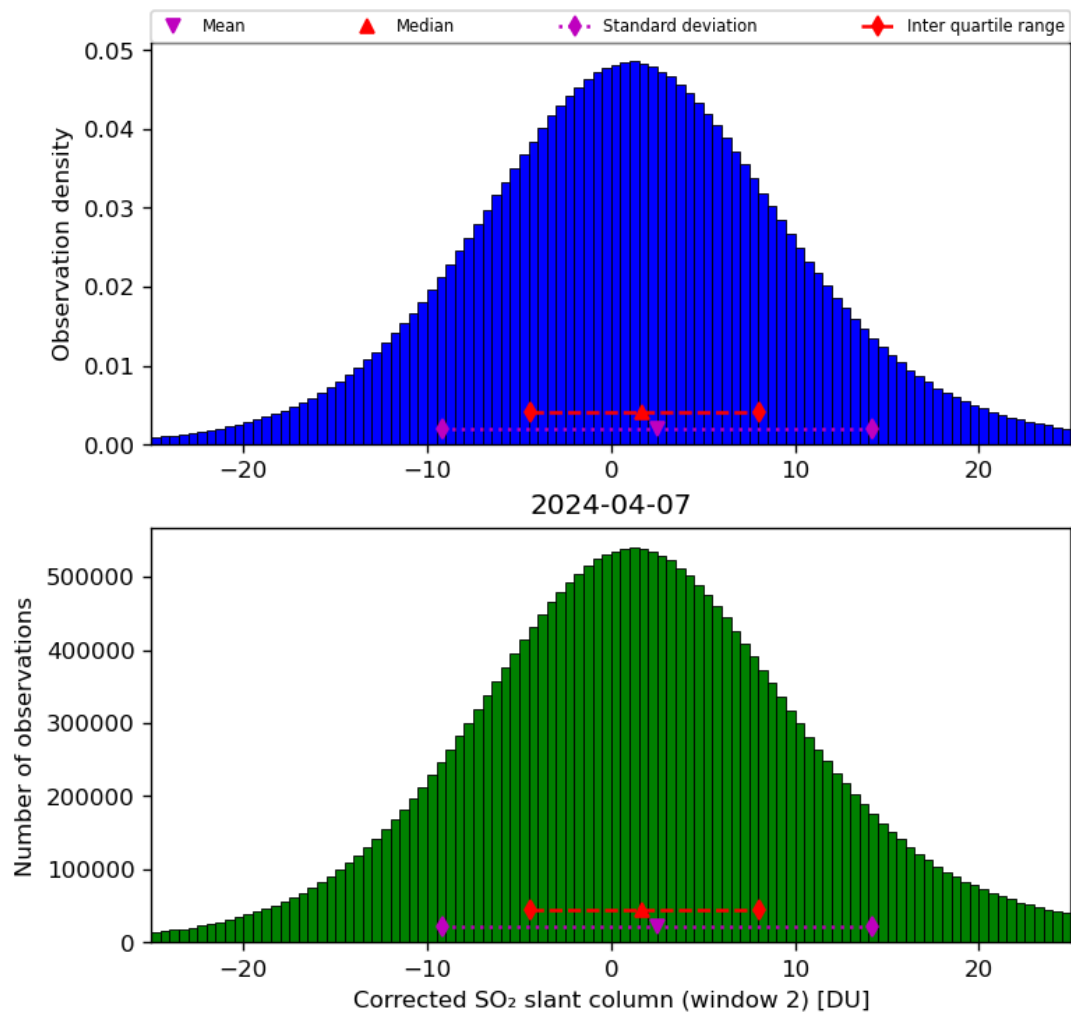
Figure 62: Histogram of “Corrected SO 2 slant column (window 2)” for 2024-04-06 to 2024-04-08
