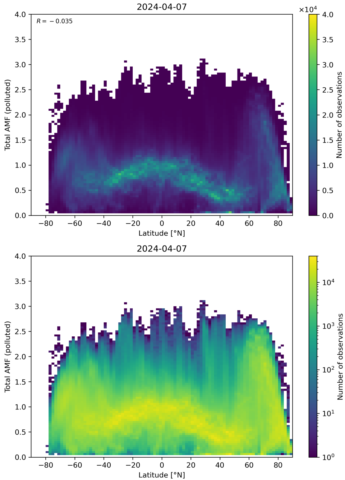
Figure 154: Scatter density plot of “Latitude” against “Total AMF (polluted)” for 2024-04-06 to 2024-04-08.
