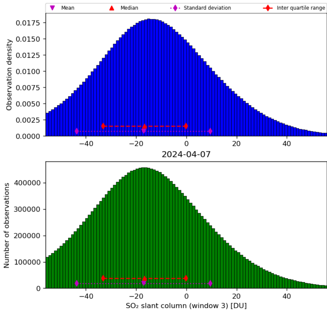
Figure 64: Histogram of “SO 2 slant column (window 3)” for 2024-04-06 to 2024-04-08
