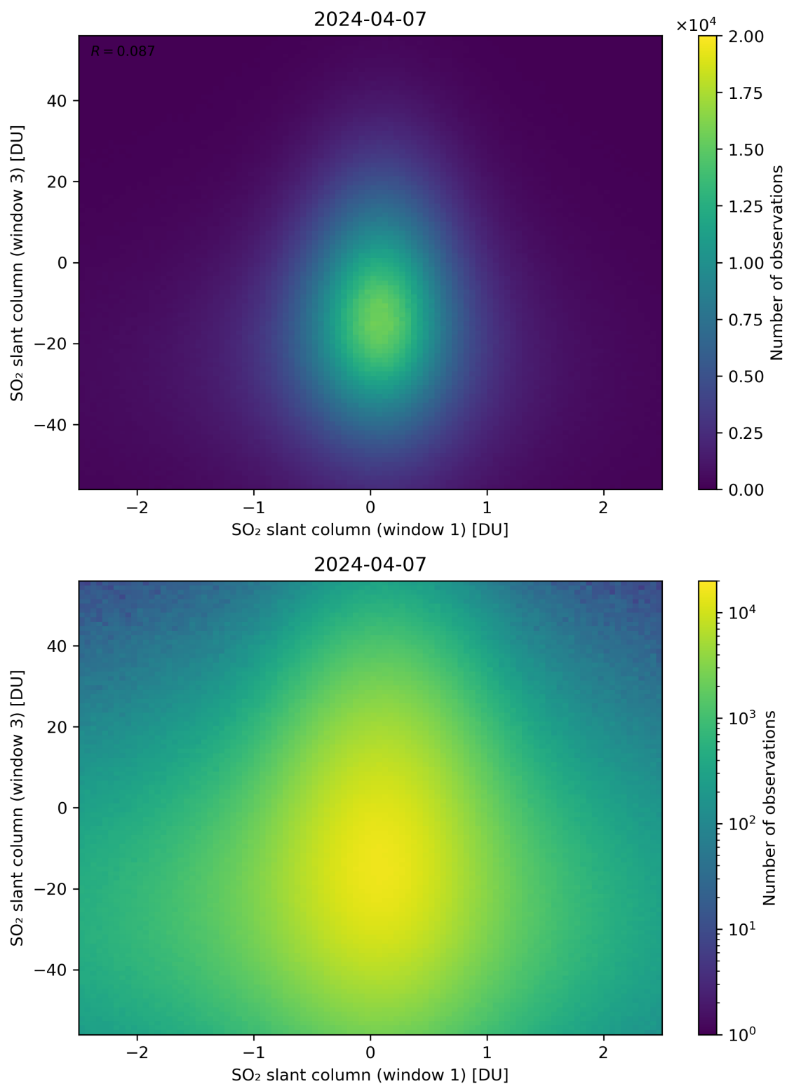
Figure 237: Scatter density plot of “SO 2 slant column (window 1)” against “SO 2 slant column (window 3)” for 2024-04-06 to 2024-04-08.
