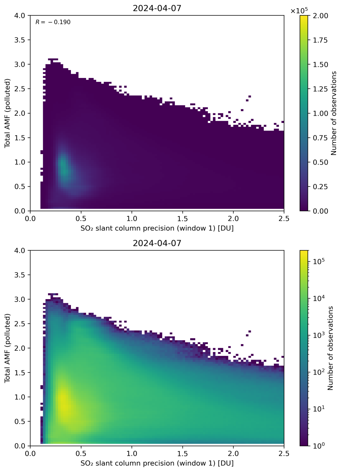
Figure 230: Scatter density plot of “SO 2 slant column precision (window 1)” against “Total AMF (polluted)” for 2024-04-06 to 2024-04-08.
