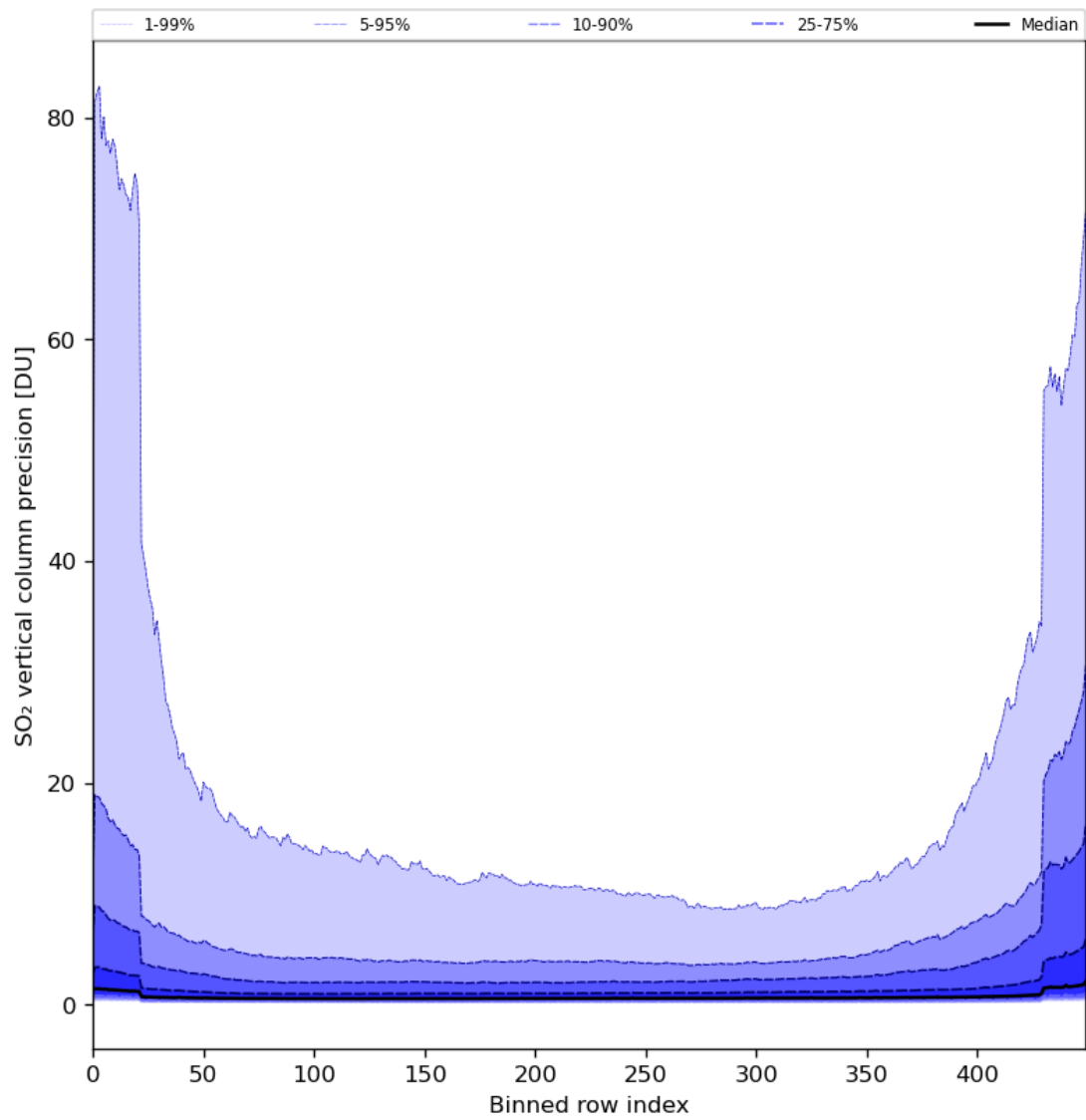
Figure 77: Along track statistics of “SO 2 vertical column precision” for 2024-04-06 to 2024-04-08
