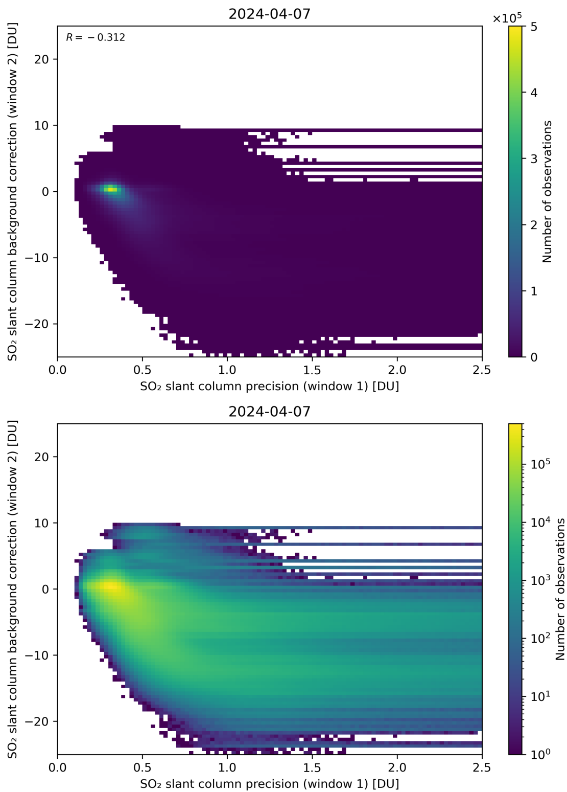
Figure 219: Scatter density plot of “SO 2 slant column precision (window 1)” against “SO 2 slant column background correction (window 2)” for 2024-04-06 to 2024-04-08.
