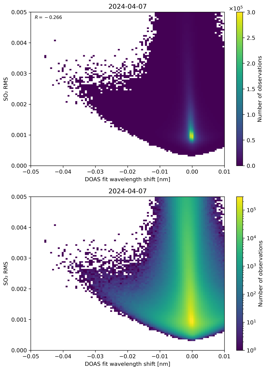
Figure 128: Scatter density plot of “DOAS fit wavelength shift” against “SO 2 RMS” for 2024-04-06 to 2024-04-08.
