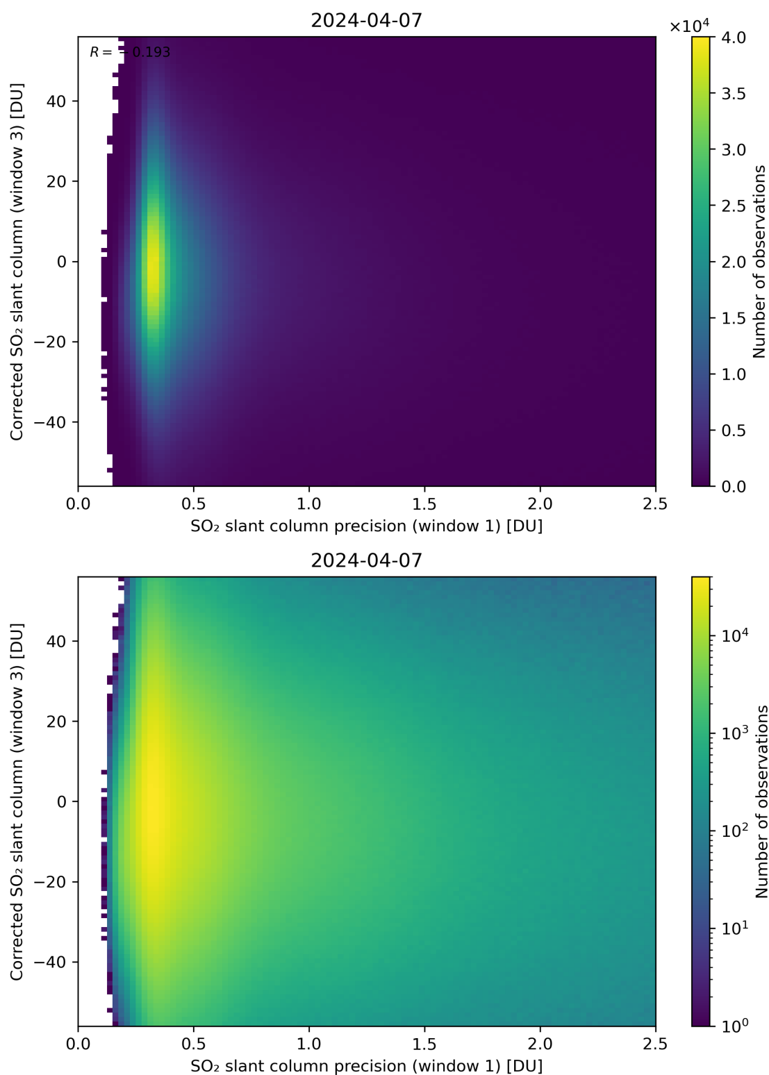
Figure 226: Scatter density plot of “SO 2 slant column precision (window 1)” against “Corrected SO 2 slant column (window 3)” for 2024-04-06 to 2024-04-08.
