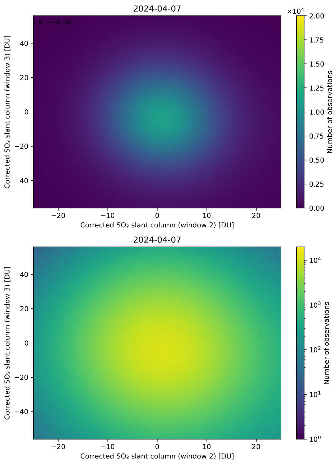
Figure 200: Scatter density plot of “Corrected SO 2 slant column (window 2)” against “Corrected SO 2 slant column (window 3)” for 2024-04-06 to 2024-04-08.
