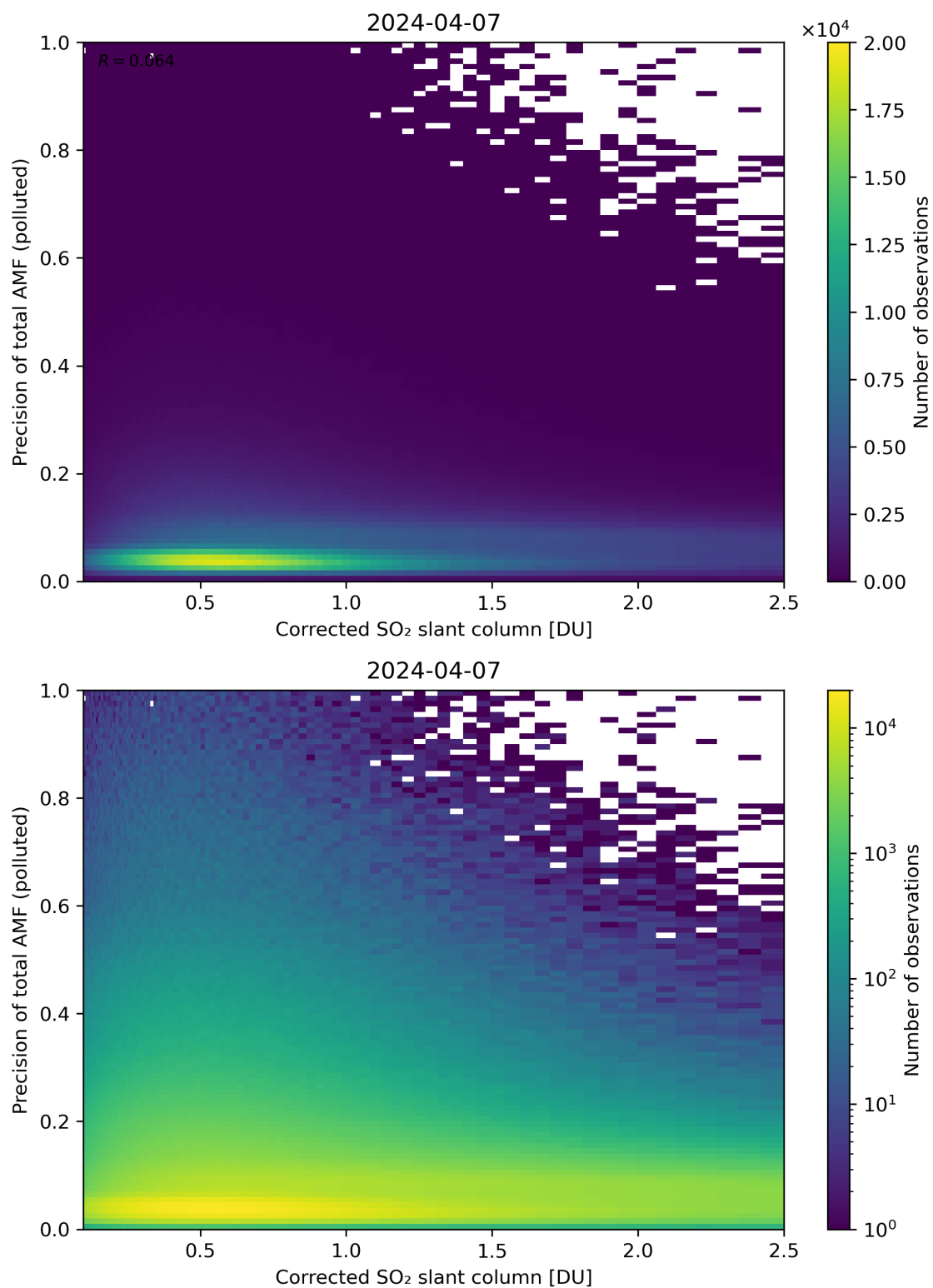
Figure 193: Scatter density plot of “Corrected SO 2 slant column” against “Precision of total AMF (polluted)” for 2024-04-06 to 2024-04-08.
