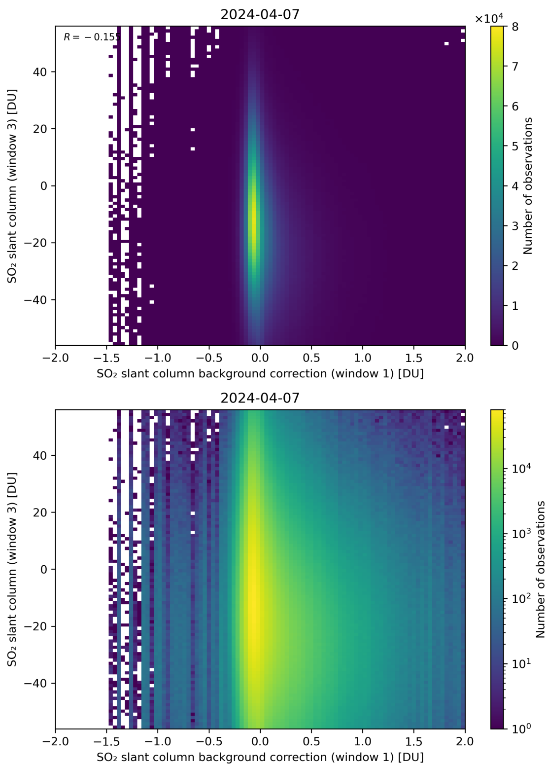
Figure 107: Scatter density plot of “SO 2 slant column background correction (window 1)” against “SO 2 slant column (window 3)” for 2024-04-06 to 2024-04-08.
