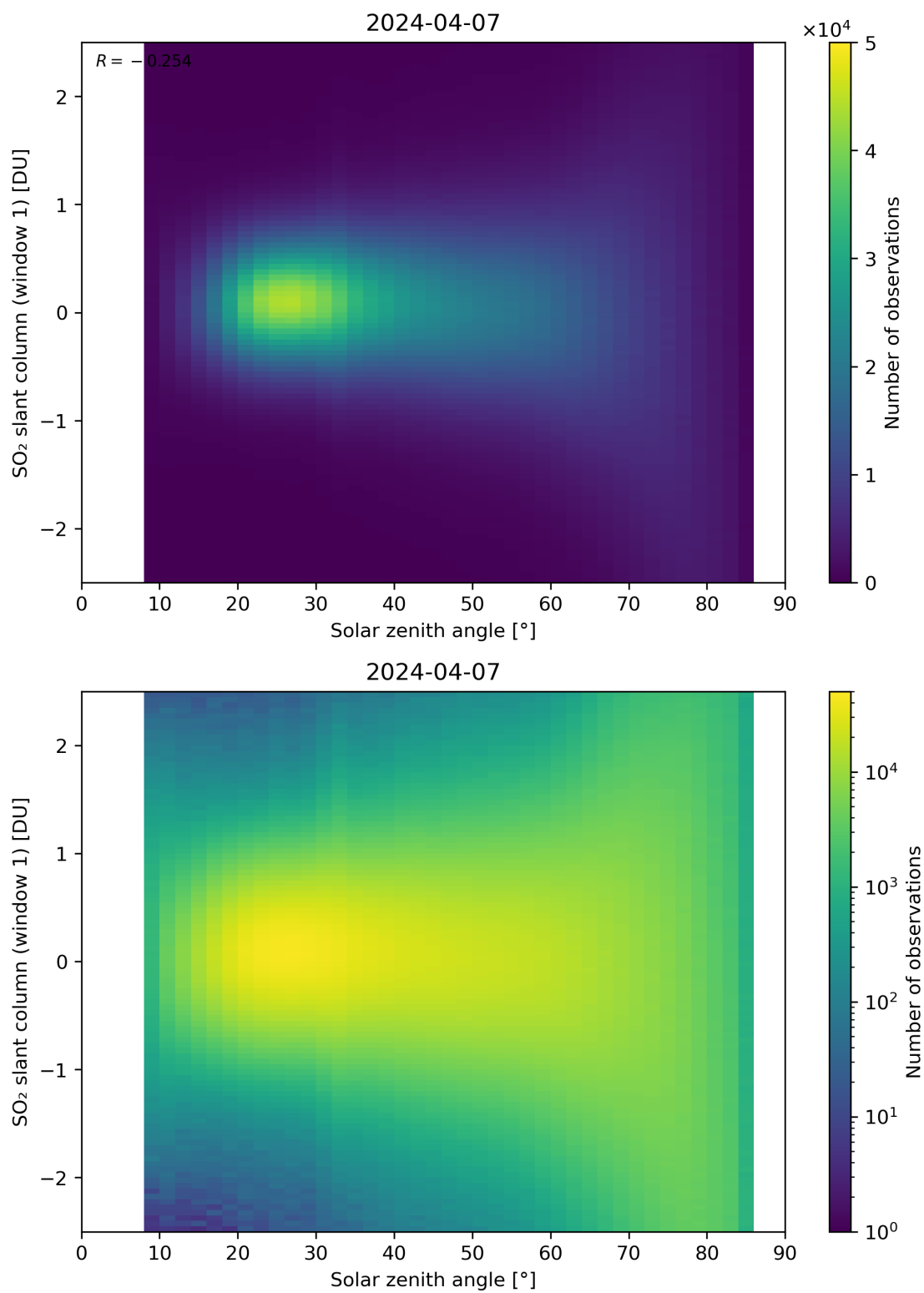
Figure 169: Scatter density plot of “Solar zenith angle” against “SO 2 slant column (window 1)” for 2024-04-06 to 2024-04-08.
