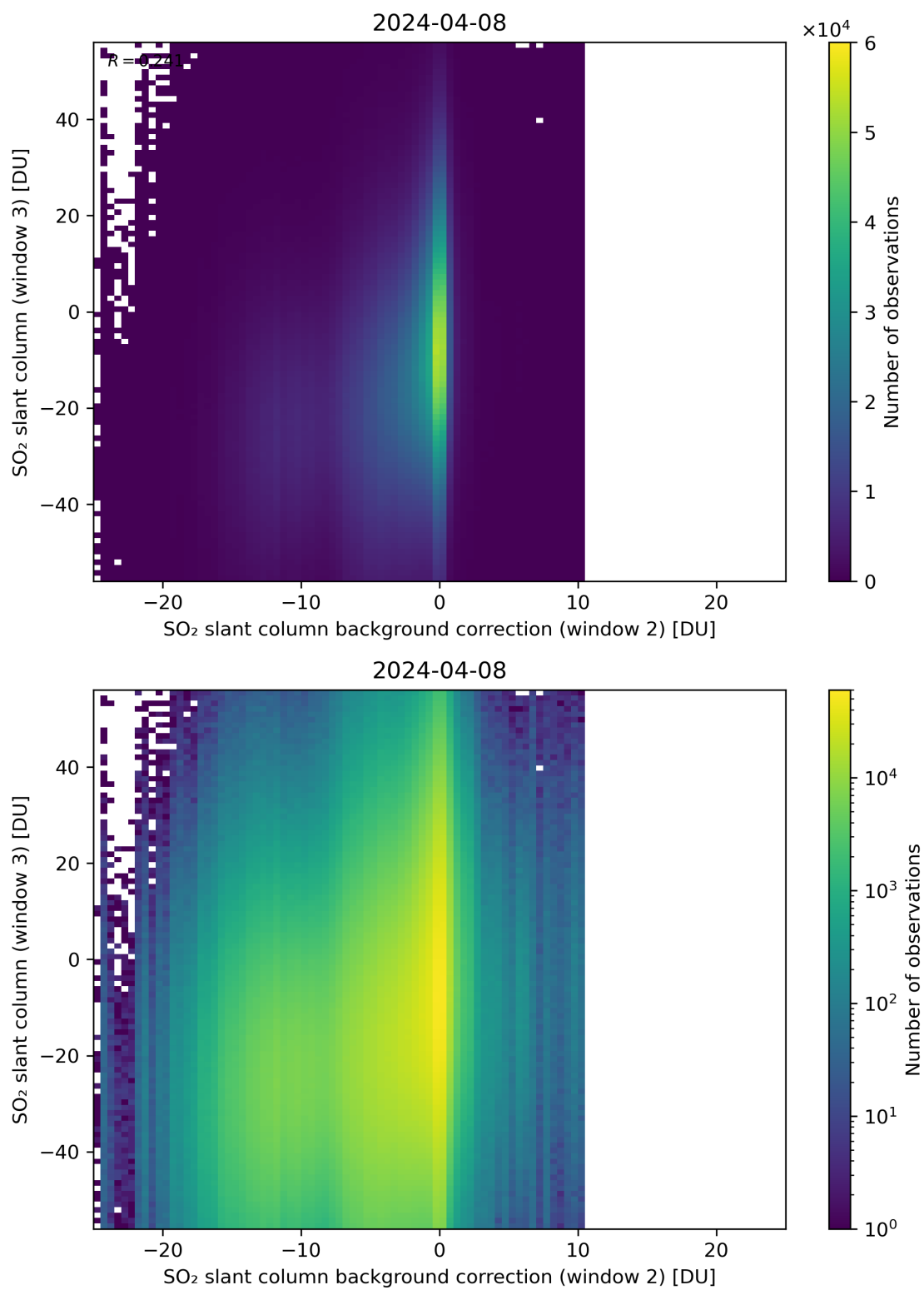
Figure 117: Scatter density plot of “SO 2 slant column background correction (window 2)” against “SO 2 slant column (window 3)” for 2024-04-07 to 2024-04-09.
