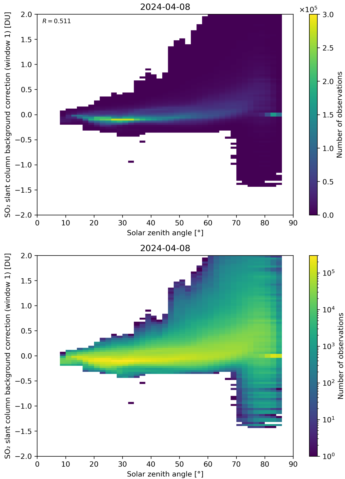
Figure 158: Scatter density plot of “Solar zenith angle” against “SO 2 slant column background correction (window 1)” for 2024-04-07 to 2024-04-09.
