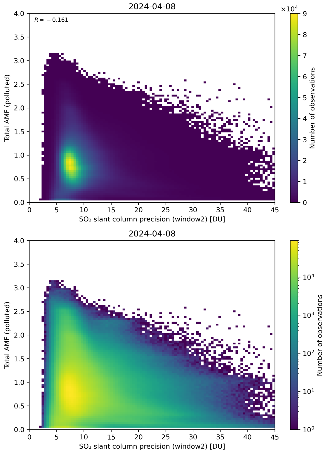
Figure 251: Scatter density plot of “SO 2 slant column precision (window2)” against “Total AMF (polluted)” for 2024-04-07 to 2024-04-09.
