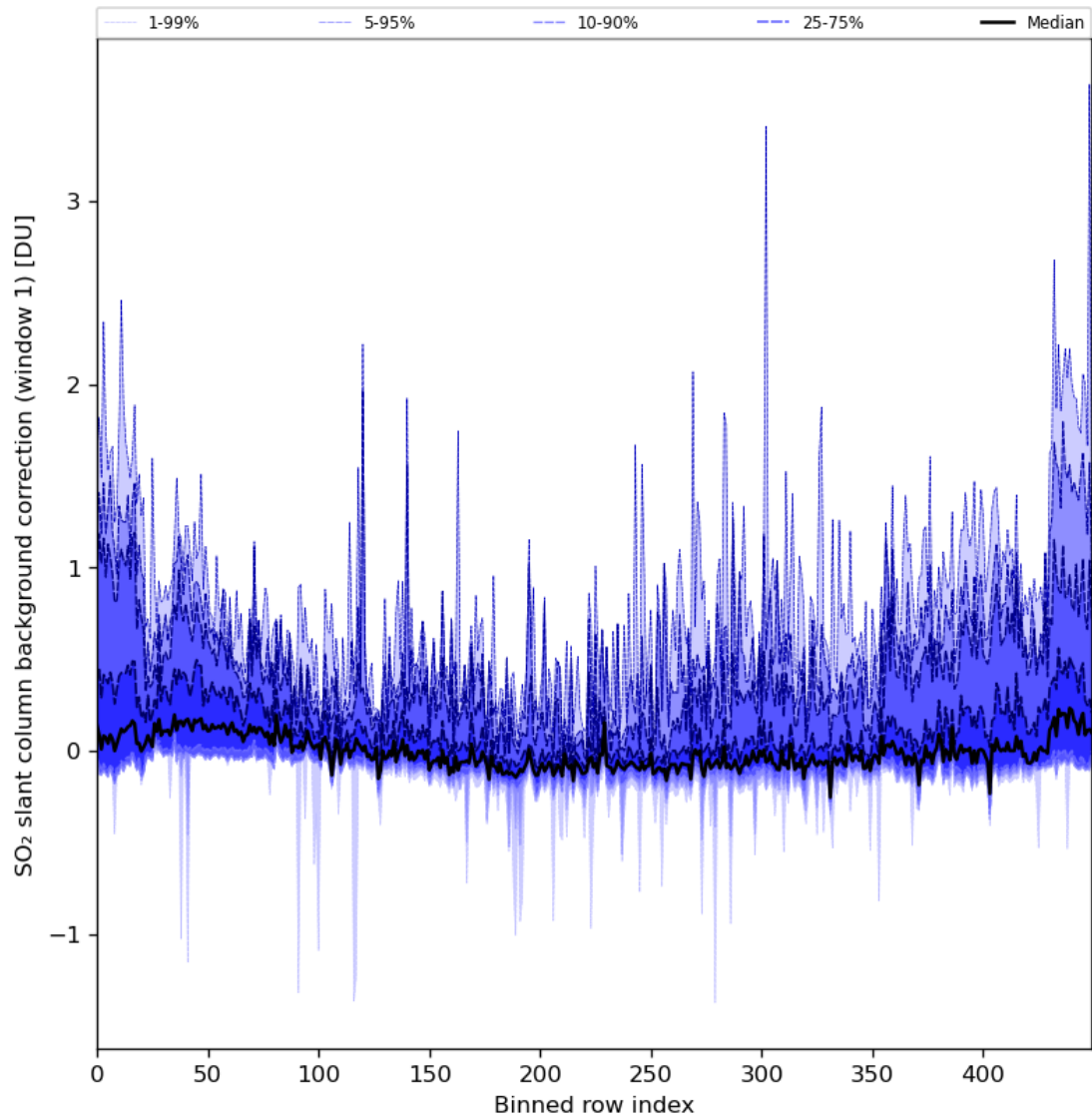
Figure 82: Along track statistics of “SO 2 slant column background correction (window 1)” for 2024-04-07 to 2024-04-09
