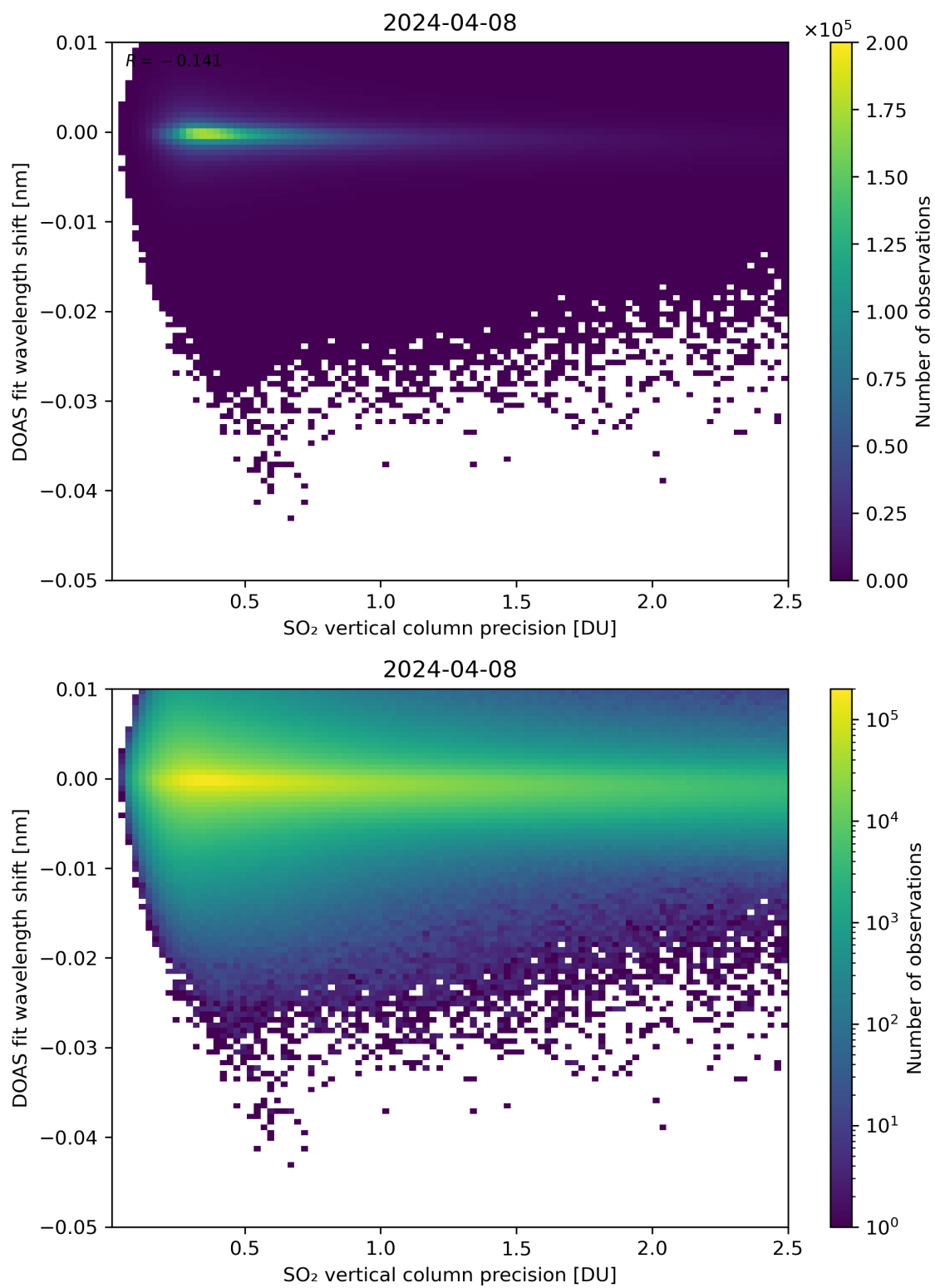
Figure 282: Scatter density plot of “SO 2 vertical column precision” against “DOAS fit wavelength shift” for 2024-04-07 to 2024-04-09.
