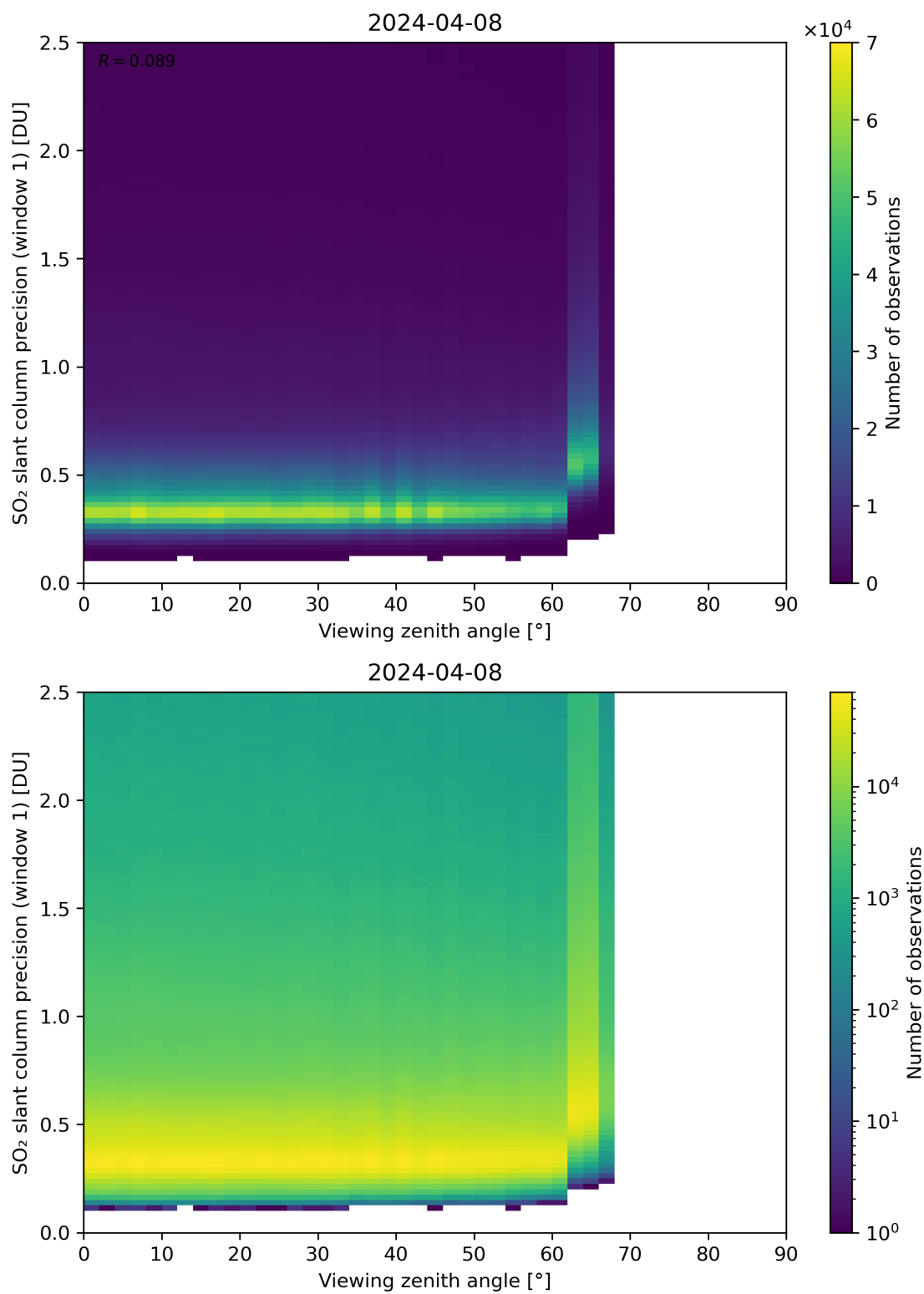
Figure 321: Scatter density plot of “Viewing zenith angle” against “SO 2 slant column precision (window 1)” for 2024-04-07 to 2024-04-09.
