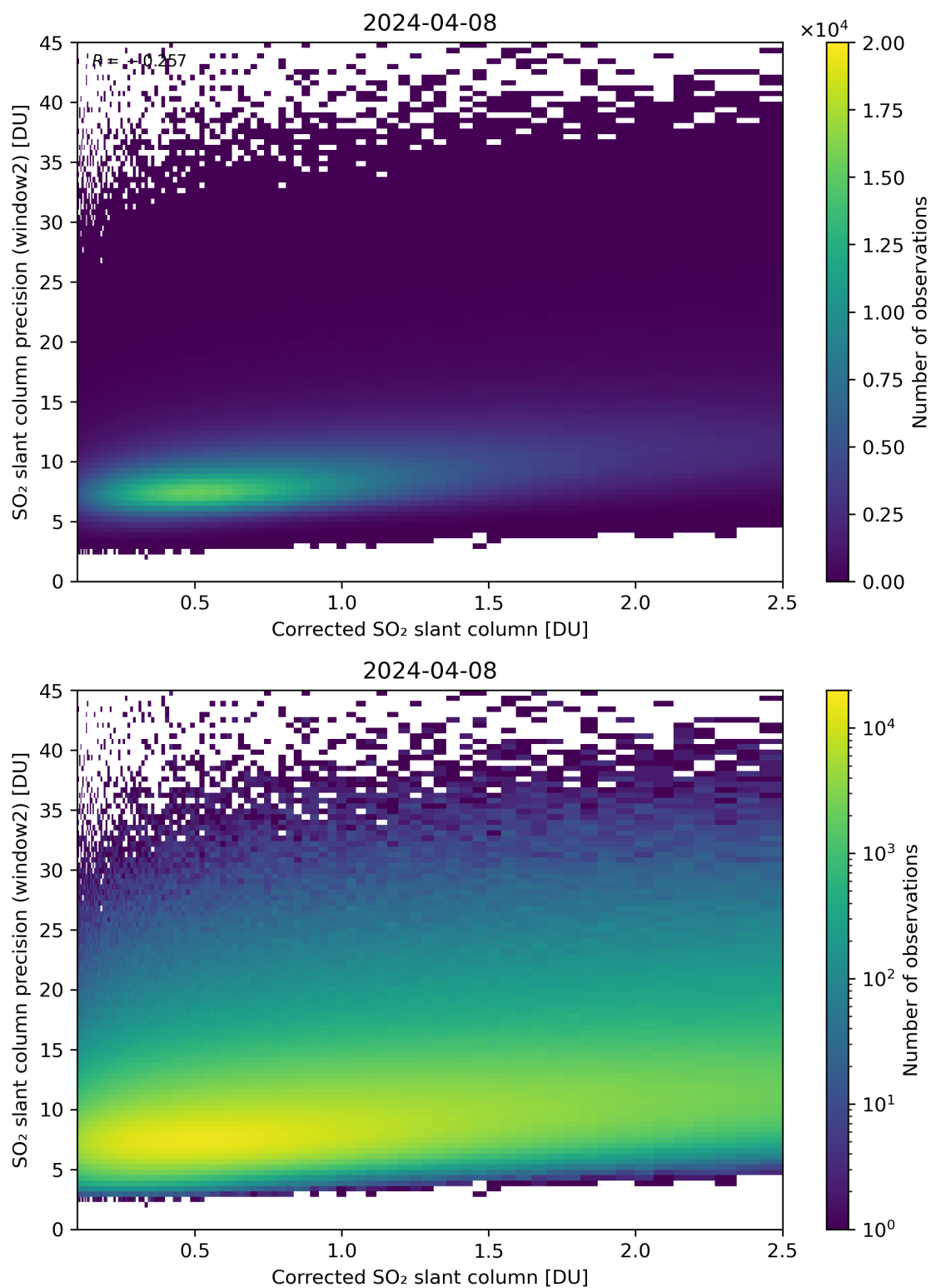
Figure 189: Scatter density plot of “Corrected SO 2 slant column” against “SO 2 slant column precision (window2)” for 2024-04-07 to 2024-04-09.
