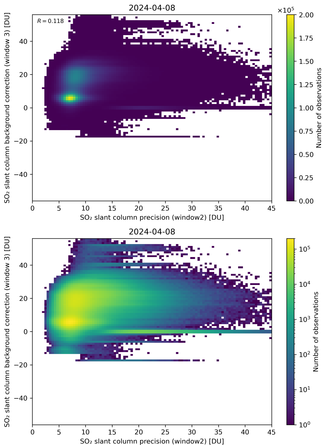
Figure 242: Scatter density plot of “SO 2 slant column precision (window2)” against “SO 2 slant column background correction (window 3)” for 2024-04-07 to 2024-04-09.
