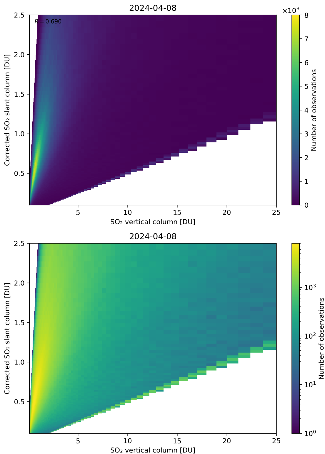
Figure 297: Scatter density plot of “SO 2 vertical column” against “Corrected SO 2 slant column” for 2024-04-07 to 2024-04-09.
