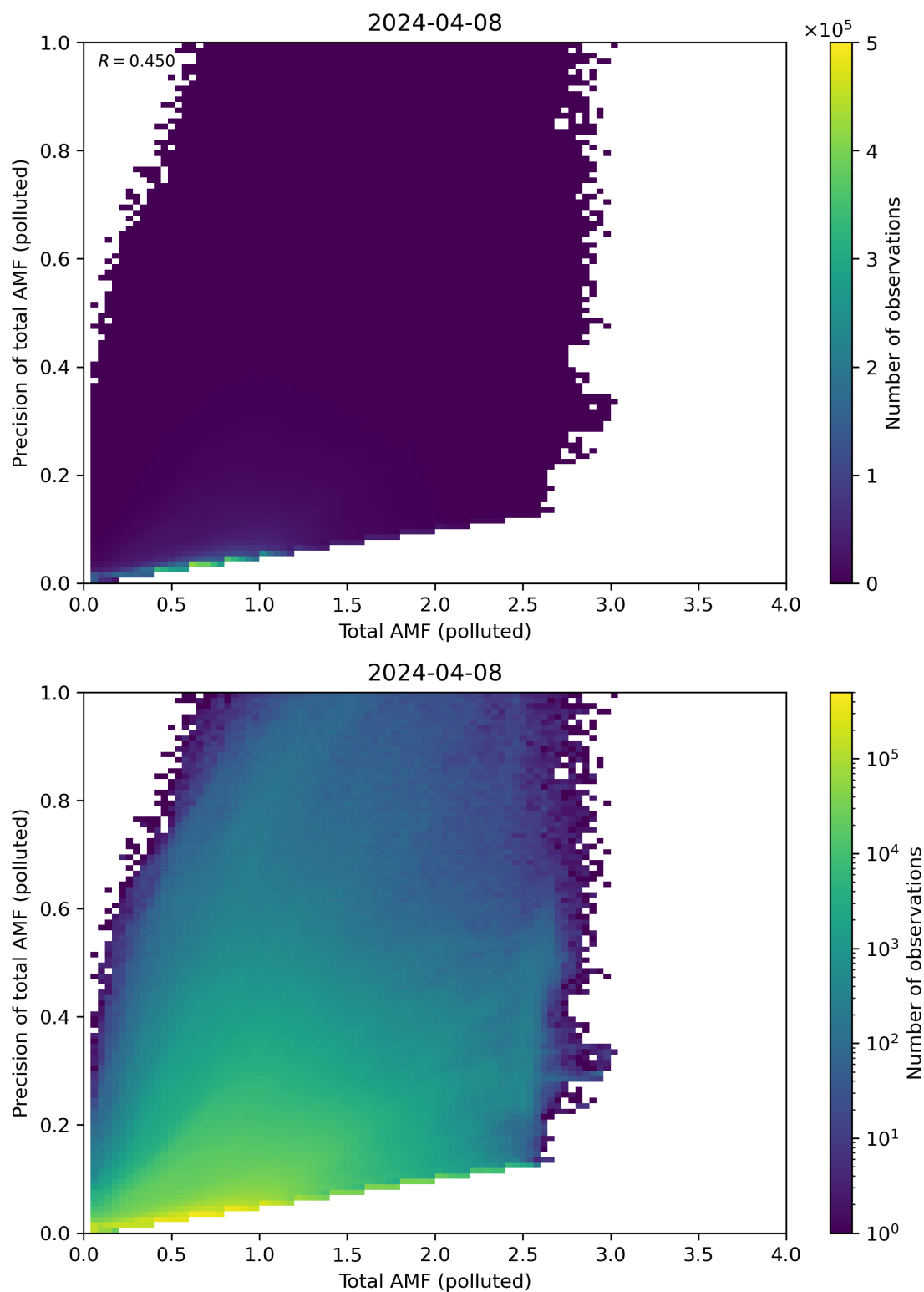
Figure 272: Scatter density plot of “Total AMF (polluted)” against “Precision of total AMF (polluted)” for 2024-04-07 to 2024-04-09.
