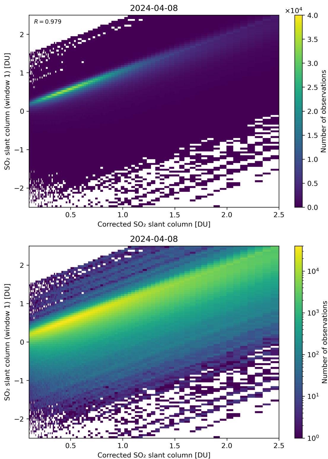
Figure 187: Scatter density plot of “Corrected SO 2 slant column” against “SO 2 slant column (window 1)” for 2024-04-07 to 2024-04-09.
