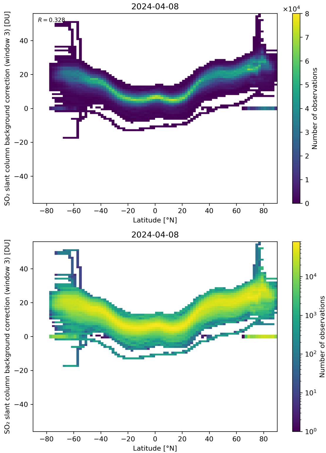
Figure 141: Scatter density plot of “Latitude” against “SO 2 slant column background correction (window 3)” for 2024-04-07 to 2024-04-09.
