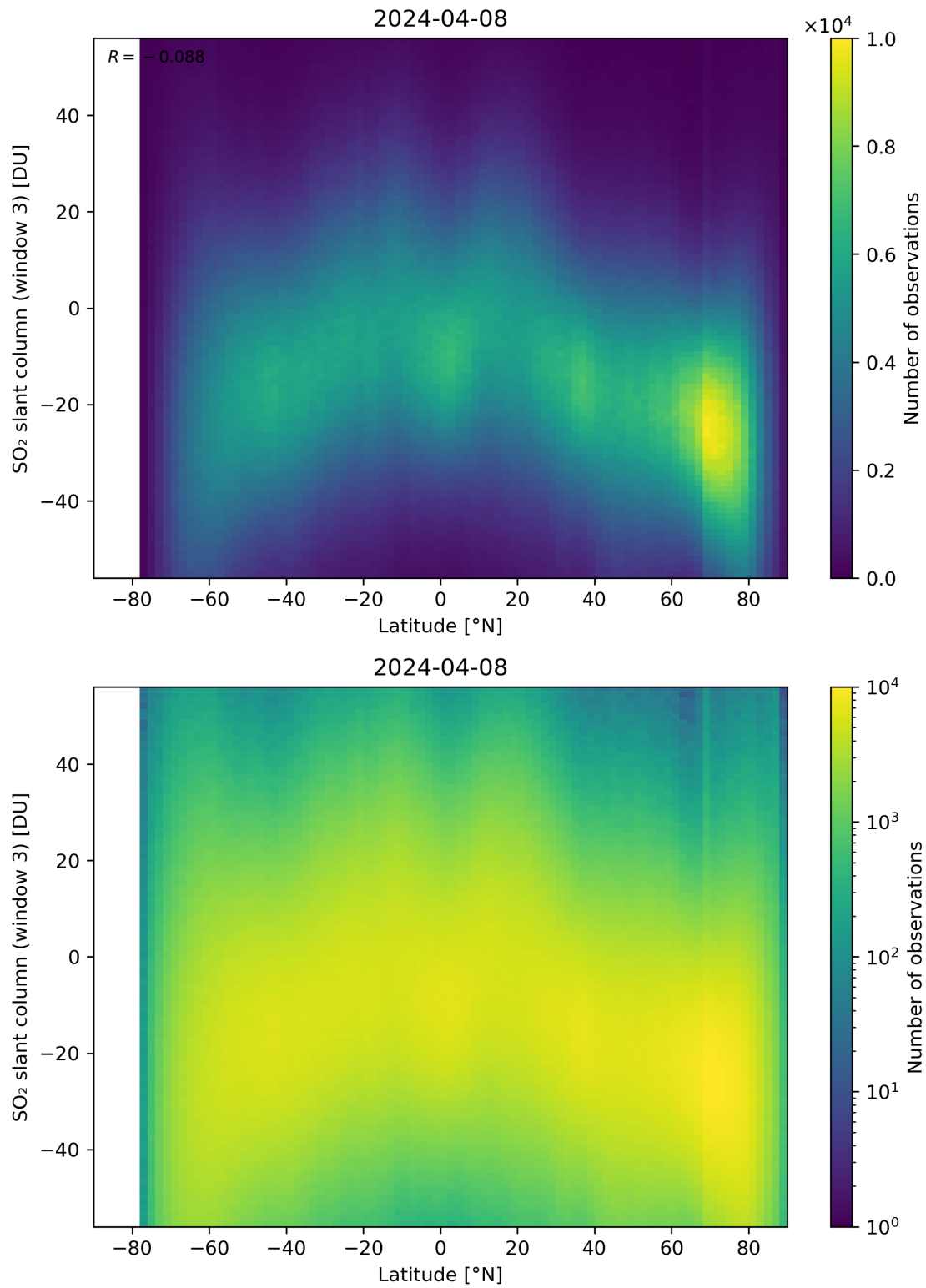
Figure 152: Scatter density plot of “Latitude” against “SO 2 slant column (window 3)” for 2024-04-07 to 2024-04-09.
