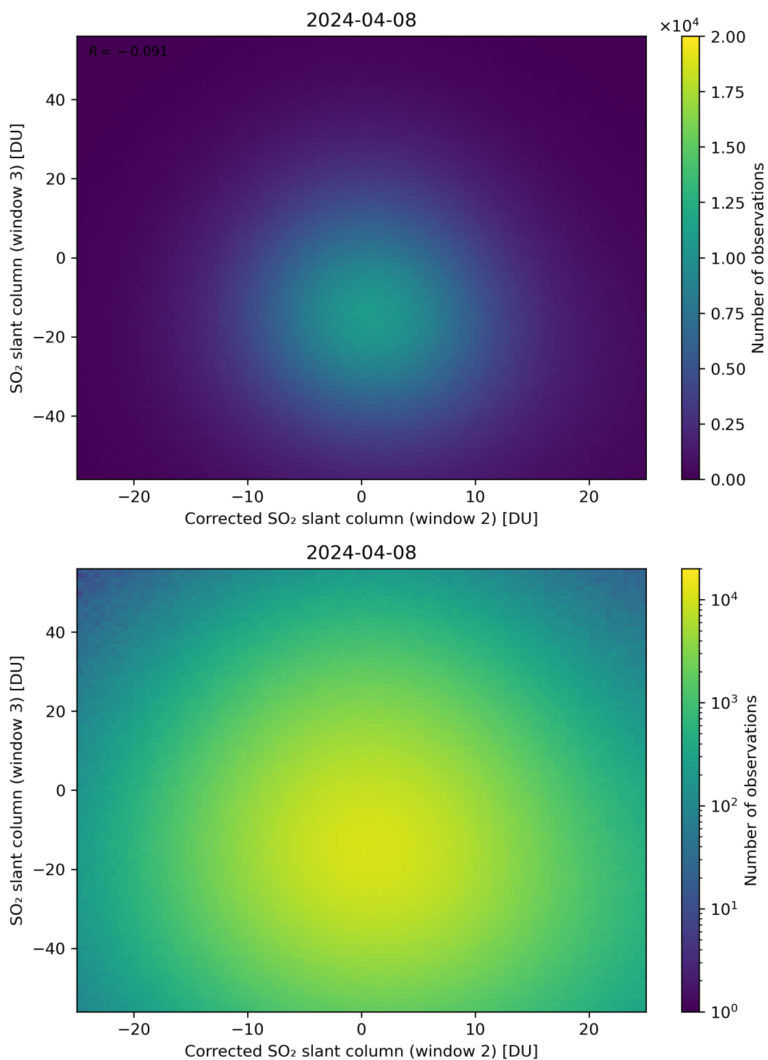
Figure 201: Scatter density plot of “Corrected SO 2 slant column (window 2)” against “SO 2 slant column (window 3)” for 2024-04-07 to 2024-04-09.
