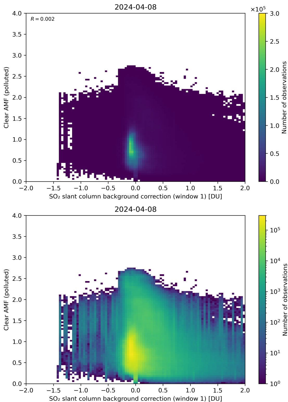
Figure 103: Scatter density plot of “SO 2 slant column background correction (window 1)” against “Clear AMF (polluted)” for 2024-04-07 to 2024-04-09.
