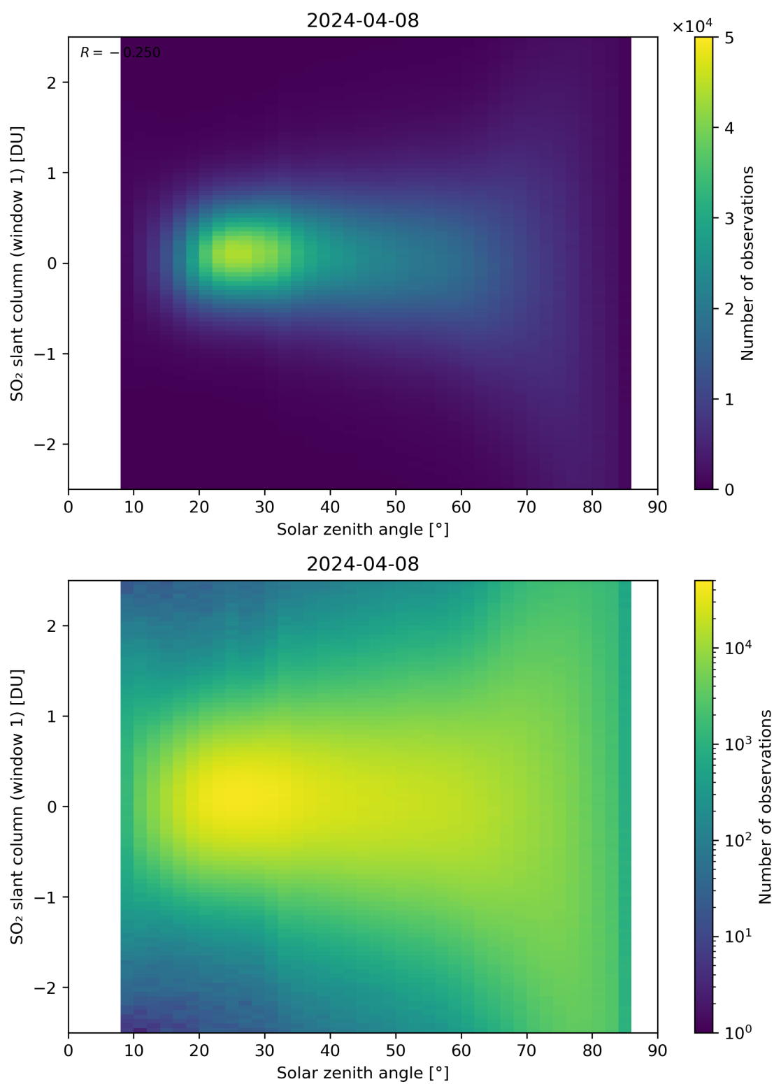
Figure 169: Scatter density plot of “Solar zenith angle” against “SO 2 slant column (window 1)” for 2024-04-07 to 2024-04-09.
