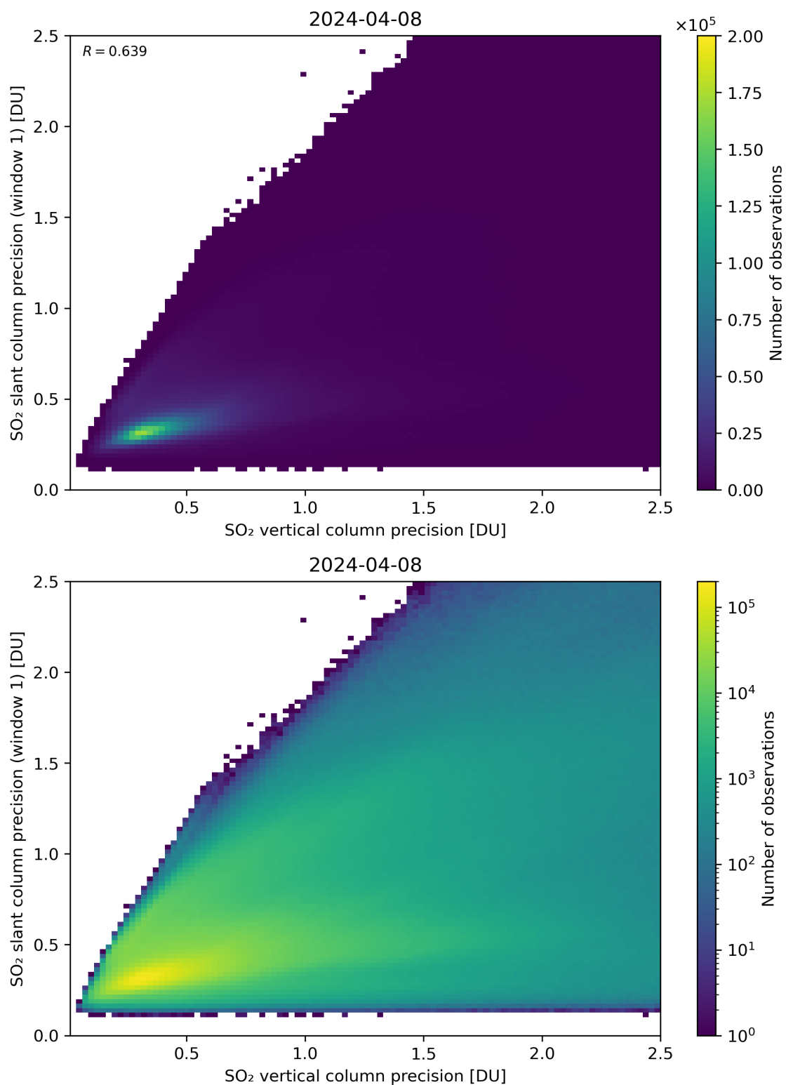
Figure 290: Scatter density plot of “SO 2 vertical column precision” against “SO 2 slant column precision (window 1)” for 2024-04-07 to 2024-04-09.
