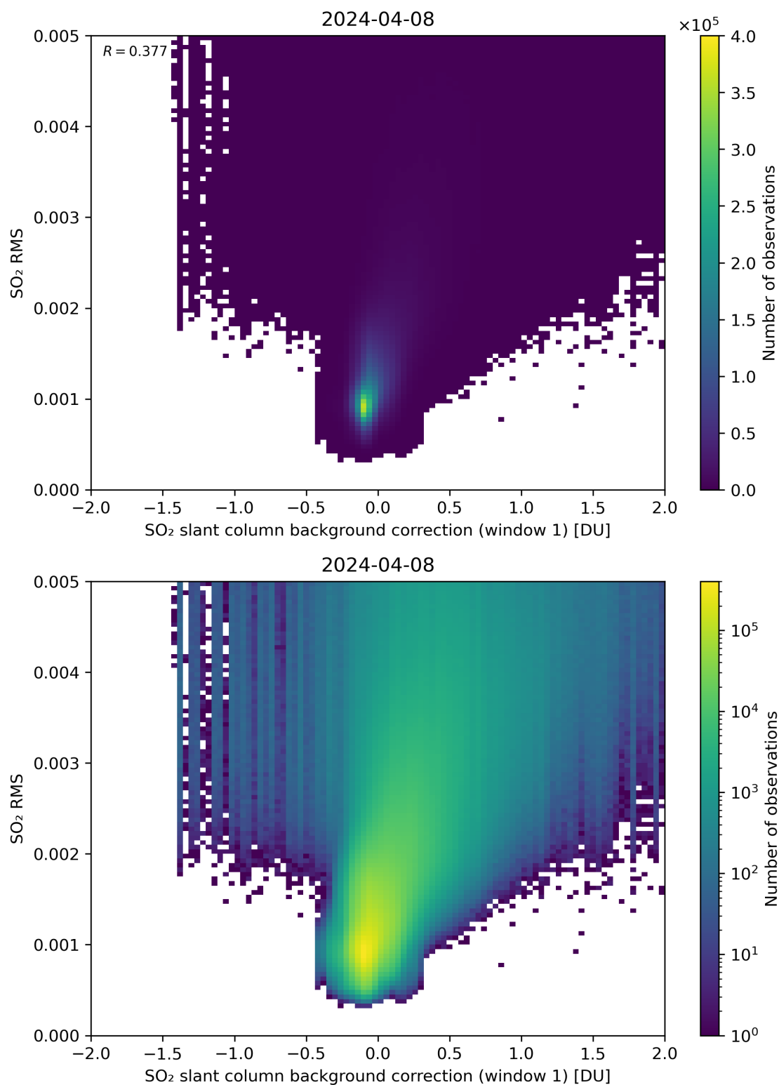
Figure 102: Scatter density plot of “SO 2 slant column background correction (window 1)” against “SO 2 RMS” for 2024-04-07 to 2024-04-09.
