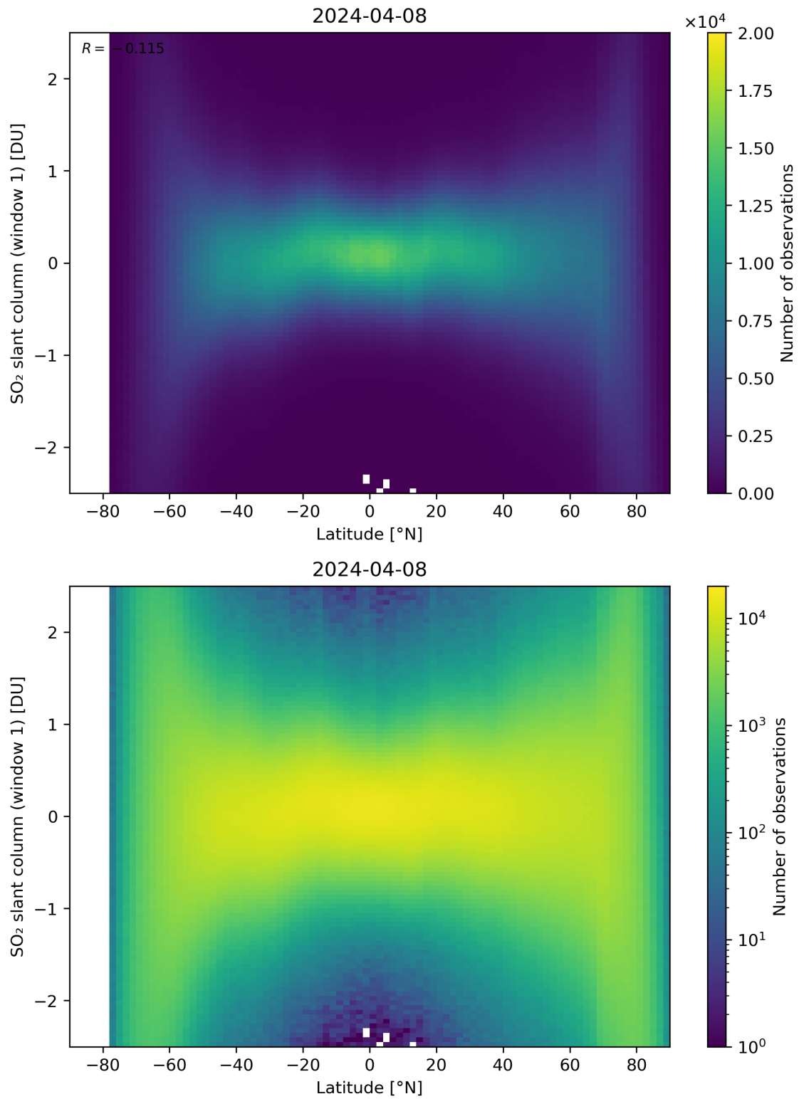
Figure 149: Scatter density plot of “Latitude” against “SO 2 slant column (window 1)” for 2024-04-07 to 2024-04-09.
