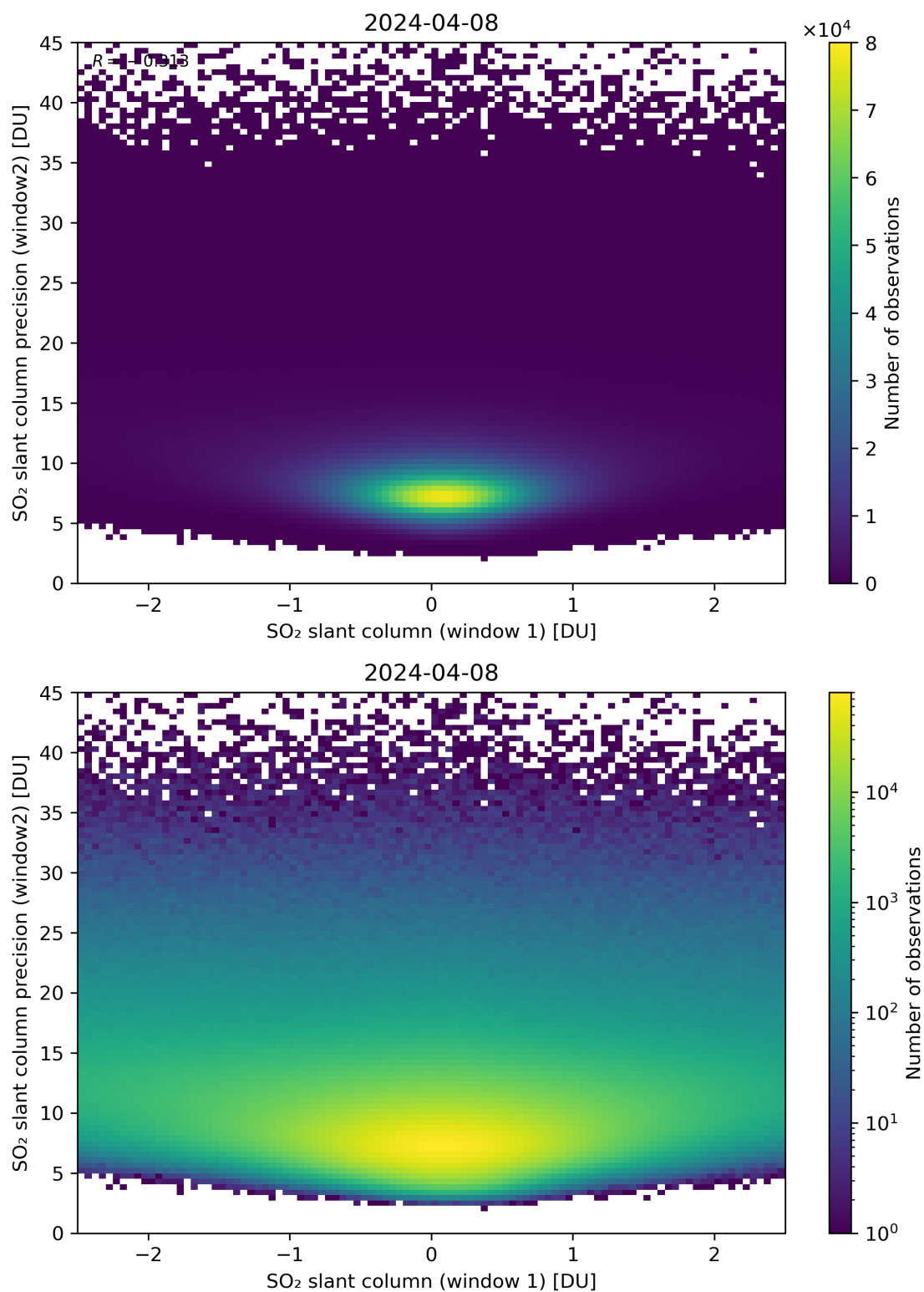
Figure 236: Scatter density plot of “SO 2 slant column (window 1)” against “SO 2 slant column precision (window2)” for 2024-04-07 to 2024-04-09.
