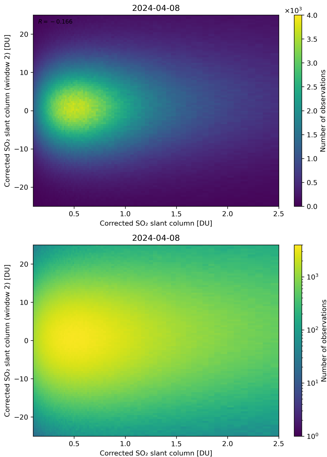
Figure 185: Scatter density plot of “Corrected SO 2 slant column” against “Corrected SO 2 slant column (window 2)” for 2024-04-07 to 2024-04-09.
