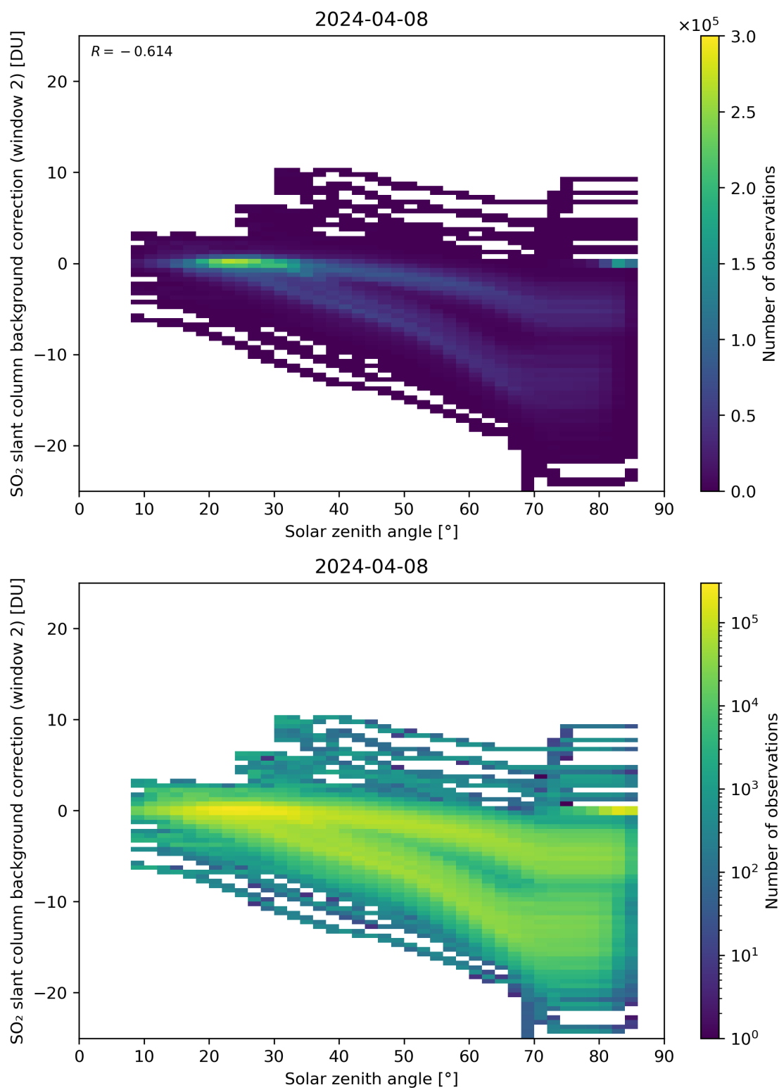
Figure 159: Scatter density plot of “Solar zenith angle” against “SO 2 slant column background correction (window 2)” for 2024-04-07 to 2024-04-09.
