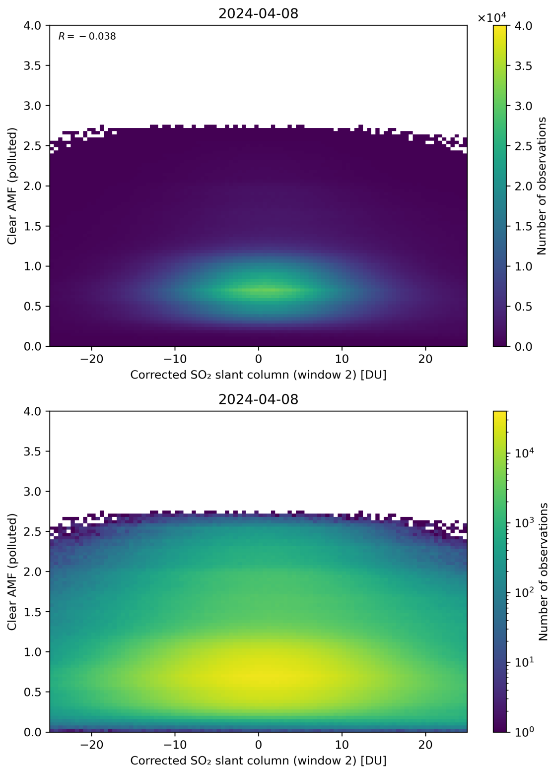
Figure 199: Scatter density plot of “Corrected SO 2 slant column (window 2)” against “Clear AMF (polluted)” for 2024-04-07 to 2024-04-09.
