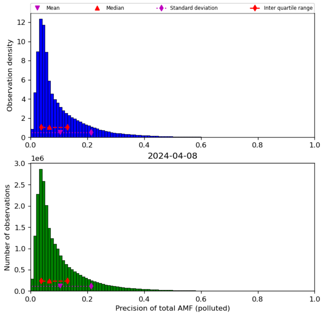
Figure 72: Histogram of “Precision of total AMF (polluted)” for 2024-04-07 to 2024-04-09
