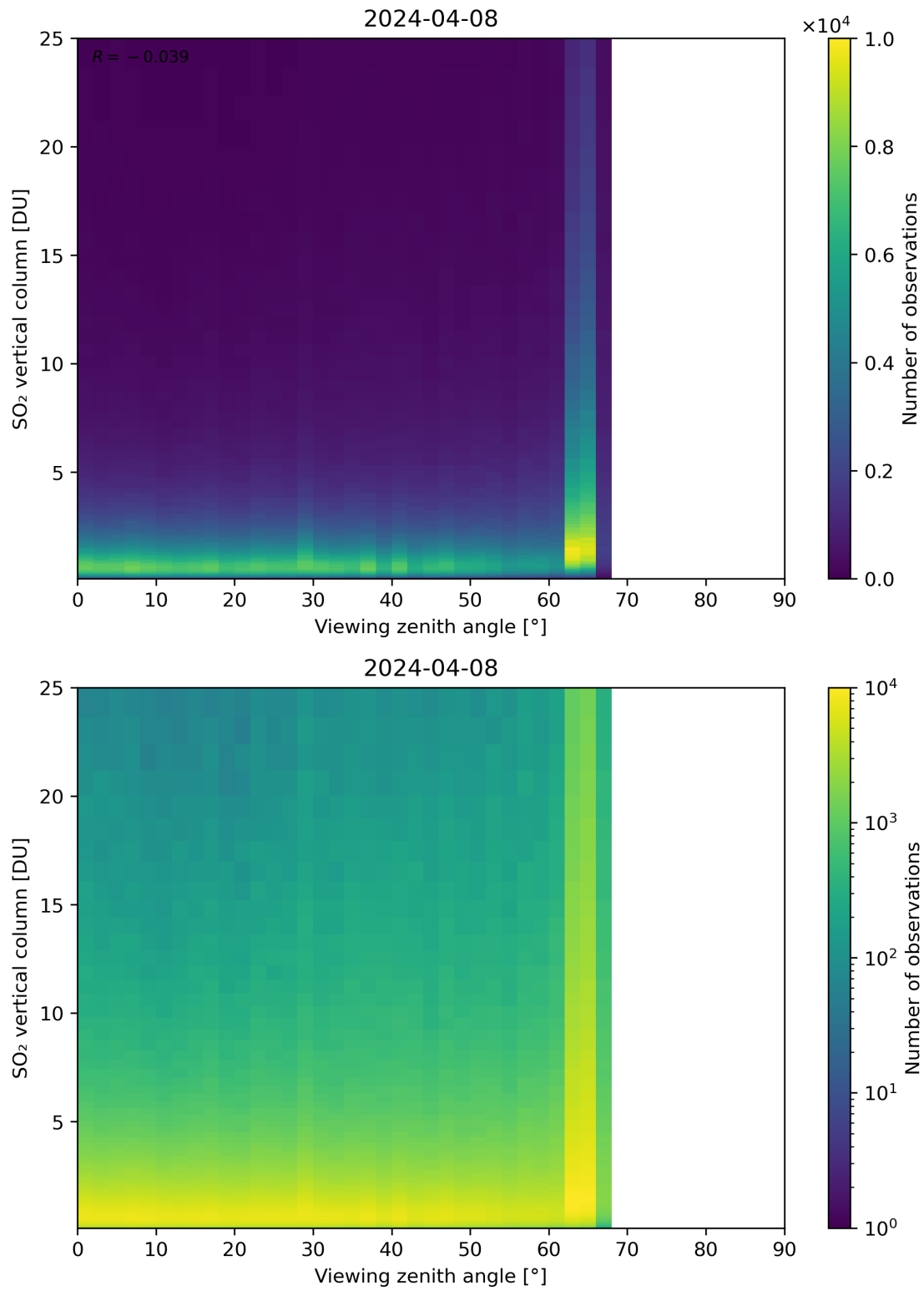
Figure 327: Scatter density plot of “Viewing zenith angle” against “SO 2 vertical column” for 2024-04-07 to 2024-04-09.
