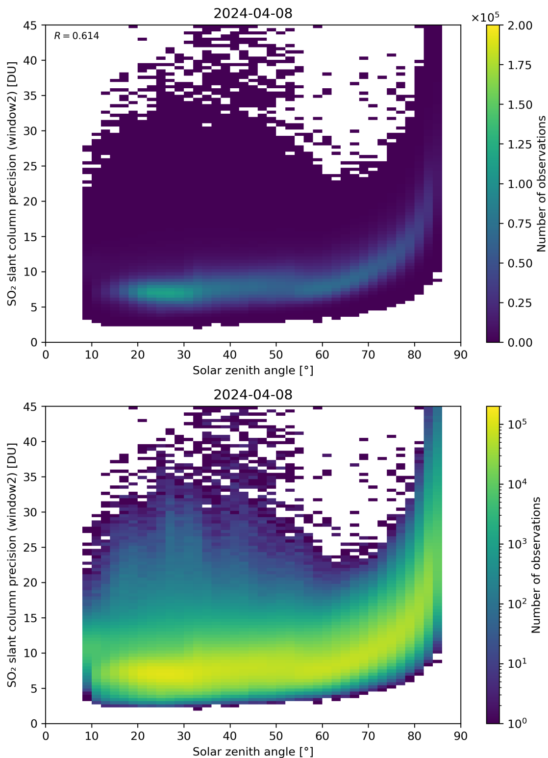
Figure 171: Scatter density plot of “Solar zenith angle” against “SO 2 slant column precision (window2)” for 2024-04-07 to 2024-04-09.
