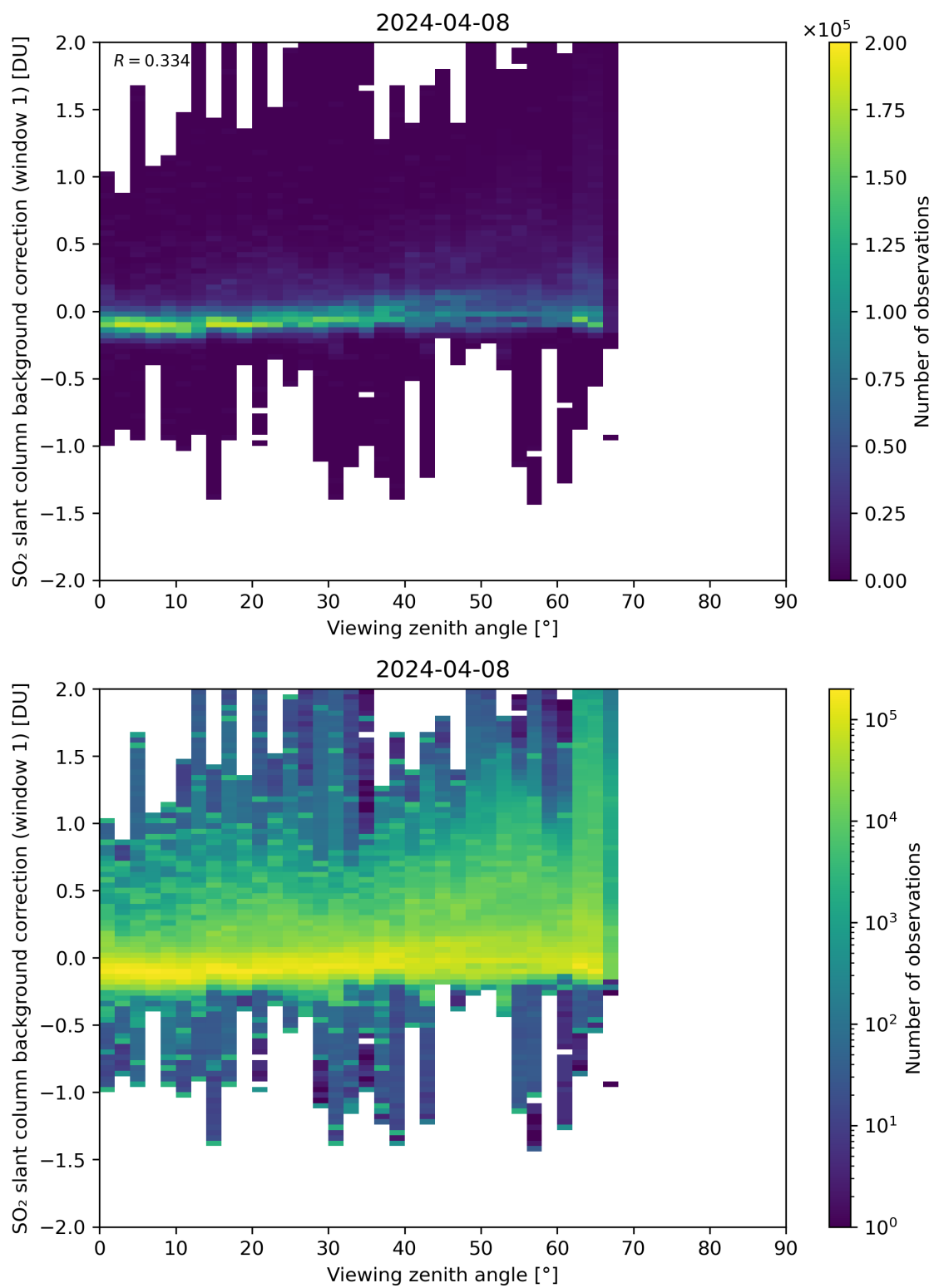
Figure 308: Scatter density plot of “Viewing zenith angle” against “SO 2 slant column background correction (window 1)” for 2024-04-07 to 2024-04-09.
