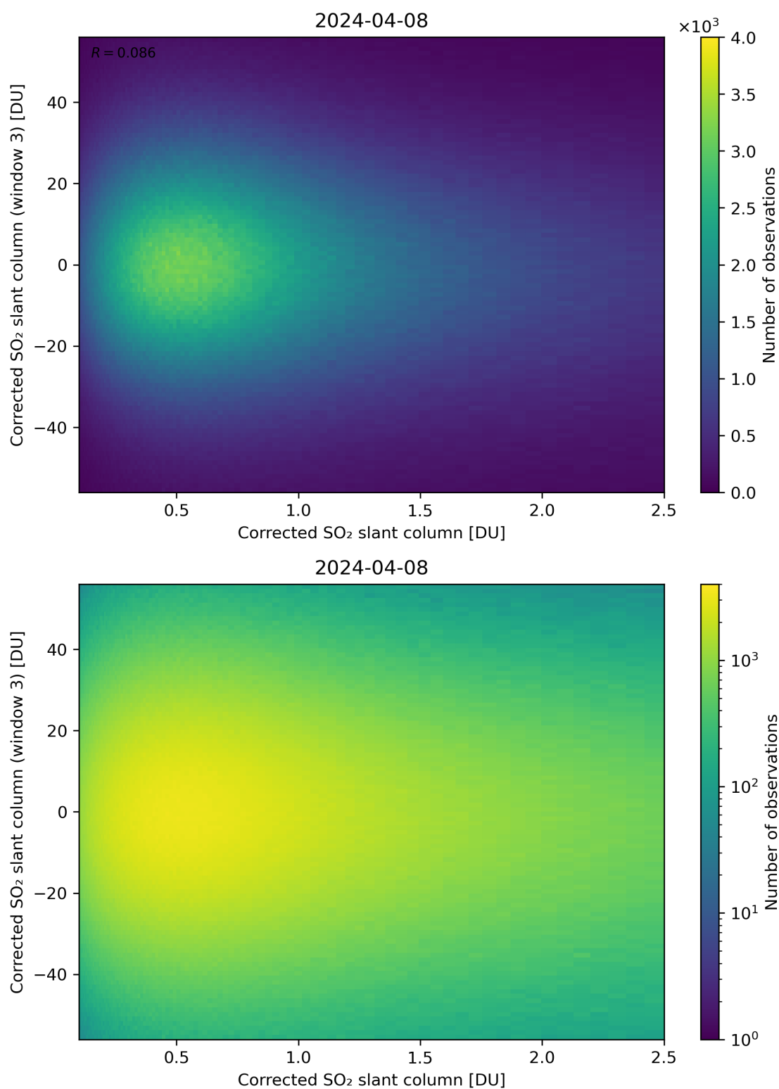
Figure 186: Scatter density plot of “Corrected SO 2 slant column” against “Corrected SO 2 slant column (window 3)” for 2024-04-07 to 2024-04-09.
