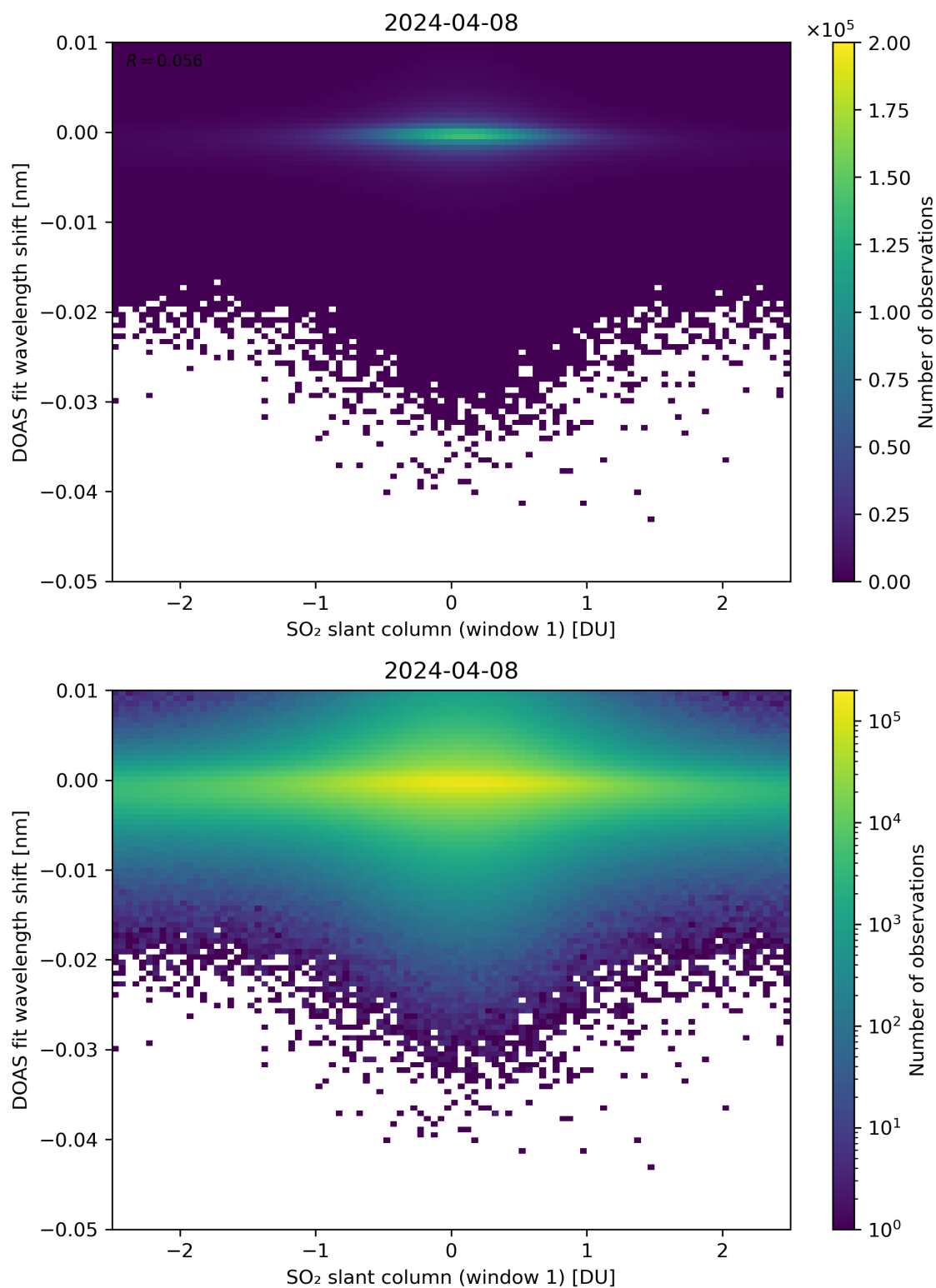
Figure 215: Scatter density plot of “SO 2 slant column (window 1)” against “DOAS fit wavelength shift” for 2024-04-07 to 2024-04-09.
