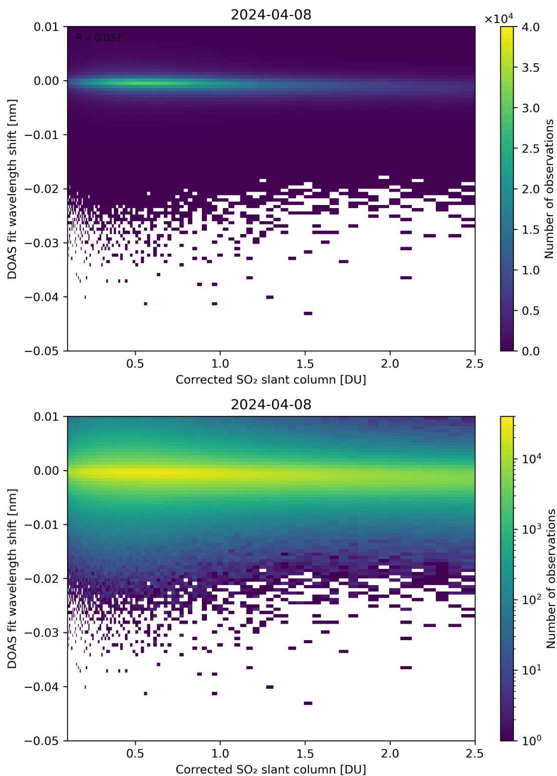
Figure 181: Scatter density plot of “Corrected SO 2 slant column” against “DOAS fit wavelength shift” for 2024-04-07 to 2024-04-09.
