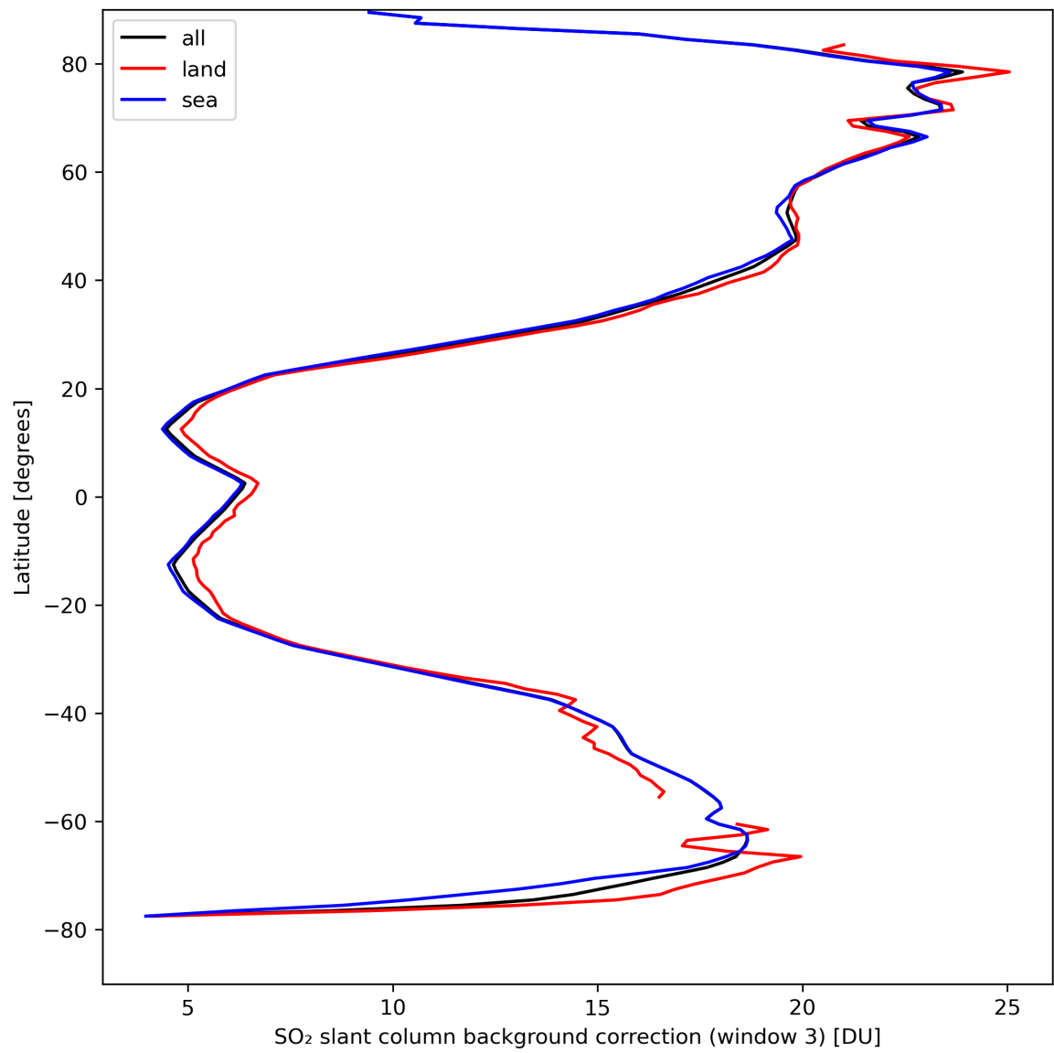
Figure 44: Zonal average of “SO 2 slant column background correction (window 3)” for 2024-04-07 to 2024-04-09.
