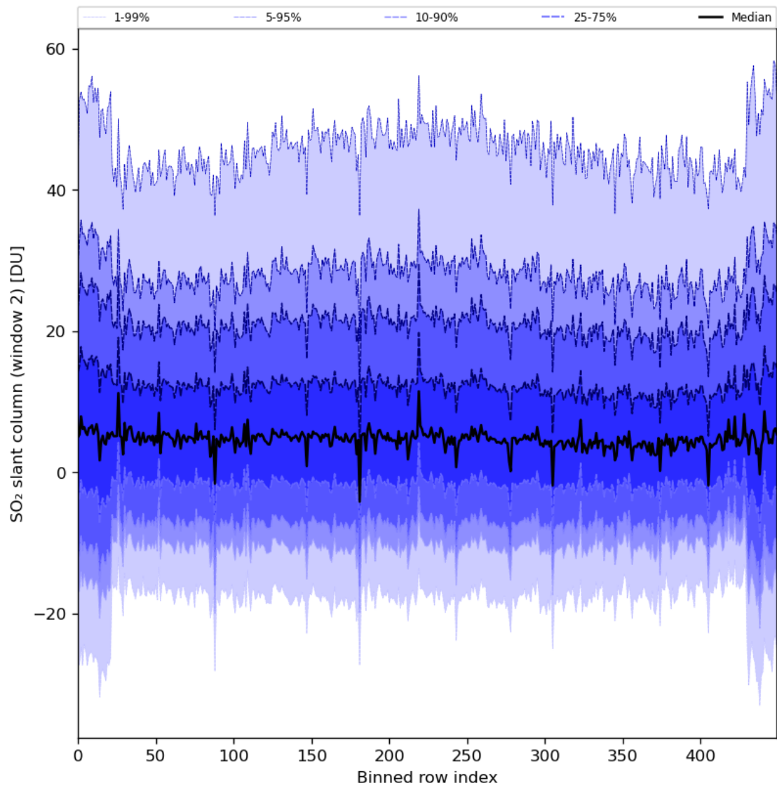
Figure 83: Along track statistics of “SO 2 slant column (window 2)” for 2024-04-07 to 2024-04-09
