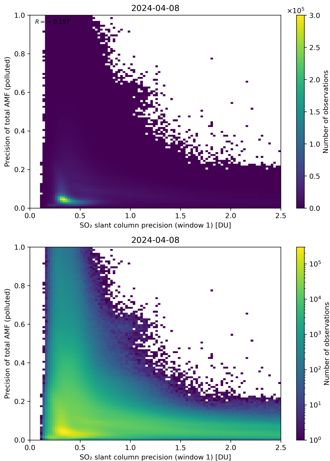
Figure 231: Scatter density plot of “SO 2 slant column precision (window 1)” against “Precision of total AMF (polluted)” for 2024-04-07 to 2024-04-09.
