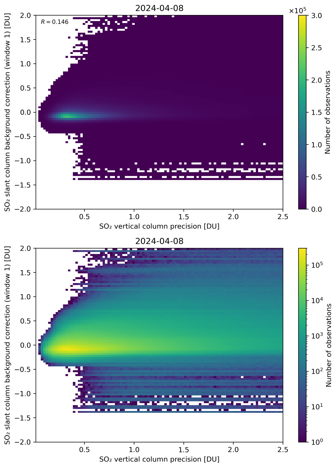
Figure 279: Scatter density plot of “SO 2 vertical column precision” against “SO 2 slant column background correction (window 1)” for 2024-04-07 to 2024-04-09.
