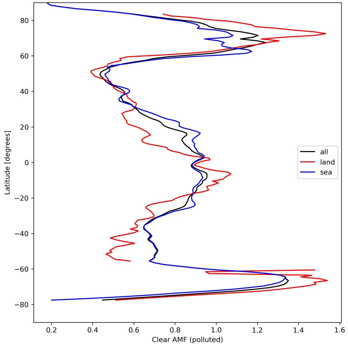
Figure 50: Zonal average of “Clear AMF (polluted)” for 2024-04-07 to 2024-04-09.
