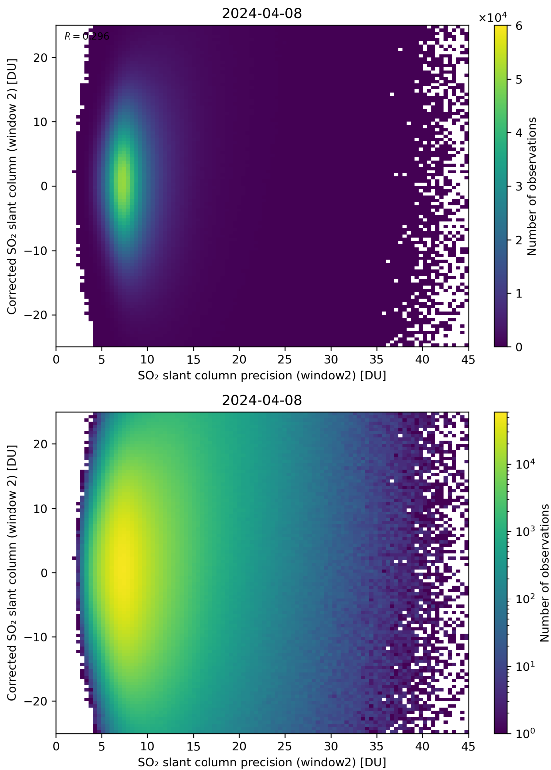
Figure 247: Scatter density plot of “SO 2 slant column precision (window2)” against “Corrected SO 2 slant column (window 2)” for 2024-04-07 to 2024-04-09.
