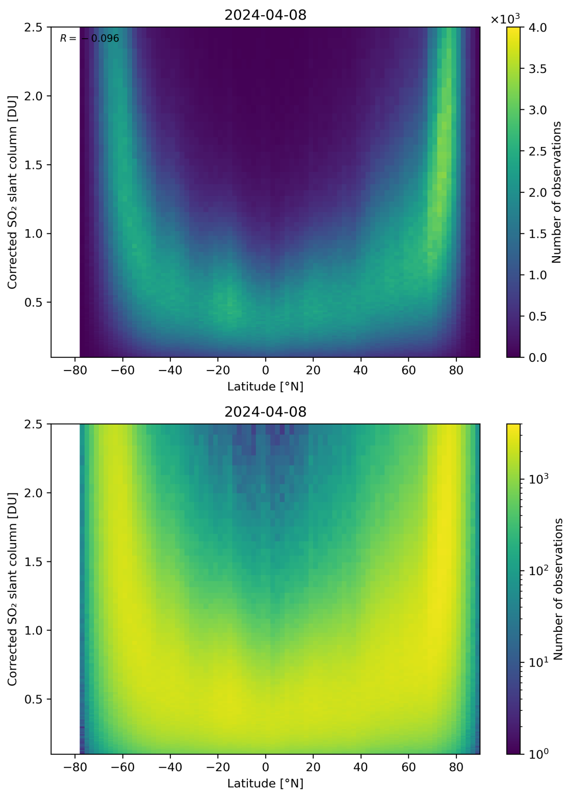
Figure 146: Scatter density plot of “Latitude” against “Corrected SO 2 slant column” for 2024-04-07 to 2024-04-09.
