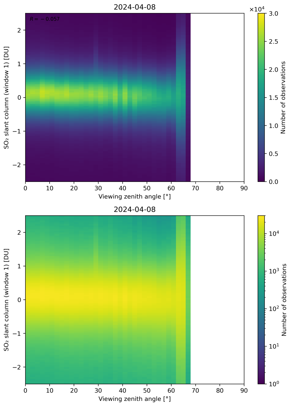
Figure 320: Scatter density plot of “Viewing zenith angle” against “SO 2 slant column (window 1)” for 2024-04-07 to 2024-04-09.
