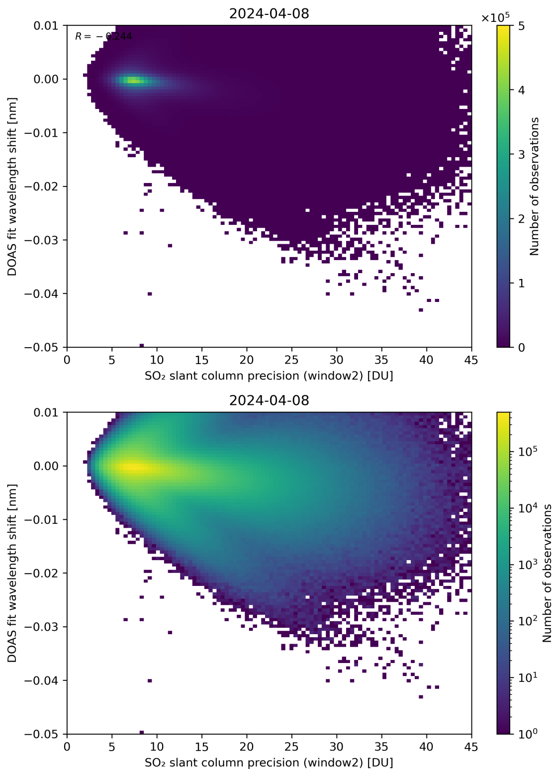
Figure 243: Scatter density plot of “SO 2 slant column precision (window2)” against “DOAS fit wavelength shift” for 2024-04-07 to 2024-04-09.
