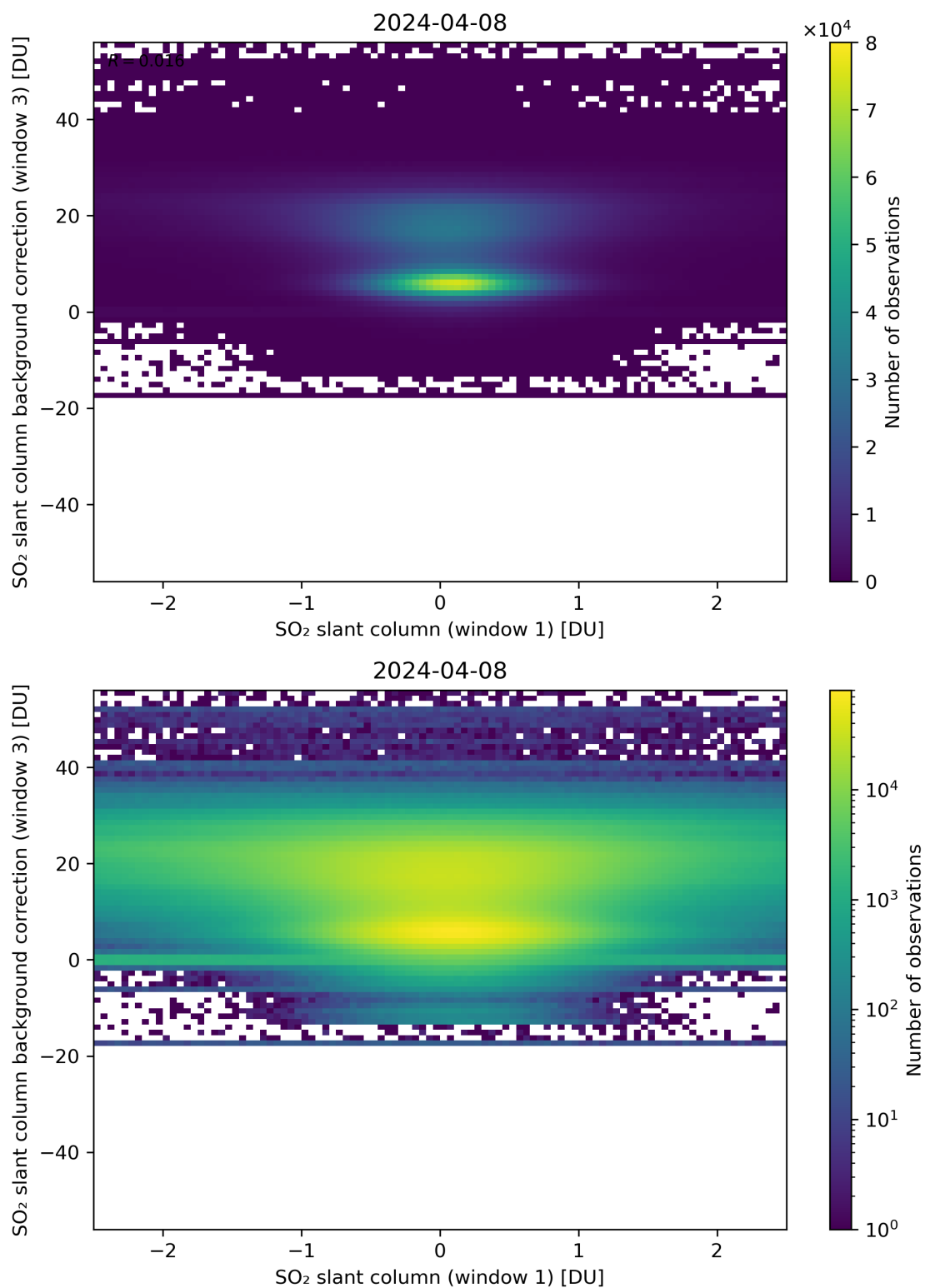
Figure 214: Scatter density plot of “SO 2 slant column (window 1)” against “SO 2 slant column background correction (window 3)” for 2024-04-07 to 2024-04-09.
