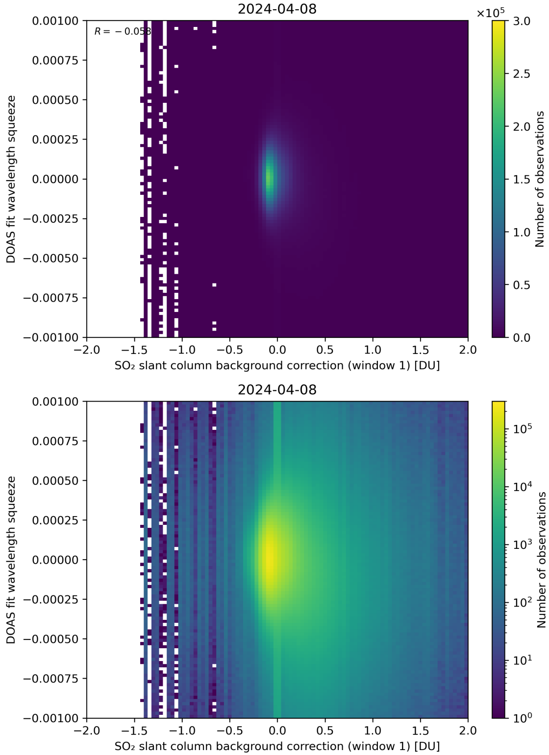
Figure 101: Scatter density plot of “SO 2 slant column background correction (window 1)” against “DOAS fit wavelength squeeze” for 2024-04-07 to 2024-04-09.
