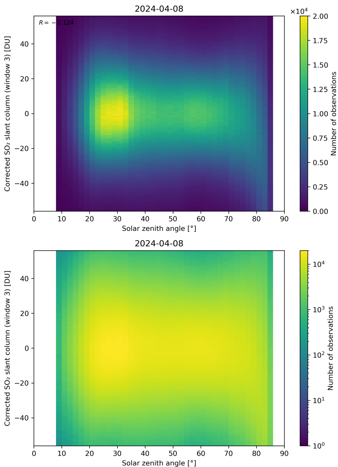
Figure 168: Scatter density plot of “Solar zenith angle” against “Corrected SO 2 slant column (window 3)” for 2024-04-07 to 2024-04-09.
