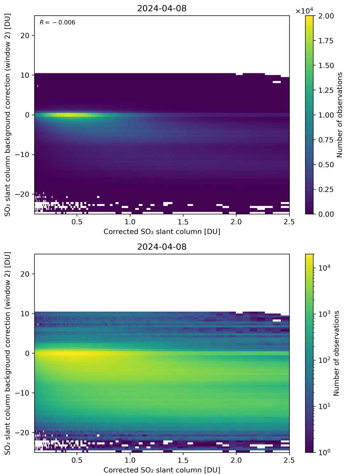
Figure 179: Scatter density plot of “Corrected SO 2 slant column” against “SO 2 slant column background correction (window 2)” for 2024-04-07 to 2024-04-09.
