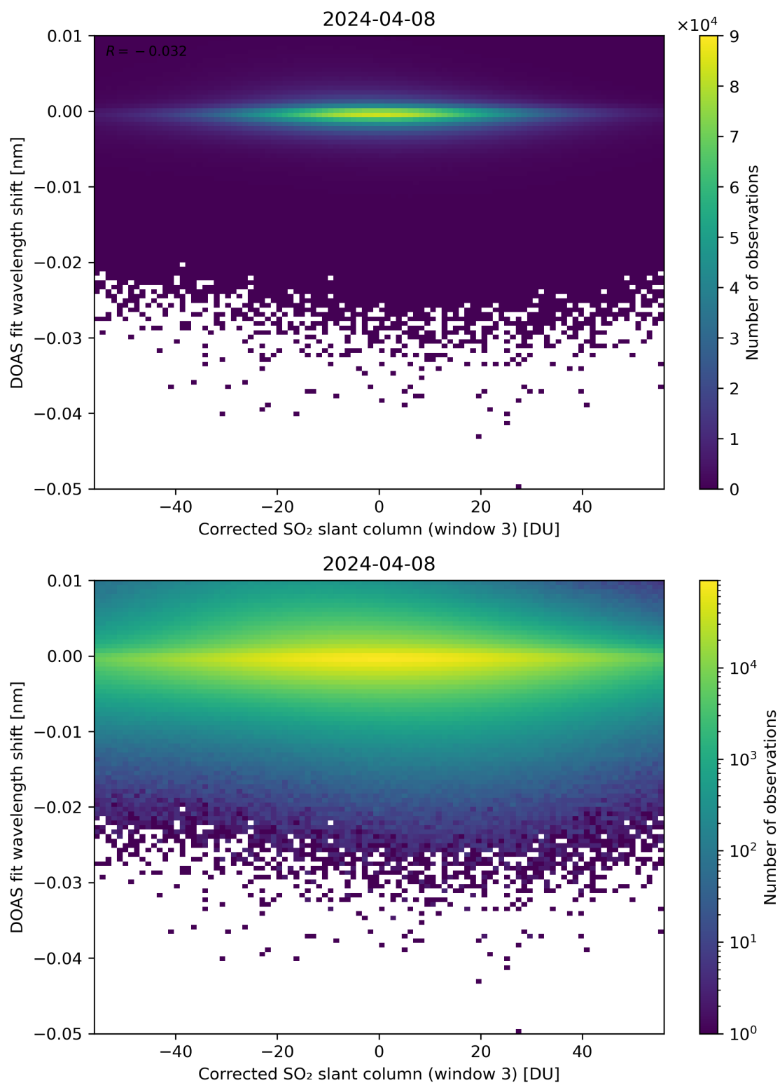
Figure 206: Scatter density plot of “Corrected SO 2 slant column (window 3)” against “DOAS fit wavelength shift” for 2024-04-07 to 2024-04-09.
