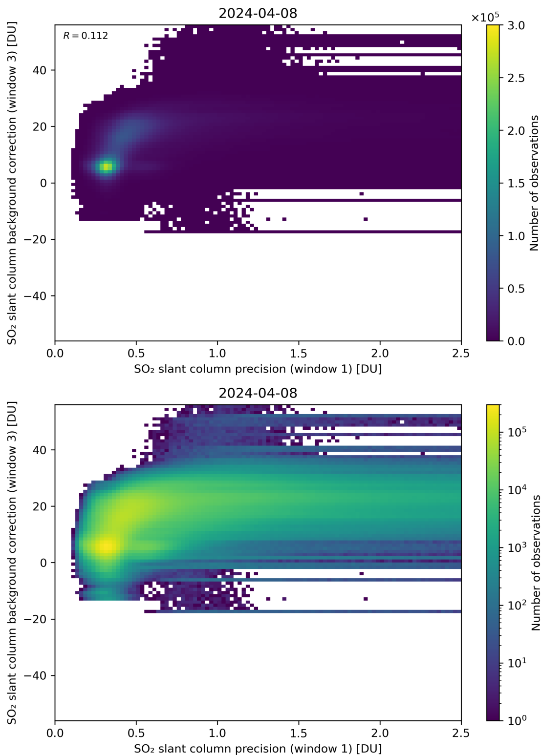
Figure 220: Scatter density plot of “SO 2 slant column precision (window 1)” against “SO 2 slant column background correction (window 3)” for 2024-04-07 to 2024-04-09.
