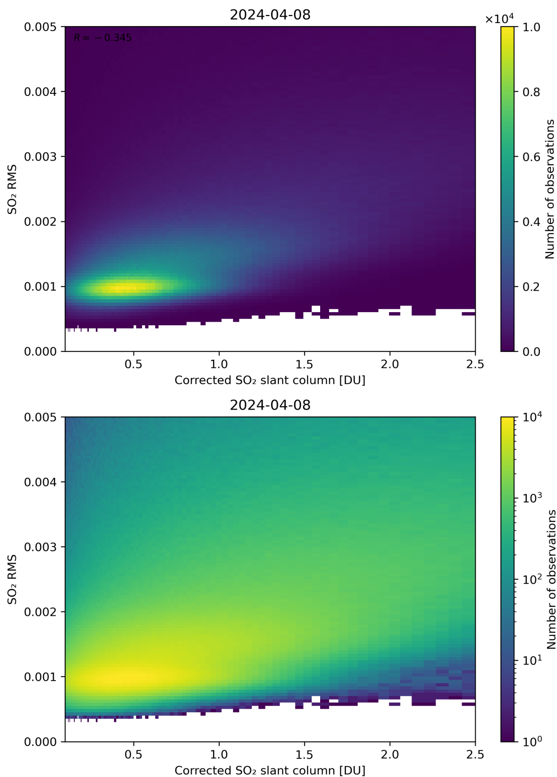
Figure 183: Scatter density plot of “Corrected SO 2 slant column” against “SO 2 RMS” for 2024-04-07 to 2024-04-09.
