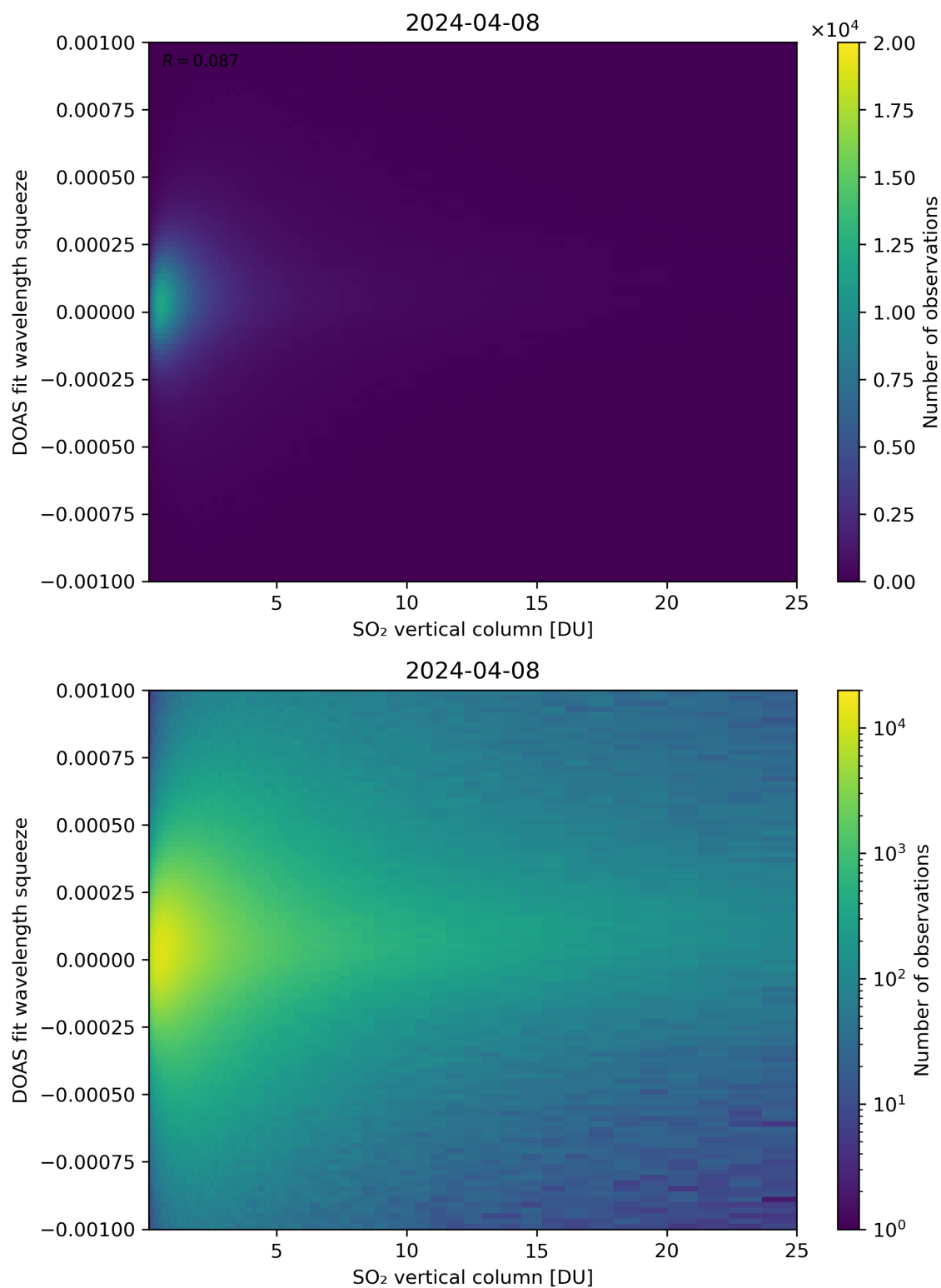
Figure 277: Scatter density plot of “SO 2 vertical column” against “DOAS fit wavelength squeeze” for 2024-04-07 to 2024-04-09.
