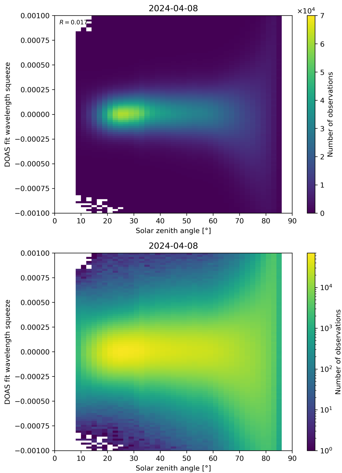
Figure 162: Scatter density plot of “Solar zenith angle” against “DOAS fit wavelength squeeze” for 2024-04-07 to 2024-04-09.
