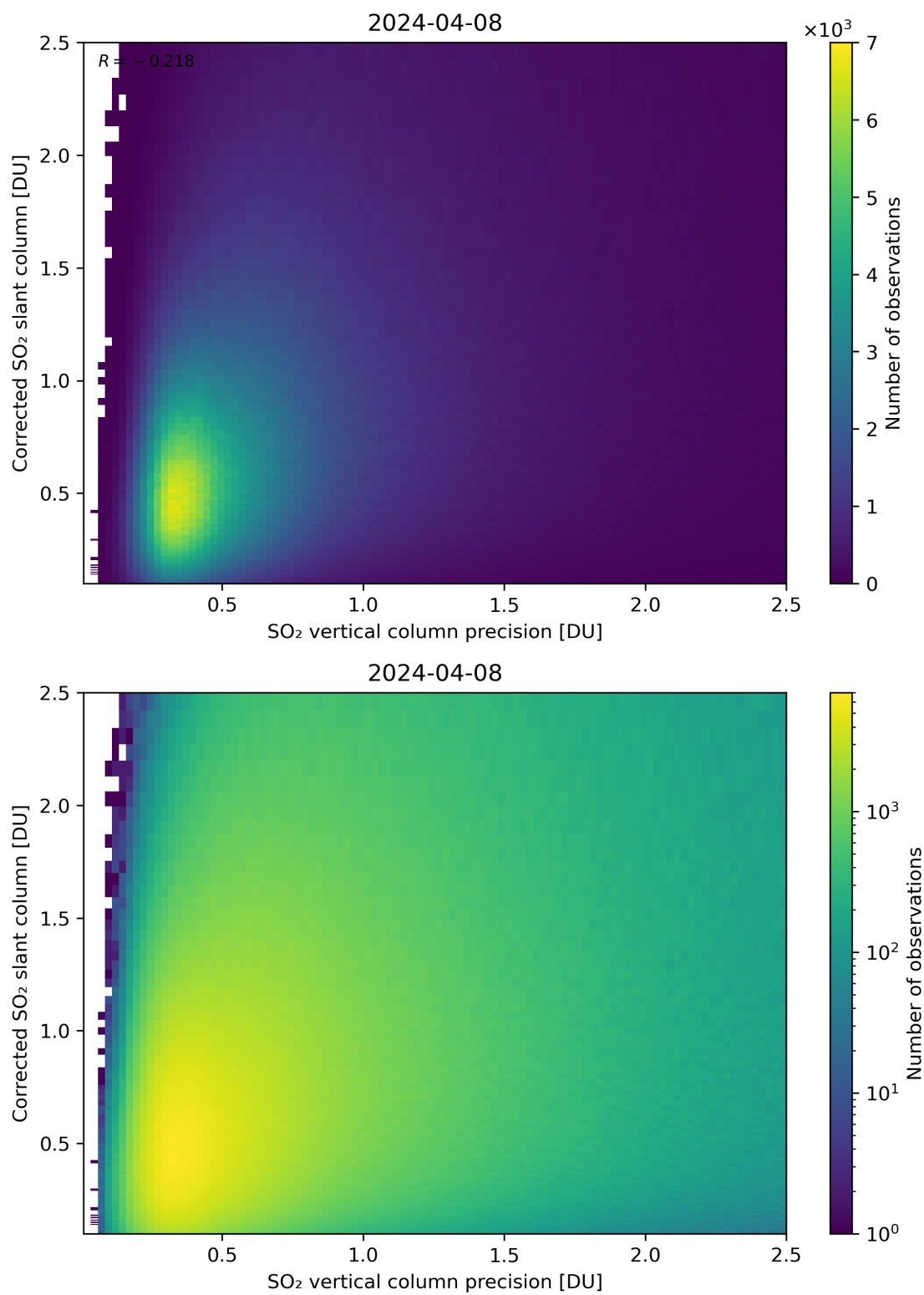
Figure 286: Scatter density plot of “SO 2 vertical column precision” against “Corrected SO 2 slant column” for 2024-04-07 to 2024-04-09.
