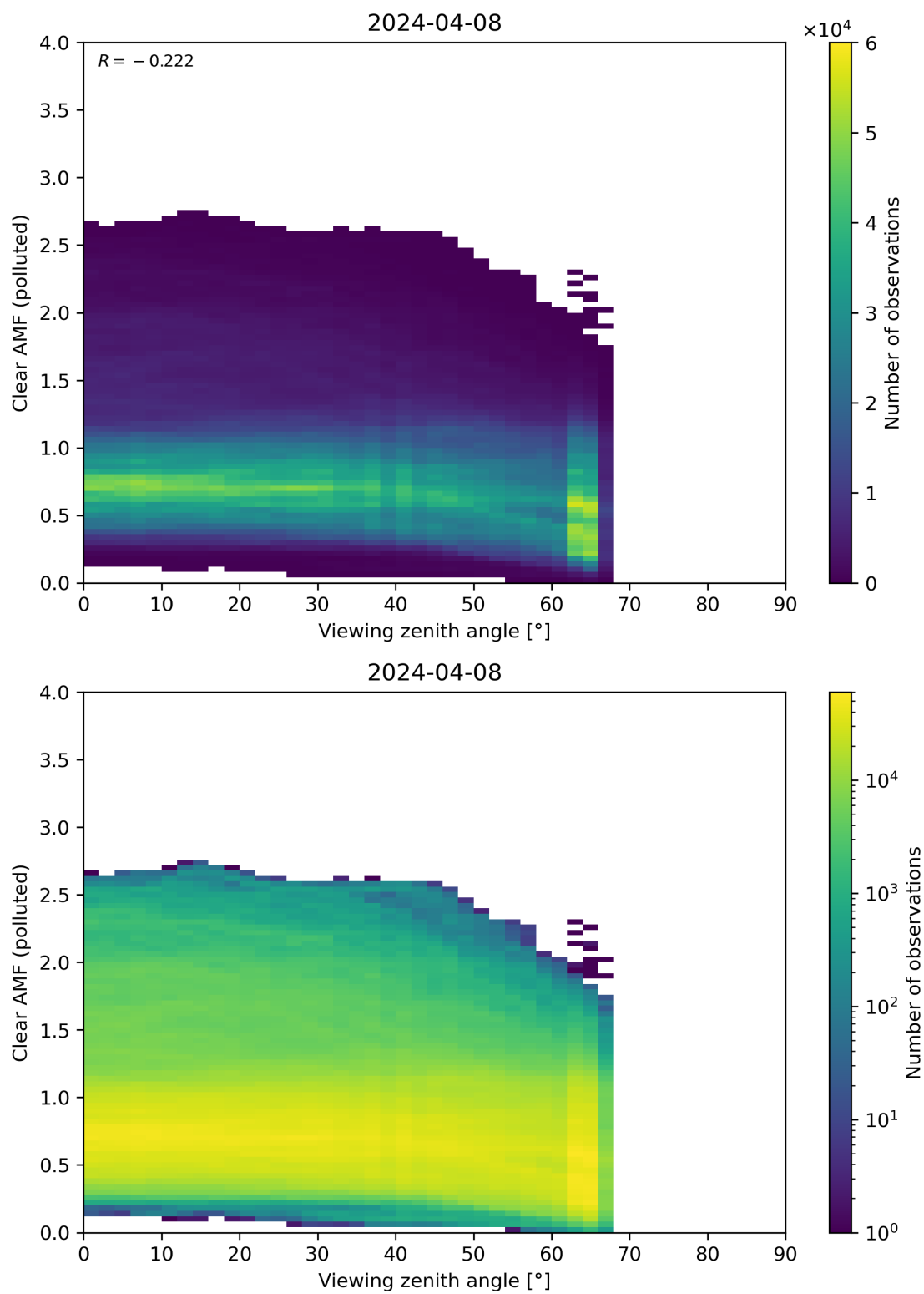
Figure 316: Scatter density plot of “Viewing zenith angle” against “Clear AMF (polluted)” for 2024-04-07 to 2024-04-09.
