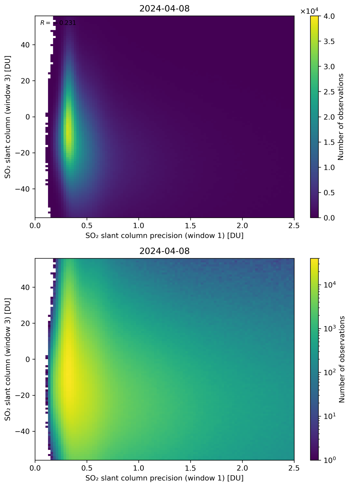
Figure 228: Scatter density plot of “SO 2 slant column precision (window 1)” against “SO 2 slant column (window 3)” for 2024-04-07 to 2024-04-09.
