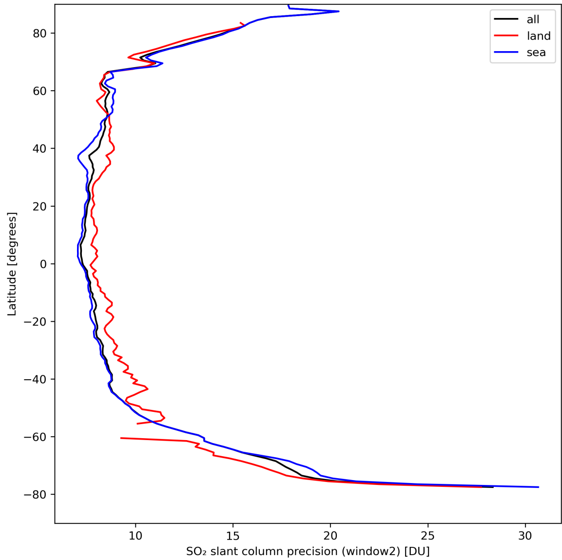
Figure 38: Zonal average of “SO 2 slant column precision (window2)” for 2024-04-07 to 2024-04-09.
