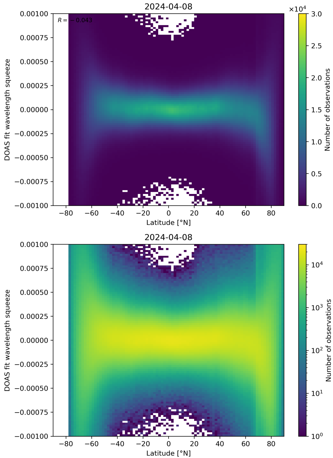
Figure 143: Scatter density plot of “Latitude” against “DOAS fit wavelength squeeze” for 2024-04-07 to 2024-04-09.
