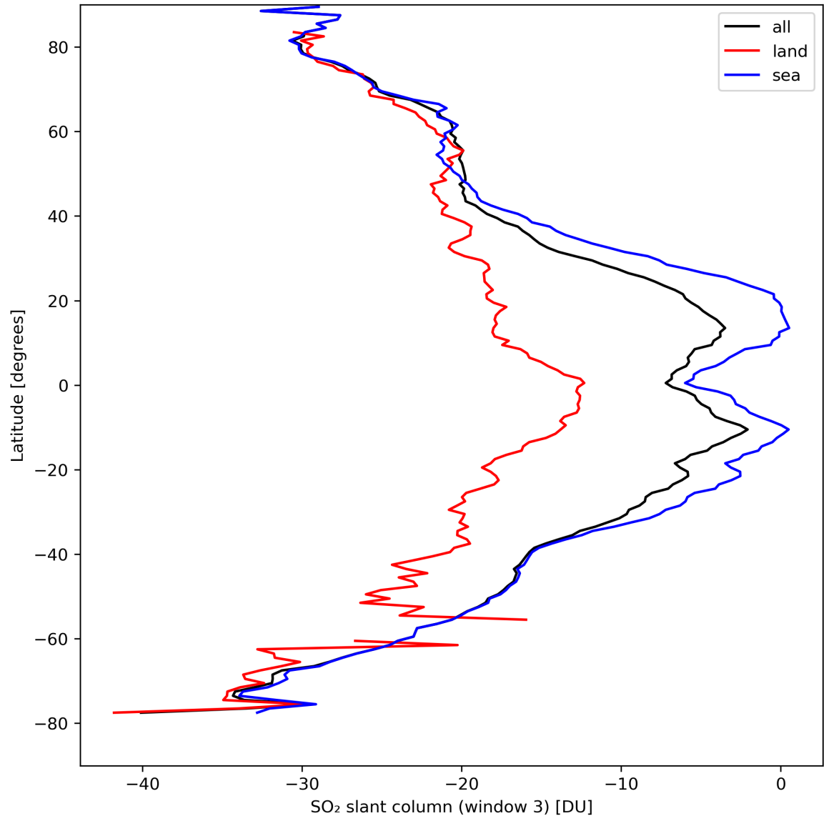
Figure 41: Zonal average of “SO 2 slant column (window 3)” for 2024-04-07 to 2024-04-09.
