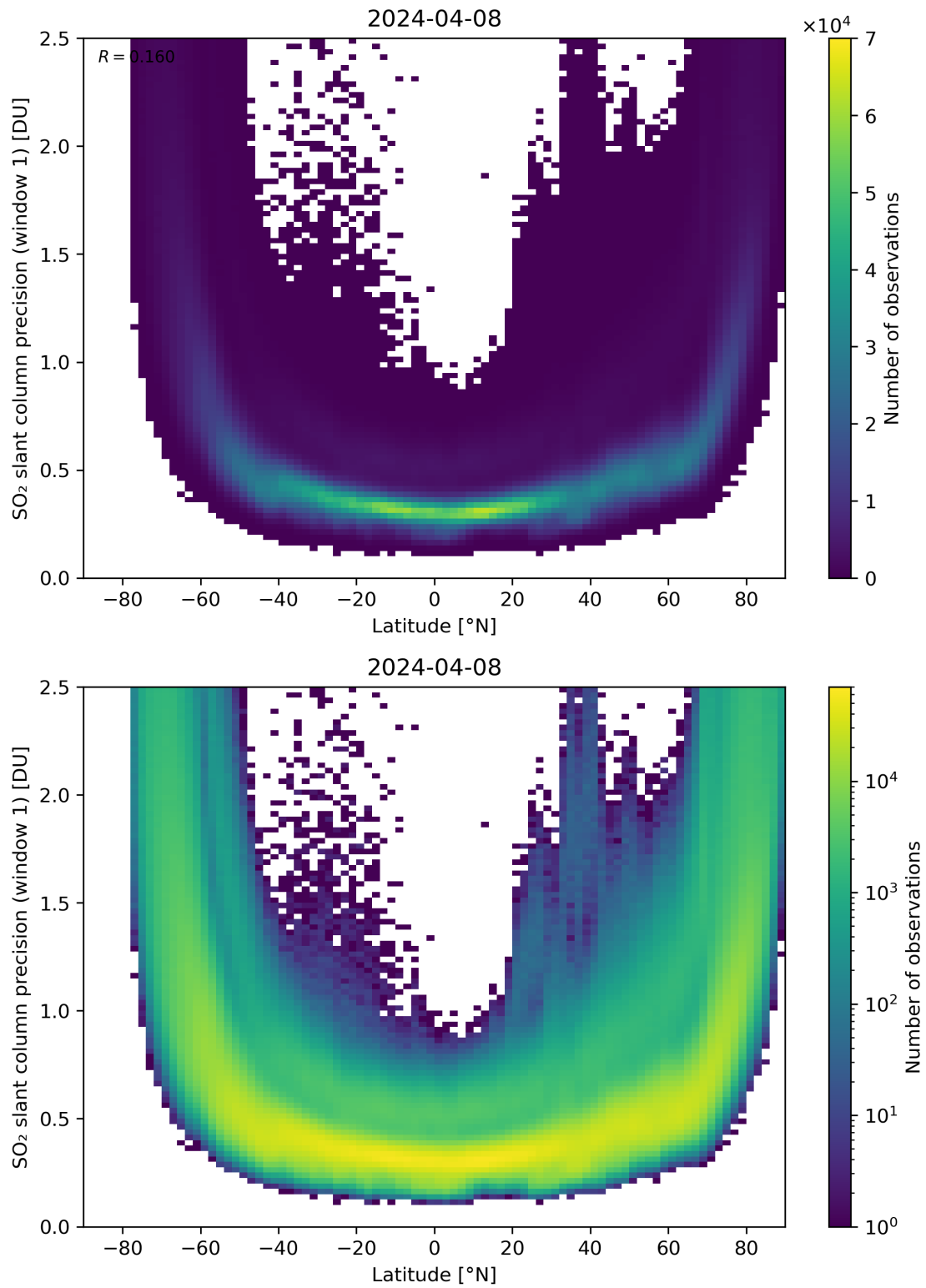
Figure 150: Scatter density plot of “Latitude” against “SO 2 slant column precision (window 1)” for 2024-04-07 to 2024-04-09.
