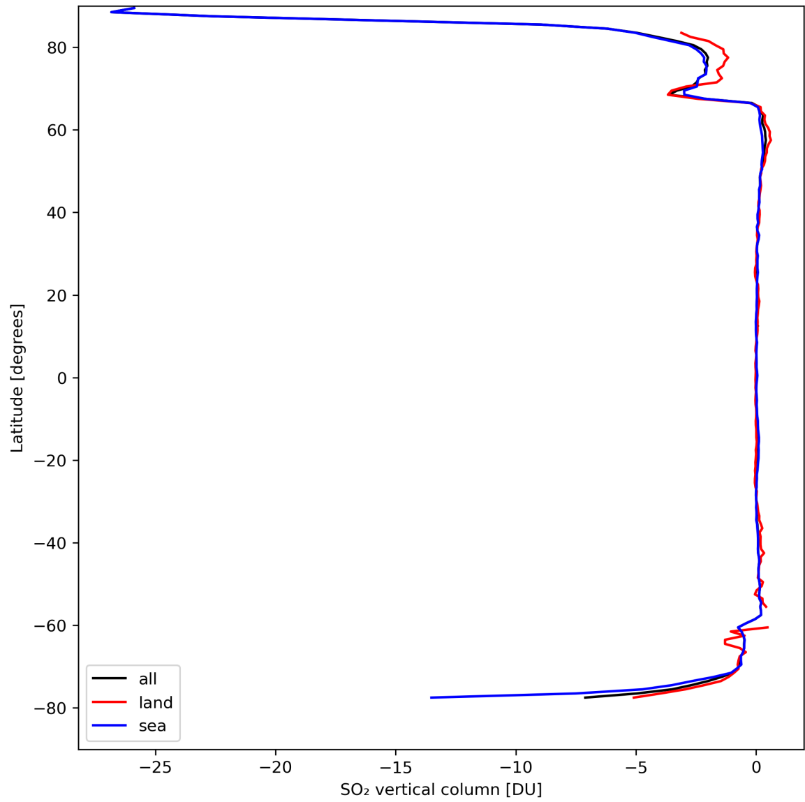
Figure 30: Zonal average of “SO 2 vertical column” for 2024-04-07 to 2024-04-09.
