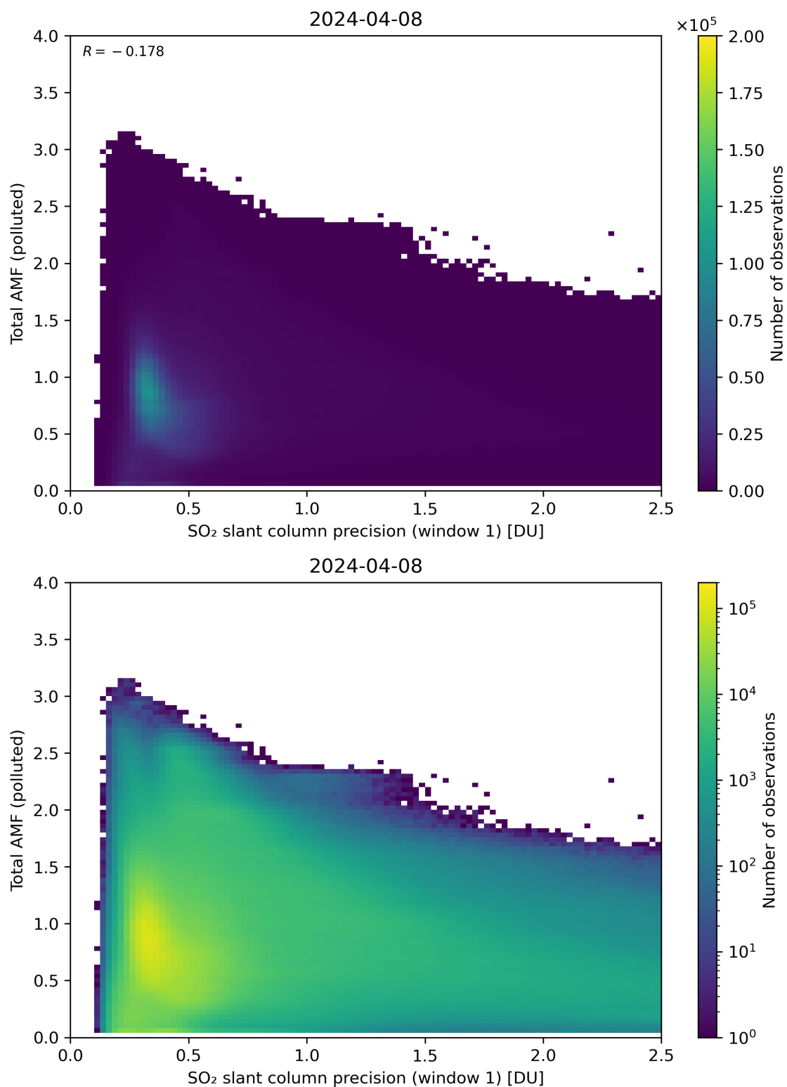
Figure 230: Scatter density plot of “SO 2 slant column precision (window 1)” against “Total AMF (polluted)” for 2024-04-07 to 2024-04-09.
