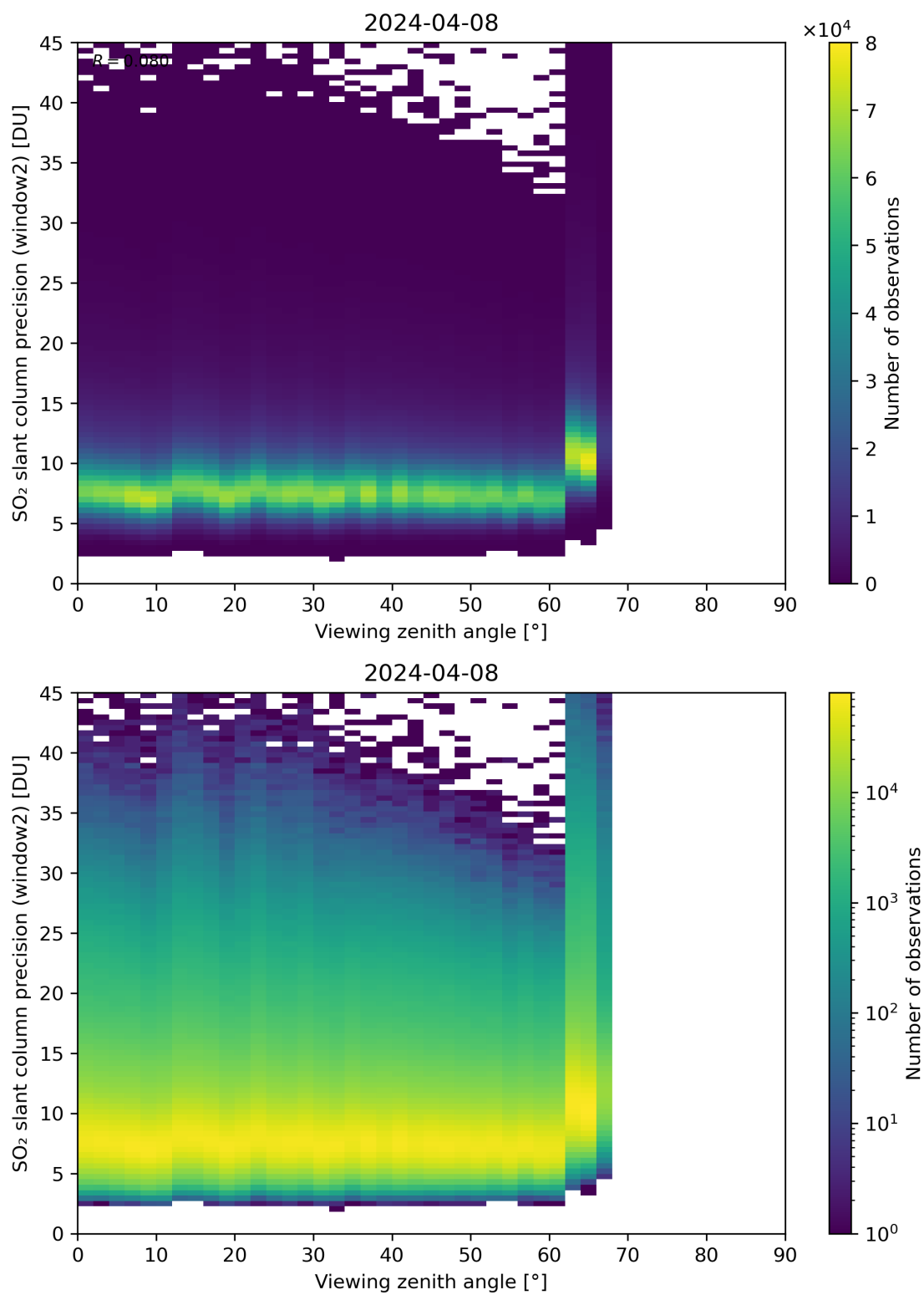
Figure 322: Scatter density plot of “Viewing zenith angle” against “SO 2 slant column precision (window2)” for 2024-04-07 to 2024-04-09.
