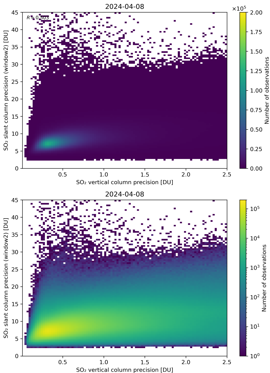
Figure 291: Scatter density plot of “SO 2 vertical column precision” against “SO 2 slant column precision (window2)” for 2024-04-07 to 2024-04-09.
