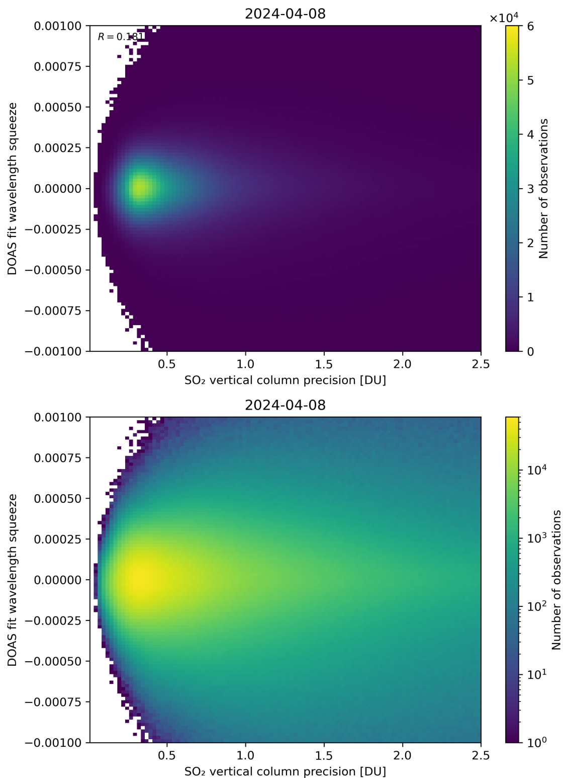
Figure 283: Scatter density plot of “SO 2 vertical column precision” against “DOAS fit wavelength squeeze” for 2024-04-07 to 2024-04-09.
