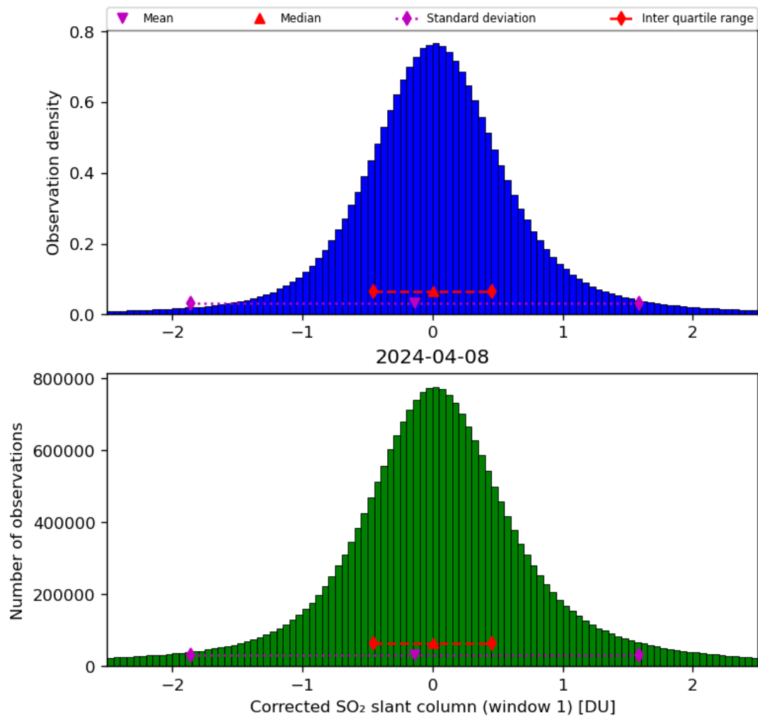
Figure 58: Histogram of “Corrected SO 2 slant column (window 1)” for 2024-04-07 to 2024-04-09
