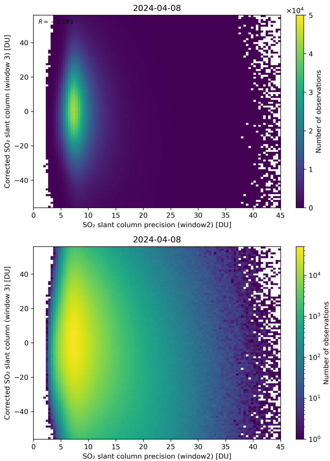
Figure 248: Scatter density plot of “SO 2 slant column precision (window2)” against “Corrected SO 2 slant column (window 3)” for 2024-04-07 to 2024-04-09.
