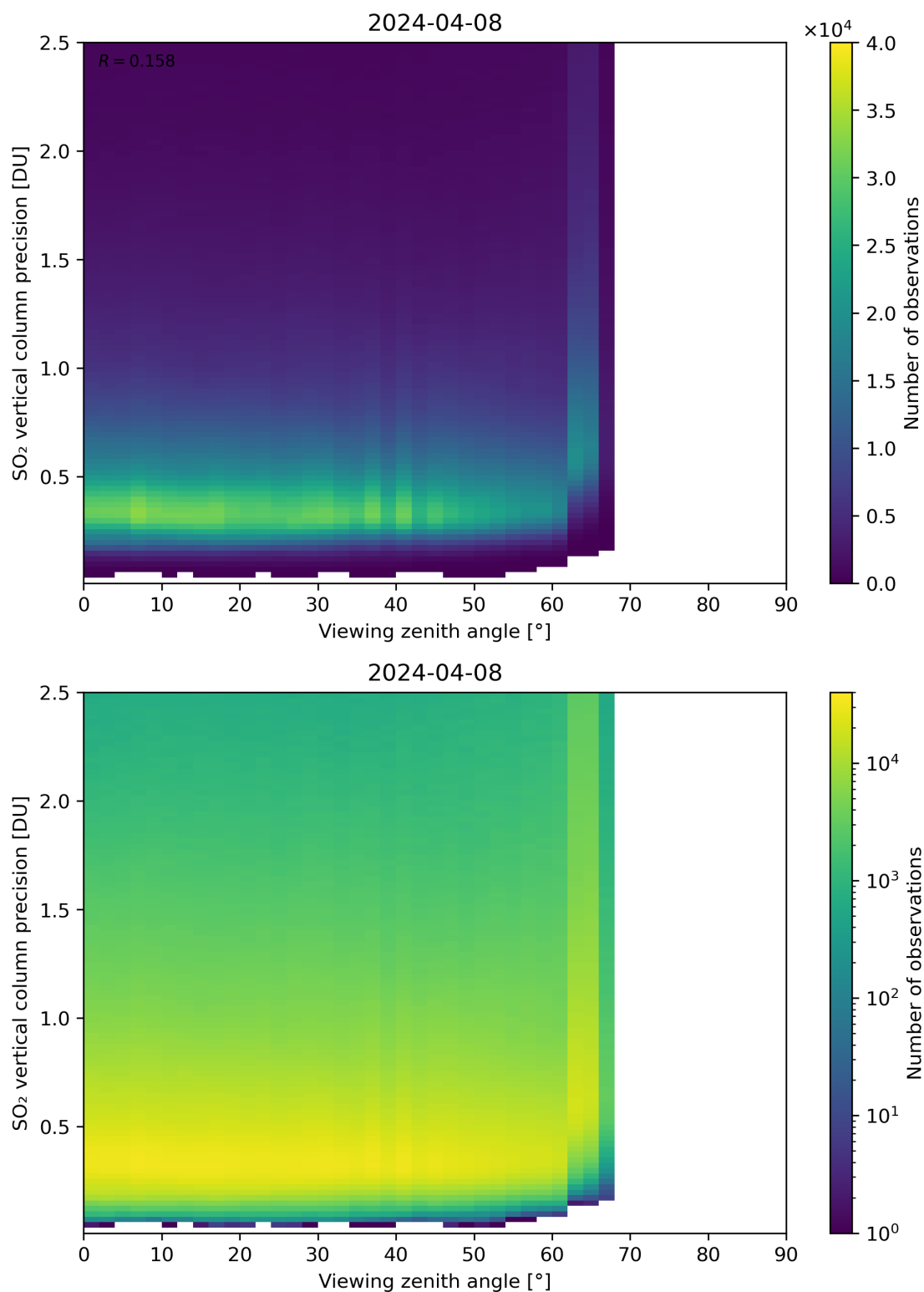
Figure 328: Scatter density plot of “Viewing zenith angle” against “SO 2 vertical column precision” for 2024-04-07 to 2024-04-09.
