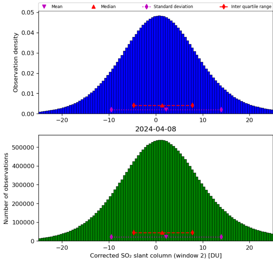
Figure 62: Histogram of “Corrected SO 2 slant column (window 2)” for 2024-04-07 to 2024-04-09
