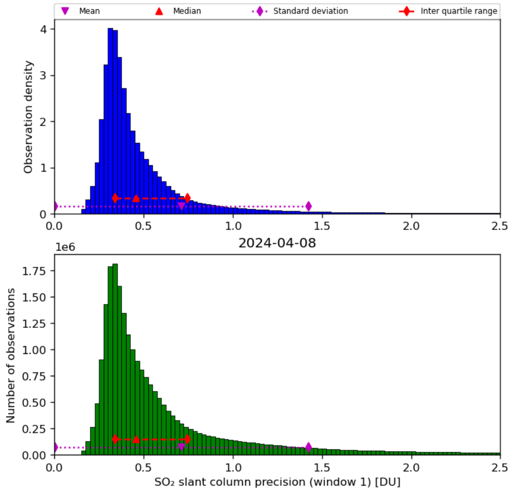
Figure 57: Histogram of “SO 2 slant column precision (window 1)” for 2024-04-07 to 2024-04-09
