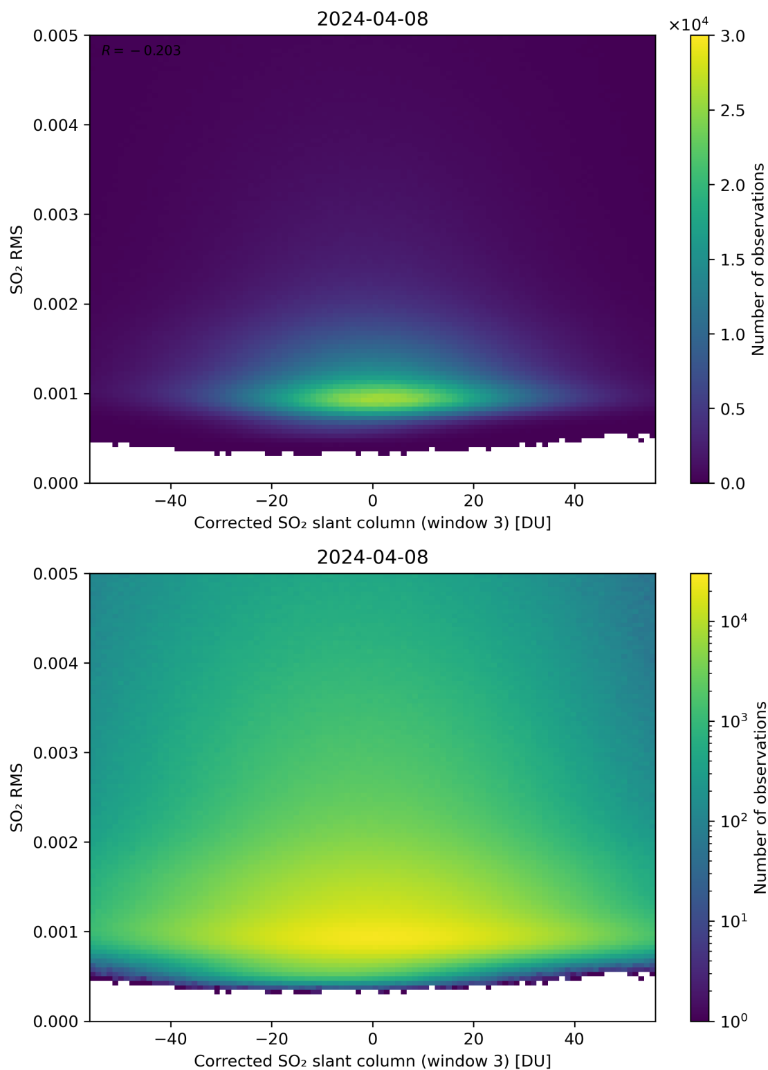
Figure 208: Scatter density plot of “Corrected SO 2 slant column (window 3)” against “SO 2 RMS” for 2024-04-07 to 2024-04-09.
