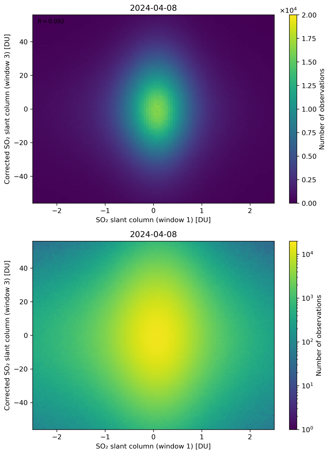
Figure 234: Scatter density plot of “SO 2 slant column (window 1)” against “Corrected SO 2 slant column (window 3)” for 2024-04-07 to 2024-04-09.
