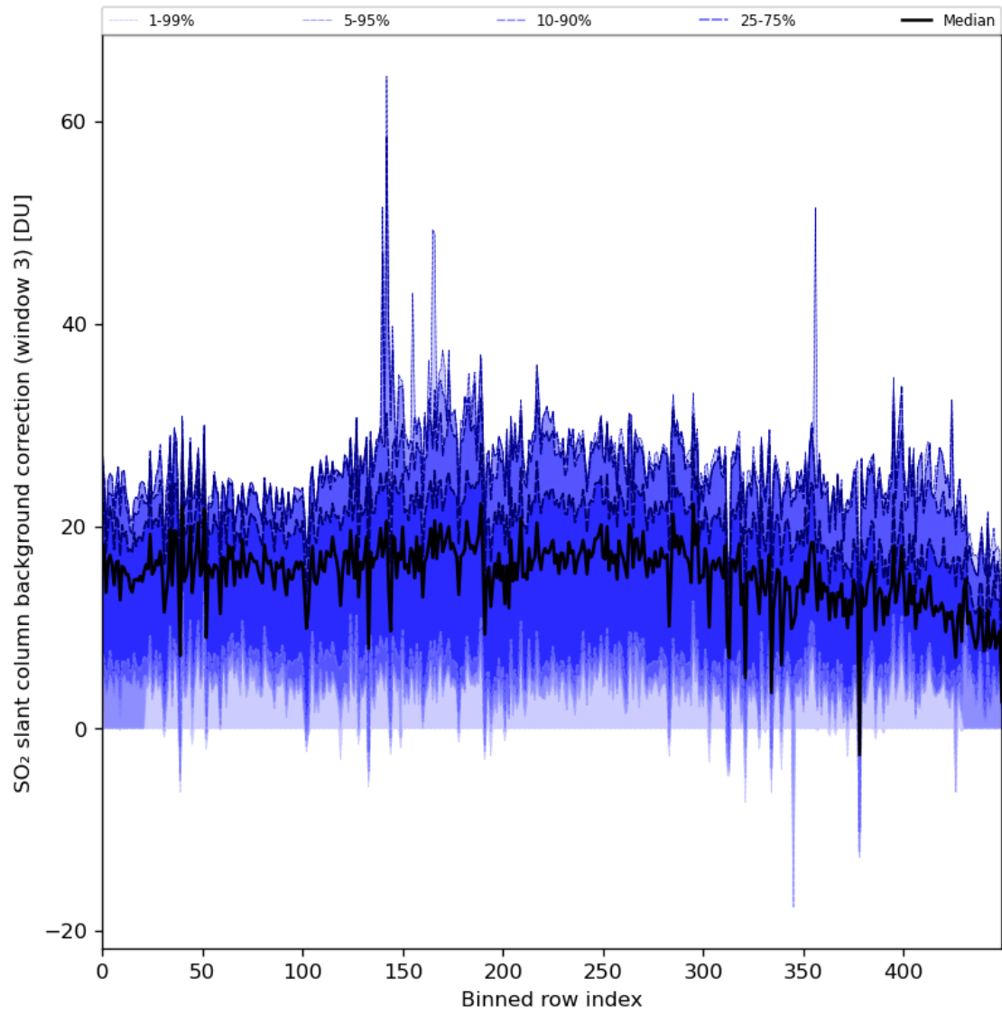
Figure 90: Along track statistics of “SO 2 slant column background correction (window 3)” for 2024-04-07 to 2024-04-09
