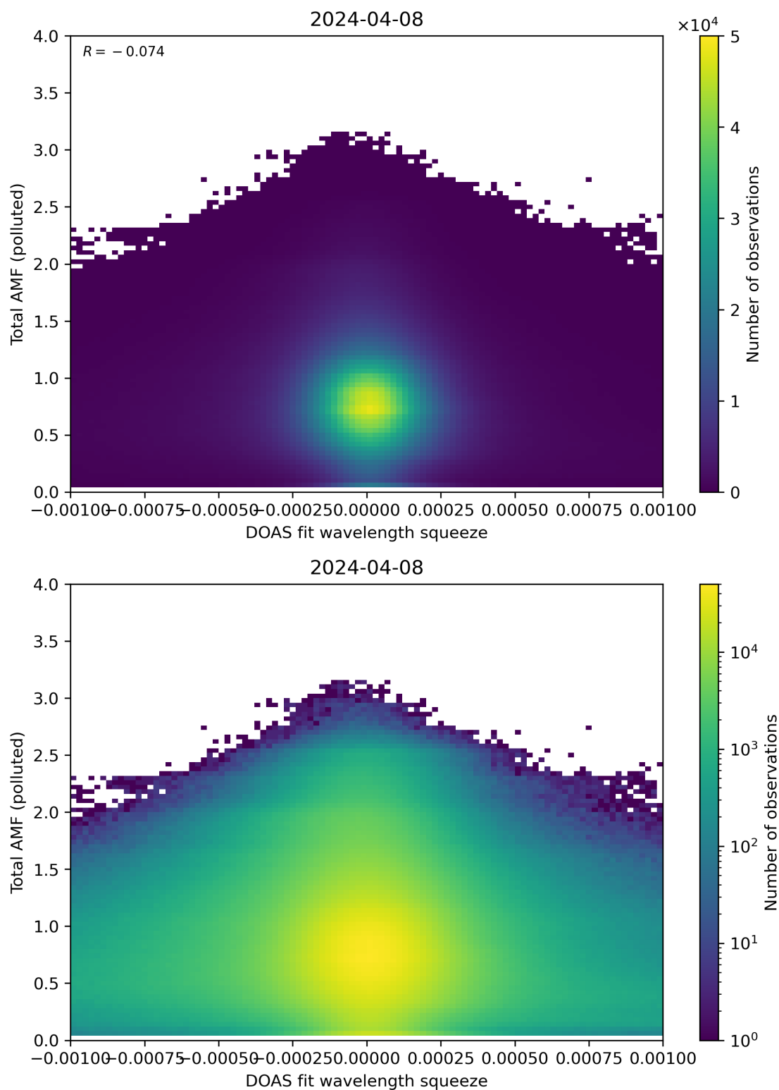
Figure 134: Scatter density plot of “DOAS fit wavelength squeeze” against “Total AMF (polluted)” for 2024-04-07 to 2024-04-09.
