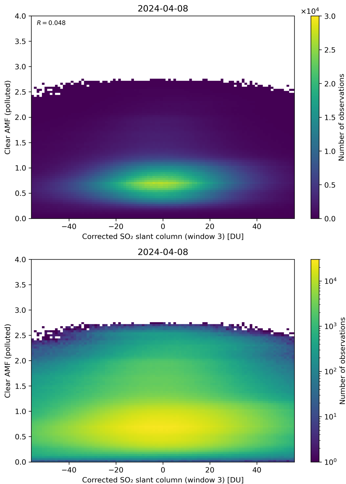
Figure 209: Scatter density plot of “Corrected SO 2 slant column (window 3)” against “Clear AMF (polluted)” for 2024-04-07 to 2024-04-09.
