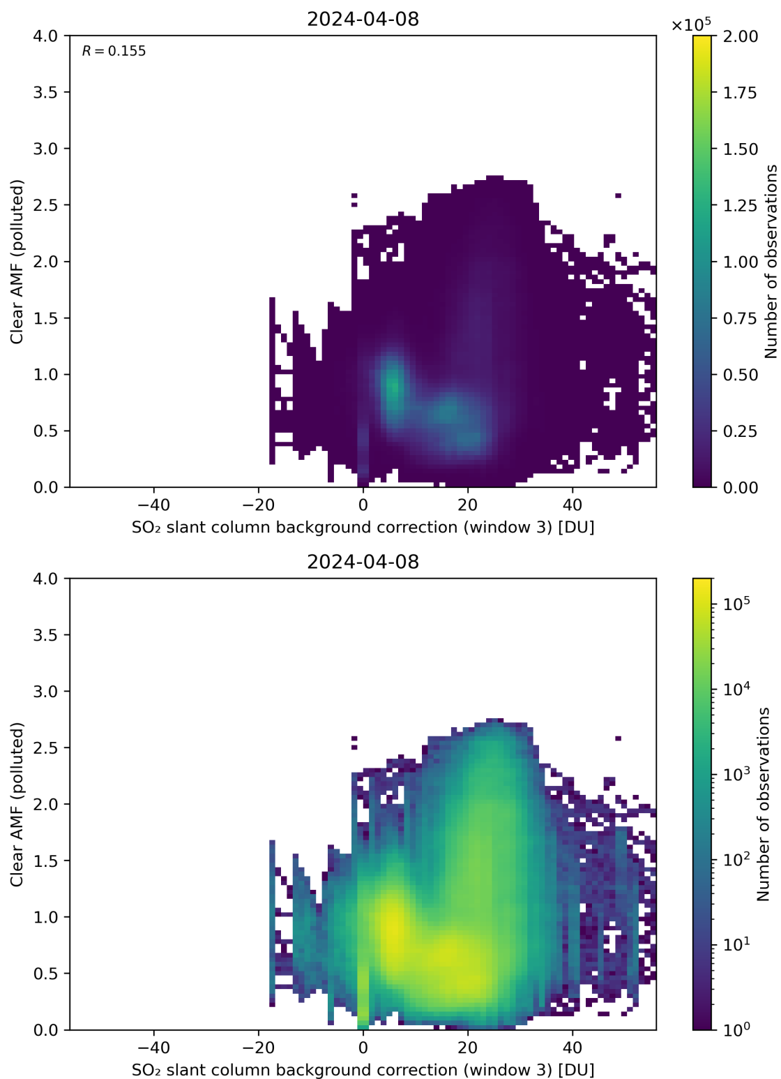
Figure 124: Scatter density plot of “SO 2 slant column background correction (window 3)” against “Clear AMF (polluted)” for 2024-04-07 to 2024-04-09.
