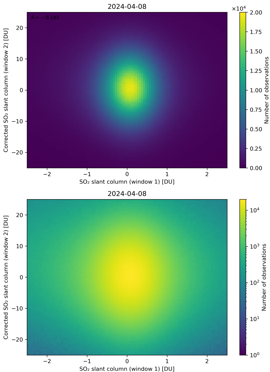
Figure 233: Scatter density plot of “SO 2 slant column (window 1)” against “Corrected SO 2 slant column (window 2)” for 2024-04-07 to 2024-04-09.
