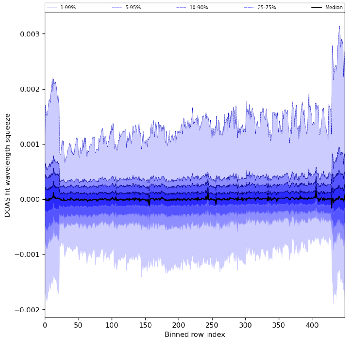
Figure 92: Along track statistics of “DOAS fit wavelength squeeze” for 2024-04-07 to 2024-04-09
