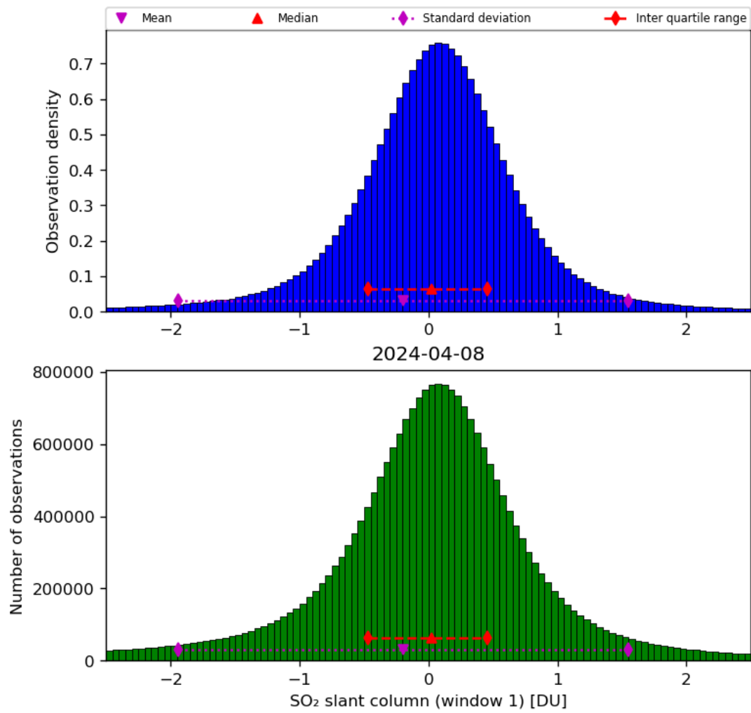
Figure 56: Histogram of “SO 2 slant column (window 1)” for 2024-04-07 to 2024-04-09
