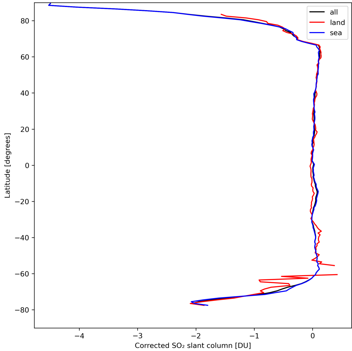
Figure 32: Zonal average of “Corrected SO 2 slant column” for 2024-04-07 to 2024-04-09.
