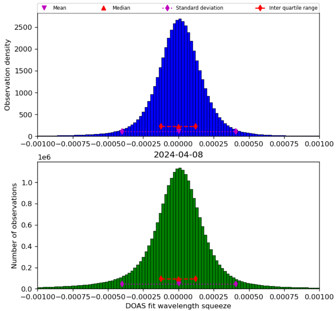
Figure 69: Histogram of “DOAS fit wavelength squeeze” for 2024-04-07 to 2024-04-09
