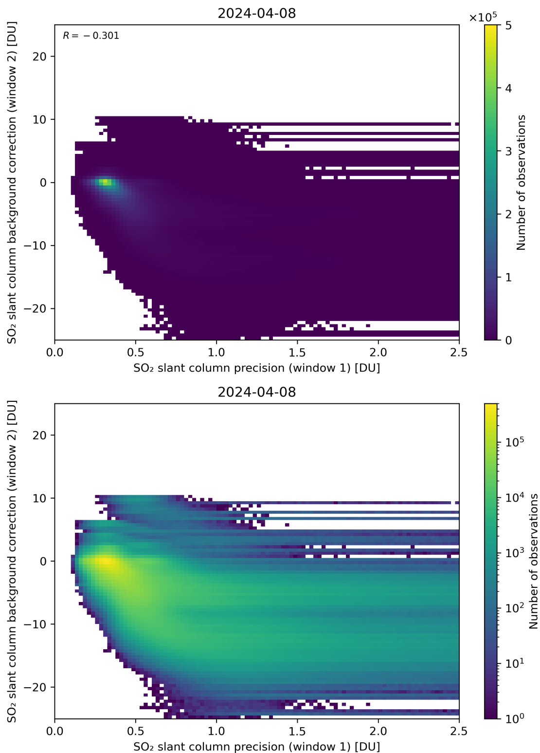
Figure 219: Scatter density plot of “SO 2 slant column precision (window 1)” against “SO 2 slant column background correction (window 2)” for 2024-04-07 to 2024-04-09.
