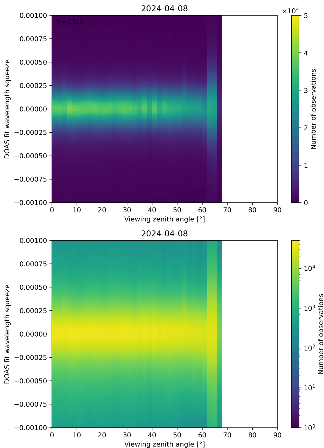
Figure 312: Scatter density plot of “Viewing zenith angle” against “DOAS fit wavelength squeeze” for 2024-04-07 to 2024-04-09.
