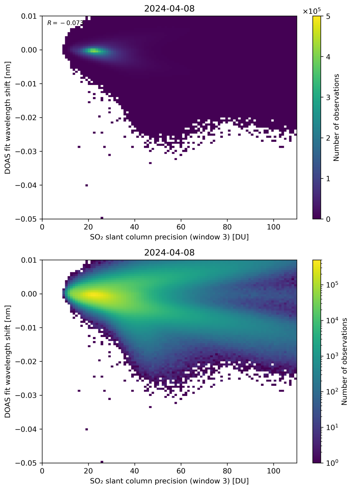
Figure 258: Scatter density plot of “SO 2 slant column precision (window 3)” against “DOAS fit wavelength shift” for 2024-04-07 to 2024-04-09.
