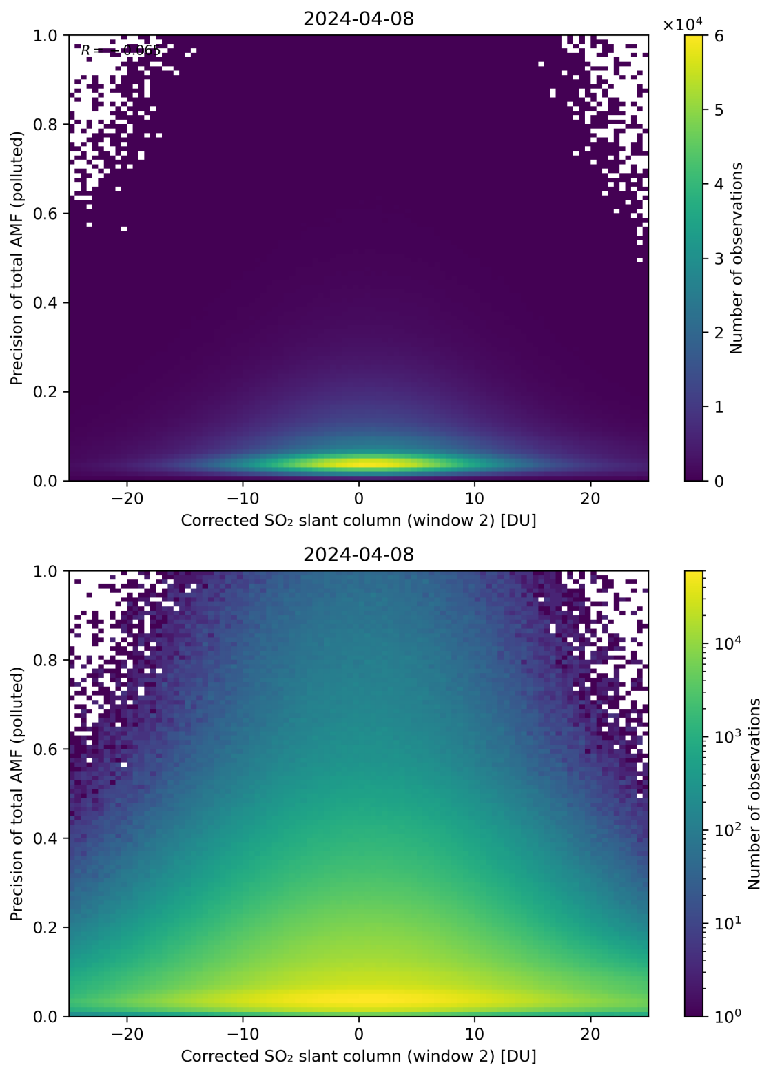
Figure 204: Scatter density plot of “Corrected SO 2 slant column (window 2)” against “Precision of total AMF (polluted)” for 2024-04-07 to 2024-04-09.
