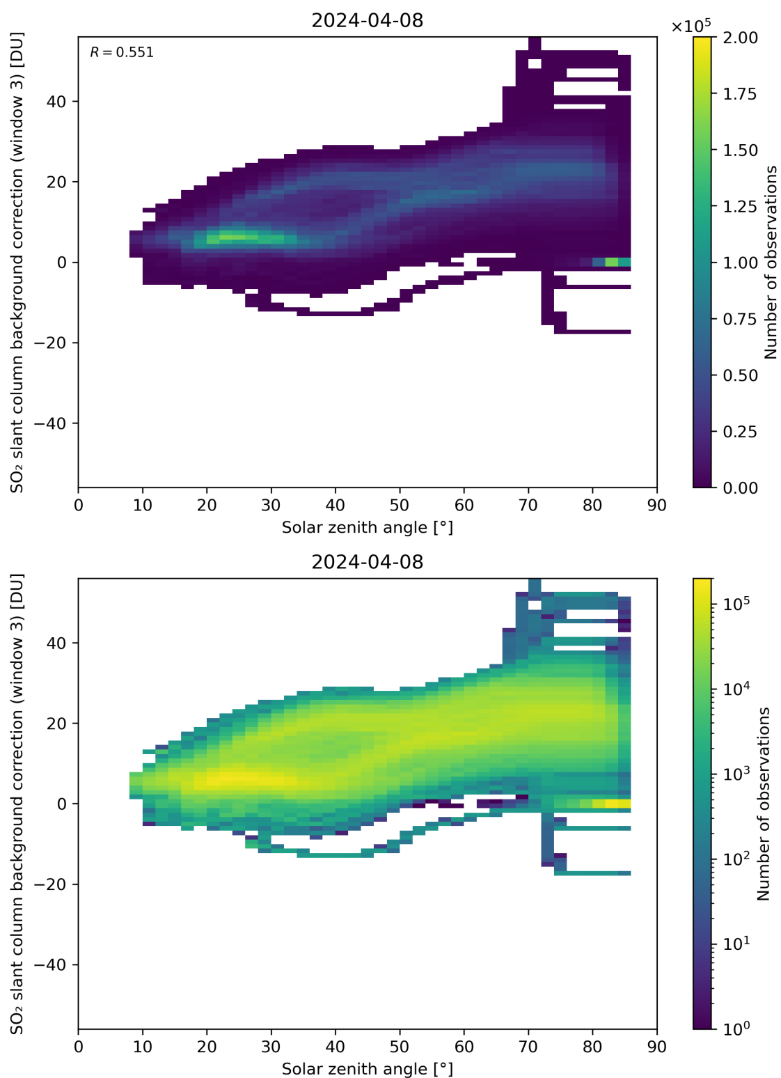
Figure 160: Scatter density plot of “Solar zenith angle” against “SO 2 slant column background correction (window 3)” for 2024-04-07 to 2024-04-09.
