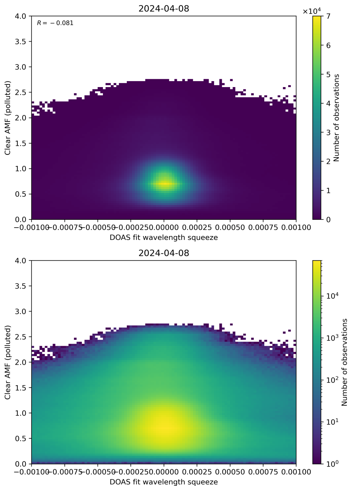
Figure 133: Scatter density plot of “DOAS fit wavelength squeeze” against “Clear AMF (polluted)” for 2024-04-07 to 2024-04-09.
