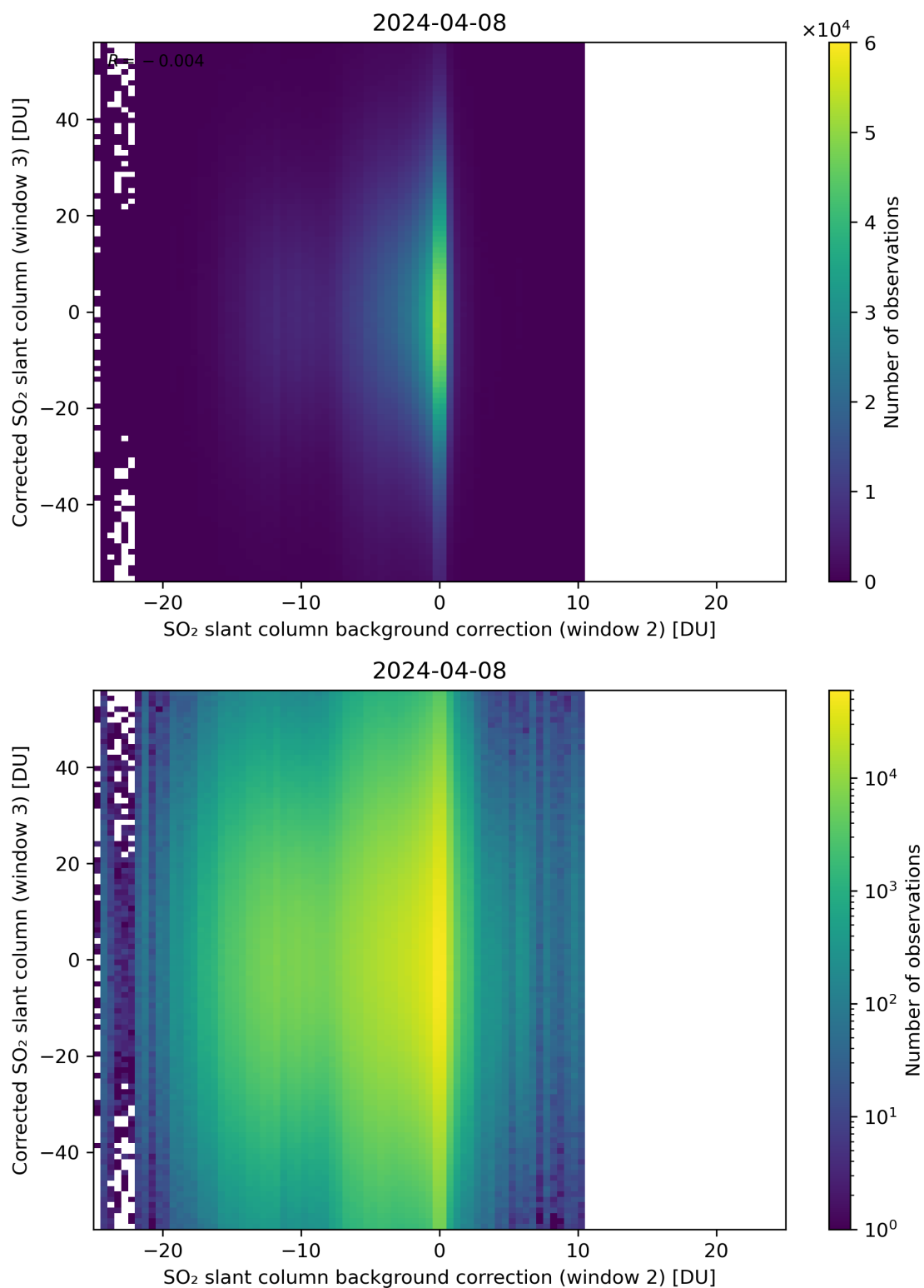
Figure 116: Scatter density plot of “SO 2 slant column background correction (window 2)” against “Corrected SO 2 slant column (window 3)” for 2024-04-07 to 2024-04-09.
