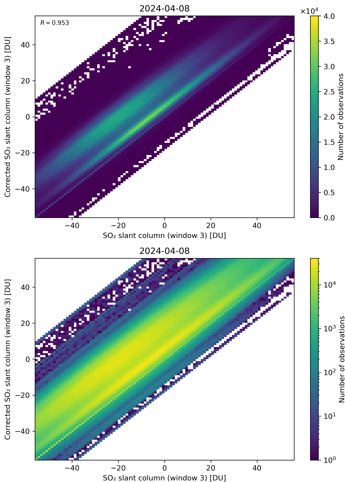
Figure 266: Scatter density plot of “SO 2 slant column (window 3)” against “Corrected SO 2 slant column (window 3)” for 2024-04-07 to 2024-04-09.
