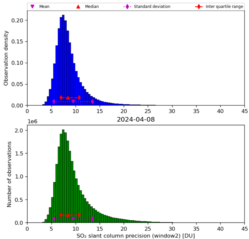
Figure 61: Histogram of “SO 2 slant column precision (window2)” for 2024-04-07 to 2024-04-09
