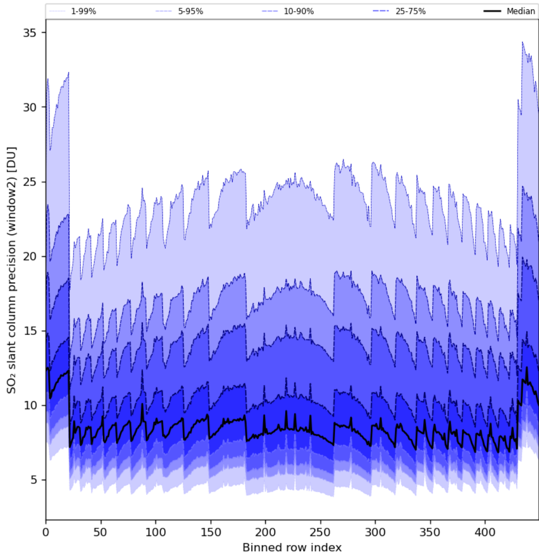
Figure 84: Along track statistics of “SO 2 slant column precision (window2)” for 2024-04-07 to 2024-04-09
