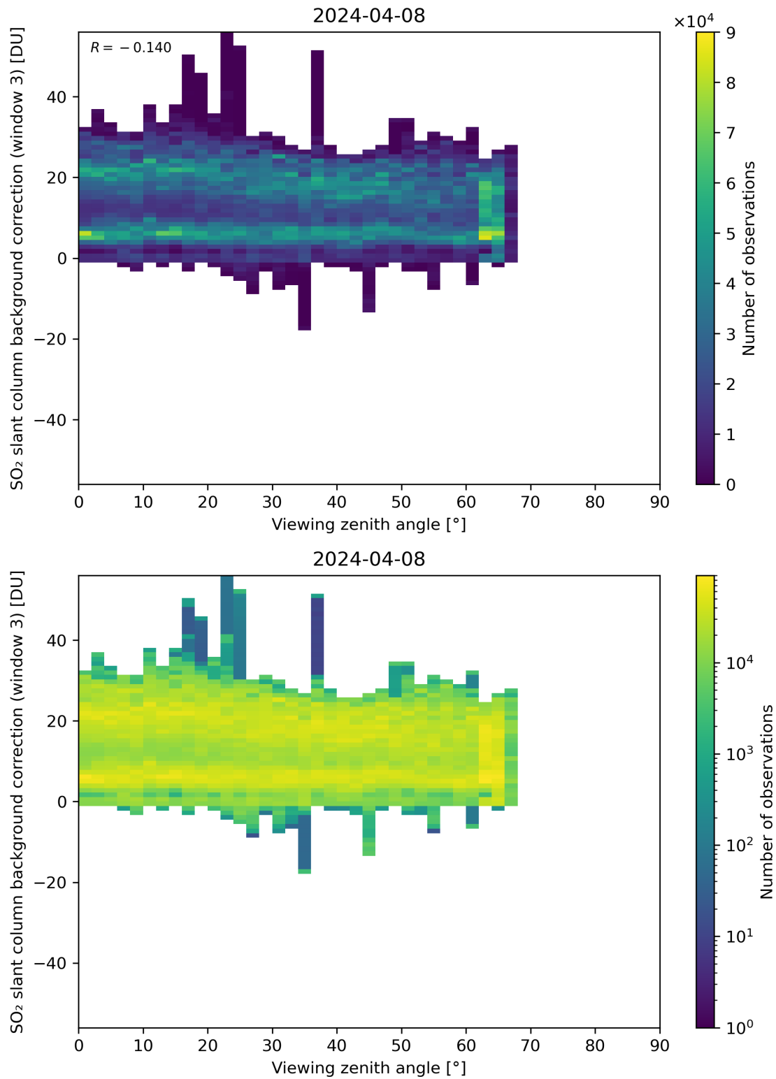
Figure 310: Scatter density plot of “Viewing zenith angle” against “SO 2 slant column background correction (window 3)” for 2024-04-07 to 2024-04-09.
