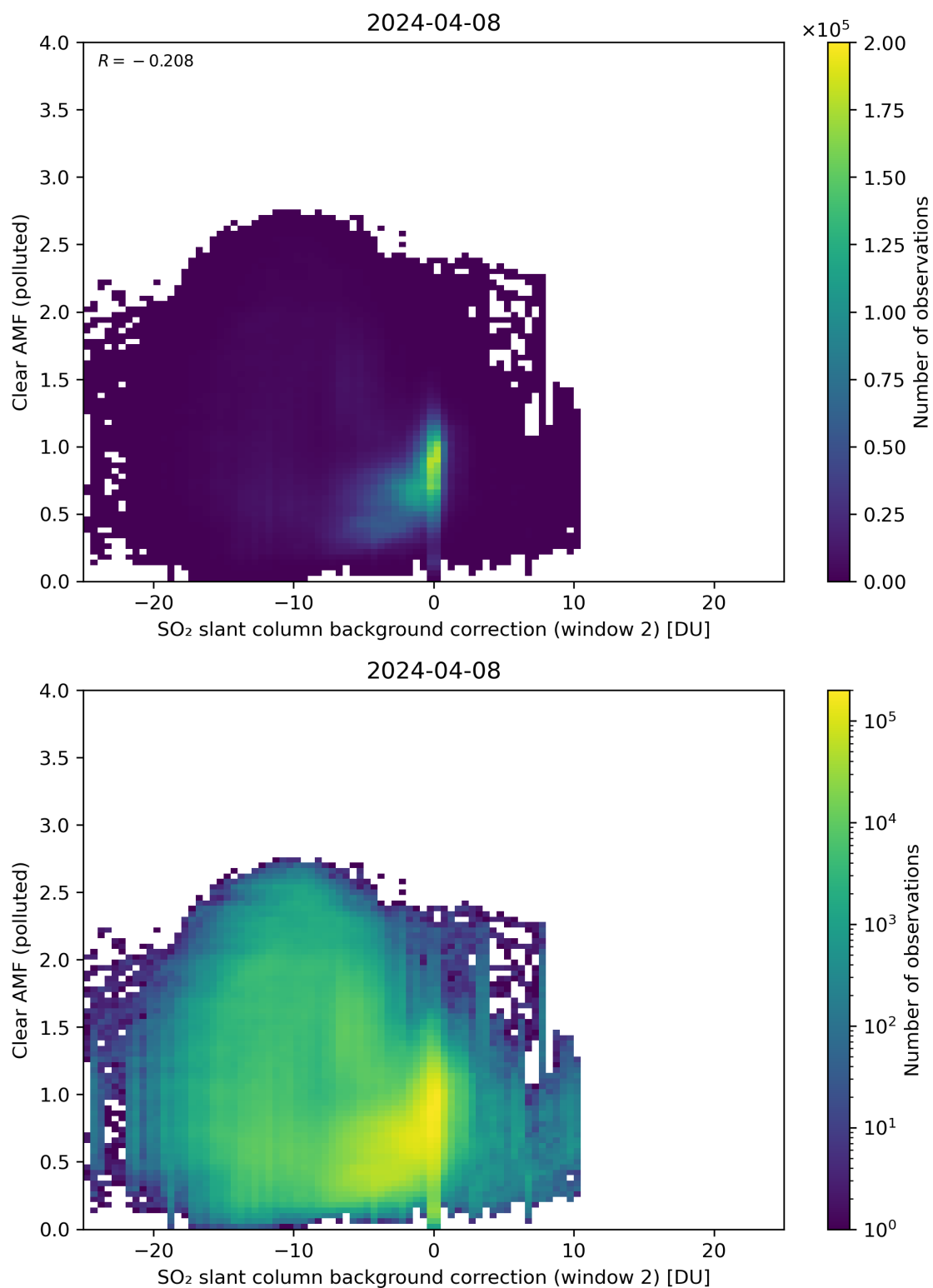
Figure 115: Scatter density plot of “SO 2 slant column background correction (window 2)” against “Clear AMF (polluted)” for 2024-04-07 to 2024-04-09.
