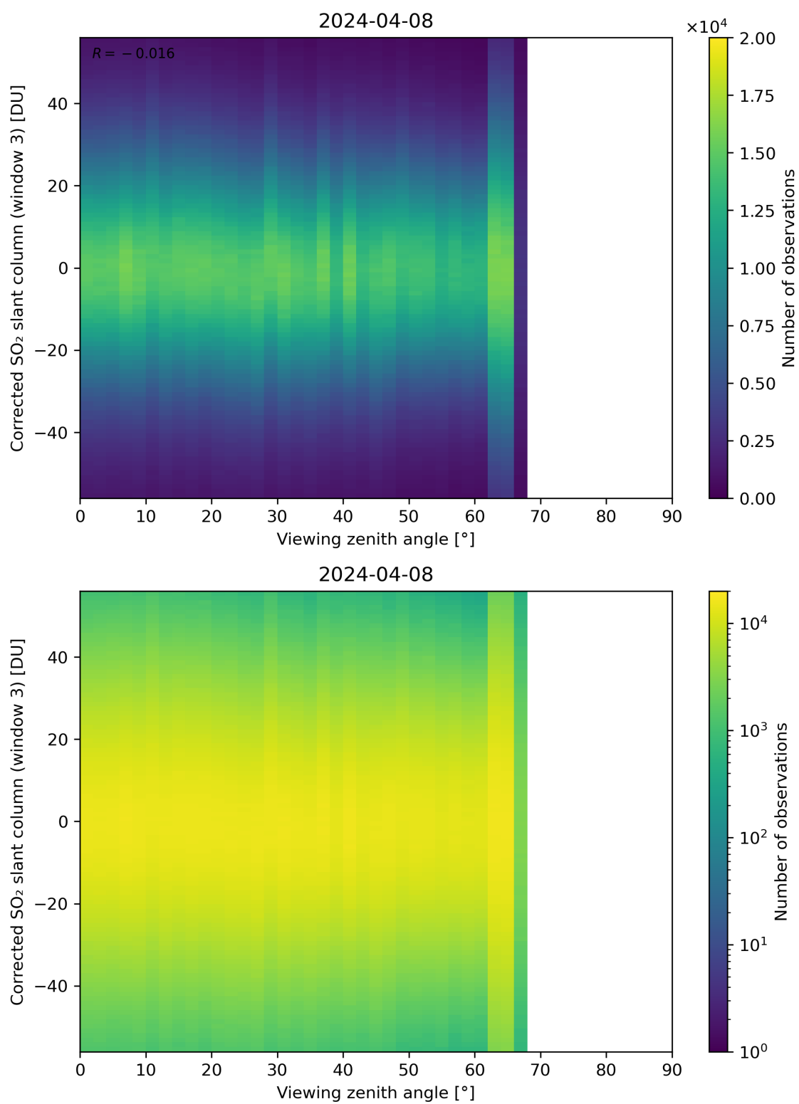
Figure 319: Scatter density plot of “Viewing zenith angle” against “Corrected SO 2 slant column (window 3)” for 2024-04-07 to 2024-04-09.
