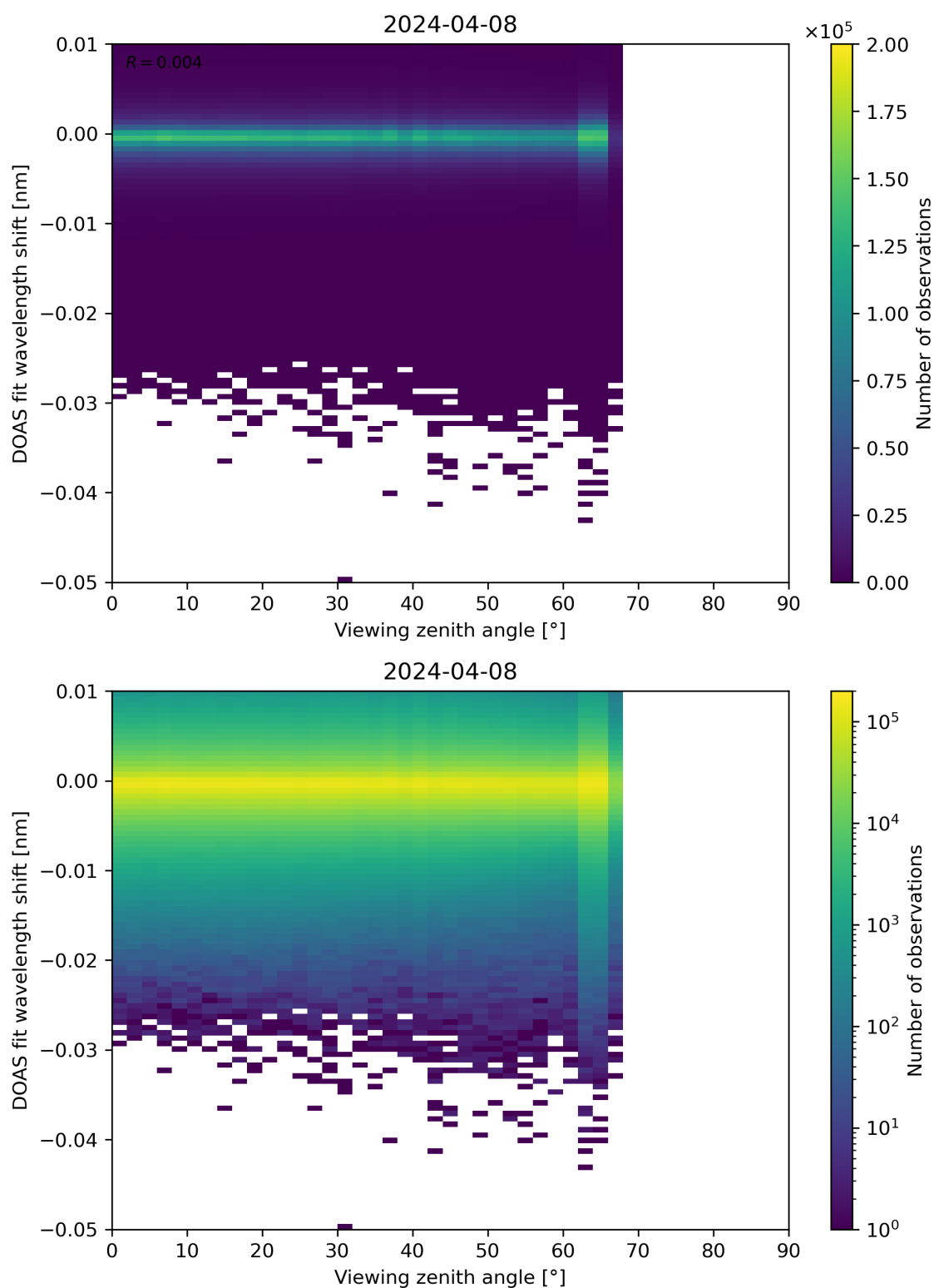
Figure 311: Scatter density plot of “Viewing zenith angle” against “DOAS fit wavelength shift” for 2024-04-07 to 2024-04-09.
