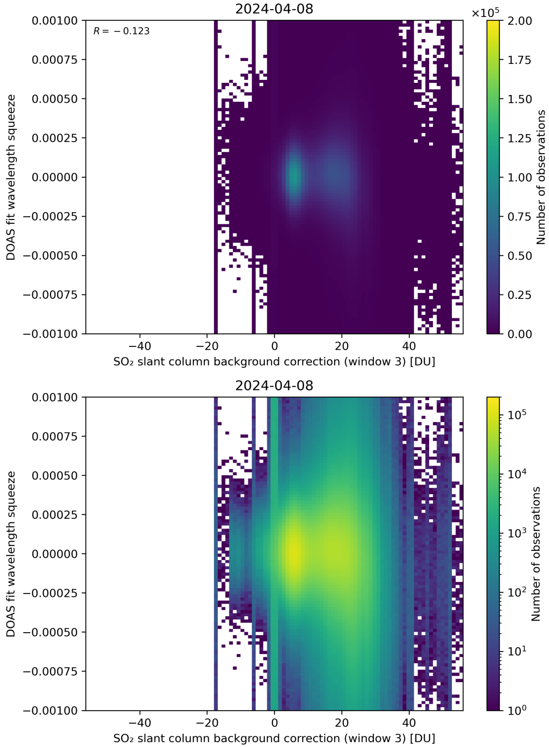
Figure 122: Scatter density plot of “SO 2 slant column background correction (window 3)” against “DOAS fit wavelength squeeze” for 2024-04-07 to 2024-04-09.
