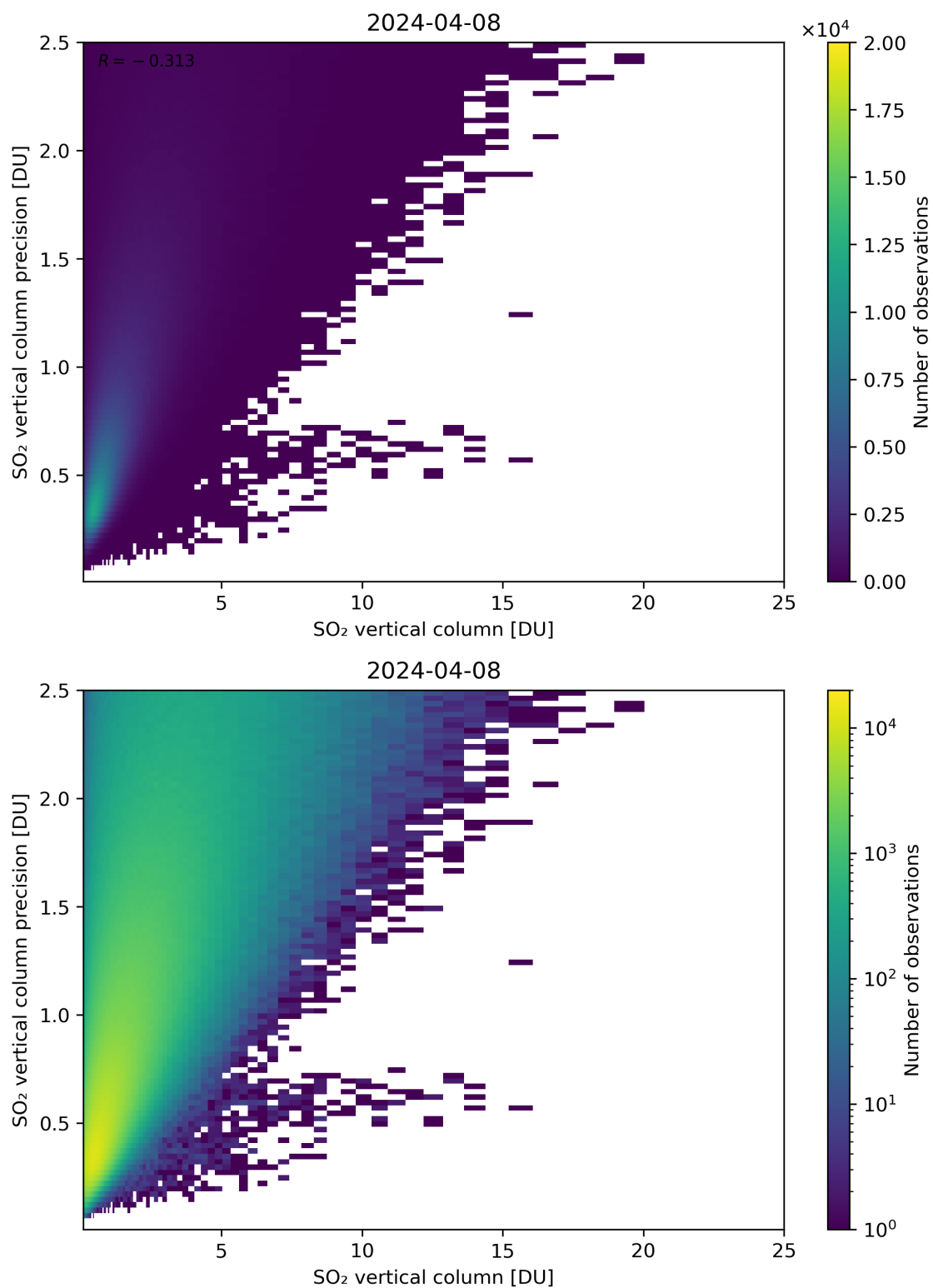
Figure 307: Scatter density plot of “SO 2 vertical column” against “SO 2 vertical column precision” for 2024-04-07 to 2024-04-09.
