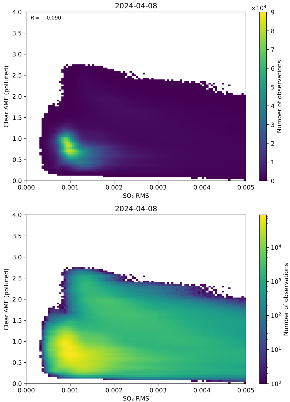
Figure 136: Scatter density plot of “SO 2 RMS” against “Clear AMF (polluted)” for 2024-04-07 to 2024-04-09.
