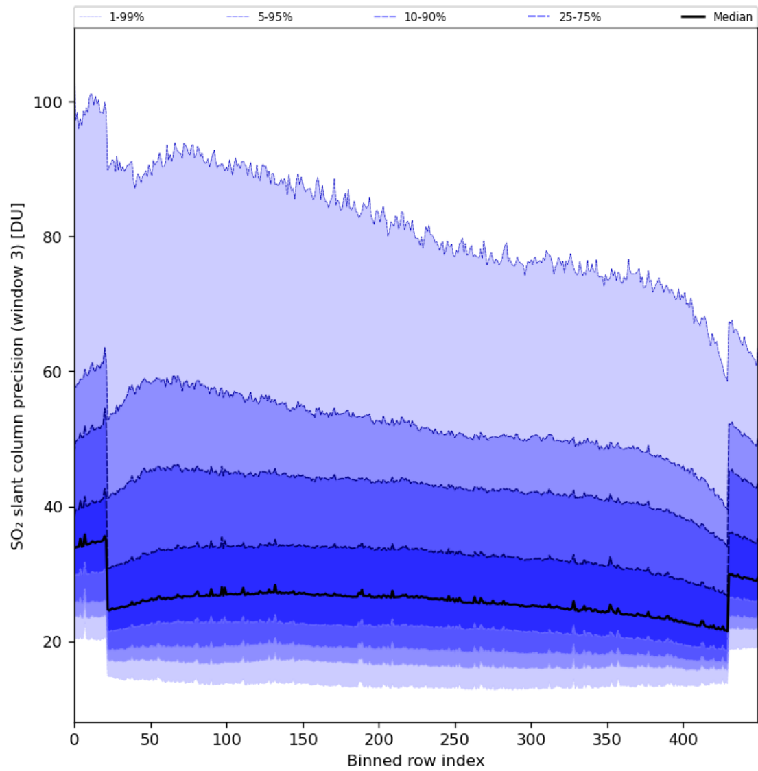
Figure 88: Along track statistics of “SO 2 slant column precision (window 3)” for 2024-04-07 to 2024-04-09
