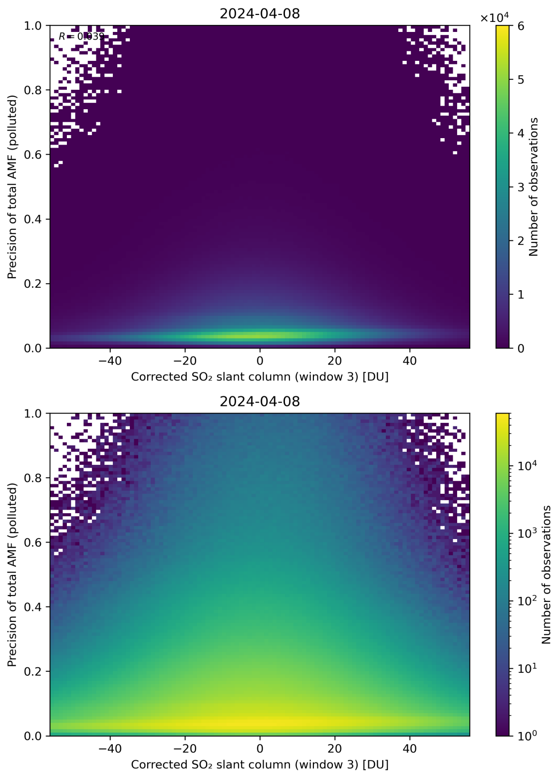
Figure 211: Scatter density plot of “Corrected SO 2 slant column (window 3)” against “Precision of total AMF (polluted)” for 2024-04-07 to 2024-04-09.
