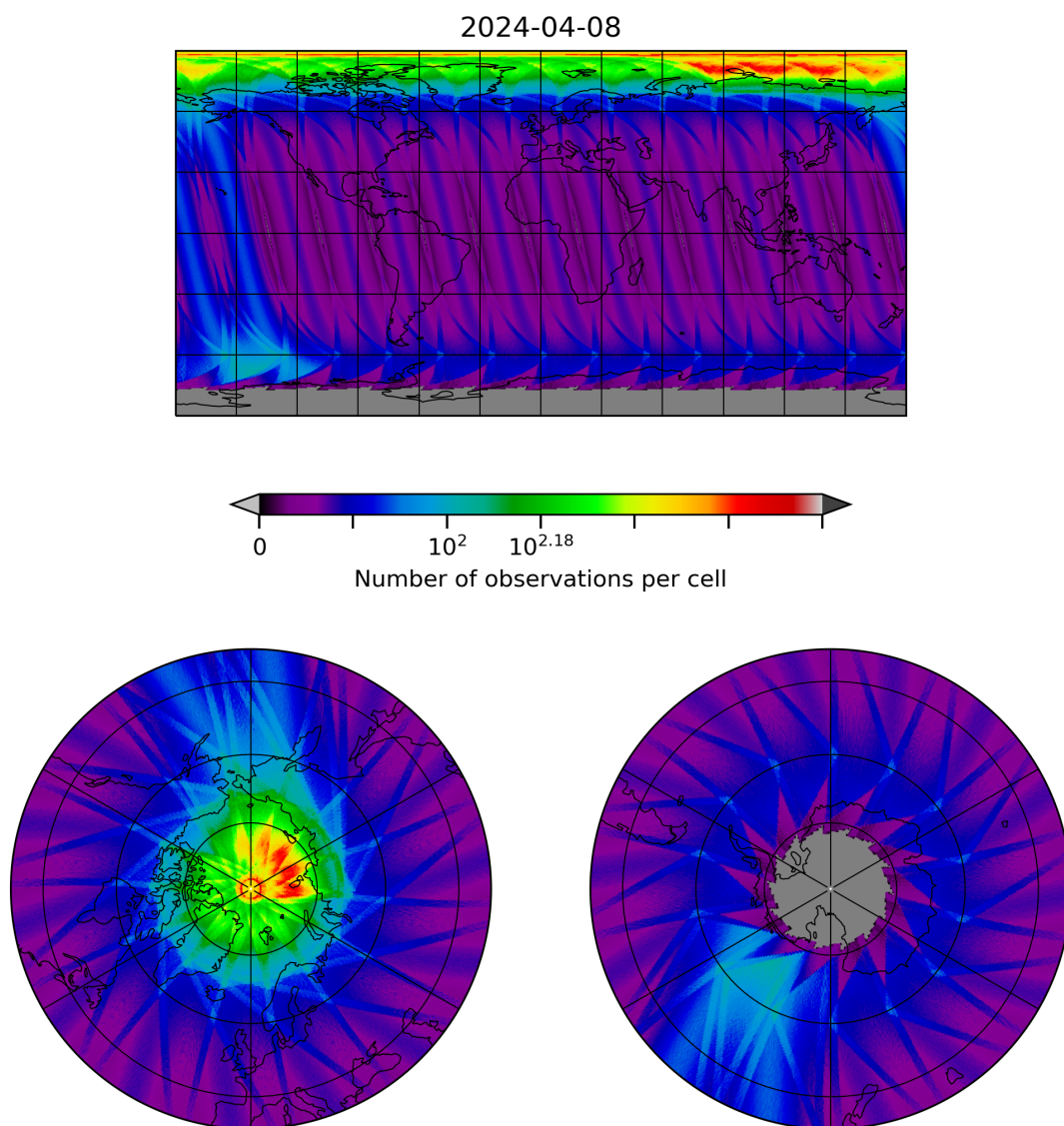
Figure 28: Map of the number of observations for 2024-04-07 to 2024-04-09
