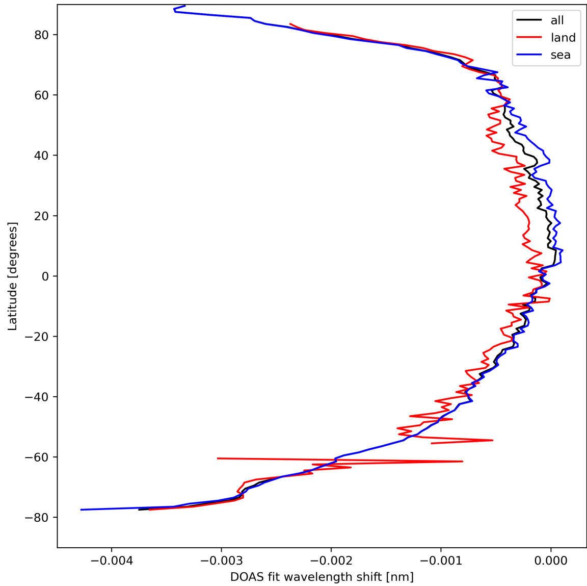
Figure 45: Zonal average of “DOAS fit wavelength shift” for 2024-04-07 to 2024-04-09.
