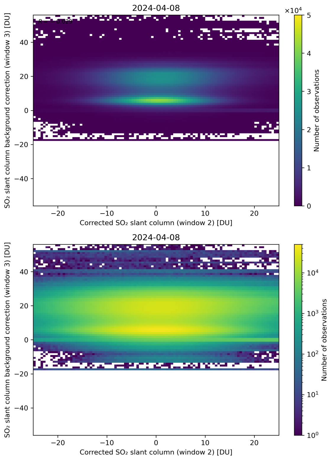
Figure 195: Scatter density plot of “Corrected SO 2 slant column (window 2)” against “SO 2 slant column background correction (window 3)” for 2024-04-07 to 2024-04-09.
