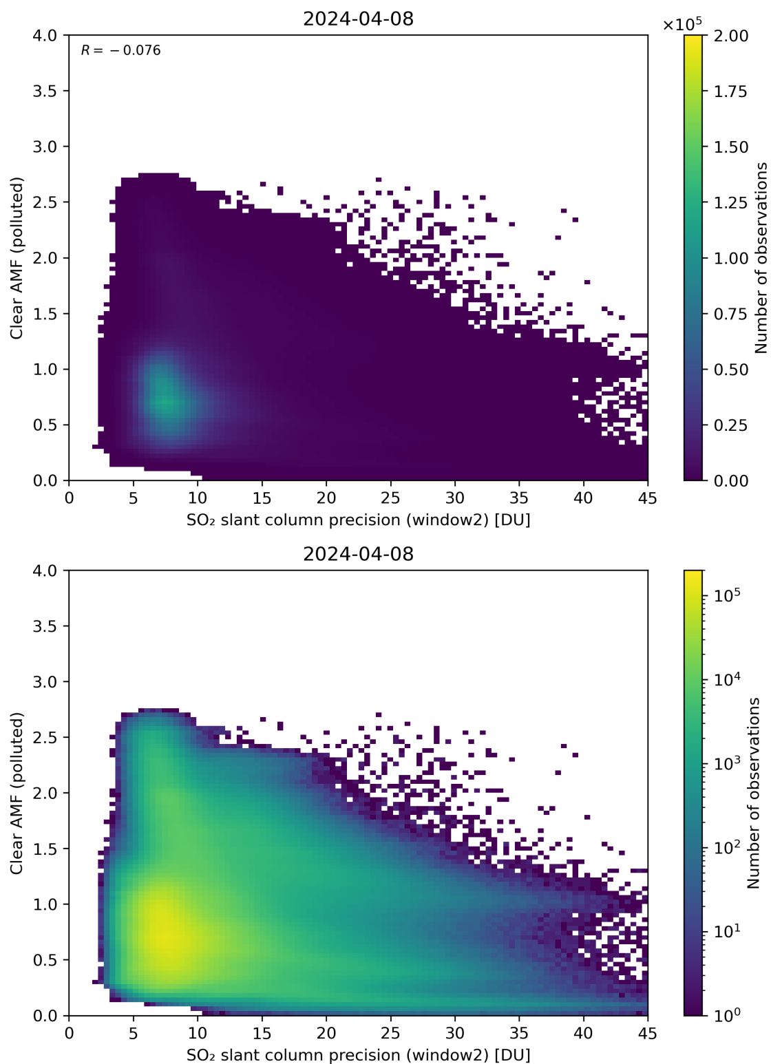
Figure 246: Scatter density plot of “SO 2 slant column precision (window2)” against “Clear AMF (polluted)” for 2024-04-07 to 2024-04-09.
