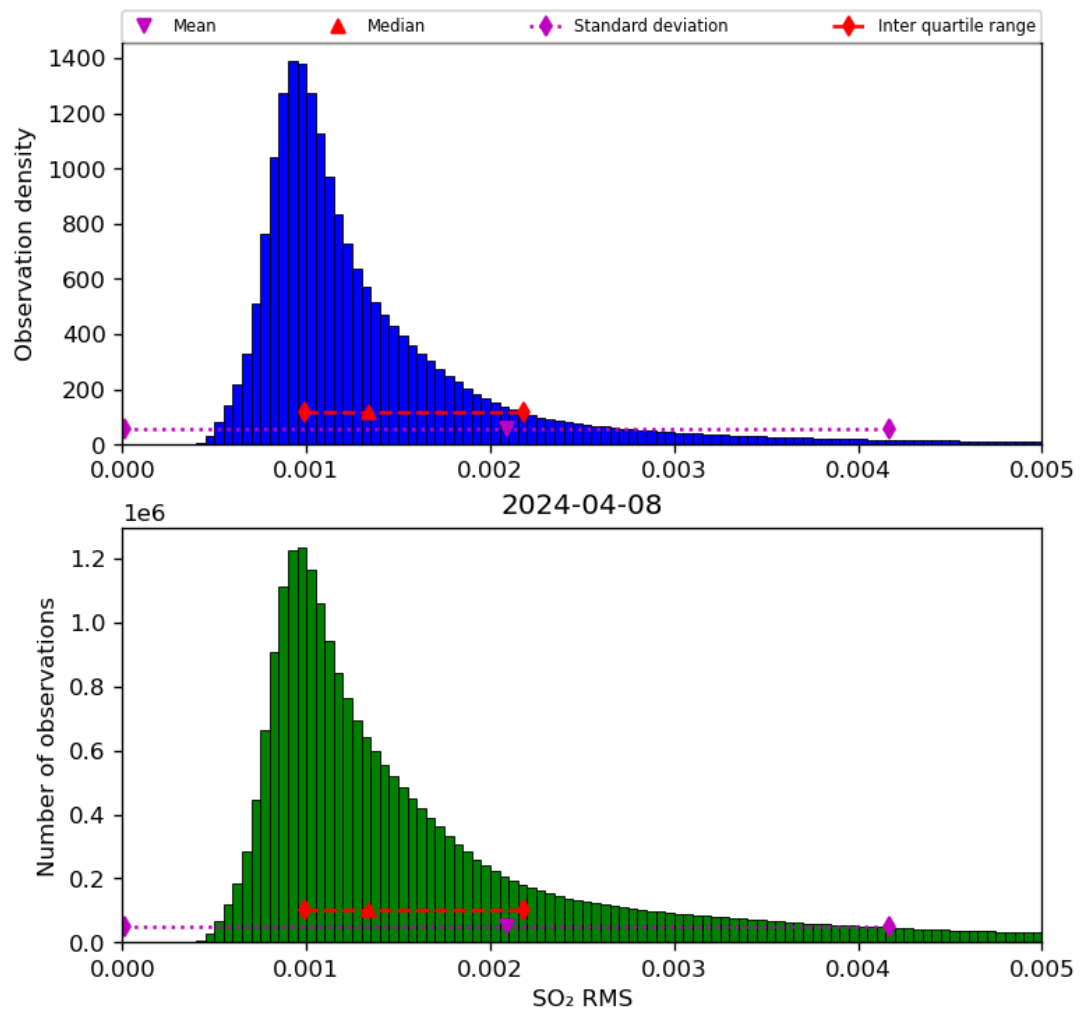
Figure 70: Histogram of “SO 2 RMS” for 2024-04-07 to 2024-04-09
