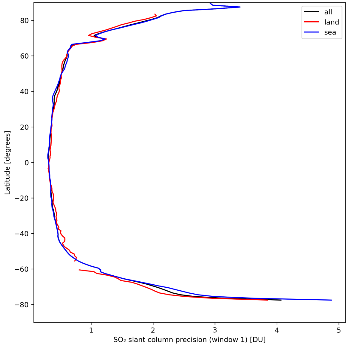
Figure 34: Zonal average of “SO 2 slant column precision (window 1)” for 2024-04-07 to 2024-04-09.
