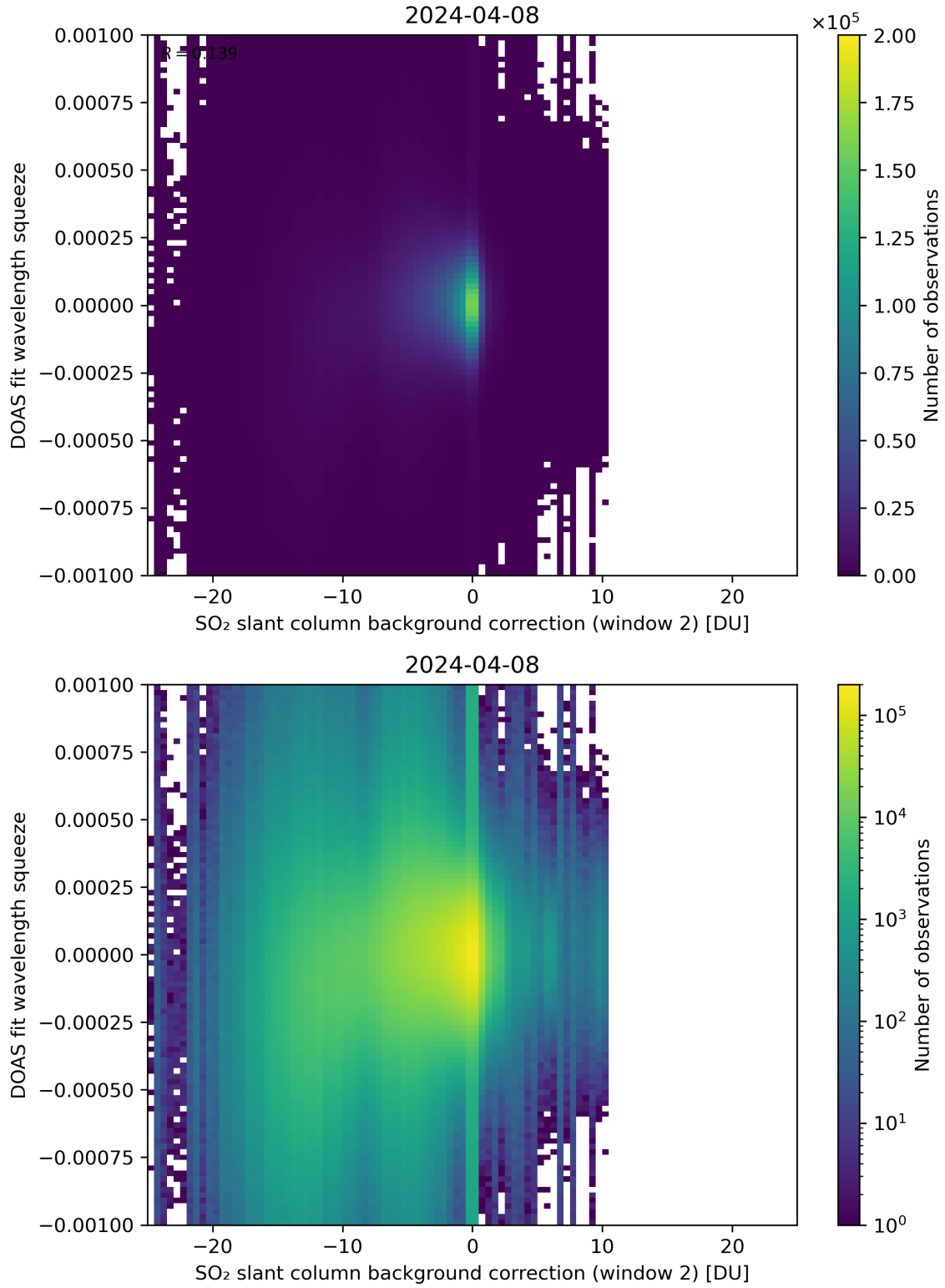
Figure 113: Scatter density plot of “SO 2 slant column background correction (window 2)” against “DOAS fit wavelength squeeze” for 2024-04-07 to 2024-04-09.
