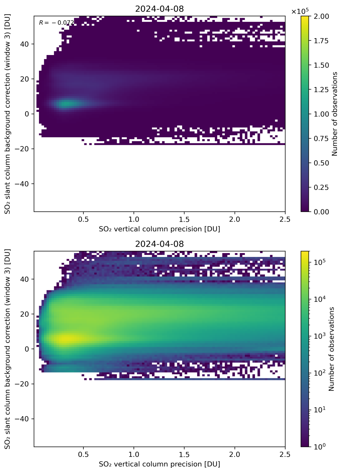
Figure 281: Scatter density plot of “SO 2 vertical column precision” against “SO 2 slant column background correction (window 3)” for 2024-04-07 to 2024-04-09.
