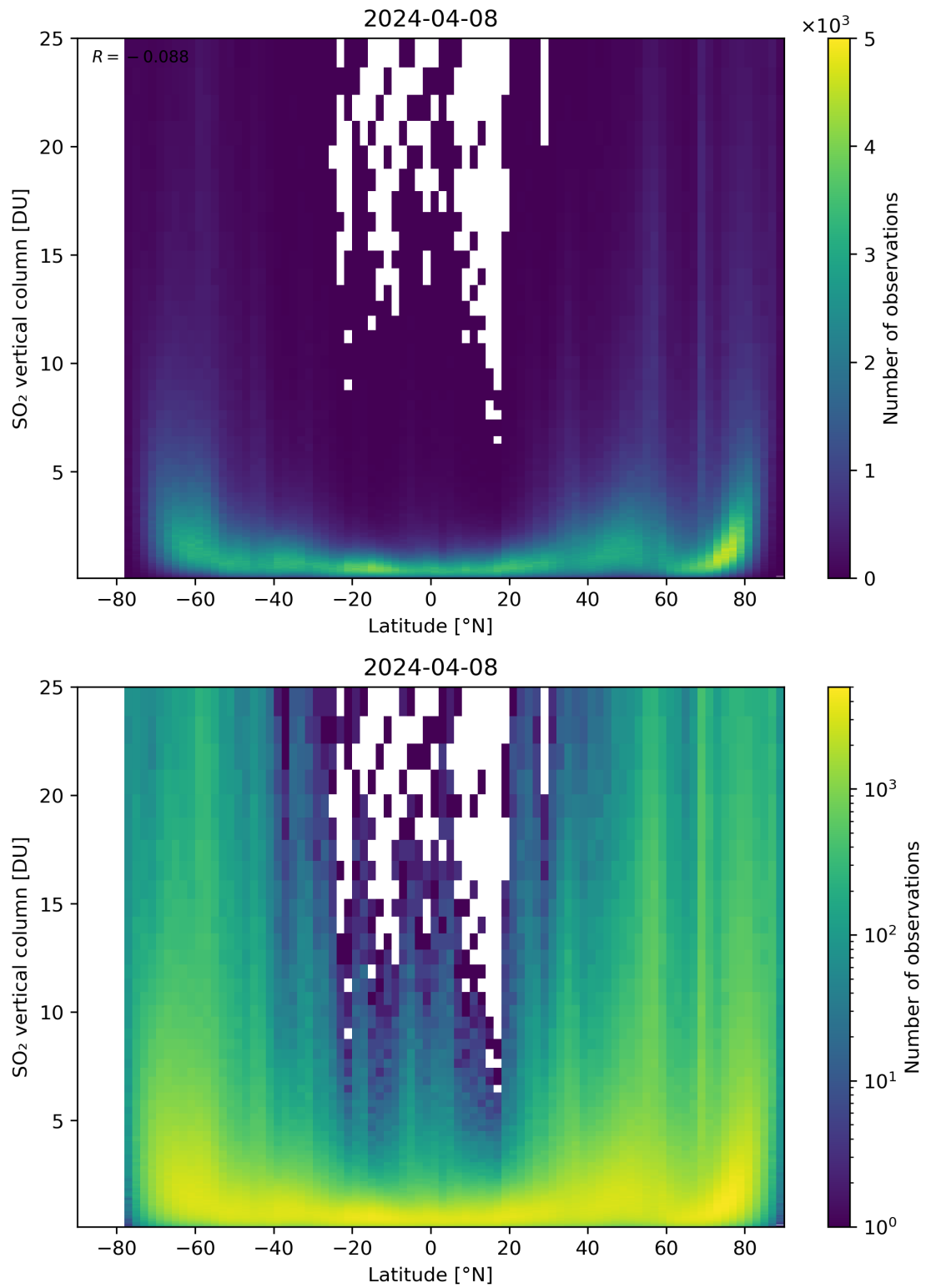
Figure 156: Scatter density plot of “Latitude” against “SO 2 vertical column” for 2024-04-07 to 2024-04-09.
