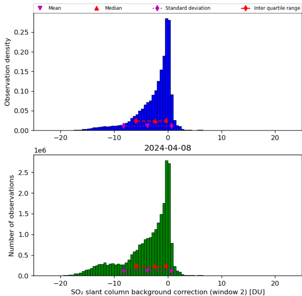
Figure 63: Histogram of “SO 2 slant column background correction (window 2)” for 2024-04-07 to 2024-04-09
