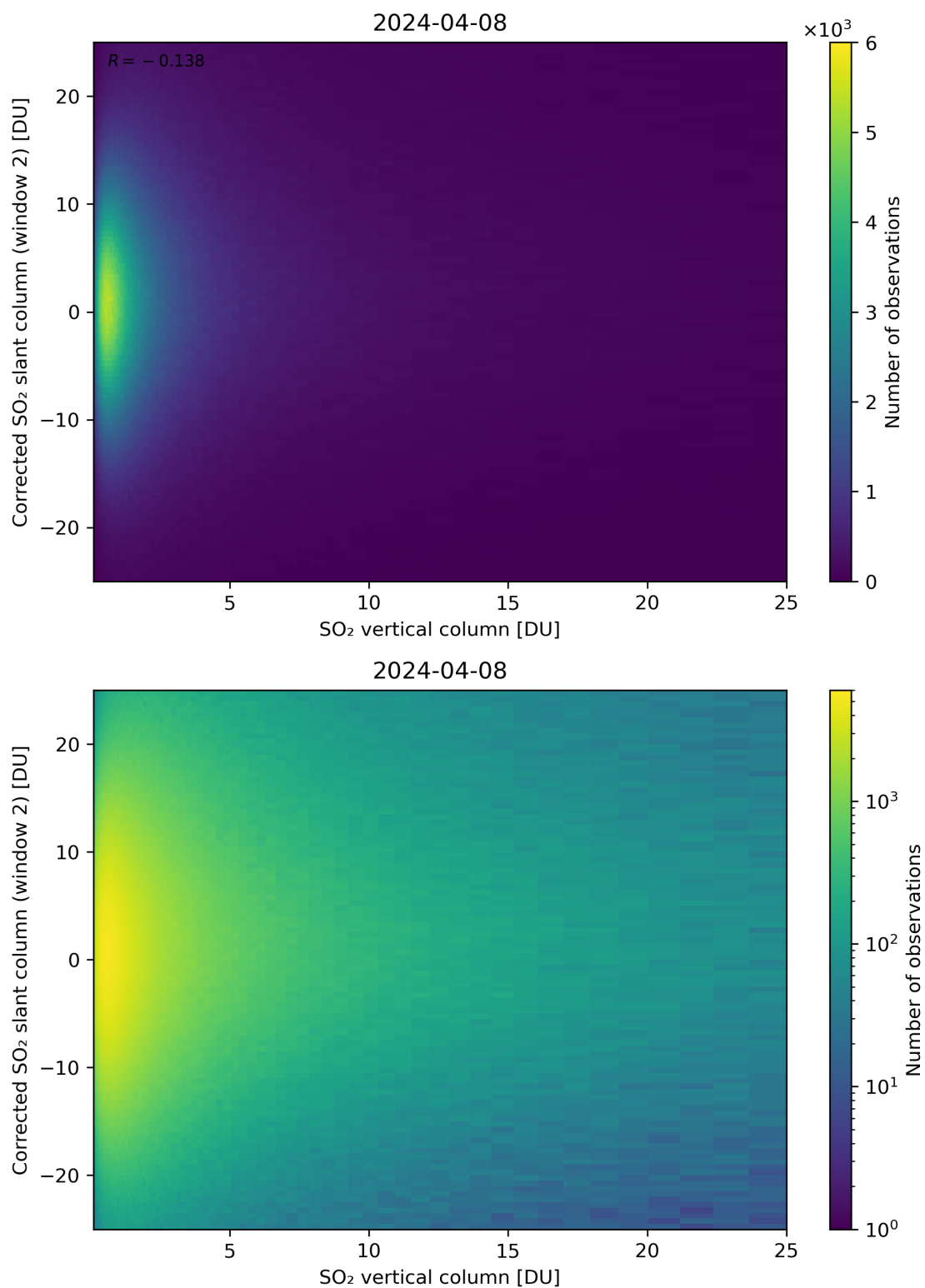
Figure 298: Scatter density plot of “SO 2 vertical column” against “Corrected SO 2 slant column (window 2)” for 2024-04-07 to 2024-04-09.
