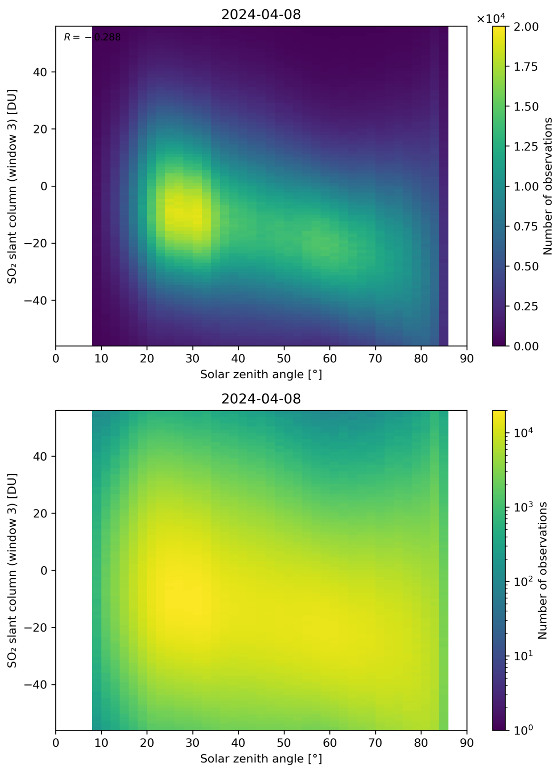
Figure 172: Scatter density plot of “Solar zenith angle” against “SO 2 slant column (window 3)” for 2024-04-07 to 2024-04-09.
