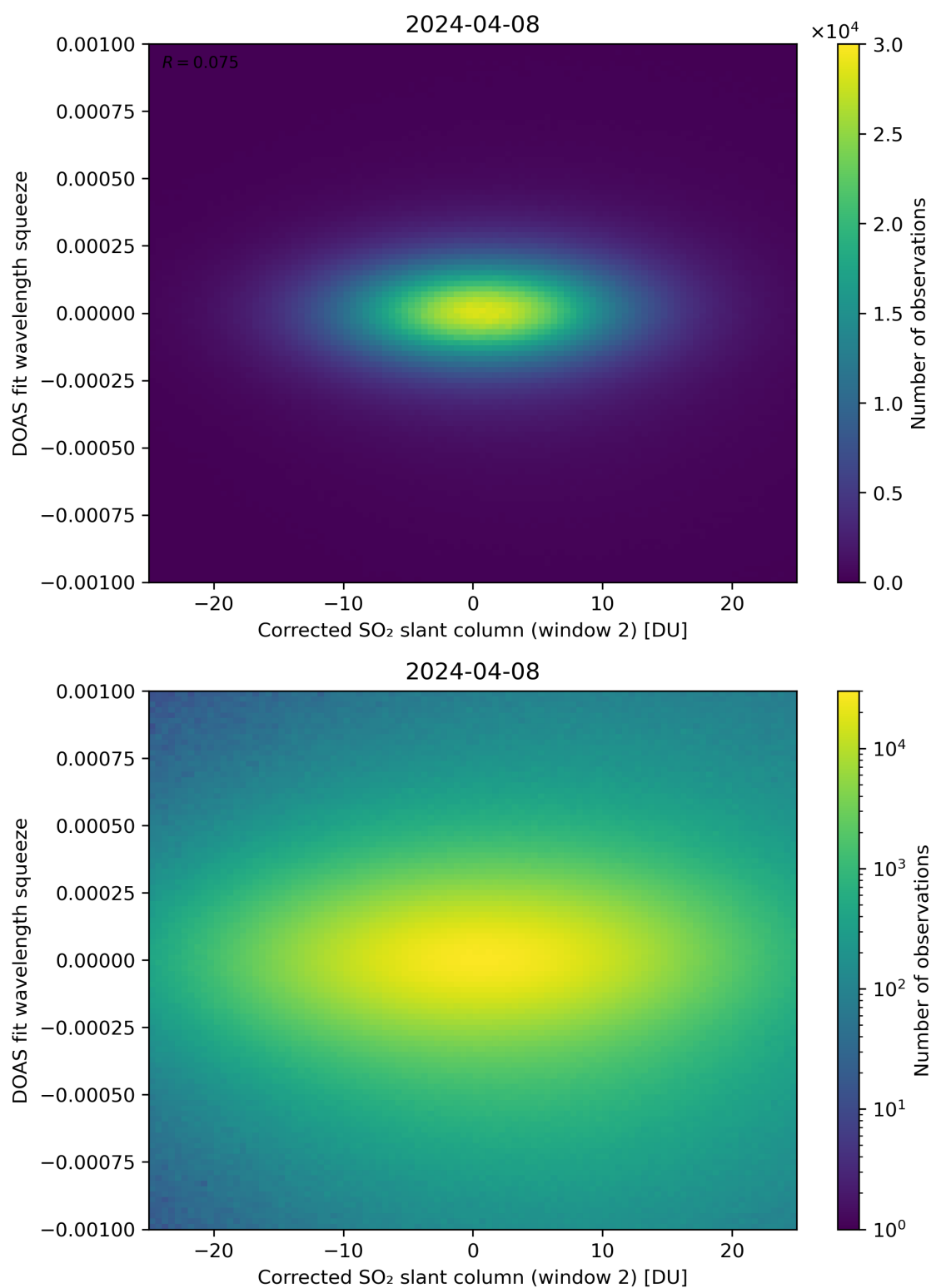
Figure 197: Scatter density plot of “Corrected SO 2 slant column (window 2)” against “DOAS fit wavelength squeeze” for 2024-04-07 to 2024-04-09.
