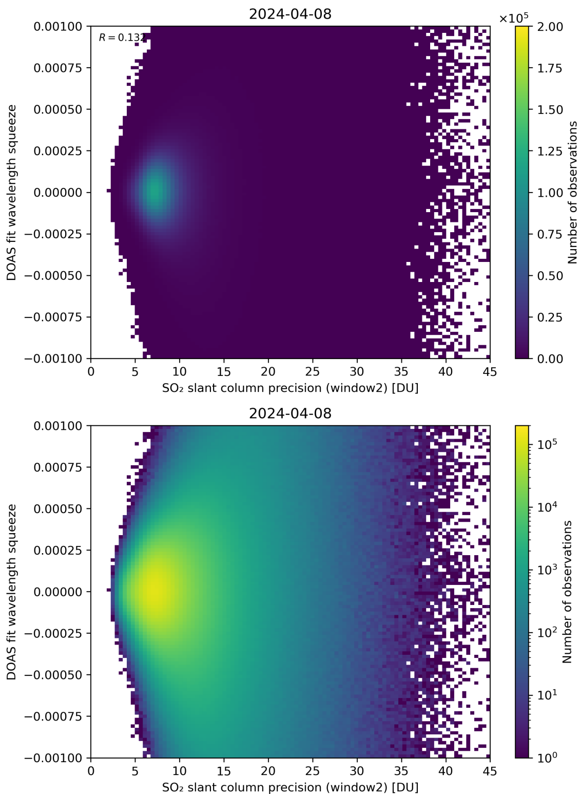
Figure 244: Scatter density plot of “SO 2 slant column precision (window2)” against “DOAS fit wavelength squeeze” for 2024-04-07 to 2024-04-09.
