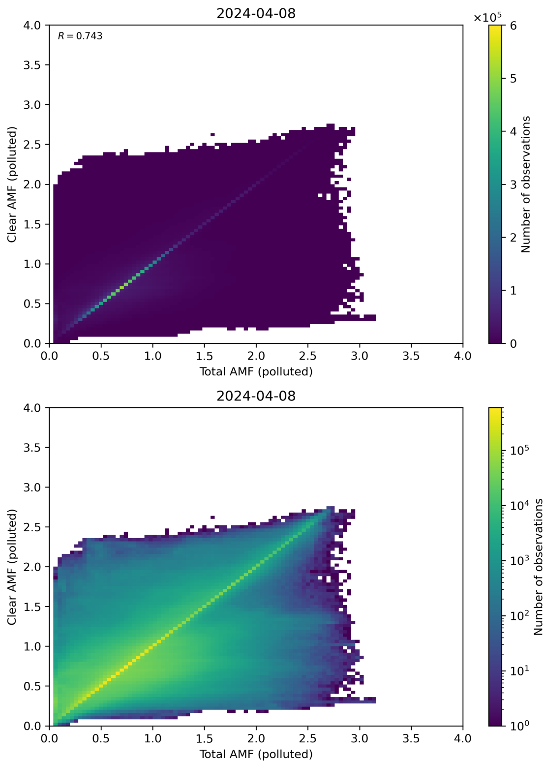
Figure 271: Scatter density plot of “Total AMF (polluted)” against “Clear AMF (polluted)” for 2024-04-07 to 2024-04-09.
