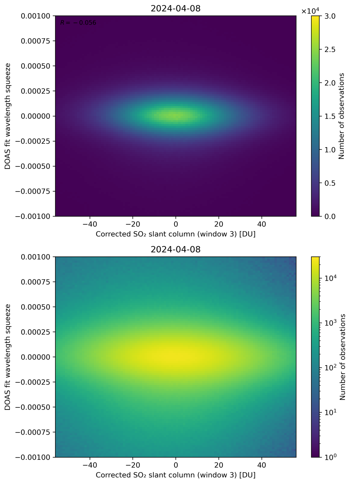
Figure 207: Scatter density plot of “Corrected SO 2 slant column (window 3)” against “DOAS fit wavelength squeeze” for 2024-04-07 to 2024-04-09.
