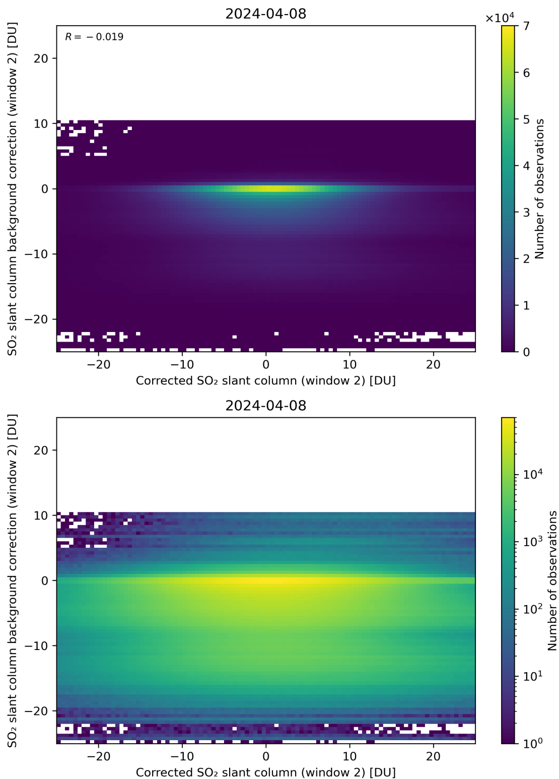
Figure 194: Scatter density plot of “Corrected SO 2 slant column (window 2)” against “SO 2 slant column background correction (window 2)” for 2024-04-07 to 2024-04-09.
