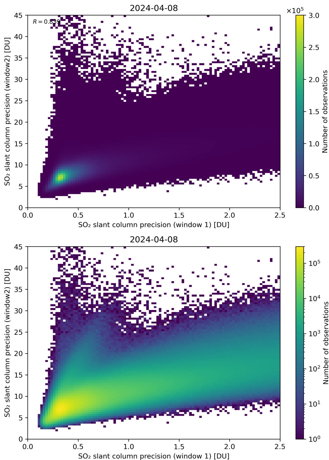
Figure 227: Scatter density plot of “SO 2 slant column precision (window 1)” against “SO 2 slant column precision (window2)” for 2024-04-07 to 2024-04-09.
