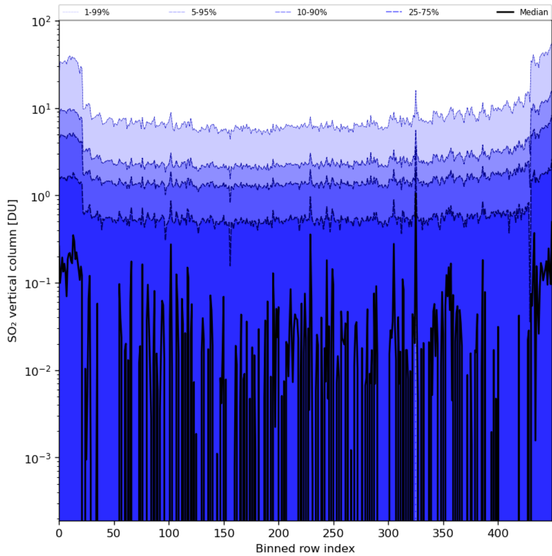
Figure 76: Along track statistics of “SO 2 vertical column” for 2024-04-07 to 2024-04-09
