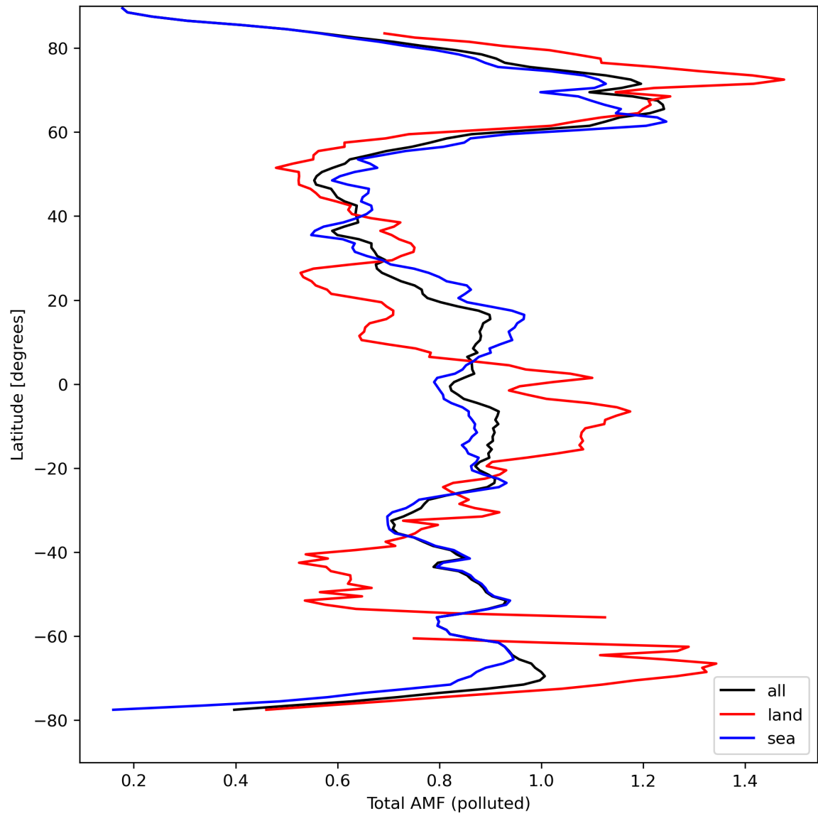
Figure 48: Zonal average of “Total AMF (polluted)” for 2024-04-07 to 2024-04-09.
