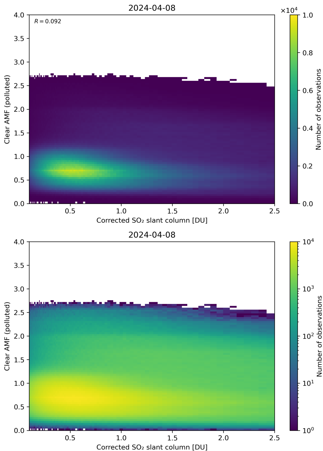
Figure 184: Scatter density plot of “Corrected SO 2 slant column” against “Clear AMF (polluted)” for 2024-04-07 to 2024-04-09.
