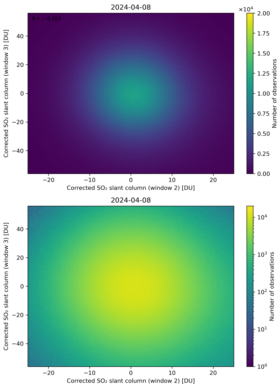
Figure 200: Scatter density plot of “Corrected SO 2 slant column (window 2)” against “Corrected SO 2 slant column (window 3)” for 2024-04-07 to 2024-04-09.
