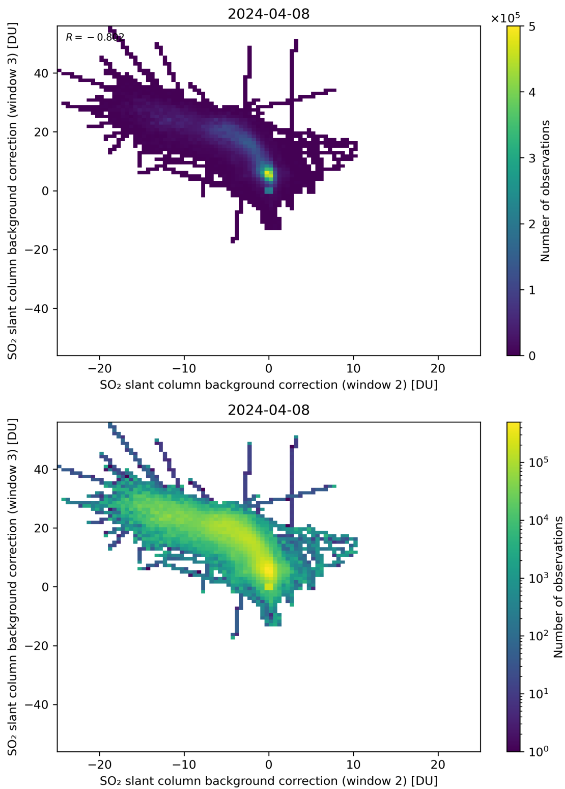
Figure 111: Scatter density plot of “SO 2 slant column background correction (window 2)” against “SO 2 slant column background correction (window 3)” for 2024-04-07 to 2024-04-09.
