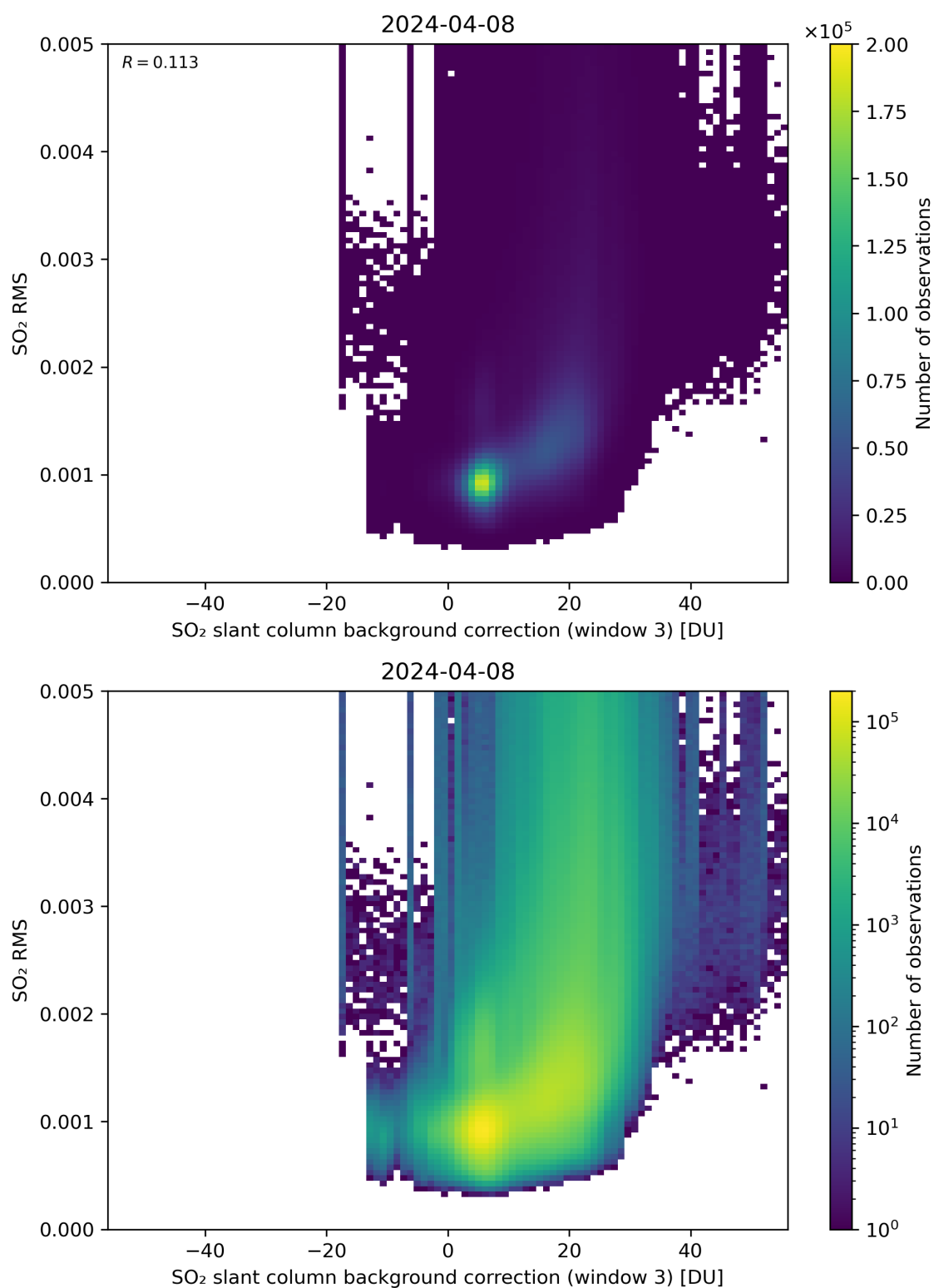
Figure 123: Scatter density plot of “SO 2 slant column background correction (window 3)” against “SO 2 RMS” for 2024-04-07 to 2024-04-09.
