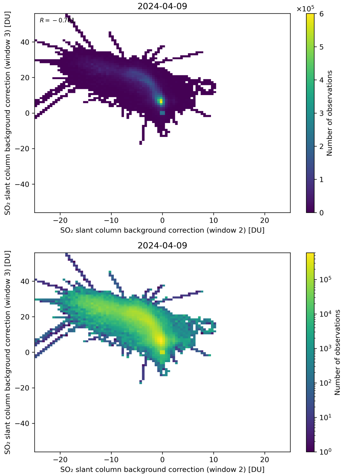
Figure 111: Scatter density plot of “SO 2 slant column background correction (window 2)” against “SO 2 slant column background correction (window 3)” for 2024-04-08 to 2024-04-10.
