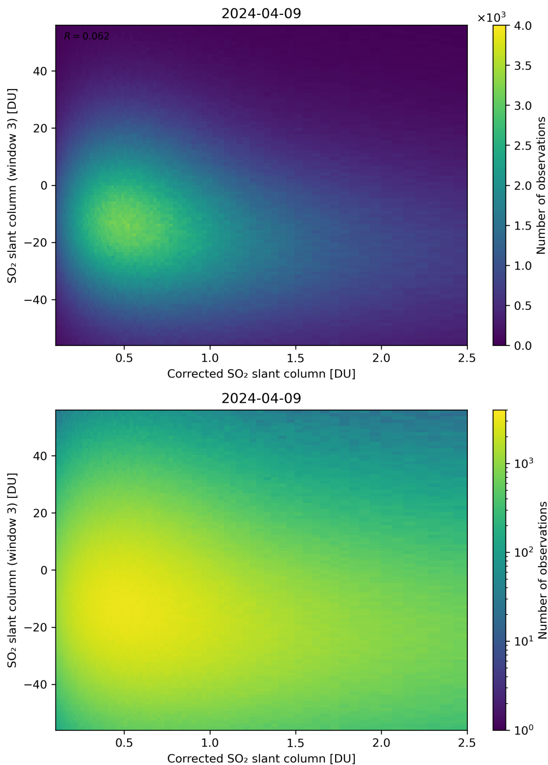
Figure 190: Scatter density plot of “Corrected SO 2 slant column” against “SO 2 slant column (window 3)” for 2024-04-08 to 2024-04-10.
