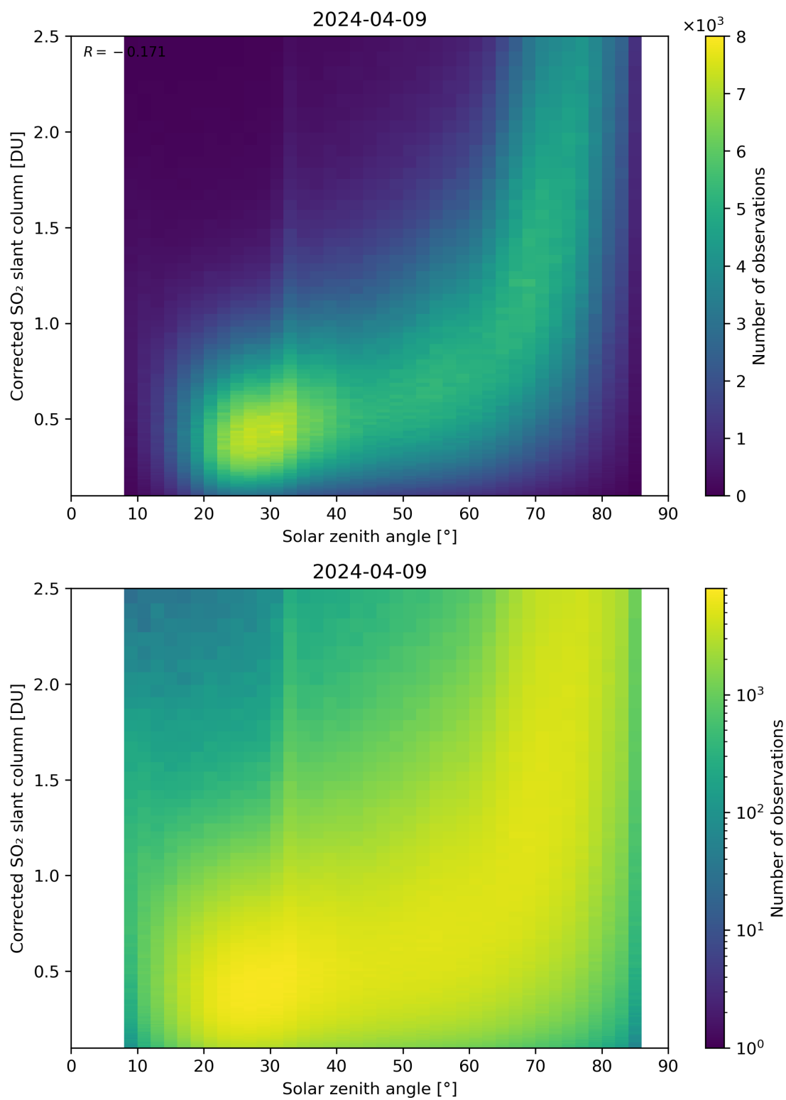
Figure 166: Scatter density plot of “Solar zenith angle” against “Corrected SO 2 slant column” for 2024-04-08 to 2024-04-10.
