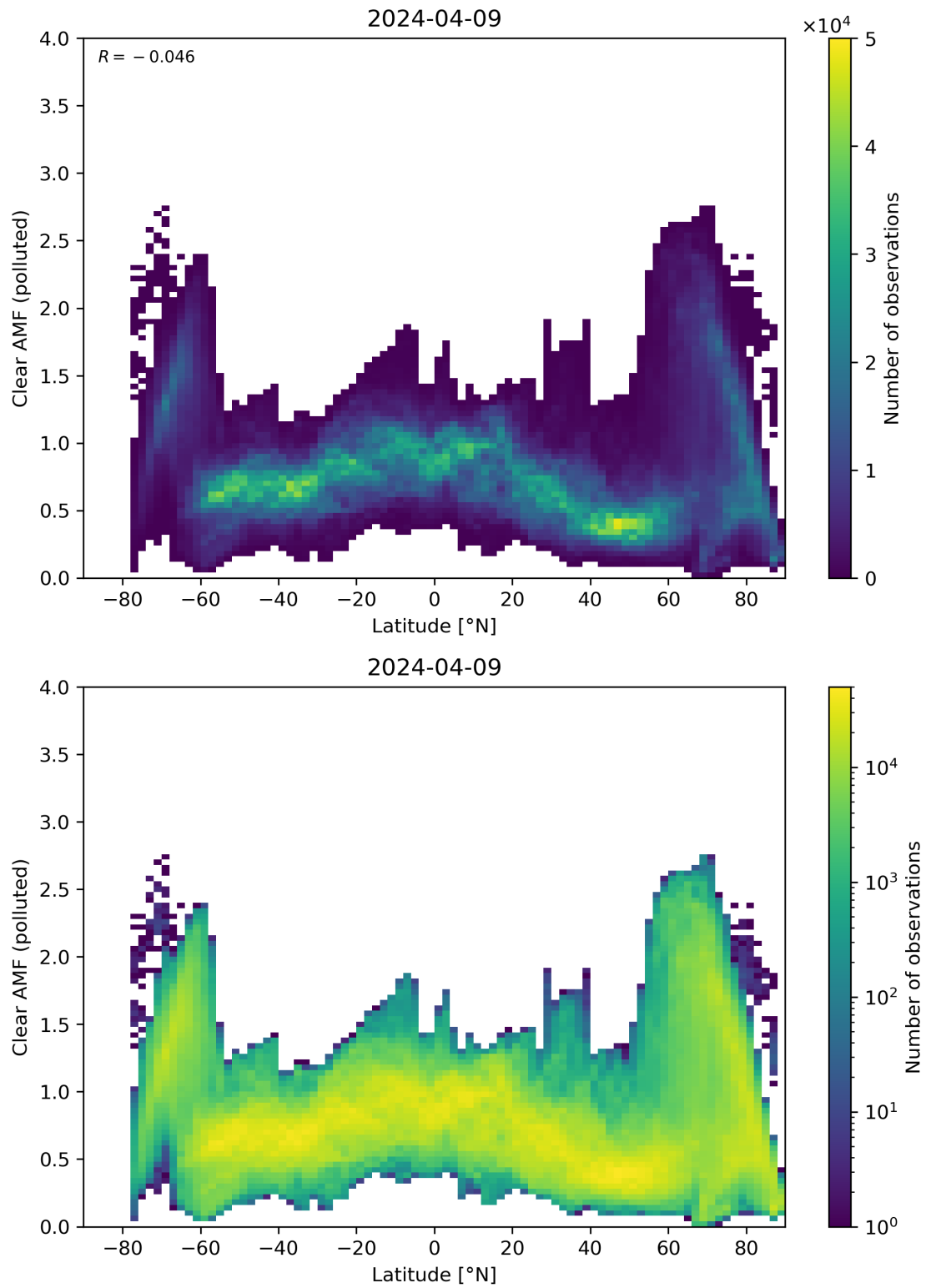
Figure 145: Scatter density plot of “Latitude” against “Clear AMF (polluted)” for 2024-04-08 to 2024-04-10.
