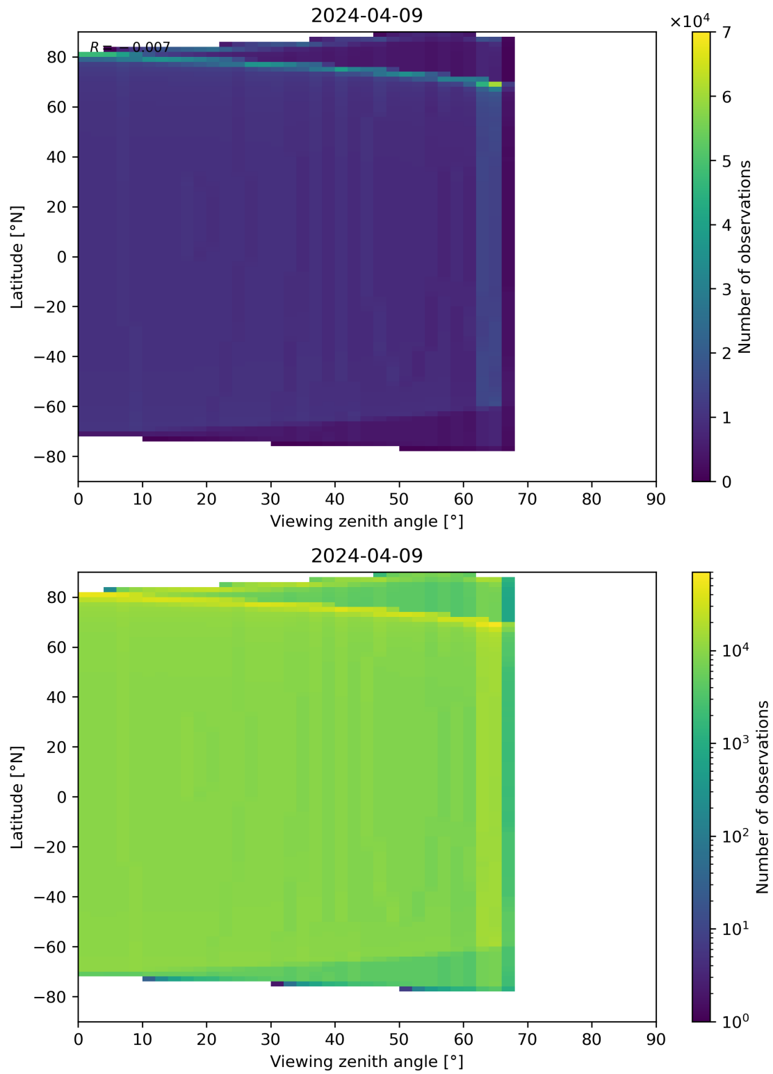
Figure 314: Scatter density plot of “Viewing zenith angle” against “Latitude” for 2024-04-08 to 2024-04-10.
