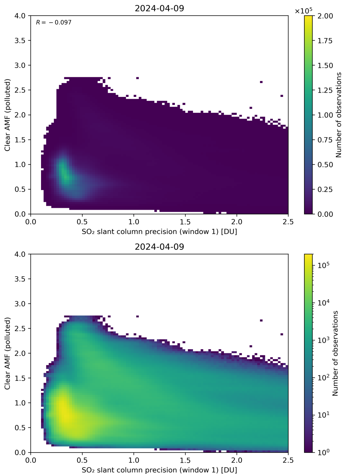
Figure 224: Scatter density plot of “SO 2 slant column precision (window 1)” against “Clear AMF (polluted)” for 2024-04-08 to 2024-04-10.
