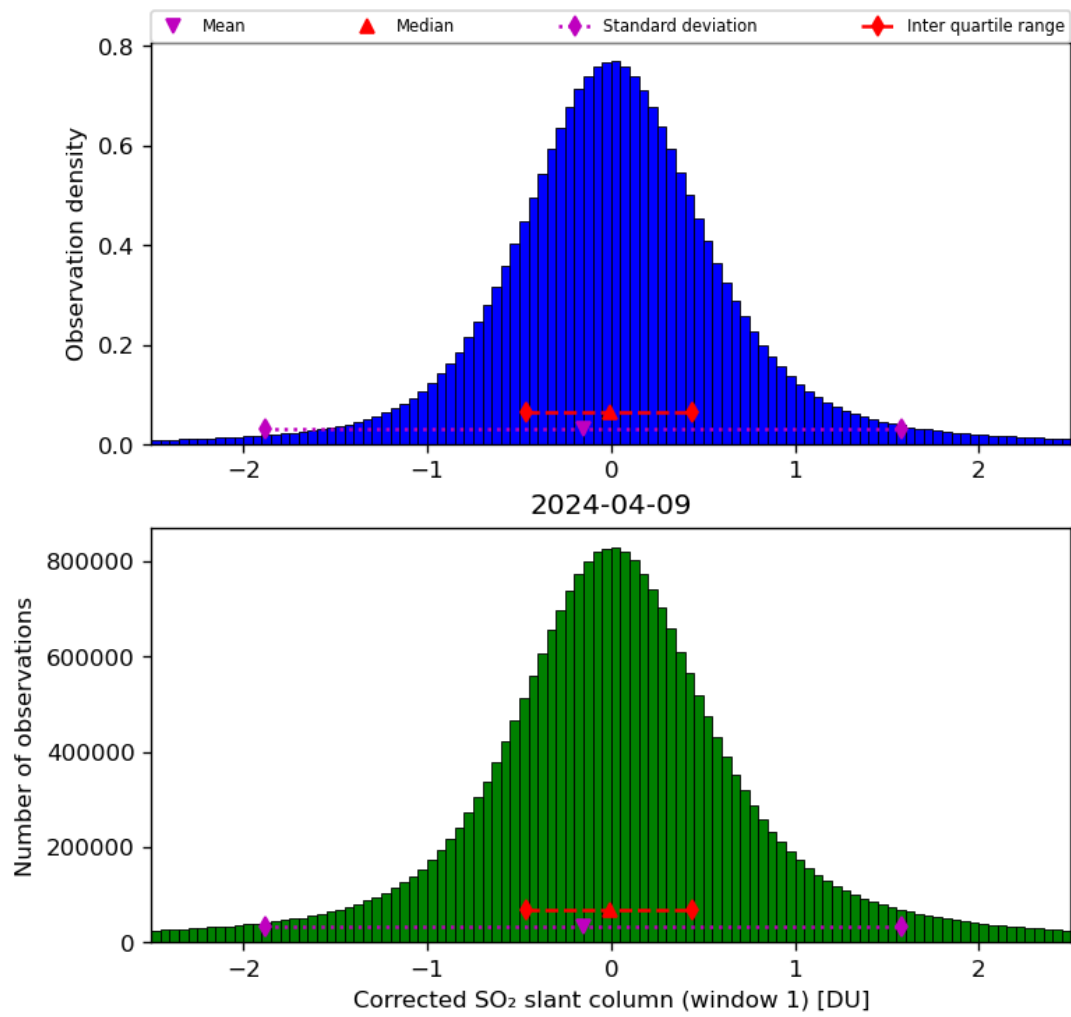
Figure 58: Histogram of “Corrected SO 2 slant column (window 1)” for 2024-04-08 to 2024-04-10
