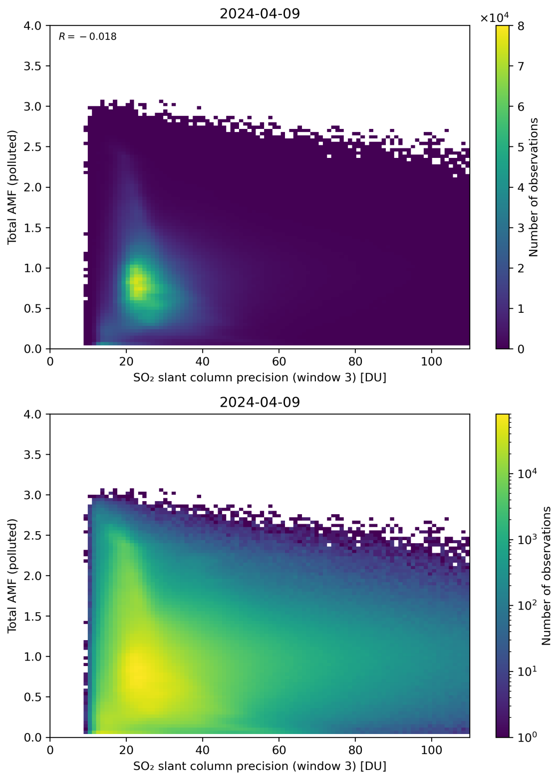
Figure 263: Scatter density plot of “SO 2 slant column precision (window 3)” against “Total AMF (polluted)” for 2024-04-08 to 2024-04-10.
