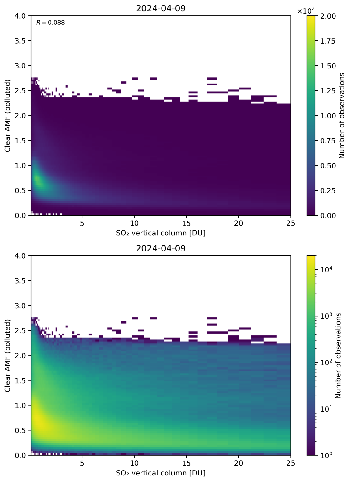
Figure 296: Scatter density plot of “SO 2 vertical column” against “Clear AMF (polluted)” for 2024-04-08 to 2024-04-10.
