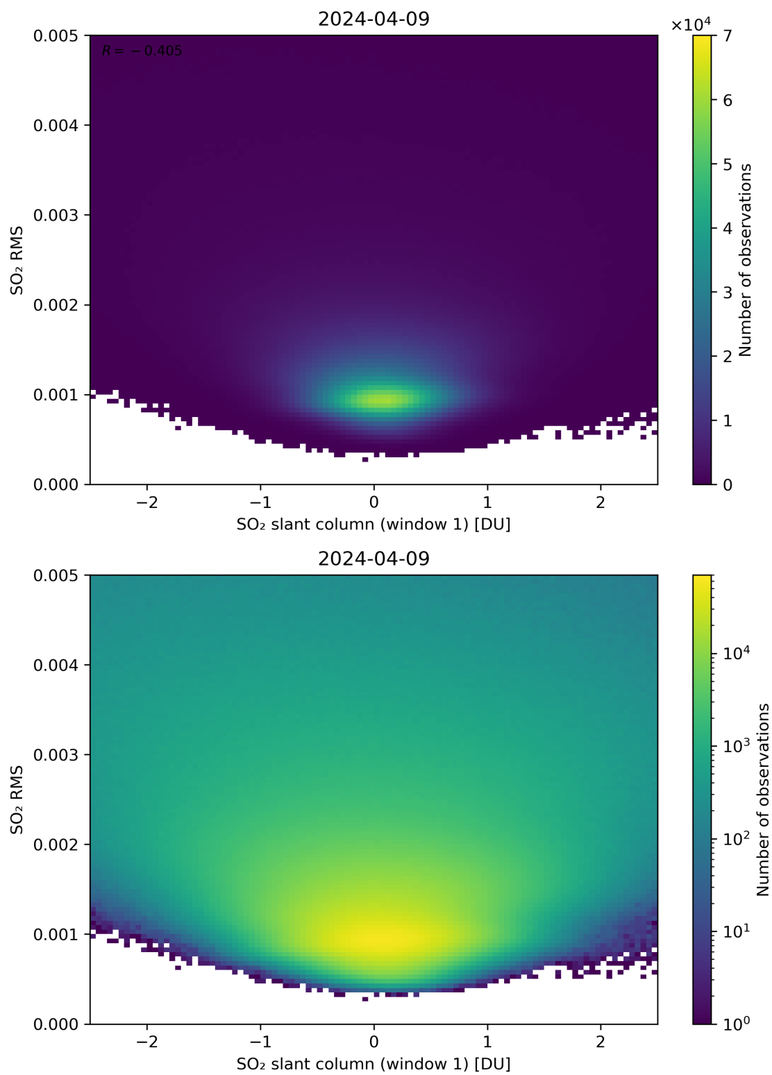
Figure 217: Scatter density plot of “SO 2 slant column (window 1)” against “SO 2 RMS” for 2024-04-08 to 2024-04-10.
