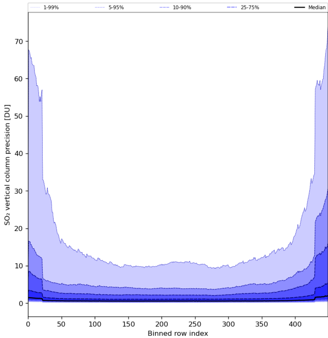
Figure 77: Along track statistics of “SO 2 vertical column precision” for 2024-04-08 to 2024-04-10
