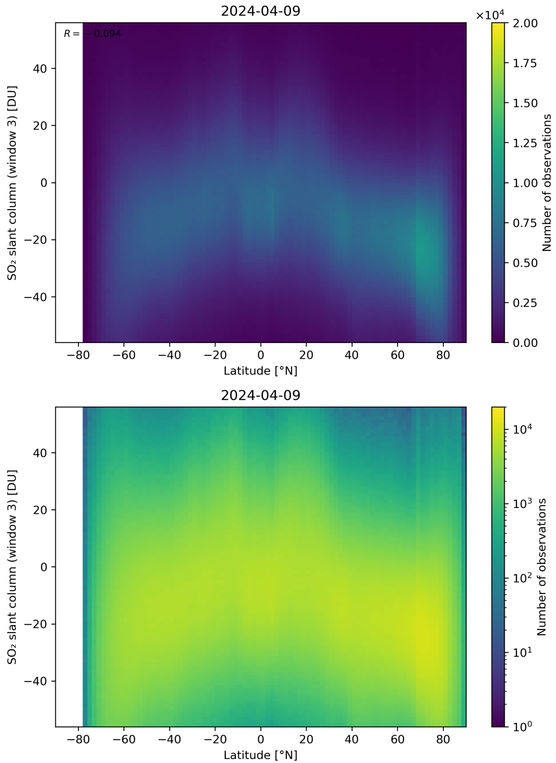
Figure 152: Scatter density plot of “Latitude” against “SO 2 slant column (window 3)” for 2024-04-08 to 2024-04-10.
