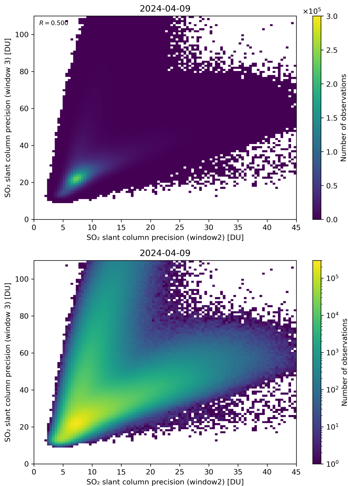
Figure 250: Scatter density plot of “SO 2 slant column precision (window2)” against “SO 2 slant column precision (window 3)” for 2024-04-08 to 2024-04-10.
