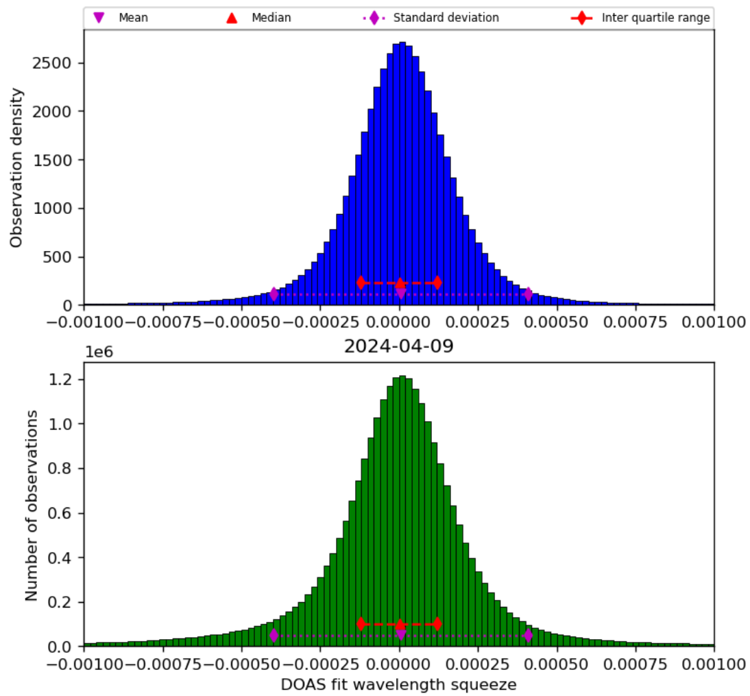
Figure 69: Histogram of “DOAS fit wavelength squeeze” for 2024-04-08 to 2024-04-10
