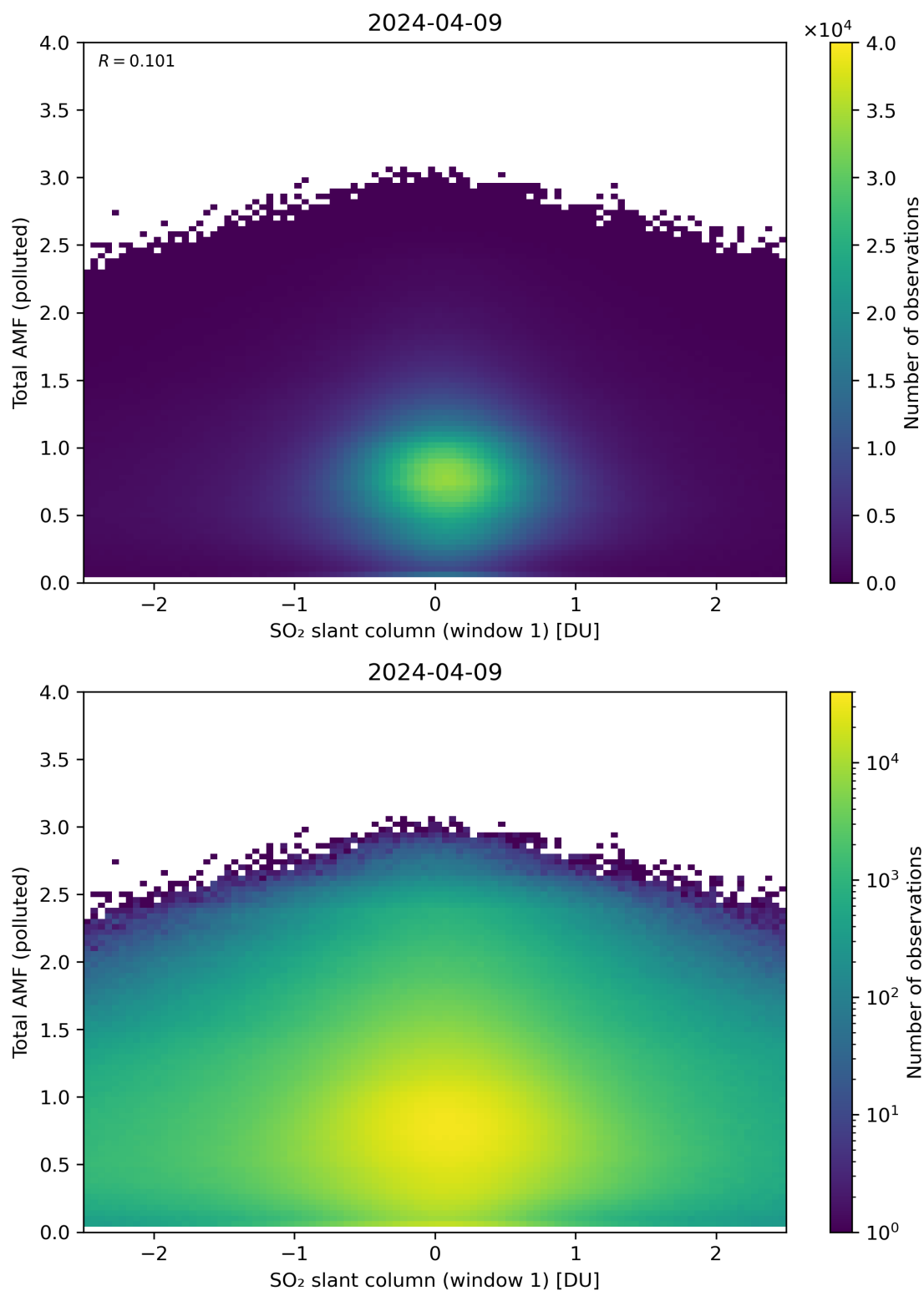
Figure 239: Scatter density plot of “SO 2 slant column (window 1)” against “Total AMF (polluted)” for 2024-04-08 to 2024-04-10.
