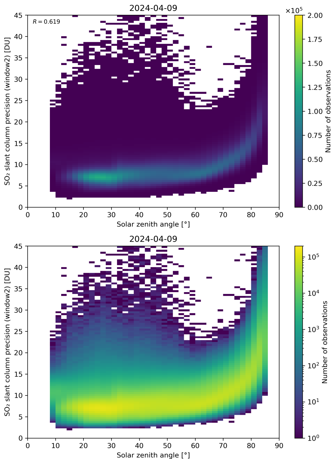
Figure 171: Scatter density plot of “Solar zenith angle” against “SO 2 slant column precision (window2)” for 2024-04-08 to 2024-04-10.
