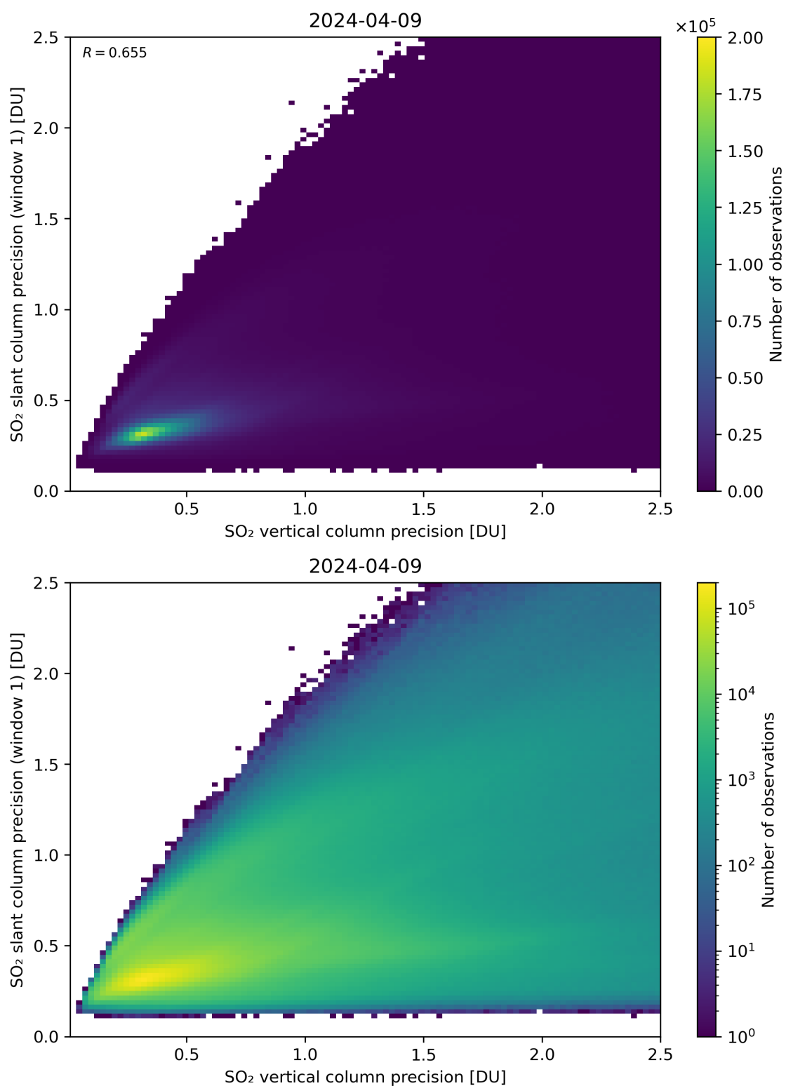
Figure 290: Scatter density plot of “SO 2 vertical column precision” against “SO 2 slant column precision (window 1)” for 2024-04-08 to 2024-04-10.
