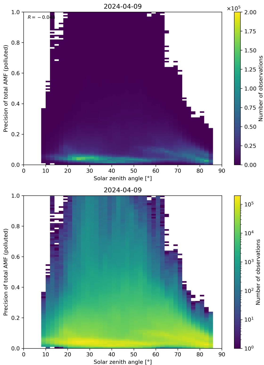
Figure 175: Scatter density plot of “Solar zenith angle” against “Precision of total AMF (polluted)” for 2024-04-08 to 2024-04-10.
