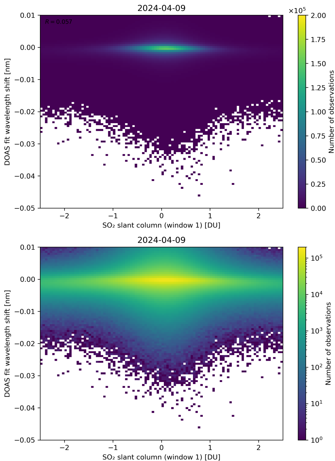
Figure 215: Scatter density plot of “SO 2 slant column (window 1)” against “DOAS fit wavelength shift” for 2024-04-08 to 2024-04-10.
