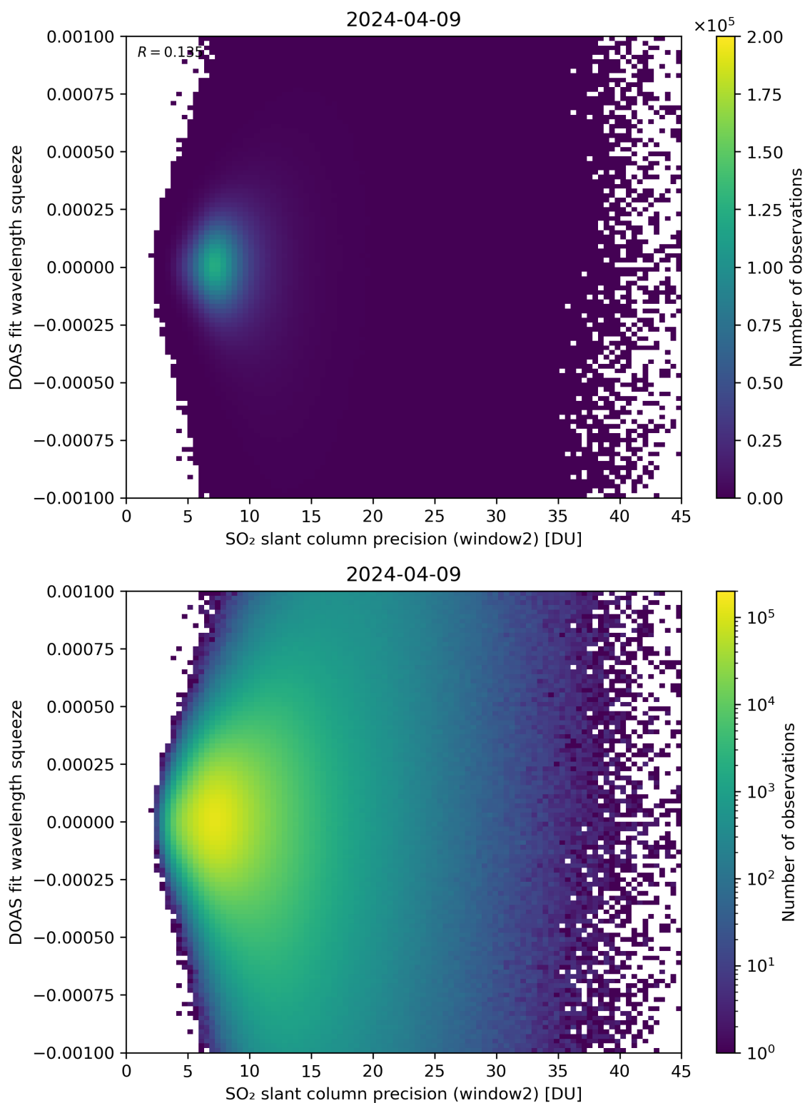
Figure 244: Scatter density plot of “SO 2 slant column precision (window2)” against “DOAS fit wavelength squeeze” for 2024-04-08 to 2024-04-10.
