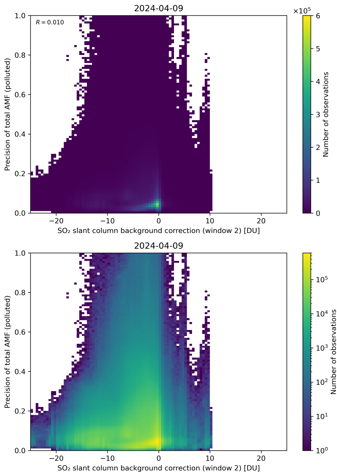
Figure 120: Scatter density plot of “SO 2 slant column background correction (window 2)” against “Precision of total AMF (polluted)” for 2024-04-08 to 2024-04-10.
