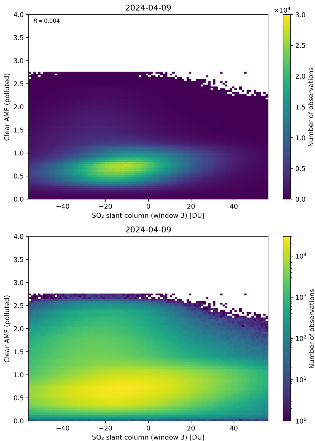
Figure 265: Scatter density plot of “SO 2 slant column (window 3)” against “Clear AMF (polluted)” for 2024-04-08 to 2024-04-10.
