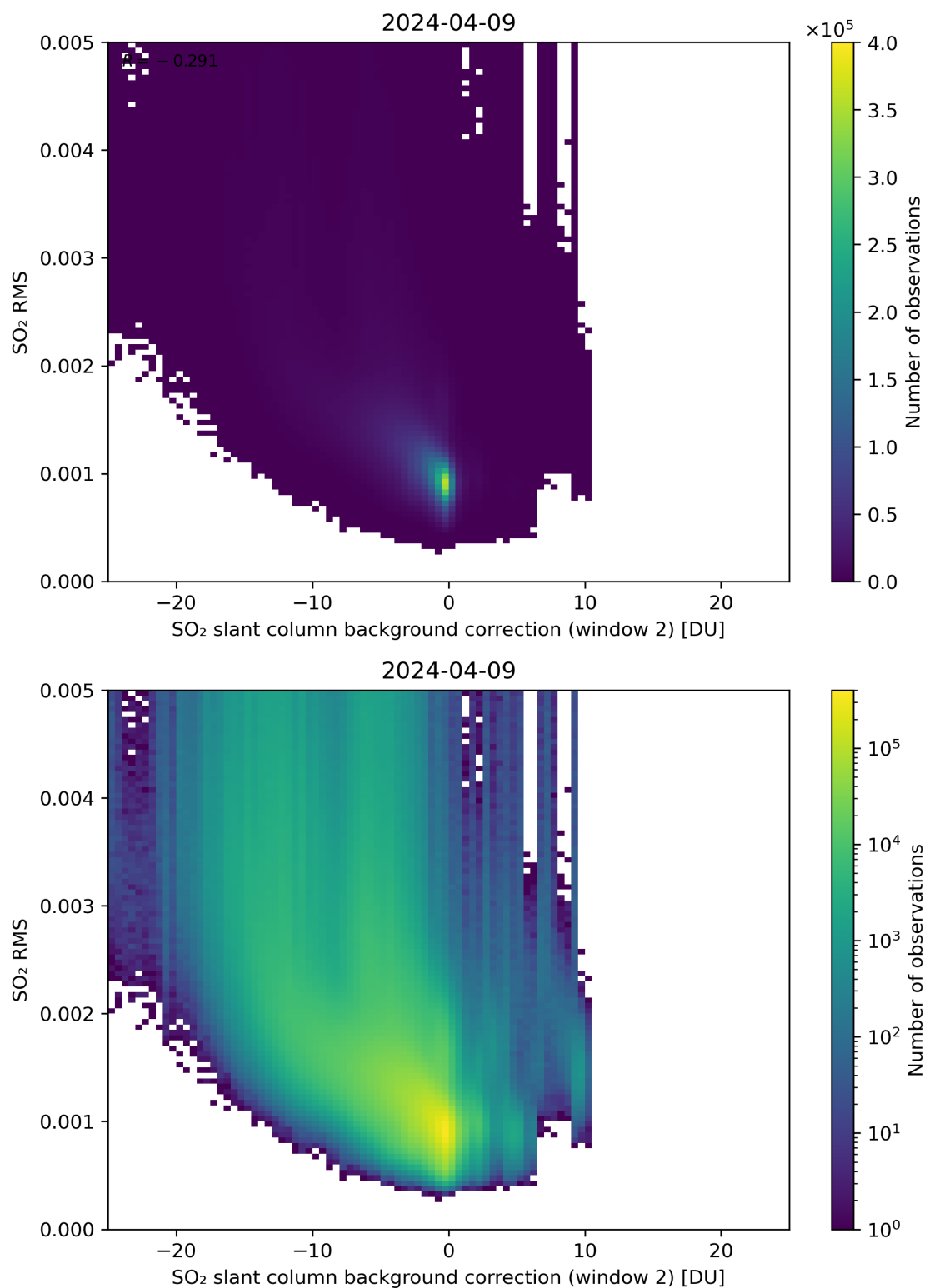
Figure 114: Scatter density plot of “SO 2 slant column background correction (window 2)” against “SO 2 RMS” for 2024-04-08 to 2024-04-10.
