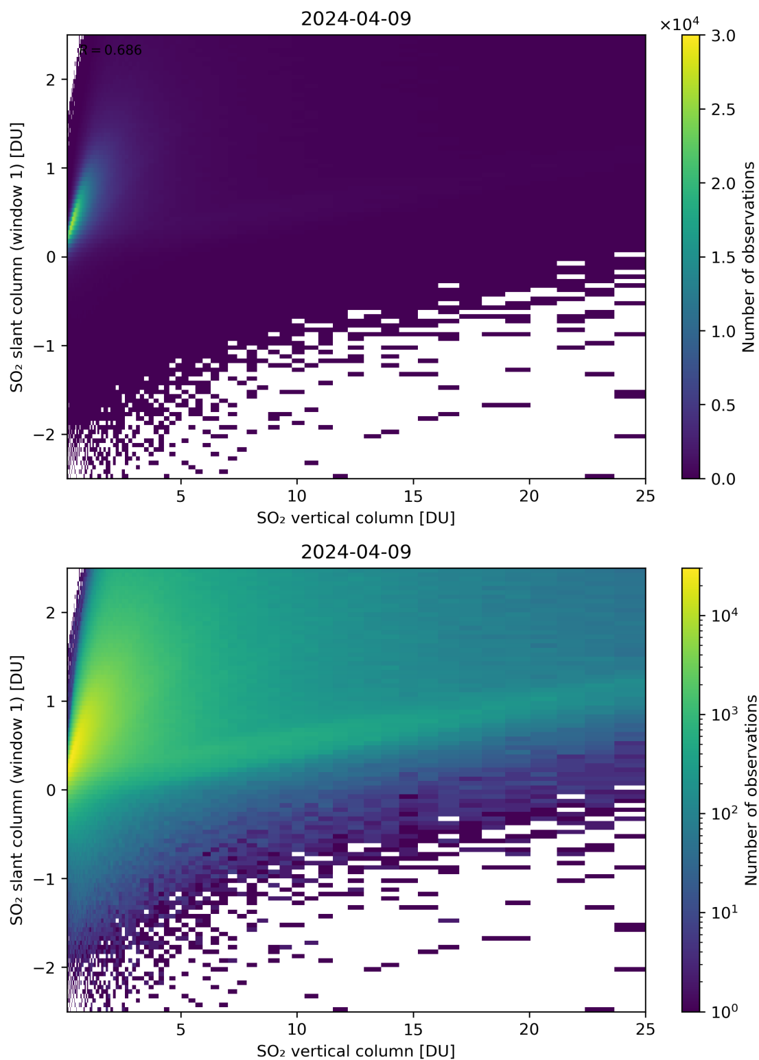
Figure 300: Scatter density plot of “SO 2 vertical column” against “SO 2 slant column (window 1)” for 2024-04-08 to 2024-04-10.
