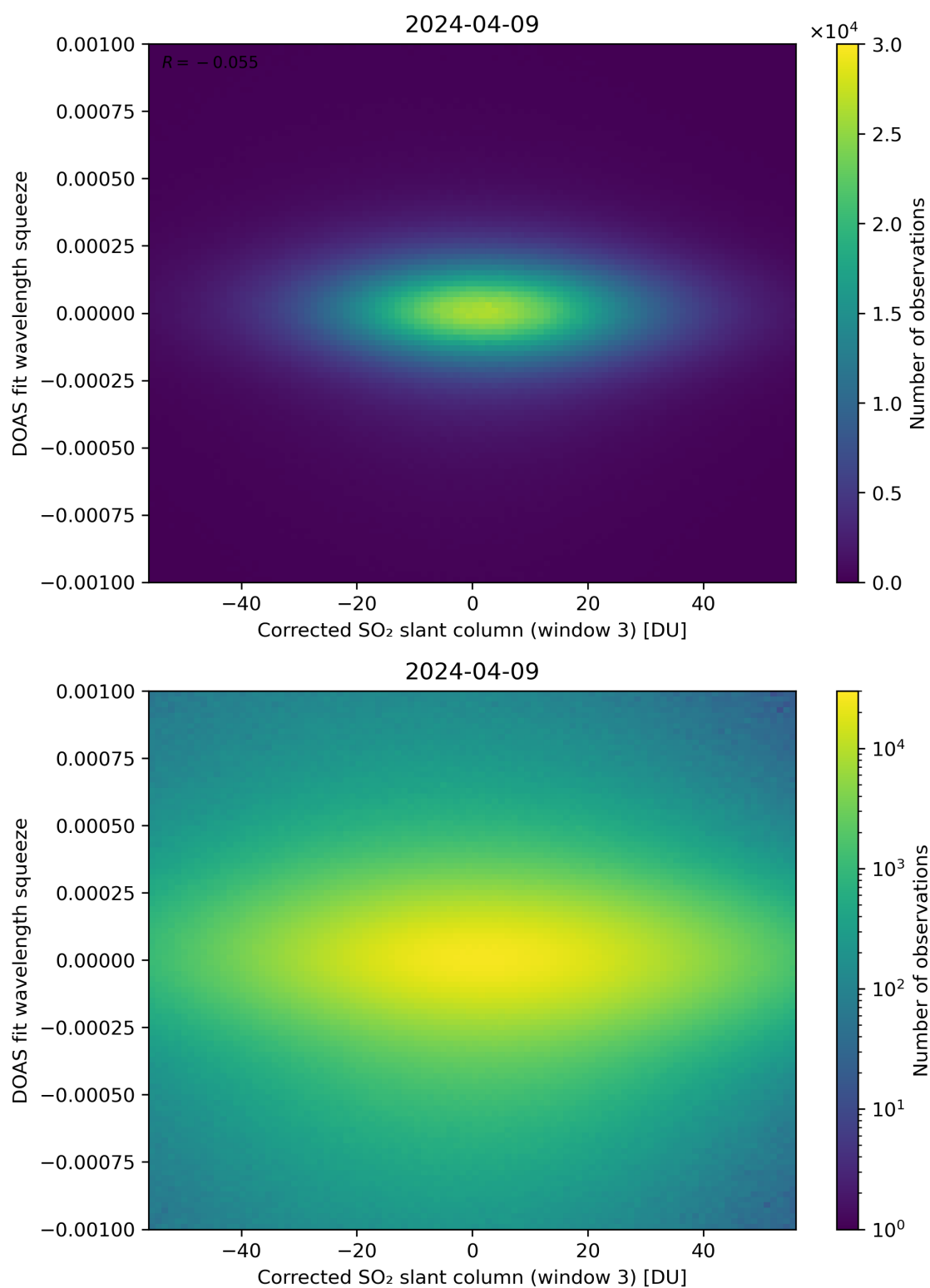
Figure 207: Scatter density plot of “Corrected SO 2 slant column (window 3)” against “DOAS fit wavelength squeeze” for 2024-04-08 to 2024-04-10.
