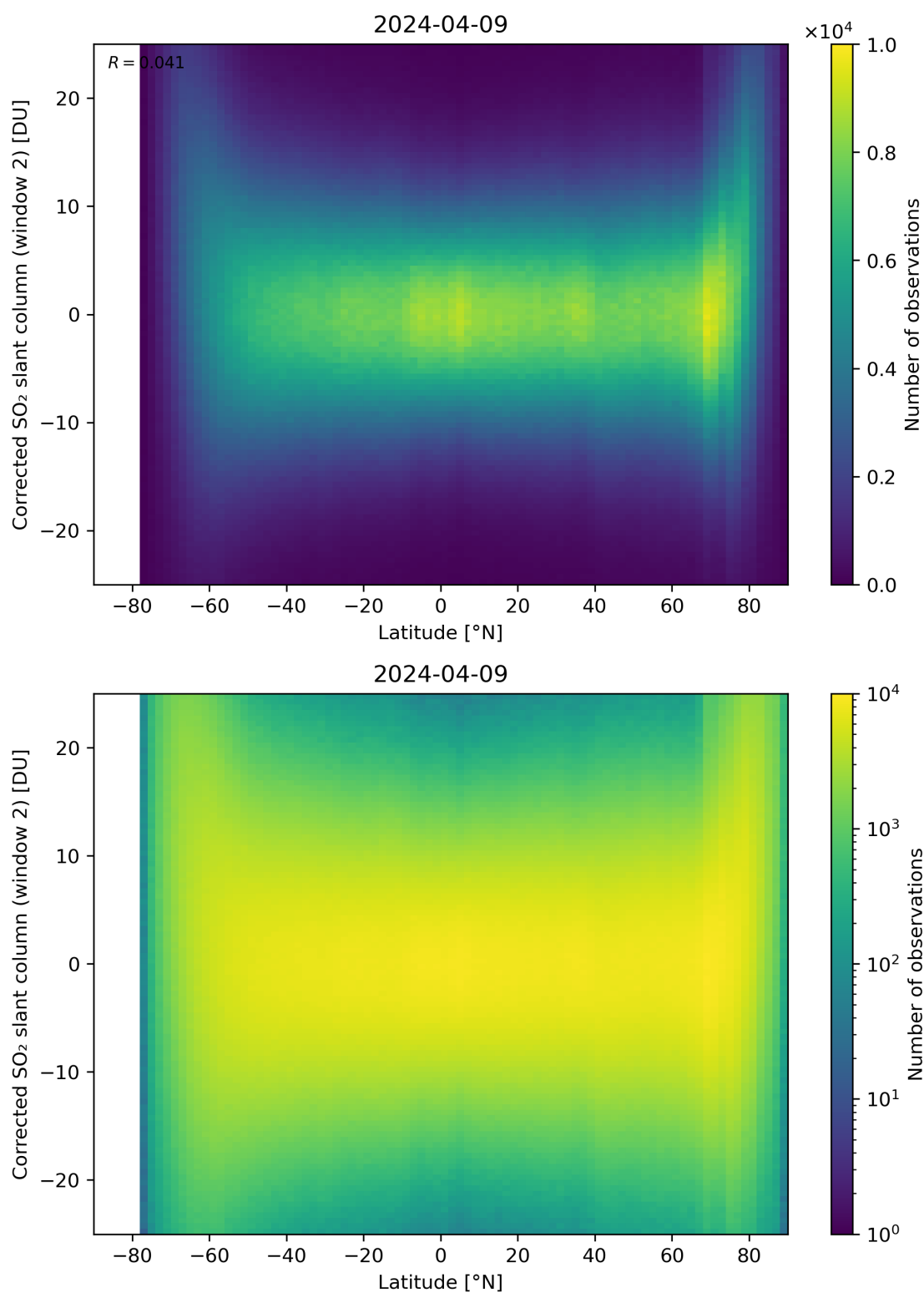
Figure 147: Scatter density plot of “Latitude” against “Corrected SO 2 slant column (window 2)” for 2024-04-08 to 2024-04-10.
