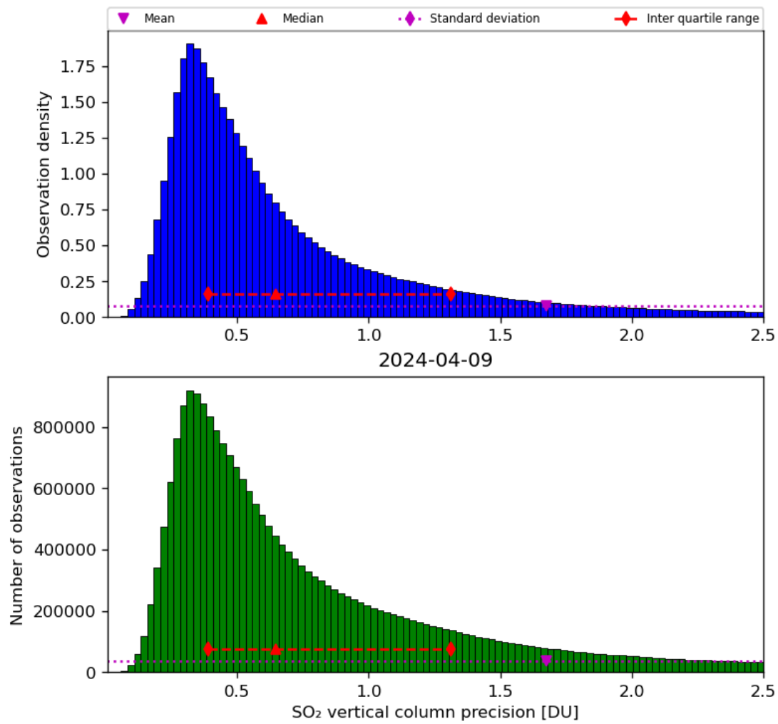
Figure 54: Histogram of “SO 2 vertical column precision” for 2024-04-08 to 2024-04-10
