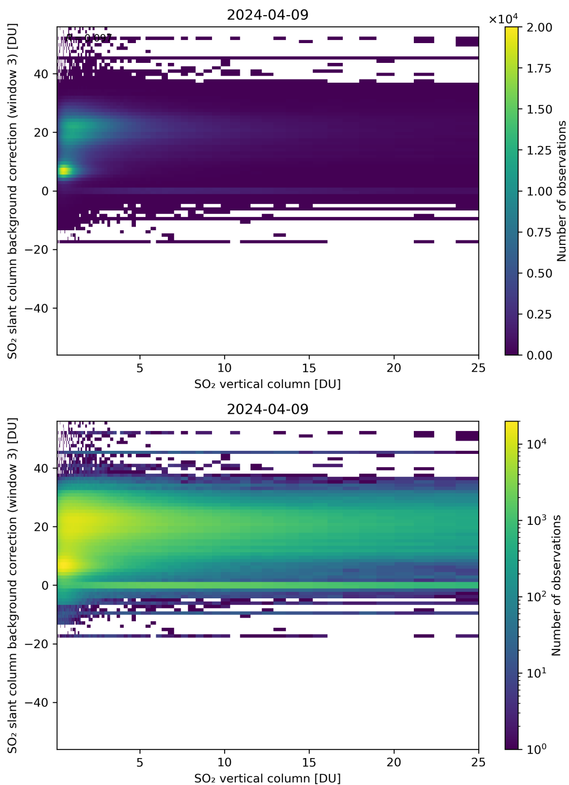
Figure 275: Scatter density plot of “SO 2 vertical column” against “SO 2 slant column background correction (window 3)” for 2024-04-08 to 2024-04-10.
