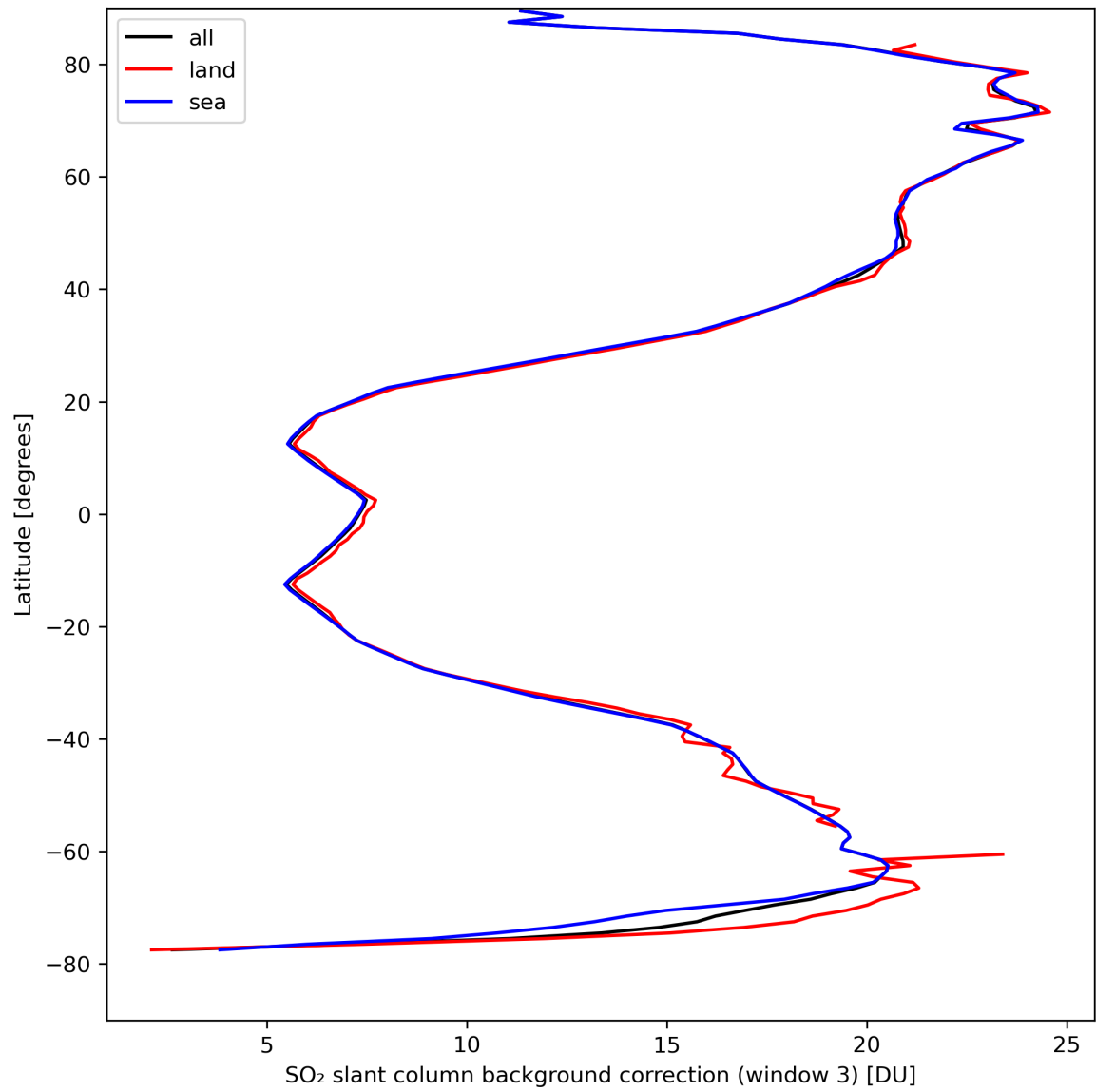
Figure 44: Zonal average of “SO 2 slant column background correction (window 3)” for 2024-04-08 to 2024-04-10.
