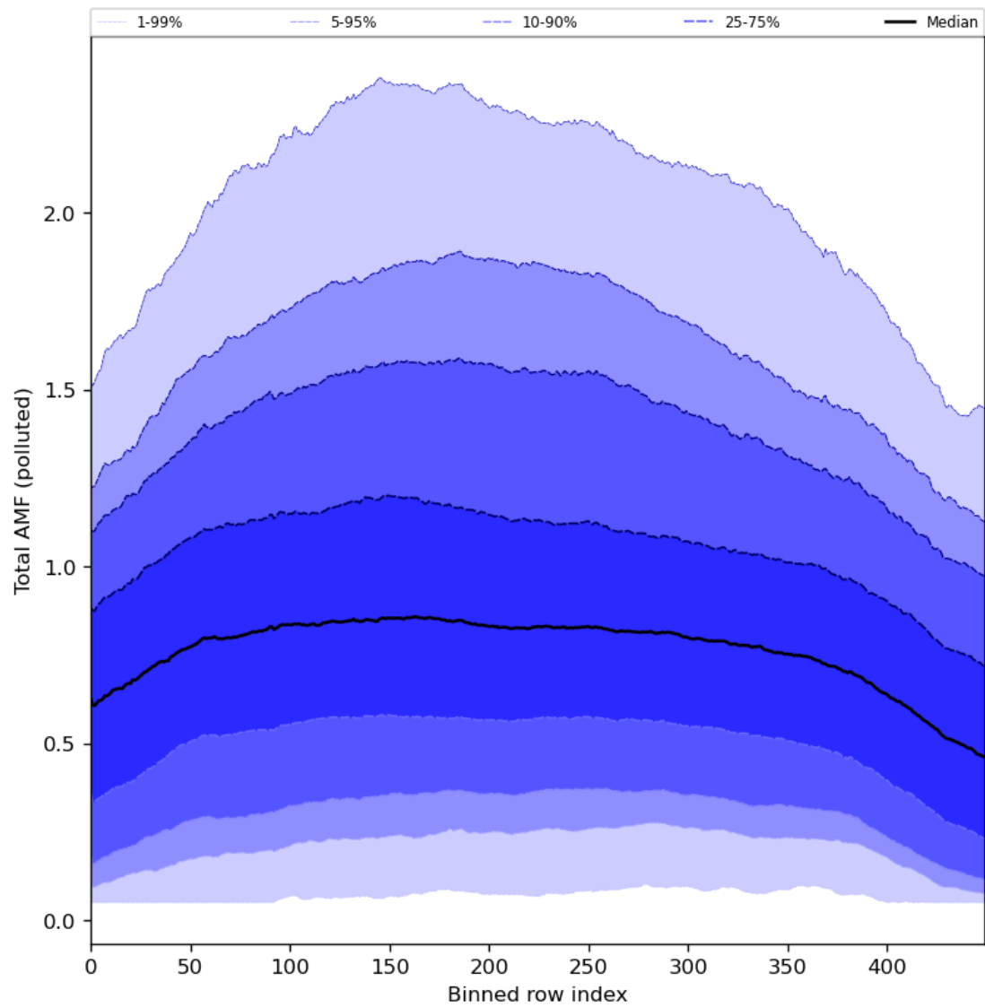
Figure 94: Along track statistics of “Total AMF (polluted)” for 2024-04-08 to 2024-04-10
