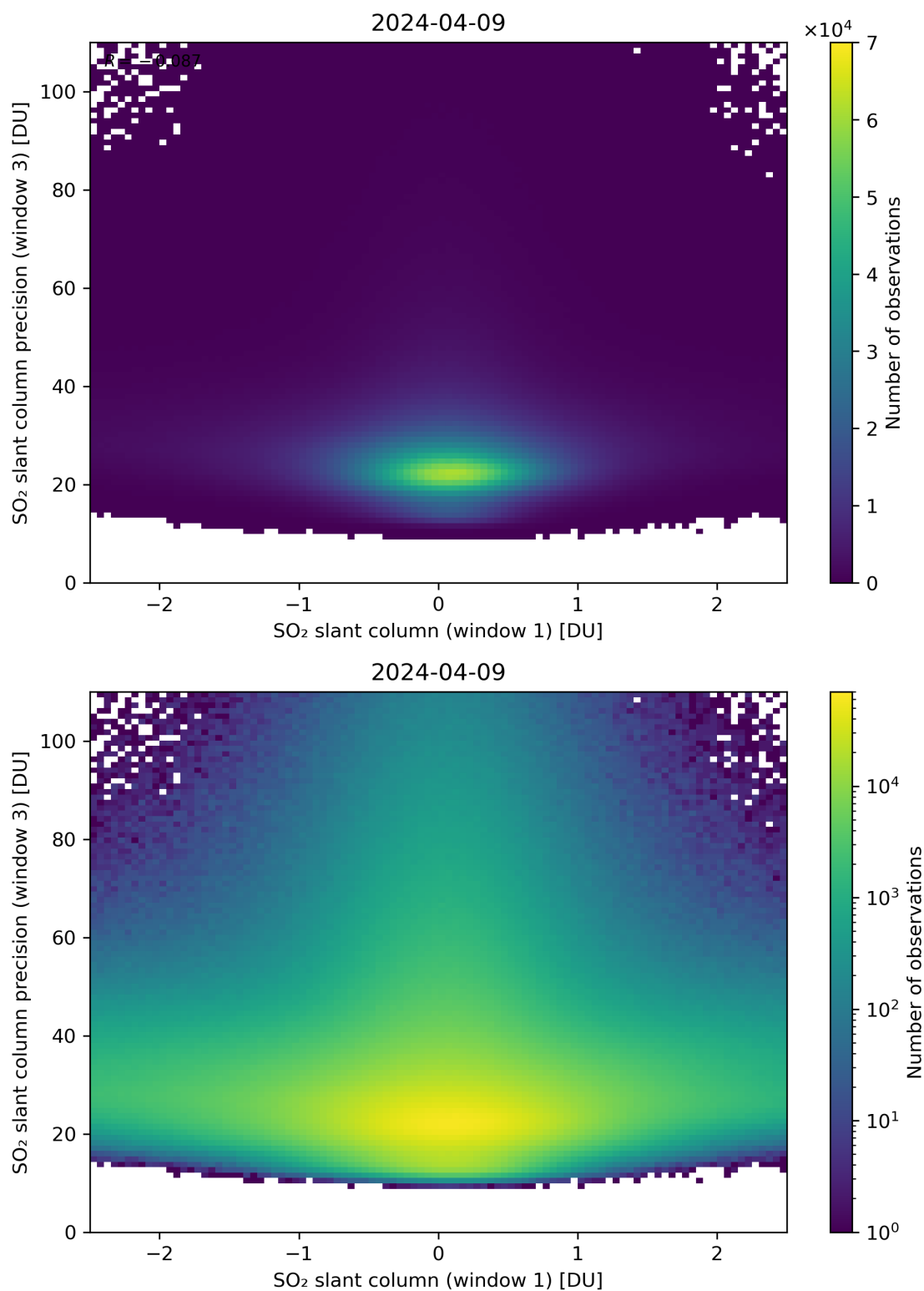
Figure 238: Scatter density plot of “SO 2 slant column (window 1)” against “SO 2 slant column precision (window 3)” for 2024-04-08 to 2024-04-10.
