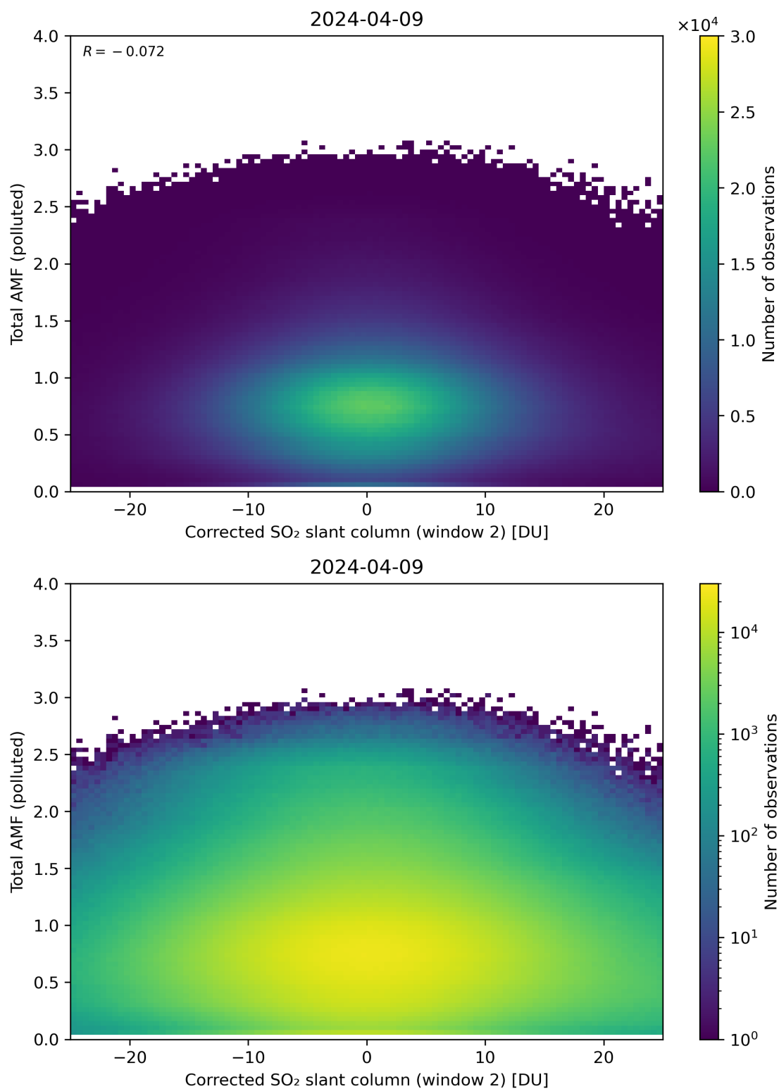
Figure 203: Scatter density plot of “Corrected SO 2 slant column (window 2)” against “Total AMF (polluted)” for 2024-04-08 to 2024-04-10.
