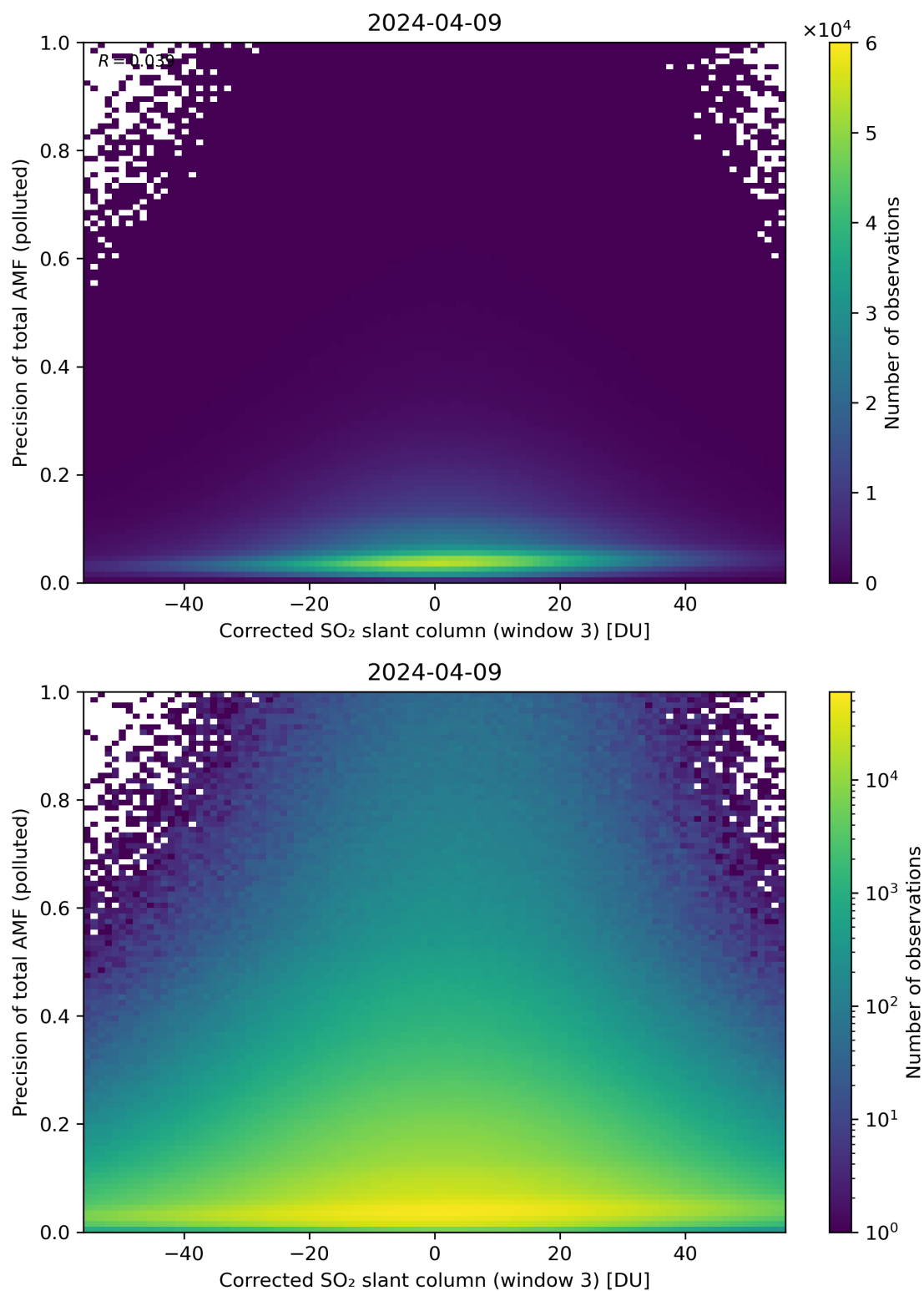
Figure 211: Scatter density plot of “Corrected SO 2 slant column (window 3)” against “Precision of total AMF (polluted)” for 2024-04-08 to 2024-04-10.
