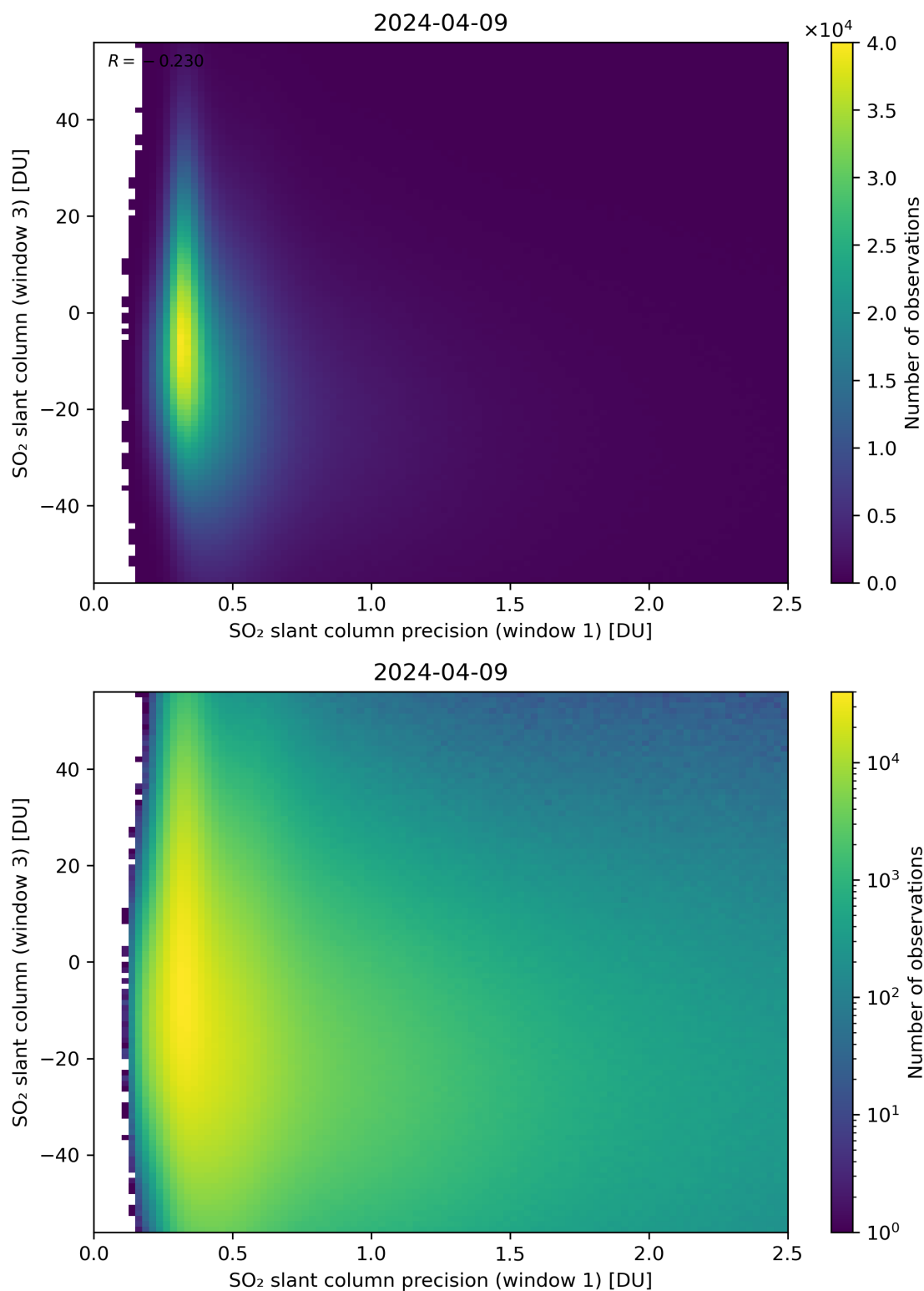
Figure 228: Scatter density plot of “SO 2 slant column precision (window 1)” against “SO 2 slant column (window 3)” for 2024-04-08 to 2024-04-10.
