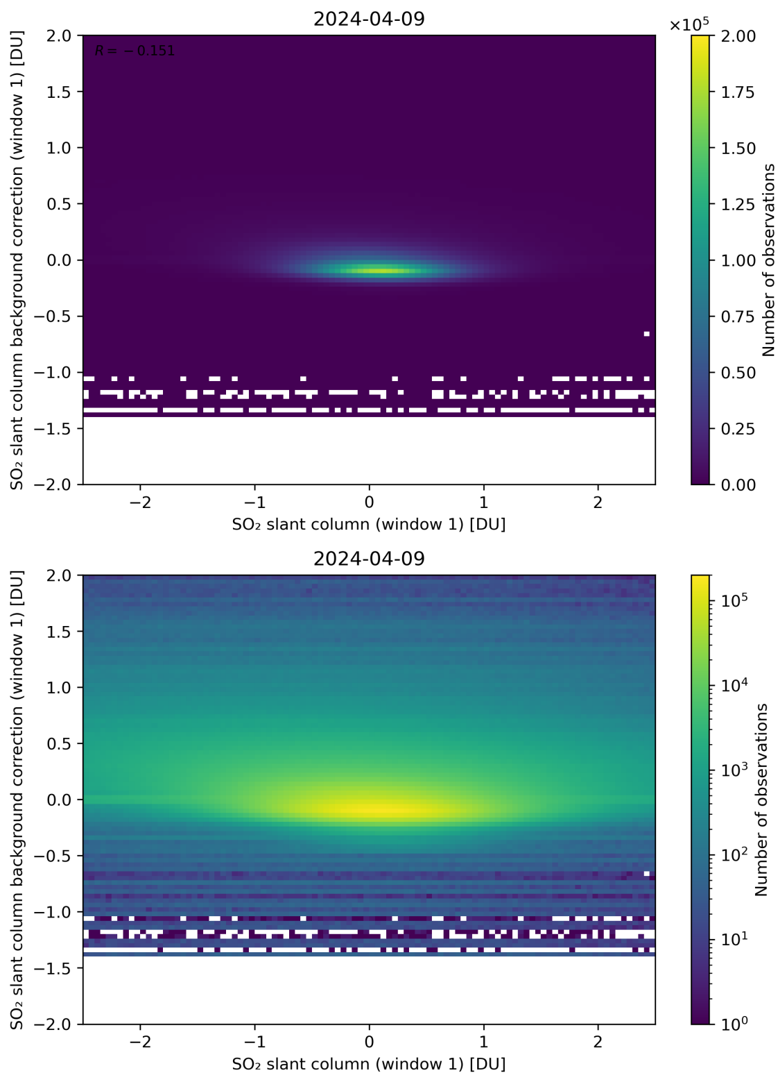
Figure 212: Scatter density plot of “SO 2 slant column (window 1)” against “SO 2 slant column background correction (window 1)” for 2024-04-08 to 2024-04-10.
