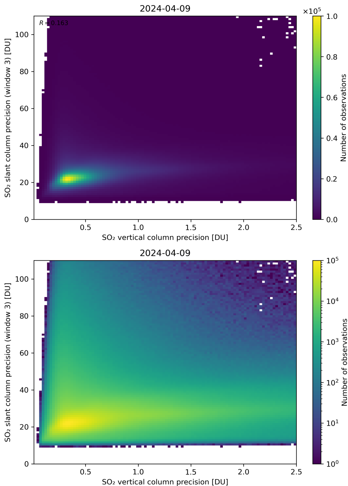
Figure 293: Scatter density plot of “SO 2 vertical column precision” against “SO 2 slant column precision (window 3)” for 2024-04-08 to 2024-04-10.
