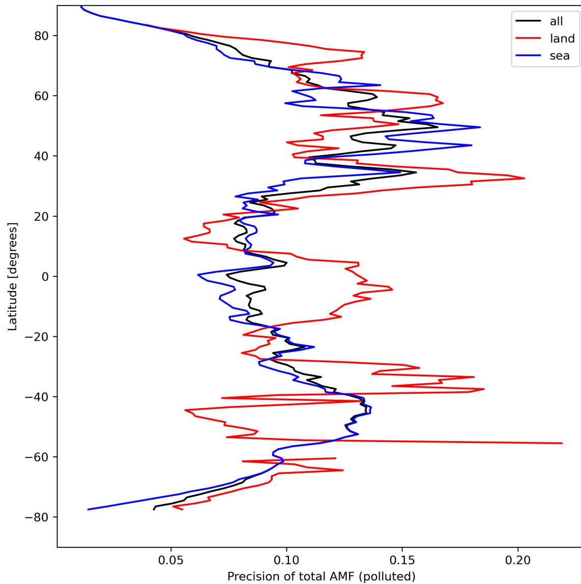
Figure 49: Zonal average of “Precision of total AMF (polluted)” for 2024-04-08 to 2024-04-10.
