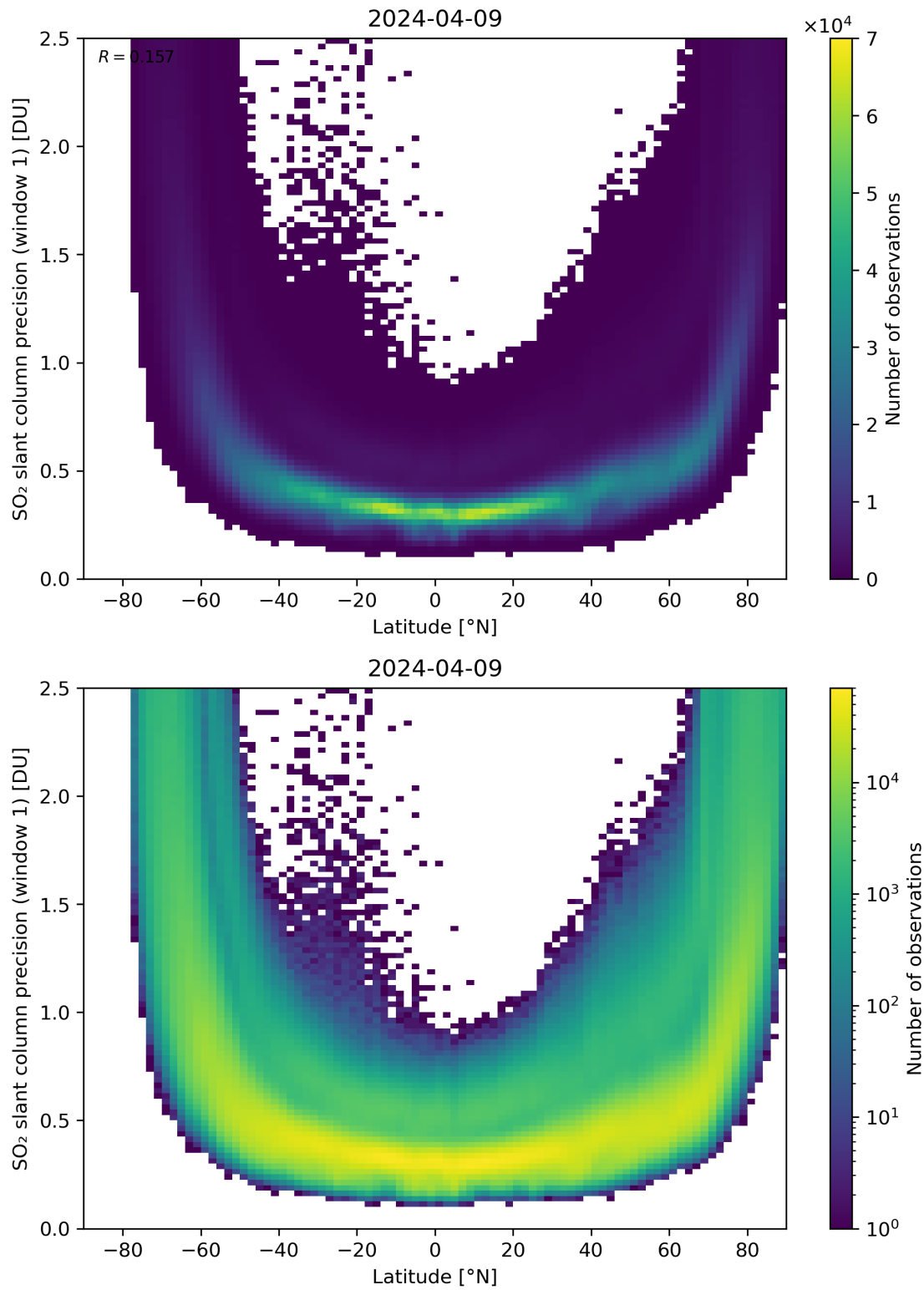
Figure 150: Scatter density plot of “Latitude” against “SO 2 slant column precision (window 1)” for 2024-04-08 to 2024-04-10.
