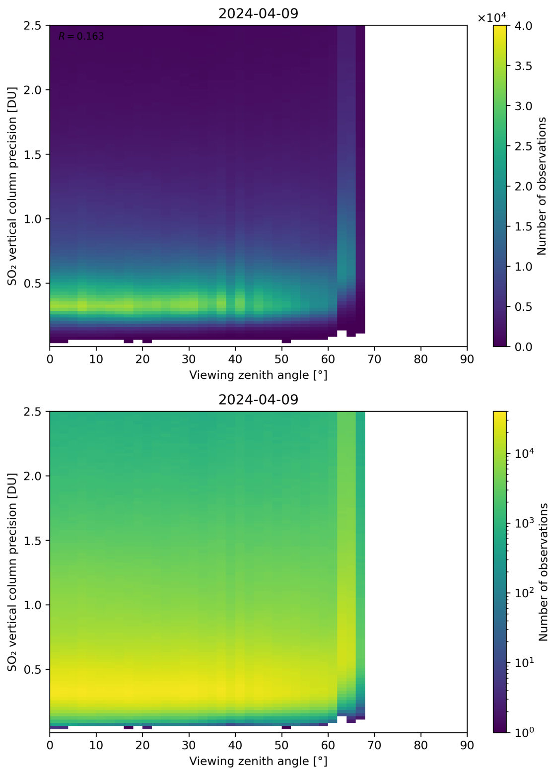
Figure 328: Scatter density plot of “Viewing zenith angle” against “SO 2 vertical column precision” for 2024-04-08 to 2024-04-10.
