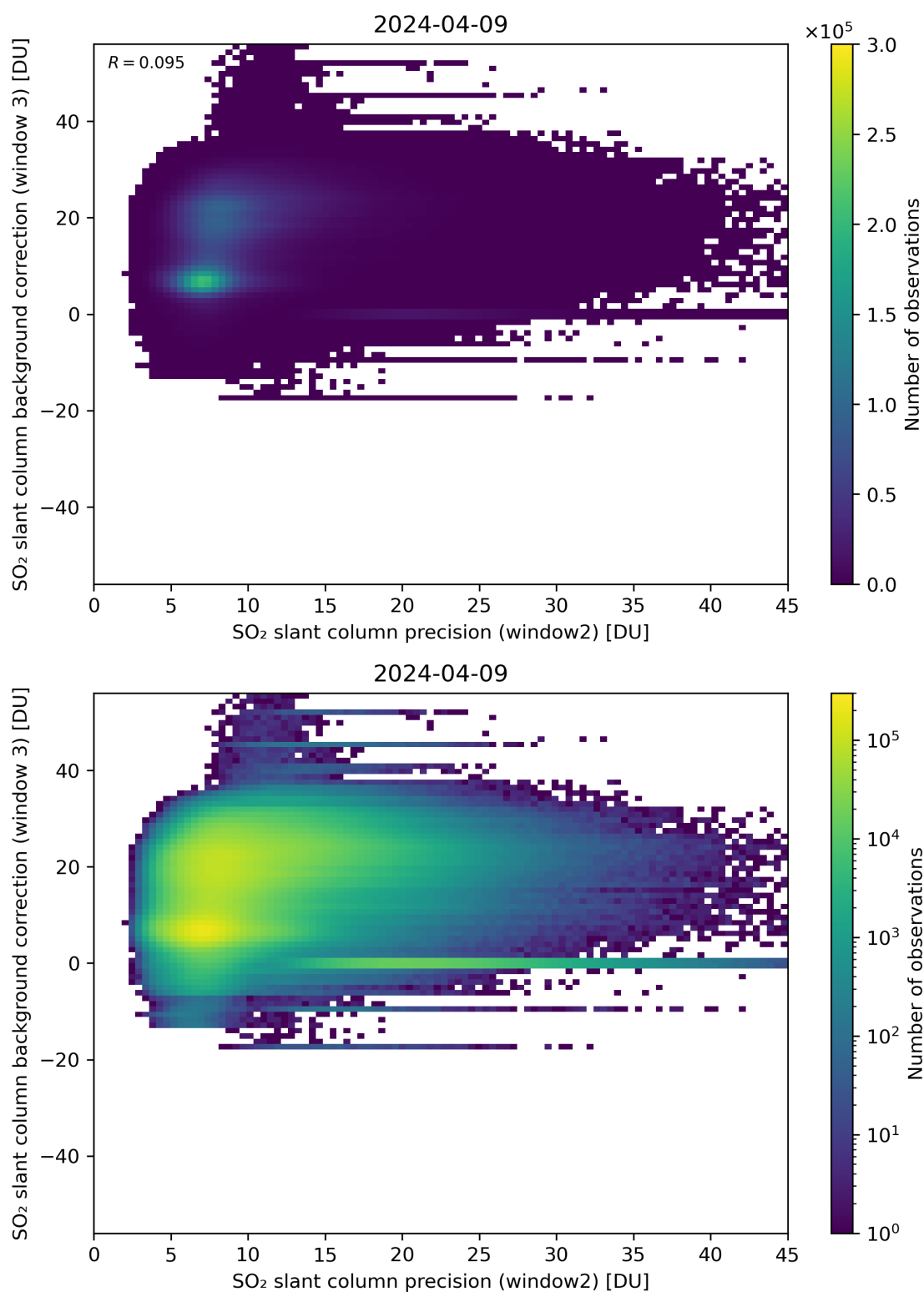
Figure 242: Scatter density plot of “SO 2 slant column precision (window2)” against “SO 2 slant column background correction (window 3)” for 2024-04-08 to 2024-04-10.
