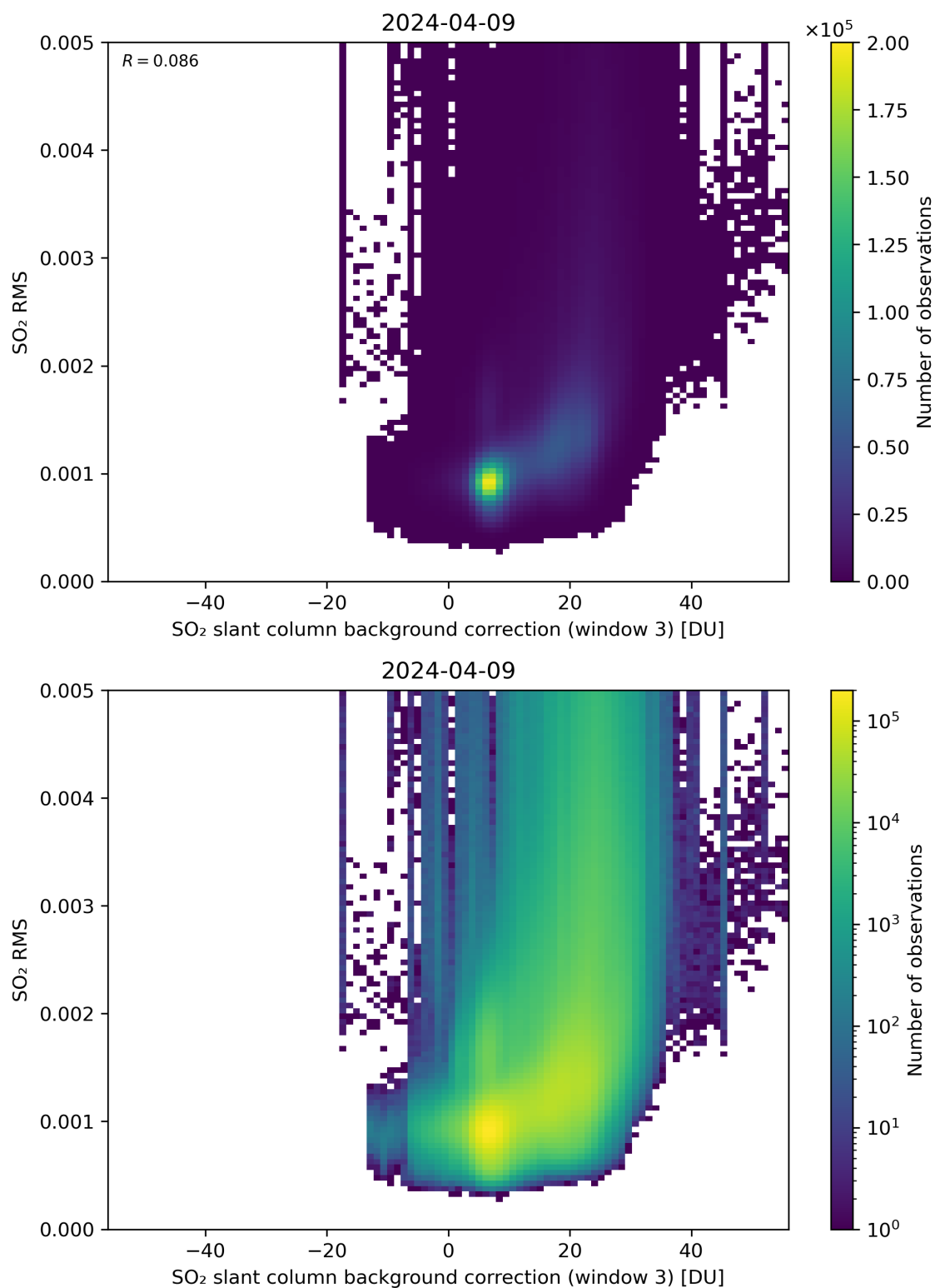
Figure 123: Scatter density plot of “SO 2 slant column background correction (window 3)” against “SO 2 RMS” for 2024-04-08 to 2024-04-10.
