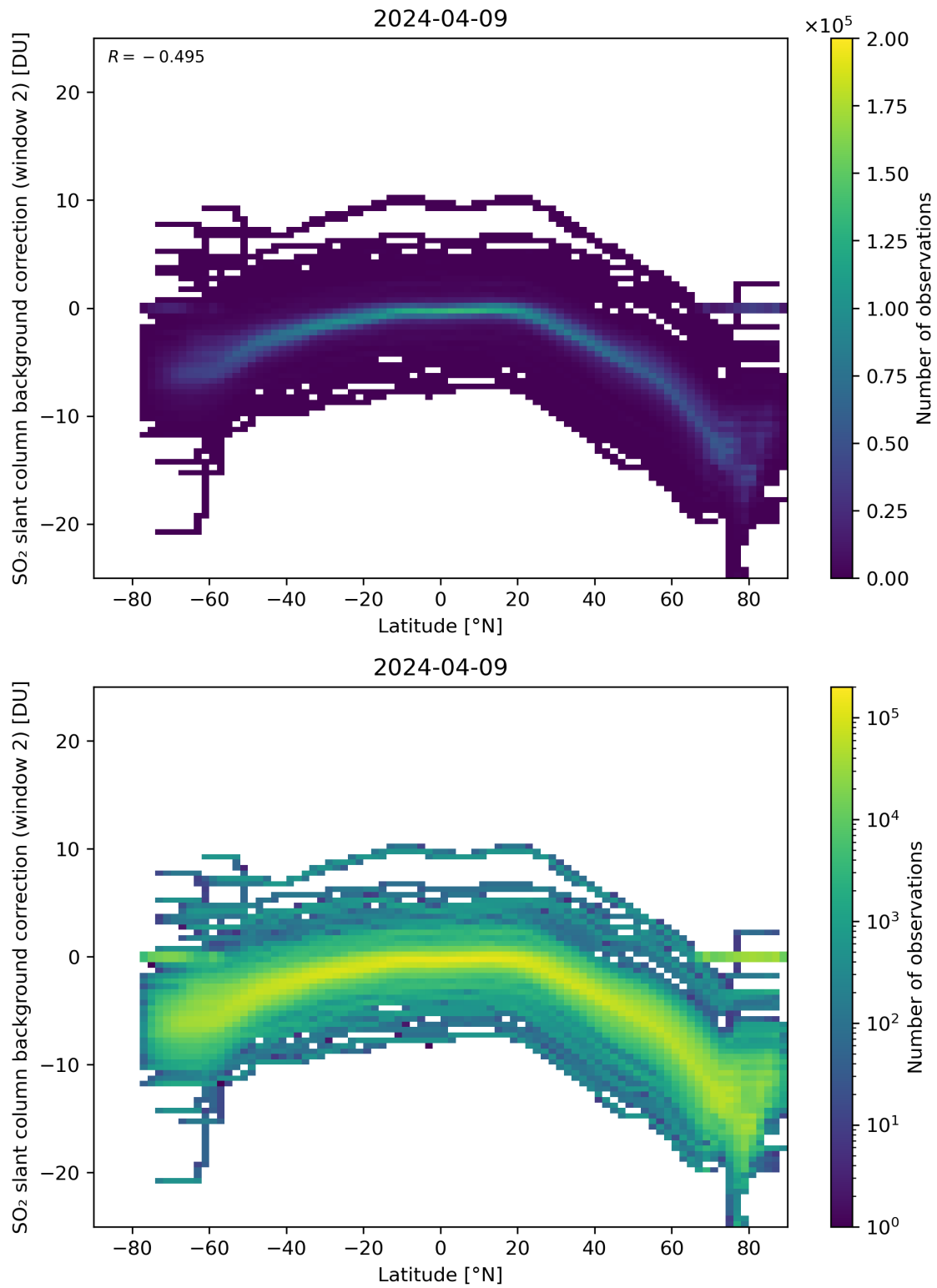
Figure 140: Scatter density plot of “Latitude” against “SO 2 slant column background correction (window 2)” for 2024-04-08 to 2024-04-10.
