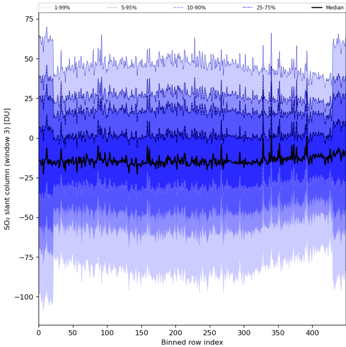
Figure 87: Along track statistics of “SO 2 slant column (window 3)” for 2024-04-08 to 2024-04-10
