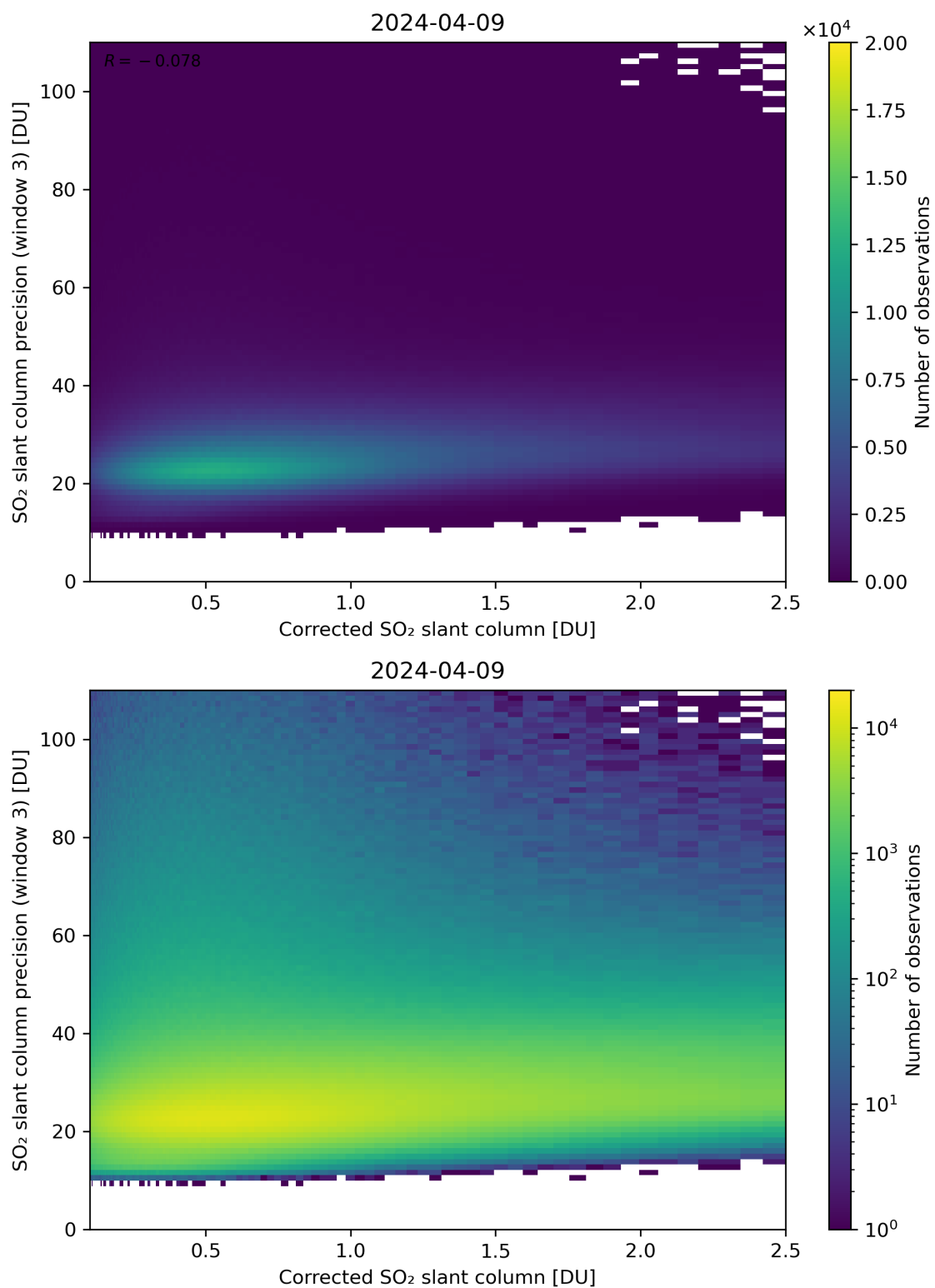
Figure 191: Scatter density plot of “Corrected SO 2 slant column” against “SO 2 slant column precision (window 3)” for 2024-04-08 to 2024-04-10.
