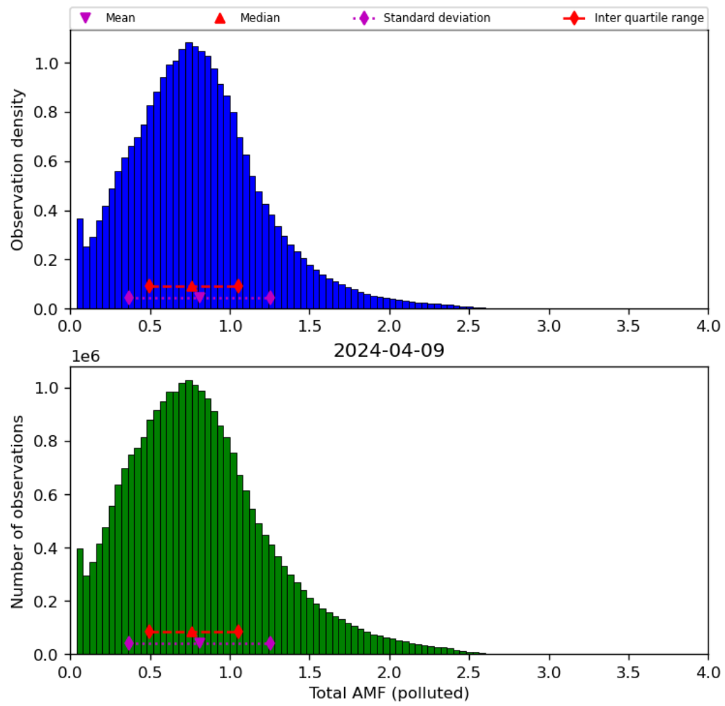
Figure 71: Histogram of “Total AMF (polluted)” for 2024-04-08 to 2024-04-10
