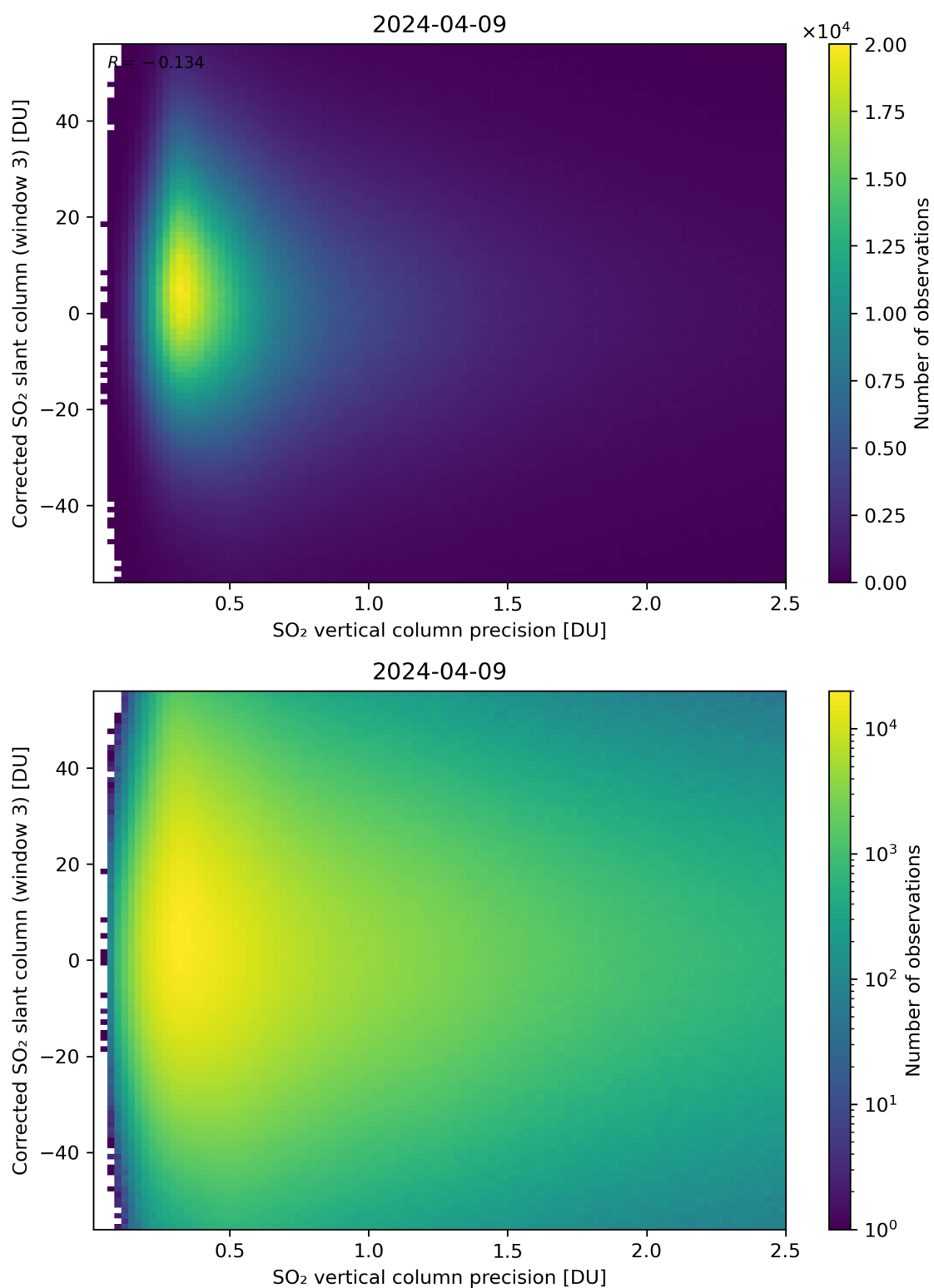
Figure 288: Scatter density plot of “SO 2 vertical column precision” against “Corrected SO 2 slant column (window 3)” for 2024-04-08 to 2024-04-10.
