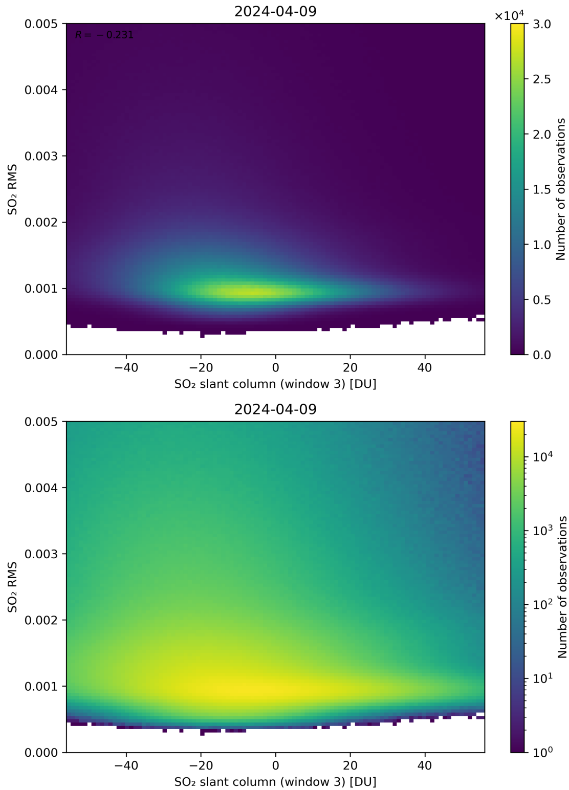
Figure 256: Scatter density plot of “SO 2 slant column (window 3)” against “SO 2 RMS” for 2024-04-08 to 2024-04-10.
