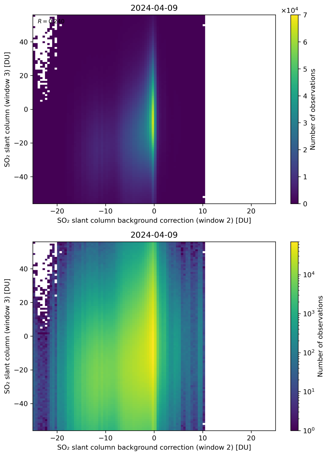
Figure 117: Scatter density plot of “SO 2 slant column background correction (window 2)” against “SO 2 slant column (window 3)” for 2024-04-08 to 2024-04-10.
