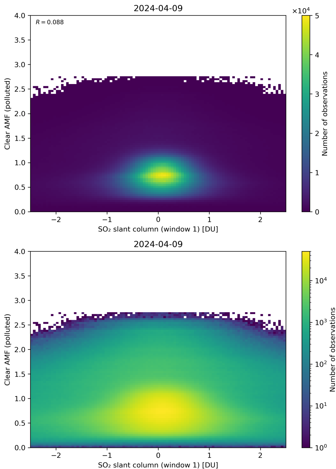
Figure 232: Scatter density plot of “SO 2 slant column (window 1)” against “Clear AMF (polluted)” for 2024-04-08 to 2024-04-10.
