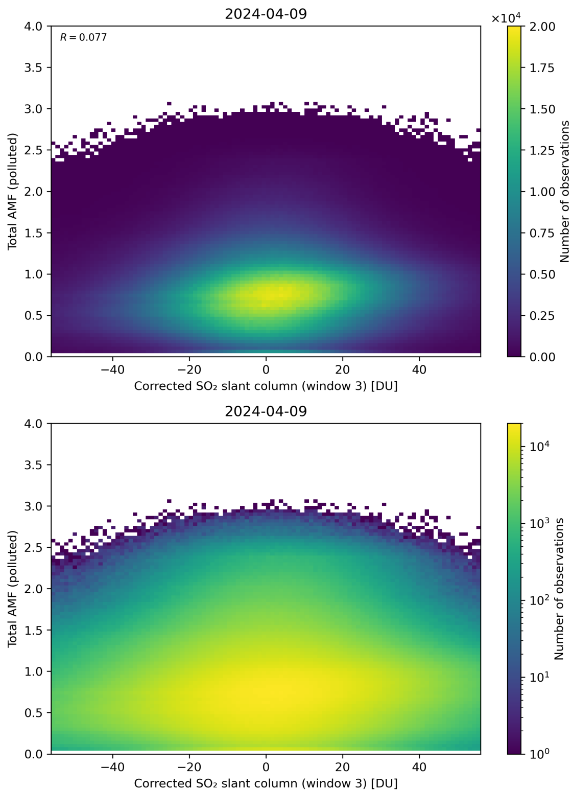
Figure 210: Scatter density plot of “Corrected SO 2 slant column (window 3)” against “Total AMF (polluted)” for 2024-04-08 to 2024-04-10.
