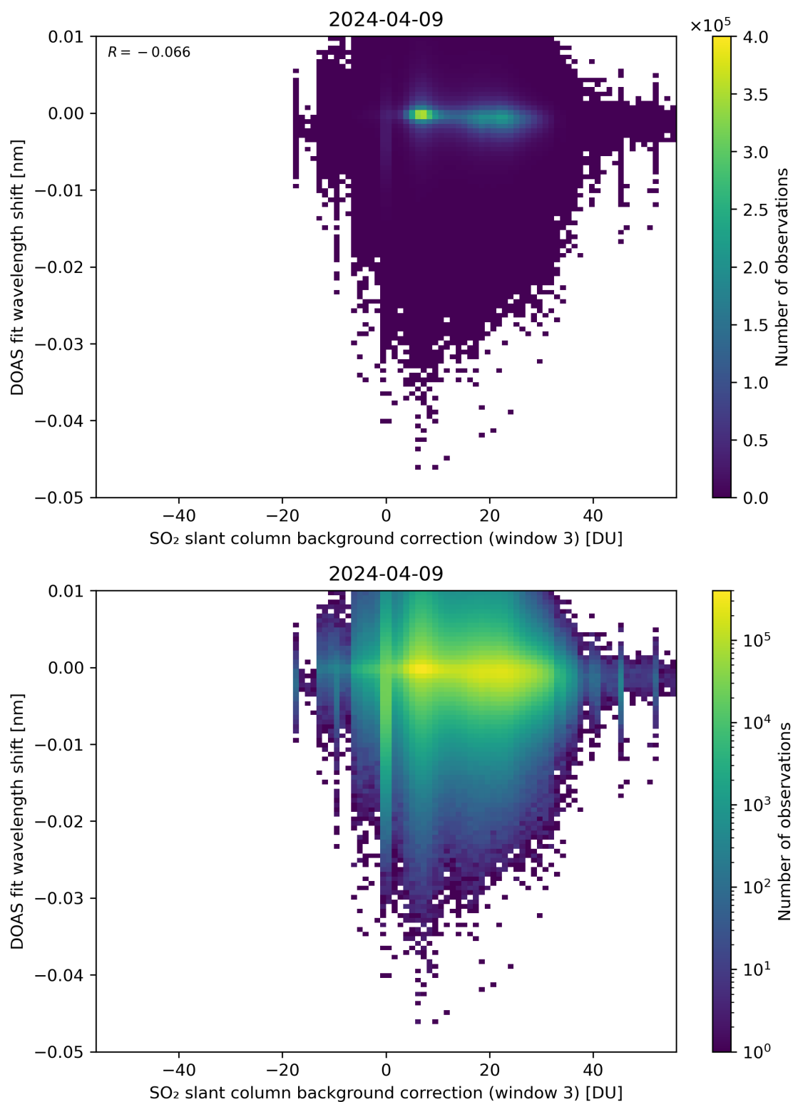
Figure 121: Scatter density plot of “SO 2 slant column background correction (window 3)” against “DOAS fit wavelength shift” for 2024-04-08 to 2024-04-10.
