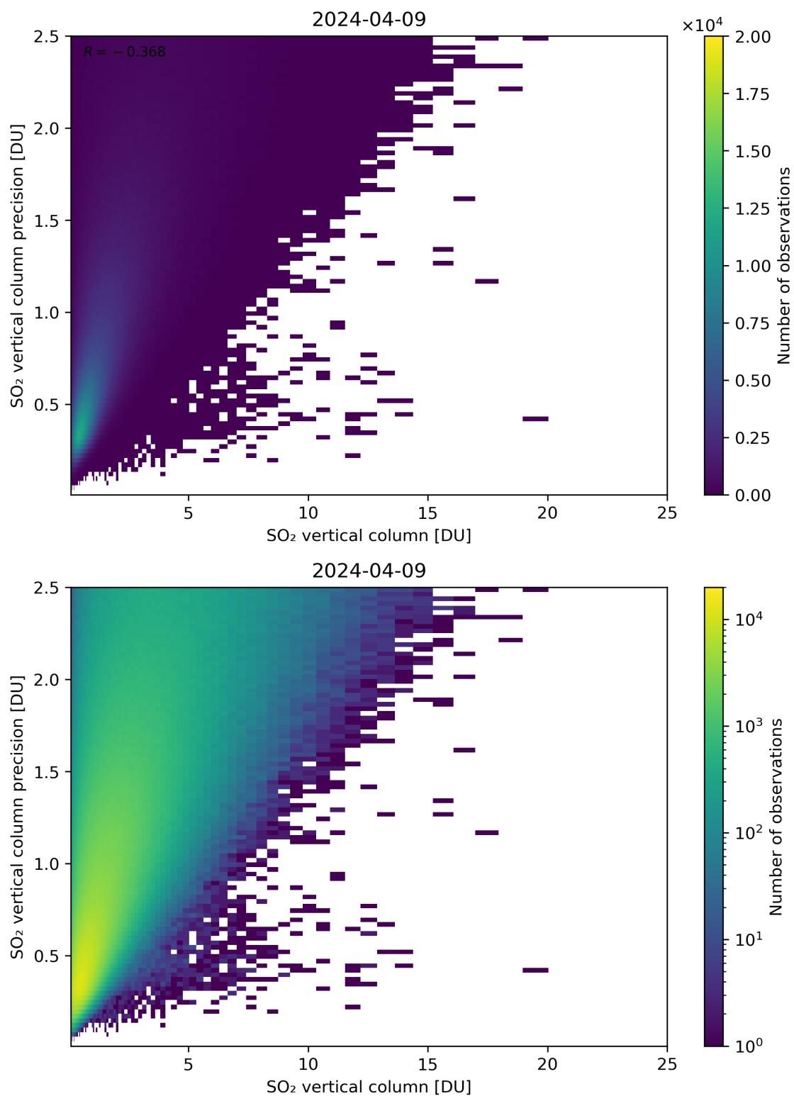
Figure 307: Scatter density plot of “SO 2 vertical column” against “SO 2 vertical column precision” for 2024-04-08 to 2024-04-10.
