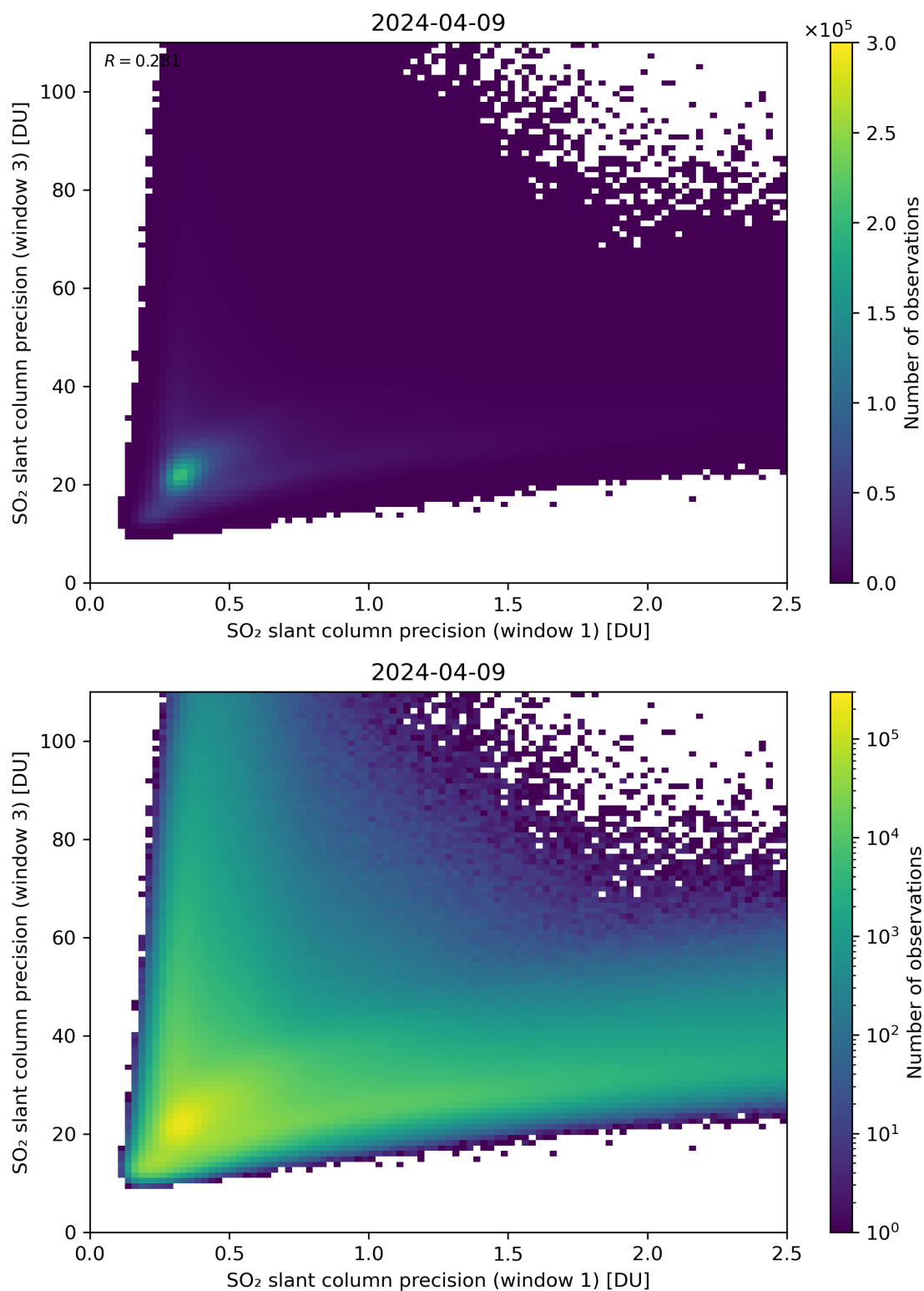
Figure 229: Scatter density plot of “SO 2 slant column precision (window 1)” against “SO 2 slant column precision (window 3)” for 2024-04-08 to 2024-04-10.
