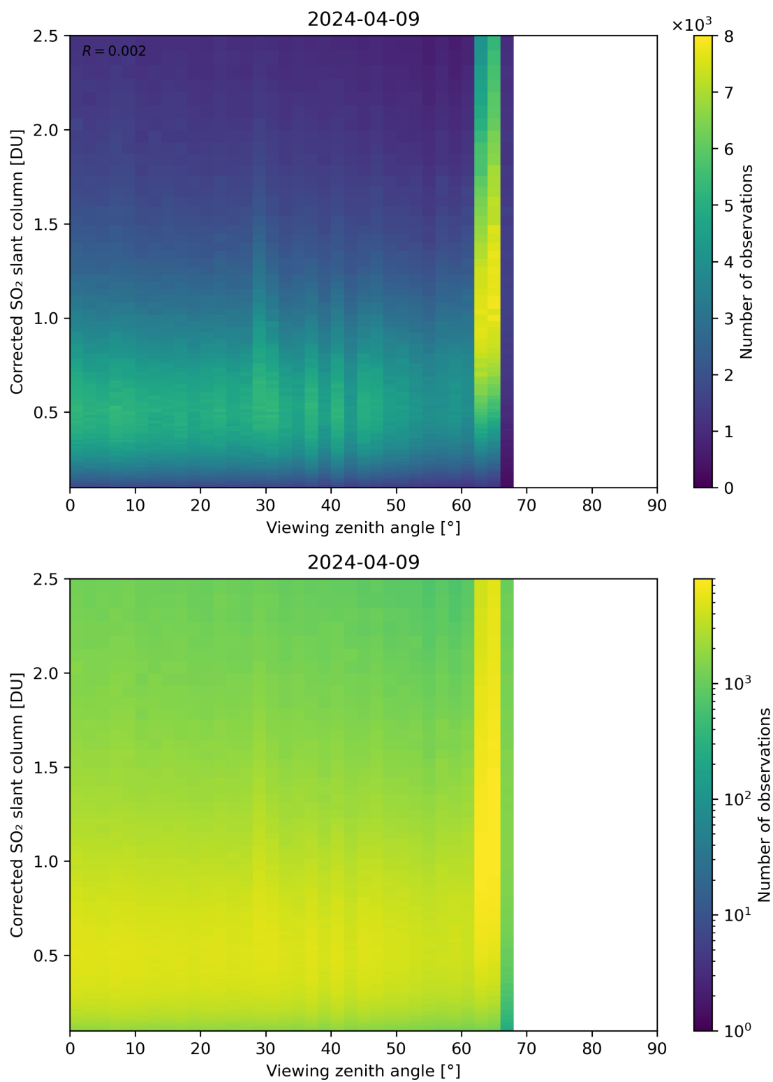
Figure 317: Scatter density plot of “Viewing zenith angle” against “Corrected SO 2 slant column” for 2024-04-08 to 2024-04-10.
