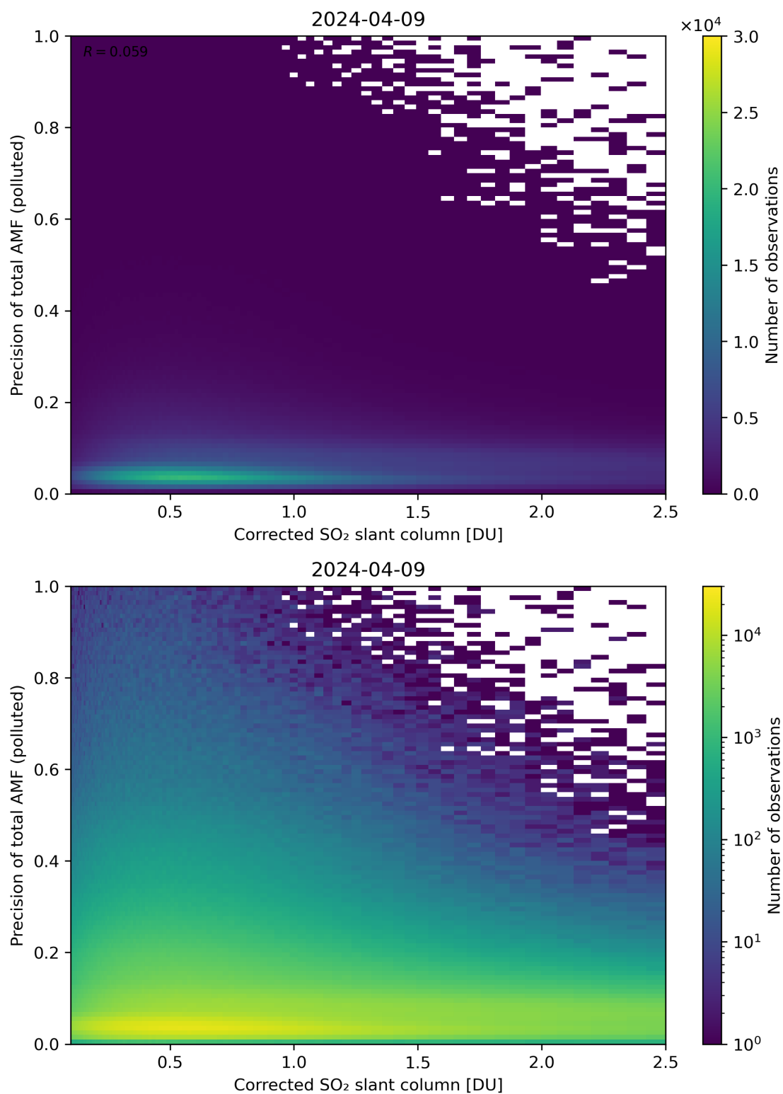
Figure 193: Scatter density plot of “Corrected SO 2 slant column” against “Precision of total AMF (polluted)” for 2024-04-08 to 2024-04-10.
