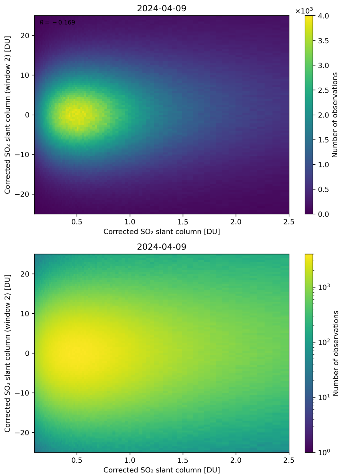
Figure 185: Scatter density plot of “Corrected SO 2 slant column” against “Corrected SO 2 slant column (window 2)” for 2024-04-08 to 2024-04-10.
