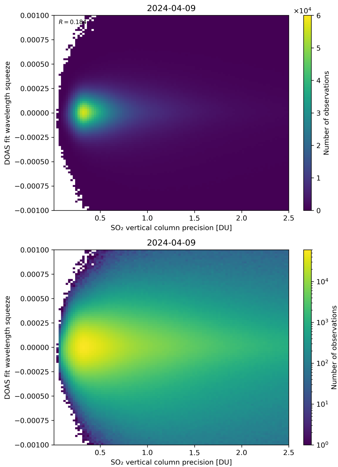
Figure 283: Scatter density plot of “SO 2 vertical column precision” against “DOAS fit wavelength squeeze” for 2024-04-08 to 2024-04-10.
