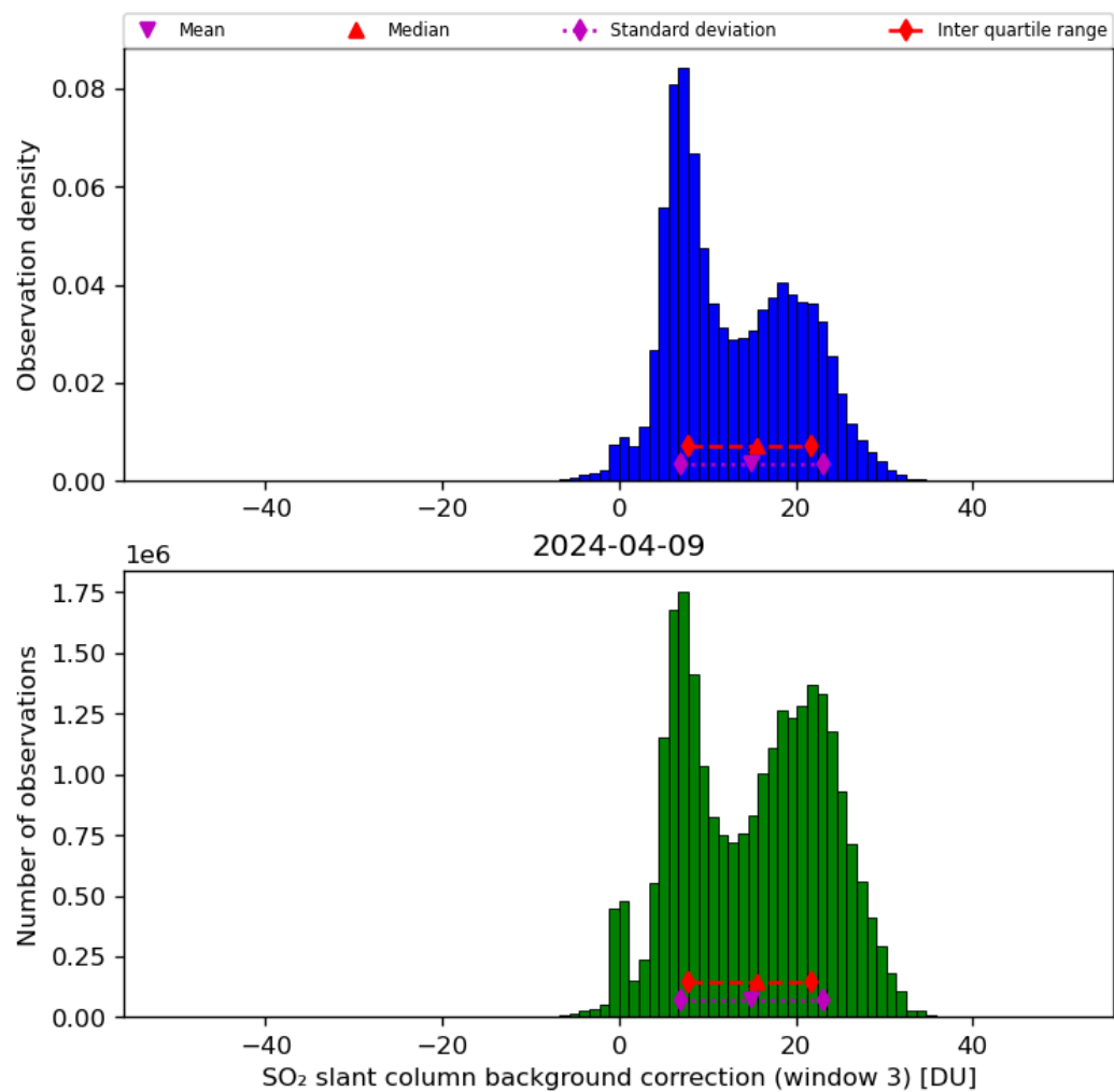
Figure 67: Histogram of “SO 2 slant column background correction (window 3)” for 2024-04-08 to 2024-04-10
