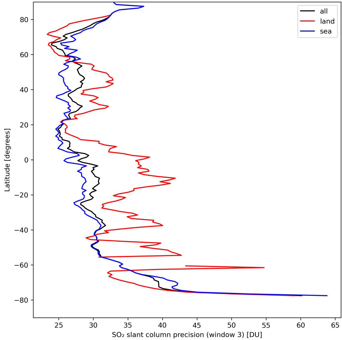
Figure 42: Zonal average of “SO 2 slant column precision (window 3)” for 2024-04-08 to 2024-04-10.
