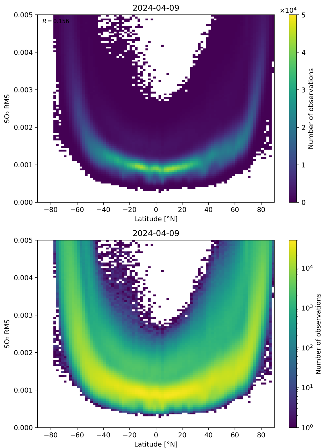
Figure 144: Scatter density plot of “Latitude” against “SO 2 RMS” for 2024-04-08 to 2024-04-10.
