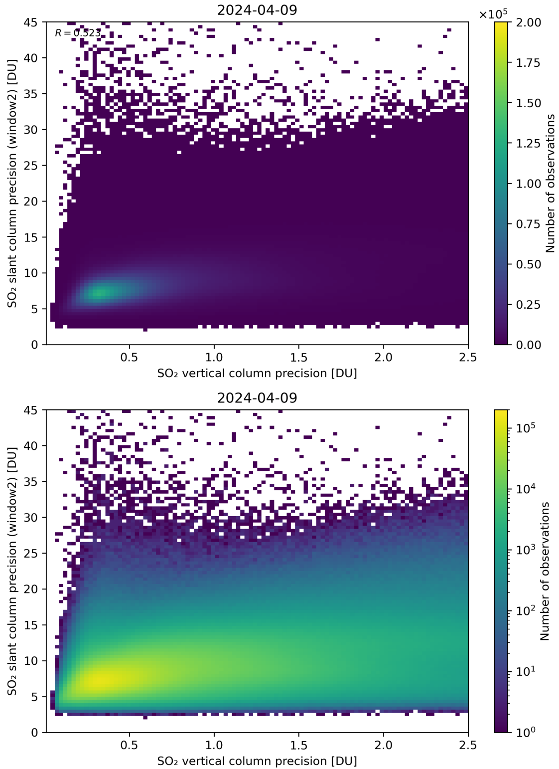
Figure 291: Scatter density plot of “SO 2 vertical column precision” against “SO 2 slant column precision (window2)” for 2024-04-08 to 2024-04-10.
