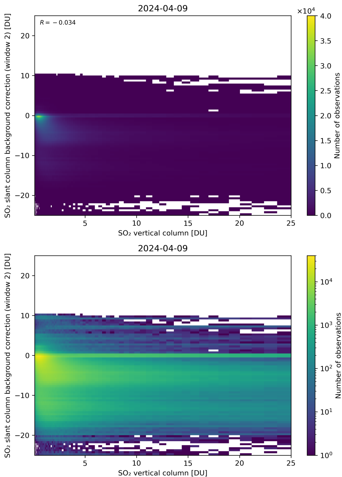
Figure 274: Scatter density plot of “SO 2 vertical column” against “SO 2 slant column background correction (window 2)” for 2024-04-08 to 2024-04-10.
