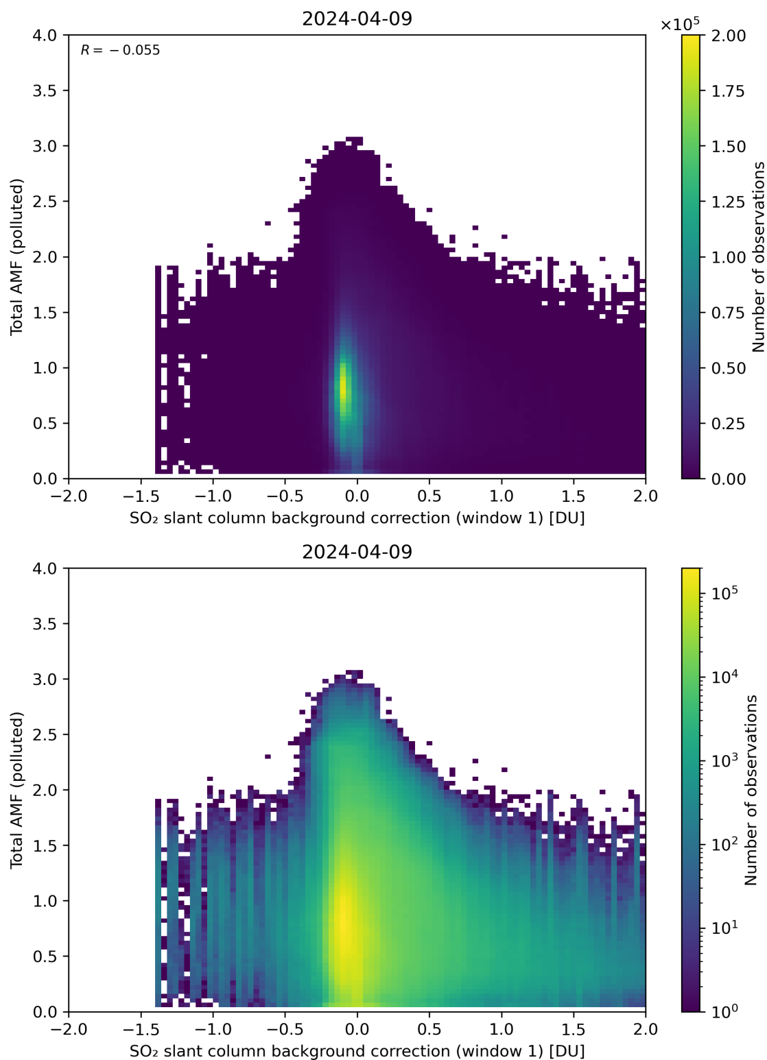
Figure 109: Scatter density plot of “SO 2 slant column background correction (window 1)” against “Total AMF (polluted)” for 2024-04-08 to 2024-04-10.
