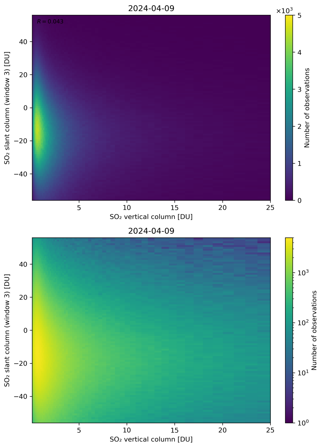
Figure 303: Scatter density plot of “SO 2 vertical column” against “SO 2 slant column (window 3)” for 2024-04-08 to 2024-04-10.
