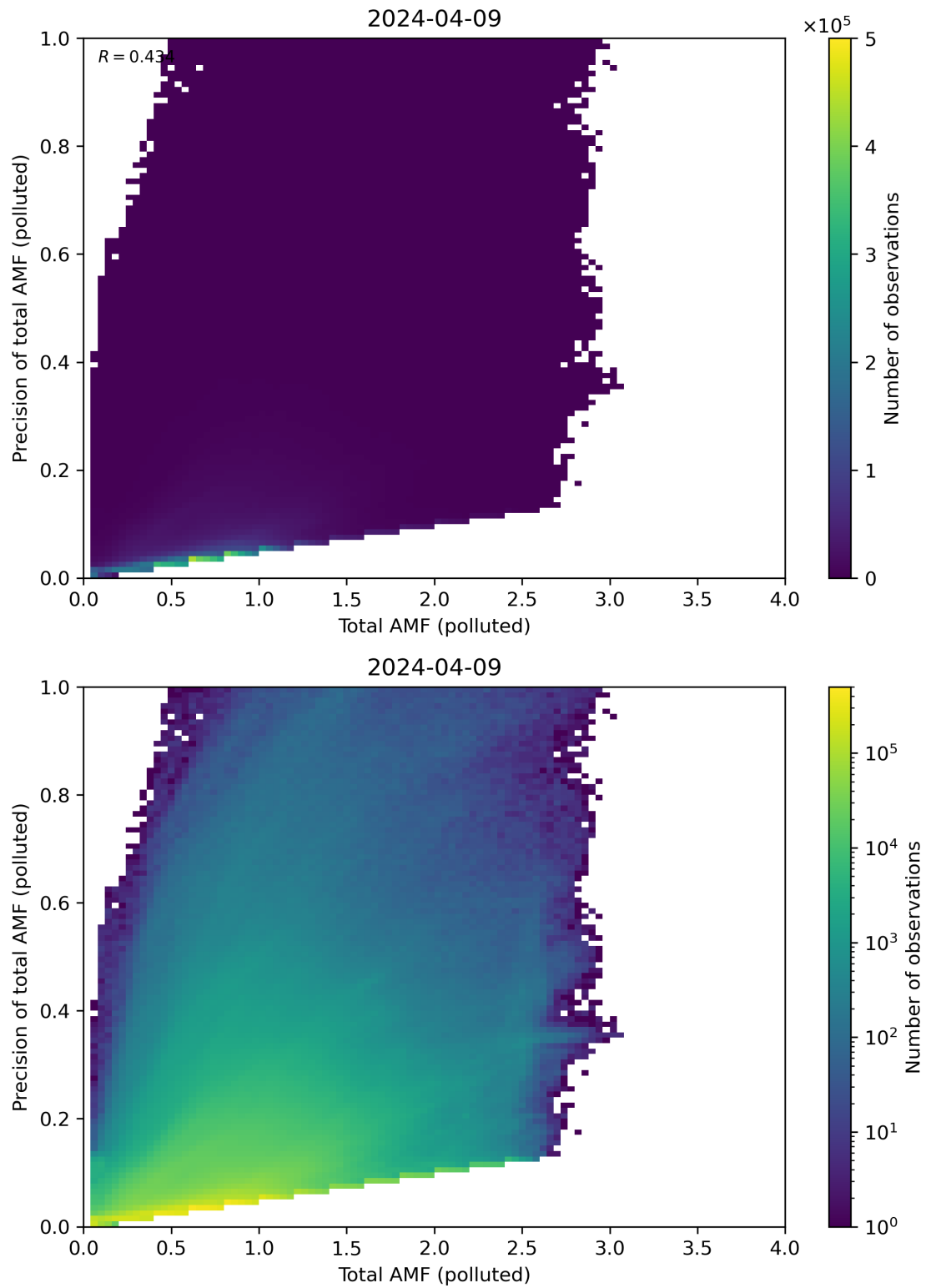
Figure 272: Scatter density plot of “Total AMF (polluted)” against “Precision of total AMF (polluted)” for 2024-04-08 to 2024-04-10.
