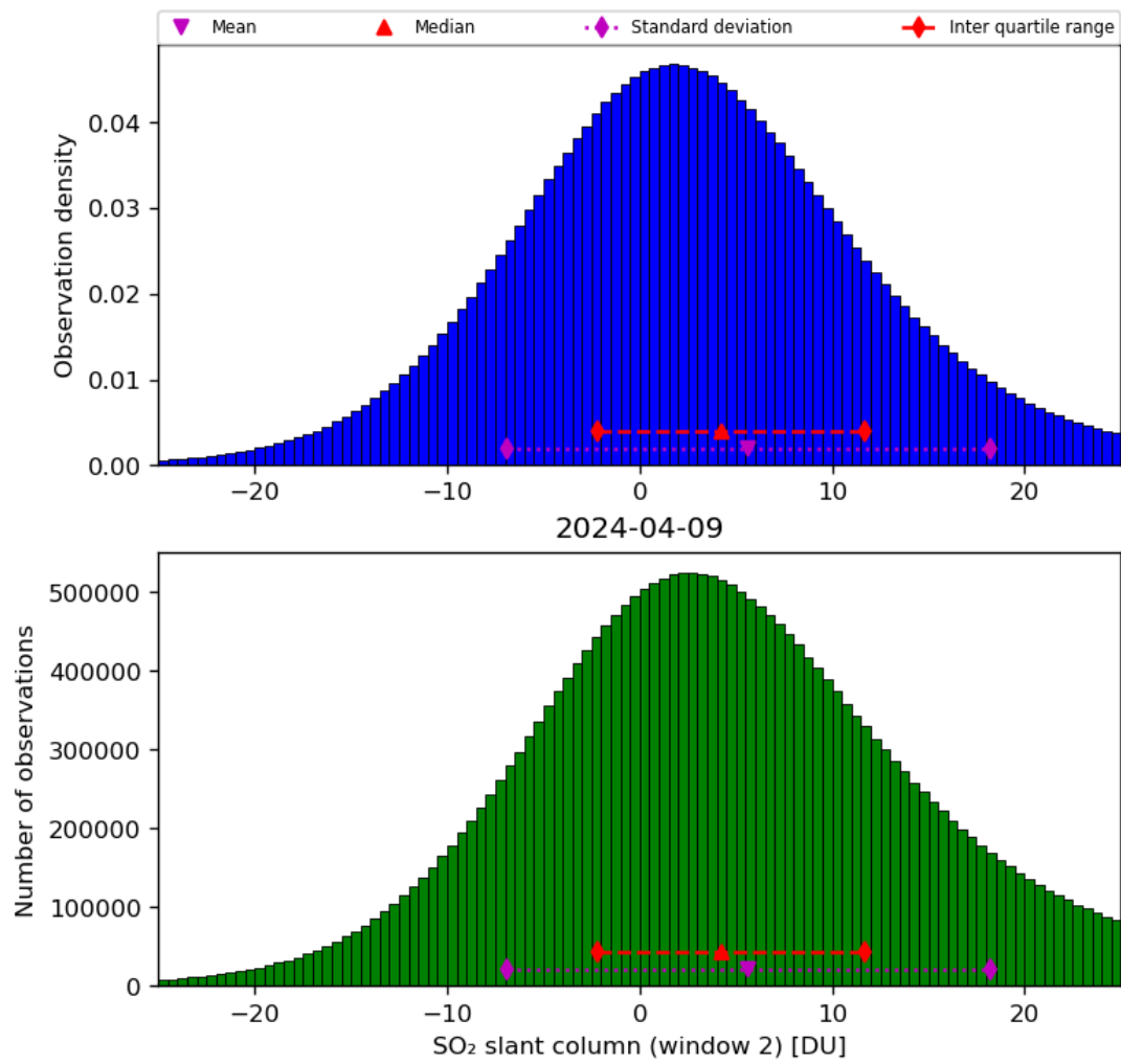
Figure 60: Histogram of “SO 2 slant column (window 2)” for 2024-04-08 to 2024-04-10
