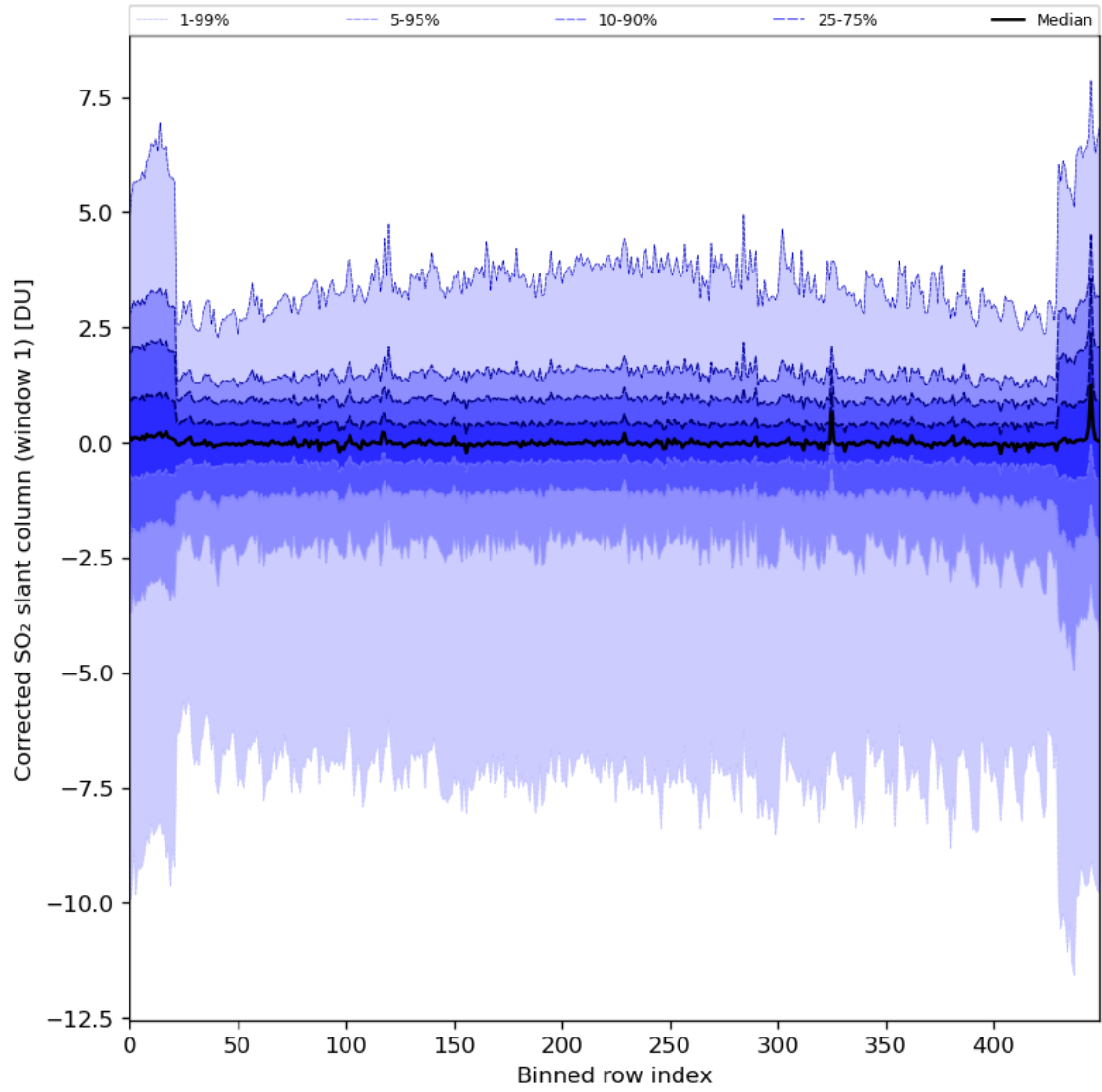
Figure 81: Along track statistics of “Corrected SO 2 slant column (window 1)” for 2024-04-08 to 2024-04-10
