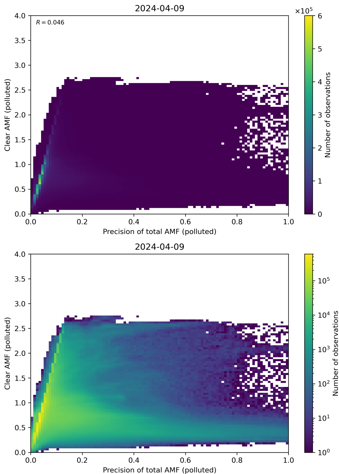
Figure 270: Scatter density plot of “Precision of total AMF (polluted)” against “Clear AMF (polluted)” for 2024-04-08 to 2024-04-10.
