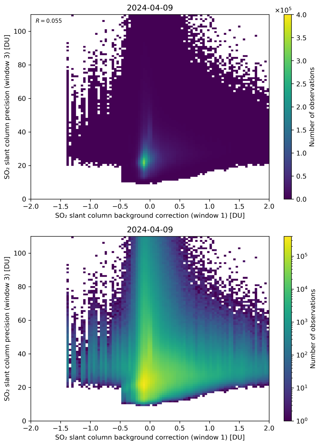
Figure 108: Scatter density plot of “SO 2 slant column background correction (window 1)” against “SO 2 slant column precision (window 3)” for 2024-04-08 to 2024-04-10.
