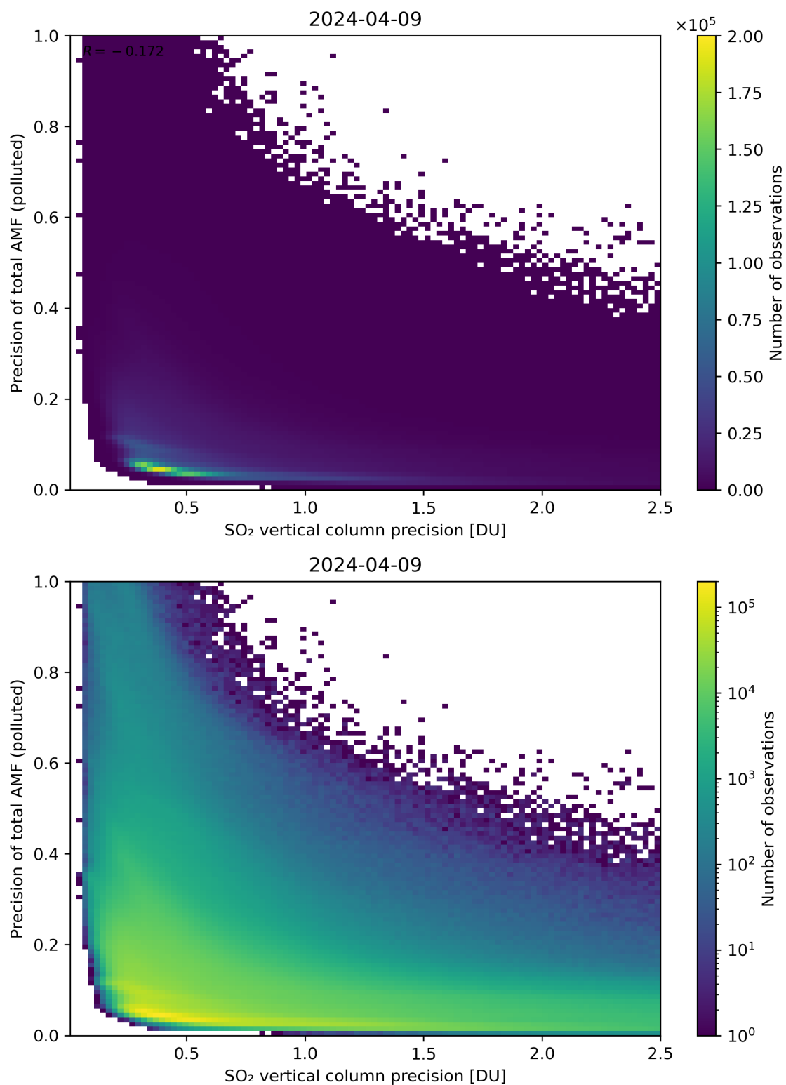
Figure 295: Scatter density plot of “SO 2 vertical column precision” against “Precision of total AMF (polluted)” for 2024-04-08 to 2024-04-10.
