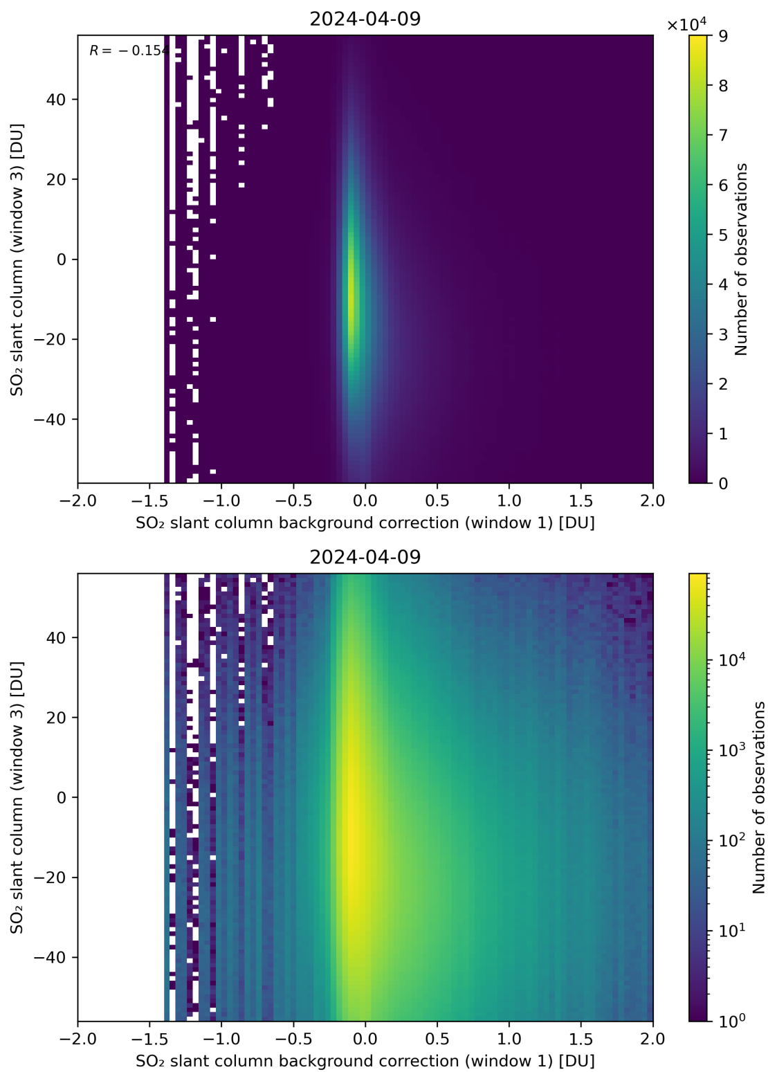
Figure 107: Scatter density plot of “SO 2 slant column background correction (window 1)” against “SO 2 slant column (window 3)” for 2024-04-08 to 2024-04-10.
