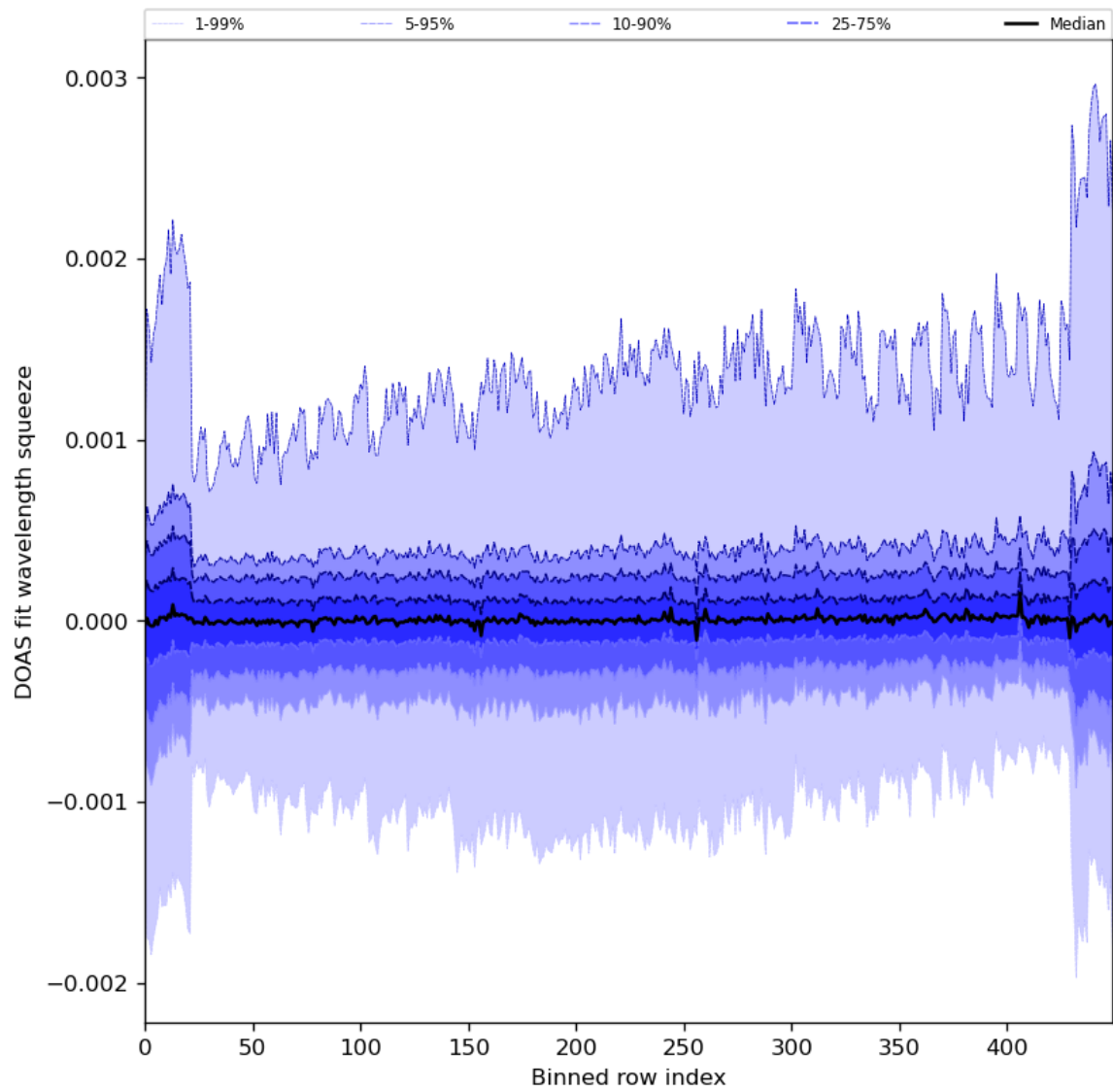
Figure 92: Along track statistics of “DOAS fit wavelength squeeze” for 2024-04-08 to 2024-04-10
