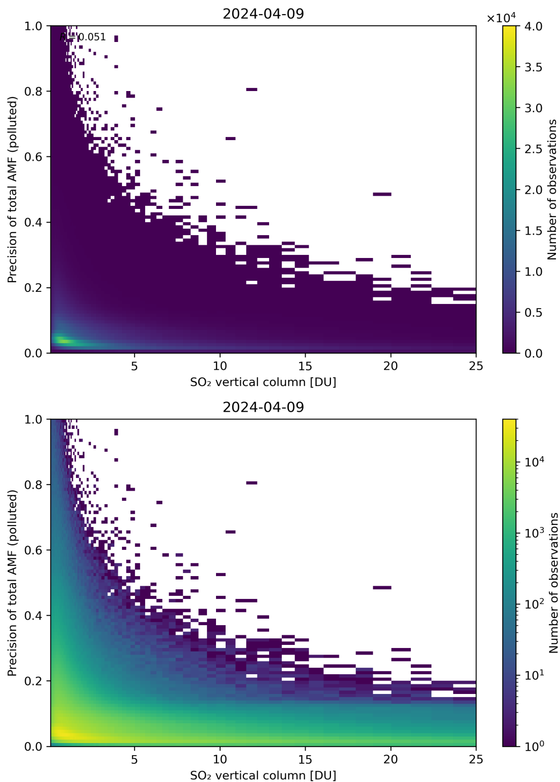
Figure 306: Scatter density plot of “SO 2 vertical column” against “Precision of total AMF (polluted)” for 2024-04-08 to 2024-04-10.
