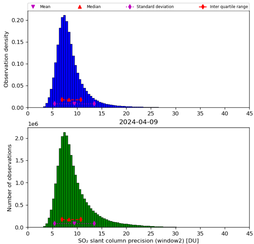
Figure 61: Histogram of “SO 2 slant column precision (window2)” for 2024-04-08 to 2024-04-10
