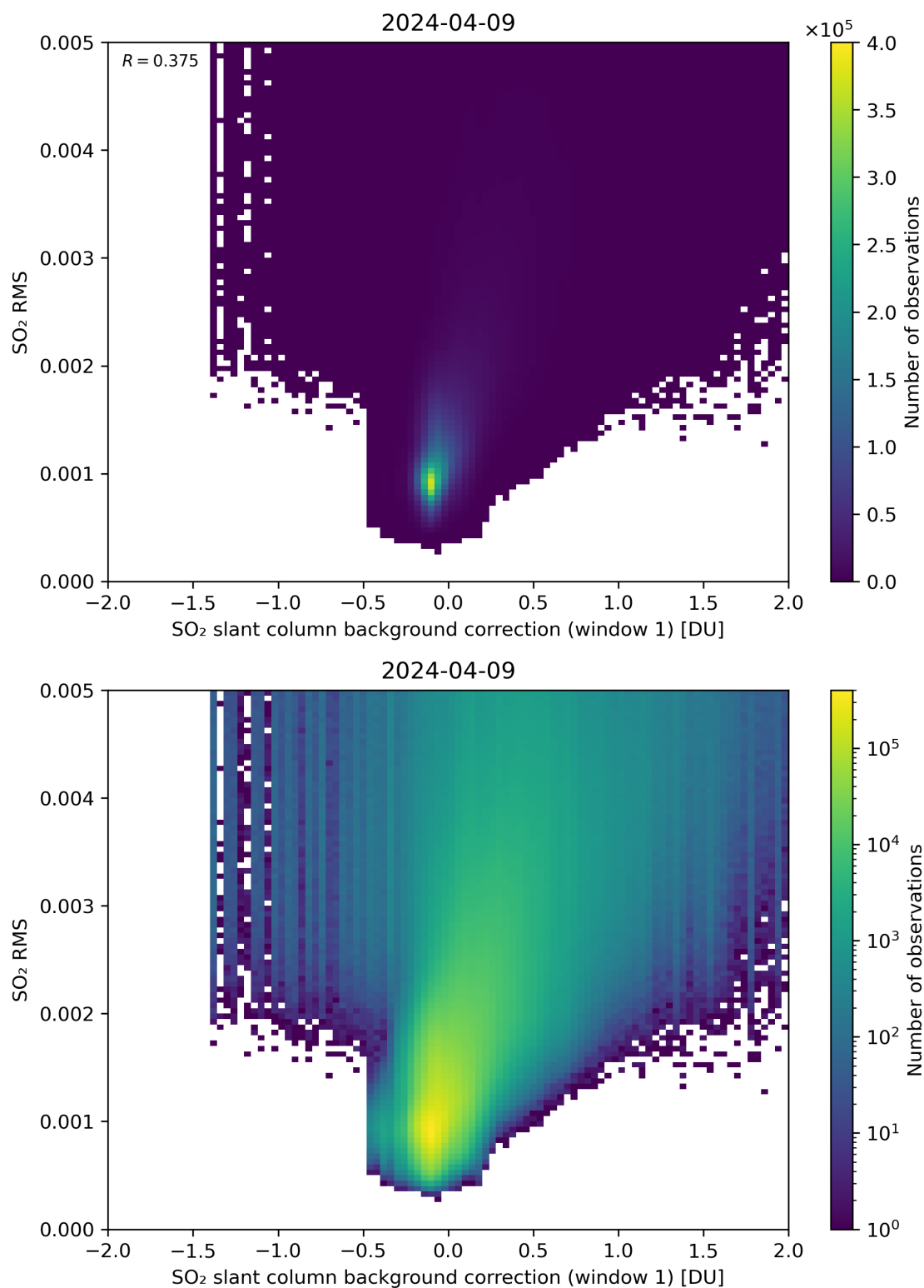
Figure 102: Scatter density plot of “SO 2 slant column background correction (window 1)” against “SO 2 RMS” for 2024-04-08 to 2024-04-10.
