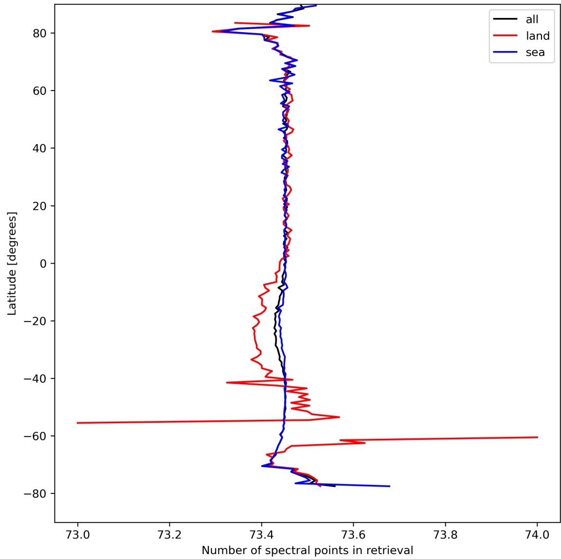
Figure 51: Zonal average of “Number of spectral points in retrieval” for 2024-04-08 to 2024-04-10.
