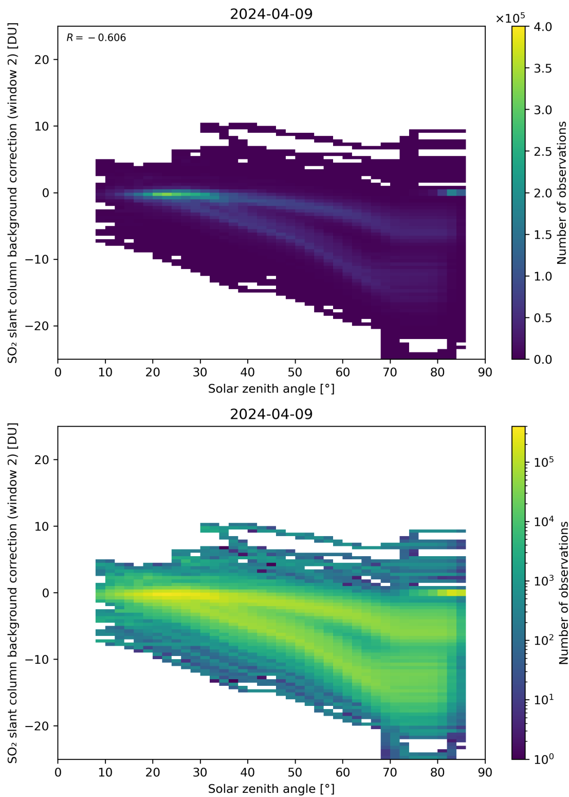
Figure 159: Scatter density plot of “Solar zenith angle” against “SO 2 slant column background correction (window 2)” for 2024-04-08 to 2024-04-10.
