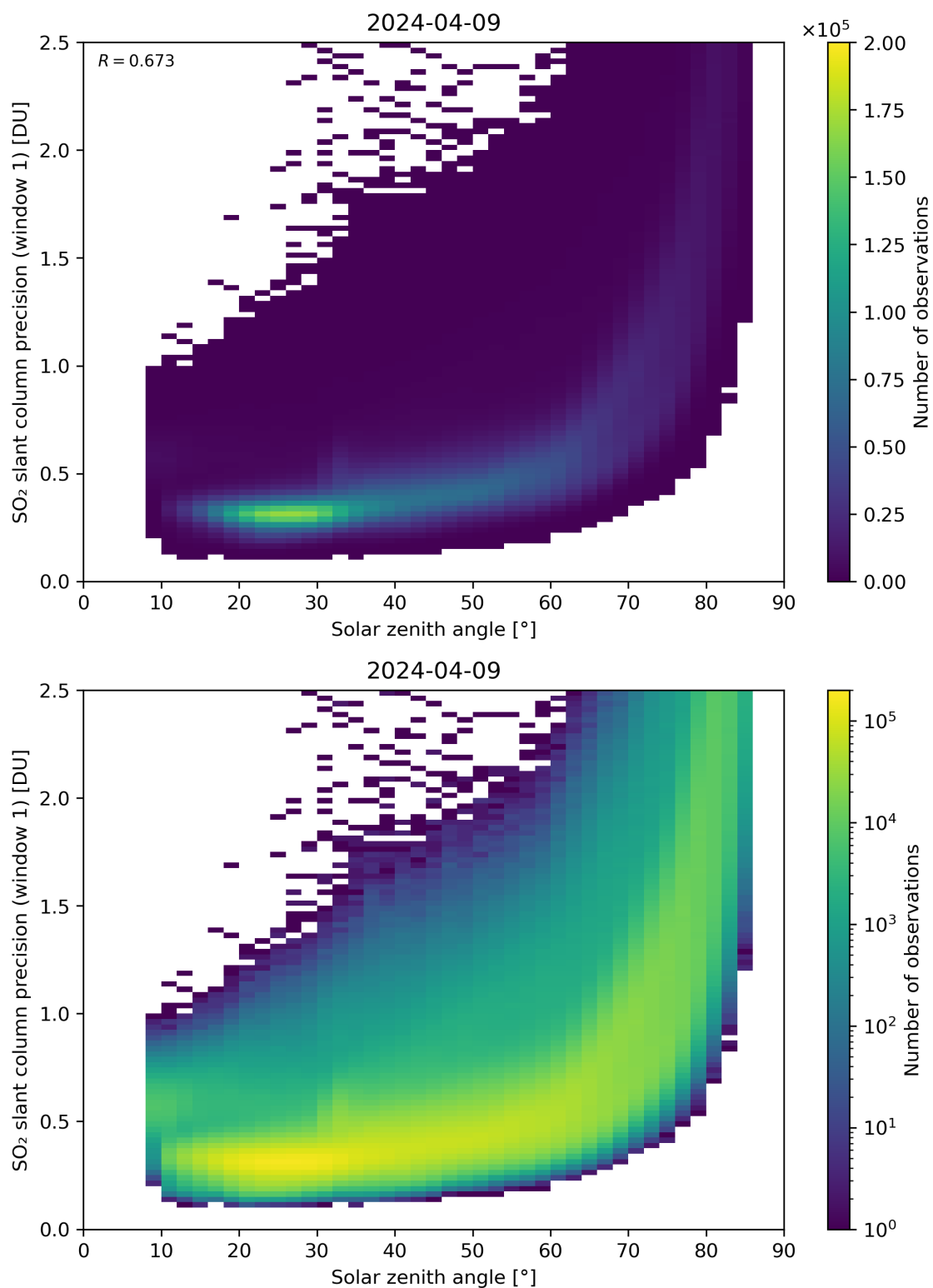
Figure 170: Scatter density plot of “Solar zenith angle” against “SO 2 slant column precision (window 1)” for 2024-04-08 to 2024-04-10.
