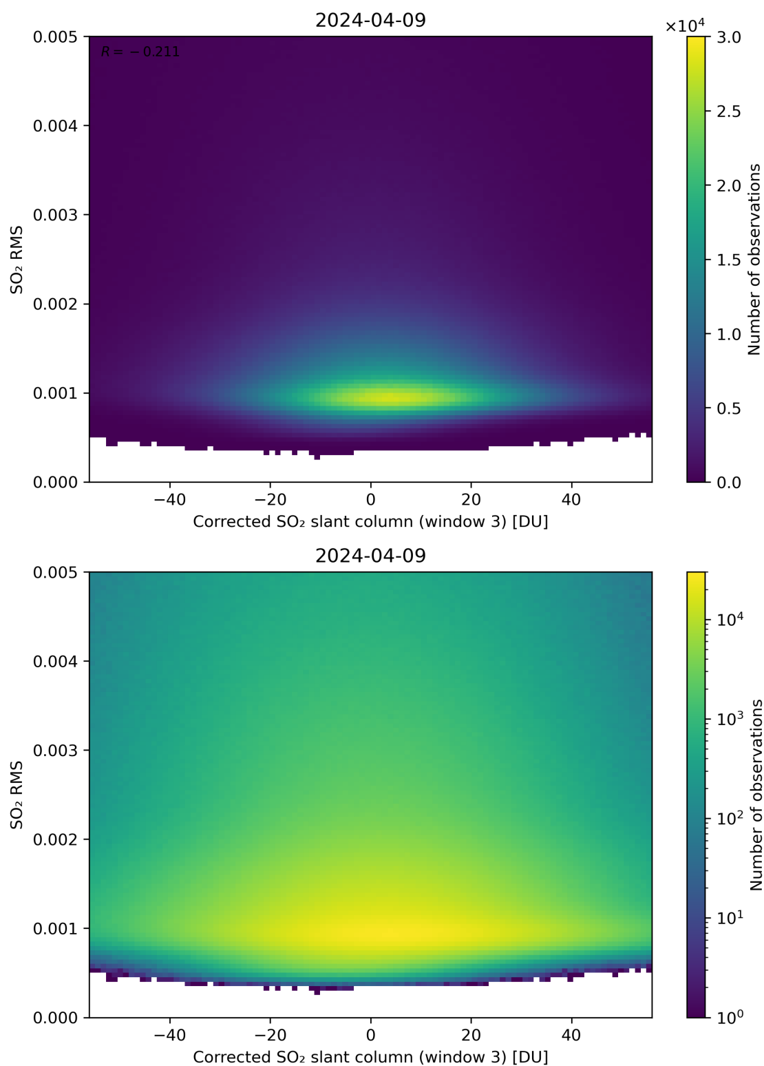
Figure 208: Scatter density plot of “Corrected SO 2 slant column (window 3)” against “SO 2 RMS” for 2024-04-08 to 2024-04-10.
