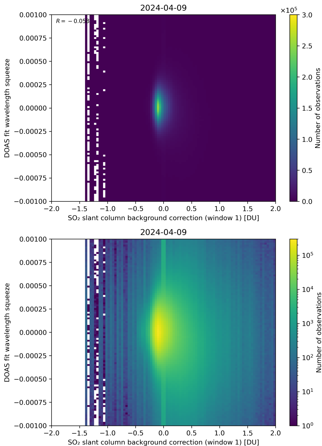
Figure 101: Scatter density plot of “SO 2 slant column background correction (window 1)” against “DOAS fit wavelength squeeze” for 2024-04-08 to 2024-04-10.
