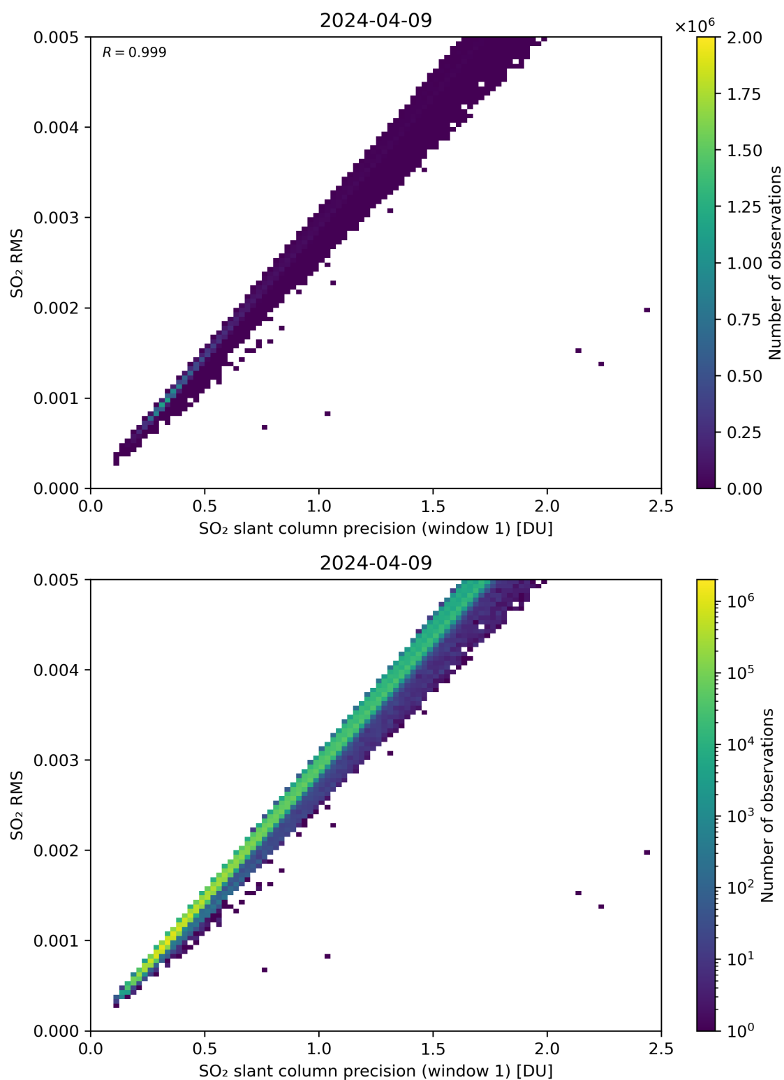
Figure 223: Scatter density plot of “SO 2 slant column precision (window 1)” against “SO 2 RMS” for 2024-04-08 to 2024-04-10.
