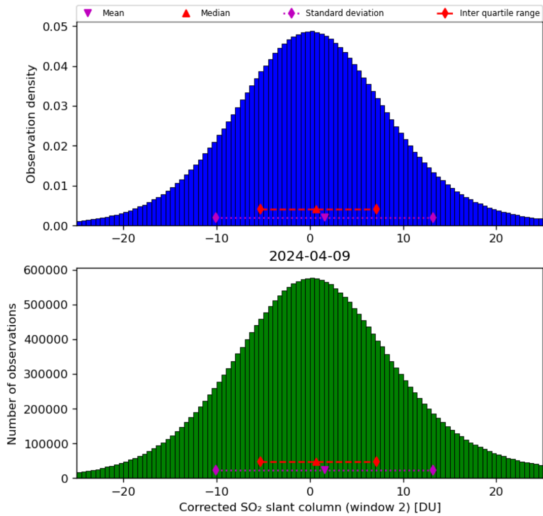
Figure 62: Histogram of “Corrected SO 2 slant column (window 2)” for 2024-04-08 to 2024-04-10
