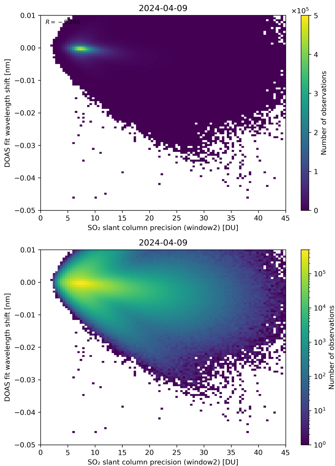
Figure 243: Scatter density plot of “SO 2 slant column precision (window2)” against “DOAS fit wavelength shift” for 2024-04-08 to 2024-04-10.
