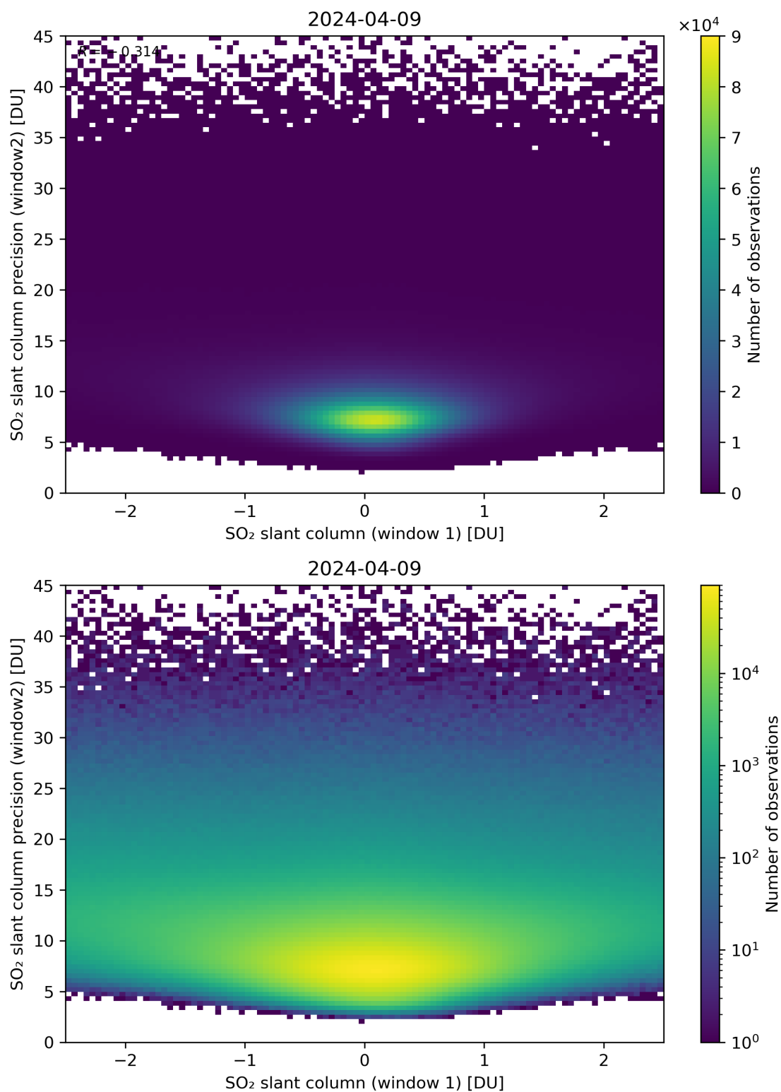
Figure 236: Scatter density plot of “SO 2 slant column (window 1)” against “SO 2 slant column precision (window2)” for 2024-04-08 to 2024-04-10.
