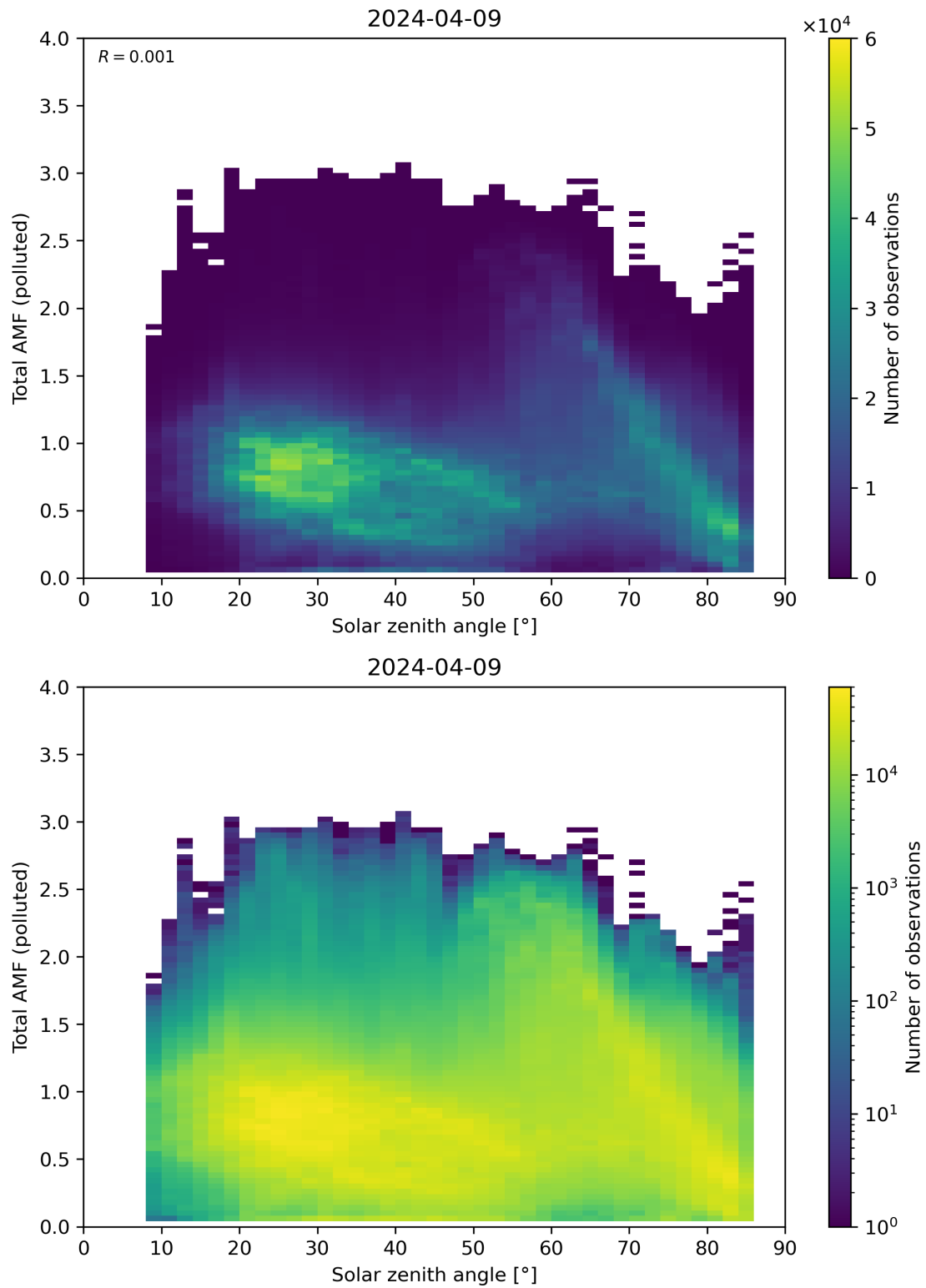
Figure 174: Scatter density plot of “Solar zenith angle” against “Total AMF (polluted)” for 2024-04-08 to 2024-04-10.
