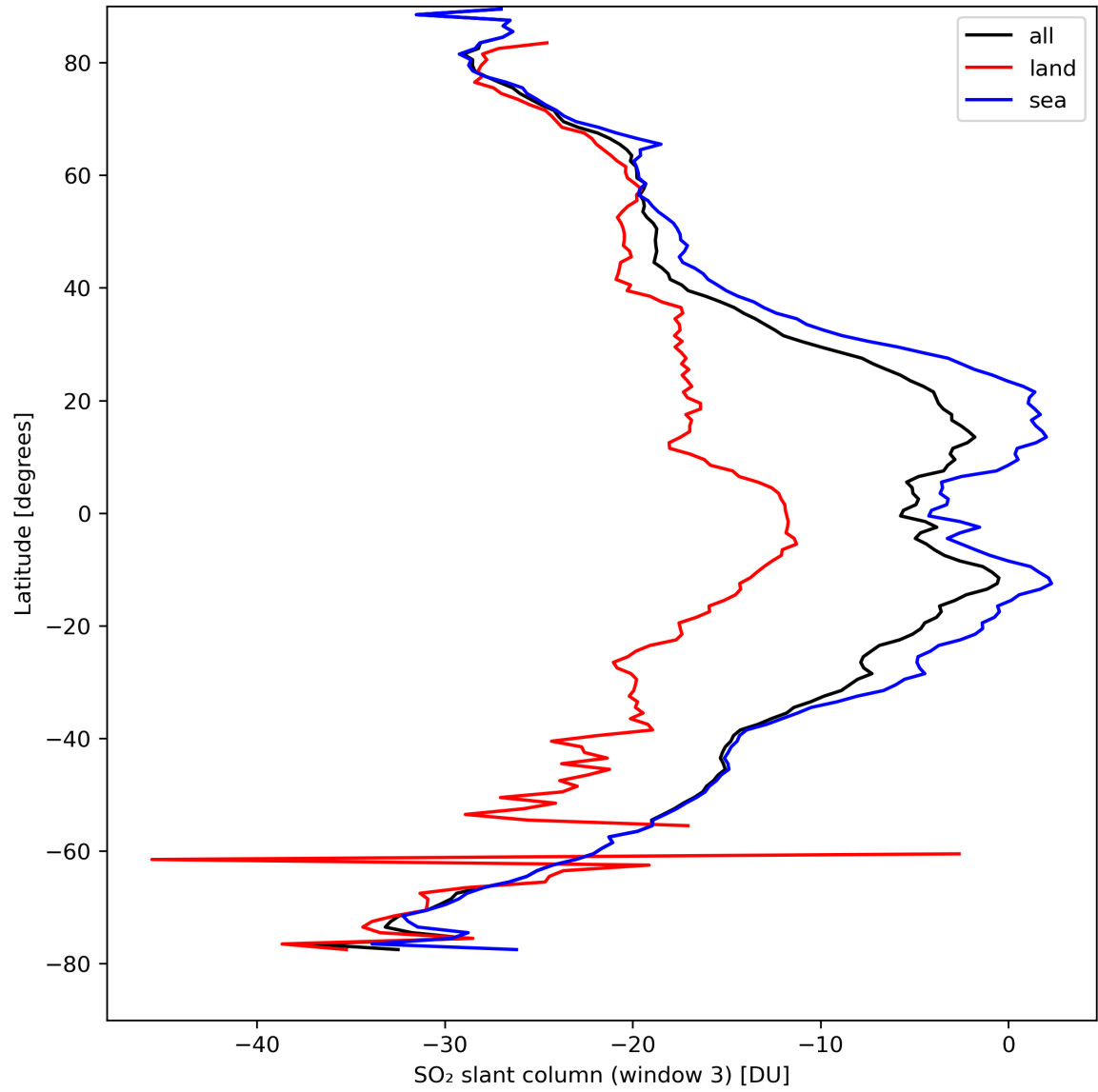
Figure 41: Zonal average of “SO 2 slant column (window 3)” for 2024-04-08 to 2024-04-10.
