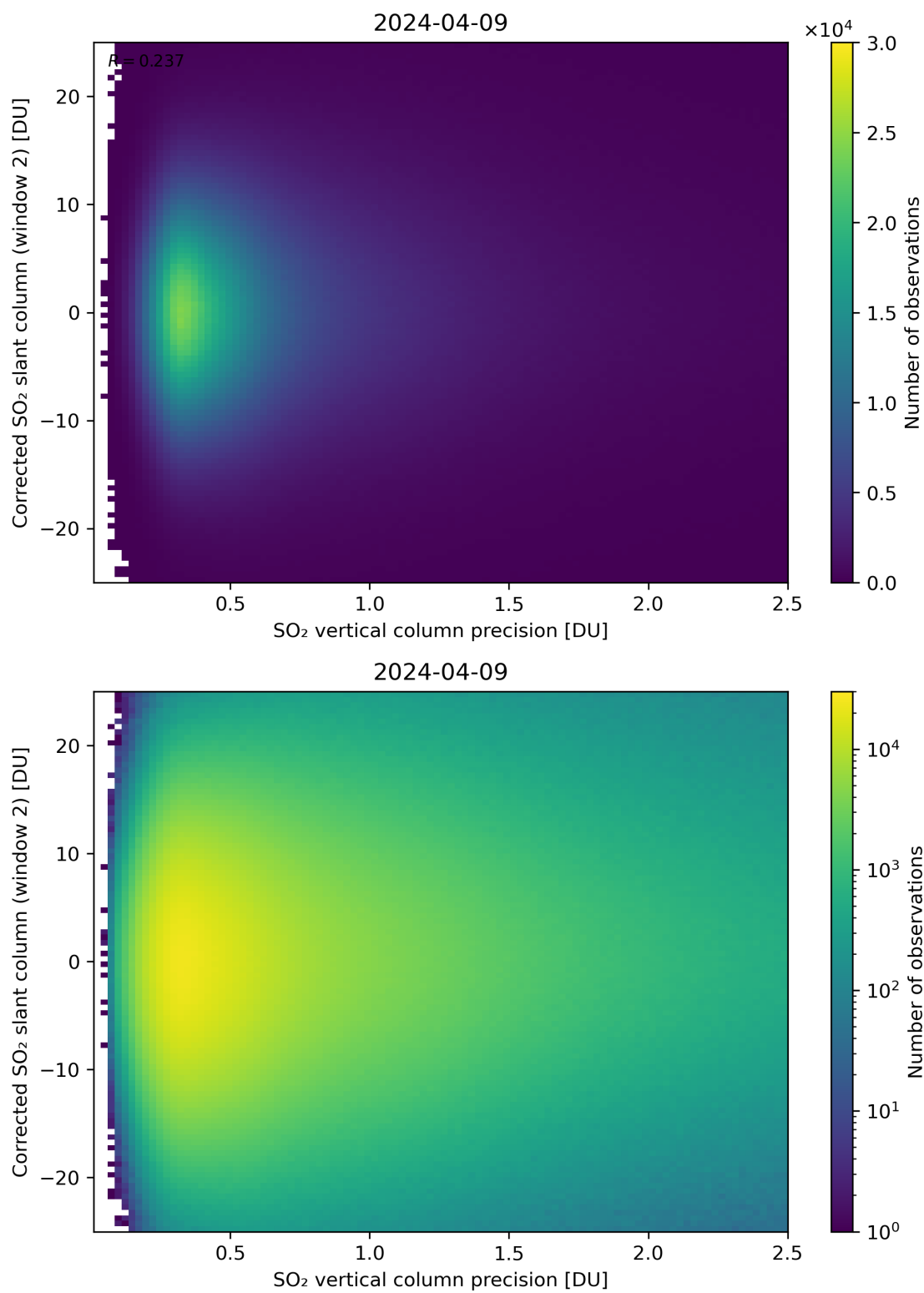
Figure 287: Scatter density plot of “SO 2 vertical column precision” against “Corrected SO 2 slant column (window 2)” for 2024-04-08 to 2024-04-10.
