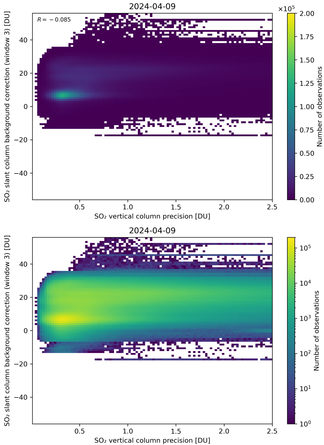
Figure 281: Scatter density plot of “SO 2 vertical column precision” against “SO 2 slant column background correction (window 3)” for 2024-04-08 to 2024-04-10.
