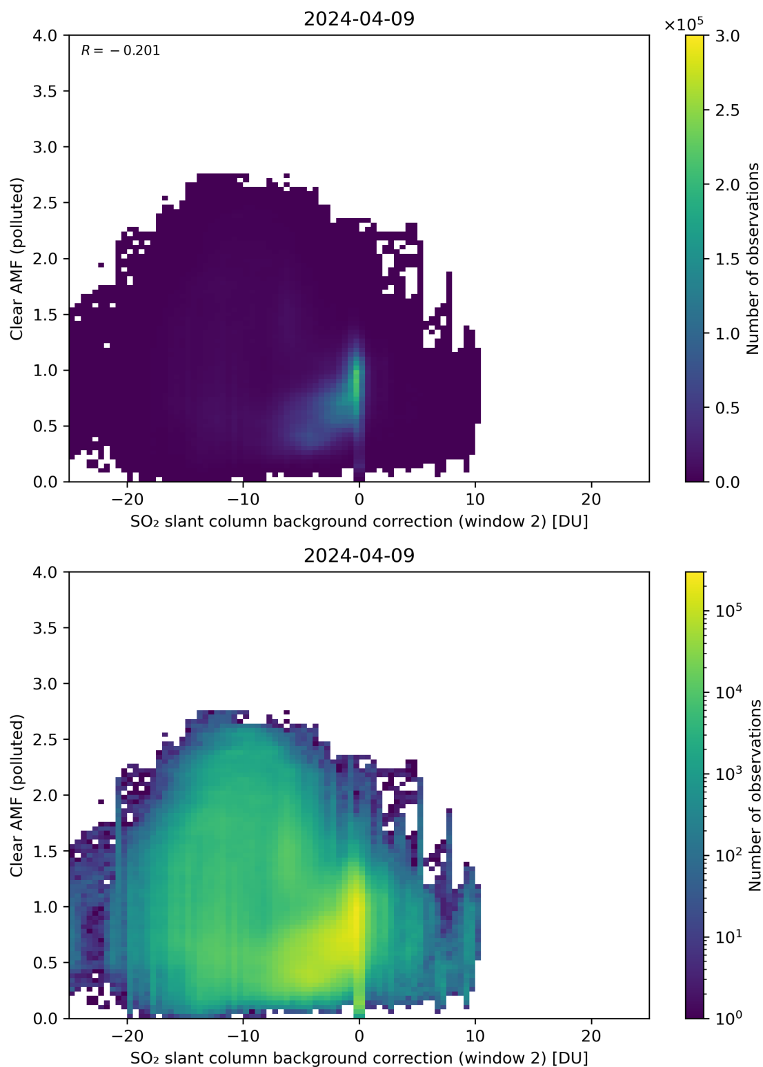
Figure 115: Scatter density plot of “SO 2 slant column background correction (window 2)” against “Clear AMF (polluted)” for 2024-04-08 to 2024-04-10.
