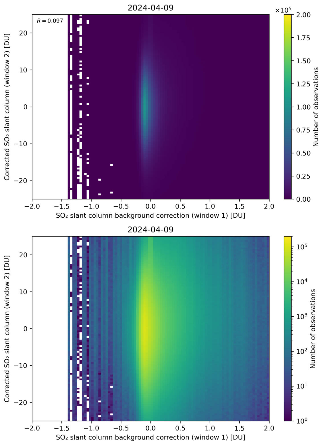
Figure 104: Scatter density plot of “SO 2 slant column background correction (window 1)” against “Corrected SO 2 slant column (window 2)” for 2024-04-08 to 2024-04-10.
