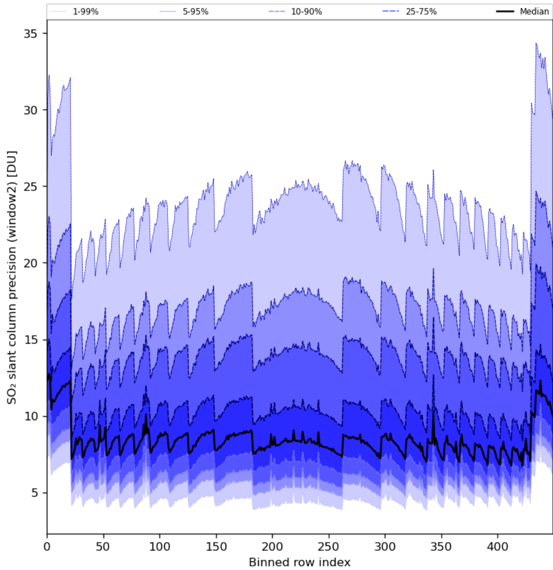
Figure 84: Along track statistics of “SO 2 slant column precision (window2)” for 2024-04-08 to 2024-04-10
