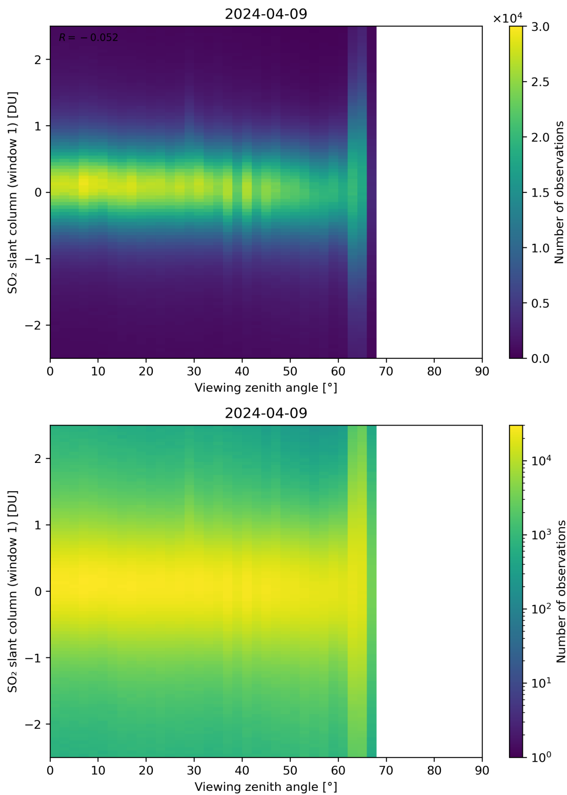
Figure 320: Scatter density plot of “Viewing zenith angle” against “SO 2 slant column (window 1)” for 2024-04-08 to 2024-04-10.
