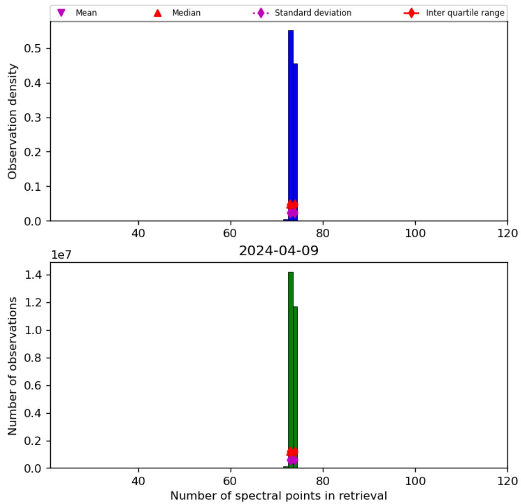
Figure 74: Histogram of “Number of spectral points in retrieval” for 2024-04-08 to 2024-04-10
