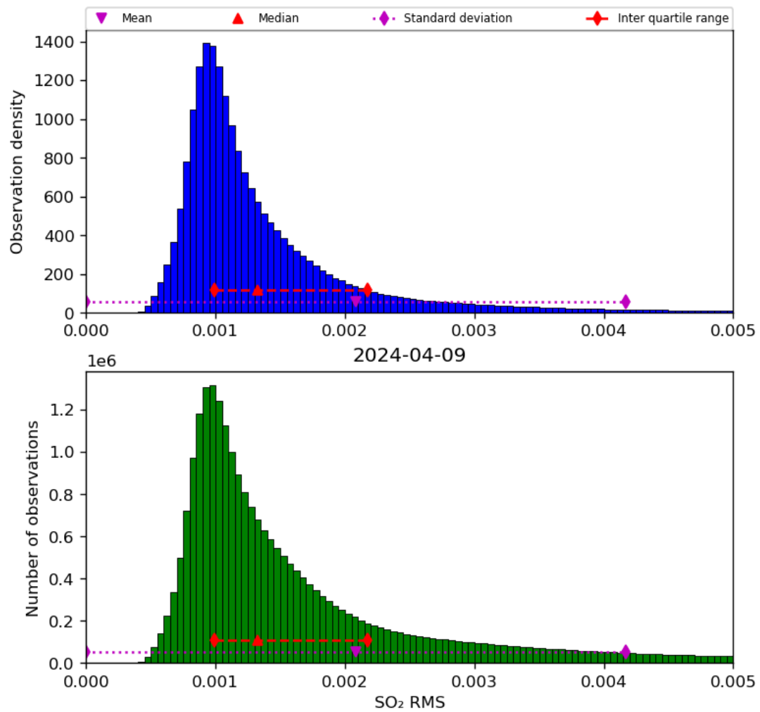
Figure 70: Histogram of “SO 2 RMS” for 2024-04-08 to 2024-04-10
