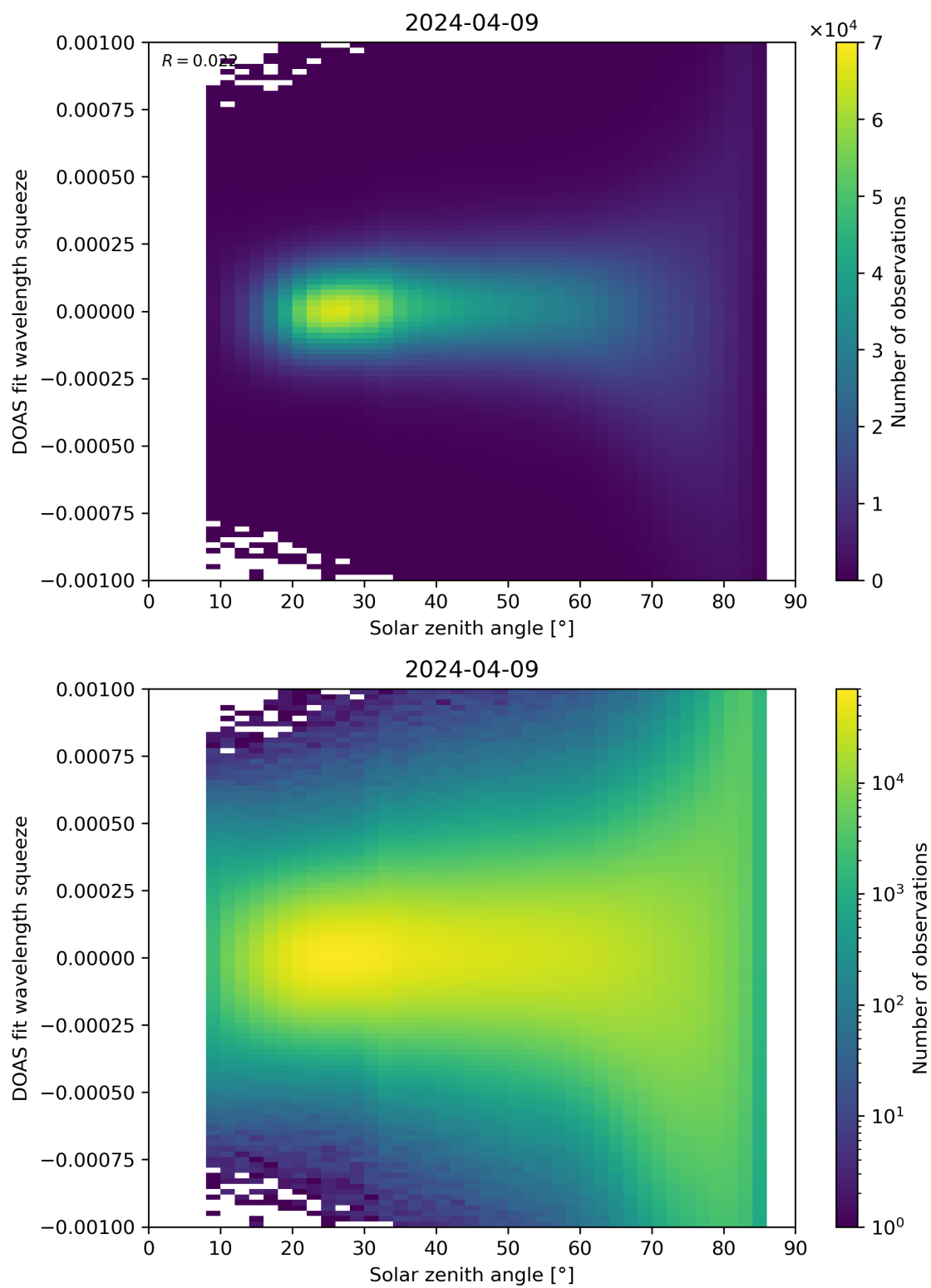
Figure 162: Scatter density plot of “Solar zenith angle” against “DOAS fit wavelength squeeze” for 2024-04-08 to 2024-04-10.
