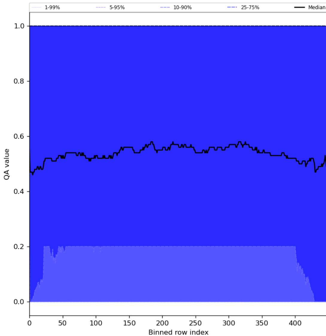
Figure 75: Along track statistics of “QA value” for 2024-04-08 to 2024-04-10
