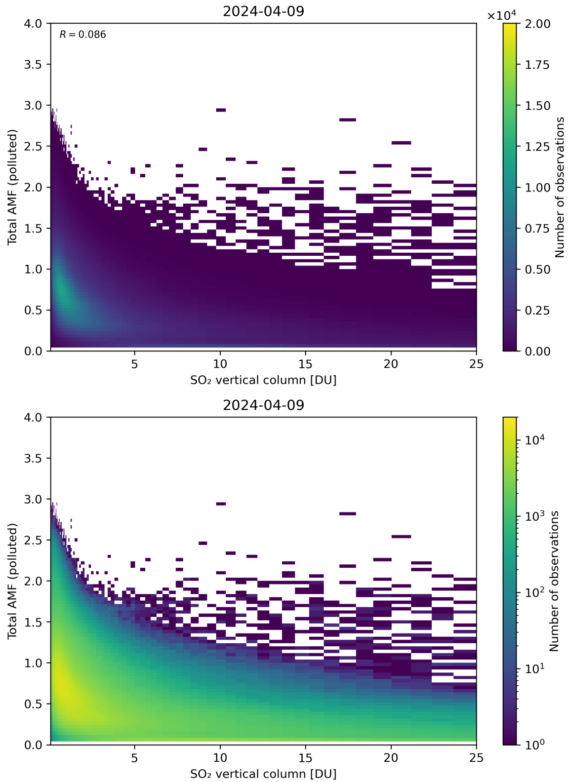
Figure 305: Scatter density plot of “SO 2 vertical column” against “Total AMF (polluted)” for 2024-04-08 to 2024-04-10.
