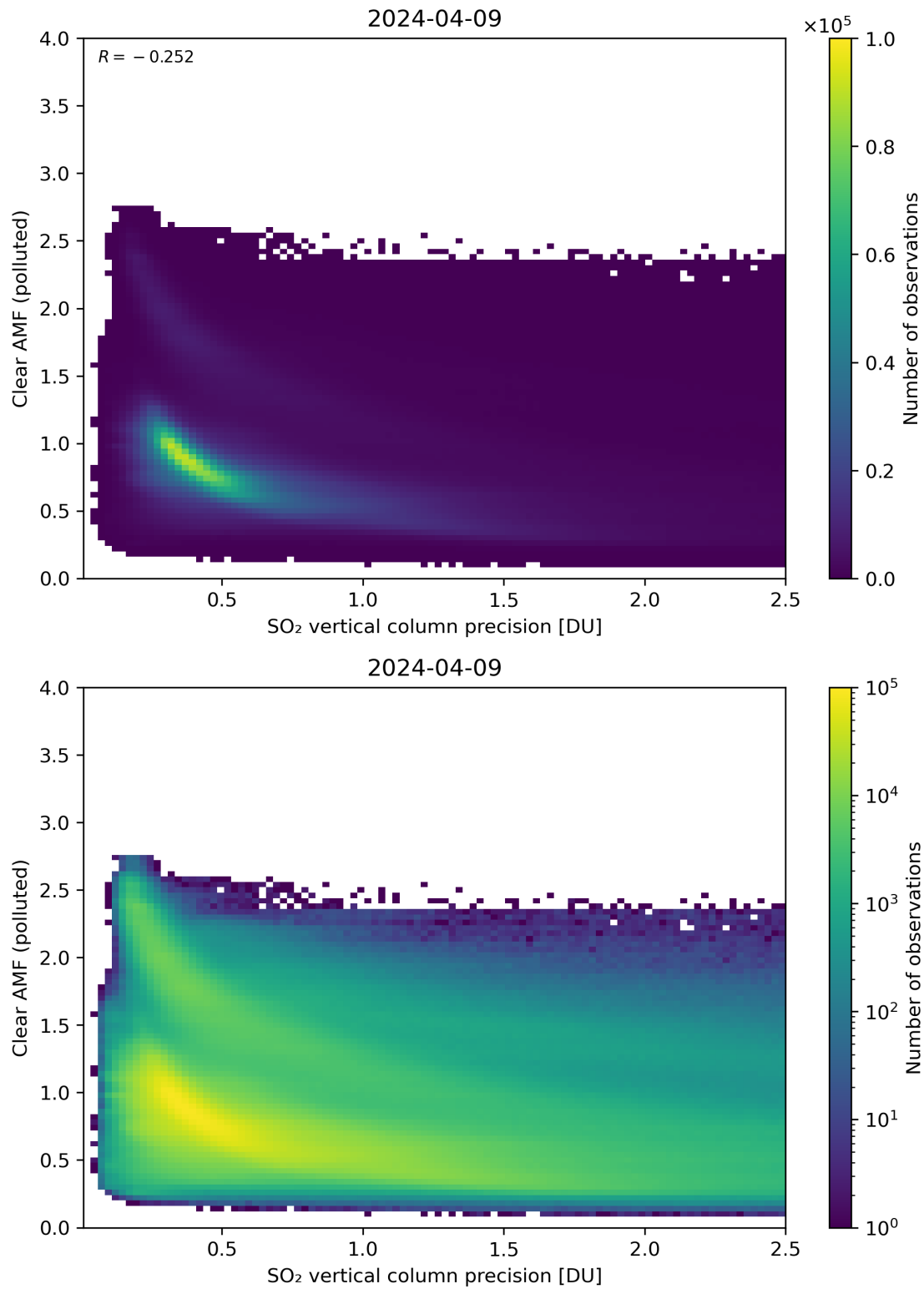
Figure 285: Scatter density plot of “SO 2 vertical column precision” against “Clear AMF (polluted)” for 2024-04-08 to 2024-04-10.
