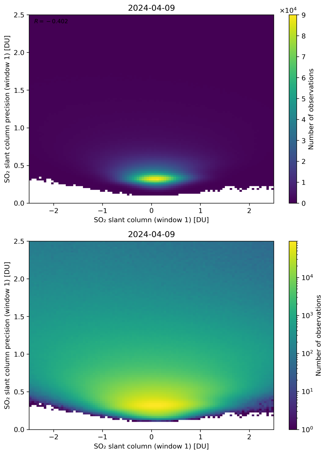
Figure 235: Scatter density plot of “SO 2 slant column (window 1)” against “SO 2 slant column precision (window 1)” for 2024-04-08 to 2024-04-10.
