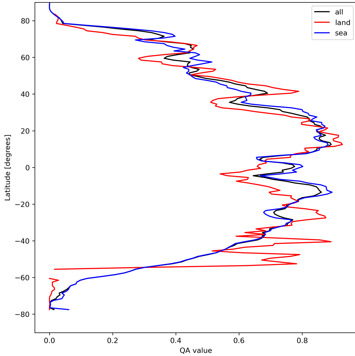
Figure 29: Zonal average of “QA value” for 2024-04-08 to 2024-04-10.
