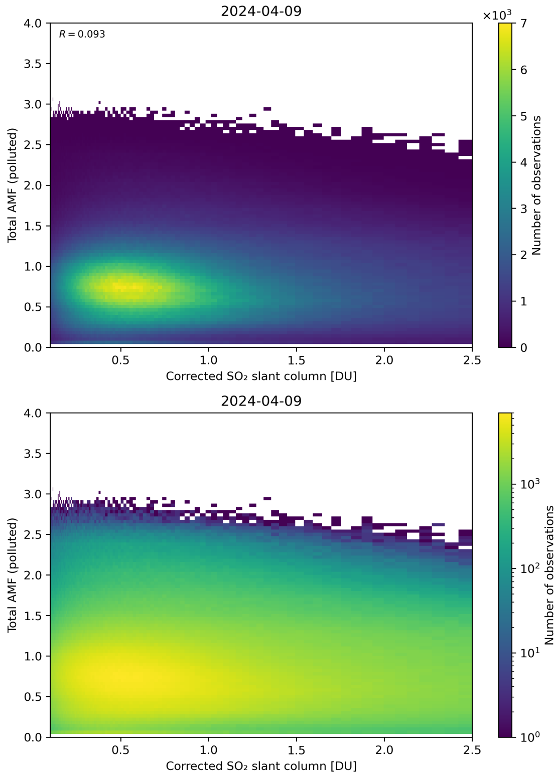
Figure 192: Scatter density plot of “Corrected SO 2 slant column” against “Total AMF (polluted)” for 2024-04-08 to 2024-04-10.
