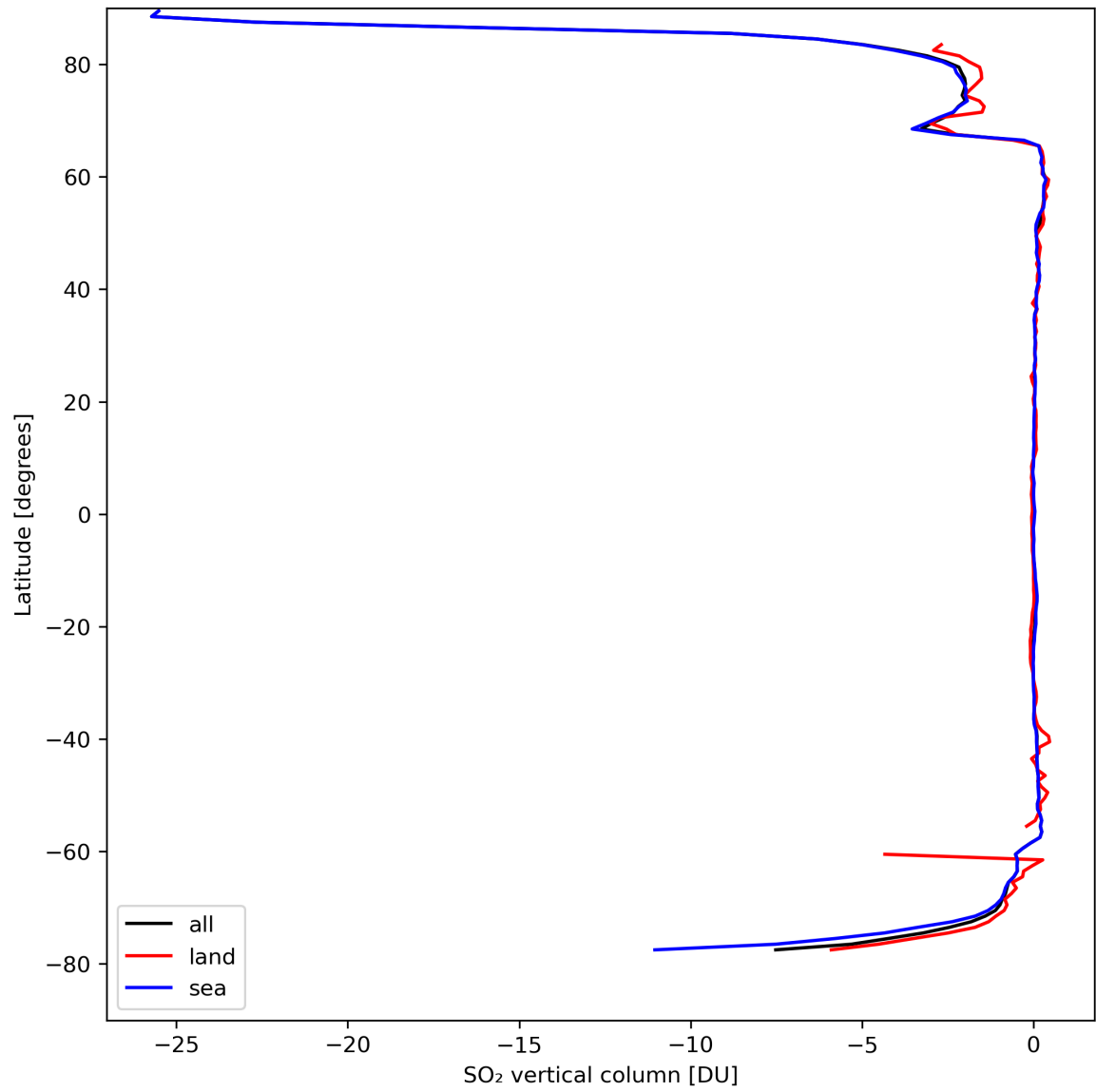
Figure 30: Zonal average of “SO 2 vertical column” for 2024-04-08 to 2024-04-10.
