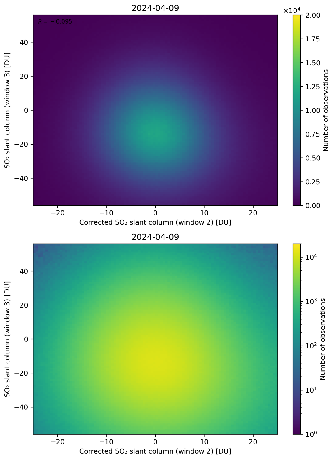
Figure 201: Scatter density plot of “Corrected SO 2 slant column (window 2)” against “SO 2 slant column (window 3)” for 2024-04-08 to 2024-04-10.
