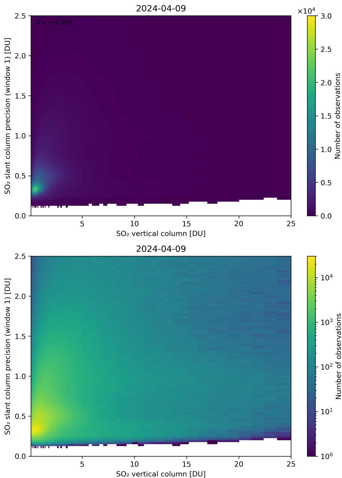
Figure 301: Scatter density plot of “SO 2 vertical column” against “SO 2 slant column precision (window 1)” for 2024-04-08 to 2024-04-10.
