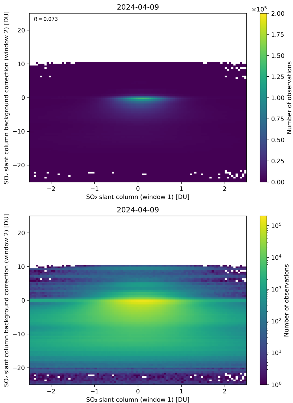
Figure 213: Scatter density plot of “SO 2 slant column (window 1)” against “SO 2 slant column background correction (window 2)” for 2024-04-08 to 2024-04-10.
