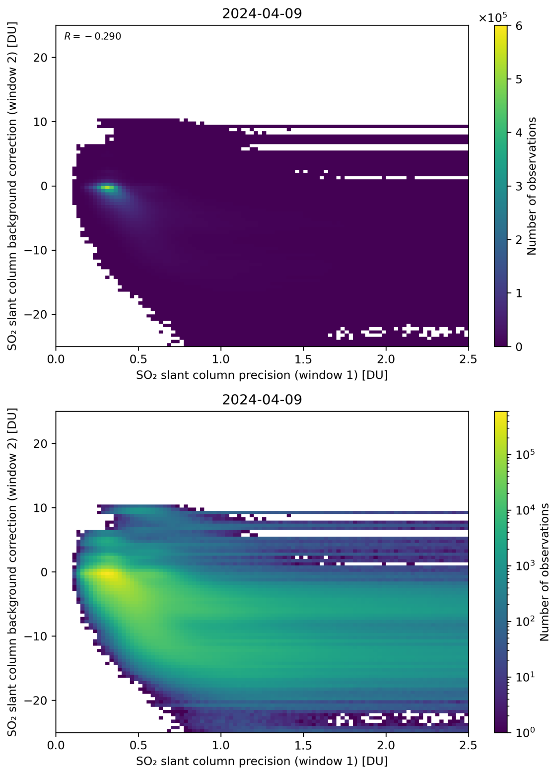
Figure 219: Scatter density plot of “SO 2 slant column precision (window 1)” against “SO 2 slant column background correction (window 2)” for 2024-04-08 to 2024-04-10.
