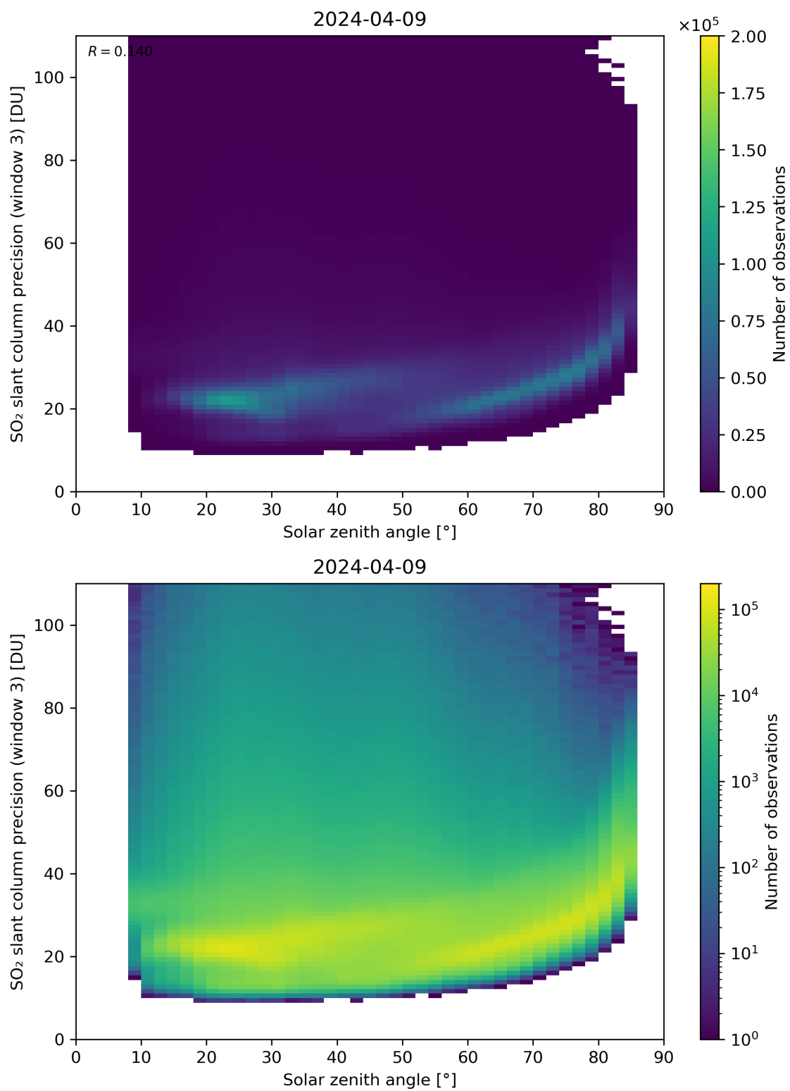
Figure 173: Scatter density plot of “Solar zenith angle” against “SO 2 slant column precision (window 3)” for 2024-04-08 to 2024-04-10.
