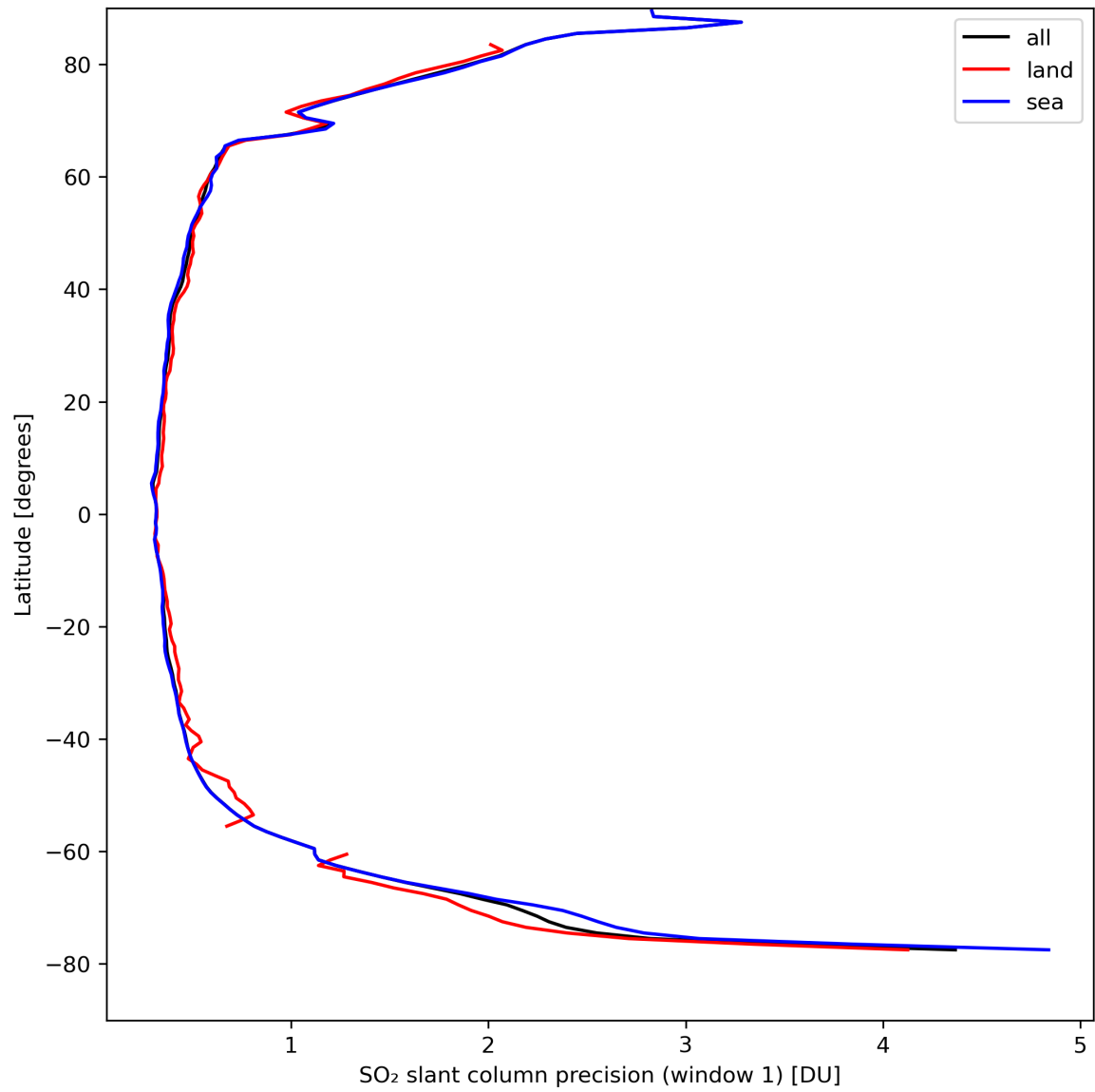
Figure 34: Zonal average of “SO 2 slant column precision (window 1)” for 2024-04-08 to 2024-04-10.
