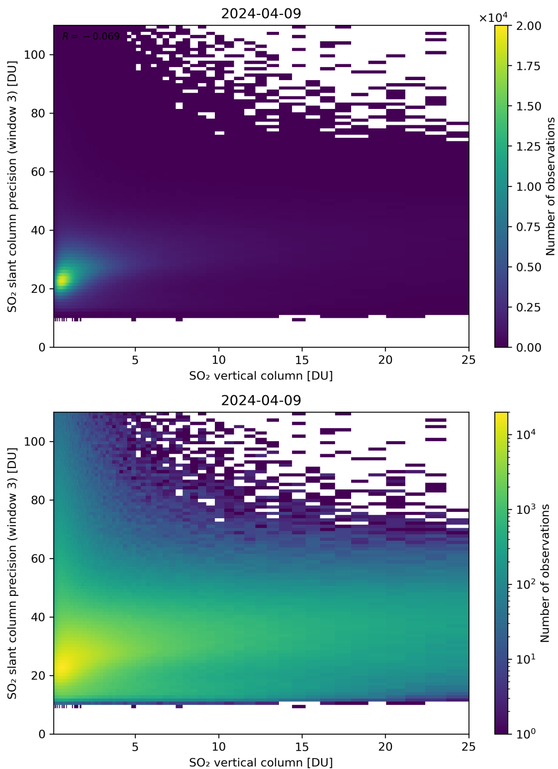
Figure 304: Scatter density plot of “SO 2 vertical column” against “SO 2 slant column precision (window 3)” for 2024-04-08 to 2024-04-10.
