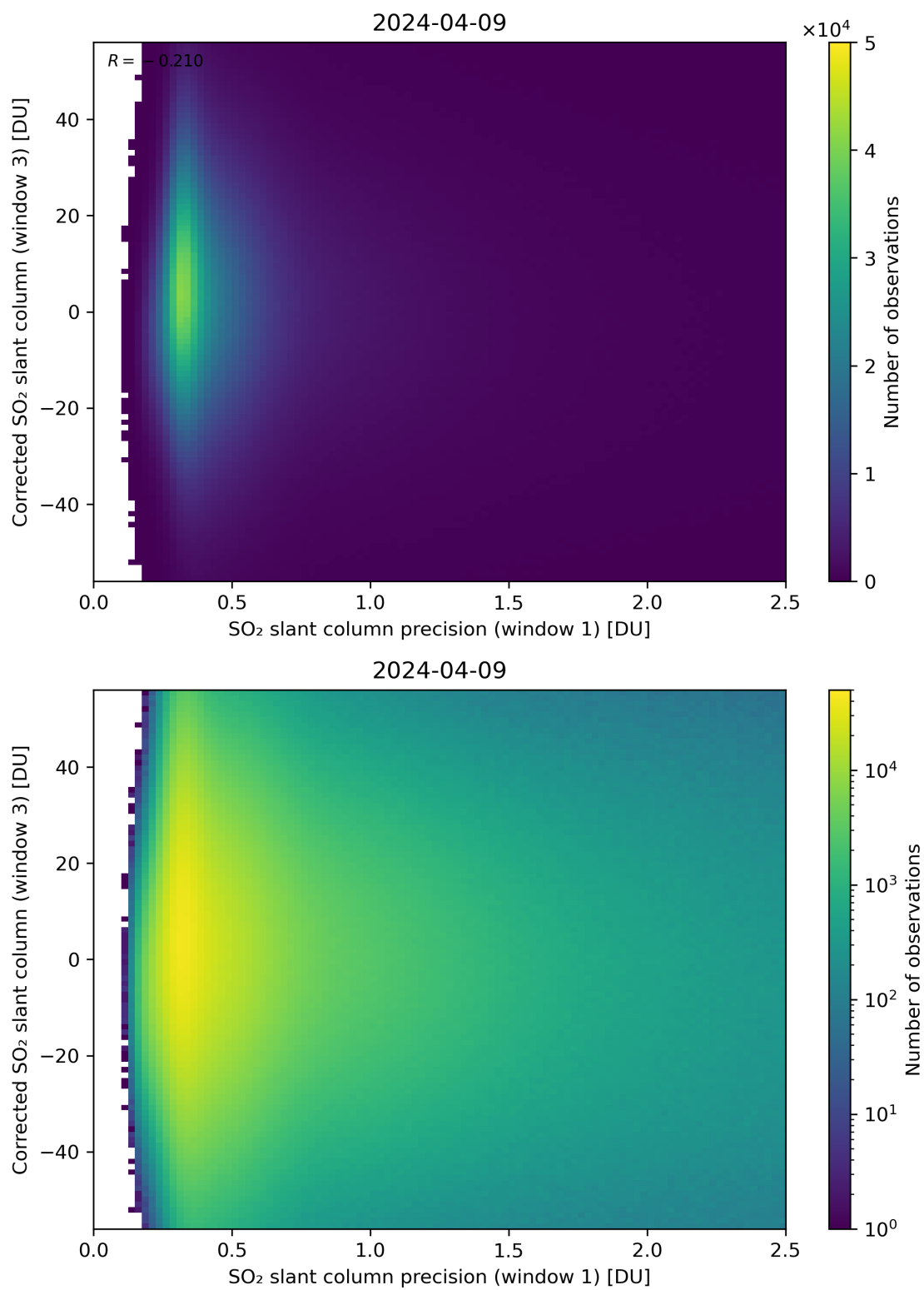
Figure 226: Scatter density plot of “SO 2 slant column precision (window 1)” against “Corrected SO 2 slant column (window 3)” for 2024-04-08 to 2024-04-10.
