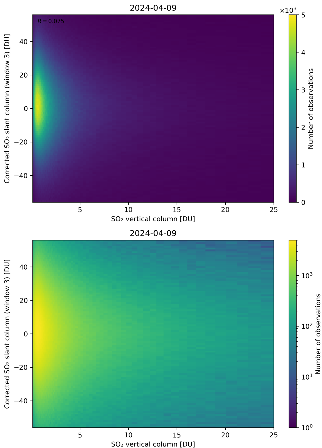
Figure 299: Scatter density plot of “SO 2 vertical column” against “Corrected SO 2 slant column (window 3)” for 2024-04-08 to 2024-04-10.
