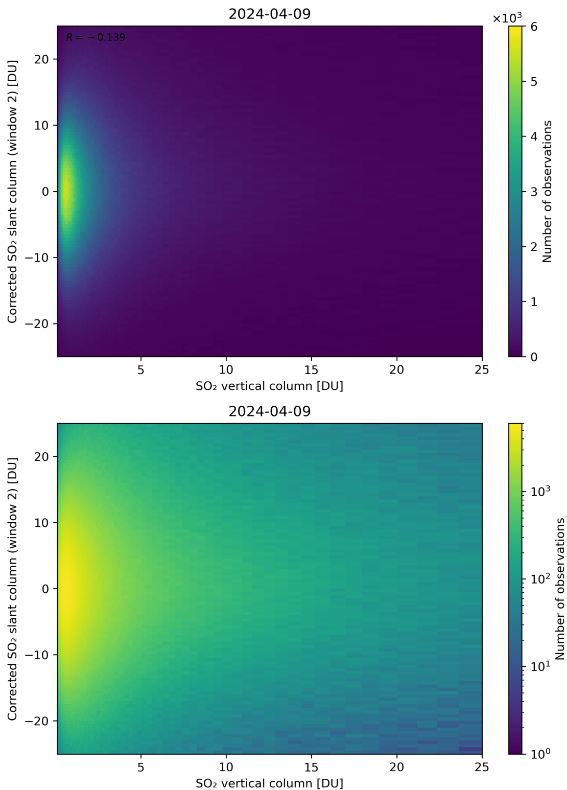
Figure 298: Scatter density plot of “SO 2 vertical column” against “Corrected SO 2 slant column (window 2)” for 2024-04-08 to 2024-04-10.
