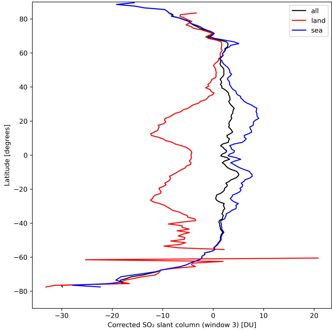
Figure 43: Zonal average of “Corrected SO 2 slant column (window 3)” for 2024-04-08 to 2024-04-10.
