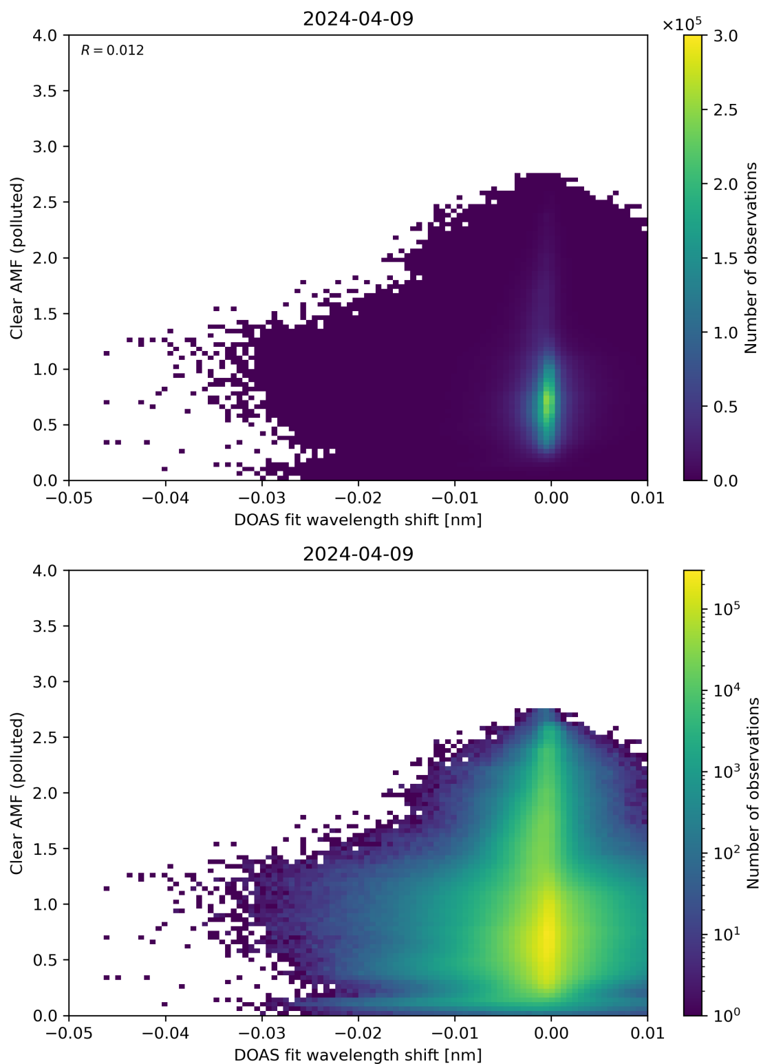
Figure 129: Scatter density plot of “DOAS fit wavelength shift” against “Clear AMF (polluted)” for 2024-04-08 to 2024-04-10.
