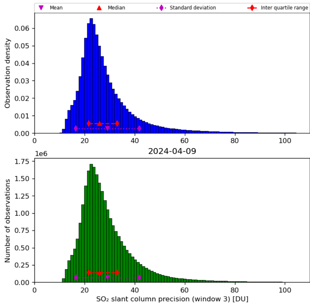
Figure 65: Histogram of “SO 2 slant column precision (window 3)” for 2024-04-08 to 2024-04-10
