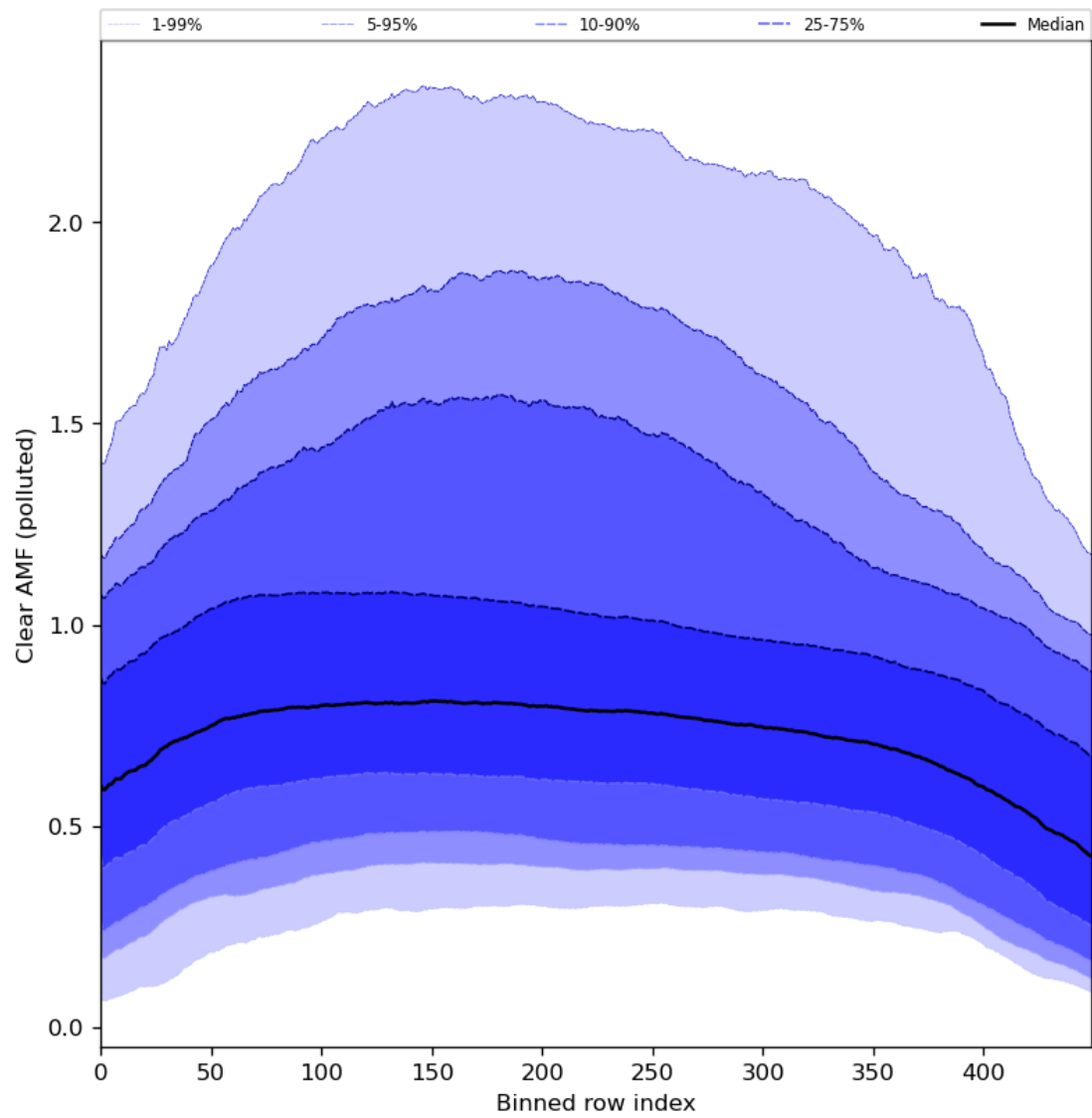
Figure 96: Along track statistics of “Clear AMF (polluted)” for 2024-04-08 to 2024-04-10
