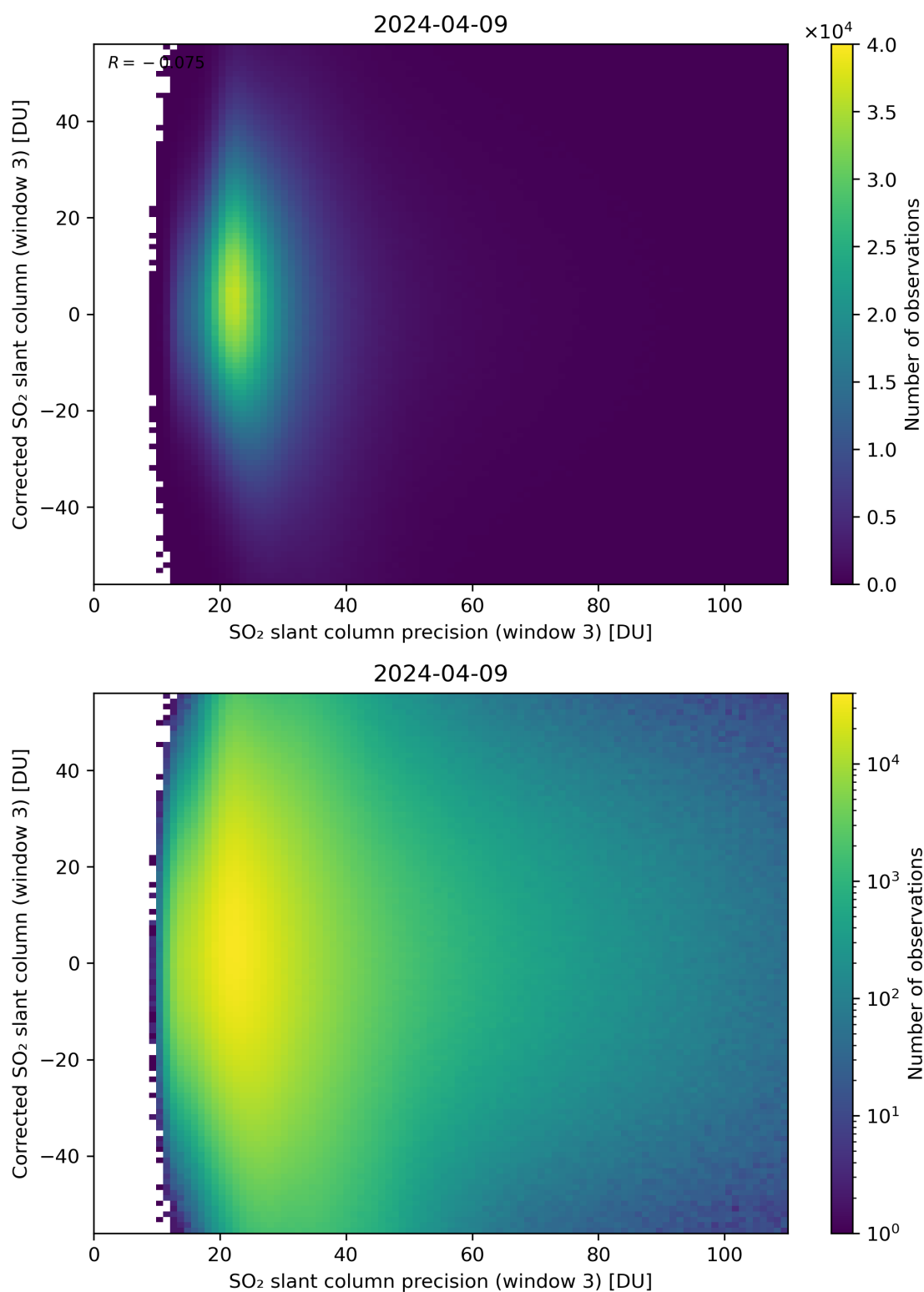
Figure 262: Scatter density plot of “SO 2 slant column precision (window 3)” against “Corrected SO 2 slant column (window 3)” for 2024-04-08 to 2024-04-10.
