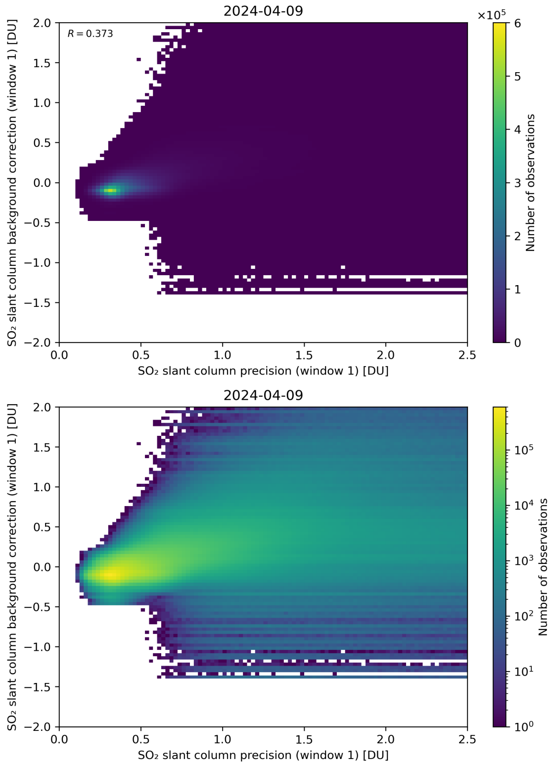
Figure 218: Scatter density plot of “SO 2 slant column precision (window 1)” against “SO 2 slant column background correction (window 1)” for 2024-04-08 to 2024-04-10.
