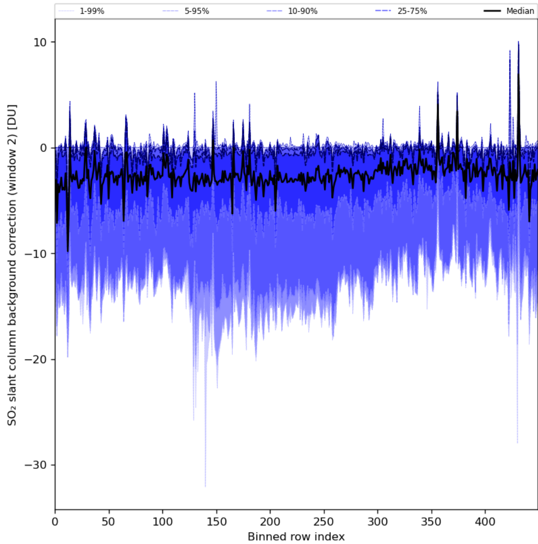
Figure 86: Along track statistics of “SO 2 slant column background correction (window 2)” for 2024-04-08 to 2024-04-10
