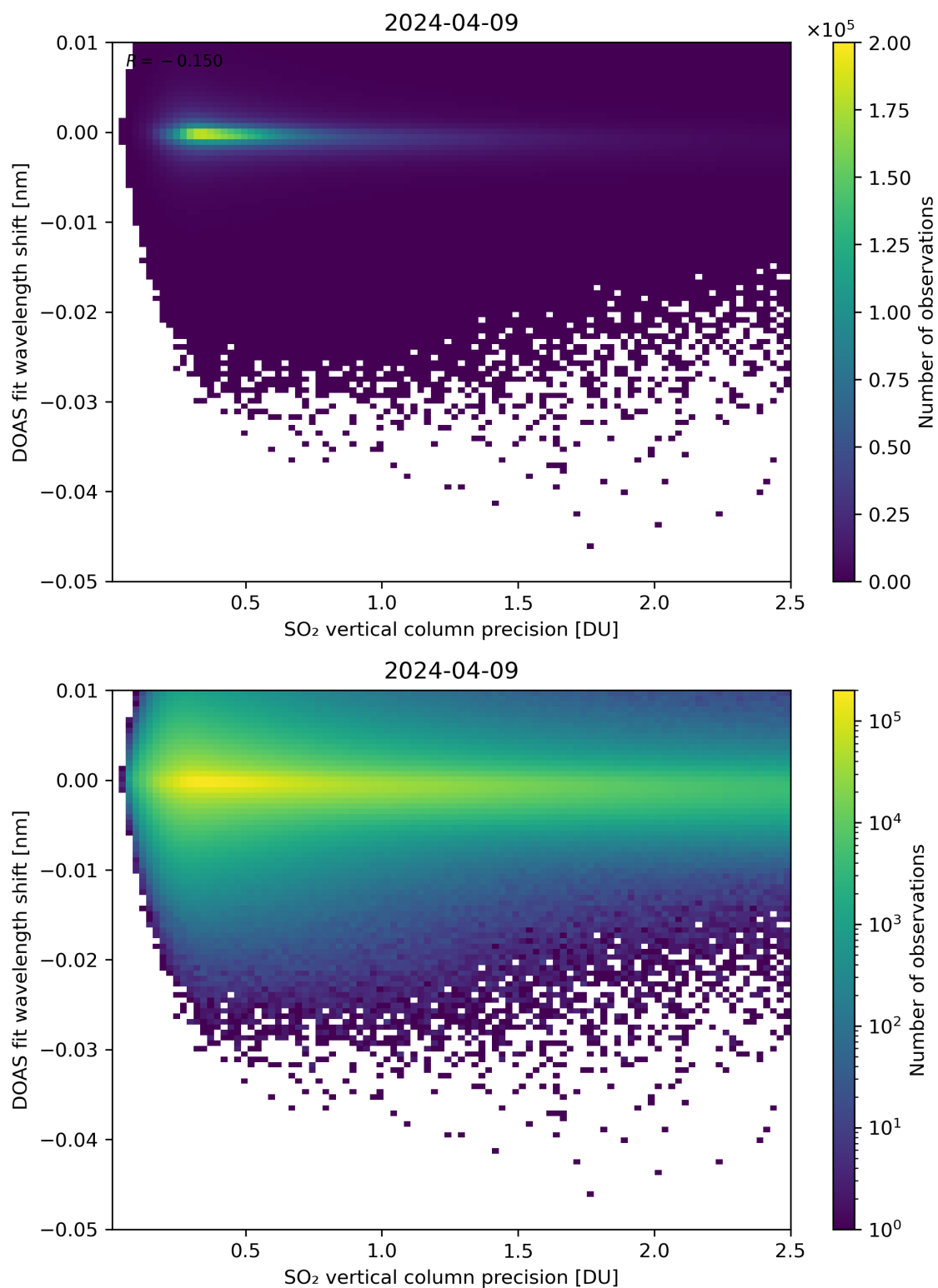
Figure 282: Scatter density plot of “SO 2 vertical column precision” against “DOAS fit wavelength shift” for 2024-04-08 to 2024-04-10.
