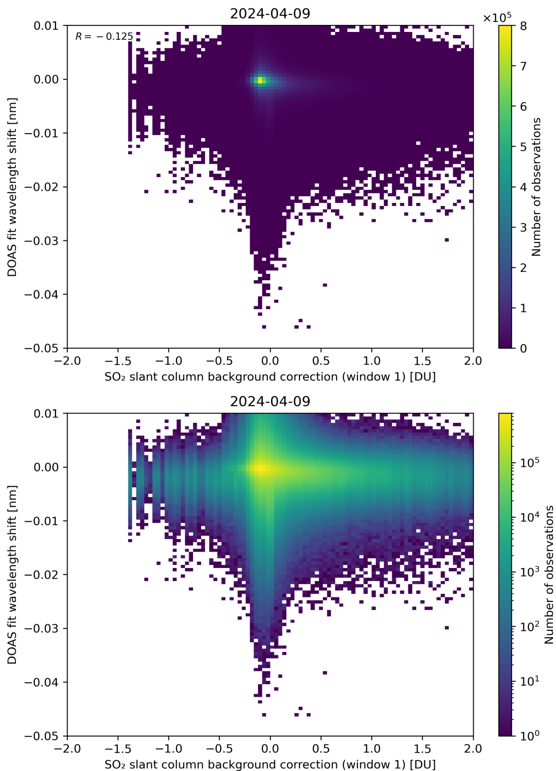
Figure 100: Scatter density plot of “SO 2 slant column background correction (window 1)” against “DOAS fit wavelength shift” for 2024-04-08 to 2024-04-10.
