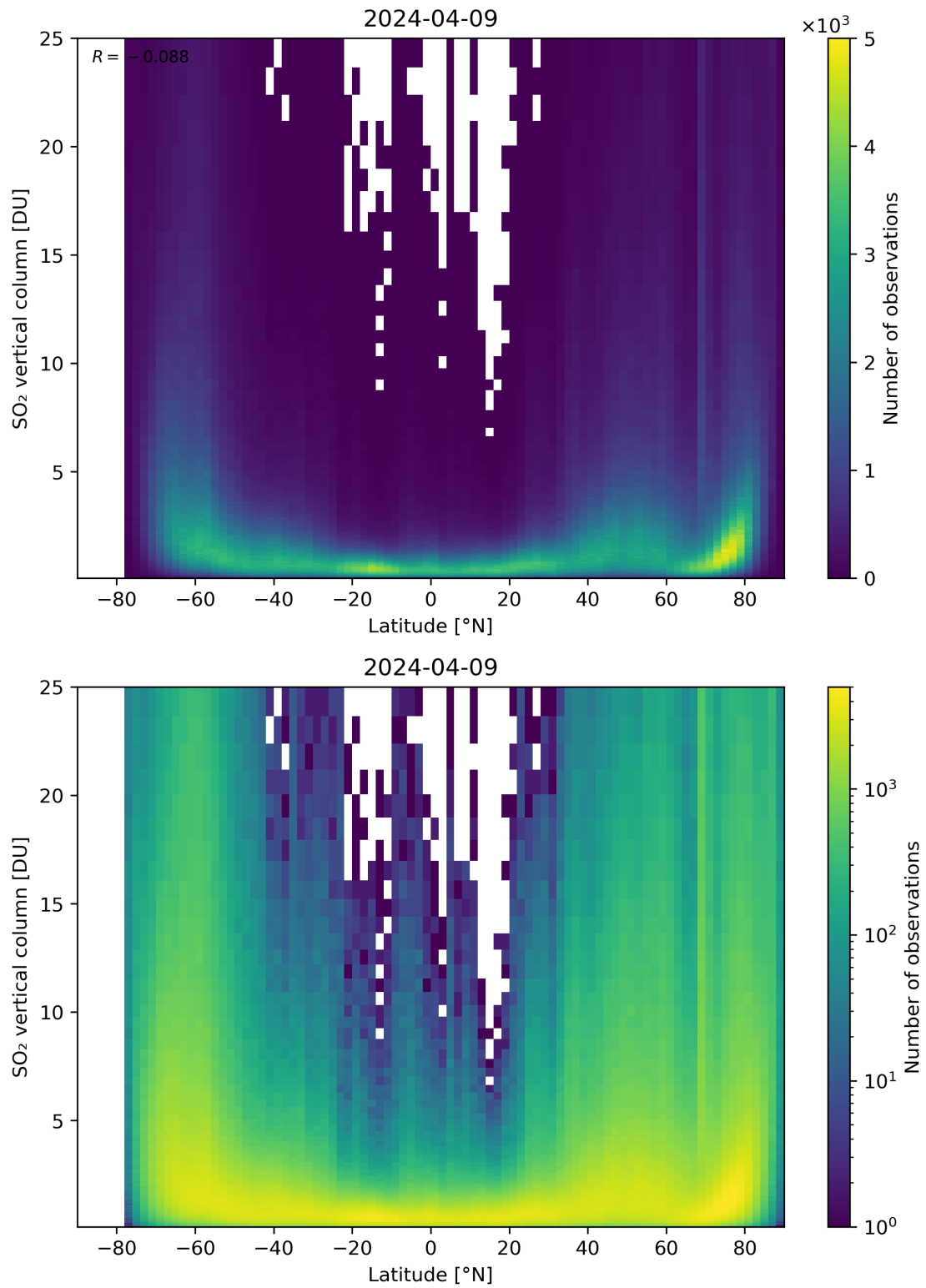
Figure 156: Scatter density plot of “Latitude” against “SO 2 vertical column” for 2024-04-08 to 2024-04-10.
