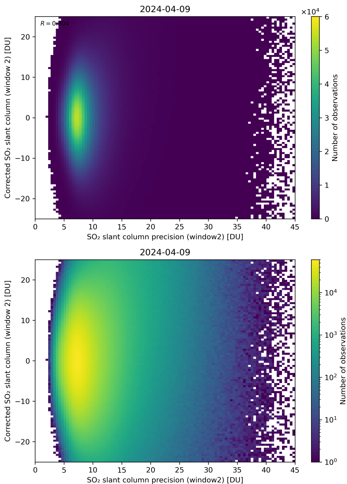
Figure 247: Scatter density plot of “SO 2 slant column precision (window2)” against “Corrected SO 2 slant column (window 2)” for 2024-04-08 to 2024-04-10.
