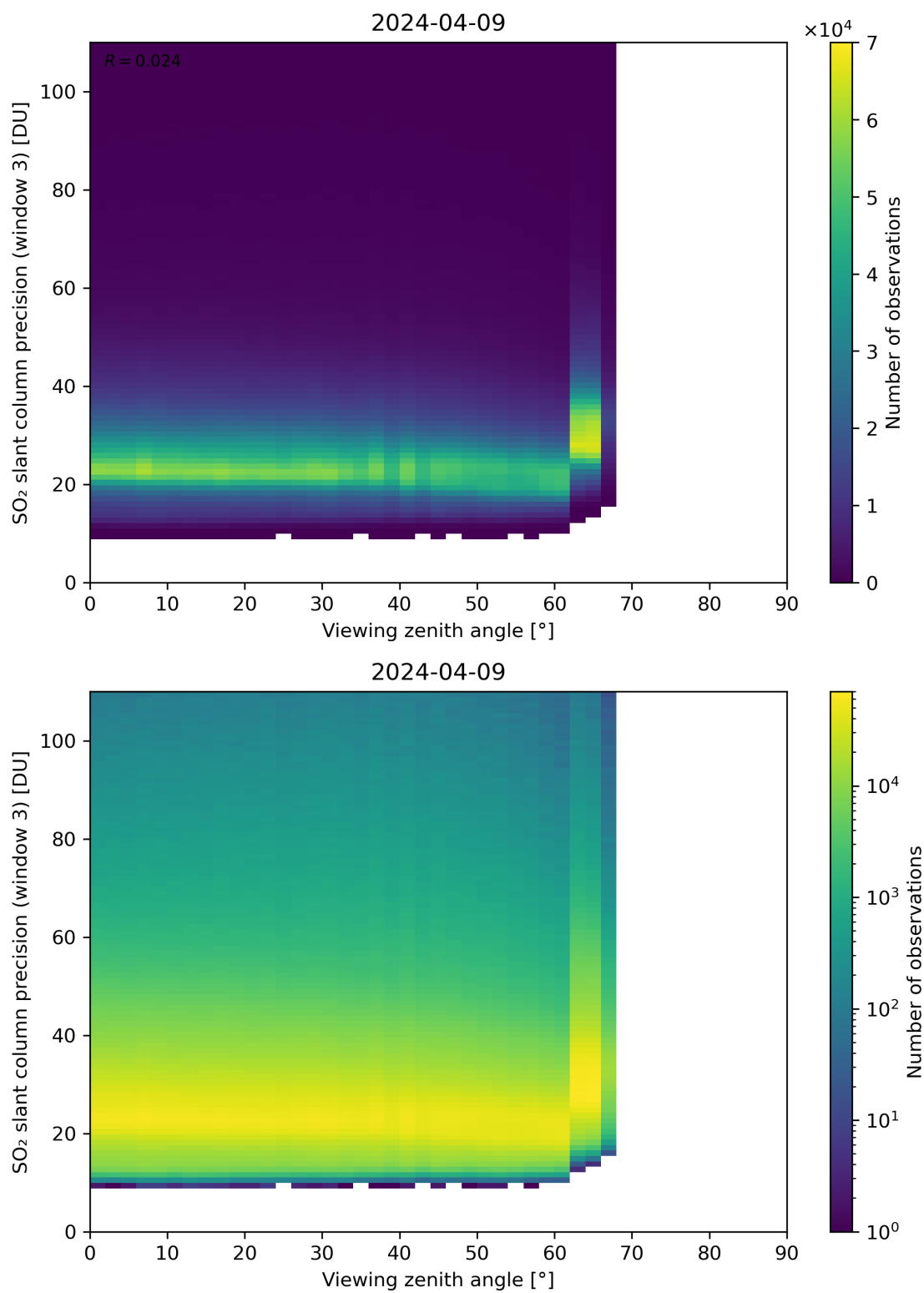
Figure 324: Scatter density plot of “Viewing zenith angle” against “SO 2 slant column precision (window 3)” for 2024-04-08 to 2024-04-10.
