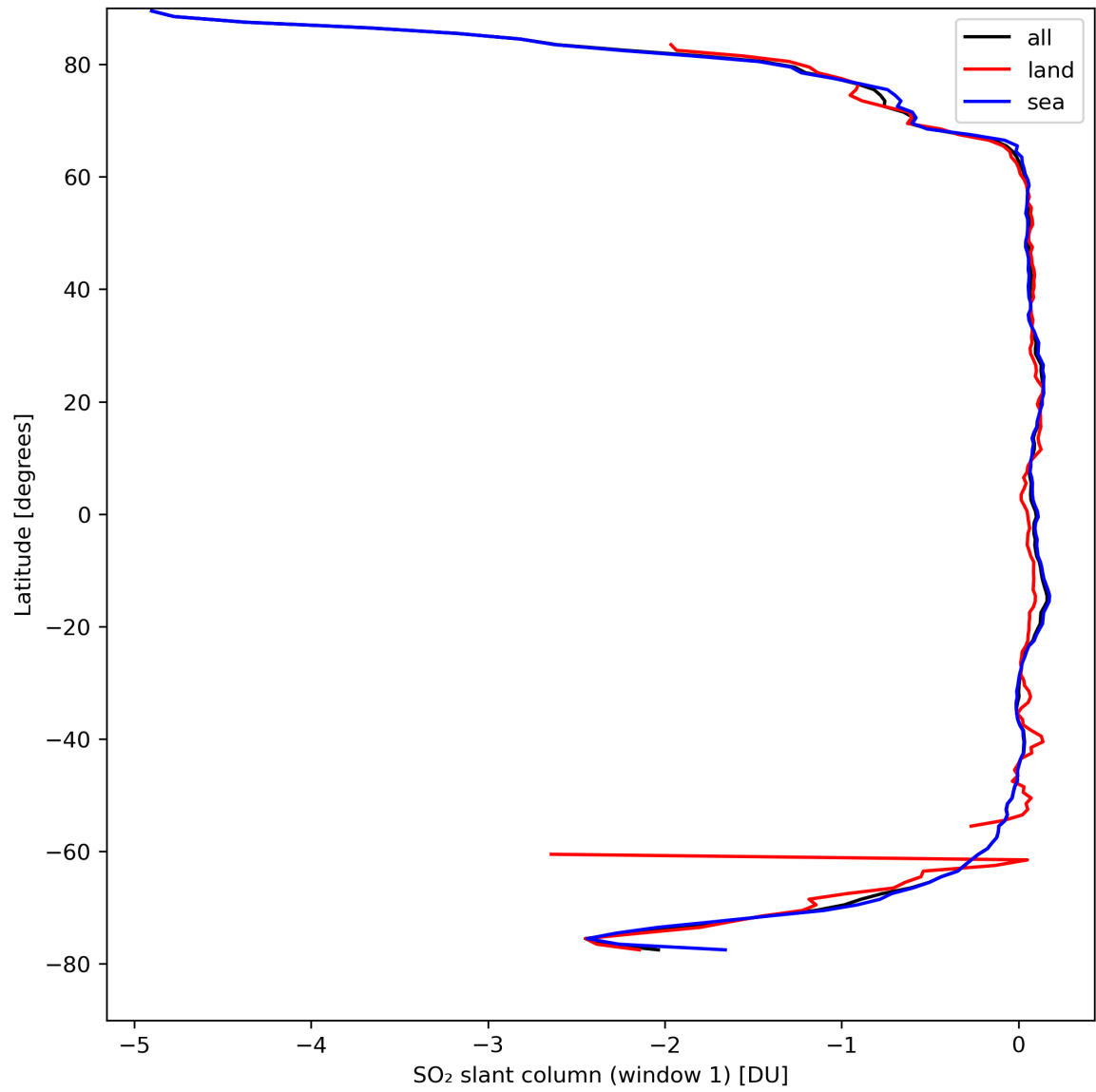
Figure 33: Zonal average of “SO 2 slant column (window 1)” for 2024-04-08 to 2024-04-10.
