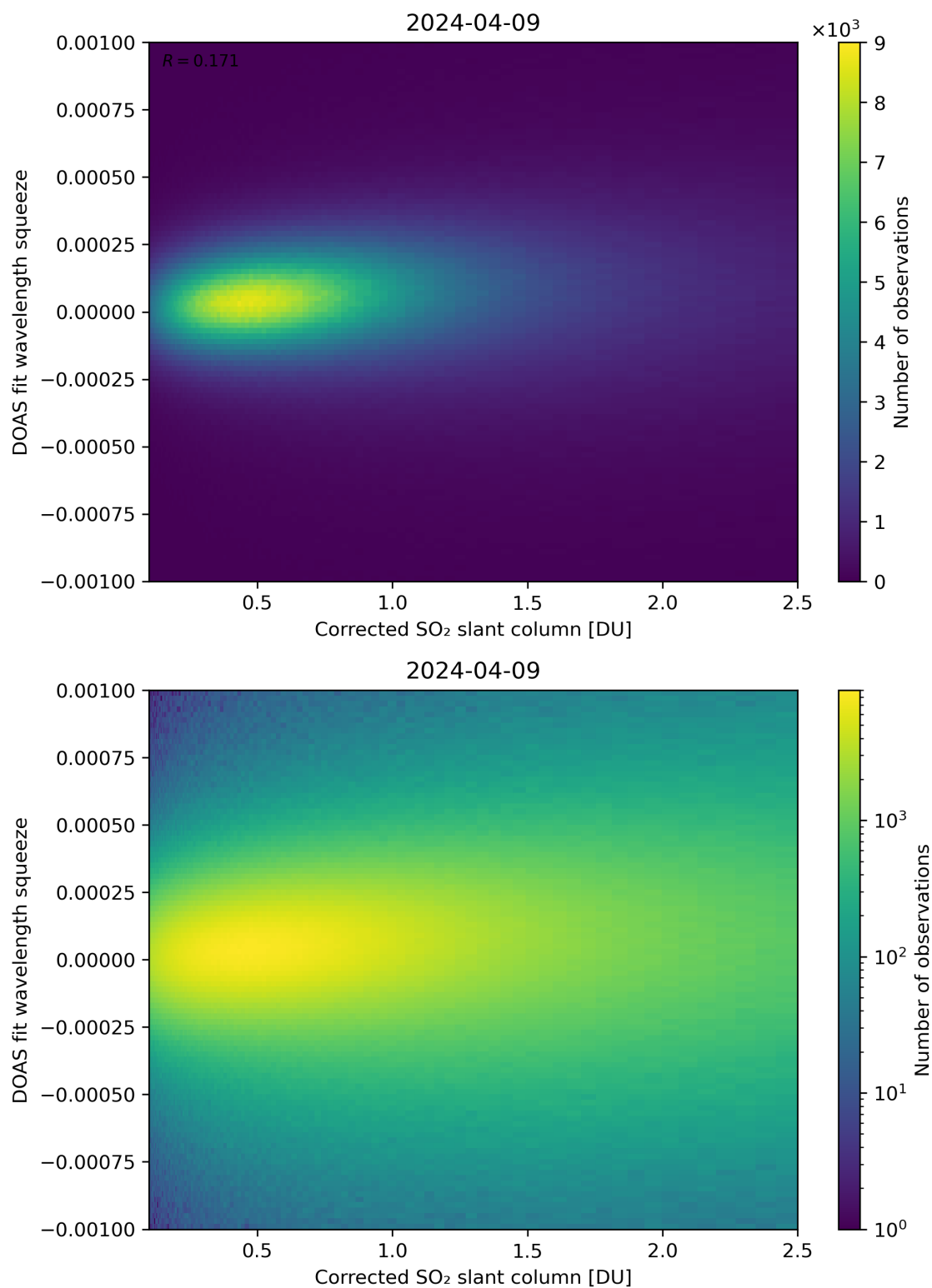
Figure 182: Scatter density plot of “Corrected SO 2 slant column” against “DOAS fit wavelength squeeze” for 2024-04-08 to 2024-04-10.
