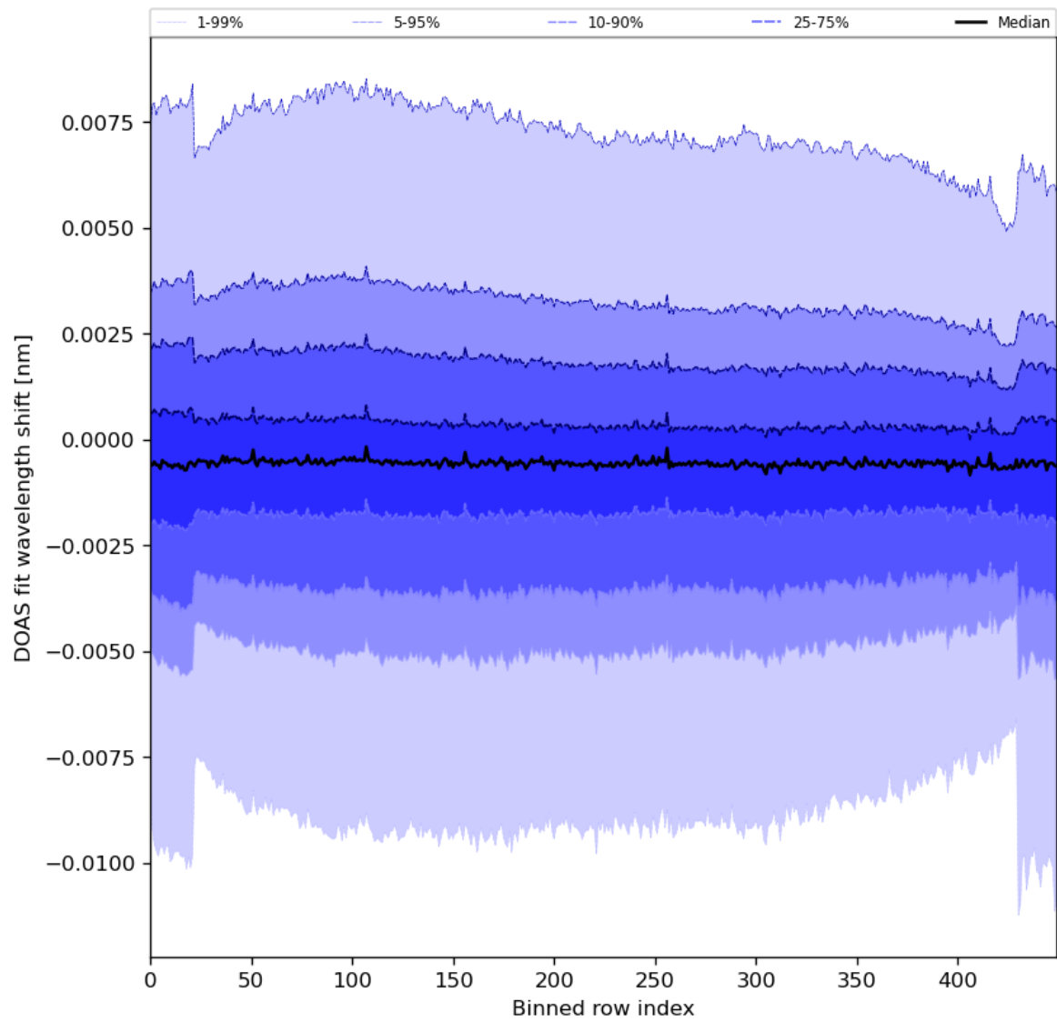
Figure 91: Along track statistics of “DOAS fit wavelength shift” for 2024-04-08 to 2024-04-10
