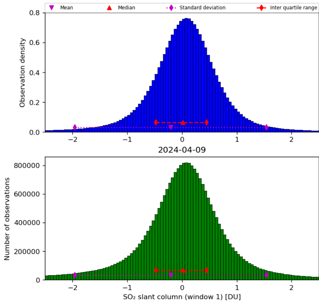
Figure 56: Histogram of “SO 2 slant column (window 1)” for 2024-04-08 to 2024-04-10
