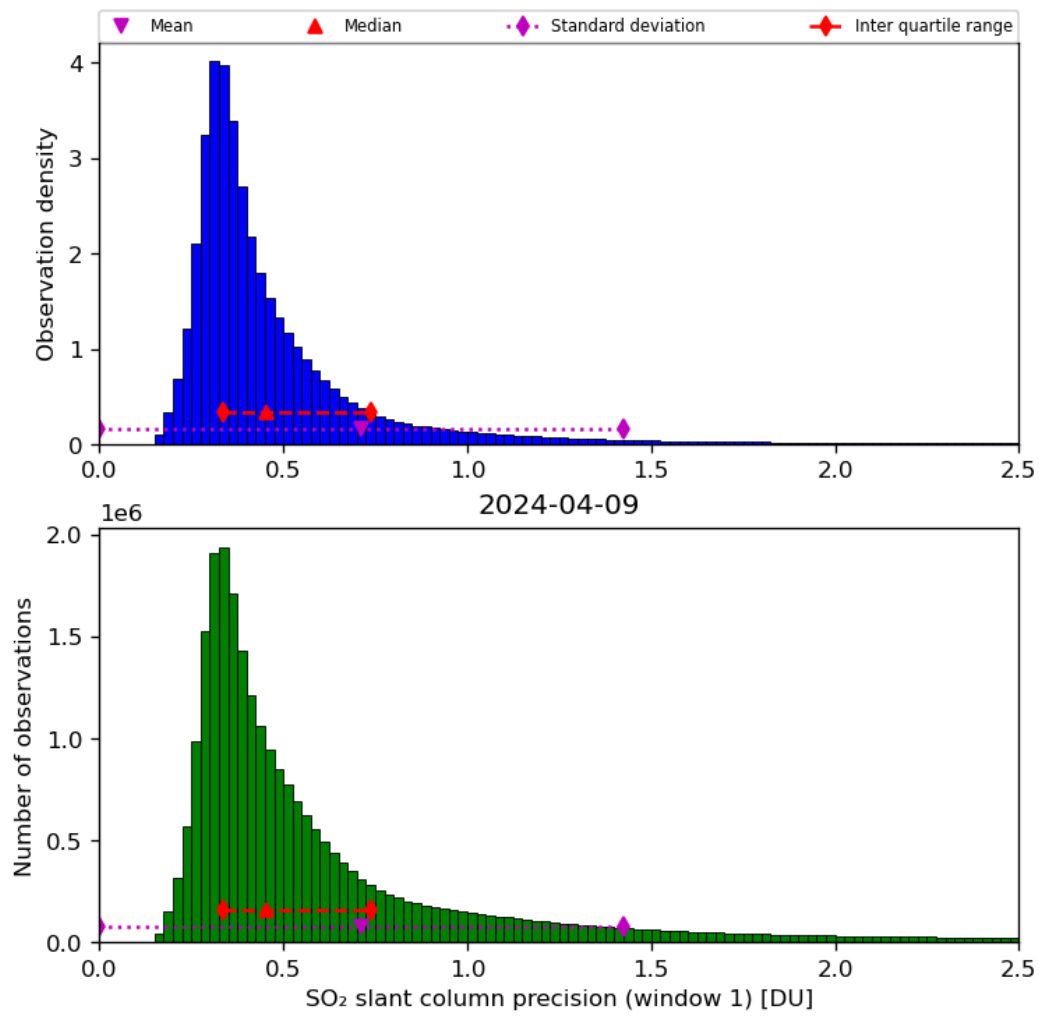
Figure 57: Histogram of “SO 2 slant column precision (window 1)” for 2024-04-08 to 2024-04-10
