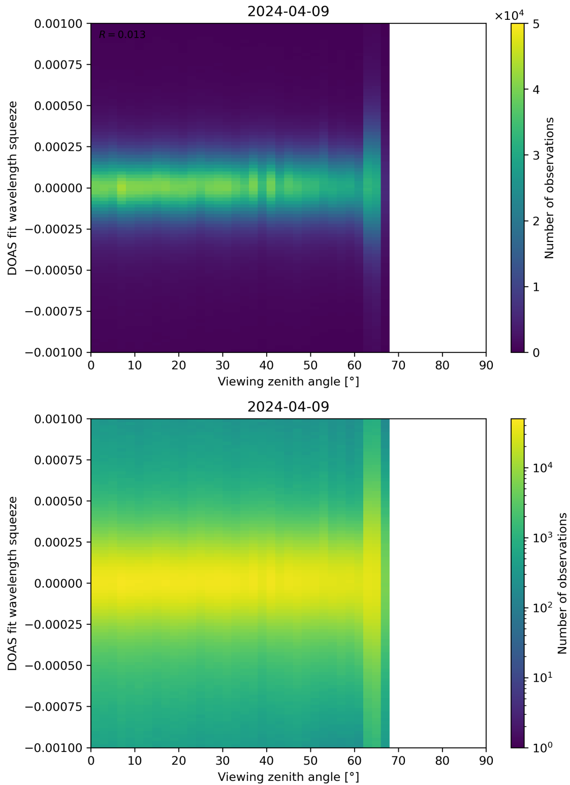
Figure 312: Scatter density plot of “Viewing zenith angle” against “DOAS fit wavelength squeeze” for 2024-04-08 to 2024-04-10.
