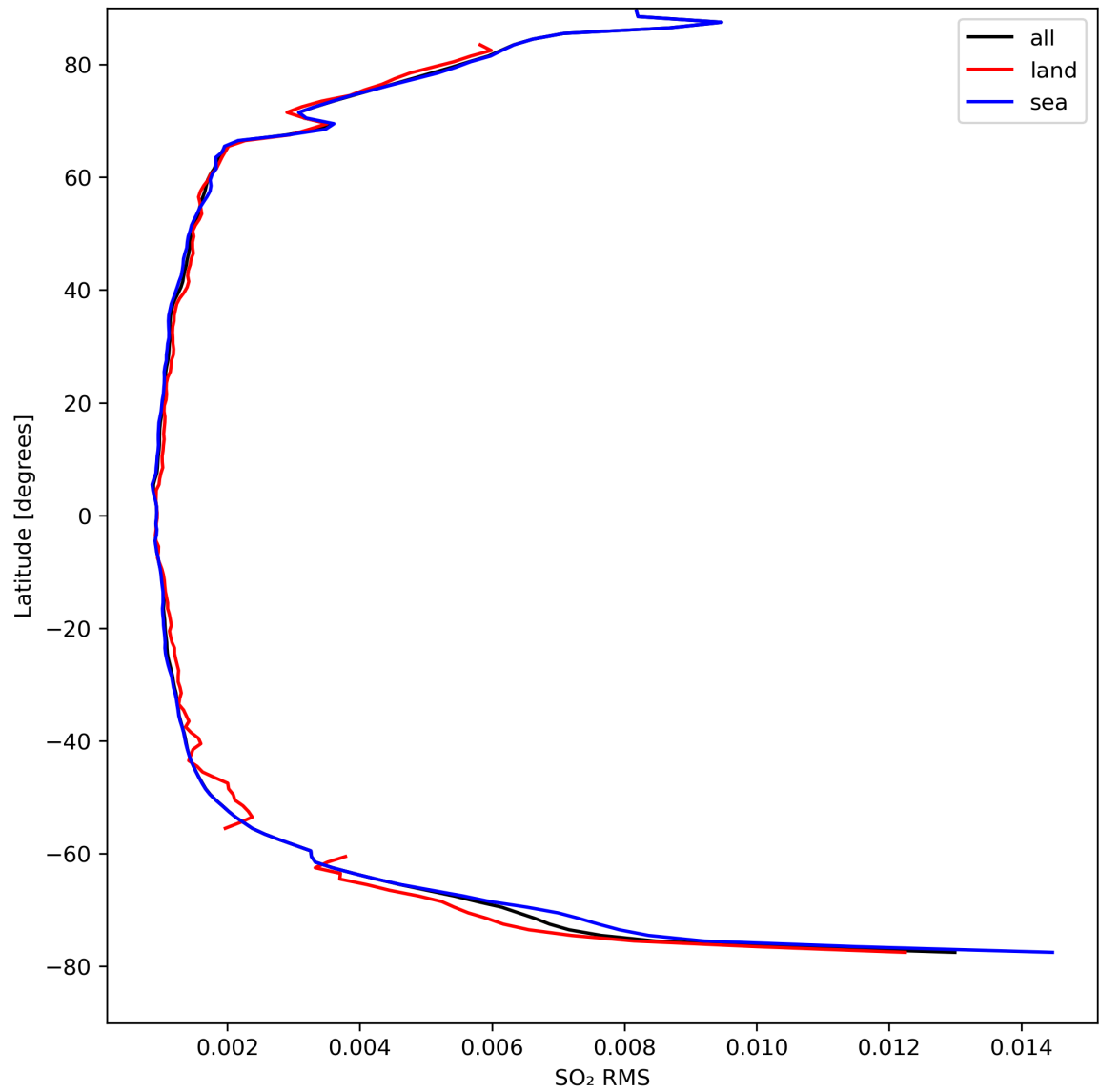
Figure 47: Zonal average of “SO 2 RMS” for 2024-04-08 to 2024-04-10.
