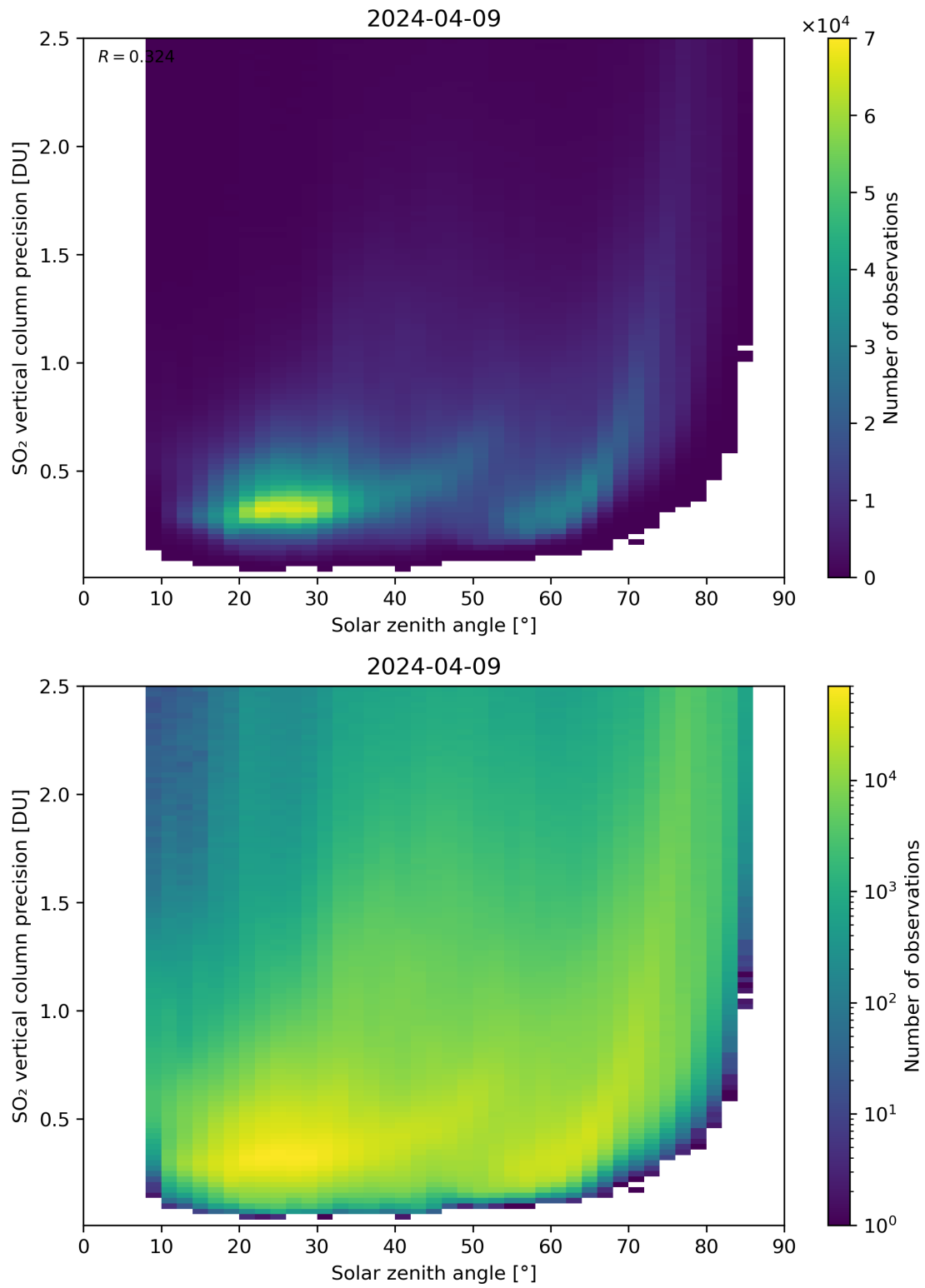
Figure 177: Scatter density plot of “Solar zenith angle” against “SO 2 vertical column precision” for 2024-04-08 to 2024-04-10.
