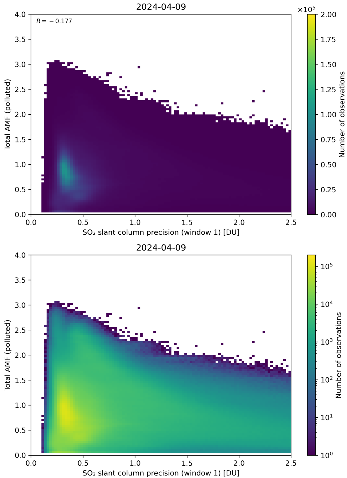
Figure 230: Scatter density plot of “SO 2 slant column precision (window 1)” against “Total AMF (polluted)” for 2024-04-08 to 2024-04-10.
