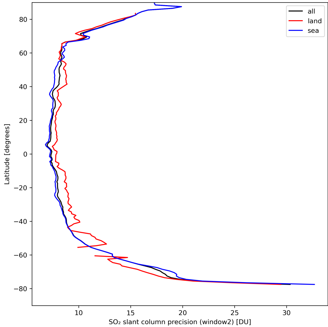
Figure 38: Zonal average of “SO 2 slant column precision (window2)” for 2024-04-08 to 2024-04-10.
