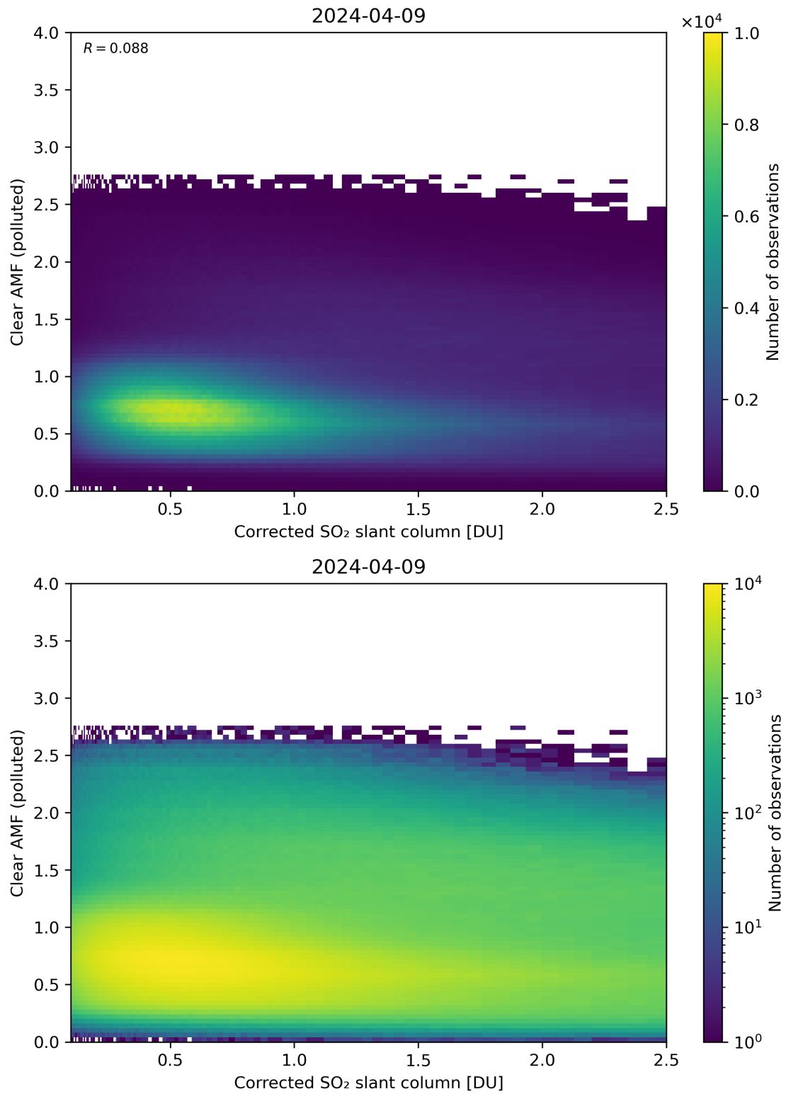
Figure 184: Scatter density plot of “Corrected SO 2 slant column” against “Clear AMF (polluted)” for 2024-04-08 to 2024-04-10.
