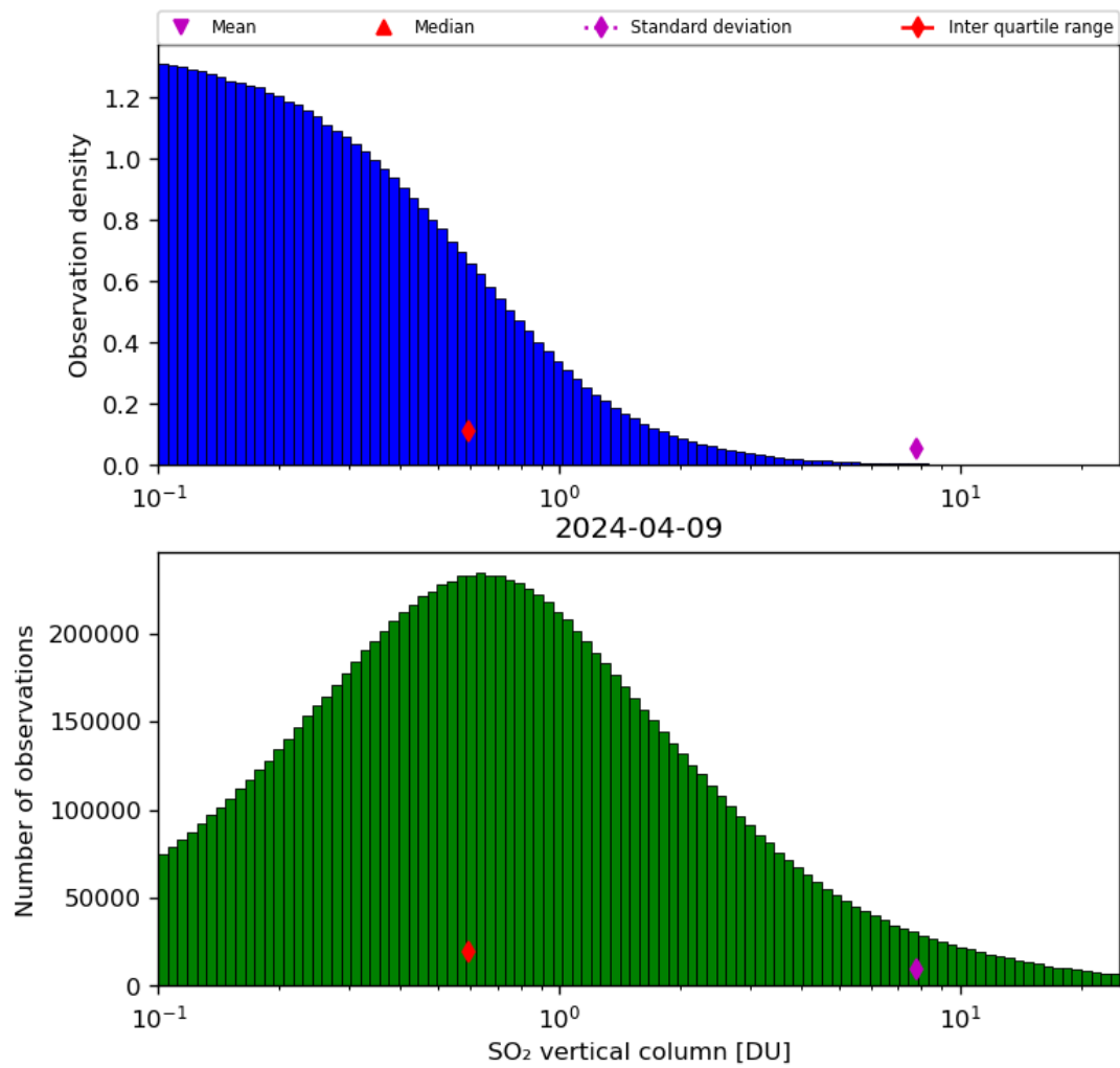
Figure 53: Histogram of “SO 2 vertical column” for 2024-04-08 to 2024-04-10
