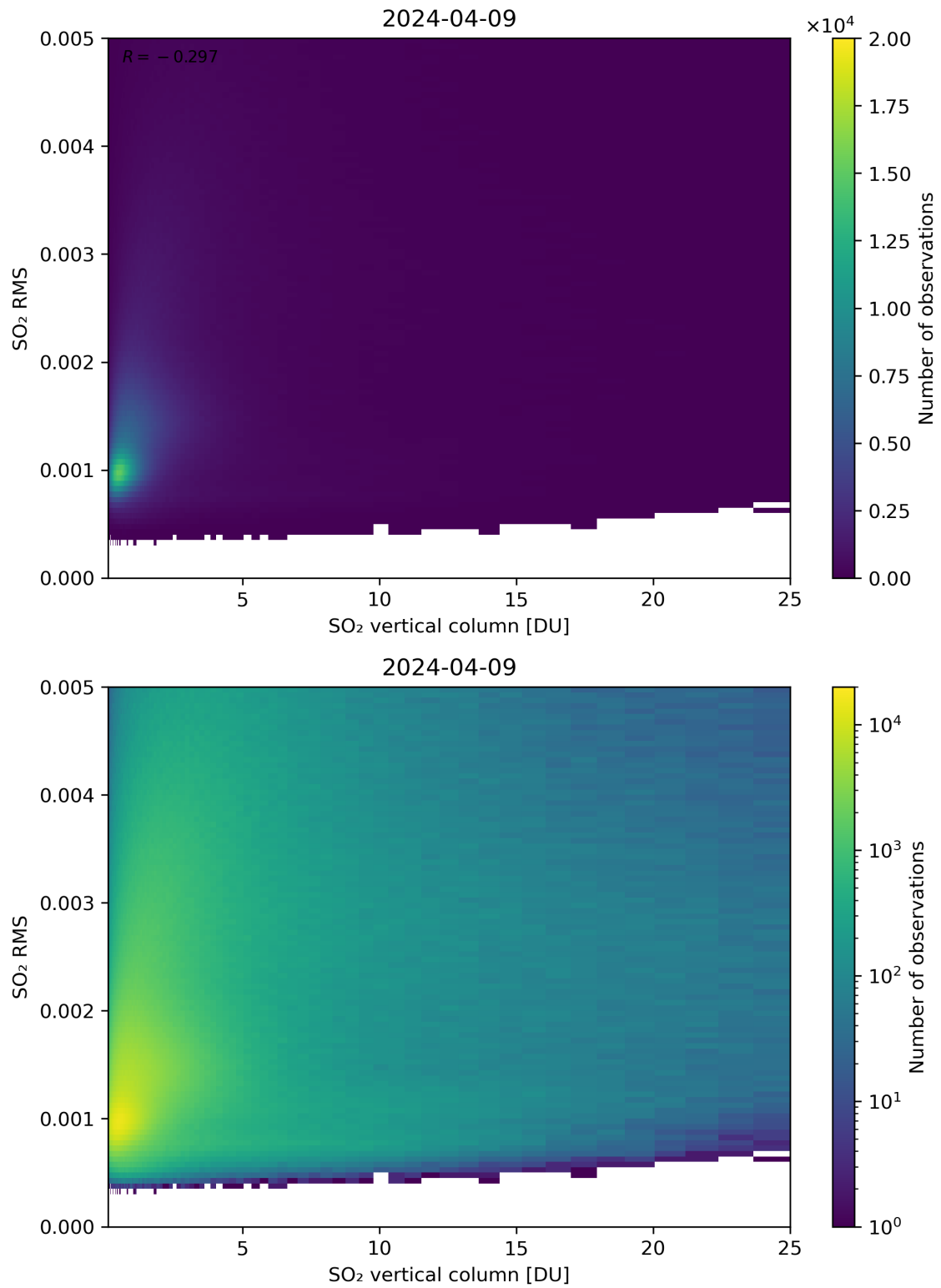
Figure 278: Scatter density plot of “SO 2 vertical column” against “SO 2 RMS” for 2024-04-08 to 2024-04-10.
