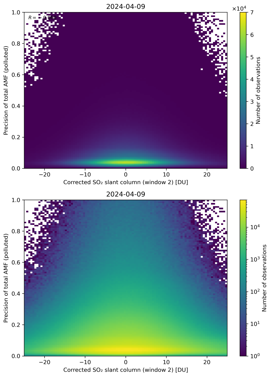
Figure 204: Scatter density plot of “Corrected SO 2 slant column (window 2)” against “Precision of total AMF (polluted)” for 2024-04-08 to 2024-04-10.
