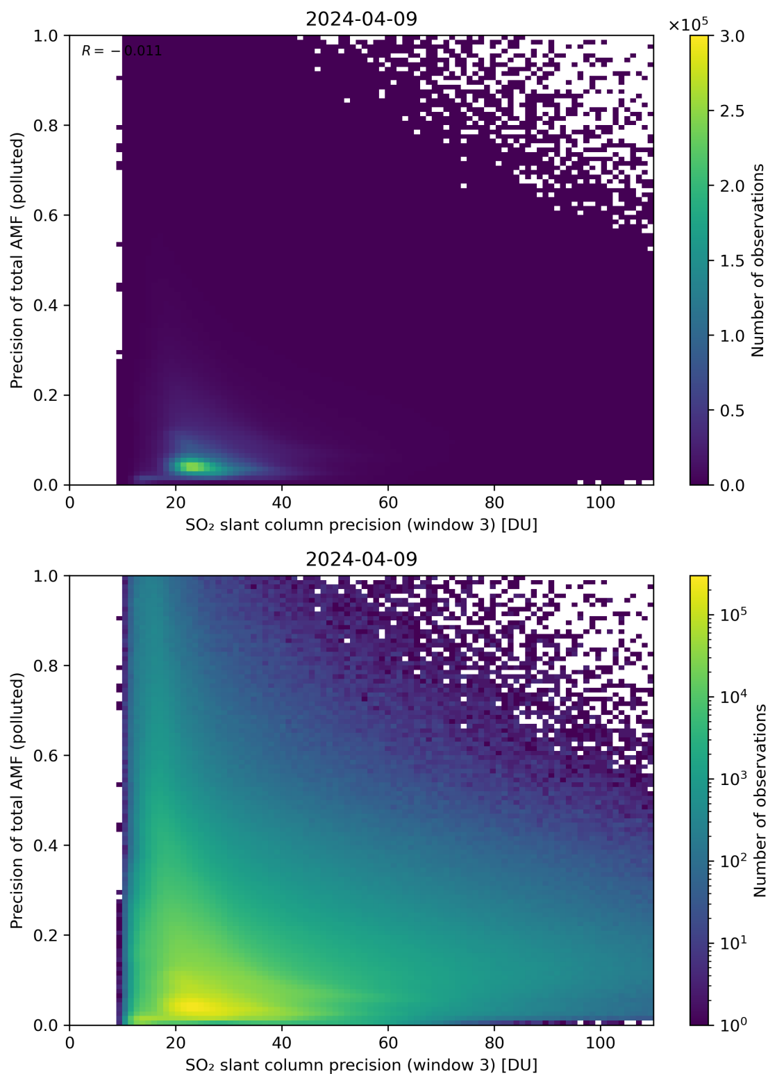
Figure 264: Scatter density plot of “SO 2 slant column precision (window 3)” against “Precision of total AMF (polluted)” for 2024-04-08 to 2024-04-10.
