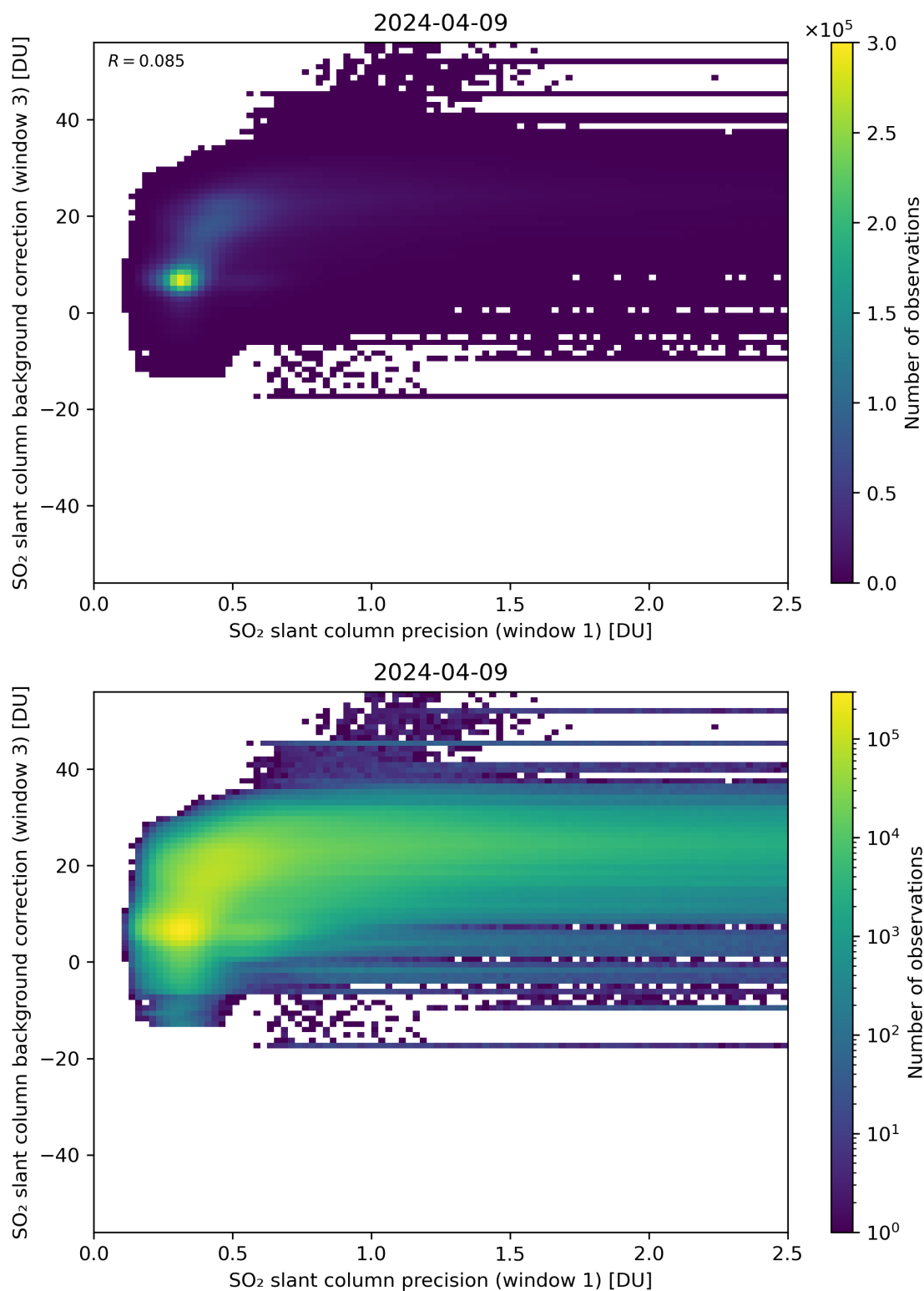
Figure 220: Scatter density plot of “SO 2 slant column precision (window 1)” against “SO 2 slant column background correction (window 3)” for 2024-04-08 to 2024-04-10.
