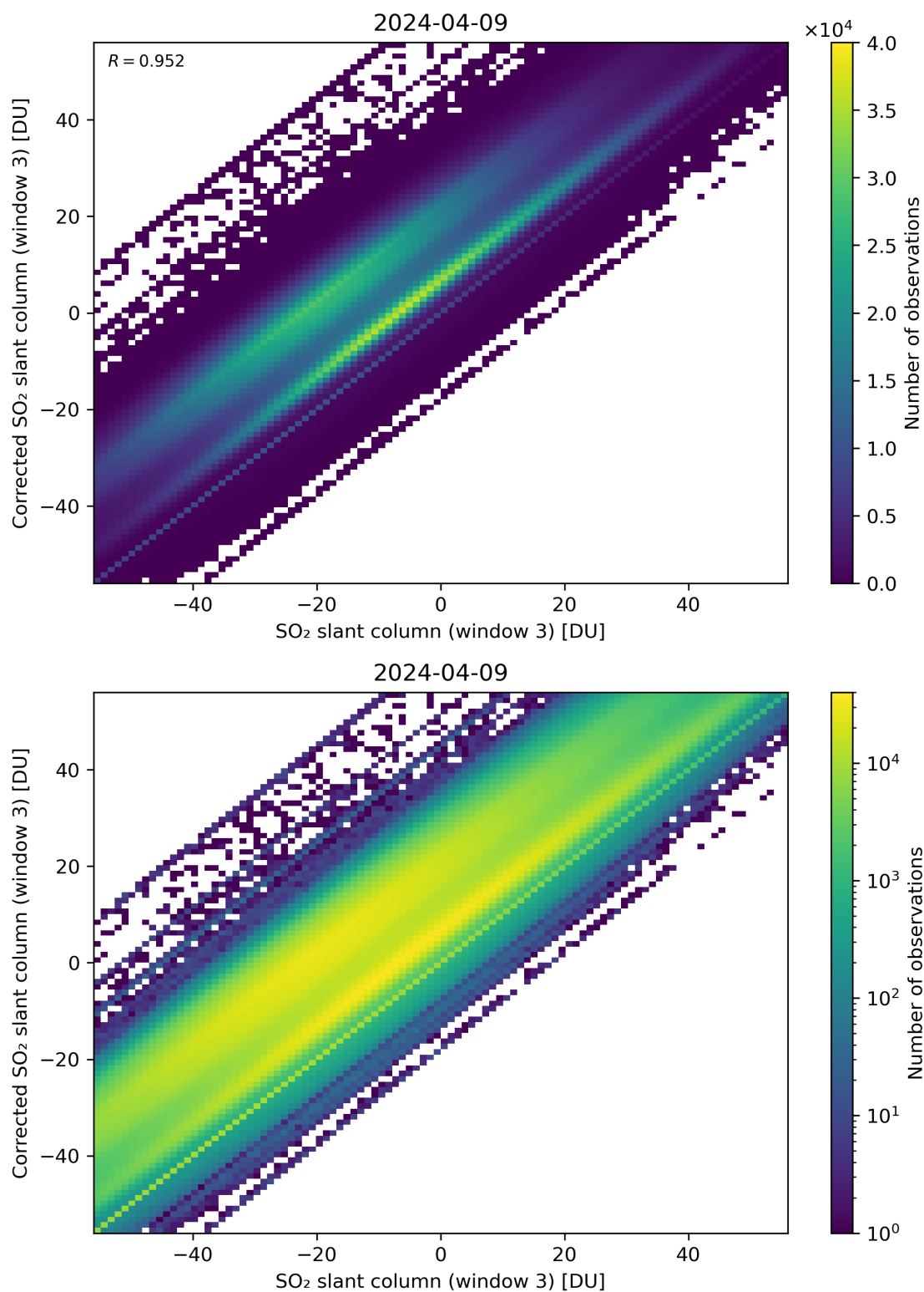
Figure 266: Scatter density plot of “SO 2 slant column (window 3)” against “Corrected SO 2 slant column (window 3)” for 2024-04-08 to 2024-04-10.
