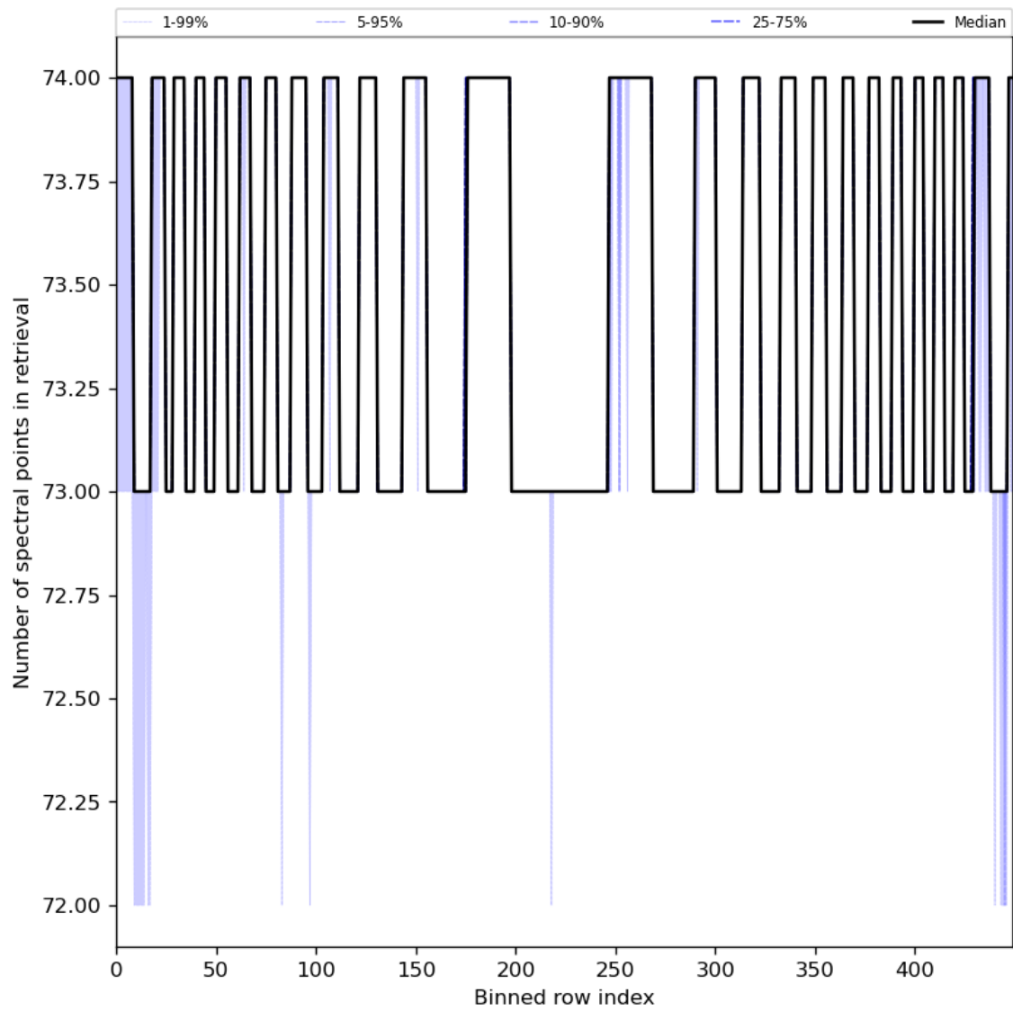
Figure 97: Along track statistics of “Number of spectral points in retrieval” for 2024-04-08 to 2024-04-10
