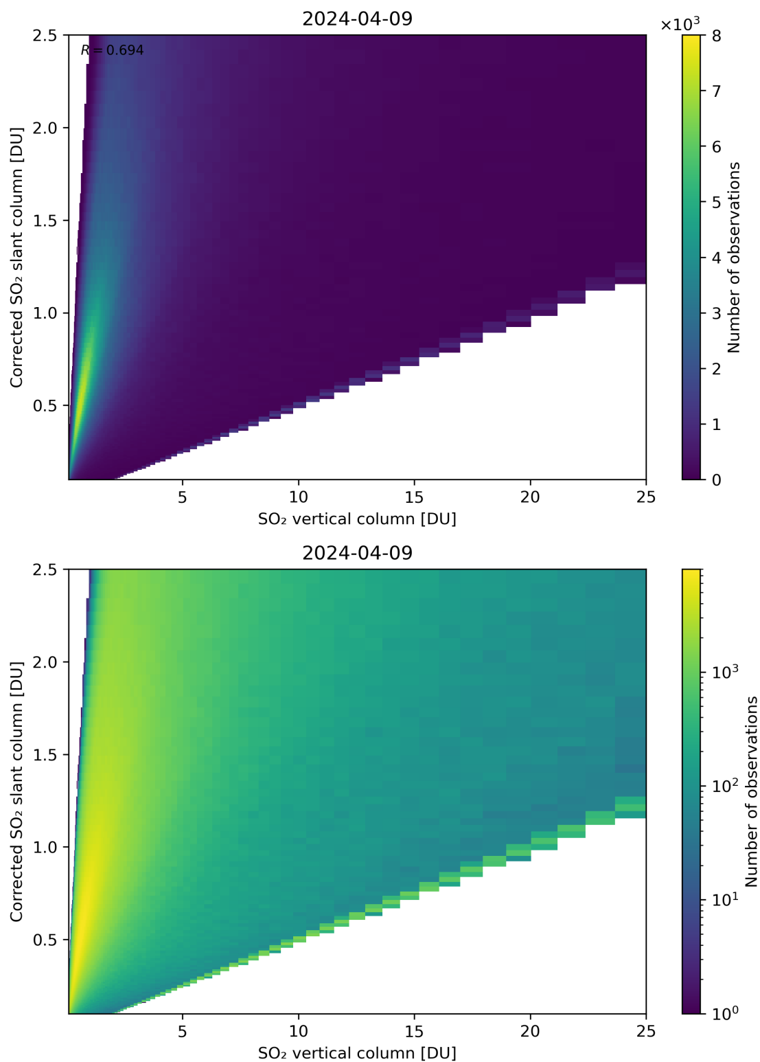
Figure 297: Scatter density plot of “SO 2 vertical column” against “Corrected SO 2 slant column” for 2024-04-08 to 2024-04-10.
