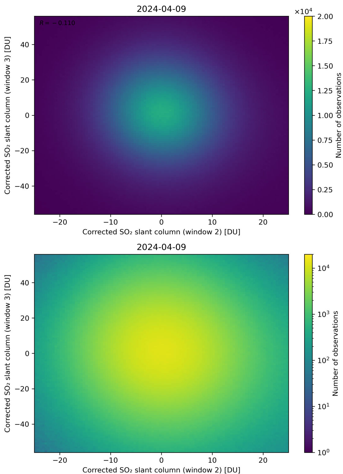
Figure 200: Scatter density plot of “Corrected SO 2 slant column (window 2)” against “Corrected SO 2 slant column (window 3)” for 2024-04-08 to 2024-04-10.
