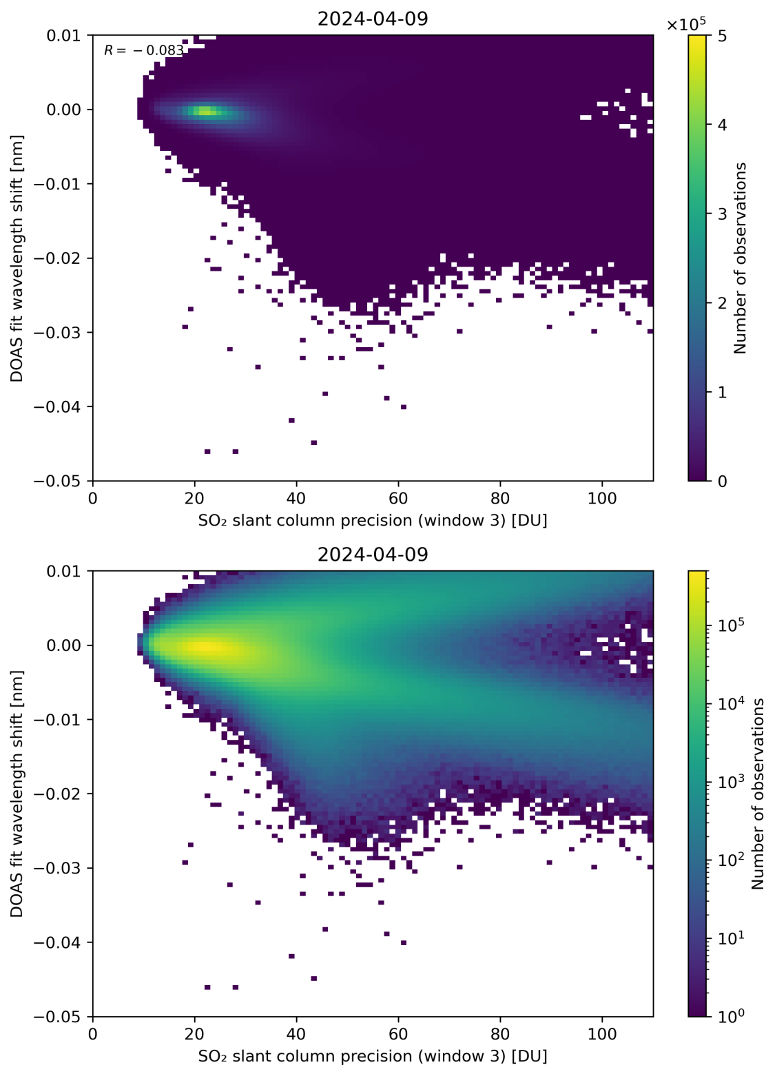
Figure 258: Scatter density plot of “SO 2 slant column precision (window 3)” against “DOAS fit wavelength shift” for 2024-04-08 to 2024-04-10.
