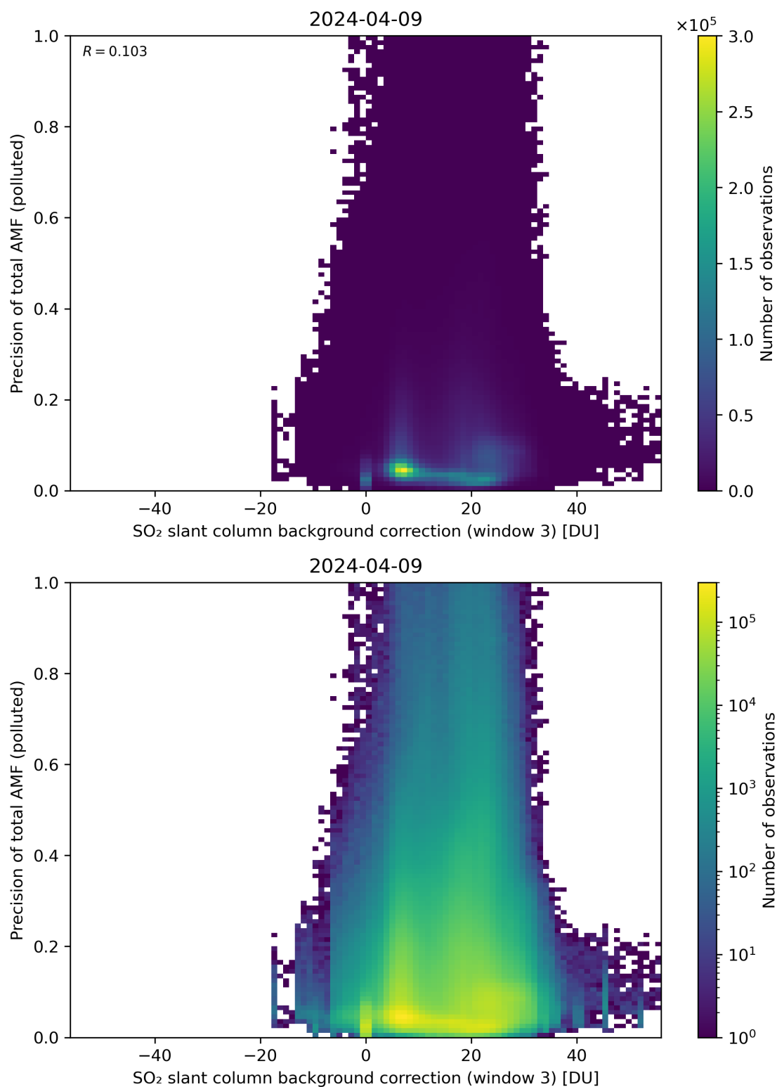
Figure 126: Scatter density plot of “SO 2 slant column background correction (window 3)” against “Precision of total AMF (polluted)” for 2024-04-08 to 2024-04-10.
