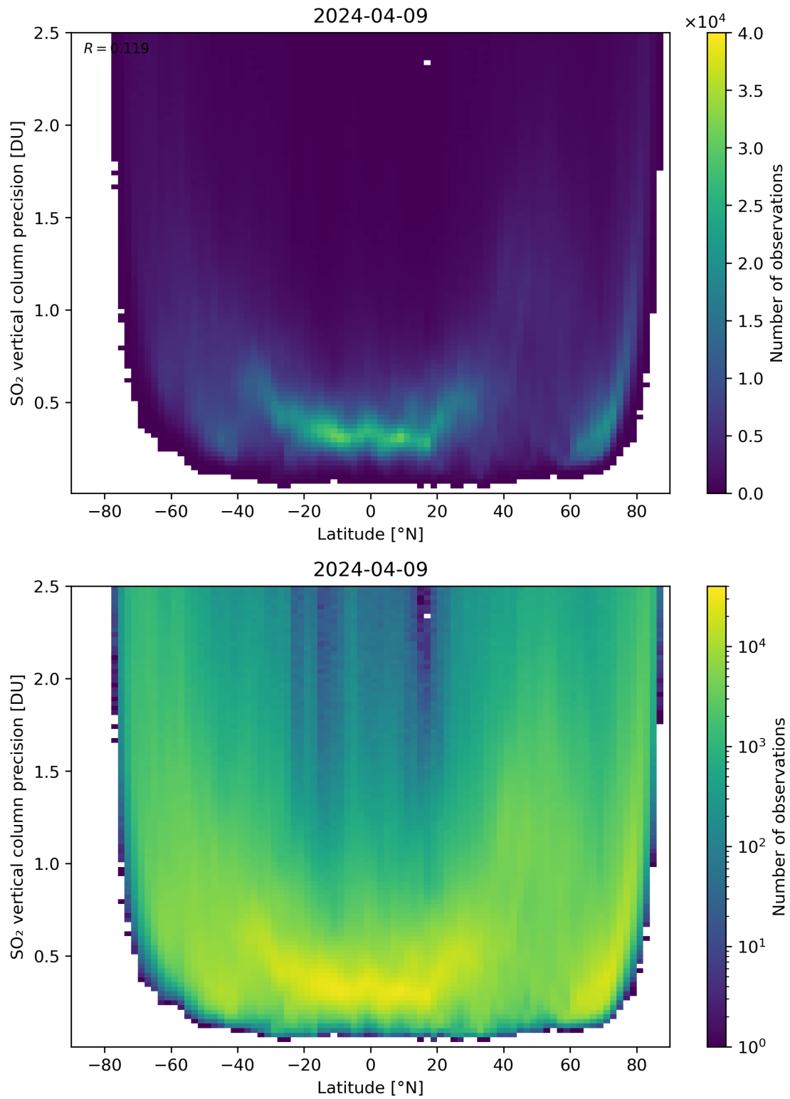
Figure 157: Scatter density plot of “Latitude” against “SO 2 vertical column precision” for 2024-04-08 to 2024-04-10.
