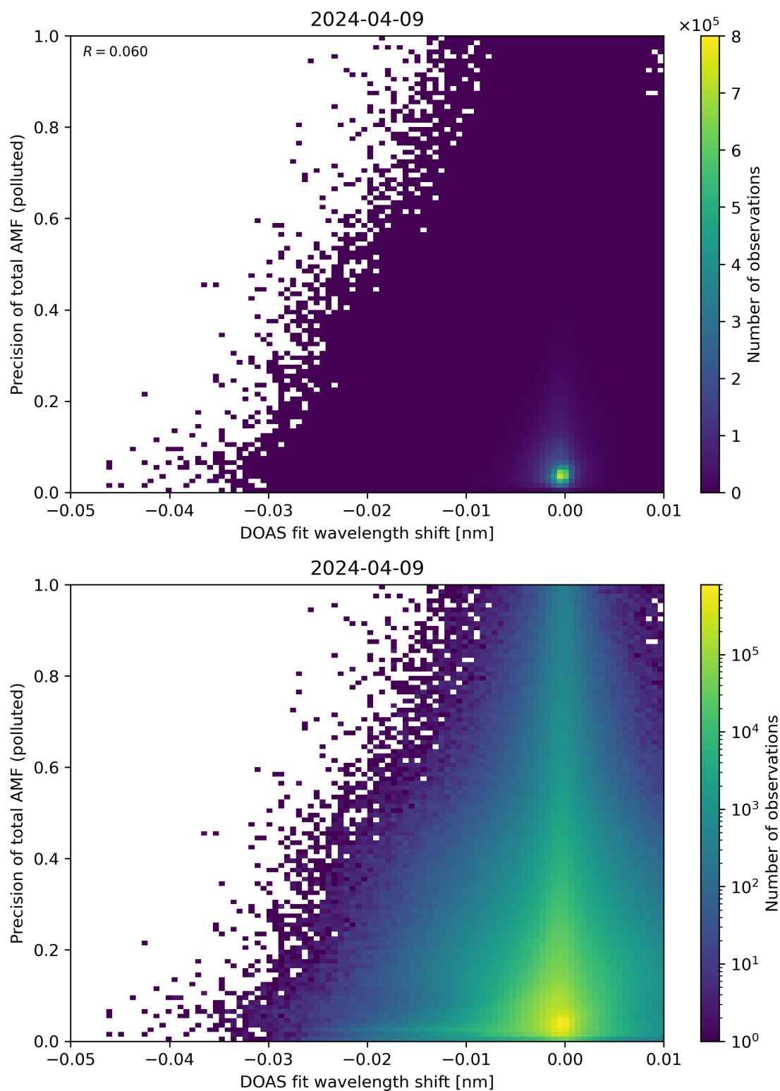
Figure 131: Scatter density plot of “DOAS fit wavelength shift” against “Precision of total AMF (polluted)” for 2024-04-08 to 2024-04-10.
