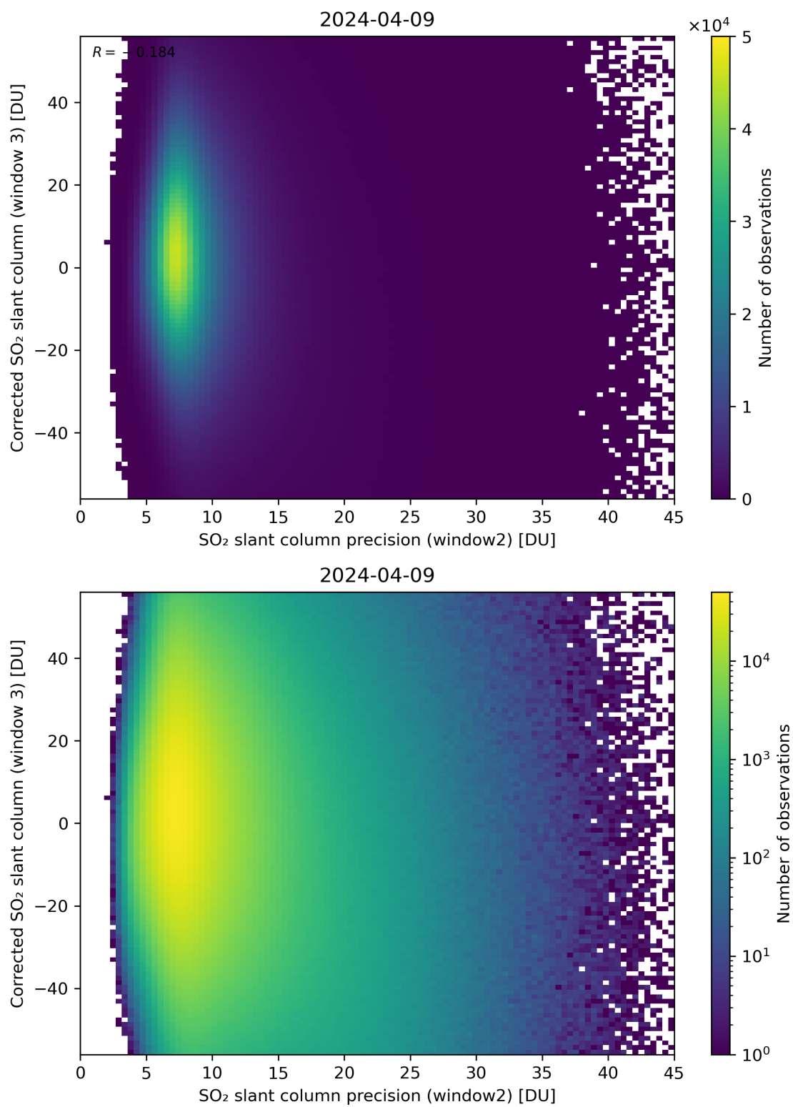
Figure 248: Scatter density plot of “SO 2 slant column precision (window2)” against “Corrected SO 2 slant column (window 3)” for 2024-04-08 to 2024-04-10.
