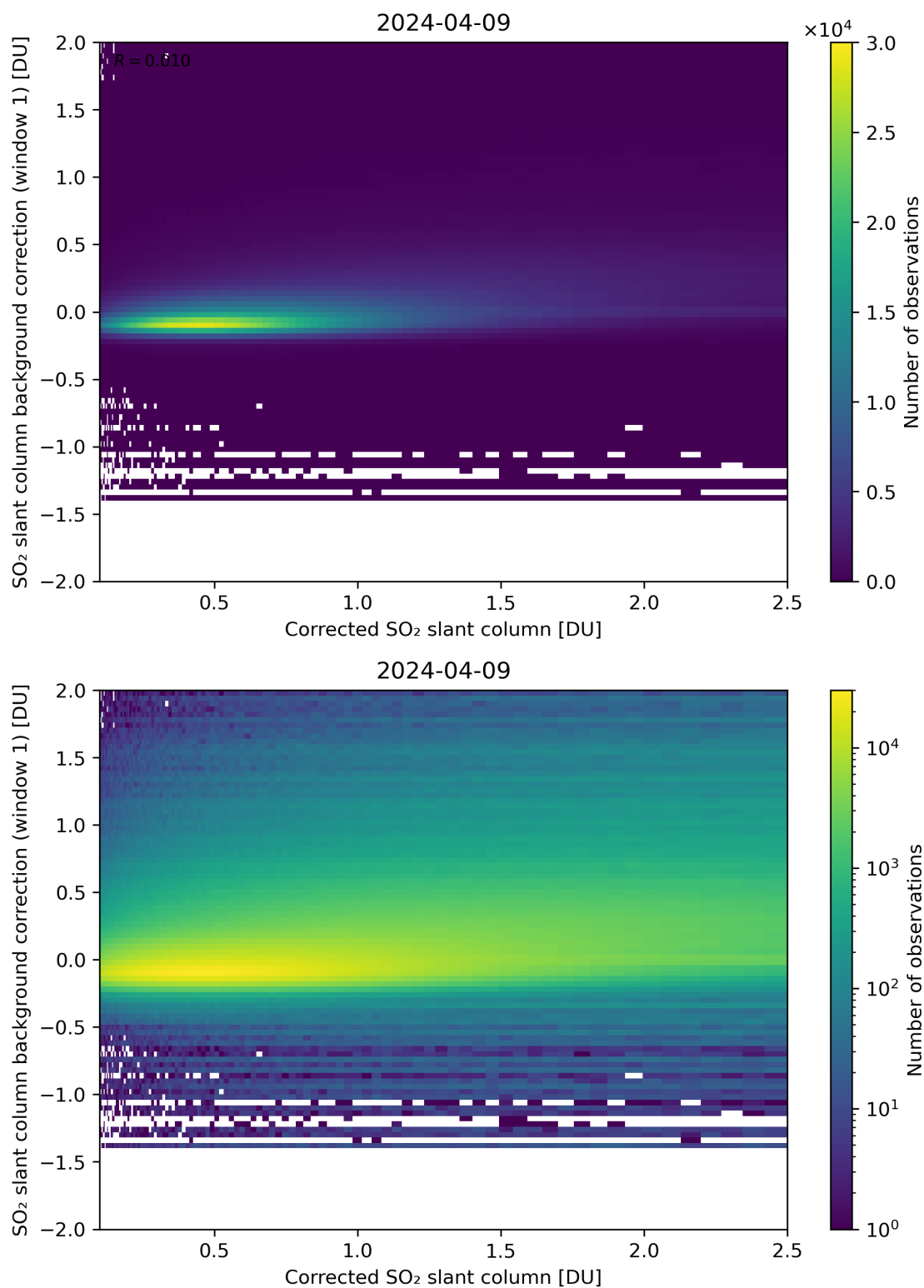
Figure 178: Scatter density plot of “Corrected SO 2 slant column” against “SO 2 slant column background correction (window 1)” for 2024-04-08 to 2024-04-10.
