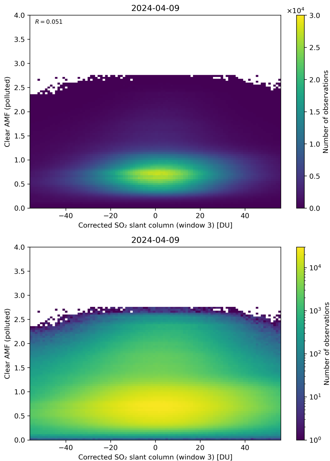
Figure 209: Scatter density plot of “Corrected SO 2 slant column (window 3)” against “Clear AMF (polluted)” for 2024-04-08 to 2024-04-10.
