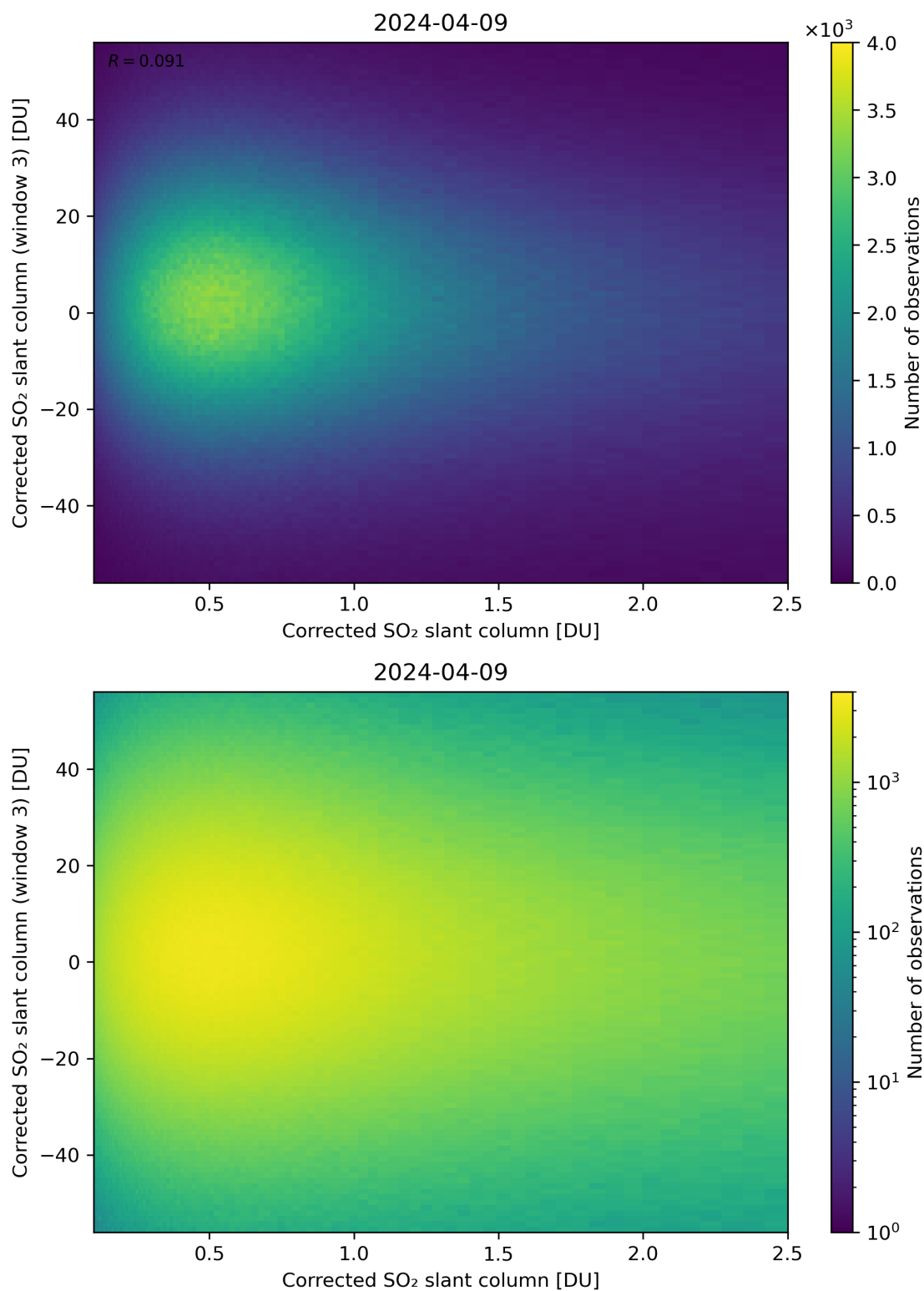
Figure 186: Scatter density plot of “Corrected SO 2 slant column” against “Corrected SO 2 slant column (window 3)” for 2024-04-08 to 2024-04-10.
