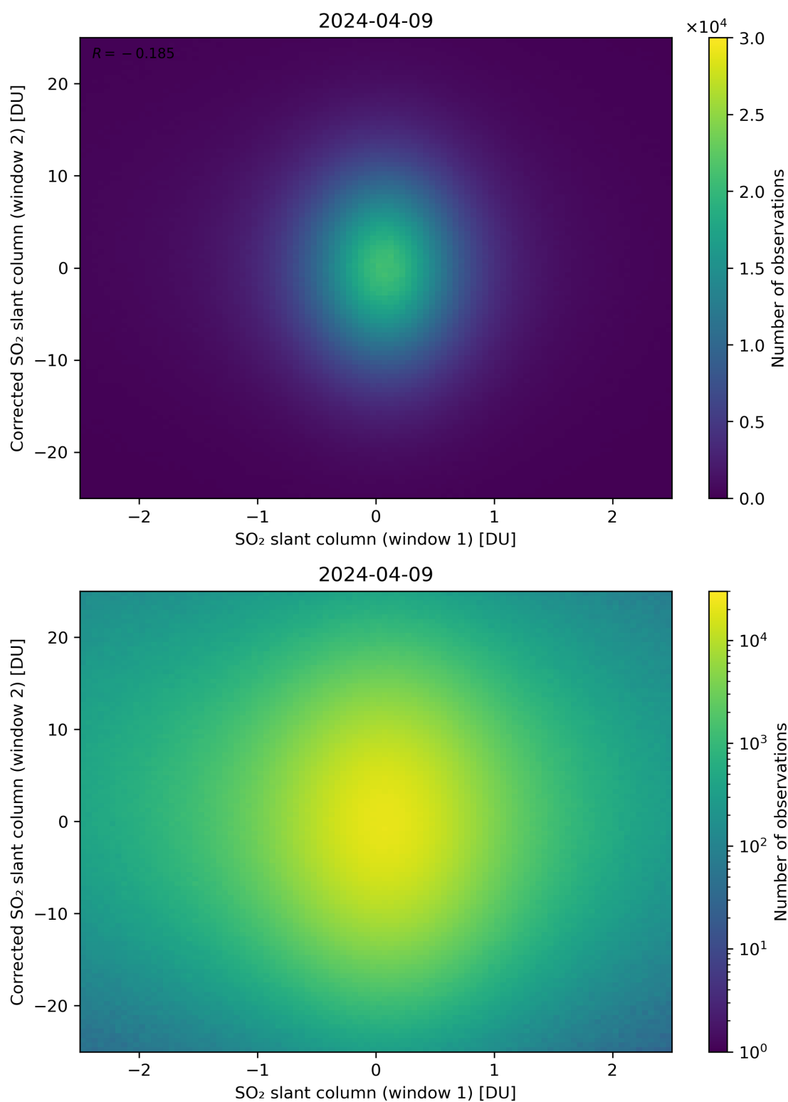
Figure 233: Scatter density plot of “SO 2 slant column (window 1)” against “Corrected SO 2 slant column (window 2)” for 2024-04-08 to 2024-04-10.
