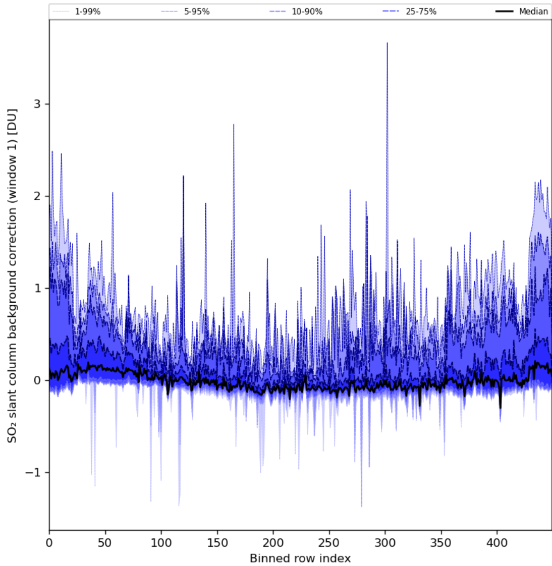
Figure 82: Along track statistics of “SO 2 slant column background correction (window 1)” for 2024-04-08 to 2024-04-10
