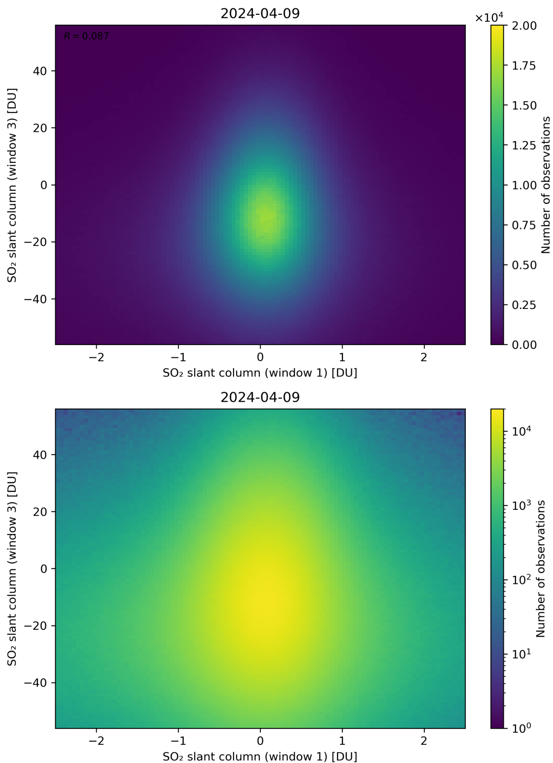
Figure 237: Scatter density plot of “SO 2 slant column (window 1)” against “SO 2 slant column (window 3)” for 2024-04-08 to 2024-04-10.
