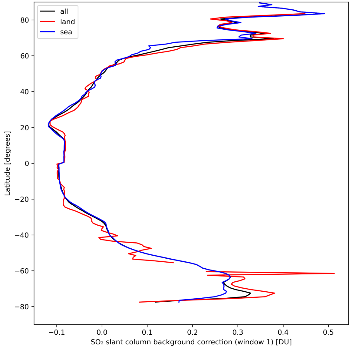
Figure 36: Zonal average of “SO 2 slant column background correction (window 1)” for 2024-04-08 to 2024-04-10.
