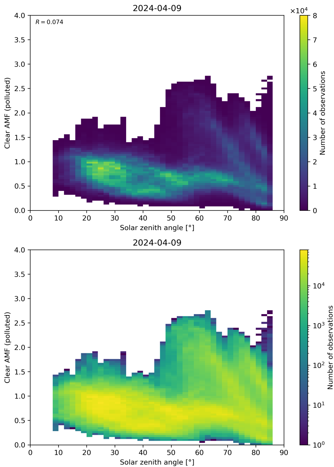
Figure 165: Scatter density plot of “Solar zenith angle” against “Clear AMF (polluted)” for 2024-04-08 to 2024-04-10.
