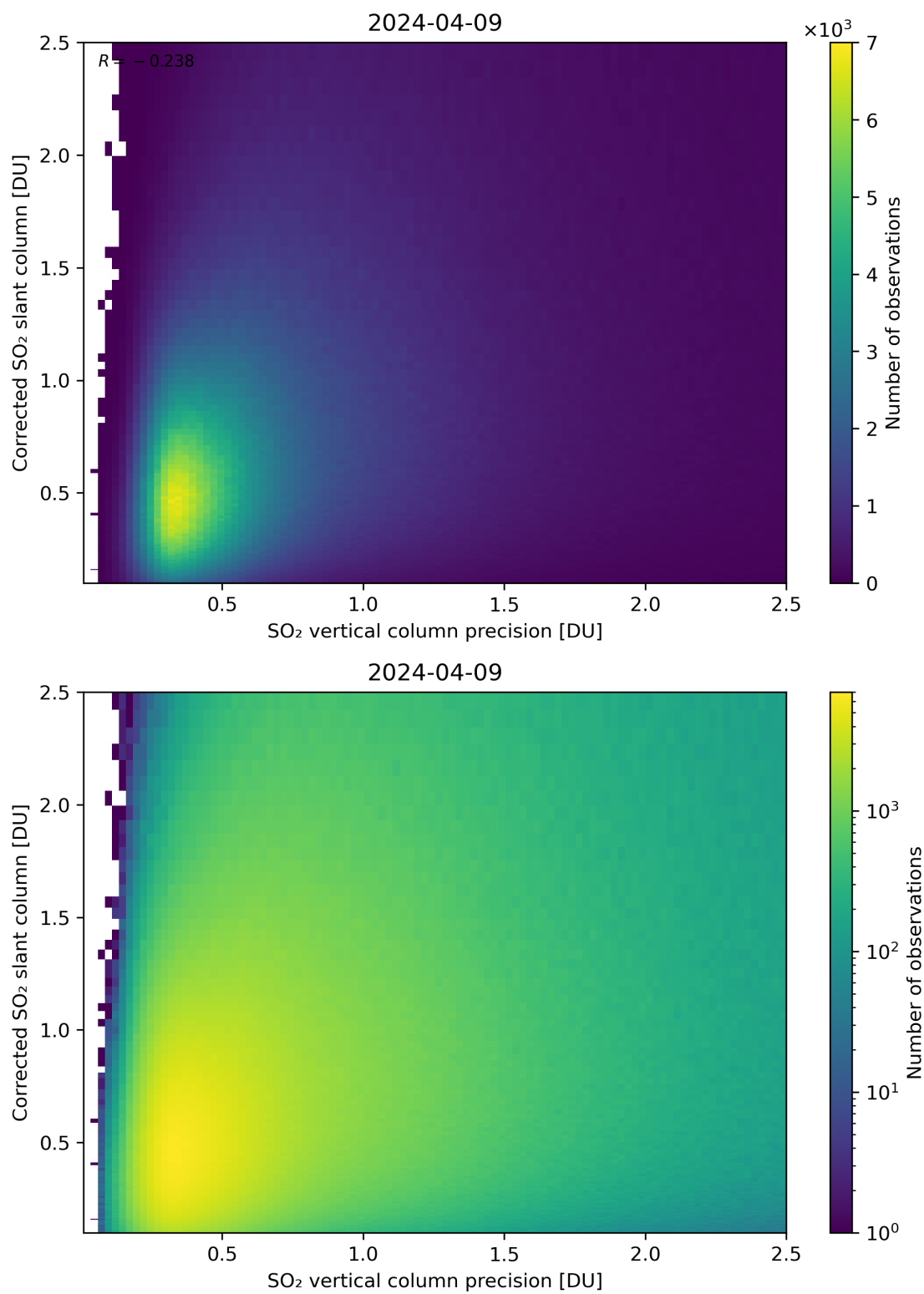
Figure 286: Scatter density plot of “SO 2 vertical column precision” against “Corrected SO 2 slant column” for 2024-04-08 to 2024-04-10.
