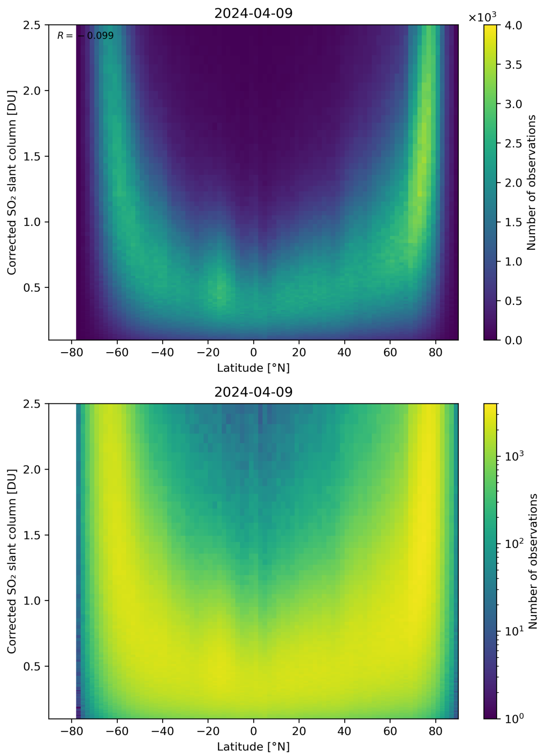
Figure 146: Scatter density plot of “Latitude” against “Corrected SO 2 slant column” for 2024-04-08 to 2024-04-10.
