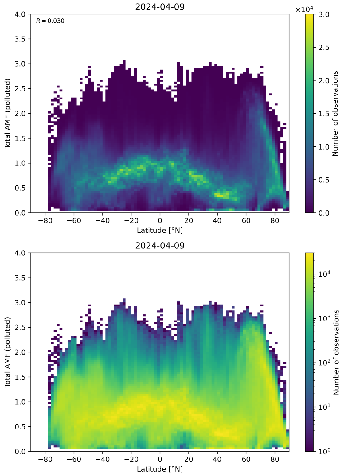
Figure 154: Scatter density plot of “Latitude” against “Total AMF (polluted)” for 2024-04-08 to 2024-04-10.
