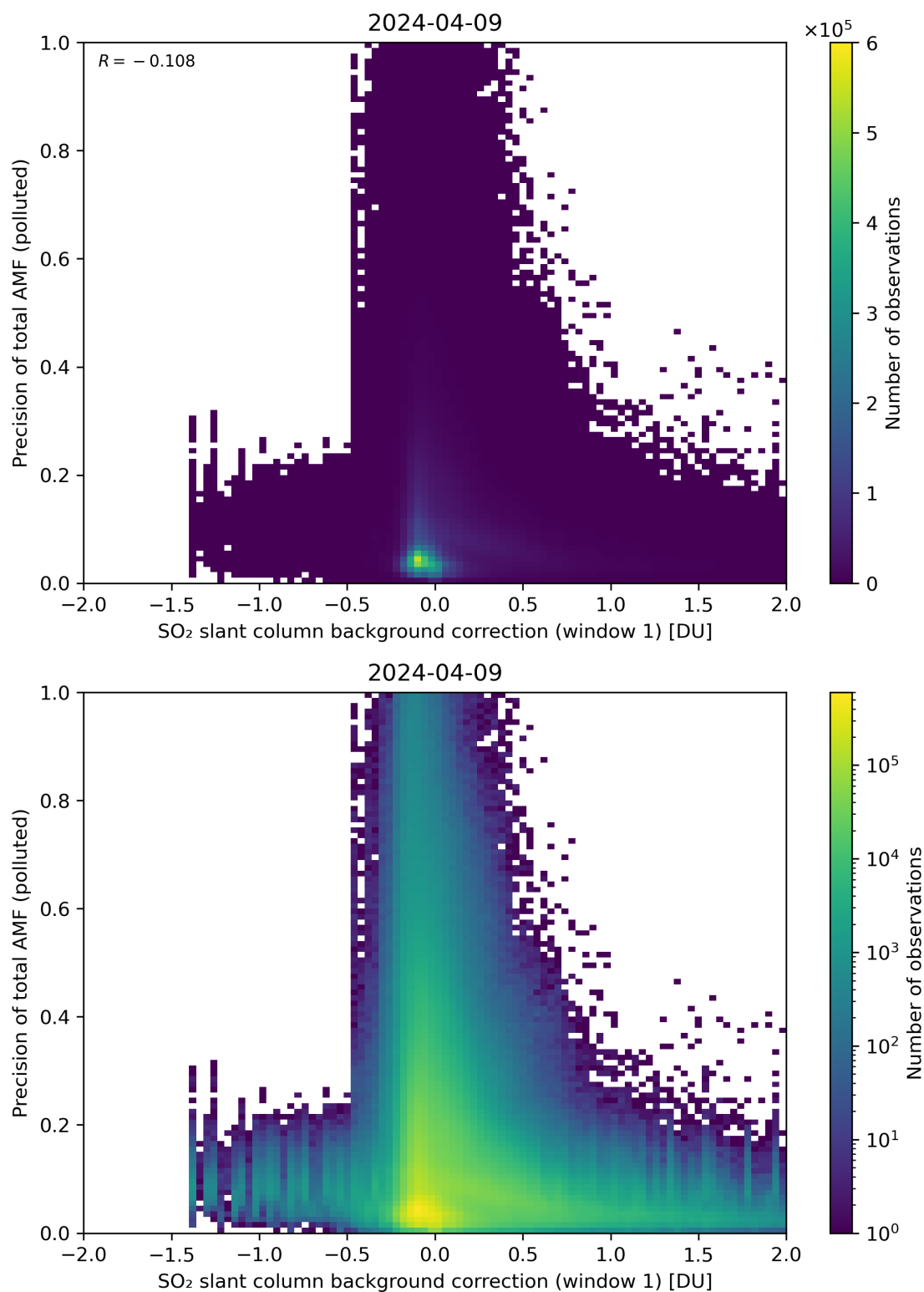
Figure 110: Scatter density plot of “SO 2 slant column background correction (window 1)” against “Precision of total AMF (polluted)” for 2024-04-08 to 2024-04-10.
