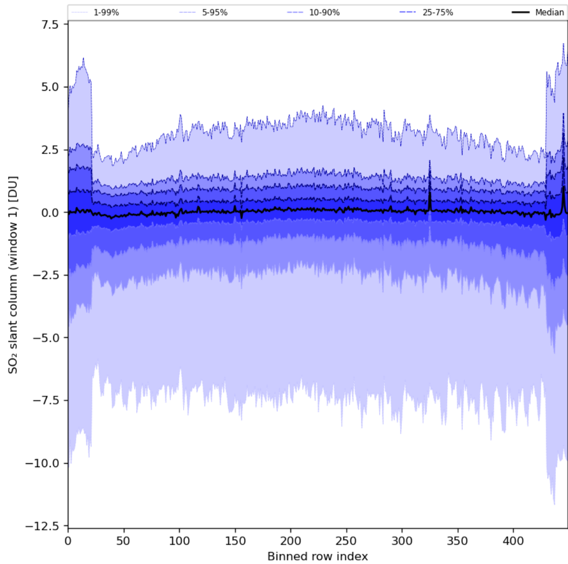
Figure 79: Along track statistics of “SO 2 slant column (window 1)” for 2024-04-08 to 2024-04-10
