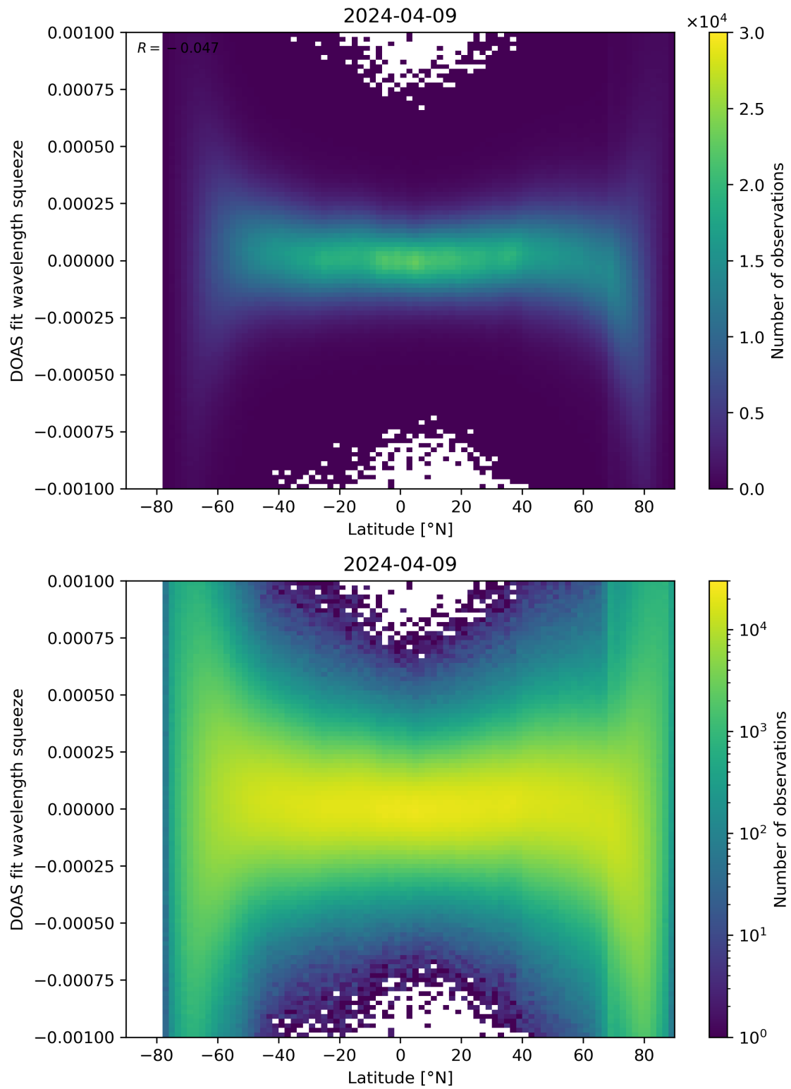
Figure 143: Scatter density plot of “Latitude” against “DOAS fit wavelength squeeze” for 2024-04-08 to 2024-04-10.
