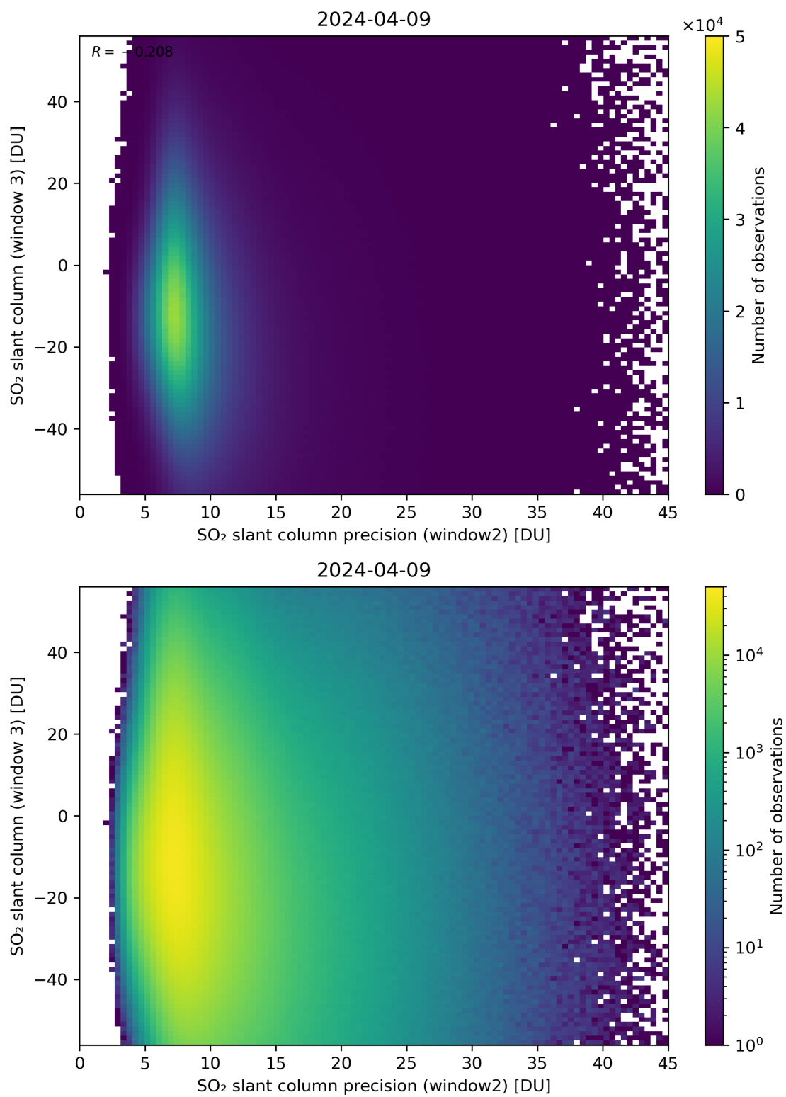
Figure 249: Scatter density plot of “SO 2 slant column precision (window2)” against “SO 2 slant column (window 3)” for 2024-04-08 to 2024-04-10.
