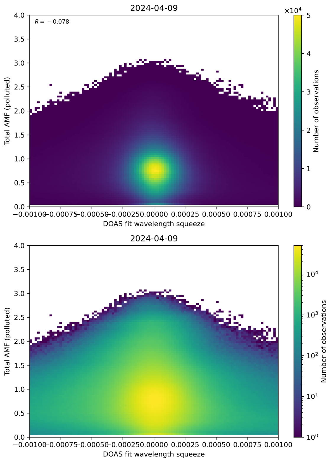
Figure 134: Scatter density plot of “DOAS fit wavelength squeeze” against “Total AMF (polluted)” for 2024-04-08 to 2024-04-10.
