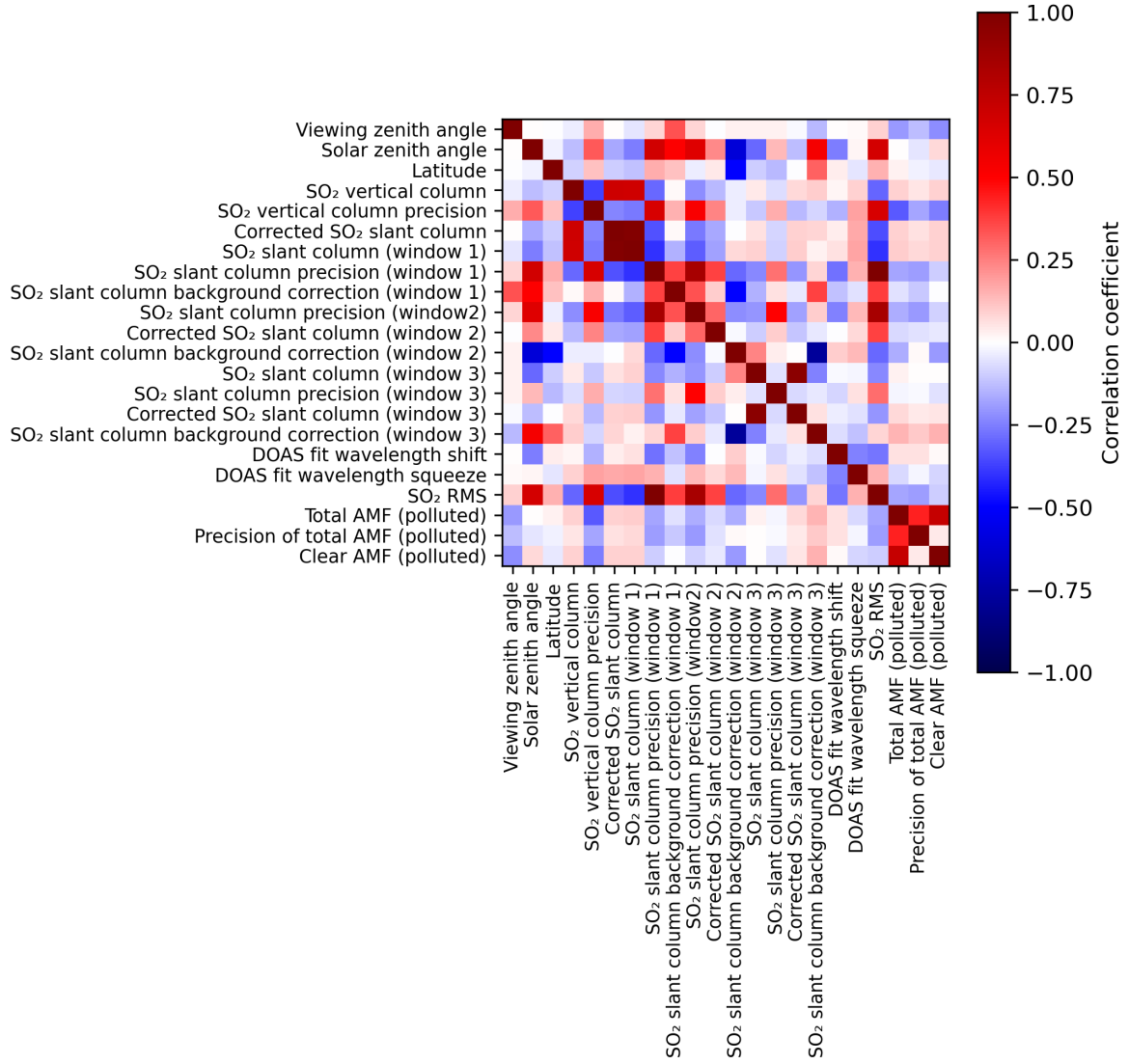
Figure 2: Map of correlation matrix for 2024-04-08 to 2024-04-10.
