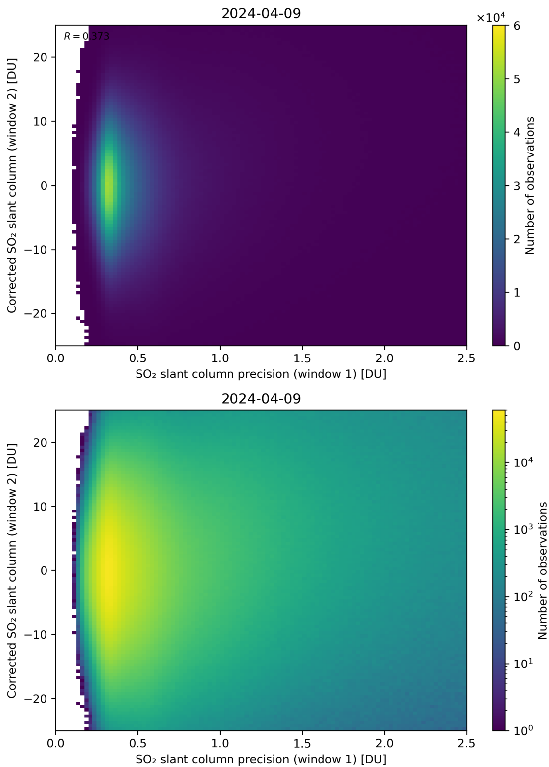
Figure 225: Scatter density plot of “SO 2 slant column precision (window 1)” against “Corrected SO 2 slant column (window 2)” for 2024-04-08 to 2024-04-10.
