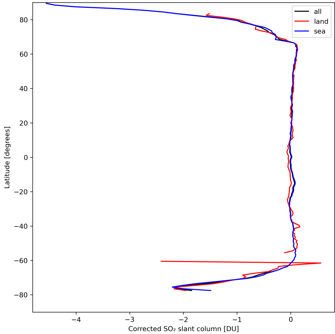
Figure 32: Zonal average of “Corrected SO 2 slant column” for 2024-04-08 to 2024-04-10.
