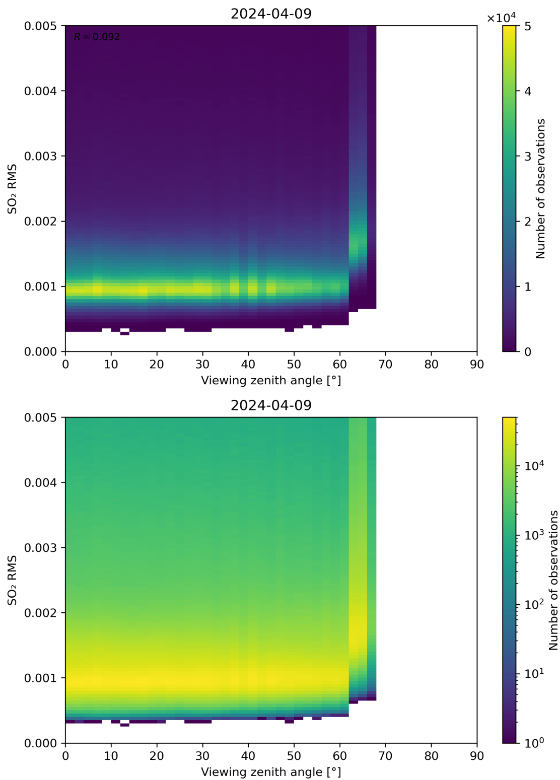
Figure 313: Scatter density plot of “Viewing zenith angle” against “SO 2 RMS” for 2024-04-08 to 2024-04-10.
