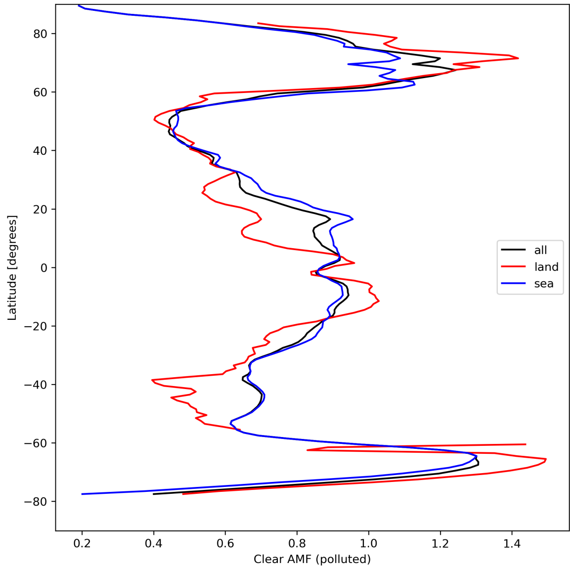
Figure 50: Zonal average of “Clear AMF (polluted)” for 2024-04-08 to 2024-04-10.
