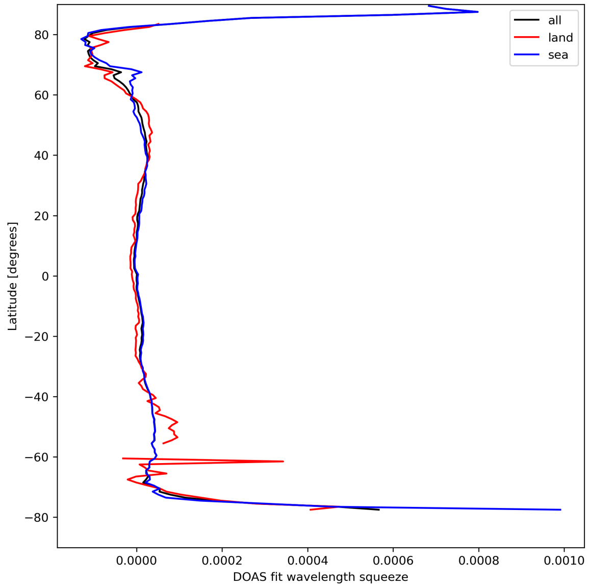
Figure 46: Zonal average of “DOAS fit wavelength squeeze” for 2024-04-08 to 2024-04-10.
