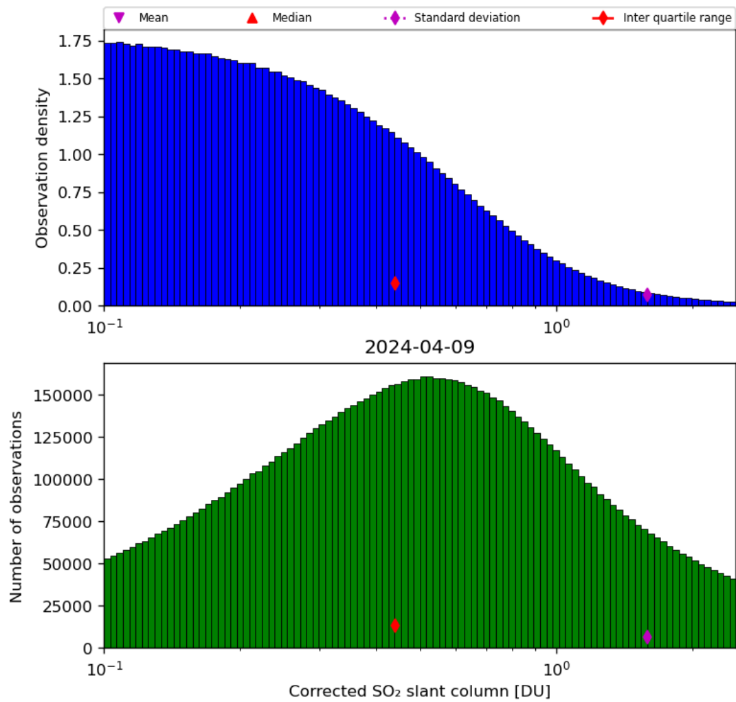
Figure 55: Histogram of “Corrected SO 2 slant column” for 2024-04-08 to 2024-04-10
