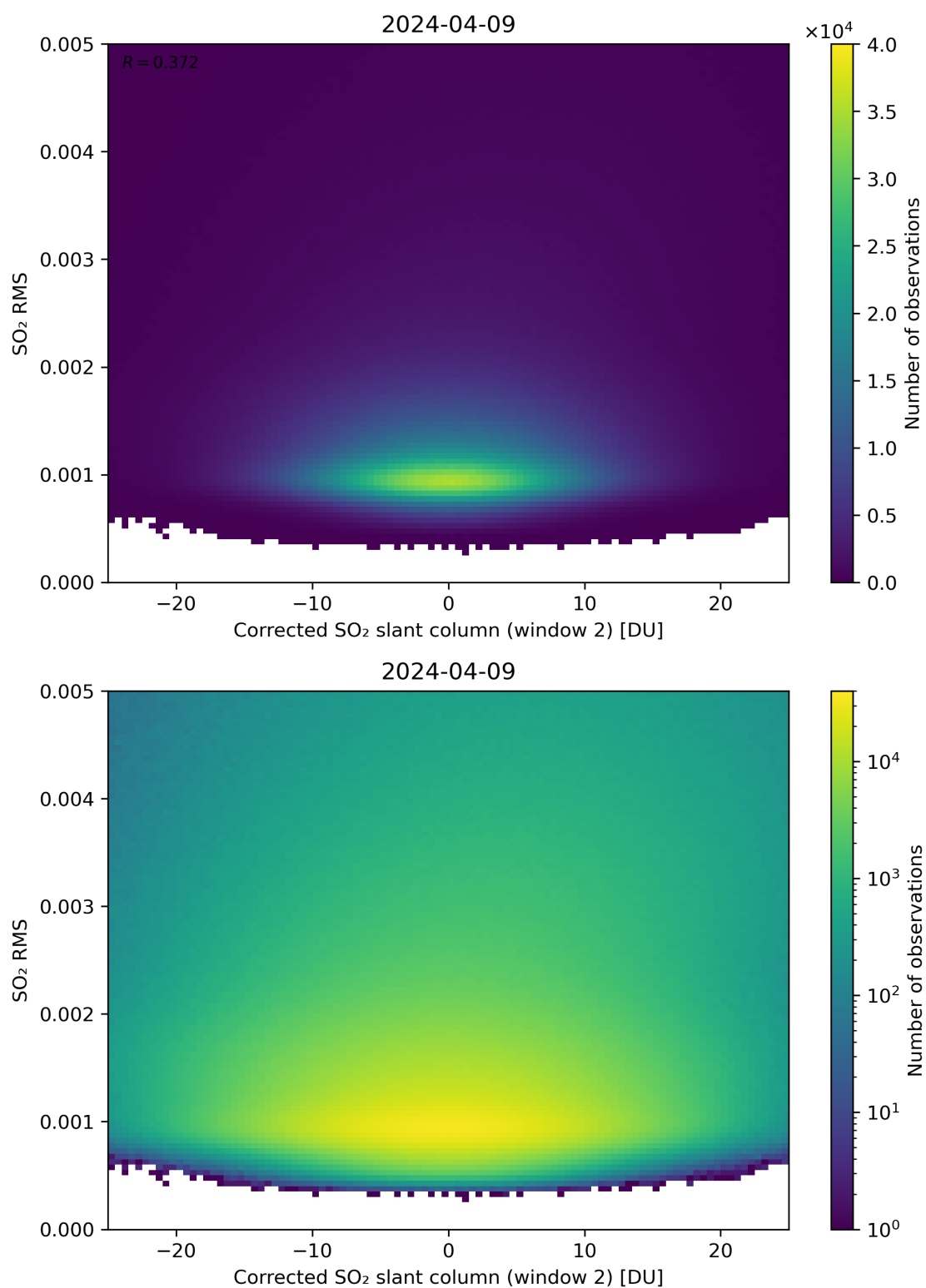
Figure 198: Scatter density plot of “Corrected SO 2 slant column (window 2)” against “SO 2 RMS” for 2024-04-08 to 2024-04-10.
