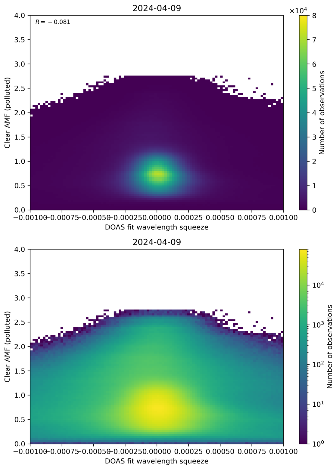
Figure 133: Scatter density plot of “DOAS fit wavelength squeeze” against “Clear AMF (polluted)” for 2024-04-08 to 2024-04-10.
