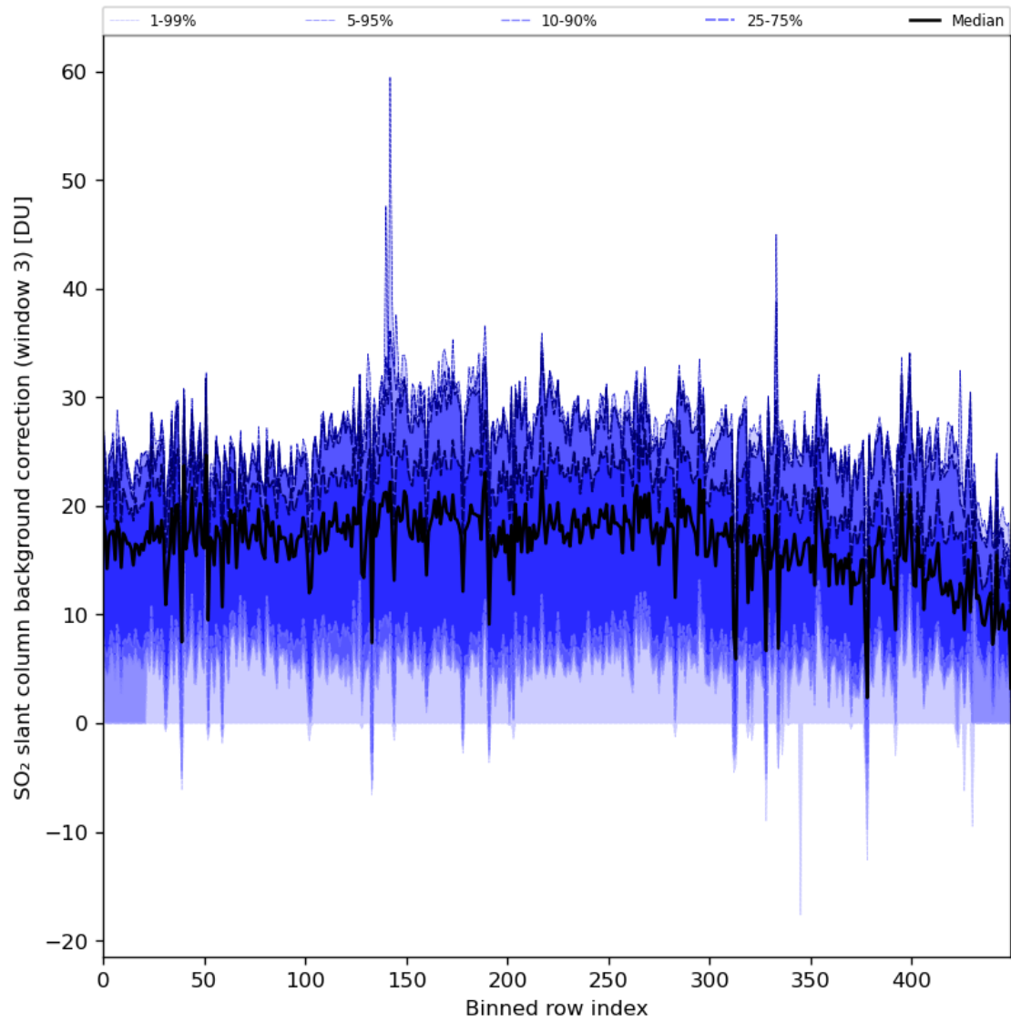
Figure 90: Along track statistics of “SO 2 slant column background correction (window 3)” for 2024-04-08 to 2024-04-10
