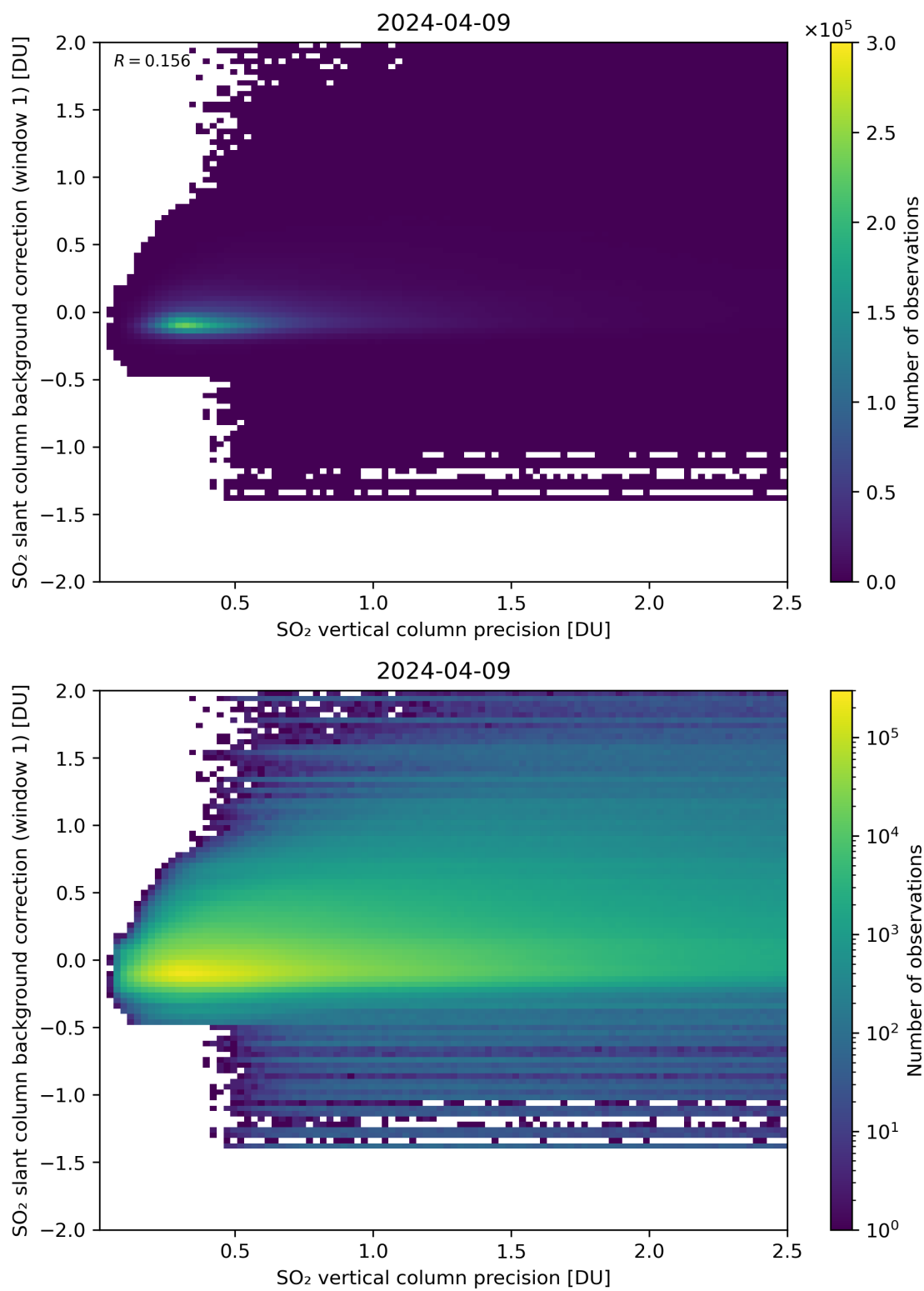
Figure 279: Scatter density plot of “SO 2 vertical column precision” against “SO 2 slant column background correction (window 1)” for 2024-04-08 to 2024-04-10.
