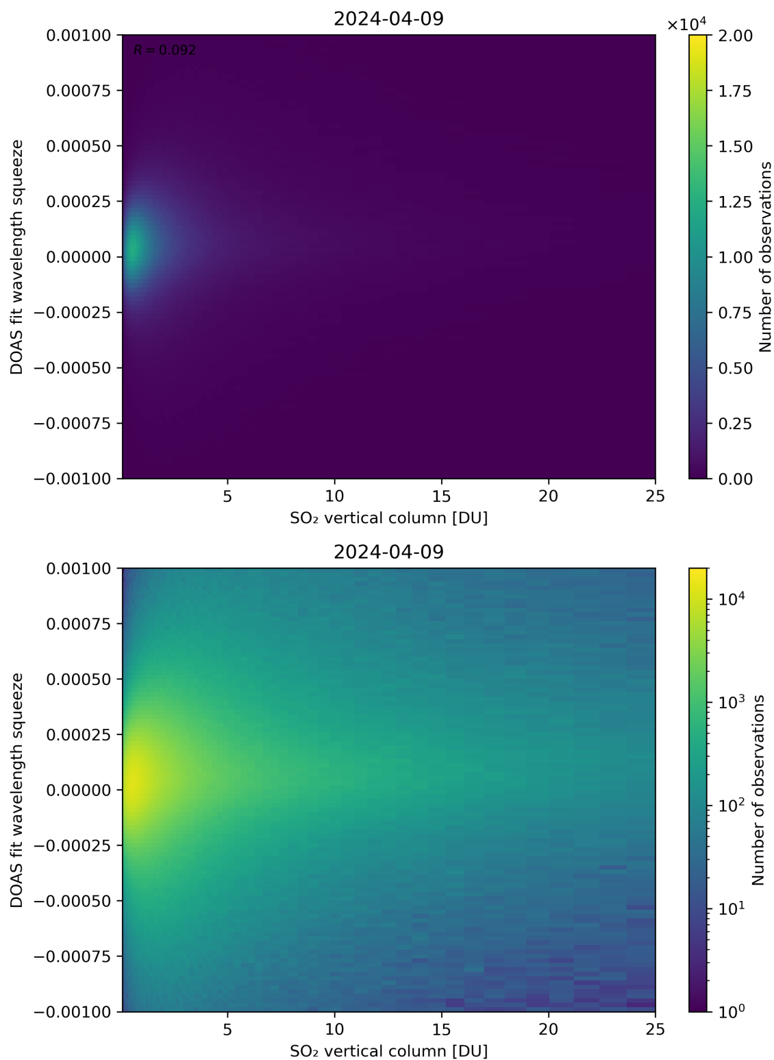
Figure 277: Scatter density plot of “SO 2 vertical column” against “DOAS fit wavelength squeeze” for 2024-04-08 to 2024-04-10.
