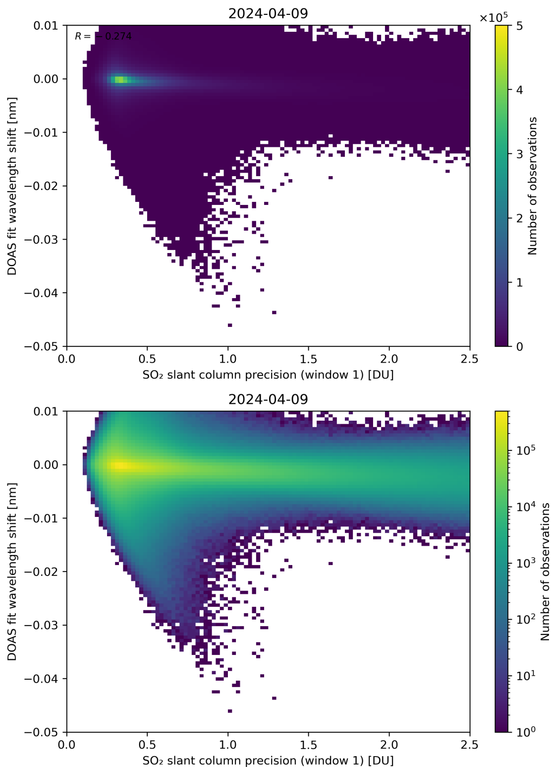
Figure 221: Scatter density plot of “SO 2 slant column precision (window 1)” against “DOAS fit wavelength shift” for 2024-04-08 to 2024-04-10.
