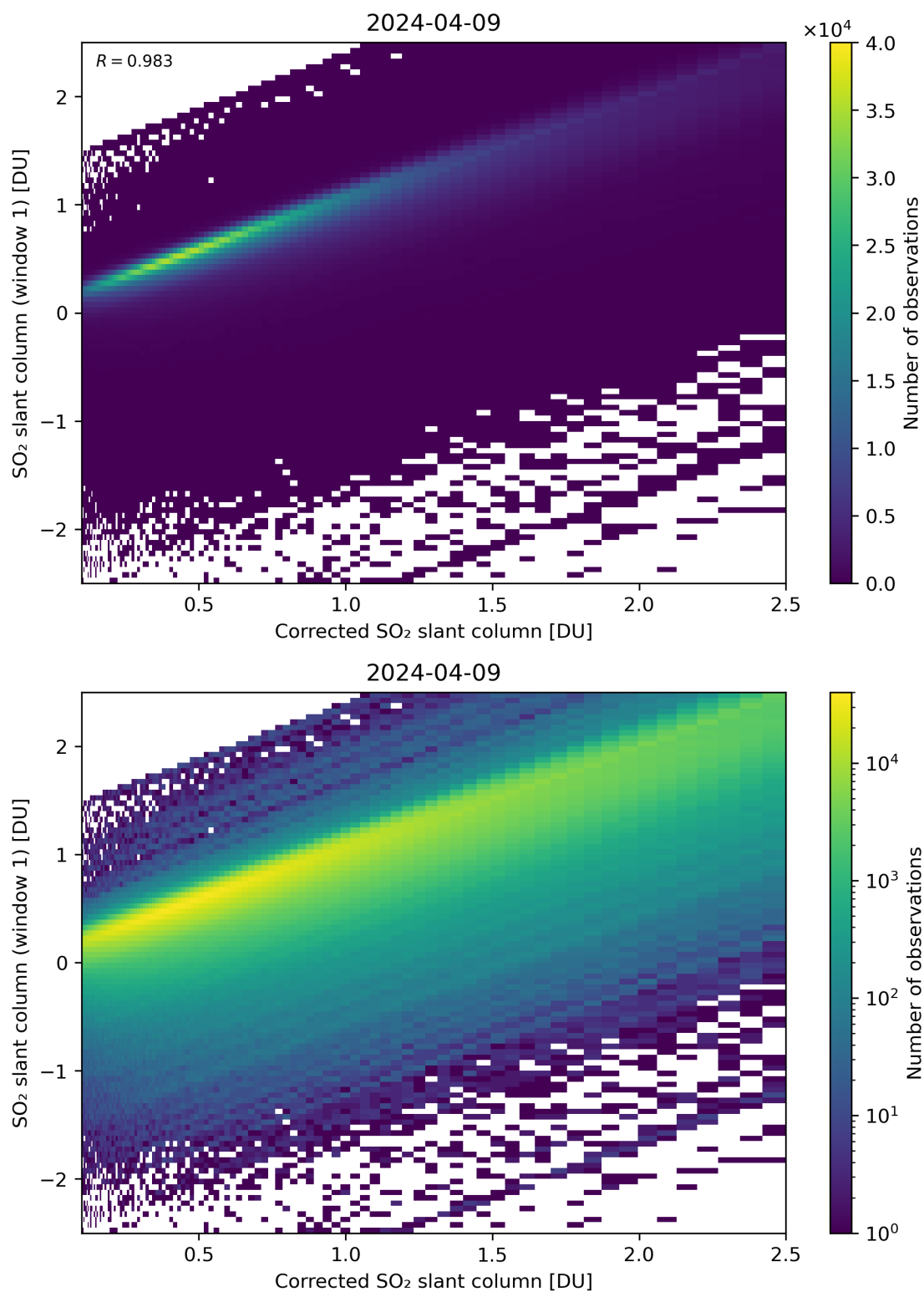
Figure 187: Scatter density plot of “Corrected SO 2 slant column” against “SO 2 slant column (window 1)” for 2024-04-08 to 2024-04-10.
