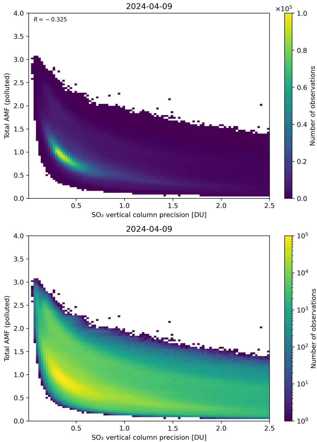
Figure 294: Scatter density plot of “SO 2 vertical column precision” against “Total AMF (polluted)” for 2024-04-08 to 2024-04-10.
