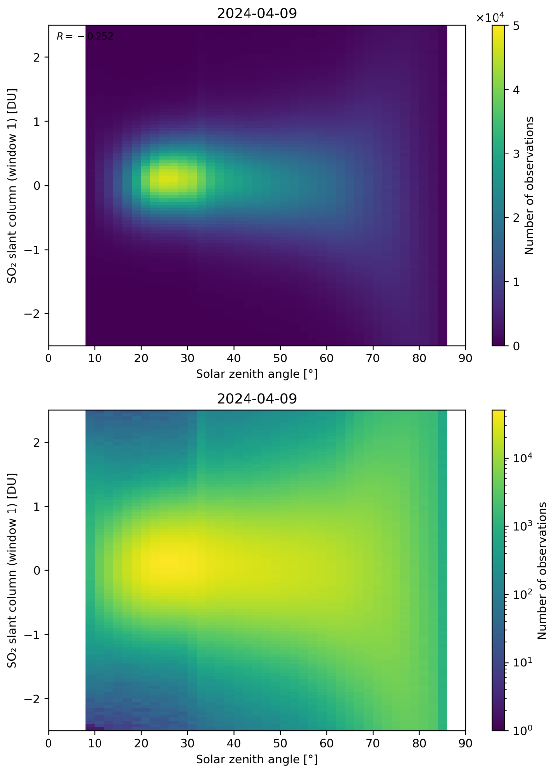
Figure 169: Scatter density plot of “Solar zenith angle” against “SO 2 slant column (window 1)” for 2024-04-08 to 2024-04-10.
