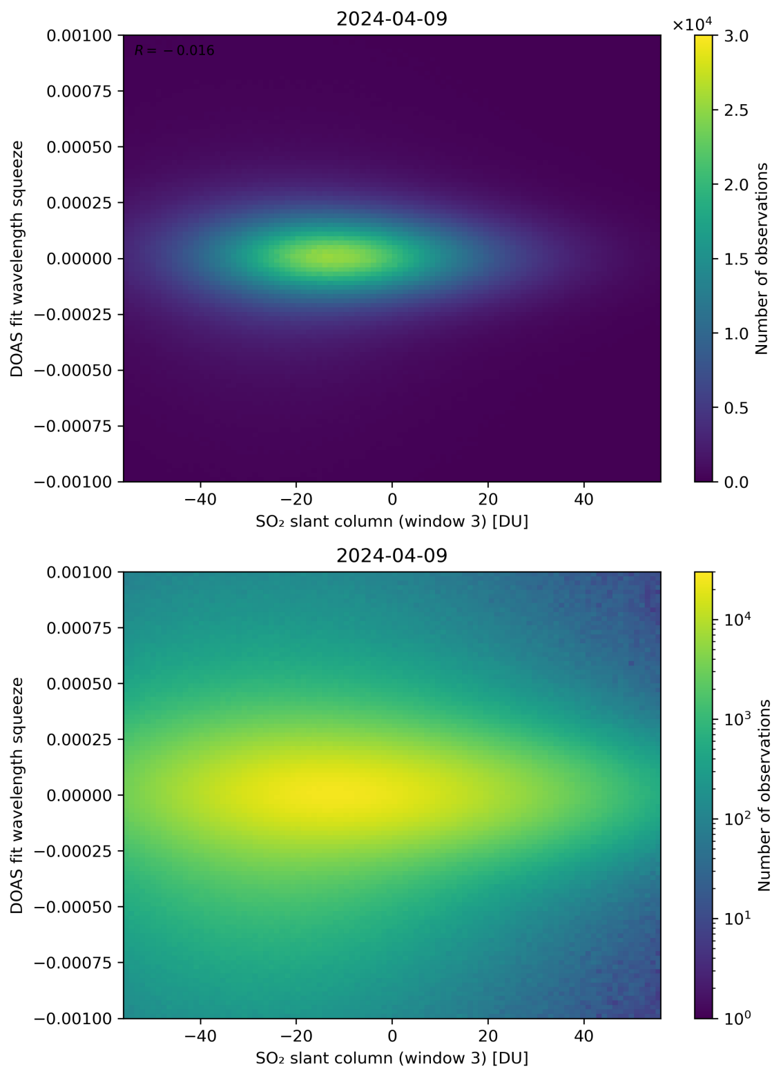
Figure 255: Scatter density plot of “SO 2 slant column (window 3)” against “DOAS fit wavelength squeeze” for 2024-04-08 to 2024-04-10.
