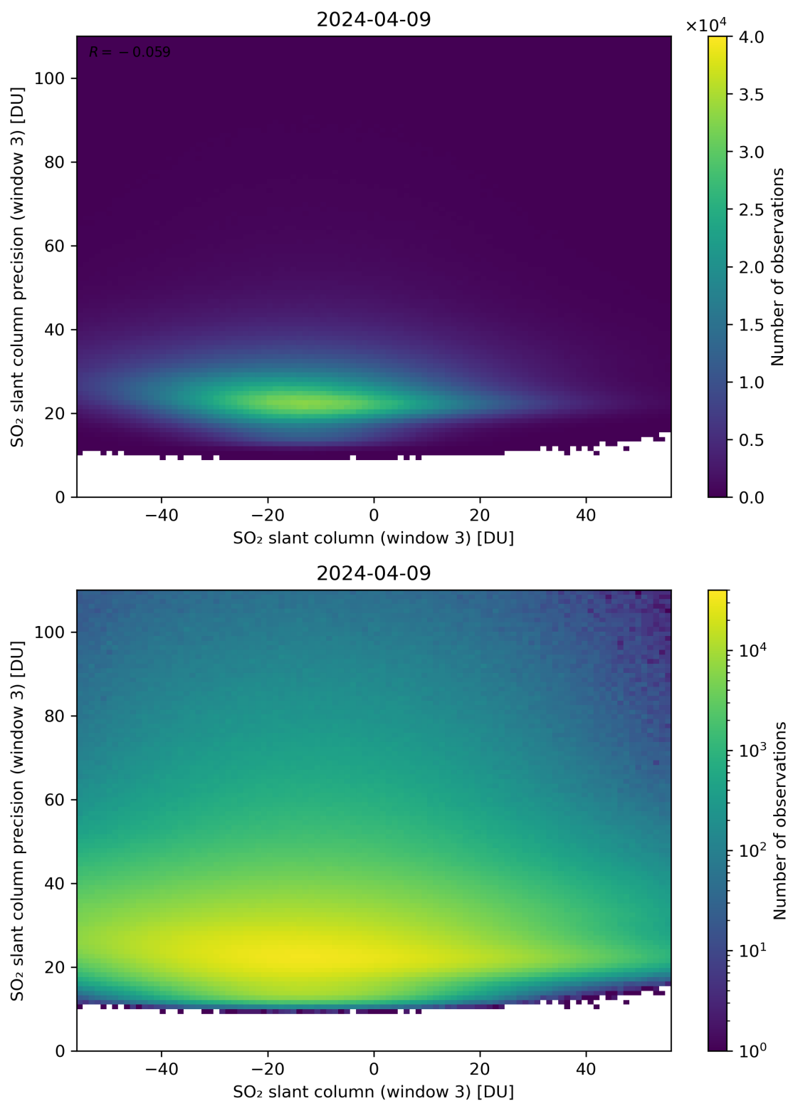
Figure 267: Scatter density plot of “SO 2 slant column (window 3)” against “SO 2 slant column precision (window 3)” for 2024-04-08 to 2024-04-10.
