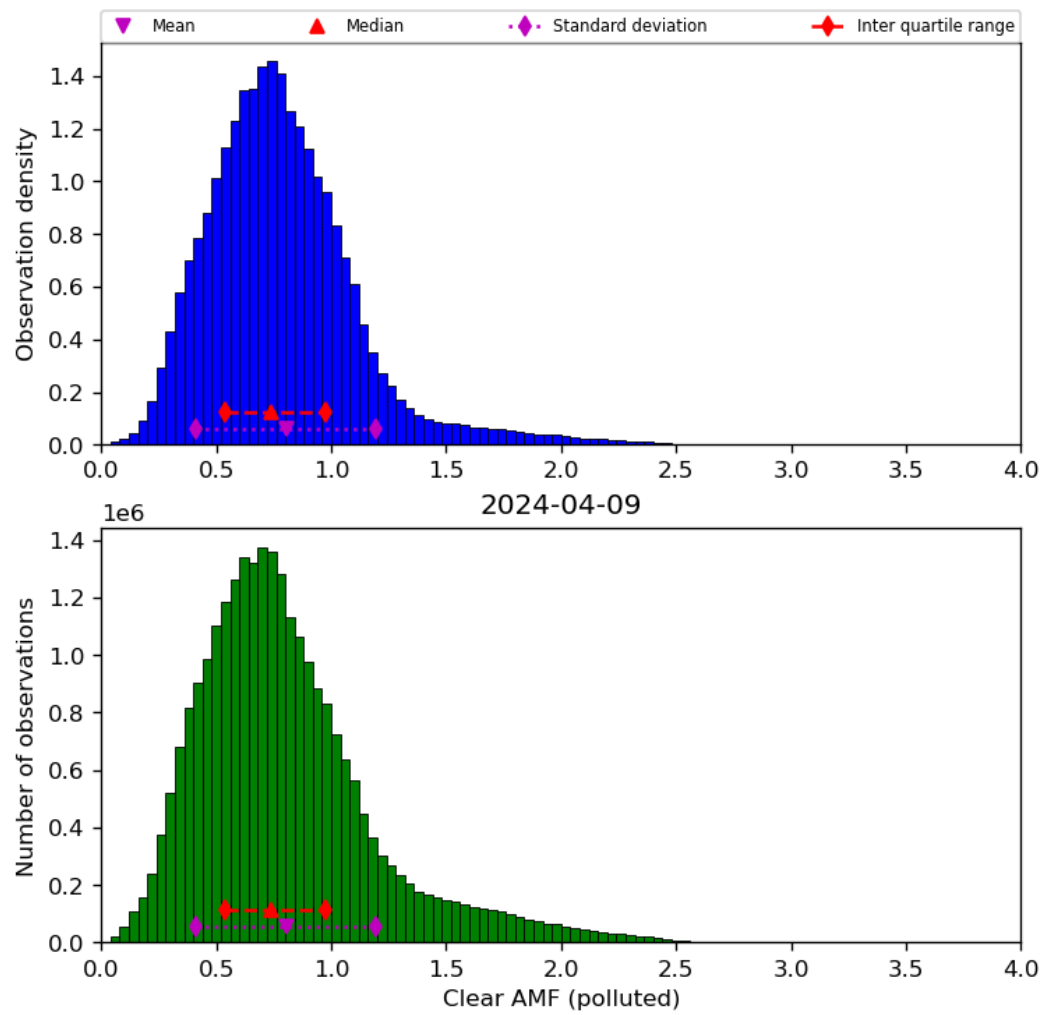
Figure 73: Histogram of “Clear AMF (polluted)” for 2024-04-08 to 2024-04-10
