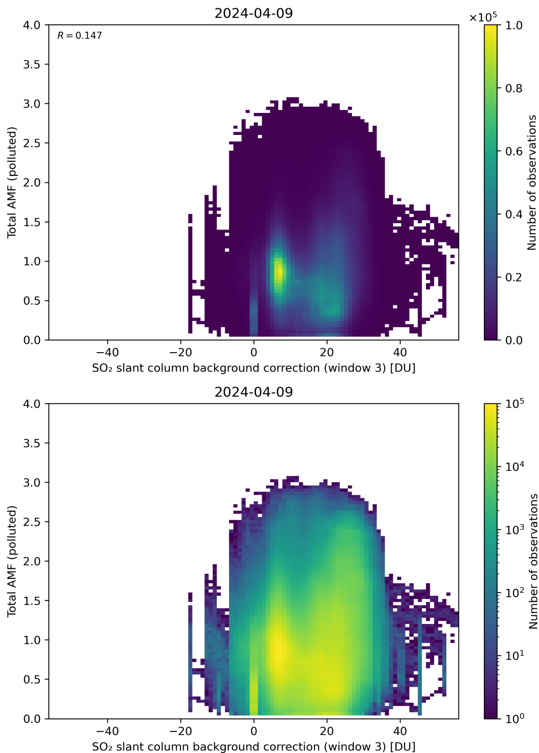
Figure 125: Scatter density plot of “SO 2 slant column background correction (window 3)” against “Total AMF (polluted)” for 2024-04-08 to 2024-04-10.
