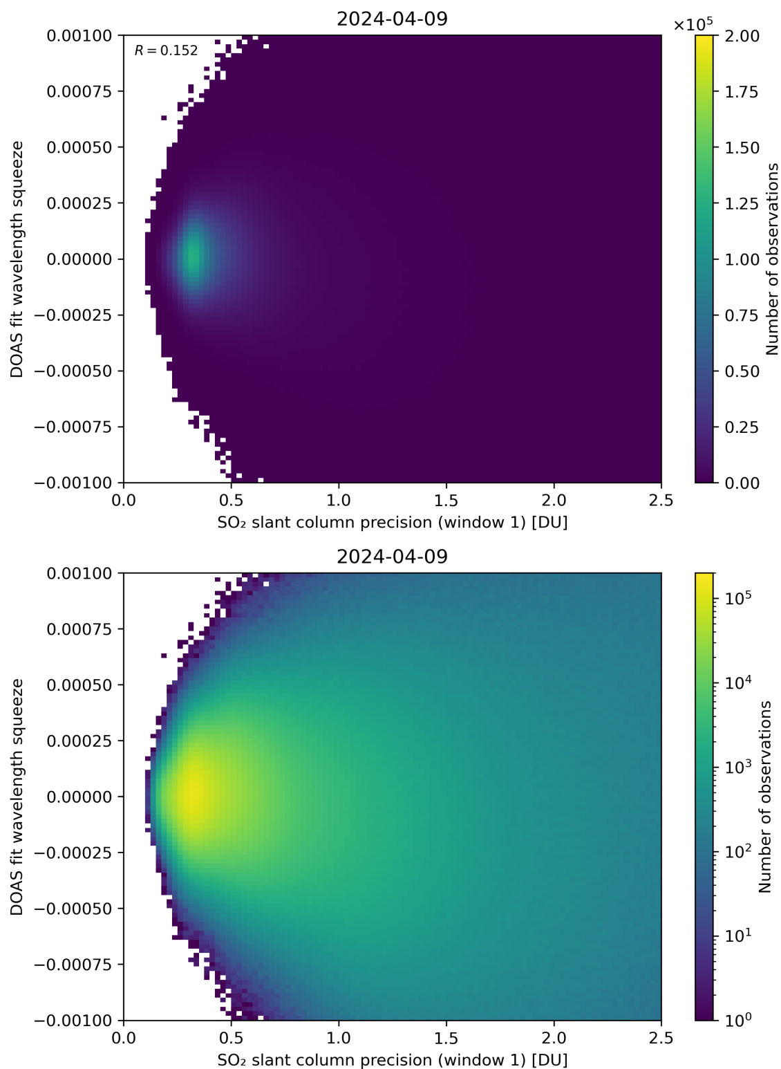
Figure 222: Scatter density plot of “SO 2 slant column precision (window 1)” against “DOAS fit wavelength squeeze” for 2024-04-08 to 2024-04-10.
