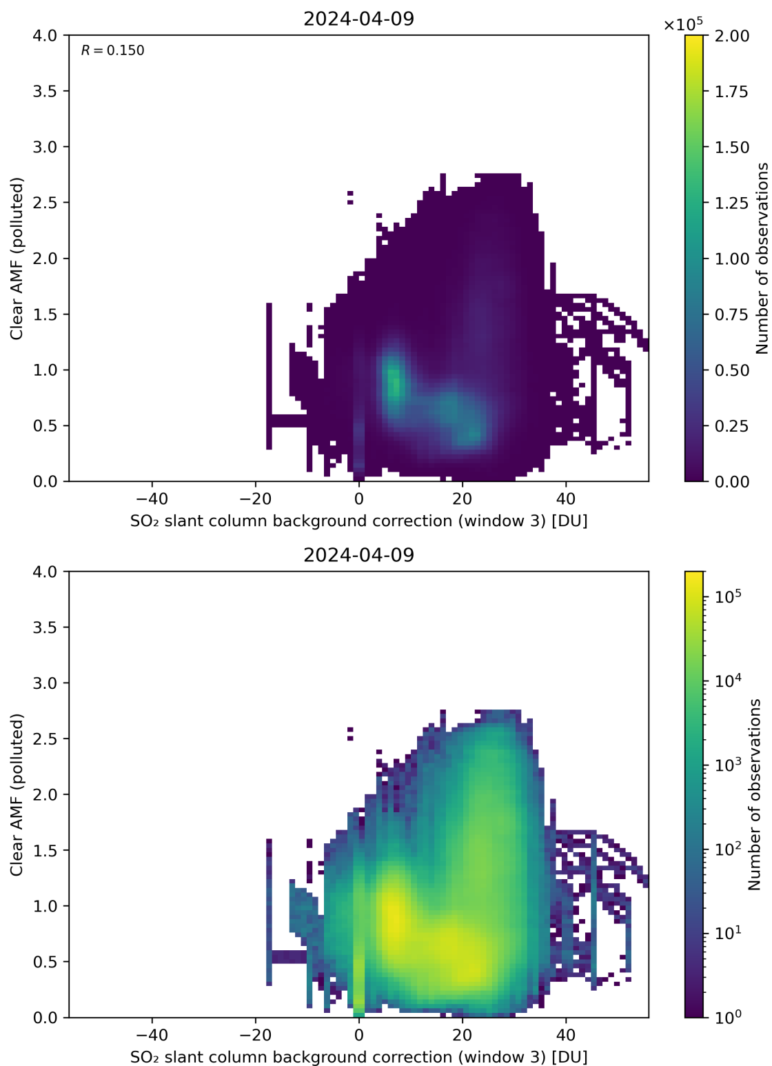
Figure 124: Scatter density plot of “SO 2 slant column background correction (window 3)” against “Clear AMF (polluted)” for 2024-04-08 to 2024-04-10.
