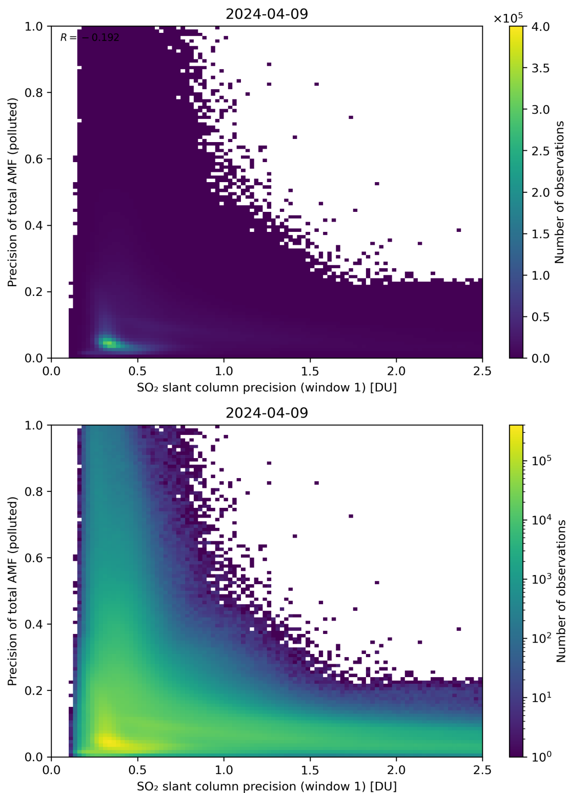
Figure 231: Scatter density plot of “SO 2 slant column precision (window 1)” against “Precision of total AMF (polluted)” for 2024-04-08 to 2024-04-10.
