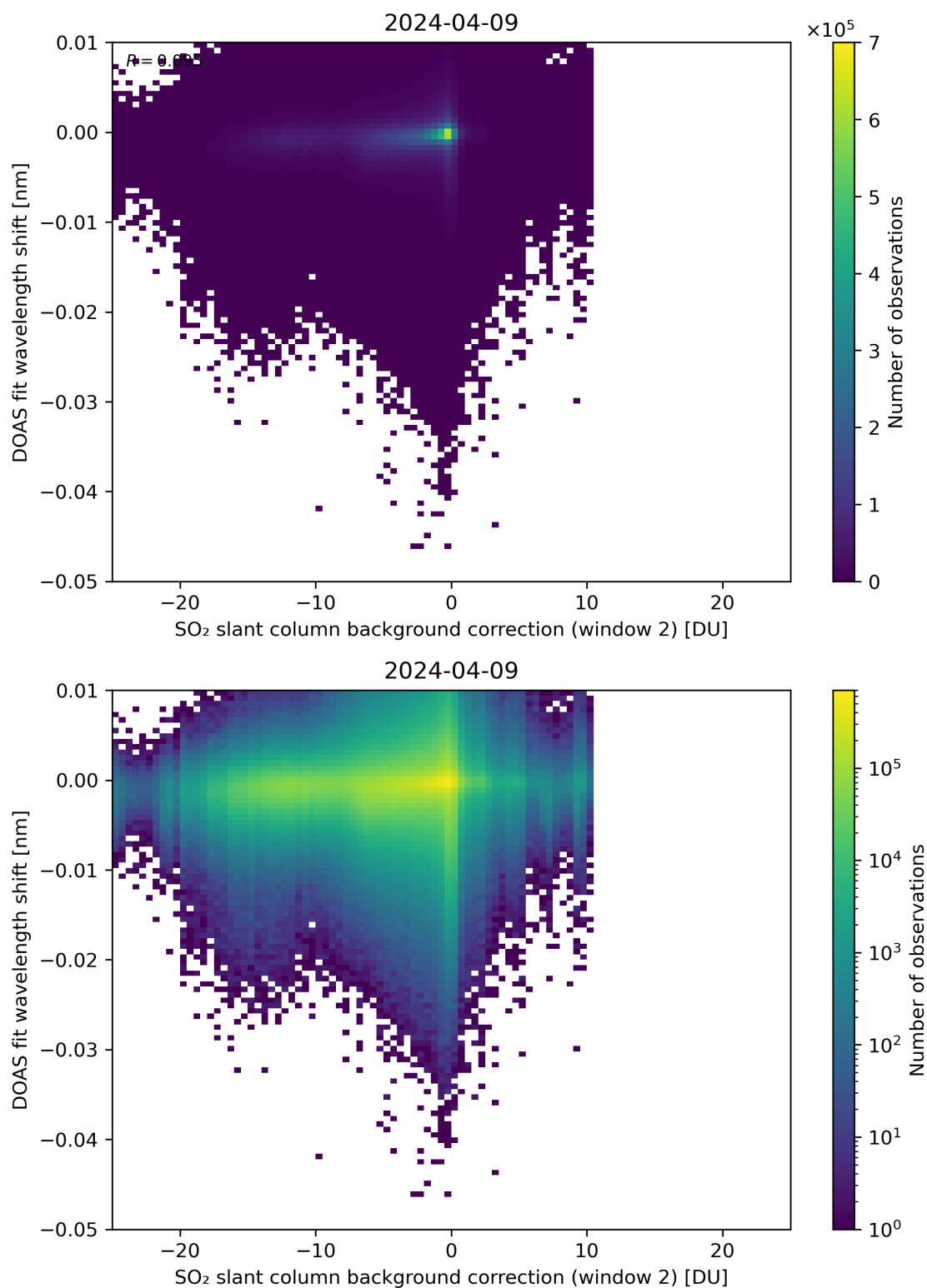
Figure 112: Scatter density plot of “SO 2 slant column background correction (window 2)” against “DOAS fit wavelength shift” for 2024-04-08 to 2024-04-10.
