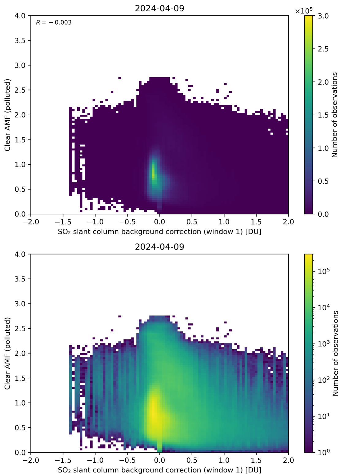
Figure 103: Scatter density plot of “SO 2 slant column background correction (window 1)” against “Clear AMF (polluted)” for 2024-04-08 to 2024-04-10.
