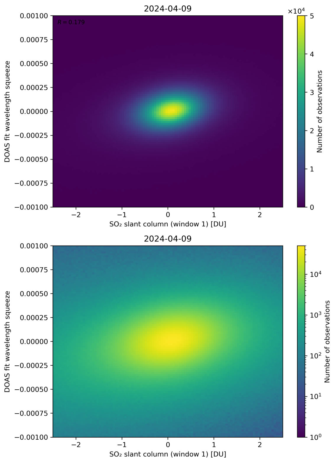
Figure 216: Scatter density plot of “SO 2 slant column (window 1)” against “DOAS fit wavelength squeeze” for 2024-04-08 to 2024-04-10.
