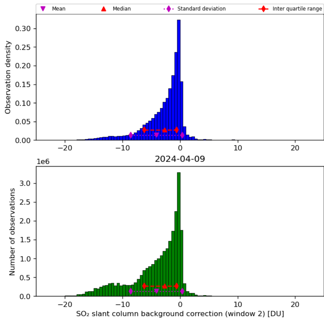
Figure 63: Histogram of “SO 2 slant column background correction (window 2)” for 2024-04-08 to 2024-04-10
