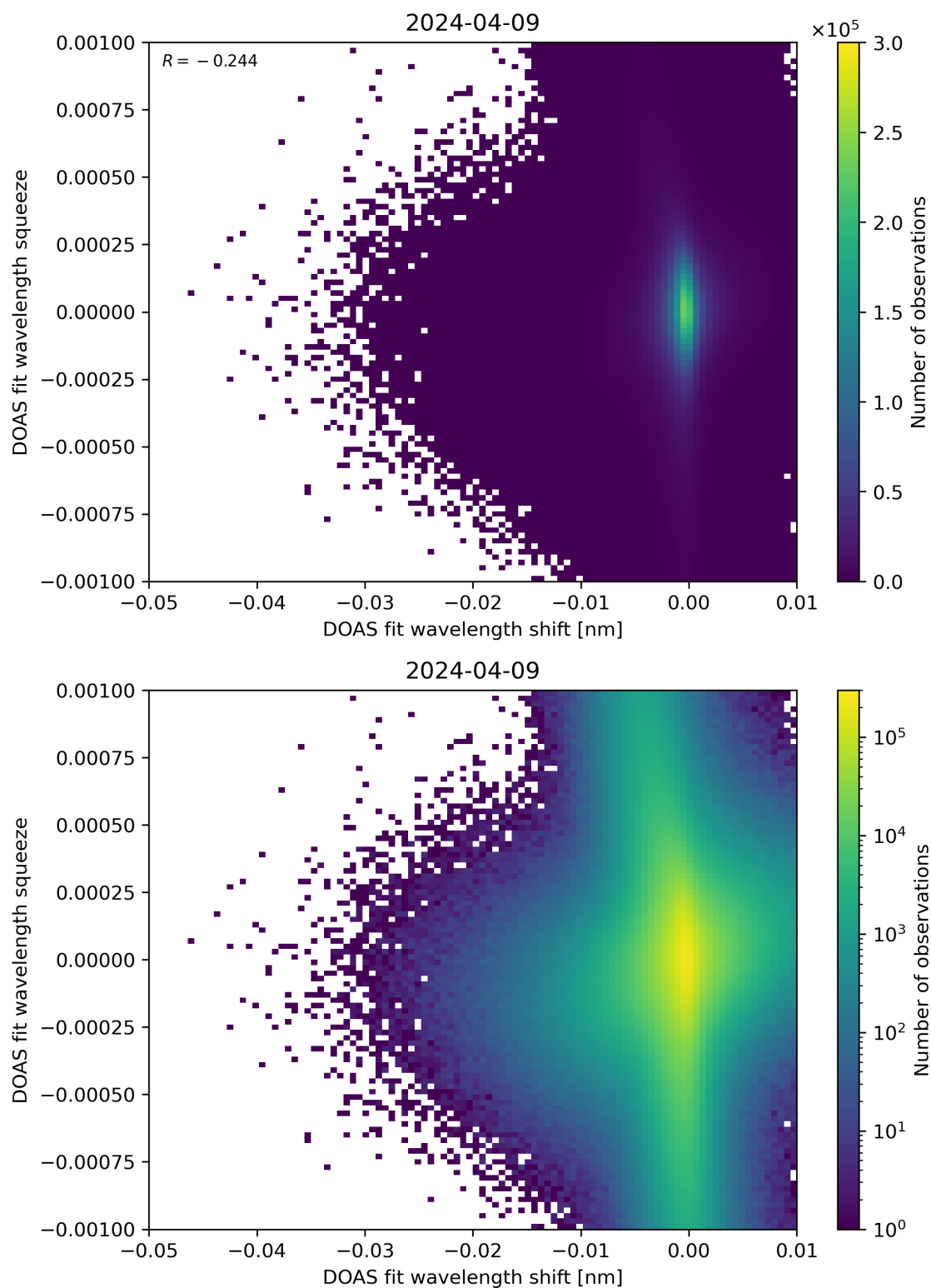
Figure 127: Scatter density plot of “DOAS fit wavelength shift” against “DOAS fit wavelength squeeze” for 2024-04-08 to 2024-04-10.
