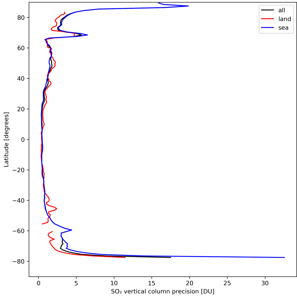
Figure 31: Zonal average of “SO 2 vertical column precision” for 2024-04-08 to 2024-04-10.
