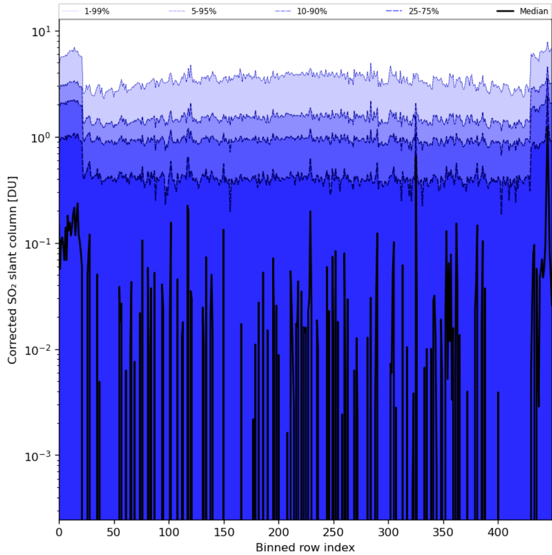
Figure 78: Along track statistics of “Corrected SO 2 slant column” for 2024-04-08 to 2024-04-10
