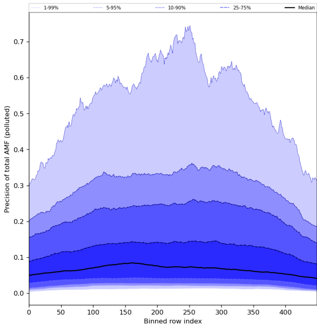
Figure 95: Along track statistics of “Precision of total AMF (polluted)” for 2024-04-08 to 2024-04-10
