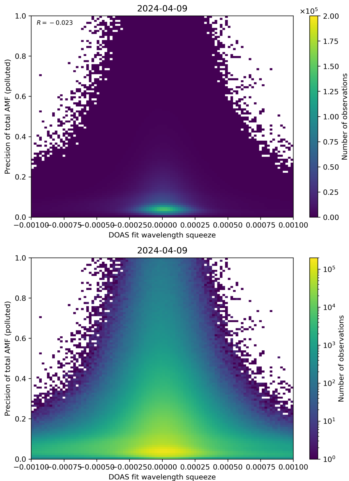
Figure 135: Scatter density plot of “DOAS fit wavelength squeeze” against “Precision of total AMF (polluted)” for 2024-04-08 to 2024-04-10.
