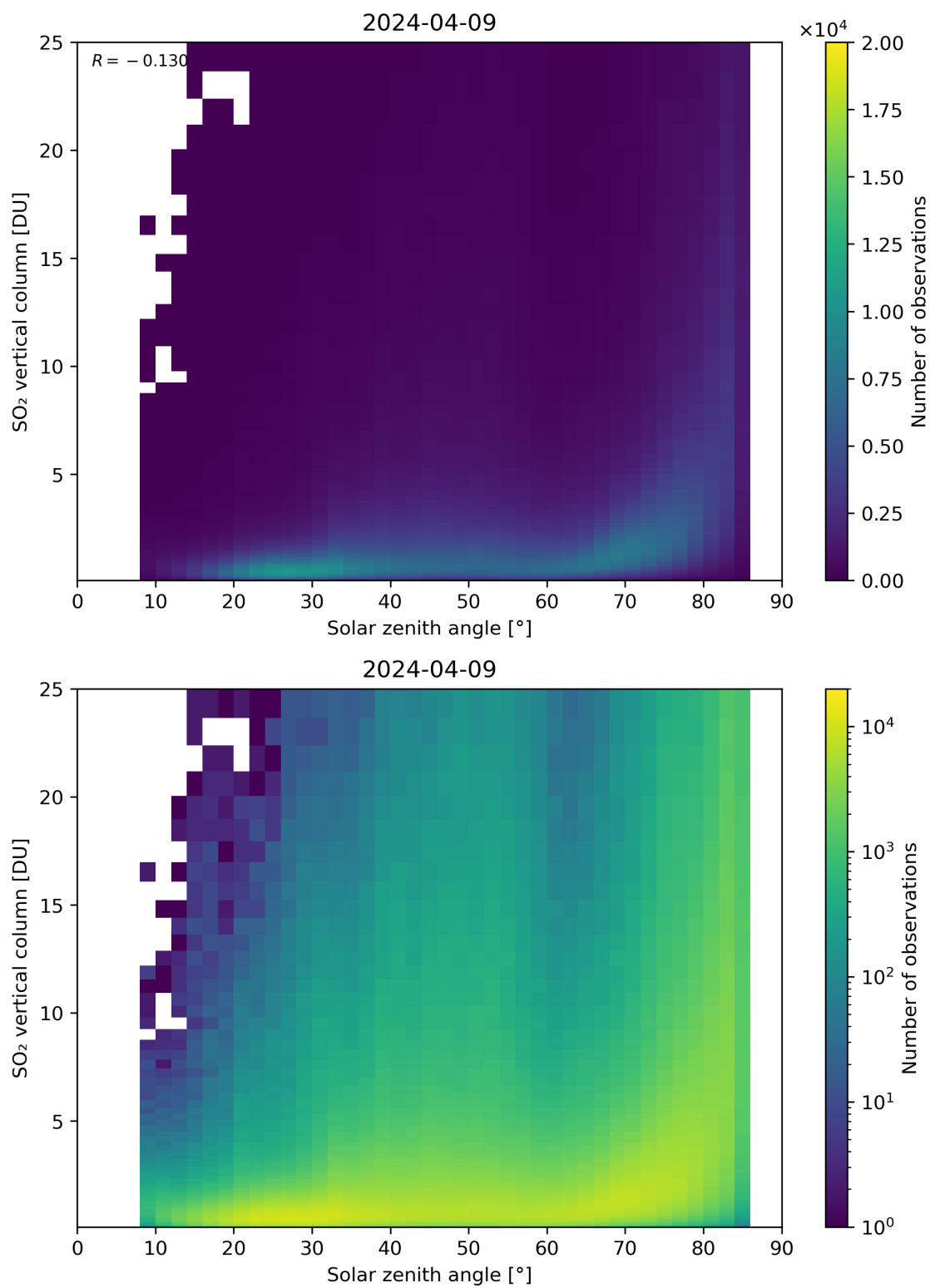
Figure 176: Scatter density plot of “Solar zenith angle” against “SO 2 vertical column” for 2024-04-08 to 2024-04-10.
