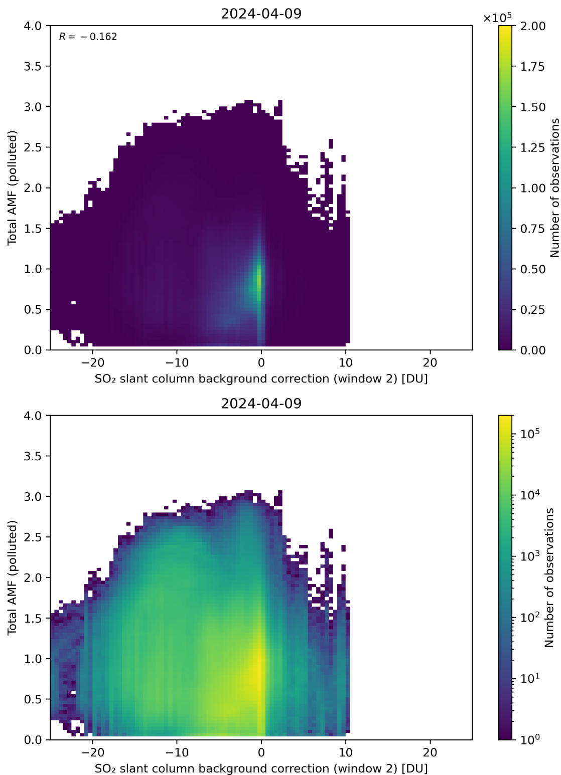
Figure 119: Scatter density plot of “SO 2 slant column background correction (window 2)” against “Total AMF (polluted)” for 2024-04-08 to 2024-04-10.
