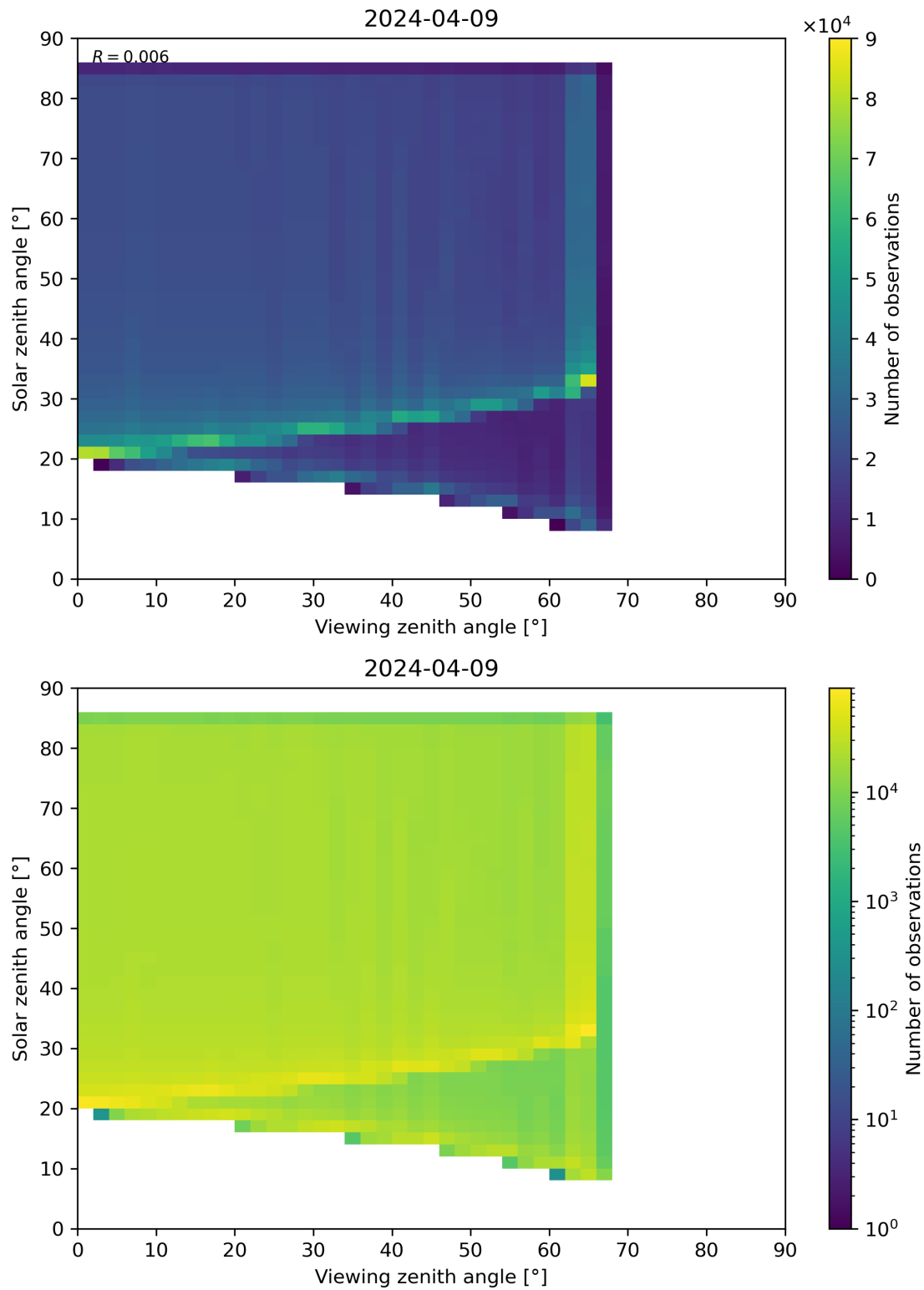
Figure 315: Scatter density plot of “Viewing zenith angle” against “Solar zenith angle” for 2024-04-08 to 2024-04-10.
