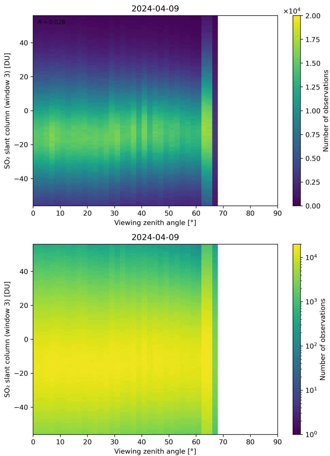
Figure 323: Scatter density plot of “Viewing zenith angle” against “SO 2 slant column (window 3)” for 2024-04-08 to 2024-04-10.
