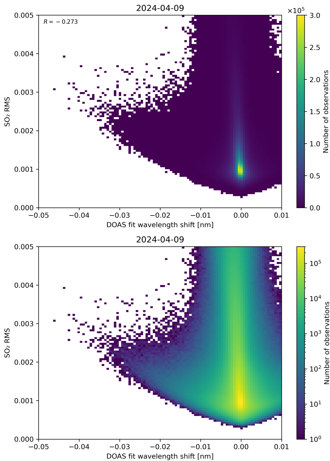
Figure 128: Scatter density plot of “DOAS fit wavelength shift” against “SO 2 RMS” for 2024-04-08 to 2024-04-10.
