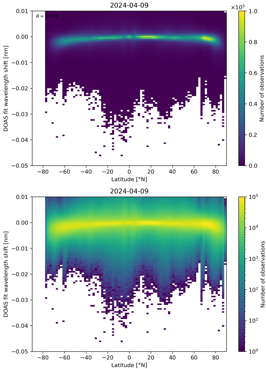
Figure 142: Scatter density plot of “Latitude” against “DOAS fit wavelength shift” for 2024-04-08 to 2024-04-10.
