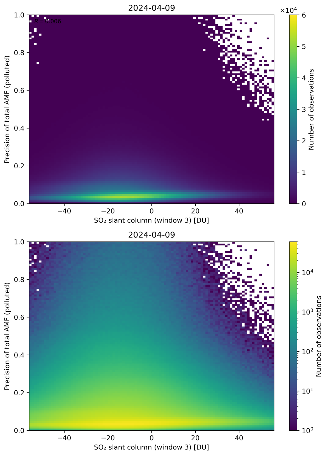
Figure 269: Scatter density plot of “SO 2 slant column (window 3)” against “Precision of total AMF (polluted)” for 2024-04-08 to 2024-04-10.
