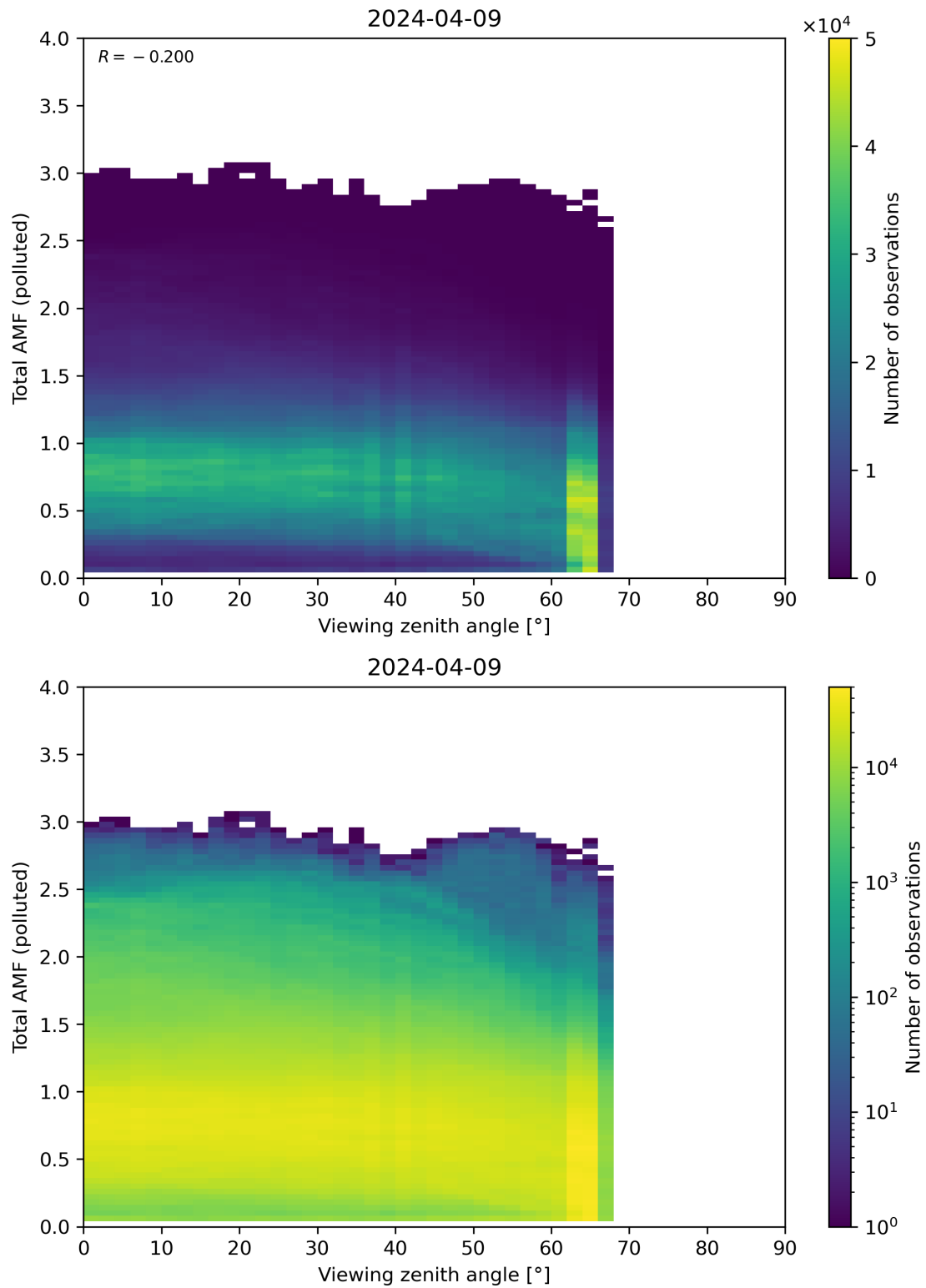
Figure 325: Scatter density plot of “Viewing zenith angle” against “Total AMF (polluted)” for 2024-04-08 to 2024-04-10.
