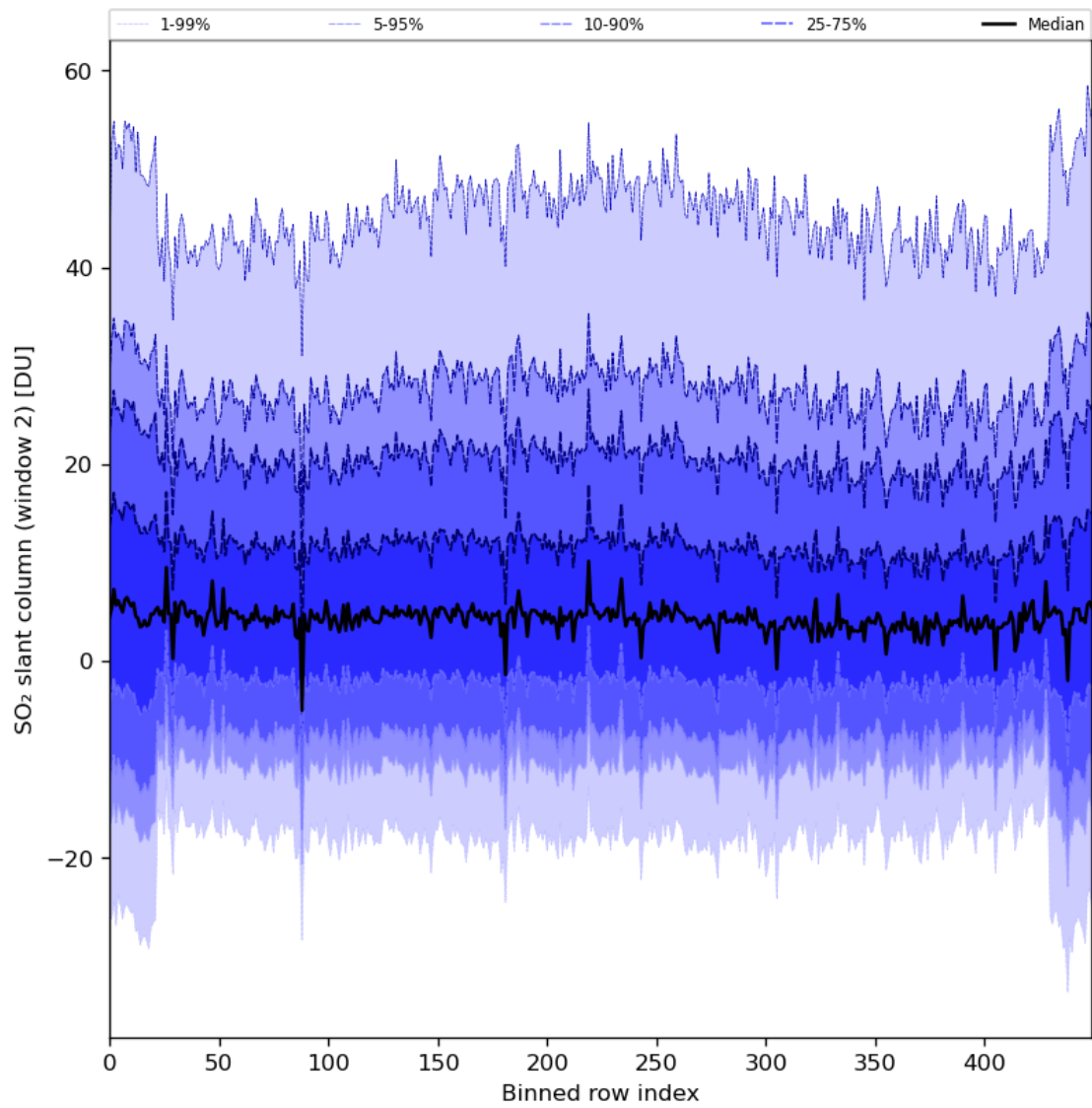
Figure 83: Along track statistics of “SO 2 slant column (window 2)” for 2024-04-08 to 2024-04-10
