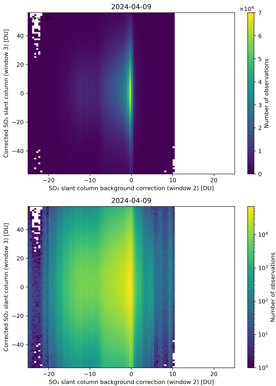
Figure 116: Scatter density plot of “SO 2 slant column background correction (window 2)” against “Corrected SO 2 slant column (window 3)” for 2024-04-08 to 2024-04-10.
