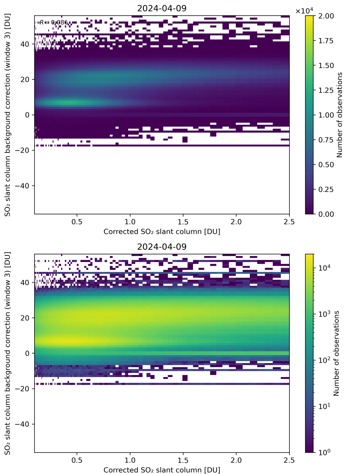
Figure 180: Scatter density plot of “Corrected SO 2 slant column” against “SO 2 slant column background correction (window 3)” for 2024-04-08 to 2024-04-10.
