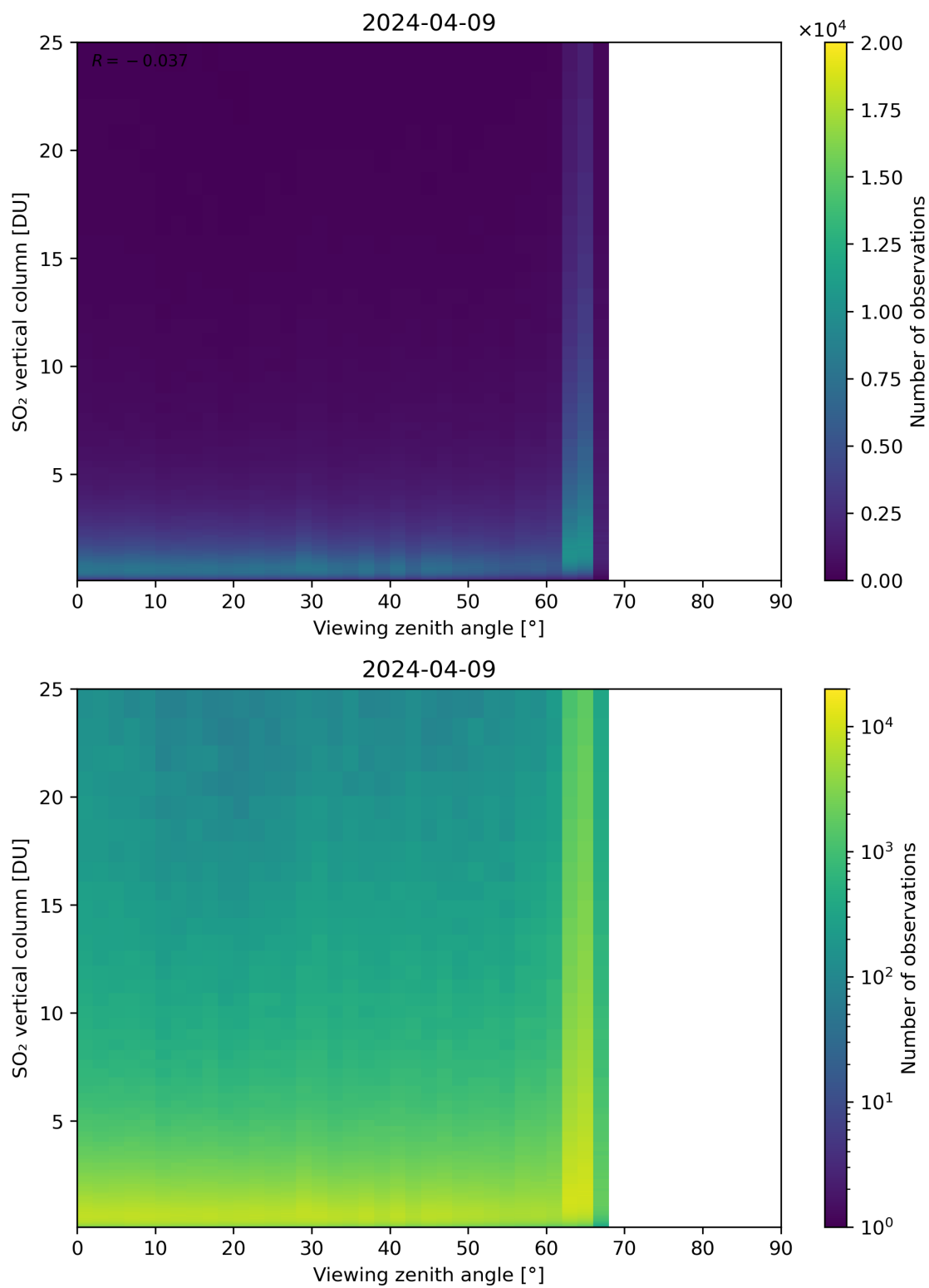
Figure 327: Scatter density plot of “Viewing zenith angle” against “SO 2 vertical column” for 2024-04-08 to 2024-04-10.
