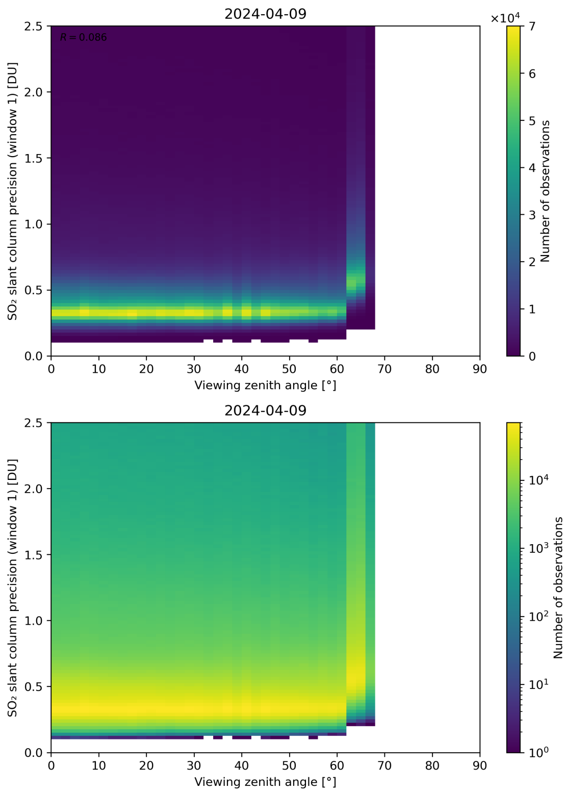
Figure 321: Scatter density plot of “Viewing zenith angle” against “SO 2 slant column precision (window 1)” for 2024-04-08 to 2024-04-10.
