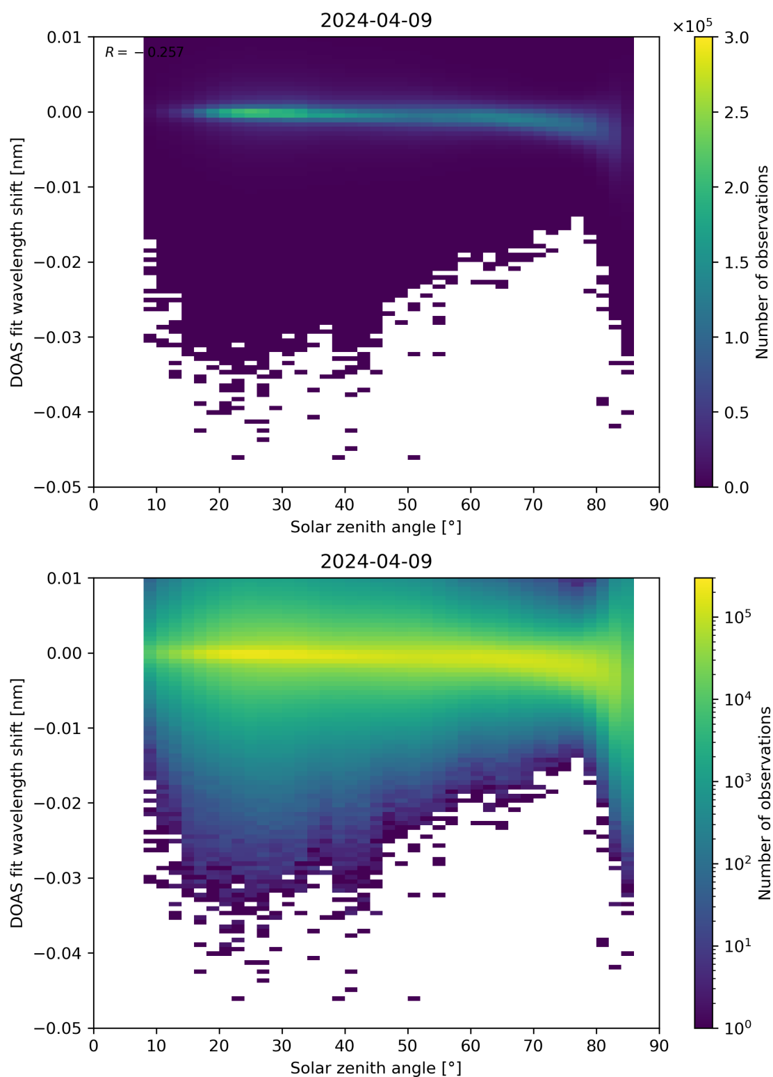
Figure 161: Scatter density plot of “Solar zenith angle” against “DOAS fit wavelength shift” for 2024-04-08 to 2024-04-10.
