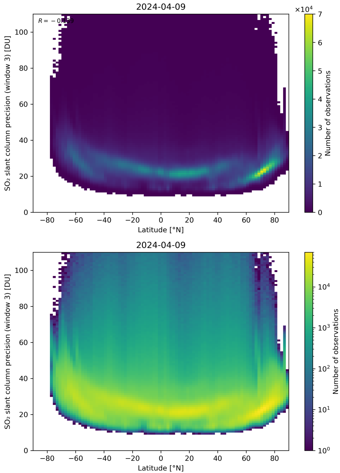
Figure 153: Scatter density plot of “Latitude” against “SO 2 slant column precision (window 3)” for 2024-04-08 to 2024-04-10.
