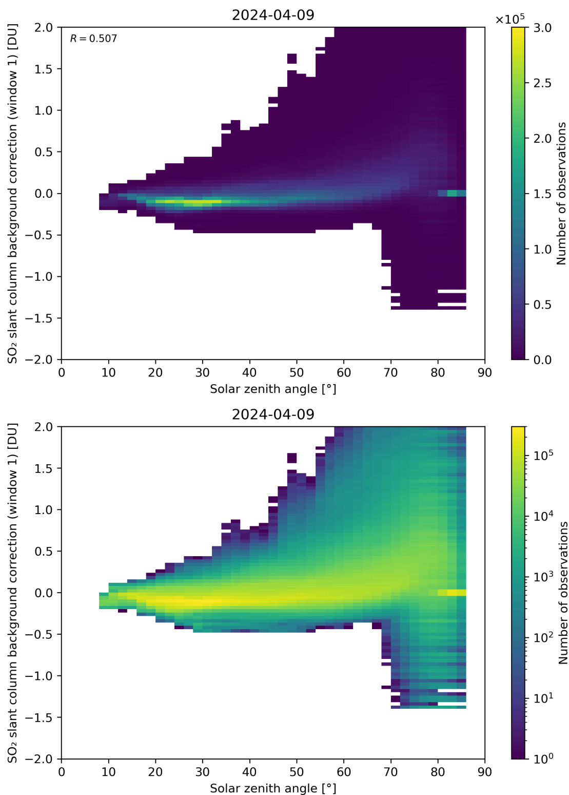
Figure 158: Scatter density plot of “Solar zenith angle” against “SO 2 slant column background correction (window 1)” for 2024-04-08 to 2024-04-10.
