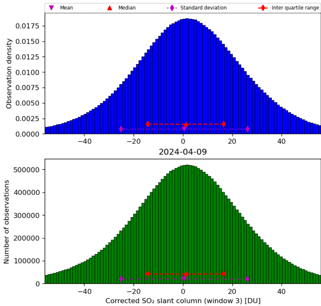
Figure 66: Histogram of “Corrected SO 2 slant column (window 3)” for 2024-04-08 to 2024-04-10
