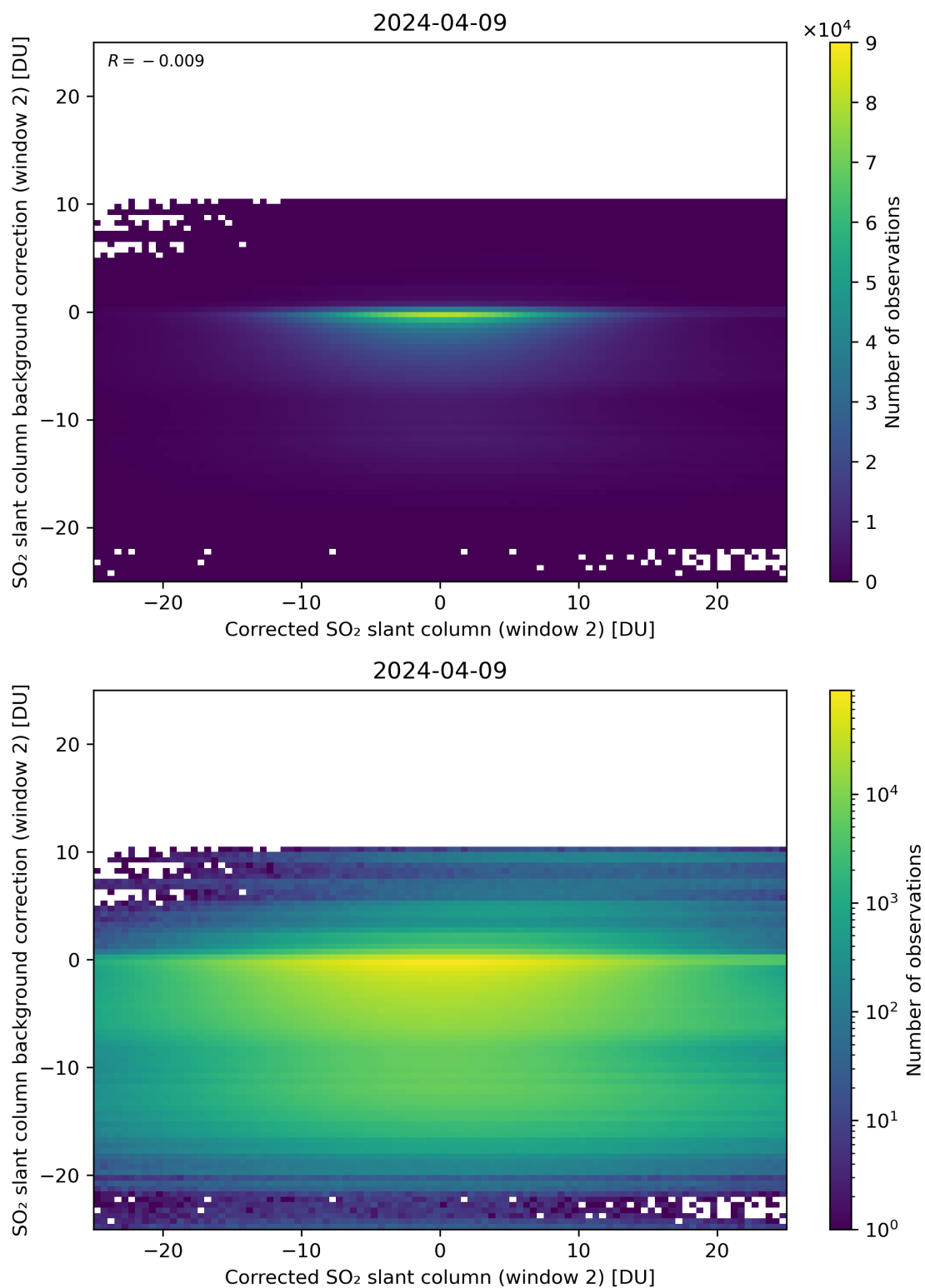
Figure 194: Scatter density plot of “Corrected SO 2 slant column (window 2)” against “SO 2 slant column background correction (window 2)” for 2024-04-08 to 2024-04-10.
