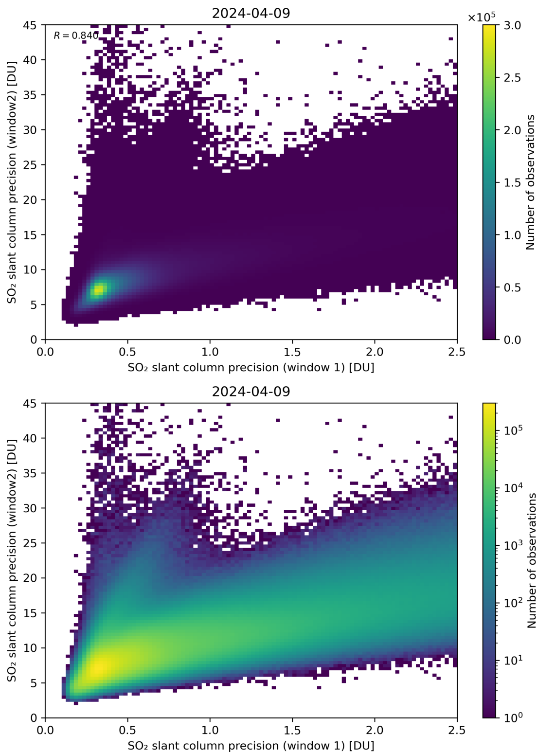
Figure 227: Scatter density plot of “SO 2 slant column precision (window 1)” against “SO 2 slant column precision (window2)” for 2024-04-08 to 2024-04-10.
