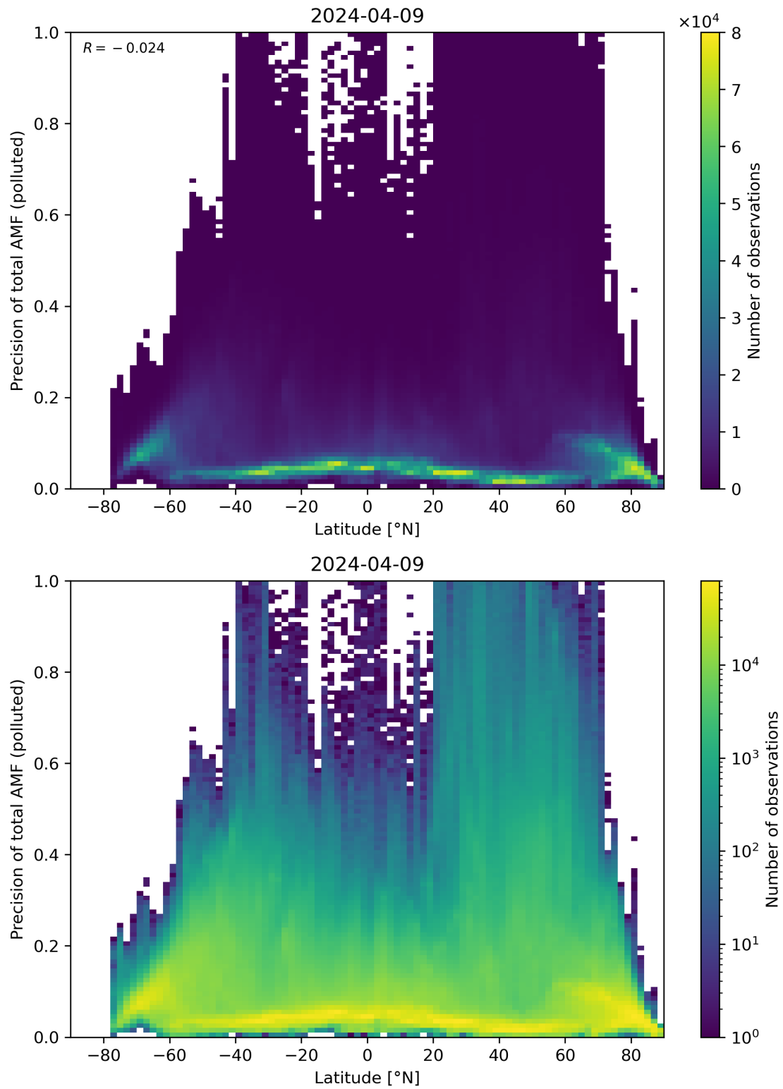
Figure 155: Scatter density plot of “Latitude” against “Precision of total AMF (polluted)” for 2024-04-08 to 2024-04-10.
