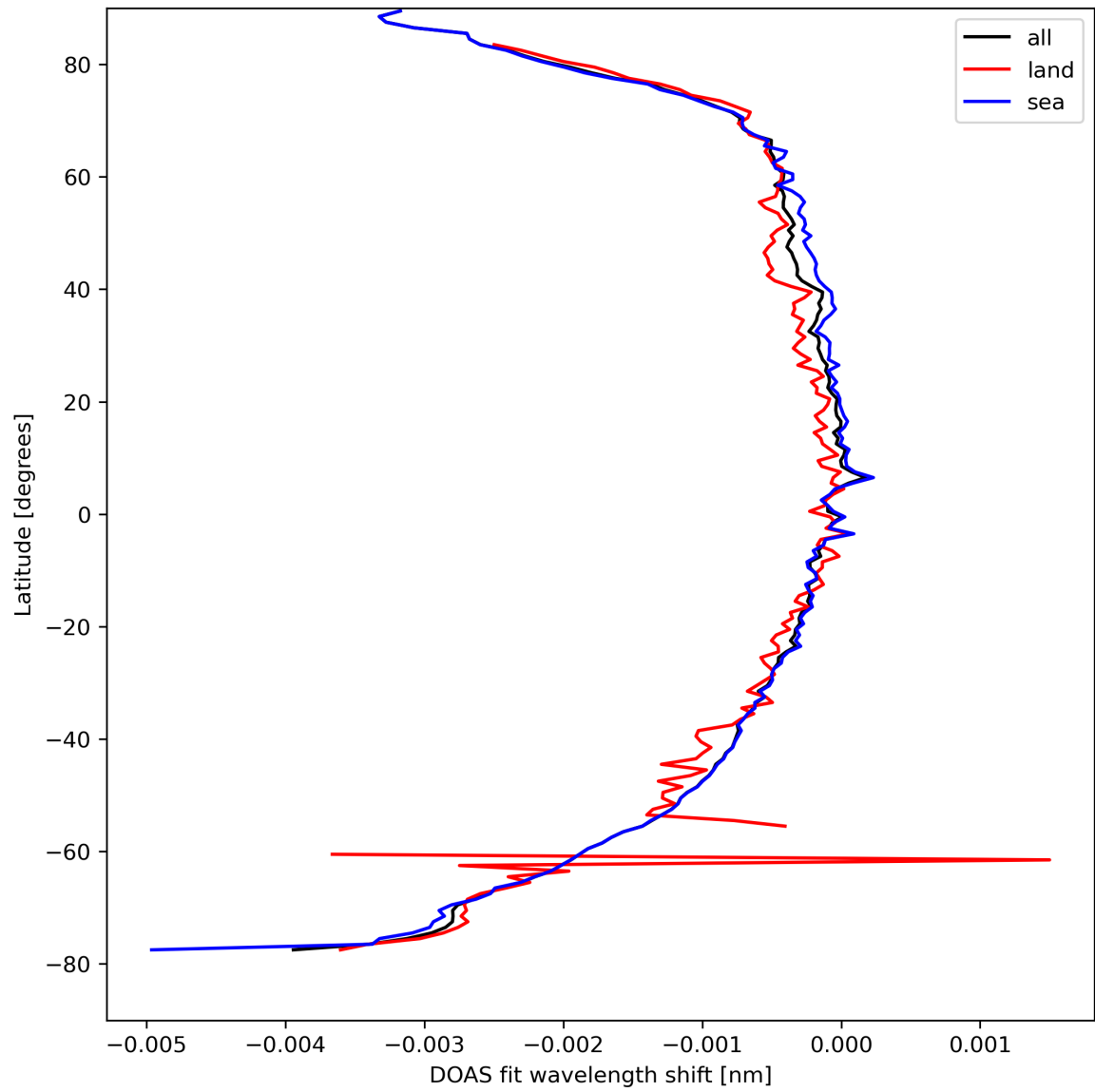
Figure 45: Zonal average of “DOAS fit wavelength shift” for 2024-04-08 to 2024-04-10.
