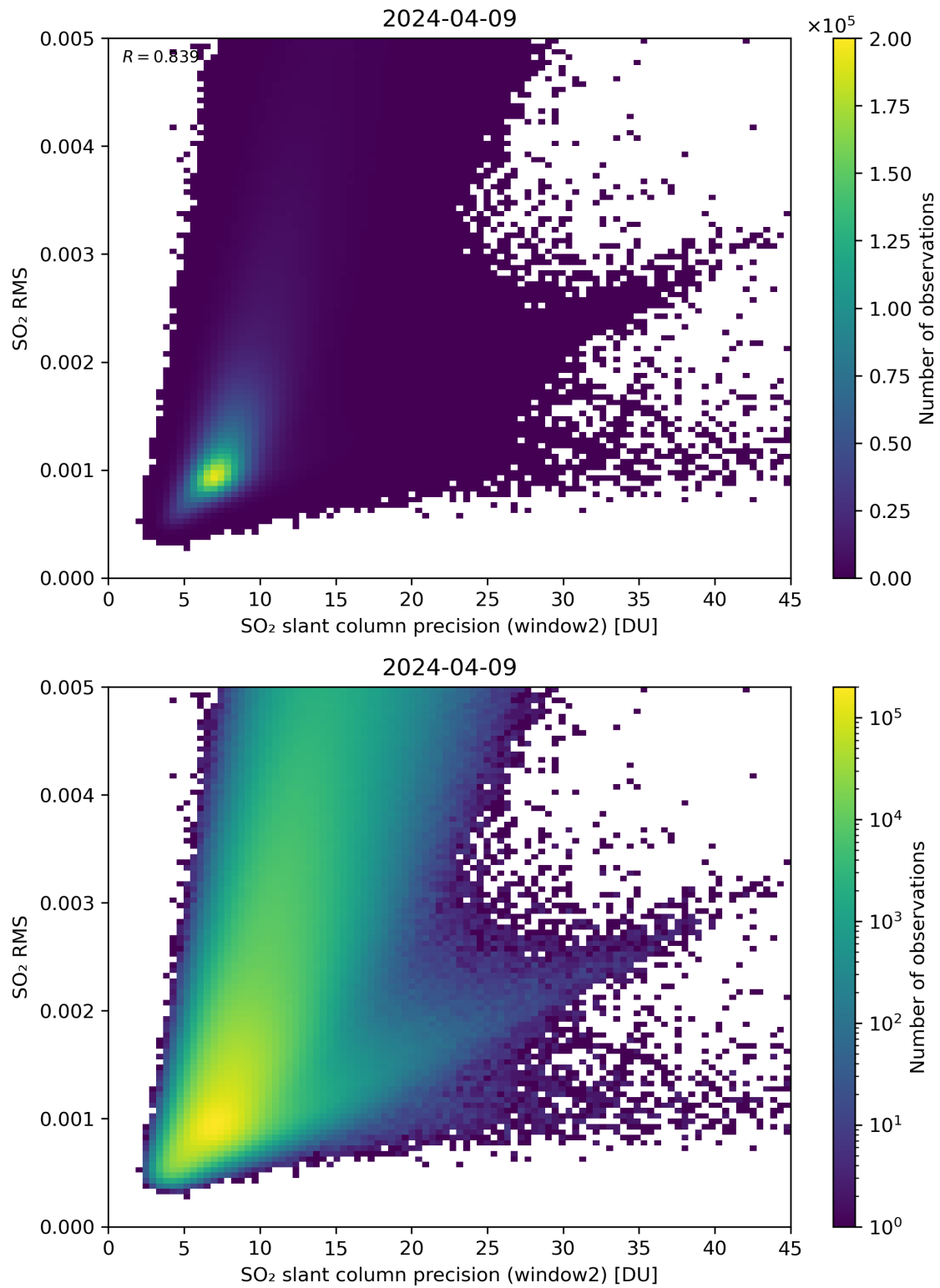
Figure 245: Scatter density plot of “SO 2 slant column precision (window2)” against “SO 2 RMS” for 2024-04-08 to 2024-04-10.
