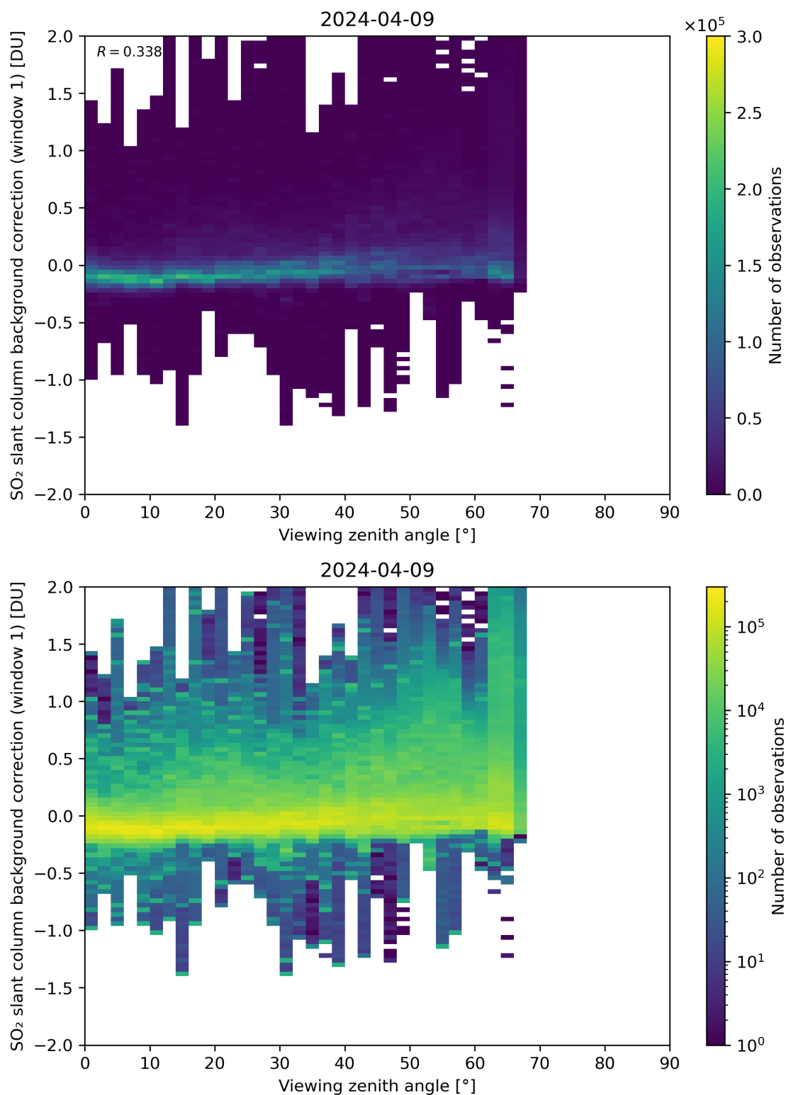
Figure 308: Scatter density plot of “Viewing zenith angle” against “SO 2 slant column background correction (window 1)” for 2024-04-08 to 2024-04-10.
