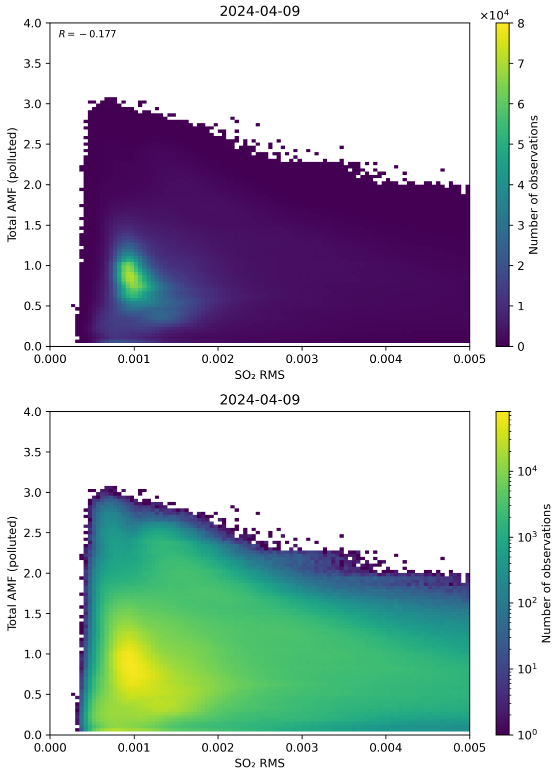
Figure 137: Scatter density plot of “SO 2 RMS” against “Total AMF (polluted)” for 2024-04-08 to 2024-04-10.
