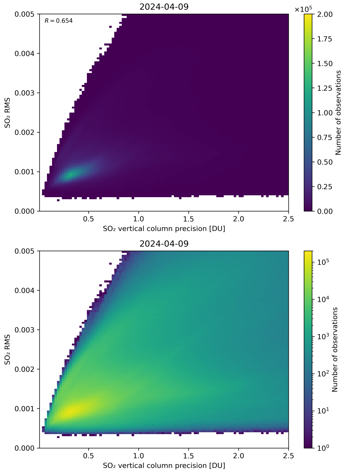
Figure 284: Scatter density plot of “SO 2 vertical column precision” against “SO 2 RMS” for 2024-04-08 to 2024-04-10.
