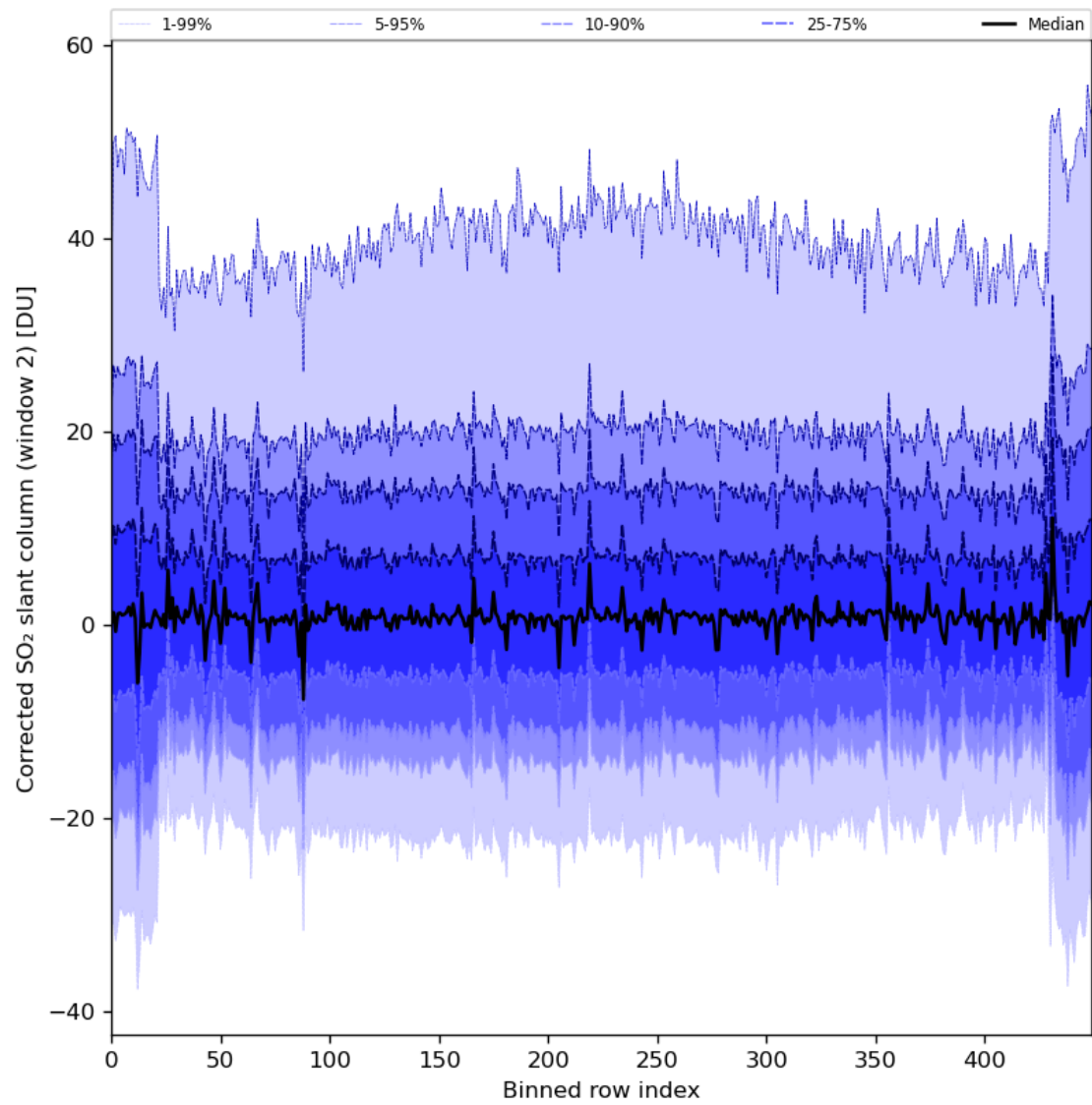
Figure 85: Along track statistics of “Corrected SO 2 slant column (window 2)” for 2024-04-08 to 2024-04-10
