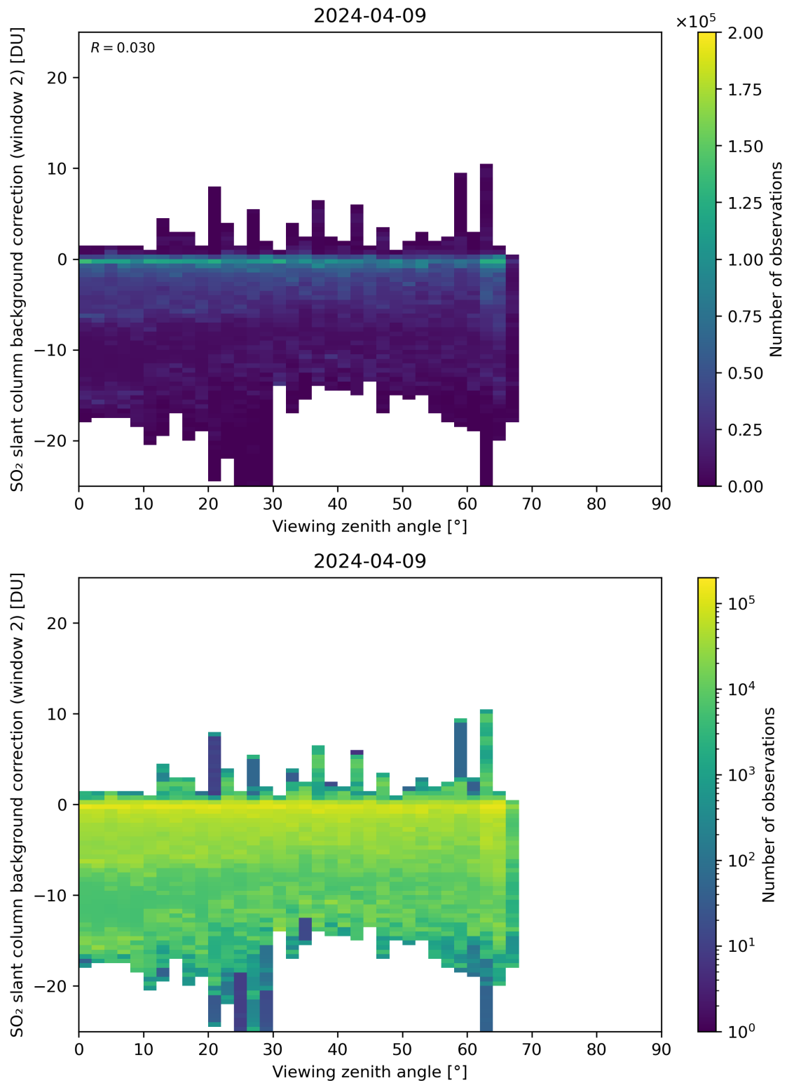
Figure 309: Scatter density plot of “Viewing zenith angle” against “SO 2 slant column background correction (window 2)” for 2024-04-08 to 2024-04-10.
