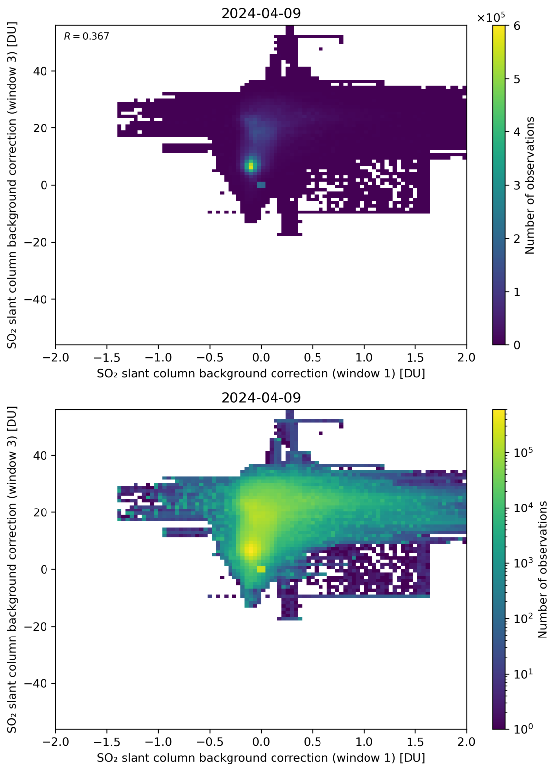
Figure 99: Scatter density plot of “SO 2 slant column background correction (window 1)” against “SO 2 slant column background correction (window 3)” for 2024-04-08 to 2024-04-10.
