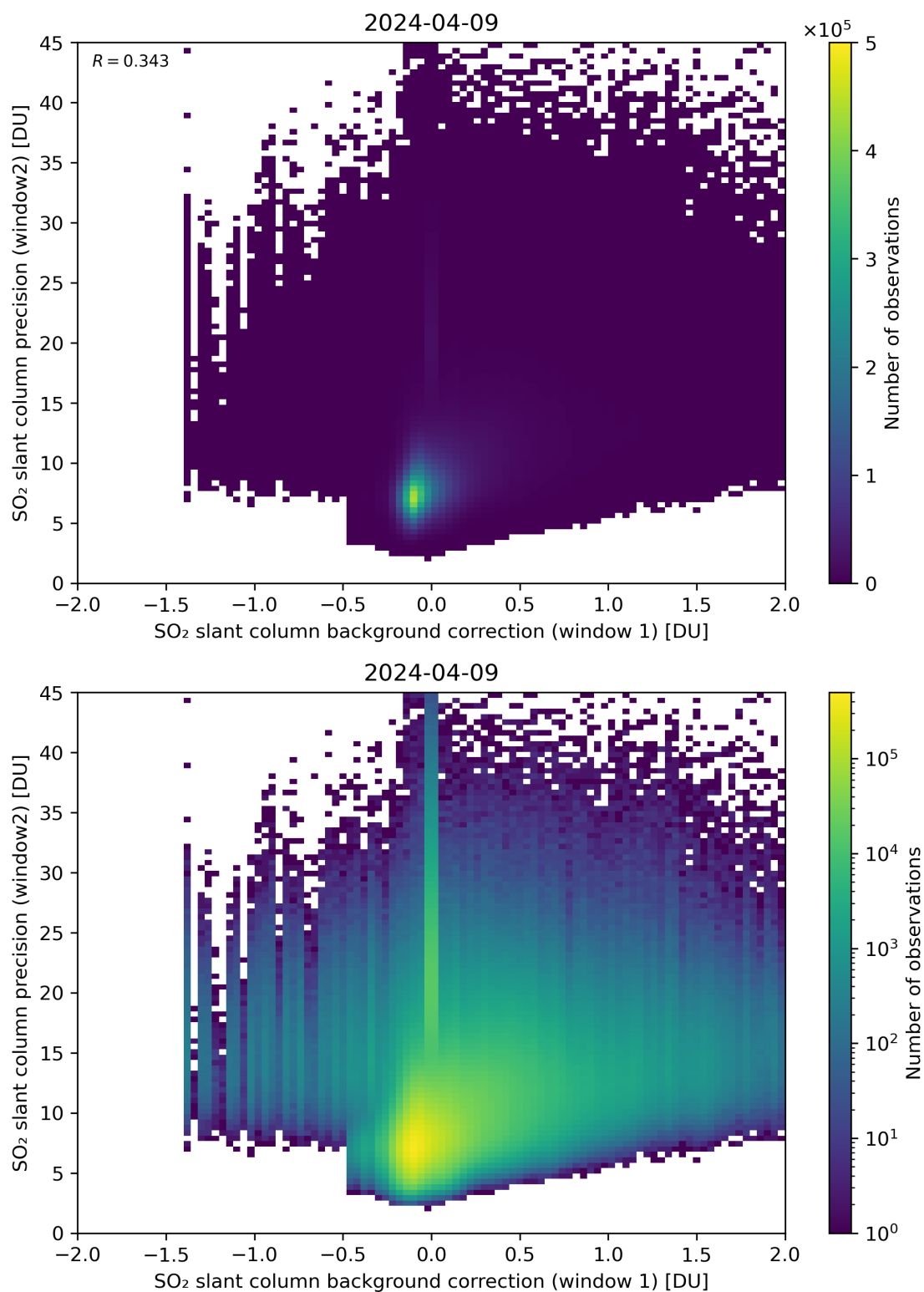
Figure 106: Scatter density plot of “SO 2 slant column background correction (window 1)” against “SO 2 slant column precision (window2)” for 2024-04-08 to 2024-04-10.
