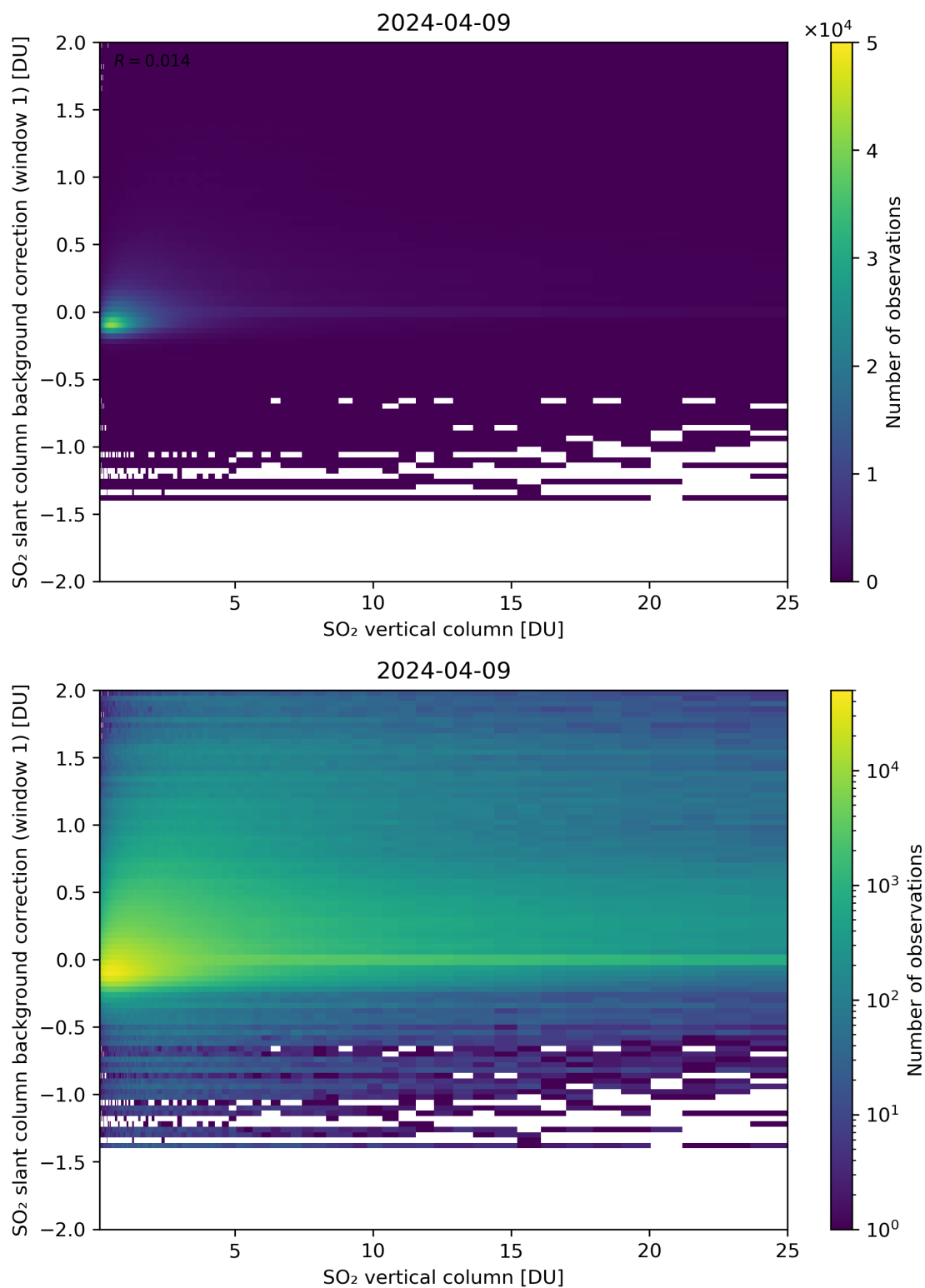
Figure 273: Scatter density plot of “SO 2 vertical column” against “SO 2 slant column background correction (window 1)” for 2024-04-08 to 2024-04-10.
