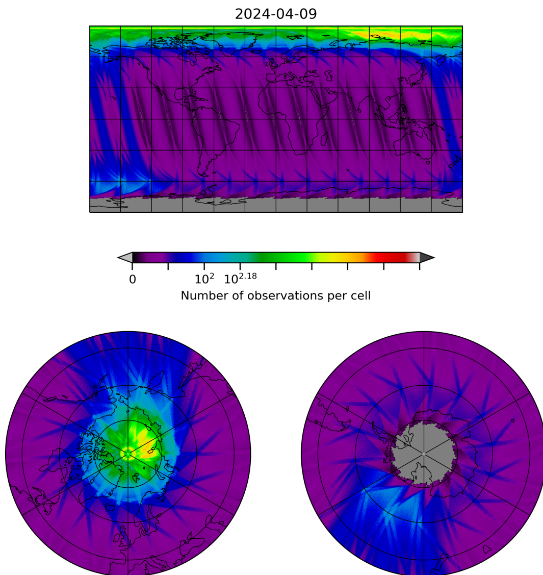
Figure 28: Map of the number of observations for 2024-04-08 to 2024-04-10
