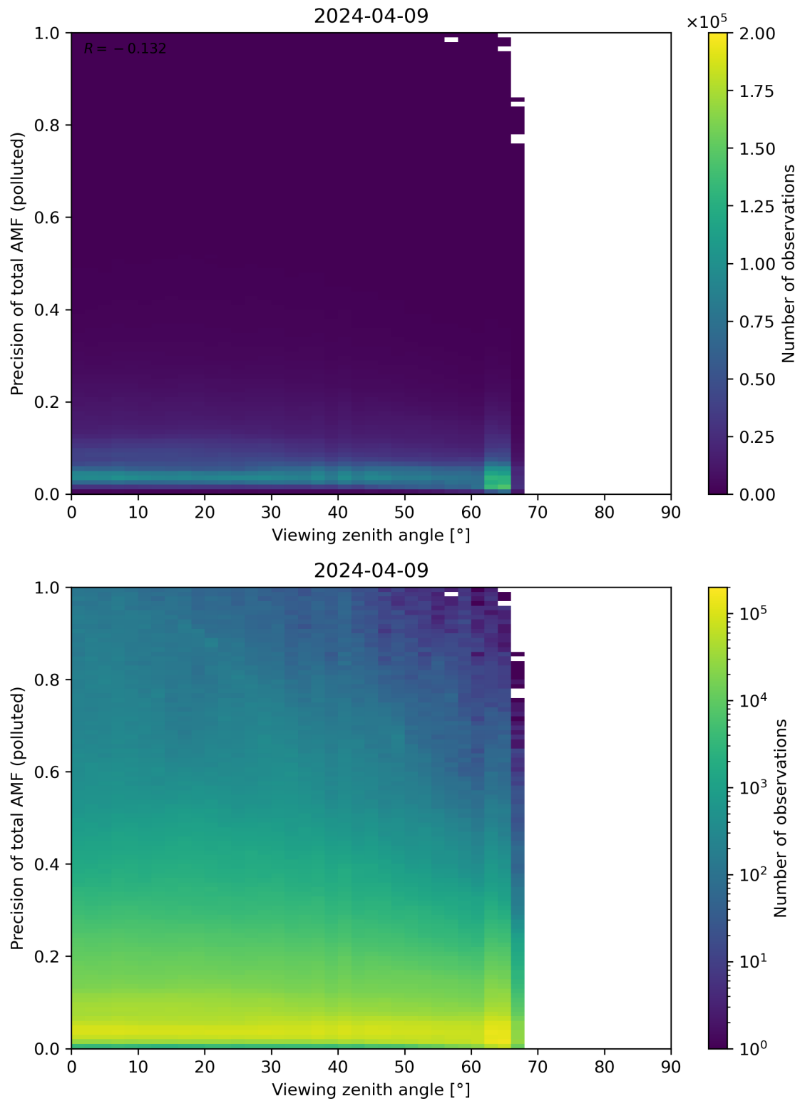
Figure 326: Scatter density plot of “Viewing zenith angle” against “Precision of total AMF (polluted)” for 2024-04-08 to 2024-04-10.
