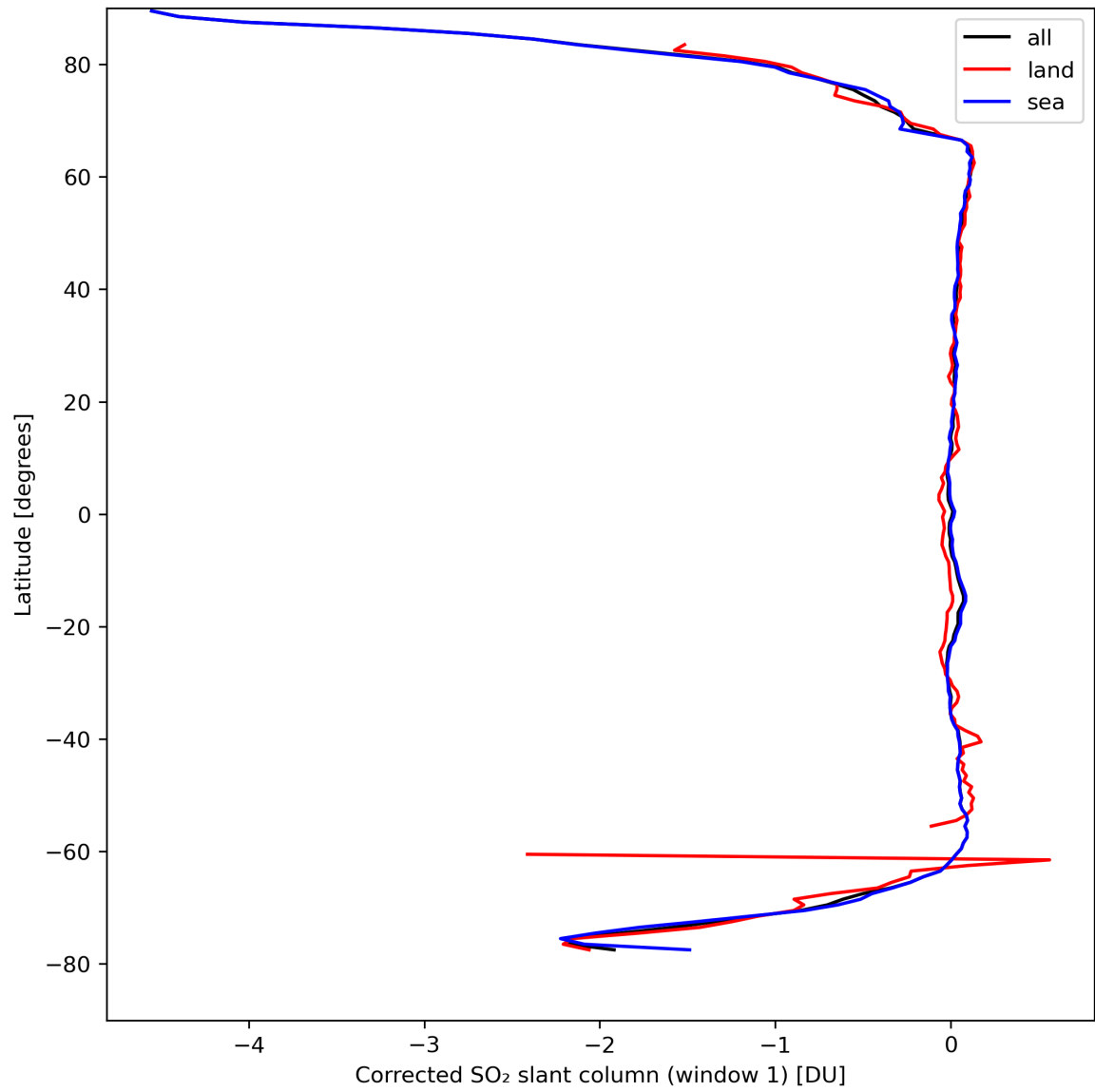
Figure 35: Zonal average of “Corrected SO 2 slant column (window 1)” for 2024-04-08 to 2024-04-10.
