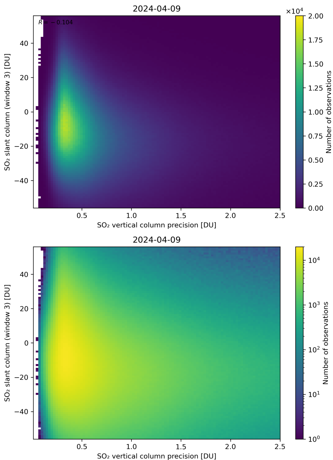
Figure 292: Scatter density plot of “SO 2 vertical column precision” against “SO 2 slant column (window 3)” for 2024-04-08 to 2024-04-10.
