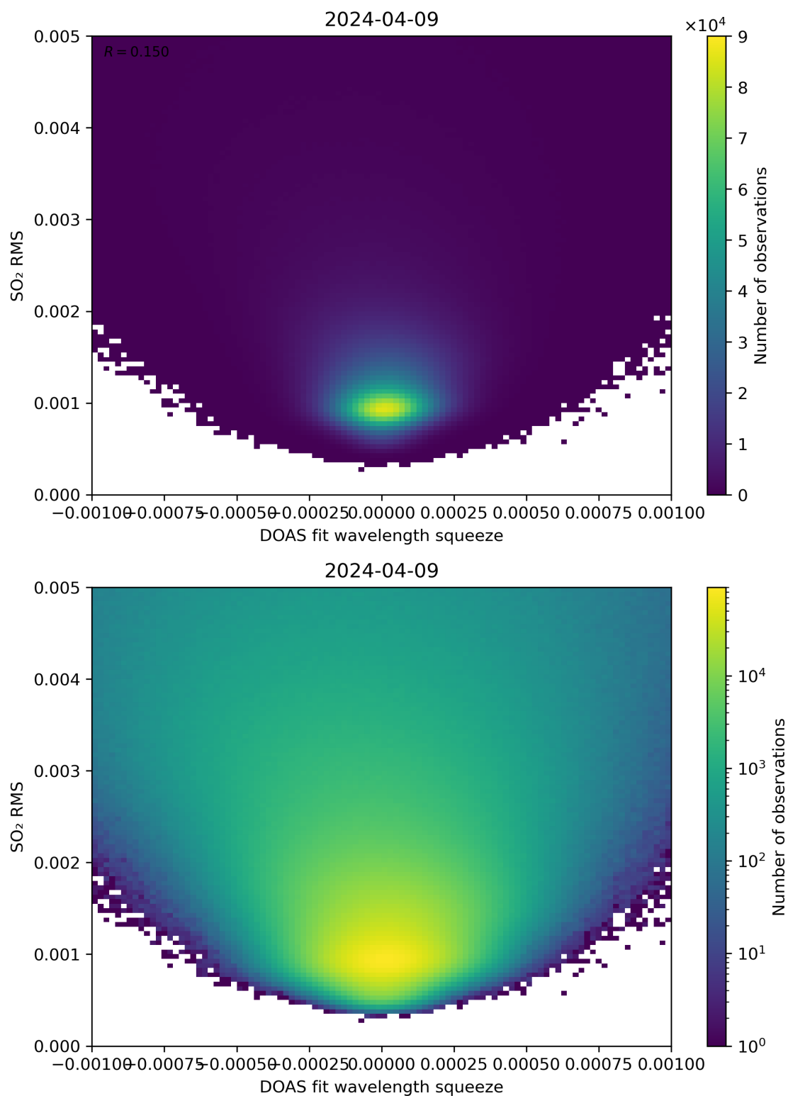
Figure 132: Scatter density plot of “DOAS fit wavelength squeeze” against “SO 2 RMS” for 2024-04-08 to 2024-04-10.
