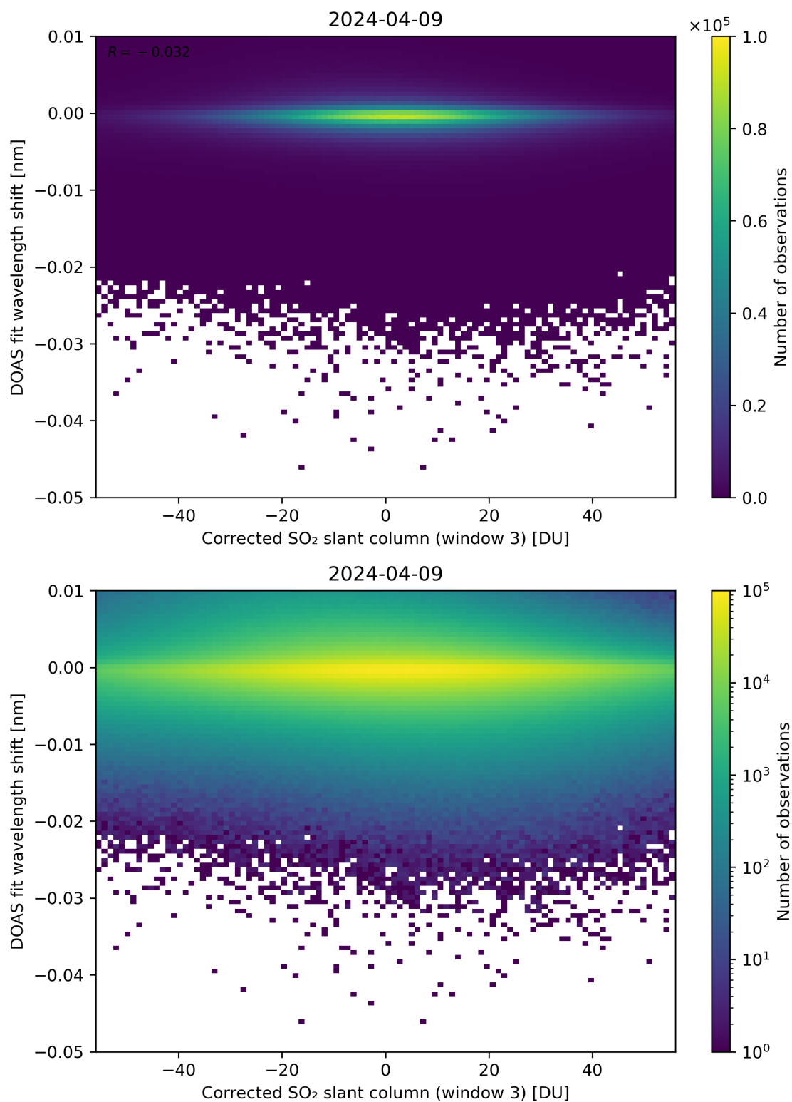
Figure 206: Scatter density plot of “Corrected SO 2 slant column (window 3)” against “DOAS fit wavelength shift” for 2024-04-08 to 2024-04-10.
