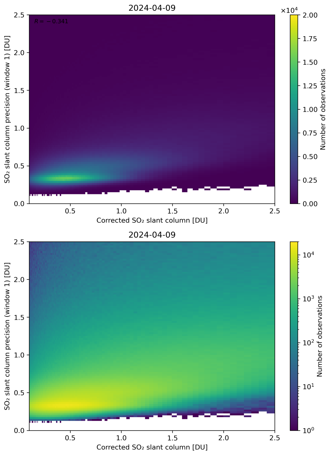
Figure 188: Scatter density plot of “Corrected SO 2 slant column” against “SO 2 slant column precision (window 1)” for 2024-04-08 to 2024-04-10.
