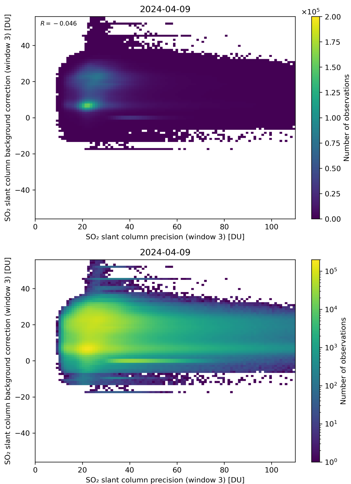
Figure 257: Scatter density plot of “SO 2 slant column precision (window 3)” against “SO 2 slant column background correction (window 3)” for 2024-04-08 to 2024-04-10.
