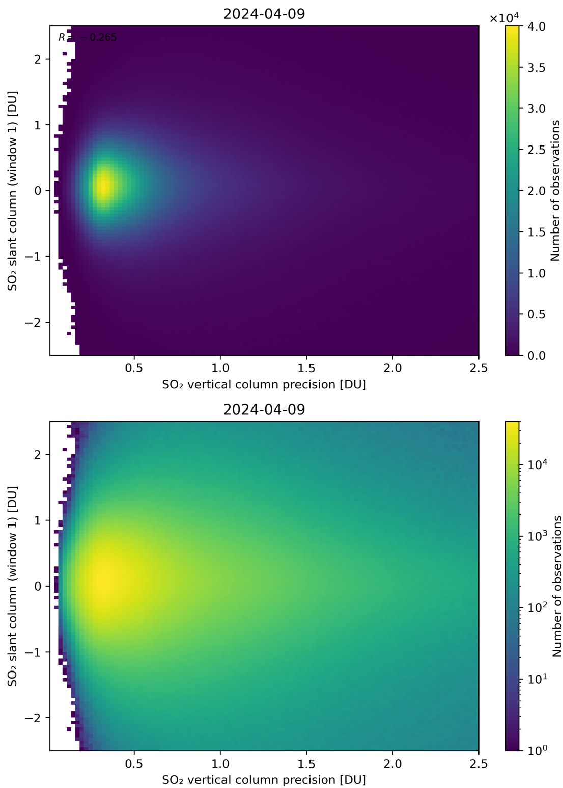
Figure 289: Scatter density plot of “SO 2 vertical column precision” against “SO 2 slant column (window 1)” for 2024-04-08 to 2024-04-10.
