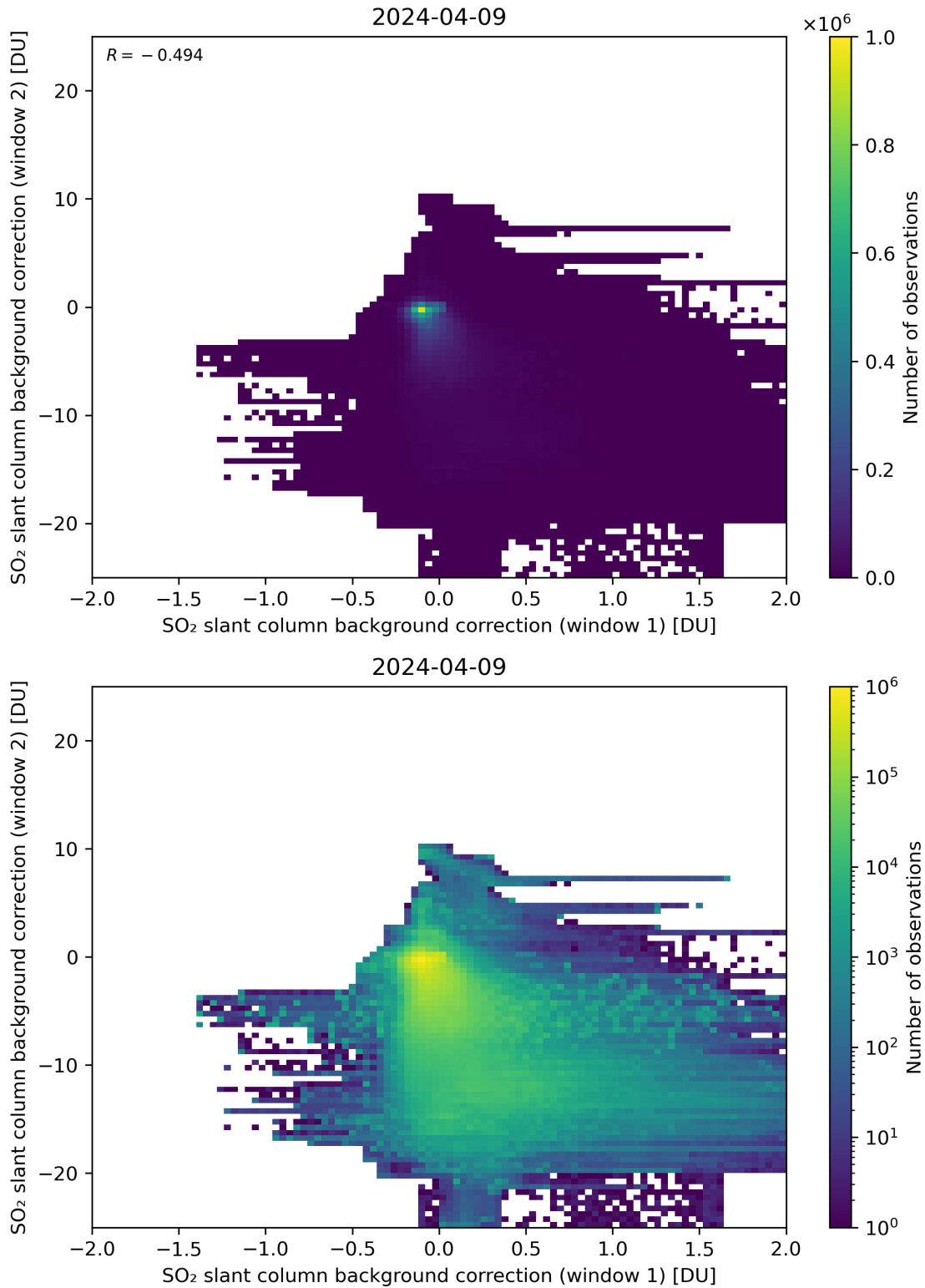
Figure 98: Scatter density plot of “SO 2 slant column background correction (window 1)” against “SO 2 slant column background correction (window 2)” for 2024-04-08 to 2024-04-10.
