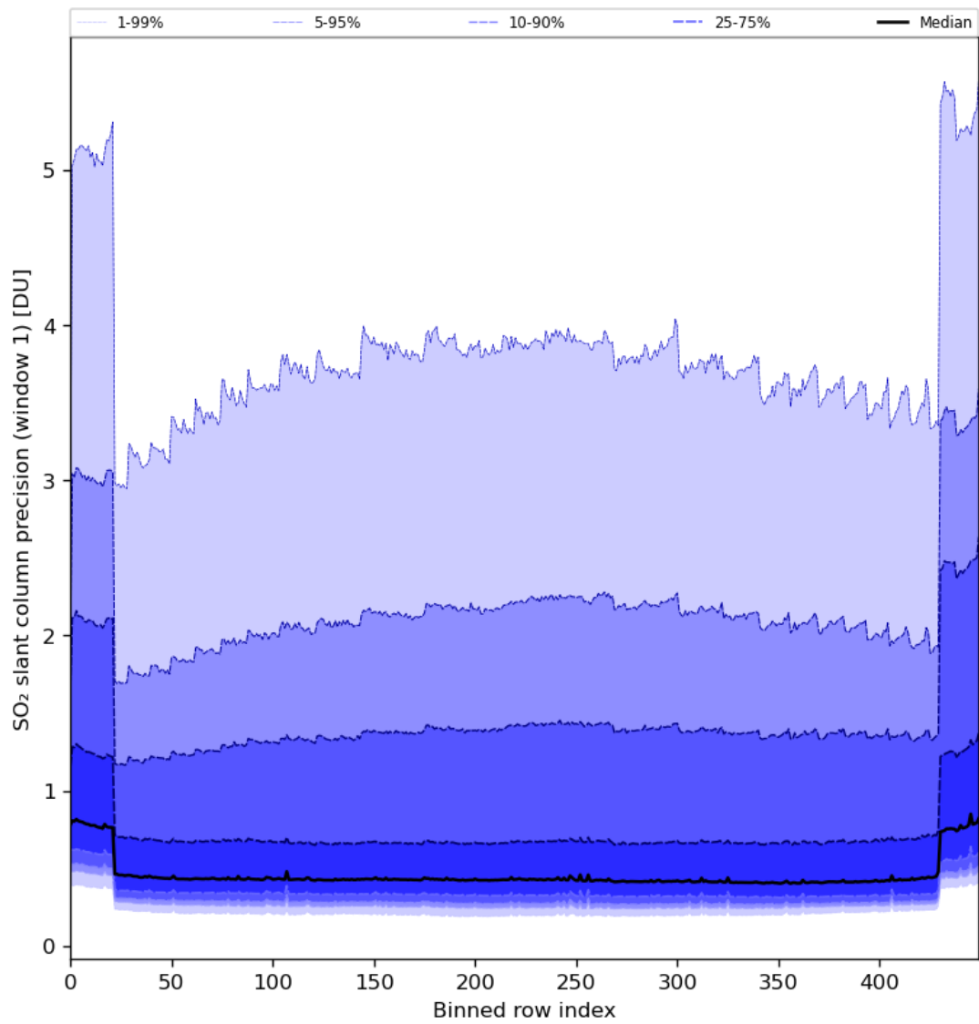
Figure 80: Along track statistics of “SO 2 slant column precision (window 1)” for 2024-04-08 to 2024-04-10
