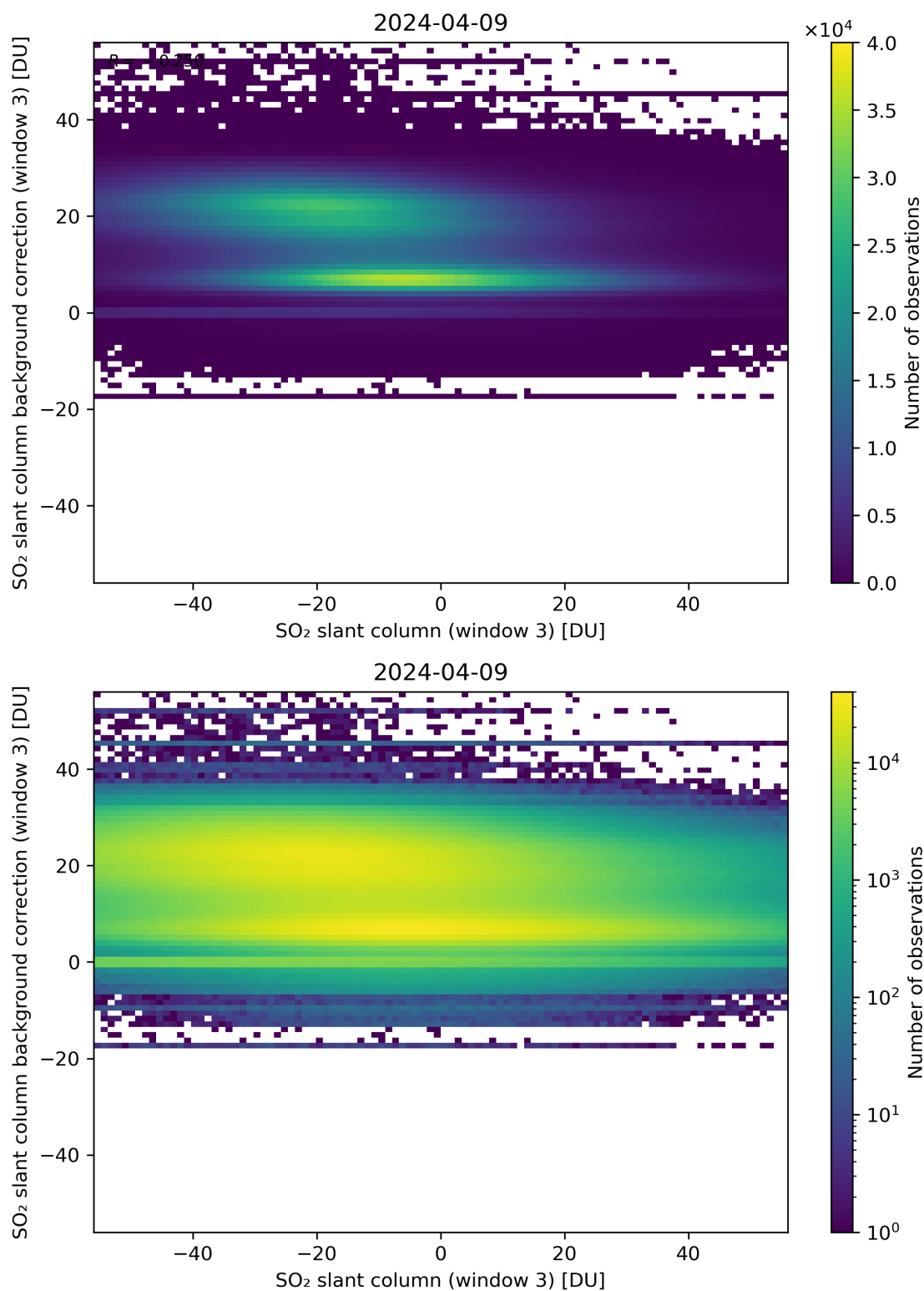
Figure 253: Scatter density plot of “SO 2 slant column (window 3)” against “SO 2 slant column background correction (window 3)” for 2024-04-08 to 2024-04-10.
