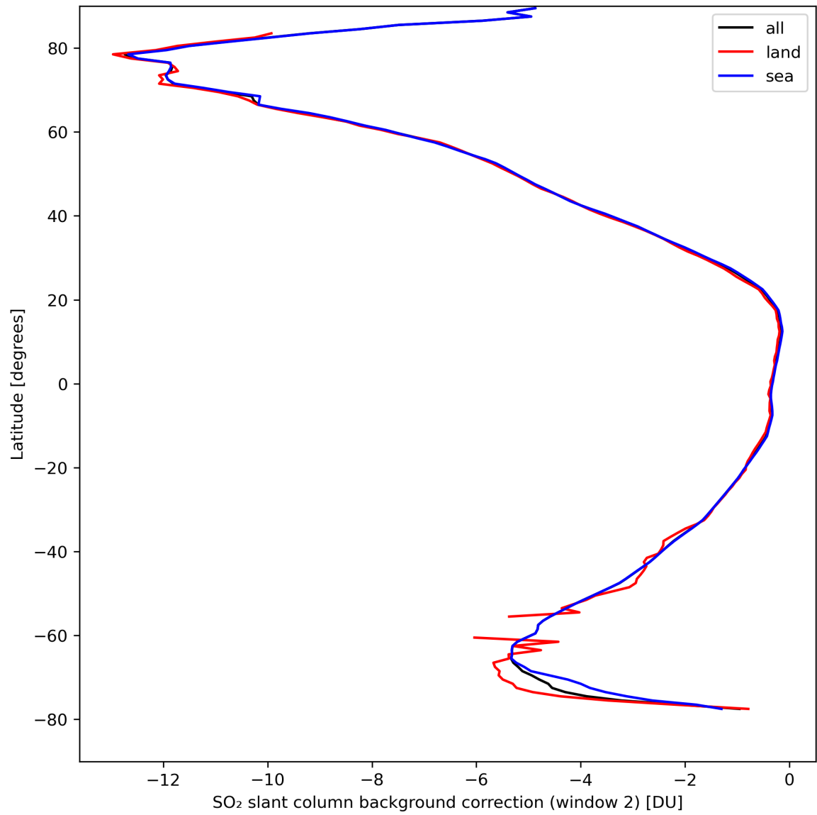
Figure 40: Zonal average of “SO 2 slant column background correction (window 2)” for 2024-04-08 to 2024-04-10.
