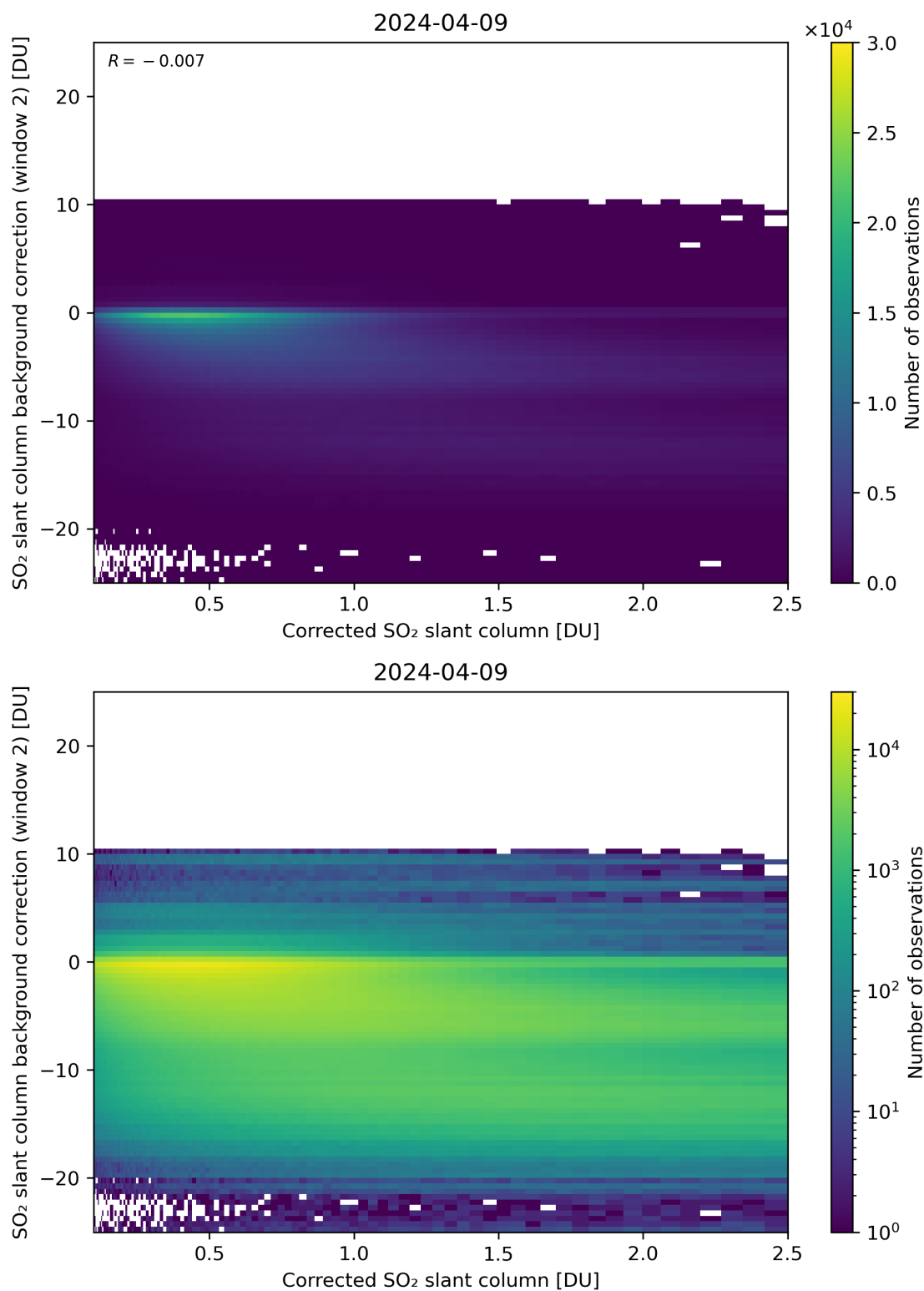
Figure 179: Scatter density plot of “Corrected SO 2 slant column” against “SO 2 slant column background correction (window 2)” for 2024-04-08 to 2024-04-10.
