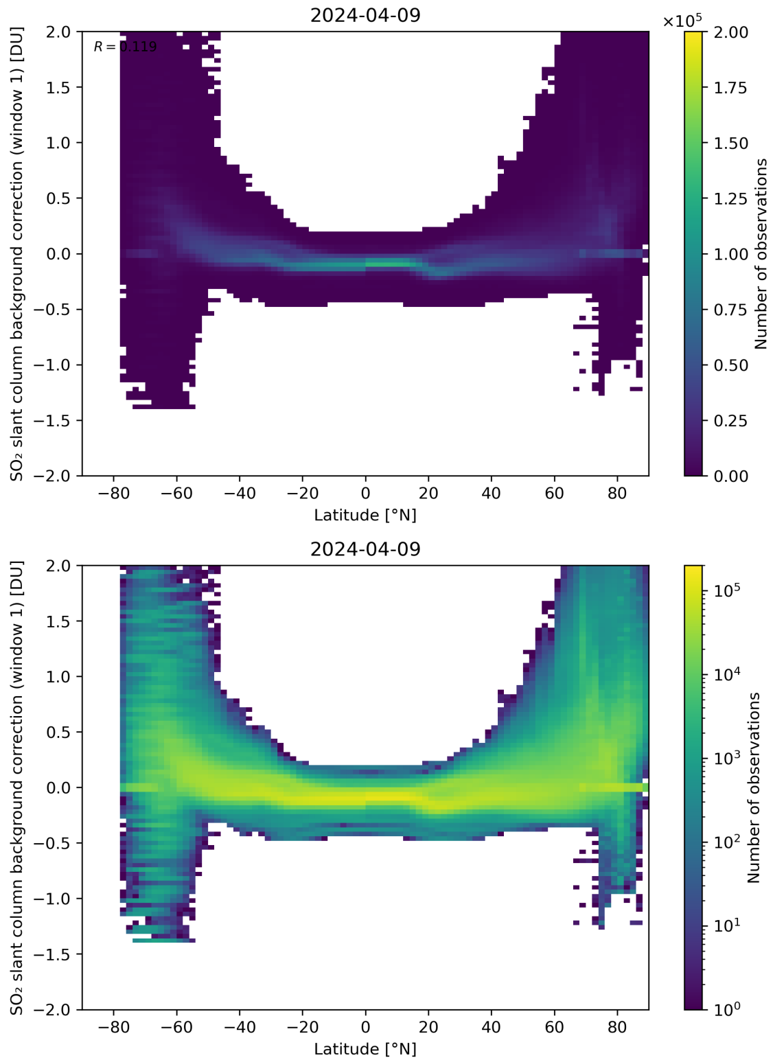
Figure 139: Scatter density plot of “Latitude” against “SO 2 slant column background correction (window 1)” for 2024-04-08 to 2024-04-10.
