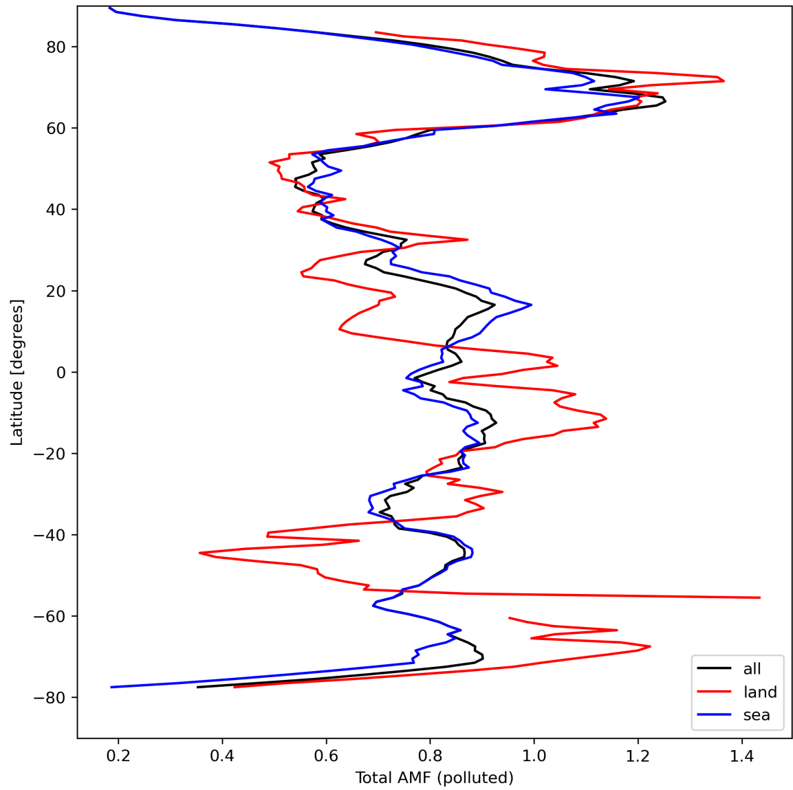
Figure 48: Zonal average of “Total AMF (polluted)” for 2024-04-08 to 2024-04-10.
