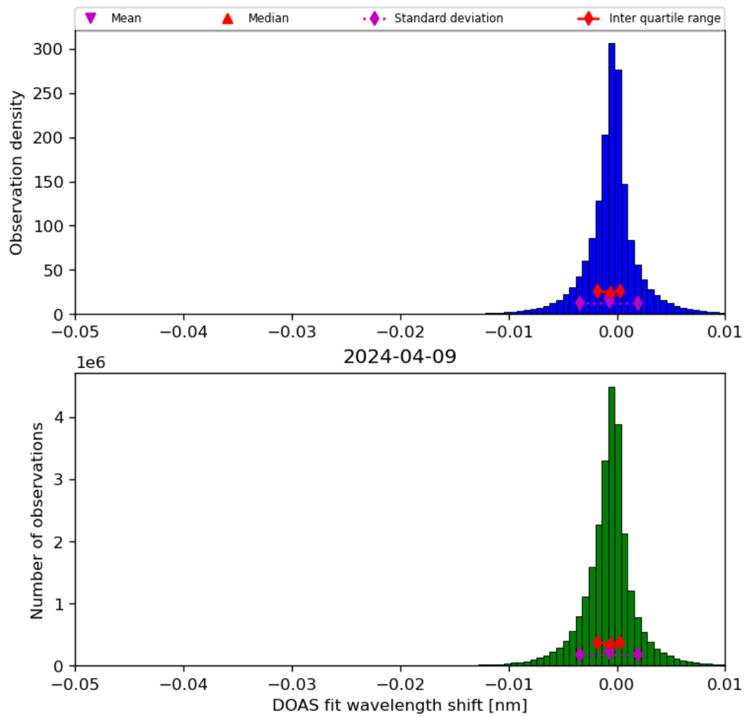
Figure 68: Histogram of “DOAS fit wavelength shift” for 2024-04-08 to 2024-04-10
