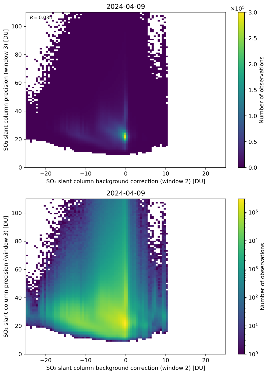
Figure 118: Scatter density plot of “SO 2 slant column background correction (window 2)” against “SO 2 slant column precision (window 3)” for 2024-04-08 to 2024-04-10.
