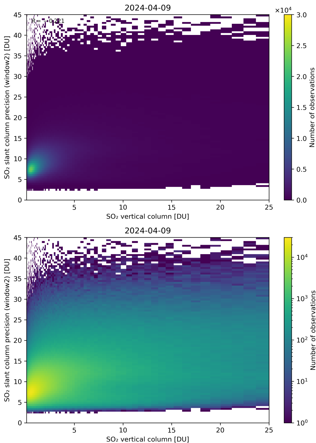
Figure 302: Scatter density plot of “SO 2 vertical column” against “SO 2 slant column precision (window2)” for 2024-04-08 to 2024-04-10.
