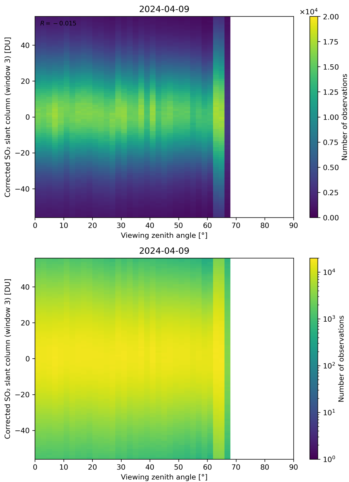
Figure 319: Scatter density plot of “Viewing zenith angle” against “Corrected SO 2 slant column (window 3)” for 2024-04-08 to 2024-04-10.
