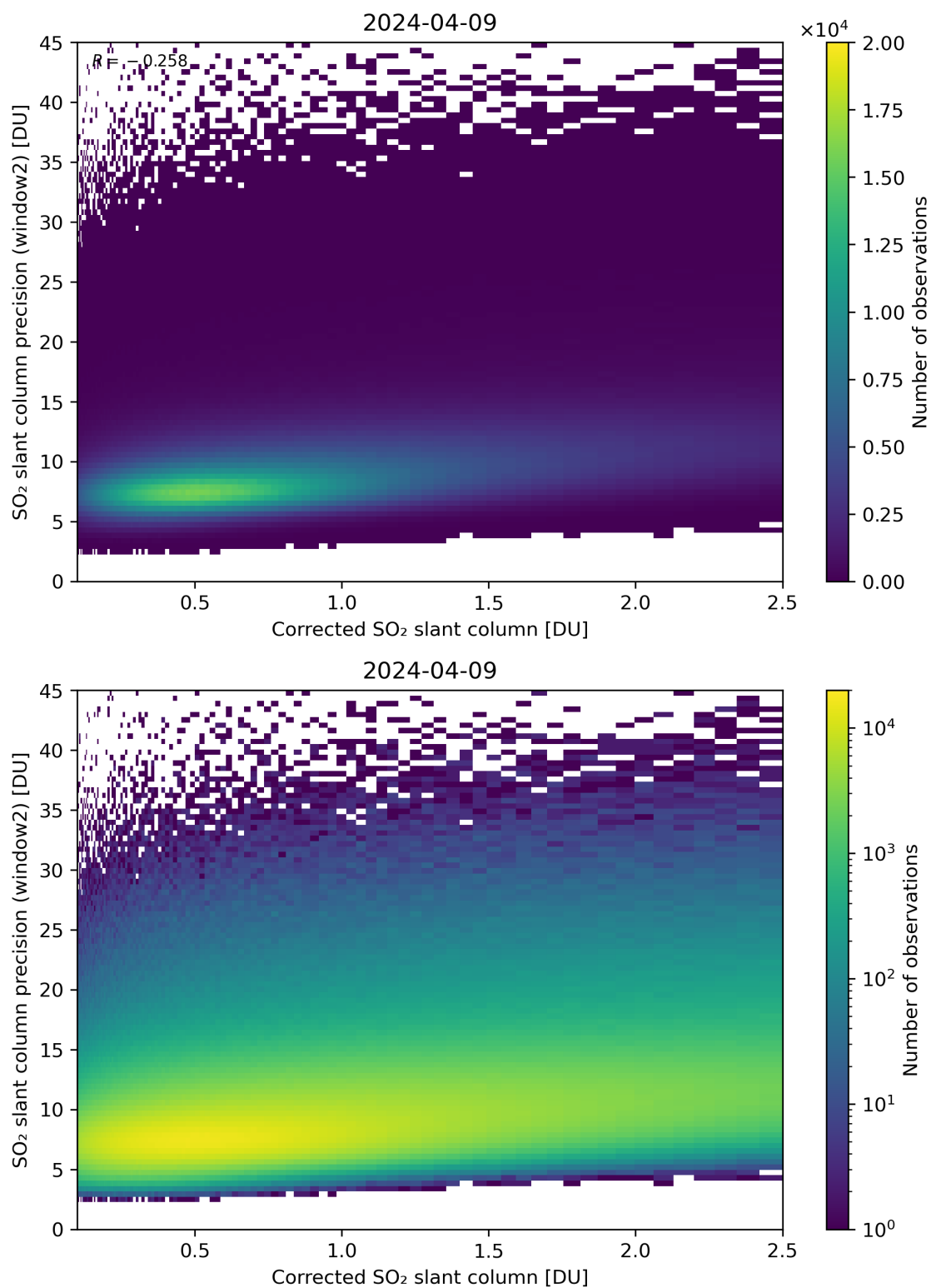
Figure 189: Scatter density plot of “Corrected SO 2 slant column” against “SO 2 slant column precision (window2)” for 2024-04-08 to 2024-04-10.
