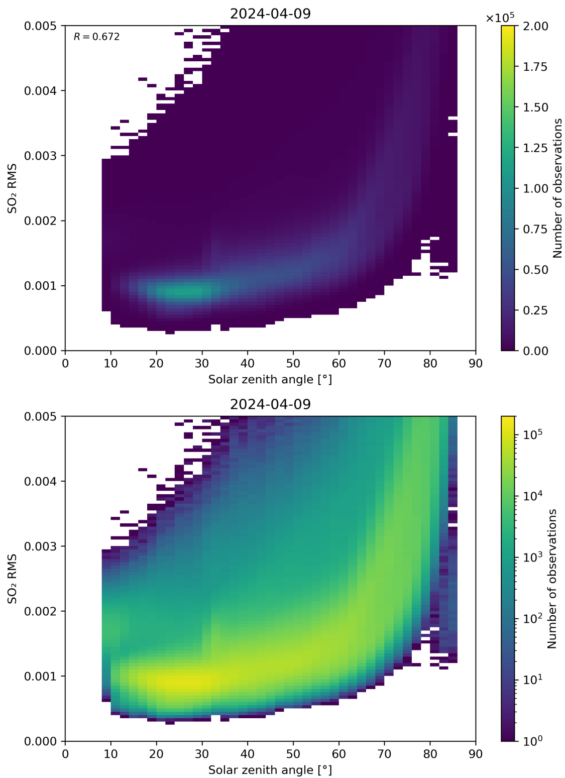
Figure 163: Scatter density plot of “Solar zenith angle” against “SO 2 RMS” for 2024-04-08 to 2024-04-10.
