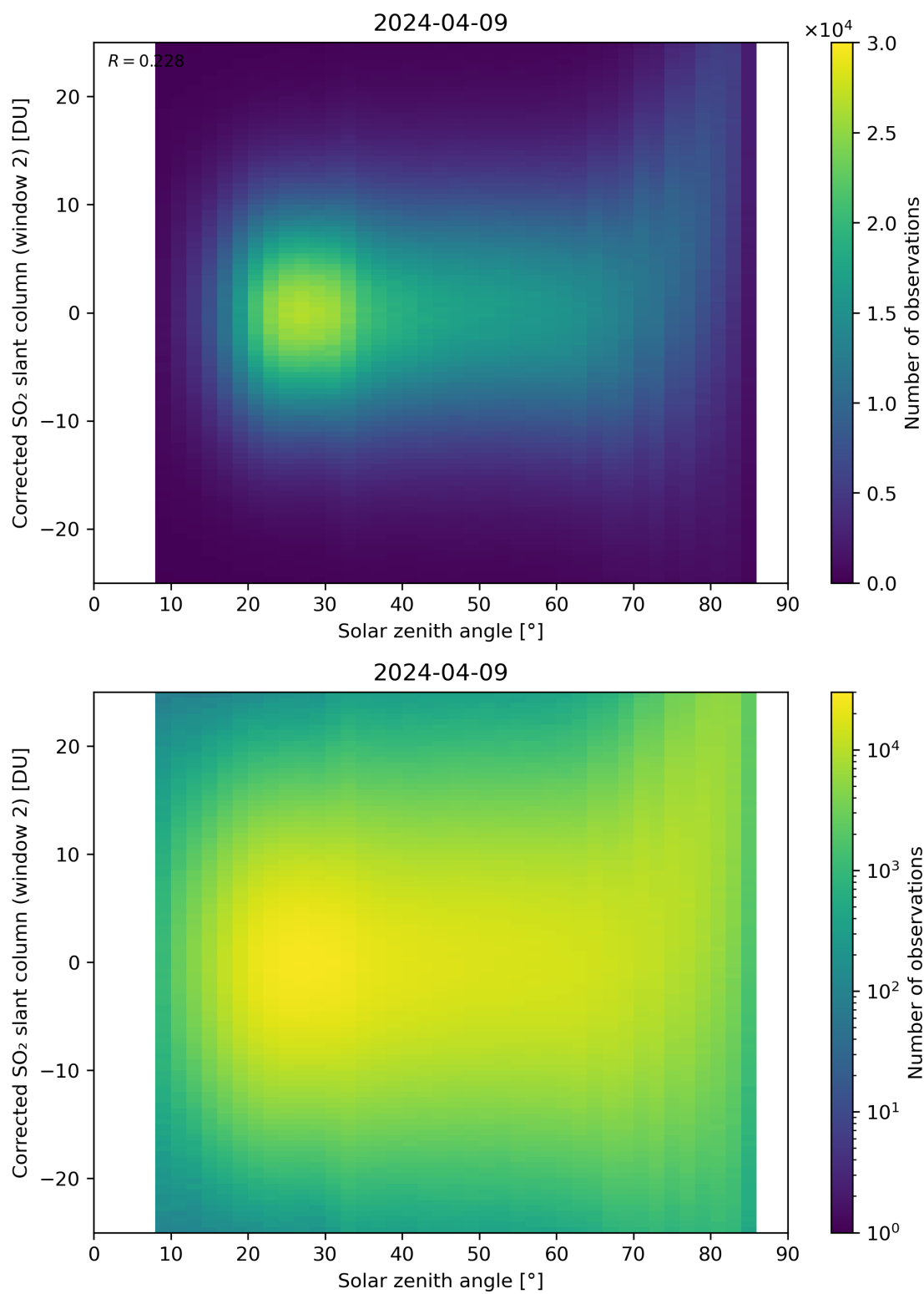
Figure 167: Scatter density plot of “Solar zenith angle” against “Corrected SO 2 slant column (window 2)” for 2024-04-08 to 2024-04-10.
