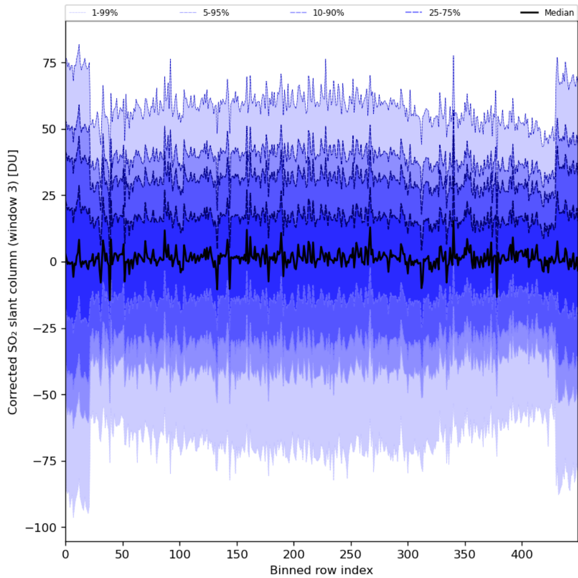
Figure 89: Along track statistics of “Corrected SO 2 slant column (window 3)” for 2024-04-08 to 2024-04-10
