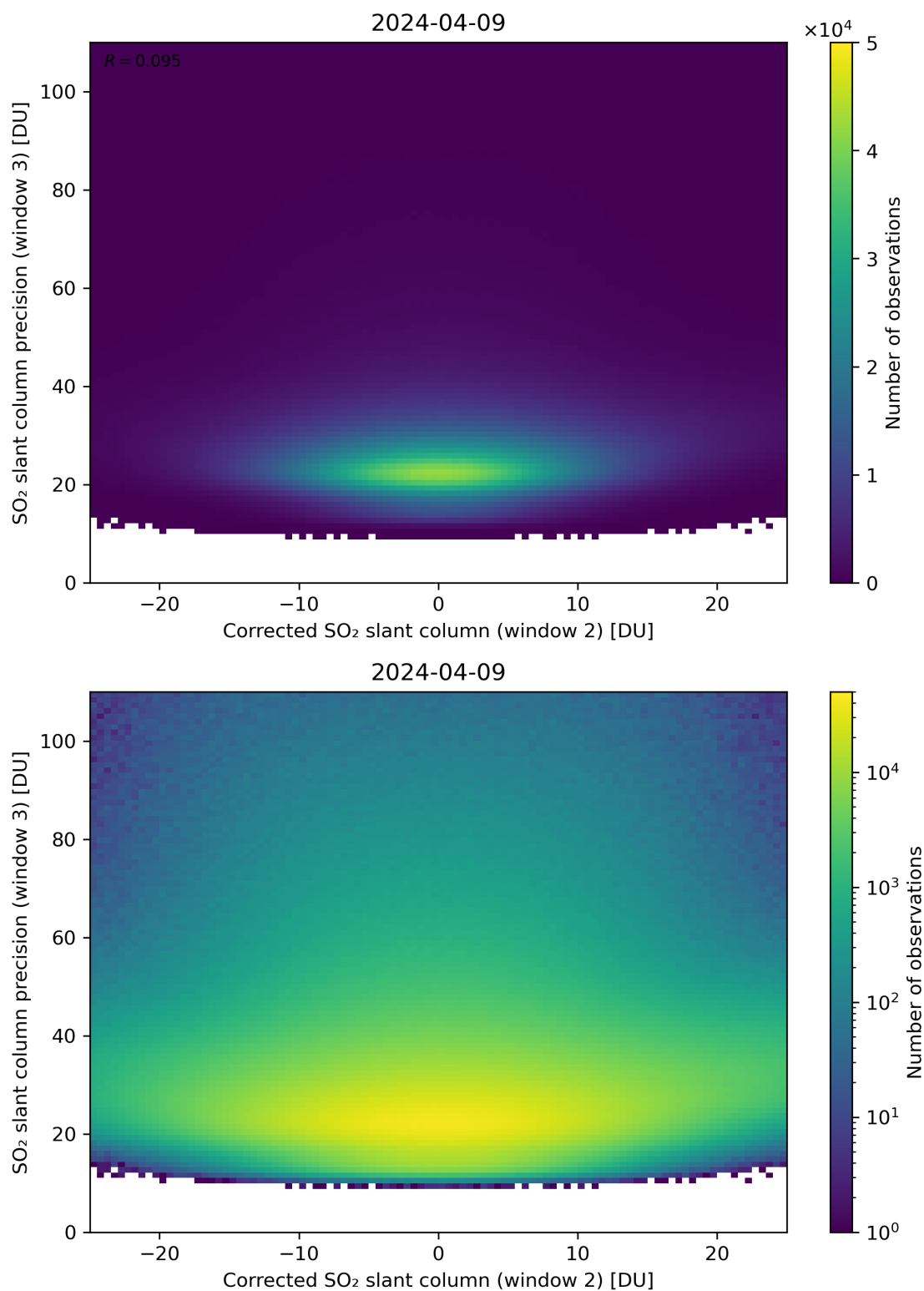
Figure 202: Scatter density plot of “Corrected SO 2 slant column (window 2)” against “SO 2 slant column precision (window 3)” for 2024-04-08 to 2024-04-10.
