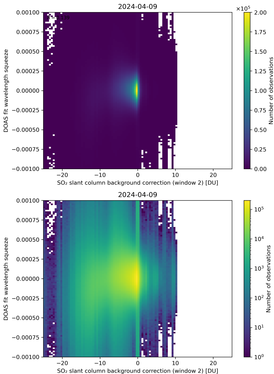
Figure 113: Scatter density plot of “SO 2 slant column background correction (window 2)” against “DOAS fit wavelength squeeze” for 2024-04-08 to 2024-04-10.
