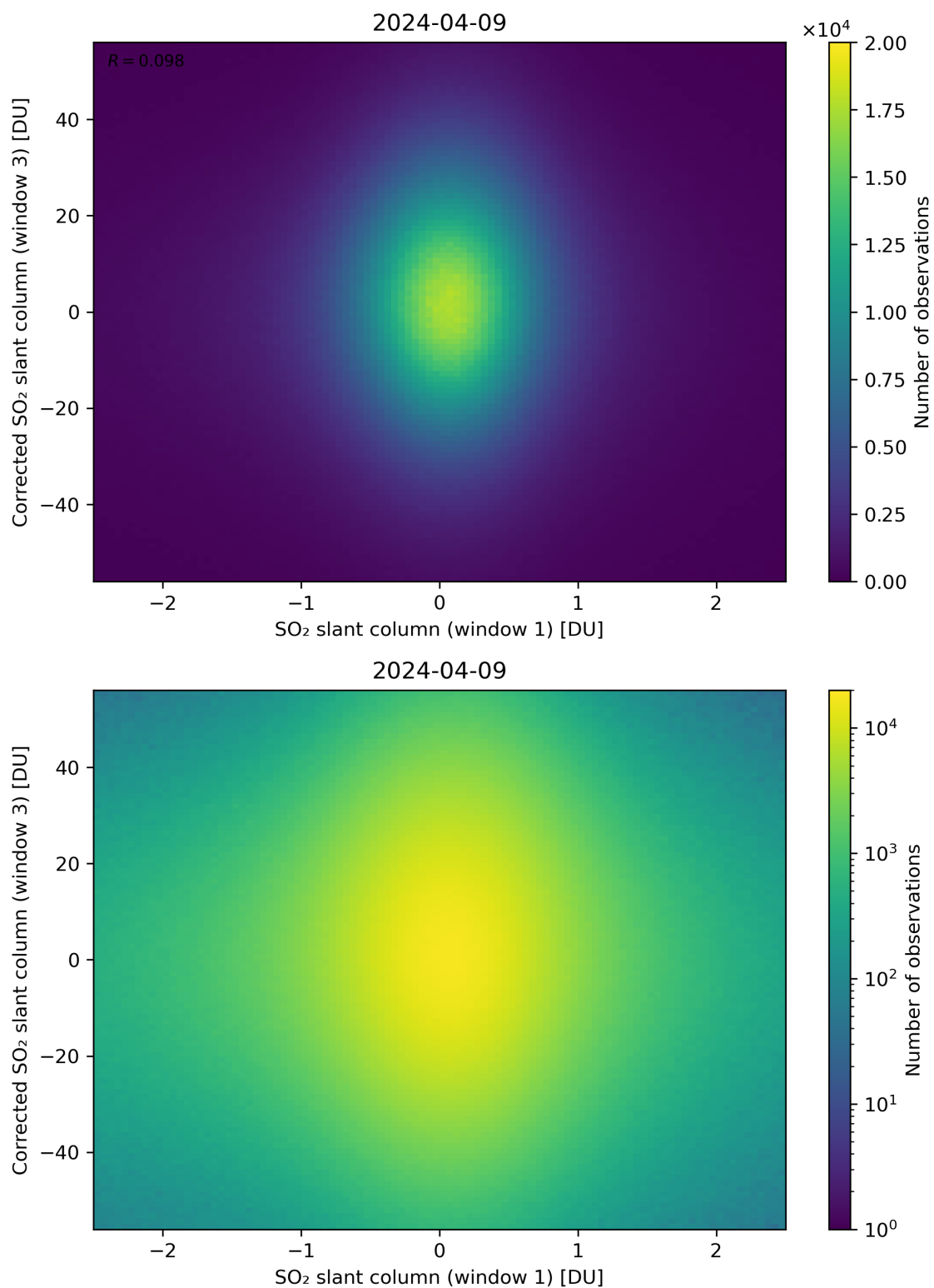
Figure 234: Scatter density plot of “SO 2 slant column (window 1)” against “Corrected SO 2 slant column (window 3)” for 2024-04-08 to 2024-04-10.
