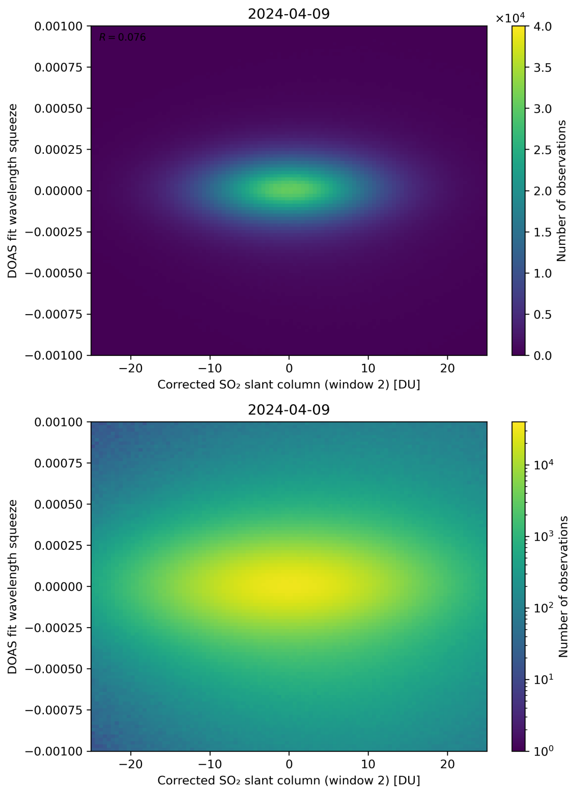
Figure 197: Scatter density plot of “Corrected SO 2 slant column (window 2)” against “DOAS fit wavelength squeeze” for 2024-04-08 to 2024-04-10.
