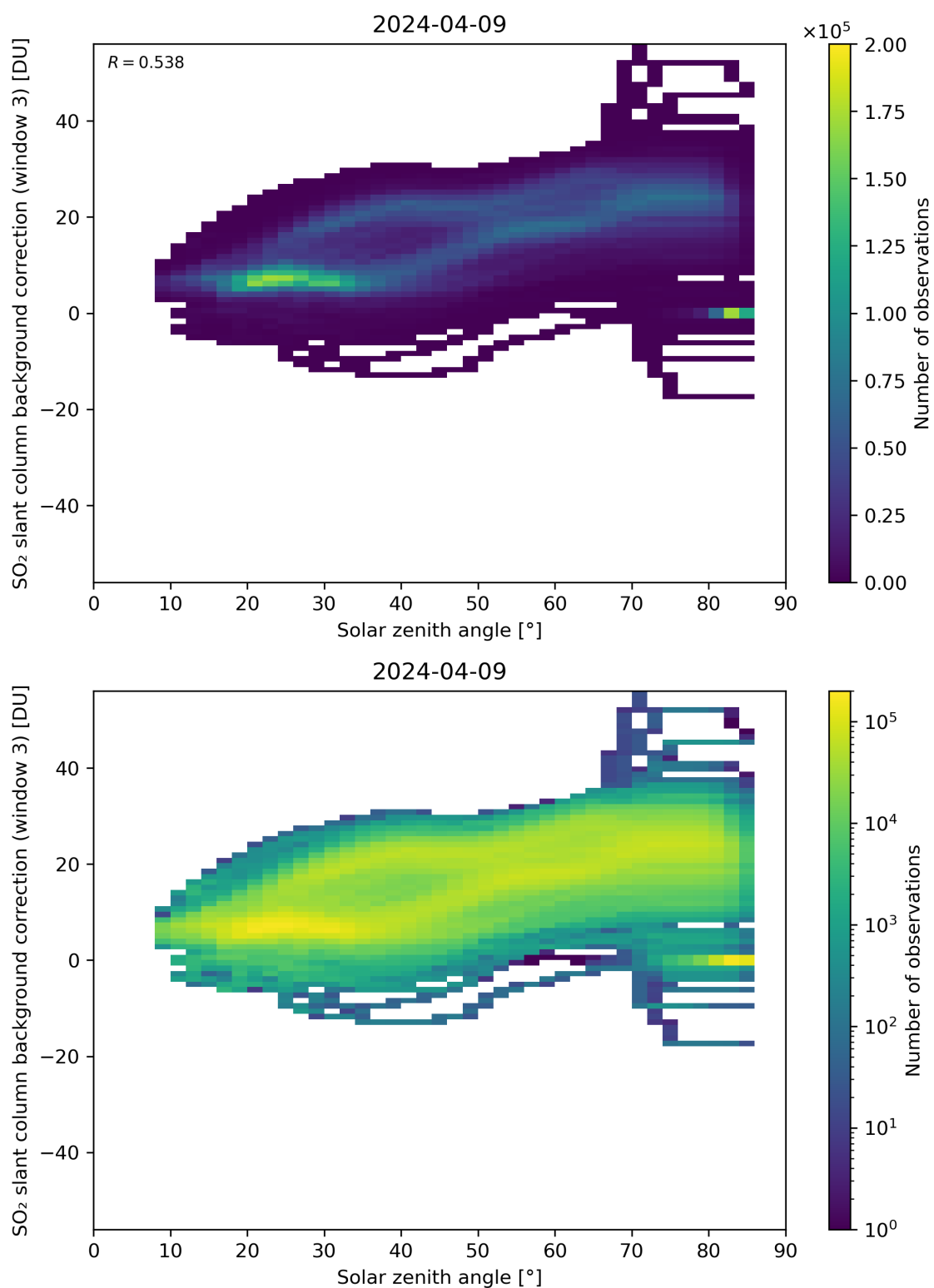
Figure 160: Scatter density plot of “Solar zenith angle” against “SO 2 slant column background correction (window 3)” for 2024-04-08 to 2024-04-10.
