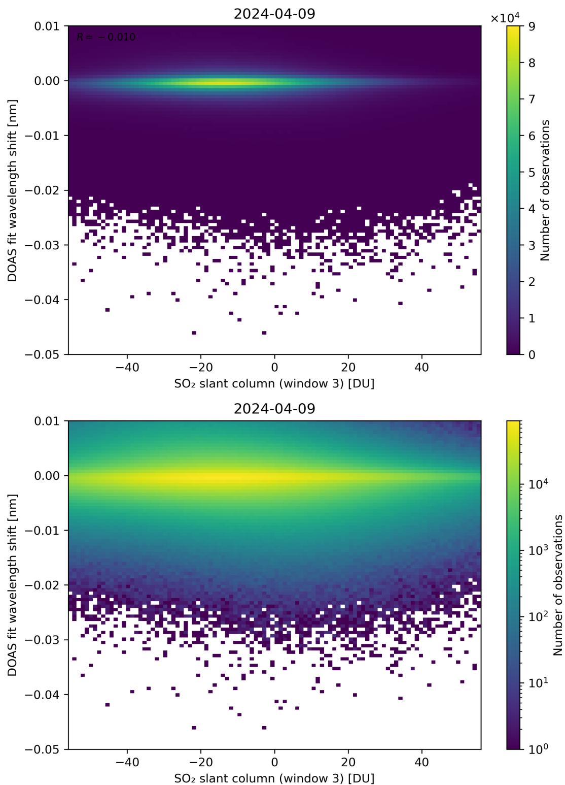
Figure 254: Scatter density plot of “SO 2 slant column (window 3)” against “DOAS fit wavelength shift” for 2024-04-08 to 2024-04-10.
