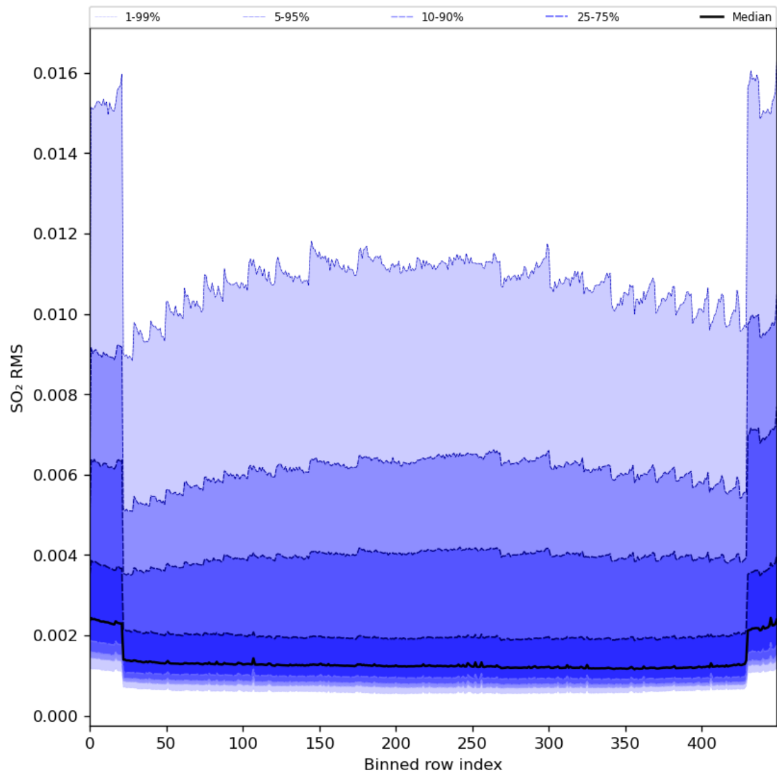
Figure 93: Along track statistics of “SO 2 RMS” for 2024-04-08 to 2024-04-10
