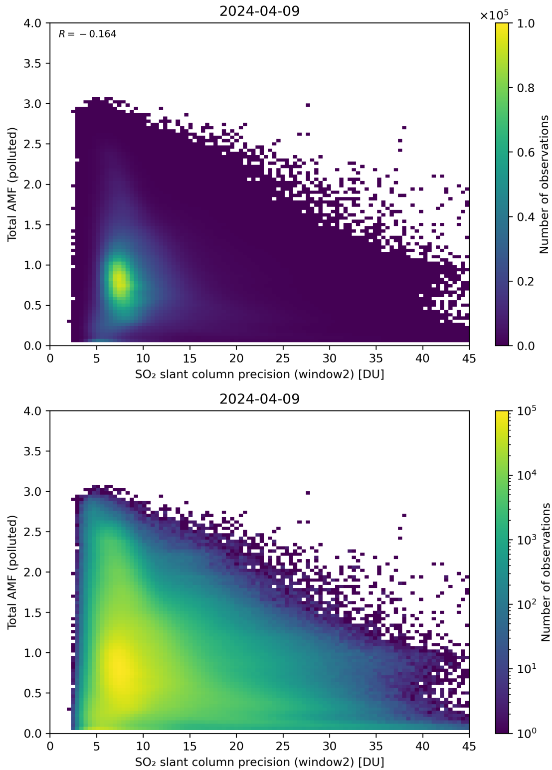
Figure 251: Scatter density plot of “SO 2 slant column precision (window2)” against “Total AMF (polluted)” for 2024-04-08 to 2024-04-10.
