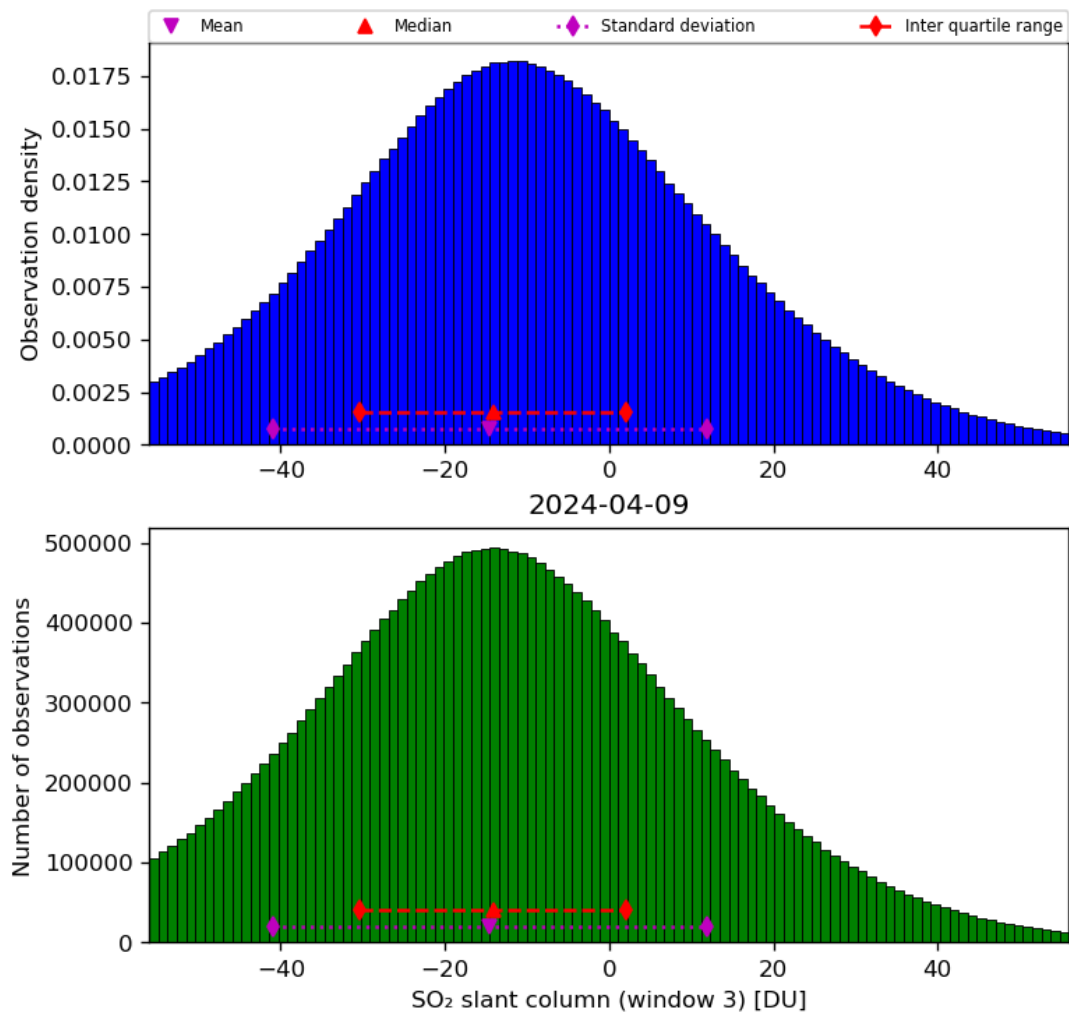
Figure 64: Histogram of “SO 2 slant column (window 3)” for 2024-04-08 to 2024-04-10
