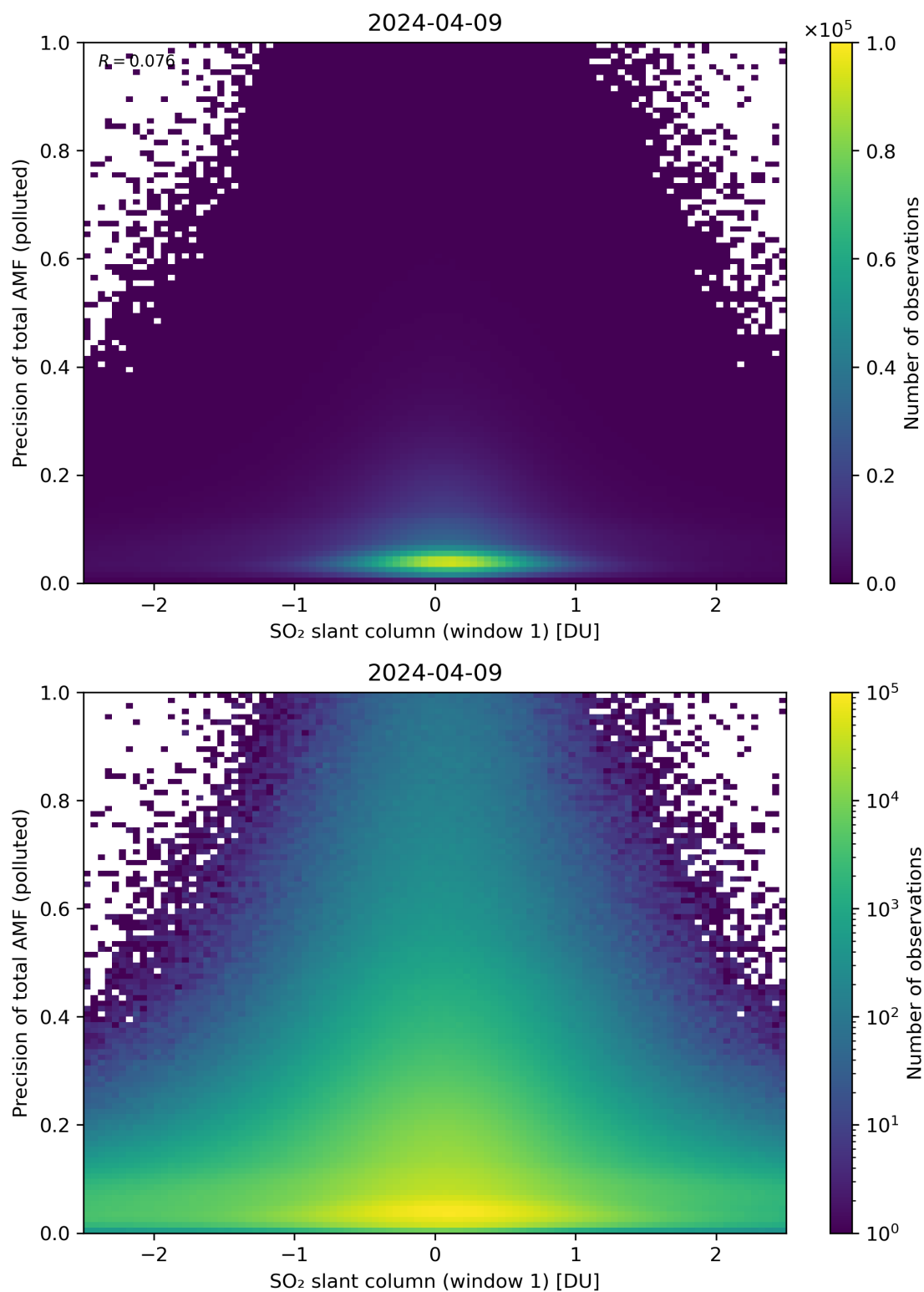
Figure 240: Scatter density plot of “SO 2 slant column (window 1)” against “Precision of total AMF (polluted)” for 2024-04-08 to 2024-04-10.
