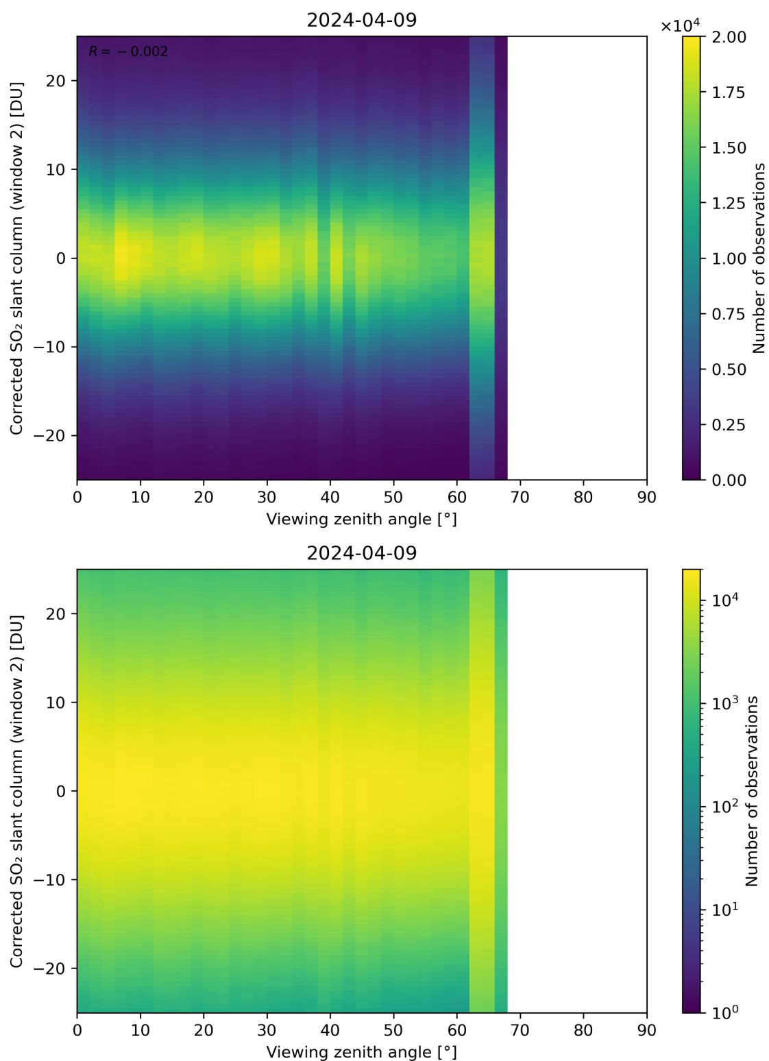
Figure 318: Scatter density plot of “Viewing zenith angle” against “Corrected SO 2 slant column (window 2)” for 2024-04-08 to 2024-04-10.
