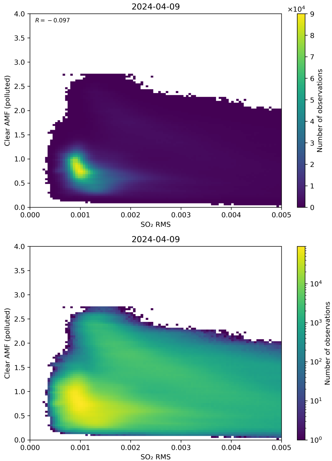
Figure 136: Scatter density plot of “SO 2 RMS” against “Clear AMF (polluted)” for 2024-04-08 to 2024-04-10.
