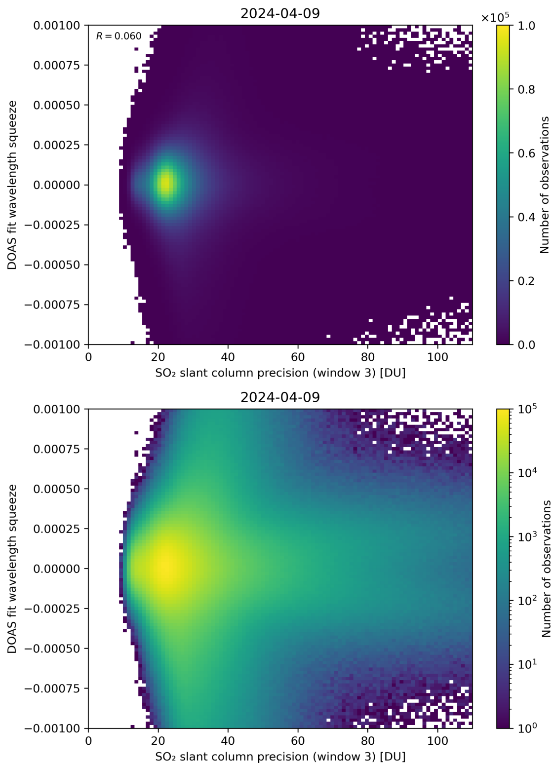
Figure 259: Scatter density plot of “SO 2 slant column precision (window 3)” against “DOAS fit wavelength squeeze” for 2024-04-08 to 2024-04-10.
