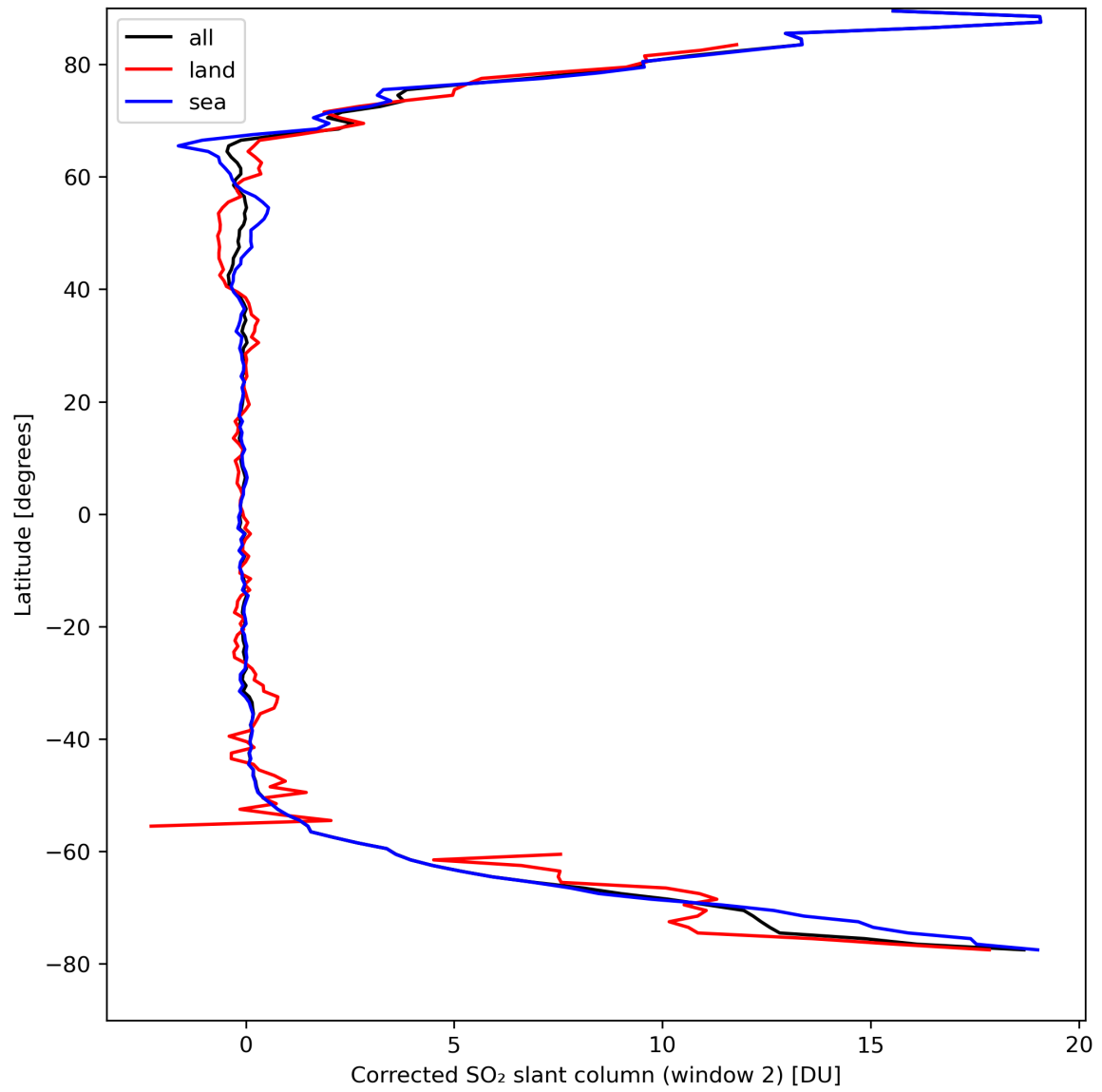
Figure 39: Zonal average of “Corrected SO 2 slant column (window 2)” for 2024-04-08 to 2024-04-10.
