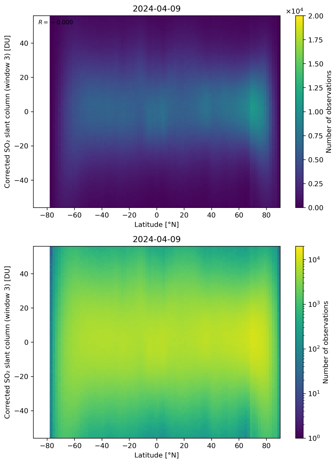
Figure 148: Scatter density plot of “Latitude” against “Corrected SO 2 slant column (window 3)” for 2024-04-08 to 2024-04-10.
