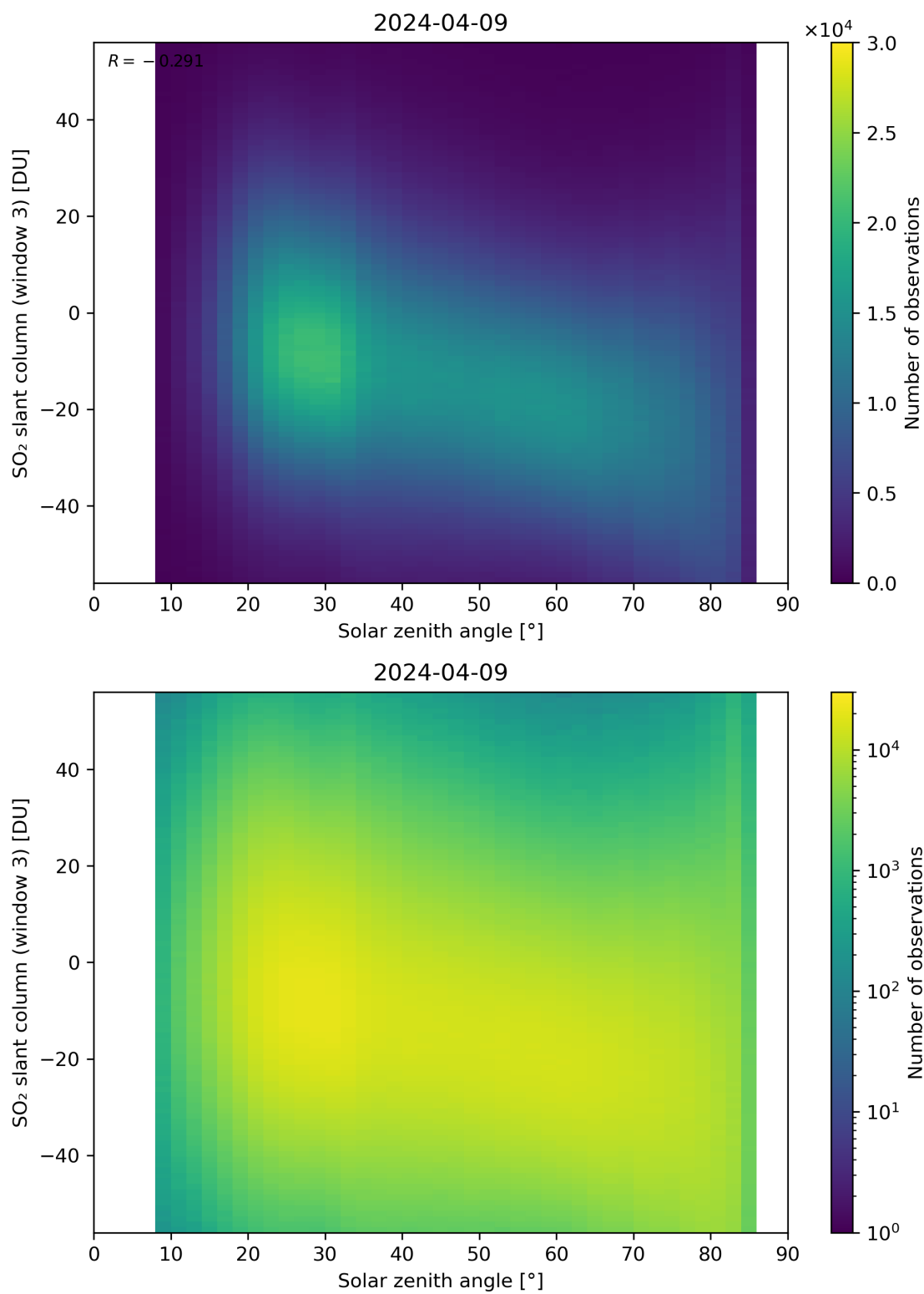
Figure 172: Scatter density plot of “Solar zenith angle” against “SO 2 slant column (window 3)” for 2024-04-08 to 2024-04-10.
