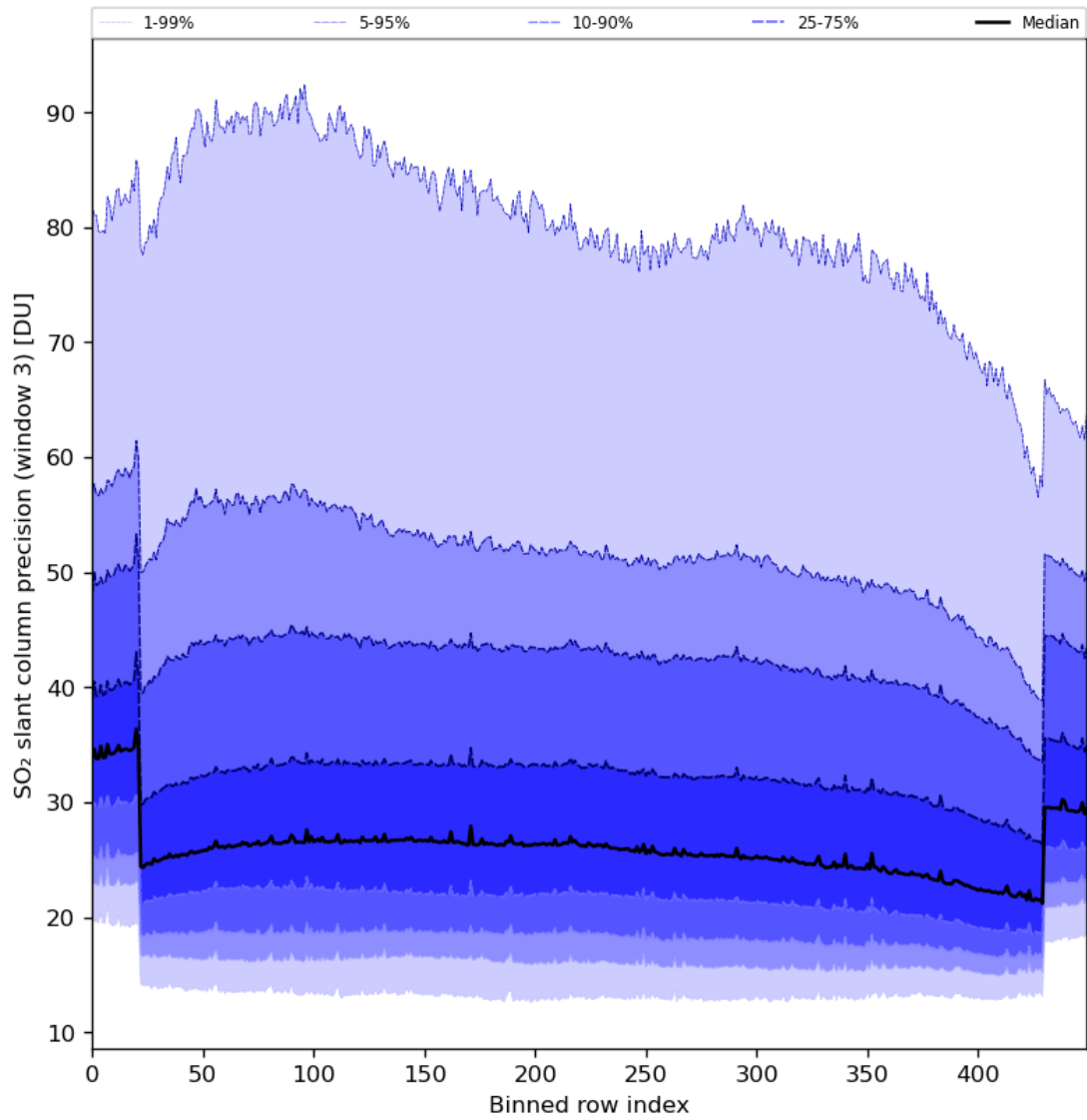
Figure 88: Along track statistics of “SO 2 slant column precision (window 3)” for 2024-04-08 to 2024-04-10
