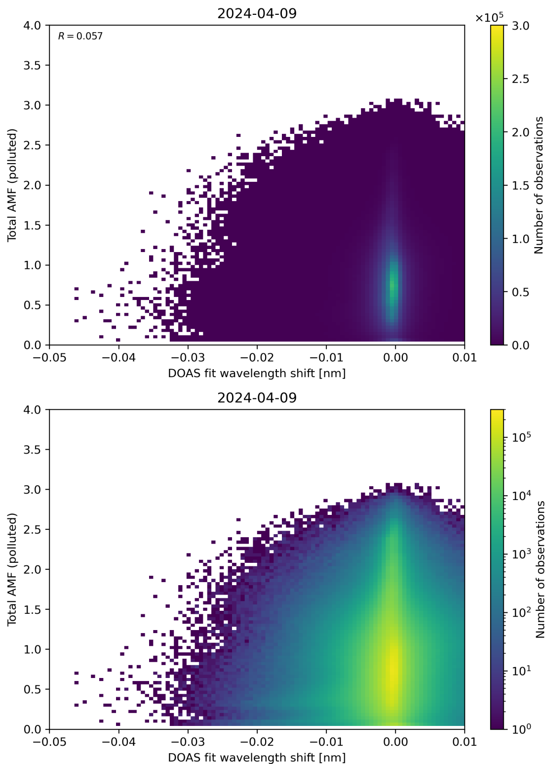
Figure 130: Scatter density plot of “DOAS fit wavelength shift” against “Total AMF (polluted)” for 2024-04-08 to 2024-04-10.
