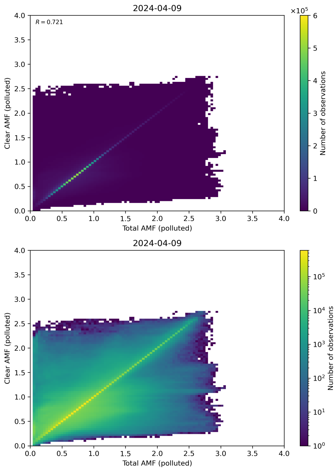
Figure 271: Scatter density plot of “Total AMF (polluted)” against “Clear AMF (polluted)” for 2024-04-08 to 2024-04-10.
