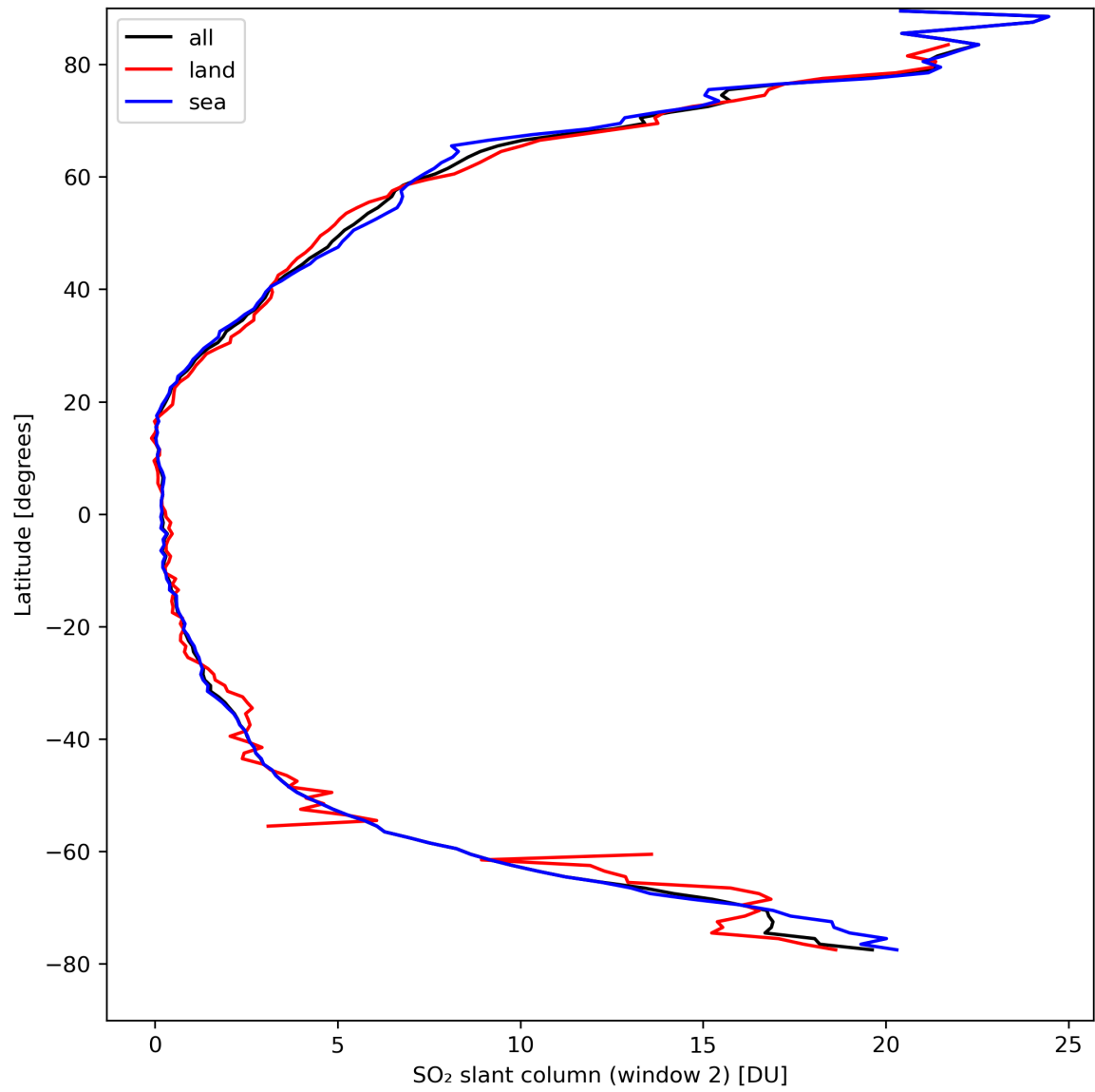
Figure 37: Zonal average of “SO 2 slant column (window 2)” for 2024-04-08 to 2024-04-10.
