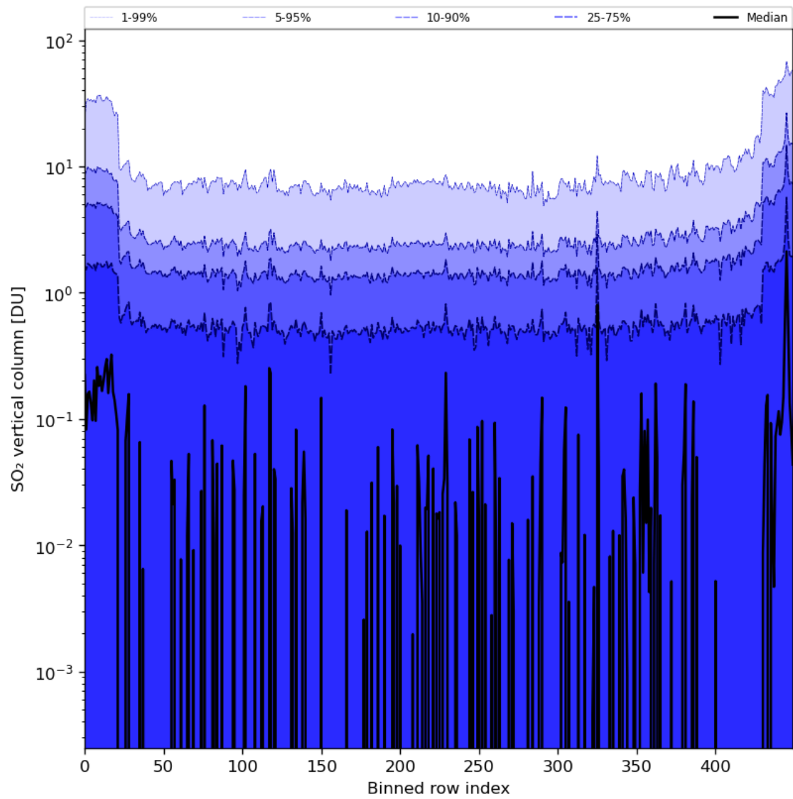
Figure 76: Along track statistics of “SO 2 vertical column” for 2024-04-08 to 2024-04-10
