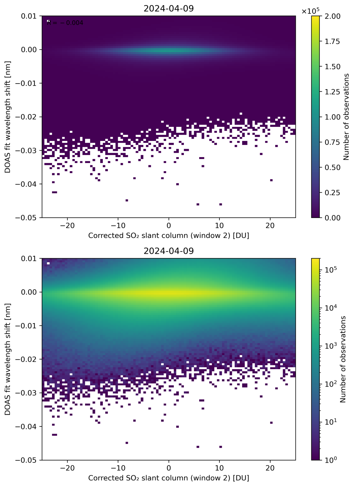
Figure 196: Scatter density plot of “Corrected SO 2 slant column (window 2)” against “DOAS fit wavelength shift” for 2024-04-08 to 2024-04-10.
