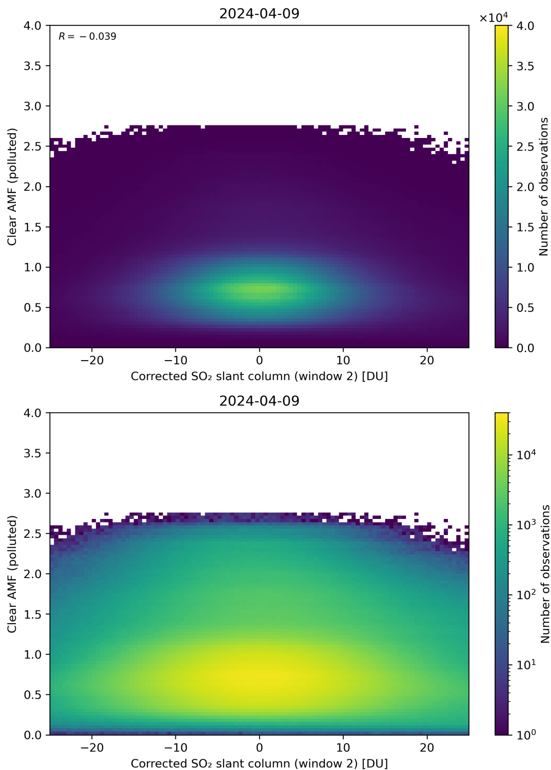
Figure 199: Scatter density plot of “Corrected SO 2 slant column (window 2)” against “Clear AMF (polluted)” for 2024-04-08 to 2024-04-10.
