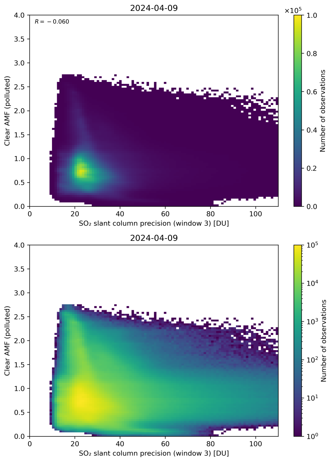
Figure 261: Scatter density plot of “SO 2 slant column precision (window 3)” against “Clear AMF (polluted)” for 2024-04-08 to 2024-04-10.
