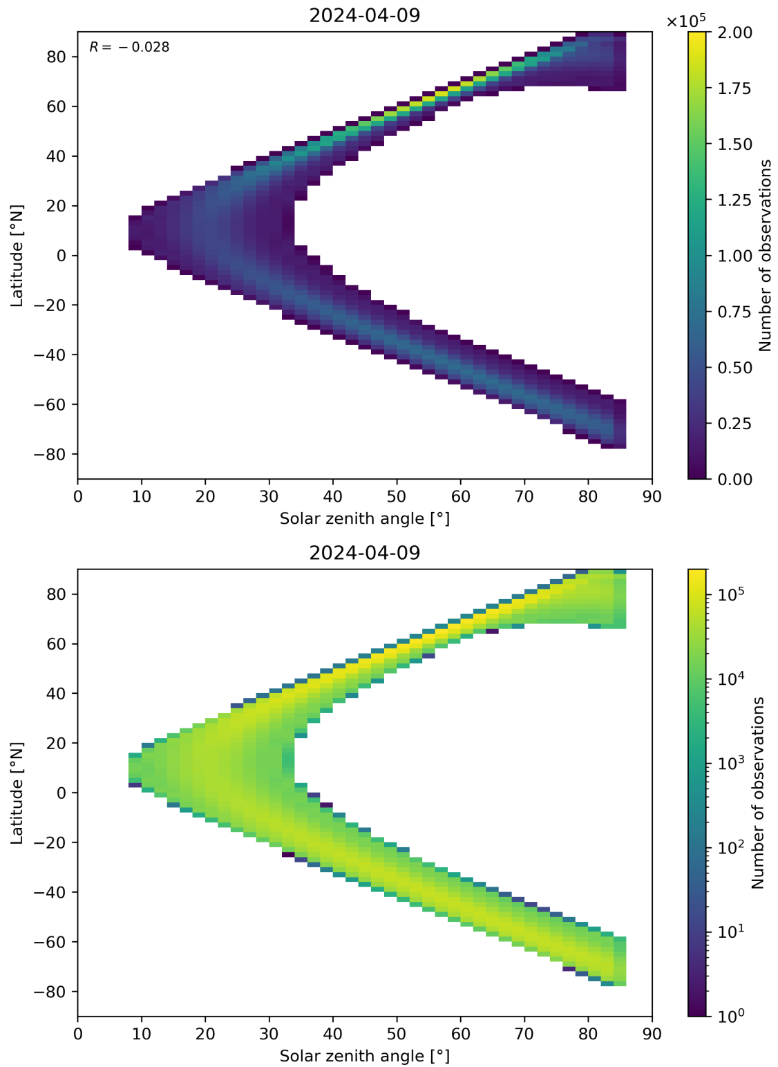
Figure 164: Scatter density plot of “Solar zenith angle” against “Latitude” for 2024-04-08 to 2024-04-10.
