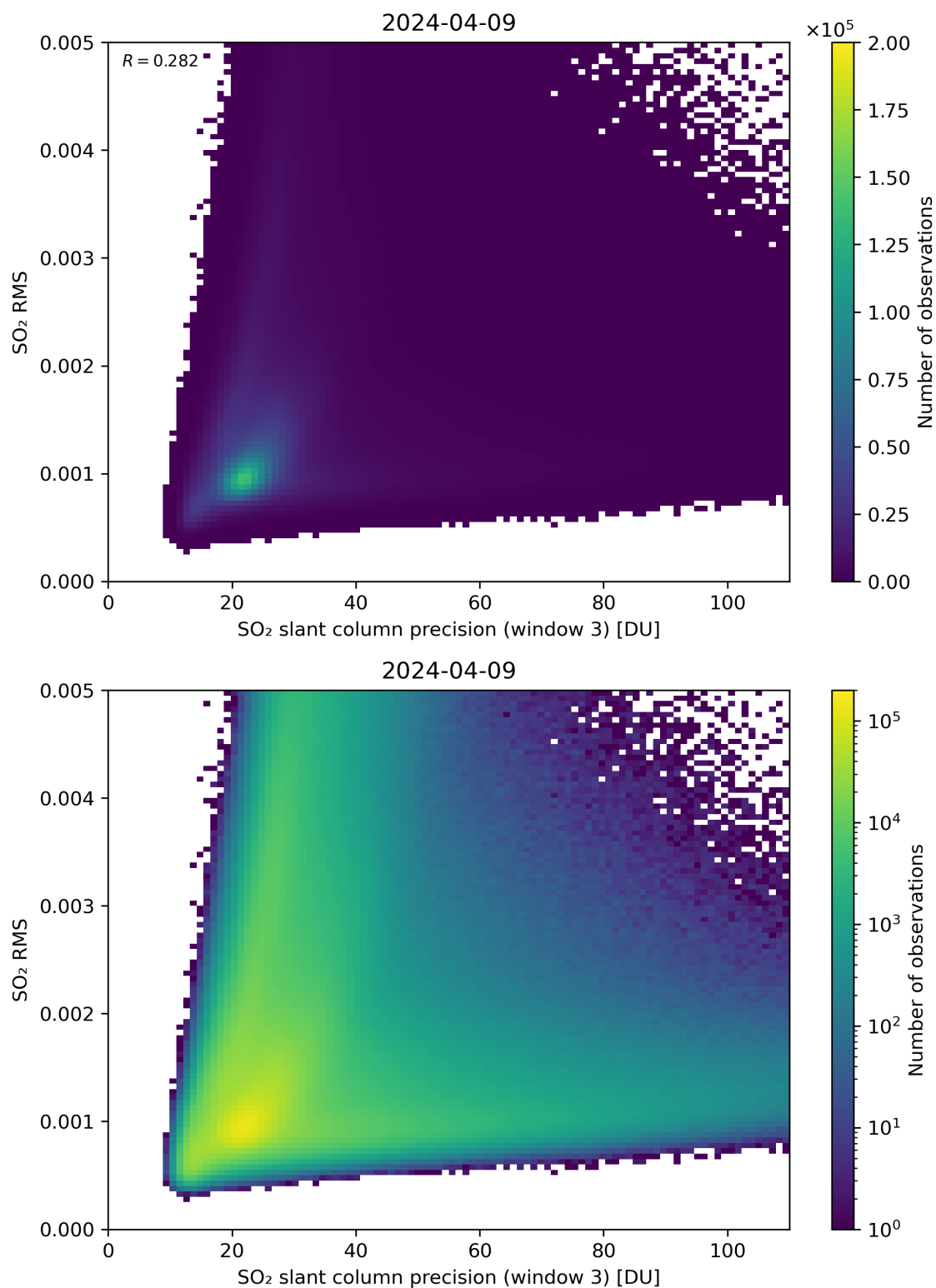
Figure 260: Scatter density plot of “SO 2 slant column precision (window 3)” against “SO 2 RMS” for 2024-04-08 to 2024-04-10.
