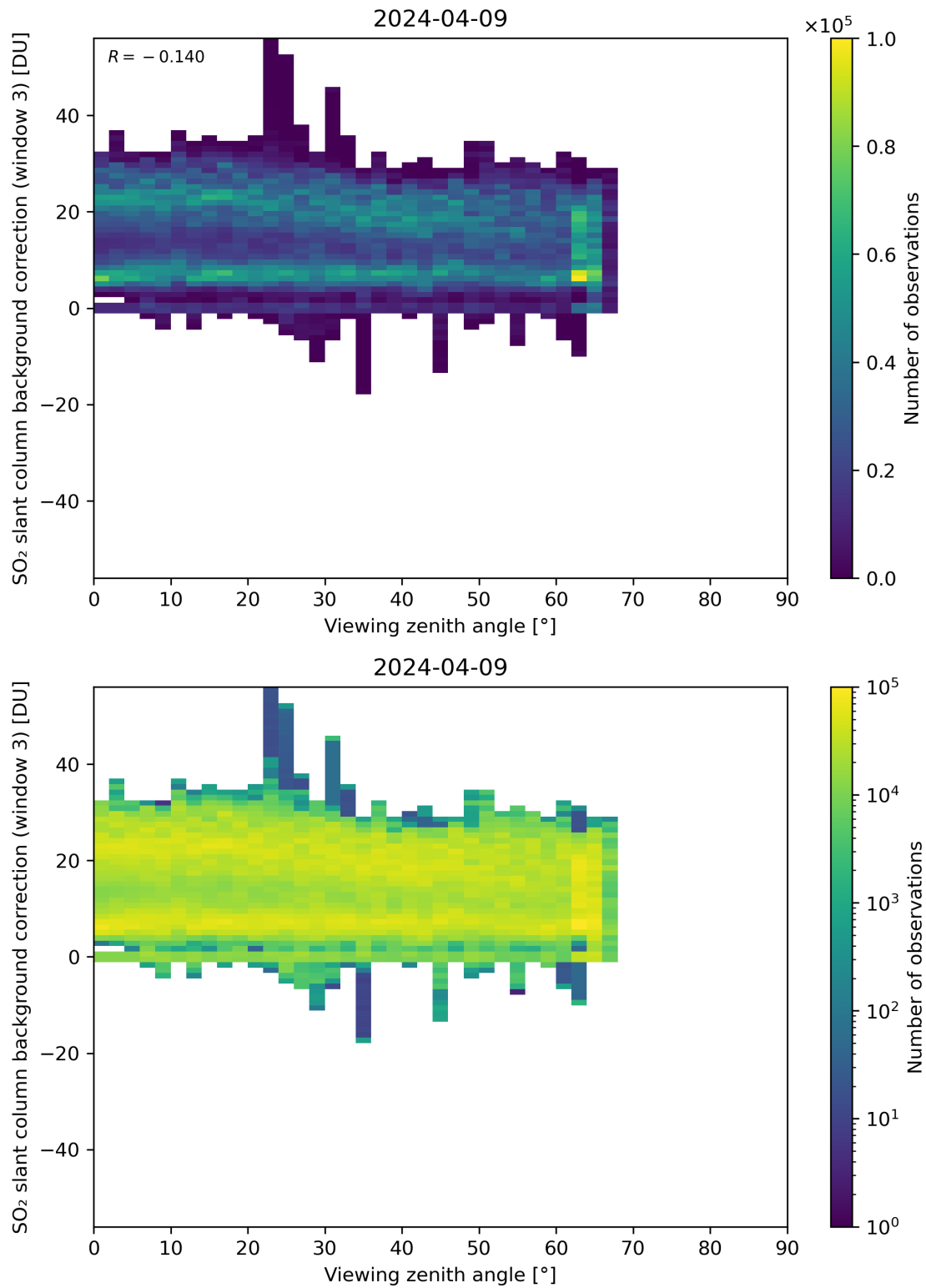
Figure 310: Scatter density plot of “Viewing zenith angle” against “SO 2 slant column background correction (window 3)” for 2024-04-08 to 2024-04-10.
