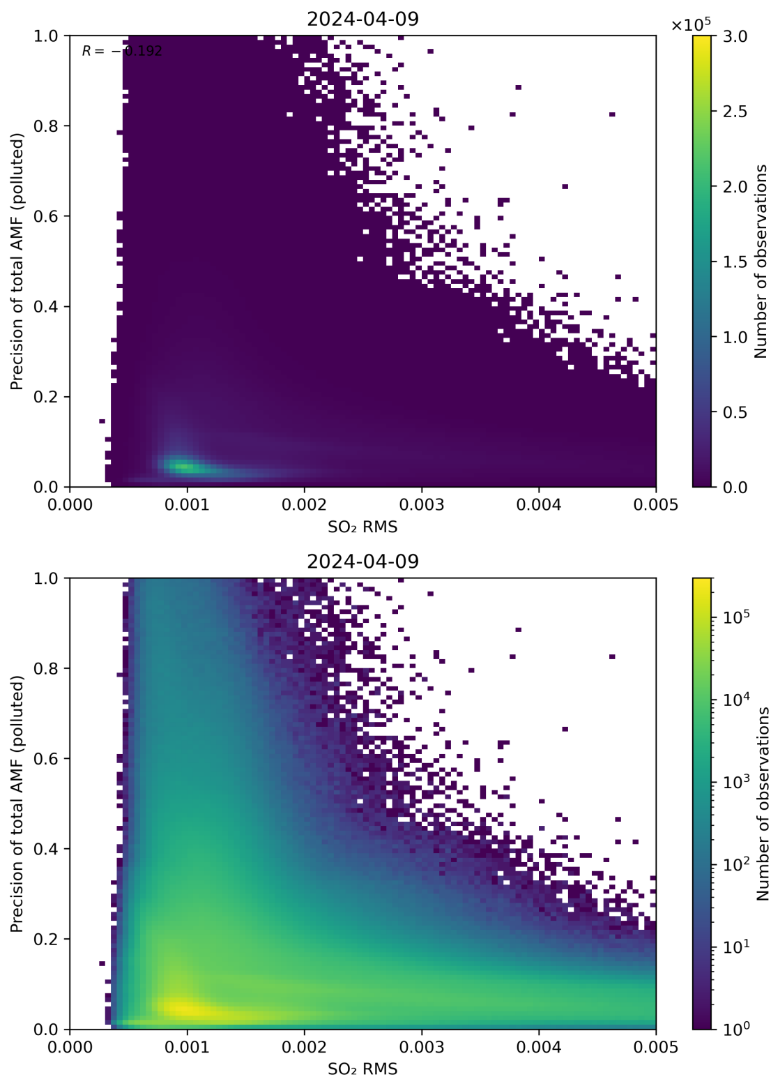
Figure 138: Scatter density plot of “SO 2 RMS” against “Precision of total AMF (polluted)” for 2024-04-08 to 2024-04-10.
