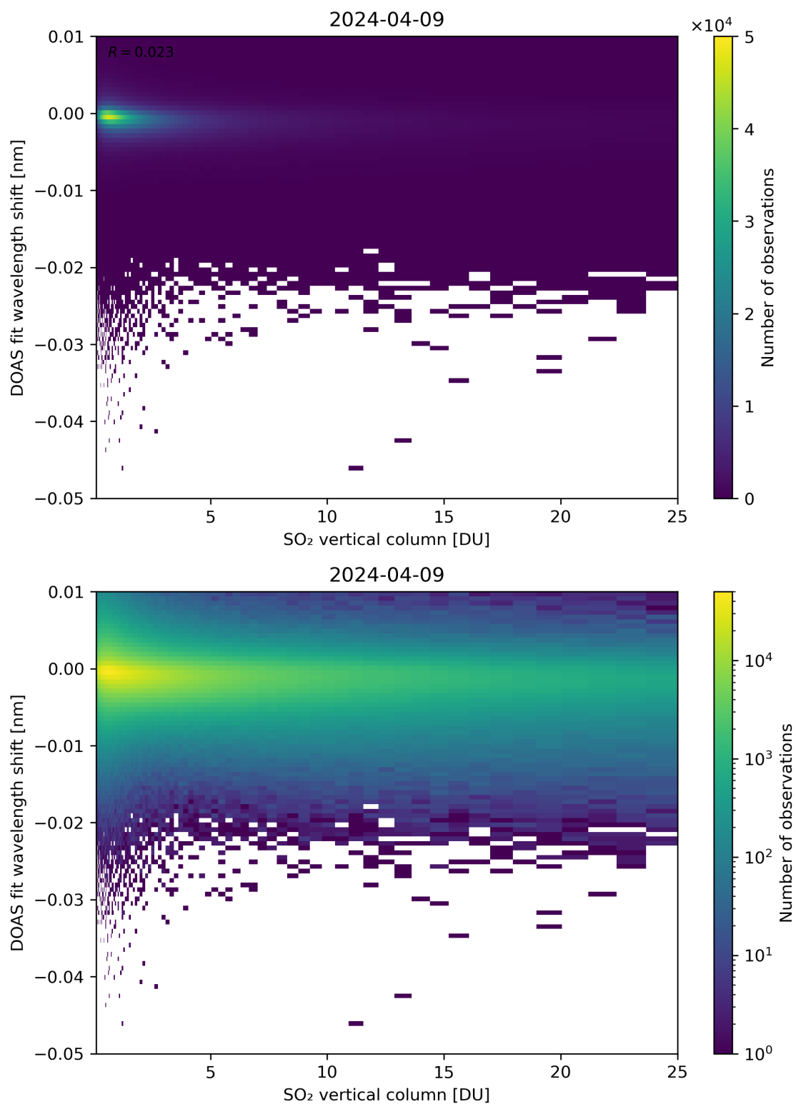
Figure 276: Scatter density plot of “SO 2 vertical column” against “DOAS fit wavelength shift” for 2024-04-08 to 2024-04-10.
