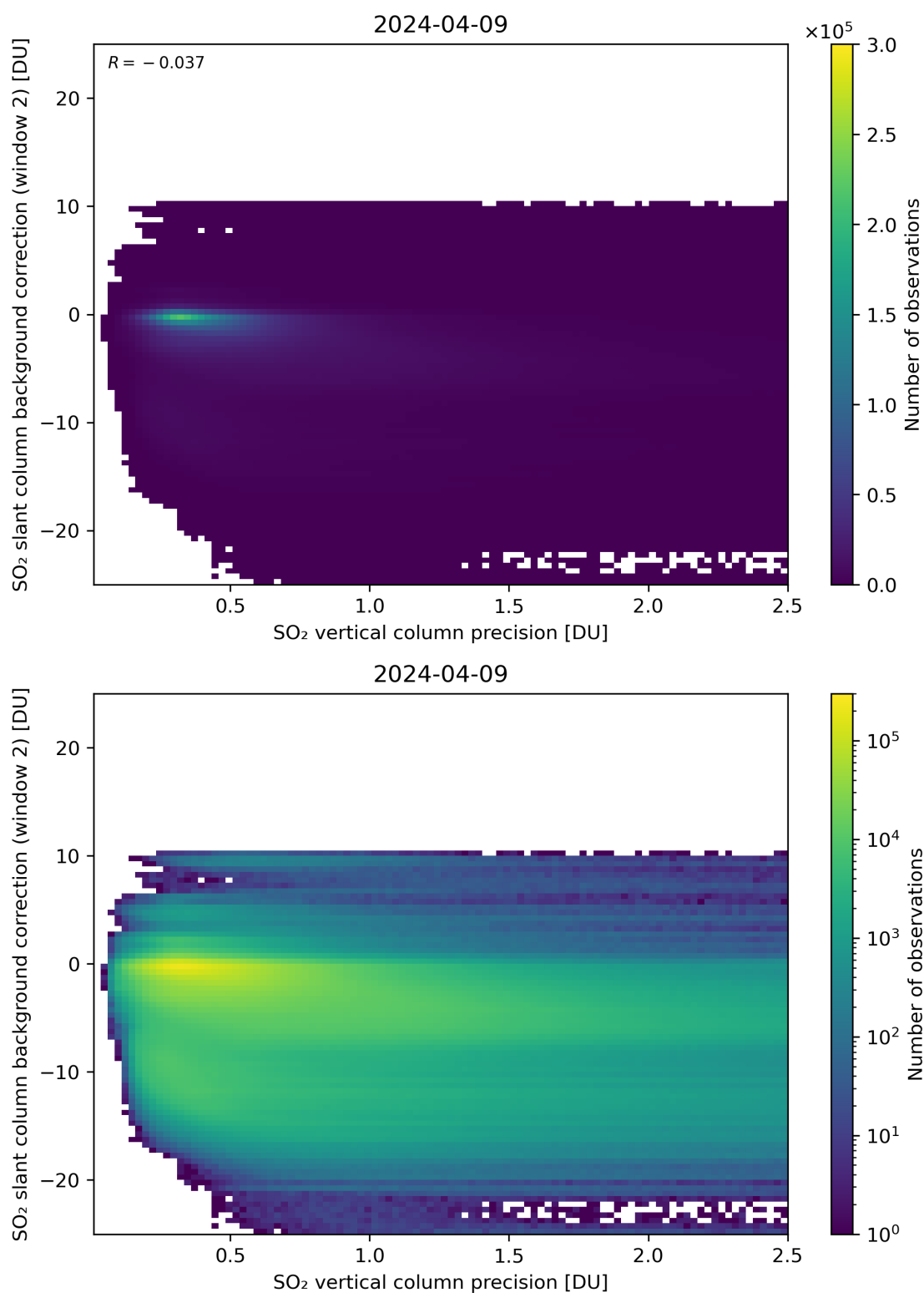
Figure 280: Scatter density plot of “SO 2 vertical column precision” against “SO 2 slant column background correction (window 2)” for 2024-04-08 to 2024-04-10.
