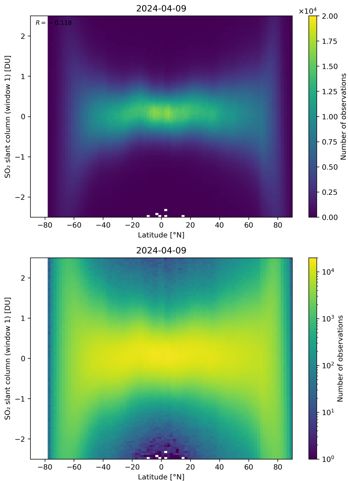
Figure 149: Scatter density plot of “Latitude” against “SO 2 slant column (window 1)” for 2024-04-08 to 2024-04-10.
