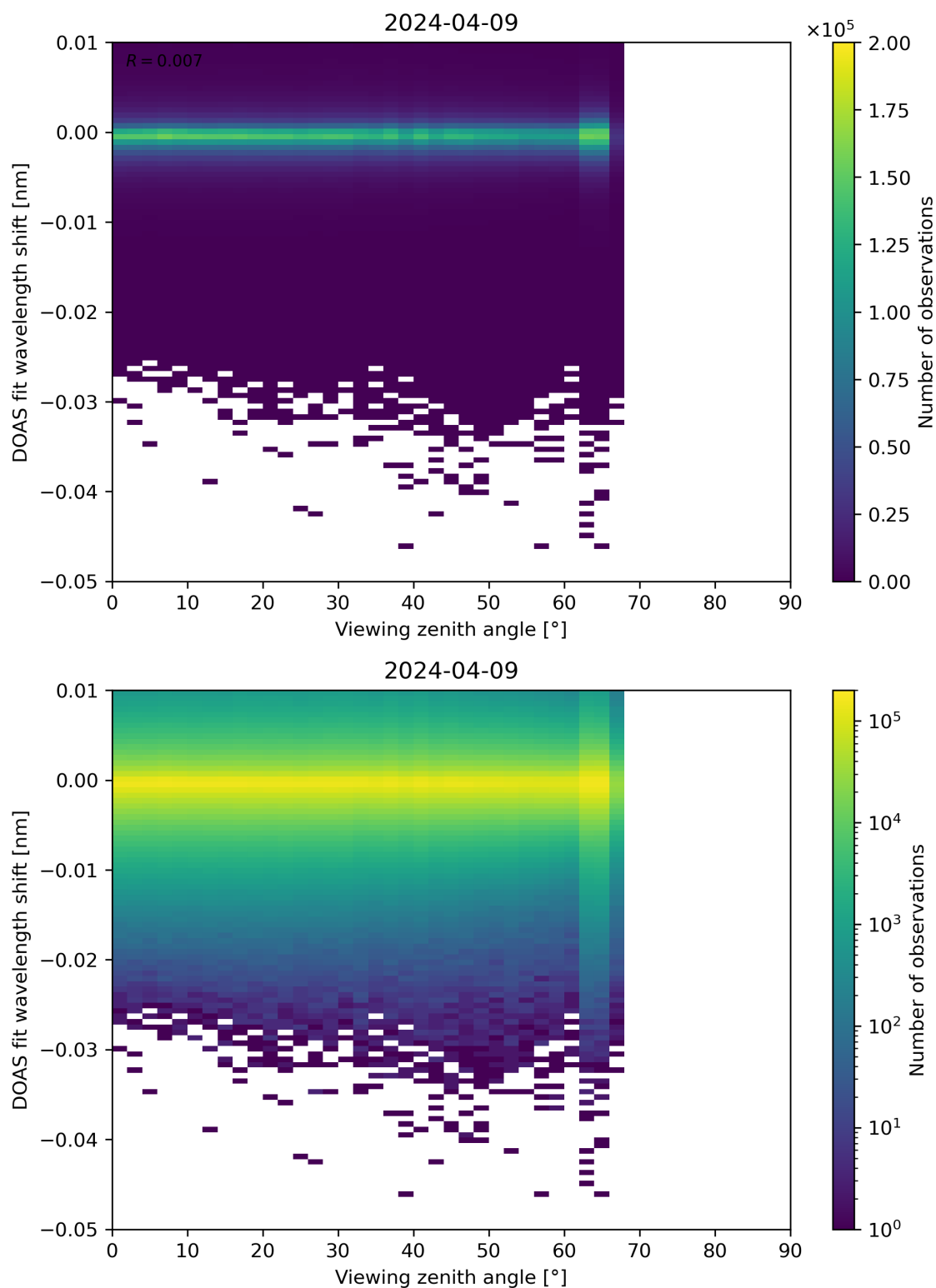
Figure 311: Scatter density plot of “Viewing zenith angle” against “DOAS fit wavelength shift” for 2024-04-08 to 2024-04-10.
