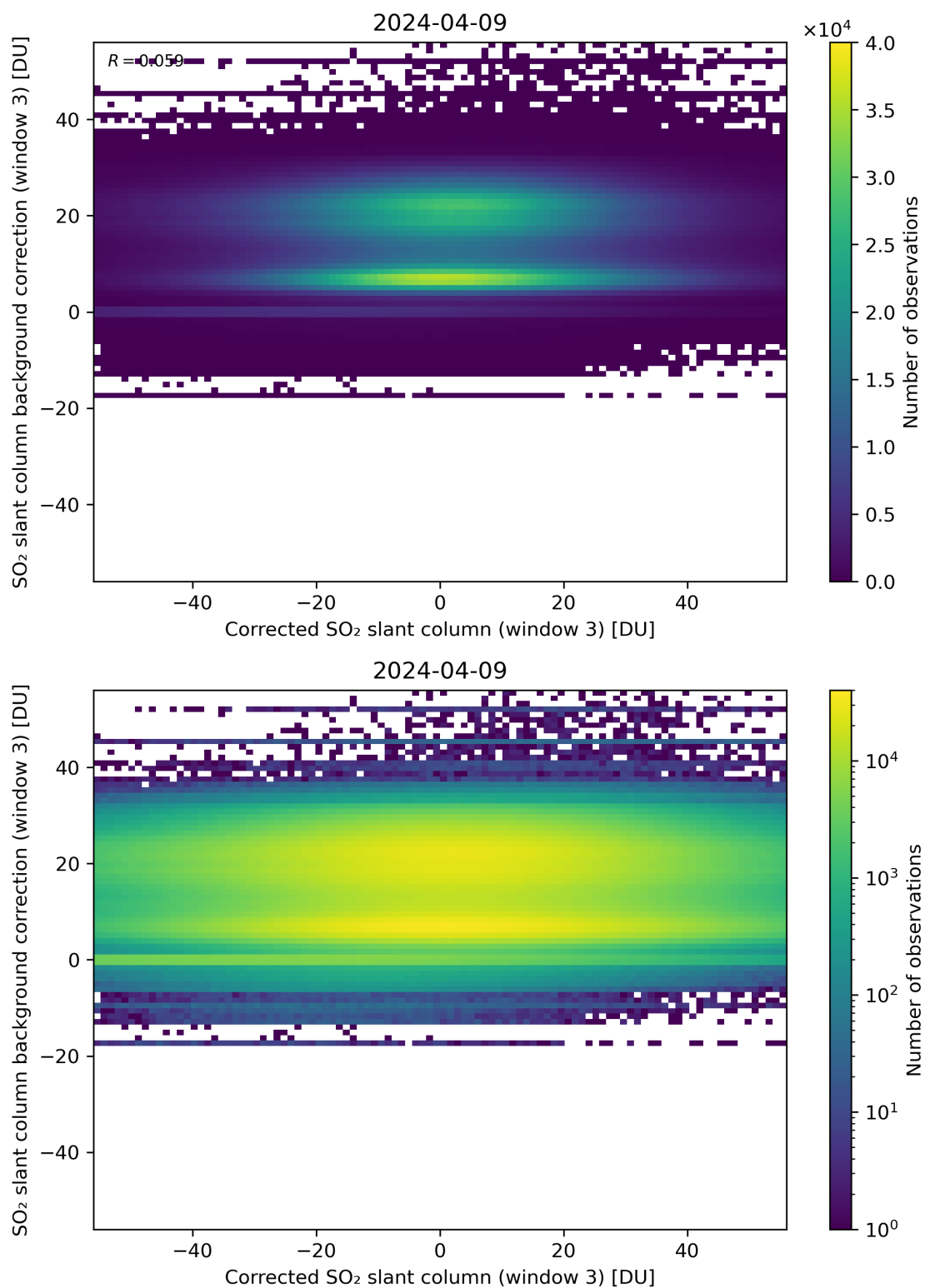
Figure 205: Scatter density plot of “Corrected SO 2 slant column (window 3)” against “SO 2 slant column background correction (window 3)” for 2024-04-08 to 2024-04-10.
