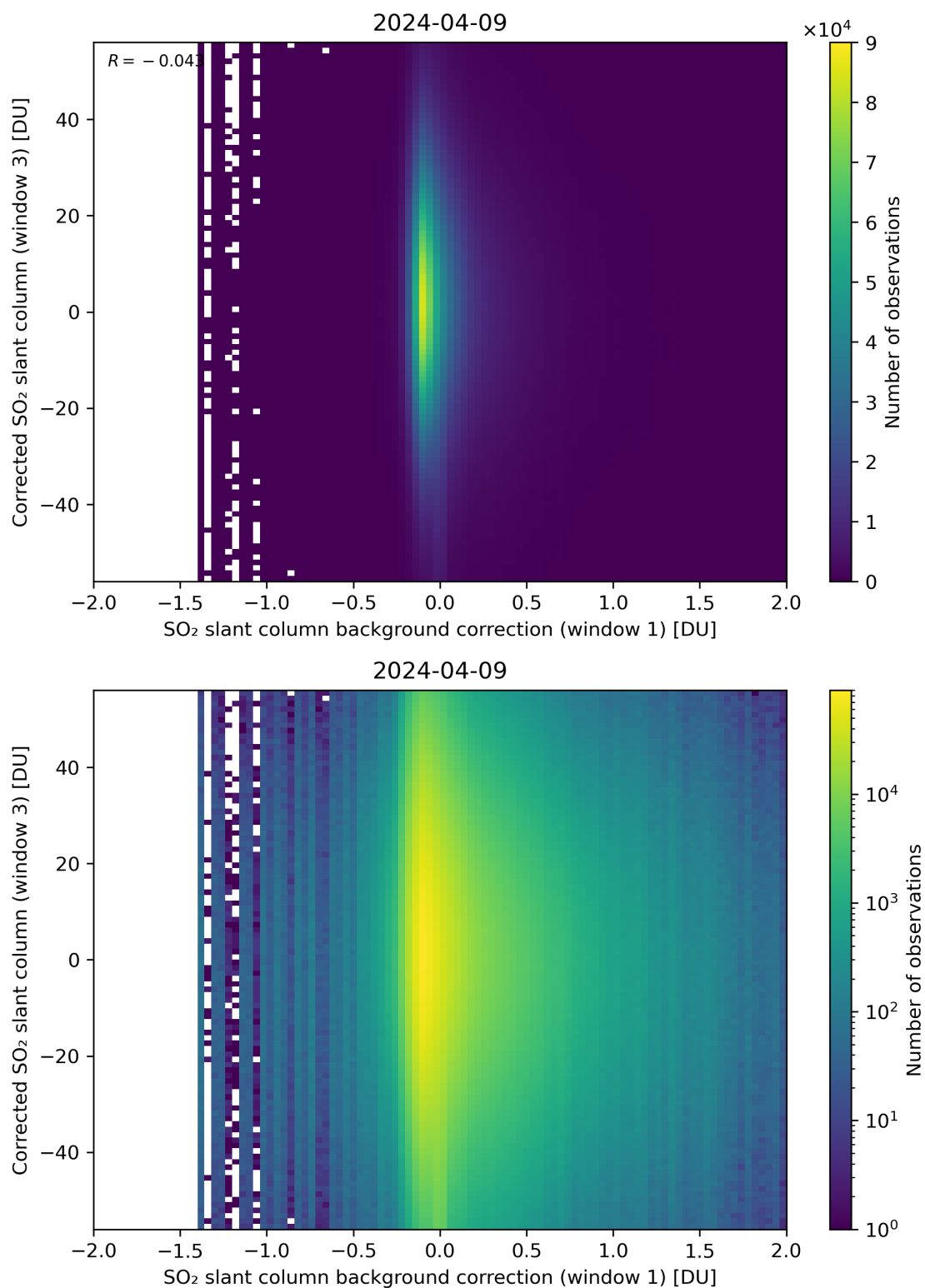
Figure 105: Scatter density plot of “SO 2 slant column background correction (window 1)” against “Corrected SO 2 slant column (window 3)” for 2024-04-08 to 2024-04-10.
