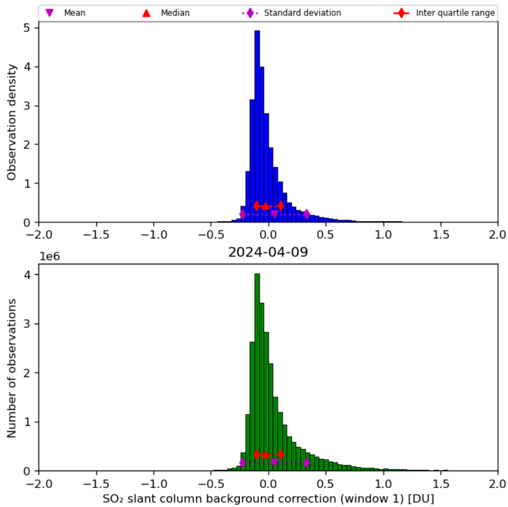
Figure 59: Histogram of “SO 2 slant column background correction (window 1)” for 2024-04-08 to 2024-04-10
