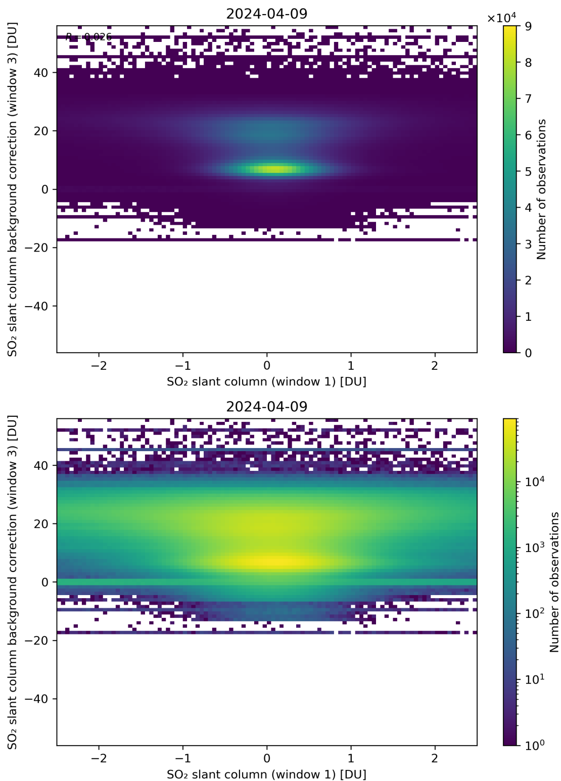
Figure 214: Scatter density plot of “SO 2 slant column (window 1)” against “SO 2 slant column background correction (window 3)” for 2024-04-08 to 2024-04-10.
