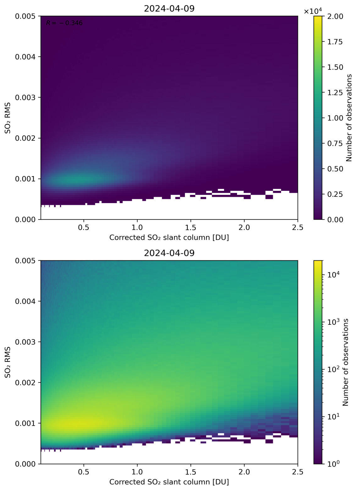
Figure 183: Scatter density plot of “Corrected SO 2 slant column” against “SO 2 RMS” for 2024-04-08 to 2024-04-10.
