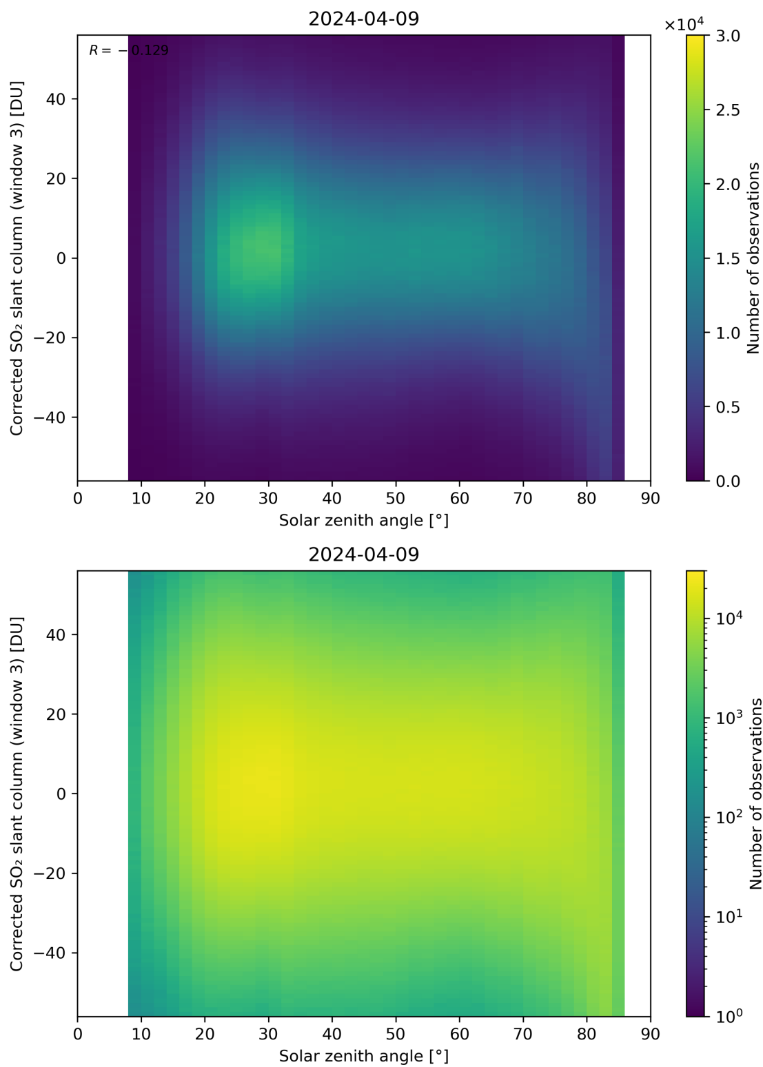
Figure 168: Scatter density plot of “Solar zenith angle” against “Corrected SO 2 slant column (window 3)” for 2024-04-08 to 2024-04-10.
