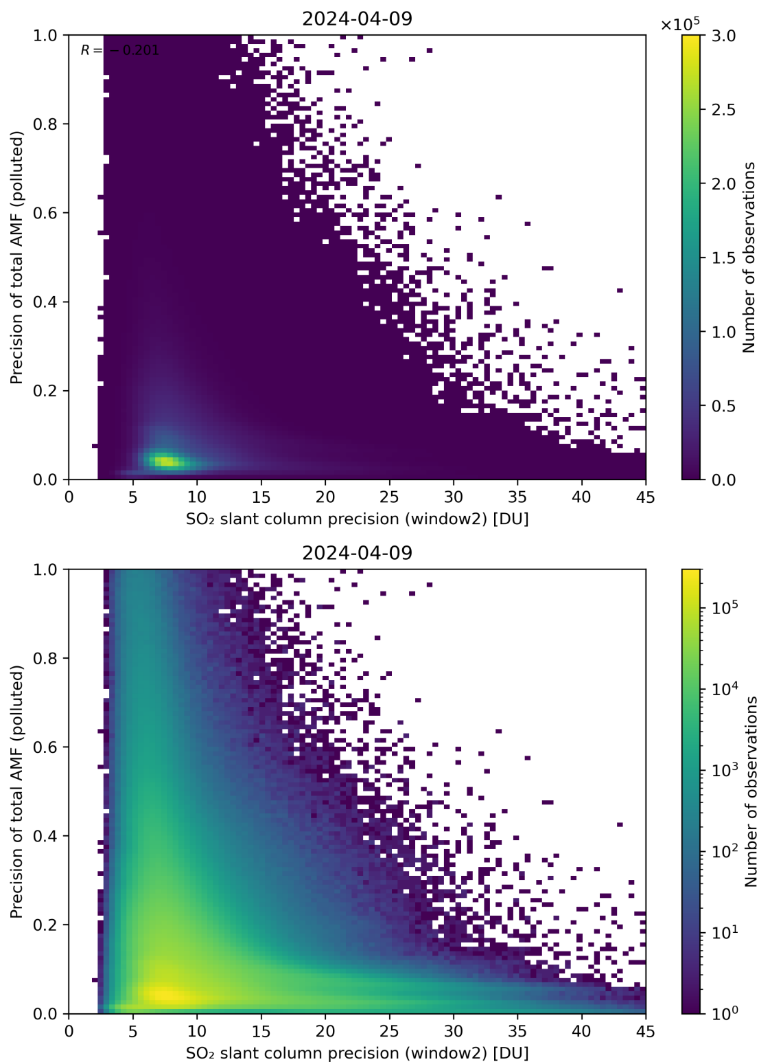
Figure 252: Scatter density plot of “SO 2 slant column precision (window2)” against “Precision of total AMF (polluted)” for 2024-04-08 to 2024-04-10.
