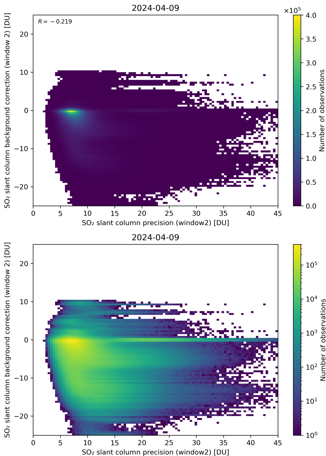
Figure 241: Scatter density plot of “SO 2 slant column precision (window2)” against “SO 2 slant column background correction (window 2)” for 2024-04-08 to 2024-04-10.
