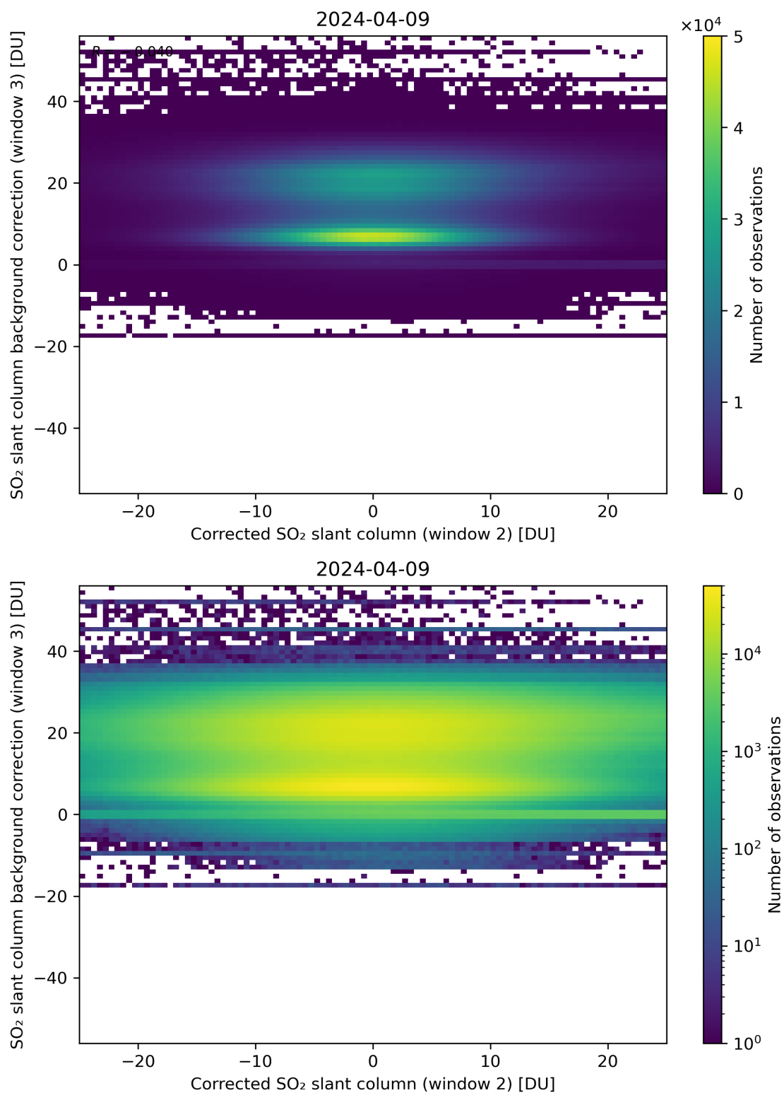
Figure 195: Scatter density plot of “Corrected SO 2 slant column (window 2)” against “SO 2 slant column background correction (window 3)” for 2024-04-08 to 2024-04-10.
