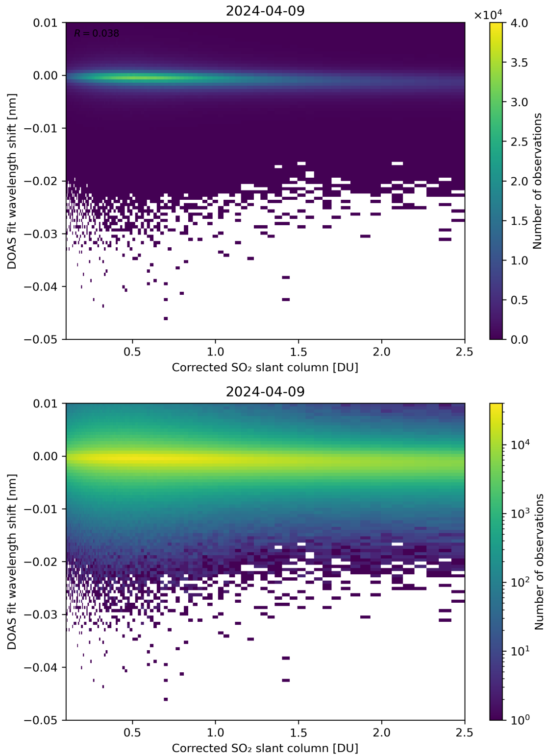
Figure 181: Scatter density plot of “Corrected SO 2 slant column” against “DOAS fit wavelength shift” for 2024-04-08 to 2024-04-10.
