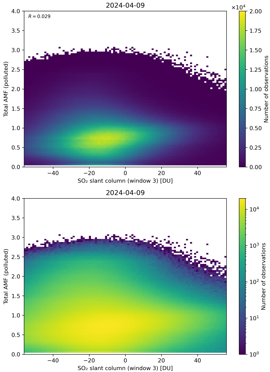
Figure 268: Scatter density plot of “SO 2 slant column (window 3)” against “Total AMF (polluted)” for 2024-04-08 to 2024-04-10.
