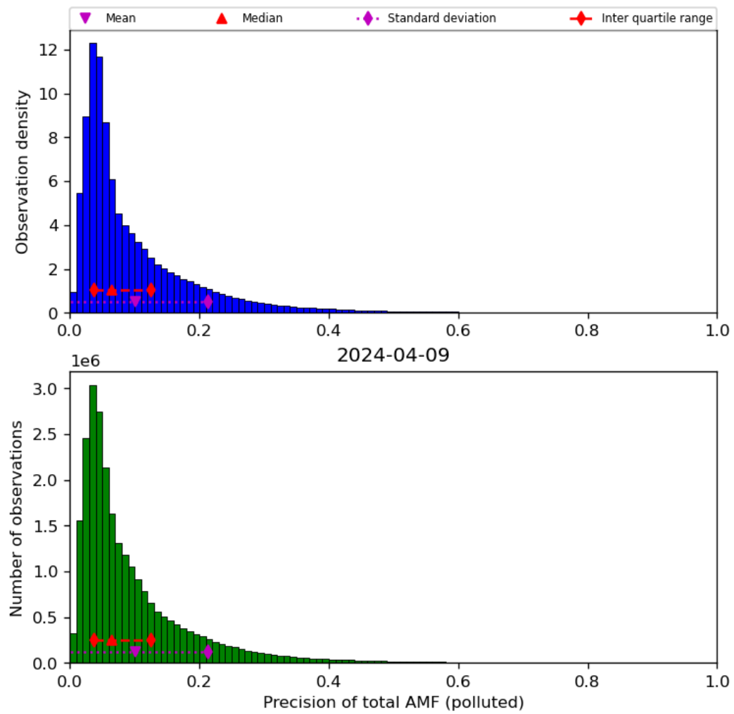
Figure 72: Histogram of “Precision of total AMF (polluted)” for 2024-04-08 to 2024-04-10
