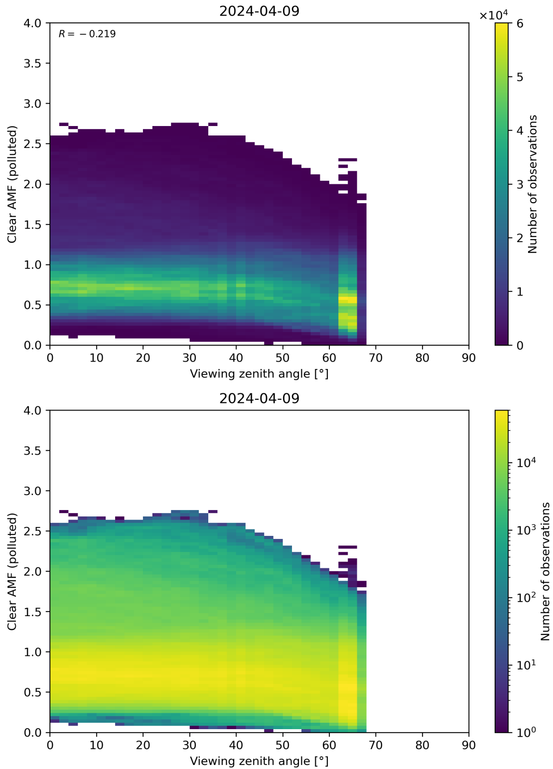
Figure 316: Scatter density plot of “Viewing zenith angle” against “Clear AMF (polluted)” for 2024-04-08 to 2024-04-10.
