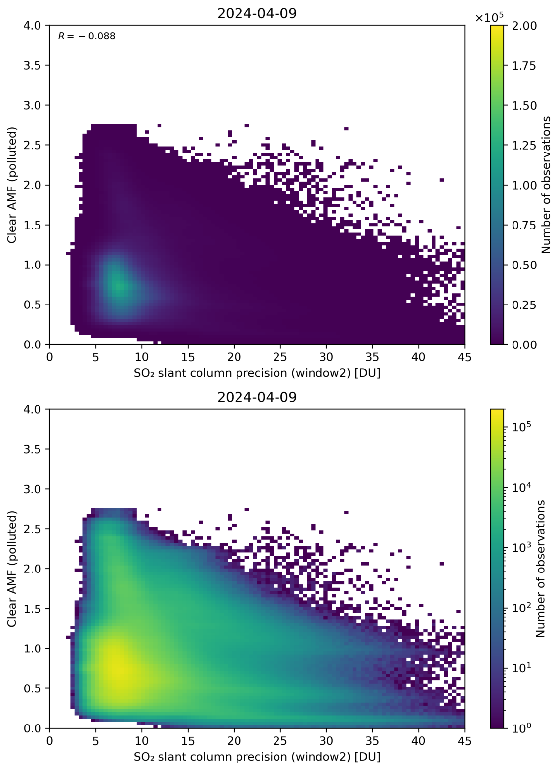
Figure 246: Scatter density plot of “SO 2 slant column precision (window2)” against “Clear AMF (polluted)” for 2024-04-08 to 2024-04-10.
