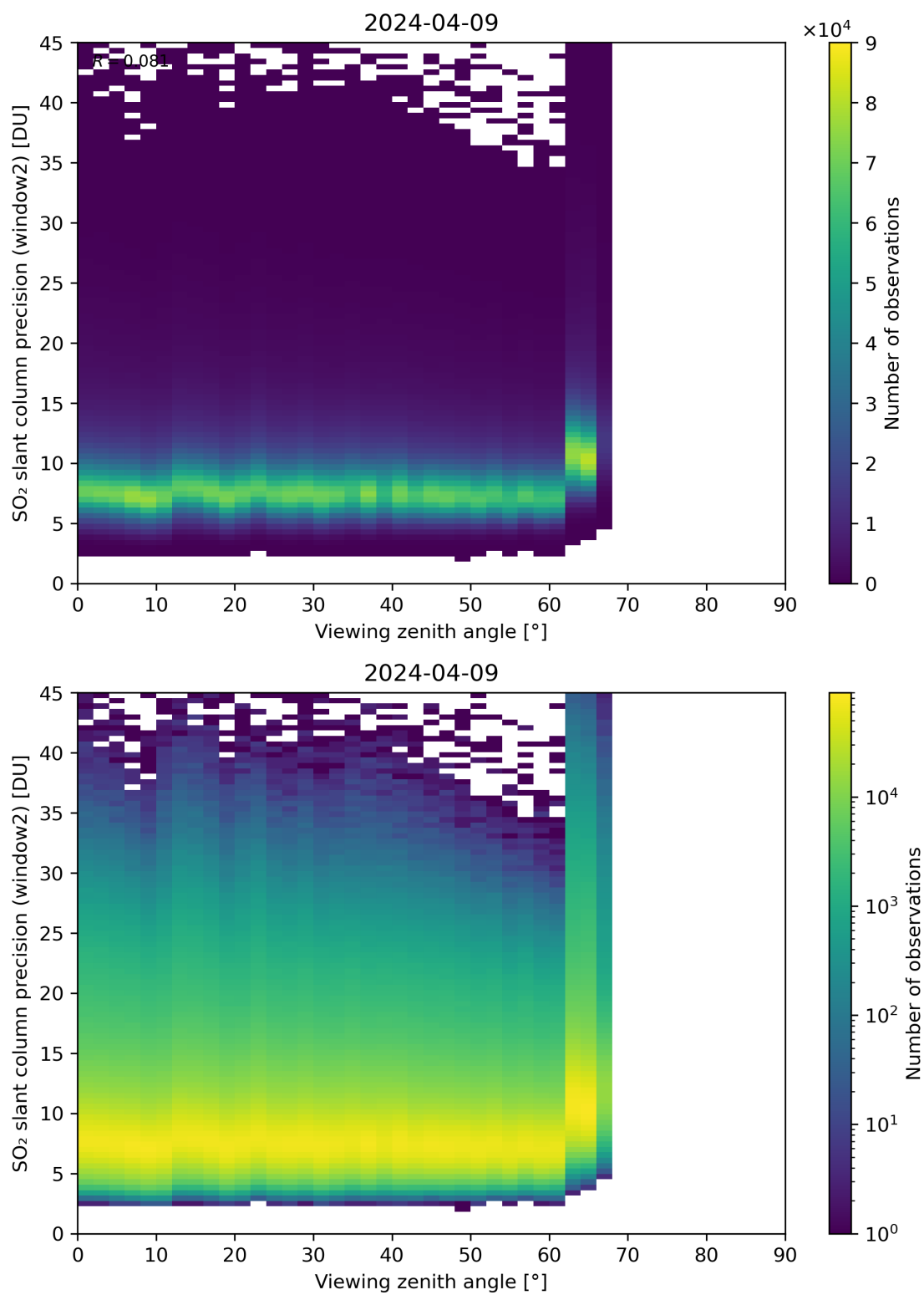
Figure 322: Scatter density plot of “Viewing zenith angle” against “SO 2 slant column precision (window2)” for 2024-04-08 to 2024-04-10.
