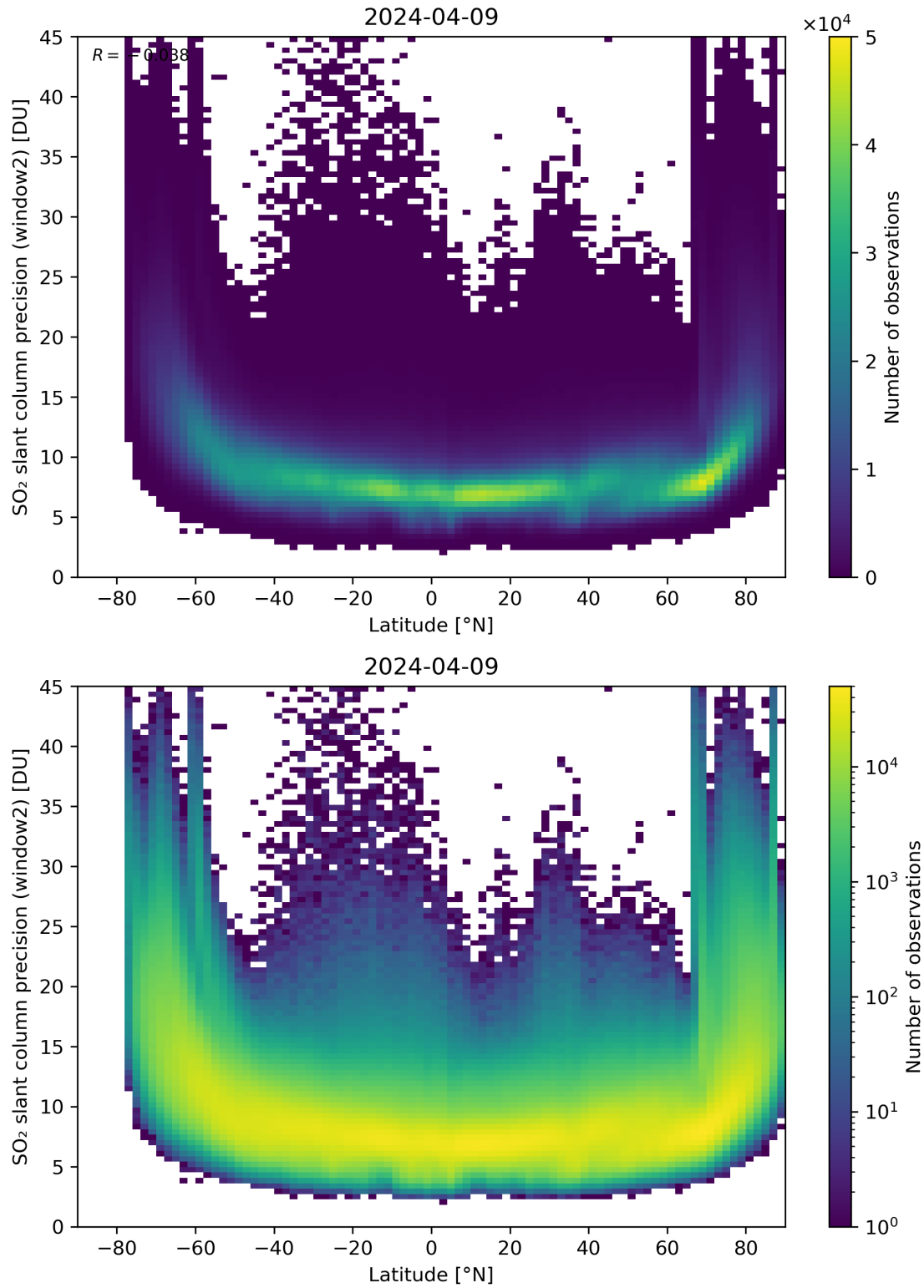
Figure 151: Scatter density plot of “Latitude” against “SO 2 slant column precision (window2)” for 2024-04-08 to 2024-04-10.
