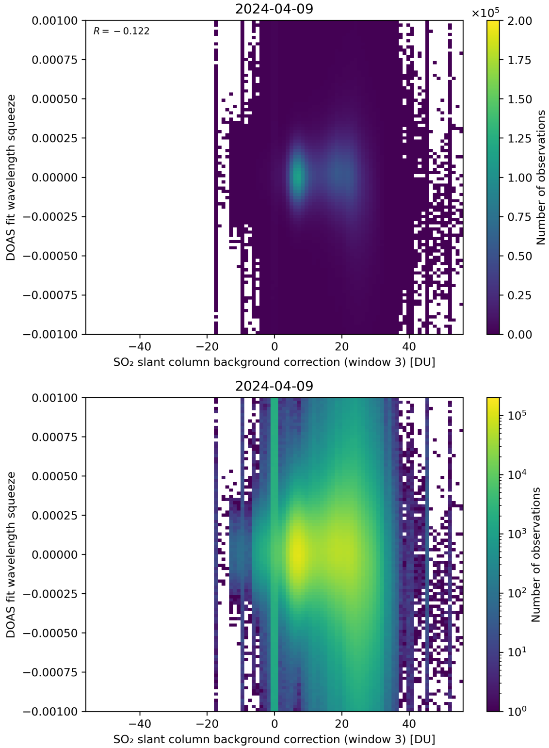
Figure 122: Scatter density plot of “SO 2 slant column background correction (window 3)” against “DOAS fit wavelength squeeze” for 2024-04-08 to 2024-04-10.
