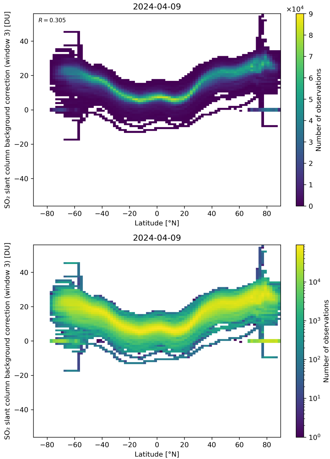
Figure 141: Scatter density plot of “Latitude” against “SO 2 slant column background correction (window 3)” for 2024-04-08 to 2024-04-10.
