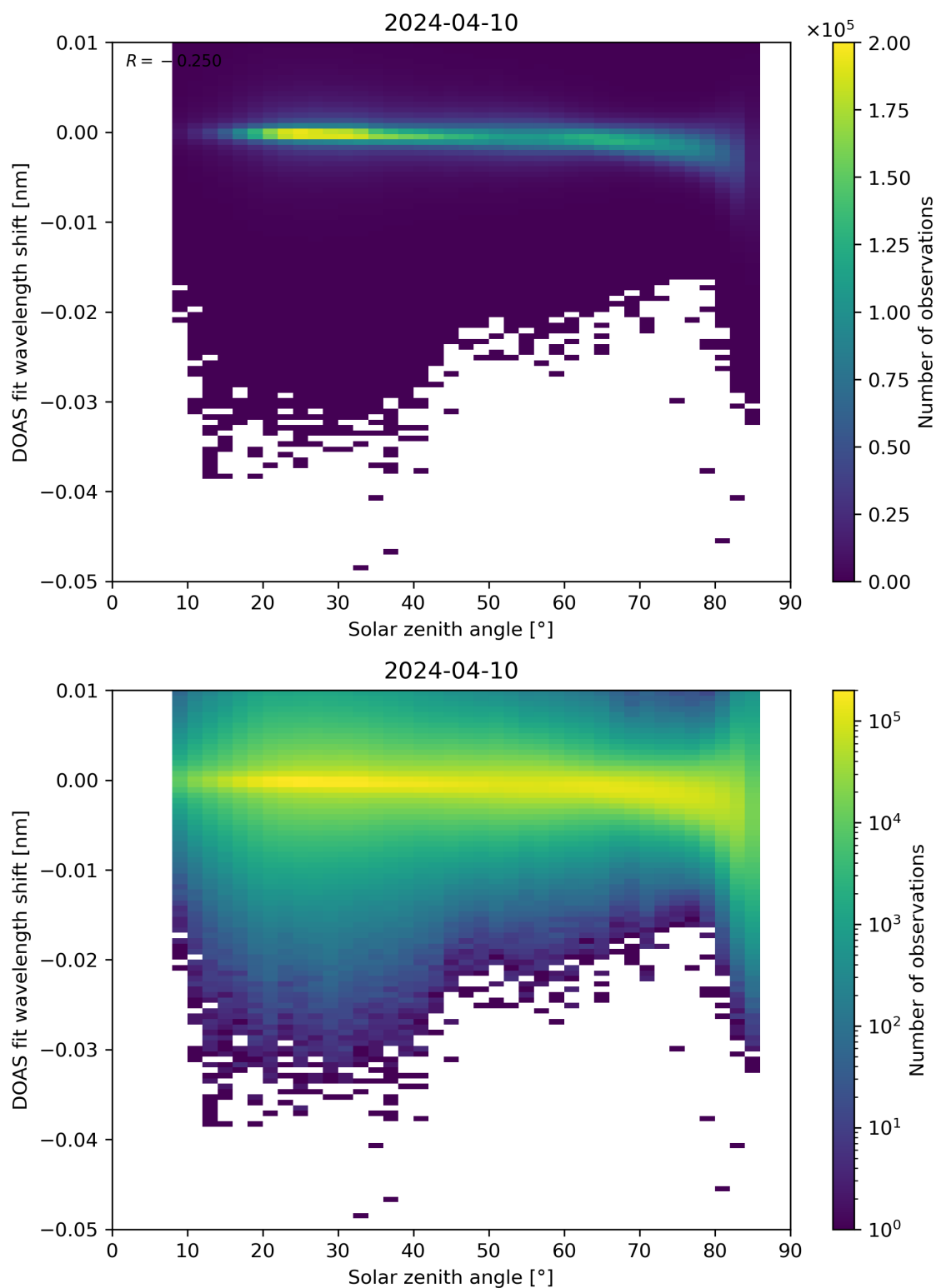
Figure 161: Scatter density plot of “Solar zenith angle” against “DOAS fit wavelength shift” for 2024-04-10 to 2024-04-11.
