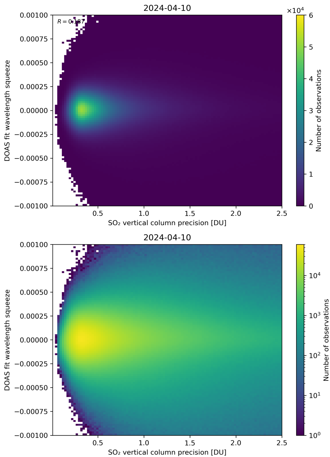
Figure 283: Scatter density plot of “SO 2 vertical column precision” against “DOAS fit wavelength squeeze” for 2024-04-10 to 2024-04-11.
