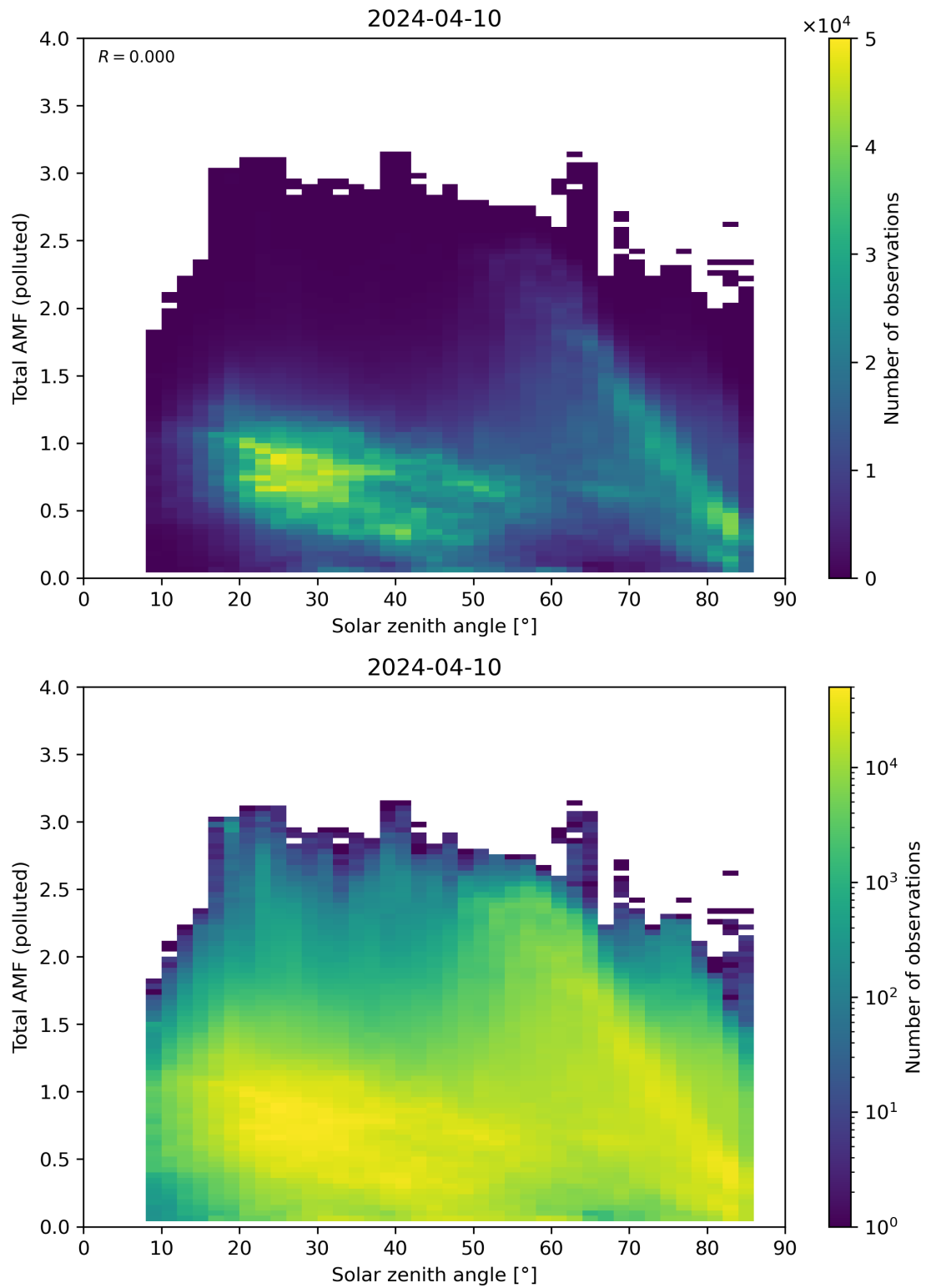
Figure 174: Scatter density plot of “Solar zenith angle” against “Total AMF (polluted)” for 2024-04-10 to 2024-04-11.
