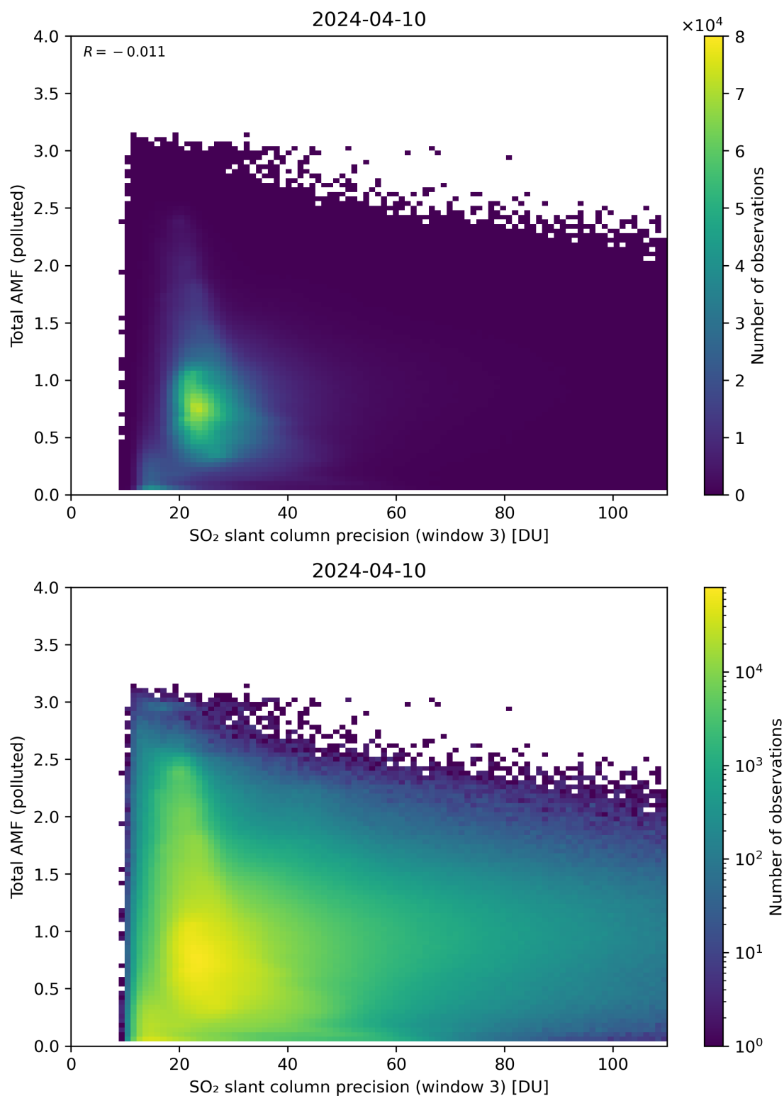
Figure 263: Scatter density plot of “SO 2 slant column precision (window 3)” against “Total AMF (polluted)” for 2024-04-10 to 2024-04-11.
