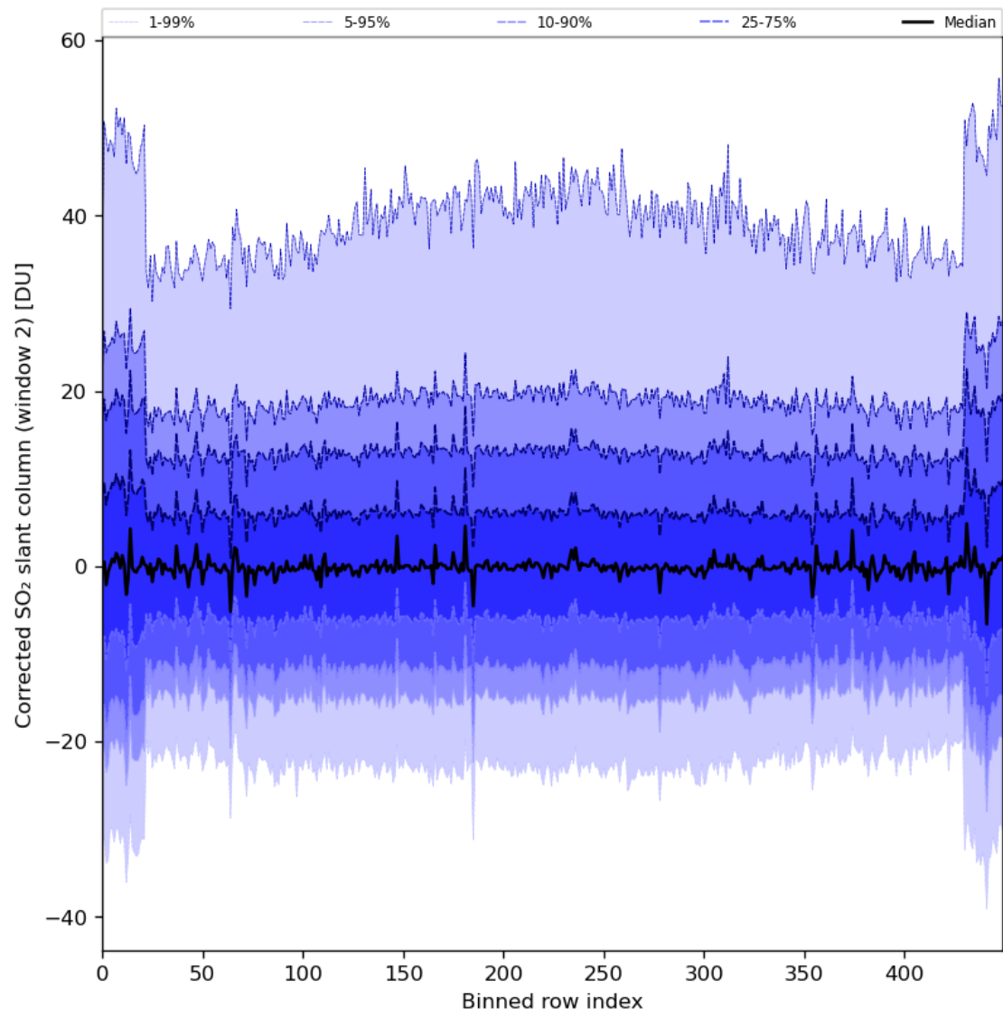
Figure 85: Along track statistics of “Corrected SO 2 slant column (window 2)” for 2024-04-10 to 2024-04-11
