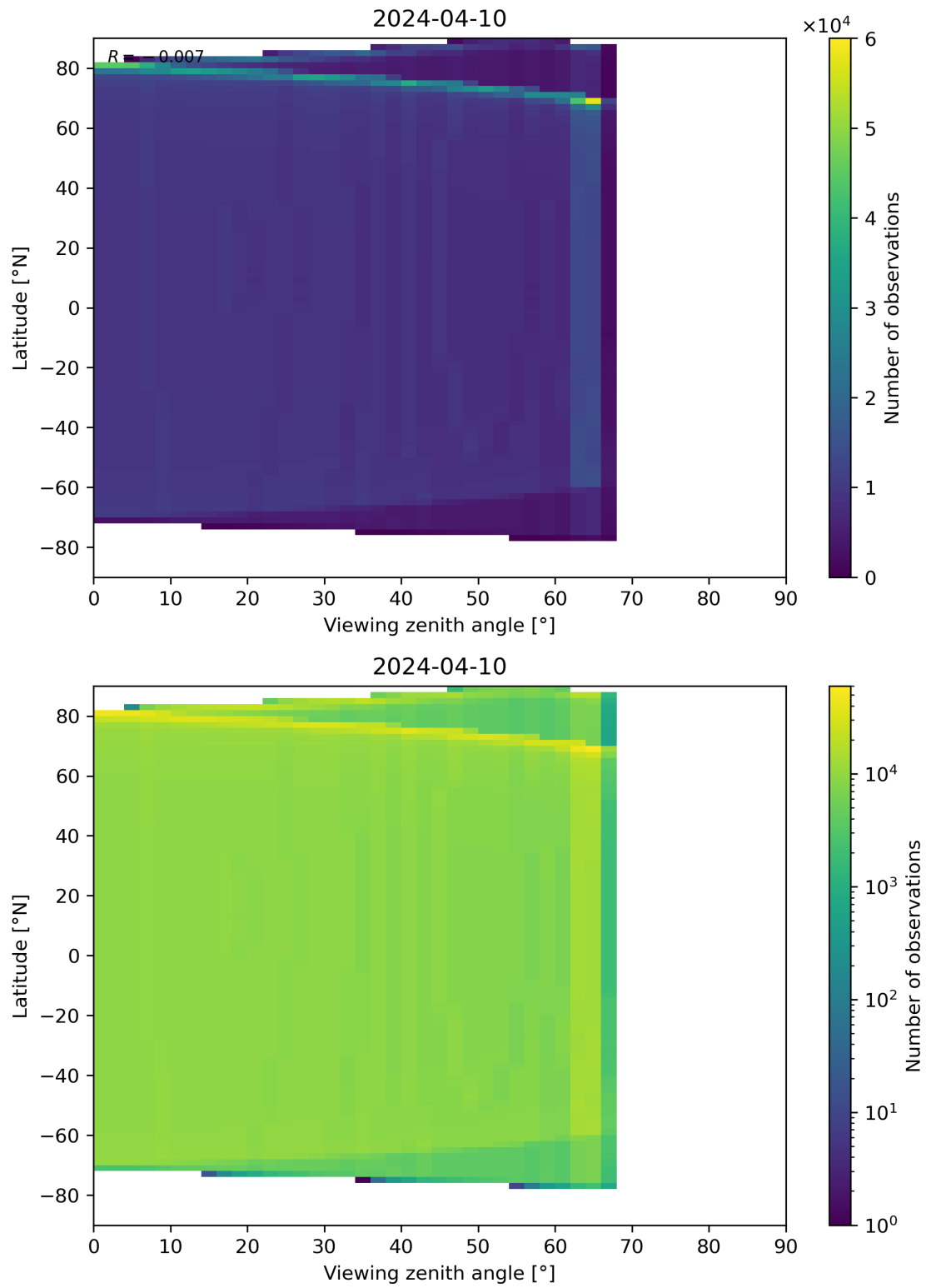
Figure 314: Scatter density plot of “Viewing zenith angle” against “Latitude” for 2024-04-10 to 2024-04-11.
