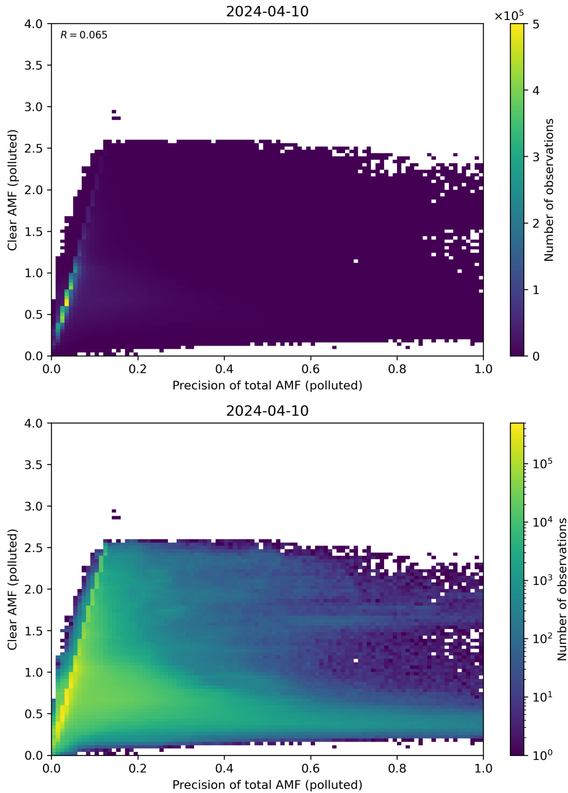
Figure 270: Scatter density plot of “Precision of total AMF (polluted)” against “Clear AMF (polluted)” for 2024-04-10 to 2024-04-11.
