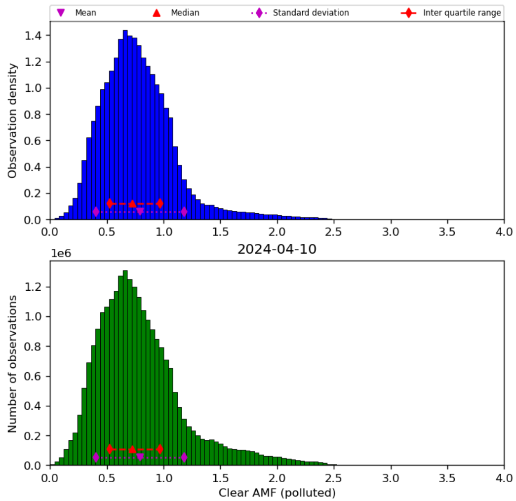
Figure 73: Histogram of “Clear AMF (polluted)” for 2024-04-10 to 2024-04-11
