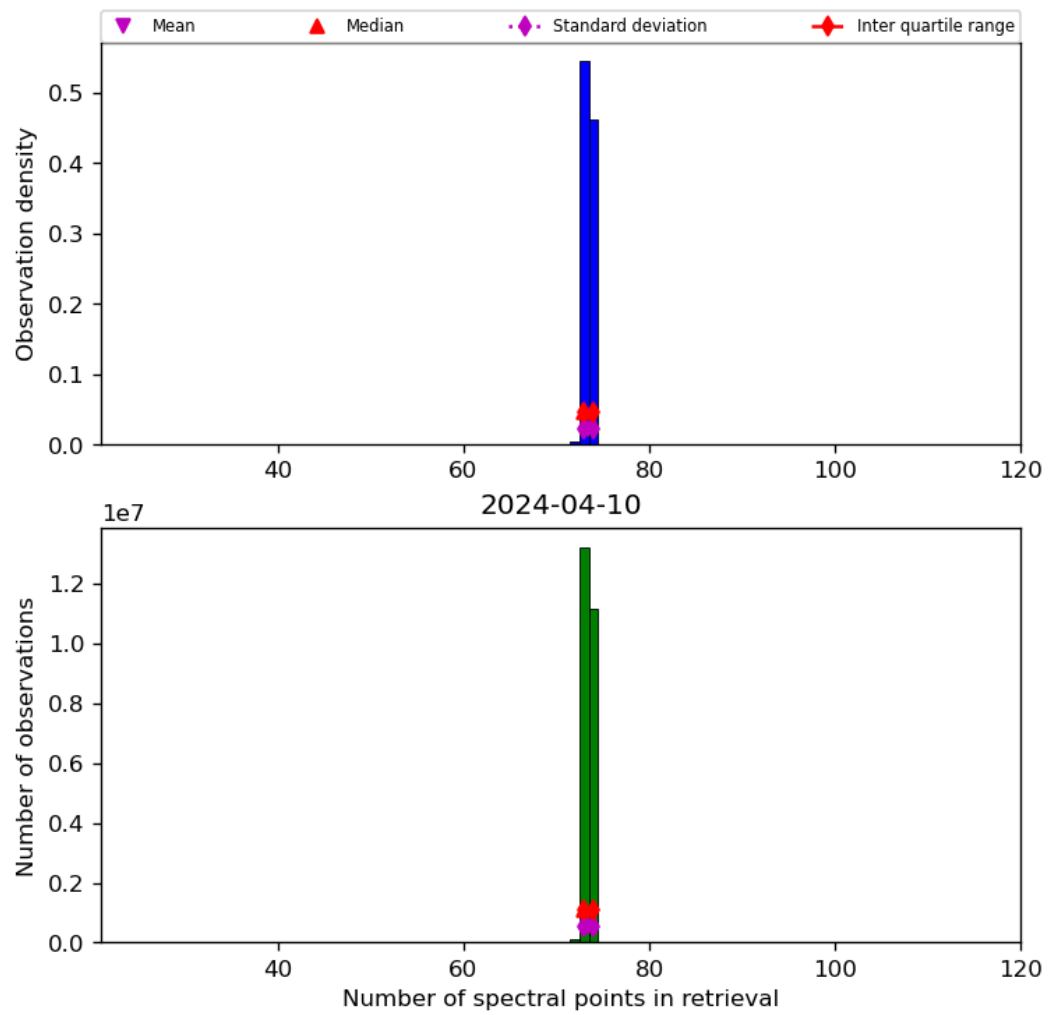
Figure 74: Histogram of “Number of spectral points in retrieval” for 2024-04-10 to 2024-04-11
