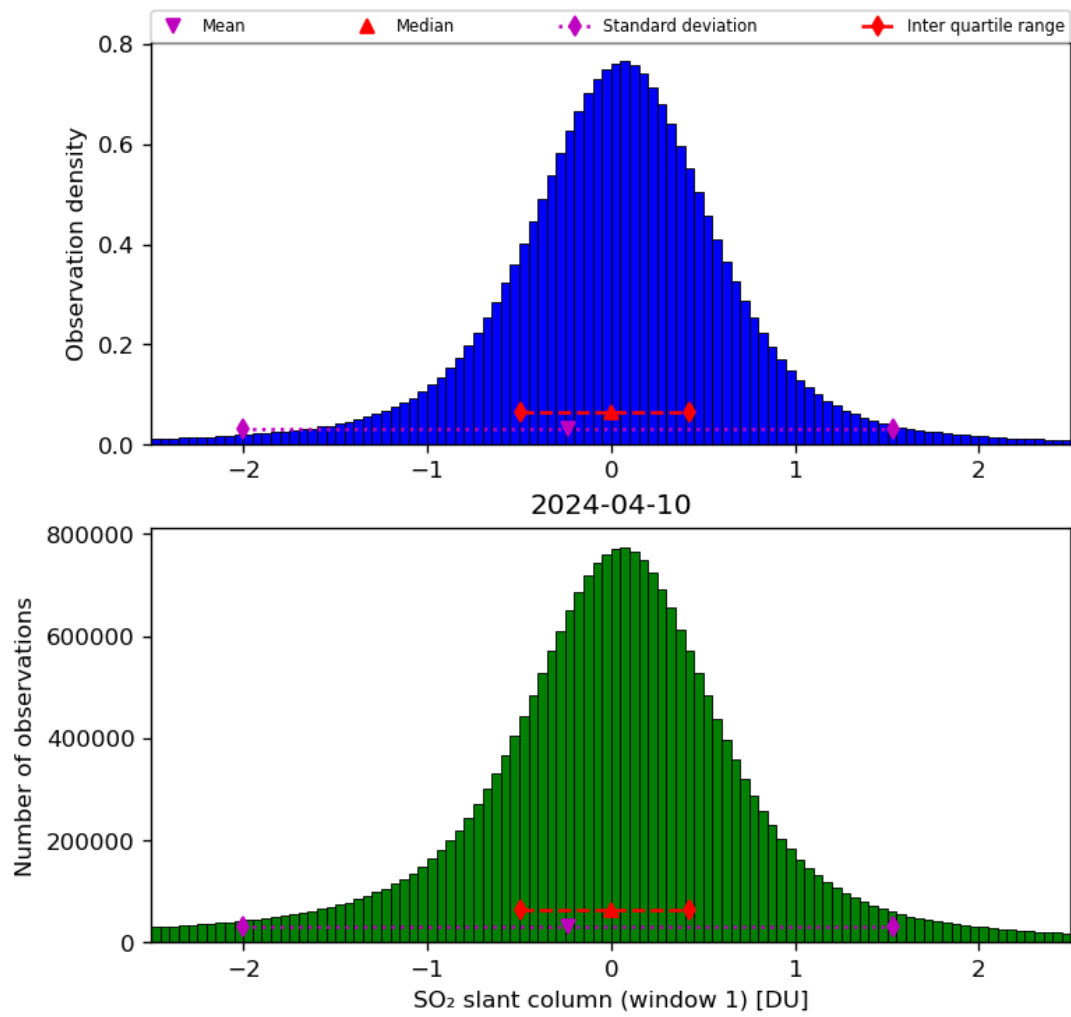
Figure 56: Histogram of “SO 2 slant column (window 1)” for 2024-04-10 to 2024-04-11
