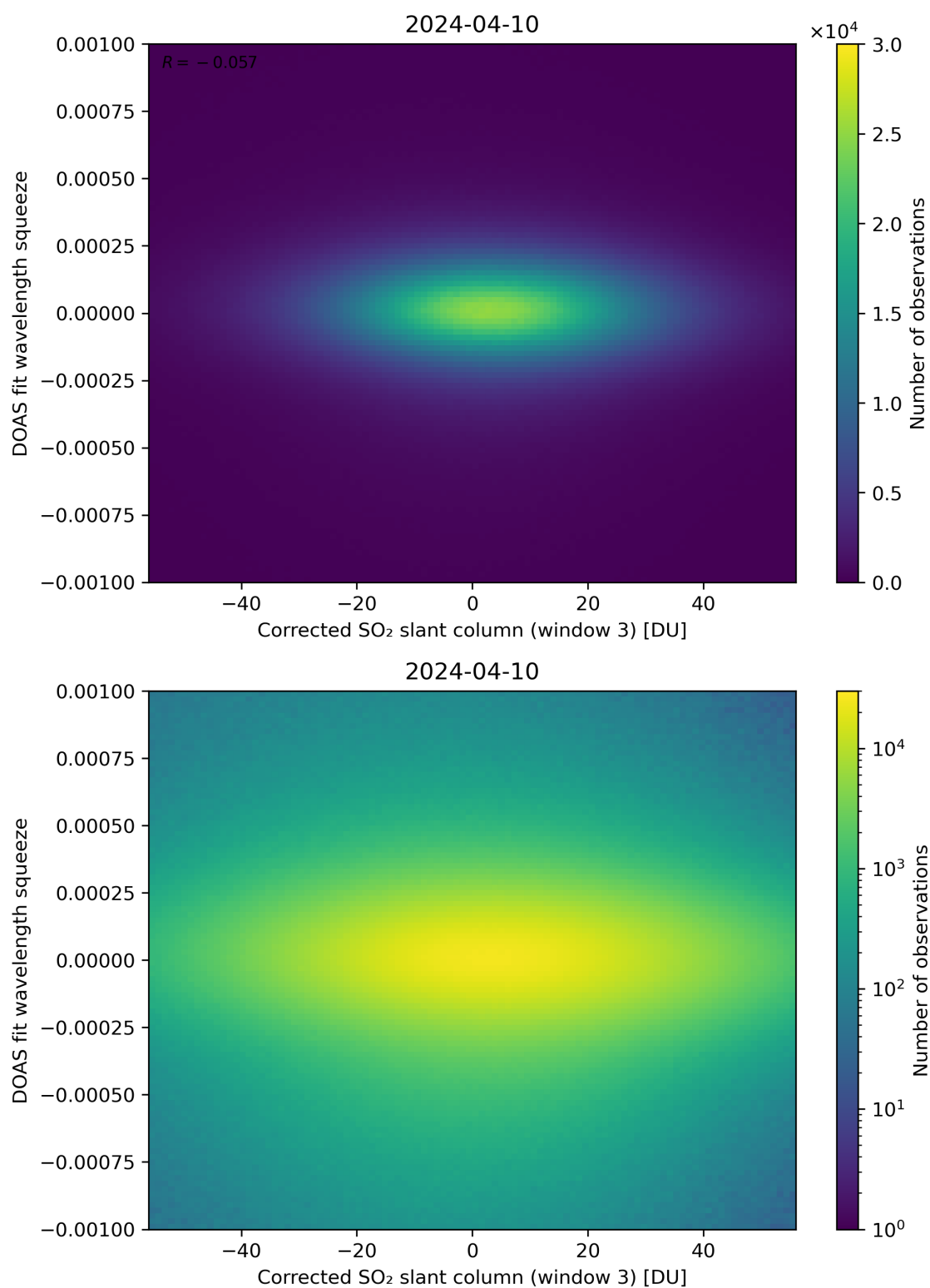
Figure 207: Scatter density plot of “Corrected SO 2 slant column (window 3)” against “DOAS fit wavelength squeeze” for 2024-04-10 to 2024-04-11.
