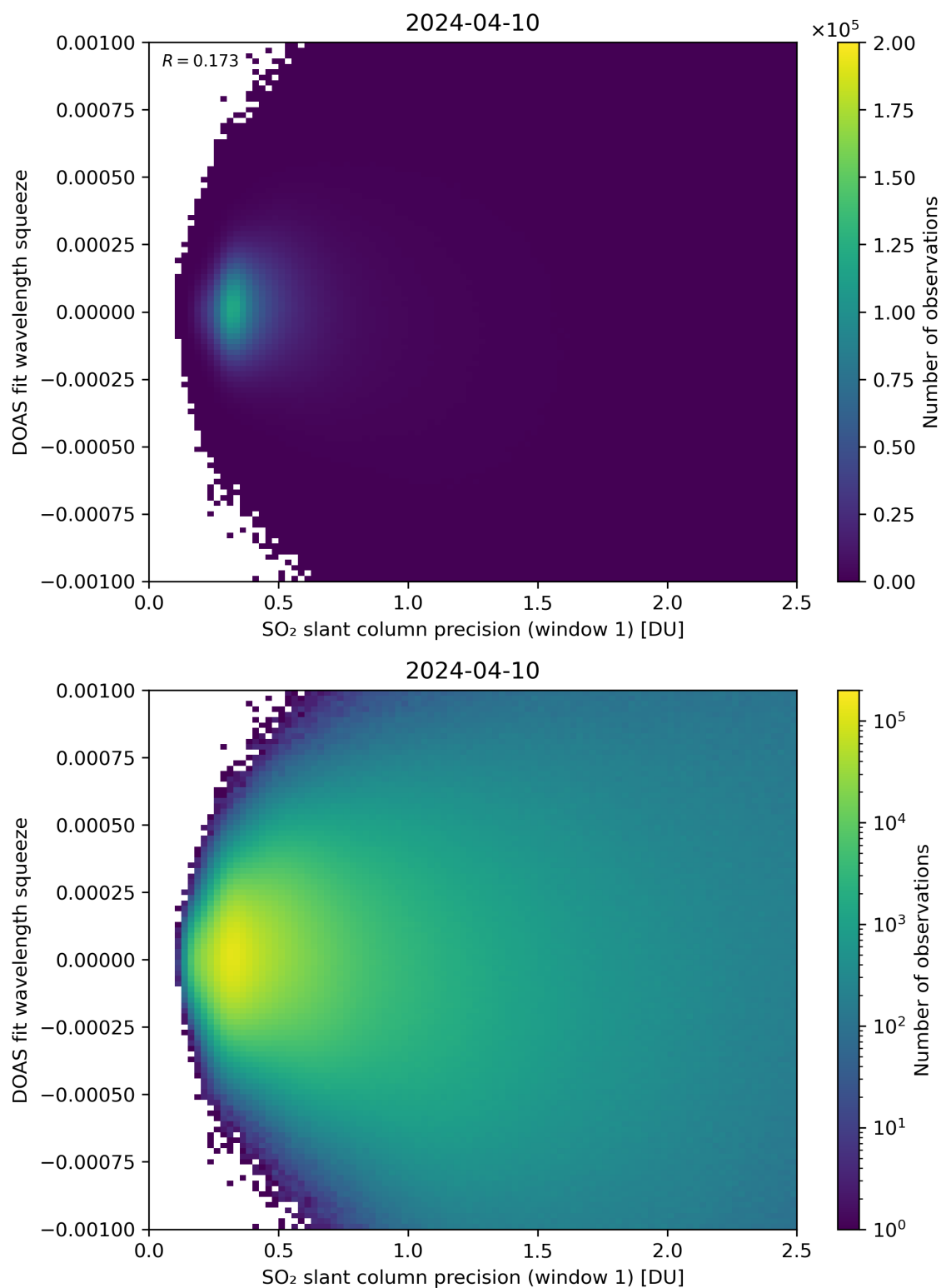
Figure 222: Scatter density plot of “SO 2 slant column precision (window 1)” against “DOAS fit wavelength squeeze” for 2024-04-10 to 2024-04-11.
