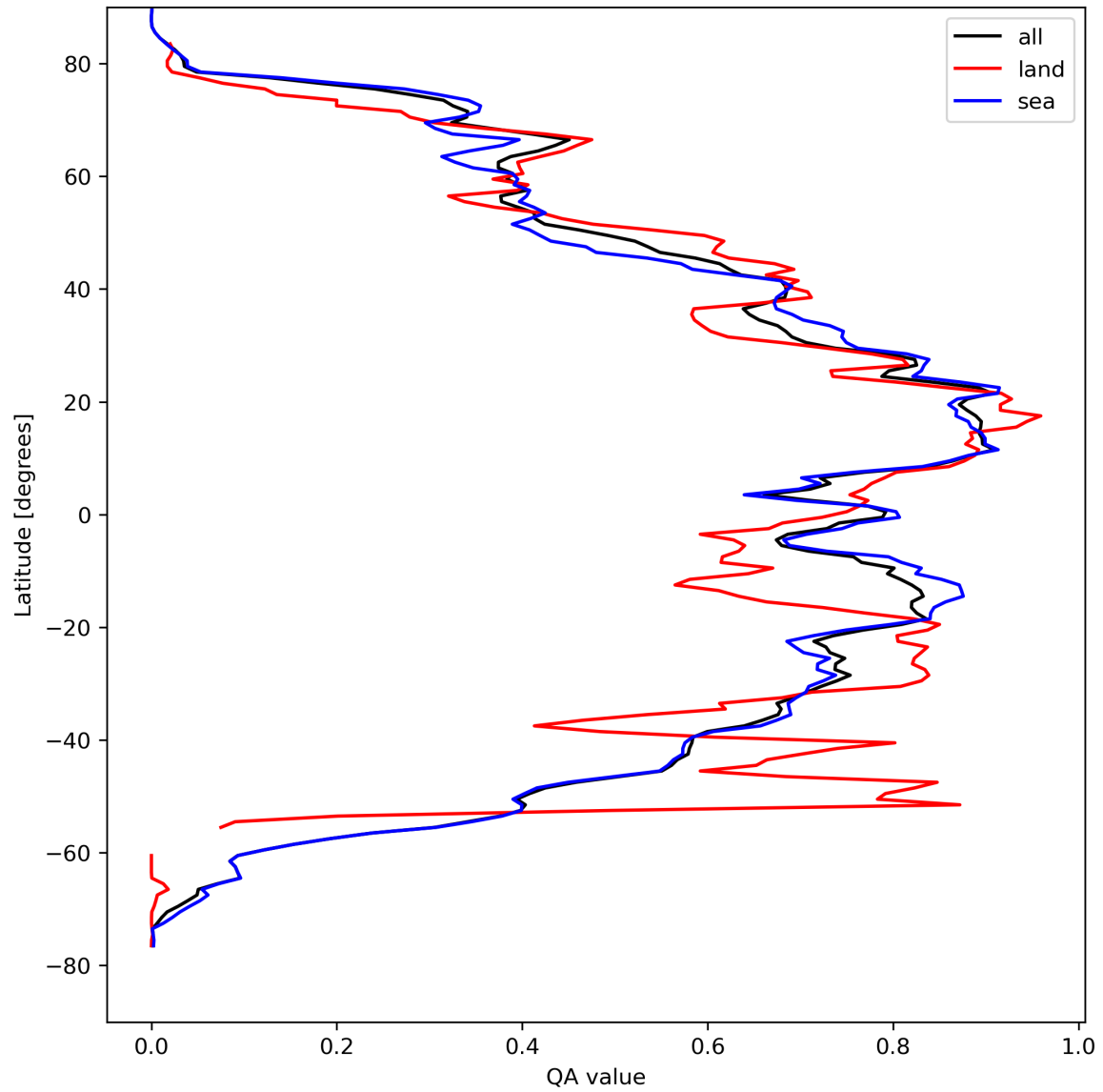
Figure 29: Zonal average of “QA value” for 2024-04-10 to 2024-04-11.
