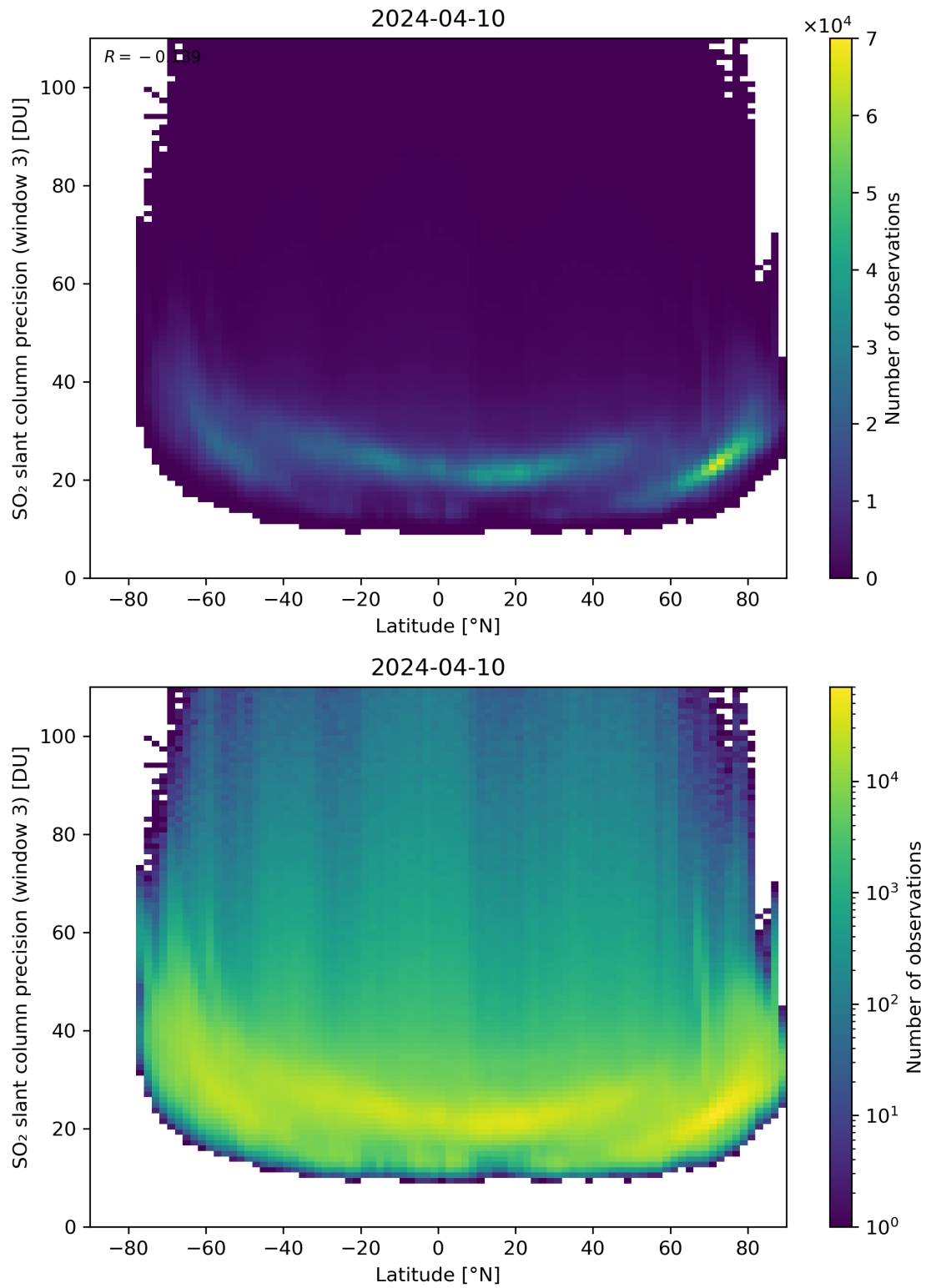
Figure 153: Scatter density plot of “Latitude” against “SO 2 slant column precision (window 3)” for 2024-04-10 to 2024-04-11.
