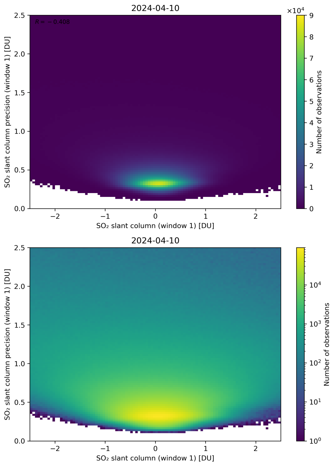
Figure 235: Scatter density plot of “SO 2 slant column (window 1)” against “SO 2 slant column precision (window 1)” for 2024-04-10 to 2024-04-11.
