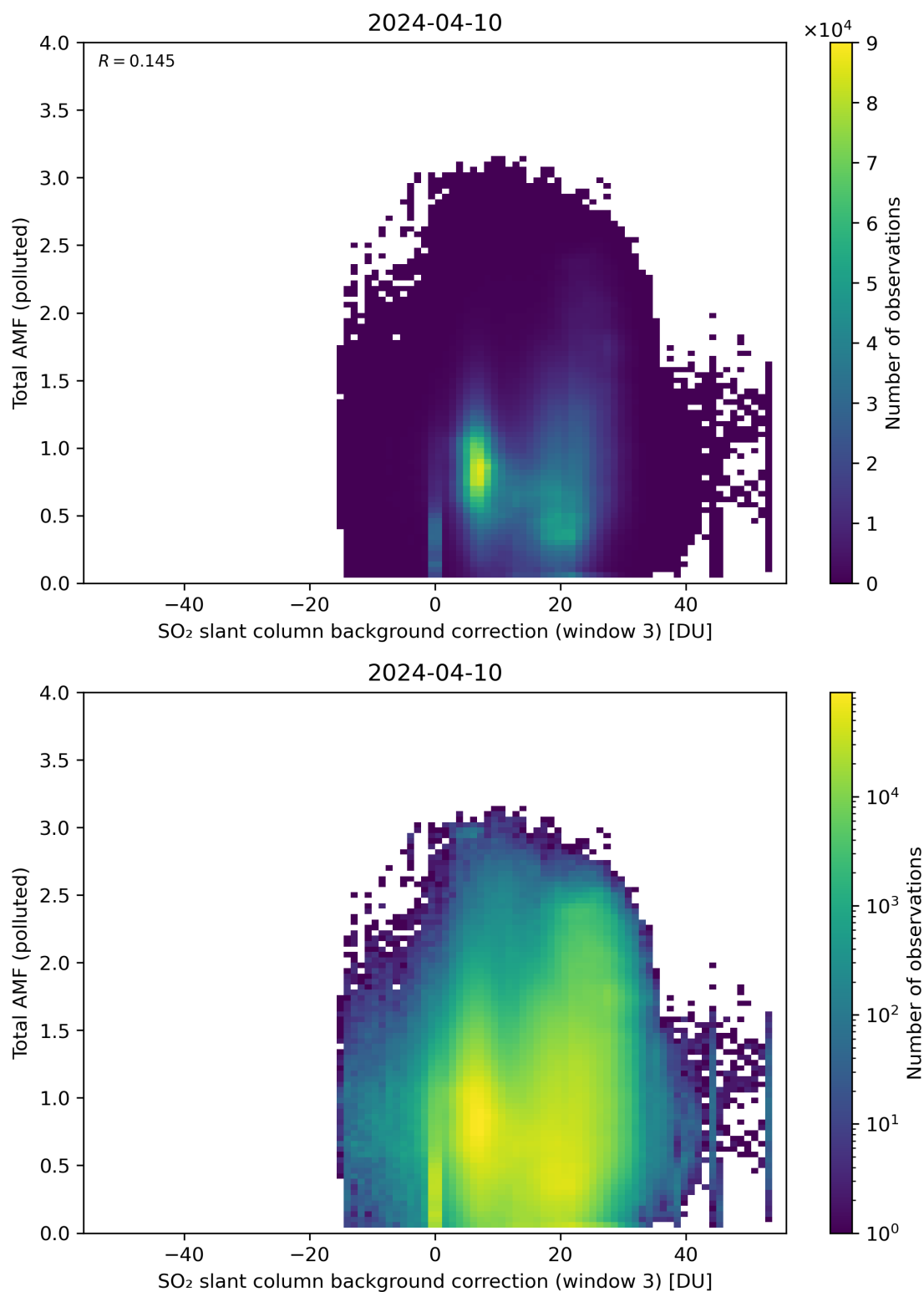
Figure 125: Scatter density plot of “SO 2 slant column background correction (window 3)” against “Total AMF (polluted)” for 2024-04-10 to 2024-04-11.
