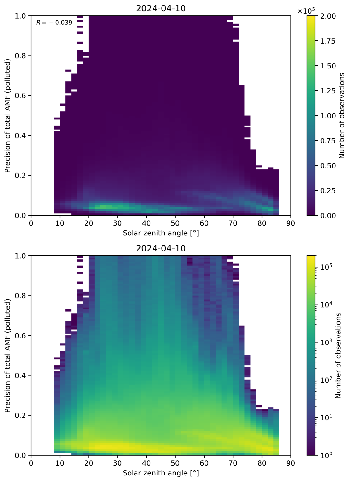
Figure 175: Scatter density plot of “Solar zenith angle” against “Precision of total AMF (polluted)” for 2024-04-10 to 2024-04-11.
