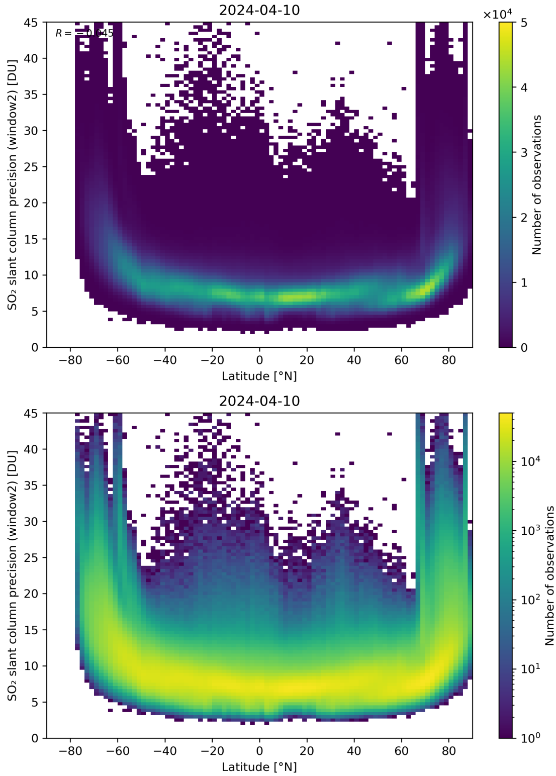
Figure 151: Scatter density plot of “Latitude” against “SO 2 slant column precision (window2)” for 2024-04-10 to 2024-04-11.
