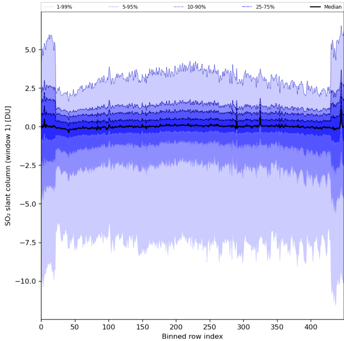
Figure 79: Along track statistics of “SO 2 slant column (window 1)” for 2024-04-10 to 2024-04-11
