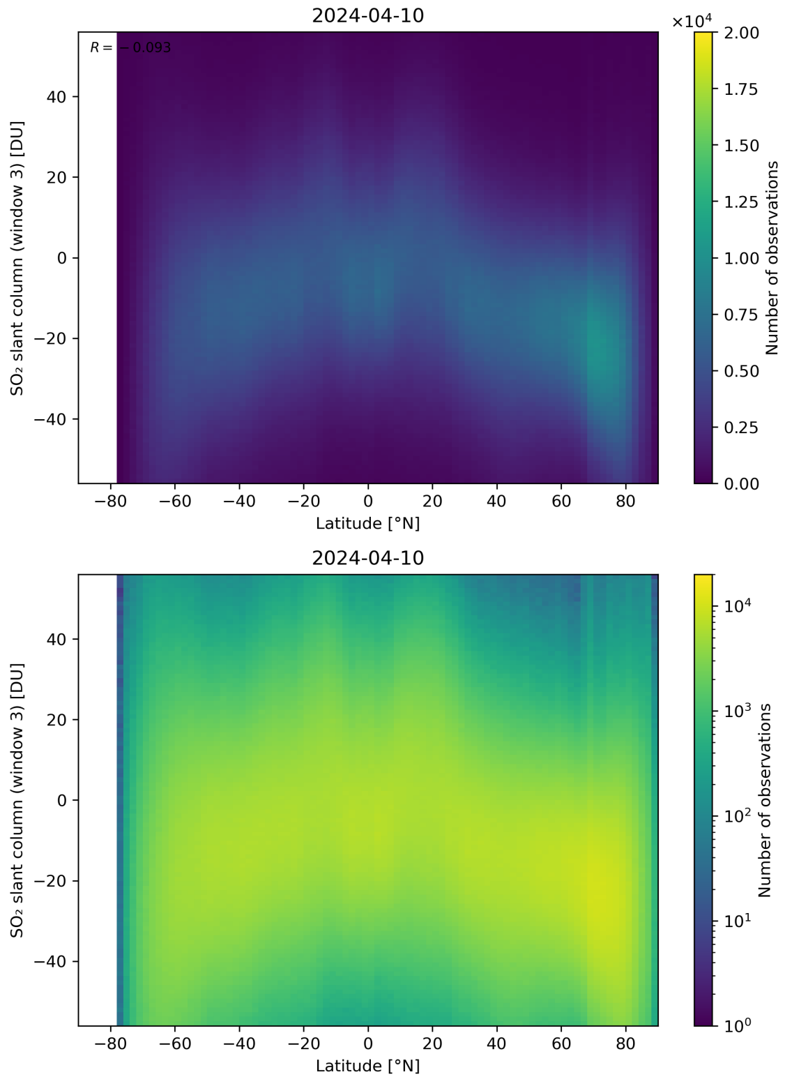
Figure 152: Scatter density plot of “Latitude” against “SO 2 slant column (window 3)” for 2024-04-10 to 2024-04-11.
