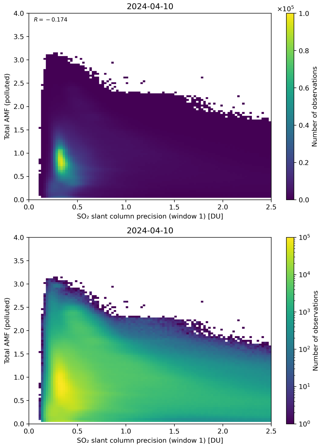
Figure 230: Scatter density plot of “SO 2 slant column precision (window 1)” against “Total AMF (polluted)” for 2024-04-10 to 2024-04-11.
