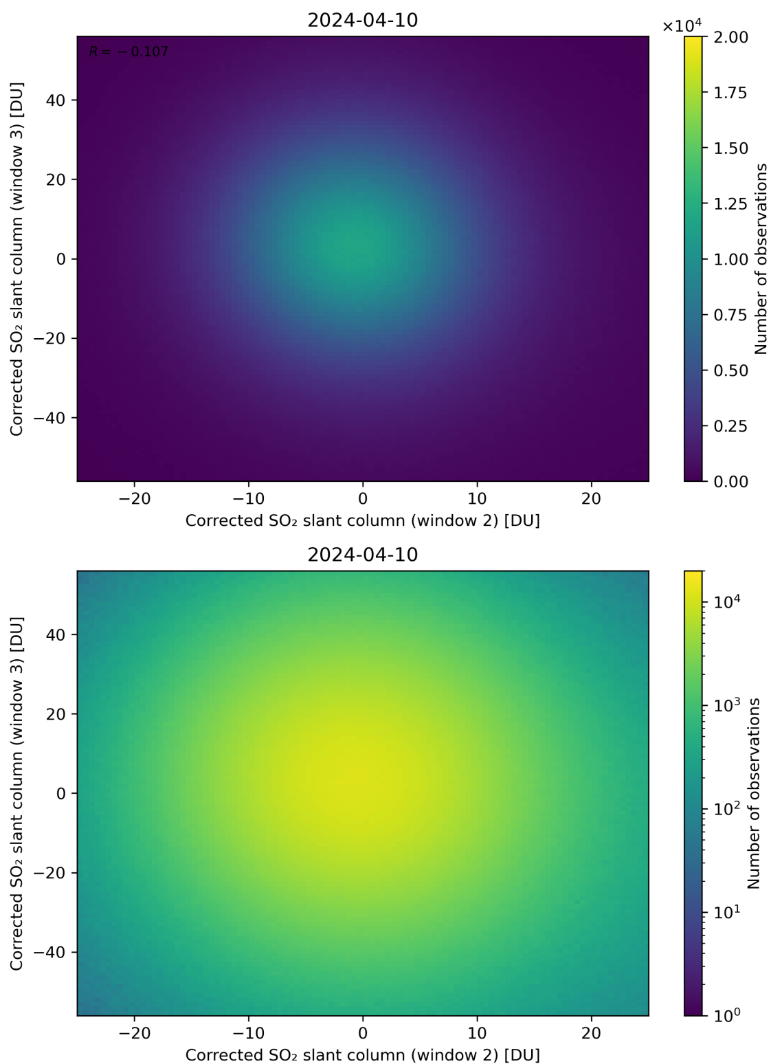
Figure 200: Scatter density plot of “Corrected SO 2 slant column (window 2)” against “Corrected SO 2 slant column (window 3)” for 2024-04-10 to 2024-04-11.
