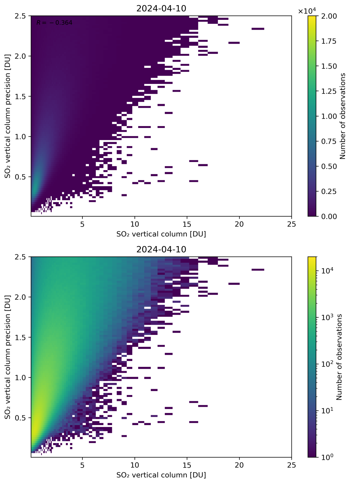
Figure 307: Scatter density plot of “SO 2 vertical column” against “SO 2 vertical column precision” for 2024-04-10 to 2024-04-11.
