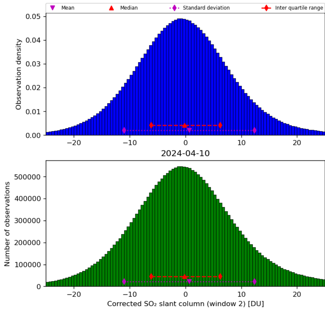
Figure 62: Histogram of “Corrected SO 2 slant column (window 2)” for 2024-04-10 to 2024-04-11
