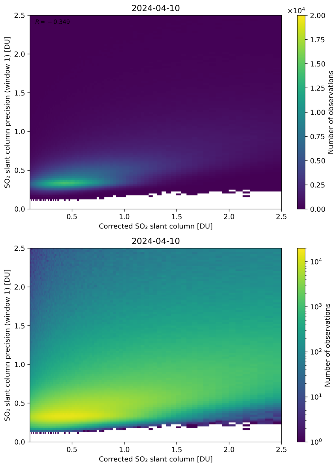
Figure 188: Scatter density plot of “Corrected SO 2 slant column” against “SO 2 slant column precision (window 1)” for 2024-04-10 to 2024-04-11.
