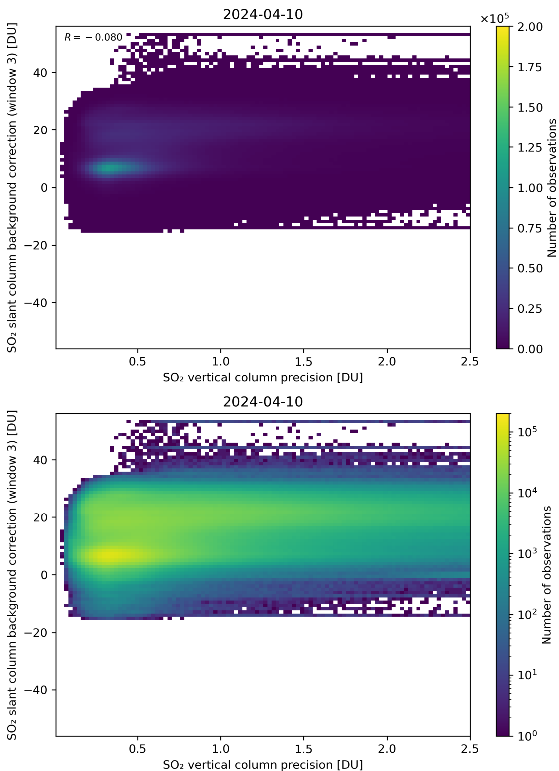
Figure 281: Scatter density plot of “SO 2 vertical column precision” against “SO 2 slant column background correction (window 3)” for 2024-04-10 to 2024-04-11.
