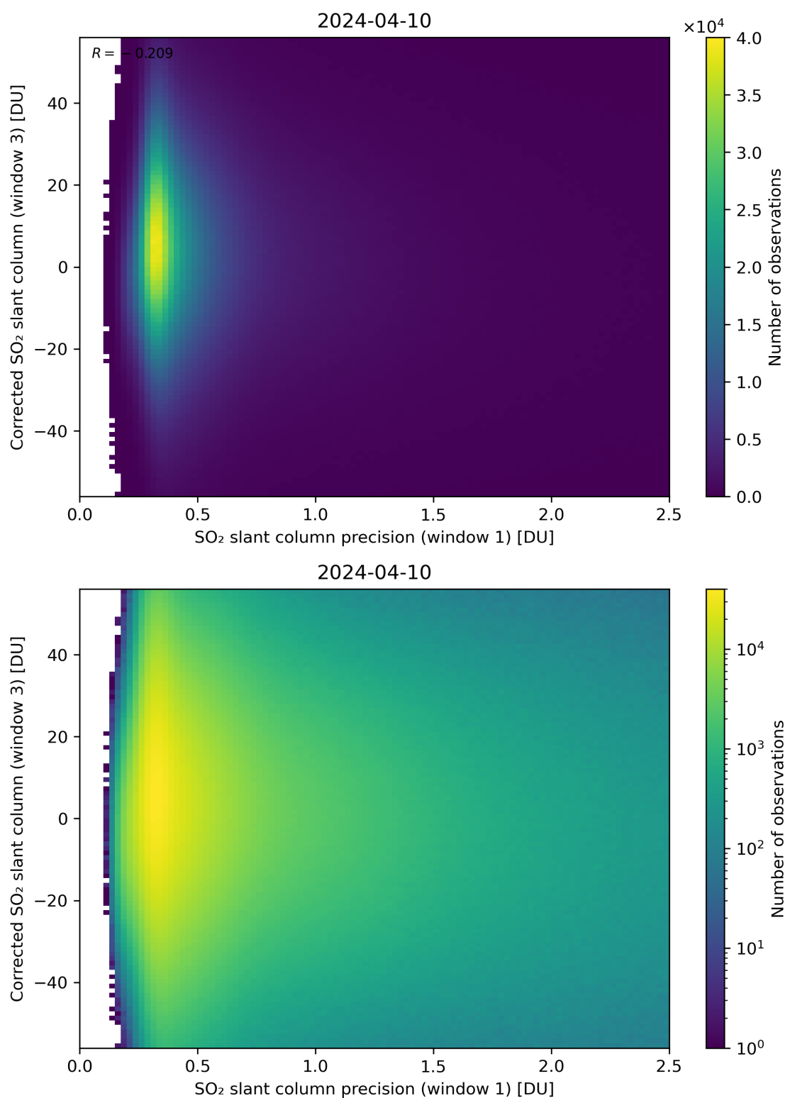
Figure 226: Scatter density plot of “SO 2 slant column precision (window 1)” against “Corrected SO 2 slant column (window 3)” for 2024-04-10 to 2024-04-11.
