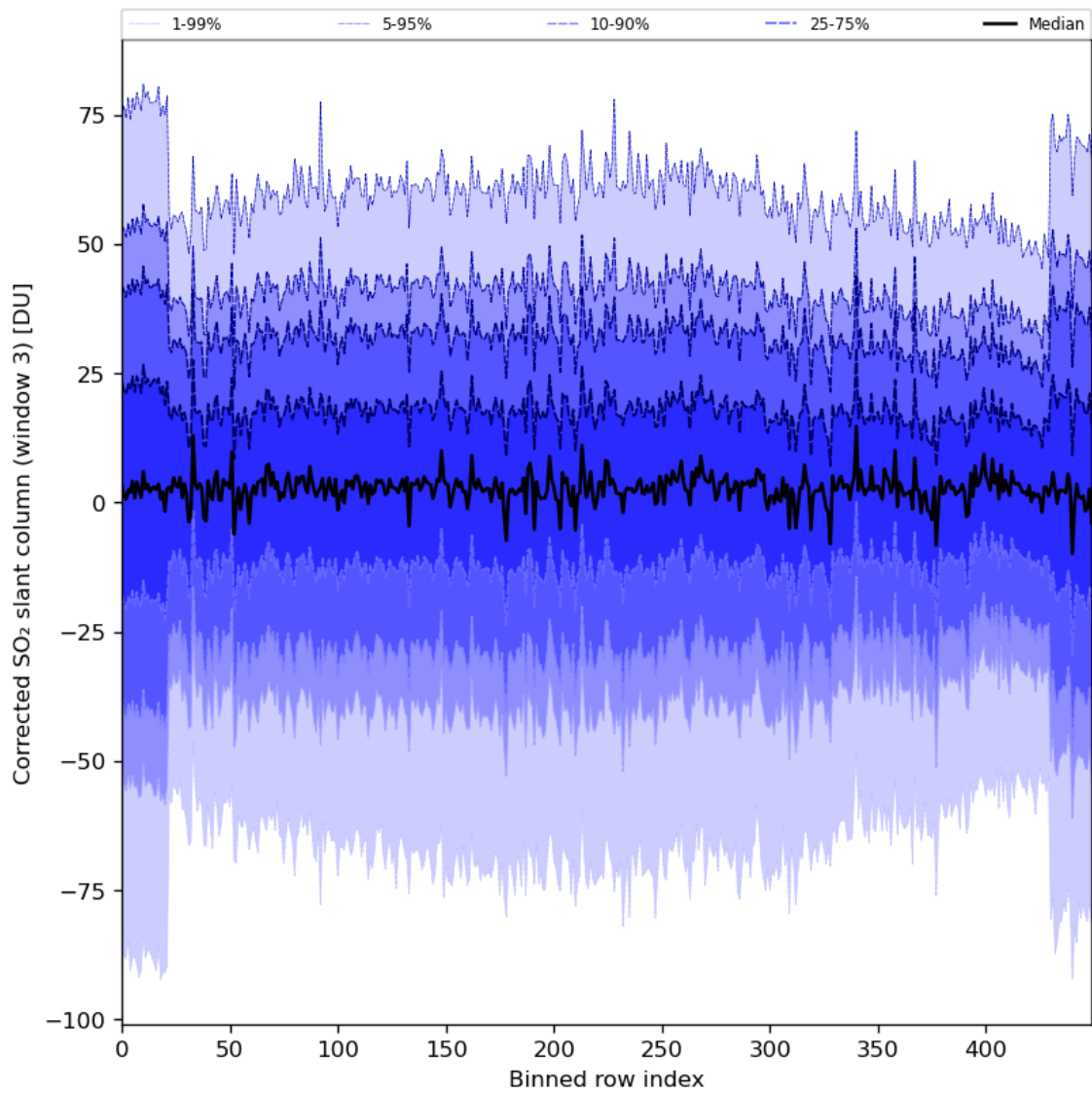
Figure 89: Along track statistics of “Corrected SO 2 slant column (window 3)” for 2024-04-10 to 2024-04-11
