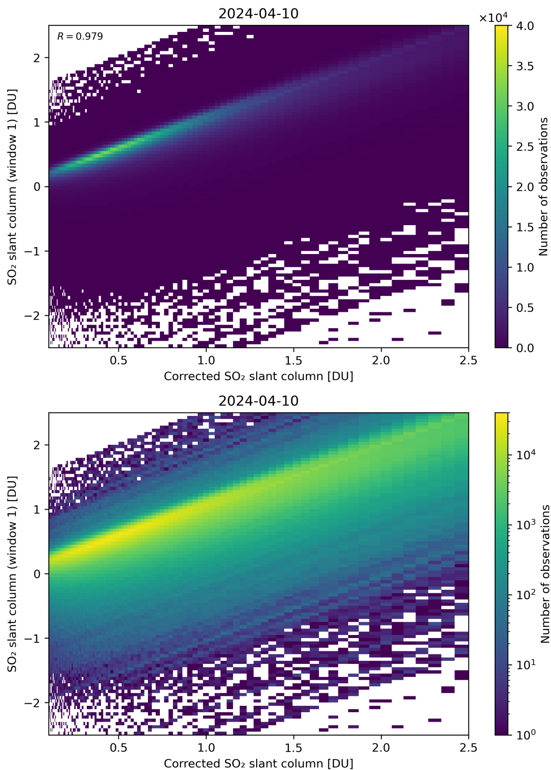
Figure 187: Scatter density plot of “Corrected SO 2 slant column” against “SO 2 slant column (window 1)” for 2024-04-10 to 2024-04-11.
