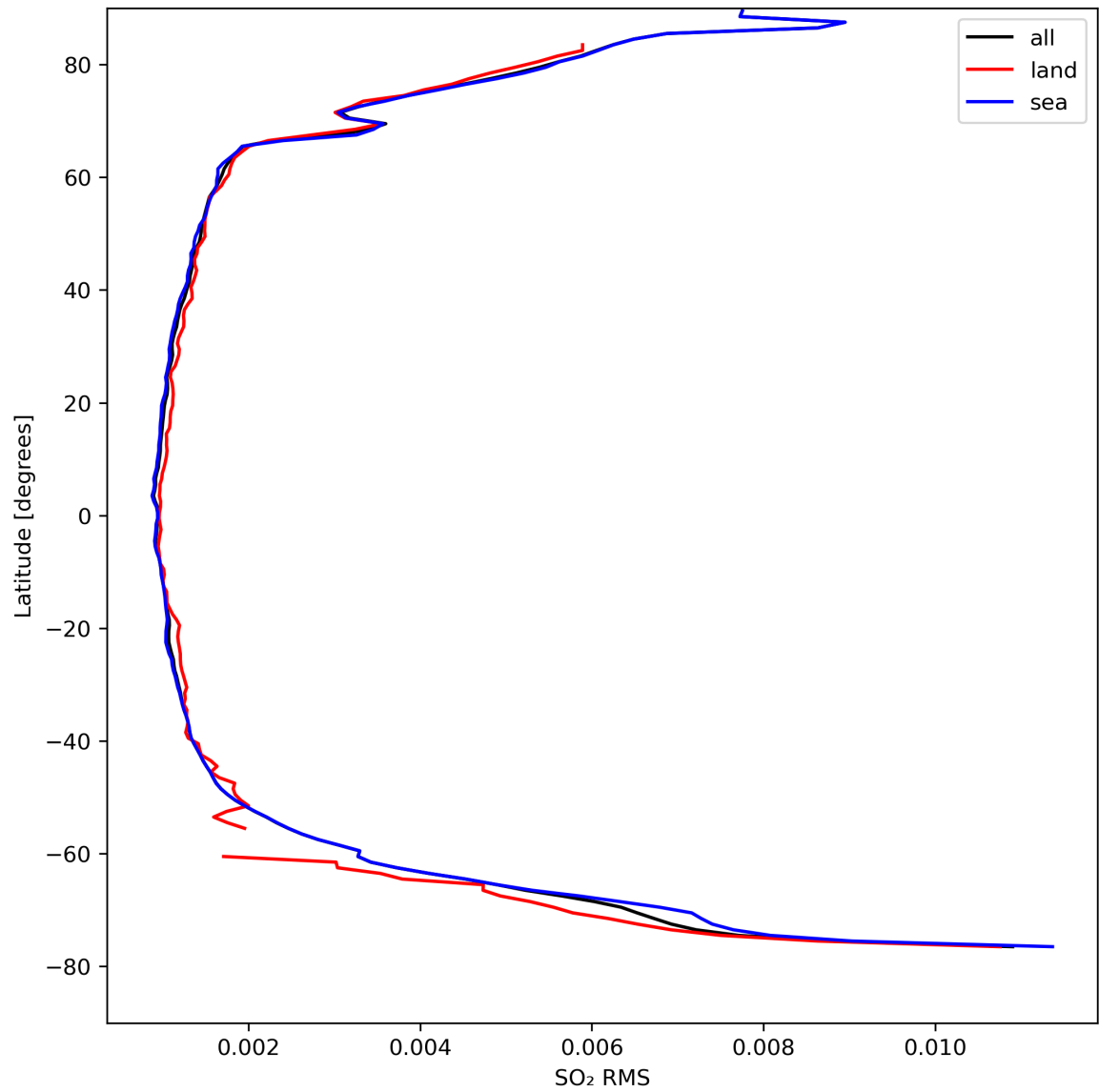
Figure 47: Zonal average of “SO 2 RMS” for 2024-04-10 to 2024-04-11.
