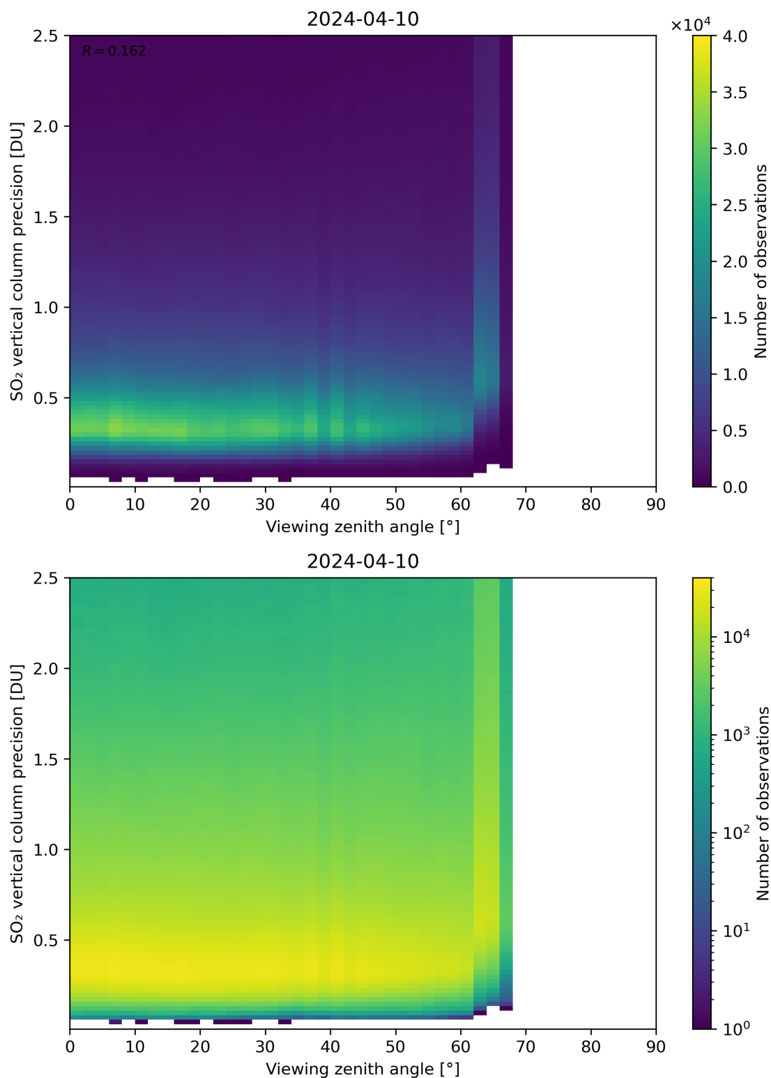
Figure 328: Scatter density plot of “Viewing zenith angle” against “SO 2 vertical column precision” for 2024-04-10 to 2024-04-11.
