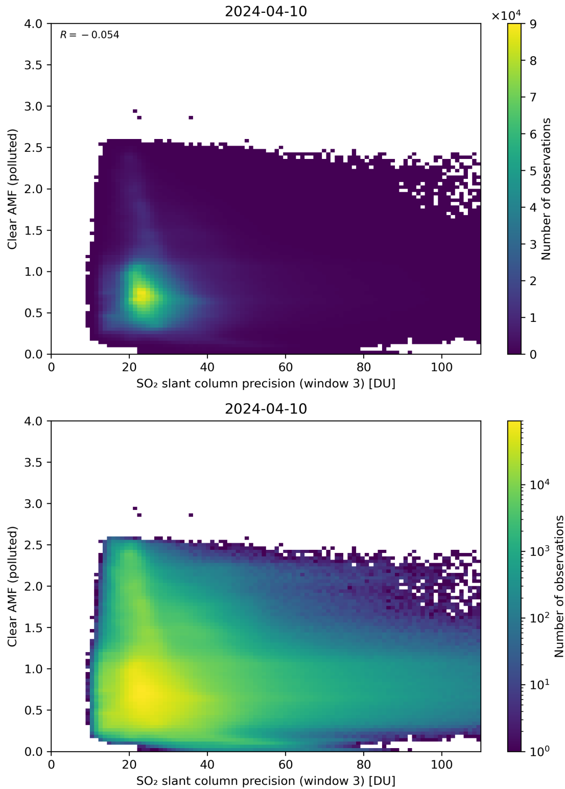
Figure 261: Scatter density plot of “SO 2 slant column precision (window 3)” against “Clear AMF (polluted)” for 2024-04-10 to 2024-04-11.
