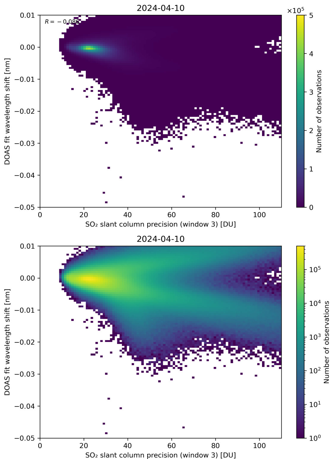
Figure 258: Scatter density plot of “SO 2 slant column precision (window 3)” against “DOAS fit wavelength shift” for 2024-04-10 to 2024-04-11.
