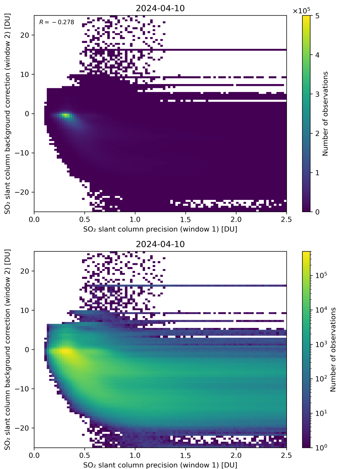
Figure 219: Scatter density plot of “SO 2 slant column precision (window 1)” against “SO 2 slant column background correction (window 2)” for 2024-04-10 to 2024-04-11.
