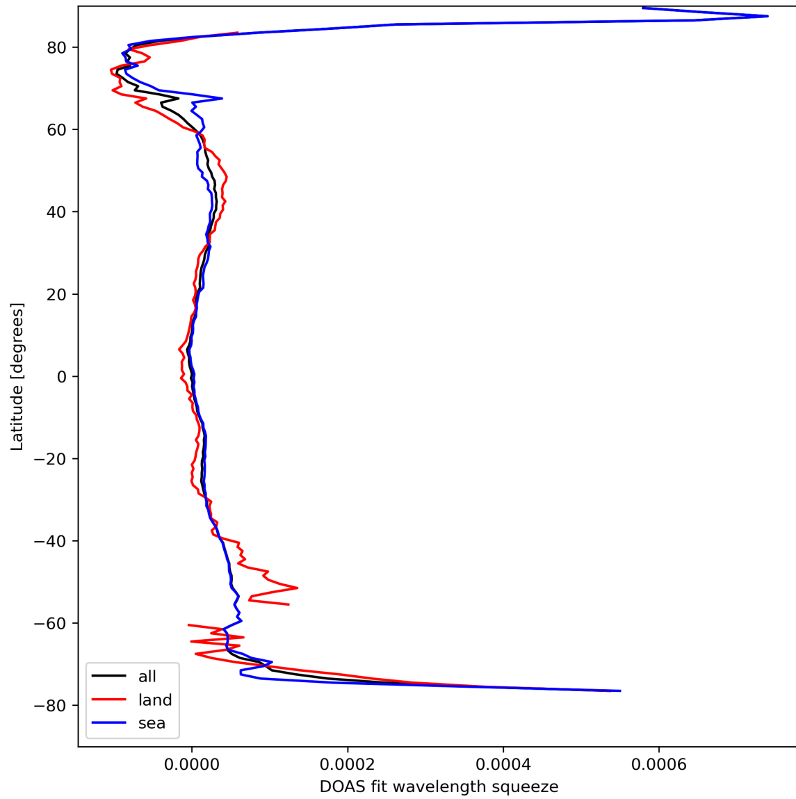
Figure 46: Zonal average of “DOAS fit wavelength squeeze” for 2024-04-10 to 2024-04-11.
