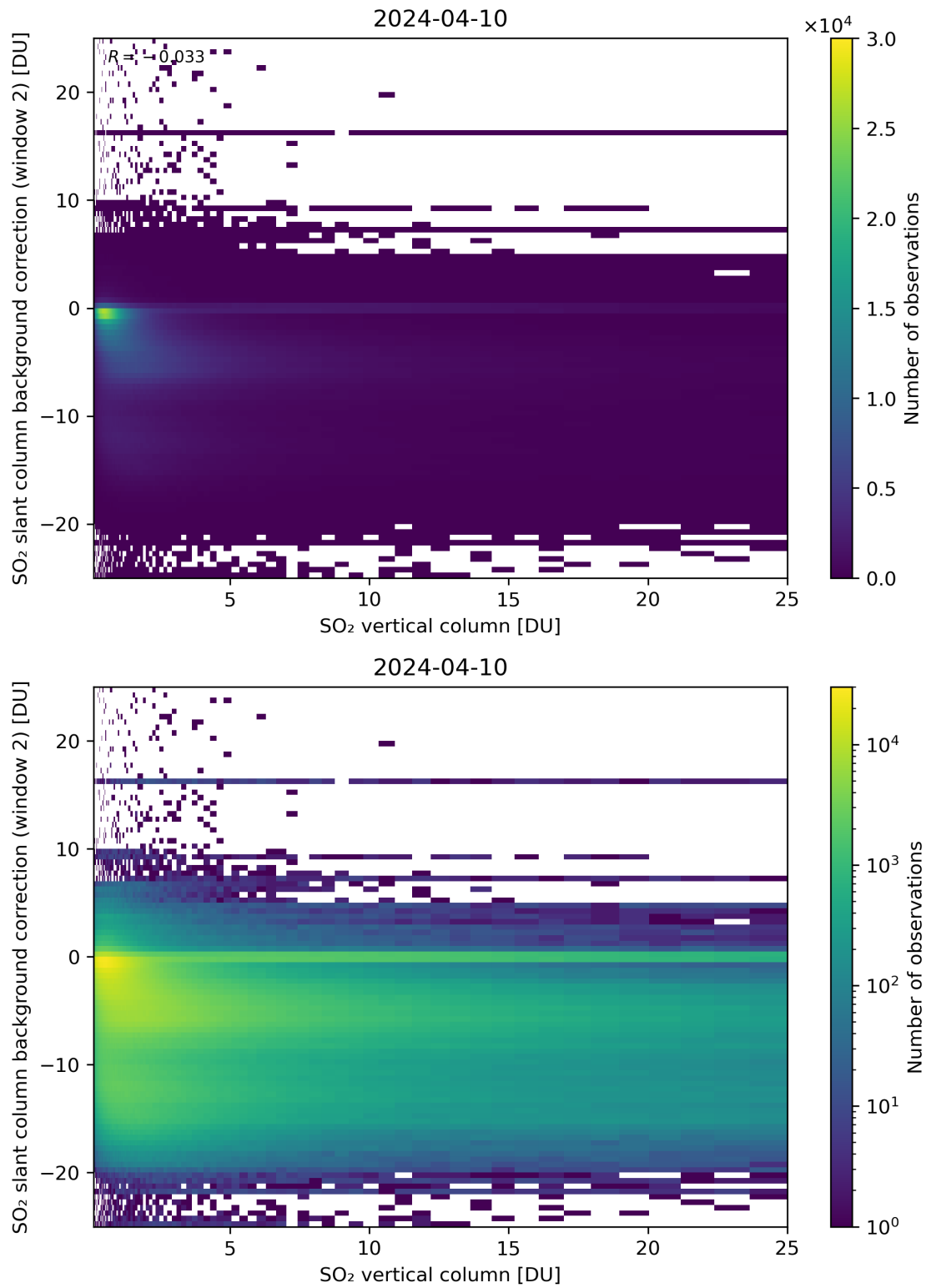
Figure 274: Scatter density plot of “SO 2 vertical column” against “SO 2 slant column background correction (window 2)” for 2024-04-10 to 2024-04-11.
