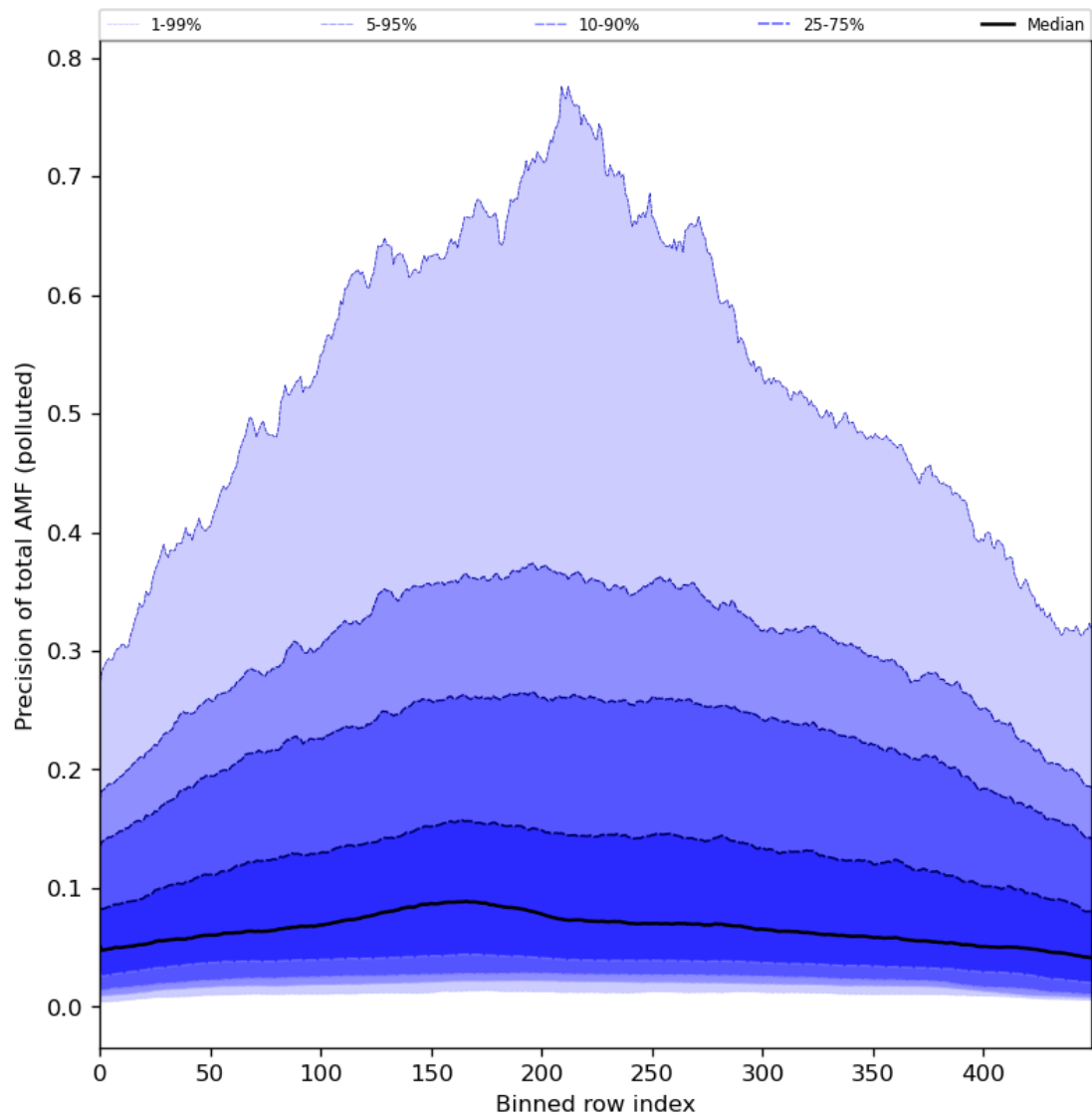
Figure 95: Along track statistics of “Precision of total AMF (polluted)” for 2024-04-10 to 2024-04-11
