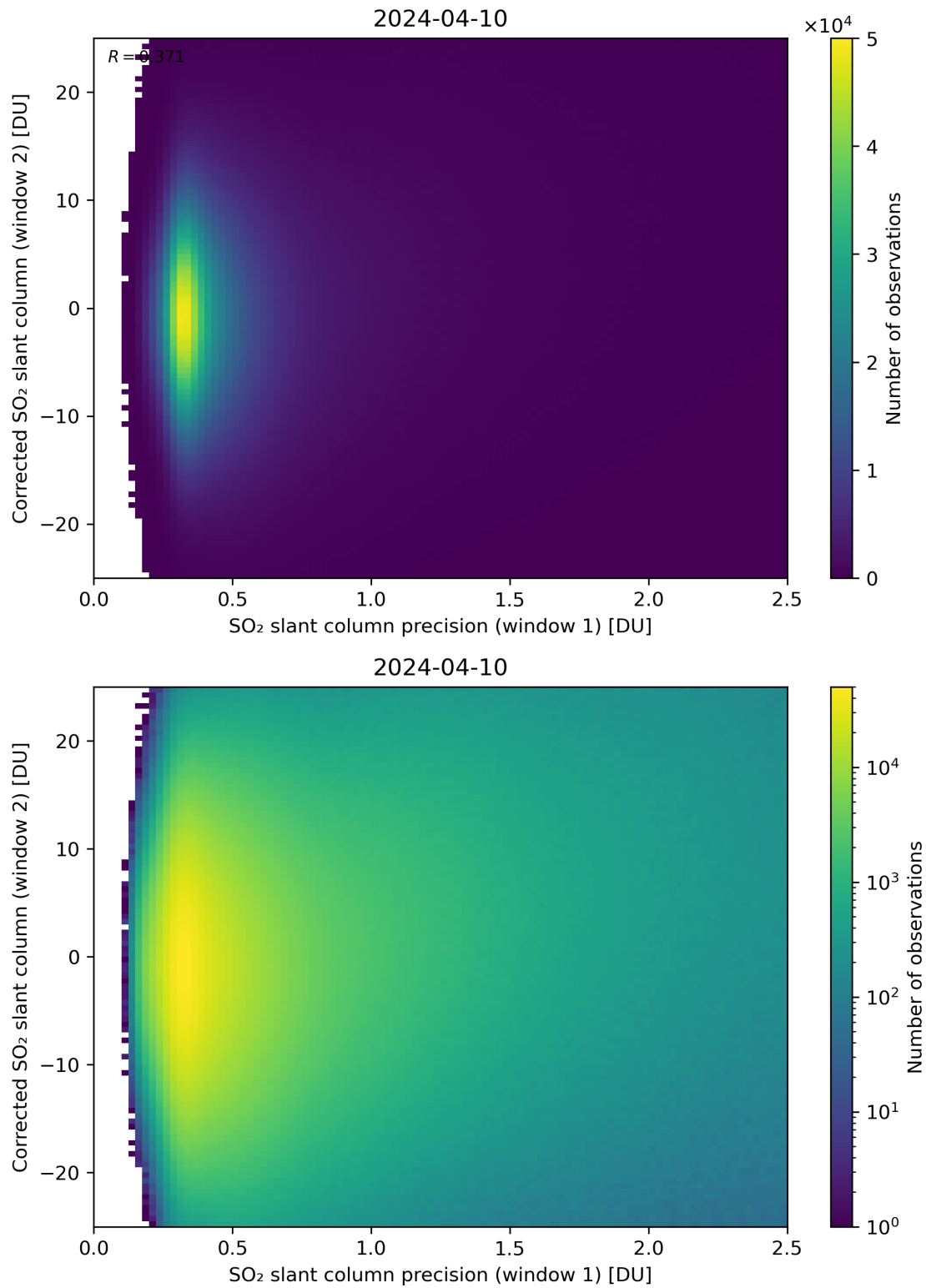
Figure 225: Scatter density plot of “SO 2 slant column precision (window 1)” against “Corrected SO 2 slant column (window 2)” for 2024-04-10 to 2024-04-11.
