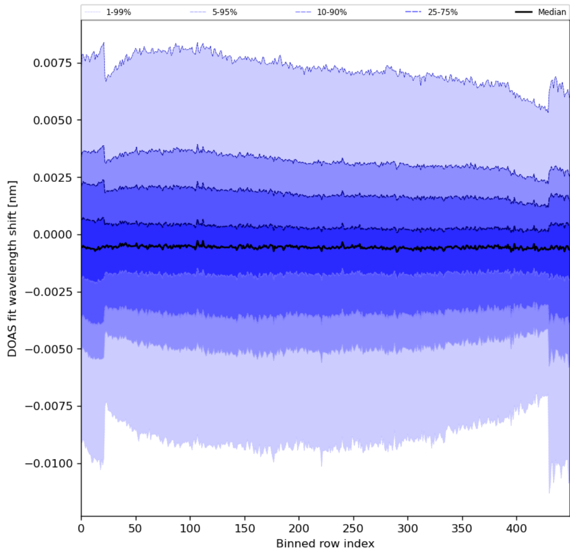
Figure 91: Along track statistics of “DOAS fit wavelength shift” for 2024-04-10 to 2024-04-11
