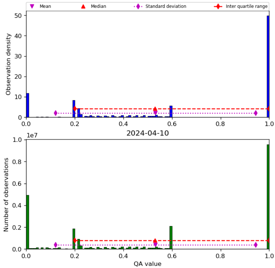
Figure 52: Histogram of “QA value” for 2024-04-10 to 2024-04-11
