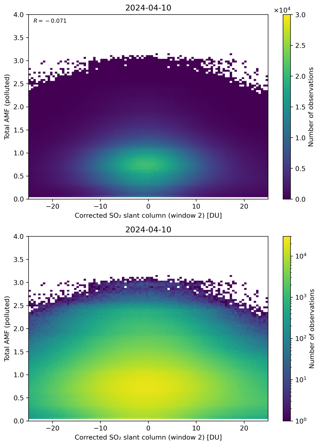
Figure 203: Scatter density plot of “Corrected SO 2 slant column (window 2)” against “Total AMF (polluted)” for 2024-04-10 to 2024-04-11.
