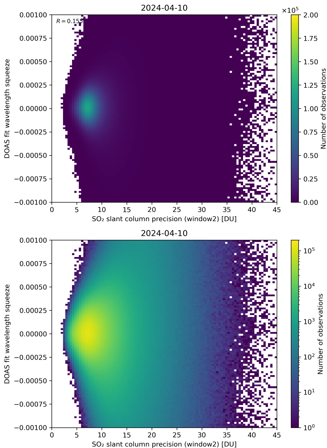
Figure 244: Scatter density plot of “SO 2 slant column precision (window2)” against “DOAS fit wavelength squeeze” for 2024-04-10 to 2024-04-11.
