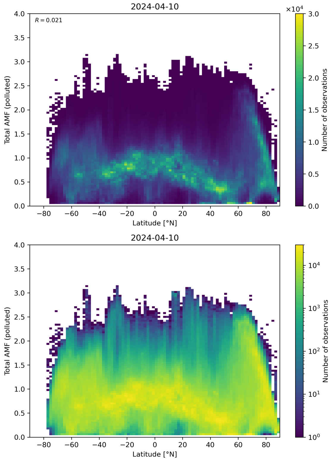
Figure 154: Scatter density plot of “Latitude” against “Total AMF (polluted)” for 2024-04-10 to 2024-04-11.
