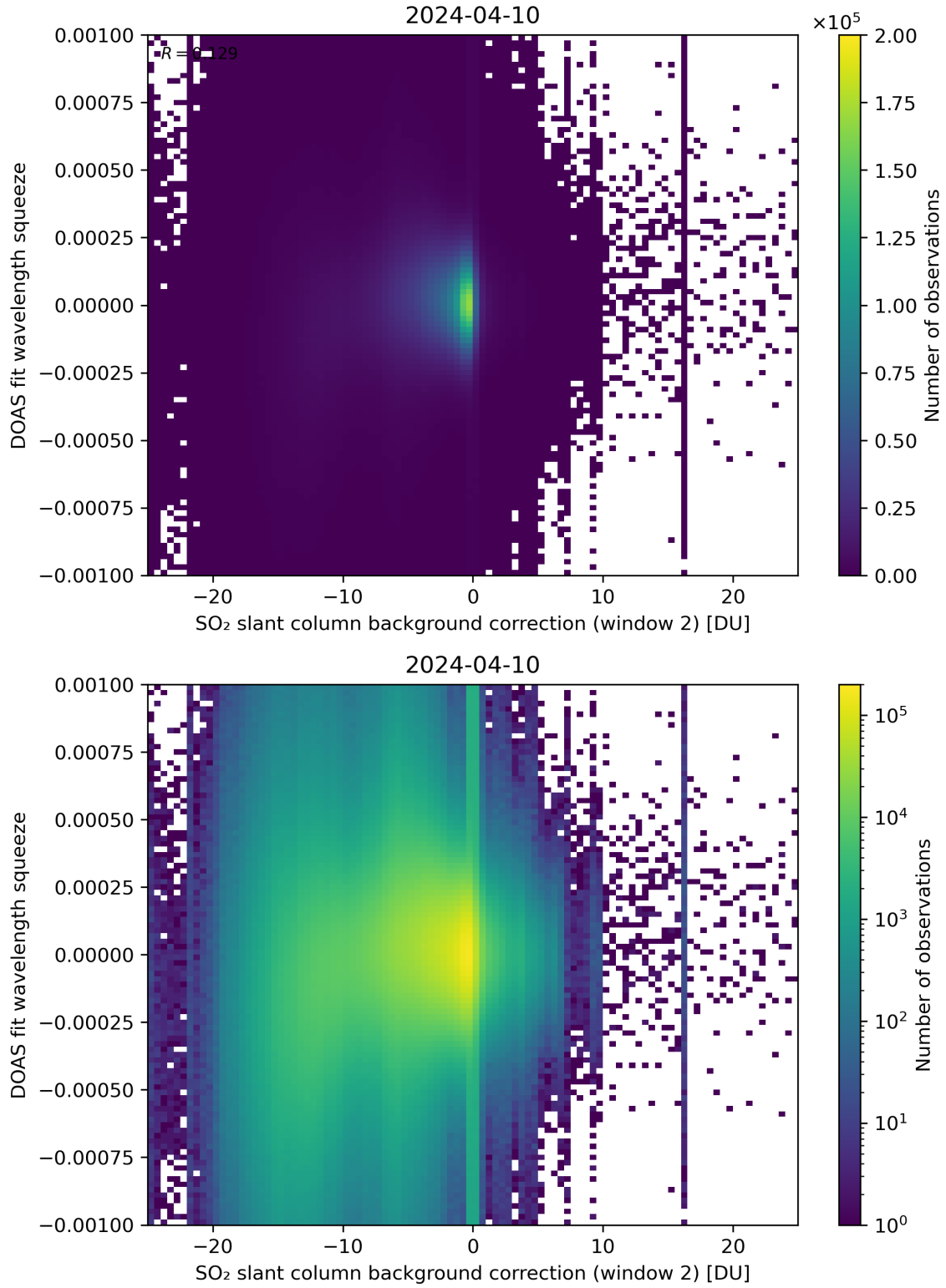
Figure 113: Scatter density plot of “SO 2 slant column background correction (window 2)” against “DOAS fit wavelength squeeze” for 2024-04-10 to 2024-04-11.
