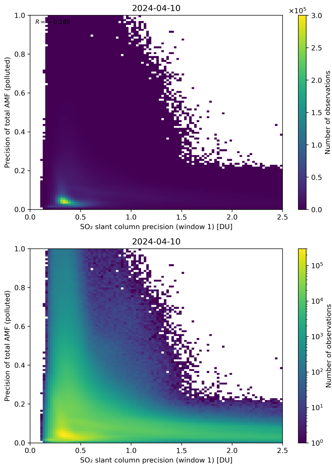
Figure 231: Scatter density plot of “SO 2 slant column precision (window 1)” against “Precision of total AMF (polluted)” for 2024-04-10 to 2024-04-11.
