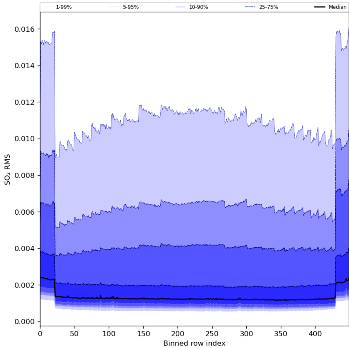
Figure 93: Along track statistics of “SO 2 RMS” for 2024-04-10 to 2024-04-11
