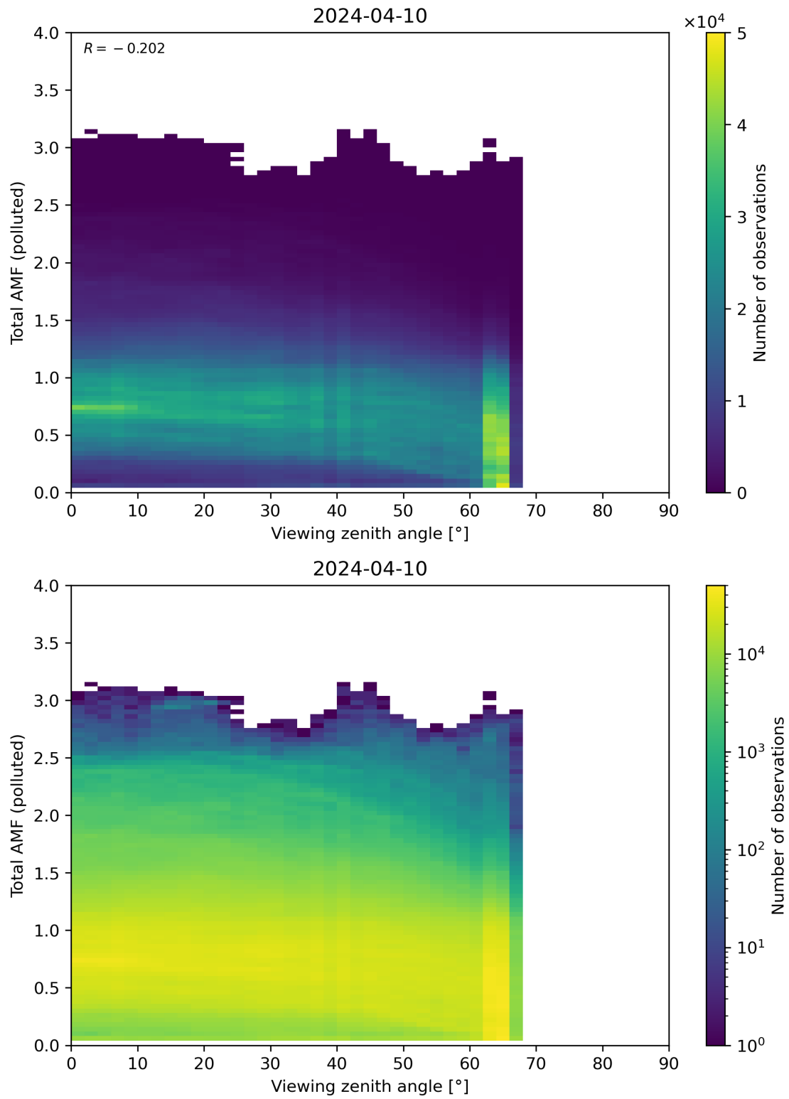
Figure 325: Scatter density plot of “Viewing zenith angle” against “Total AMF (polluted)” for 2024-04-10 to 2024-04-11.
