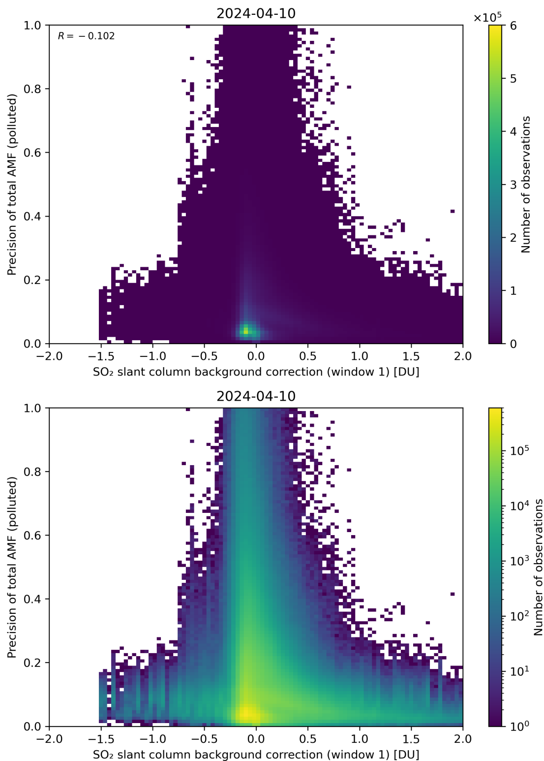
Figure 110: Scatter density plot of “SO 2 slant column background correction (window 1)” against “Precision of total AMF (polluted)” for 2024-04-10 to 2024-04-11.
