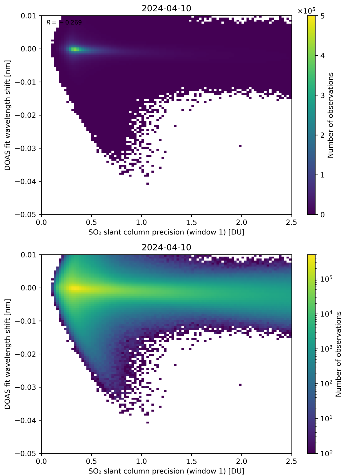
Figure 221: Scatter density plot of “SO 2 slant column precision (window 1)” against “DOAS fit wavelength shift” for 2024-04-10 to 2024-04-11.
