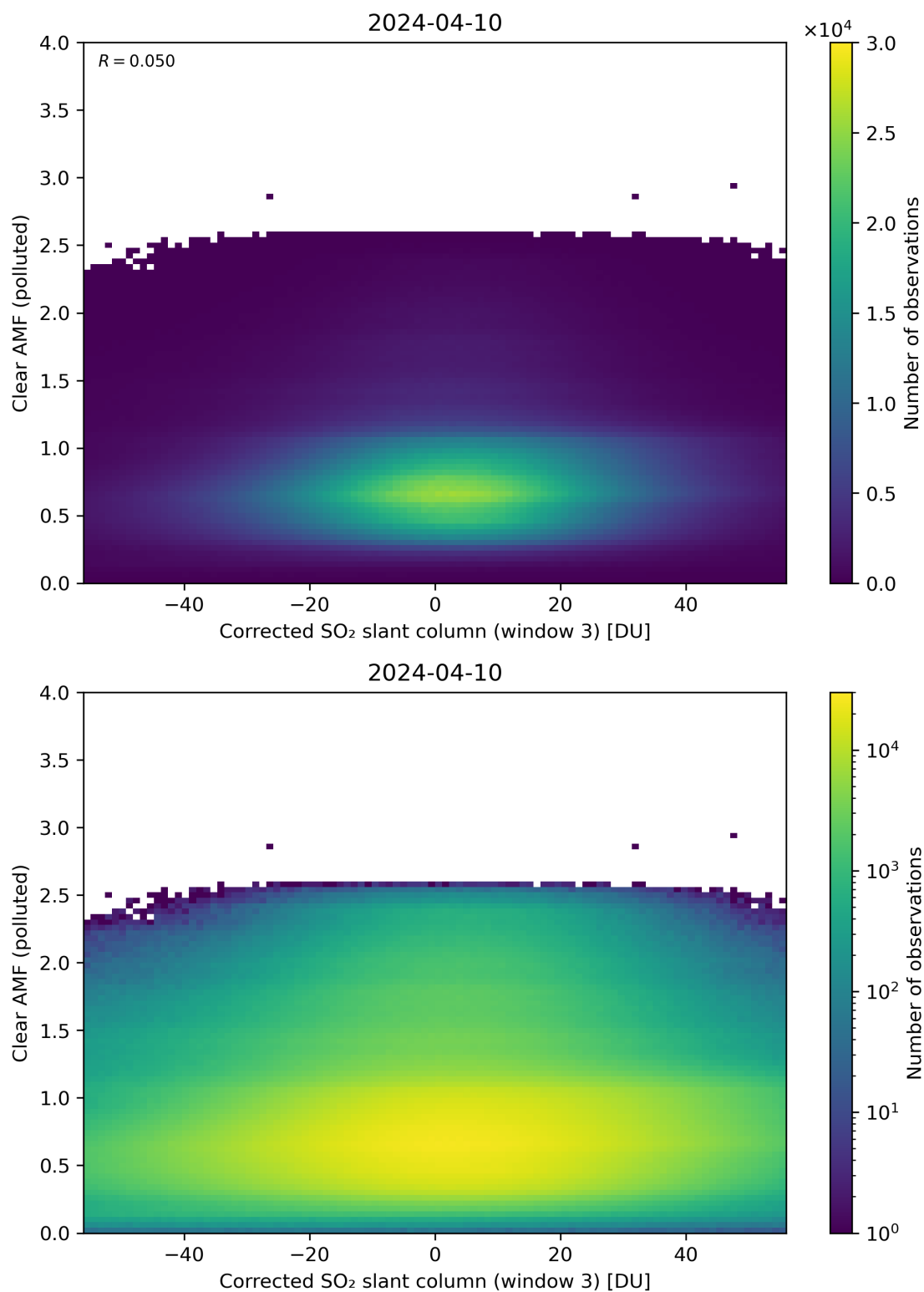
Figure 209: Scatter density plot of “Corrected SO 2 slant column (window 3)” against “Clear AMF (polluted)” for 2024-04-10 to 2024-04-11.
