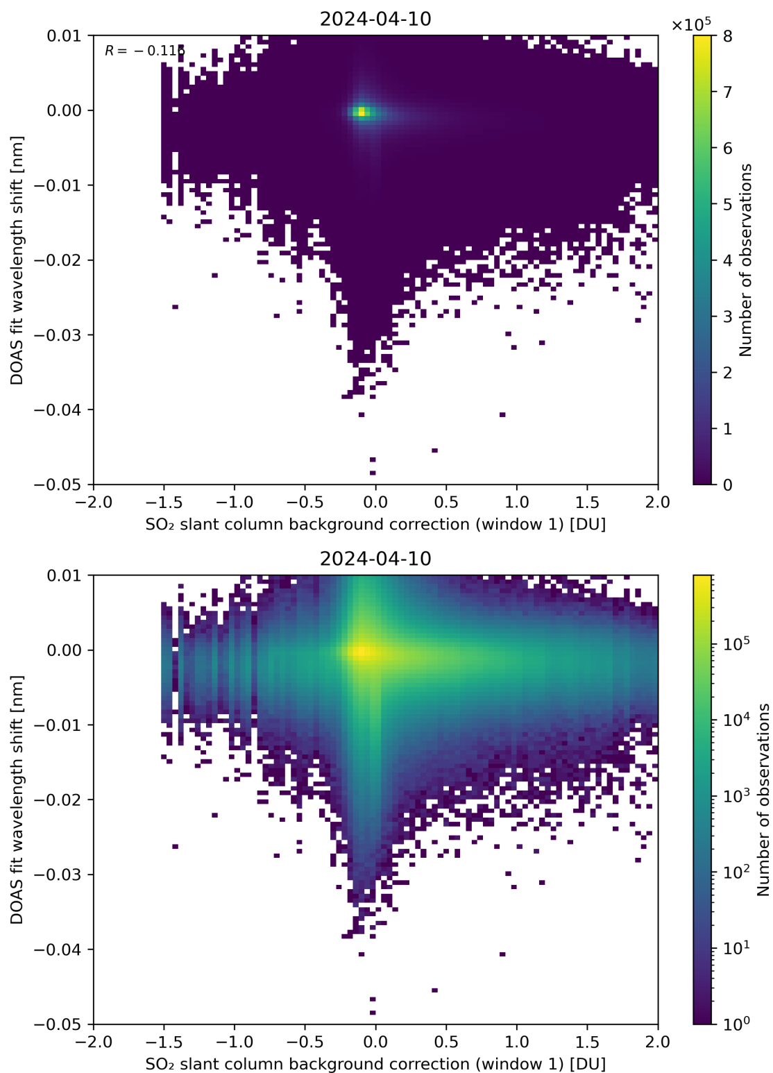
Figure 100: Scatter density plot of “SO 2 slant column background correction (window 1)” against “DOAS fit wavelength shift” for 2024-04-10 to 2024-04-11.
