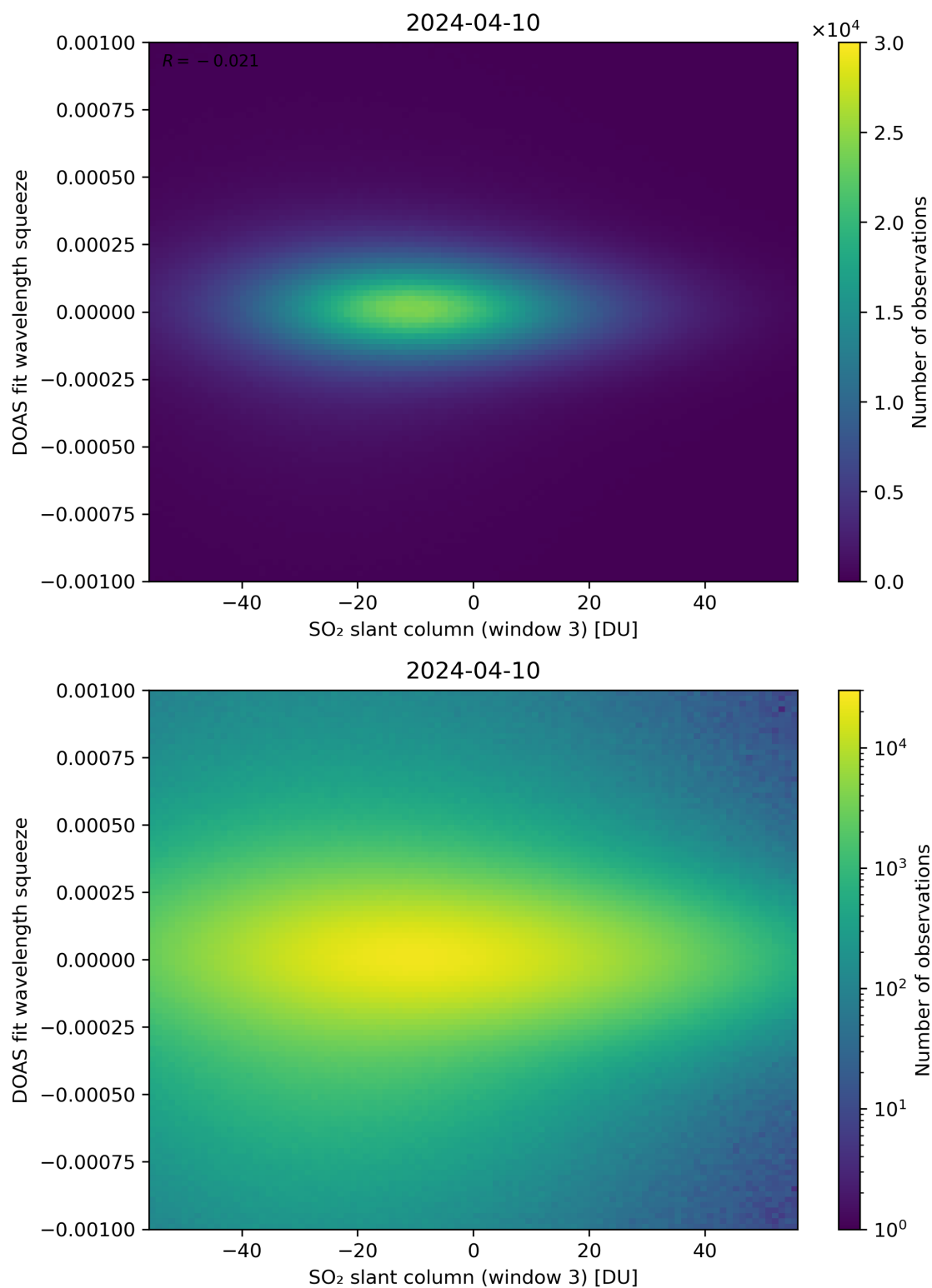
Figure 255: Scatter density plot of “SO 2 slant column (window 3)” against “DOAS fit wavelength squeeze” for 2024-04-10 to 2024-04-11.
