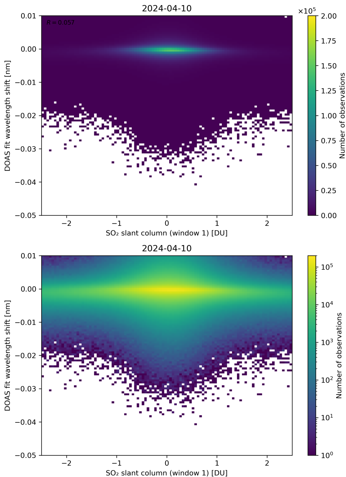
Figure 215: Scatter density plot of “SO 2 slant column (window 1)” against “DOAS fit wavelength shift” for 2024-04-10 to 2024-04-11.
