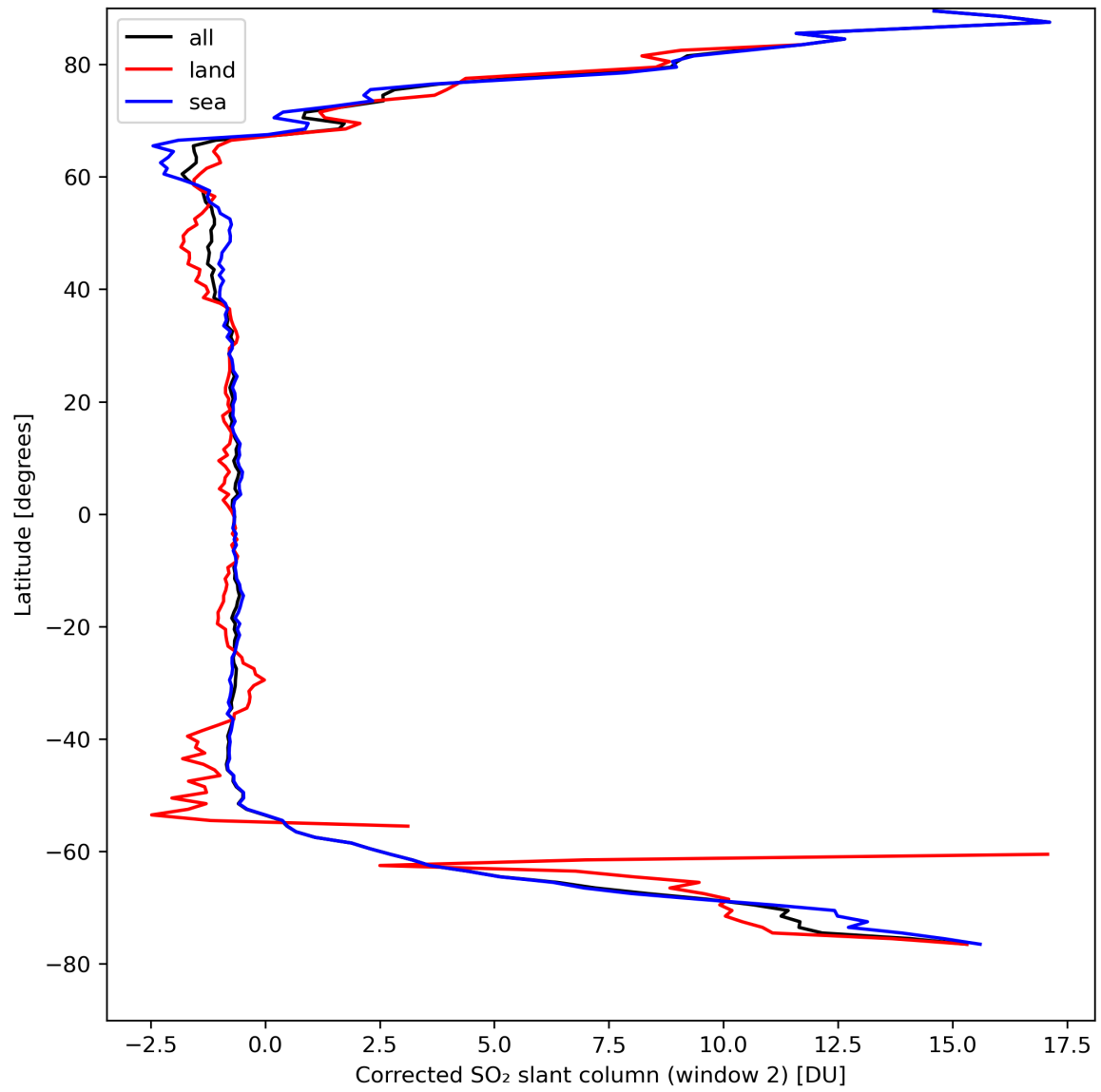
Figure 39: Zonal average of “Corrected SO 2 slant column (window 2)” for 2024-04-10 to 2024-04-11.
