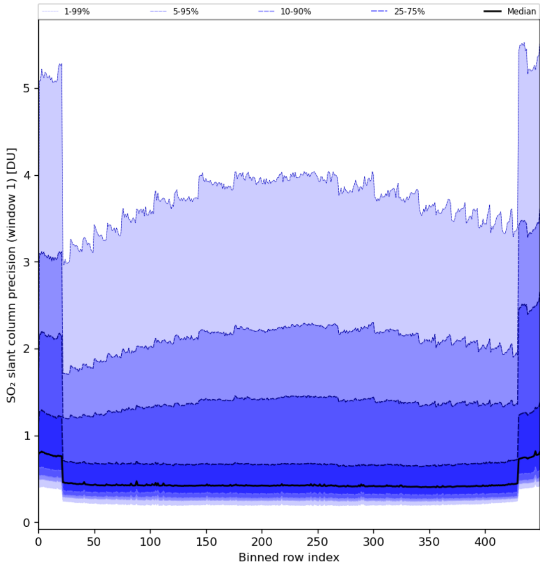
Figure 80: Along track statistics of “SO 2 slant column precision (window 1)” for 2024-04-10 to 2024-04-11
