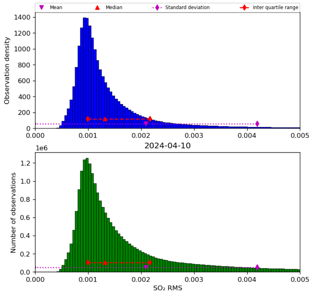
Figure 70: Histogram of “SO 2 RMS” for 2024-04-10 to 2024-04-11
