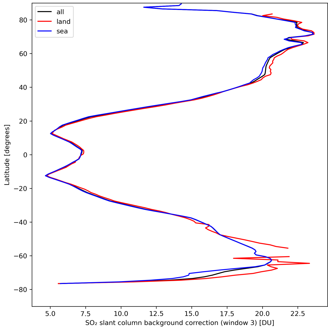
Figure 44: Zonal average of “SO 2 slant column background correction (window 3)” for 2024-04-10 to 2024-04-11.
