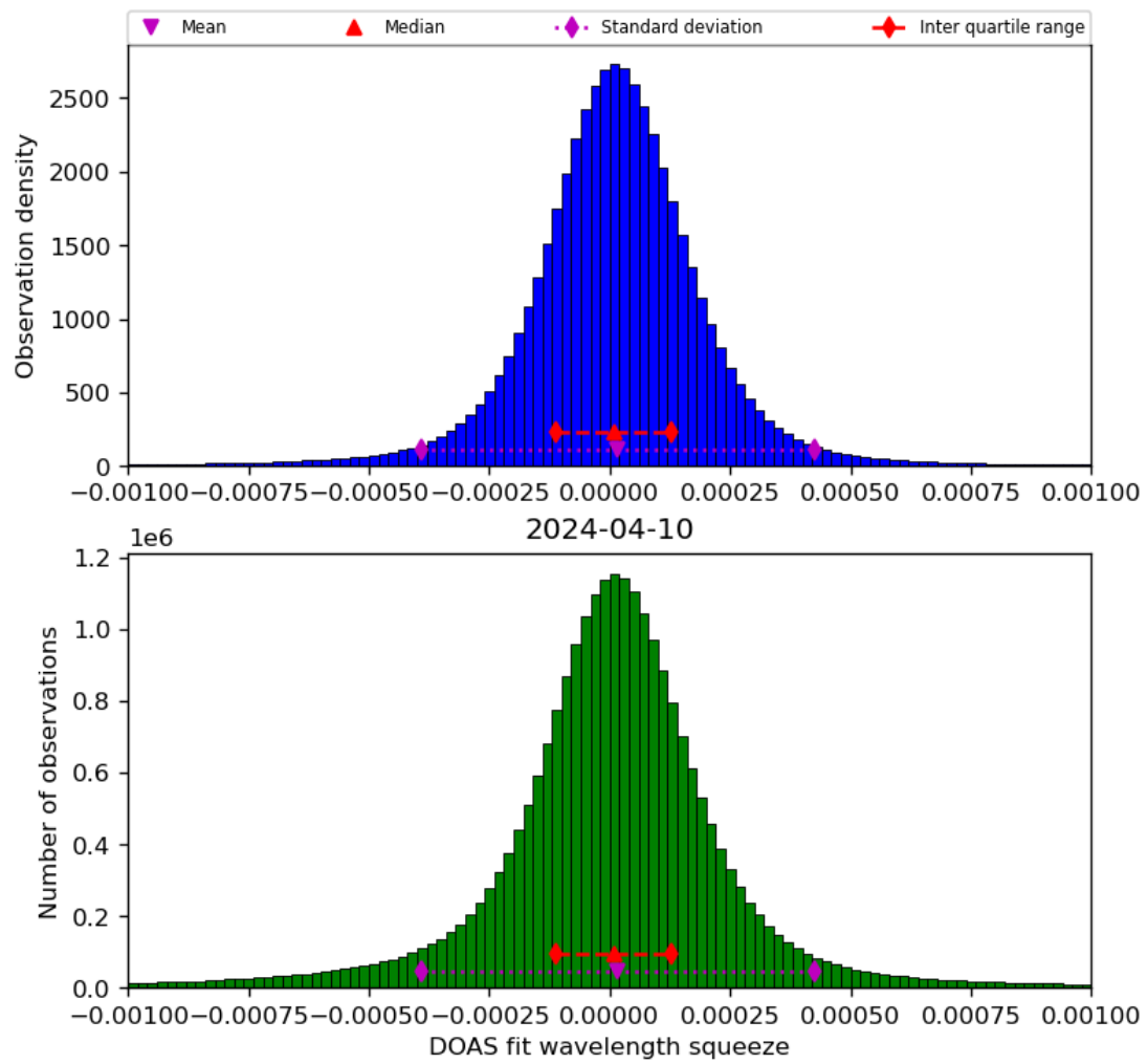
Figure 69: Histogram of “DOAS fit wavelength squeeze” for 2024-04-10 to 2024-04-11
