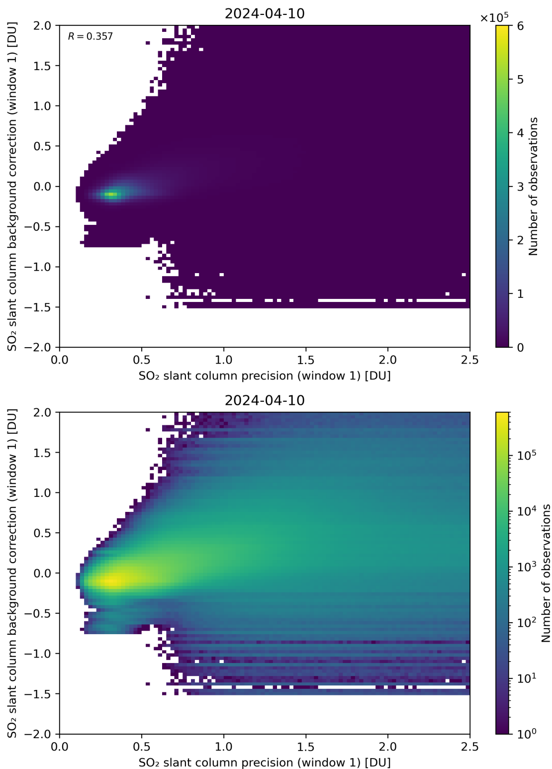
Figure 218: Scatter density plot of “SO 2 slant column precision (window 1)” against “SO 2 slant column background correction (window 1)” for 2024-04-10 to 2024-04-11.
