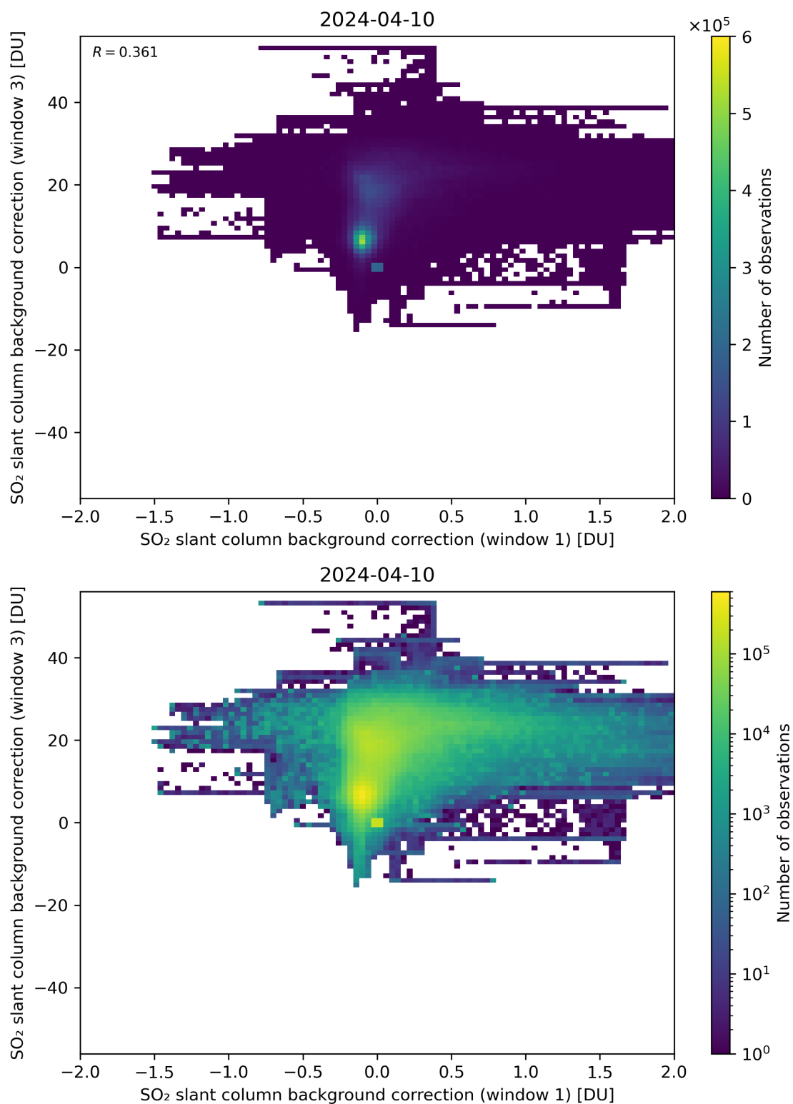
Figure 99: Scatter density plot of “SO 2 slant column background correction (window 1)” against “SO 2 slant column background correction (window 3)” for 2024-04-10 to 2024-04-11.
