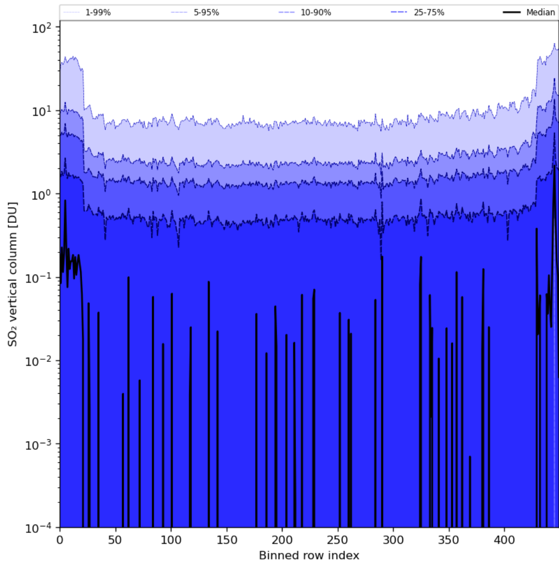
Figure 76: Along track statistics of “SO 2 vertical column” for 2024-04-10 to 2024-04-11
