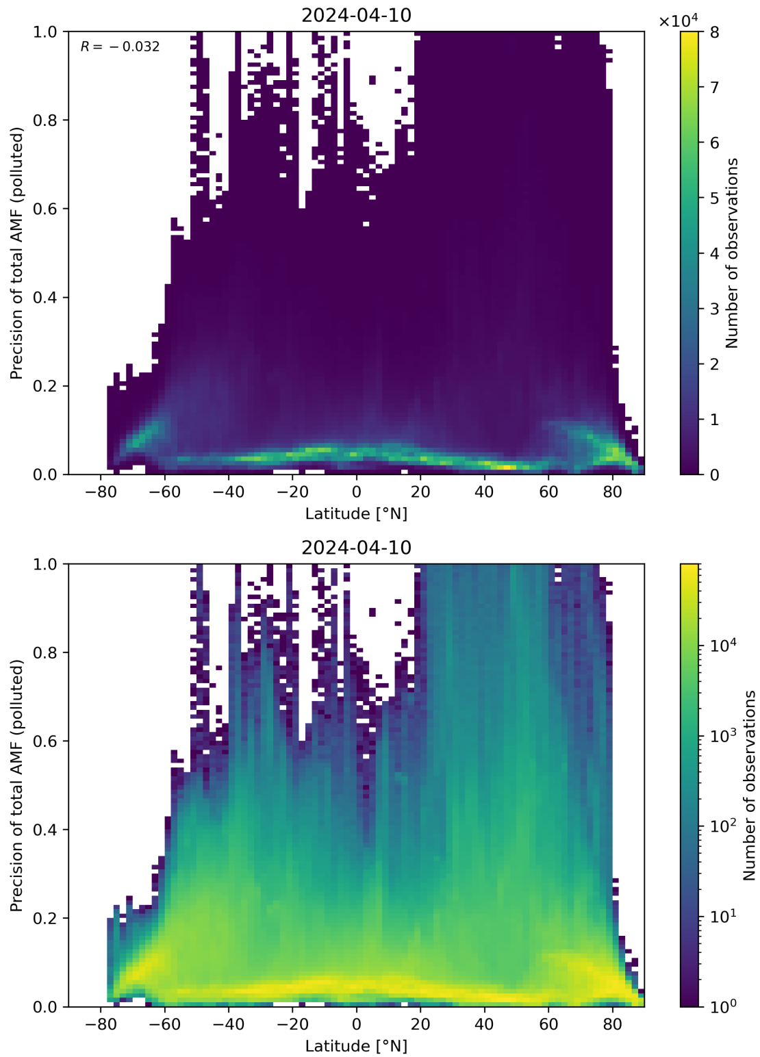
Figure 155: Scatter density plot of “Latitude” against “Precision of total AMF (polluted)” for 2024-04-10 to 2024-04-11.
