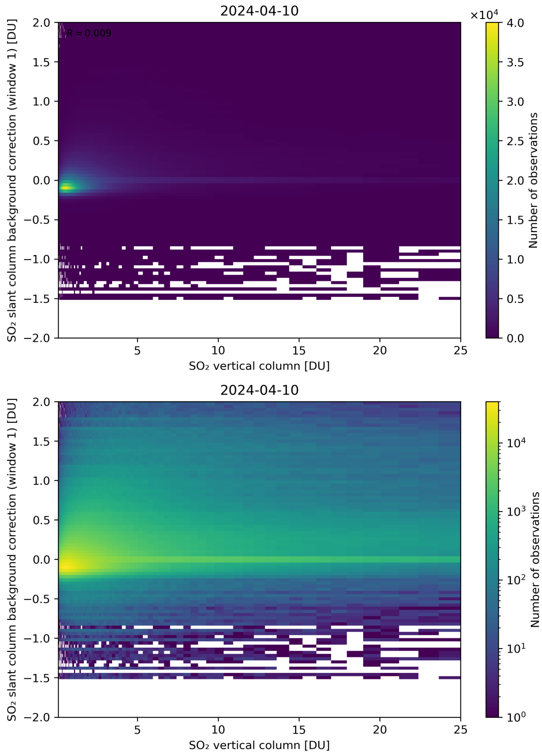
Figure 273: Scatter density plot of “SO 2 vertical column” against “SO 2 slant column background correction (window 1)” for 2024-04-10 to 2024-04-11.
