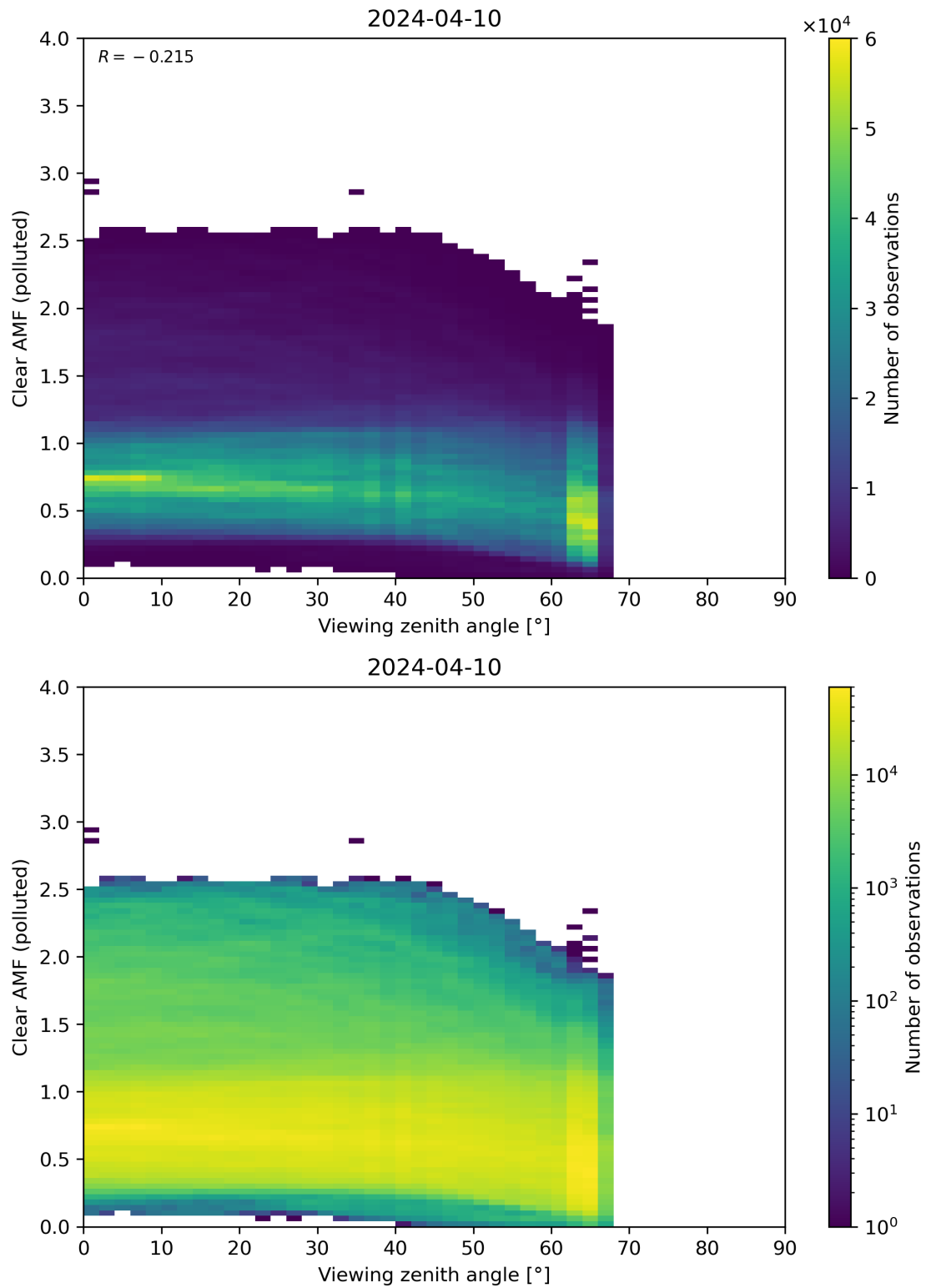
Figure 316: Scatter density plot of “Viewing zenith angle” against “Clear AMF (polluted)” for 2024-04-10 to 2024-04-11.
