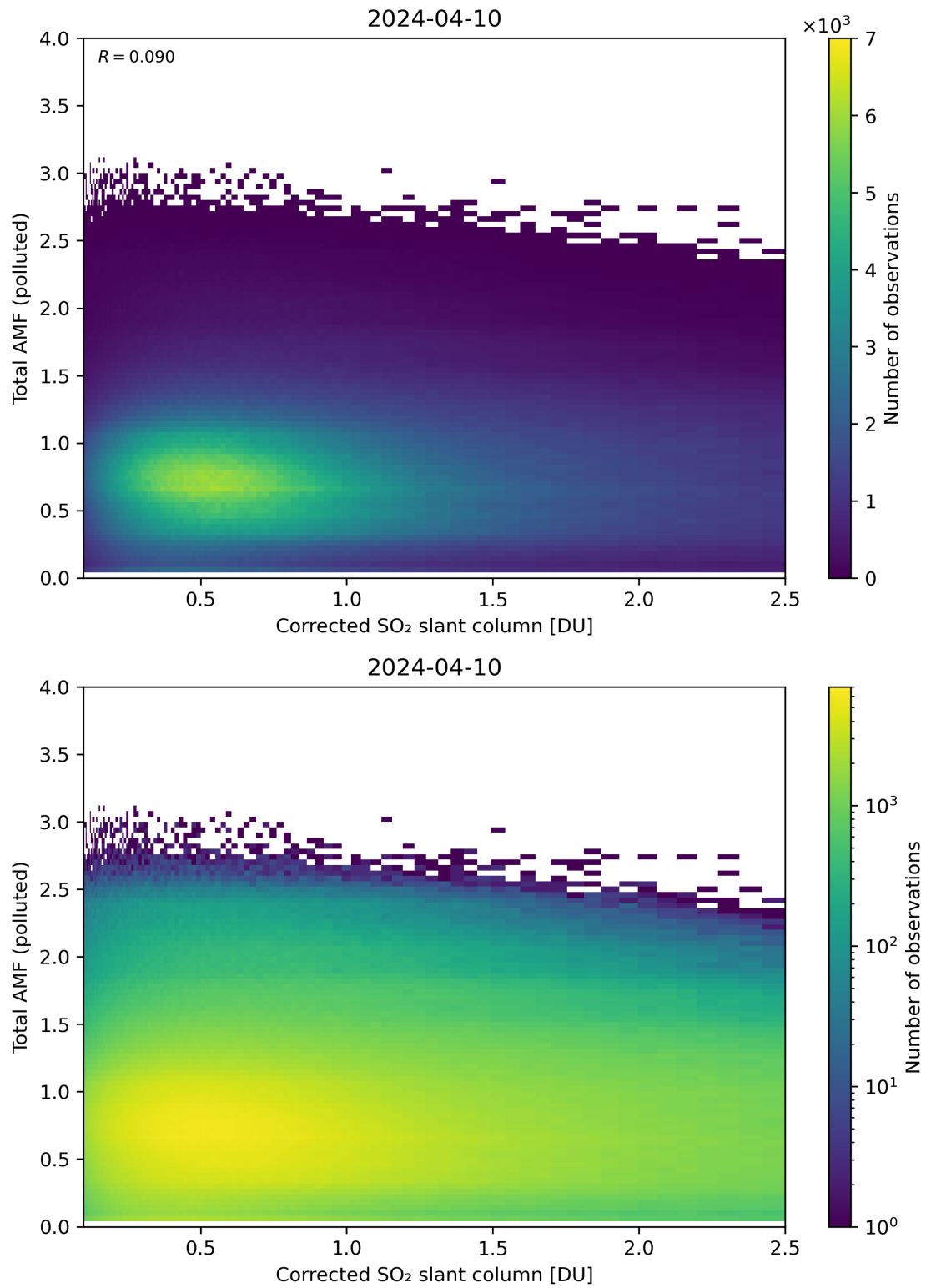
Figure 192: Scatter density plot of “Corrected SO 2 slant column” against “Total AMF (polluted)” for 2024-04-10 to 2024-04-11.
