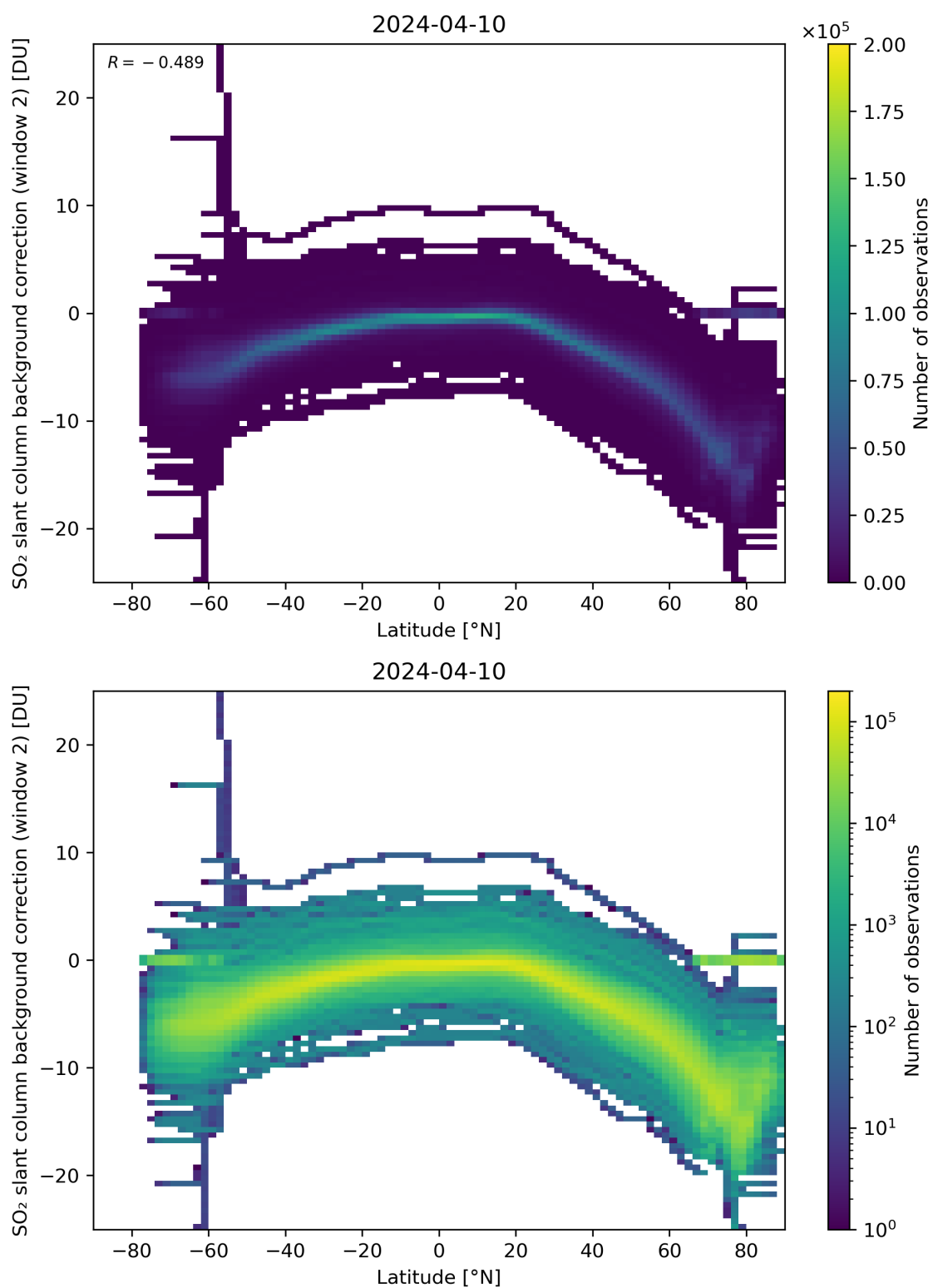
Figure 140: Scatter density plot of “Latitude” against “SO 2 slant column background correction (window 2)” for 2024-04-10 to 2024-04-11.
