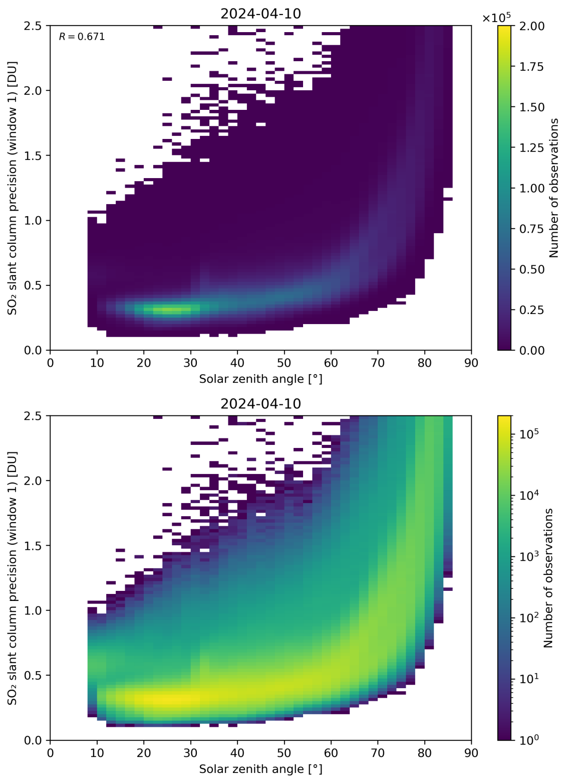
Figure 170: Scatter density plot of “Solar zenith angle” against “SO 2 slant column precision (window 1)” for 2024-04-10 to 2024-04-11.
