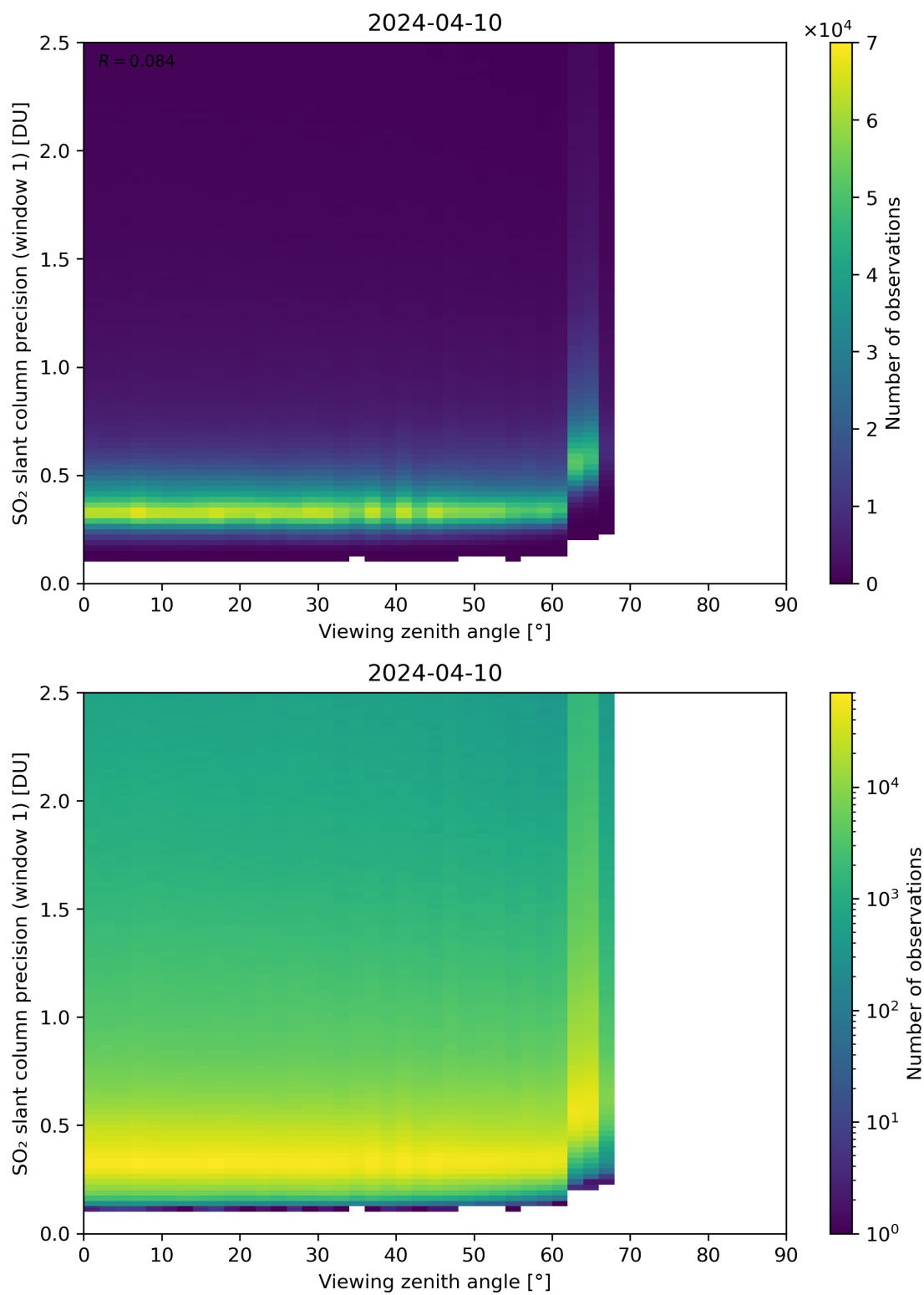
Figure 321: Scatter density plot of “Viewing zenith angle” against “SO 2 slant column precision (window 1)” for 2024-04-10 to 2024-04-11.
