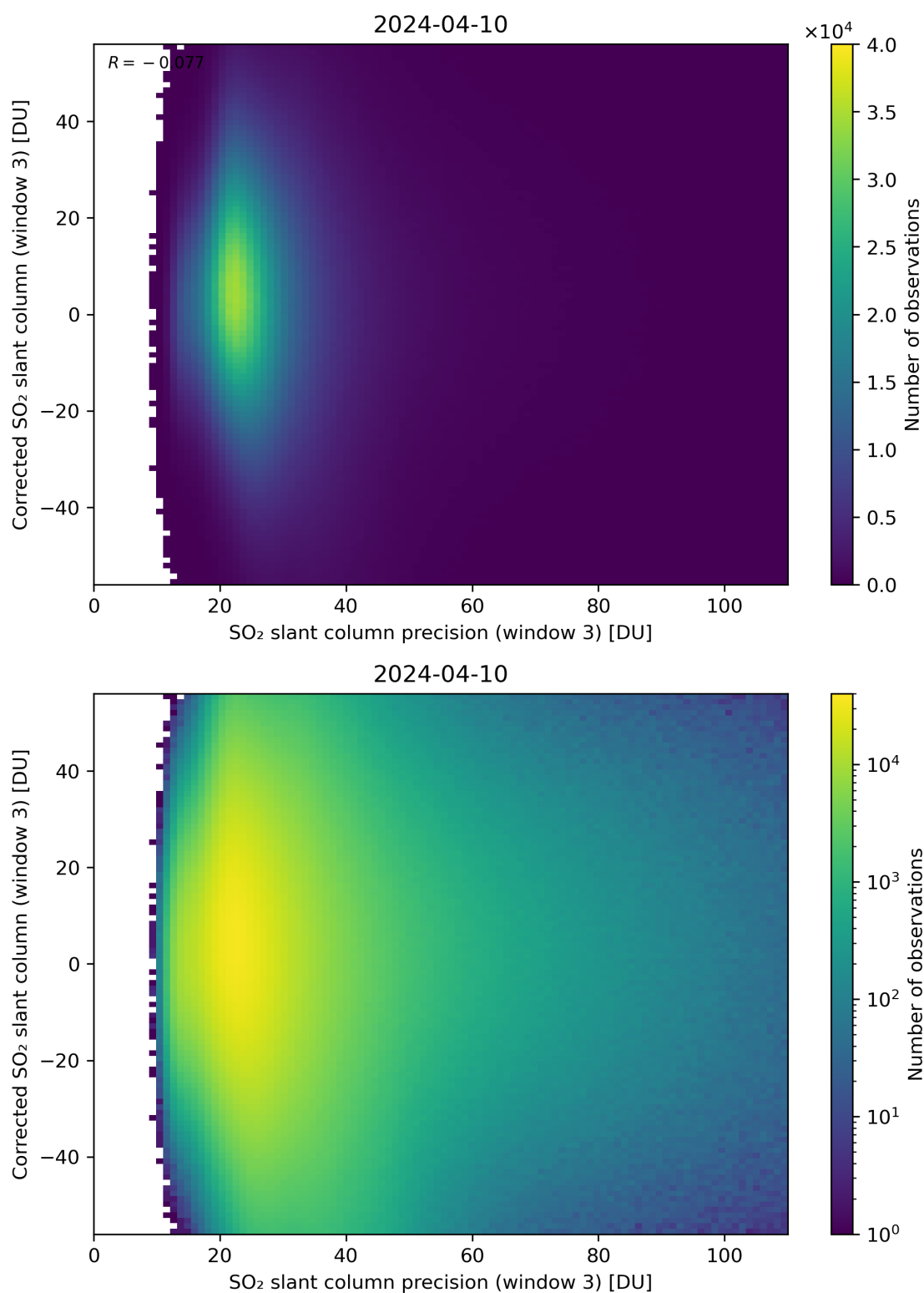
Figure 262: Scatter density plot of “SO 2 slant column precision (window 3)” against “Corrected SO 2 slant column (window 3)” for 2024-04-10 to 2024-04-11.
