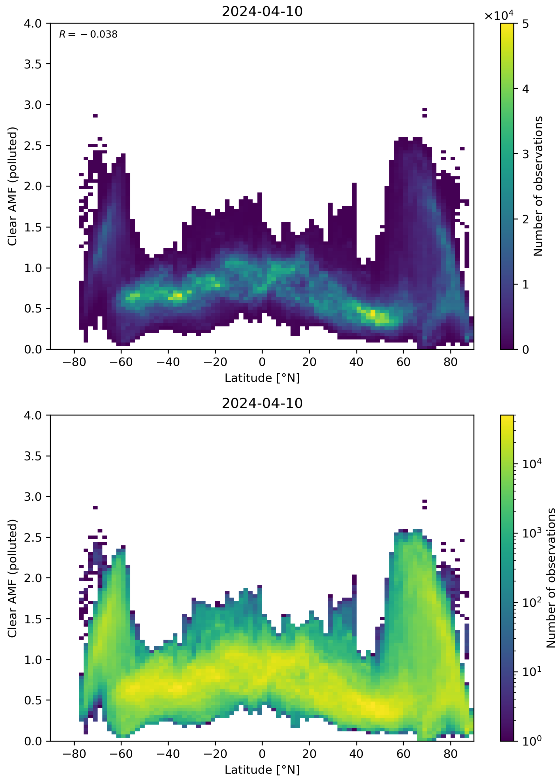
Figure 145: Scatter density plot of “Latitude” against “Clear AMF (polluted)” for 2024-04-10 to 2024-04-11.
