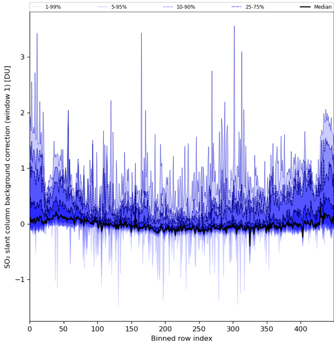
Figure 82: Along track statistics of “SO 2 slant column background correction (window 1)” for 2024-04-10 to 2024-04-11
