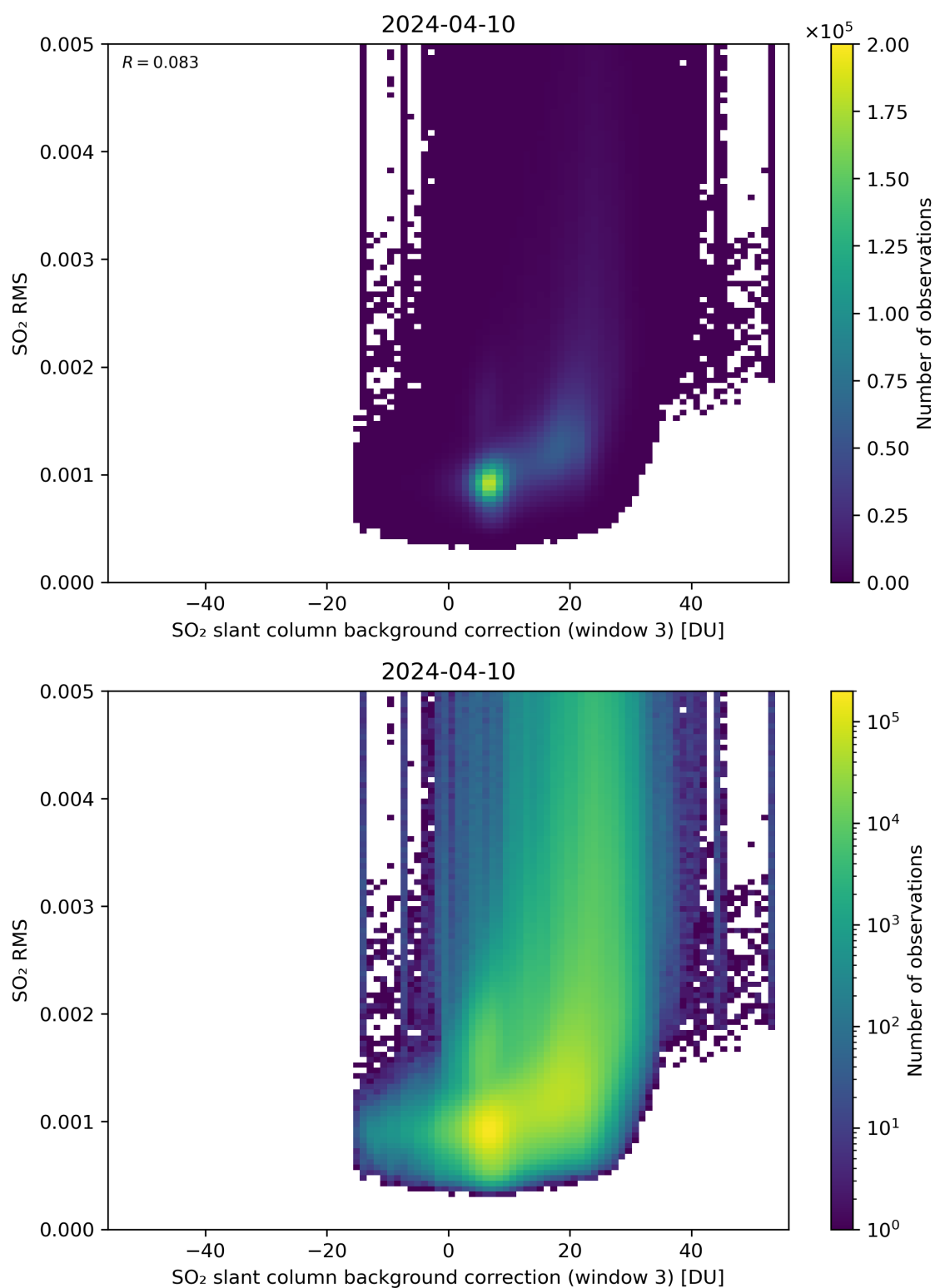
Figure 123: Scatter density plot of “SO 2 slant column background correction (window 3)” against “SO 2 RMS” for 2024-04-10 to 2024-04-11.
