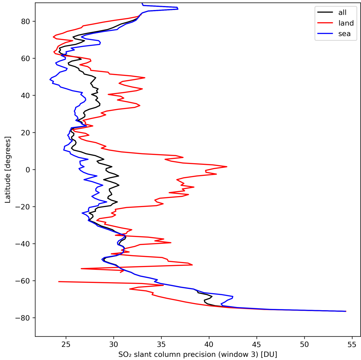
Figure 42: Zonal average of “SO 2 slant column precision (window 3)” for 2024-04-10 to 2024-04-11.
