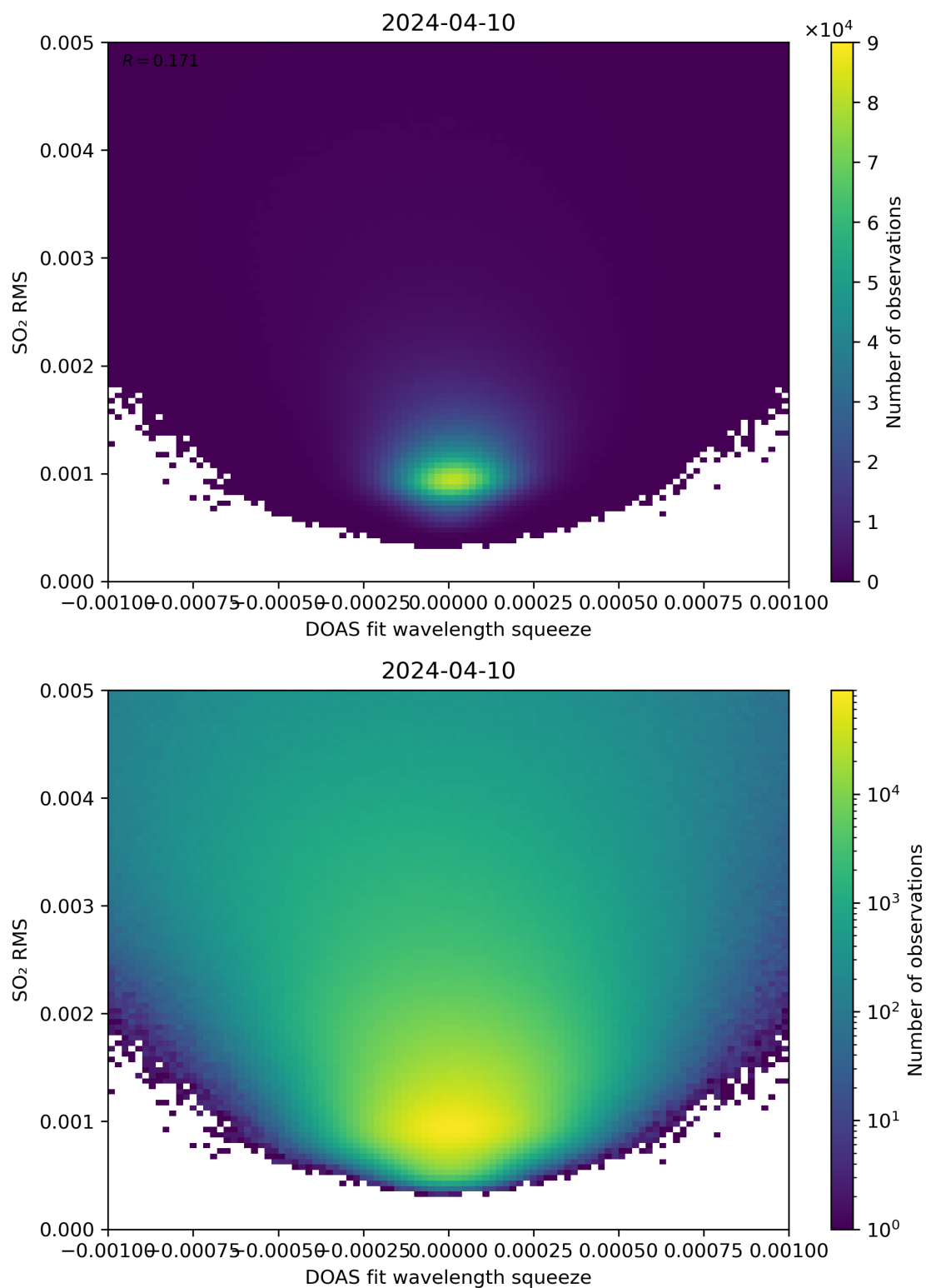
Figure 132: Scatter density plot of “DOAS fit wavelength squeeze” against “SO 2 RMS” for 2024-04-10 to 2024-04-11.
