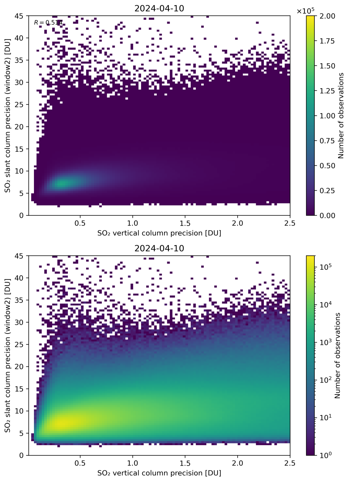
Figure 291: Scatter density plot of “SO 2 vertical column precision” against “SO 2 slant column precision (window2)” for 2024-04-10 to 2024-04-11.
