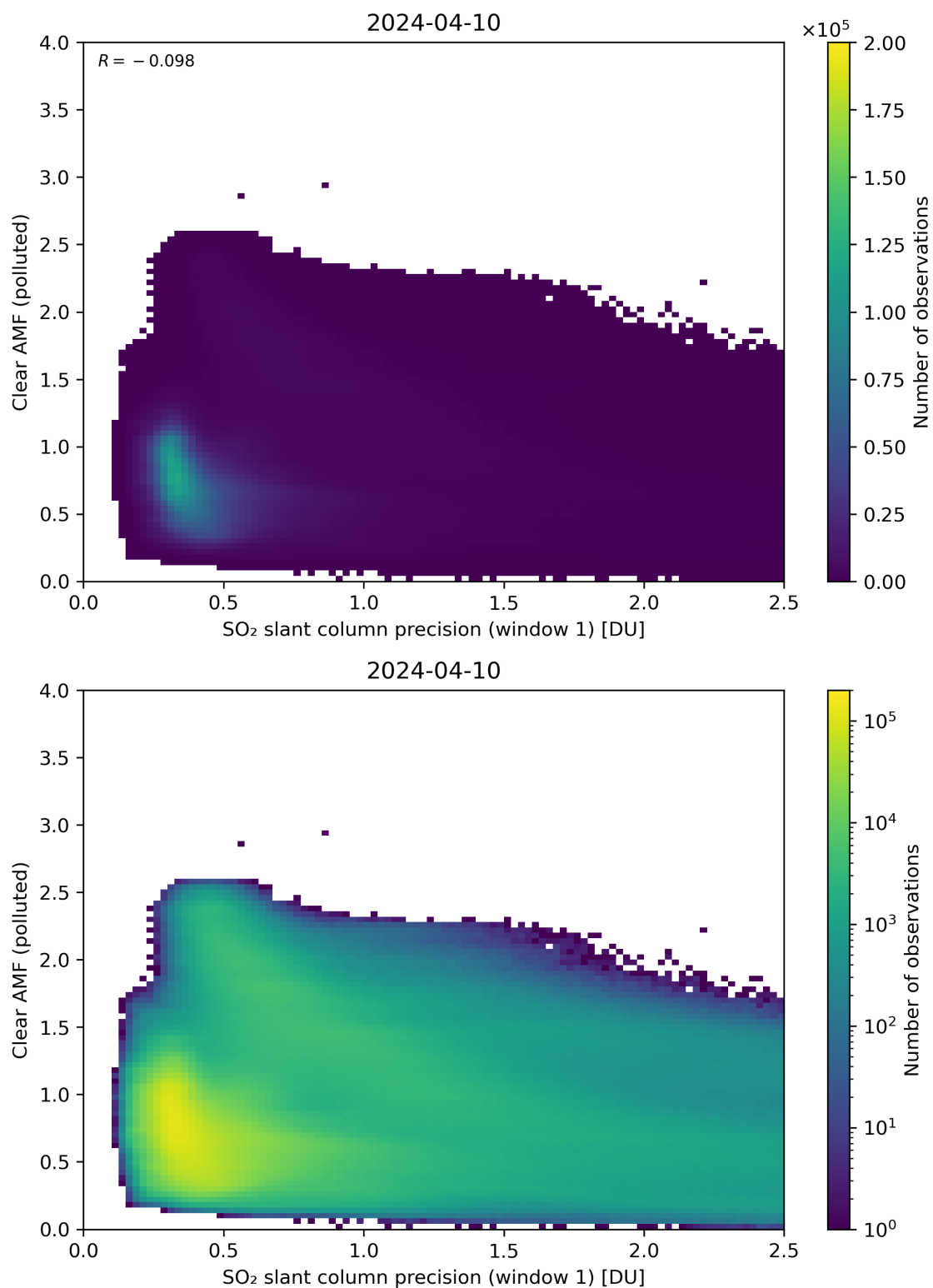
Figure 224: Scatter density plot of “SO 2 slant column precision (window 1)” against “Clear AMF (polluted)” for 2024-04-10 to 2024-04-11.
