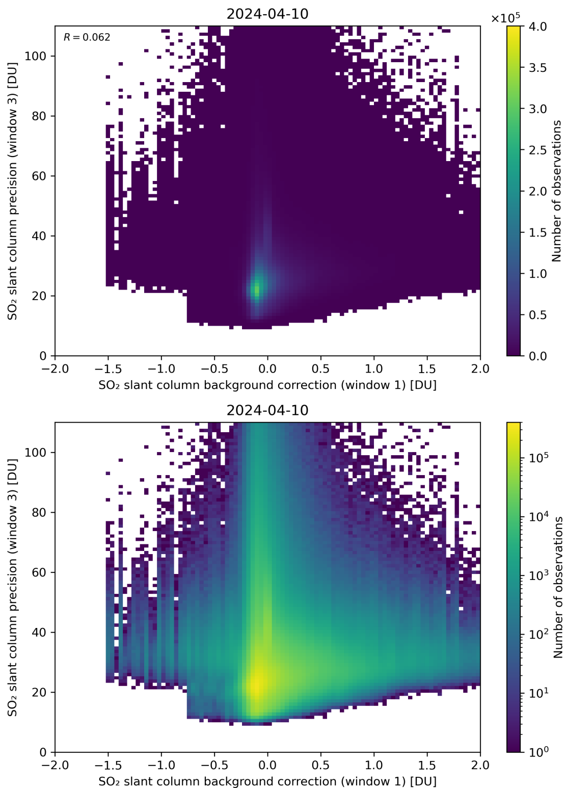
Figure 108: Scatter density plot of “SO 2 slant column background correction (window 1)” against “SO 2 slant column precision (window 3)” for 2024-04-10 to 2024-04-11.
