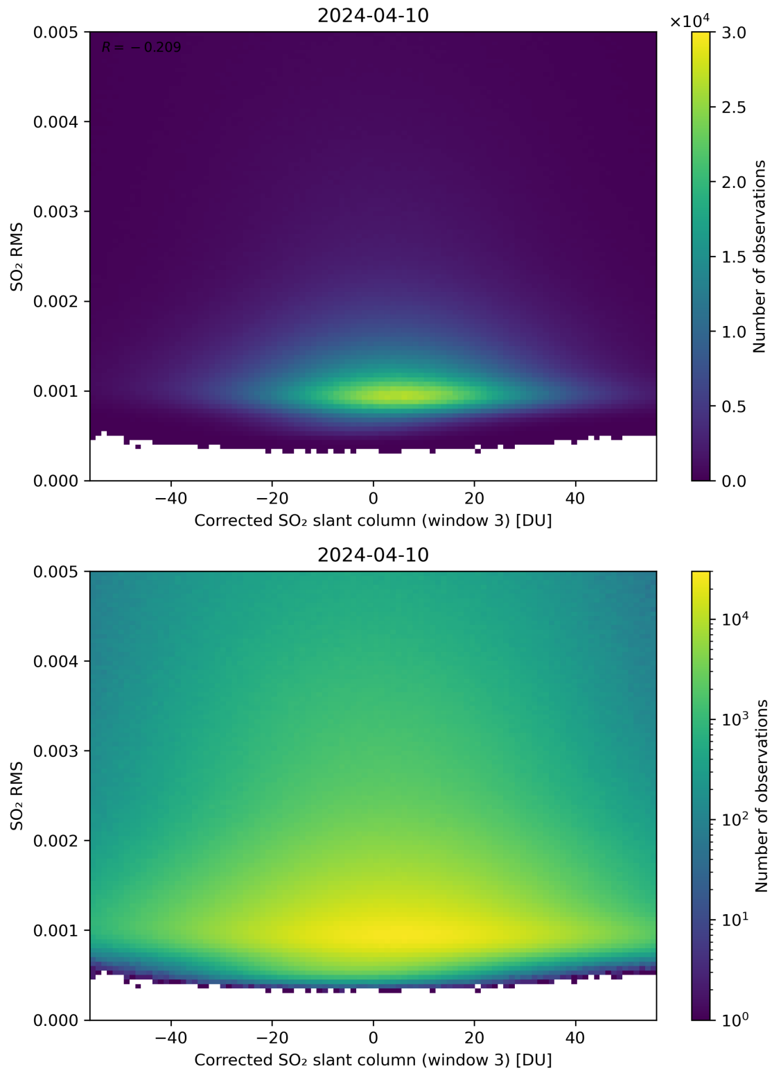
Figure 208: Scatter density plot of “Corrected SO 2 slant column (window 3)” against “SO 2 RMS” for 2024-04-10 to 2024-04-11.
