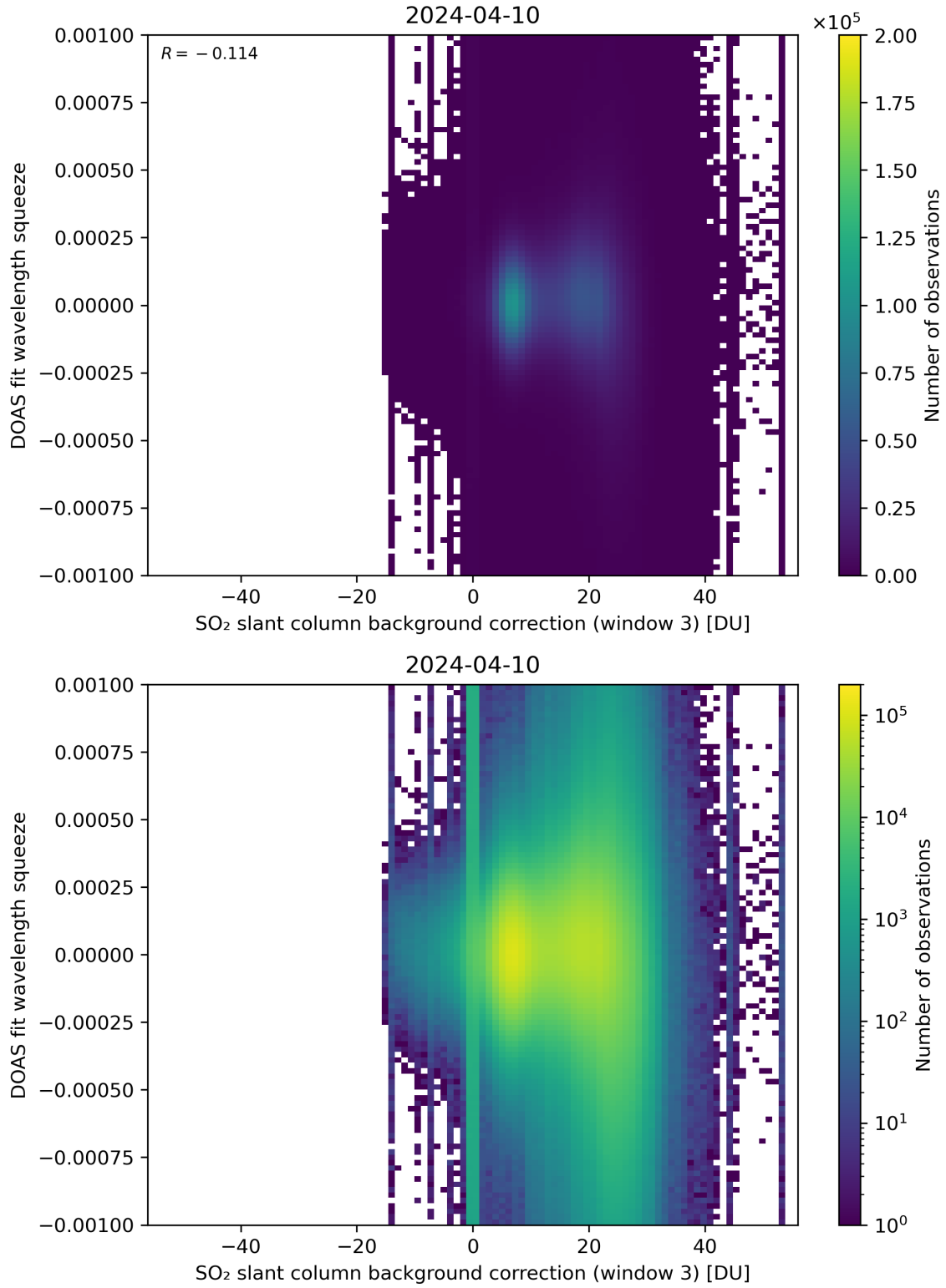
Figure 122: Scatter density plot of “SO 2 slant column background correction (window 3)” against “DOAS fit wavelength squeeze” for 2024-04-10 to 2024-04-11.
