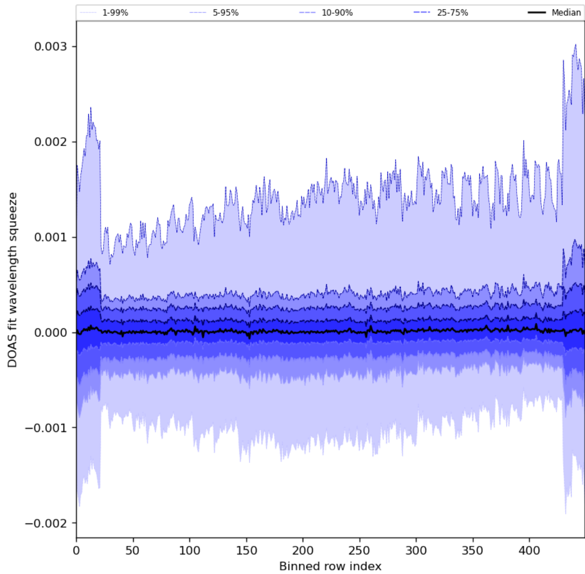
Figure 92: Along track statistics of “DOAS fit wavelength squeeze” for 2024-04-10 to 2024-04-11
