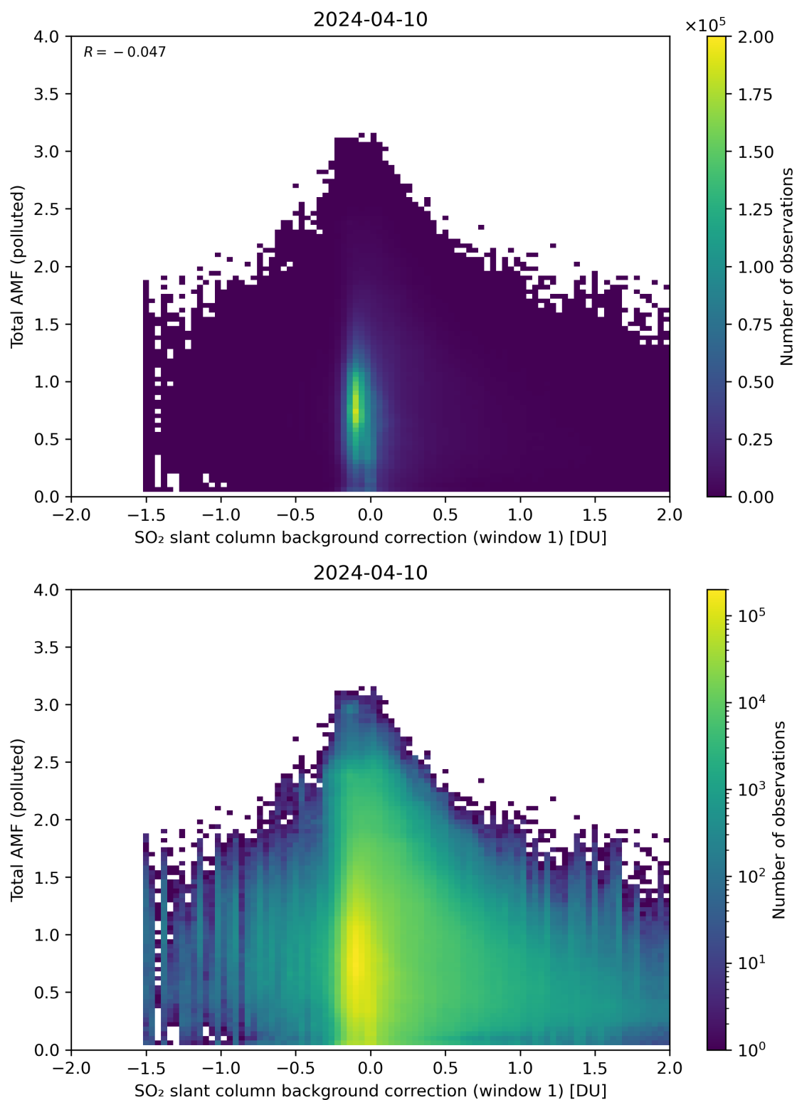
Figure 109: Scatter density plot of “SO 2 slant column background correction (window 1)” against “Total AMF (polluted)” for 2024-04-10 to 2024-04-11.
