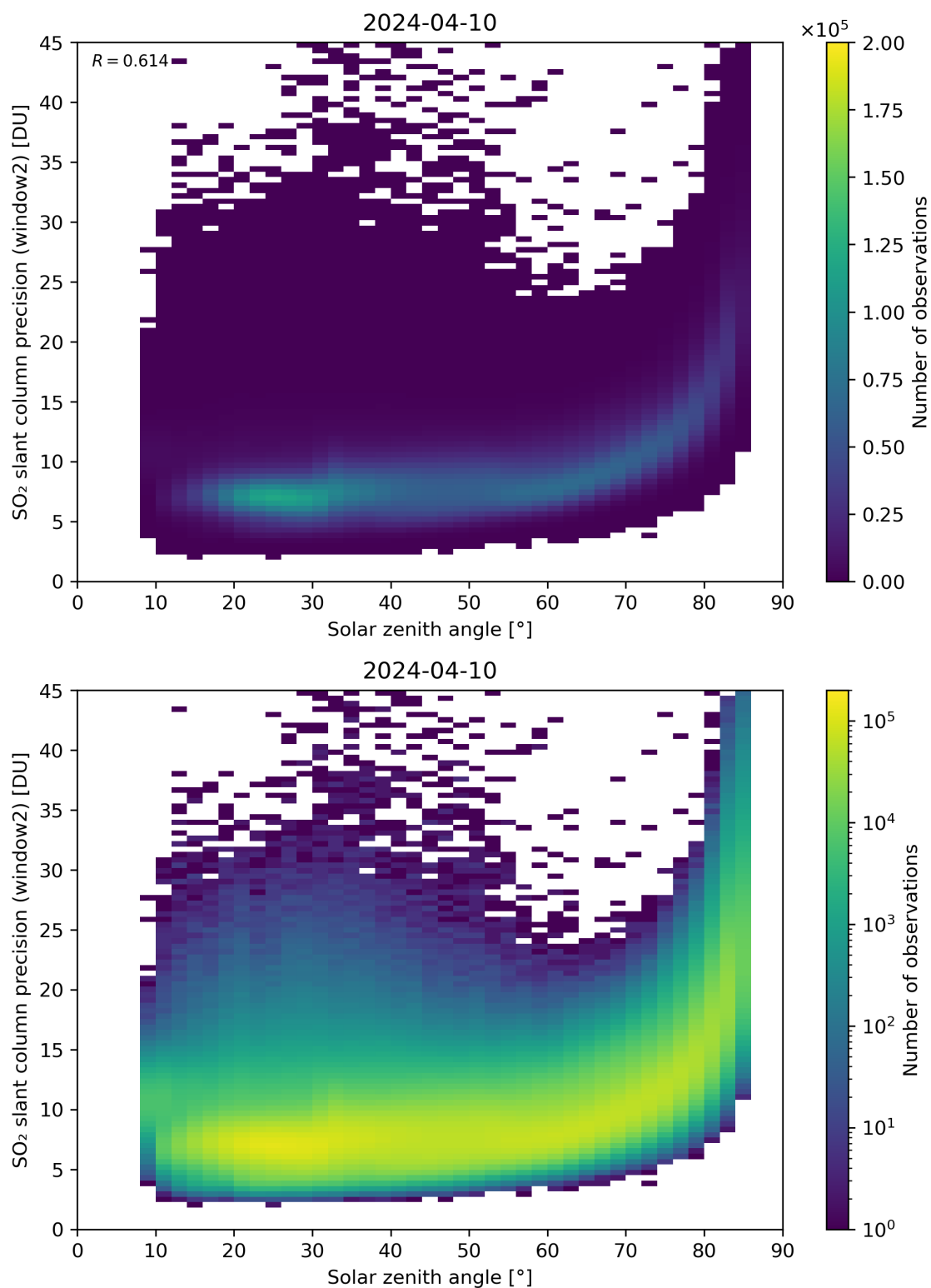
Figure 171: Scatter density plot of “Solar zenith angle” against “SO 2 slant column precision (window2)” for 2024-04-10 to 2024-04-11.
