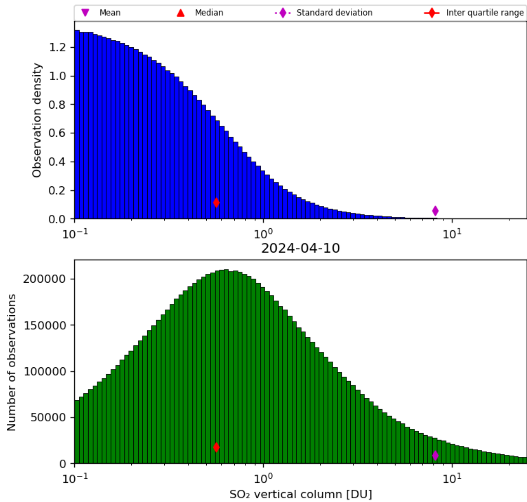
Figure 53: Histogram of “SO 2 vertical column” for 2024-04-10 to 2024-04-11
