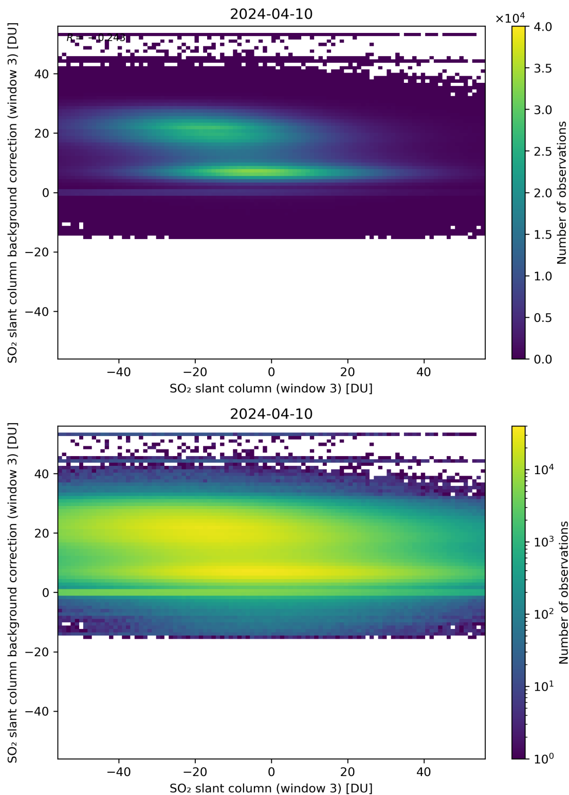
Figure 253: Scatter density plot of “SO 2 slant column (window 3)” against “SO 2 slant column background correction (window 3)” for 2024-04-10 to 2024-04-11.
