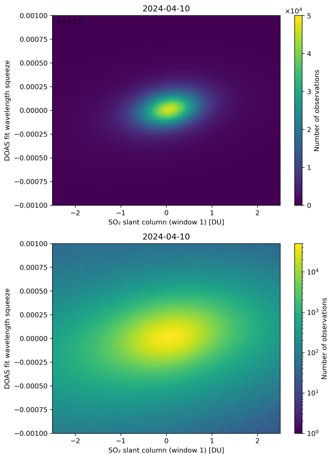
Figure 216: Scatter density plot of “SO 2 slant column (window 1)” against “DOAS fit wavelength squeeze” for 2024-04-10 to 2024-04-11.
