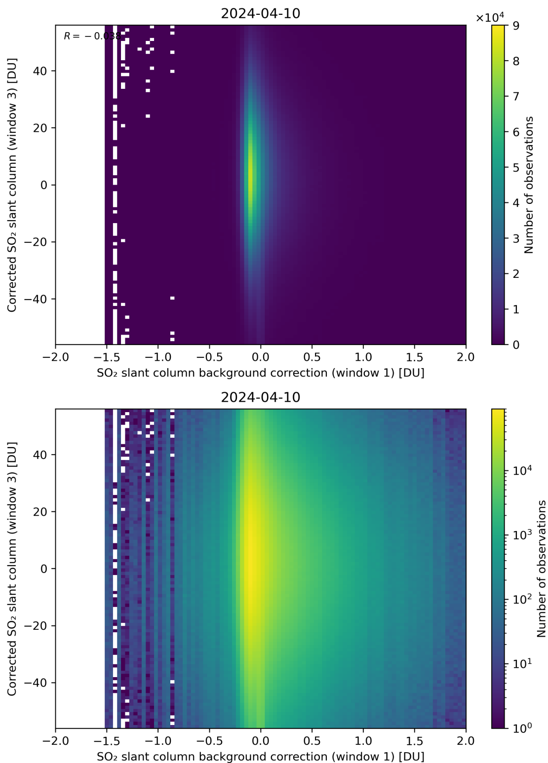
Figure 105: Scatter density plot of “SO 2 slant column background correction (window 1)” against “Corrected SO 2 slant column (window 3)” for 2024-04-10 to 2024-04-11.
