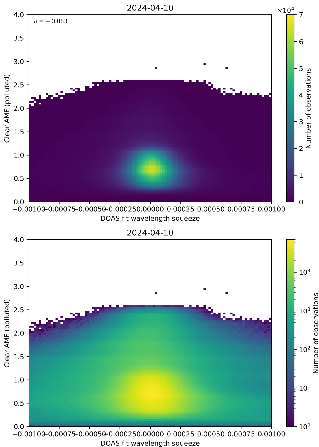
Figure 133: Scatter density plot of “DOAS fit wavelength squeeze” against “Clear AMF (polluted)” for 2024-04-10 to 2024-04-11.
