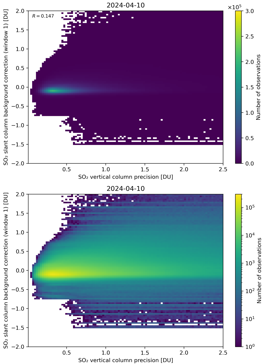
Figure 279: Scatter density plot of “SO 2 vertical column precision” against “SO 2 slant column background correction (window 1)” for 2024-04-10 to 2024-04-11.
