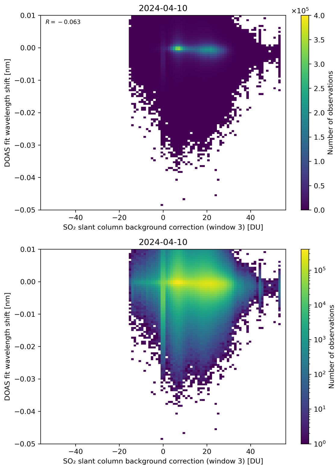
Figure 121: Scatter density plot of “SO 2 slant column background correction (window 3)” against “DOAS fit wavelength shift” for 2024-04-10 to 2024-04-11.
