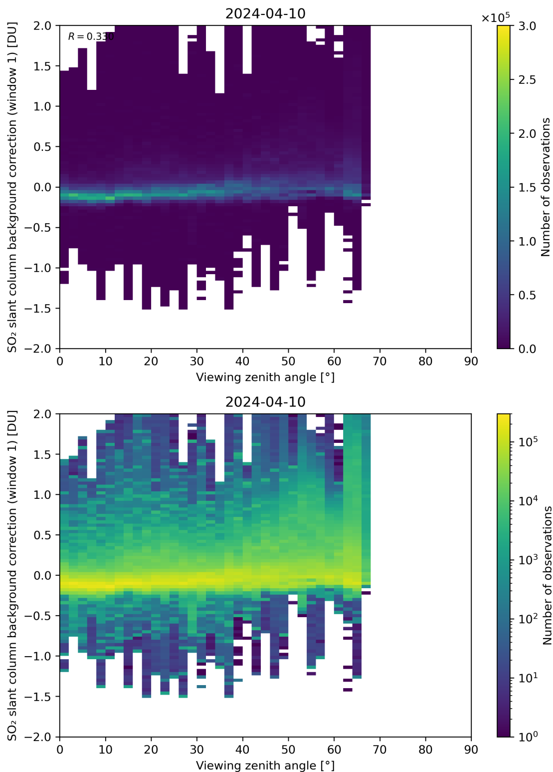
Figure 308: Scatter density plot of “Viewing zenith angle” against “SO 2 slant column background correction (window 1)” for 2024-04-10 to 2024-04-11.
