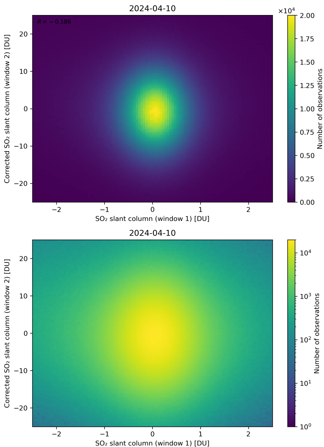
Figure 233: Scatter density plot of “SO 2 slant column (window 1)” against “Corrected SO 2 slant column (window 2)” for 2024-04-10 to 2024-04-11.
