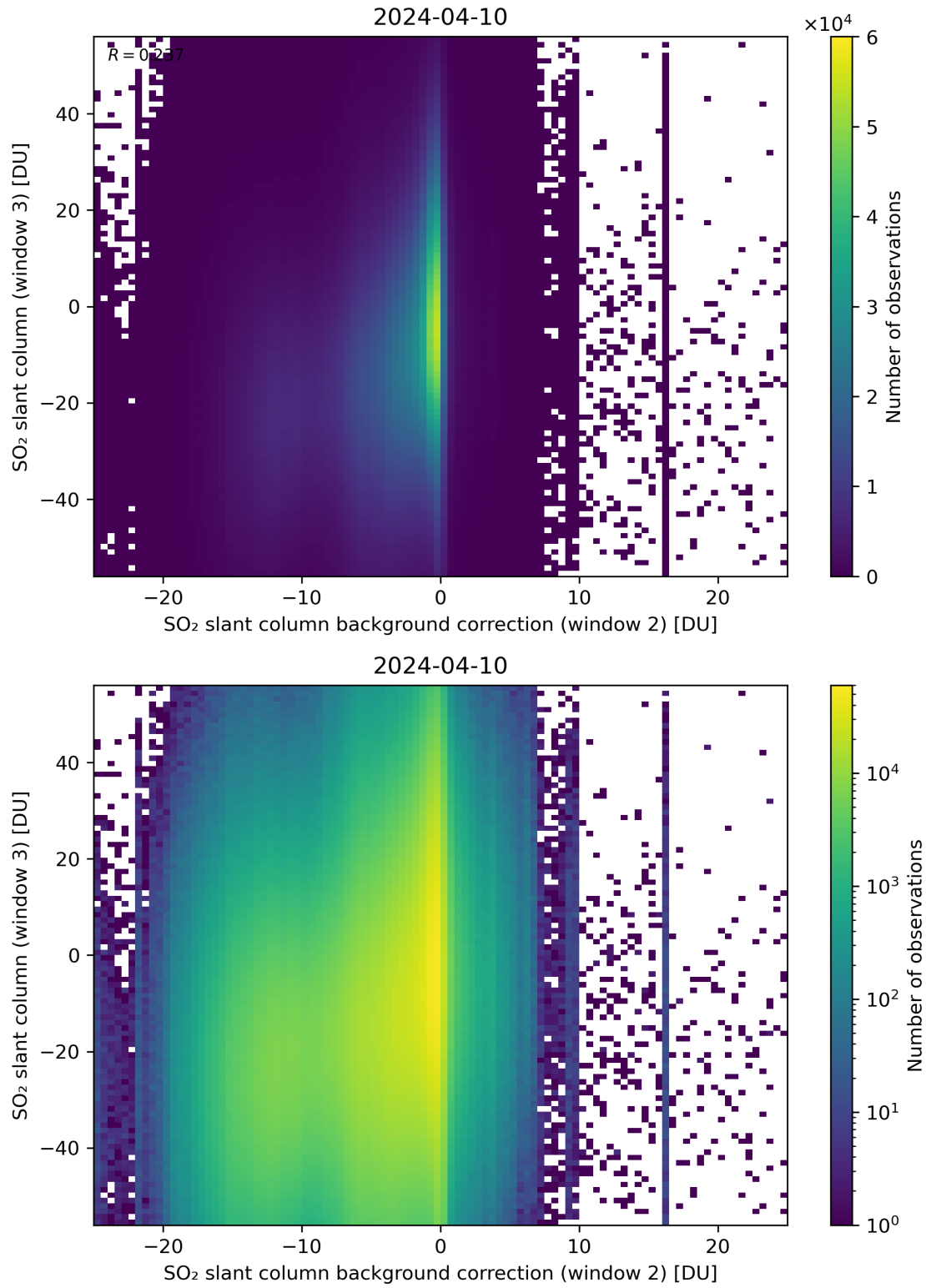
Figure 117: Scatter density plot of “SO 2 slant column background correction (window 2)” against “SO 2 slant column (window 3)” for 2024-04-10 to 2024-04-11.
