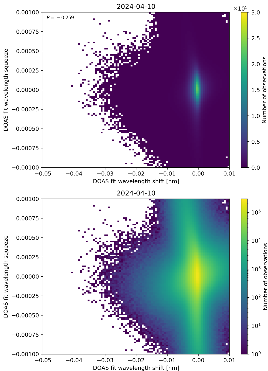
Figure 127: Scatter density plot of “DOAS fit wavelength shift” against “DOAS fit wavelength squeeze” for 2024-04-10 to 2024-04-11.
