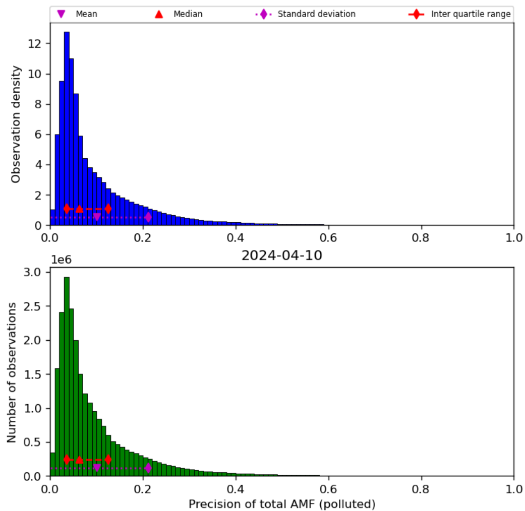
Figure 72: Histogram of “Precision of total AMF (polluted)” for 2024-04-10 to 2024-04-11
