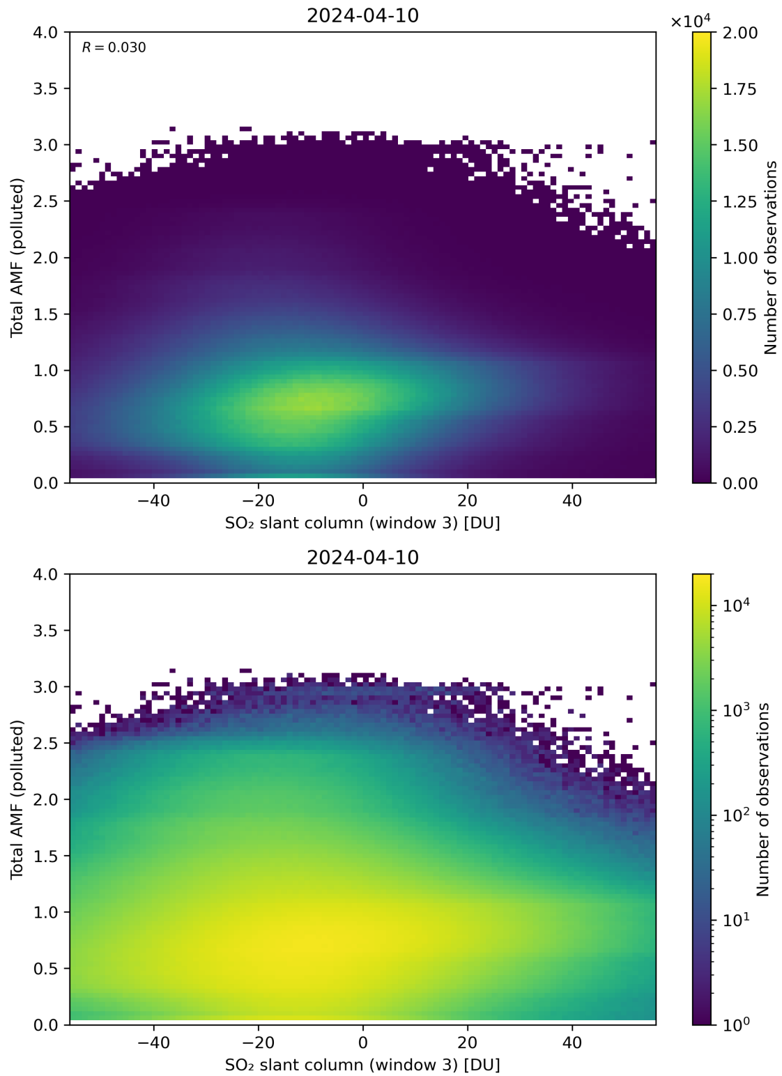
Figure 268: Scatter density plot of “SO 2 slant column (window 3)” against “Total AMF (polluted)” for 2024-04-10 to 2024-04-11.
