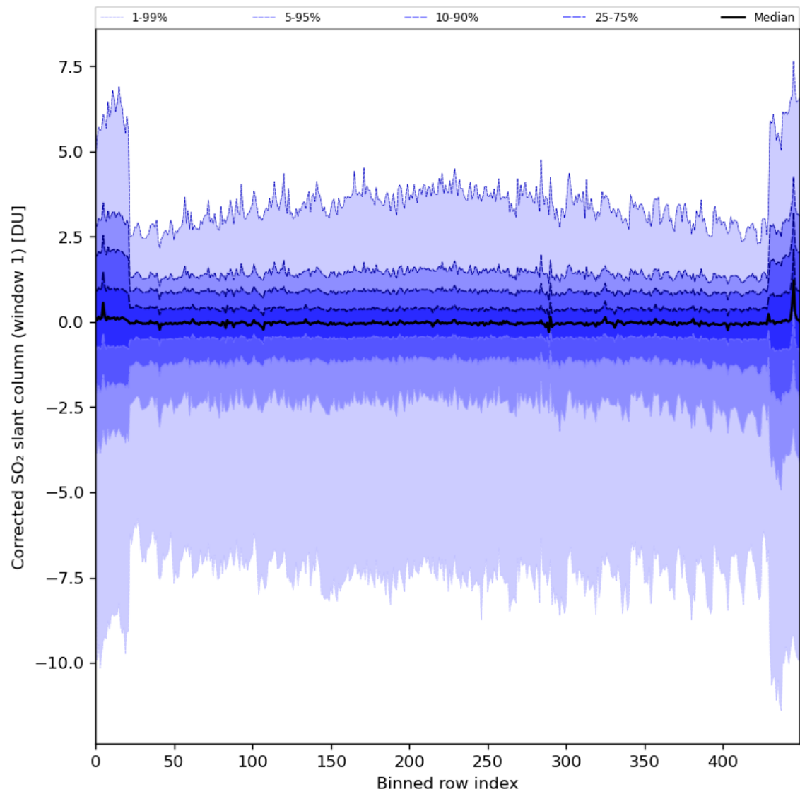
Figure 81: Along track statistics of “Corrected SO 2 slant column (window 1)” for 2024-04-10 to 2024-04-11
