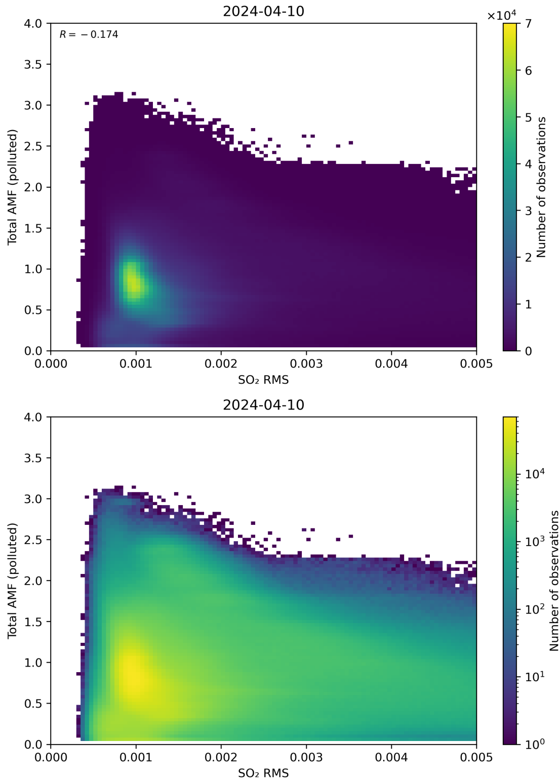
Figure 137: Scatter density plot of “SO 2 RMS” against “Total AMF (polluted)” for 2024-04-10 to 2024-04-11.
