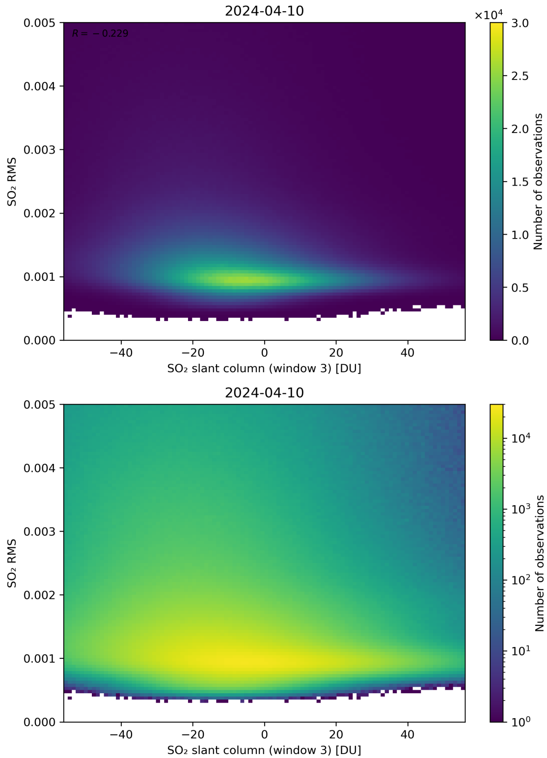
Figure 256: Scatter density plot of “SO 2 slant column (window 3)” against “SO 2 RMS” for 2024-04-10 to 2024-04-11.
