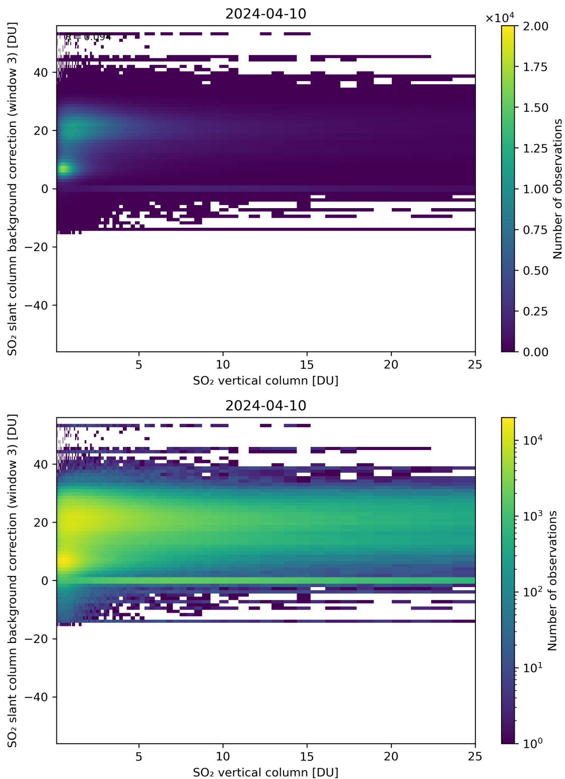
Figure 275: Scatter density plot of “SO 2 vertical column” against “SO 2 slant column background correction (window 3)” for 2024-04-10 to 2024-04-11.
