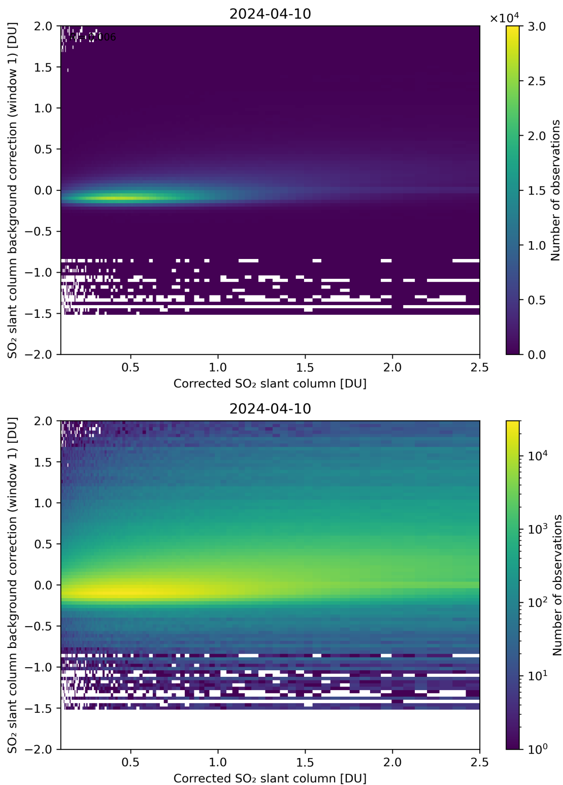
Figure 178: Scatter density plot of “Corrected SO 2 slant column” against “SO 2 slant column background correction (window 1)” for 2024-04-10 to 2024-04-11.
