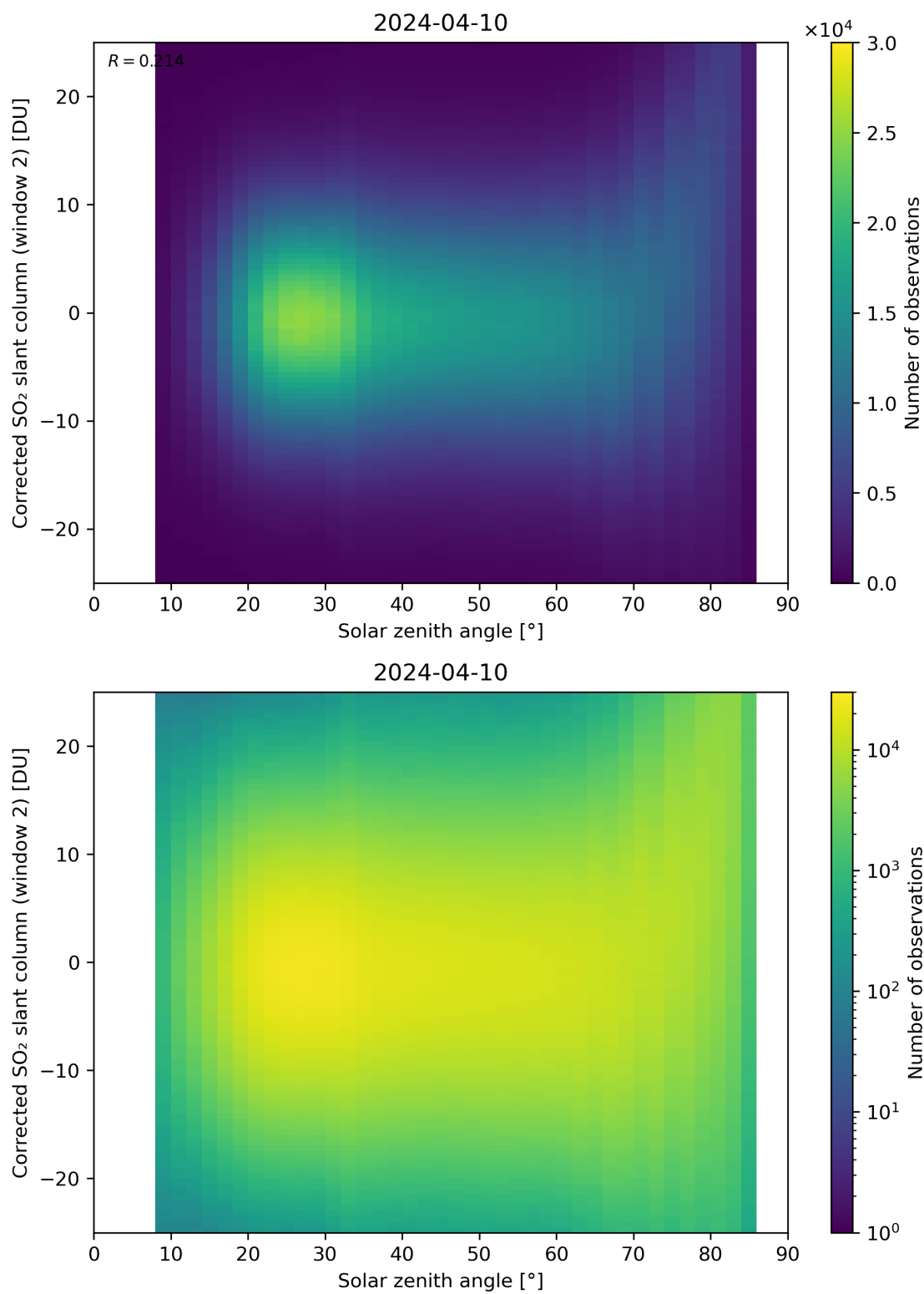
Figure 167: Scatter density plot of “Solar zenith angle” against “Corrected SO 2 slant column (window 2)” for 2024-04-10 to 2024-04-11.
