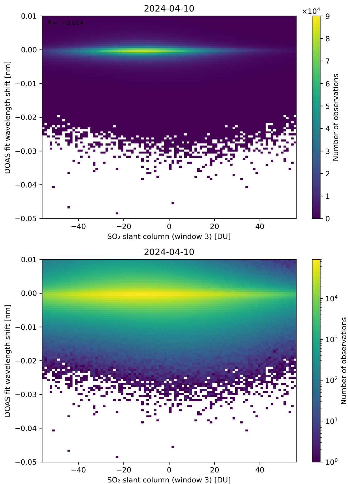
Figure 254: Scatter density plot of “SO 2 slant column (window 3)” against “DOAS fit wavelength shift” for 2024-04-10 to 2024-04-11.
