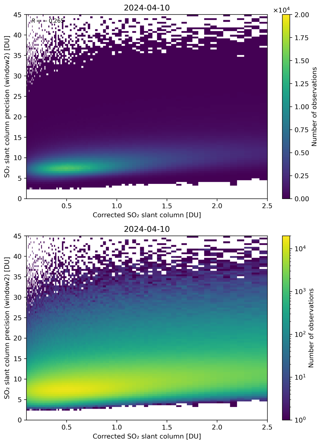
Figure 189: Scatter density plot of “Corrected SO 2 slant column” against “SO 2 slant column precision (window2)” for 2024-04-10 to 2024-04-11.
