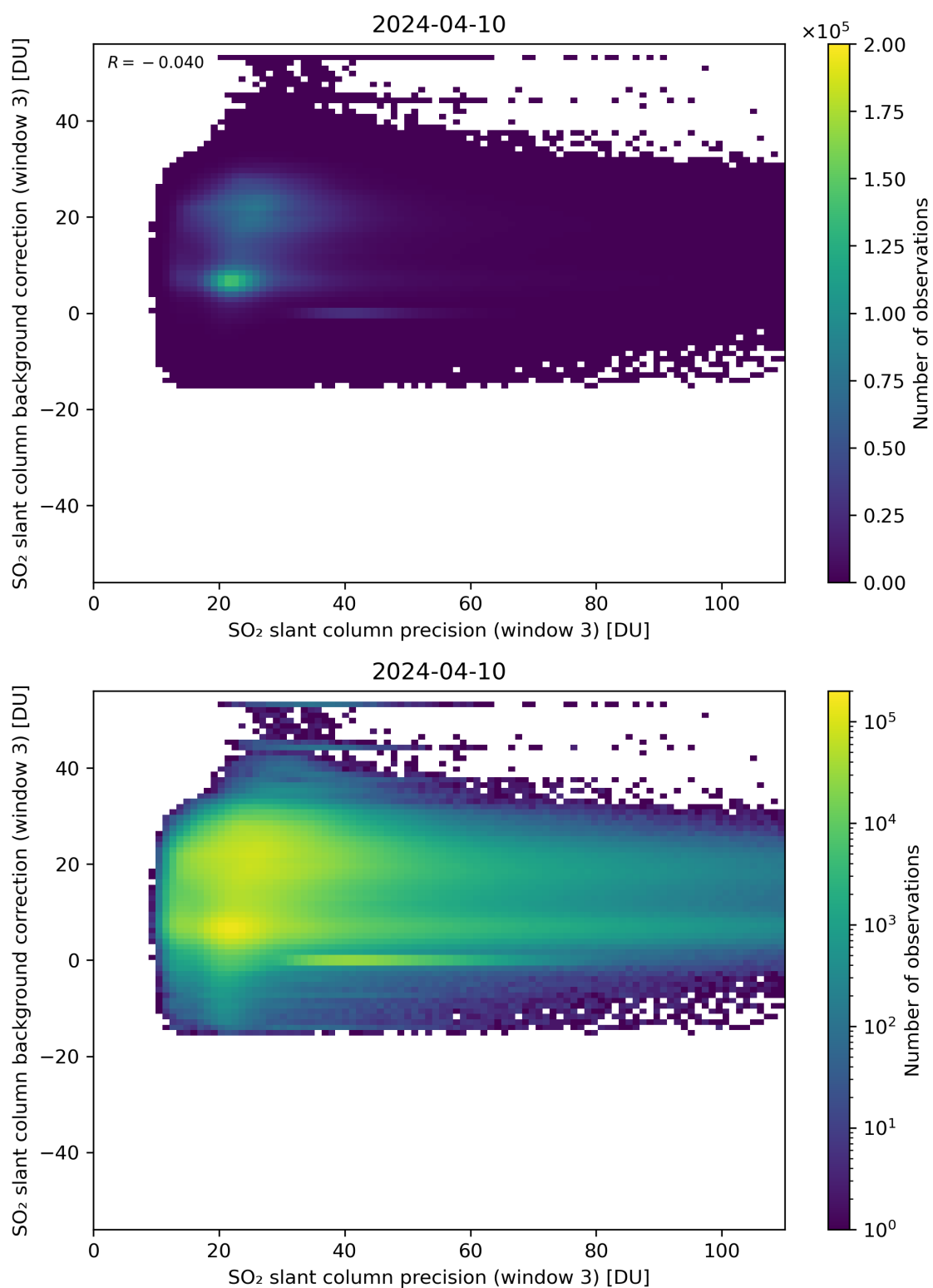
Figure 257: Scatter density plot of “SO 2 slant column precision (window 3)” against “SO 2 slant column background correction (window 3)” for 2024-04-10 to 2024-04-11.
