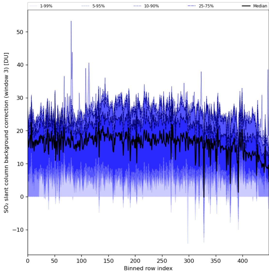
Figure 90: Along track statistics of “SO 2 slant column background correction (window 3)” for 2024-04-10 to 2024-04-11
