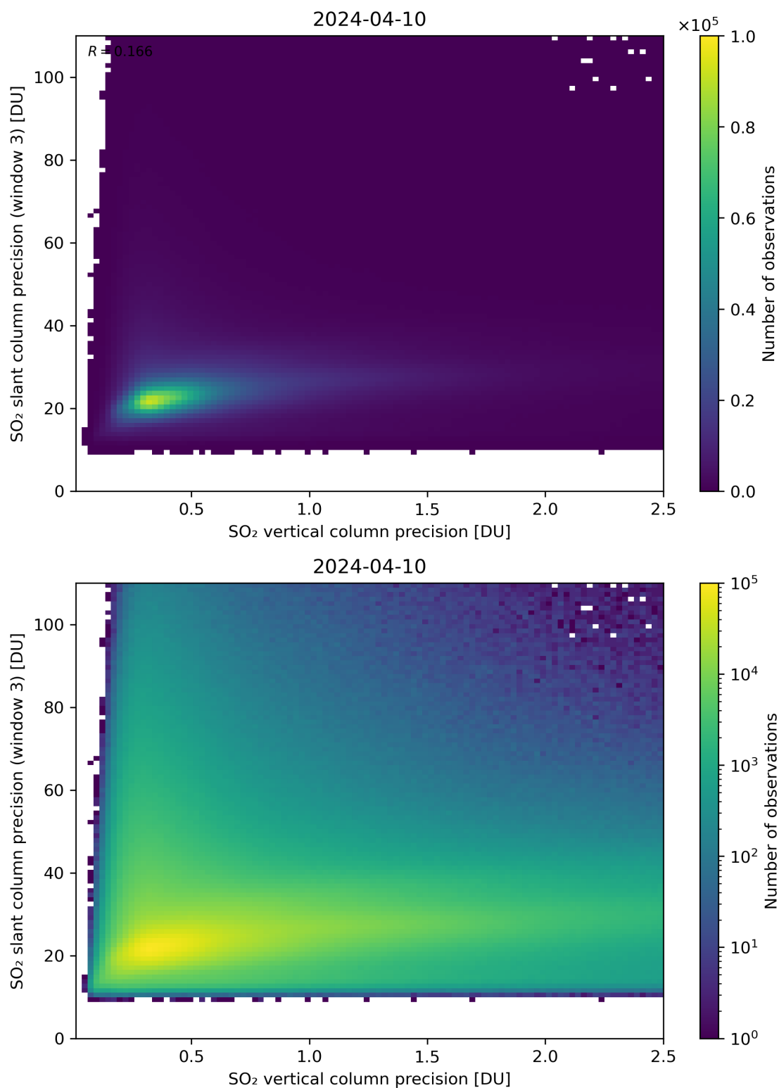
Figure 293: Scatter density plot of “SO 2 vertical column precision” against “SO 2 slant column precision (window 3)” for 2024-04-10 to 2024-04-11.
