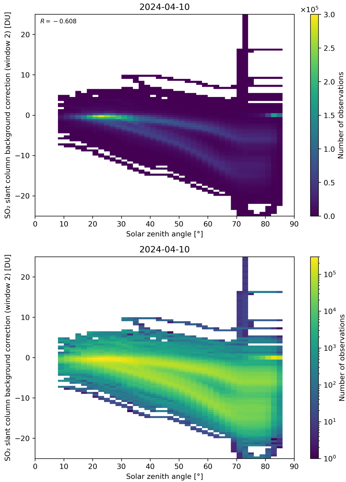
Figure 159: Scatter density plot of “Solar zenith angle” against “SO 2 slant column background correction (window 2)” for 2024-04-10 to 2024-04-11.
