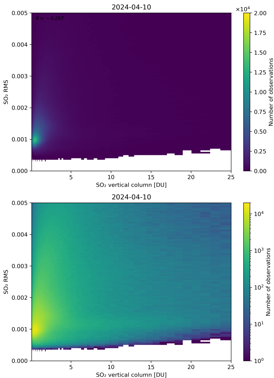
Figure 278: Scatter density plot of “SO 2 vertical column” against “SO 2 RMS” for 2024-04-10 to 2024-04-11.
