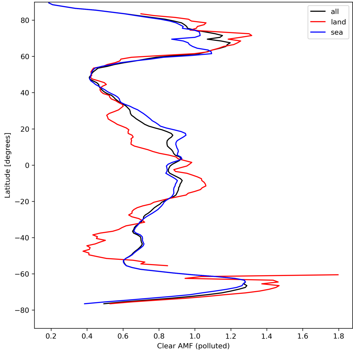
Figure 50: Zonal average of “Clear AMF (polluted)” for 2024-04-10 to 2024-04-11.
