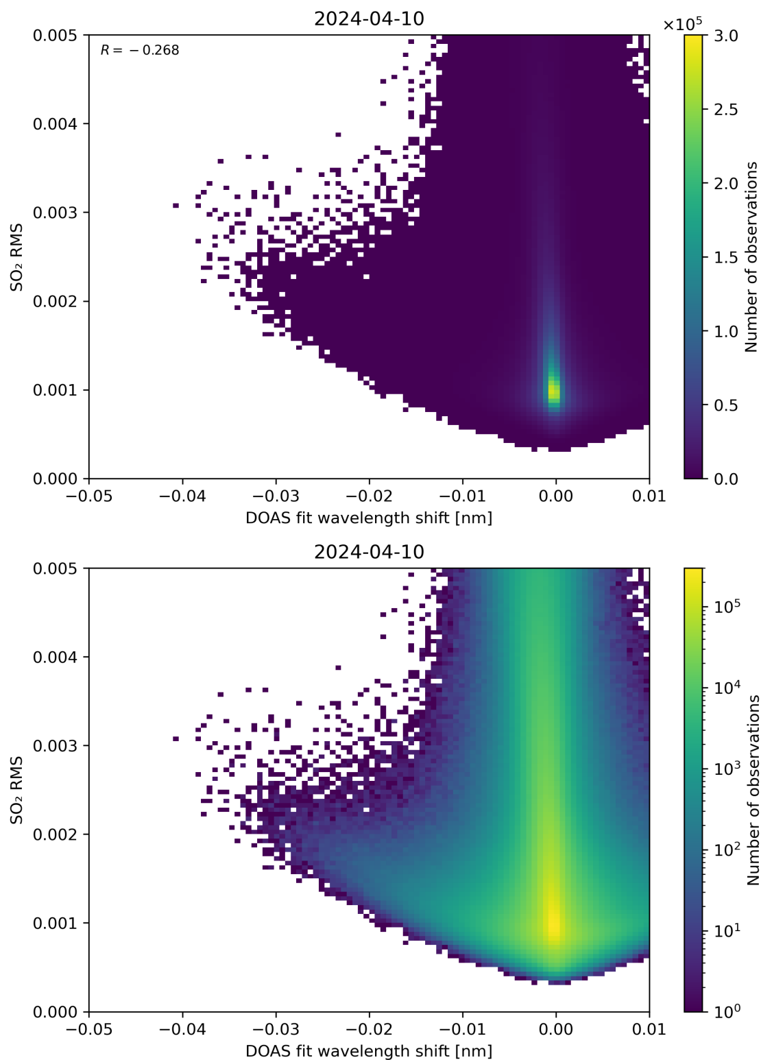
Figure 128: Scatter density plot of “DOAS fit wavelength shift” against “SO 2 RMS” for 2024-04-10 to 2024-04-11.
