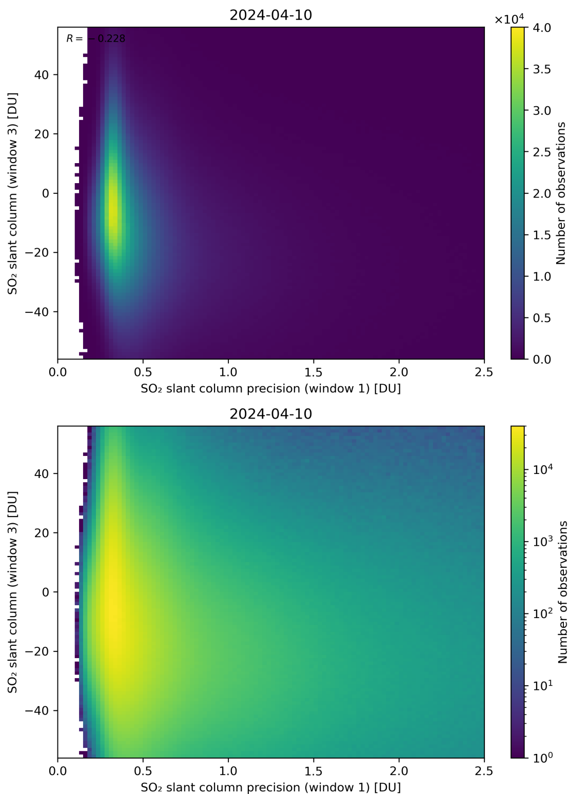
Figure 228: Scatter density plot of “SO 2 slant column precision (window 1)” against “SO 2 slant column (window 3)” for 2024-04-10 to 2024-04-11.
