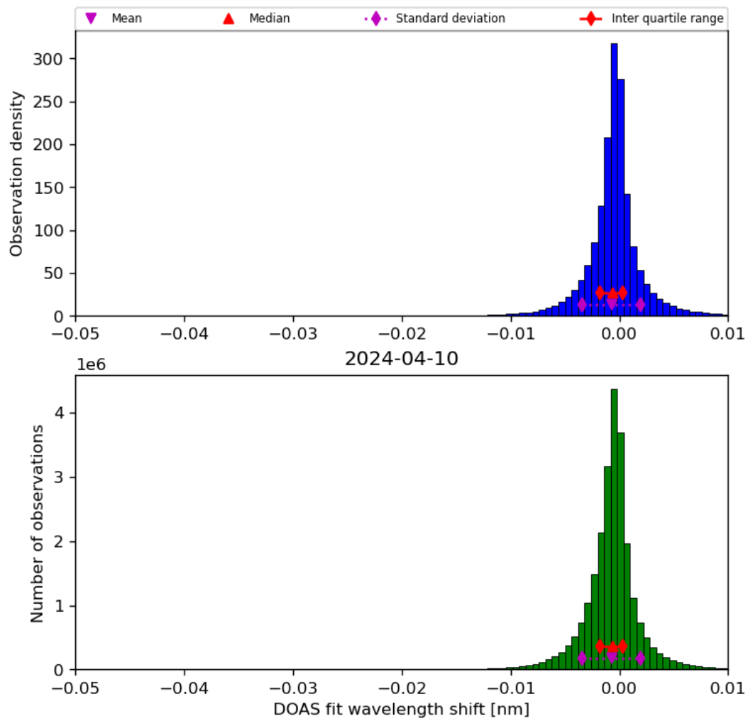
Figure 68: Histogram of “DOAS fit wavelength shift” for 2024-04-10 to 2024-04-11
