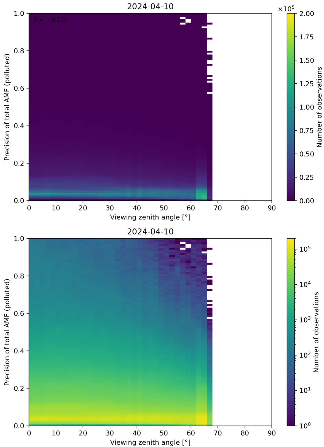
Figure 326: Scatter density plot of “Viewing zenith angle” against “Precision of total AMF (polluted)” for 2024-04-10 to 2024-04-11.
