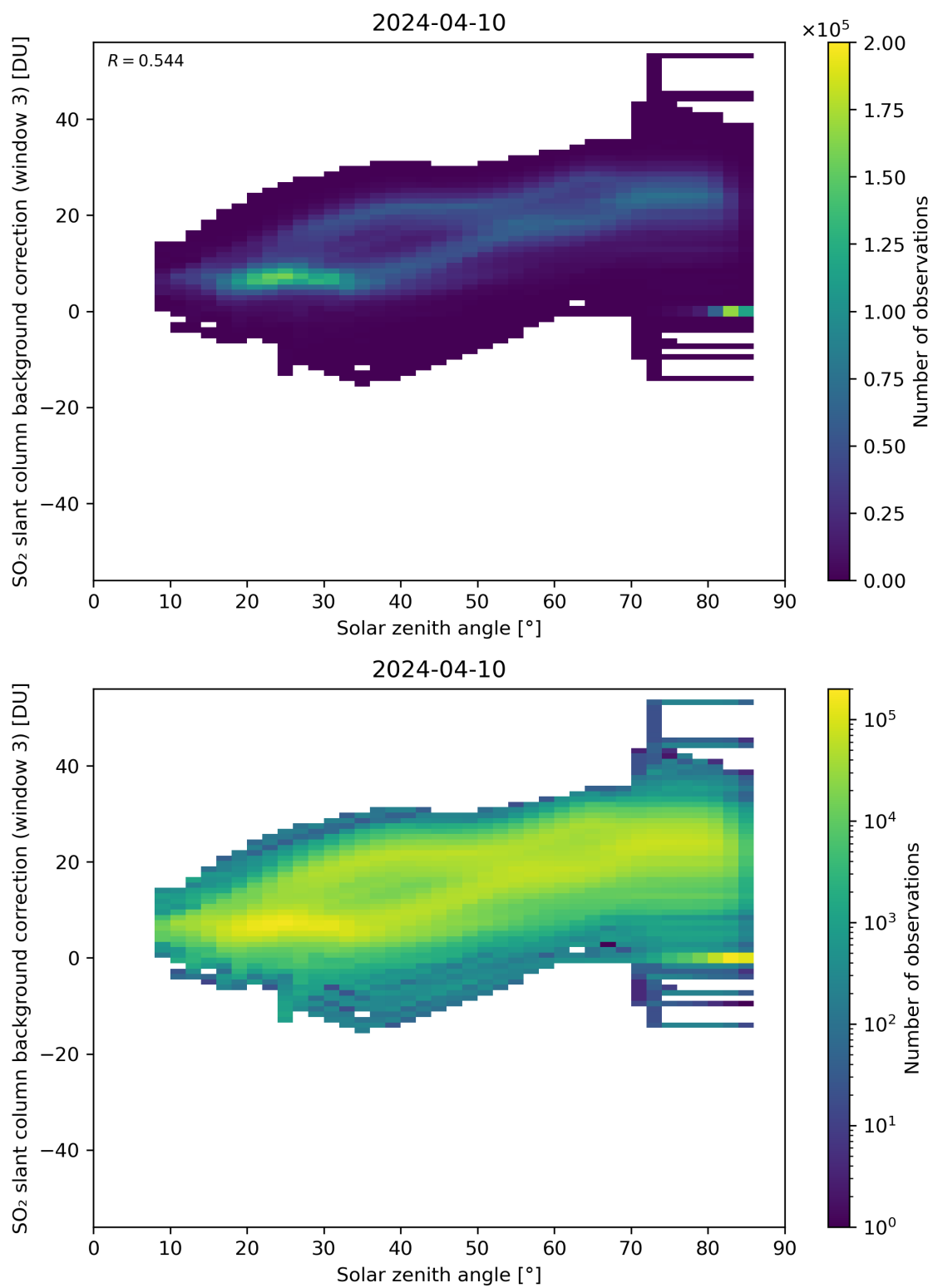
Figure 160: Scatter density plot of “Solar zenith angle” against “SO 2 slant column background correction (window 3)” for 2024-04-10 to 2024-04-11.
