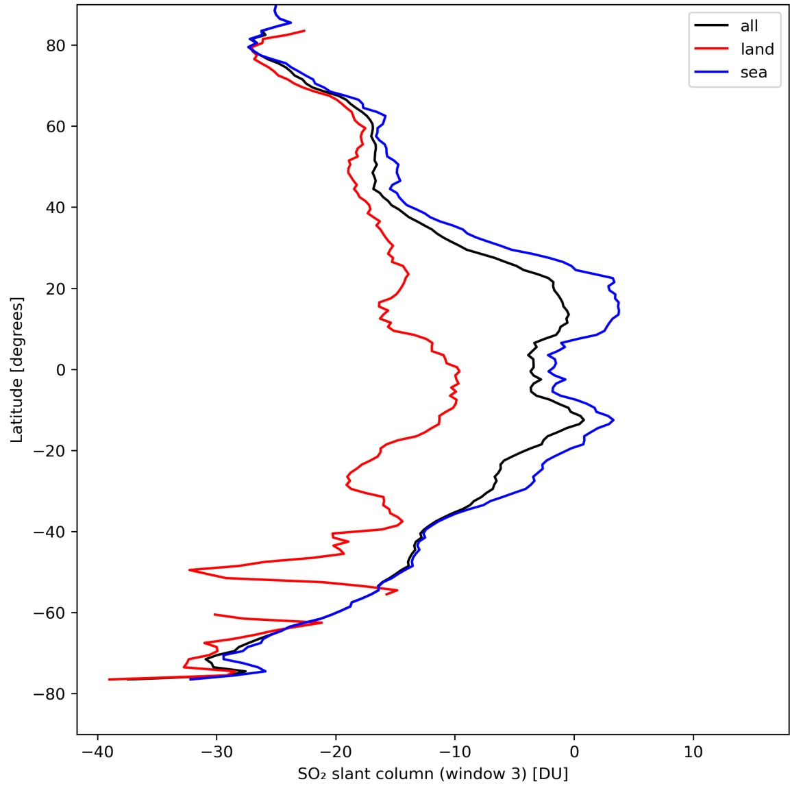
Figure 41: Zonal average of “SO 2 slant column (window 3)” for 2024-04-10 to 2024-04-11.
