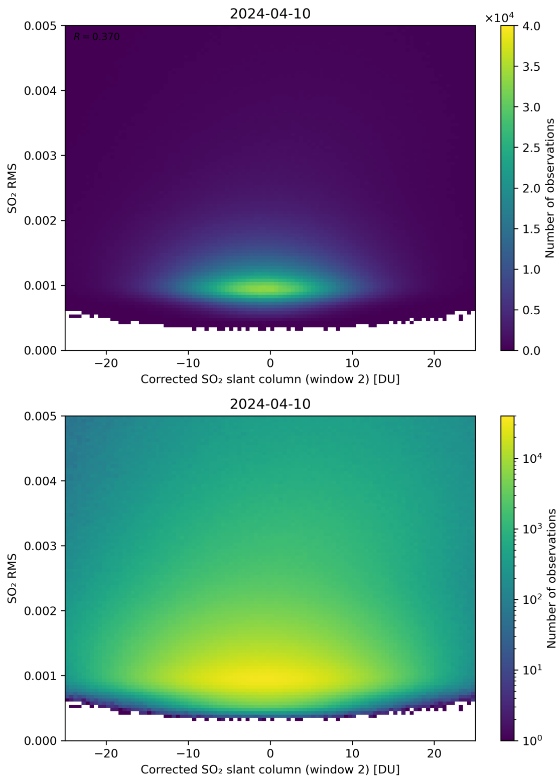
Figure 198: Scatter density plot of “Corrected SO 2 slant column (window 2)” against “SO 2 RMS” for 2024-04-10 to 2024-04-11.
