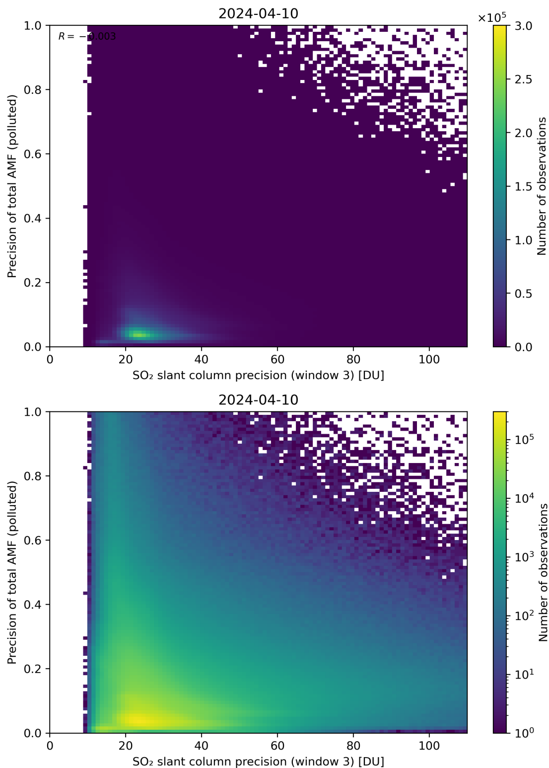
Figure 264: Scatter density plot of “SO 2 slant column precision (window 3)” against “Precision of total AMF (polluted)” for 2024-04-10 to 2024-04-11.
