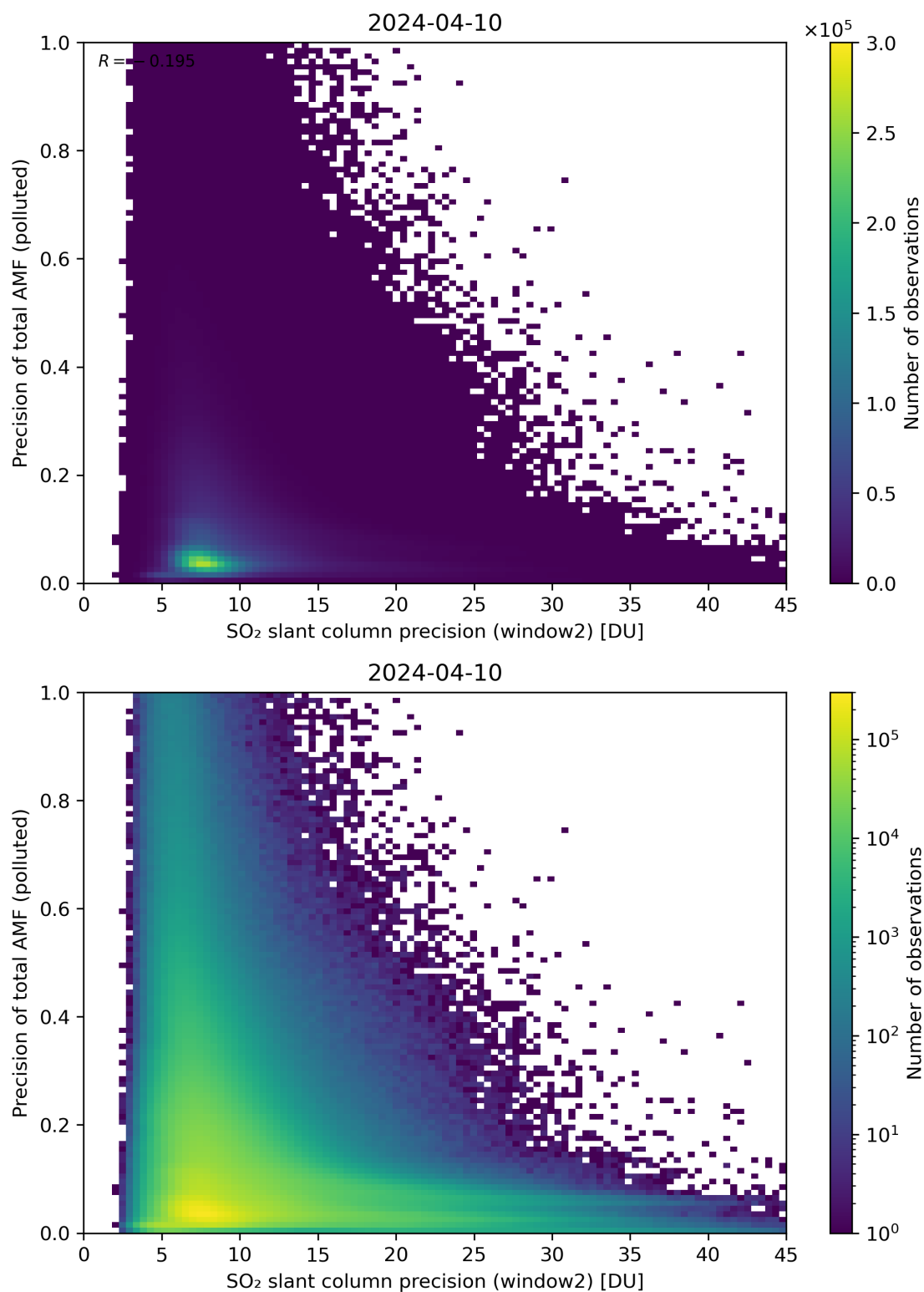
Figure 252: Scatter density plot of “SO 2 slant column precision (window2)” against “Precision of total AMF (polluted)” for 2024-04-10 to 2024-04-11.
