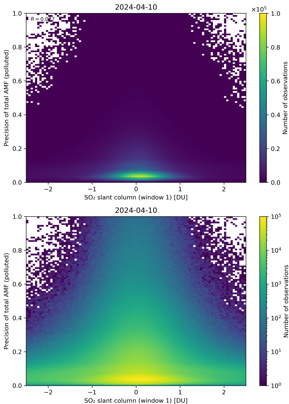
Figure 240: Scatter density plot of “SO 2 slant column (window 1)” against “Precision of total AMF (polluted)” for 2024-04-10 to 2024-04-11.
