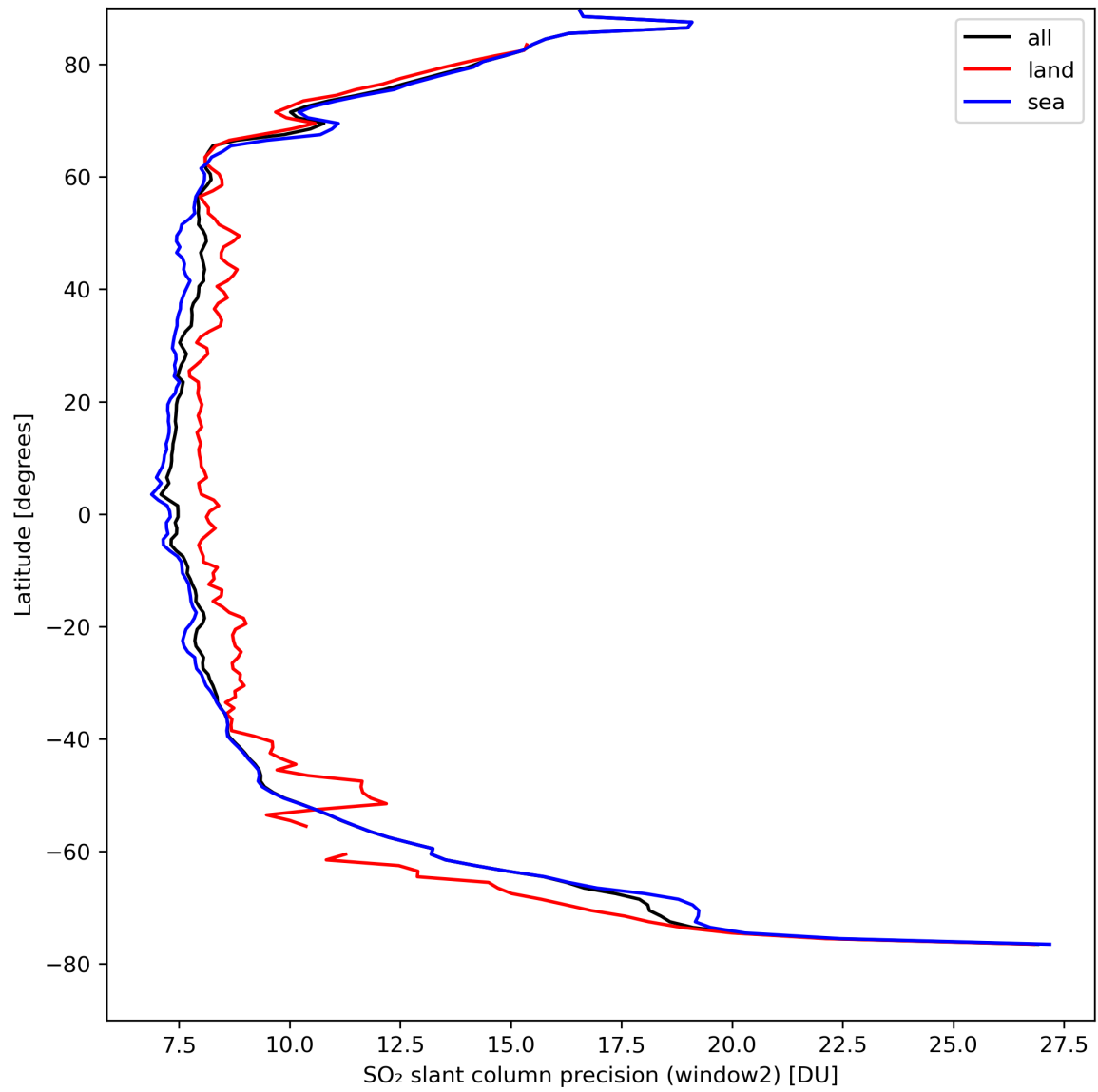
Figure 38: Zonal average of “SO 2 slant column precision (window2)” for 2024-04-10 to 2024-04-11.
