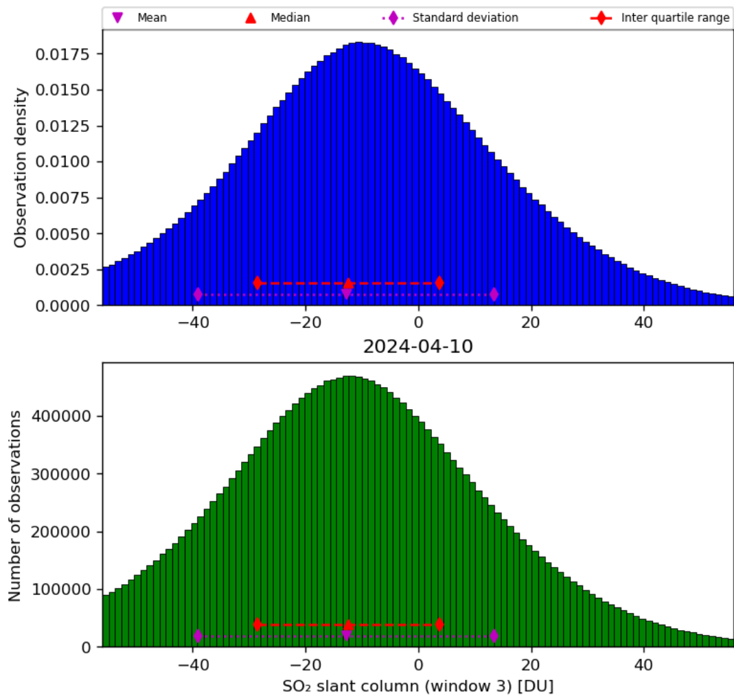
Figure 64: Histogram of “SO 2 slant column (window 3)” for 2024-04-10 to 2024-04-11
