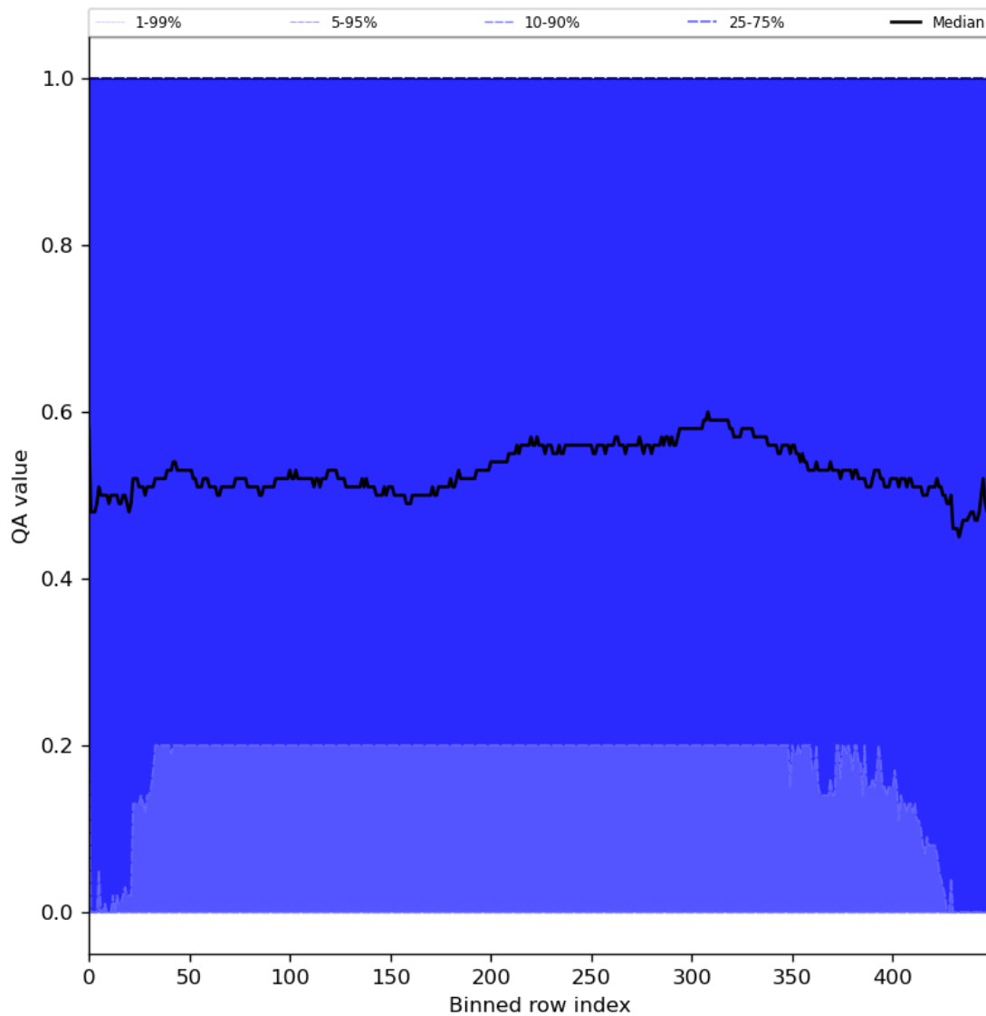
Figure 75: Along track statistics of “QA value” for 2024-04-10 to 2024-04-11
