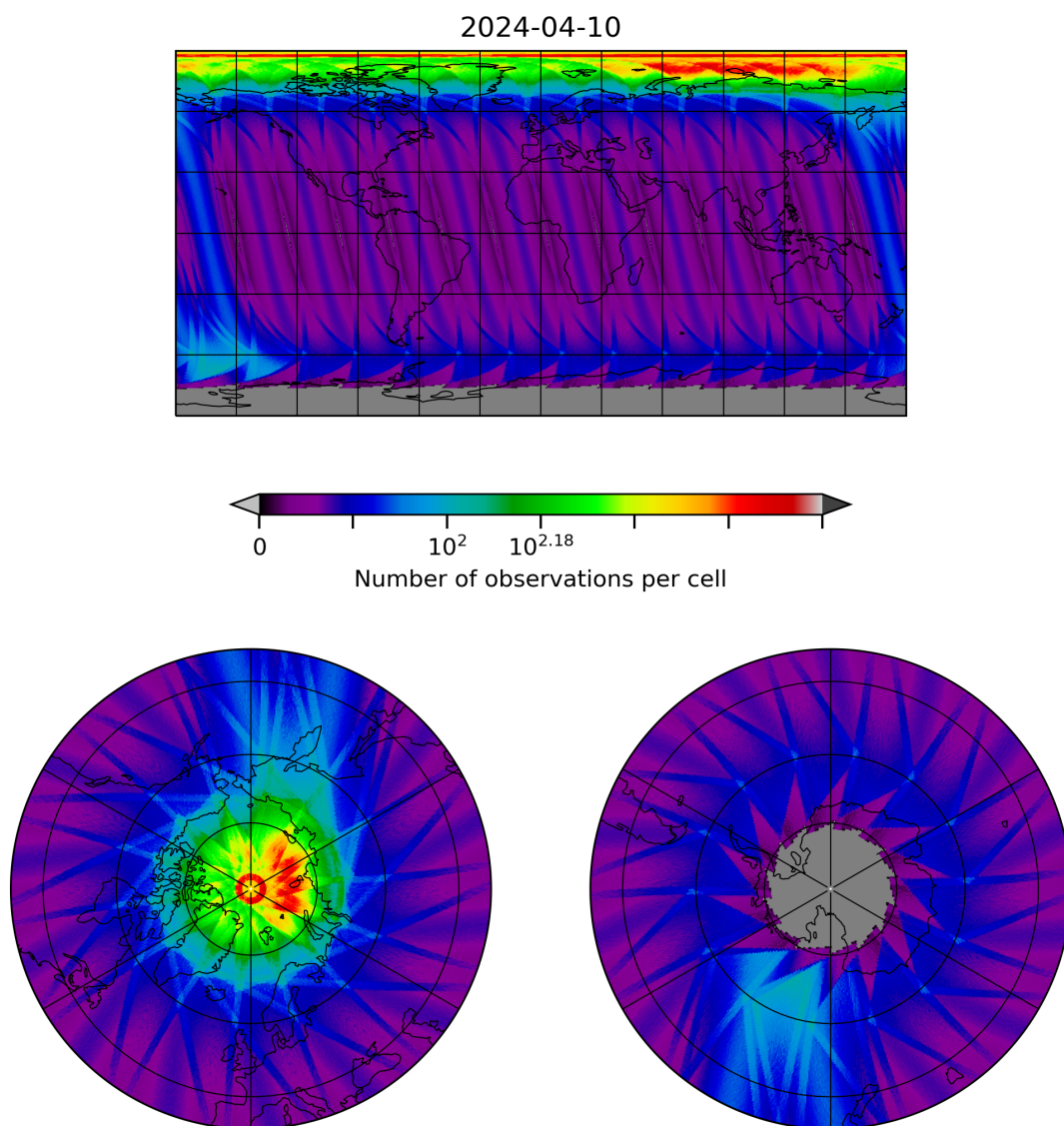
Figure 28: Map of the number of observations for 2024-04-10 to 2024-04-11
