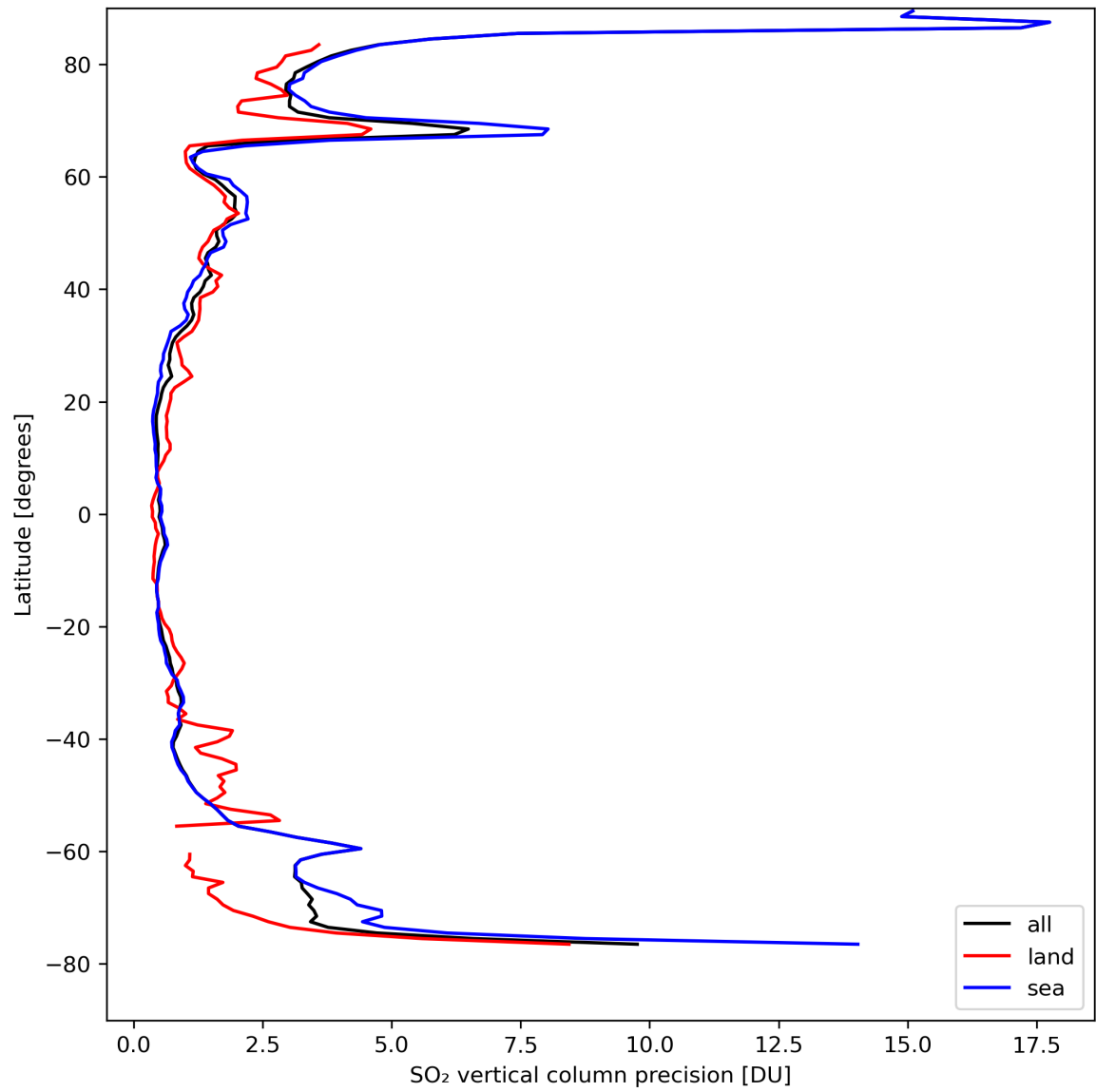
Figure 31: Zonal average of “SO 2 vertical column precision” for 2024-04-10 to 2024-04-11.
