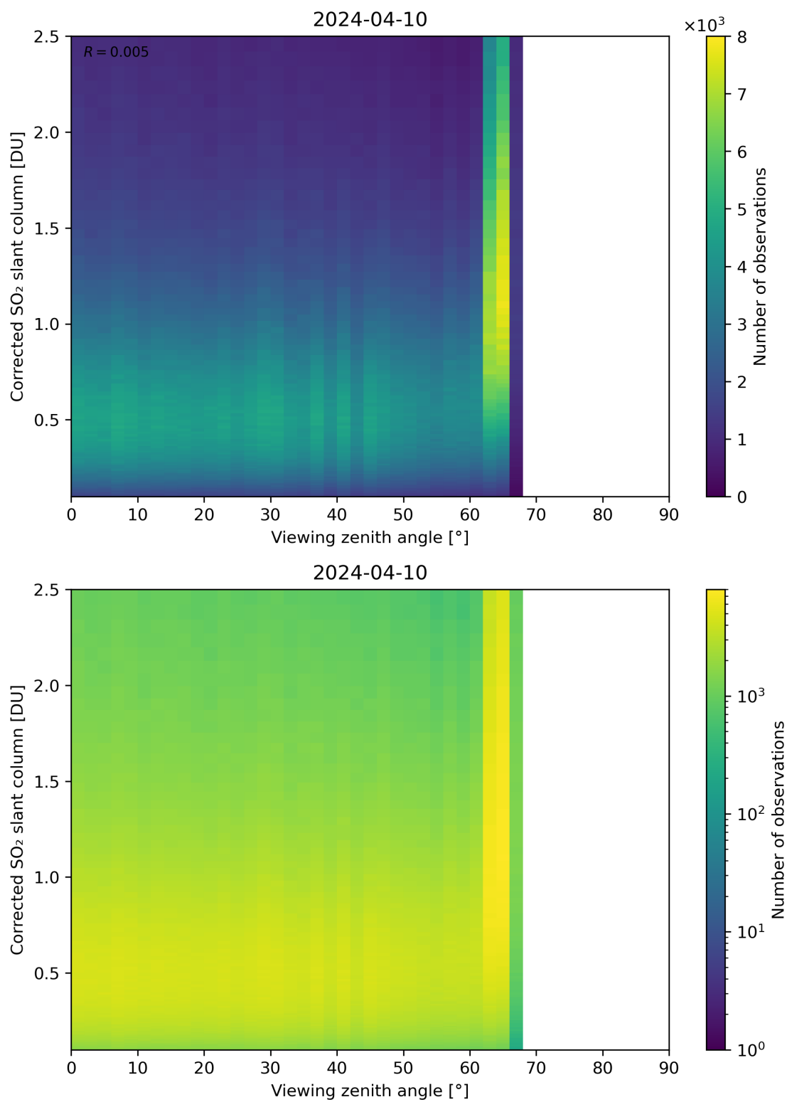
Figure 317: Scatter density plot of “Viewing zenith angle” against “Corrected SO 2 slant column” for 2024-04-10 to 2024-04-11.
