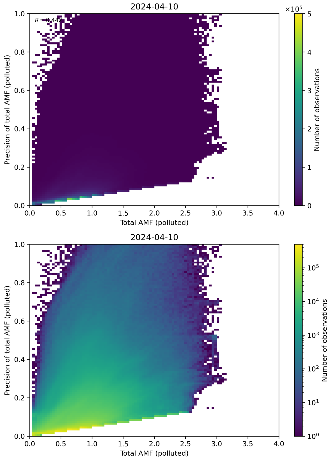
Figure 272: Scatter density plot of “Total AMF (polluted)” against “Precision of total AMF (polluted)” for 2024-04-10 to 2024-04-11.
