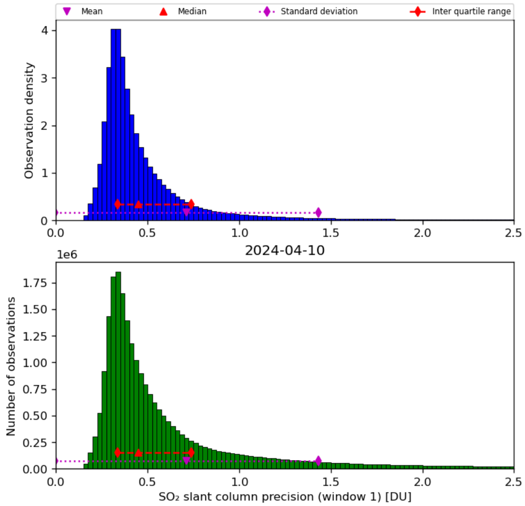
Figure 57: Histogram of “SO 2 slant column precision (window 1)” for 2024-04-10 to 2024-04-11
