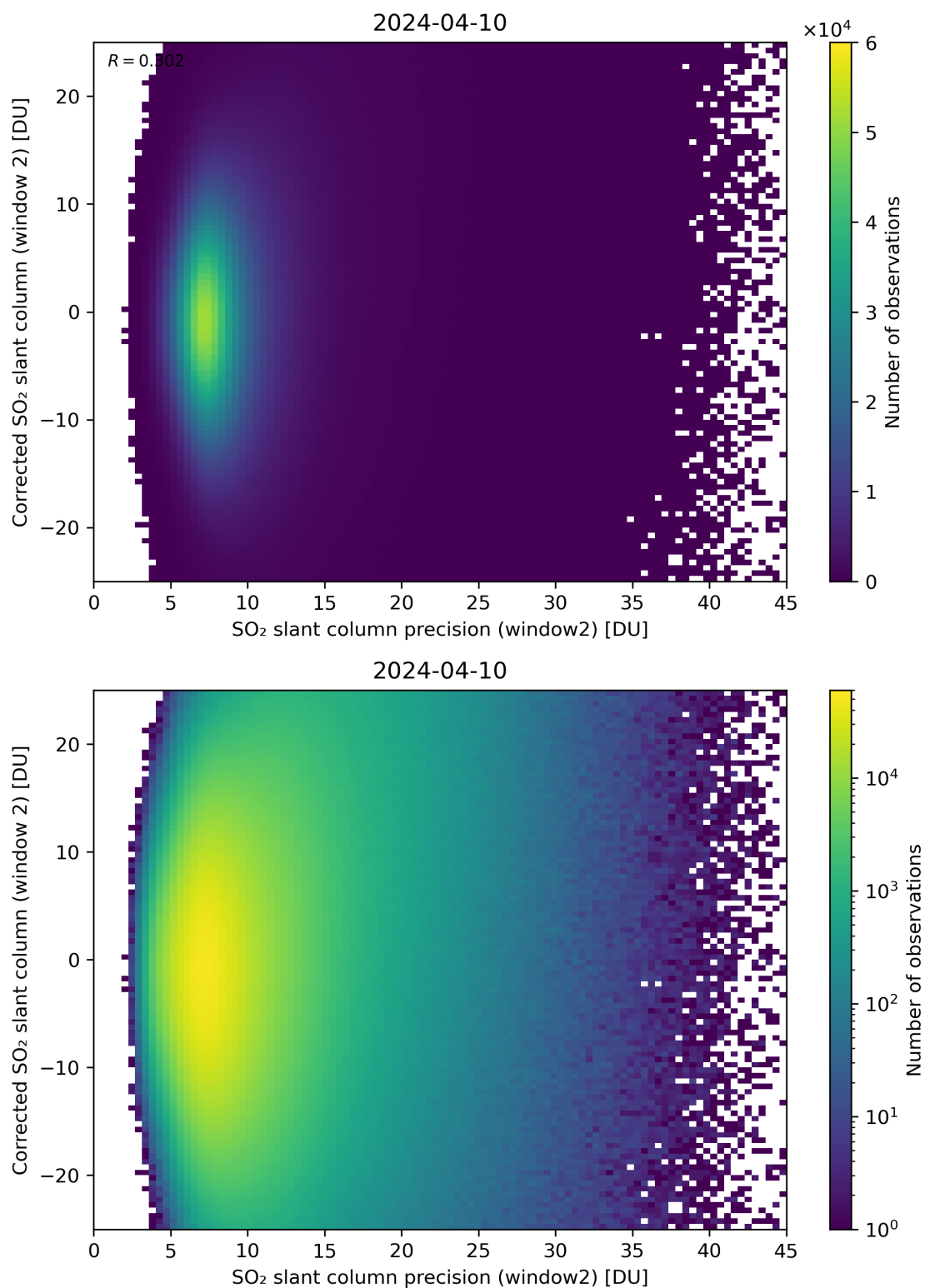
Figure 247: Scatter density plot of “SO 2 slant column precision (window2)” against “Corrected SO 2 slant column (window 2)” for 2024-04-10 to 2024-04-11.
