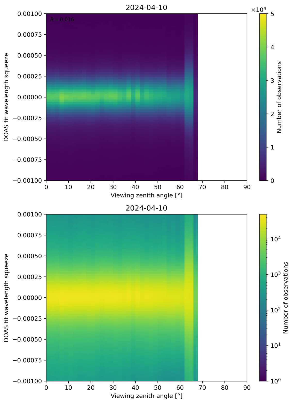
Figure 312: Scatter density plot of “Viewing zenith angle” against “DOAS fit wavelength squeeze” for 2024-04-10 to 2024-04-11.
