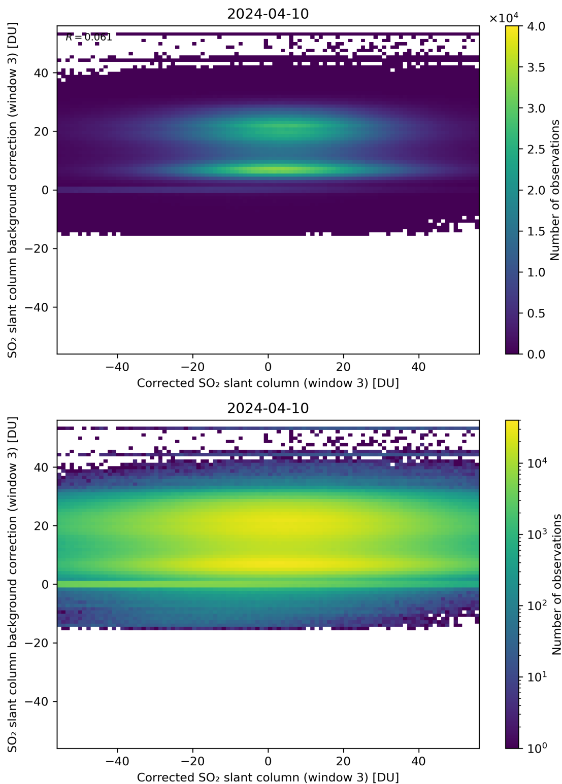
Figure 205: Scatter density plot of “Corrected SO 2 slant column (window 3)” against “SO 2 slant column background correction (window 3)” for 2024-04-10 to 2024-04-11.
