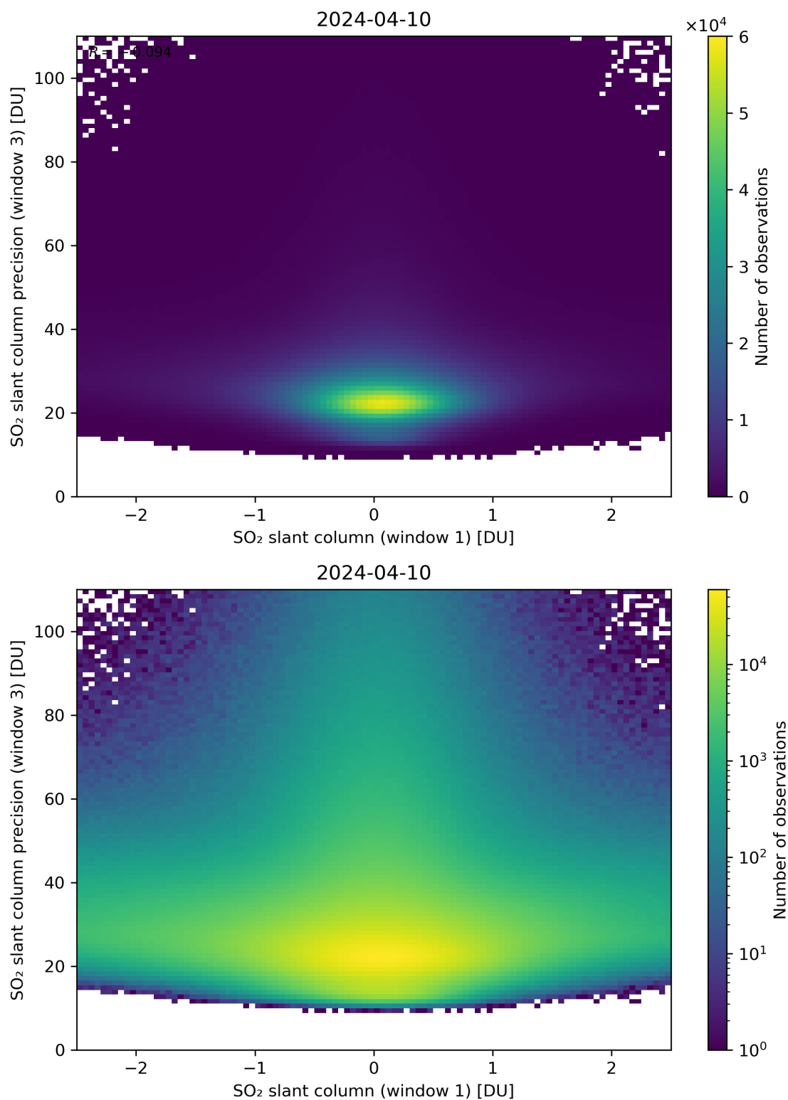
Figure 238: Scatter density plot of “SO 2 slant column (window 1)” against “SO 2 slant column precision (window 3)” for 2024-04-10 to 2024-04-11.
