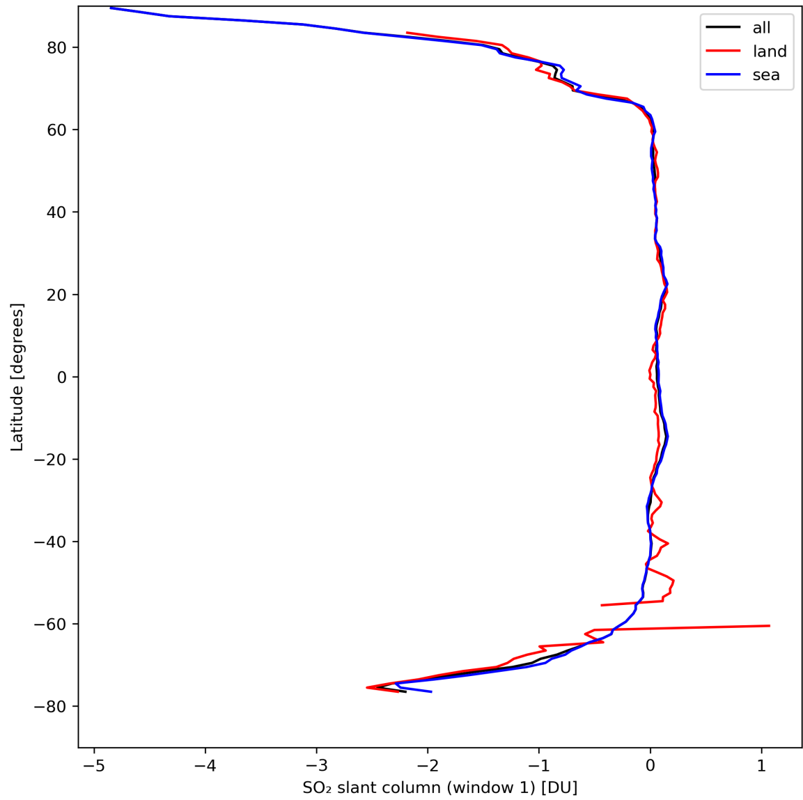
Figure 33: Zonal average of “SO 2 slant column (window 1)” for 2024-04-10 to 2024-04-11.
