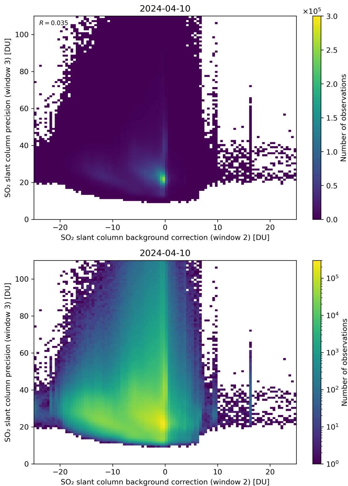
Figure 118: Scatter density plot of “SO 2 slant column background correction (window 2)” against “SO 2 slant column precision (window 3)” for 2024-04-10 to 2024-04-11.
