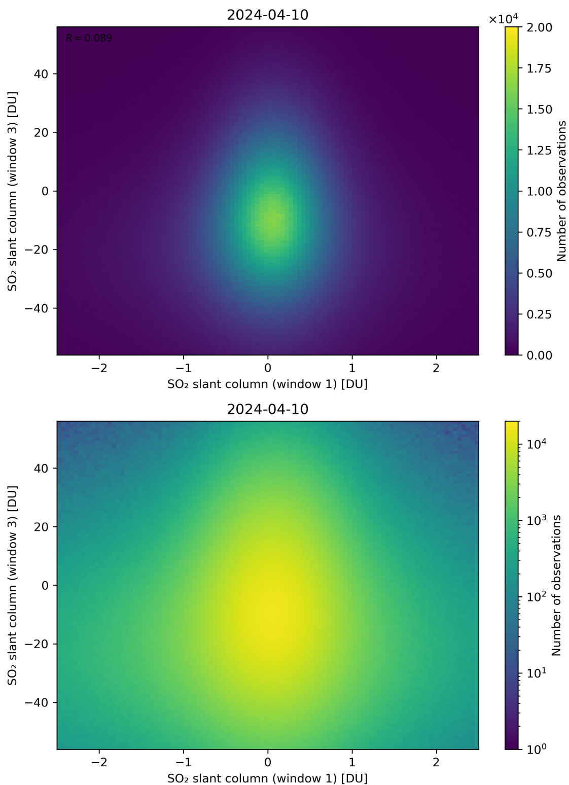
Figure 237: Scatter density plot of “SO 2 slant column (window 1)” against “SO 2 slant column (window 3)” for 2024-04-10 to 2024-04-11.
