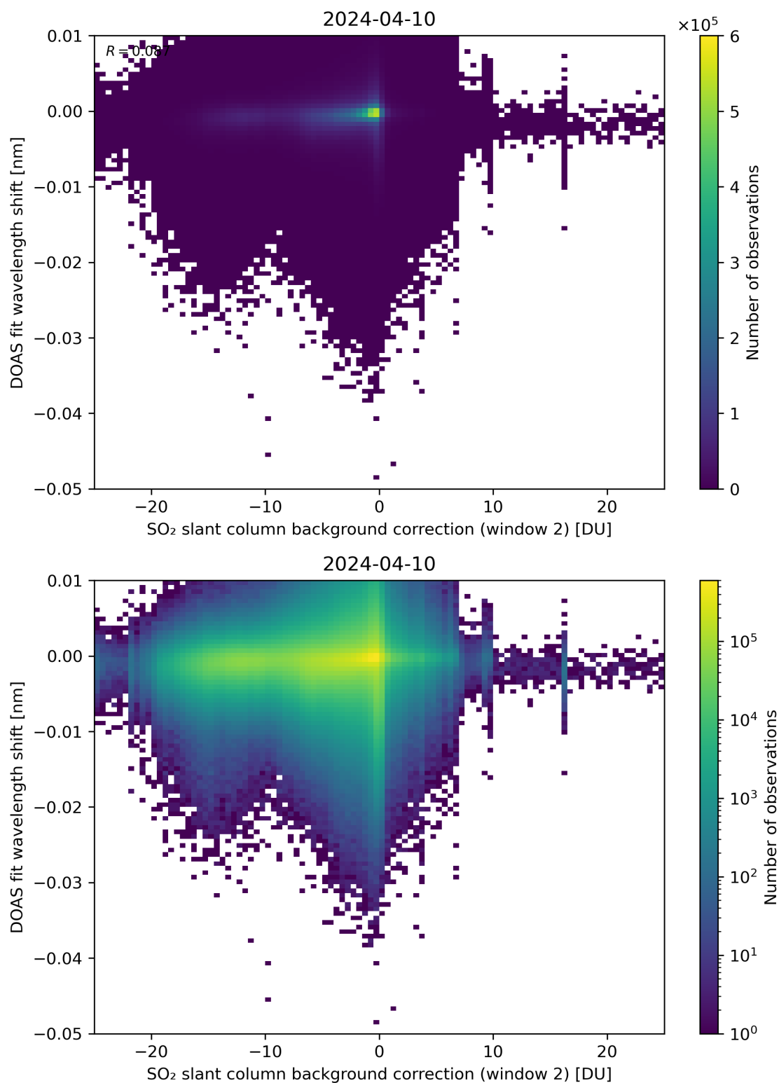
Figure 112: Scatter density plot of “SO 2 slant column background correction (window 2)” against “DOAS fit wavelength shift” for 2024-04-10 to 2024-04-11.
