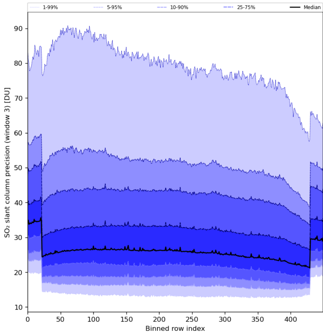
Figure 88: Along track statistics of “SO 2 slant column precision (window 3)” for 2024-04-10 to 2024-04-11
