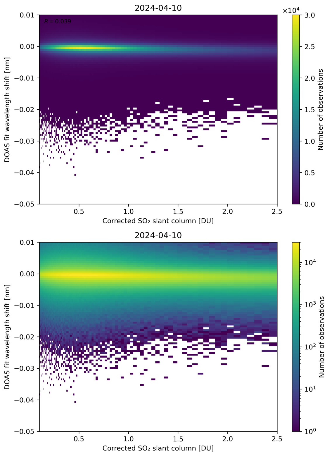
Figure 181: Scatter density plot of “Corrected SO 2 slant column” against “DOAS fit wavelength shift” for 2024-04-10 to 2024-04-11.
