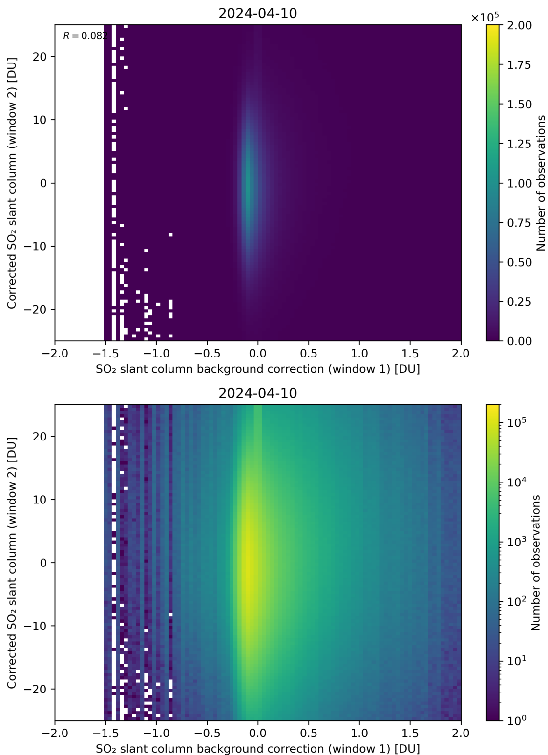
Figure 104: Scatter density plot of “SO 2 slant column background correction (window 1)” against “Corrected SO 2 slant column (window 2)” for 2024-04-10 to 2024-04-11.
