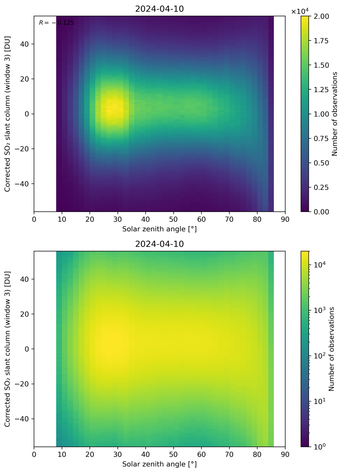
Figure 168: Scatter density plot of “Solar zenith angle” against “Corrected SO 2 slant column (window 3)” for 2024-04-10 to 2024-04-11.
