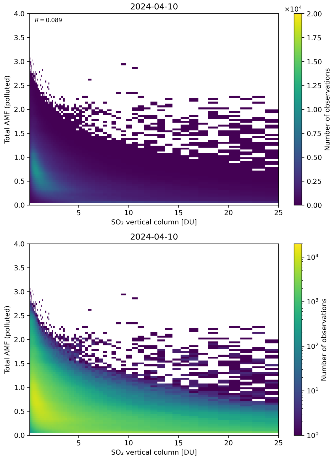
Figure 305: Scatter density plot of “SO 2 vertical column” against “Total AMF (polluted)” for 2024-04-10 to 2024-04-11.
