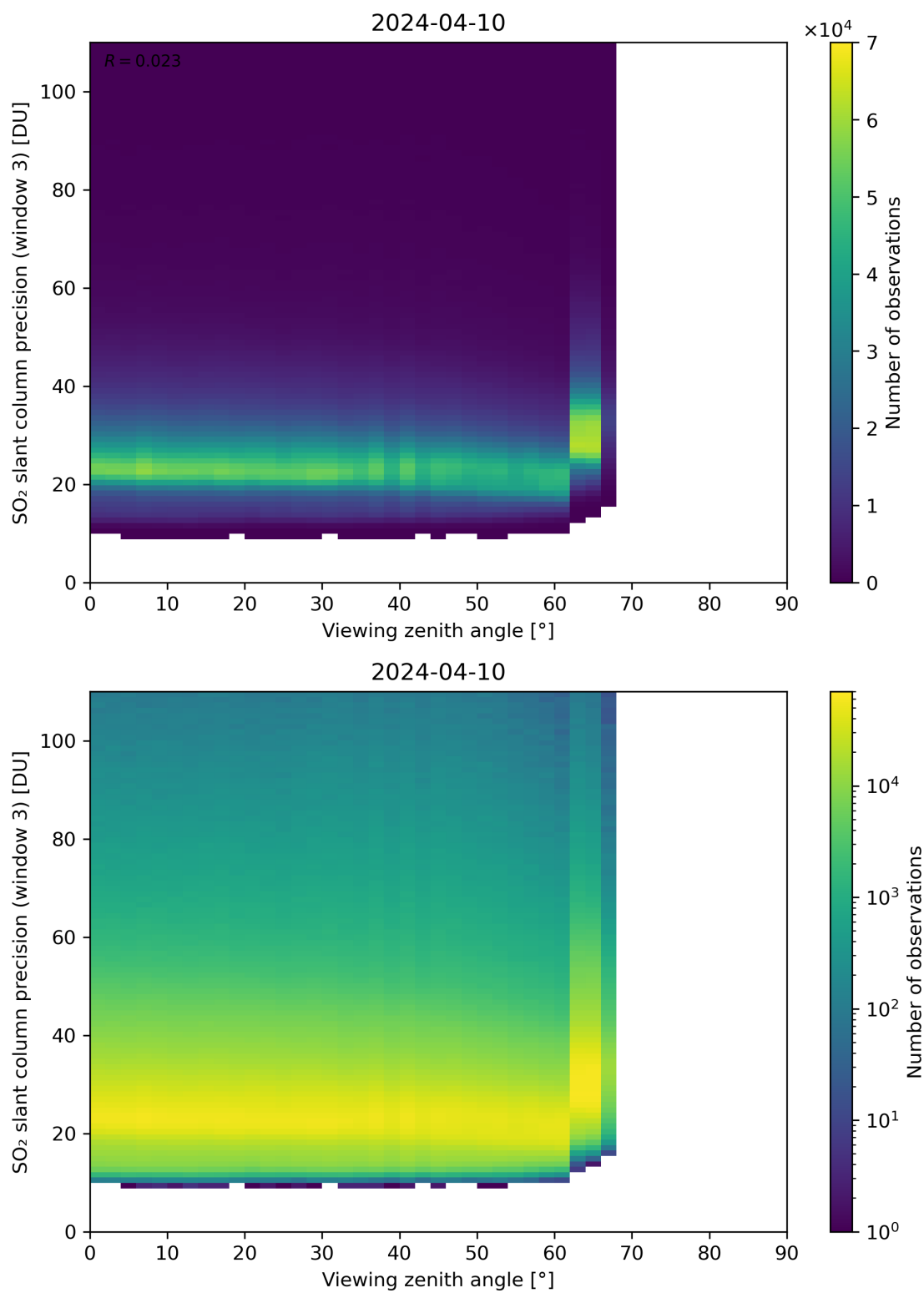
Figure 324: Scatter density plot of “Viewing zenith angle” against “SO 2 slant column precision (window 3)” for 2024-04-10 to 2024-04-11.
