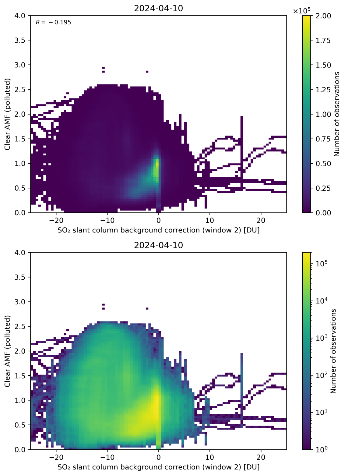
Figure 115: Scatter density plot of “SO 2 slant column background correction (window 2)” against “Clear AMF (polluted)” for 2024-04-10 to 2024-04-11.
