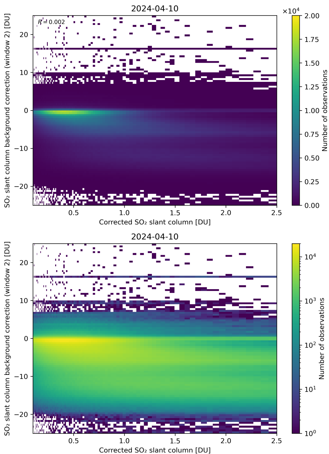
Figure 179: Scatter density plot of “Corrected SO 2 slant column” against “SO 2 slant column background correction (window 2)” for 2024-04-10 to 2024-04-11.
