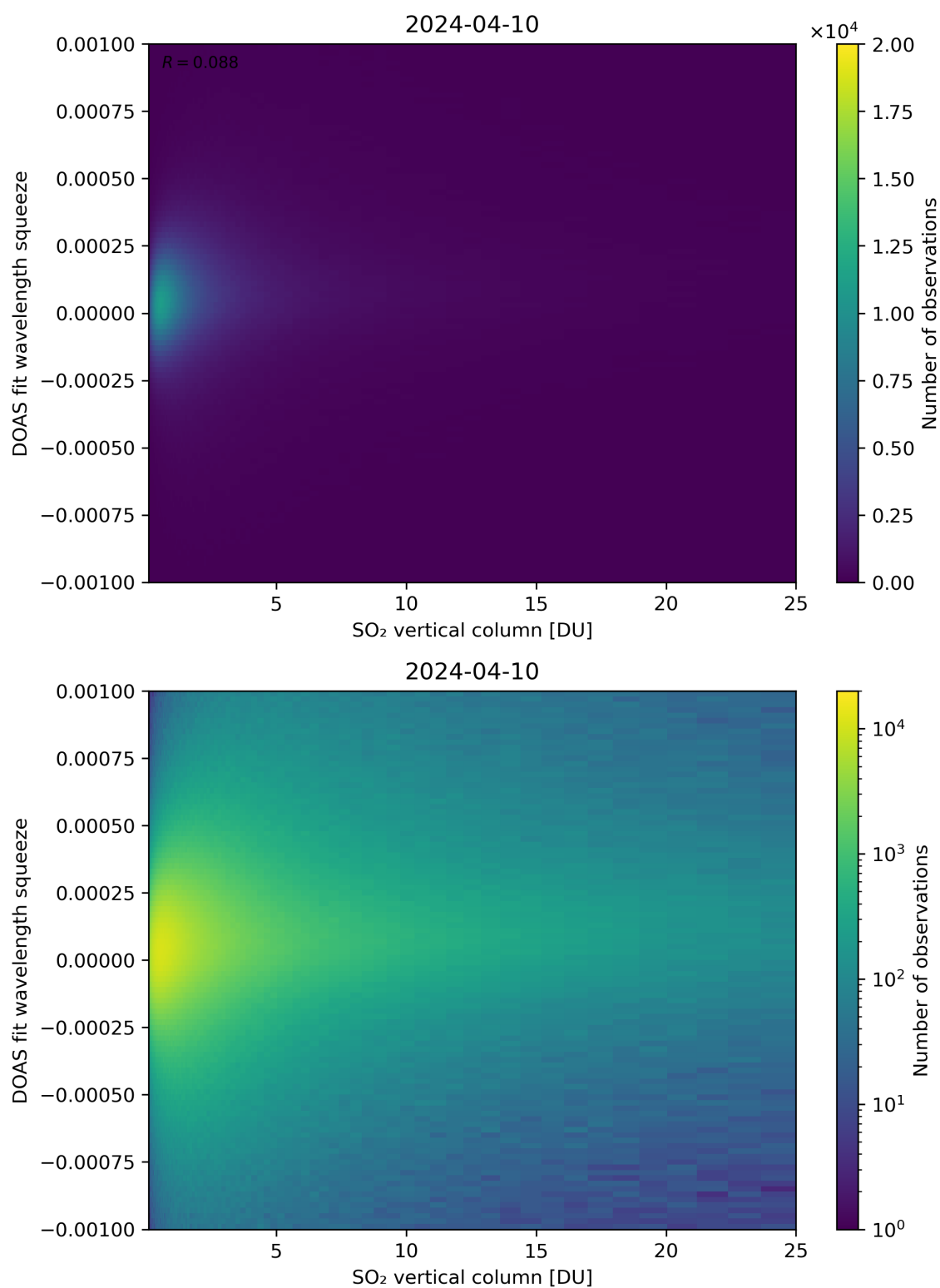
Figure 277: Scatter density plot of “SO 2 vertical column” against “DOAS fit wavelength squeeze” for 2024-04-10 to 2024-04-11.
