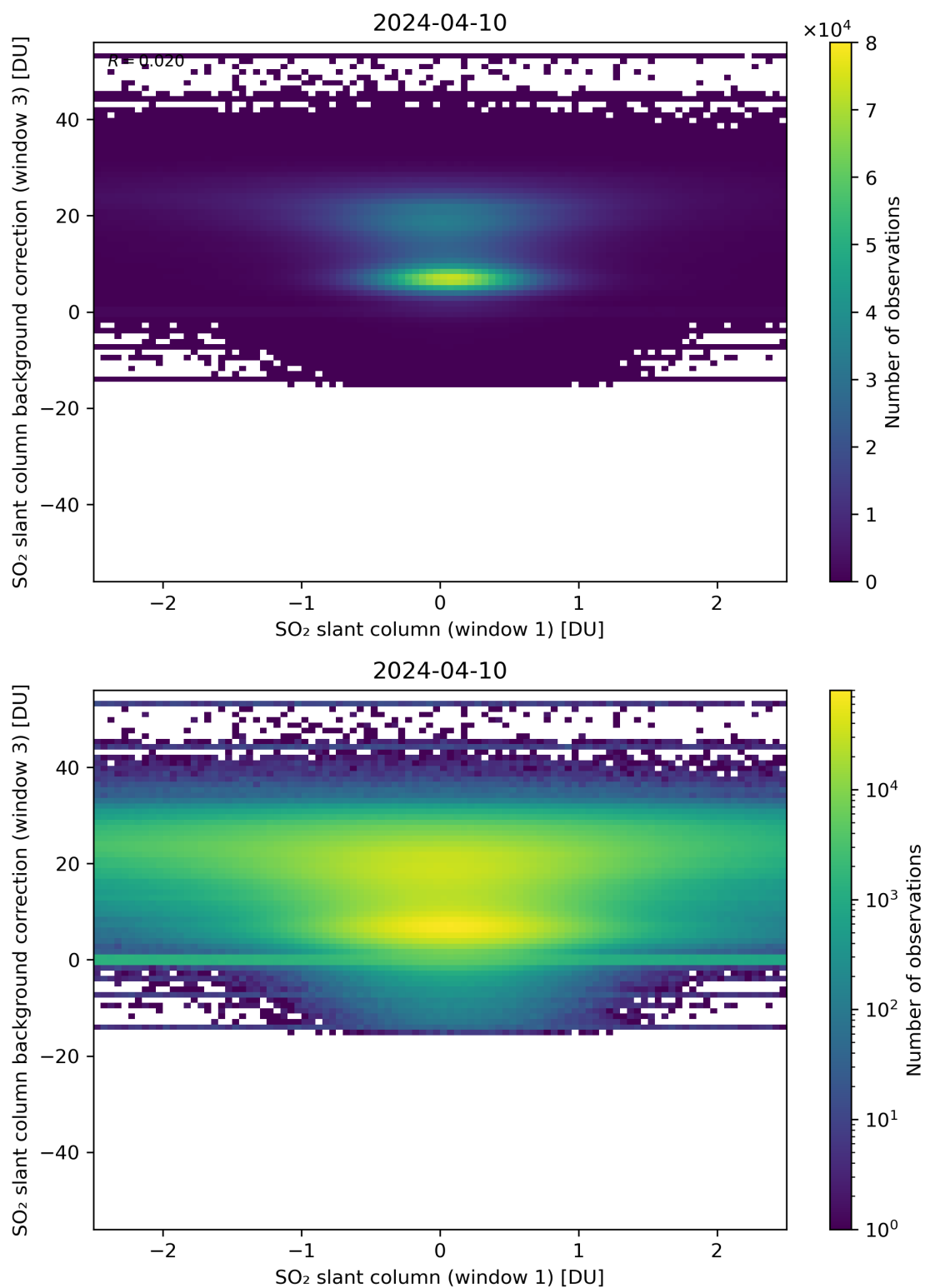
Figure 214: Scatter density plot of “SO 2 slant column (window 1)” against “SO 2 slant column background correction (window 3)” for 2024-04-10 to 2024-04-11.
