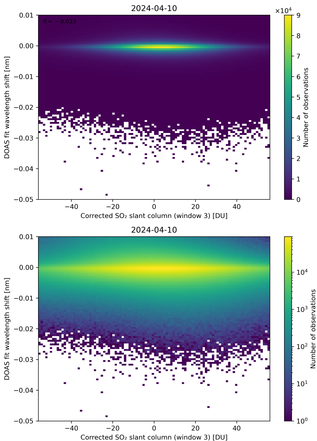
Figure 206: Scatter density plot of “Corrected SO 2 slant column (window 3)” against “DOAS fit wavelength shift” for 2024-04-10 to 2024-04-11.
