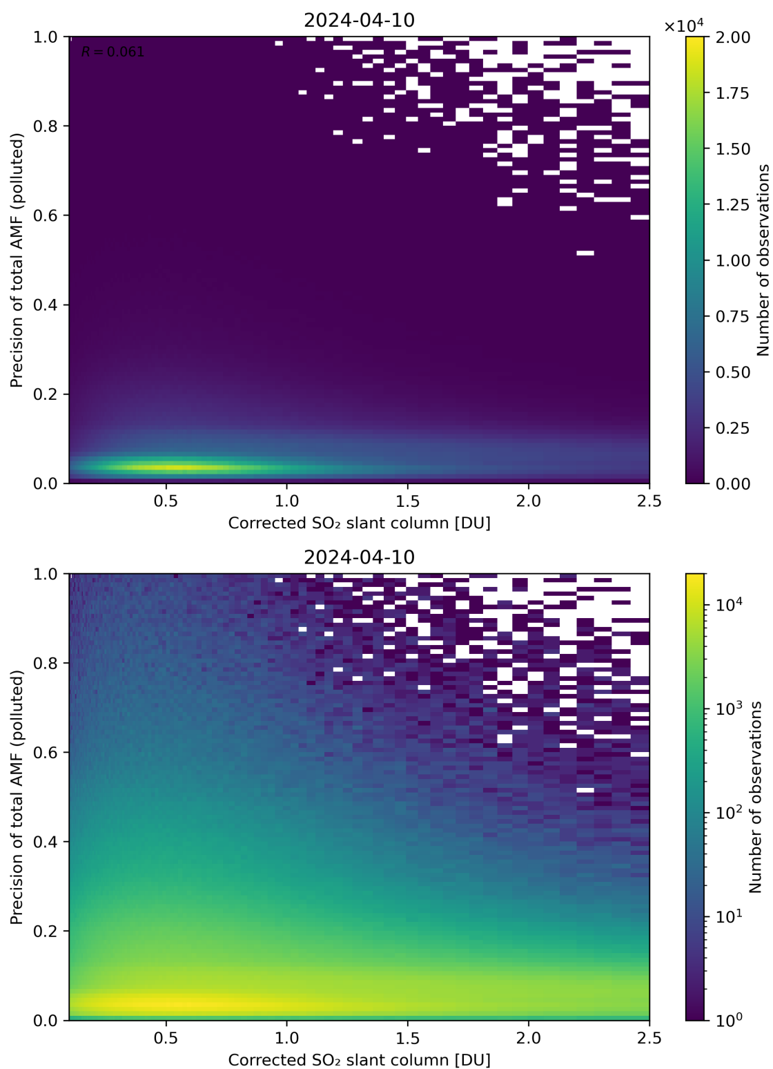
Figure 193: Scatter density plot of “Corrected SO 2 slant column” against “Precision of total AMF (polluted)” for 2024-04-10 to 2024-04-11.
