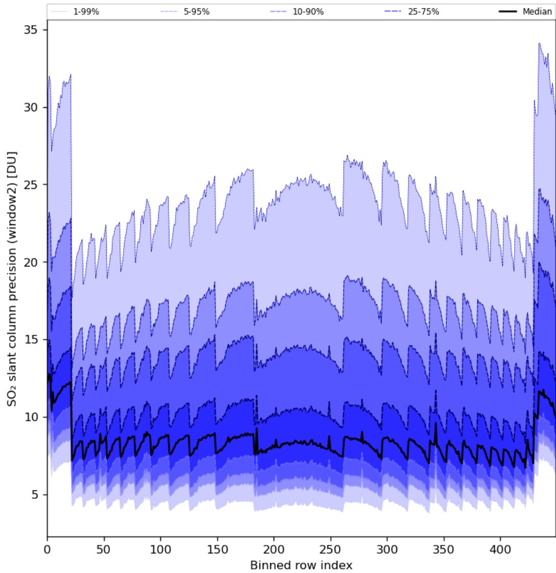
Figure 84: Along track statistics of “SO 2 slant column precision (window2)” for 2024-04-10 to 2024-04-11
