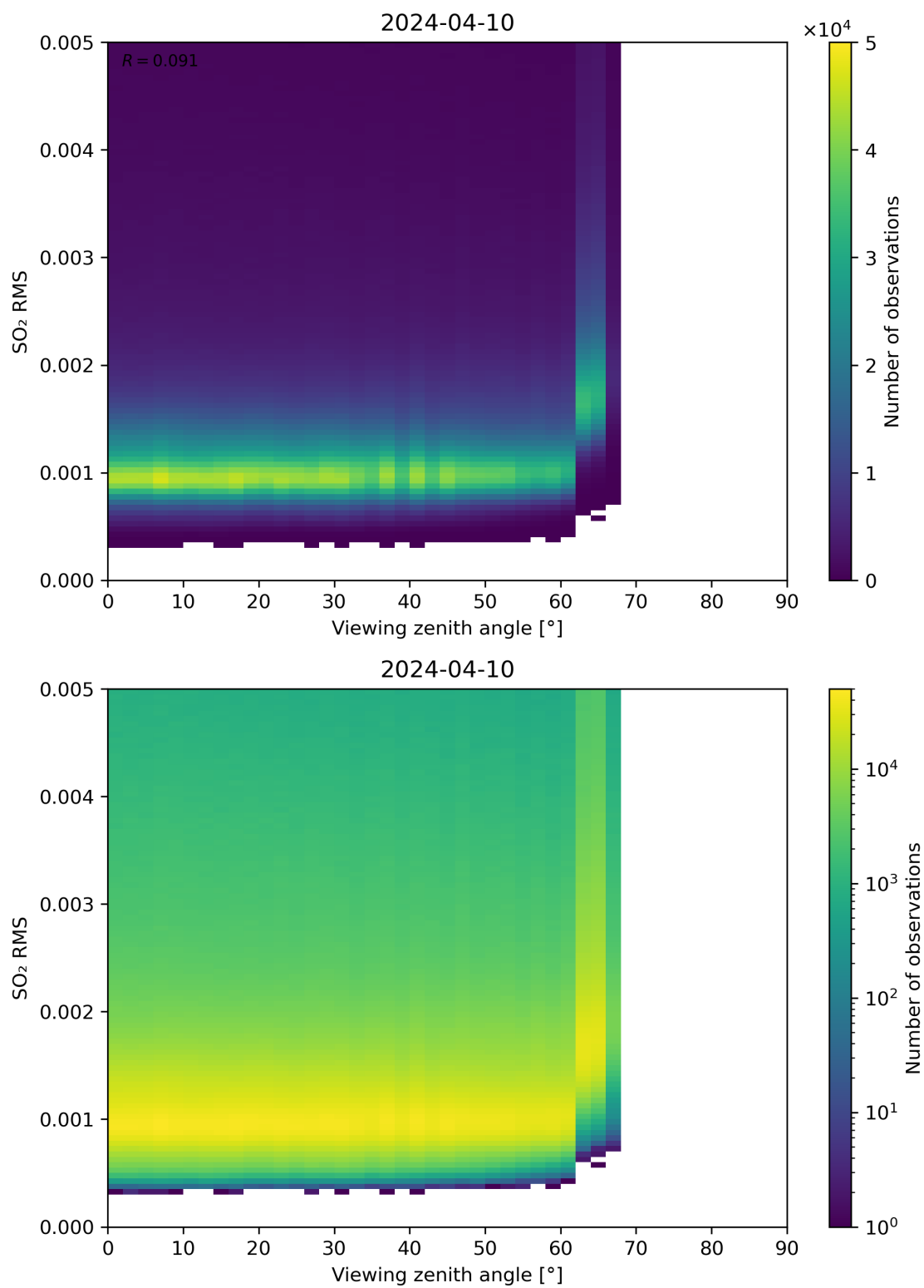
Figure 313: Scatter density plot of “Viewing zenith angle” against “SO 2 RMS” for 2024-04-10 to 2024-04-11.
