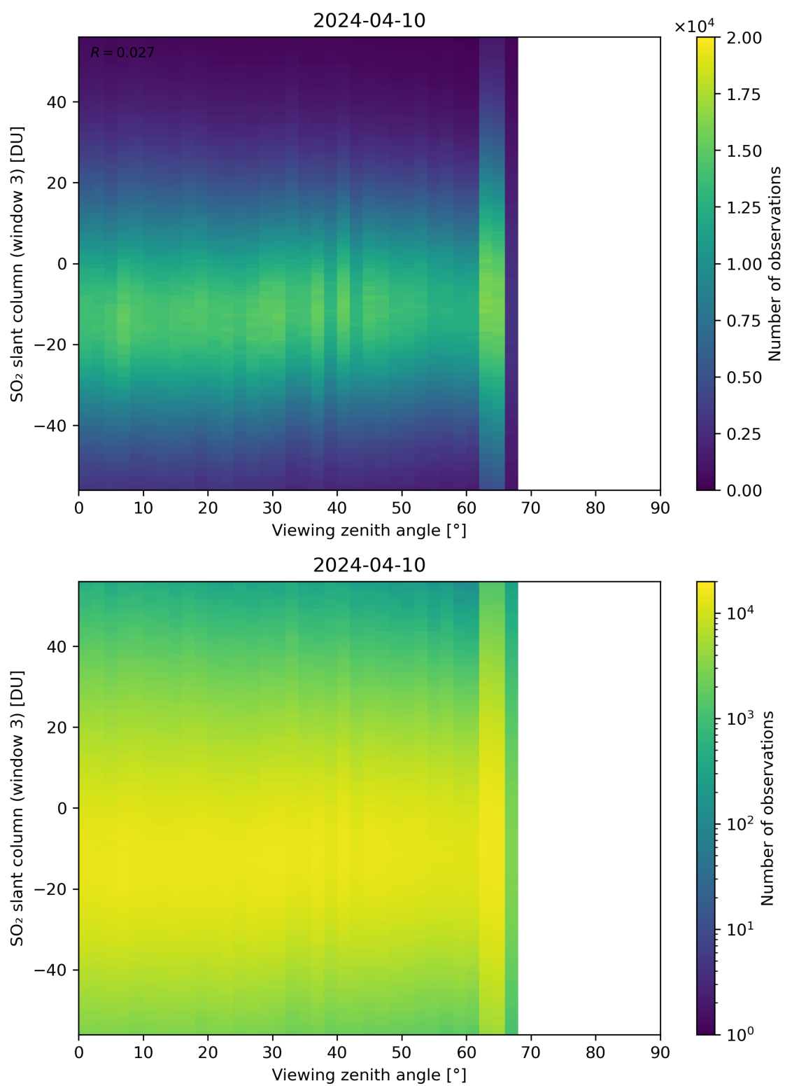
Figure 323: Scatter density plot of “Viewing zenith angle” against “SO 2 slant column (window 3)” for 2024-04-10 to 2024-04-11.
