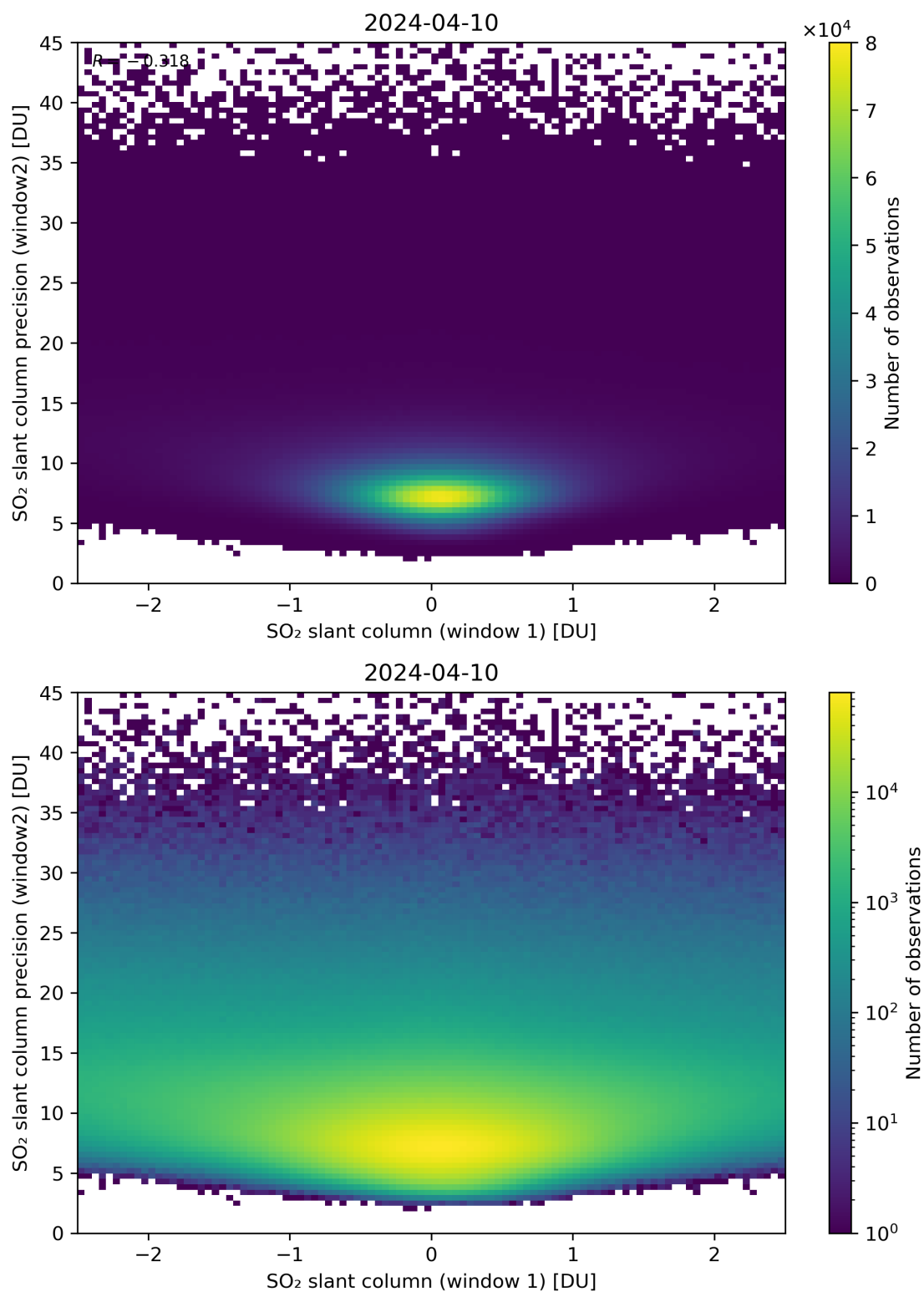
Figure 236: Scatter density plot of “SO 2 slant column (window 1)” against “SO 2 slant column precision (window2)” for 2024-04-10 to 2024-04-11.
