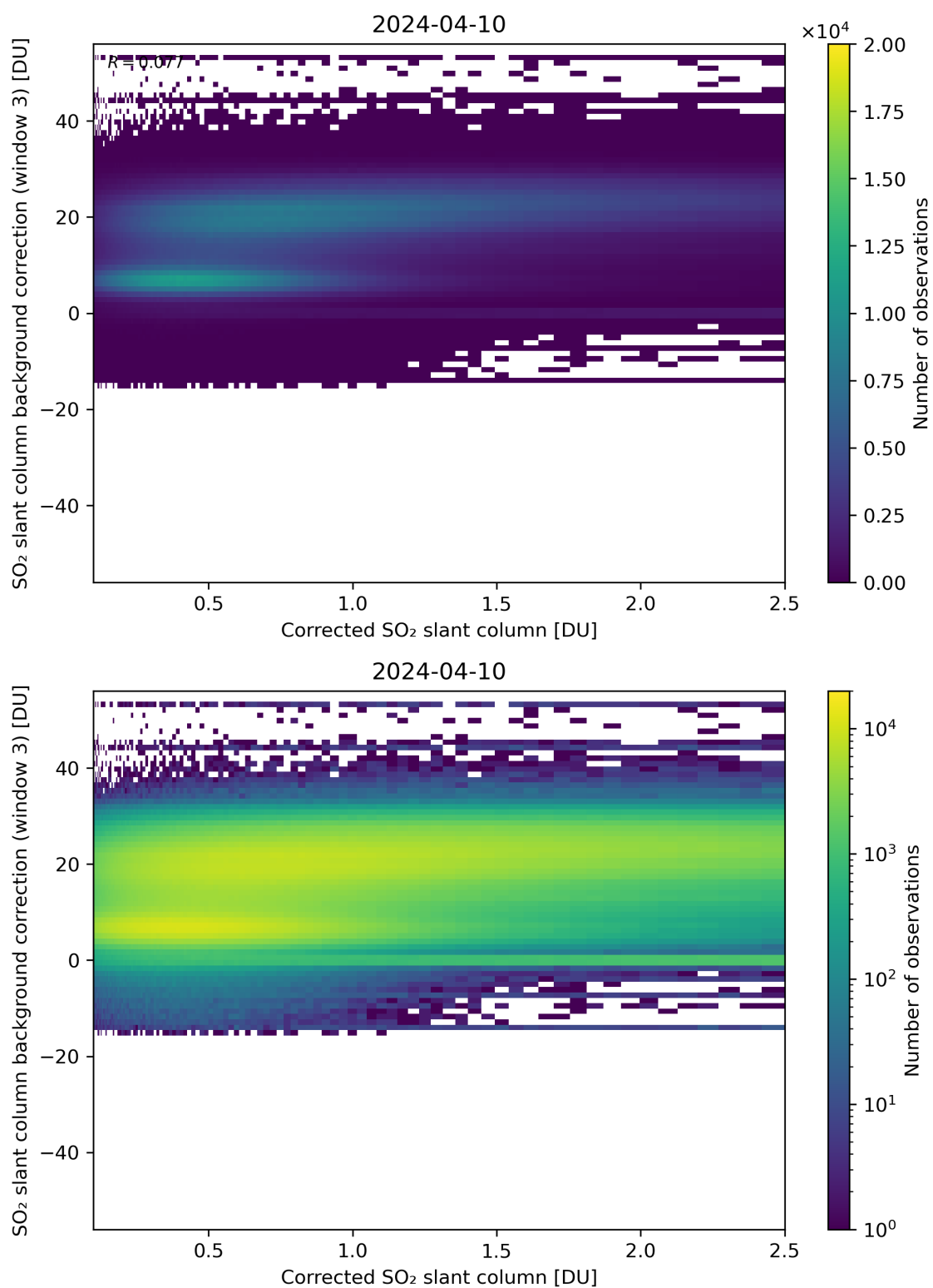
Figure 180: Scatter density plot of “Corrected SO 2 slant column” against “SO 2 slant column background correction (window 3)” for 2024-04-10 to 2024-04-11.
