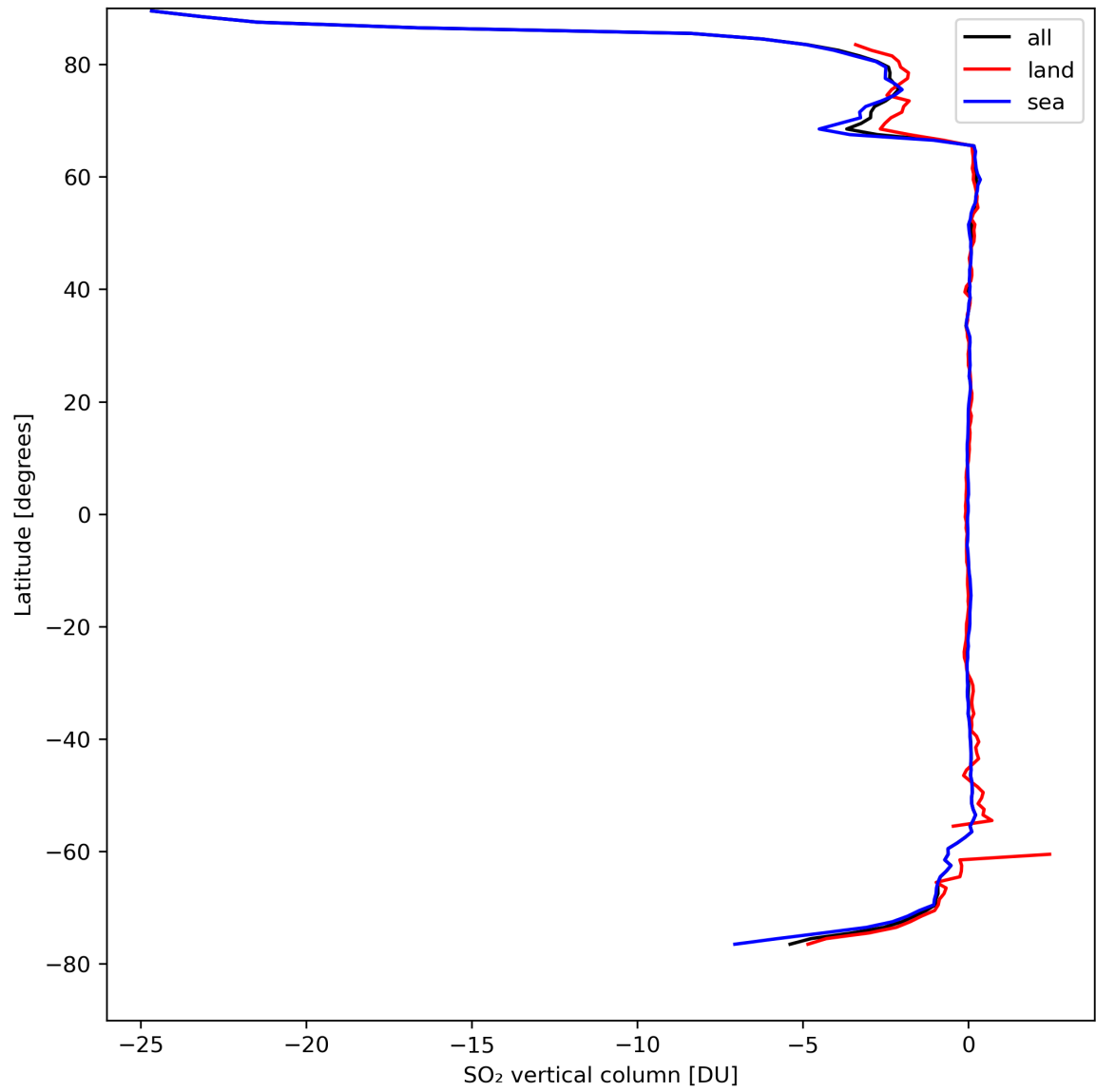
Figure 30: Zonal average of “SO 2 vertical column” for 2024-04-10 to 2024-04-11.
