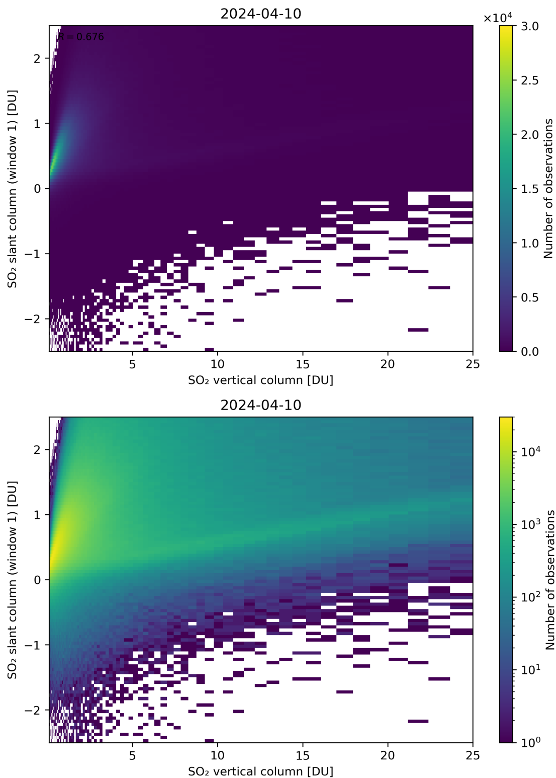
Figure 300: Scatter density plot of “SO 2 vertical column” against “SO 2 slant column (window 1)” for 2024-04-10 to 2024-04-11.
