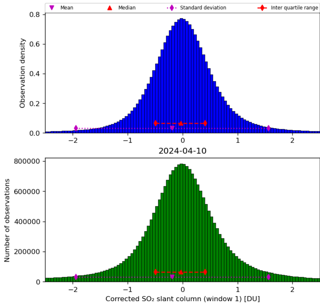
Figure 58: Histogram of “Corrected SO 2 slant column (window 1)” for 2024-04-10 to 2024-04-11
