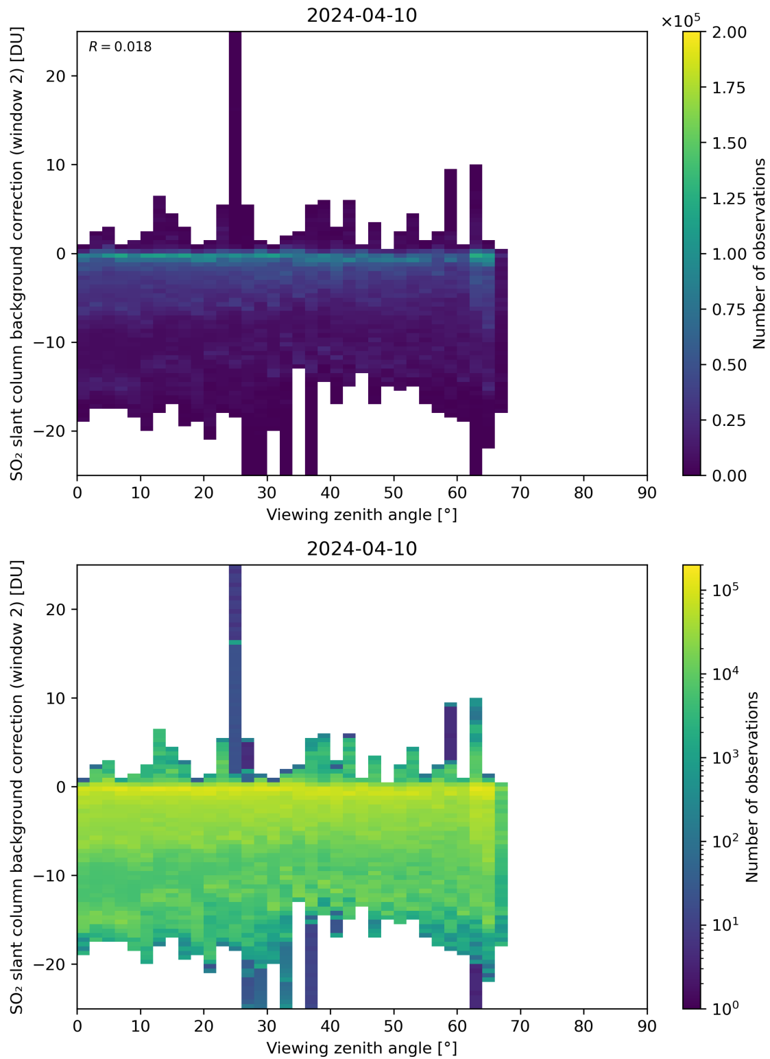
Figure 309: Scatter density plot of “Viewing zenith angle” against “SO 2 slant column background correction (window 2)” for 2024-04-10 to 2024-04-11.
