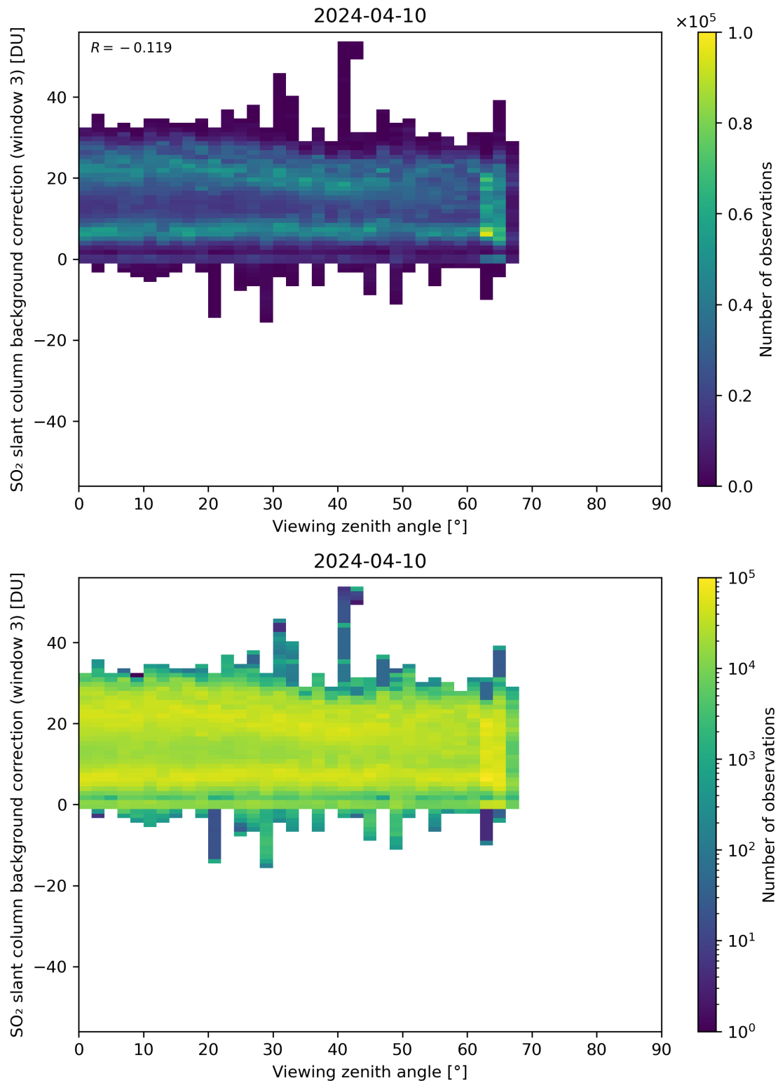
Figure 310: Scatter density plot of “Viewing zenith angle” against “SO 2 slant column background correction (window 3)” for 2024-04-10 to 2024-04-11.
