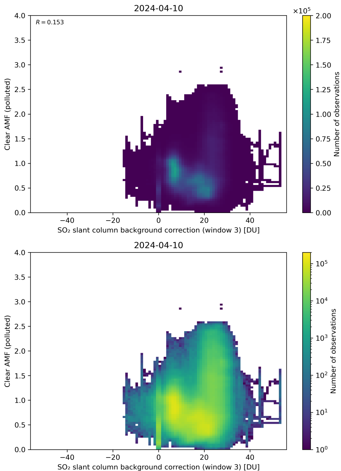
Figure 124: Scatter density plot of “SO 2 slant column background correction (window 3)” against “Clear AMF (polluted)” for 2024-04-10 to 2024-04-11.
