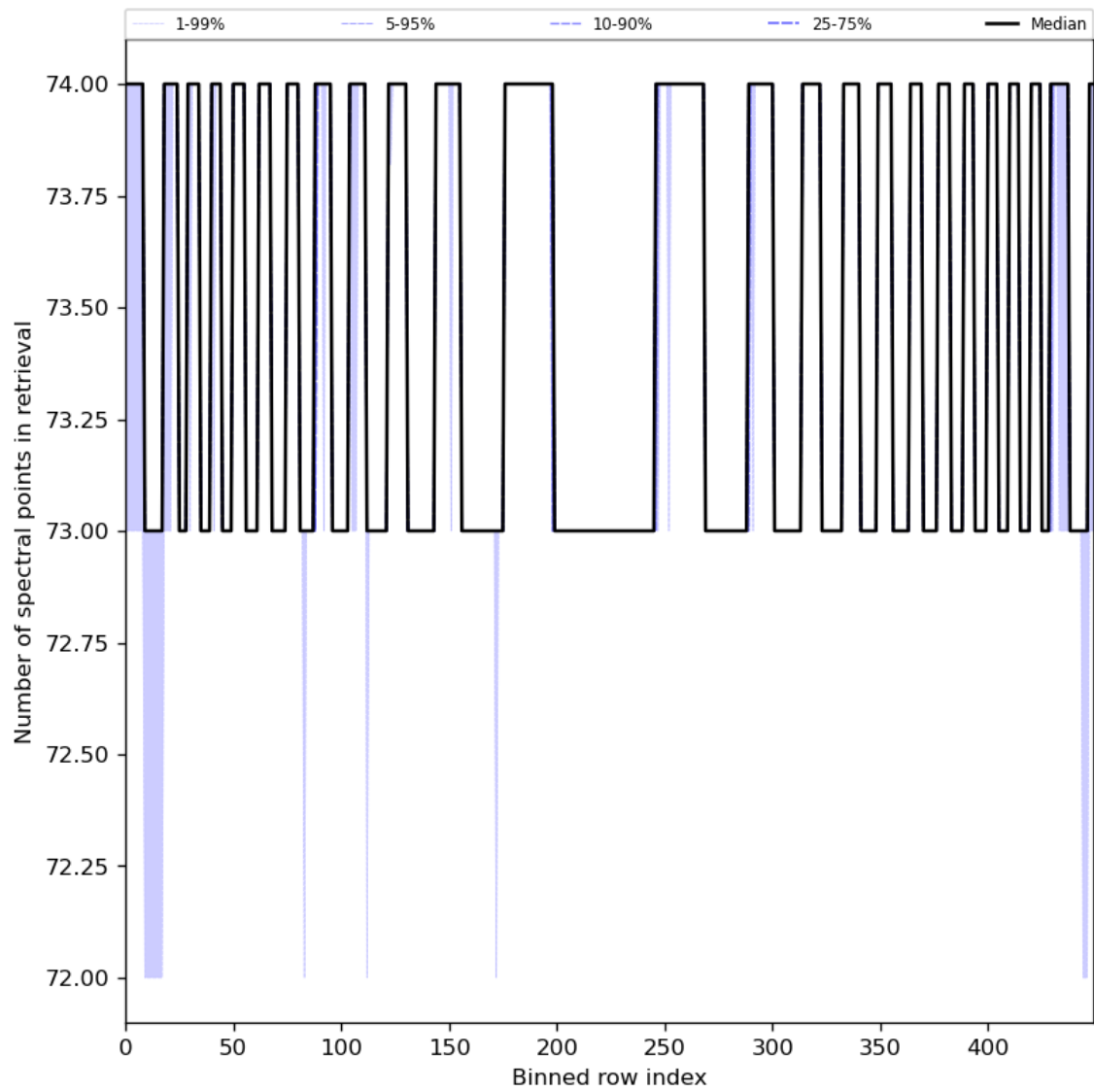
Figure 97: Along track statistics of “Number of spectral points in retrieval” for 2024-04-10 to 2024-04-11
