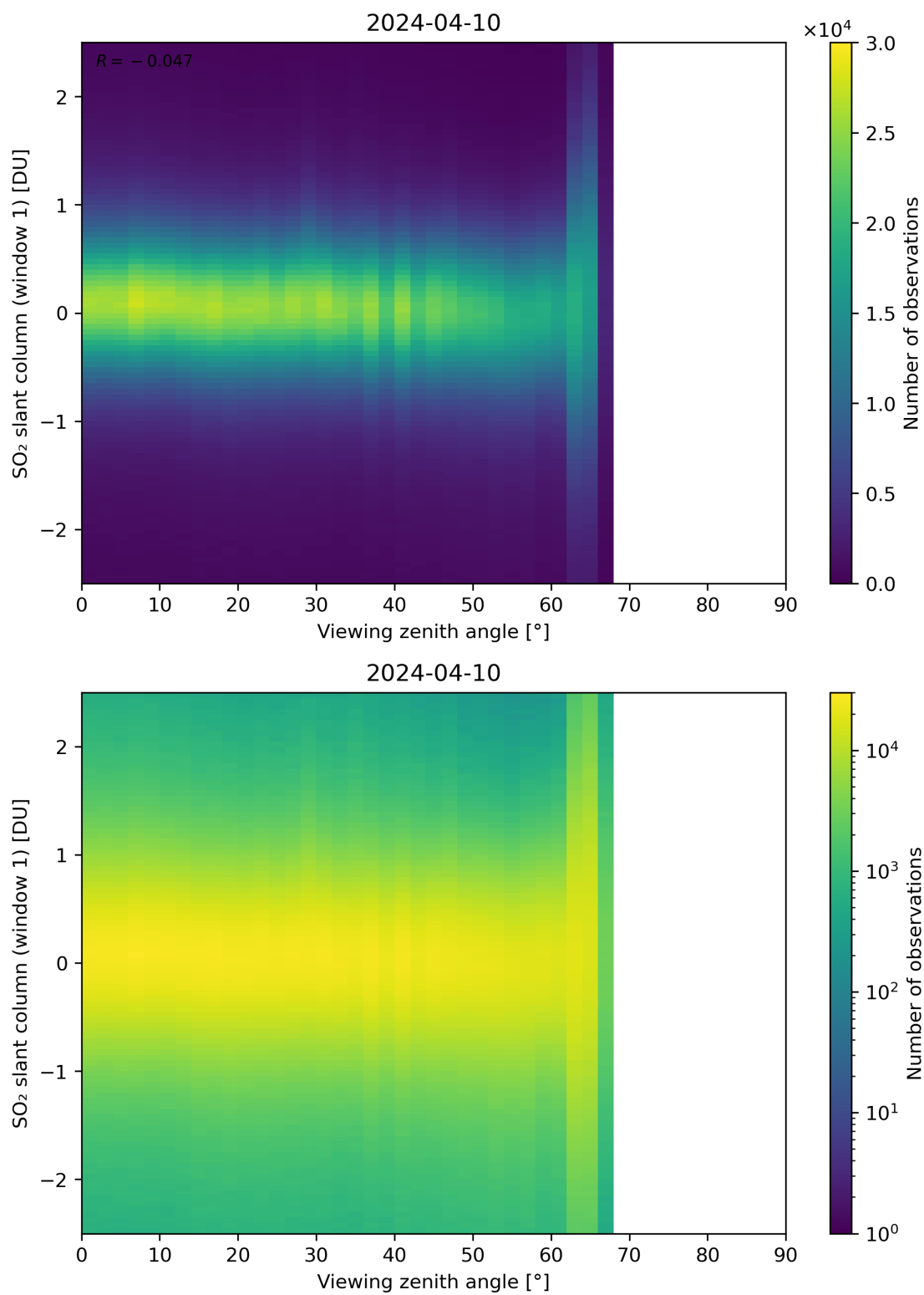
Figure 320: Scatter density plot of “Viewing zenith angle” against “SO 2 slant column (window 1)” for 2024-04-10 to 2024-04-11.
