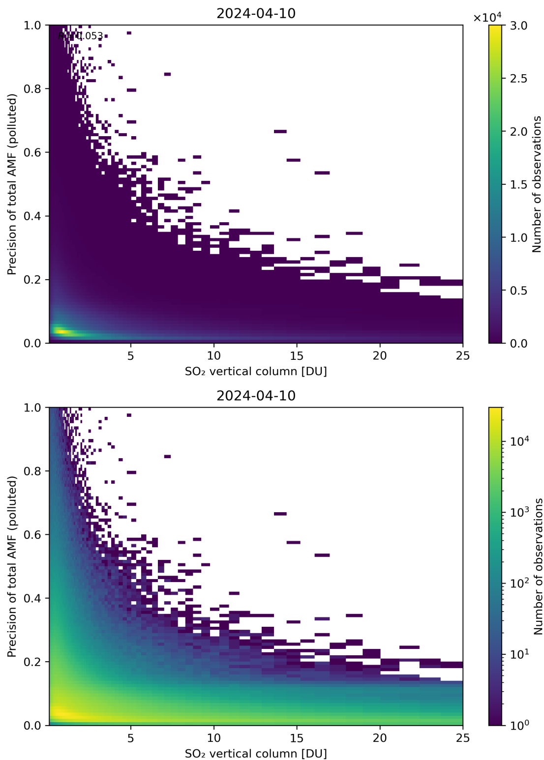
Figure 306: Scatter density plot of “SO 2 vertical column” against “Precision of total AMF (polluted)” for 2024-04-10 to 2024-04-11.
