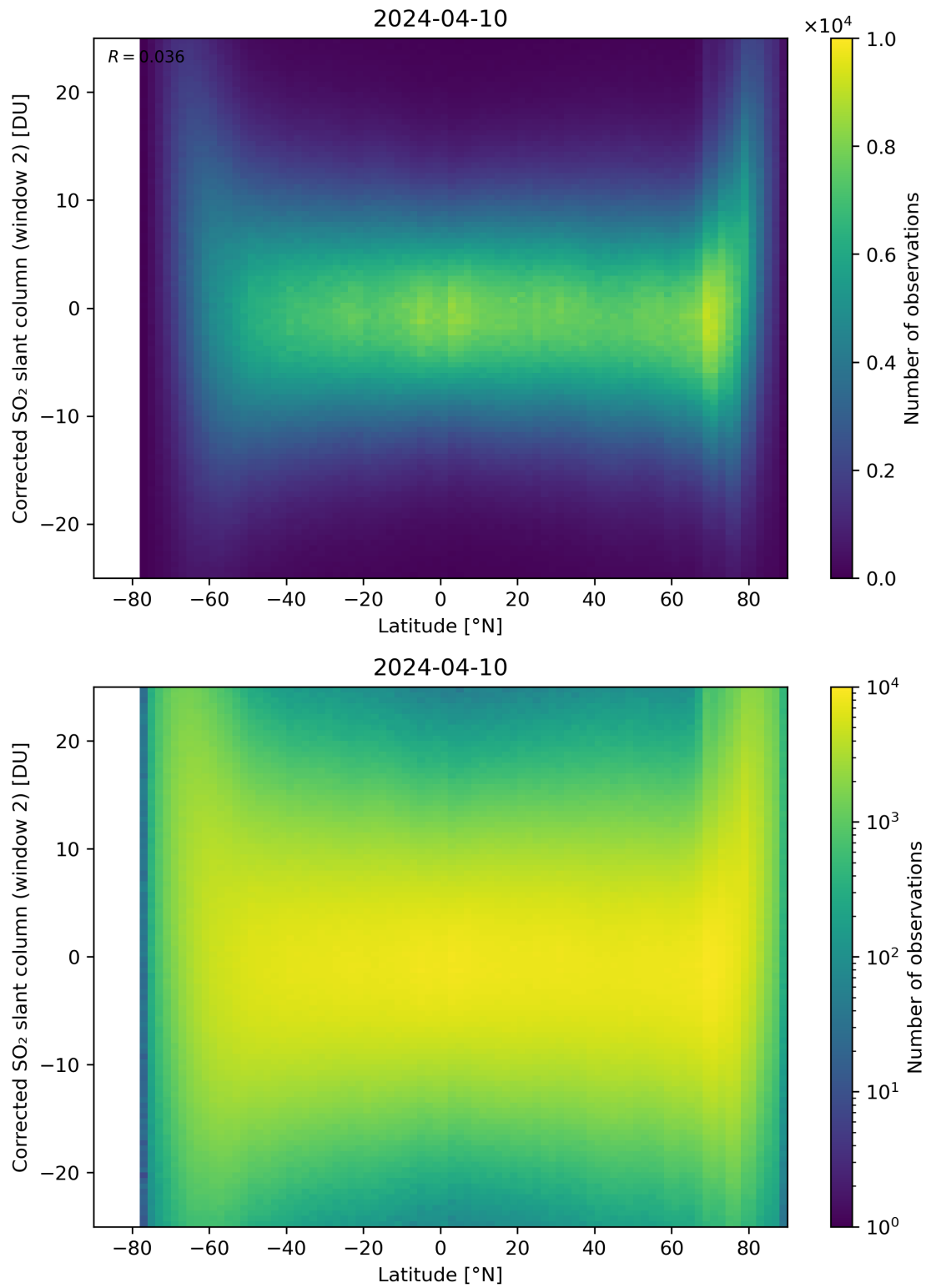
Figure 147: Scatter density plot of “Latitude” against “Corrected SO 2 slant column (window 2)” for 2024-04-10 to 2024-04-11.
