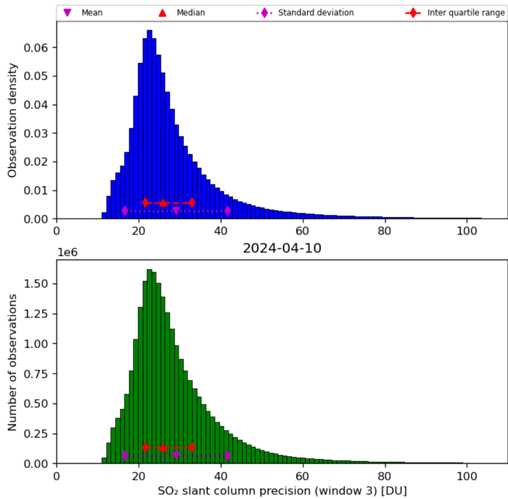
Figure 65: Histogram of “SO 2 slant column precision (window 3)” for 2024-04-10 to 2024-04-11
