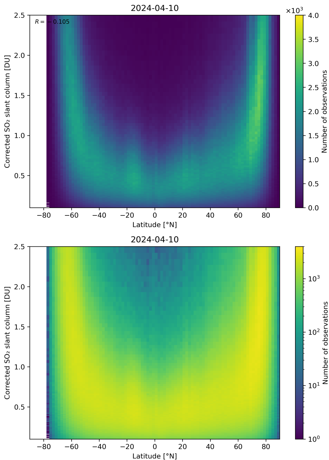
Figure 146: Scatter density plot of “Latitude” against “Corrected SO 2 slant column” for 2024-04-10 to 2024-04-11.
