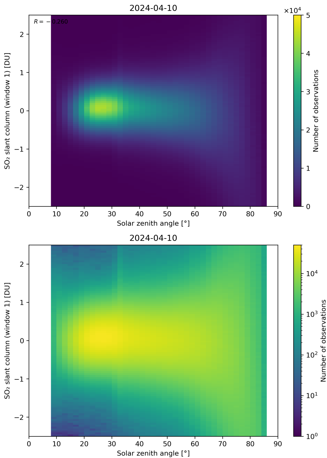
Figure 169: Scatter density plot of “Solar zenith angle” against “SO 2 slant column (window 1)” for 2024-04-10 to 2024-04-11.
