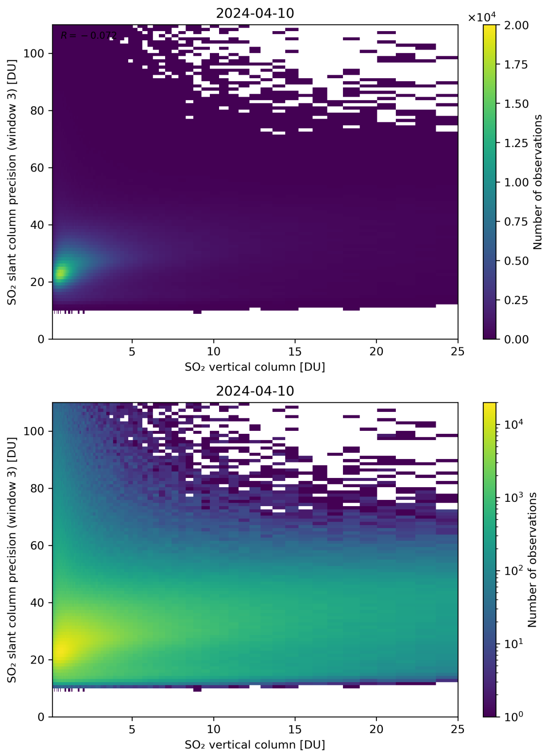
Figure 304: Scatter density plot of “SO 2 vertical column” against “SO 2 slant column precision (window 3)” for 2024-04-10 to 2024-04-11.
