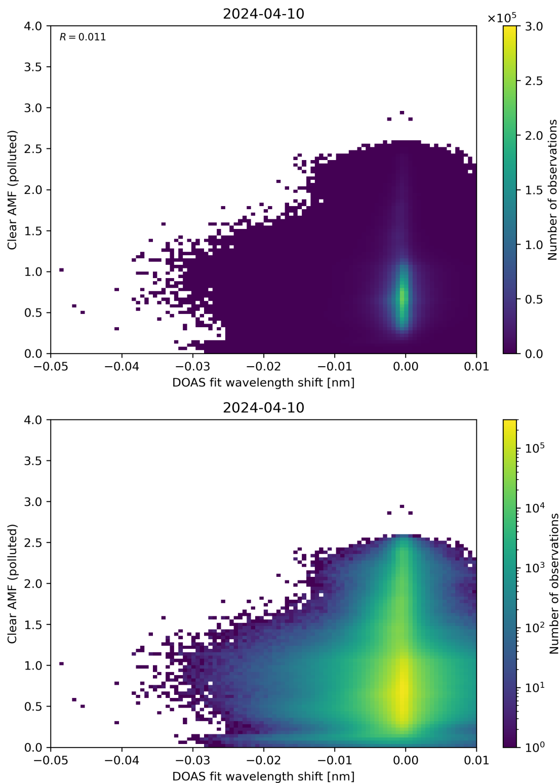
Figure 129: Scatter density plot of “DOAS fit wavelength shift” against “Clear AMF (polluted)” for 2024-04-10 to 2024-04-11.
