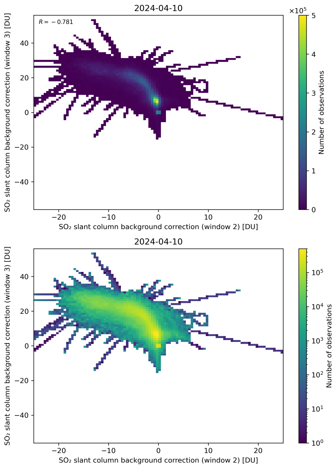
Figure 111: Scatter density plot of “SO 2 slant column background correction (window 2)” against “SO 2 slant column background correction (window 3)” for 2024-04-10 to 2024-04-11.
