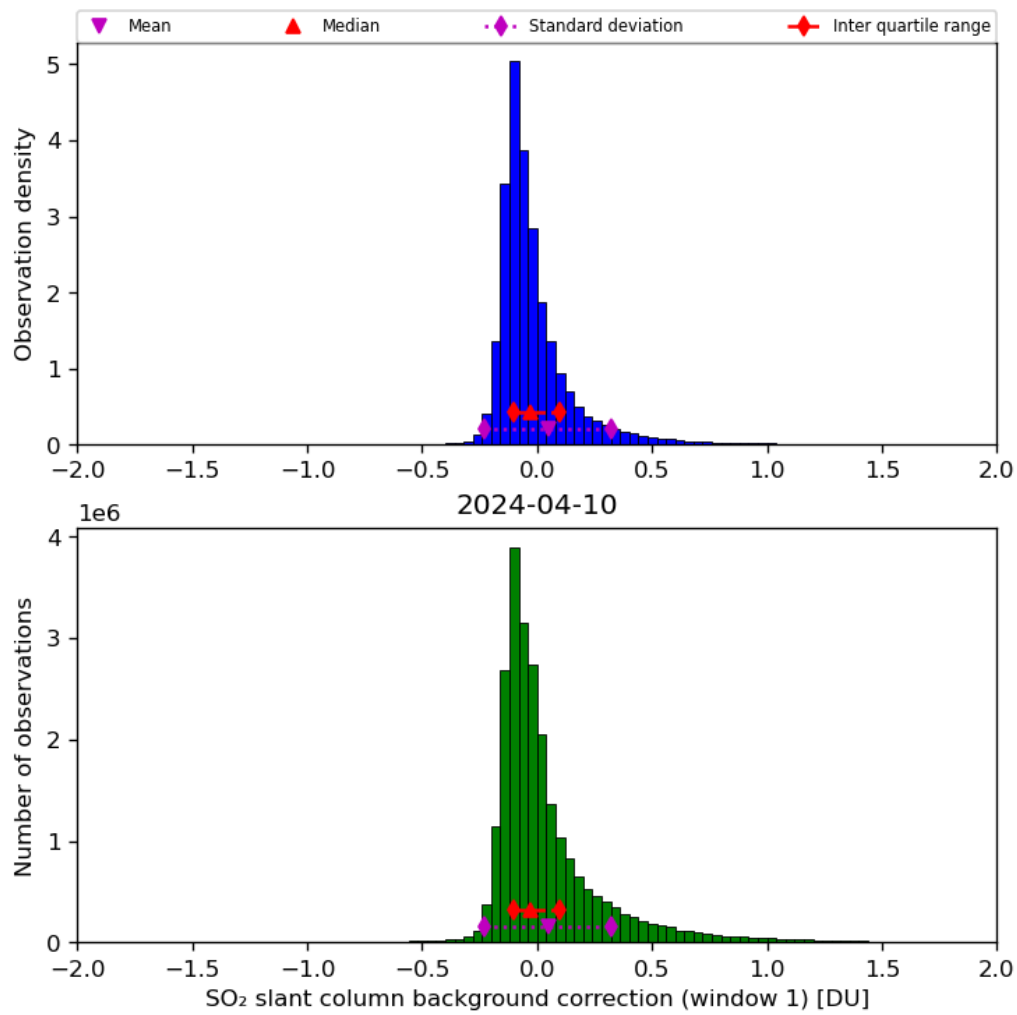
Figure 59: Histogram of “SO 2 slant column background correction (window 1)” for 2024-04-10 to 2024-04-11
