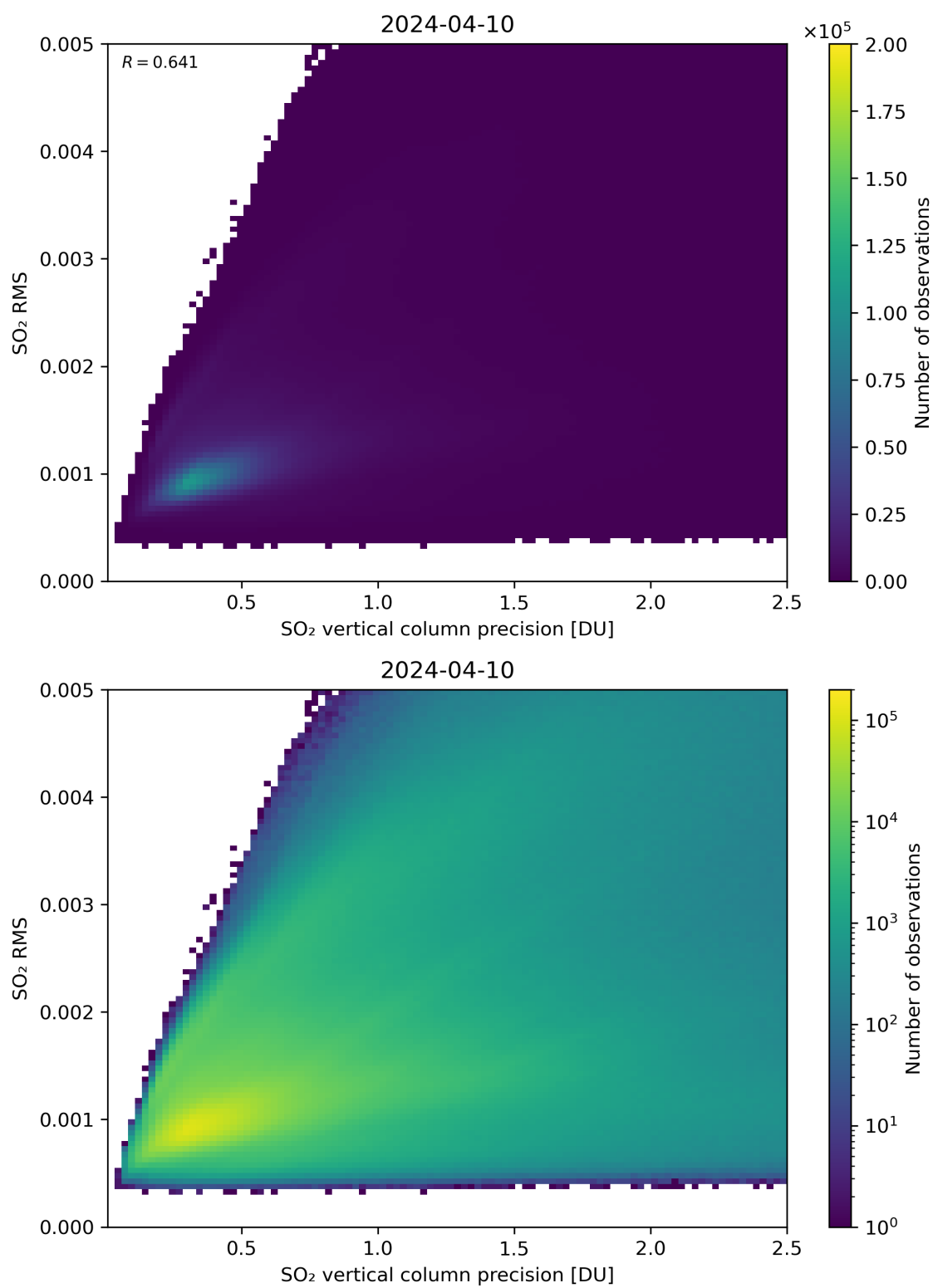
Figure 284: Scatter density plot of “SO 2 vertical column precision” against “SO 2 RMS” for 2024-04-10 to 2024-04-11.
