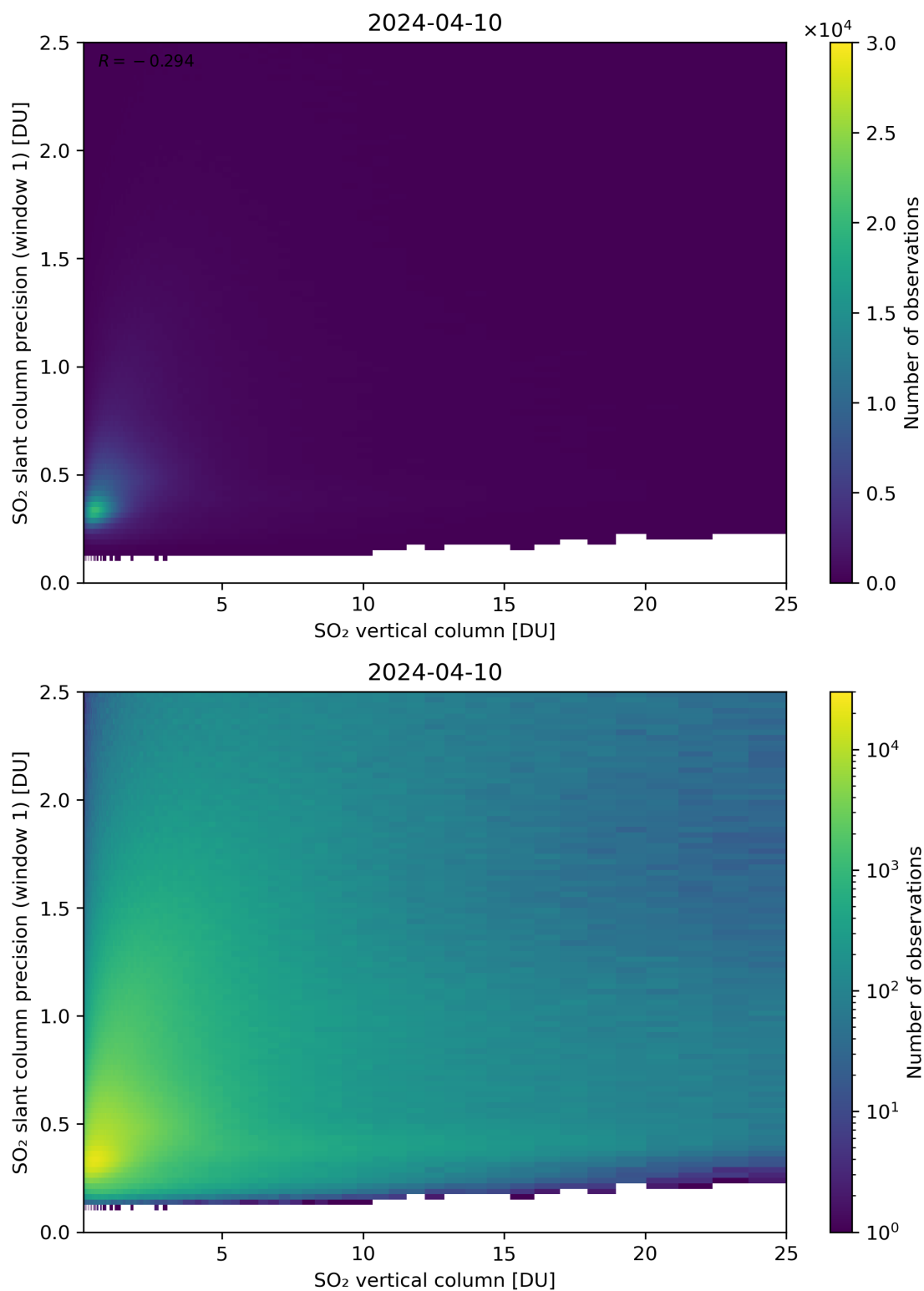
Figure 301: Scatter density plot of “SO 2 vertical column” against “SO 2 slant column precision (window 1)” for 2024-04-10 to 2024-04-11.
