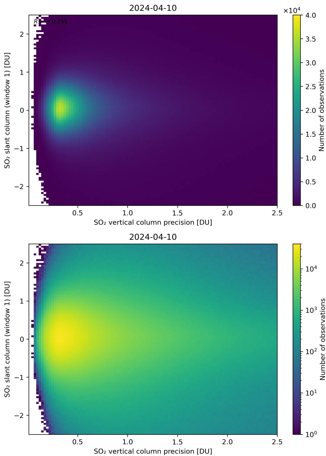
Figure 289: Scatter density plot of “SO 2 vertical column precision” against “SO 2 slant column (window 1)” for 2024-04-10 to 2024-04-11.
