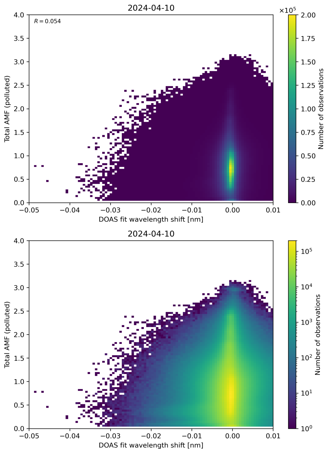
Figure 130: Scatter density plot of “DOAS fit wavelength shift” against “Total AMF (polluted)” for 2024-04-10 to 2024-04-11.
