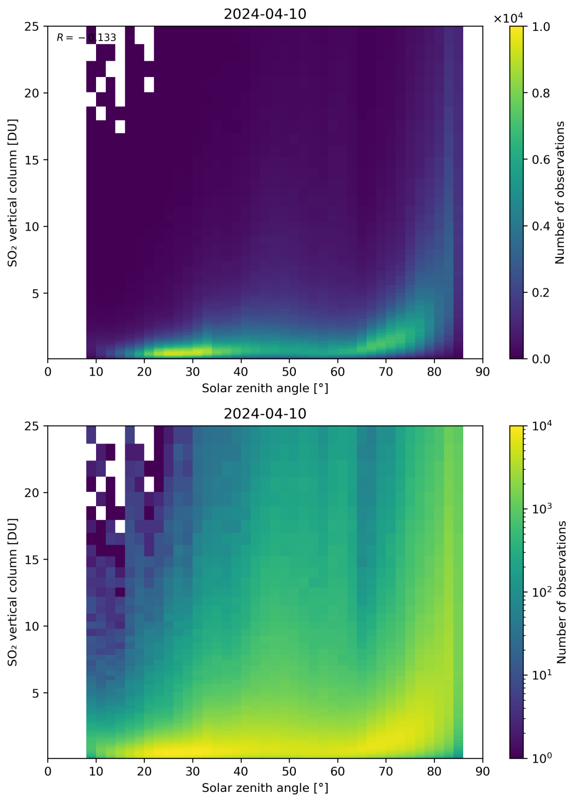
Figure 176: Scatter density plot of “Solar zenith angle” against “SO 2 vertical column” for 2024-04-10 to 2024-04-11.
