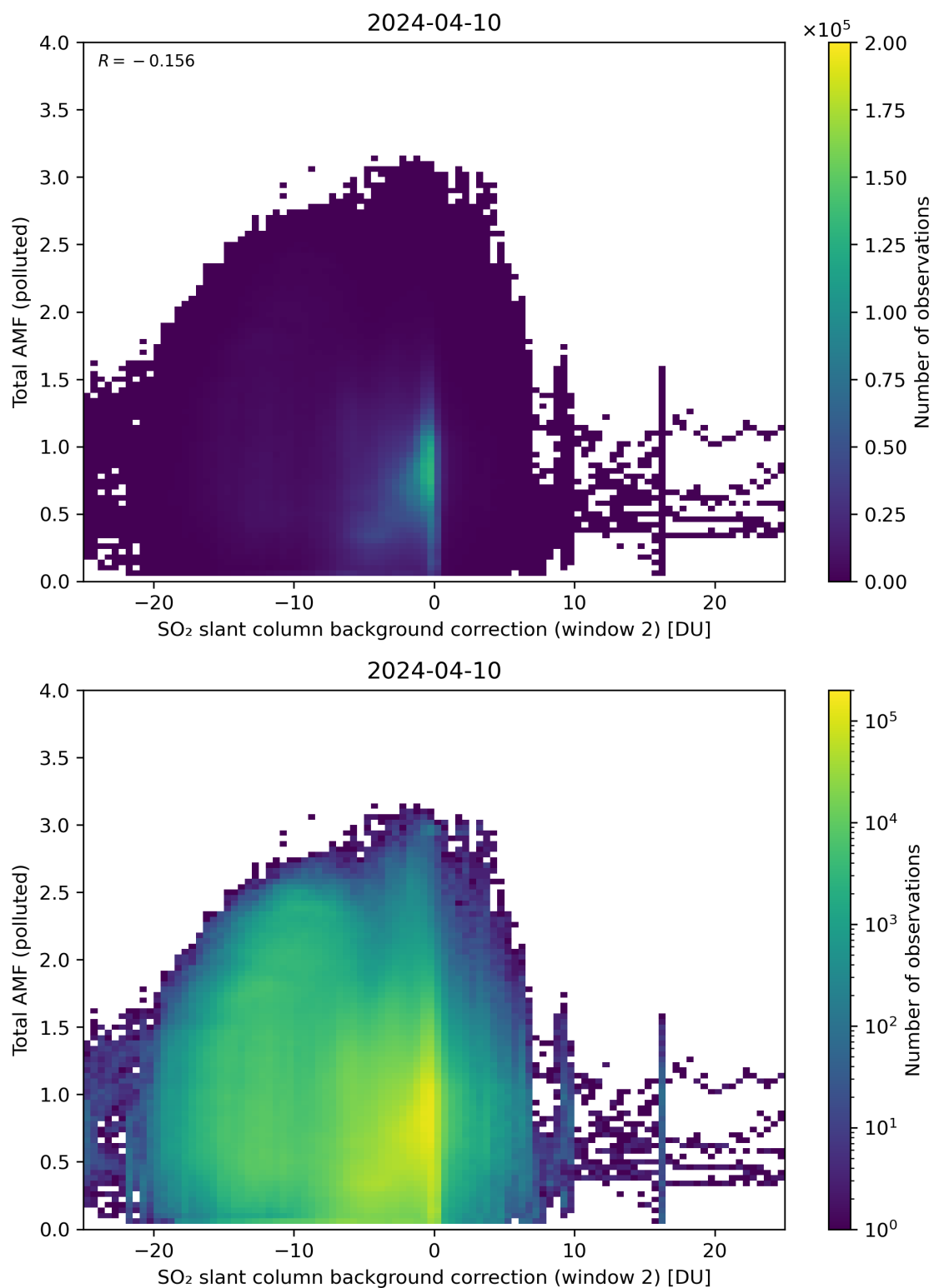
Figure 119: Scatter density plot of “SO 2 slant column background correction (window 2)” against “Total AMF (polluted)” for 2024-04-10 to 2024-04-11.
