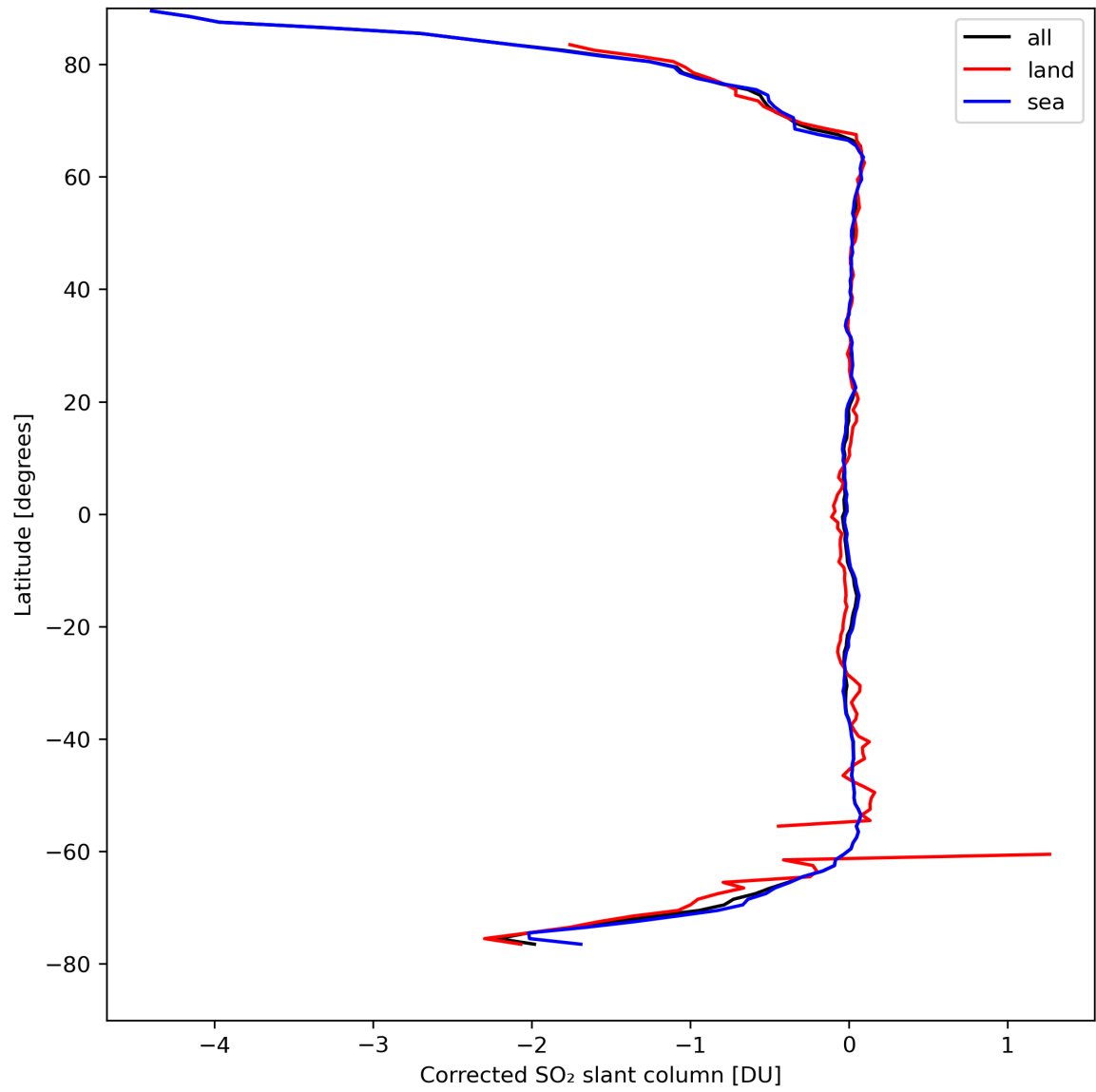
Figure 32: Zonal average of “Corrected SO 2 slant column” for 2024-04-10 to 2024-04-11.
