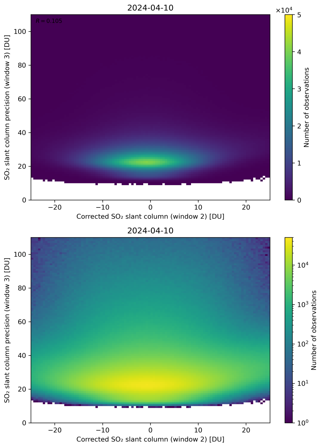
Figure 202: Scatter density plot of “Corrected SO 2 slant column (window 2)” against “SO 2 slant column precision (window 3)” for 2024-04-10 to 2024-04-11.
