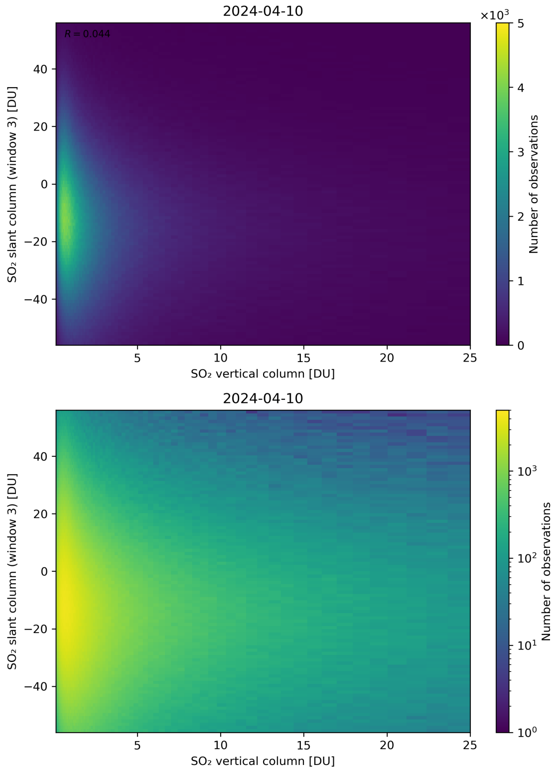
Figure 303: Scatter density plot of “SO 2 vertical column” against “SO 2 slant column (window 3)” for 2024-04-10 to 2024-04-11.
