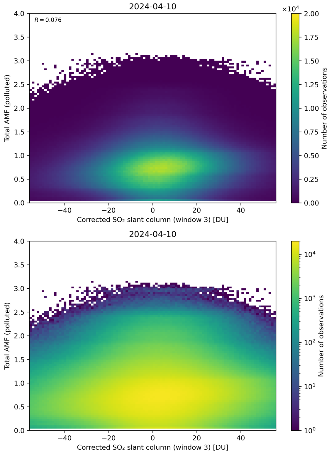
Figure 210: Scatter density plot of “Corrected SO 2 slant column (window 3)” against “Total AMF (polluted)” for 2024-04-10 to 2024-04-11.
