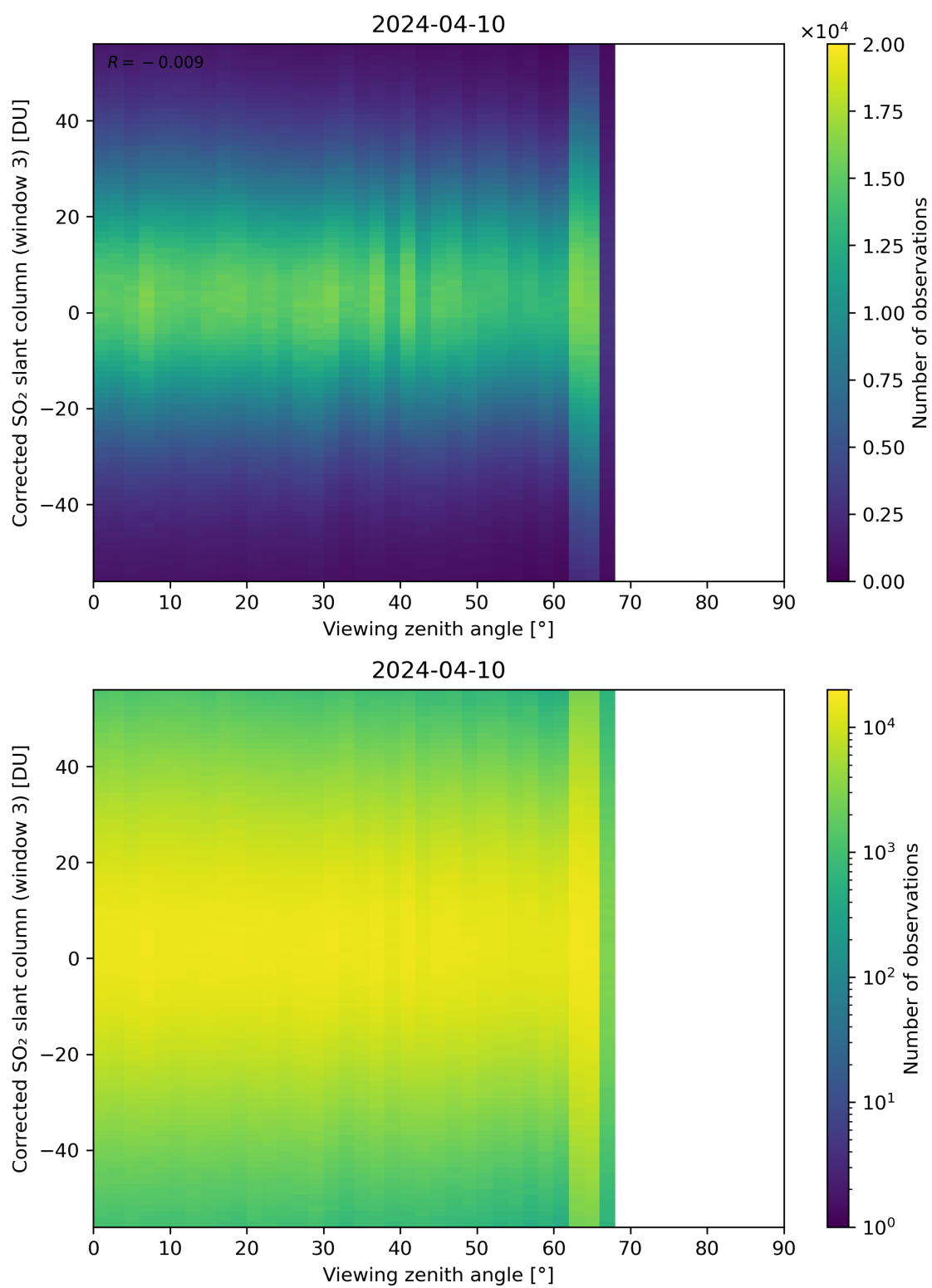
Figure 319: Scatter density plot of “Viewing zenith angle” against “Corrected SO 2 slant column (window 3)” for 2024-04-10 to 2024-04-11.
