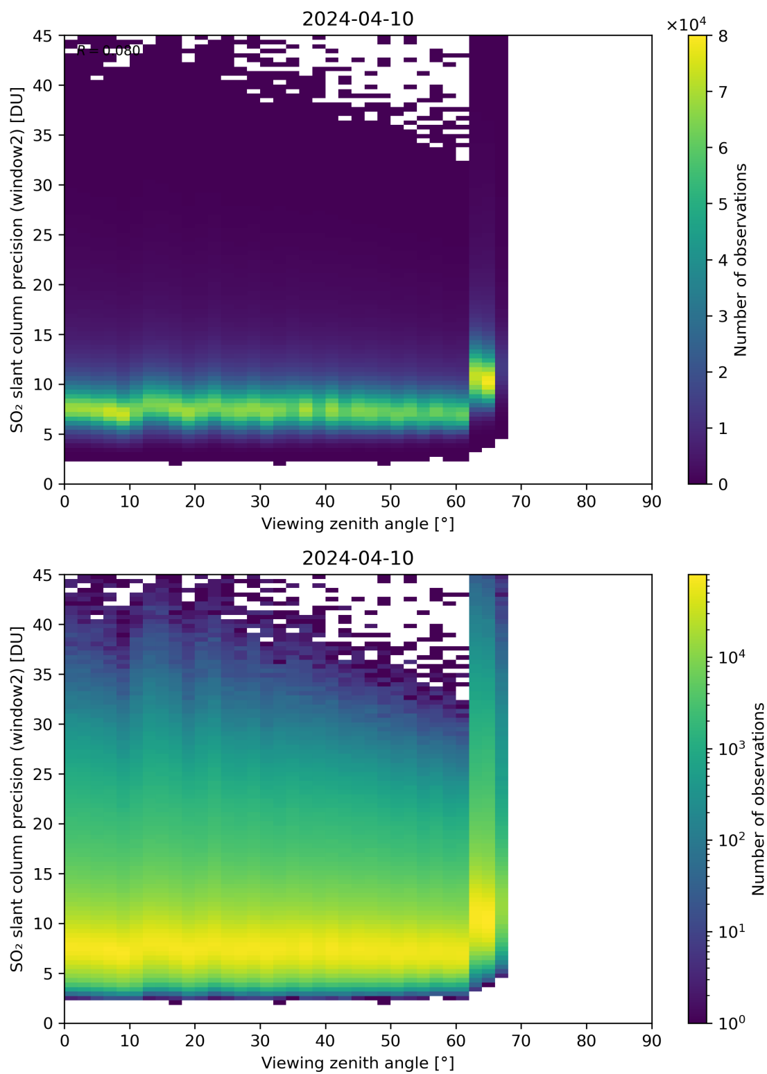
Figure 322: Scatter density plot of “Viewing zenith angle” against “SO 2 slant column precision (window2)” for 2024-04-10 to 2024-04-11.
