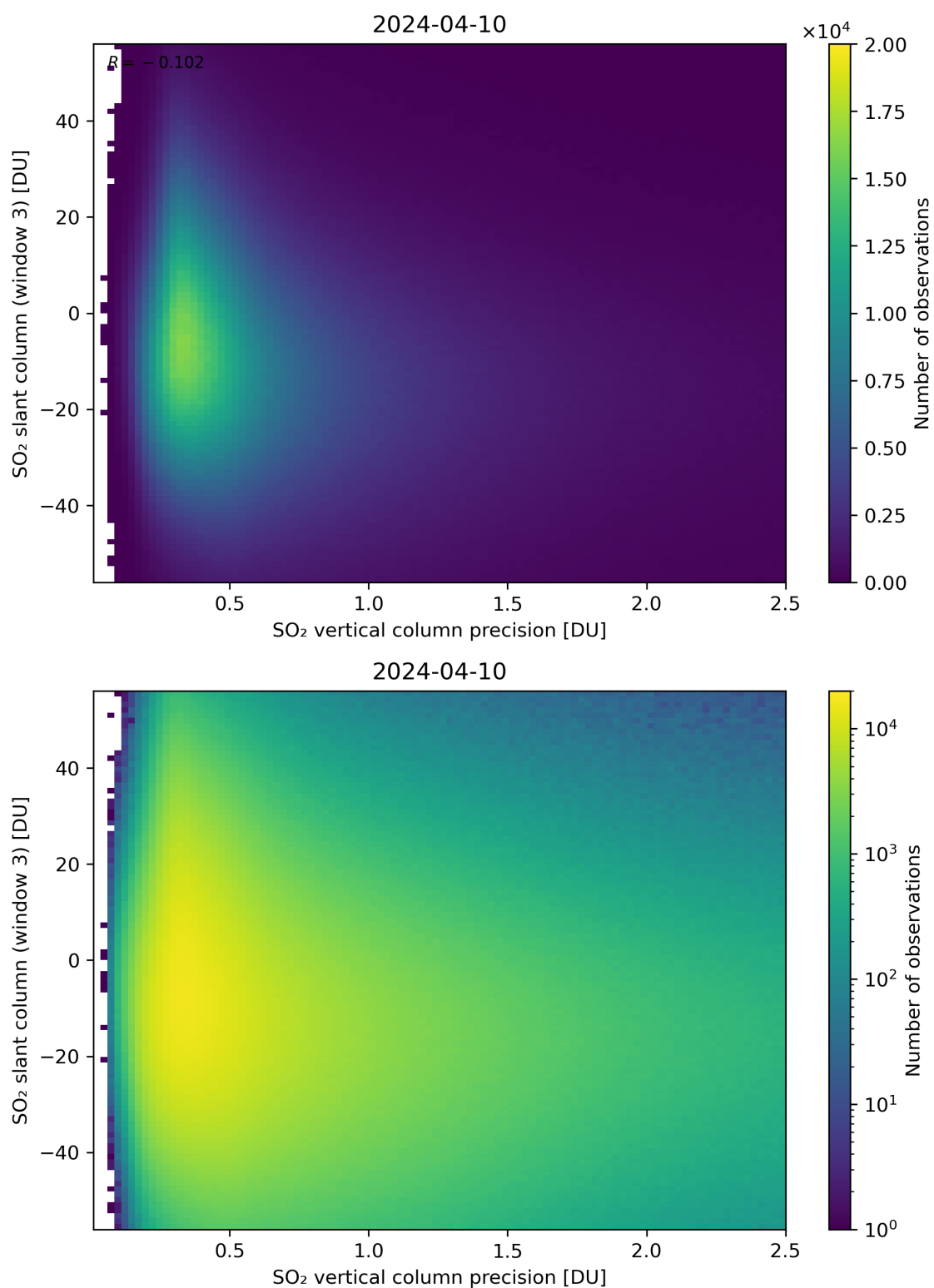
Figure 292: Scatter density plot of “SO 2 vertical column precision” against “SO 2 slant column (window 3)” for 2024-04-10 to 2024-04-11.
