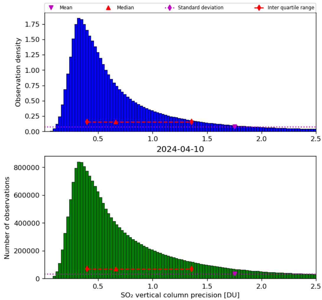
Figure 54: Histogram of “SO 2 vertical column precision” for 2024-04-10 to 2024-04-11
