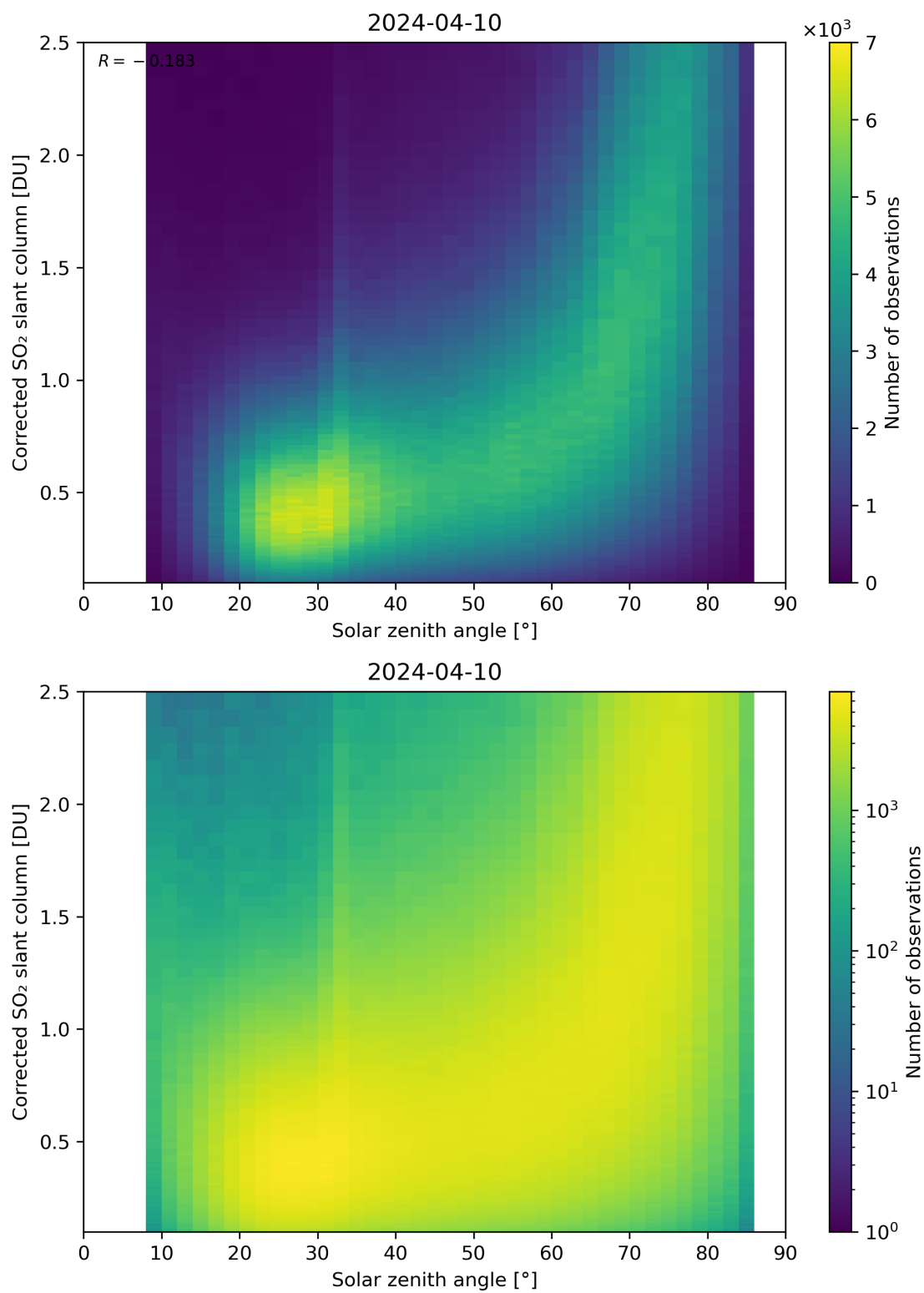
Figure 166: Scatter density plot of “Solar zenith angle” against “Corrected SO 2 slant column” for 2024-04-10 to 2024-04-11.
