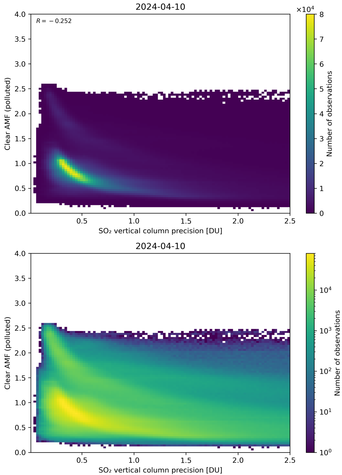
Figure 285: Scatter density plot of “SO 2 vertical column precision” against “Clear AMF (polluted)” for 2024-04-10 to 2024-04-11.
