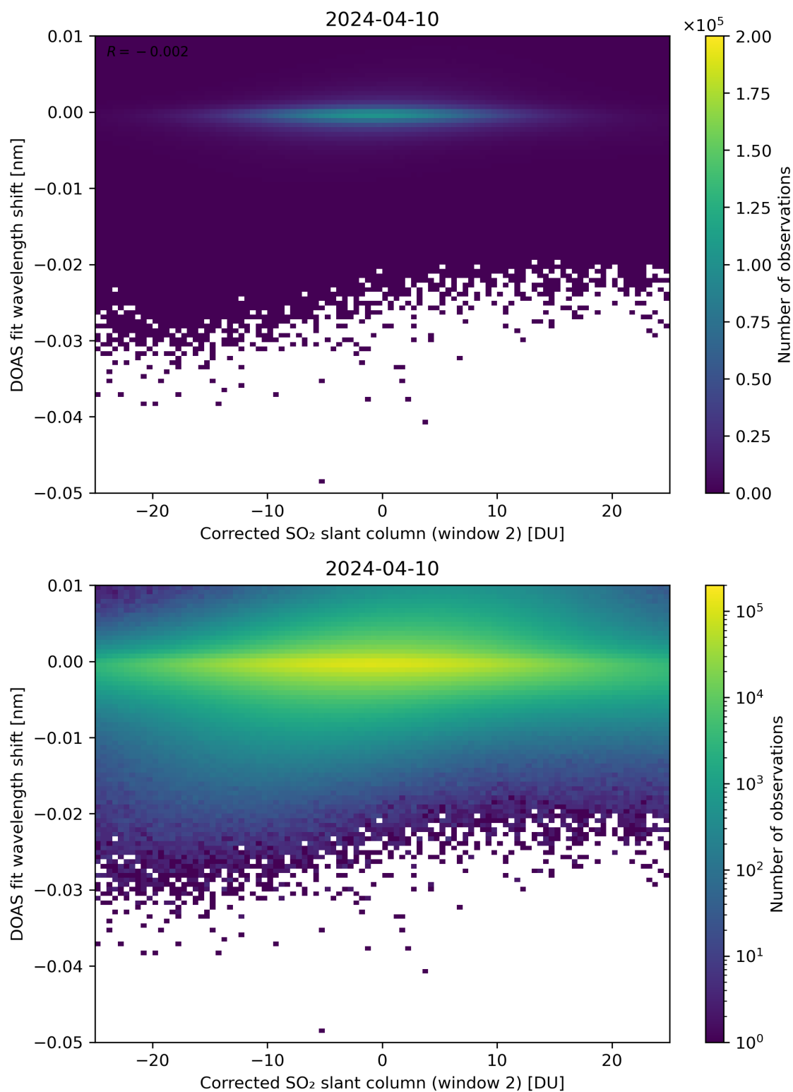
Figure 196: Scatter density plot of “Corrected SO 2 slant column (window 2)” against “DOAS fit wavelength shift” for 2024-04-10 to 2024-04-11.
