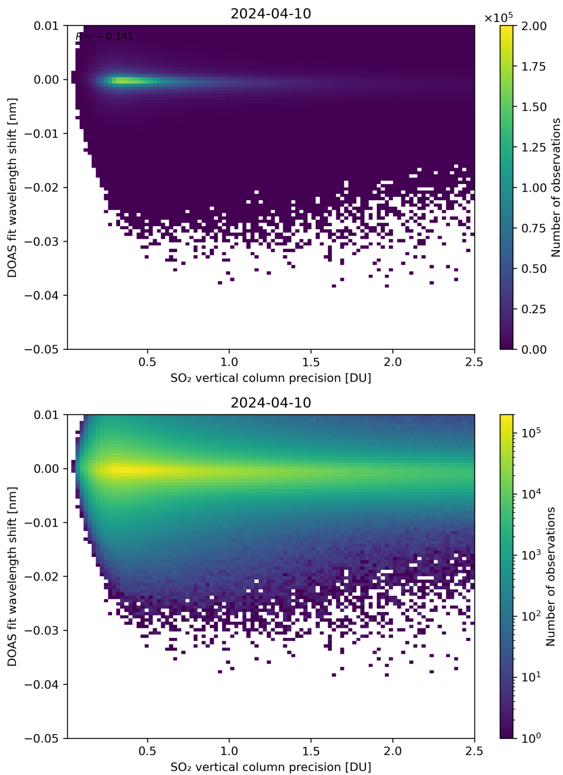
Figure 282: Scatter density plot of “SO 2 vertical column precision” against “DOAS fit wavelength shift” for 2024-04-10 to 2024-04-11.
