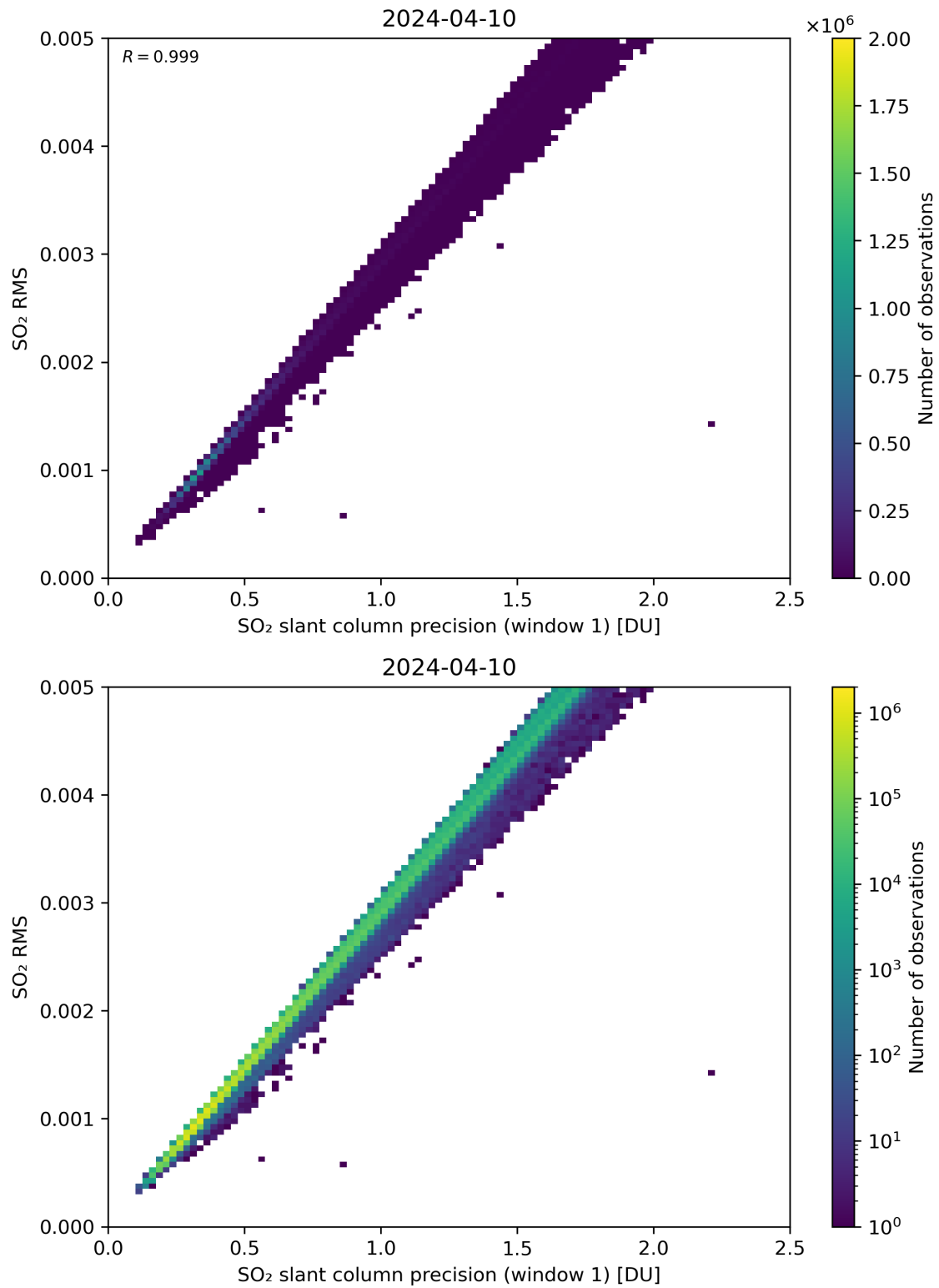
Figure 223: Scatter density plot of “SO 2 slant column precision (window 1)” against “SO 2 RMS” for 2024-04-10 to 2024-04-11.
