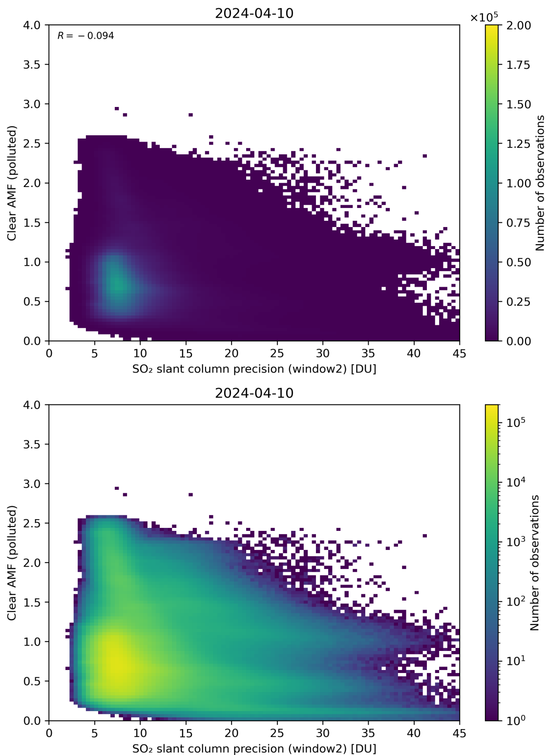
Figure 246: Scatter density plot of “SO 2 slant column precision (window2)” against “Clear AMF (polluted)” for 2024-04-10 to 2024-04-11.
