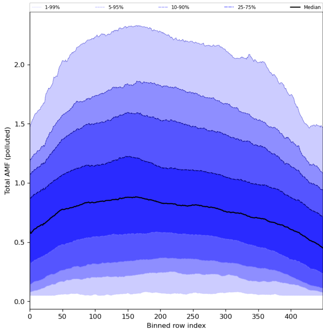
Figure 94: Along track statistics of “Total AMF (polluted)” for 2024-04-10 to 2024-04-11
