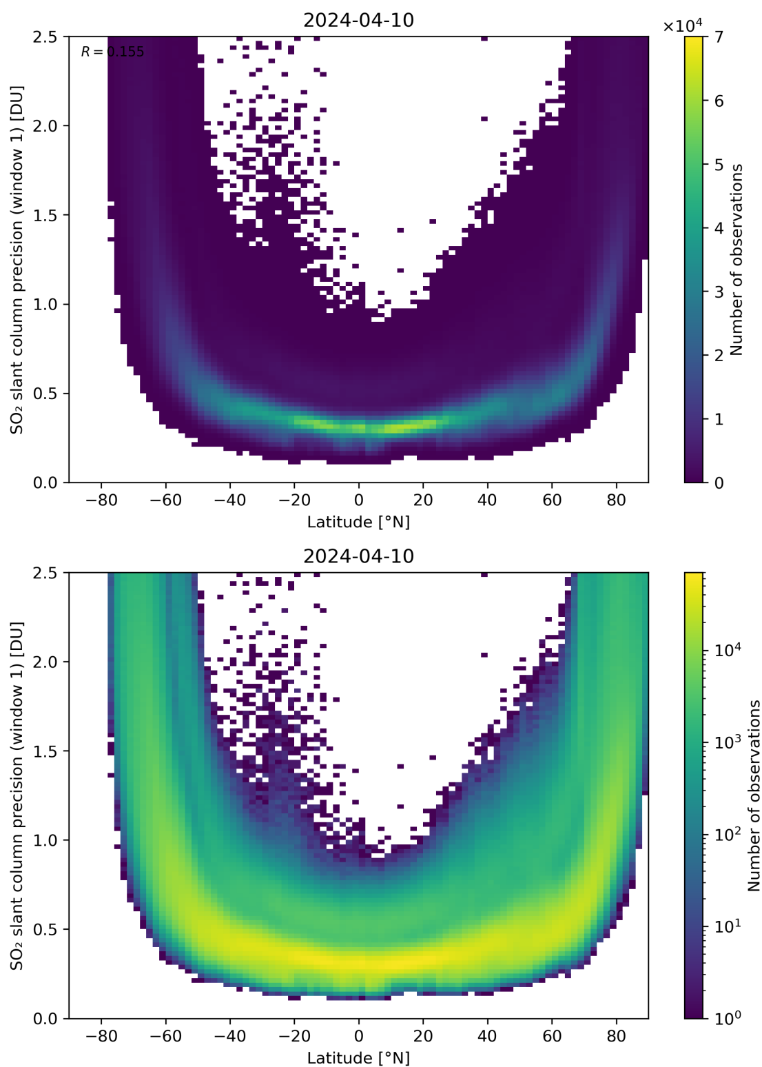
Figure 150: Scatter density plot of “Latitude” against “SO 2 slant column precision (window 1)” for 2024-04-10 to 2024-04-11.
