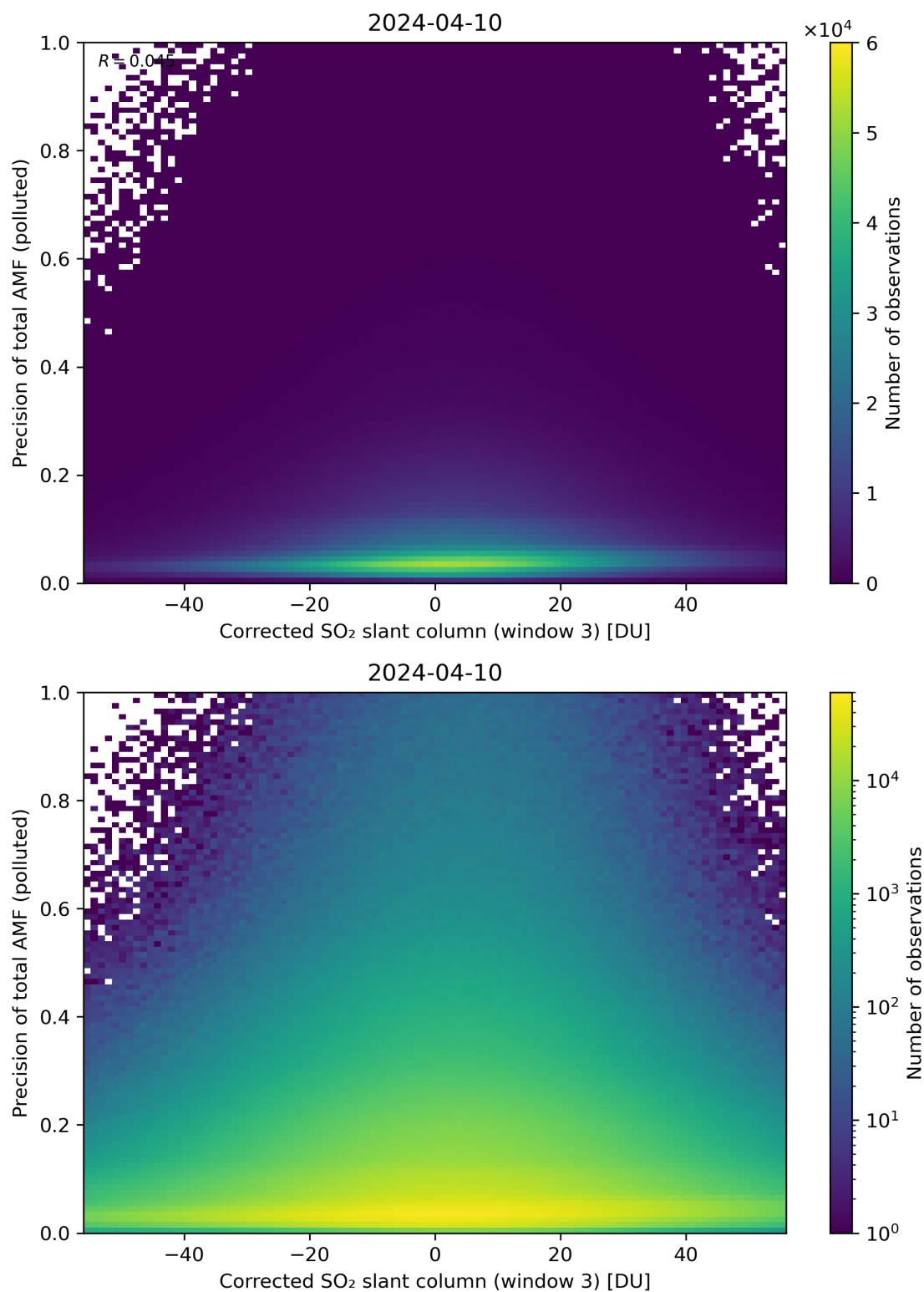
Figure 211: Scatter density plot of “Corrected SO 2 slant column (window 3)” against “Precision of total AMF (polluted)” for 2024-04-10 to 2024-04-11.
