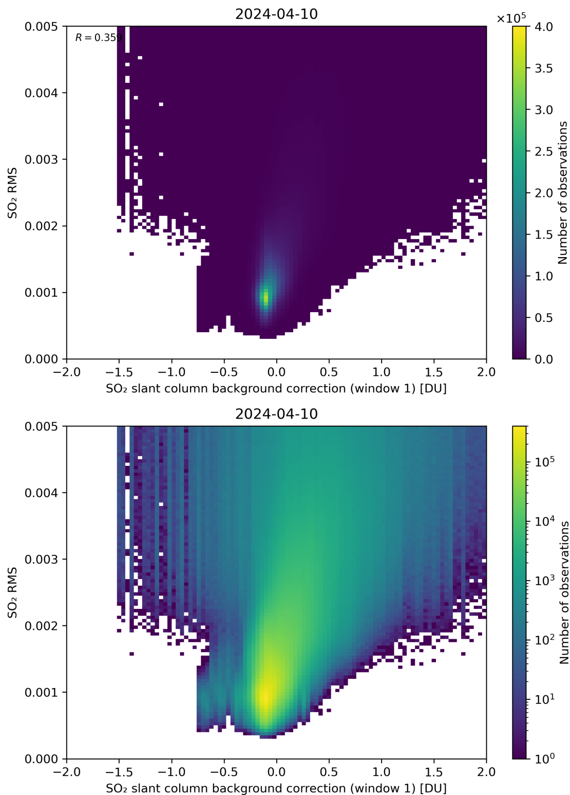
Figure 102: Scatter density plot of “SO 2 slant column background correction (window 1)” against “SO 2 RMS” for 2024-04-10 to 2024-04-11.
