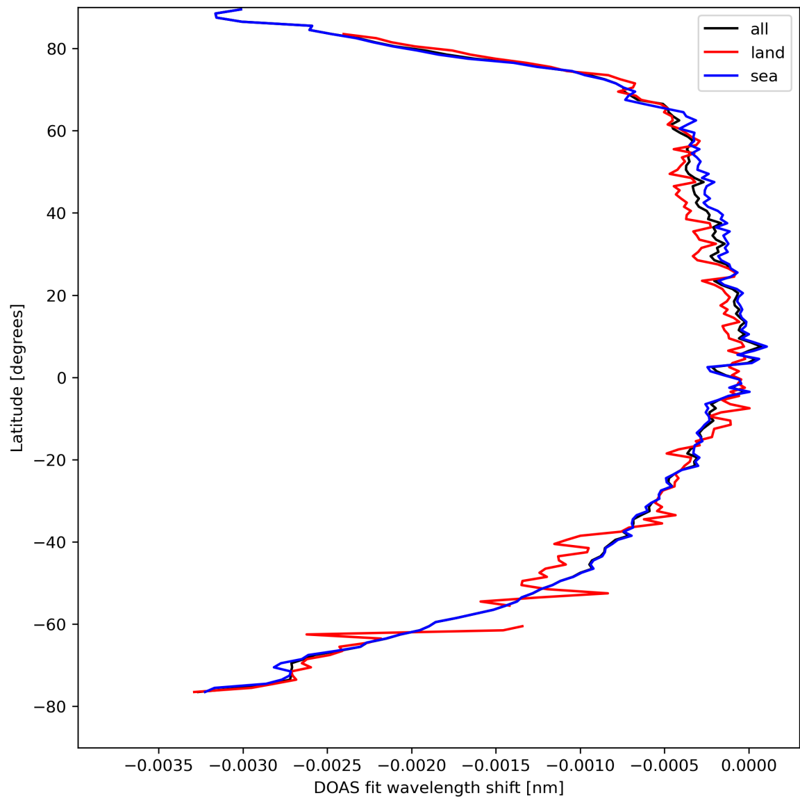
Figure 45: Zonal average of “DOAS fit wavelength shift” for 2024-04-10 to 2024-04-11.
