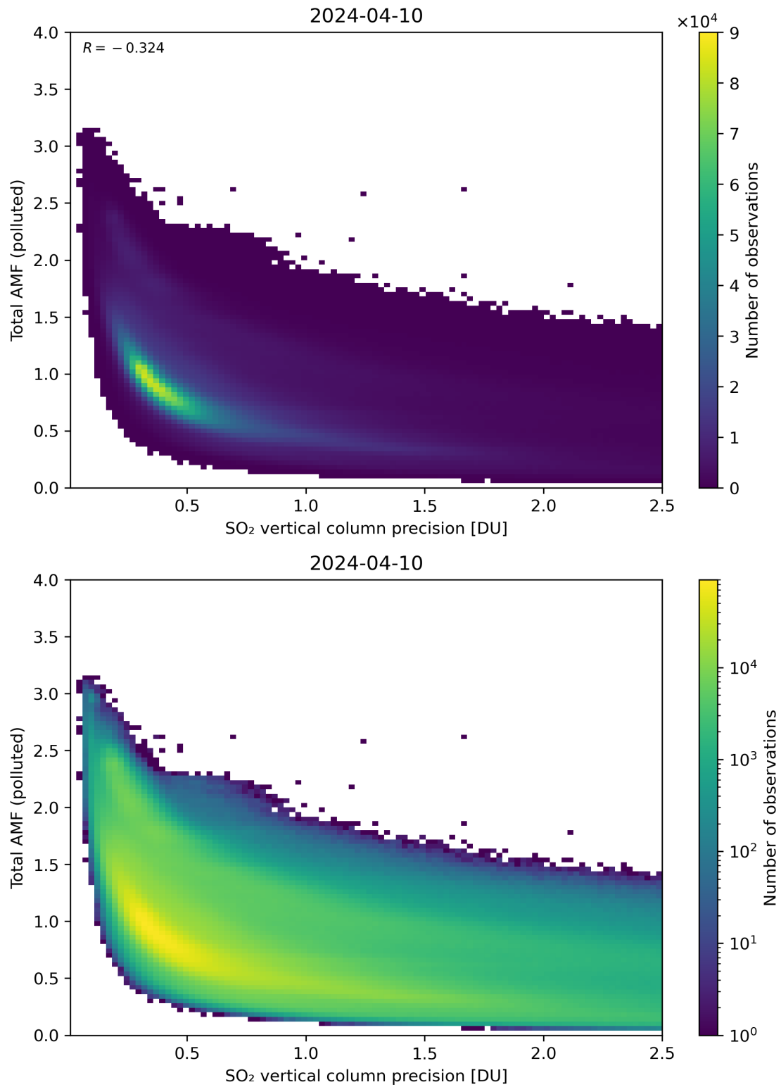
Figure 294: Scatter density plot of “SO 2 vertical column precision” against “Total AMF (polluted)” for 2024-04-10 to 2024-04-11.
