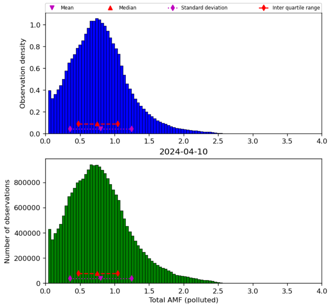
Figure 71: Histogram of “Total AMF (polluted)” for 2024-04-10 to 2024-04-11
