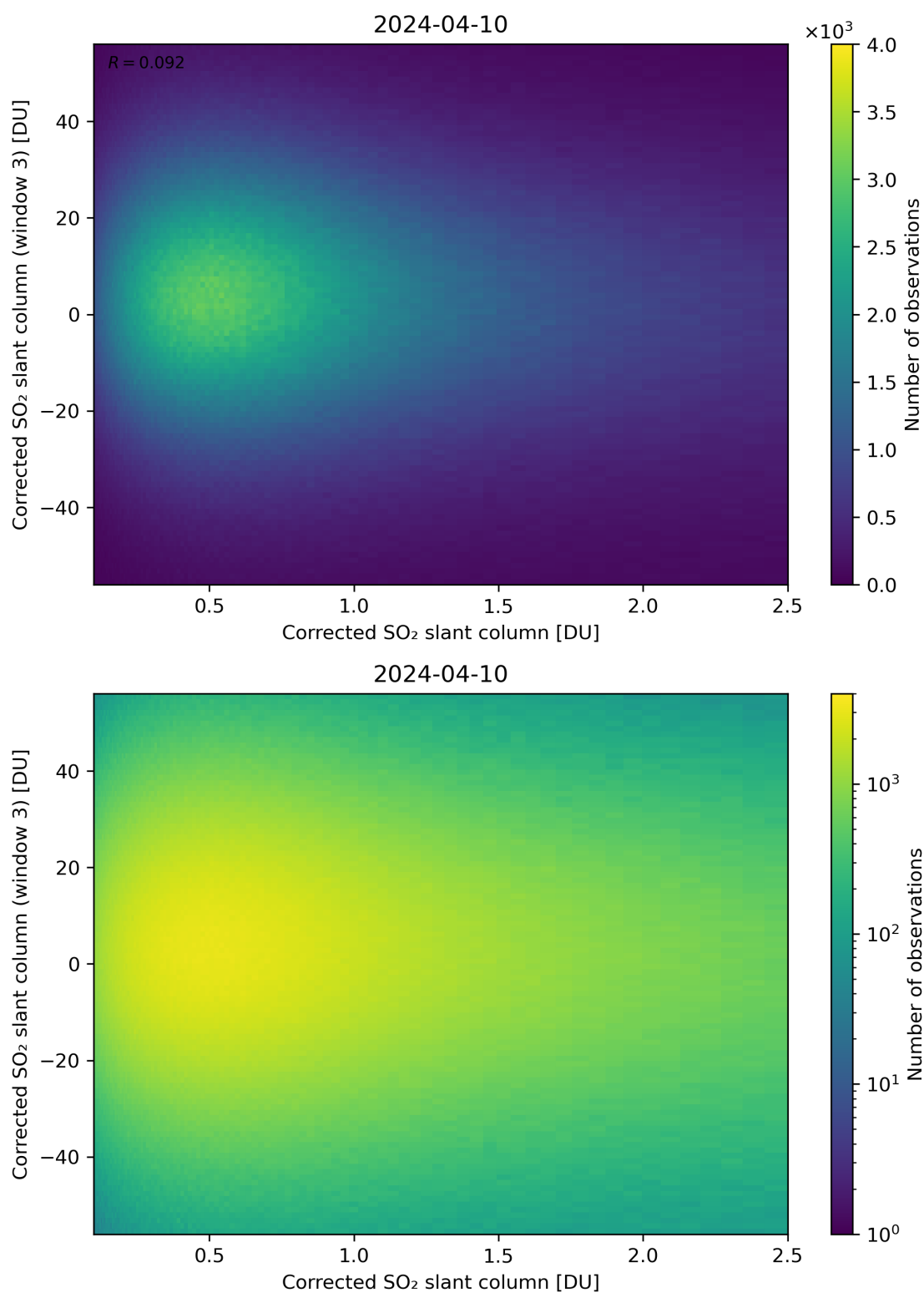
Figure 186: Scatter density plot of “Corrected SO 2 slant column” against “Corrected SO 2 slant column (window 3)” for 2024-04-10 to 2024-04-11.
