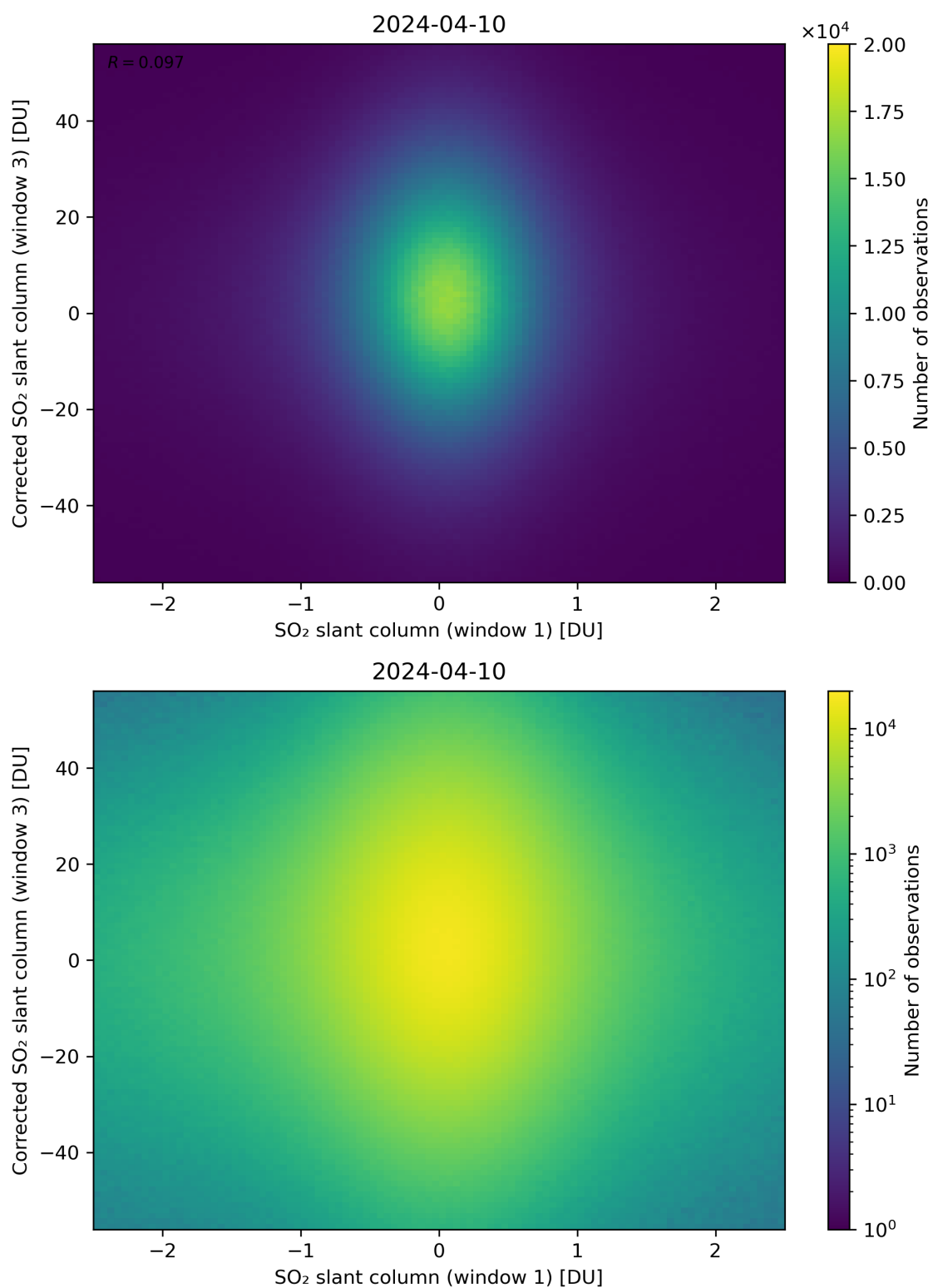
Figure 234: Scatter density plot of “SO 2 slant column (window 1)” against “Corrected SO 2 slant column (window 3)” for 2024-04-10 to 2024-04-11.
