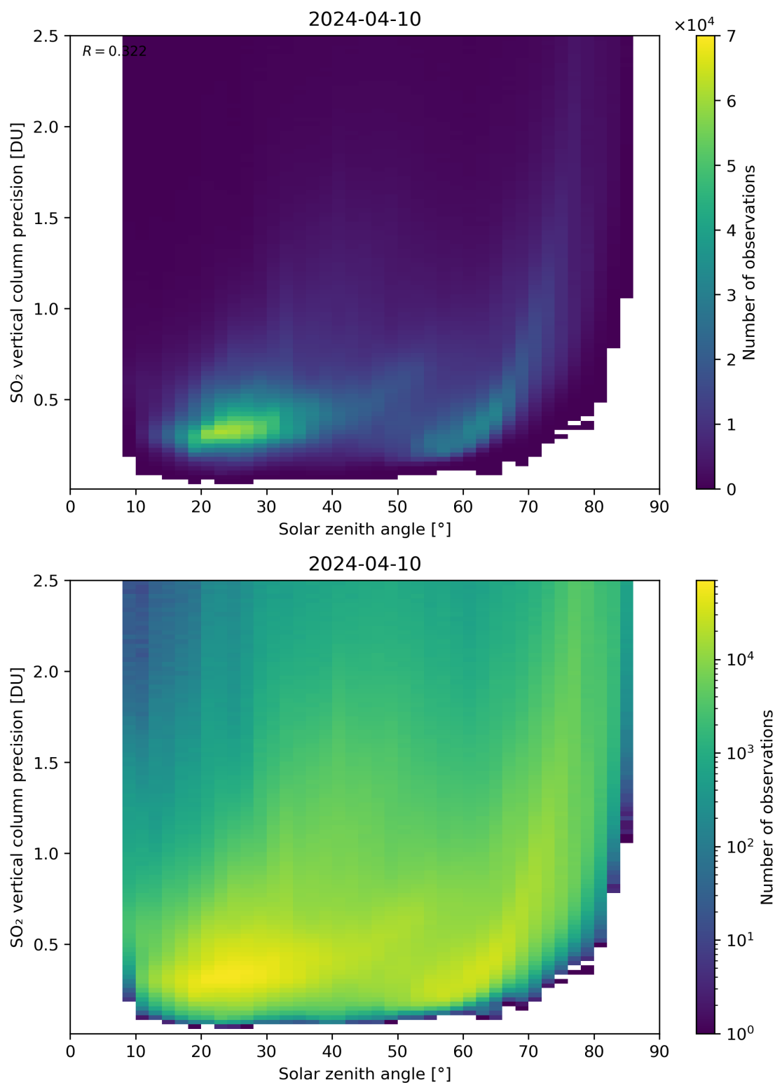
Figure 177: Scatter density plot of “Solar zenith angle” against “SO 2 vertical column precision” for 2024-04-10 to 2024-04-11.
