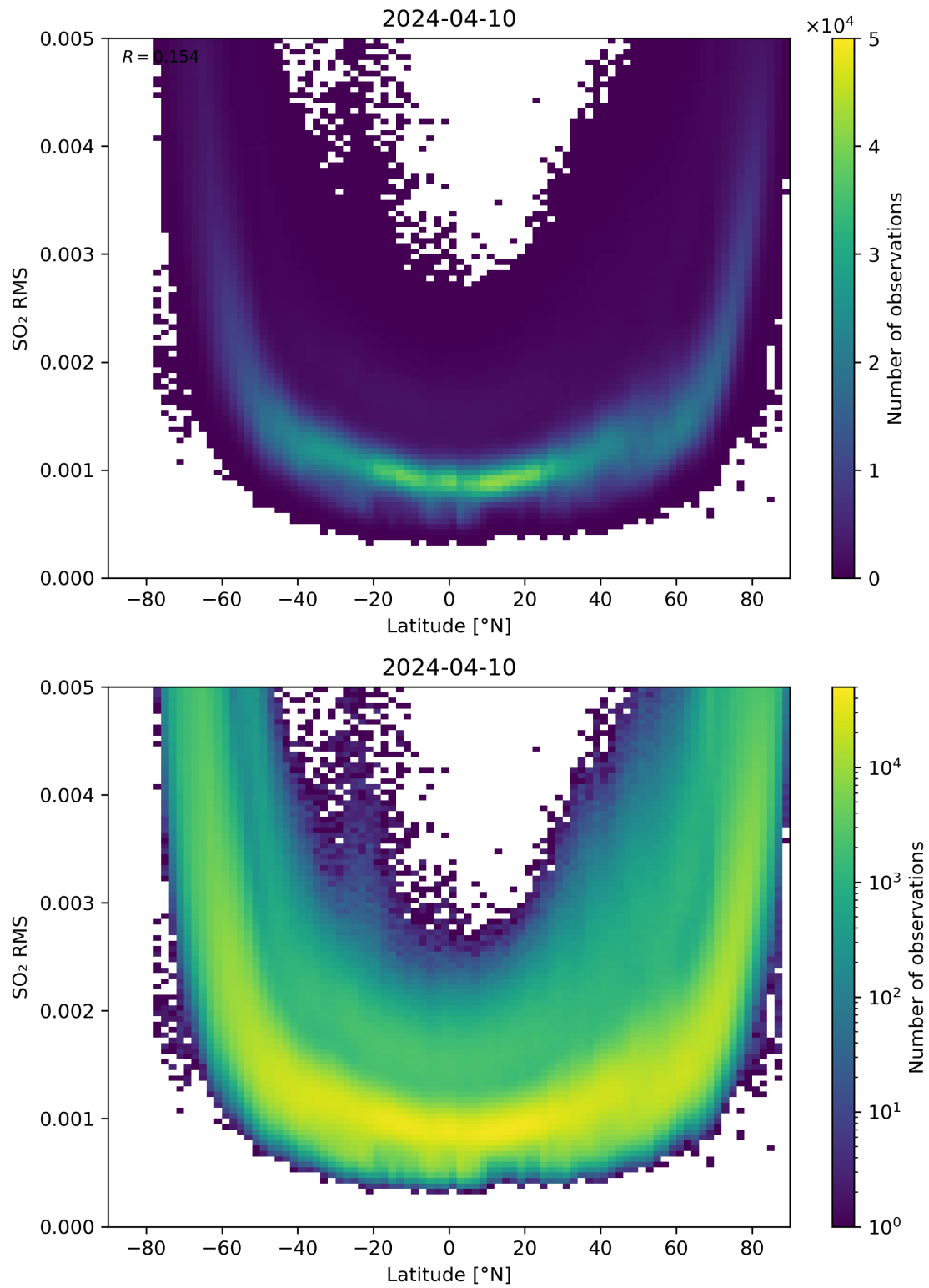
Figure 144: Scatter density plot of “Latitude” against “SO 2 RMS” for 2024-04-10 to 2024-04-11.
