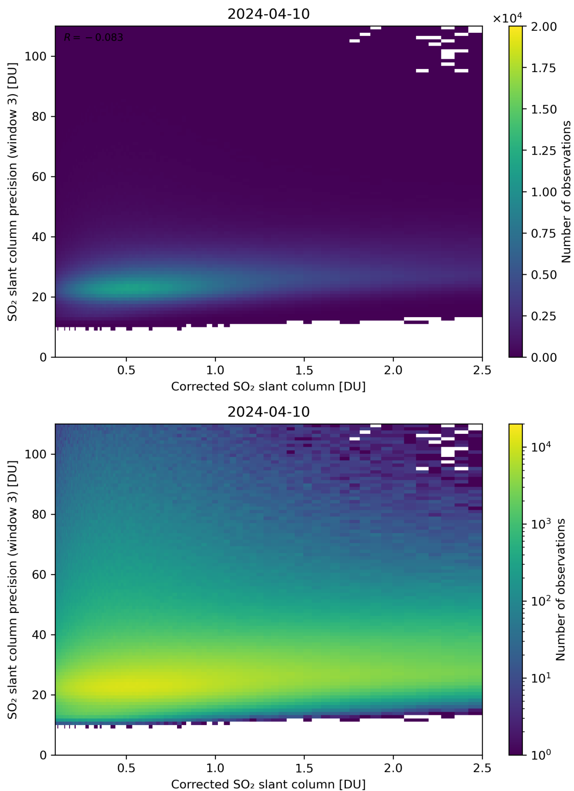
Figure 191: Scatter density plot of “Corrected SO 2 slant column” against “SO 2 slant column precision (window 3)” for 2024-04-10 to 2024-04-11.
