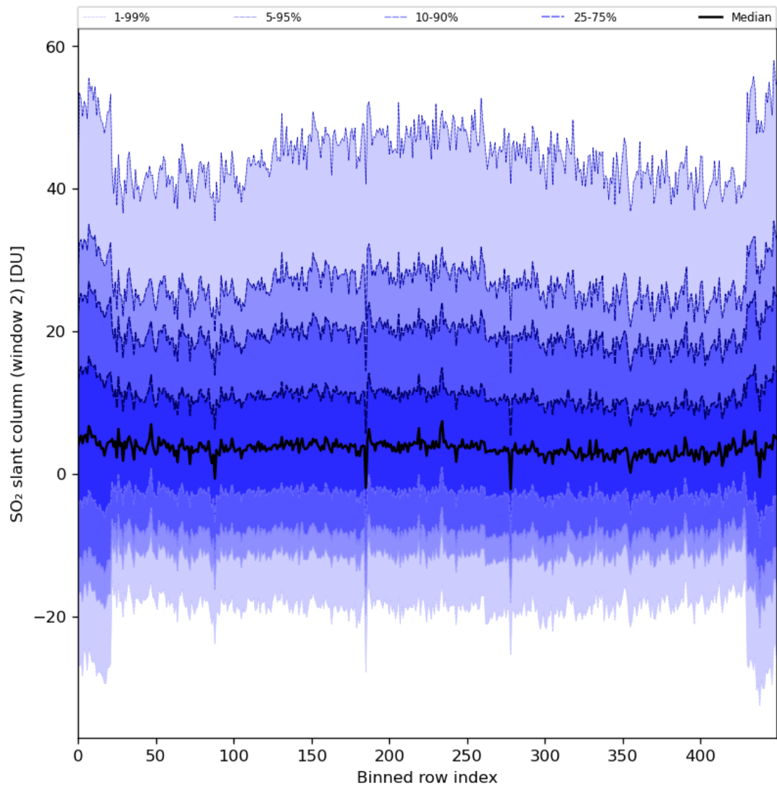
Figure 83: Along track statistics of “SO 2 slant column (window 2)” for 2024-04-10 to 2024-04-11
