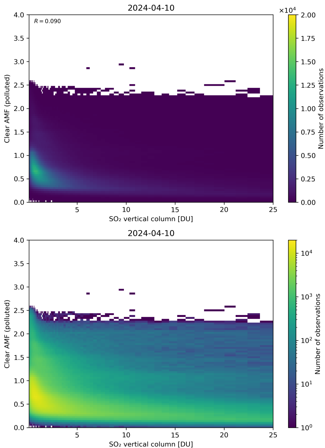
Figure 296: Scatter density plot of “SO 2 vertical column” against “Clear AMF (polluted)” for 2024-04-10 to 2024-04-11.
