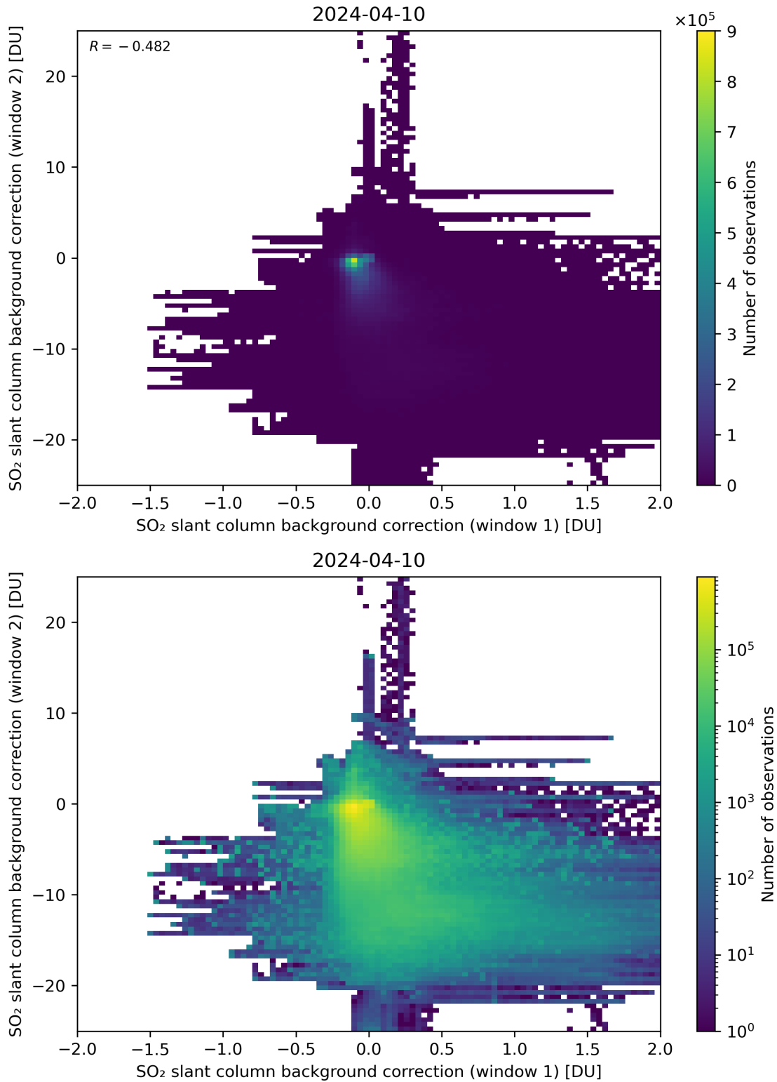
Figure 98: Scatter density plot of “SO 2 slant column background correction (window 1)” against “SO 2 slant column background correction (window 2)” for 2024-04-10 to 2024-04-11.
