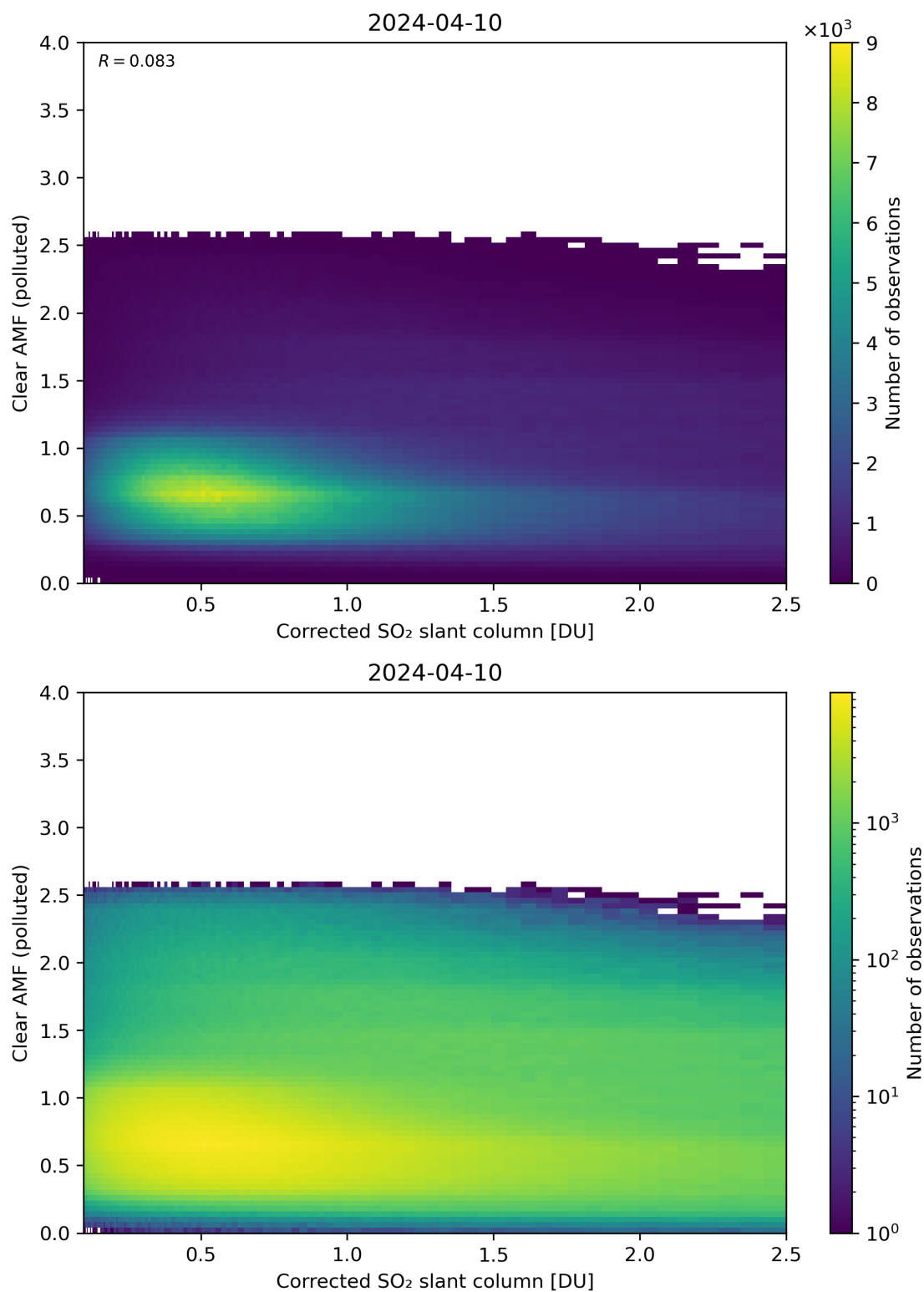
Figure 184: Scatter density plot of “Corrected SO 2 slant column” against “Clear AMF (polluted)” for 2024-04-10 to 2024-04-11.
