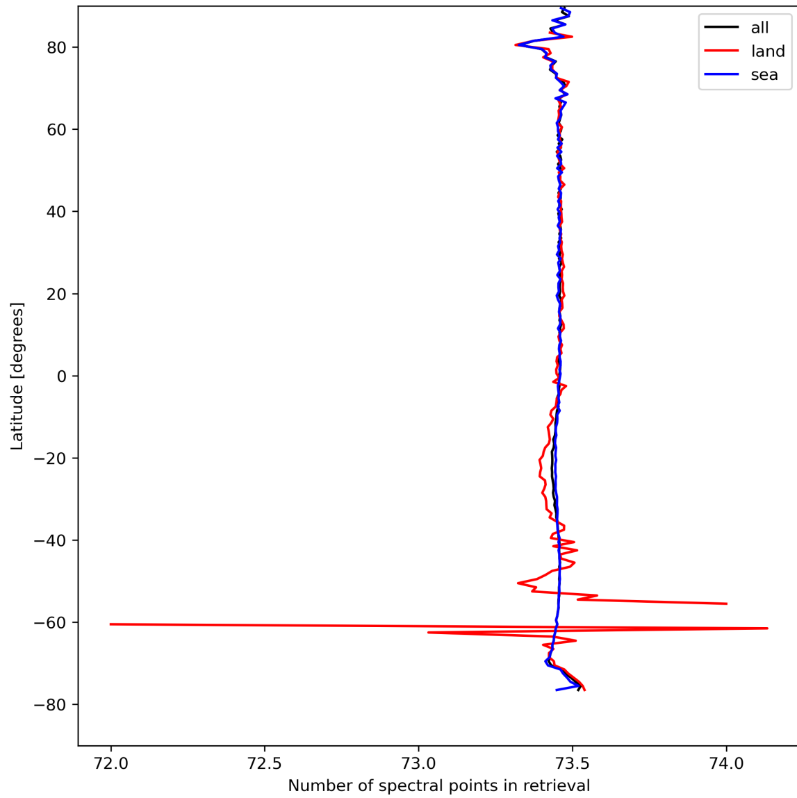
Figure 51: Zonal average of “Number of spectral points in retrieval” for 2024-04-10 to 2024-04-11.
