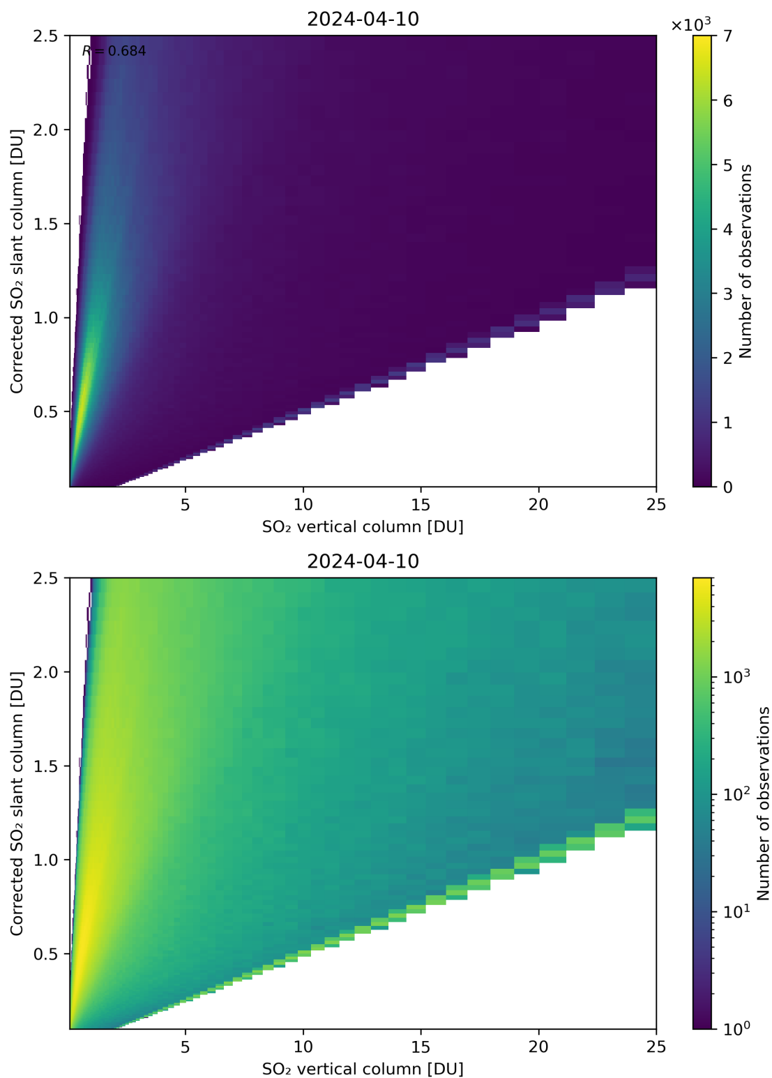
Figure 297: Scatter density plot of “SO 2 vertical column” against “Corrected SO 2 slant column” for 2024-04-10 to 2024-04-11.
