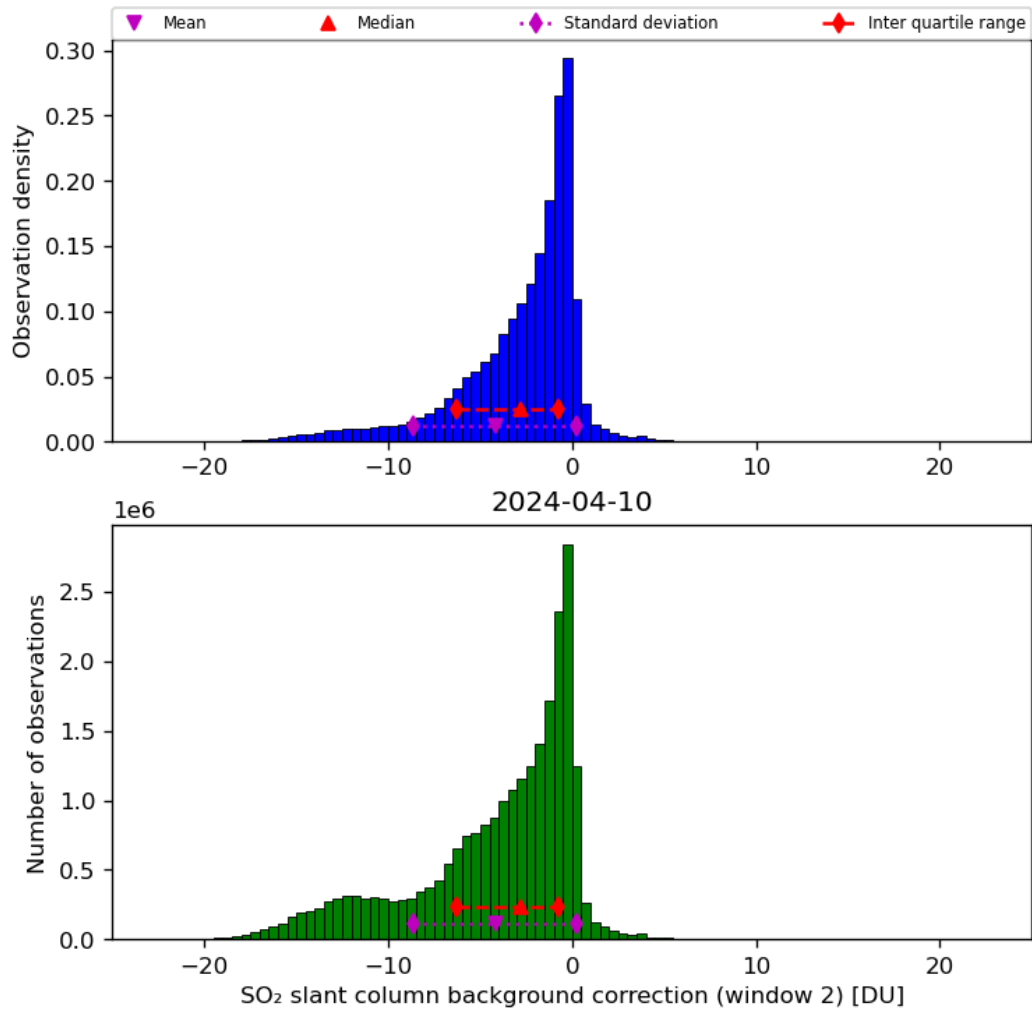
Figure 63: Histogram of “SO 2 slant column background correction (window 2)” for 2024-04-10 to 2024-04-11
