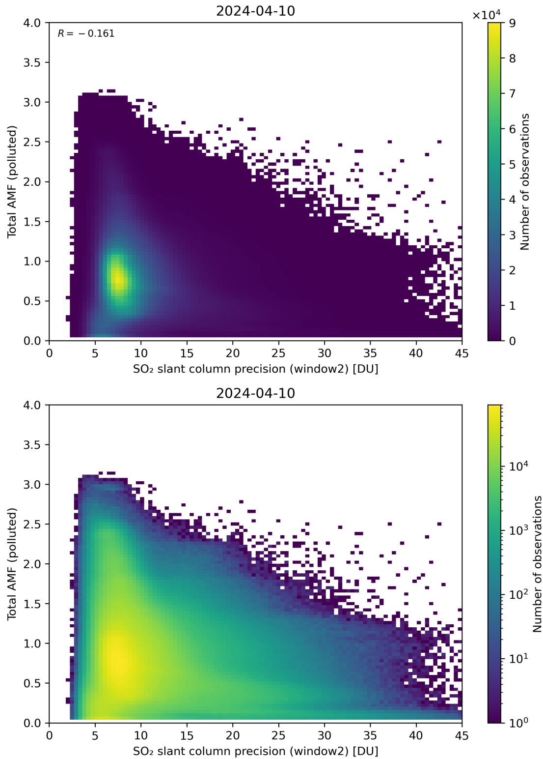
Figure 251: Scatter density plot of “SO 2 slant column precision (window2)” against “Total AMF (polluted)” for 2024-04-10 to 2024-04-11.
