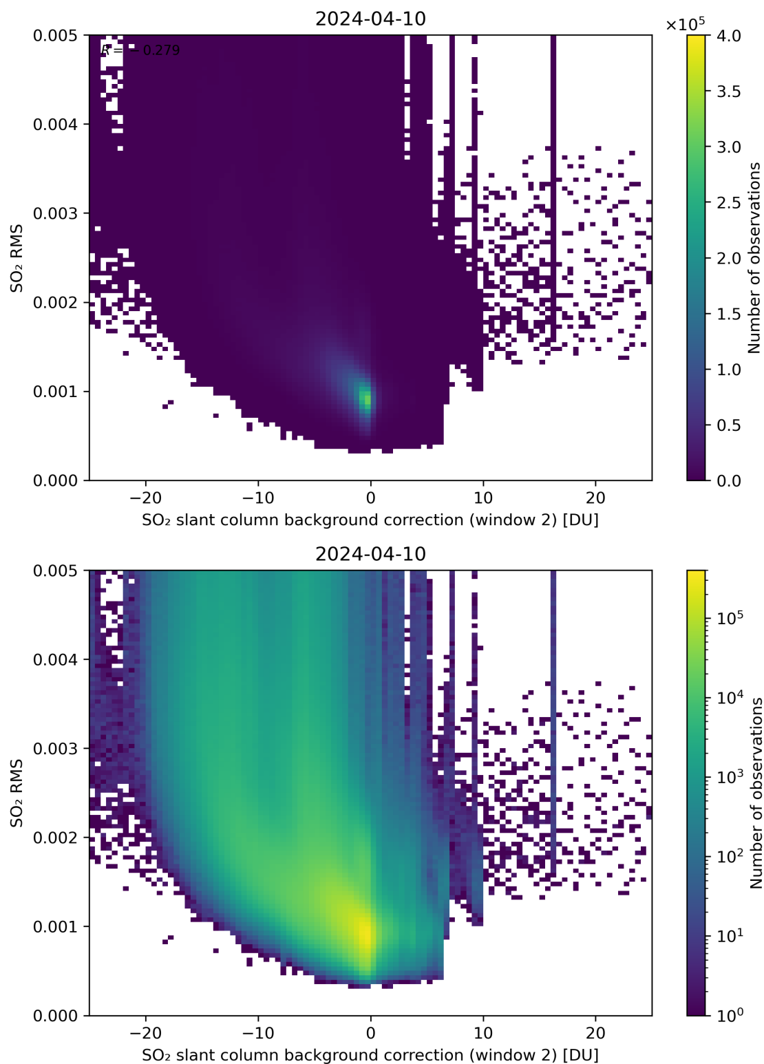
Figure 114: Scatter density plot of “SO 2 slant column background correction (window 2)” against “SO 2 RMS” for 2024-04-10 to 2024-04-11.
