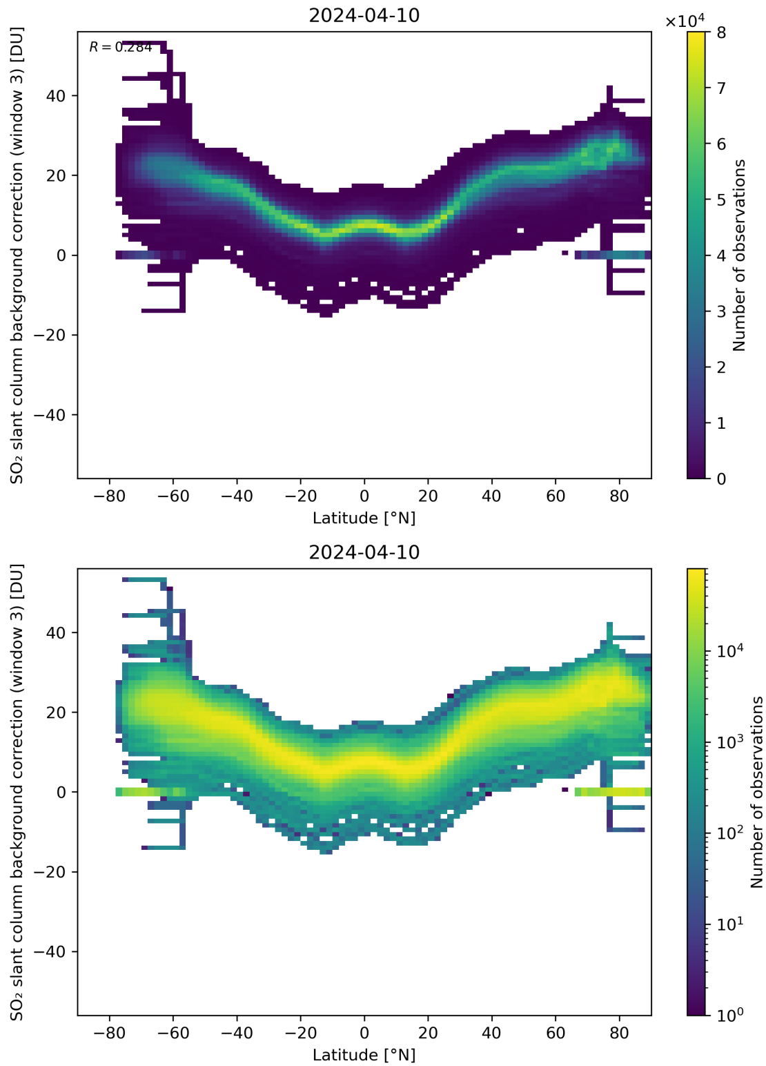
Figure 141: Scatter density plot of “Latitude” against “SO 2 slant column background correction (window 3)” for 2024-04-10 to 2024-04-11.
