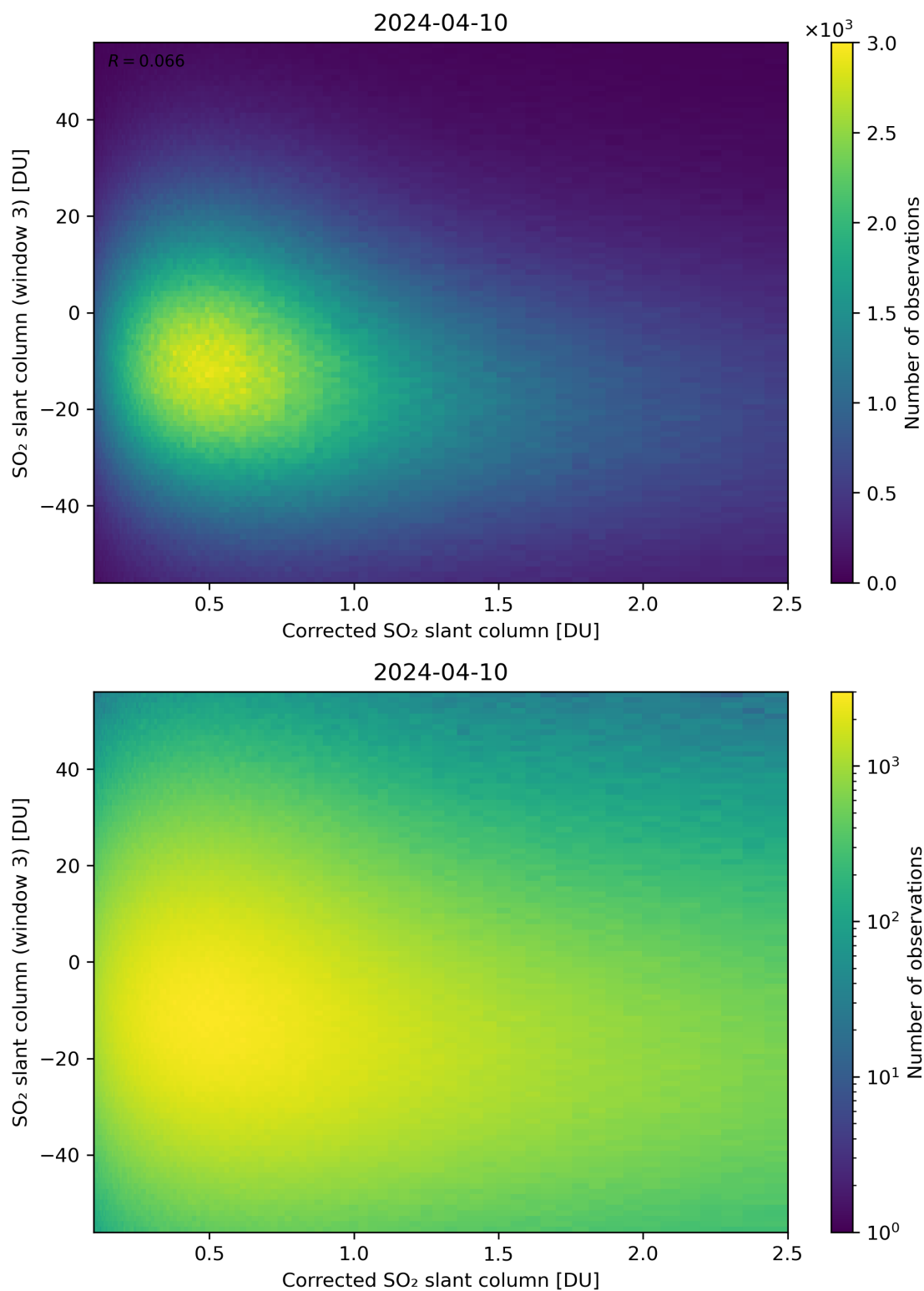
Figure 190: Scatter density plot of “Corrected SO 2 slant column” against “SO 2 slant column (window 3)” for 2024-04-10 to 2024-04-11.
