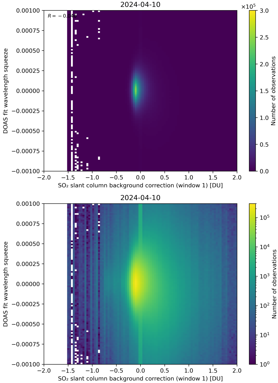
Figure 101: Scatter density plot of “SO 2 slant column background correction (window 1)” against “DOAS fit wavelength squeeze” for 2024-04-10 to 2024-04-11.
