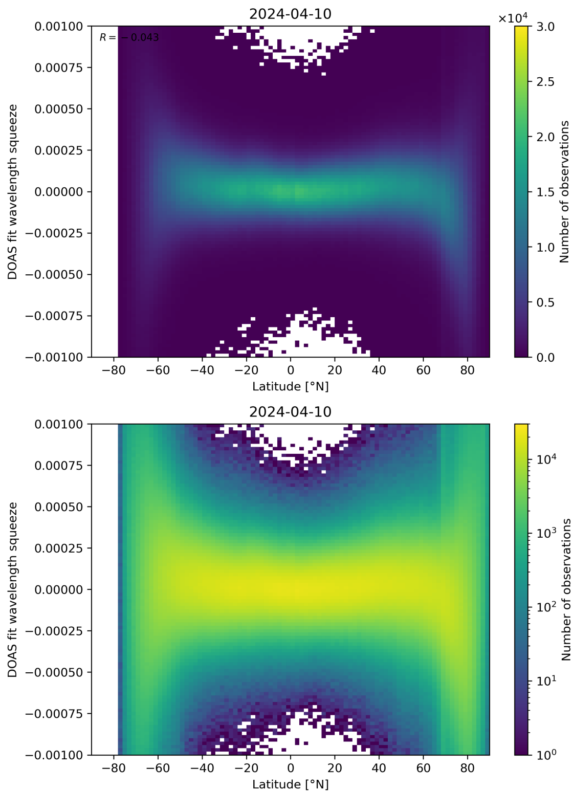
Figure 143: Scatter density plot of “Latitude” against “DOAS fit wavelength squeeze” for 2024-04-10 to 2024-04-11.
