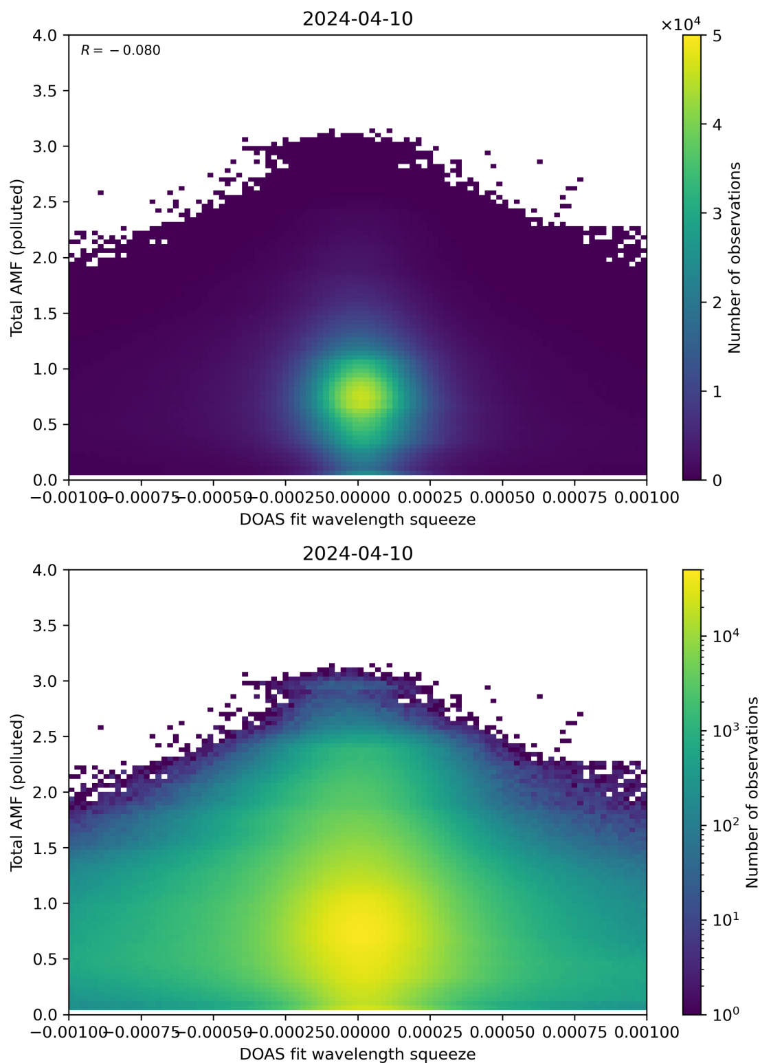
Figure 134: Scatter density plot of “DOAS fit wavelength squeeze” against “Total AMF (polluted)” for 2024-04-10 to 2024-04-11.
