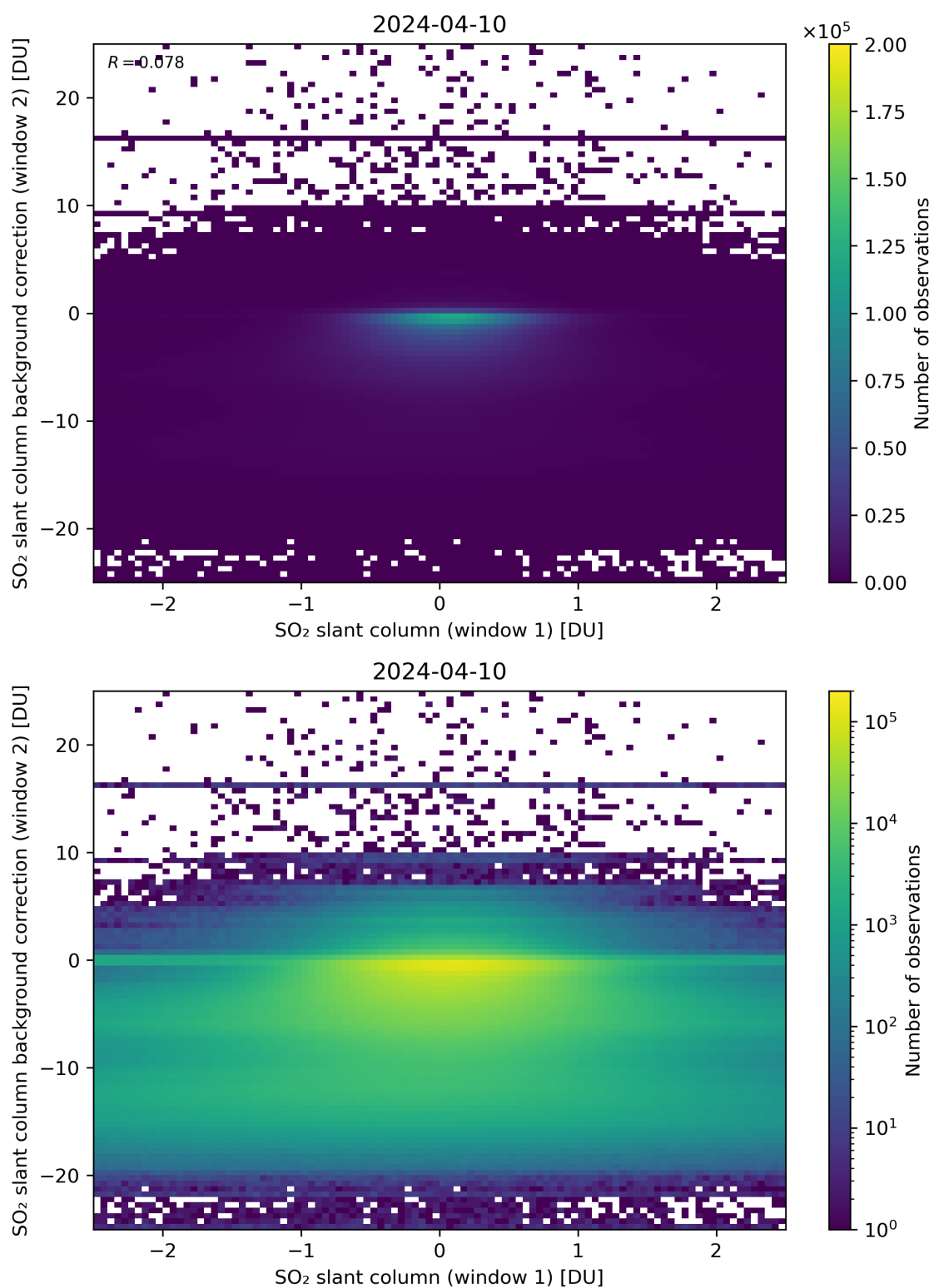
Figure 213: Scatter density plot of “SO 2 slant column (window 1)” against “SO 2 slant column background correction (window 2)” for 2024-04-10 to 2024-04-11.
