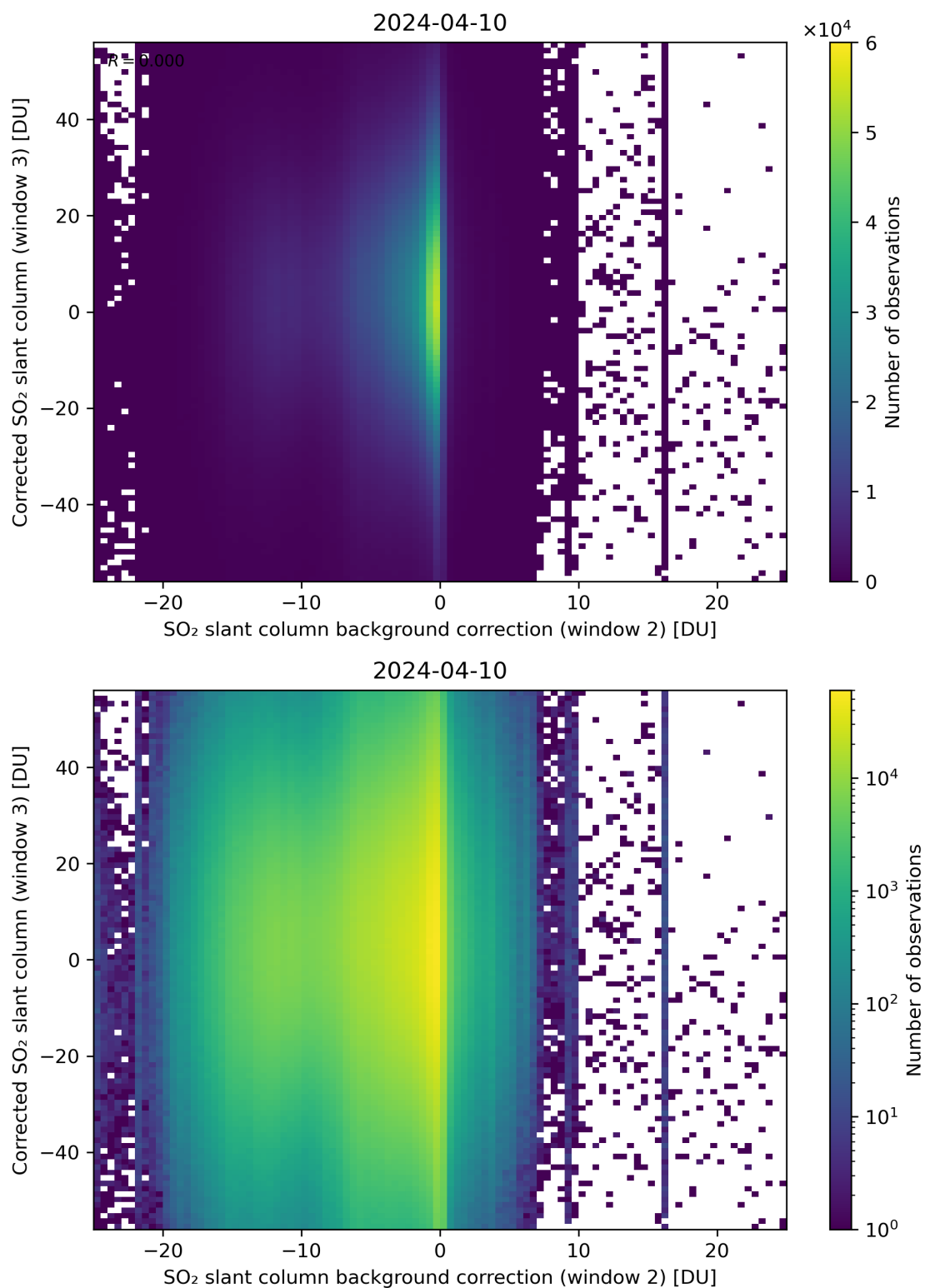
Figure 116: Scatter density plot of “SO 2 slant column background correction (window 2)” against “Corrected SO 2 slant column (window 3)” for 2024-04-10 to 2024-04-11.
