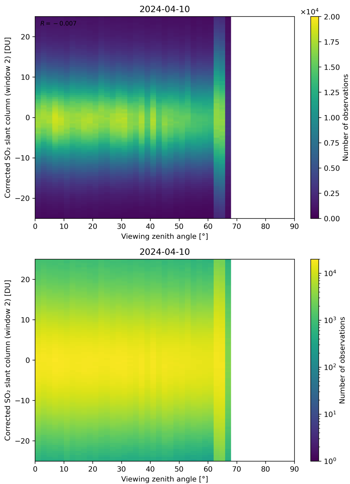
Figure 318: Scatter density plot of “Viewing zenith angle” against “Corrected SO 2 slant column (window 2)” for 2024-04-10 to 2024-04-11.
