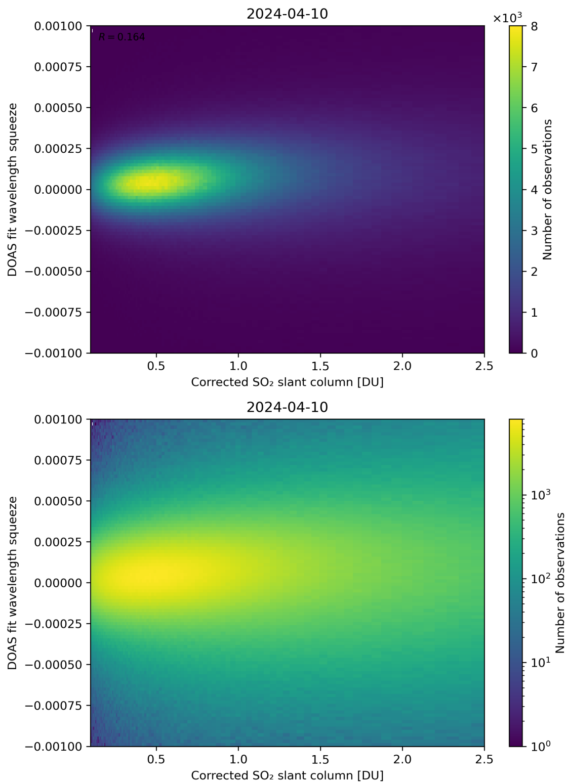
Figure 182: Scatter density plot of “Corrected SO 2 slant column” against “DOAS fit wavelength squeeze” for 2024-04-10 to 2024-04-11.
