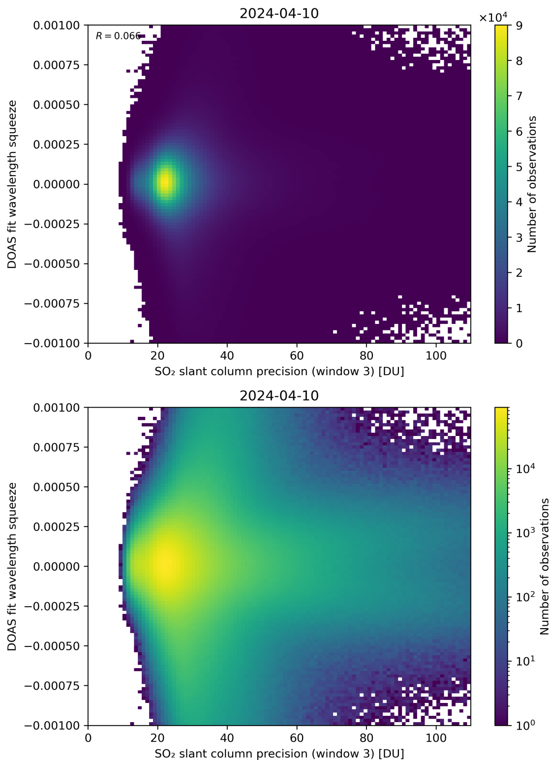
Figure 259: Scatter density plot of “SO 2 slant column precision (window 3)” against “DOAS fit wavelength squeeze” for 2024-04-10 to 2024-04-11.
