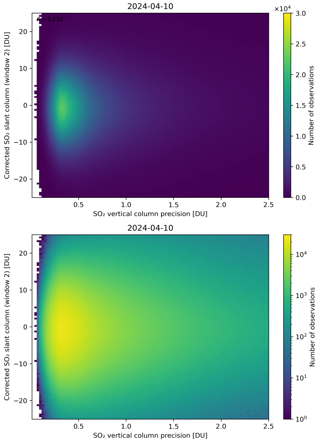
Figure 287: Scatter density plot of “SO 2 vertical column precision” against “Corrected SO 2 slant column (window 2)” for 2024-04-10 to 2024-04-11.
