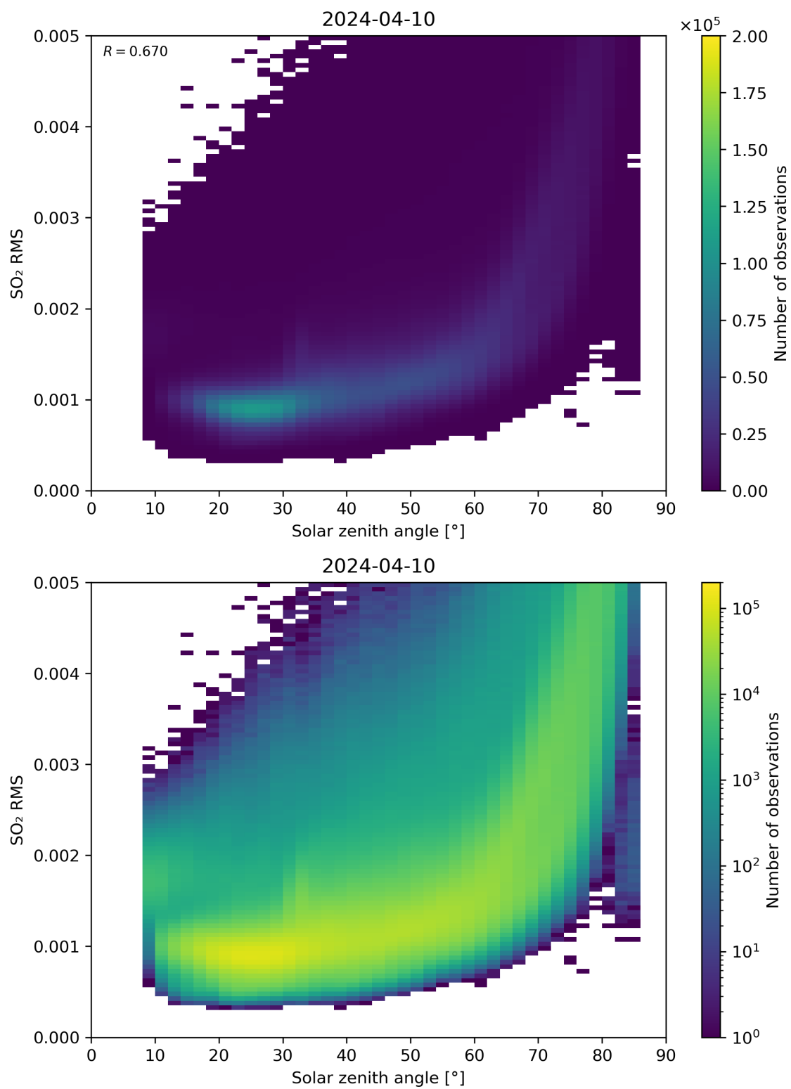
Figure 163: Scatter density plot of “Solar zenith angle” against “SO 2 RMS” for 2024-04-10 to 2024-04-11.
