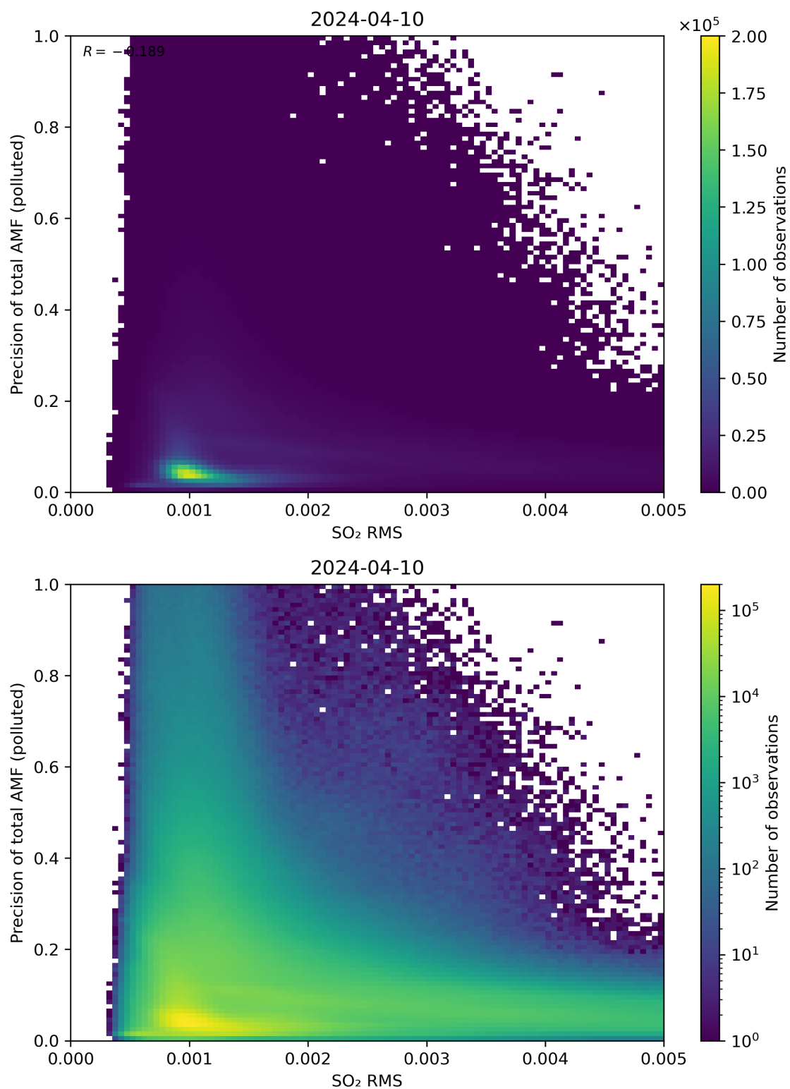
Figure 138: Scatter density plot of “SO 2 RMS” against “Precision of total AMF (polluted)” for 2024-04-10 to 2024-04-11.
