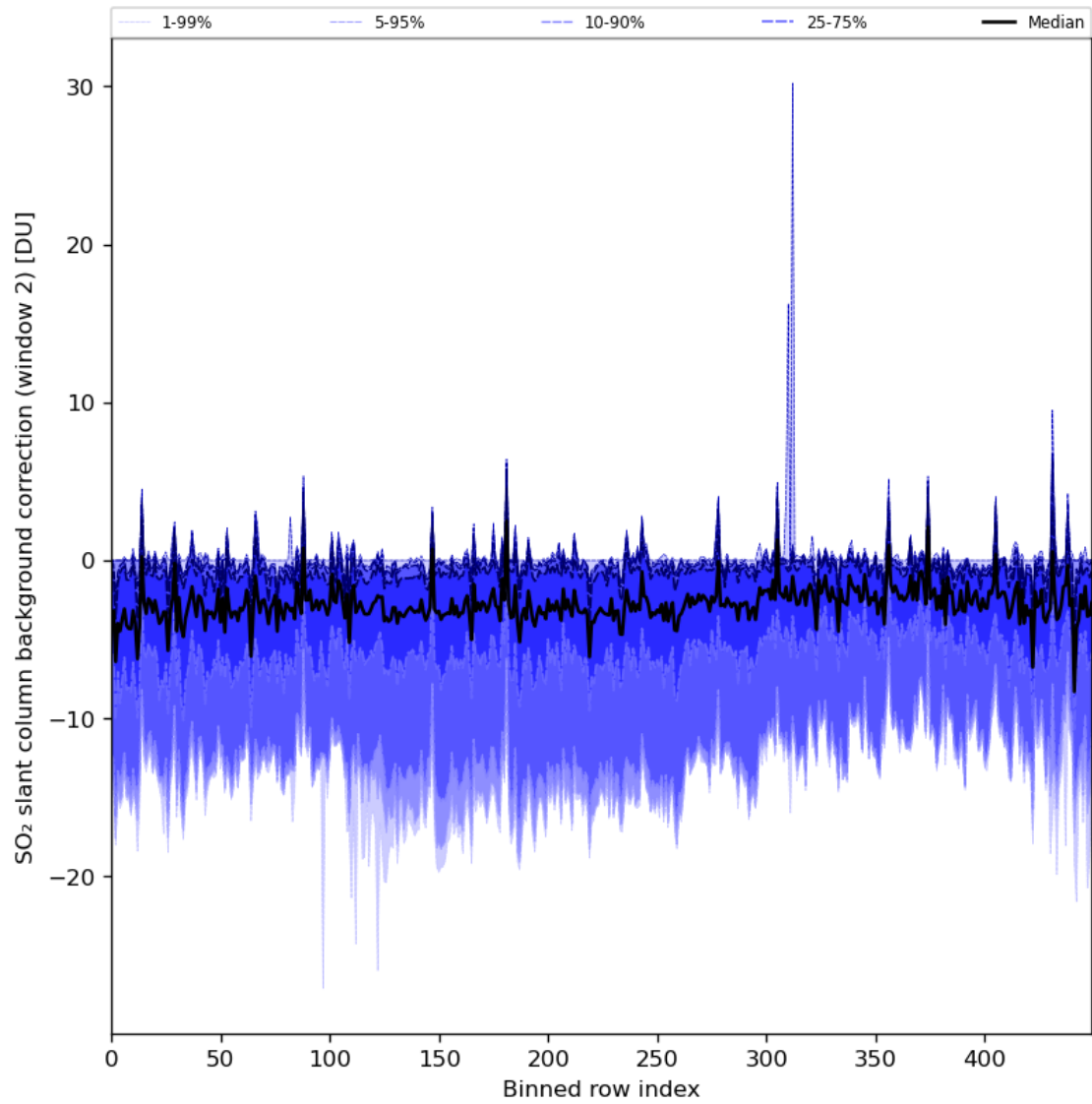
Figure 86: Along track statistics of “SO 2 slant column background correction (window 2)” for 2024-04-10 to 2024-04-11
