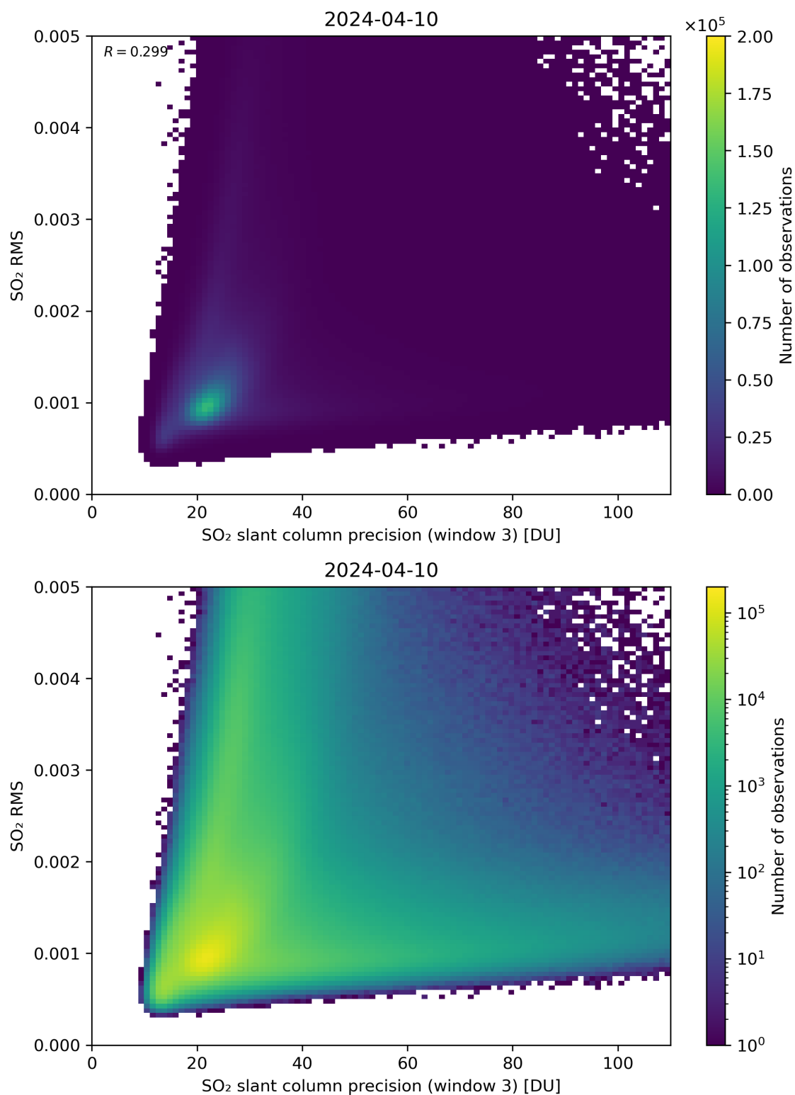
Figure 260: Scatter density plot of “SO 2 slant column precision (window 3)” against “SO 2 RMS” for 2024-04-10 to 2024-04-11.
