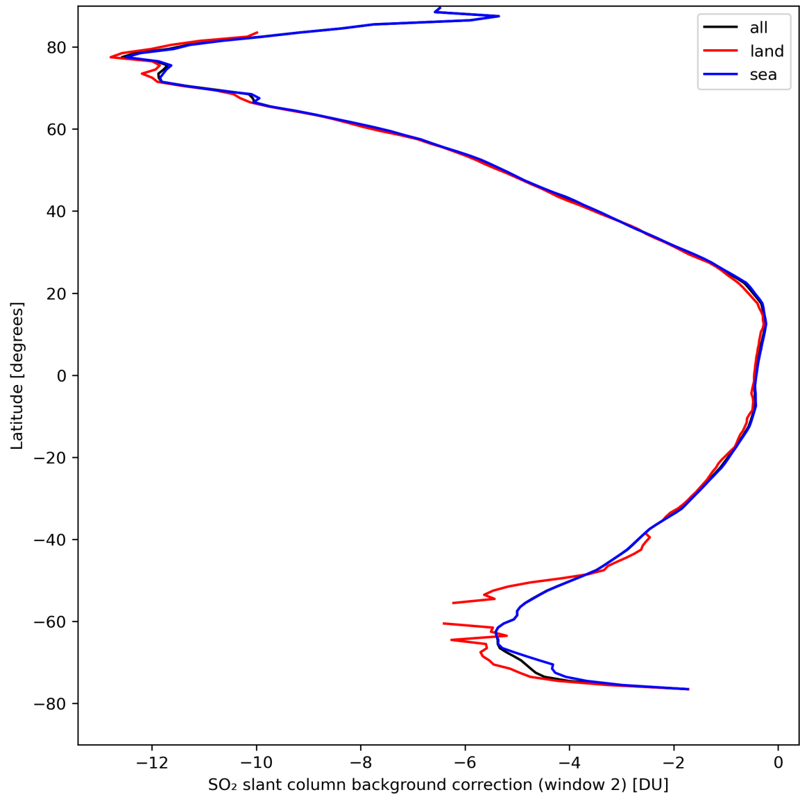
Figure 40: Zonal average of “SO 2 slant column background correction (window 2)” for 2024-04-10 to 2024-04-11.
