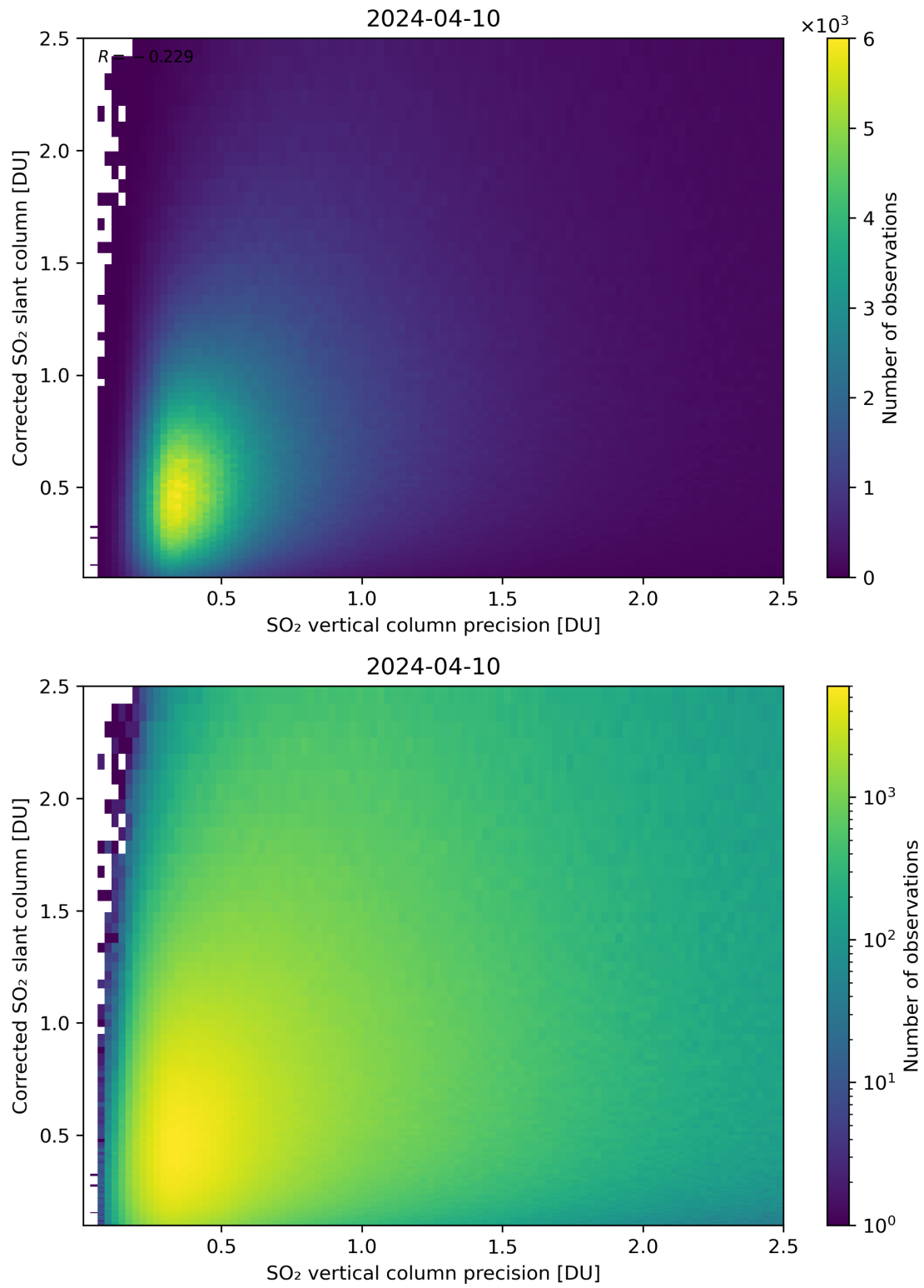
Figure 286: Scatter density plot of “SO 2 vertical column precision” against “Corrected SO 2 slant column” for 2024-04-10 to 2024-04-11.
