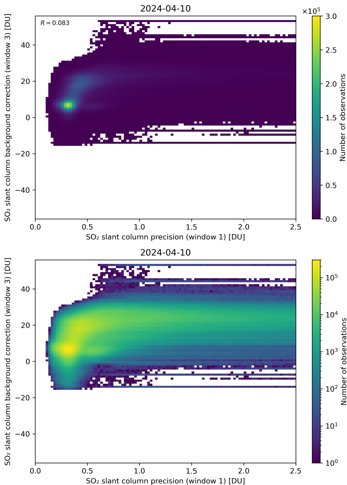
Figure 220: Scatter density plot of “SO 2 slant column precision (window 1)” against “SO 2 slant column background correction (window 3)” for 2024-04-10 to 2024-04-11.
