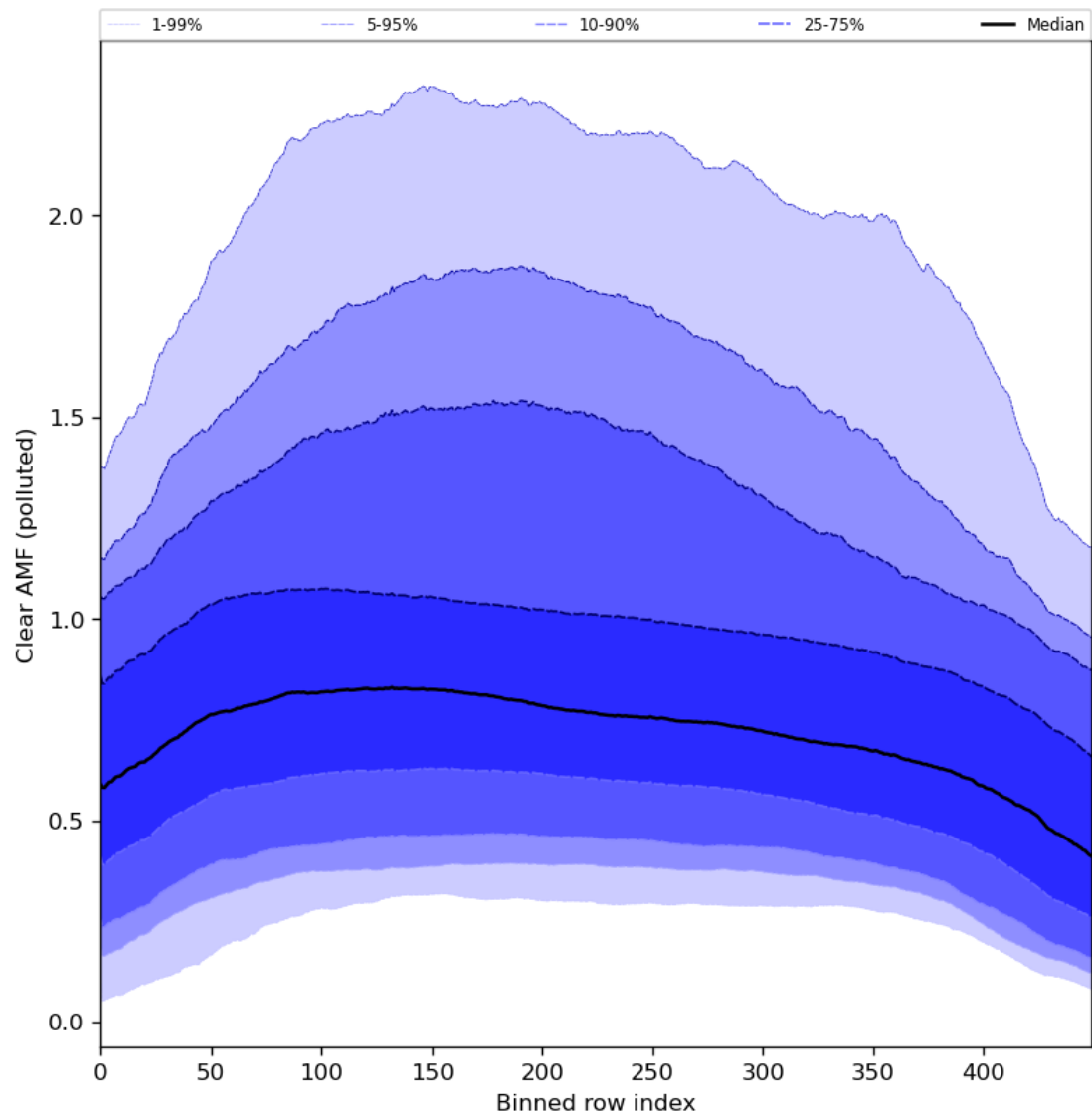
Figure 96: Along track statistics of “Clear AMF (polluted)” for 2024-04-10 to 2024-04-11
