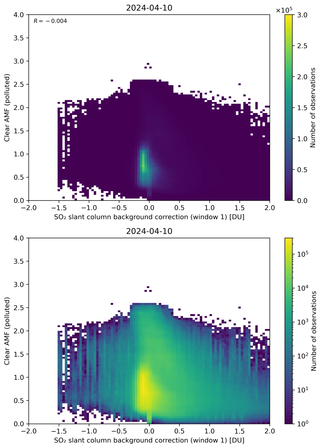
Figure 103: Scatter density plot of “SO 2 slant column background correction (window 1)” against “Clear AMF (polluted)” for 2024-04-10 to 2024-04-11.
