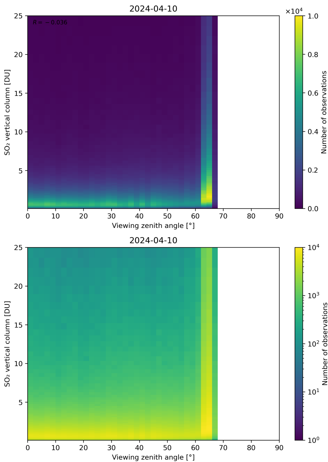
Figure 327: Scatter density plot of “Viewing zenith angle” against “SO 2 vertical column” for 2024-04-10 to 2024-04-11.
