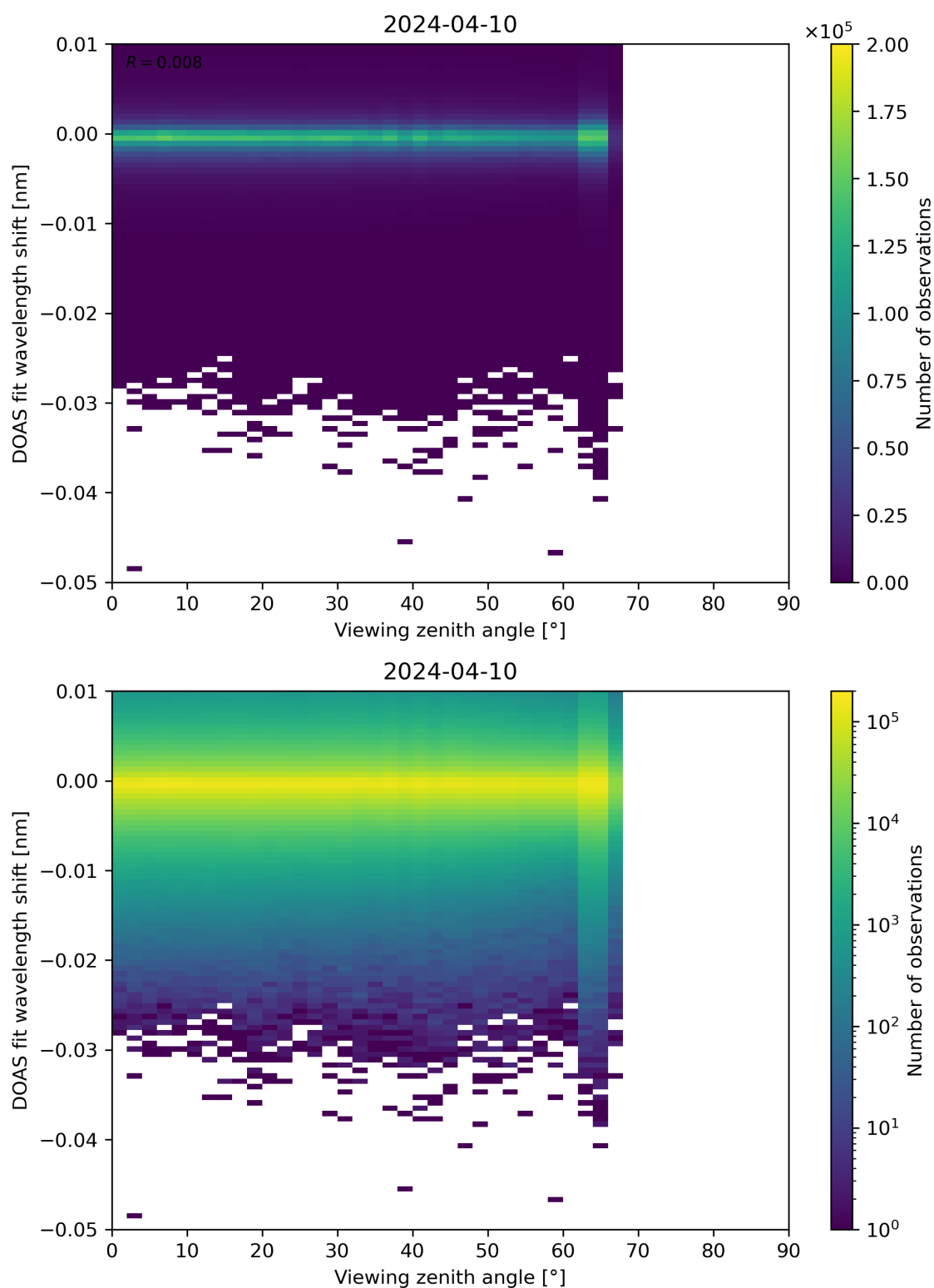
Figure 311: Scatter density plot of “Viewing zenith angle” against “DOAS fit wavelength shift” for 2024-04-10 to 2024-04-11.
