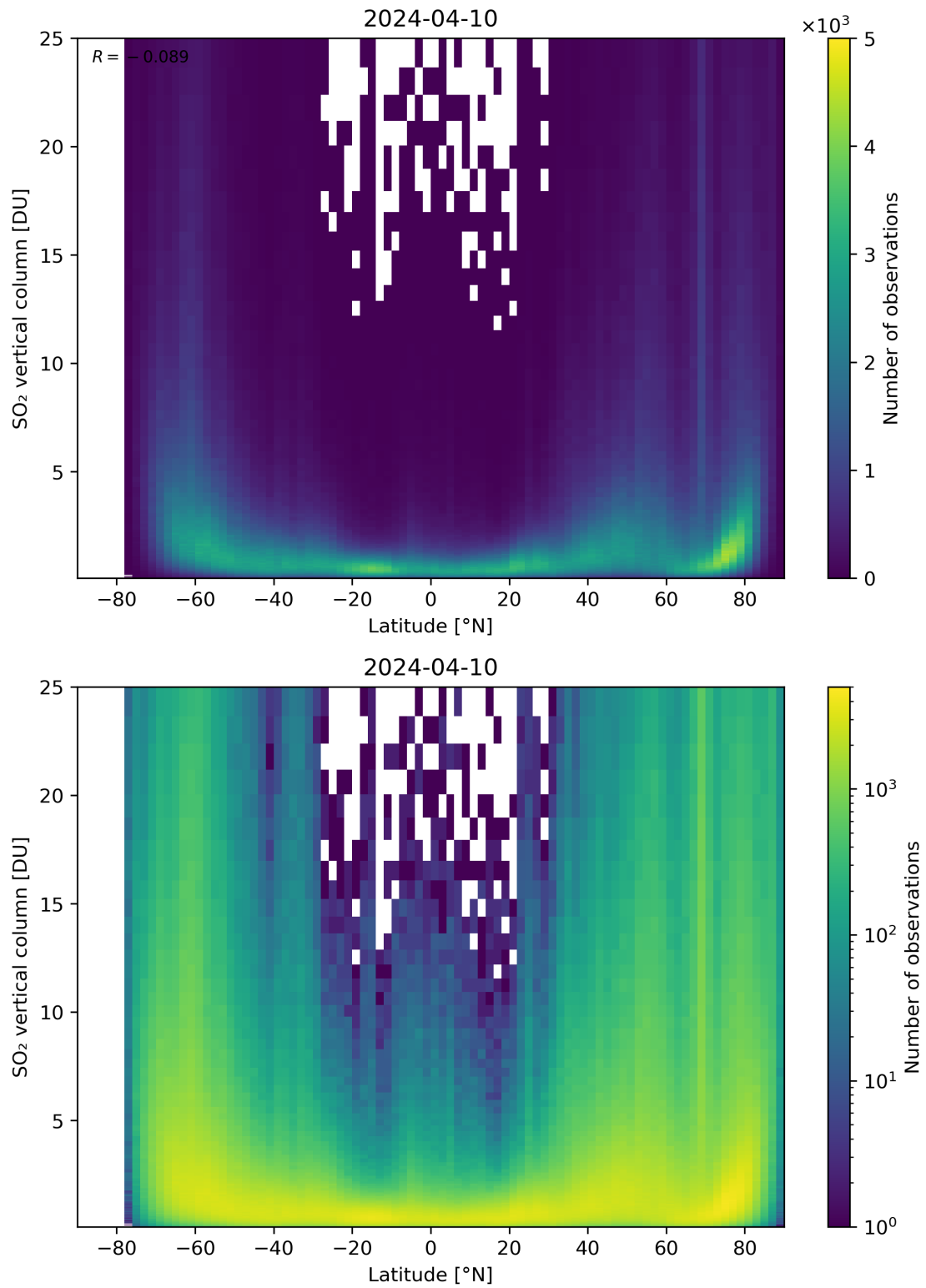
Figure 156: Scatter density plot of “Latitude” against “SO 2 vertical column” for 2024-04-10 to 2024-04-11.
