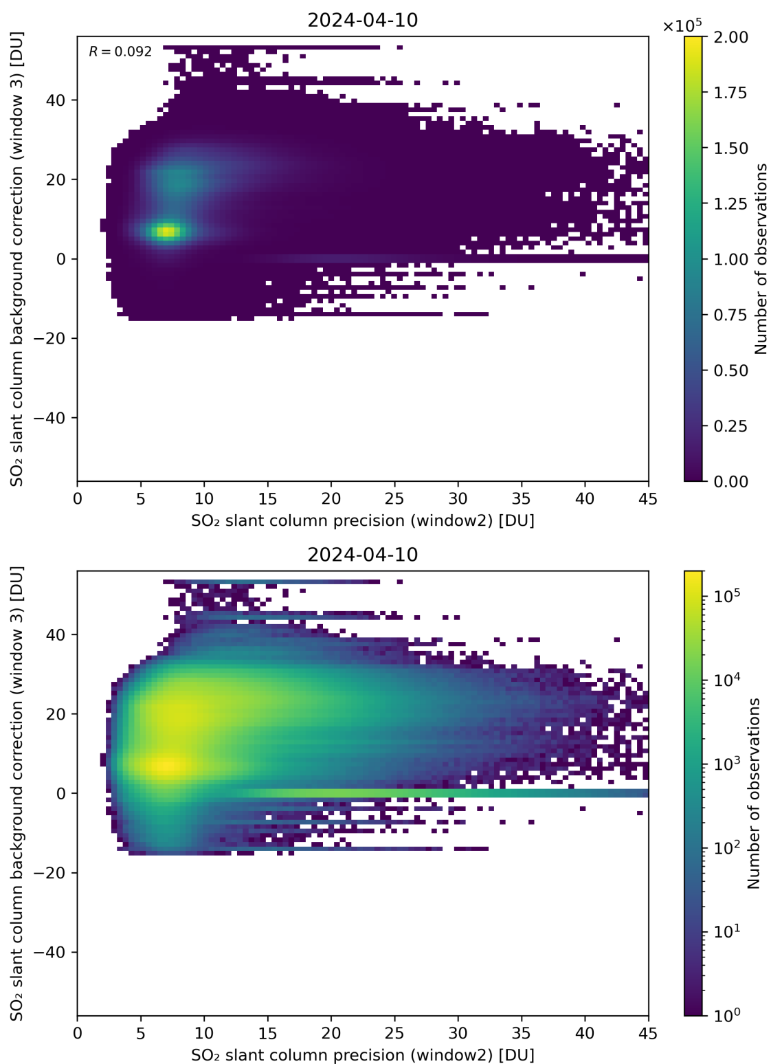
Figure 242: Scatter density plot of “SO 2 slant column precision (window2)” against “SO 2 slant column background correction (window 3)” for 2024-04-10 to 2024-04-11.
