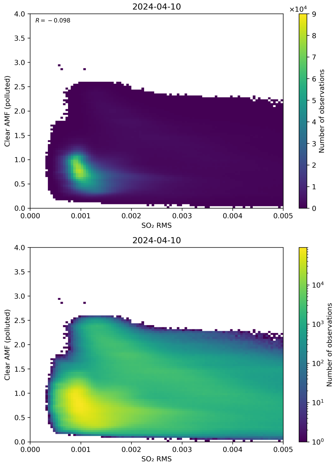
Figure 136: Scatter density plot of “SO 2 RMS” against “Clear AMF (polluted)” for 2024-04-10 to 2024-04-11.
