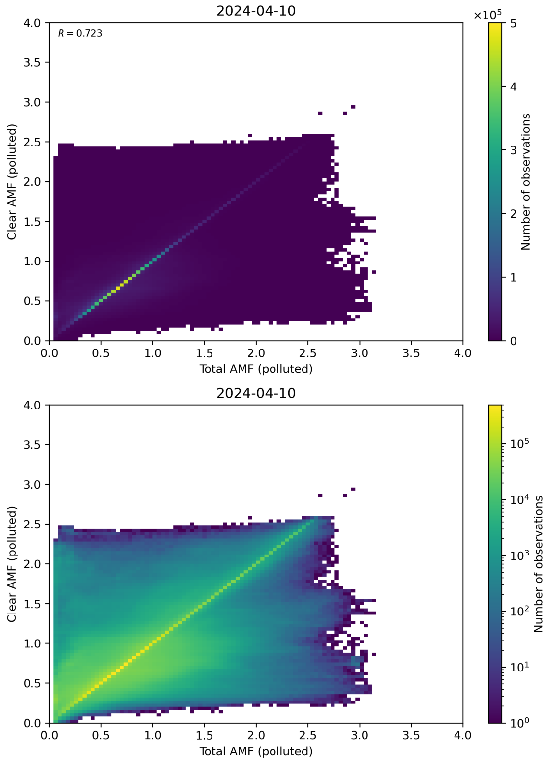
Figure 271: Scatter density plot of “Total AMF (polluted)” against “Clear AMF (polluted)” for 2024-04-10 to 2024-04-11.
