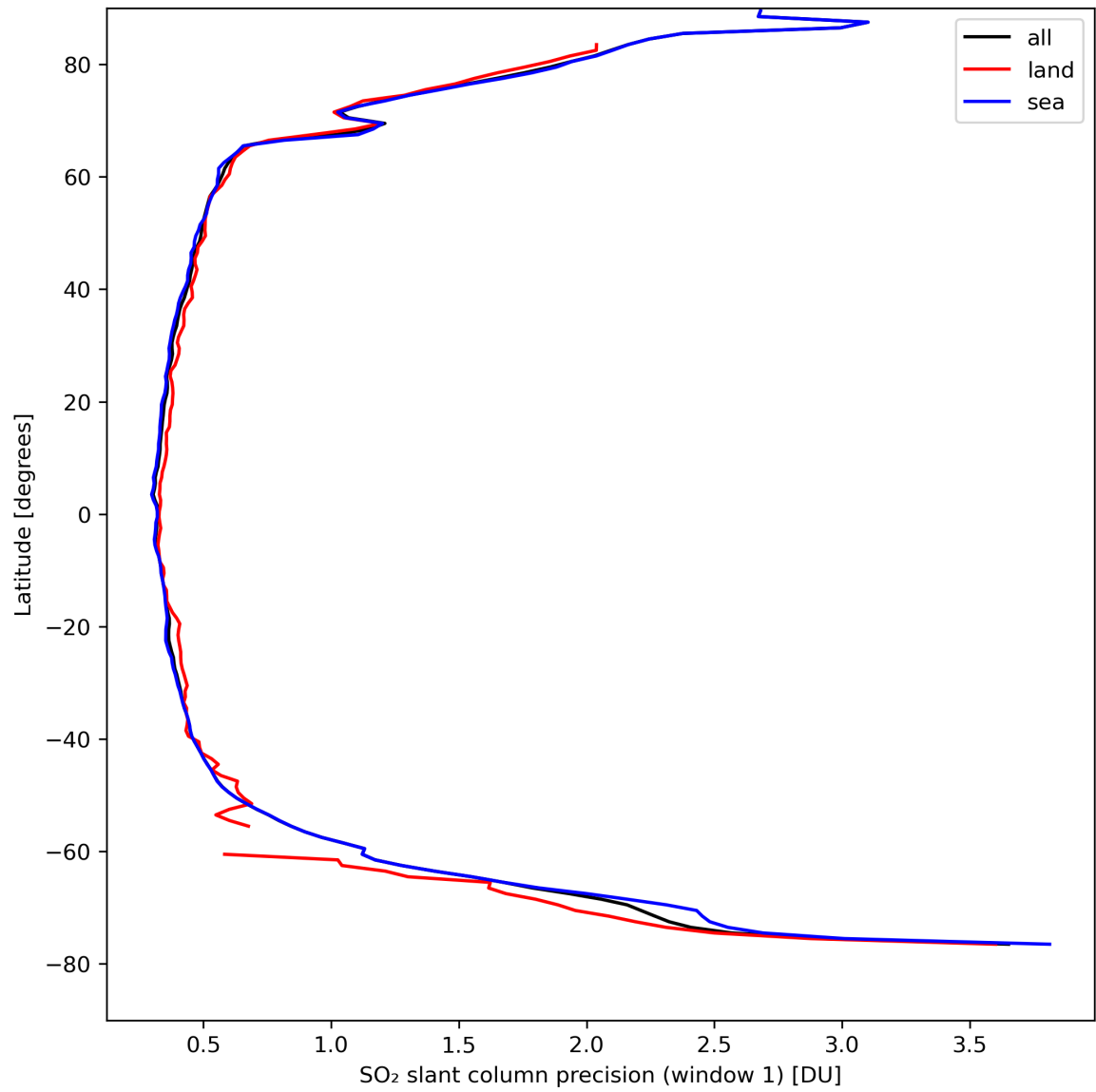
Figure 34: Zonal average of “SO 2 slant column precision (window 1)” for 2024-04-10 to 2024-04-11.
