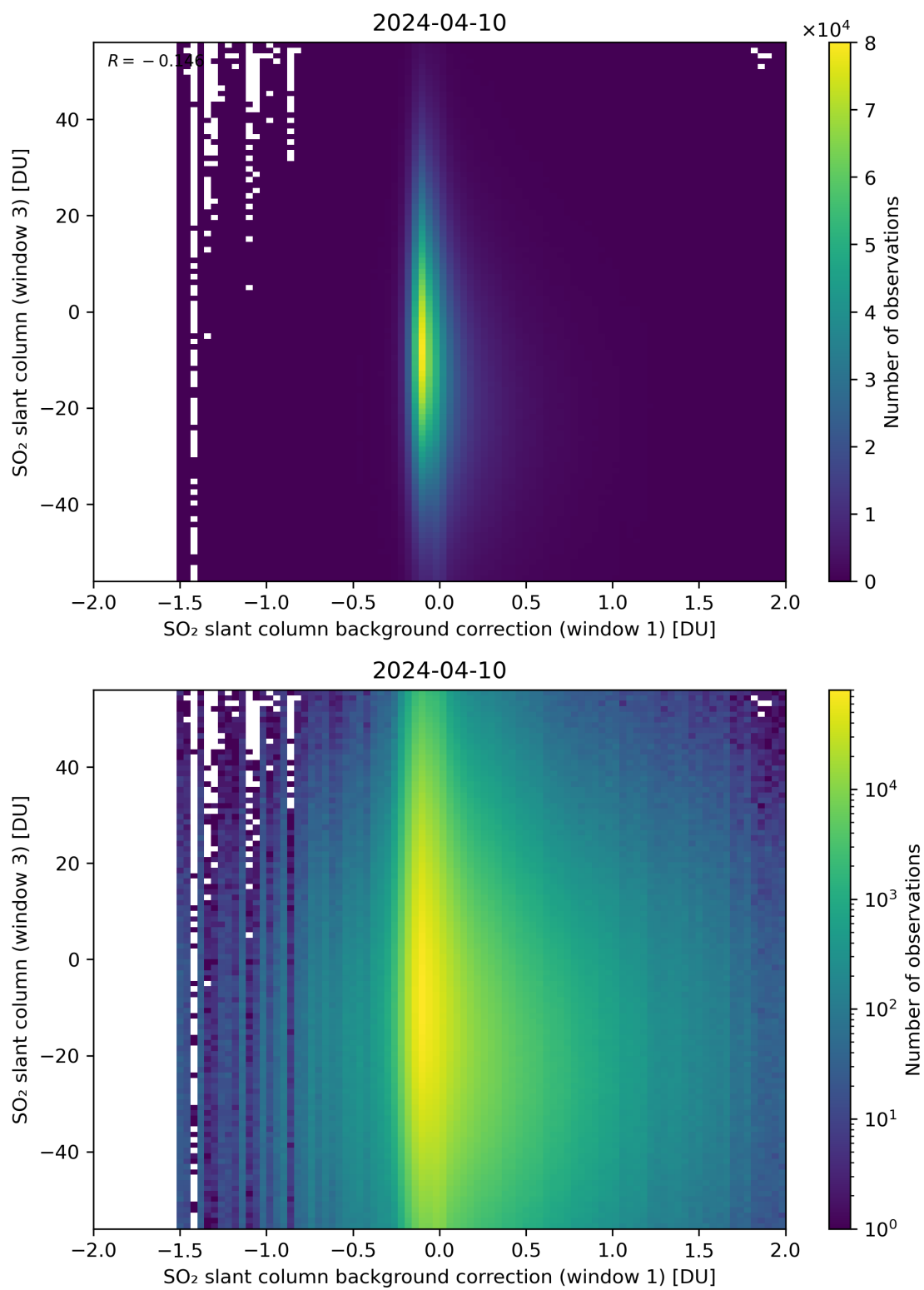
Figure 107: Scatter density plot of “SO 2 slant column background correction (window 1)” against “SO 2 slant column (window 3)” for 2024-04-10 to 2024-04-11.
