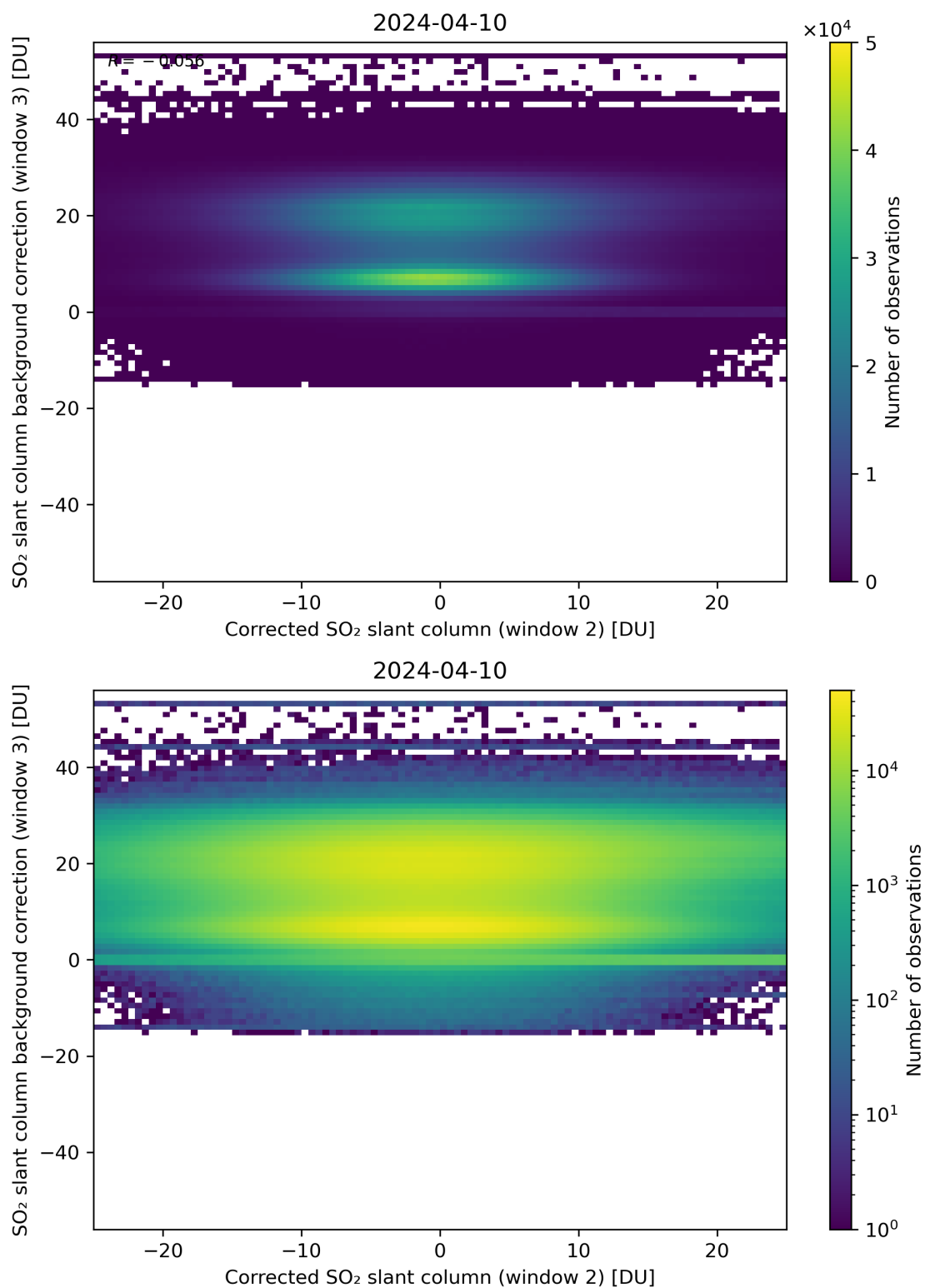
Figure 195: Scatter density plot of “Corrected SO 2 slant column (window 2)” against “SO 2 slant column background correction (window 3)” for 2024-04-10 to 2024-04-11.
