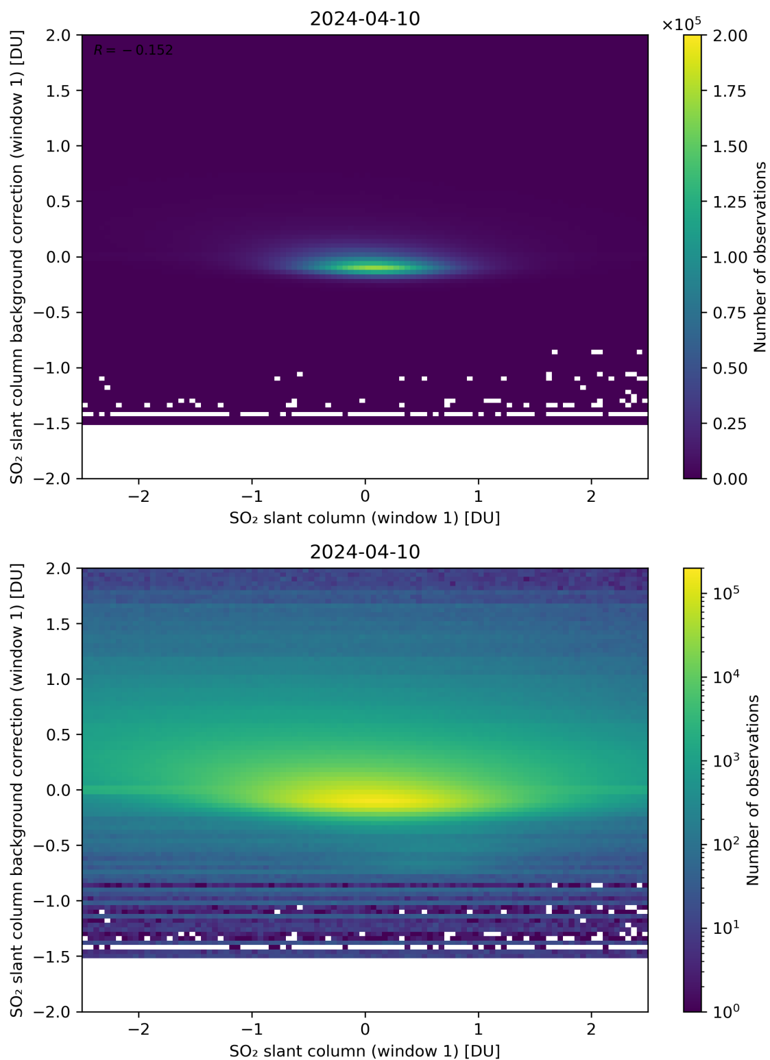
Figure 212: Scatter density plot of “SO 2 slant column (window 1)” against “SO 2 slant column background correction (window 1)” for 2024-04-10 to 2024-04-11.
