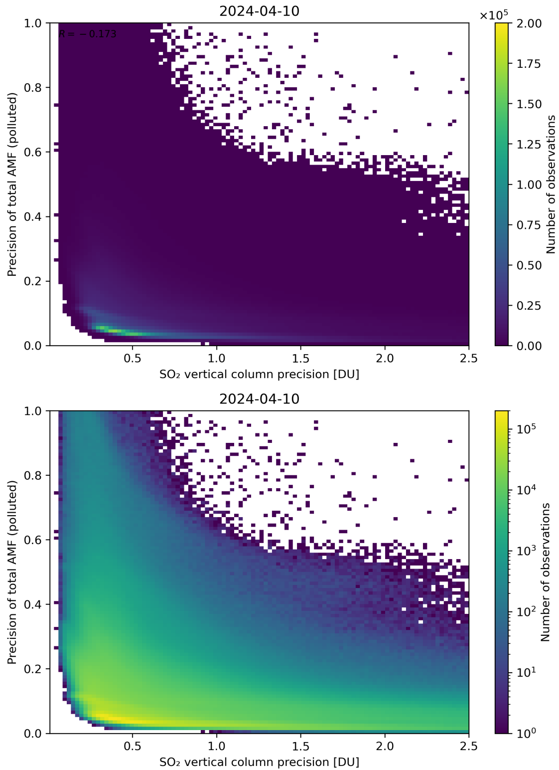
Figure 295: Scatter density plot of “SO 2 vertical column precision” against “Precision of total AMF (polluted)” for 2024-04-10 to 2024-04-11.
