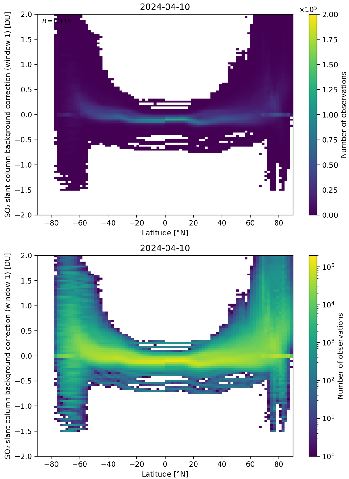
Figure 139: Scatter density plot of “Latitude” against “SO 2 slant column background correction (window 1)” for 2024-04-10 to 2024-04-11.
