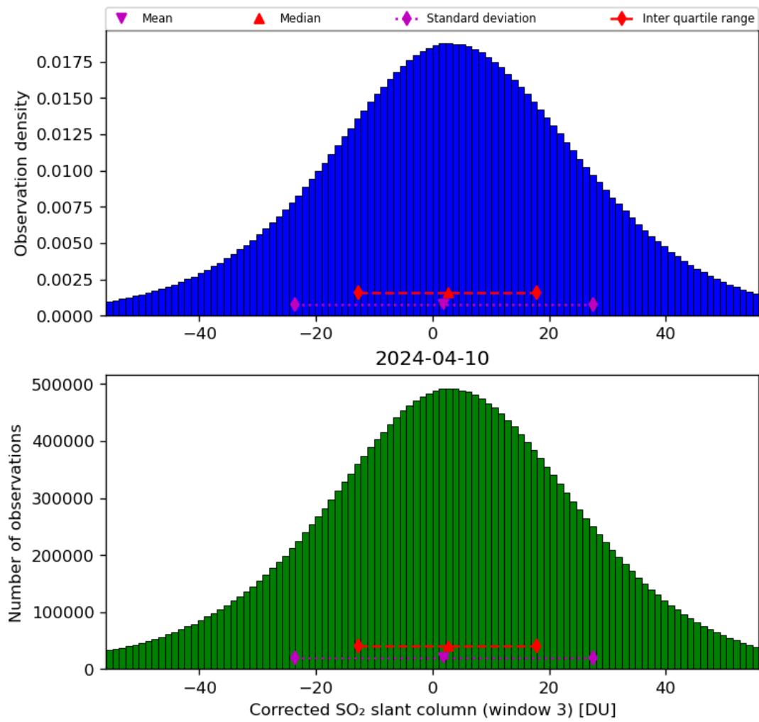
Figure 66: Histogram of “Corrected SO 2 slant column (window 3)” for 2024-04-10 to 2024-04-11
