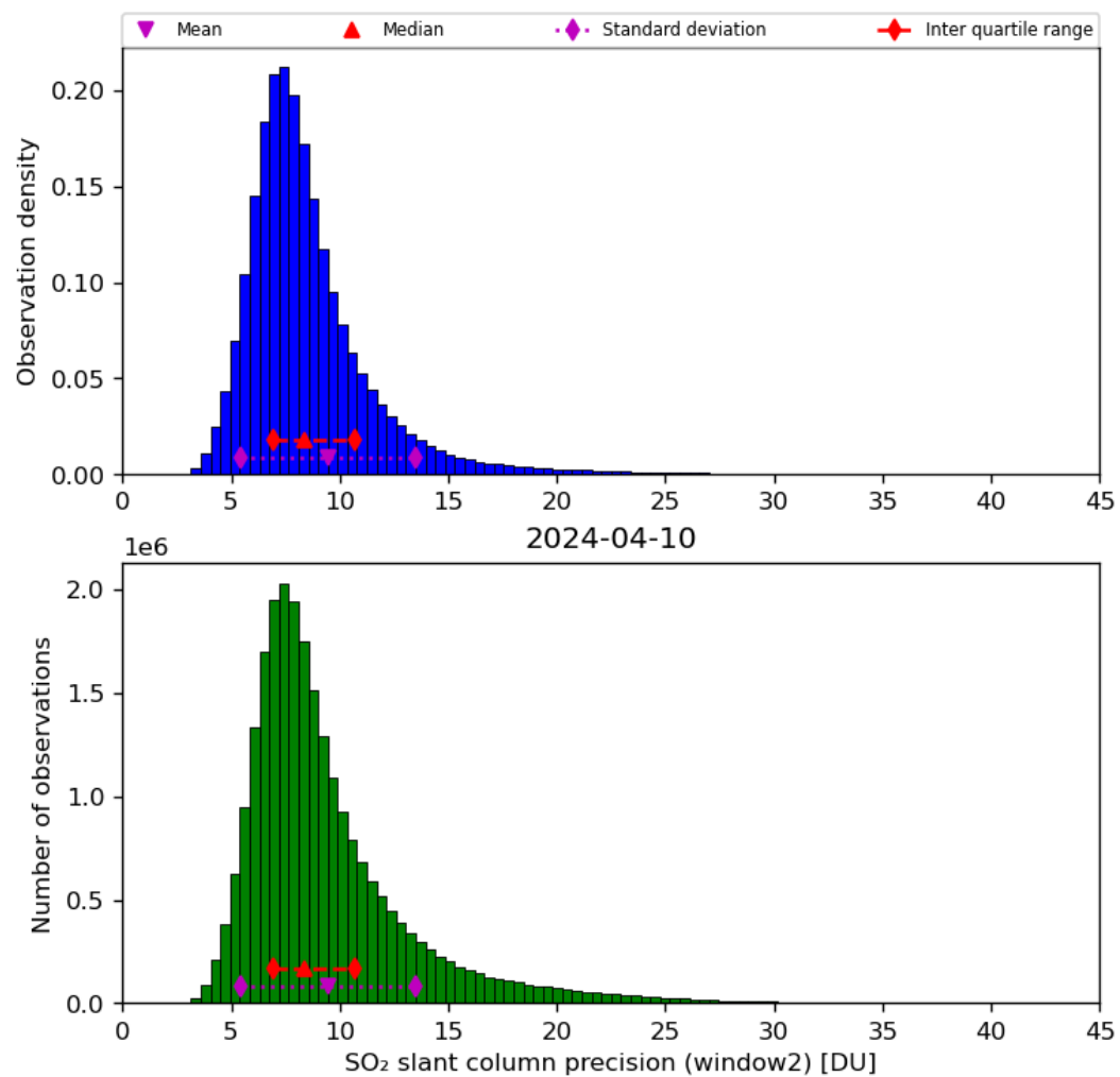
Figure 61: Histogram of “SO 2 slant column precision (window2)” for 2024-04-10 to 2024-04-11
