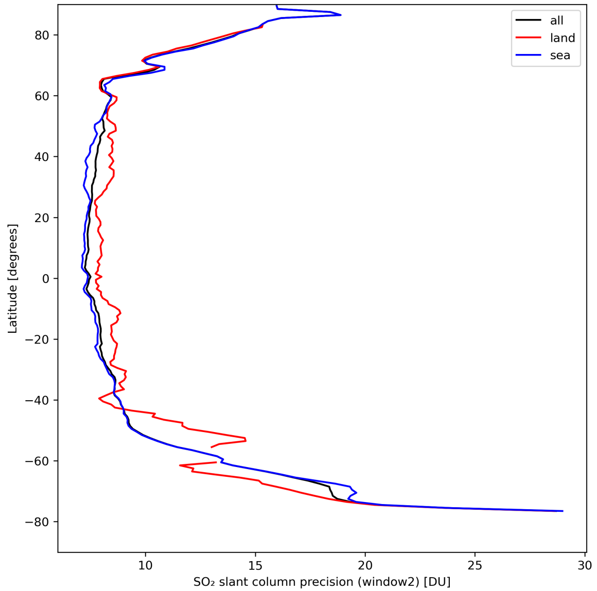
Figure 38: Zonal average of “SO 2 slant column precision (window2)” for 2024-04-10 to 2024-04-12.
