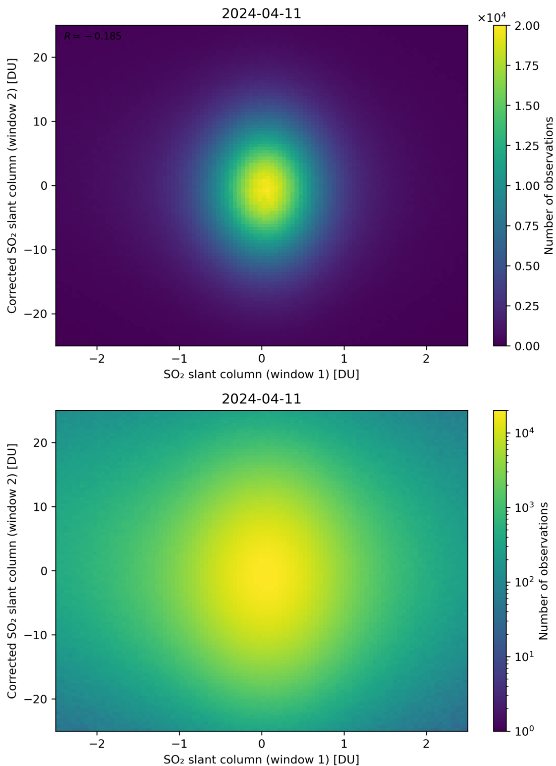
Figure 233: Scatter density plot of “SO 2 slant column (window 1)” against “Corrected SO 2 slant column (window 2)” for 2024-04-10 to 2024-04-12.
