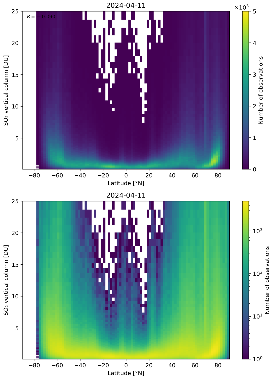
Figure 156: Scatter density plot of “Latitude” against “SO 2 vertical column” for 2024-04-10 to 2024-04-12.
