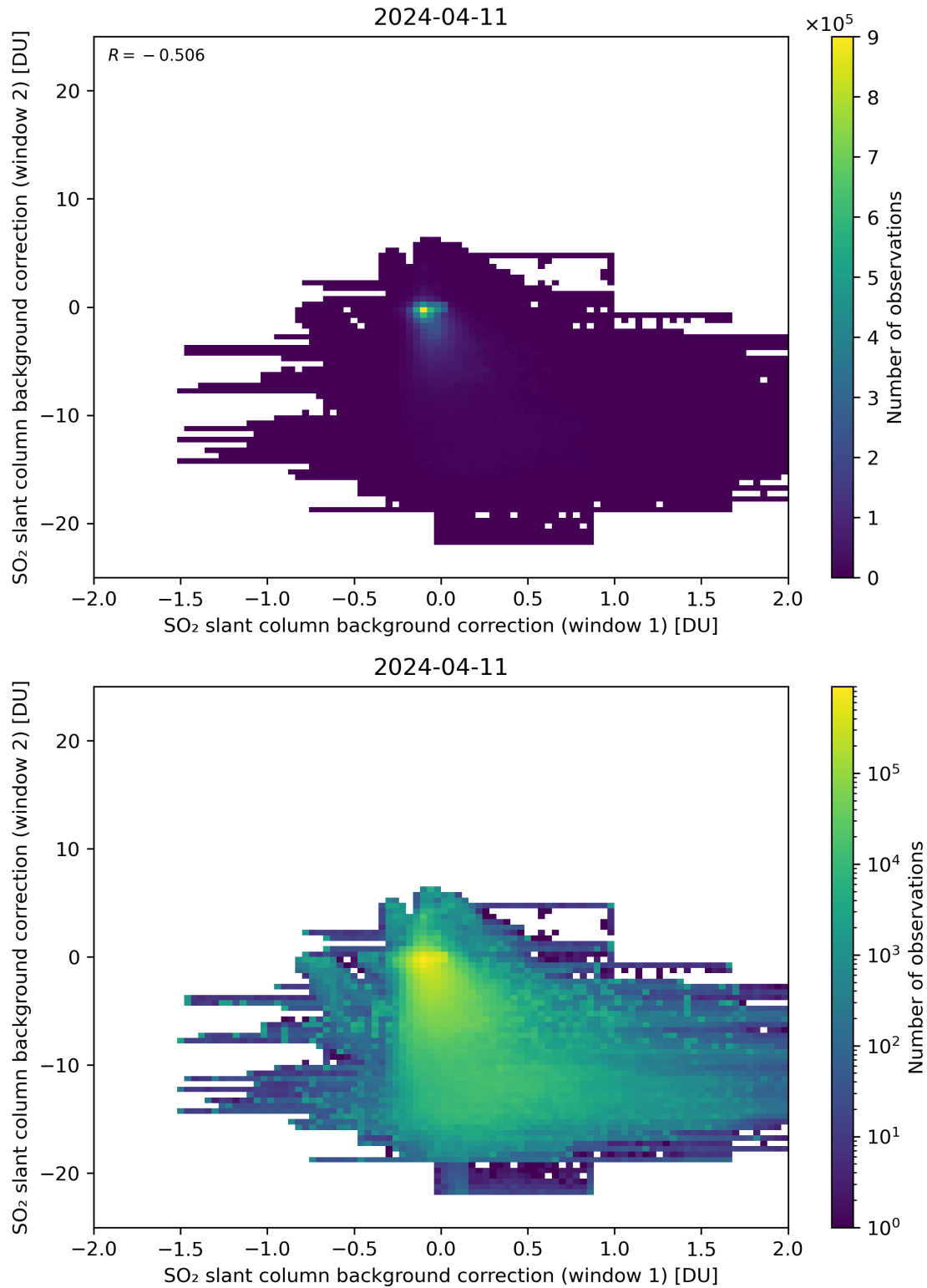
Figure 98: Scatter density plot of “SO 2 slant column background correction (window 1)” against “SO 2 slant column background correction (window 2)” for 2024-04-10 to 2024-04-12.
