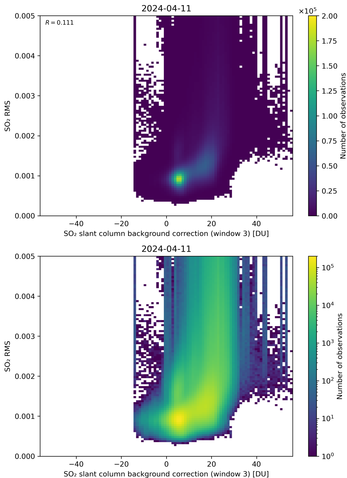
Figure 123: Scatter density plot of “SO 2 slant column background correction (window 3)” against “SO 2 RMS” for 2024-04-10 to 2024-04-12.
