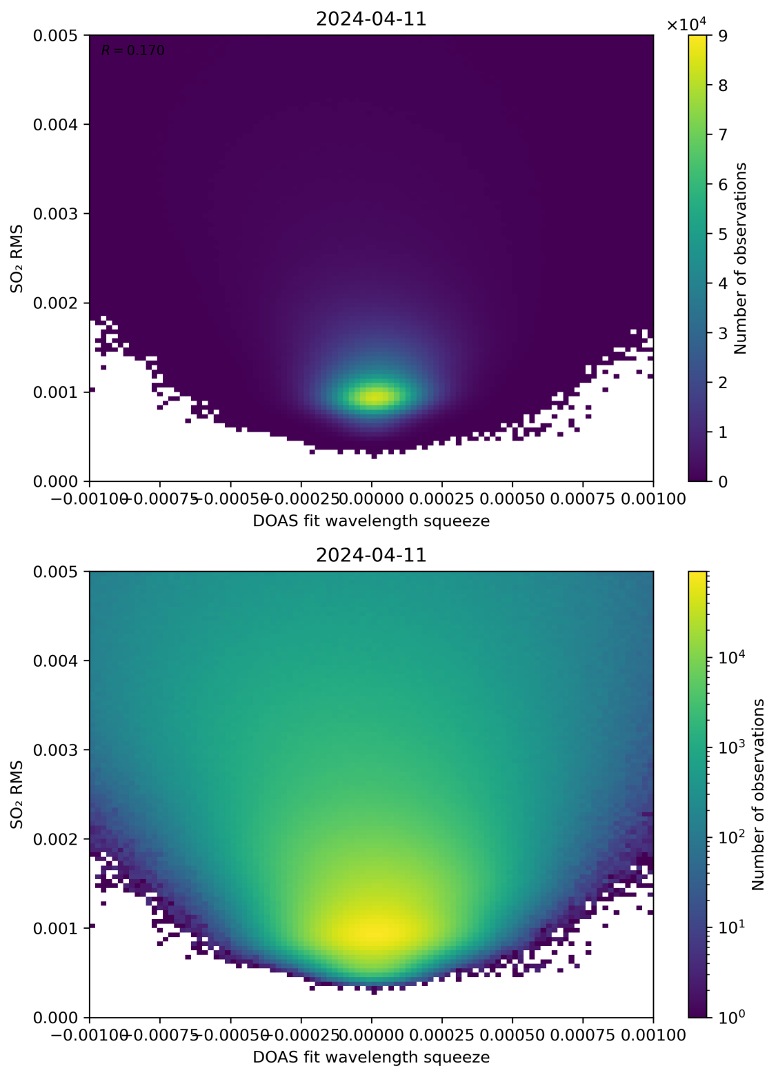
Figure 132: Scatter density plot of “DOAS fit wavelength squeeze” against “SO 2 RMS” for 2024-04-10 to 2024-04-12.
