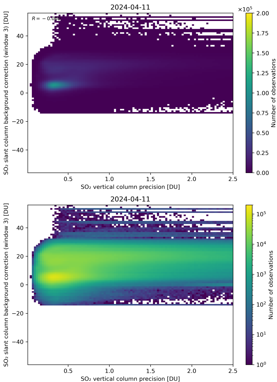
Figure 281: Scatter density plot of “SO 2 vertical column precision” against “SO 2 slant column background correction (window 3)” for 2024-04-10 to 2024-04-12.
