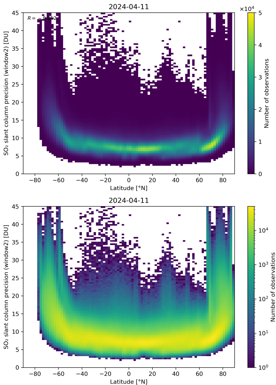
Figure 151: Scatter density plot of “Latitude” against “SO 2 slant column precision (window2)” for 2024-04-10 to 2024-04-12.
