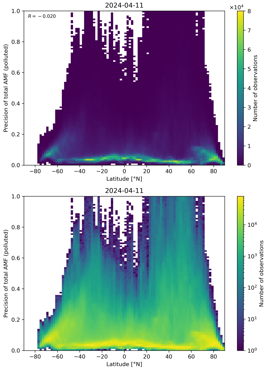
Figure 155: Scatter density plot of “Latitude” against “Precision of total AMF (polluted)” for 2024-04-10 to 2024-04-12.
