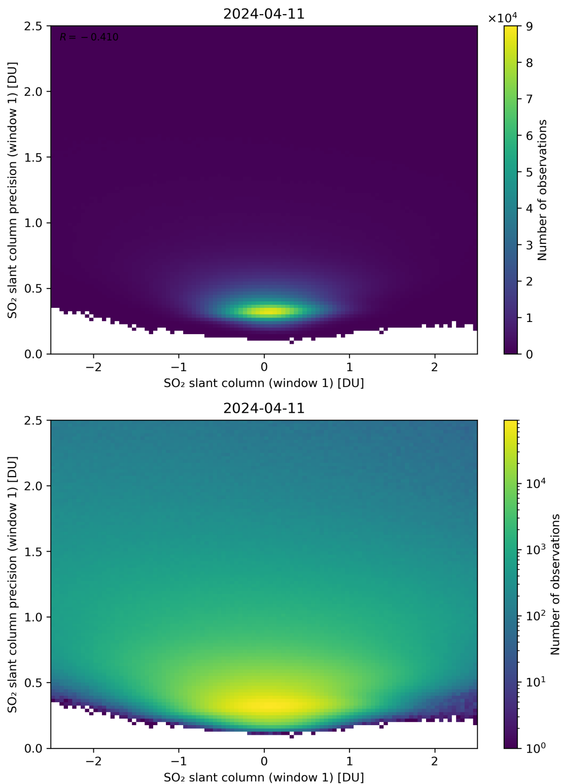
Figure 235: Scatter density plot of “SO 2 slant column (window 1)” against “SO 2 slant column precision (window 1)” for 2024-04-10 to 2024-04-12.
