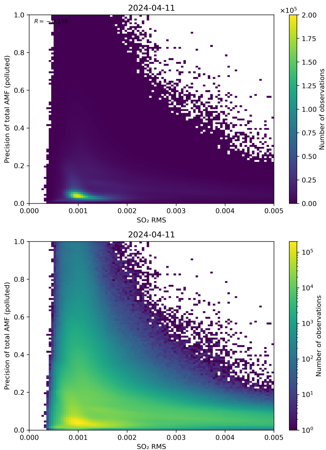
Figure 138: Scatter density plot of “SO 2 RMS” against “Precision of total AMF (polluted)” for 2024-04-10 to 2024-04-12.
