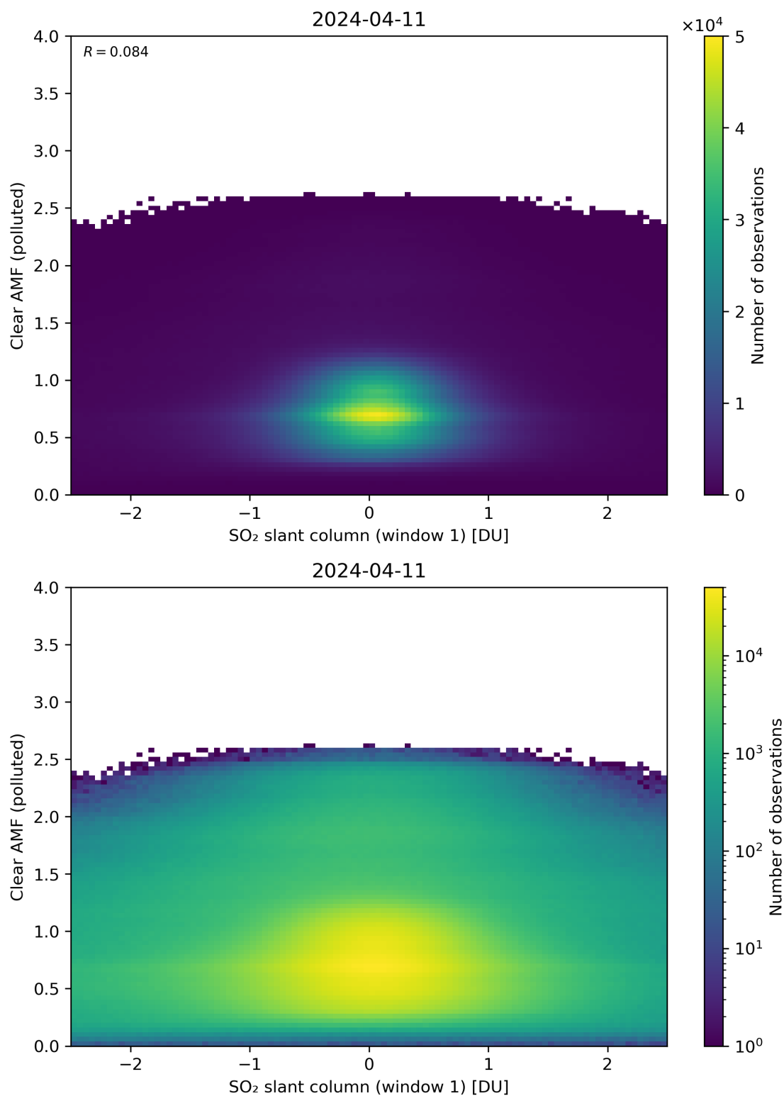
Figure 232: Scatter density plot of “SO 2 slant column (window 1)” against “Clear AMF (polluted)” for 2024-04-10 to 2024-04-12.
