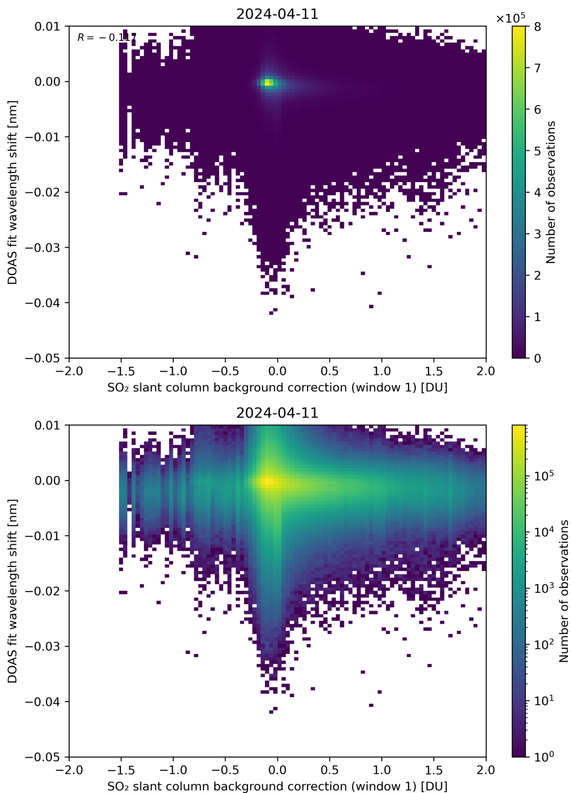
Figure 100: Scatter density plot of “SO 2 slant column background correction (window 1)” against “DOAS fit wavelength shift” for 2024-04-10 to 2024-04-12.
