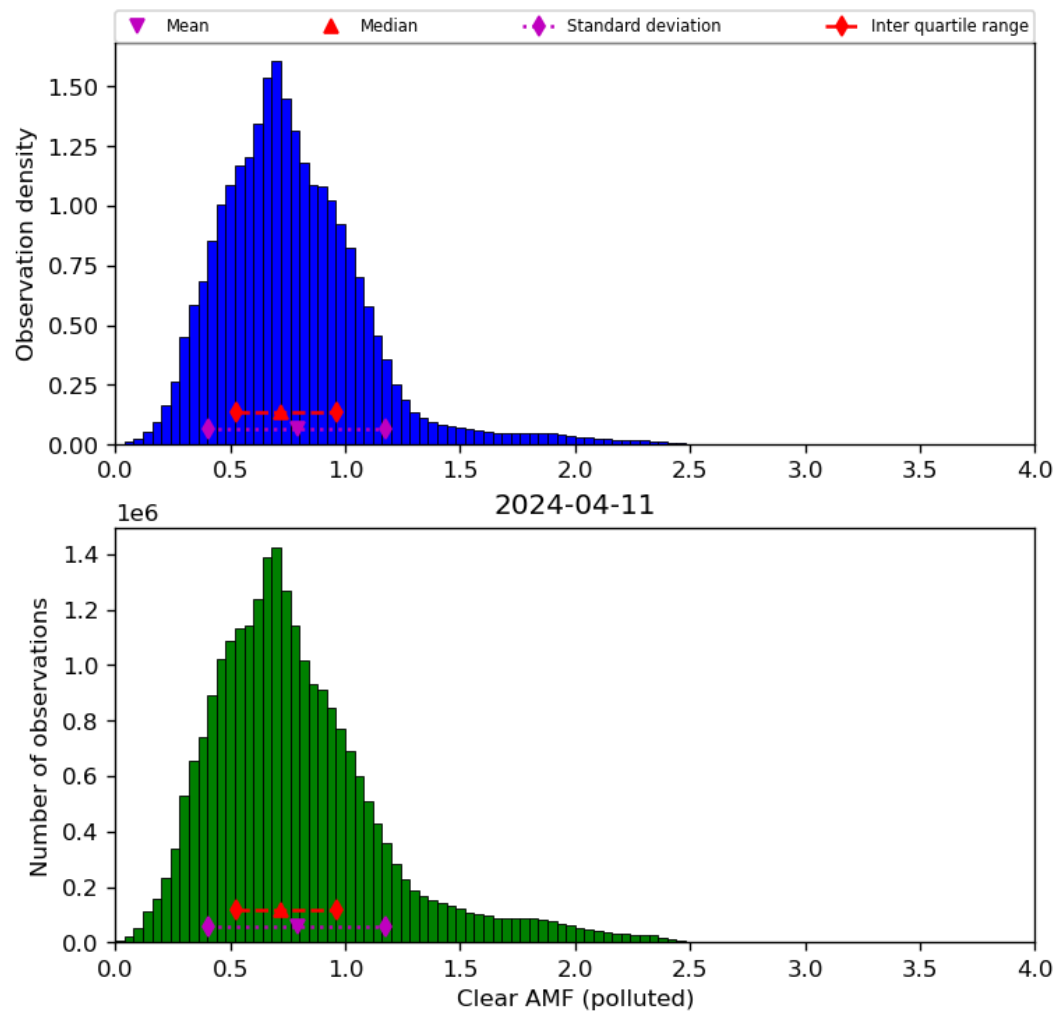
Figure 73: Histogram of “Clear AMF (polluted)” for 2024-04-10 to 2024-04-12
