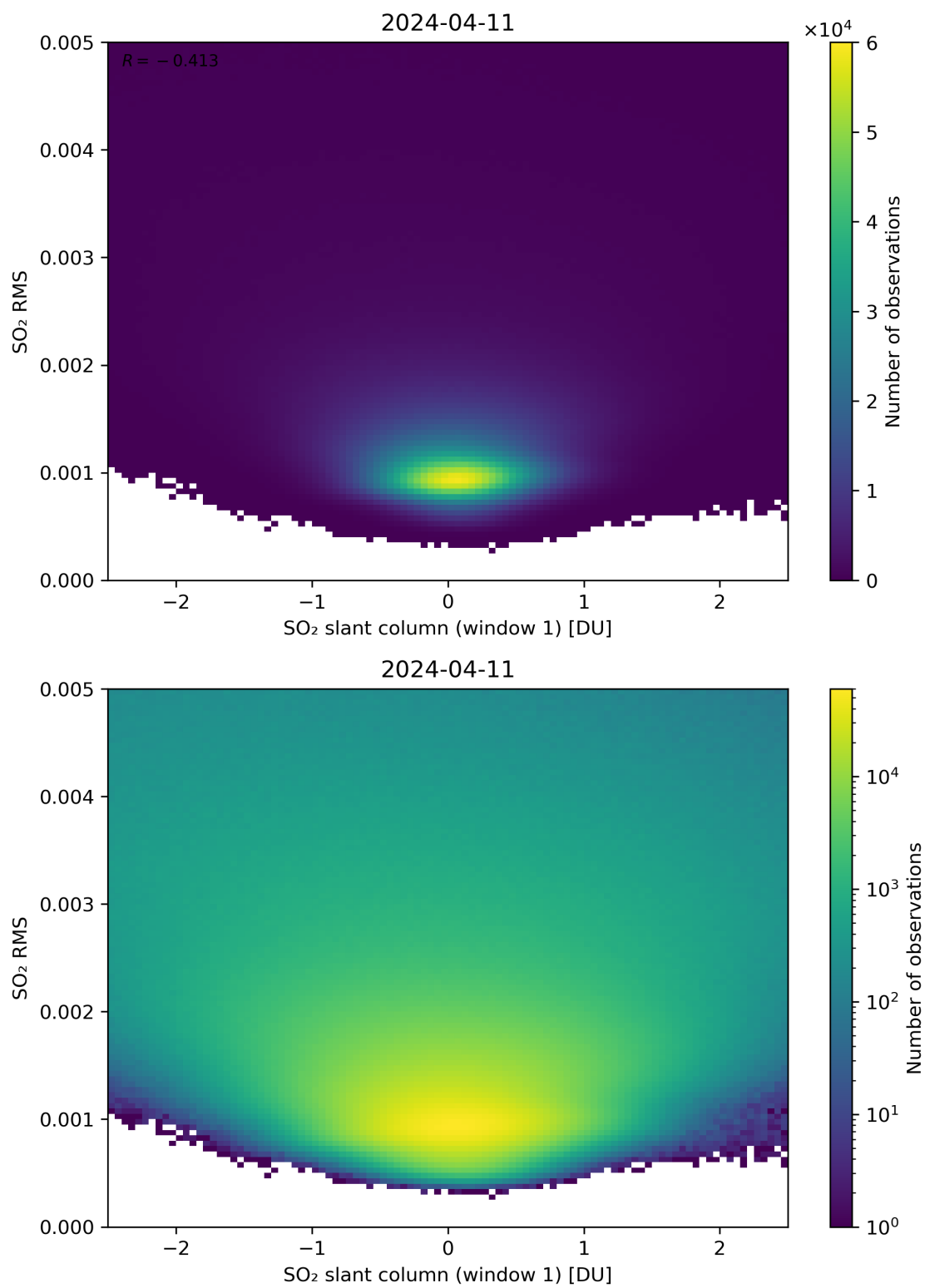
Figure 217: Scatter density plot of “SO 2 slant column (window 1)” against “SO 2 RMS” for 2024-04-10 to 2024-04-12.
