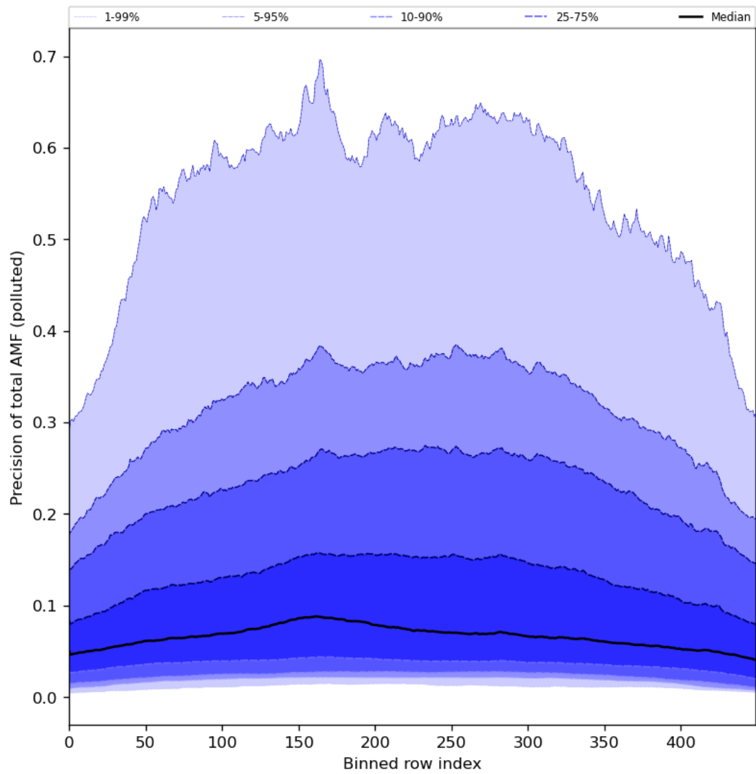
Figure 95: Along track statistics of “Precision of total AMF (polluted)” for 2024-04-10 to 2024-04-12
