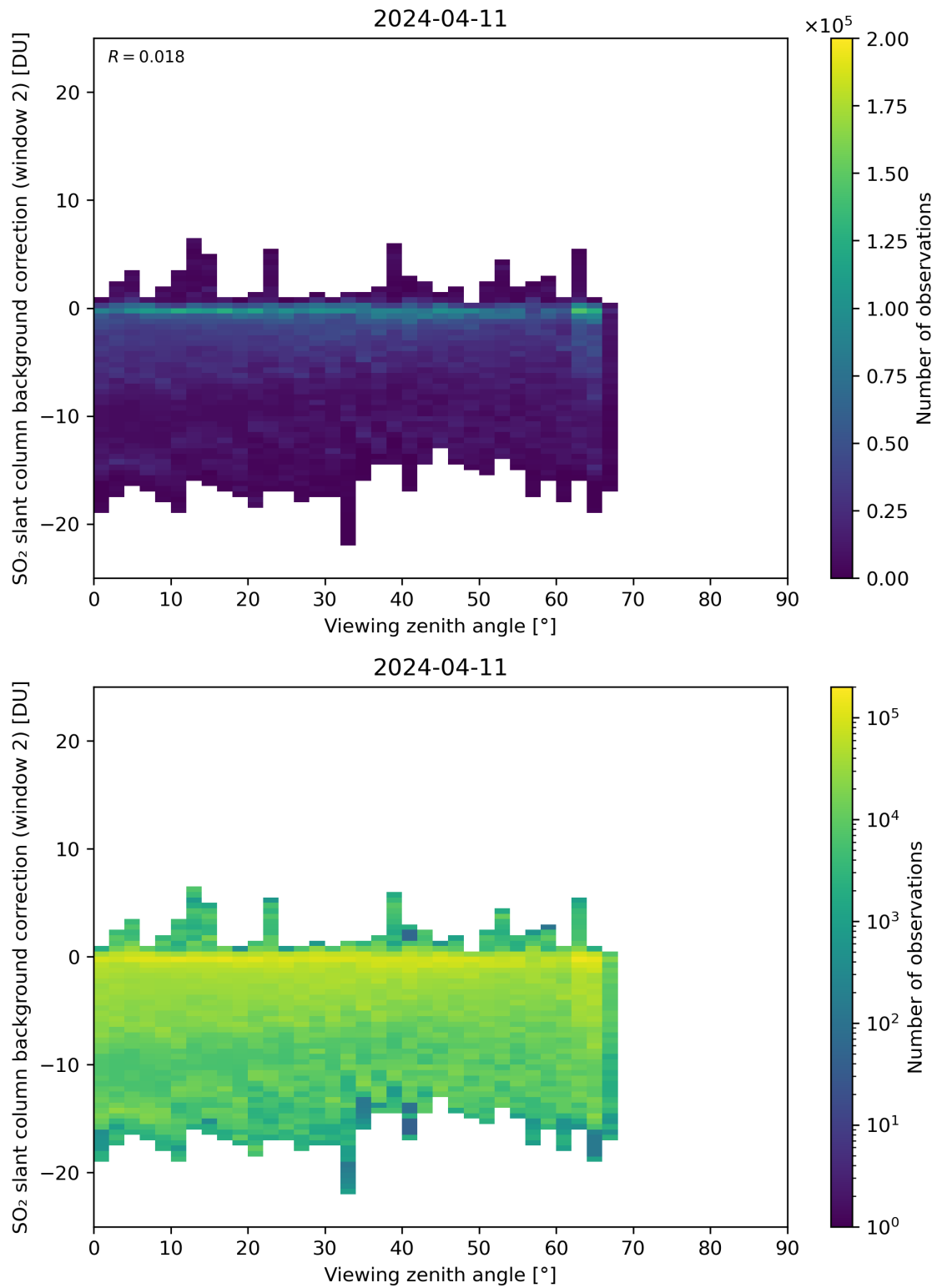
Figure 309: Scatter density plot of “Viewing zenith angle” against “SO 2 slant column background correction (window 2)” for 2024-04-10 to 2024-04-12.
