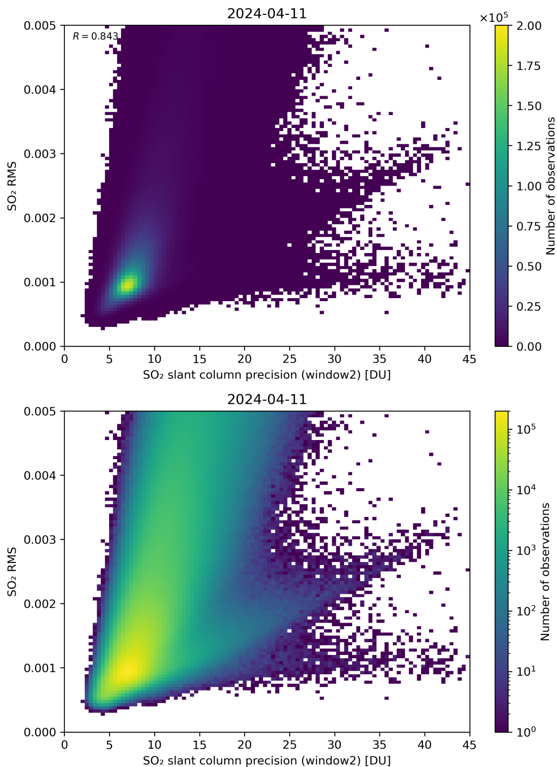
Figure 245: Scatter density plot of “SO 2 slant column precision (window2)” against “SO 2 RMS” for 2024-04-10 to 2024-04-12.
