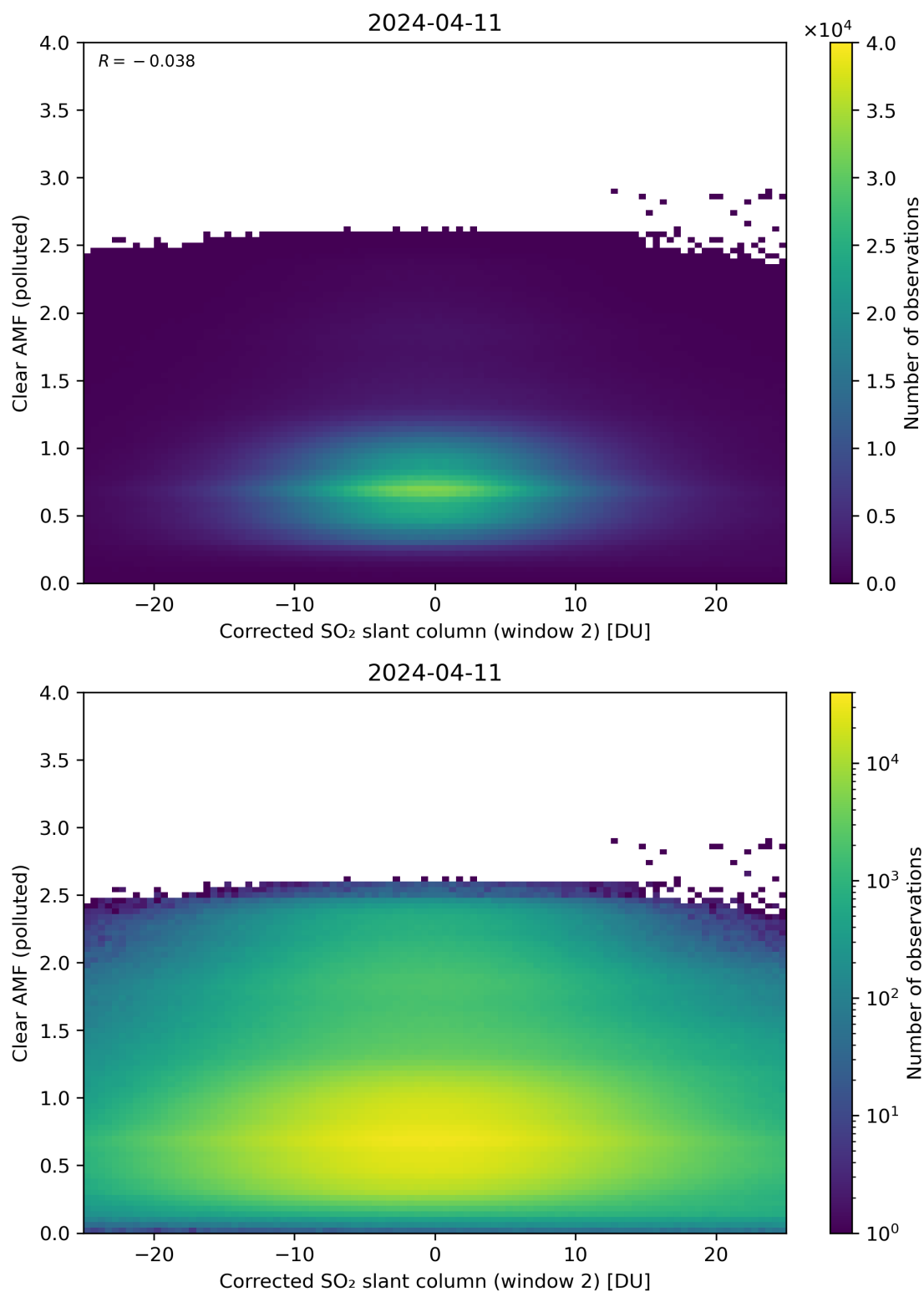
Figure 199: Scatter density plot of “Corrected SO 2 slant column (window 2)” against “Clear AMF (polluted)” for 2024-04-10 to 2024-04-12.
