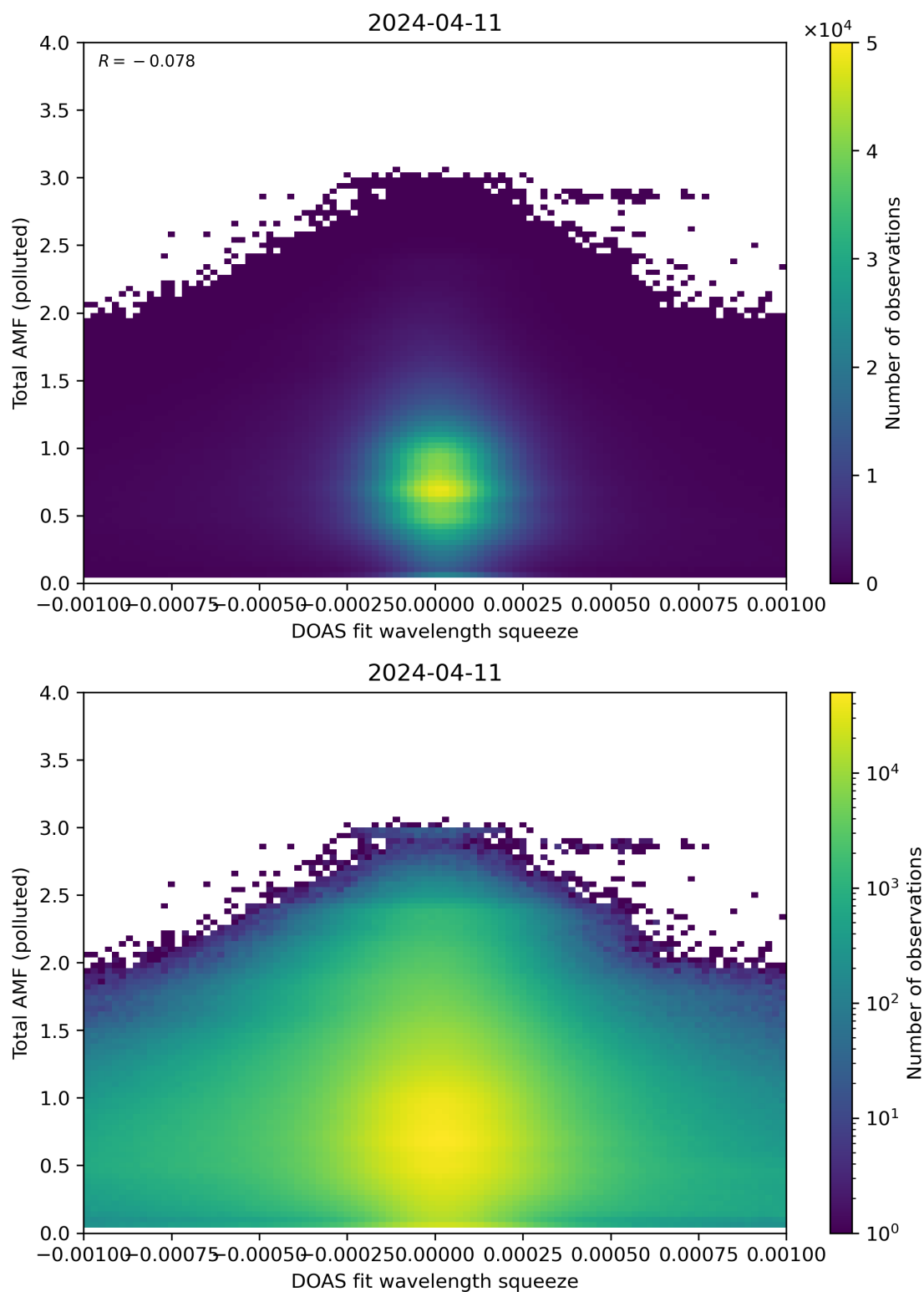
Figure 134: Scatter density plot of “DOAS fit wavelength squeeze” against “Total AMF (polluted)” for 2024-04-10 to 2024-04-12.
