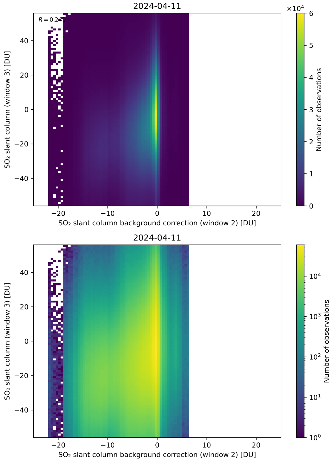
Figure 117: Scatter density plot of “SO 2 slant column background correction (window 2)” against “SO 2 slant column (window 3)” for 2024-04-10 to 2024-04-12.
