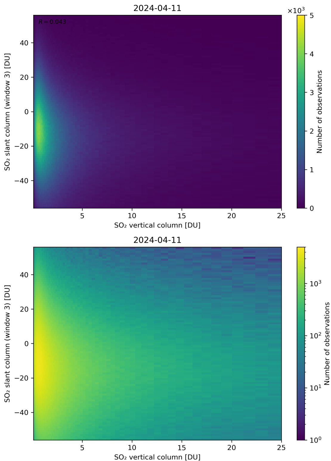
Figure 303: Scatter density plot of “SO 2 vertical column” against “SO 2 slant column (window 3)” for 2024-04-10 to 2024-04-12.
