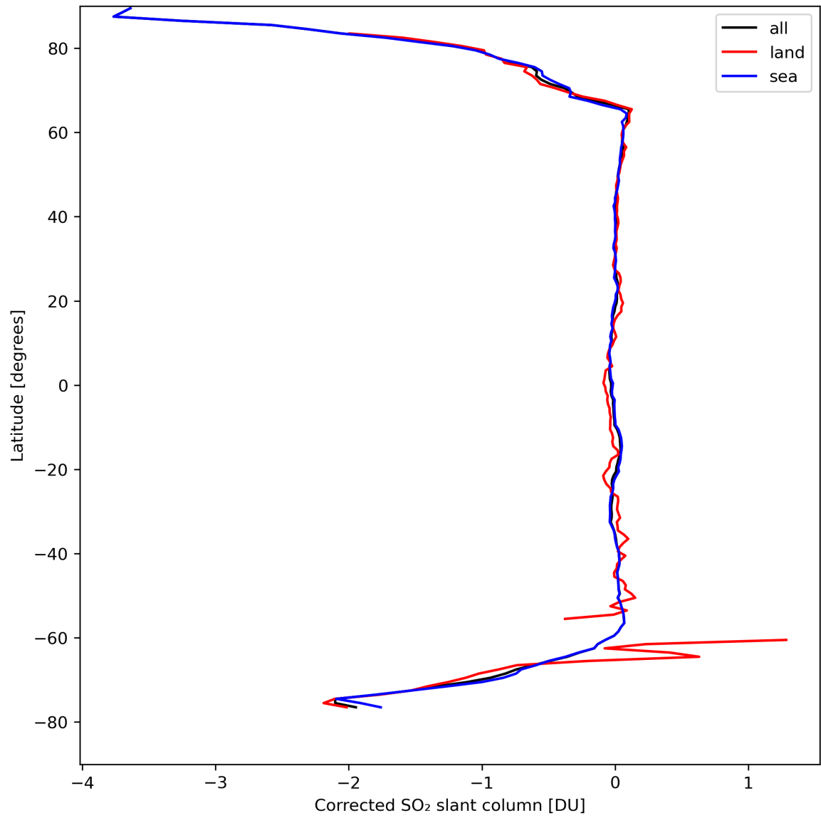
Figure 32: Zonal average of “Corrected SO 2 slant column” for 2024-04-10 to 2024-04-12.
