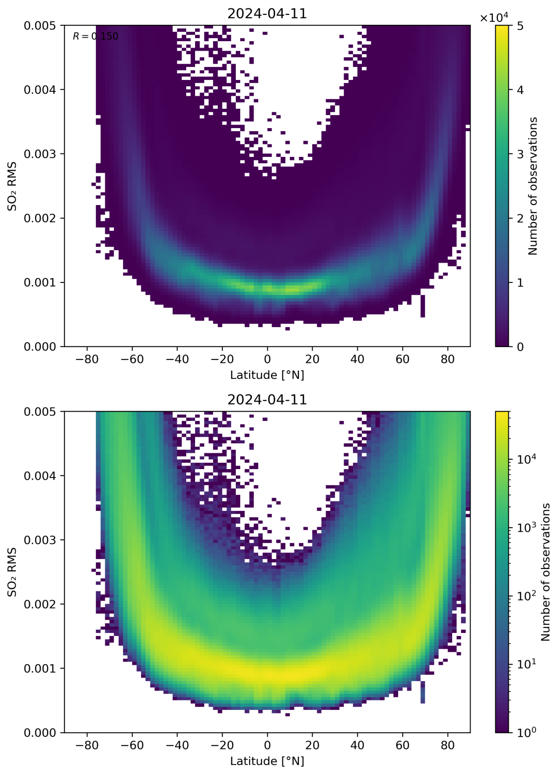
Figure 144: Scatter density plot of “Latitude” against “SO 2 RMS” for 2024-04-10 to 2024-04-12.
