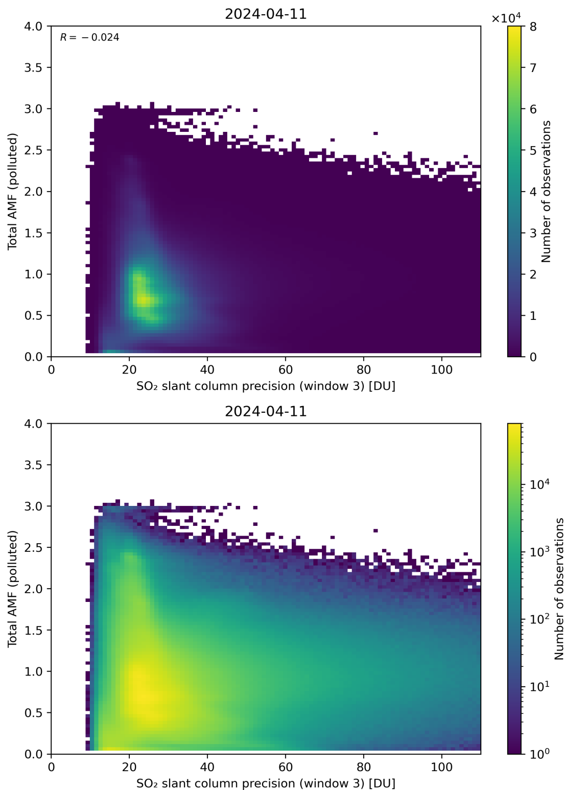
Figure 263: Scatter density plot of “SO 2 slant column precision (window 3)” against “Total AMF (polluted)” for 2024-04-10 to 2024-04-12.
