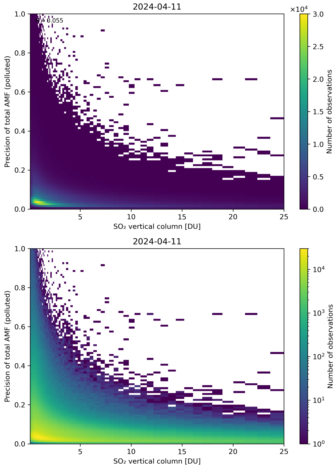
Figure 306: Scatter density plot of “SO 2 vertical column” against “Precision of total AMF (polluted)” for 2024-04-10 to 2024-04-12.
