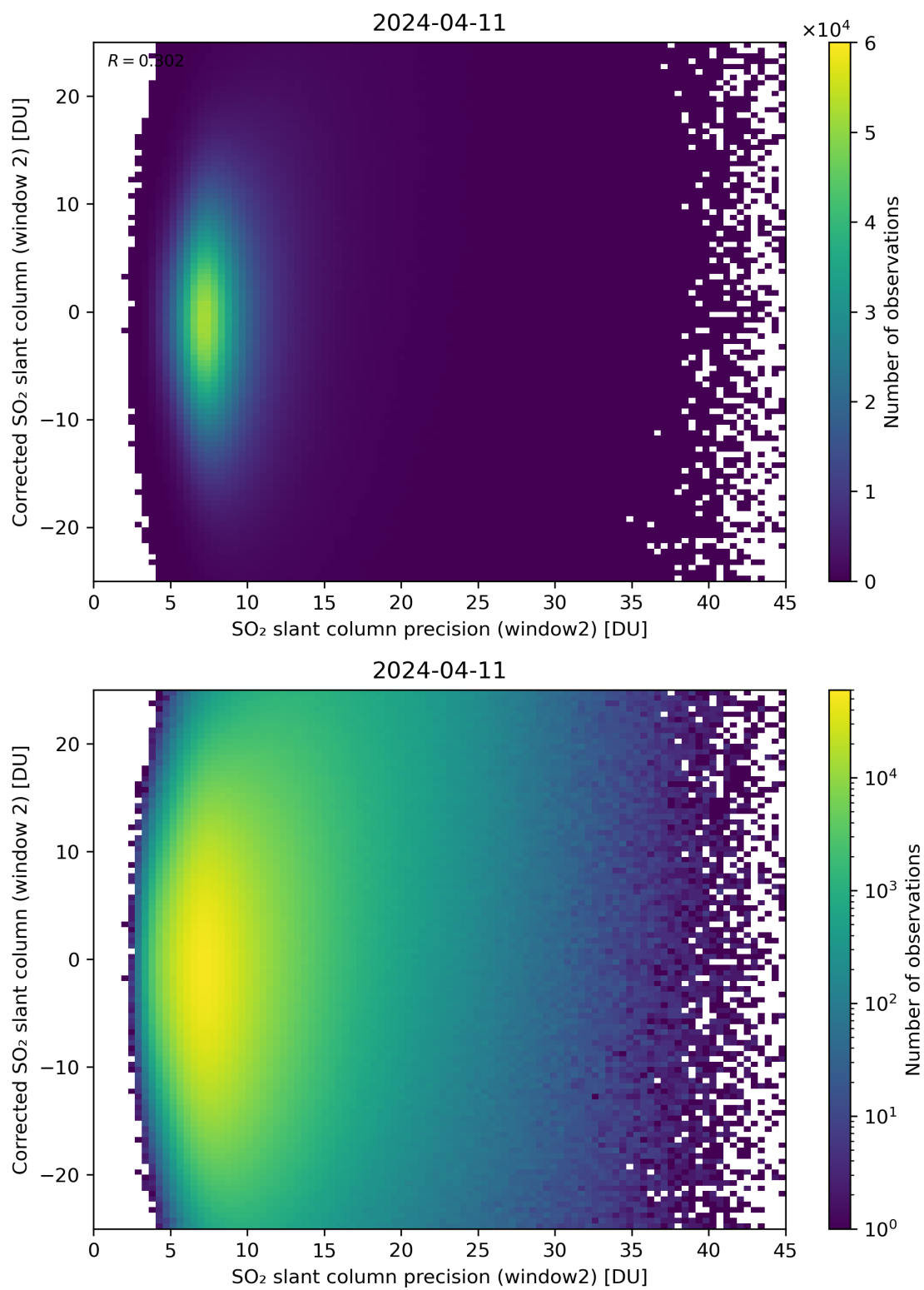
Figure 247: Scatter density plot of “SO 2 slant column precision (window2)” against “Corrected SO 2 slant column (window 2)” for 2024-04-10 to 2024-04-12.
