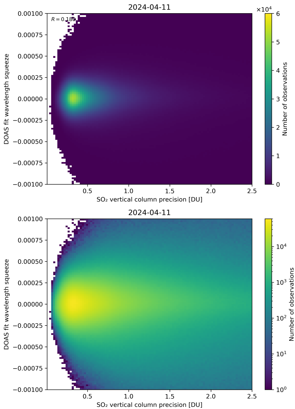
Figure 283: Scatter density plot of “SO 2 vertical column precision” against “DOAS fit wavelength squeeze” for 2024-04-10 to 2024-04-12.
