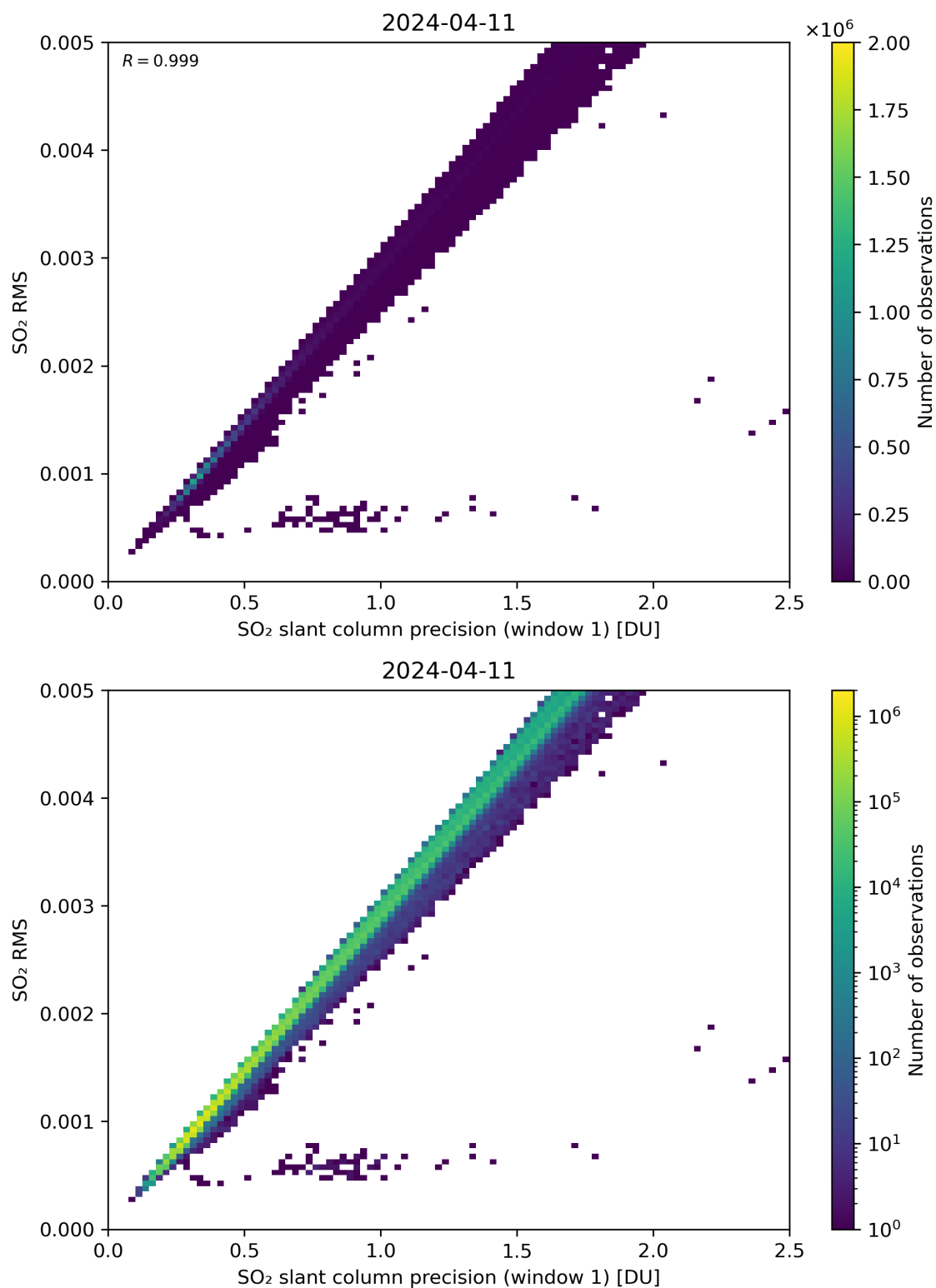
Figure 223: Scatter density plot of “SO 2 slant column precision (window 1)” against “SO 2 RMS” for 2024-04-10 to 2024-04-12.
