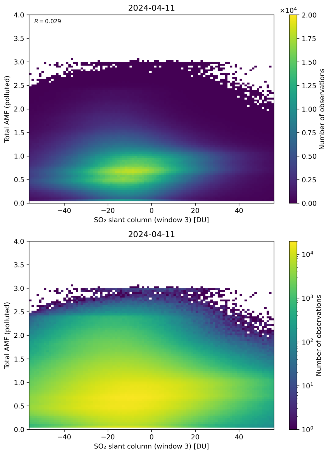
Figure 268: Scatter density plot of “SO 2 slant column (window 3)” against “Total AMF (polluted)” for 2024-04-10 to 2024-04-12.
