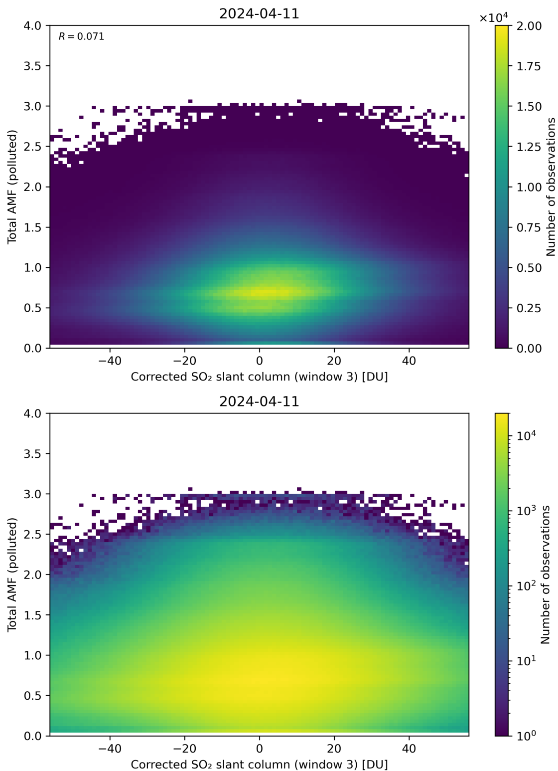
Figure 210: Scatter density plot of “Corrected SO 2 slant column (window 3)” against “Total AMF (polluted)” for 2024-04-10 to 2024-04-12.
