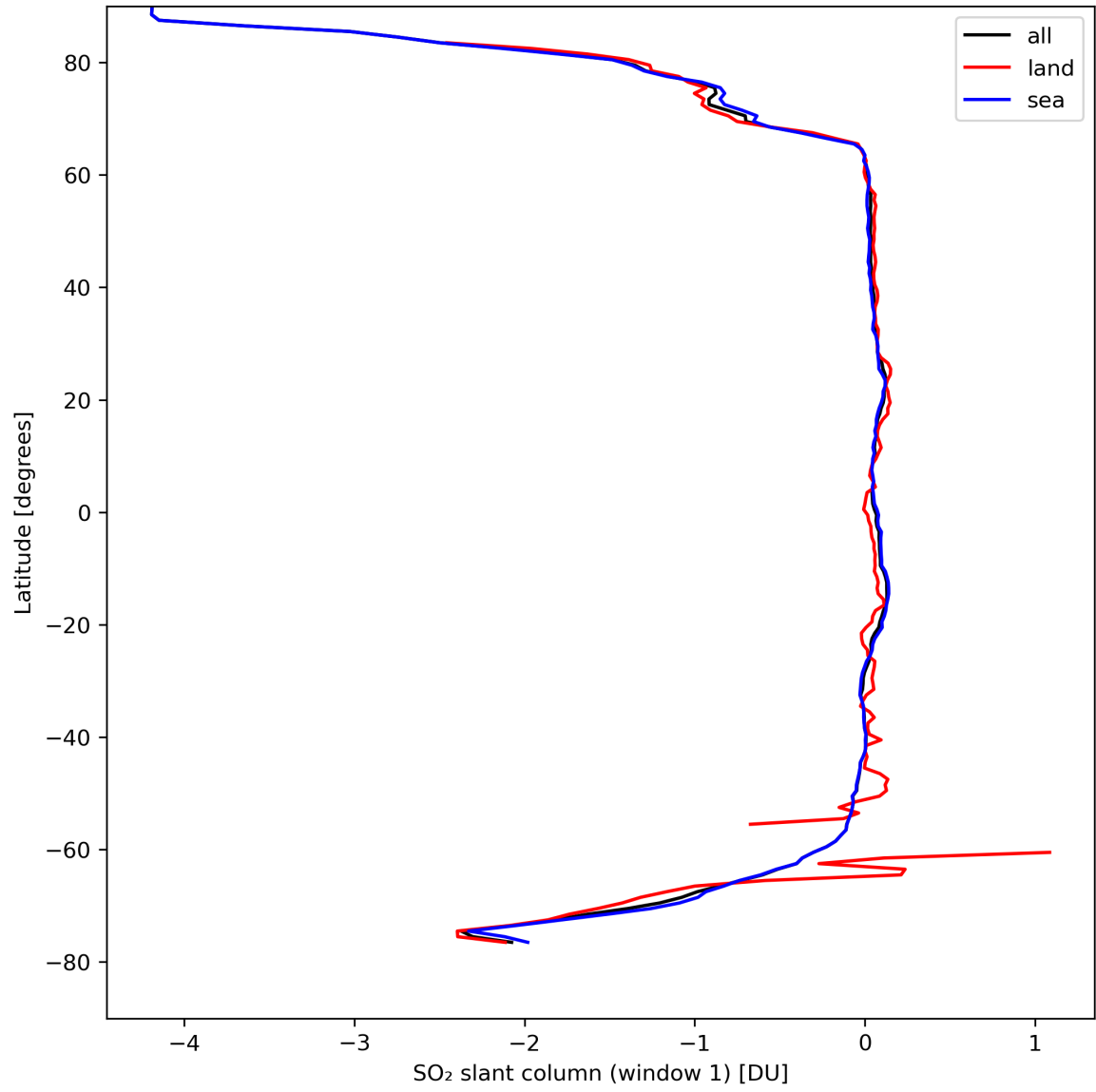
Figure 33: Zonal average of “SO 2 slant column (window 1)” for 2024-04-10 to 2024-04-12.
