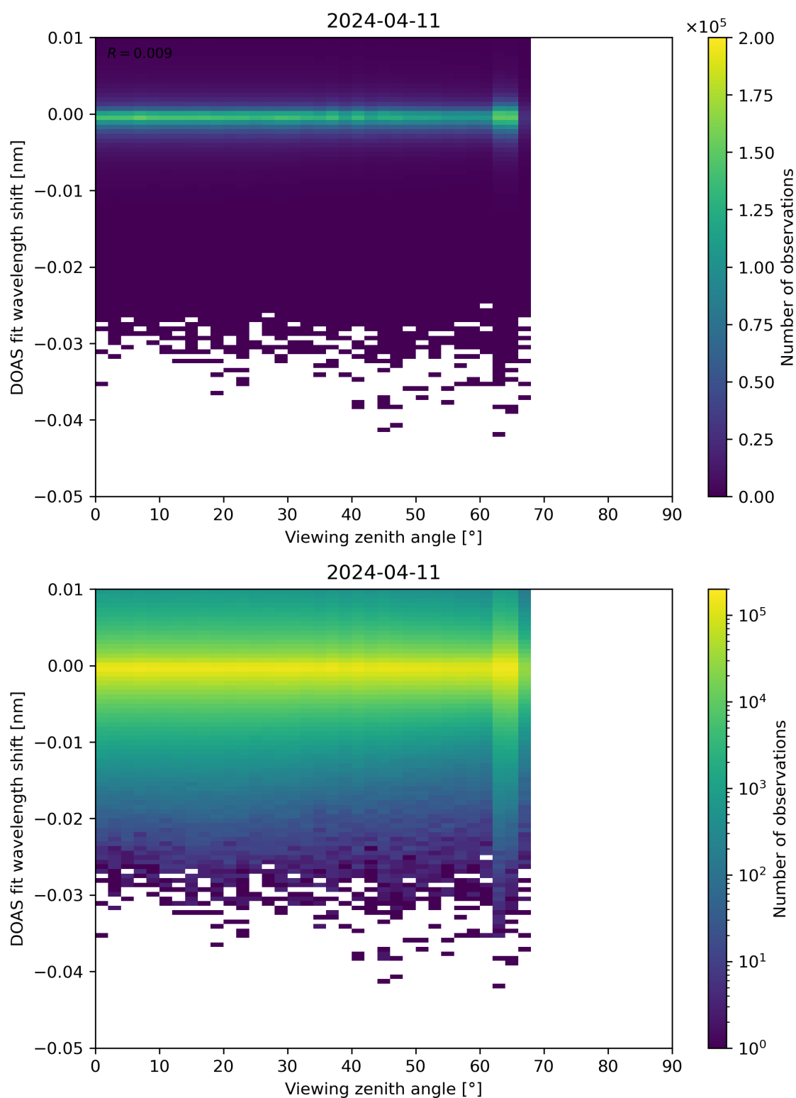
Figure 311: Scatter density plot of “Viewing zenith angle” against “DOAS fit wavelength shift” for 2024-04-10 to 2024-04-12.
