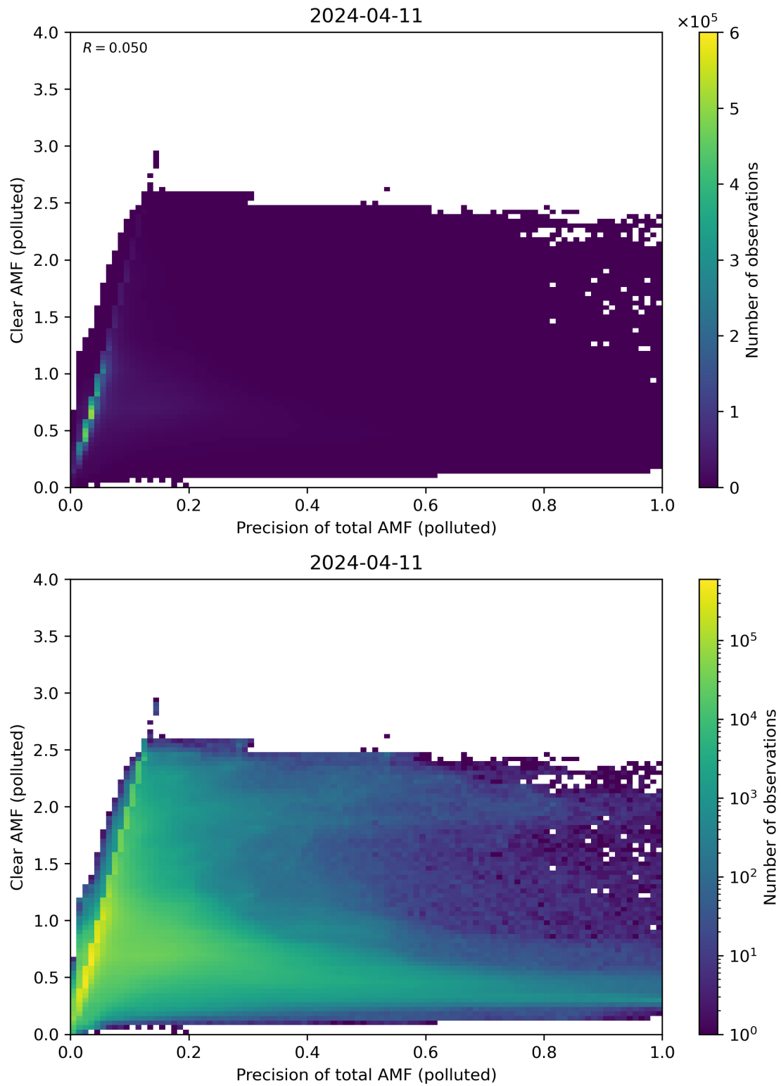
Figure 270: Scatter density plot of “Precision of total AMF (polluted)” against “Clear AMF (polluted)” for 2024-04-10 to 2024-04-12.
