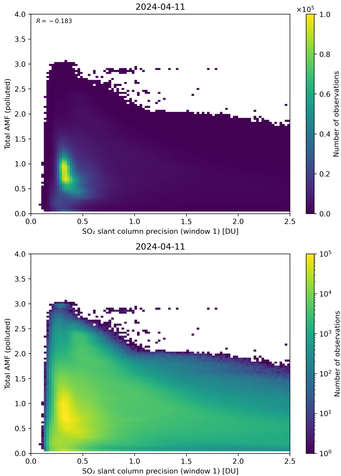
Figure 230: Scatter density plot of “SO 2 slant column precision (window 1)” against “Total AMF (polluted)” for 2024-04-10 to 2024-04-12.
