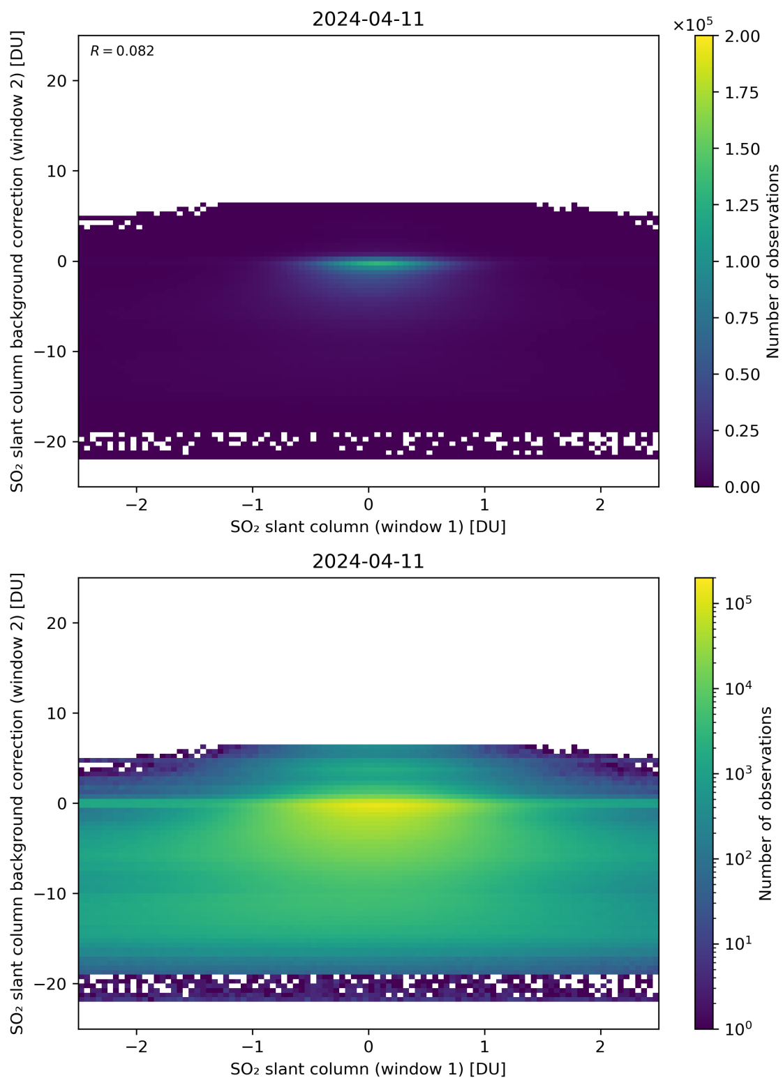
Figure 213: Scatter density plot of “SO 2 slant column (window 1)” against “SO 2 slant column background correction (window 2)” for 2024-04-10 to 2024-04-12.
