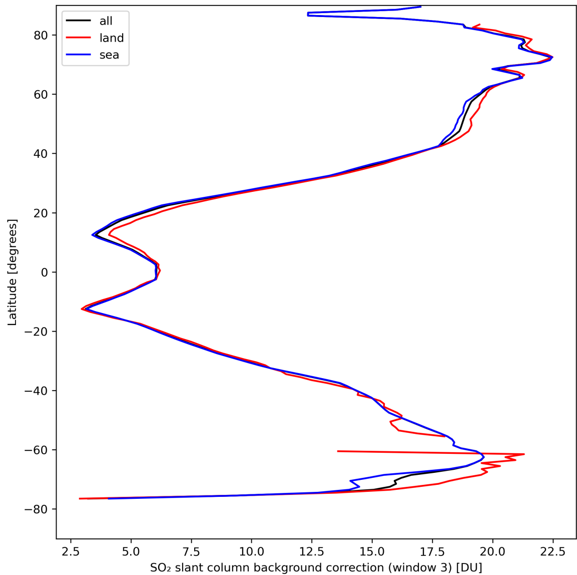
Figure 44: Zonal average of “SO 2 slant column background correction (window 3)” for 2024-04-10 to 2024-04-12.
