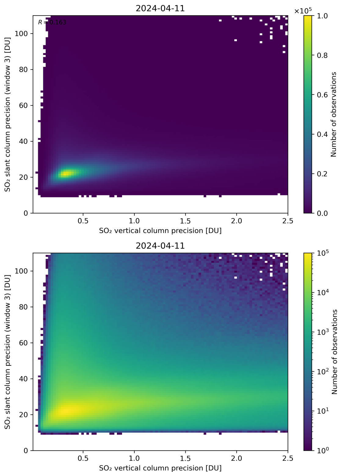
Figure 293: Scatter density plot of “SO 2 vertical column precision” against “SO 2 slant column precision (window 3)” for 2024-04-10 to 2024-04-12.
