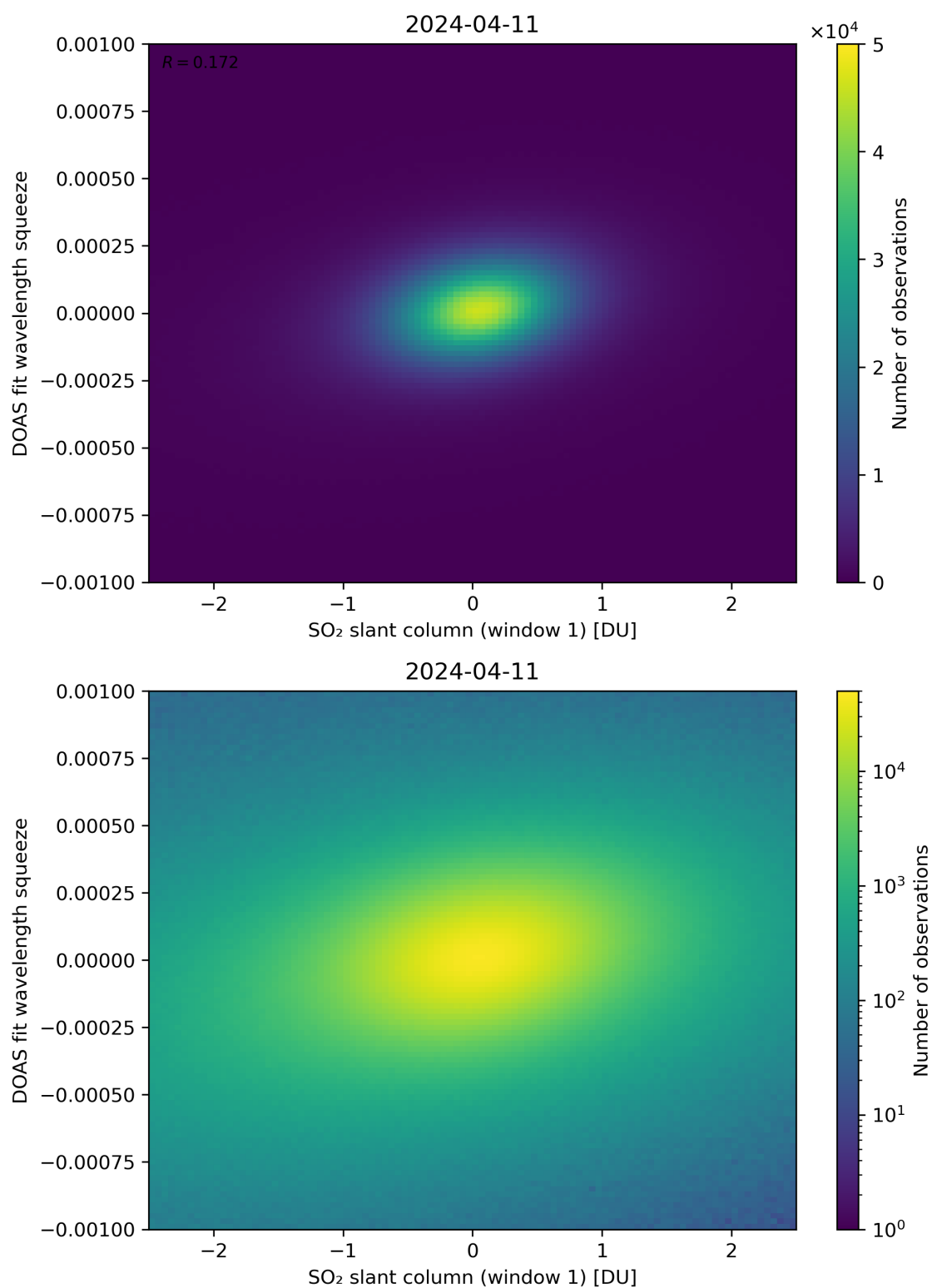
Figure 216: Scatter density plot of “SO 2 slant column (window 1)” against “DOAS fit wavelength squeeze” for 2024-04-10 to 2024-04-12.
