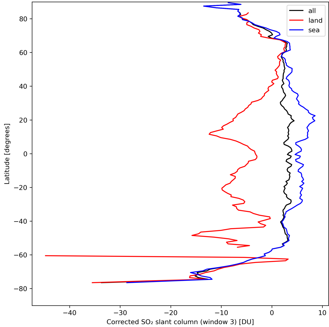
Figure 43: Zonal average of “Corrected SO 2 slant column (window 3)” for 2024-04-10 to 2024-04-12.
