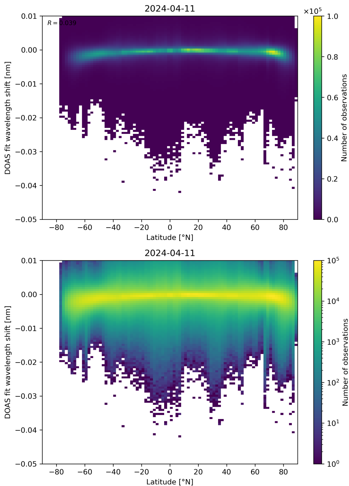
Figure 142: Scatter density plot of “Latitude” against “DOAS fit wavelength shift” for 2024-04-10 to 2024-04-12.
