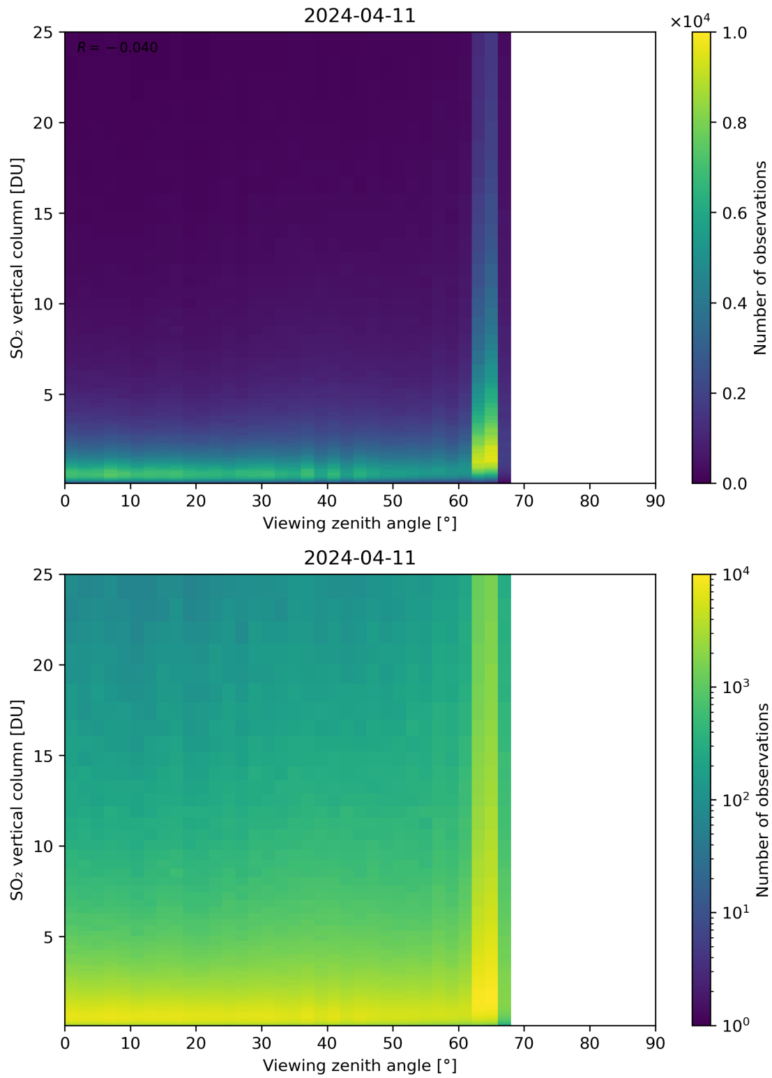
Figure 327: Scatter density plot of “Viewing zenith angle” against “SO 2 vertical column” for 2024-04-10 to 2024-04-12.
