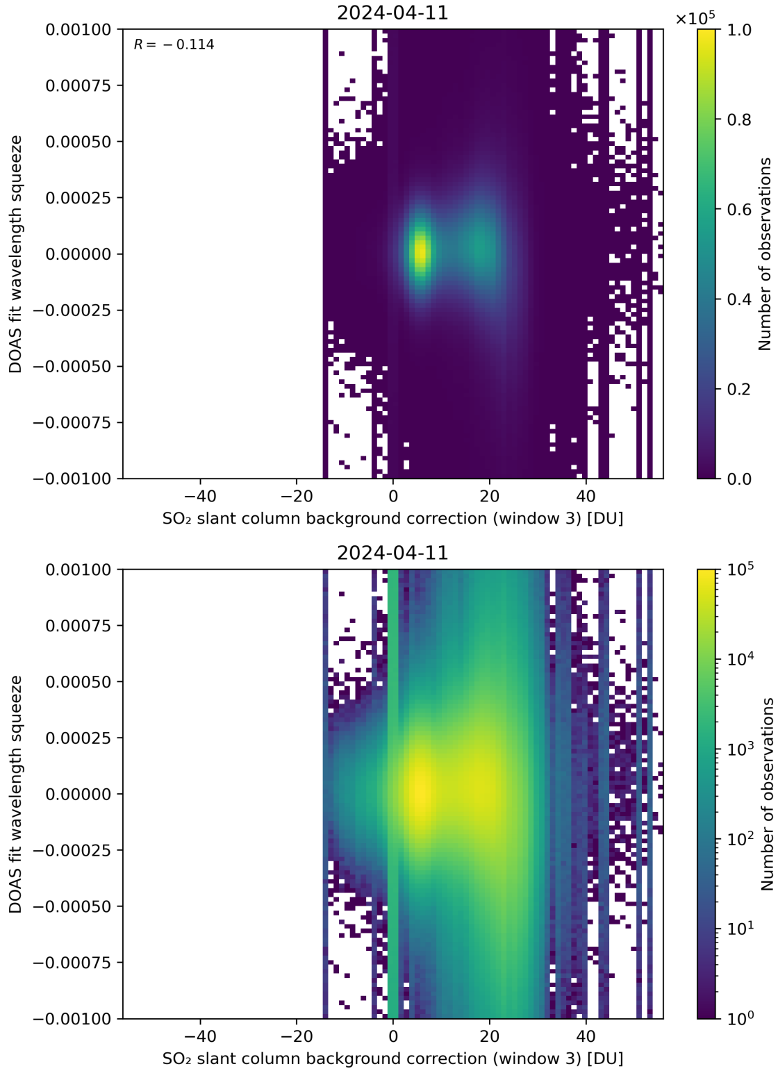
Figure 122: Scatter density plot of “SO 2 slant column background correction (window 3)” against “DOAS fit wavelength squeeze” for 2024-04-10 to 2024-04-12.
