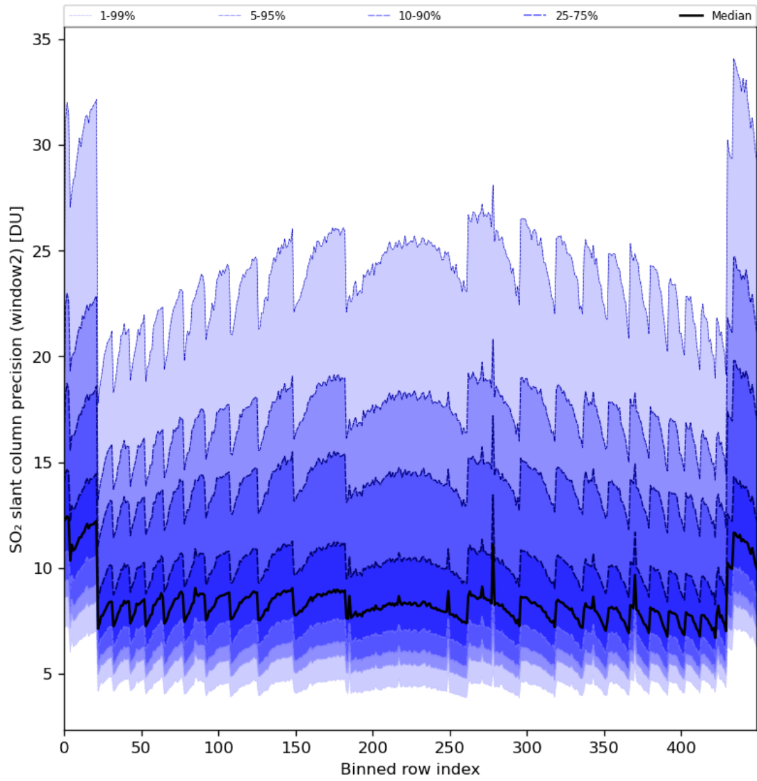
Figure 84: Along track statistics of “SO 2 slant column precision (window2)” for 2024-04-10 to 2024-04-12
