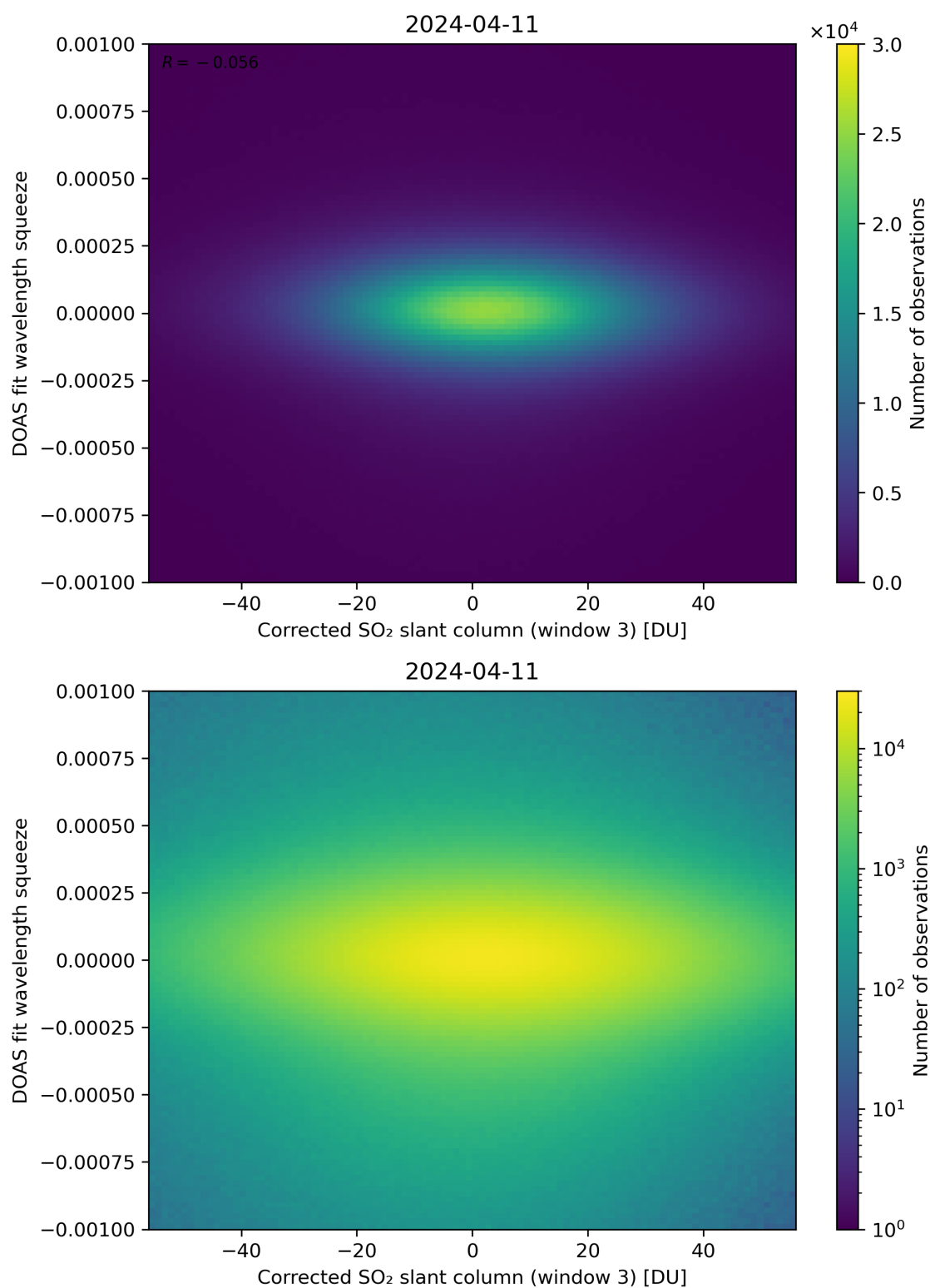
Figure 207: Scatter density plot of “Corrected SO 2 slant column (window 3)” against “DOAS fit wavelength squeeze” for 2024-04-10 to 2024-04-12.
