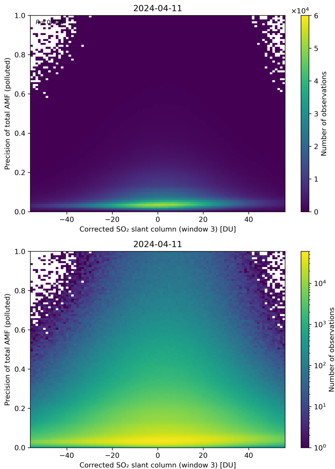
Figure 211: Scatter density plot of “Corrected SO 2 slant column (window 3)” against “Precision of total AMF (polluted)” for 2024-04-10 to 2024-04-12.
