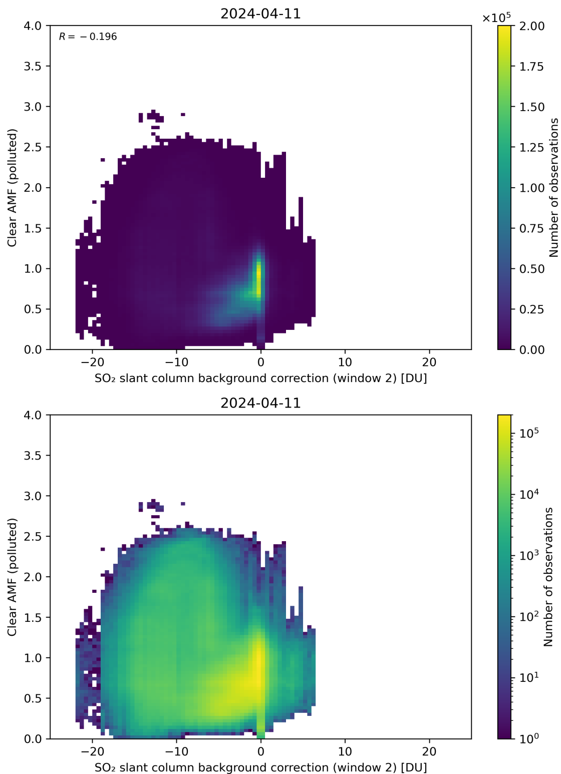
Figure 115: Scatter density plot of “SO 2 slant column background correction (window 2)” against “Clear AMF (polluted)” for 2024-04-10 to 2024-04-12.
