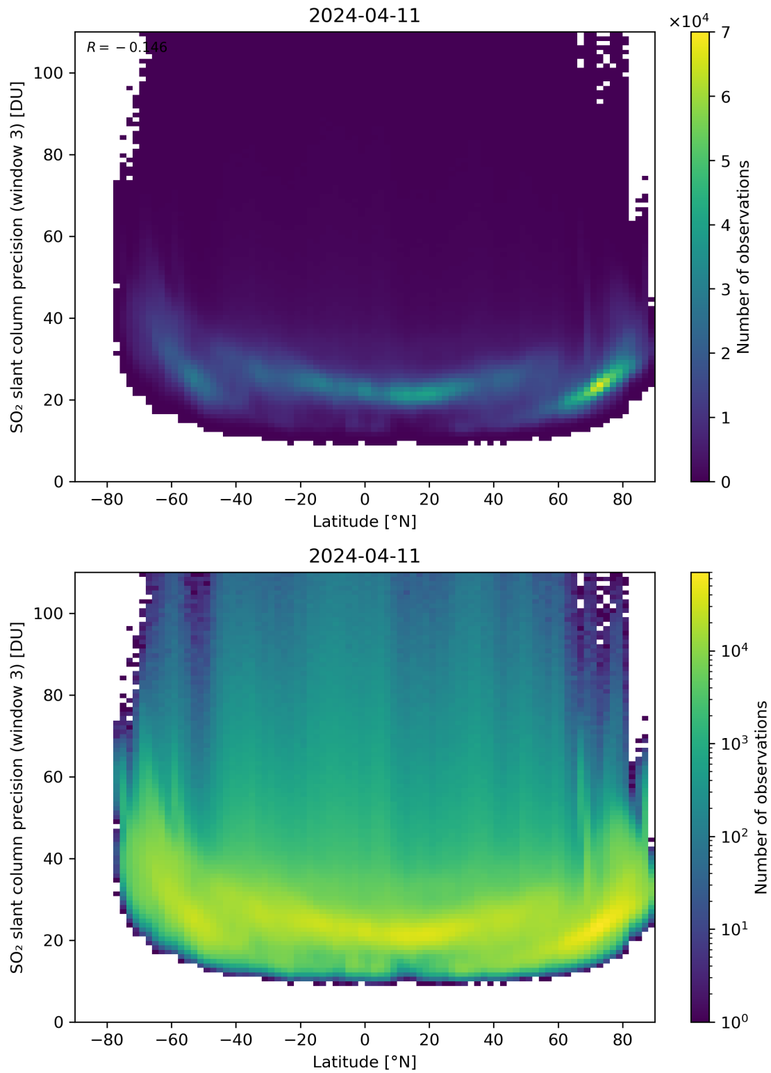
Figure 153: Scatter density plot of “Latitude” against “SO 2 slant column precision (window 3)” for 2024-04-10 to 2024-04-12.
