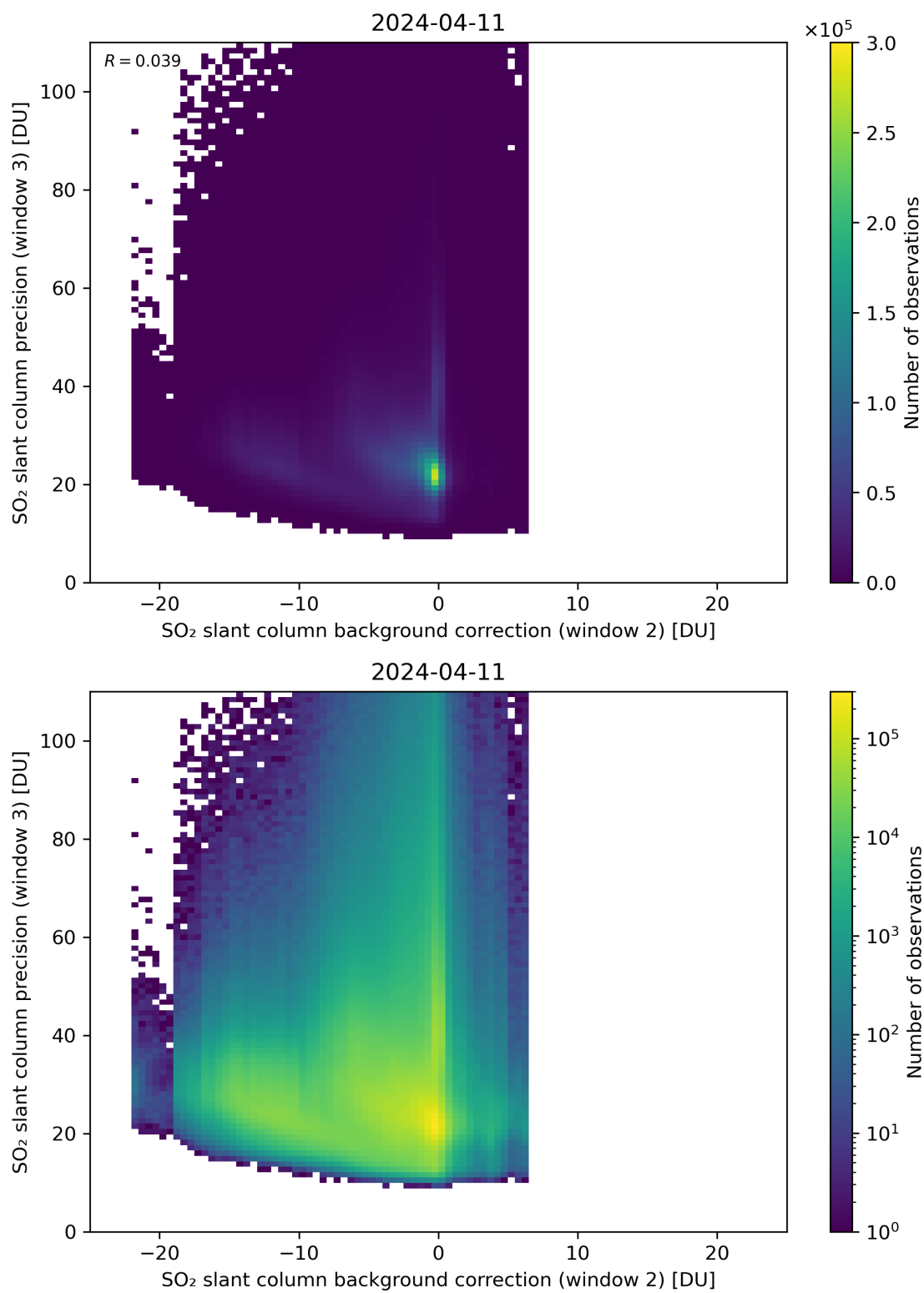
Figure 118: Scatter density plot of “SO 2 slant column background correction (window 2)” against “SO 2 slant column precision (window 3)” for 2024-04-10 to 2024-04-12.
