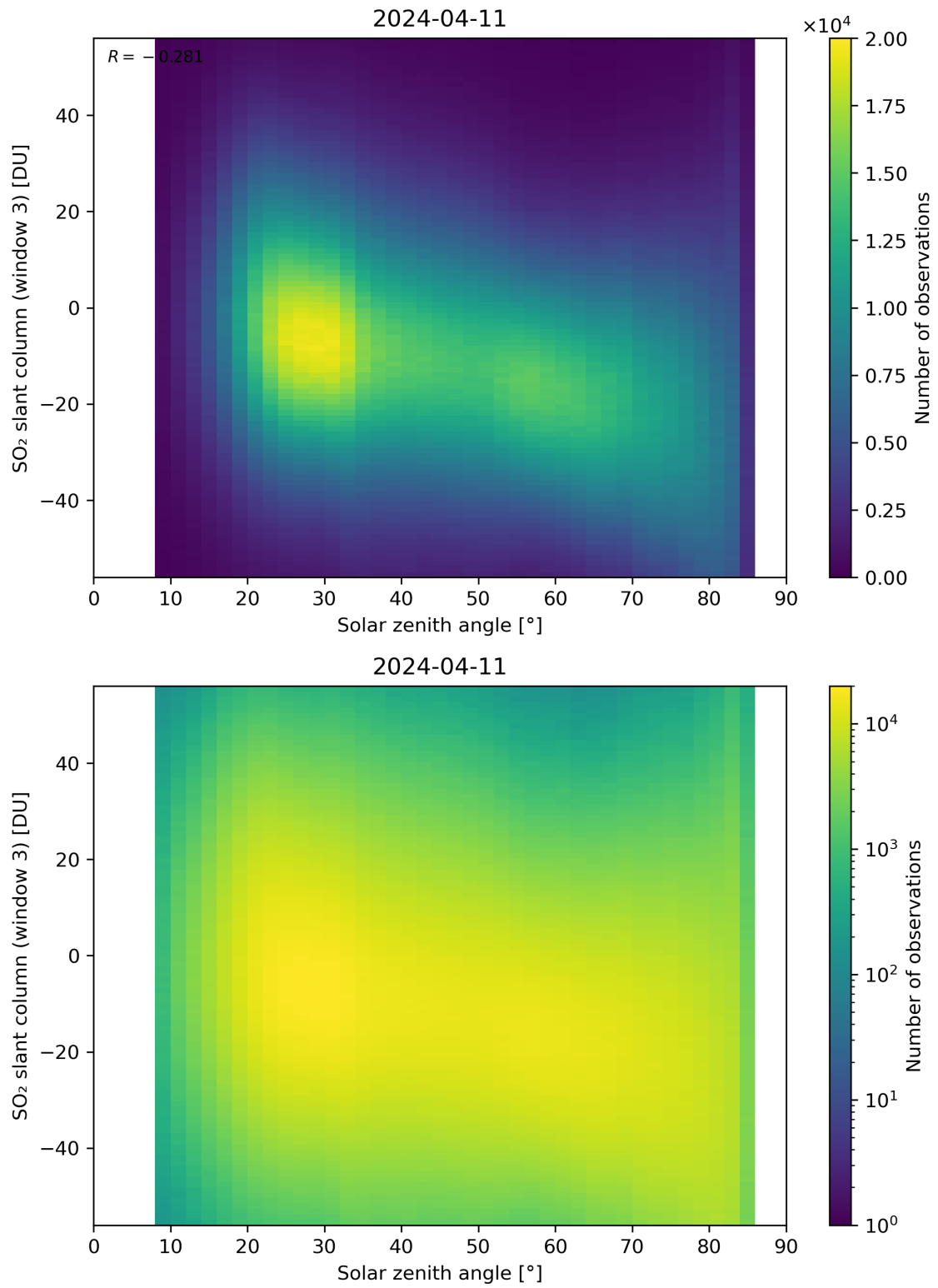
Figure 172: Scatter density plot of “Solar zenith angle” against “SO 2 slant column (window 3)” for 2024-04-10 to 2024-04-12.
