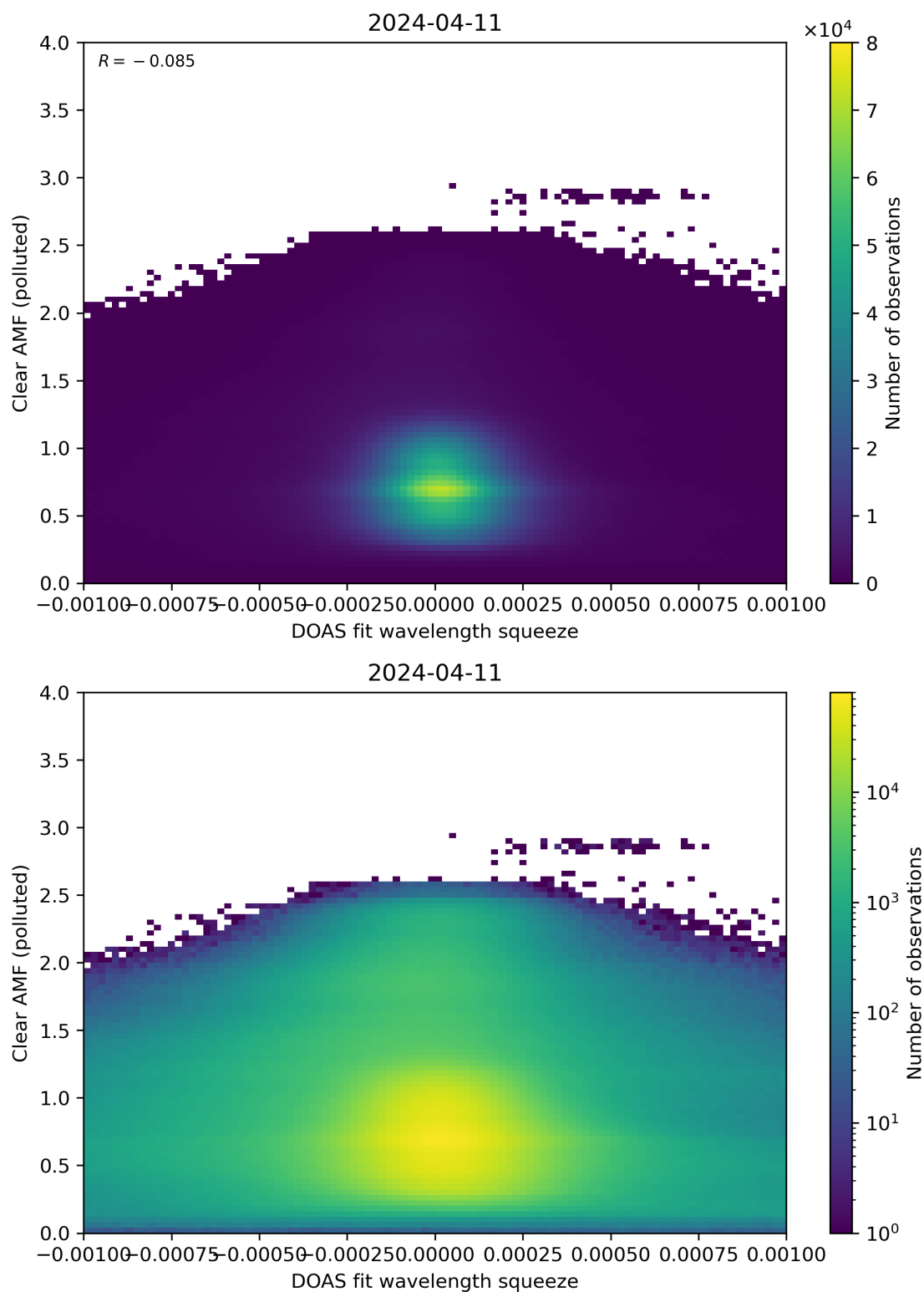
Figure 133: Scatter density plot of “DOAS fit wavelength squeeze” against “Clear AMF (polluted)” for 2024-04-10 to 2024-04-12.
