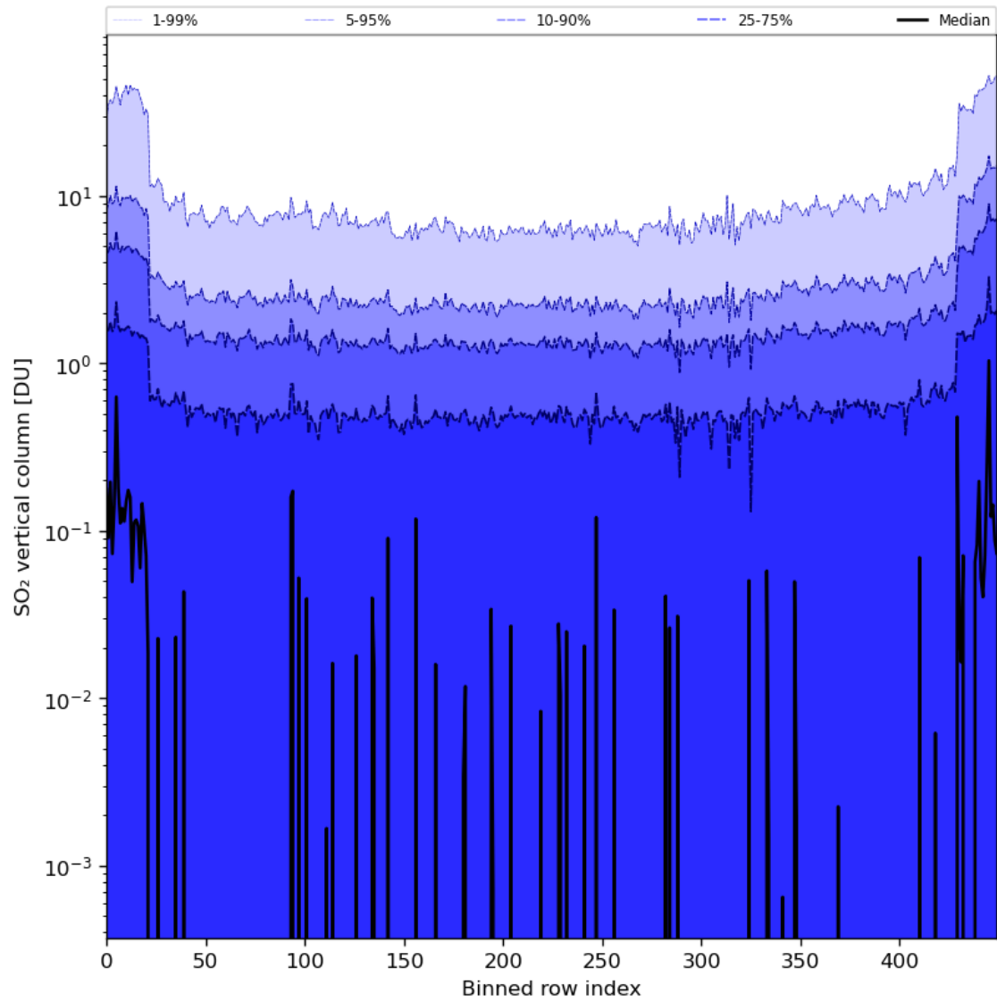
Figure 76: Along track statistics of “SO 2 vertical column” for 2024-04-10 to 2024-04-12
