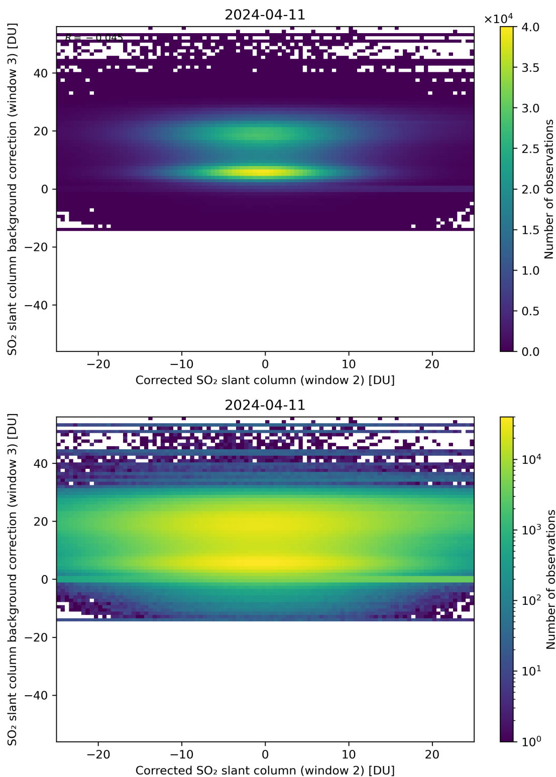
Figure 195: Scatter density plot of “Corrected SO 2 slant column (window 2)” against “SO 2 slant column background correction (window 3)” for 2024-04-10 to 2024-04-12.
