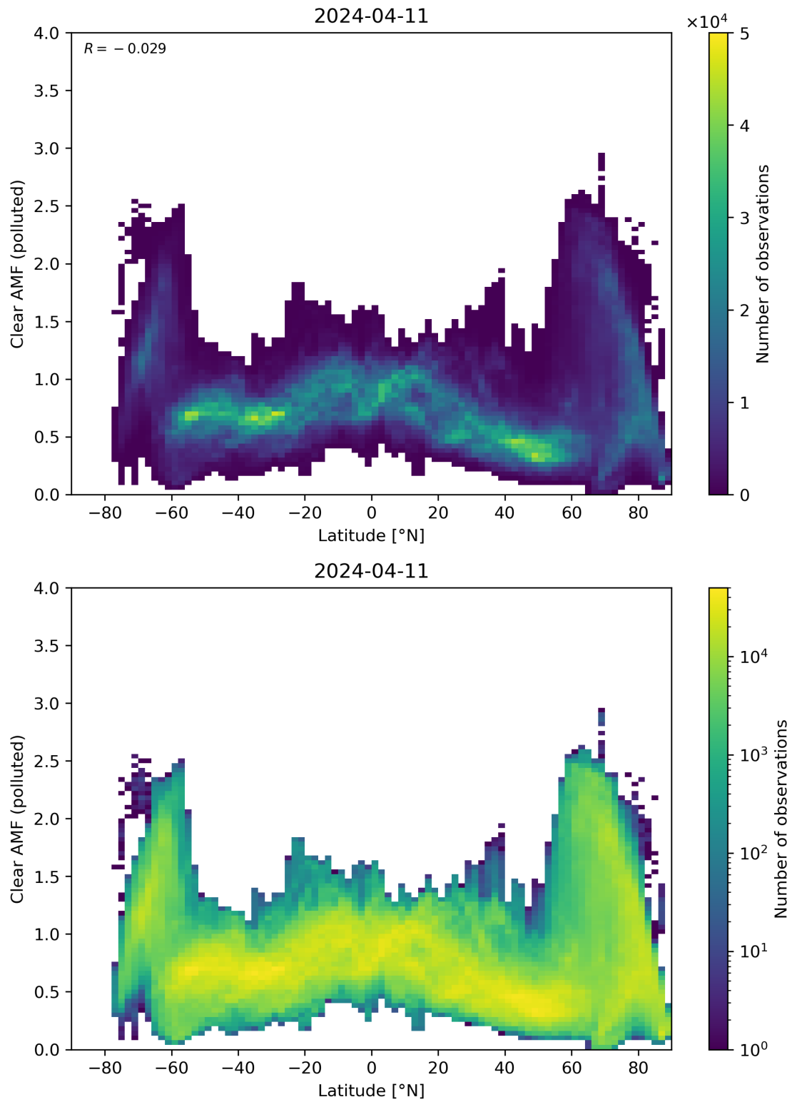
Figure 145: Scatter density plot of “Latitude” against “Clear AMF (polluted)” for 2024-04-10 to 2024-04-12.
