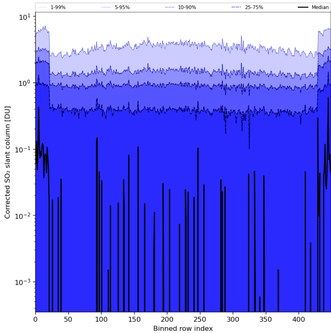
Figure 78: Along track statistics of “Corrected SO 2 slant column” for 2024-04-10 to 2024-04-12
