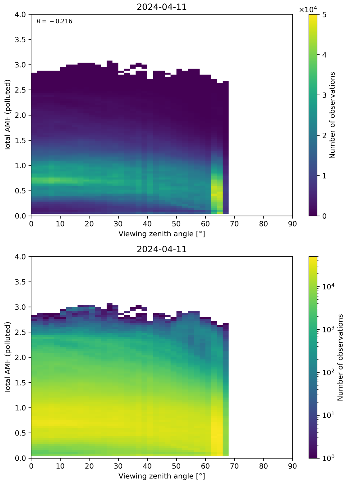
Figure 325: Scatter density plot of “Viewing zenith angle” against “Total AMF (polluted)” for 2024-04-10 to 2024-04-12.
