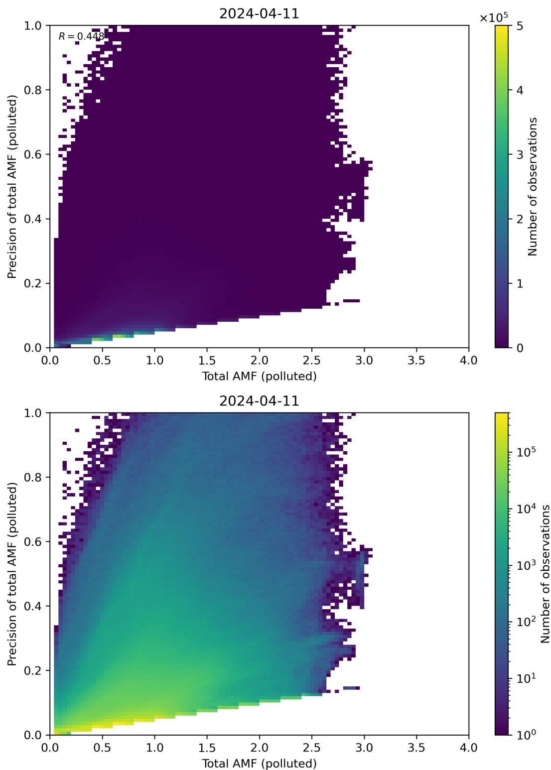
Figure 272: Scatter density plot of “Total AMF (polluted)” against “Precision of total AMF (polluted)” for 2024-04-10 to 2024-04-12.
