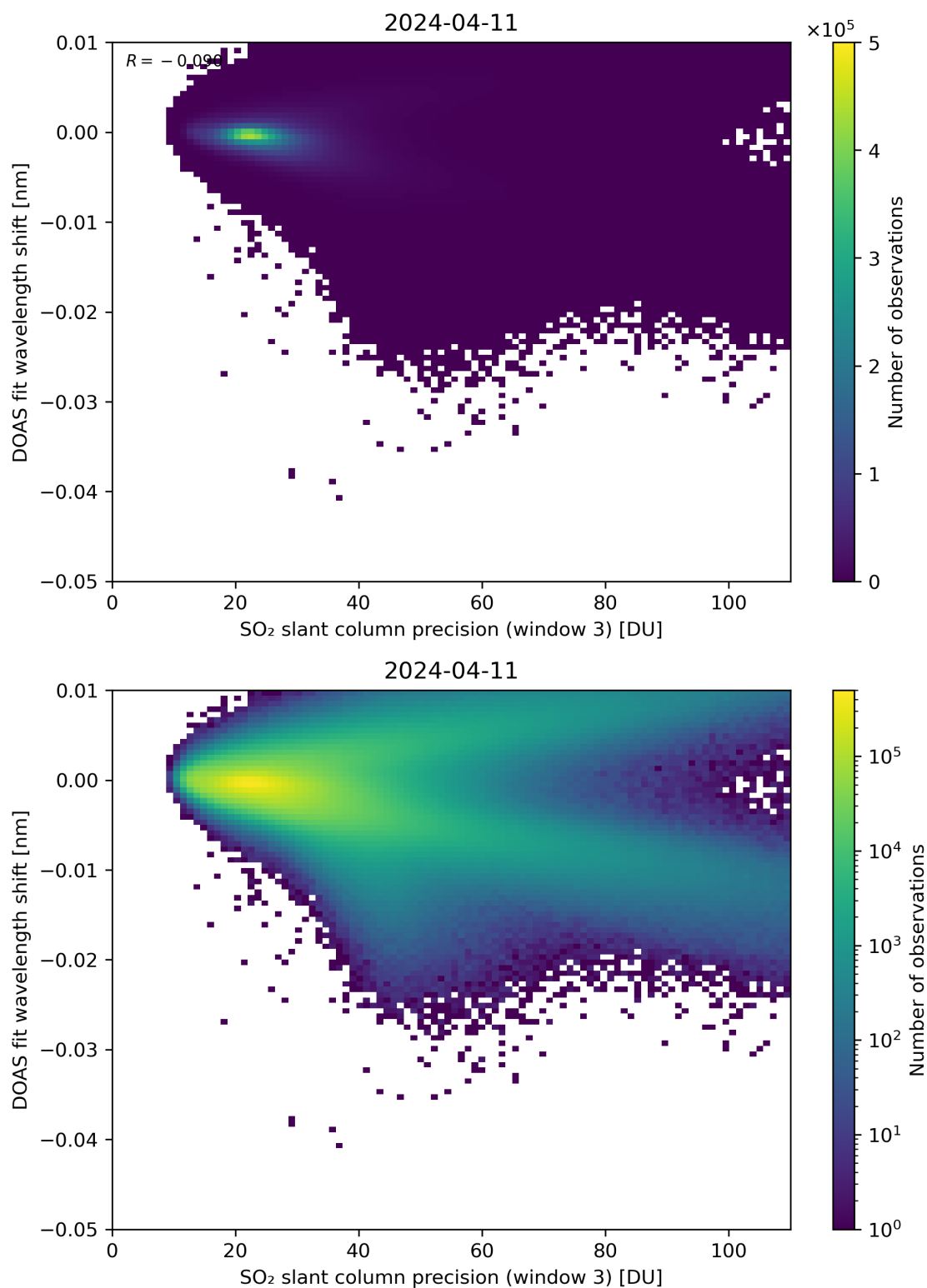
Figure 258: Scatter density plot of “SO 2 slant column precision (window 3)” against “DOAS fit wavelength shift” for 2024-04-10 to 2024-04-12.
