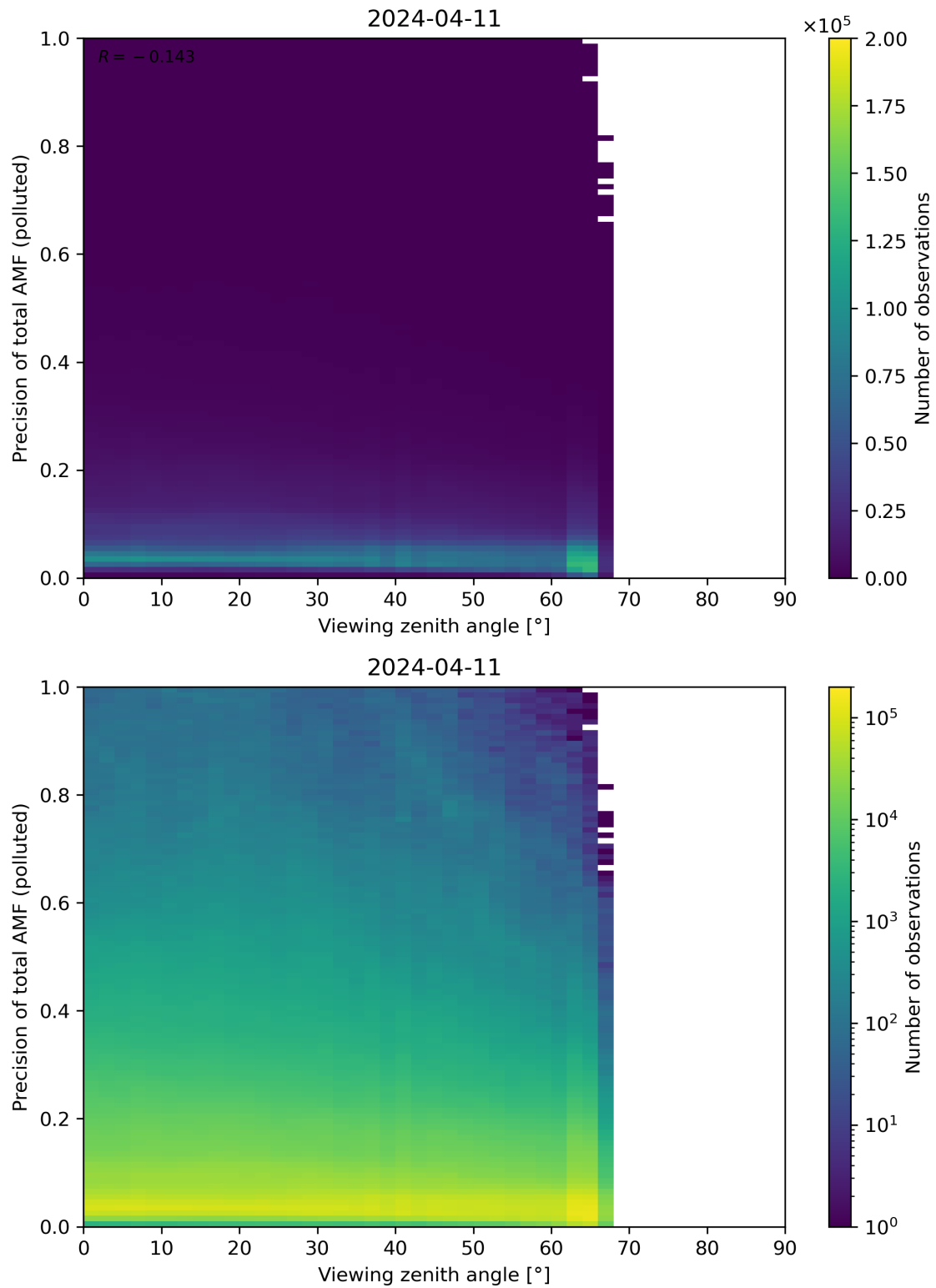
Figure 326: Scatter density plot of “Viewing zenith angle” against “Precision of total AMF (polluted)” for 2024-04-10 to 2024-04-12.
