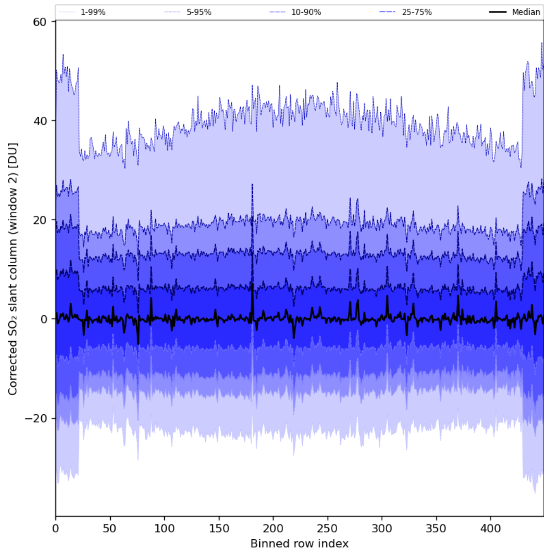
Figure 85: Along track statistics of “Corrected SO 2 slant column (window 2)” for 2024-04-10 to 2024-04-12
