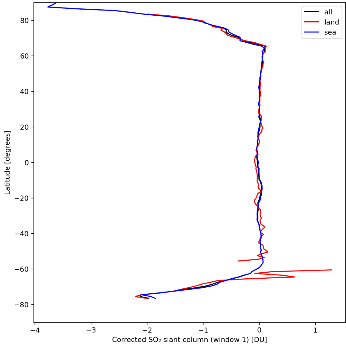
Figure 35: Zonal average of “Corrected SO 2 slant column (window 1)” for 2024-04-10 to 2024-04-12.
