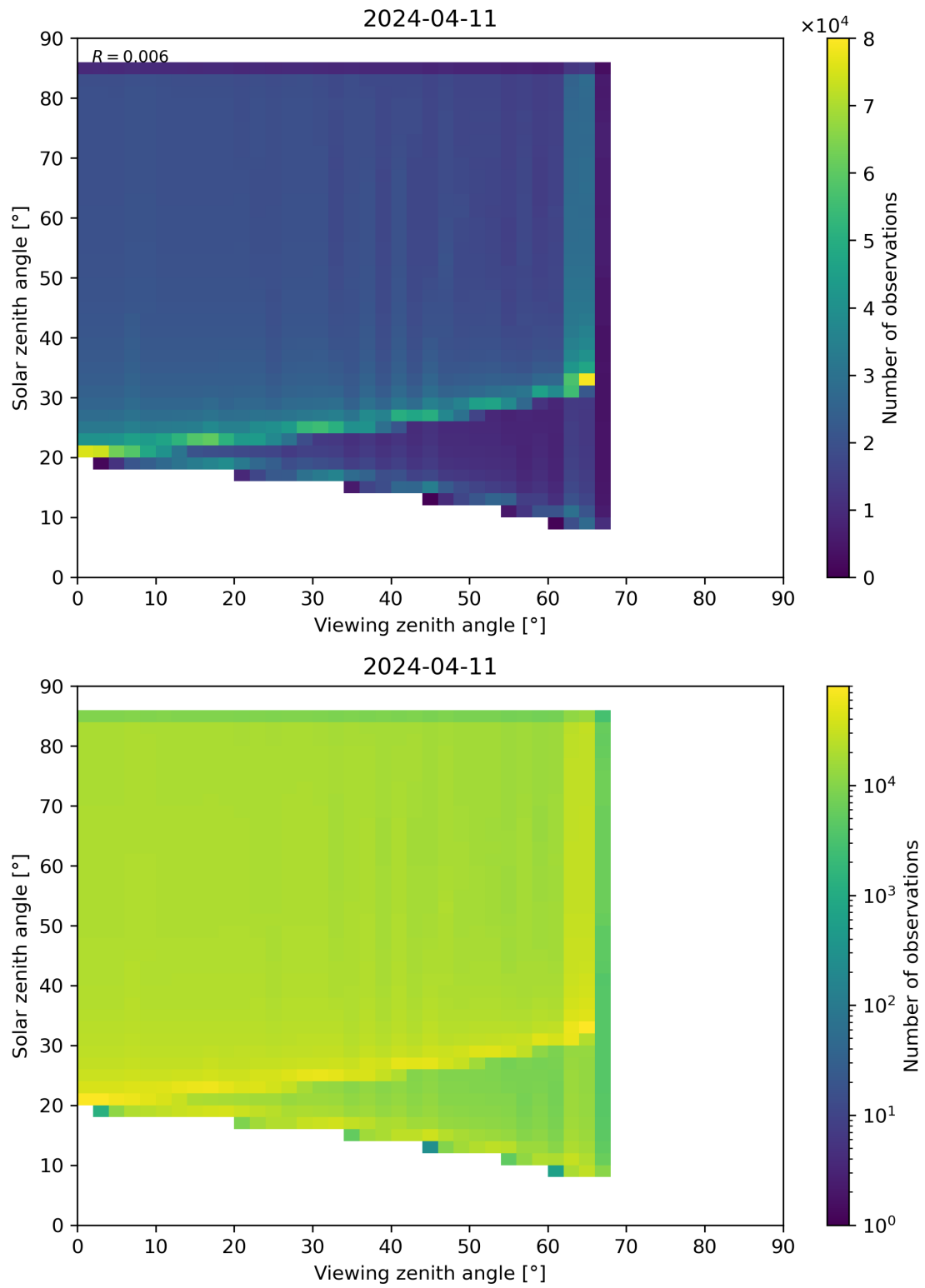
Figure 315: Scatter density plot of “Viewing zenith angle” against “Solar zenith angle” for 2024-04-10 to 2024-04-12.
