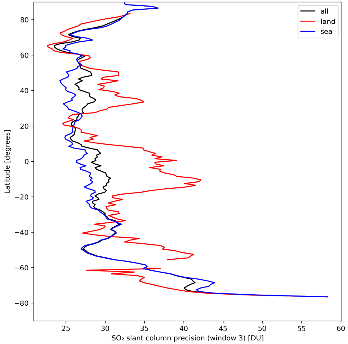
Figure 42: Zonal average of “SO 2 slant column precision (window 3)” for 2024-04-10 to 2024-04-12.
