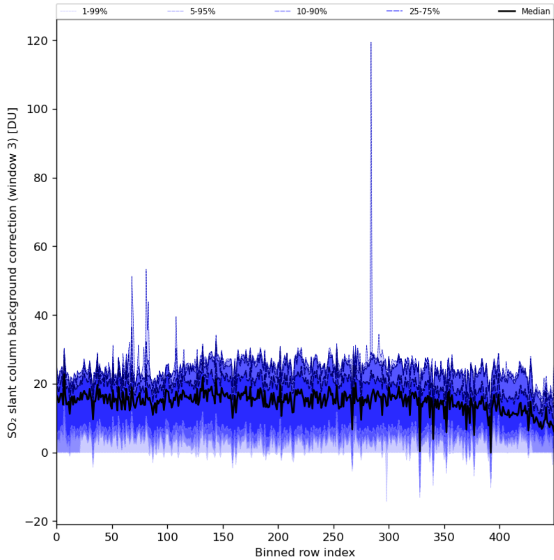
Figure 90: Along track statistics of “SO 2 slant column background correction (window 3)” for 2024-04-10 to 2024-04-12
