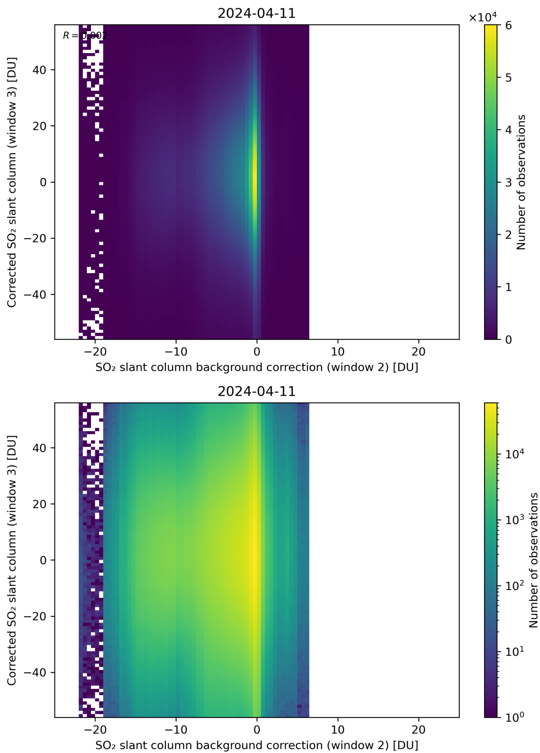
Figure 116: Scatter density plot of “SO 2 slant column background correction (window 2)” against “Corrected SO 2 slant column (window 3)” for 2024-04-10 to 2024-04-12.
