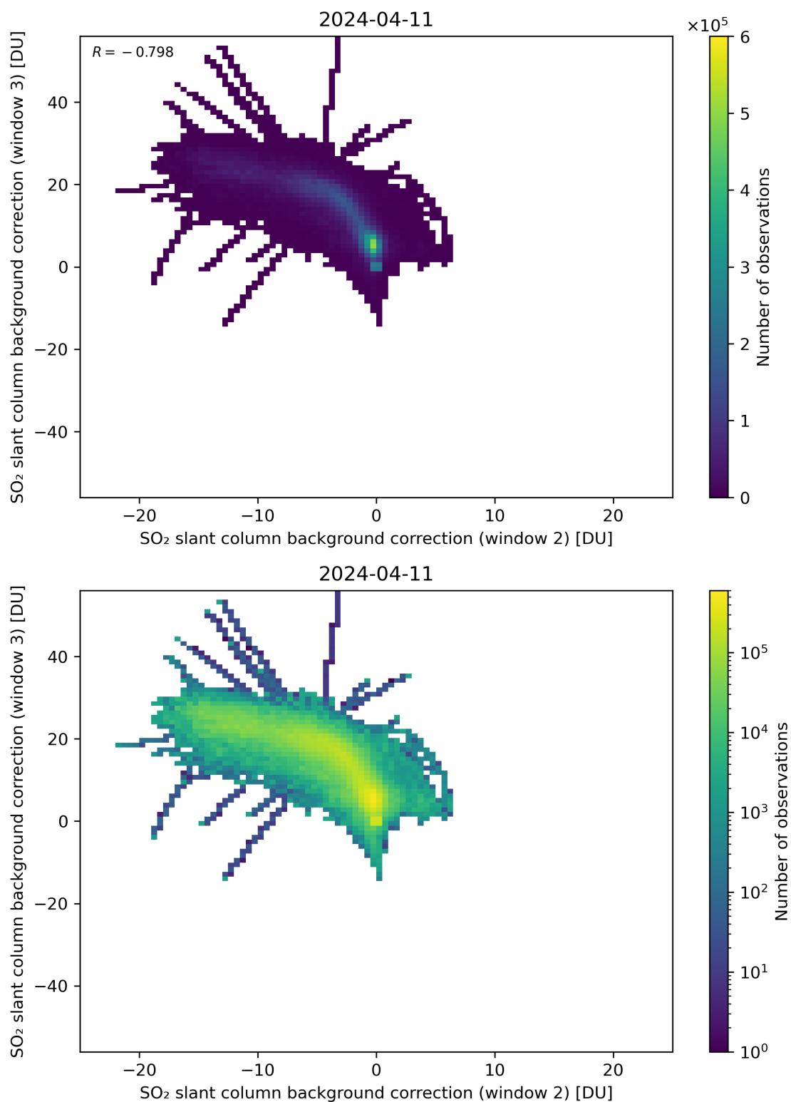
Figure 111: Scatter density plot of “SO 2 slant column background correction (window 2)” against “SO 2 slant column background correction (window 3)” for 2024-04-10 to 2024-04-12.
