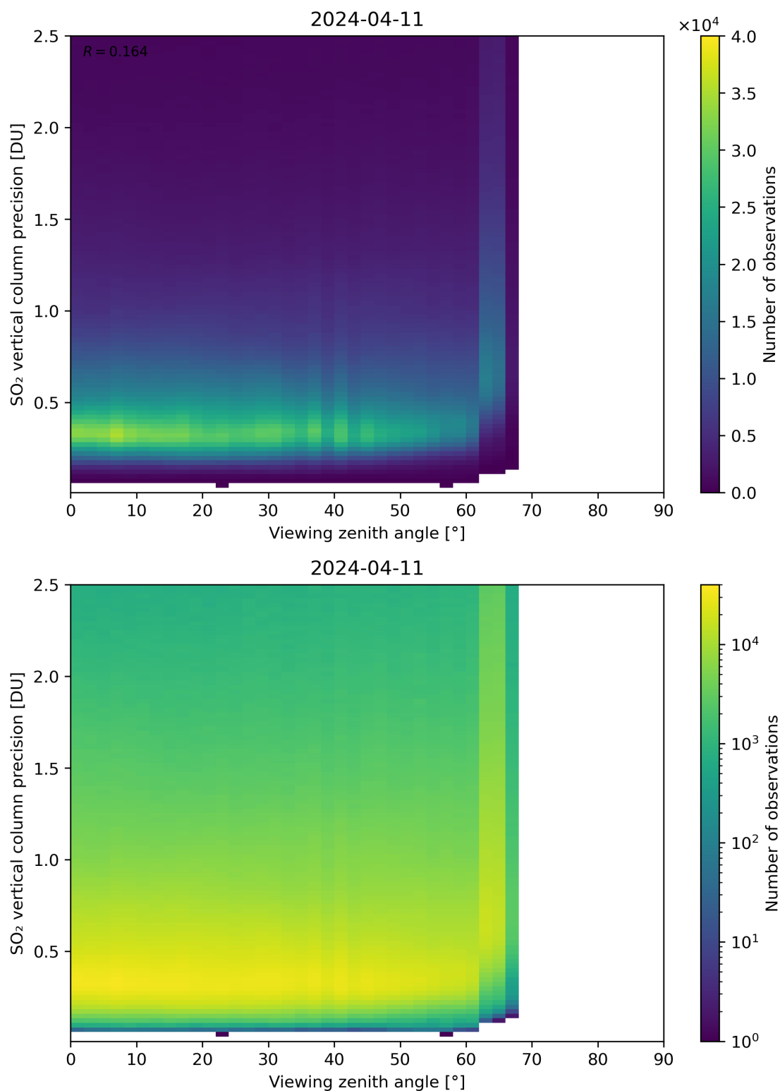
Figure 328: Scatter density plot of “Viewing zenith angle” against “SO 2 vertical column precision” for 2024-04-10 to 2024-04-12.
