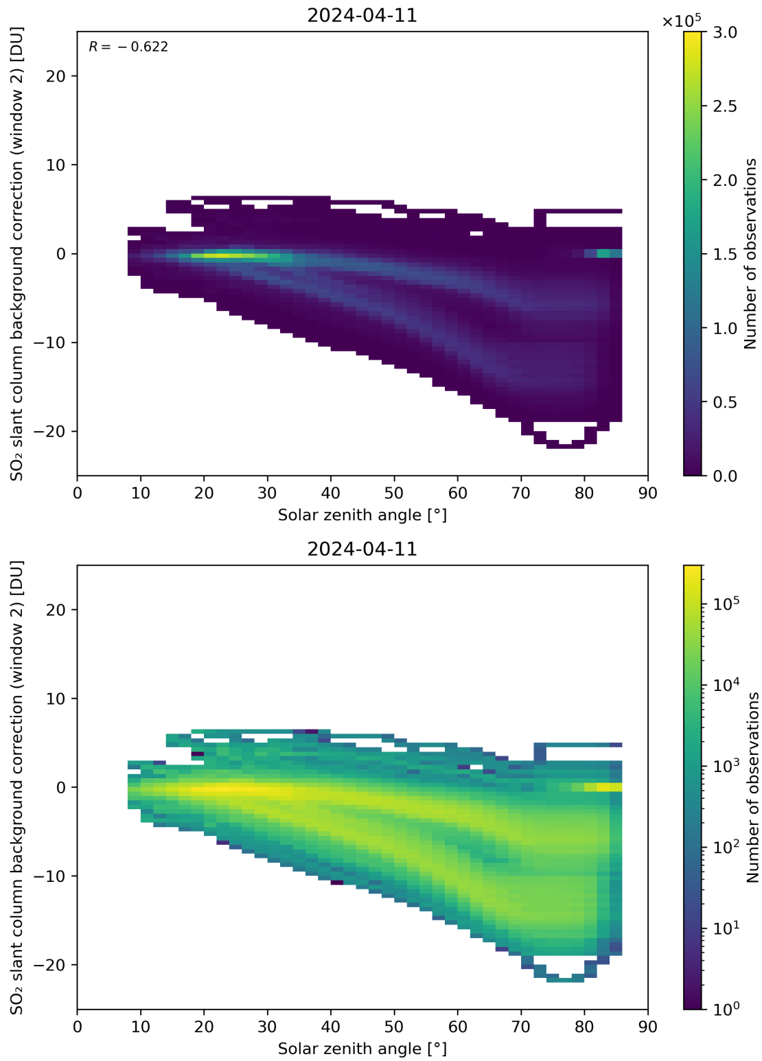
Figure 159: Scatter density plot of “Solar zenith angle” against “SO 2 slant column background correction (window 2)” for 2024-04-10 to 2024-04-12.
