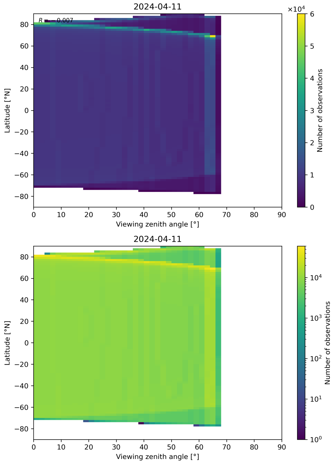
Figure 314: Scatter density plot of “Viewing zenith angle” against “Latitude” for 2024-04-10 to 2024-04-12.
