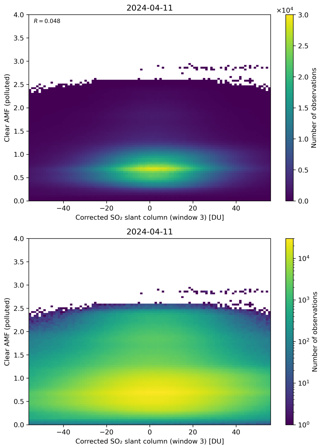
Figure 209: Scatter density plot of “Corrected SO 2 slant column (window 3)” against “Clear AMF (polluted)” for 2024-04-10 to 2024-04-12.
