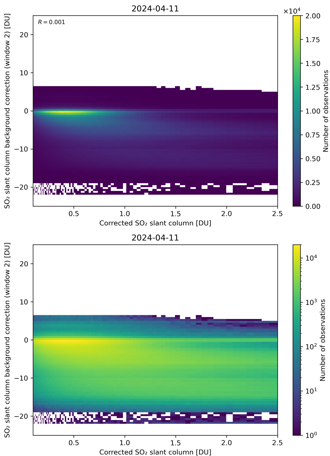
Figure 179: Scatter density plot of “Corrected SO 2 slant column” against “SO 2 slant column background correction (window 2)” for 2024-04-10 to 2024-04-12.
