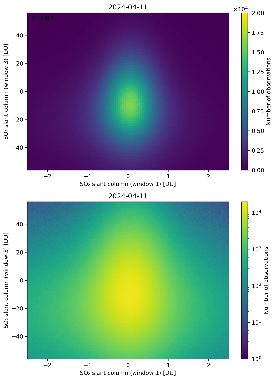
Figure 237: Scatter density plot of “SO 2 slant column (window 1)” against “SO 2 slant column (window 3)” for 2024-04-10 to 2024-04-12.
