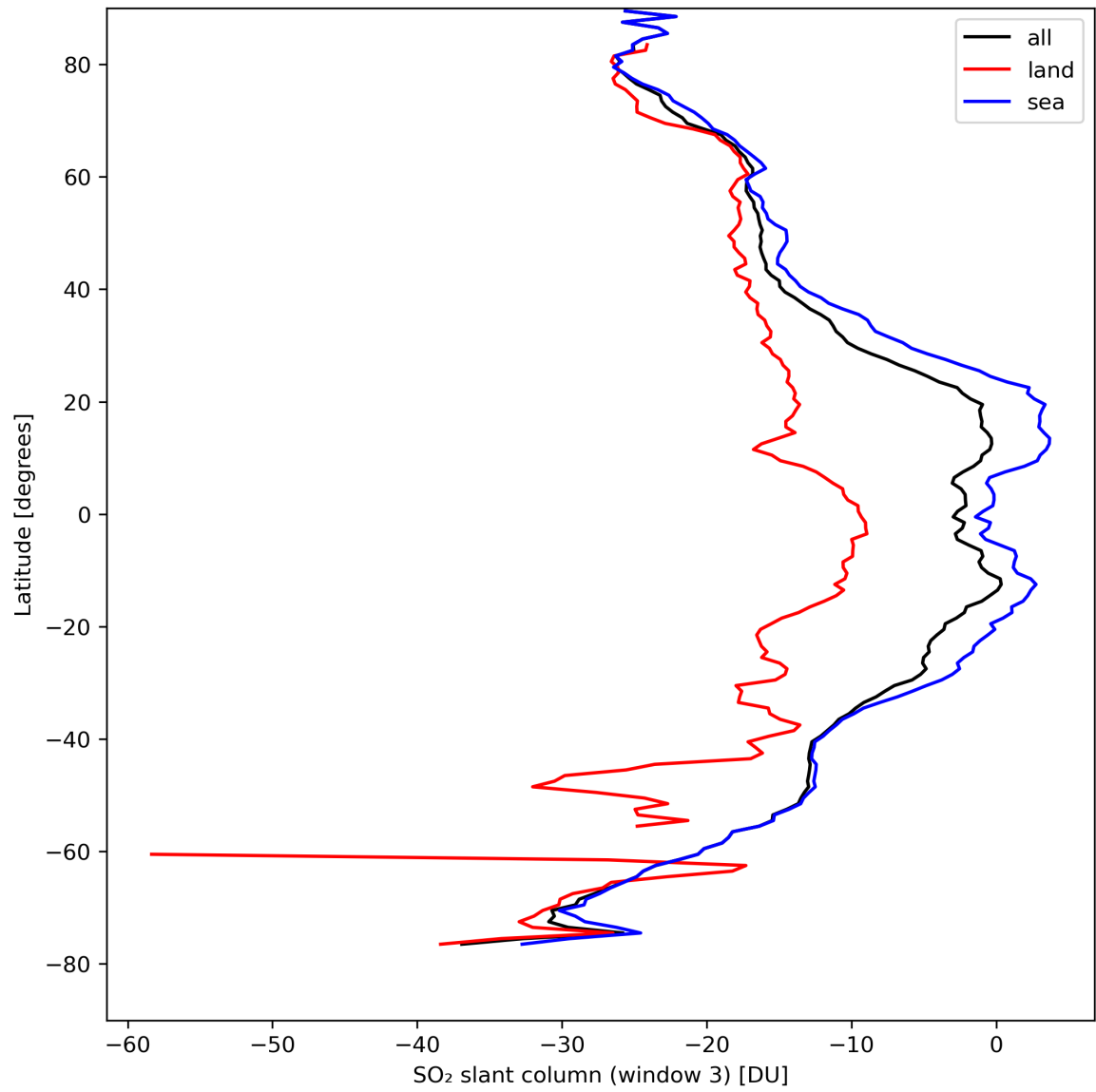
Figure 41: Zonal average of “SO 2 slant column (window 3)” for 2024-04-10 to 2024-04-12.
