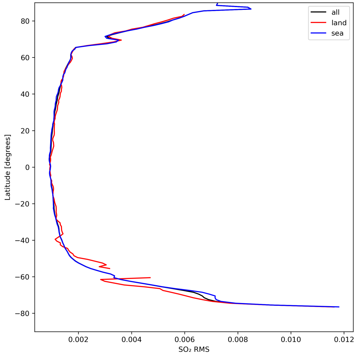
Figure 47: Zonal average of “SO 2 RMS” for 2024-04-10 to 2024-04-12.
