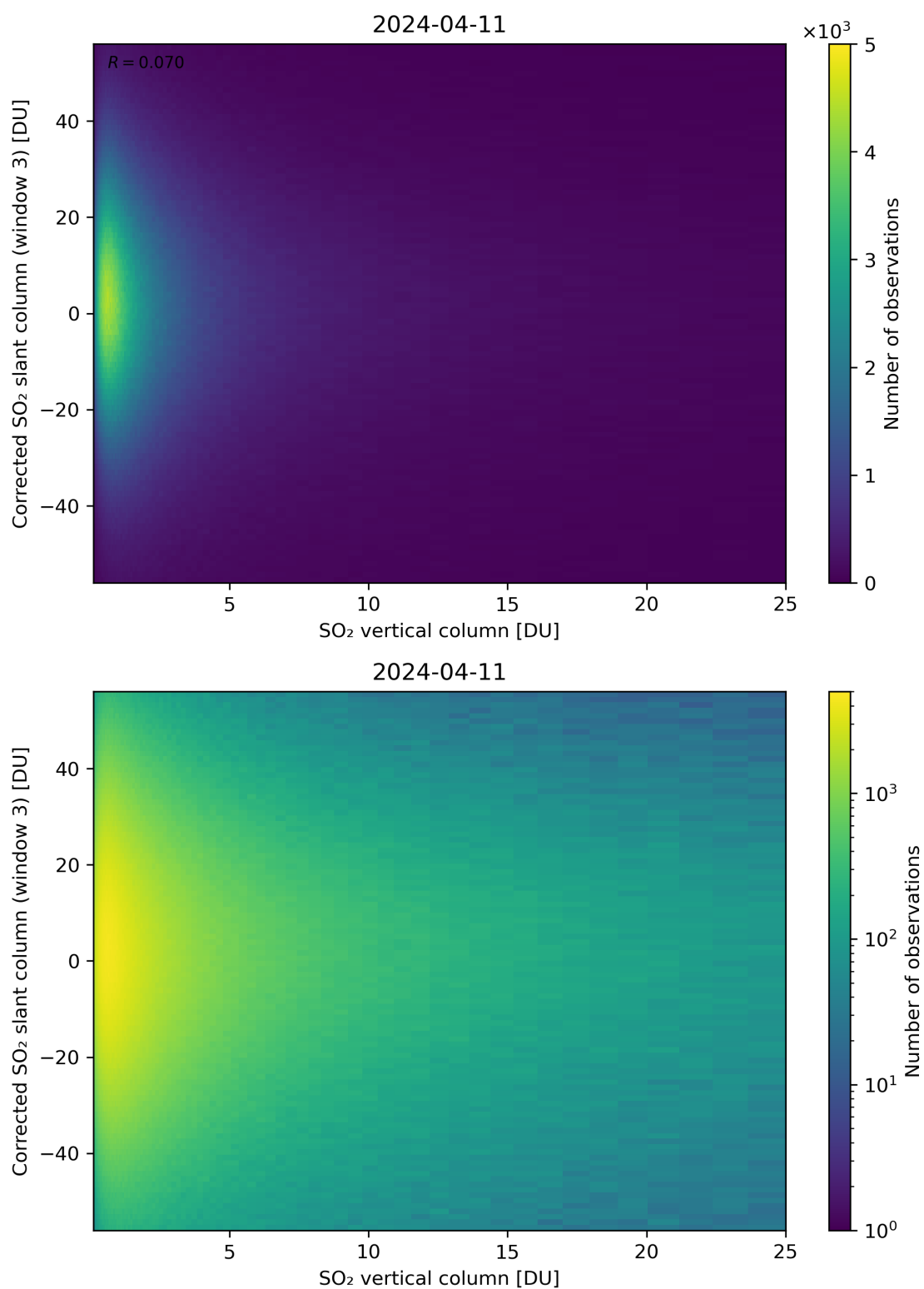
Figure 299: Scatter density plot of “SO 2 vertical column” against “Corrected SO 2 slant column (window 3)” for 2024-04-10 to 2024-04-12.
