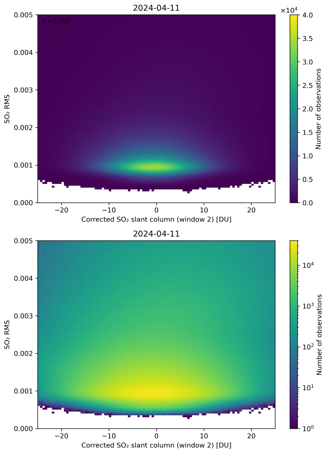
Figure 198: Scatter density plot of “Corrected SO 2 slant column (window 2)” against “SO 2 RMS” for 2024-04-10 to 2024-04-12.
