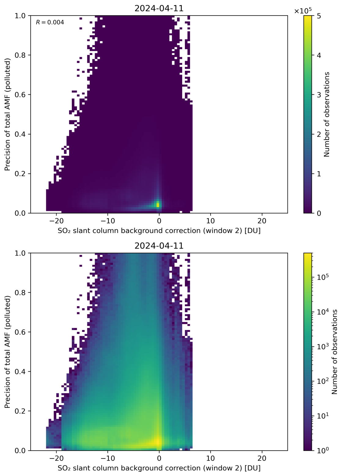
Figure 120: Scatter density plot of “SO 2 slant column background correction (window 2)” against “Precision of total AMF (polluted)” for 2024-04-10 to 2024-04-12.
