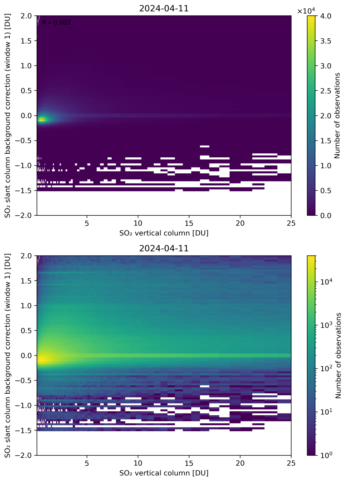
Figure 273: Scatter density plot of “SO 2 vertical column” against “SO 2 slant column background correction (window 1)” for 2024-04-10 to 2024-04-12.
