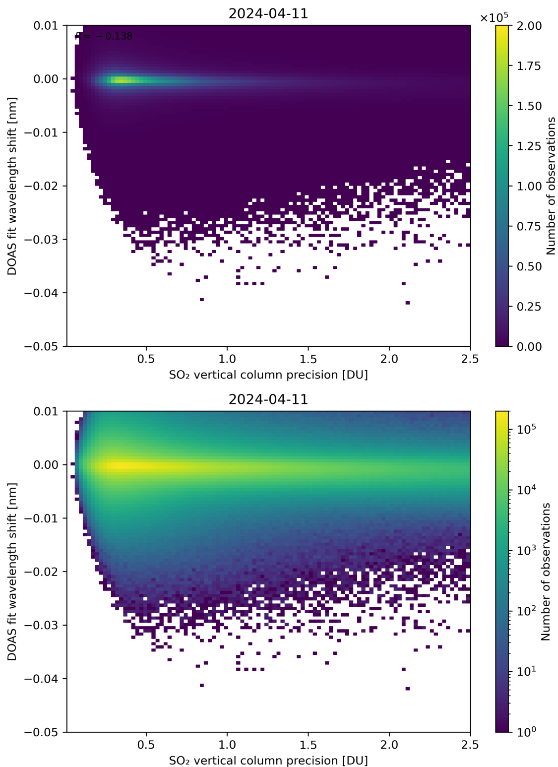
Figure 282: Scatter density plot of “SO 2 vertical column precision” against “DOAS fit wavelength shift” for 2024-04-10 to 2024-04-12.
