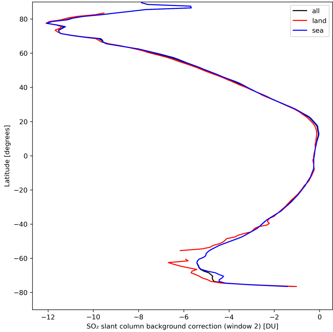
Figure 40: Zonal average of “SO 2 slant column background correction (window 2)” for 2024-04-10 to 2024-04-12.
