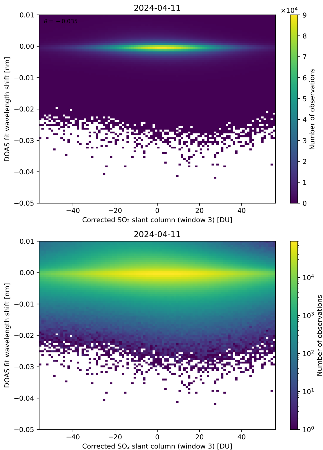
Figure 206: Scatter density plot of “Corrected SO 2 slant column (window 3)” against “DOAS fit wavelength shift” for 2024-04-10 to 2024-04-12.
