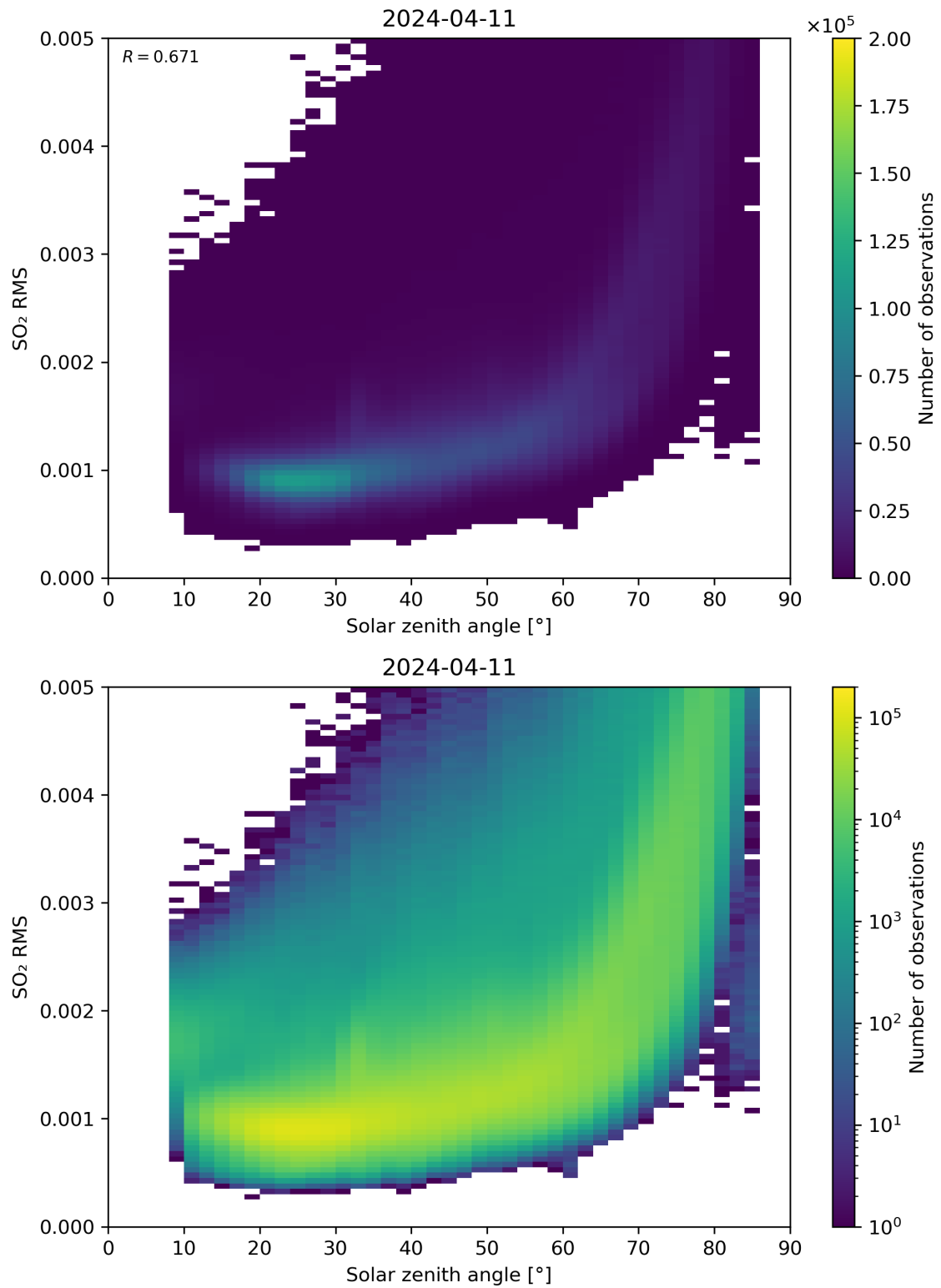
Figure 163: Scatter density plot of “Solar zenith angle” against “SO 2 RMS” for 2024-04-10 to 2024-04-12.
