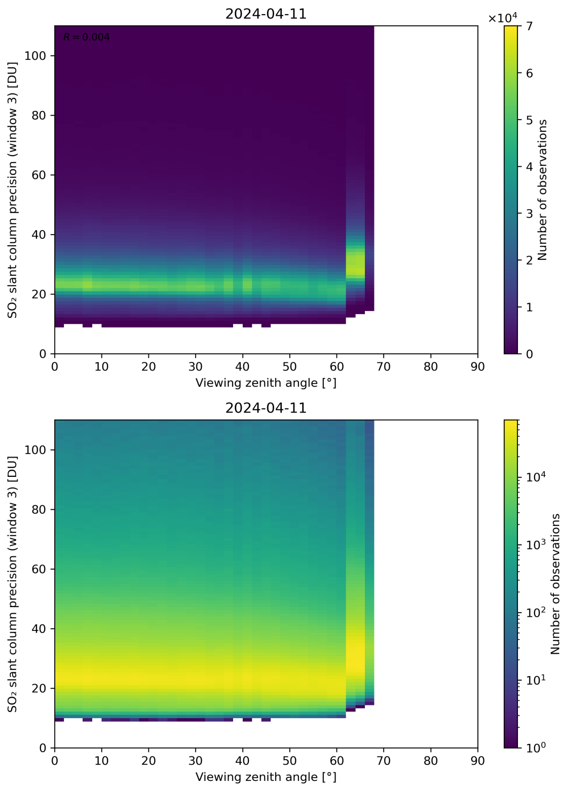
Figure 324: Scatter density plot of “Viewing zenith angle” against “SO 2 slant column precision (window 3)” for 2024-04-10 to 2024-04-12.
