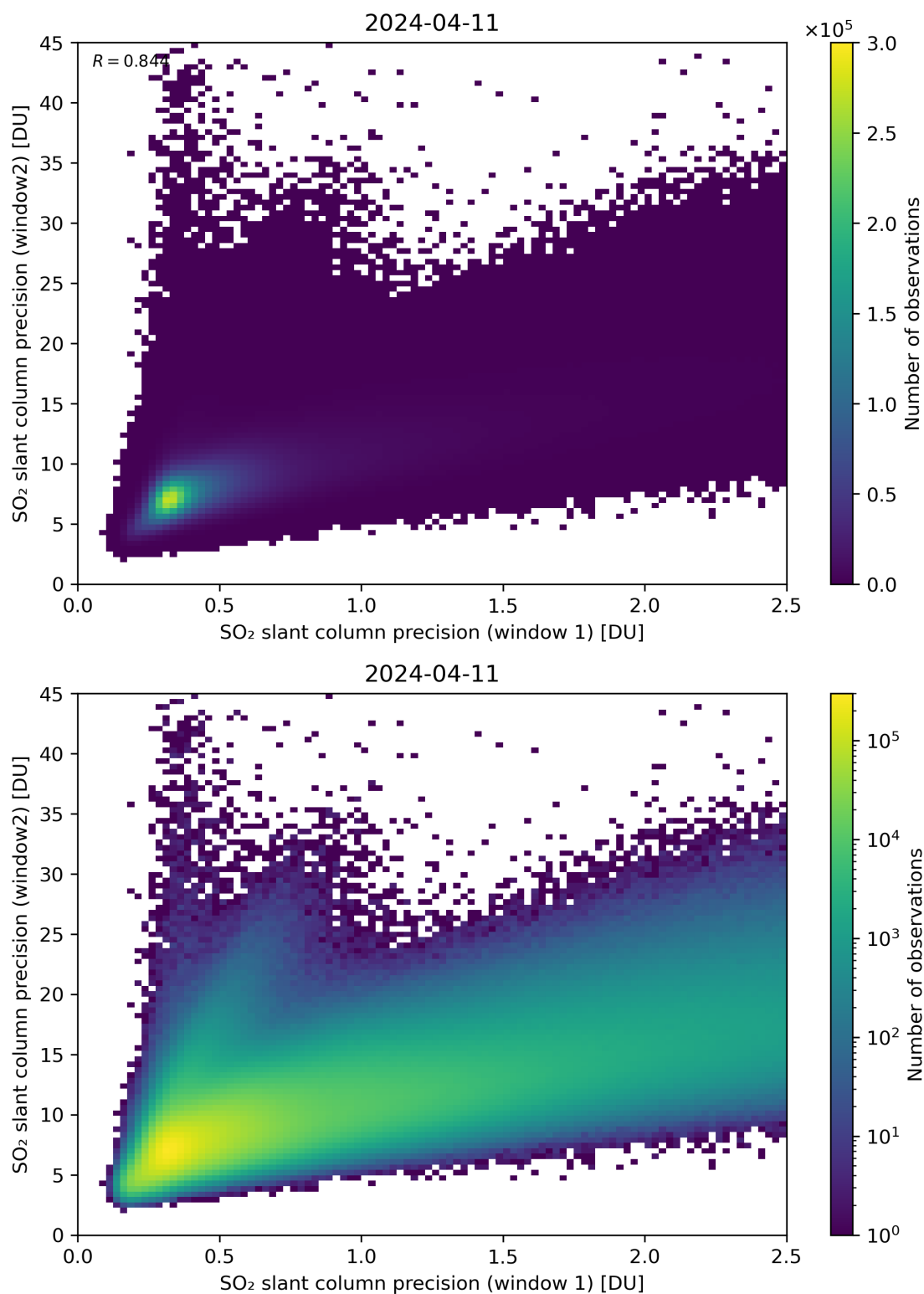
Figure 227: Scatter density plot of “SO 2 slant column precision (window 1)” against “SO 2 slant column precision (window2)” for 2024-04-10 to 2024-04-12.
