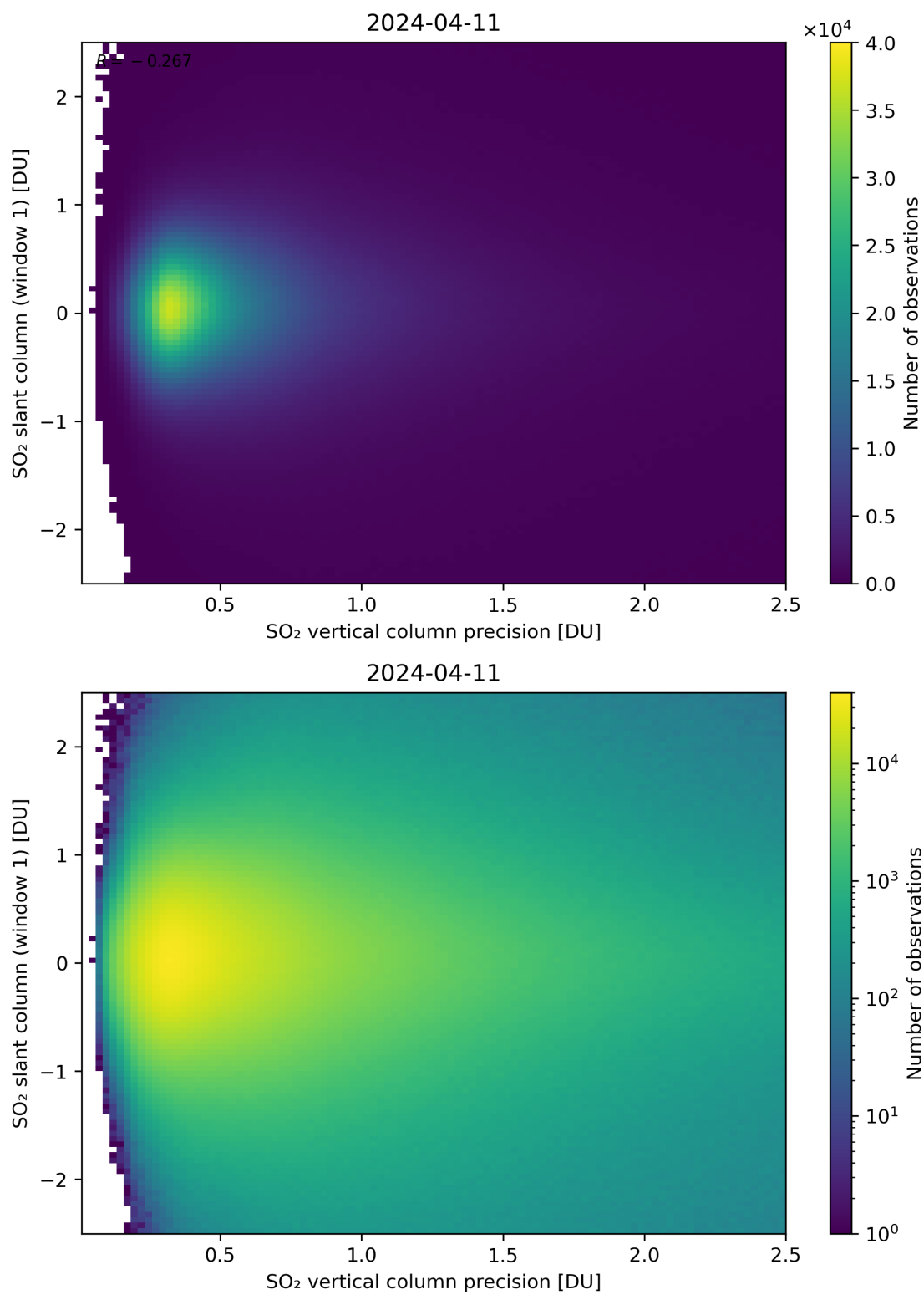
Figure 289: Scatter density plot of “SO 2 vertical column precision” against “SO 2 slant column (window 1)” for 2024-04-10 to 2024-04-12.
