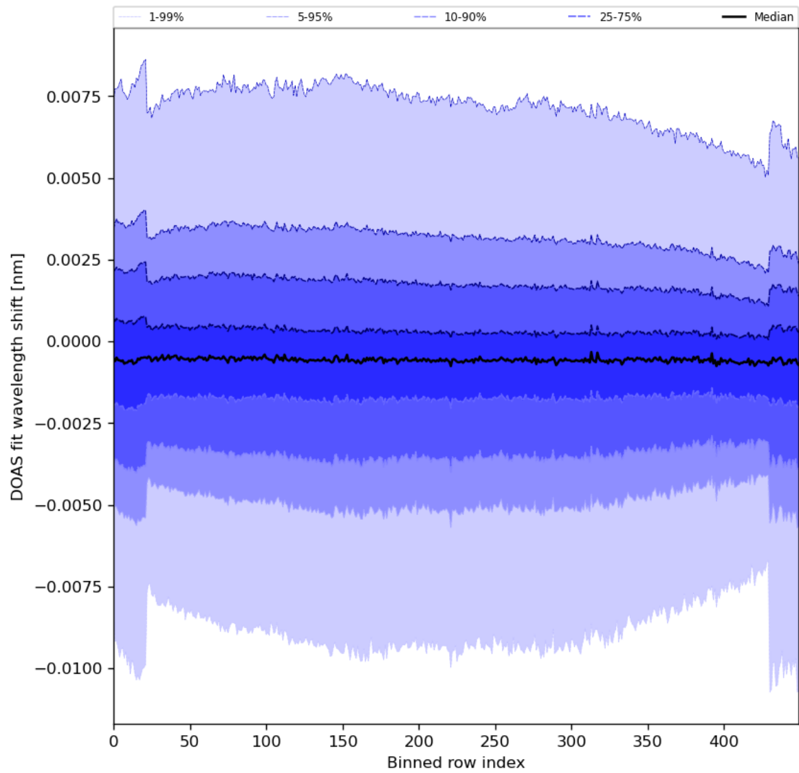
Figure 91: Along track statistics of “DOAS fit wavelength shift” for 2024-04-10 to 2024-04-12
