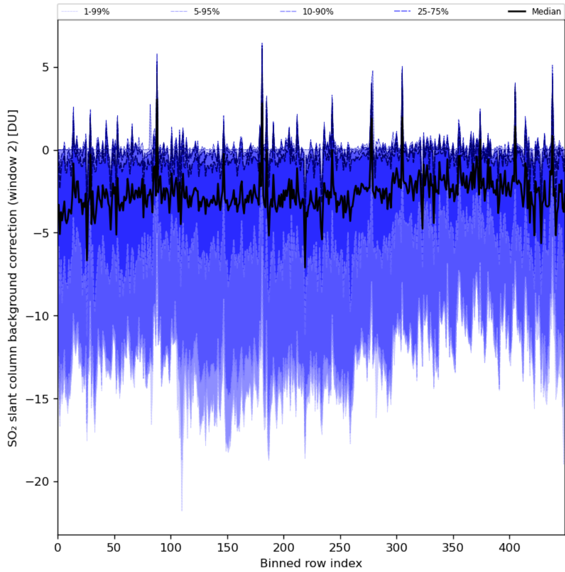
Figure 86: Along track statistics of “SO 2 slant column background correction (window 2)” for 2024-04-10 to 2024-04-12
