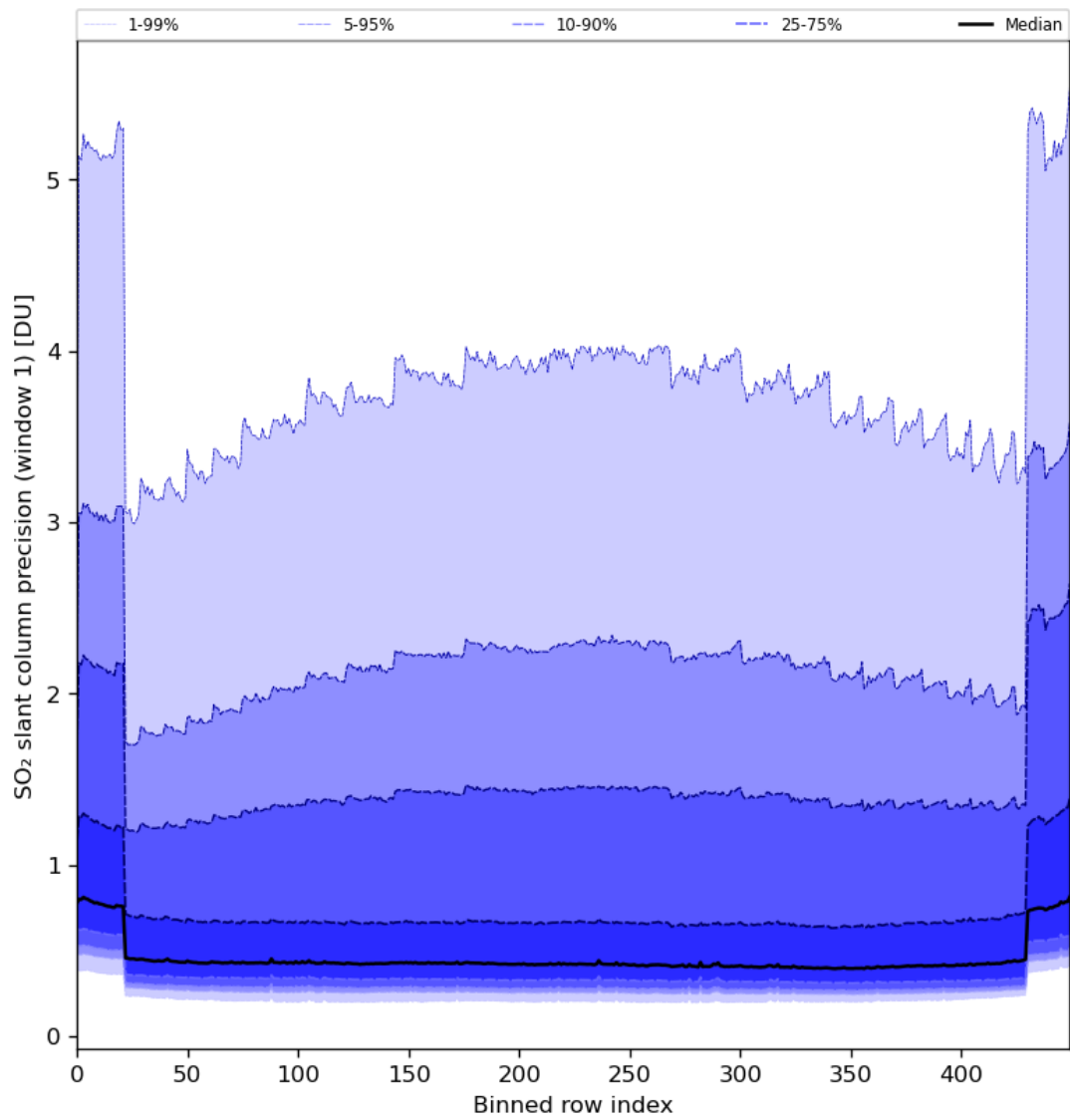
Figure 80: Along track statistics of “SO 2 slant column precision (window 1)” for 2024-04-10 to 2024-04-12
