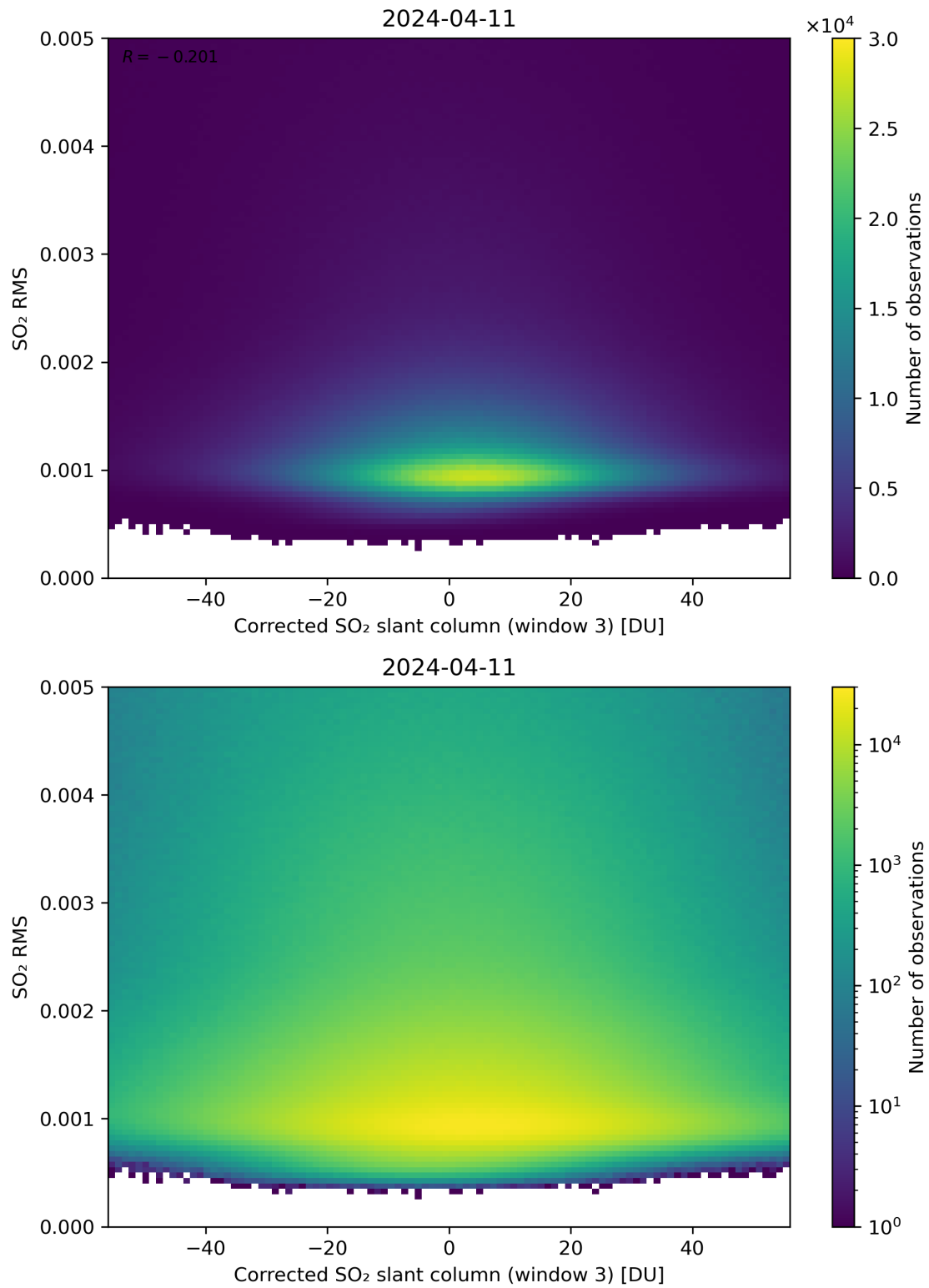
Figure 208: Scatter density plot of “Corrected SO 2 slant column (window 3)” against “SO 2 RMS” for 2024-04-10 to 2024-04-12.
