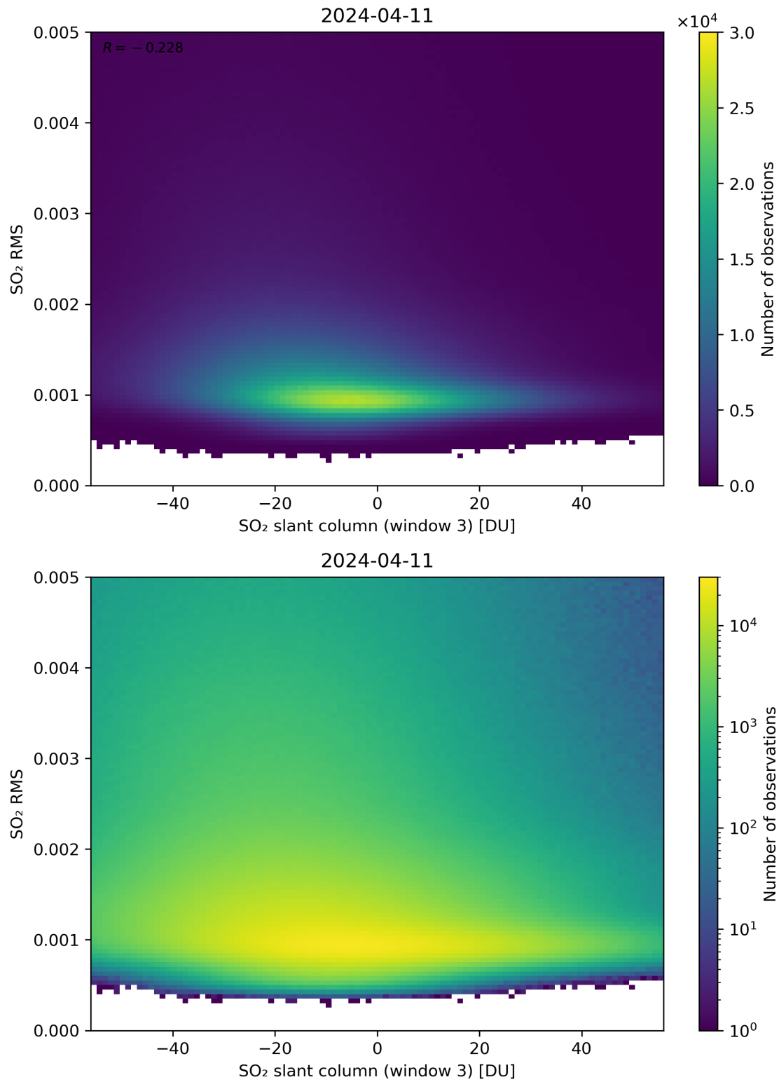
Figure 256: Scatter density plot of “SO 2 slant column (window 3)” against “SO 2 RMS” for 2024-04-10 to 2024-04-12.
