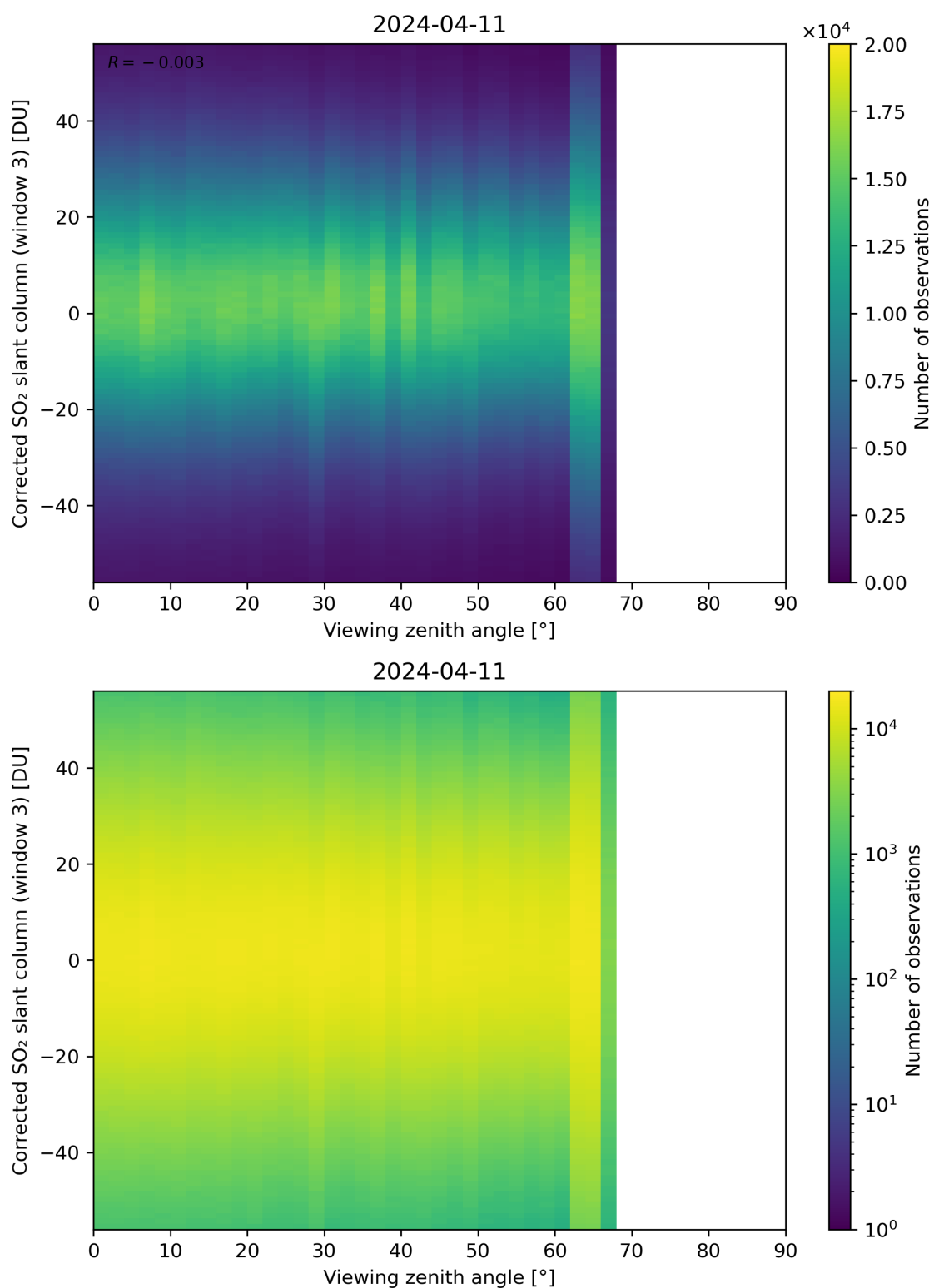
Figure 319: Scatter density plot of “Viewing zenith angle” against “Corrected SO 2 slant column (window 3)” for 2024-04-10 to 2024-04-12.
