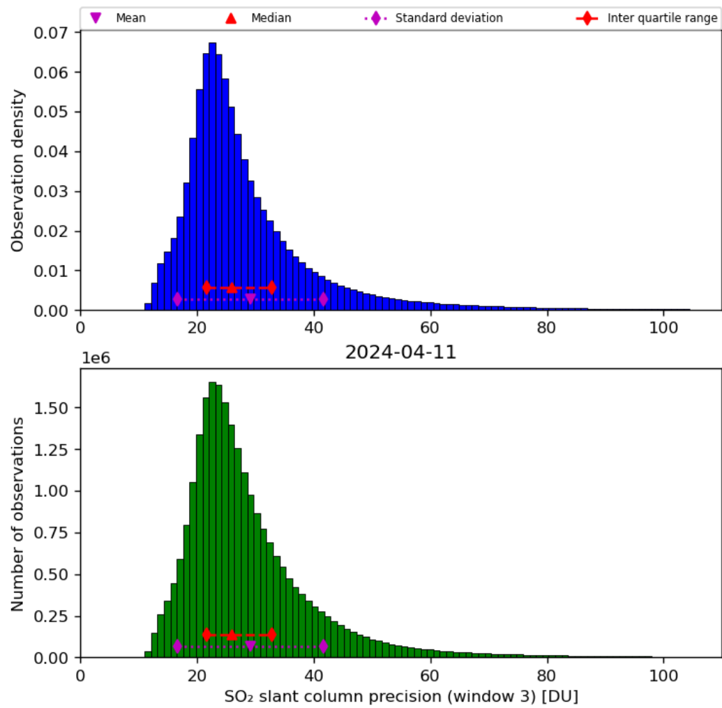
Figure 65: Histogram of “SO 2 slant column precision (window 3)” for 2024-04-10 to 2024-04-12
