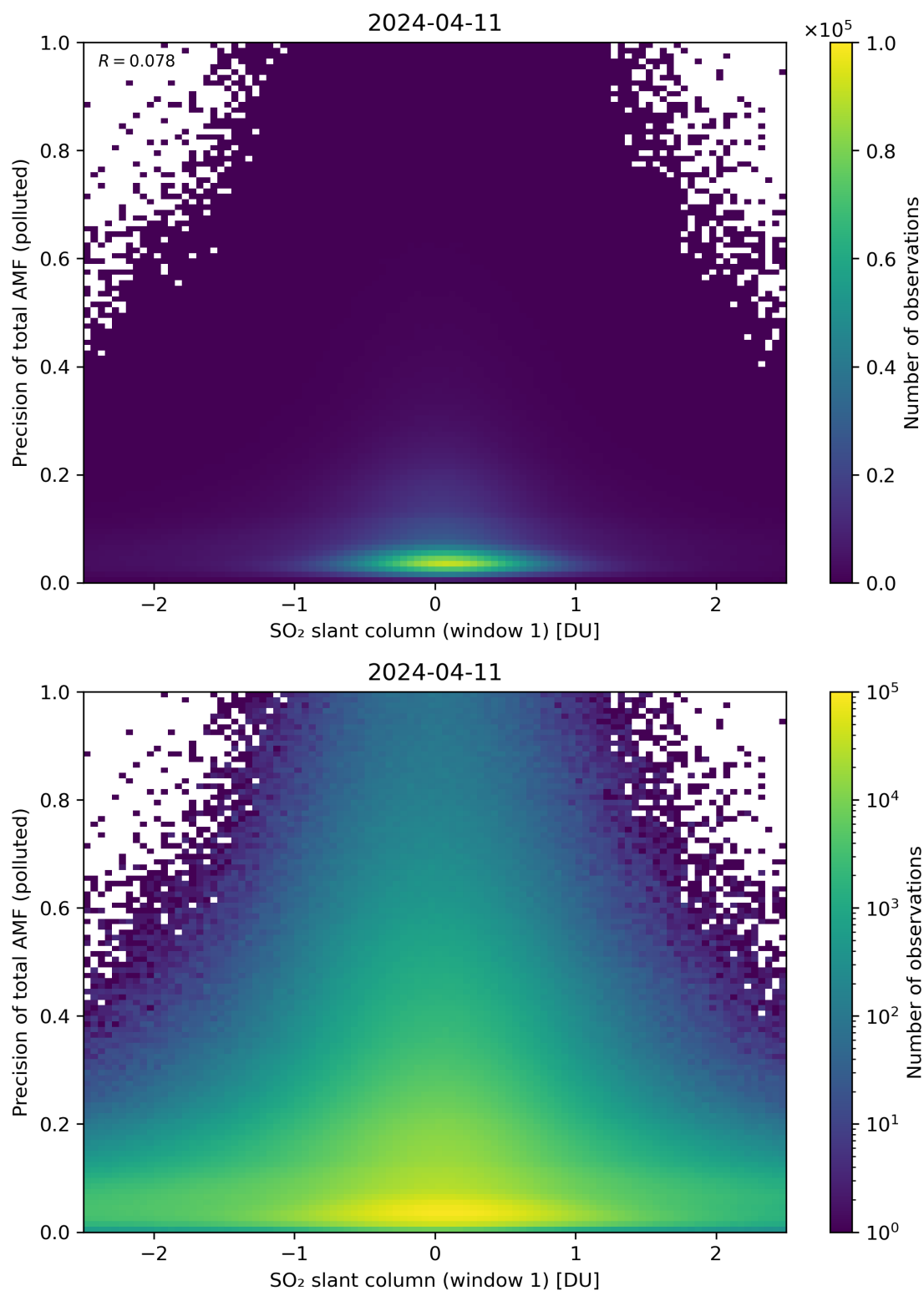
Figure 240: Scatter density plot of “SO 2 slant column (window 1)” against “Precision of total AMF (polluted)” for 2024-04-10 to 2024-04-12.
