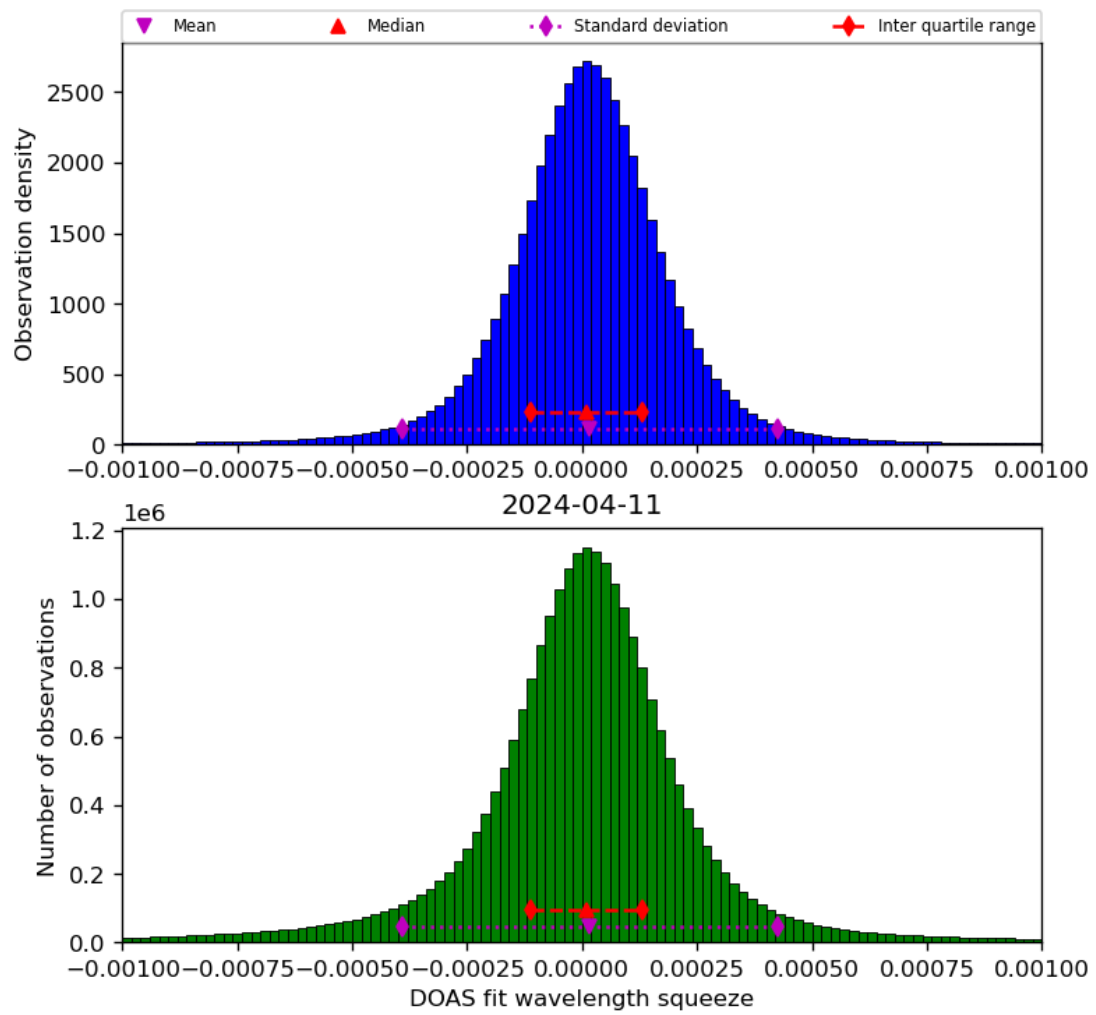
Figure 69: Histogram of “DOAS fit wavelength squeeze” for 2024-04-10 to 2024-04-12
