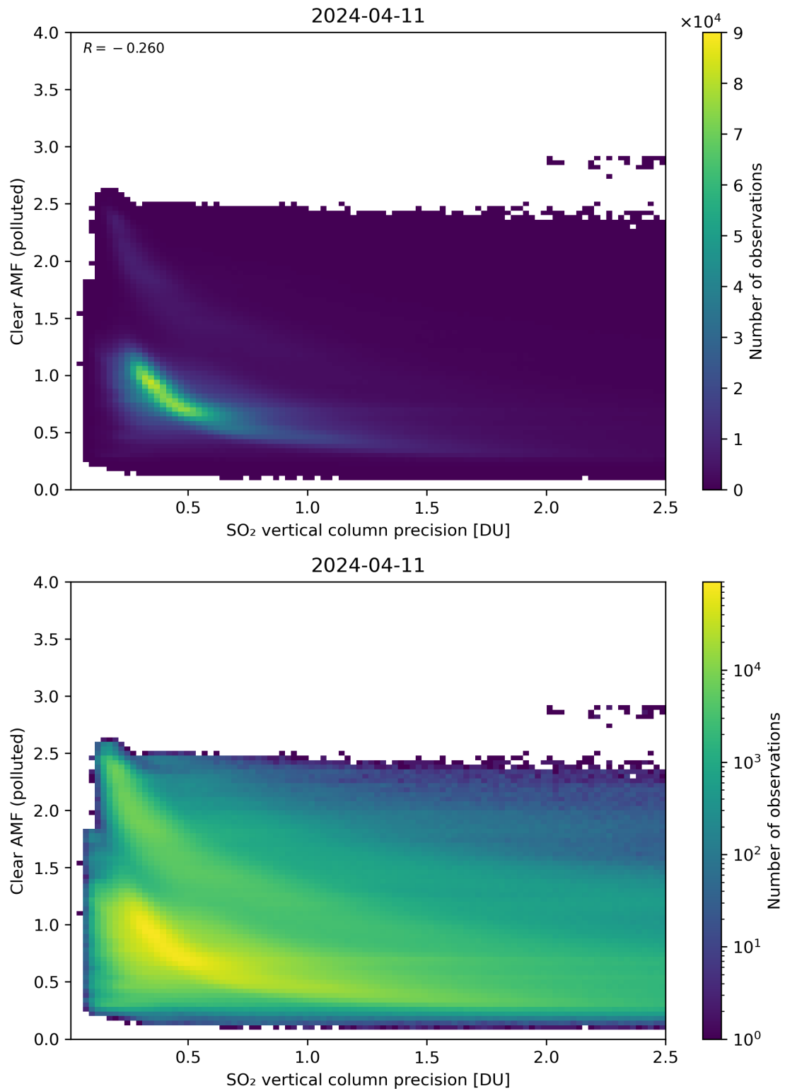
Figure 285: Scatter density plot of “SO 2 vertical column precision” against “Clear AMF (polluted)” for 2024-04-10 to 2024-04-12.
