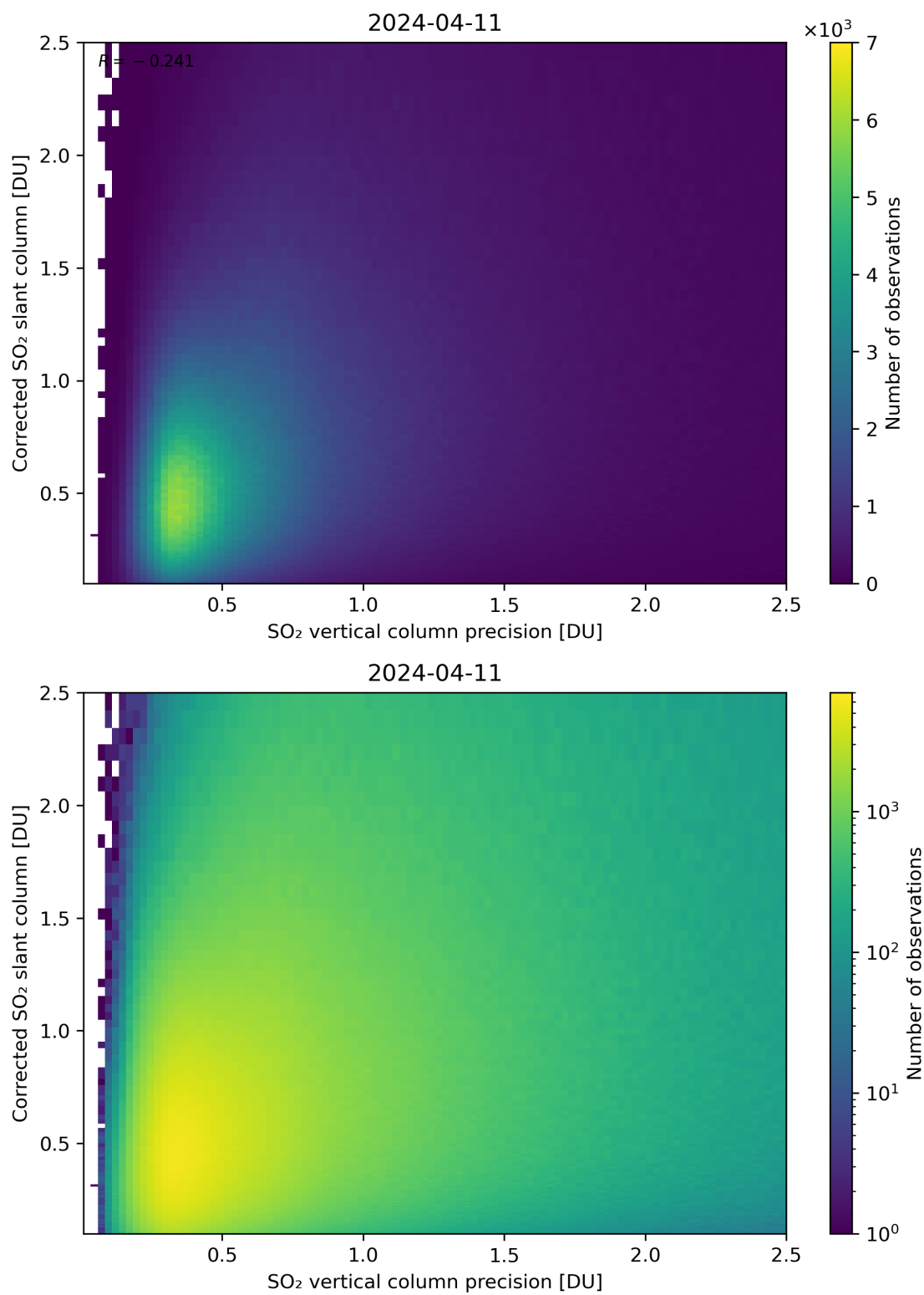
Figure 286: Scatter density plot of “SO 2 vertical column precision” against “Corrected SO 2 slant column” for 2024-04-10 to 2024-04-12.
