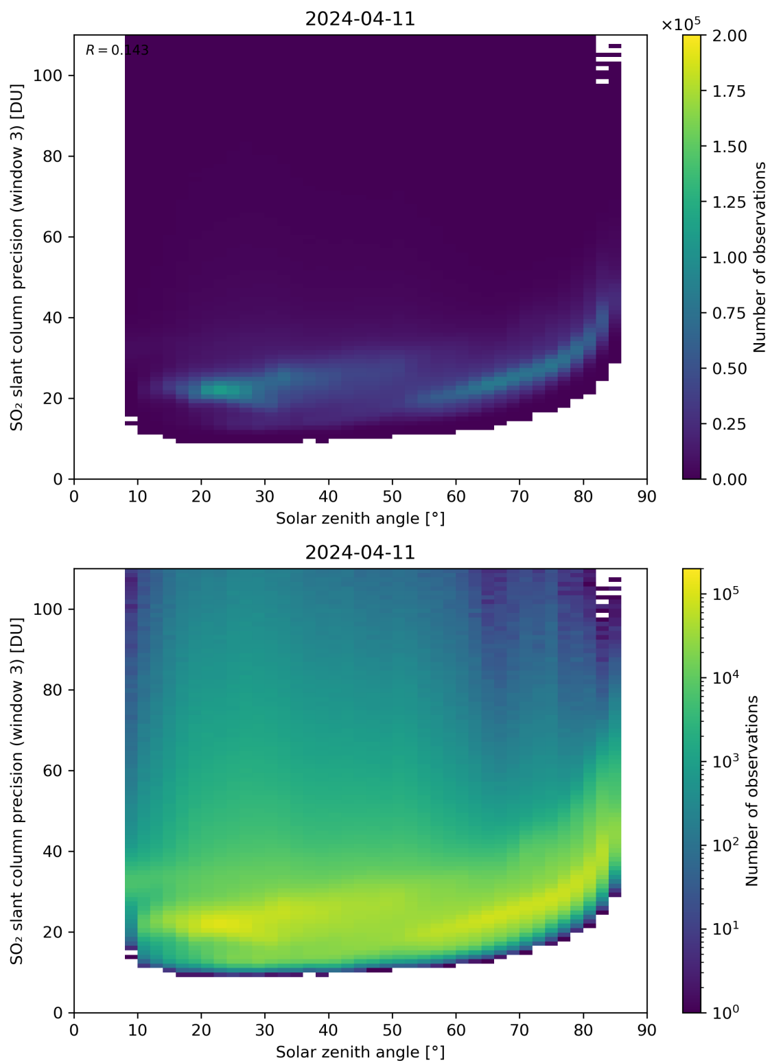
Figure 173: Scatter density plot of “Solar zenith angle” against “SO 2 slant column precision (window 3)” for 2024-04-10 to 2024-04-12.
