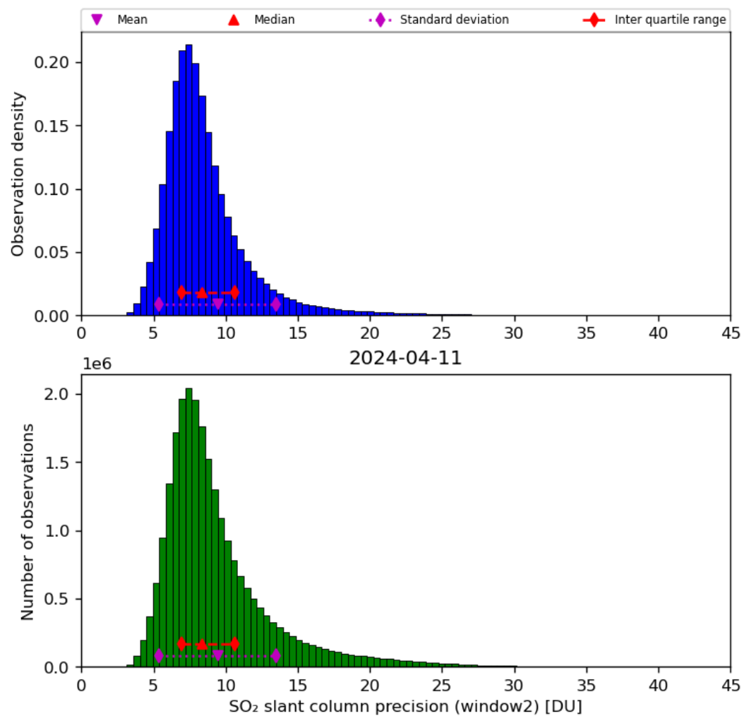
Figure 61: Histogram of “SO 2 slant column precision (window2)” for 2024-04-10 to 2024-04-12
