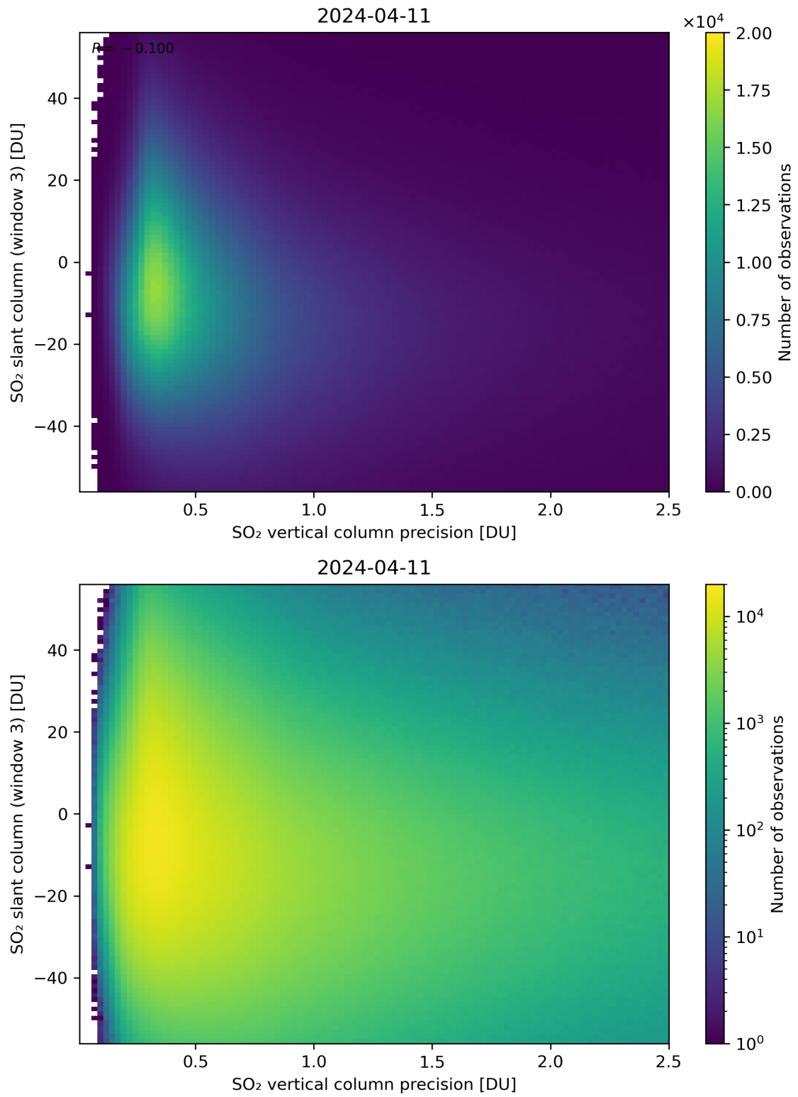
Figure 292: Scatter density plot of “SO 2 vertical column precision” against “SO 2 slant column (window 3)” for 2024-04-10 to 2024-04-12.
