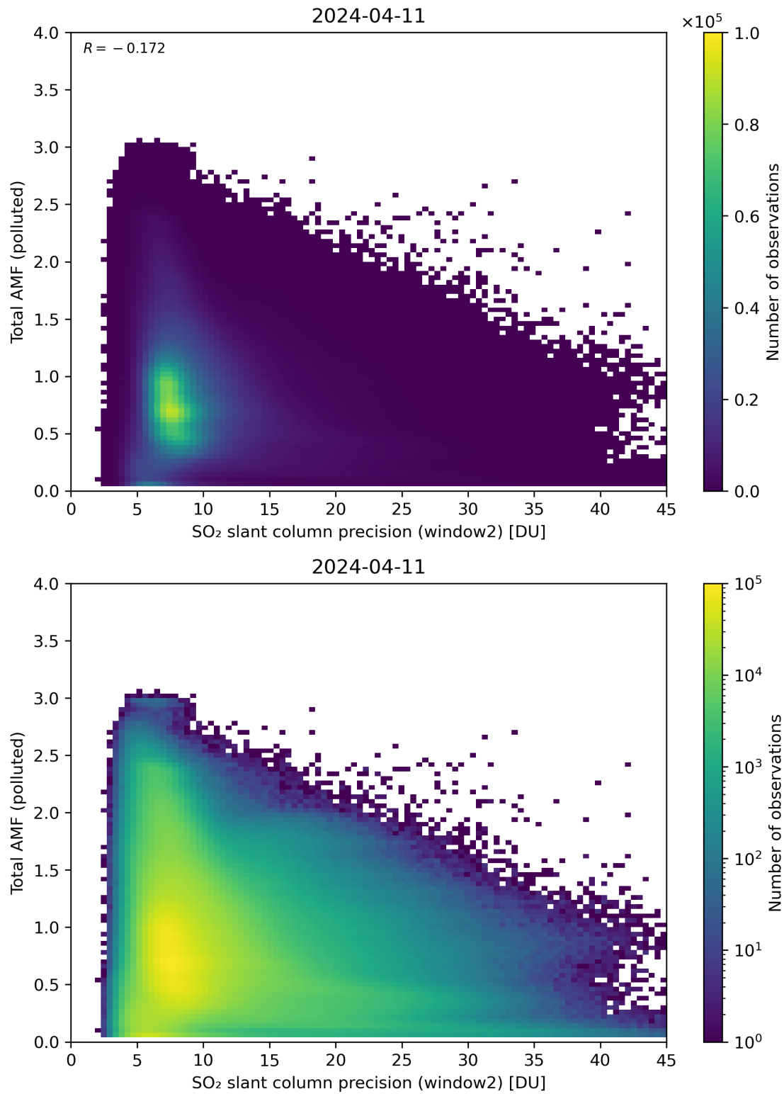
Figure 251: Scatter density plot of “SO 2 slant column precision (window2)” against “Total AMF (polluted)” for 2024-04-10 to 2024-04-12.
