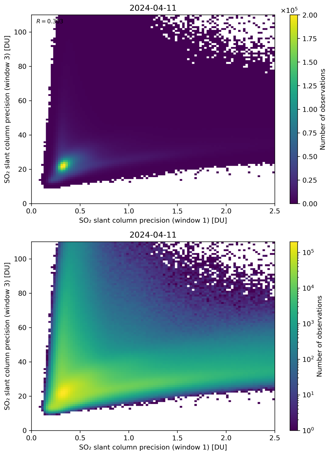
Figure 229: Scatter density plot of “SO 2 slant column precision (window 1)” against “SO 2 slant column precision (window 3)” for 2024-04-10 to 2024-04-12.
