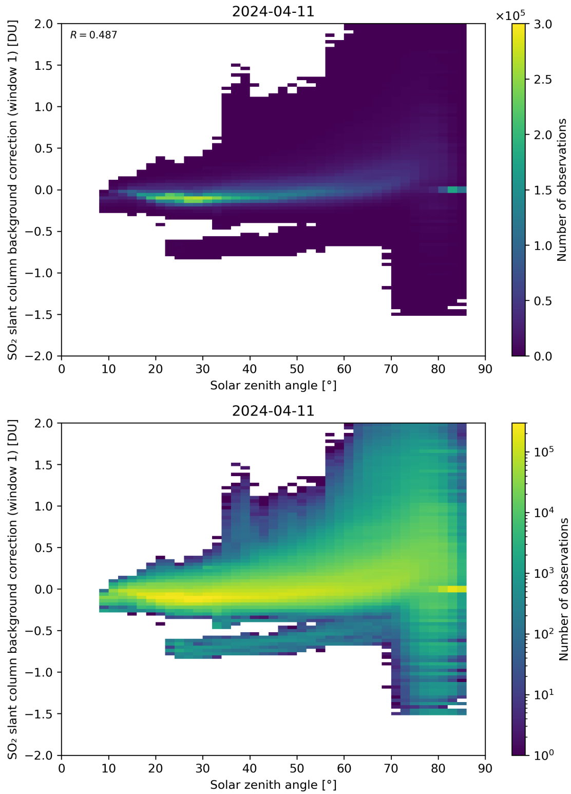
Figure 158: Scatter density plot of “Solar zenith angle” against “SO 2 slant column background correction (window 1)” for 2024-04-10 to 2024-04-12.
