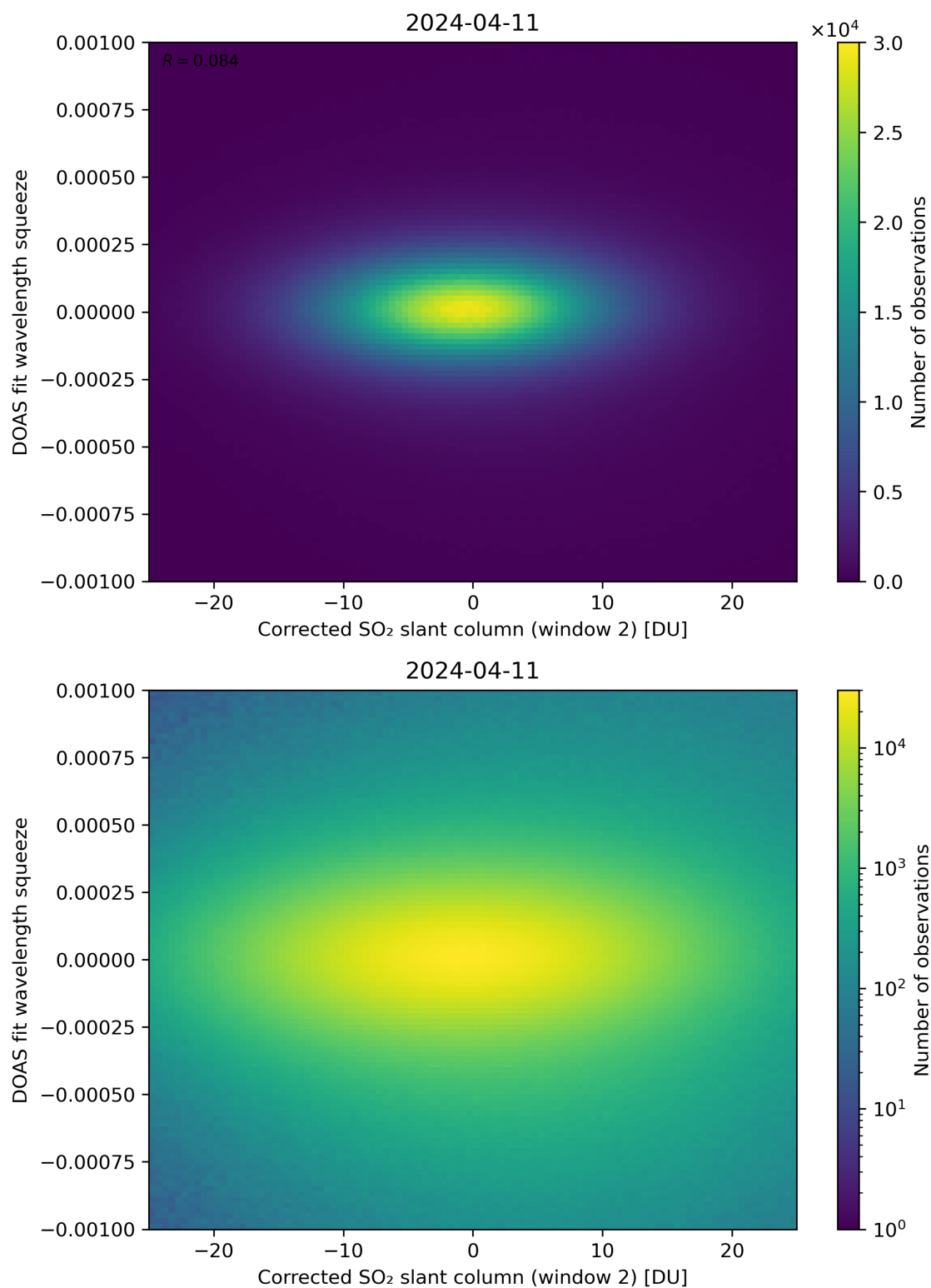
Figure 197: Scatter density plot of “Corrected SO 2 slant column (window 2)” against “DOAS fit wavelength squeeze” for 2024-04-10 to 2024-04-12.
