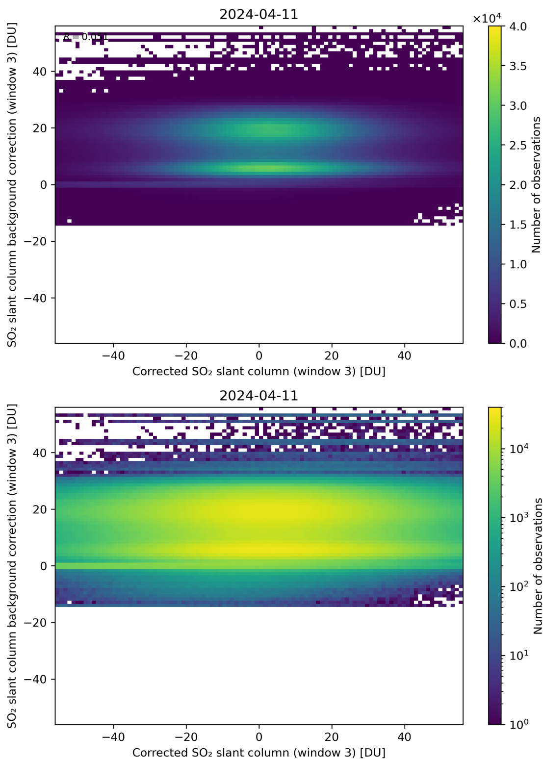
Figure 205: Scatter density plot of “Corrected SO 2 slant column (window 3)” against “SO 2 slant column background correction (window 3)” for 2024-04-10 to 2024-04-12.
