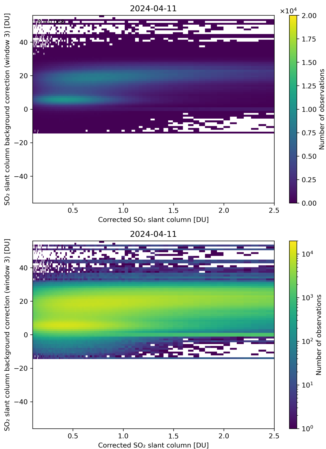
Figure 180: Scatter density plot of “Corrected SO 2 slant column” against “SO 2 slant column background correction (window 3)” for 2024-04-10 to 2024-04-12.
