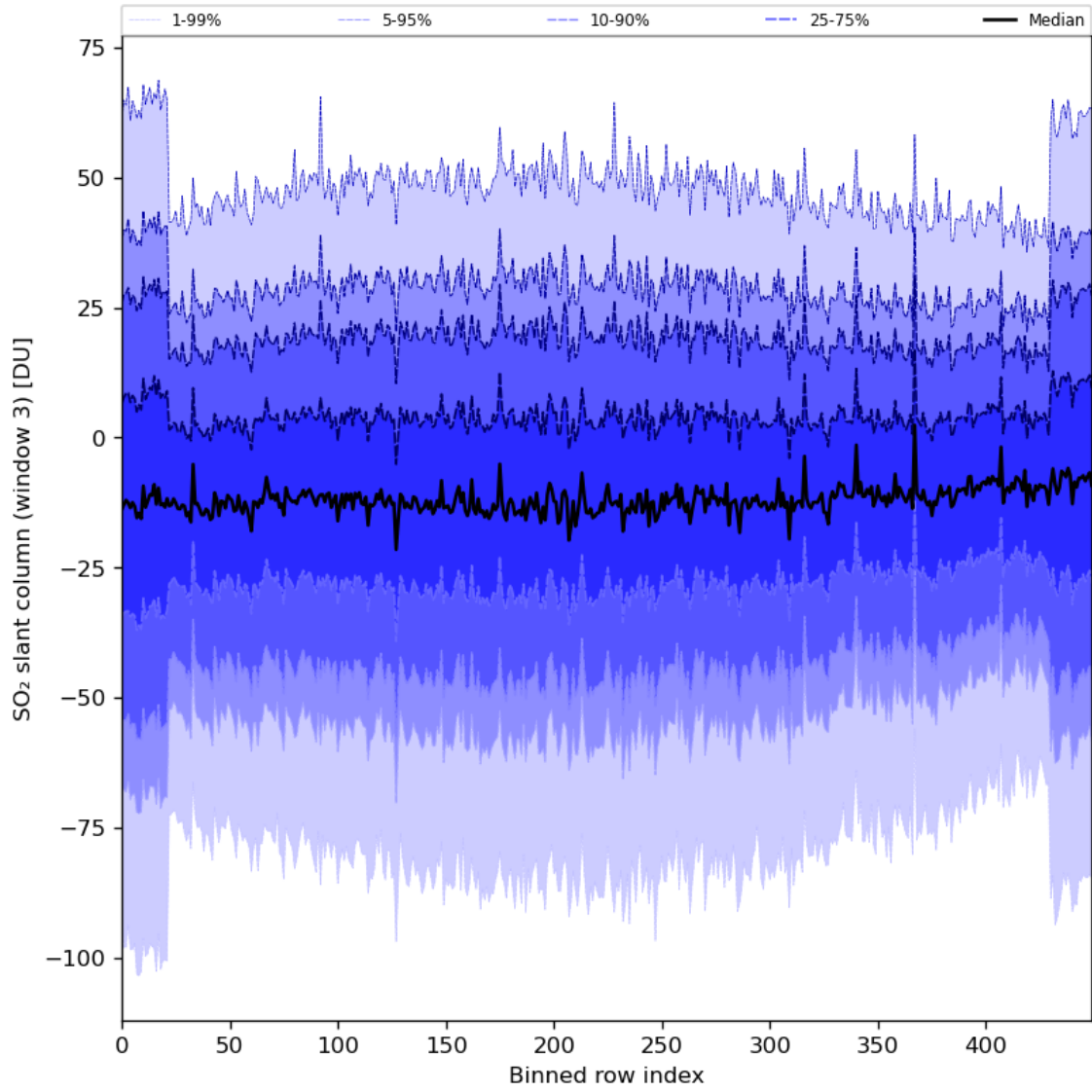
Figure 87: Along track statistics of “SO 2 slant column (window 3)” for 2024-04-10 to 2024-04-12
