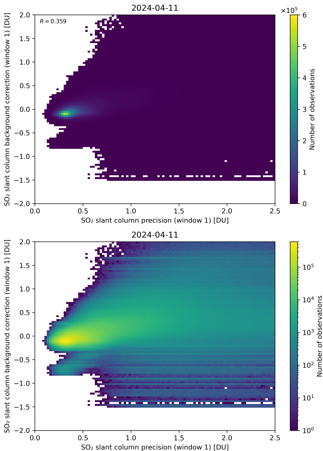
Figure 218: Scatter density plot of “SO 2 slant column precision (window 1)” against “SO 2 slant column background correction (window 1)” for 2024-04-10 to 2024-04-12.
