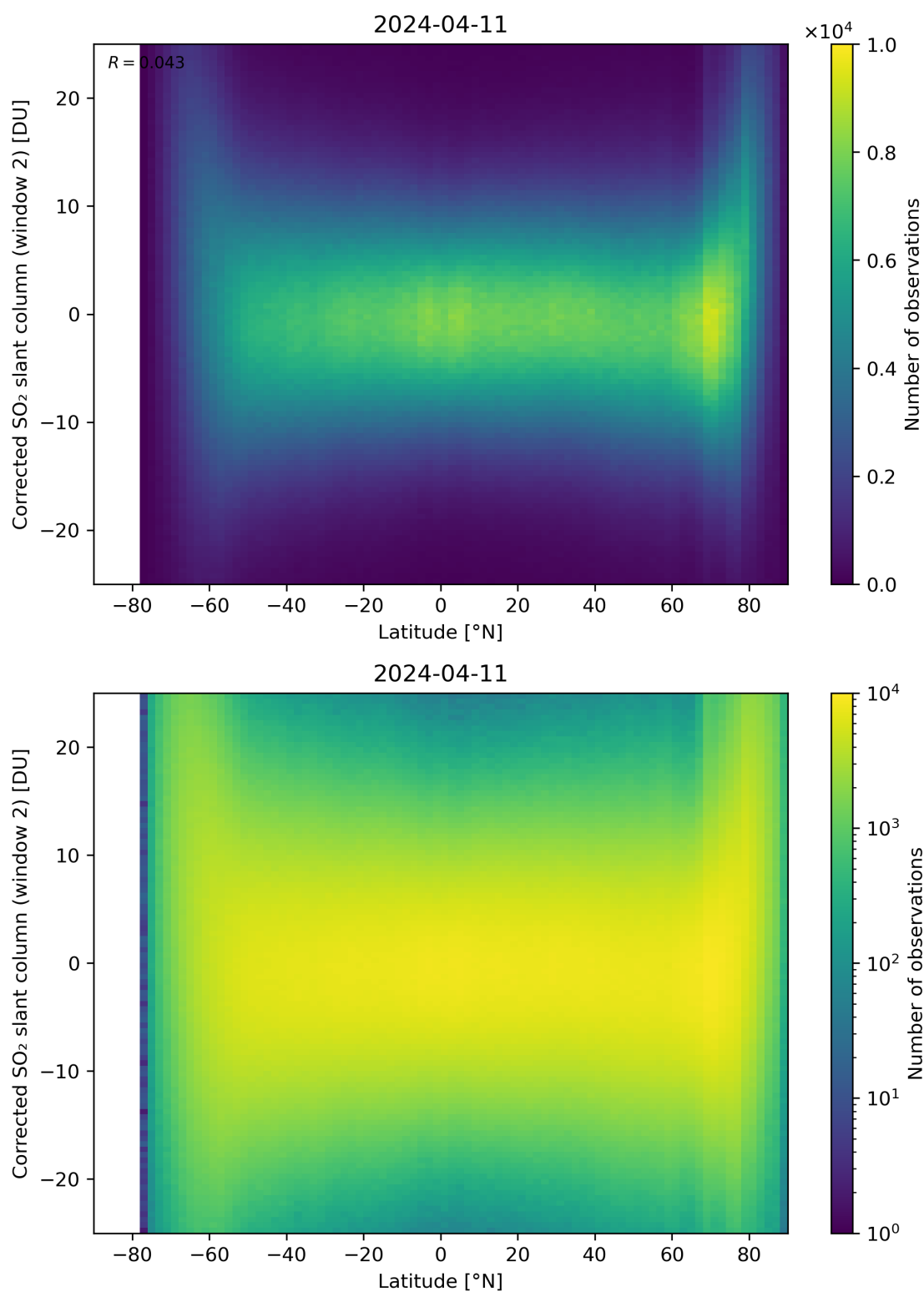
Figure 147: Scatter density plot of “Latitude” against “Corrected SO 2 slant column (window 2)” for 2024-04-10 to 2024-04-12.
