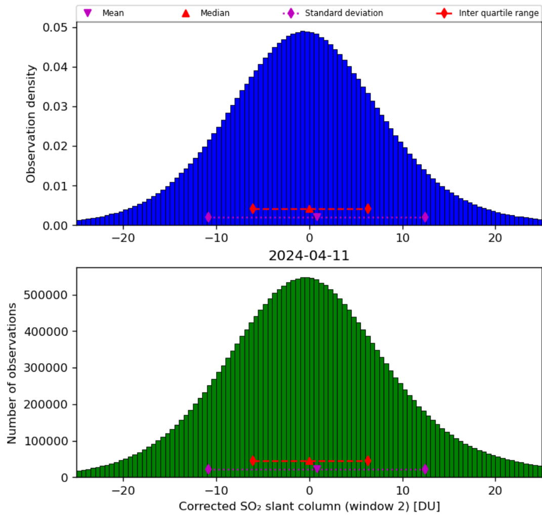
Figure 62: Histogram of “Corrected SO 2 slant column (window 2)” for 2024-04-10 to 2024-04-12
