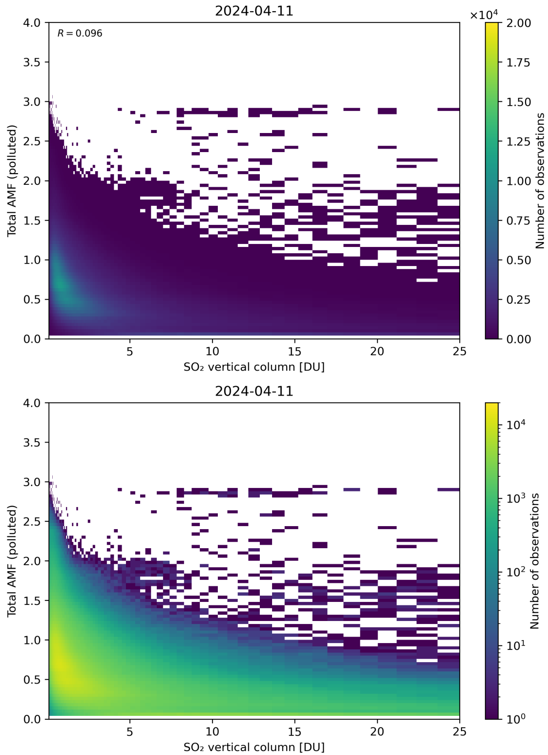
Figure 305: Scatter density plot of “SO 2 vertical column” against “Total AMF (polluted)” for 2024-04-10 to 2024-04-12.
