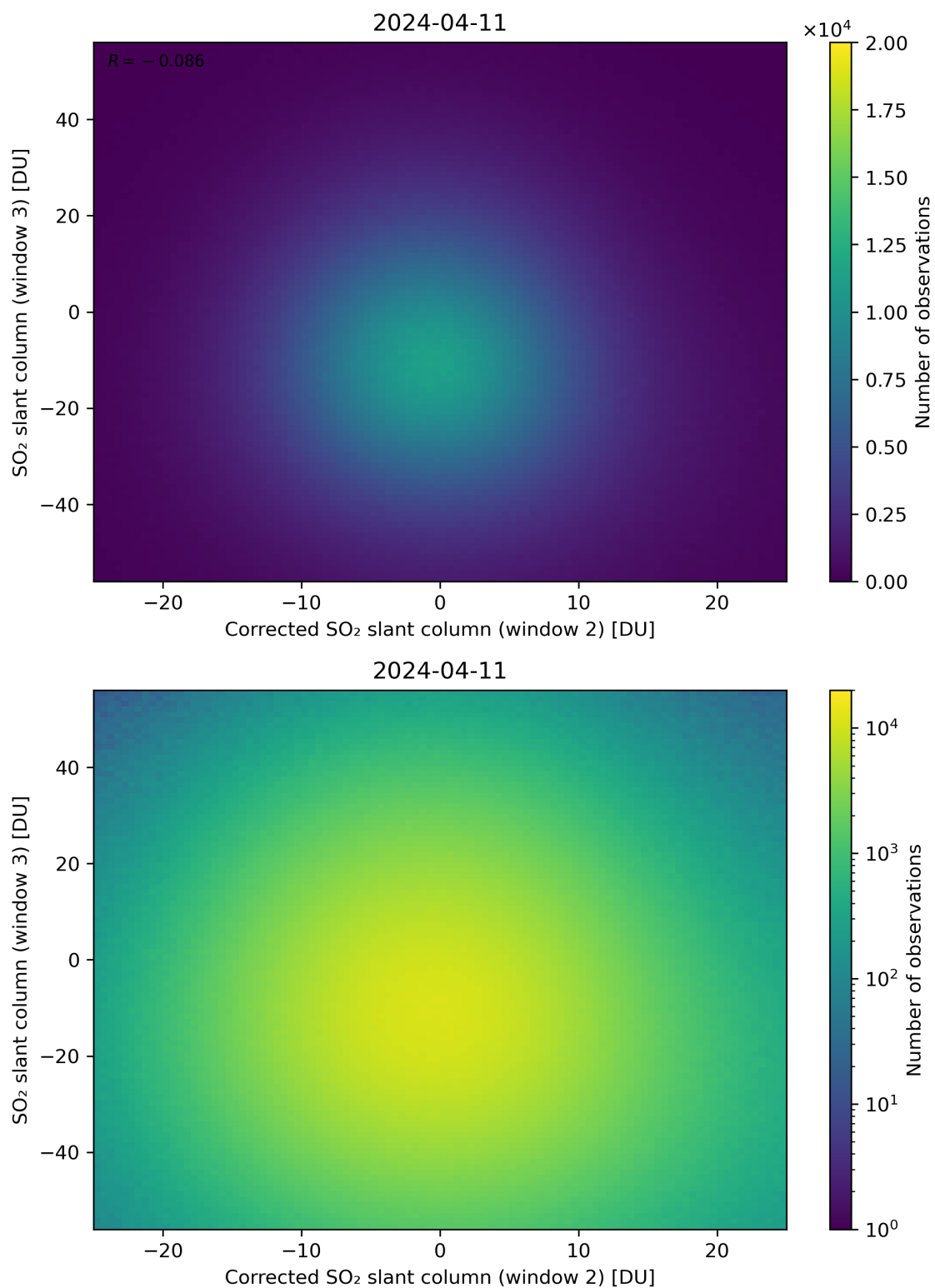
Figure 201: Scatter density plot of “Corrected SO 2 slant column (window 2)” against “SO 2 slant column (window 3)” for 2024-04-10 to 2024-04-12.
