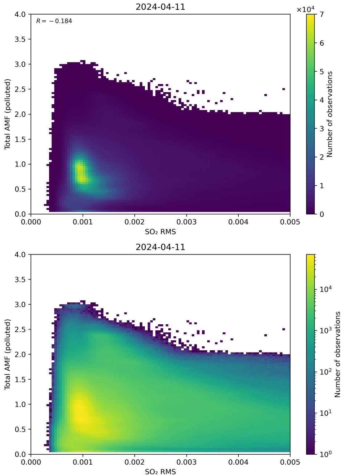
Figure 137: Scatter density plot of “SO 2 RMS” against “Total AMF (polluted)” for 2024-04-10 to 2024-04-12.
