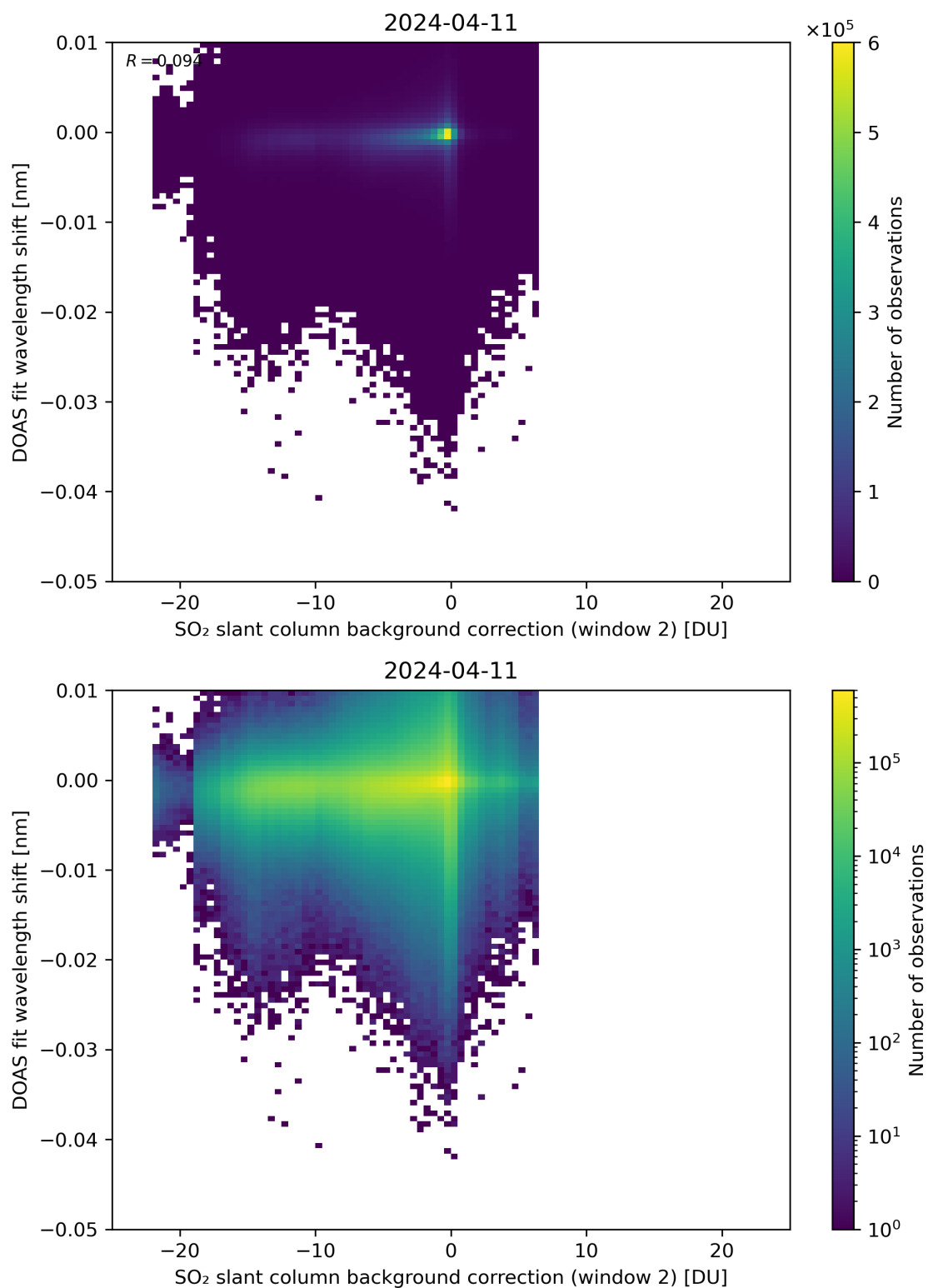
Figure 112: Scatter density plot of “SO 2 slant column background correction (window 2)” against “DOAS fit wavelength shift” for 2024-04-10 to 2024-04-12.
