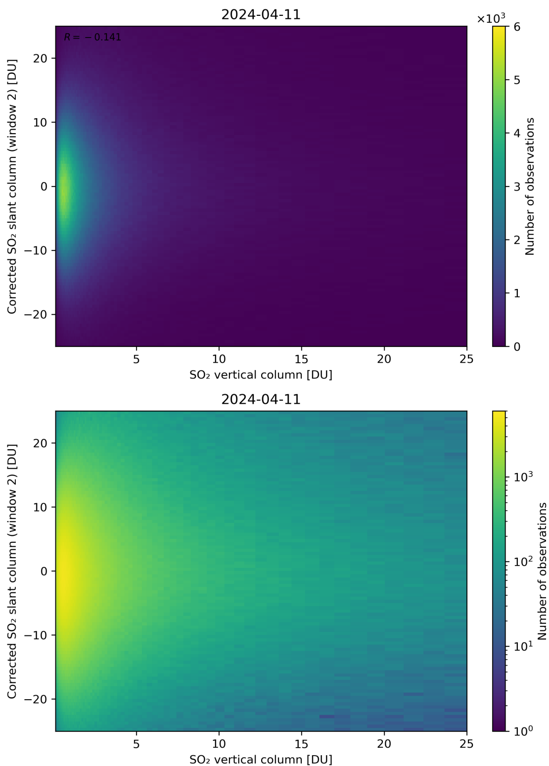
Figure 298: Scatter density plot of “SO 2 vertical column” against “Corrected SO 2 slant column (window 2)” for 2024-04-10 to 2024-04-12.
