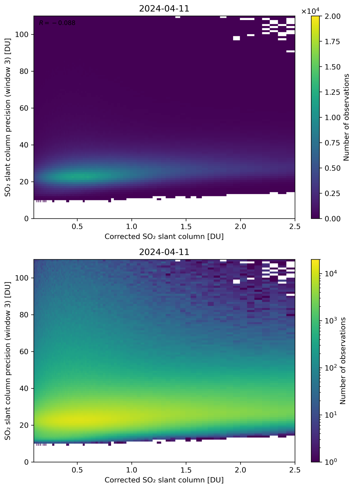
Figure 191: Scatter density plot of “Corrected SO 2 slant column” against “SO 2 slant column precision (window 3)” for 2024-04-10 to 2024-04-12.
