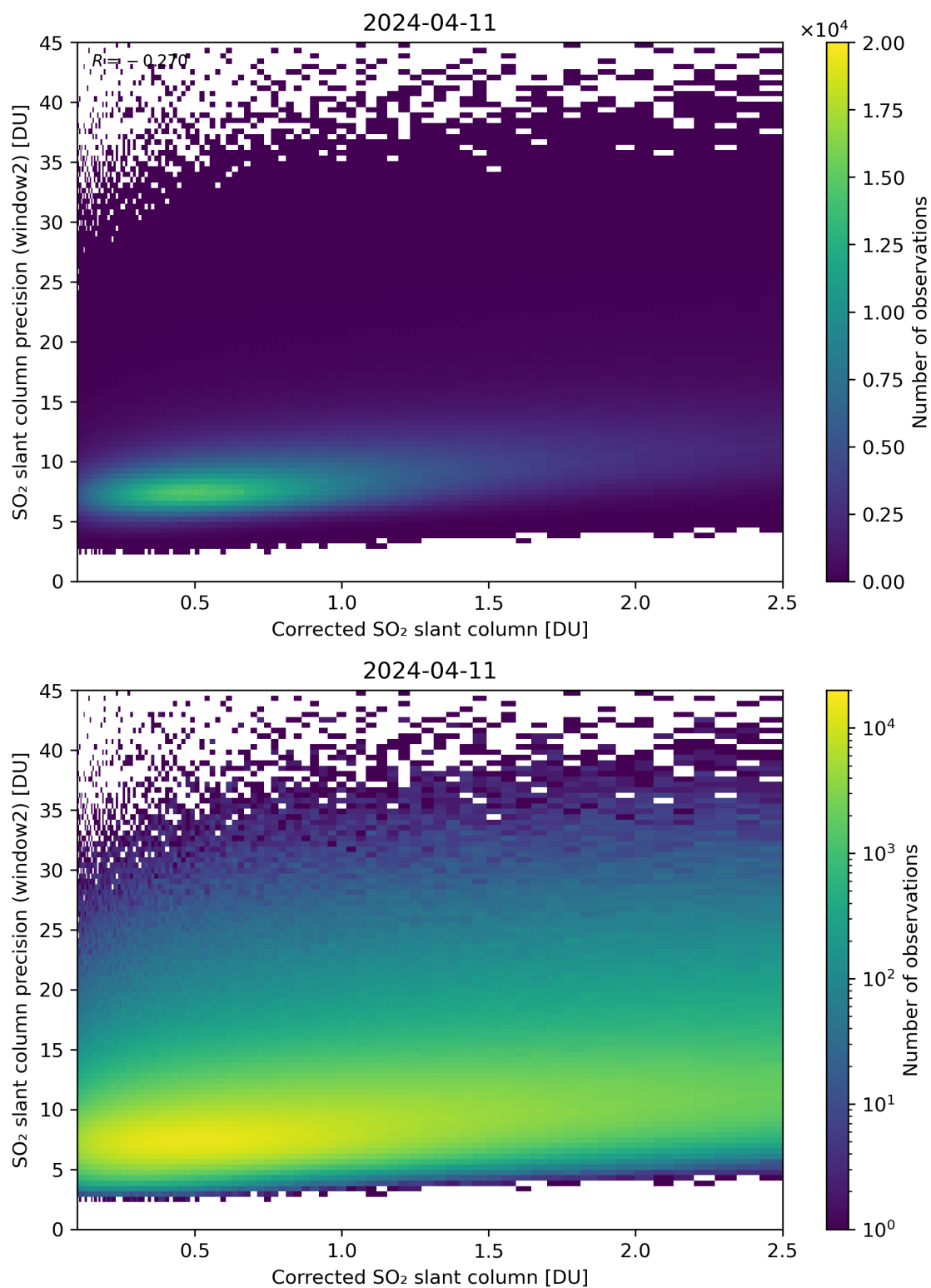
Figure 189: Scatter density plot of “Corrected SO 2 slant column” against “SO 2 slant column precision (window2)” for 2024-04-10 to 2024-04-12.
