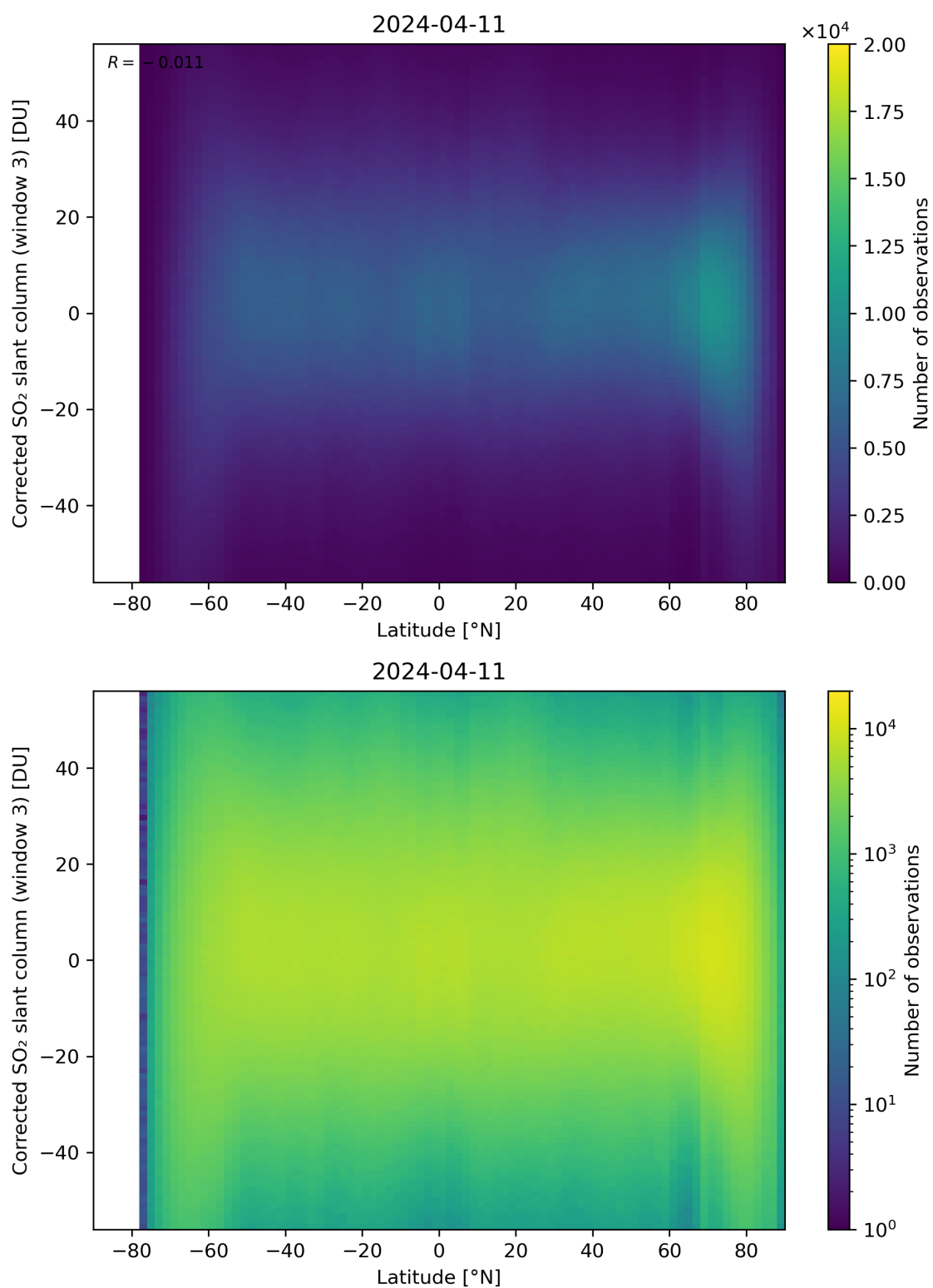
Figure 148: Scatter density plot of “Latitude” against “Corrected SO 2 slant column (window 3)” for 2024-04-10 to 2024-04-12.
