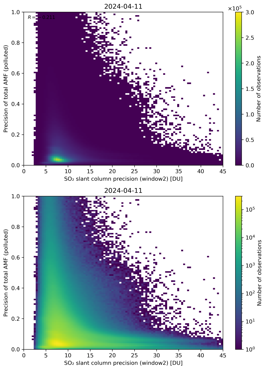
Figure 252: Scatter density plot of “SO 2 slant column precision (window2)” against “Precision of total AMF (polluted)” for 2024-04-10 to 2024-04-12.
