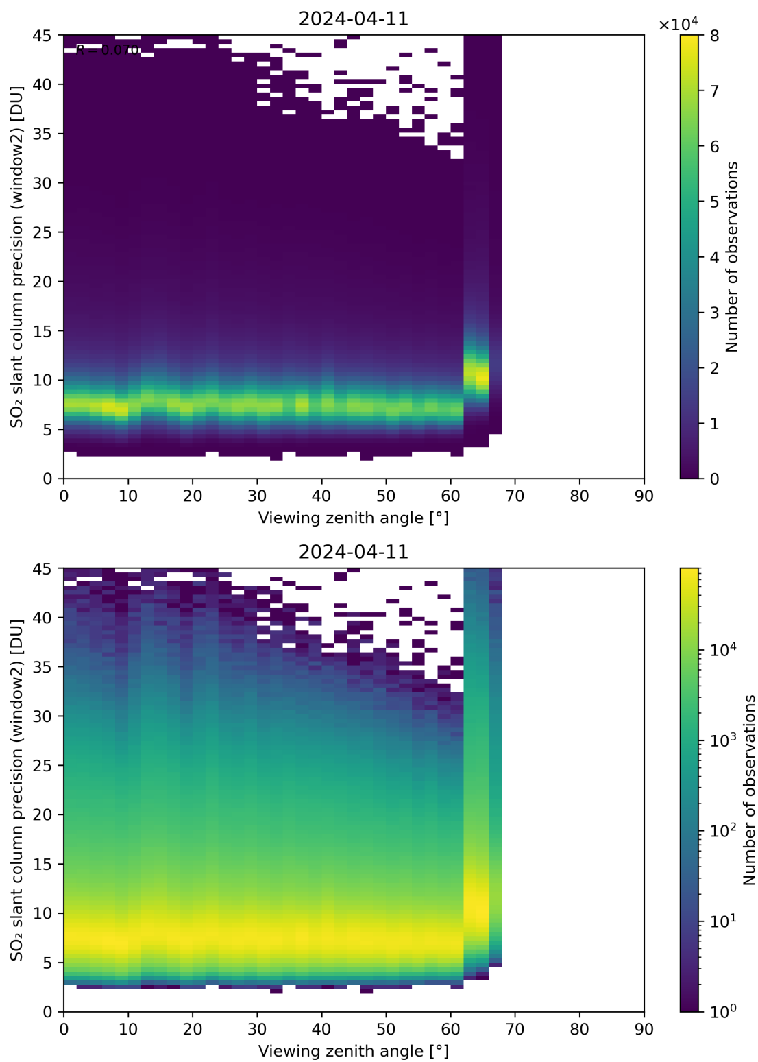
Figure 322: Scatter density plot of “Viewing zenith angle” against “SO 2 slant column precision (window2)” for 2024-04-10 to 2024-04-12.
