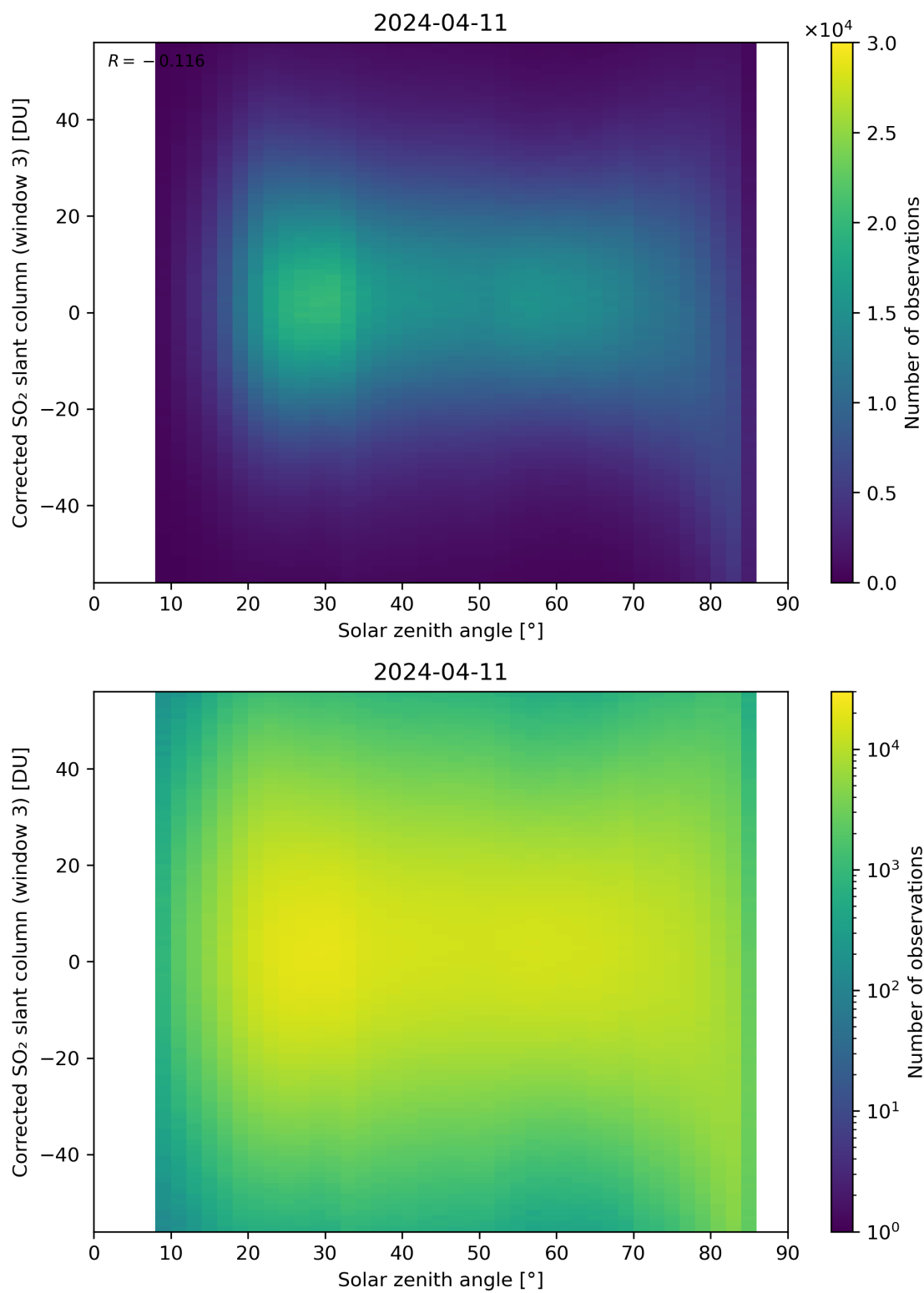
Figure 168: Scatter density plot of “Solar zenith angle” against “Corrected SO 2 slant column (window 3)” for 2024-04-10 to 2024-04-12.
