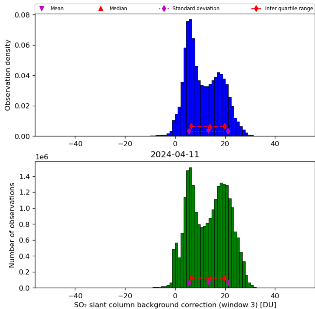
Figure 67: Histogram of “SO 2 slant column background correction (window 3)” for 2024-04-10 to 2024-04-12
