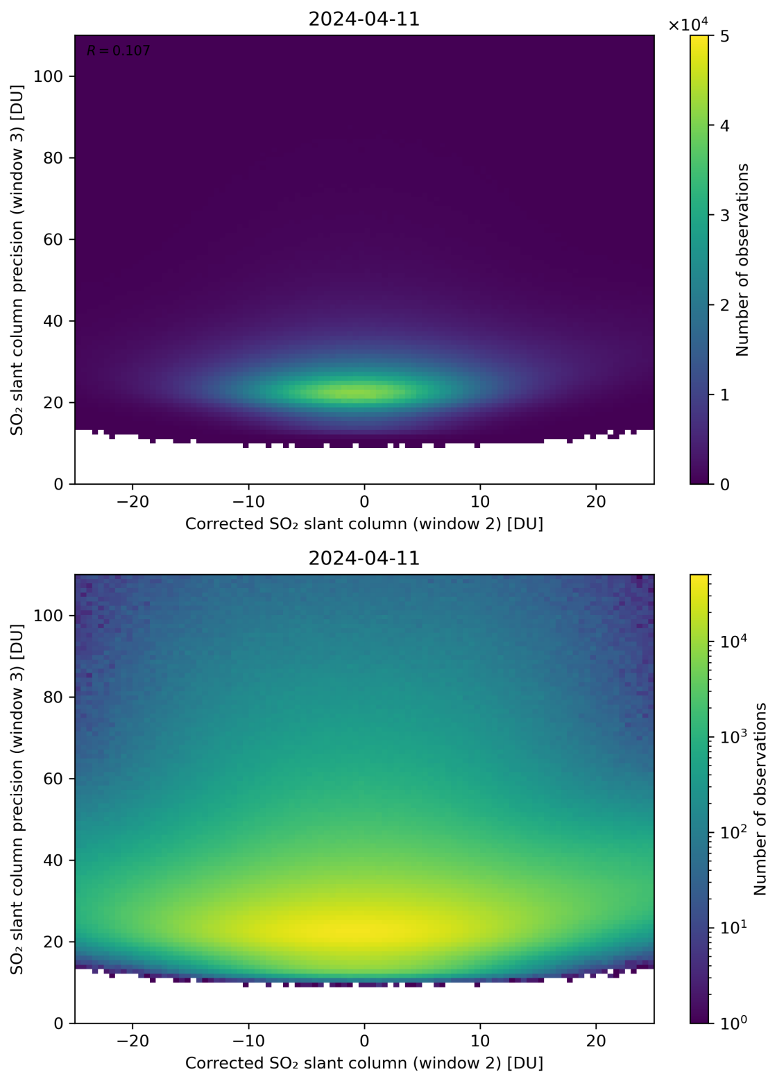
Figure 202: Scatter density plot of “Corrected SO 2 slant column (window 2)” against “SO 2 slant column precision (window 3)” for 2024-04-10 to 2024-04-12.
