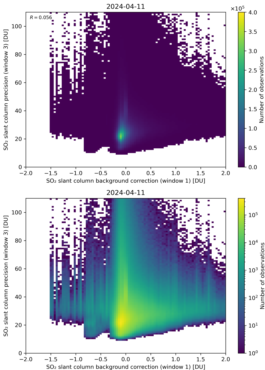
Figure 108: Scatter density plot of “SO 2 slant column background correction (window 1)” against “SO 2 slant column precision (window 3)” for 2024-04-10 to 2024-04-12.
