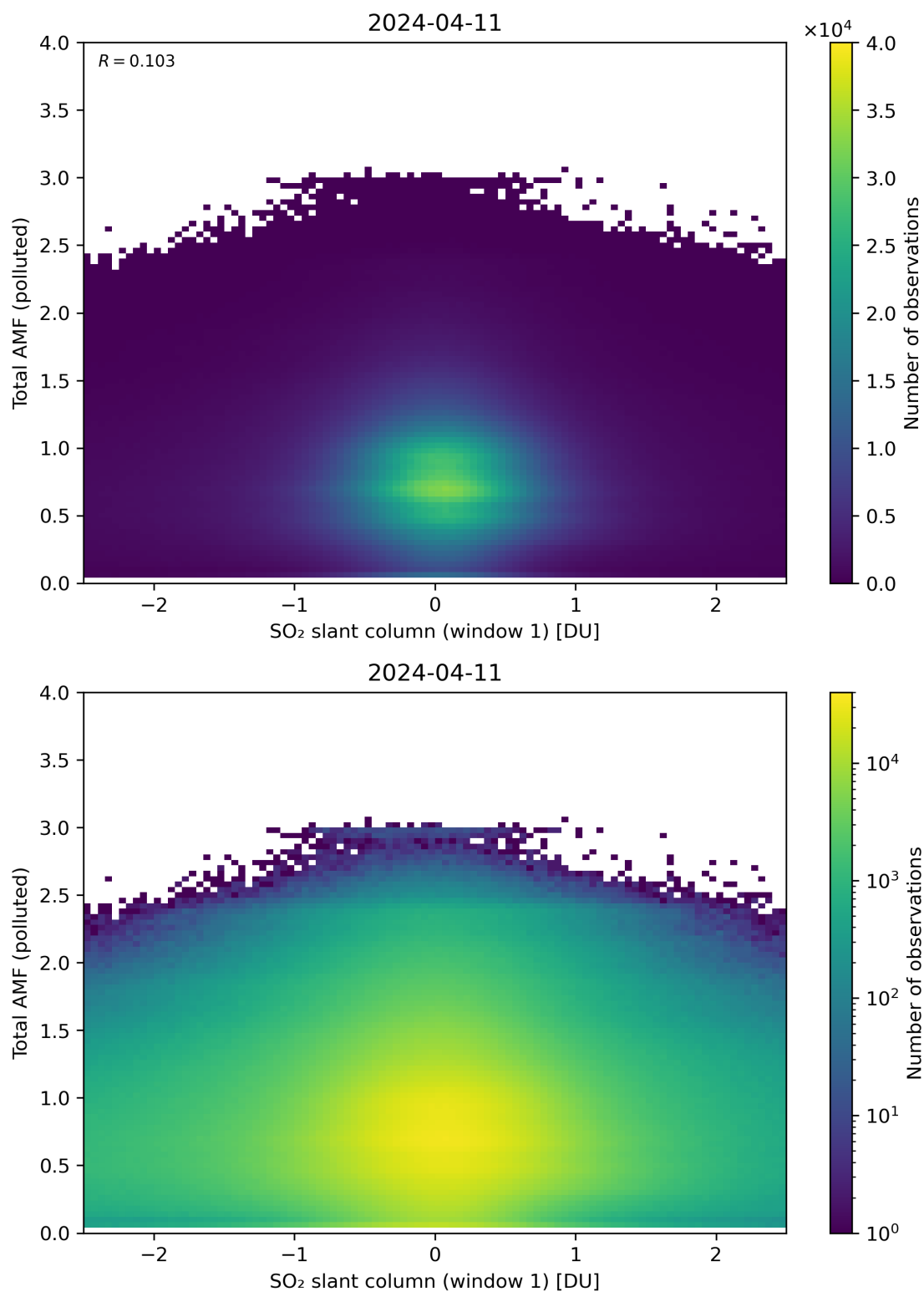
Figure 239: Scatter density plot of “SO 2 slant column (window 1)” against “Total AMF (polluted)” for 2024-04-10 to 2024-04-12.
