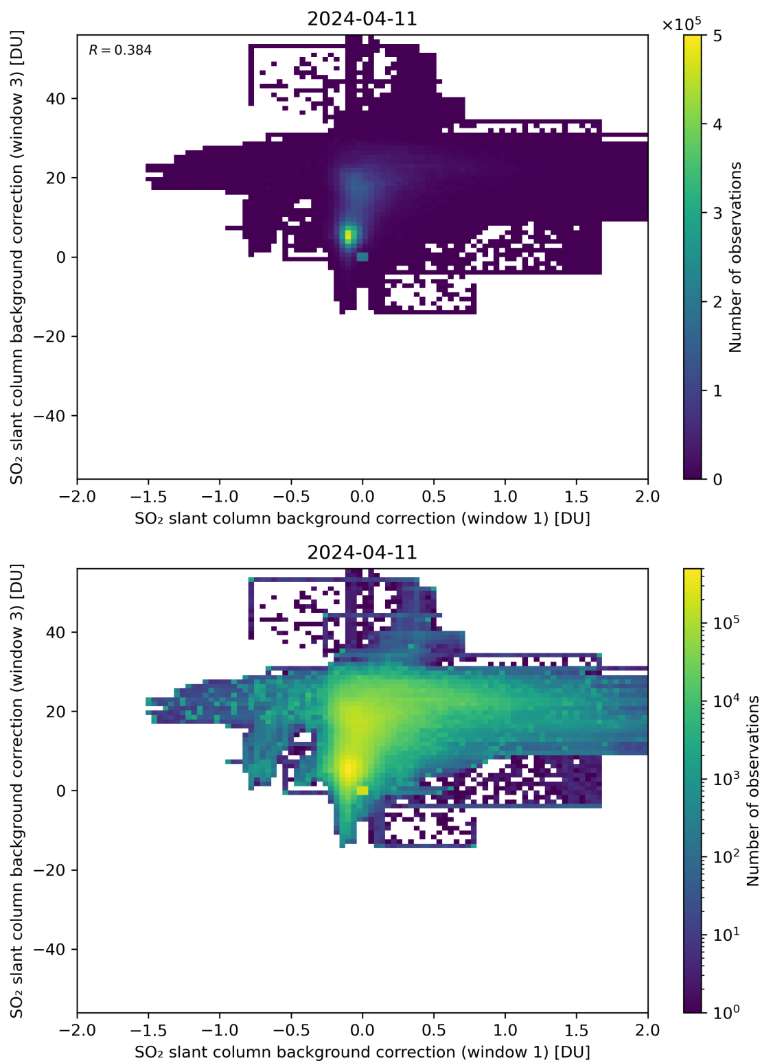
Figure 99: Scatter density plot of “SO 2 slant column background correction (window 1)” against “SO 2 slant column background correction (window 3)” for 2024-04-10 to 2024-04-12.
