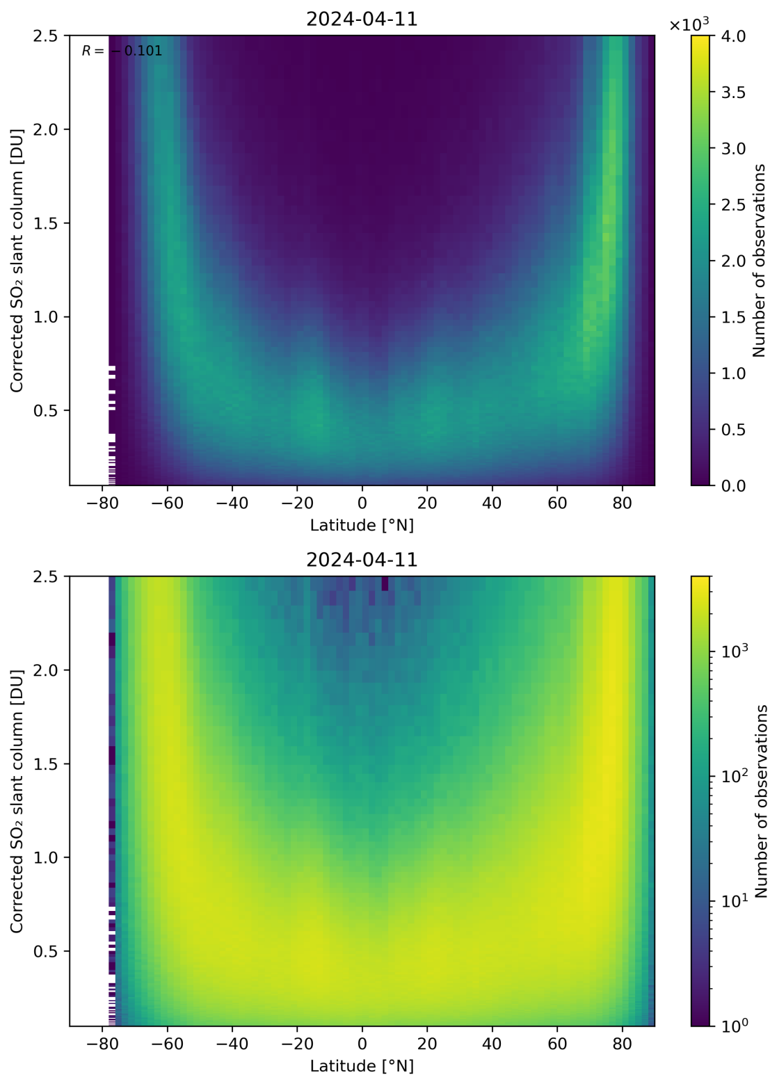
Figure 146: Scatter density plot of “Latitude” against “Corrected SO 2 slant column” for 2024-04-10 to 2024-04-12.
