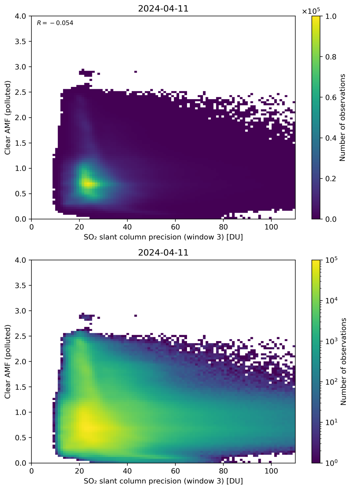
Figure 261: Scatter density plot of “SO 2 slant column precision (window 3)” against “Clear AMF (polluted)” for 2024-04-10 to 2024-04-12.
