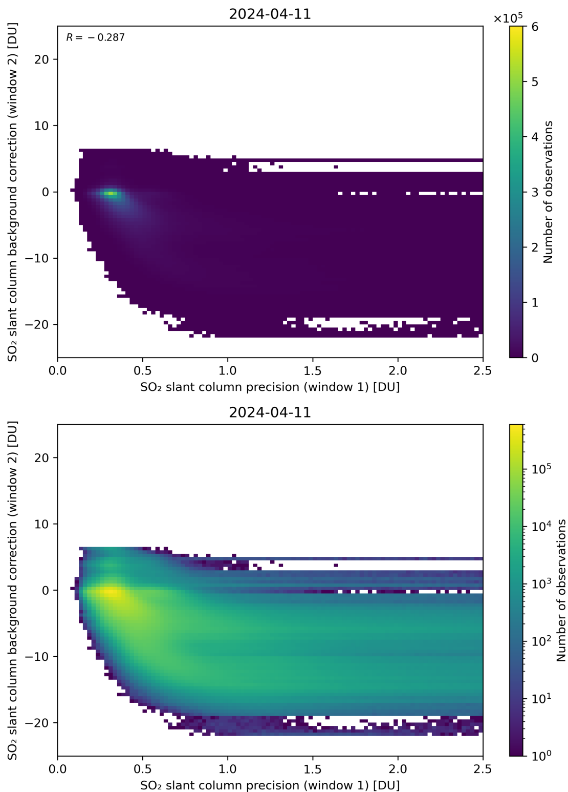
Figure 219: Scatter density plot of “SO 2 slant column precision (window 1)” against “SO 2 slant column background correction (window 2)” for 2024-04-10 to 2024-04-12.
