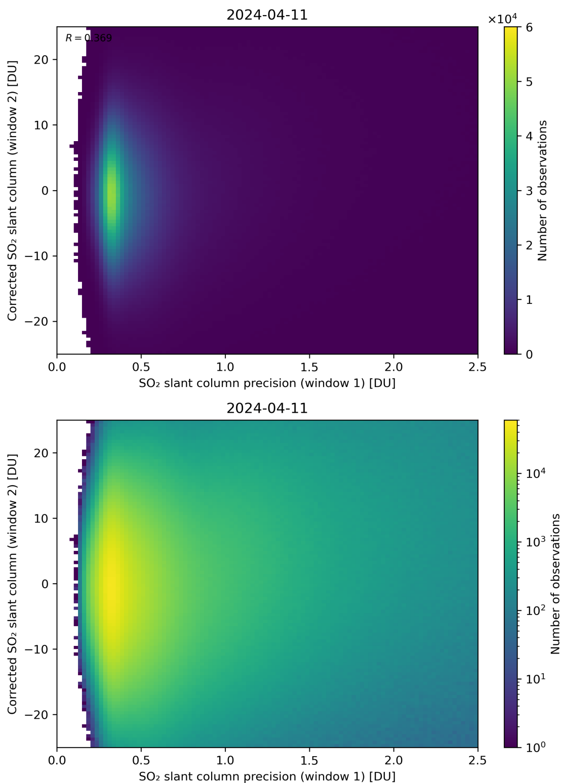
Figure 225: Scatter density plot of “SO 2 slant column precision (window 1)” against “Corrected SO 2 slant column (window 2)” for 2024-04-10 to 2024-04-12.
