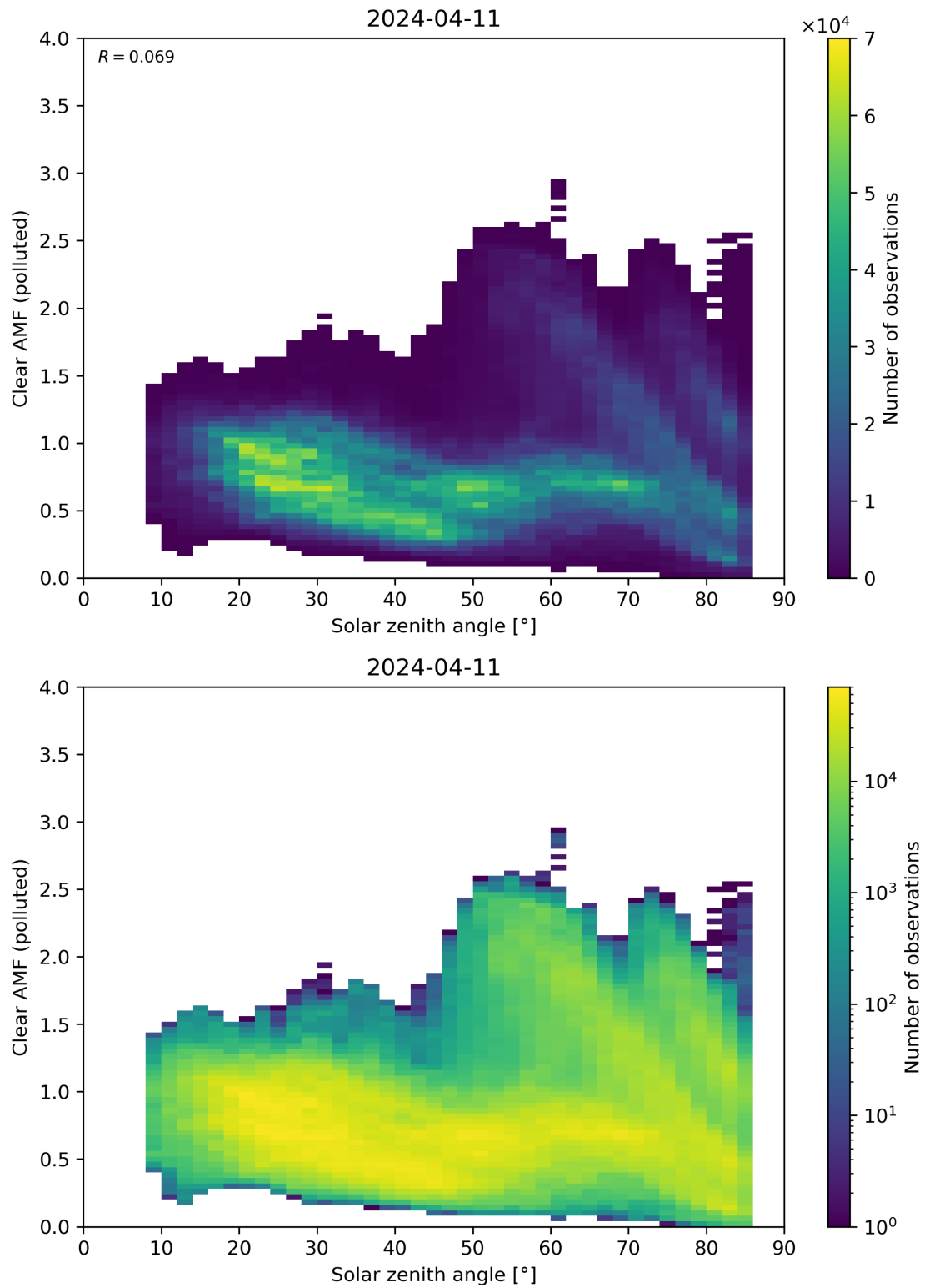
Figure 165: Scatter density plot of “Solar zenith angle” against “Clear AMF (polluted)” for 2024-04-10 to 2024-04-12.
