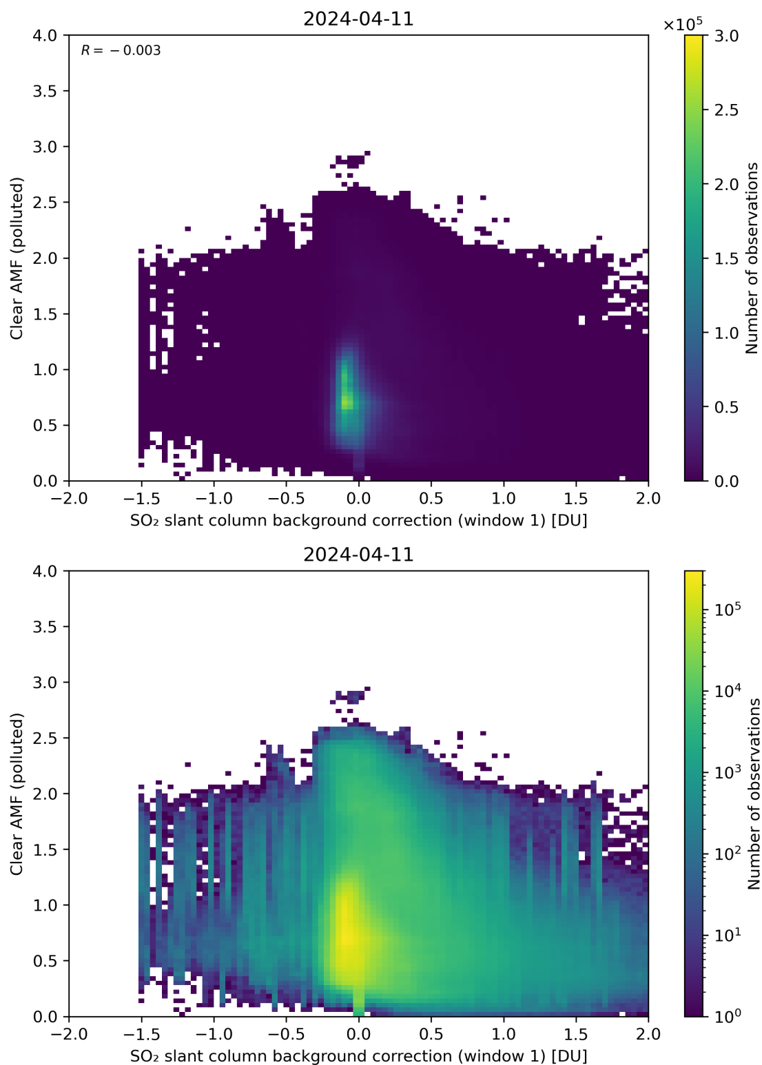
Figure 103: Scatter density plot of “SO 2 slant column background correction (window 1)” against “Clear AMF (polluted)” for 2024-04-10 to 2024-04-12.
