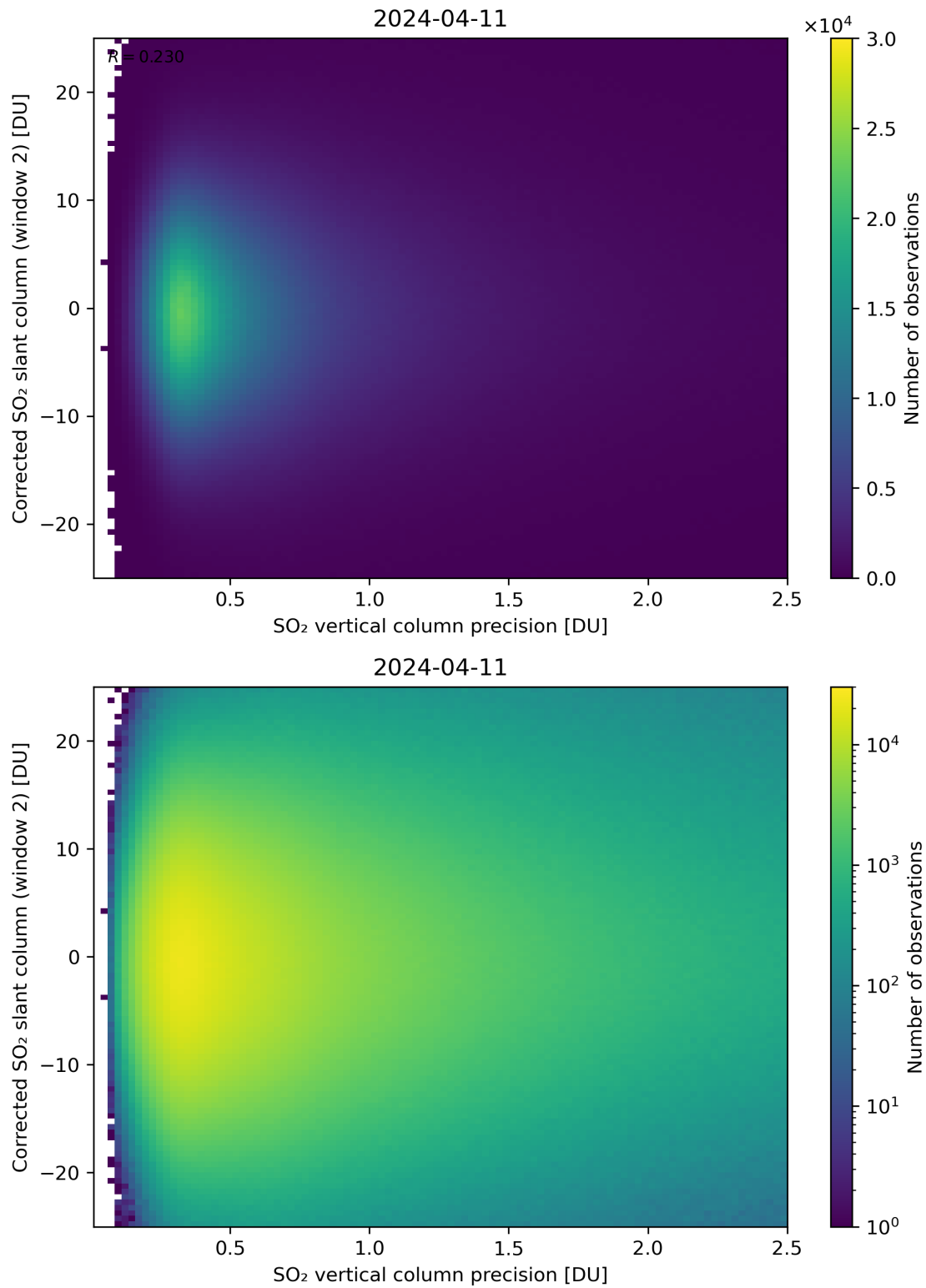
Figure 287: Scatter density plot of “SO 2 vertical column precision” against “Corrected SO 2 slant column (window 2)” for 2024-04-10 to 2024-04-12.
