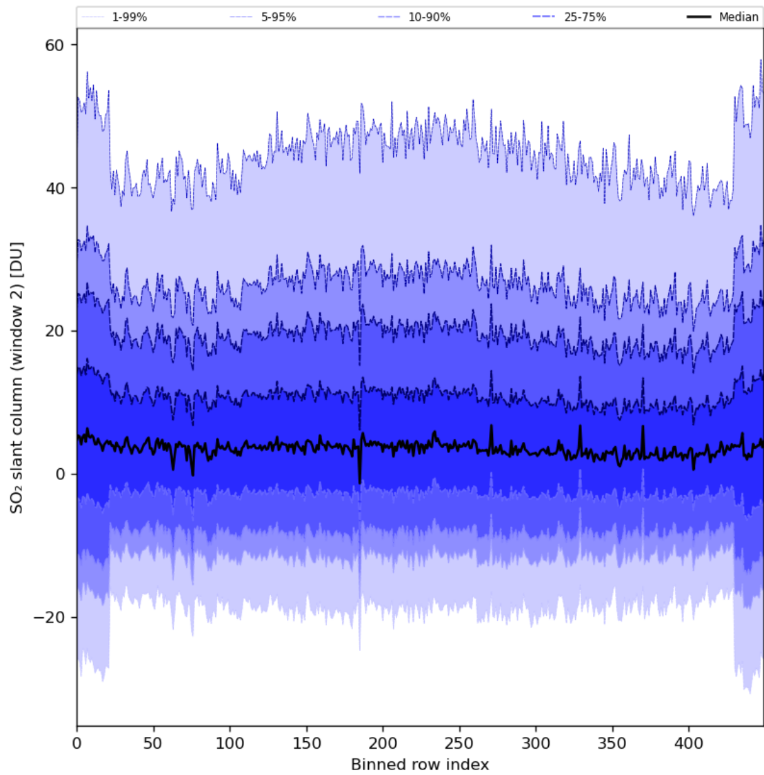
Figure 83: Along track statistics of “SO 2 slant column (window 2)” for 2024-04-10 to 2024-04-12
