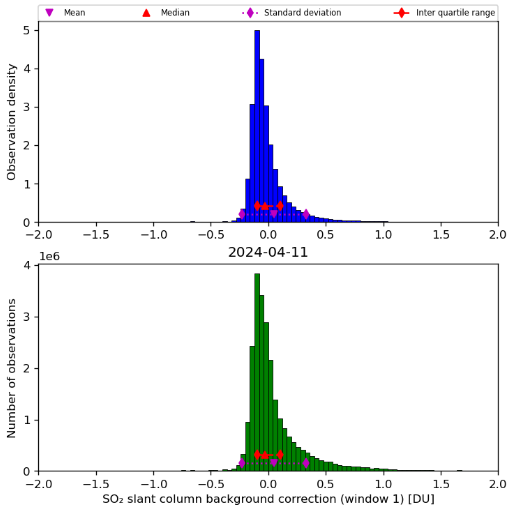
Figure 59: Histogram of “SO 2 slant column background correction (window 1)” for 2024-04-10 to 2024-04-12
