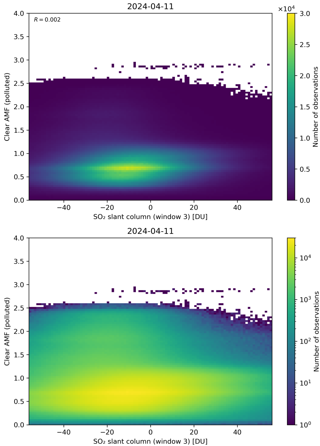
Figure 265: Scatter density plot of “SO 2 slant column (window 3)” against “Clear AMF (polluted)” for 2024-04-10 to 2024-04-12.
