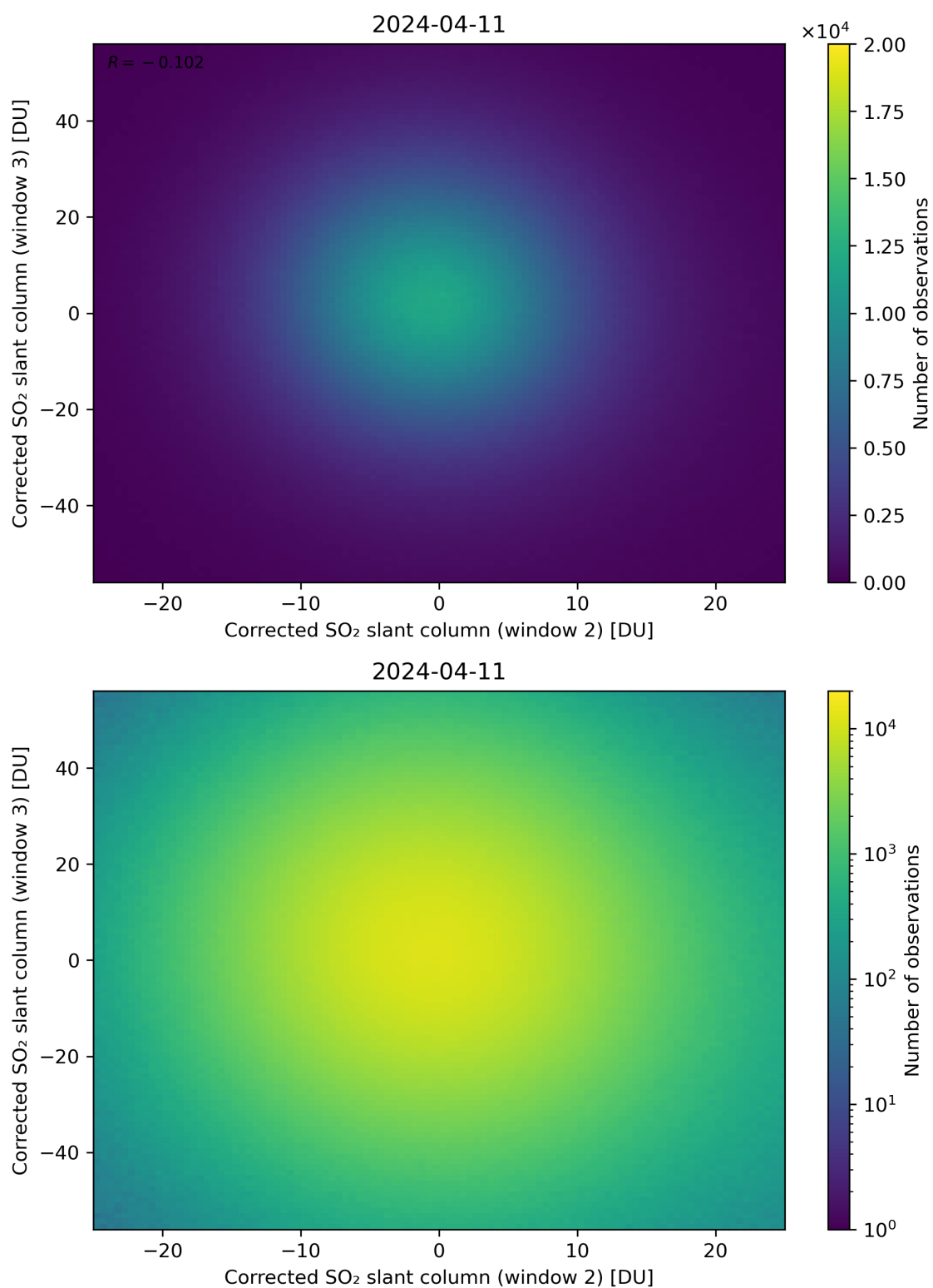
Figure 200: Scatter density plot of “Corrected SO 2 slant column (window 2)” against “Corrected SO 2 slant column (window 3)” for 2024-04-10 to 2024-04-12.
