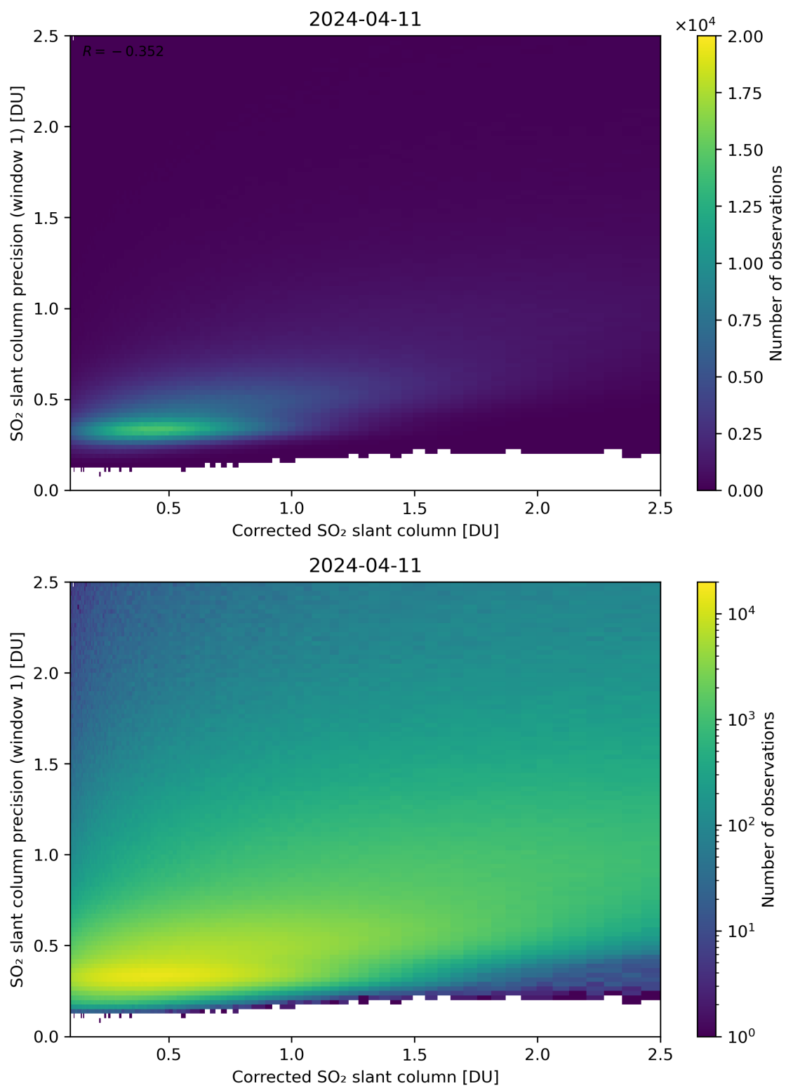
Figure 188: Scatter density plot of “Corrected SO 2 slant column” against “SO 2 slant column precision (window 1)” for 2024-04-10 to 2024-04-12.
