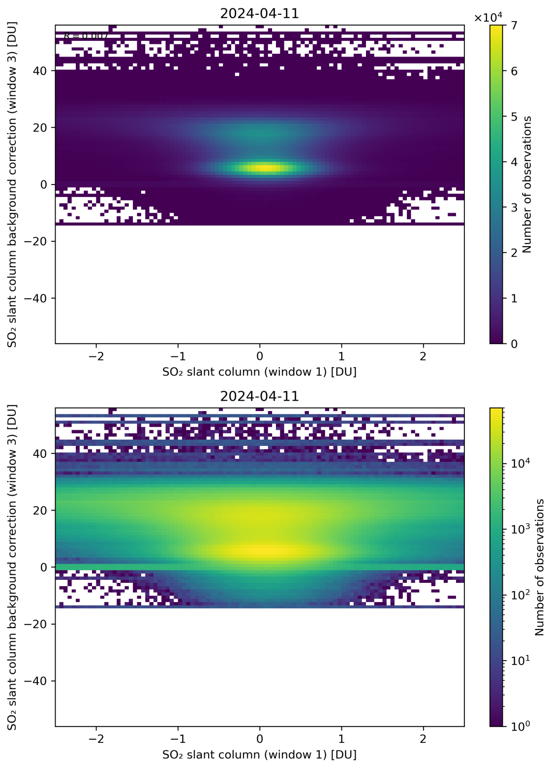
Figure 214: Scatter density plot of “SO 2 slant column (window 1)” against “SO 2 slant column background correction (window 3)” for 2024-04-10 to 2024-04-12.
