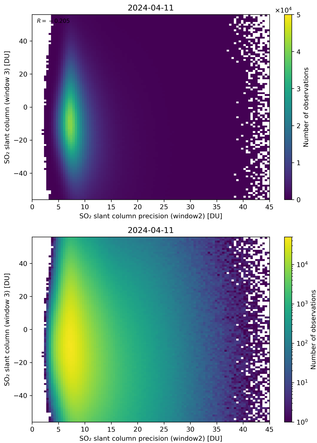
Figure 249: Scatter density plot of “SO 2 slant column precision (window2)” against “SO 2 slant column (window 3)” for 2024-04-10 to 2024-04-12.
