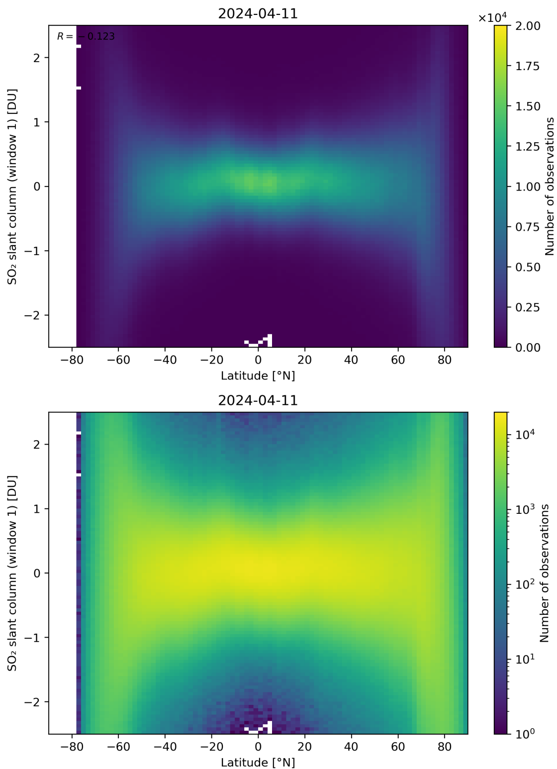
Figure 149: Scatter density plot of “Latitude” against “SO 2 slant column (window 1)” for 2024-04-10 to 2024-04-12.
