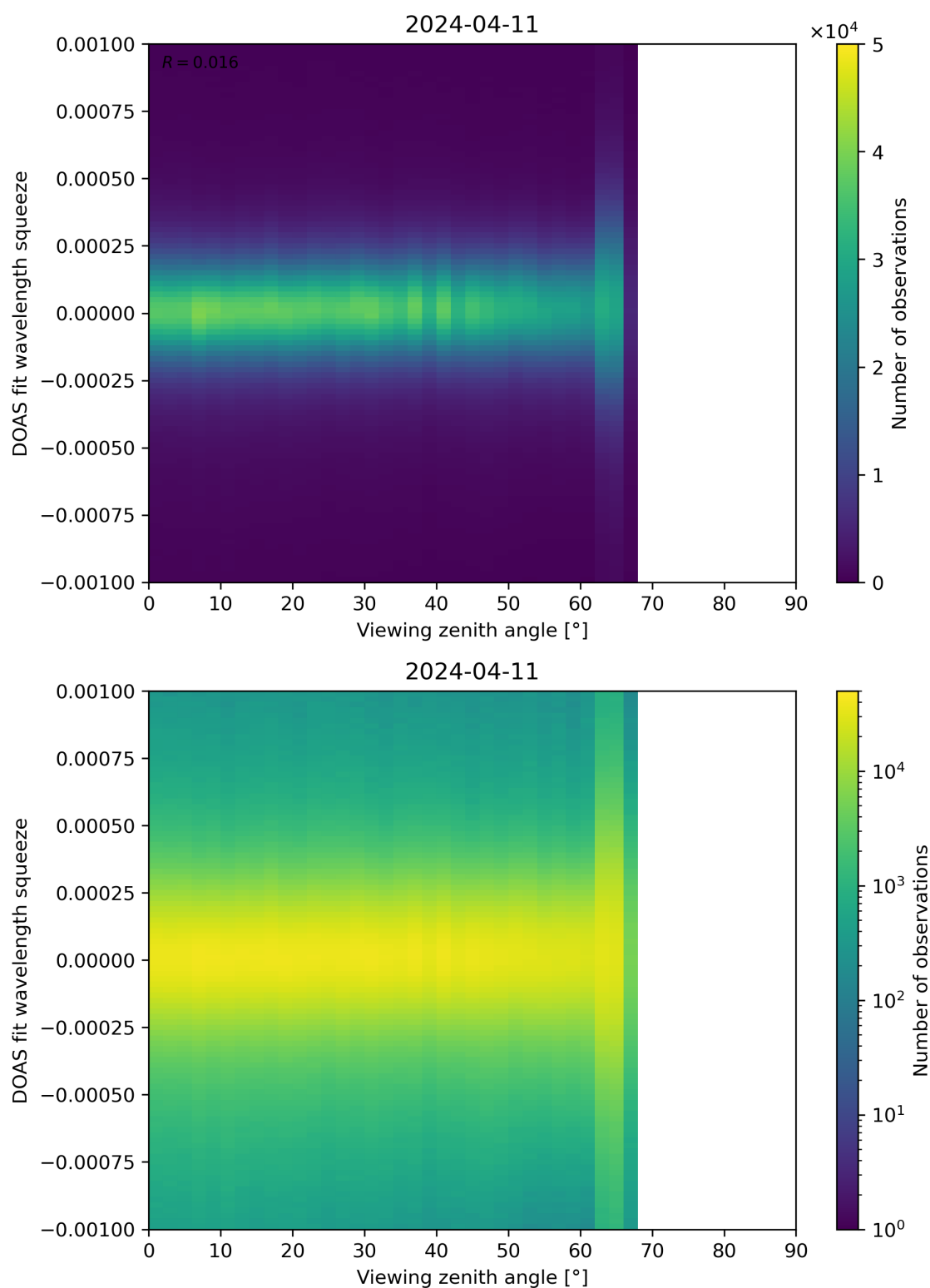
Figure 312: Scatter density plot of “Viewing zenith angle” against “DOAS fit wavelength squeeze” for 2024-04-10 to 2024-04-12.
