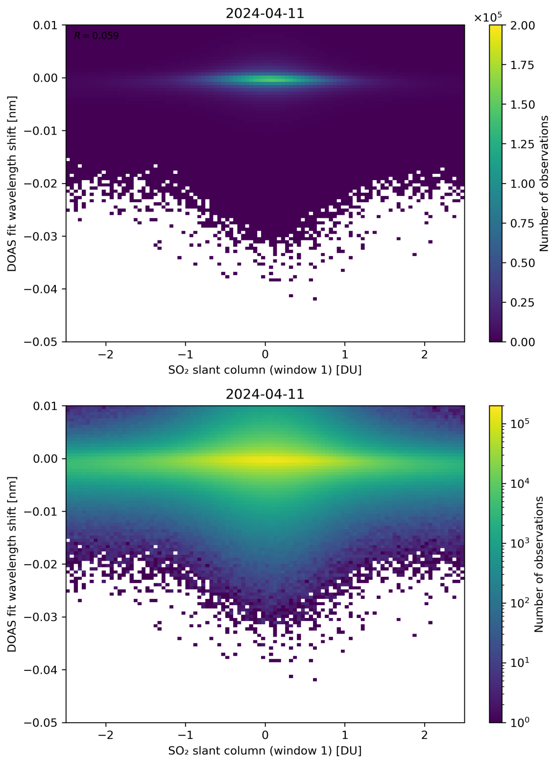
Figure 215: Scatter density plot of “SO 2 slant column (window 1)” against “DOAS fit wavelength shift” for 2024-04-10 to 2024-04-12.
