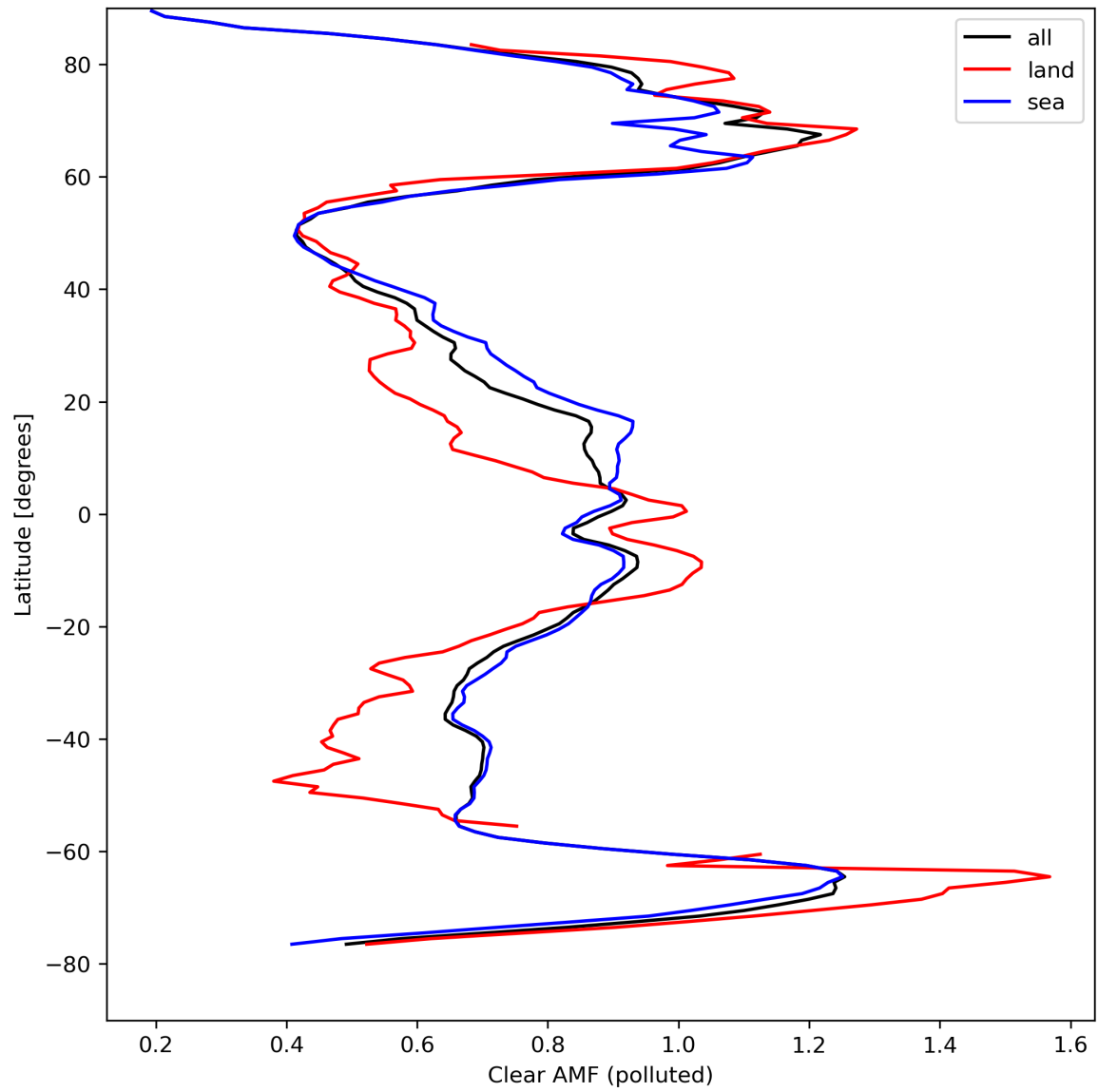
Figure 50: Zonal average of “Clear AMF (polluted)” for 2024-04-10 to 2024-04-12.
