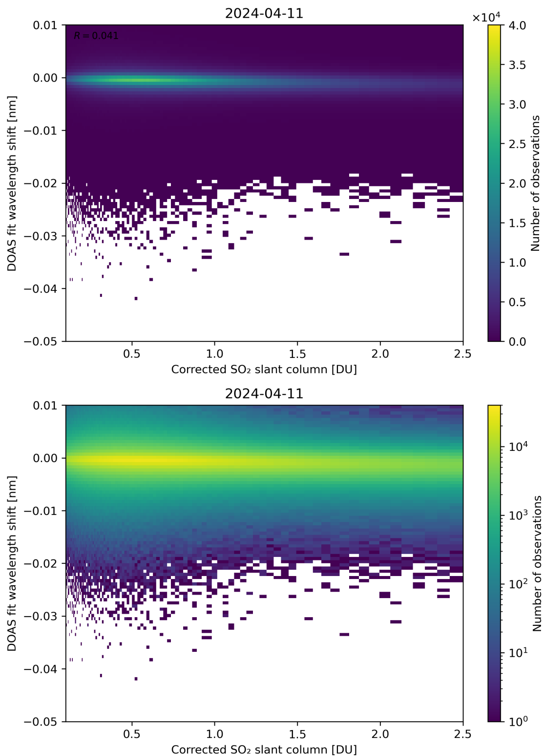
Figure 181: Scatter density plot of “Corrected SO 2 slant column” against “DOAS fit wavelength shift” for 2024-04-10 to 2024-04-12.
