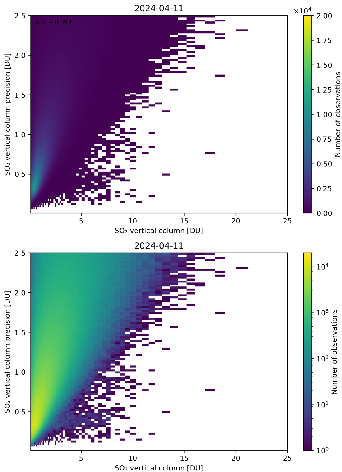
Figure 307: Scatter density plot of “SO 2 vertical column” against “SO 2 vertical column precision” for 2024-04-10 to 2024-04-12.
