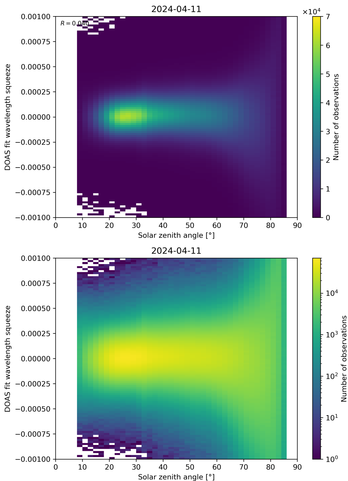
Figure 162: Scatter density plot of “Solar zenith angle” against “DOAS fit wavelength squeeze” for 2024-04-10 to 2024-04-12.
