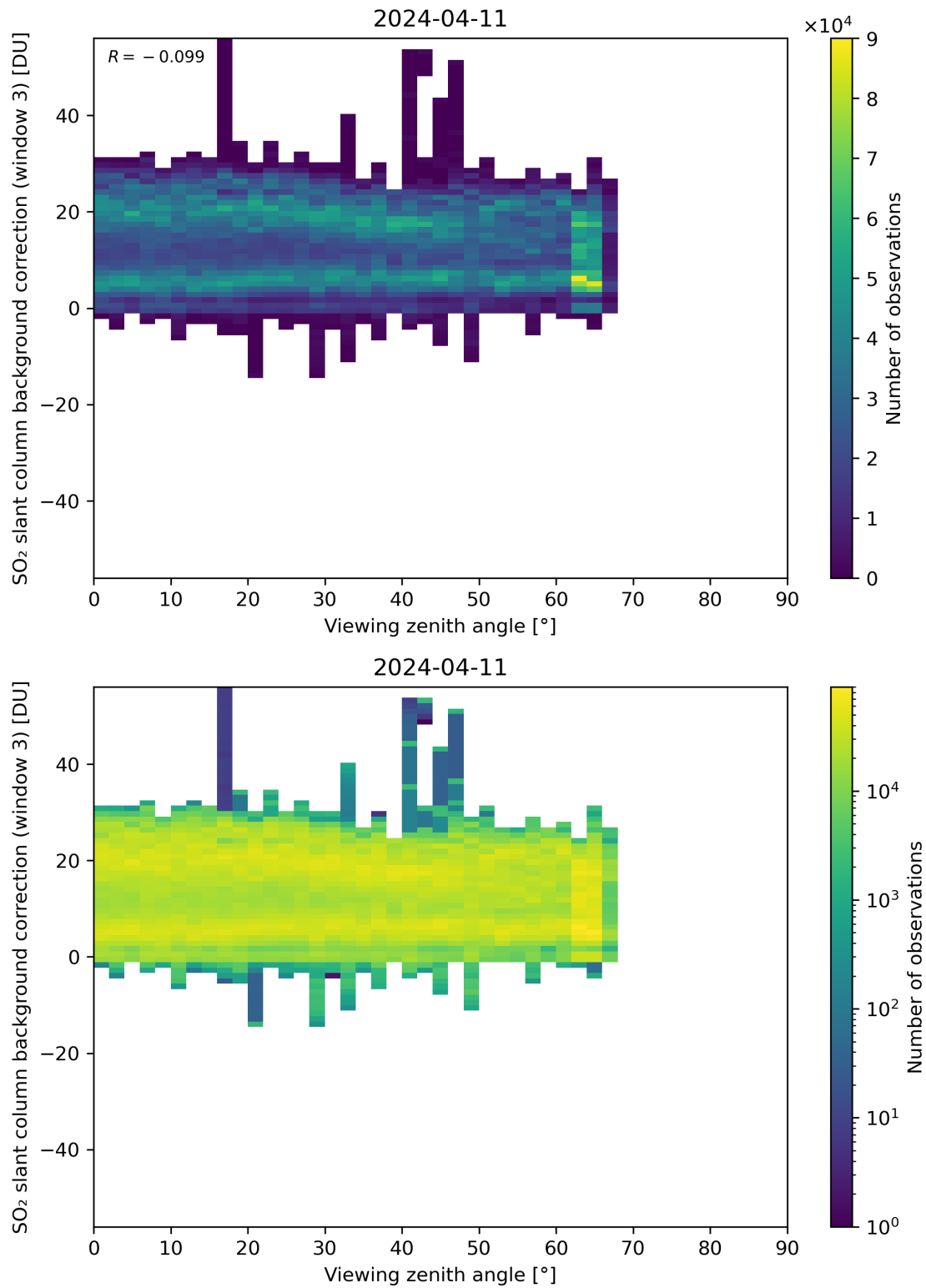
Figure 310: Scatter density plot of “Viewing zenith angle” against “SO 2 slant column background correction (window 3)” for 2024-04-10 to 2024-04-12.
