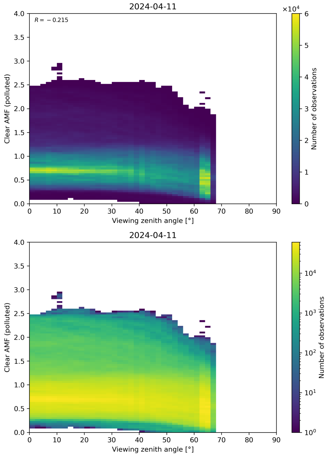
Figure 316: Scatter density plot of “Viewing zenith angle” against “Clear AMF (polluted)” for 2024-04-10 to 2024-04-12.
