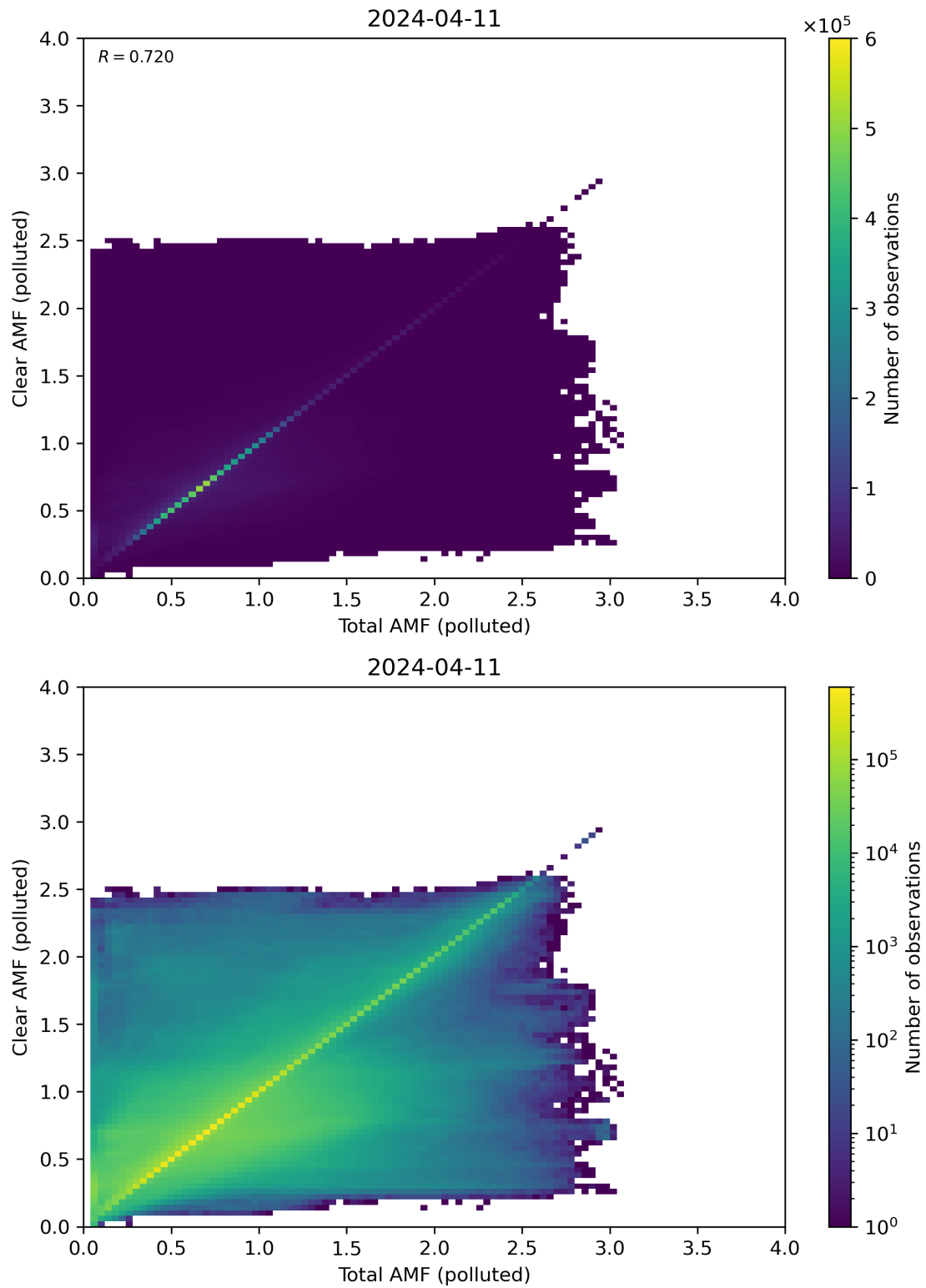
Figure 271: Scatter density plot of “Total AMF (polluted)” against “Clear AMF (polluted)” for 2024-04-10 to 2024-04-12.
