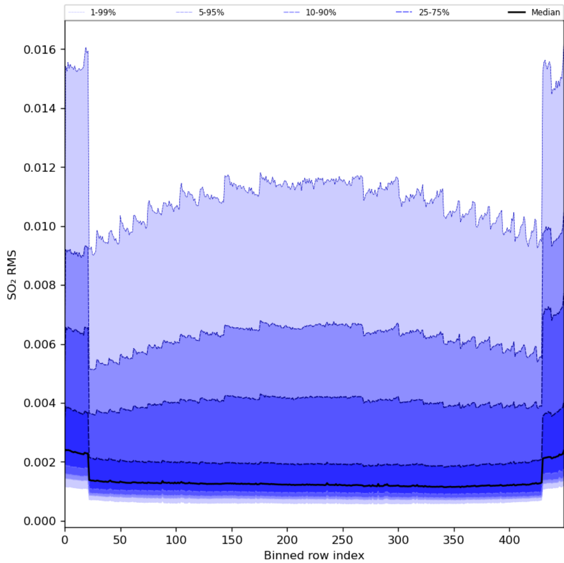
Figure 93: Along track statistics of “SO 2 RMS” for 2024-04-10 to 2024-04-12
