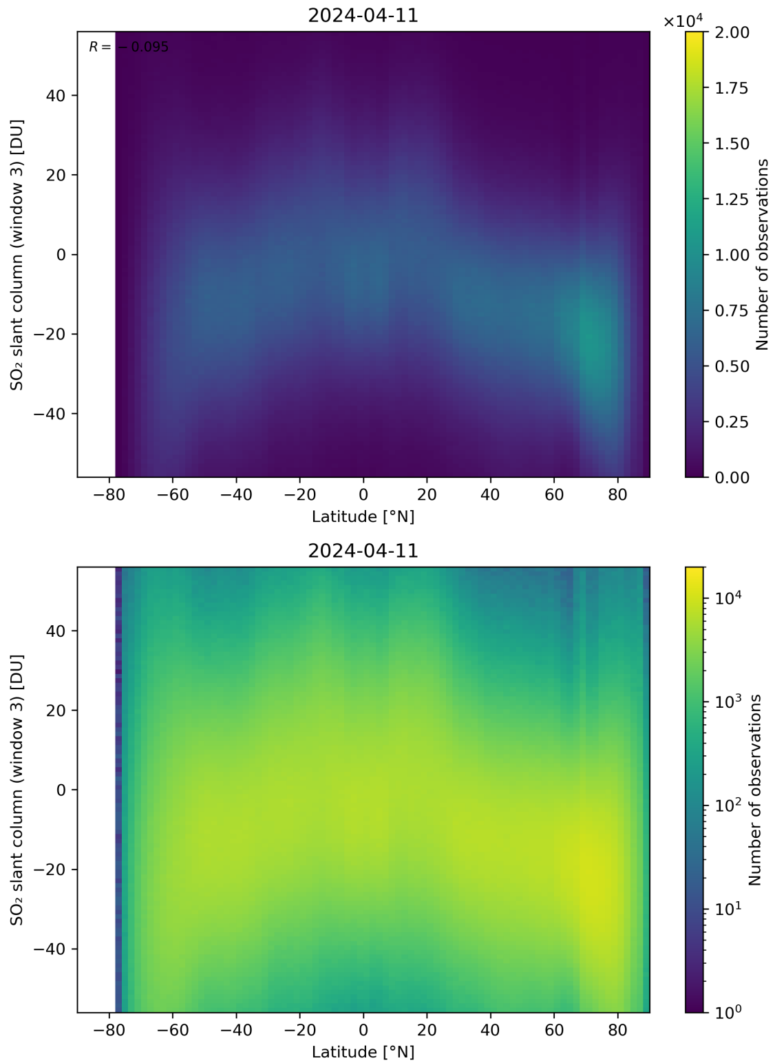
Figure 152: Scatter density plot of “Latitude” against “SO 2 slant column (window 3)” for 2024-04-10 to 2024-04-12.
