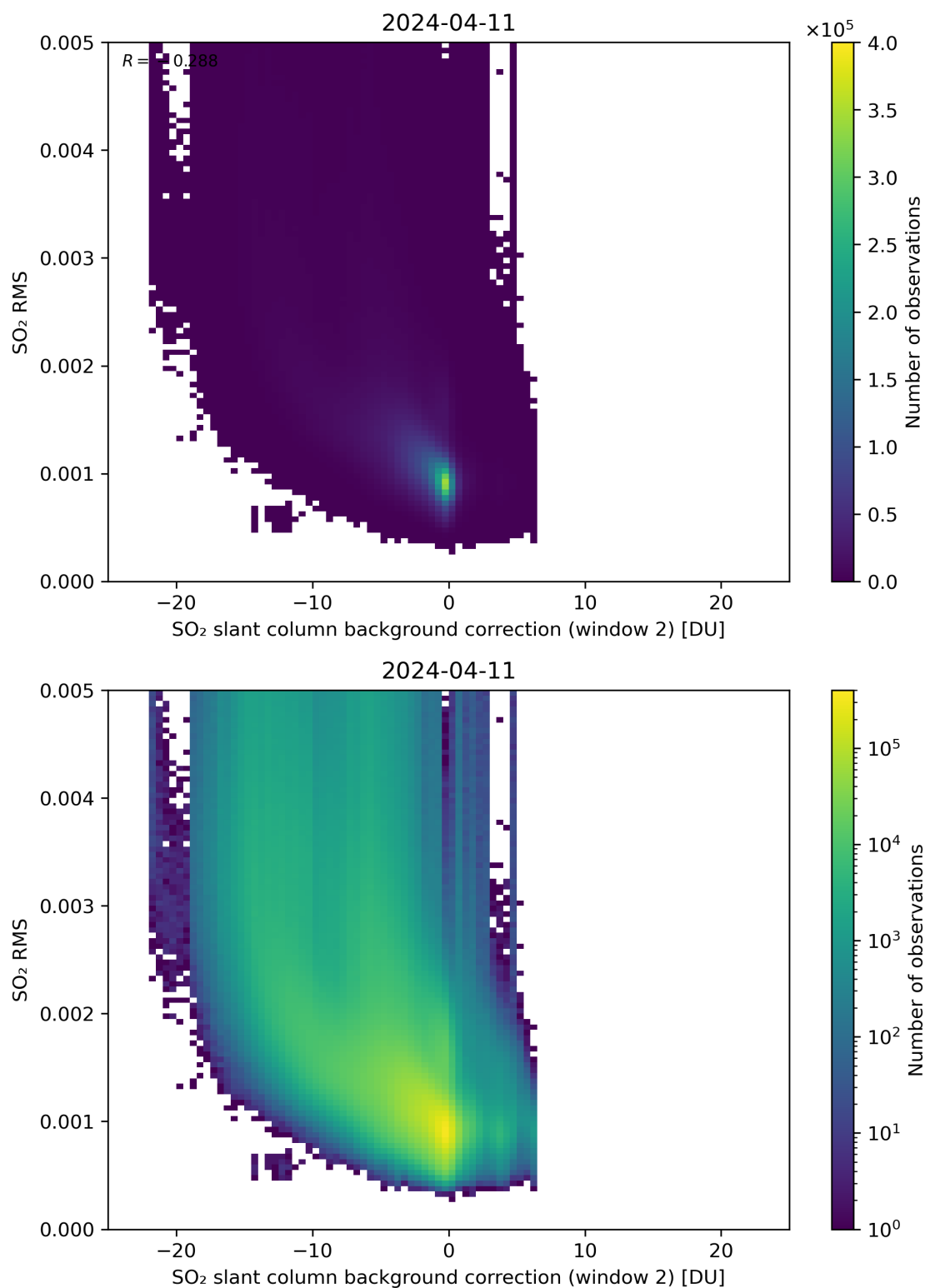
Figure 114: Scatter density plot of “SO 2 slant column background correction (window 2)” against “SO 2 RMS” for 2024-04-10 to 2024-04-12.
