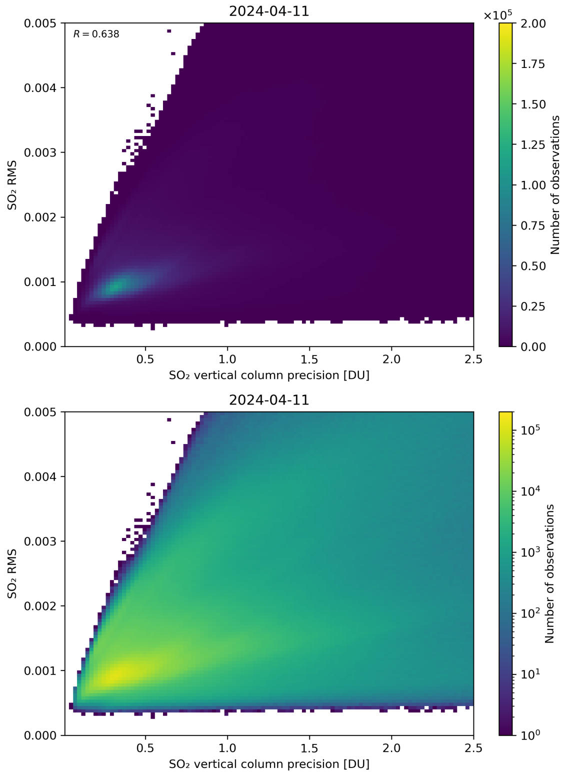
Figure 284: Scatter density plot of “SO 2 vertical column precision” against “SO 2 RMS” for 2024-04-10 to 2024-04-12.
