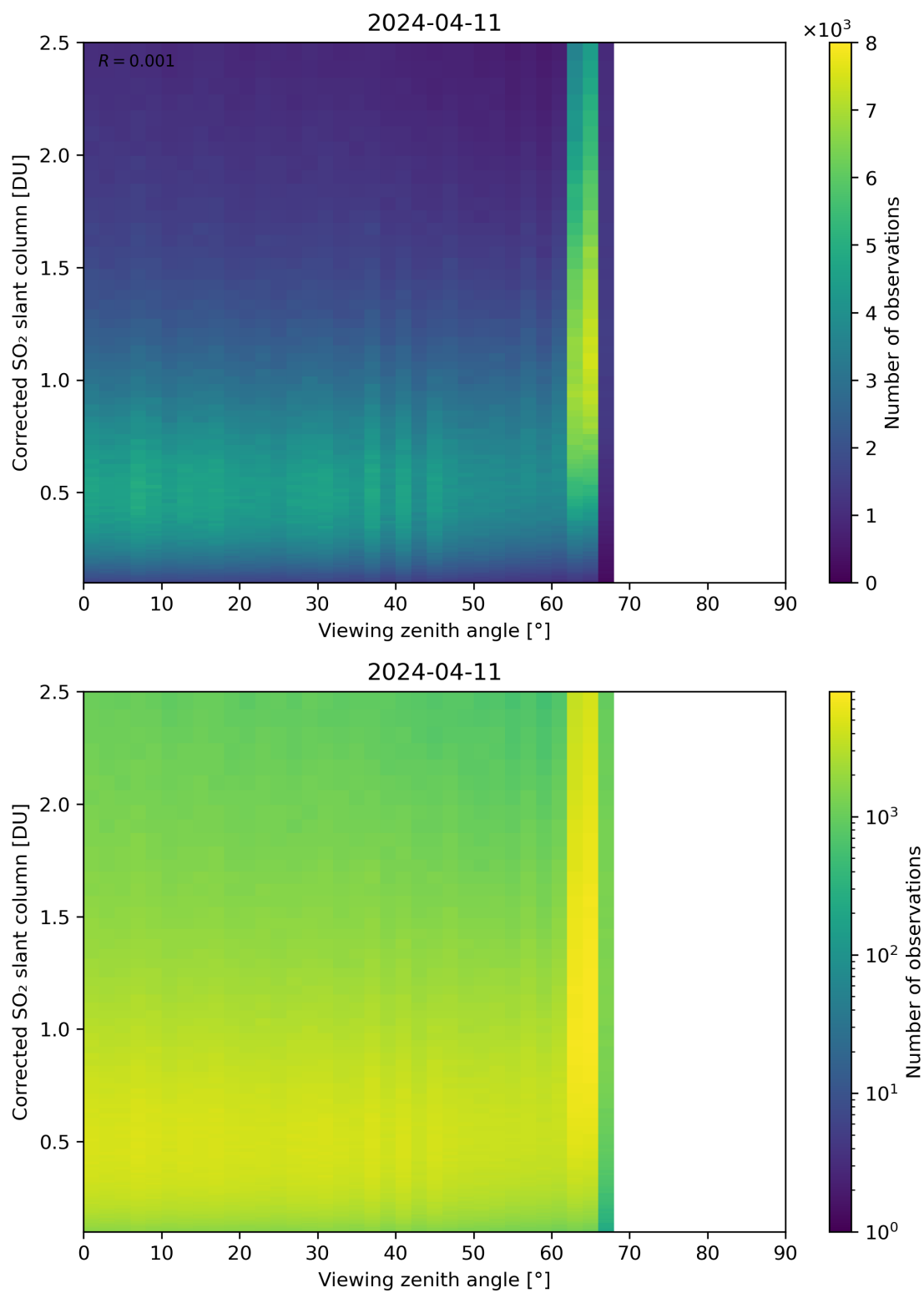
Figure 317: Scatter density plot of “Viewing zenith angle” against “Corrected SO 2 slant column” for 2024-04-10 to 2024-04-12.
