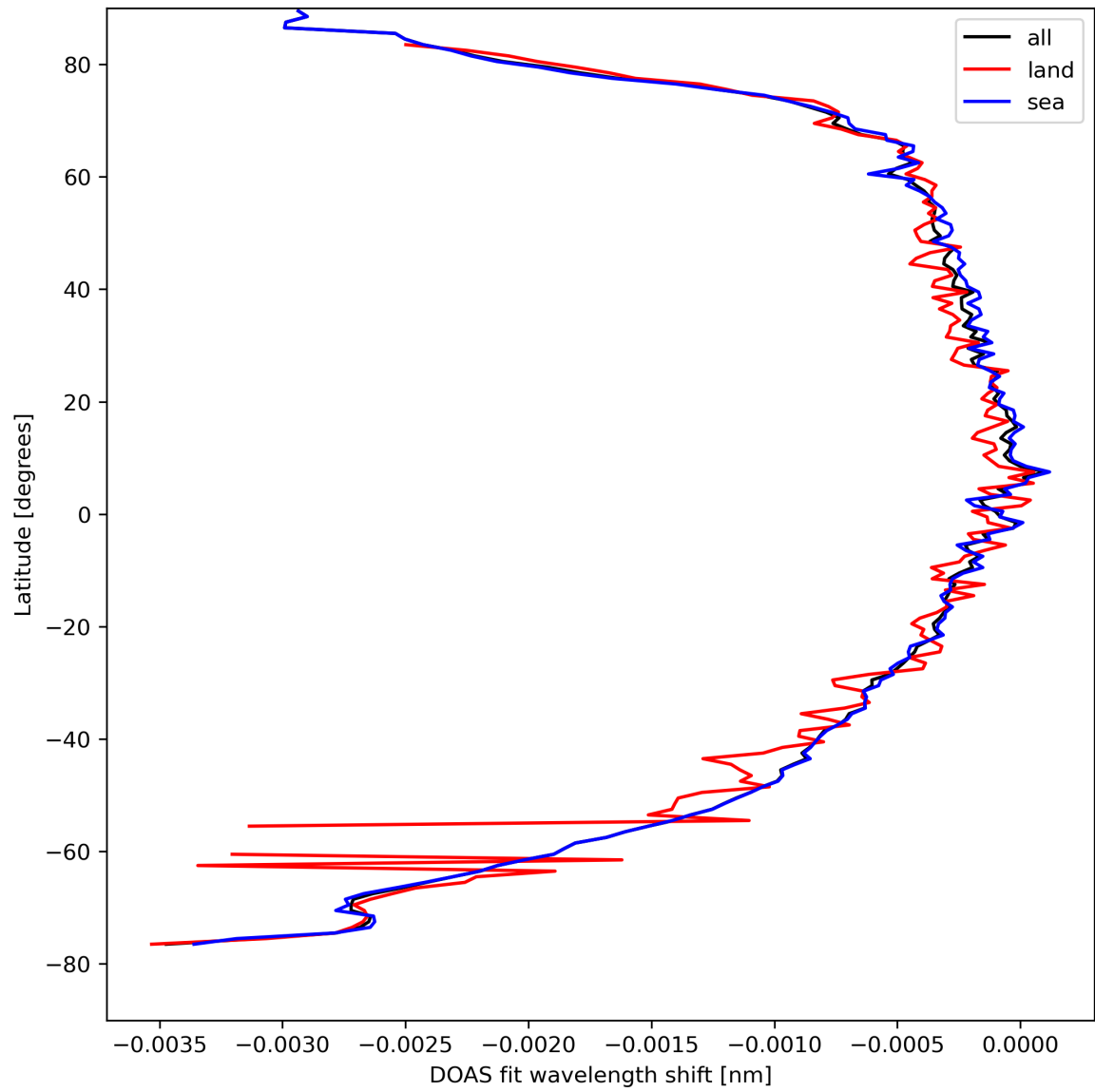
Figure 45: Zonal average of “DOAS fit wavelength shift” for 2024-04-10 to 2024-04-12.
