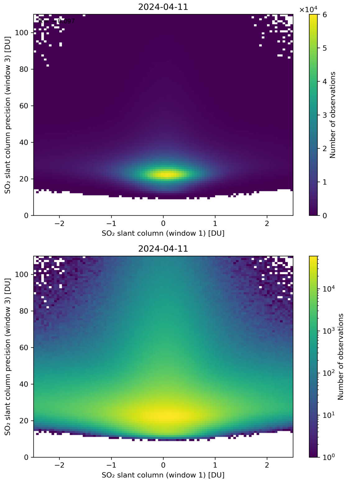
Figure 238: Scatter density plot of “SO 2 slant column (window 1)” against “SO 2 slant column precision (window 3)” for 2024-04-10 to 2024-04-12.
