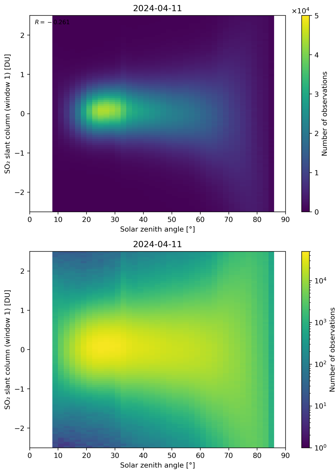
Figure 169: Scatter density plot of “Solar zenith angle” against “SO 2 slant column (window 1)” for 2024-04-10 to 2024-04-12.
