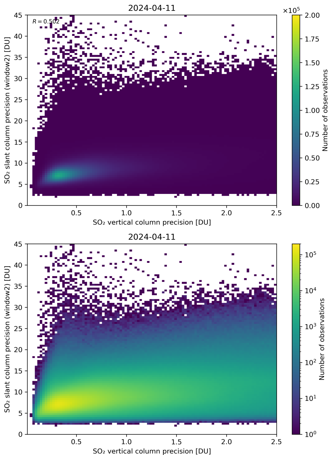
Figure 291: Scatter density plot of “SO 2 vertical column precision” against “SO 2 slant column precision (window2)” for 2024-04-10 to 2024-04-12.
