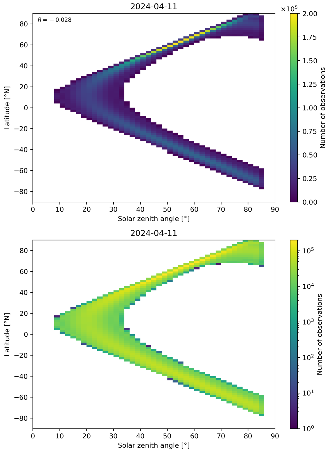
Figure 164: Scatter density plot of “Solar zenith angle” against “Latitude” for 2024-04-10 to 2024-04-12.
