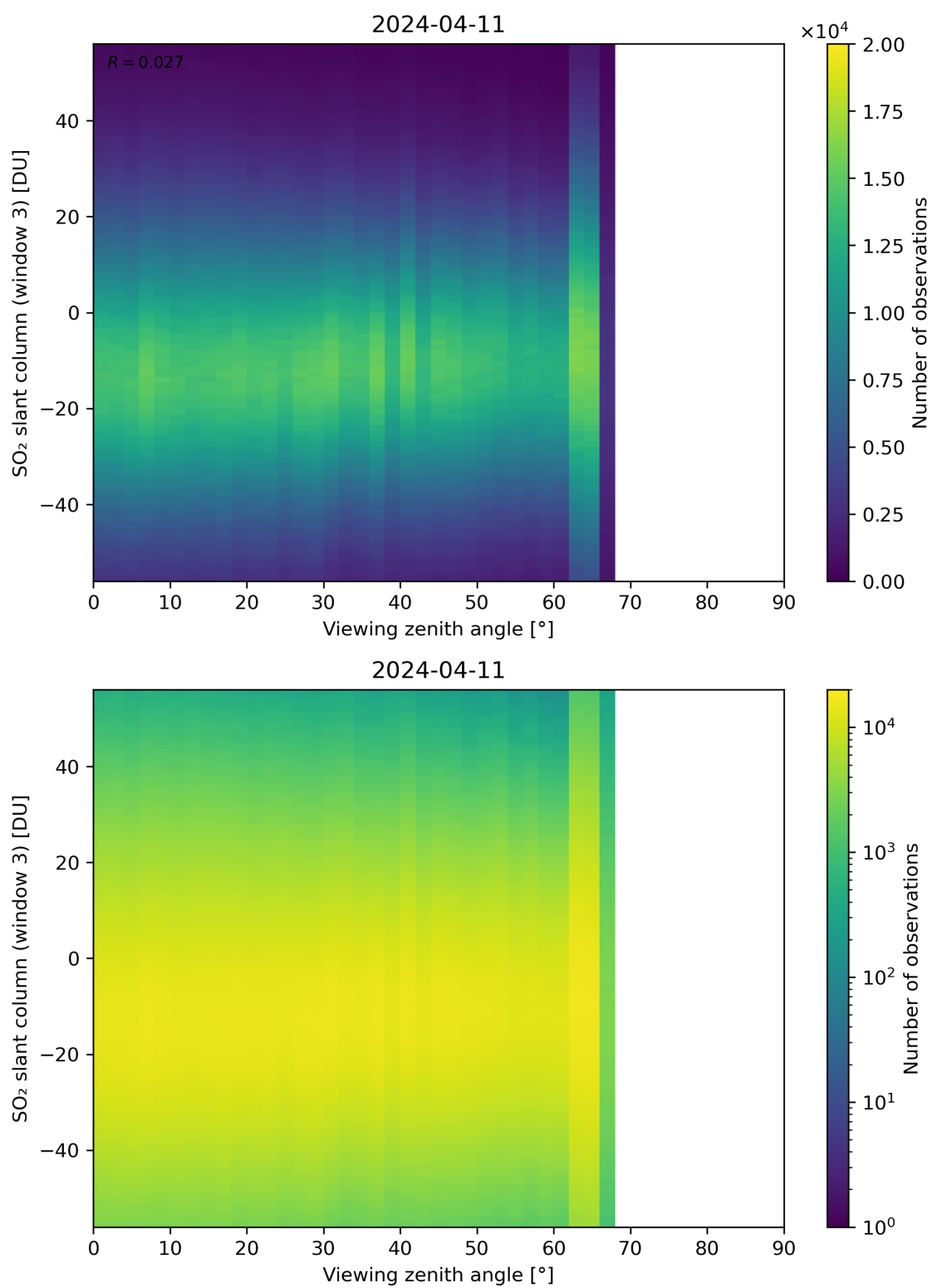
Figure 323: Scatter density plot of “Viewing zenith angle” against “SO 2 slant column (window 3)” for 2024-04-10 to 2024-04-12.
