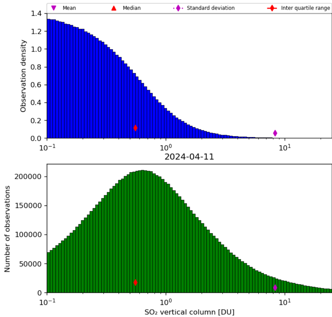
Figure 53: Histogram of “SO 2 vertical column” for 2024-04-10 to 2024-04-12
