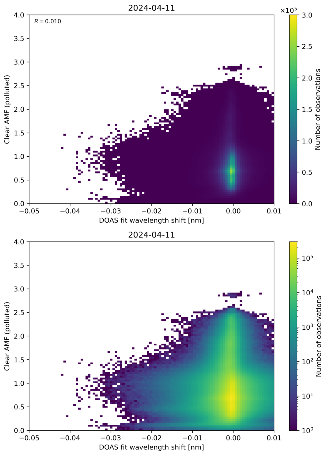
Figure 129: Scatter density plot of “DOAS fit wavelength shift” against “Clear AMF (polluted)” for 2024-04-10 to 2024-04-12.
