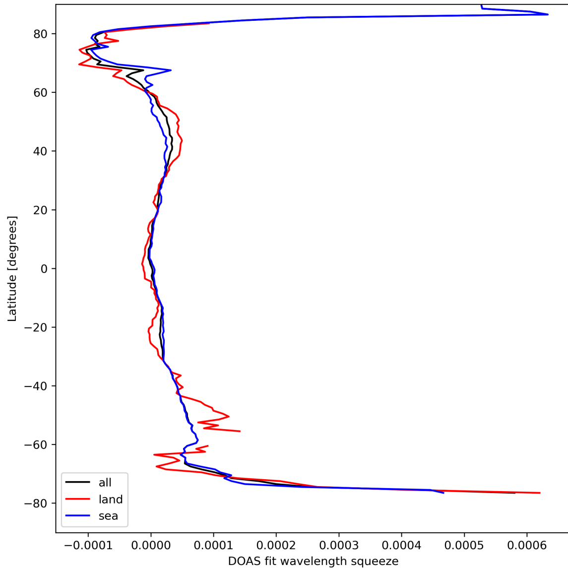
Figure 46: Zonal average of “DOAS fit wavelength squeeze” for 2024-04-10 to 2024-04-12.
