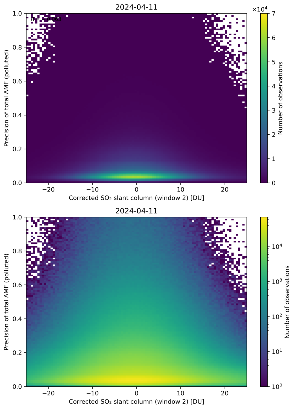
Figure 204: Scatter density plot of “Corrected SO 2 slant column (window 2)” against “Precision of total AMF (polluted)” for 2024-04-10 to 2024-04-12.
