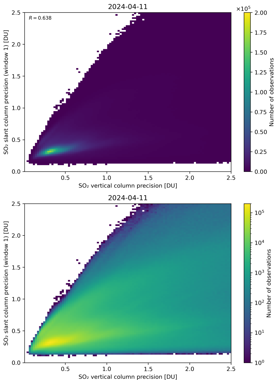
Figure 290: Scatter density plot of “SO 2 vertical column precision” against “SO 2 slant column precision (window 1)” for 2024-04-10 to 2024-04-12.
