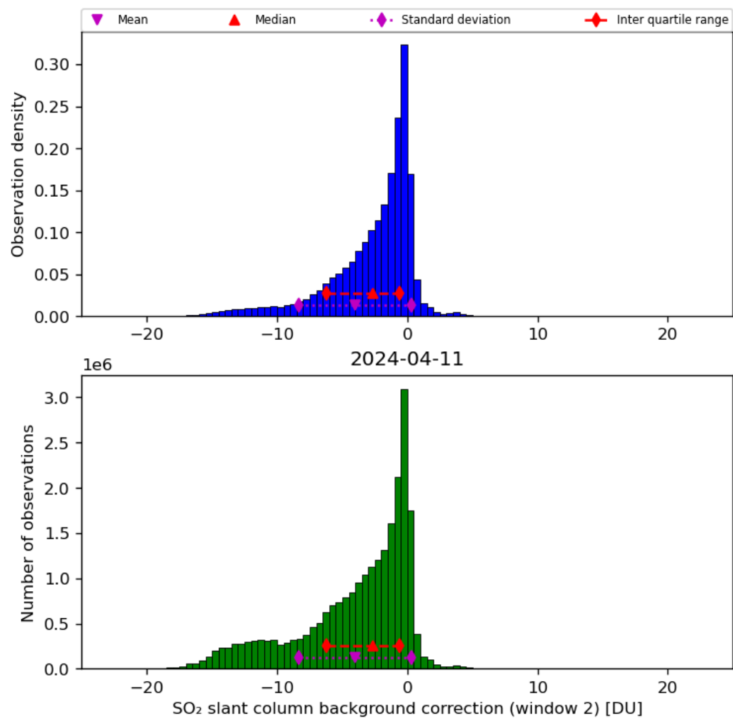
Figure 63: Histogram of “SO 2 slant column background correction (window 2)” for 2024-04-10 to 2024-04-12
