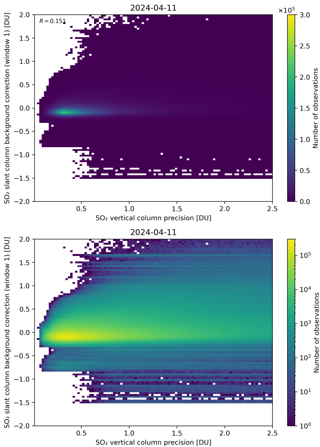
Figure 279: Scatter density plot of “SO 2 vertical column precision” against “SO 2 slant column background correction (window 1)” for 2024-04-10 to 2024-04-12.
