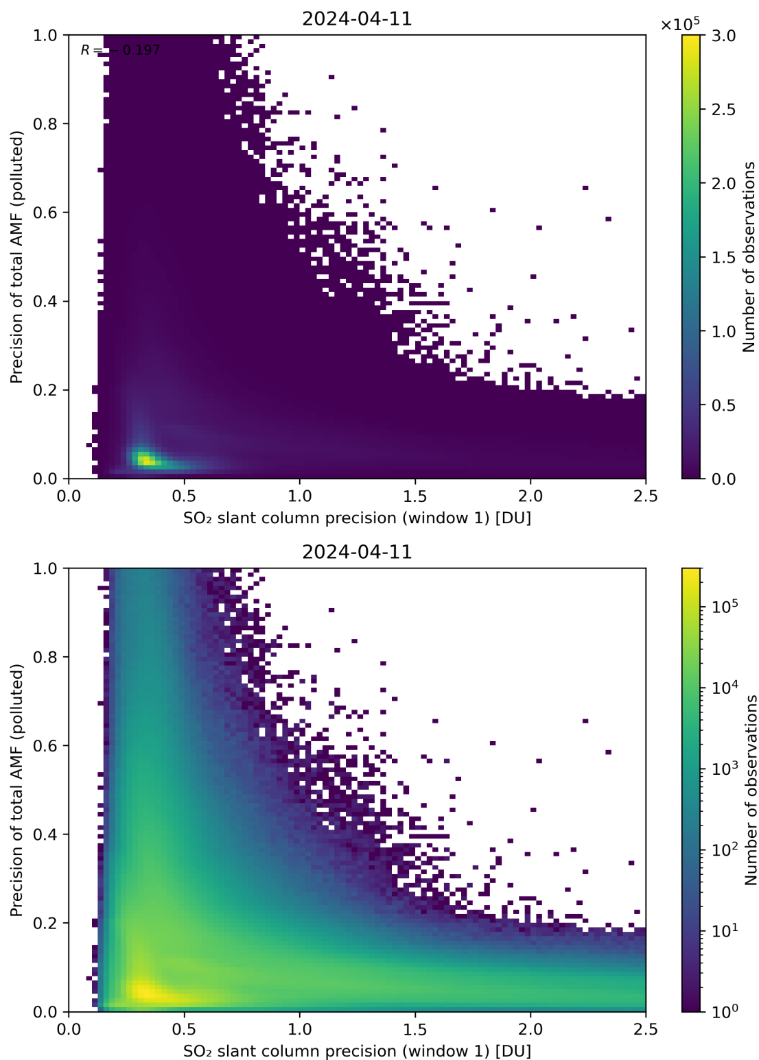
Figure 231: Scatter density plot of “SO 2 slant column precision (window 1)” against “Precision of total AMF (polluted)” for 2024-04-10 to 2024-04-12.
