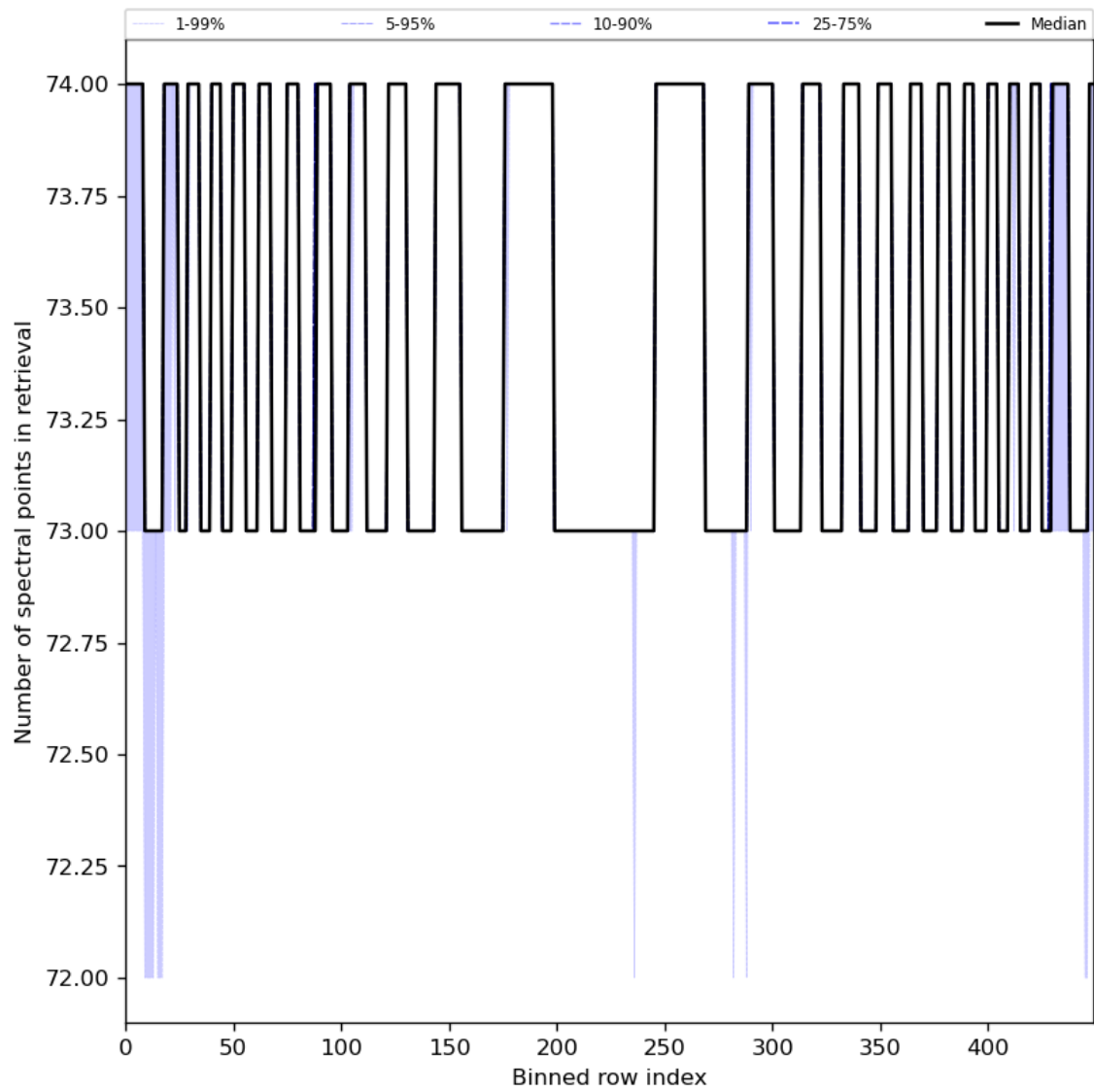
Figure 97: Along track statistics of “Number of spectral points in retrieval” for 2024-04-10 to 2024-04-12
