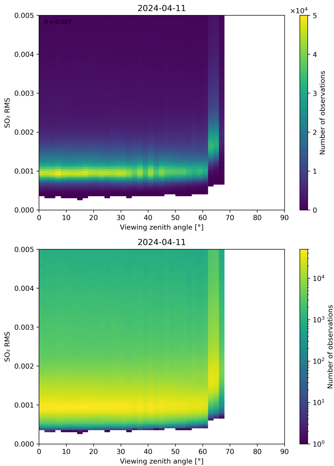
Figure 313: Scatter density plot of “Viewing zenith angle” against “SO 2 RMS” for 2024-04-10 to 2024-04-12.
