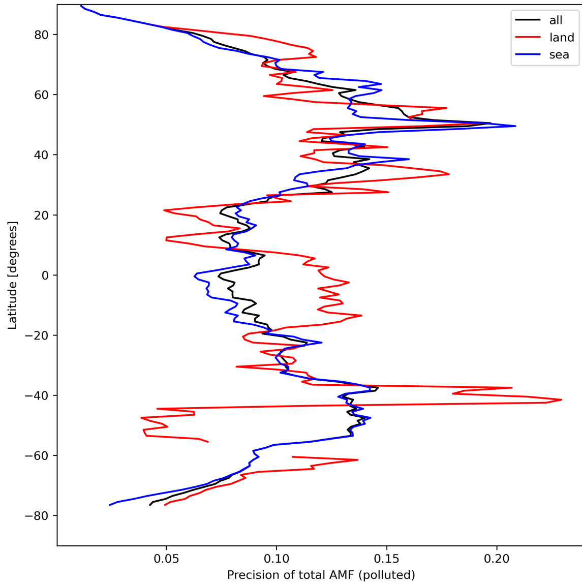
Figure 49: Zonal average of “Precision of total AMF (polluted)” for 2024-04-10 to 2024-04-12.
