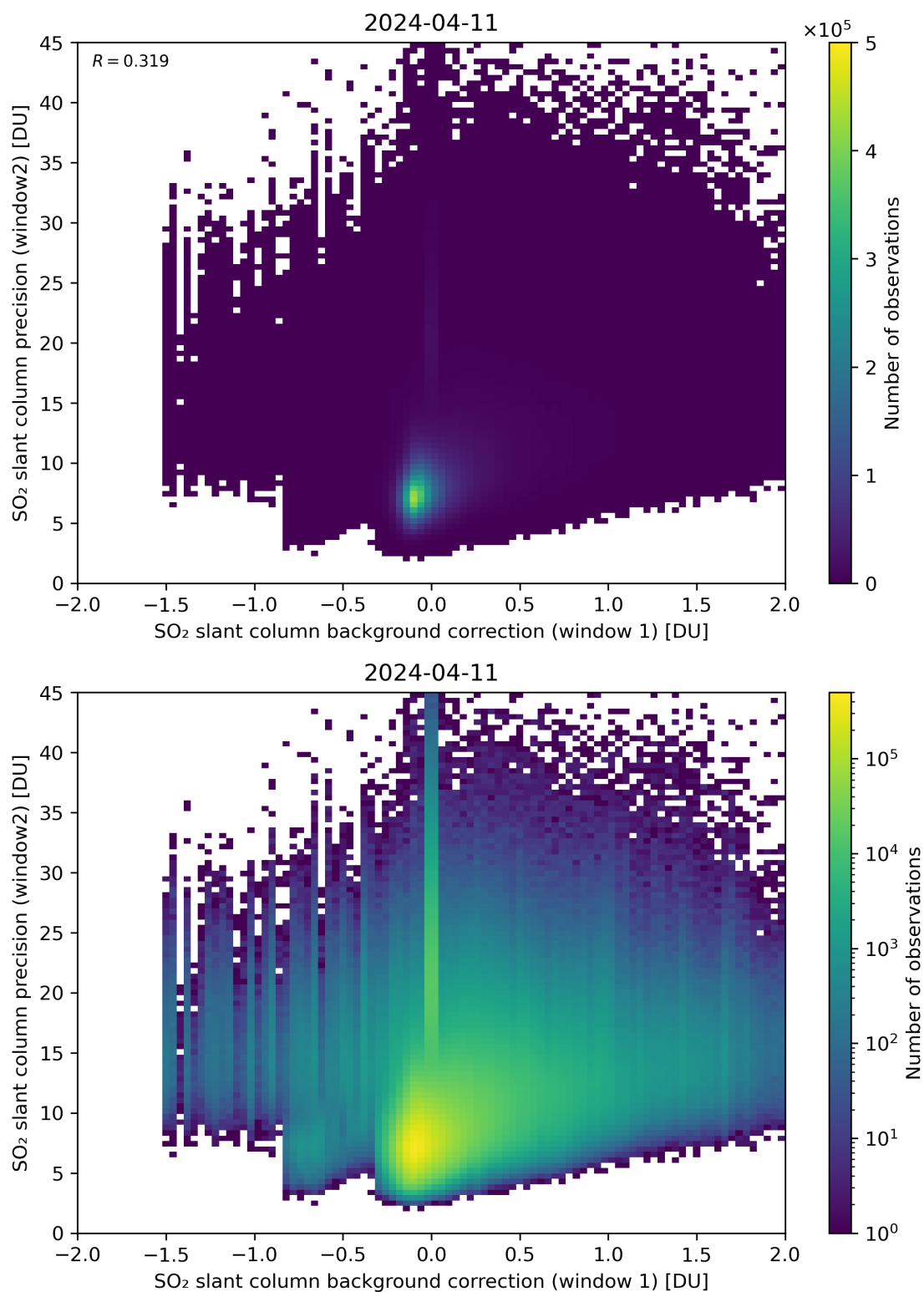
Figure 106: Scatter density plot of “SO 2 slant column background correction (window 1)” against “SO 2 slant column precision (window2)” for 2024-04-10 to 2024-04-12.
