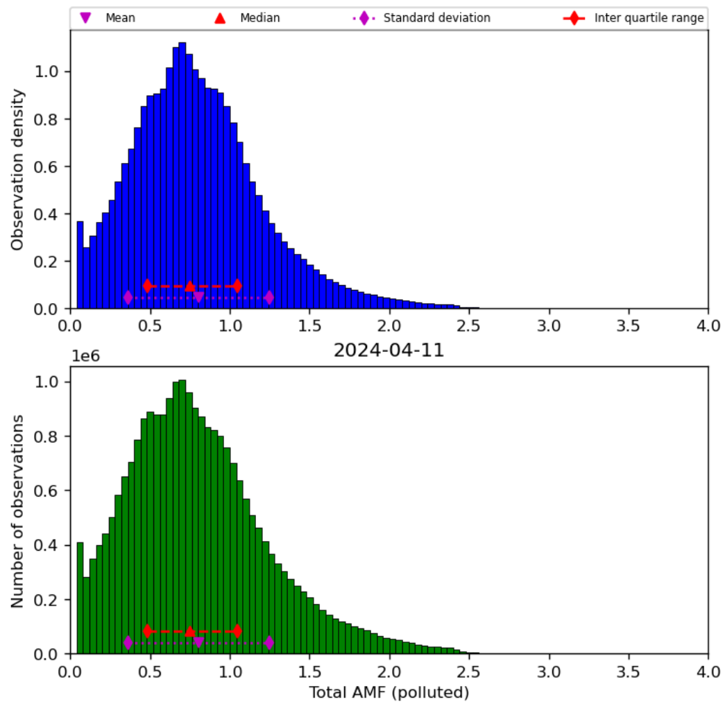
Figure 71: Histogram of “Total AMF (polluted)” for 2024-04-10 to 2024-04-12
