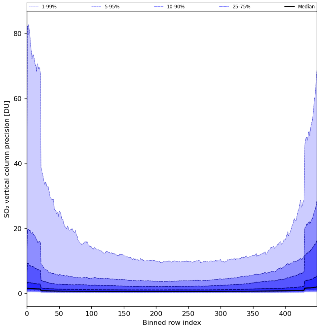
Figure 77: Along track statistics of “SO 2 vertical column precision” for 2024-04-10 to 2024-04-12
