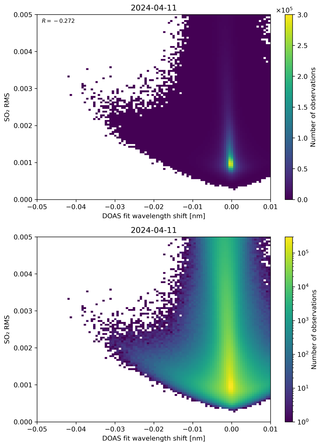
Figure 128: Scatter density plot of “DOAS fit wavelength shift” against “SO 2 RMS” for 2024-04-10 to 2024-04-12.
