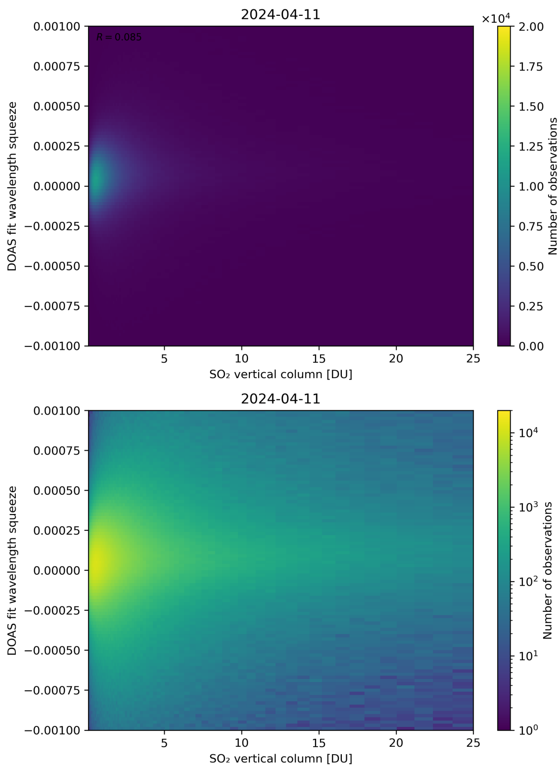
Figure 277: Scatter density plot of “SO 2 vertical column” against “DOAS fit wavelength squeeze” for 2024-04-10 to 2024-04-12.
