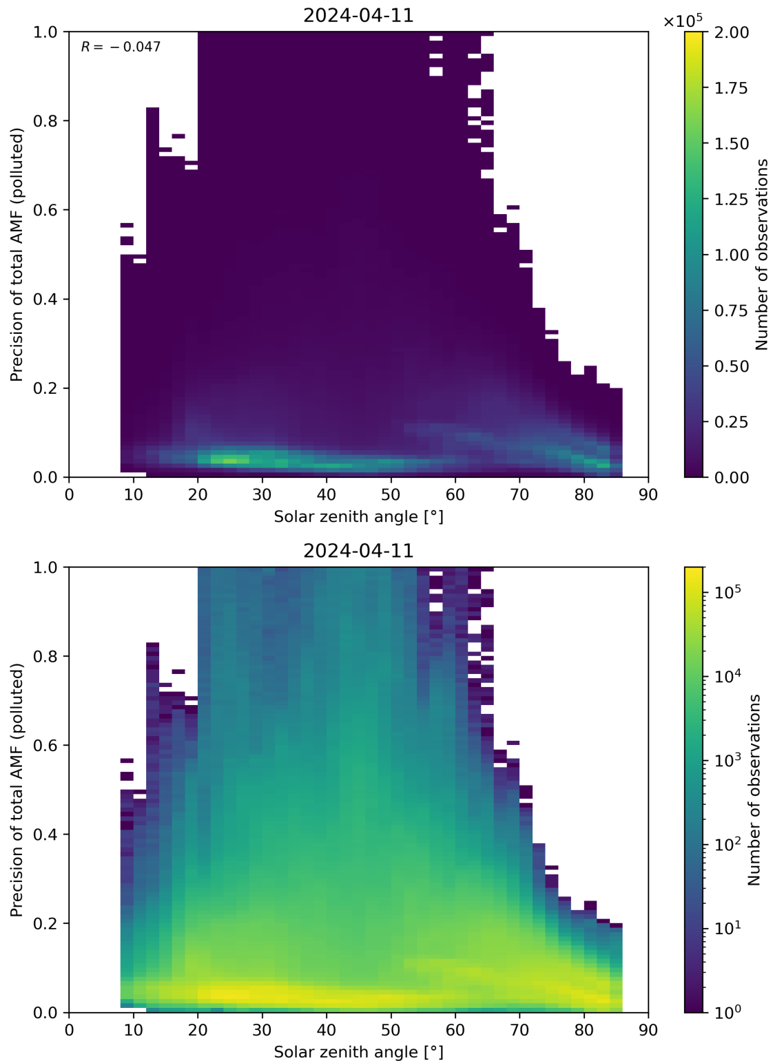
Figure 175: Scatter density plot of “Solar zenith angle” against “Precision of total AMF (polluted)” for 2024-04-10 to 2024-04-12.
