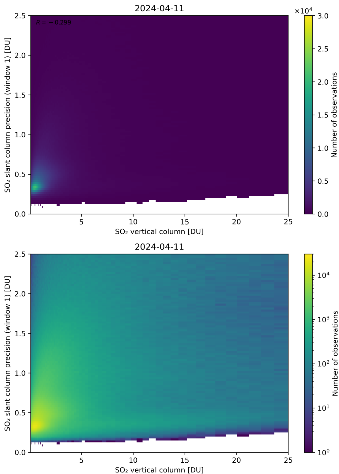
Figure 301: Scatter density plot of “SO 2 vertical column” against “SO 2 slant column precision (window 1)” for 2024-04-10 to 2024-04-12.
