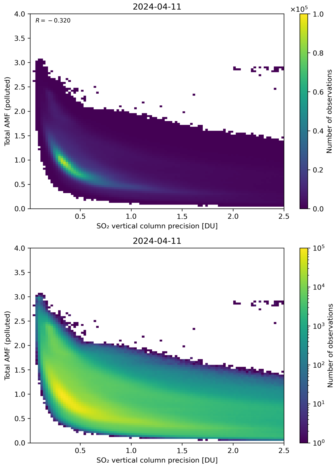
Figure 294: Scatter density plot of “SO 2 vertical column precision” against “Total AMF (polluted)” for 2024-04-10 to 2024-04-12.
