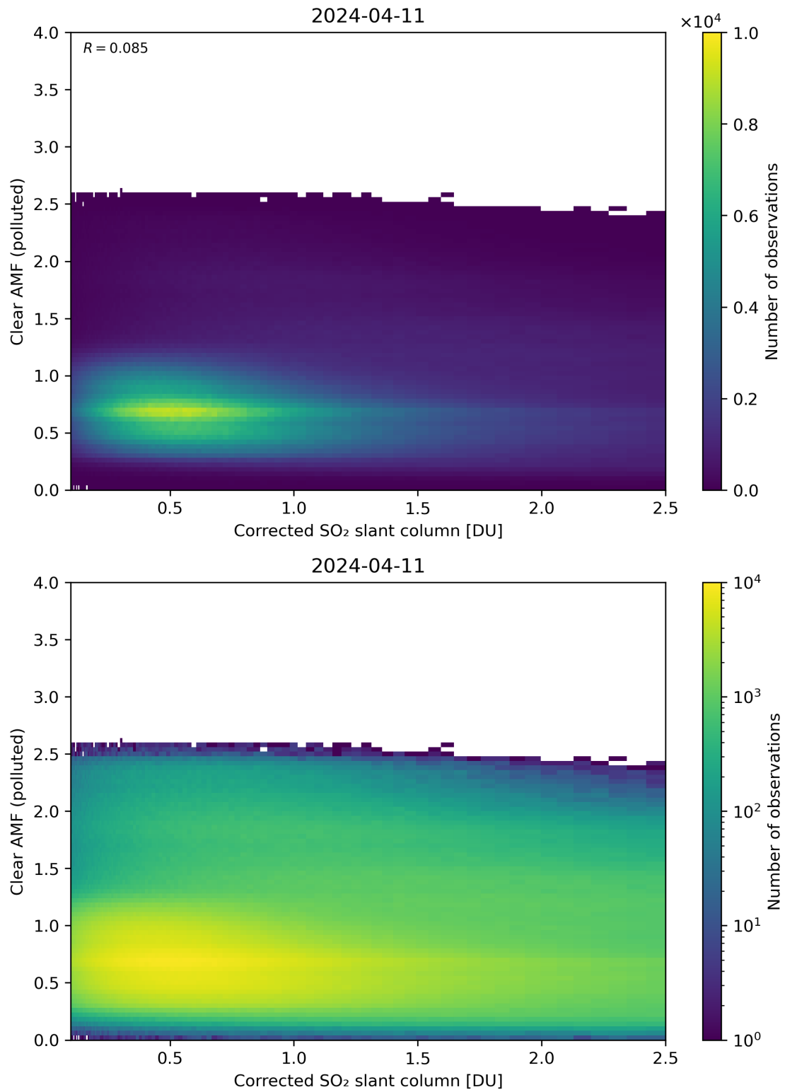
Figure 184: Scatter density plot of “Corrected SO 2 slant column” against “Clear AMF (polluted)” for 2024-04-10 to 2024-04-12.
