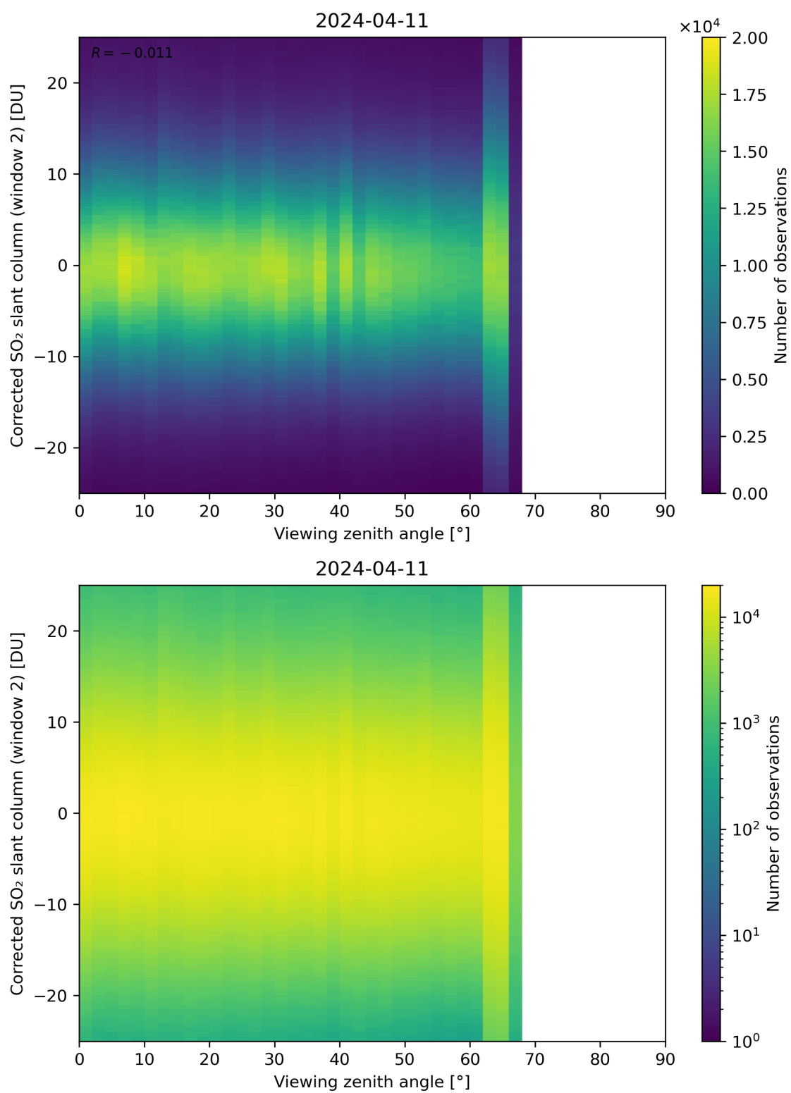
Figure 318: Scatter density plot of “Viewing zenith angle” against “Corrected SO 2 slant column (window 2)” for 2024-04-10 to 2024-04-12.
