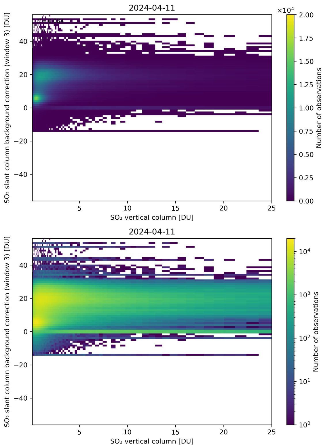
Figure 275: Scatter density plot of “SO 2 vertical column” against “SO 2 slant column background correction (window 3)” for 2024-04-10 to 2024-04-12.
