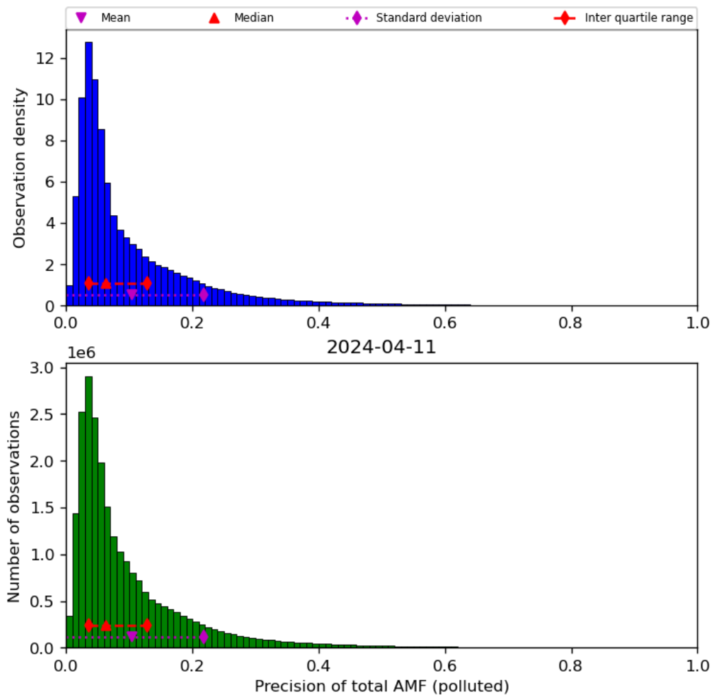
Figure 72: Histogram of “Precision of total AMF (polluted)” for 2024-04-10 to 2024-04-12
