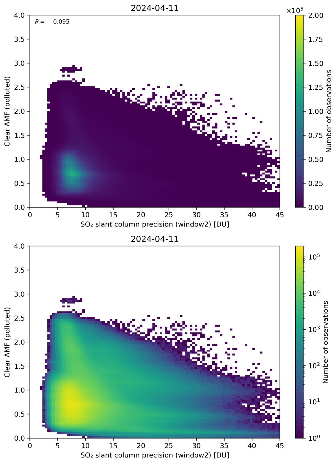
Figure 246: Scatter density plot of “SO 2 slant column precision (window2)” against “Clear AMF (polluted)” for 2024-04-10 to 2024-04-12.
