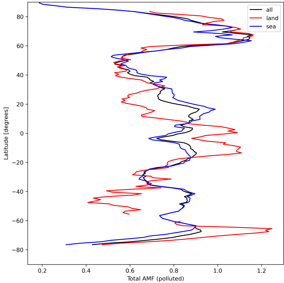
Figure 48: Zonal average of “Total AMF (polluted)” for 2024-04-10 to 2024-04-12.
