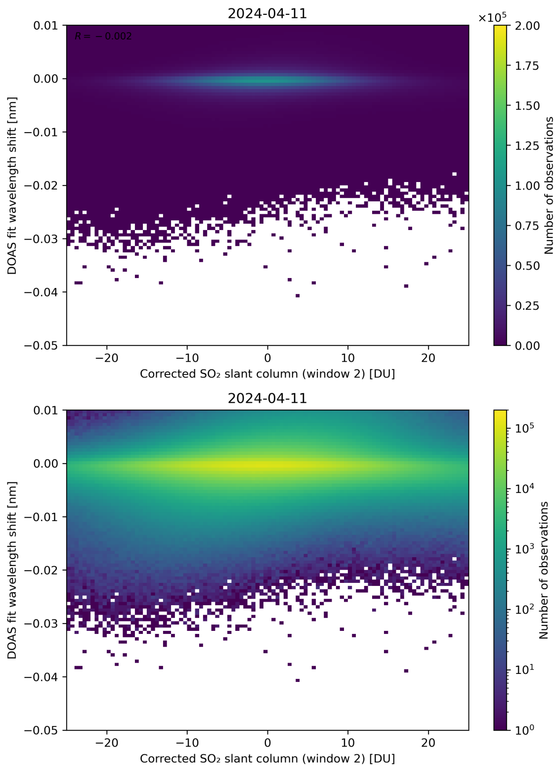
Figure 196: Scatter density plot of “Corrected SO 2 slant column (window 2)” against “DOAS fit wavelength shift” for 2024-04-10 to 2024-04-12.
