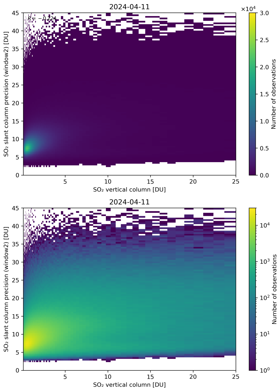
Figure 302: Scatter density plot of “SO 2 vertical column” against “SO 2 slant column precision (window2)” for 2024-04-10 to 2024-04-12.
