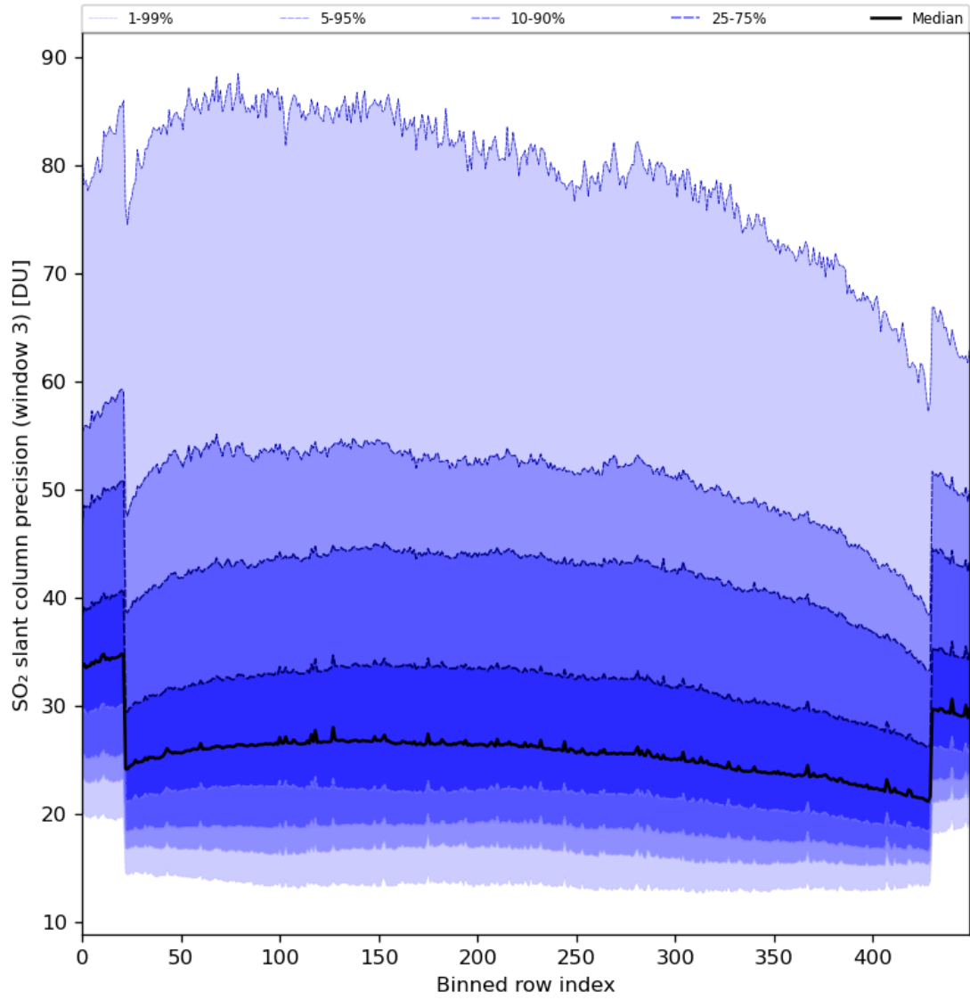
Figure 88: Along track statistics of “SO 2 slant column precision (window 3)” for 2024-04-10 to 2024-04-12
