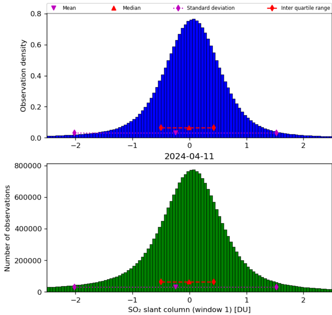
Figure 56: Histogram of “SO 2 slant column (window 1)” for 2024-04-10 to 2024-04-12
