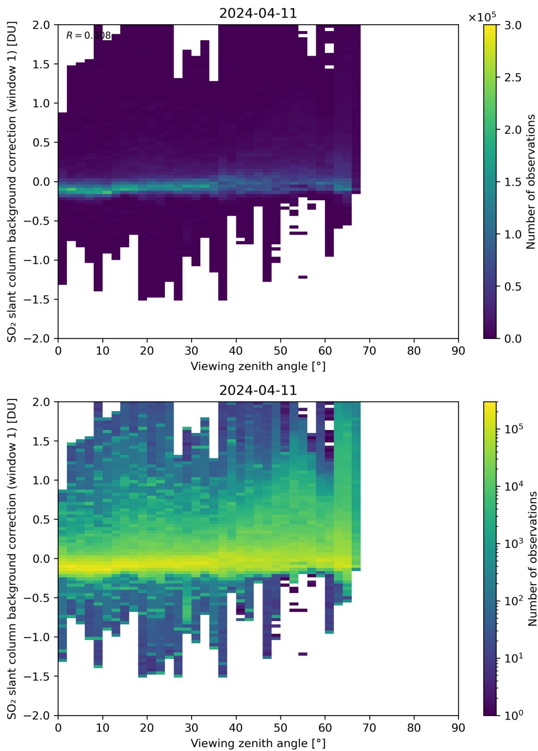
Figure 308: Scatter density plot of “Viewing zenith angle” against “SO 2 slant column background correction (window 1)” for 2024-04-10 to 2024-04-12.
