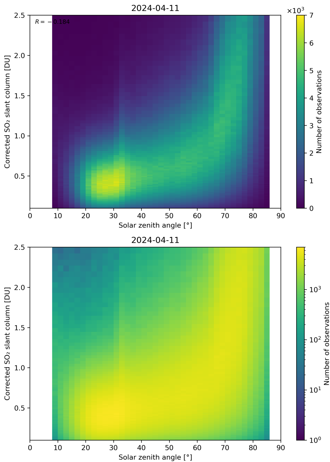
Figure 166: Scatter density plot of “Solar zenith angle” against “Corrected SO 2 slant column” for 2024-04-10 to 2024-04-12.
