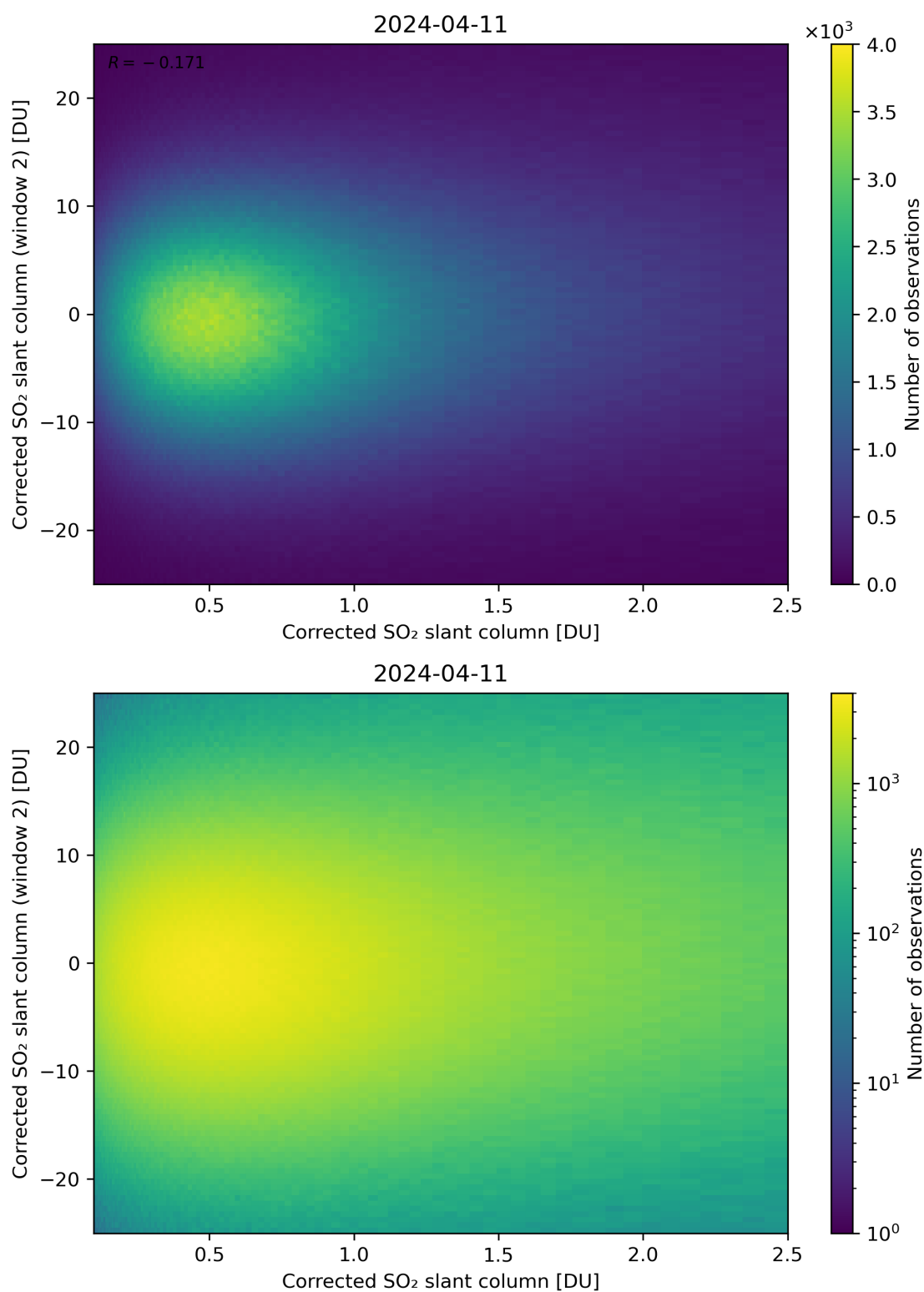
Figure 185: Scatter density plot of “Corrected SO 2 slant column” against “Corrected SO 2 slant column (window 2)” for 2024-04-10 to 2024-04-12.
