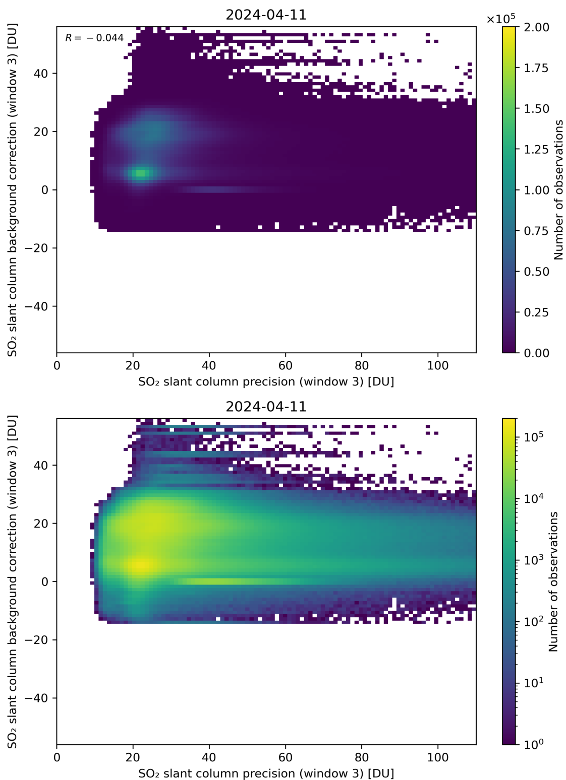
Figure 257: Scatter density plot of “SO 2 slant column precision (window 3)” against “SO 2 slant column background correction (window 3)” for 2024-04-10 to 2024-04-12.
