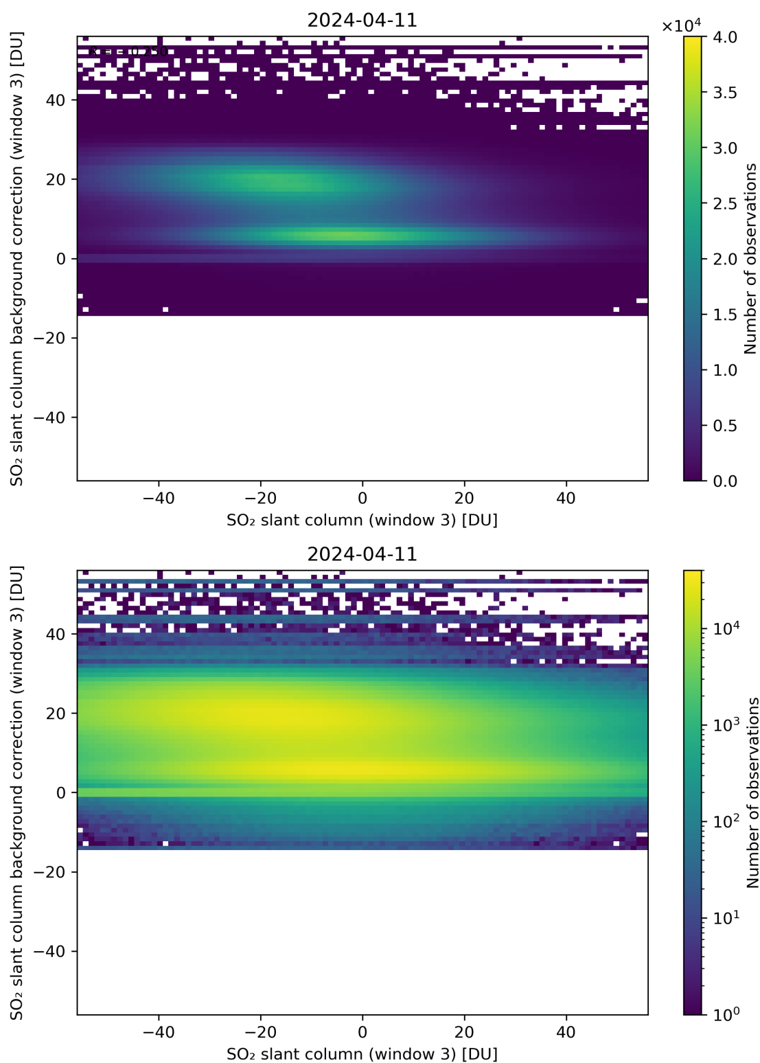
Figure 253: Scatter density plot of “SO 2 slant column (window 3)” against “SO 2 slant column background correction (window 3)” for 2024-04-10 to 2024-04-12.
