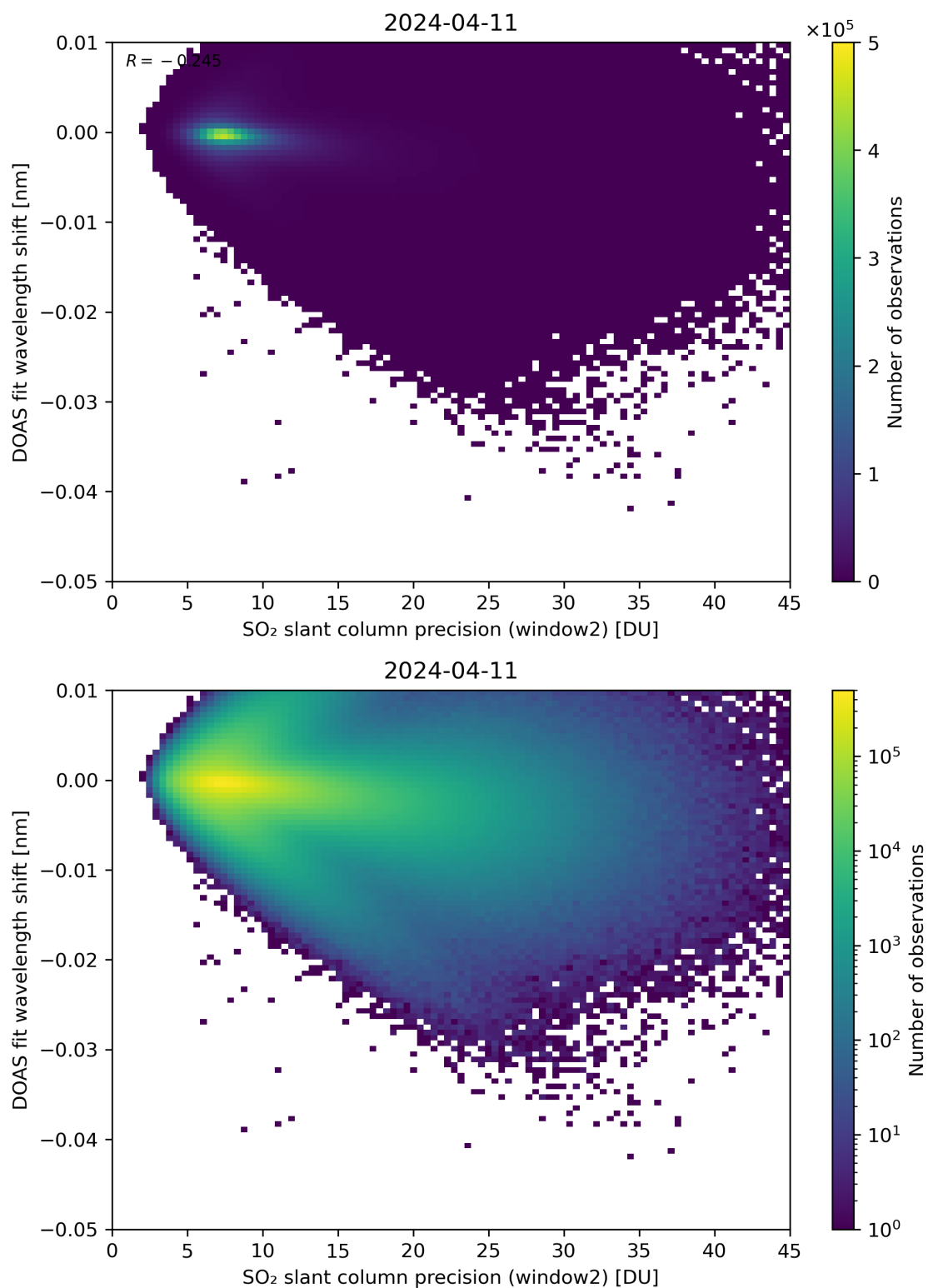
Figure 243: Scatter density plot of “SO 2 slant column precision (window2)” against “DOAS fit wavelength shift” for 2024-04-10 to 2024-04-12.
