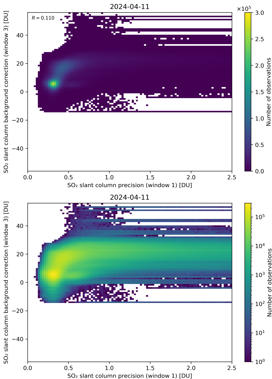
Figure 220: Scatter density plot of “SO 2 slant column precision (window 1)” against “SO 2 slant column background correction (window 3)” for 2024-04-10 to 2024-04-12.
