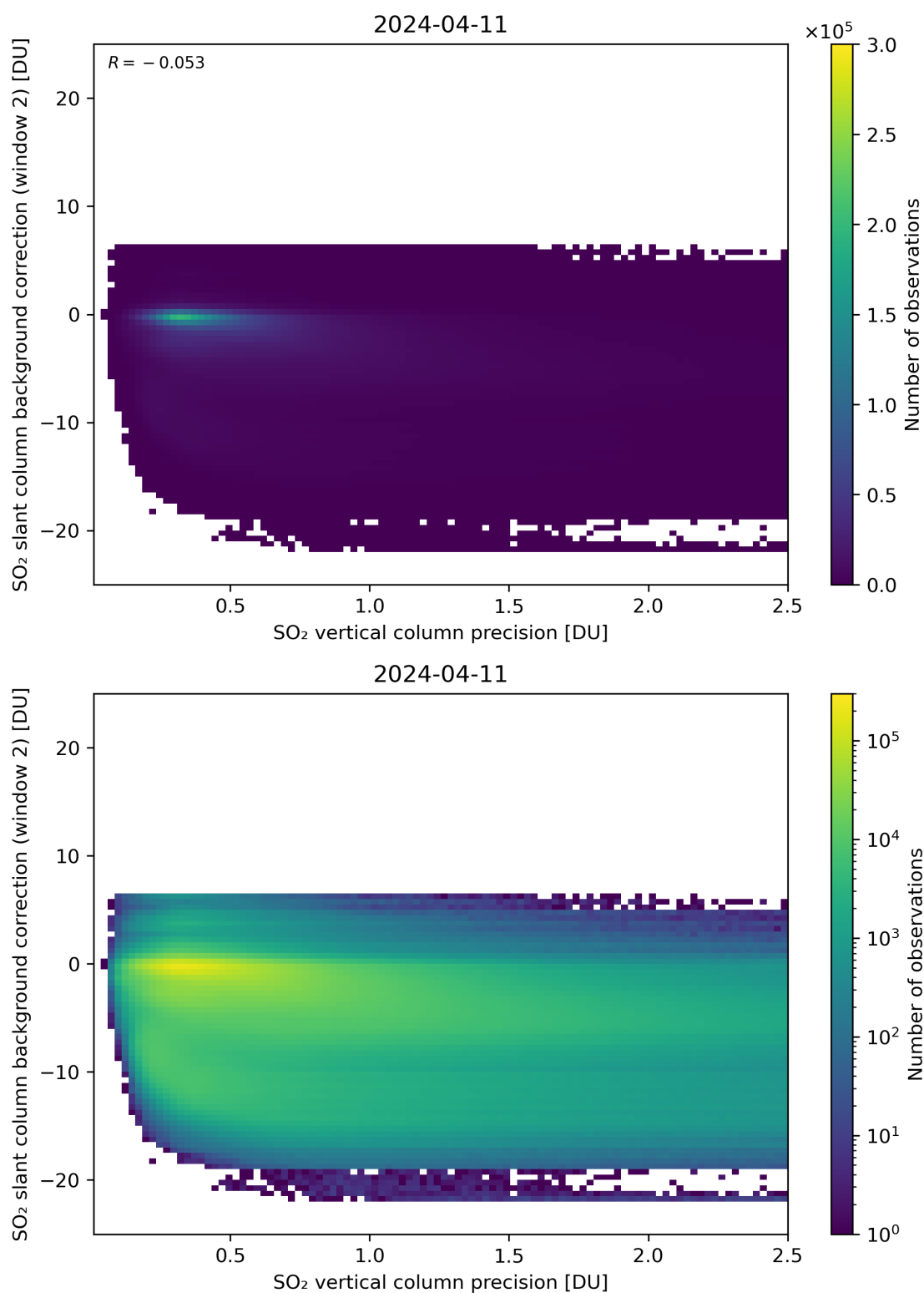
Figure 280: Scatter density plot of “SO 2 vertical column precision” against “SO 2 slant column background correction (window 2)” for 2024-04-10 to 2024-04-12.
