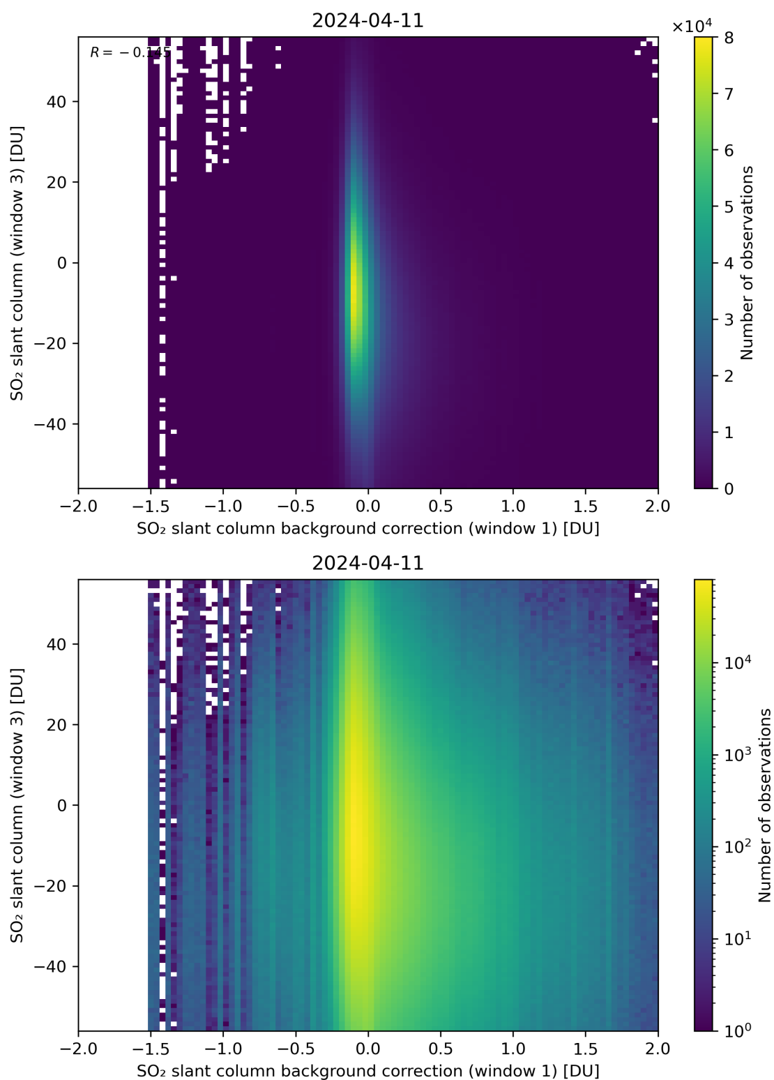
Figure 107: Scatter density plot of “SO 2 slant column background correction (window 1)” against “SO 2 slant column (window 3)” for 2024-04-10 to 2024-04-12.
