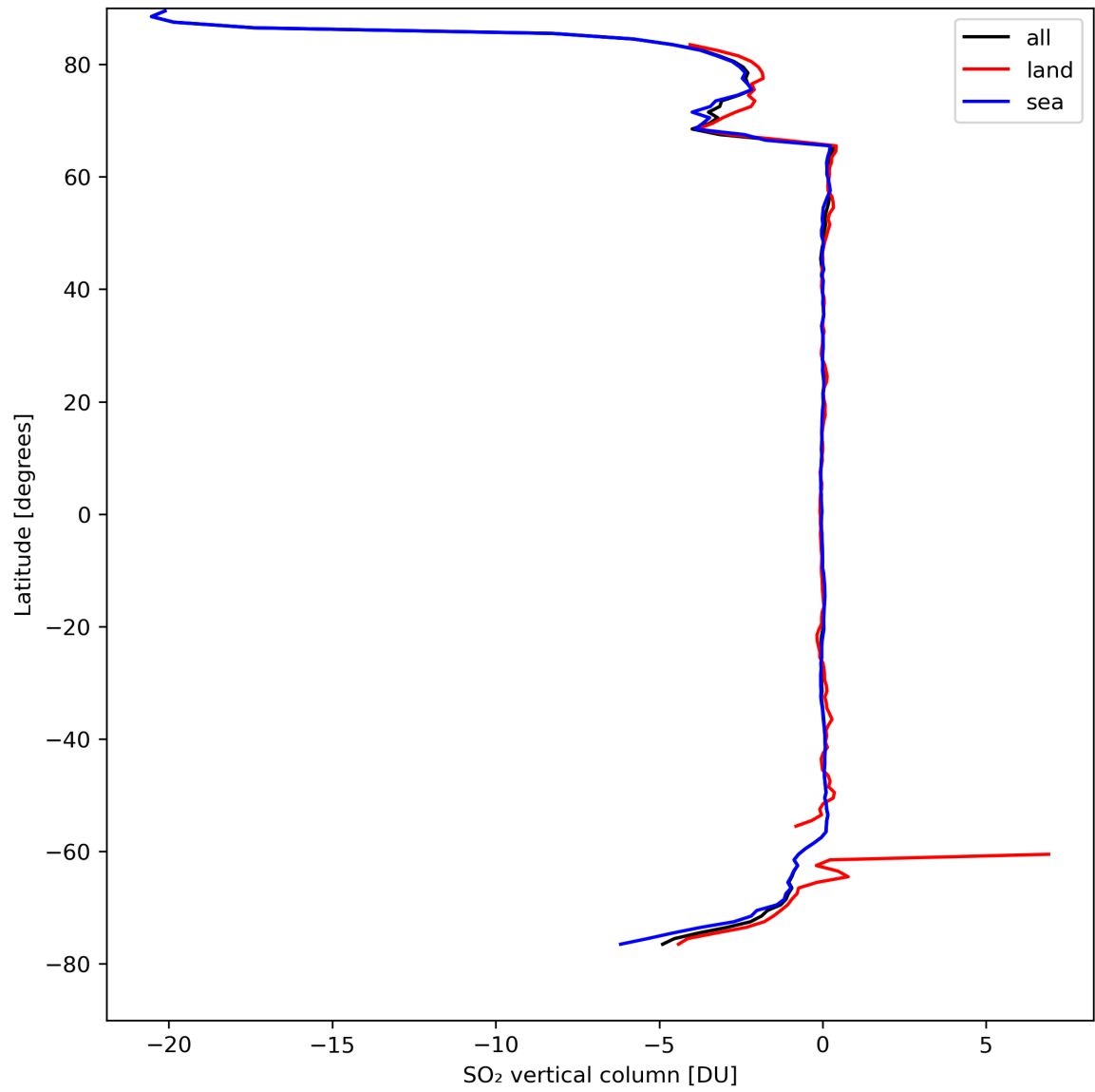
Figure 30: Zonal average of “SO 2 vertical column” for 2024-04-10 to 2024-04-12.
