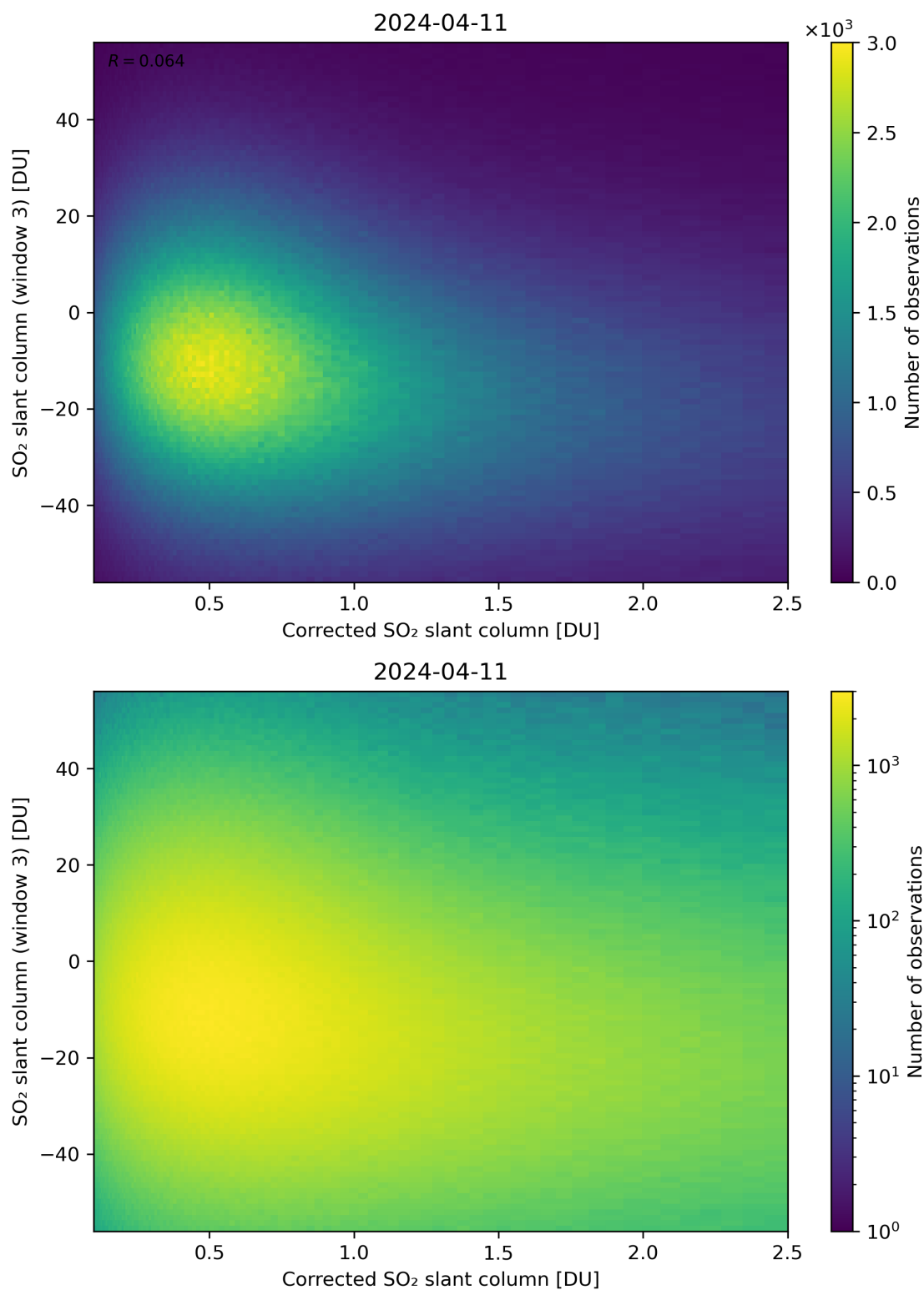
Figure 190: Scatter density plot of “Corrected SO 2 slant column” against “SO 2 slant column (window 3)” for 2024-04-10 to 2024-04-12.
