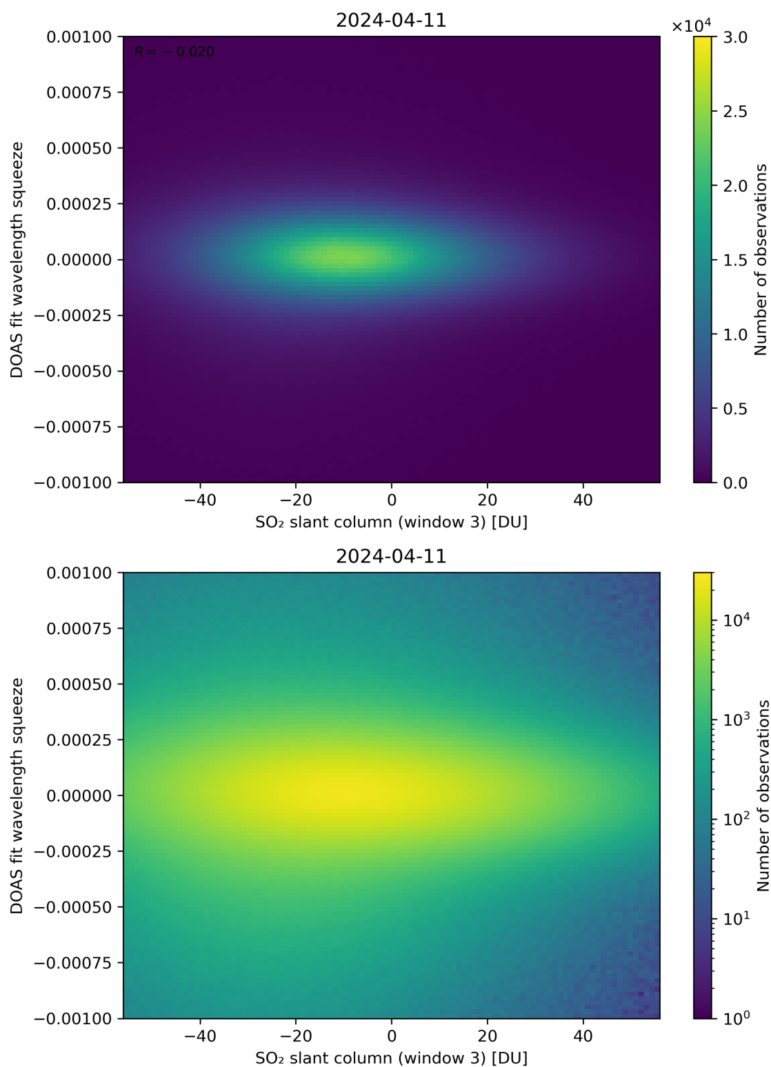
Figure 255: Scatter density plot of “SO 2 slant column (window 3)” against “DOAS fit wavelength squeeze” for 2024-04-10 to 2024-04-12.
