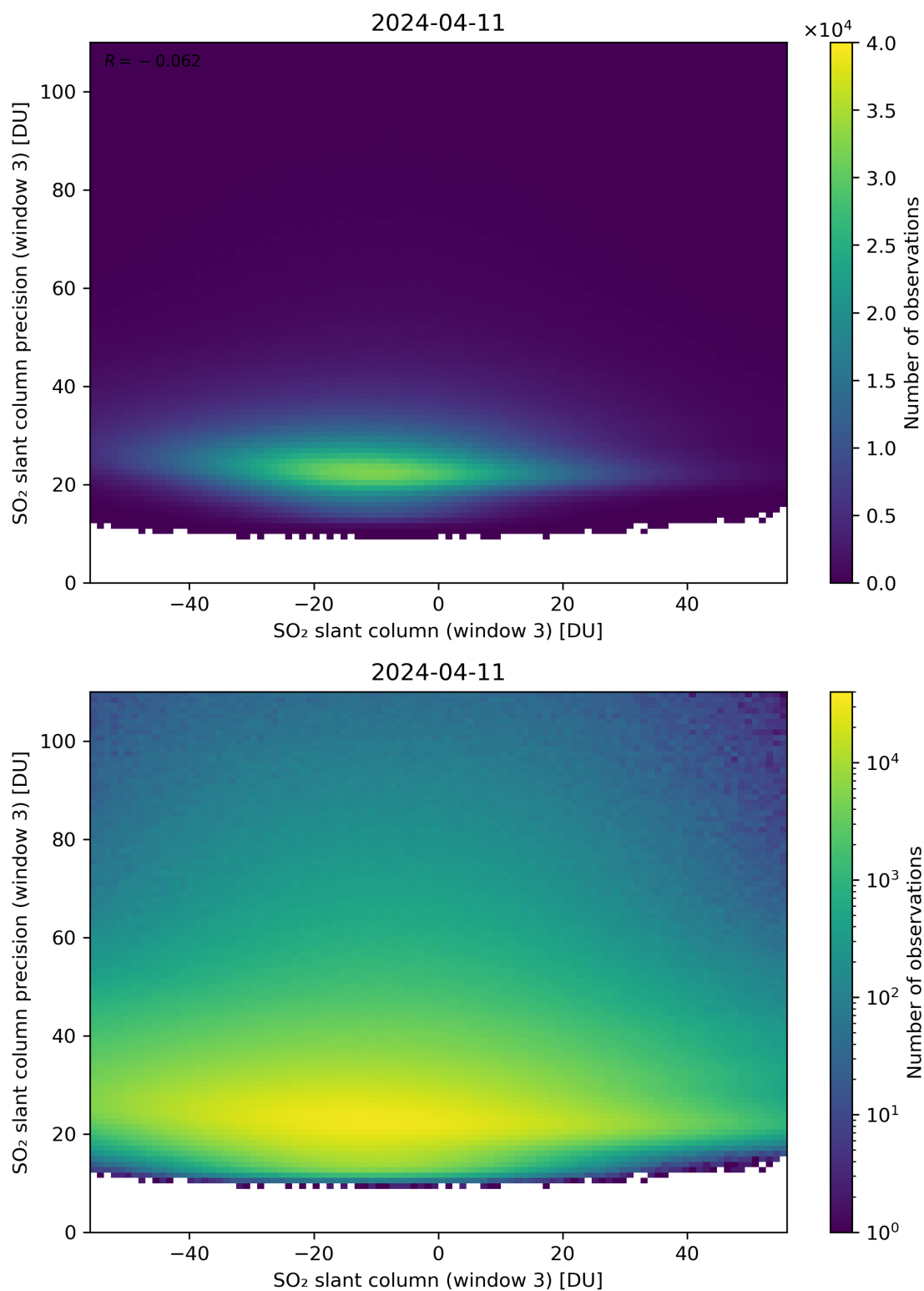
Figure 267: Scatter density plot of “SO 2 slant column (window 3)” against “SO 2 slant column precision (window 3)” for 2024-04-10 to 2024-04-12.
