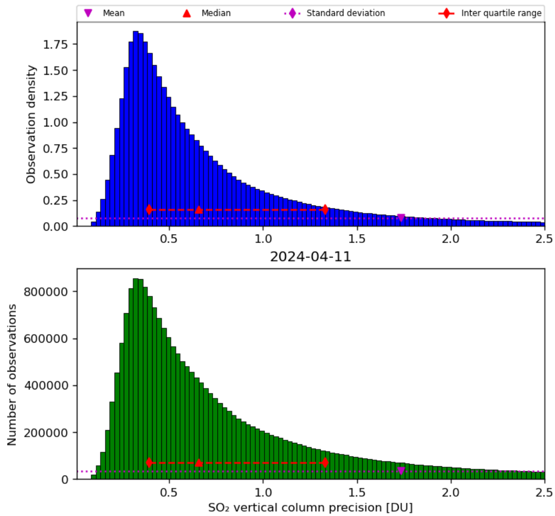
Figure 54: Histogram of “SO 2 vertical column precision” for 2024-04-10 to 2024-04-12
