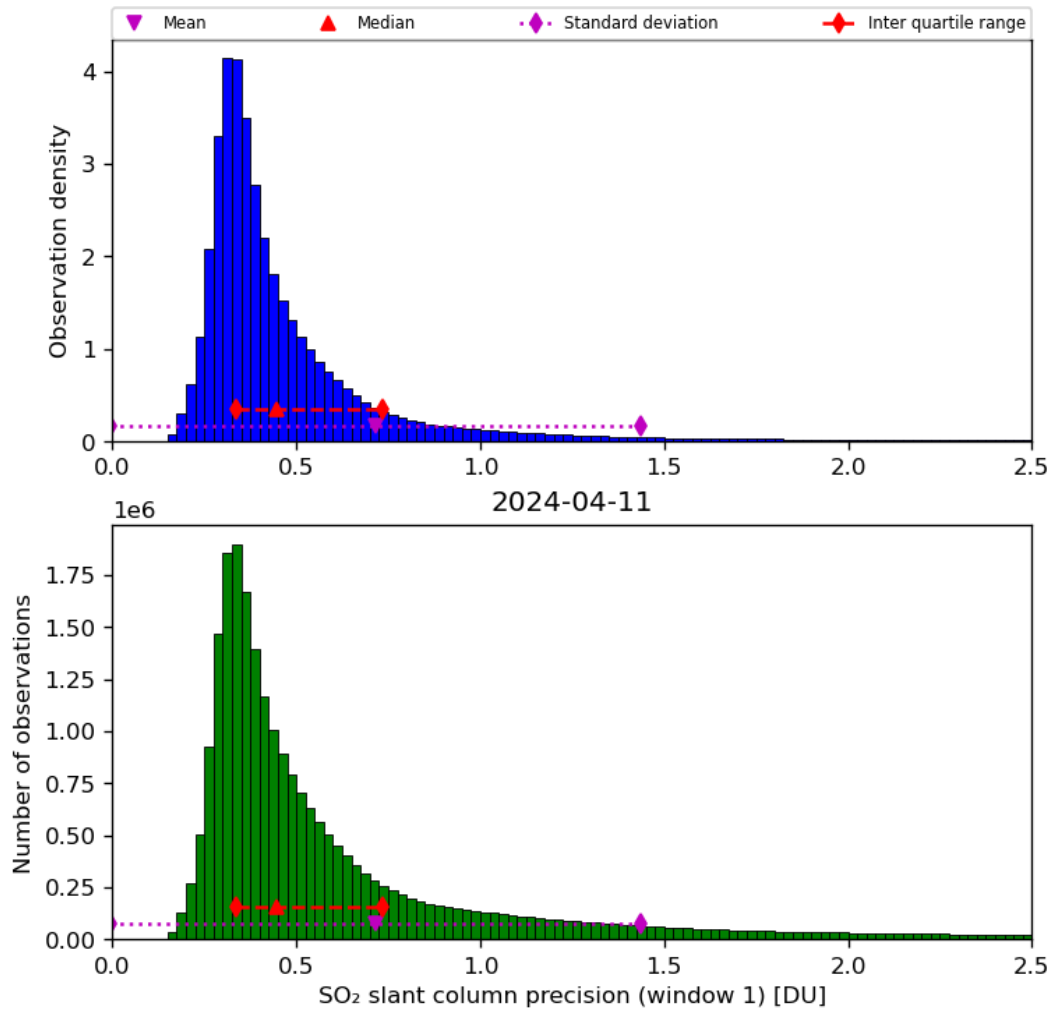
Figure 57: Histogram of “SO 2 slant column precision (window 1)” for 2024-04-10 to 2024-04-12
