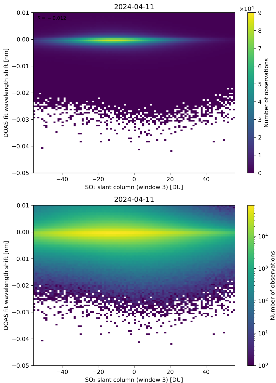
Figure 254: Scatter density plot of “SO 2 slant column (window 3)” against “DOAS fit wavelength shift” for 2024-04-10 to 2024-04-12.
