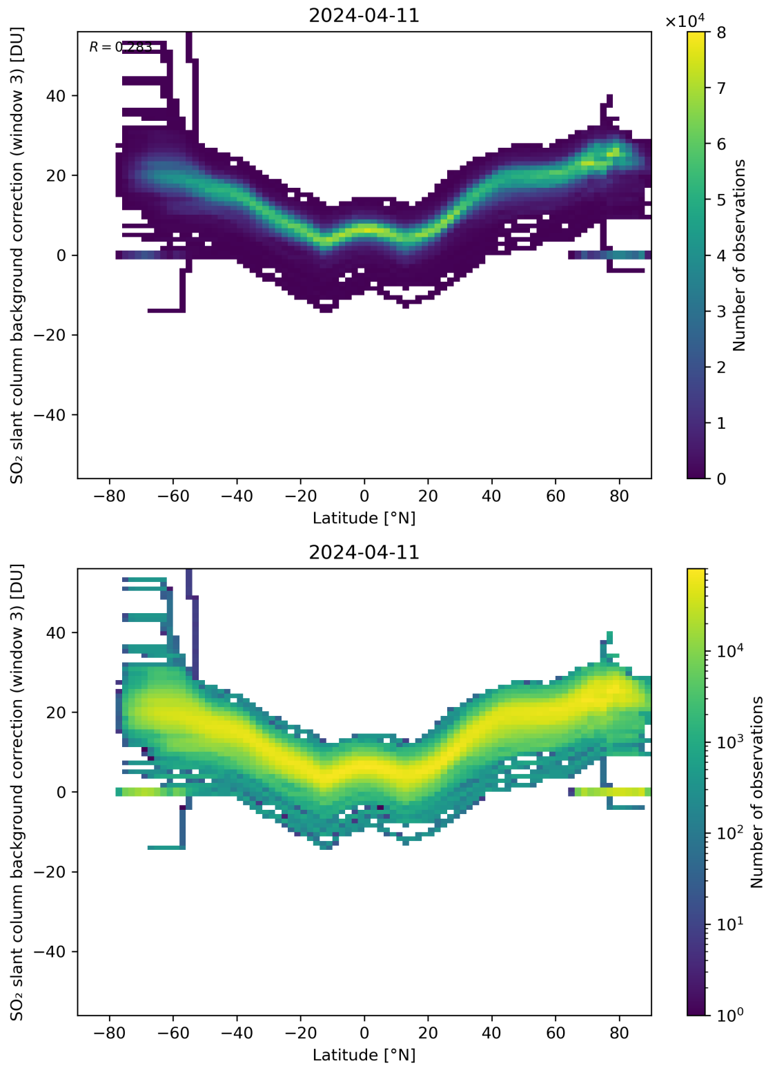
Figure 141: Scatter density plot of “Latitude” against “SO 2 slant column background correction (window 3)” for 2024-04-10 to 2024-04-12.
