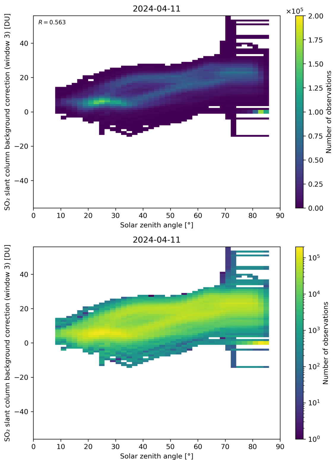
Figure 160: Scatter density plot of “Solar zenith angle” against “SO 2 slant column background correction (window 3)” for 2024-04-10 to 2024-04-12.
