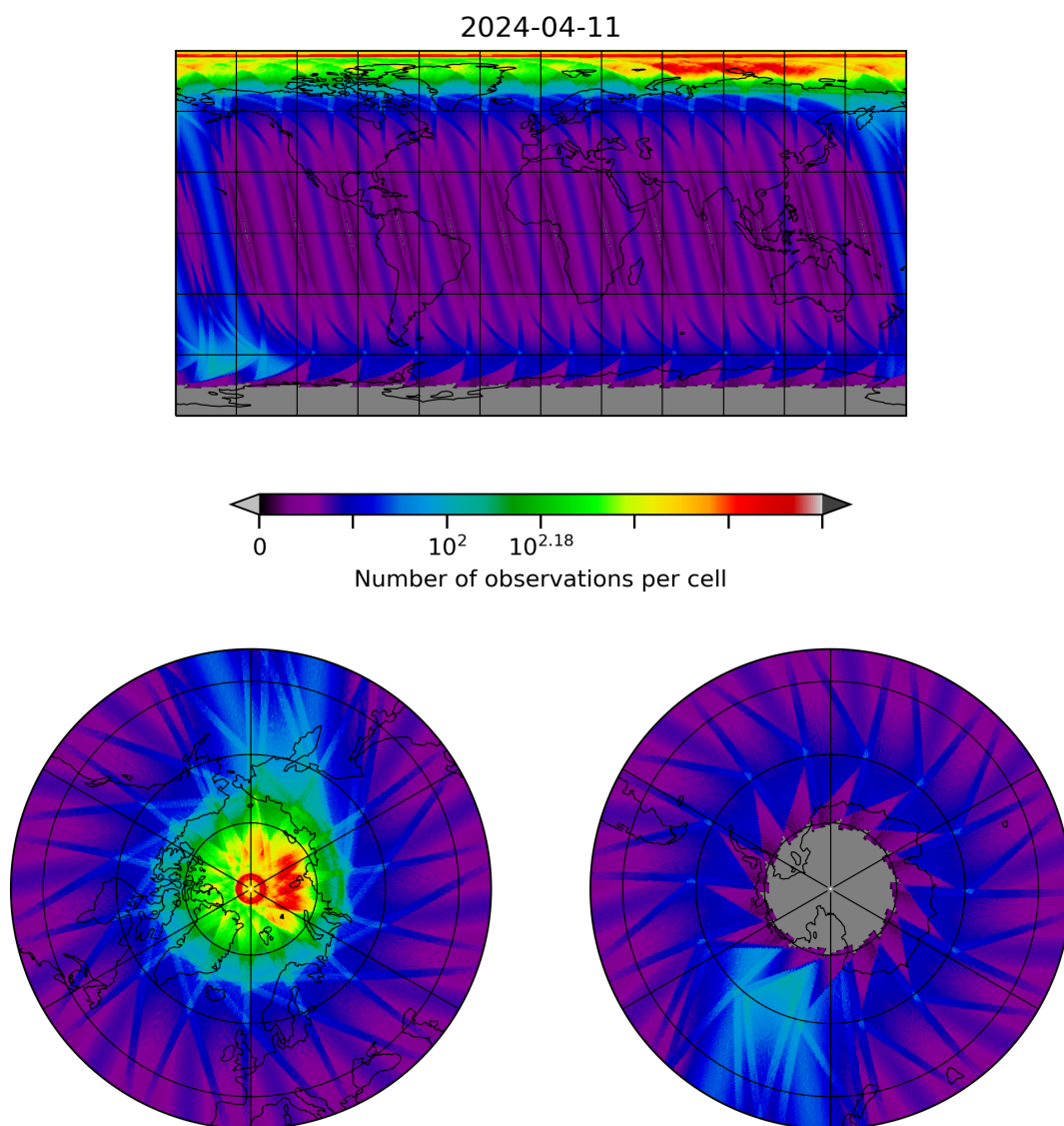
Figure 28: Map of the number of observations for 2024-04-10 to 2024-04-12
