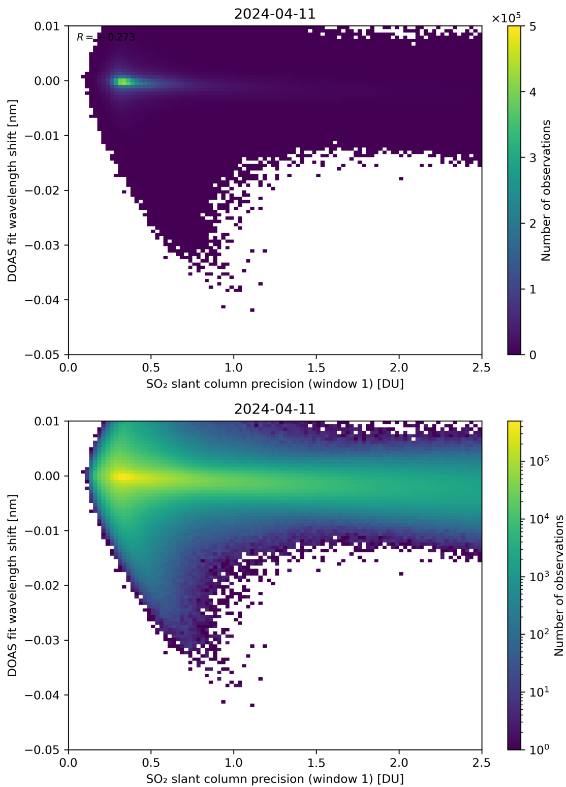
Figure 221: Scatter density plot of “SO 2 slant column precision (window 1)” against “DOAS fit wavelength shift” for 2024-04-10 to 2024-04-12.
