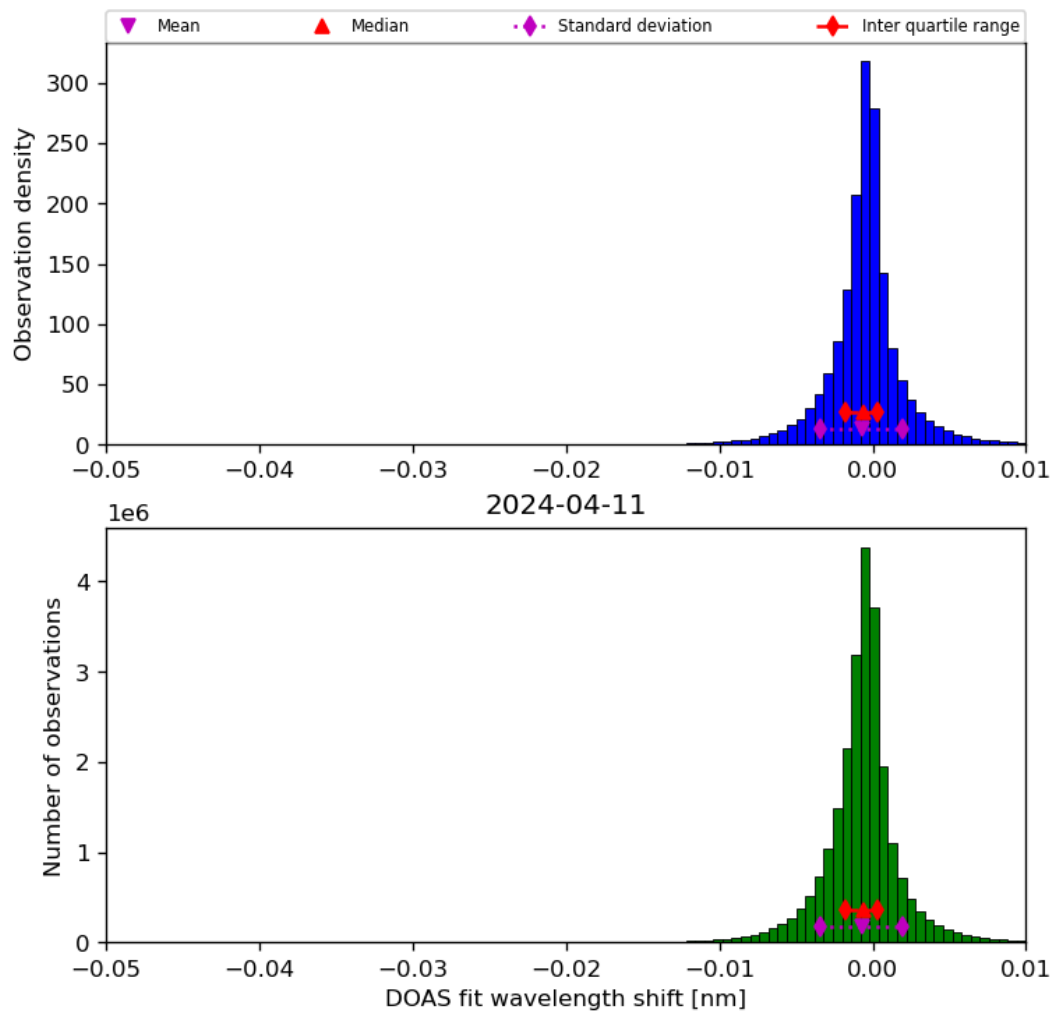
Figure 68: Histogram of “DOAS fit wavelength shift” for 2024-04-10 to 2024-04-12
