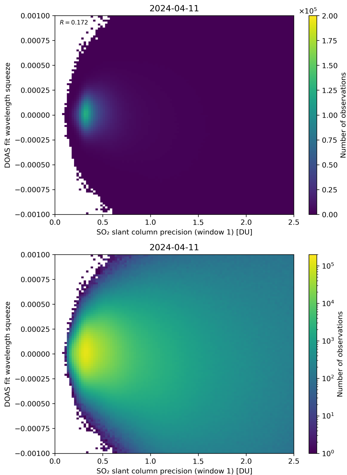
Figure 222: Scatter density plot of “SO 2 slant column precision (window 1)” against “DOAS fit wavelength squeeze” for 2024-04-10 to 2024-04-12.
