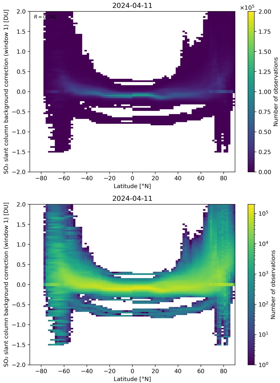
Figure 139: Scatter density plot of “Latitude” against “SO 2 slant column background correction (window 1)” for 2024-04-10 to 2024-04-12.
