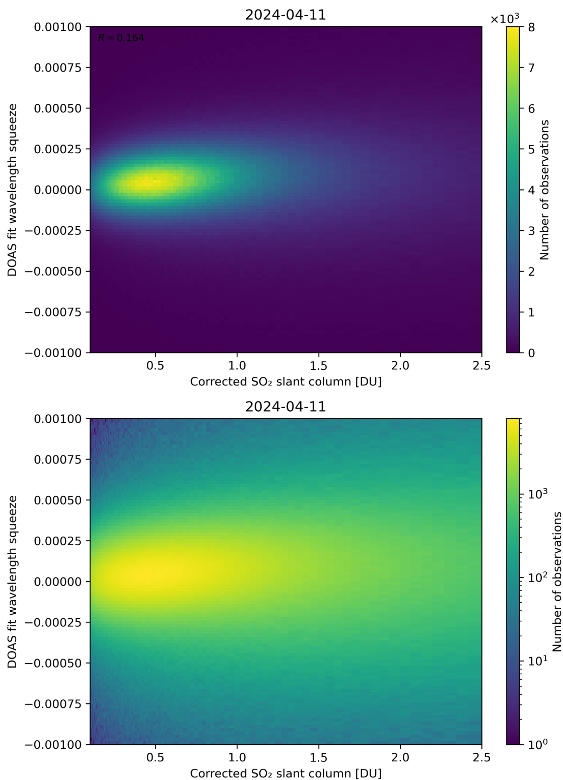
Figure 182: Scatter density plot of “Corrected SO 2 slant column” against “DOAS fit wavelength squeeze” for 2024-04-10 to 2024-04-12.
