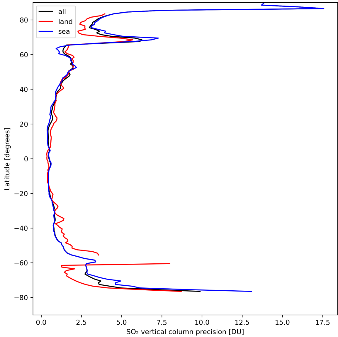
Figure 31: Zonal average of “SO 2 vertical column precision” for 2024-04-10 to 2024-04-12.
