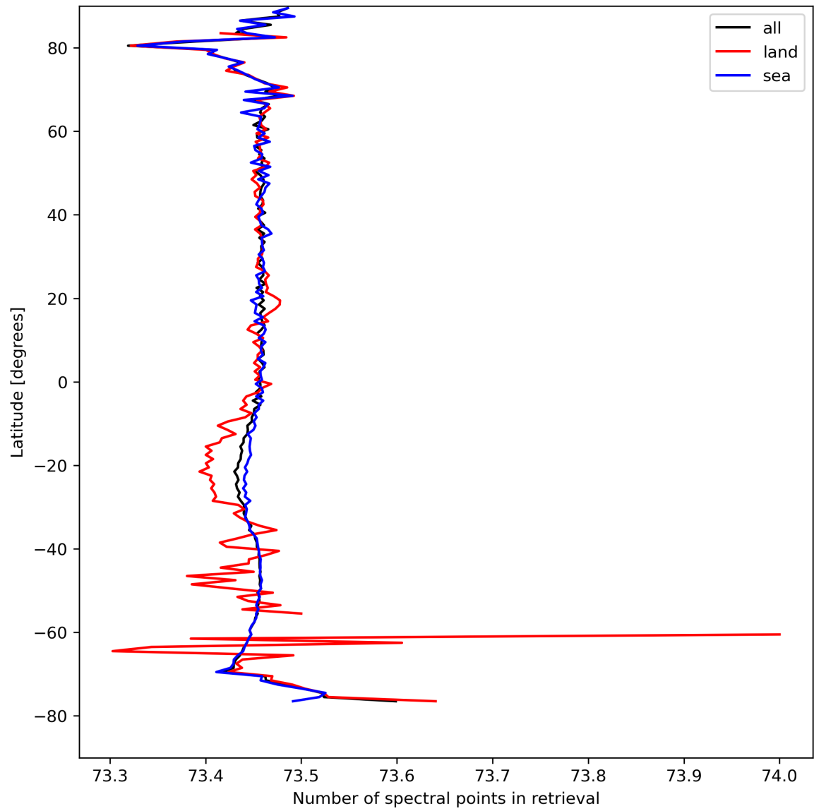
Figure 51: Zonal average of “Number of spectral points in retrieval” for 2024-04-10 to 2024-04-12.
