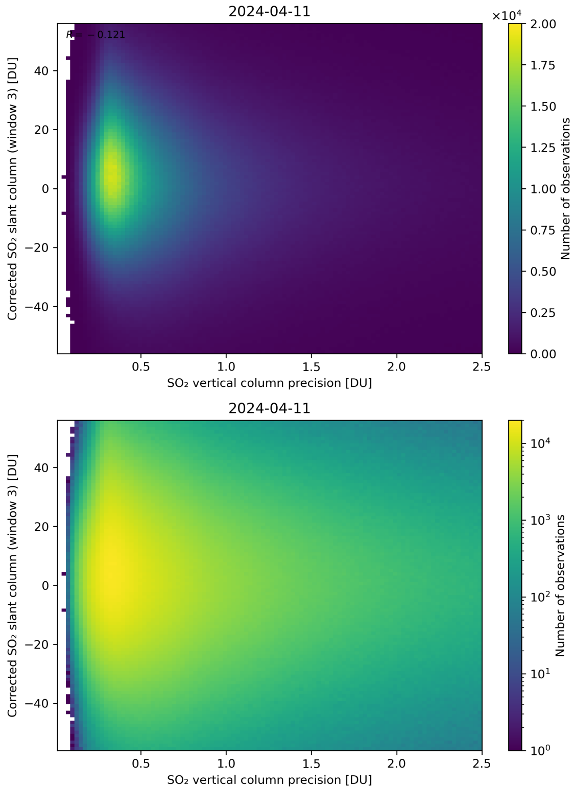
Figure 288: Scatter density plot of “SO 2 vertical column precision” against “Corrected SO 2 slant column (window 3)” for 2024-04-10 to 2024-04-12.
