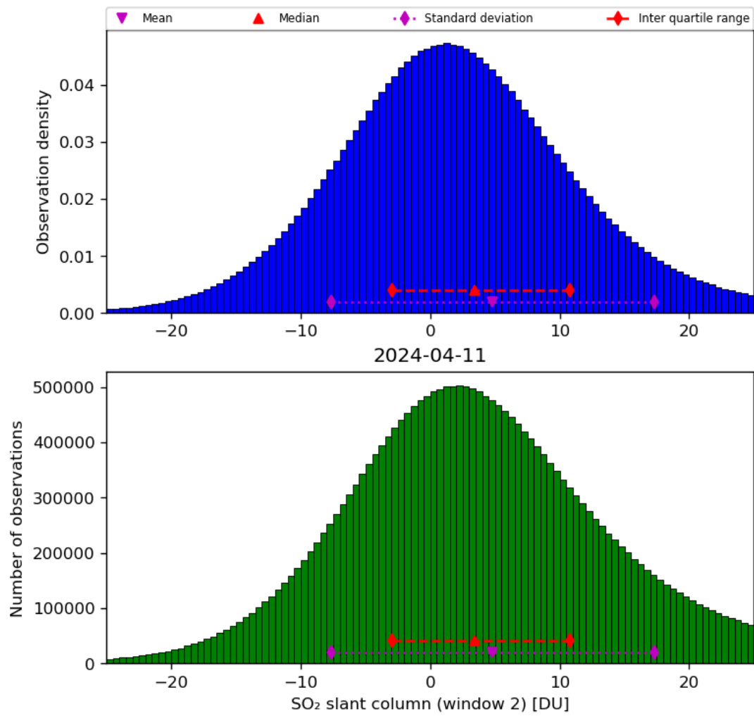
Figure 60: Histogram of “SO 2 slant column (window 2)” for 2024-04-10 to 2024-04-12
