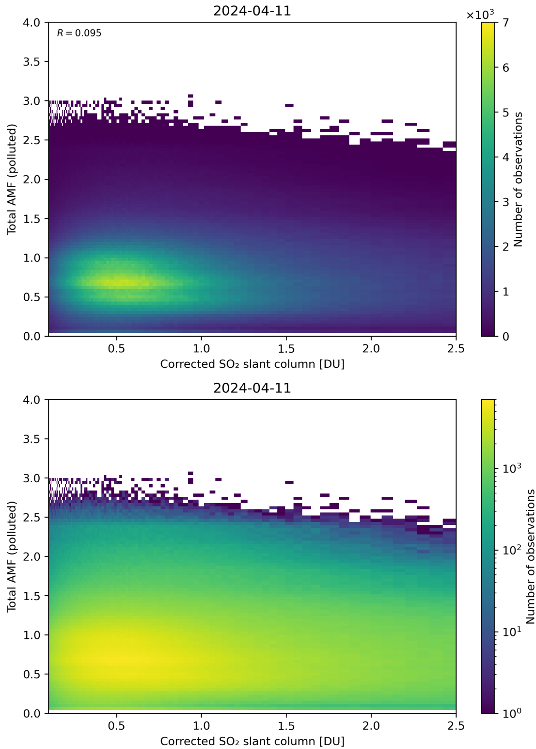
Figure 192: Scatter density plot of “Corrected SO 2 slant column” against “Total AMF (polluted)” for 2024-04-10 to 2024-04-12.
