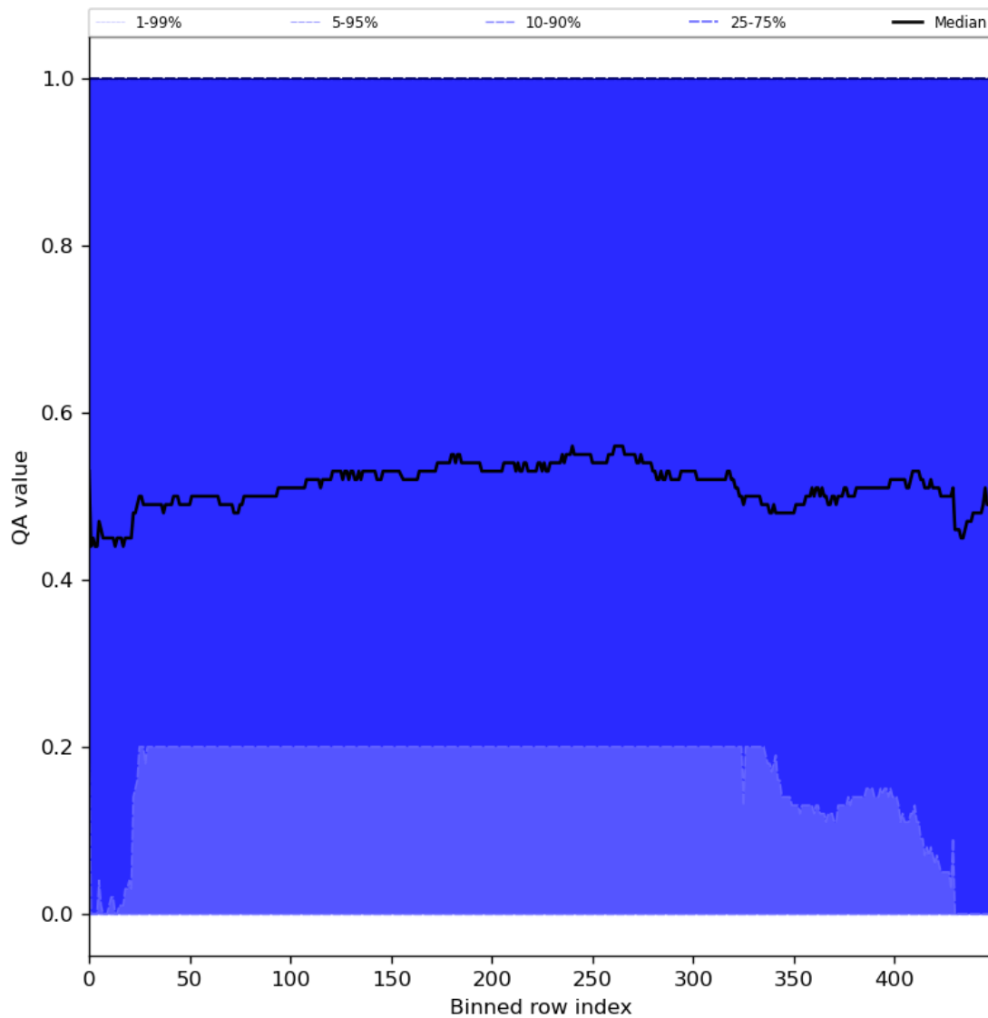
Figure 75: Along track statistics of “QA value” for 2024-04-10 to 2024-04-12
