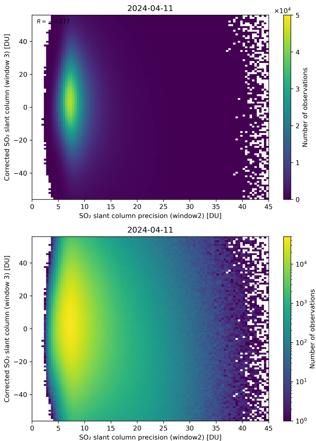
Figure 248: Scatter density plot of “SO 2 slant column precision (window2)” against “Corrected SO 2 slant column (window 3)” for 2024-04-10 to 2024-04-12.
