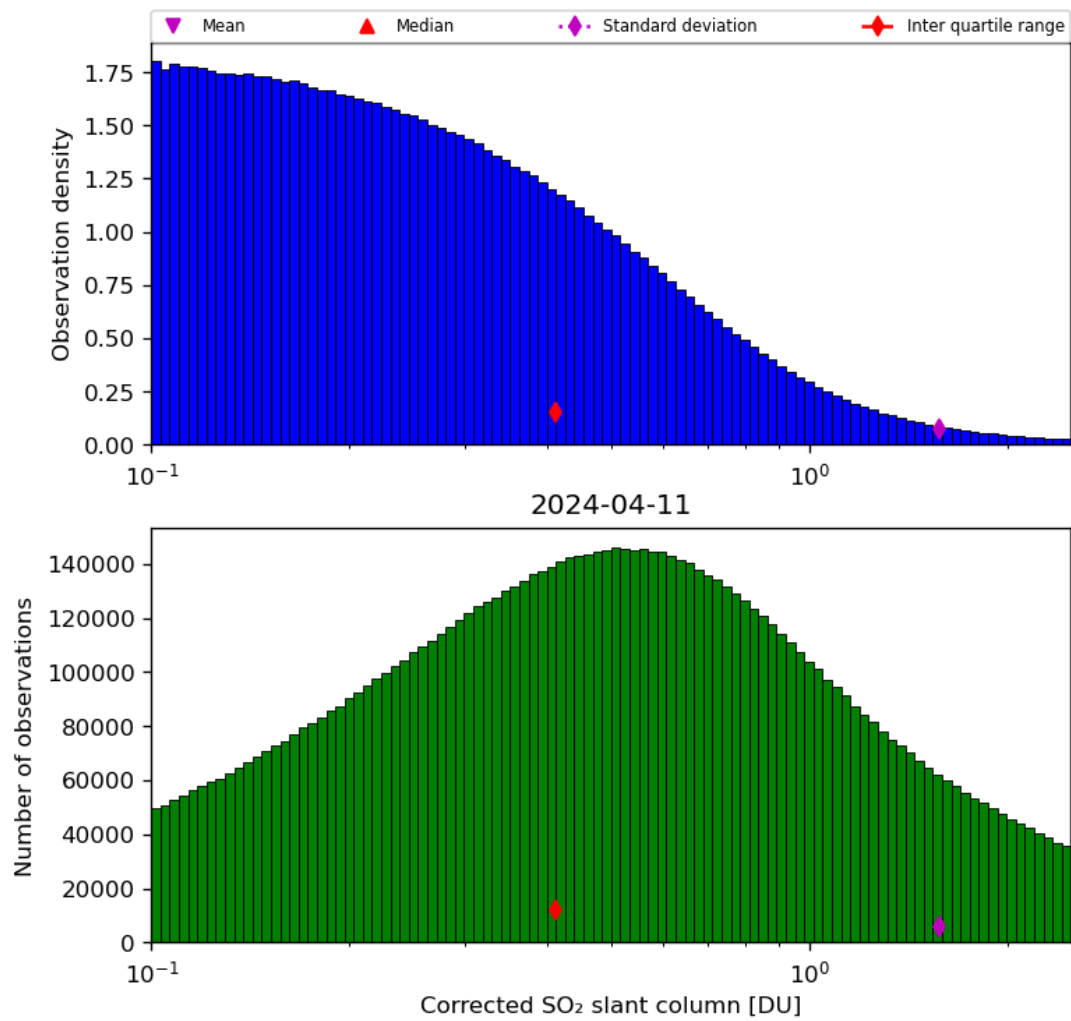
Figure 55: Histogram of “Corrected SO 2 slant column” for 2024-04-10 to 2024-04-12
