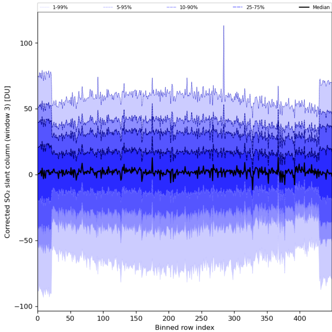
Figure 89: Along track statistics of “Corrected SO 2 slant column (window 3)” for 2024-04-10 to 2024-04-12
