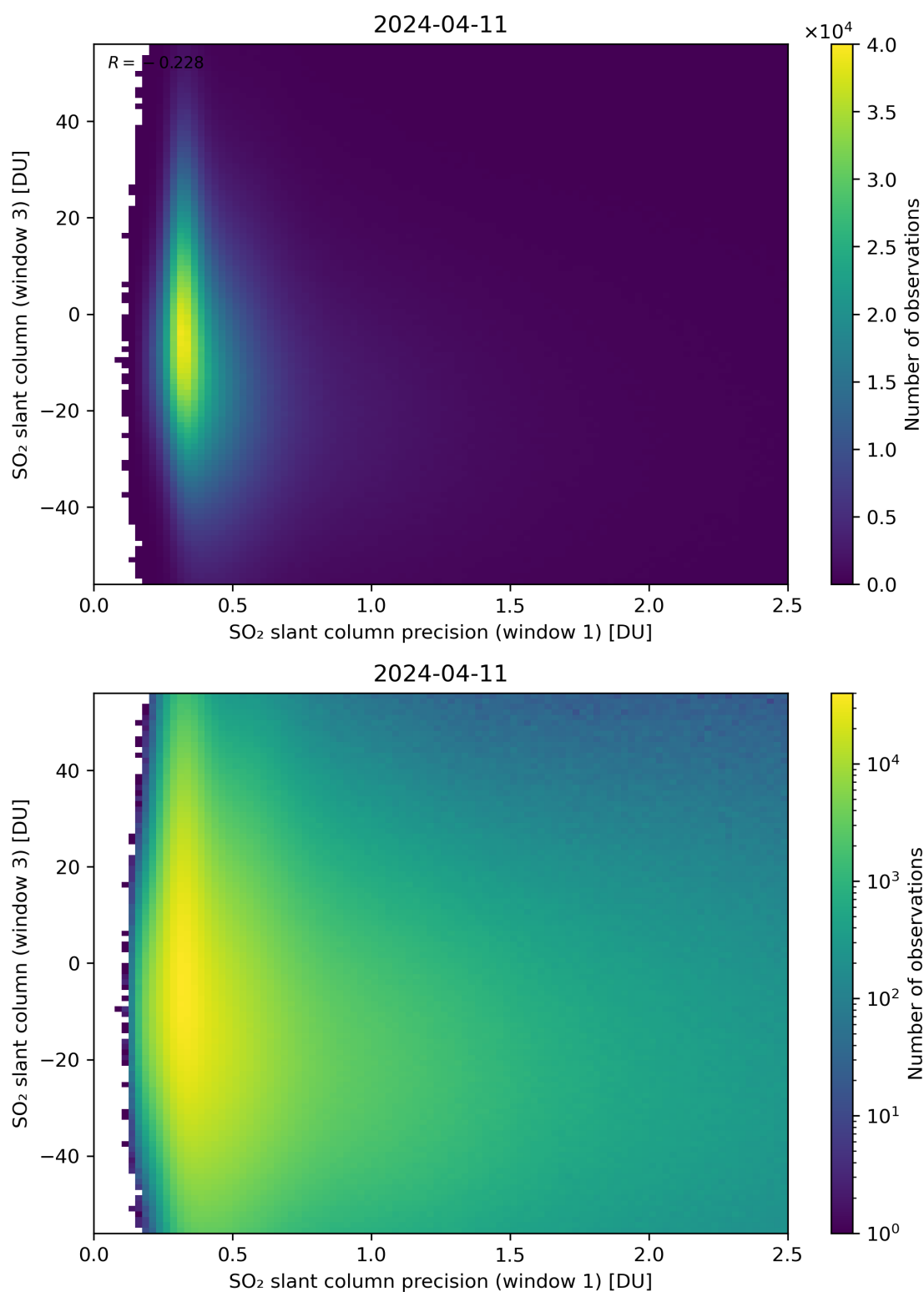
Figure 228: Scatter density plot of “SO 2 slant column precision (window 1)” against “SO 2 slant column (window 3)” for 2024-04-10 to 2024-04-12.
