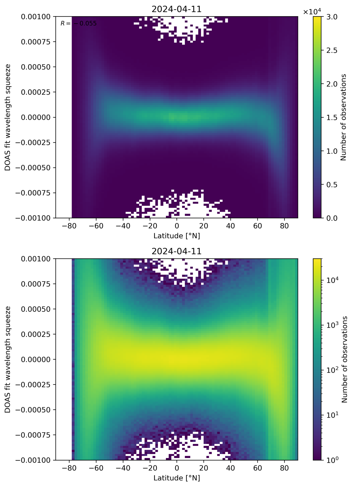
Figure 143: Scatter density plot of “Latitude” against “DOAS fit wavelength squeeze” for 2024-04-10 to 2024-04-12.
