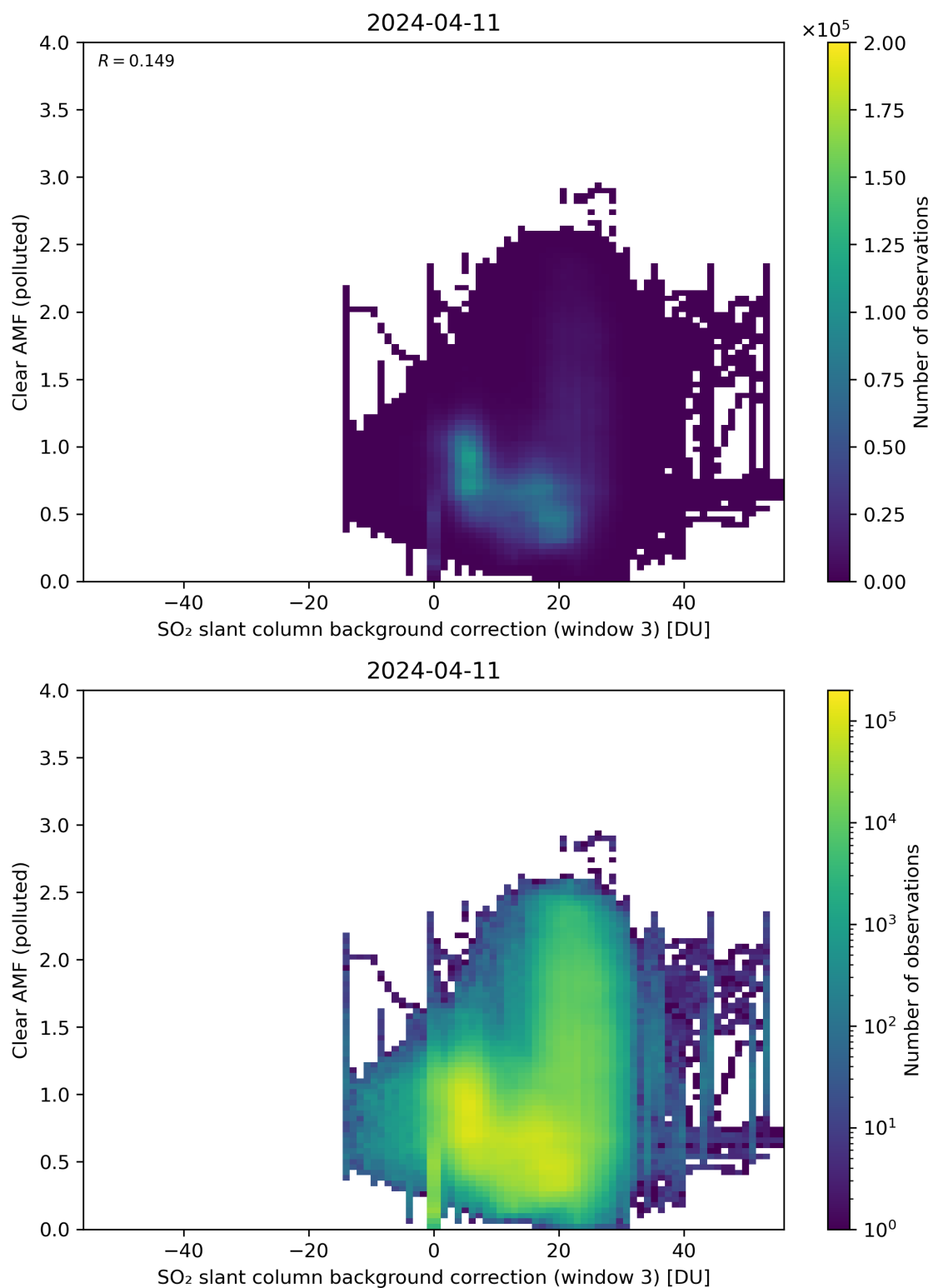
Figure 124: Scatter density plot of “SO 2 slant column background correction (window 3)” against “Clear AMF (polluted)” for 2024-04-10 to 2024-04-12.
