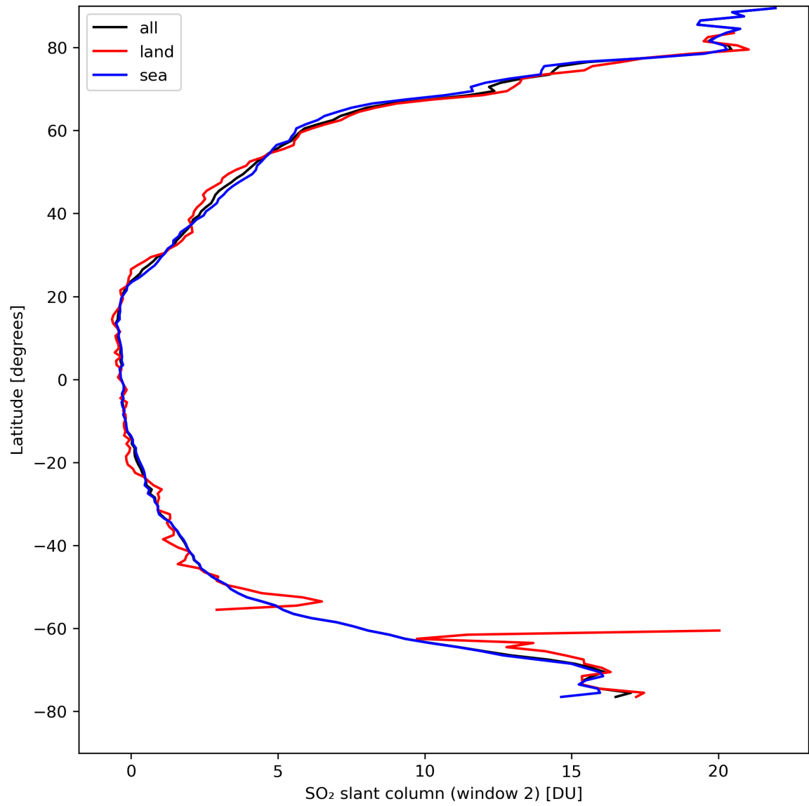
Figure 37: Zonal average of “SO 2 slant column (window 2)” for 2024-04-10 to 2024-04-12.
