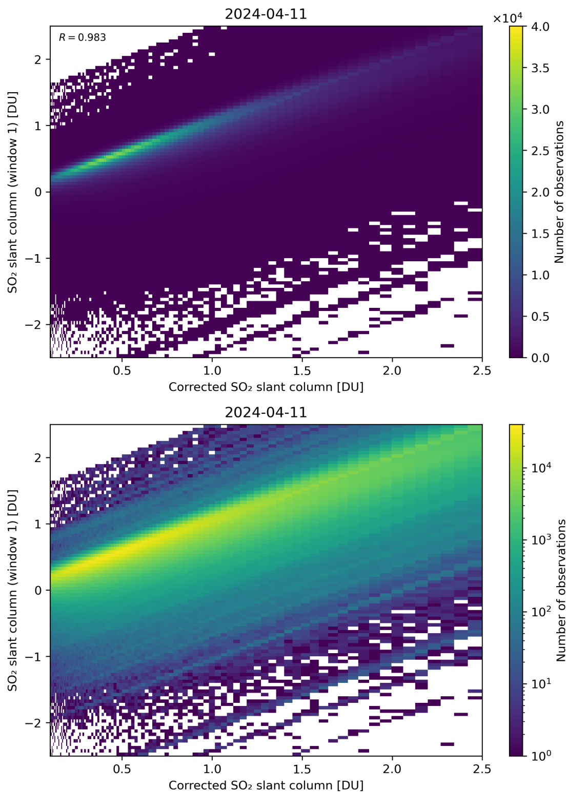
Figure 187: Scatter density plot of “Corrected SO 2 slant column” against “SO 2 slant column (window 1)” for 2024-04-10 to 2024-04-12.
