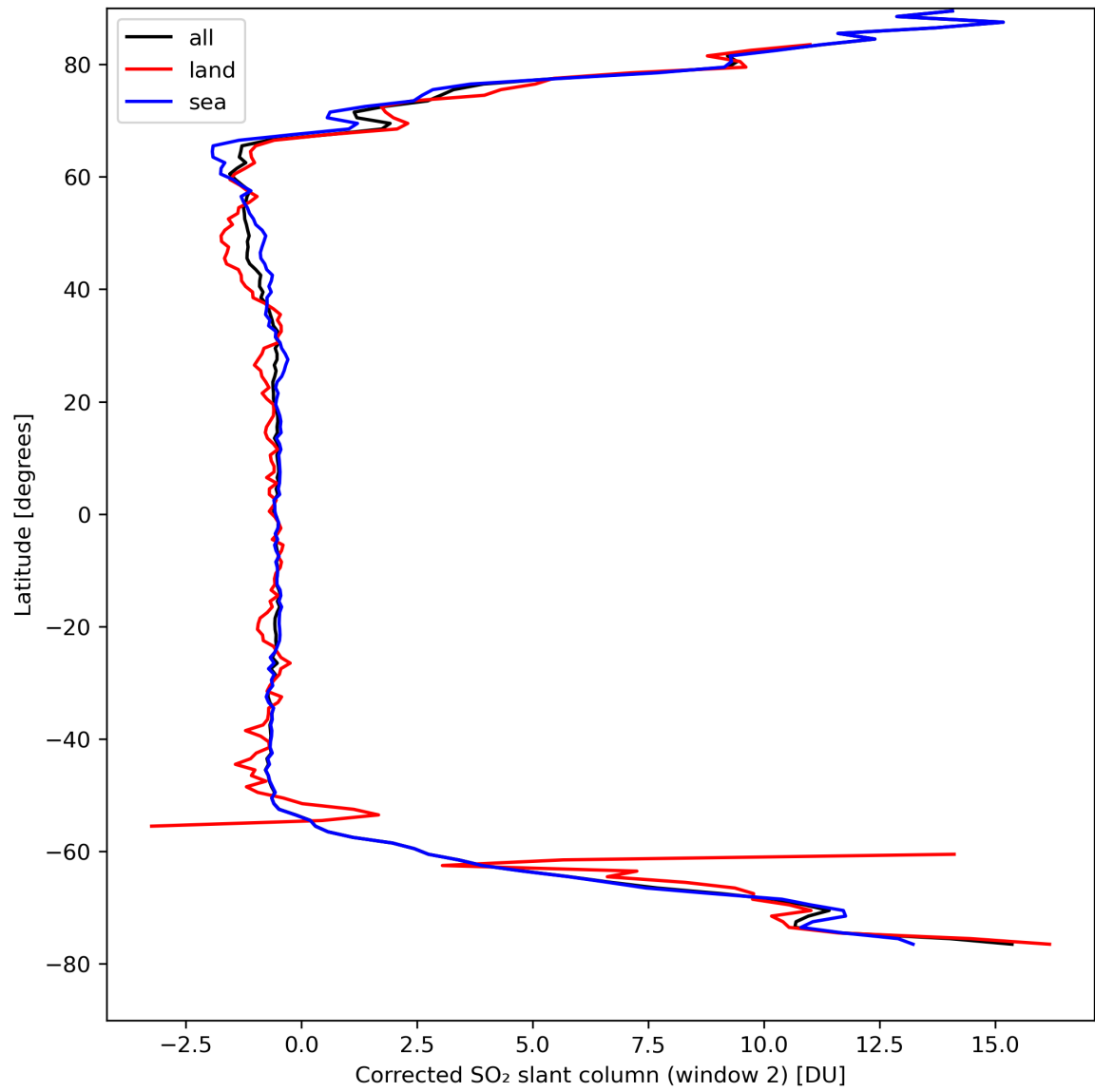
Figure 39: Zonal average of “Corrected SO 2 slant column (window 2)” for 2024-04-10 to 2024-04-12.
