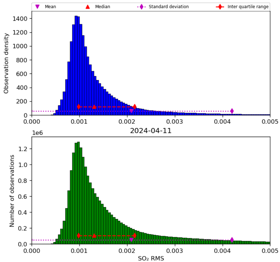
Figure 70: Histogram of “SO 2 RMS” for 2024-04-10 to 2024-04-12
