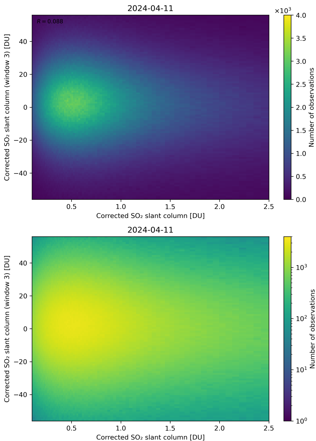
Figure 186: Scatter density plot of “Corrected SO 2 slant column” against “Corrected SO 2 slant column (window 3)” for 2024-04-10 to 2024-04-12.
