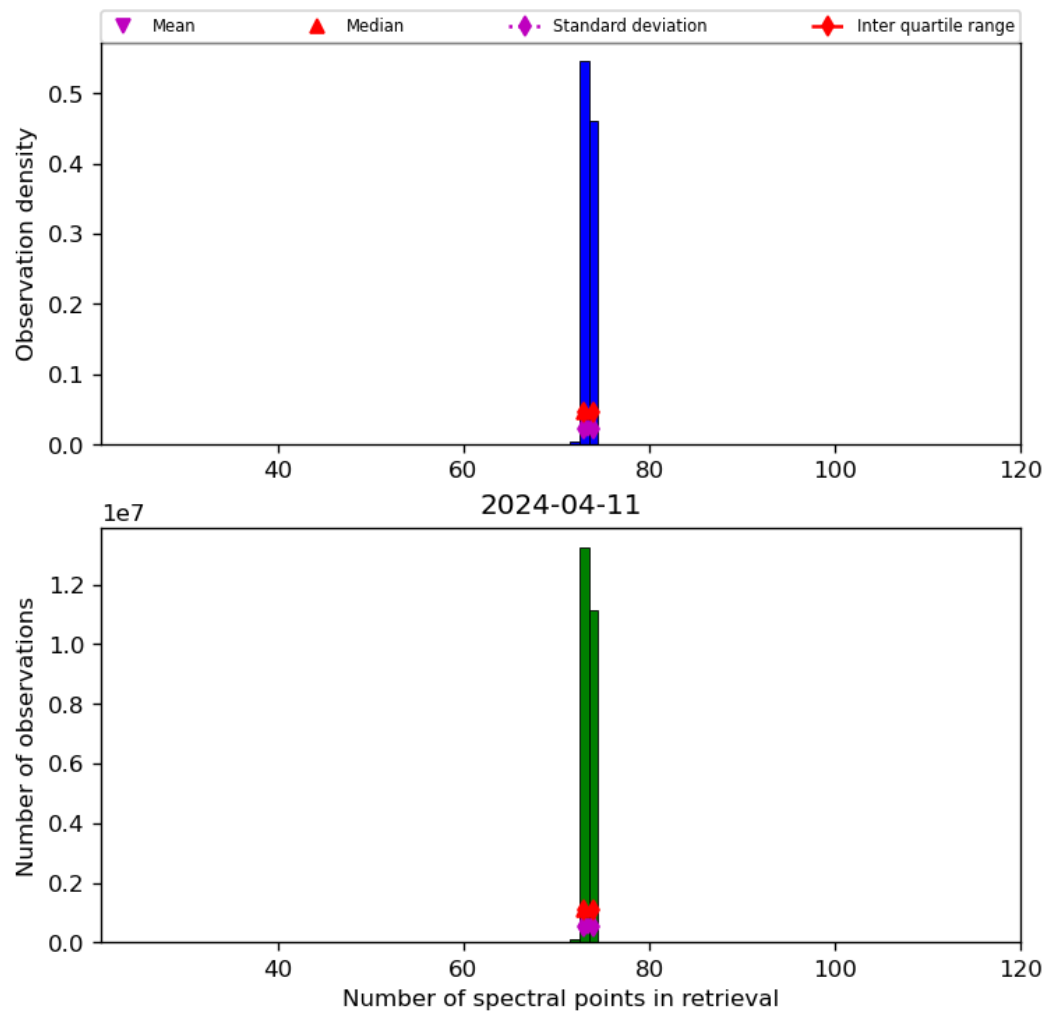
Figure 74: Histogram of “Number of spectral points in retrieval” for 2024-04-10 to 2024-04-12
