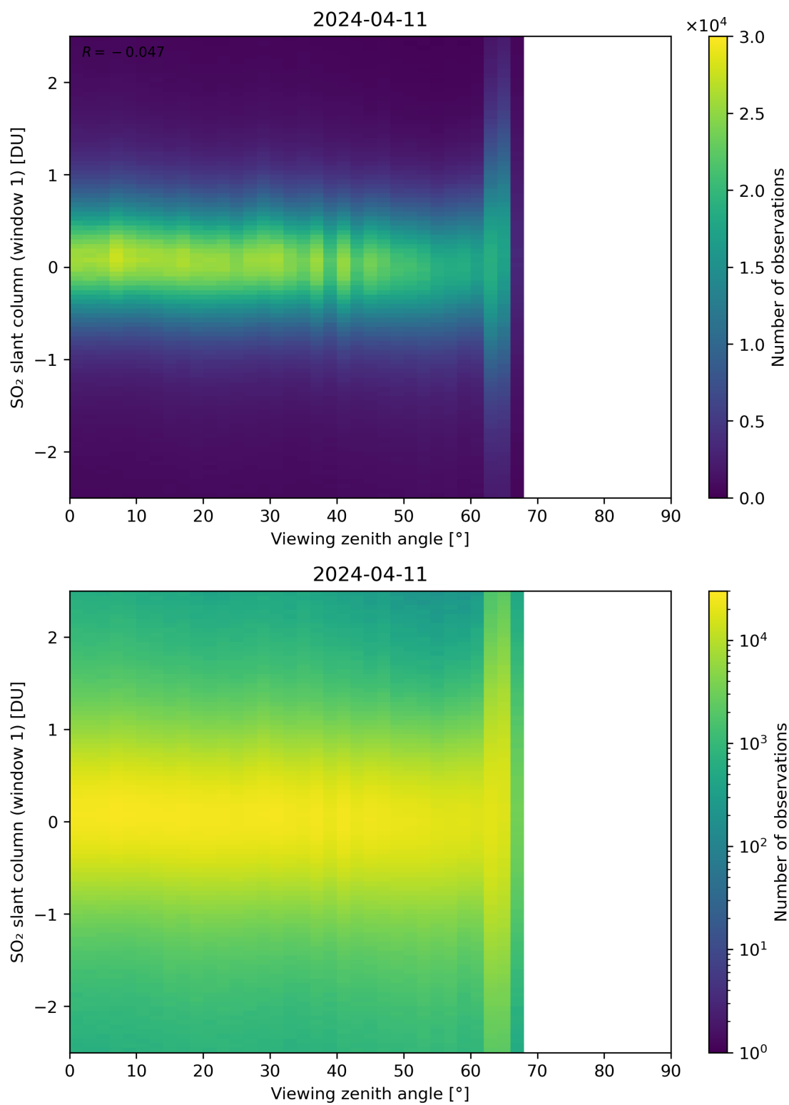
Figure 320: Scatter density plot of “Viewing zenith angle” against “SO 2 slant column (window 1)” for 2024-04-10 to 2024-04-12.
