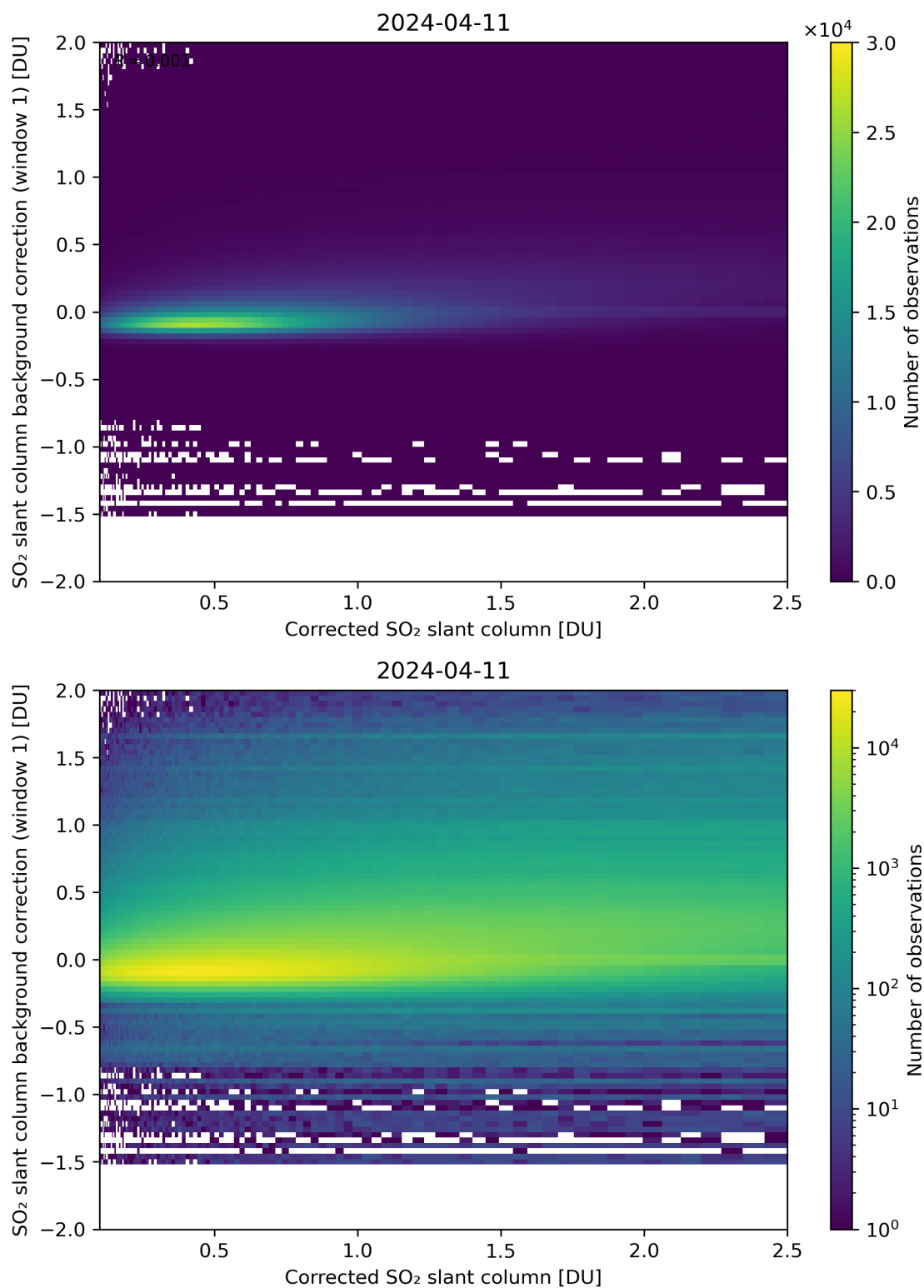
Figure 178: Scatter density plot of “Corrected SO 2 slant column” against “SO 2 slant column background correction (window 1)” for 2024-04-10 to 2024-04-12.
