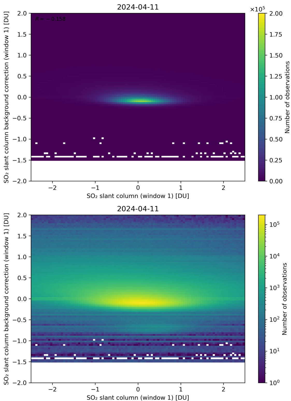
Figure 212: Scatter density plot of “SO 2 slant column (window 1)” against “SO 2 slant column background correction (window 1)” for 2024-04-10 to 2024-04-12.
