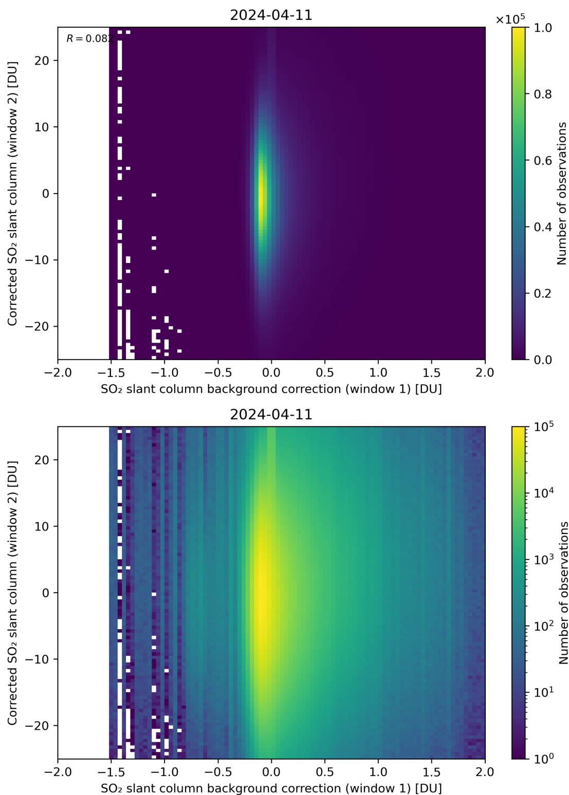
Figure 104: Scatter density plot of “SO 2 slant column background correction (window 1)” against “Corrected SO 2 slant column (window 2)” for 2024-04-10 to 2024-04-12.
