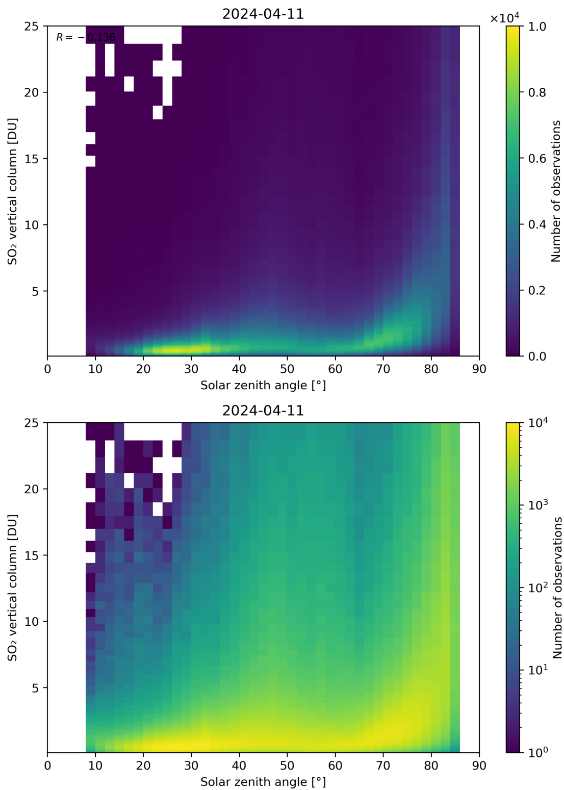
Figure 176: Scatter density plot of “Solar zenith angle” against “SO 2 vertical column” for 2024-04-10 to 2024-04-12.
