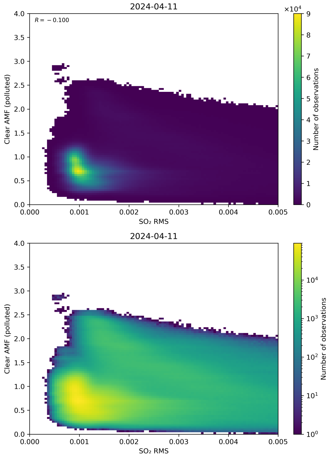
Figure 136: Scatter density plot of “SO 2 RMS” against “Clear AMF (polluted)” for 2024-04-10 to 2024-04-12.
