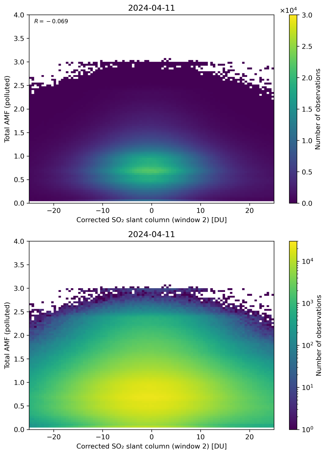
Figure 203: Scatter density plot of “Corrected SO 2 slant column (window 2)” against “Total AMF (polluted)” for 2024-04-10 to 2024-04-12.
