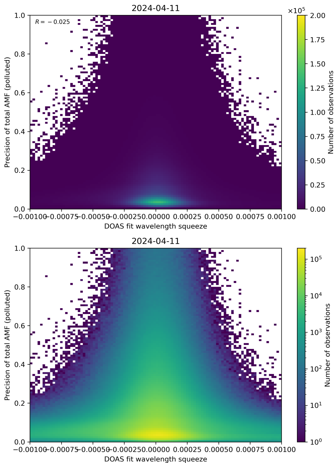
Figure 135: Scatter density plot of “DOAS fit wavelength squeeze” against “Precision of total AMF (polluted)” for 2024-04-10 to 2024-04-12.
