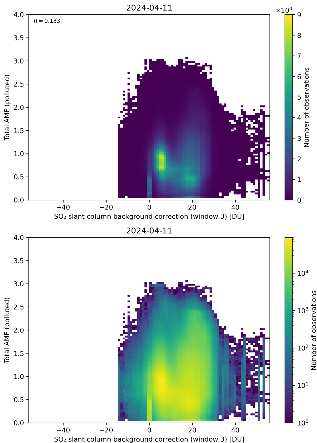
Figure 125: Scatter density plot of “SO 2 slant column background correction (window 3)” against “Total AMF (polluted)” for 2024-04-10 to 2024-04-12.
