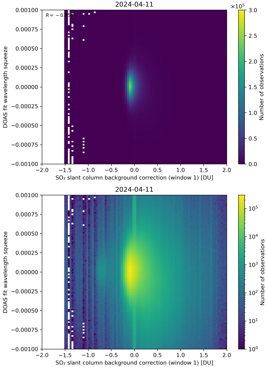
Figure 101: Scatter density plot of “SO 2 slant column background correction (window 1)” against “DOAS fit wavelength squeeze” for 2024-04-10 to 2024-04-12.
