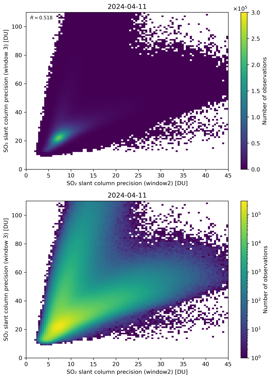
Figure 250: Scatter density plot of “SO 2 slant column precision (window2)” against “SO 2 slant column precision (window 3)” for 2024-04-10 to 2024-04-12.
