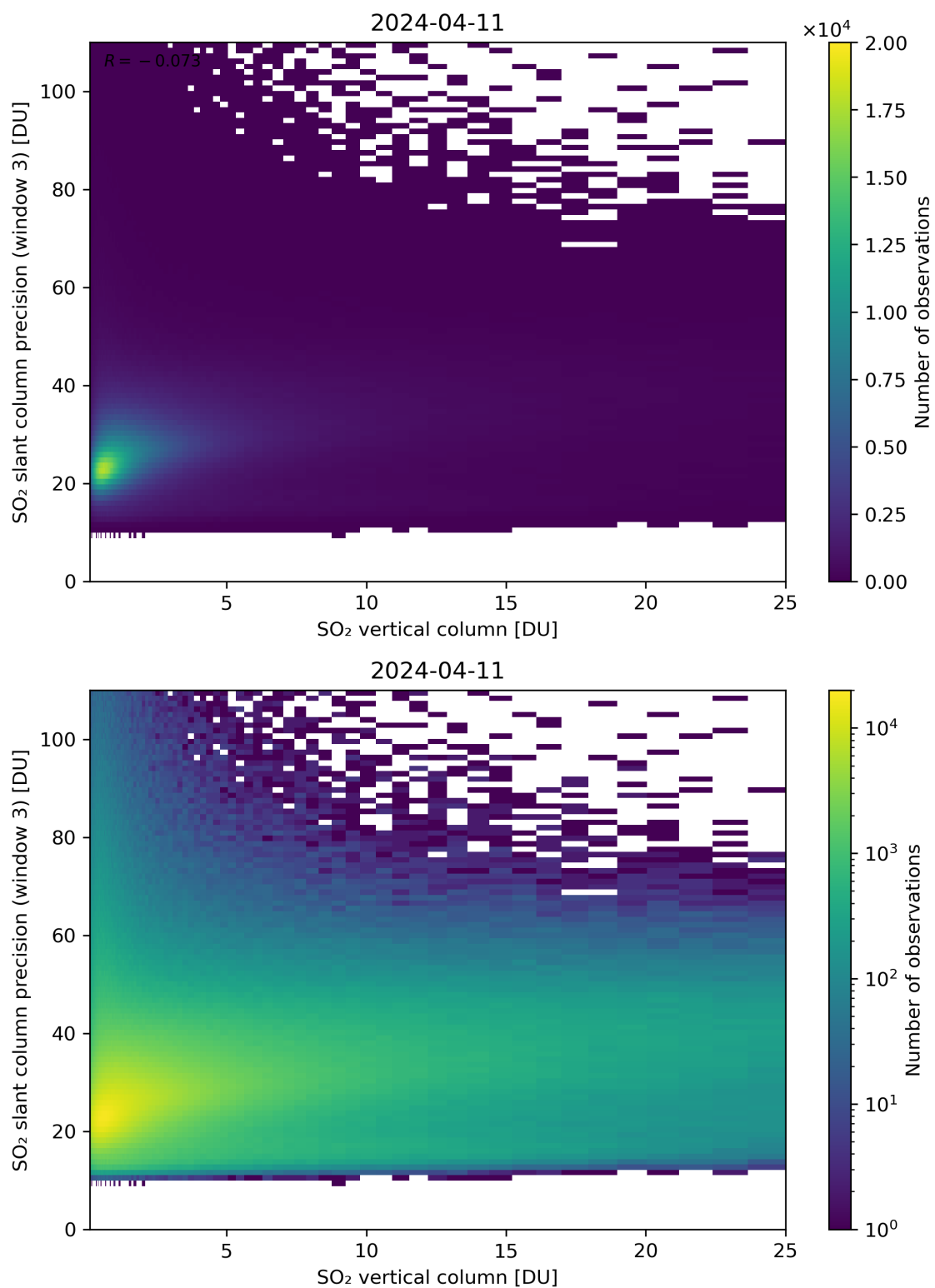
Figure 304: Scatter density plot of “SO 2 vertical column” against “SO 2 slant column precision (window 3)” for 2024-04-10 to 2024-04-12.
