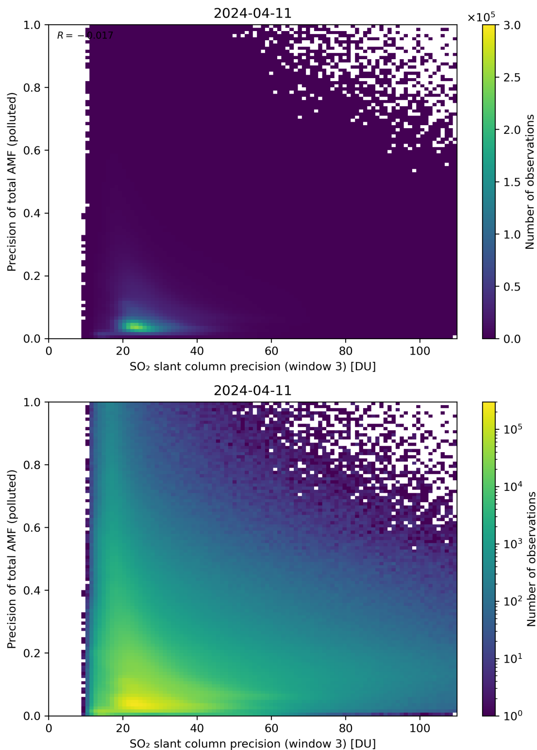
Figure 264: Scatter density plot of “SO 2 slant column precision (window 3)” against “Precision of total AMF (polluted)” for 2024-04-10 to 2024-04-12.
