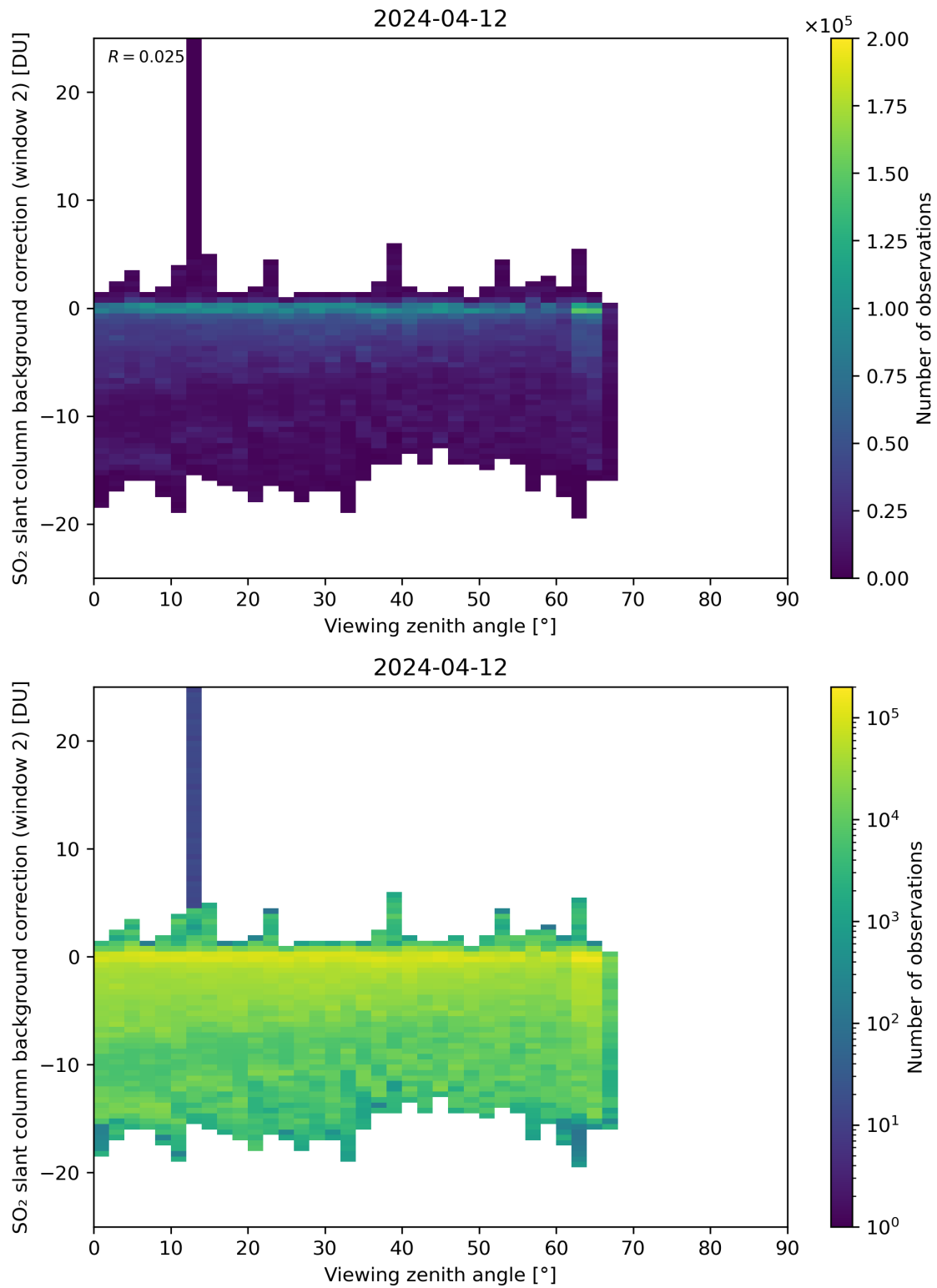
Figure 309: Scatter density plot of “Viewing zenith angle” against “SO 2 slant column background correction (window 2)” for 2024-04-11 to 2024-04-13.
