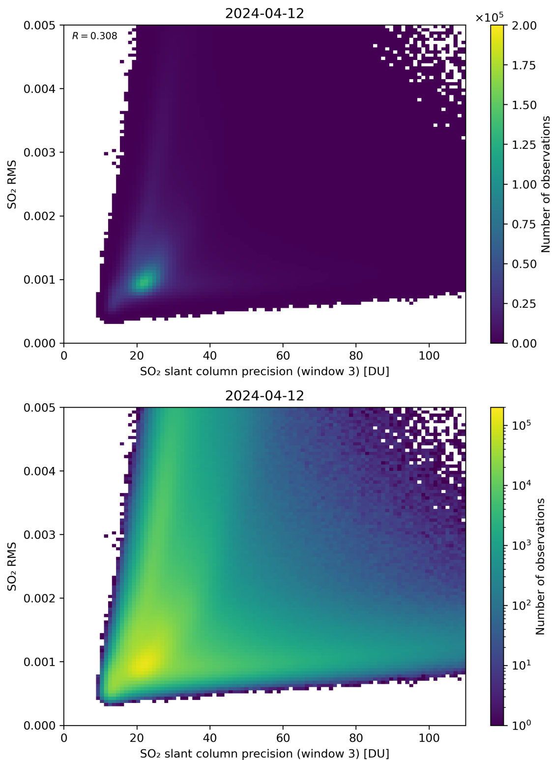
Figure 260: Scatter density plot of “SO 2 slant column precision (window 3)” against “SO 2 RMS” for 2024-04-11 to 2024-04-13.
