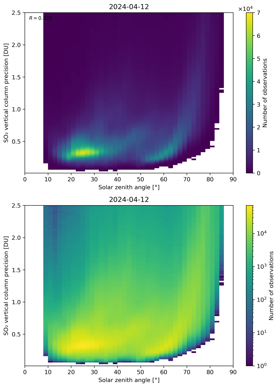
Figure 177: Scatter density plot of “Solar zenith angle” against “SO 2 vertical column precision” for 2024-04-11 to 2024-04-13.
