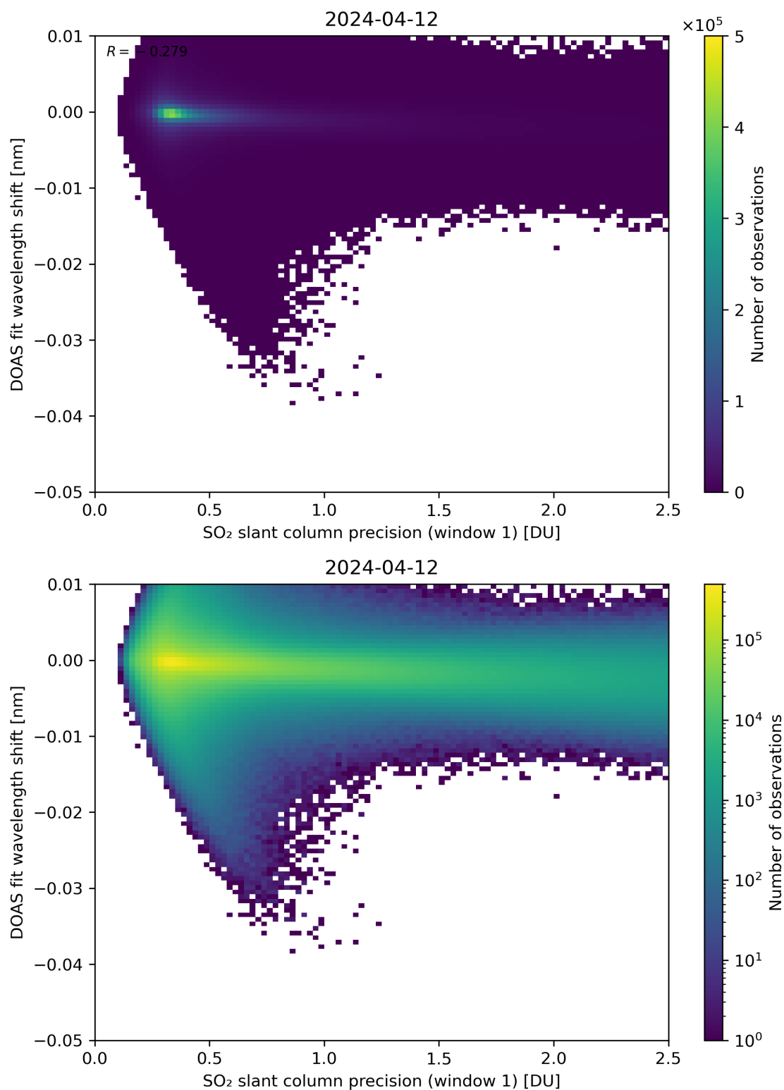
Figure 221: Scatter density plot of “SO 2 slant column precision (window 1)” against “DOAS fit wavelength shift” for 2024-04-11 to 2024-04-13.
