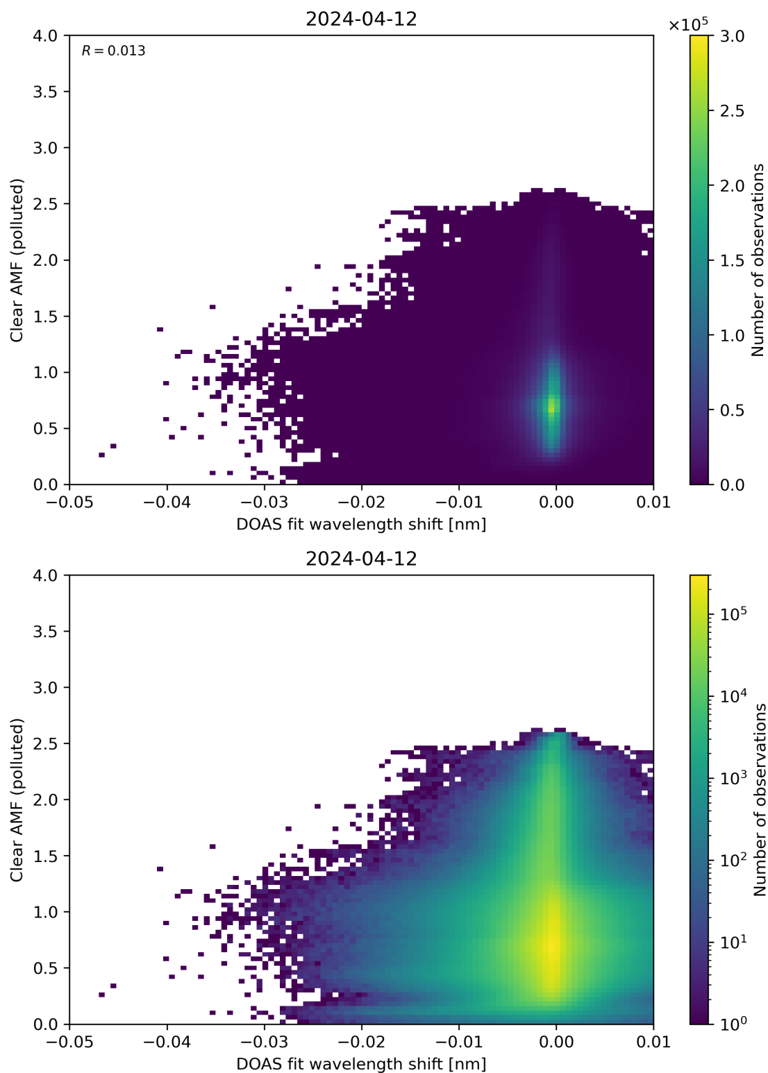
Figure 129: Scatter density plot of “DOAS fit wavelength shift” against “Clear AMF (polluted)” for 2024-04-11 to 2024-04-13.
