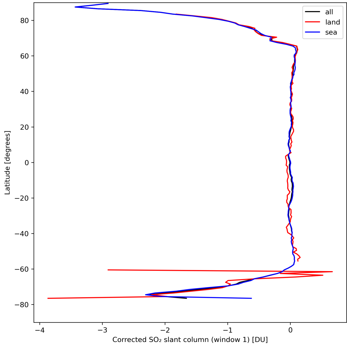
Figure 35: Zonal average of “Corrected SO 2 slant column (window 1)” for 2024-04-11 to 2024-04-13.
