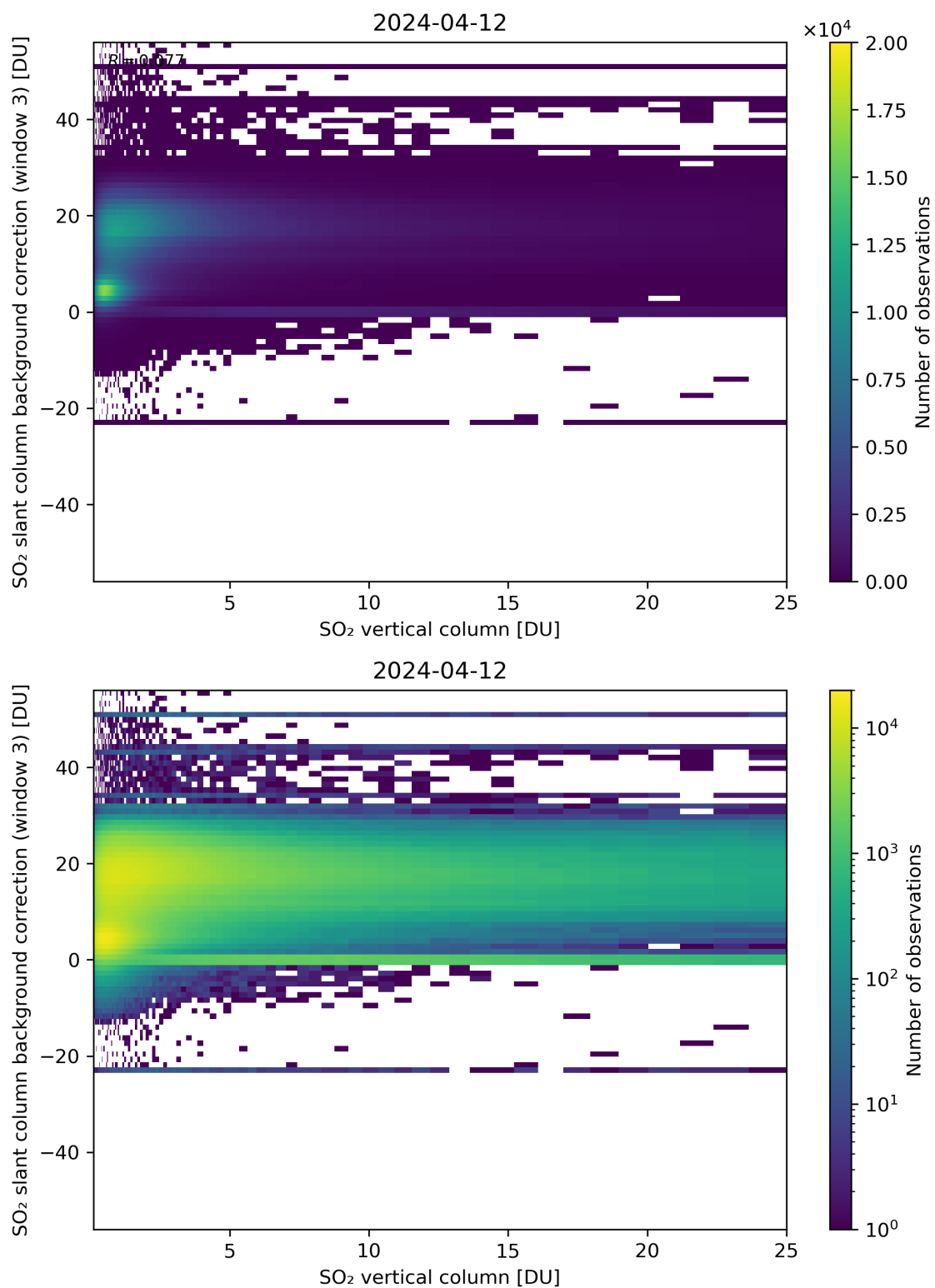
Figure 275: Scatter density plot of “SO 2 vertical column” against “SO 2 slant column background correction (window 3)” for 2024-04-11 to 2024-04-13.
