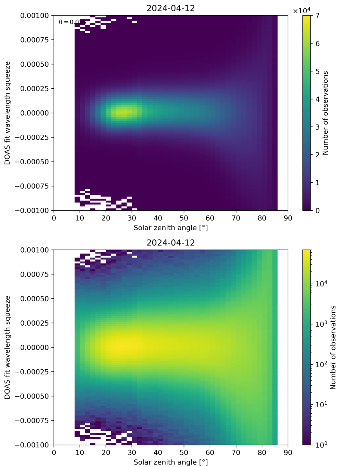
Figure 162: Scatter density plot of “Solar zenith angle” against “DOAS fit wavelength squeeze” for 2024-04-11 to 2024-04-13.
