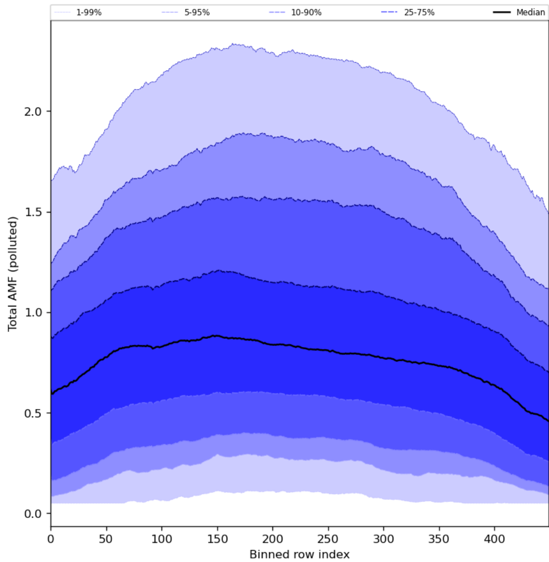
Figure 94: Along track statistics of “Total AMF (polluted)” for 2024-04-11 to 2024-04-13
