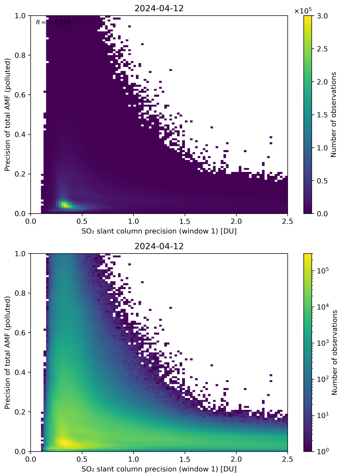
Figure 231: Scatter density plot of “SO 2 slant column precision (window 1)” against “Precision of total AMF (polluted)” for 2024-04-11 to 2024-04-13.
