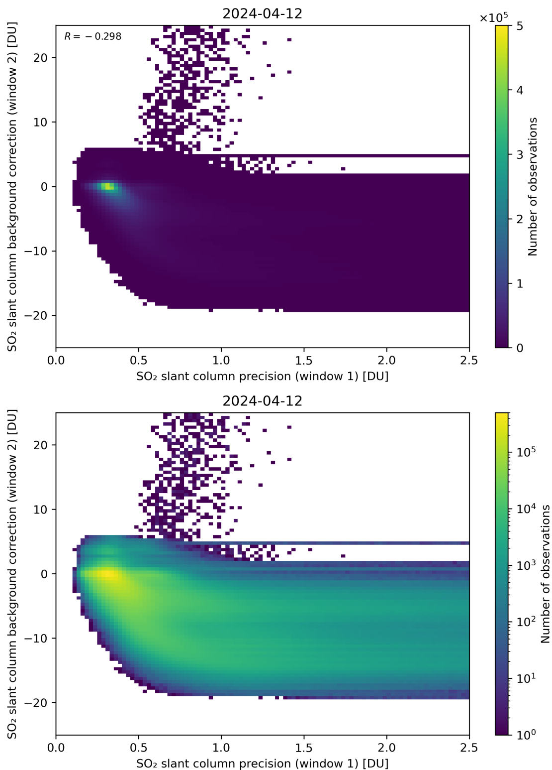
Figure 219: Scatter density plot of “SO 2 slant column precision (window 1)” against “SO 2 slant column background correction (window 2)” for 2024-04-11 to 2024-04-13.
