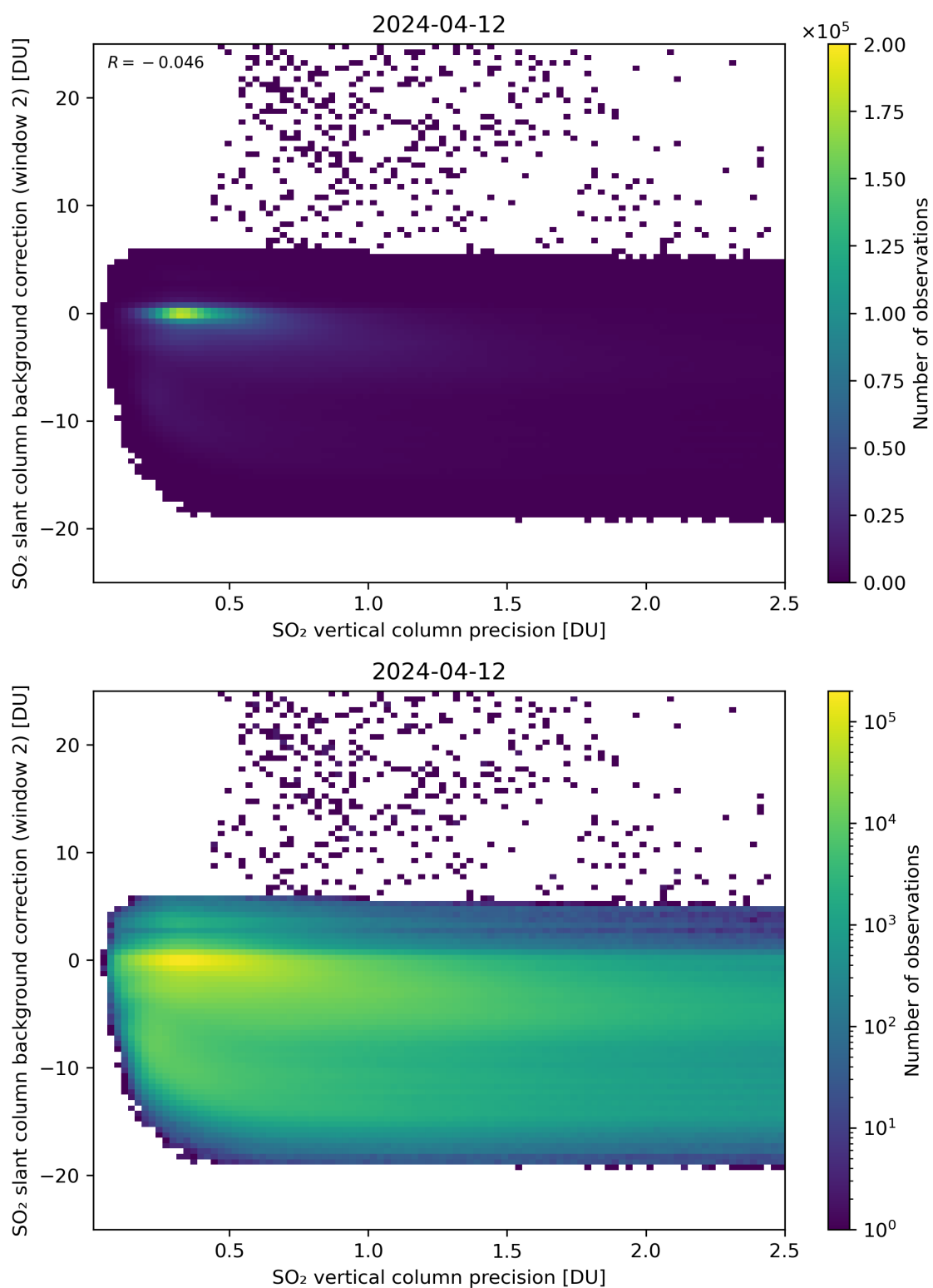
Figure 280: Scatter density plot of “SO 2 vertical column precision” against “SO 2 slant column background correction (window 2)” for 2024-04-11 to 2024-04-13.
