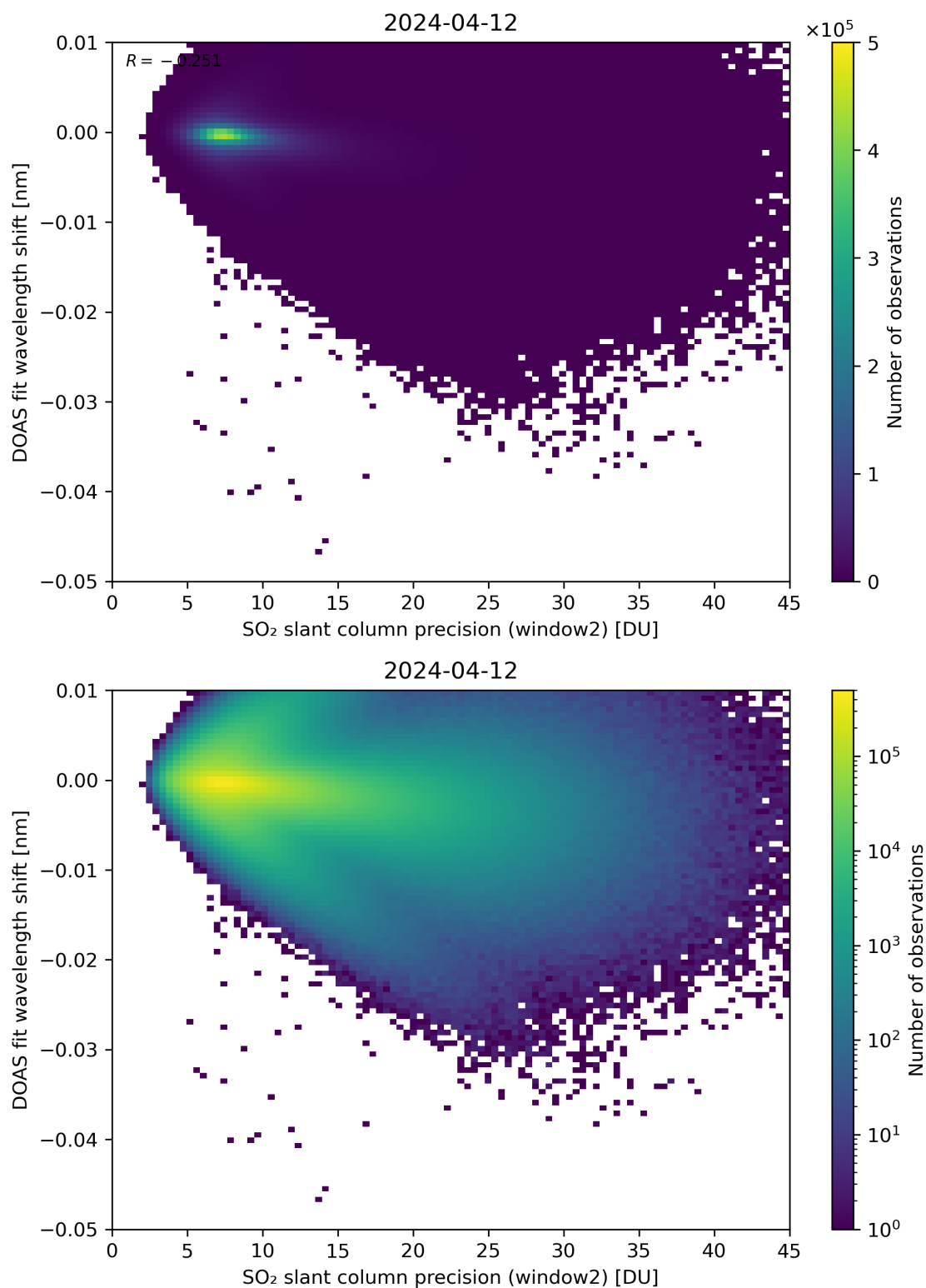
Figure 243: Scatter density plot of “SO 2 slant column precision (window2)” against “DOAS fit wavelength shift” for 2024-04-11 to 2024-04-13.
