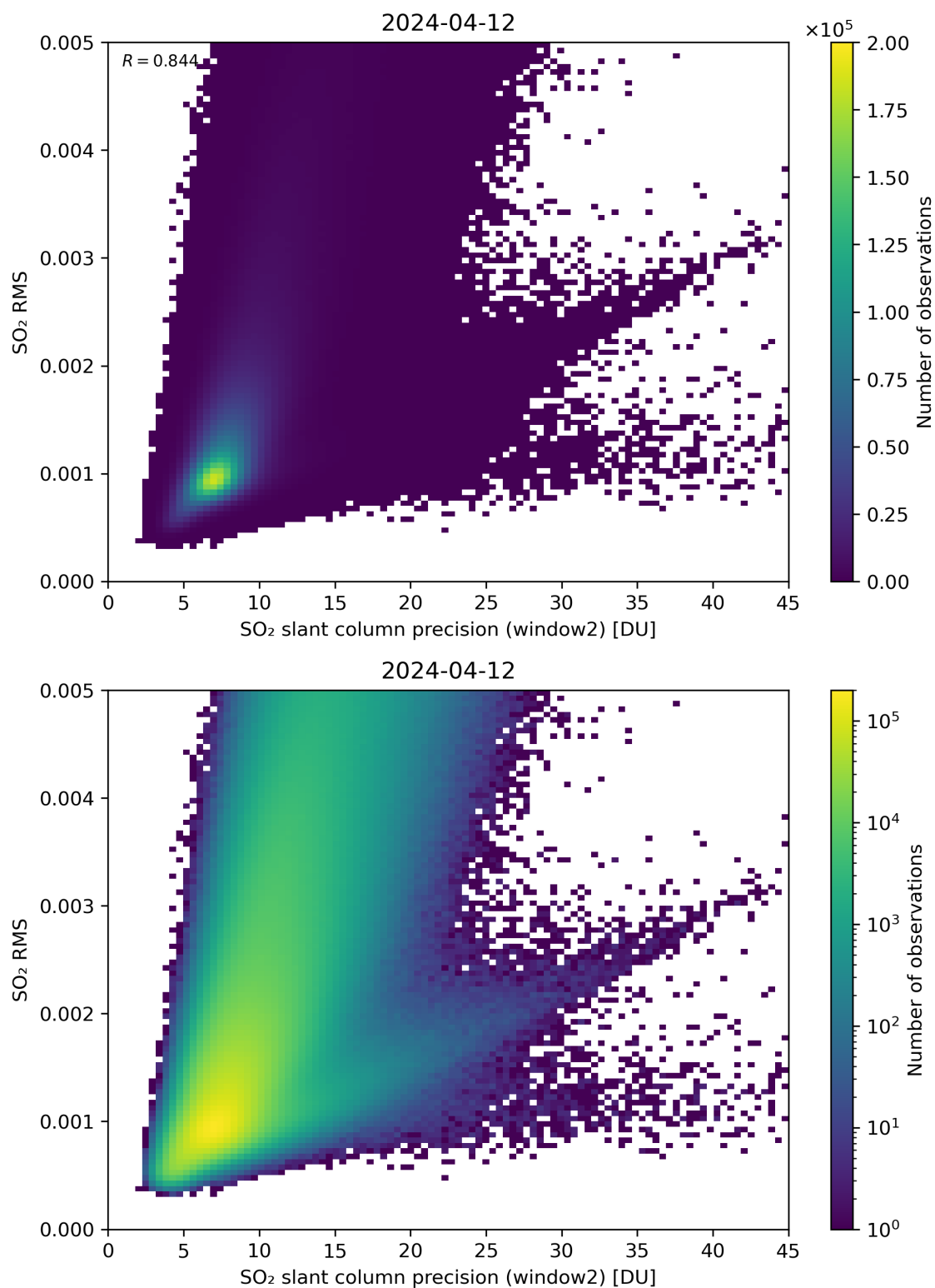
Figure 245: Scatter density plot of “SO 2 slant column precision (window2)” against “SO 2 RMS” for 2024-04-11 to 2024-04-13.
