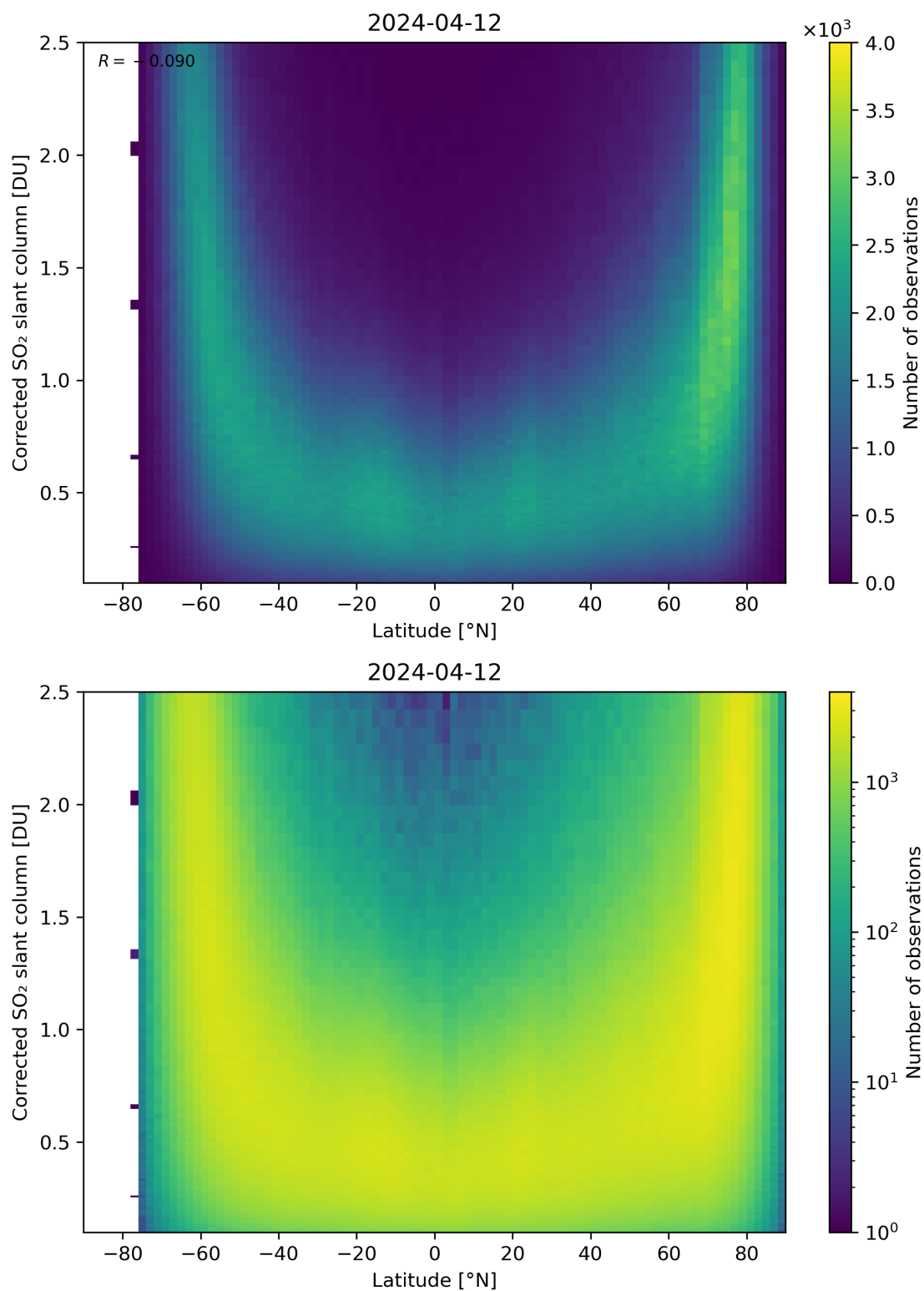
Figure 146: Scatter density plot of “Latitude” against “Corrected SO 2 slant column” for 2024-04-11 to 2024-04-13.
