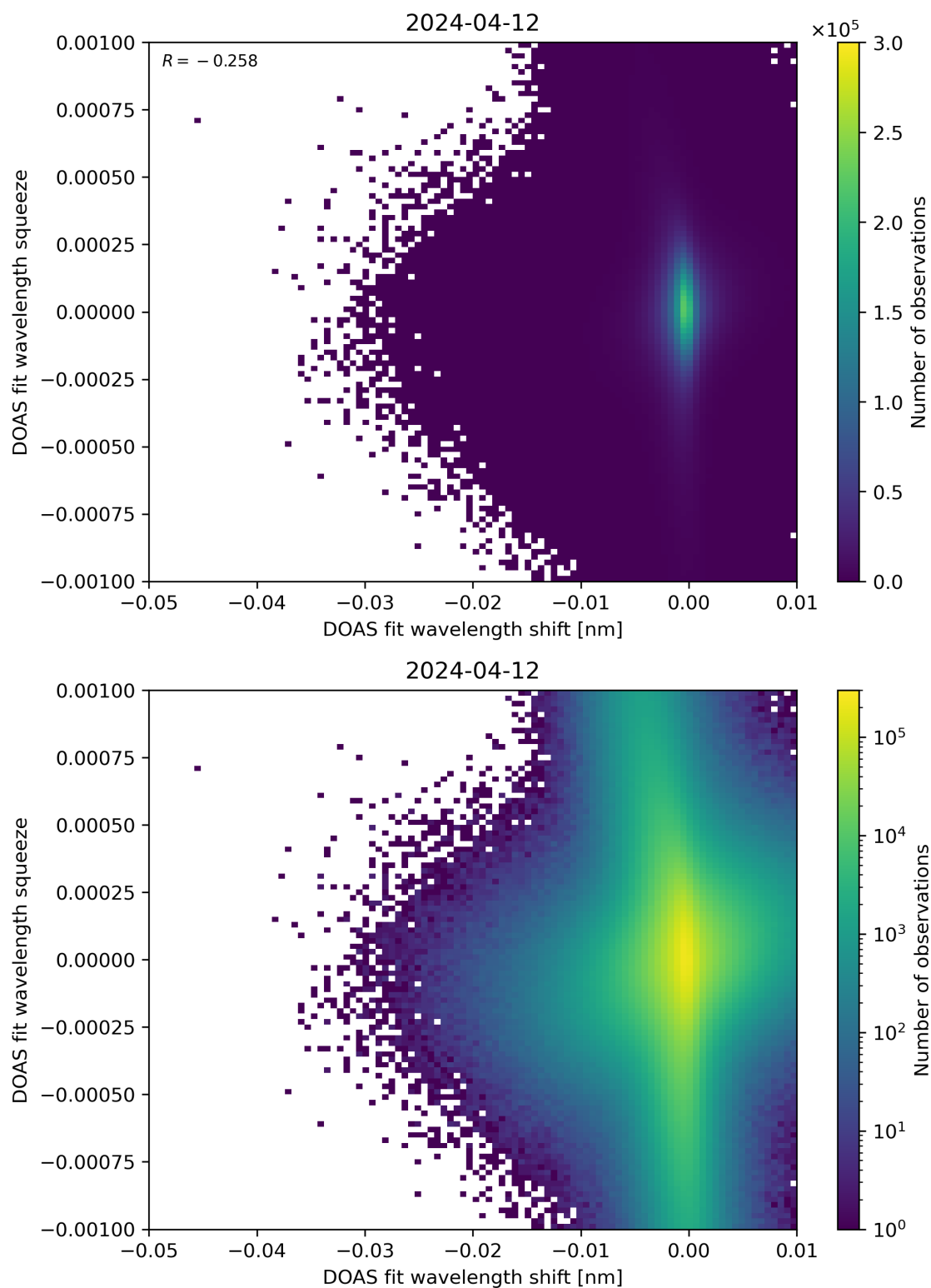
Figure 127: Scatter density plot of “DOAS fit wavelength shift” against “DOAS fit wavelength squeeze” for 2024-04-11 to 2024-04-13.
