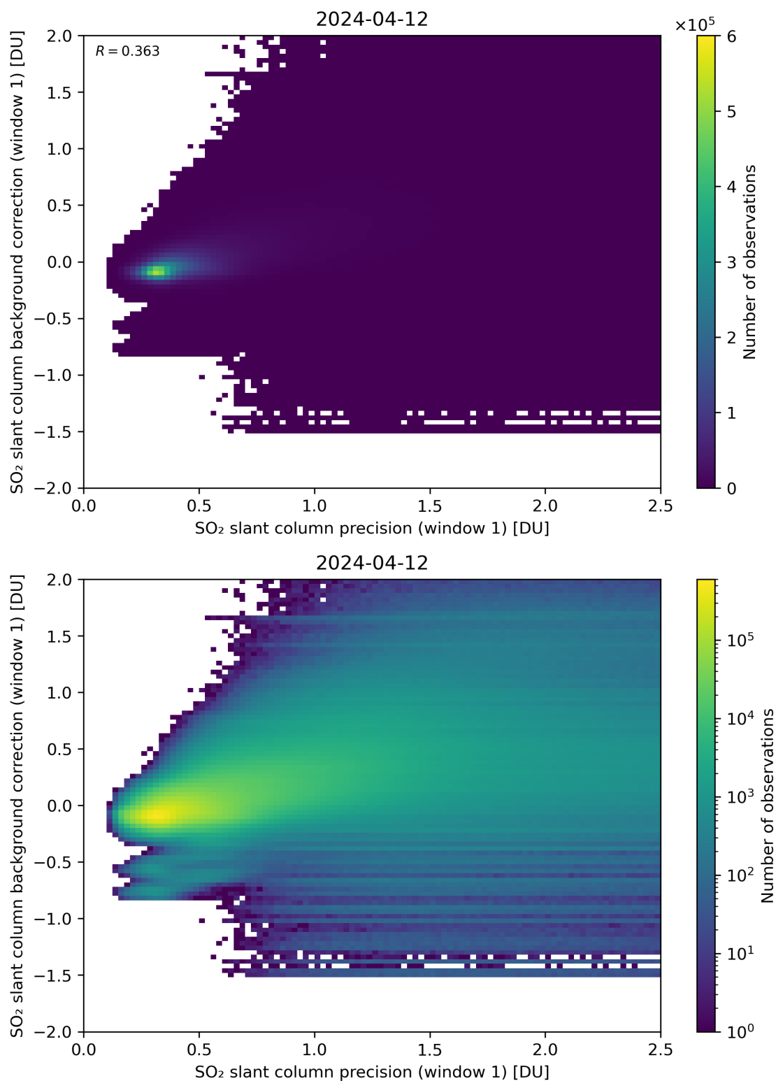
Figure 218: Scatter density plot of “SO 2 slant column precision (window 1)” against “SO 2 slant column background correction (window 1)” for 2024-04-11 to 2024-04-13.
