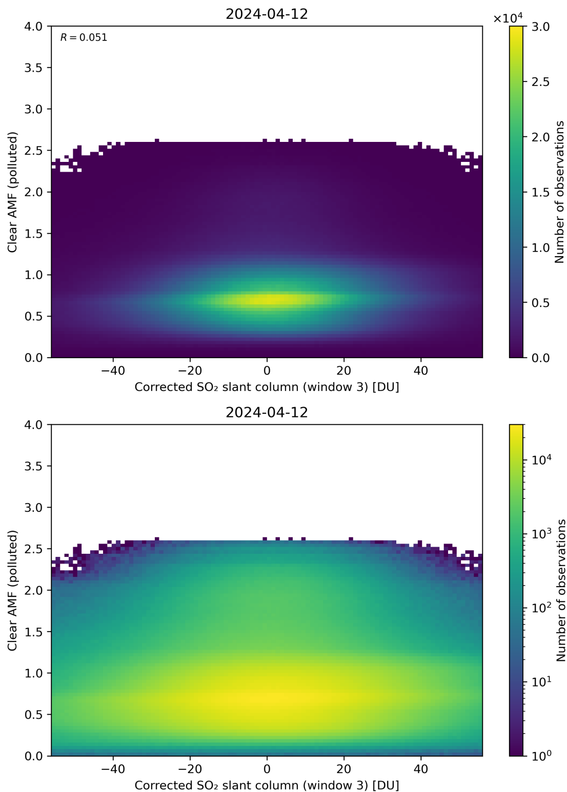
Figure 209: Scatter density plot of “Corrected SO 2 slant column (window 3)” against “Clear AMF (polluted)” for 2024-04-11 to 2024-04-13.
