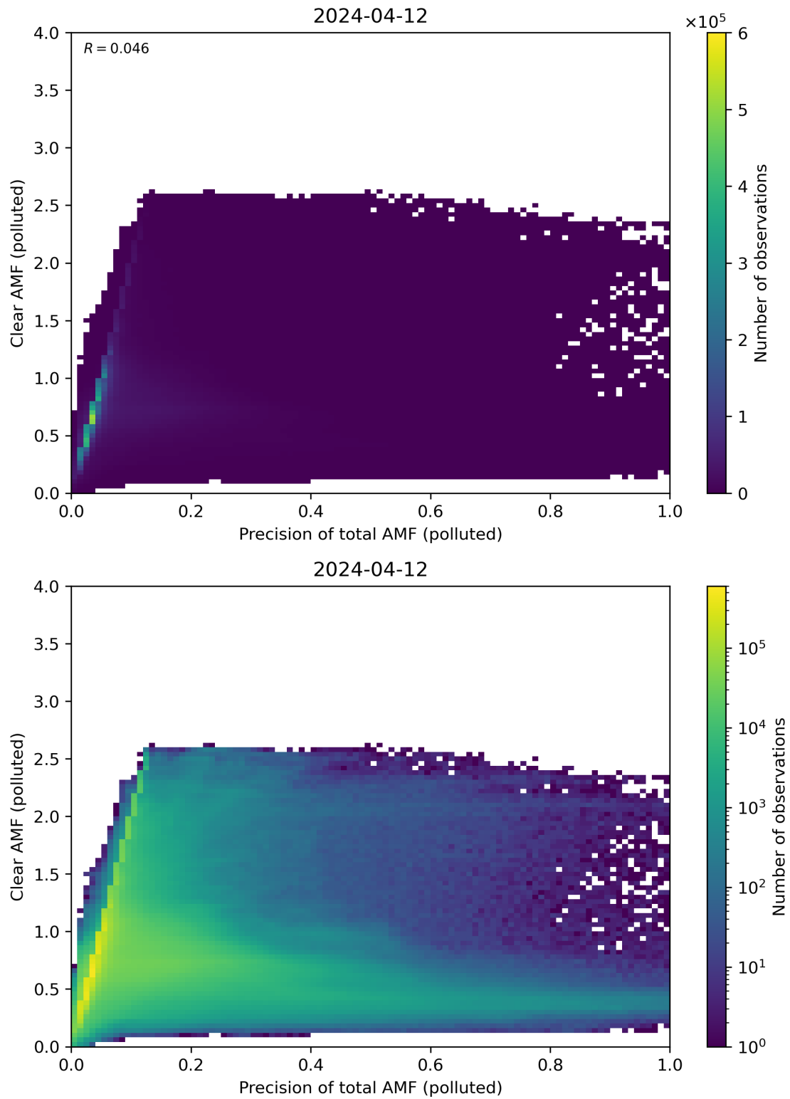
Figure 270: Scatter density plot of “Precision of total AMF (polluted)” against “Clear AMF (polluted)” for 2024-04-11 to 2024-04-13.
