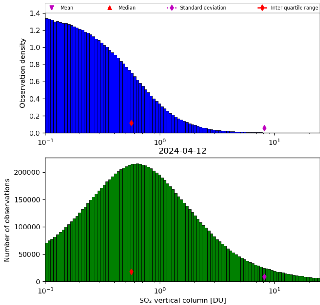
Figure 53: Histogram of “SO 2 vertical column” for 2024-04-11 to 2024-04-13
