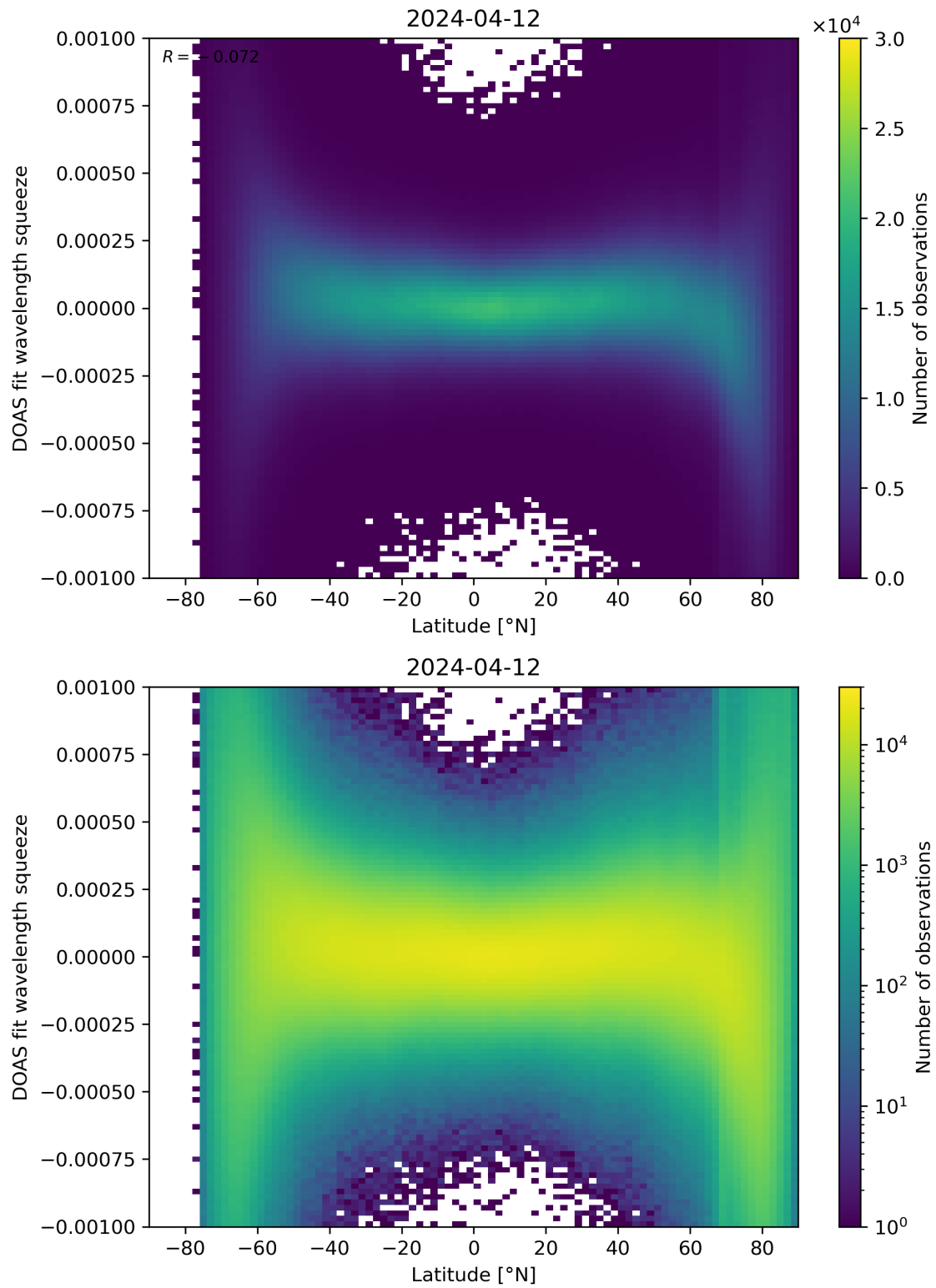
Figure 143: Scatter density plot of “Latitude” against “DOAS fit wavelength squeeze” for 2024-04-11 to 2024-04-13.
