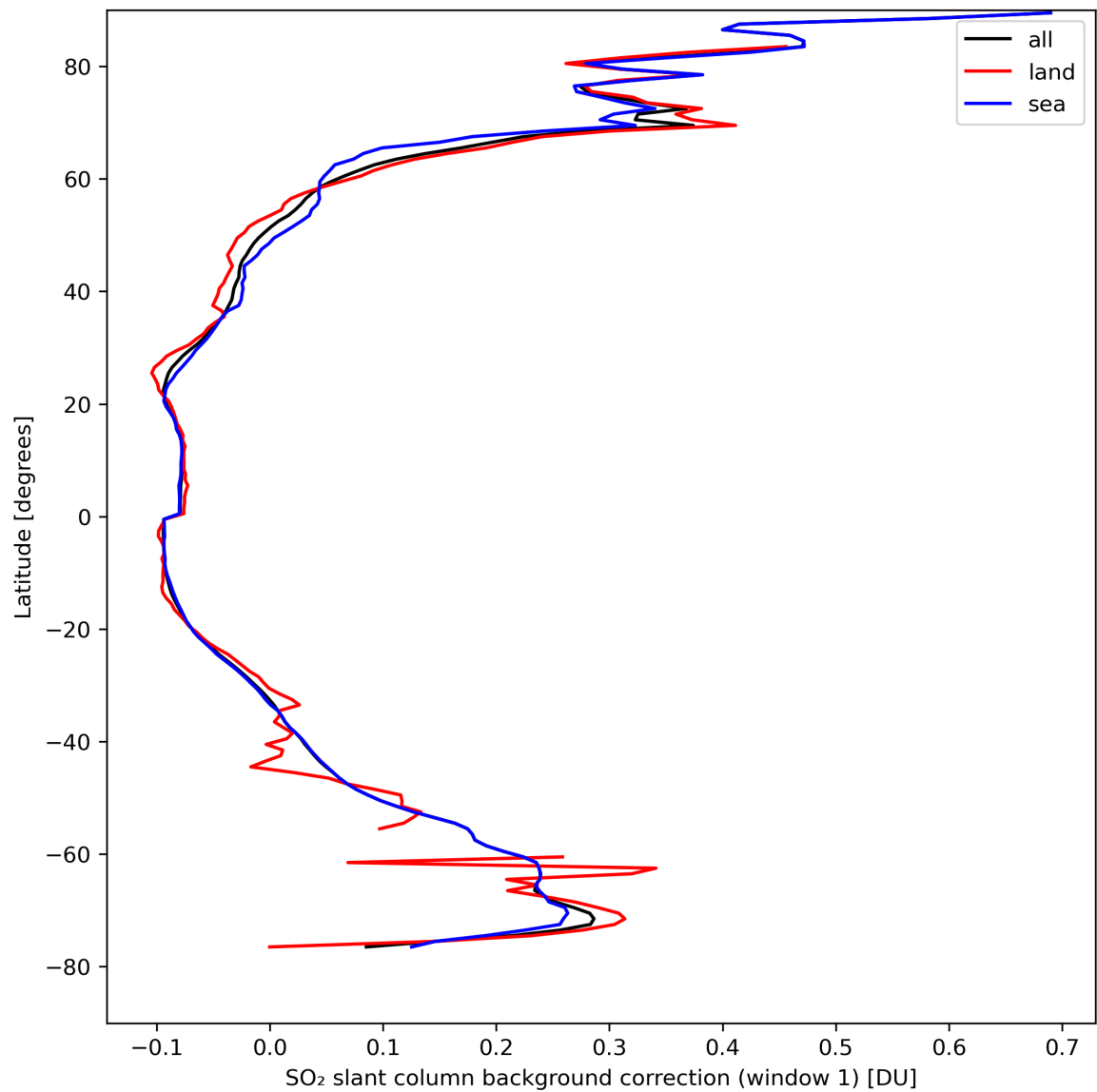
Figure 36: Zonal average of “SO 2 slant column background correction (window 1)” for 2024-04-11 to 2024-04-13.
