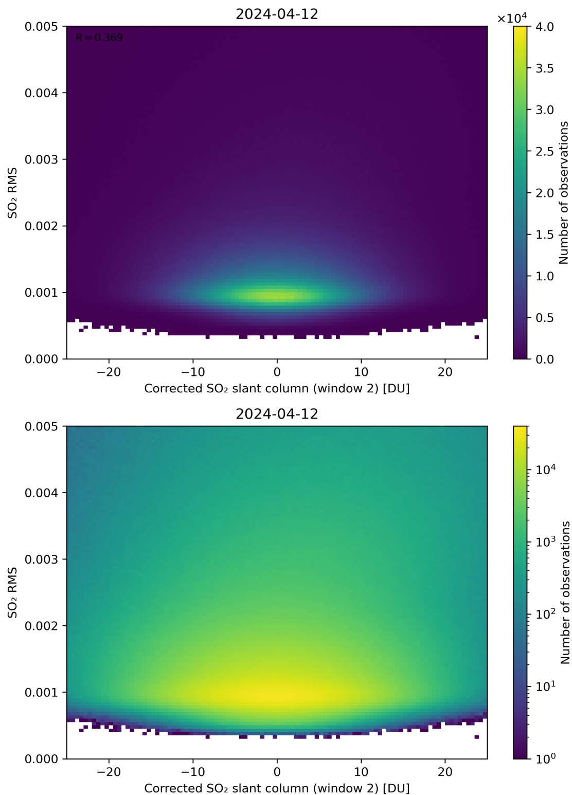
Figure 198: Scatter density plot of “Corrected SO 2 slant column (window 2)” against “SO 2 RMS” for 2024-04-11 to 2024-04-13.
