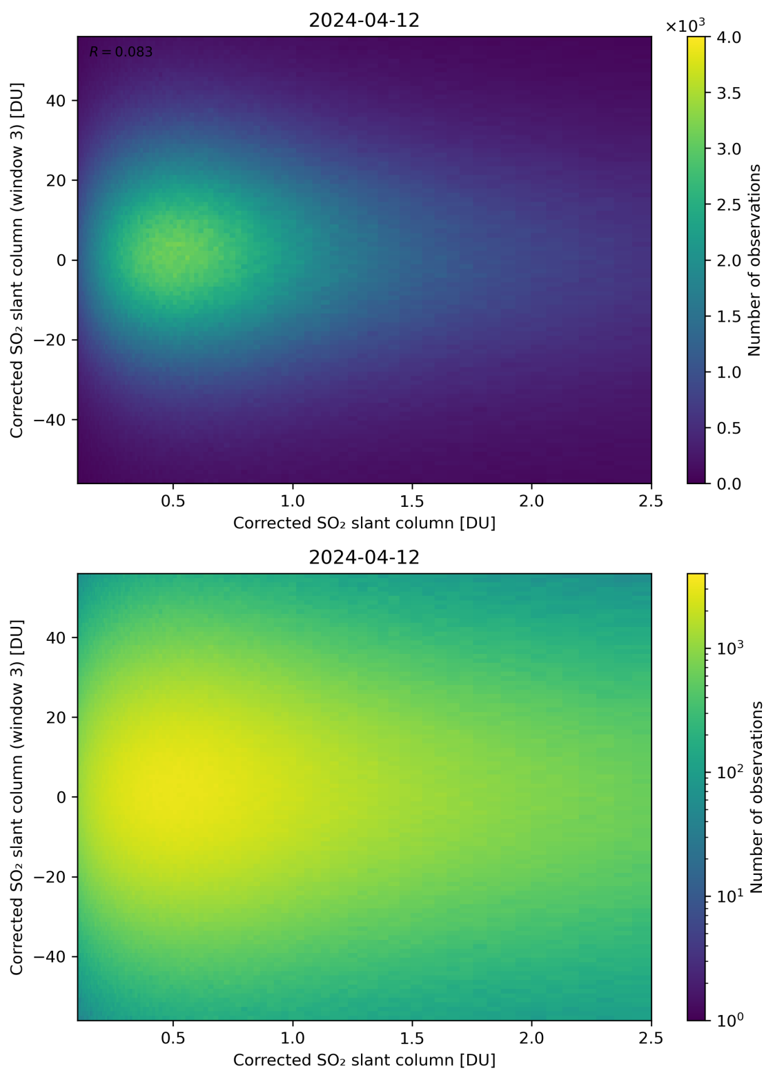
Figure 186: Scatter density plot of “Corrected SO 2 slant column” against “Corrected SO 2 slant column (window 3)” for 2024-04-11 to 2024-04-13.
