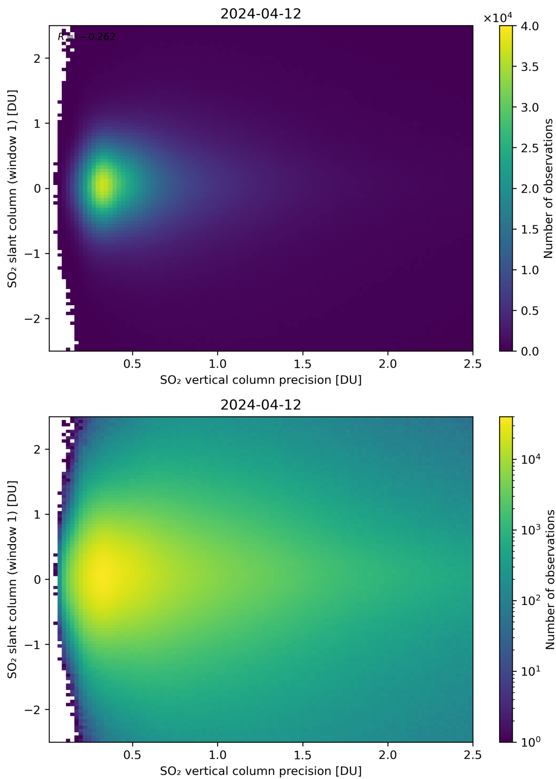
Figure 289: Scatter density plot of “SO 2 vertical column precision” against “SO 2 slant column (window 1)” for 2024-04-11 to 2024-04-13.
