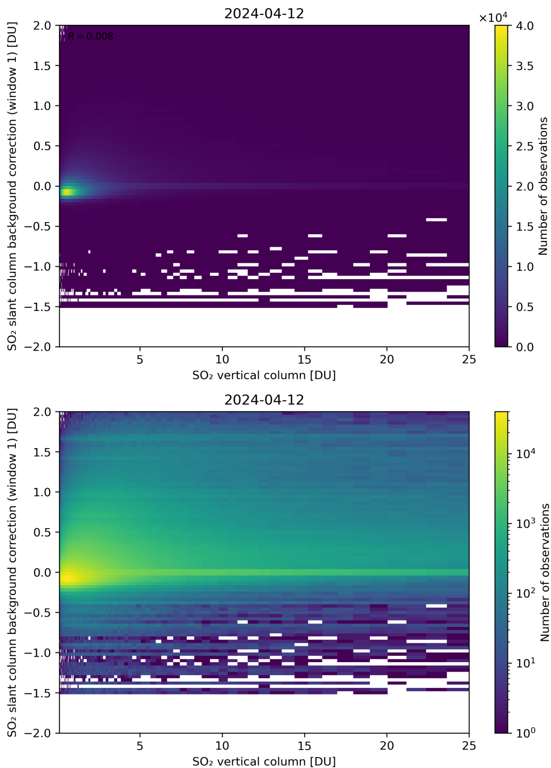
Figure 273: Scatter density plot of “SO 2 vertical column” against “SO 2 slant column background correction (window 1)” for 2024-04-11 to 2024-04-13.
