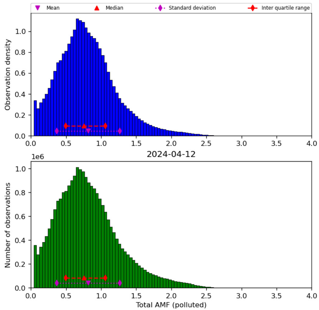
Figure 71: Histogram of “Total AMF (polluted)” for 2024-04-11 to 2024-04-13
