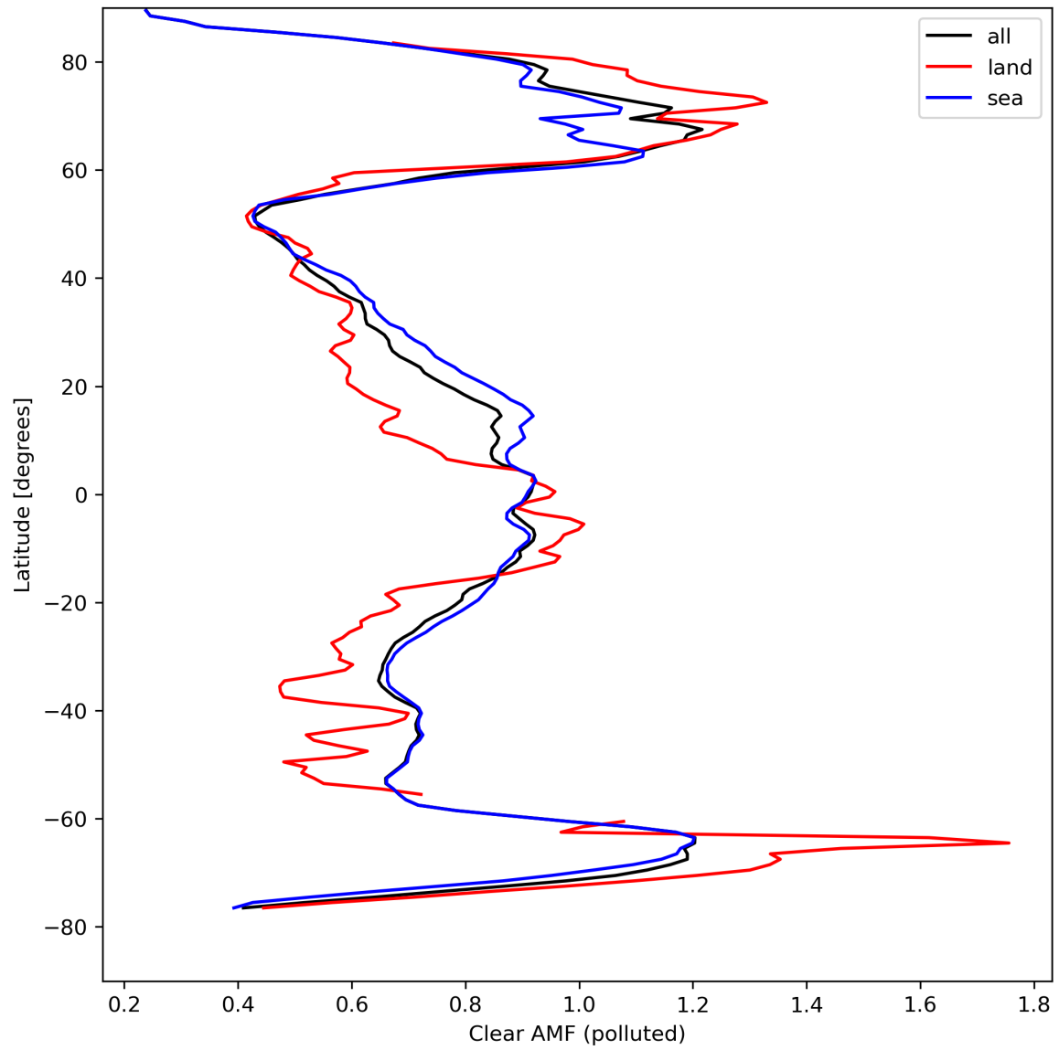
Figure 50: Zonal average of “Clear AMF (polluted)” for 2024-04-11 to 2024-04-13.
