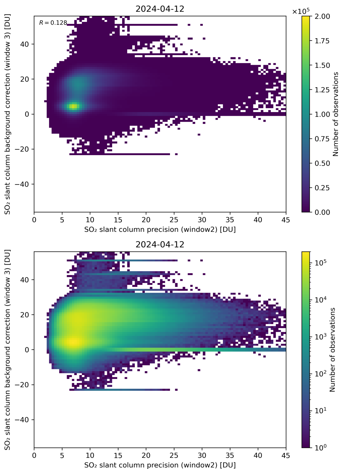
Figure 242: Scatter density plot of “SO 2 slant column precision (window2)” against “SO 2 slant column background correction (window 3)” for 2024-04-11 to 2024-04-13.
