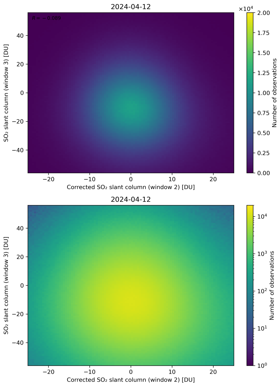
Figure 201: Scatter density plot of “Corrected SO 2 slant column (window 2)” against “SO 2 slant column (window 3)” for 2024-04-11 to 2024-04-13.
