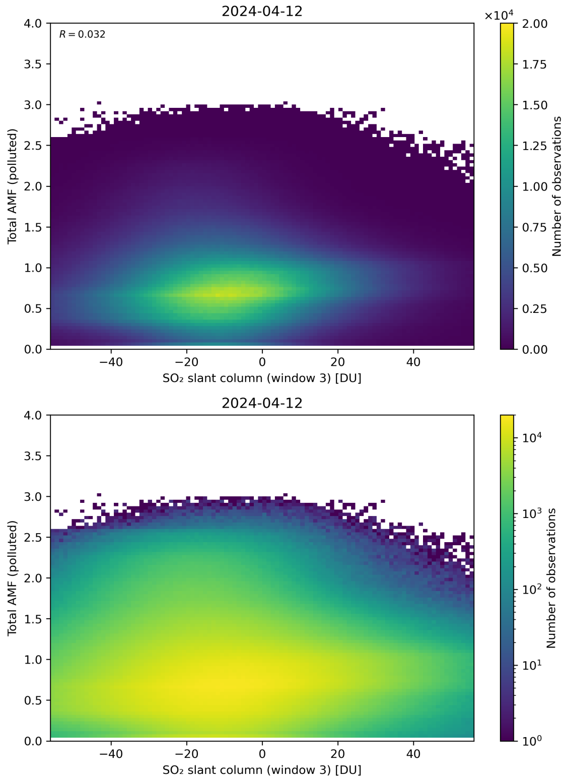
Figure 268: Scatter density plot of “SO 2 slant column (window 3)” against “Total AMF (polluted)” for 2024-04-11 to 2024-04-13.
