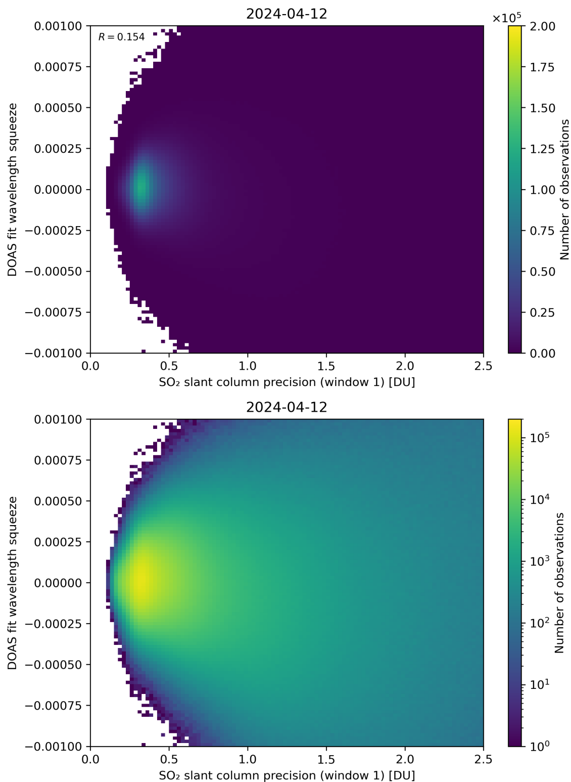
Figure 222: Scatter density plot of “SO 2 slant column precision (window 1)” against “DOAS fit wavelength squeeze” for 2024-04-11 to 2024-04-13.
