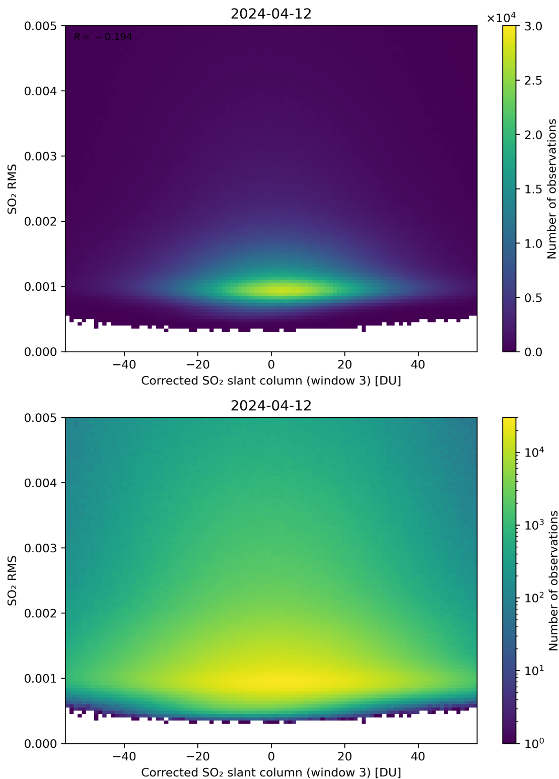
Figure 208: Scatter density plot of “Corrected SO 2 slant column (window 3)” against “SO 2 RMS” for 2024-04-11 to 2024-04-13.
