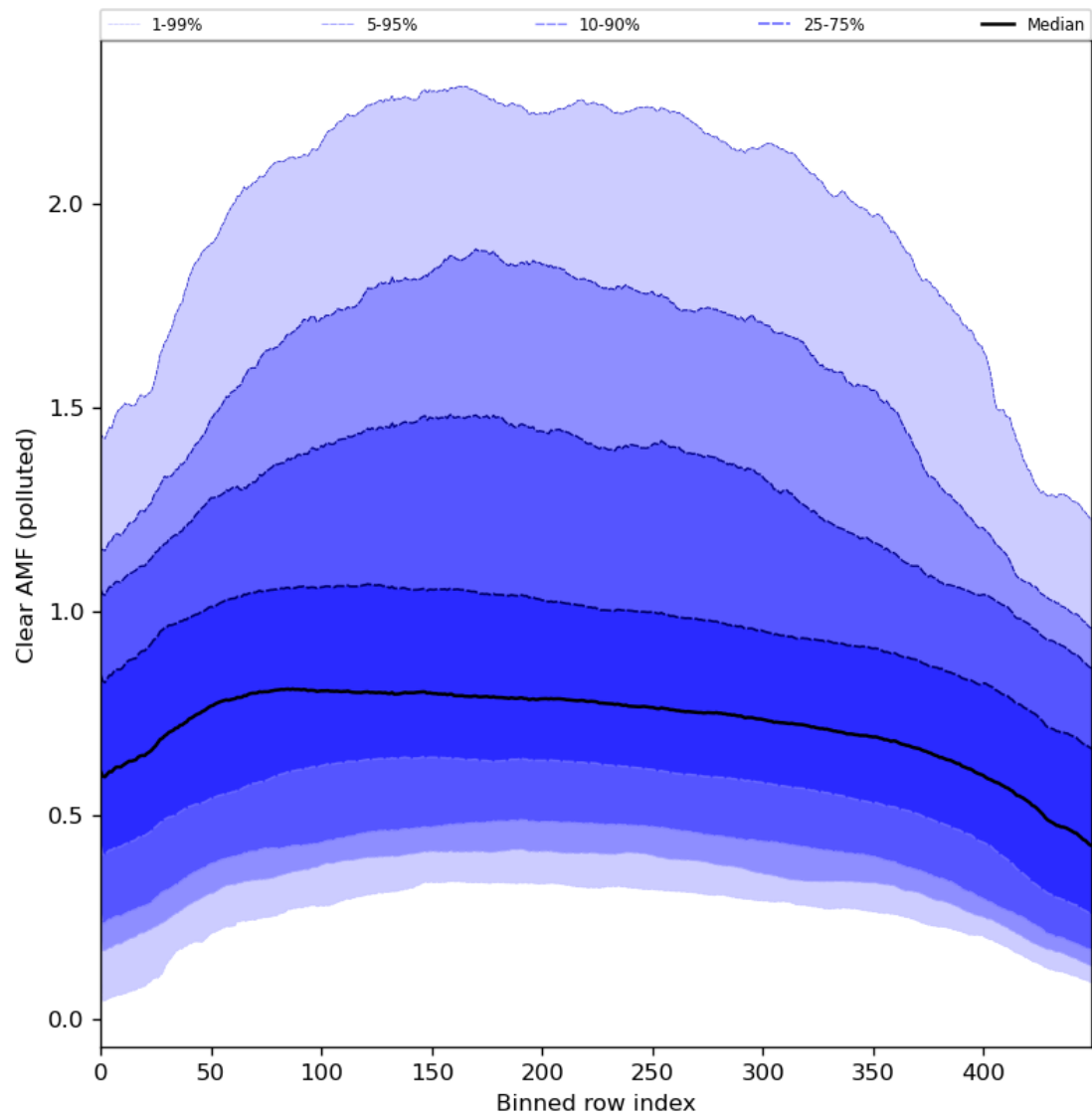
Figure 96: Along track statistics of “Clear AMF (polluted)” for 2024-04-11 to 2024-04-13
