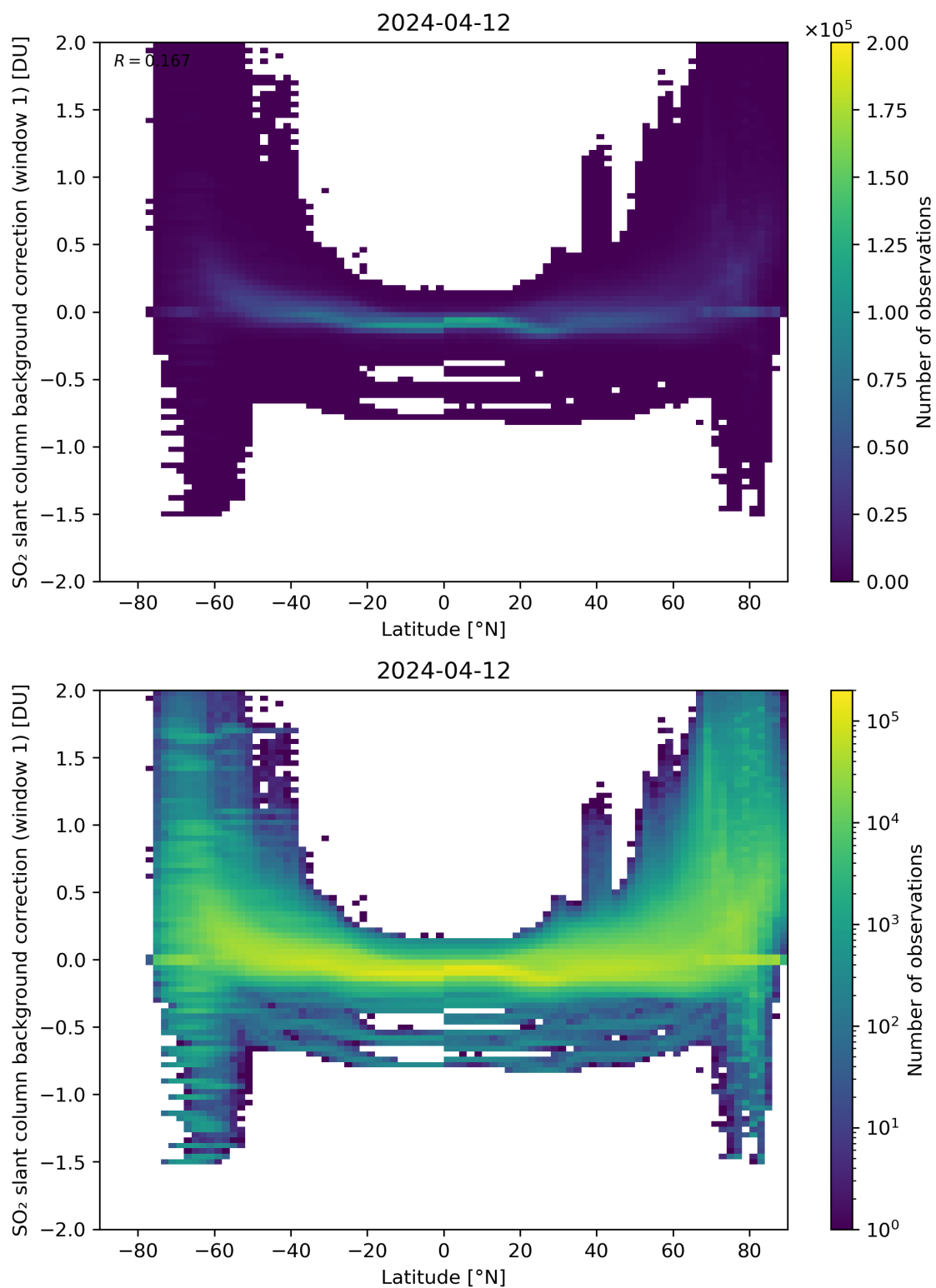
Figure 139: Scatter density plot of “Latitude” against “SO 2 slant column background correction (window 1)” for 2024-04-11 to 2024-04-13.
