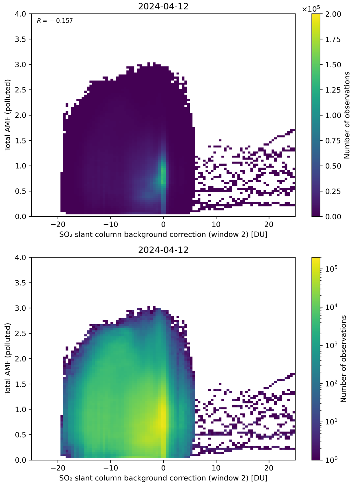
Figure 119: Scatter density plot of “SO 2 slant column background correction (window 2)” against “Total AMF (polluted)” for 2024-04-11 to 2024-04-13.
