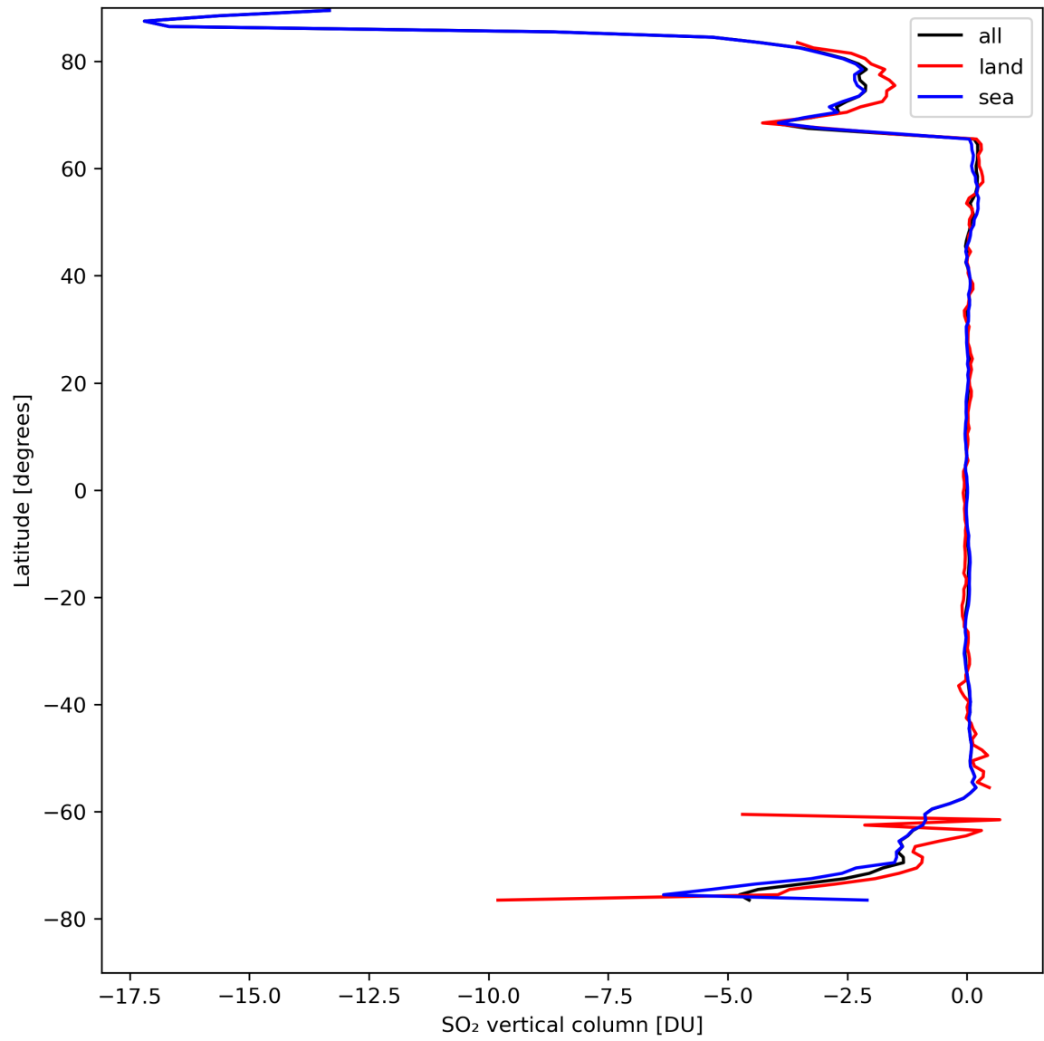
Figure 30: Zonal average of “SO 2 vertical column” for 2024-04-11 to 2024-04-13.
