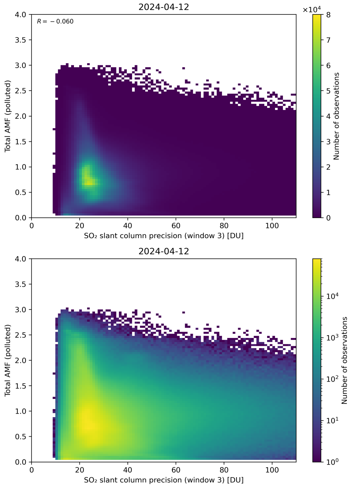
Figure 263: Scatter density plot of “SO 2 slant column precision (window 3)” against “Total AMF (polluted)” for 2024-04-11 to 2024-04-13.
