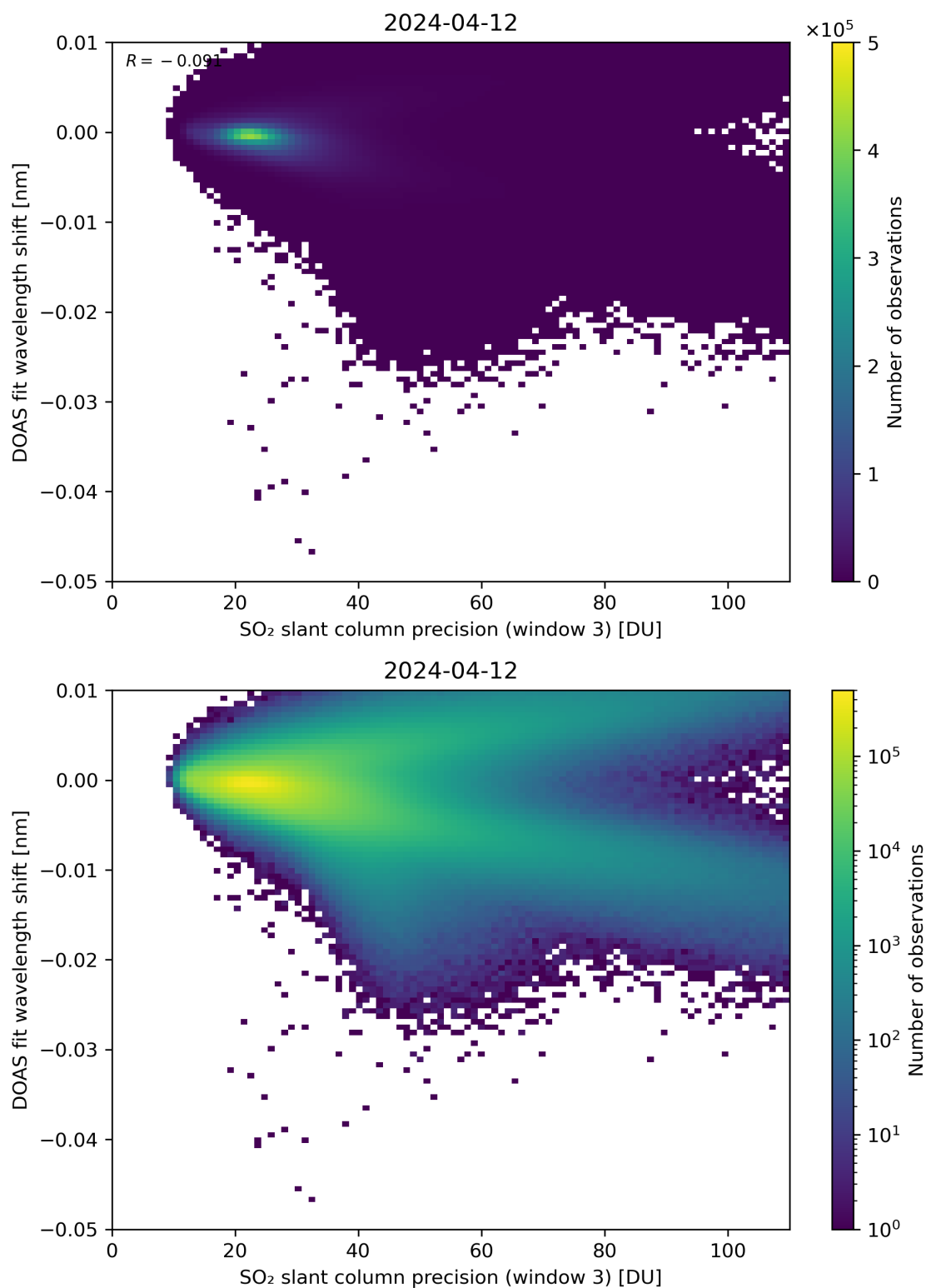
Figure 258: Scatter density plot of “SO 2 slant column precision (window 3)” against “DOAS fit wavelength shift” for 2024-04-11 to 2024-04-13.
