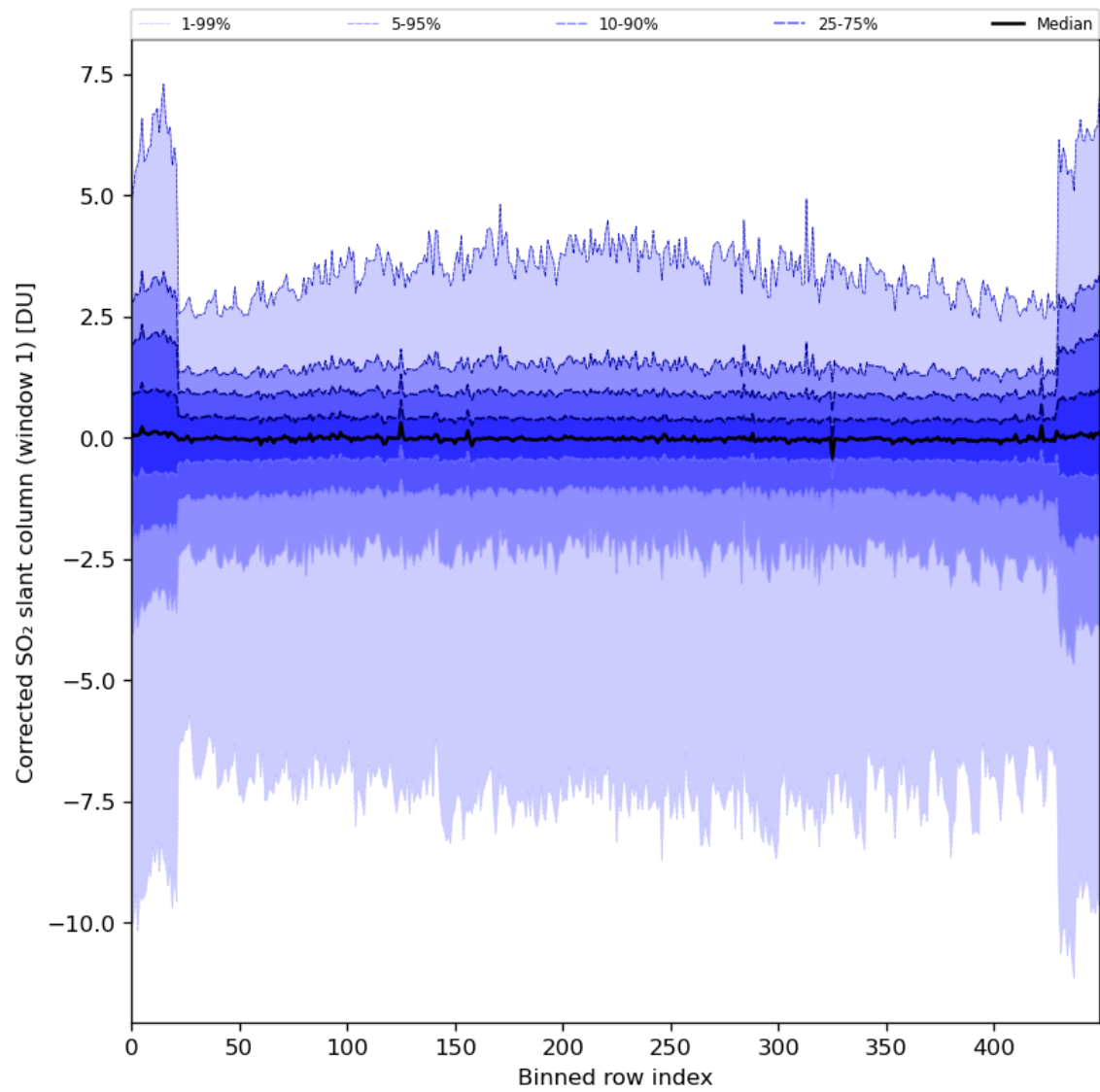
Figure 81: Along track statistics of “Corrected SO 2 slant column (window 1)” for 2024-04-11 to 2024-04-13
