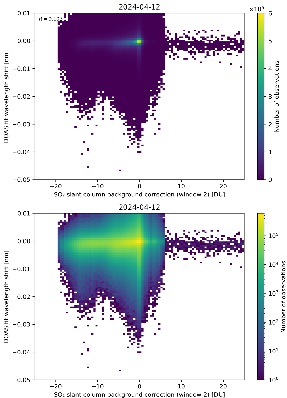
Figure 112: Scatter density plot of “SO 2 slant column background correction (window 2)” against “DOAS fit wavelength shift” for 2024-04-11 to 2024-04-13.
