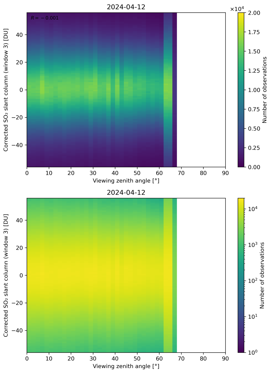
Figure 319: Scatter density plot of “Viewing zenith angle” against “Corrected SO 2 slant column (window 3)” for 2024-04-11 to 2024-04-13.
