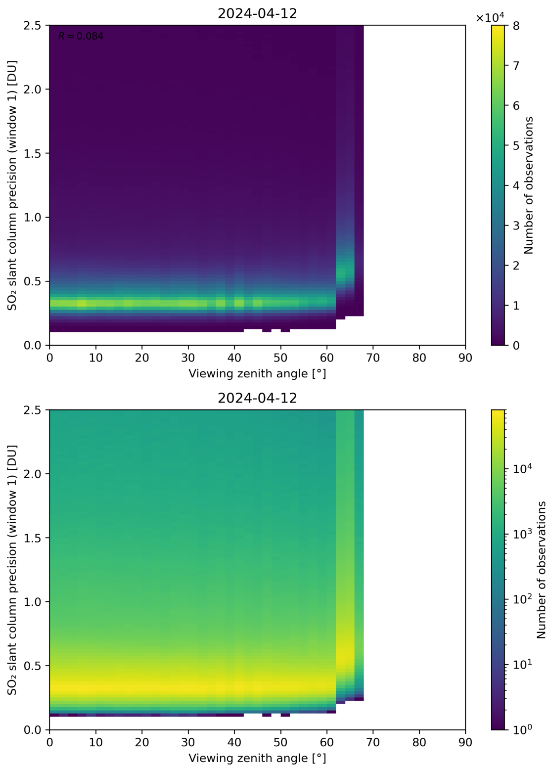
Figure 321: Scatter density plot of “Viewing zenith angle” against “SO 2 slant column precision (window 1)” for 2024-04-11 to 2024-04-13.
