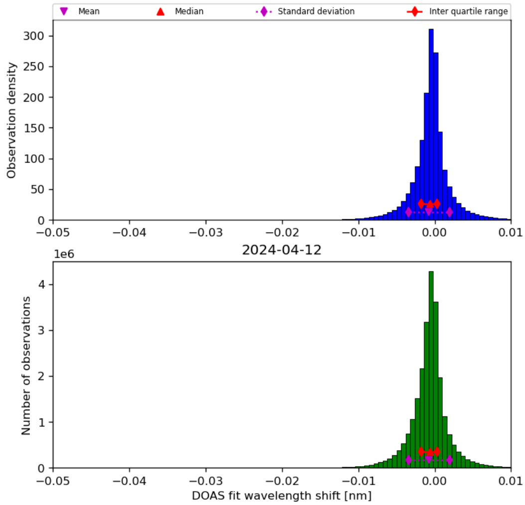
Figure 68: Histogram of “DOAS fit wavelength shift” for 2024-04-11 to 2024-04-13
