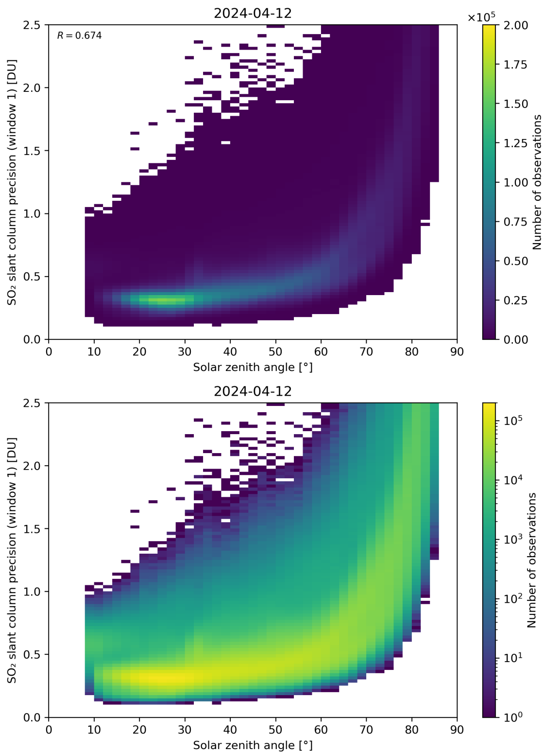
Figure 170: Scatter density plot of “Solar zenith angle” against “SO 2 slant column precision (window 1)” for 2024-04-11 to 2024-04-13.
