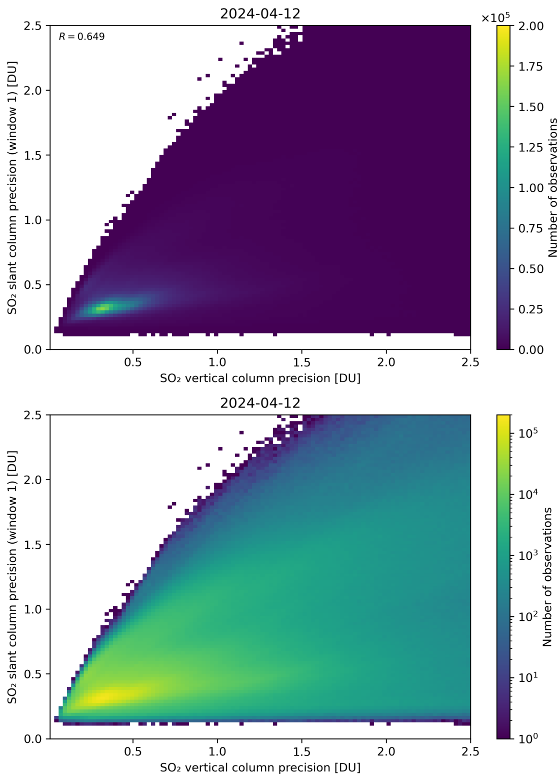
Figure 290: Scatter density plot of “SO 2 vertical column precision” against “SO 2 slant column precision (window 1)” for 2024-04-11 to 2024-04-13.
