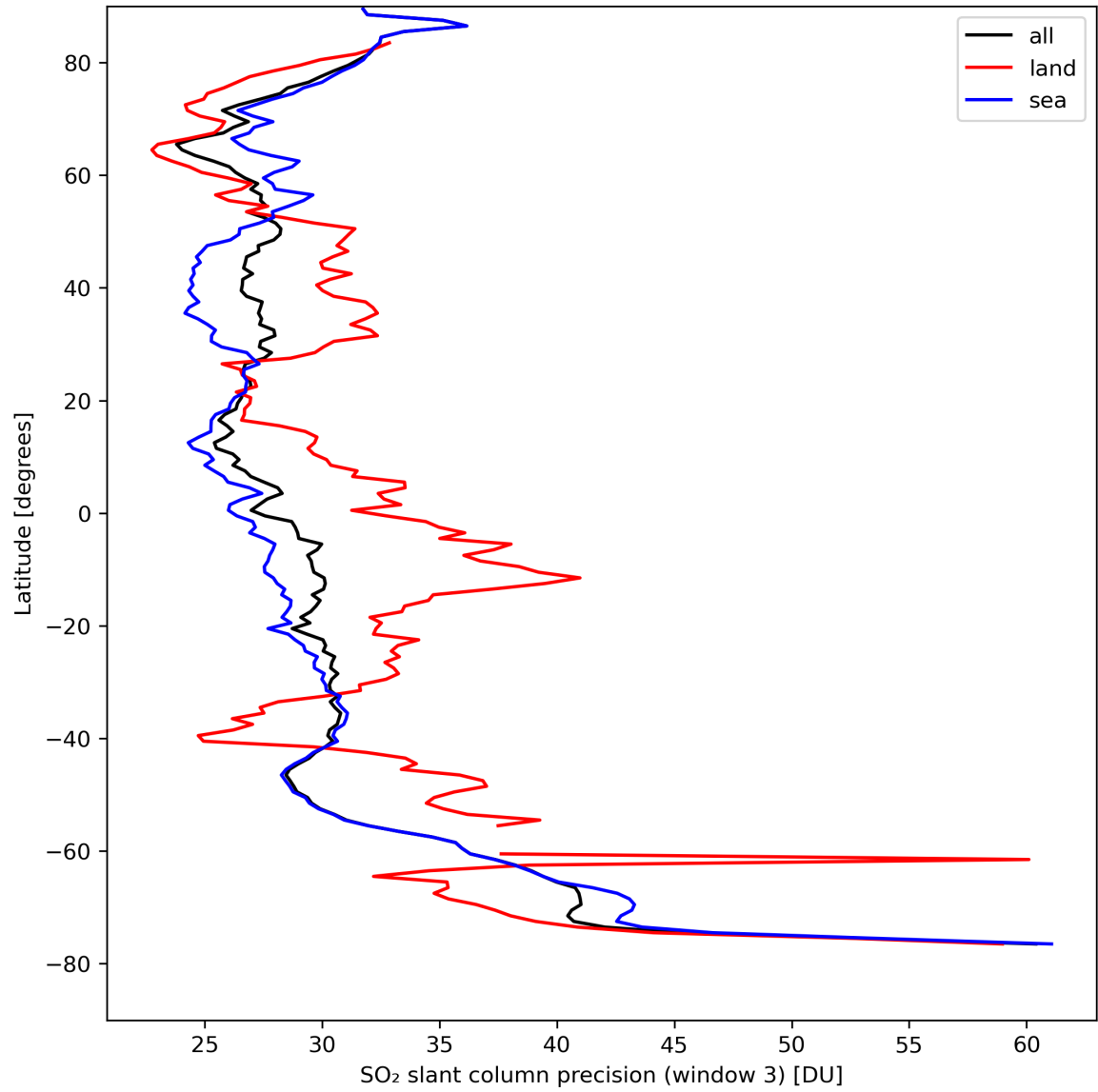
Figure 42: Zonal average of “SO 2 slant column precision (window 3)” for 2024-04-11 to 2024-04-13.
