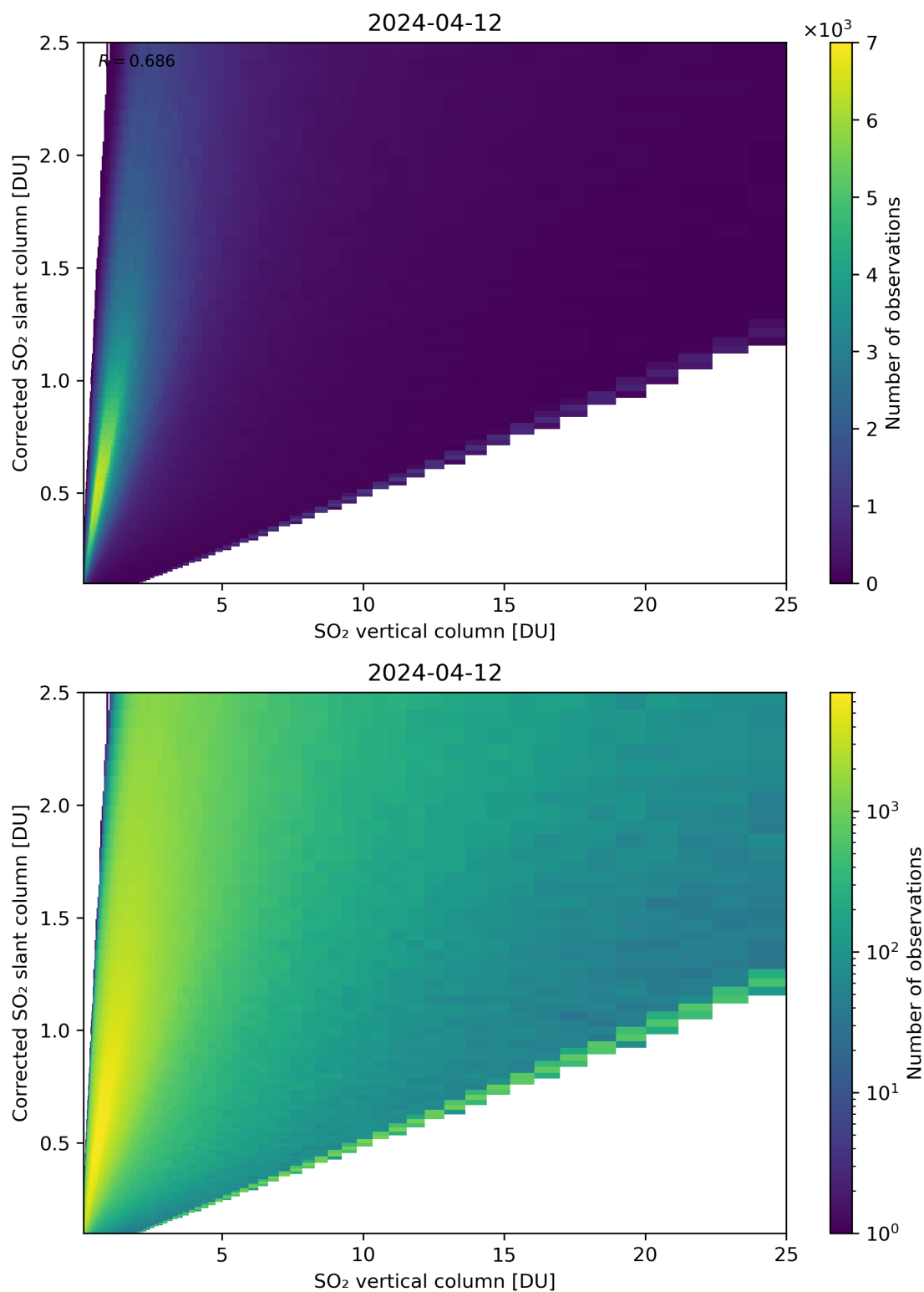
Figure 297: Scatter density plot of “SO 2 vertical column” against “Corrected SO 2 slant column” for 2024-04-11 to 2024-04-13.
