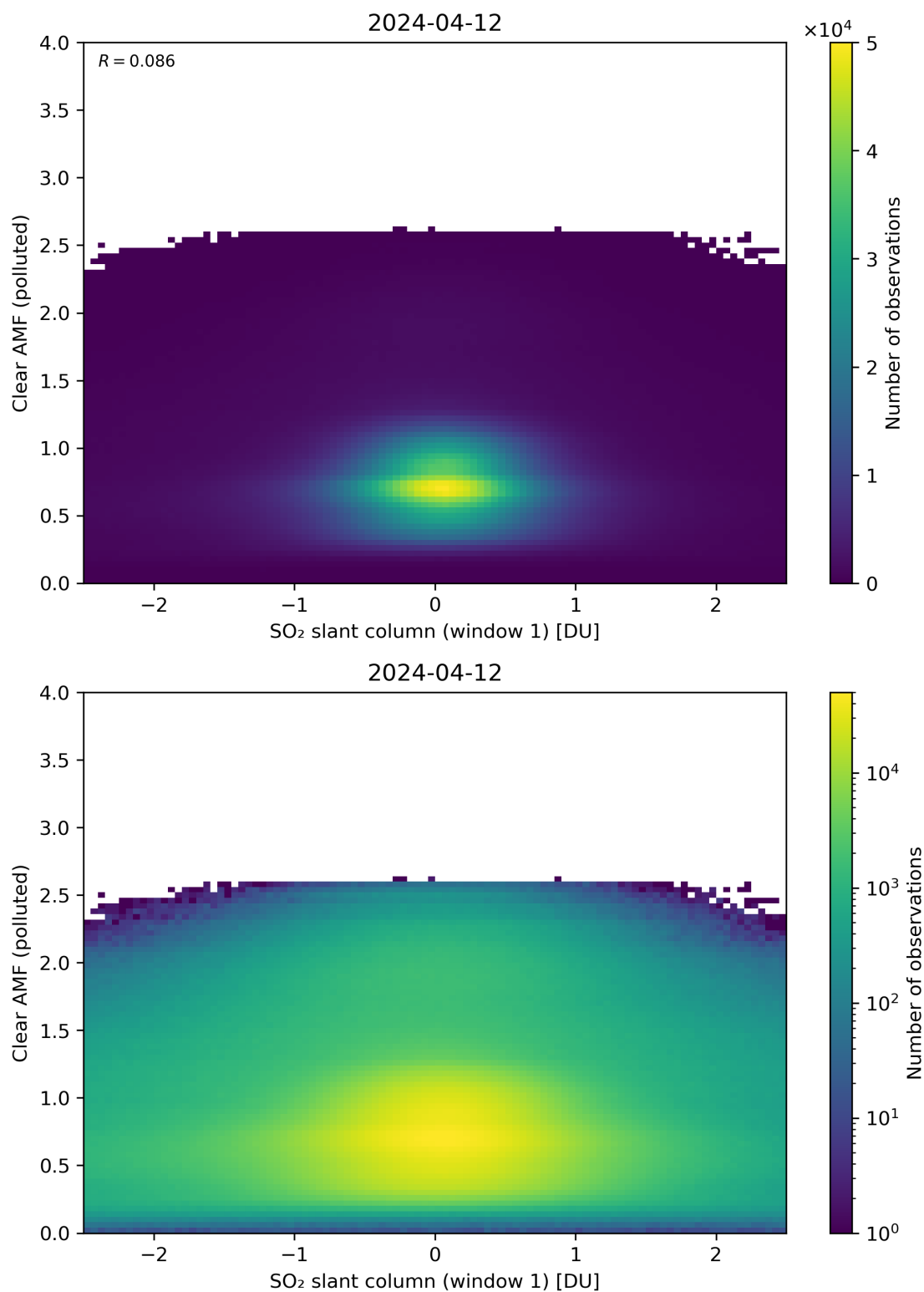
Figure 232: Scatter density plot of “SO 2 slant column (window 1)” against “Clear AMF (polluted)” for 2024-04-11 to 2024-04-13.
