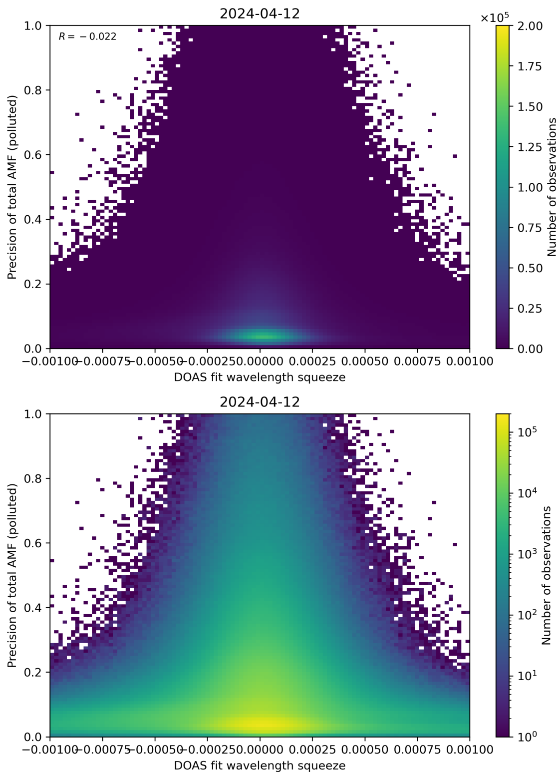
Figure 135: Scatter density plot of “DOAS fit wavelength squeeze” against “Precision of total AMF (polluted)” for 2024-04-11 to 2024-04-13.
