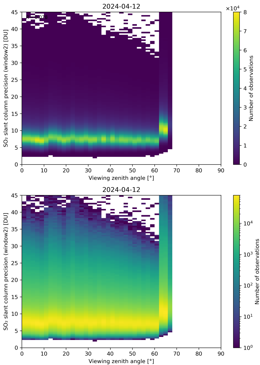
Figure 322: Scatter density plot of “Viewing zenith angle” against “SO 2 slant column precision (window2)” for 2024-04-11 to 2024-04-13.
