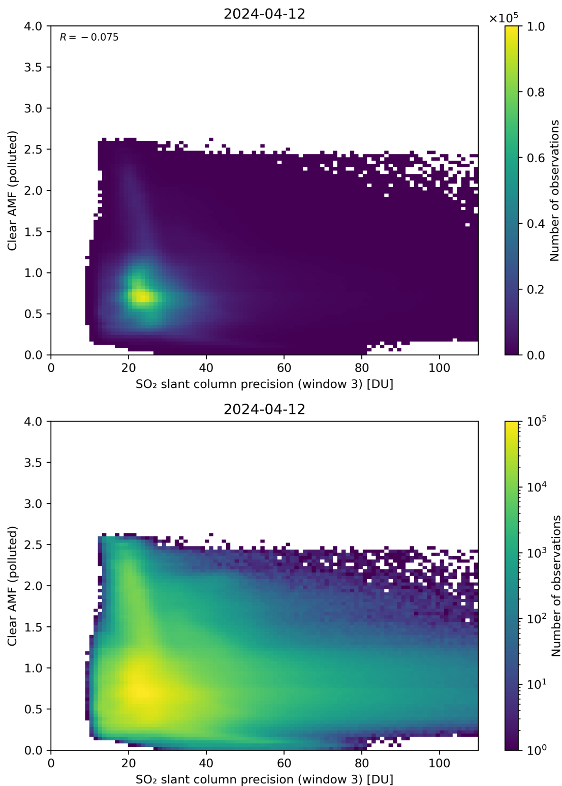
Figure 261: Scatter density plot of “SO 2 slant column precision (window 3)” against “Clear AMF (polluted)” for 2024-04-11 to 2024-04-13.
