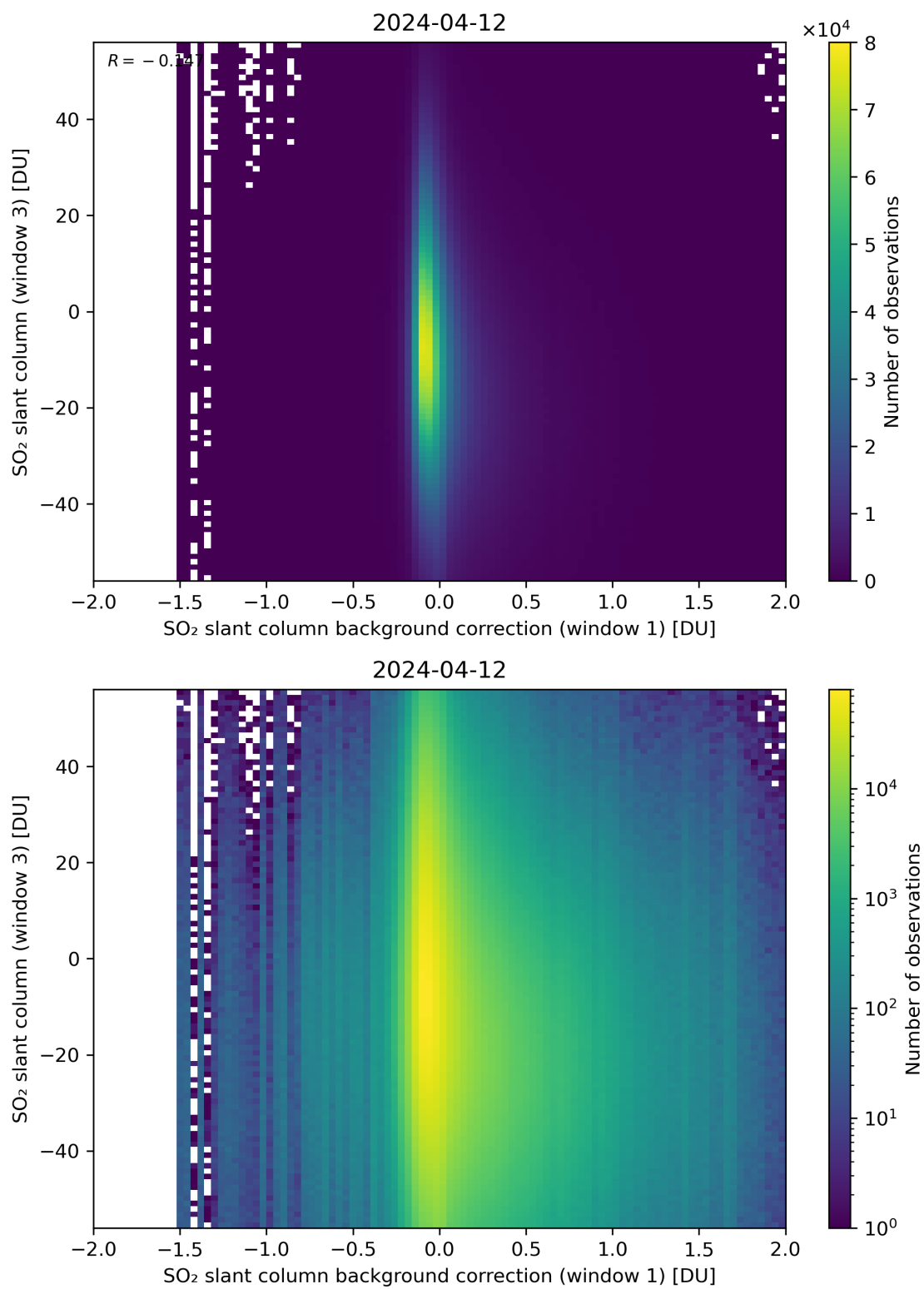
Figure 107: Scatter density plot of “SO 2 slant column background correction (window 1)” against “SO 2 slant column (window 3)” for 2024-04-11 to 2024-04-13.
