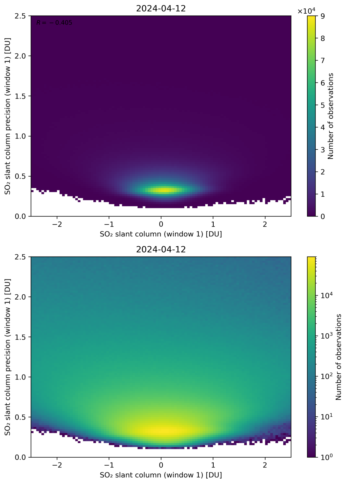
Figure 235: Scatter density plot of “SO 2 slant column (window 1)” against “SO 2 slant column precision (window 1)” for 2024-04-11 to 2024-04-13.
