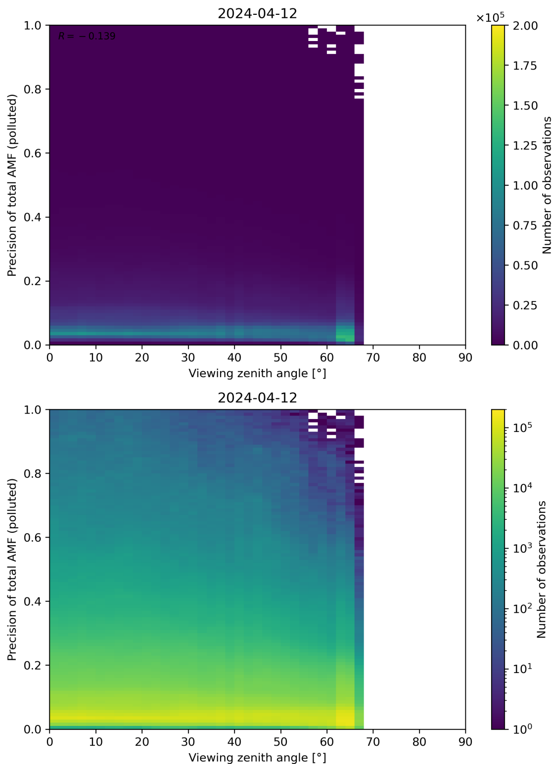
Figure 326: Scatter density plot of “Viewing zenith angle” against “Precision of total AMF (polluted)” for 2024-04-11 to 2024-04-13.
