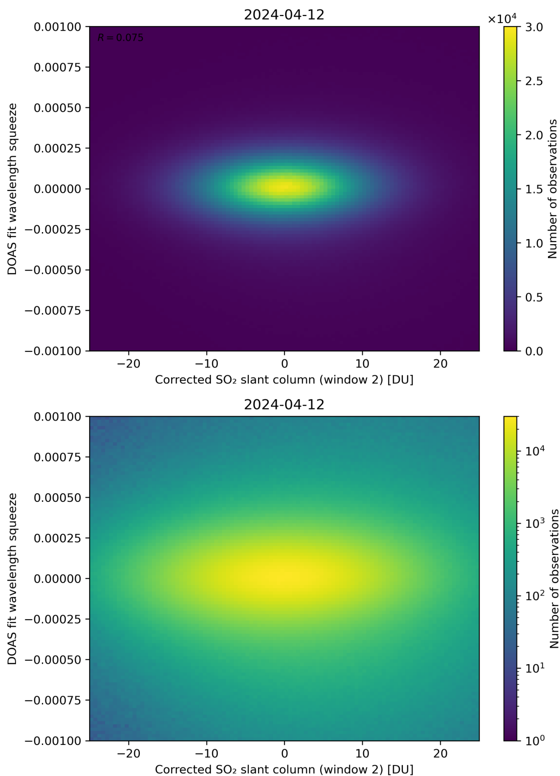
Figure 197: Scatter density plot of “Corrected SO 2 slant column (window 2)” against “DOAS fit wavelength squeeze” for 2024-04-11 to 2024-04-13.
