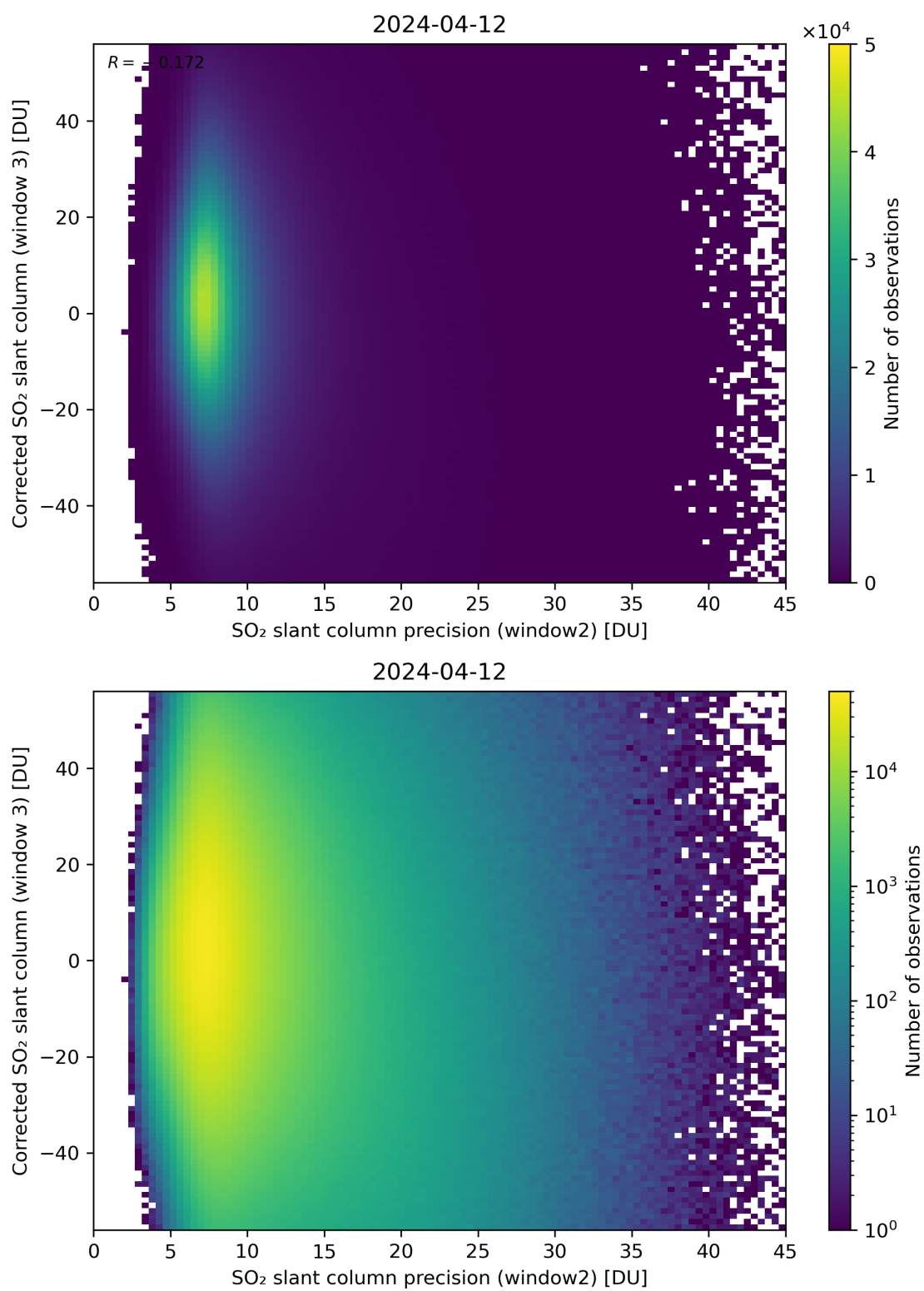
Figure 248: Scatter density plot of “SO 2 slant column precision (window2)” against “Corrected SO 2 slant column (window 3)” for 2024-04-11 to 2024-04-13.
