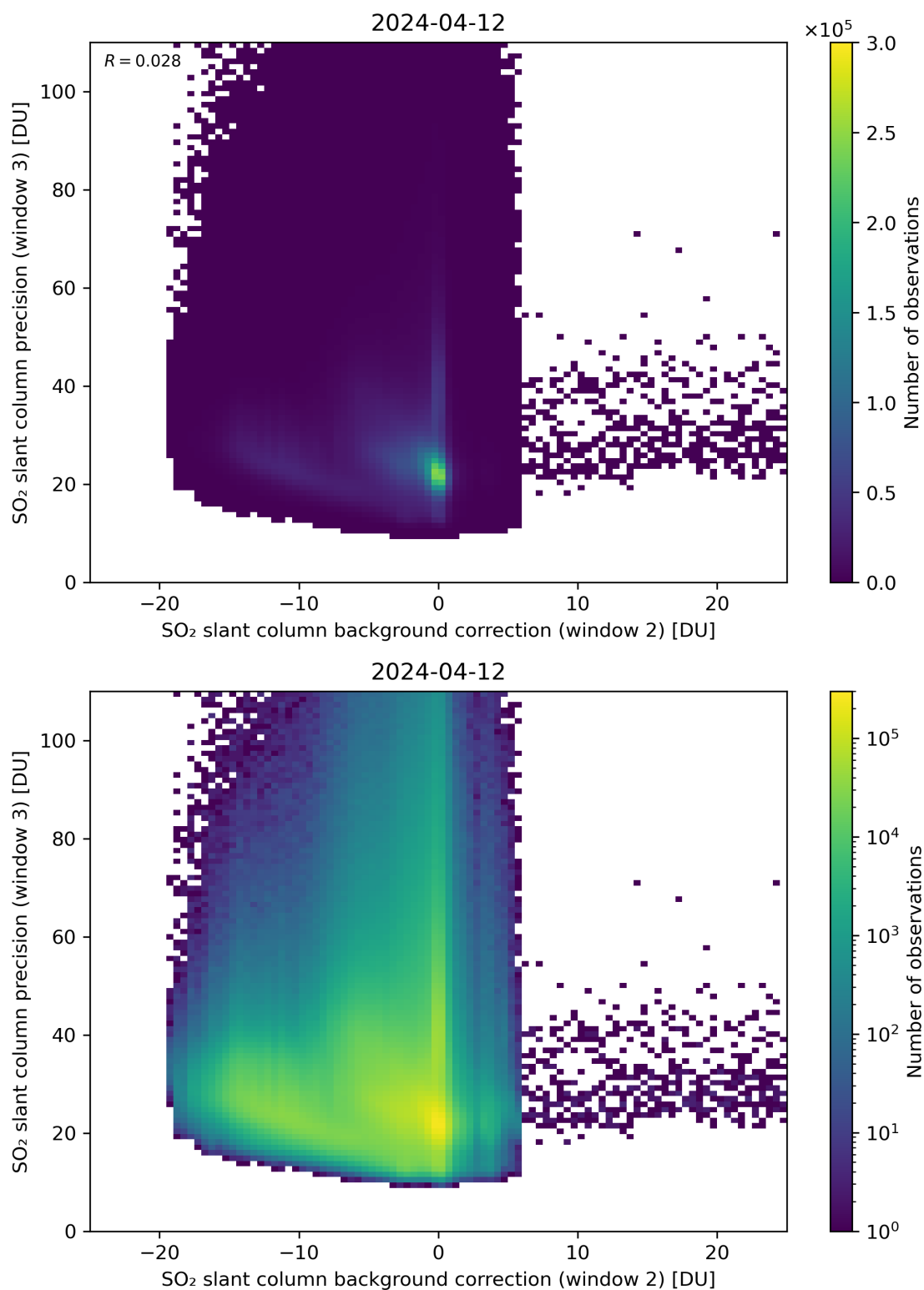
Figure 118: Scatter density plot of “SO 2 slant column background correction (window 2)” against “SO 2 slant column precision (window 3)” for 2024-04-11 to 2024-04-13.
