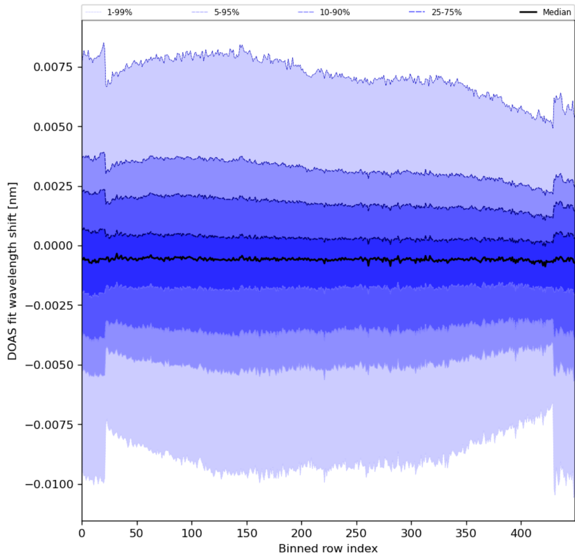
Figure 91: Along track statistics of “DOAS fit wavelength shift” for 2024-04-11 to 2024-04-13
