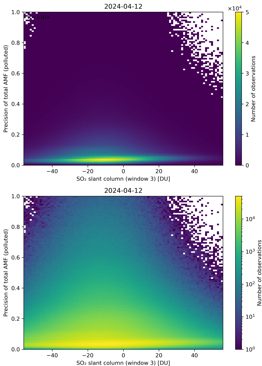
Figure 269: Scatter density plot of “SO 2 slant column (window 3)” against “Precision of total AMF (polluted)” for 2024-04-11 to 2024-04-13.
