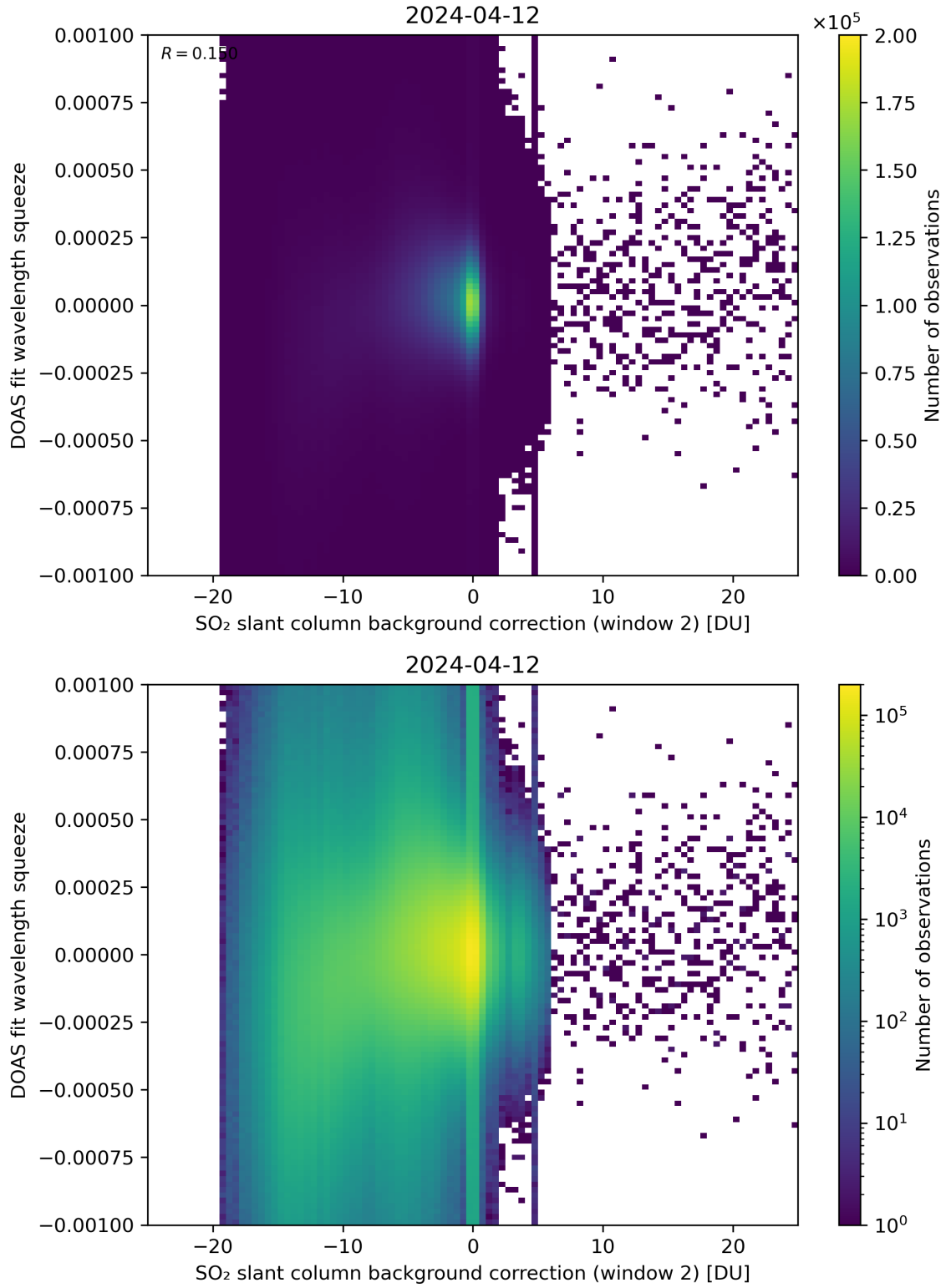
Figure 113: Scatter density plot of “SO 2 slant column background correction (window 2)” against “DOAS fit wavelength squeeze” for 2024-04-11 to 2024-04-13.
