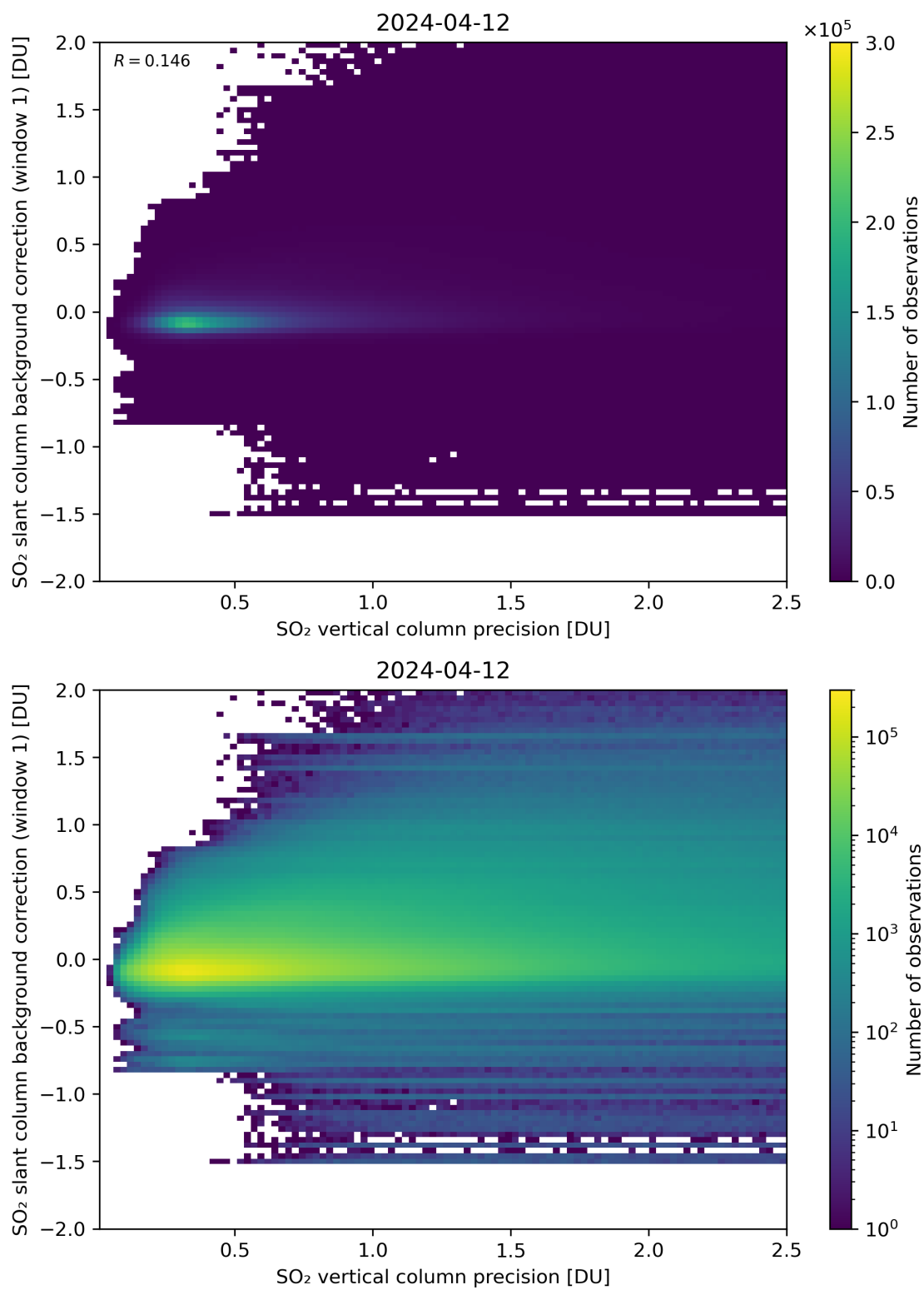
Figure 279: Scatter density plot of “SO 2 vertical column precision” against “SO 2 slant column background correction (window 1)” for 2024-04-11 to 2024-04-13.
