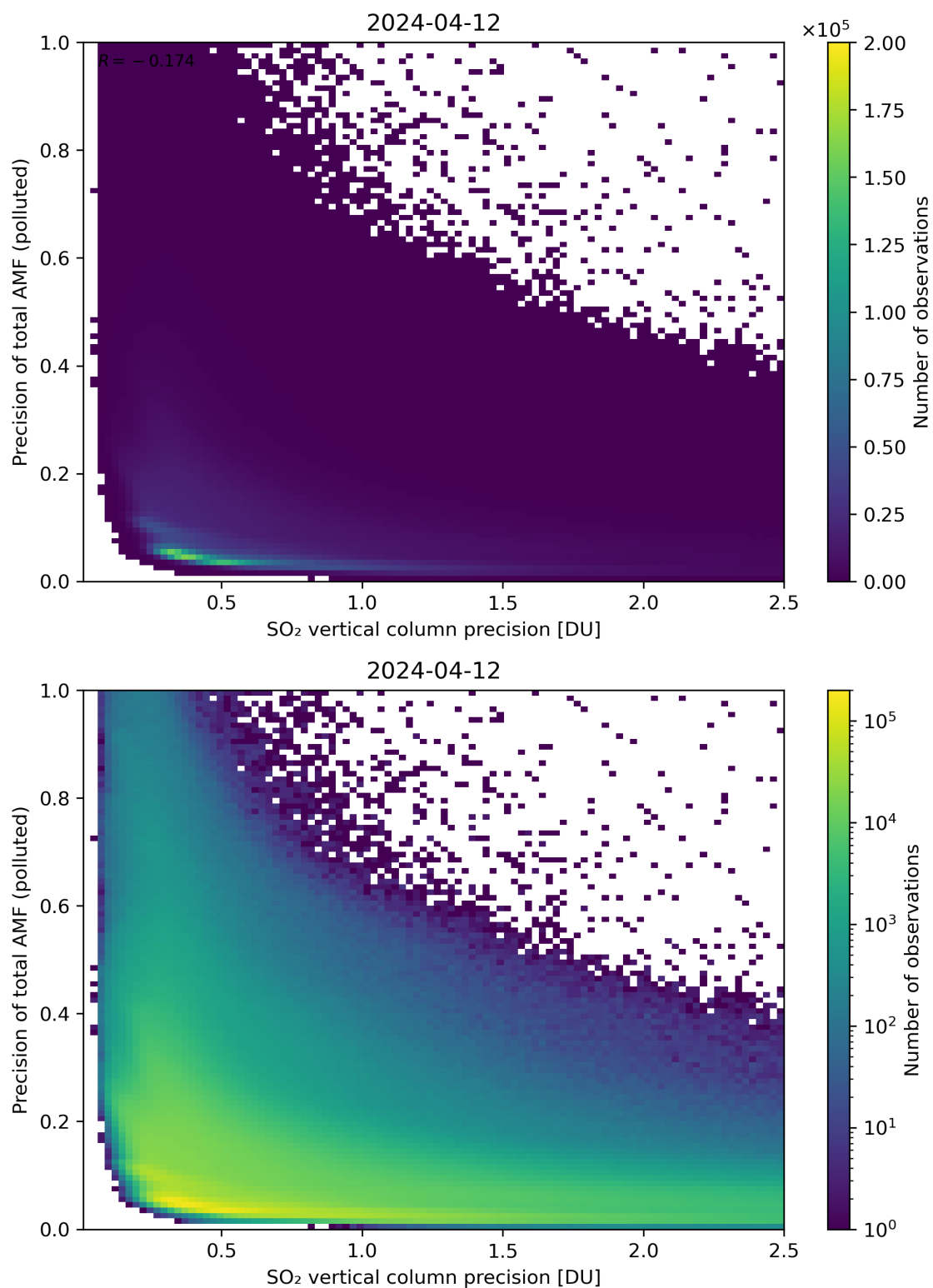
Figure 295: Scatter density plot of “SO 2 vertical column precision” against “Precision of total AMF (polluted)” for 2024-04-11 to 2024-04-13.
