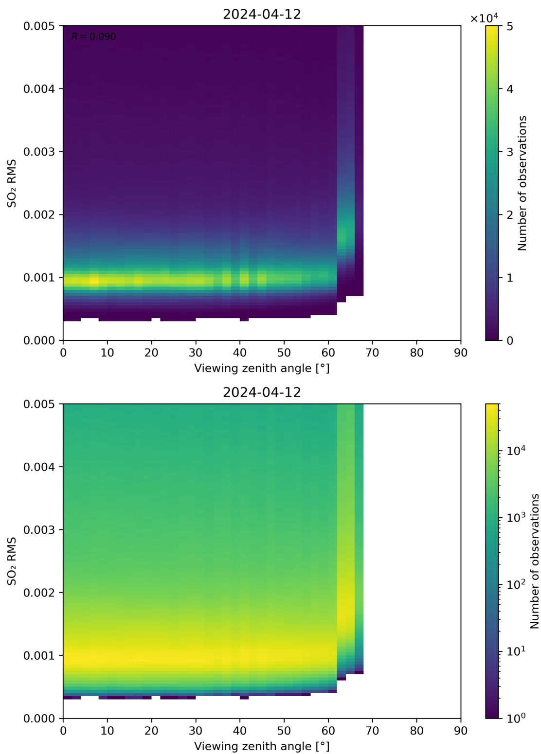
Figure 313: Scatter density plot of “Viewing zenith angle” against “SO 2 RMS” for 2024-04-11 to 2024-04-13.
