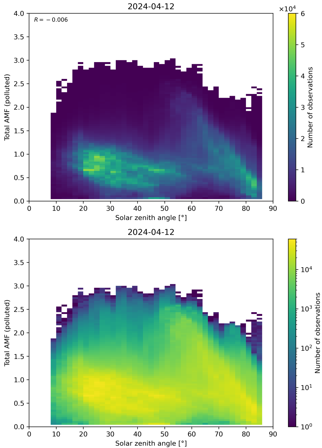
Figure 174: Scatter density plot of “Solar zenith angle” against “Total AMF (polluted)” for 2024-04-11 to 2024-04-13.
