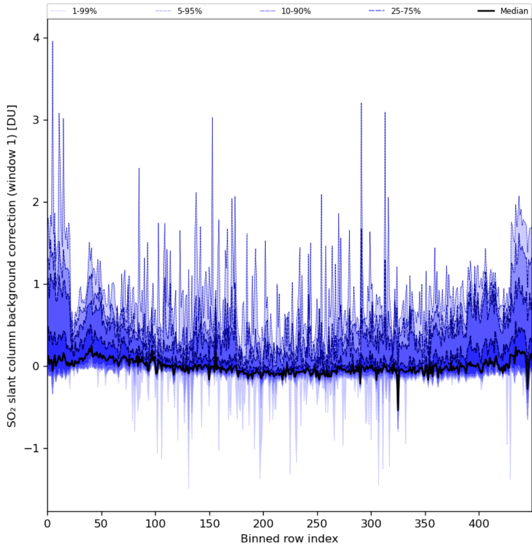
Figure 82: Along track statistics of “SO 2 slant column background correction (window 1)” for 2024-04-11 to 2024-04-13
