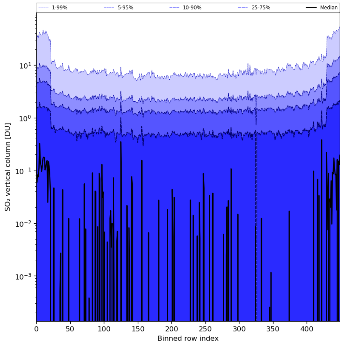
Figure 76: Along track statistics of “SO 2 vertical column” for 2024-04-11 to 2024-04-13
