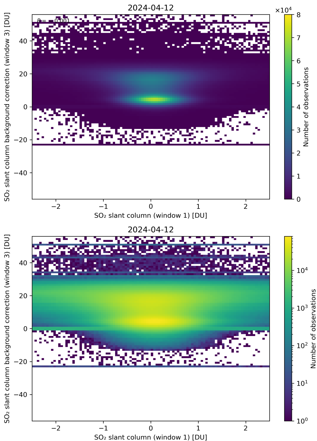
Figure 214: Scatter density plot of “SO 2 slant column (window 1)” against “SO 2 slant column background correction (window 3)” for 2024-04-11 to 2024-04-13.
