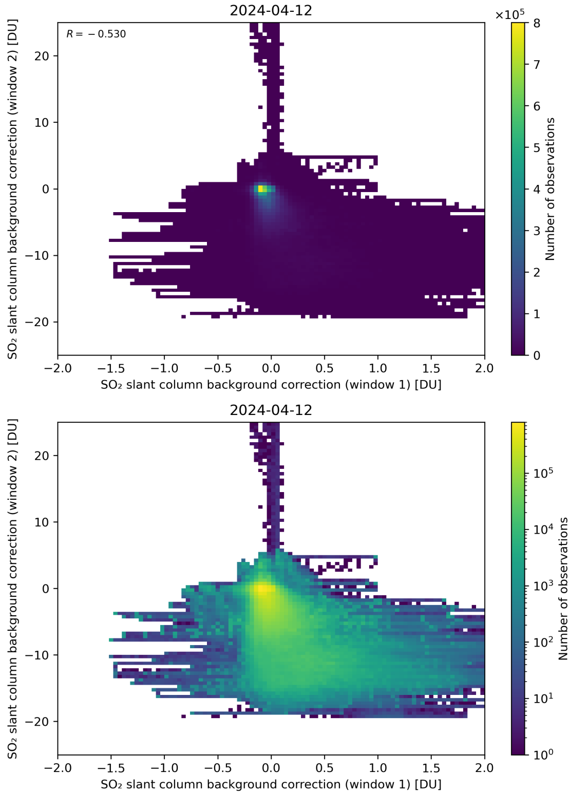
Figure 98: Scatter density plot of “SO 2 slant column background correction (window 1)” against “SO 2 slant column background correction (window 2)” for 2024-04-11 to 2024-04-13.
