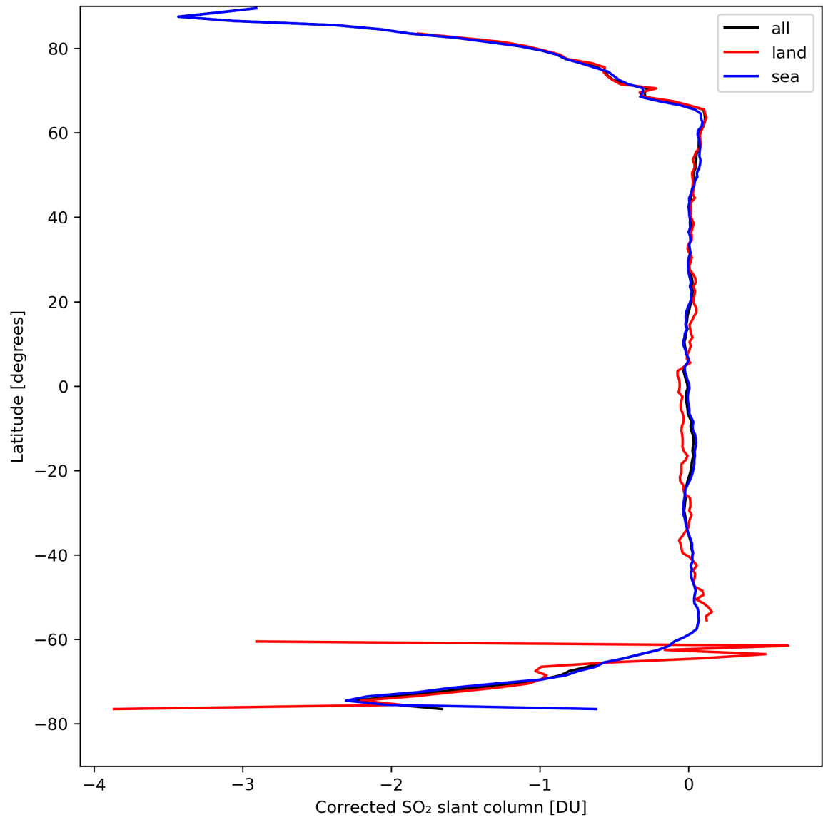
Figure 32: Zonal average of "Corrected SO 2 slant column" for 2024-04-11 to 2024-04-13.
