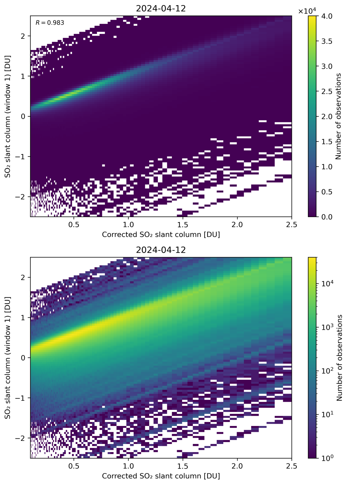
Figure 187: Scatter density plot of “Corrected SO 2 slant column” against “SO 2 slant column (window 1)” for 2024-04-11 to 2024-04-13.
