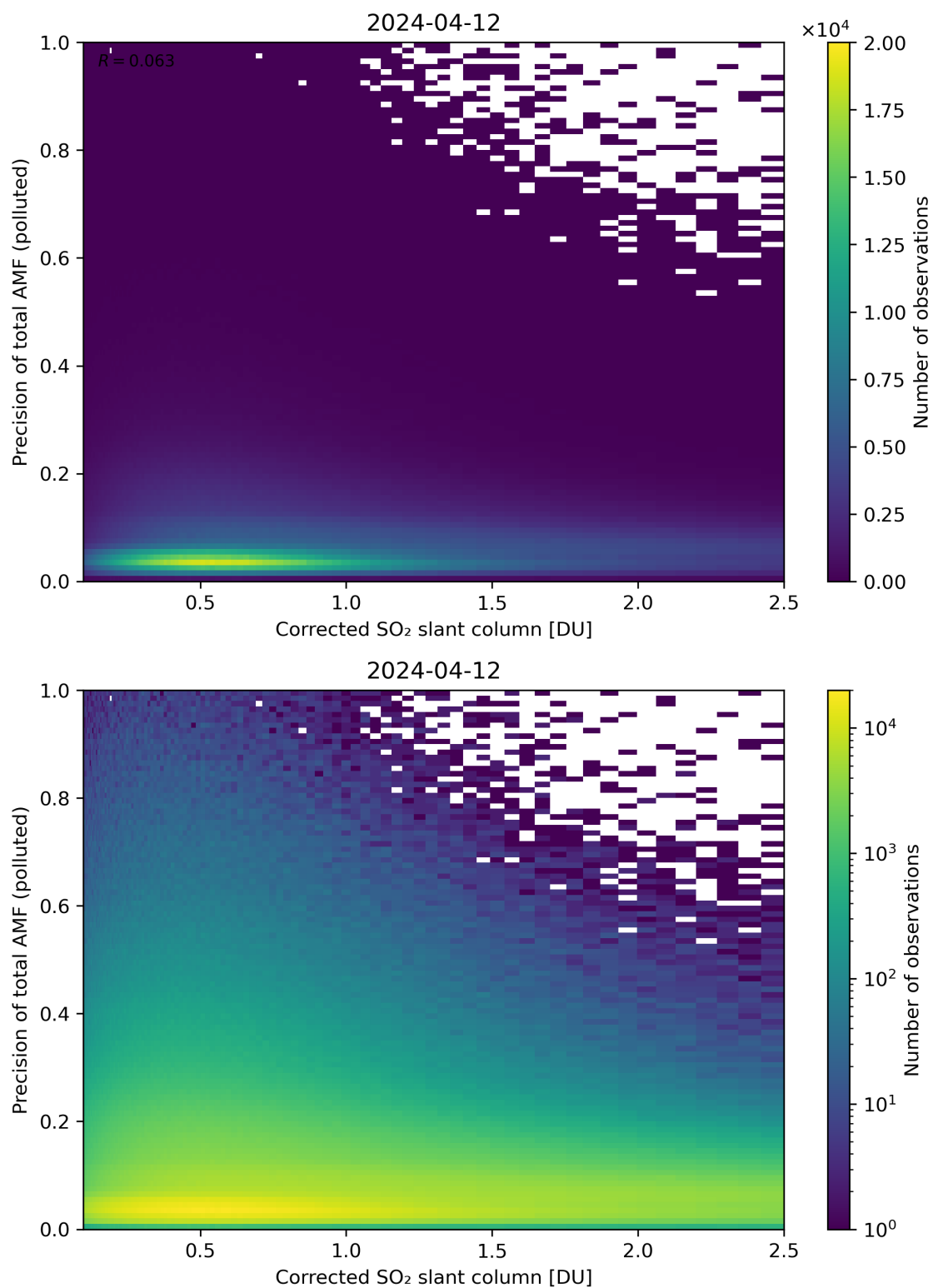
Figure 193: Scatter density plot of “Corrected SO 2 slant column” against “Precision of total AMF (polluted)” for 2024-04-11 to 2024-04-13.
