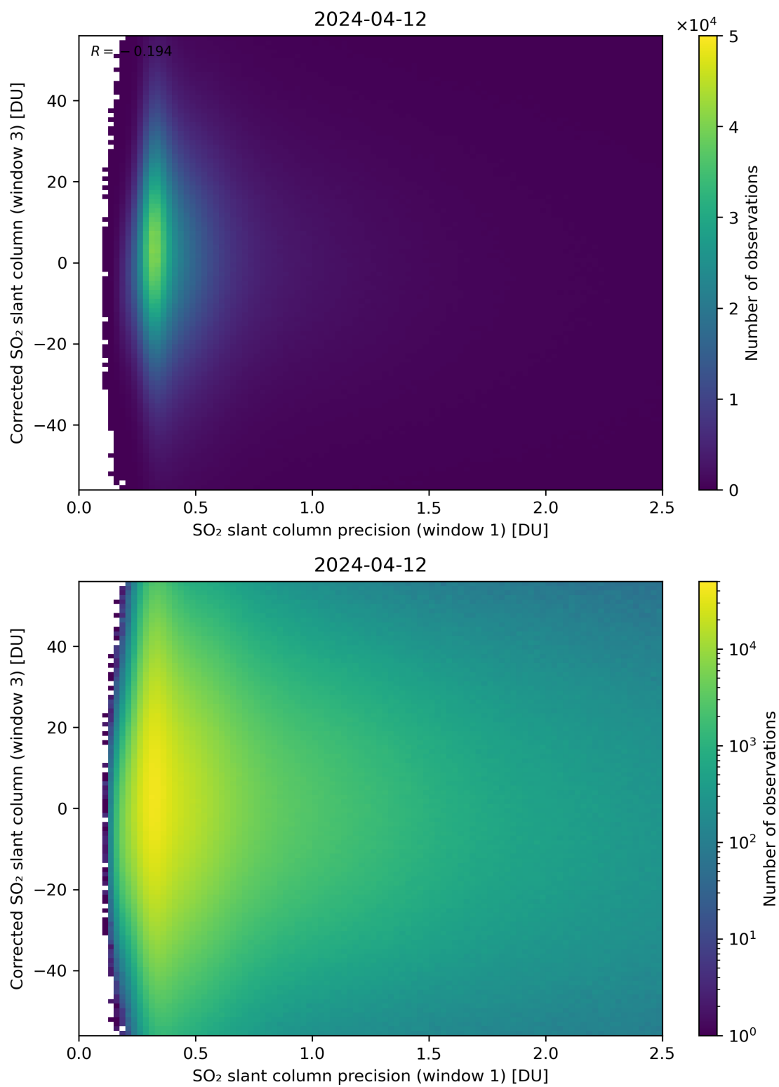
Figure 226: Scatter density plot of “SO 2 slant column precision (window 1)” against “Corrected SO 2 slant column (window 3)” for 2024-04-11 to 2024-04-13.
