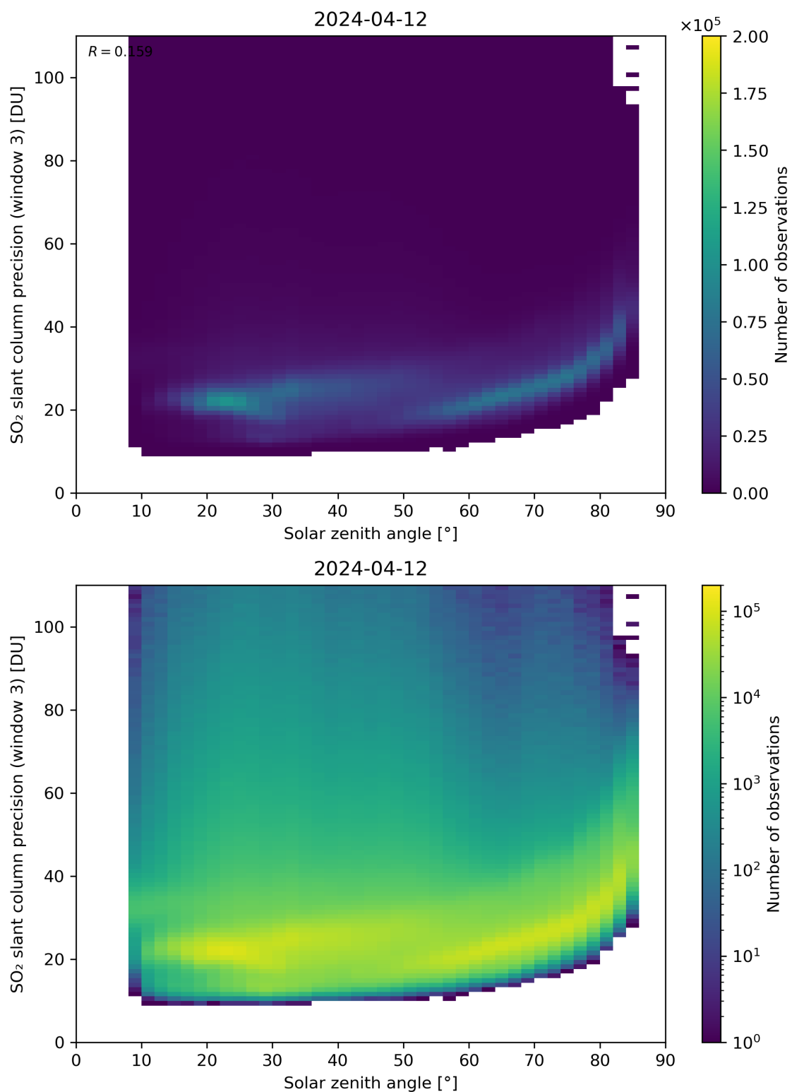
Figure 173: Scatter density plot of “Solar zenith angle” against “SO 2 slant column precision (window 3)” for 2024-04-11 to 2024-04-13.
