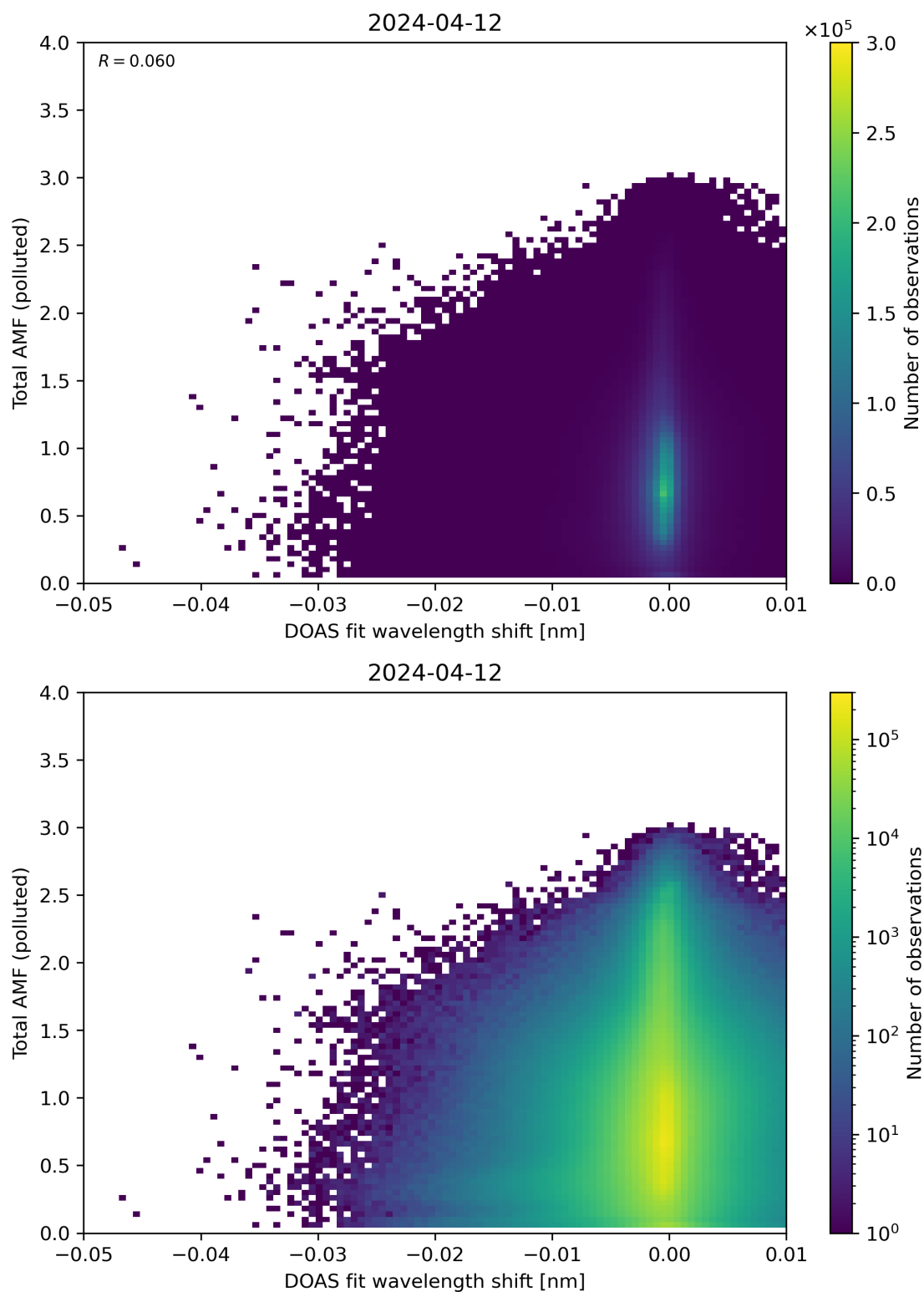
Figure 130: Scatter density plot of “DOAS fit wavelength shift” against “Total AMF (polluted)” for 2024-04-11 to 2024-04-13.
