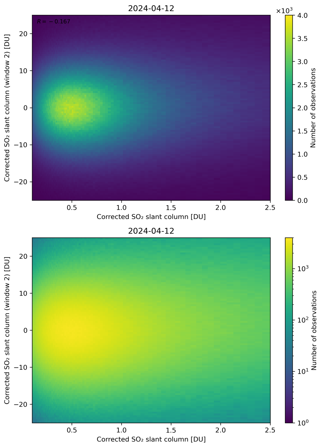
Figure 185: Scatter density plot of “Corrected SO 2 slant column” against “Corrected SO 2 slant column (window 2)” for 2024-04-11 to 2024-04-13.
