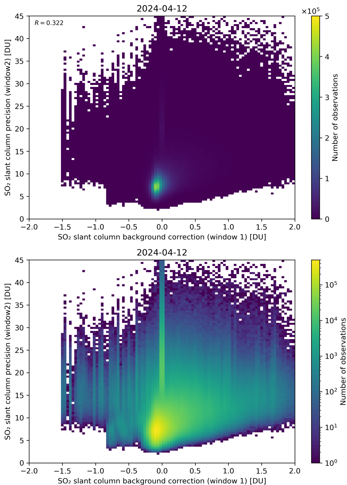
Figure 106: Scatter density plot of “SO 2 slant column background correction (window 1)” against “SO 2 slant column precision (window2)” for 2024-04-11 to 2024-04-13.
