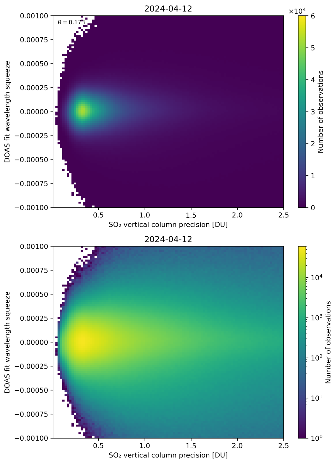
Figure 283: Scatter density plot of “SO 2 vertical column precision” against “DOAS fit wavelength squeeze” for 2024-04-11 to 2024-04-13.
