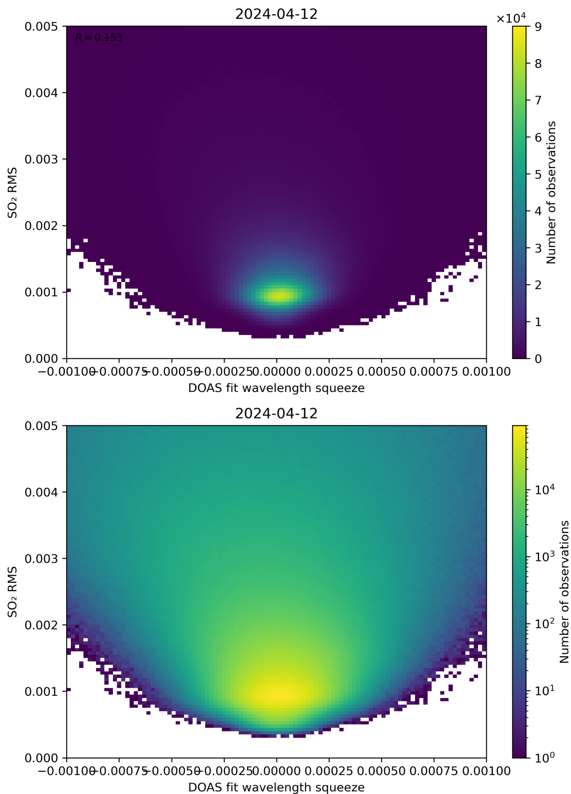
Figure 132: Scatter density plot of “DOAS fit wavelength squeeze” against “SO 2 RMS” for 2024-04-11 to 2024-04-13.
