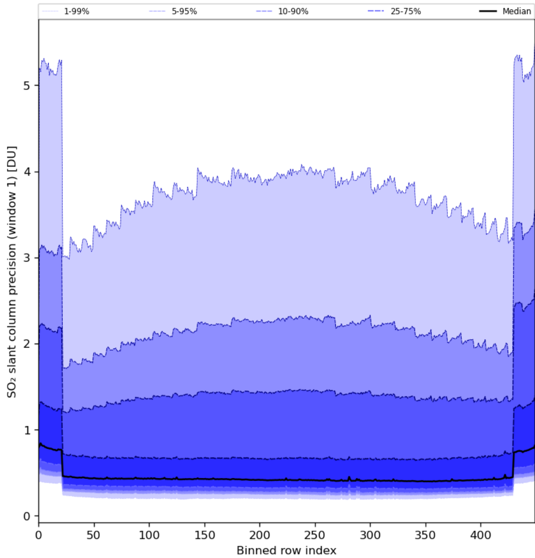
Figure 80: Along track statistics of “SO 2 slant column precision (window 1)” for 2024-04-11 to 2024-04-13
