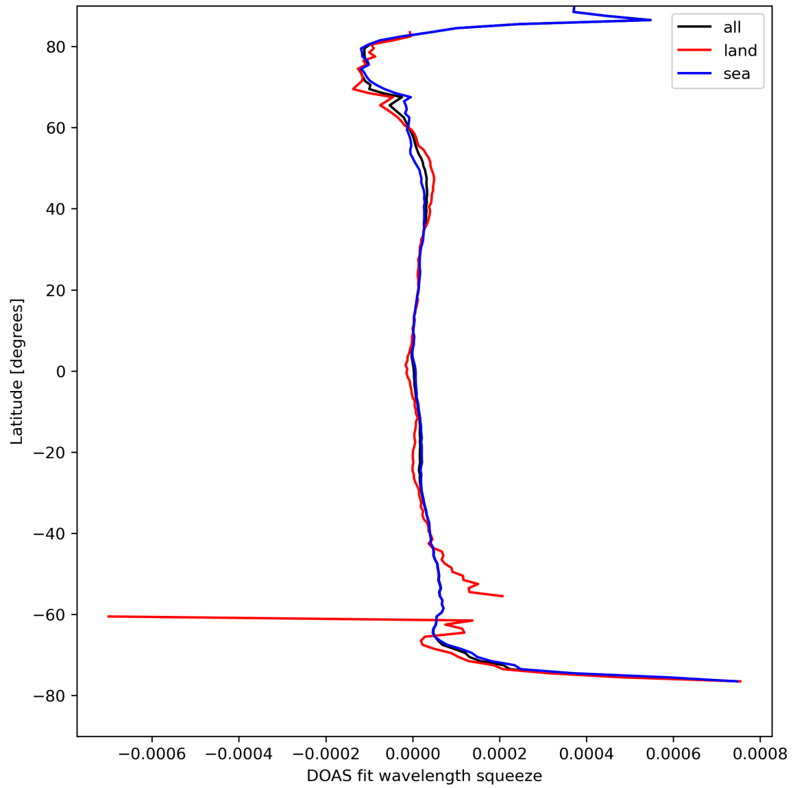
Figure 46: Zonal average of “DOAS fit wavelength squeeze” for 2024-04-11 to 2024-04-13.
