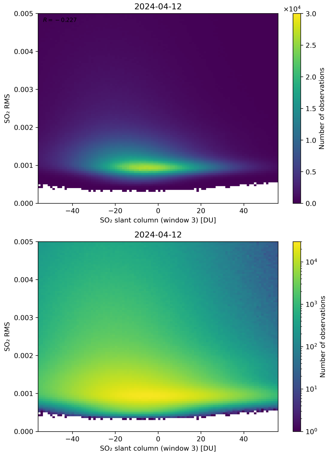
Figure 256: Scatter density plot of “SO 2 slant column (window 3)” against “SO 2 RMS” for 2024-04-11 to 2024-04-13.
