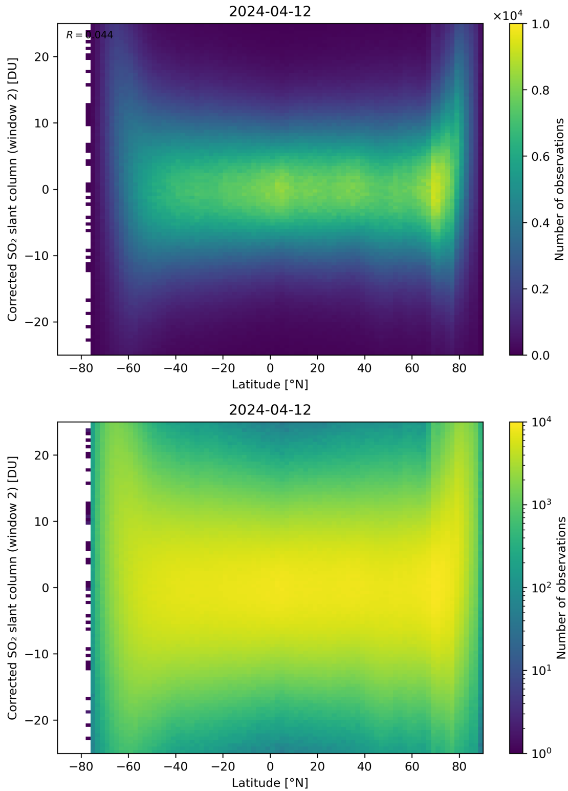
Figure 147: Scatter density plot of “Latitude” against “Corrected SO 2 slant column (window 2)” for 2024-04-11 to 2024-04-13.
