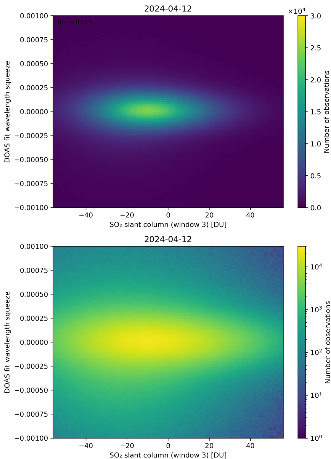
Figure 255: Scatter density plot of “SO 2 slant column (window 3)” against “DOAS fit wavelength squeeze” for 2024-04-11 to 2024-04-13.
