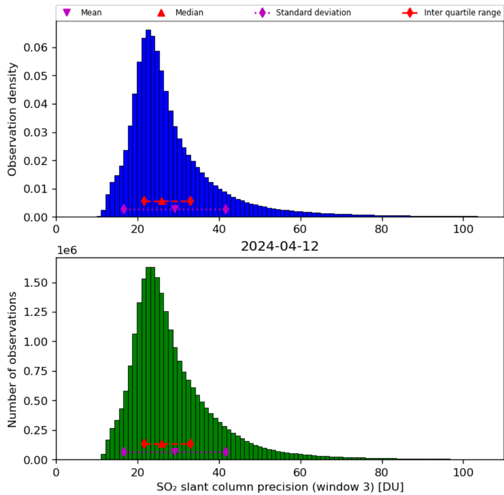
Figure 65: Histogram of “SO 2 slant column precision (window 3)” for 2024-04-11 to 2024-04-13
