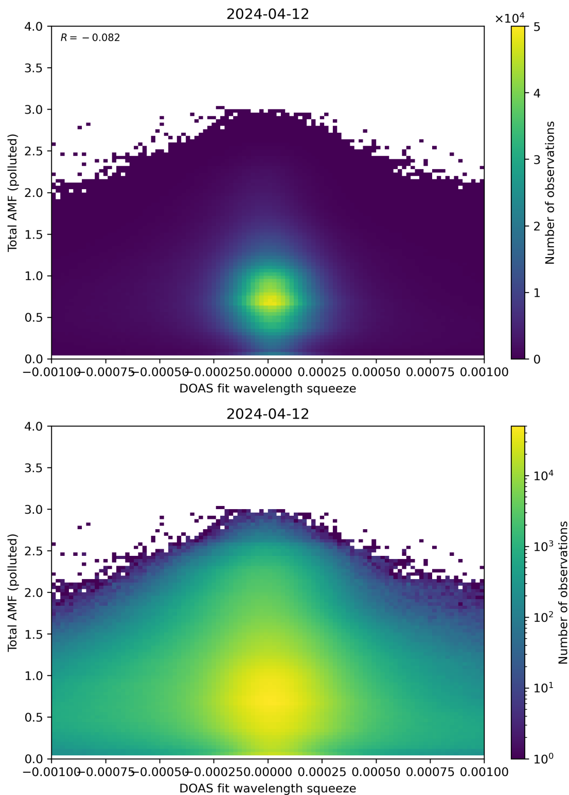
Figure 134: Scatter density plot of “DOAS fit wavelength squeeze” against “Total AMF (polluted)” for 2024-04-11 to 2024-04-13.
