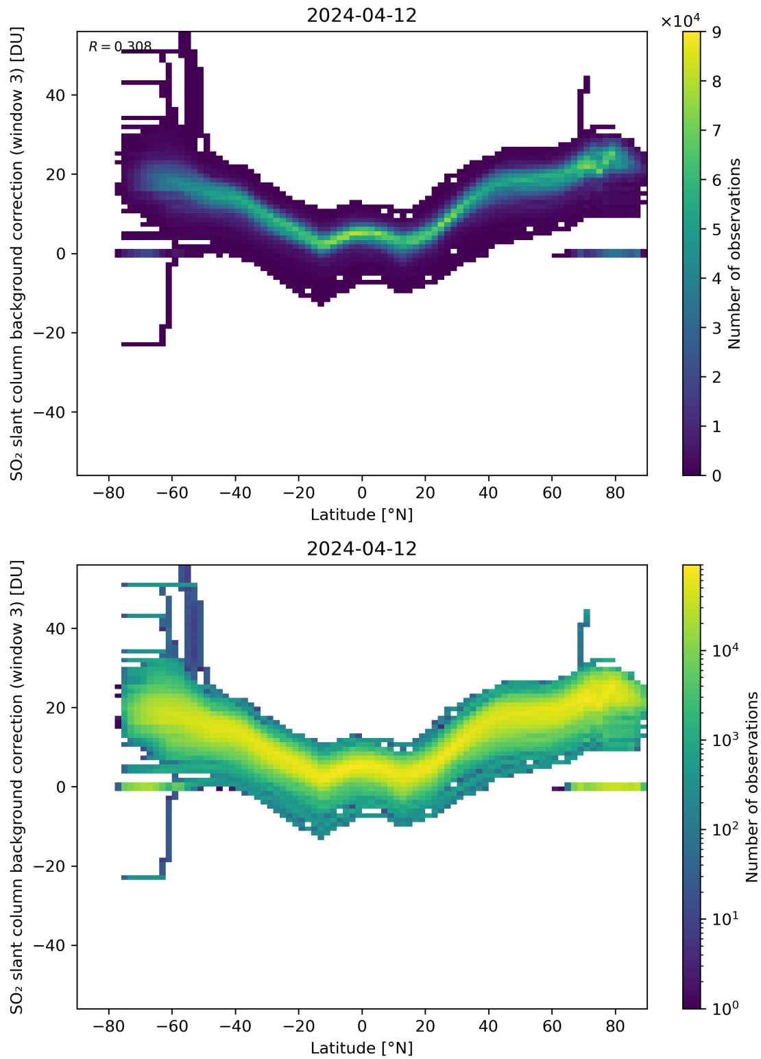
Figure 141: Scatter density plot of “Latitude” against “SO 2 slant column background correction (window 3)” for 2024-04-11 to 2024-04-13.
