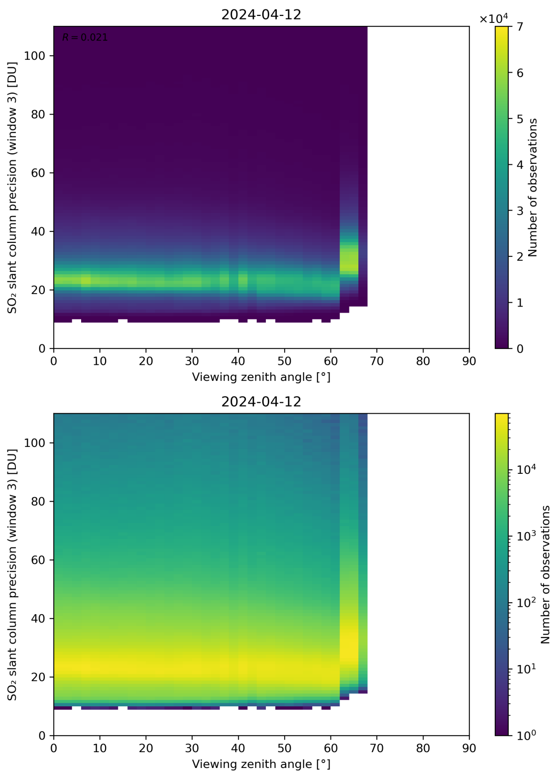
Figure 324: Scatter density plot of “Viewing zenith angle” against “SO 2 slant column precision (window 3)” for 2024-04-11 to 2024-04-13.
