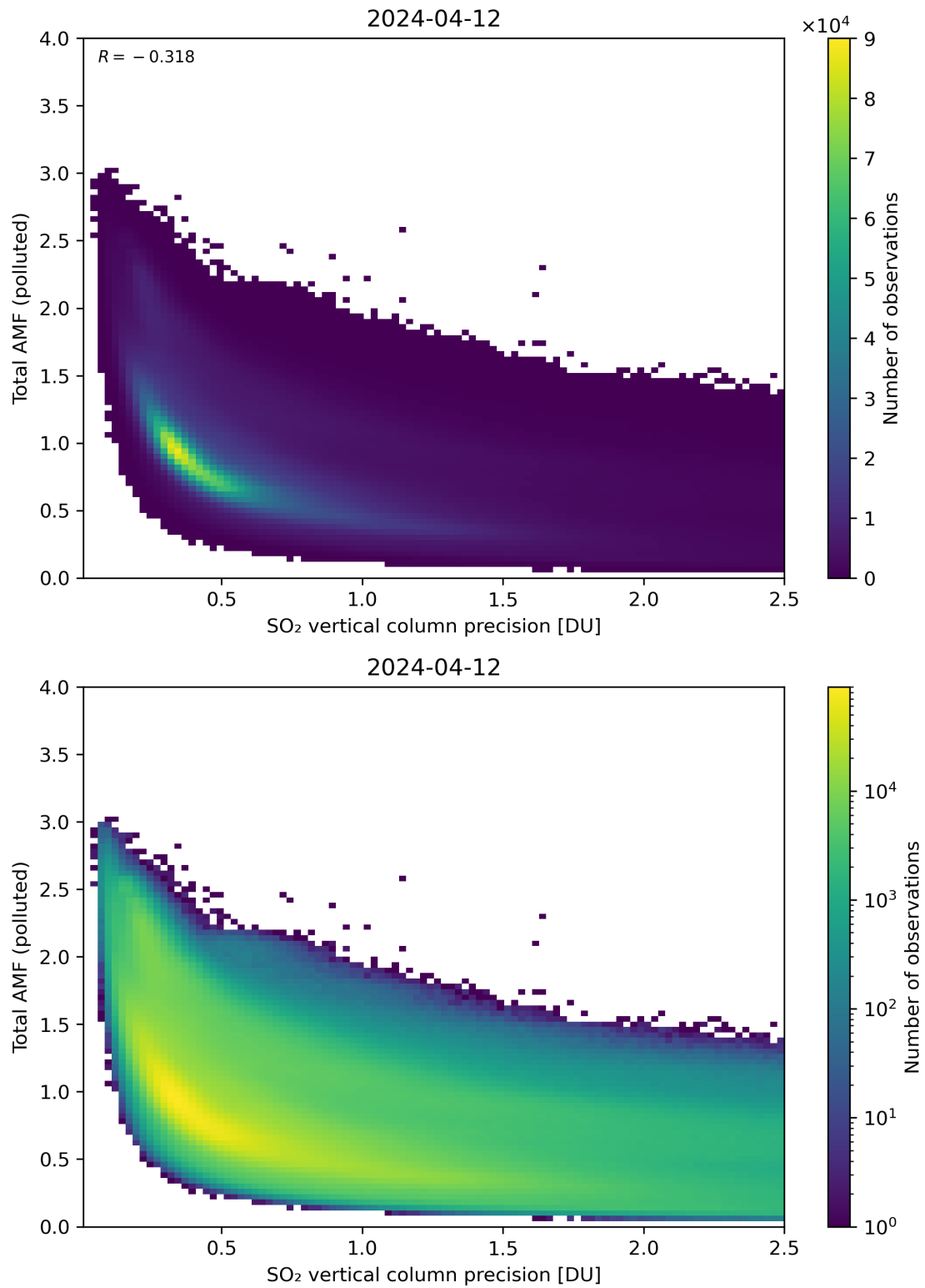
Figure 294: Scatter density plot of “SO 2 vertical column precision” against “Total AMF (polluted)” for 2024-04-11 to 2024-04-13.
