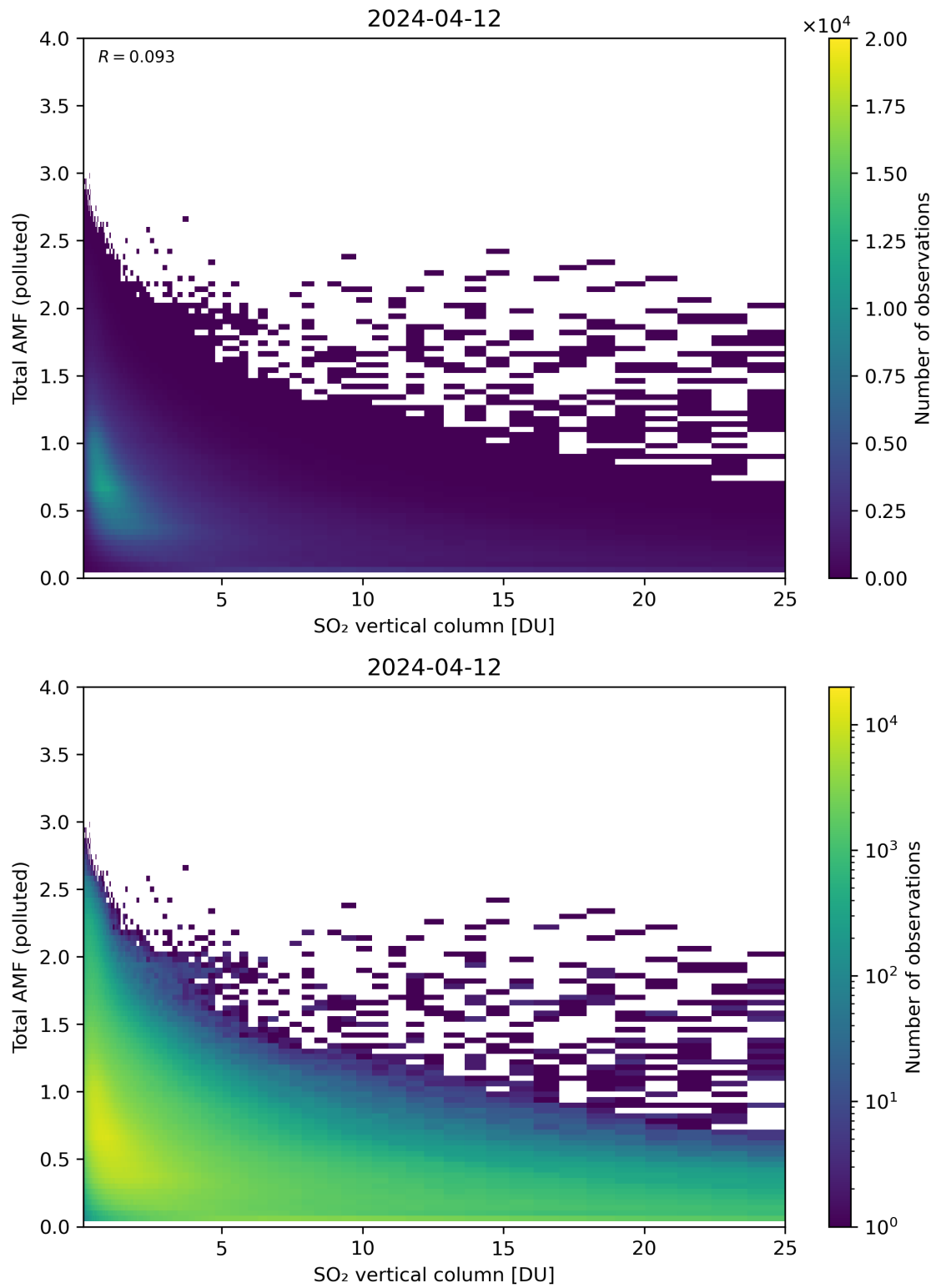
Figure 305: Scatter density plot of “SO 2 vertical column” against “Total AMF (polluted)” for 2024-04-11 to 2024-04-13.
