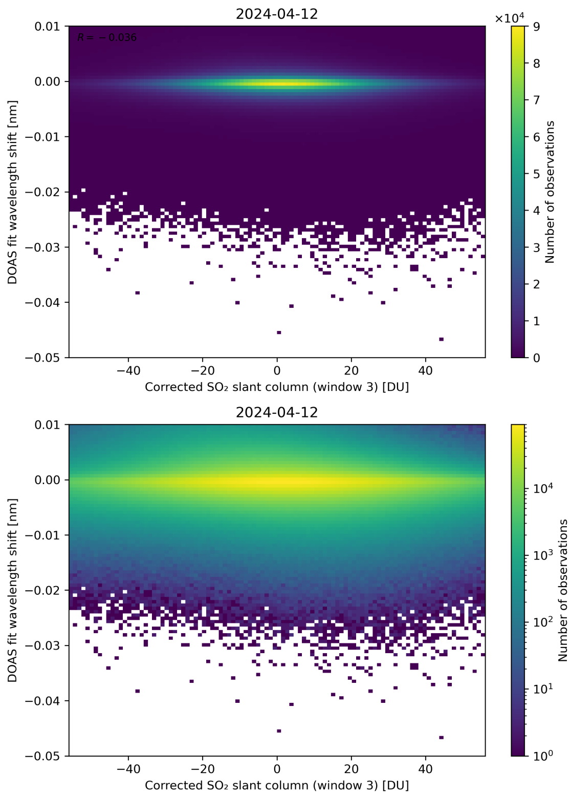
Figure 206: Scatter density plot of “Corrected SO 2 slant column (window 3)” against “DOAS fit wavelength shift” for 2024-04-11 to 2024-04-13.
