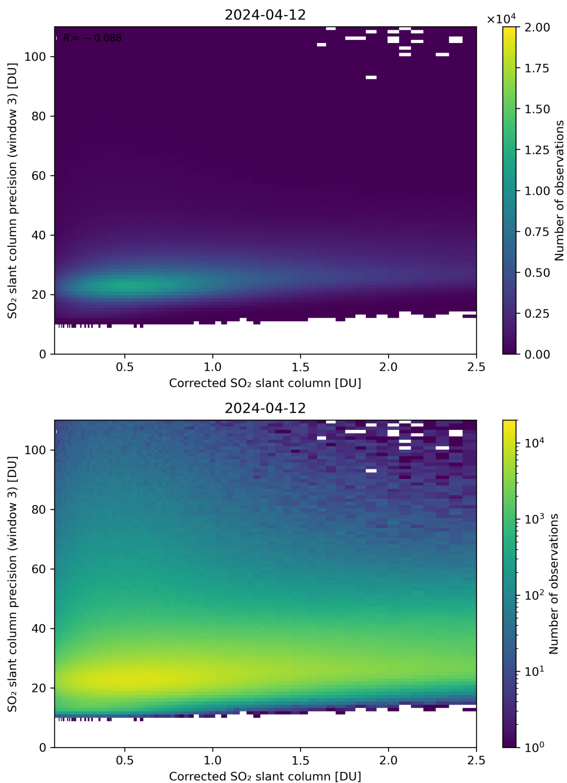
Figure 191: Scatter density plot of “Corrected SO 2 slant column” against “SO 2 slant column precision (window 3)” for 2024-04-11 to 2024-04-13.
