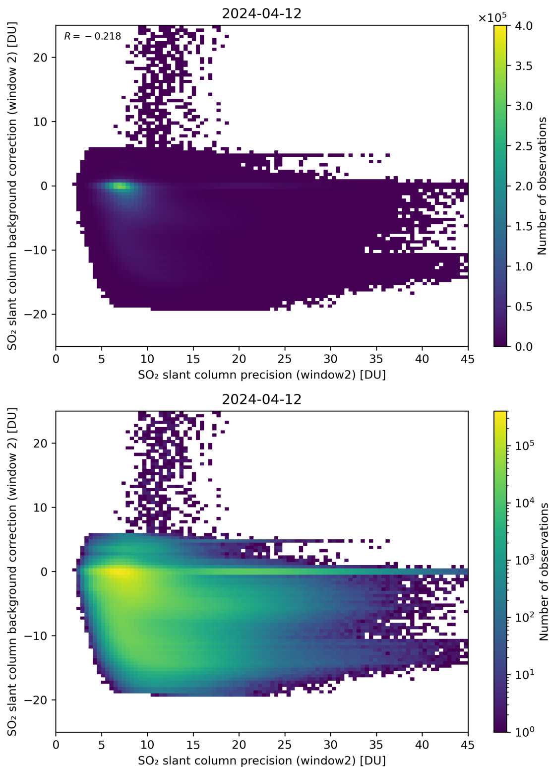
Figure 241: Scatter density plot of “SO 2 slant column precision (window2)” against “SO 2 slant column background correction (window 2)” for 2024-04-11 to 2024-04-13.
