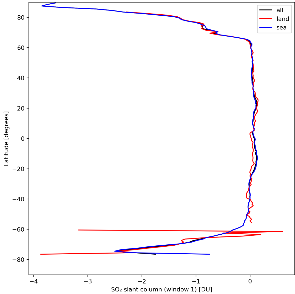
Figure 33: Zonal average of “SO 2 slant column (window 1)” for 2024-04-11 to 2024-04-13.
