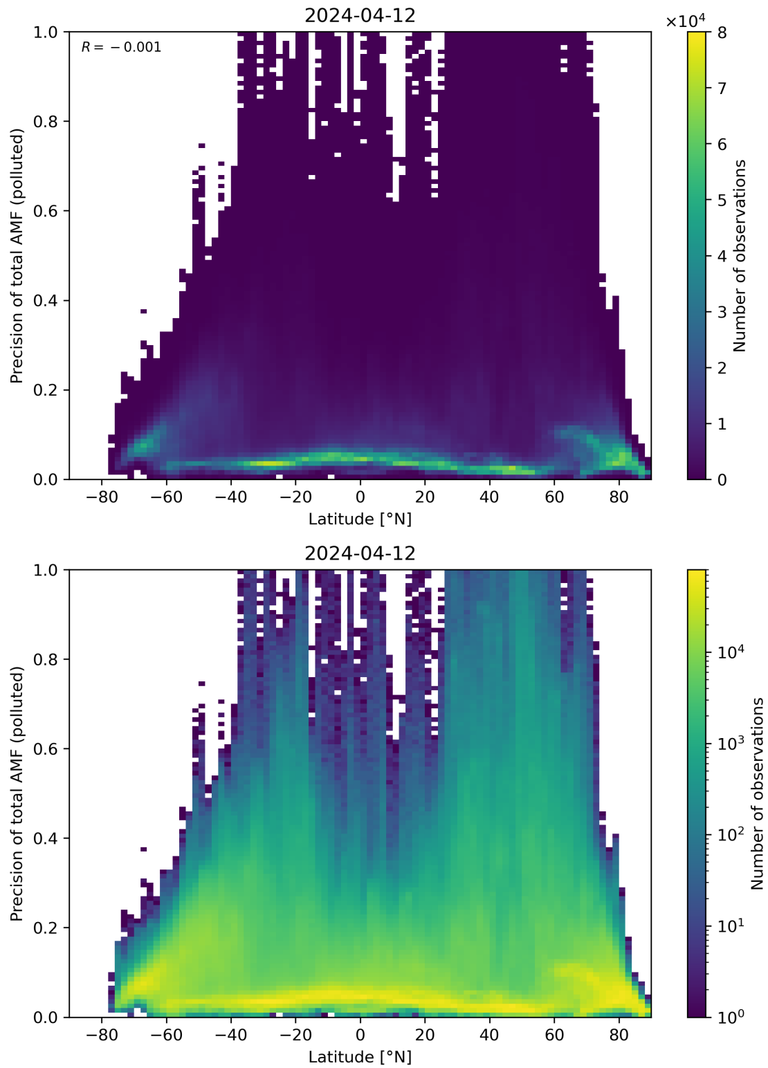
Figure 155: Scatter density plot of “Latitude” against “Precision of total AMF (polluted)” for 2024-04-11 to 2024-04-13.
