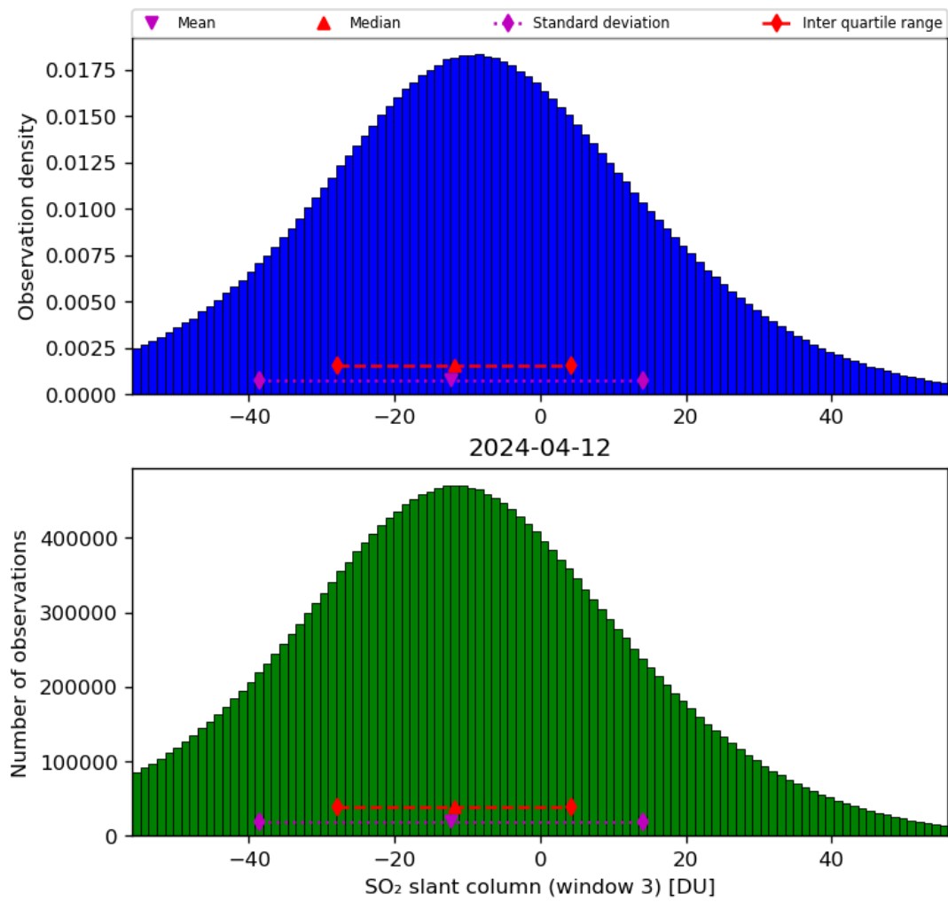
Figure 64: Histogram of “SO 2 slant column (window 3)” for 2024-04-11 to 2024-04-13
