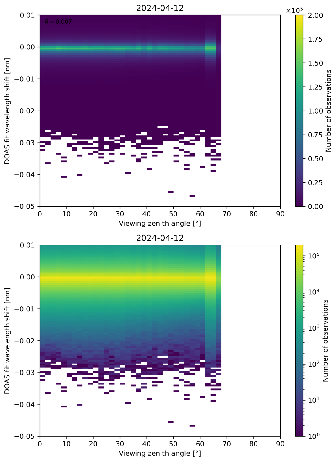
Figure 311: Scatter density plot of “Viewing zenith angle” against “DOAS fit wavelength shift” for 2024-04-11 to 2024-04-13.
