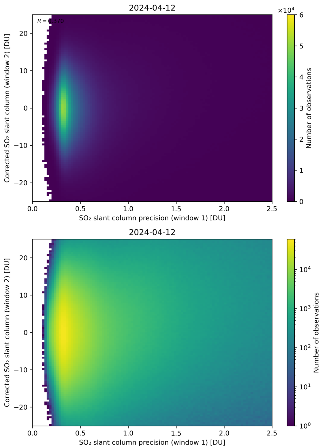
Figure 225: Scatter density plot of “SO 2 slant column precision (window 1)” against “Corrected SO 2 slant column (window 2)” for 2024-04-11 to 2024-04-13.
