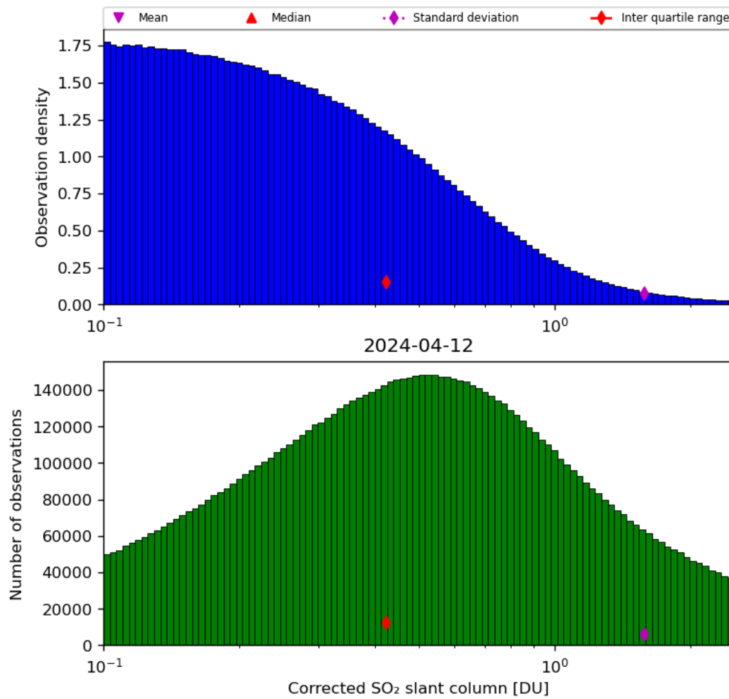
Figure 55: Histogram of “Corrected SO 2 slant column” for 2024-04-11 to 2024-04-13
