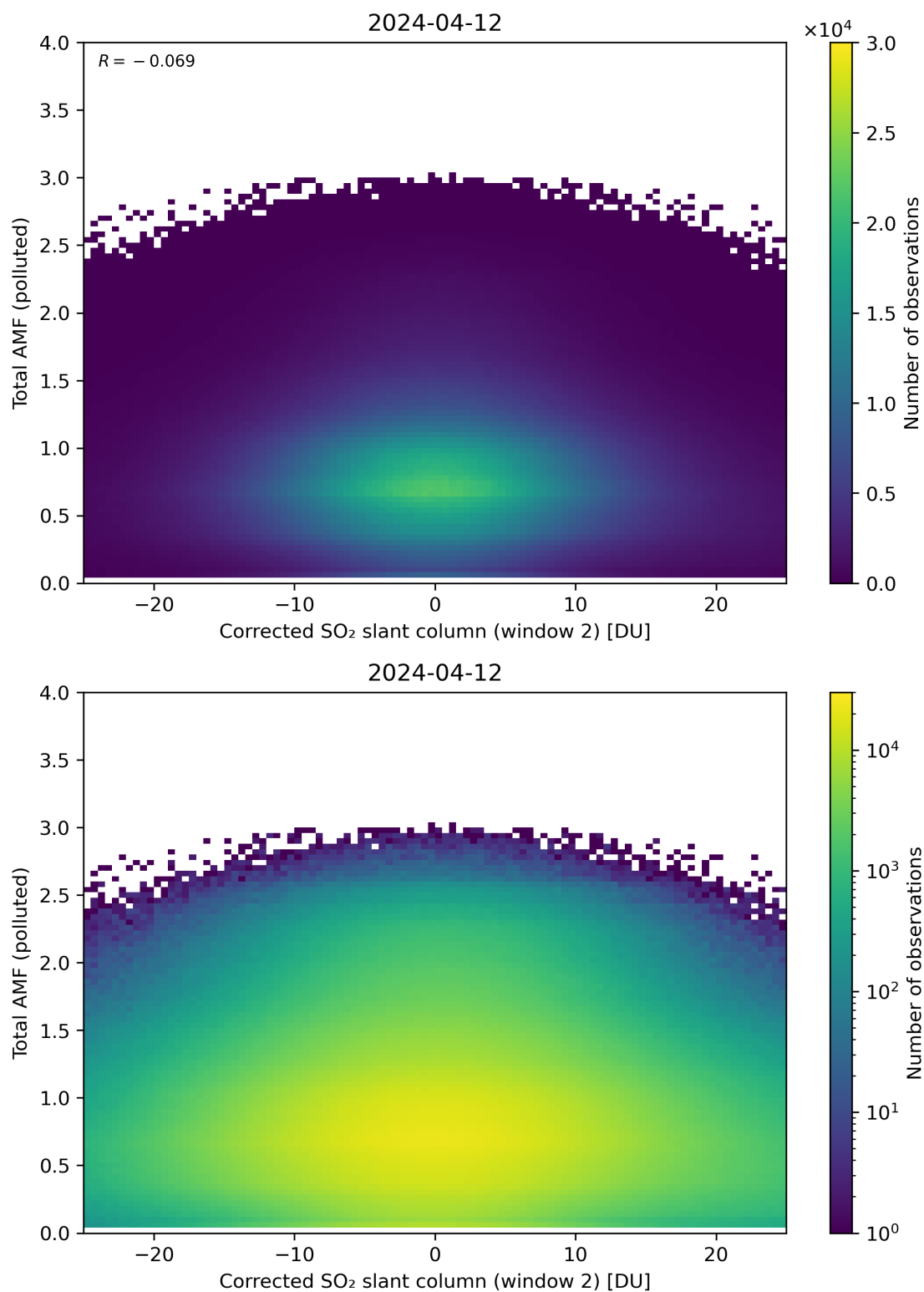
Figure 203: Scatter density plot of “Corrected SO 2 slant column (window 2)” against “Total AMF (polluted)” for 2024-04-11 to 2024-04-13.
