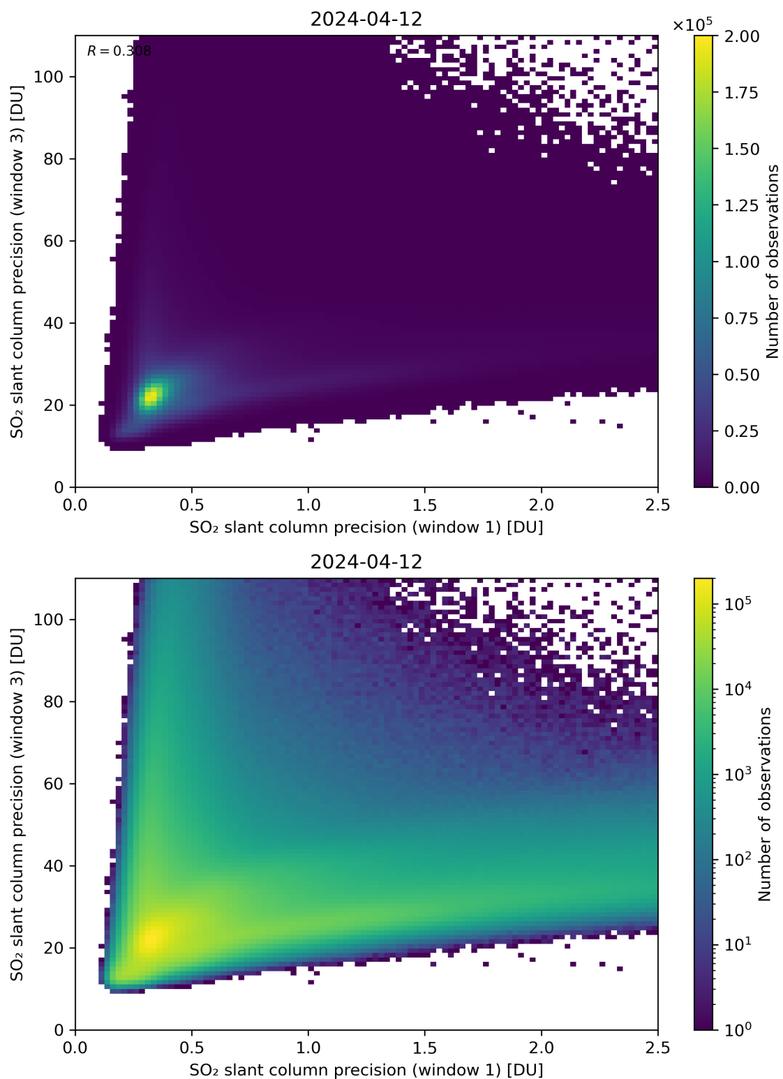
Figure 229: Scatter density plot of “SO 2 slant column precision (window 1)” against “SO 2 slant column precision (window 3)” for 2024-04-11 to 2024-04-13.
