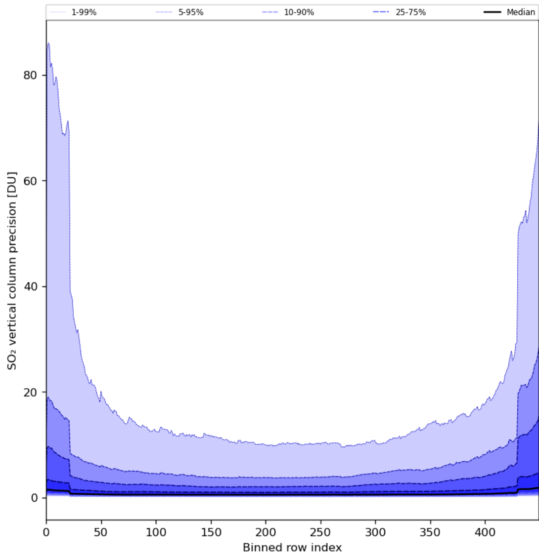
Figure 77: Along track statistics of “SO 2 vertical column precision” for 2024-04-11 to 2024-04-13
