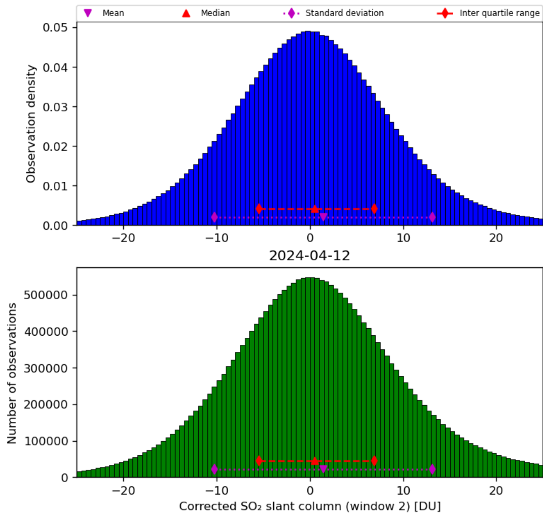
Figure 62: Histogram of “Corrected SO 2 slant column (window 2)” for 2024-04-11 to 2024-04-13
