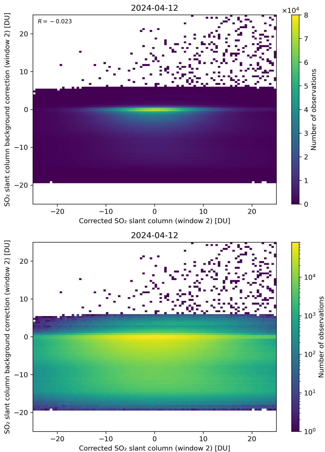
Figure 194: Scatter density plot of “Corrected SO 2 slant column (window 2)” against “SO 2 slant column background correction (window 2)” for 2024-04-11 to 2024-04-13.
