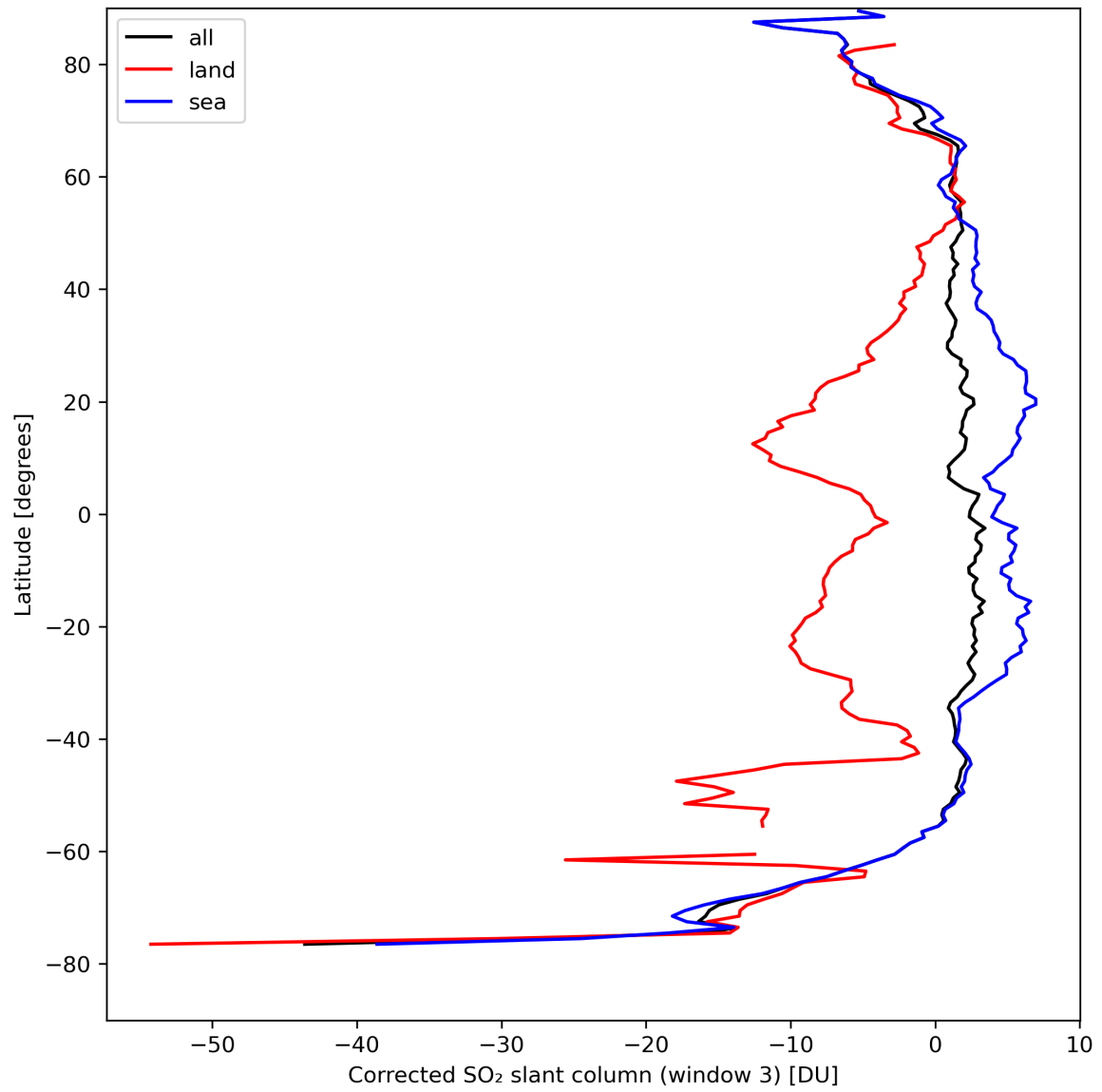
Figure 43: Zonal average of “Corrected SO 2 slant column (window 3)” for 2024-04-11 to 2024-04-13.
