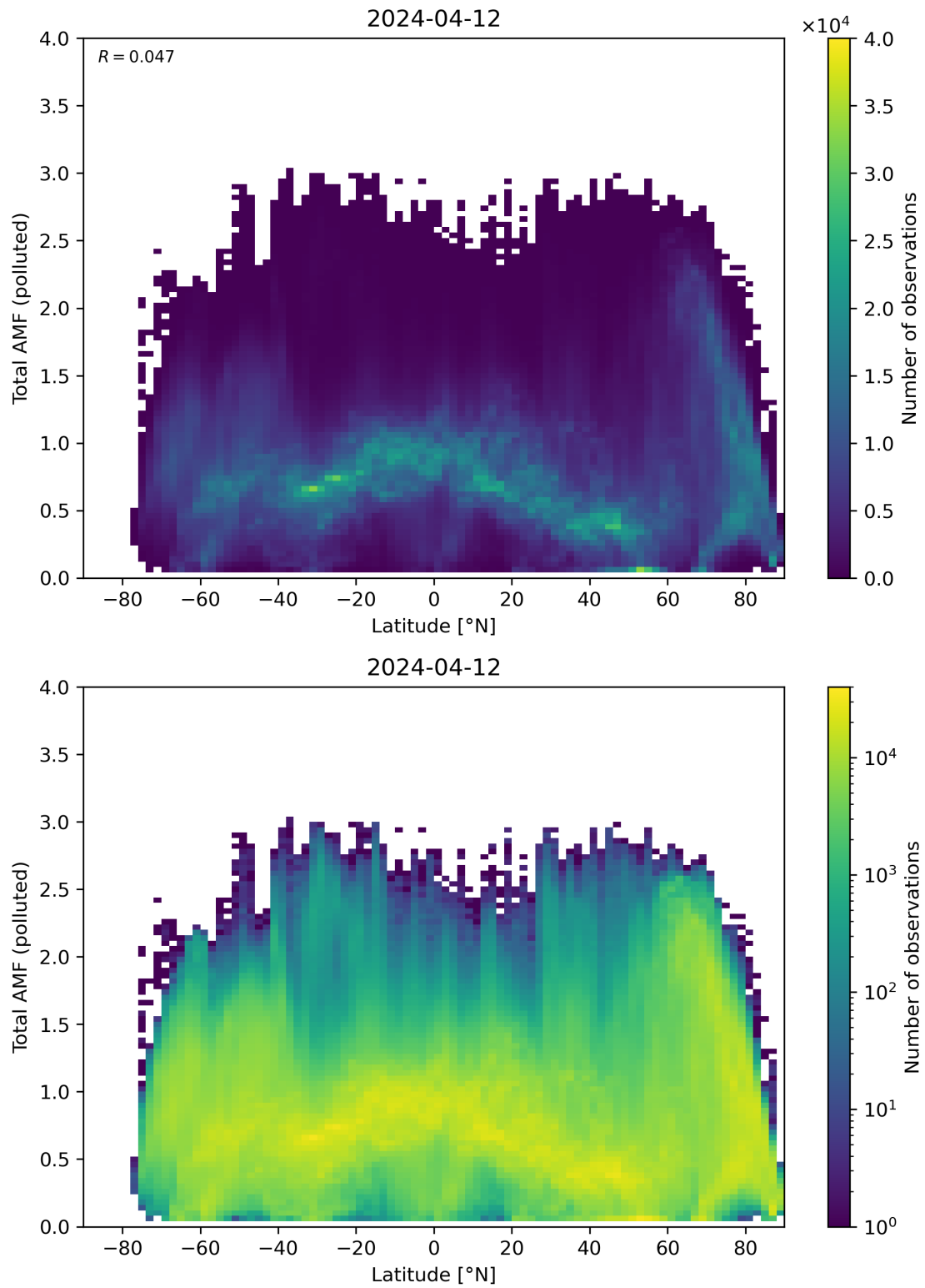
Figure 154: Scatter density plot of “Latitude” against “Total AMF (polluted)” for 2024-04-11 to 2024-04-13.
