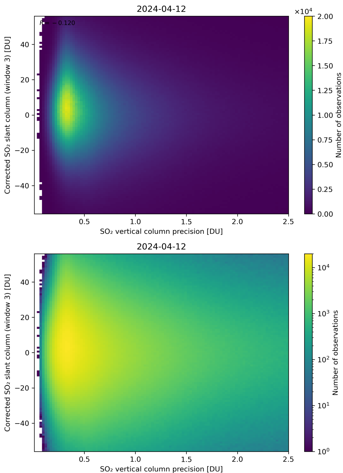
Figure 288: Scatter density plot of “SO 2 vertical column precision” against “Corrected SO 2 slant column (window 3)” for 2024-04-11 to 2024-04-13.
