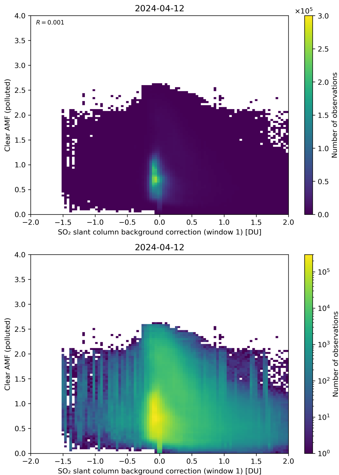
Figure 103: Scatter density plot of “SO 2 slant column background correction (window 1)” against “Clear AMF (polluted)” for 2024-04-11 to 2024-04-13.
