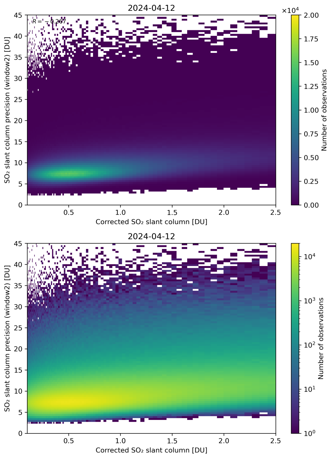
Figure 189: Scatter density plot of “Corrected SO 2 slant column” against “SO 2 slant column precision (window2)” for 2024-04-11 to 2024-04-13.
