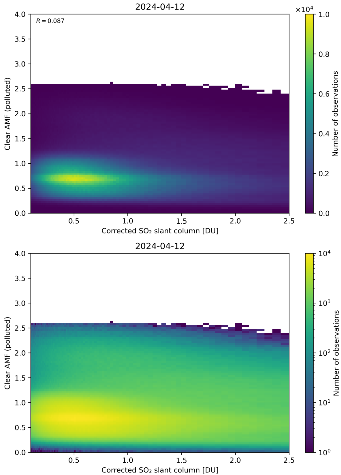
Figure 184: Scatter density plot of “Corrected SO 2 slant column” against “Clear AMF (polluted)” for 2024-04-11 to 2024-04-13.
