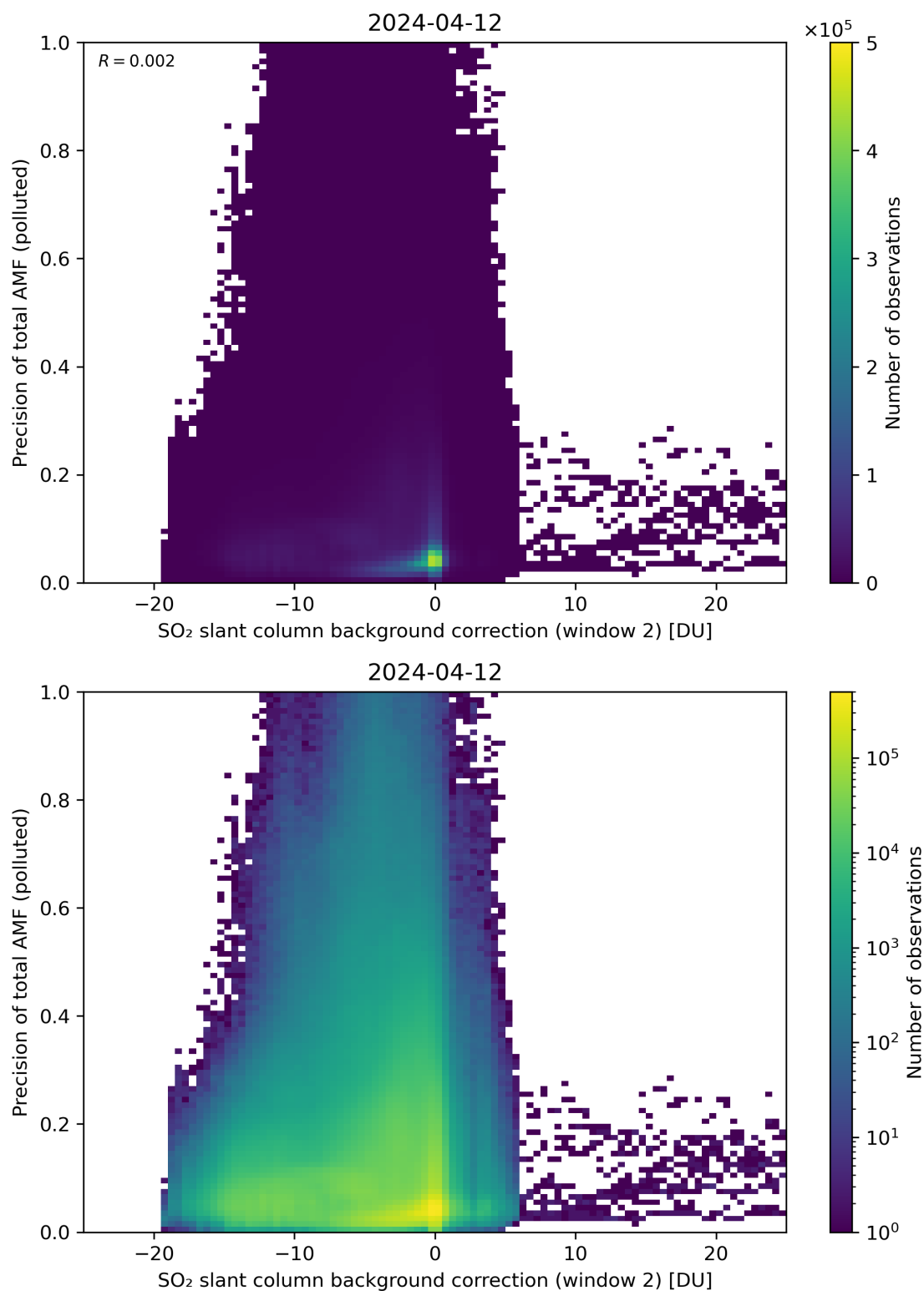
Figure 120: Scatter density plot of “SO 2 slant column background correction (window 2)” against “Precision of total AMF (polluted)” for 2024-04-11 to 2024-04-13.
