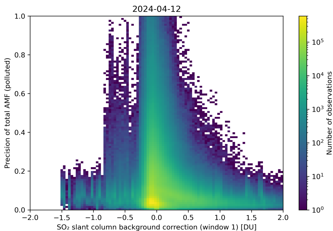
Figure 110: Scatter density plot of “SO 2 slant column background correction (window 1)” against “Precision of total AMF (polluted)” for 2024-04-11 to 2024-04-13.
