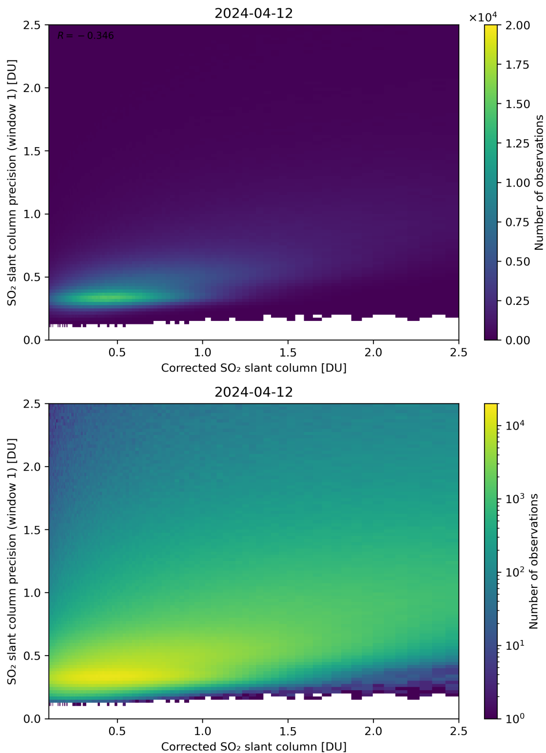
Figure 188: Scatter density plot of “Corrected SO 2 slant column” against “SO 2 slant column precision (window 1)” for 2024-04-11 to 2024-04-13.
