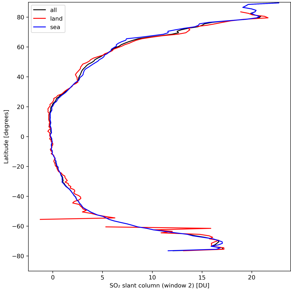
Figure 37: Zonal average of “SO 2 slant column (window 2)” for 2024-04-11 to 2024-04-13.
