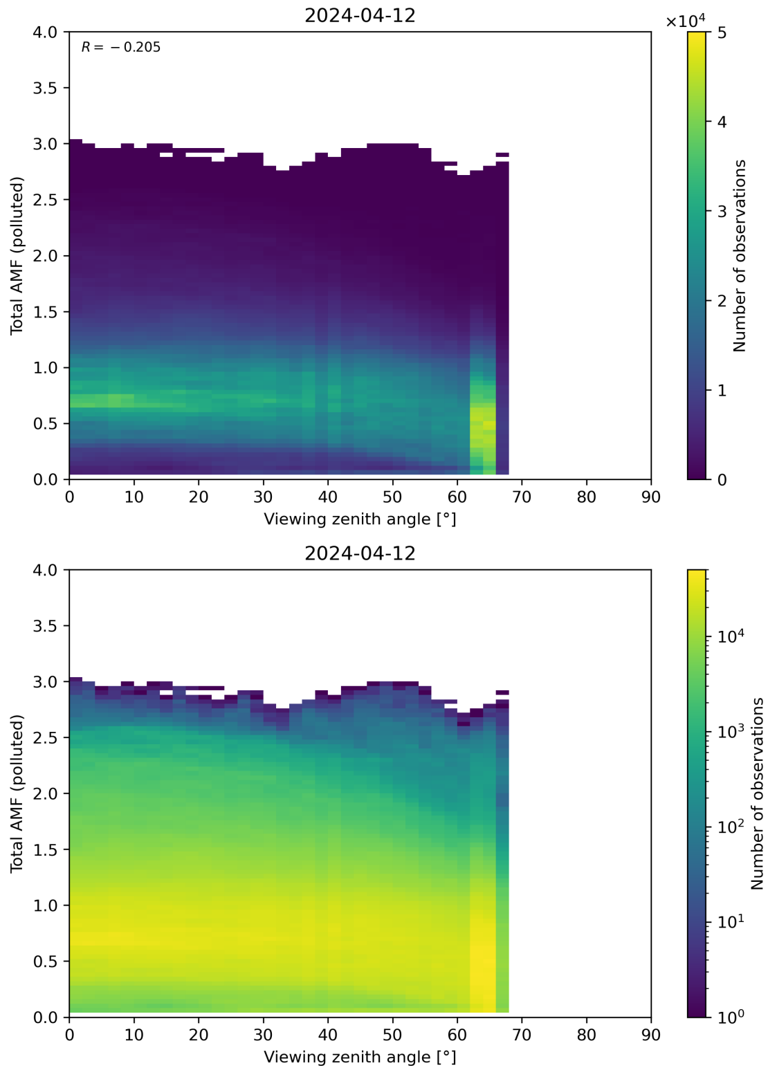
Figure 325: Scatter density plot of “Viewing zenith angle” against “Total AMF (polluted)” for 2024-04-11 to 2024-04-13.
