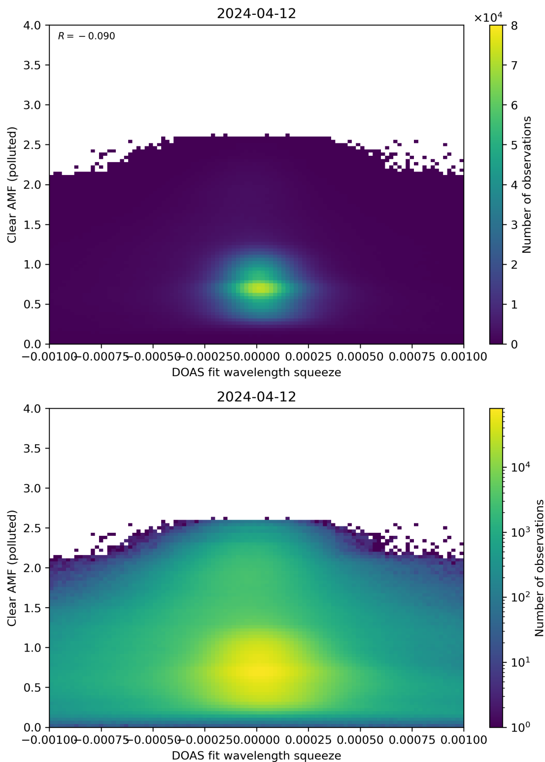
Figure 133: Scatter density plot of “DOAS fit wavelength squeeze” against “Clear AMF (polluted)” for 2024-04-11 to 2024-04-13.
