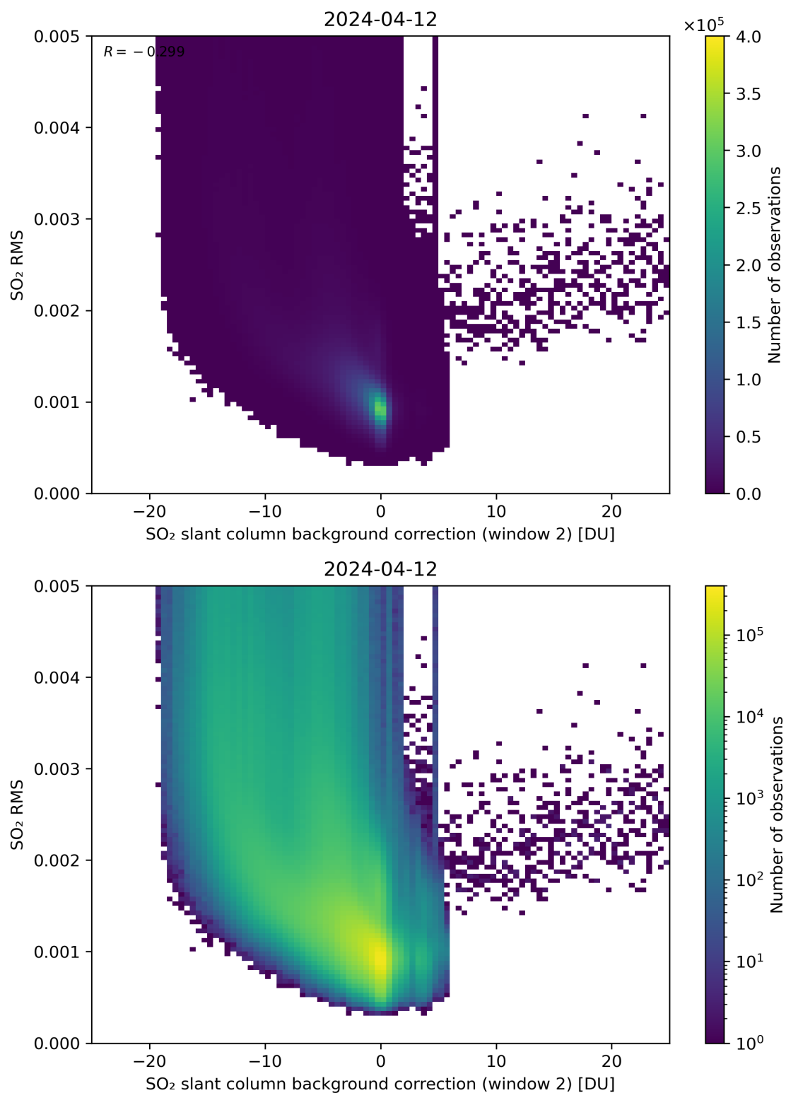
Figure 114: Scatter density plot of “SO 2 slant column background correction (window 2)” against “SO 2 RMS” for 2024-04-11 to 2024-04-13.
