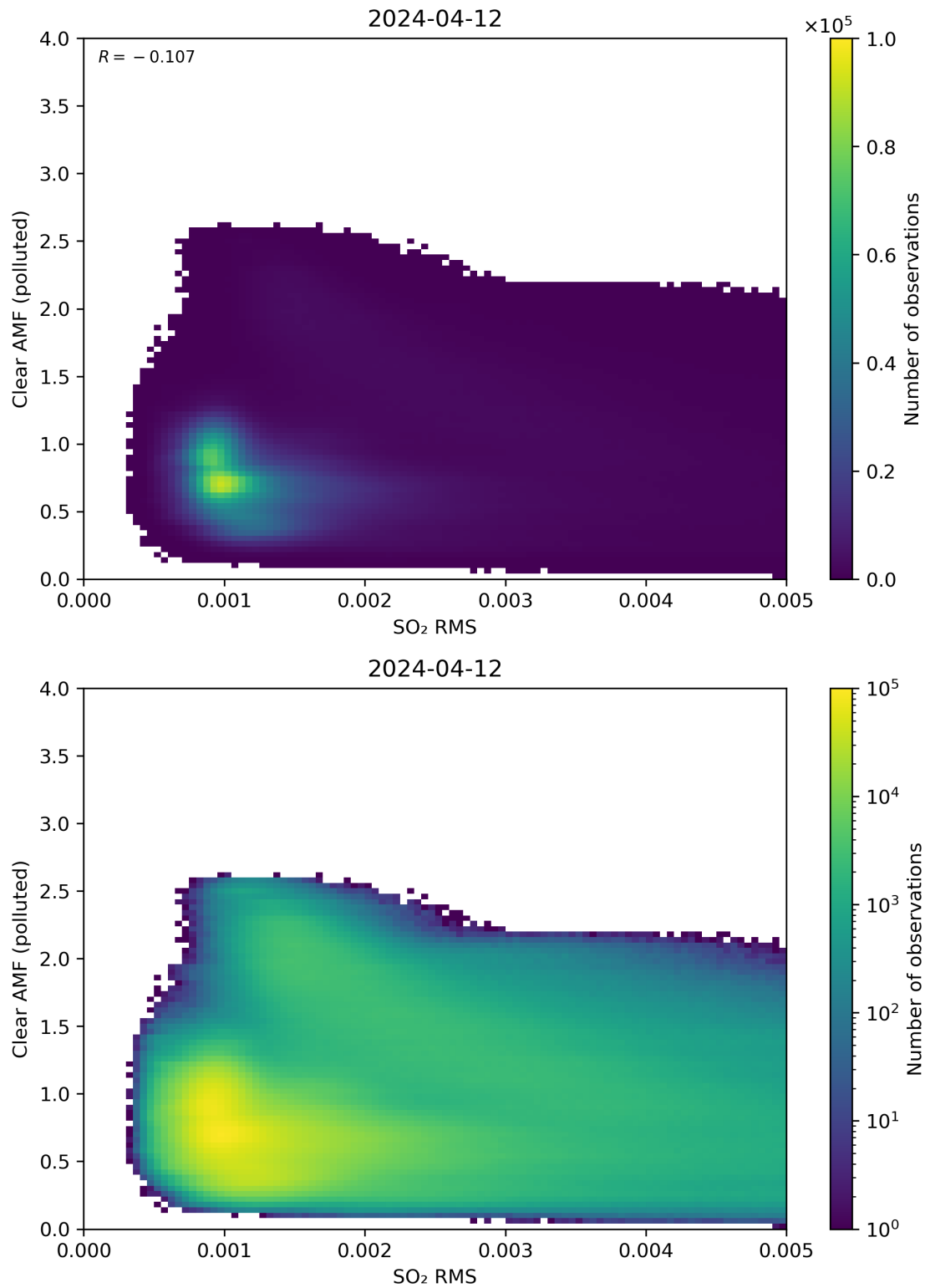
Figure 136: Scatter density plot of “SO 2 RMS” against “Clear AMF (polluted)” for 2024-04-11 to 2024-04-13.
