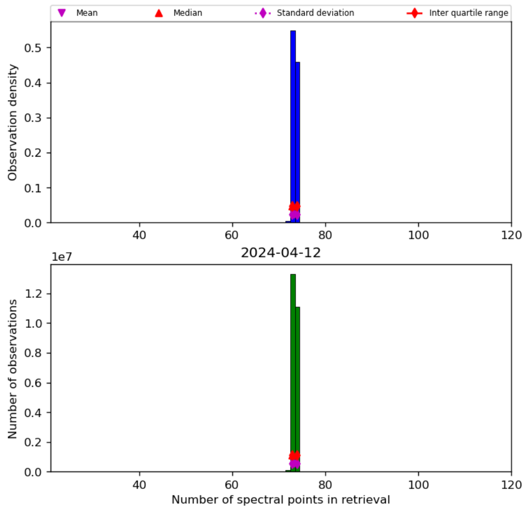
Figure 74: Histogram of “Number of spectral points in retrieval” for 2024-04-11 to 2024-04-13
