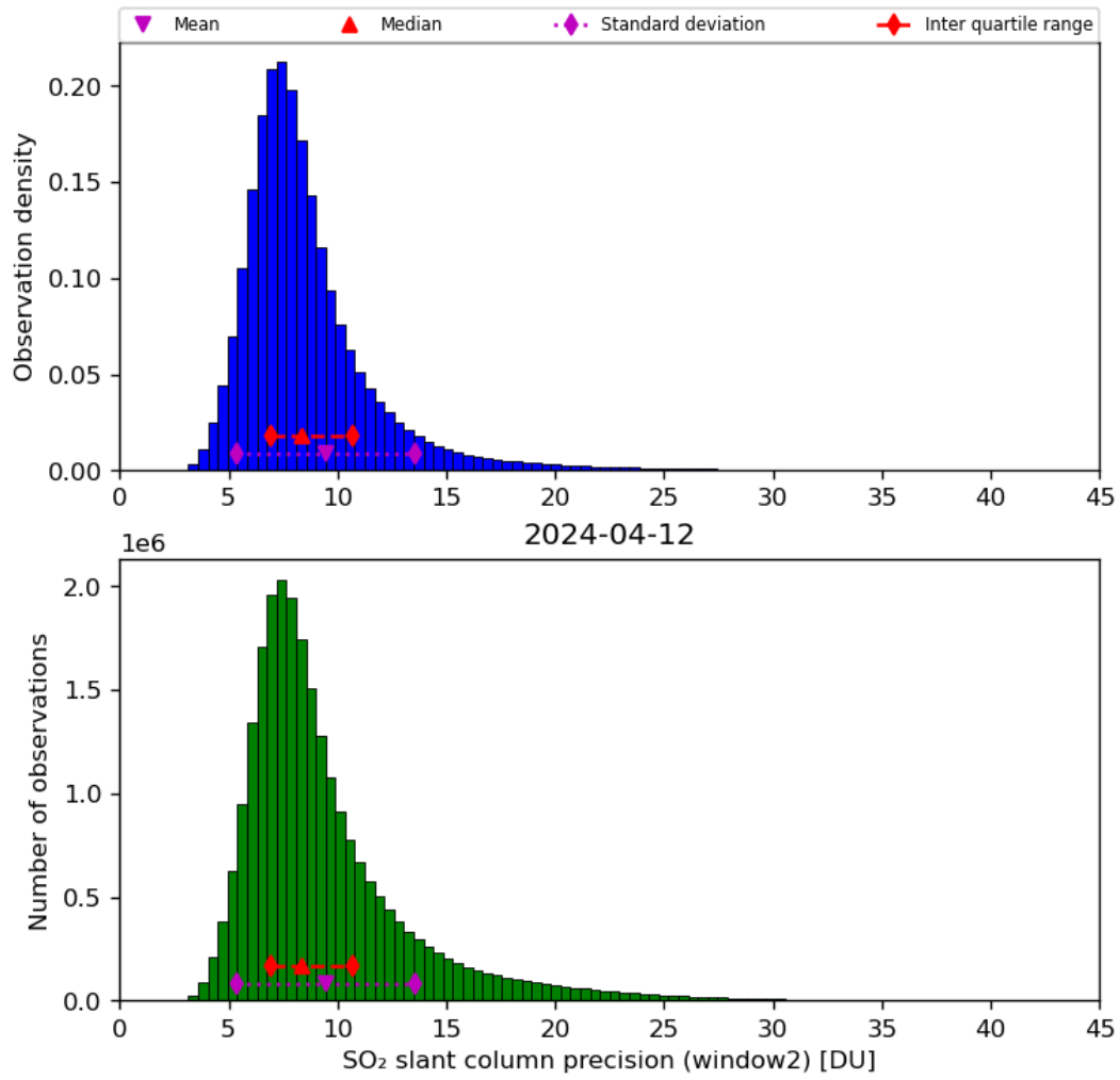
Figure 61: Histogram of “SO 2 slant column precision (window2)” for 2024-04-11 to 2024-04-13
