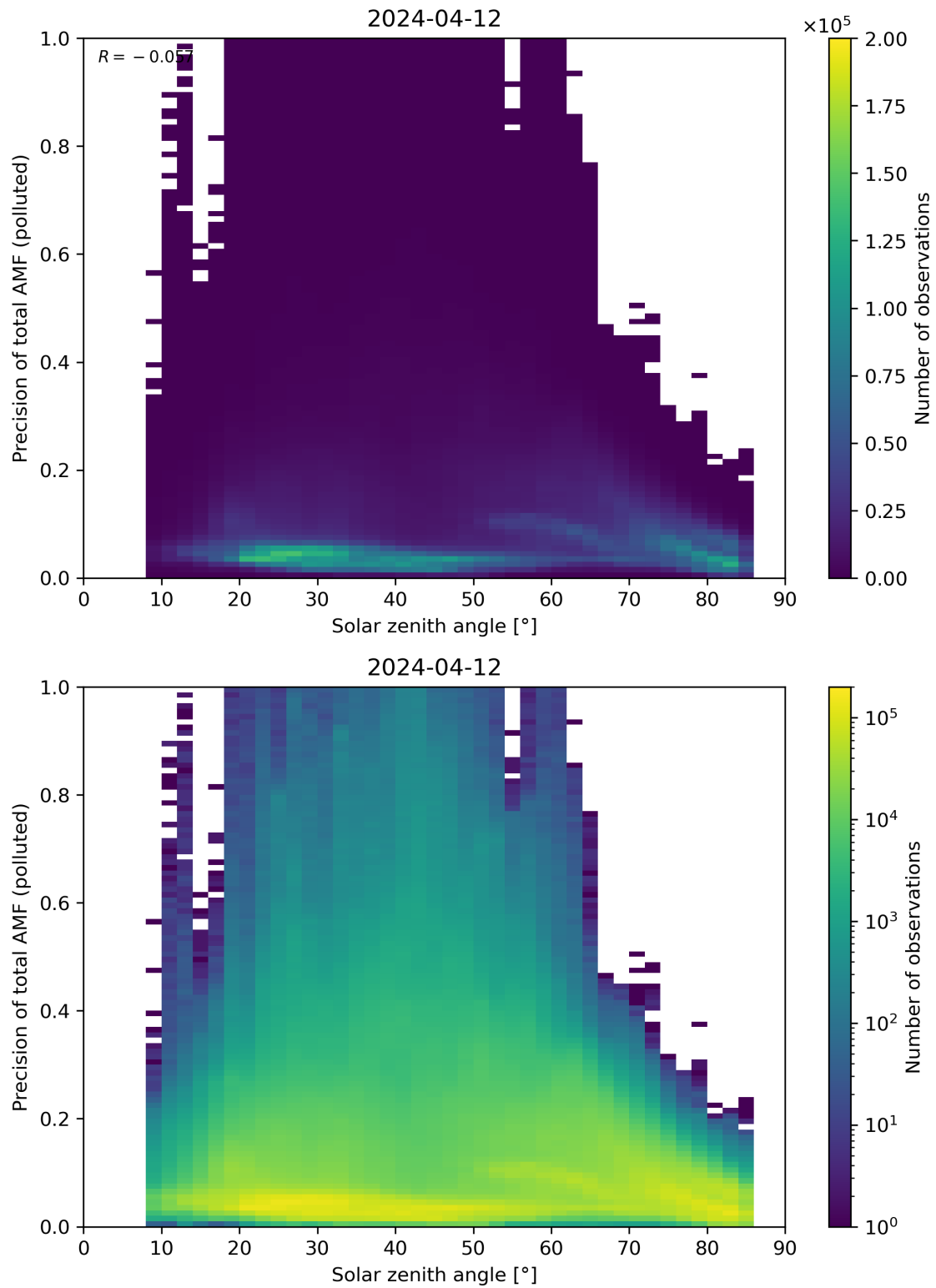
Figure 175: Scatter density plot of “Solar zenith angle” against “Precision of total AMF (polluted)” for 2024-04-11 to 2024-04-13.
