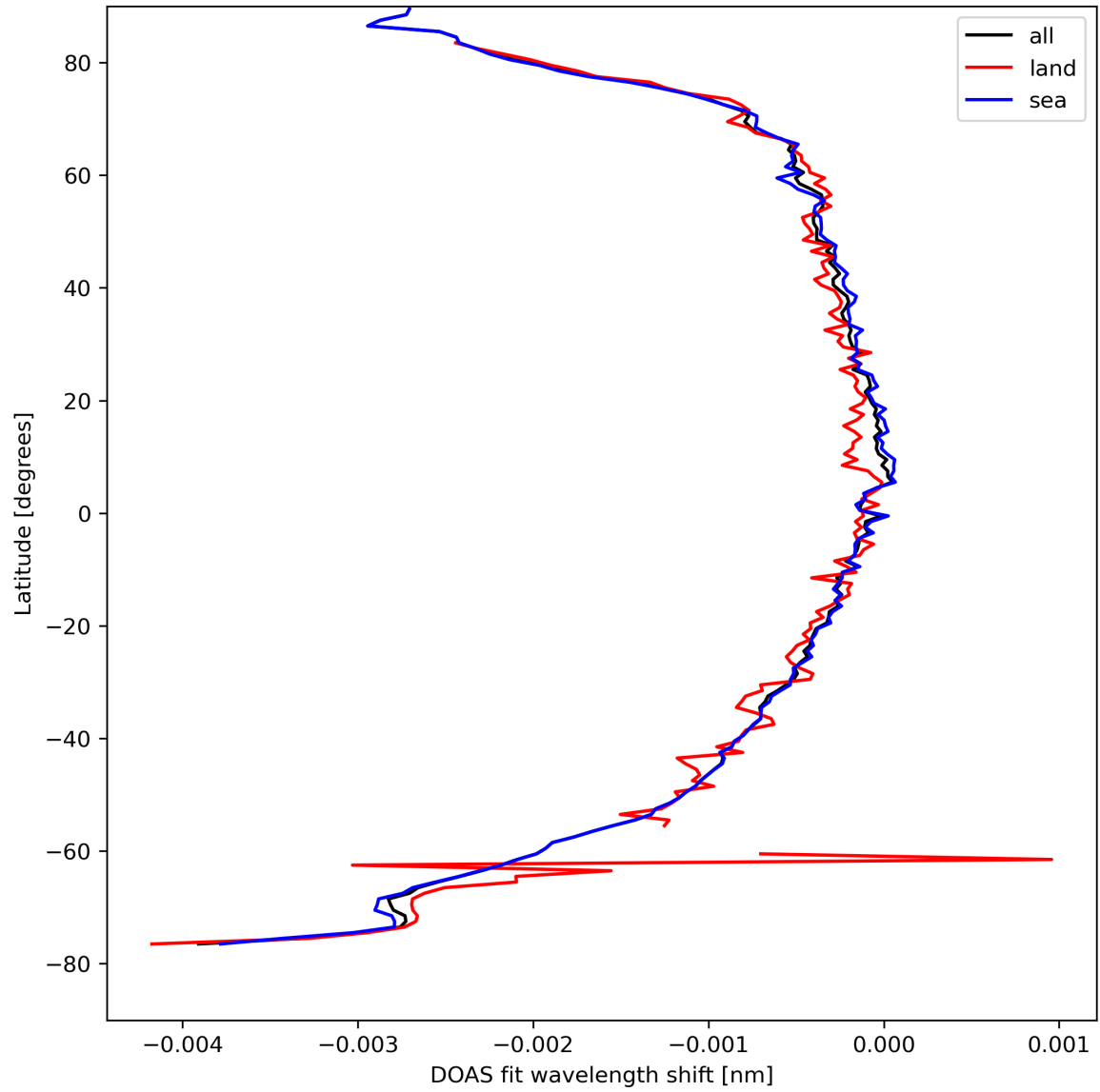
Figure 45: Zonal average of “DOAS fit wavelength shift” for 2024-04-11 to 2024-04-13.
