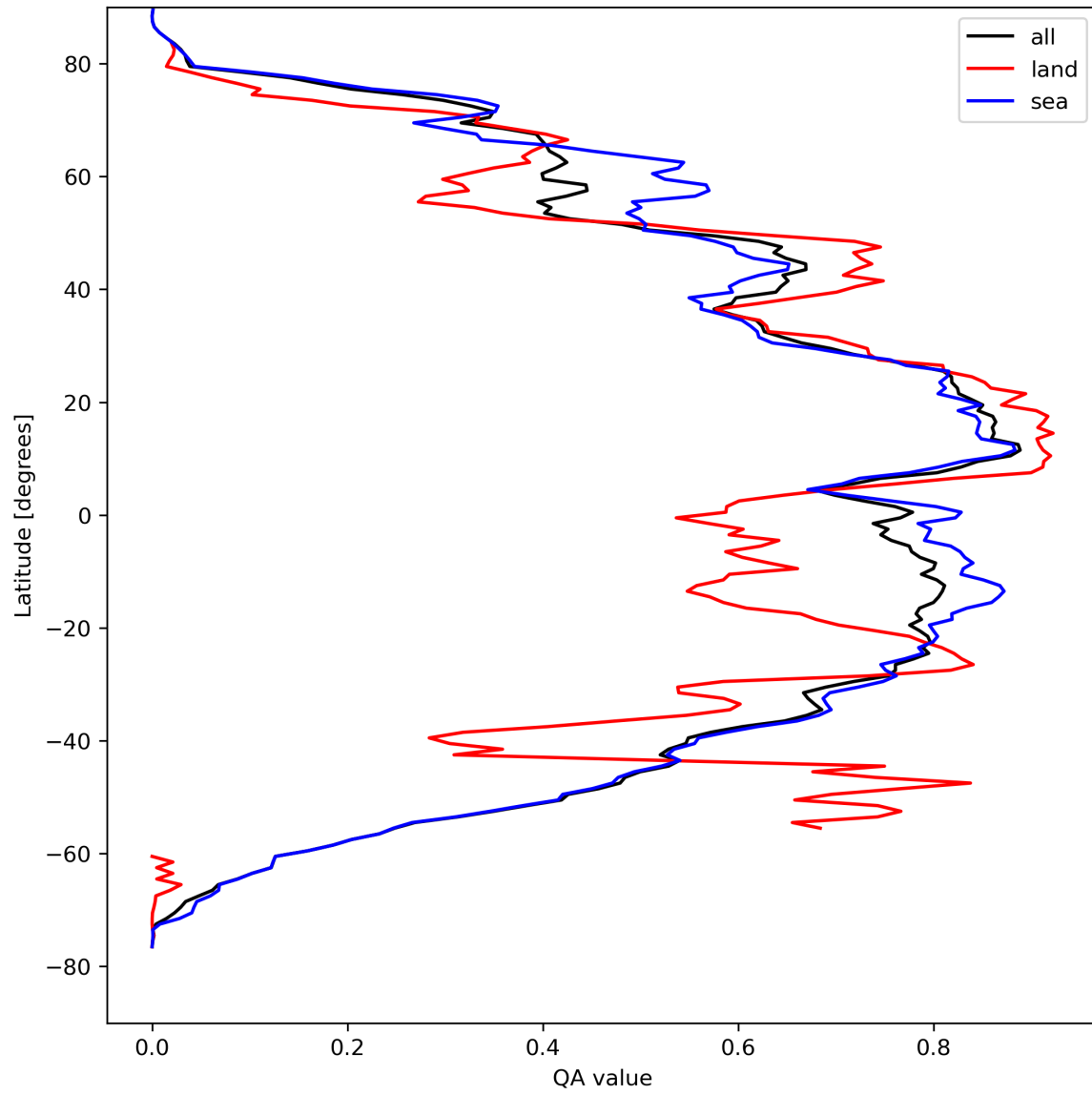
Figure 29: Zonal average of “QA value” for 2024-04-11 to 2024-04-13.
