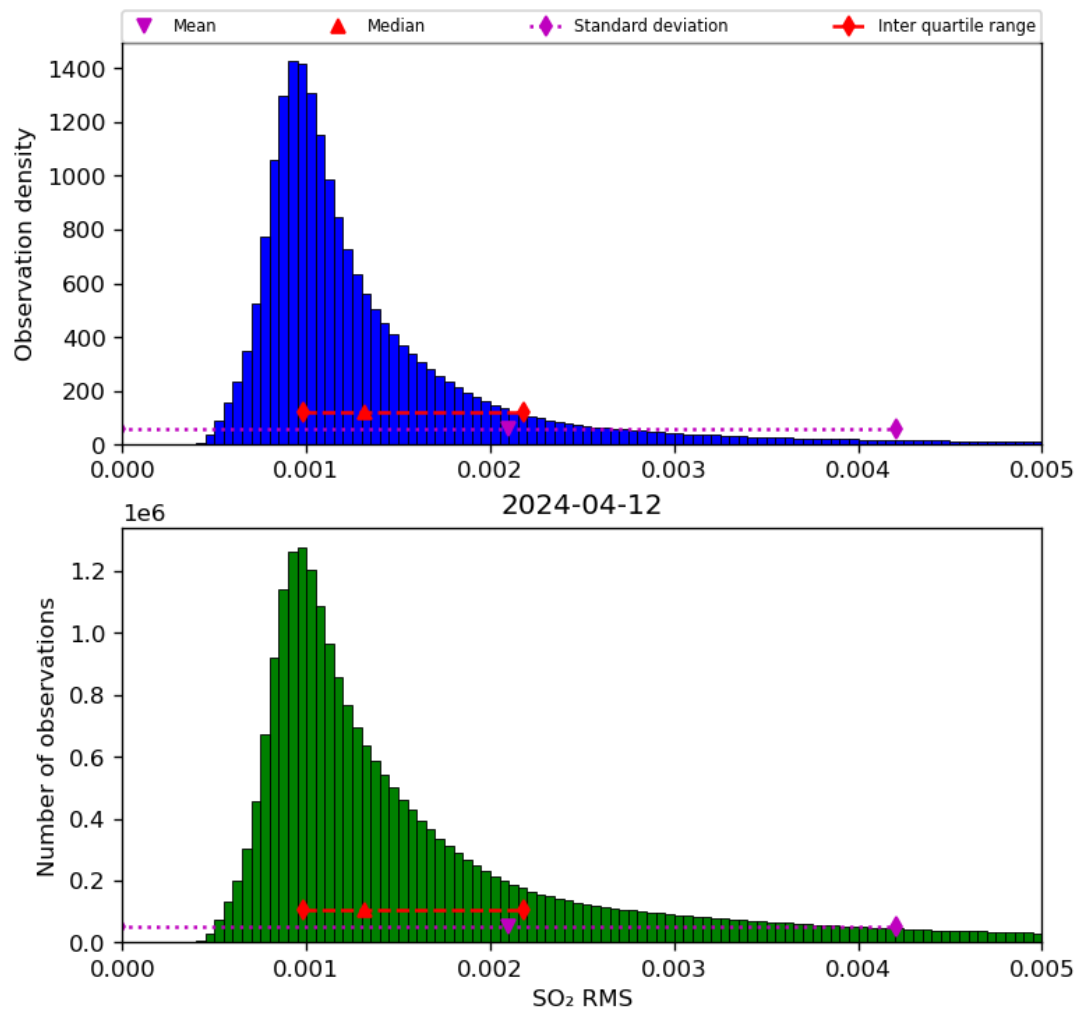
Figure 70: Histogram of “SO 2 RMS” for 2024-04-11 to 2024-04-13
