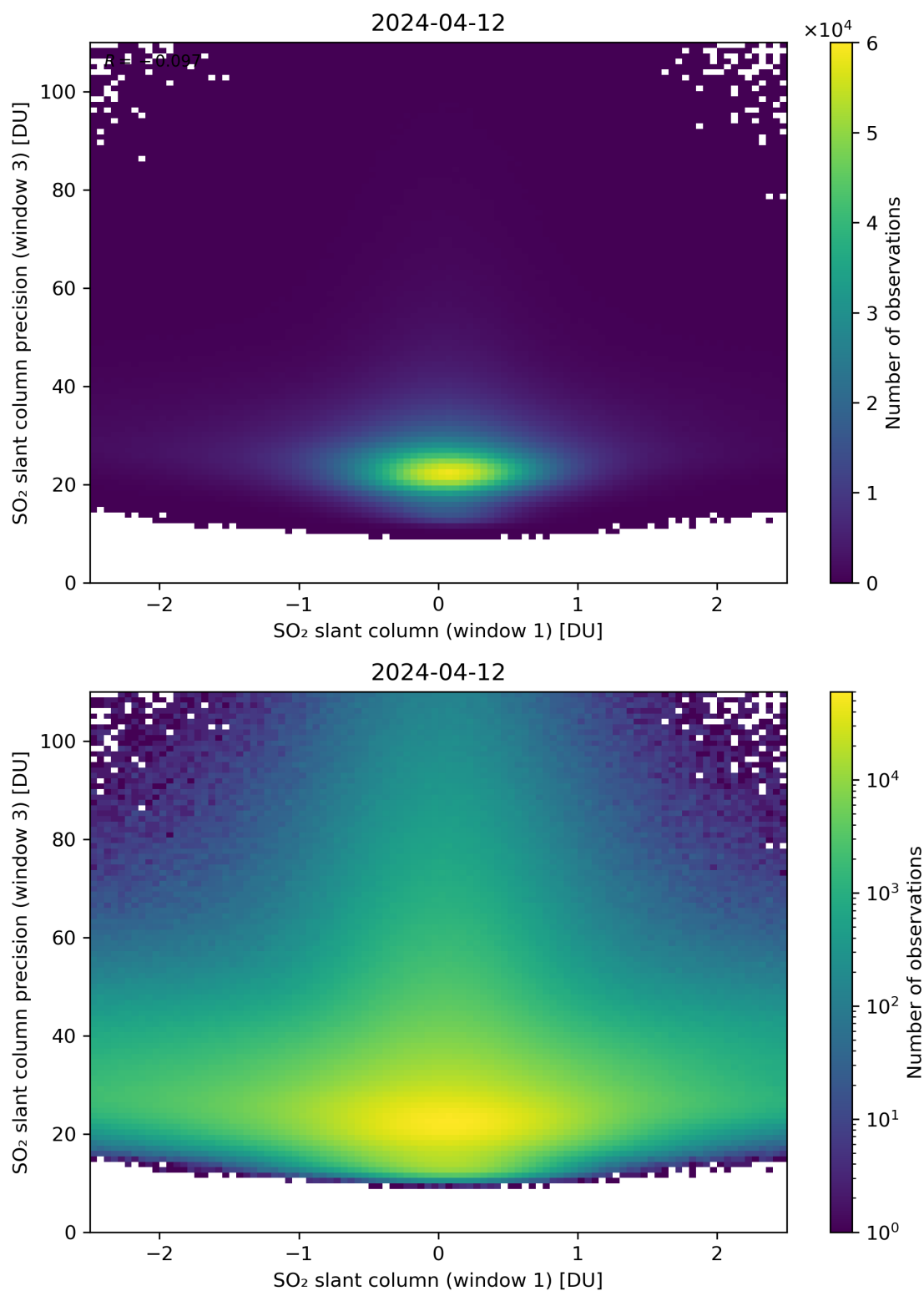
Figure 238: Scatter density plot of “SO 2 slant column (window 1)” against “SO 2 slant column precision (window 3)” for 2024-04-11 to 2024-04-13.
