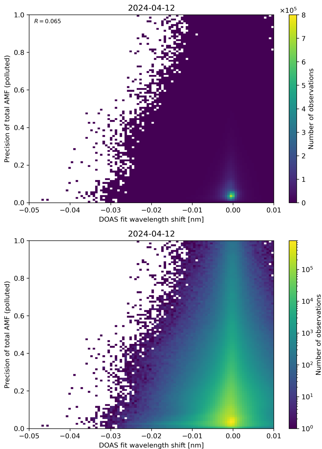
Figure 131: Scatter density plot of “DOAS fit wavelength shift” against “Precision of total AMF (polluted)” for 2024-04-11 to 2024-04-13.
