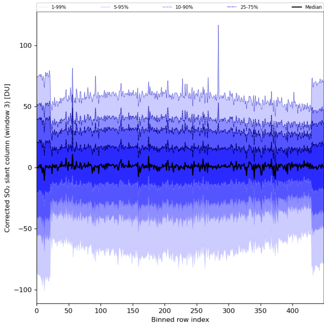
Figure 89: Along track statistics of “Corrected SO 2 slant column (window 3)” for 2024-04-11 to 2024-04-13
