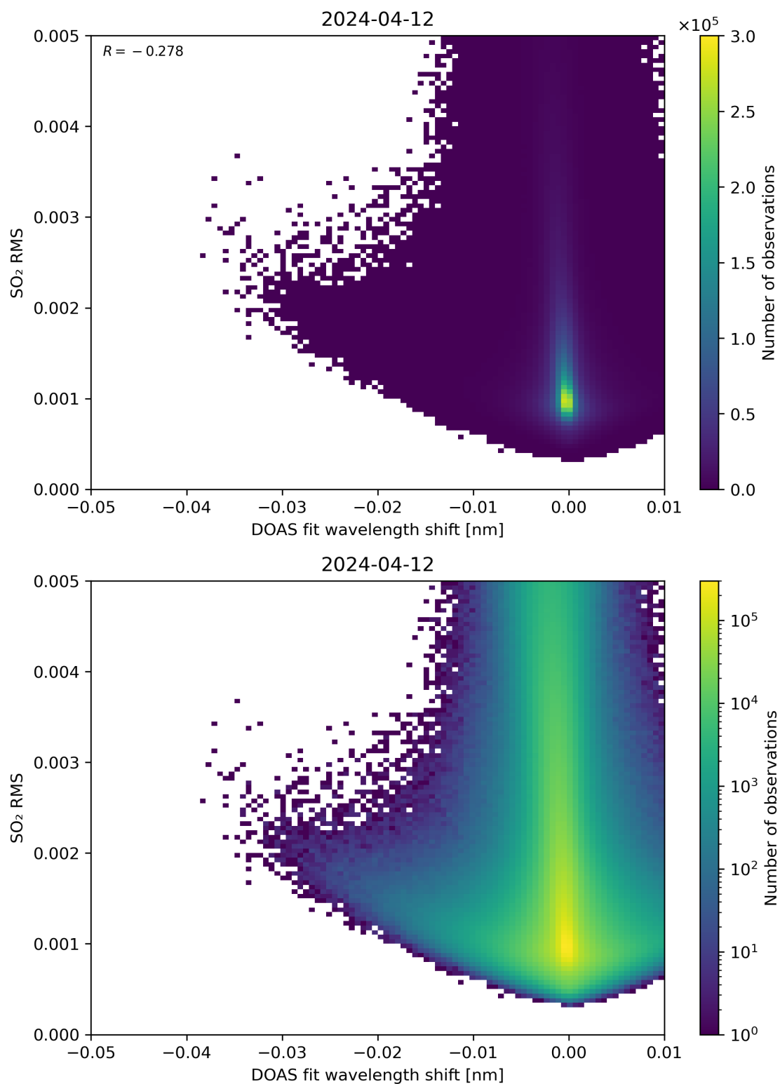
Figure 128: Scatter density plot of “DOAS fit wavelength shift” against “SO 2 RMS” for 2024-04-11 to 2024-04-13.
