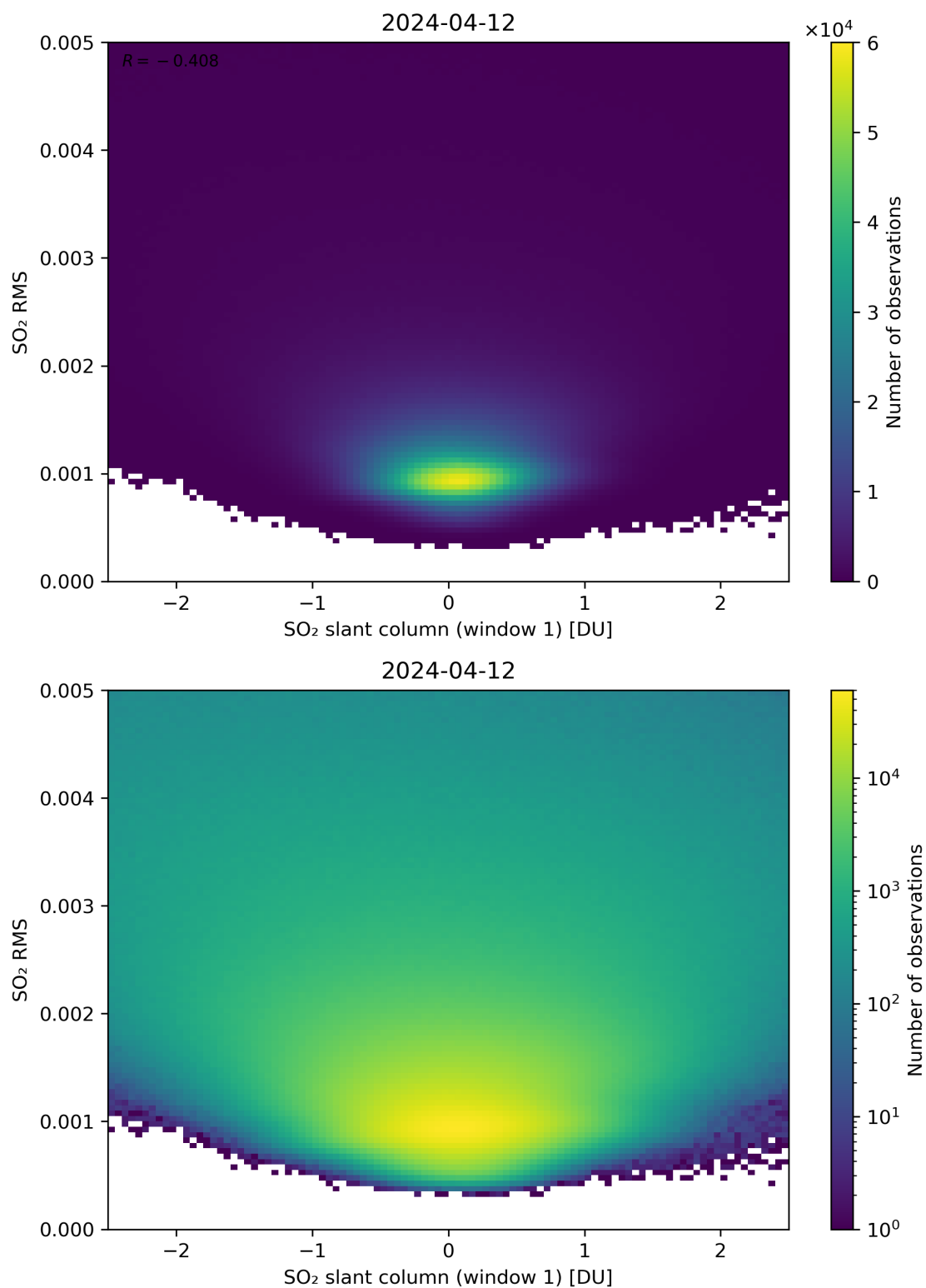
Figure 217: Scatter density plot of “SO 2 slant column (window 1)” against “SO 2 RMS” for 2024-04-11 to 2024-04-13.
