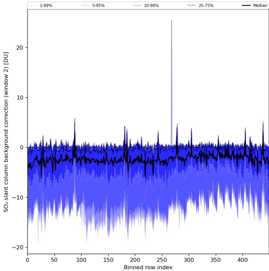
Figure 86: Along track statistics of “SO 2 slant column background correction (window 2)” for 2024-04-11 to 2024-04-13
