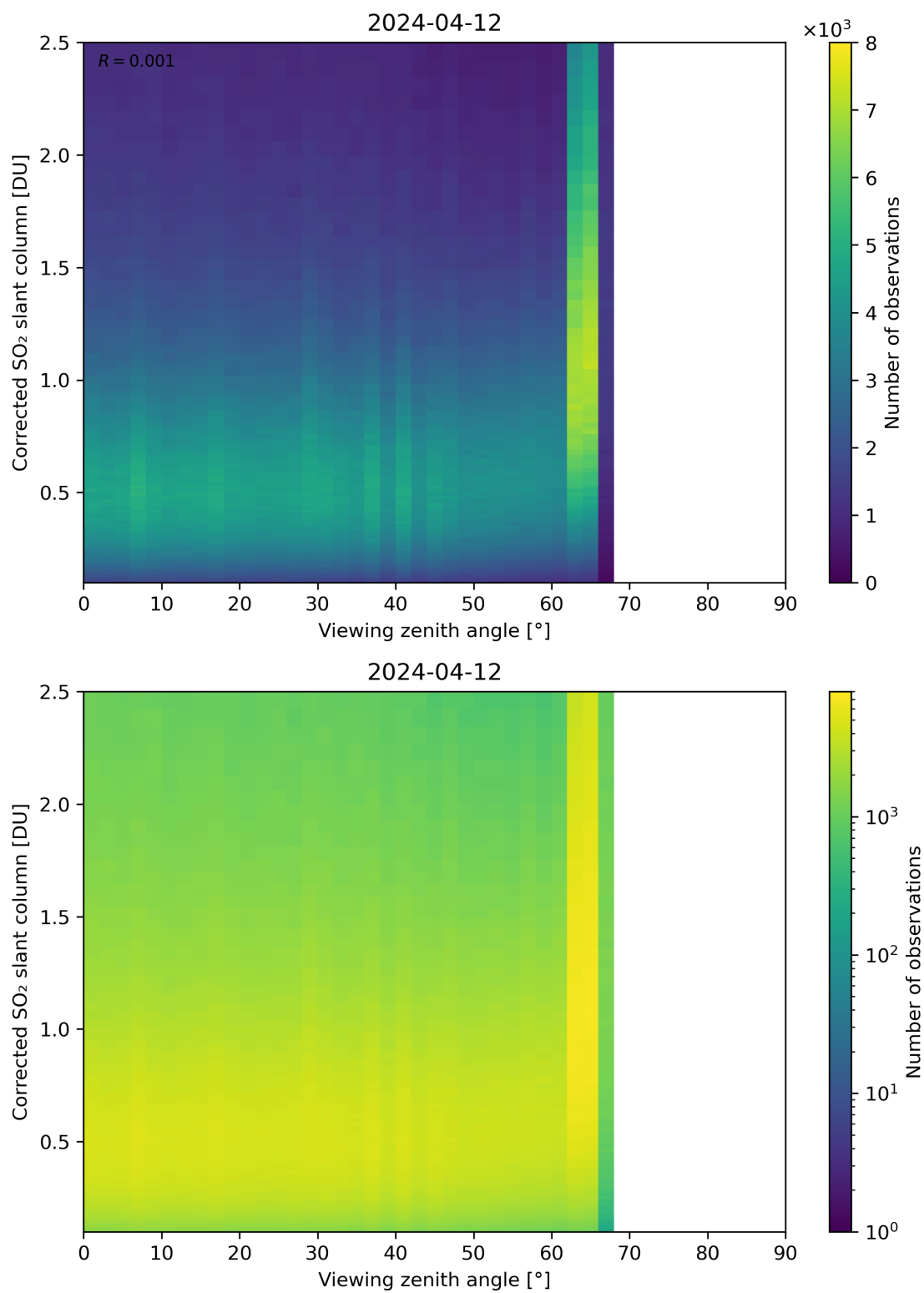
Figure 317: Scatter density plot of “Viewing zenith angle” against “Corrected SO 2 slant column” for 2024-04-11 to 2024-04-13.
