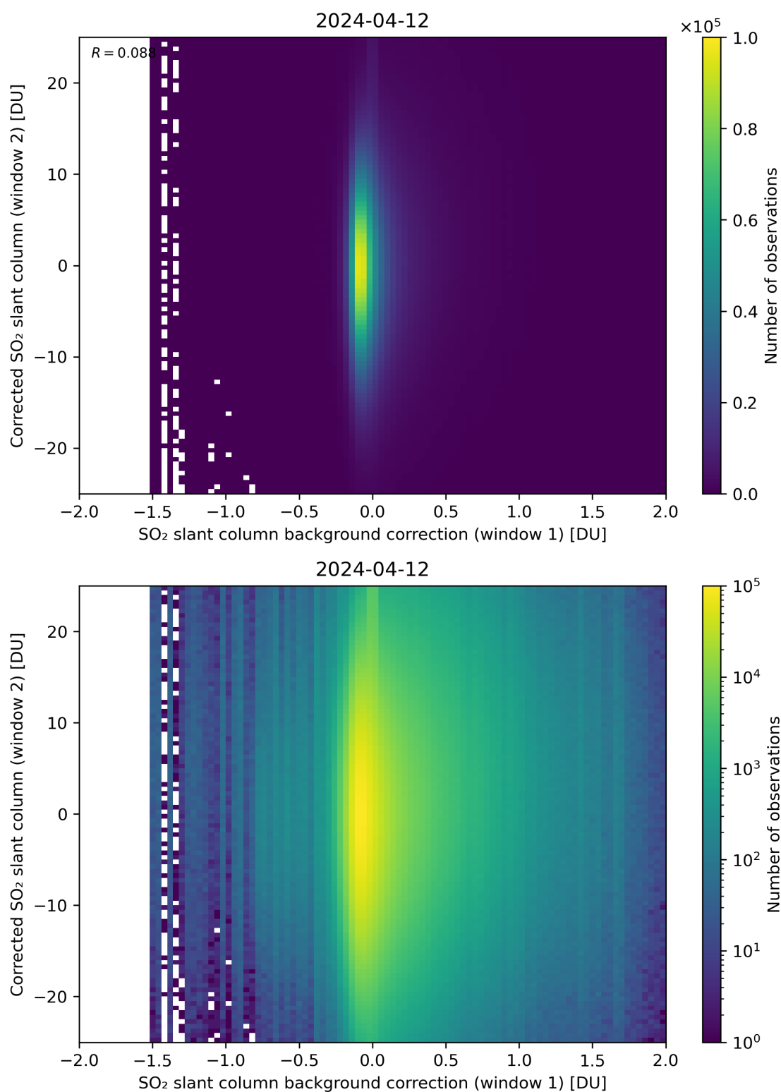
Figure 104: Scatter density plot of “SO 2 slant column background correction (window 1)” against “Corrected SO 2 slant column (window 2)” for 2024-04-11 to 2024-04-13.
