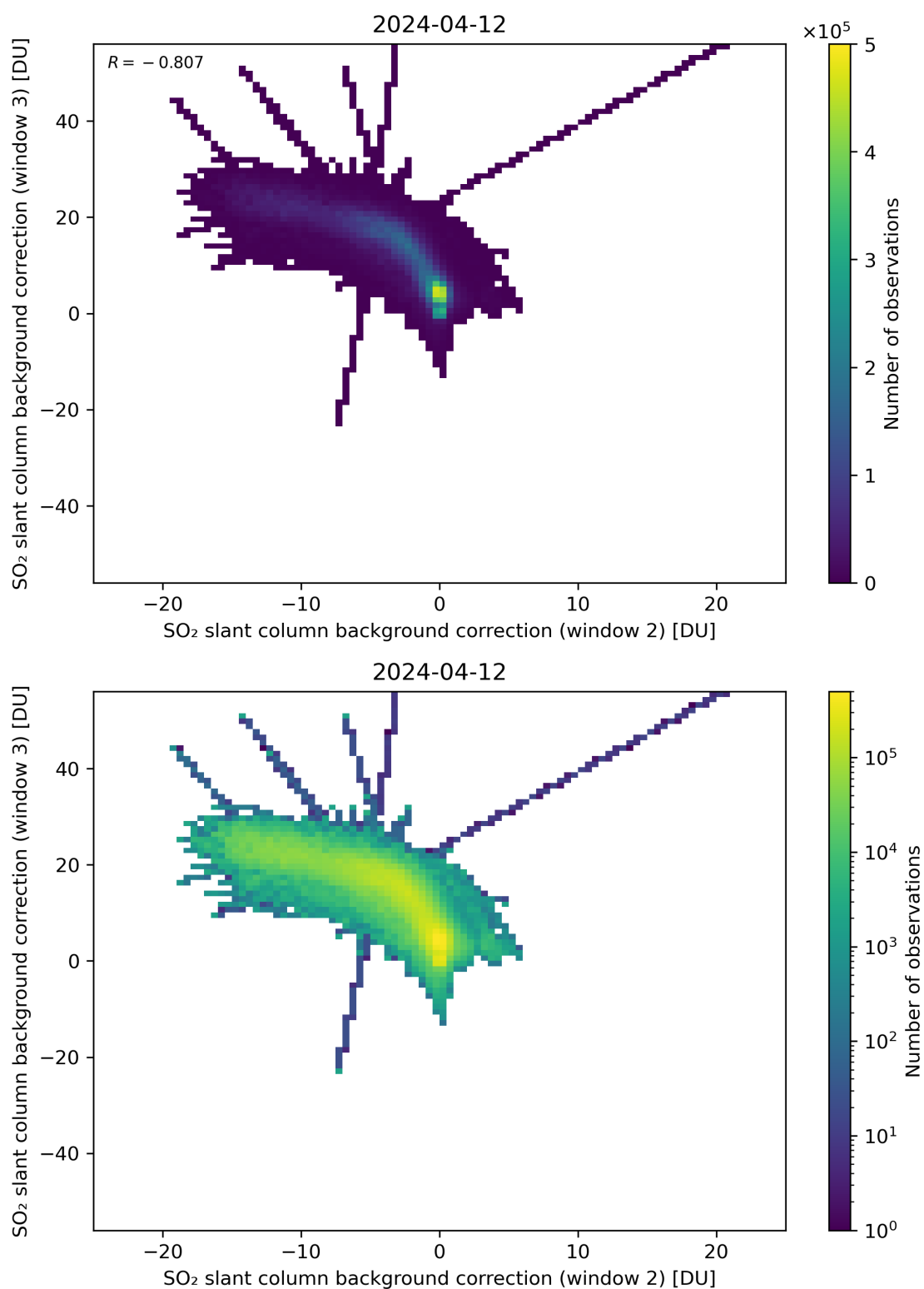
Figure 111: Scatter density plot of “SO 2 slant column background correction (window 2)” against “SO 2 slant column background correction (window 3)” for 2024-04-11 to 2024-04-13.
