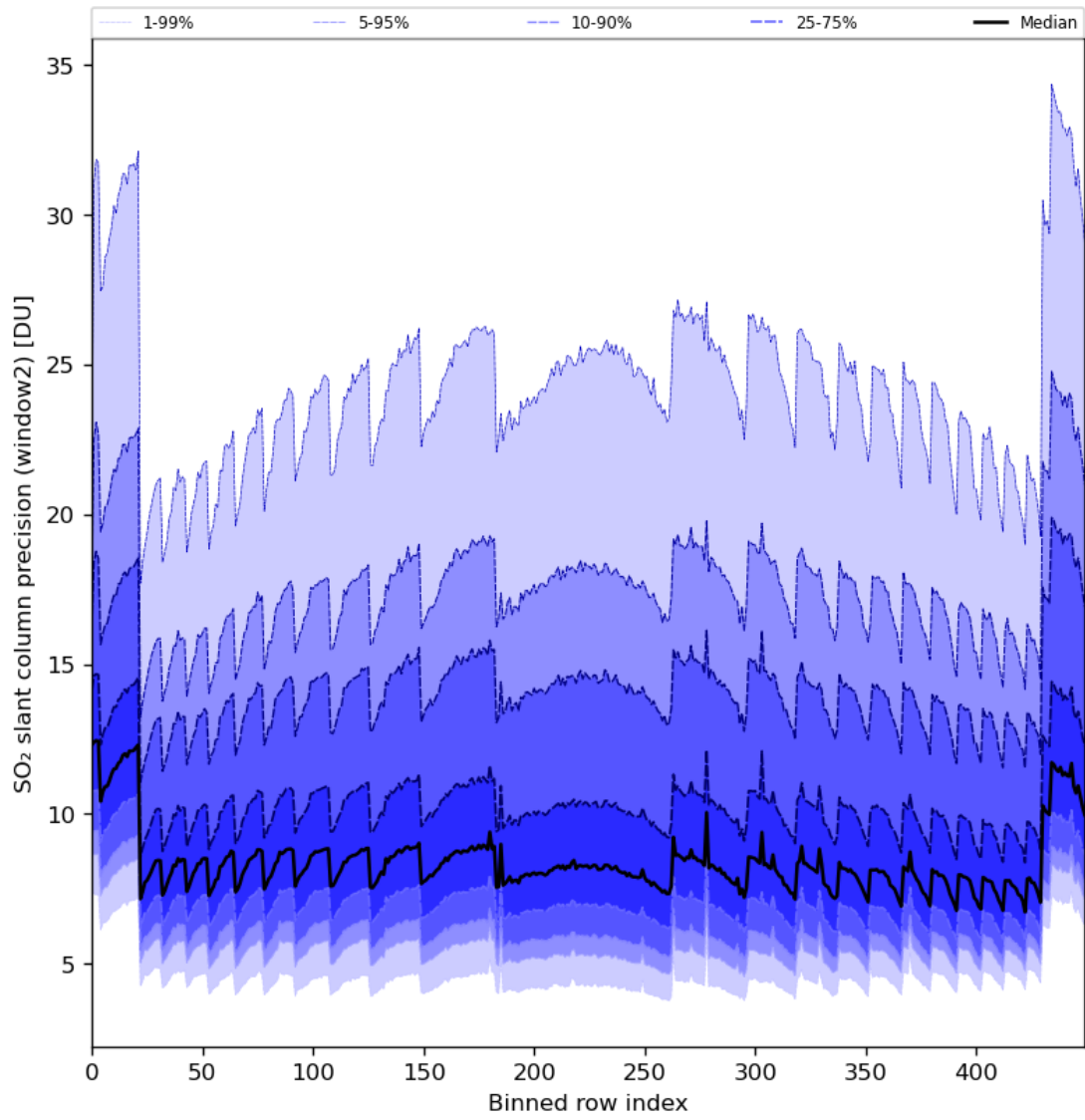
Figure 84: Along track statistics of “SO 2 slant column precision (window2)” for 2024-04-11 to 2024-04-13
