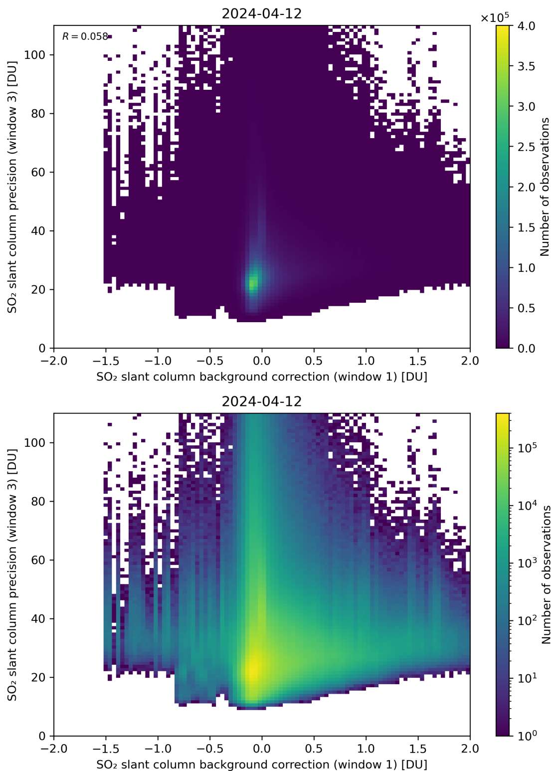
Figure 108: Scatter density plot of “SO 2 slant column background correction (window 1)” against “SO 2 slant column precision (window 3)” for 2024-04-11 to 2024-04-13.
