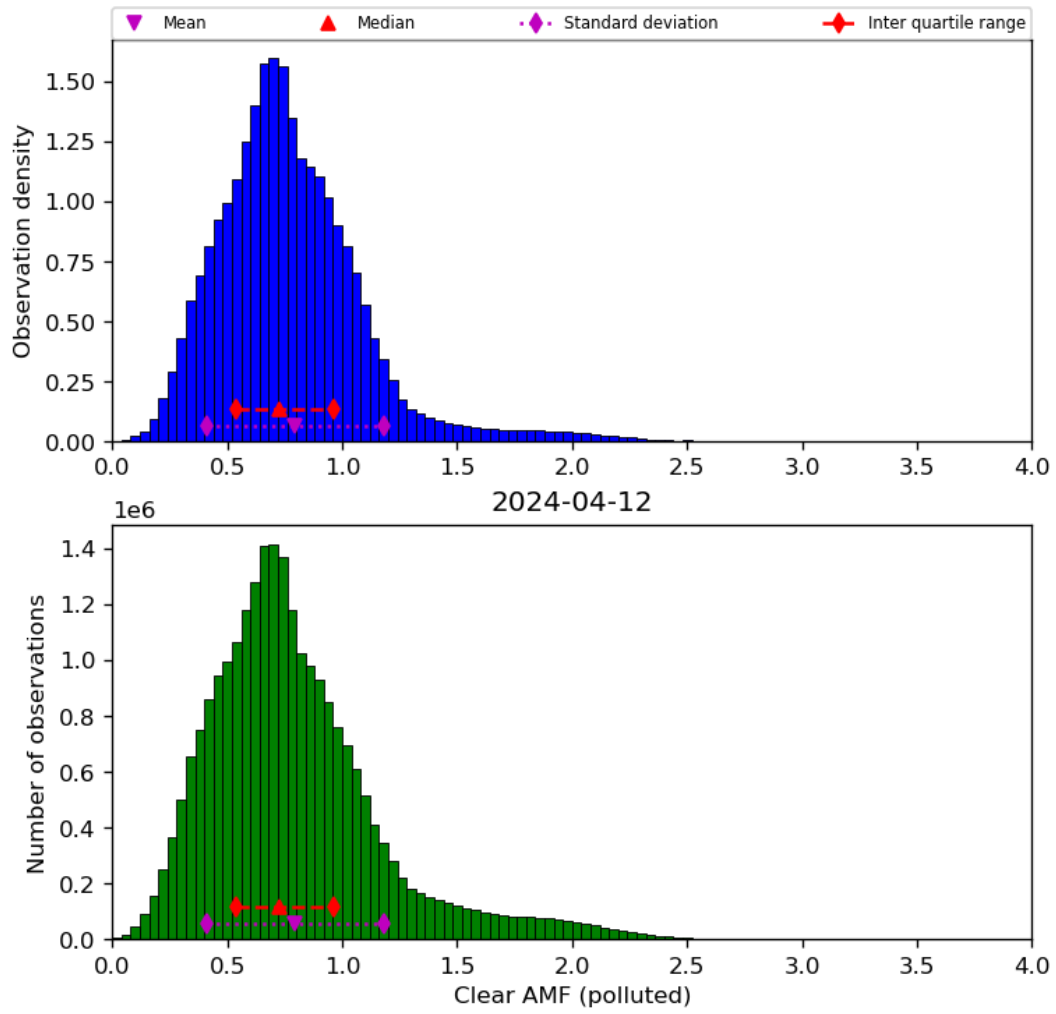
Figure 73: Histogram of "Clear AMF (polluted)" for 2024-04-11 to 2024-04-13
