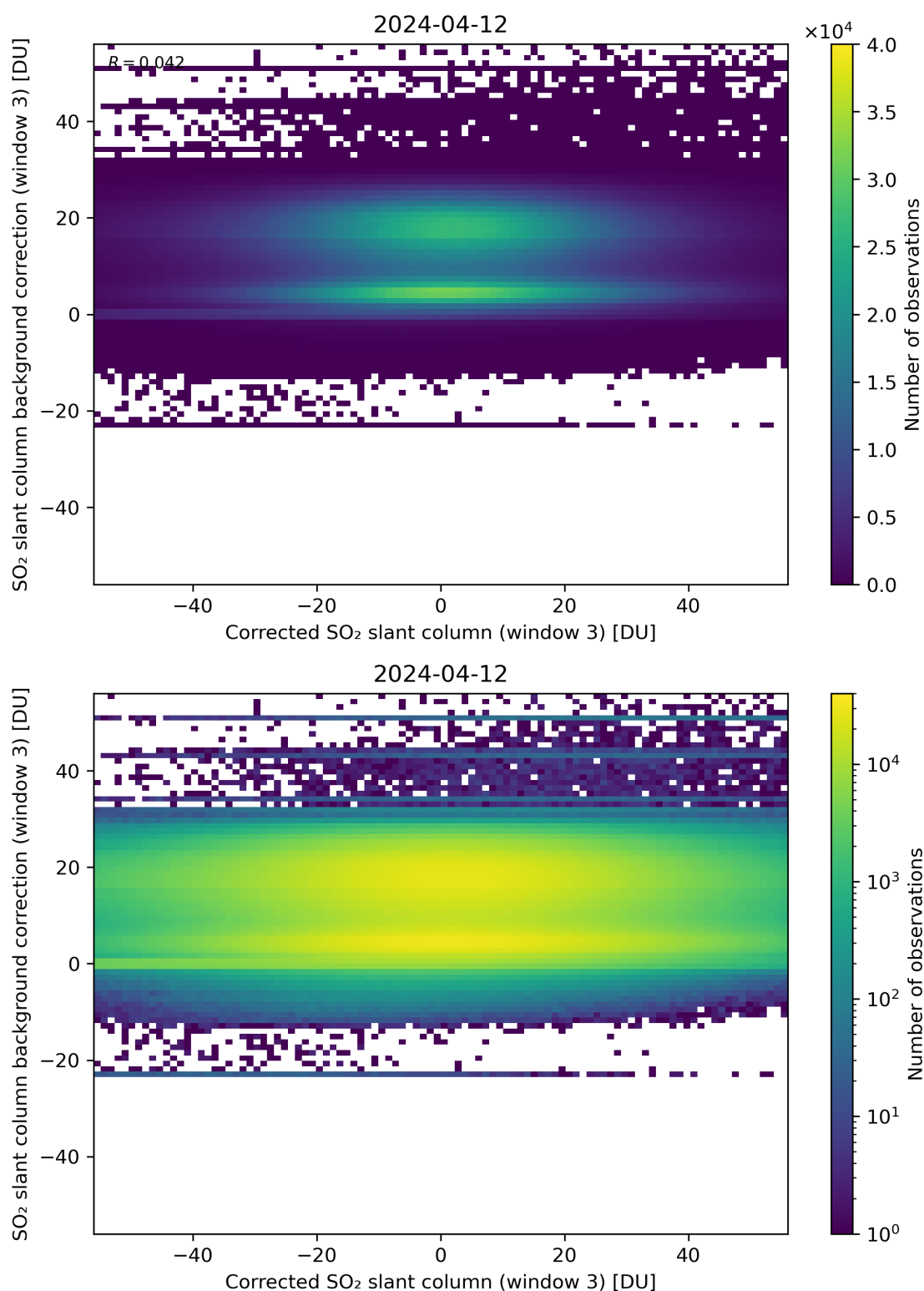
Figure 205: Scatter density plot of “Corrected SO 2 slant column (window 3)” against “SO 2 slant column background correction (window 3)” for 2024-04-11 to 2024-04-13.
