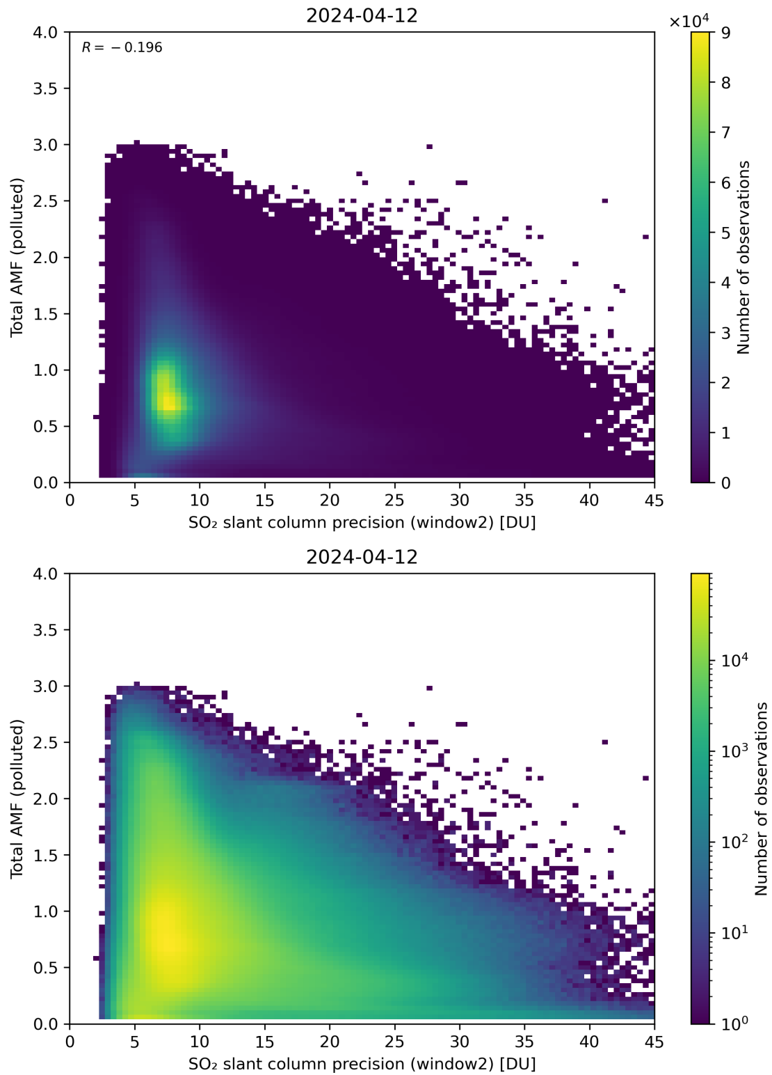
Figure 251: Scatter density plot of “SO 2 slant column precision (window2)” against “Total AMF (polluted)” for 2024-04-11 to 2024-04-13.
