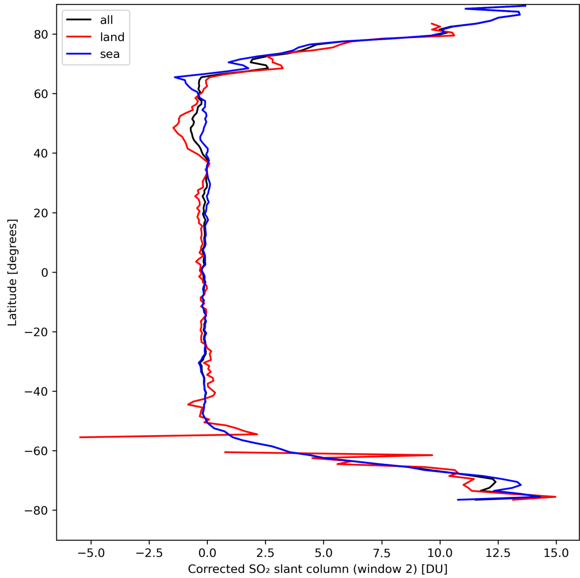
Figure 39: Zonal average of “Corrected SO 2 slant column (window 2)” for 2024-04-11 to 2024-04-13.
