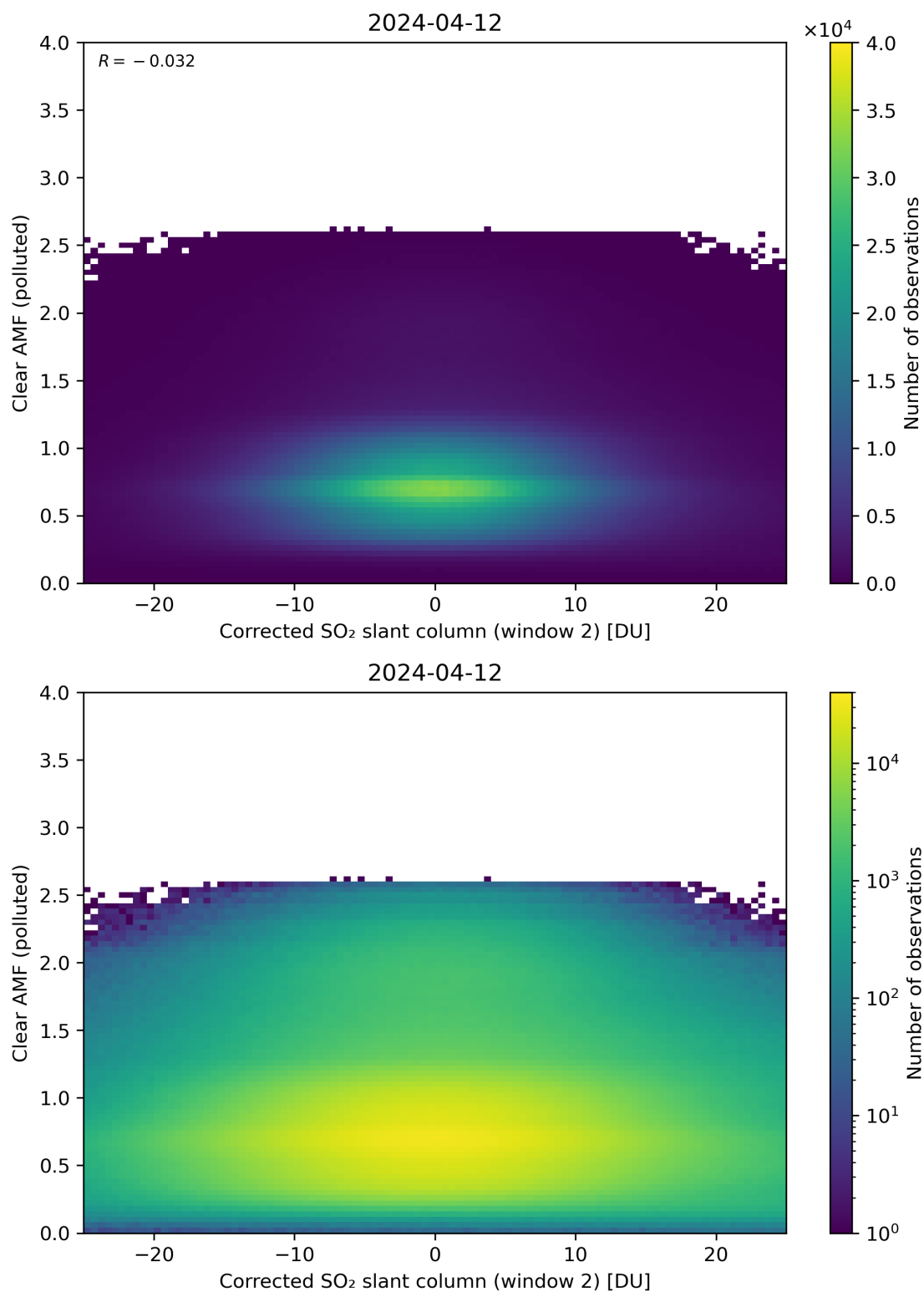
Figure 199: Scatter density plot of “Corrected SO 2 slant column (window 2)” against “Clear AMF (polluted)” for 2024-04-11 to 2024-04-13.
