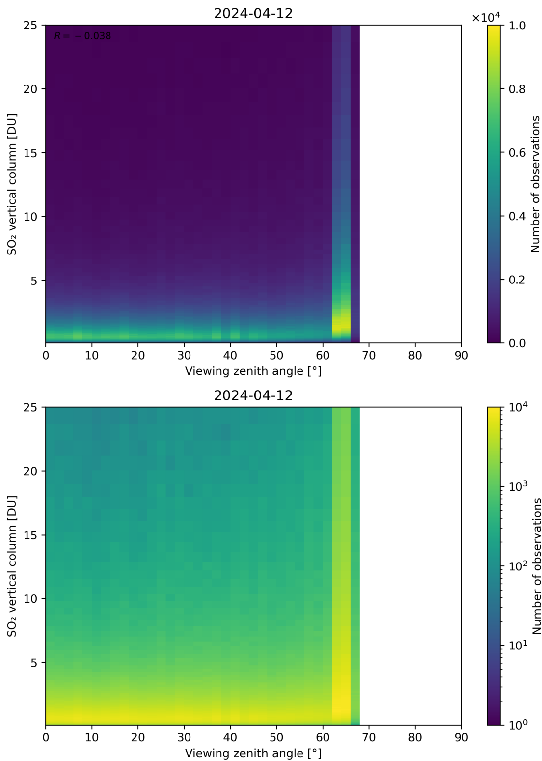
Figure 327: Scatter density plot of “Viewing zenith angle” against “SO 2 vertical column” for 2024-04-11 to 2024-04-13.
