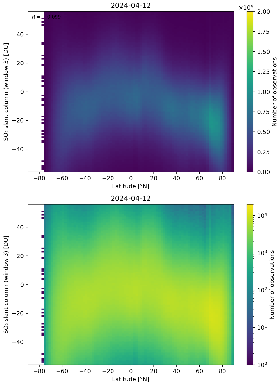
Figure 152: Scatter density plot of “Latitude” against “SO 2 slant column (window 3)” for 2024-04-11 to 2024-04-13.
