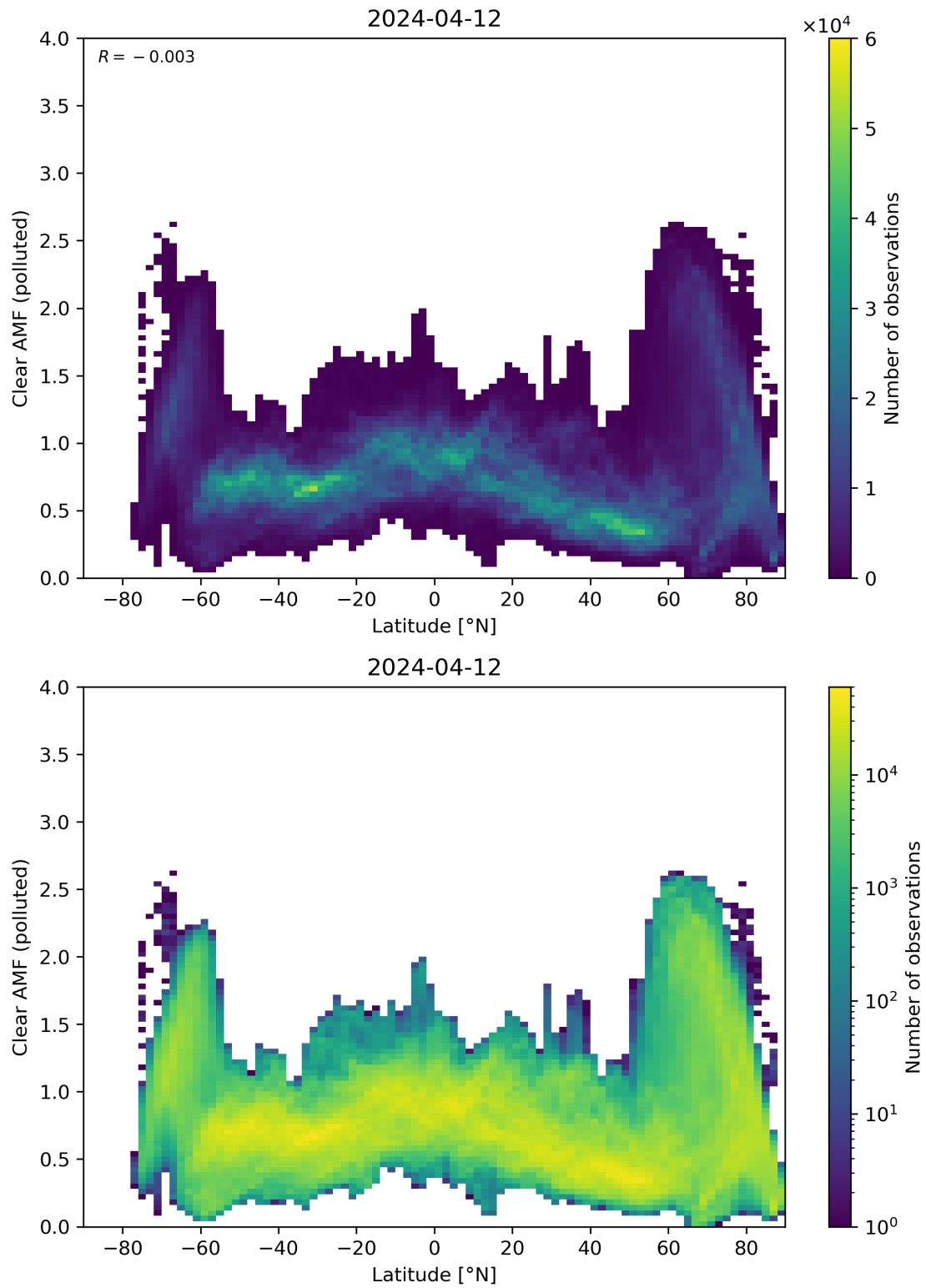
Figure 145: Scatter density plot of “Latitude” against “Clear AMF (polluted)” for 2024-04-11 to 2024-04-13.
