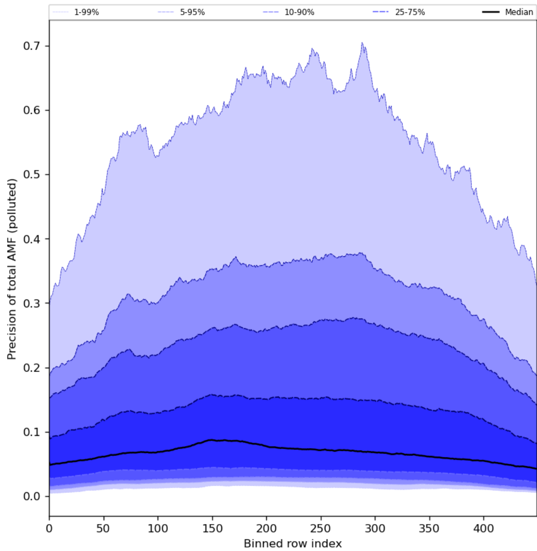
Figure 95: Along track statistics of “Precision of total AMF (polluted)” for 2024-04-11 to 2024-04-13
