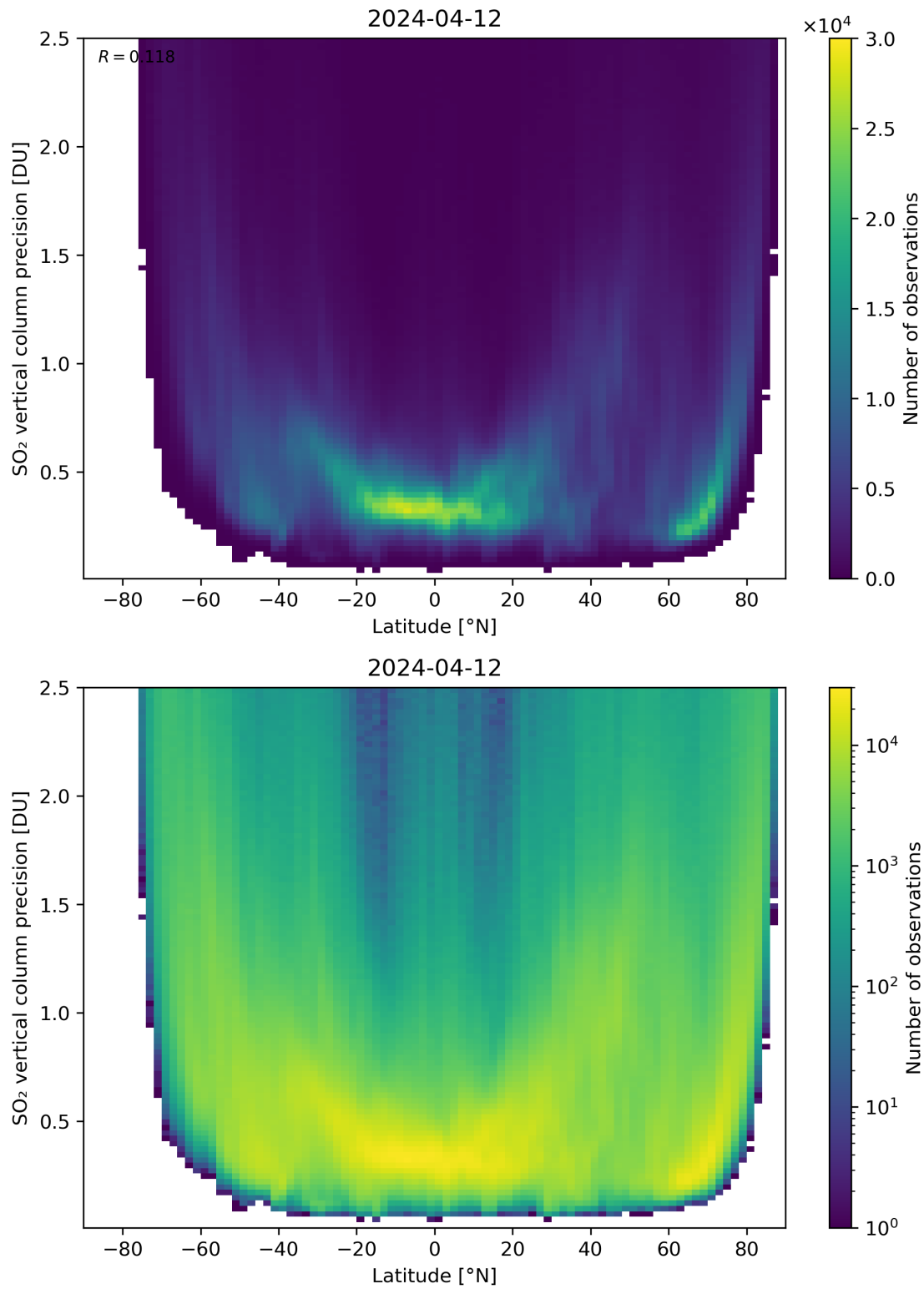
Figure 157: Scatter density plot of “Latitude” against “SO 2 vertical column precision” for 2024-04-11 to 2024-04-13.
