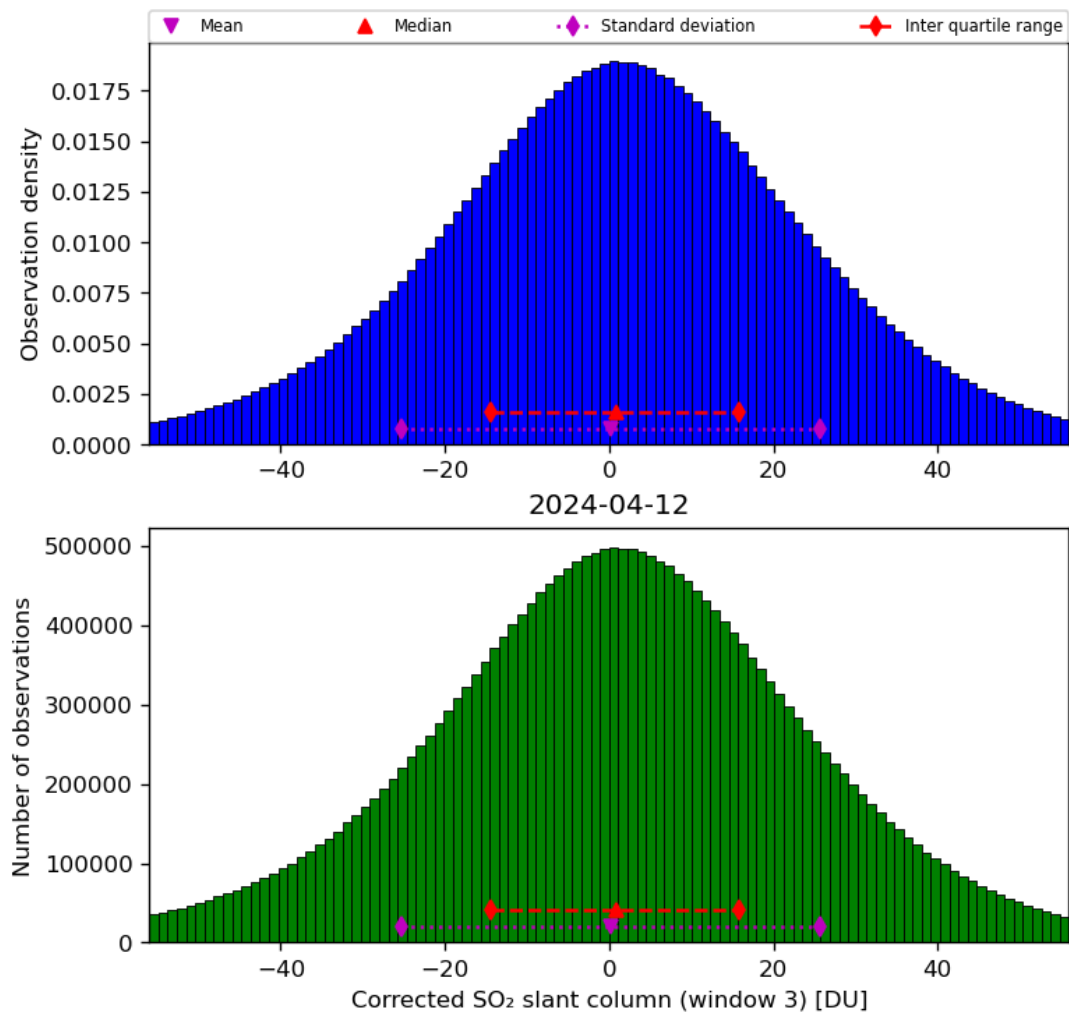
Figure 66: Histogram of “Corrected SO 2 slant column (window 3)” for 2024-04-11 to 2024-04-13
