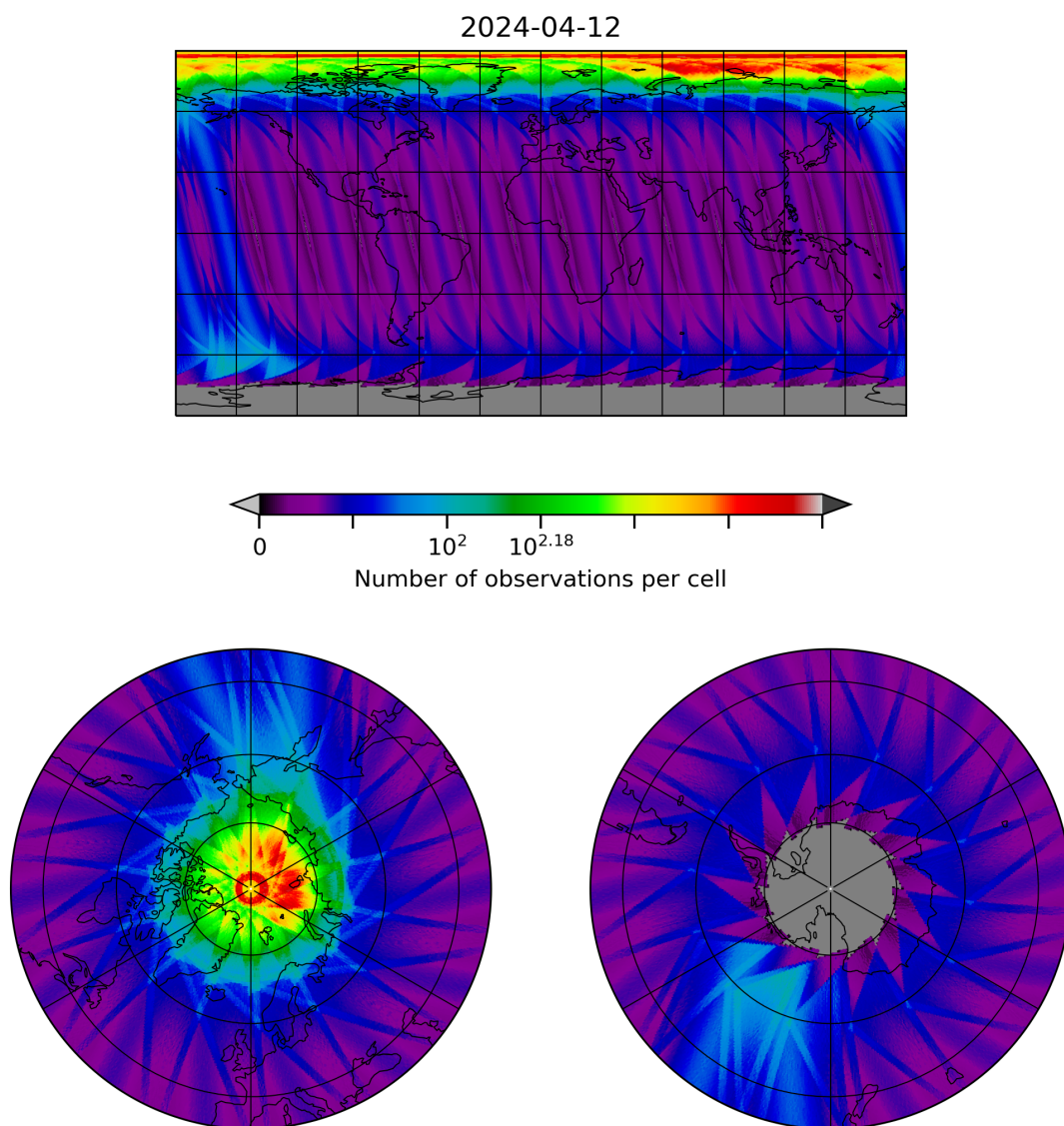
Figure 28: Map of the number of observations for 2024-04-11 to 2024-04-13
