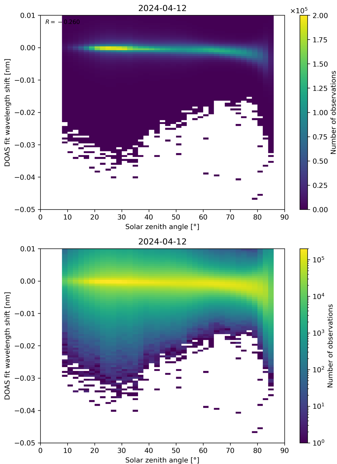
Figure 161: Scatter density plot of “Solar zenith angle” against “DOAS fit wavelength shift” for 2024-04-11 to 2024-04-13.
