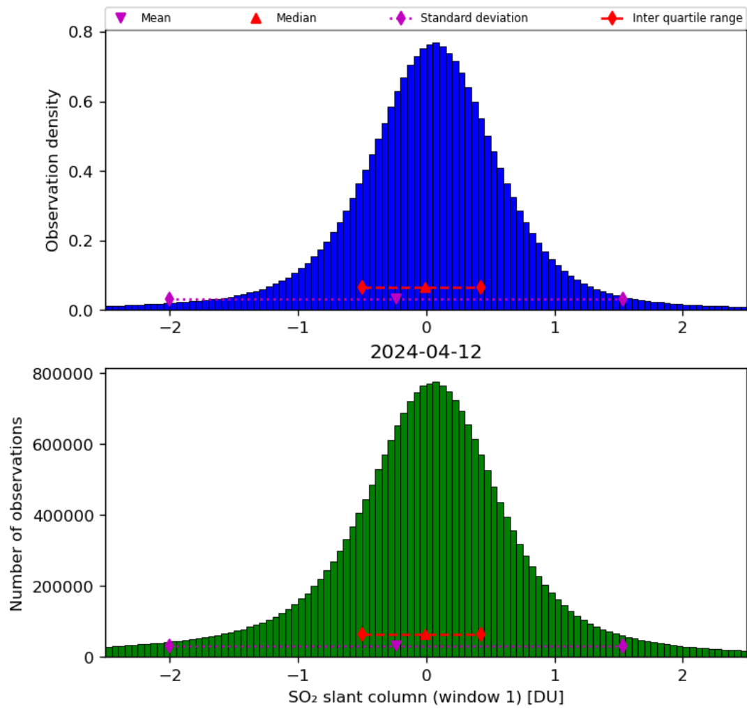
Figure 56: Histogram of “SO 2 slant column (window 1)” for 2024-04-11 to 2024-04-13
