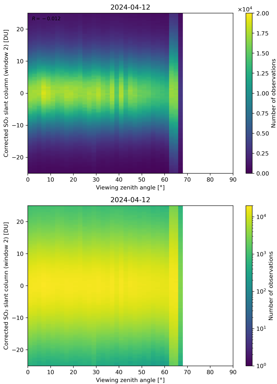
Figure 318: Scatter density plot of “Viewing zenith angle” against “Corrected SO 2 slant column (window 2)” for 2024-04-11 to 2024-04-13.
