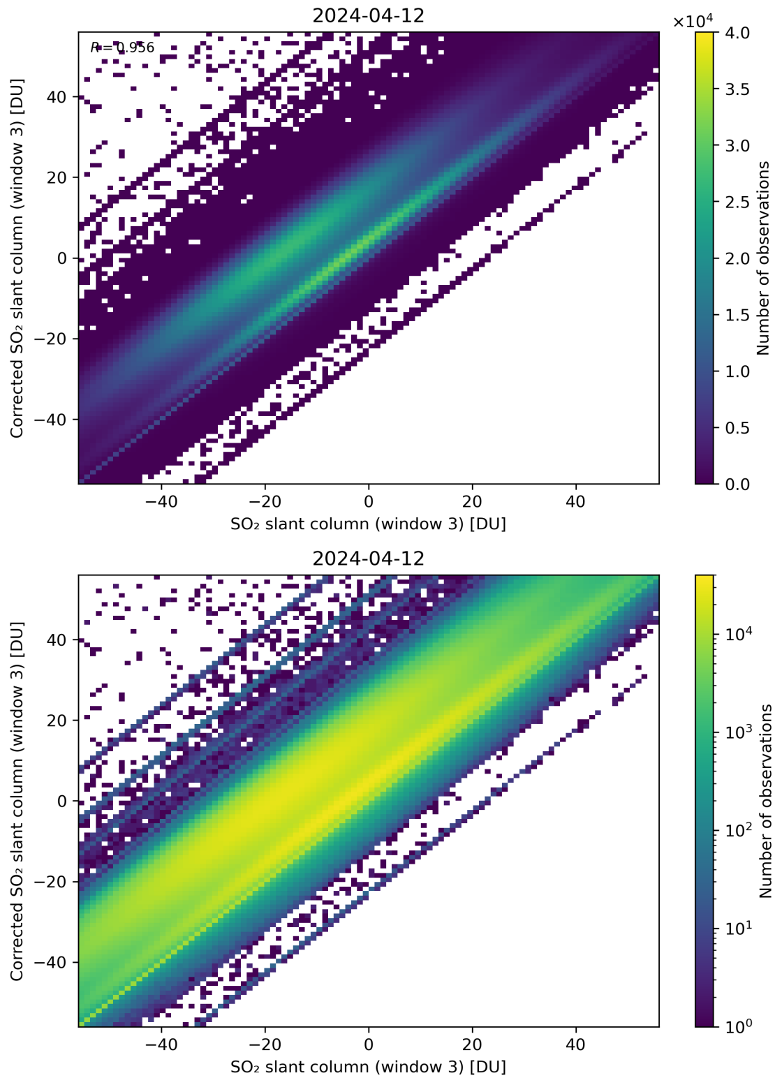
Figure 266: Scatter density plot of “SO 2 slant column (window 3)” against “Corrected SO 2 slant column (window 3)” for 2024-04-11 to 2024-04-13.
