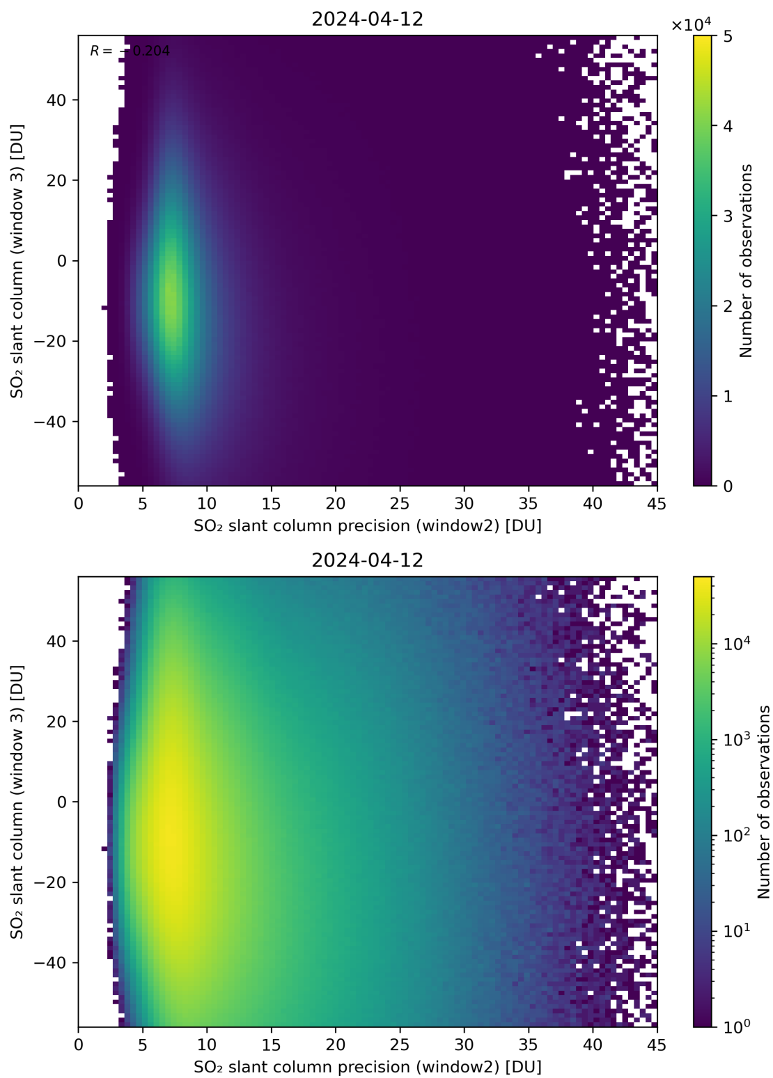
Figure 249: Scatter density plot of “SO 2 slant column precision (window2)” against “SO 2 slant column (window 3)” for 2024-04-11 to 2024-04-13.
