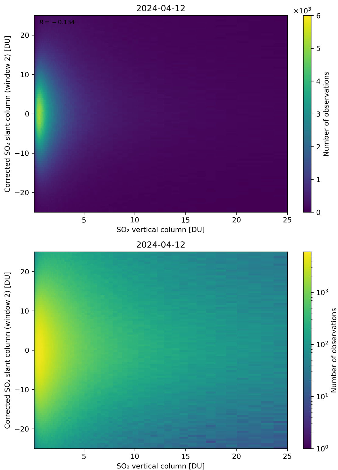
Figure 298: Scatter density plot of “SO 2 vertical column” against “Corrected SO 2 slant column (window 2)” for 2024-04-11 to 2024-04-13.
