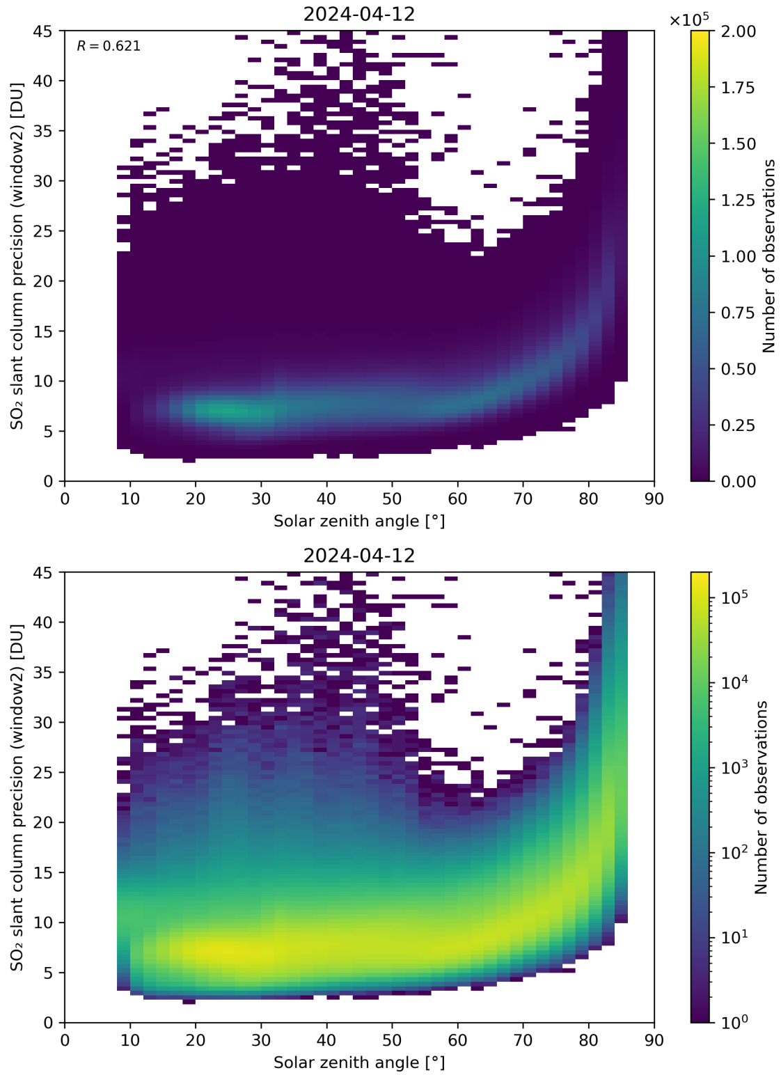
Figure 171: Scatter density plot of “Solar zenith angle” against “SO 2 slant column precision (window2)” for 2024-04-11 to 2024-04-13.
