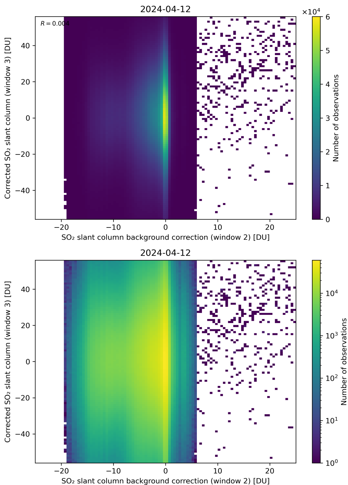
Figure 116: Scatter density plot of “SO 2 slant column background correction (window 2)” against “Corrected SO 2 slant column (window 3)” for 2024-04-11 to 2024-04-13.
