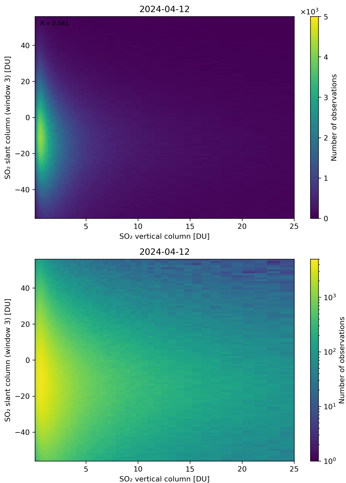
Figure 303: Scatter density plot of “SO 2 vertical column” against “SO 2 slant column (window 3)” for 2024-04-11 to 2024-04-13.
