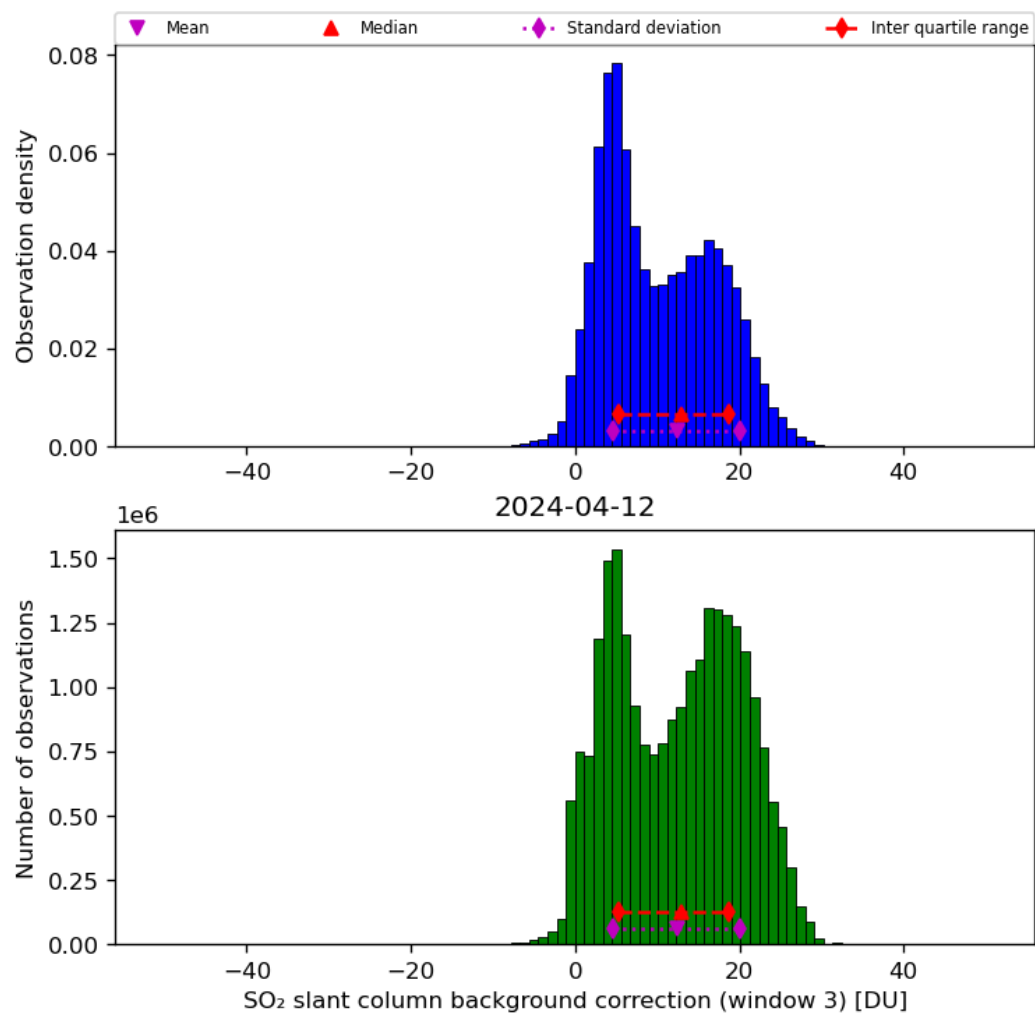
Figure 67: Histogram of "SO 2 slant column background correction (window 3)" for 2024-04-11 to 2024-04-13
