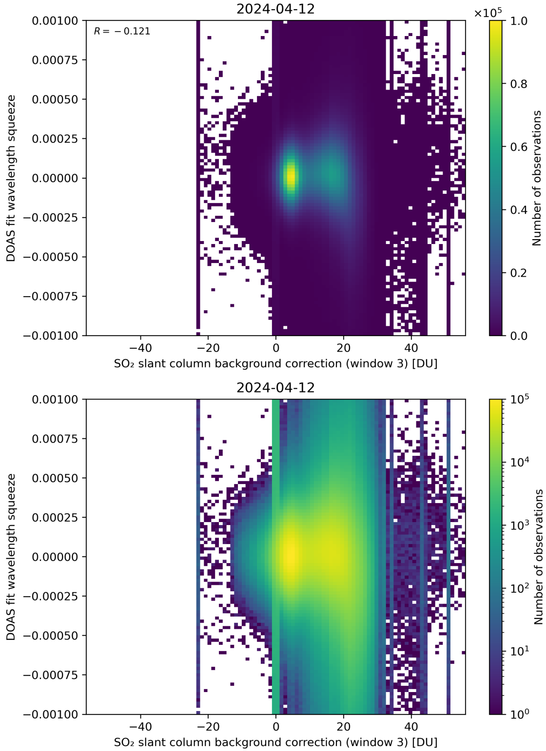
Figure 122: Scatter density plot of “SO 2 slant column background correction (window 3)” against “DOAS fit wavelength squeeze” for 2024-04-11 to 2024-04-13.
