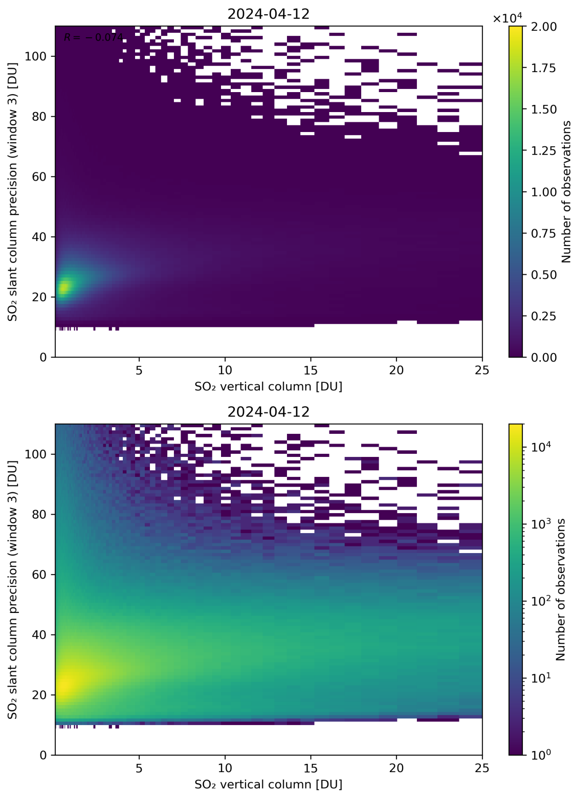
Figure 304: Scatter density plot of “SO 2 vertical column” against “SO 2 slant column precision (window 3)” for 2024-04-11 to 2024-04-13.
