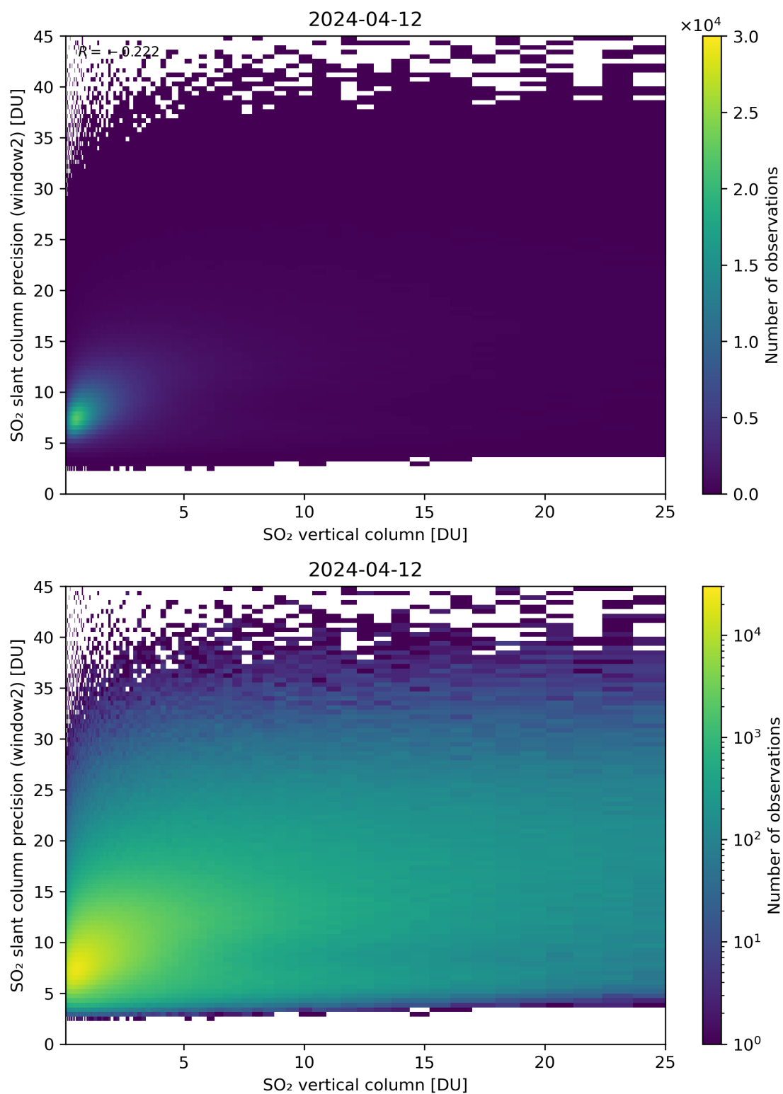
Figure 302: Scatter density plot of “SO 2 vertical column” against “SO 2 slant column precision (window2)” for 2024-04-11 to 2024-04-13.
