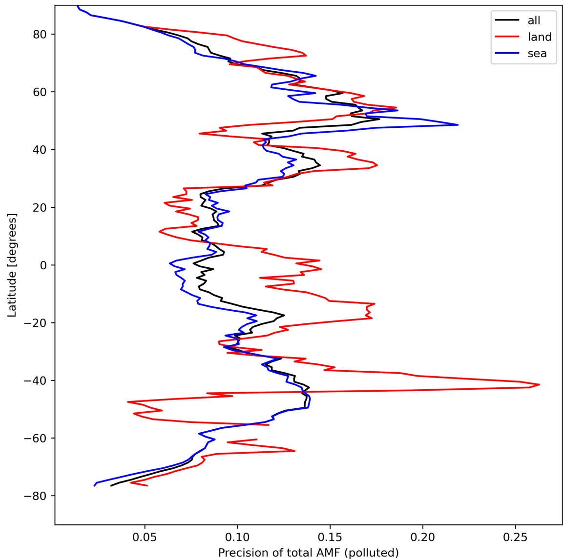
Figure 49: Zonal average of “Precision of total AMF (polluted)” for 2024-04-11 to 2024-04-13.
