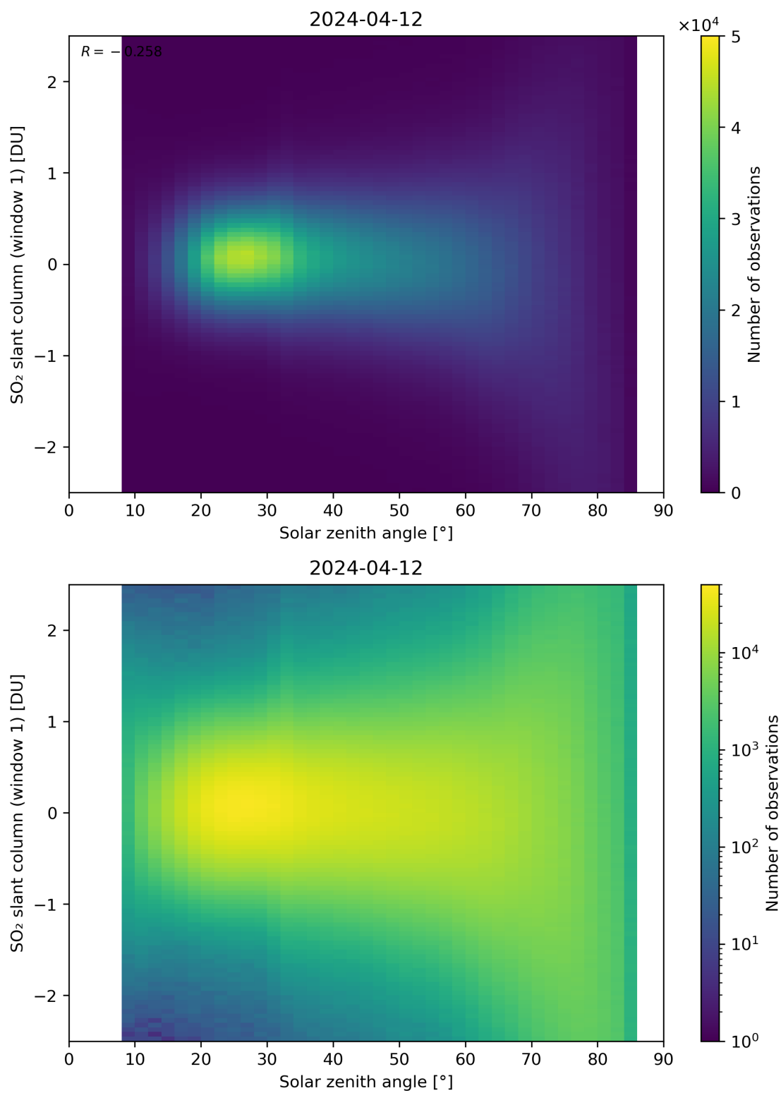
Figure 169: Scatter density plot of “Solar zenith angle” against “SO 2 slant column (window 1)” for 2024-04-11 to 2024-04-13.
