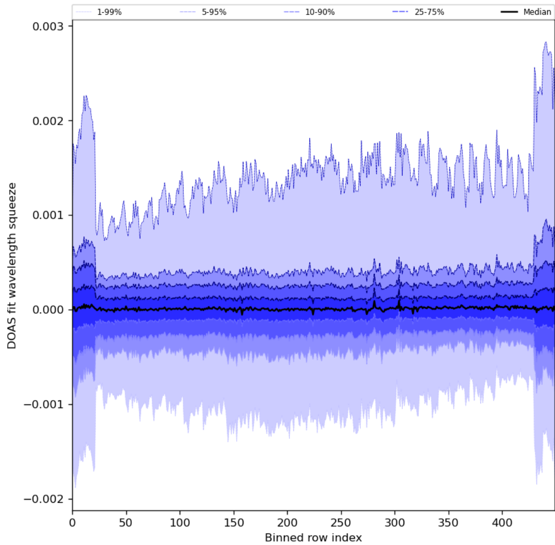
Figure 92: Along track statistics of “DOAS fit wavelength squeeze” for 2024-04-11 to 2024-04-13
