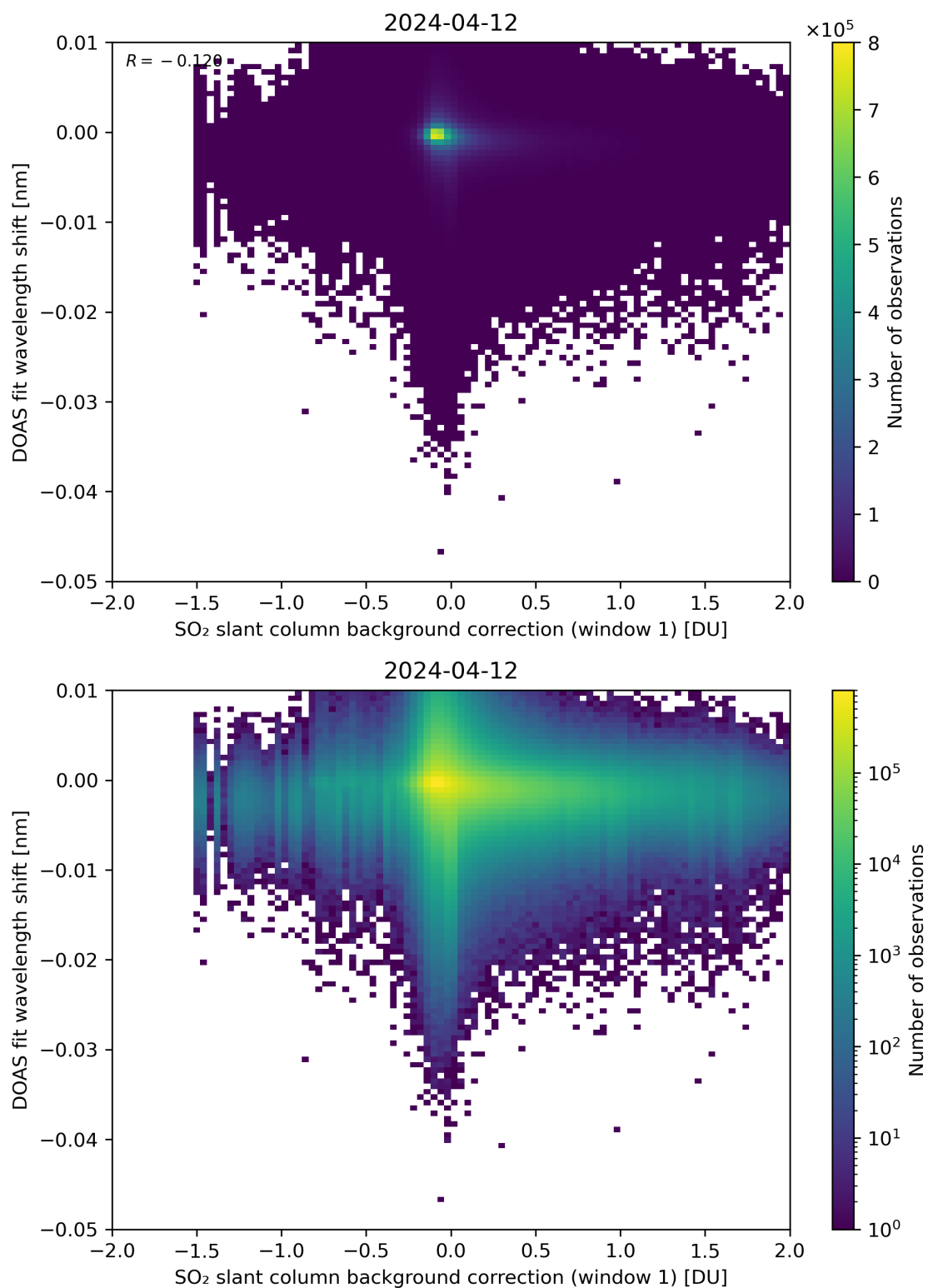
Figure 100: Scatter density plot of “SO 2 slant column background correction (window 1)” against “DOAS fit wavelength shift” for 2024-04-11 to 2024-04-13.
