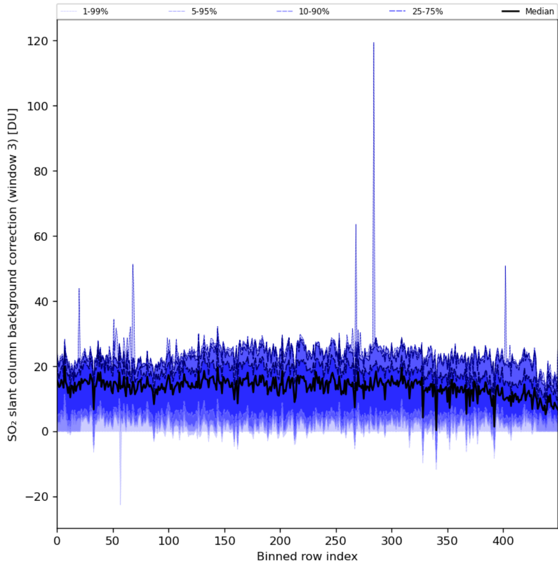
Figure 90: Along track statistics of “SO 2 slant column background correction (window 3)” for 2024-04-11 to 2024-04-13
