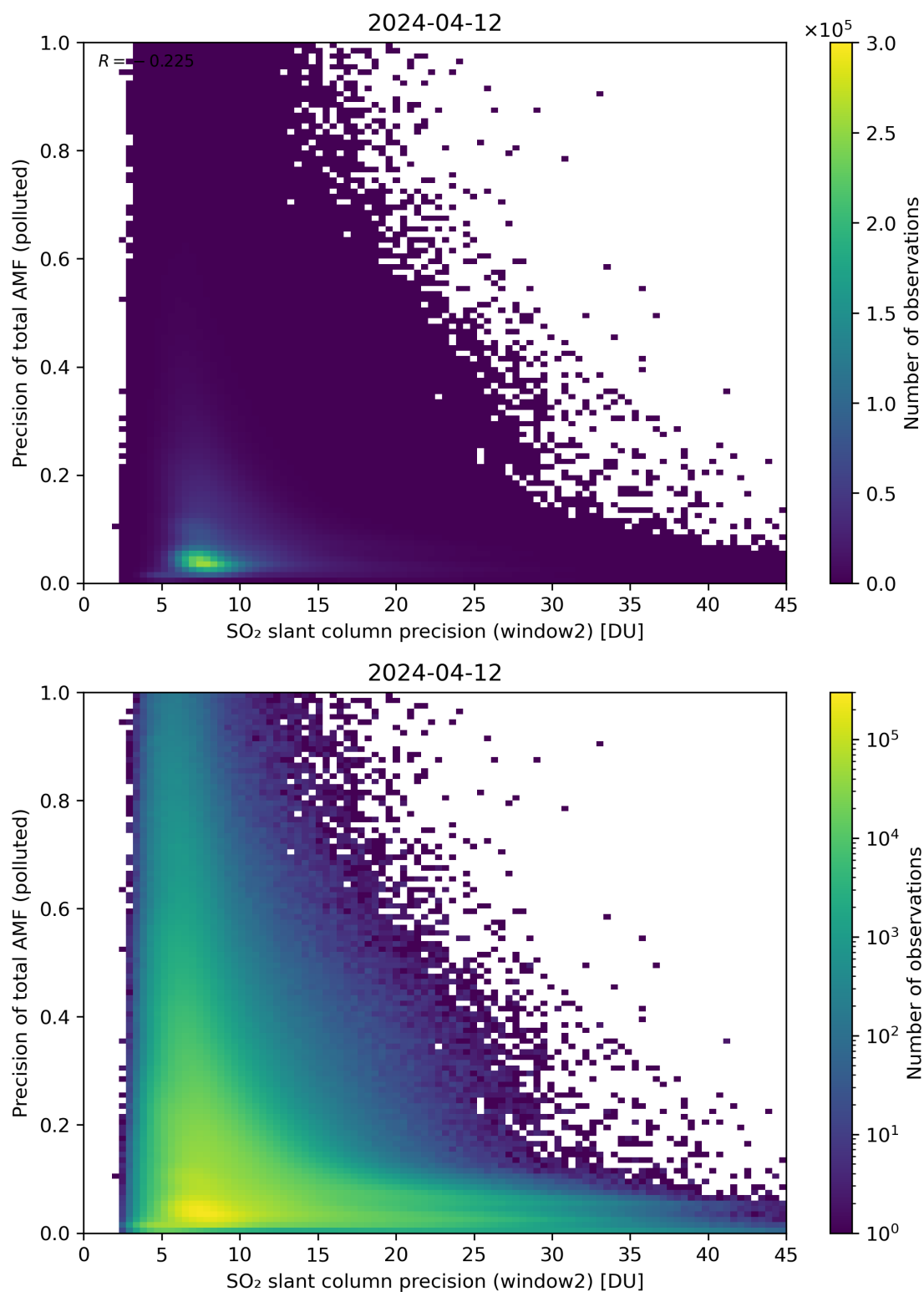
Figure 252: Scatter density plot of “SO 2 slant column precision (window2)” against “Precision of total AMF (polluted)” for 2024-04-11 to 2024-04-13.
