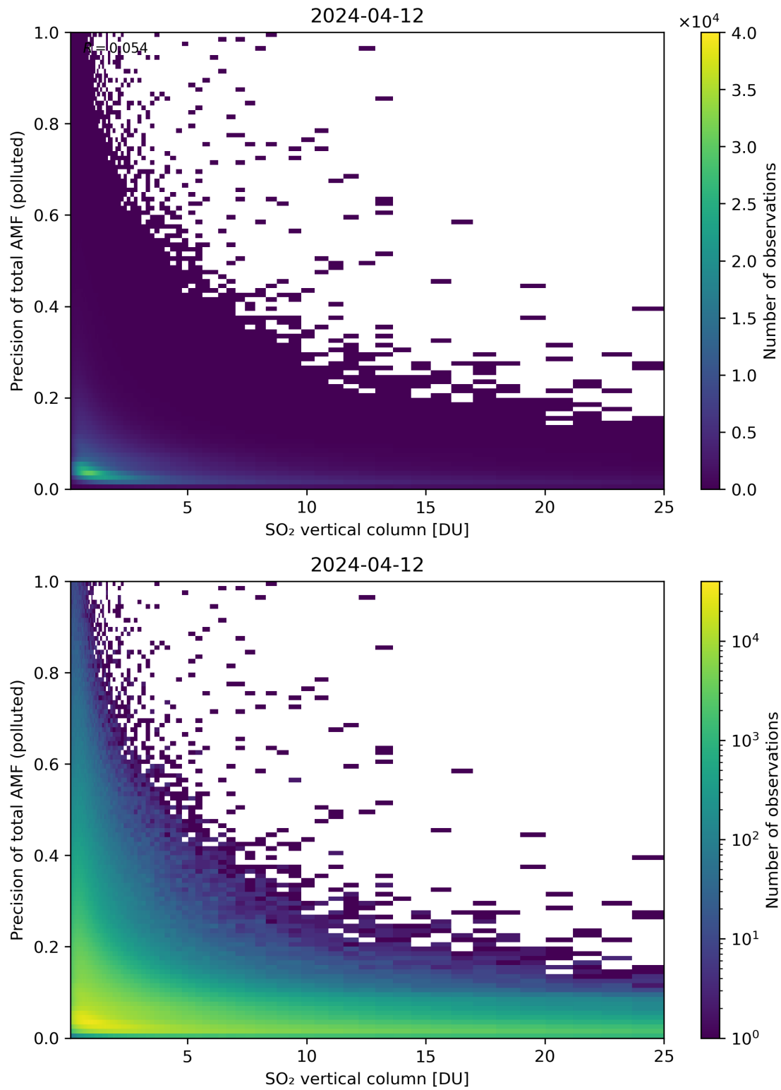
Figure 306: Scatter density plot of “SO 2 vertical column” against “Precision of total AMF (polluted)” for 2024-04-11 to 2024-04-13.
