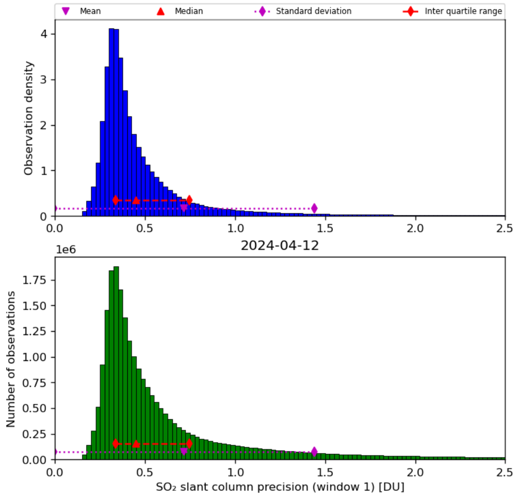
Figure 57: Histogram of “SO 2 slant column precision (window 1)” for 2024-04-11 to 2024-04-13
