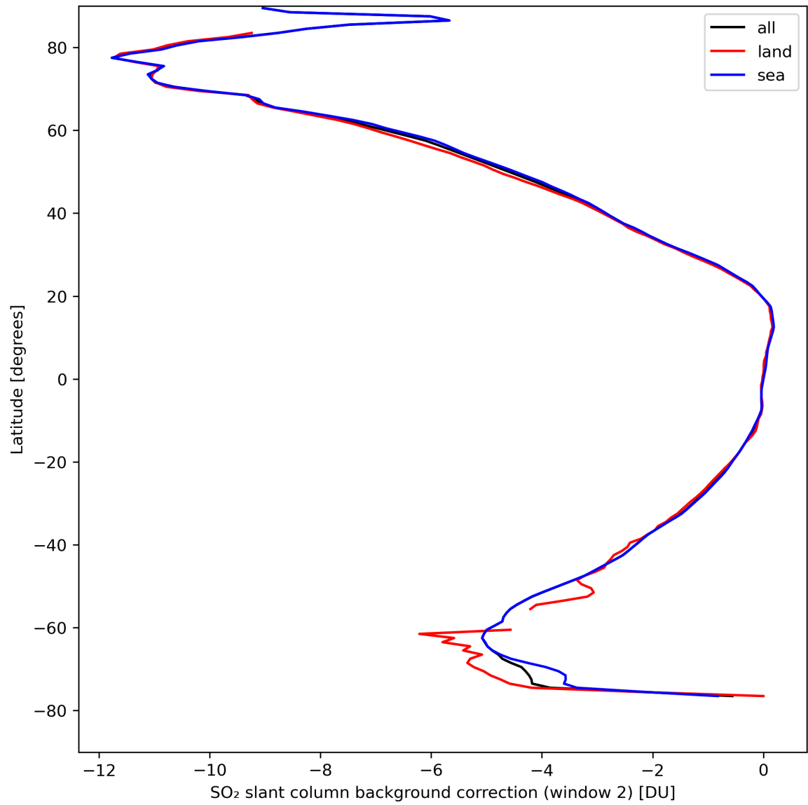
Figure 40: Zonal average of “SO 2 slant column background correction (window 2)” for 2024-04-11 to 2024-04-13.
