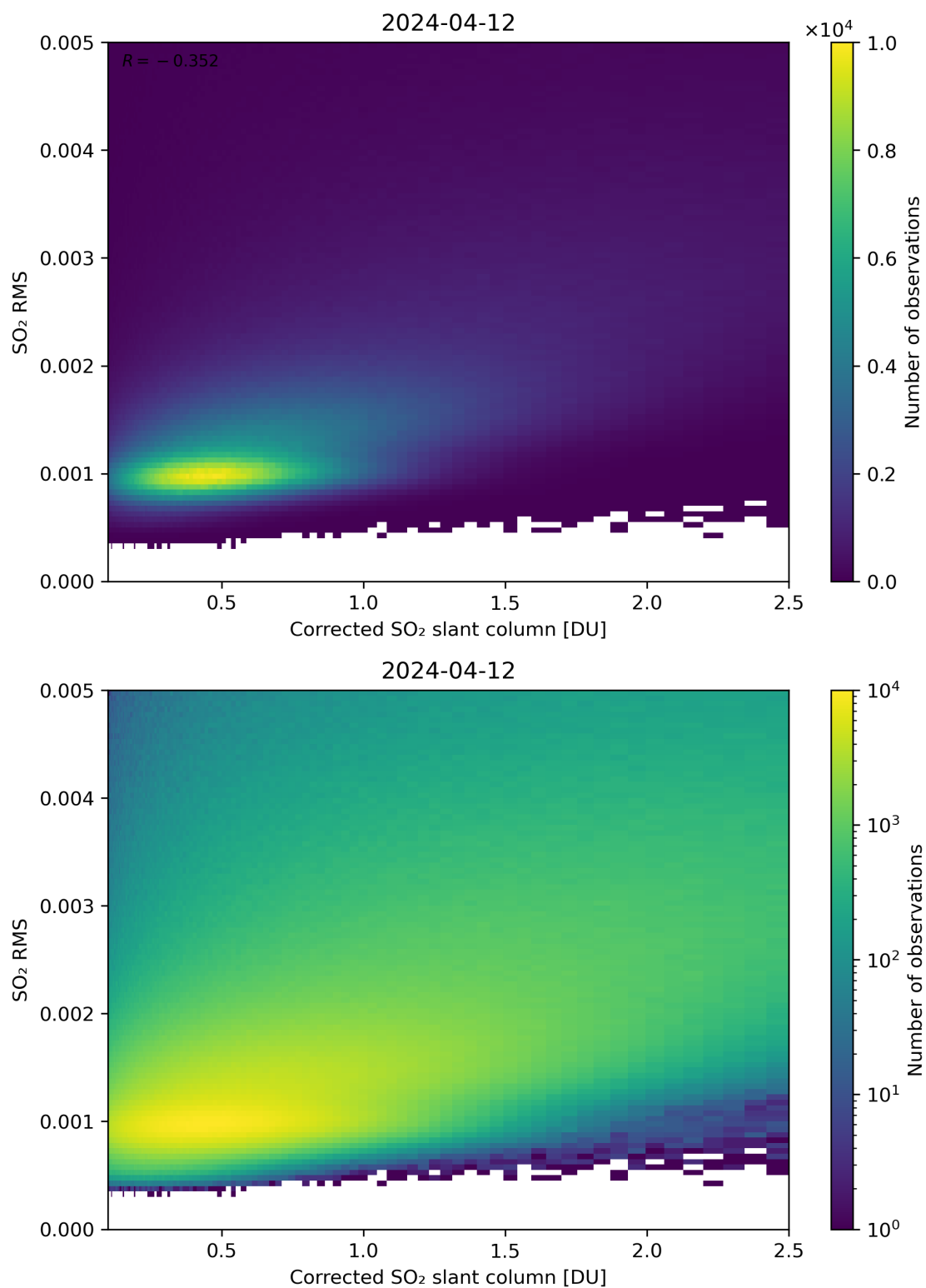
Figure 183: Scatter density plot of “Corrected SO 2 slant column” against “SO 2 RMS” for 2024-04-11 to 2024-04-13.
