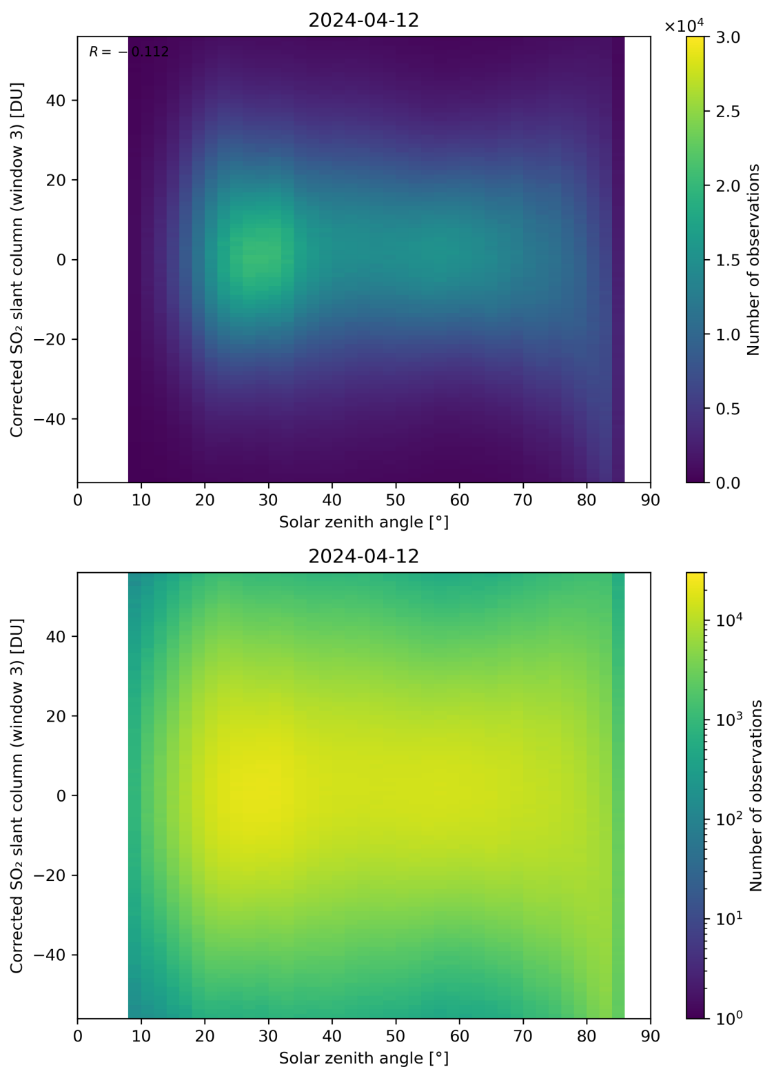
Figure 168: Scatter density plot of “Solar zenith angle” against “Corrected SO 2 slant column (window 3)” for 2024-04-11 to 2024-04-13.
