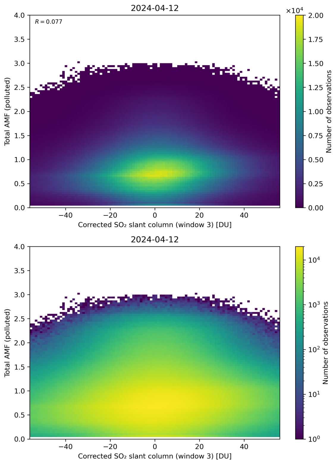
Figure 210: Scatter density plot of “Corrected SO 2 slant column (window 3)” against “Total AMF (polluted)” for 2024-04-11 to 2024-04-13.
