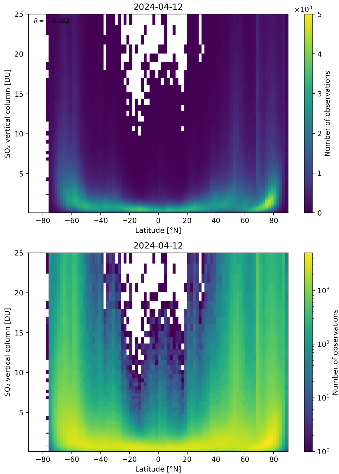
Figure 156: Scatter density plot of “Latitude” against “SO 2 vertical column” for 2024-04-11 to 2024-04-13.
