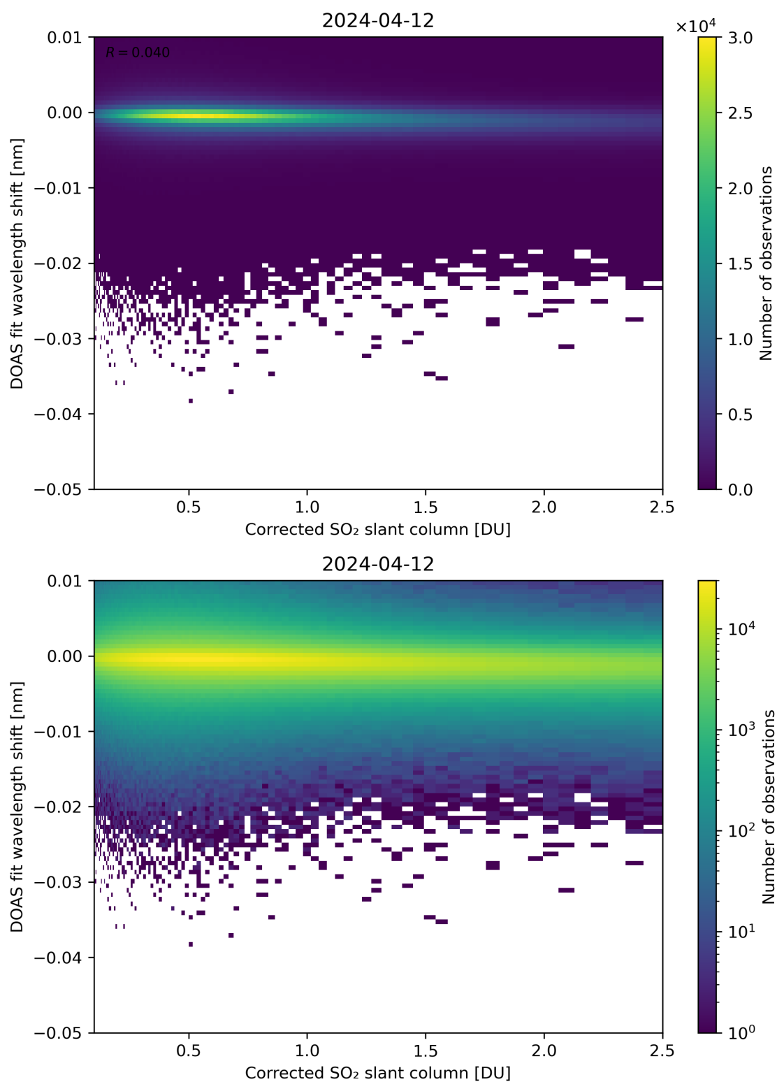
Figure 181: Scatter density plot of “Corrected SO 2 slant column” against “DOAS fit wavelength shift” for 2024-04-11 to 2024-04-13.
