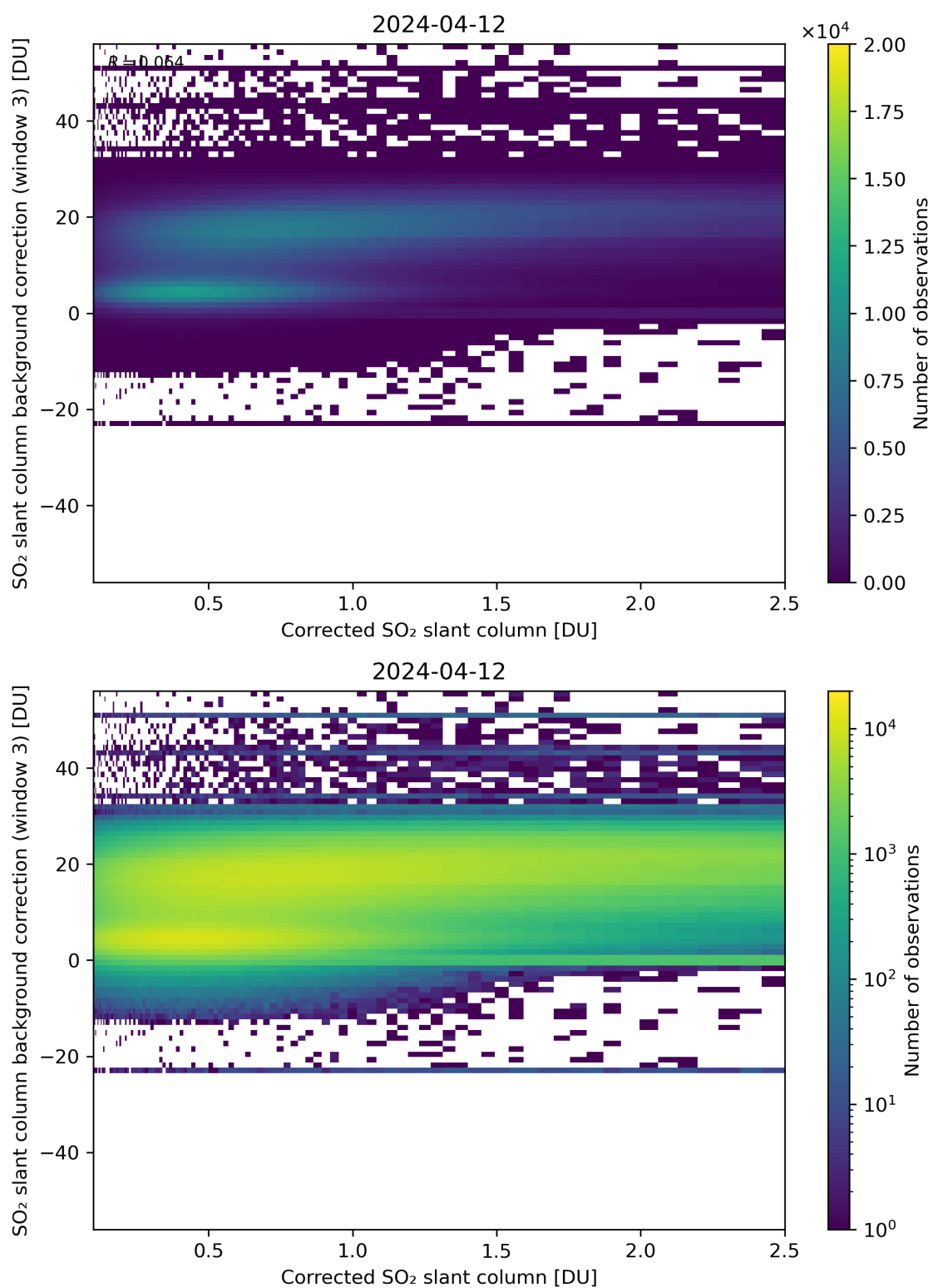
Figure 180: Scatter density plot of “Corrected SO 2 slant column” against “SO 2 slant column background correction (window 3)” for 2024-04-11 to 2024-04-13.
