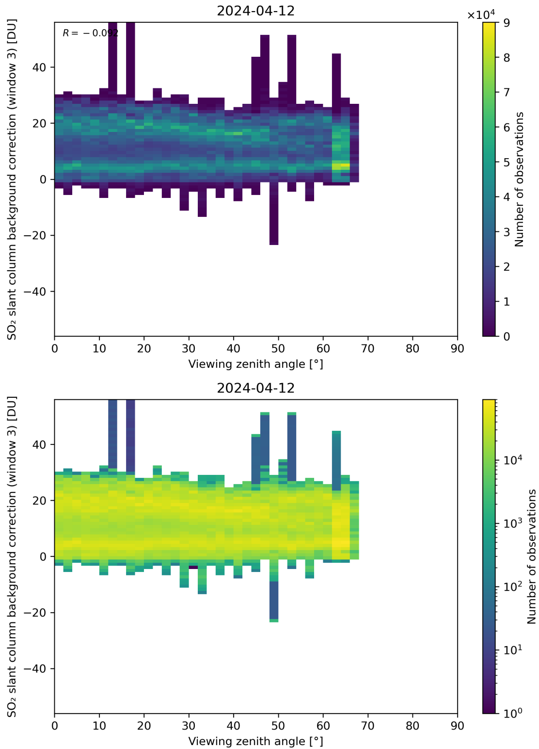
Figure 310: Scatter density plot of “Viewing zenith angle” against “SO 2 slant column background correction (window 3)” for 2024-04-11 to 2024-04-13.
