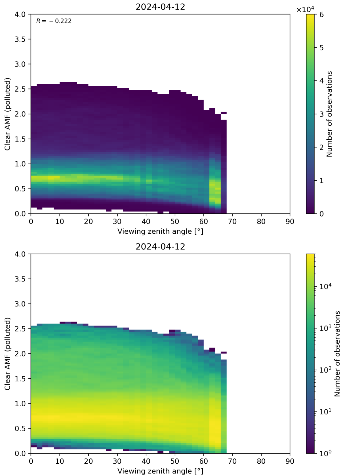
Figure 316: Scatter density plot of “Viewing zenith angle” against “Clear AMF (polluted)” for 2024-04-11 to 2024-04-13.
