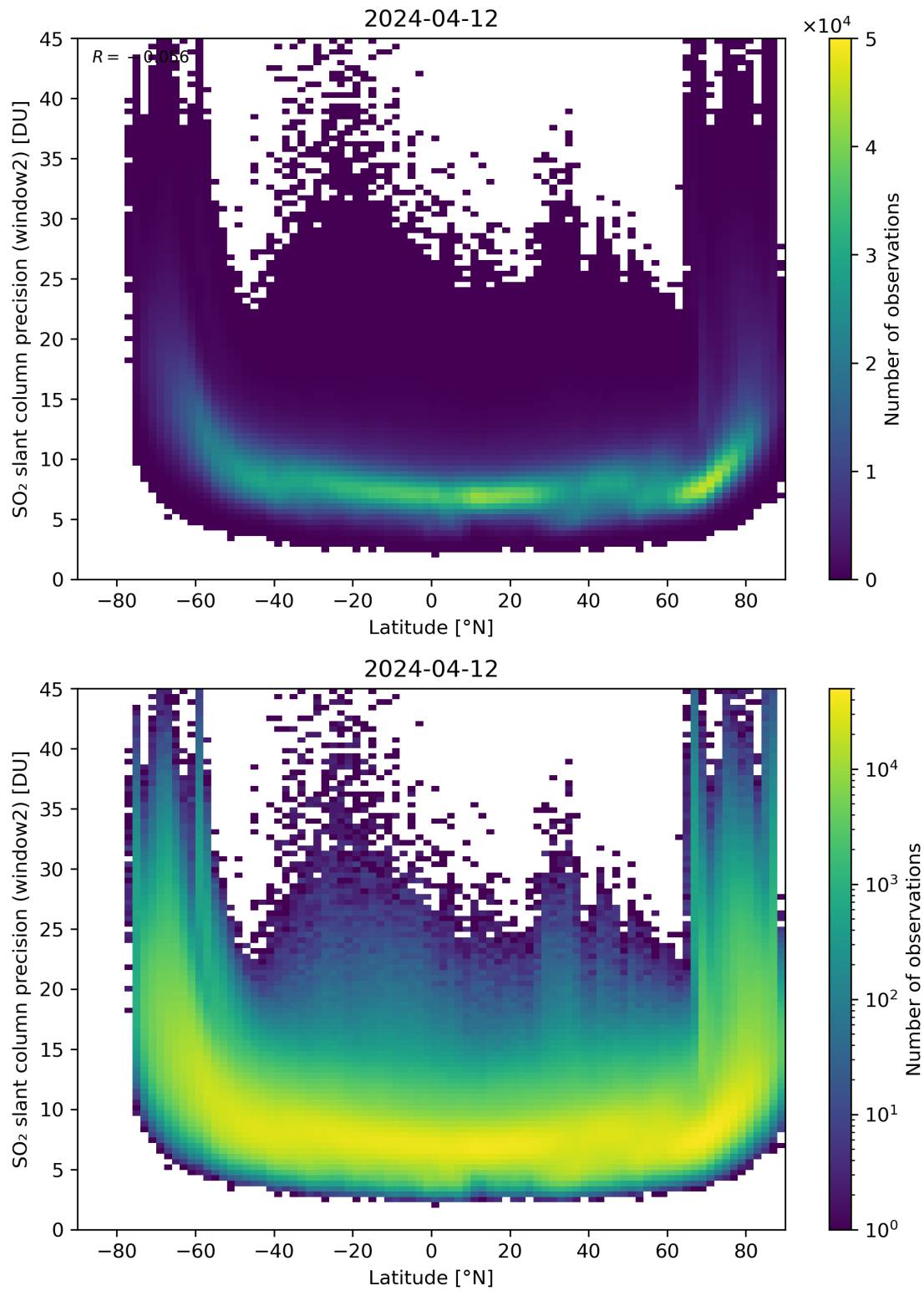
Figure 151: Scatter density plot of “Latitude” against “SO 2 slant column precision (window2)” for 2024-04-11 to 2024-04-13.
