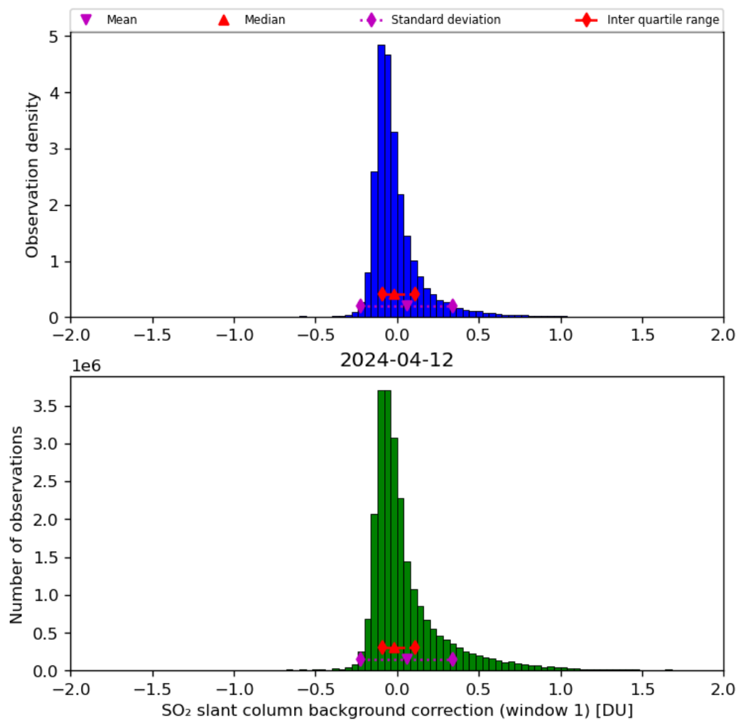
Figure 59: Histogram of “SO 2 slant column background correction (window 1)” for 2024-04-11 to 2024-04-13
