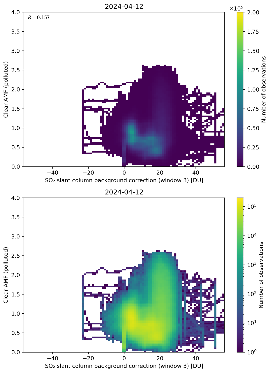
Figure 124: Scatter density plot of “SO 2 slant column background correction (window 3)” against “Clear AMF (polluted)” for 2024-04-11 to 2024-04-13.
