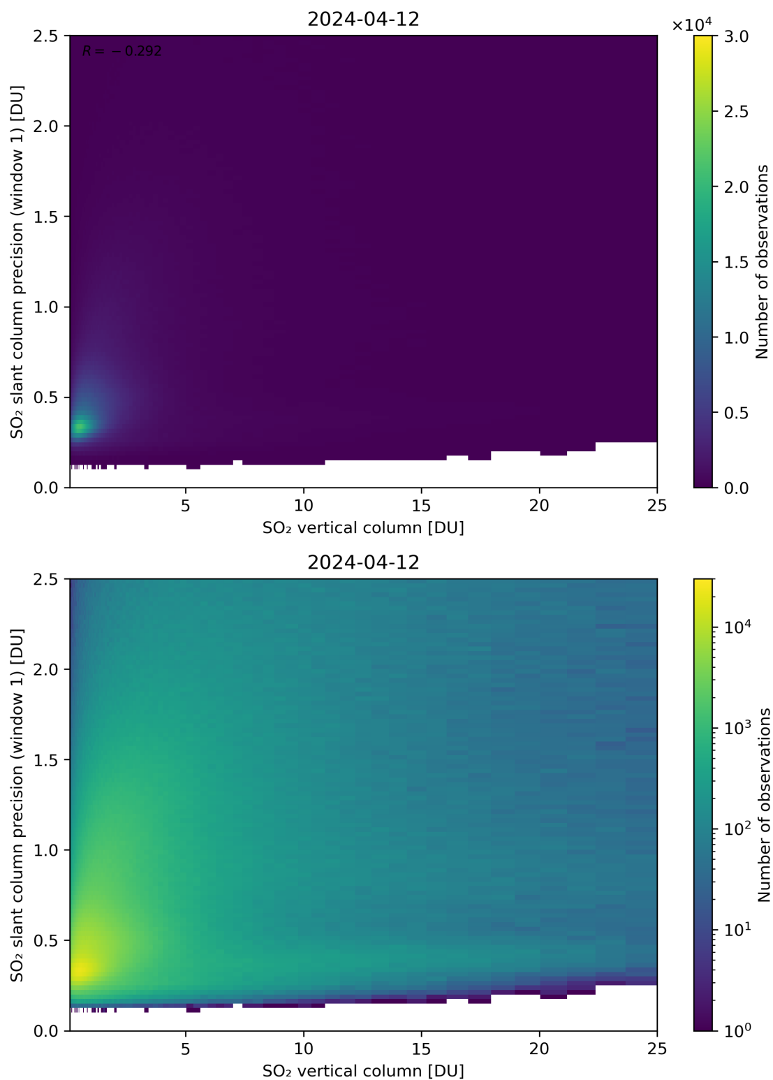
Figure 301: Scatter density plot of “SO 2 vertical column” against “SO 2 slant column precision (window 1)” for 2024-04-11 to 2024-04-13.
