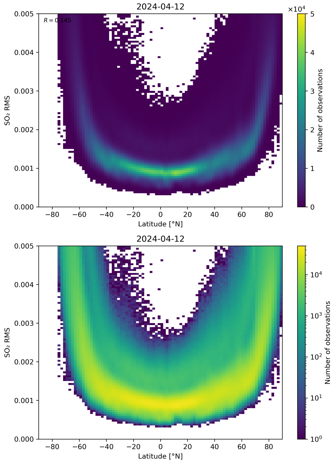
Figure 144: Scatter density plot of “Latitude” against “SO 2 RMS” for 2024-04-11 to 2024-04-13.
