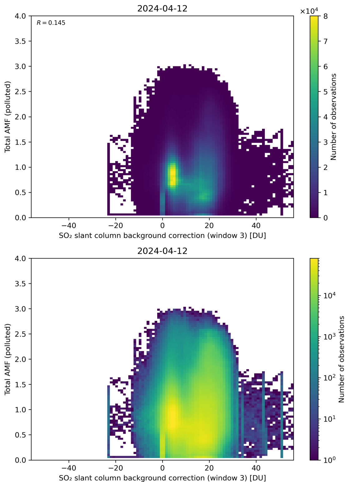
Figure 125: Scatter density plot of “SO 2 slant column background correction (window 3)” against “Total AMF (polluted)” for 2024-04-11 to 2024-04-13.
