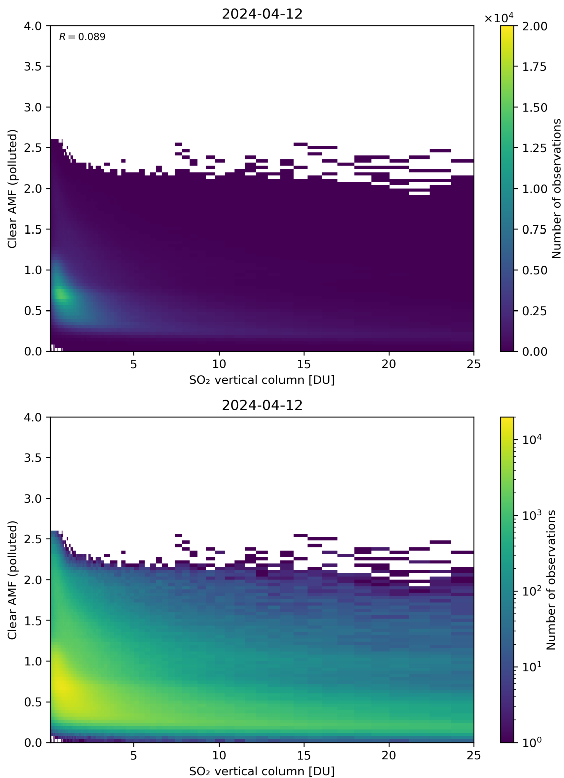
Figure 296: Scatter density plot of “SO 2 vertical column” against “Clear AMF (polluted)” for 2024-04-11 to 2024-04-13.
