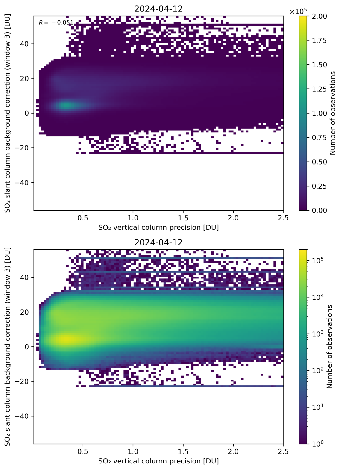
Figure 281: Scatter density plot of “SO 2 vertical column precision” against “SO 2 slant column background correction (window 3)” for 2024-04-11 to 2024-04-13.
