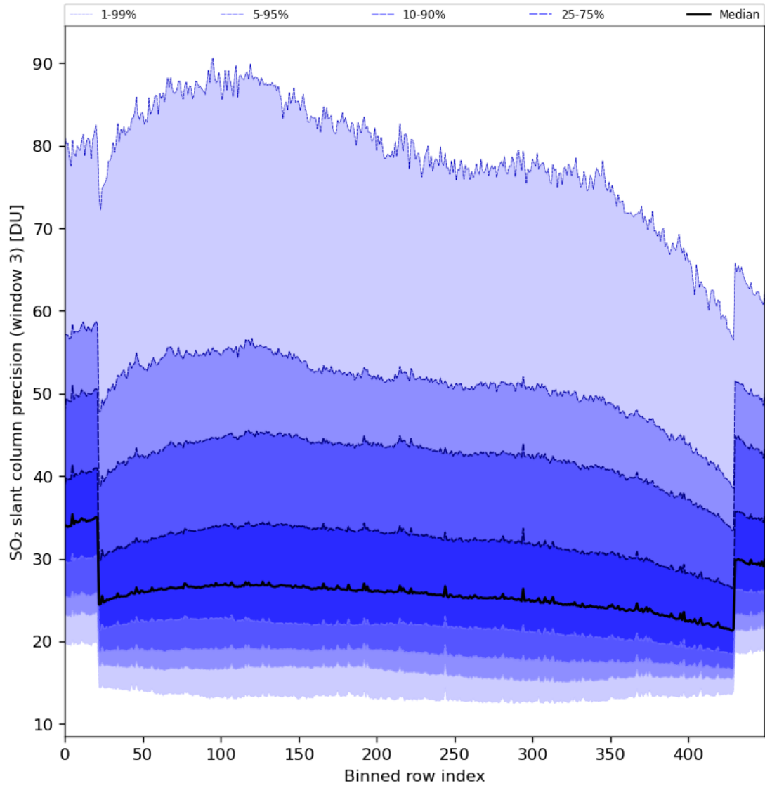
Figure 88: Along track statistics of “SO 2 slant column precision (window 3)” for 2024-04-11 to 2024-04-13
