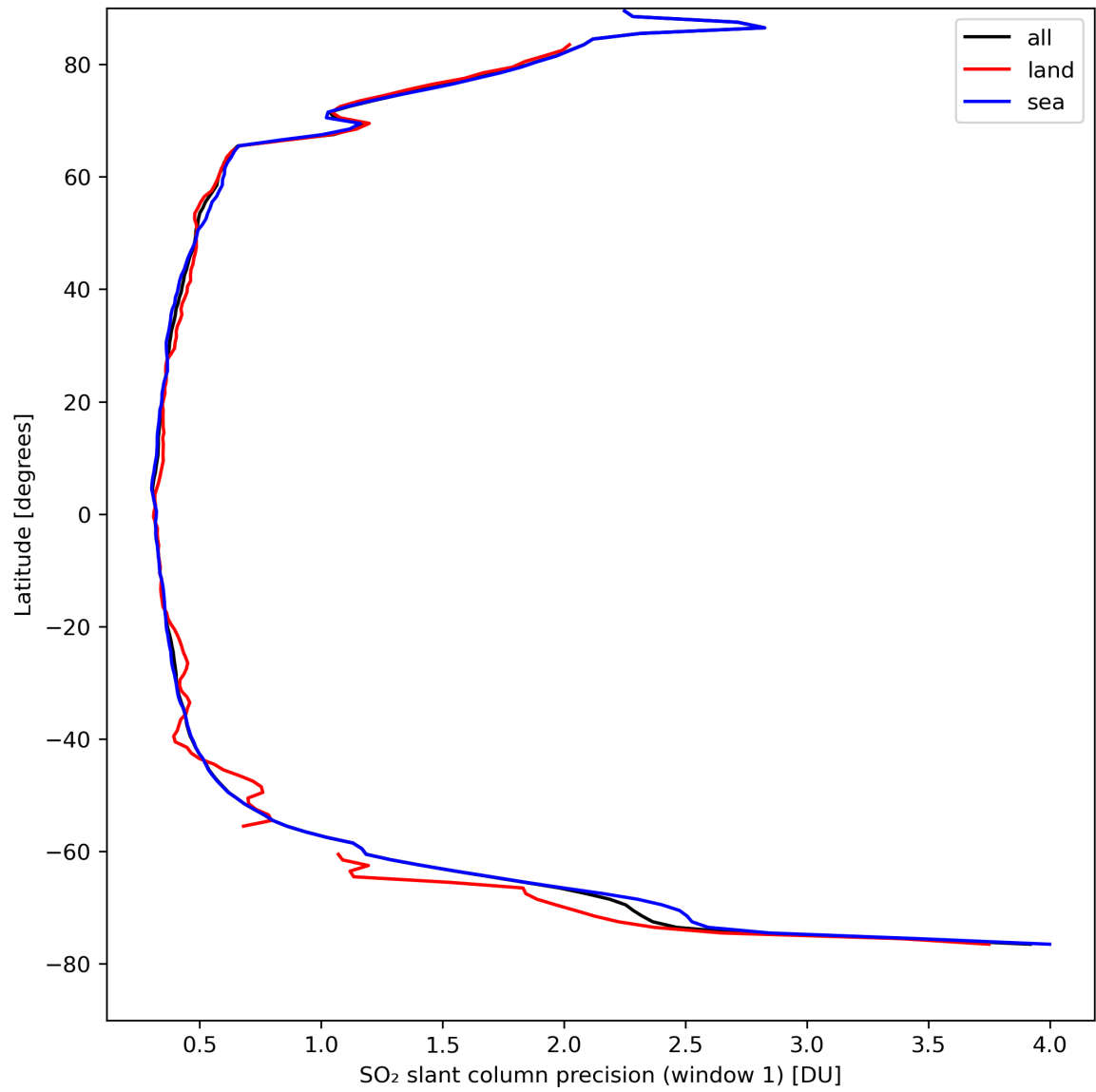
Figure 34: Zonal average of “SO 2 slant column precision (window 1)” for 2024-04-11 to 2024-04-13.
