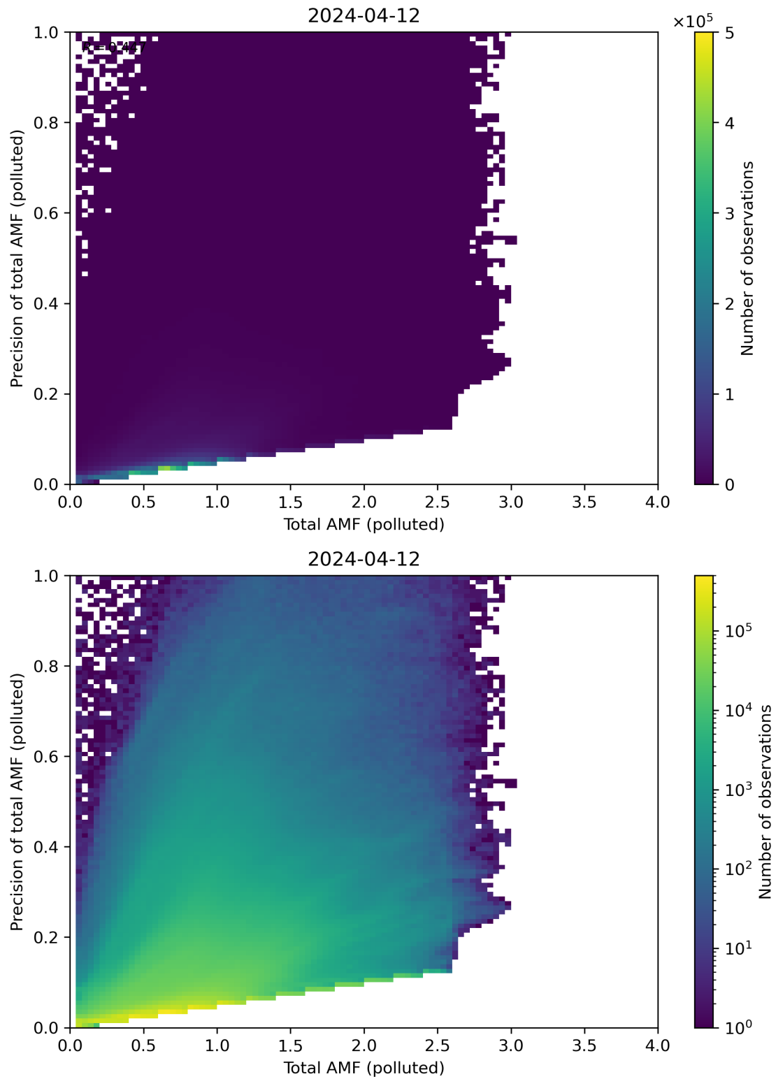
Figure 272: Scatter density plot of “Total AMF (polluted)” against “Precision of total AMF (polluted)” for 2024-04-11 to 2024-04-13.
