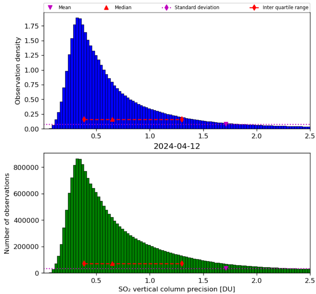
Figure 54: Histogram of “SO 2 vertical column precision” for 2024-04-11 to 2024-04-13
