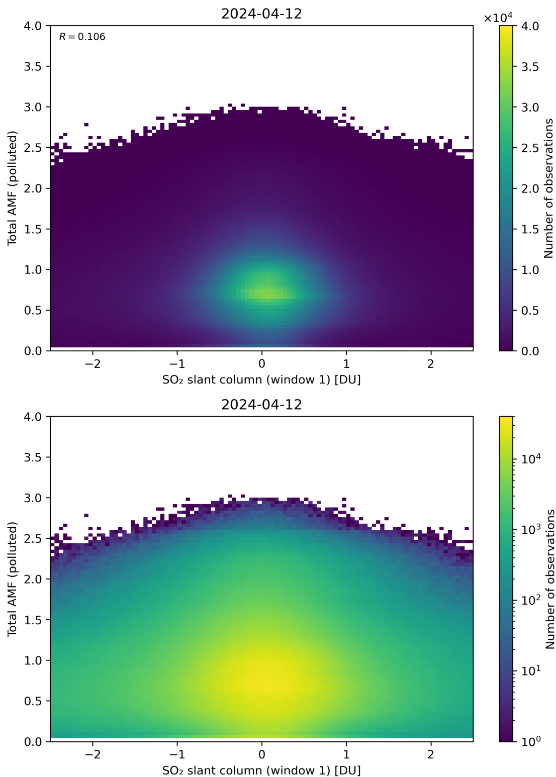
Figure 239: Scatter density plot of “SO 2 slant column (window 1)” against “Total AMF (polluted)” for 2024-04-11 to 2024-04-13.
