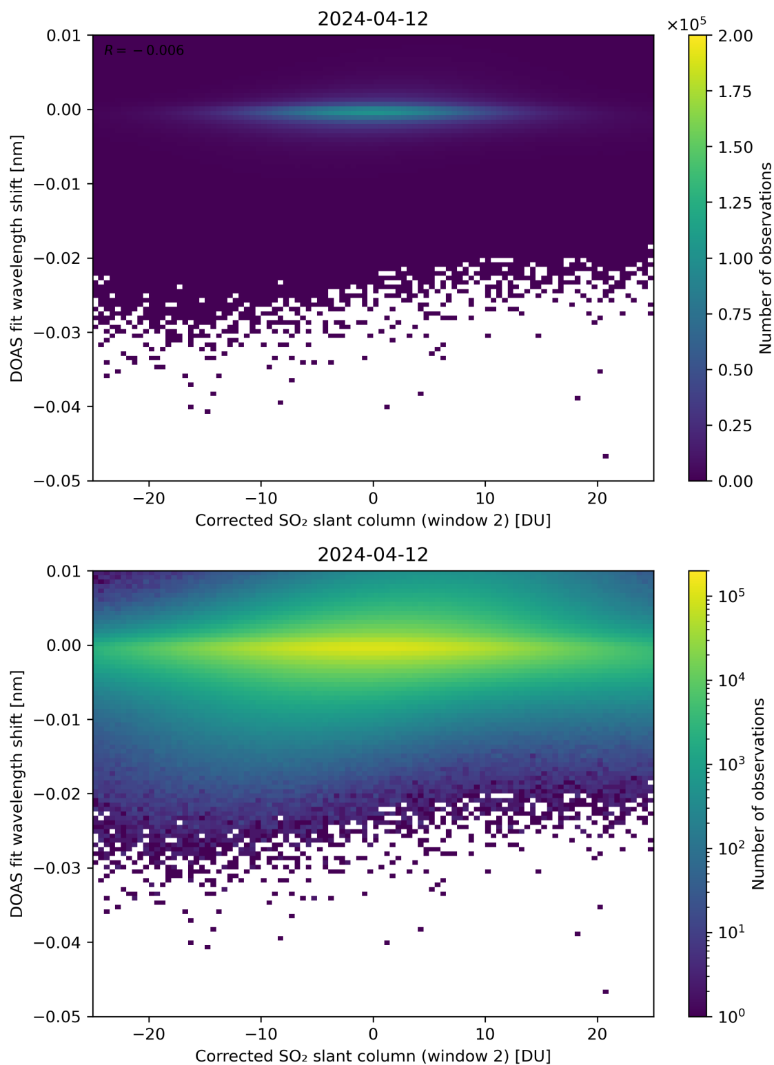
Figure 196: Scatter density plot of “Corrected SO 2 slant column (window 2)” against “DOAS fit wavelength shift” for 2024-04-11 to 2024-04-13.
