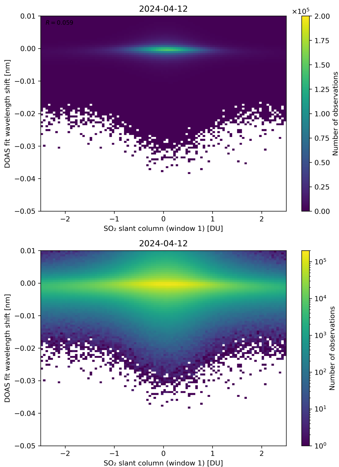
Figure 215: Scatter density plot of “SO 2 slant column (window 1)” against “DOAS fit wavelength shift” for 2024-04-11 to 2024-04-13.
