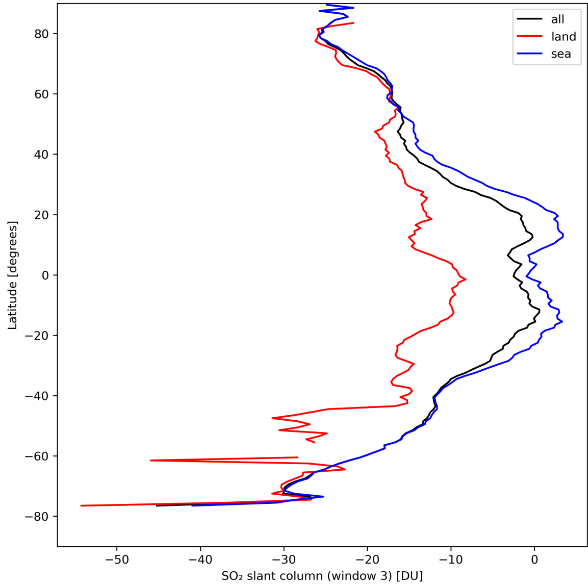
Figure 41: Zonal average of “SO 2 slant column (window 3)” for 2024-04-11 to 2024-04-13.
