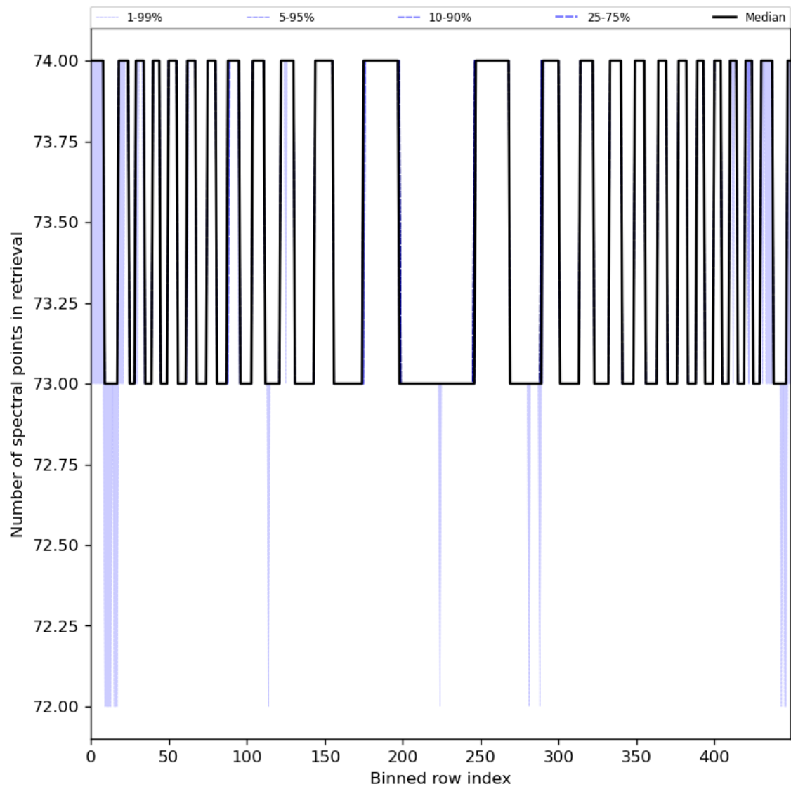
Figure 97: Along track statistics of “Number of spectral points in retrieval” for 2024-04-11 to 2024-04-13
