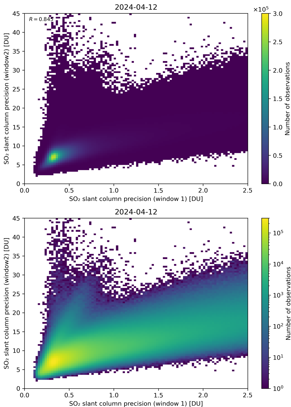
Figure 227: Scatter density plot of “SO 2 slant column precision (window 1)” against “SO 2 slant column precision (window2)” for 2024-04-11 to 2024-04-13.
