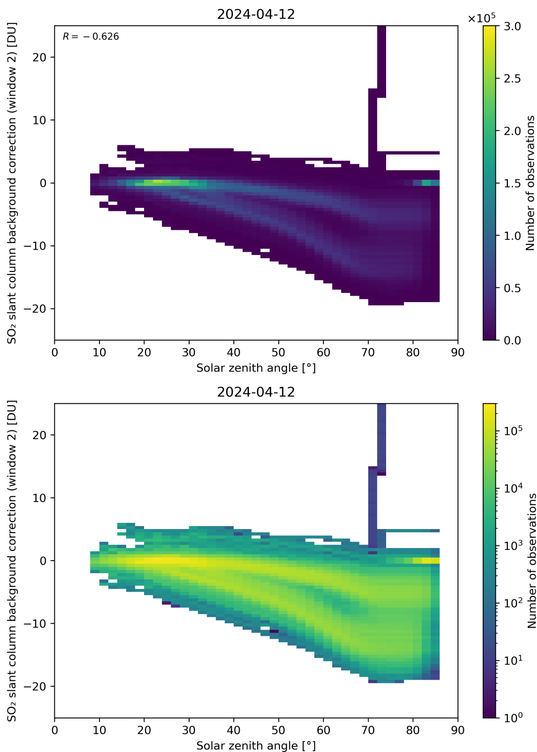
Figure 159: Scatter density plot of “Solar zenith angle” against “SO 2 slant column background correction (window 2)” for 2024-04-11 to 2024-04-13.
