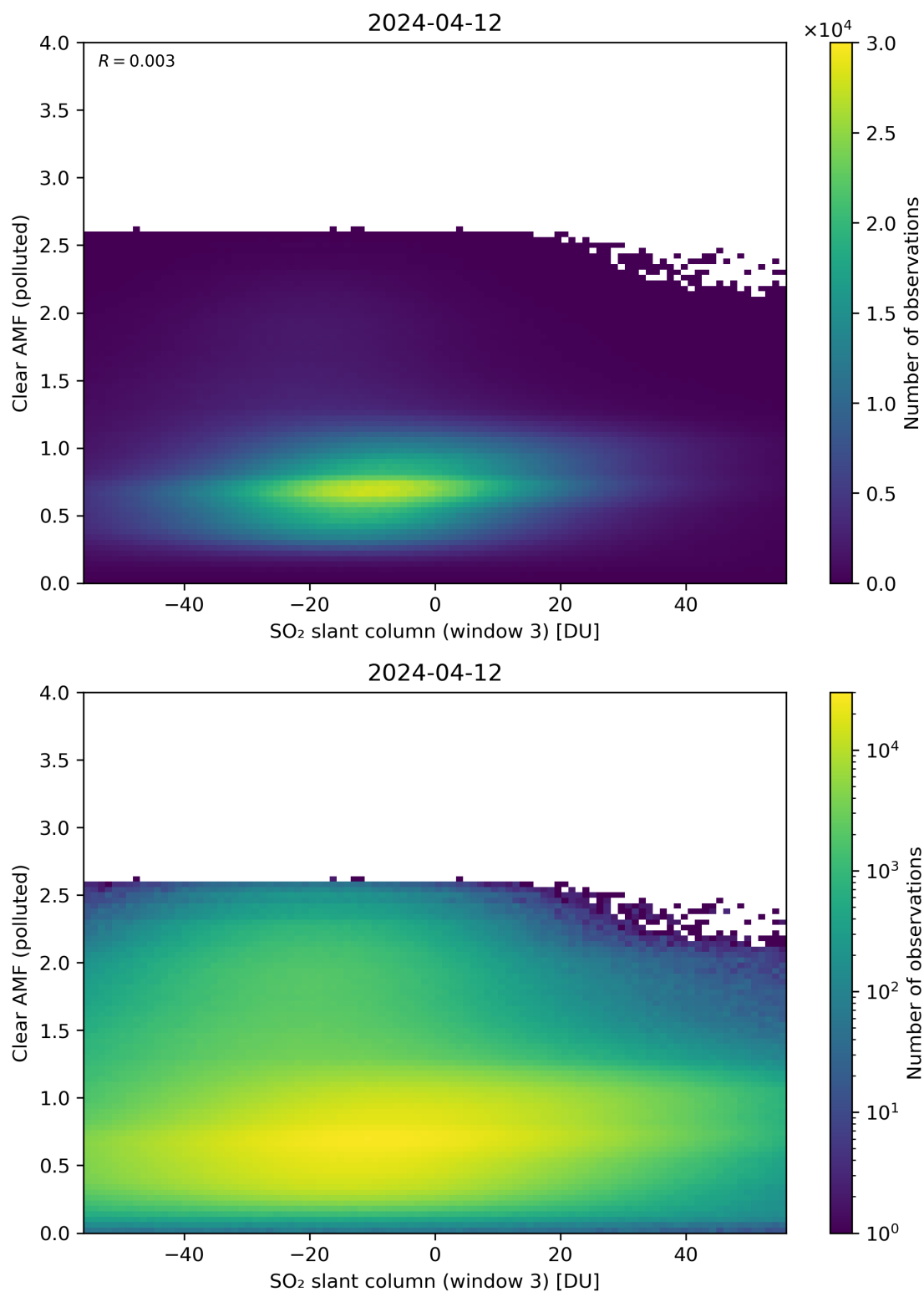
Figure 265: Scatter density plot of “SO 2 slant column (window 3)” against “Clear AMF (polluted)” for 2024-04-11 to 2024-04-13.
