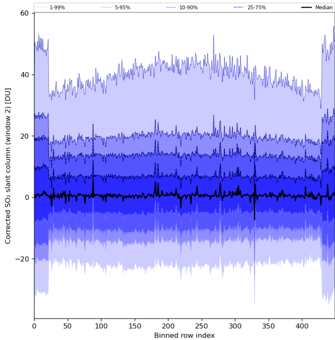
Figure 85: Along track statistics of "Corrected SO 2 slant column (window 2)" for 2024-04-11 to 2024-04-13
