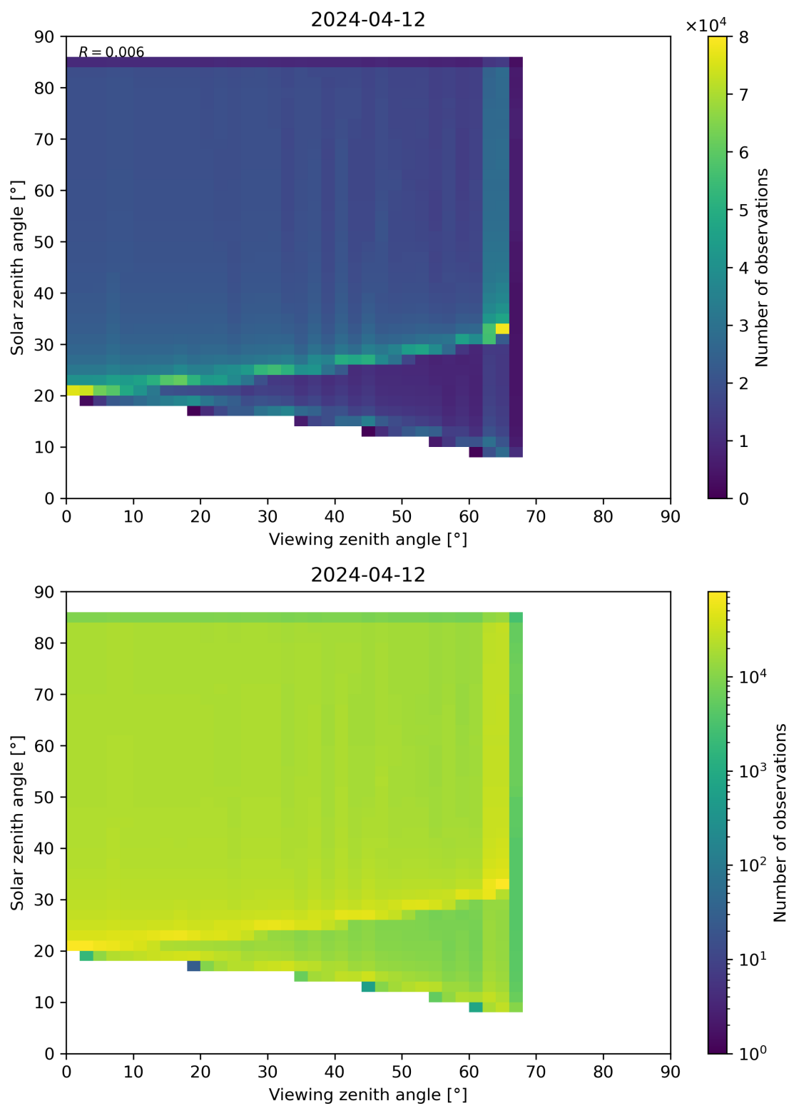
Figure 315: Scatter density plot of “Viewing zenith angle” against “Solar zenith angle” for 2024-04-11 to 2024-04-13.
