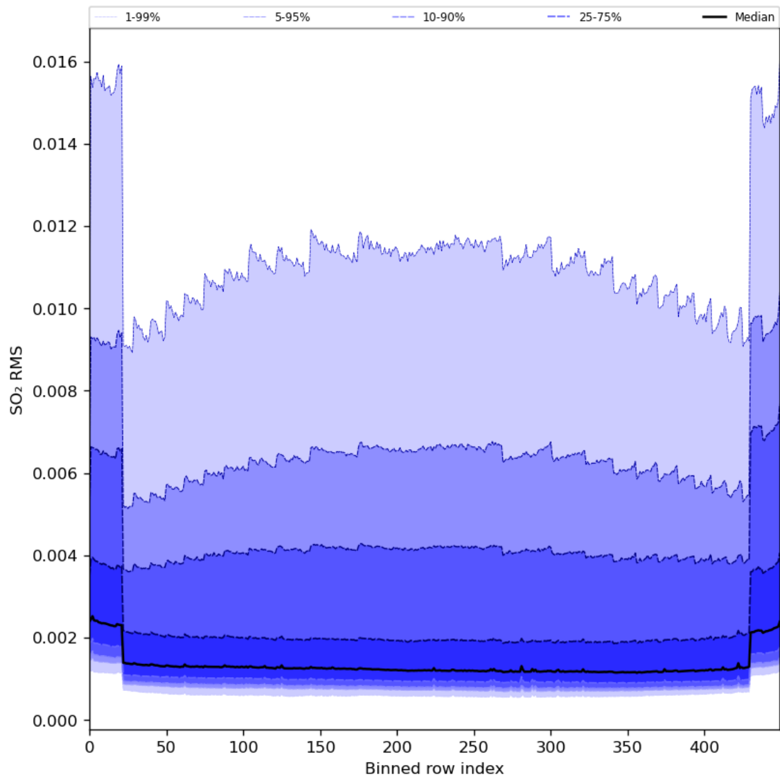
Figure 93: Along track statistics of “SO 2 RMS” for 2024-04-11 to 2024-04-13
