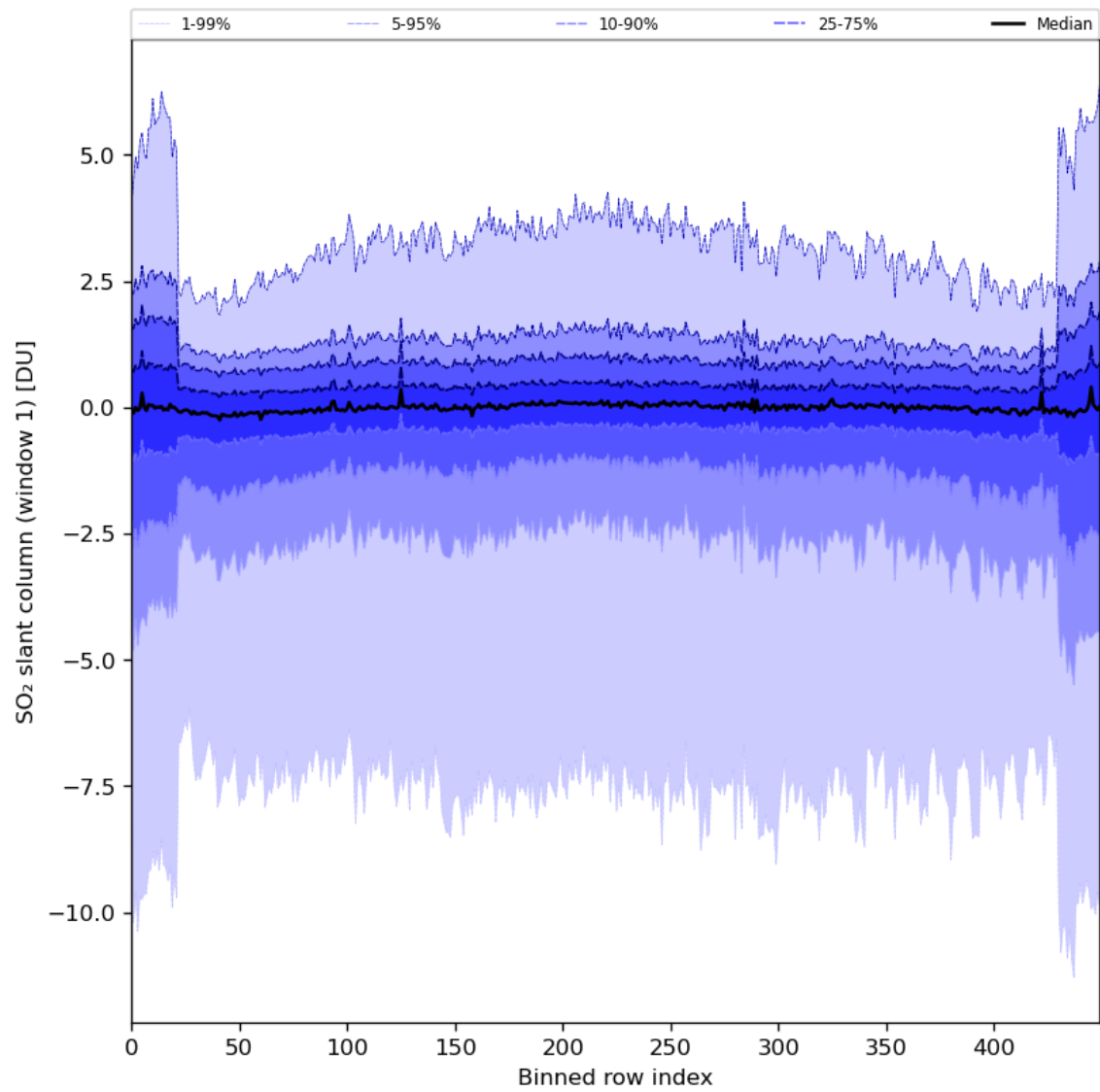
Figure 79: Along track statistics of “SO 2 slant column (window 1)” for 2024-04-11 to 2024-04-13
