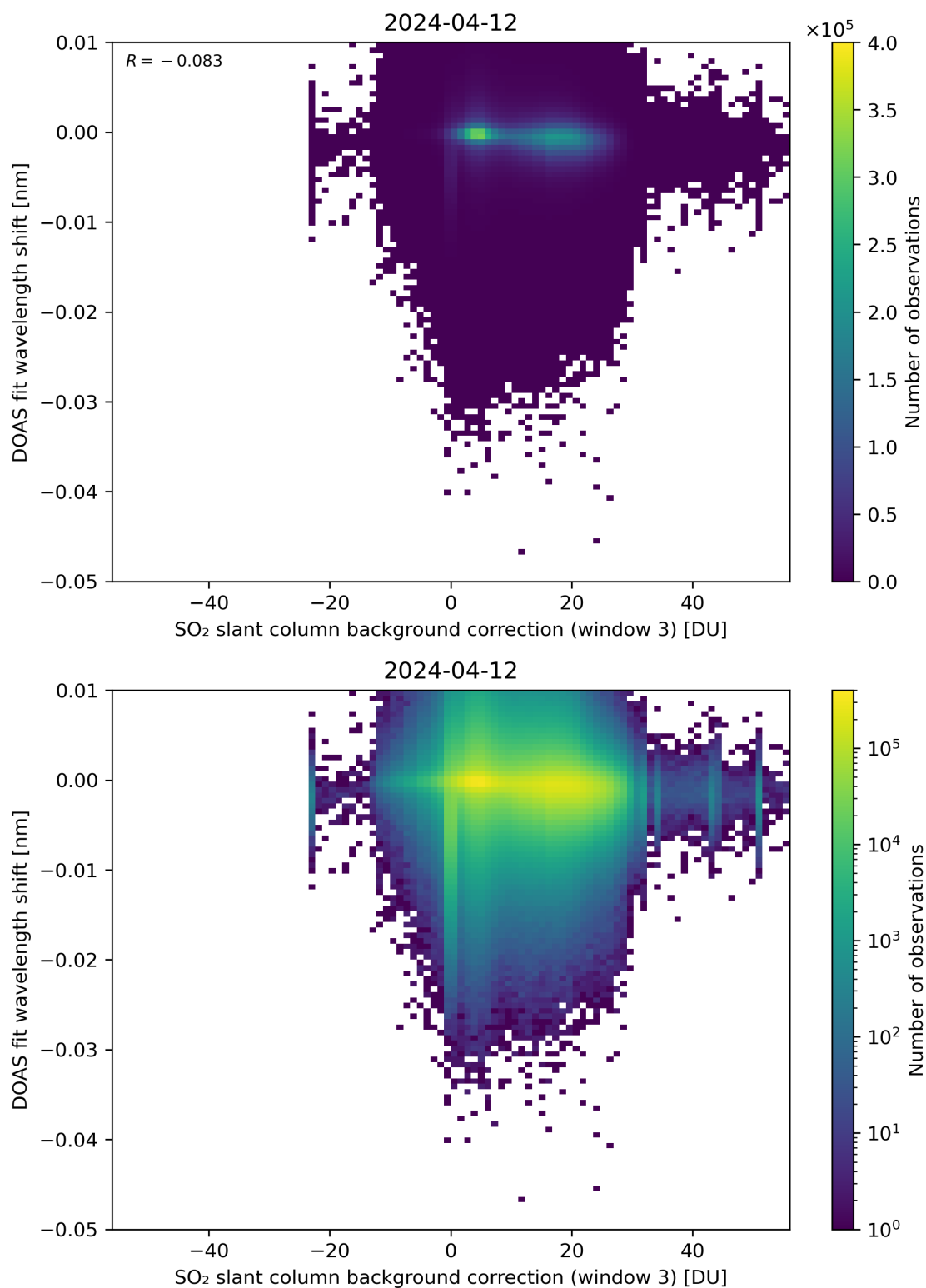
Figure 121: Scatter density plot of “SO 2 slant column background correction (window 3)” against “DOAS fit wavelength shift” for 2024-04-11 to 2024-04-13.
