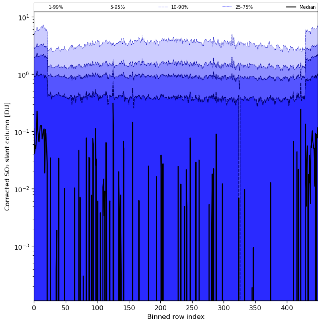
Figure 78: Along track statistics of “Corrected SO 2 slant column” for 2024-04-11 to 2024-04-13
