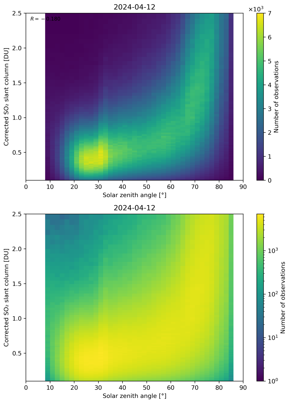
Figure 166: Scatter density plot of “Solar zenith angle” against “Corrected SO 2 slant column” for 2024-04-11 to 2024-04-13.
