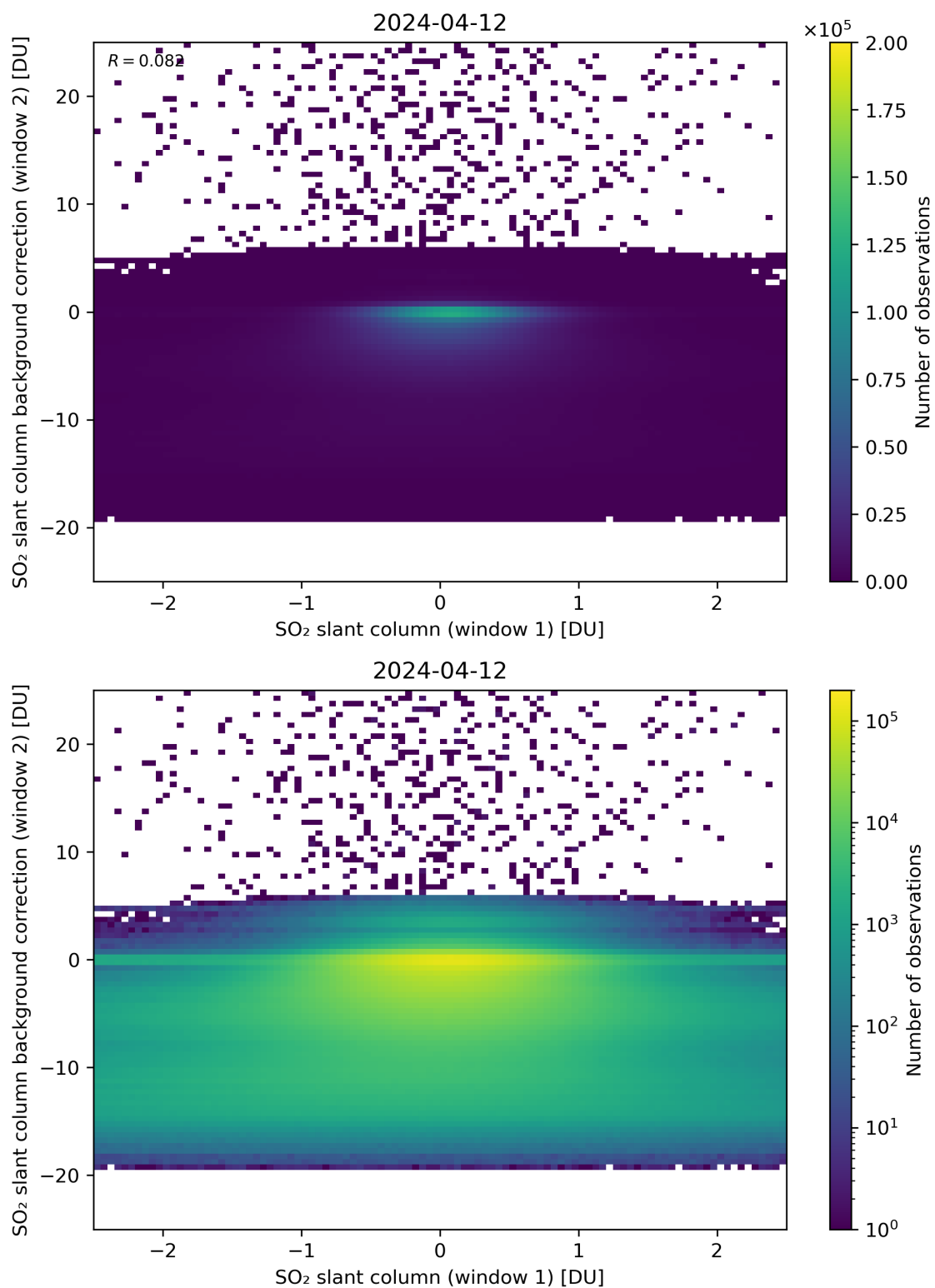
Figure 213: Scatter density plot of “SO 2 slant column (window 1)” against “SO 2 slant column background correction (window 2)” for 2024-04-11 to 2024-04-13.
