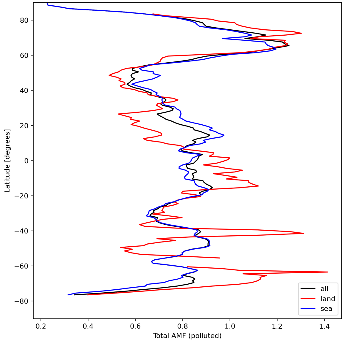
Figure 48: Zonal average of “Total AMF (polluted)” for 2024-04-11 to 2024-04-13.
