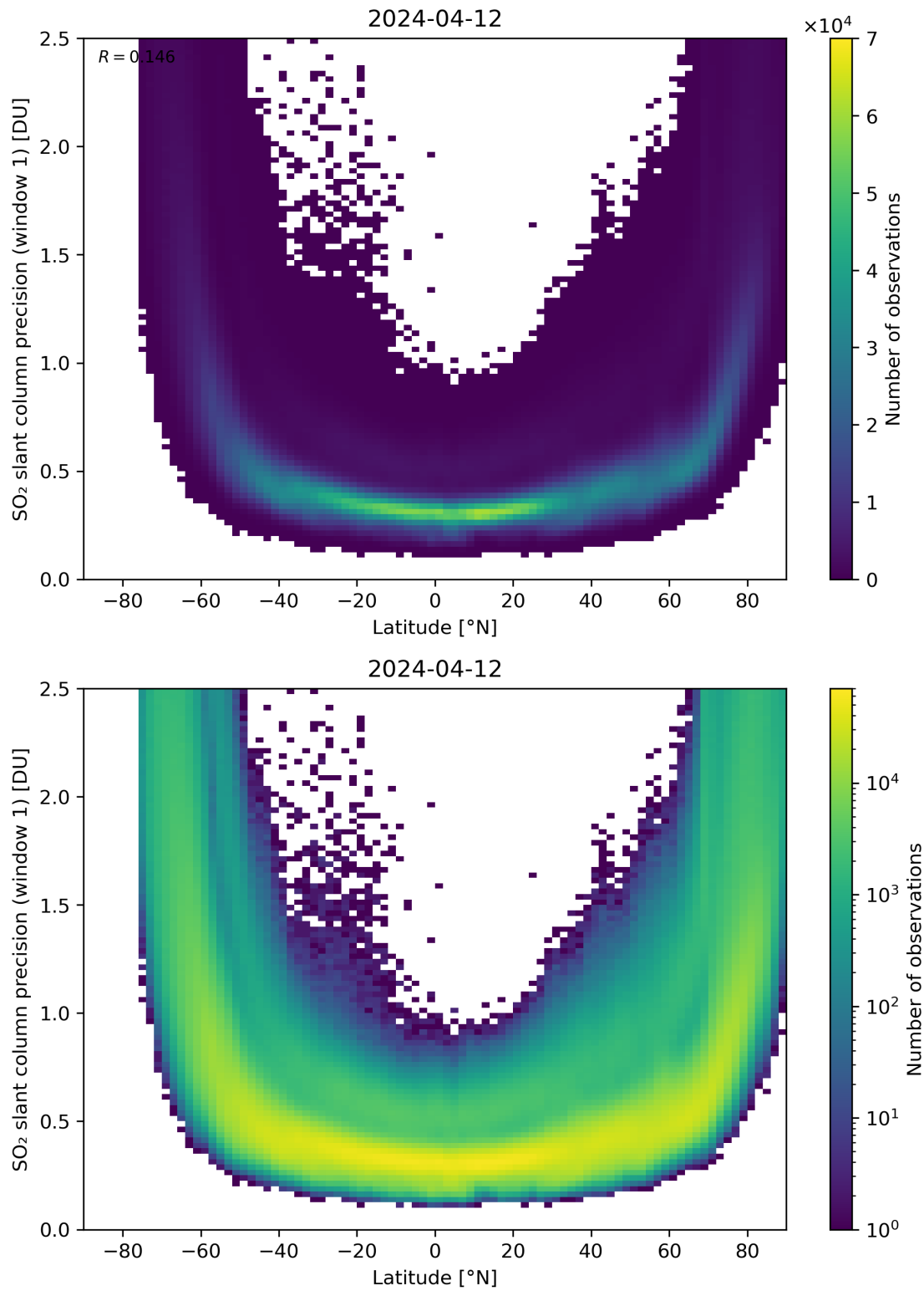
Figure 150: Scatter density plot of “Latitude” against “SO 2 slant column precision (window 1)” for 2024-04-11 to 2024-04-13.
