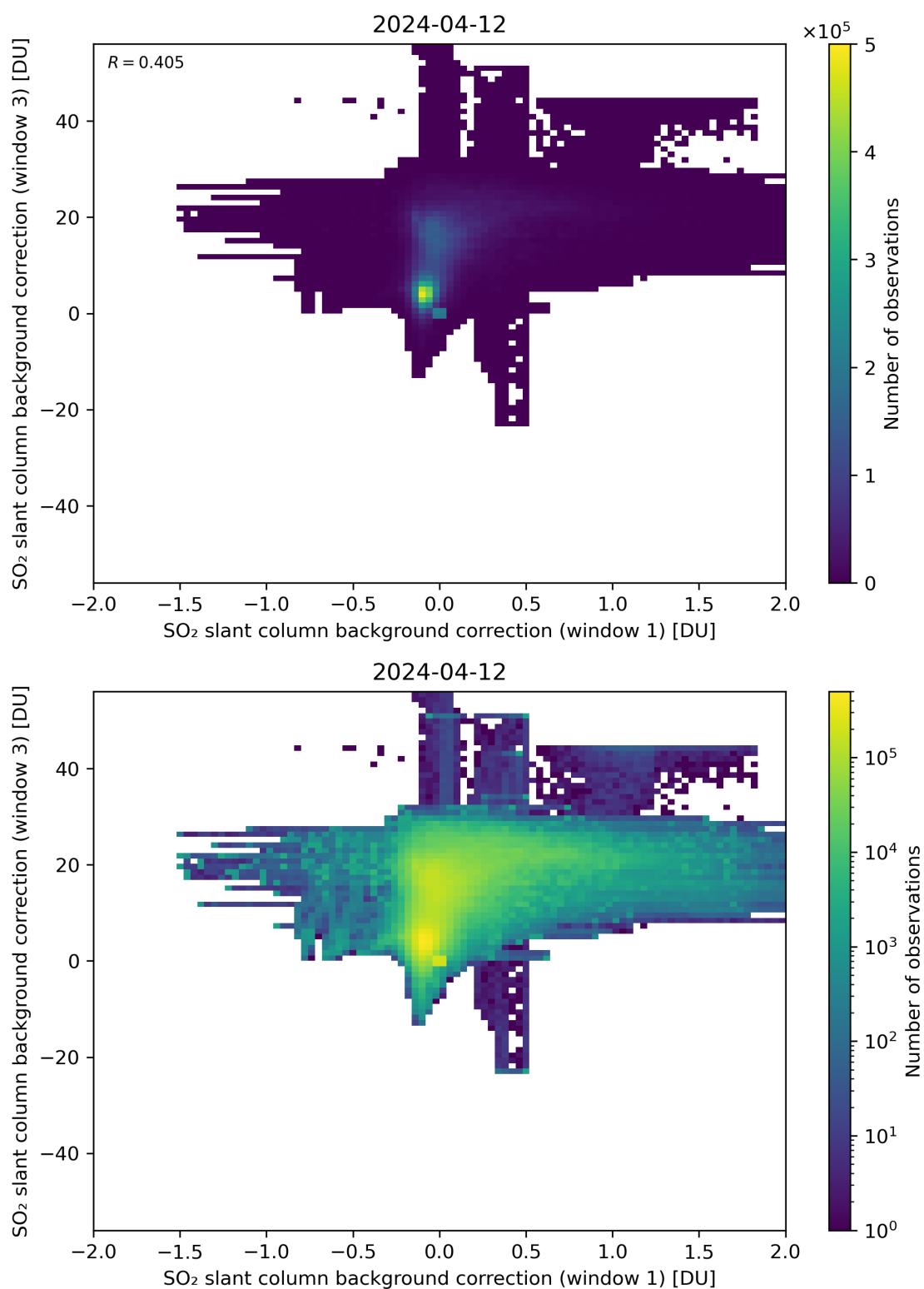
Figure 99: Scatter density plot of “SO 2 slant column background correction (window 1)” against “SO 2 slant column background correction (window 3)” for 2024-04-11 to 2024-04-13.
