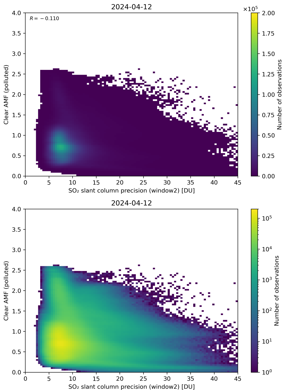
Figure 246: Scatter density plot of “SO 2 slant column precision (window2)” against “Clear AMF (polluted)” for 2024-04-11 to 2024-04-13.
