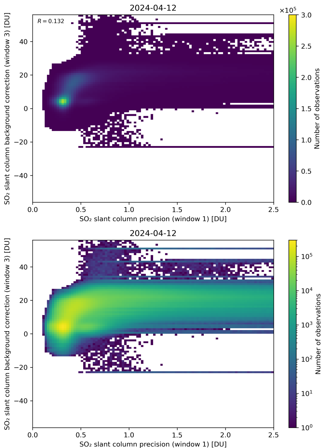
Figure 220: Scatter density plot of “SO 2 slant column precision (window 1)” against “SO 2 slant column background correction (window 3)” for 2024-04-11 to 2024-04-13.
