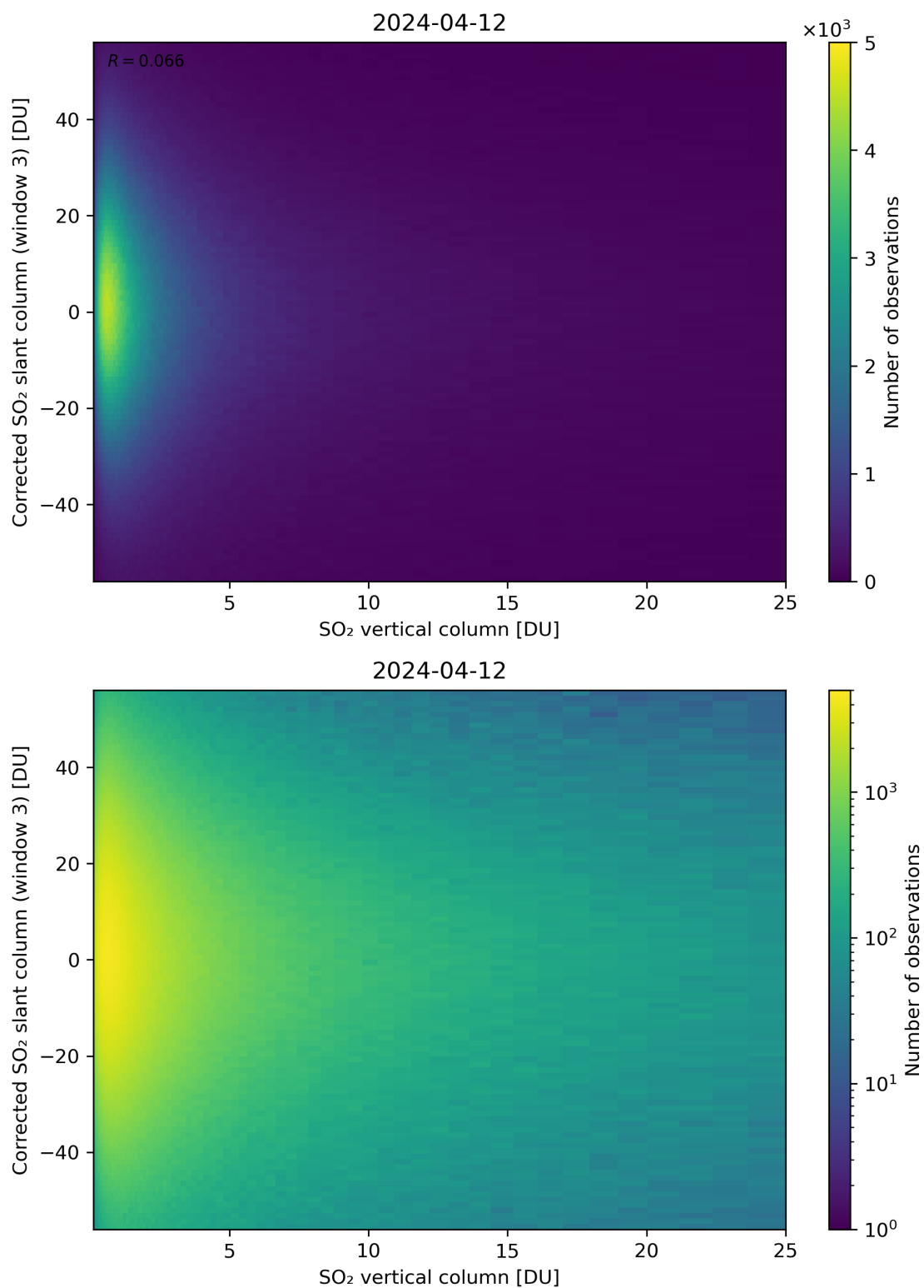
Figure 299: Scatter density plot of “SO 2 vertical column” against “Corrected SO 2 slant column (window 3)” for 2024-04-11 to 2024-04-13.
