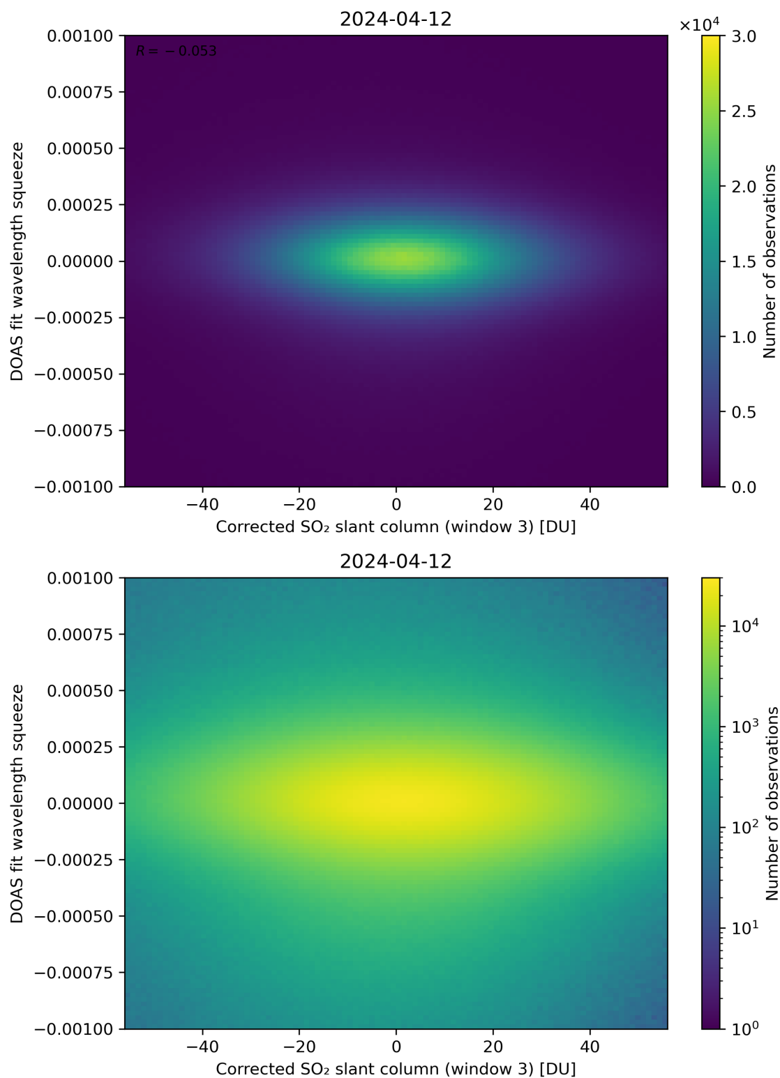
Figure 207: Scatter density plot of “Corrected SO 2 slant column (window 3)” against “DOAS fit wavelength squeeze” for 2024-04-11 to 2024-04-13.
