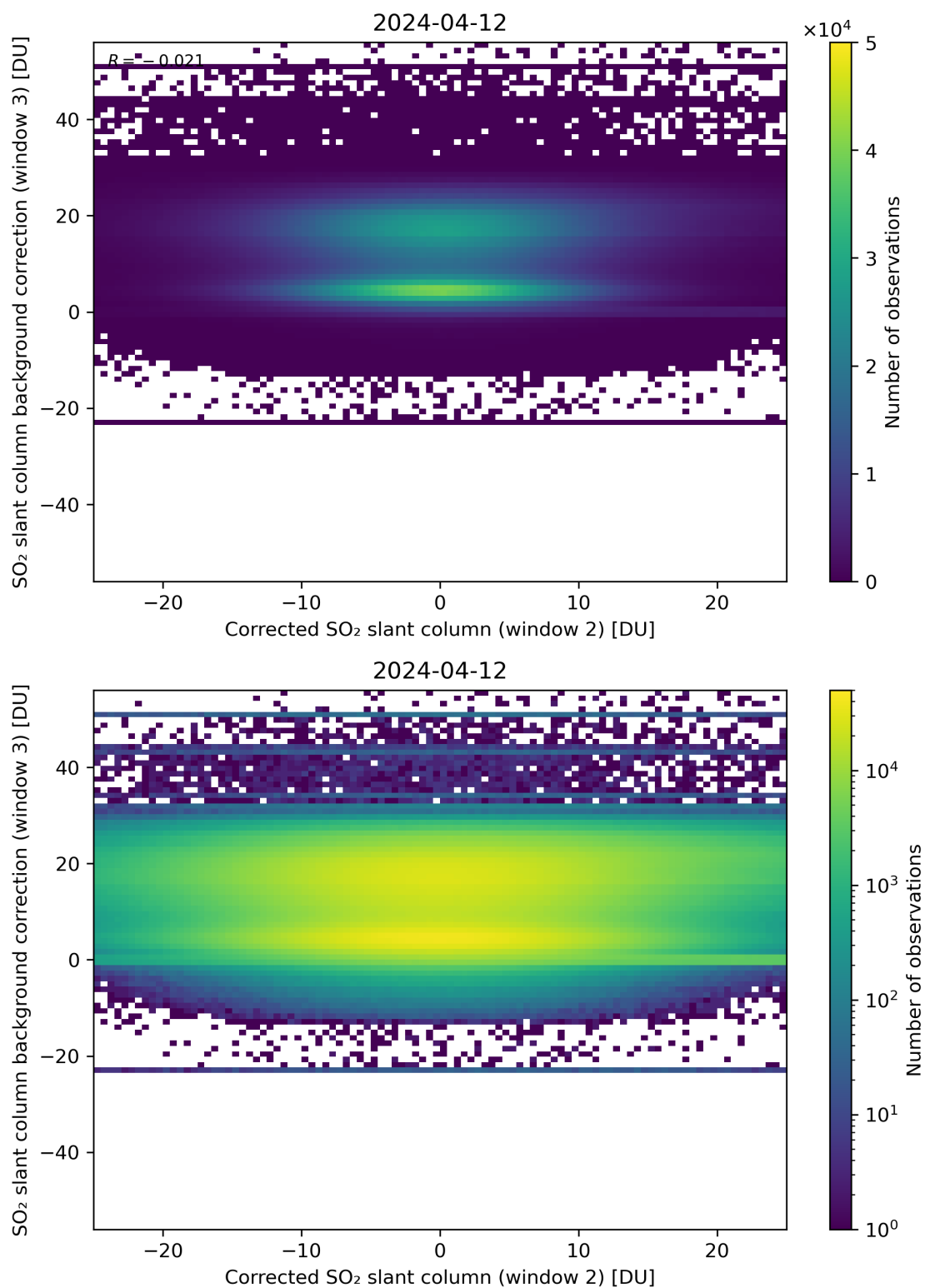
Figure 195: Scatter density plot of “Corrected SO 2 slant column (window 2)” against “SO 2 slant column background correction (window 3)” for 2024-04-11 to 2024-04-13.
