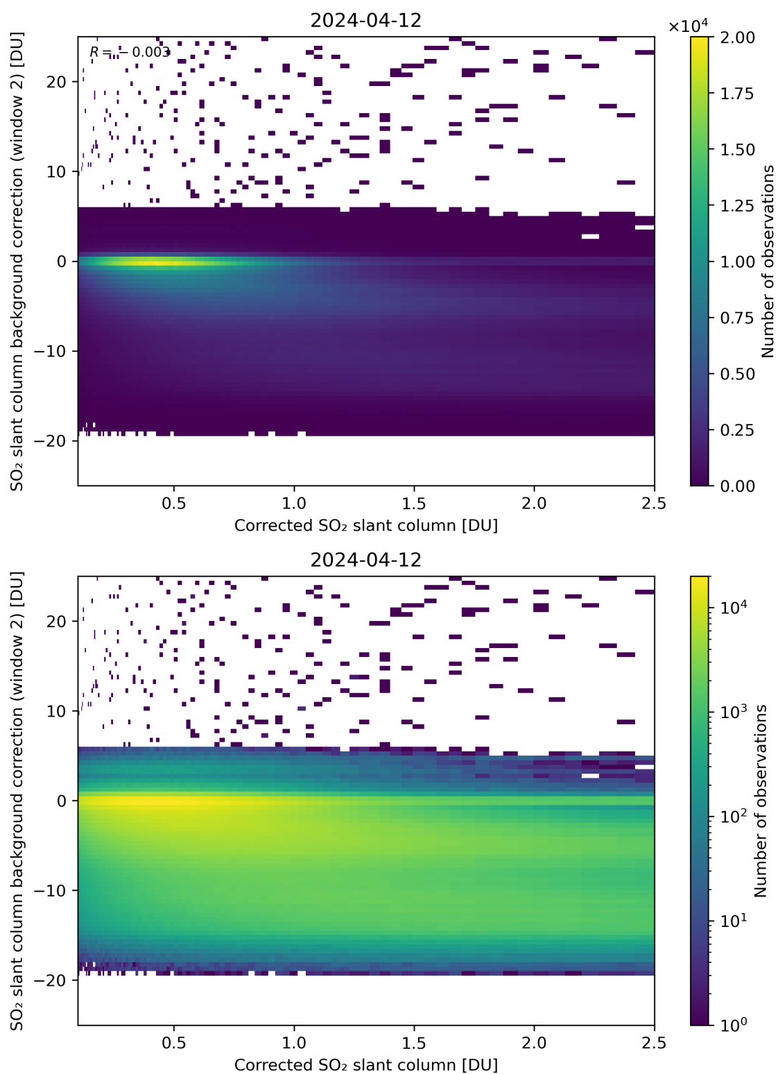
Figure 179: Scatter density plot of “Corrected SO 2 slant column” against “SO 2 slant column background correction (window 2)” for 2024-04-11 to 2024-04-13.
