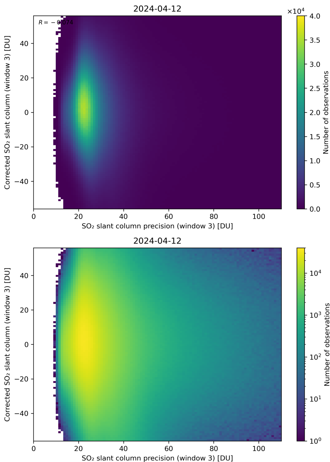
Figure 262: Scatter density plot of “SO 2 slant column precision (window 3)” against “Corrected SO 2 slant column (window 3)” for 2024-04-11 to 2024-04-13.
