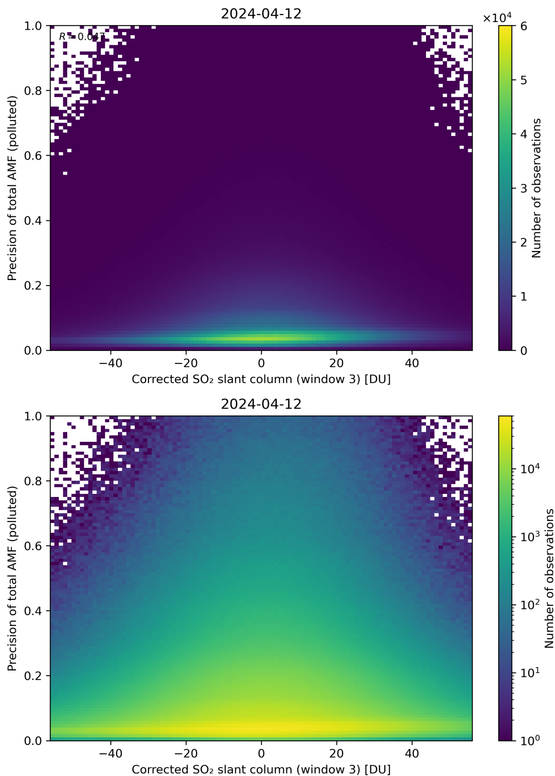
Figure 211: Scatter density plot of “Corrected SO 2 slant column (window 3)” against “Precision of total AMF (polluted)” for 2024-04-11 to 2024-04-13.
