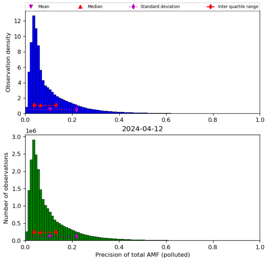
Figure 72: Histogram of “Precision of total AMF (polluted)” for 2024-04-11 to 2024-04-13
