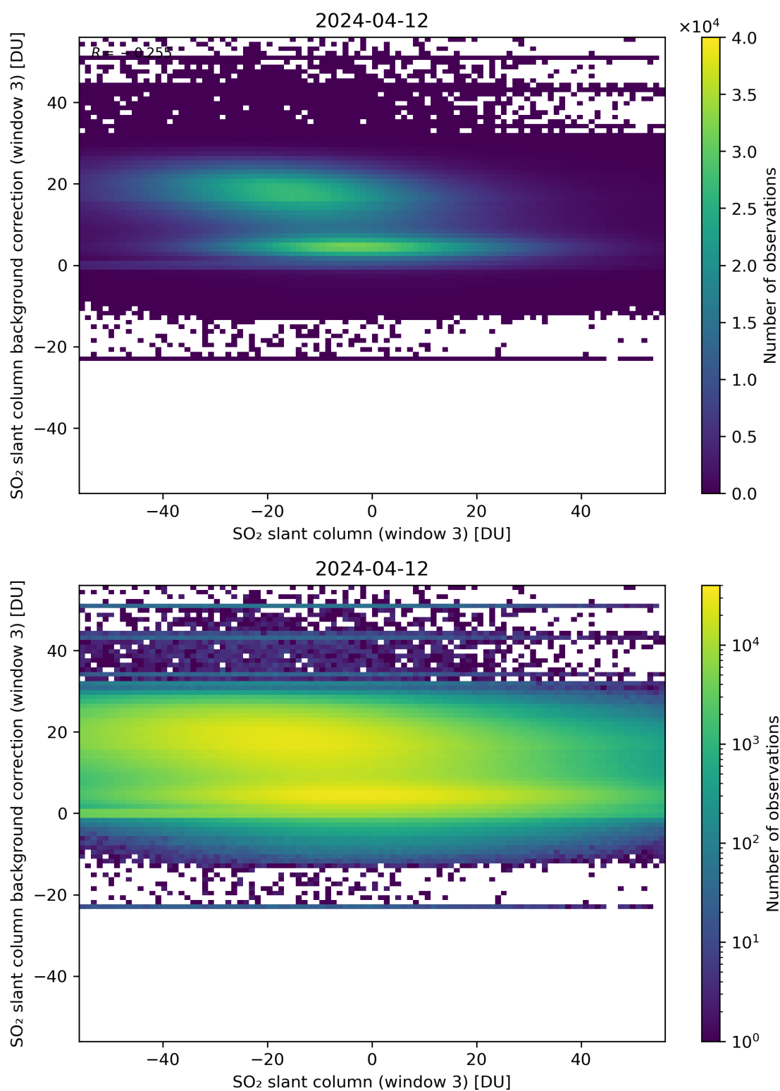
Figure 253: Scatter density plot of “SO 2 slant column (window 3)” against “SO 2 slant column background correction (window 3)” for 2024-04-11 to 2024-04-13.
