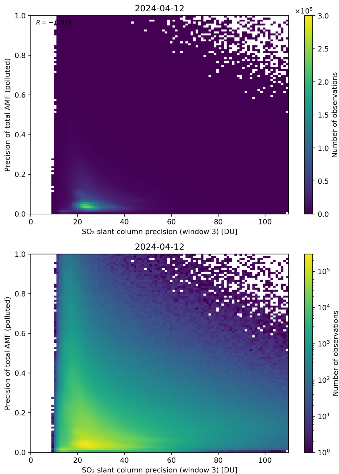
Figure 264: Scatter density plot of “SO 2 slant column precision (window 3)” against “Precision of total AMF (polluted)” for 2024-04-11 to 2024-04-13.
