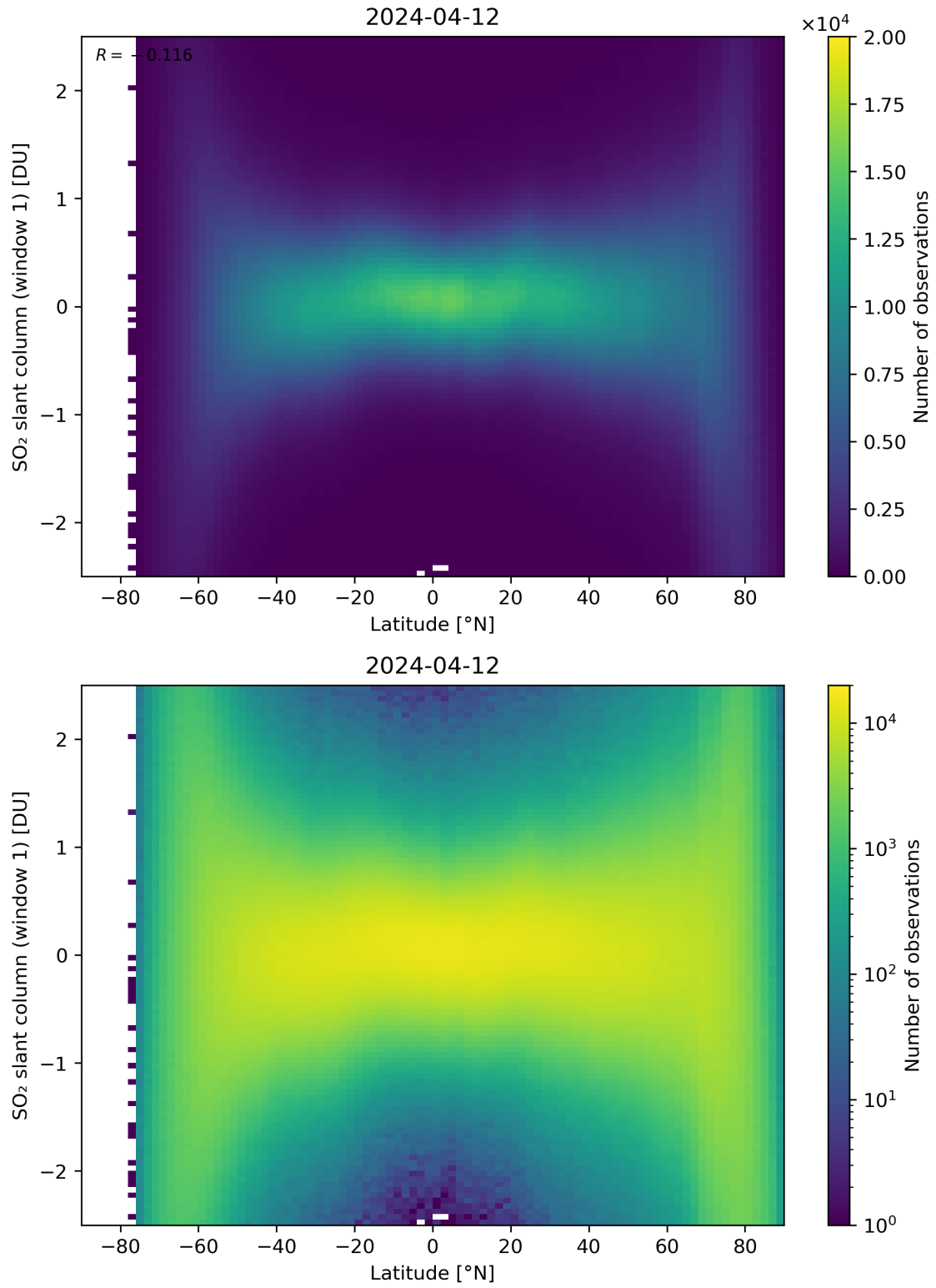
Figure 149: Scatter density plot of “Latitude” against “SO 2 slant column (window 1)” for 2024-04-11 to 2024-04-13.
