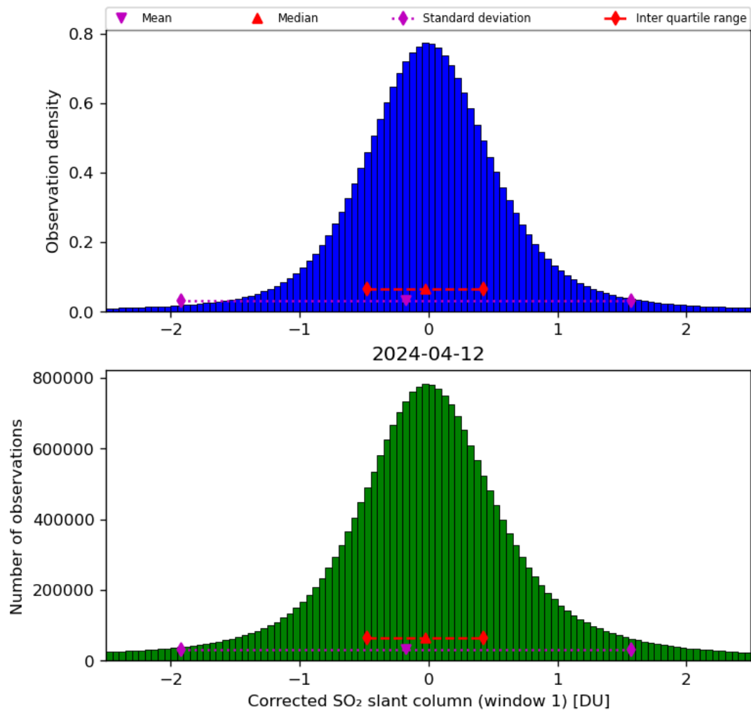
Figure 58: Histogram of “Corrected SO 2 slant column (window 1)” for 2024-04-11 to 2024-04-13
