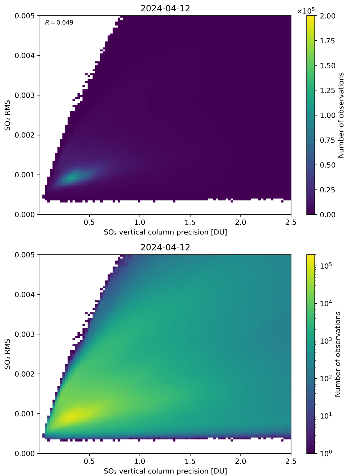
Figure 284: Scatter density plot of “SO 2 vertical column precision” against “SO 2 RMS” for 2024-04-11 to 2024-04-13.
