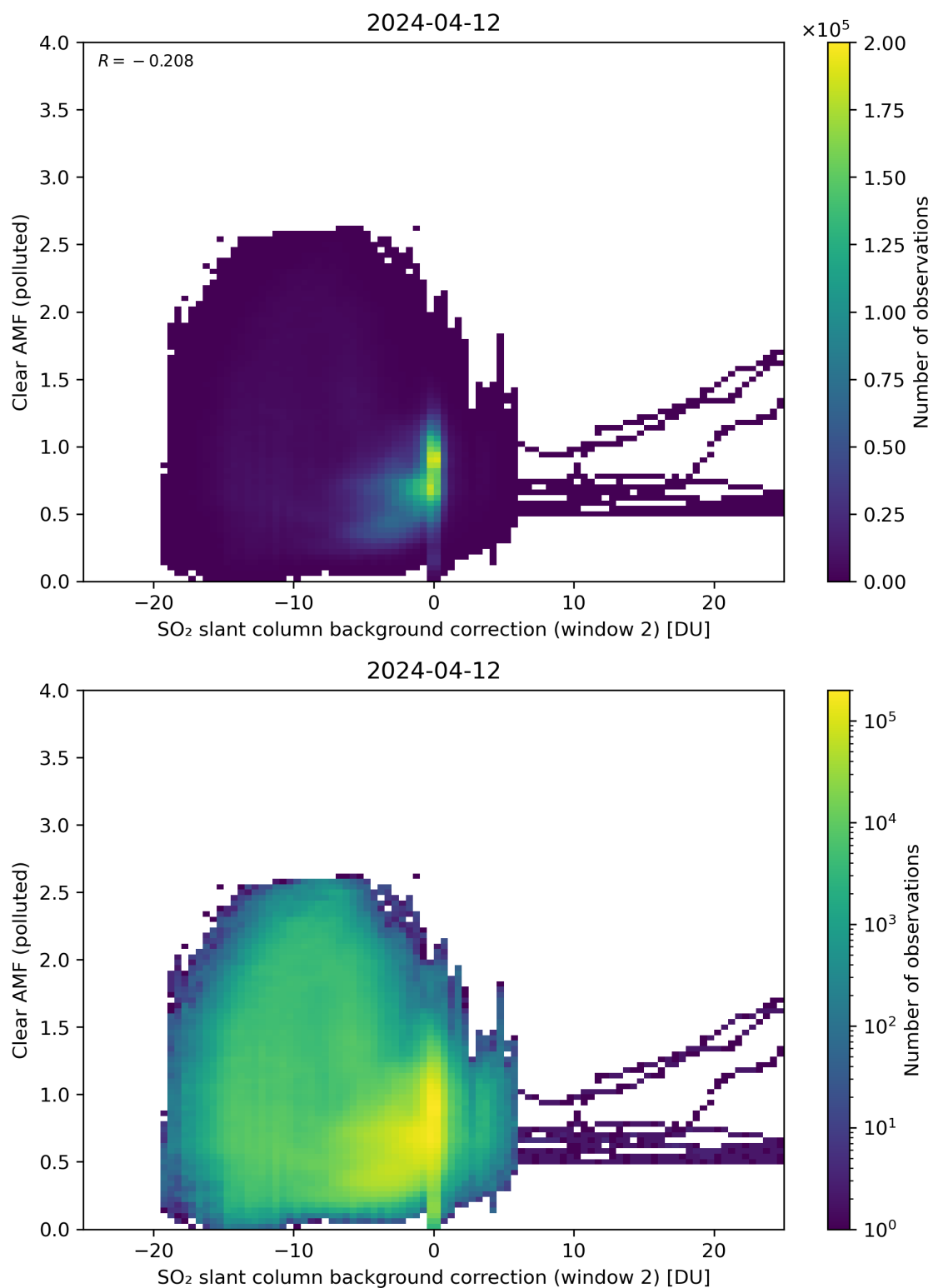
Figure 115: Scatter density plot of “SO 2 slant column background correction (window 2)” against “Clear AMF (polluted)” for 2024-04-11 to 2024-04-13.
