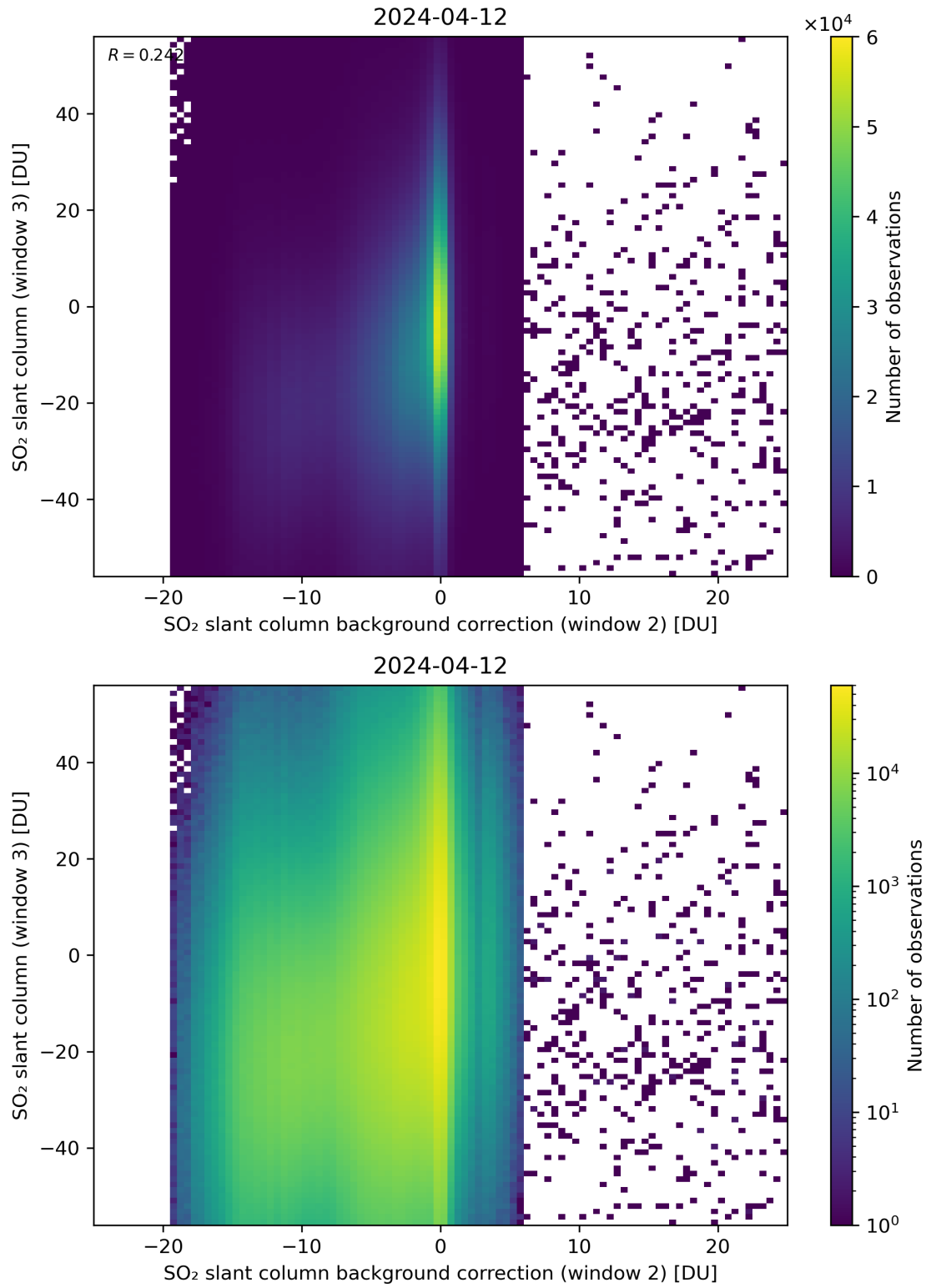
Figure 117: Scatter density plot of “SO 2 slant column background correction (window 2)” against “SO 2 slant column (window 3)” for 2024-04-11 to 2024-04-13.
