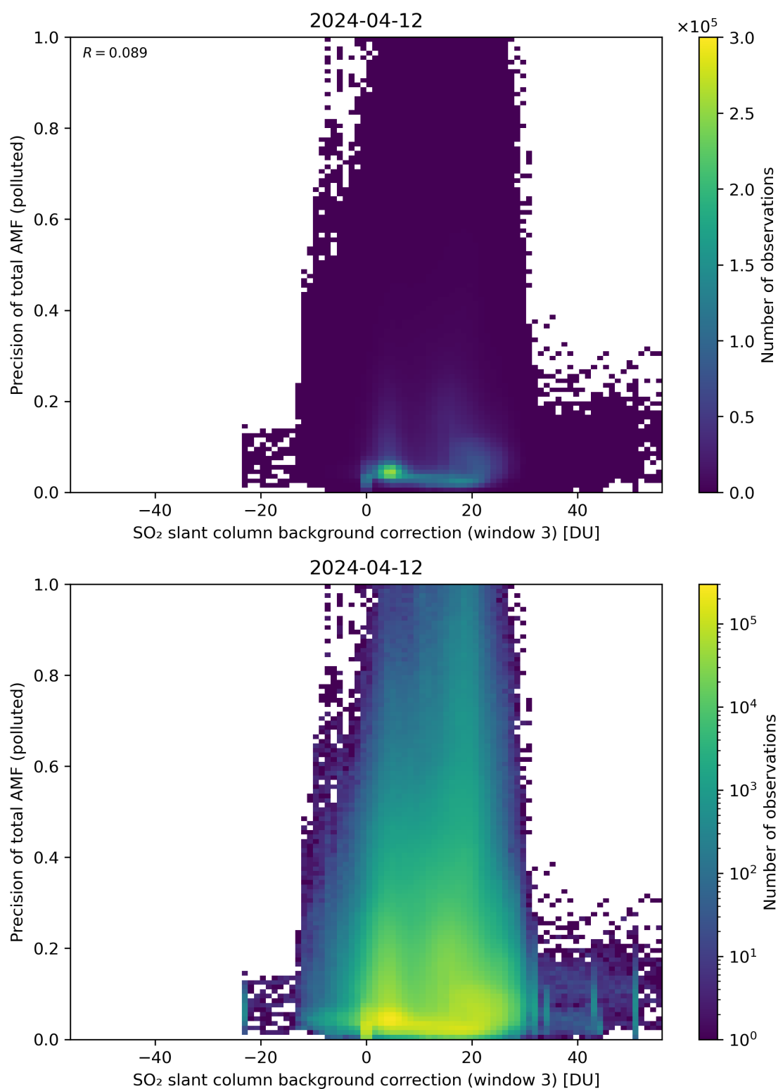
Figure 126: Scatter density plot of “SO 2 slant column background correction (window 3)” against “Precision of total AMF (polluted)” for 2024-04-11 to 2024-04-13.
