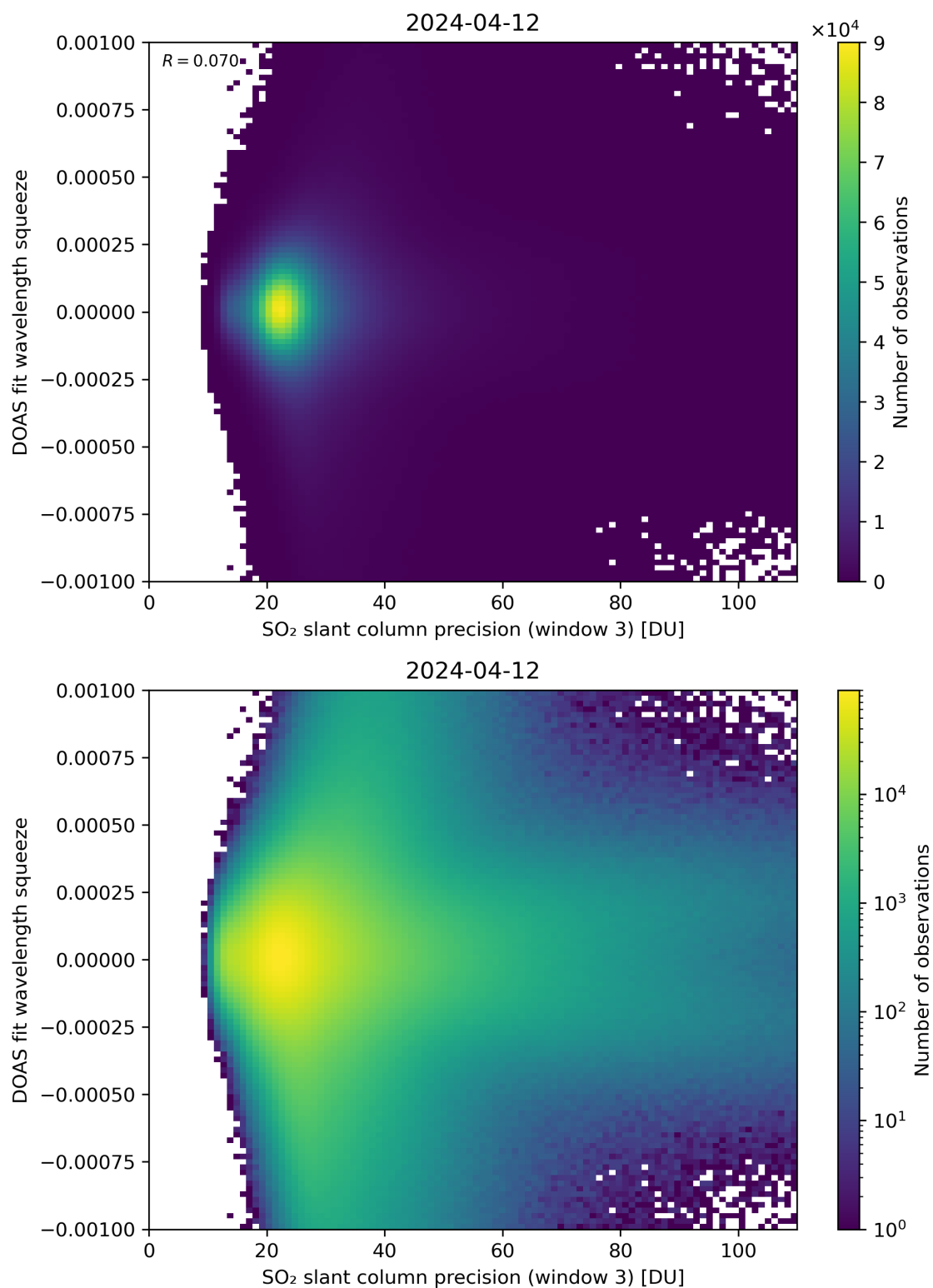
Figure 259: Scatter density plot of “SO 2 slant column precision (window 3)” against “DOAS fit wavelength squeeze” for 2024-04-11 to 2024-04-13.
