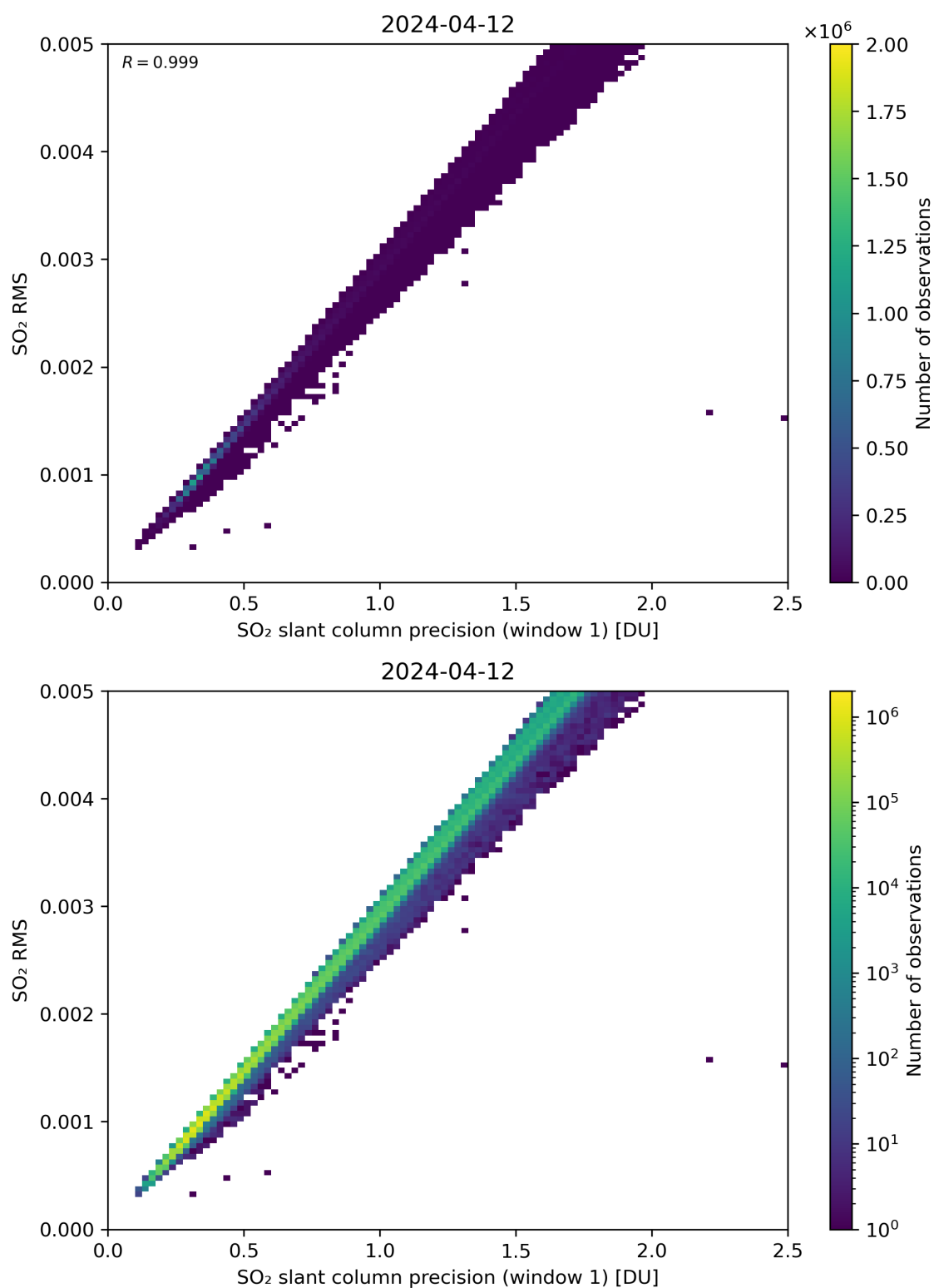
Figure 223: Scatter density plot of “SO 2 slant column precision (window 1)” against “SO 2 RMS” for 2024-04-11 to 2024-04-13.
