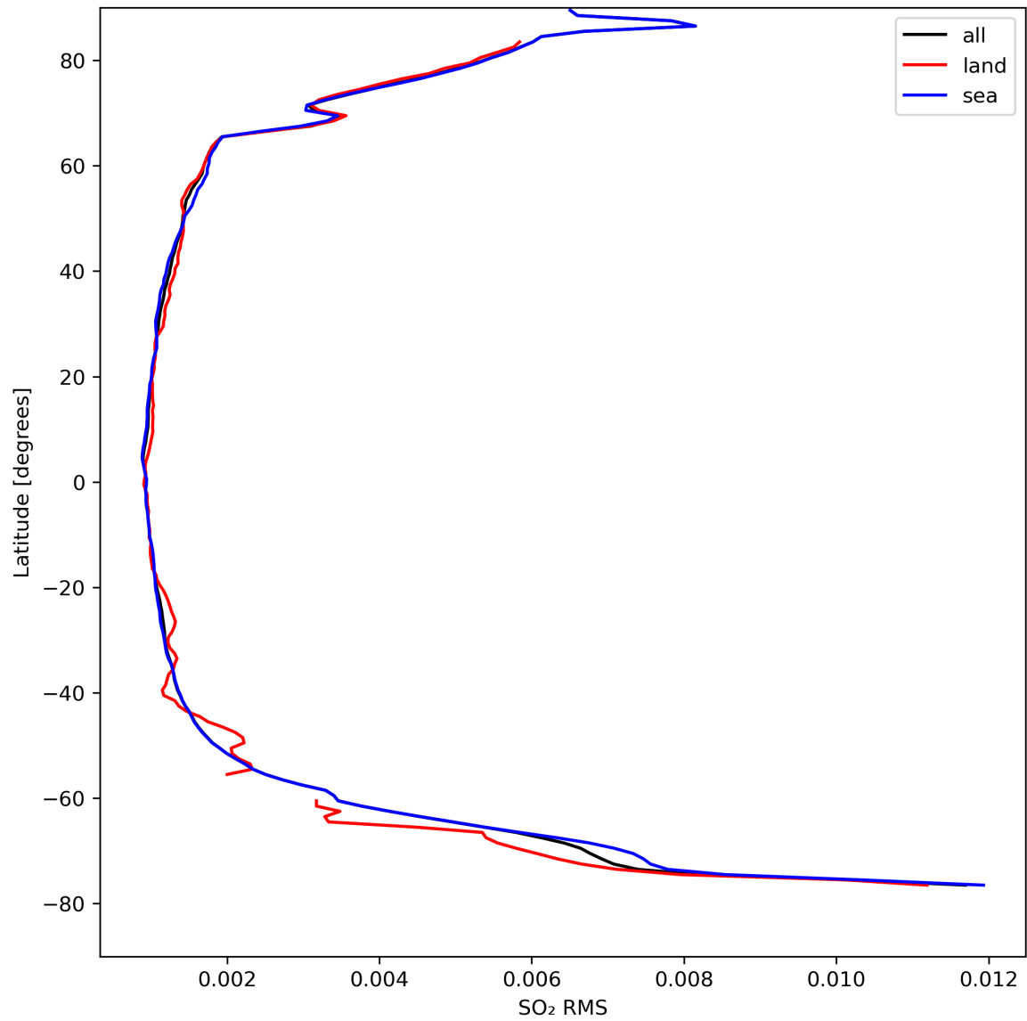
Figure 47: Zonal average of “SO 2 RMS” for 2024-04-11 to 2024-04-13.
