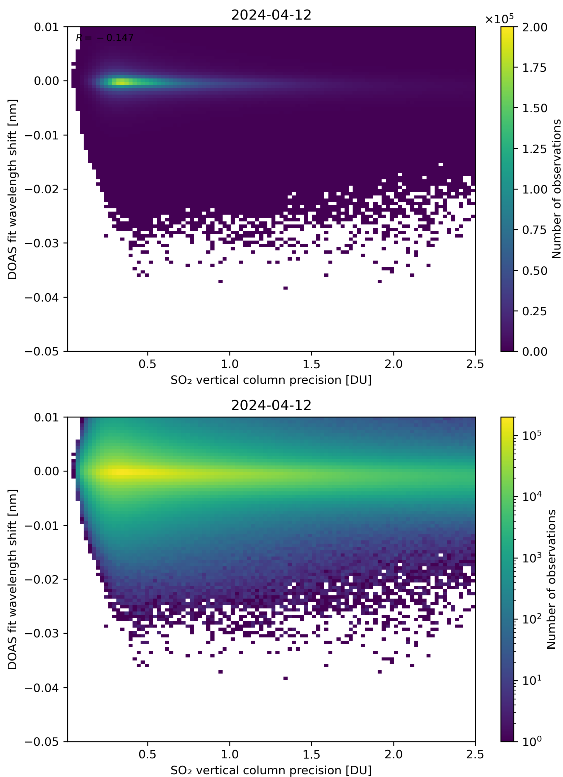
Figure 282: Scatter density plot of “SO 2 vertical column precision” against “DOAS fit wavelength shift” for 2024-04-11 to 2024-04-13.
