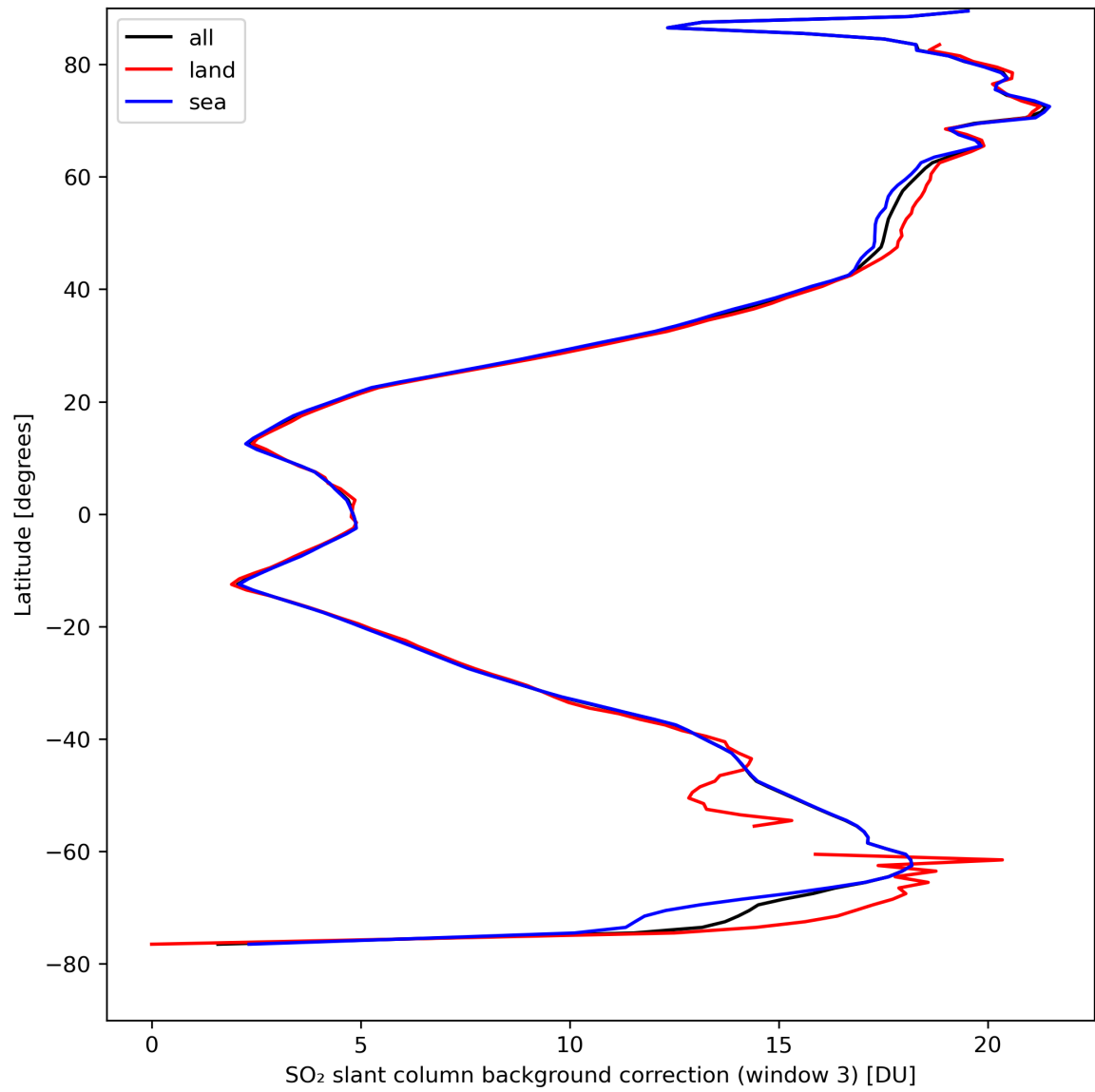
Figure 44: Zonal average of “SO 2 slant column background correction (window 3)” for 2024-04-11 to 2024-04-13.
