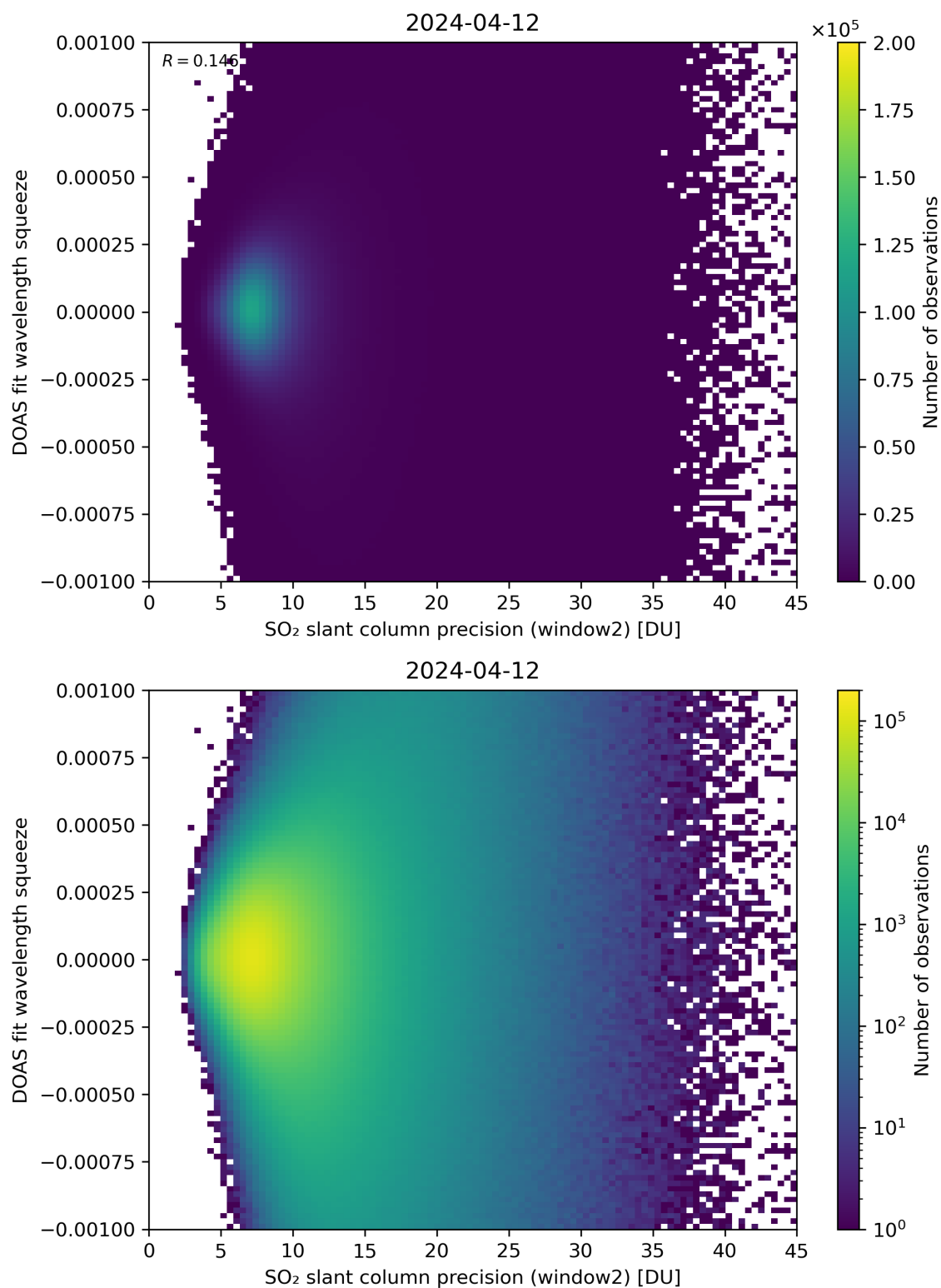
Figure 244: Scatter density plot of “SO 2 slant column precision (window2)” against “DOAS fit wavelength squeeze” for 2024-04-11 to 2024-04-13.
