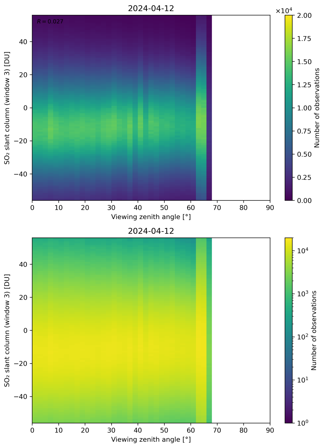
Figure 323: Scatter density plot of “Viewing zenith angle” against “SO 2 slant column (window 3)” for 2024-04-11 to 2024-04-13.
