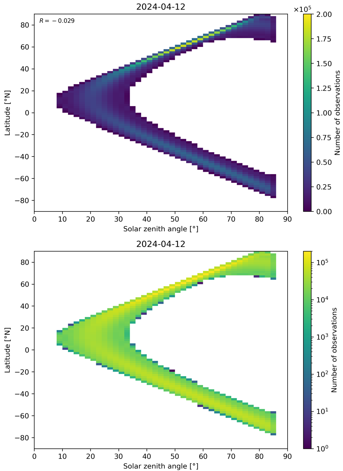
Figure 164: Scatter density plot of “Solar zenith angle” against “Latitude” for 2024-04-11 to 2024-04-13.
