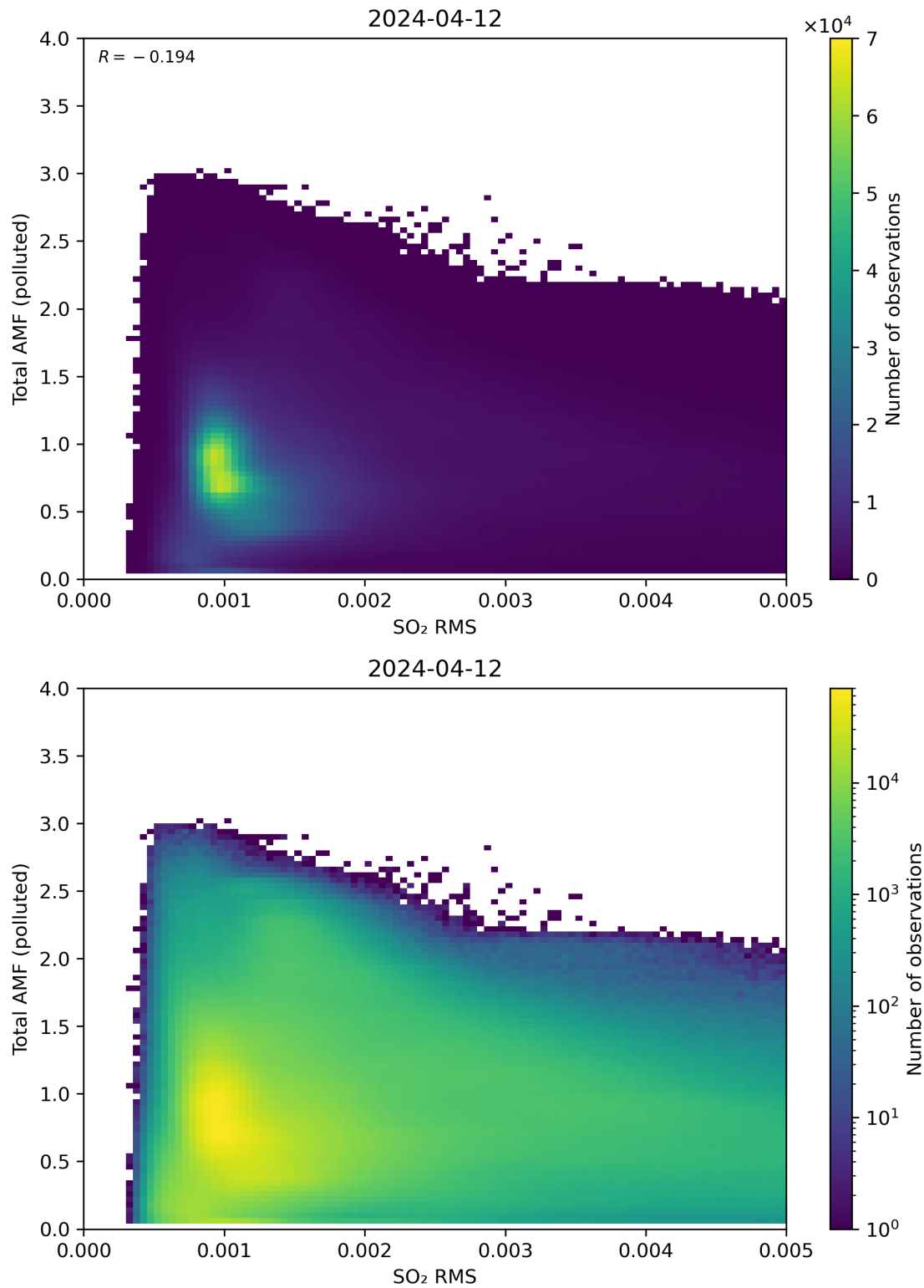
Figure 137: Scatter density plot of “SO 2 RMS” against “Total AMF (polluted)” for 2024-04-11 to 2024-04-13.
