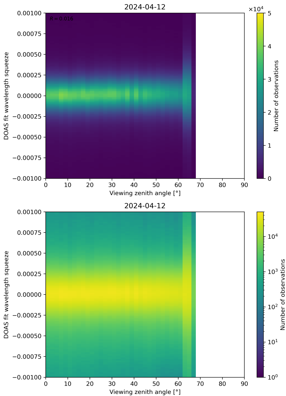
Figure 312: Scatter density plot of “Viewing zenith angle” against “DOAS fit wavelength squeeze” for 2024-04-11 to 2024-04-13.
