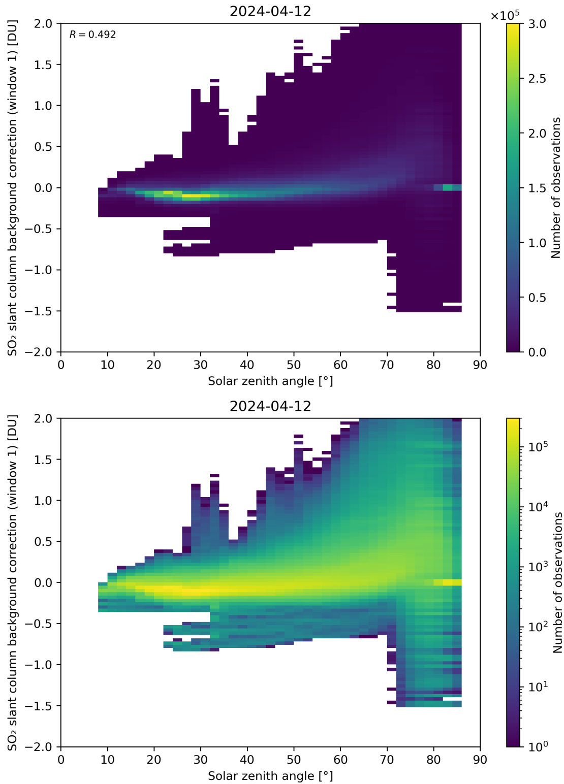
Figure 158: Scatter density plot of “Solar zenith angle” against “SO 2 slant column background correction (window 1)” for 2024-04-11 to 2024-04-13.
