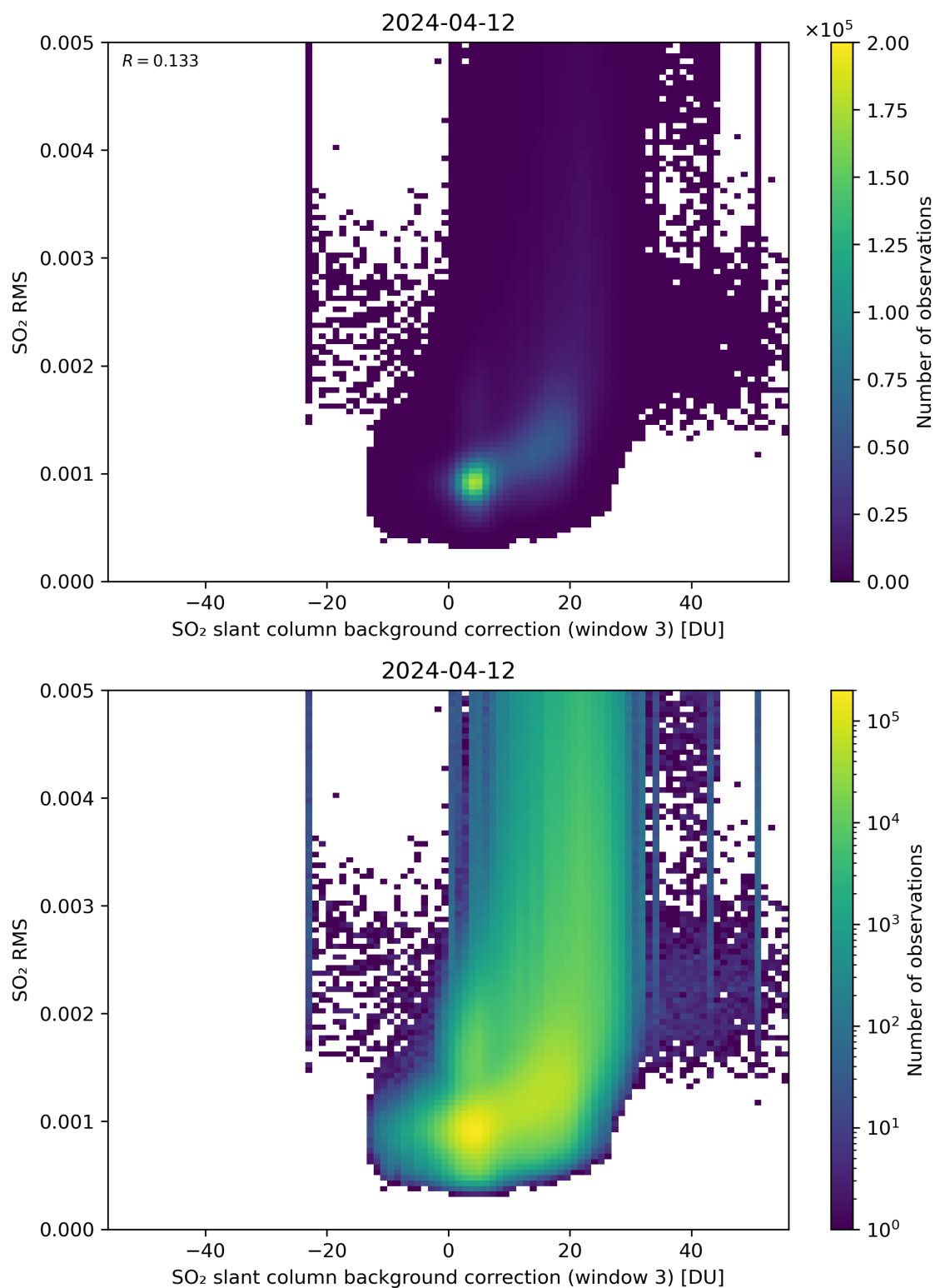
Figure 123: Scatter density plot of “SO 2 slant column background correction (window 3)” against “SO 2 RMS” for 2024-04-11 to 2024-04-13.
