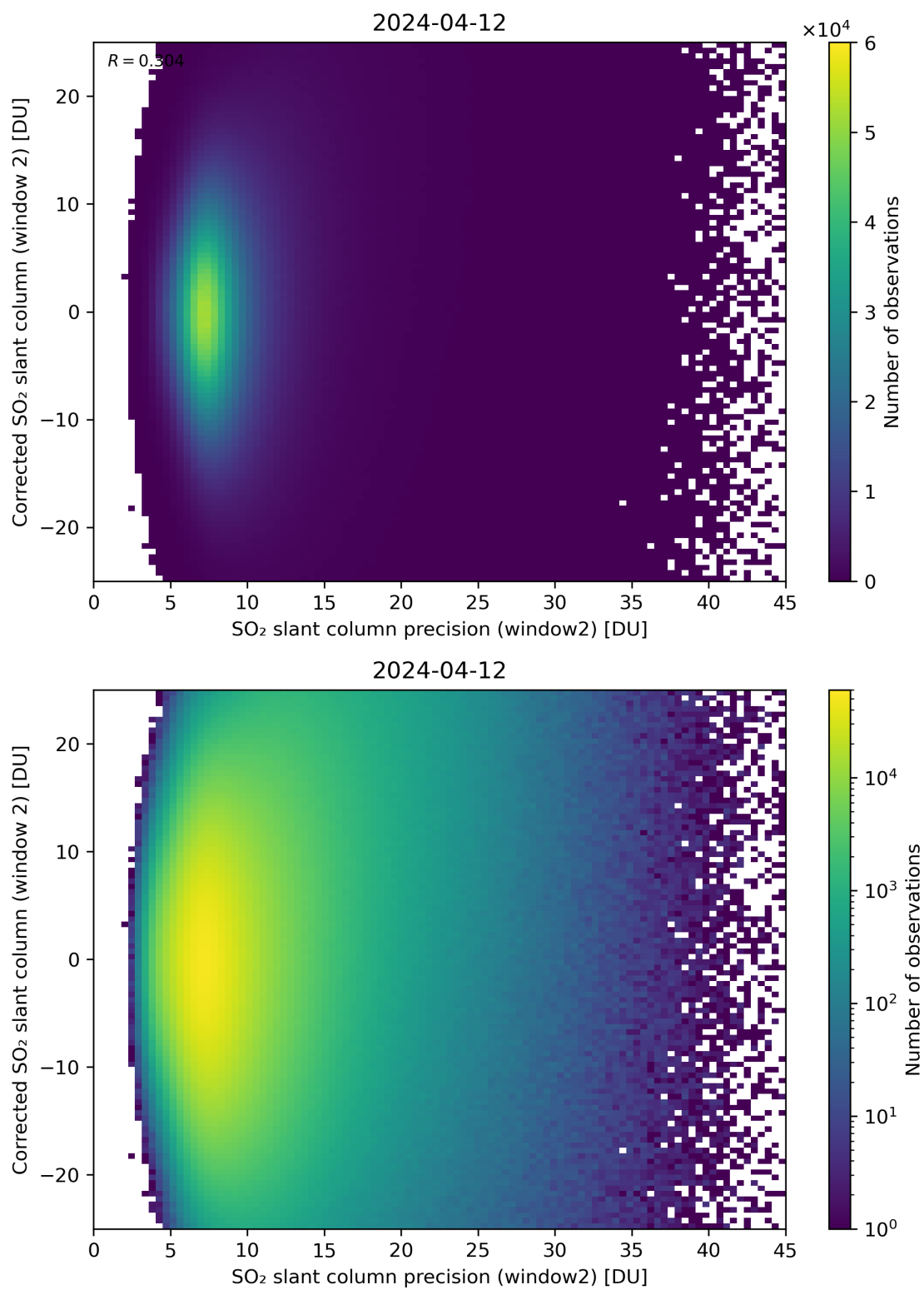
Figure 247: Scatter density plot of “SO 2 slant column precision (window2)” against “Corrected SO 2 slant column (window 2)” for 2024-04-11 to 2024-04-13.
