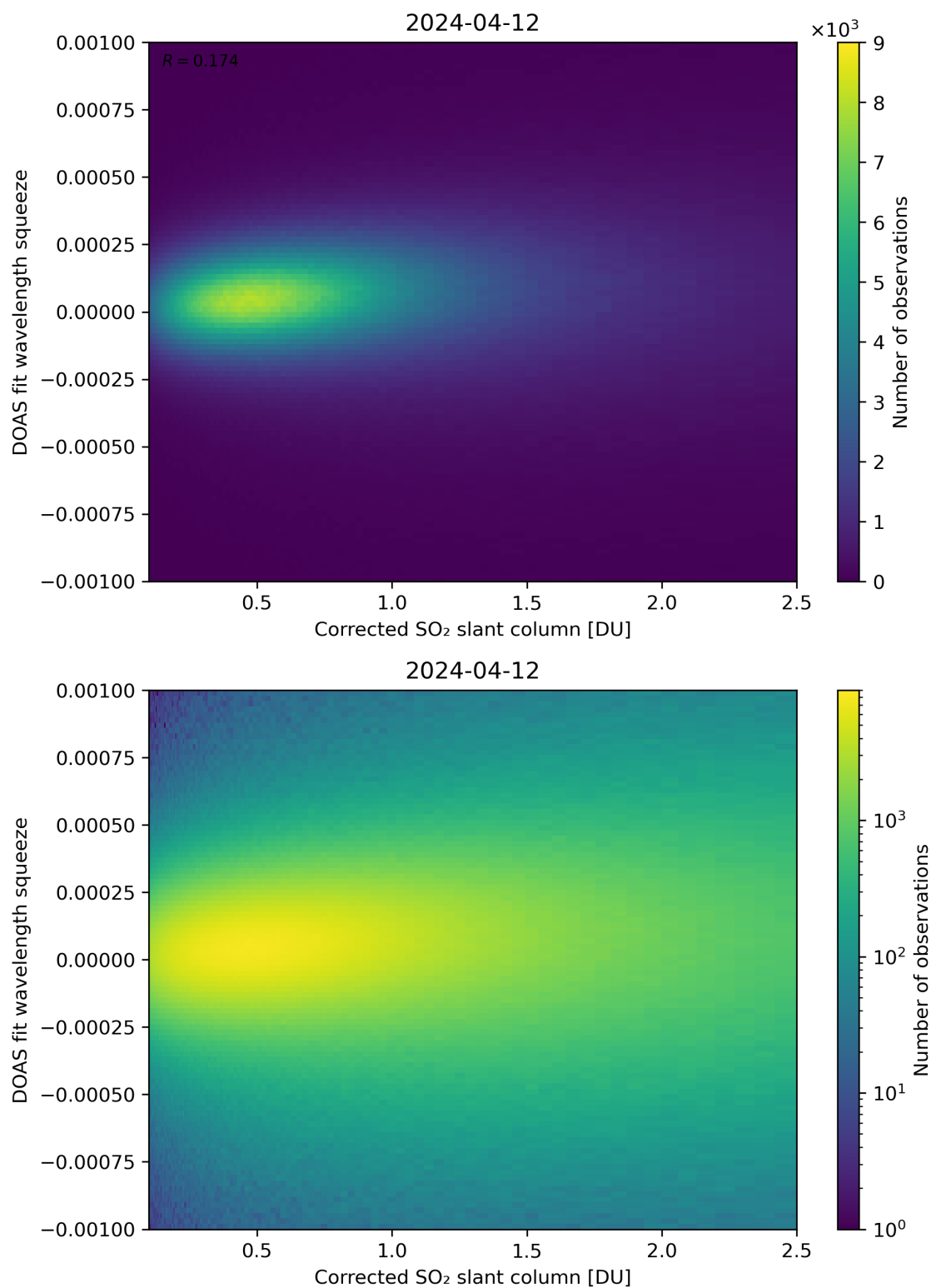
Figure 182: Scatter density plot of “Corrected SO 2 slant column” against “DOAS fit wavelength squeeze” for 2024-04-11 to 2024-04-13.
