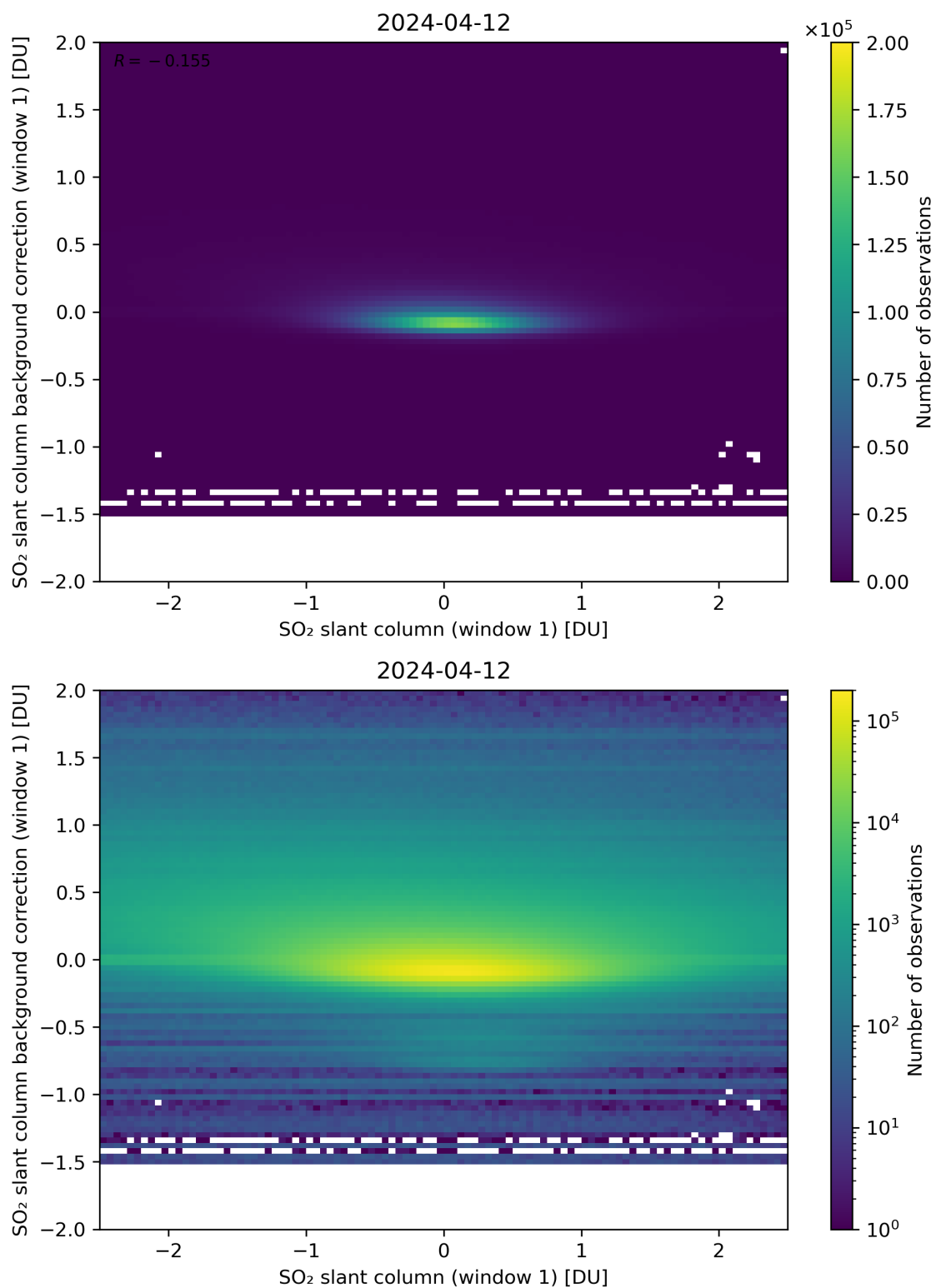
Figure 212: Scatter density plot of “SO 2 slant column (window 1)” against “SO 2 slant column background correction (window 1)” for 2024-04-11 to 2024-04-13.
