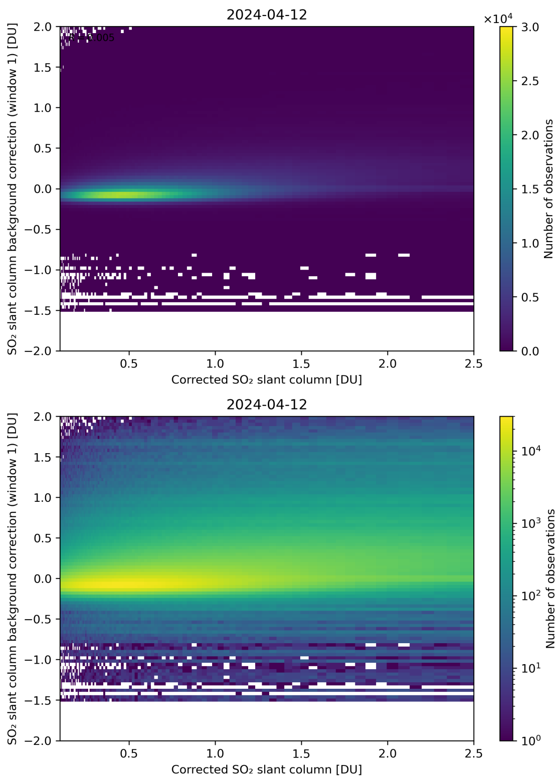
Figure 178: Scatter density plot of “Corrected SO 2 slant column” against “SO 2 slant column background correction (window 1)” for 2024-04-11 to 2024-04-13.
