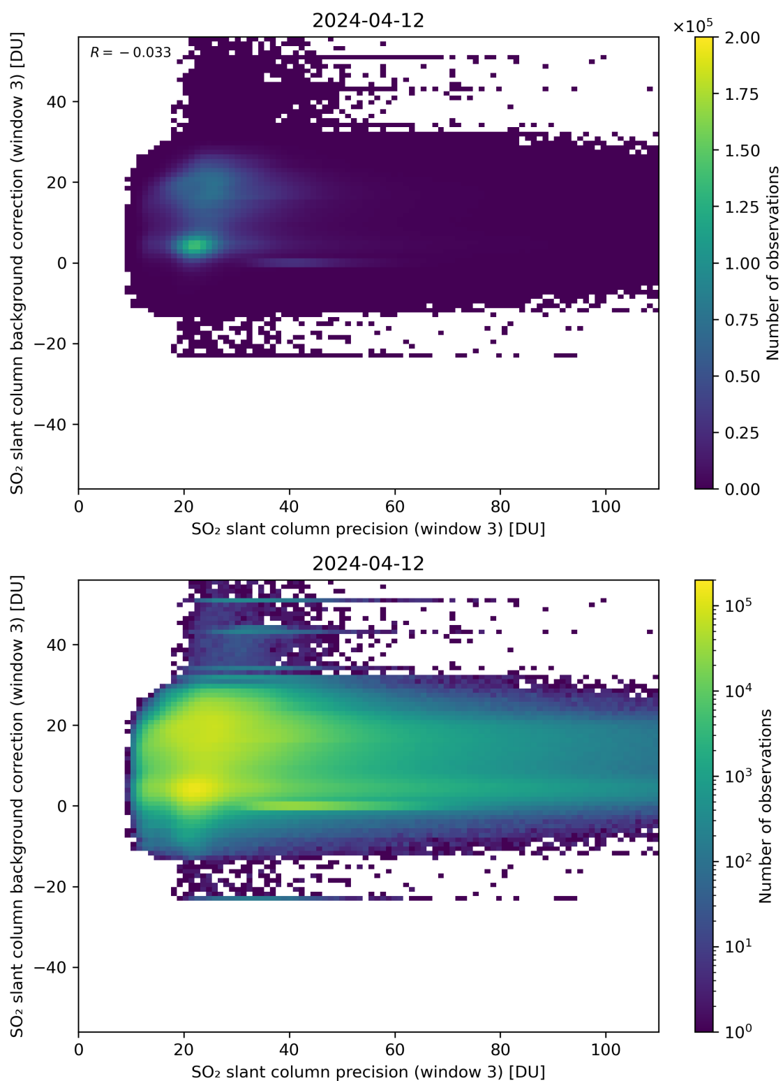
Figure 257: Scatter density plot of “SO 2 slant column precision (window 3)” against “SO 2 slant column background correction (window 3)” for 2024-04-11 to 2024-04-13.
