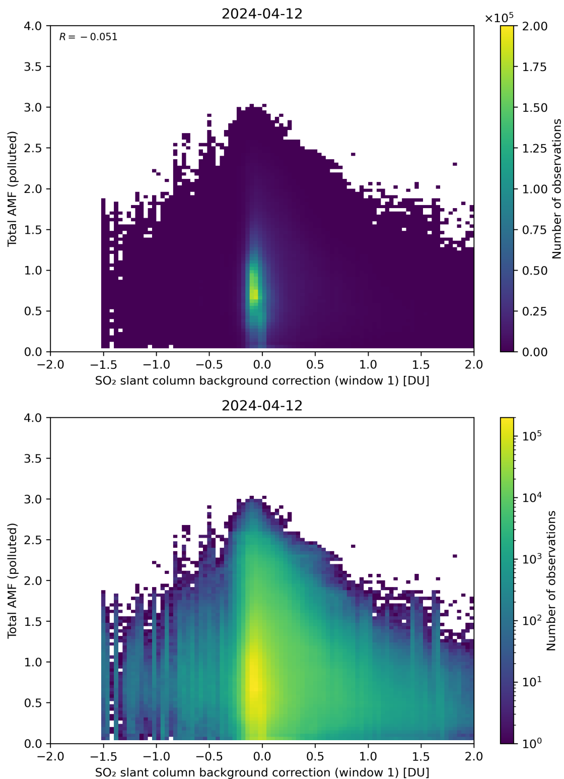
Figure 109: Scatter density plot of “SO 2 slant column background correction (window 1)” against “Total AMF (polluted)” for 2024-04-11 to 2024-04-13.
