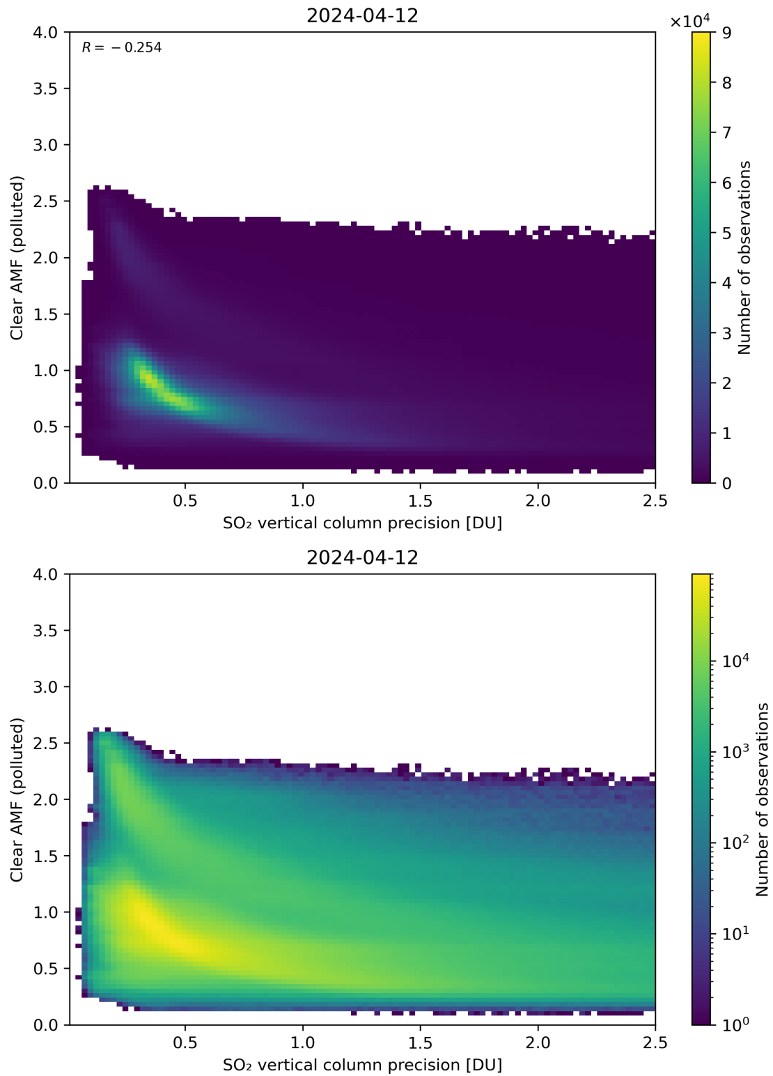
Figure 285: Scatter density plot of “SO 2 vertical column precision” against “Clear AMF (polluted)” for 2024-04-11 to 2024-04-13.
