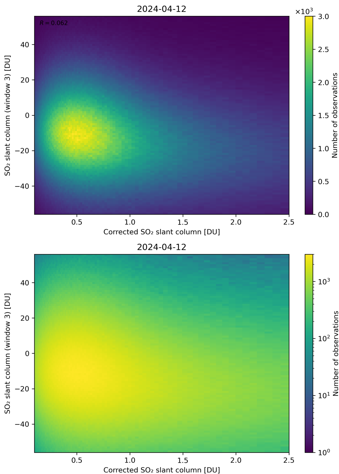
Figure 190: Scatter density plot of “Corrected SO 2 slant column” against “SO 2 slant column (window 3)” for 2024-04-11 to 2024-04-13.
