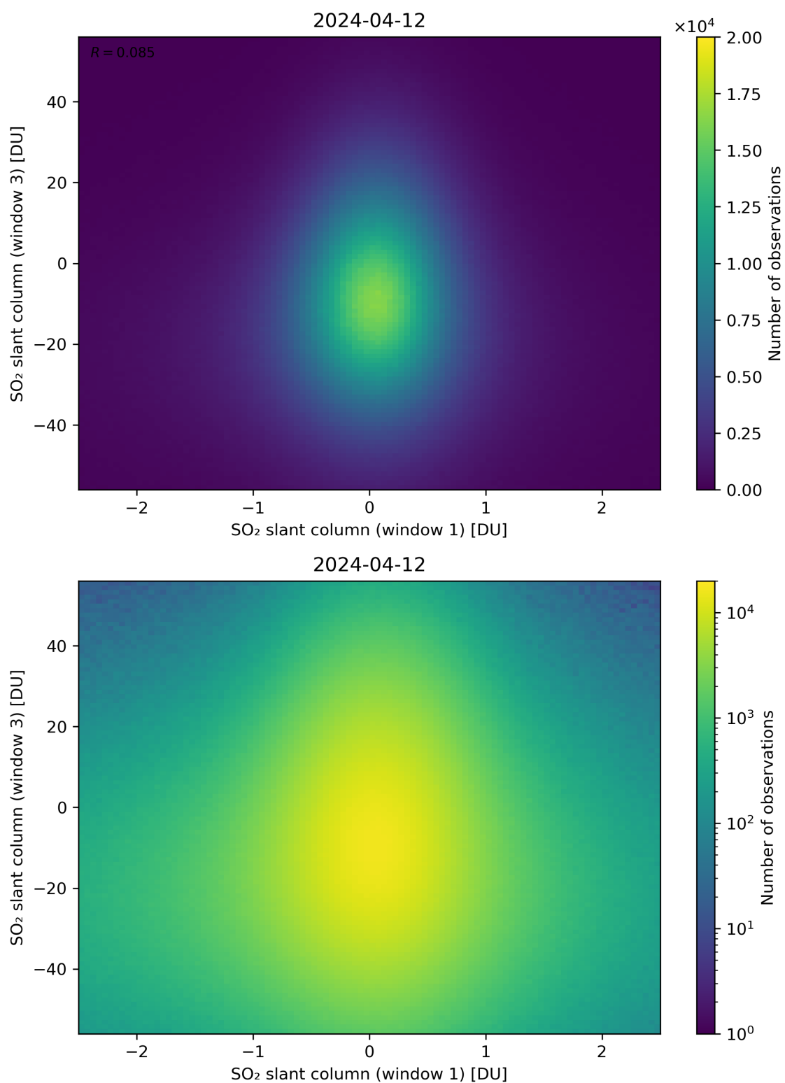
Figure 237: Scatter density plot of “SO 2 slant column (window 1)” against “SO 2 slant column (window 3)” for 2024-04-11 to 2024-04-13.
