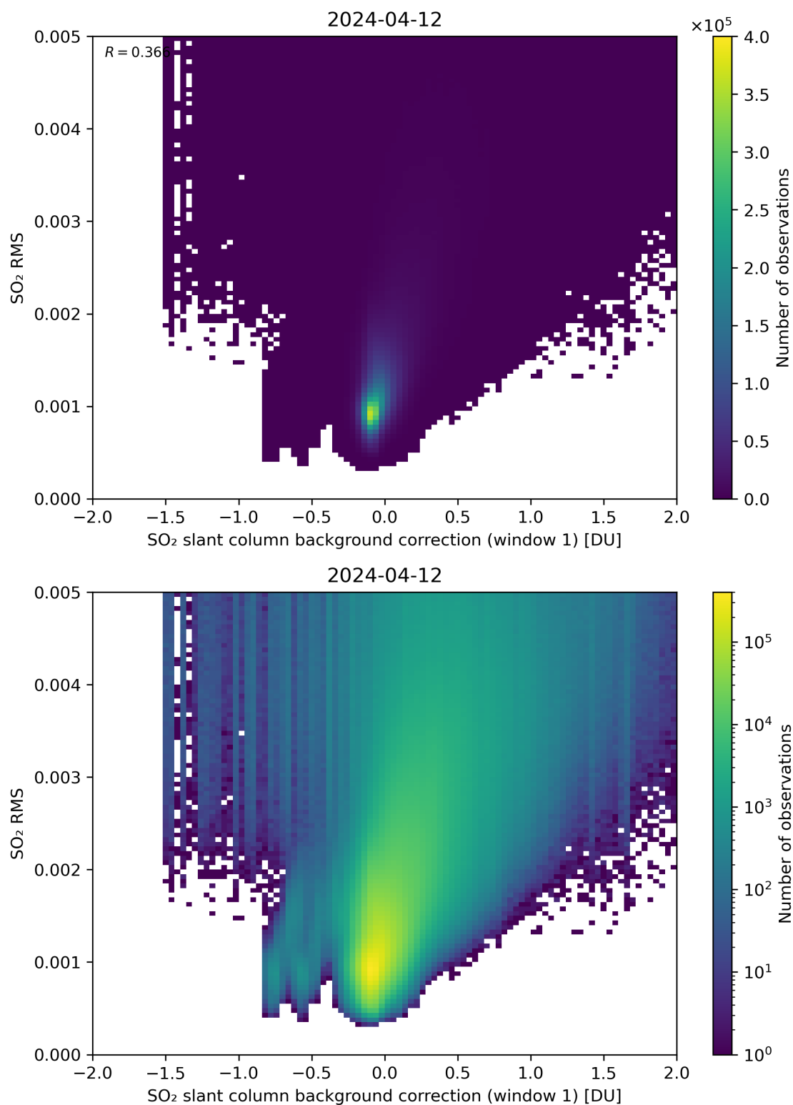
Figure 102: Scatter density plot of “SO 2 slant column background correction (window 1)” against “SO 2 RMS” for 2024-04-11 to 2024-04-13.
