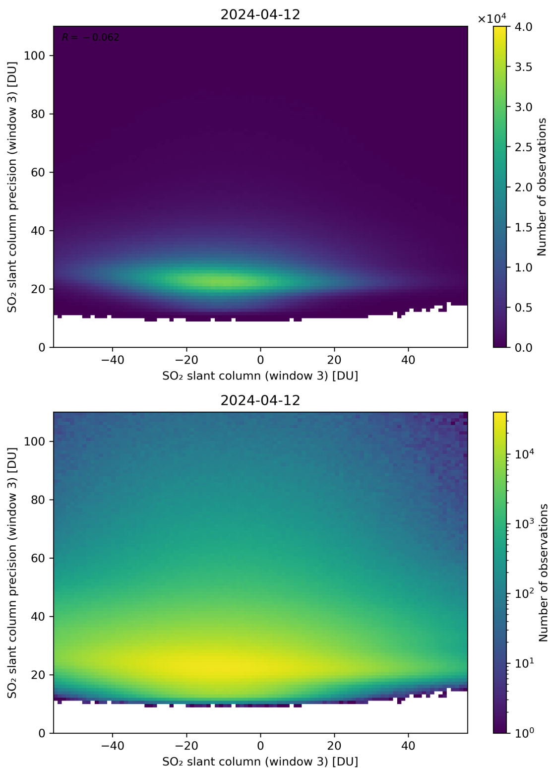
Figure 267: Scatter density plot of “SO 2 slant column (window 3)” against “SO 2 slant column precision (window 3)” for 2024-04-11 to 2024-04-13.
