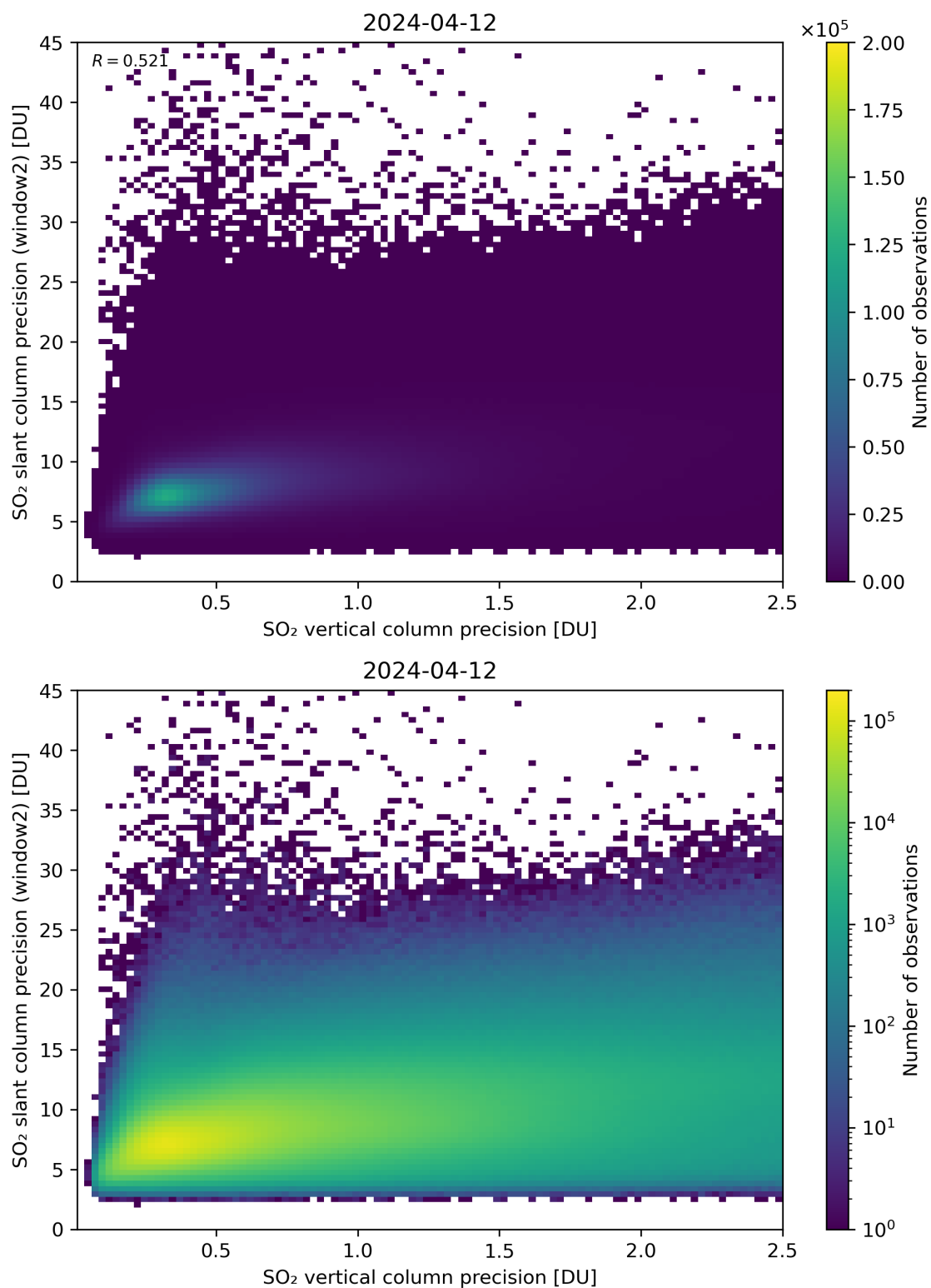
Figure 291: Scatter density plot of “SO 2 vertical column precision” against “SO 2 slant column precision (window2)” for 2024-04-11 to 2024-04-13.
