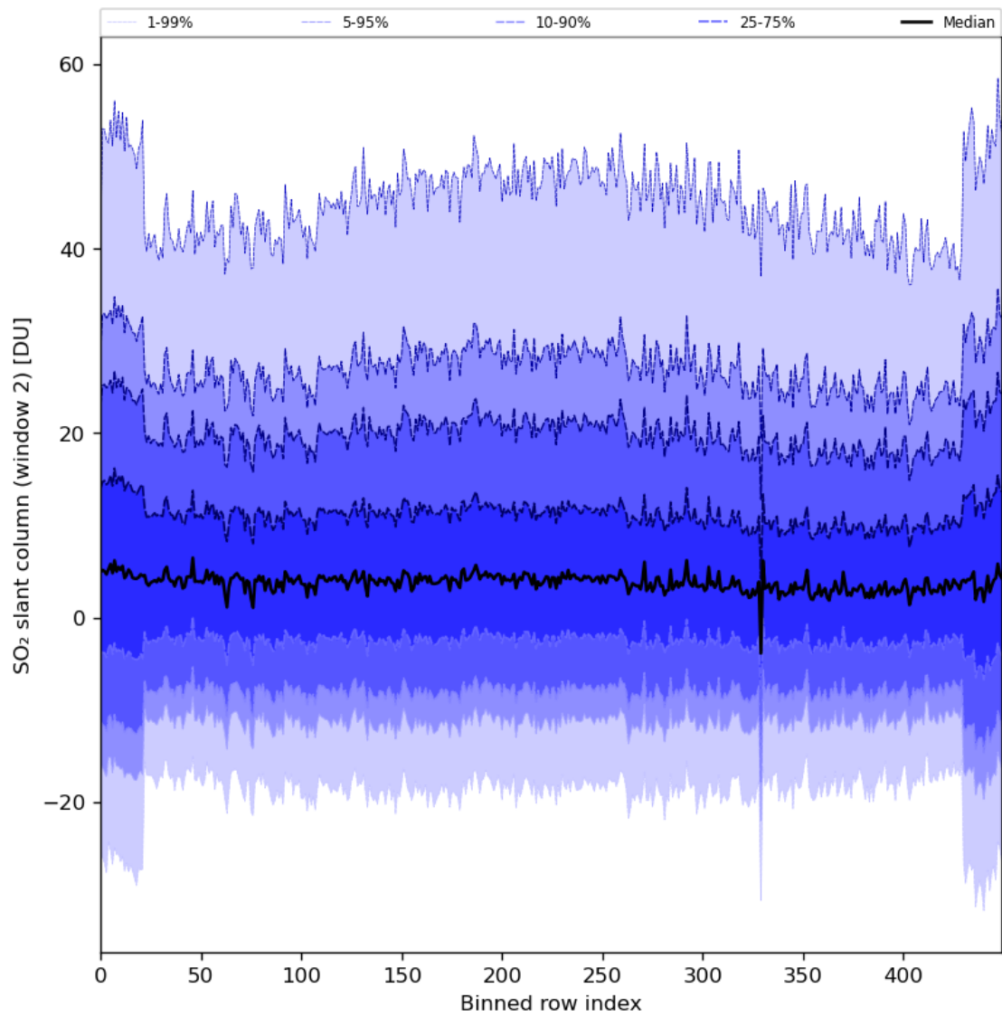
Figure 83: Along track statistics of “SO 2 slant column (window 2)” for 2024-04-11 to 2024-04-13
