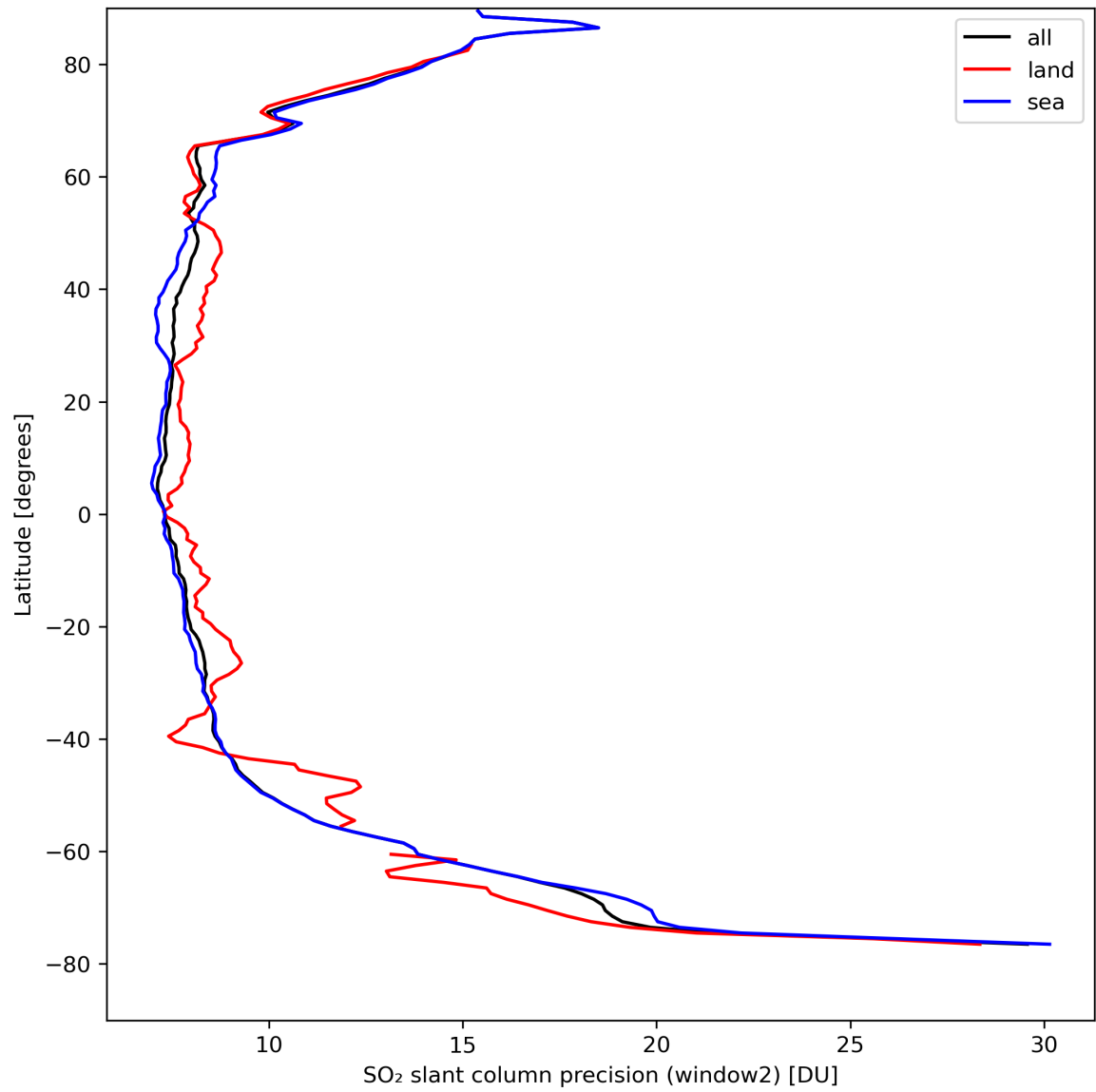
Figure 38: Zonal average of “SO 2 slant column precision (window2)” for 2024-04-11 to 2024-04-13.
