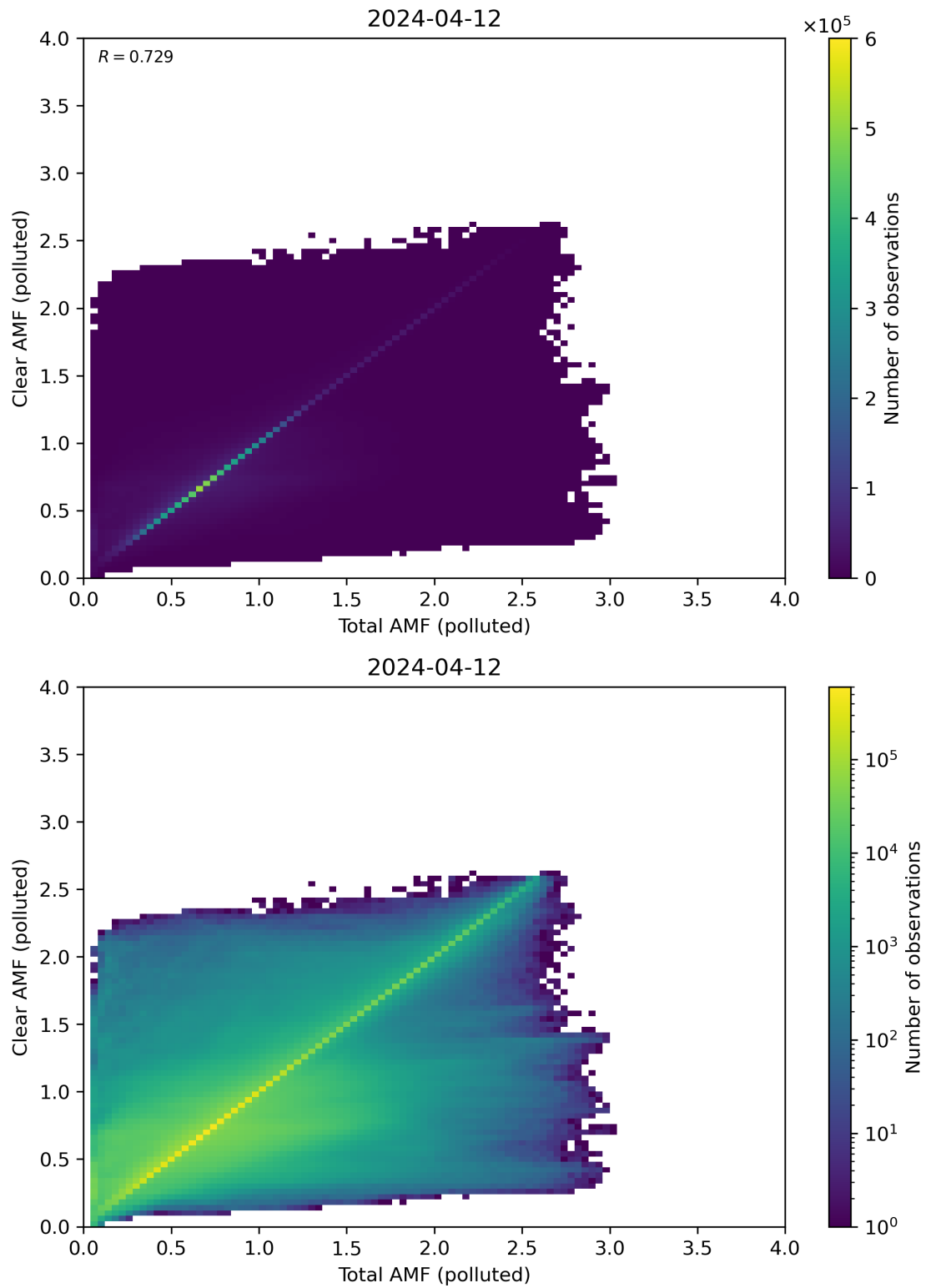
Figure 271: Scatter density plot of “Total AMF (polluted)” against “Clear AMF (polluted)” for 2024-04-11 to 2024-04-13.
