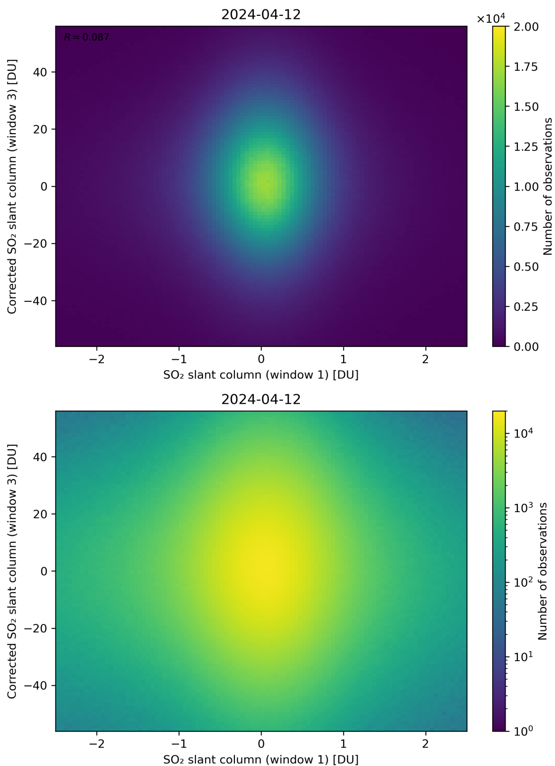
Figure 234: Scatter density plot of “SO 2 slant column (window 1)” against “Corrected SO 2 slant column (window 3)” for 2024-04-11 to 2024-04-13.
