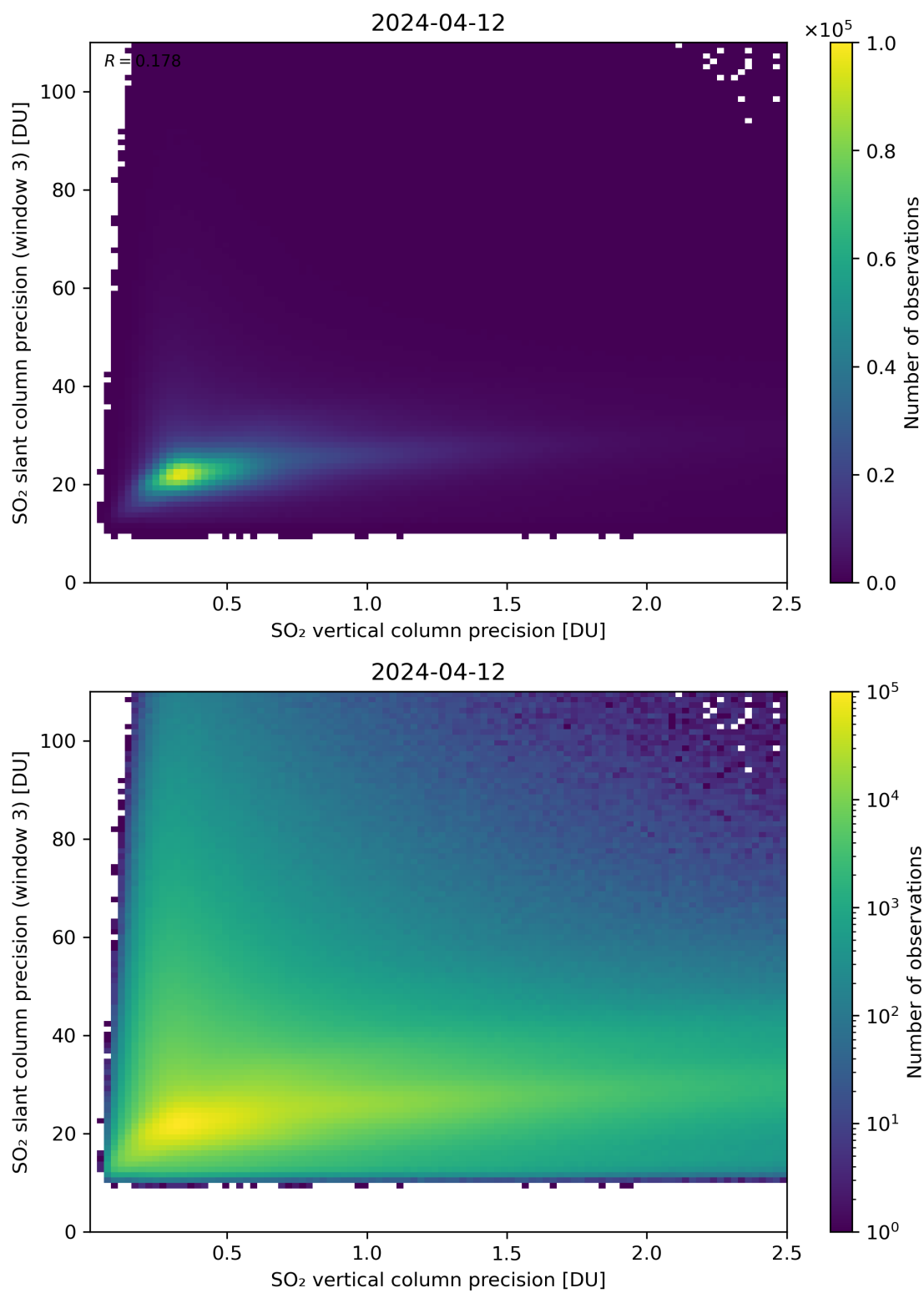
Figure 293: Scatter density plot of “SO 2 vertical column precision” against “SO 2 slant column precision (window 3)” for 2024-04-11 to 2024-04-13.
