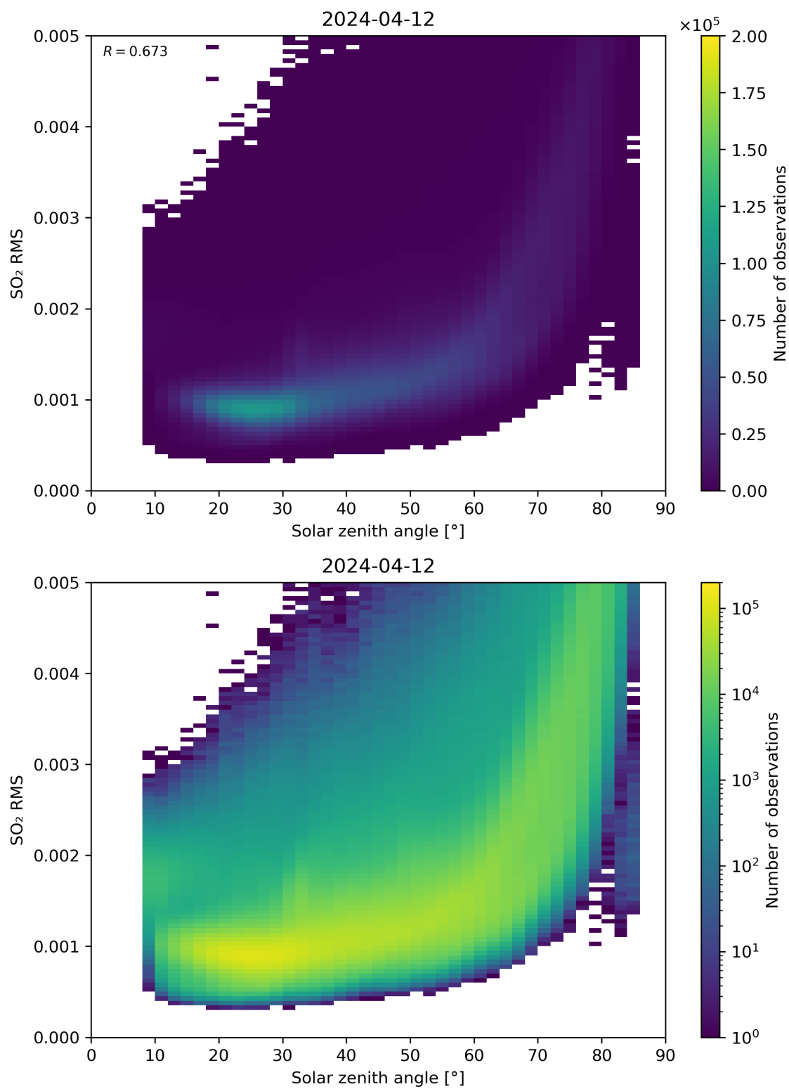
Figure 163: Scatter density plot of “Solar zenith angle” against “SO 2 RMS” for 2024-04-11 to 2024-04-13.
