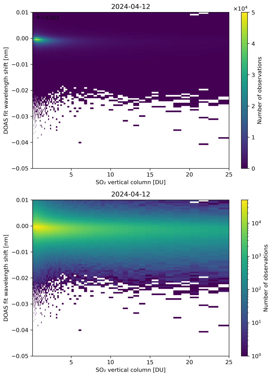
Figure 276: Scatter density plot of “SO 2 vertical column” against “DOAS fit wavelength shift” for 2024-04-11 to 2024-04-13.
