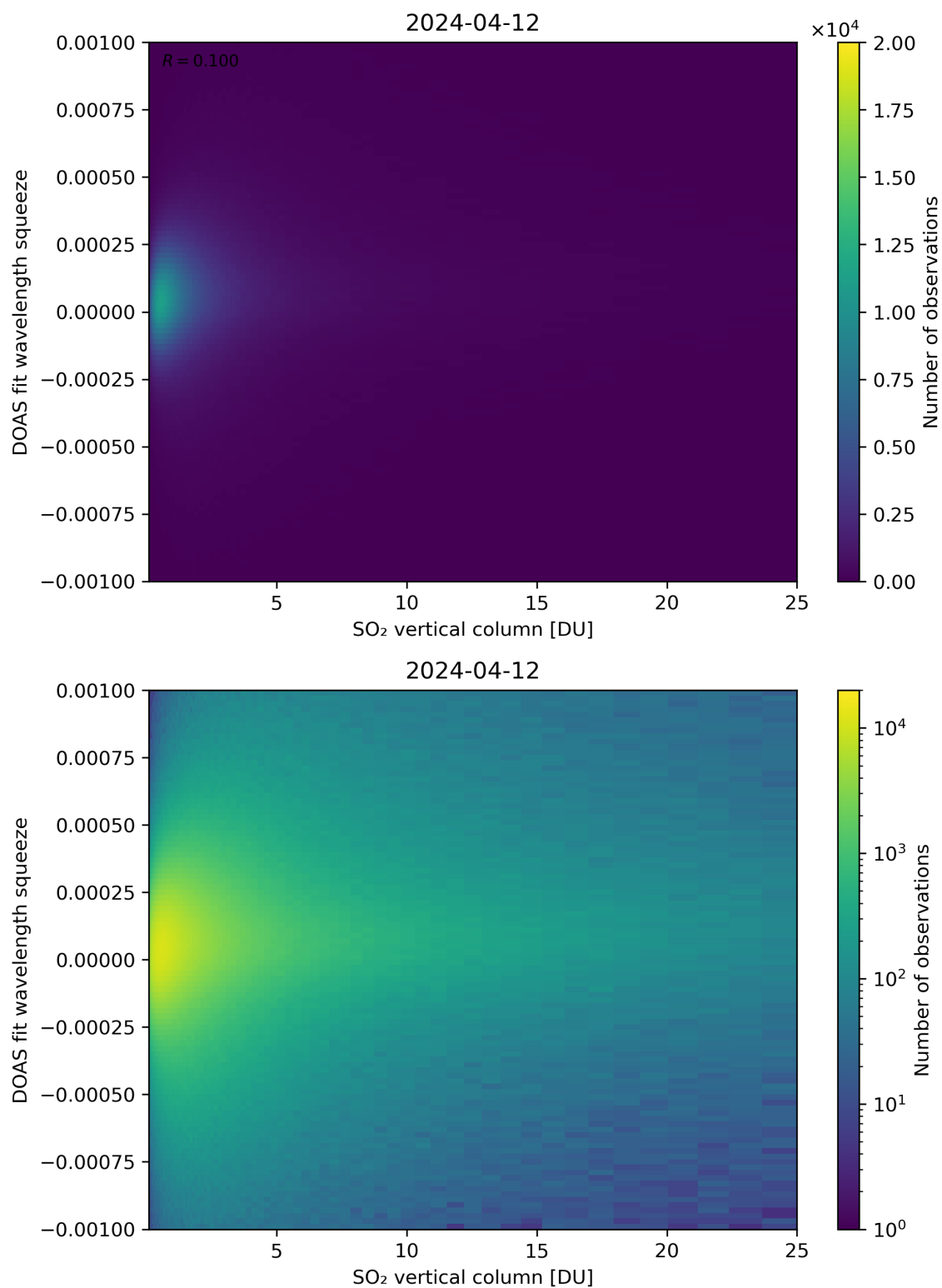
Figure 277: Scatter density plot of “SO 2 vertical column” against “DOAS fit wavelength squeeze” for 2024-04-11 to 2024-04-13.
