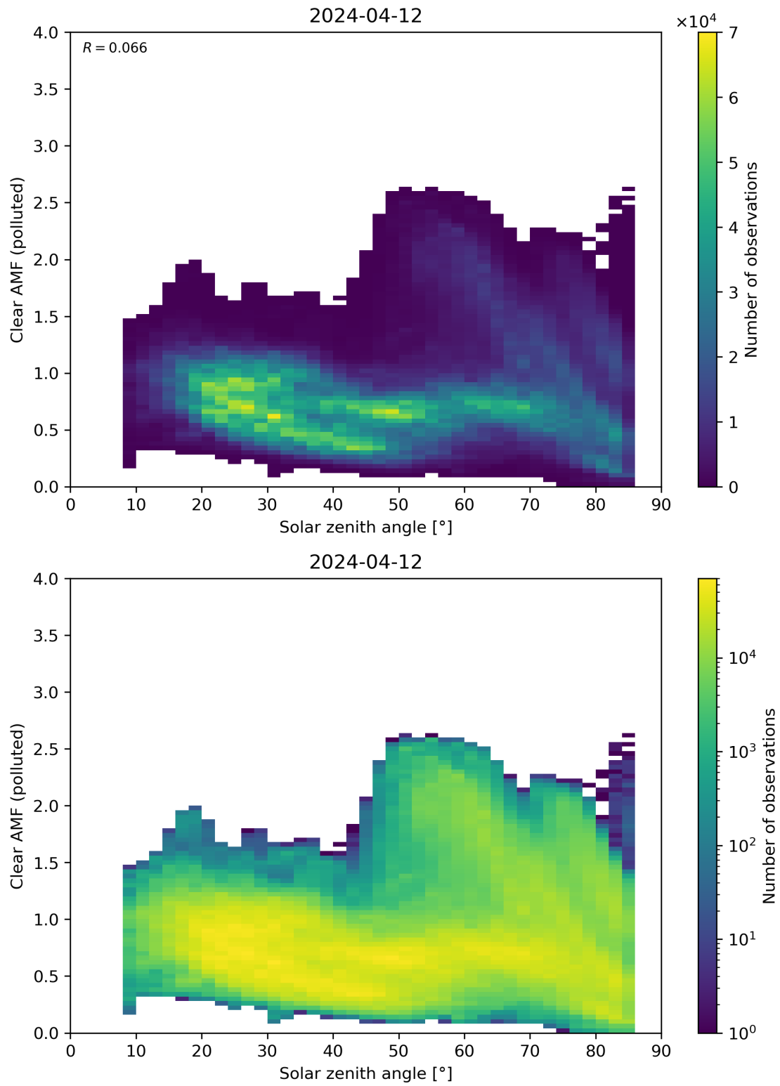
Figure 165: Scatter density plot of “Solar zenith angle” against “Clear AMF (polluted)” for 2024-04-11 to 2024-04-13.
