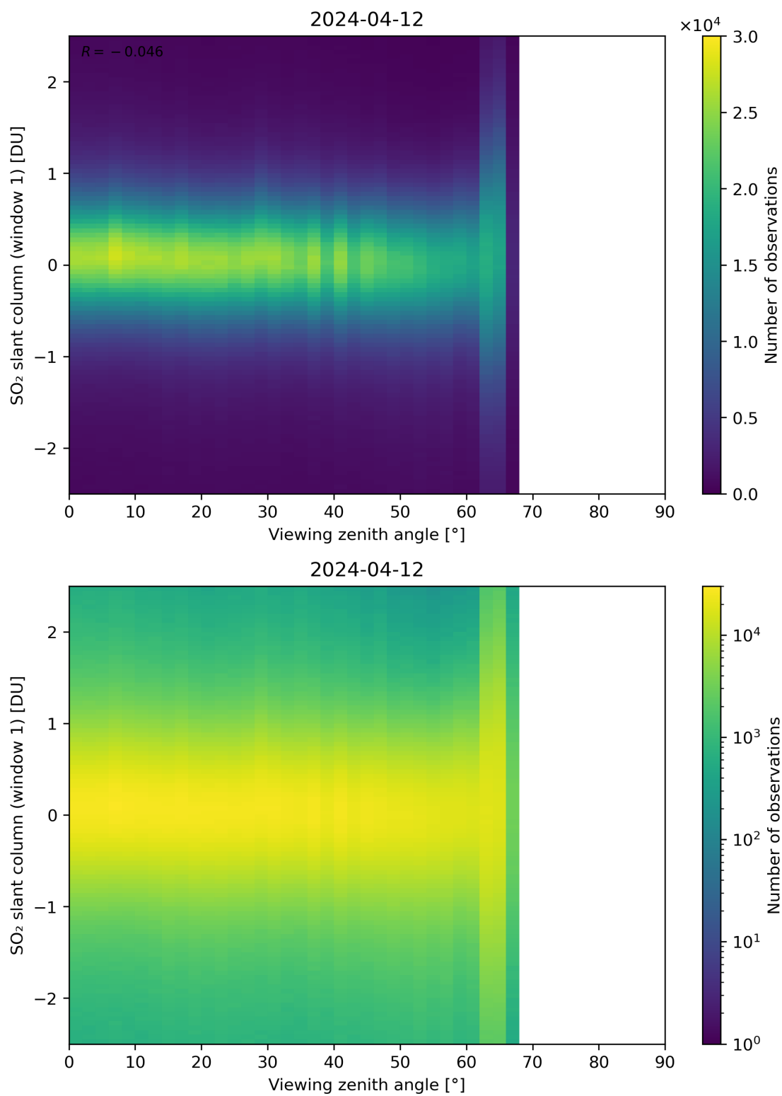
Figure 320: Scatter density plot of “Viewing zenith angle” against “SO 2 slant column (window 1)” for 2024-04-11 to 2024-04-13.
