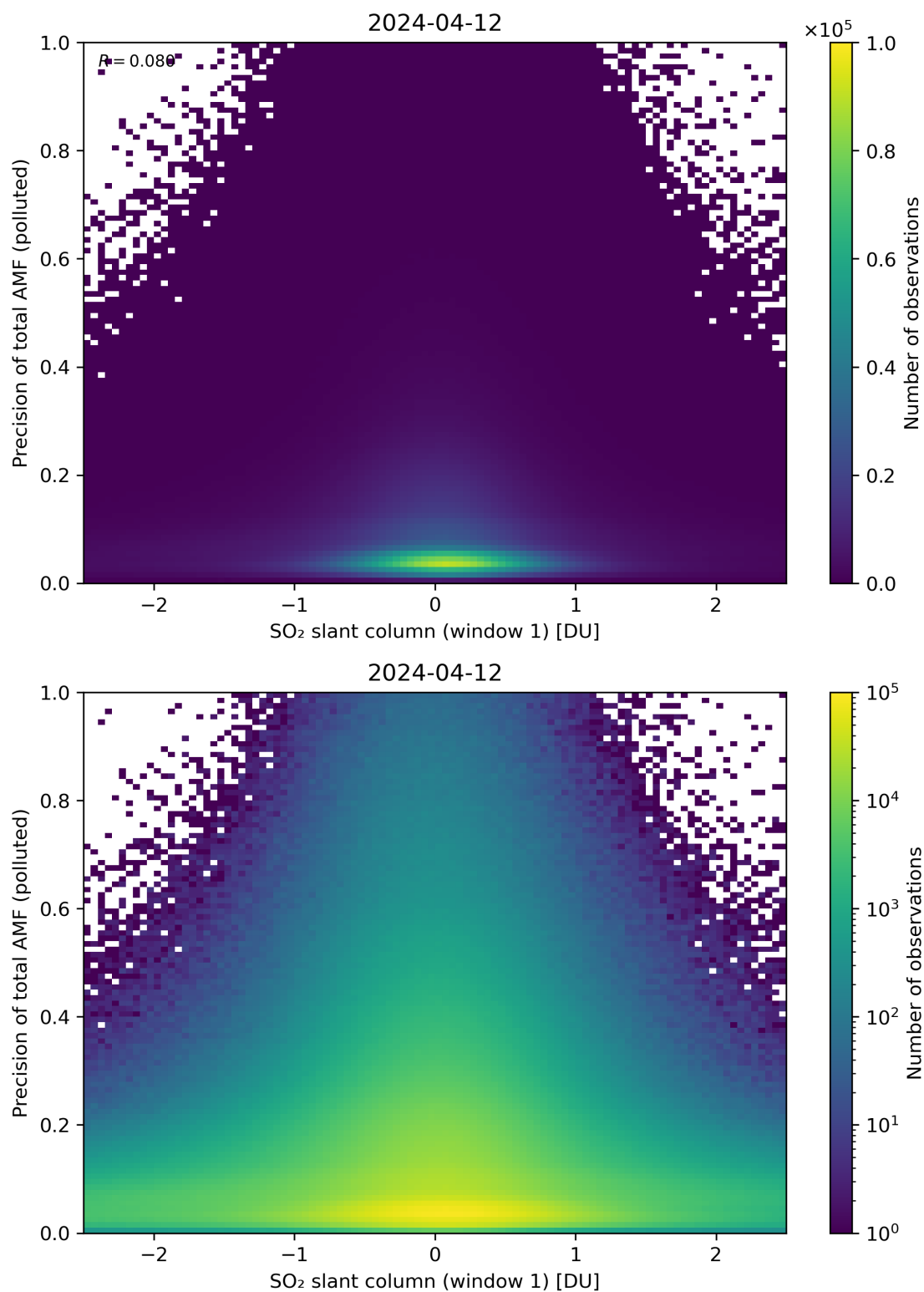
Figure 240: Scatter density plot of “SO 2 slant column (window 1)” against “Precision of total AMF (polluted)” for 2024-04-11 to 2024-04-13.
