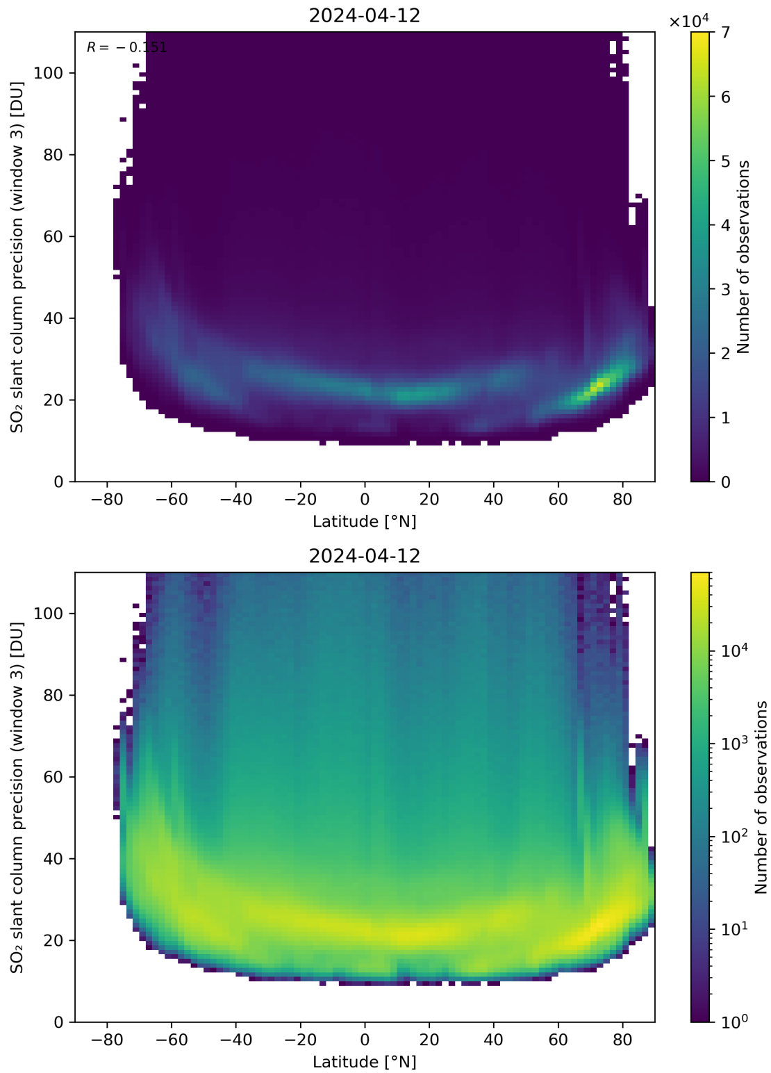
Figure 153: Scatter density plot of “Latitude” against “SO 2 slant column precision (window 3)” for 2024-04-11 to 2024-04-13.
