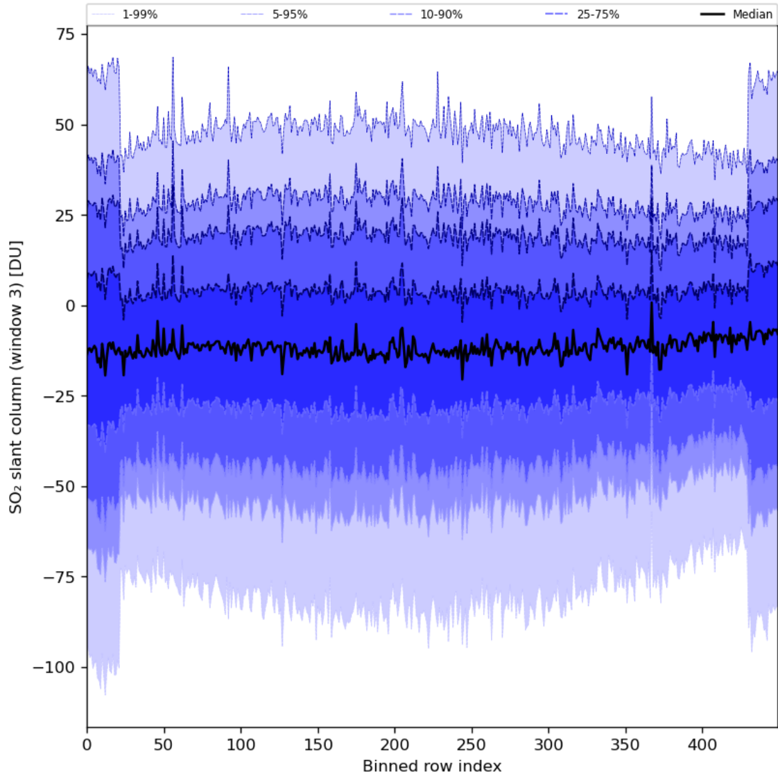
Figure 87: Along track statistics of “SO 2 slant column (window 3)” for 2024-04-11 to 2024-04-13
