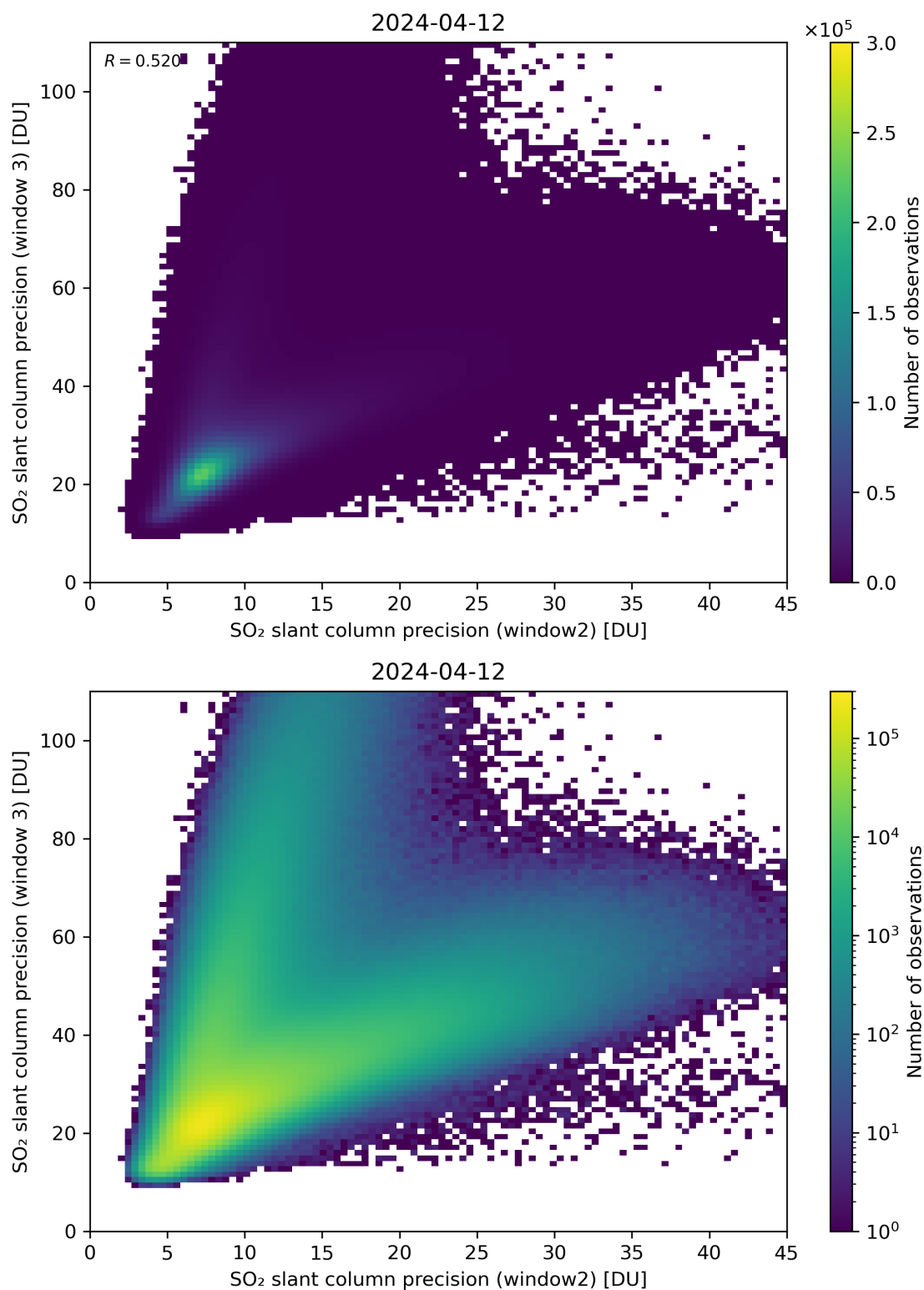
Figure 250: Scatter density plot of “SO 2 slant column precision (window2)” against “SO 2 slant column precision (window 3)” for 2024-04-11 to 2024-04-13.
