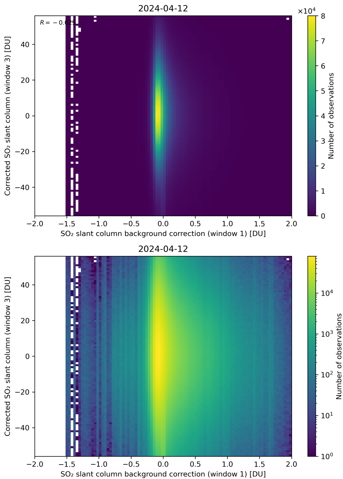
Figure 105: Scatter density plot of “SO 2 slant column background correction (window 1)” against “Corrected SO 2 slant column (window 3)” for 2024-04-11 to 2024-04-13.
