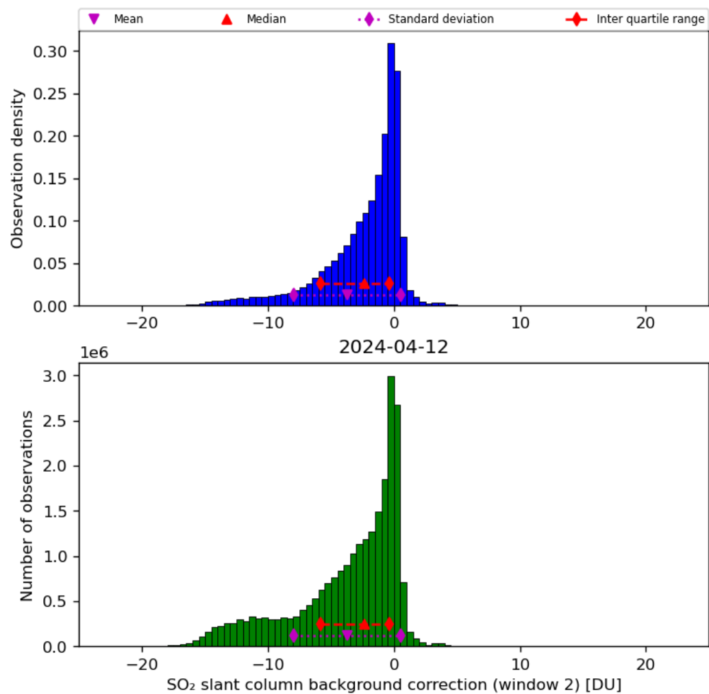
Figure 63: Histogram of “SO 2 slant column background correction (window 2)” for 2024-04-11 to 2024-04-13
