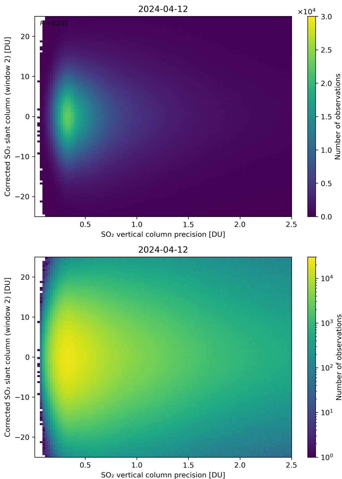
Figure 287: Scatter density plot of “SO 2 vertical column precision” against “Corrected SO 2 slant column (window 2)” for 2024-04-11 to 2024-04-13.
