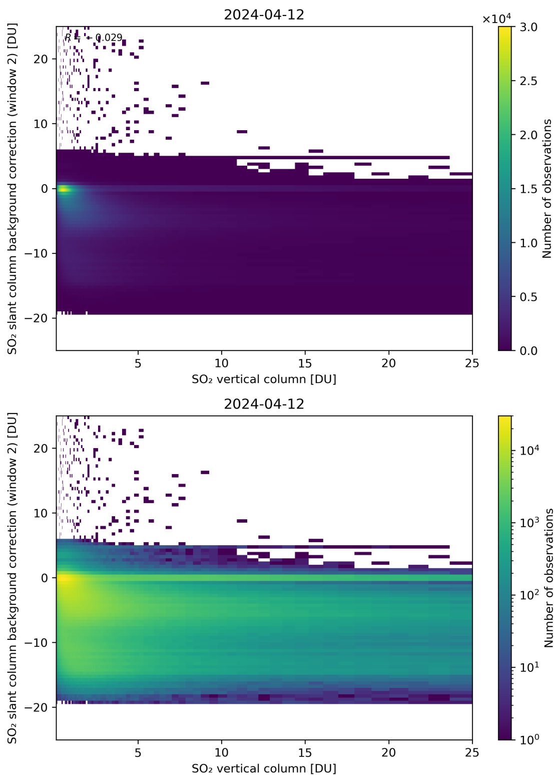
Figure 274: Scatter density plot of “SO 2 vertical column” against “SO 2 slant column background correction (window 2)” for 2024-04-11 to 2024-04-13.
