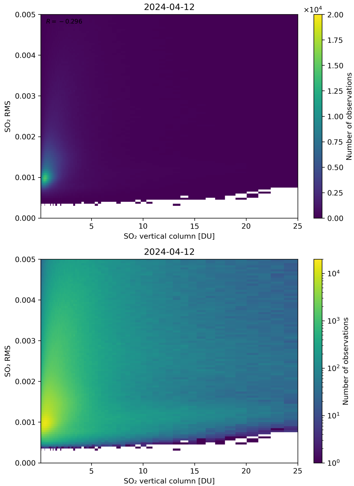
Figure 278: Scatter density plot of “SO 2 vertical column” against “SO 2 RMS” for 2024-04-11 to 2024-04-13.
