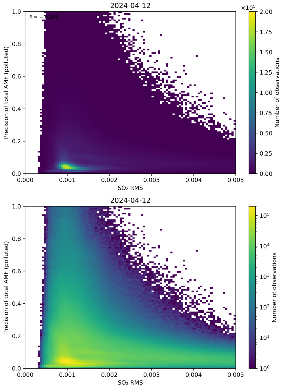
Figure 138: Scatter density plot of “SO 2 RMS” against “Precision of total AMF (polluted)” for 2024-04-11 to 2024-04-13.
