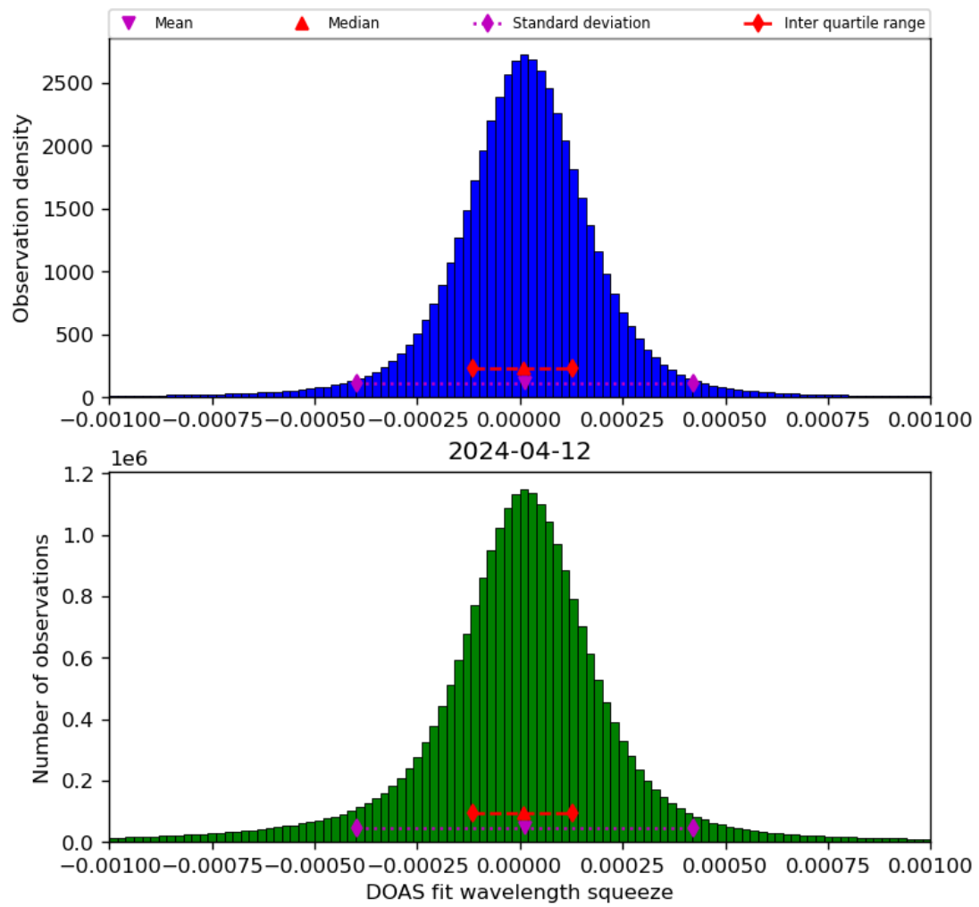
Figure 69: Histogram of “DOAS fit wavelength squeeze” for 2024-04-11 to 2024-04-13
