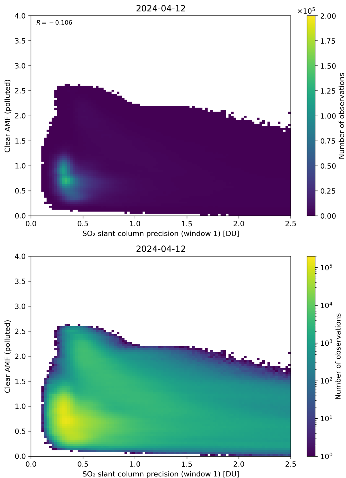
Figure 224: Scatter density plot of “SO 2 slant column precision (window 1)” against “Clear AMF (polluted)” for 2024-04-11 to 2024-04-13.
