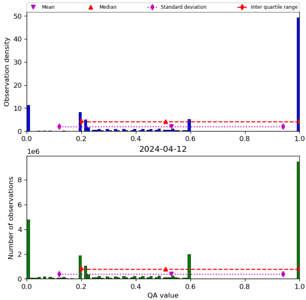
Figure 52: Histogram of “QA value” for 2024-04-11 to 2024-04-13
