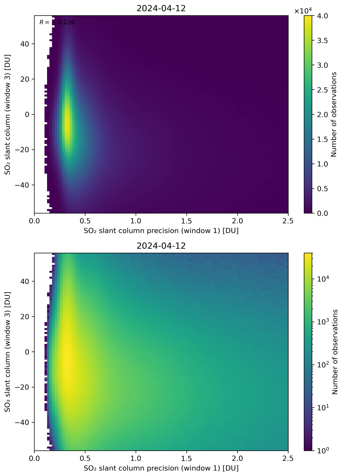
Figure 228: Scatter density plot of “SO 2 slant column precision (window 1)” against “SO 2 slant column (window 3)” for 2024-04-11 to 2024-04-13.
