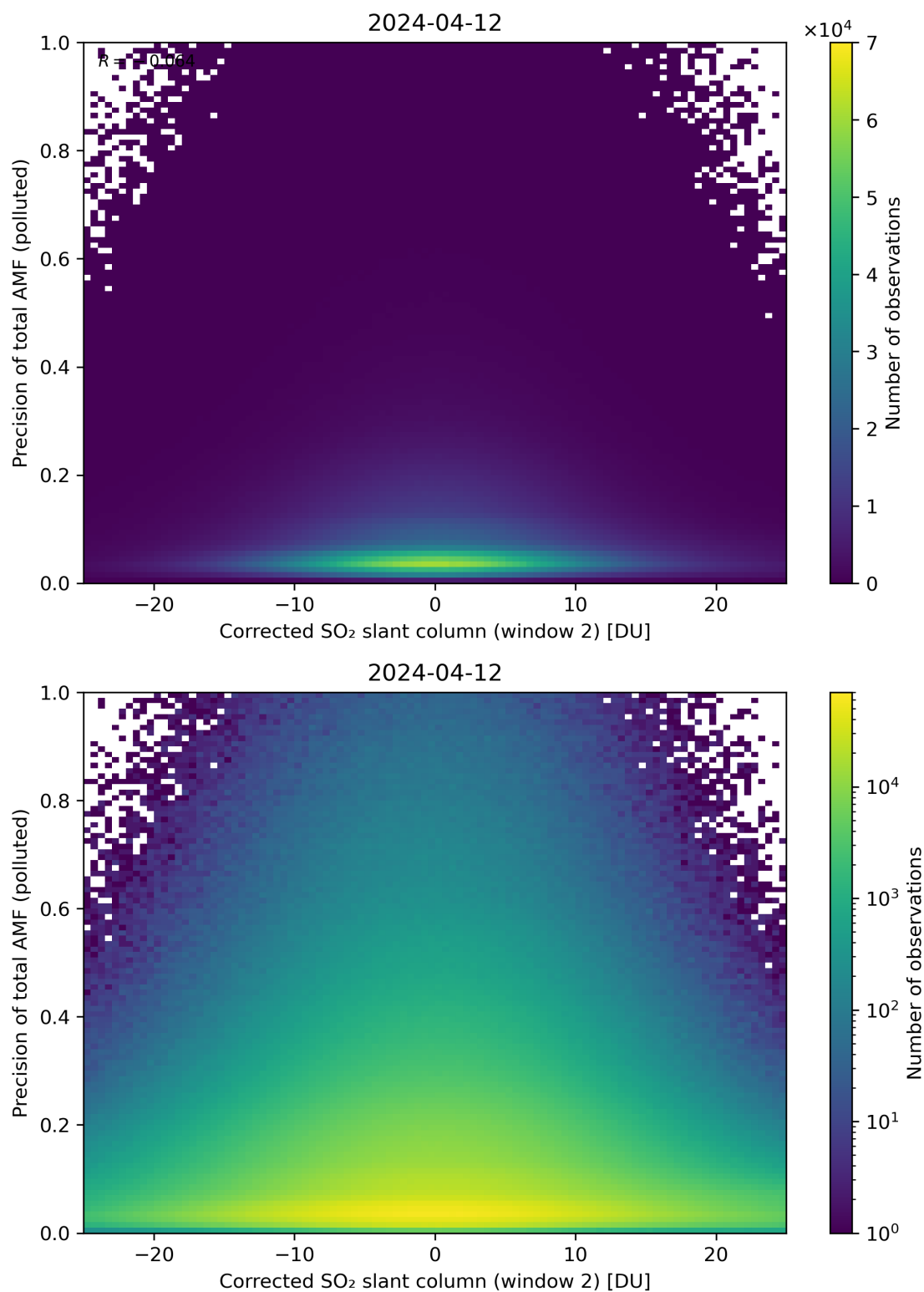
Figure 204: Scatter density plot of “Corrected SO 2 slant column (window 2)” against “Precision of total AMF (polluted)” for 2024-04-11 to 2024-04-13.
