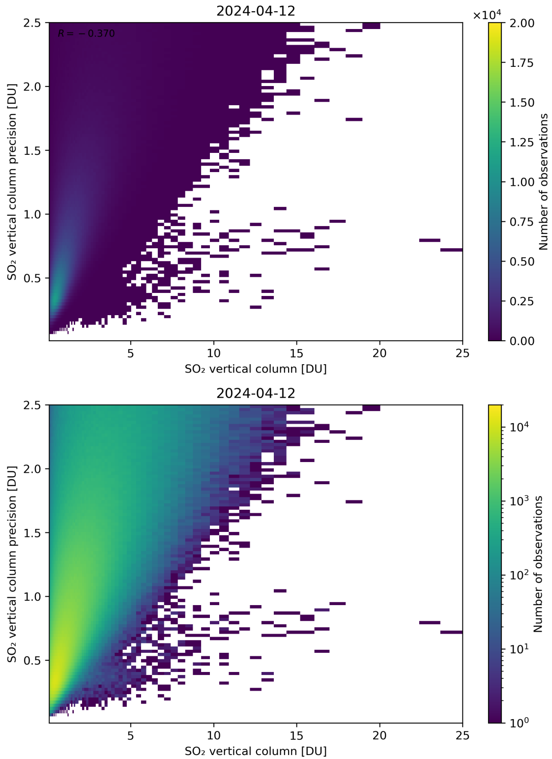
Figure 307: Scatter density plot of “SO 2 vertical column” against “SO 2 vertical column precision” for 2024-04-11 to 2024-04-13.
