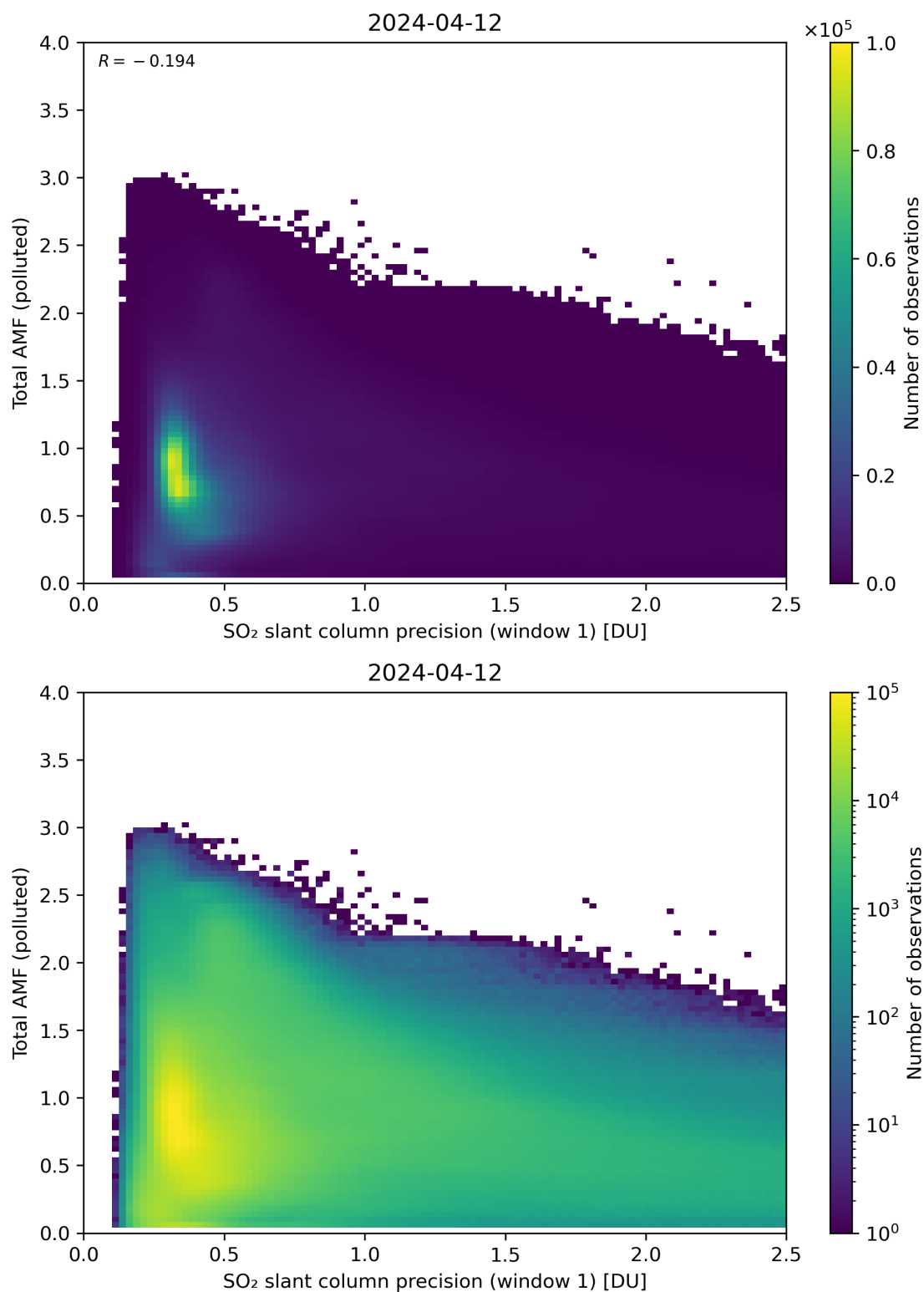
Figure 230: Scatter density plot of “SO 2 slant column precision (window 1)” against “Total AMF (polluted)” for 2024-04-11 to 2024-04-13.
