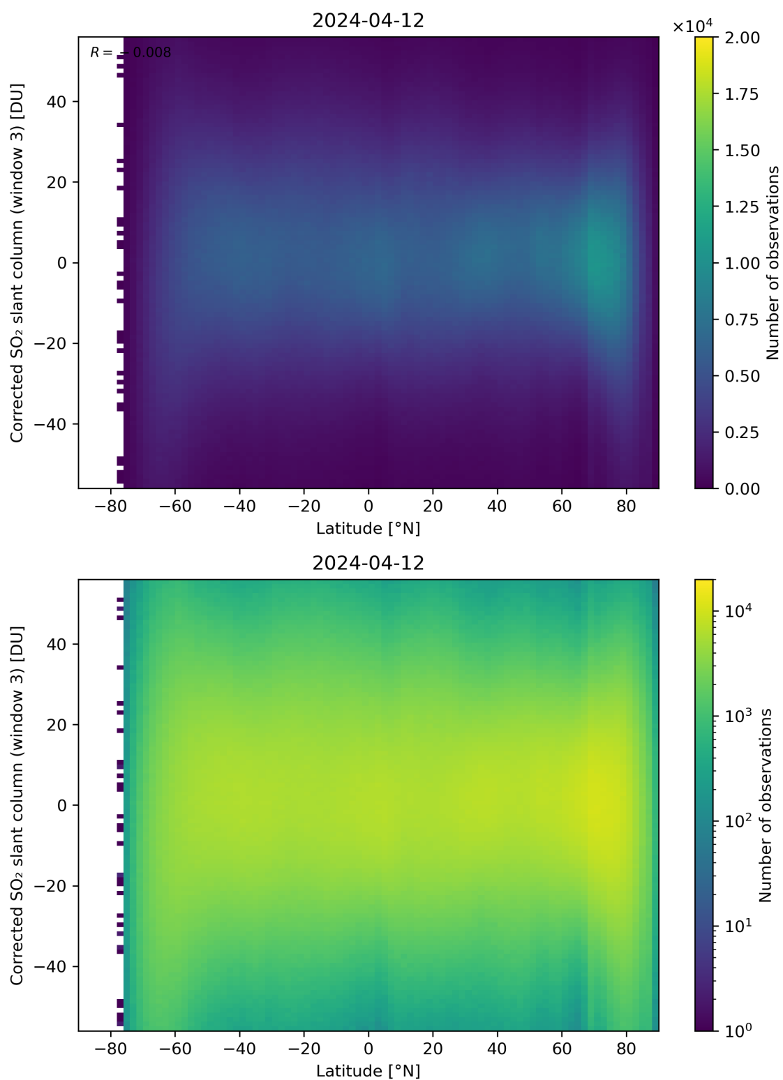
Figure 148: Scatter density plot of “Latitude” against “Corrected SO 2 slant column (window 3)” for 2024-04-11 to 2024-04-13.
