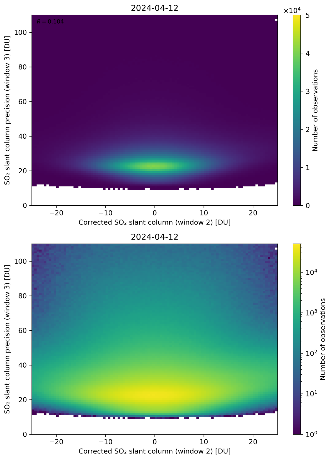
Figure 202: Scatter density plot of “Corrected SO 2 slant column (window 2)” against “SO 2 slant column precision (window 3)” for 2024-04-11 to 2024-04-13.
