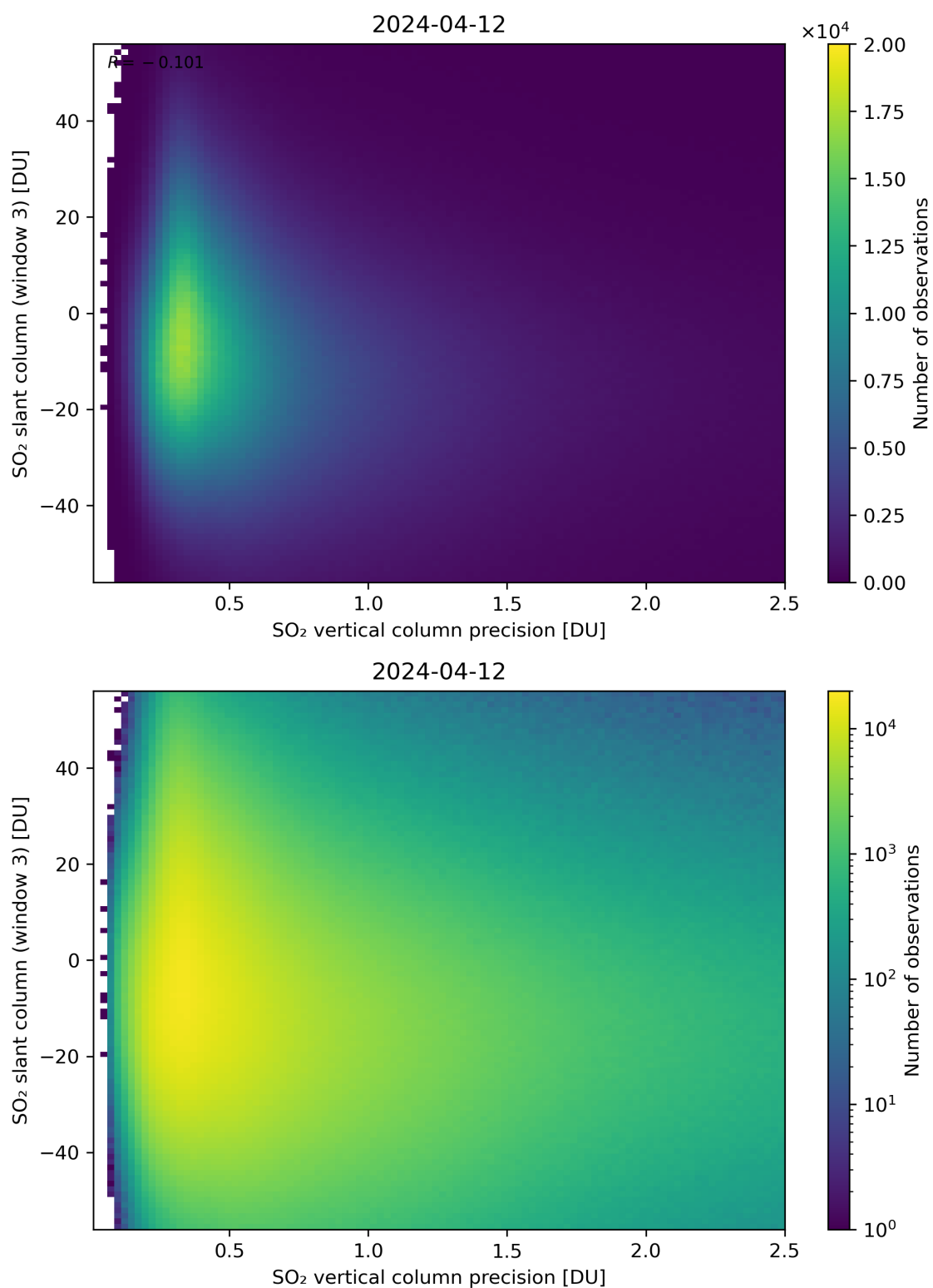
Figure 292: Scatter density plot of “SO 2 vertical column precision” against “SO 2 slant column (window 3)” for 2024-04-11 to 2024-04-13.
