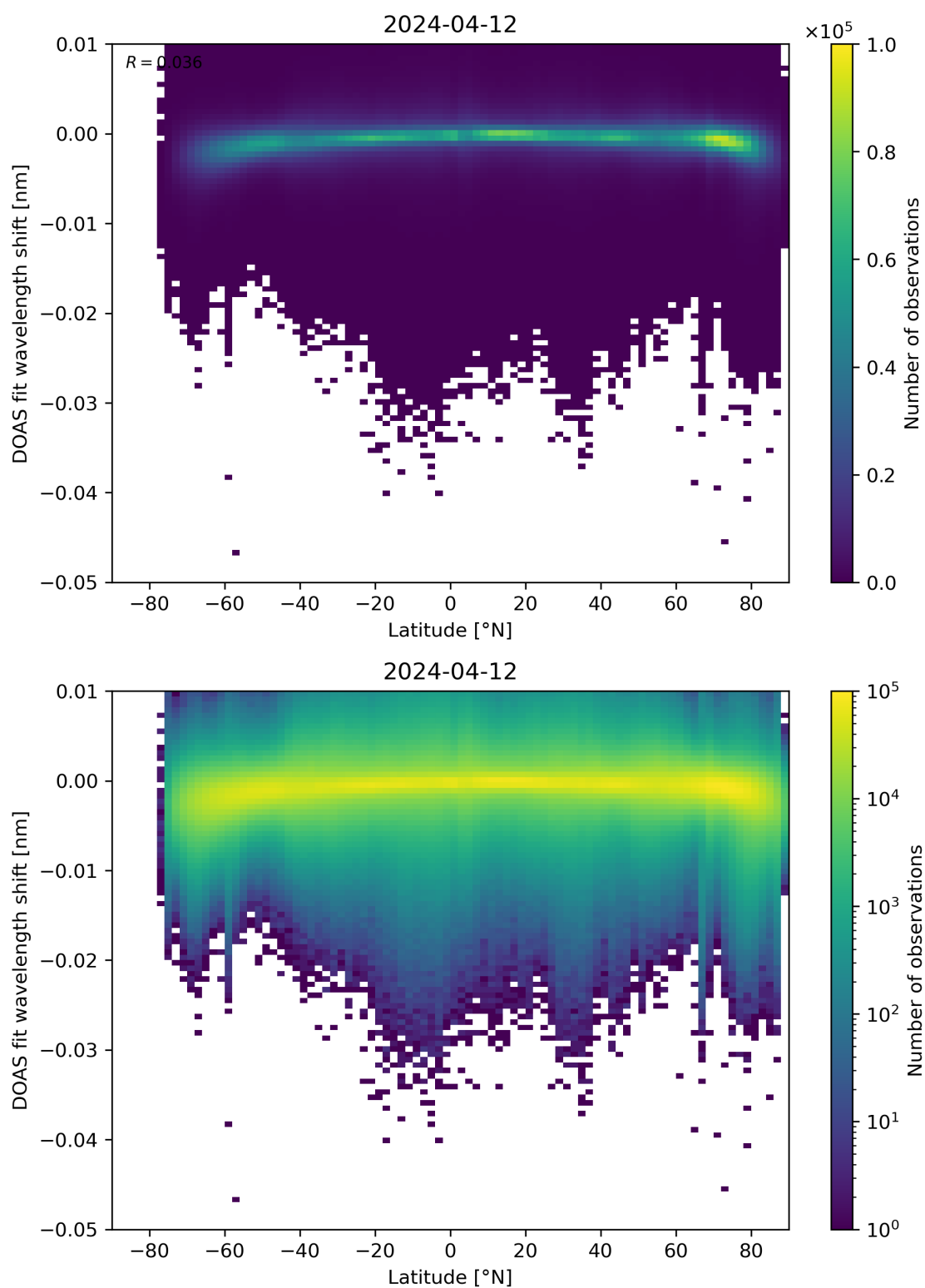
Figure 142: Scatter density plot of “Latitude” against “DOAS fit wavelength shift” for 2024-04-11 to 2024-04-13.
