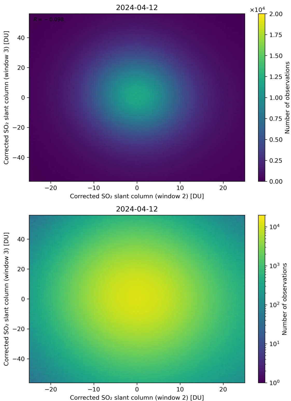
Figure 200: Scatter density plot of “Corrected SO 2 slant column (window 2)” against “Corrected SO 2 slant column (window 3)” for 2024-04-11 to 2024-04-13.
