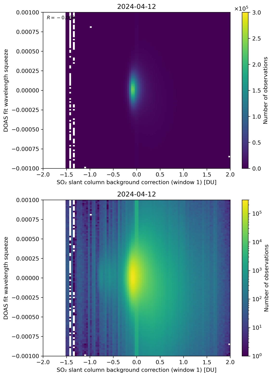
Figure 101: Scatter density plot of “SO 2 slant column background correction (window 1)” against “DOAS fit wavelength squeeze” for 2024-04-11 to 2024-04-13.
