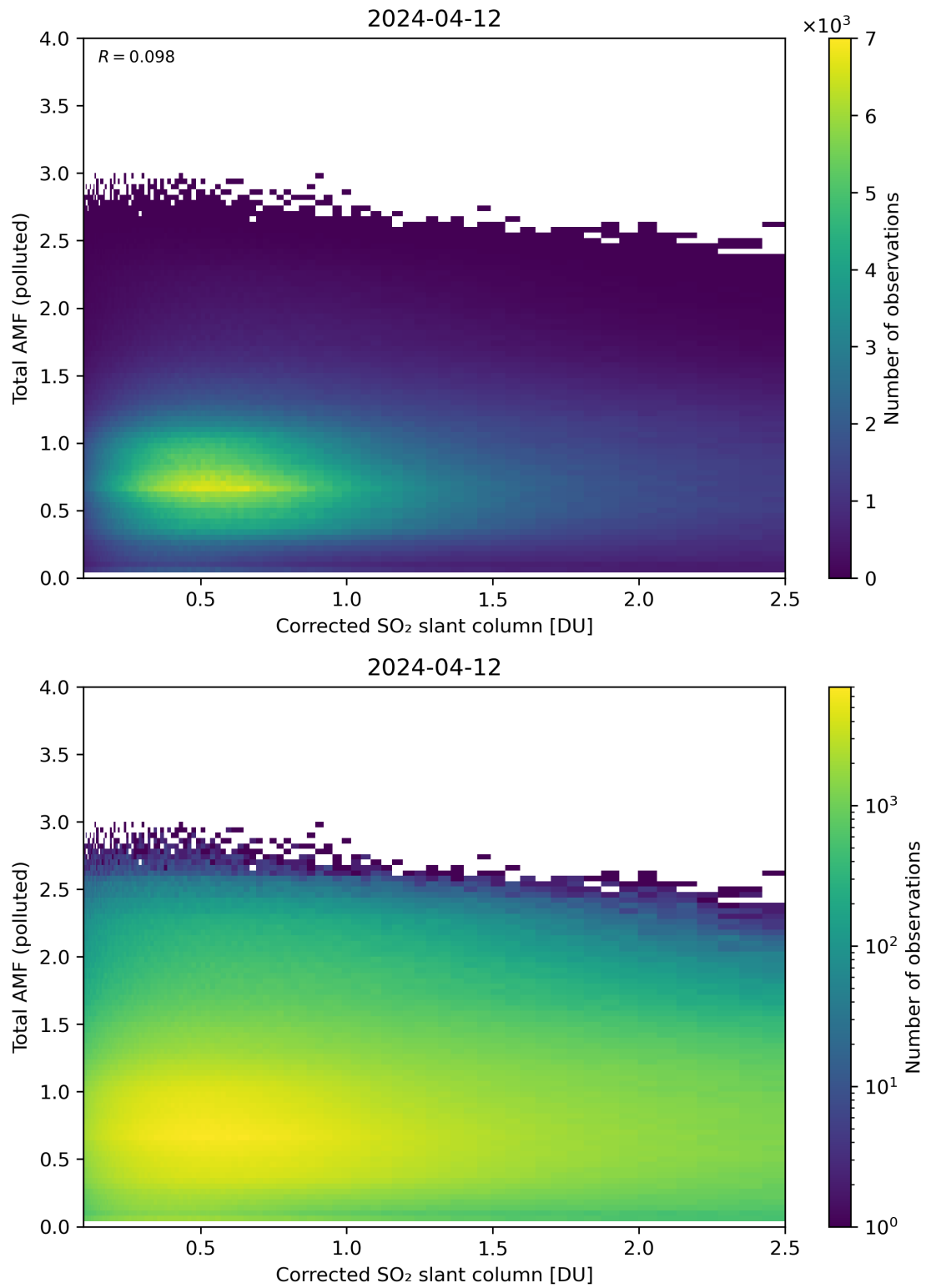
Figure 192: Scatter density plot of “Corrected SO 2 slant column” against “Total AMF (polluted)” for 2024-04-11 to 2024-04-13.
