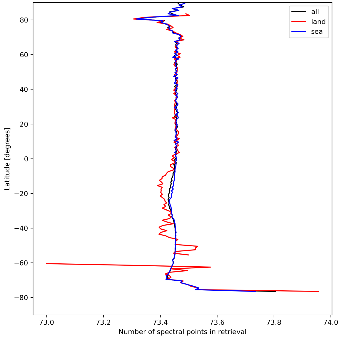
Figure 51: Zonal average of “Number of spectral points in retrieval” for 2024-04-11 to 2024-04-13.
