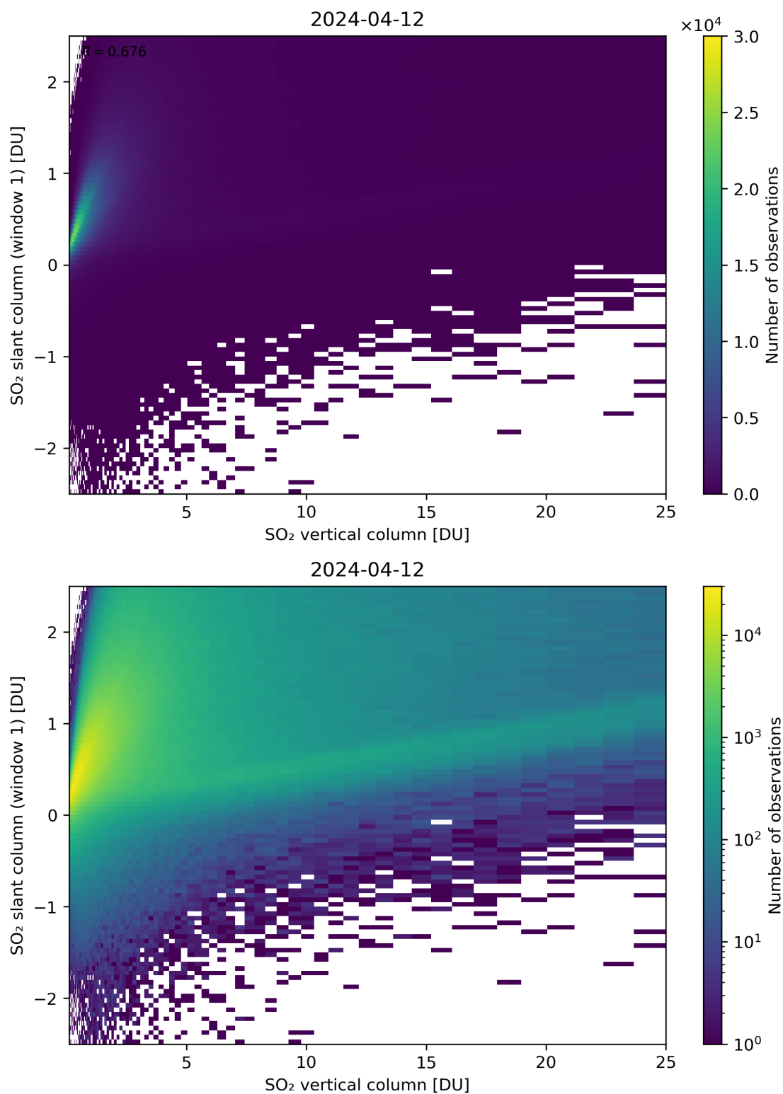
Figure 300: Scatter density plot of “SO 2 vertical column” against “SO 2 slant column (window 1)” for 2024-04-11 to 2024-04-13.
