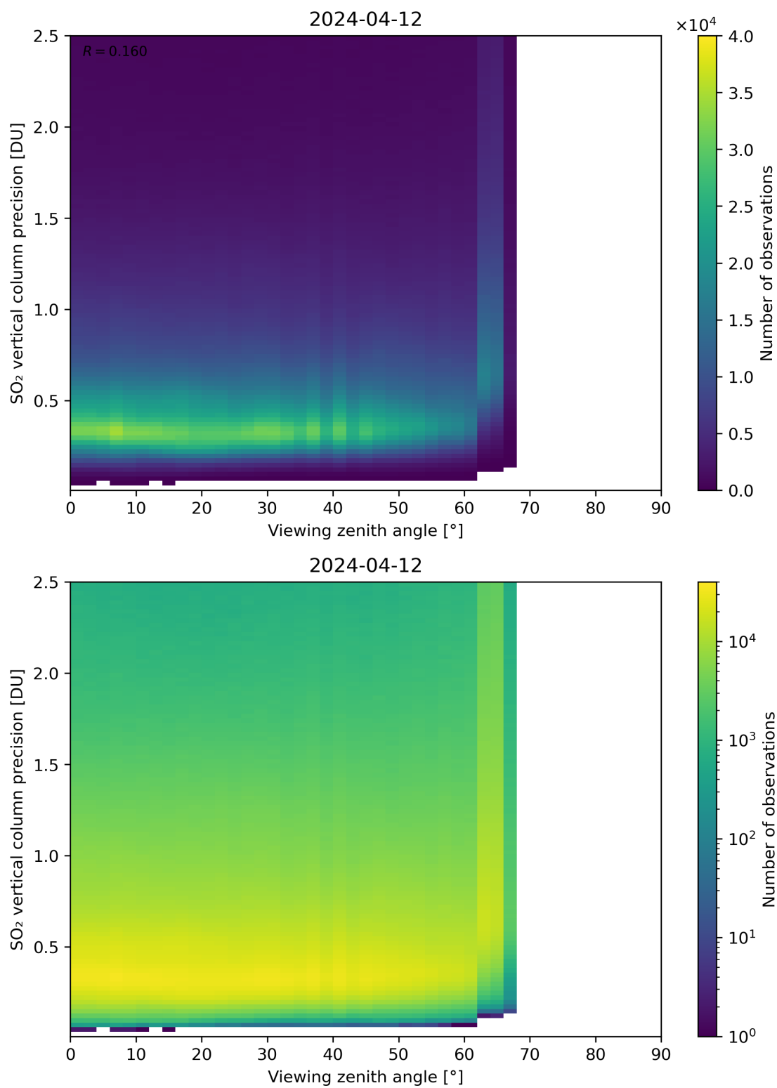
Figure 328: Scatter density plot of “Viewing zenith angle” against “SO 2 vertical column precision” for 2024-04-11 to 2024-04-13.
