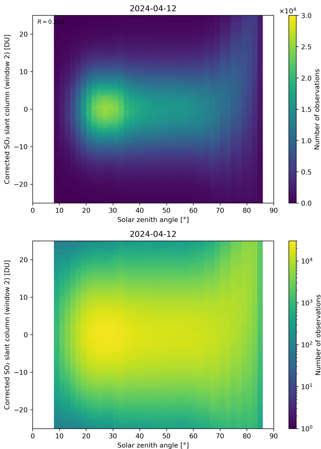
Figure 167: Scatter density plot of “Solar zenith angle” against “Corrected SO 2 slant column (window 2)” for 2024-04-11 to 2024-04-13.
