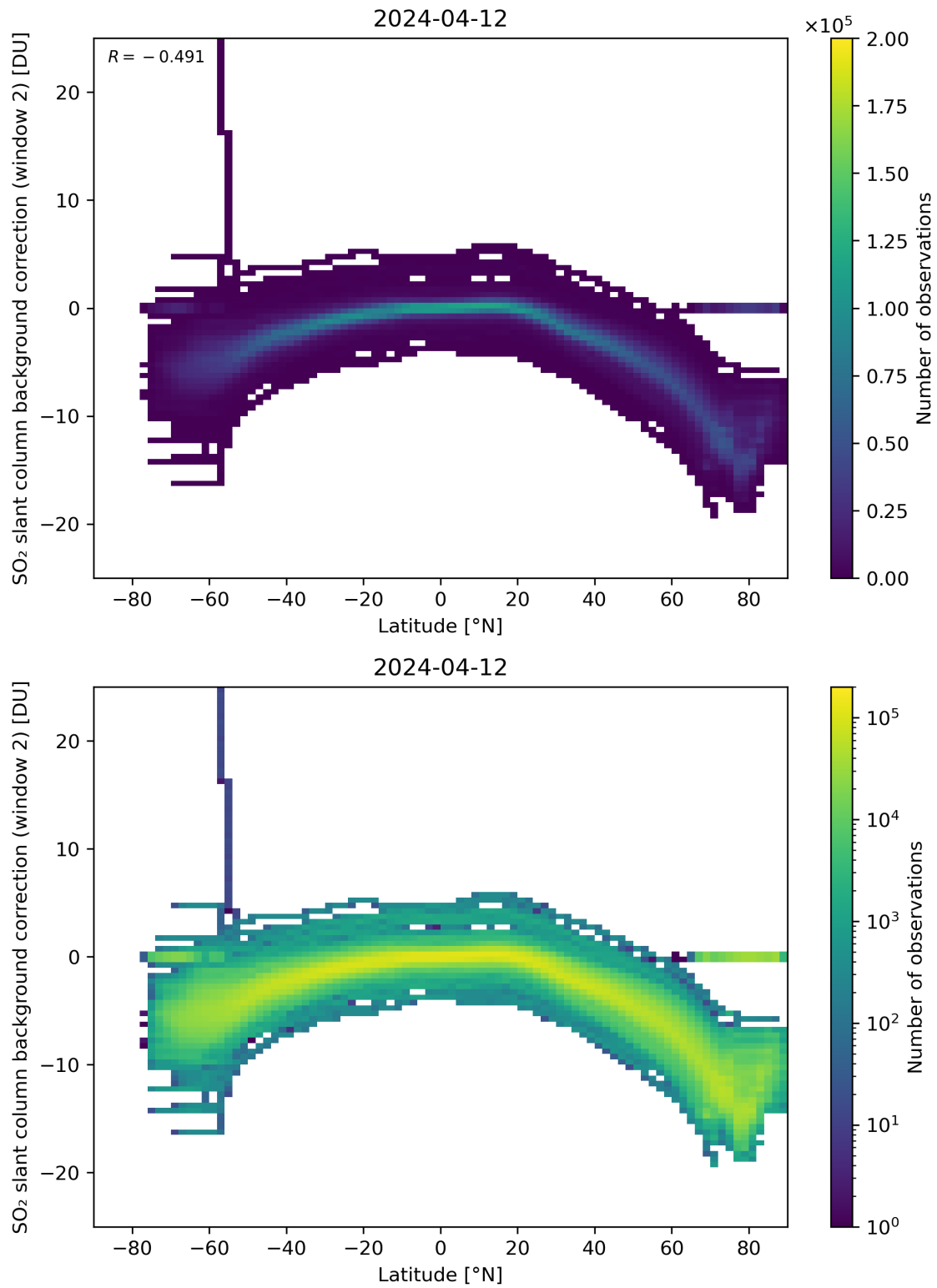
Figure 140: Scatter density plot of “Latitude” against “SO 2 slant column background correction (window 2)” for 2024-04-11 to 2024-04-13.
