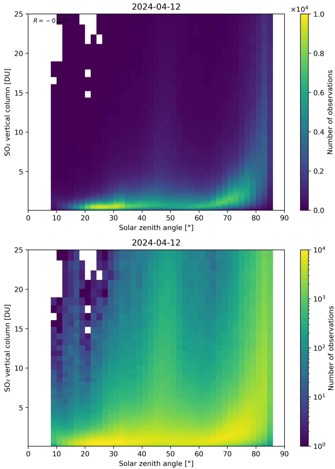
Figure 176: Scatter density plot of “Solar zenith angle” against “SO 2 vertical column” for 2024-04-11 to 2024-04-13.
