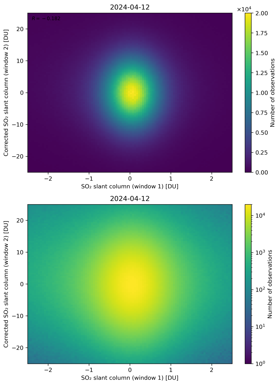
Figure 233: Scatter density plot of “SO 2 slant column (window 1)” against “Corrected SO 2 slant column (window 2)” for 2024-04-11 to 2024-04-13.
