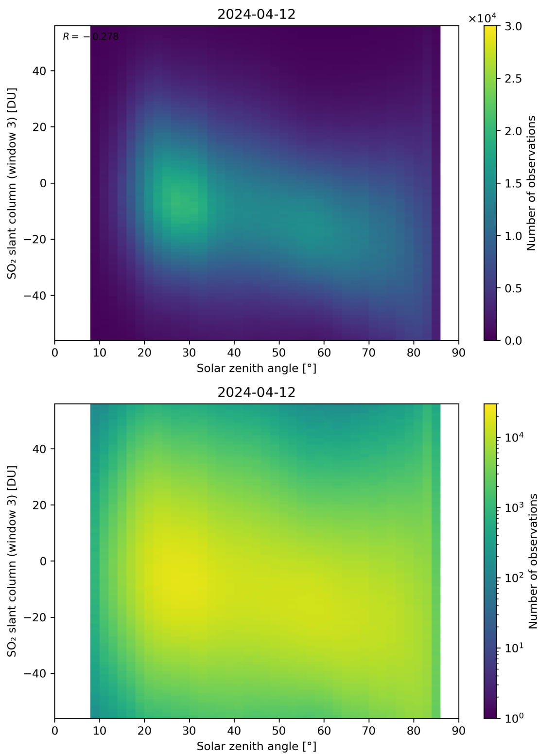
Figure 172: Scatter density plot of “Solar zenith angle” against “SO 2 slant column (window 3)” for 2024-04-11 to 2024-04-13.
