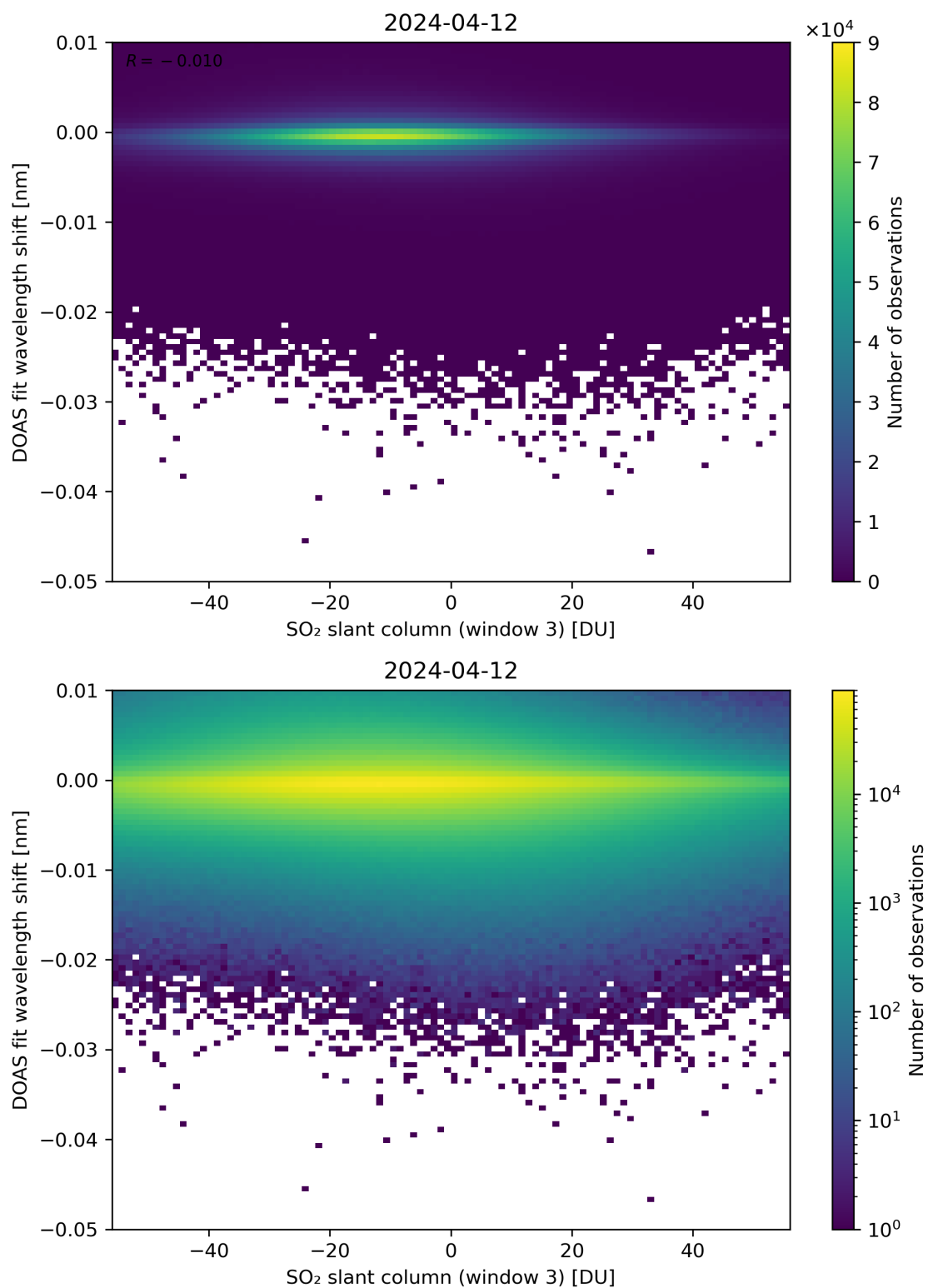
Figure 254: Scatter density plot of “SO 2 slant column (window 3)” against “DOAS fit wavelength shift” for 2024-04-11 to 2024-04-13.
