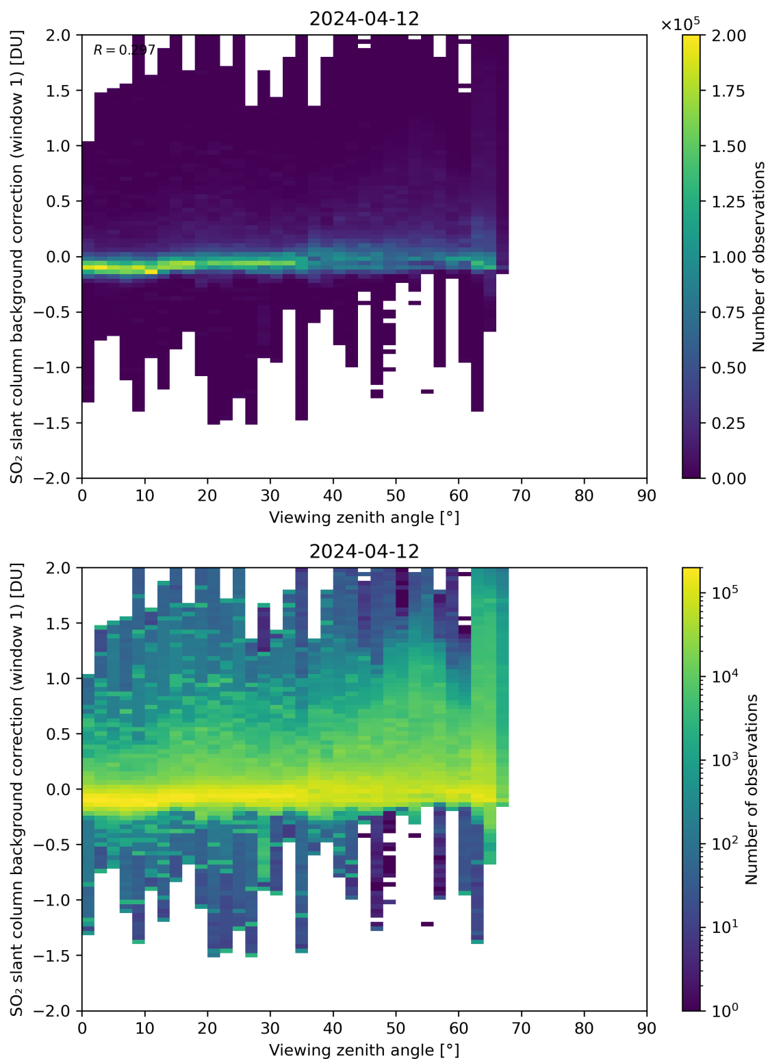
Figure 308: Scatter density plot of “Viewing zenith angle” against “SO 2 slant column background correction (window 1)” for 2024-04-11 to 2024-04-13.
