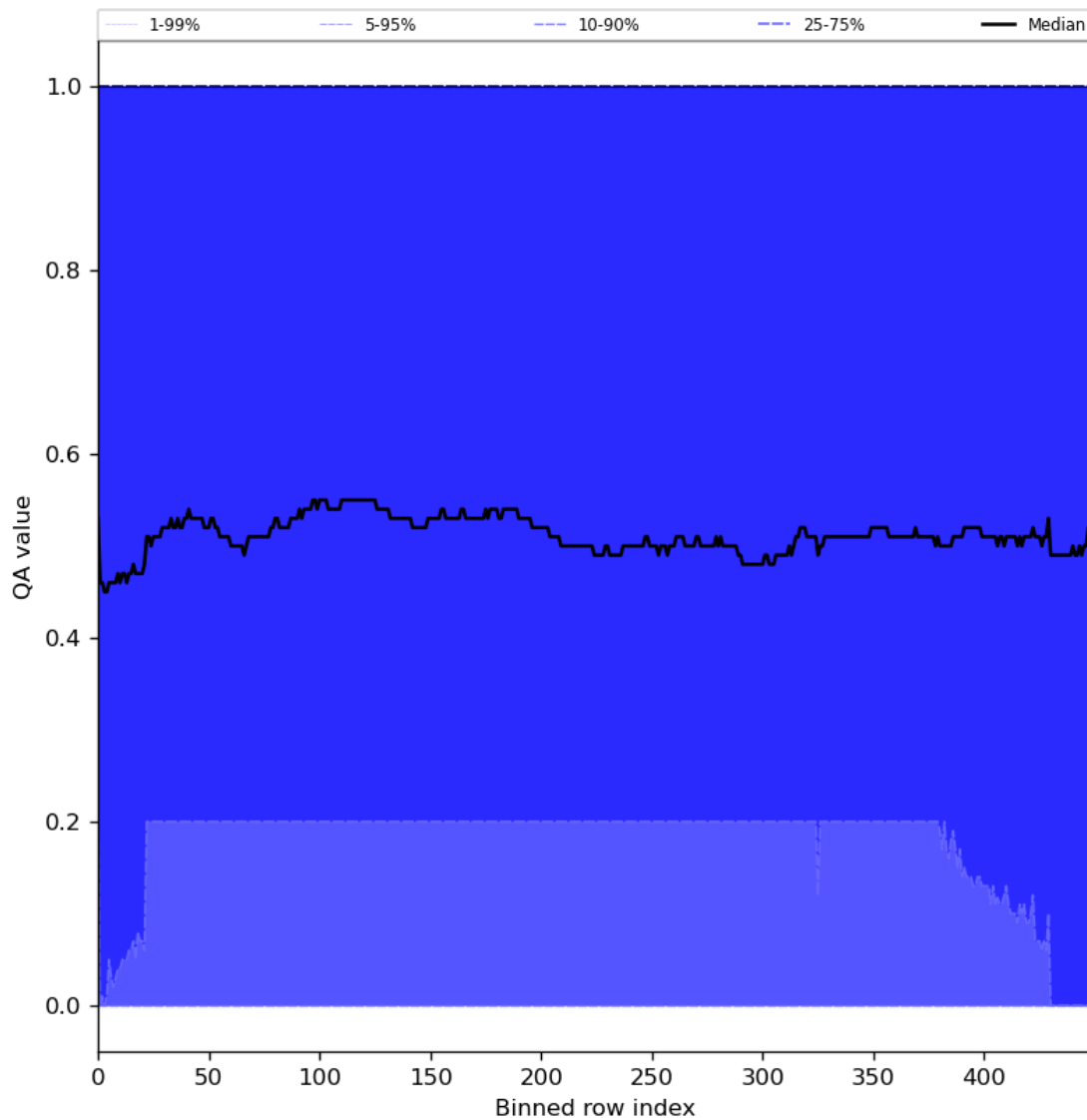
Figure 75: Along track statistics of “QA value” for 2024-04-11 to 2024-04-13
