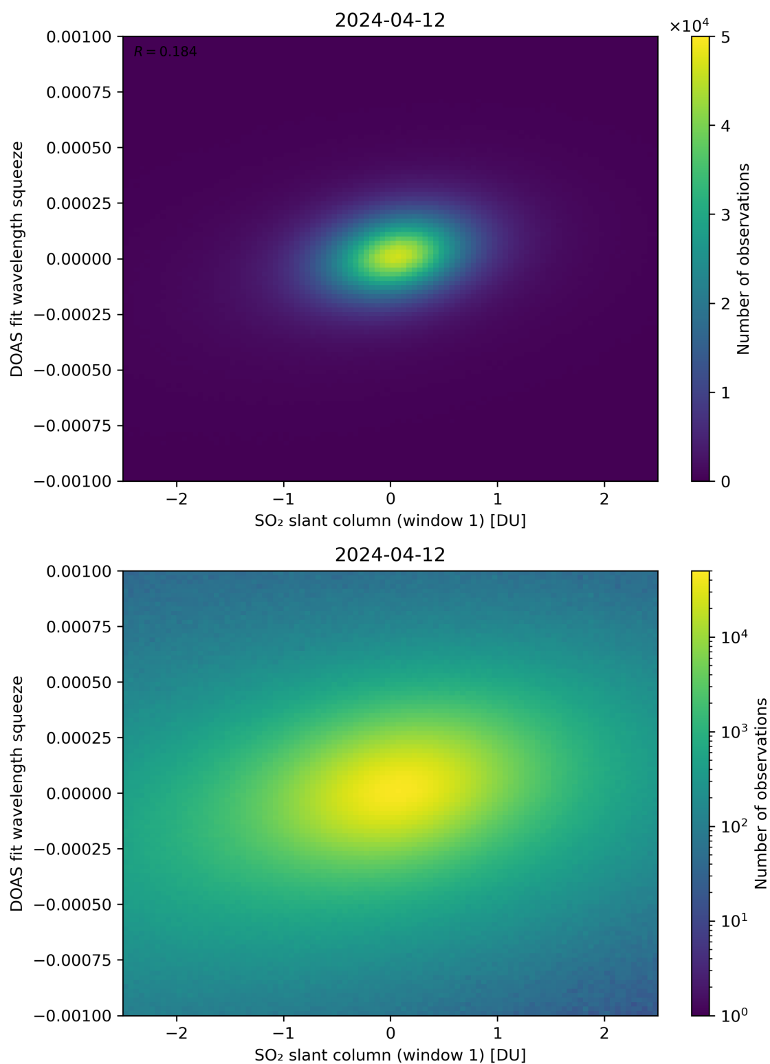
Figure 216: Scatter density plot of “SO 2 slant column (window 1)” against “DOAS fit wavelength squeeze” for 2024-04-11 to 2024-04-13.
