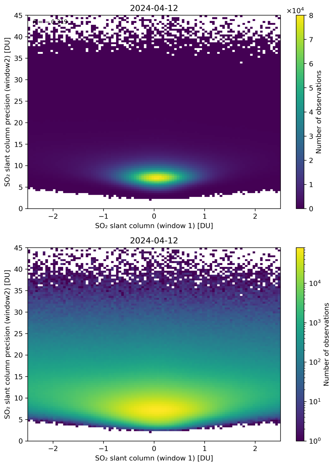
Figure 236: Scatter density plot of “SO 2 slant column (window 1)” against “SO 2 slant column precision (window2)” for 2024-04-11 to 2024-04-13.
