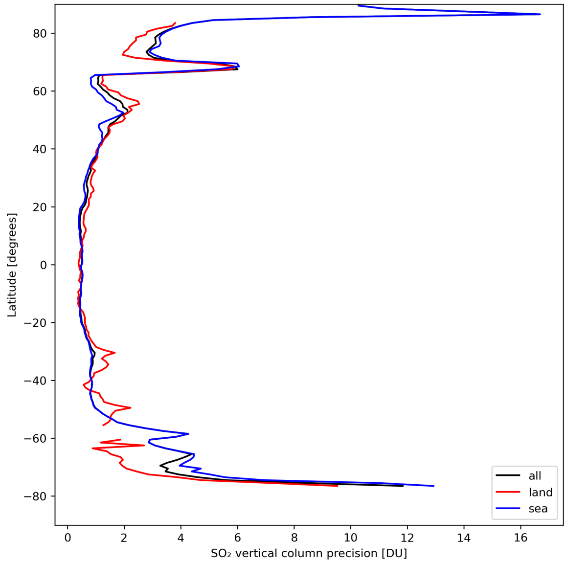
Figure 31: Zonal average of “SO 2 vertical column precision” for 2024-04-11 to 2024-04-13.
