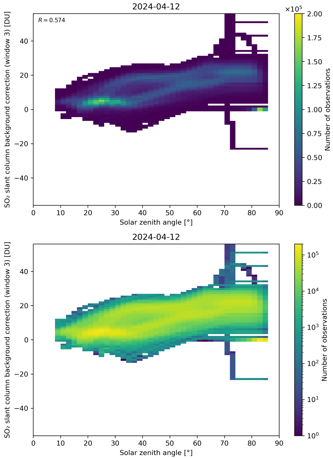
Figure 160: Scatter density plot of “Solar zenith angle” against “SO 2 slant column background correction (window 3)” for 2024-04-11 to 2024-04-13.
