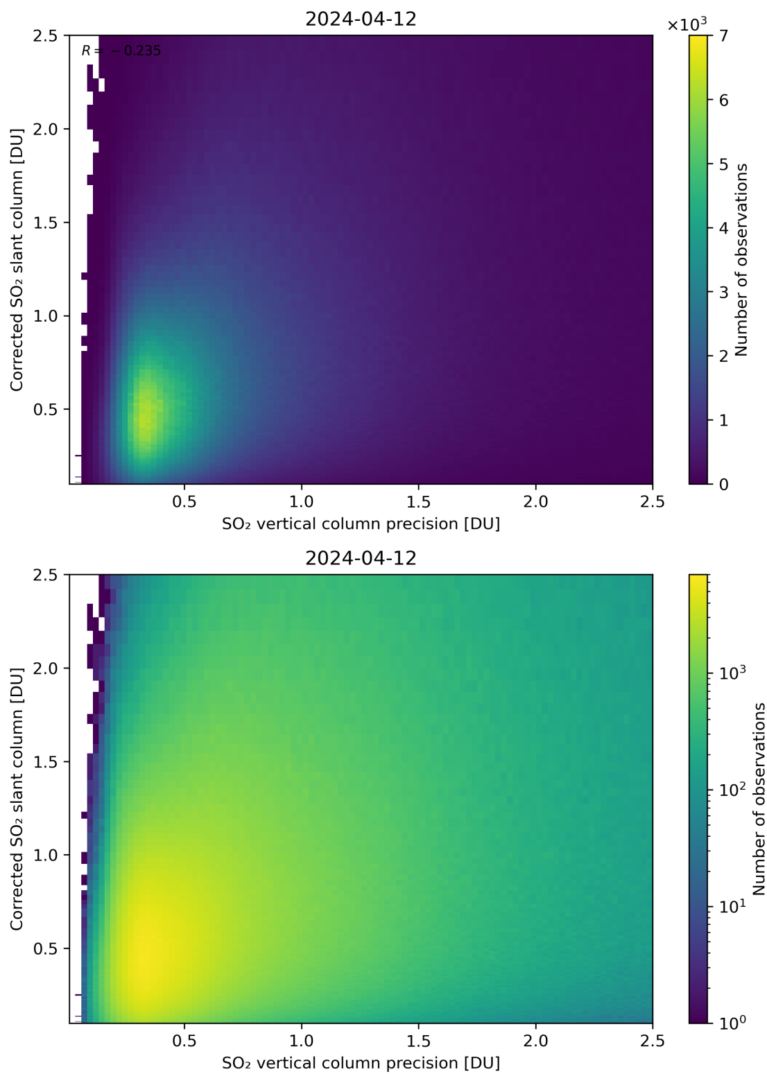
Figure 286: Scatter density plot of “SO 2 vertical column precision” against “Corrected SO 2 slant column” for 2024-04-11 to 2024-04-13.
