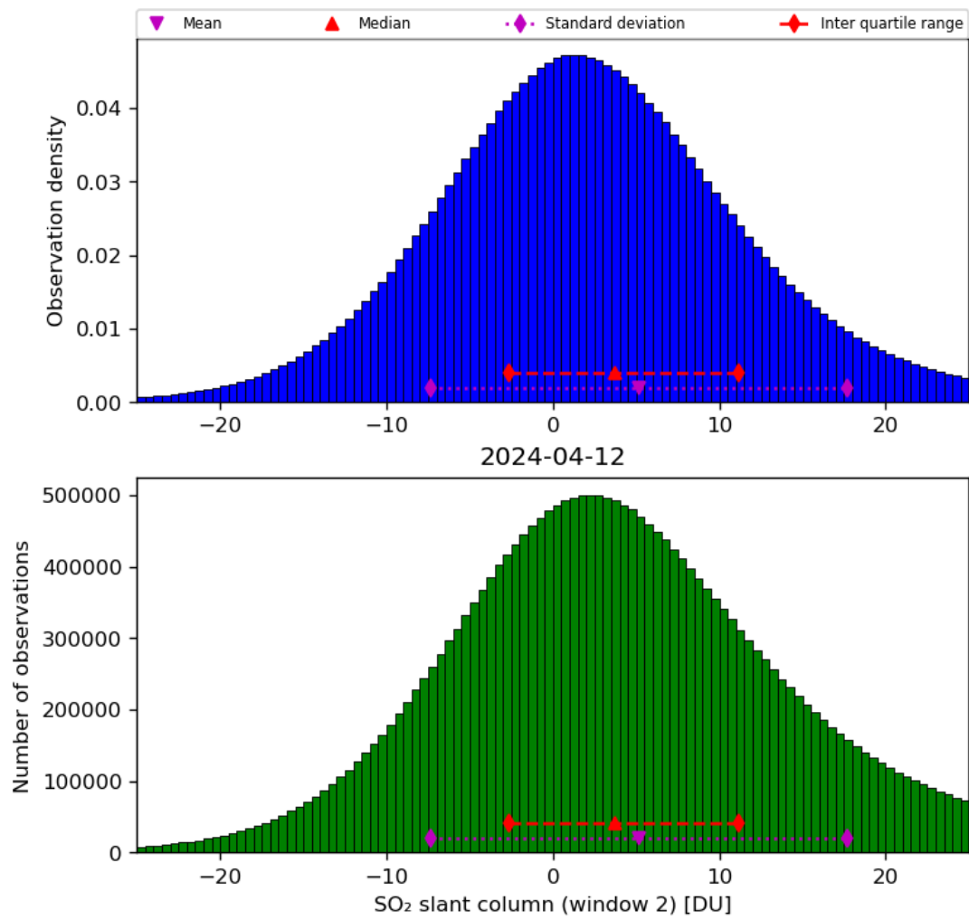
Figure 60: Histogram of “SO 2 slant column (window 2)” for 2024-04-11 to 2024-04-13
