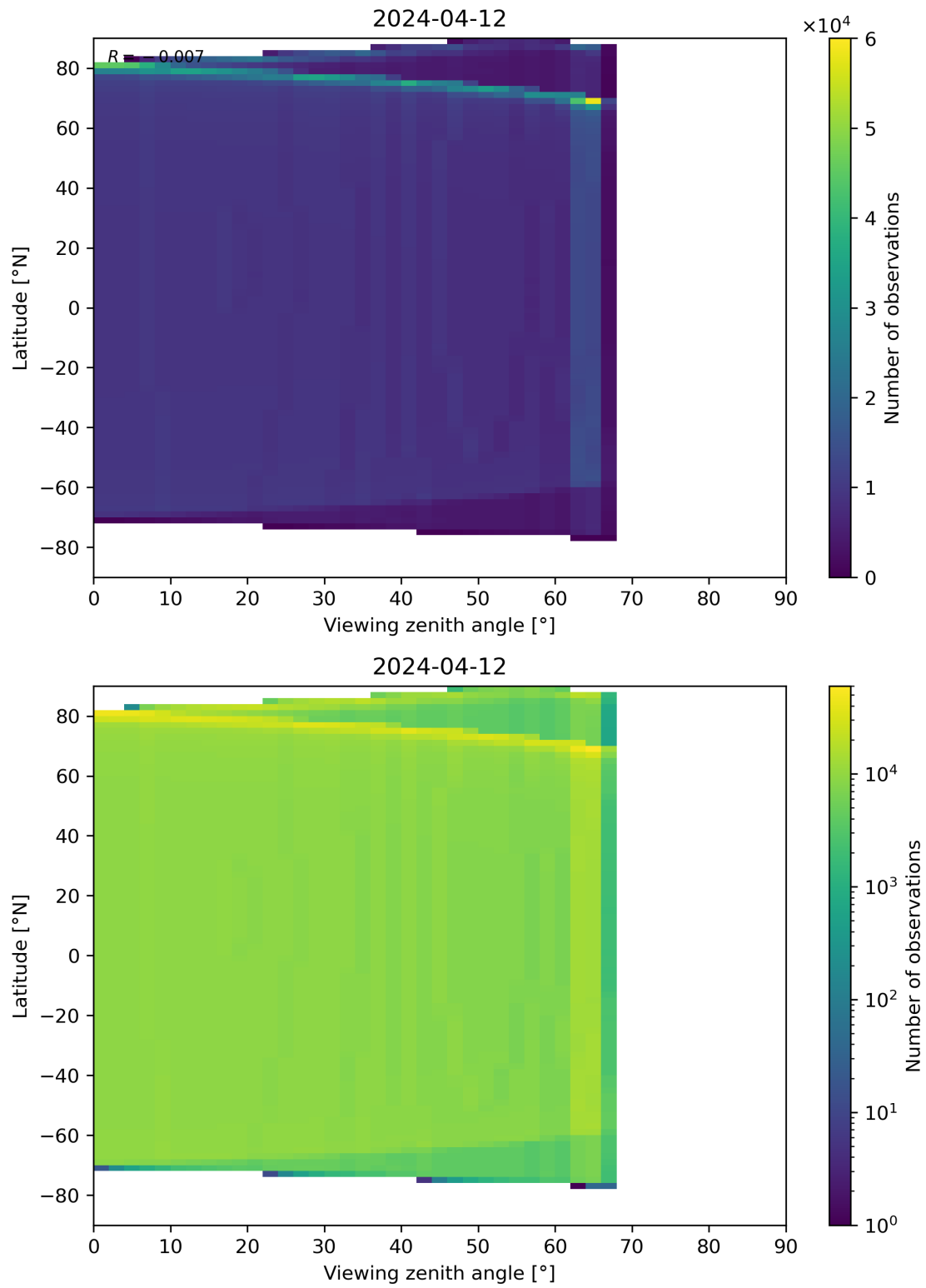
Figure 314: Scatter density plot of “Viewing zenith angle” against “Latitude” for 2024-04-11 to 2024-04-13.
