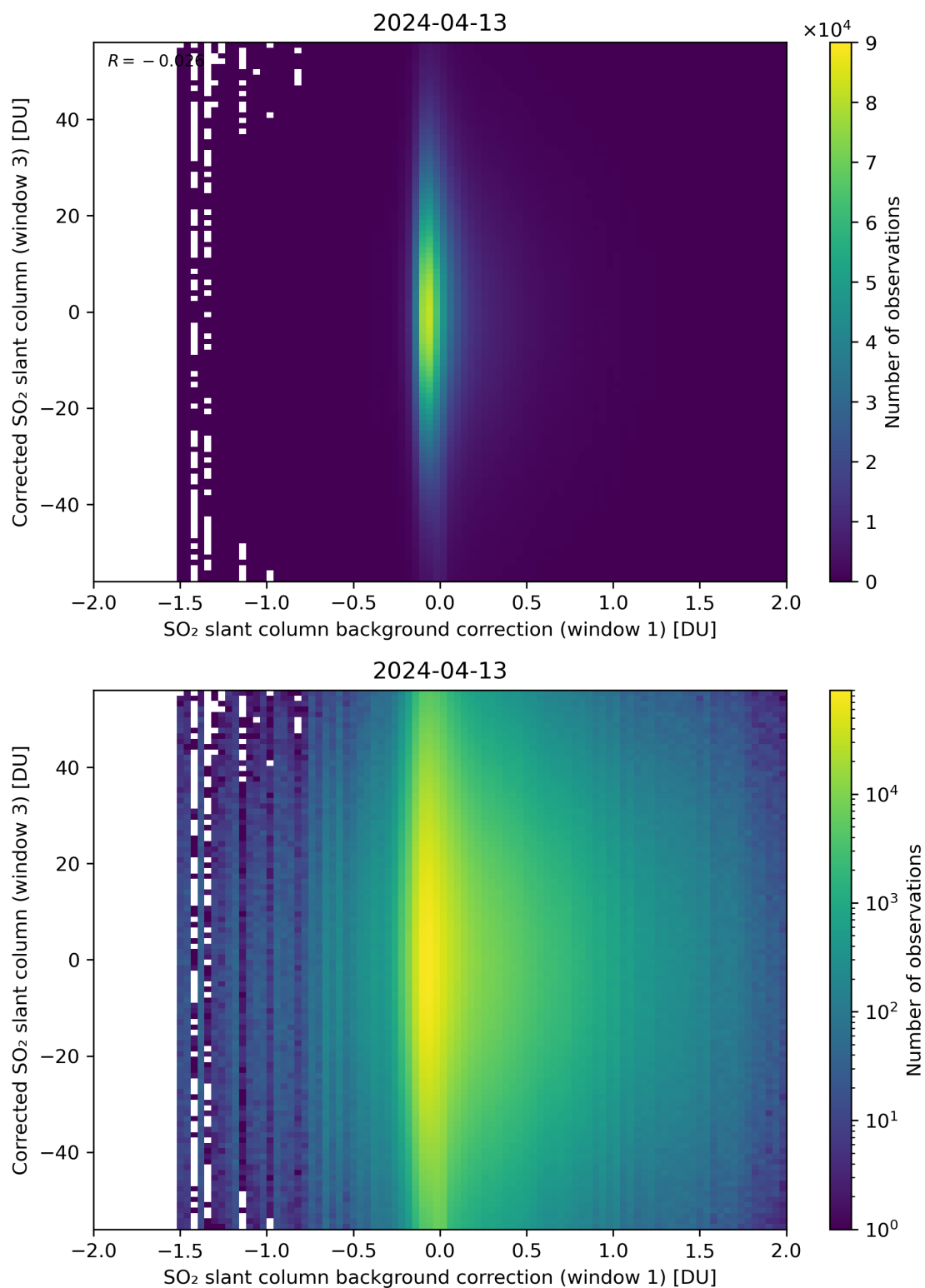
Figure 105: Scatter density plot of “SO 2 slant column background correction (window 1)” against “Corrected SO 2 slant column (window 3)” for 2024-04-12 to 2024-04-14.
