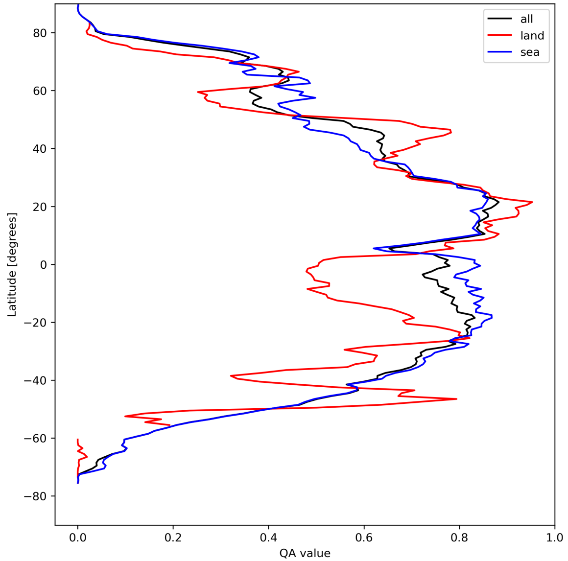
Figure 29: Zonal average of “QA value” for 2024-04-12 to 2024-04-14.
