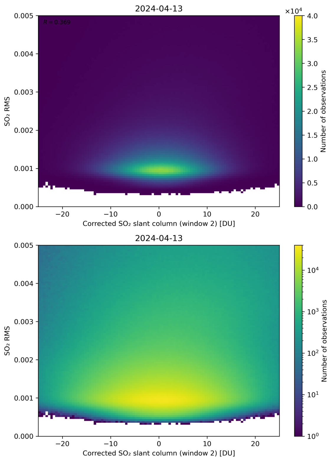
Figure 198: Scatter density plot of “Corrected SO 2 slant column (window 2)” against “SO 2 RMS” for 2024-04-12 to 2024-04-14.
