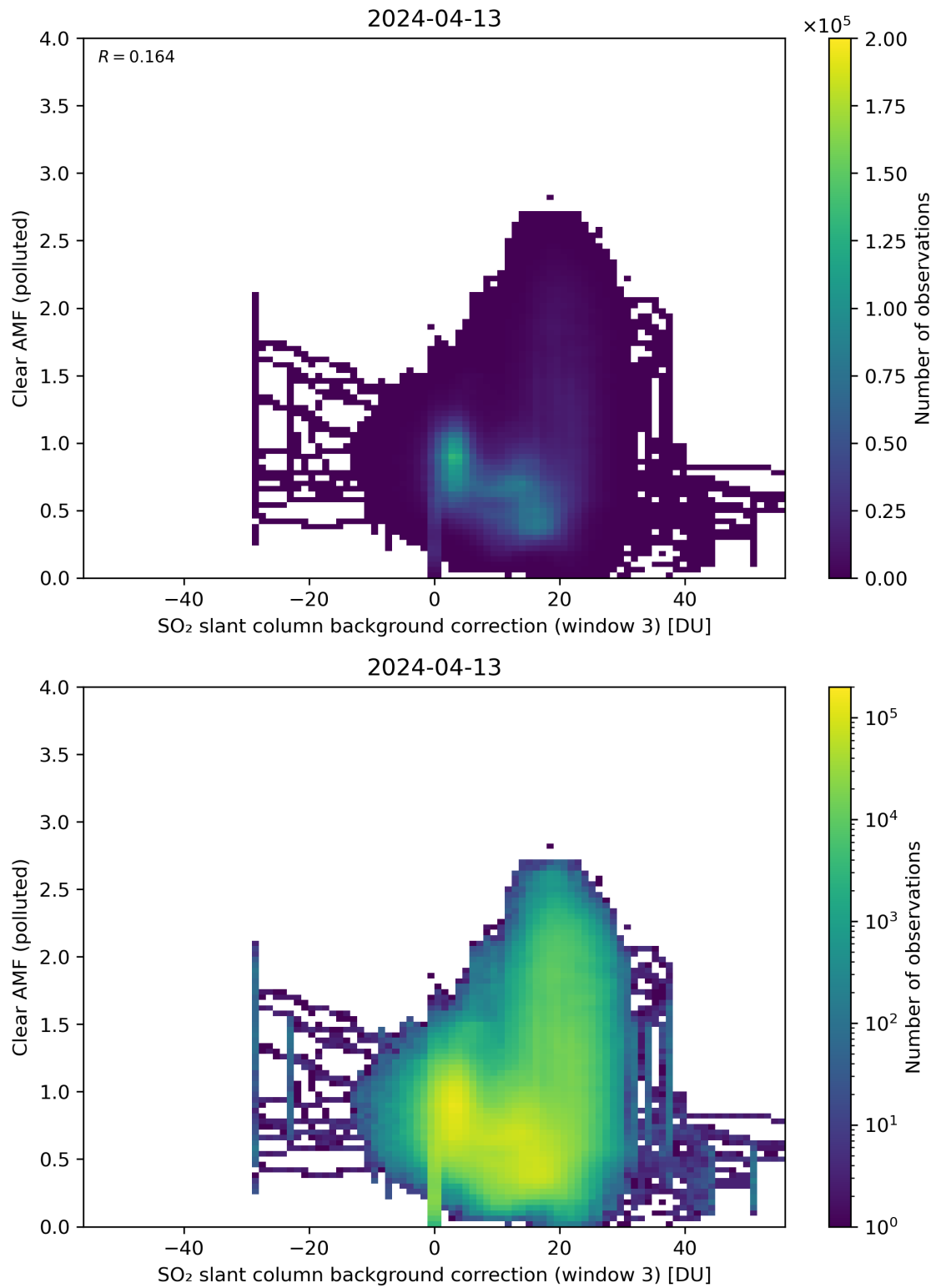
Figure 124: Scatter density plot of “SO 2 slant column background correction (window 3)” against “Clear AMF (polluted)” for 2024-04-12 to 2024-04-14.
