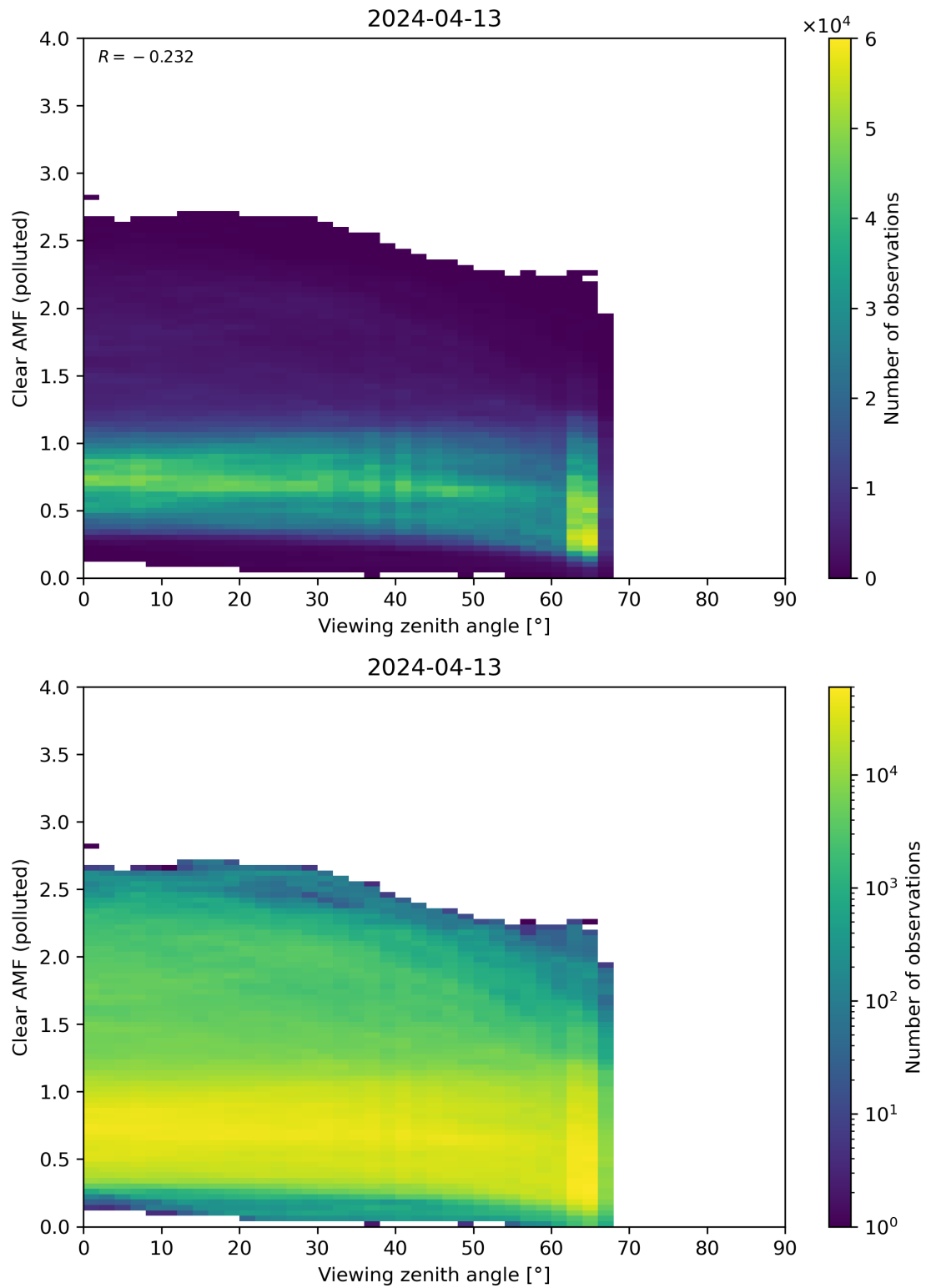
Figure 316: Scatter density plot of “Viewing zenith angle” against “Clear AMF (polluted)” for 2024-04-12 to 2024-04-14.
