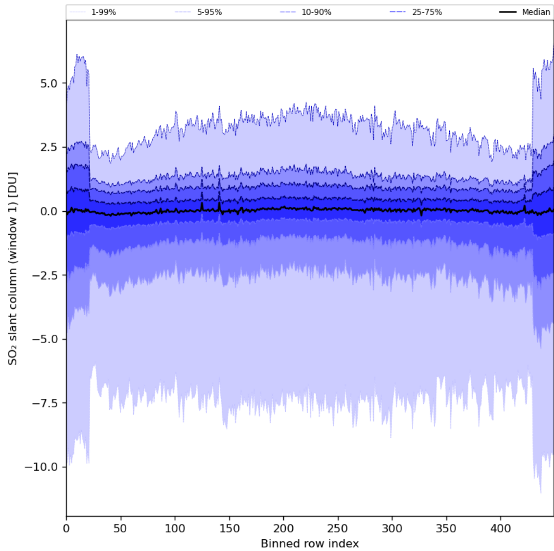
Figure 79: Along track statistics of “SO 2 slant column (window 1)” for 2024-04-12 to 2024-04-14
