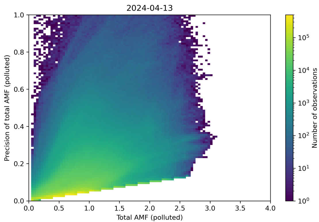
Figure 272: Scatter density plot of “Total AMF (polluted)” against “Precision of total AMF (polluted)” for 2024-04-12 to 2024-04-14.
