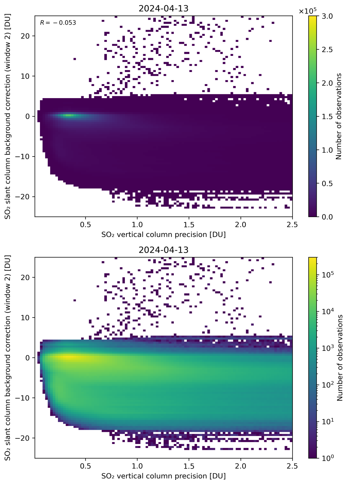
Figure 280: Scatter density plot of “SO 2 vertical column precision” against “SO 2 slant column background correction (window 2)” for 2024-04-12 to 2024-04-14.
