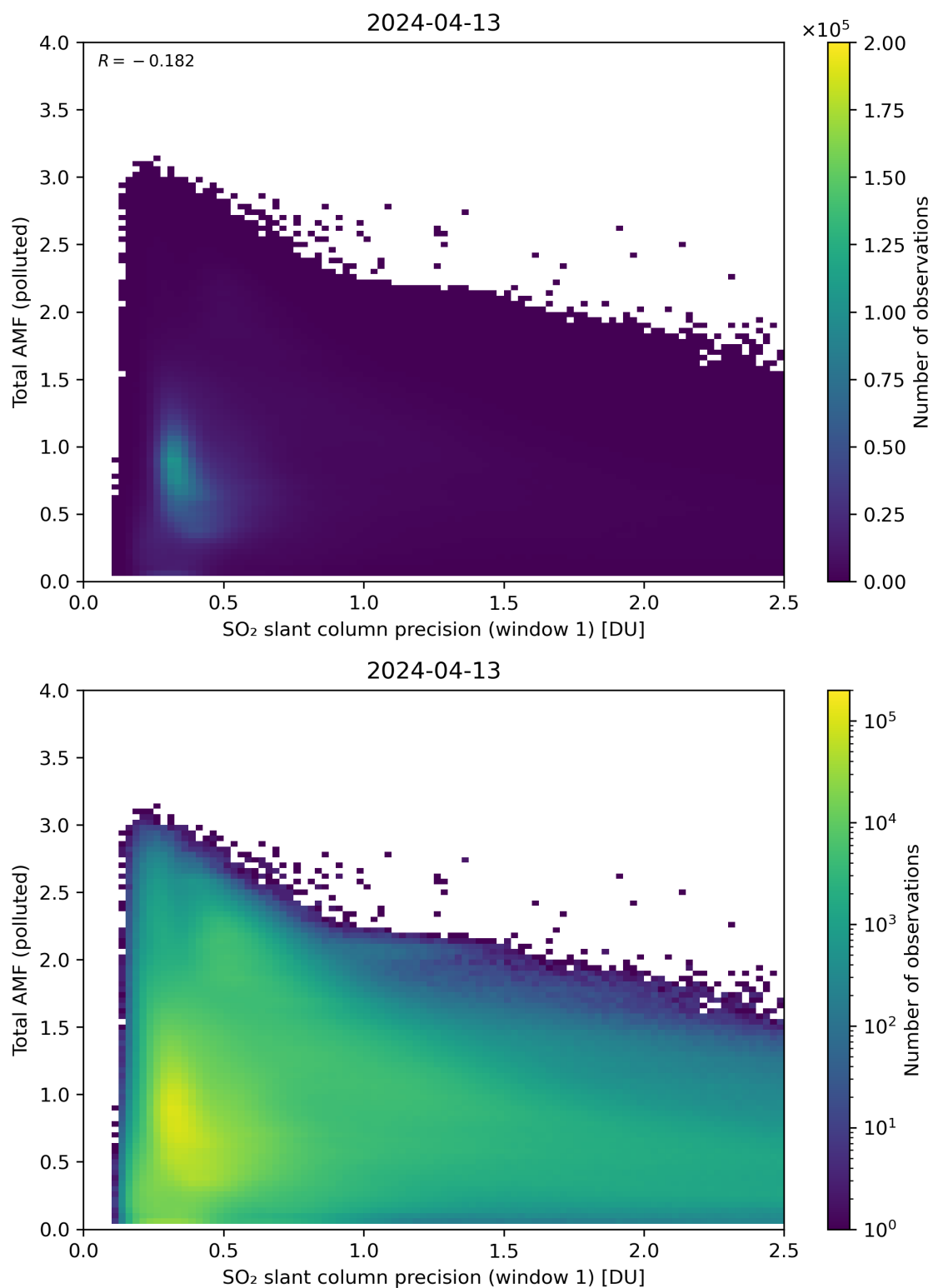
Figure 230: Scatter density plot of “SO 2 slant column precision (window 1)” against “Total AMF (polluted)” for 2024-04-12 to 2024-04-14.
