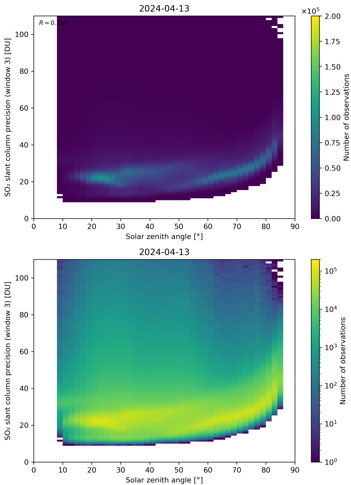
Figure 173: Scatter density plot of “Solar zenith angle” against “SO 2 slant column precision (window 3)” for 2024-04-12 to 2024-04-14.
