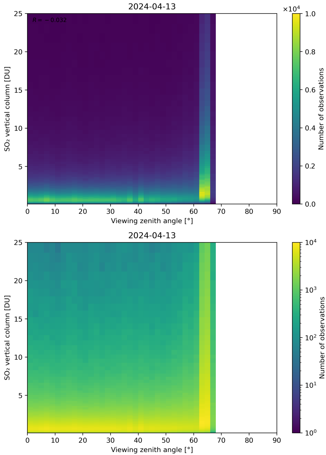
Figure 327: Scatter density plot of “Viewing zenith angle” against “SO 2 vertical column” for 2024-04-12 to 2024-04-14.
