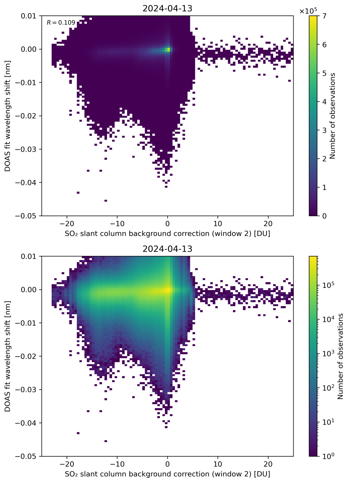
Figure 112: Scatter density plot of “SO 2 slant column background correction (window 2)” against “DOAS fit wavelength shift” for 2024-04-12 to 2024-04-14.
