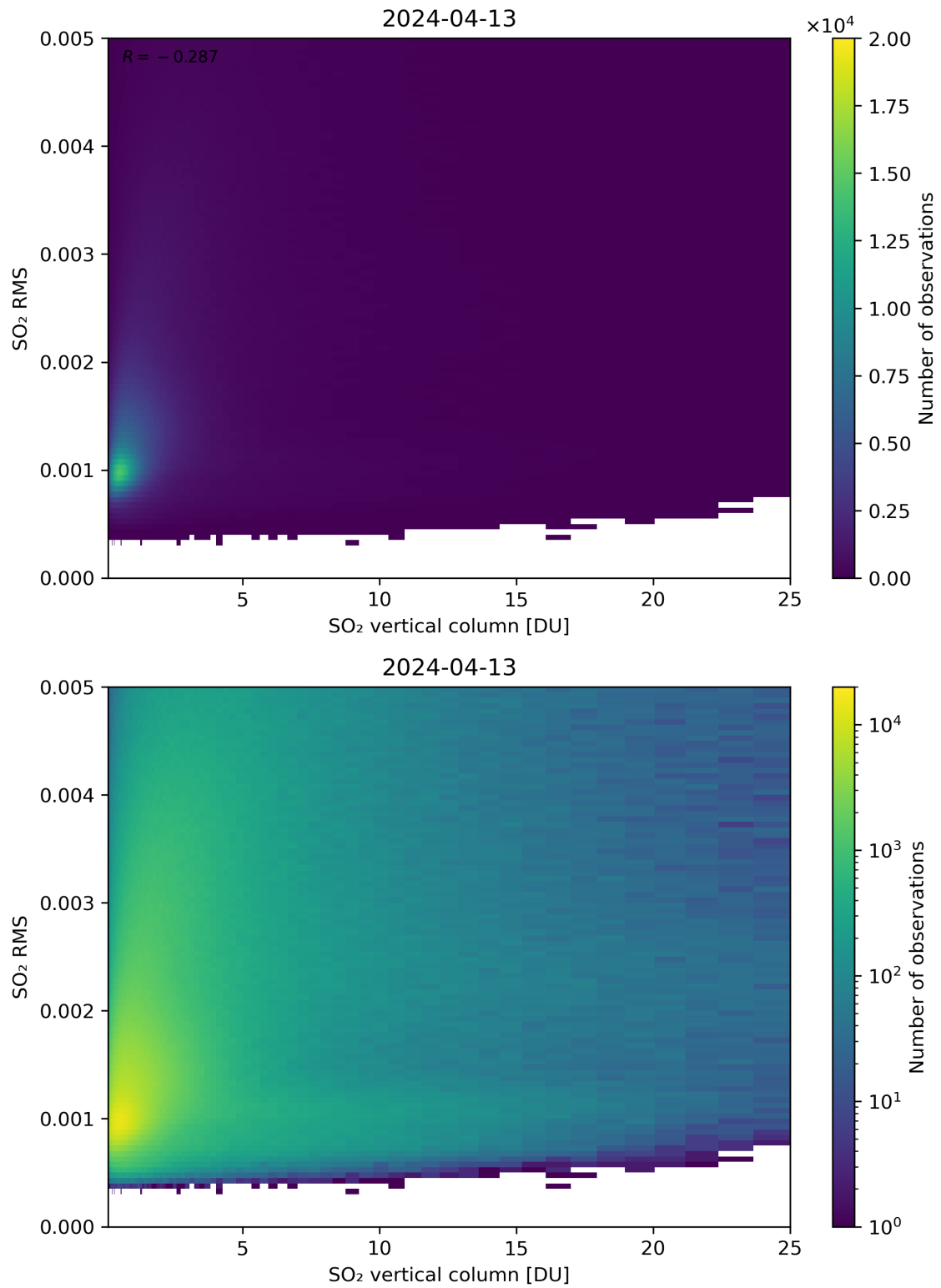
Figure 278: Scatter density plot of “SO 2 vertical column” against “SO 2 RMS” for 2024-04-12 to 2024-04-14.
