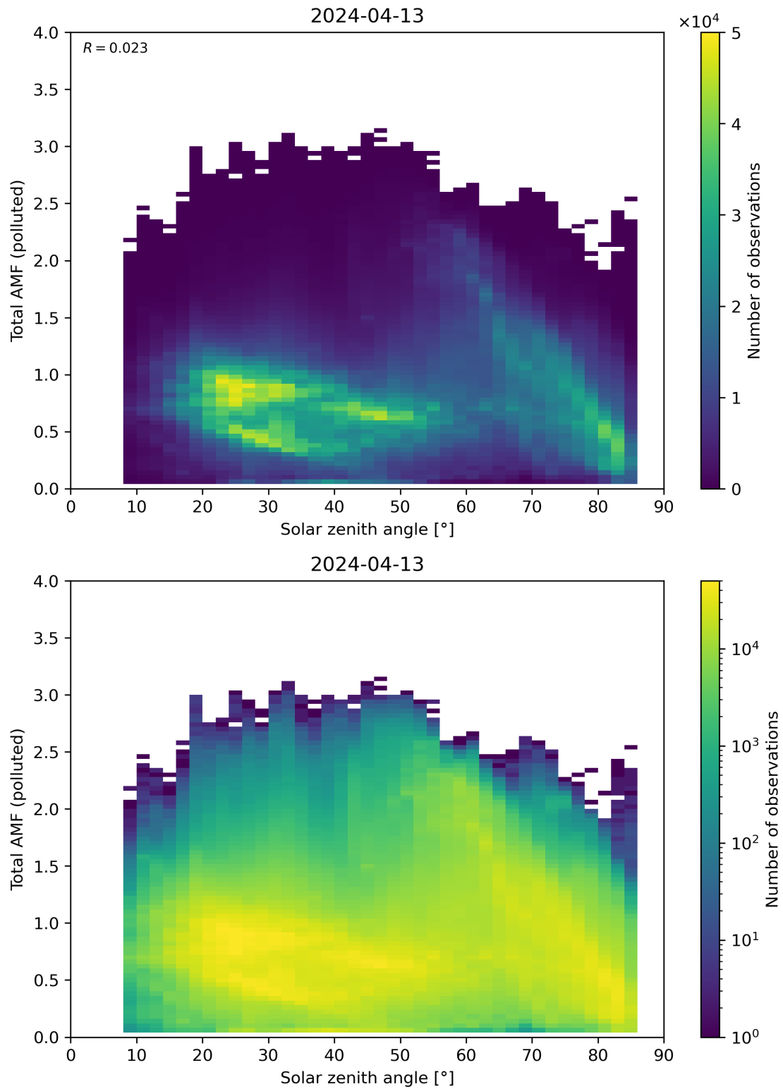
Figure 174: Scatter density plot of “Solar zenith angle” against “Total AMF (polluted)” for 2024-04-12 to 2024-04-14.
