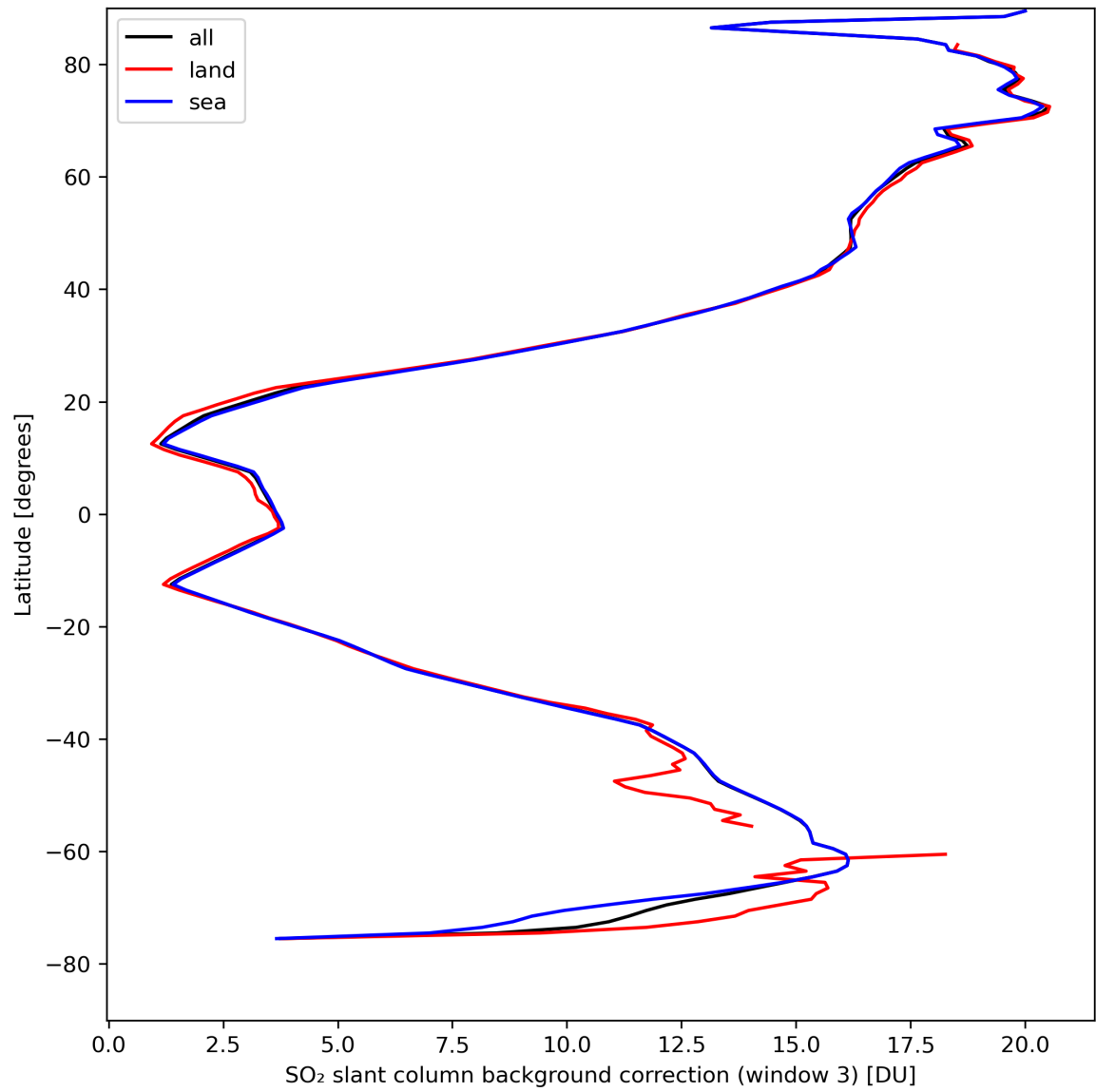
Figure 44: Zonal average of “SO 2 slant column background correction (window 3)” for 2024-04-12 to 2024-04-14.
