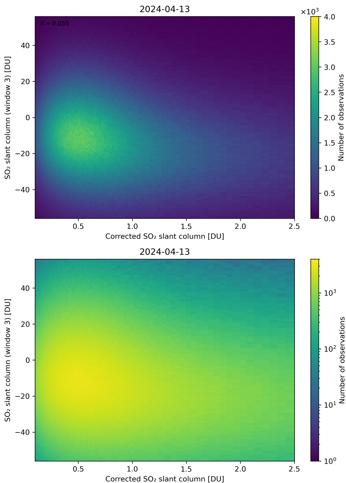
Figure 190: Scatter density plot of “Corrected SO 2 slant column” against “SO 2 slant column (window 3)” for 2024-04-12 to 2024-04-14.
