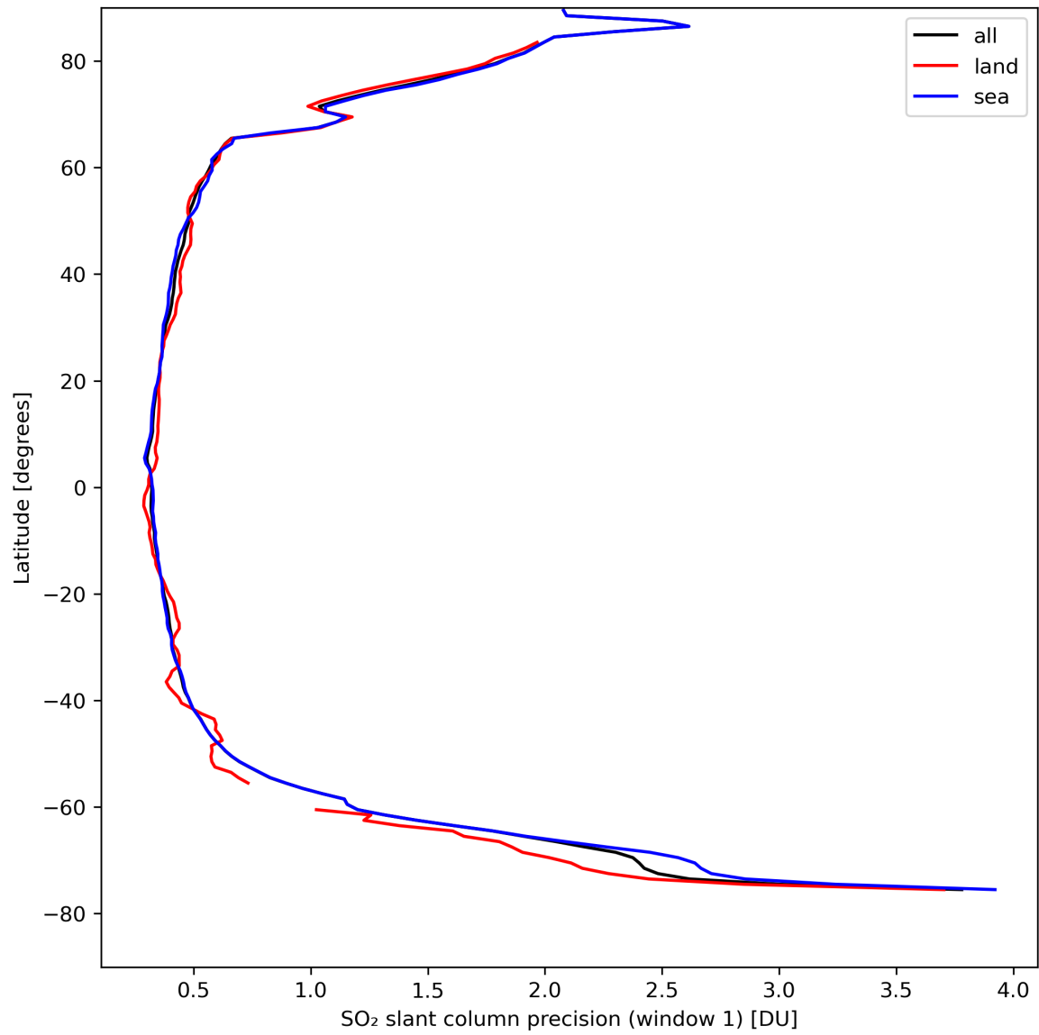
Figure 34: Zonal average of “SO 2 slant column precision (window 1)” for 2024-04-12 to 2024-04-14.
