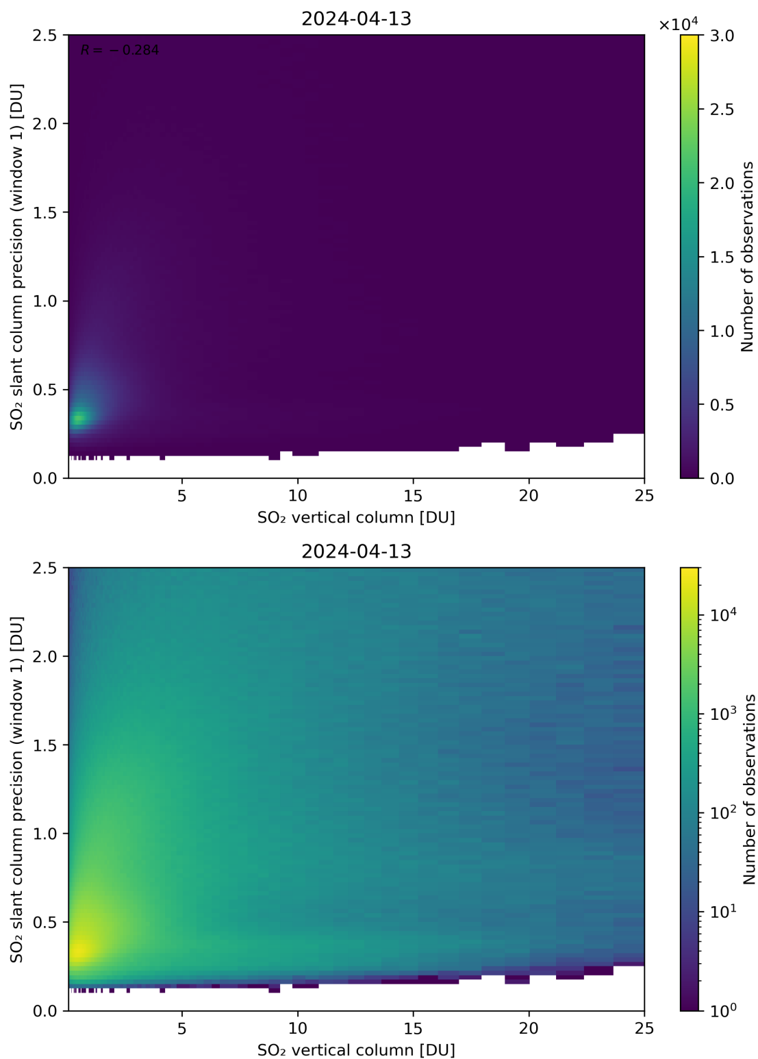
Figure 301: Scatter density plot of “SO 2 vertical column” against “SO 2 slant column precision (window 1)” for 2024-04-12 to 2024-04-14.
