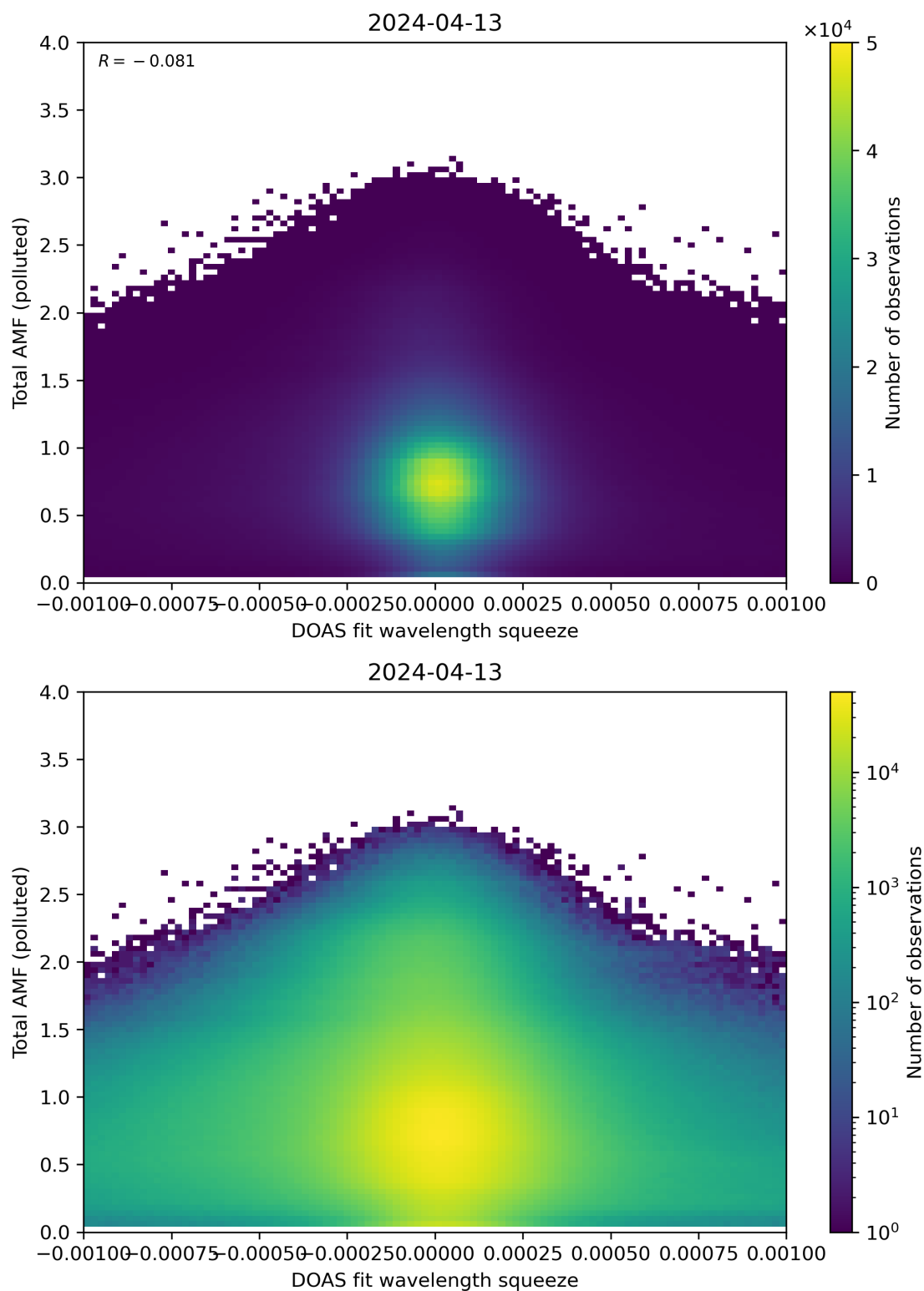
Figure 134: Scatter density plot of “DOAS fit wavelength squeeze” against “Total AMF (polluted)” for 2024-04-12 to 2024-04-14.
