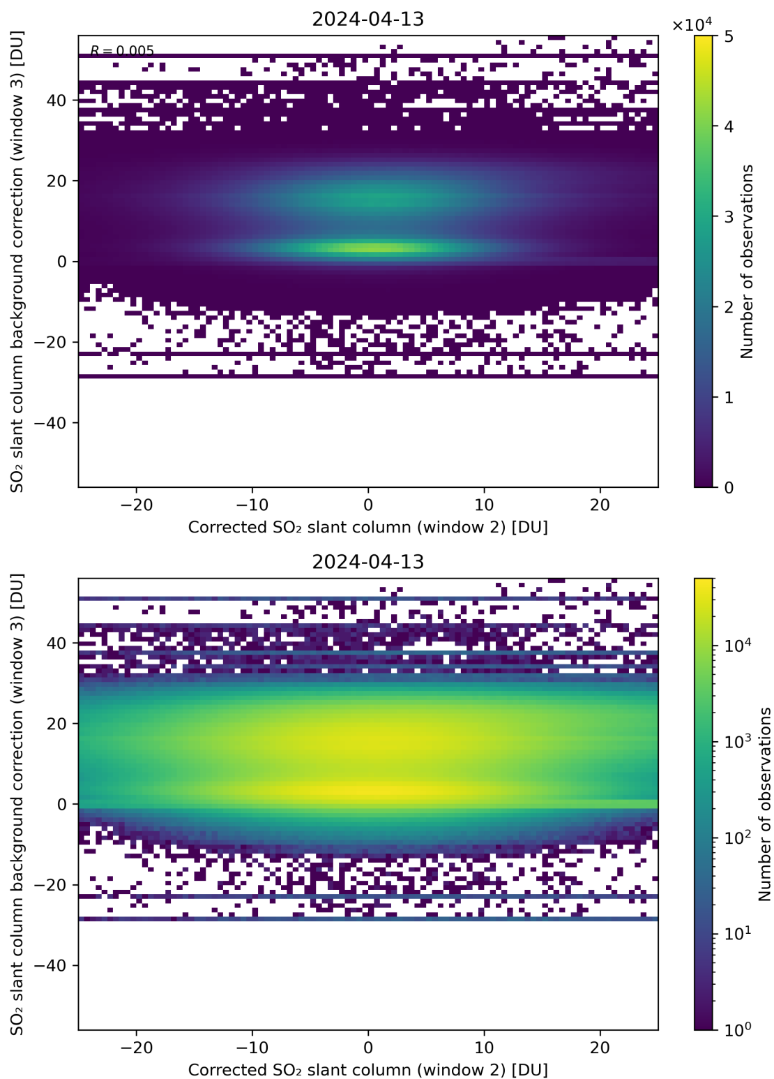
Figure 195: Scatter density plot of “Corrected SO 2 slant column (window 2)” against “SO 2 slant column background correction (window 3)” for 2024-04-12 to 2024-04-14.
