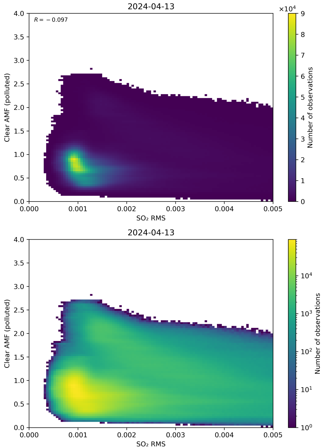
Figure 136: Scatter density plot of “SO 2 RMS” against “Clear AMF (polluted)” for 2024-04-12 to 2024-04-14.
