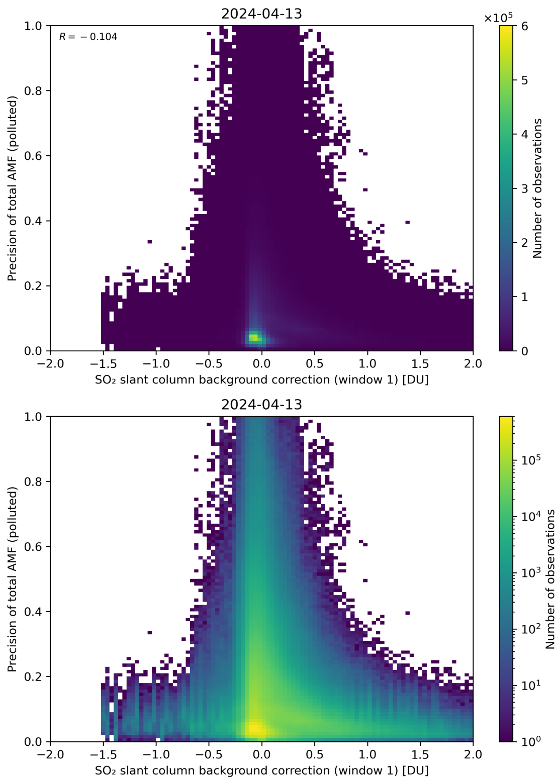
Figure 110: Scatter density plot of “SO 2 slant column background correction (window 1)” against “Precision of total AMF (polluted)” for 2024-04-12 to 2024-04-14.
