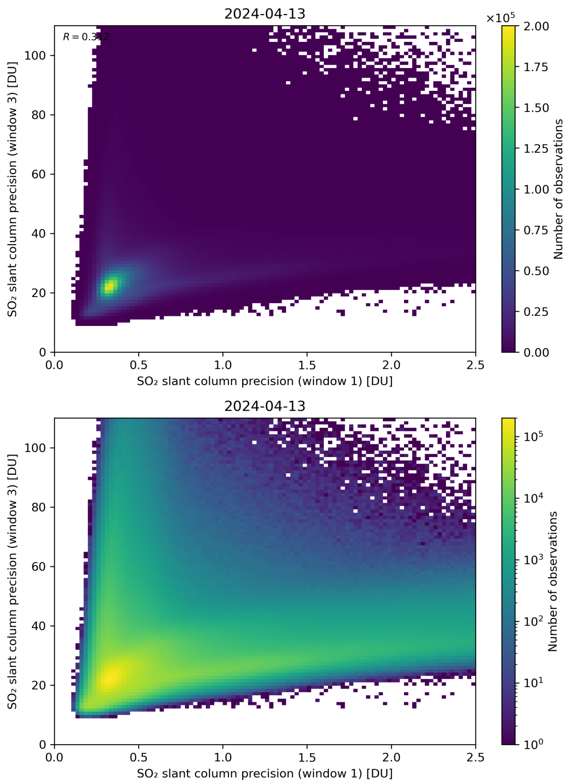
Figure 229: Scatter density plot of “SO 2 slant column precision (window 1)” against “SO 2 slant column precision (window 3)” for 2024-04-12 to 2024-04-14.
