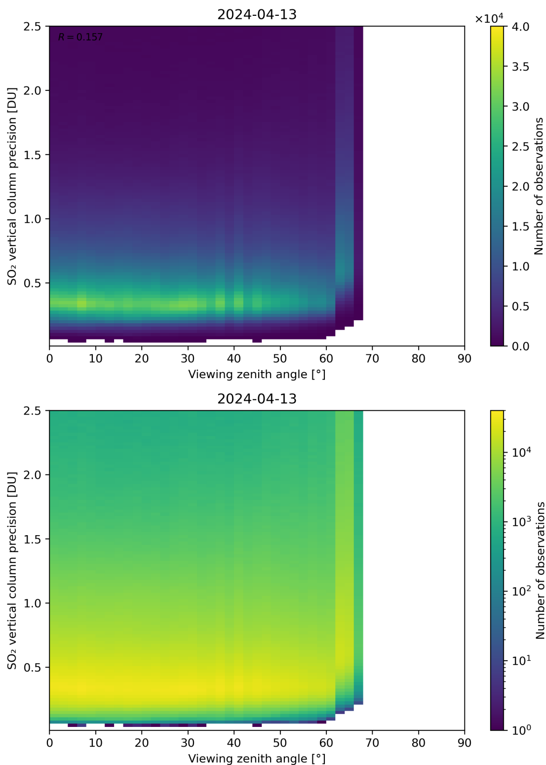
Figure 328: Scatter density plot of “Viewing zenith angle” against “SO 2 vertical column precision” for 2024-04-12 to 2024-04-14.
