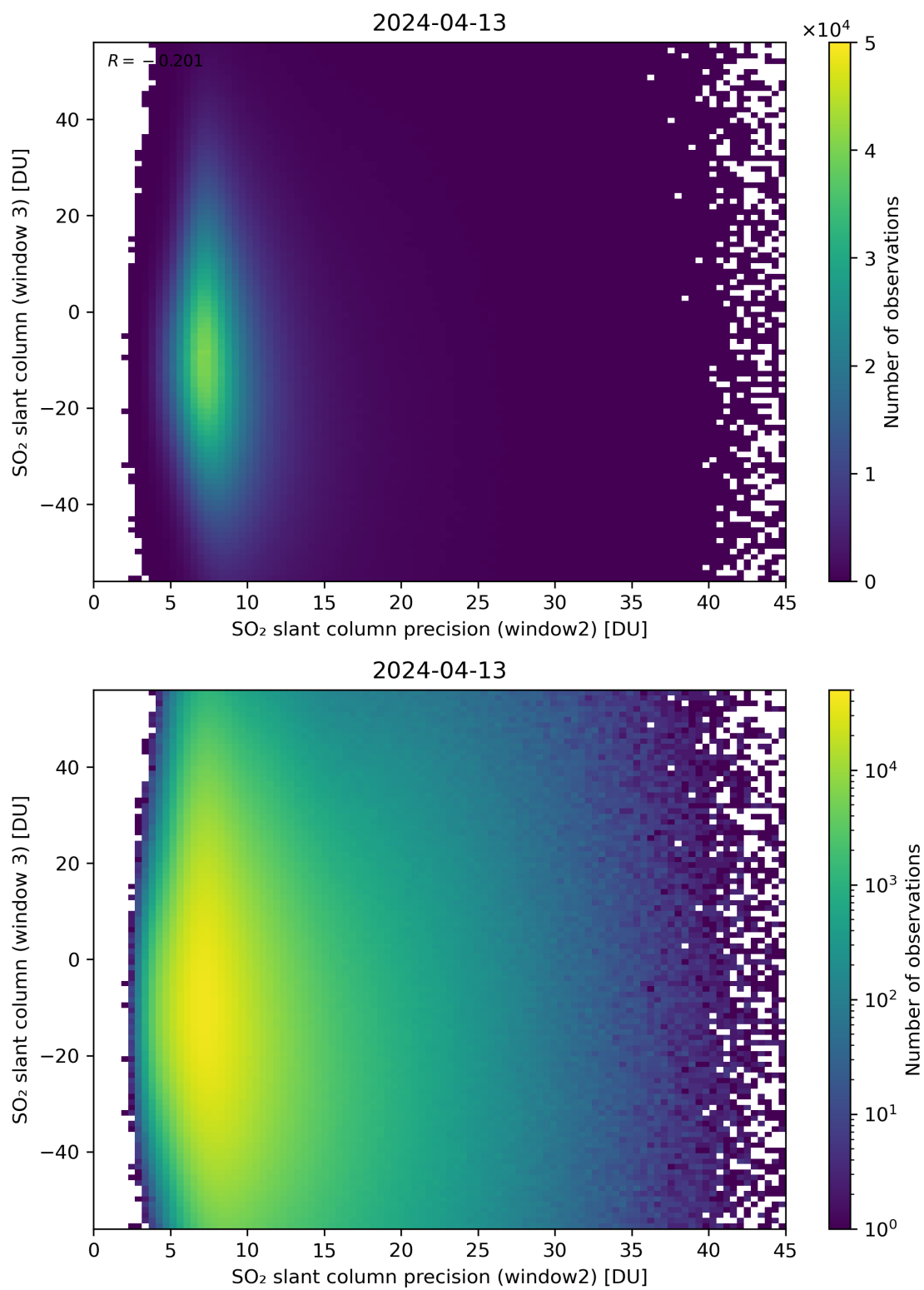
Figure 249: Scatter density plot of “SO 2 slant column precision (window2)” against “SO 2 slant column (window 3)” for 2024-04-12 to 2024-04-14.
