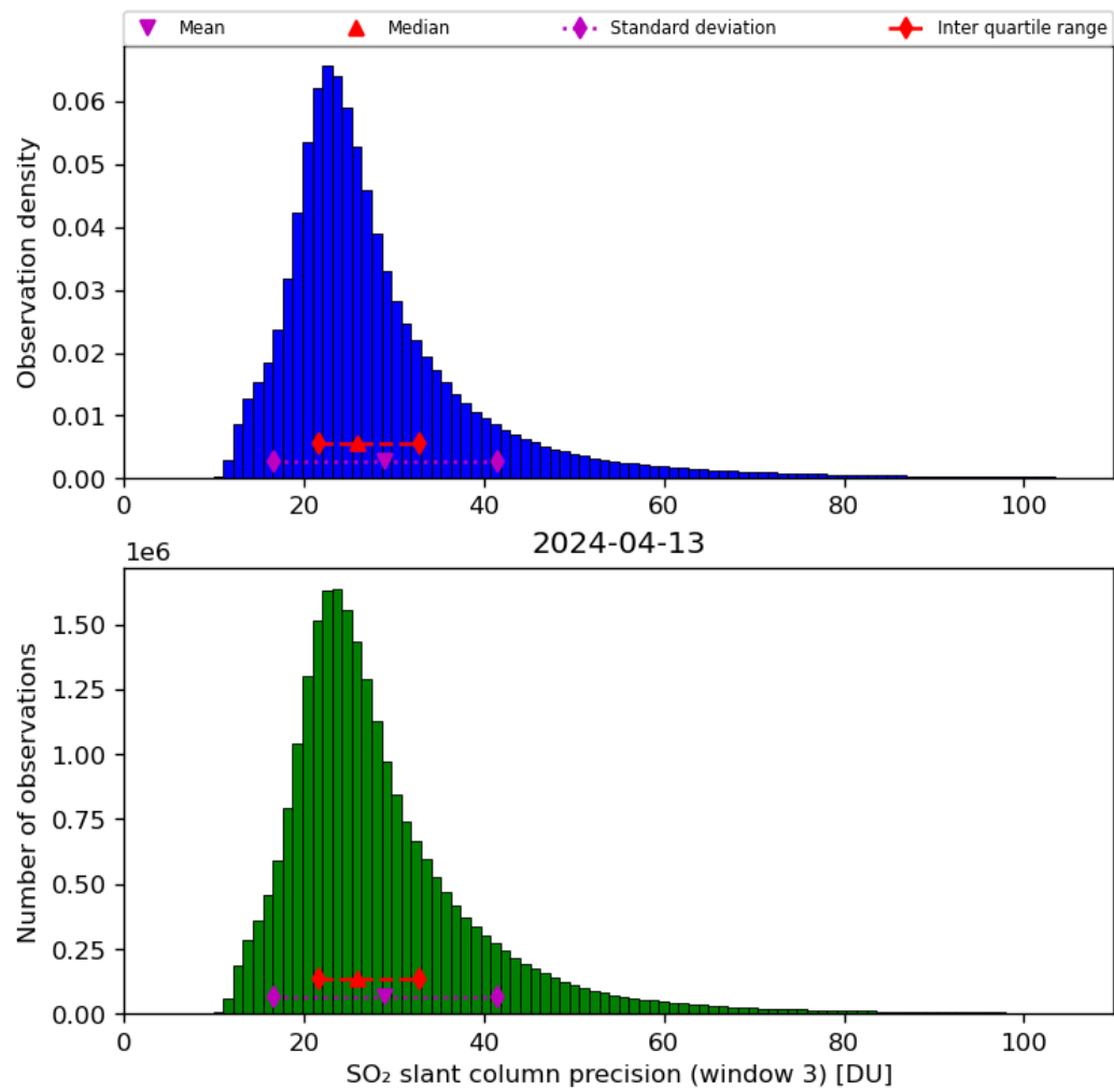
Figure 65: Histogram of “SO 2 slant column precision (window 3)” for 2024-04-12 to 2024-04-14
