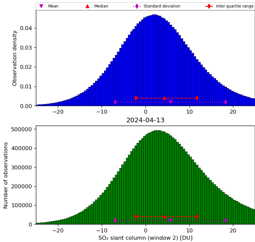
Figure 60: Histogram of “SO 2 slant column (window 2)” for 2024-04-12 to 2024-04-14
