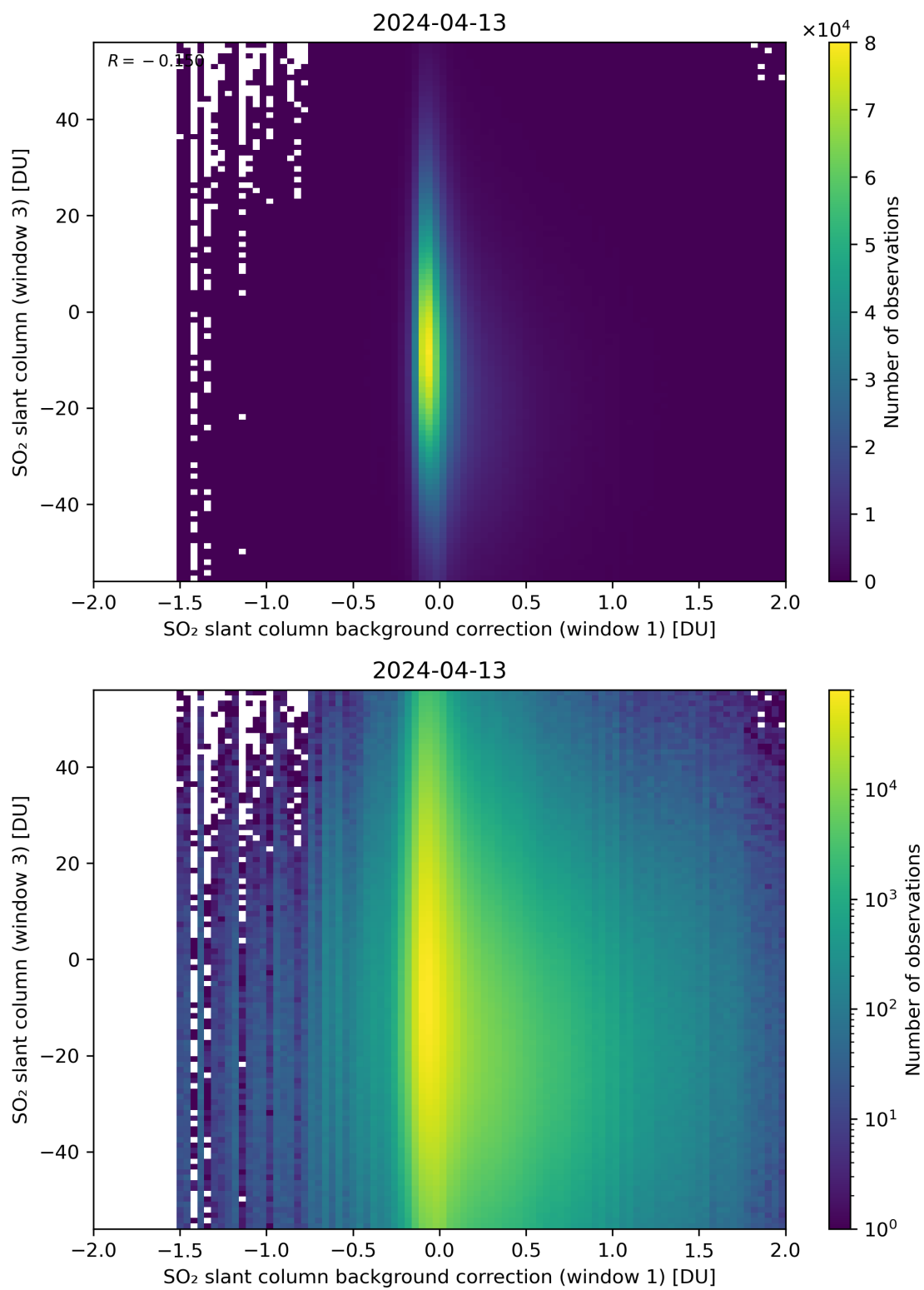
Figure 107: Scatter density plot of “SO 2 slant column background correction (window 1)” against “SO 2 slant column (window 3)” for 2024-04-12 to 2024-04-14.
