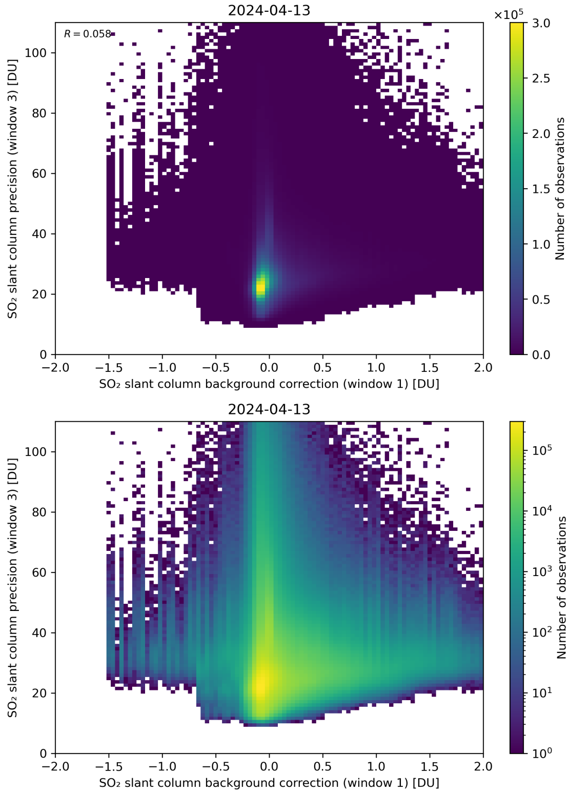
Figure 108: Scatter density plot of “SO 2 slant column background correction (window 1)” against “SO 2 slant column precision (window 3)” for 2024-04-12 to 2024-04-14.
