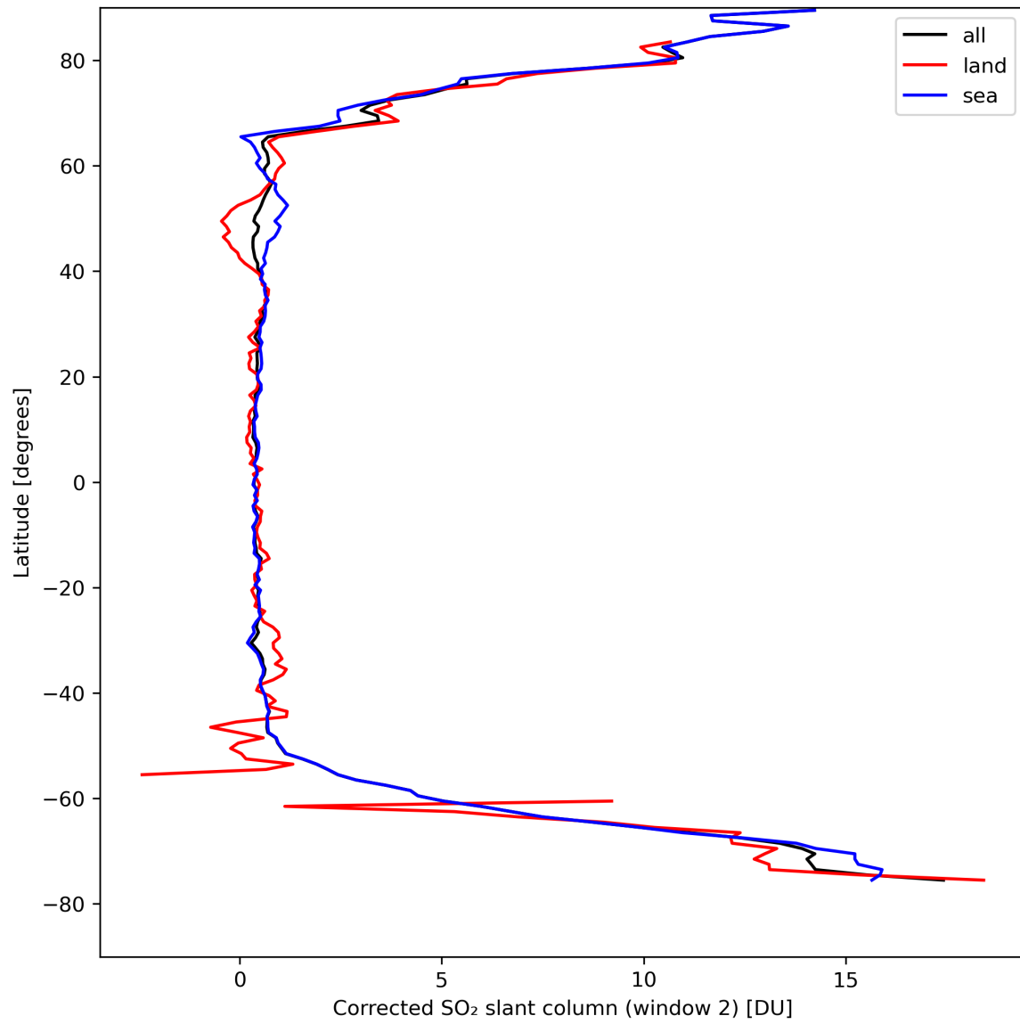
Figure 39: Zonal average of “Corrected SO 2 slant column (window 2)” for 2024-04-12 to 2024-04-14.
