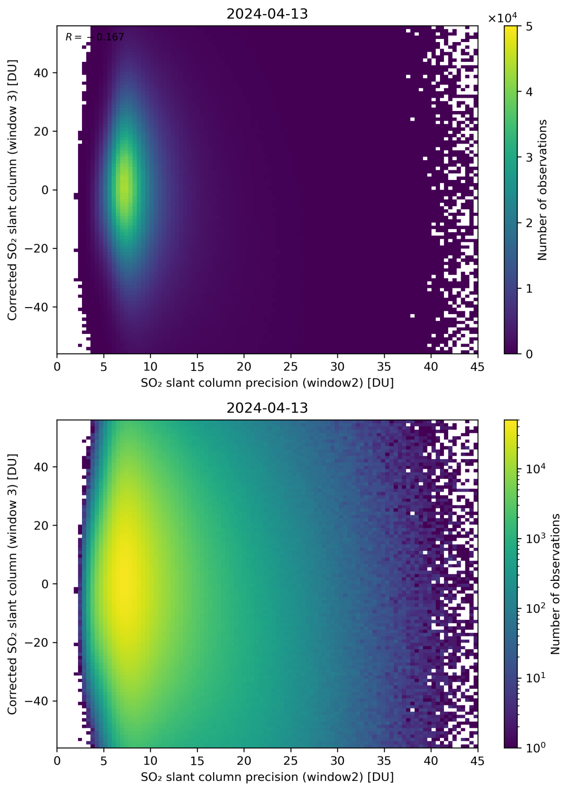
Figure 248: Scatter density plot of “SO 2 slant column precision (window2)” against “Corrected SO 2 slant column (window 3)” for 2024-04-12 to 2024-04-14.
