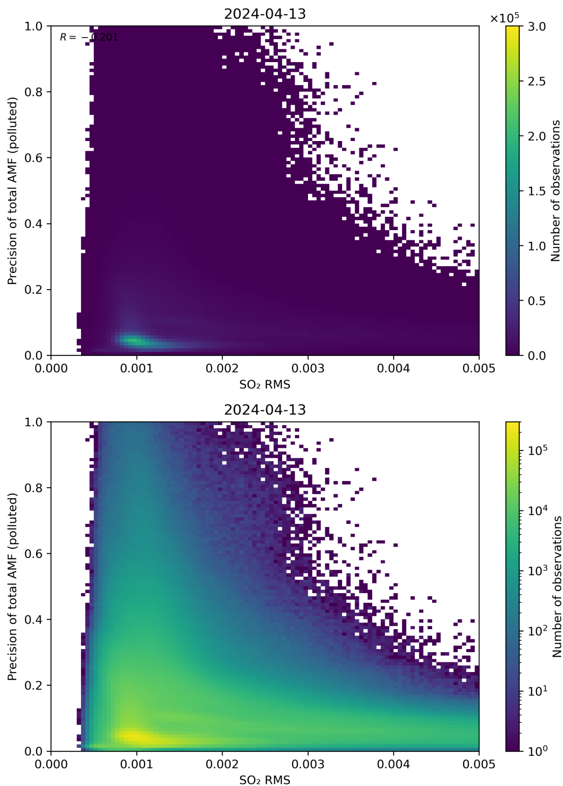
Figure 138: Scatter density plot of “SO 2 RMS” against “Precision of total AMF (polluted)” for 2024-04-12 to 2024-04-14.
