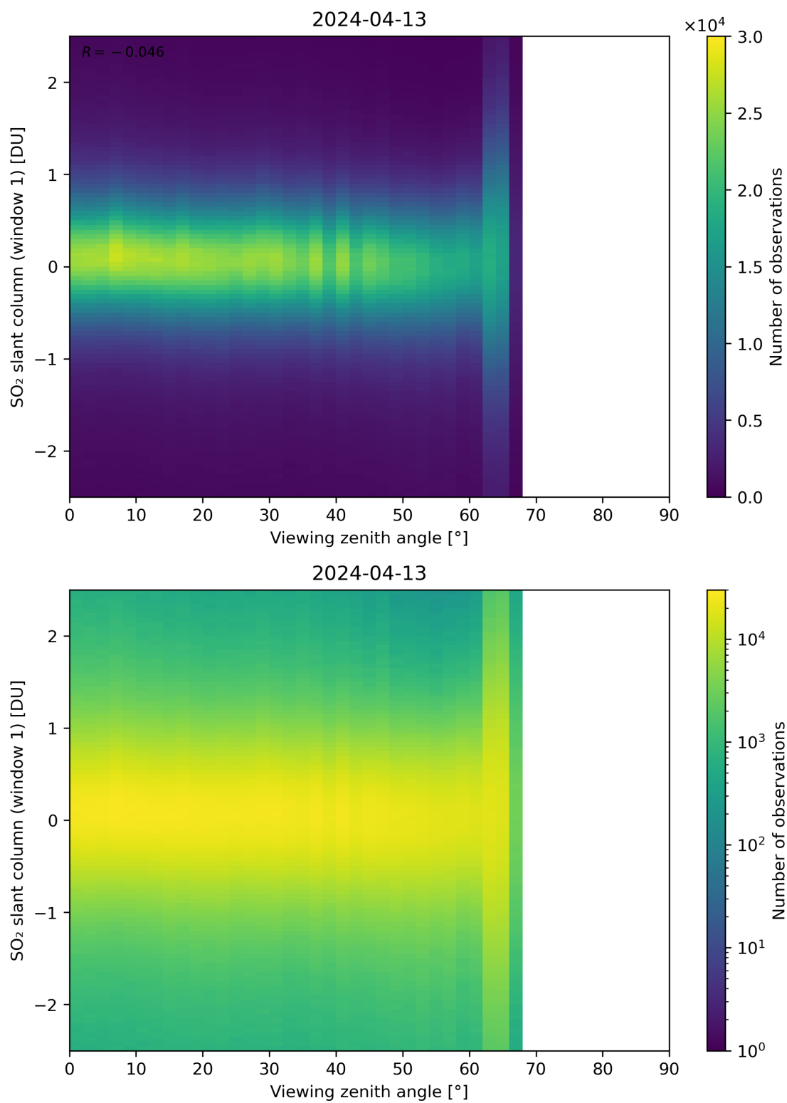
Figure 320: Scatter density plot of “Viewing zenith angle” against “SO 2 slant column (window 1)” for 2024-04-12 to 2024-04-14.
