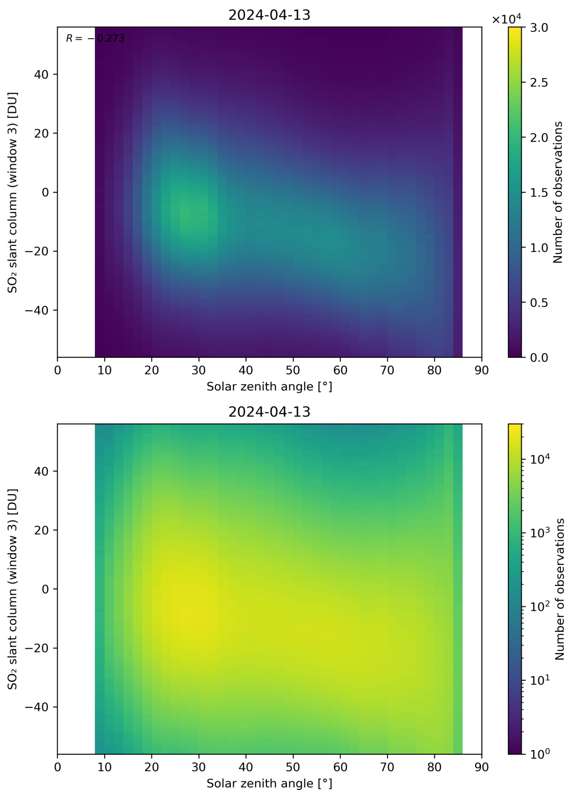
Figure 172: Scatter density plot of “Solar zenith angle” against “SO 2 slant column (window 3)” for 2024-04-12 to 2024-04-14.
