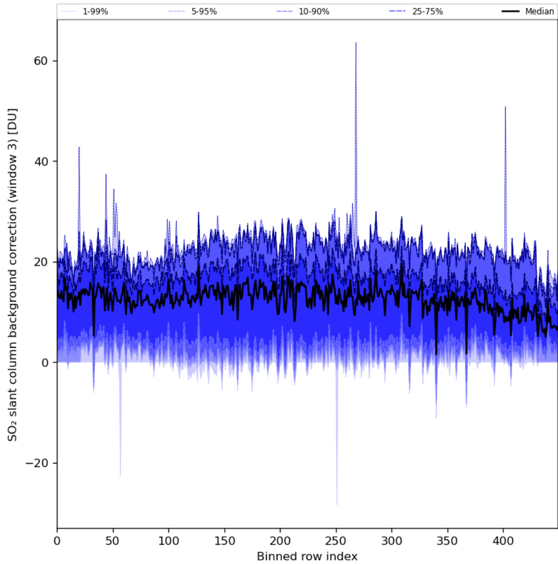
Figure 90: Along track statistics of “SO 2 slant column background correction (window 3)” for 2024-04-12 to 2024-04-14
