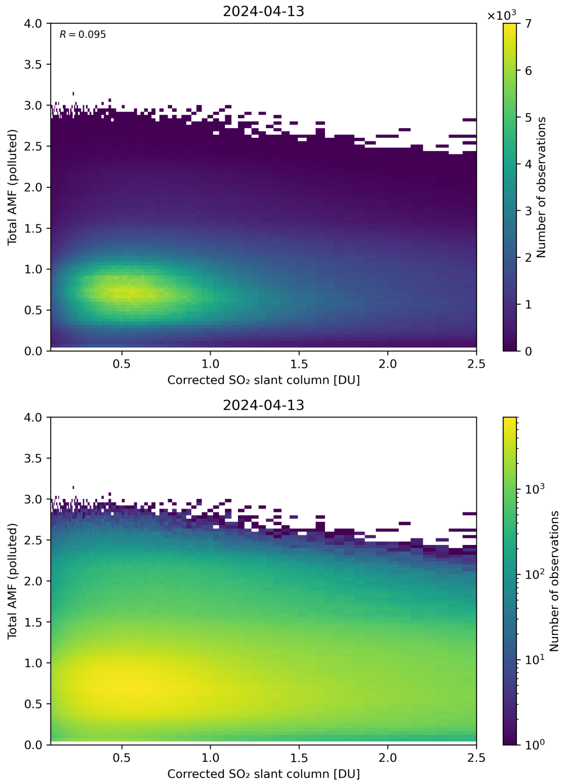
Figure 192: Scatter density plot of “Corrected SO 2 slant column” against “Total AMF (polluted)” for 2024-04-12 to 2024-04-14.
