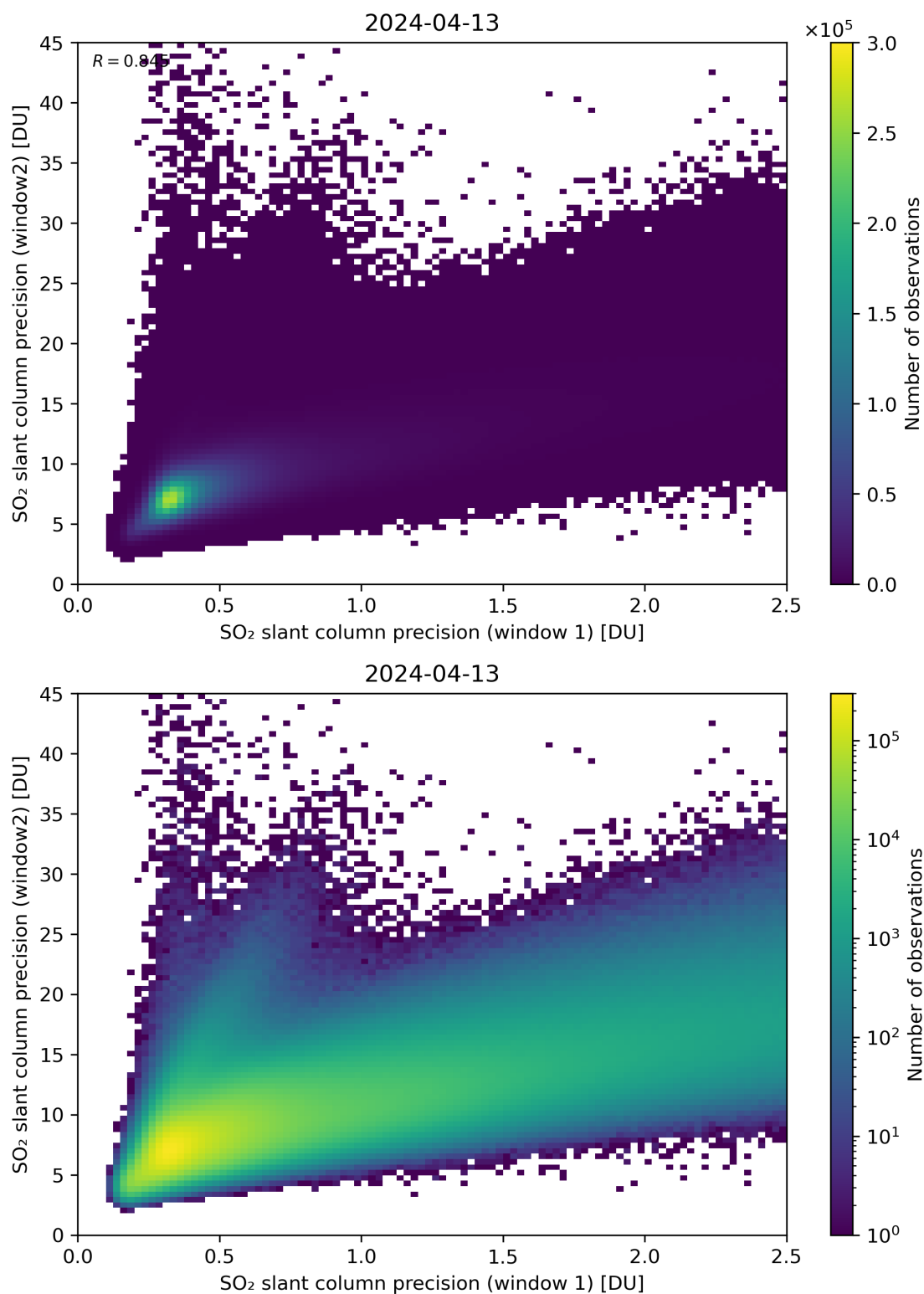
Figure 227: Scatter density plot of “SO 2 slant column precision (window 1)” against “SO 2 slant column precision (window 2)” for 2024-04-12 to 2024-04-14.
