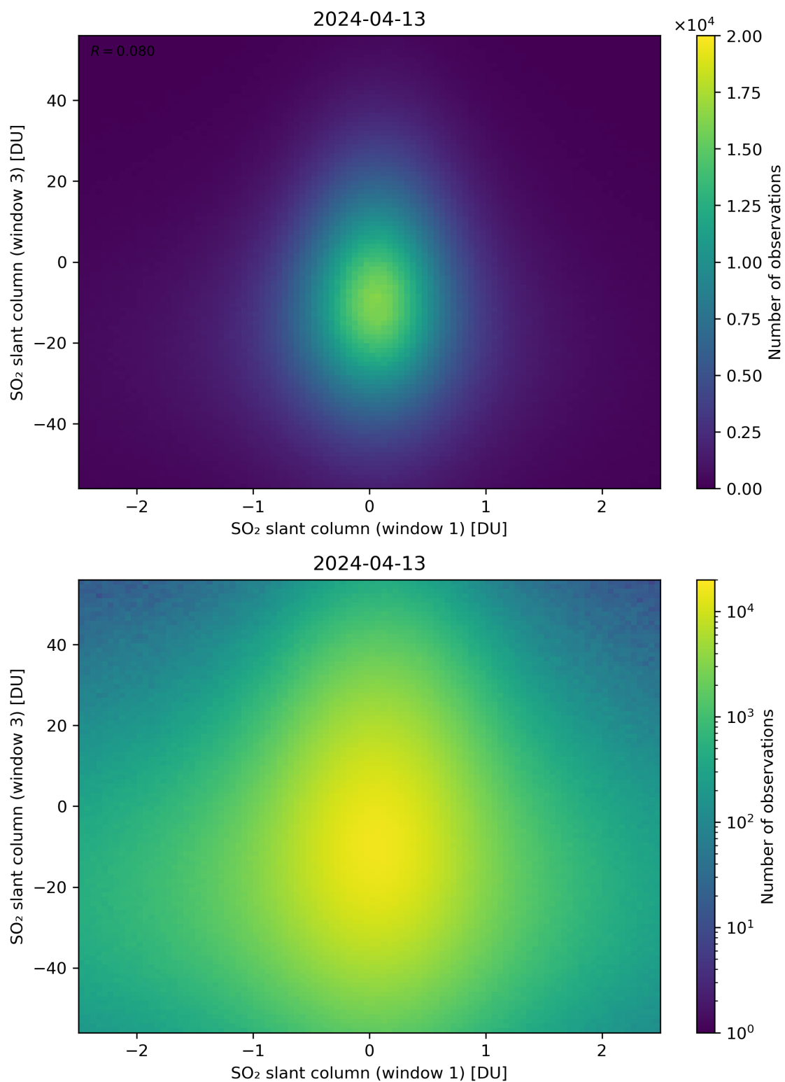
Figure 237: Scatter density plot of “SO 2 slant column (window 1)” against “SO 2 slant column (window 3)” for 2024-04-12 to 2024-04-14.
