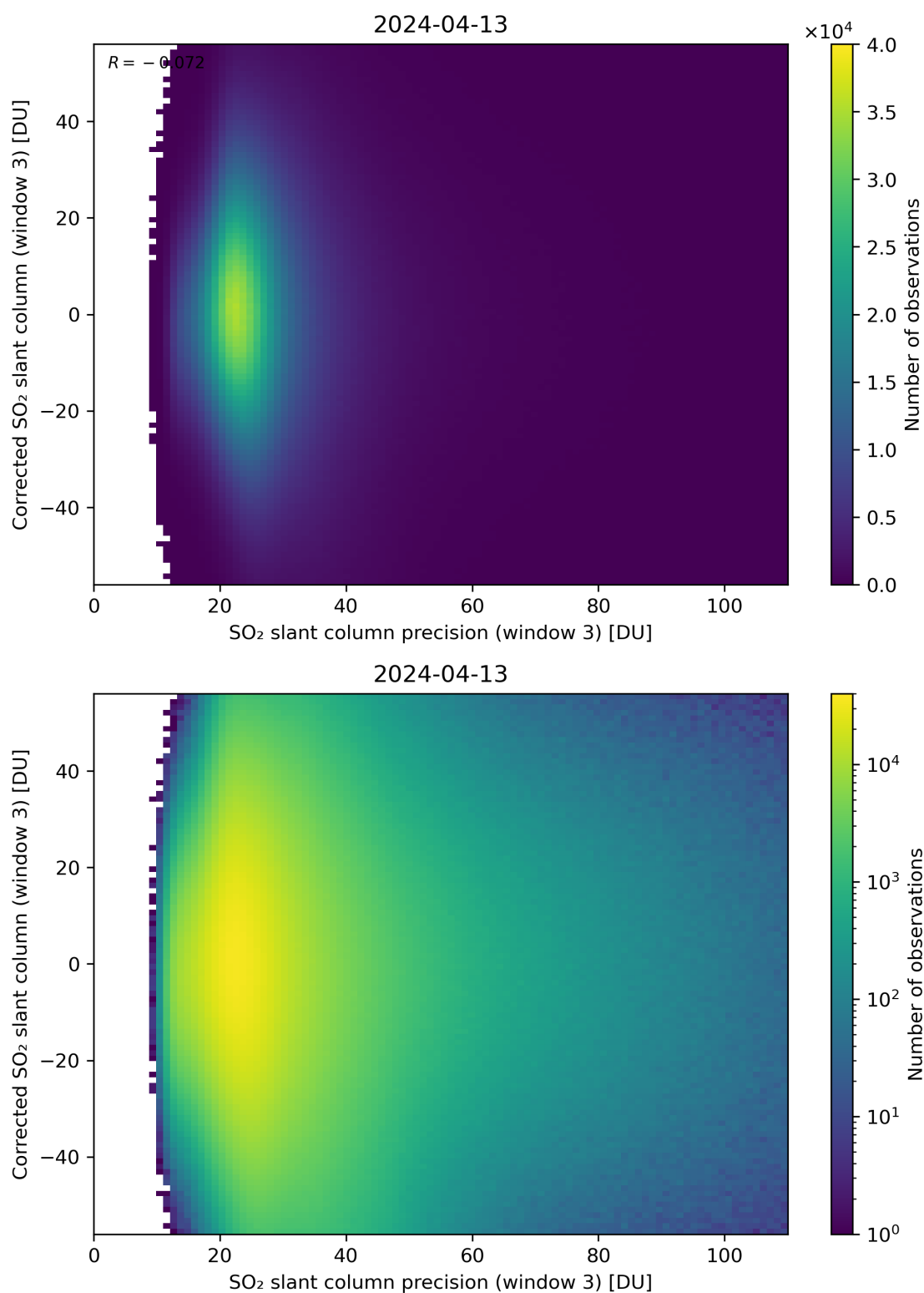
Figure 262: Scatter density plot of “SO 2 slant column precision (window 3)” against “Corrected SO 2 slant column (window 3)” for 2024-04-12 to 2024-04-14.
