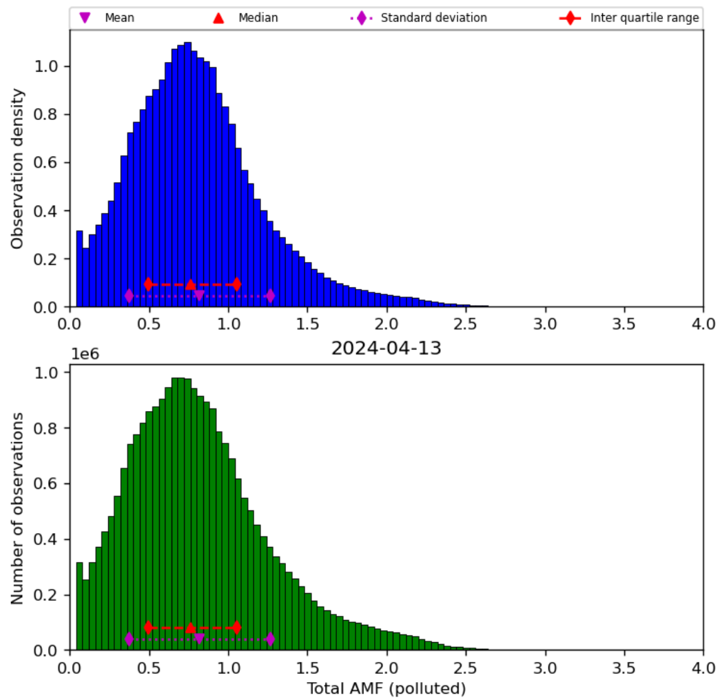
Figure 71: Histogram of “Total AMF (polluted)” for 2024-04-12 to 2024-04-14
