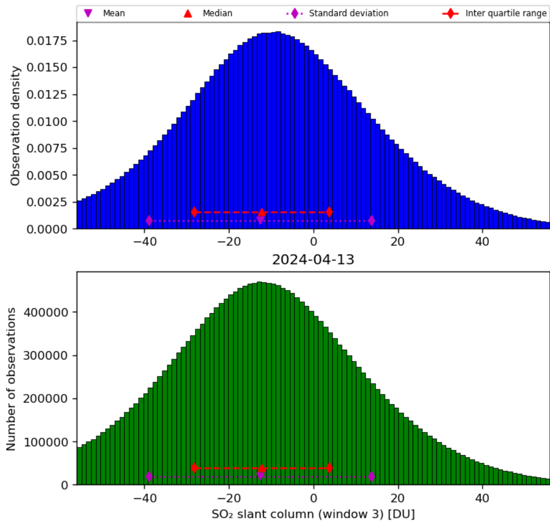
Figure 64: Histogram of “SO 2 slant column (window 3)” for 2024-04-12 to 2024-04-14
