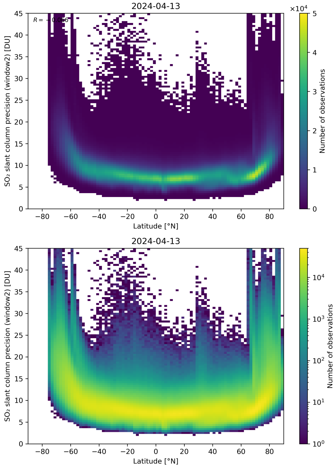
Figure 151: Scatter density plot of “Latitude” against “SO 2 slant column precision (window2)” for 2024-04-12 to 2024-04-14.
