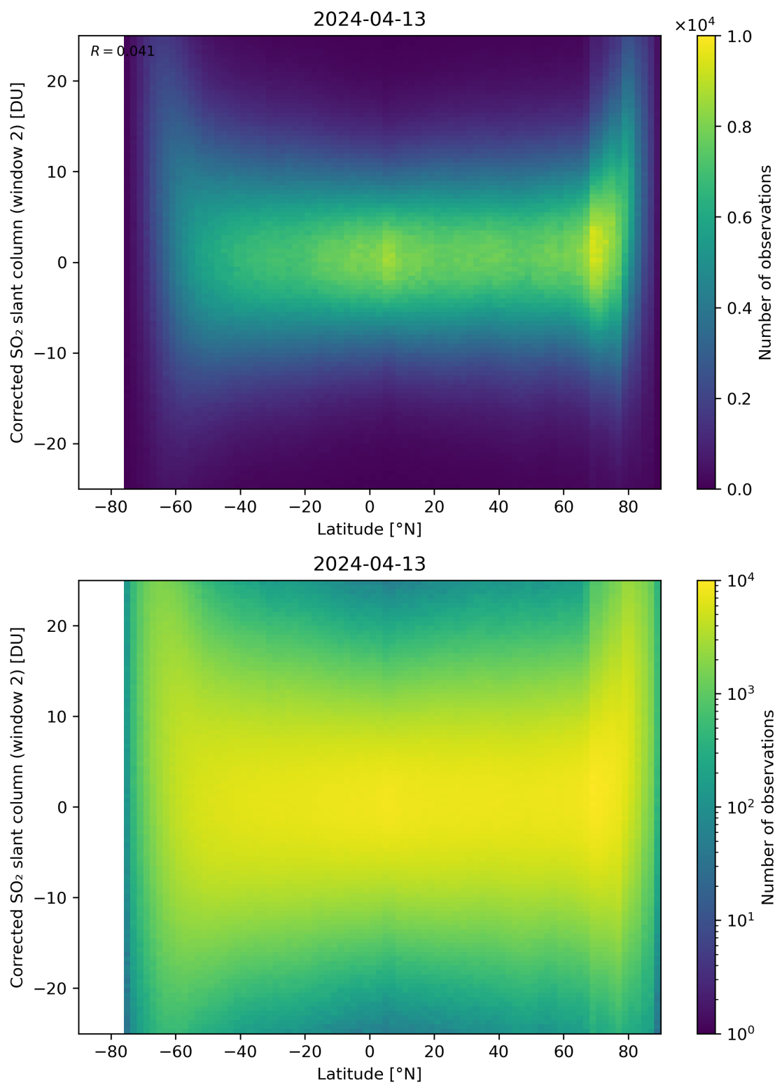
Figure 147: Scatter density plot of “Latitude” against “Corrected SO 2 slant column (window 2)” for 2024-04-12 to 2024-04-14.
