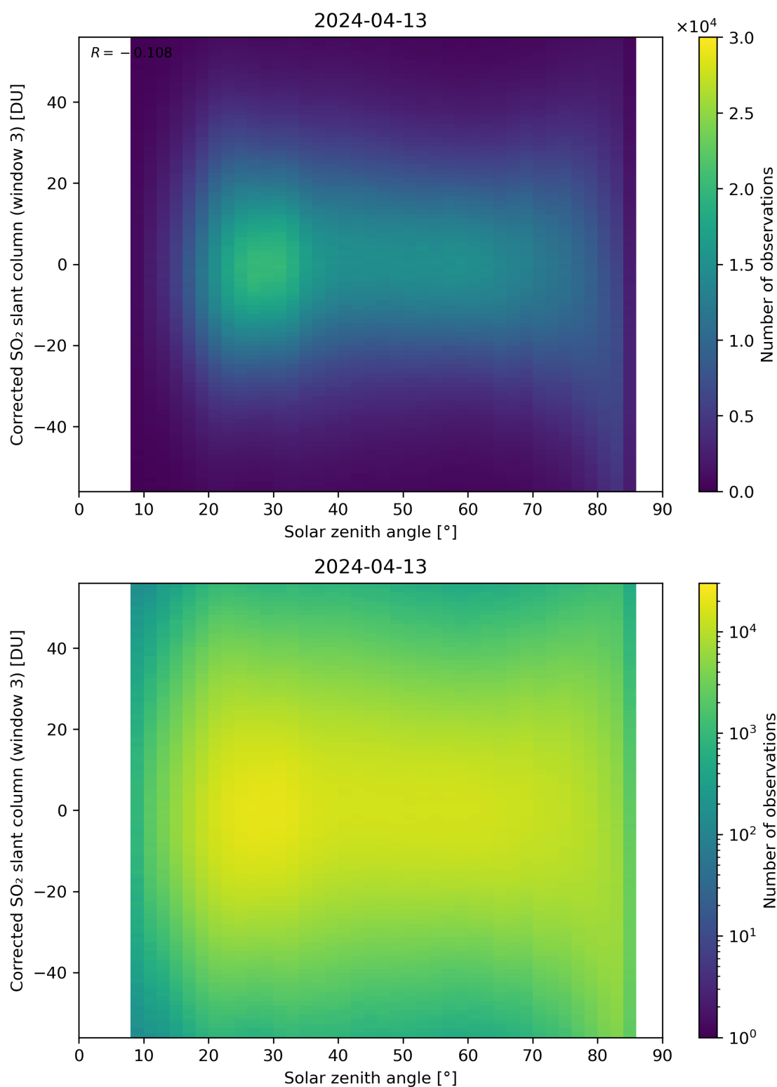
Figure 168: Scatter density plot of “Solar zenith angle” against “Corrected SO 2 slant column (window 3)” for 2024-04-12 to 2024-04-14.
