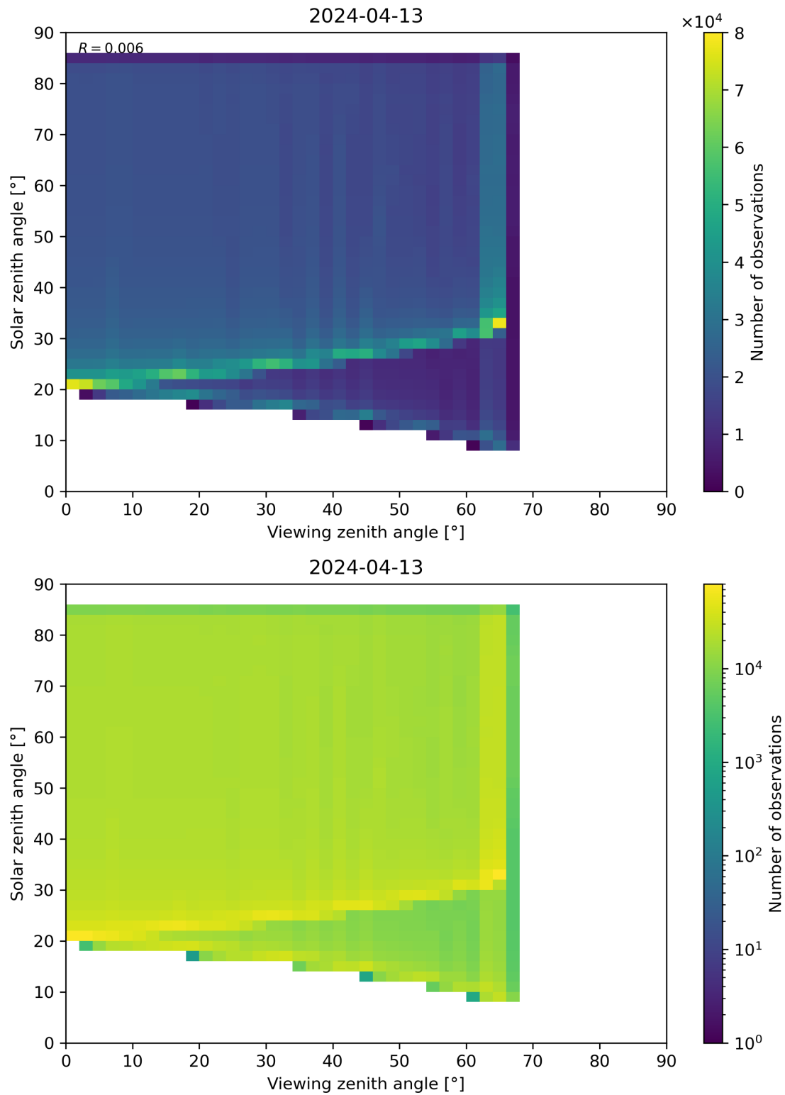
Figure 315: Scatter density plot of “Viewing zenith angle” against “Solar zenith angle” for 2024-04-12 to 2024-04-14.
