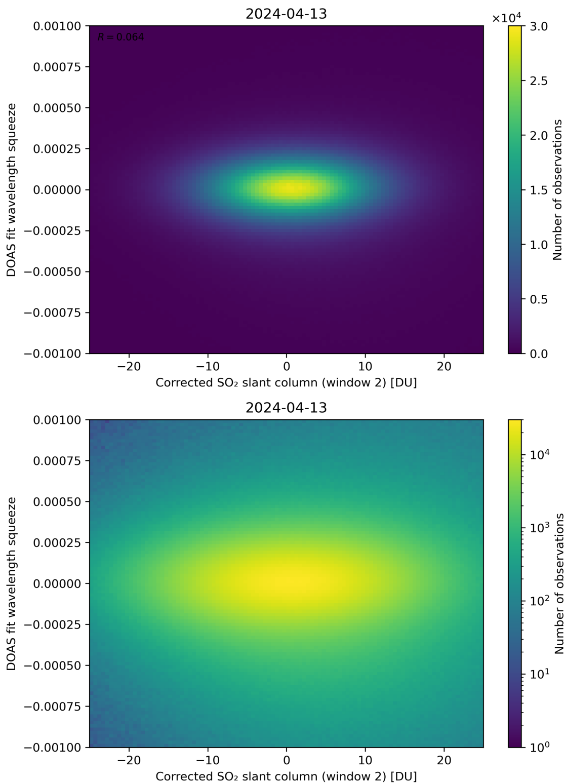
Figure 197: Scatter density plot of “Corrected SO 2 slant column (window 2)” against “DOAS fit wavelength squeeze” for 2024-04-12 to 2024-04-14.
