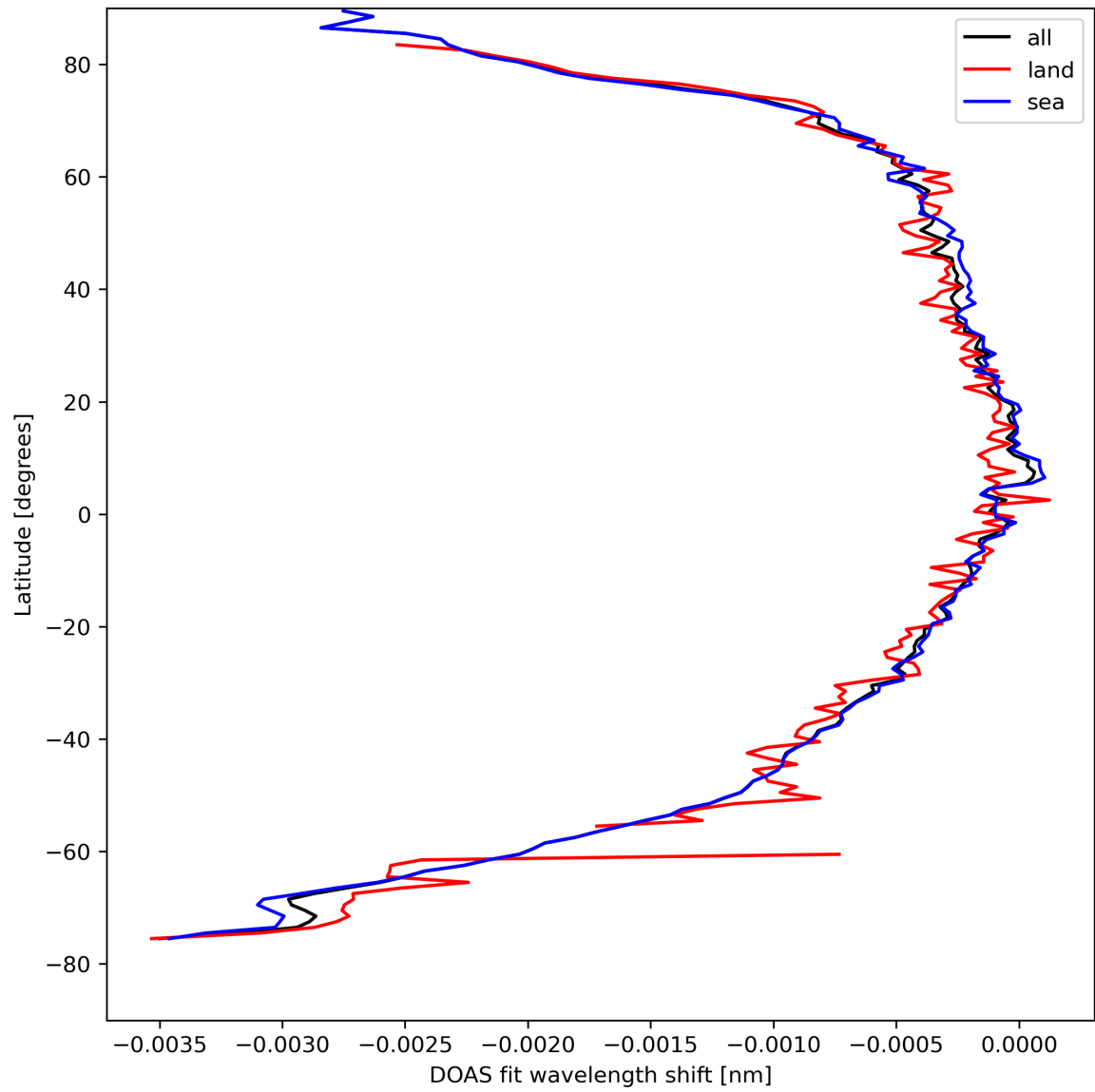
Figure 45: Zonal average of “DOAS fit wavelength shift” for 2024-04-12 to 2024-04-14.
