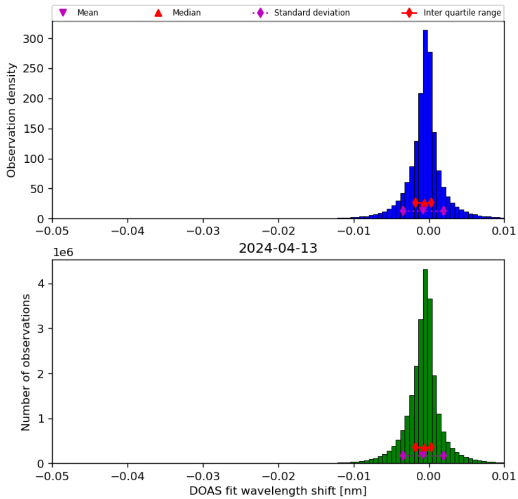
Figure 68: Histogram of “DOAS fit wavelength shift” for 2024-04-12 to 2024-04-14
