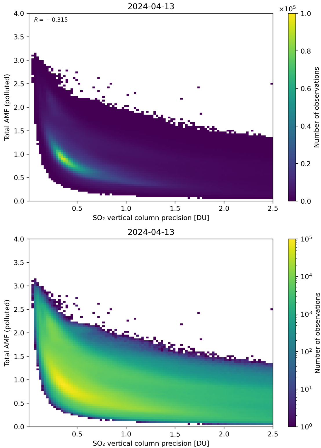
Figure 294: Scatter density plot of “SO 2 vertical column precision” against “Total AMF (polluted)” for 2024-04-12 to 2024-04-14.
