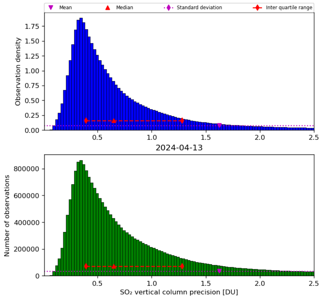
Figure 54: Histogram of “SO 2 vertical column precision” for 2024-04-12 to 2024-04-14
