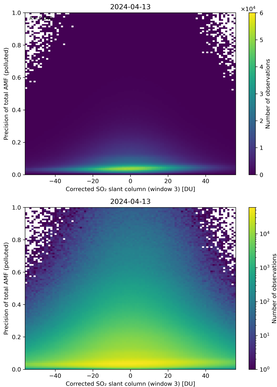
Figure 211: Scatter density plot of “Corrected SO 2 slant column (window 3)” against “Precision of total AMF (polluted)” for 2024-04-12 to 2024-04-14.
