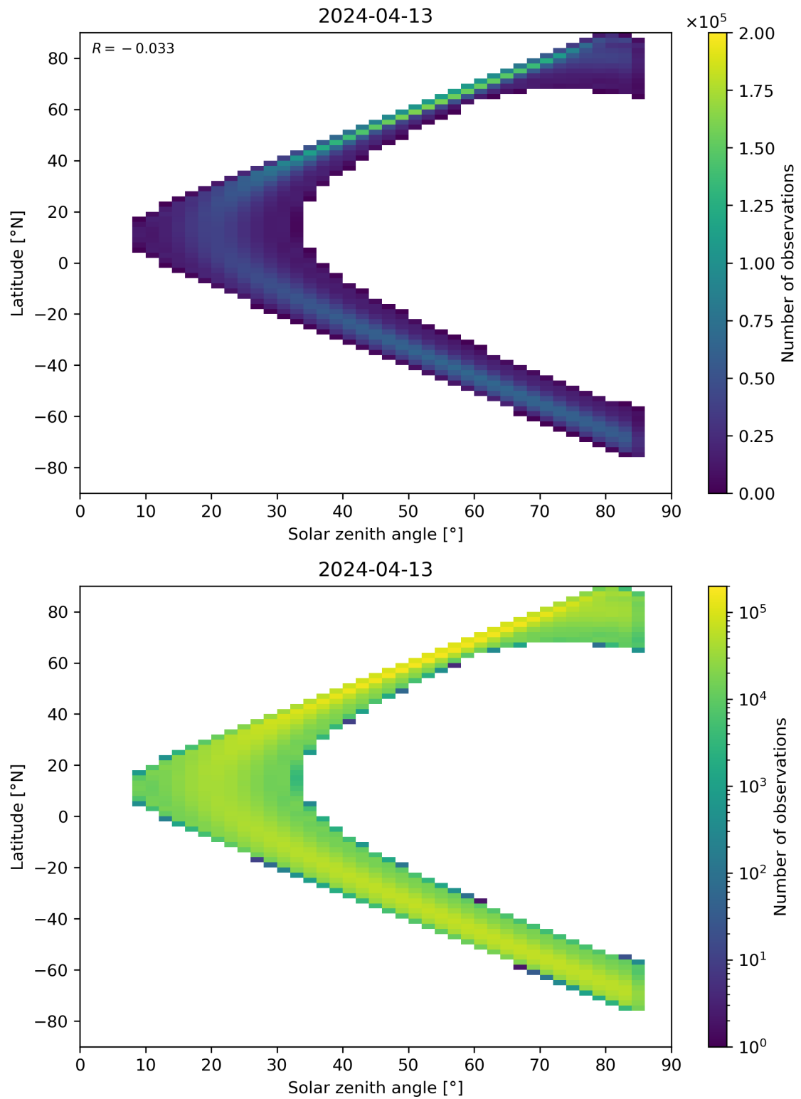
Figure 164: Scatter density plot of “Solar zenith angle” against “Latitude” for 2024-04-12 to 2024-04-14.
