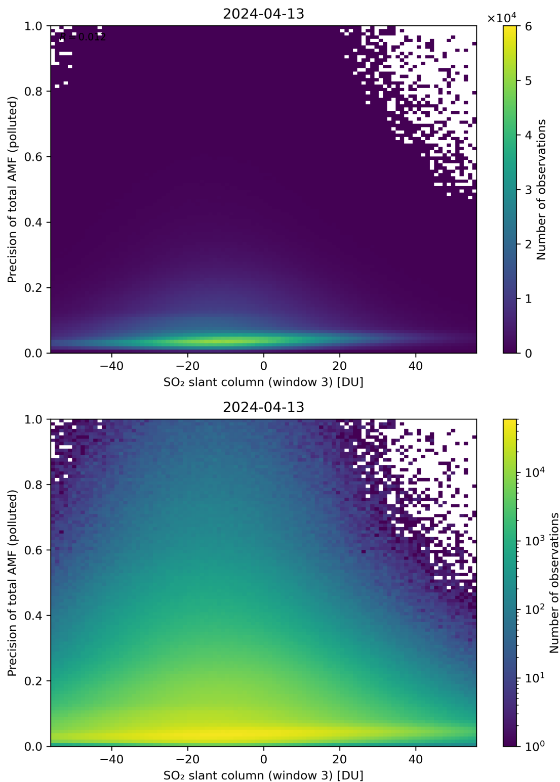
Figure 269: Scatter density plot of “SO 2 slant column (window 3)” against “Precision of total AMF (polluted)” for 2024-04-12 to 2024-04-14.
