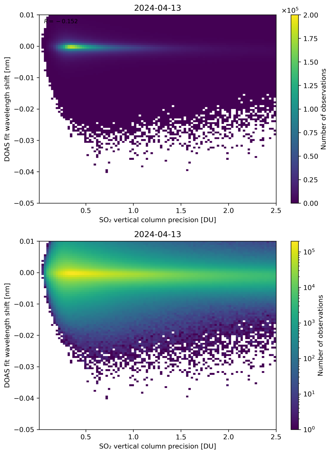
Figure 282: Scatter density plot of “SO 2 vertical column precision” against “DOAS fit wavelength shift” for 2024-04-12 to 2024-04-14.
