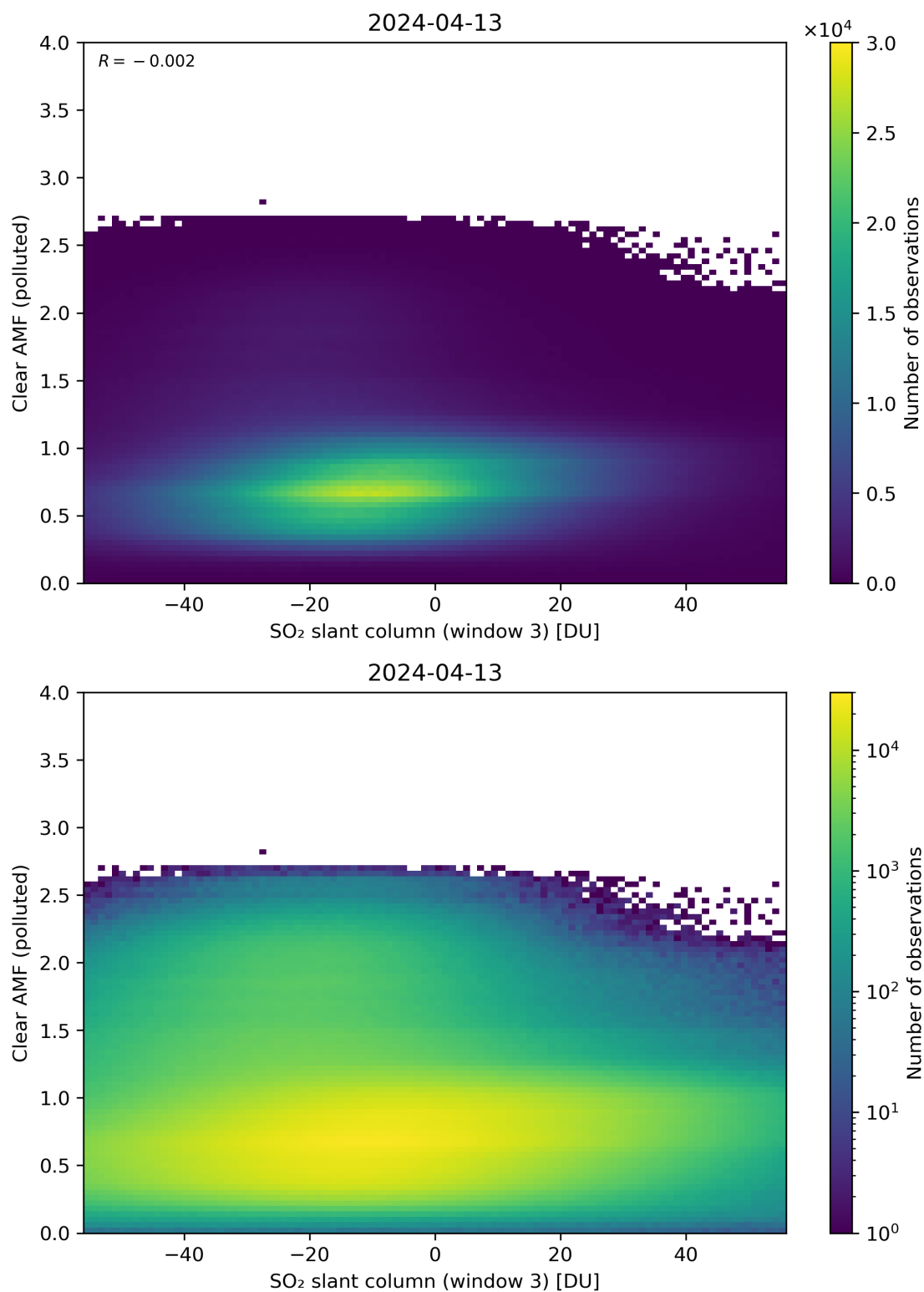
Figure 265: Scatter density plot of “SO 2 slant column (window 3)” against “Clear AMF (polluted)” for 2024-04-12 to 2024-04-14.
