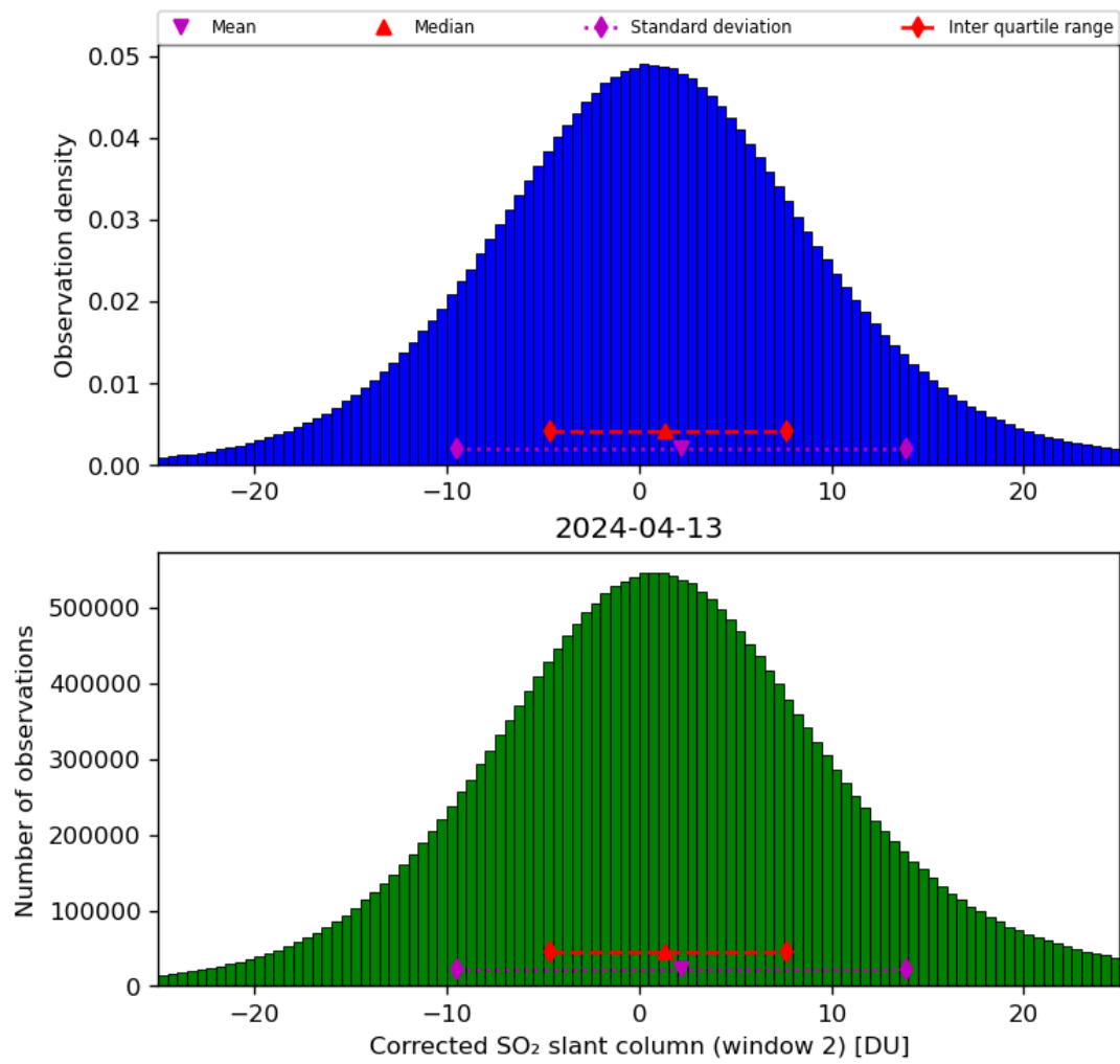
Figure 62: Histogram of “Corrected SO 2 slant column (window 2)” for 2024-04-12 to 2024-04-14
