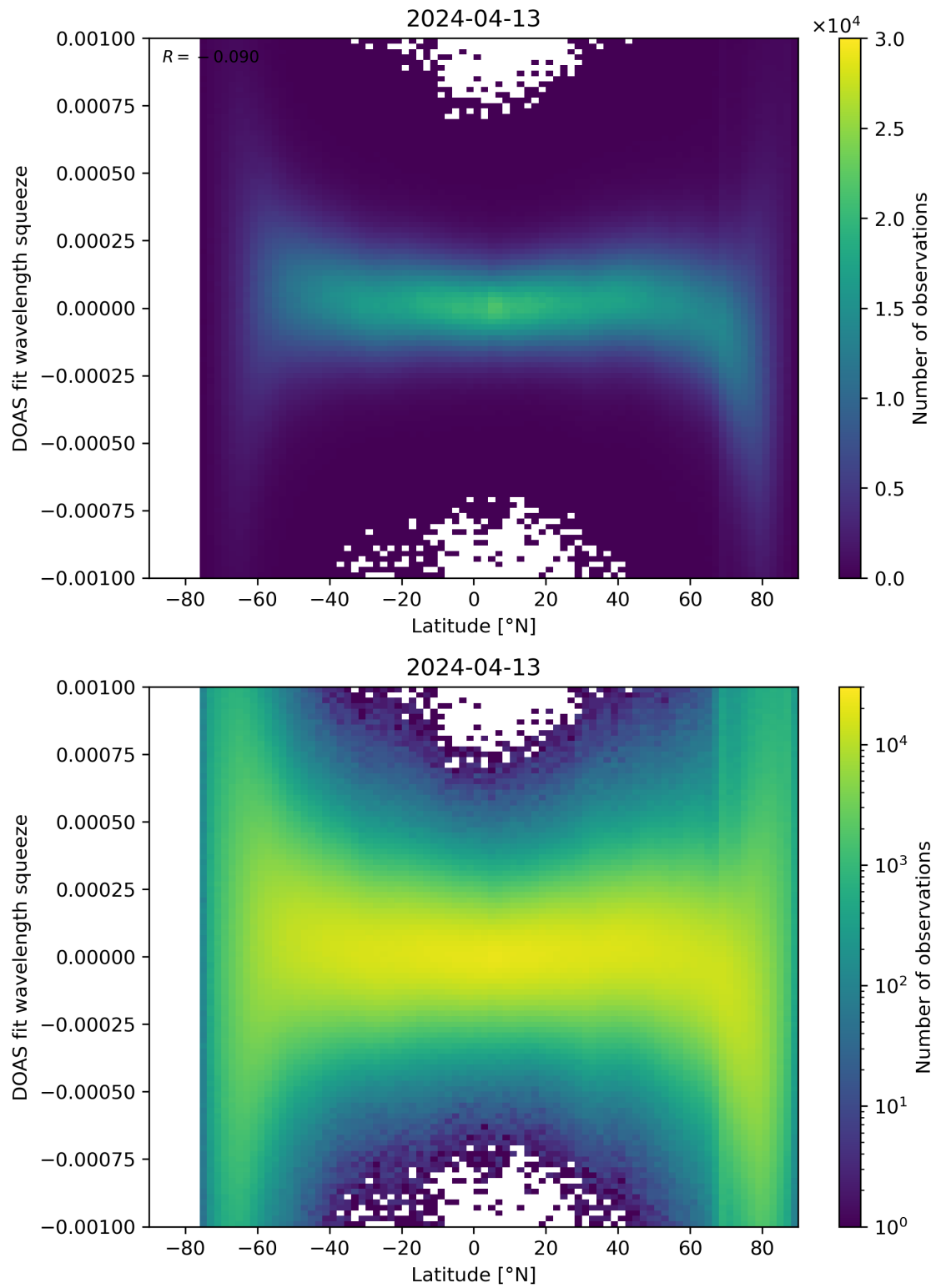
Figure 143: Scatter density plot of “Latitude” against “DOAS fit wavelength squeeze” for 2024-04-12 to 2024-04-14.
