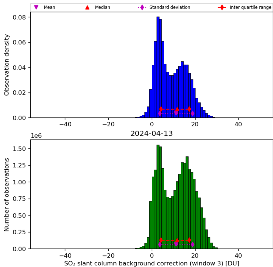
Figure 67: Histogram of “SO 2 slant column background correction (window 3)” for 2024-04-12 to 2024-04-14
