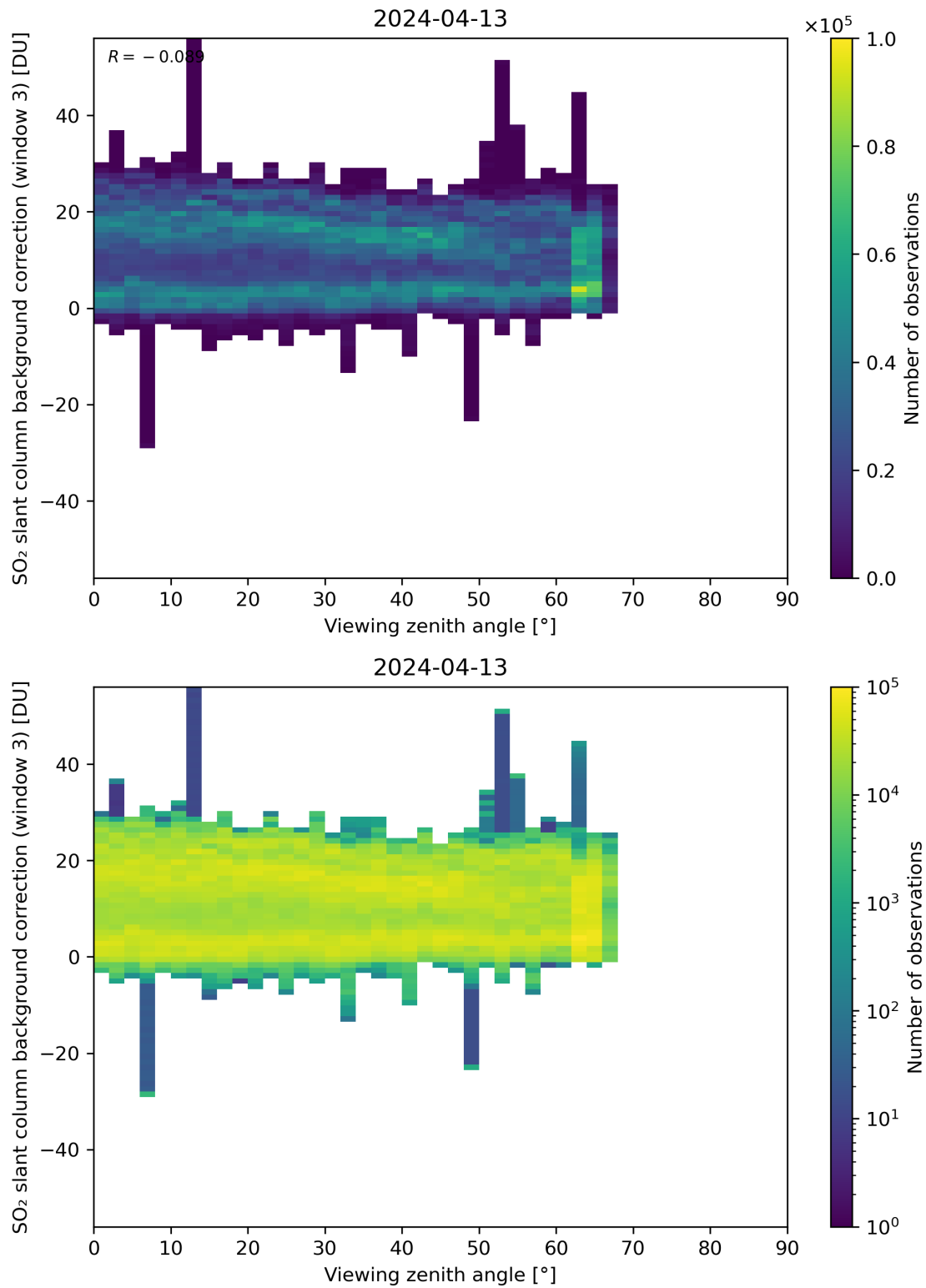
Figure 310: Scatter density plot of “Viewing zenith angle” against “SO 2 slant column background correction (window 3)” for 2024-04-12 to 2024-04-14.
