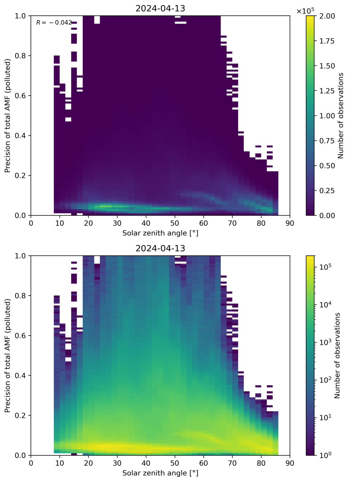
Figure 175: Scatter density plot of “Solar zenith angle” against “Precision of total AMF (polluted)” for 2024-04-12 to 2024-04-14.
