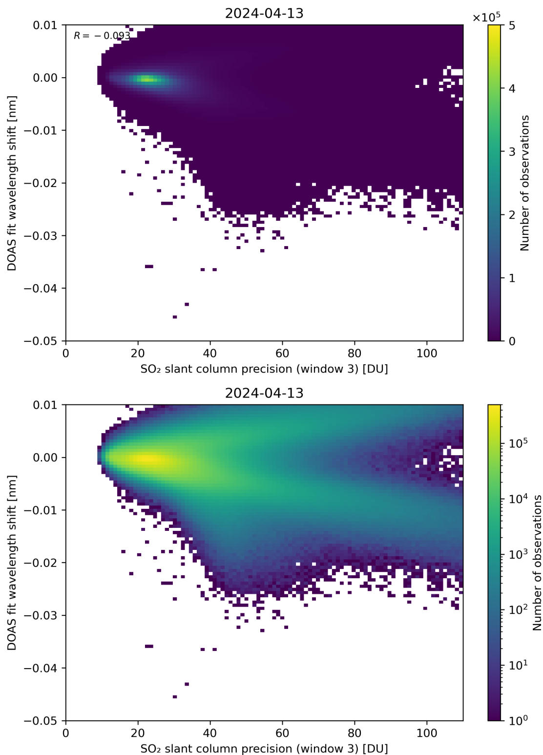
Figure 258: Scatter density plot of “SO 2 slant column precision (window 3)” against “DOAS fit wavelength shift” for 2024-04-12 to 2024-04-14.
