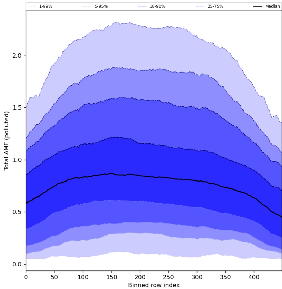
Figure 94: Along track statistics of “Total AMF (polluted)” for 2024-04-12 to 2024-04-14
