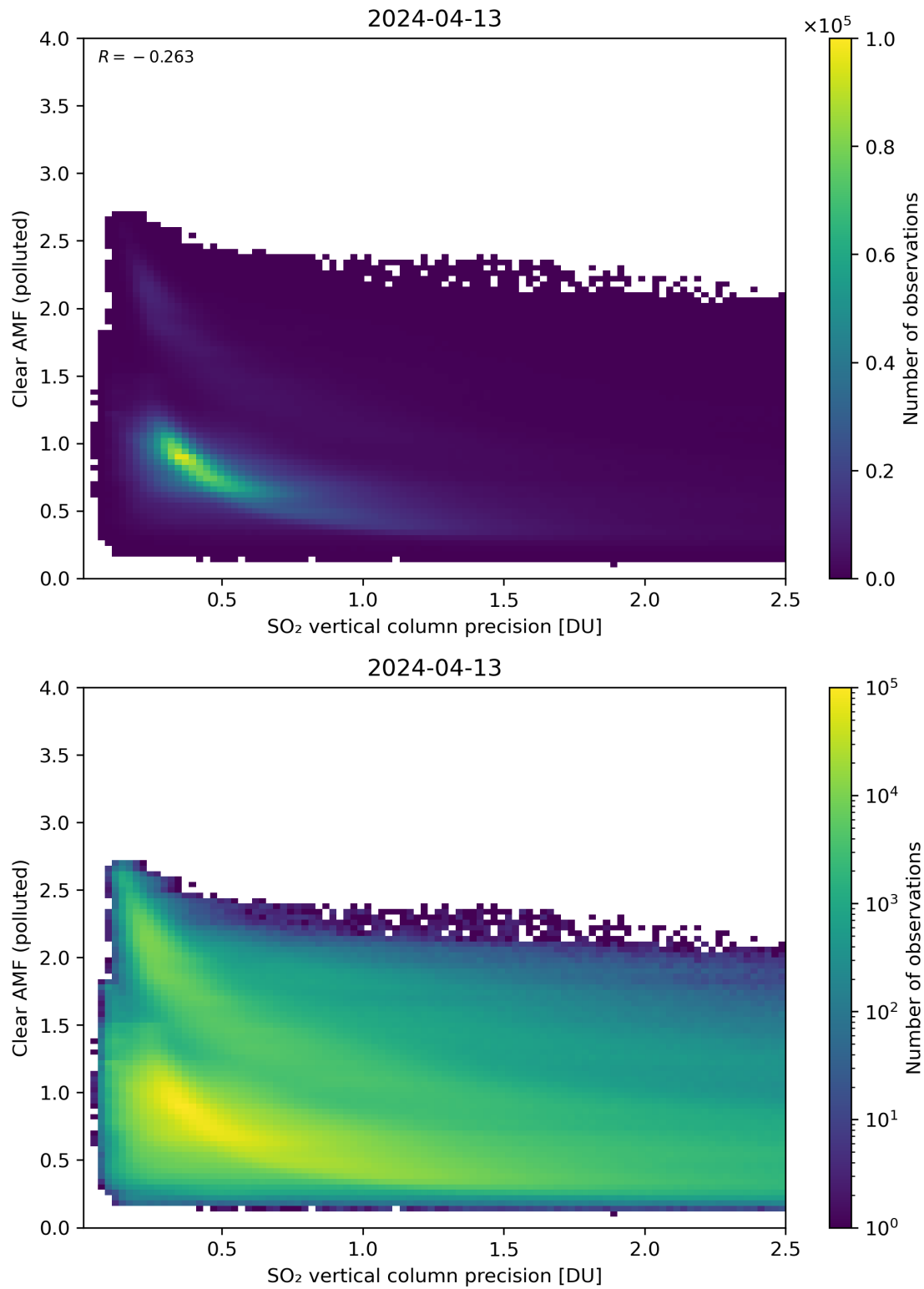
Figure 285: Scatter density plot of “SO 2 vertical column precision” against “Clear AMF (polluted)” for 2024-04-12 to 2024-04-14.
