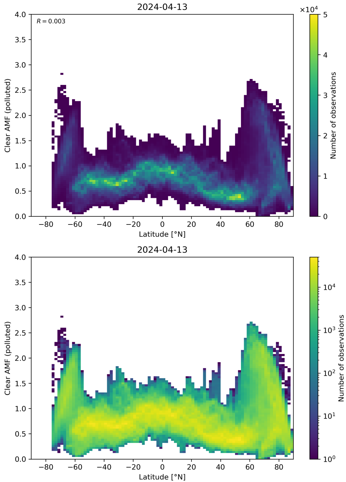
Figure 145: Scatter density plot of “Latitude” against “Clear AMF (polluted)” for 2024-04-12 to 2024-04-14.
