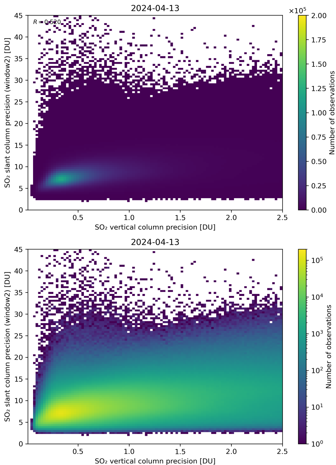
Figure 291: Scatter density plot of “SO 2 vertical column precision” against “SO 2 slant column precision (window2)” for 2024-04-12 to 2024-04-14.
