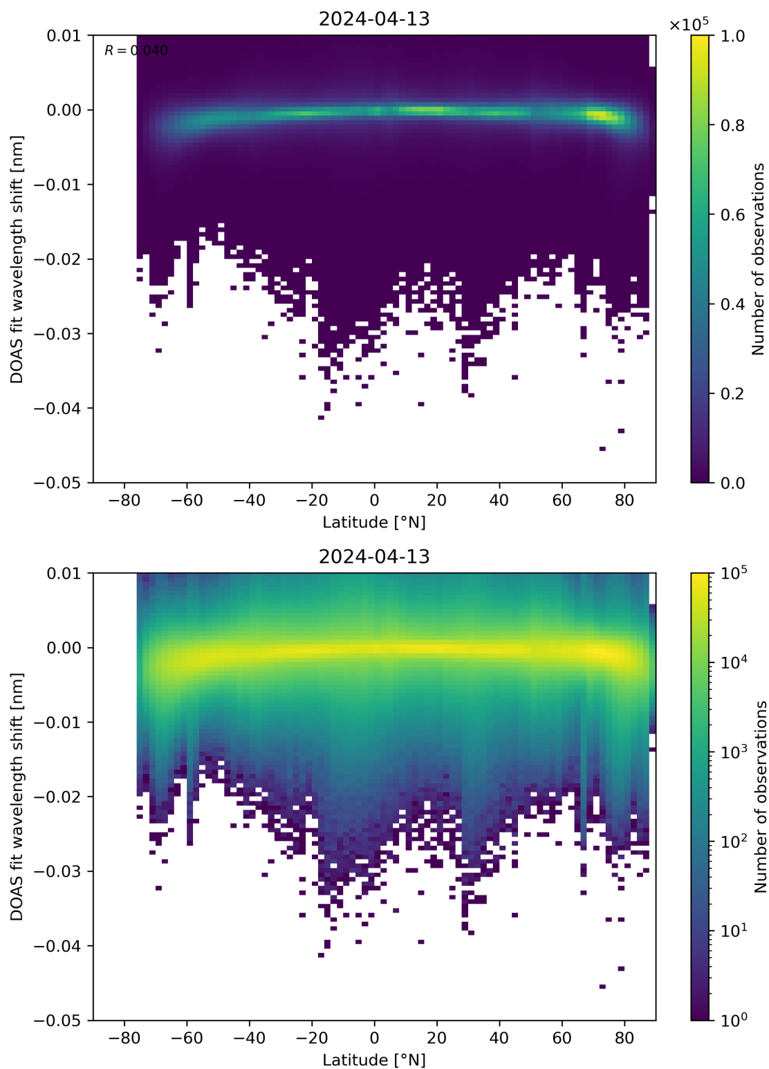
Figure 142: Scatter density plot of “Latitude” against “DOAS fit wavelength shift” for 2024-04-12 to 2024-04-14.
