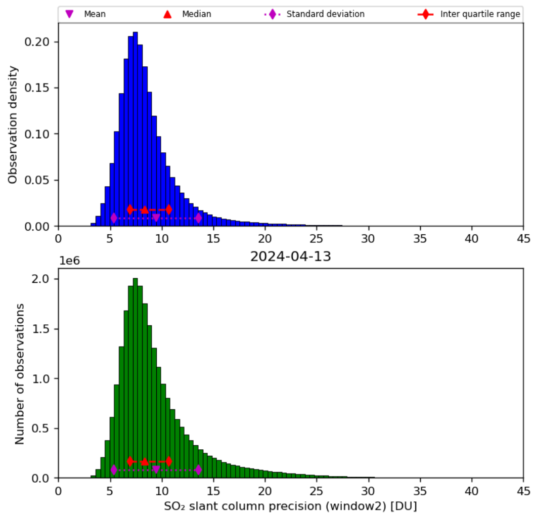
Figure 61: Histogram of “SO 2 slant column precision (window2)” for 2024-04-12 to 2024-04-14
