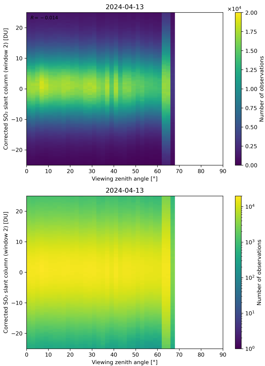
Figure 318: Scatter density plot of “Viewing zenith angle” against “Corrected SO 2 slant column (window 2)” for 2024-04-12 to 2024-04-14.
