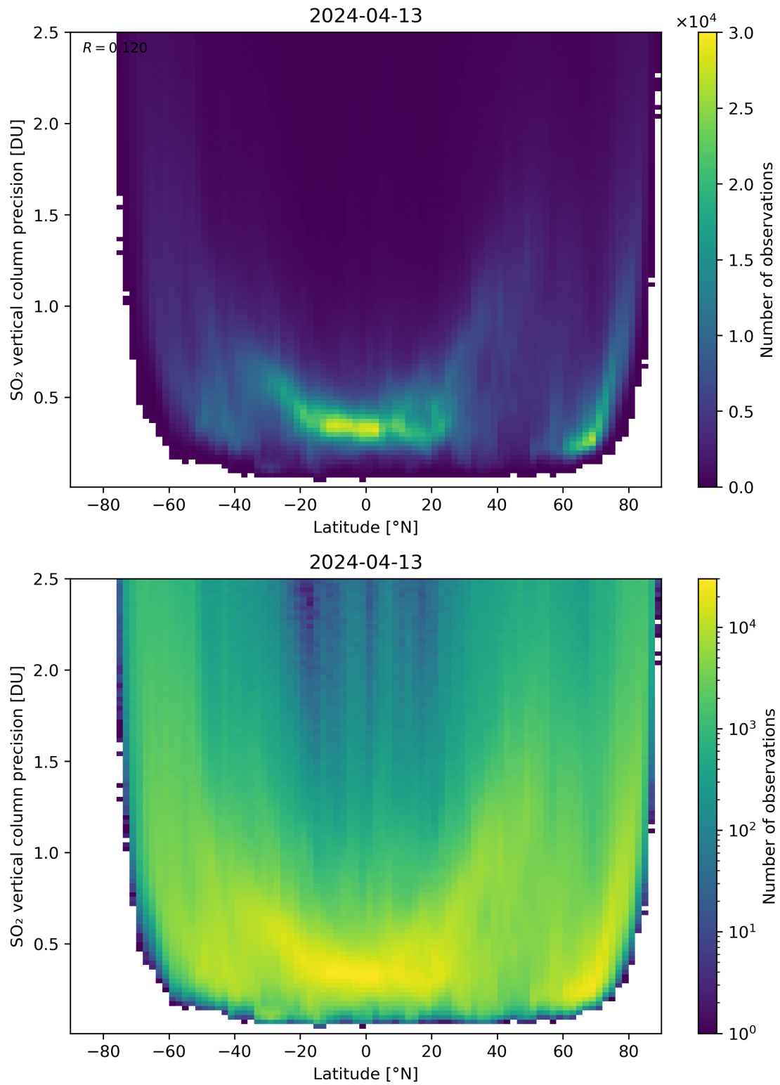
Figure 157: Scatter density plot of “Latitude” against “SO 2 vertical column precision” for 2024-04-12 to 2024-04-14.
