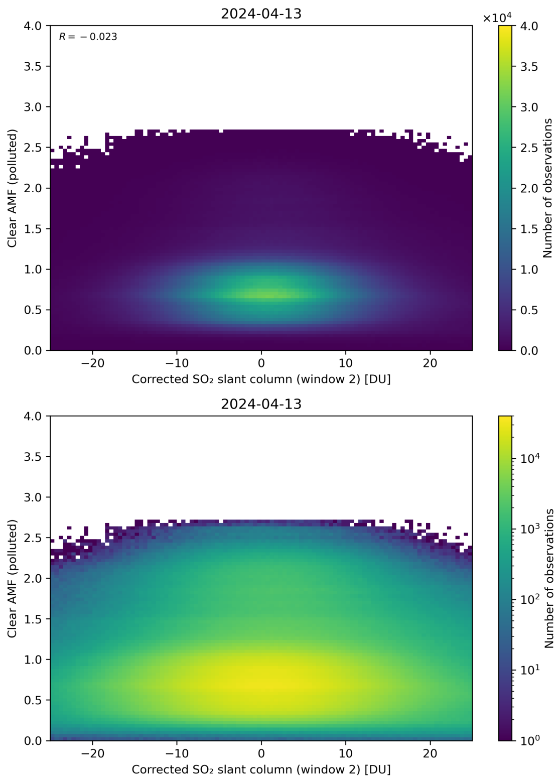
Figure 199: Scatter density plot of “Corrected SO 2 slant column (window 2)” against “Clear AMF (polluted)” for 2024-04-12 to 2024-04-14.
