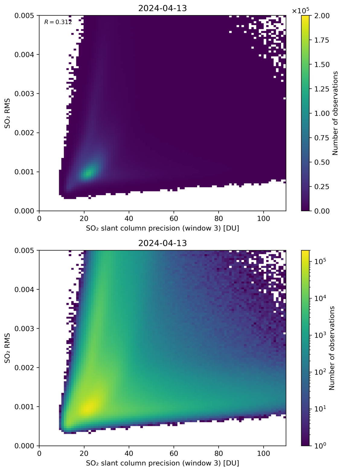
Figure 260: Scatter density plot of “SO 2 slant column precision (window 3)” against “SO 2 RMS” for 2024-04-12 to 2024-04-14.
