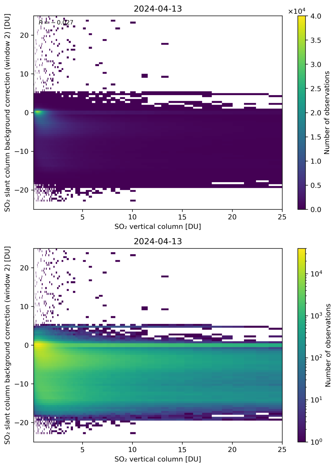
Figure 274: Scatter density plot of “SO 2 vertical column” against “SO 2 slant column background correction (window 2)” for 2024-04-12 to 2024-04-14.
