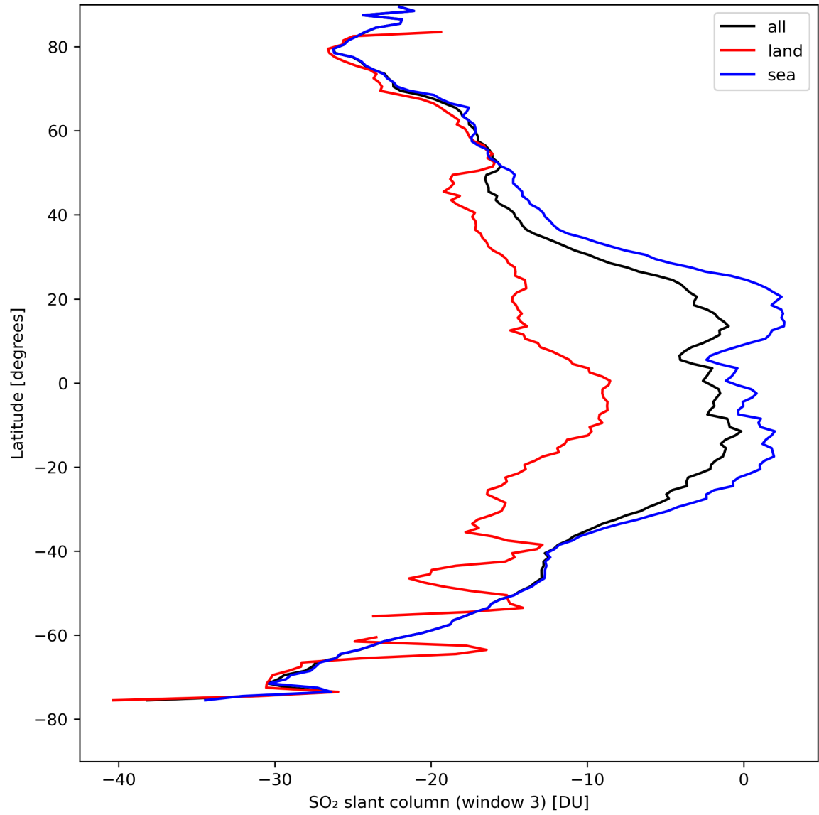
Figure 41: Zonal average of “SO 2 slant column (window 3)” for 2024-04-12 to 2024-04-14.
