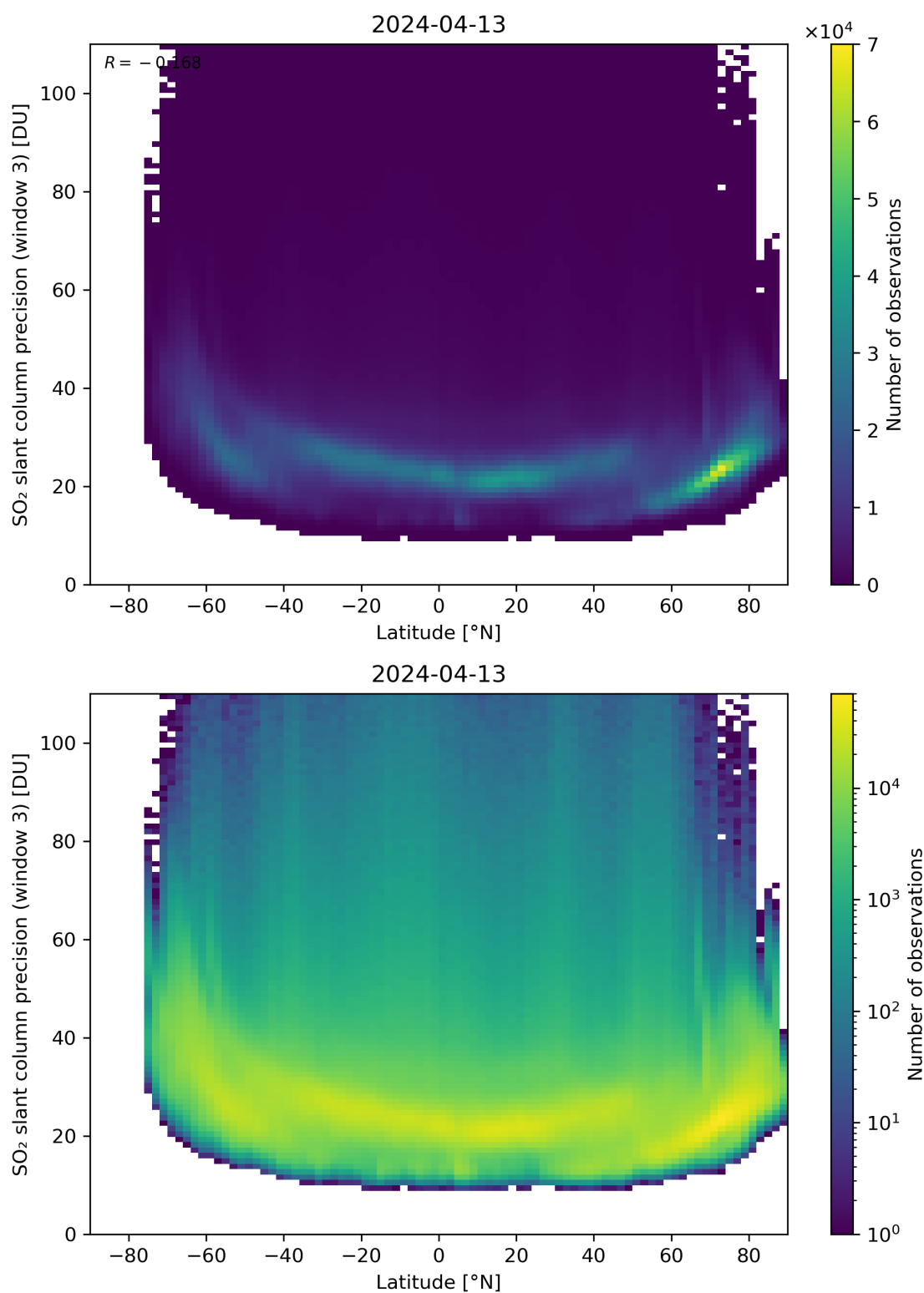
Figure 153: Scatter density plot of “Latitude” against “SO 2 slant column precision (window 3)” for 2024-04-12 to 2024-04-14.
