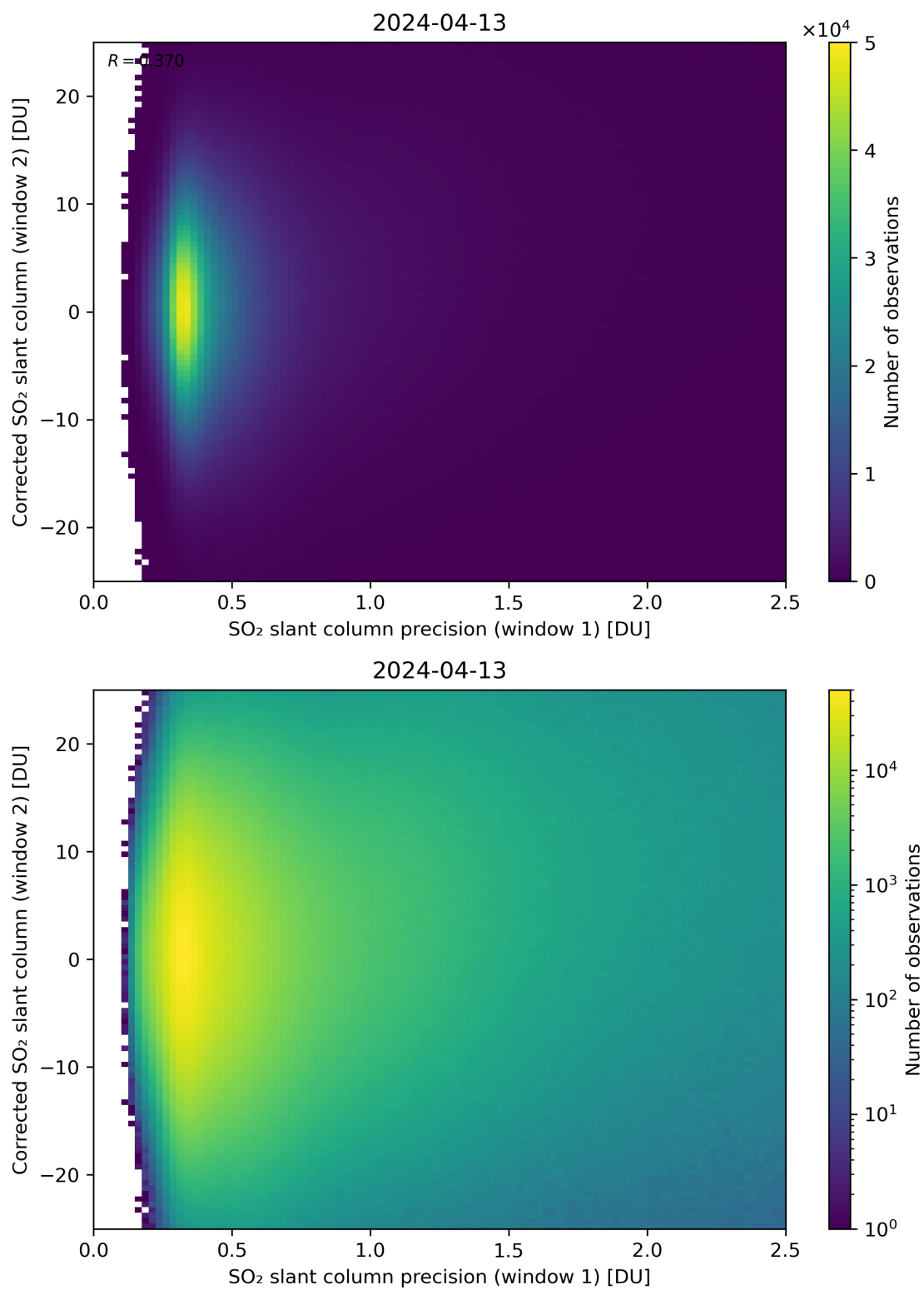
Figure 225: Scatter density plot of “SO 2 slant column precision (window 1)” against “Corrected SO 2 slant column (window 2)” for 2024-04-12 to 2024-04-14.
