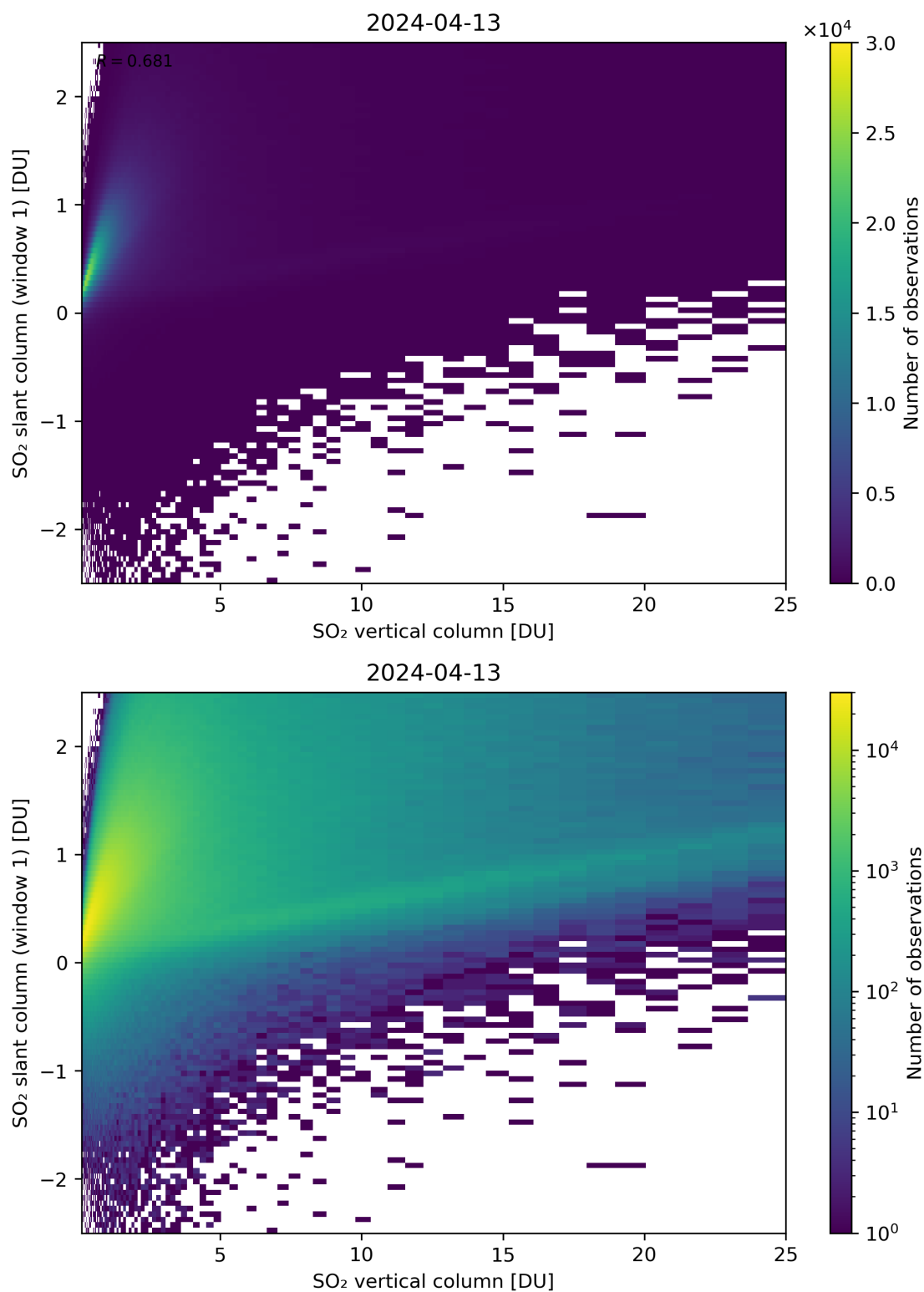
Figure 300: Scatter density plot of “SO 2 vertical column” against “SO 2 slant column (window 1)” for 2024-04-12 to 2024-04-14.
