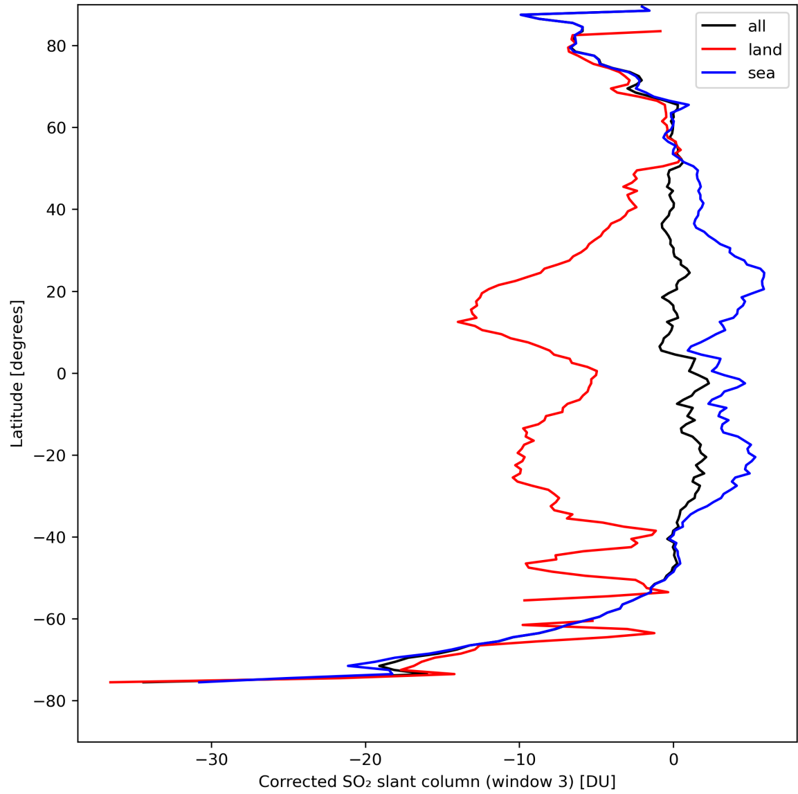
Figure 43: Zonal average of “Corrected SO 2 slant column (window 3)” for 2024-04-12 to 2024-04-14.
