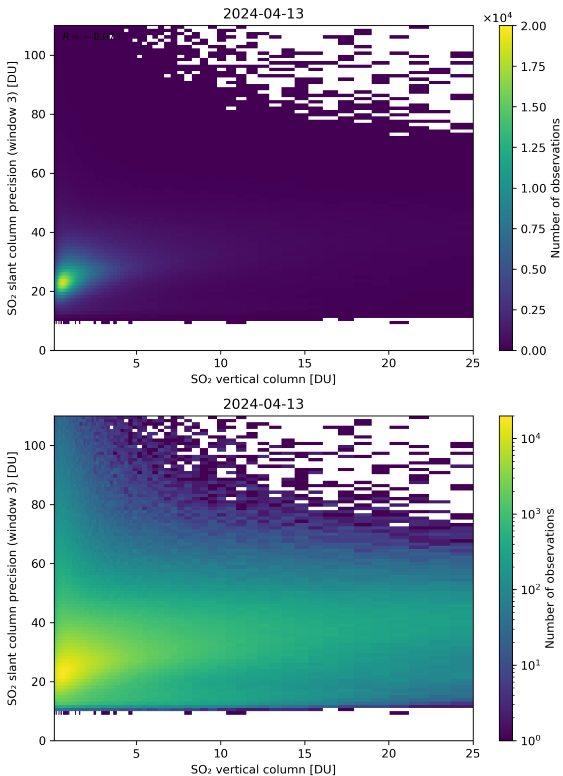
Figure 304: Scatter density plot of “SO 2 vertical column” against “SO 2 slant column precision (window 3)” for 2024-04-12 to 2024-04-14.
