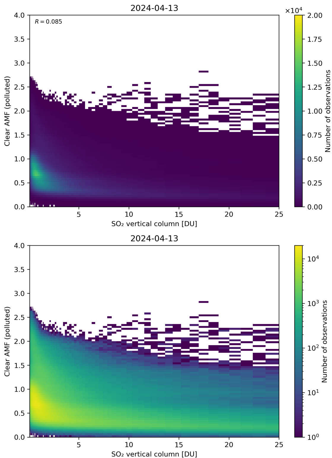
Figure 296: Scatter density plot of “SO 2 vertical column” against “Clear AMF (polluted)” for 2024-04-12 to 2024-04-14.
