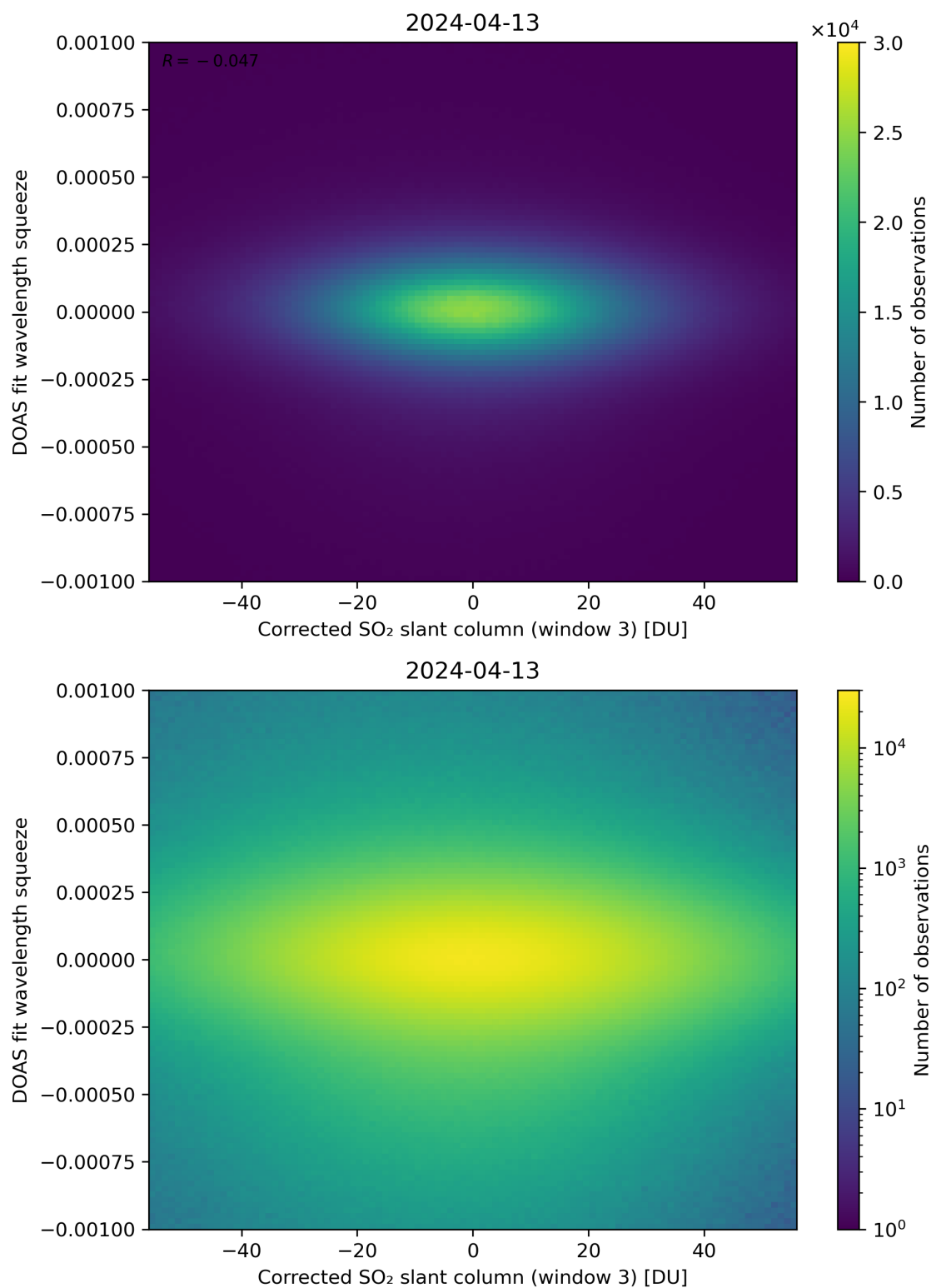
Figure 207: Scatter density plot of “Corrected SO 2 slant column (window 3)” against “DOAS fit wavelength squeeze” for 2024-04-12 to 2024-04-14.
