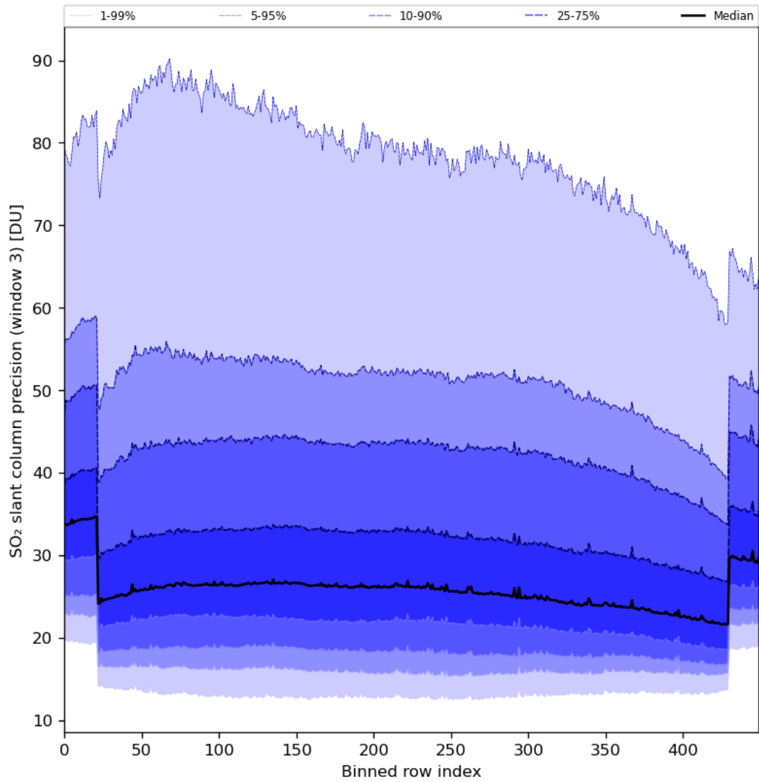
Figure 88: Along track statistics of “SO 2 slant column precision (window 3)” for 2024-04-12 to 2024-04-14
