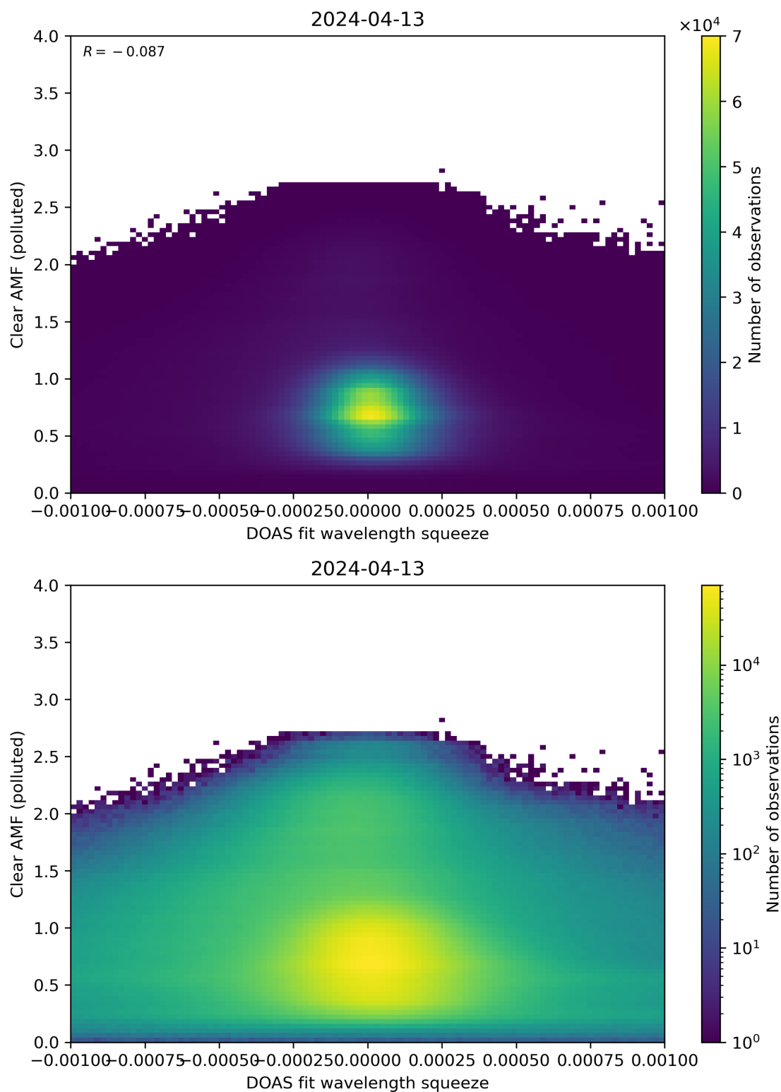
Figure 133: Scatter density plot of “DOAS fit wavelength squeeze” against “Clear AMF (polluted)” for 2024-04-12 to 2024-04-14.
