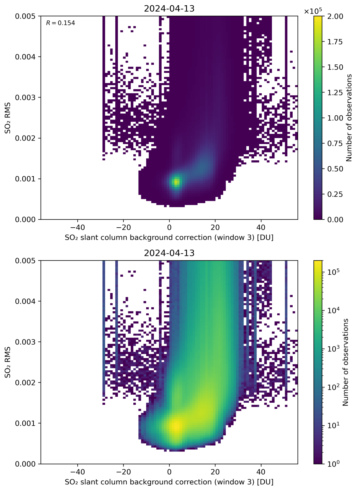
Figure 123: Scatter density plot of “SO 2 slant column background correction (window 3)” against “SO 2 RMS” for 2024-04-12 to 2024-04-14.
