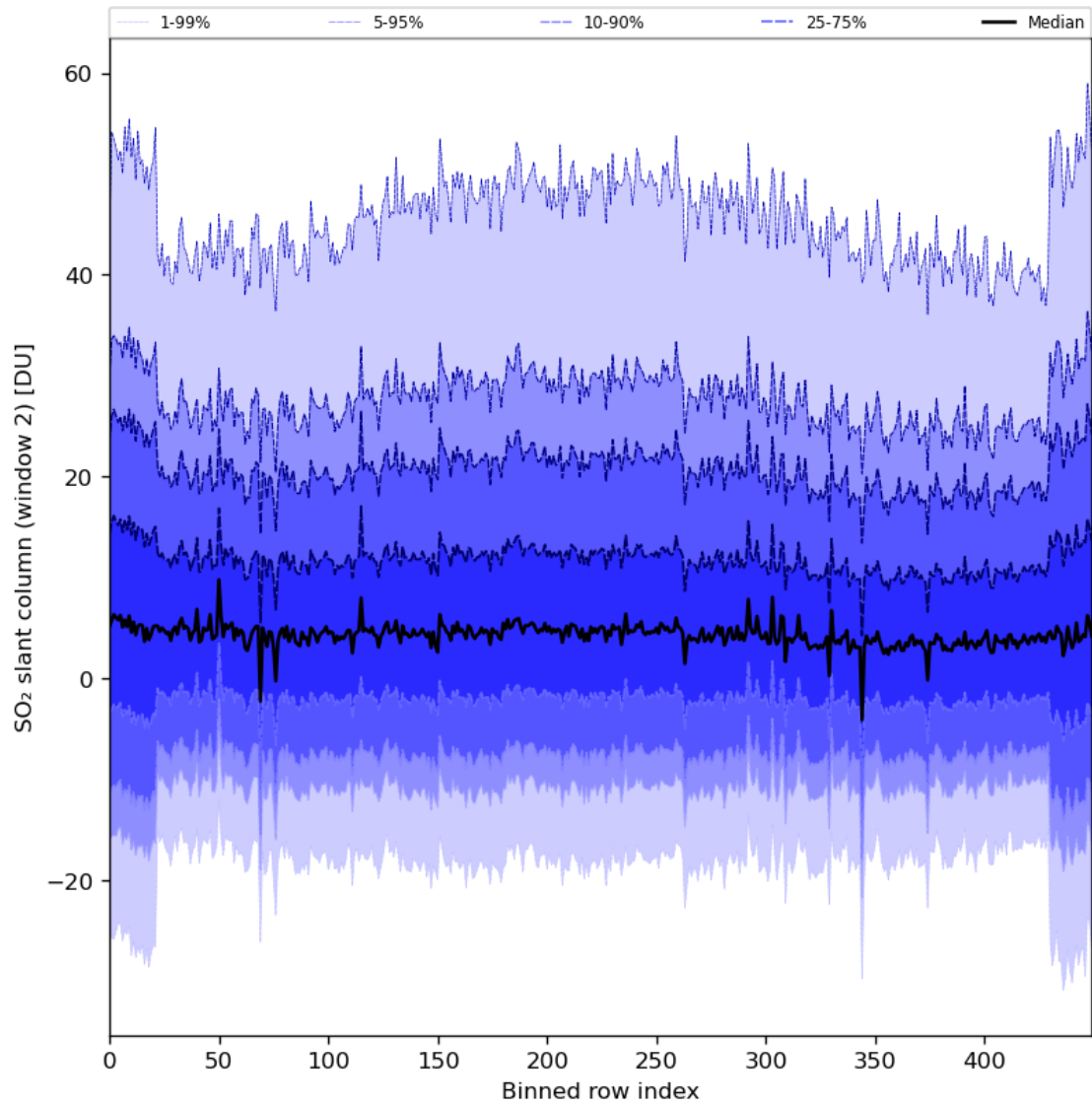
Figure 83: Along track statistics of “SO 2 slant column (window 2)” for 2024-04-12 to 2024-04-14
