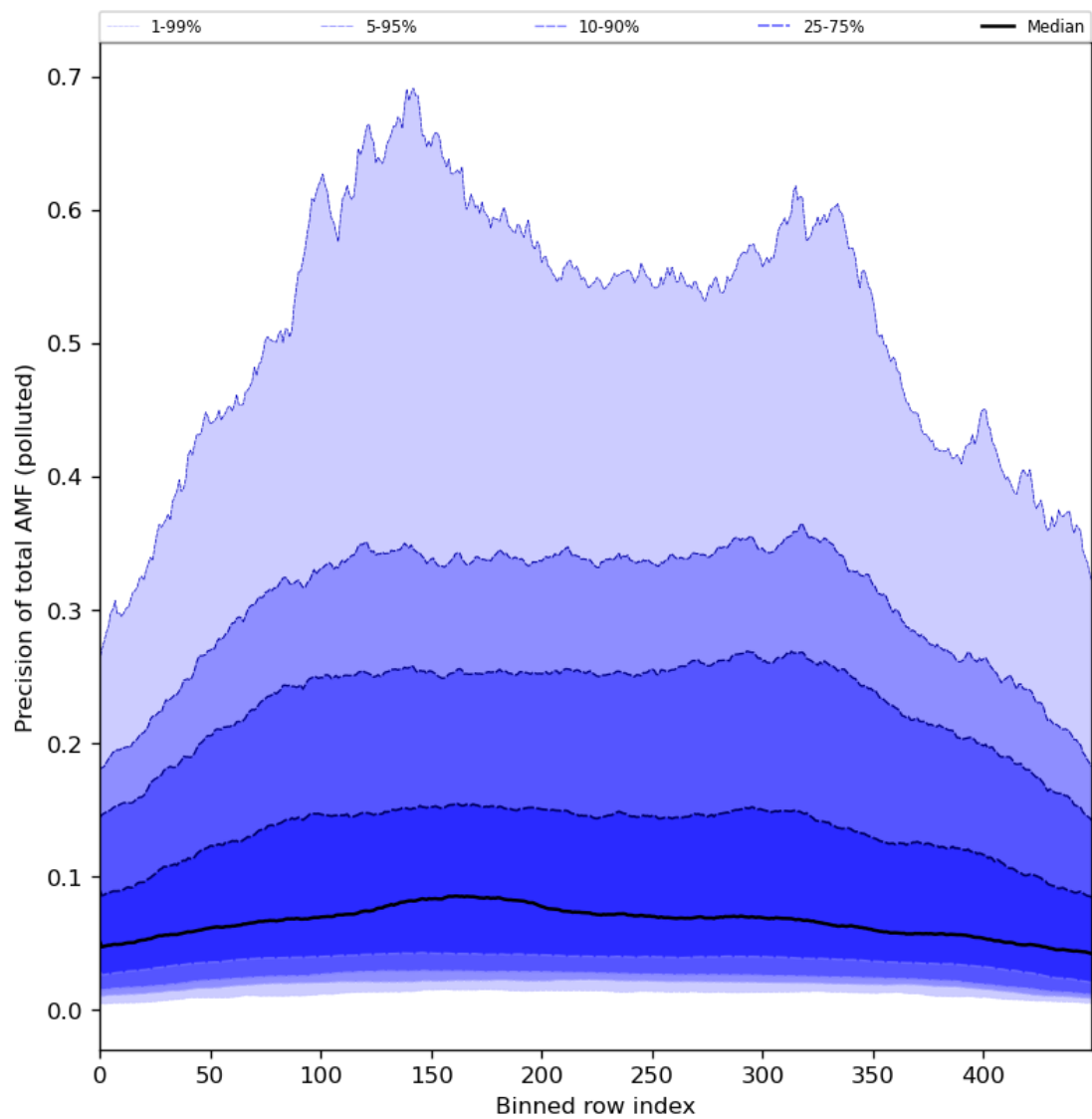
Figure 95: Along track statistics of “Precision of total AMF (polluted)” for 2024-04-12 to 2024-04-14
