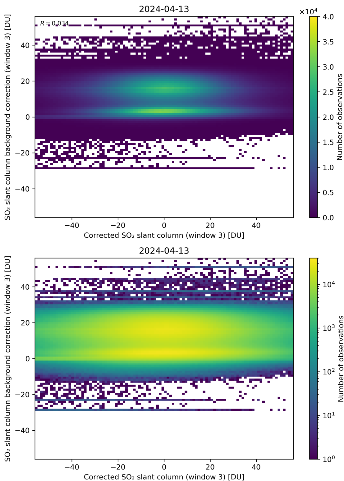
Figure 205: Scatter density plot of “Corrected SO 2 slant column (window 3)” against “SO 2 slant column background correction (window 3)” for 2024-04-12 to 2024-04-14.
