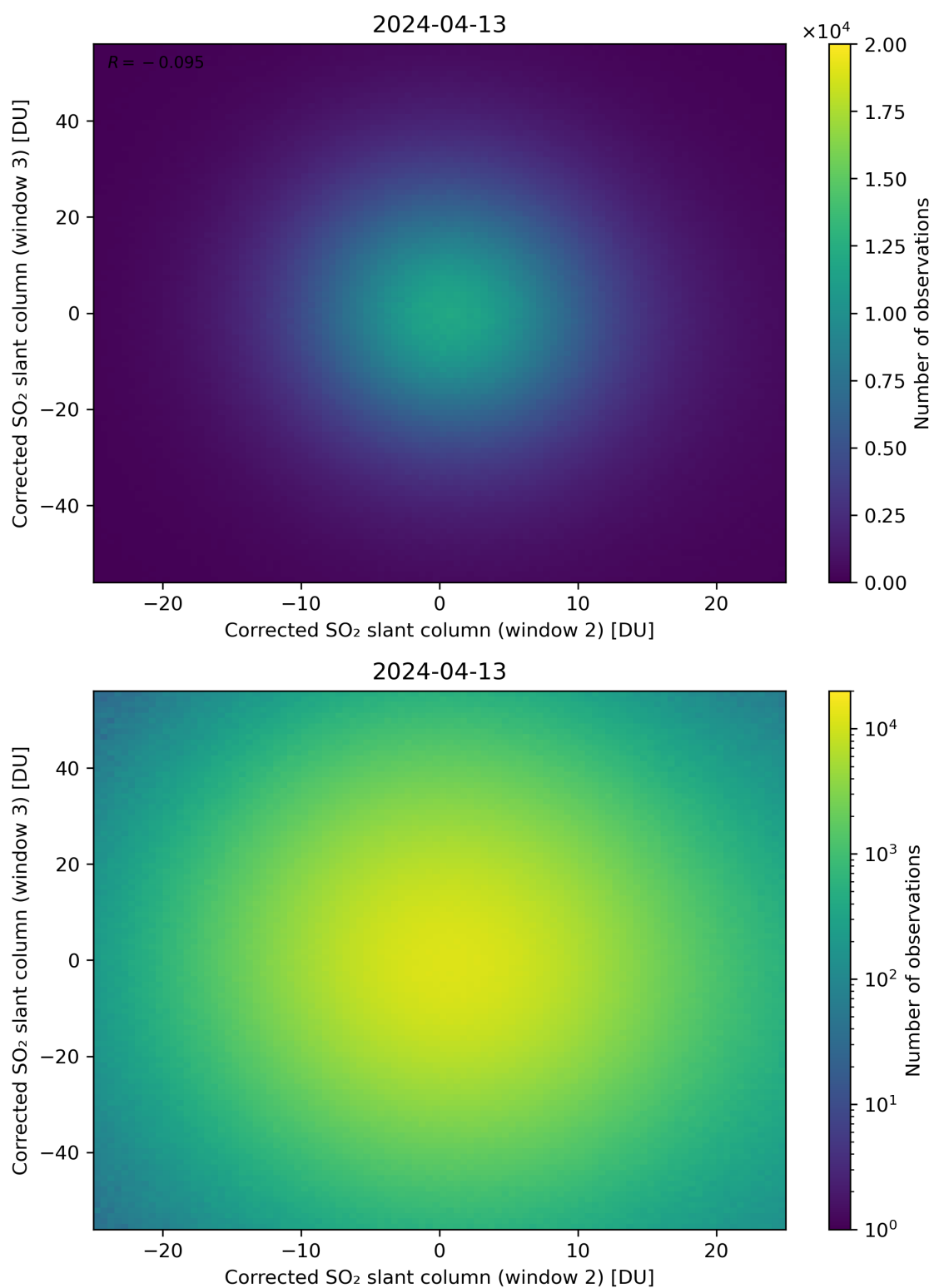
Figure 200: Scatter density plot of “Corrected SO 2 slant column (window 2)” against “Corrected SO 2 slant column (window 3)” for 2024-04-12 to 2024-04-14.
