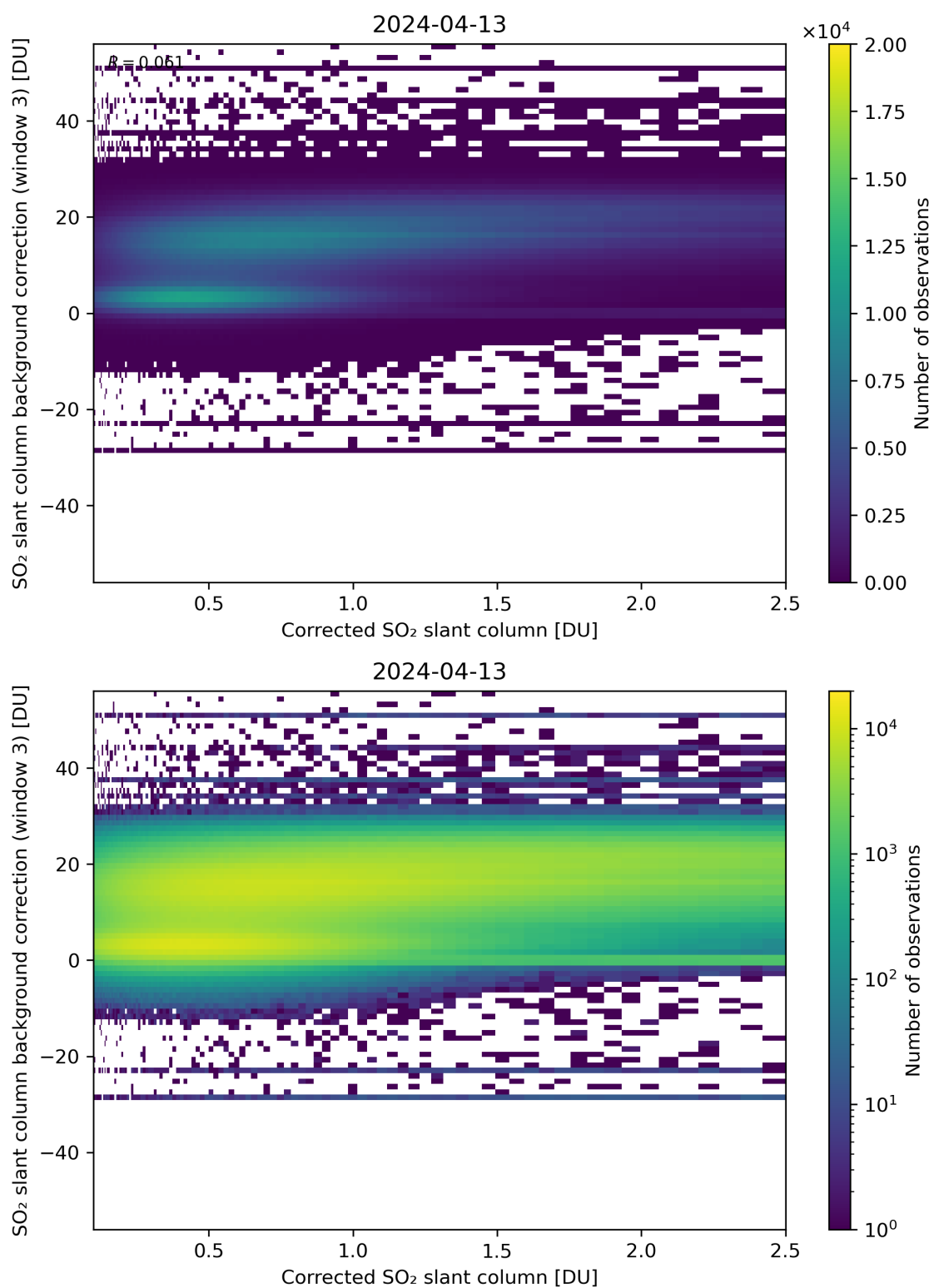
Figure 180: Scatter density plot of “Corrected SO 2 slant column” against “SO 2 slant column background correction (window 3)” for 2024-04-12 to 2024-04-14.
