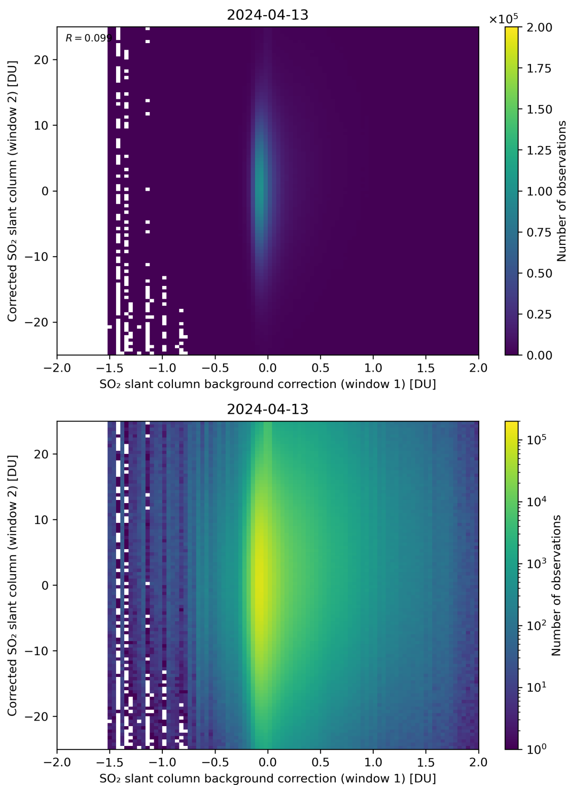
Figure 104: Scatter density plot of “SO 2 slant column background correction (window 1)” against “Corrected SO 2 slant column (window 2)” for 2024-04-12 to 2024-04-14.
