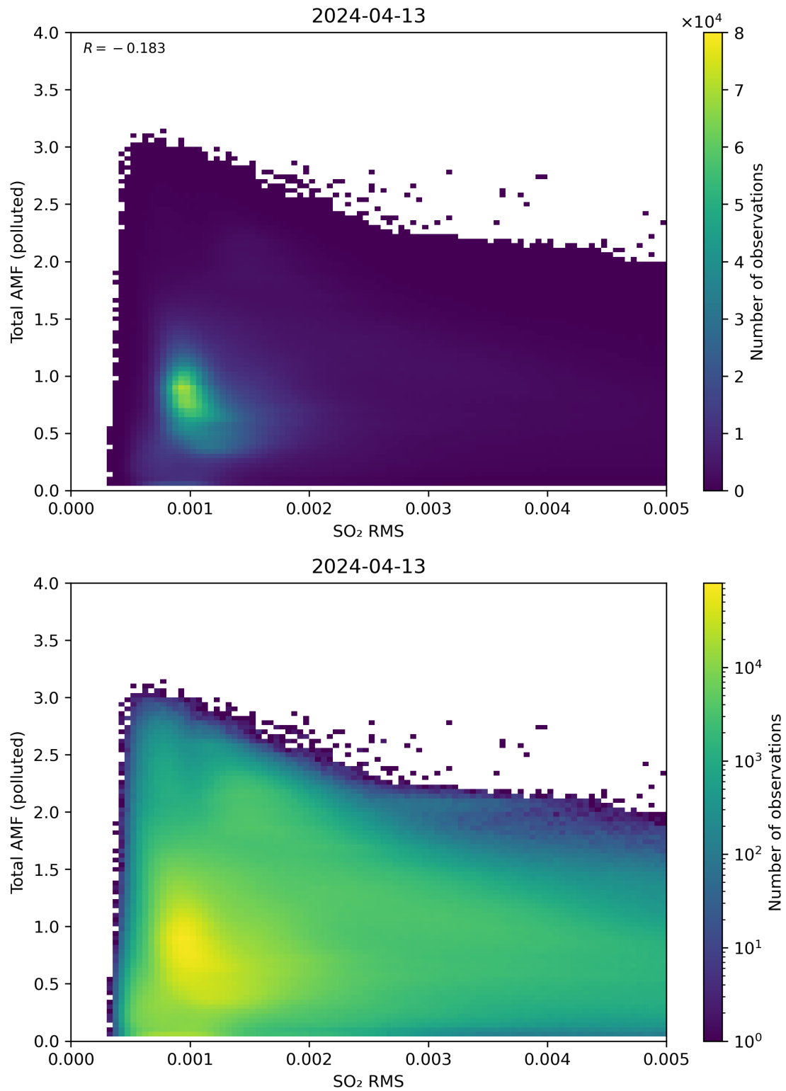
Figure 137: Scatter density plot of “SO 2 RMS” against “Total AMF (polluted)” for 2024-04-12 to 2024-04-14.
