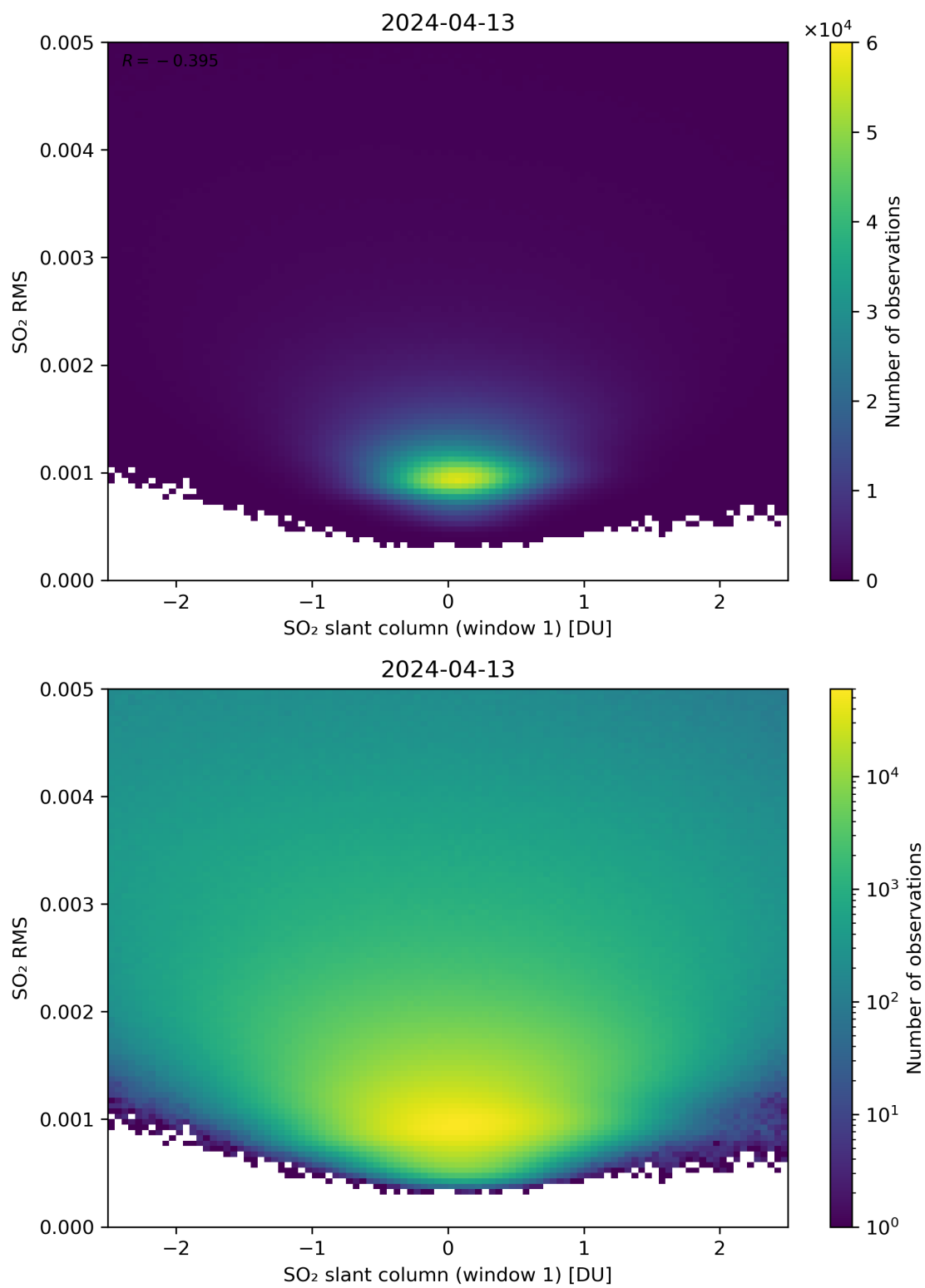
Figure 217: Scatter density plot of “SO 2 slant column (window 1)” against “SO 2 RMS” for 2024-04-12 to 2024-04-14.
