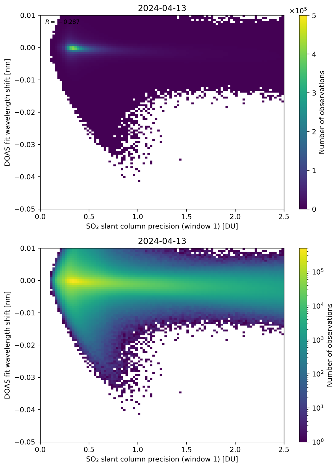
Figure 221: Scatter density plot of “SO 2 slant column precision (window 1)” against “DOAS fit wavelength shift” for 2024-04-12 to 2024-04-14.
