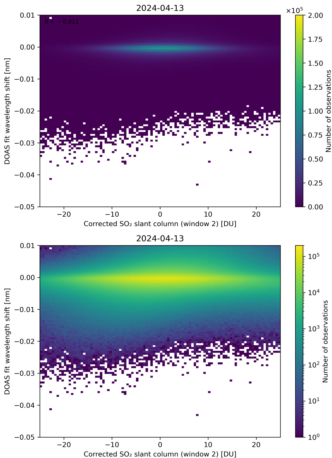
Figure 196: Scatter density plot of “Corrected SO 2 slant column (window 2)” against “DOAS fit wavelength shift” for 2024-04-12 to 2024-04-14.
