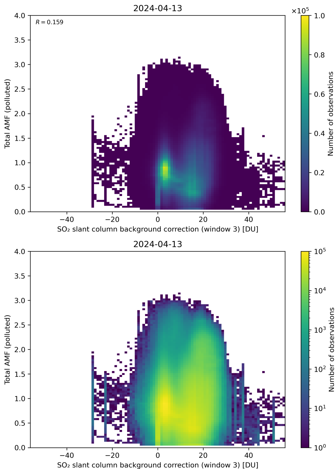
Figure 125: Scatter density plot of “SO 2 slant column background correction (window 3)” against “Total AMF (polluted)” for 2024-04-12 to 2024-04-14.
