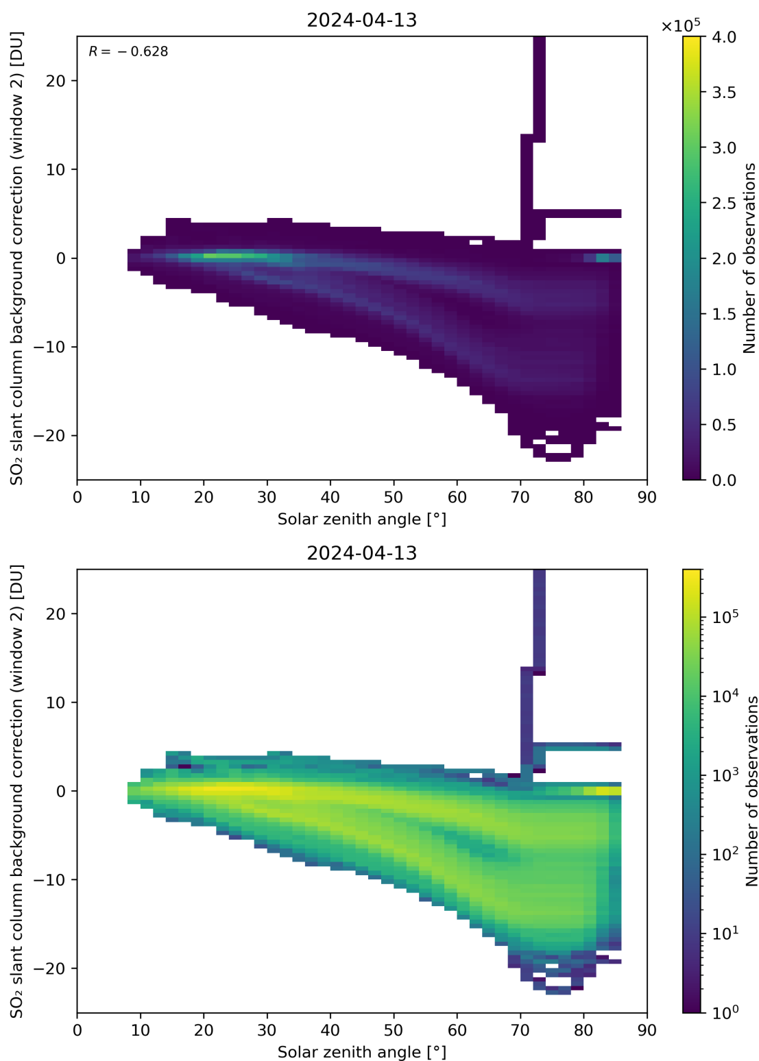
Figure 159: Scatter density plot of “Solar zenith angle” against “SO 2 slant column background correction (window 2)” for 2024-04-12 to 2024-04-14.
