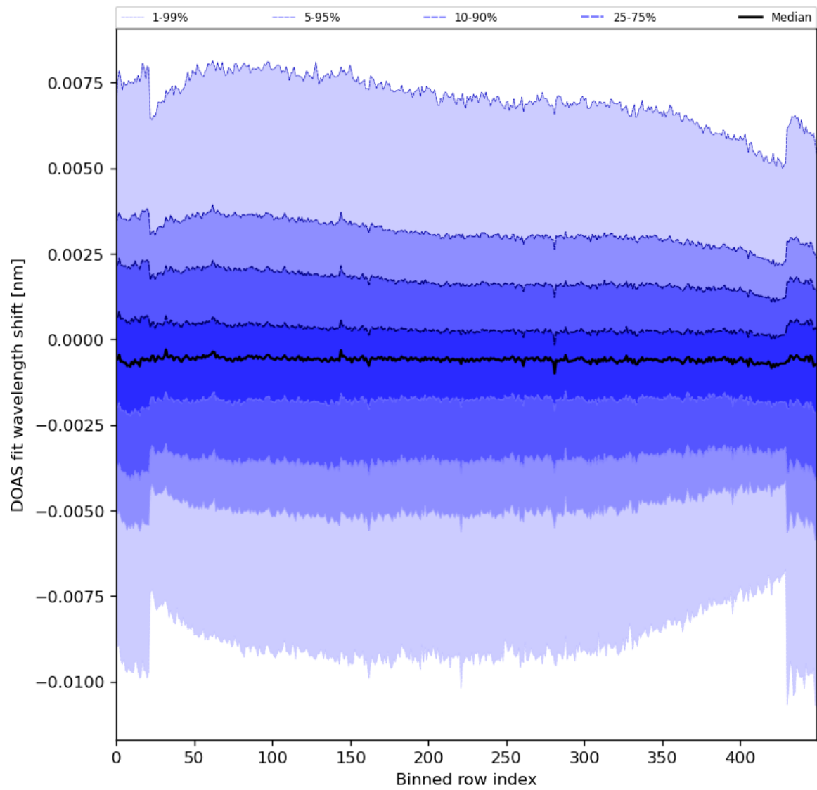
Figure 91: Along track statistics of “DOAS fit wavelength shift” for 2024-04-12 to 2024-04-14
