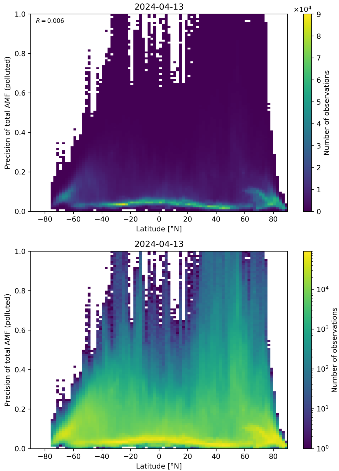
Figure 155: Scatter density plot of “Latitude” against “Precision of total AMF (polluted)” for 2024-04-12 to 2024-04-14.
