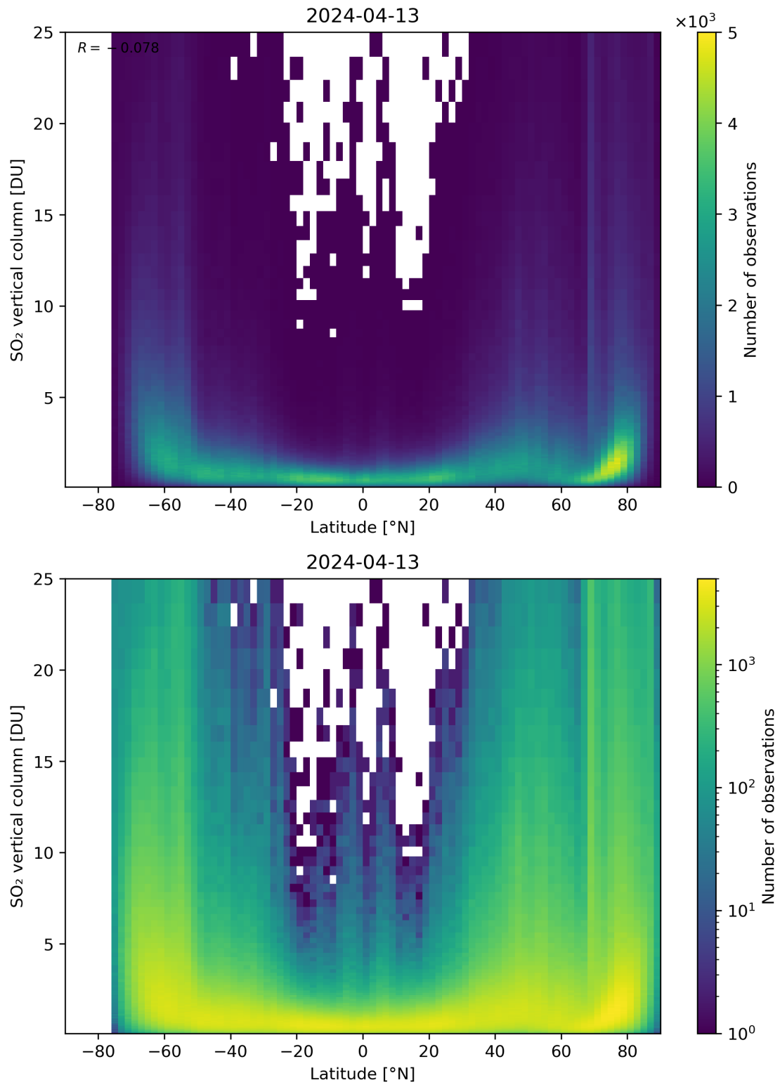
Figure 156: Scatter density plot of “Latitude” against “SO 2 vertical column” for 2024-04-12 to 2024-04-14.
