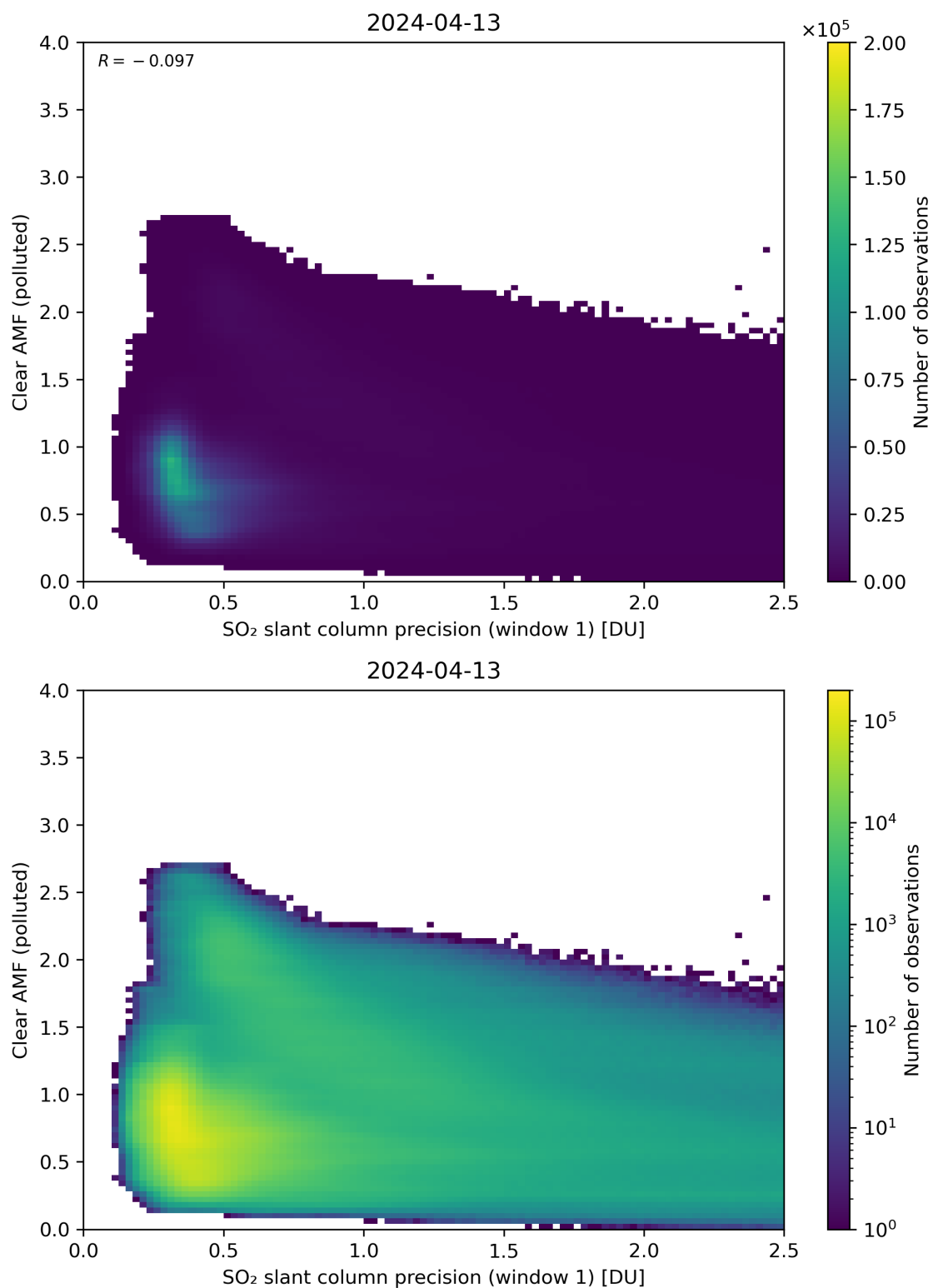
Figure 224: Scatter density plot of “SO 2 slant column precision (window 1)” against “Clear AMF (polluted)” for 2024-04-12 to 2024-04-14.
