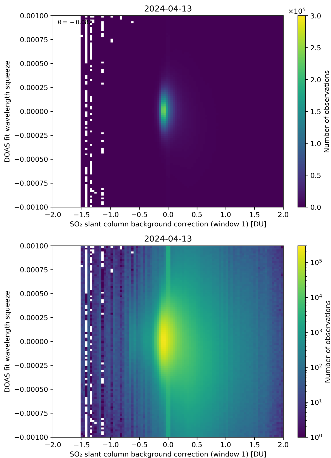
Figure 101: Scatter density plot of “SO 2 slant column background correction (window 1)” against “DOAS fit wavelength squeeze” for 2024-04-12 to 2024-04-14.
