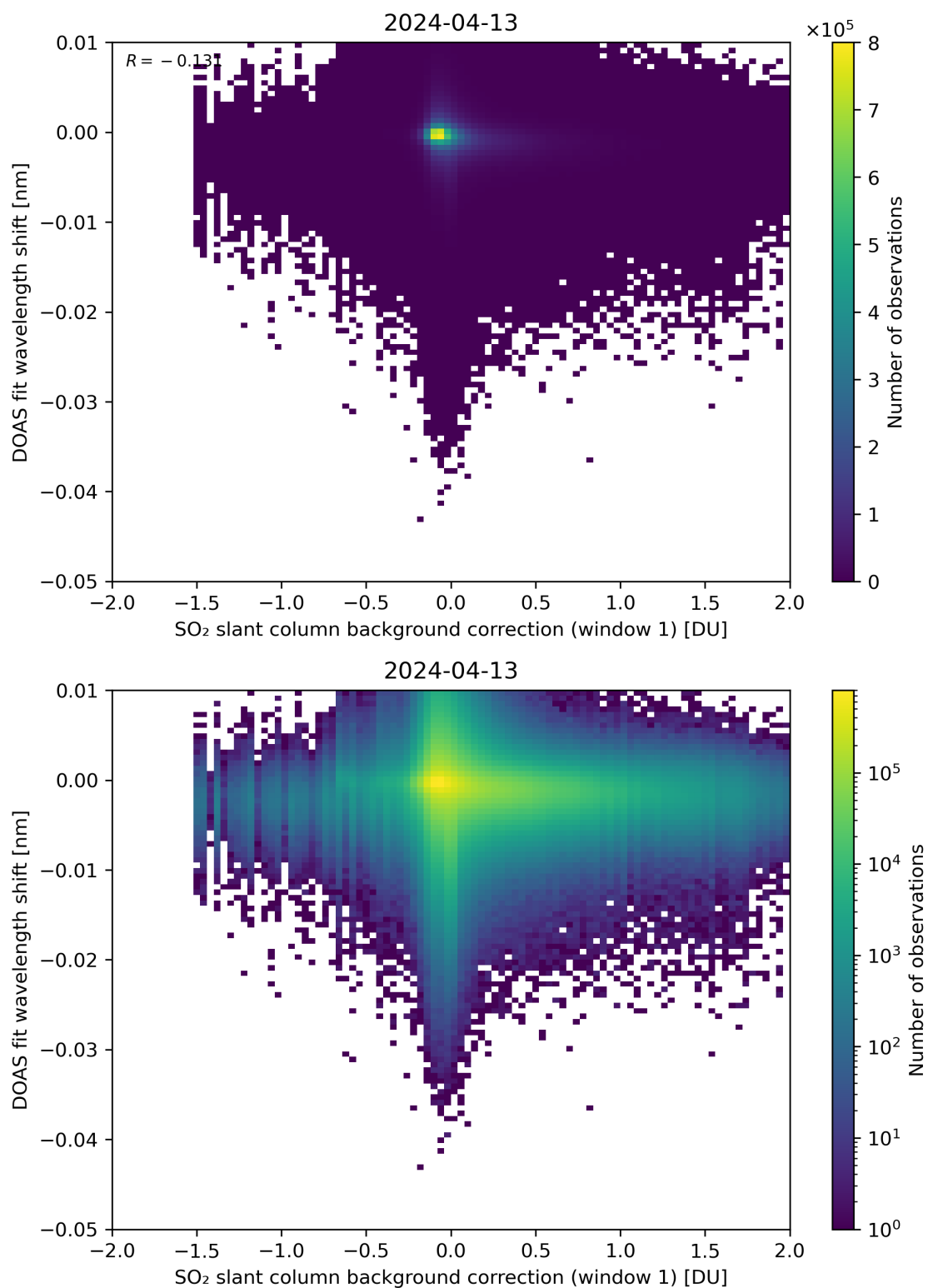
Figure 100: Scatter density plot of “SO 2 slant column background correction (window 1)” against “DOAS fit wavelength shift” for 2024-04-12 to 2024-04-14.
