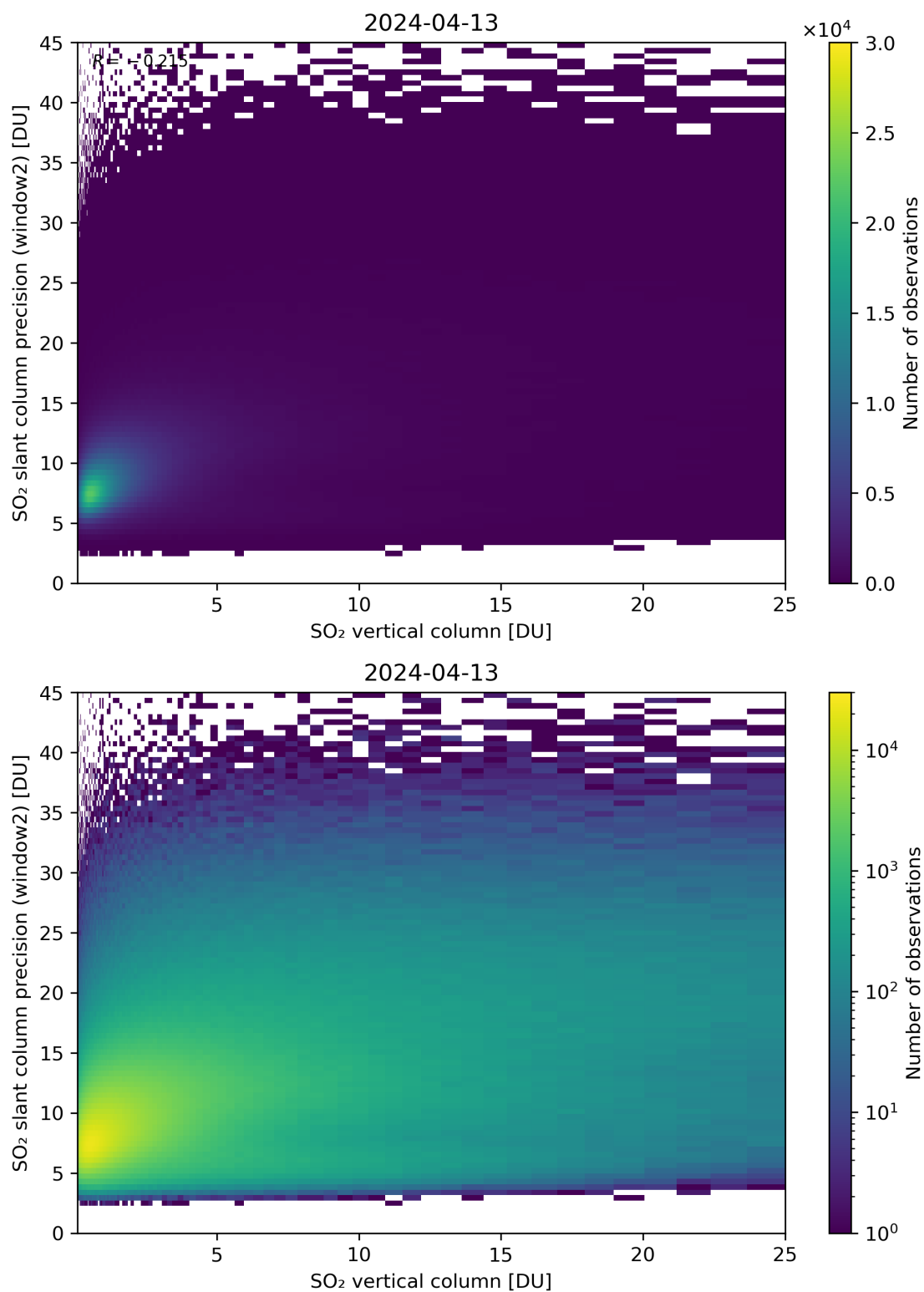
Figure 302: Scatter density plot of “SO 2 vertical column” against “SO 2 slant column precision (window2)” for 2024-04-12 to 2024-04-14.
