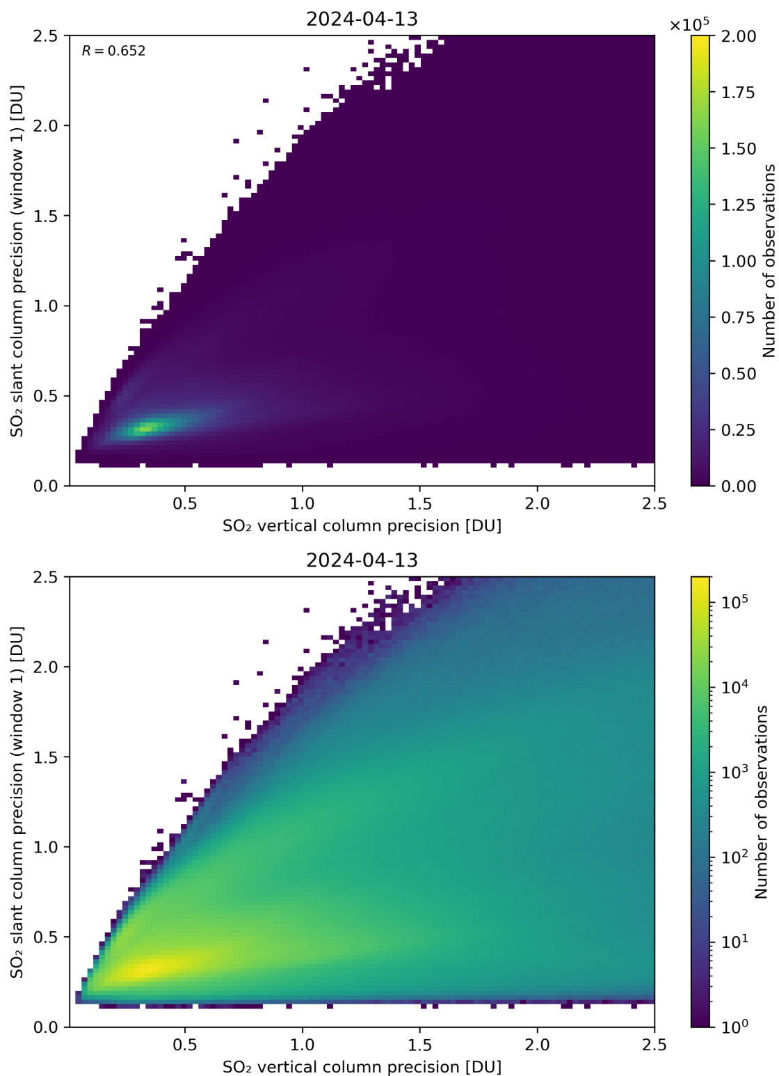
Figure 290: Scatter density plot of “SO 2 vertical column precision” against “SO 2 slant column precision (window 1)” for 2024-04-12 to 2024-04-14.
