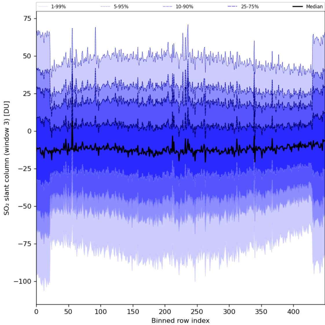
Figure 87: Along track statistics of “SO 2 slant column (window 3)” for 2024-04-12 to 2024-04-14
