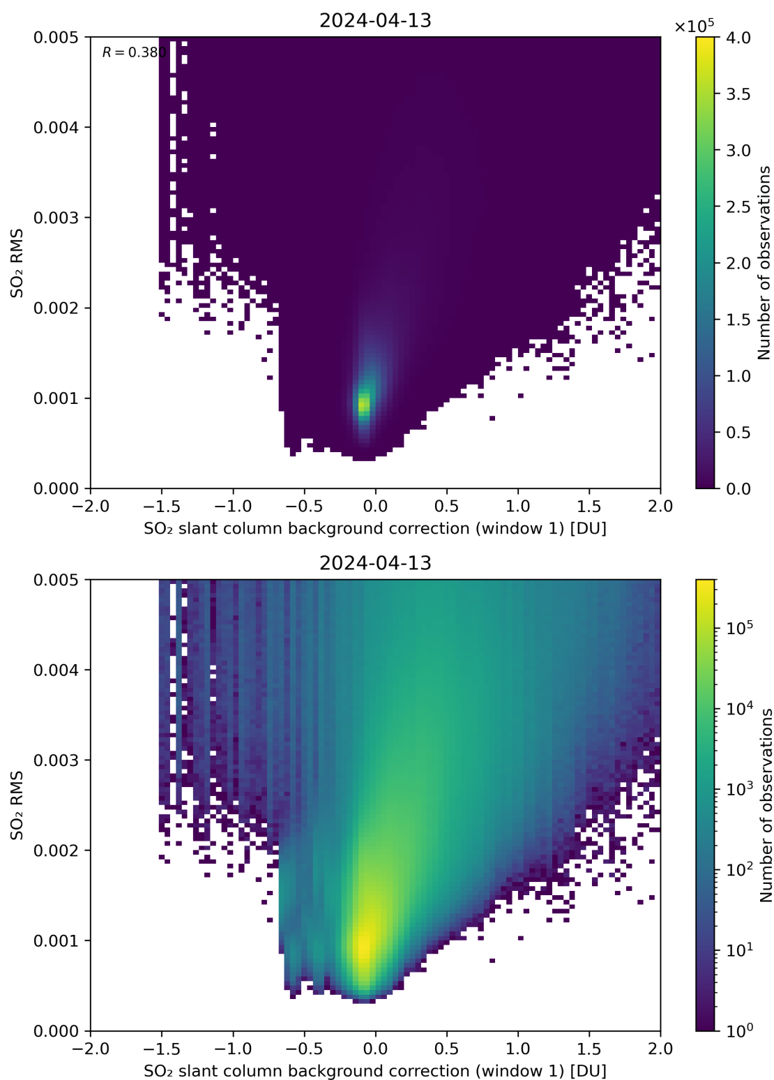
Figure 102: Scatter density plot of “SO 2 slant column background correction (window 1)” against “SO 2 RMS” for 2024-04-12 to 2024-04-14.
