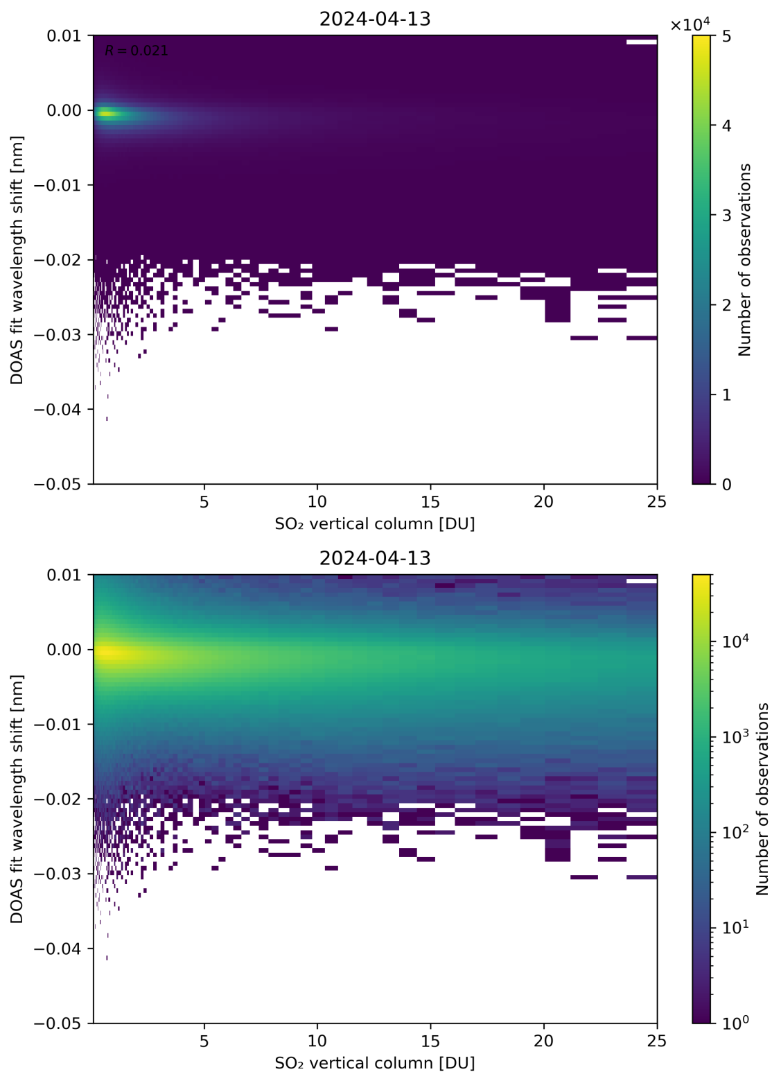
Figure 276: Scatter density plot of “SO 2 vertical column” against “DOAS fit wavelength shift” for 2024-04-12 to 2024-04-14.
