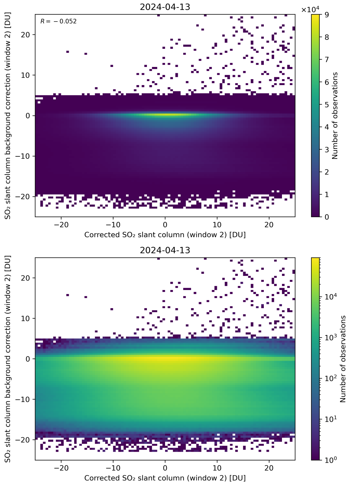
Figure 194: Scatter density plot of “Corrected SO 2 slant column (window 2)” against “SO 2 slant column background correction (window 2)” for 2024-04-12 to 2024-04-14.
