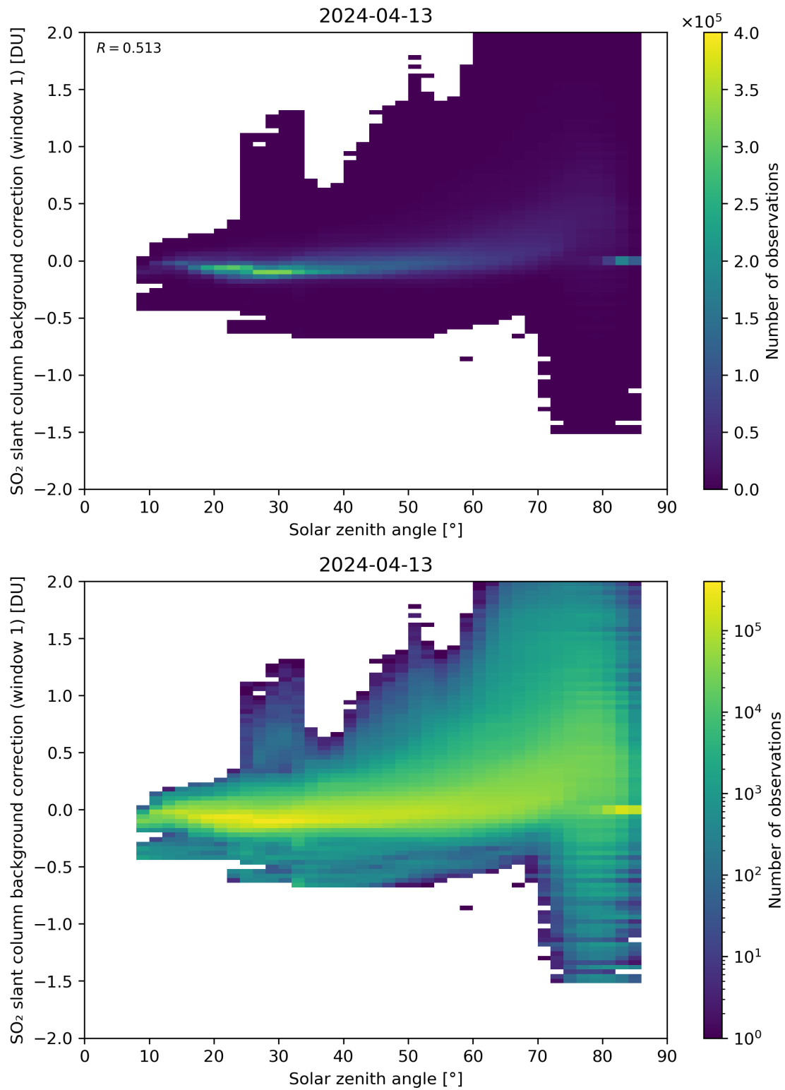
Figure 158: Scatter density plot of “Solar zenith angle” against “SO 2 slant column background correction (window 1)” for 2024-04-12 to 2024-04-14.
