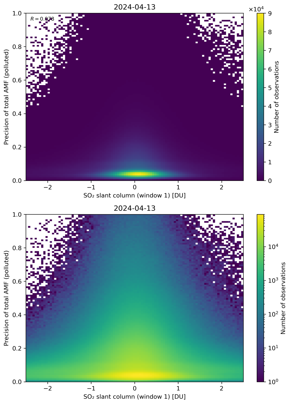
Figure 240: Scatter density plot of “SO 2 slant column (window 1)” against “Precision of total AMF (polluted)” for 2024-04-12 to 2024-04-14.
