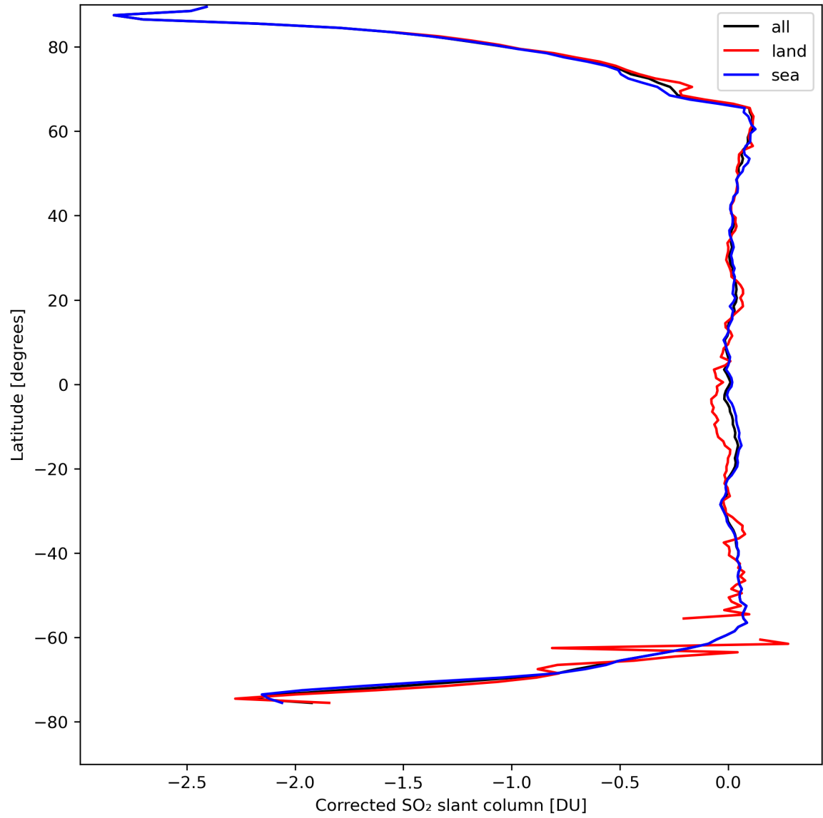
Figure 32: Zonal average of “Corrected SO 2 slant column” for 2024-04-12 to 2024-04-14.
