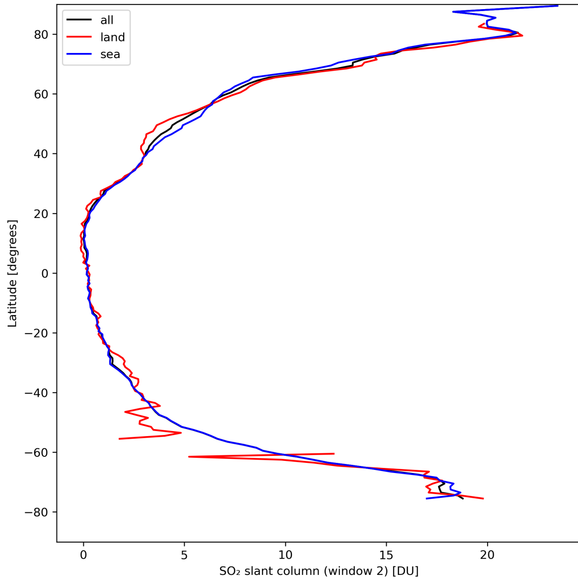
Figure 37: Zonal average of “SO 2 slant column (window 2)” for 2024-04-12 to 2024-04-14.
