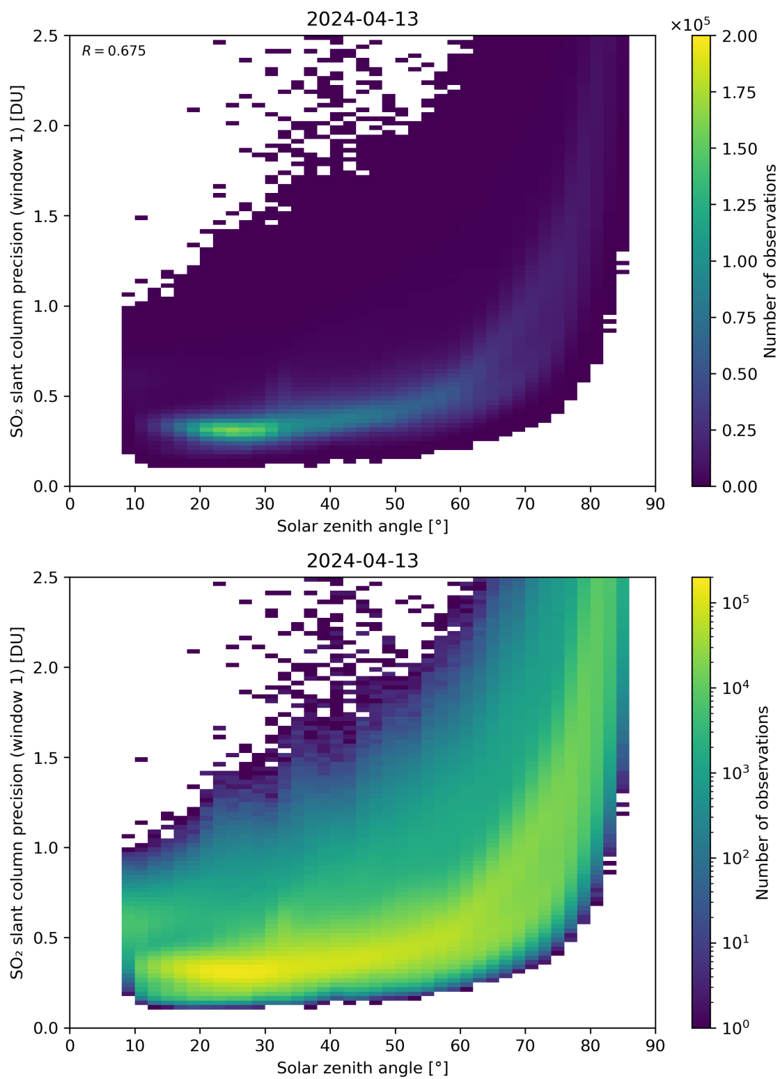
Figure 170: Scatter density plot of “Solar zenith angle” against “SO 2 slant column precision (window 1)” for 2024-04-12 to 2024-04-14.
