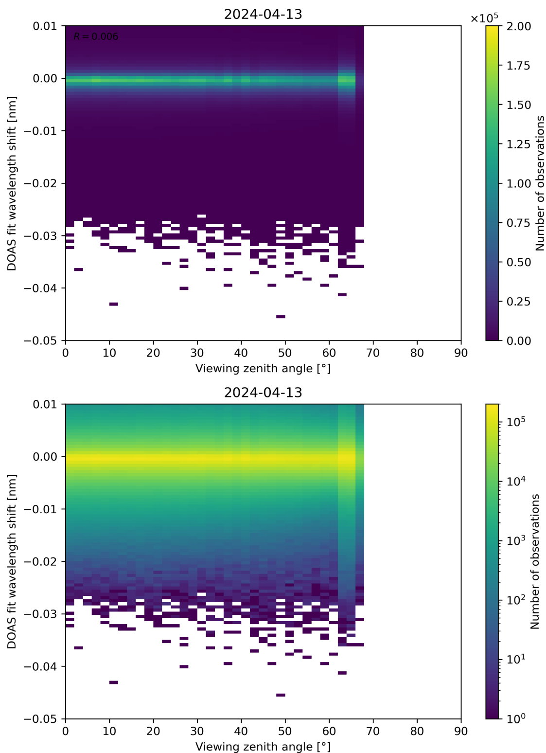
Figure 311: Scatter density plot of “Viewing zenith angle” against “DOAS fit wavelength shift” for 2024-04-12 to 2024-04-14.
