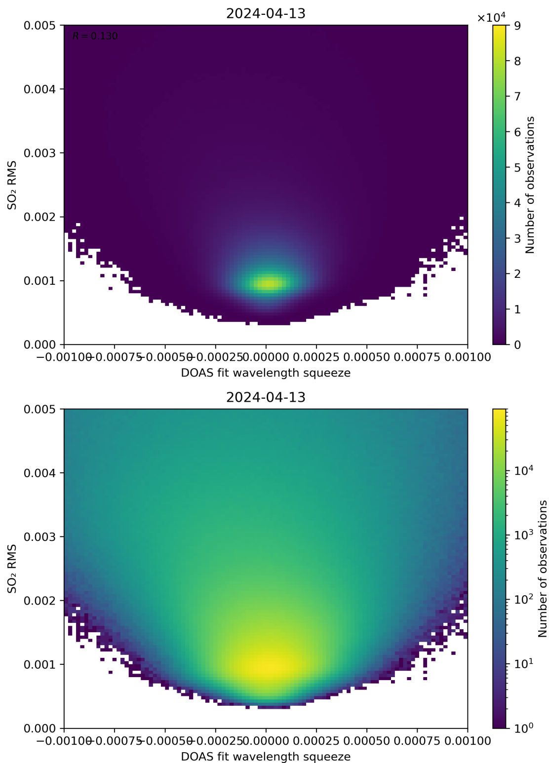
Figure 132: Scatter density plot of “DOAS fit wavelength squeeze” against “SO 2 RMS” for 2024-04-12 to 2024-04-14.
