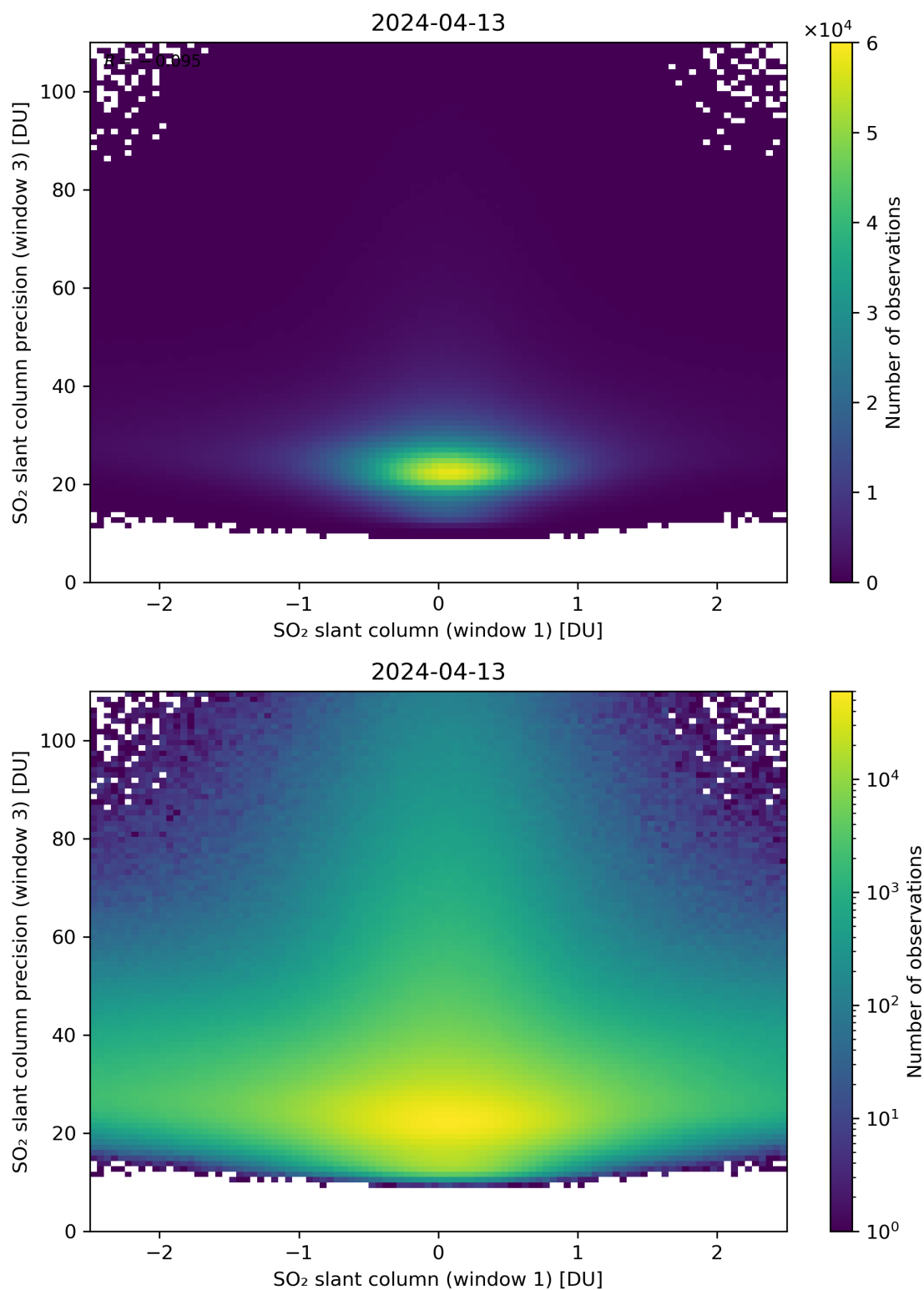
Figure 238: Scatter density plot of “SO 2 slant column (window 1)” against “SO 2 slant column precision (window 3)” for 2024-04-12 to 2024-04-14.
