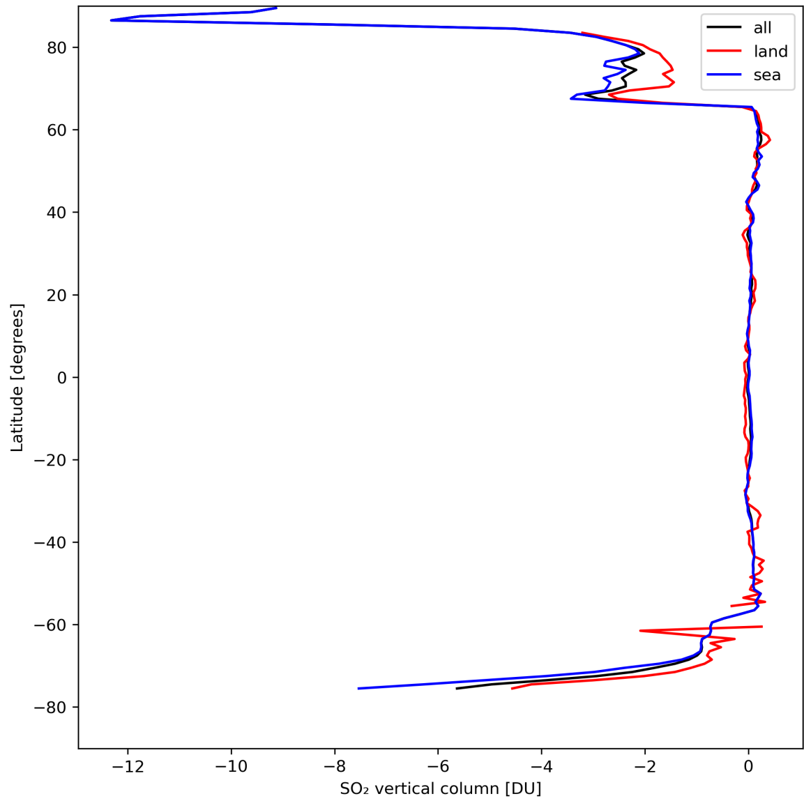
Figure 30: Zonal average of “SO 2 vertical column” for 2024-04-12 to 2024-04-14.
