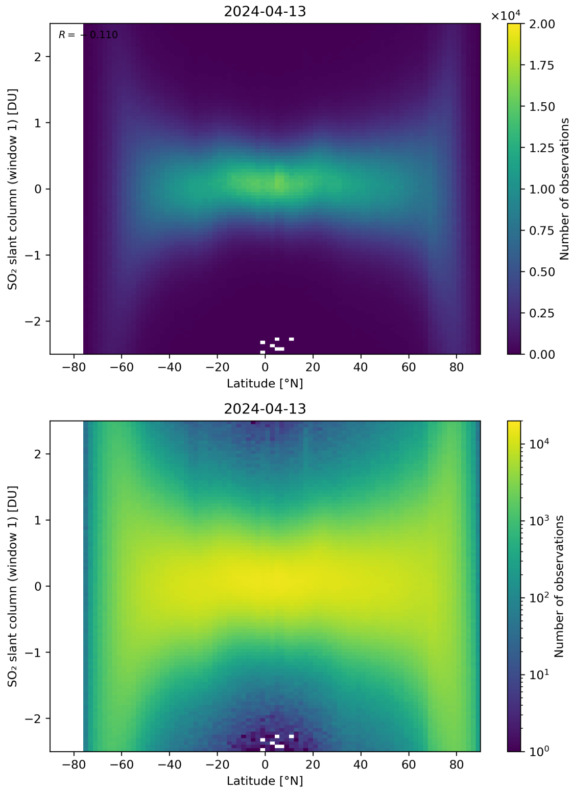
Figure 149: Scatter density plot of “Latitude” against “SO 2 slant column (window 1)” for 2024-04-12 to 2024-04-14.
