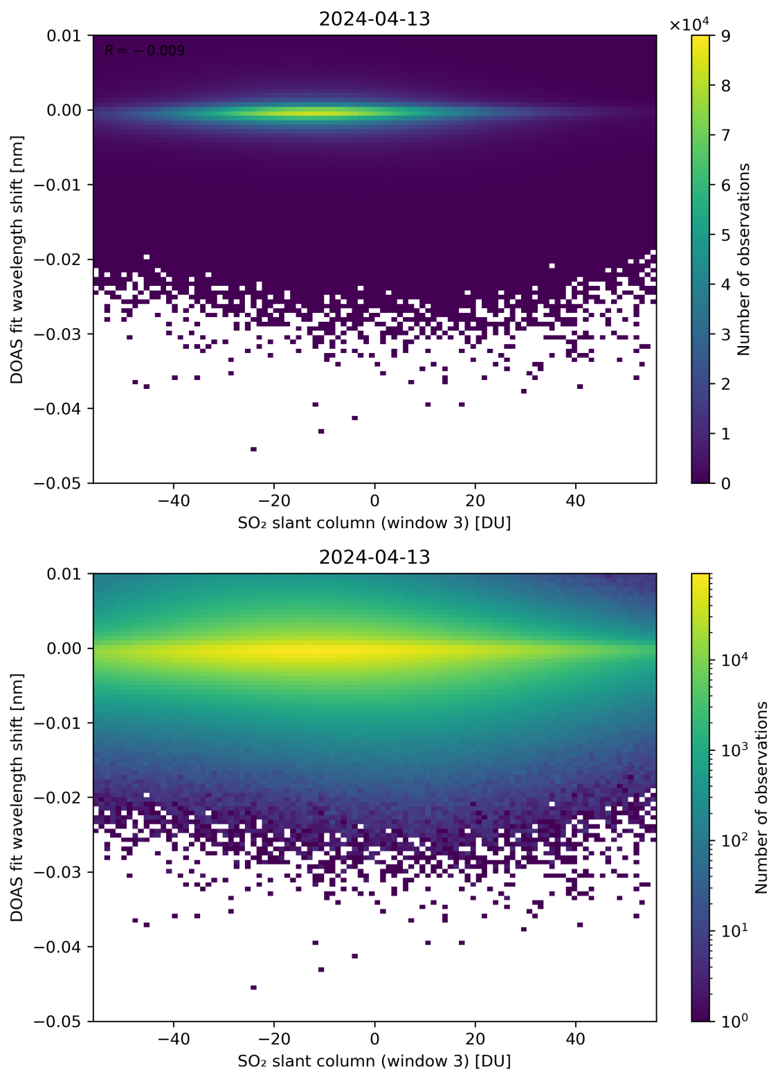
Figure 254: Scatter density plot of “SO 2 slant column (window 3)” against “DOAS fit wavelength shift” for 2024-04-12 to 2024-04-14.
