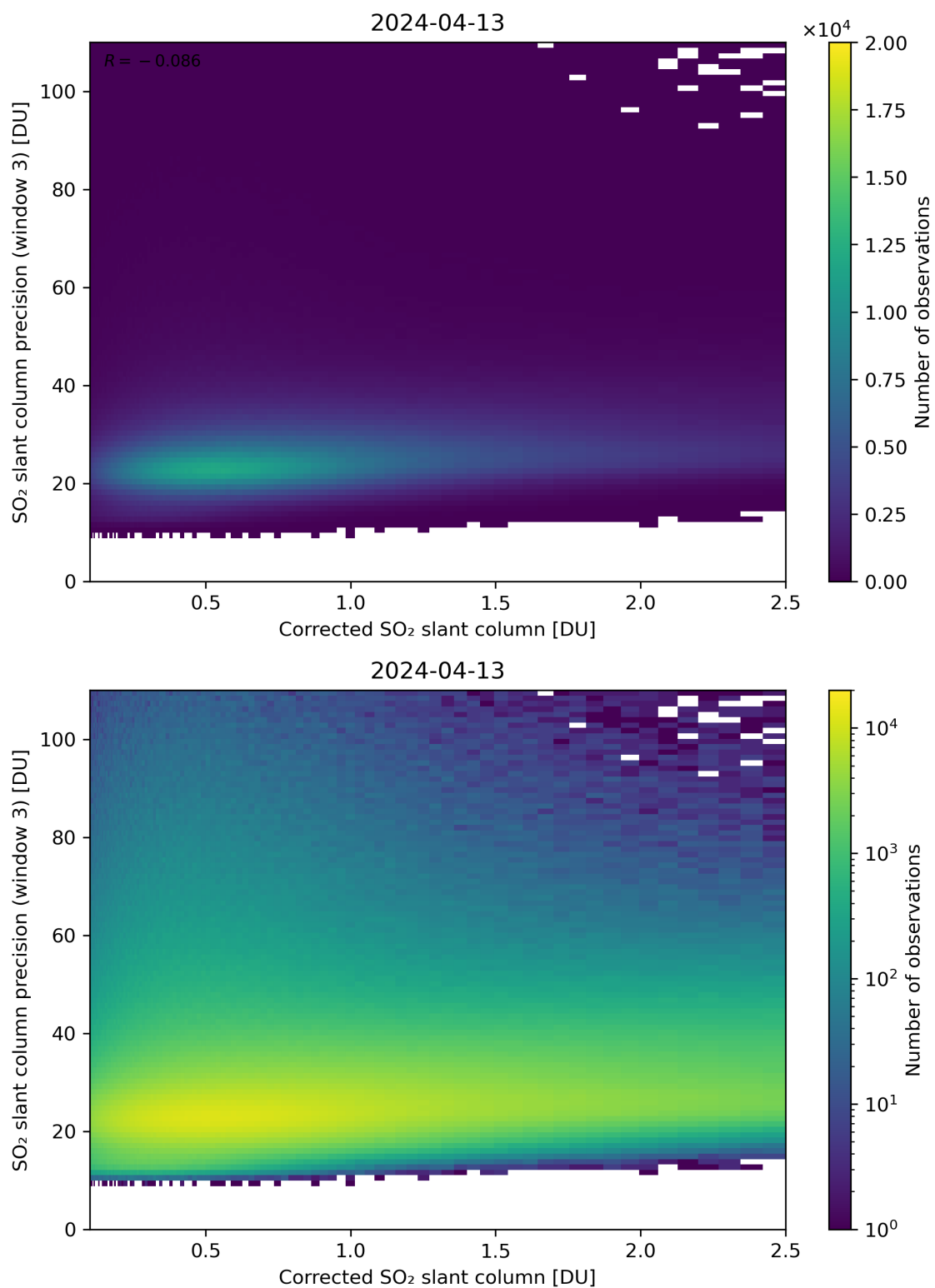
Figure 191: Scatter density plot of “Corrected SO 2 slant column” against “SO 2 slant column precision (window 3)” for 2024-04-12 to 2024-04-14.
