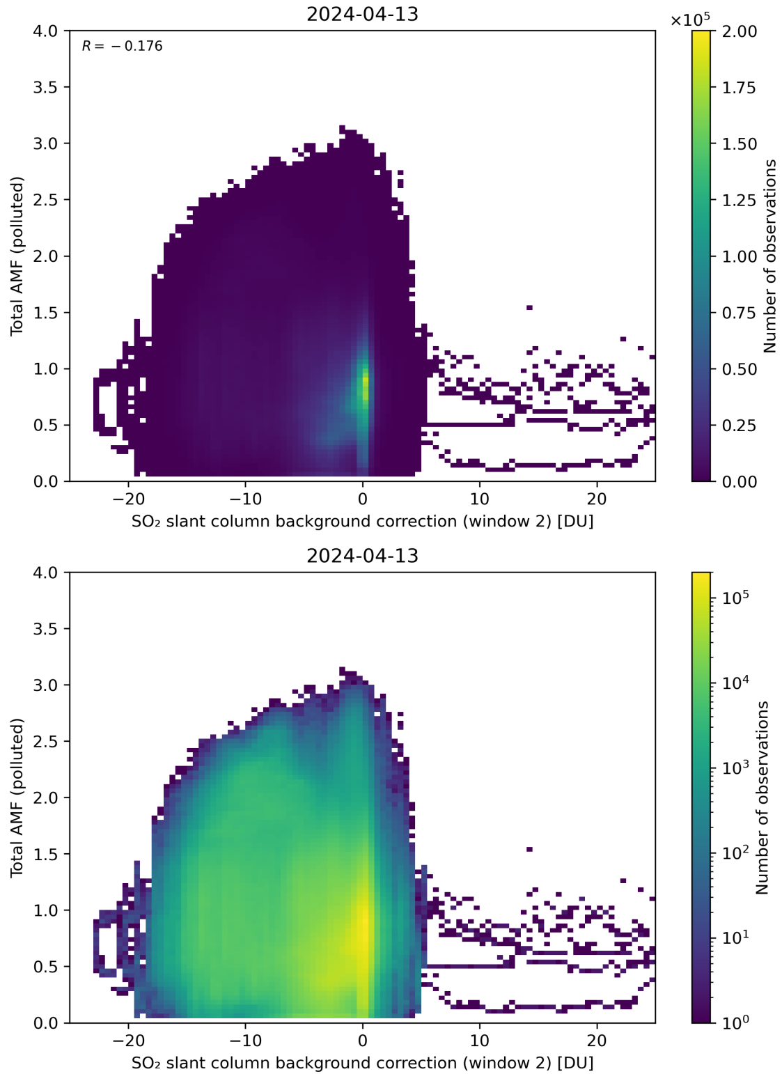
Figure 119: Scatter density plot of “SO 2 slant column background correction (window 2)” against “Total AMF (polluted)” for 2024-04-12 to 2024-04-14.
