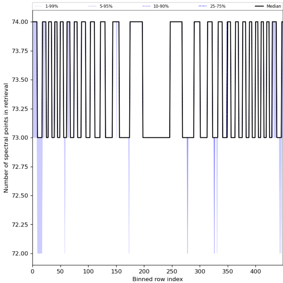
Figure 97: Along track statistics of “Number of spectral points in retrieval” for 2024-04-12 to 2024-04-14
