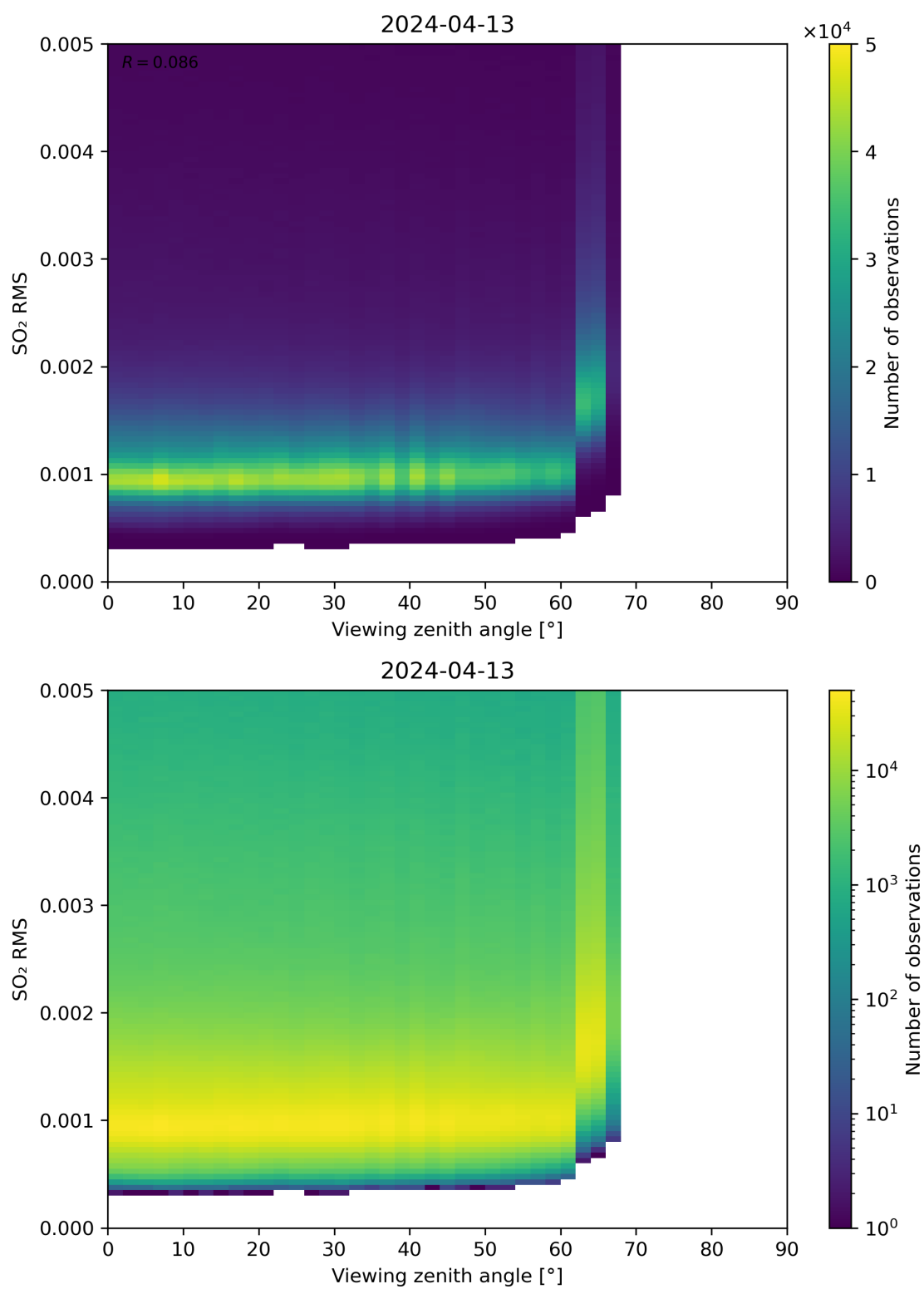
Figure 313: Scatter density plot of “Viewing zenith angle” against “SO 2 RMS” for 2024-04-12 to 2024-04-14.
