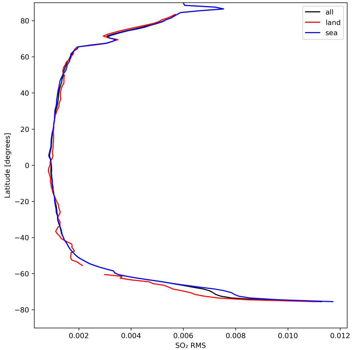
Figure 47: Zonal average of “SO 2 RMS” for 2024-04-12 to 2024-04-14.
