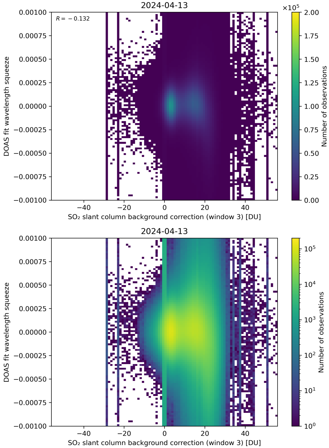
Figure 122: Scatter density plot of “SO 2 slant column background correction (window 3)” against “DOAS fit wavelength squeeze” for 2024-04-12 to 2024-04-14.
