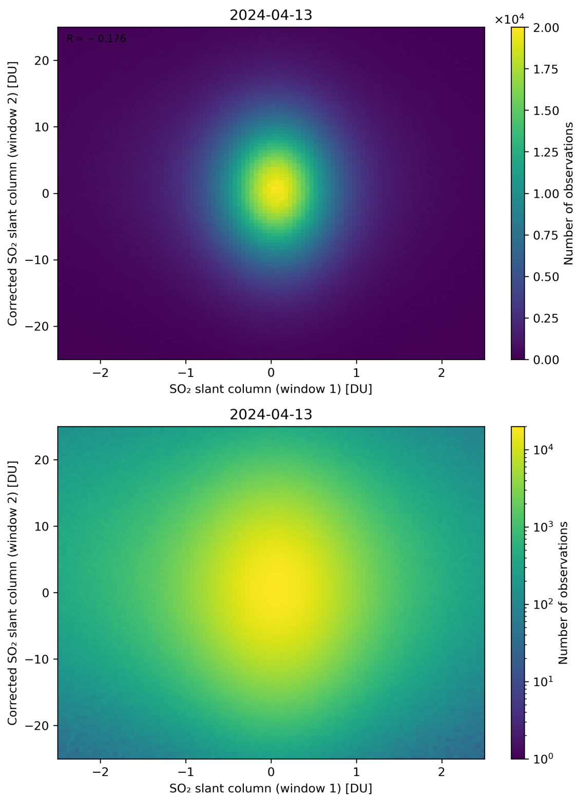
Figure 233: Scatter density plot of “SO 2 slant column (window 1)” against “Corrected SO 2 slant column (window 2)” for 2024-04-12 to 2024-04-14.
