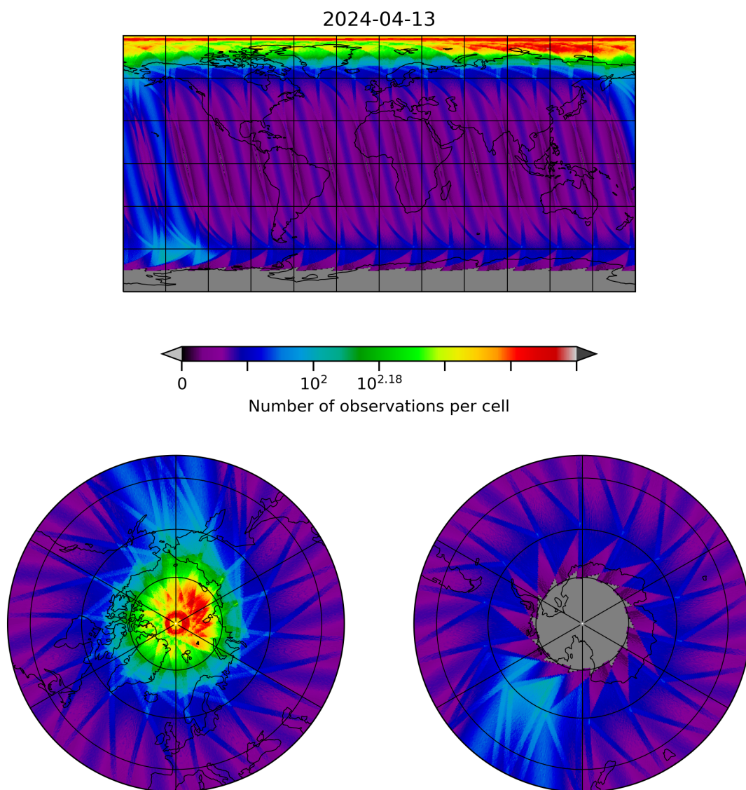
Figure 28: Map of the number of observations for 2024-04-12 to 2024-04-14
