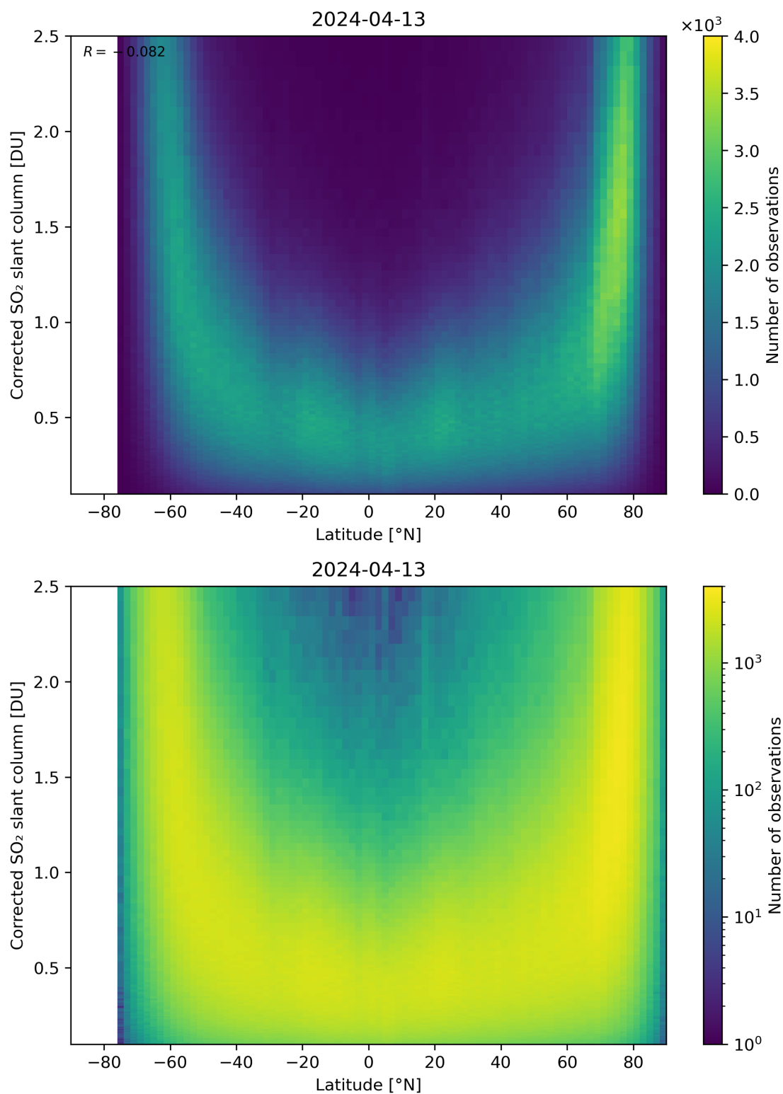
Figure 146: Scatter density plot of “Latitude” against “Corrected SO 2 slant column” for 2024-04-12 to 2024-04-14.
