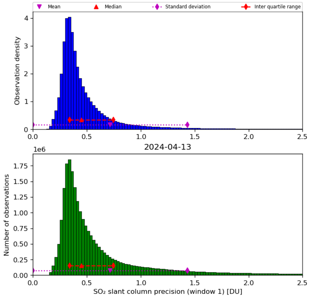
Figure 57: Histogram of “SO 2 slant column precision (window 1)” for 2024-04-12 to 2024-04-14
