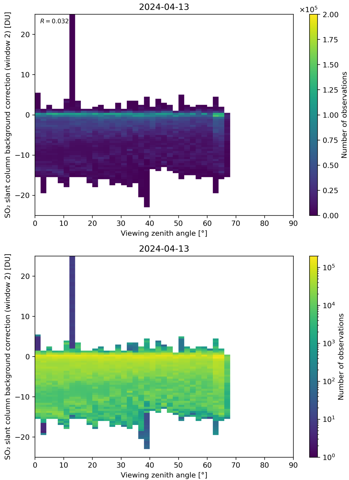
Figure 309: Scatter density plot of “Viewing zenith angle” against “SO 2 slant column background correction (window 2)” for 2024-04-12 to 2024-04-14.
