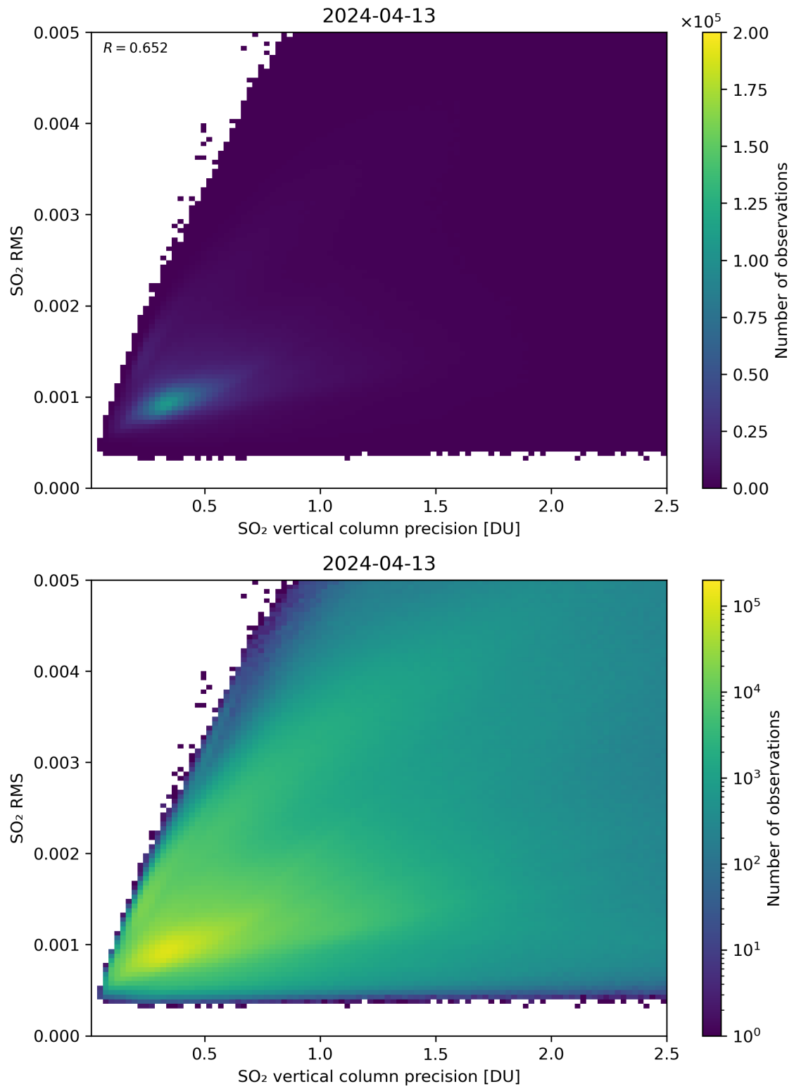
Figure 284: Scatter density plot of “SO 2 vertical column precision” against “SO 2 RMS” for 2024-04-12 to 2024-04-14.
