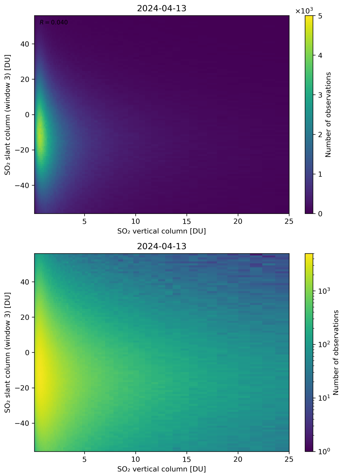
Figure 303: Scatter density plot of “SO 2 vertical column” against “SO 2 slant column (window 3)” for 2024-04-12 to 2024-04-14.
