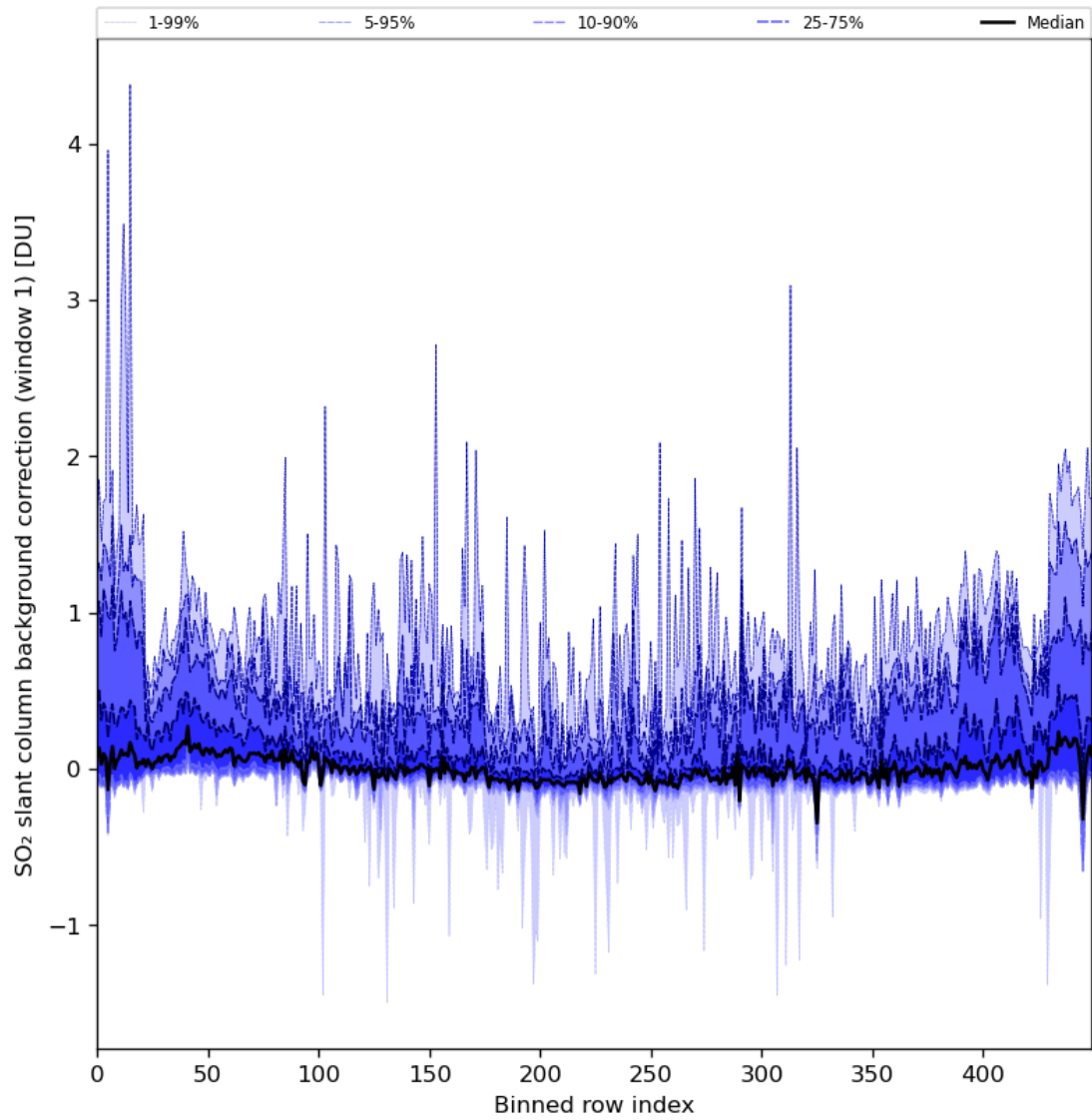
Figure 82: Along track statistics of “SO 2 slant column background correction (window 1)” for 2024-04-12 to 2024-04-14
