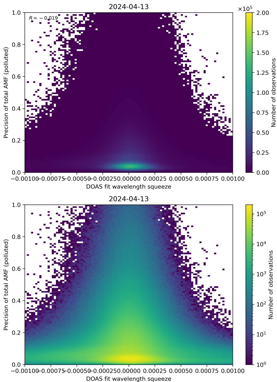
Figure 135: Scatter density plot of “DOAS fit wavelength squeeze” against “Precision of total AMF (polluted)” for 2024-04-12 to 2024-04-14.
