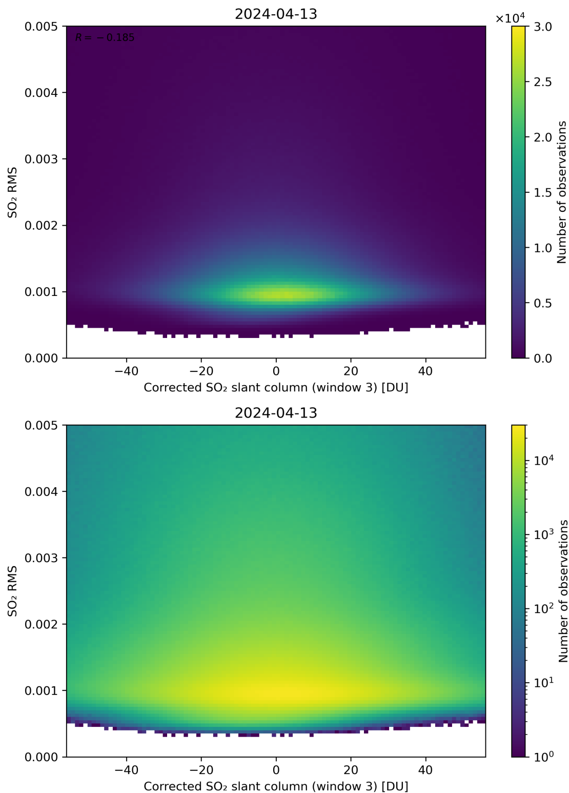
Figure 208: Scatter density plot of “Corrected SO 2 slant column (window 3)” against “SO 2 RMS” for 2024-04-12 to 2024-04-14.
