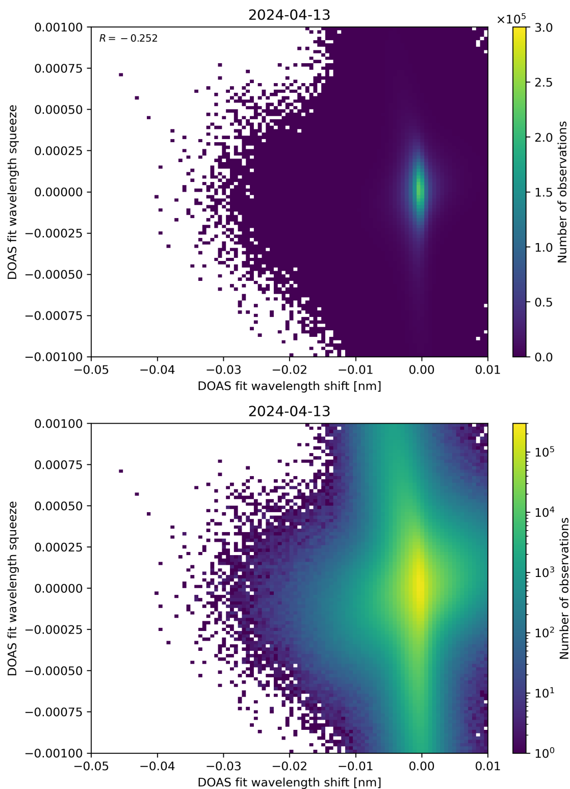
Figure 127: Scatter density plot of “DOAS fit wavelength shift” against “DOAS fit wavelength squeeze” for 2024-04-12 to 2024-04-14.
