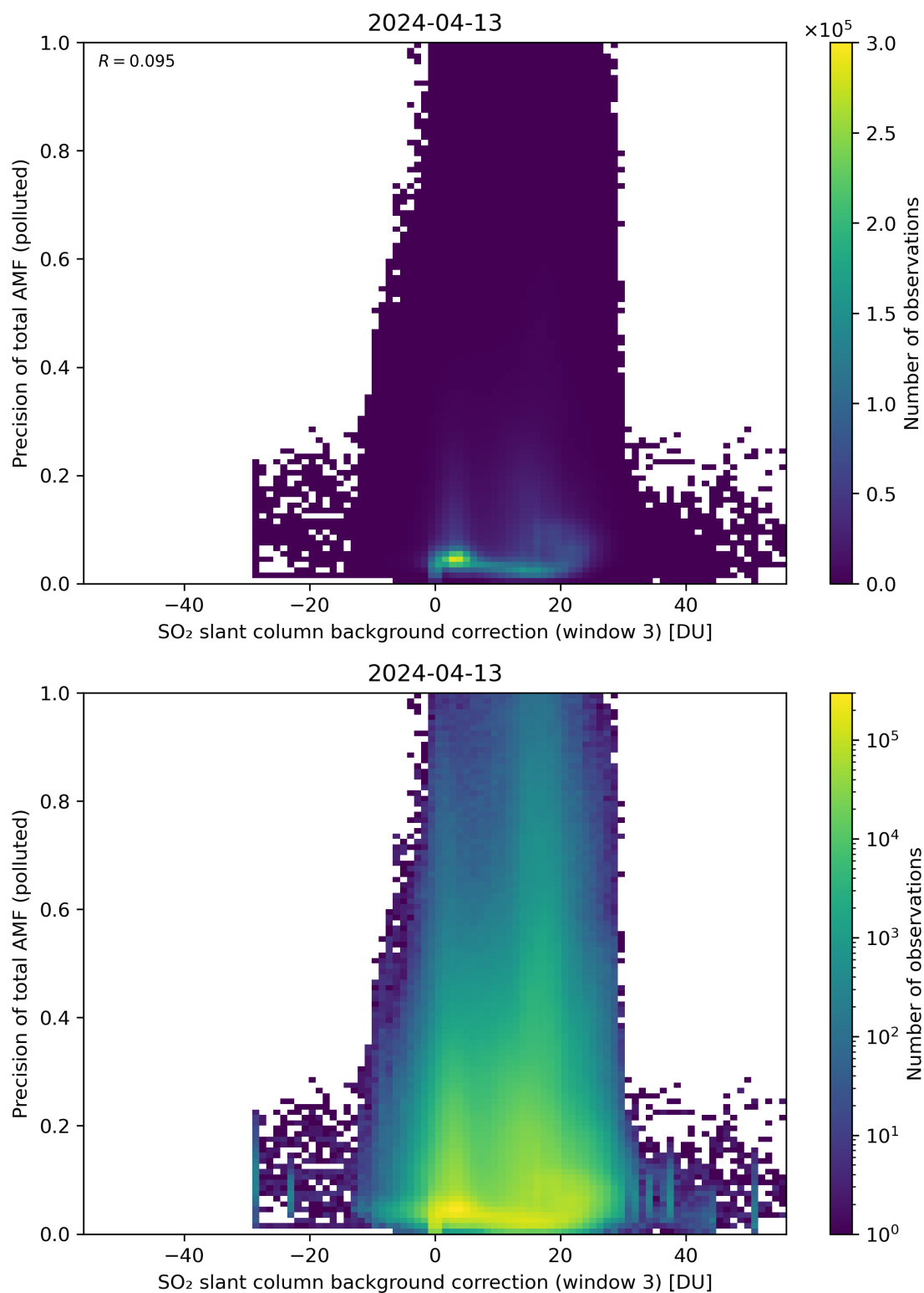
Figure 126: Scatter density plot of “SO 2 slant column background correction (window 3)” against “Precision of total AMF (polluted)” for 2024-04-12 to 2024-04-14.
