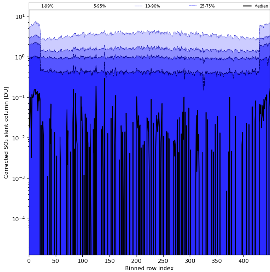
Figure 78: Along track statistics of “Corrected SO 2 slant column” for 2024-04-12 to 2024-04-14
