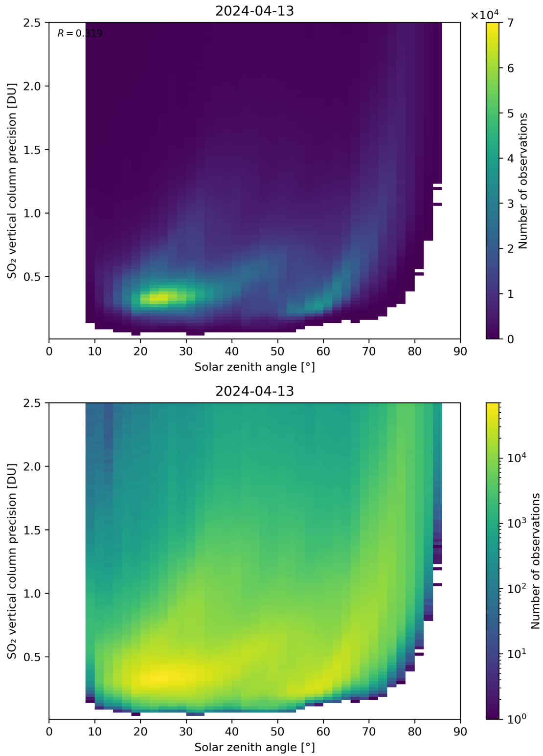
Figure 177: Scatter density plot of “Solar zenith angle” against “SO 2 vertical column precision” for 2024-04-12 to 2024-04-14.
