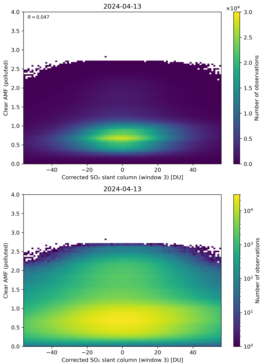
Figure 209: Scatter density plot of “Corrected SO 2 slant column (window 3)” against “Clear AMF (polluted)” for 2024-04-12 to 2024-04-14.
