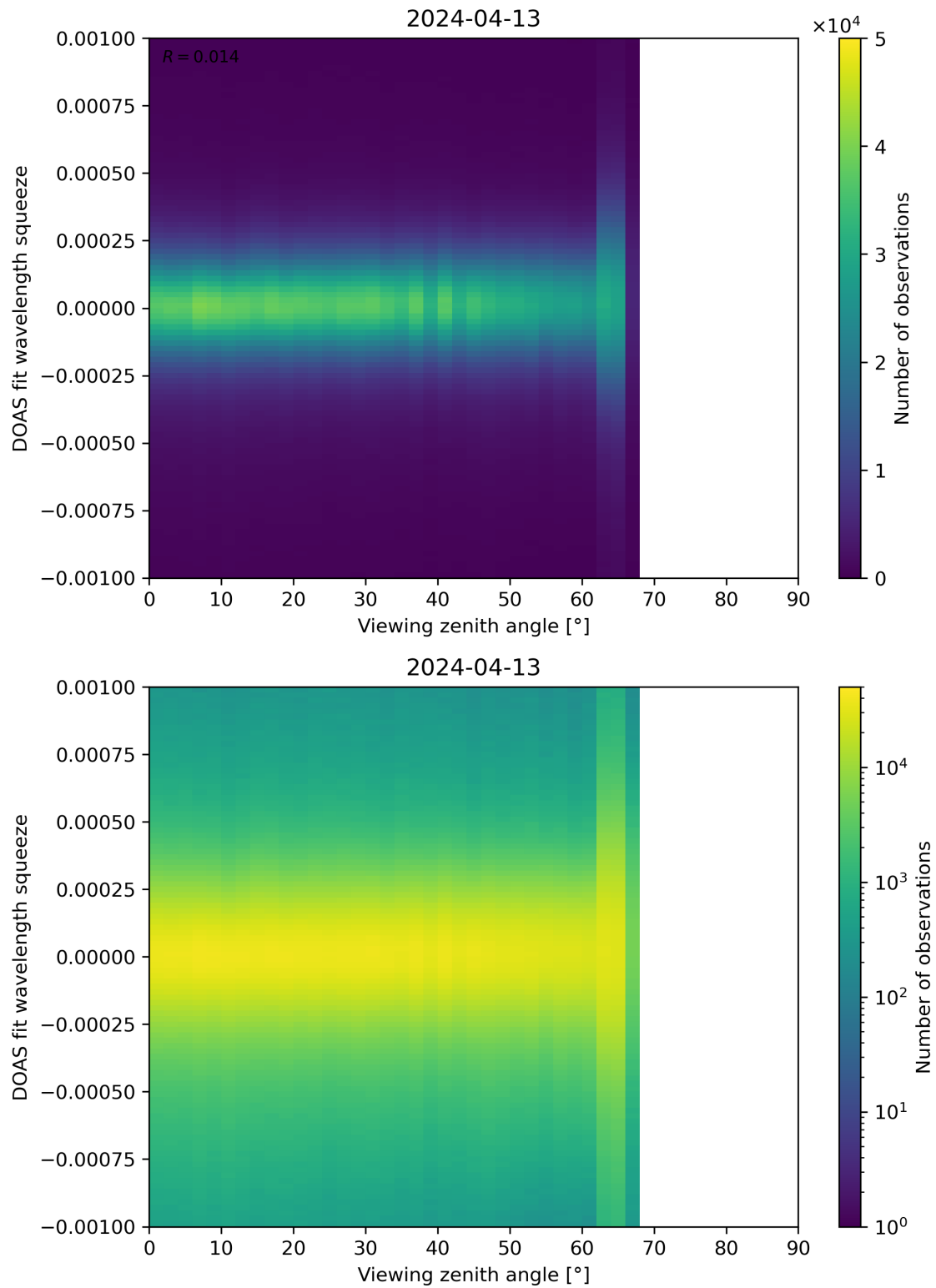
Figure 312: Scatter density plot of “Viewing zenith angle” against “DOAS fit wavelength squeeze” for 2024-04-12 to 2024-04-14.
