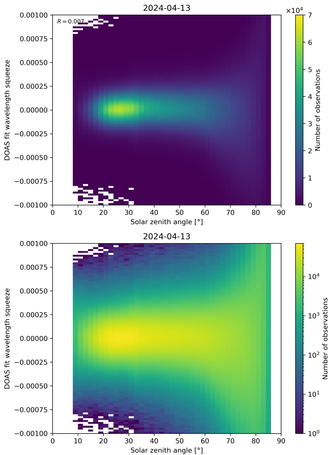
Figure 162: Scatter density plot of “Solar zenith angle” against “DOAS fit wavelength squeeze” for 2024-04-12 to 2024-04-14.
