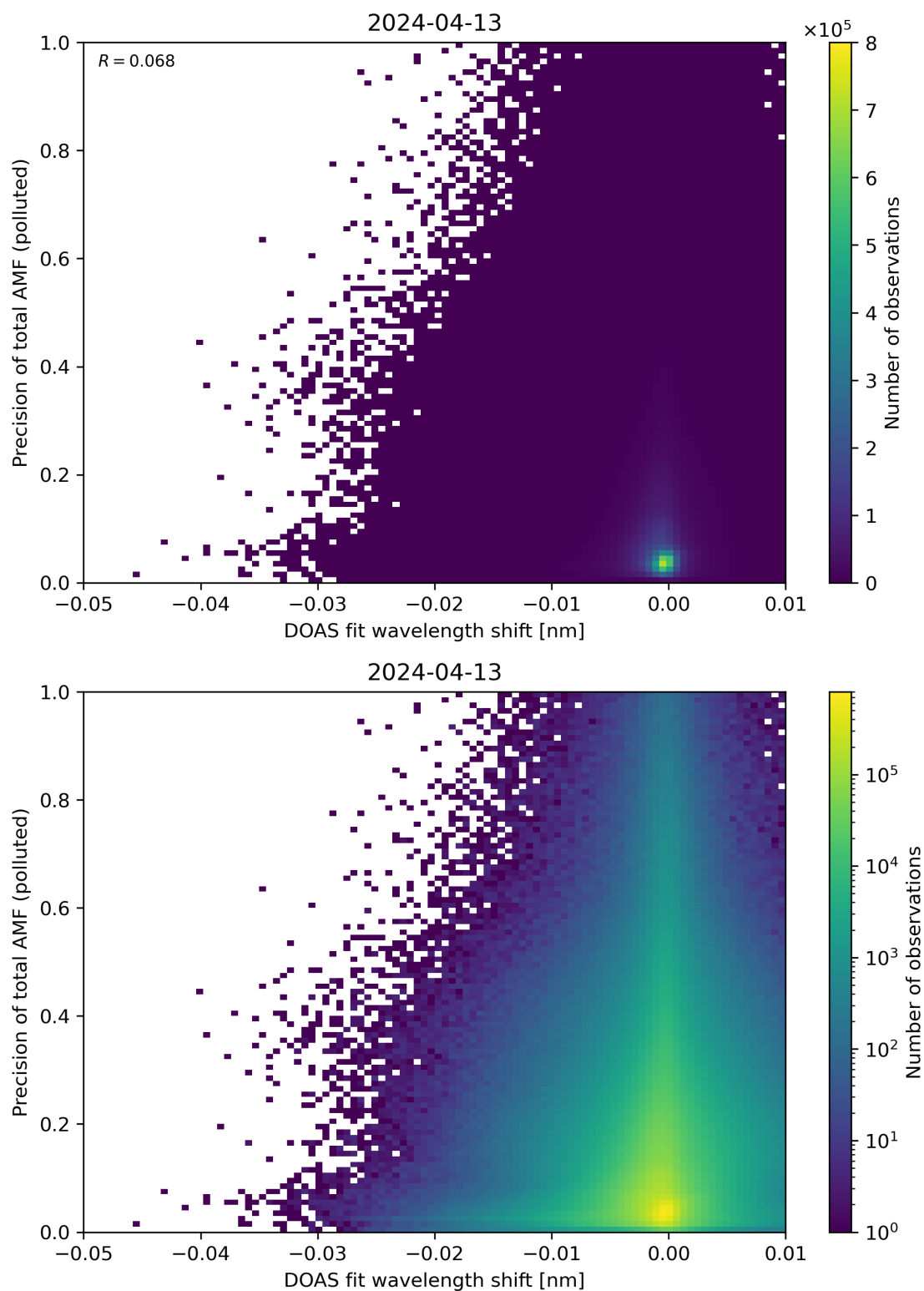
Figure 131: Scatter density plot of “DOAS fit wavelength shift” against “Precision of total AMF (polluted)” for 2024-04-12 to 2024-04-14.
