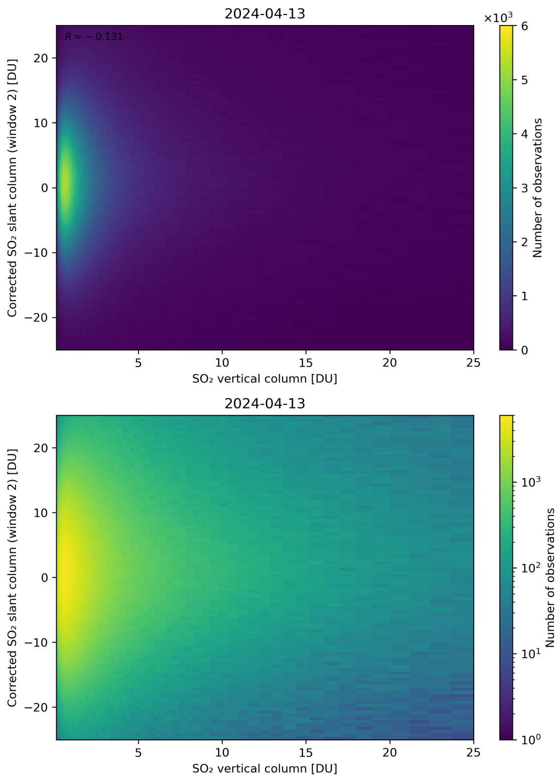
Figure 298: Scatter density plot of “SO 2 vertical column” against “Corrected SO 2 slant column (window 2)” for 2024-04-12 to 2024-04-14.
