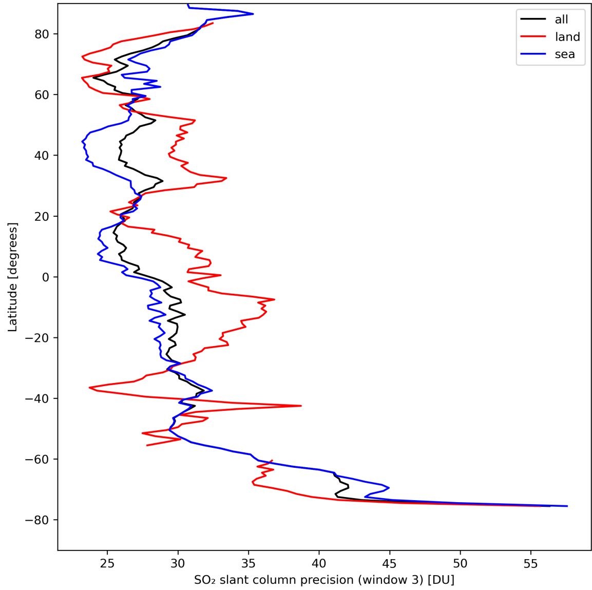
Figure 42: Zonal average of “SO 2 slant column precision (window 3)” for 2024-04-12 to 2024-04-14.
