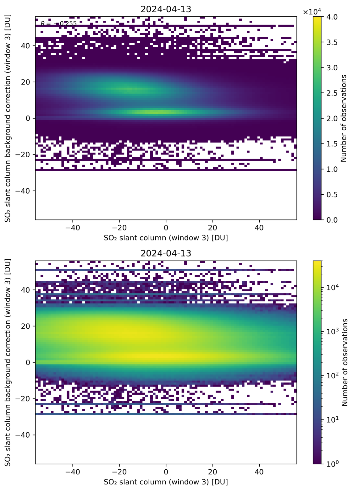
Figure 253: Scatter density plot of “SO 2 slant column (window 3)” against “SO 2 slant column background correction (window 3)” for 2024-04-12 to 2024-04-14.
