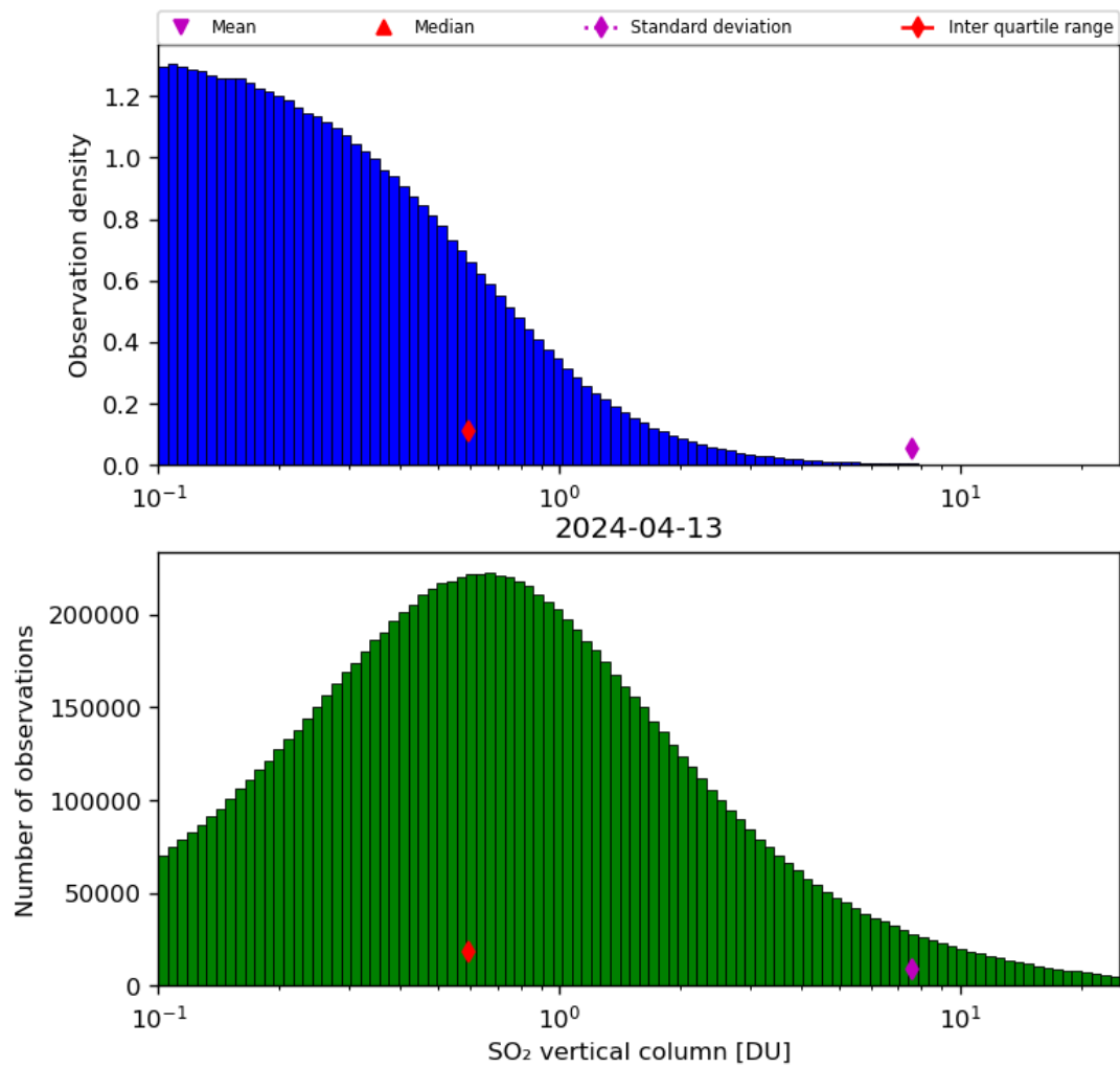
Figure 53: Histogram of “SO 2 vertical column” for 2024-04-12 to 2024-04-14
