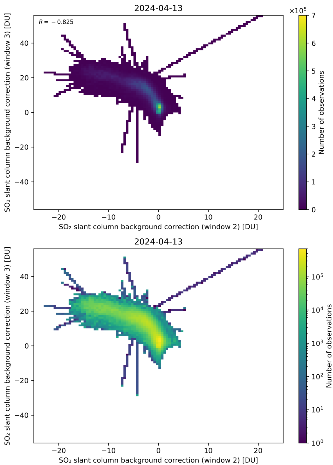
Figure 111: Scatter density plot of “SO 2 slant column background correction (window 2)” against “SO 2 slant column background correction (window 3)” for 2024-04-12 to 2024-04-14.
