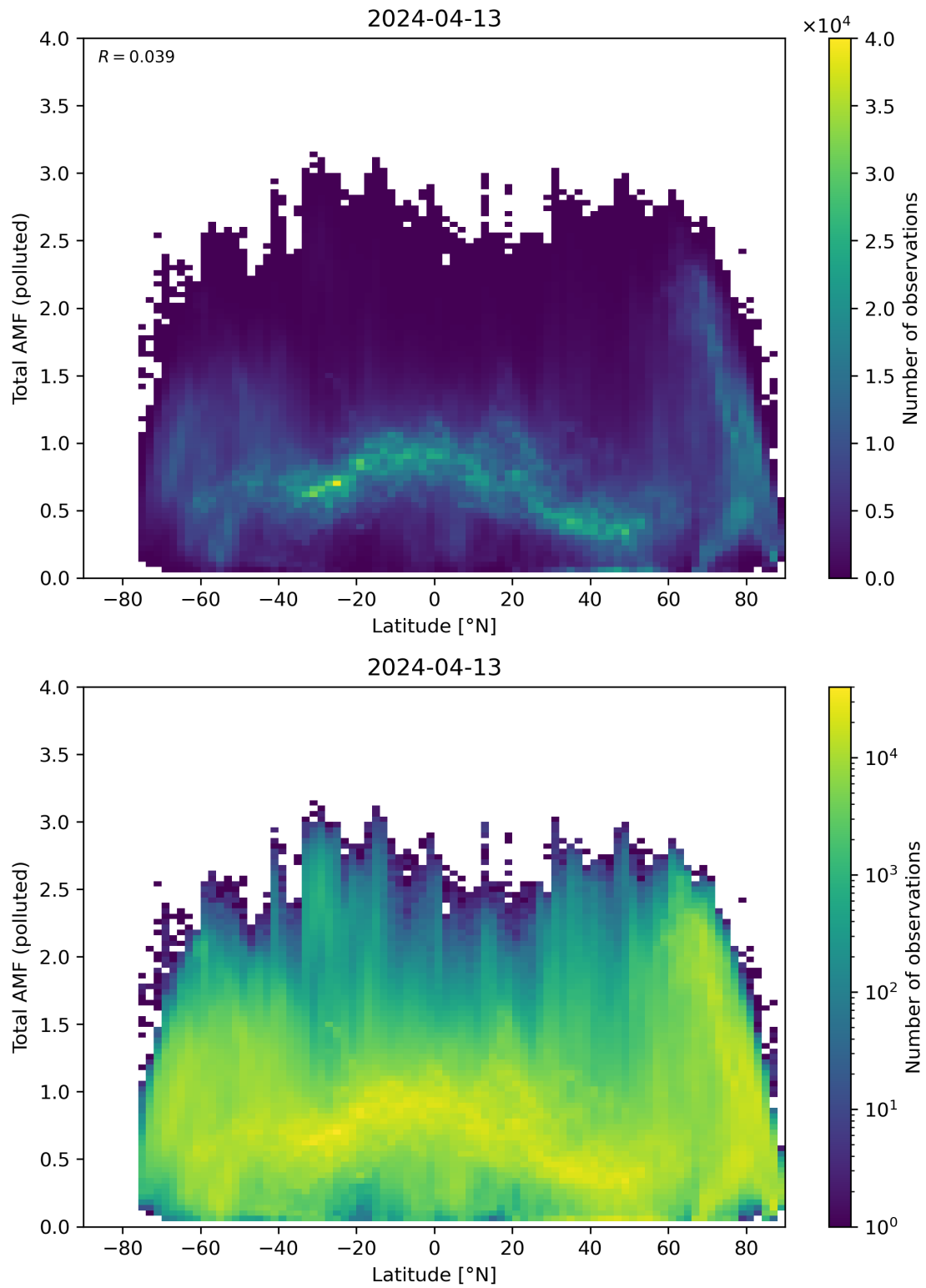
Figure 154: Scatter density plot of “Latitude” against “Total AMF (polluted)” for 2024-04-12 to 2024-04-14.
