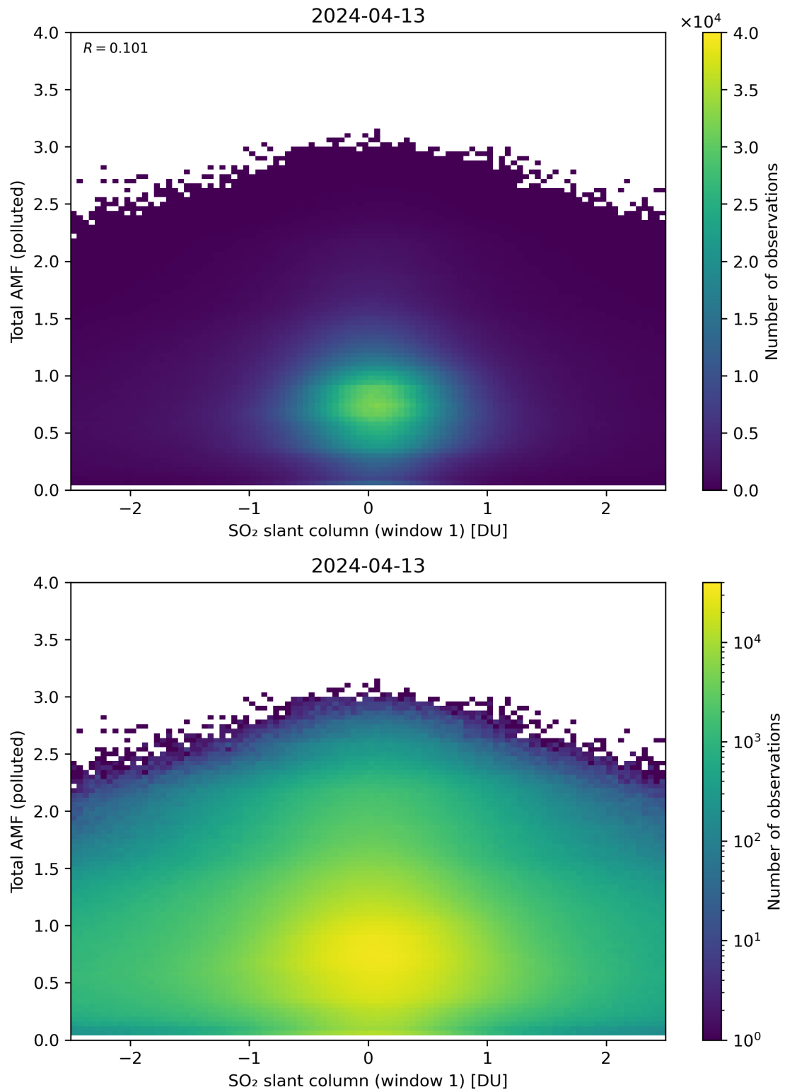
Figure 239: Scatter density plot of “SO 2 slant column (window 1)” against “Total AMF (polluted)” for 2024-04-12 to 2024-04-14.
