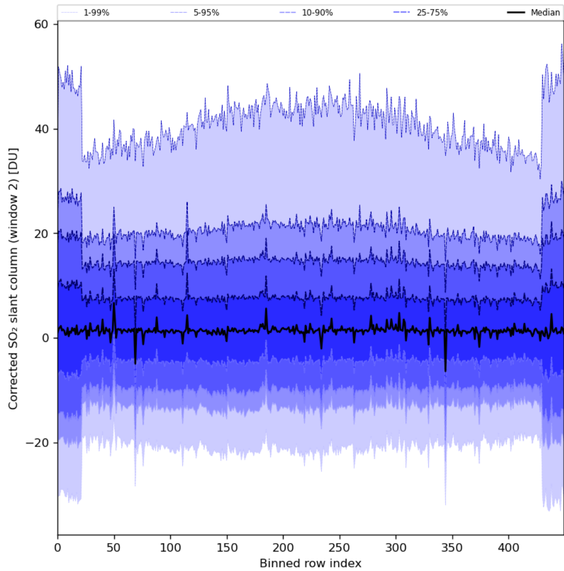
Figure 85: Along track statistics of “Corrected SO 2 slant column (window 2)” for 2024-04-12 to 2024-04-14
