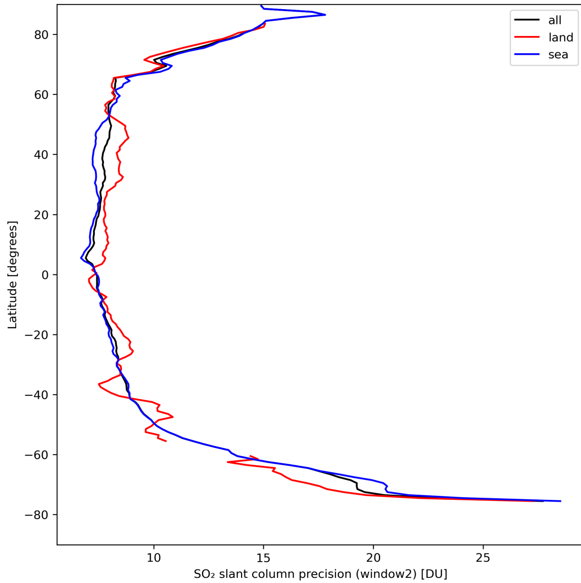
Figure 38: Zonal average of “SO 2 slant column precision (window2)” for 2024-04-12 to 2024-04-14.
