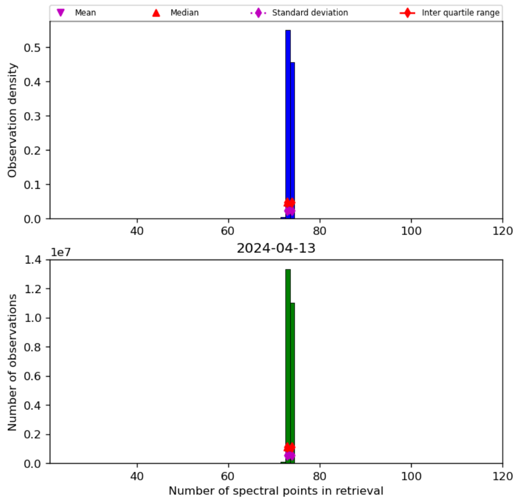
Figure 74: Histogram of “Number of spectral points in retrieval” for 2024-04-12 to 2024-04-14
