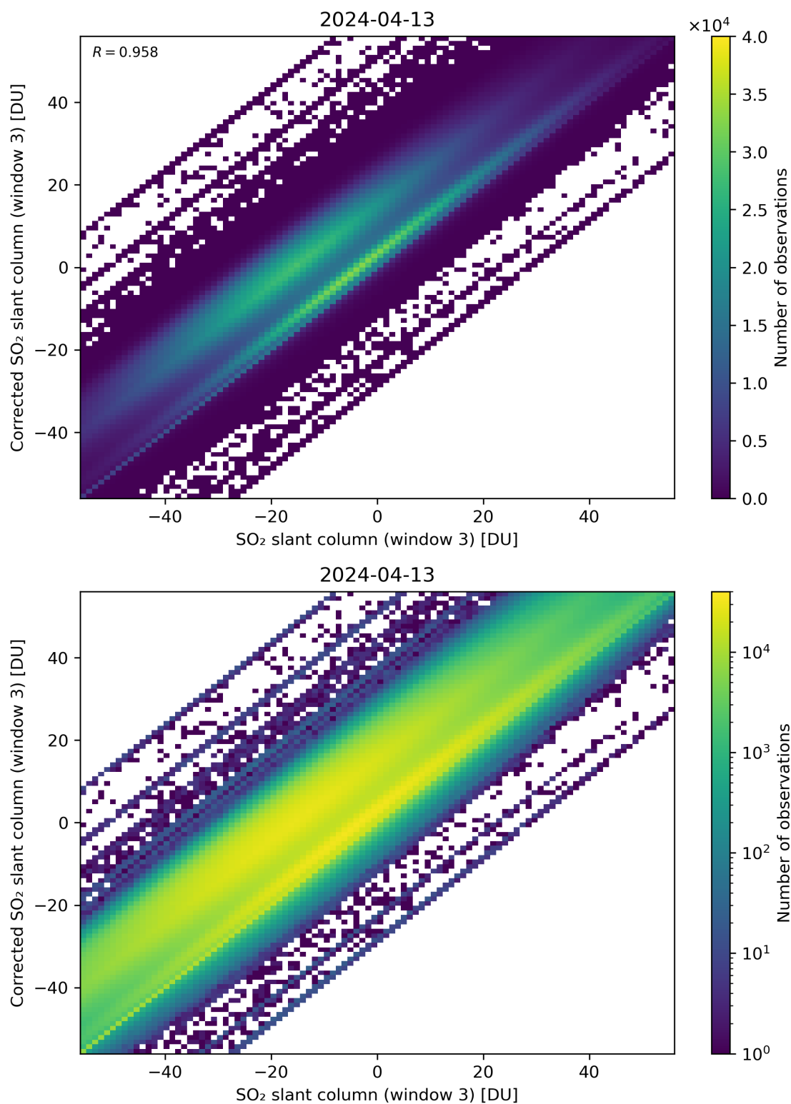
Figure 266: Scatter density plot of “SO 2 slant column (window 3)” against “Corrected SO 2 slant column (window 3)” for 2024-04-12 to 2024-04-14.
