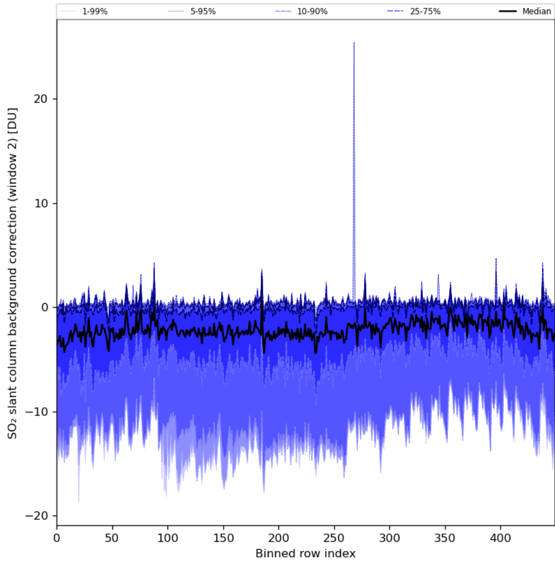
Figure 86: Along track statistics of “SO 2 slant column background correction (window 2)” for 2024-04-12 to 2024-04-14
