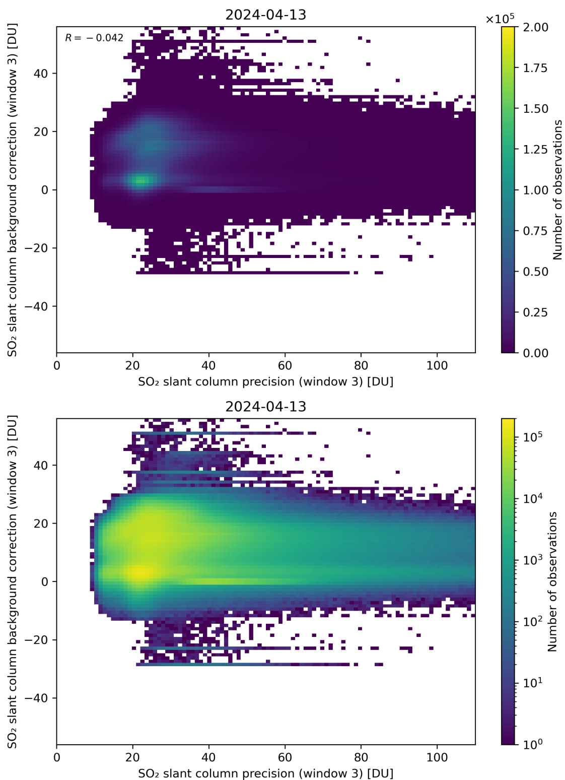
Figure 257: Scatter density plot of “SO 2 slant column precision (window 3)” against “SO 2 slant column background correction (window 3)” for 2024-04-12 to 2024-04-14.
