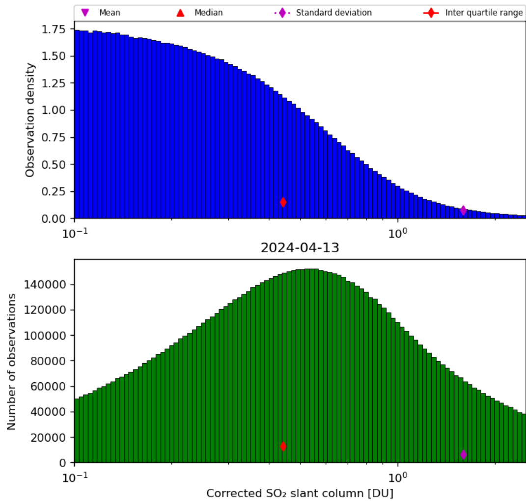
Figure 55: Histogram of “Corrected SO 2 slant column” for 2024-04-12 to 2024-04-14
