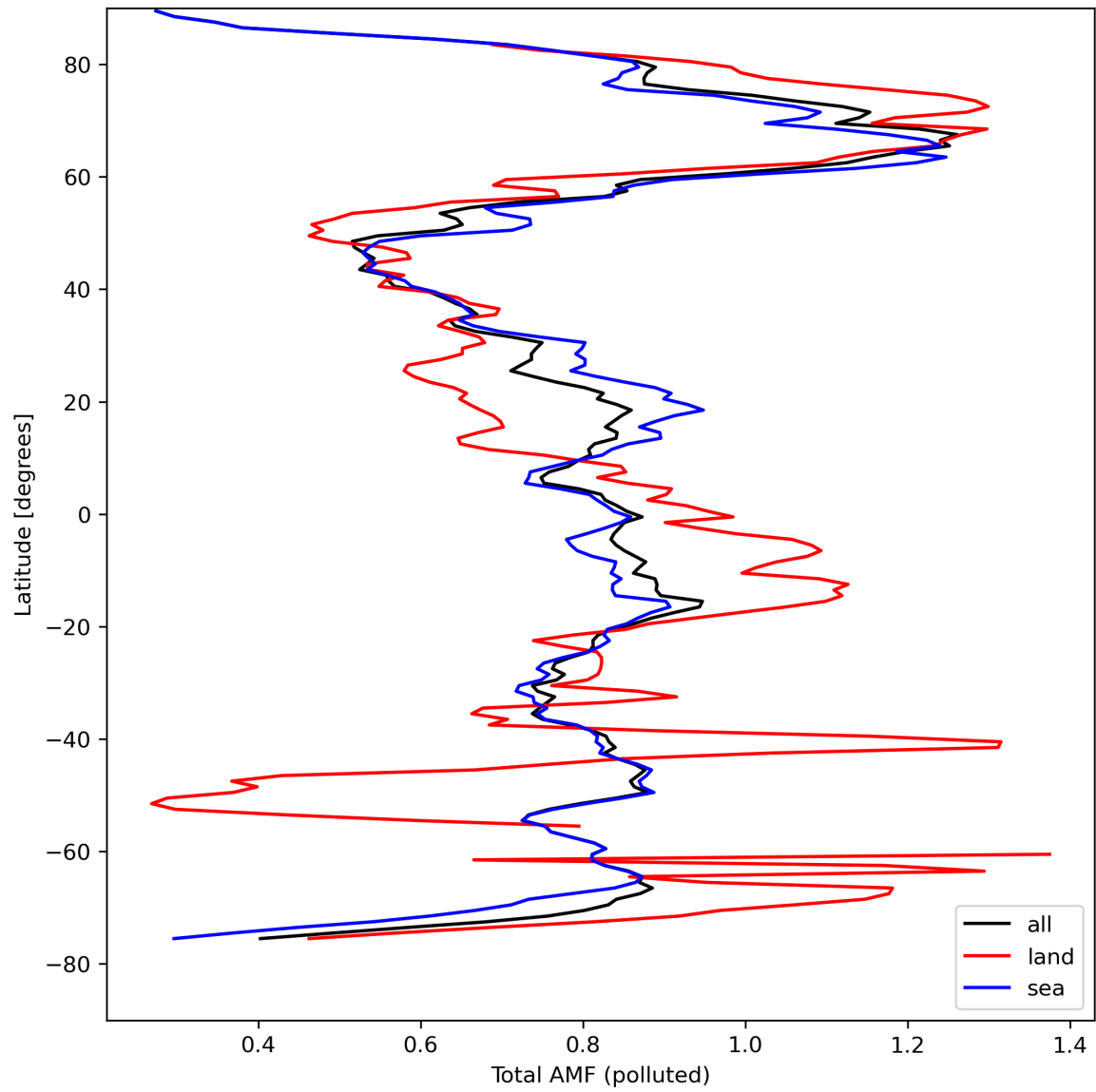
Figure 48: Zonal average of “Total AMF (polluted)” for 2024-04-12 to 2024-04-14.
