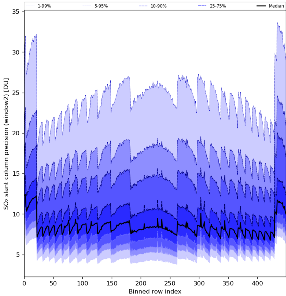
Figure 84: Along track statistics of “SO 2 slant column precision (window2)” for 2024-04-12 to 2024-04-14
