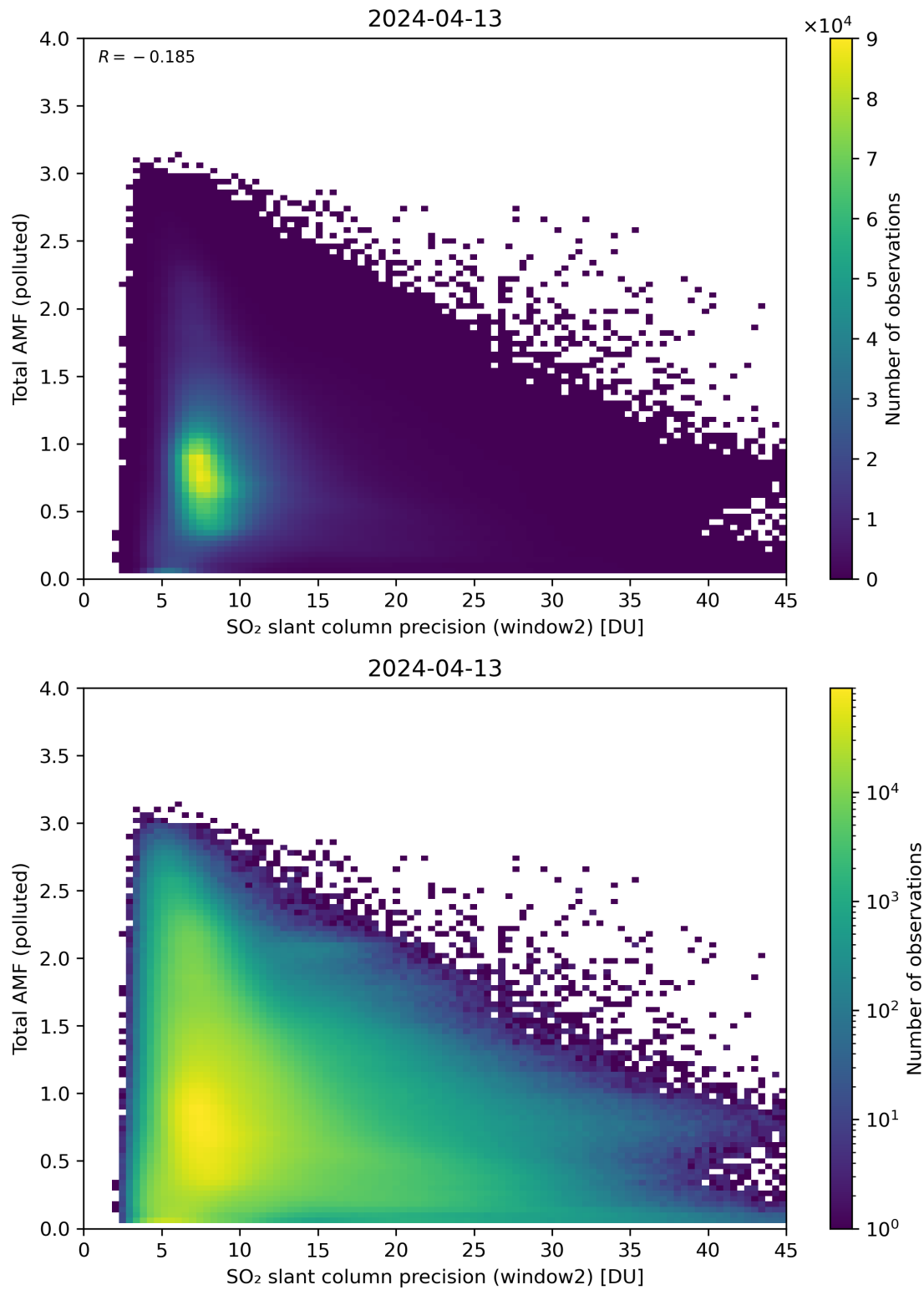
Figure 251: Scatter density plot of “SO 2 slant column precision (window2)” against “Total AMF (polluted)” for 2024-04-12 to 2024-04-14.
