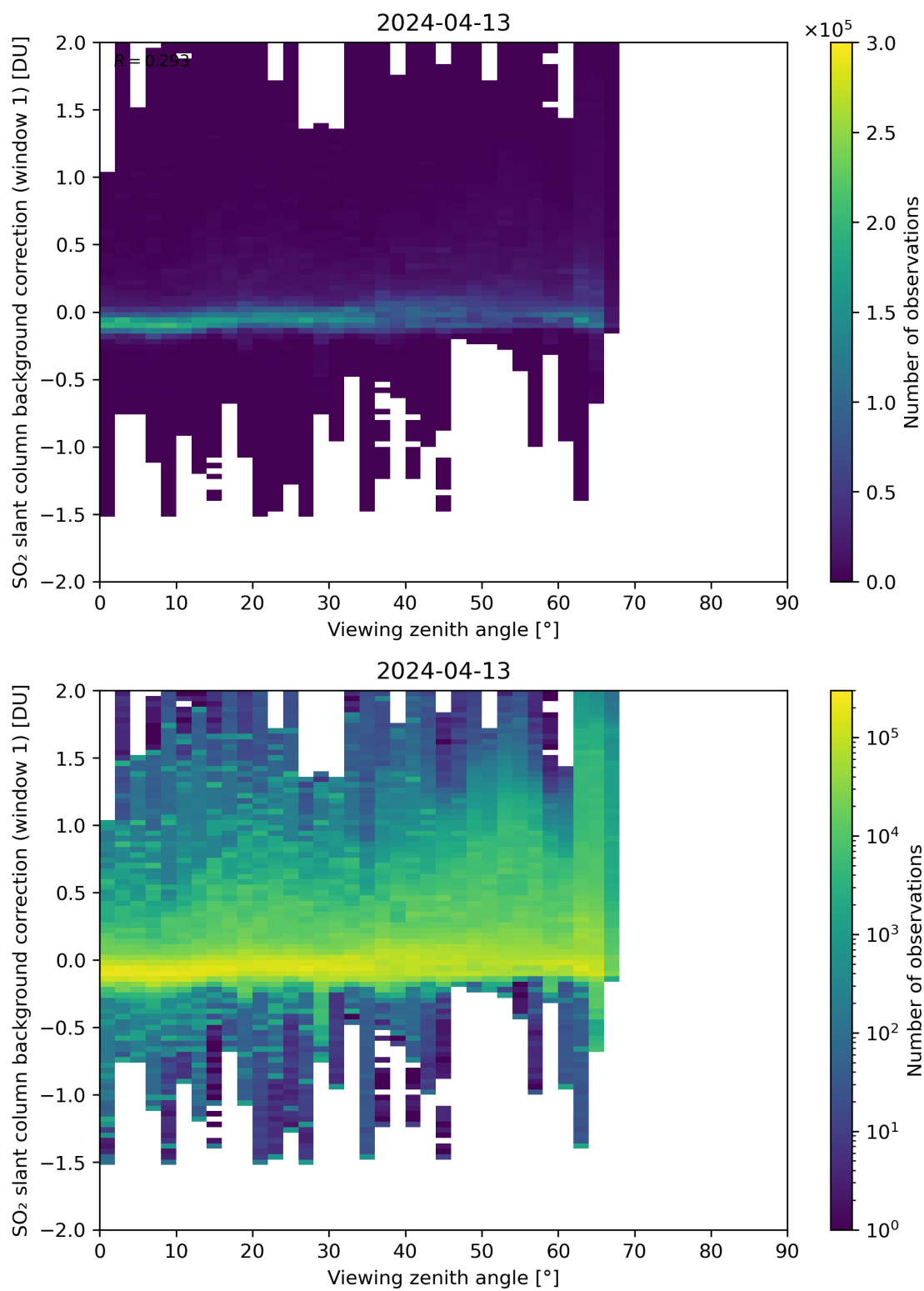
Figure 308: Scatter density plot of “Viewing zenith angle” against “SO 2 slant column background correction (window 1)” for 2024-04-12 to 2024-04-14.
