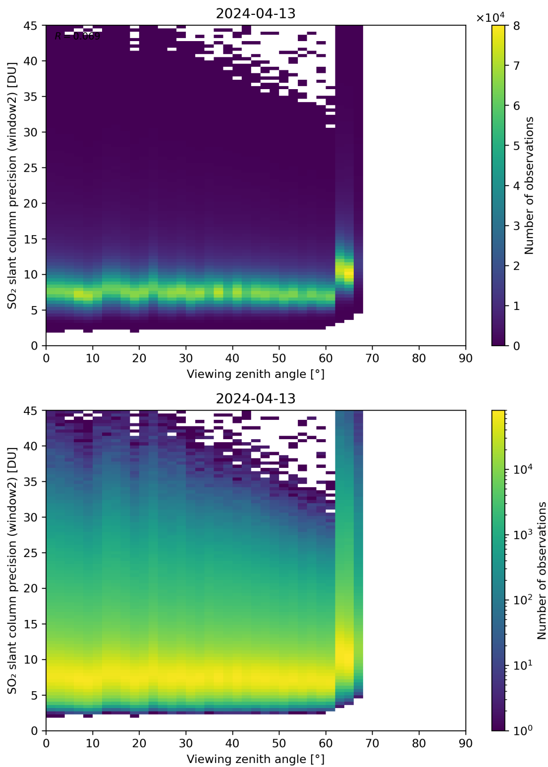
Figure 322: Scatter density plot of “Viewing zenith angle” against “SO 2 slant column precision (window2)” for 2024-04-12 to 2024-04-14.
