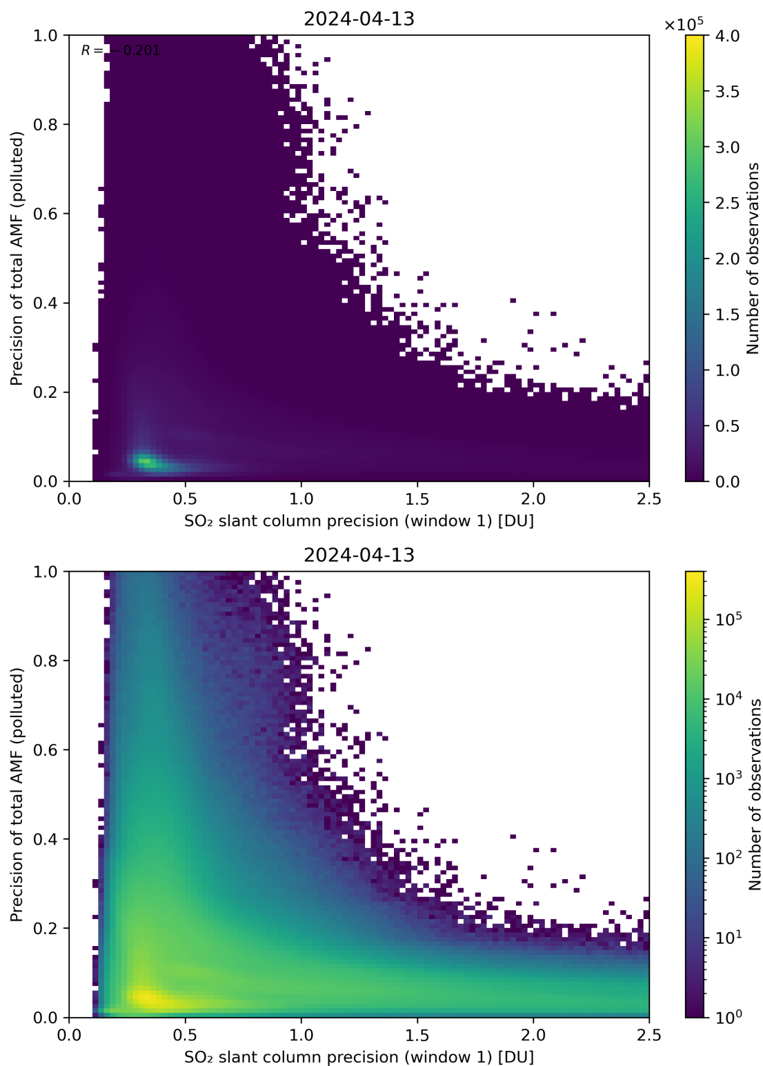
Figure 231: Scatter density plot of “SO 2 slant column precision (window 1)” against “Precision of total AMF (polluted)” for 2024-04-12 to 2024-04-14.
