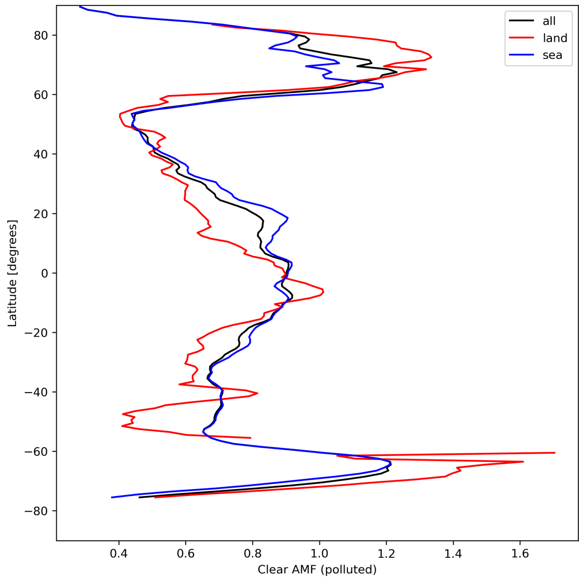
Figure 50: Zonal average of “Clear AMF (polluted)” for 2024-04-12 to 2024-04-14.
