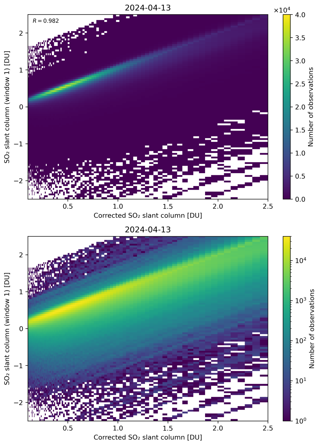
Figure 187: Scatter density plot of “Corrected SO 2 slant column” against “SO 2 slant column (window 1)” for 2024-04-12 to 2024-04-14.
