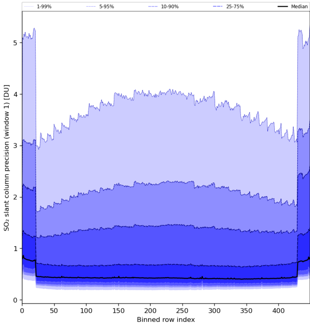
Figure 80: Along track statistics of “SO 2 slant column precision (window 1)” for 2024-04-12 to 2024-04-14
