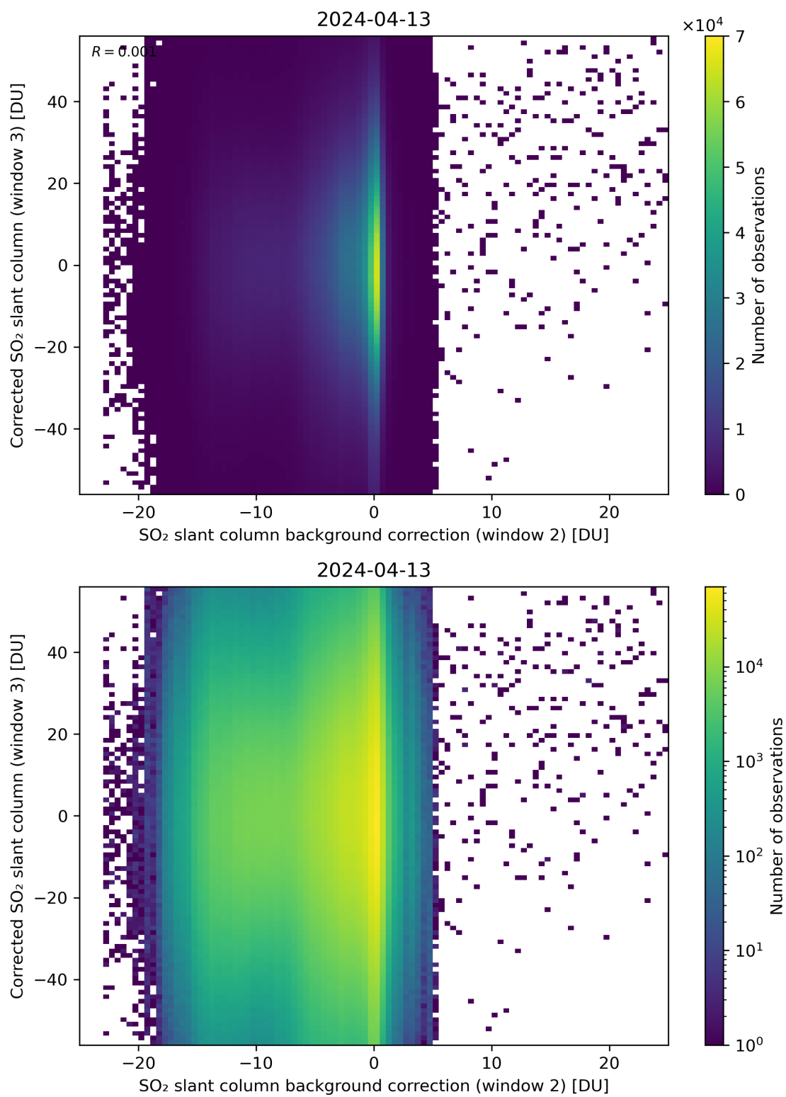
Figure 116: Scatter density plot of “SO 2 slant column background correction (window 2)” against “Corrected SO 2 slant column (window 3)” for 2024-04-12 to 2024-04-14.
