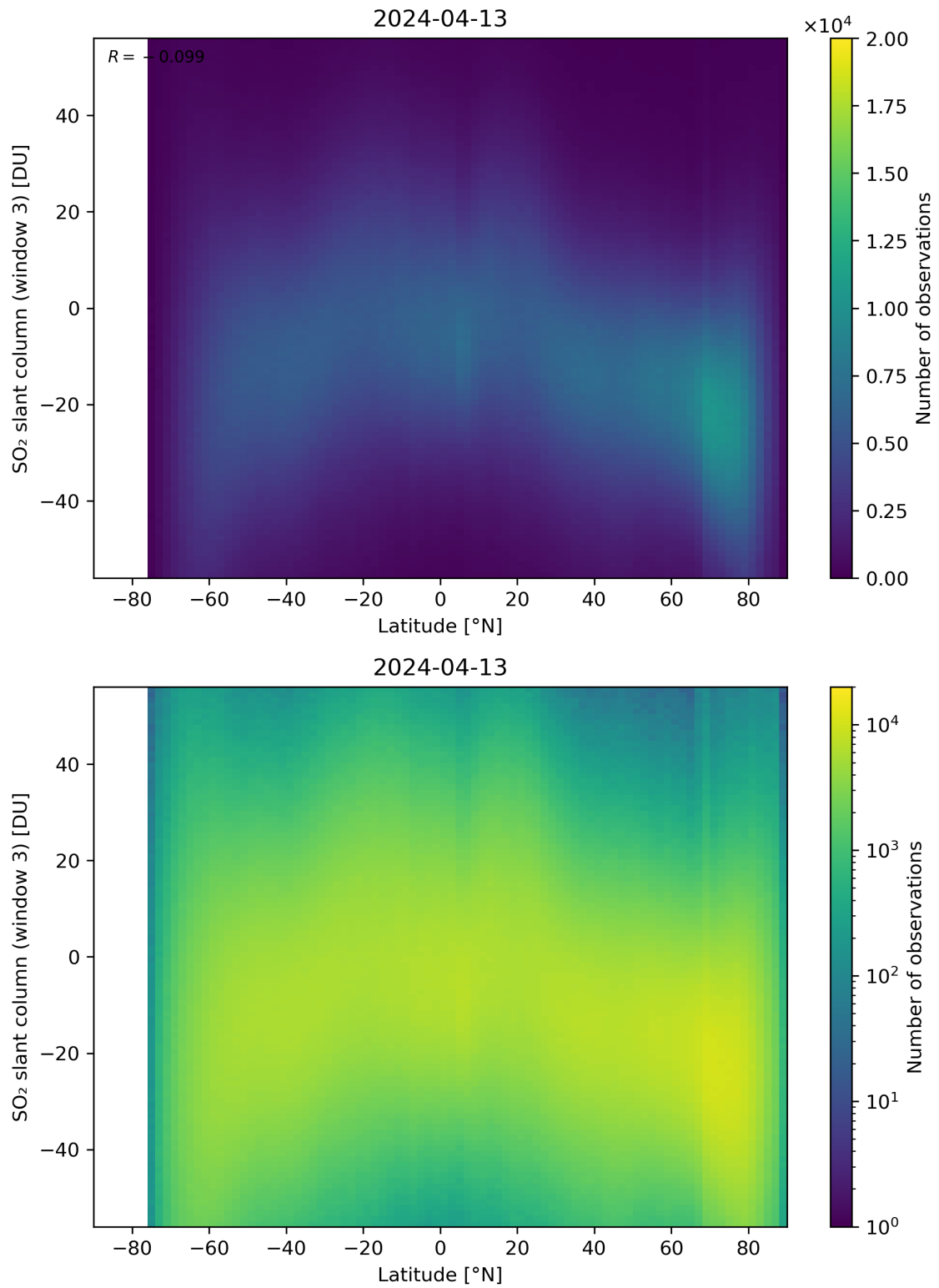
Figure 152: Scatter density plot of “Latitude” against “SO 2 slant column (window 3)” for 2024-04-12 to 2024-04-14.
