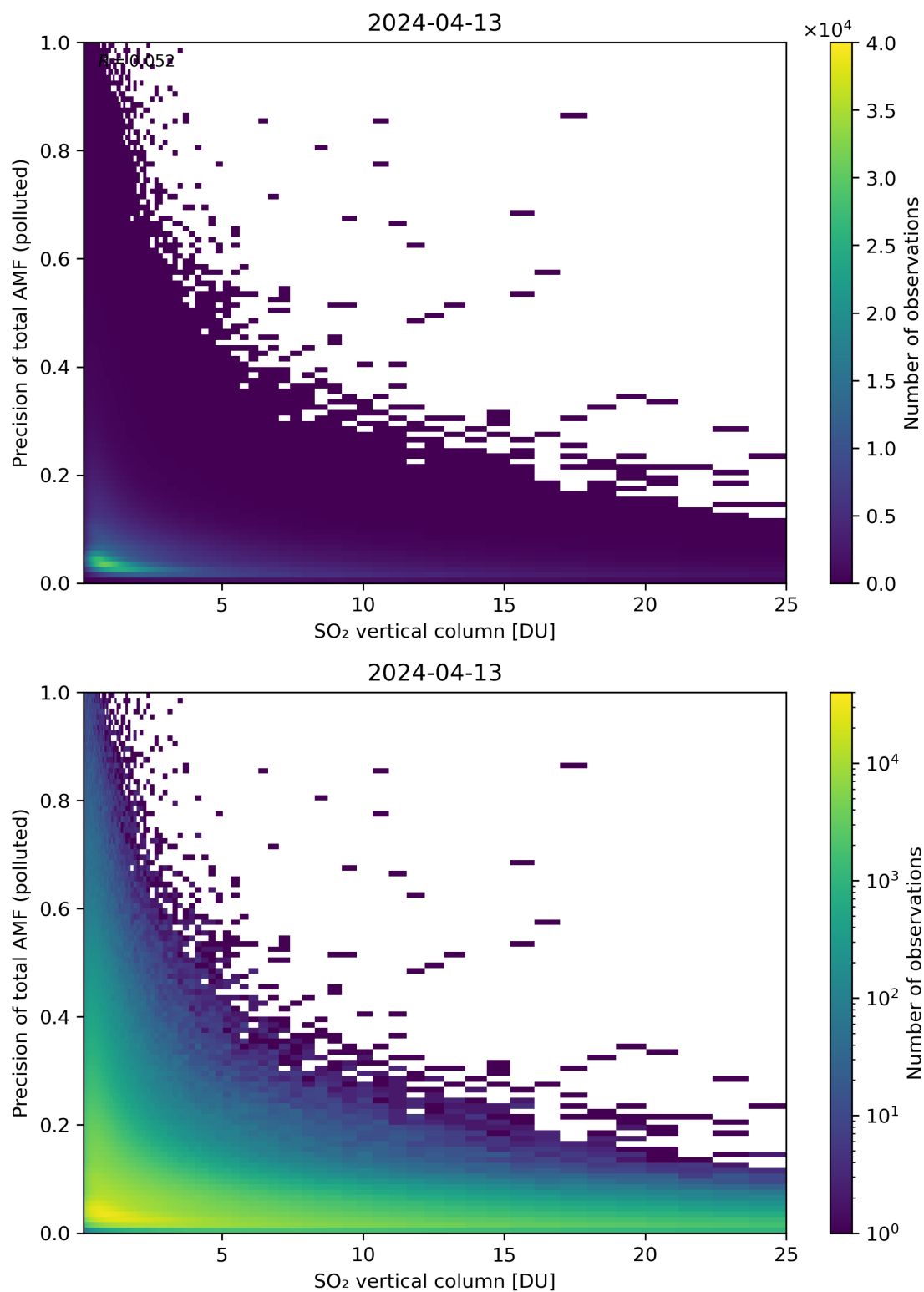
Figure 306: Scatter density plot of “SO 2 vertical column” against “Precision of total AMF (polluted)” for 2024-04-12 to 2024-04-14.
