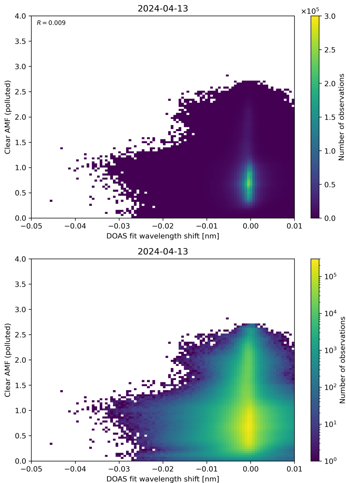
Figure 129: Scatter density plot of “DOAS fit wavelength shift” against “Clear AMF (polluted)” for 2024-04-12 to 2024-04-14.
