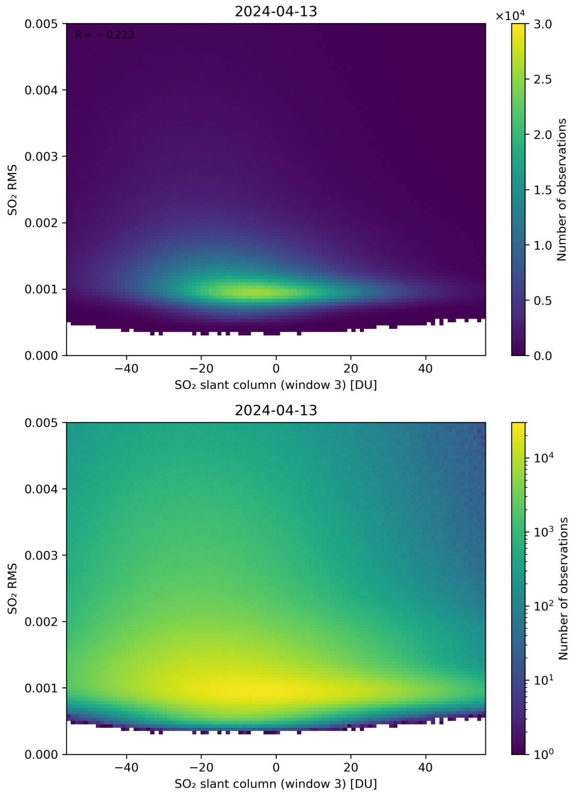
Figure 256: Scatter density plot of “SO 2 slant column (window 3)” against “SO 2 RMS” for 2024-04-12 to 2024-04-14.
