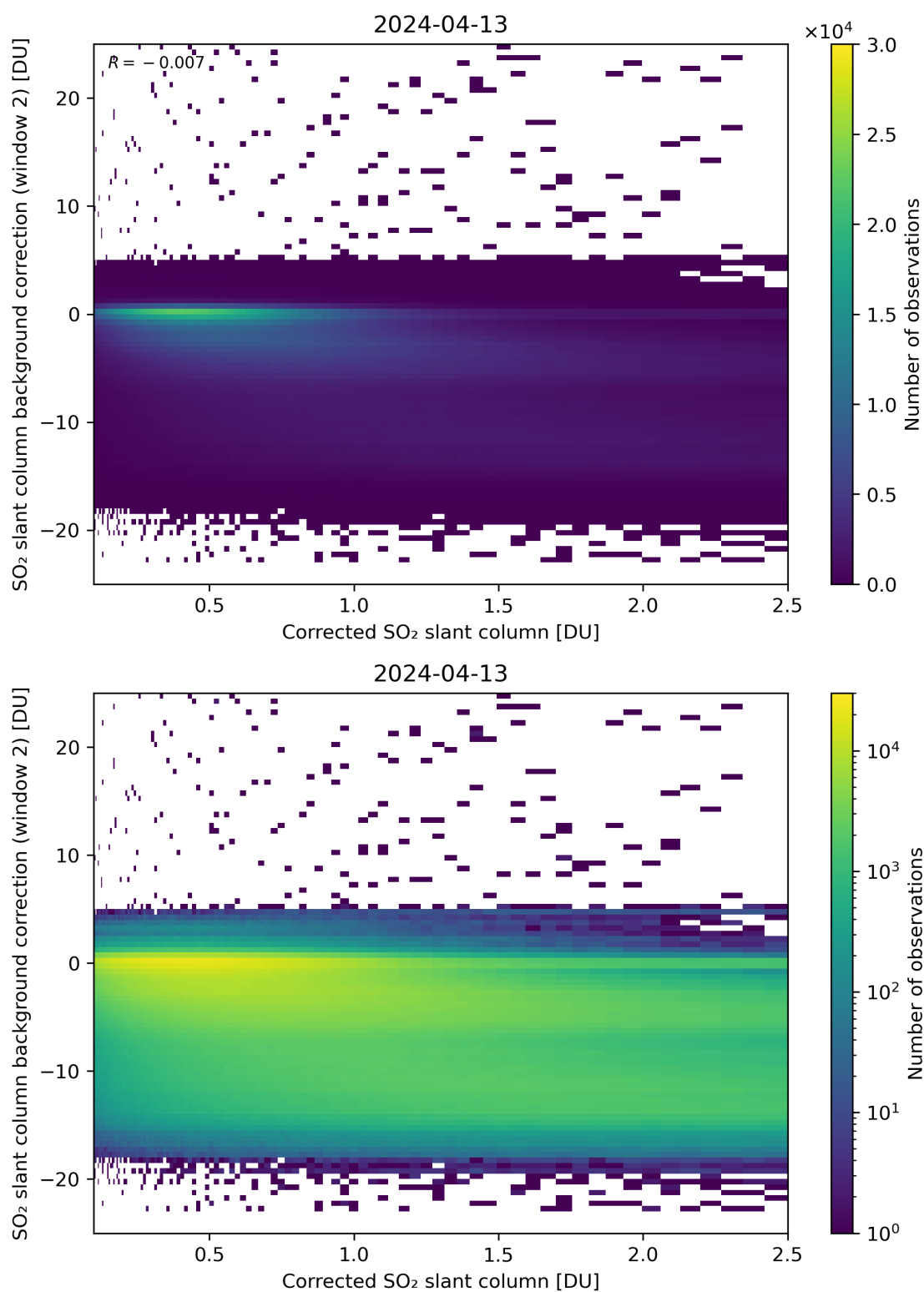
Figure 179: Scatter density plot of “Corrected SO 2 slant column” against “SO 2 slant column background correction (window 2)” for 2024-04-12 to 2024-04-14.
