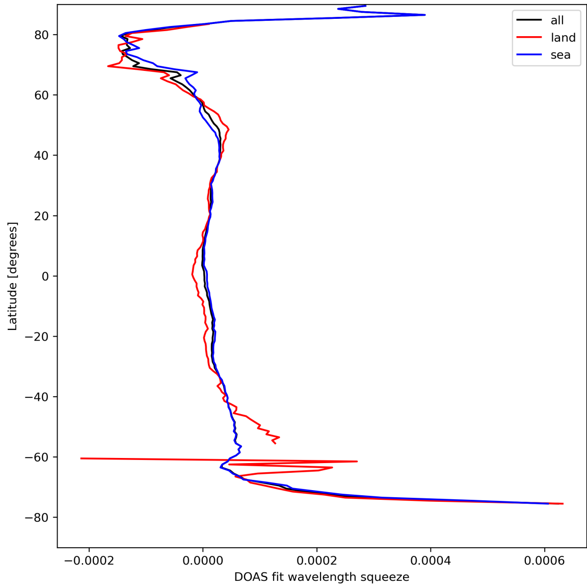
Figure 46: Zonal average of “DOAS fit wavelength squeeze” for 2024-04-12 to 2024-04-14.
