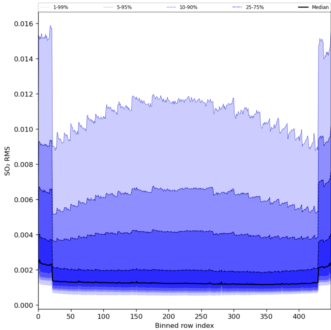
Figure 93: Along track statistics of “SO 2 RMS” for 2024-04-12 to 2024-04-14
