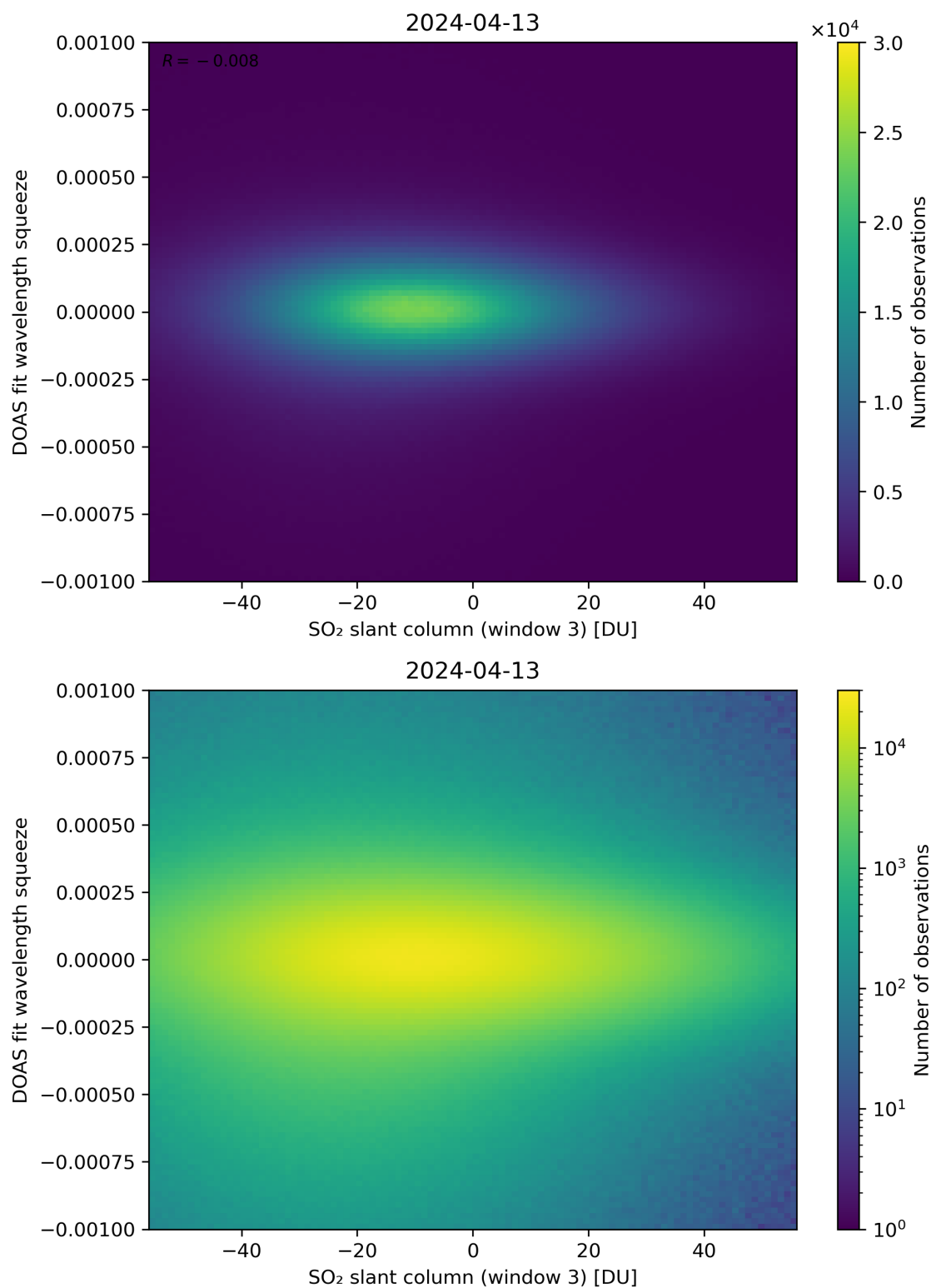
Figure 255: Scatter density plot of “SO 2 slant column (window 3)” against “DOAS fit wavelength squeeze” for 2024-04-12 to 2024-04-14.
