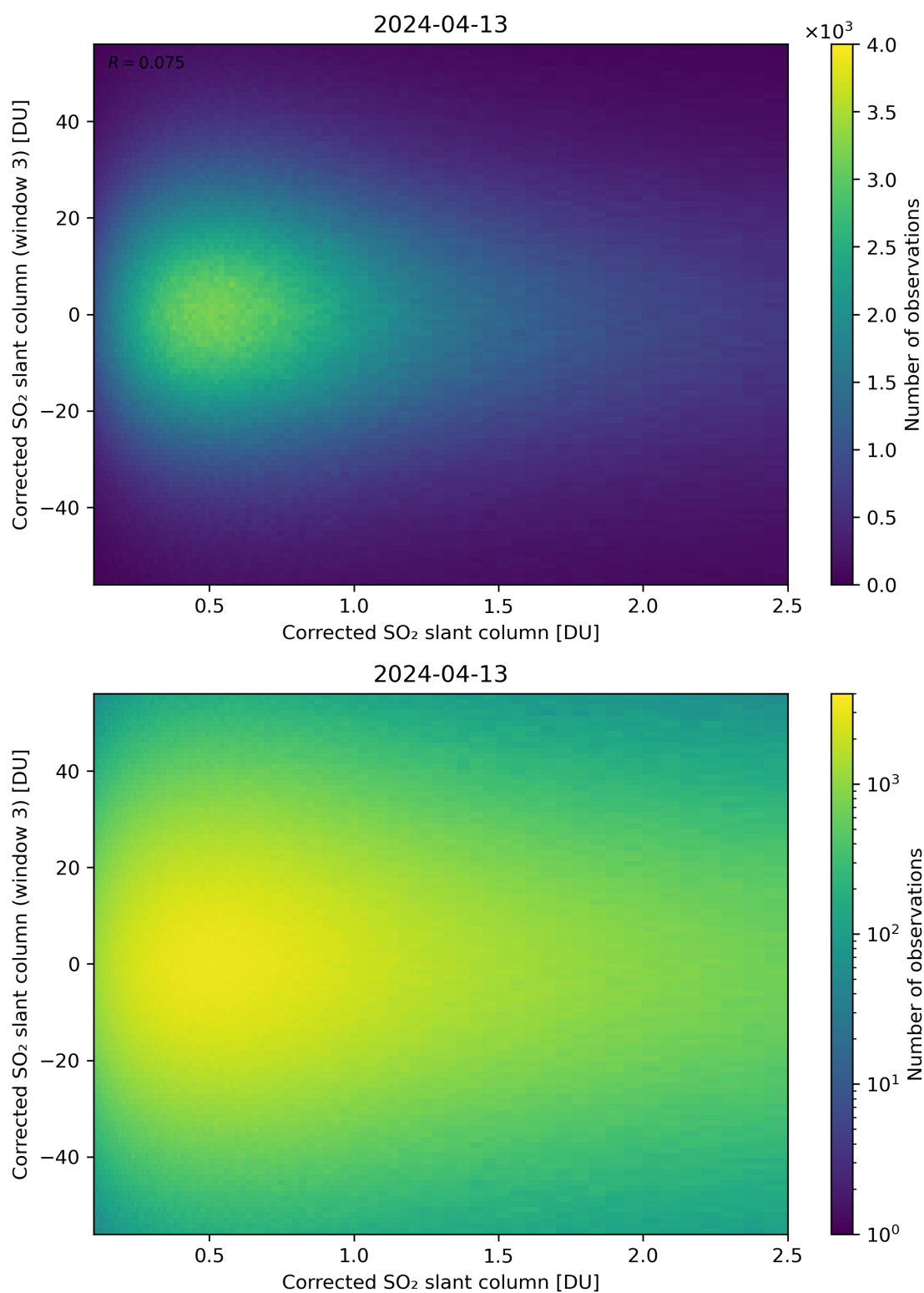
Figure 186: Scatter density plot of “Corrected SO 2 slant column” against “Corrected SO 2 slant column (window 3)” for 2024-04-12 to 2024-04-14.
