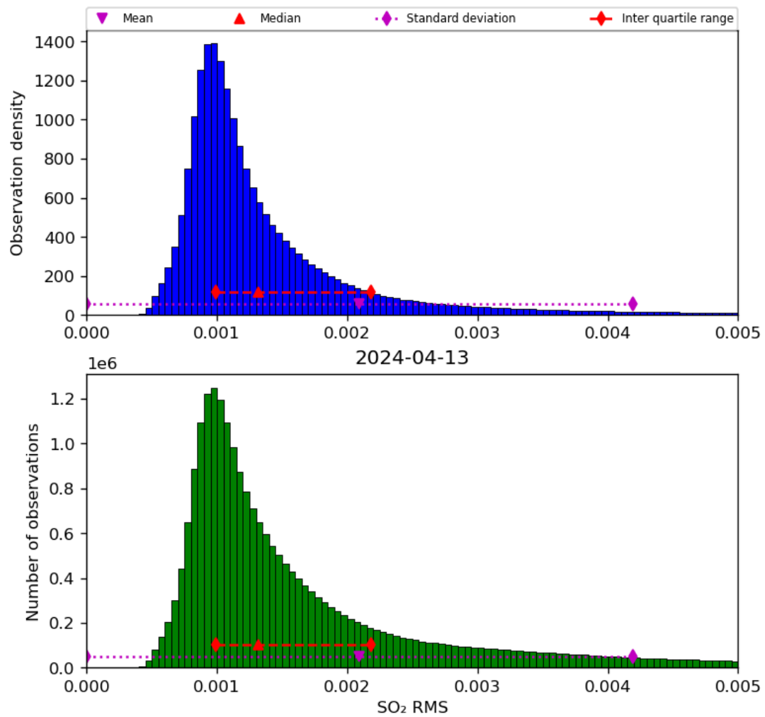
Figure 70: Histogram of “SO 2 RMS” for 2024-04-12 to 2024-04-14
