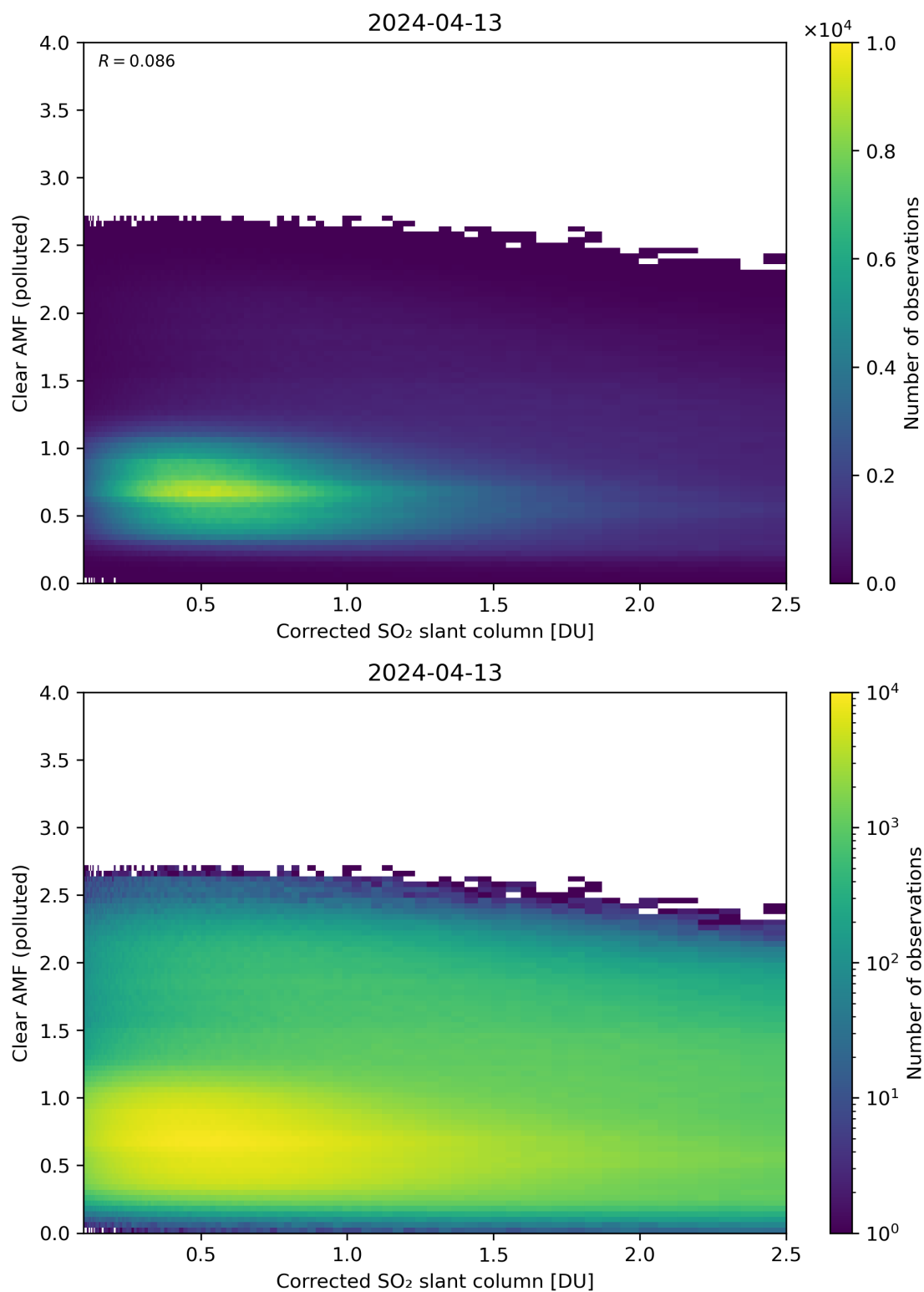
Figure 184: Scatter density plot of “Corrected SO 2 slant column” against “Clear AMF (polluted)” for 2024-04-12 to 2024-04-14.
