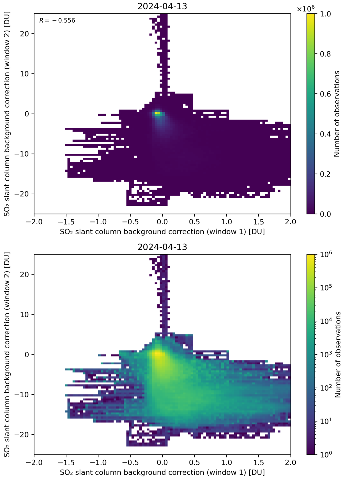
Figure 98: Scatter density plot of “SO 2 slant column background correction (window 1)” against “SO 2 slant column background correction (window 2)” for 2024-04-12 to 2024-04-14.
