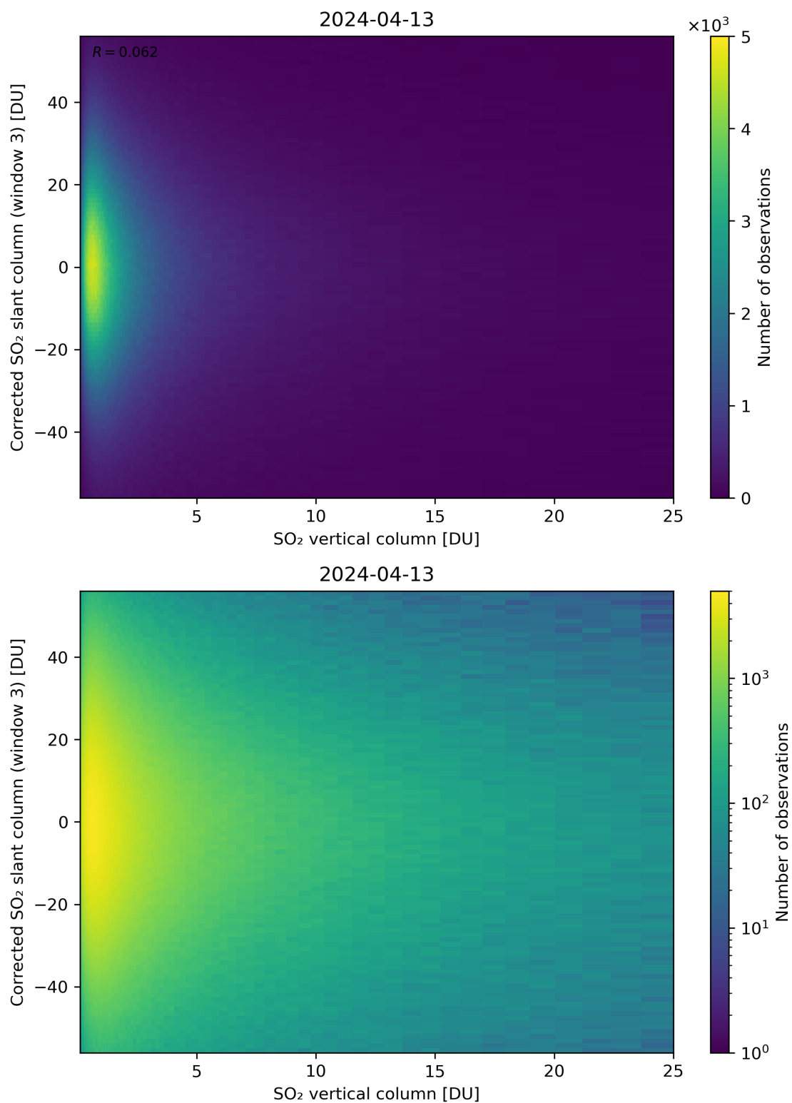
Figure 299: Scatter density plot of “SO 2 vertical column” against “Corrected SO 2 slant column (window 3)” for 2024-04-12 to 2024-04-14.
