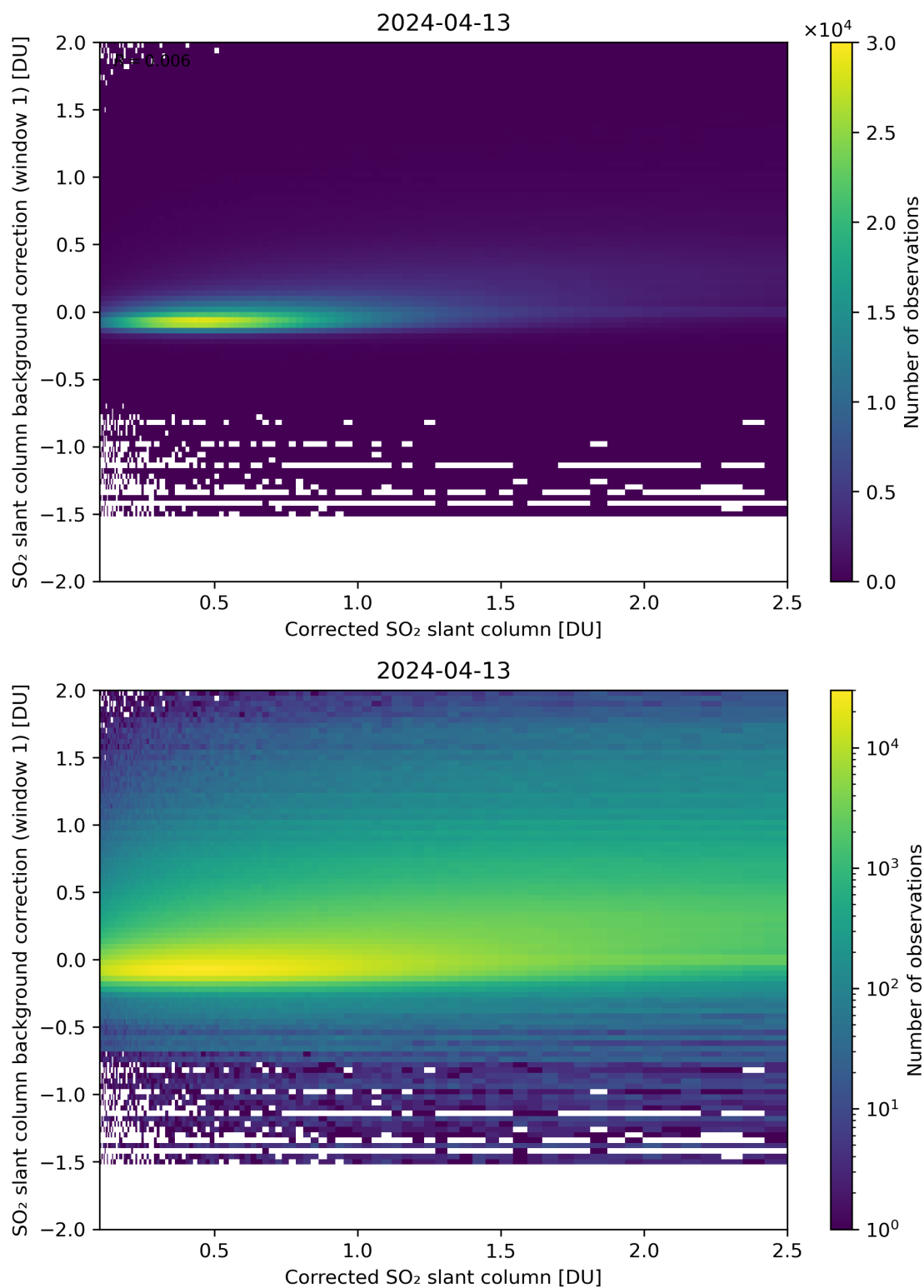
Figure 178: Scatter density plot of “Corrected SO 2 slant column” against “SO 2 slant column background correction (window 1)” for 2024-04-12 to 2024-04-14.
