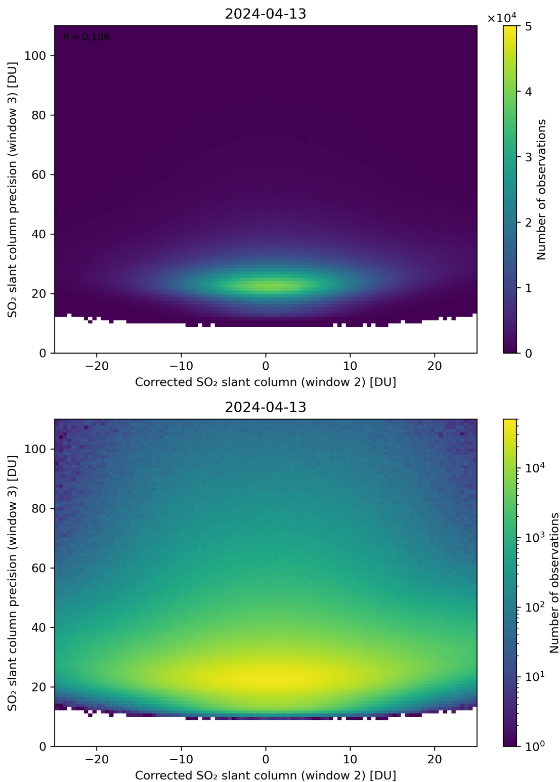
Figure 202: Scatter density plot of “Corrected SO 2 slant column (window 2)” against “SO 2 slant column precision (window 3)” for 2024-04-12 to 2024-04-14.
