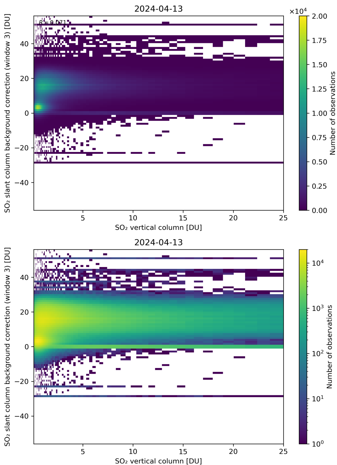
Figure 275: Scatter density plot of “SO 2 vertical column” against “SO 2 slant column background correction (window 3)” for 2024-04-12 to 2024-04-14.
