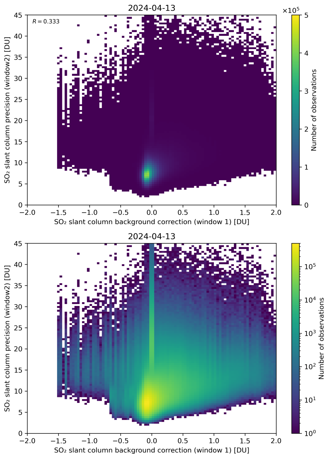
Figure 106: Scatter density plot of “SO 2 slant column background correction (window 1)” against “SO 2 slant column precision (window2)” for 2024-04-12 to 2024-04-14.
