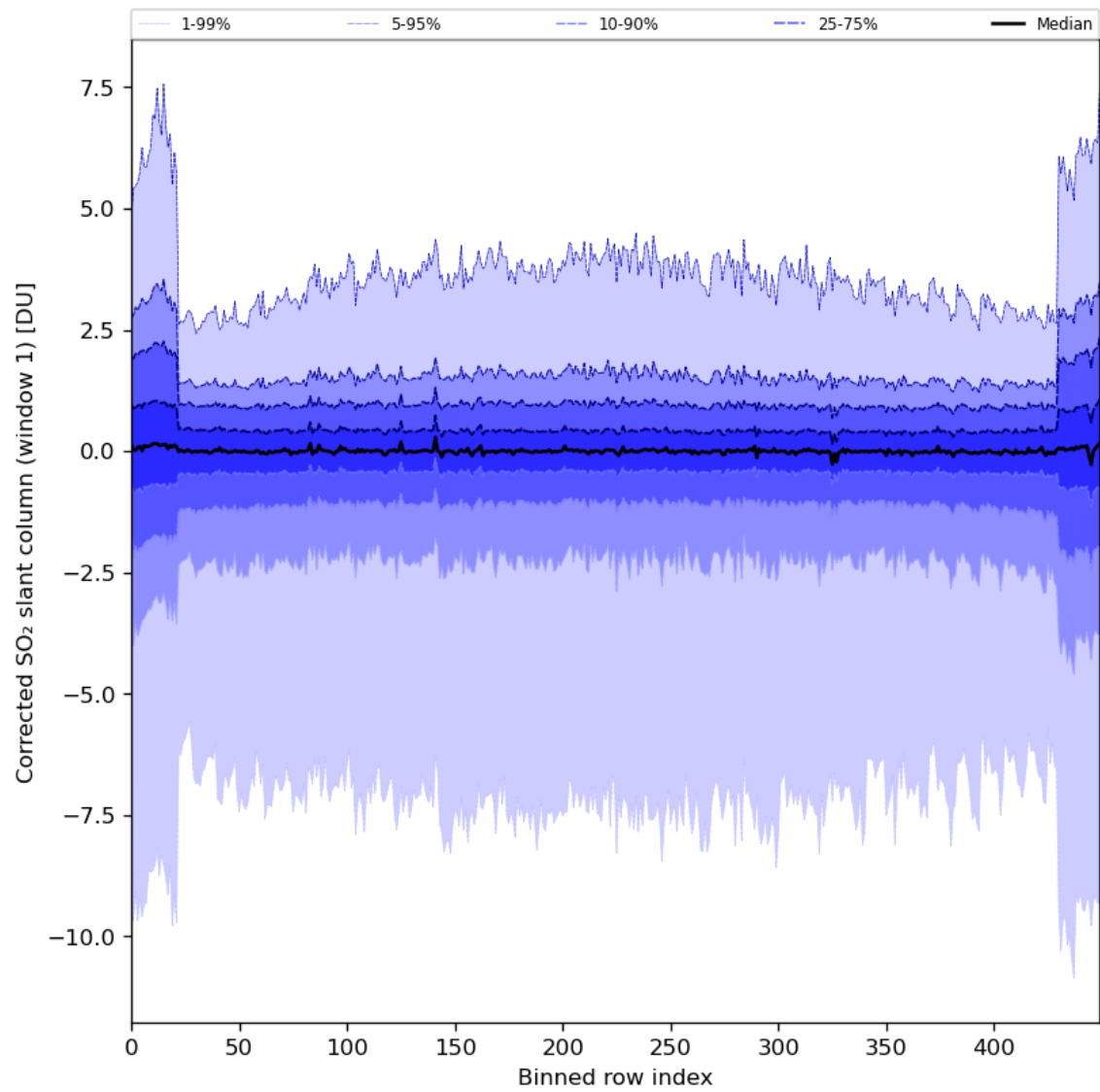
Figure 81: Along track statistics of “Corrected SO 2 slant column (window 1)” for 2024-04-12 to 2024-04-14
