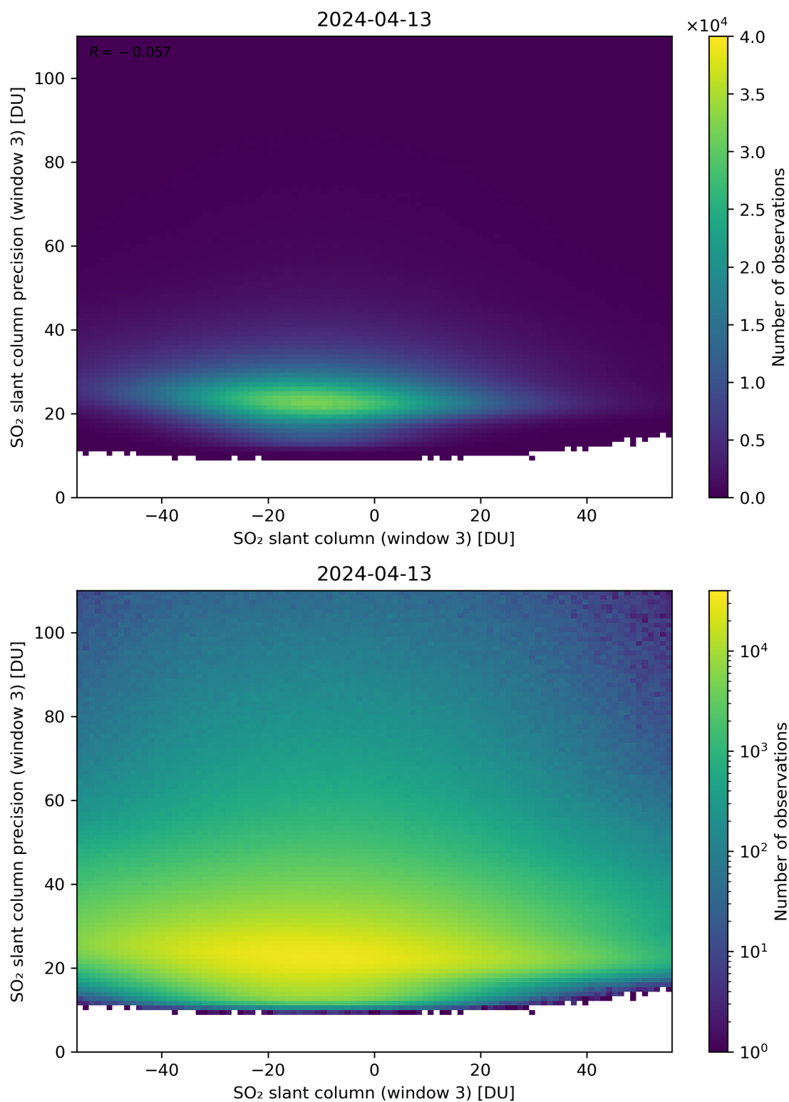
Figure 267: Scatter density plot of “SO 2 slant column (window 3)” against “SO 2 slant column precision (window 3)” for 2024-04-12 to 2024-04-14.
