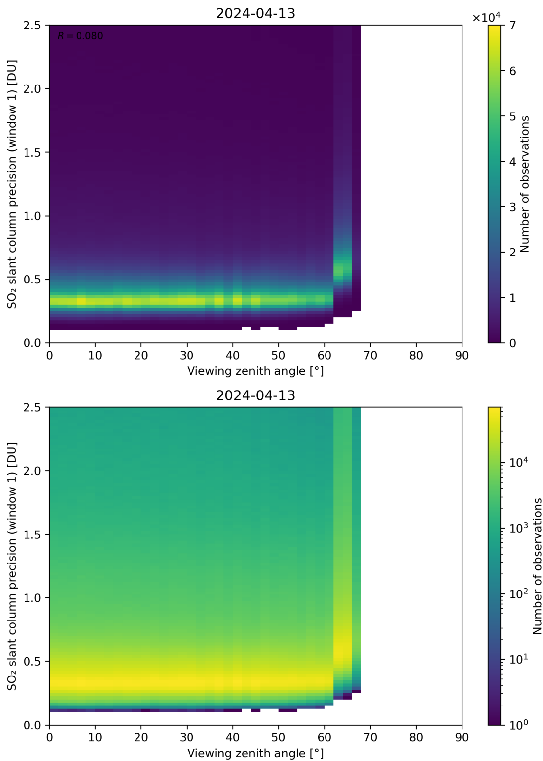
Figure 321: Scatter density plot of “Viewing zenith angle” against “SO 2 slant column precision (window 1)” for 2024-04-12 to 2024-04-14.
