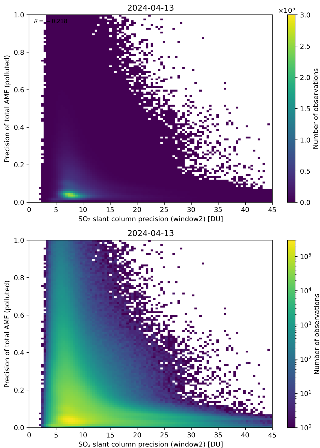
Figure 252: Scatter density plot of “SO 2 slant column precision (window2)” against “Precision of total AMF (polluted)” for 2024-04-12 to 2024-04-14.
