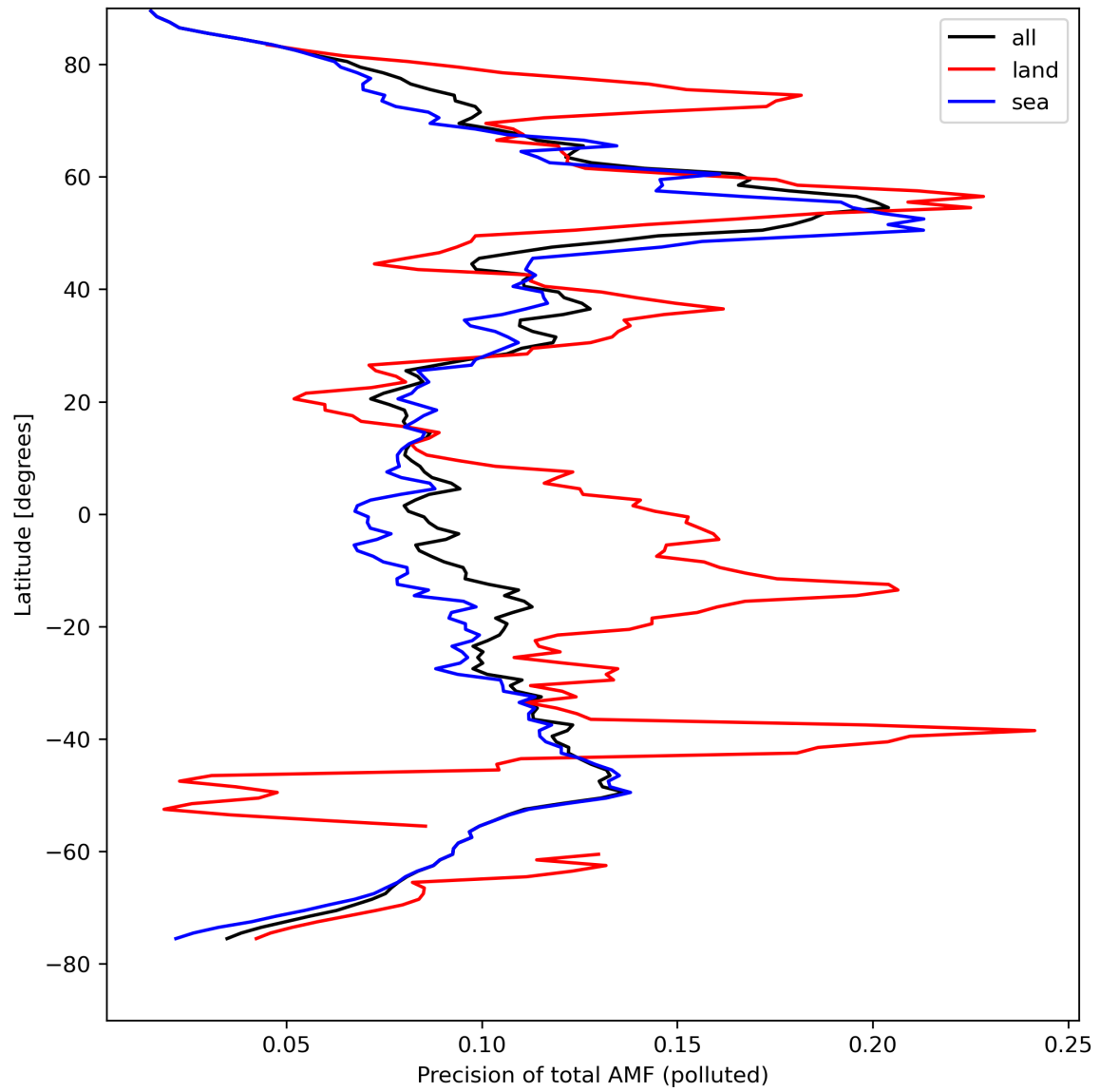
Figure 49: Zonal average of “Precision of total AMF (polluted)” for 2024-04-12 to 2024-04-14.
