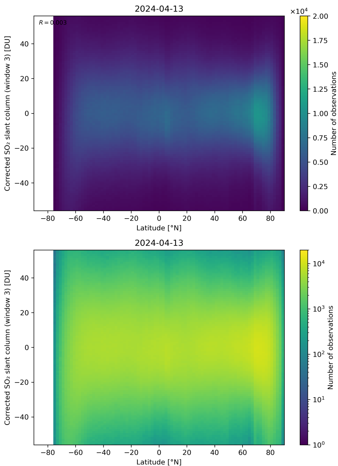
Figure 148: Scatter density plot of “Latitude” against “Corrected SO 2 slant column (window 3)” for 2024-04-12 to 2024-04-14.
