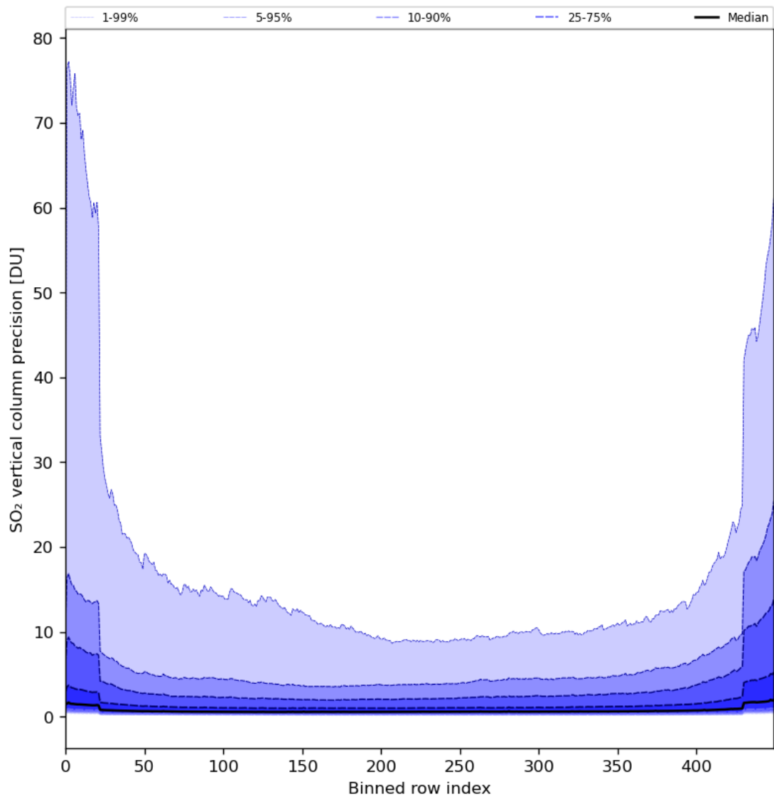
Figure 77: Along track statistics of “SO 2 vertical column precision” for 2024-04-12 to 2024-04-14
