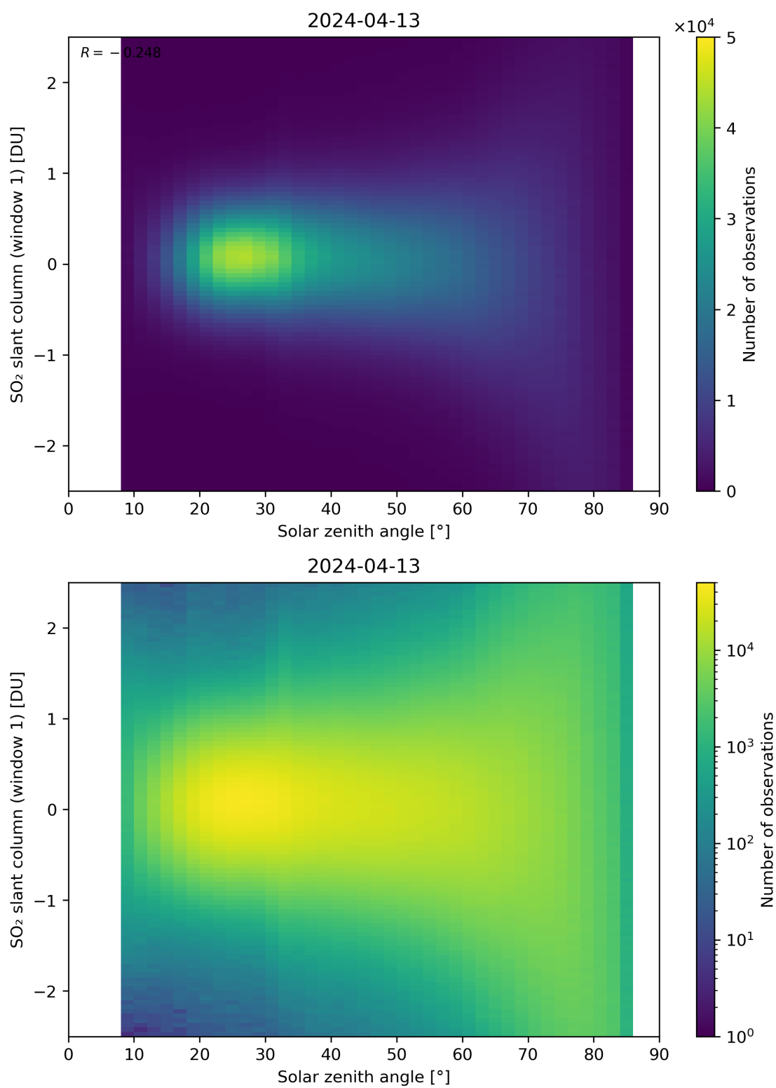
Figure 169: Scatter density plot of “Solar zenith angle” against “SO 2 slant column (window 1)” for 2024-04-12 to 2024-04-14.
