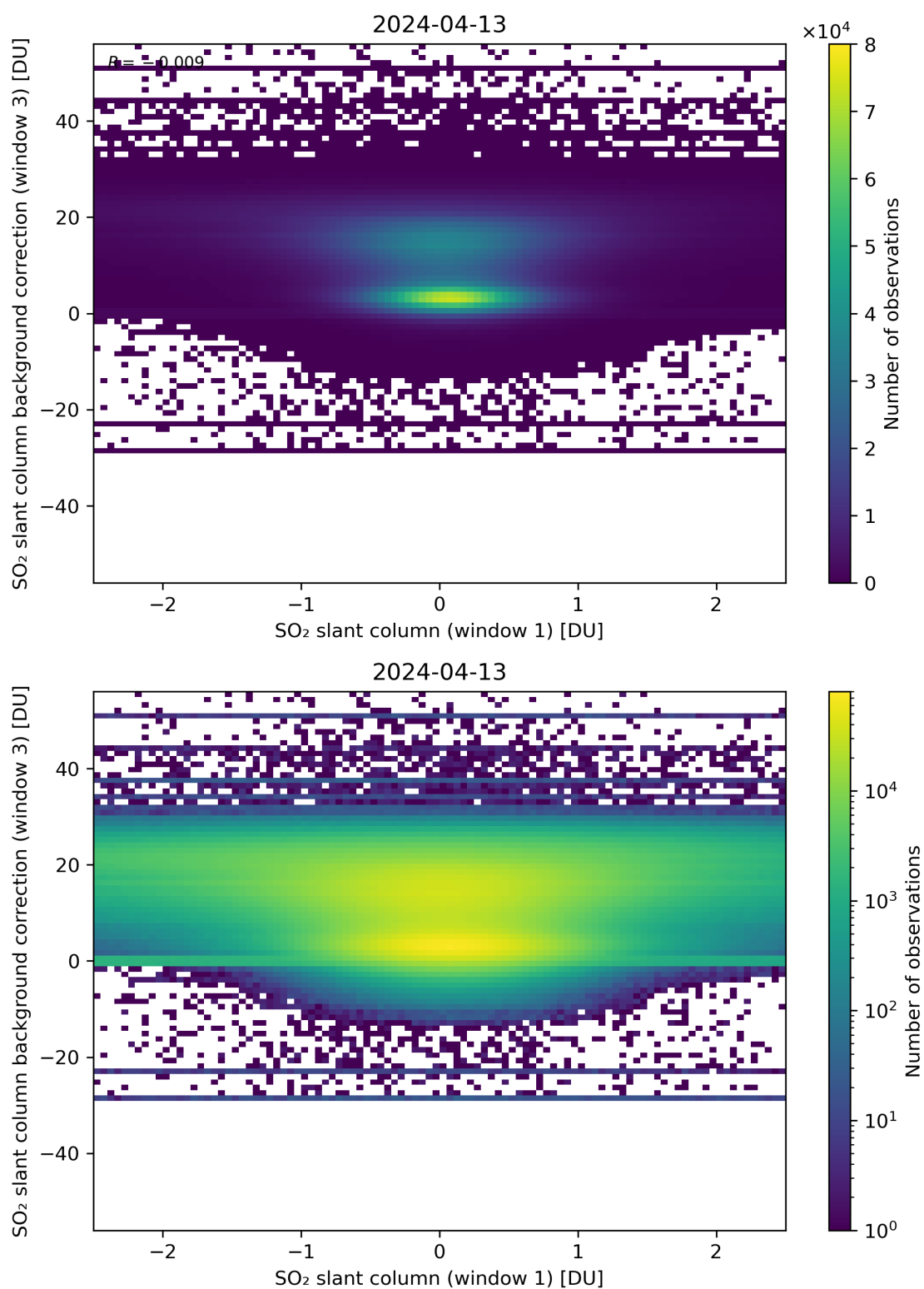
Figure 214: Scatter density plot of “SO 2 slant column (window 1)” against “SO 2 slant column background correction (window 3)” for 2024-04-12 to 2024-04-14.
