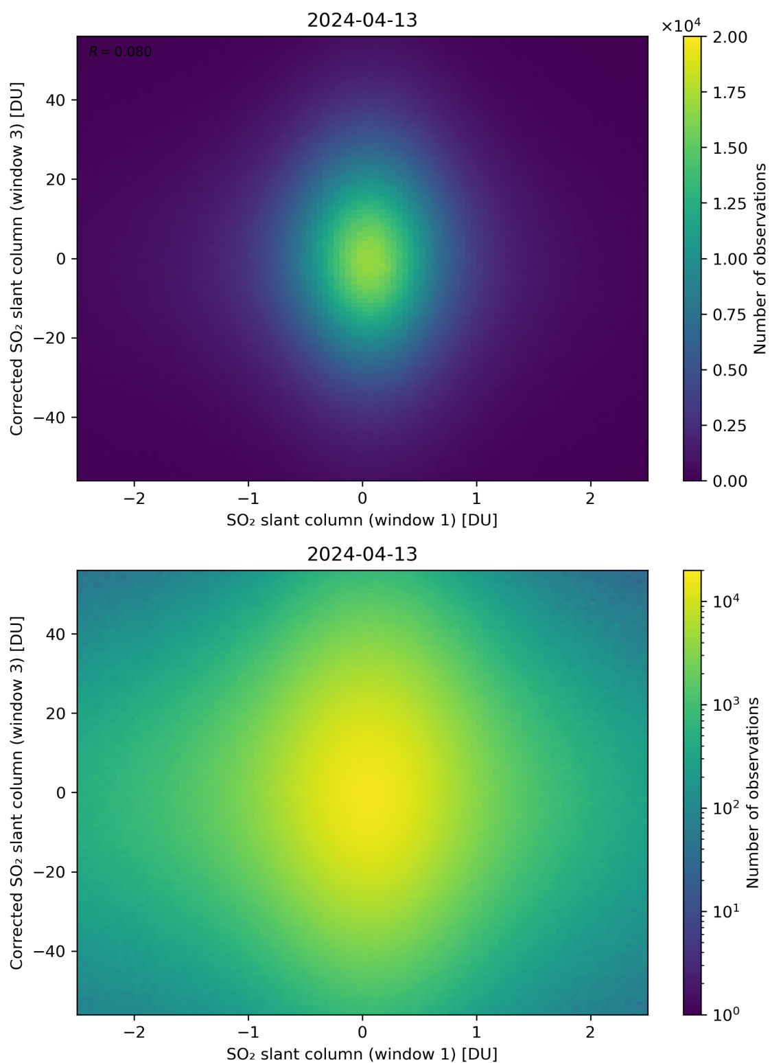
Figure 234: Scatter density plot of “SO 2 slant column (window 1)” against “Corrected SO 2 slant column (window 3)” for 2024-04-12 to 2024-04-14.
