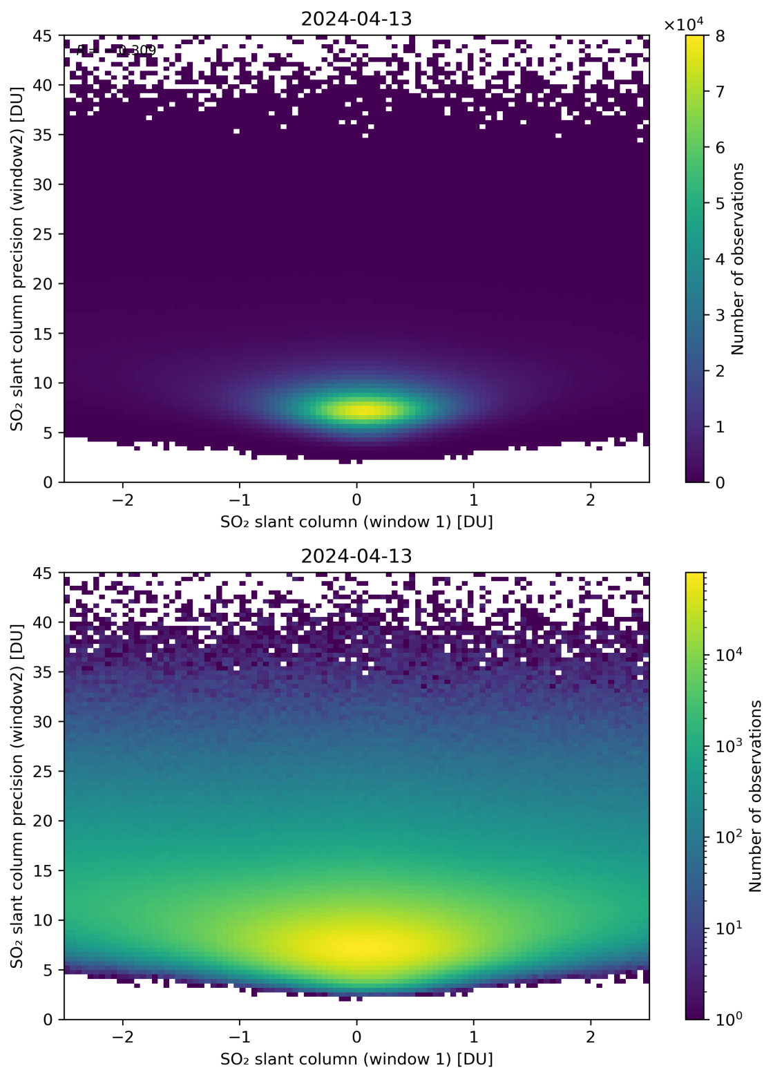
Figure 236: Scatter density plot of “SO 2 slant column (window 1)” against “SO 2 slant column precision (window2)” for 2024-04-12 to 2024-04-14.
