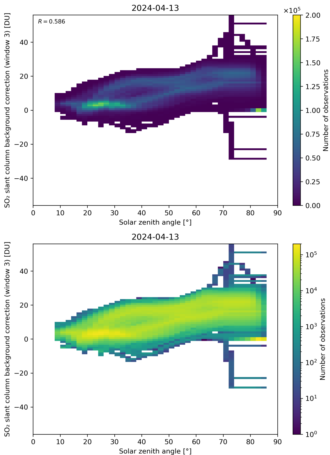
Figure 160: Scatter density plot of “Solar zenith angle” against “SO 2 slant column background correction (window 3)” for 2024-04-12 to 2024-04-14.
