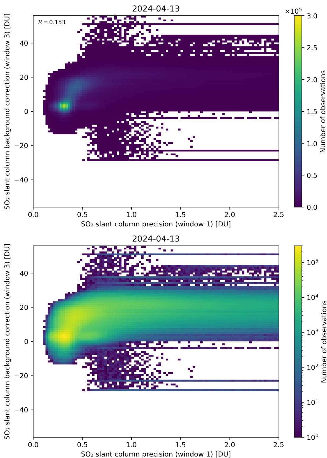
Figure 220: Scatter density plot of “SO 2 slant column precision (window 1)” against “SO 2 slant column background correction (window 3)” for 2024-04-12 to 2024-04-14.
