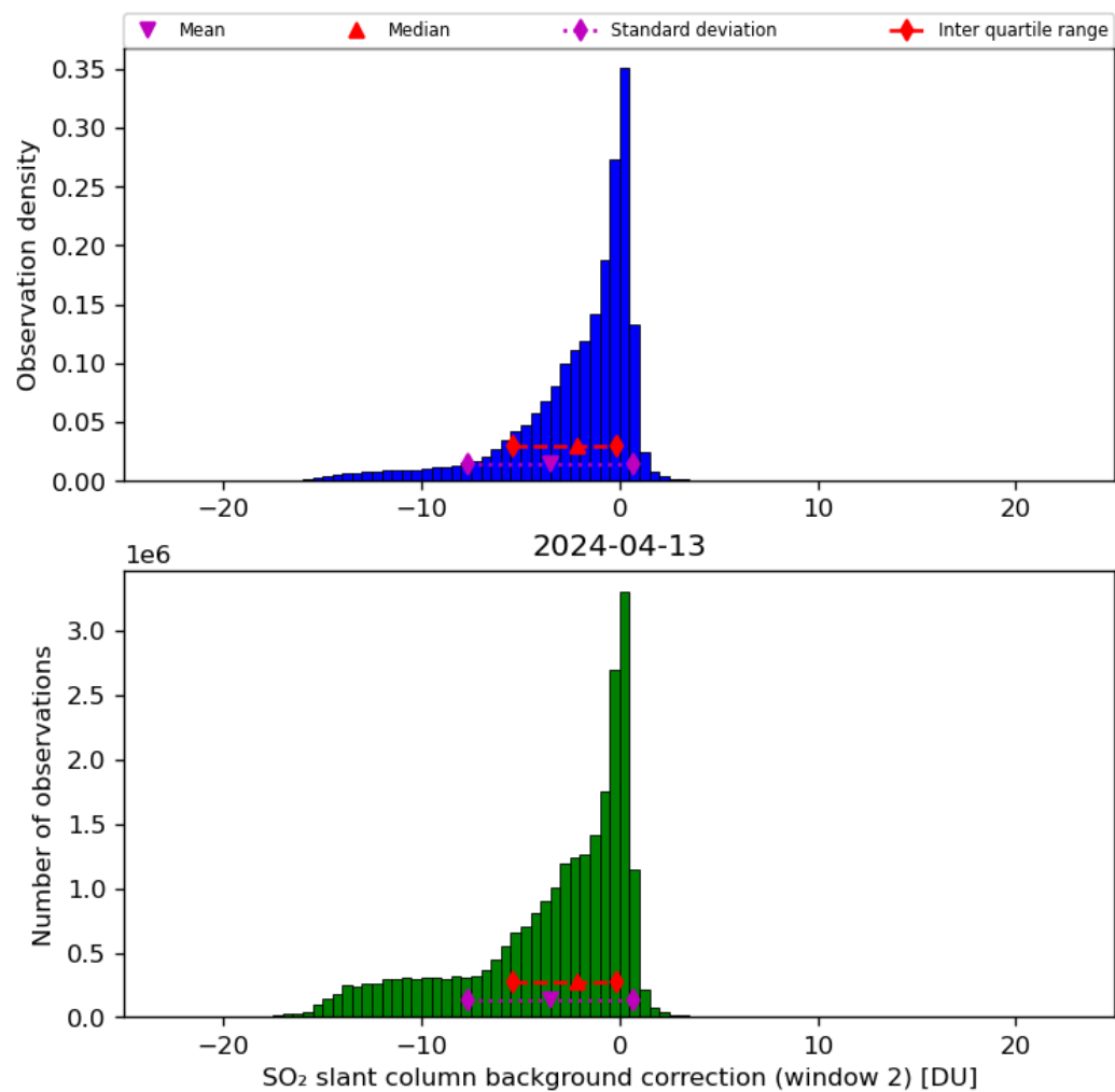
Figure 63: Histogram of “SO 2 slant column background correction (window 2)” for 2024-04-12 to 2024-04-14
