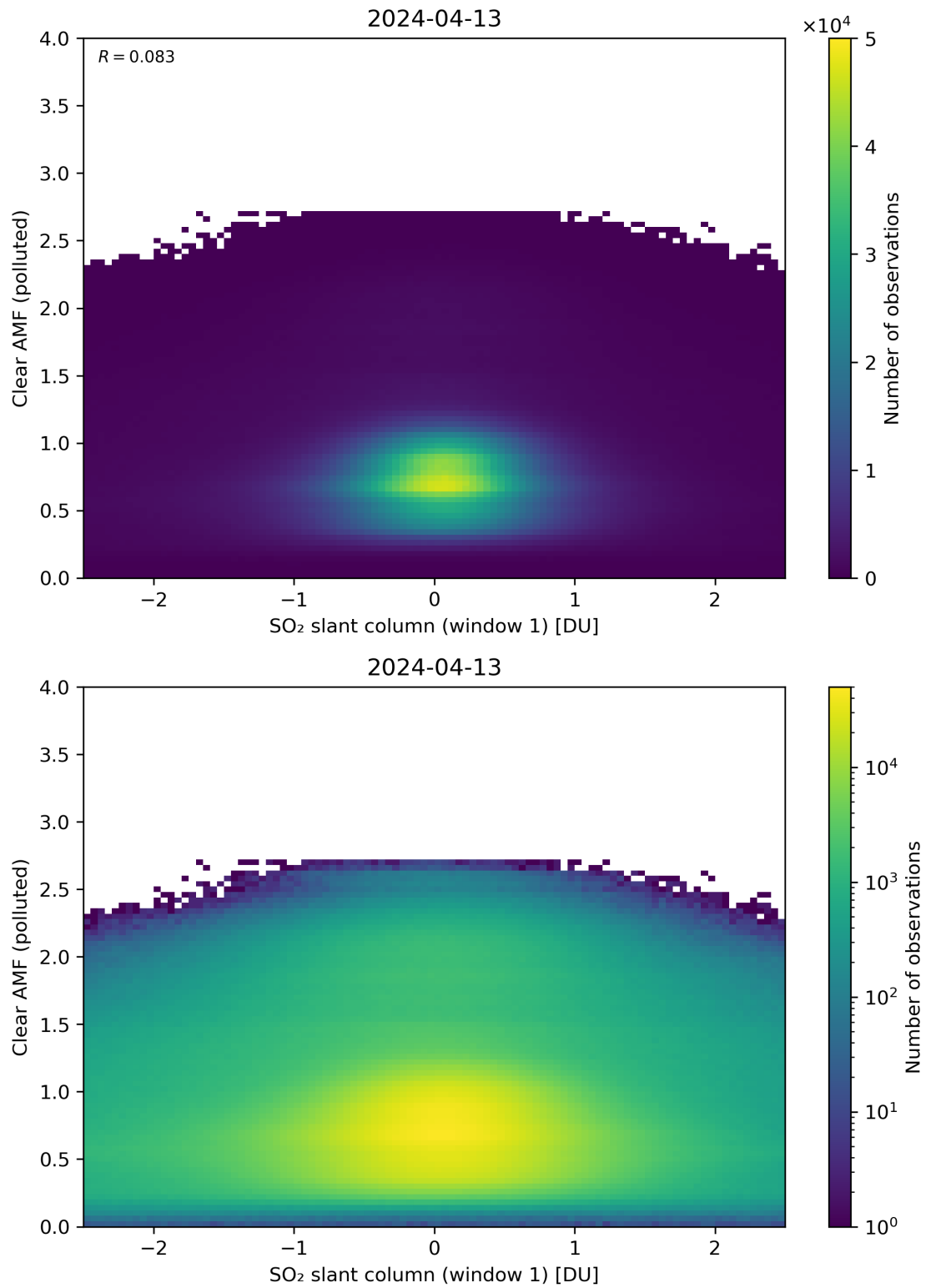
Figure 232: Scatter density plot of “SO 2 slant column (window 1)” against “Clear AMF (polluted)” for 2024-04-12 to 2024-04-14.
