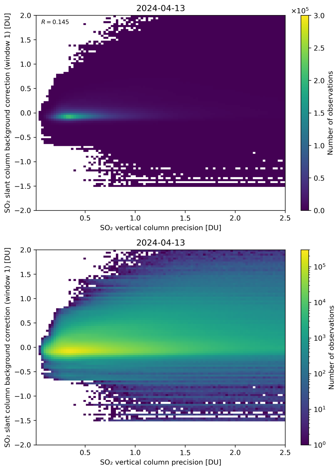
Figure 279: Scatter density plot of “SO 2 vertical column precision” against “SO 2 slant column background correction (window 1)” for 2024-04-12 to 2024-04-14.
