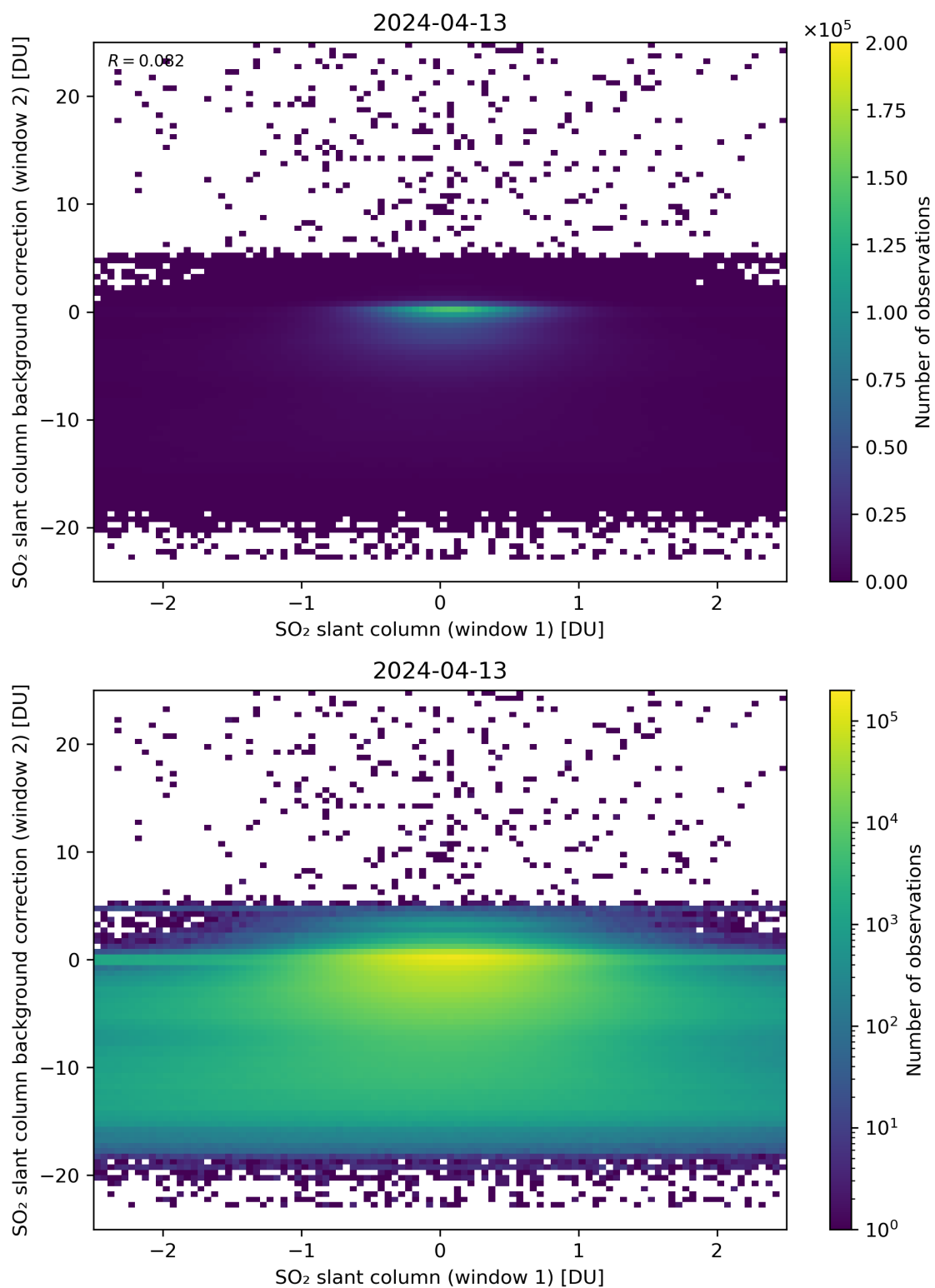
Figure 213: Scatter density plot of “SO 2 slant column (window 1)” against “SO 2 slant column background correction (window 2)” for 2024-04-12 to 2024-04-14.
