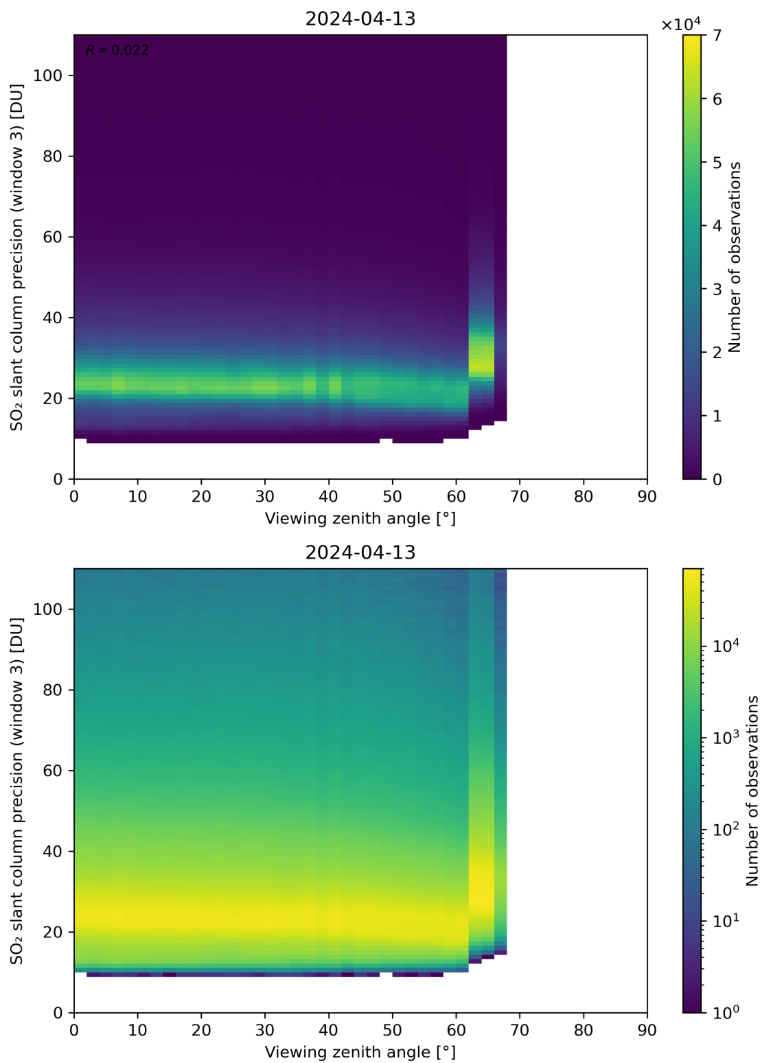
Figure 324: Scatter density plot of “Viewing zenith angle” against “SO 2 slant column precision (window 3)” for 2024-04-12 to 2024-04-14.
