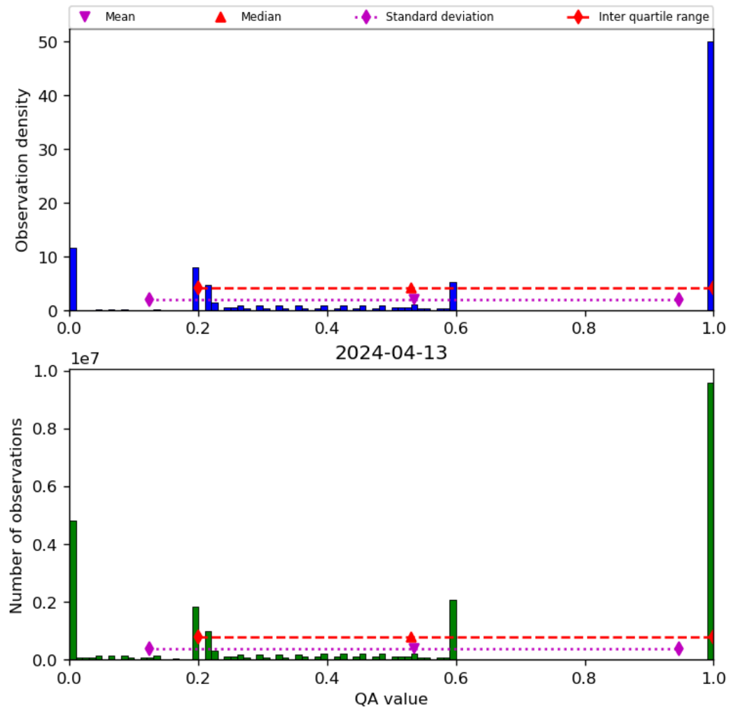
Figure 52: Histogram of “QA value” for 2024-04-12 to 2024-04-14
