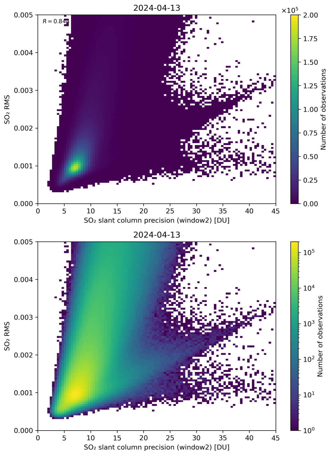
Figure 245: Scatter density plot of “SO 2 slant column precision (window2)” against “SO 2 RMS” for 2024-04-12 to 2024-04-14.
