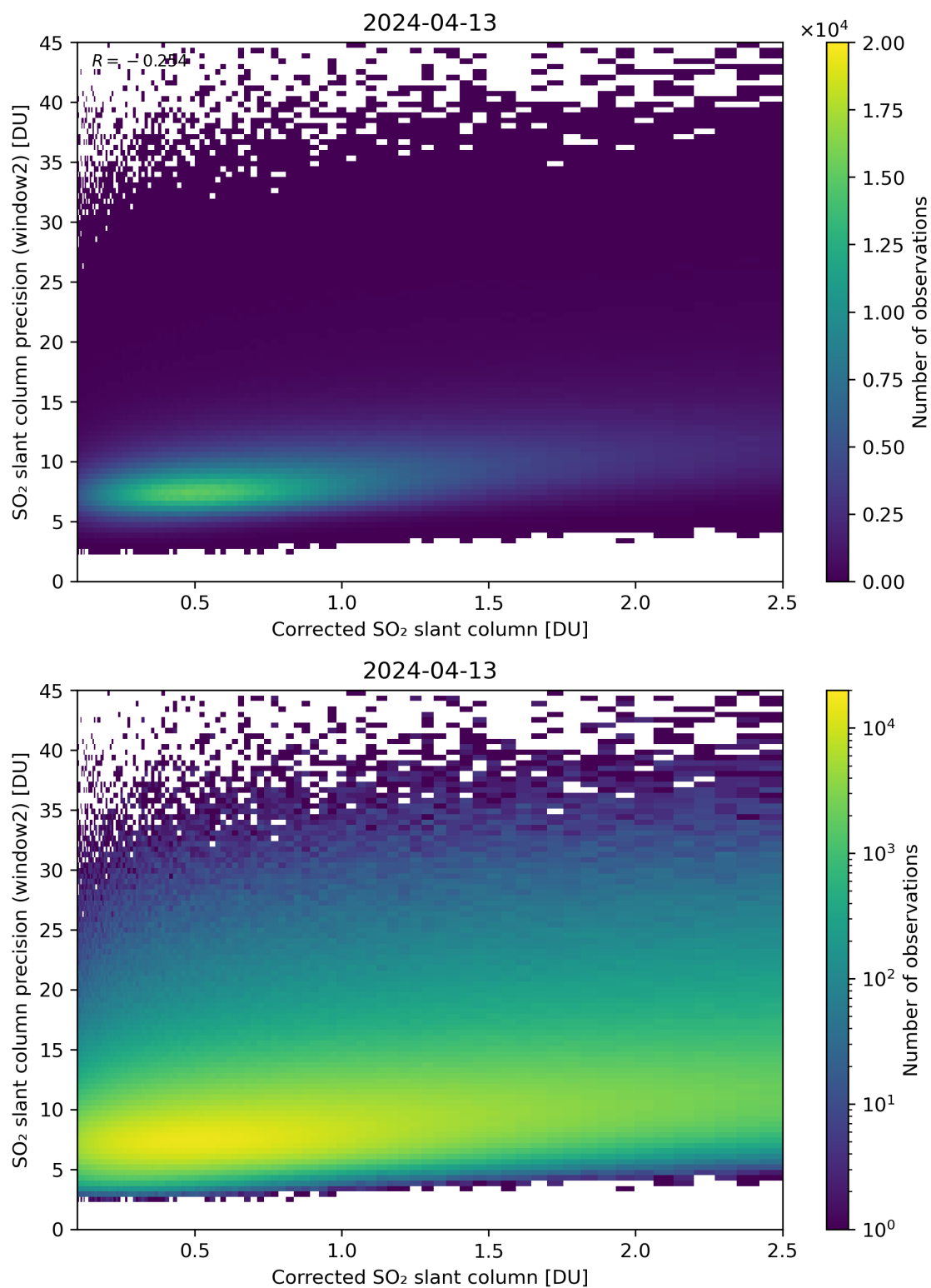
Figure 189: Scatter density plot of “Corrected SO 2 slant column” against “SO 2 slant column precision (window2)” for 2024-04-12 to 2024-04-14.
