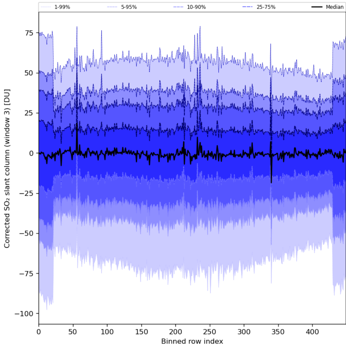
Figure 89: Along track statistics of “Corrected SO 2 slant column (window 3)” for 2024-04-12 to 2024-04-14
