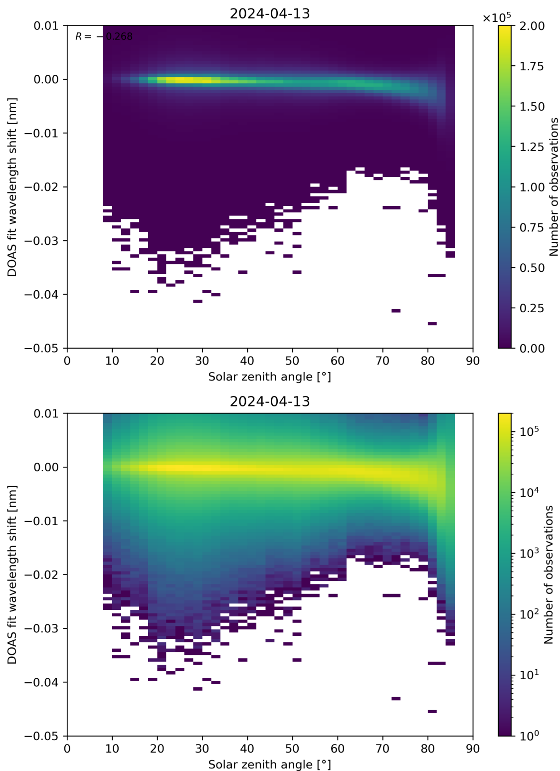
Figure 161: Scatter density plot of “Solar zenith angle” against “DOAS fit wavelength shift” for 2024-04-12 to 2024-04-14.
