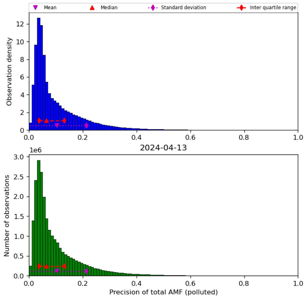
Figure 72: Histogram of “Precision of total AMF (polluted)” for 2024-04-12 to 2024-04-14
