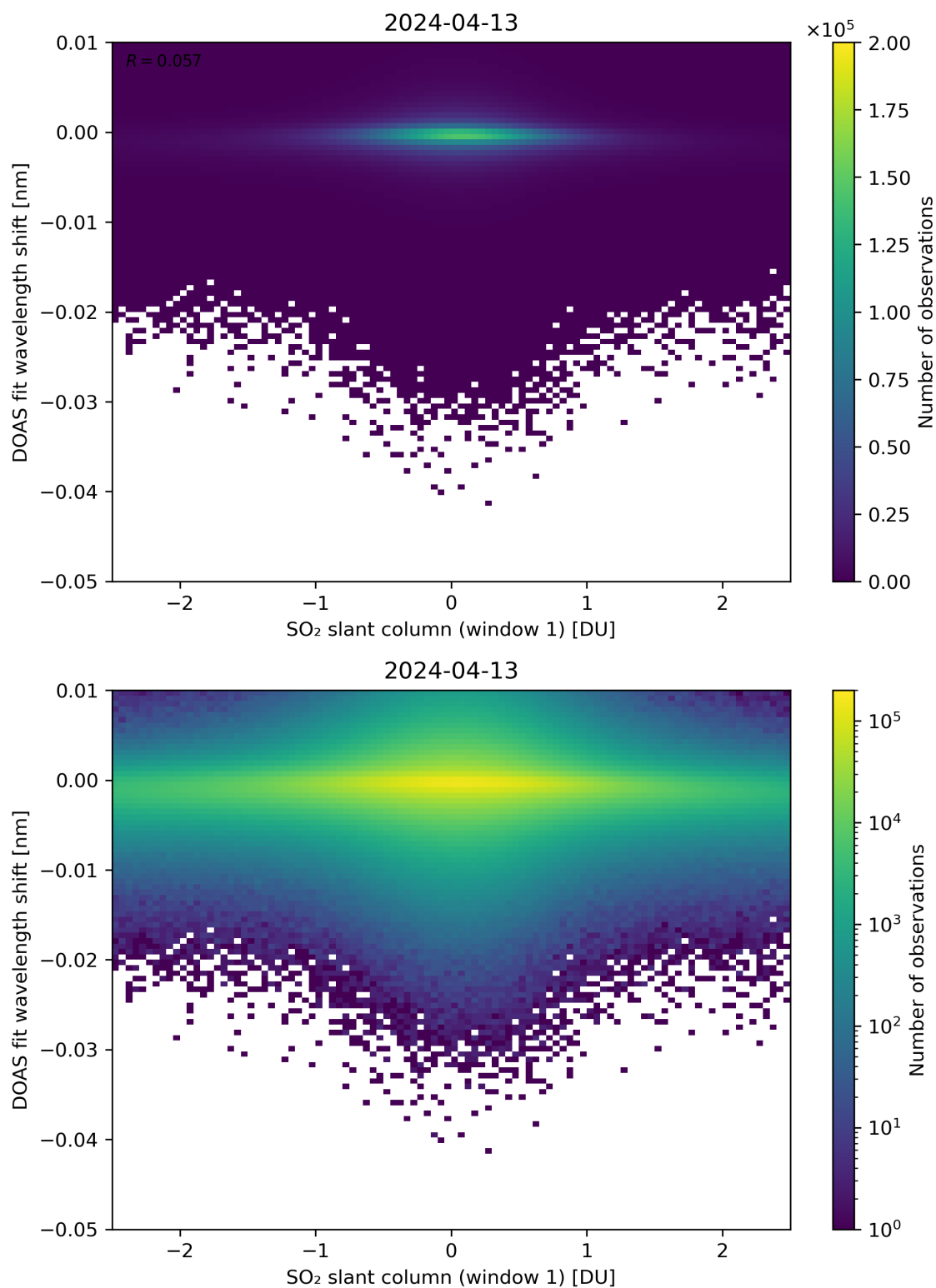
Figure 215: Scatter density plot of “SO 2 slant column (window 1)” against “DOAS fit wavelength shift” for 2024-04-12 to 2024-04-14.
