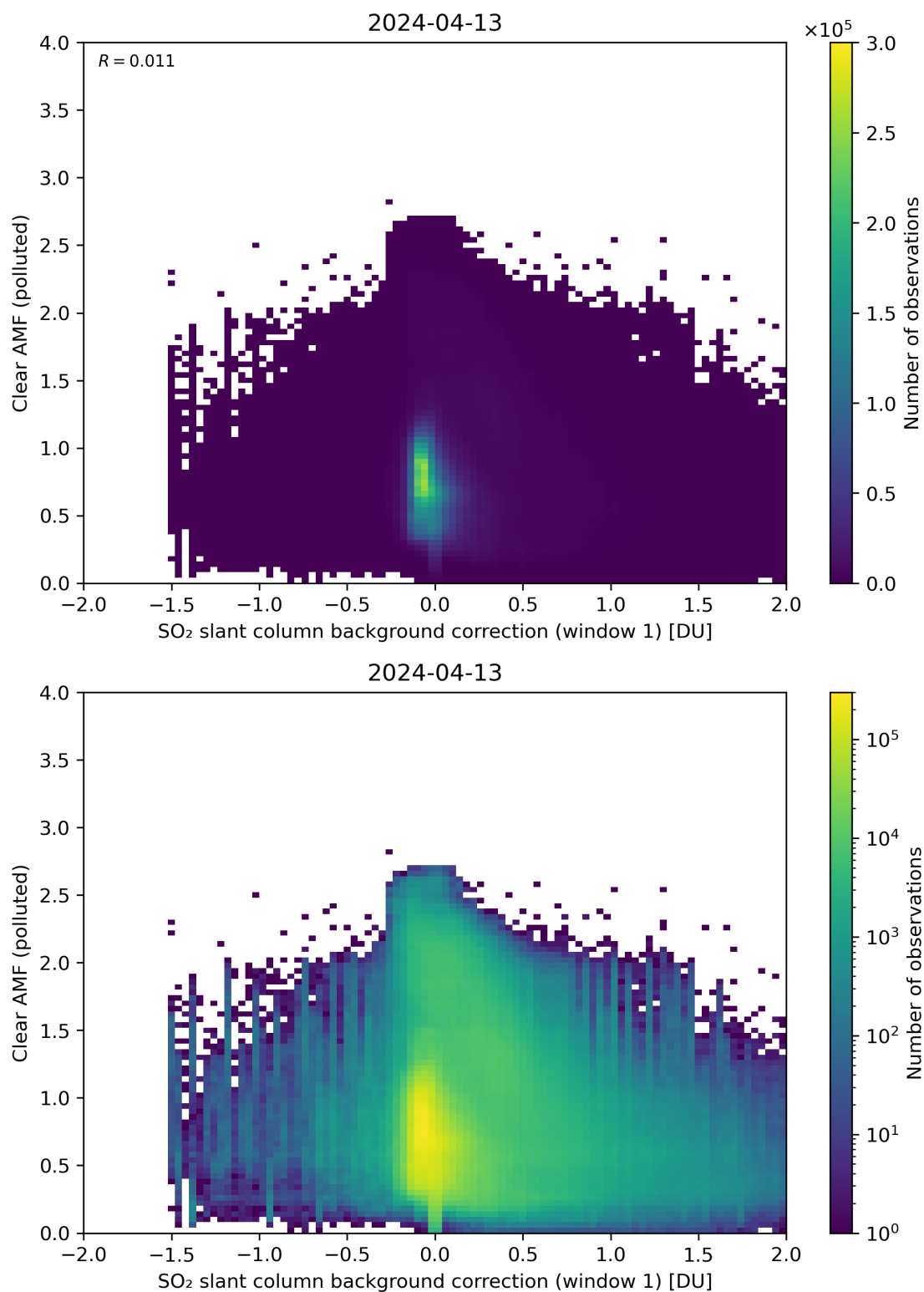
Figure 103: Scatter density plot of “SO 2 slant column background correction (window 1)” against “Clear AMF (polluted)” for 2024-04-12 to 2024-04-14.
