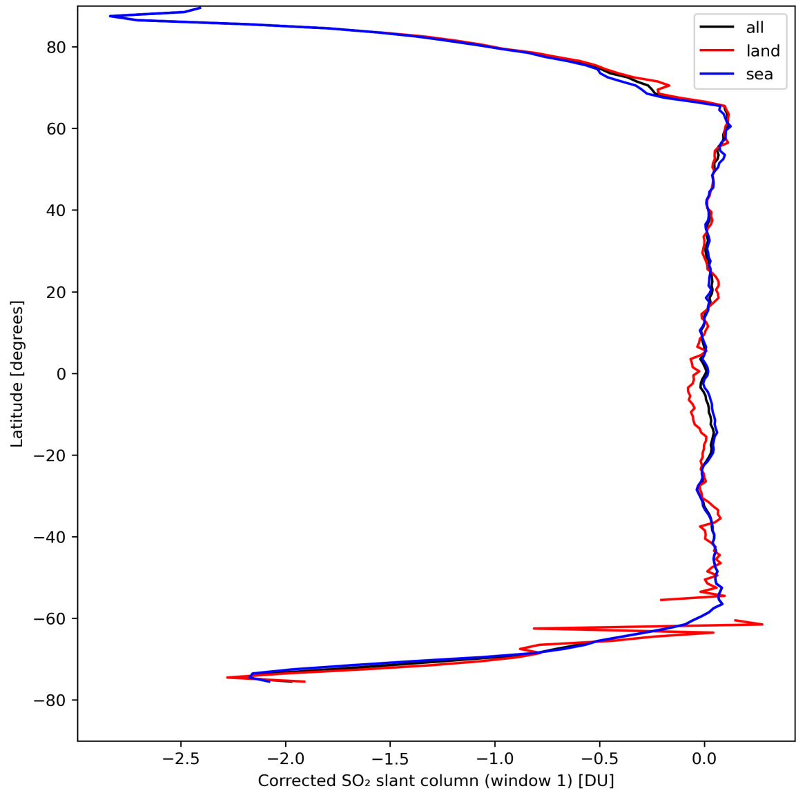
Figure 35: Zonal average of “Corrected SO 2 slant column (window 1)” for 2024-04-12 to 2024-04-14.
