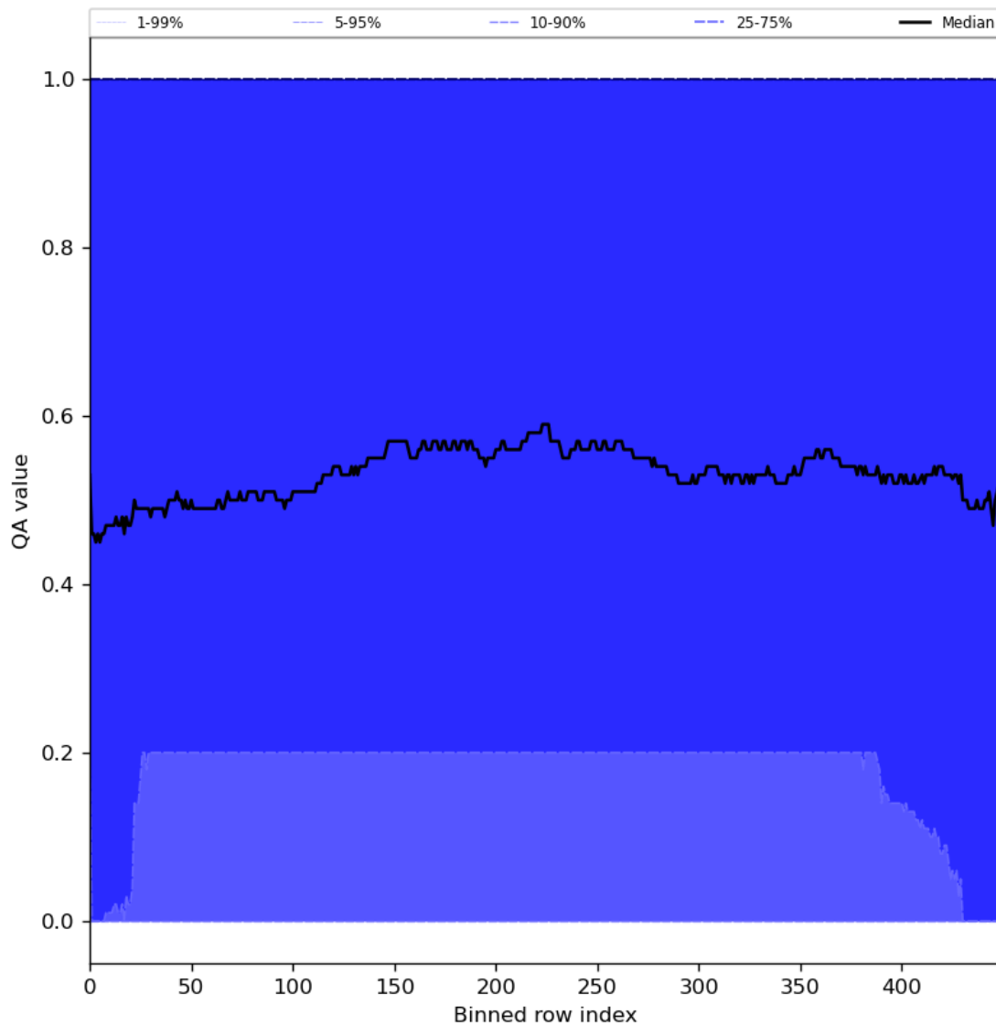
Figure 75: Along track statistics of "QA value" for 2024-04-12 to 2024-04-14
