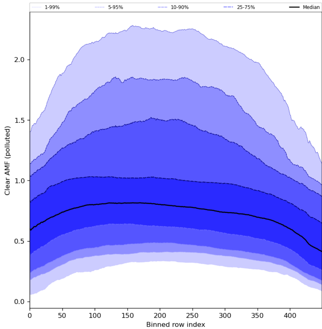
Figure 96: Along track statistics of “Clear AMF (polluted)” for 2024-04-12 to 2024-04-14
