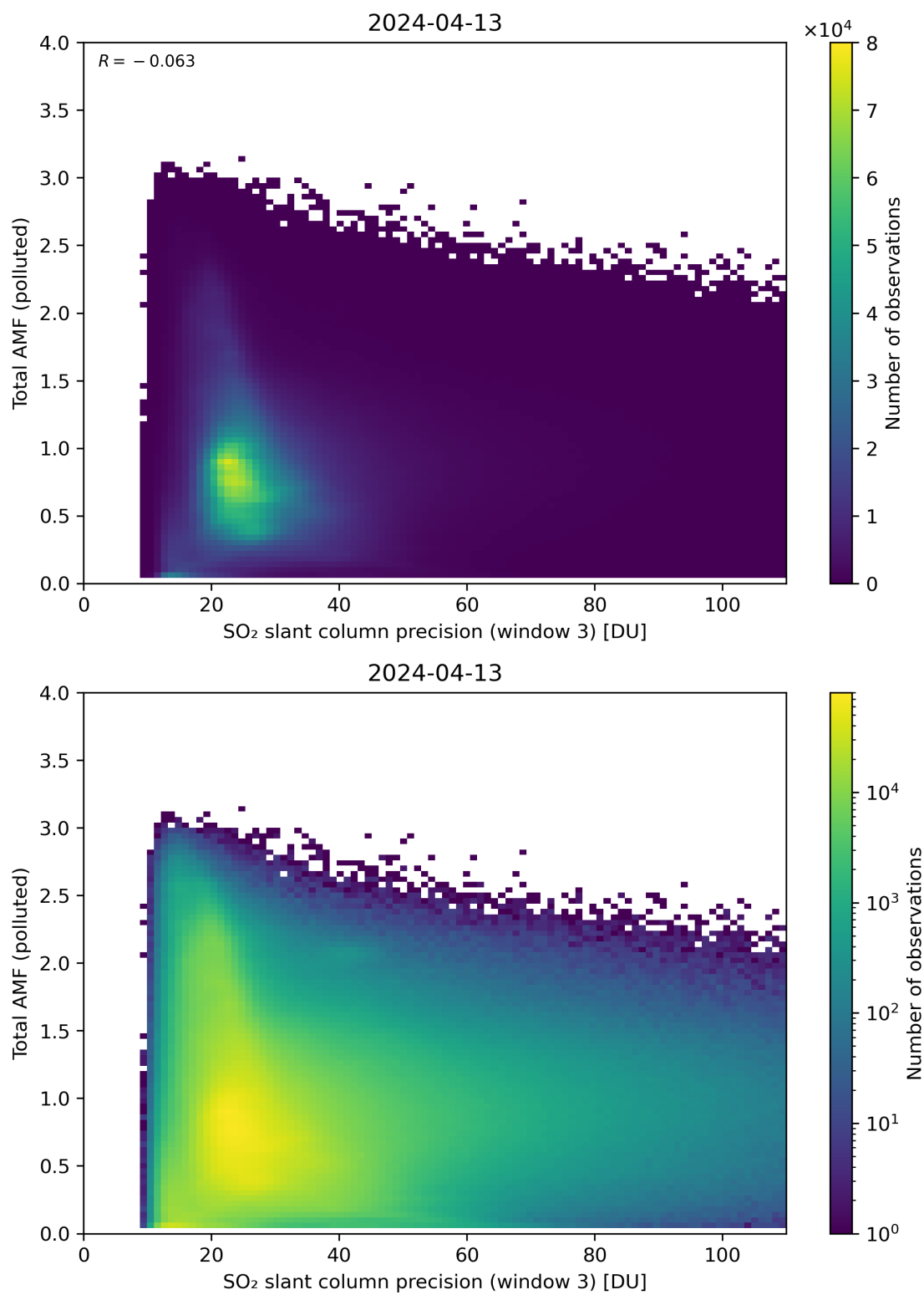
Figure 263: Scatter density plot of “SO 2 slant column precision (window 3)” against “Total AMF (polluted)” for 2024-04-12 to 2024-04-14.
