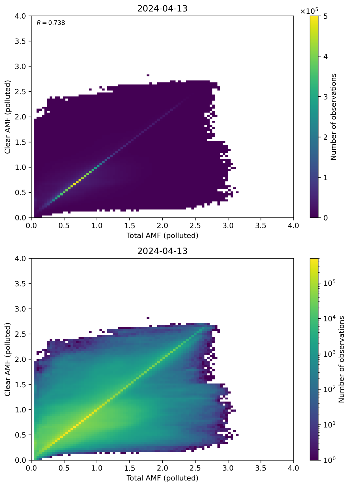
Figure 271: Scatter density plot of “Total AMF (polluted)” against “Clear AMF (polluted)” for 2024-04-12 to 2024-04-14.
