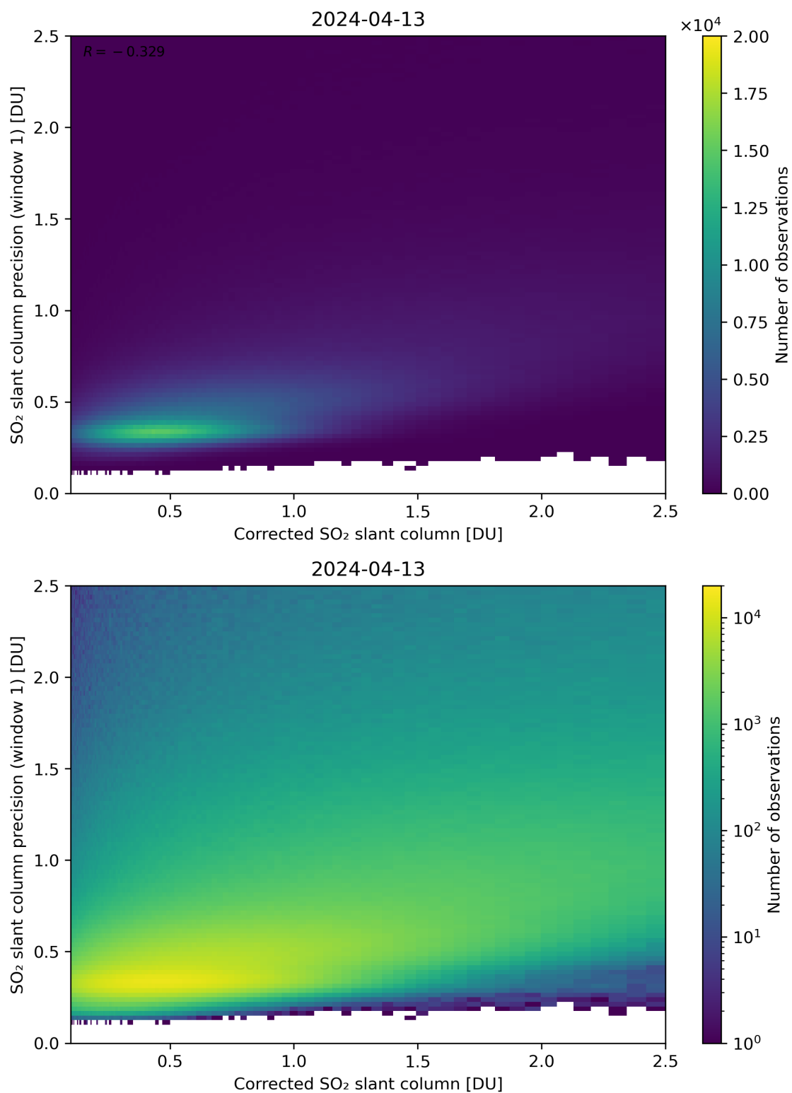
Figure 188: Scatter density plot of “Corrected SO 2 slant column” against “SO 2 slant column precision (window 1)” for 2024-04-12 to 2024-04-14.
