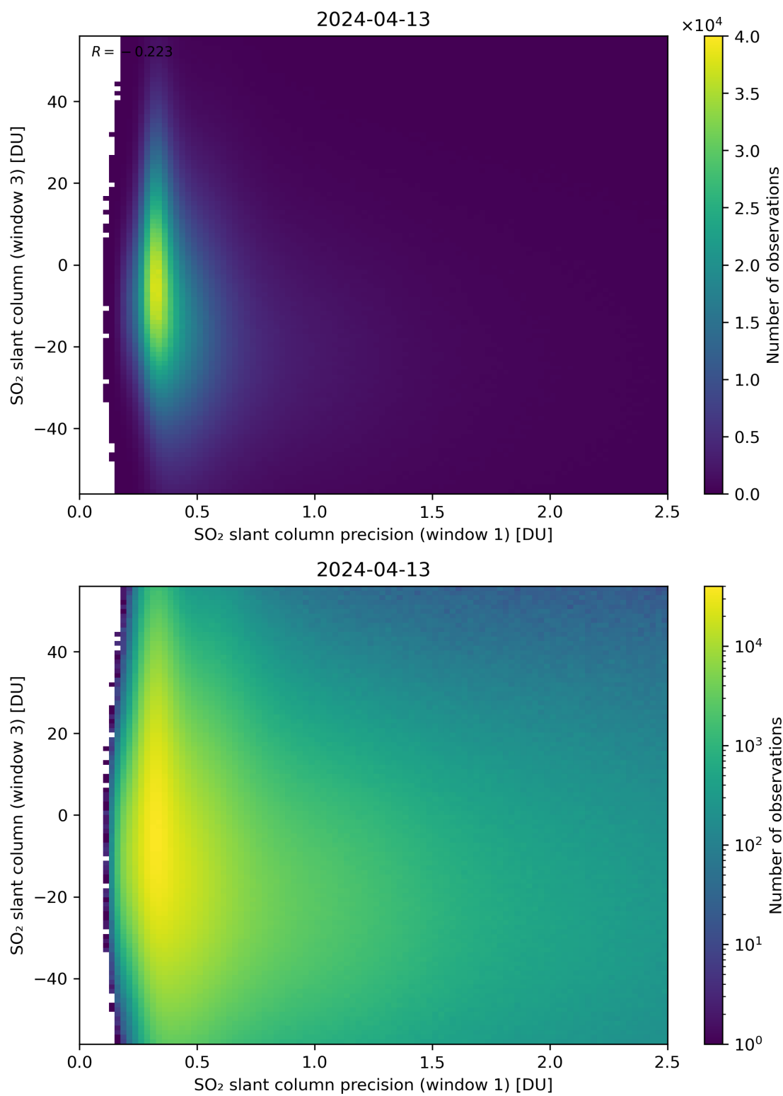
Figure 228: Scatter density plot of “SO 2 slant column precision (window 1)” against “SO 2 slant column (window 3)” for 2024-04-12 to 2024-04-14.
