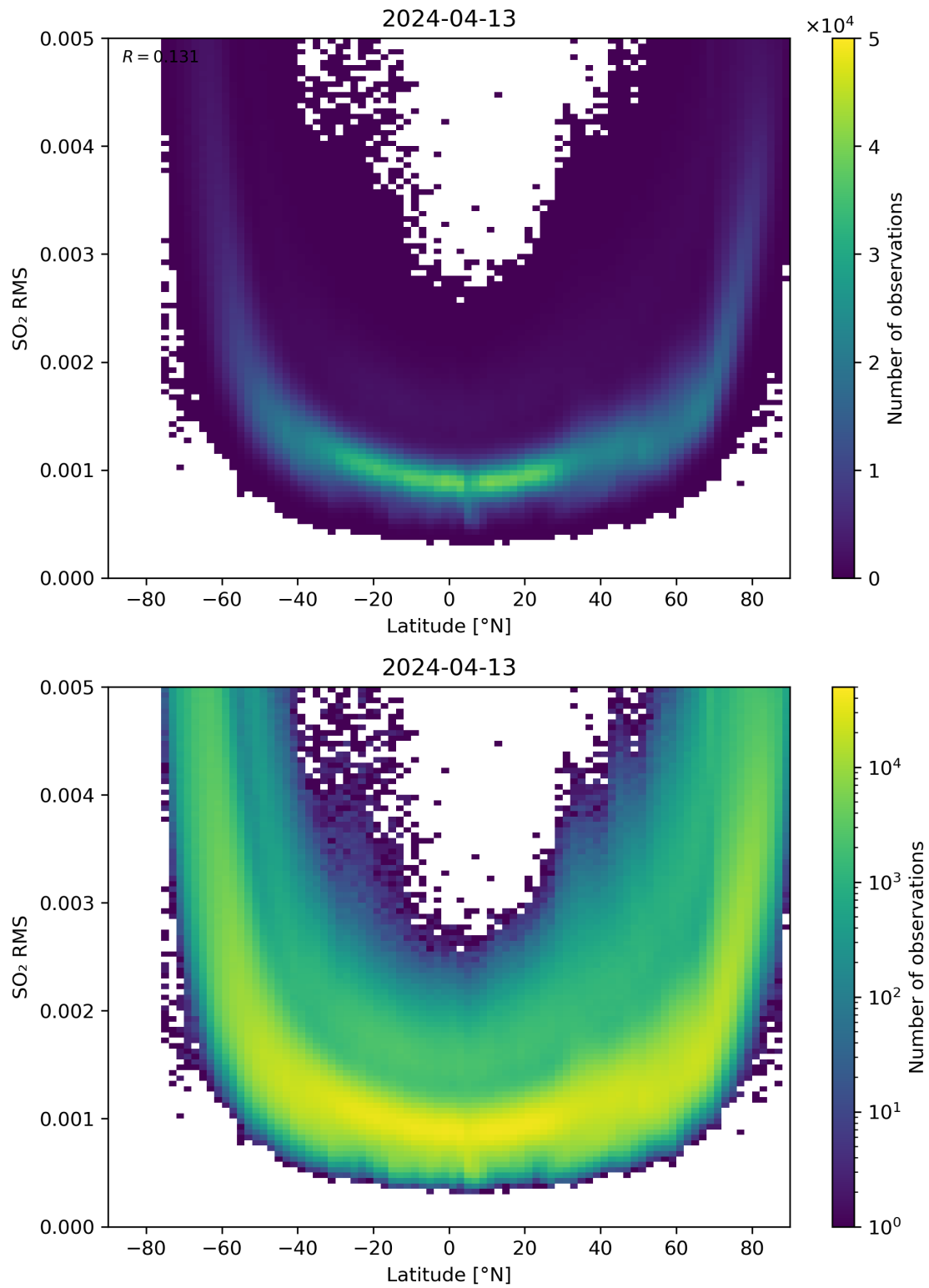
Figure 144: Scatter density plot of “Latitude” against “SO 2 RMS” for 2024-04-12 to 2024-04-14.
