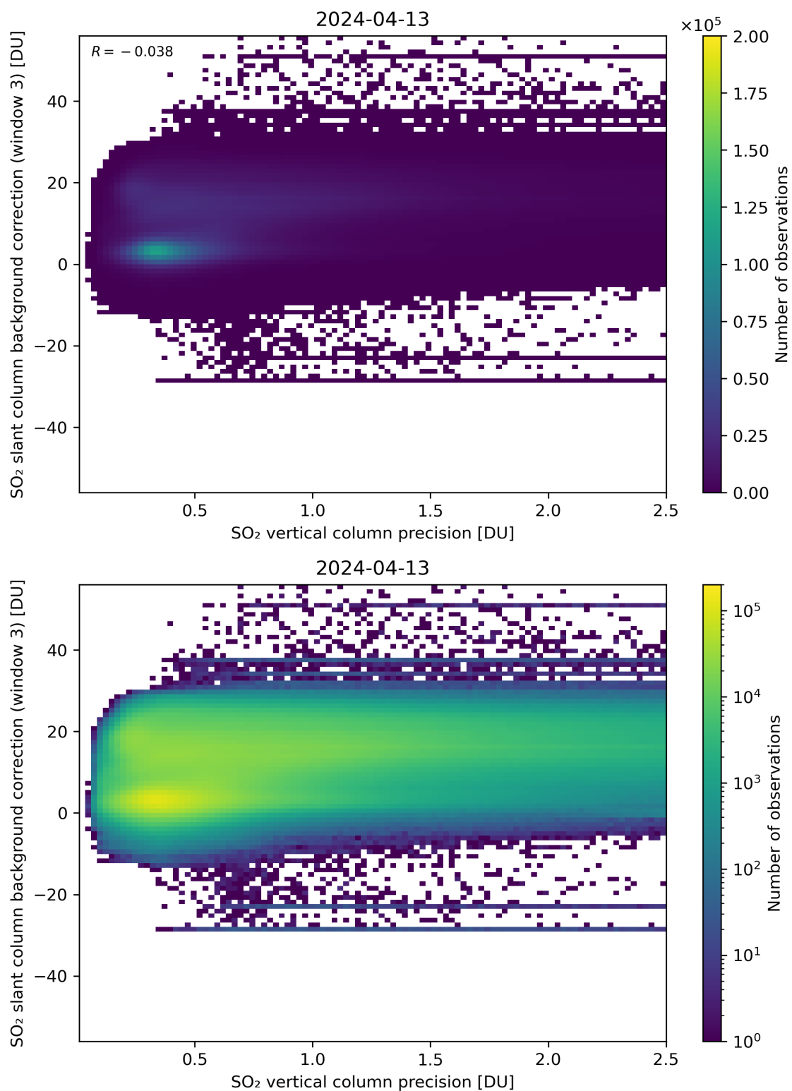
Figure 281: Scatter density plot of “SO 2 vertical column precision” against “SO 2 slant column background correction (window 3)” for 2024-04-12 to 2024-04-14.
