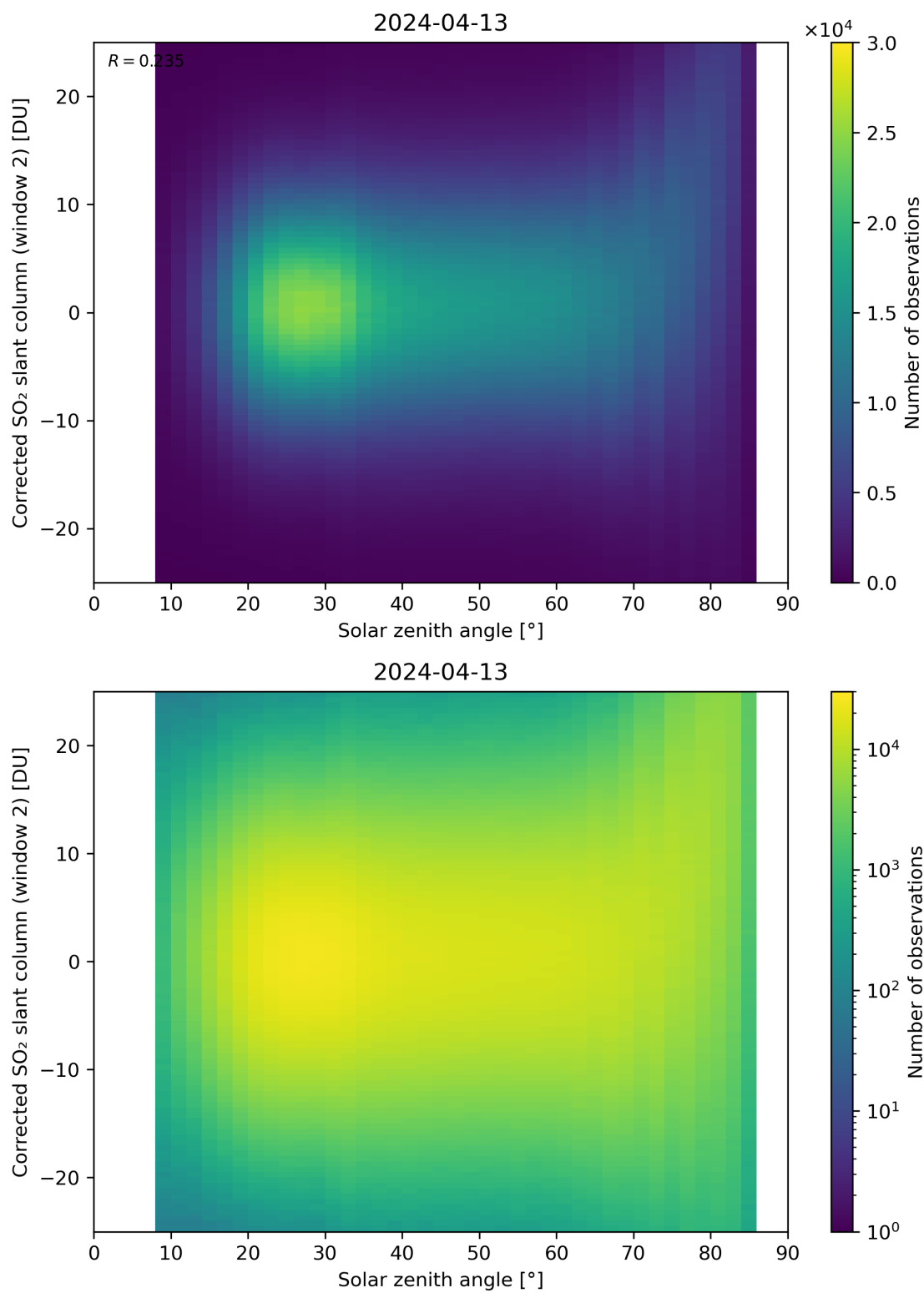
Figure 167: Scatter density plot of “Solar zenith angle” against “Corrected SO 2 slant column (window 2)” for 2024-04-12 to 2024-04-14.
