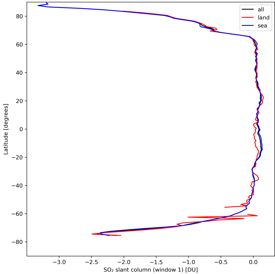
Figure 33: Zonal average of “SO 2 slant column (window 1)” for 2024-04-12 to 2024-04-14.
