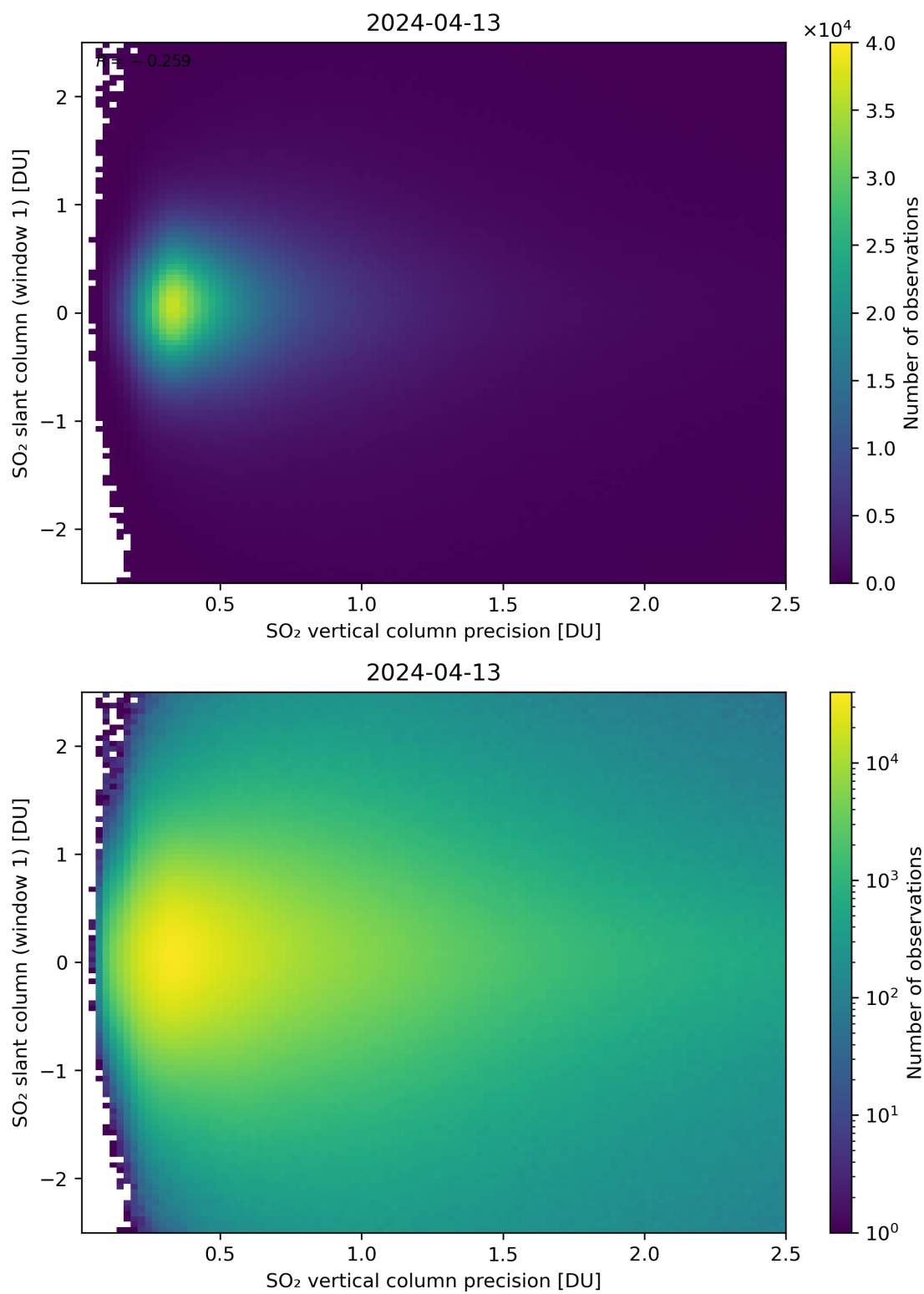
Figure 289: Scatter density plot of “SO 2 vertical column precision” against “SO 2 slant column (window 1)” for 2024-04-12 to 2024-04-14.
