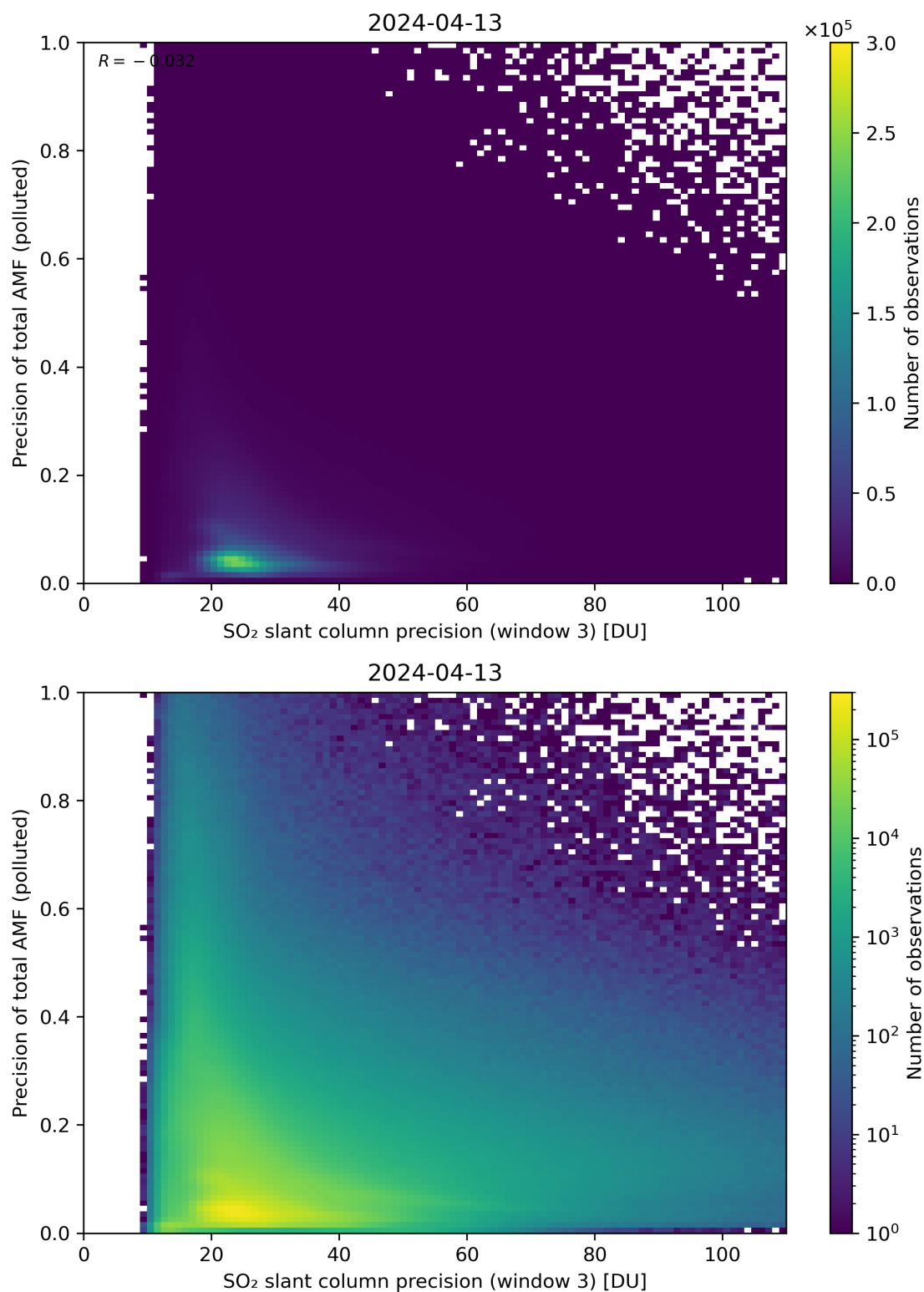
Figure 264: Scatter density plot of “SO 2 slant column precision (window 3)” against “Precision of total AMF (polluted)” for 2024-04-12 to 2024-04-14.
