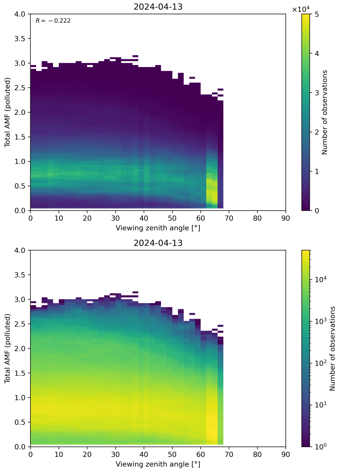
Figure 325: Scatter density plot of “Viewing zenith angle” against “Total AMF (polluted)” for 2024-04-12 to 2024-04-14.
