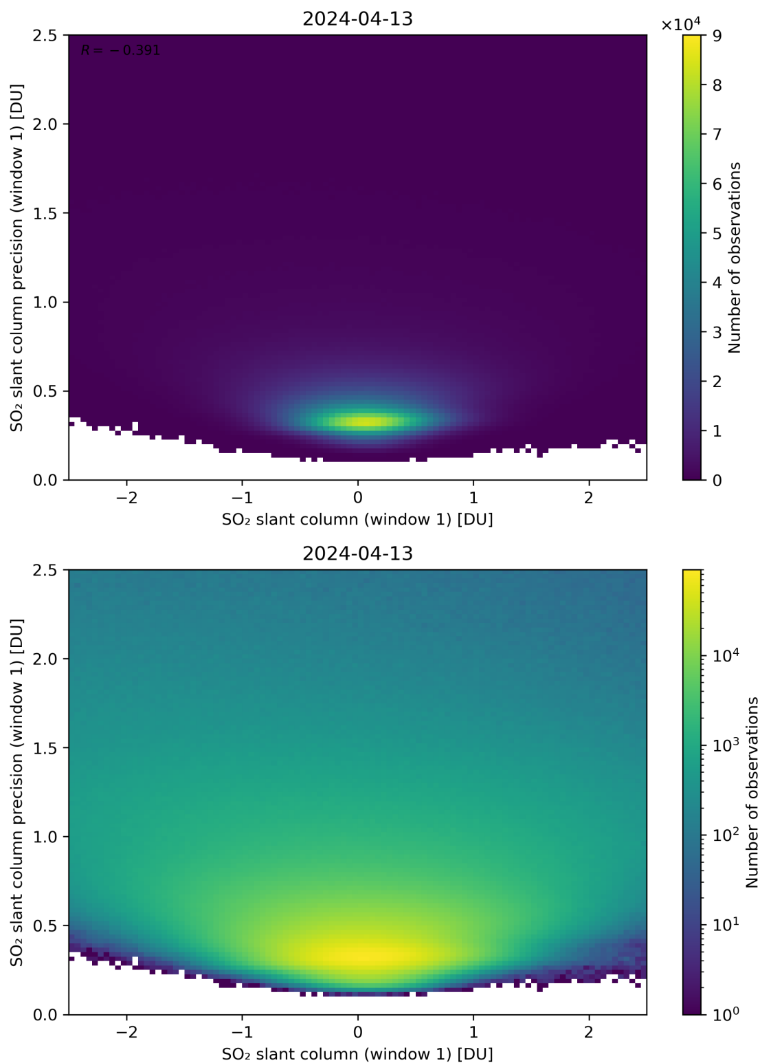
Figure 235: Scatter density plot of “SO 2 slant column (window 1)” against “SO 2 slant column precision (window 1)” for 2024-04-12 to 2024-04-14.
