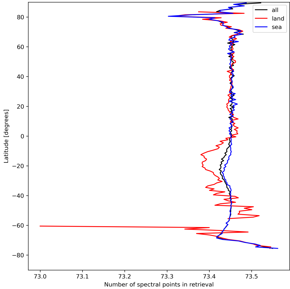
Figure 51: Zonal average of “Number of spectral points in retrieval” for 2024-04-12 to 2024-04-14.
