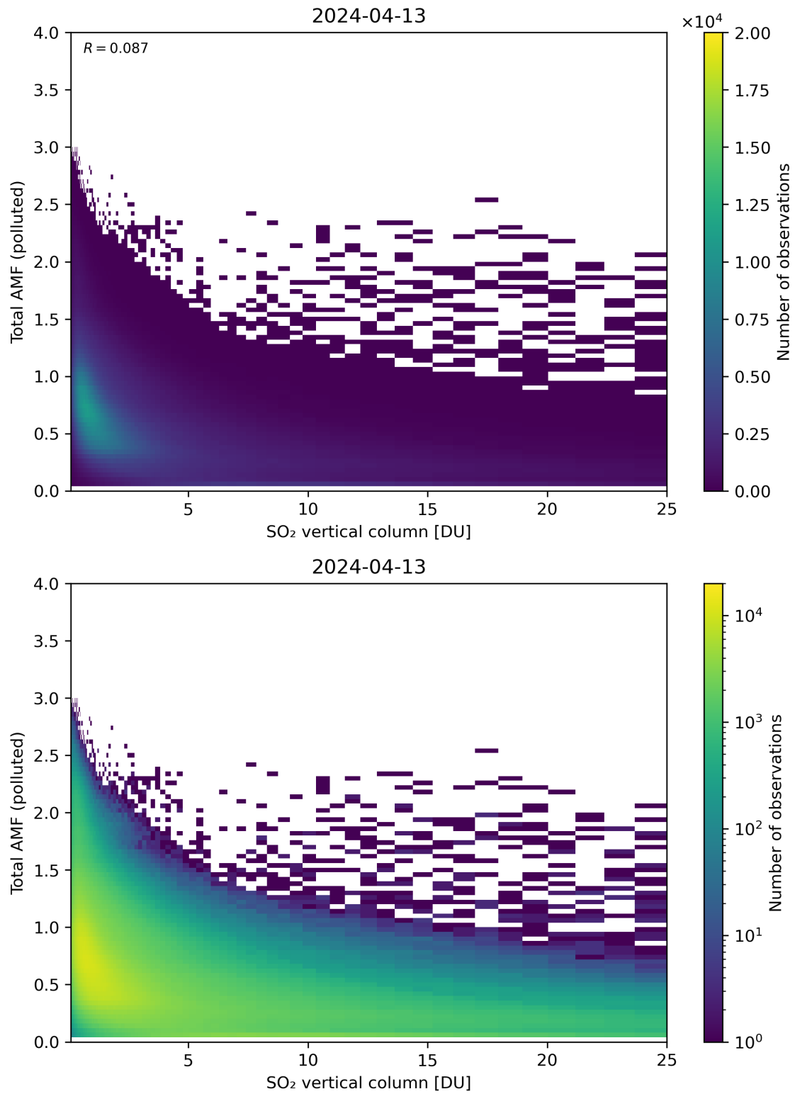
Figure 305: Scatter density plot of “SO 2 vertical column” against “Total AMF (polluted)” for 2024-04-12 to 2024-04-14.
