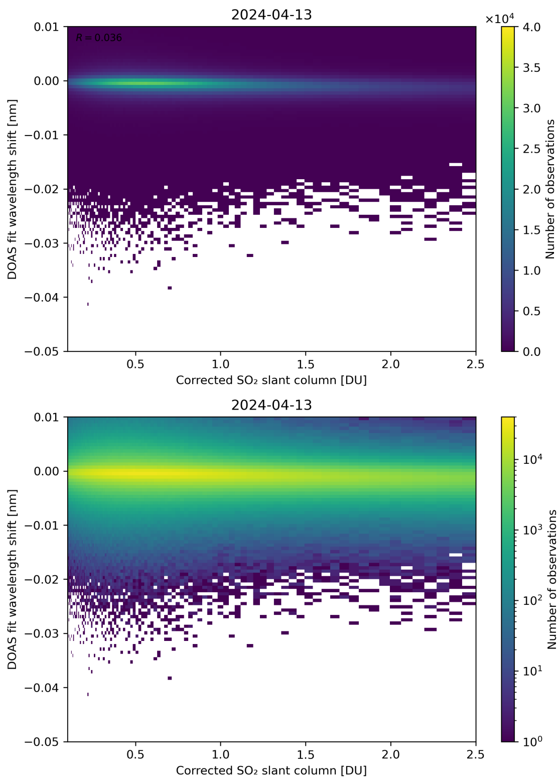
Figure 181: Scatter density plot of “Corrected SO 2 slant column” against “DOAS fit wavelength shift” for 2024-04-12 to 2024-04-14.
