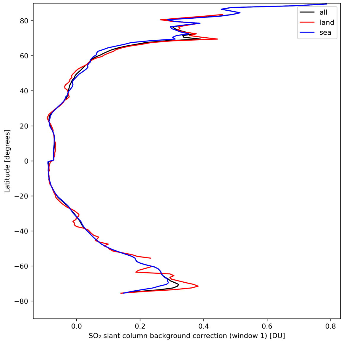
Figure 36: Zonal average of “SO 2 slant column background correction (window 1)” for 2024-04-12 to 2024-04-14.
