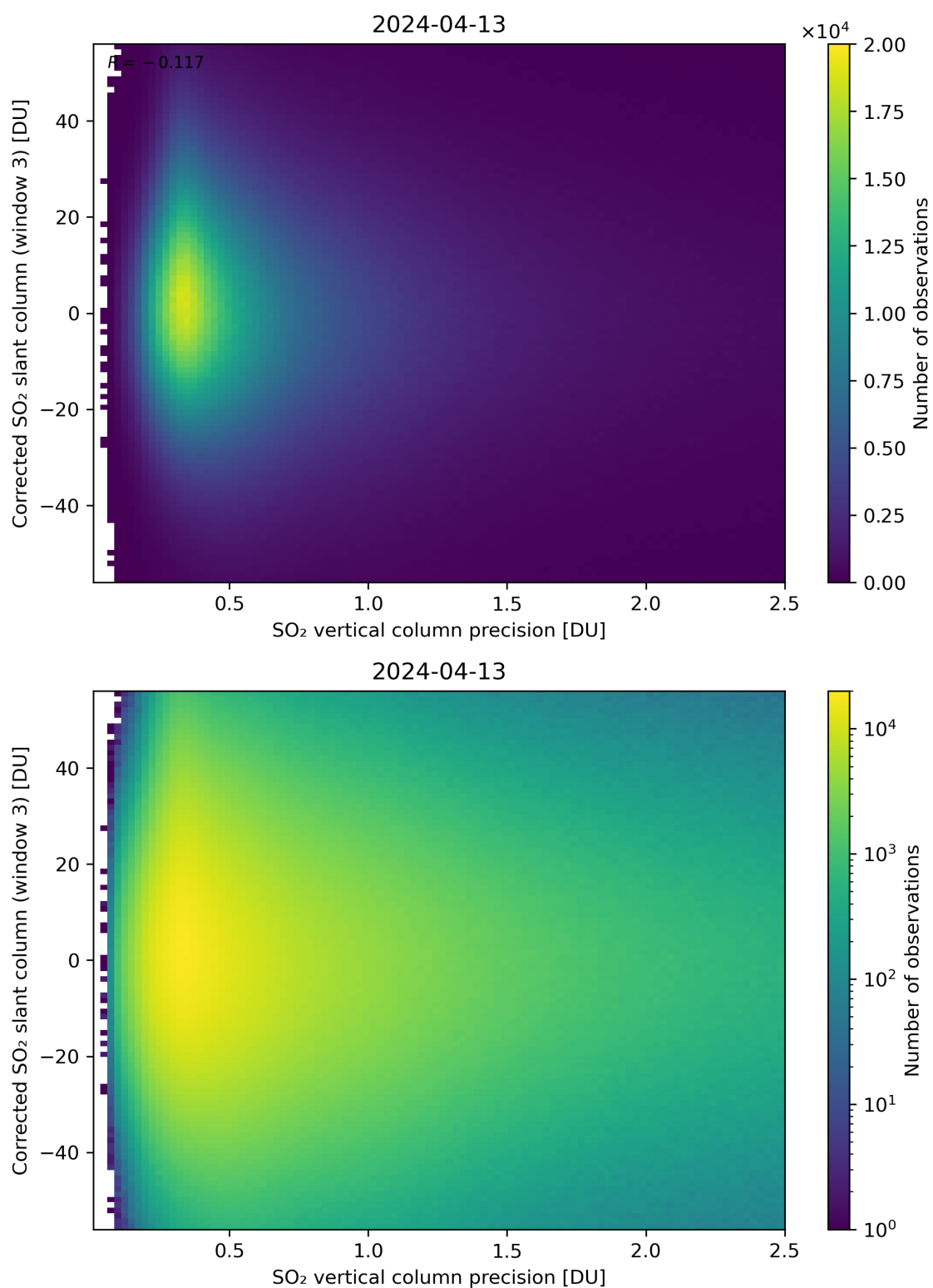
Figure 288: Scatter density plot of “SO 2 vertical column precision” against “Corrected SO 2 slant column (window 3)” for 2024-04-12 to 2024-04-14.
