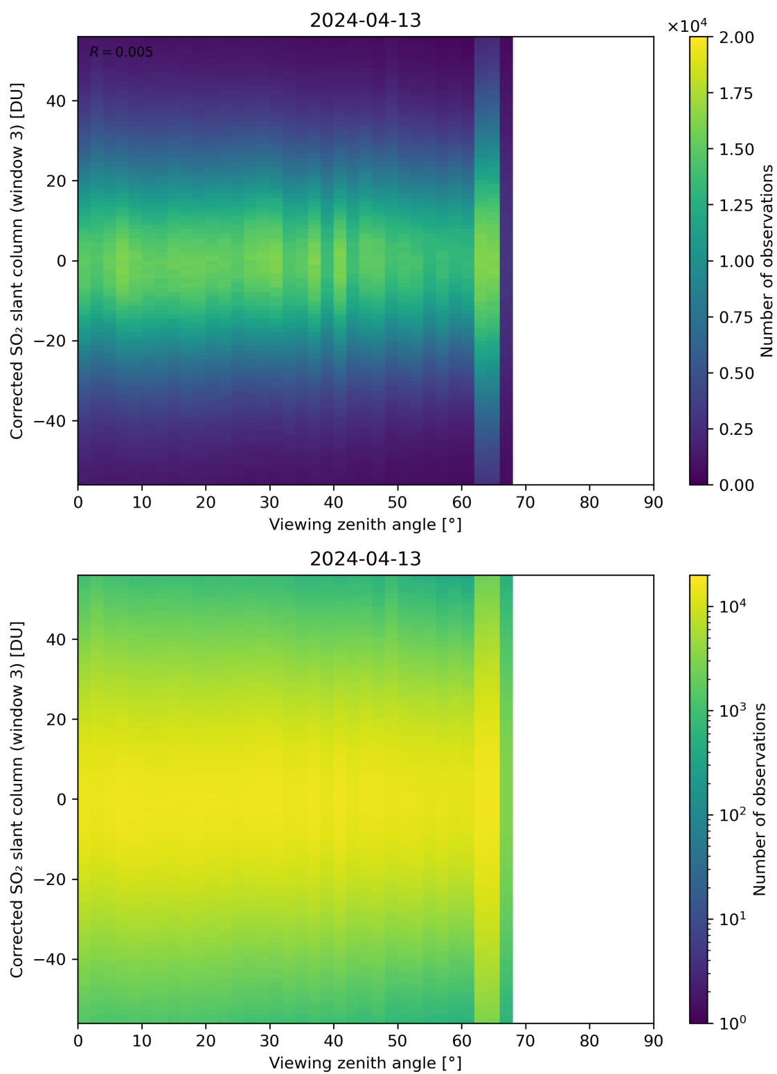
Figure 319: Scatter density plot of “Viewing zenith angle” against “Corrected SO 2 slant column (window 3)” for 2024-04-12 to 2024-04-14.
