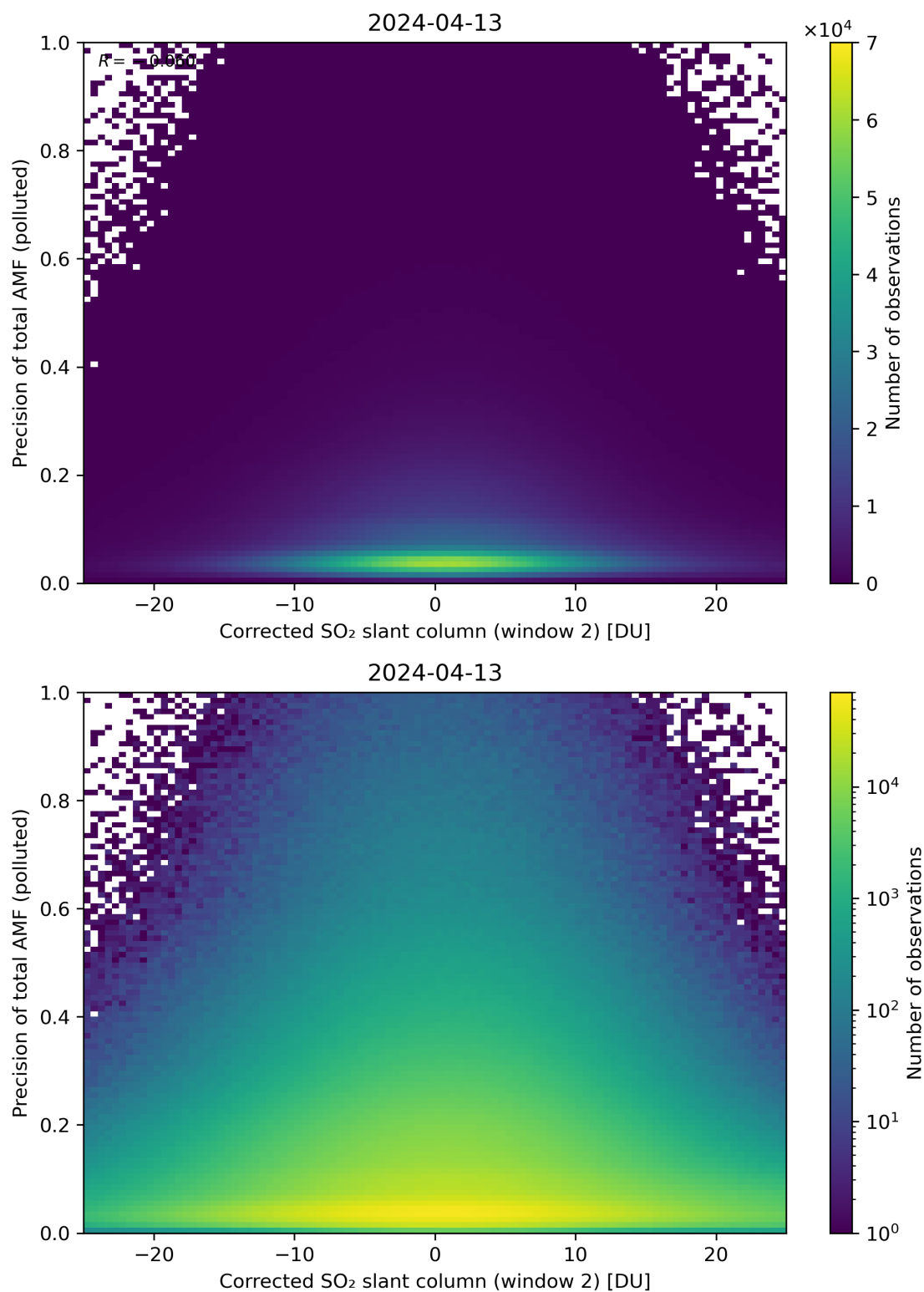
Figure 204: Scatter density plot of “Corrected SO 2 slant column (window 2)” against “Precision of total AMF (polluted)” for 2024-04-12 to 2024-04-14.
