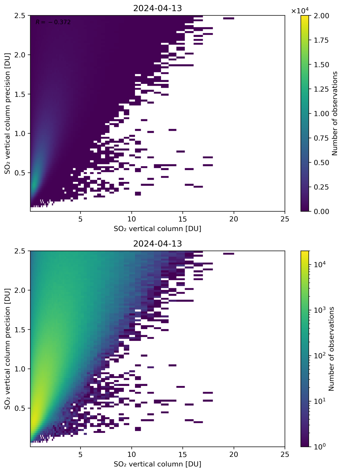
Figure 307: Scatter density plot of “SO 2 vertical column” against “SO 2 vertical column precision” for 2024-04-12 to 2024-04-14.
