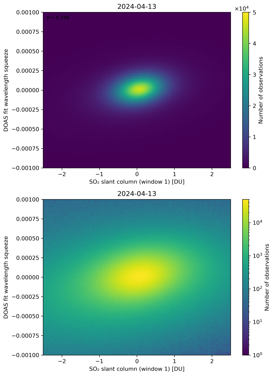
Figure 216: Scatter density plot of “SO 2 slant column (window 1)” against “DOAS fit wavelength squeeze” for 2024-04-12 to 2024-04-14.
