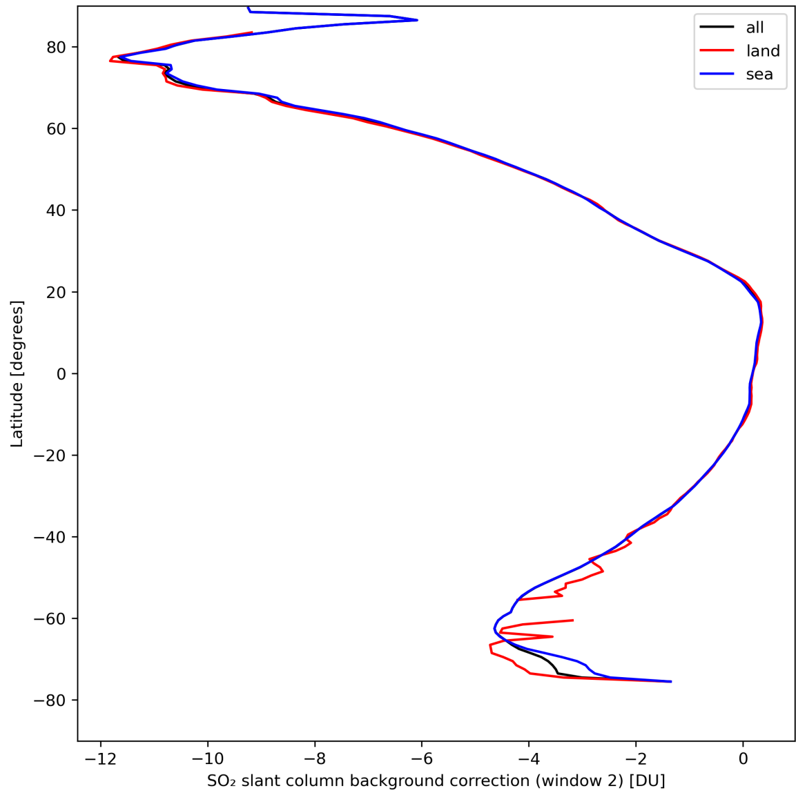
Figure 40: Zonal average of “SO 2 slant column background correction (window 2)” for 2024-04-12 to 2024-04-14.
