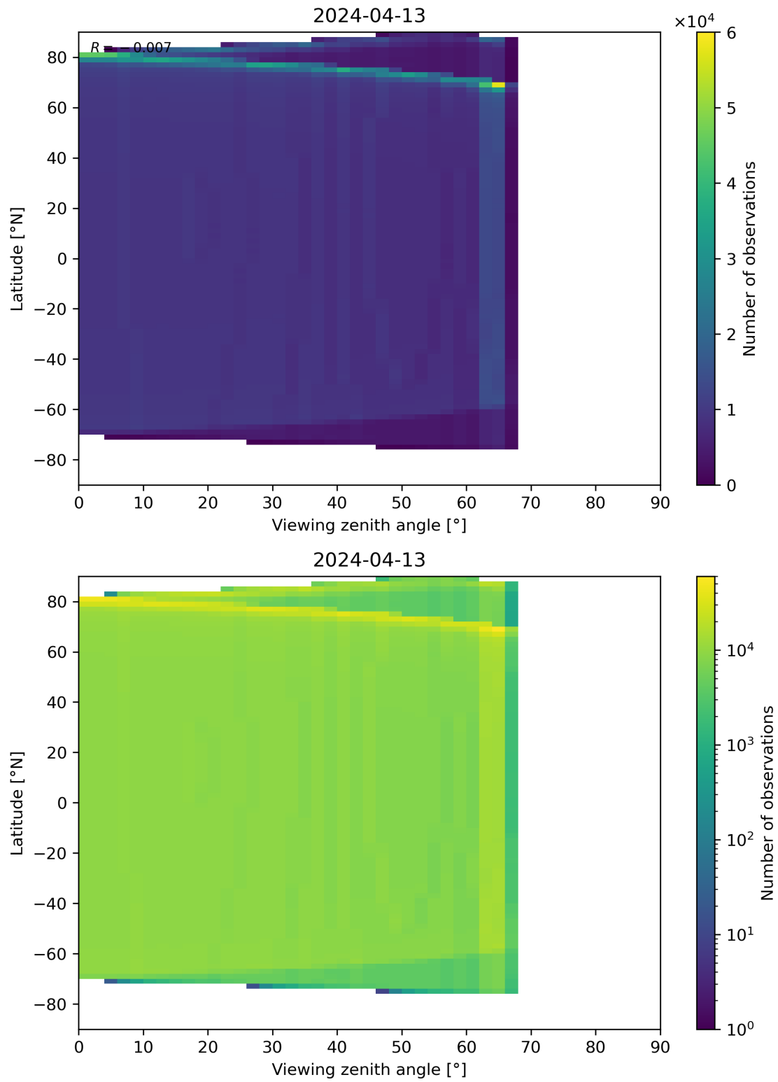
Figure 314: Scatter density plot of “Viewing zenith angle” against “Latitude” for 2024-04-12 to 2024-04-14.
