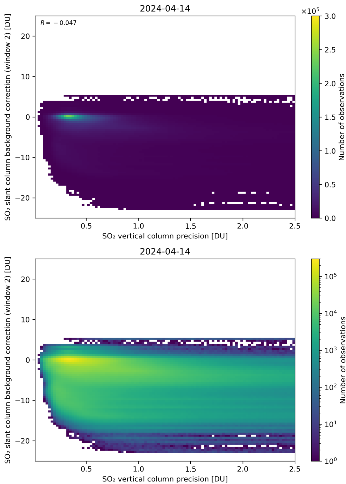
Figure 280: Scatter density plot of “SO 2 vertical column precision” against “SO 2 slant column background correction (window 2)” for 2024-04-13 to 2024-04-15.
