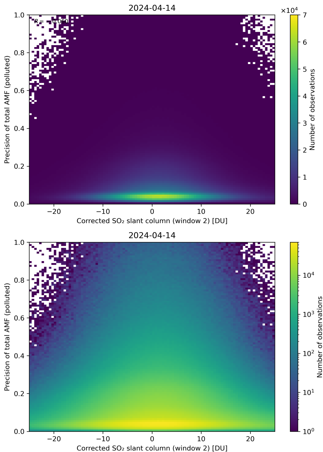
Figure 204: Scatter density plot of “Corrected SO 2 slant column (window 2)” against “Precision of total AMF (polluted)” for 2024-04-13 to 2024-04-15.
