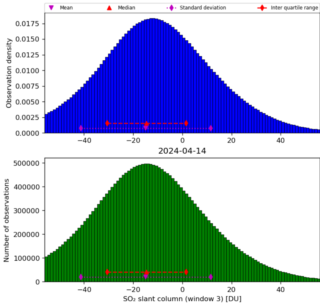
Figure 64: Histogram of “SO 2 slant column (window 3)” for 2024-04-13 to 2024-04-15
