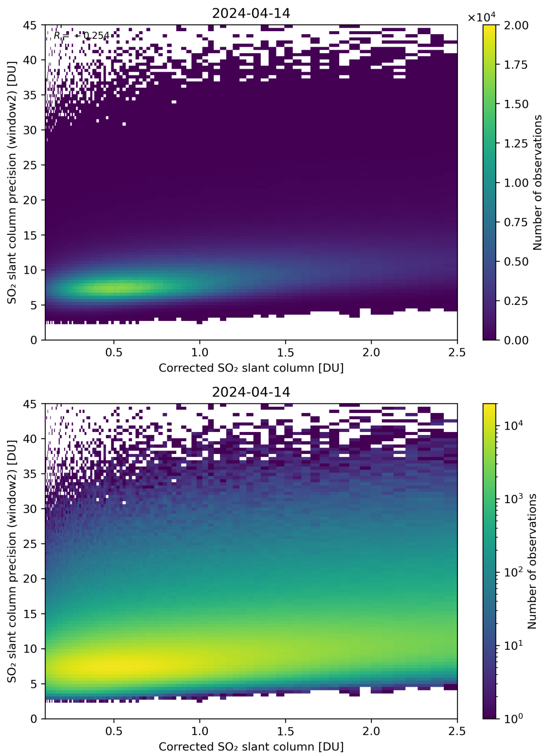
Figure 189: Scatter density plot of “Corrected SO 2 slant column” against “SO 2 slant column precision (window2)” for 2024-04-13 to 2024-04-15.
