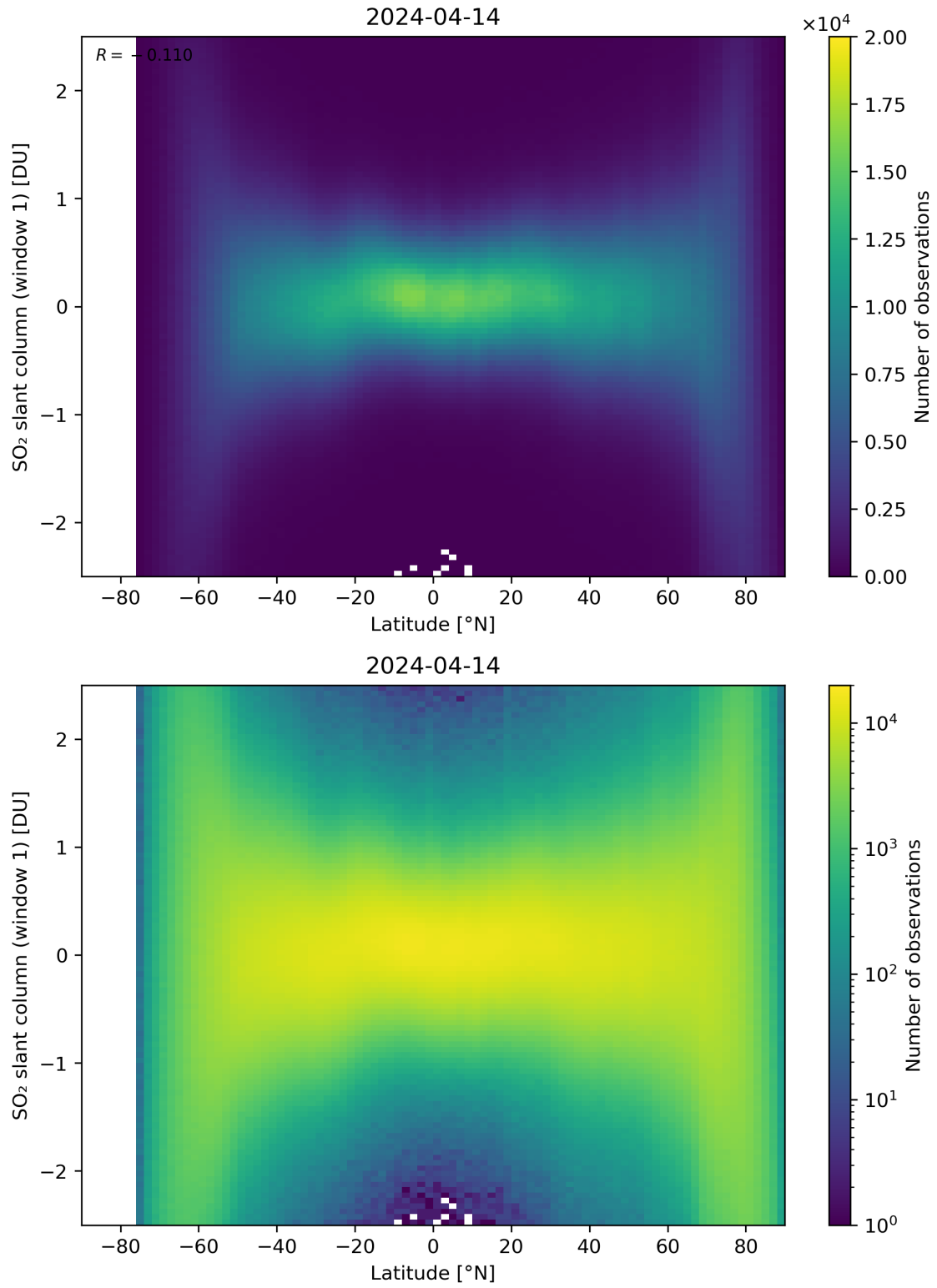
Figure 149: Scatter density plot of “Latitude” against “SO 2 slant column (window 1)” for 2024-04-13 to 2024-04-15.
