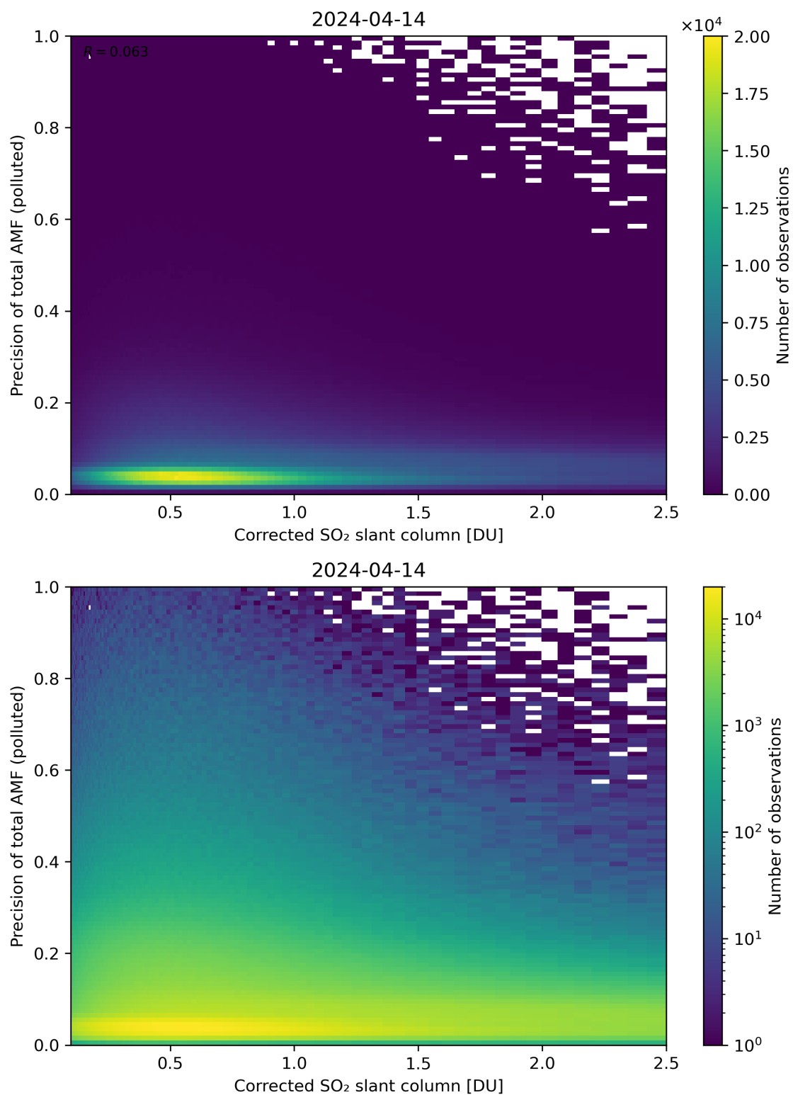
Figure 193: Scatter density plot of “Corrected SO 2 slant column” against “Precision of total AMF (polluted)” for 2024-04-13 to 2024-04-15.
