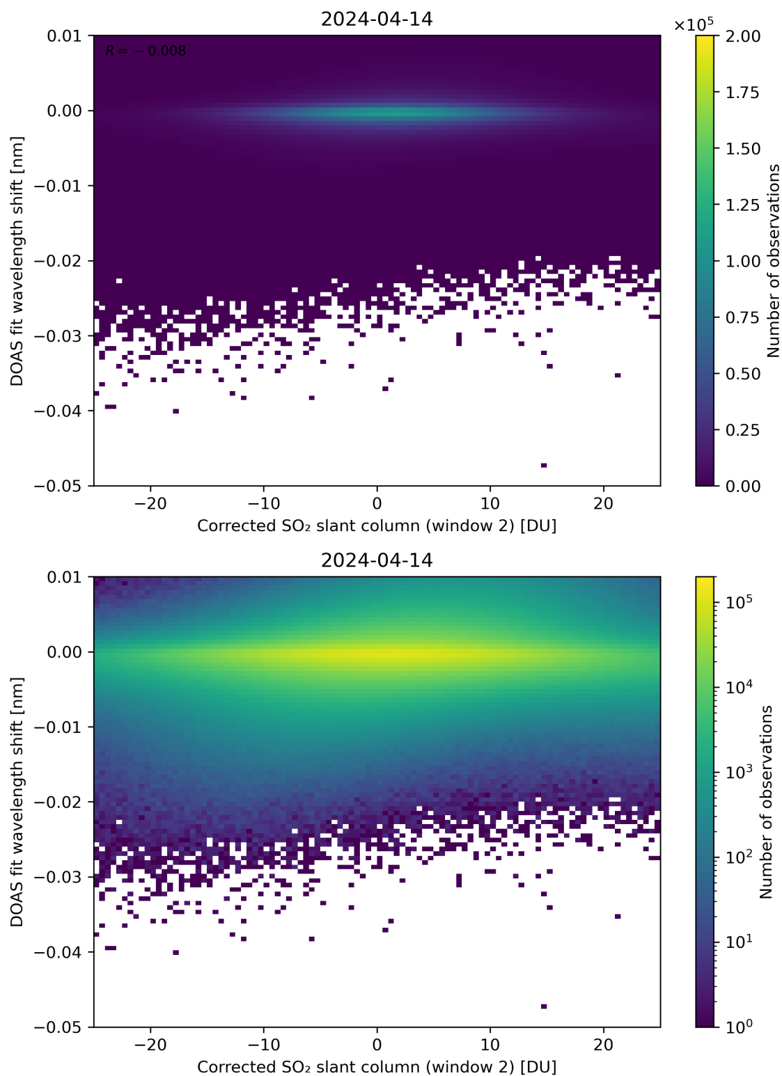
Figure 196: Scatter density plot of “Corrected SO 2 slant column (window 2)” against “DOAS fit wavelength shift” for 2024-04-13 to 2024-04-15.
