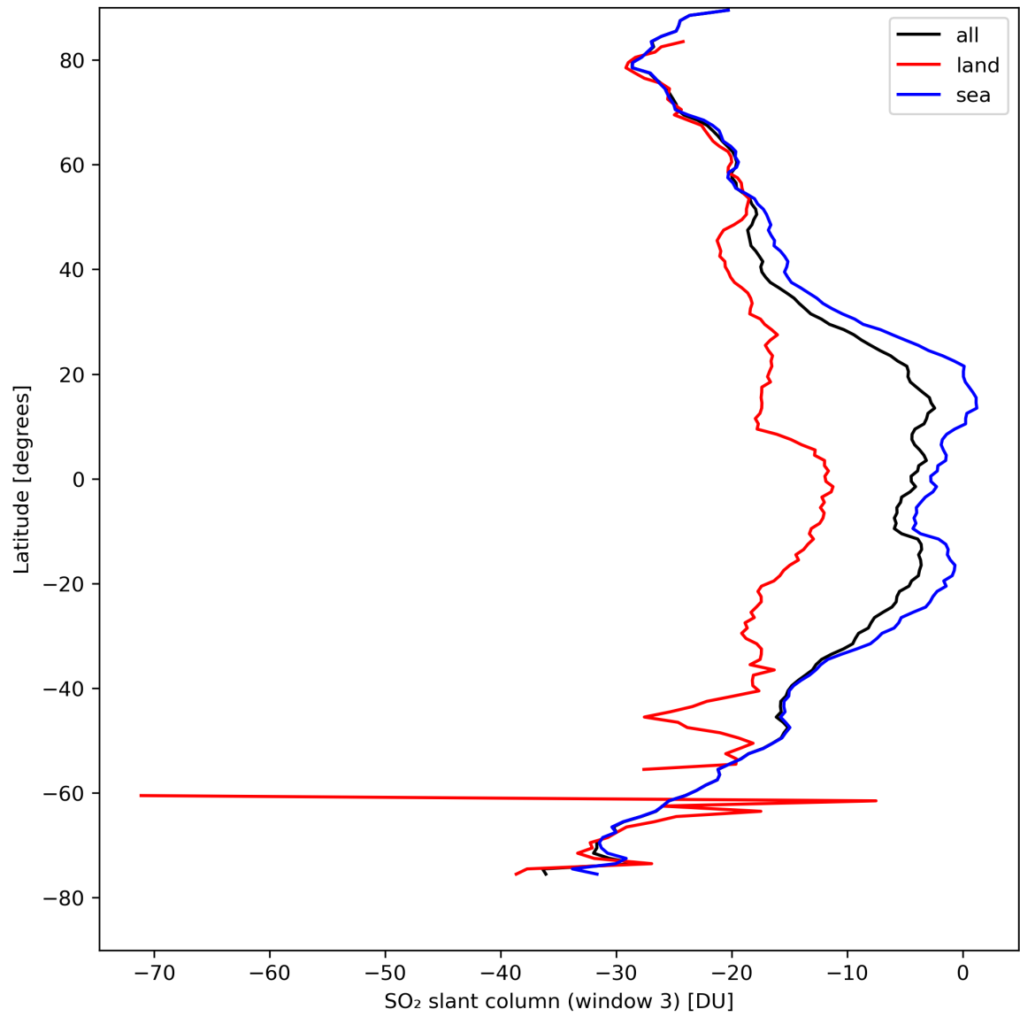
Figure 41: Zonal average of “SO 2 slant column (window 3)” for 2024-04-13 to 2024-04-15.
