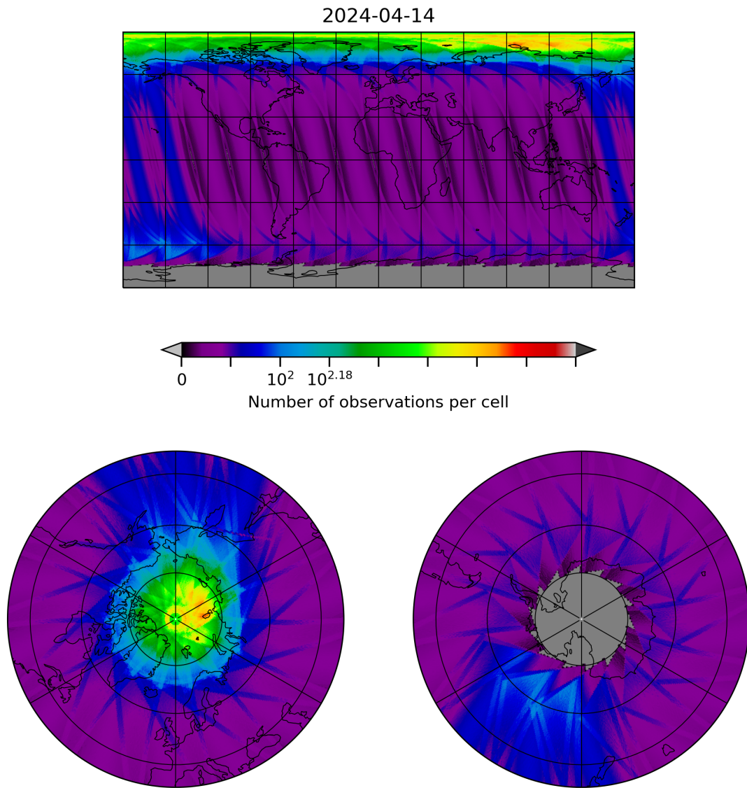
Figure 28: Map of the number of observations for 2024-04-13 to 2024-04-15
