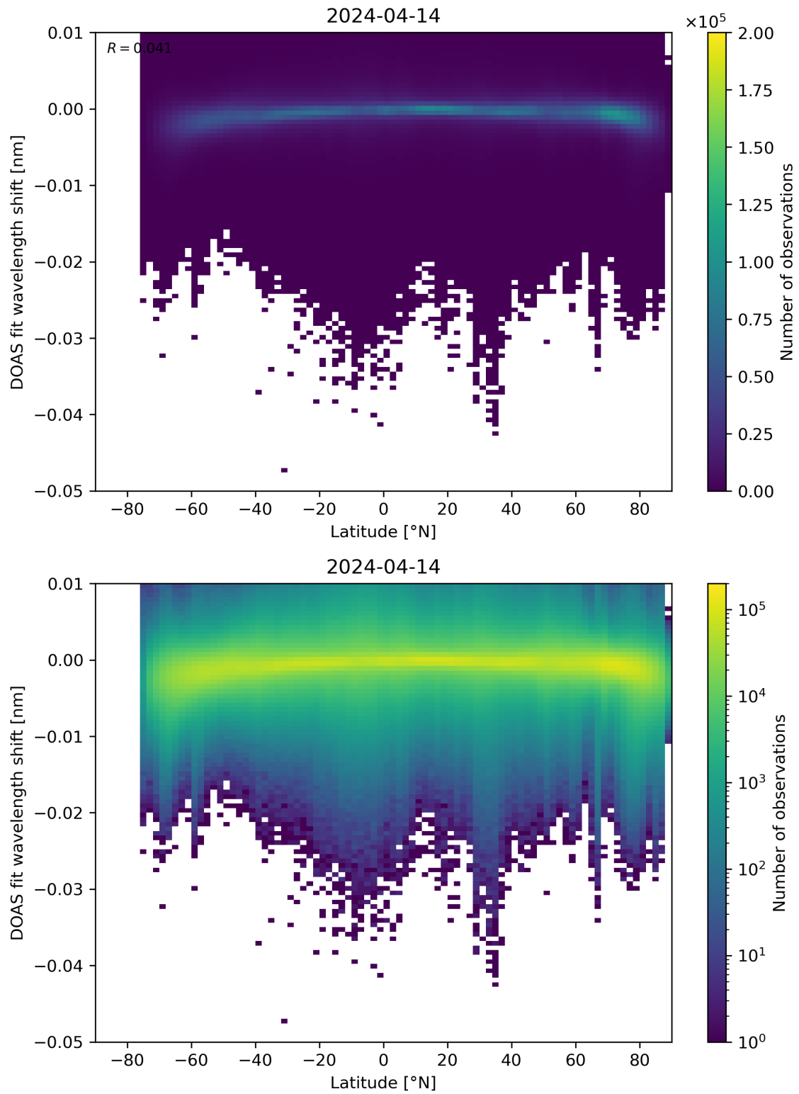
Figure 142: Scatter density plot of “Latitude” against “DOAS fit wavelength shift” for 2024-04-13 to 2024-04-15.
