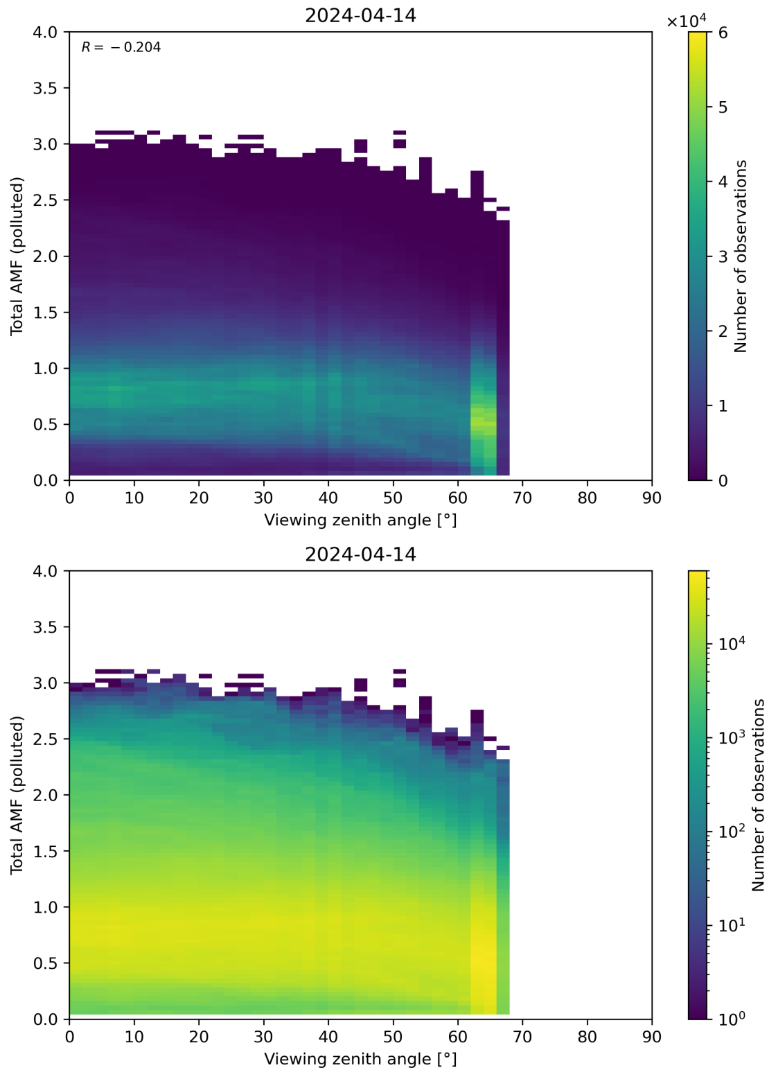
Figure 325: Scatter density plot of “Viewing zenith angle” against “Total AMF (polluted)” for 2024-04-13 to 2024-04-15.
