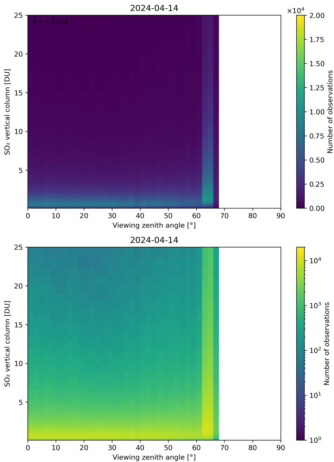
Figure 327: Scatter density plot of “Viewing zenith angle” against “SO 2 vertical column” for 2024-04-13 to 2024-04-15.
