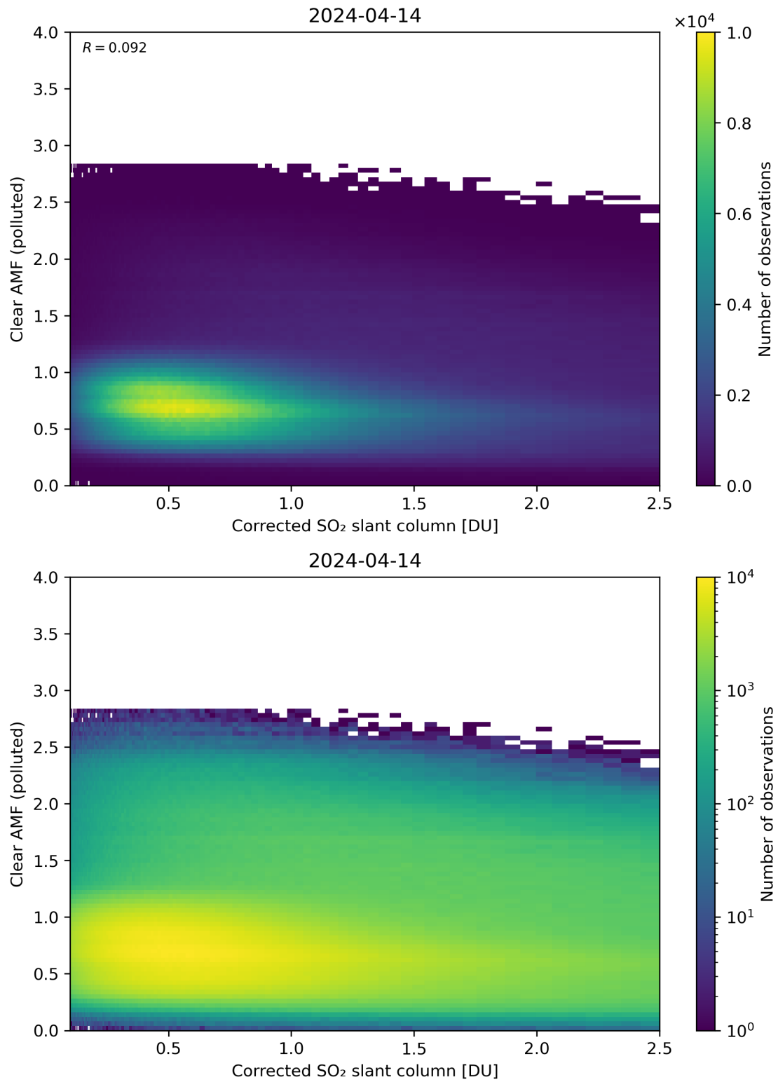
Figure 184: Scatter density plot of “Corrected SO 2 slant column” against “Clear AMF (polluted)” for 2024-04-13 to 2024-04-15.
