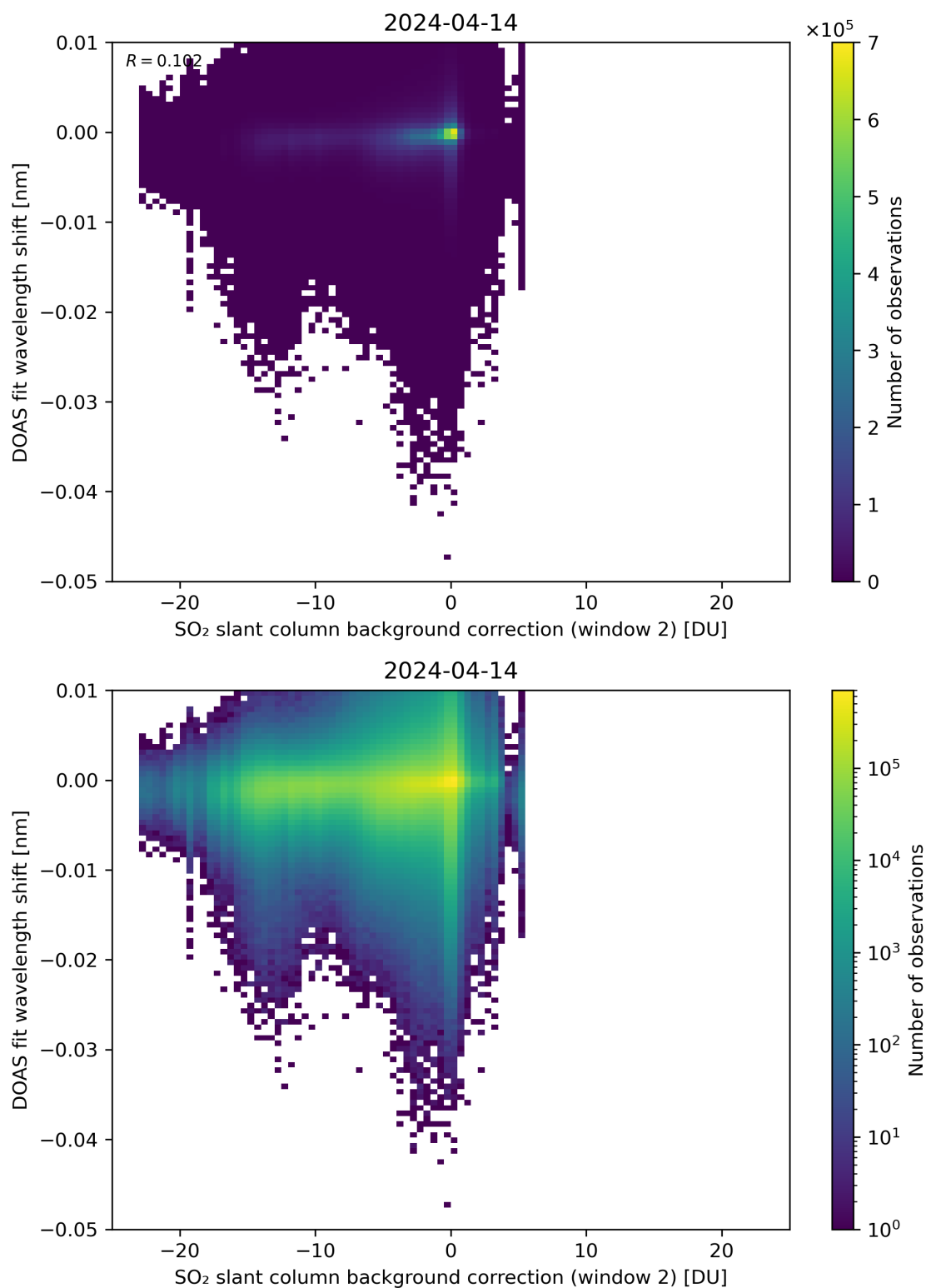
Figure 112: Scatter density plot of “SO 2 slant column background correction (window 2)” against “DOAS fit wavelength shift” for 2024-04-13 to 2024-04-15.
