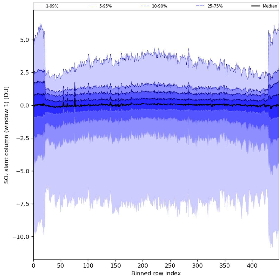
Figure 79: Along track statistics of “SO 2 slant column (window 1)” for 2024-04-13 to 2024-04-15
