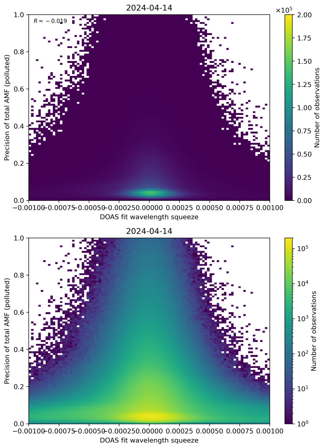
Figure 135: Scatter density plot of “DOAS fit wavelength squeeze” against “Precision of total AMF (polluted)” for 2024-04-13 to 2024-04-15.
