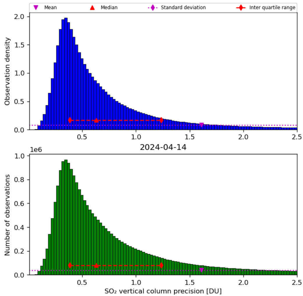
Figure 54: Histogram of “SO 2 vertical column precision” for 2024-04-13 to 2024-04-15
