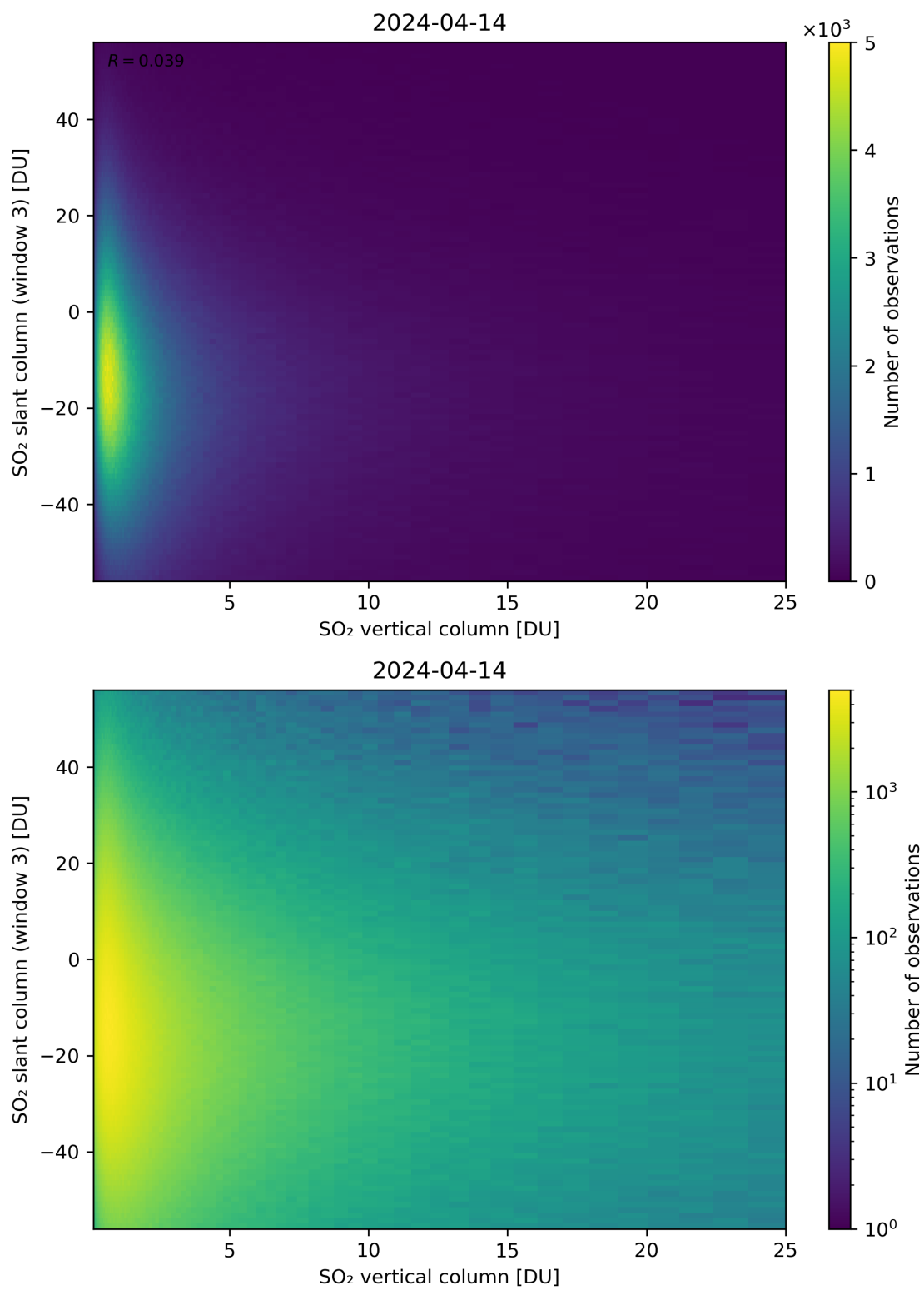
Figure 303: Scatter density plot of “SO 2 vertical column” against “SO 2 slant column (window 3)” for 2024-04-13 to 2024-04-15.
