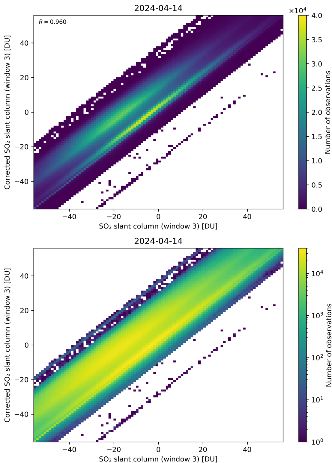
Figure 266: Scatter density plot of “SO 2 slant column (window 3)” against “Corrected SO 2 slant column (window 3)” for 2024-04-13 to 2024-04-15.
