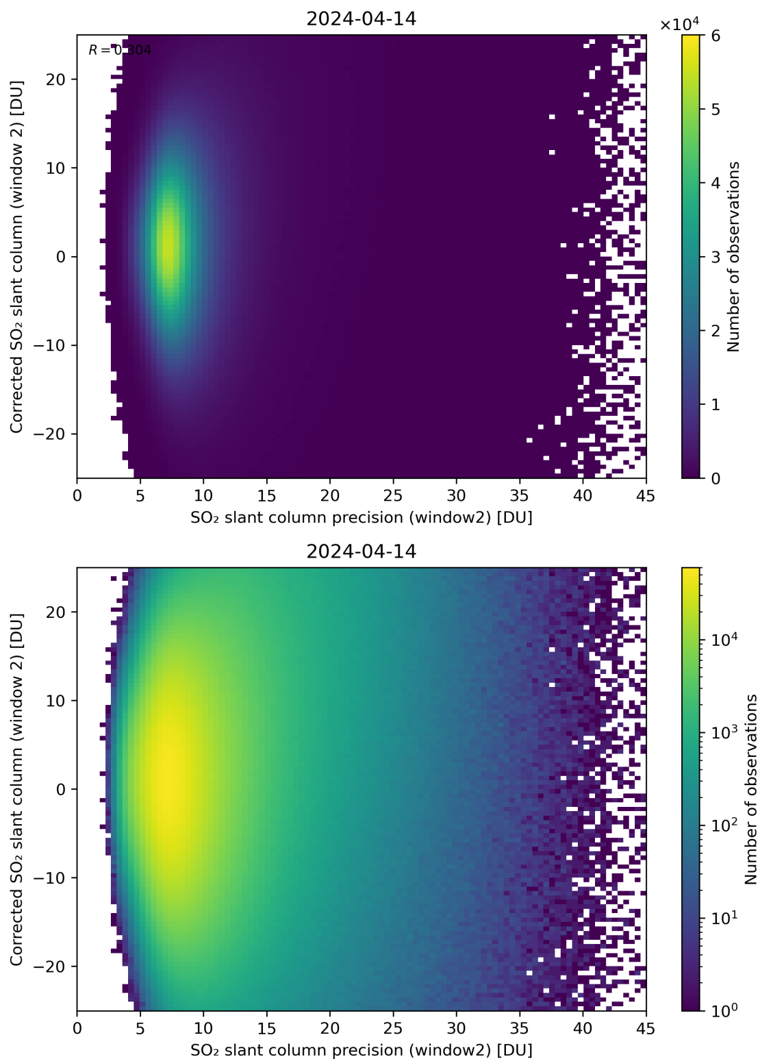
Figure 247: Scatter density plot of “SO 2 slant column precision (window2)” against “Corrected SO 2 slant column (window 2)” for 2024-04-13 to 2024-04-15.
