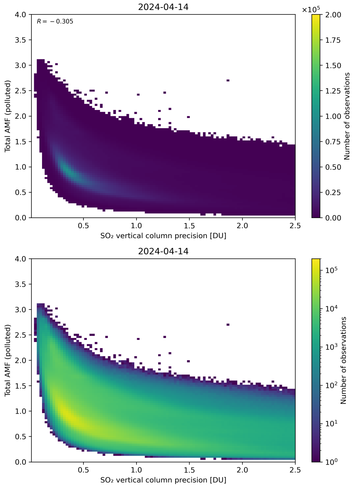
Figure 294: Scatter density plot of “SO 2 vertical column precision” against “Total AMF (polluted)” for 2024-04-13 to 2024-04-15.
