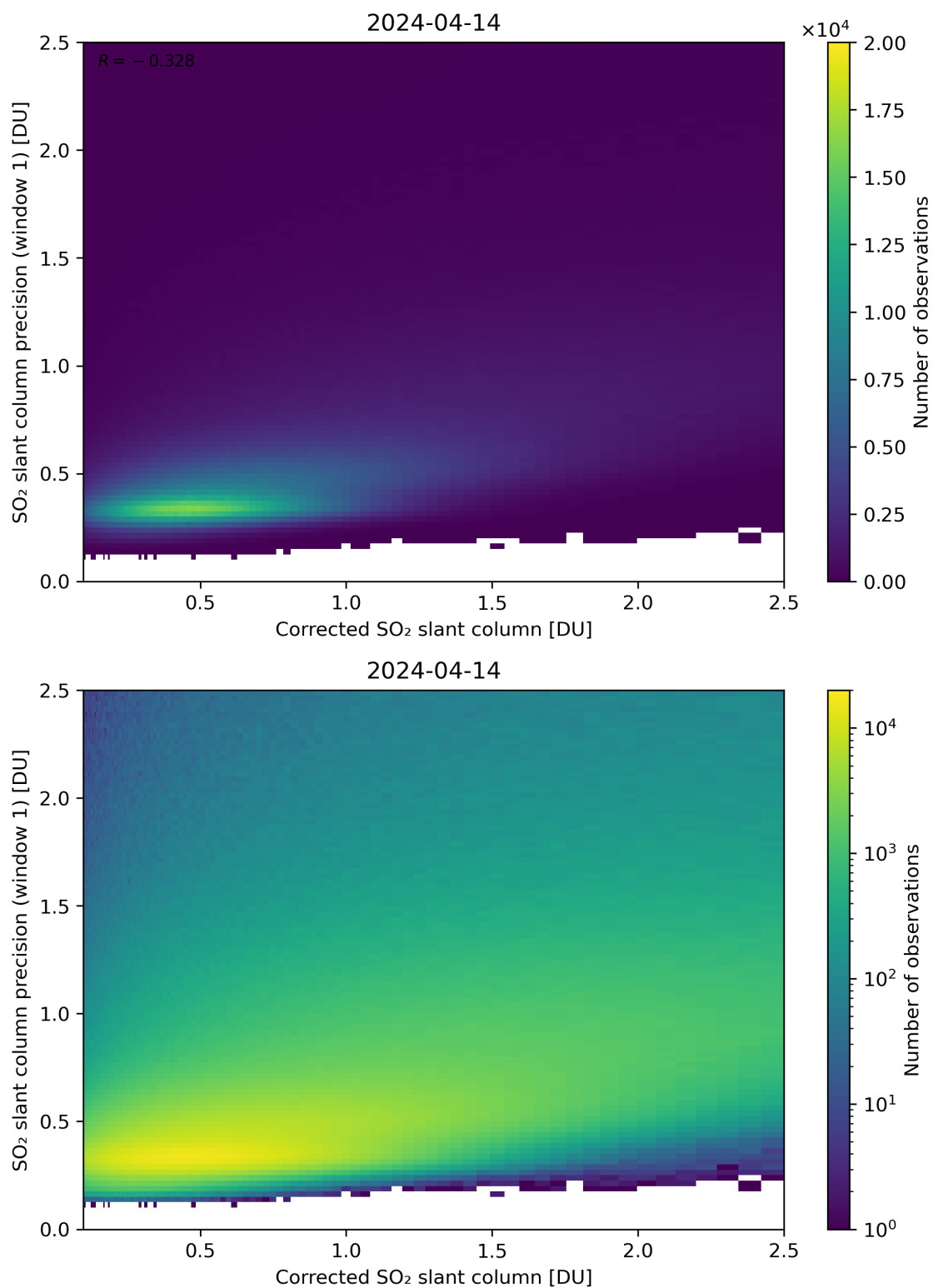
Figure 188: Scatter density plot of “Corrected SO 2 slant column” against “SO 2 slant column precision (window 1)” for 2024-04-13 to 2024-04-15.
