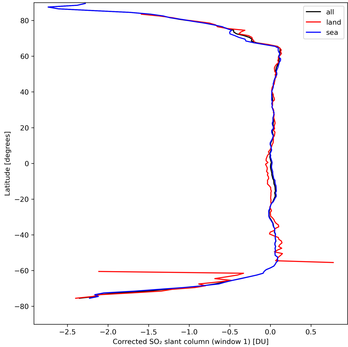
Figure 35: Zonal average of “Corrected SO 2 slant column (window 1)” for 2024-04-13 to 2024-04-15.
