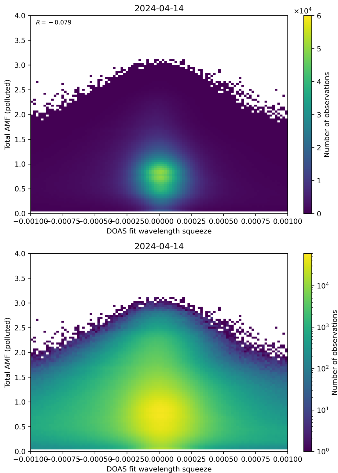
Figure 134: Scatter density plot of “DOAS fit wavelength squeeze” against “Total AMF (polluted)” for 2024-04-13 to 2024-04-15.
