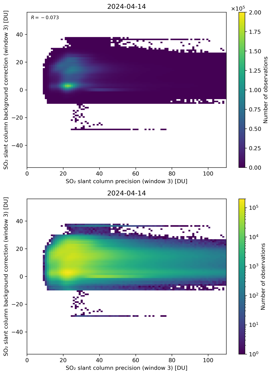
Figure 257: Scatter density plot of “SO 2 slant column precision (window 3)” against “SO 2 slant column background correction (window 3)” for 2024-04-13 to 2024-04-15.
