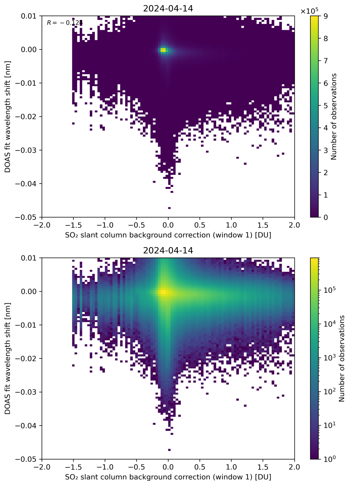
Figure 100: Scatter density plot of “SO 2 slant column background correction (window 1)” against “DOAS fit wavelength shift” for 2024-04-13 to 2024-04-15.
