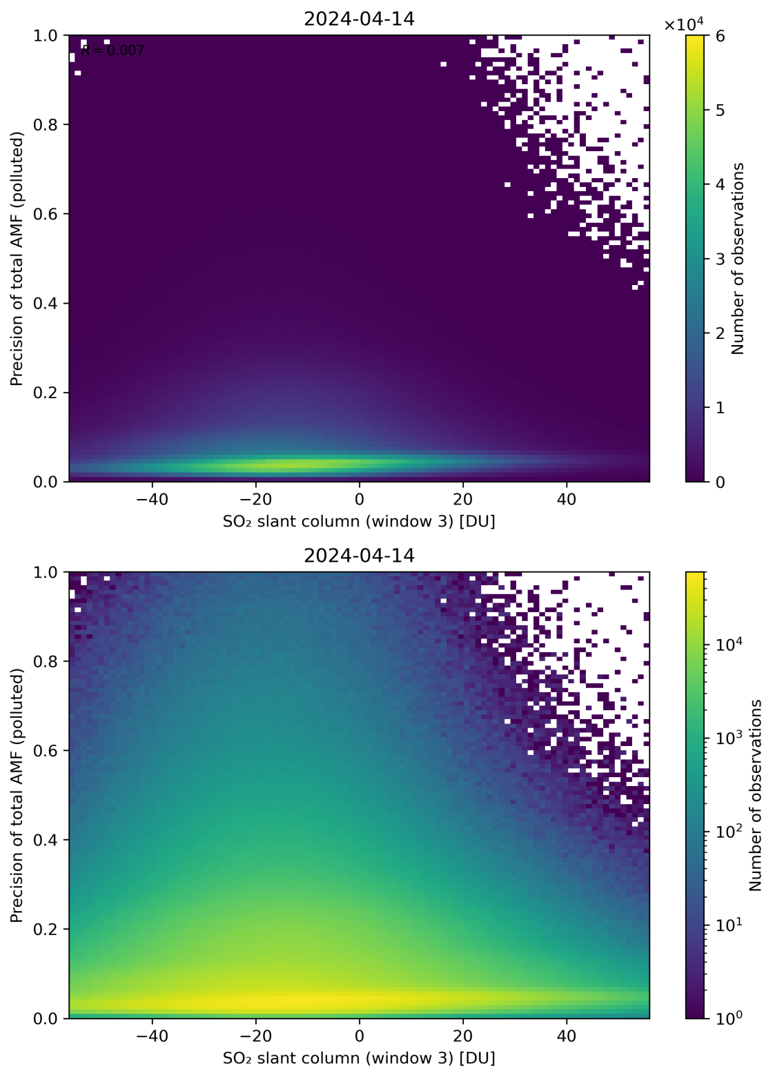
Figure 269: Scatter density plot of “SO 2 slant column (window 3)” against “Precision of total AMF (polluted)” for 2024-04-13 to 2024-04-15.
