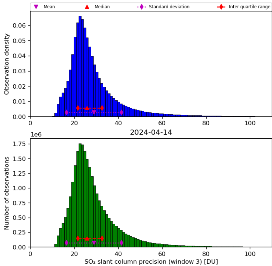
Figure 65: Histogram of “SO 2 slant column precision (window 3)” for 2024-04-13 to 2024-04-15
