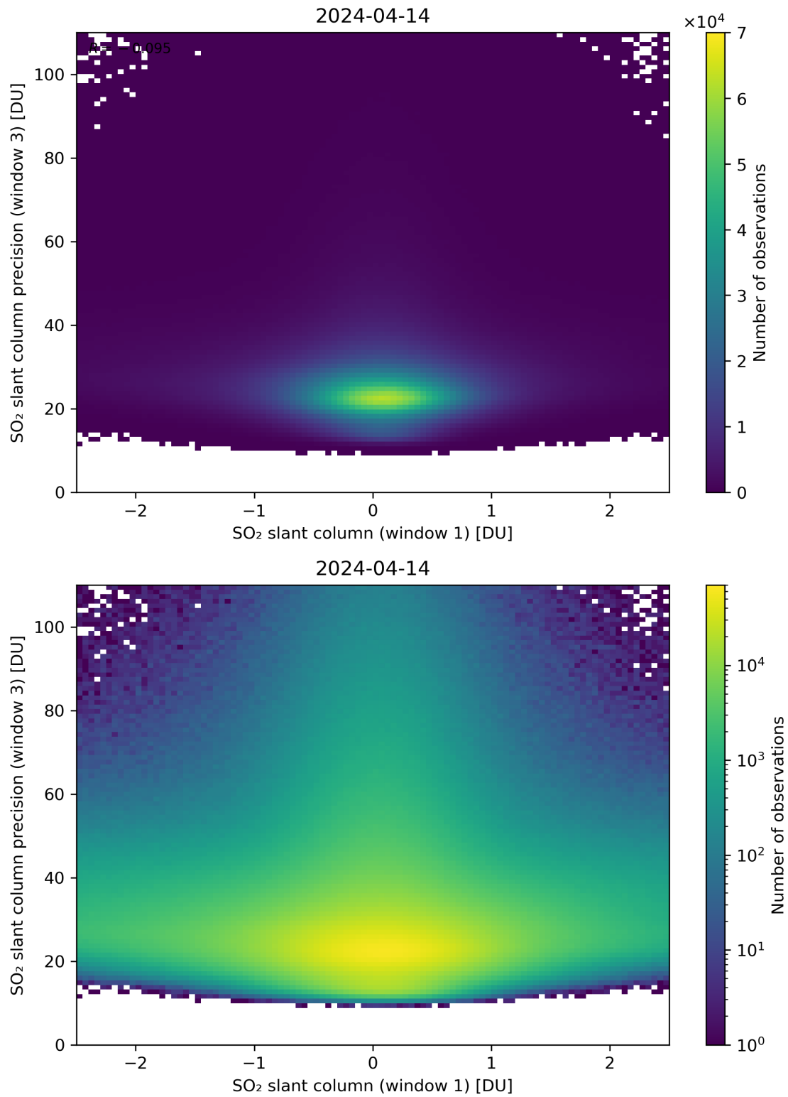
Figure 238: Scatter density plot of “SO 2 slant column (window 1)” against “SO 2 slant column precision (window 3)” for 2024-04-13 to 2024-04-15.
