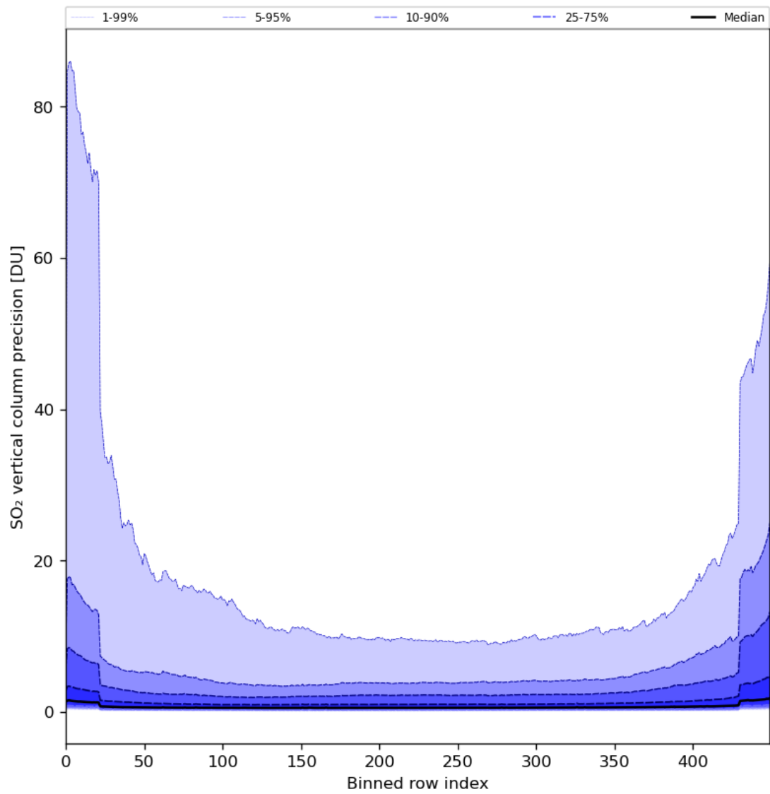
Figure 77: Along track statistics of “SO 2 vertical column precision” for 2024-04-13 to 2024-04-15
