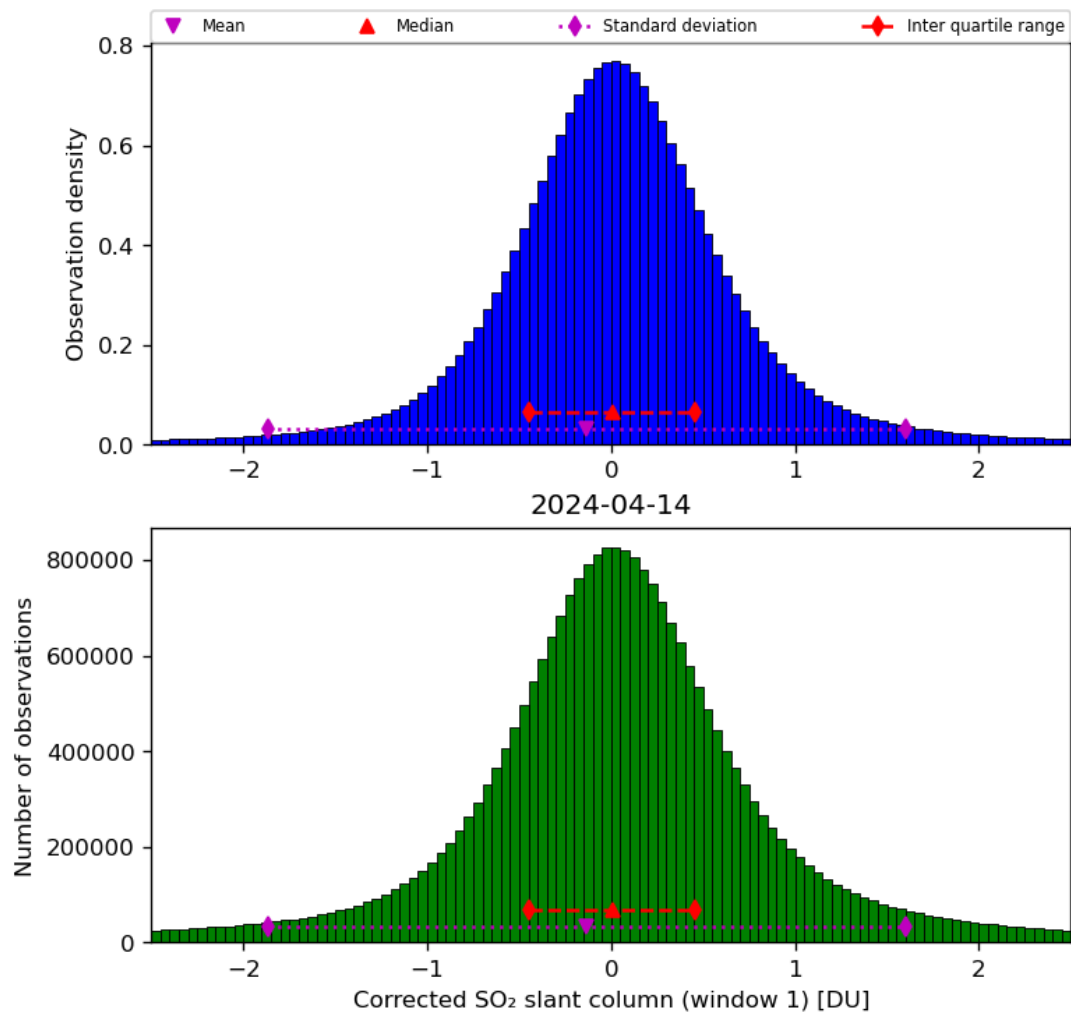
Figure 58: Histogram of “Corrected SO 2 slant column (window 1)” for 2024-04-13 to 2024-04-15
