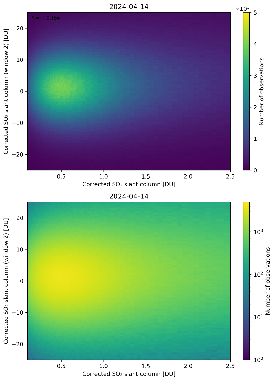
Figure 185: Scatter density plot of “Corrected SO 2 slant column” against “Corrected SO 2 slant column (window 2)” for 2024-04-13 to 2024-04-15.
