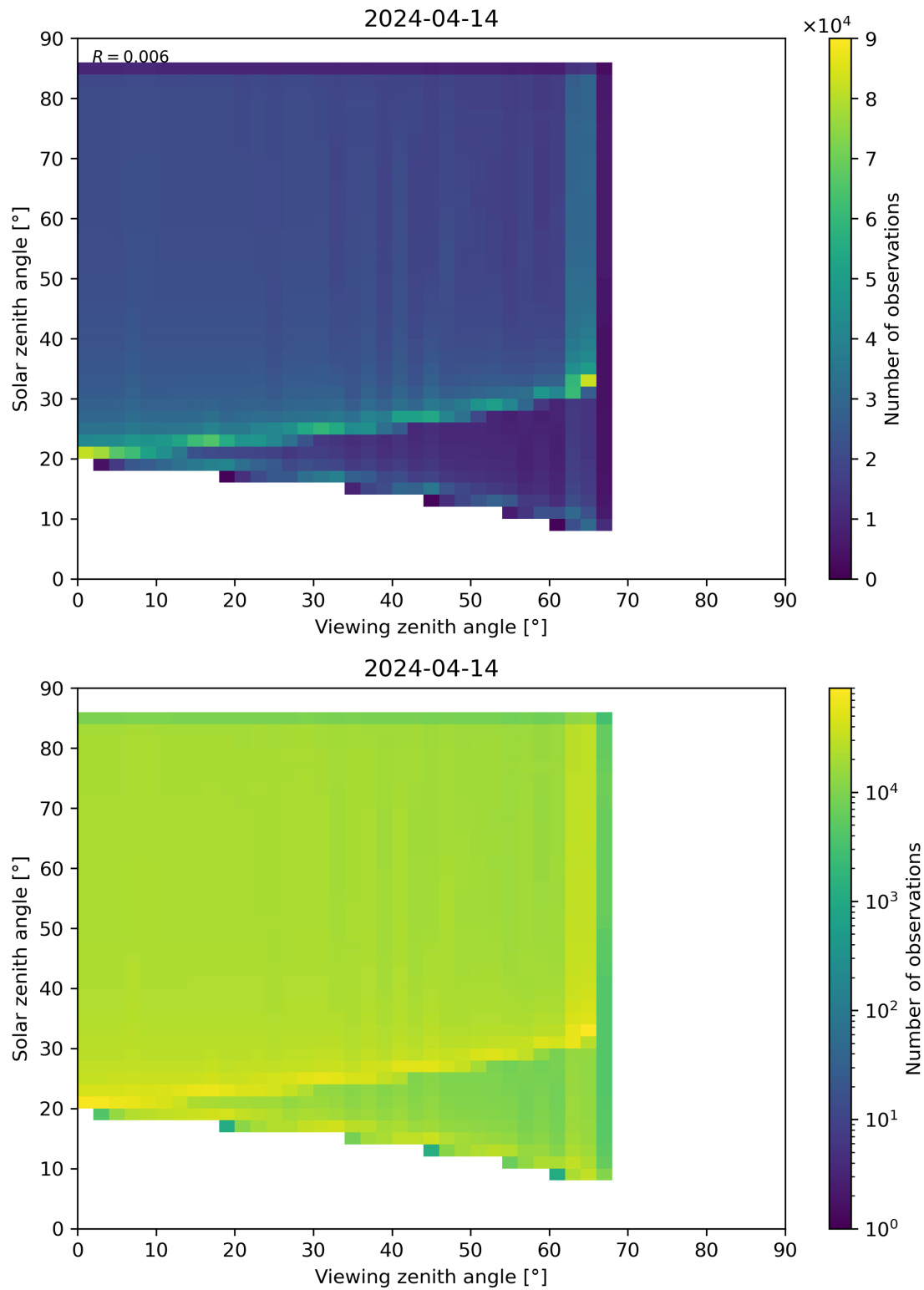
Figure 315: Scatter density plot of “Viewing zenith angle” against “Solar zenith angle” for 2024-04-13 to 2024-04-15.
