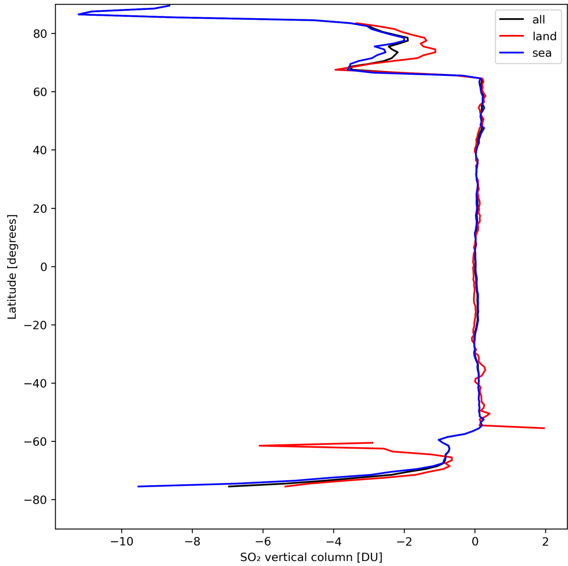
Figure 30: Zonal average of “SO 2 vertical column” for 2024-04-13 to 2024-04-15.
