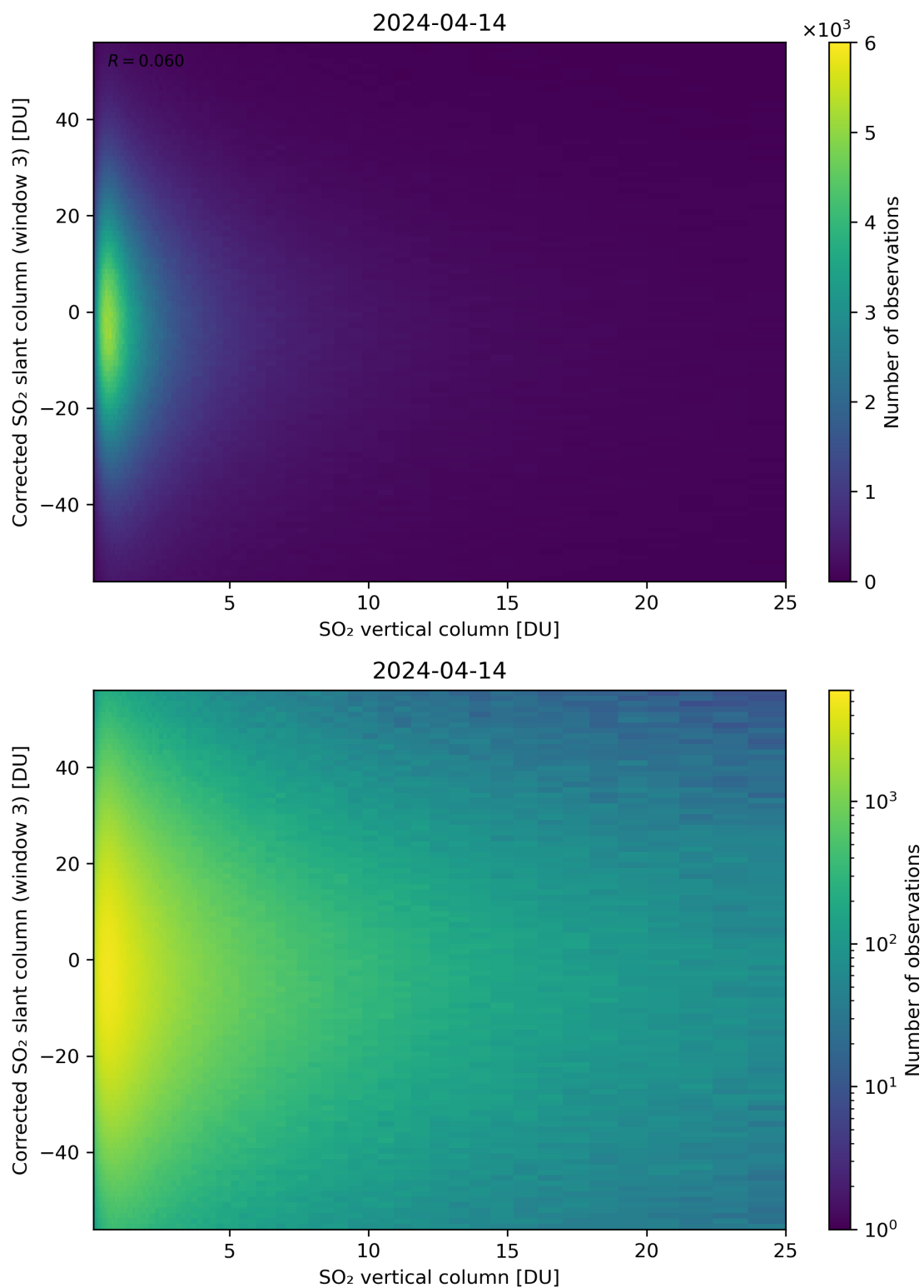
Figure 299: Scatter density plot of “SO 2 vertical column” against “Corrected SO 2 slant column (window 3)” for 2024-04-13 to 2024-04-15.
