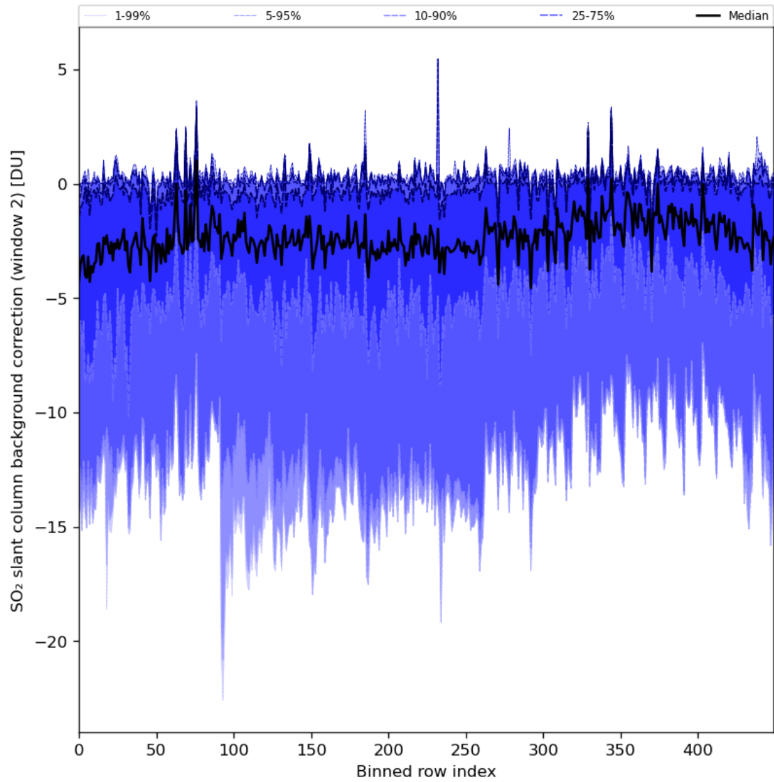
Figure 86: Along track statistics of “SO 2 slant column background correction (window 2)” for 2024-04-13 to 2024-04-15
