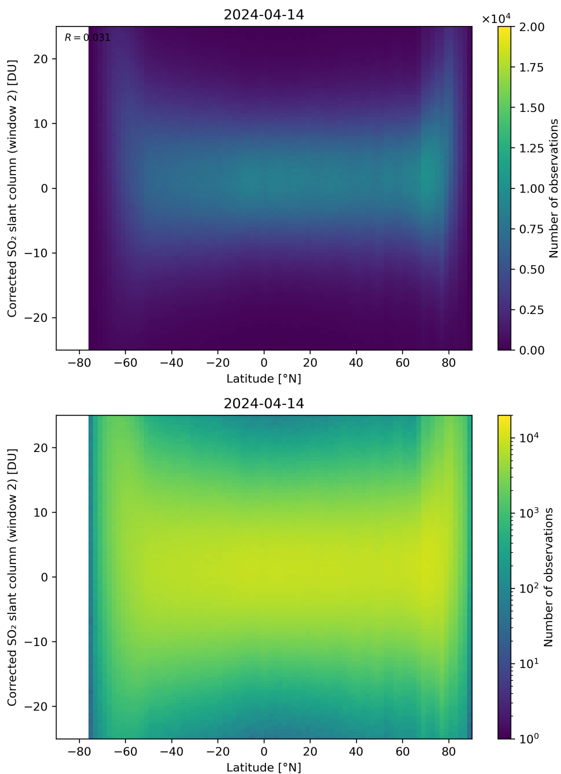
Figure 147: Scatter density plot of “Latitude” against “Corrected SO 2 slant column (window 2)” for 2024-04-13 to 2024-04-15.
