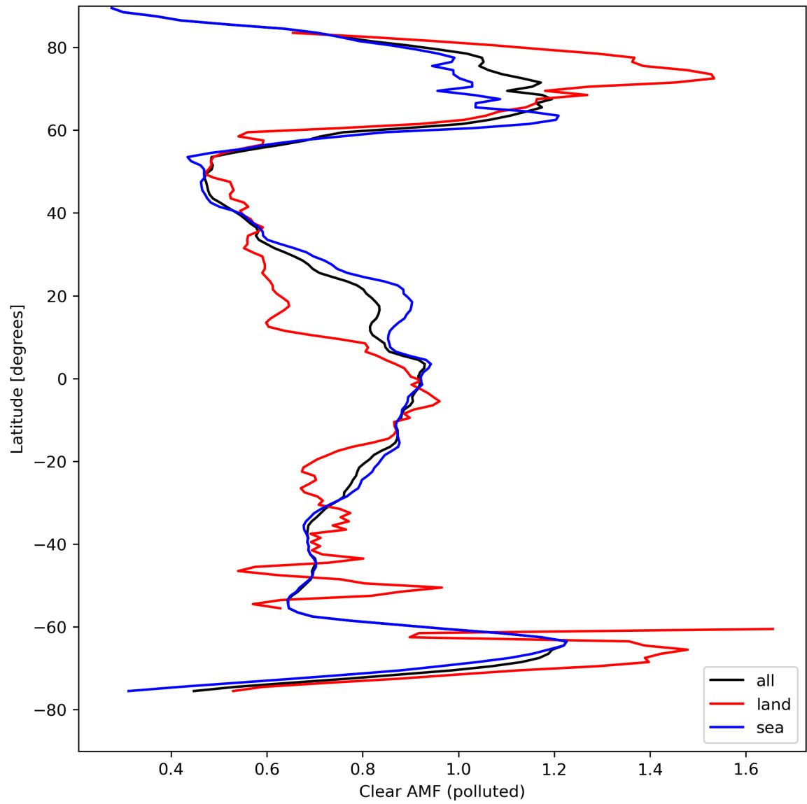
Figure 50: Zonal average of “Clear AMF (polluted)” for 2024-04-13 to 2024-04-15.
