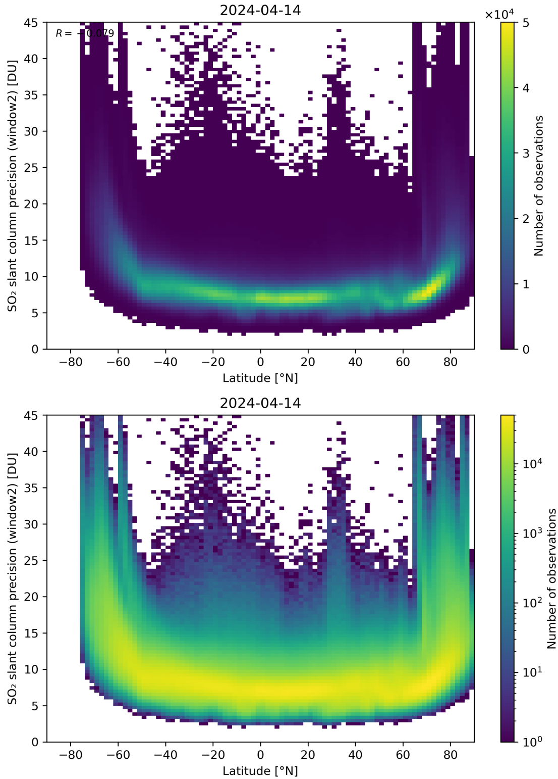
Figure 151: Scatter density plot of “Latitude” against “SO 2 slant column precision (window2)” for 2024-04-13 to 2024-04-15.
