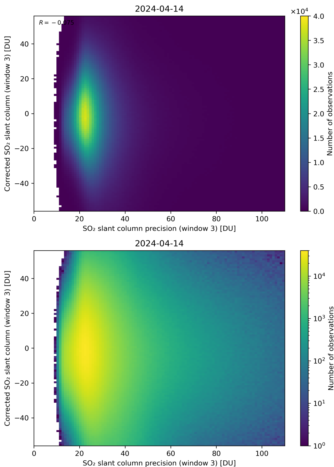
Figure 262: Scatter density plot of “SO 2 slant column precision (window 3)” against “Corrected SO 2 slant column (window 3)” for 2024-04-13 to 2024-04-15.
