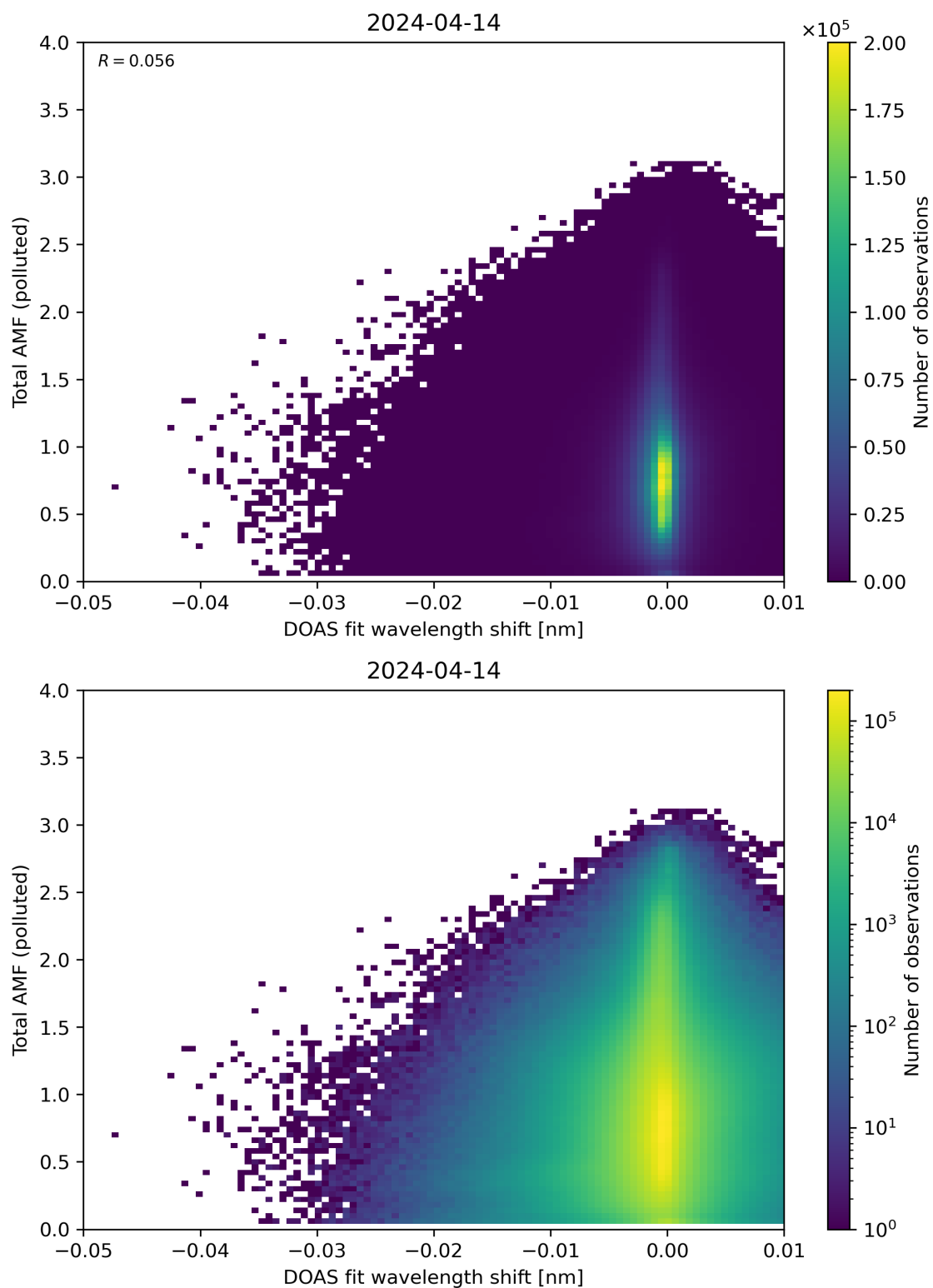
Figure 130: Scatter density plot of “DOAS fit wavelength shift” against “Total AMF (polluted)” for 2024-04-13 to 2024-04-15.
