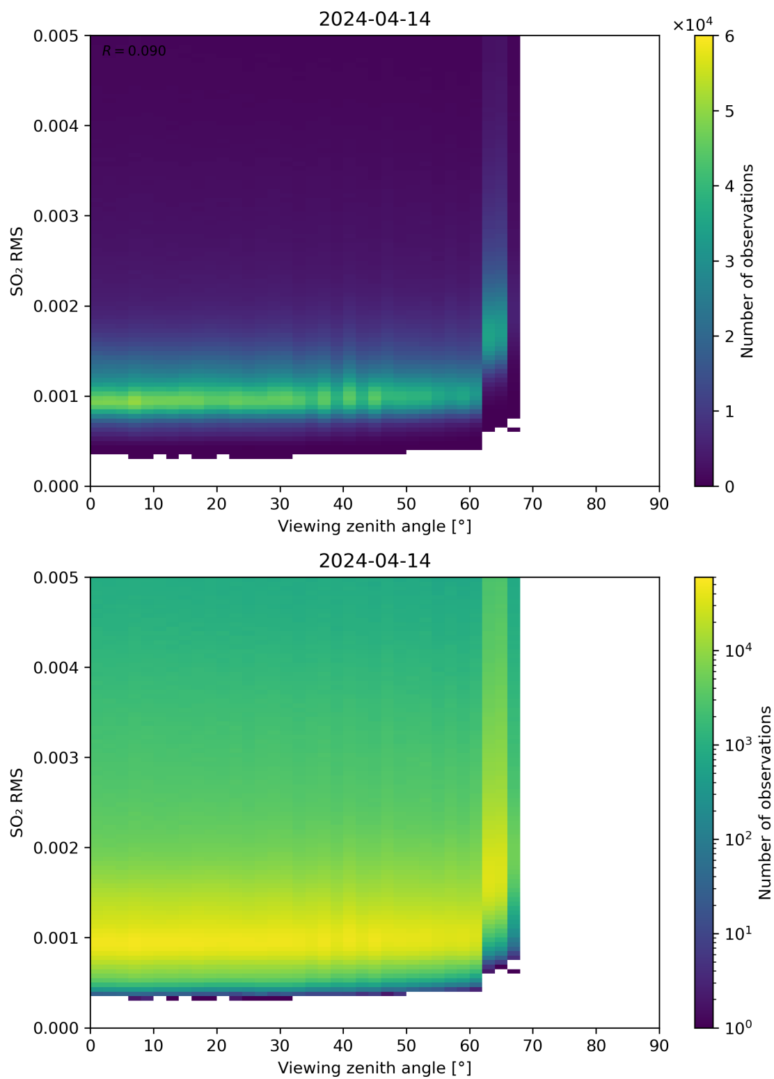
Figure 313: Scatter density plot of “Viewing zenith angle” against “SO 2 RMS” for 2024-04-13 to 2024-04-15.
