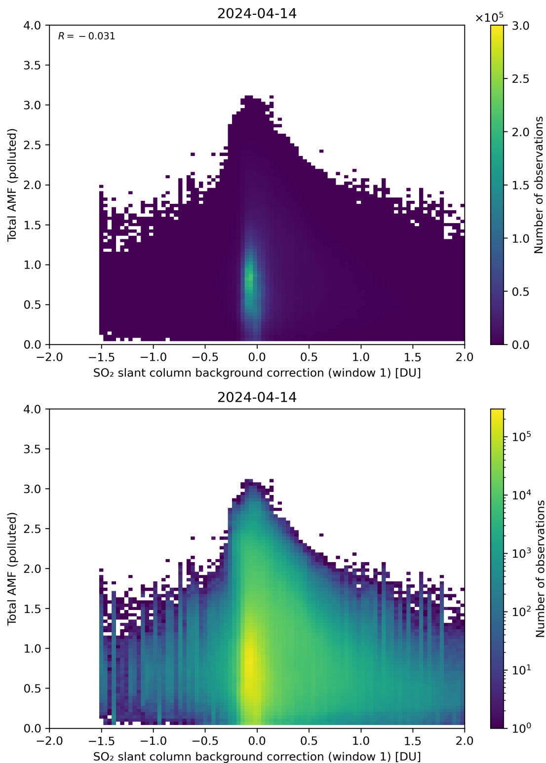
Figure 109: Scatter density plot of “SO 2 slant column background correction (window 1)” against “Total AMF (polluted)” for 2024-04-13 to 2024-04-15.
