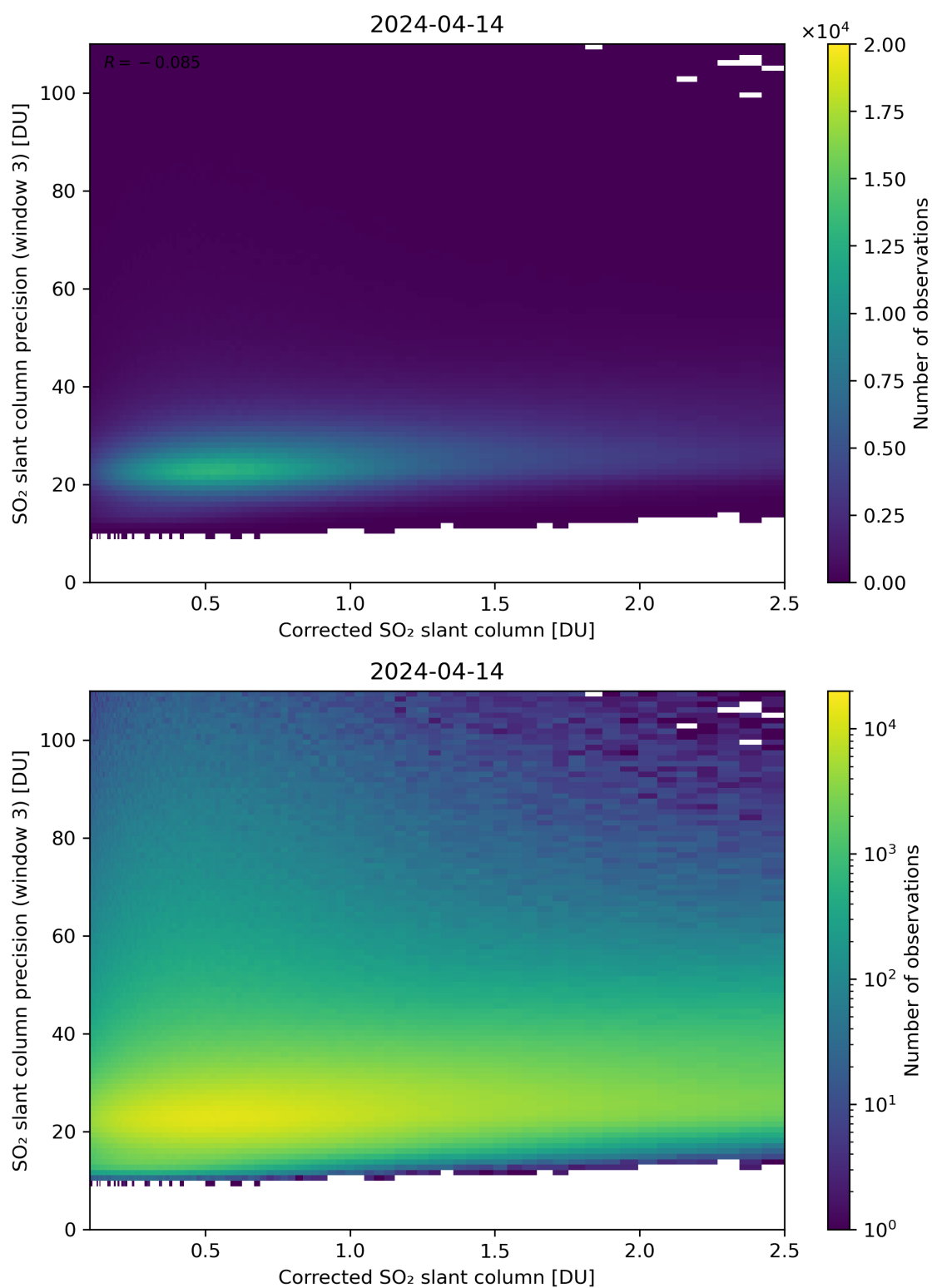
Figure 191: Scatter density plot of “Corrected SO 2 slant column” against “SO 2 slant column precision (window 3)” for 2024-04-13 to 2024-04-15.
