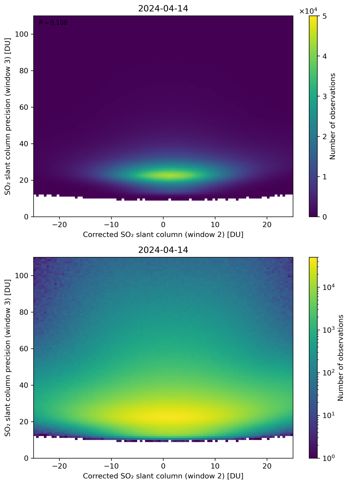
Figure 202: Scatter density plot of “Corrected SO 2 slant column (window 2)” against “SO 2 slant column precision (window 3)” for 2024-04-13 to 2024-04-15.
