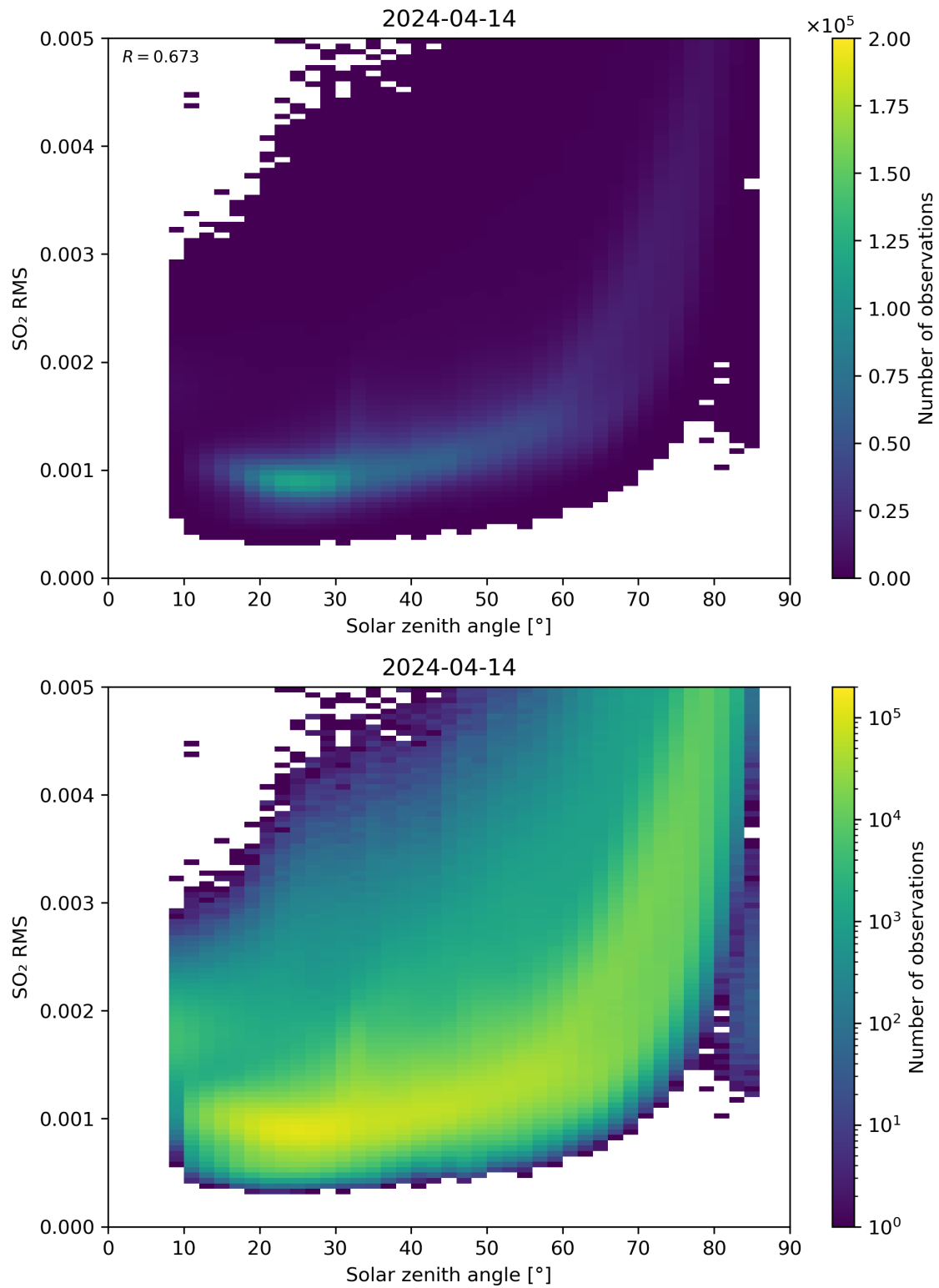
Figure 163: Scatter density plot of “Solar zenith angle” against “SO 2 RMS” for 2024-04-13 to 2024-04-15.
