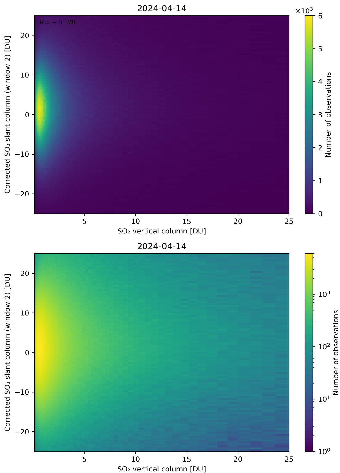
Figure 298: Scatter density plot of “SO 2 vertical column” against “Corrected SO 2 slant column (window 2)” for 2024-04-13 to 2024-04-15.
