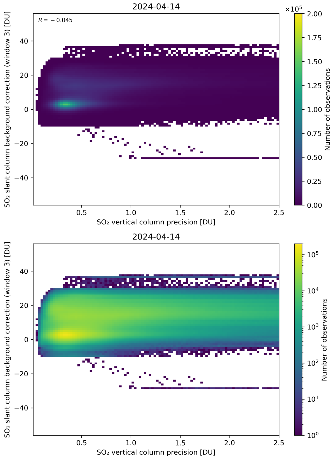
Figure 281: Scatter density plot of “SO 2 vertical column precision” against “SO 2 slant column background correction (window 3)” for 2024-04-13 to 2024-04-15.
