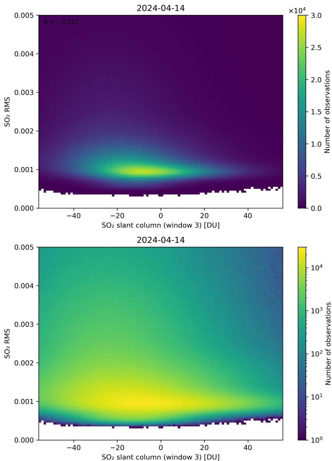
Figure 256: Scatter density plot of “SO 2 slant column (window 3)” against “SO 2 RMS” for 2024-04-13 to 2024-04-15.
