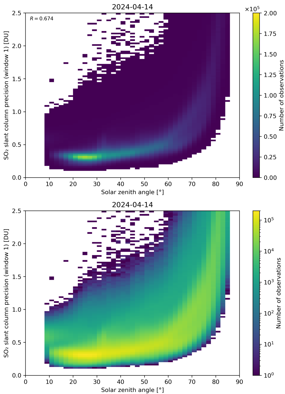
Figure 170: Scatter density plot of “Solar zenith angle” against “SO 2 slant column precision (window 1)” for 2024-04-13 to 2024-04-15.
