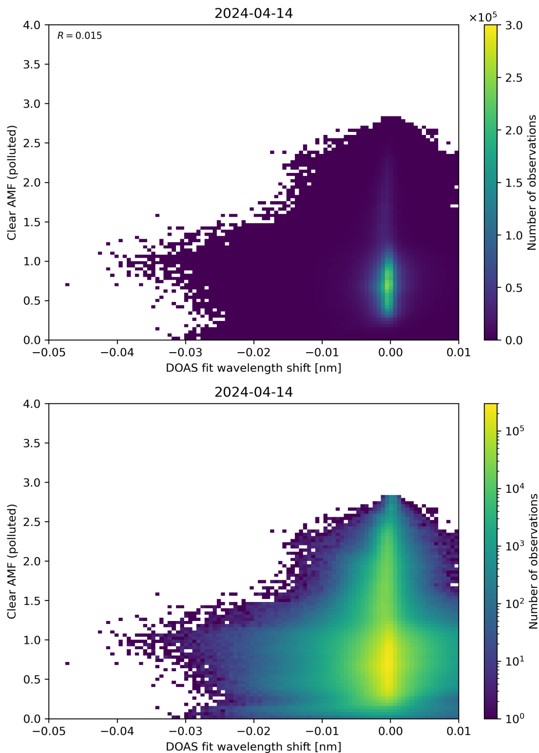
Figure 129: Scatter density plot of “DOAS fit wavelength shift” against “Clear AMF (polluted)” for 2024-04-13 to 2024-04-15.
