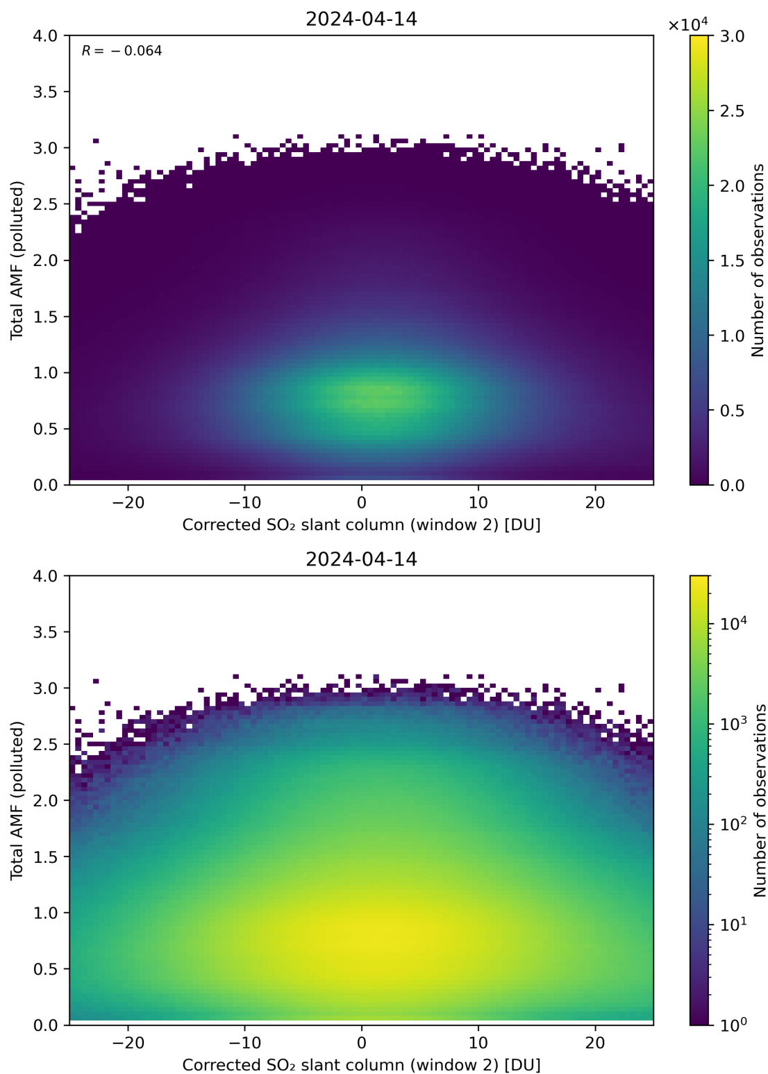
Figure 203: Scatter density plot of “Corrected SO 2 slant column (window 2)” against “Total AMF (polluted)” for 2024-04-13 to 2024-04-15.
