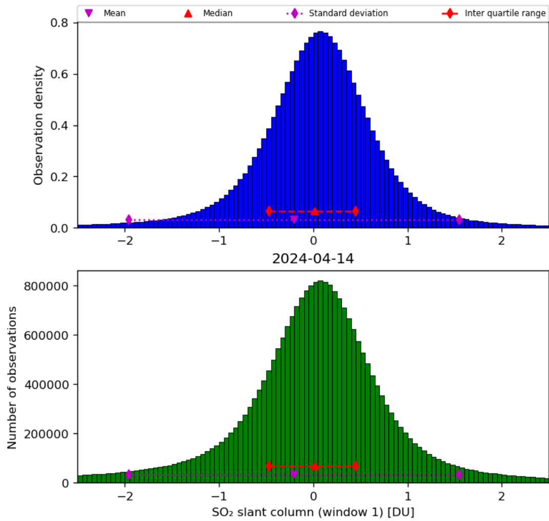
Figure 56: Histogram of “SO 2 slant column (window 1)” for 2024-04-13 to 2024-04-15
