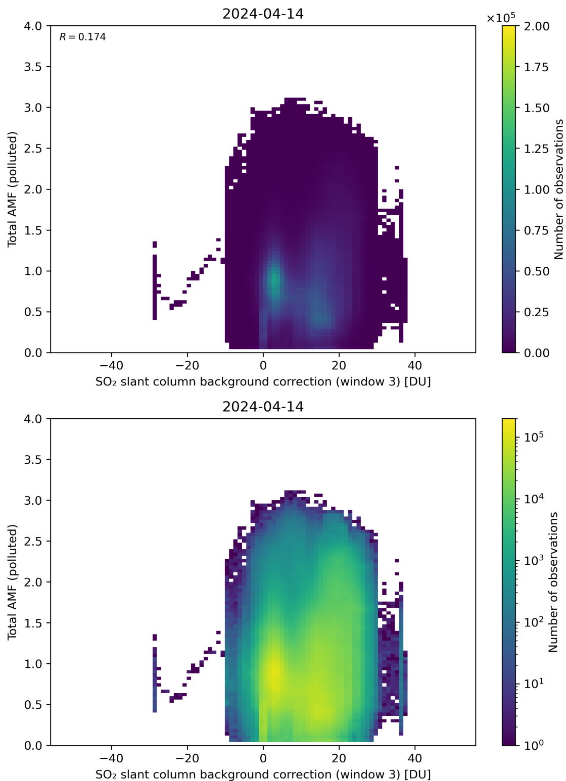
Figure 125: Scatter density plot of “SO 2 slant column background correction (window 3)” against “Total AMF (polluted)” for 2024-04-13 to 2024-04-15.
