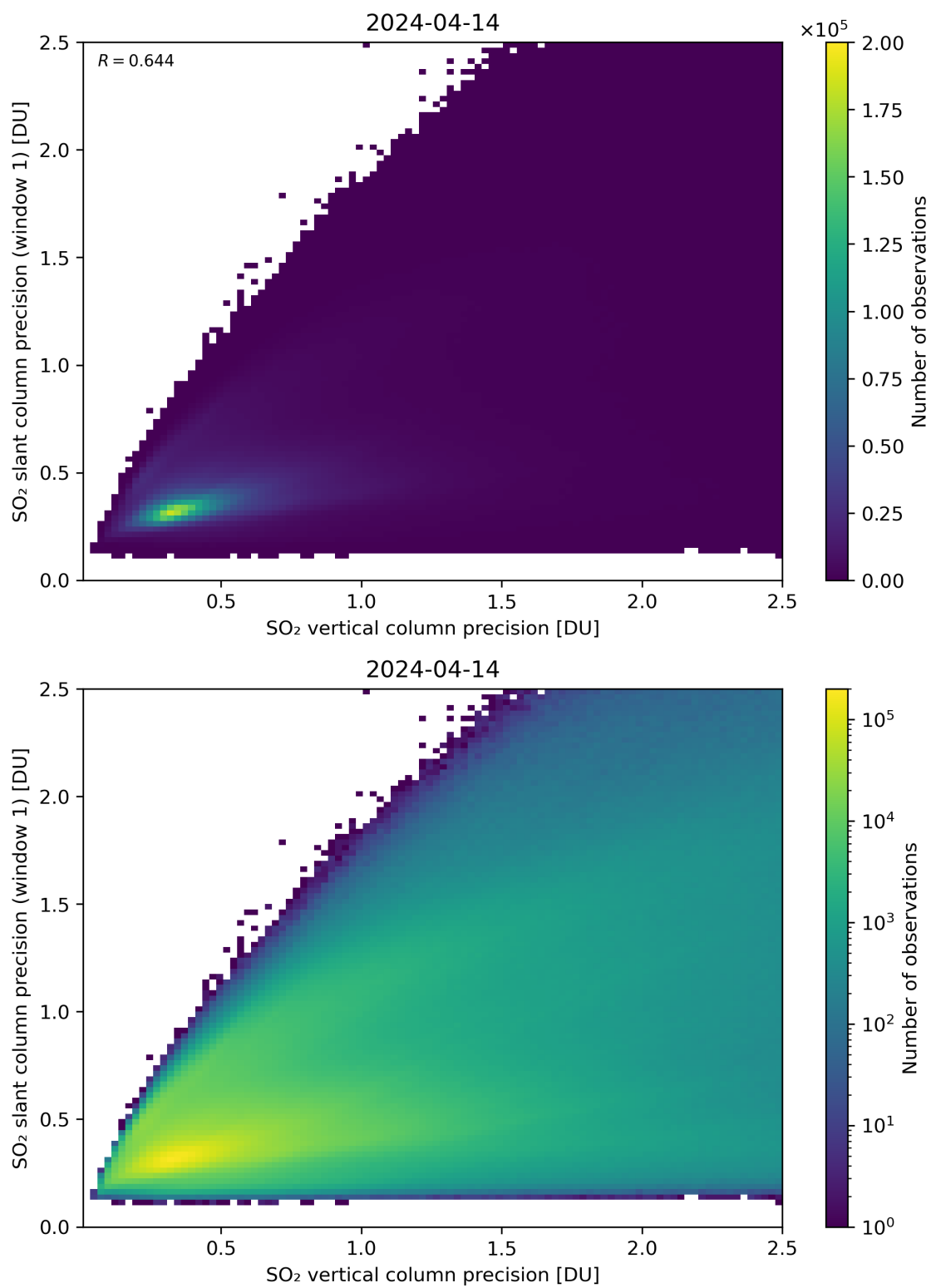
Figure 290: Scatter density plot of “SO 2 vertical column precision” against “SO 2 slant column precision (window 1)” for 2024-04-13 to 2024-04-15.
