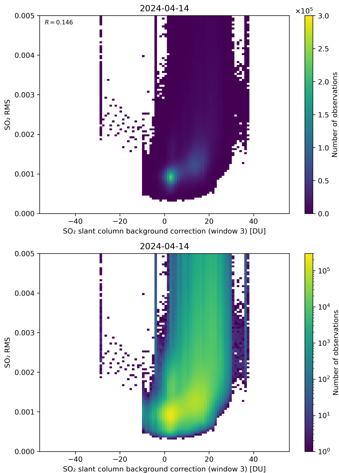
Figure 123: Scatter density plot of “SO 2 slant column background correction (window 3)” against “SO 2 RMS” for 2024-04-13 to 2024-04-15.
