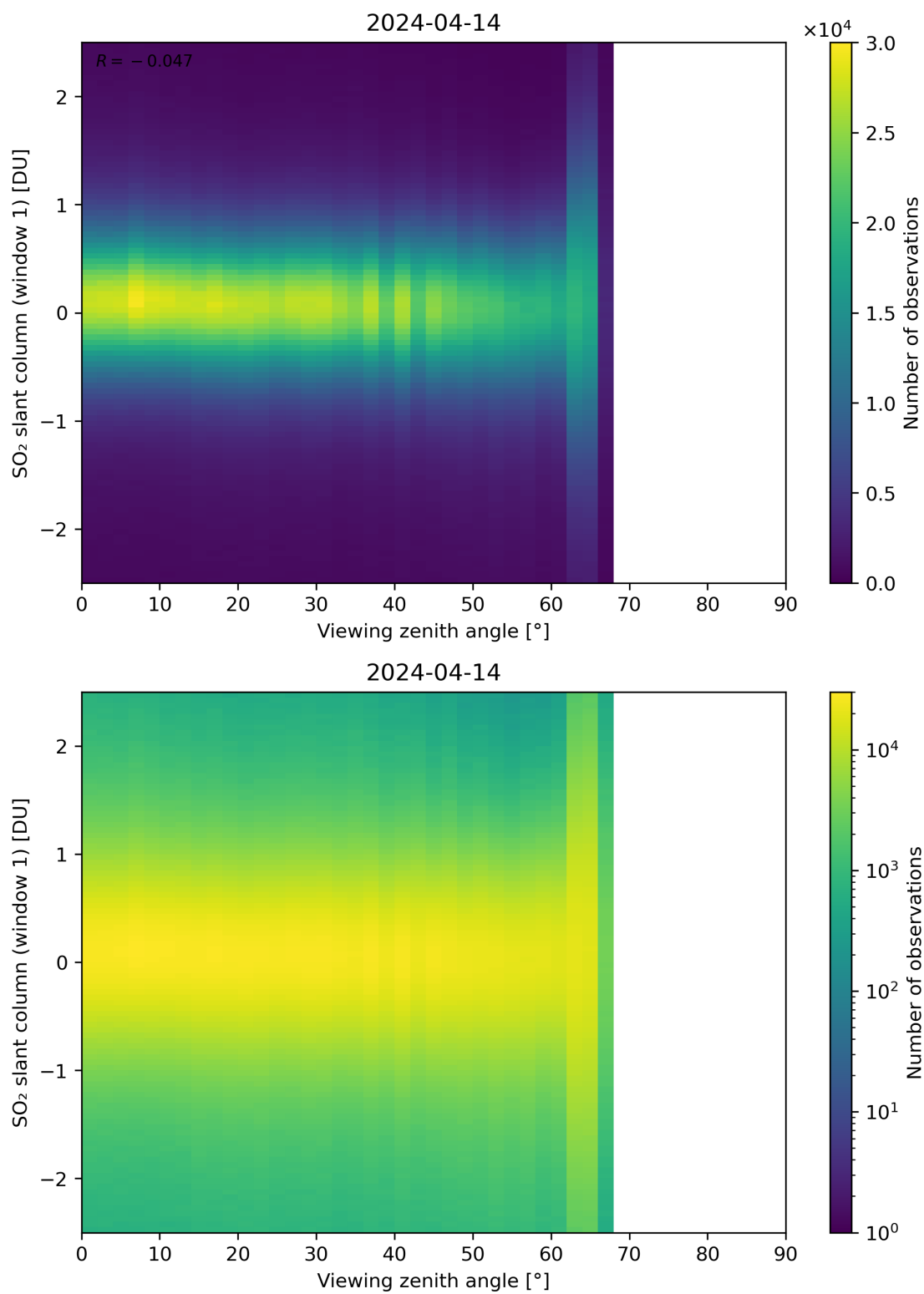
Figure 320: Scatter density plot of “Viewing zenith angle” against “SO 2 slant column (window 1)” for 2024-04-13 to 2024-04-15.
