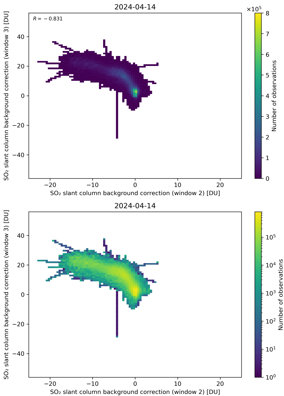
Figure 111: Scatter density plot of “SO 2 slant column background correction (window 2)” against “SO 2 slant column background correction (window 3)” for 2024-04-13 to 2024-04-15.
