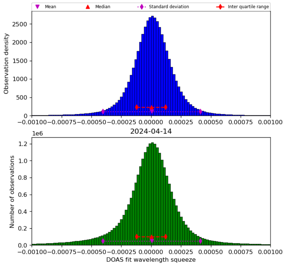
Figure 69: Histogram of “DOAS fit wavelength squeeze” for 2024-04-13 to 2024-04-15
