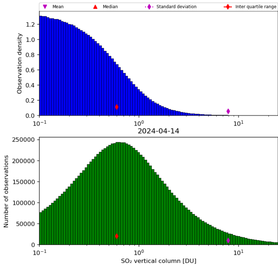
Figure 53: Histogram of “SO 2 vertical column” for 2024-04-13 to 2024-04-15
