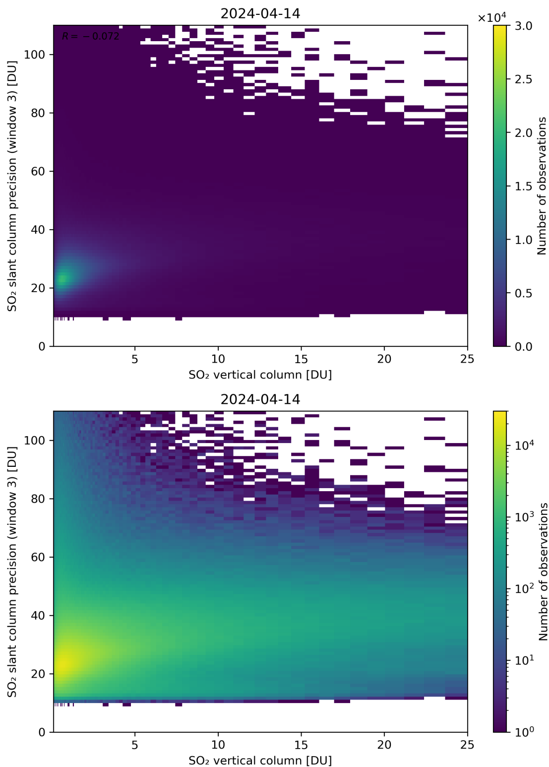
Figure 304: Scatter density plot of “SO 2 vertical column” against “SO 2 slant column precision (window 3)” for 2024-04-13 to 2024-04-15.
