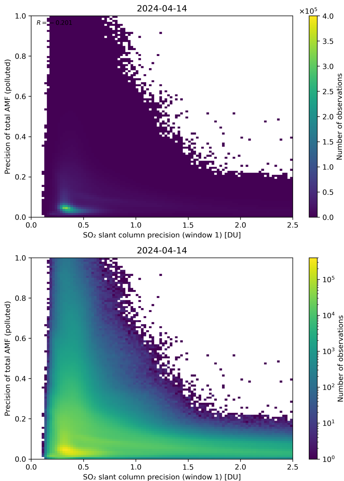
Figure 231: Scatter density plot of “SO 2 slant column precision (window 1)” against “Precision of total AMF (polluted)” for 2024-04-13 to 2024-04-15.
