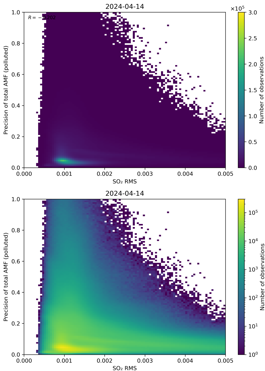
Figure 138: Scatter density plot of “SO 2 RMS” against “Precision of total AMF (polluted)” for 2024-04-13 to 2024-04-15.
