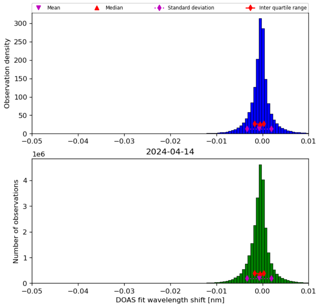
Figure 68: Histogram of “DOAS fit wavelength shift” for 2024-04-13 to 2024-04-15
