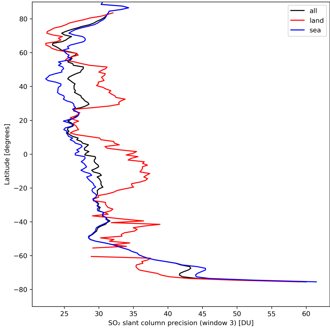
Figure 42: Zonal average of “SO 2 slant column precision (window 3)” for 2024-04-13 to 2024-04-15.
