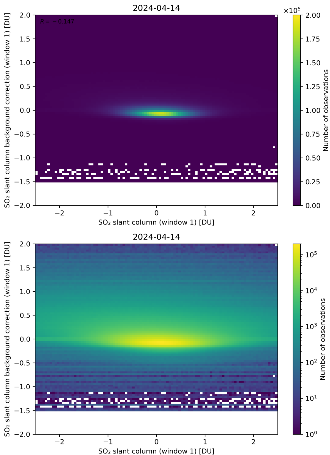
Figure 212: Scatter density plot of “SO 2 slant column (window 1)” against “SO 2 slant column background correction (window 1)” for 2024-04-13 to 2024-04-15.
