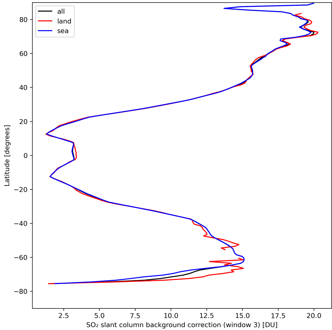
Figure 44: Zonal average of “SO 2 slant column background correction (window 3)” for 2024-04-13 to 2024-04-15.
