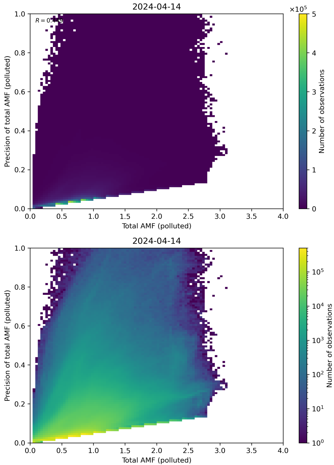
Figure 272: Scatter density plot of “Total AMF (polluted)” against “Precision of total AMF (polluted)” for 2024-04-13 to 2024-04-15.
