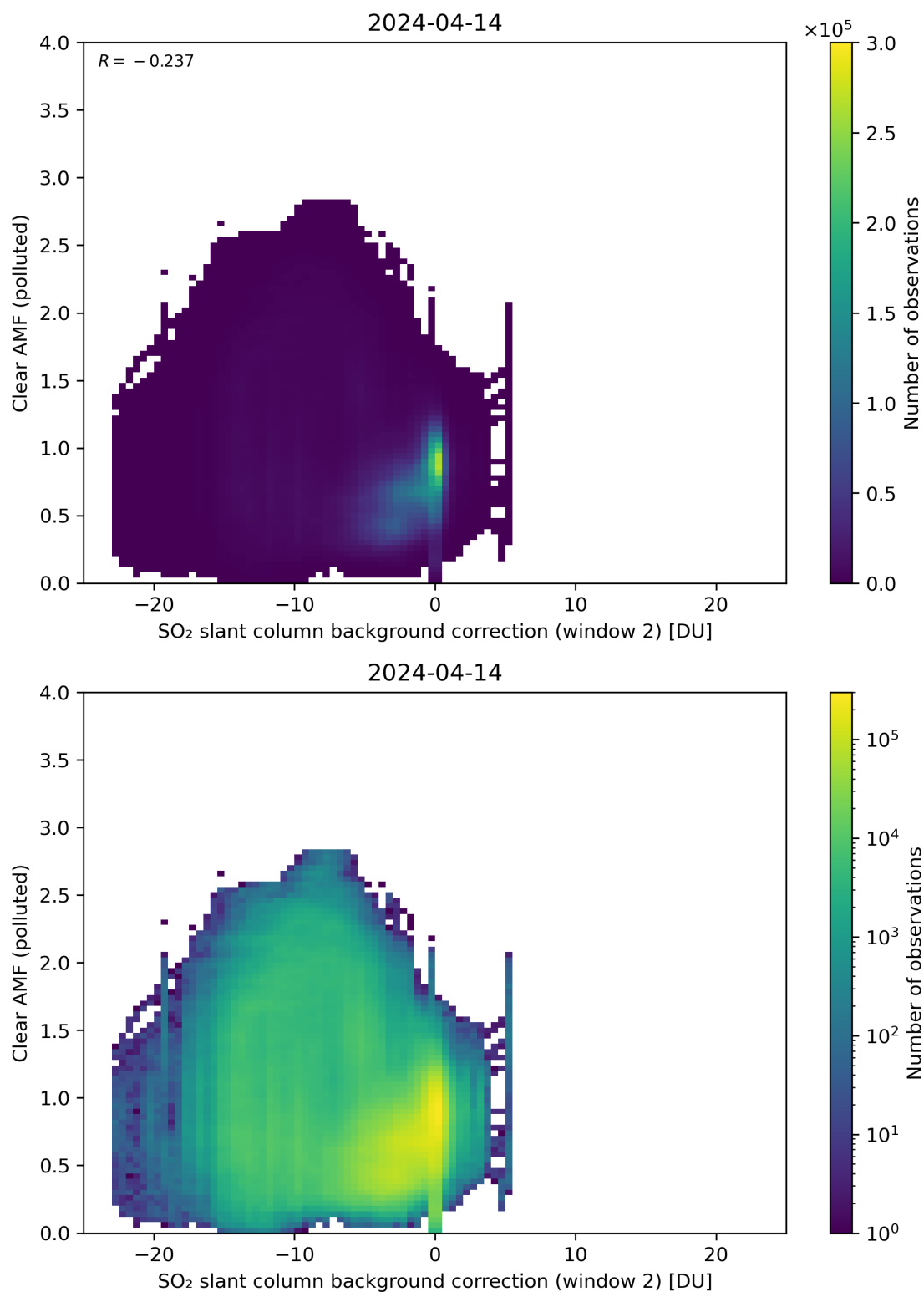
Figure 115: Scatter density plot of “SO 2 slant column background correction (window 2)” against “Clear AMF (polluted)” for 2024-04-13 to 2024-04-15.
