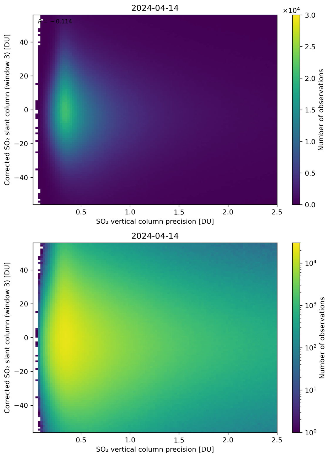
Figure 288: Scatter density plot of “SO 2 vertical column precision” against “Corrected SO 2 slant column (window 3)” for 2024-04-13 to 2024-04-15.
