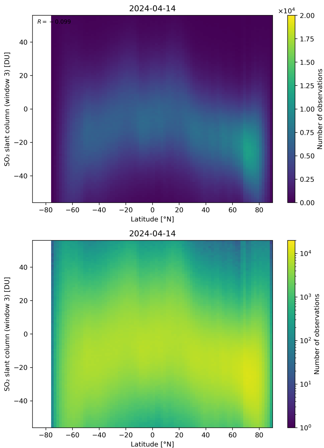
Figure 152: Scatter density plot of “Latitude” against “SO 2 slant column (window 3)” for 2024-04-13 to 2024-04-15.
