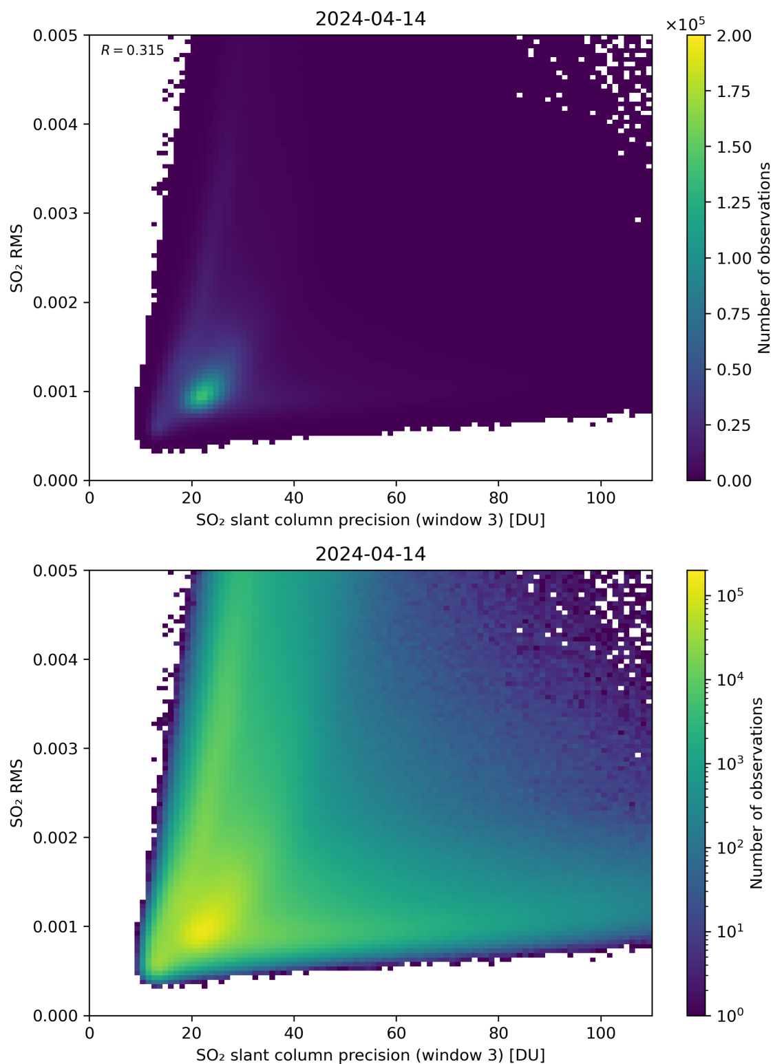
Figure 260: Scatter density plot of “SO 2 slant column precision (window 3)” against “SO 2 RMS” for 2024-04-13 to 2024-04-15.
