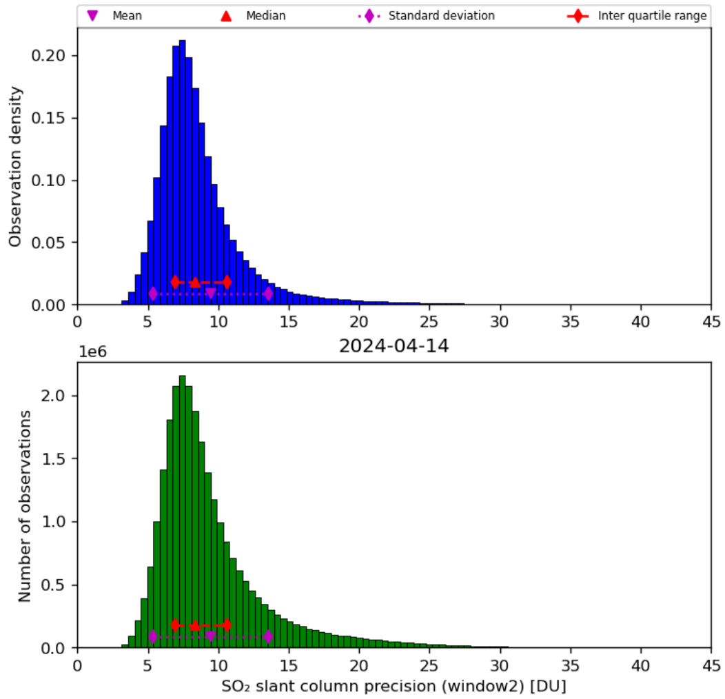
Figure 61: Histogram of “SO 2 slant column precision (window2)” for 2024-04-13 to 2024-04-15
