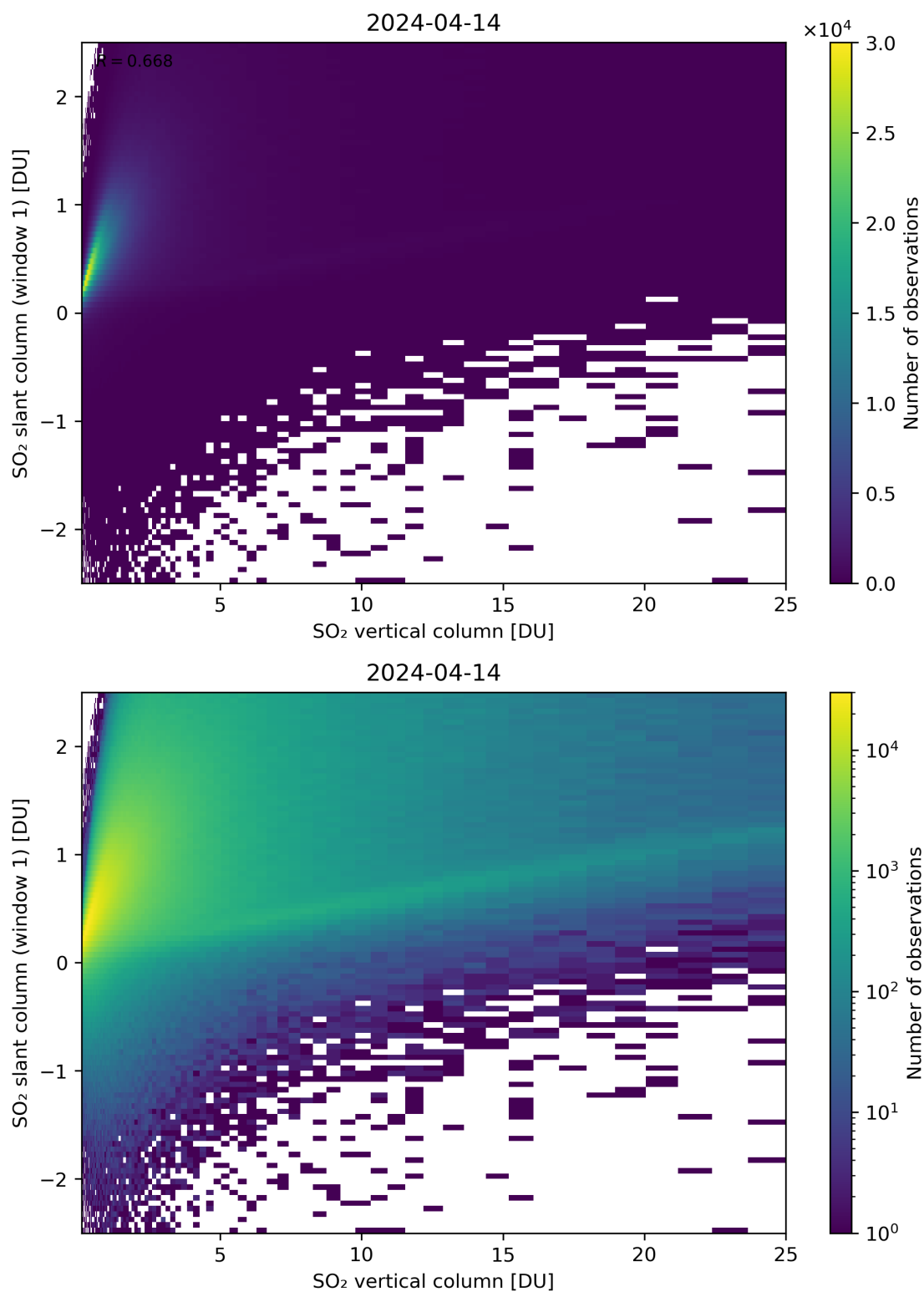
Figure 300: Scatter density plot of “SO 2 vertical column” against “SO 2 slant column (window 1)” for 2024-04-13 to 2024-04-15.
