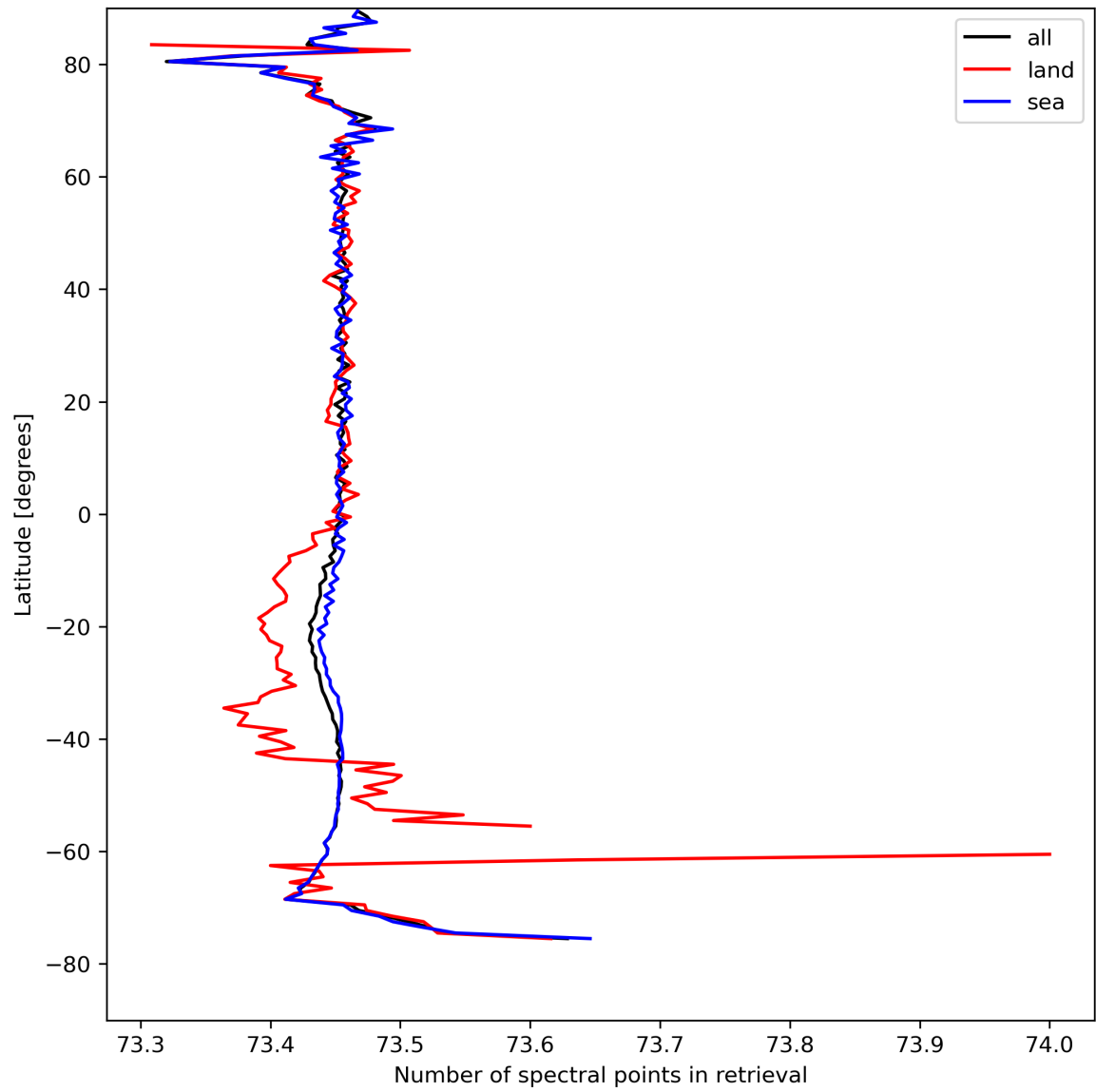
Figure 51: Zonal average of “Number of spectral points in retrieval” for 2024-04-13 to 2024-04-15.
