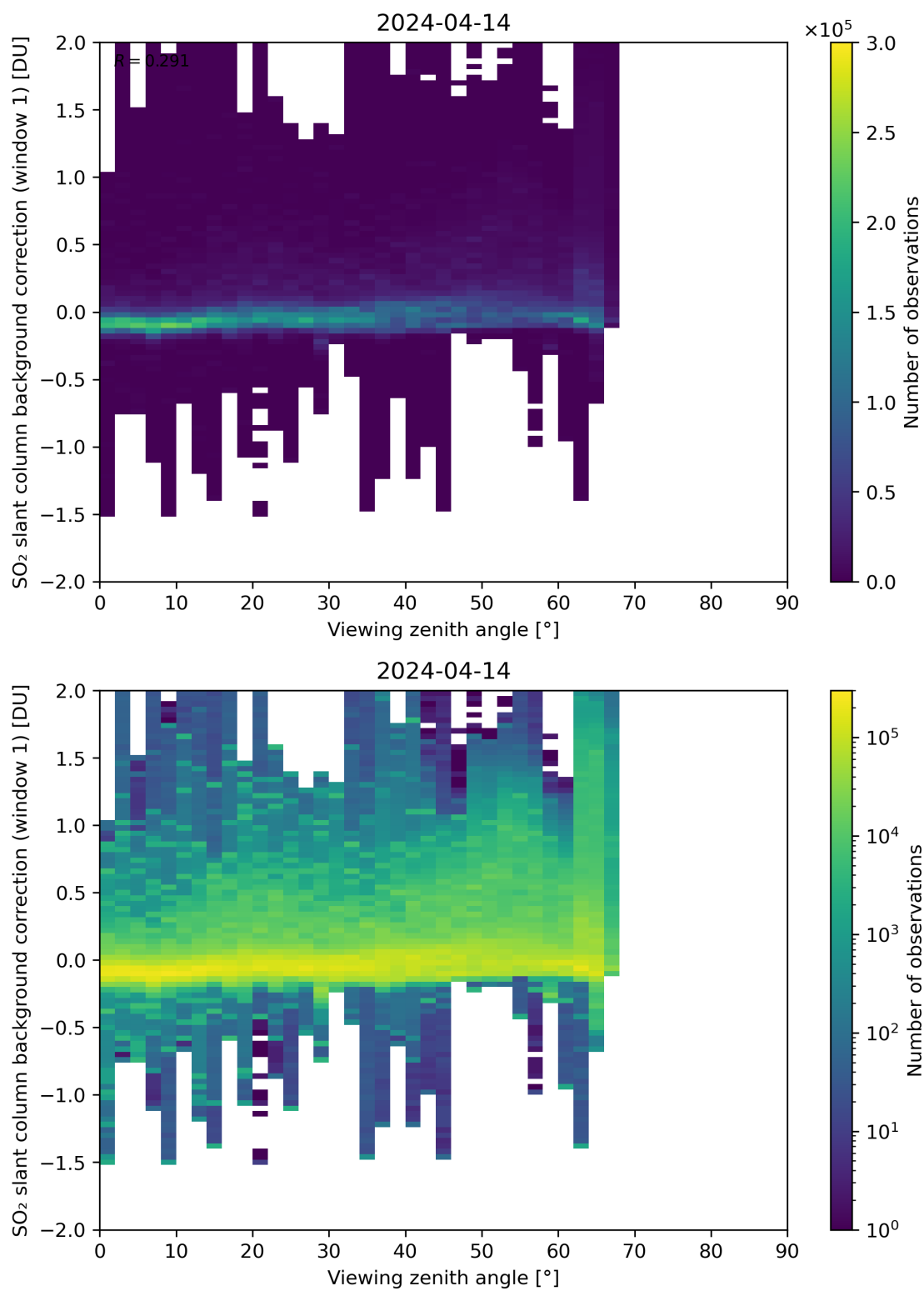
Figure 308: Scatter density plot of “Viewing zenith angle” against “SO 2 slant column background correction (window 1)” for 2024-04-13 to 2024-04-15.
