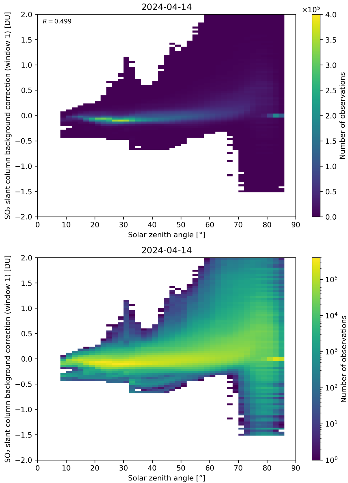
Figure 158: Scatter density plot of “Solar zenith angle” against “SO 2 slant column background correction (window 1)” for 2024-04-13 to 2024-04-15.
