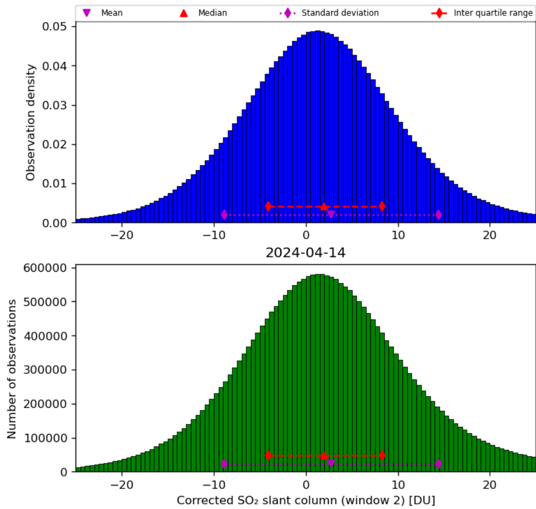
Figure 62: Histogram of “Corrected SO 2 slant column (window 2)” for 2024-04-13 to 2024-04-15
