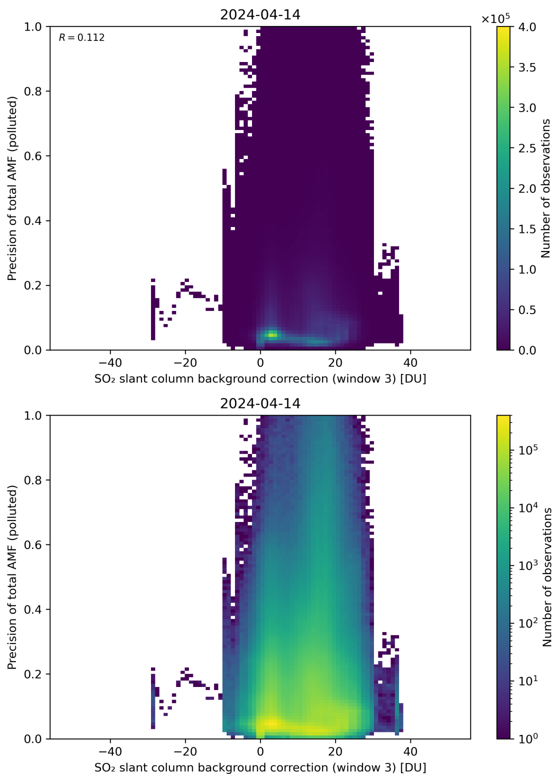
Figure 126: Scatter density plot of “SO 2 slant column background correction (window 3)” against “Precision of total AMF (polluted)” for 2024-04-13 to 2024-04-15.
