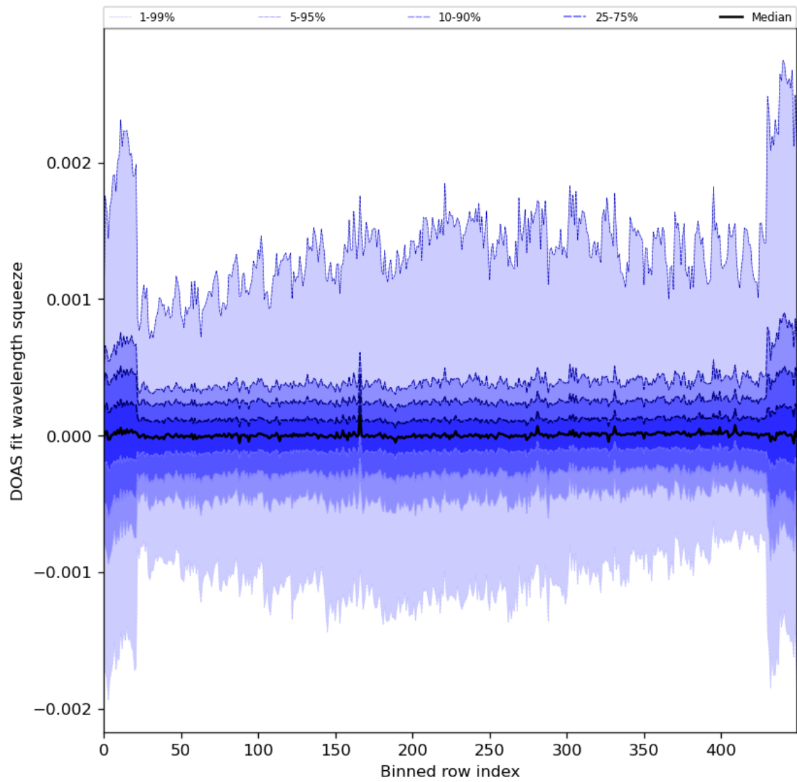
Figure 92: Along track statistics of “DOAS fit wavelength squeeze” for 2024-04-13 to 2024-04-15
