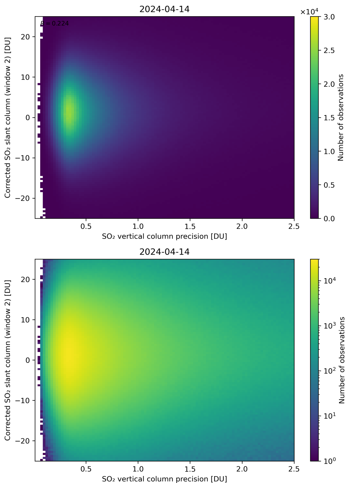
Figure 287: Scatter density plot of “SO 2 vertical column precision” against “Corrected SO 2 slant column (window 2)” for 2024-04-13 to 2024-04-15.
