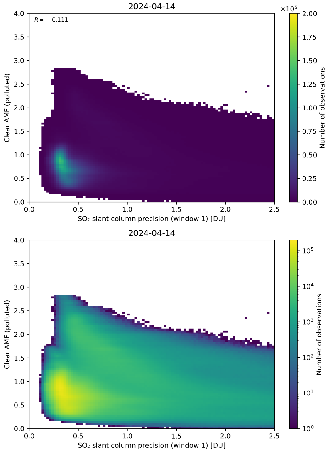
Figure 224: Scatter density plot of “SO 2 slant column precision (window 1)” against “Clear AMF (polluted)” for 2024-04-13 to 2024-04-15.
