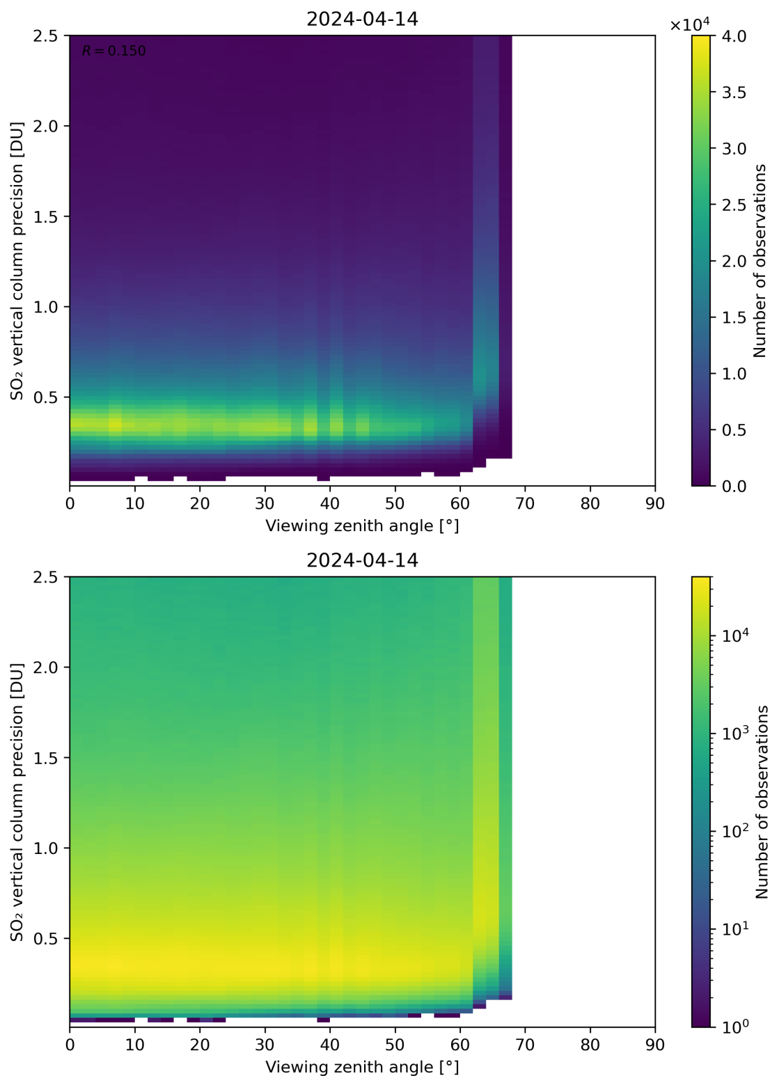
Figure 328: Scatter density plot of “Viewing zenith angle” against “SO 2 vertical column precision” for 2024-04-13 to 2024-04-15.
