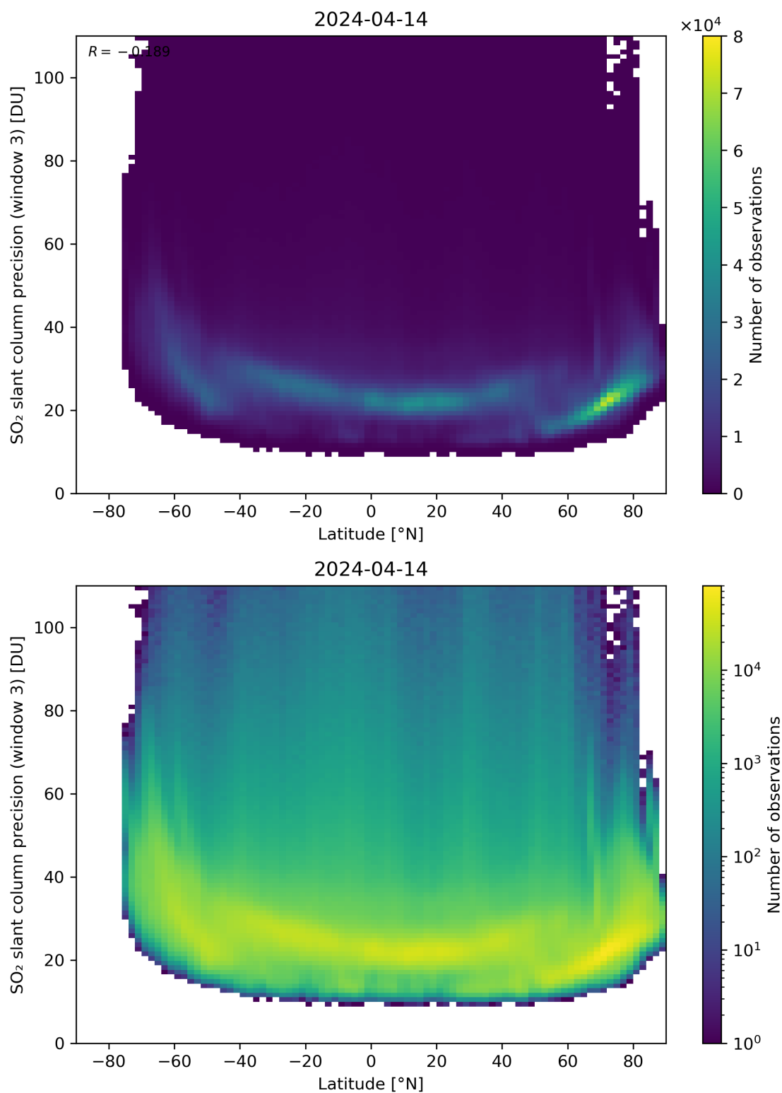
Figure 153: Scatter density plot of “Latitude” against “SO 2 slant column precision (window 3)” for 2024-04-13 to 2024-04-15.
