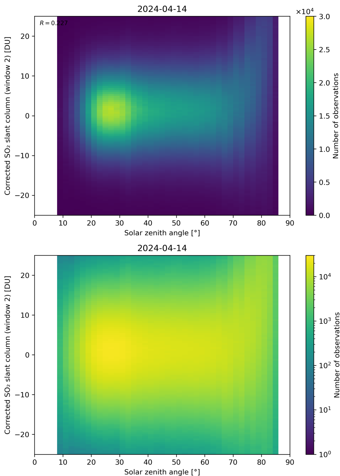
Figure 167: Scatter density plot of “Solar zenith angle” against “Corrected SO 2 slant column (window 2)” for 2024-04-13 to 2024-04-15.
