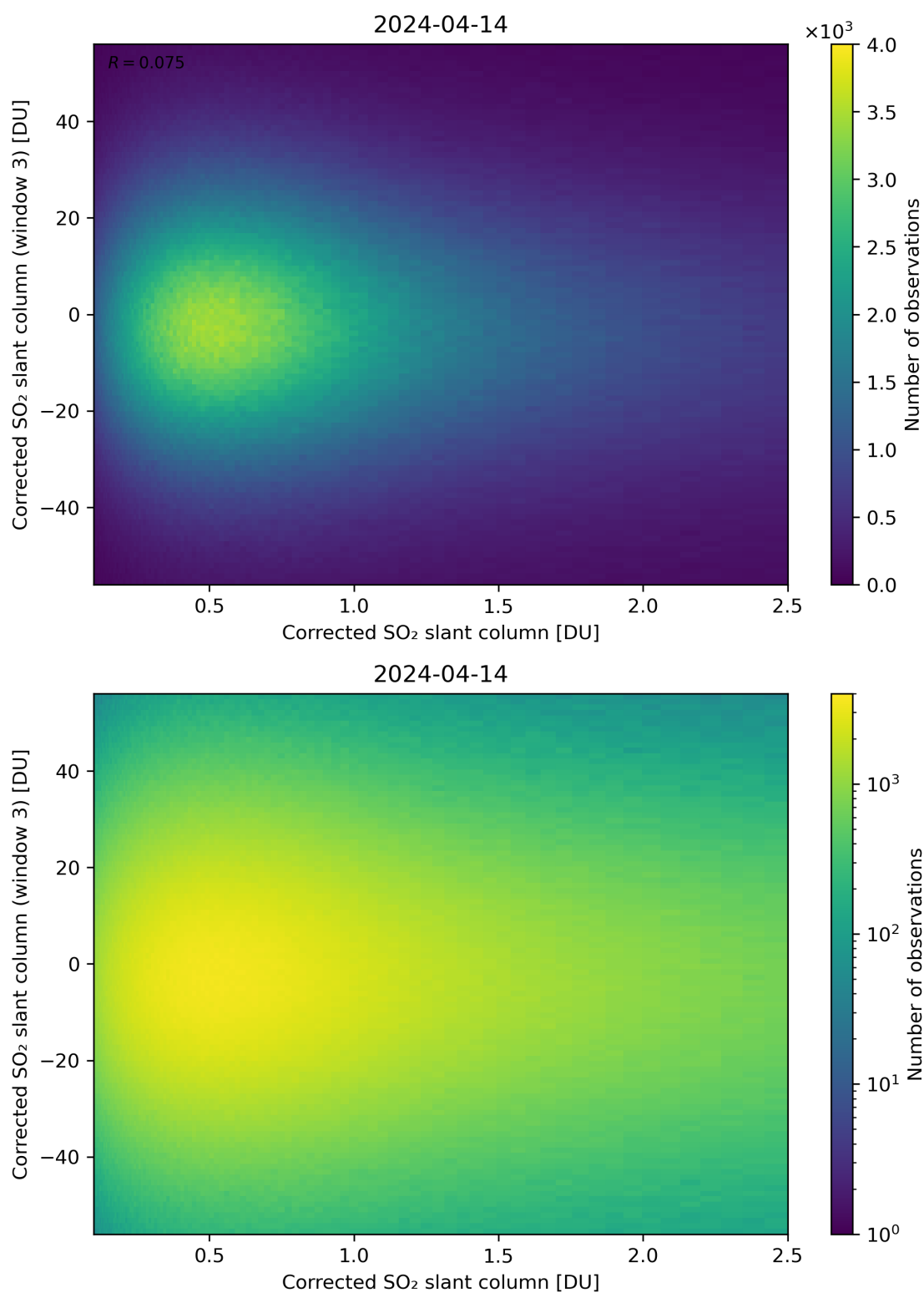
Figure 186: Scatter density plot of “Corrected SO 2 slant column” against “Corrected SO 2 slant column (window 3)” for 2024-04-13 to 2024-04-15.
