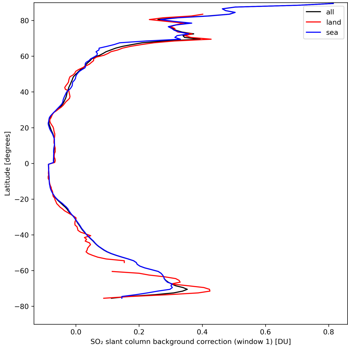
Figure 36: Zonal average of “SO 2 slant column background correction (window 1)” for 2024-04-13 to 2024-04-15.
