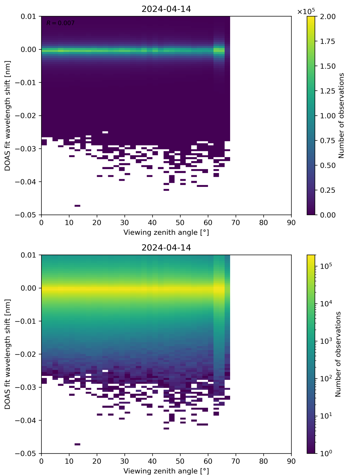
Figure 311: Scatter density plot of “Viewing zenith angle” against “DOAS fit wavelength shift” for 2024-04-13 to 2024-04-15.
