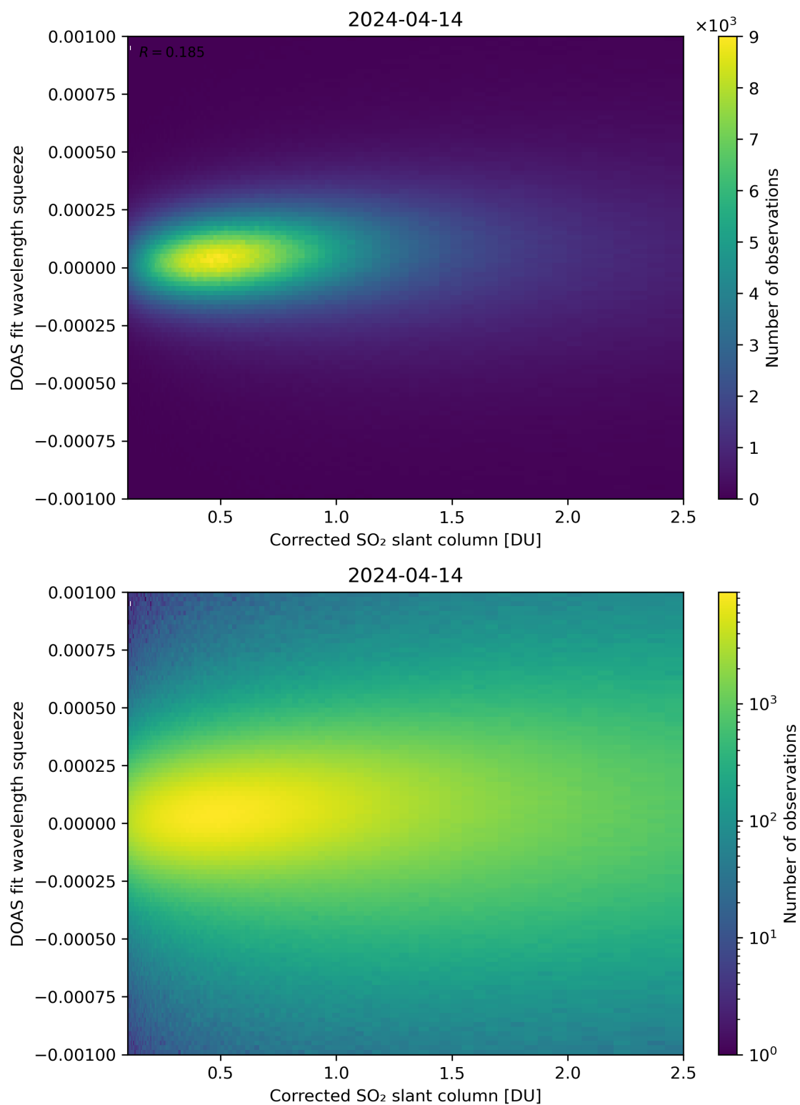
Figure 182: Scatter density plot of “Corrected SO 2 slant column” against “DOAS fit wavelength squeeze” for 2024-04-13 to 2024-04-15.
