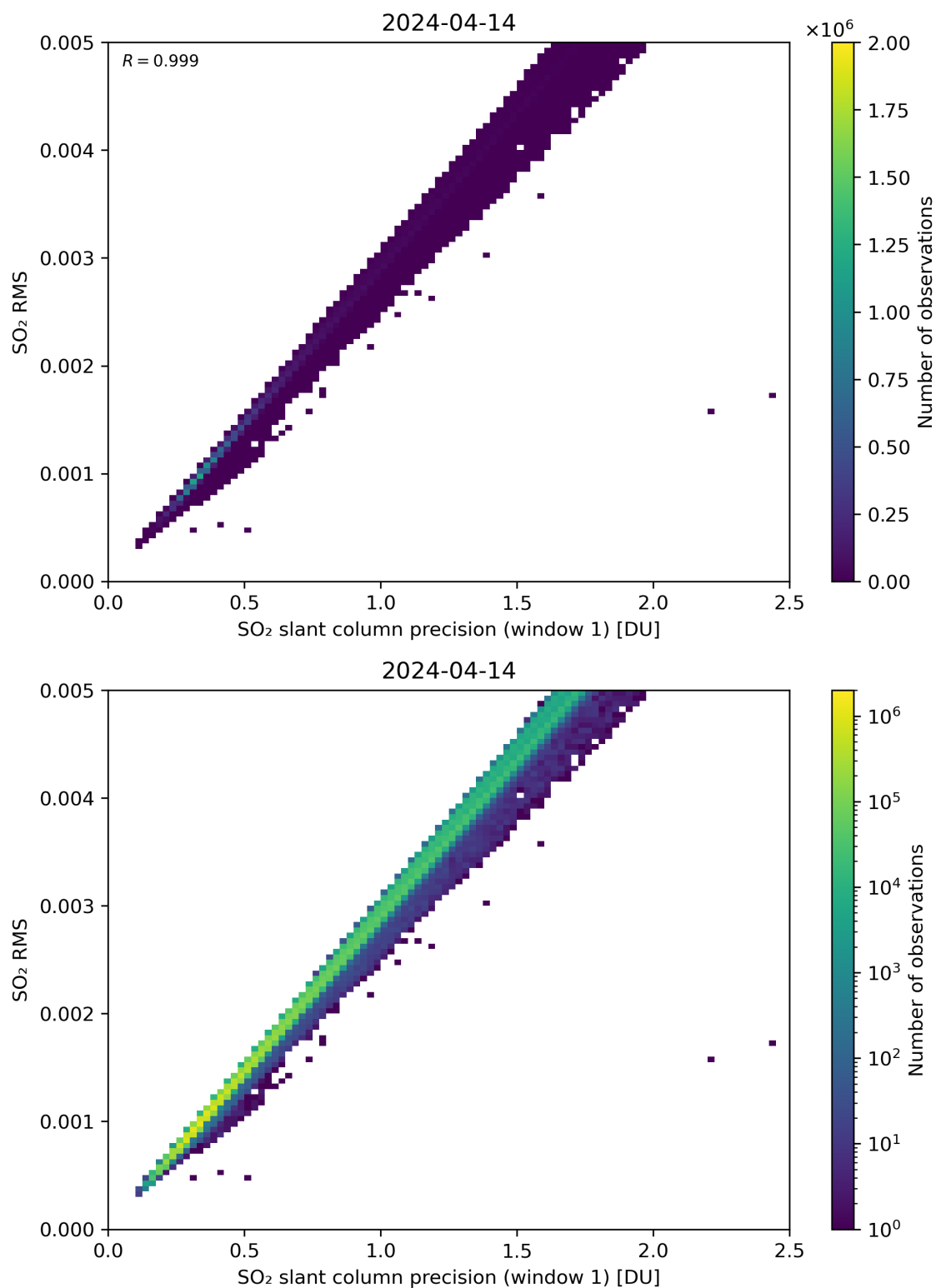
Figure 223: Scatter density plot of “SO 2 slant column precision (window 1)” against “SO 2 RMS” for 2024-04-13 to 2024-04-15.
