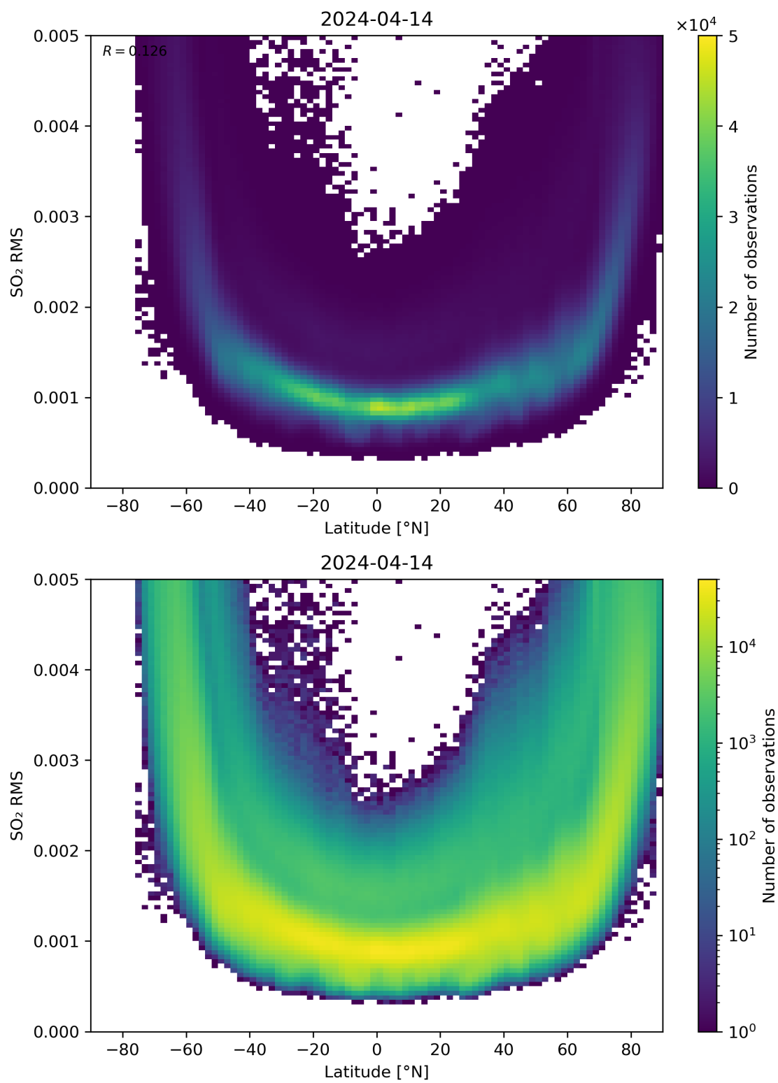
Figure 144: Scatter density plot of “Latitude” against “SO 2 RMS” for 2024-04-13 to 2024-04-15.
