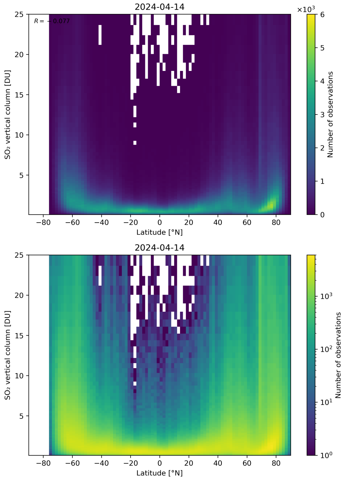
Figure 156: Scatter density plot of “Latitude” against “SO 2 vertical column” for 2024-04-13 to 2024-04-15.
