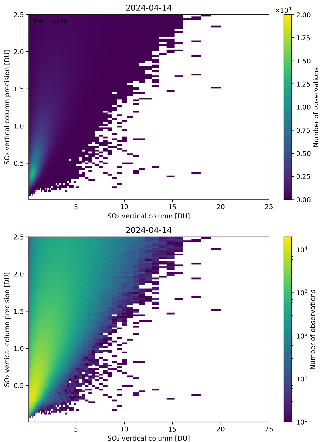
Figure 307: Scatter density plot of “SO 2 vertical column” against “SO 2 vertical column precision” for 2024-04-13 to 2024-04-15.
