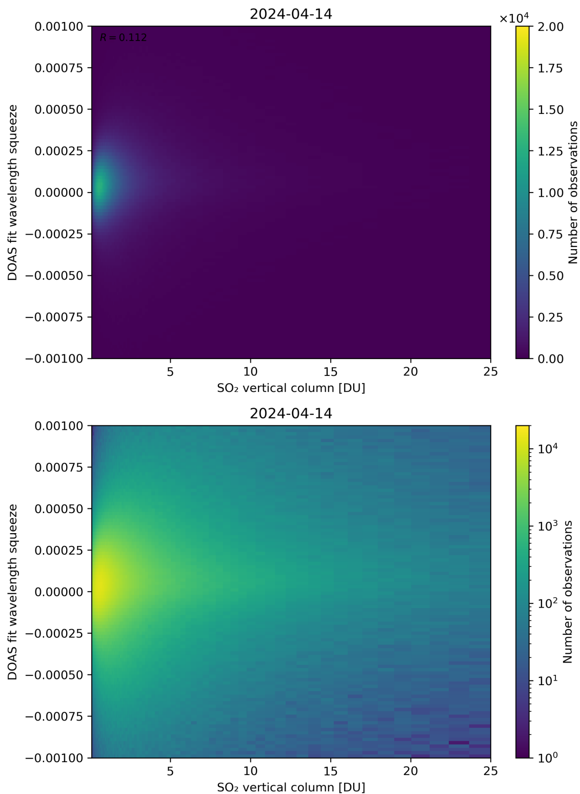
Figure 277: Scatter density plot of “SO 2 vertical column” against “DOAS fit wavelength squeeze” for 2024-04-13 to 2024-04-15.
