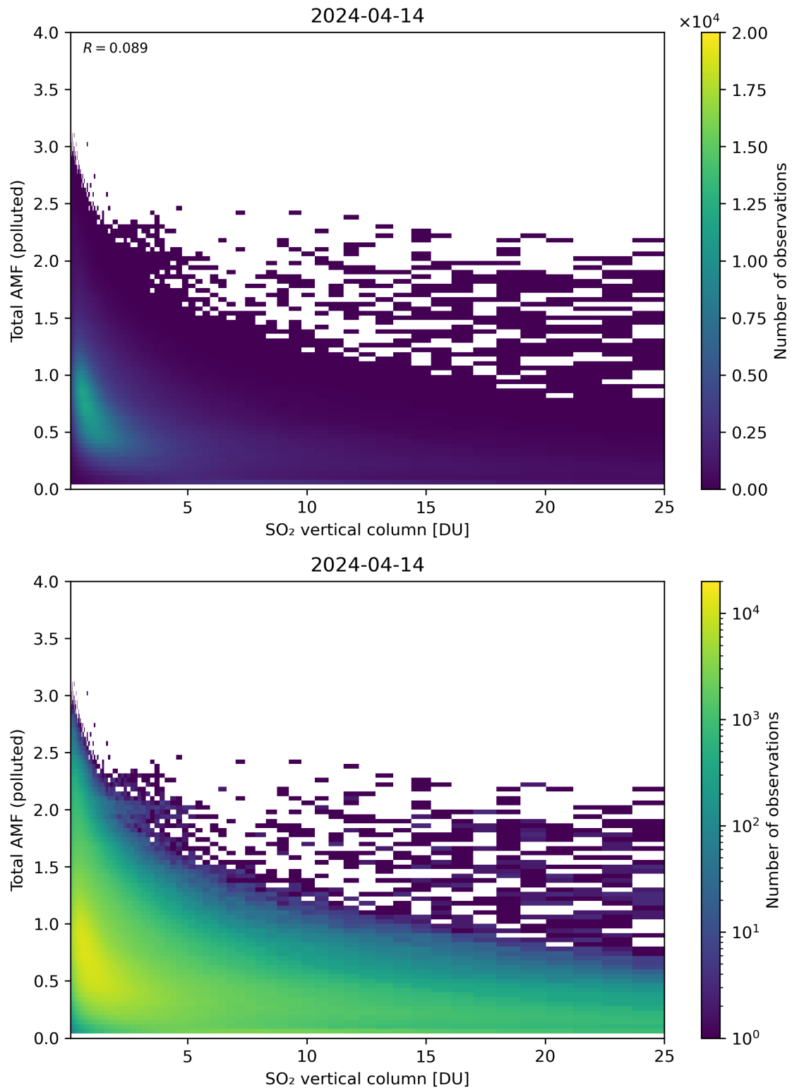
Figure 305: Scatter density plot of “SO 2 vertical column” against “Total AMF (polluted)” for 2024-04-13 to 2024-04-15.
