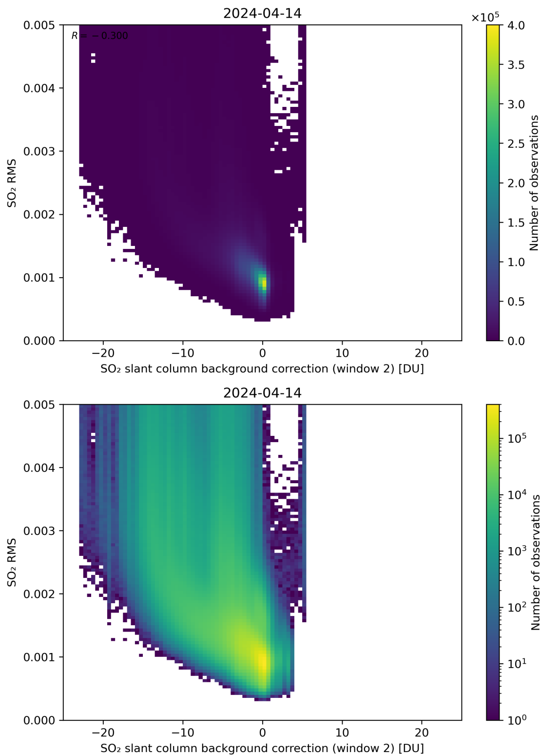
Figure 114: Scatter density plot of “SO 2 slant column background correction (window 2)” against “SO 2 RMS” for 2024-04-13 to 2024-04-15.
