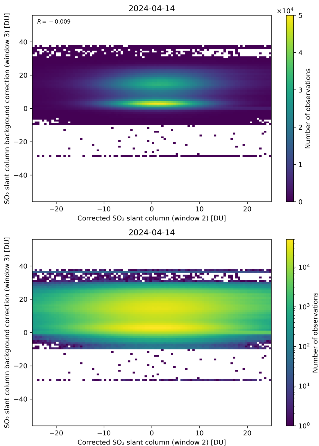
Figure 195: Scatter density plot of “Corrected SO 2 slant column (window 2)” against “SO 2 slant column background correction (window 3)” for 2024-04-13 to 2024-04-15.
