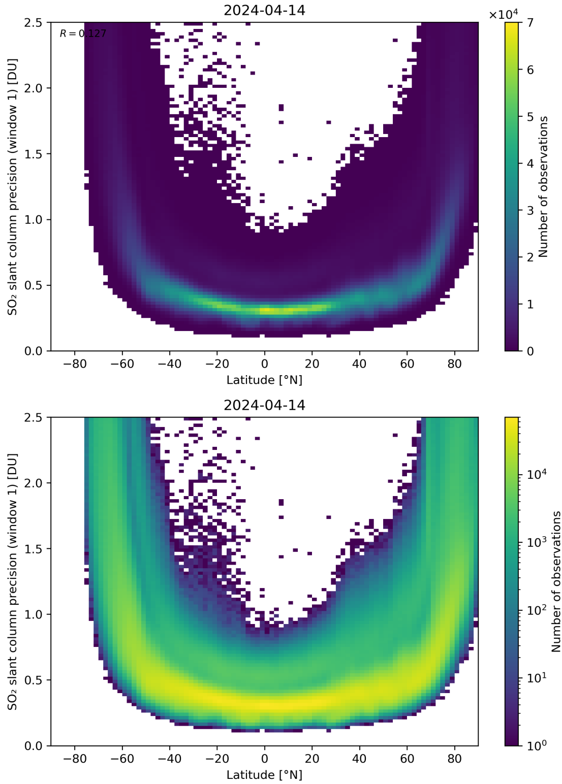
Figure 150: Scatter density plot of “Latitude” against “SO 2 slant column precision (window 1)” for 2024-04-13 to 2024-04-15.
