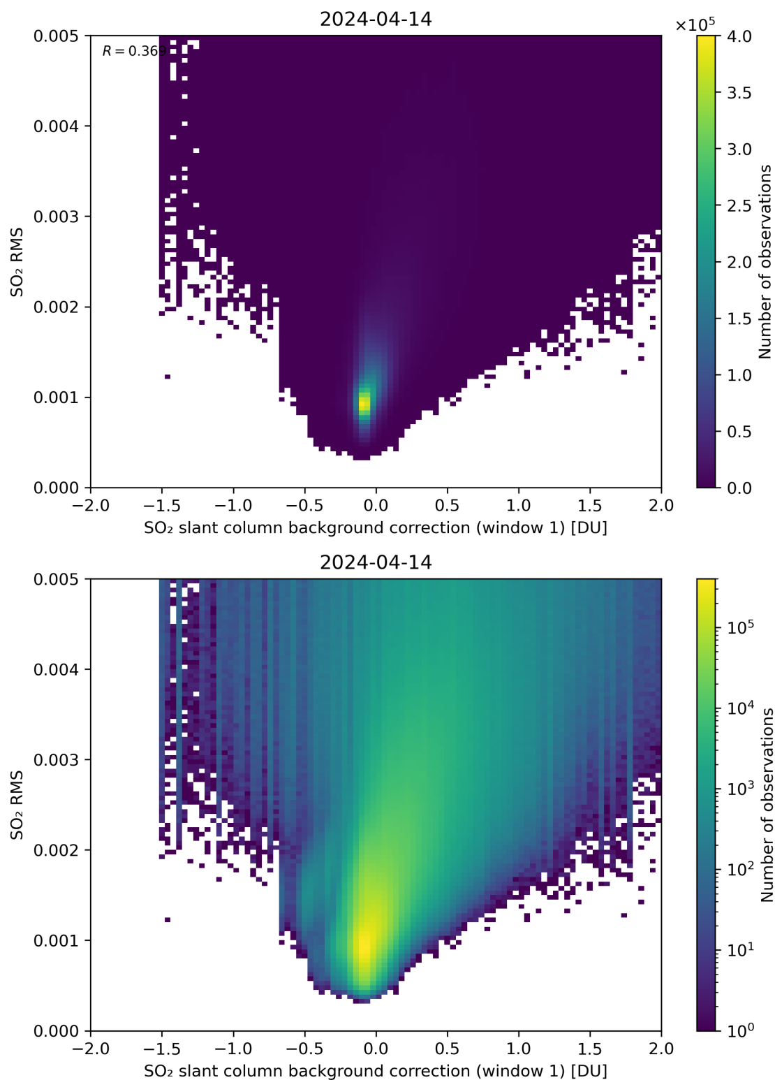
Figure 102: Scatter density plot of “SO 2 slant column background correction (window 1)” against “SO 2 RMS” for 2024-04-13 to 2024-04-15.
