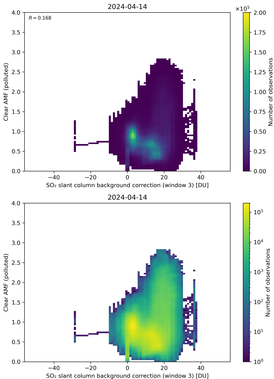
Figure 124: Scatter density plot of “SO 2 slant column background correction (window 3)” against “Clear AMF (polluted)” for 2024-04-13 to 2024-04-15.
