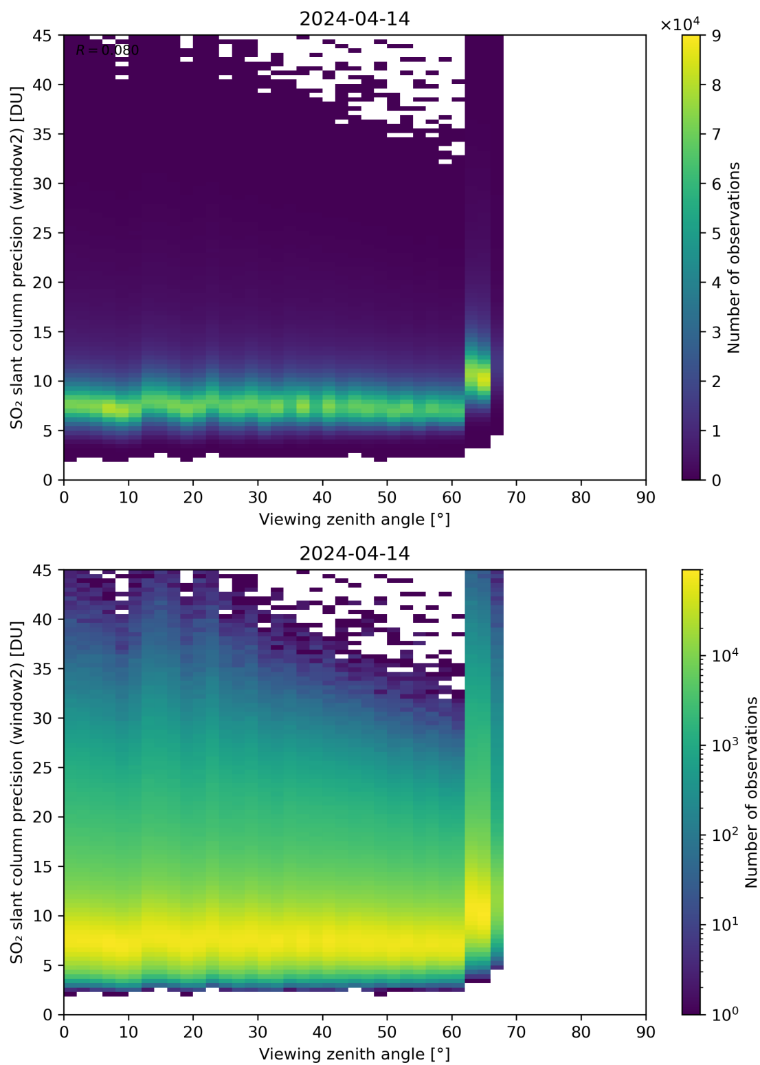
Figure 322: Scatter density plot of “Viewing zenith angle” against “SO 2 slant column precision (window2)” for 2024-04-13 to 2024-04-15.
