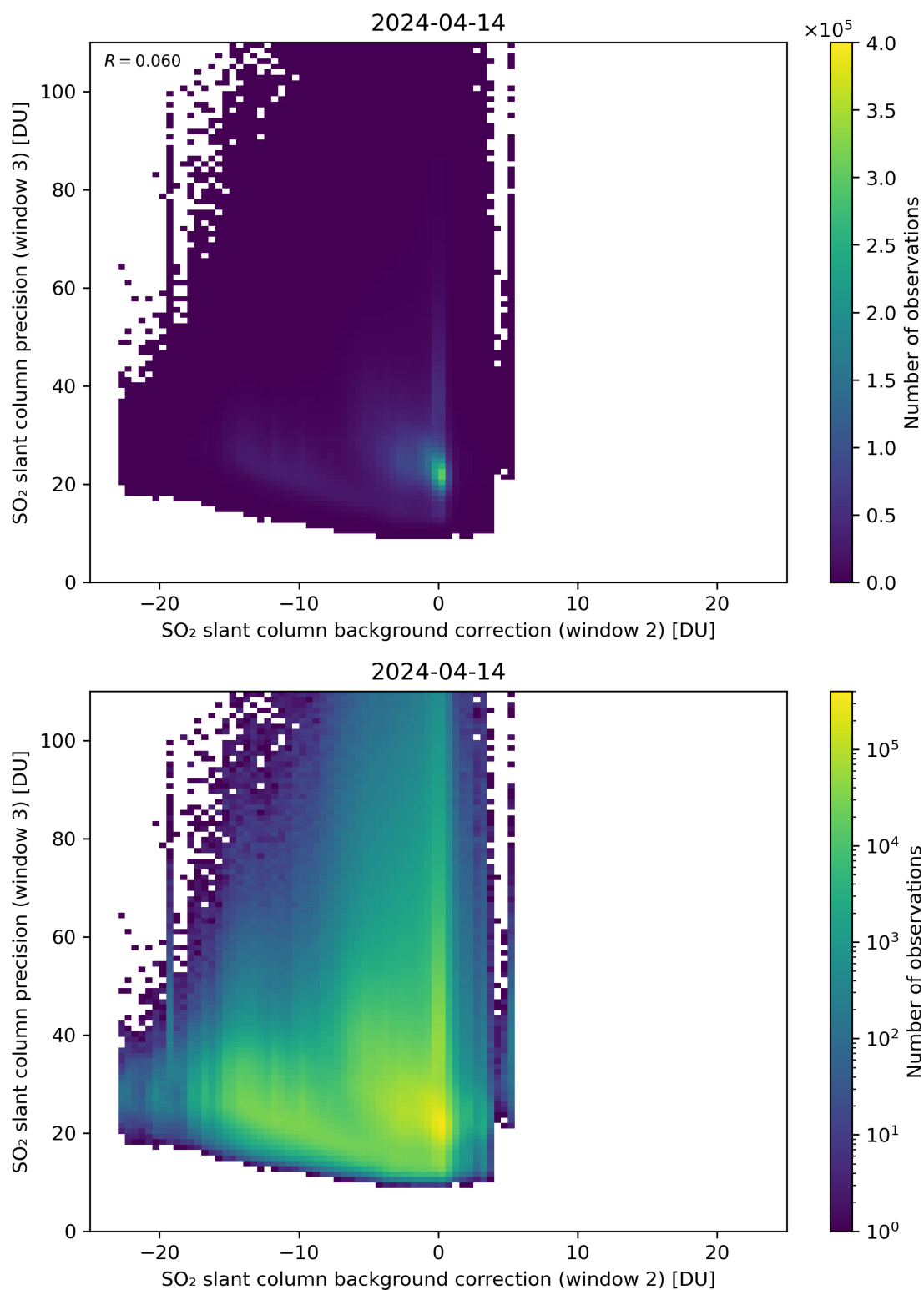
Figure 118: Scatter density plot of “SO 2 slant column background correction (window 2)” against “SO 2 slant column precision (window 3)” for 2024-04-13 to 2024-04-15.
