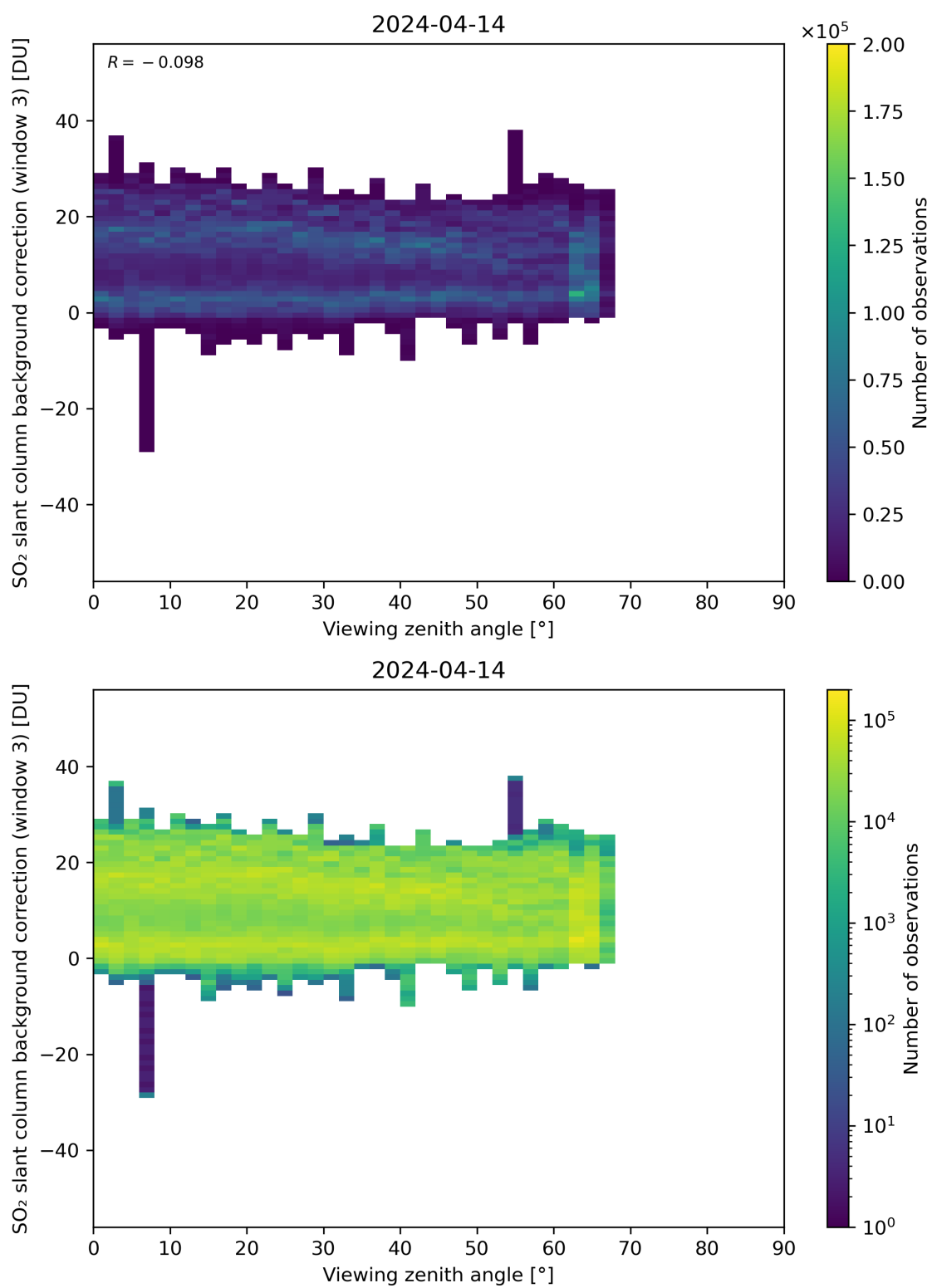
Figure 310: Scatter density plot of “Viewing zenith angle” against “SO 2 slant column background correction (window 3)” for 2024-04-13 to 2024-04-15.
