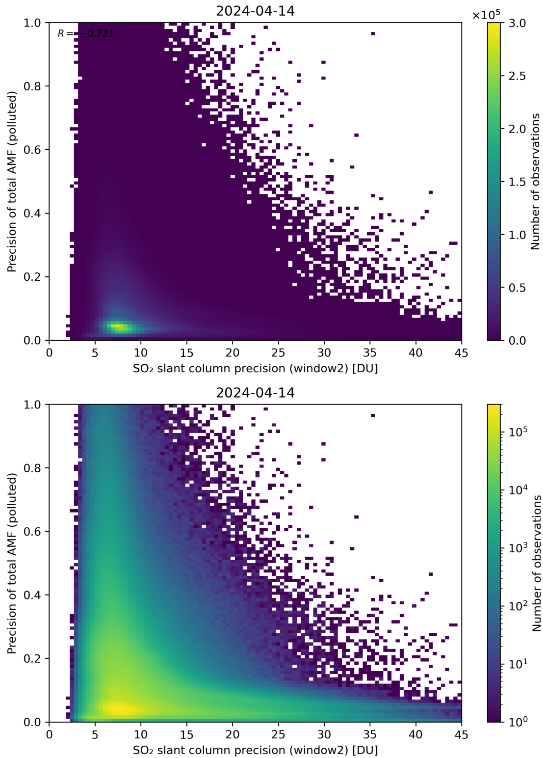
Figure 252: Scatter density plot of “SO 2 slant column precision (window2)” against “Precision of total AMF (polluted)” for 2024-04-13 to 2024-04-15.
