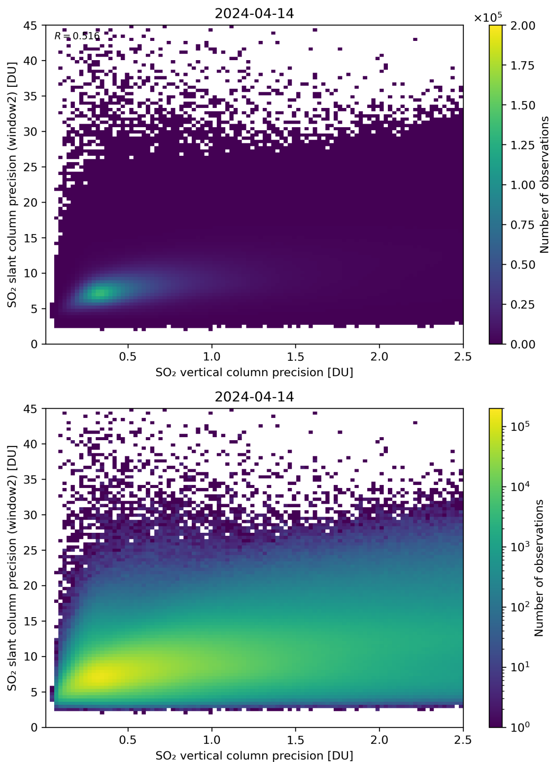
Figure 291: Scatter density plot of “SO 2 vertical column precision” against “SO 2 slant column precision (window2)” for 2024-04-13 to 2024-04-15.
