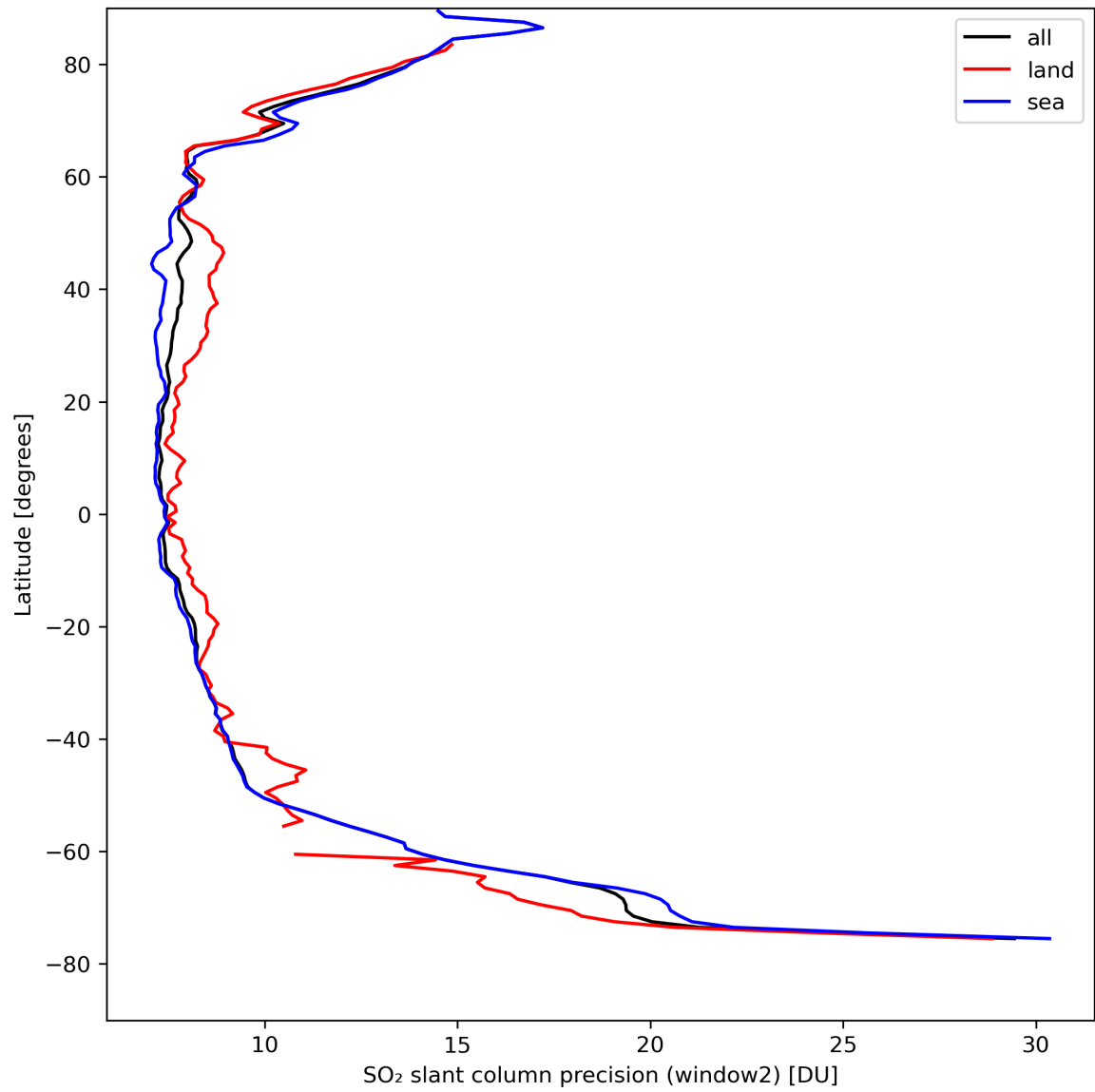
Figure 38: Zonal average of “SO 2 slant column precision (window2)” for 2024-04-13 to 2024-04-15.
