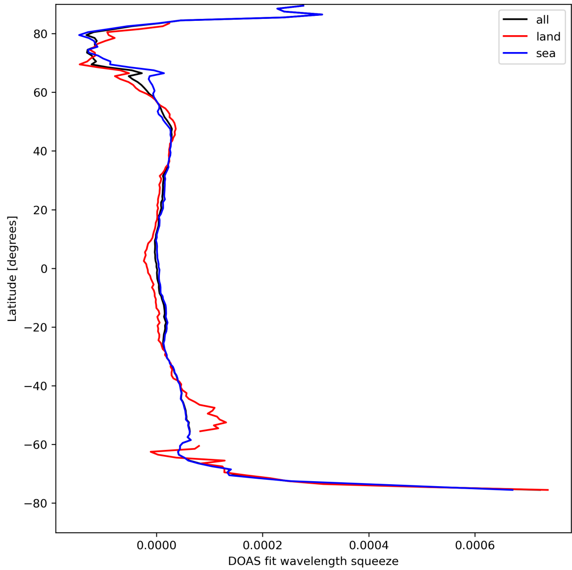
Figure 46: Zonal average of “DOAS fit wavelength squeeze” for 2024-04-13 to 2024-04-15.
