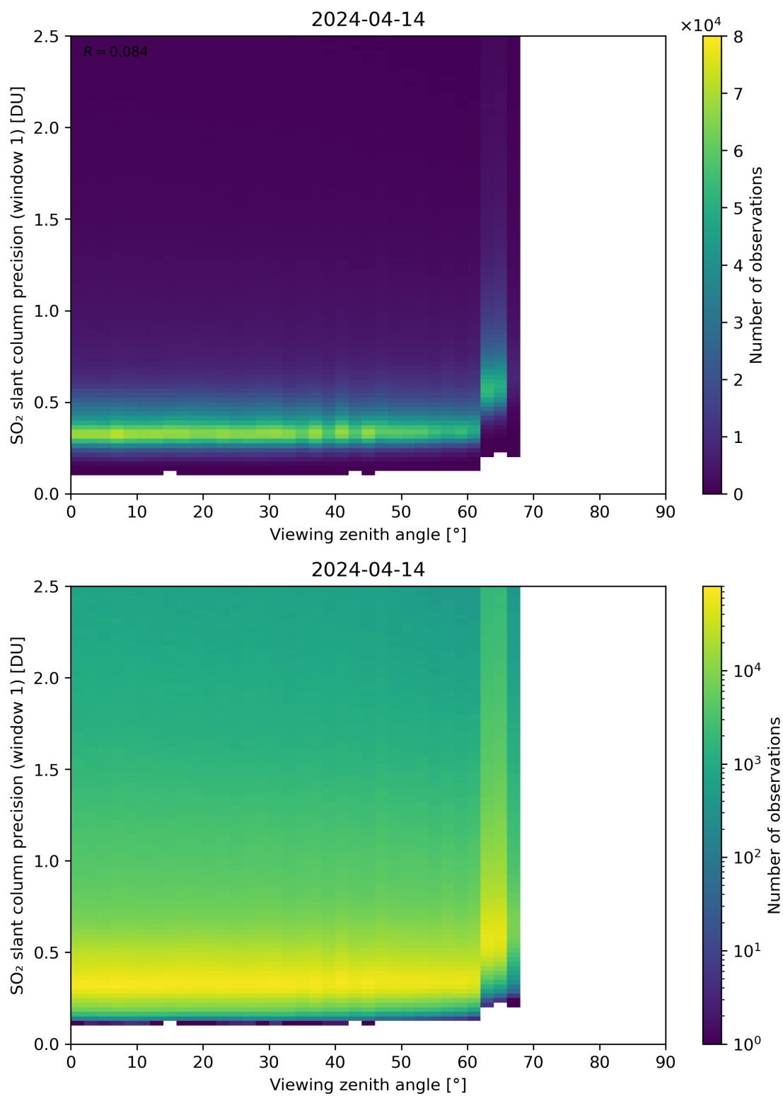
Figure 321: Scatter density plot of “Viewing zenith angle” against “SO 2 slant column precision (window 1)” for 2024-04-13 to 2024-04-15.
