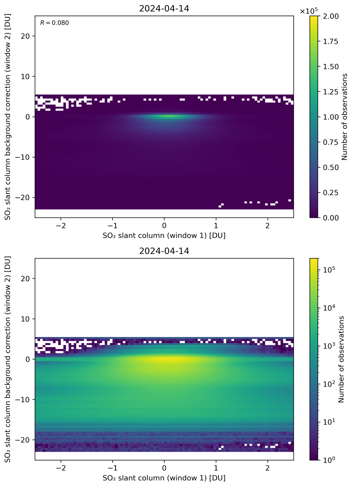
Figure 213: Scatter density plot of “SO 2 slant column (window 1)” against “SO 2 slant column background correction (window 2)” for 2024-04-13 to 2024-04-15.
