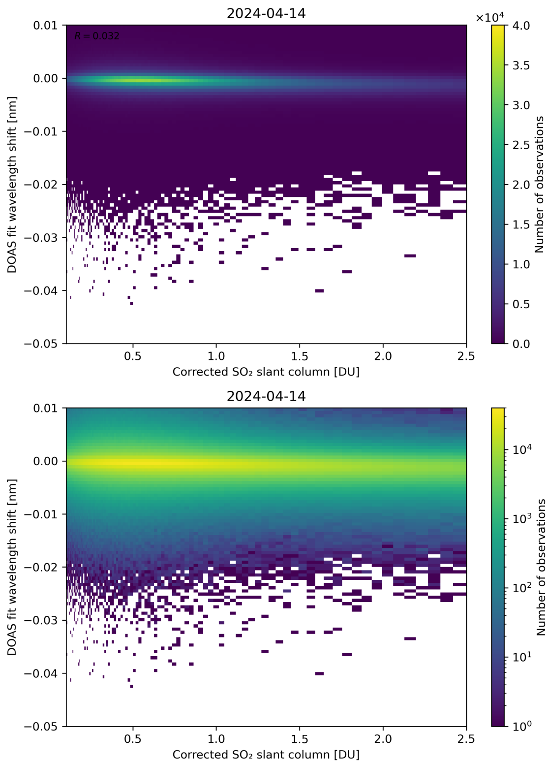
Figure 181: Scatter density plot of “Corrected SO 2 slant column” against “DOAS fit wavelength shift” for 2024-04-13 to 2024-04-15.
