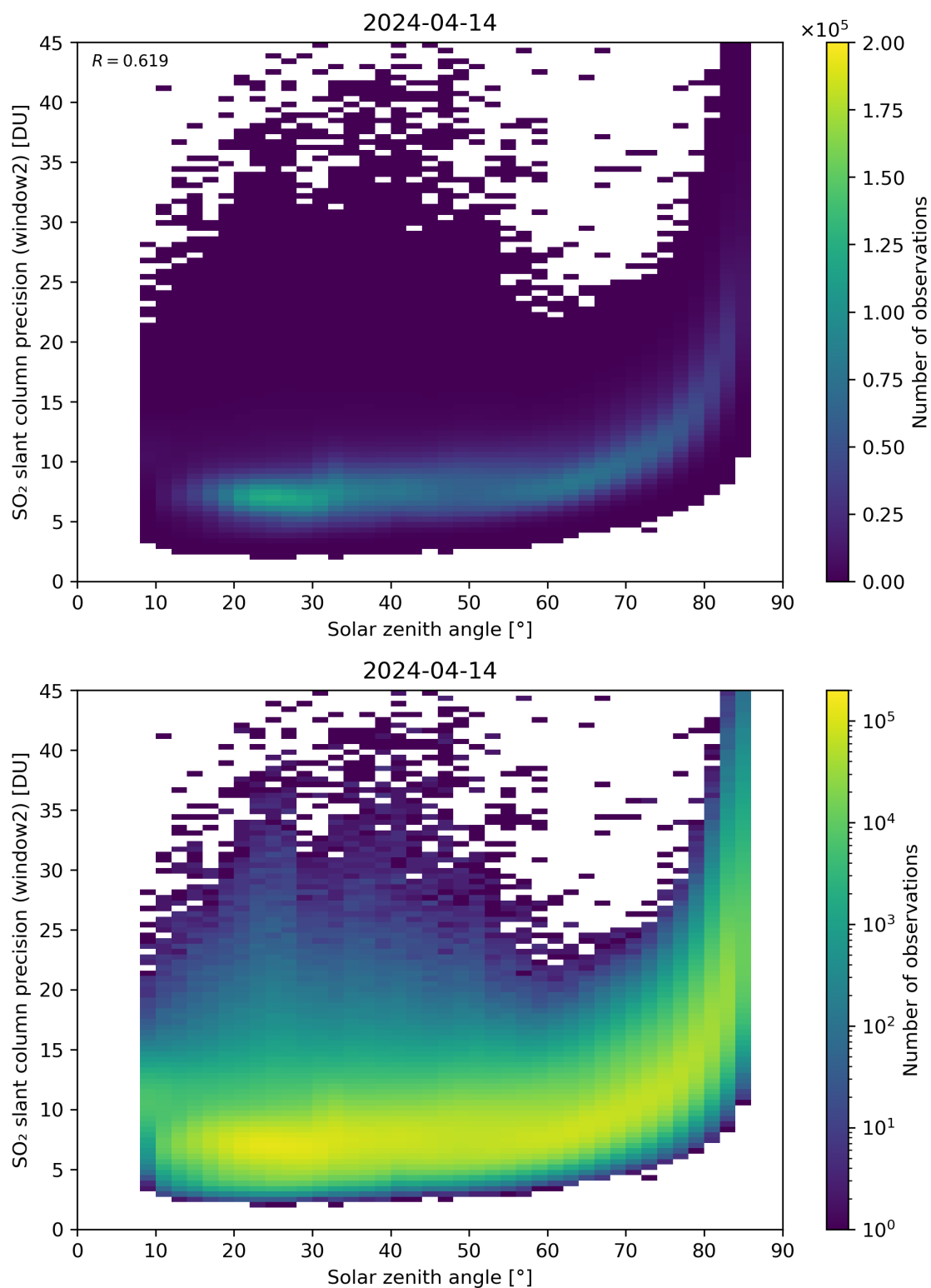
Figure 171: Scatter density plot of “Solar zenith angle” against “SO 2 slant column precision (window2)” for 2024-04-13 to 2024-04-15.
