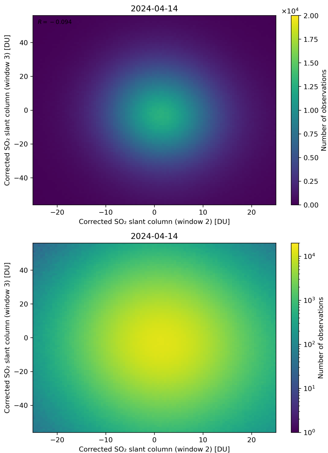
Figure 200: Scatter density plot of “Corrected SO 2 slant column (window 2)” against “Corrected SO 2 slant column (window 3)” for 2024-04-13 to 2024-04-15.
