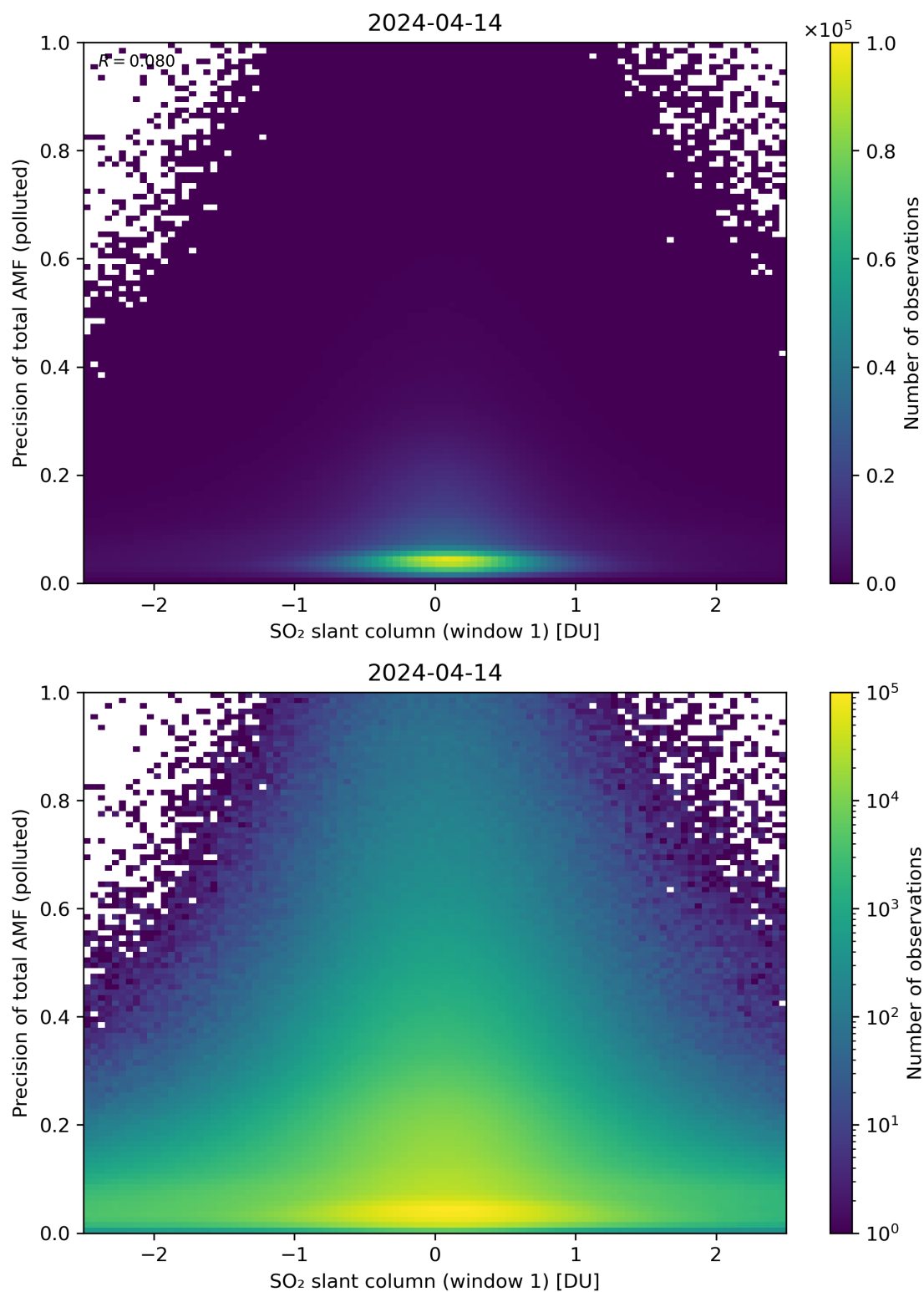
Figure 240: Scatter density plot of “SO 2 slant column (window 1)” against “Precision of total AMF (polluted)” for 2024-04-13 to 2024-04-15.
