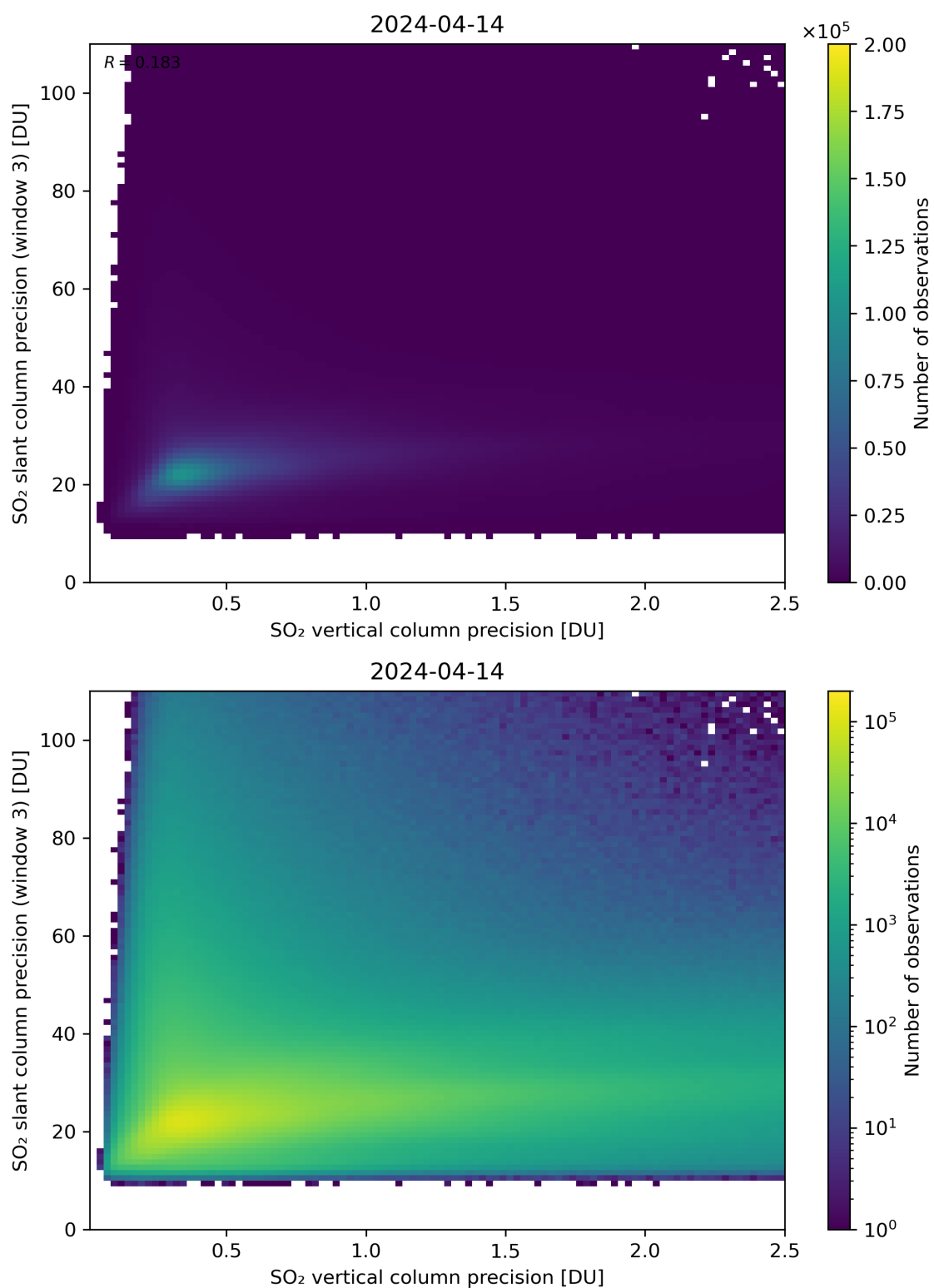
Figure 293: Scatter density plot of “SO 2 vertical column precision” against “SO 2 slant column precision (window 3)” for 2024-04-13 to 2024-04-15.
