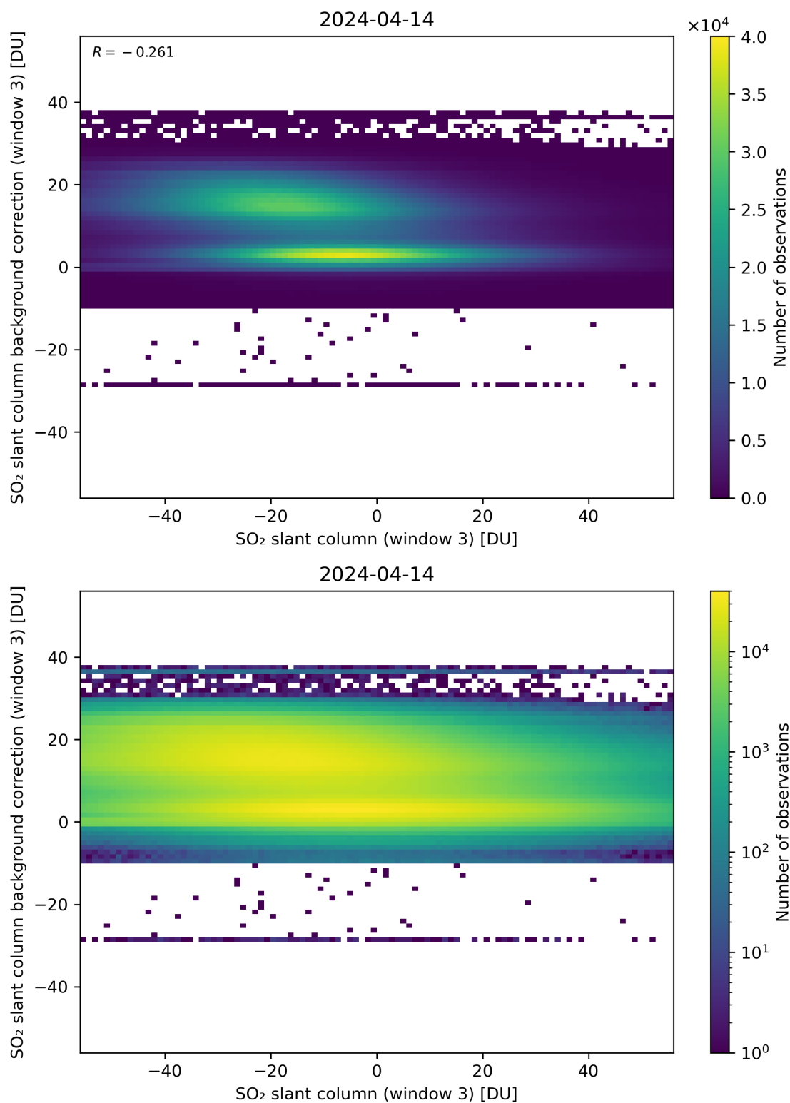
Figure 253: Scatter density plot of “SO 2 slant column (window 3)” against “SO 2 slant column background correction (window 3)” for 2024-04-13 to 2024-04-15.
