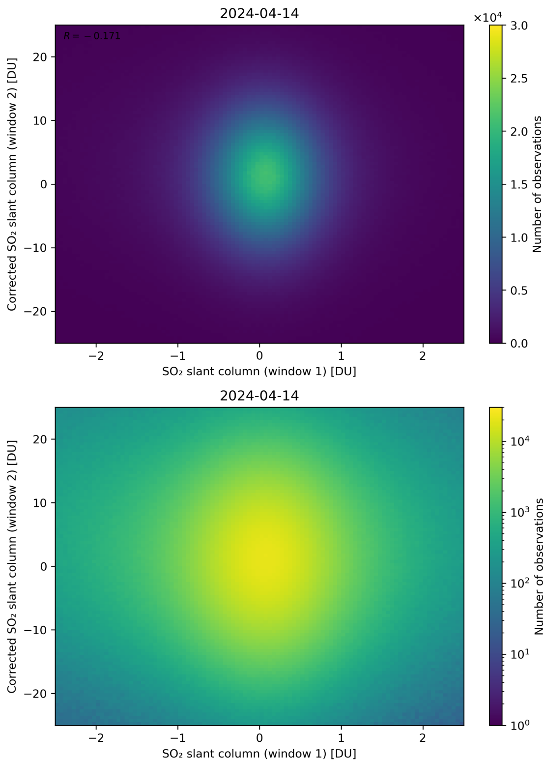
Figure 233: Scatter density plot of “SO 2 slant column (window 1)” against “Corrected SO 2 slant column (window 2)” for 2024-04-13 to 2024-04-15.
