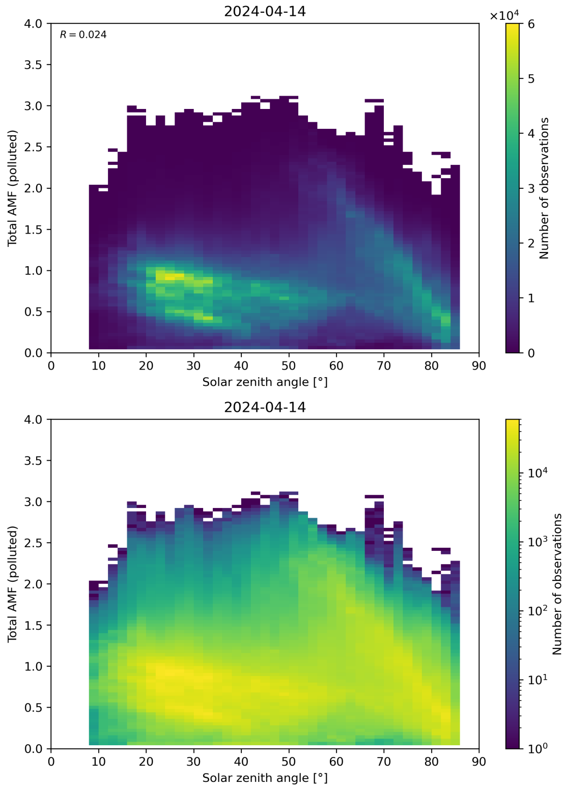
Figure 174: Scatter density plot of “Solar zenith angle” against “Total AMF (polluted)” for 2024-04-13 to 2024-04-15.
