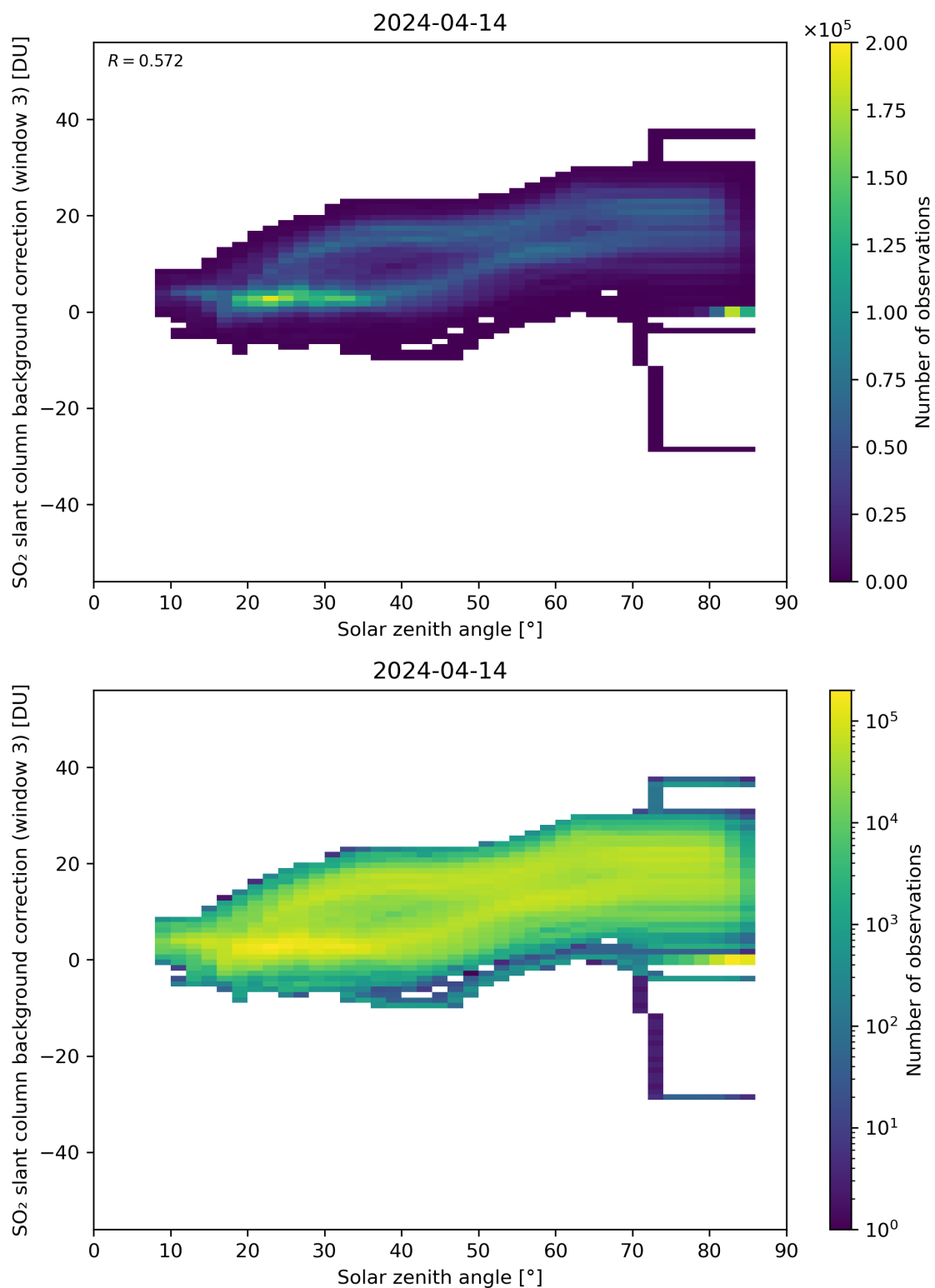
Figure 160: Scatter density plot of “Solar zenith angle” against “SO 2 slant column background correction (window 3)” for 2024-04-13 to 2024-04-15.
