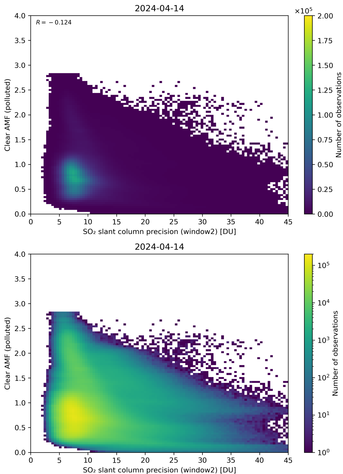
Figure 246: Scatter density plot of “SO 2 slant column precision (window2)” against “Clear AMF (polluted)” for 2024-04-13 to 2024-04-15.
