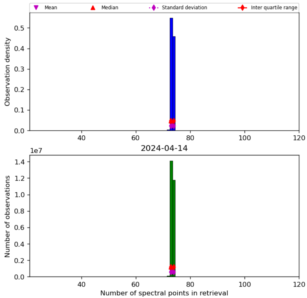
Figure 74: Histogram of “Number of spectral points in retrieval” for 2024-04-13 to 2024-04-15
