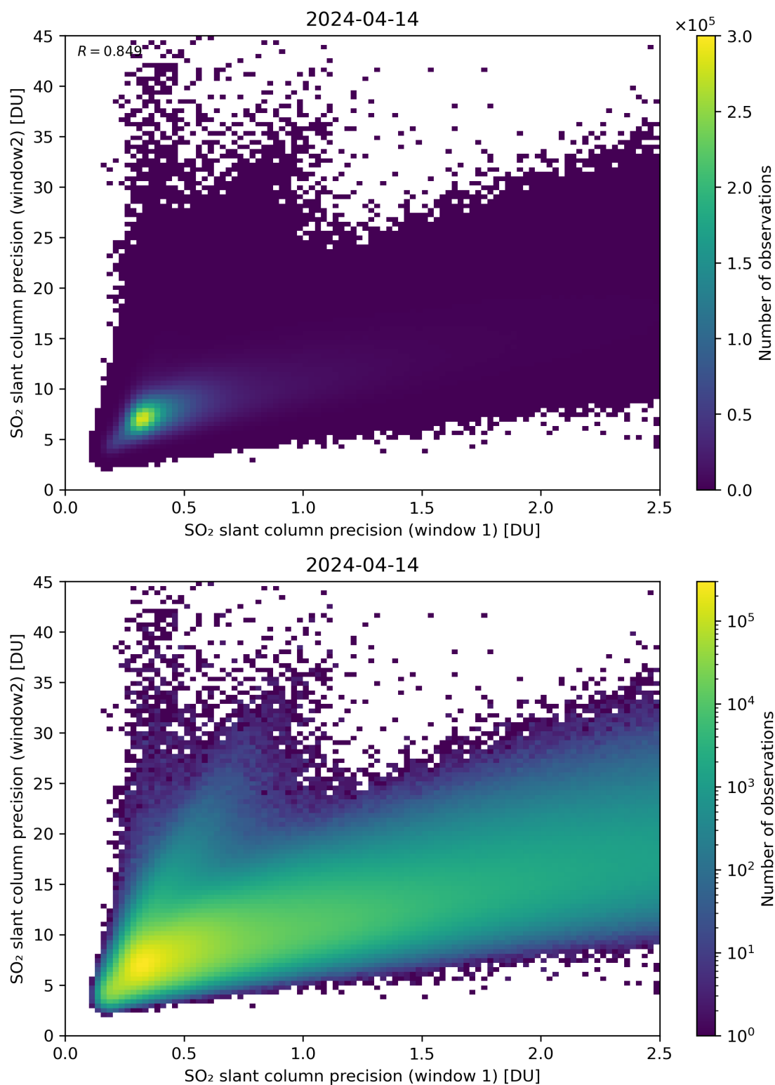
Figure 227: Scatter density plot of “SO 2 slant column precision (window 1)” against “SO 2 slant column precision (window 2)” for 2024-04-13 to 2024-04-15.
