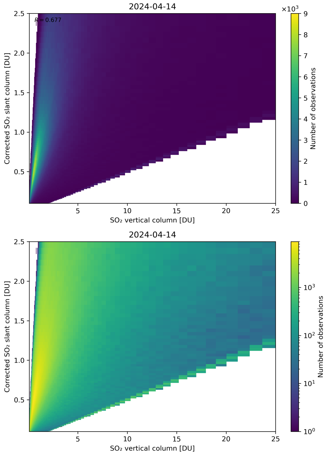
Figure 297: Scatter density plot of “SO 2 vertical column” against “Corrected SO 2 slant column” for 2024-04-13 to 2024-04-15.
