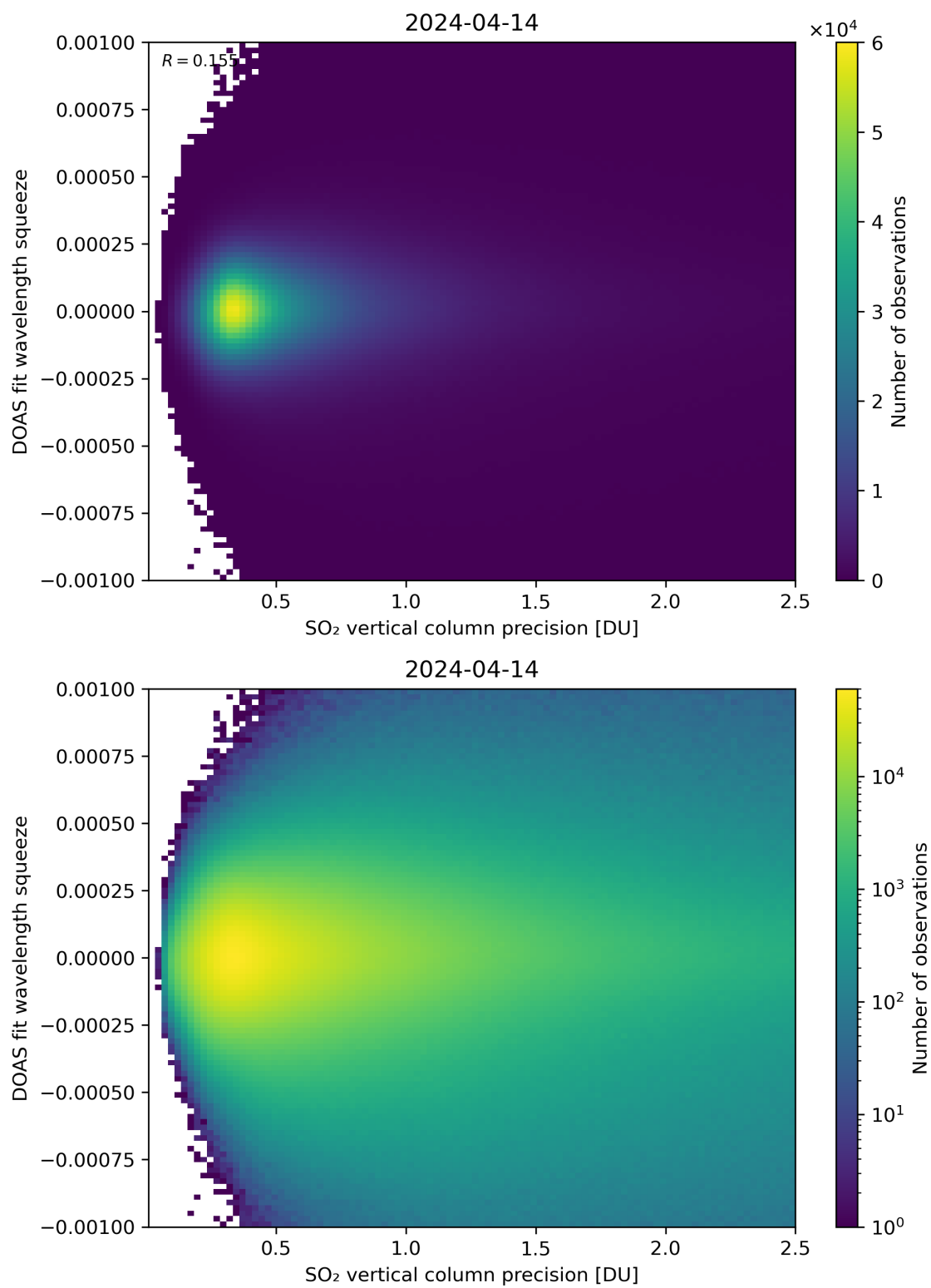
Figure 283: Scatter density plot of “SO 2 vertical column precision” against “DOAS fit wavelength squeeze” for 2024-04-13 to 2024-04-15.
