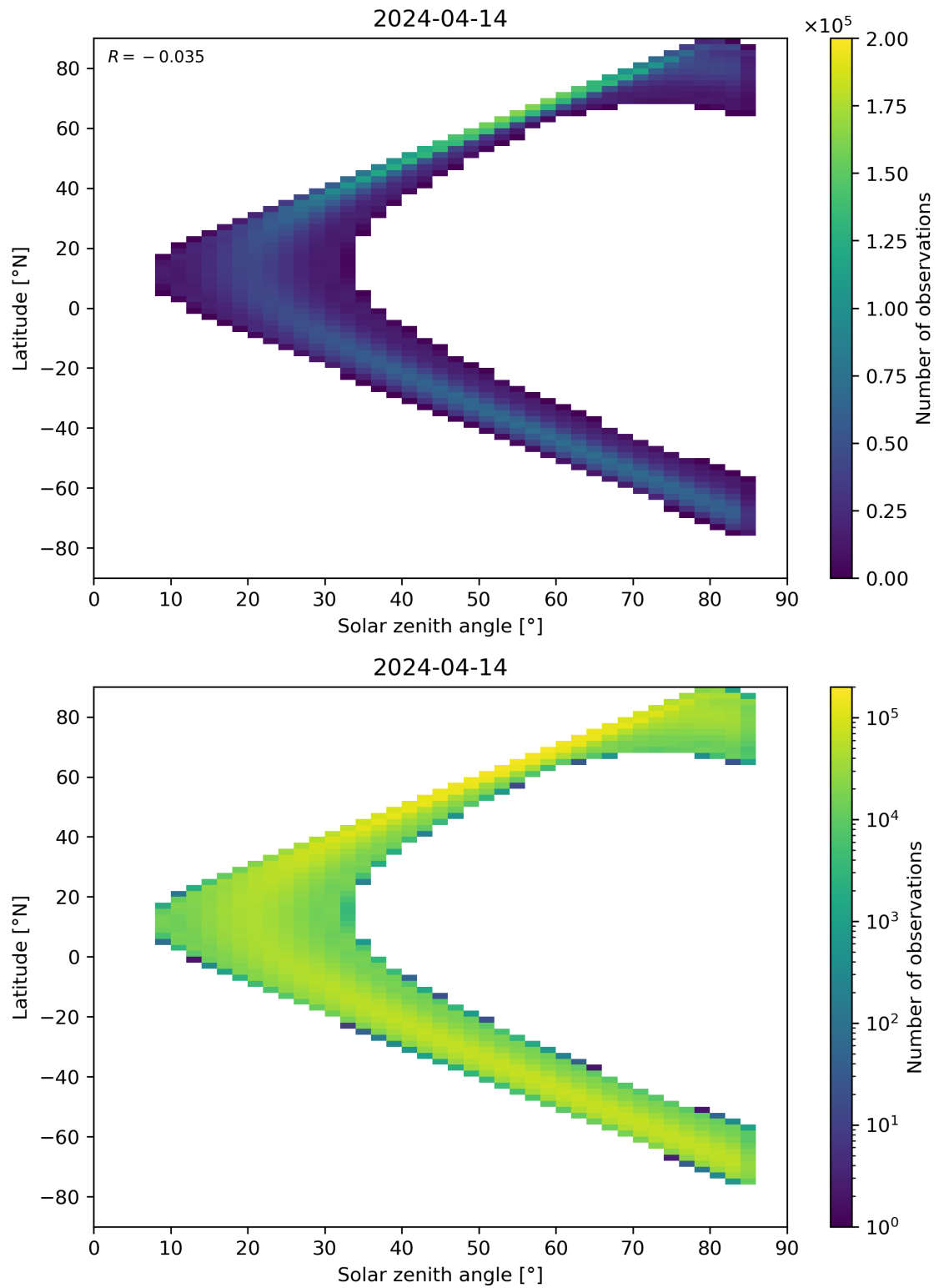
Figure 164: Scatter density plot of “Solar zenith angle” against “Latitude” for 2024-04-13 to 2024-04-15.
