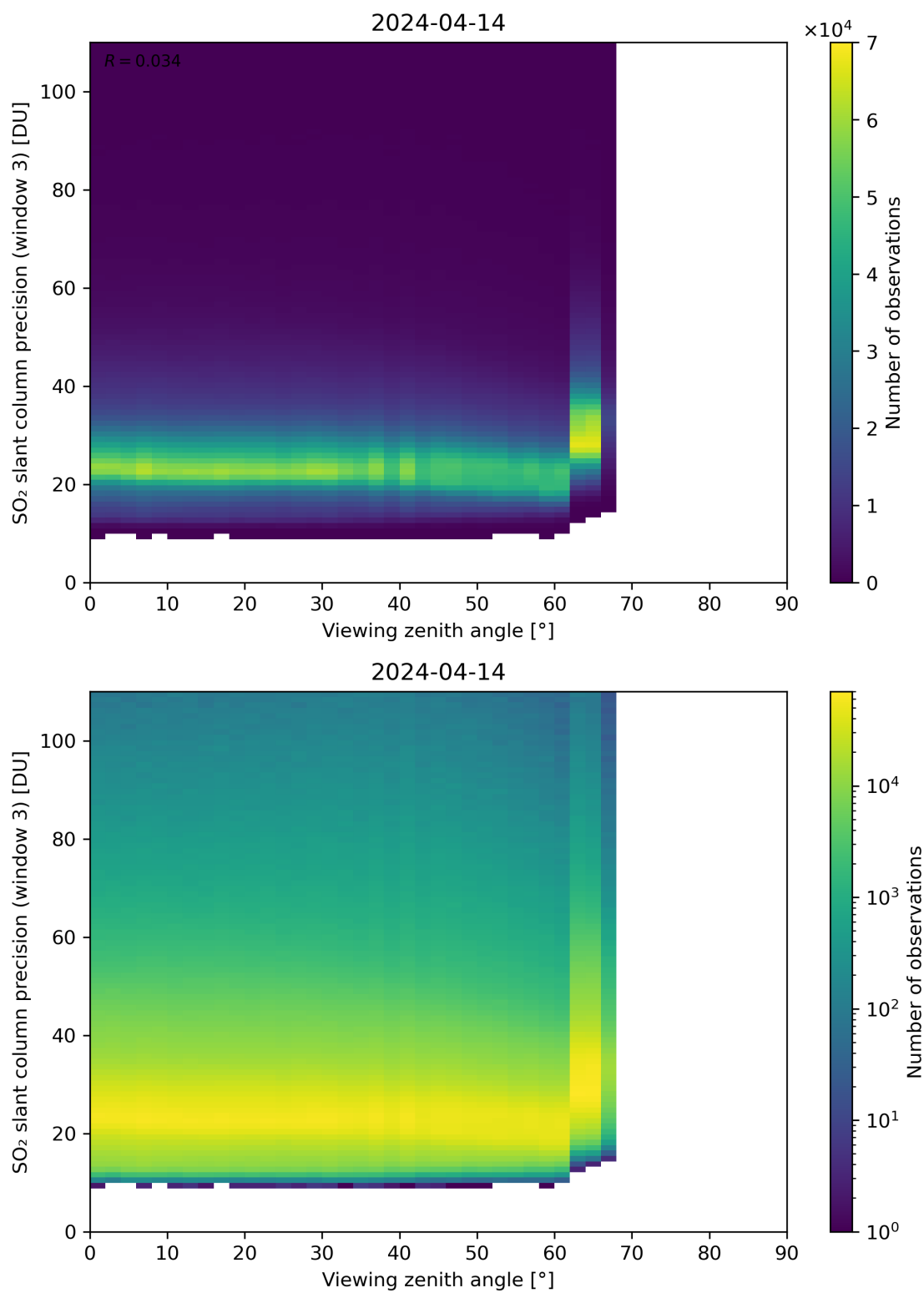
Figure 324: Scatter density plot of “Viewing zenith angle” against “SO 2 slant column precision (window 3)” for 2024-04-13 to 2024-04-15.
