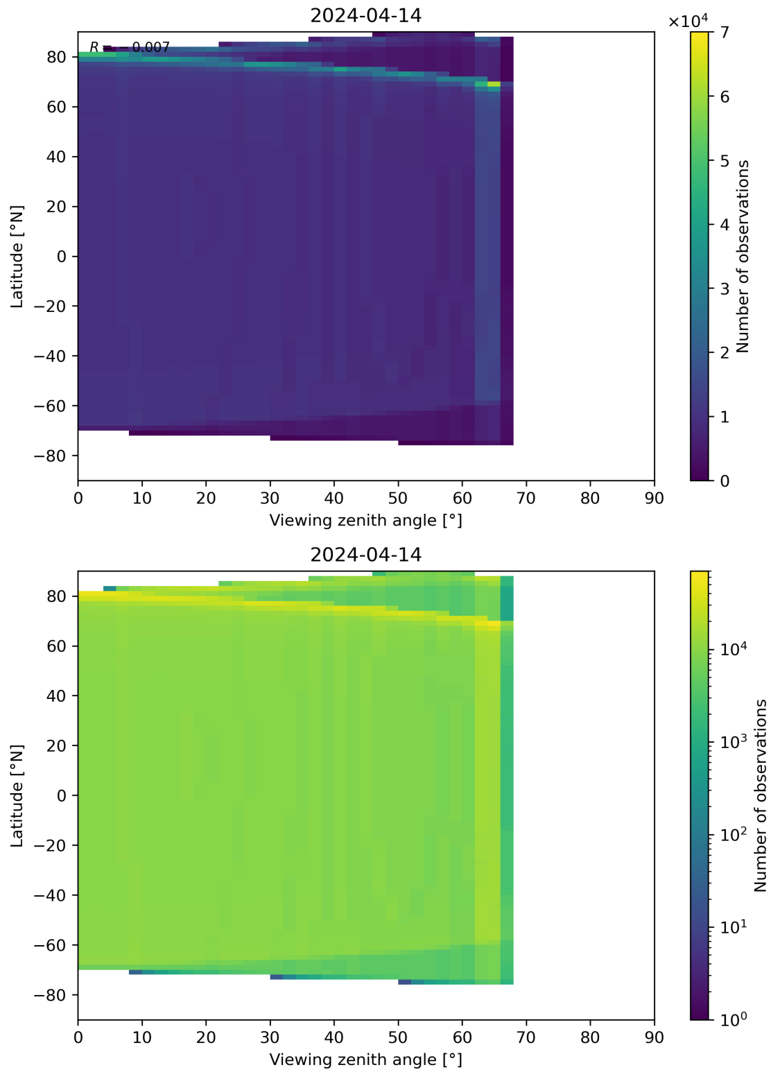
Figure 314: Scatter density plot of “Viewing zenith angle” against “Latitude” for 2024-04-13 to 2024-04-15.
