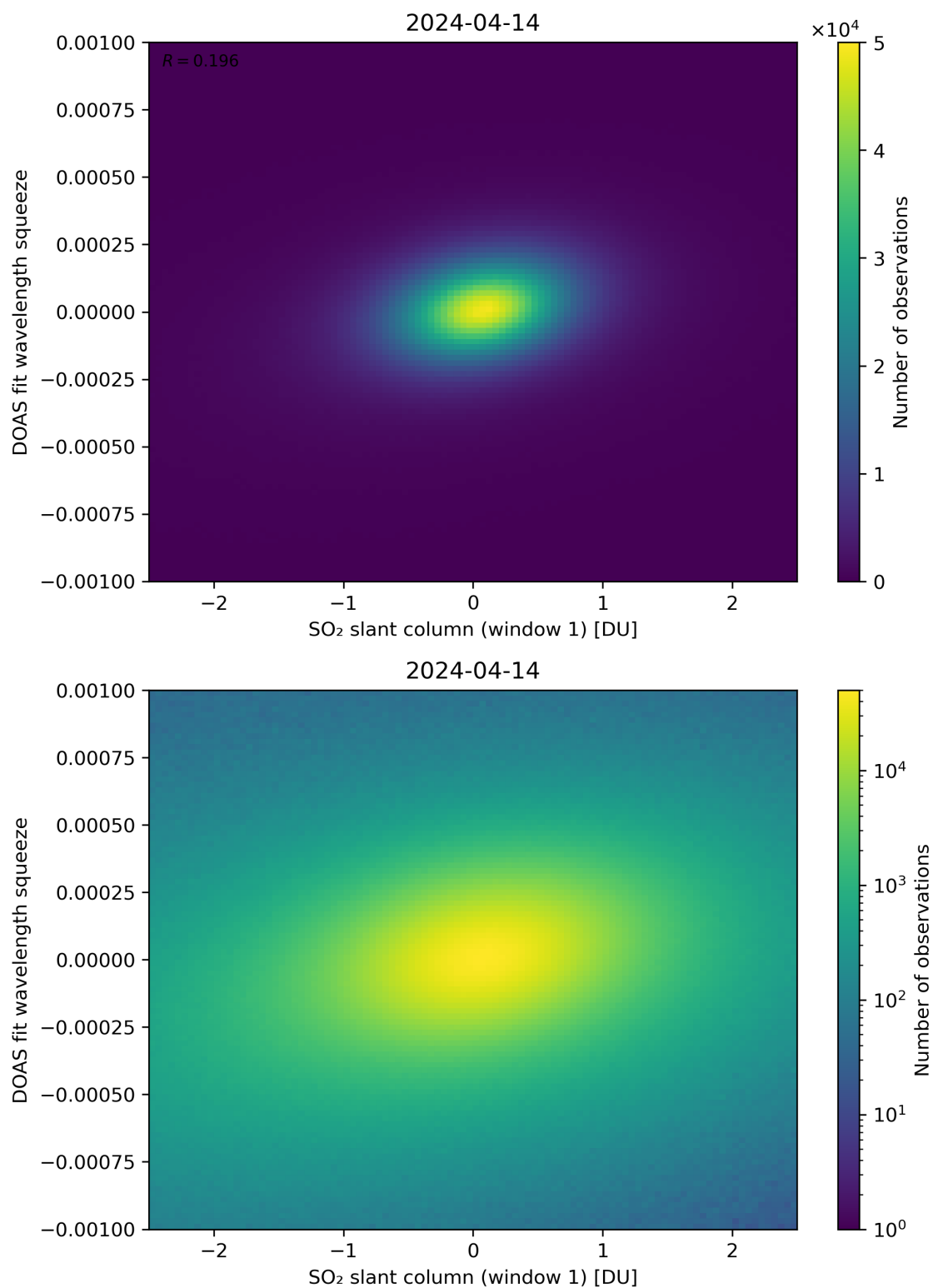
Figure 216: Scatter density plot of “SO 2 slant column (window 1)” against “DOAS fit wavelength squeeze” for 2024-04-13 to 2024-04-15.
