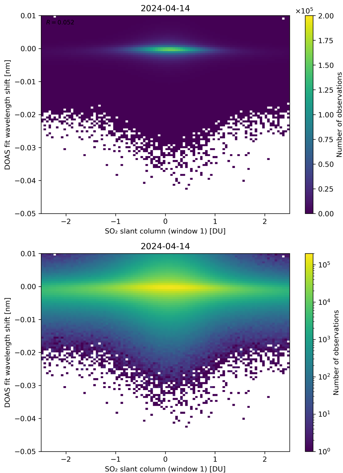
Figure 215: Scatter density plot of “SO 2 slant column (window 1)” against “DOAS fit wavelength shift” for 2024-04-13 to 2024-04-15.
