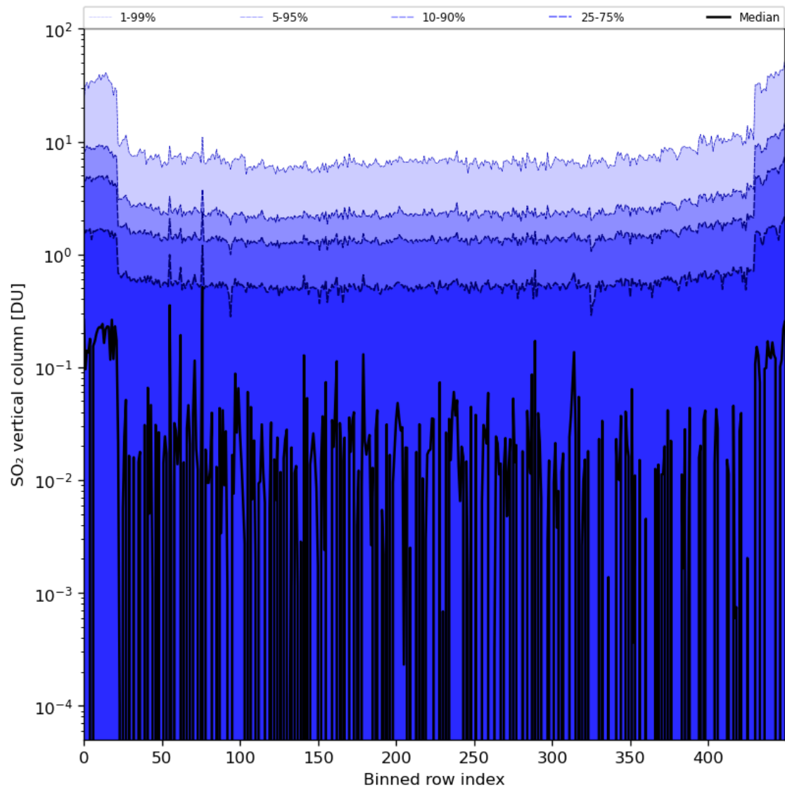
Figure 76: Along track statistics of “SO 2 vertical column” for 2024-04-13 to 2024-04-15
