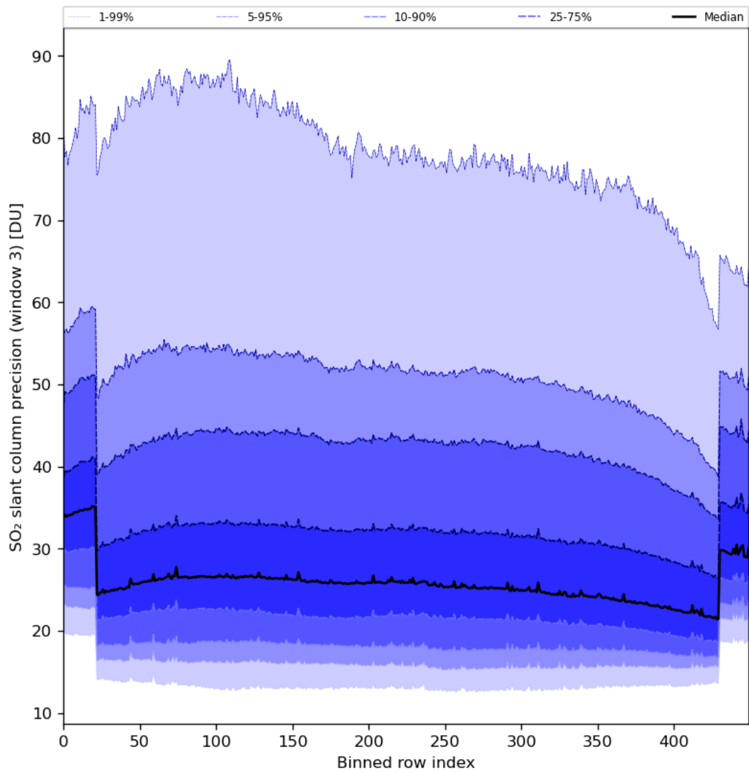
Figure 88: Along track statistics of “SO 2 slant column precision (window 3)” for 2024-04-13 to 2024-04-15
