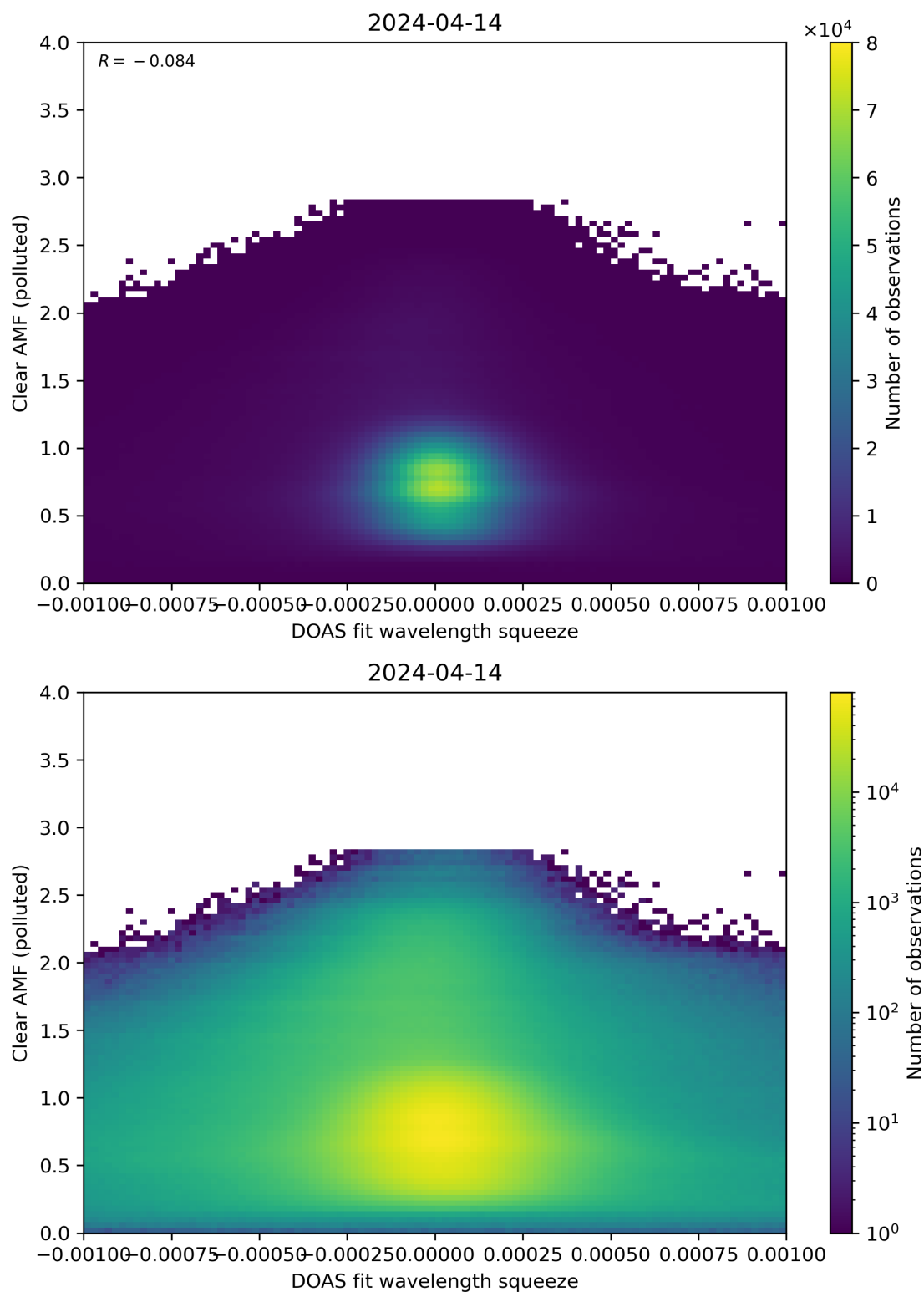
Figure 133: Scatter density plot of “DOAS fit wavelength squeeze” against “Clear AMF (polluted)” for 2024-04-13 to 2024-04-15.
