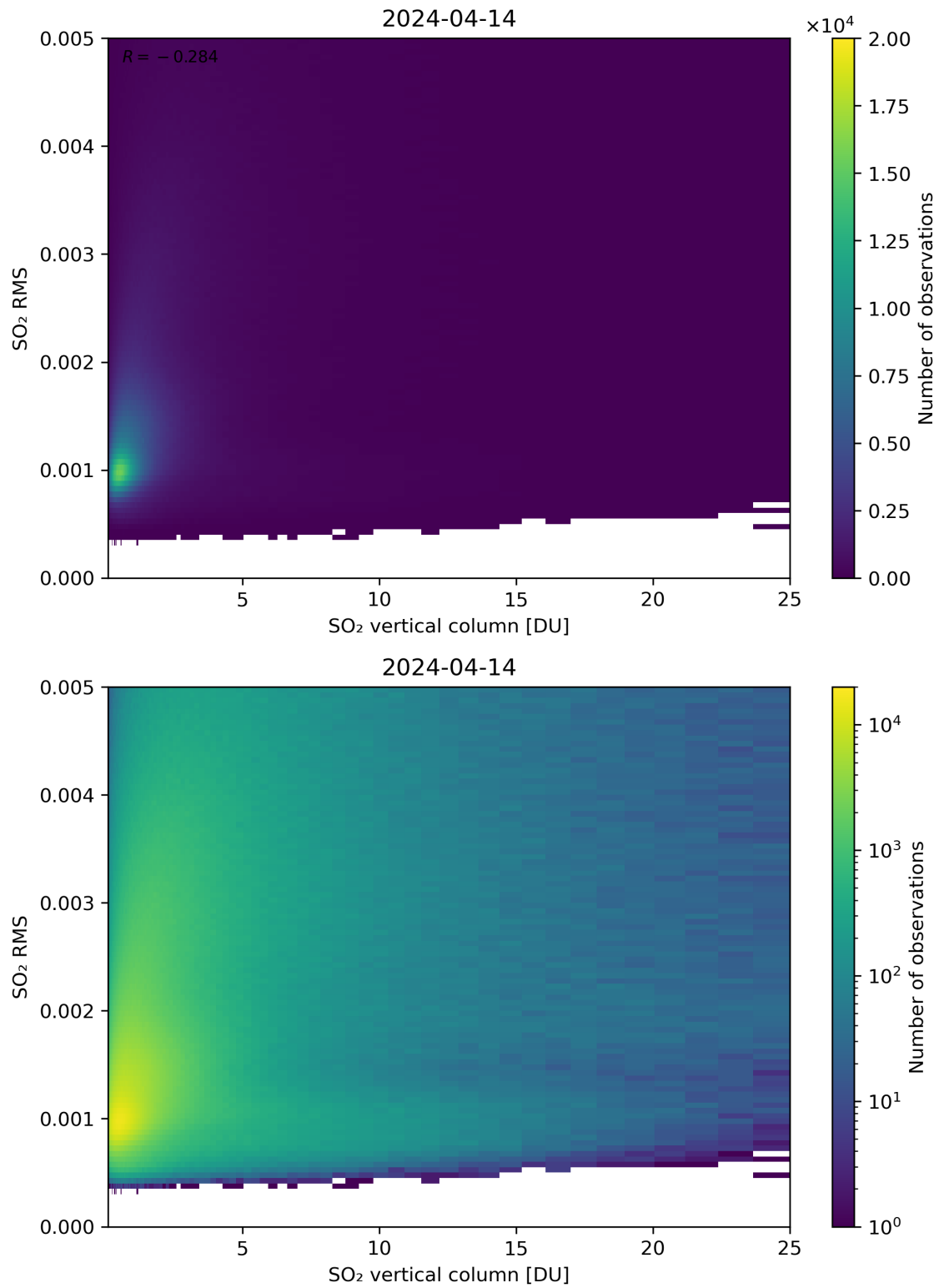
Figure 278: Scatter density plot of “SO 2 vertical column” against “SO 2 RMS” for 2024-04-13 to 2024-04-15.
