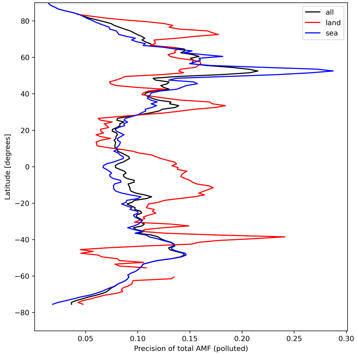
Figure 49: Zonal average of “Precision of total AMF (polluted)” for 2024-04-13 to 2024-04-15.
