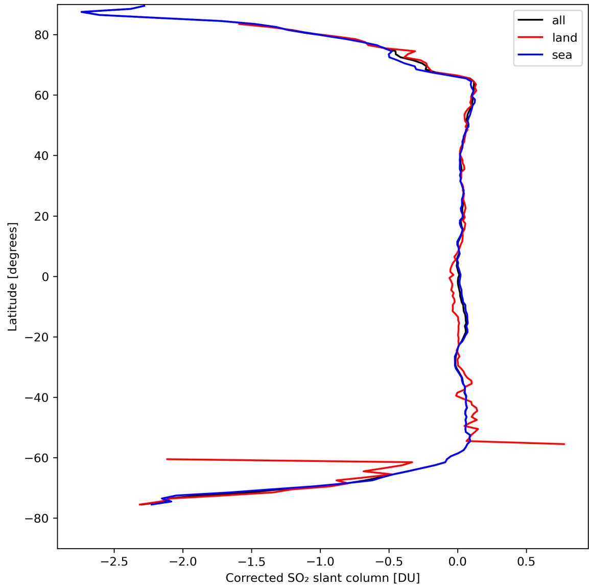
Figure 32: Zonal average of “Corrected SO 2 slant column” for 2024-04-13 to 2024-04-15.
