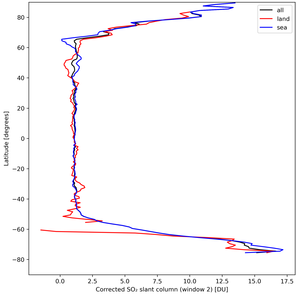
Figure 39: Zonal average of “Corrected SO 2 slant column (window 2)” for 2024-04-13 to 2024-04-15.
