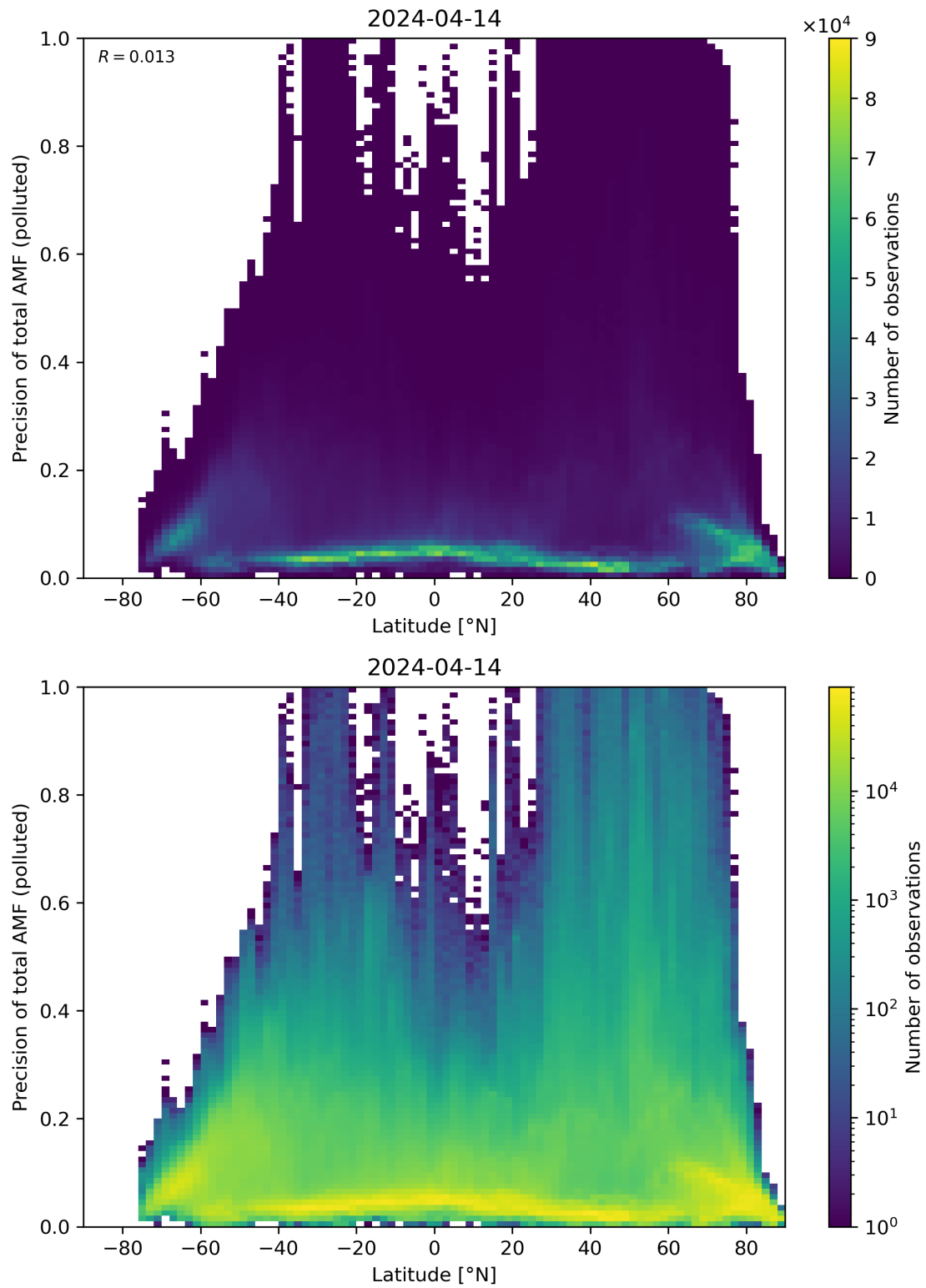
Figure 155: Scatter density plot of “Latitude” against “Precision of total AMF (polluted)” for 2024-04-13 to 2024-04-15.
