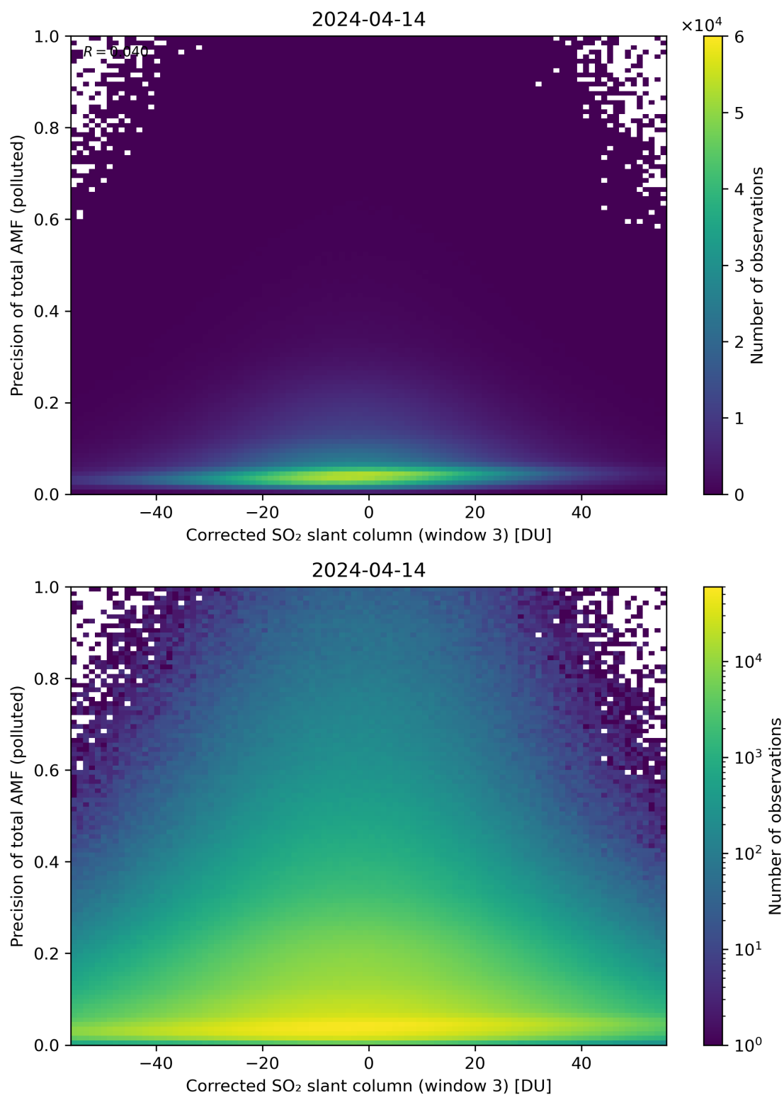
Figure 211: Scatter density plot of “Corrected SO 2 slant column (window 3)” against “Precision of total AMF (polluted)” for 2024-04-13 to 2024-04-15.
