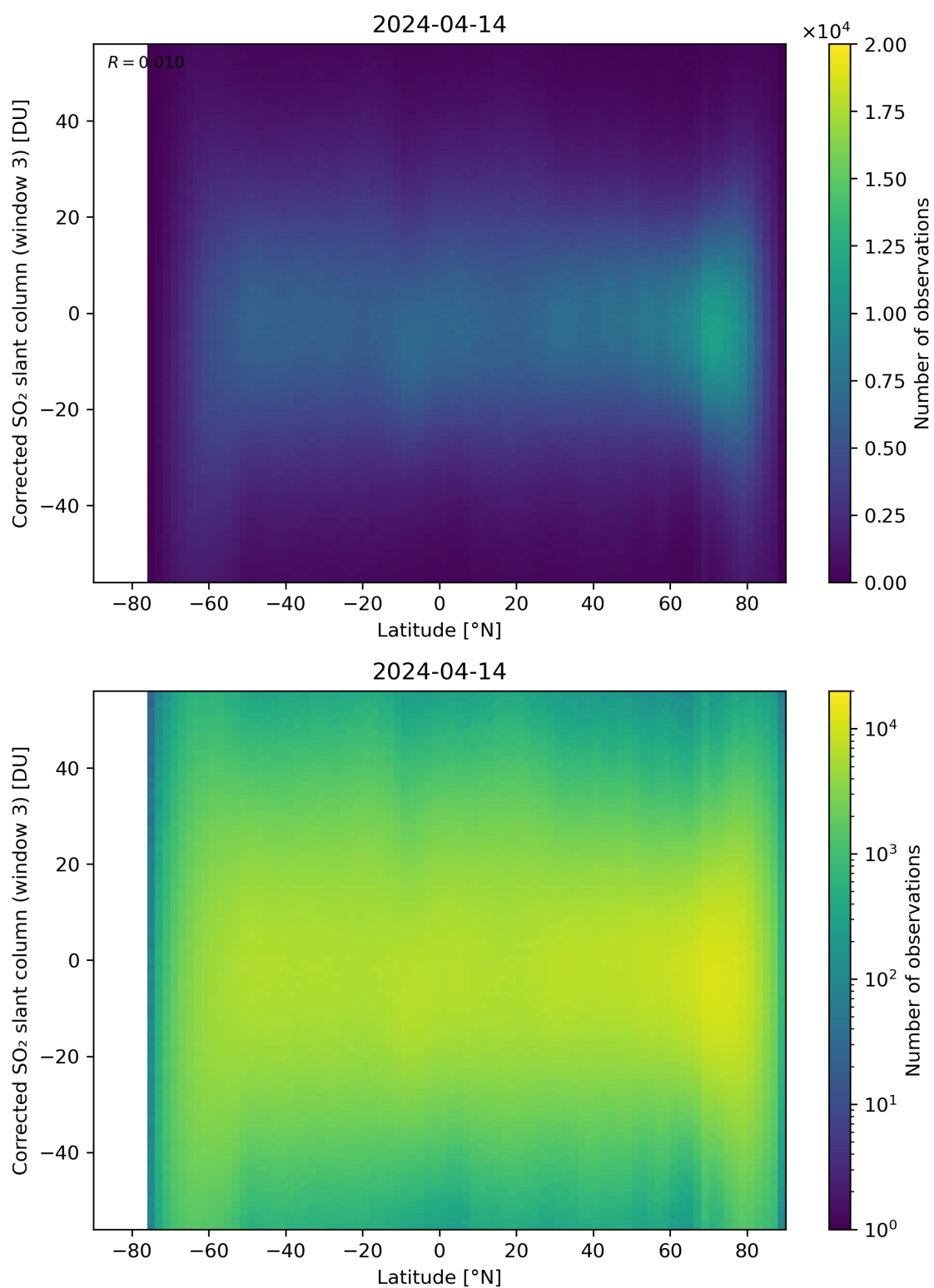
Figure 148: Scatter density plot of “Latitude” against “Corrected SO 2 slant column (window 3)” for 2024-04-13 to 2024-04-15.
