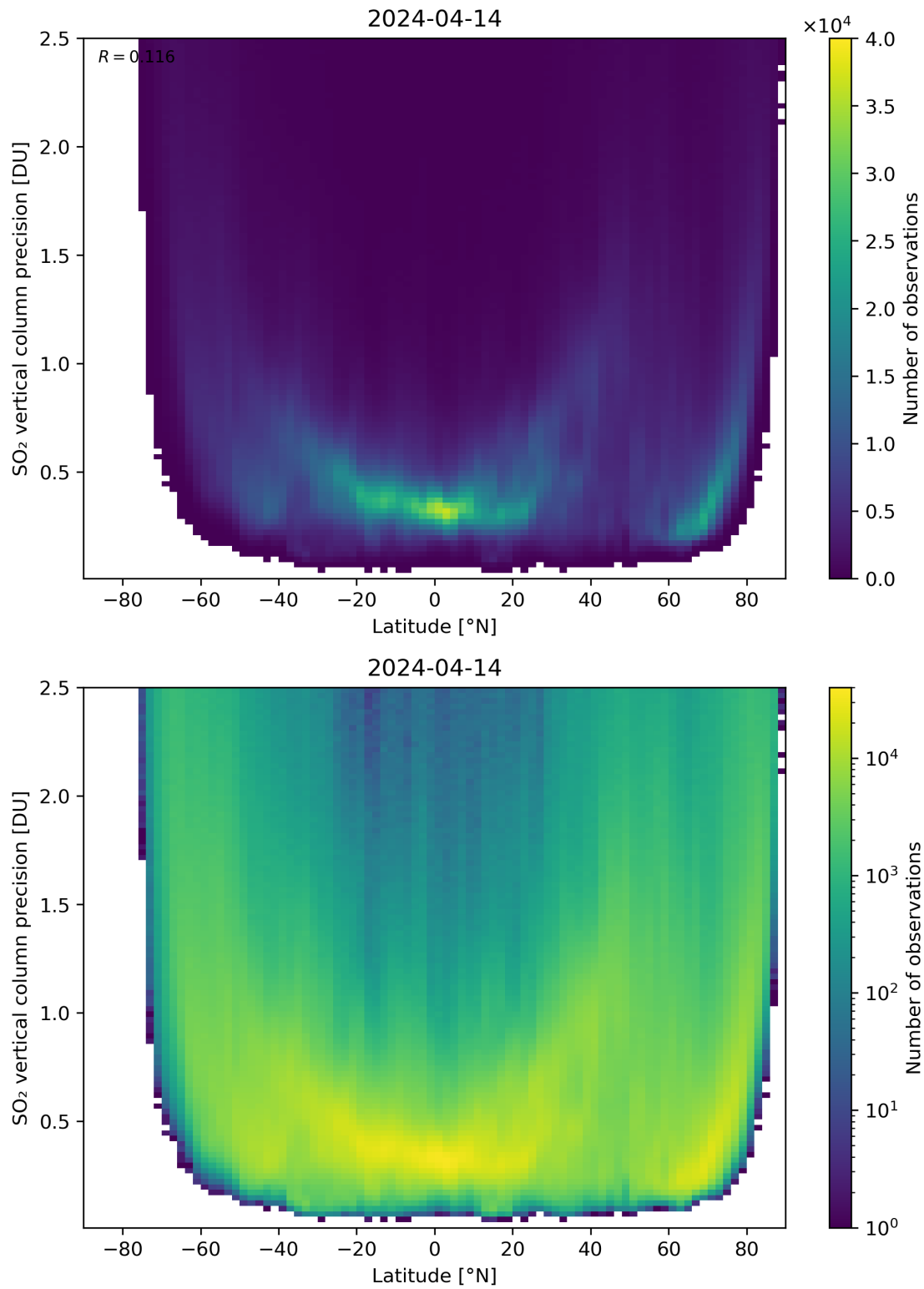
Figure 157: Scatter density plot of “Latitude” against “SO 2 vertical column precision” for 2024-04-13 to 2024-04-15.
