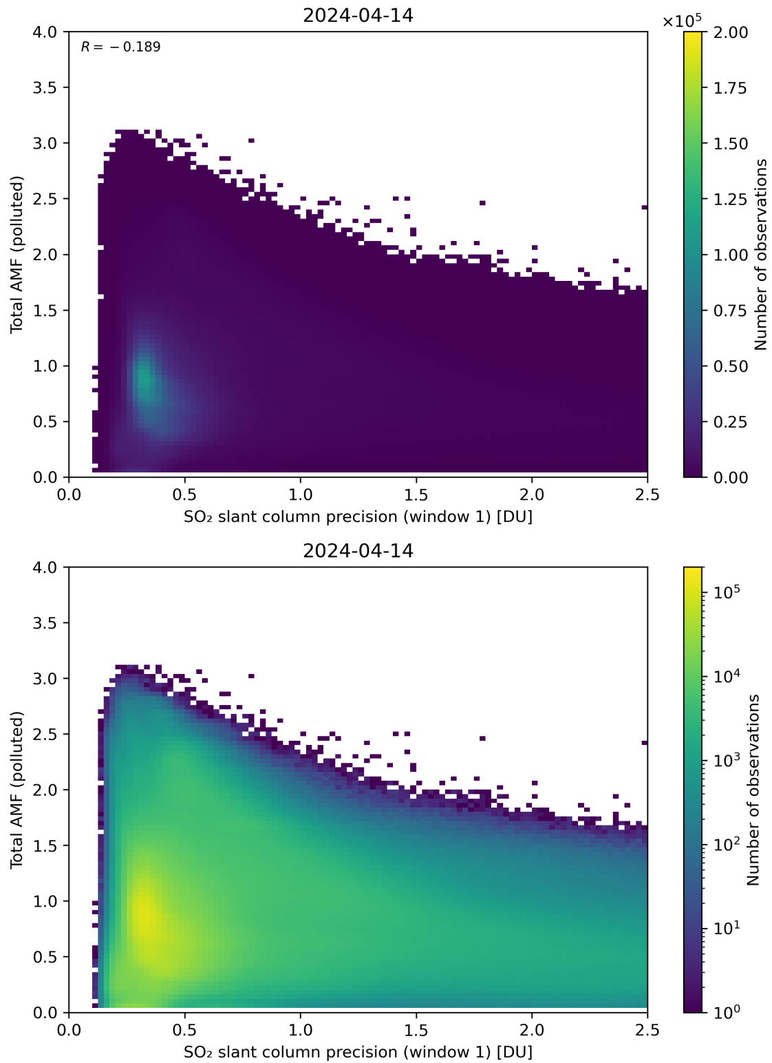
Figure 230: Scatter density plot of “SO 2 slant column precision (window 1)” against “Total AMF (polluted)” for 2024-04-13 to 2024-04-15.
