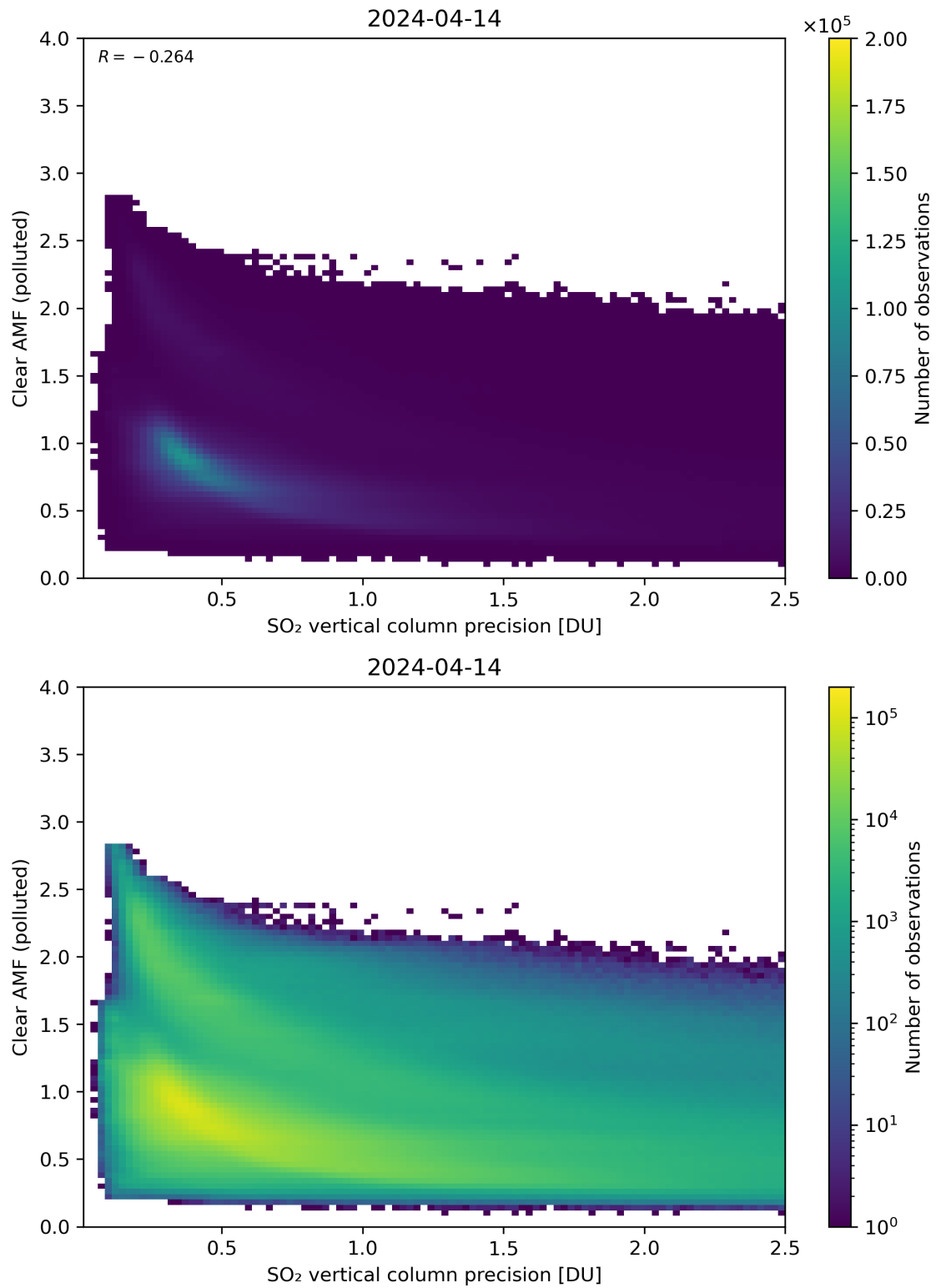
Figure 285: Scatter density plot of “SO 2 vertical column precision” against “Clear AMF (polluted)” for 2024-04-13 to 2024-04-15.
