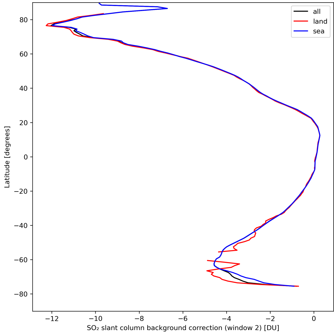
Figure 40: Zonal average of “SO 2 slant column background correction (window 2)” for 2024-04-13 to 2024-04-15.
