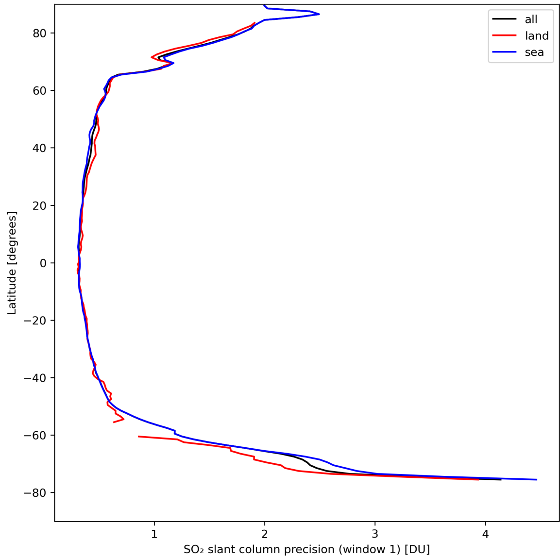
Figure 34: Zonal average of “SO 2 slant column precision (window 1)” for 2024-04-13 to 2024-04-15.
