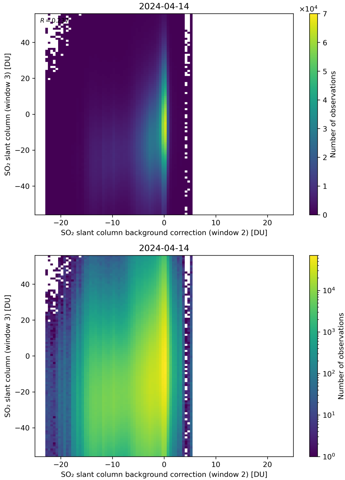
Figure 117: Scatter density plot of “SO 2 slant column background correction (window 2)” against “SO 2 slant column (window 3)” for 2024-04-13 to 2024-04-15.
