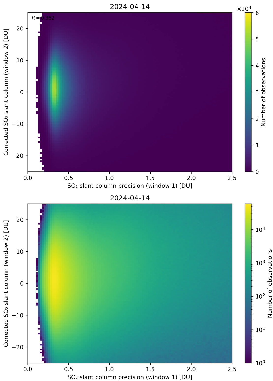
Figure 225: Scatter density plot of “SO 2 slant column precision (window 1)” against “Corrected SO 2 slant column (window 2)” for 2024-04-13 to 2024-04-15.
