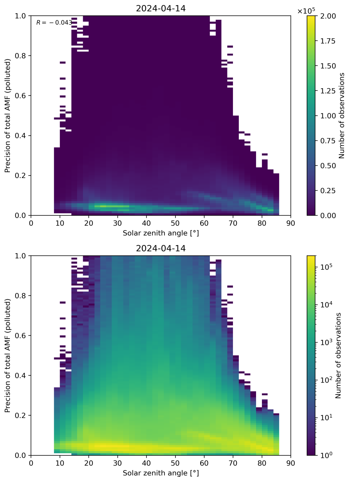
Figure 175: Scatter density plot of “Solar zenith angle” against “Precision of total AMF (polluted)” for 2024-04-13 to 2024-04-15.
