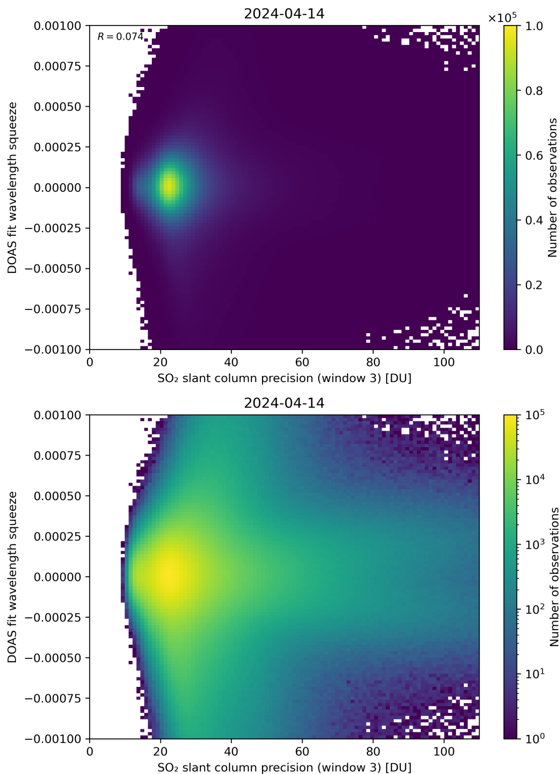
Figure 259: Scatter density plot of “SO 2 slant column precision (window 3)” against “DOAS fit wavelength squeeze” for 2024-04-13 to 2024-04-15.
