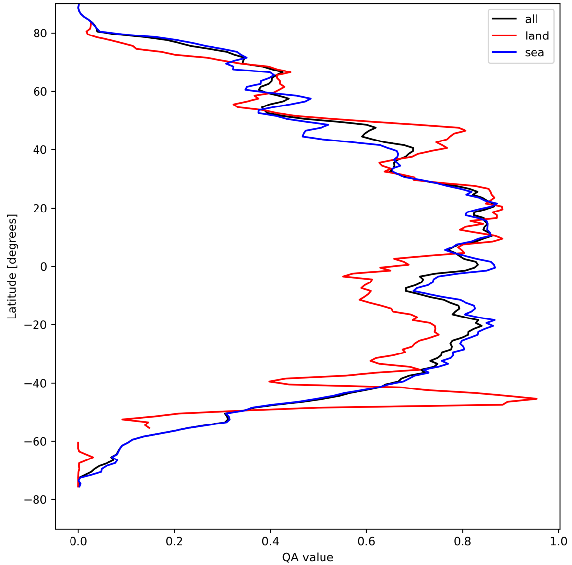
Figure 29: Zonal average of “QA value” for 2024-04-13 to 2024-04-15.
