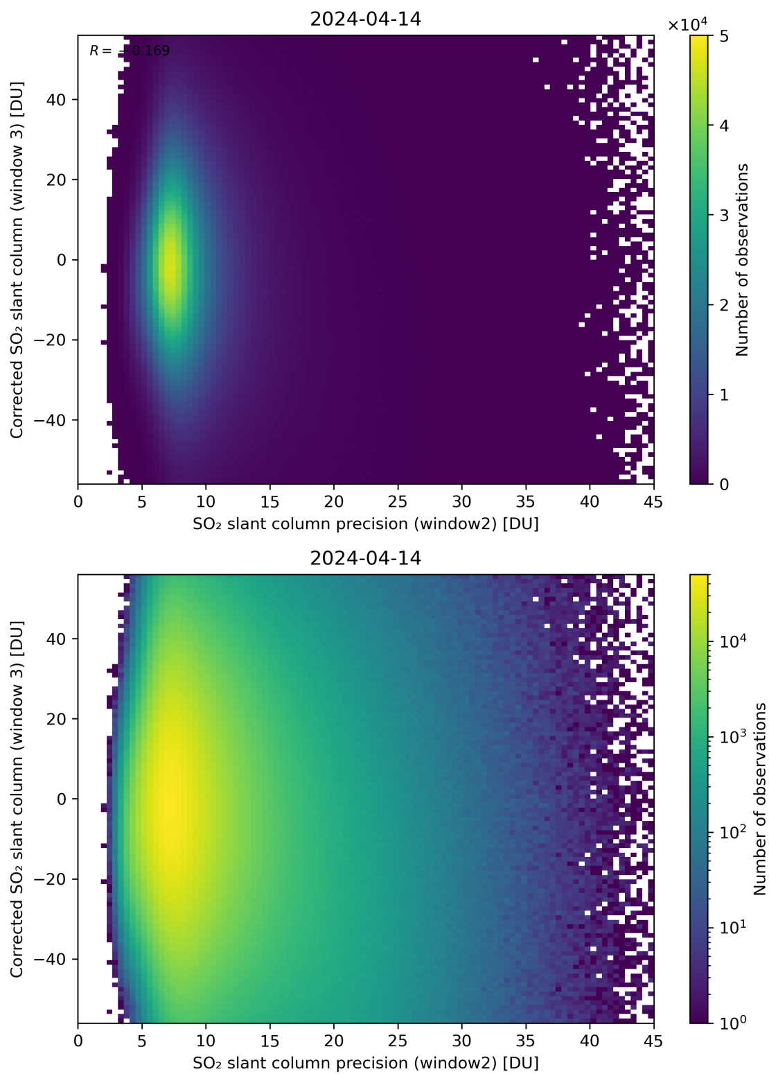
Figure 248: Scatter density plot of “SO 2 slant column precision (window2)” against “Corrected SO 2 slant column (window 3)” for 2024-04-13 to 2024-04-15.
