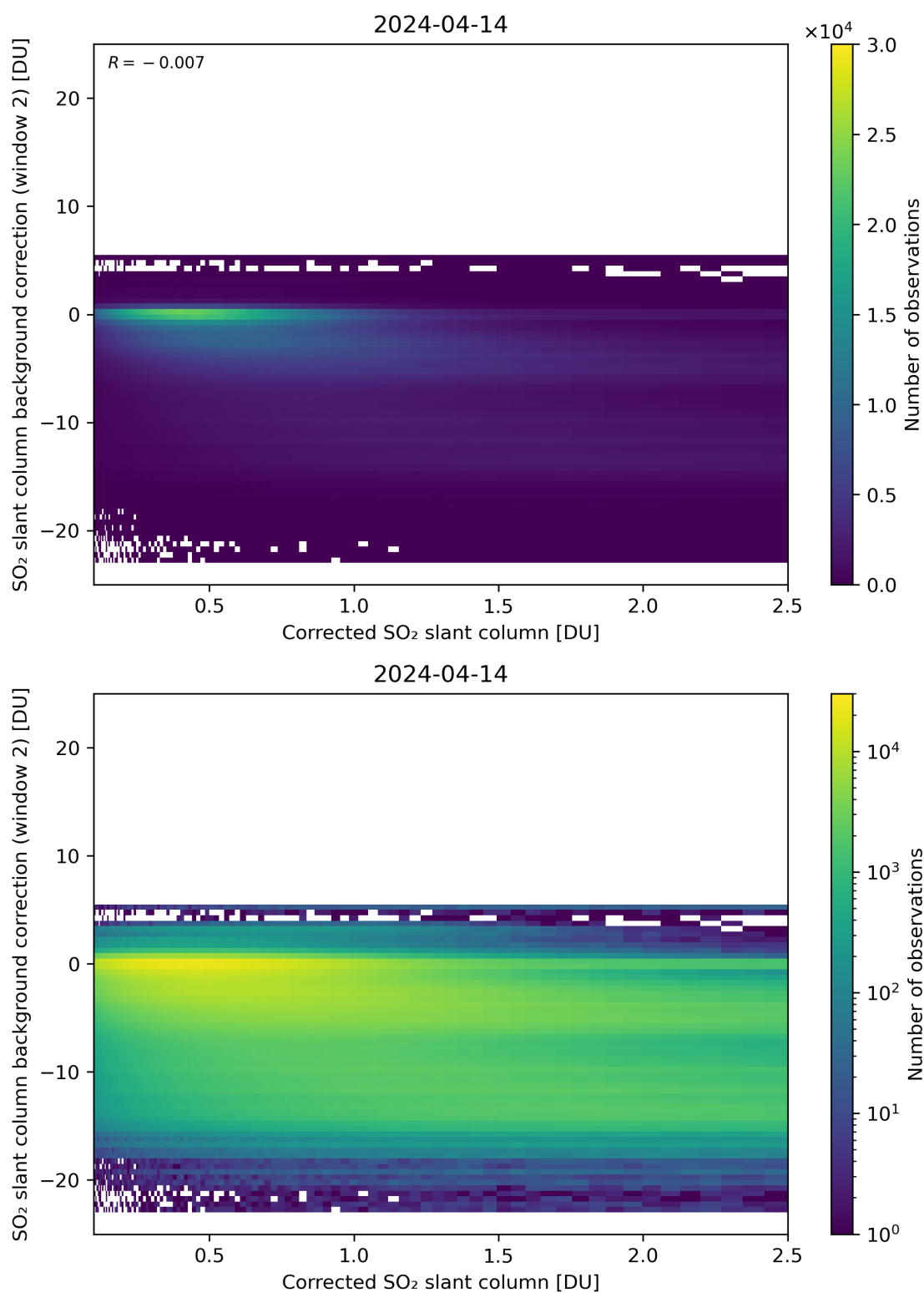
Figure 179: Scatter density plot of “Corrected SO 2 slant column” against “SO 2 slant column background correction (window 2)” for 2024-04-13 to 2024-04-15.
