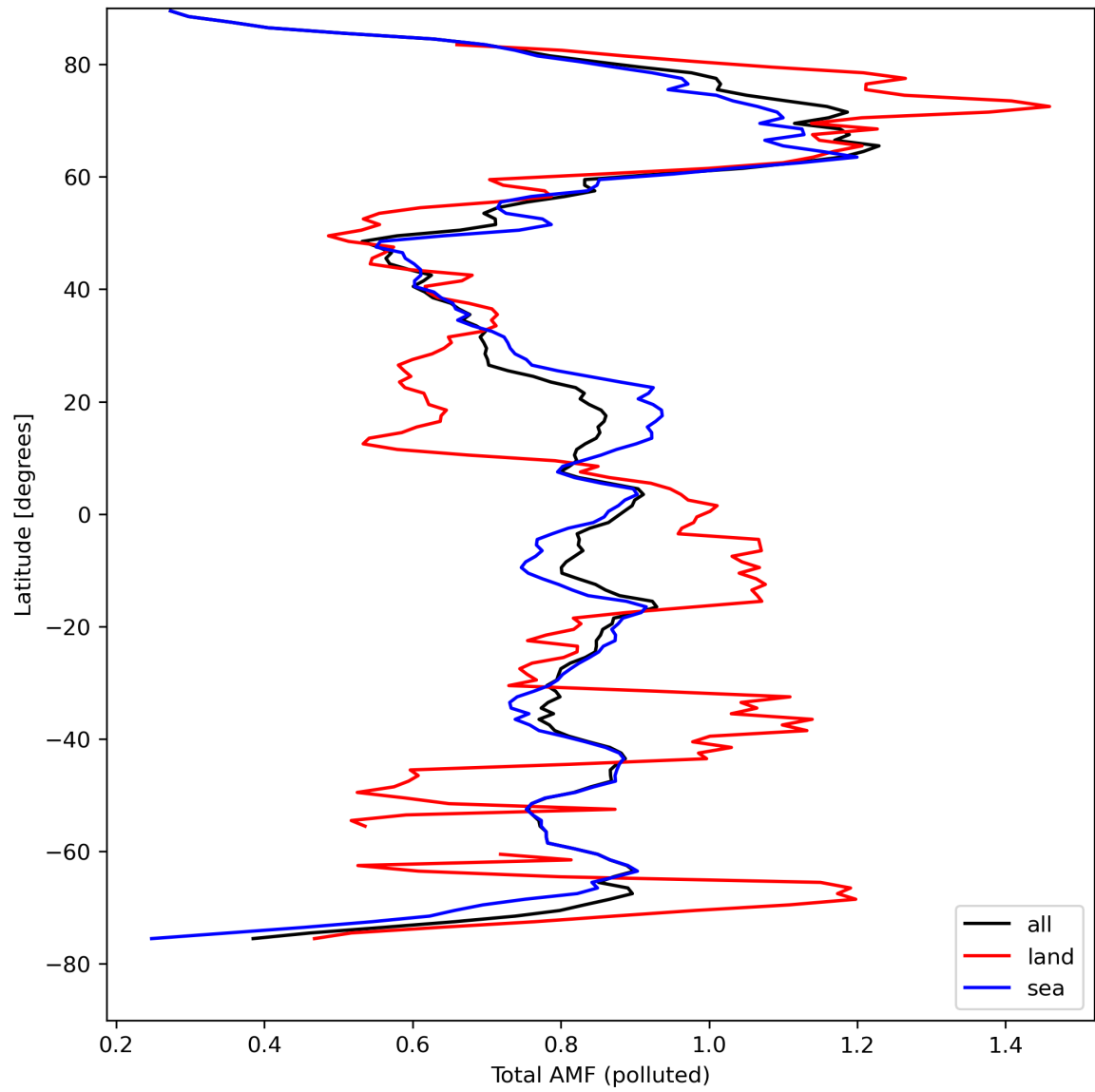
Figure 48: Zonal average of “Total AMF (polluted)” for 2024-04-13 to 2024-04-15.
