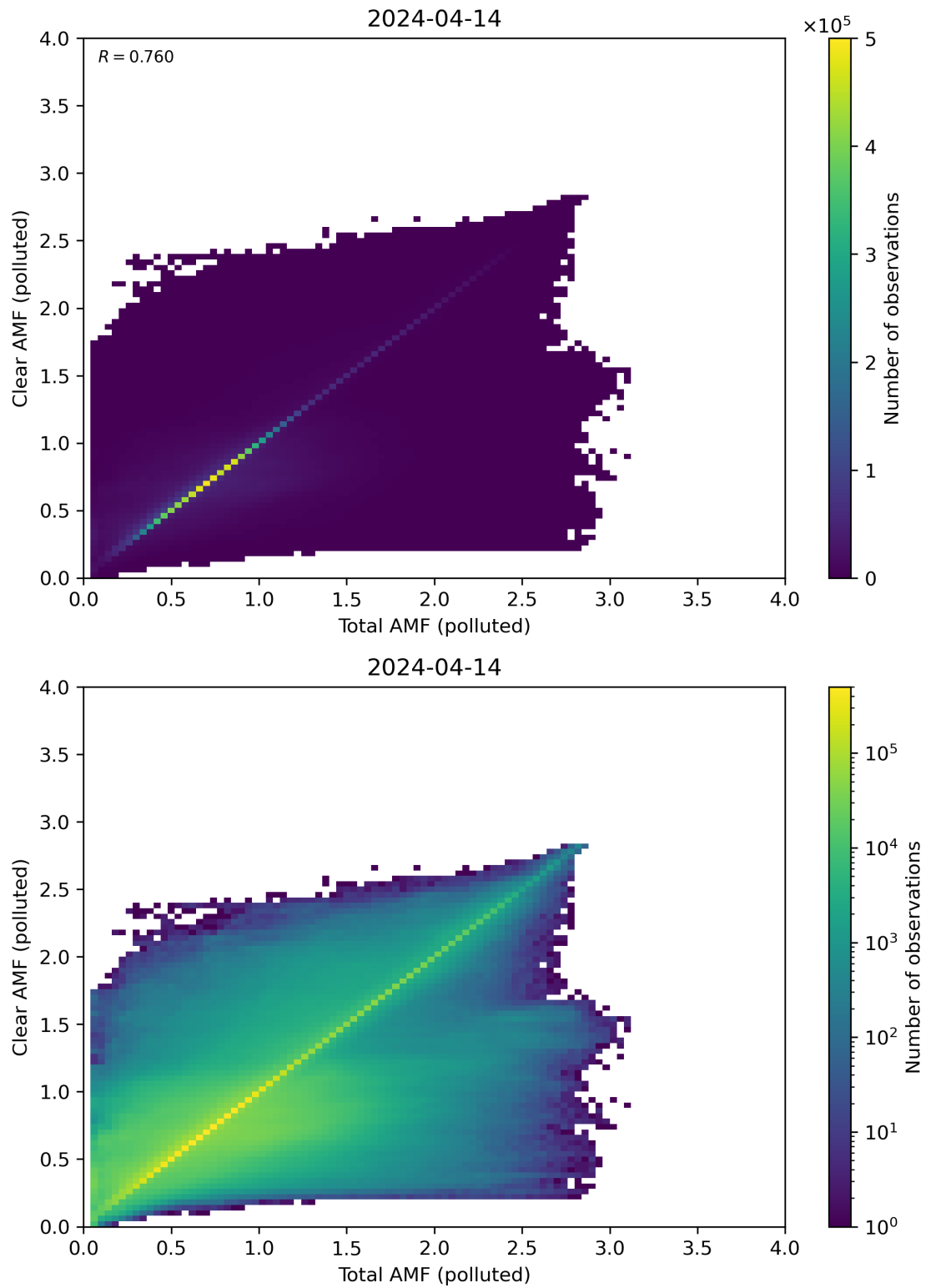
Figure 271: Scatter density plot of “Total AMF (polluted)” against “Clear AMF (polluted)” for 2024-04-13 to 2024-04-15.
