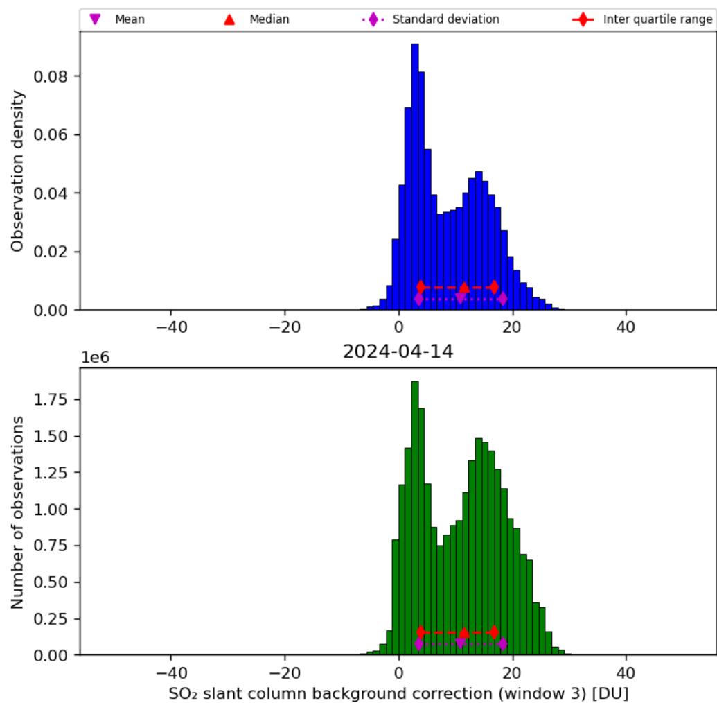
Figure 67: Histogram of “SO 2 slant column background correction (window 3)” for 2024-04-13 to 2024-04-15
