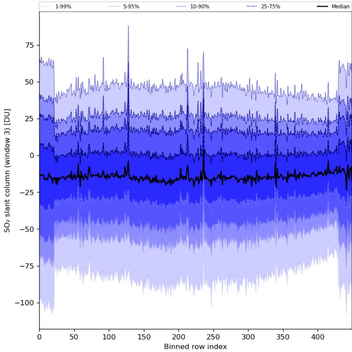
Figure 87: Along track statistics of “SO 2 slant column (window 3)” for 2024-04-13 to 2024-04-15
