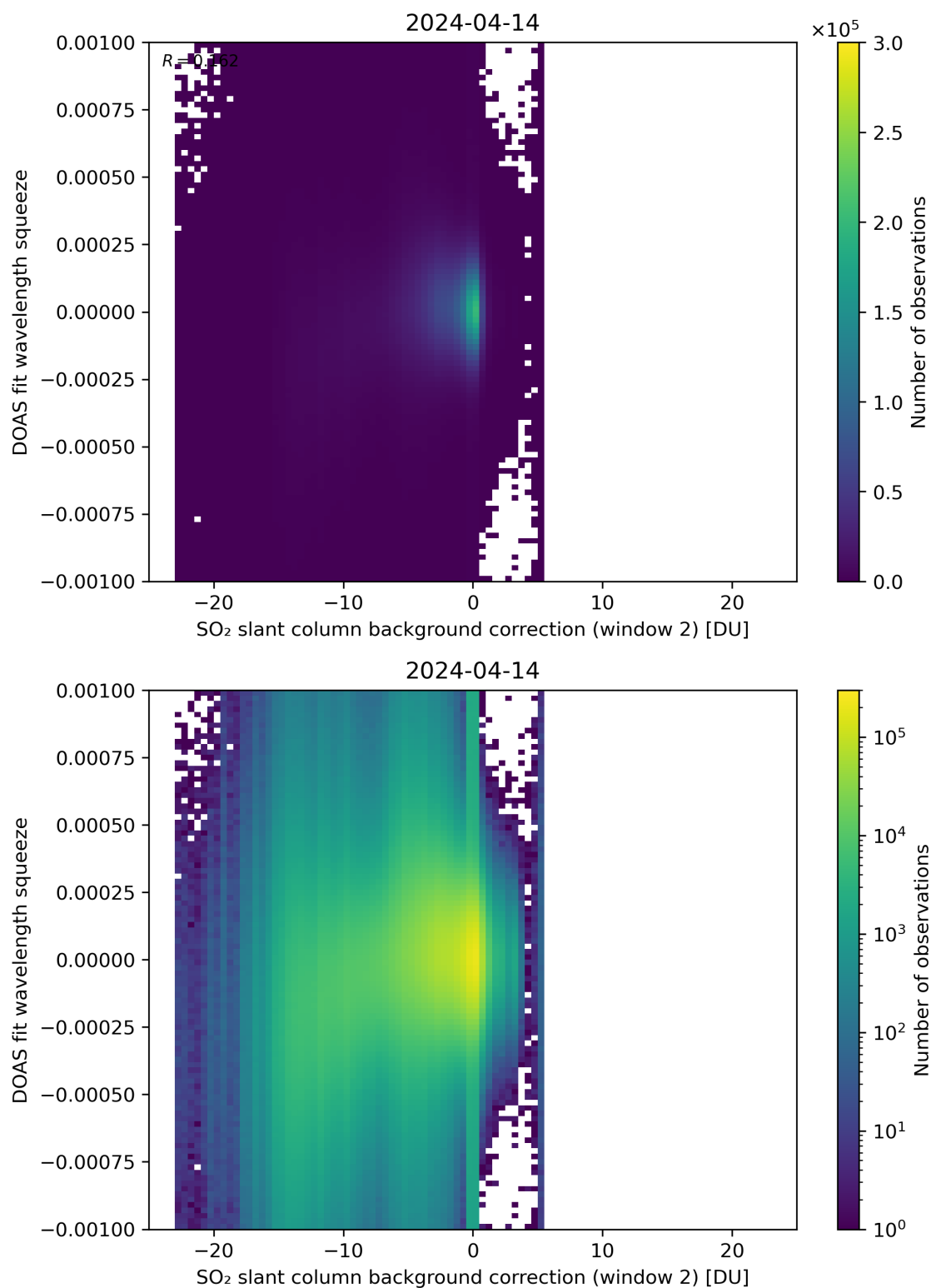
Figure 113: Scatter density plot of “SO 2 slant column background correction (window 2)” against “DOAS fit wavelength squeeze” for 2024-04-13 to 2024-04-15.
