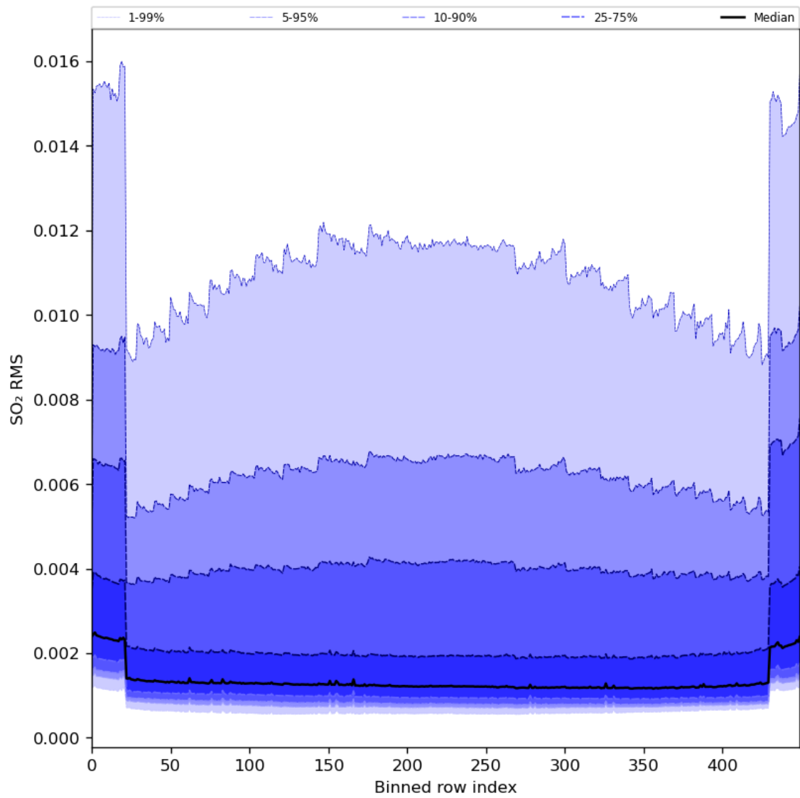
Figure 93: Along track statistics of “SO 2 RMS” for 2024-04-13 to 2024-04-15
