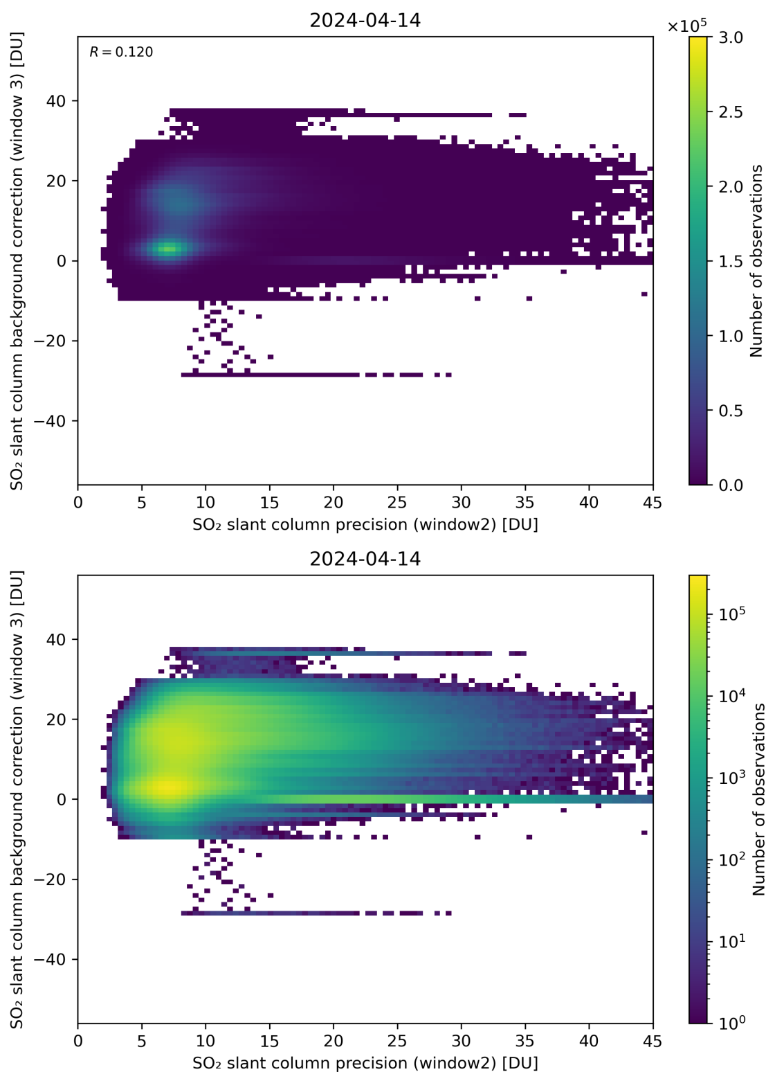
Figure 242: Scatter density plot of “SO 2 slant column precision (window2)” against “SO 2 slant column background correction (window 3)” for 2024-04-13 to 2024-04-15.
