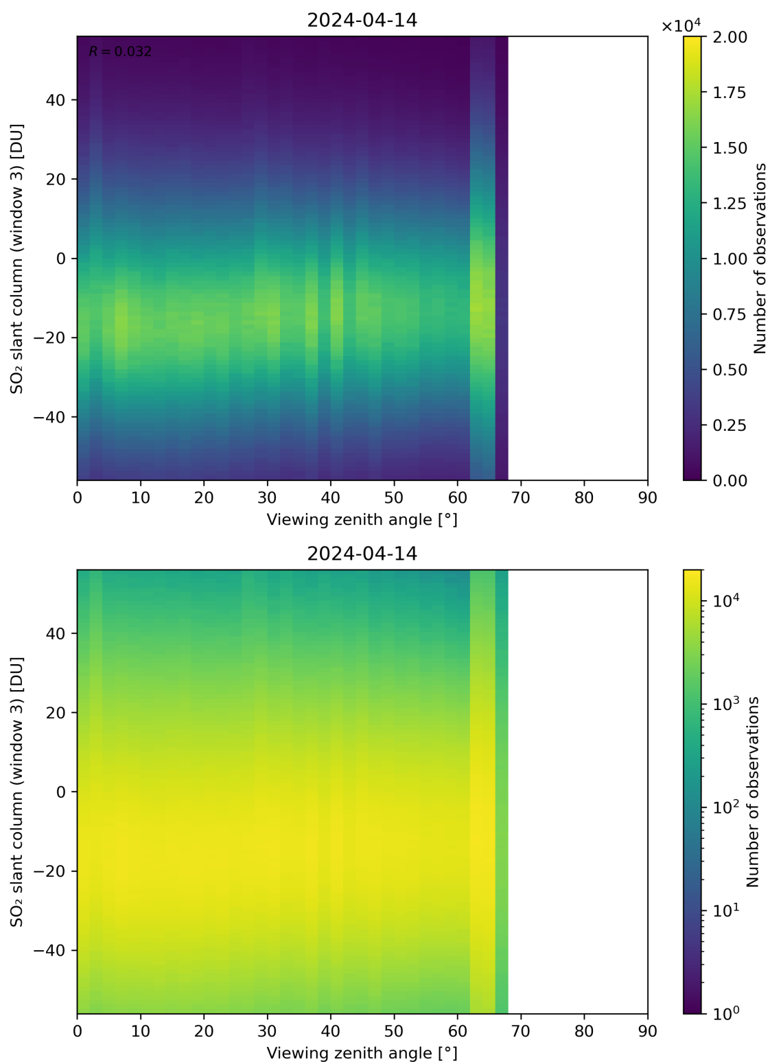
Figure 323: Scatter density plot of “Viewing zenith angle” against “SO 2 slant column (window 3)” for 2024-04-13 to 2024-04-15.
