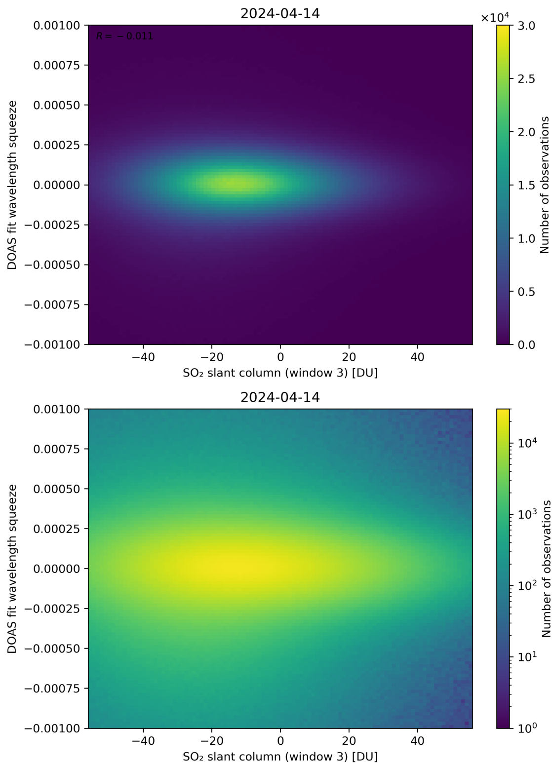
Figure 255: Scatter density plot of “SO 2 slant column (window 3)” against “DOAS fit wavelength squeeze” for 2024-04-13 to 2024-04-15.
