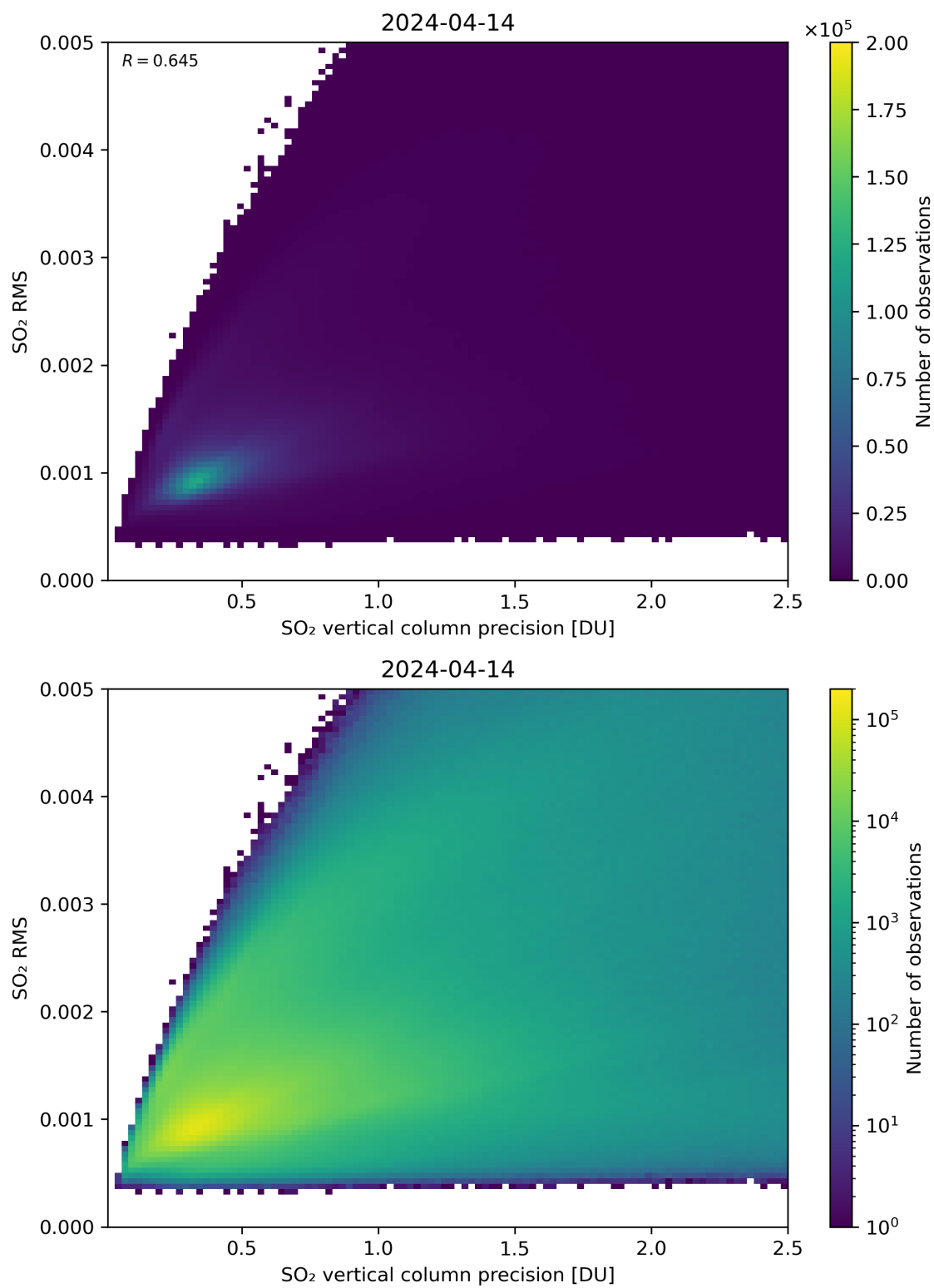
Figure 284: Scatter density plot of “SO 2 vertical column precision” against “SO 2 RMS” for 2024-04-13 to 2024-04-15.
