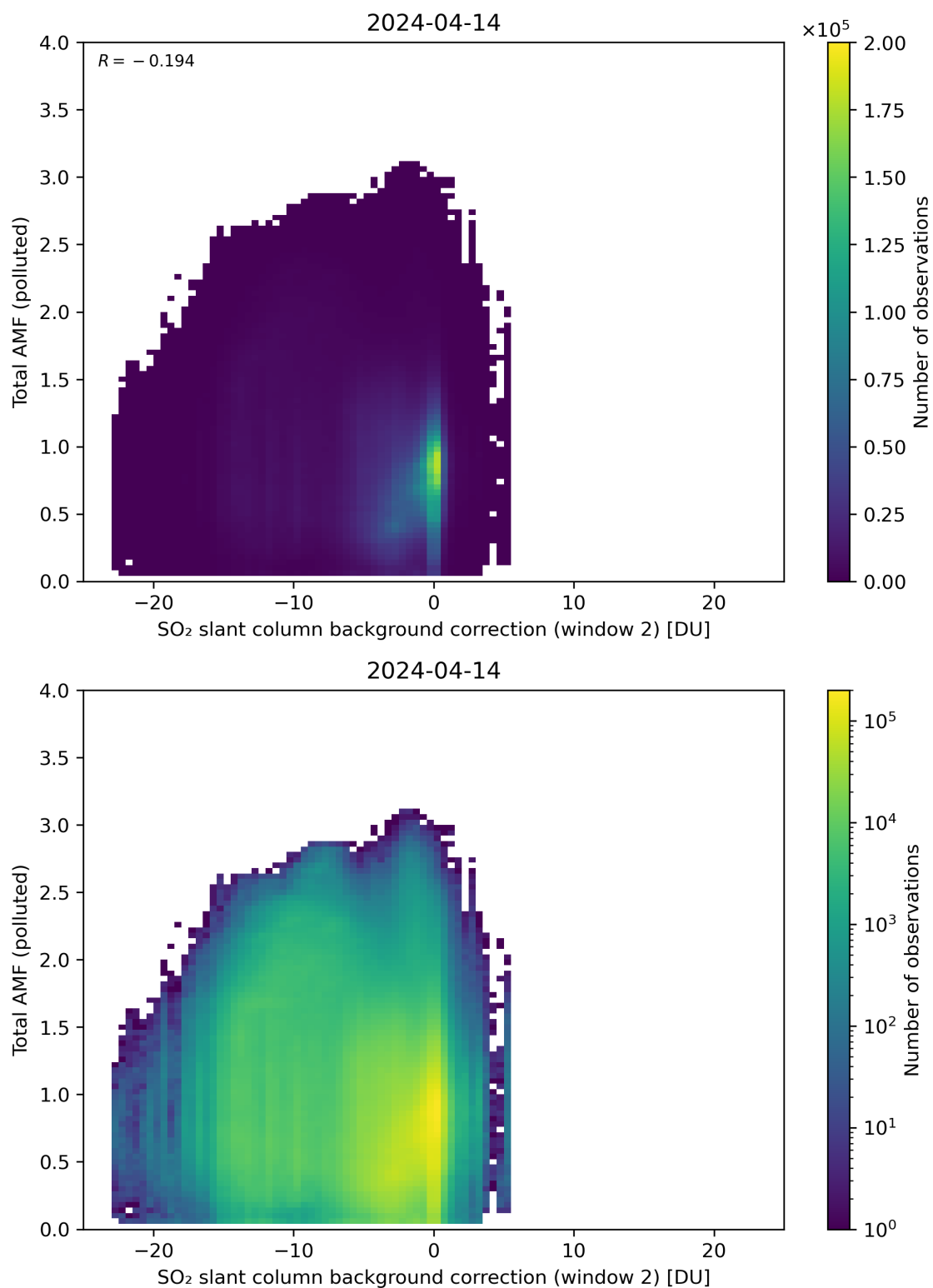
Figure 119: Scatter density plot of “SO 2 slant column background correction (window 2)” against “Total AMF (polluted)” for 2024-04-13 to 2024-04-15.
