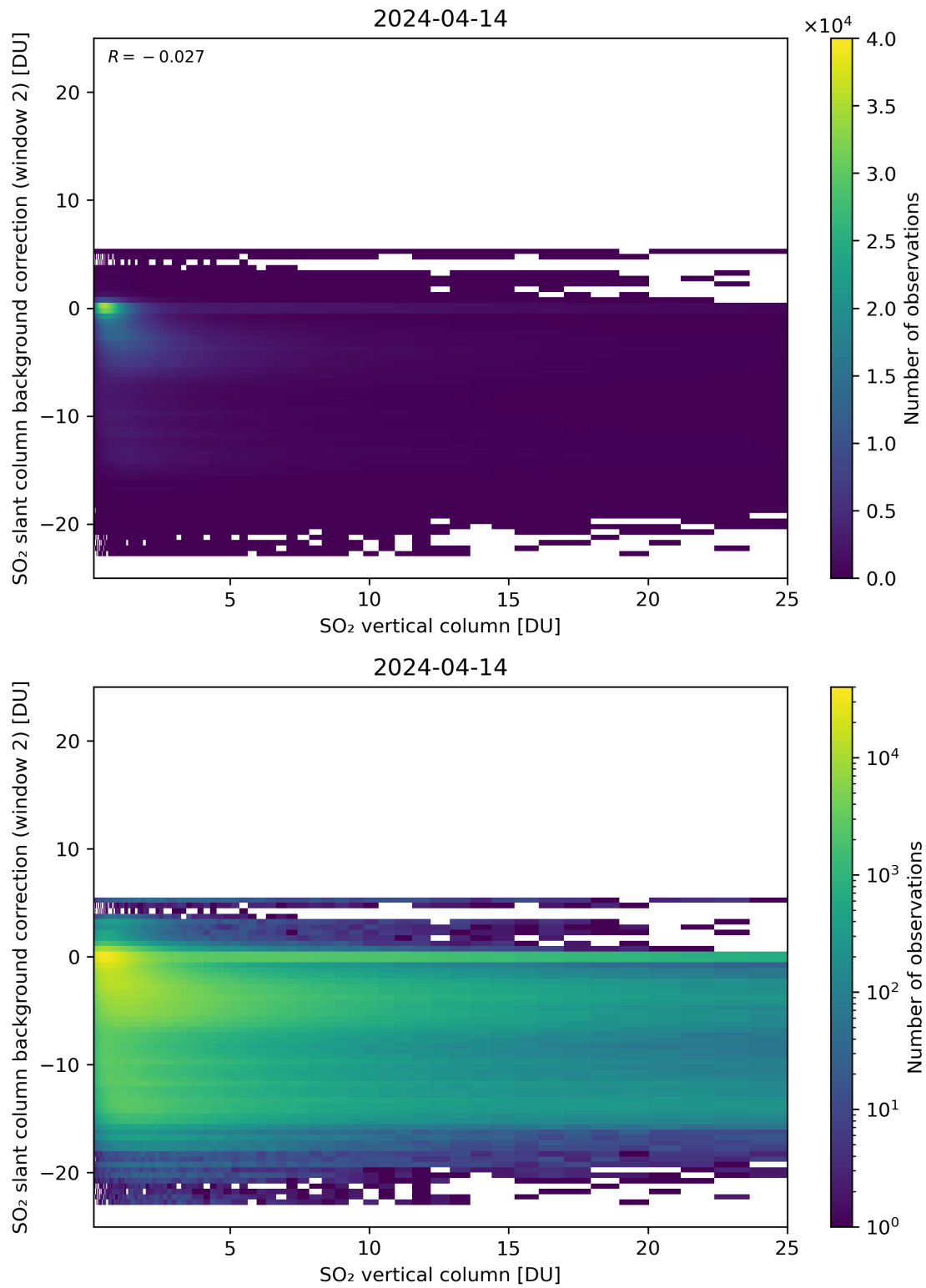
Figure 274: Scatter density plot of “SO 2 vertical column” against “SO 2 slant column background correction (window 2)” for 2024-04-13 to 2024-04-15.
