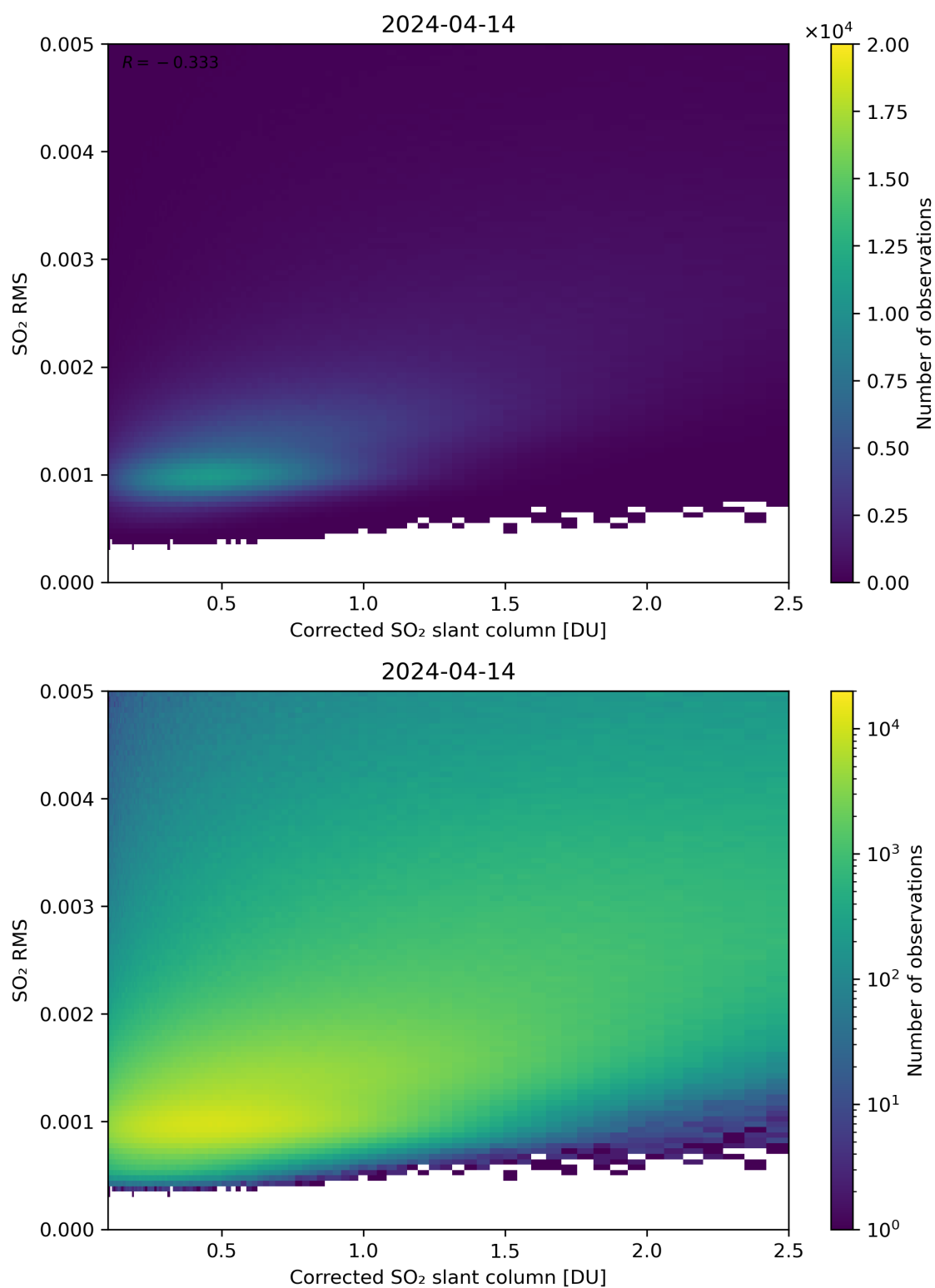
Figure 183: Scatter density plot of “Corrected SO 2 slant column” against “SO 2 RMS” for 2024-04-13 to 2024-04-15.
