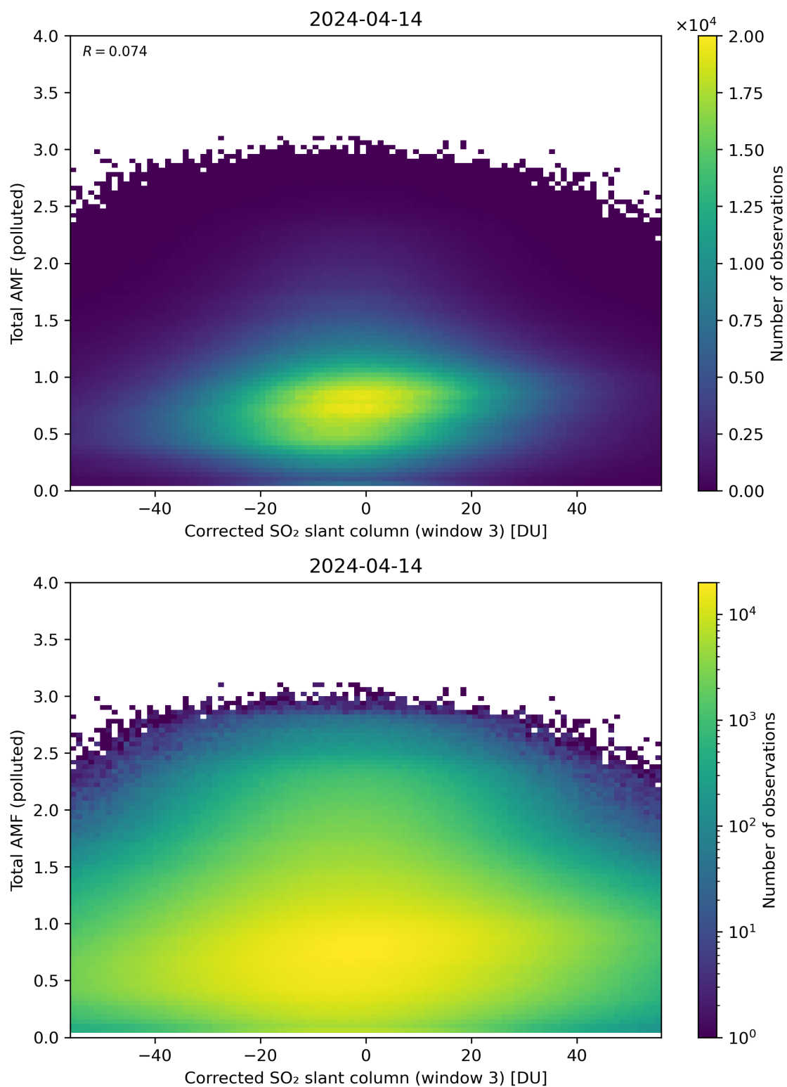
Figure 210: Scatter density plot of “Corrected SO 2 slant column (window 3)” against “Total AMF (polluted)” for 2024-04-13 to 2024-04-15.
