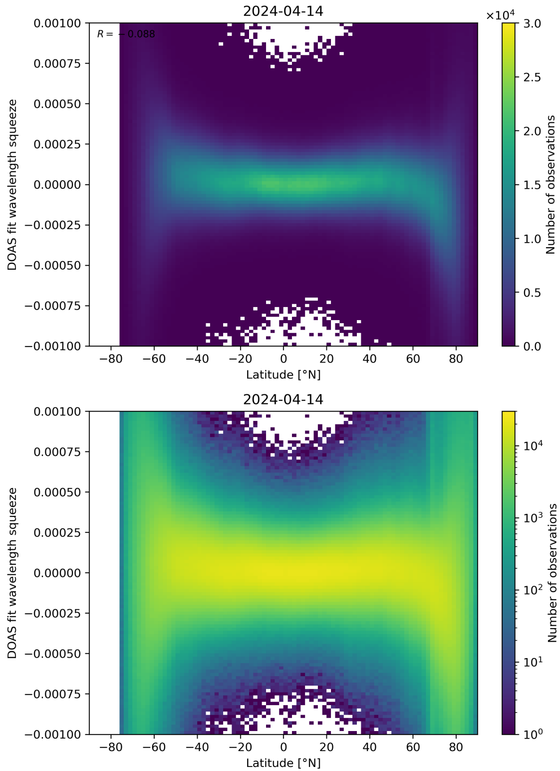
Figure 143: Scatter density plot of “Latitude” against “DOAS fit wavelength squeeze” for 2024-04-13 to 2024-04-15.
