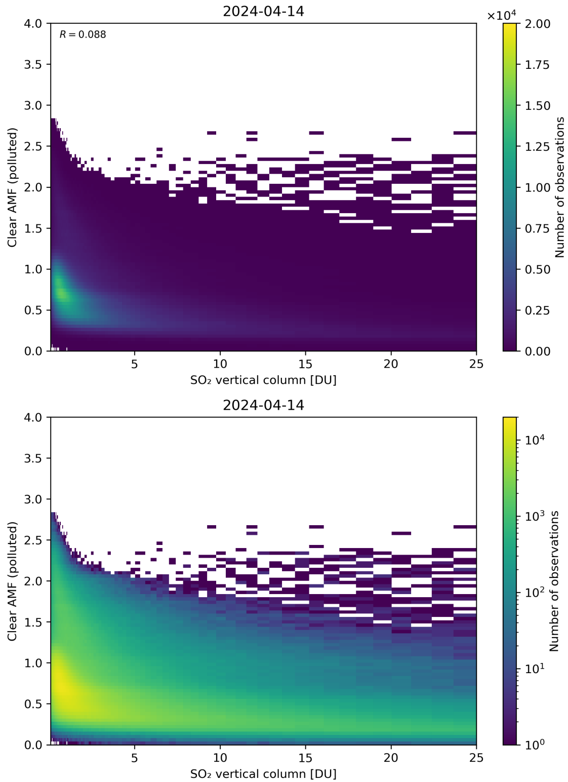
Figure 296: Scatter density plot of “SO 2 vertical column” against “Clear AMF (polluted)” for 2024-04-13 to 2024-04-15.
