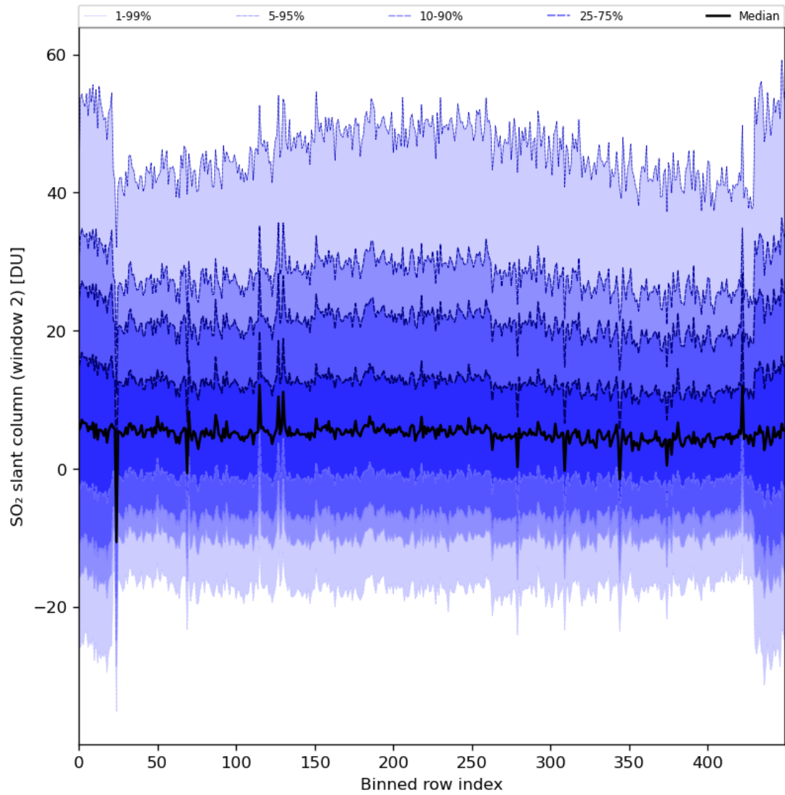
Figure 83: Along track statistics of “SO 2 slant column (window 2)” for 2024-04-13 to 2024-04-15
