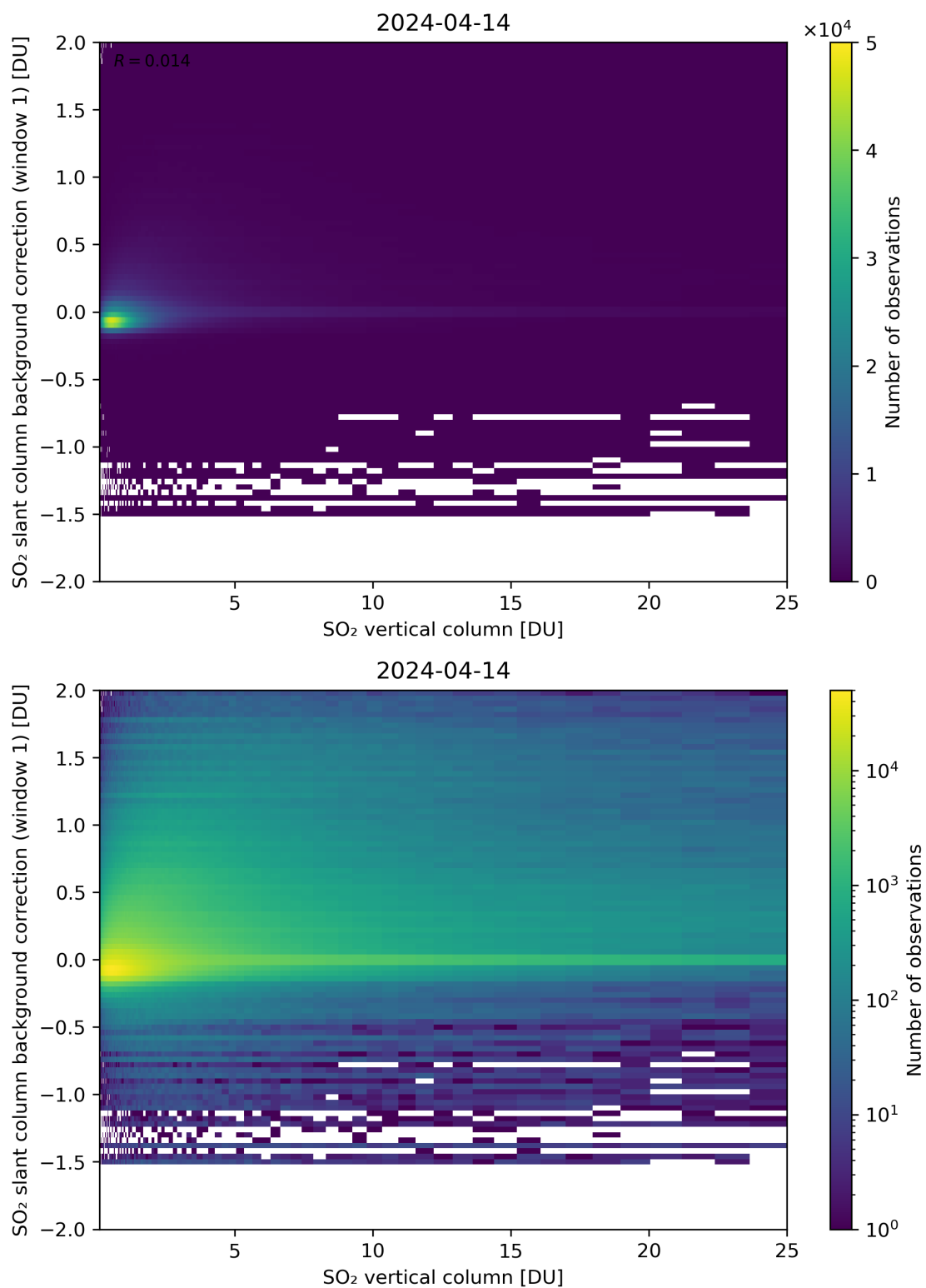
Figure 273: Scatter density plot of “SO 2 vertical column” against “SO 2 slant column background correction (window 1)” for 2024-04-13 to 2024-04-15.
