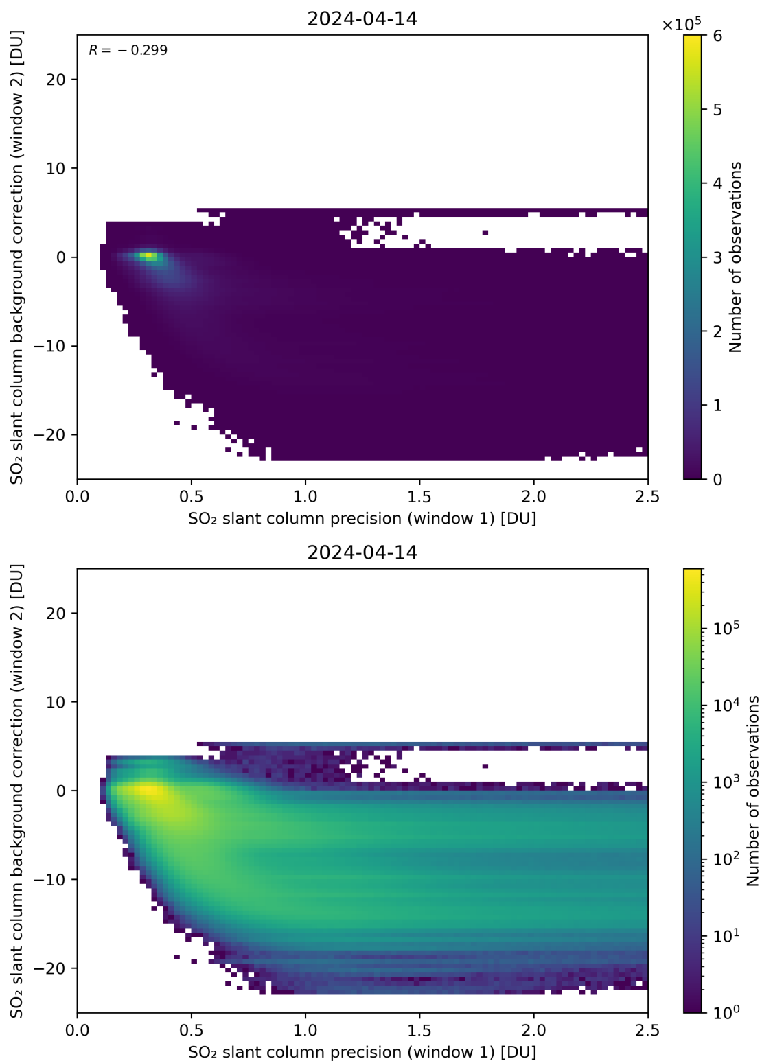
Figure 219: Scatter density plot of “SO 2 slant column precision (window 1)” against “SO 2 slant column background correction (window 2)” for 2024-04-13 to 2024-04-15.
