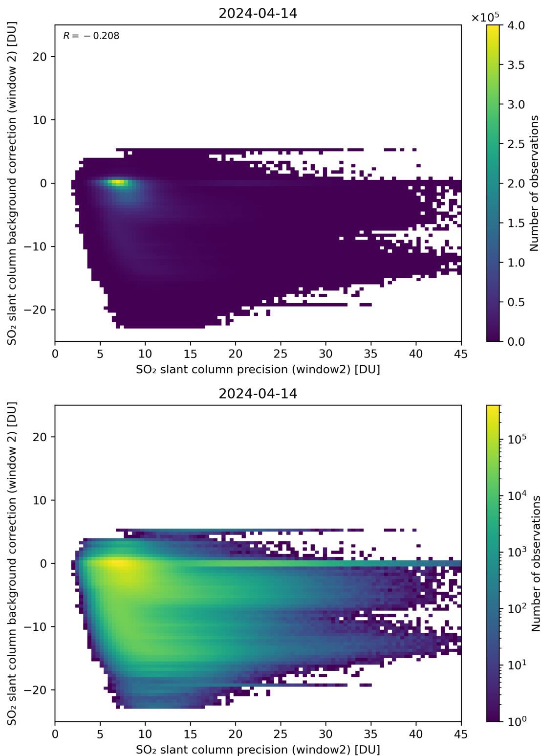
Figure 241: Scatter density plot of “SO 2 slant column precision (window2)” against “SO 2 slant column background correction (window 2)” for 2024-04-13 to 2024-04-15.
