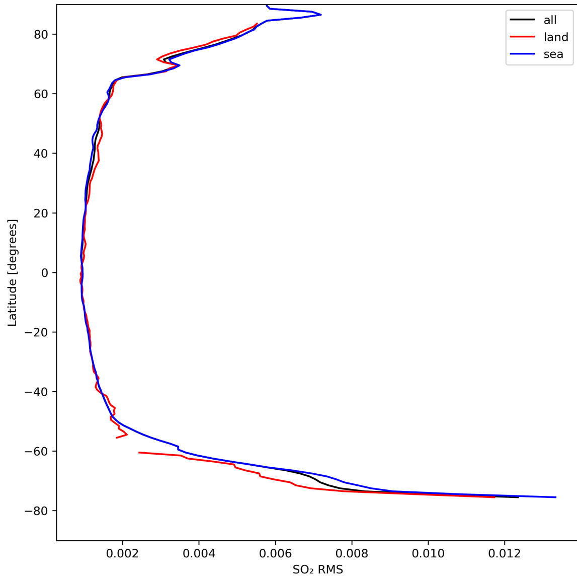
Figure 47: Zonal average of “SO 2 RMS” for 2024-04-13 to 2024-04-15.
