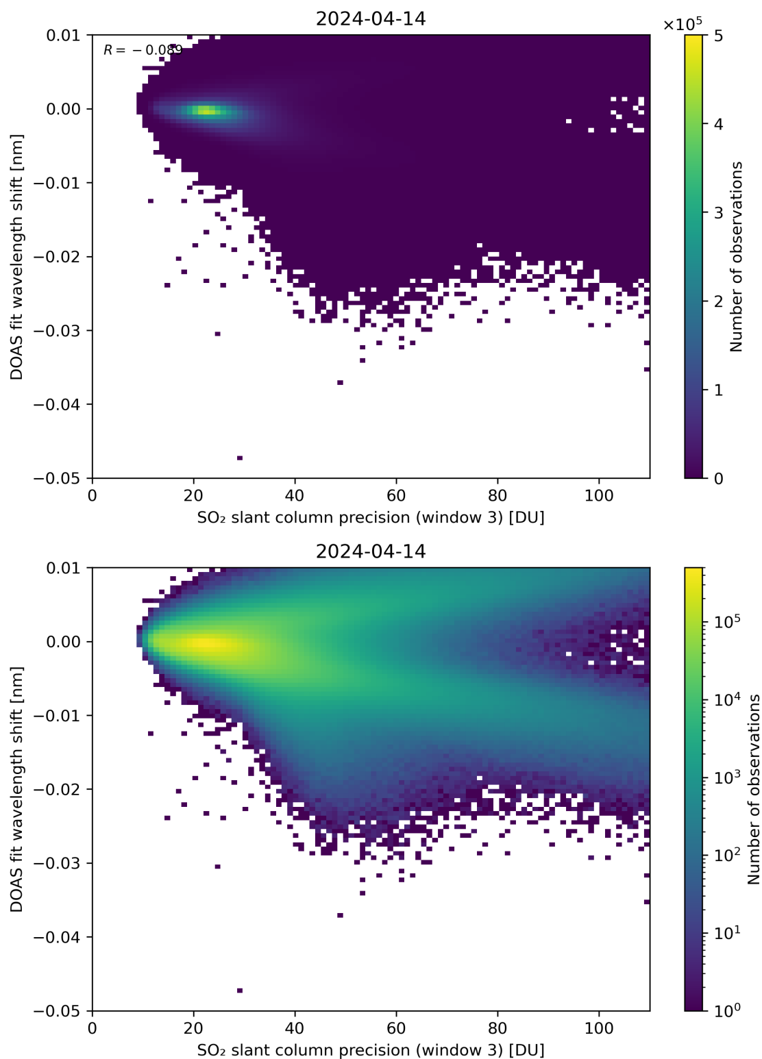
Figure 258: Scatter density plot of “SO 2 slant column precision (window 3)” against “DOAS fit wavelength shift” for 2024-04-13 to 2024-04-15.
