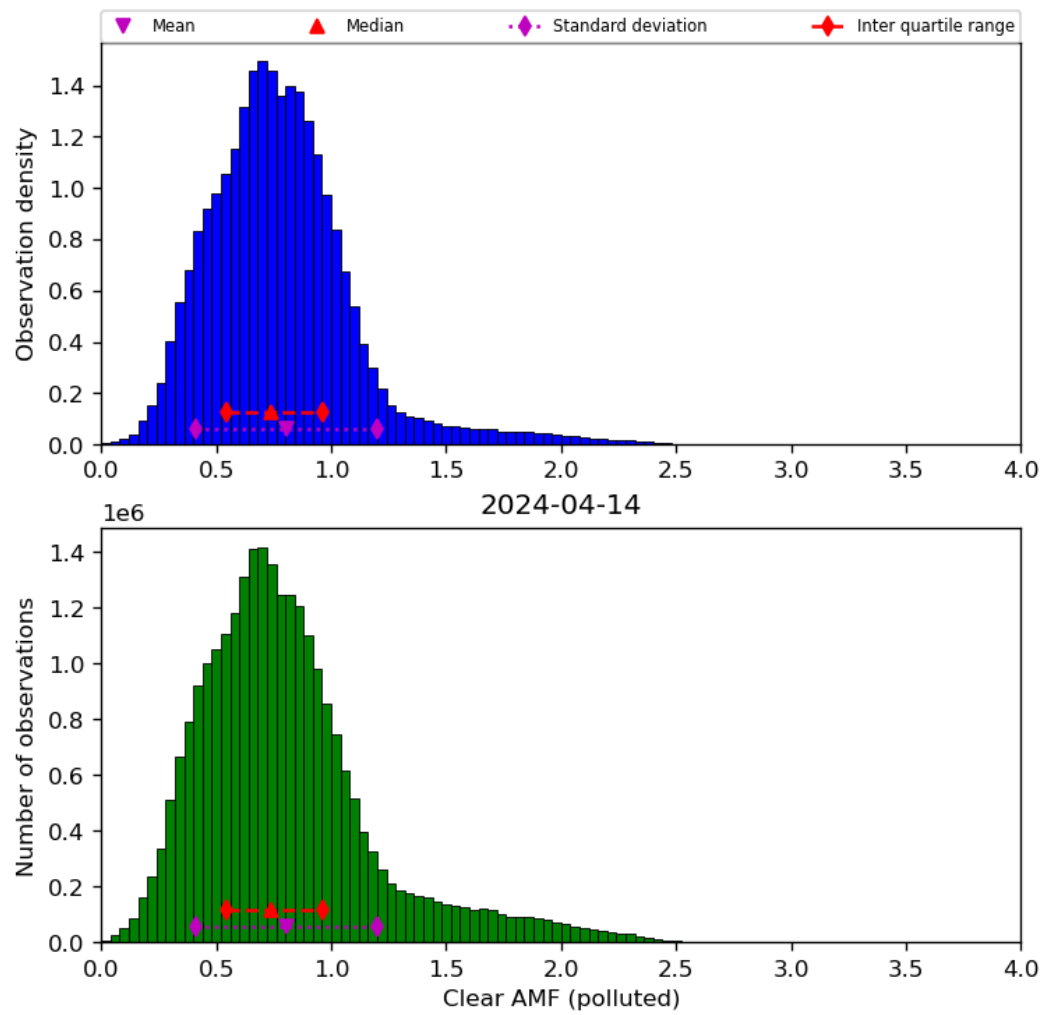
Figure 73: Histogram of “Clear AMF (polluted)” for 2024-04-13 to 2024-04-15
