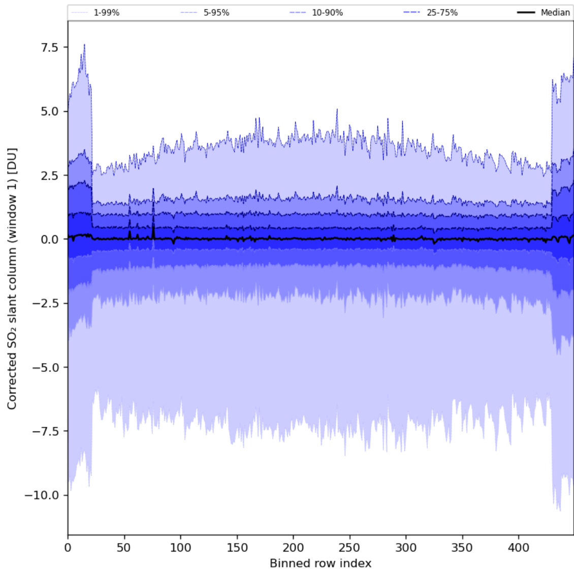
Figure 81: Along track statistics of “Corrected SO 2 slant column (window 1)” for 2024-04-13 to 2024-04-15
