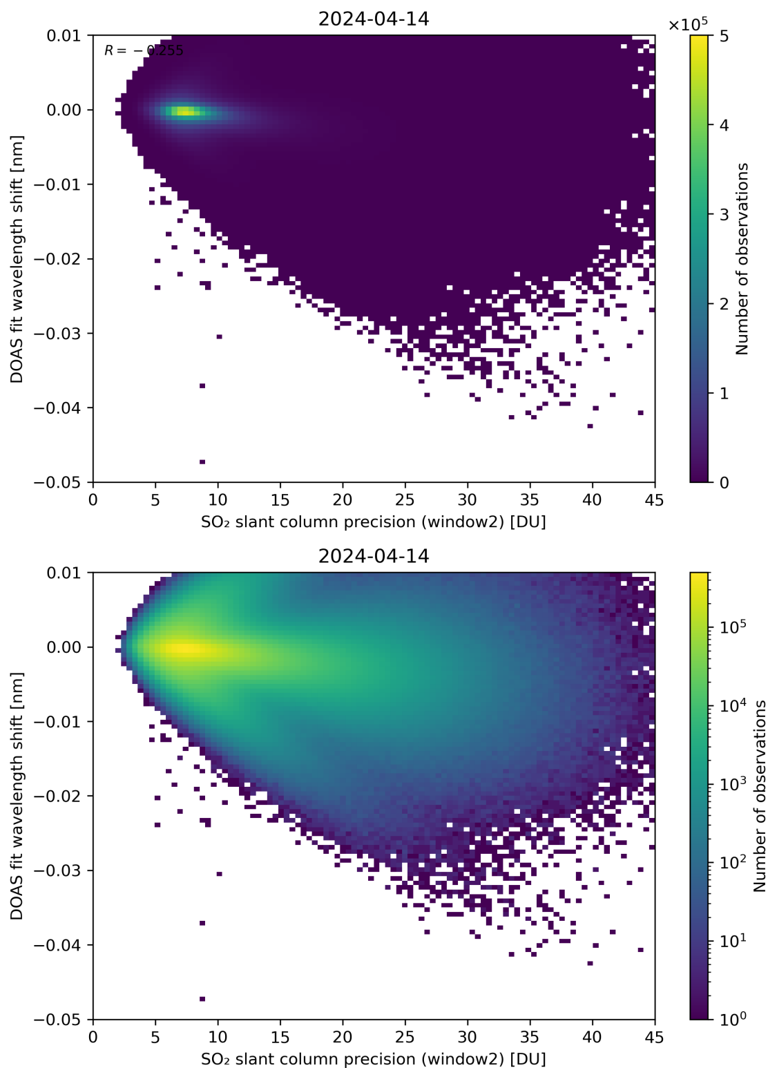
Figure 243: Scatter density plot of “SO 2 slant column precision (window2)” against “DOAS fit wavelength shift” for 2024-04-13 to 2024-04-15.
