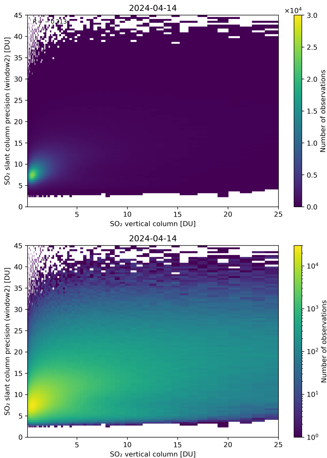
Figure 302: Scatter density plot of “SO 2 vertical column” against “SO 2 slant column precision (window2)” for 2024-04-13 to 2024-04-15.
