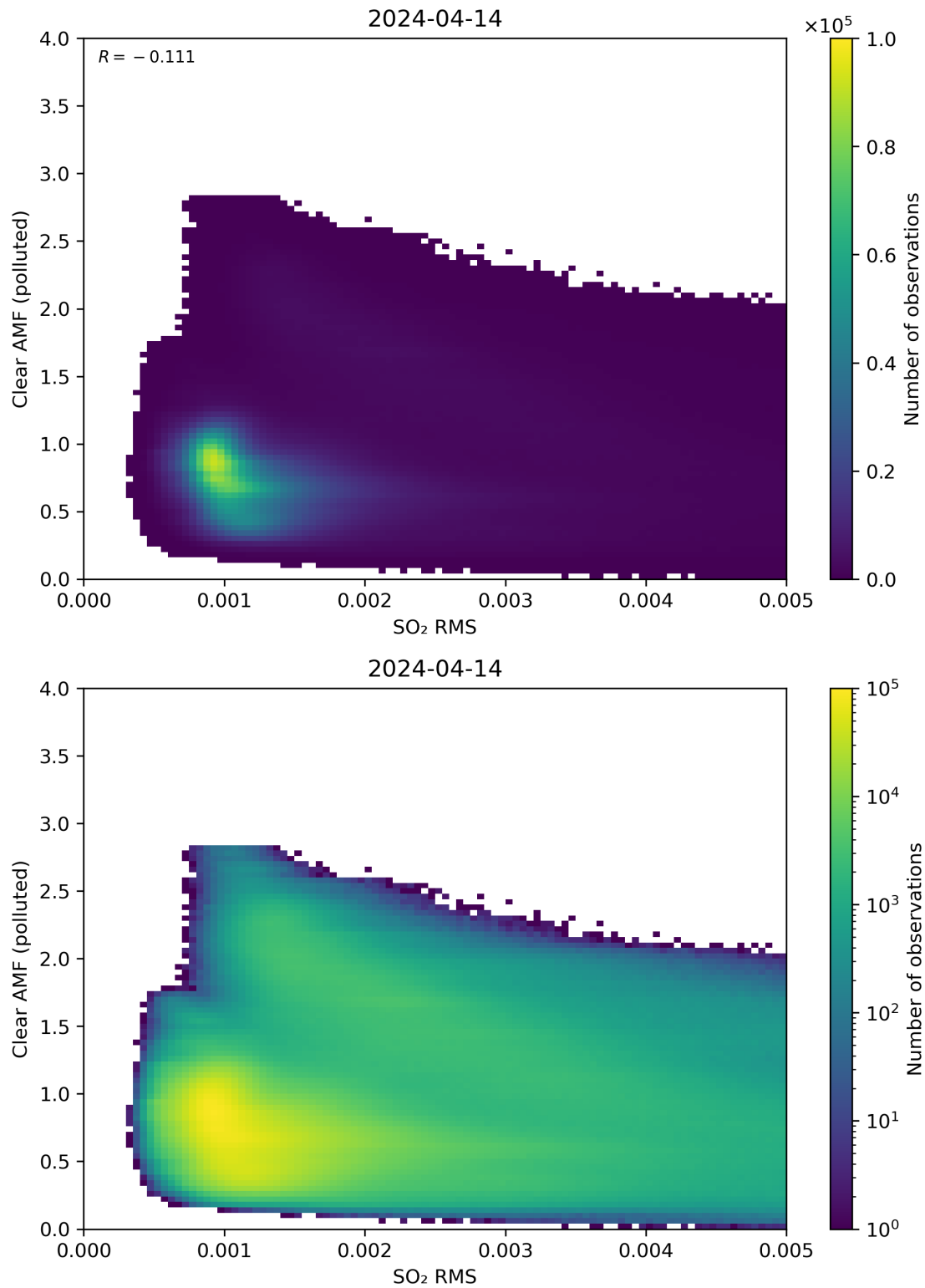
Figure 136: Scatter density plot of “SO 2 RMS” against “Clear AMF (polluted)” for 2024-04-13 to 2024-04-15.
