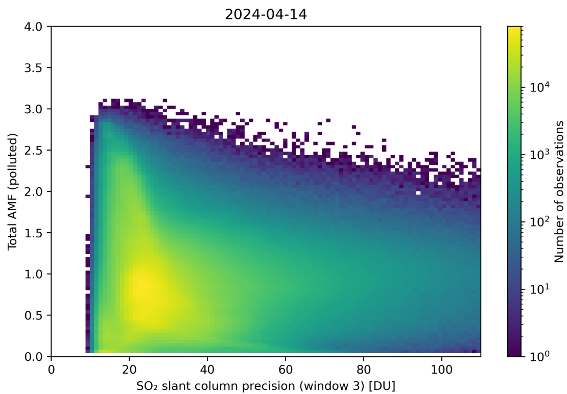
Figure 263: Scatter density plot of “SO 2 slant column precision (window 3)” against “Total AMF (polluted)” for 2024-04-13 to 2024-04-15.
