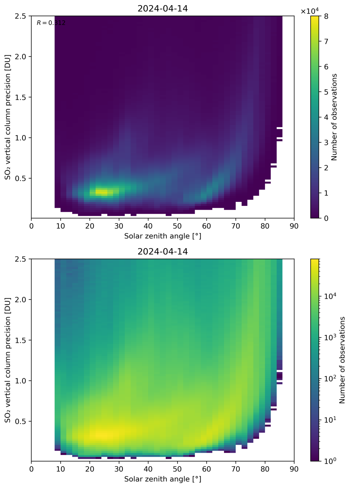
Figure 177: Scatter density plot of “Solar zenith angle” against “SO 2 vertical column precision” for 2024-04-13 to 2024-04-15.
