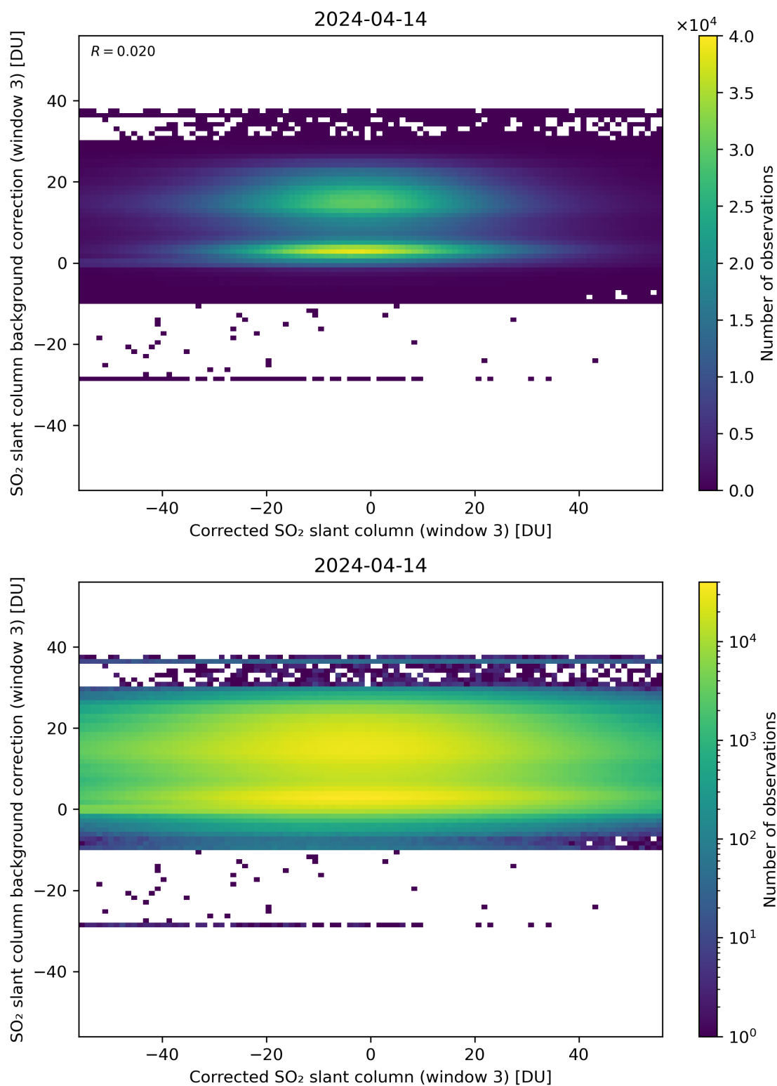
Figure 205: Scatter density plot of “Corrected SO 2 slant column (window 3)” against “SO 2 slant column background correction (window 3)” for 2024-04-13 to 2024-04-15.
