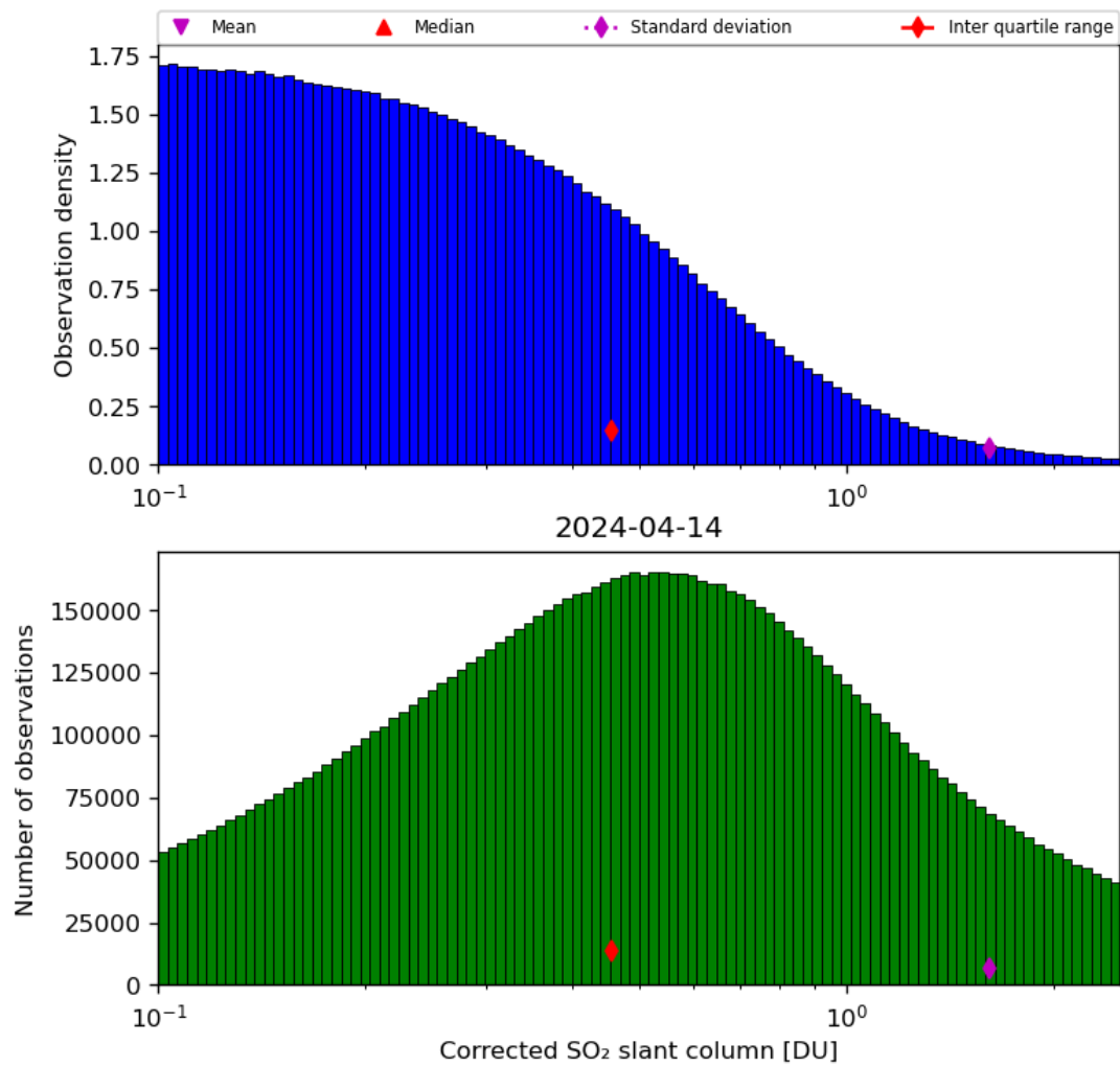
Figure 55: Histogram of “Corrected SO 2 slant column” for 2024-04-13 to 2024-04-15
