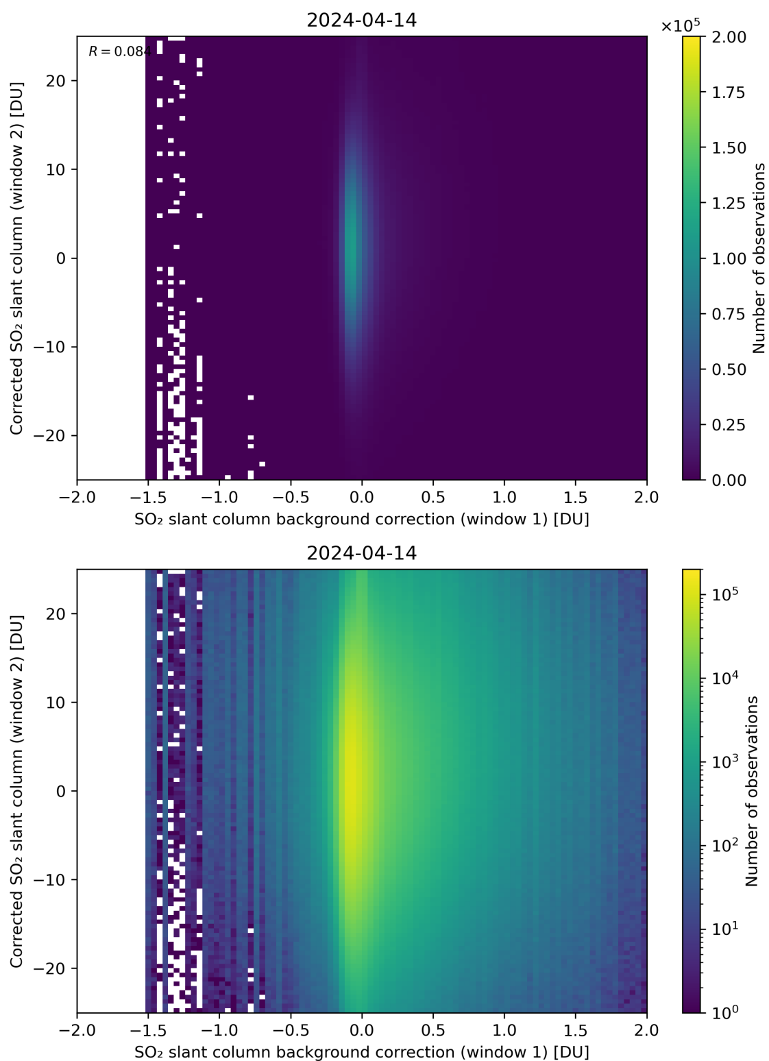
Figure 104: Scatter density plot of “SO 2 slant column background correction (window 1)” against “Corrected SO 2 slant column (window 2)” for 2024-04-13 to 2024-04-15.
