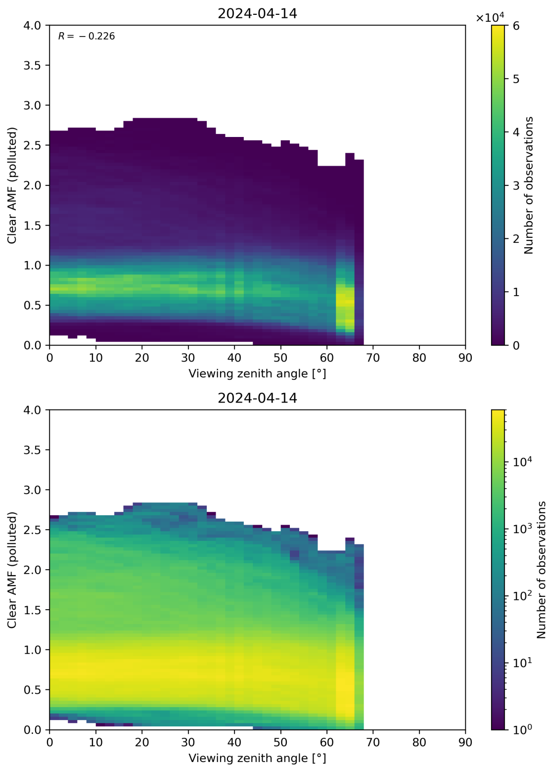
Figure 316: Scatter density plot of “Viewing zenith angle” against “Clear AMF (polluted)” for 2024-04-13 to 2024-04-15.
