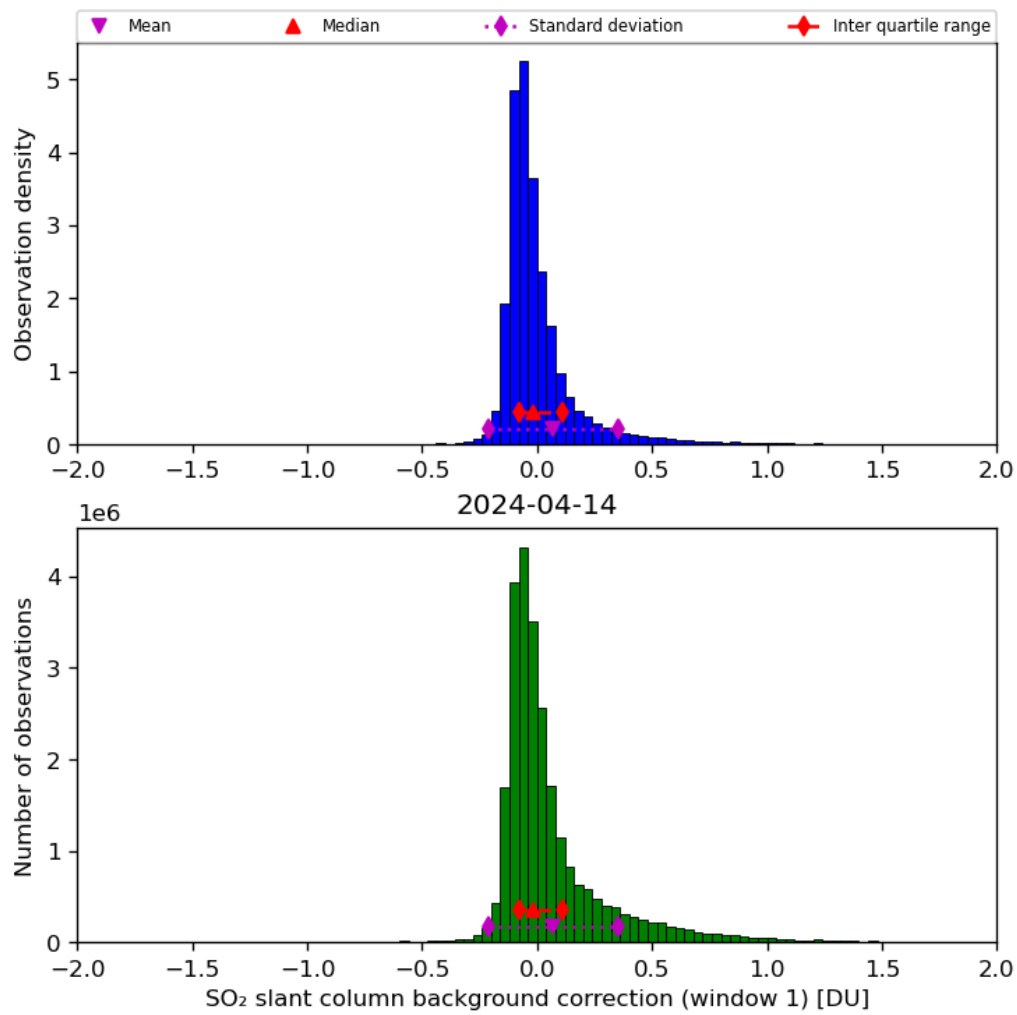
Figure 59: Histogram of “SO 2 slant column background correction (window 1)” for 2024-04-13 to 2024-04-15
