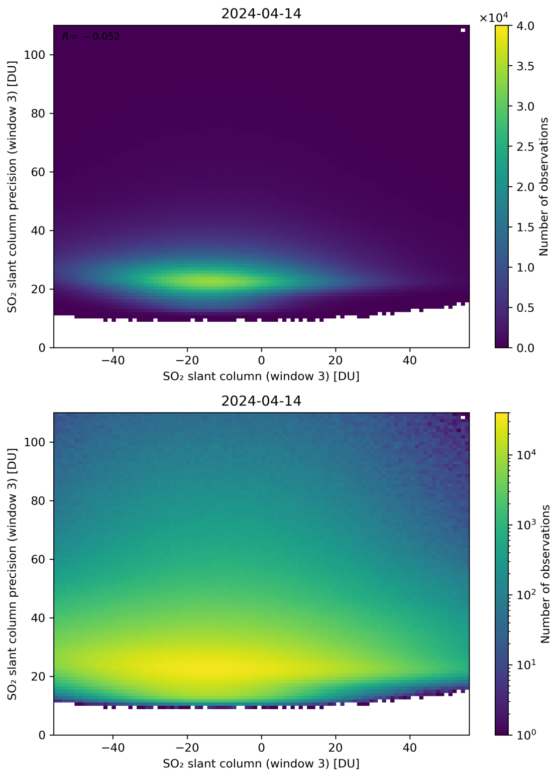
Figure 267: Scatter density plot of “SO 2 slant column (window 3)” against “SO 2 slant column precision (window 3)” for 2024-04-13 to 2024-04-15.
