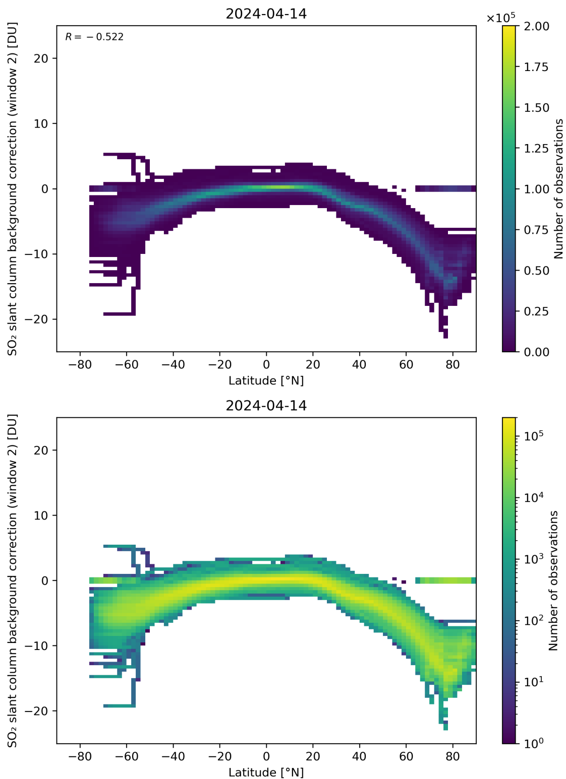
Figure 140: Scatter density plot of “Latitude” against “SO 2 slant column background correction (window 2)” for 2024-04-13 to 2024-04-15.
