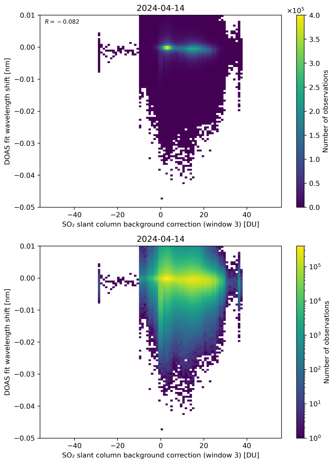
Figure 121: Scatter density plot of “SO 2 slant column background correction (window 3)” against “DOAS fit wavelength shift” for 2024-04-13 to 2024-04-15.
