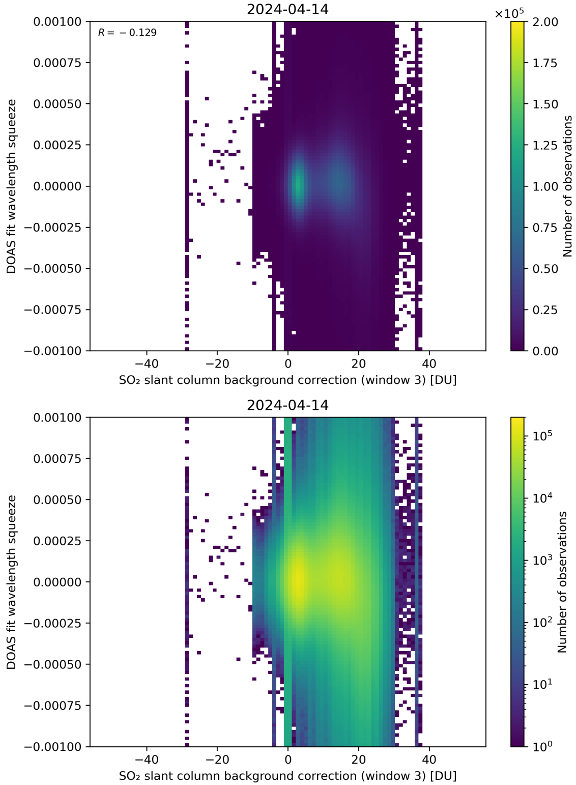
Figure 122: Scatter density plot of “SO 2 slant column background correction (window 3)” against “DOAS fit wavelength squeeze” for 2024-04-13 to 2024-04-15.
