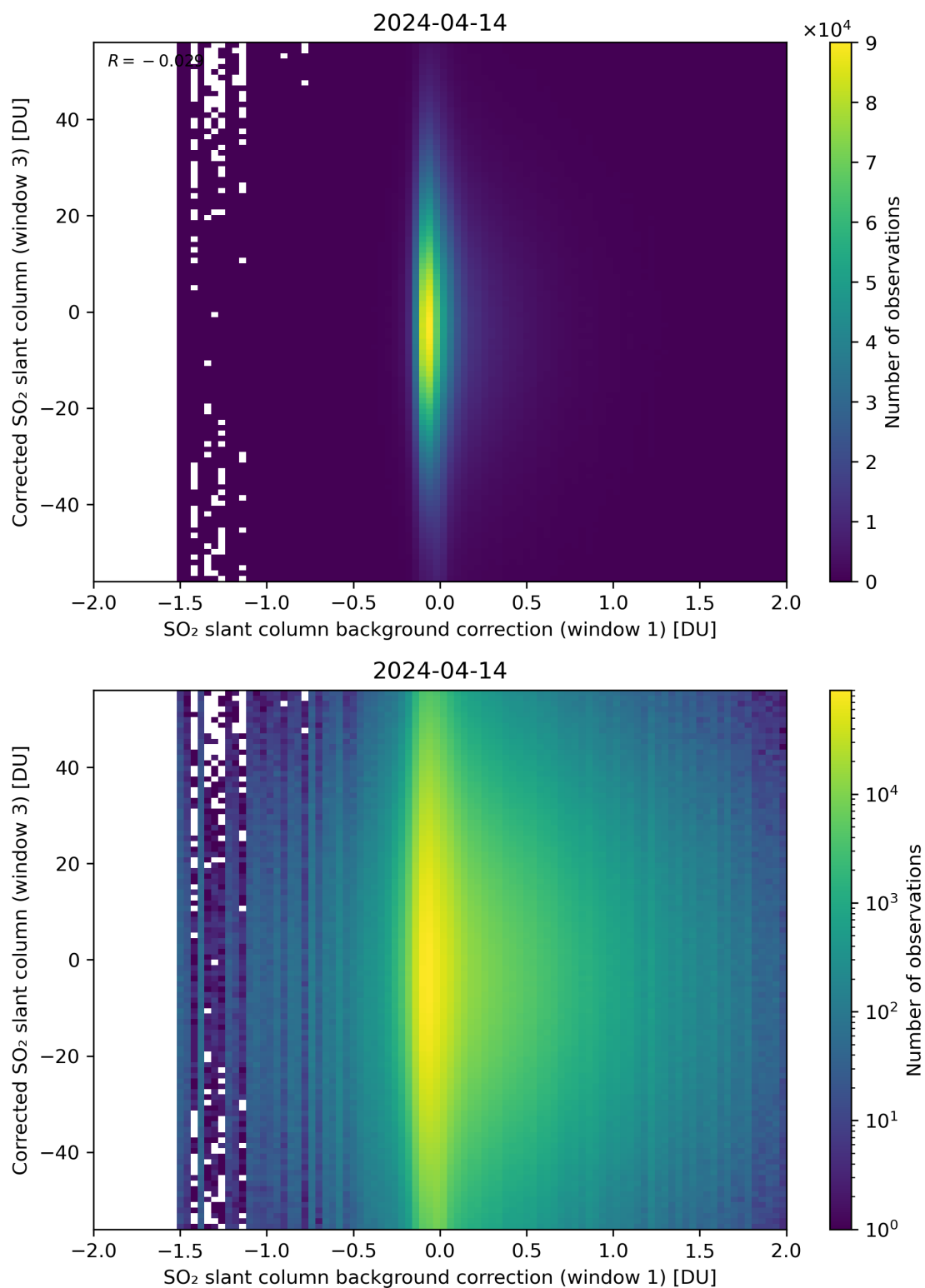
Figure 105: Scatter density plot of “SO 2 slant column background correction (window 1)” against “Corrected SO 2 slant column (window 3)” for 2024-04-13 to 2024-04-15.
