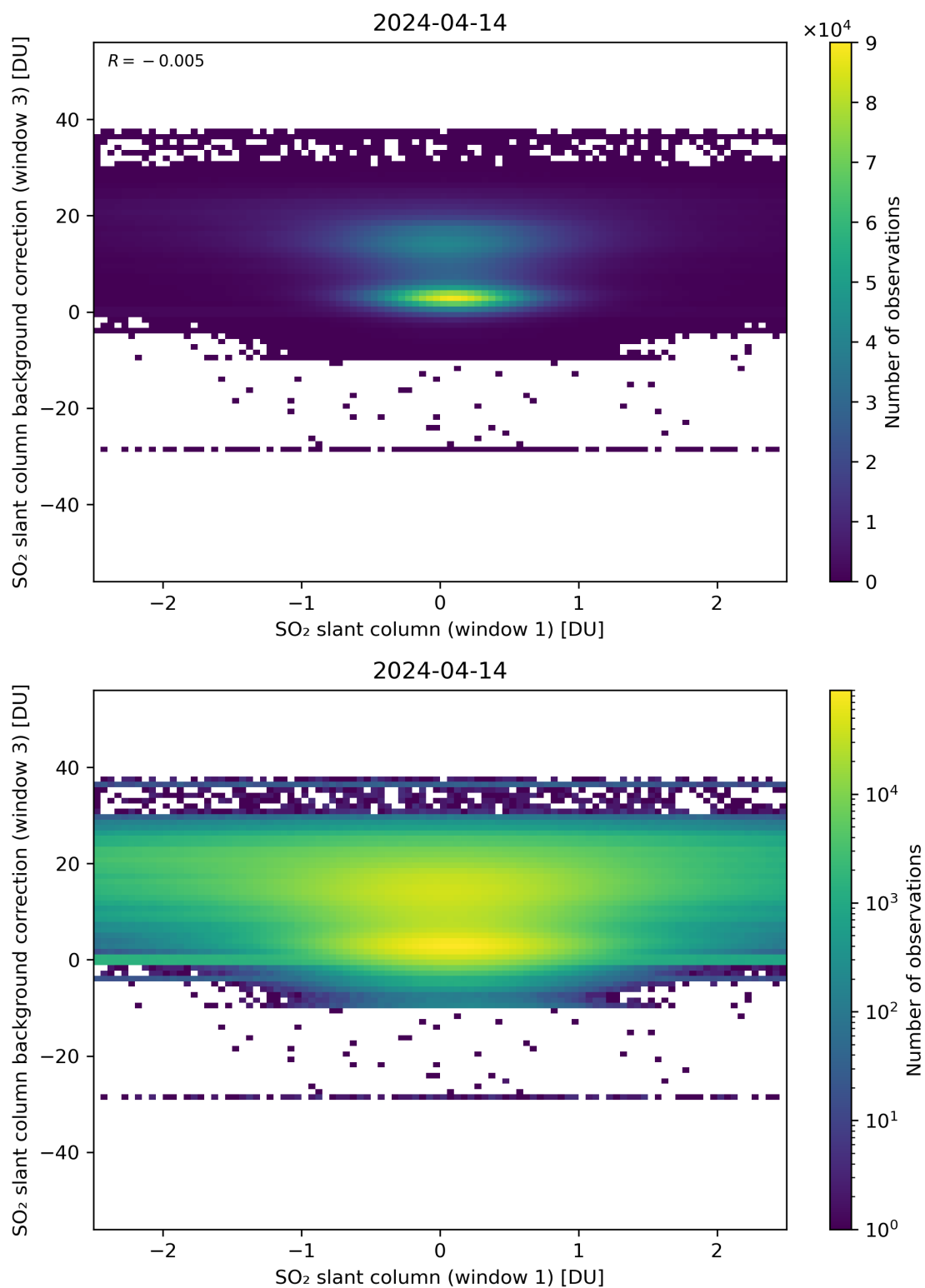
Figure 214: Scatter density plot of “SO 2 slant column (window 1)” against “SO 2 slant column background correction (window 3)” for 2024-04-13 to 2024-04-15.
