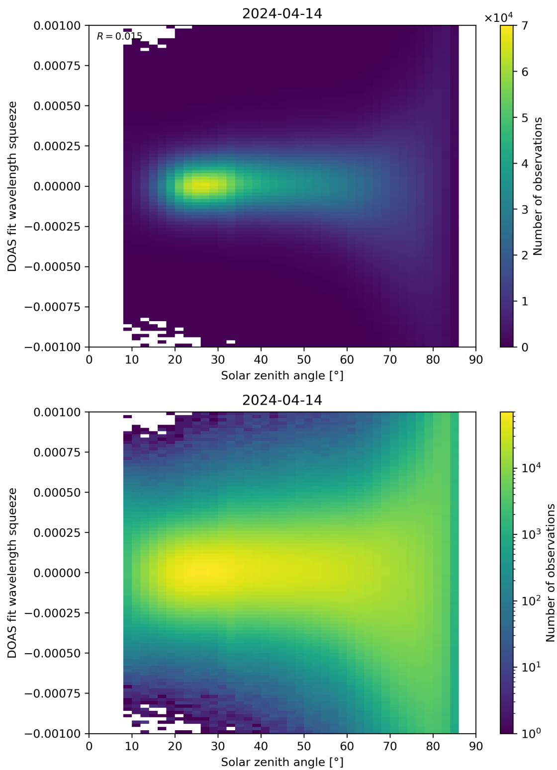
Figure 162: Scatter density plot of “Solar zenith angle” against “DOAS fit wavelength squeeze” for 2024-04-13 to 2024-04-15.
