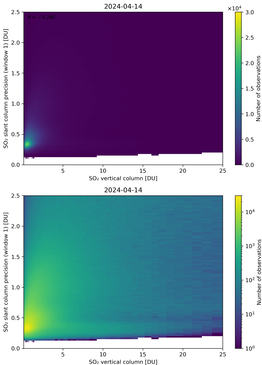
Figure 301: Scatter density plot of “SO 2 vertical column” against “SO 2 slant column precision (window 1)” for 2024-04-13 to 2024-04-15.
