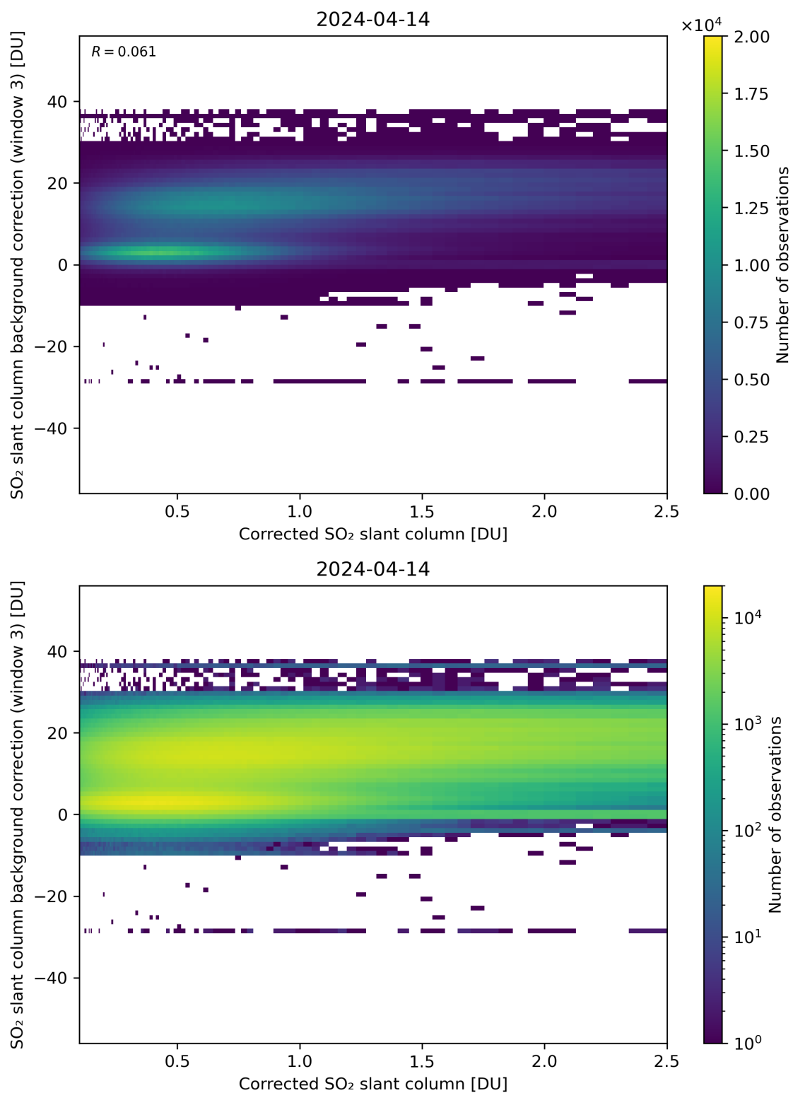
Figure 180: Scatter density plot of “Corrected SO 2 slant column” against “SO 2 slant column background correction (window 3)” for 2024-04-13 to 2024-04-15.
