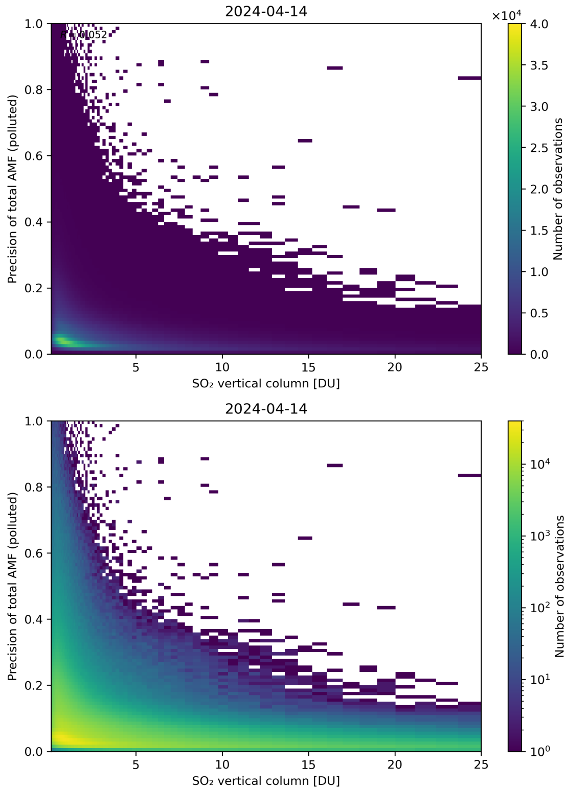
Figure 306: Scatter density plot of “SO 2 vertical column” against “Precision of total AMF (polluted)” for 2024-04-13 to 2024-04-15.
