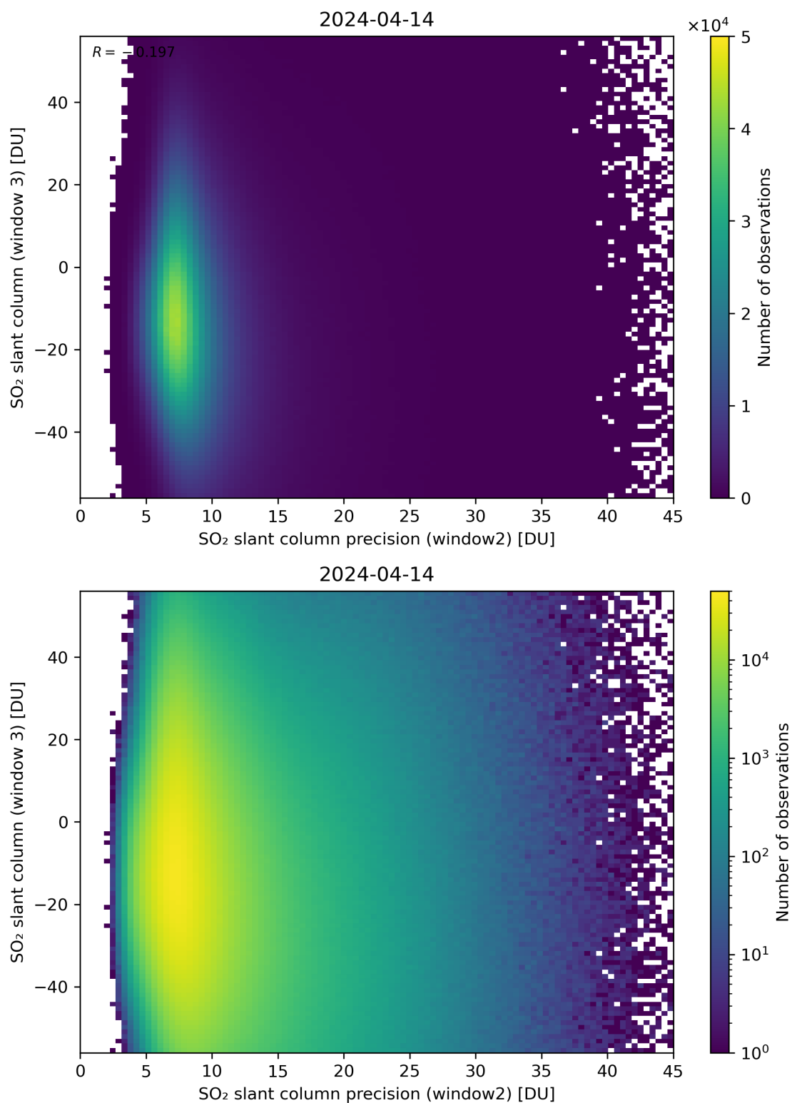
Figure 249: Scatter density plot of “SO 2 slant column precision (window2)” against “SO 2 slant column (window 3)” for 2024-04-13 to 2024-04-15.
