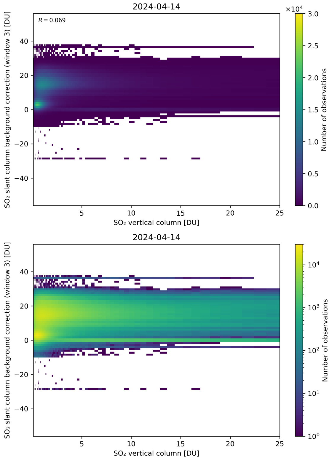
Figure 275: Scatter density plot of “SO 2 vertical column” against “SO 2 slant column background correction (window 3)” for 2024-04-13 to 2024-04-15.
