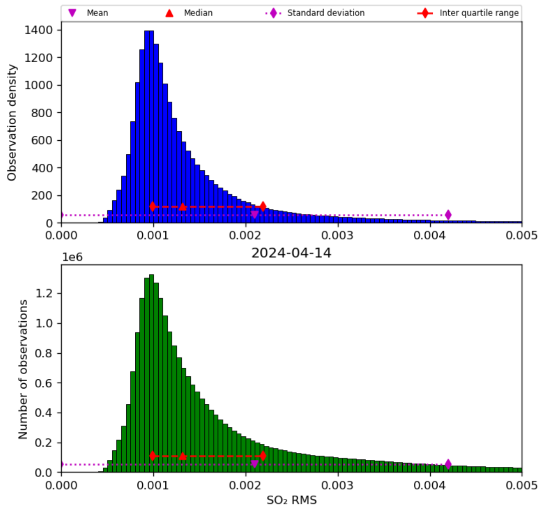
Figure 70: Histogram of “SO 2 RMS” for 2024-04-13 to 2024-04-15
