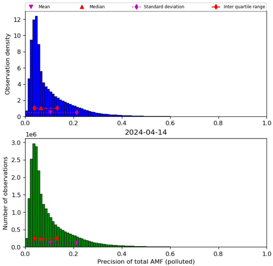
Figure 72: Histogram of “Precision of total AMF (polluted)” for 2024-04-13 to 2024-04-15
