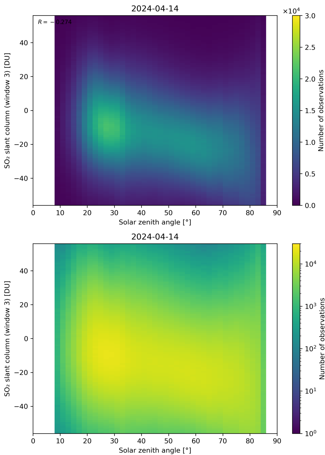
Figure 172: Scatter density plot of “Solar zenith angle” against “SO 2 slant column (window 3)” for 2024-04-13 to 2024-04-15.
