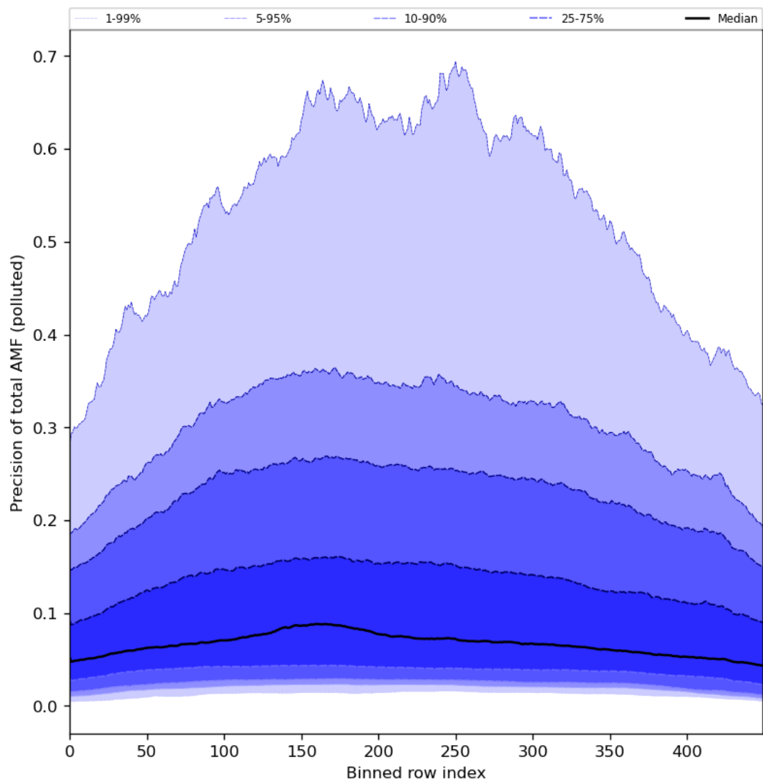
Figure 95: Along track statistics of “Precision of total AMF (polluted)” for 2024-04-13 to 2024-04-15
