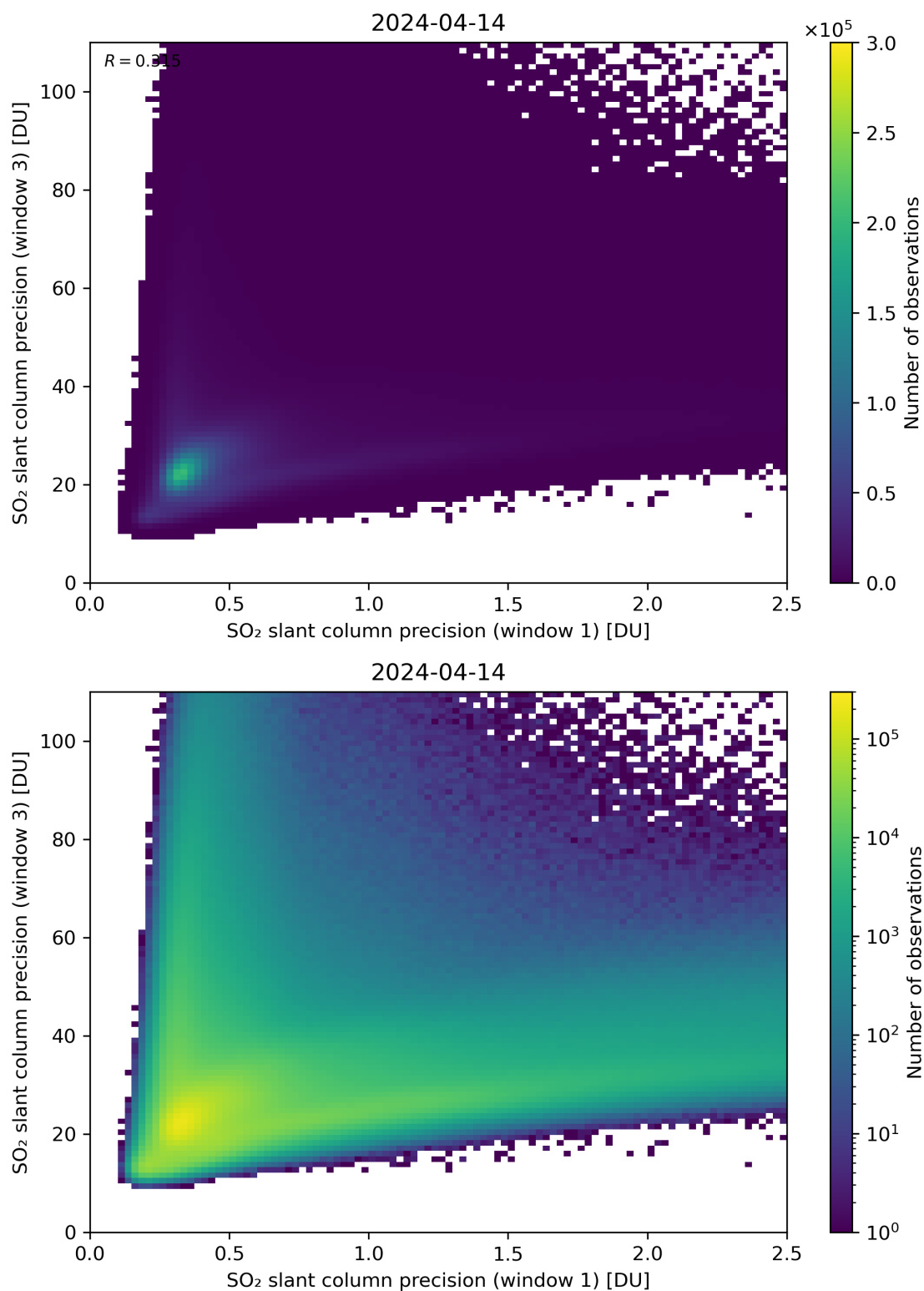
Figure 229: Scatter density plot of “SO 2 slant column precision (window 1)” against “SO 2 slant column precision (window 3)” for 2024-04-13 to 2024-04-15.
