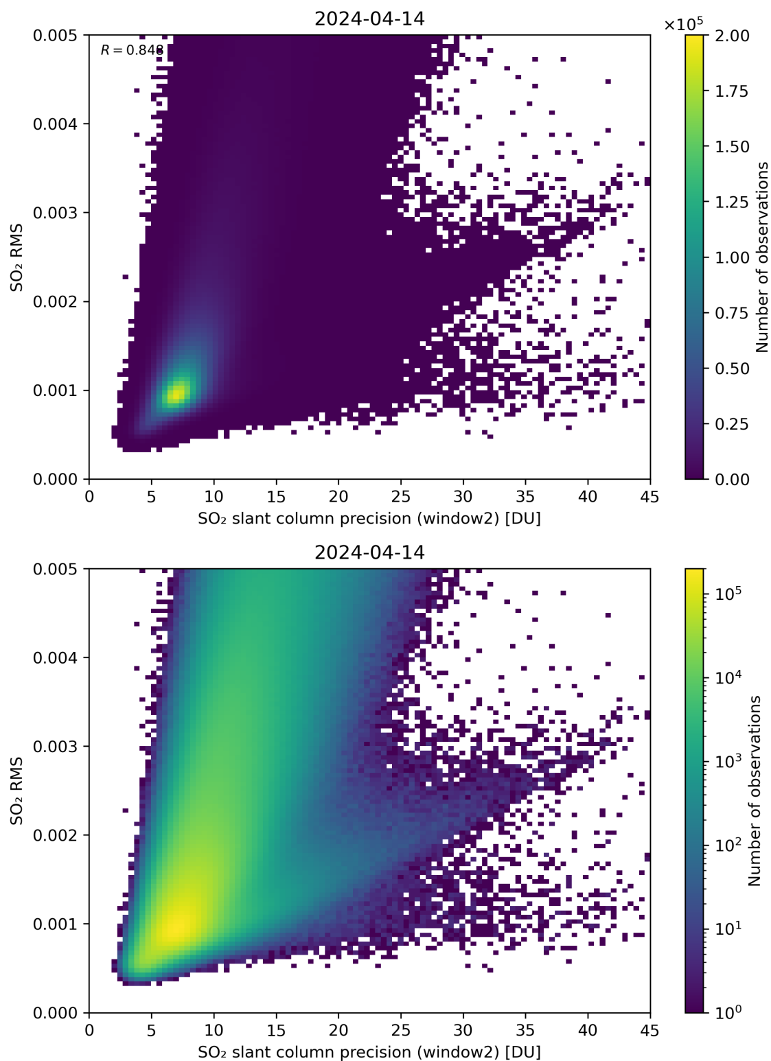
Figure 245: Scatter density plot of “SO 2 slant column precision (window2)” against “SO 2 RMS” for 2024-04-13 to 2024-04-15.
