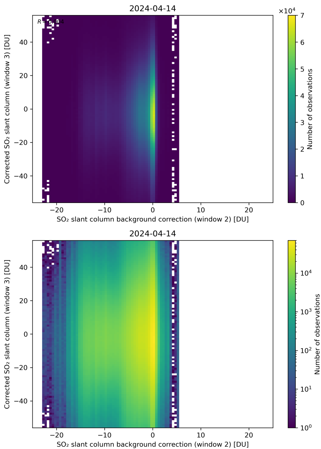
Figure 116: Scatter density plot of “SO 2 slant column background correction (window 2)” against “Corrected SO 2 slant column (window 3)” for 2024-04-13 to 2024-04-15.
