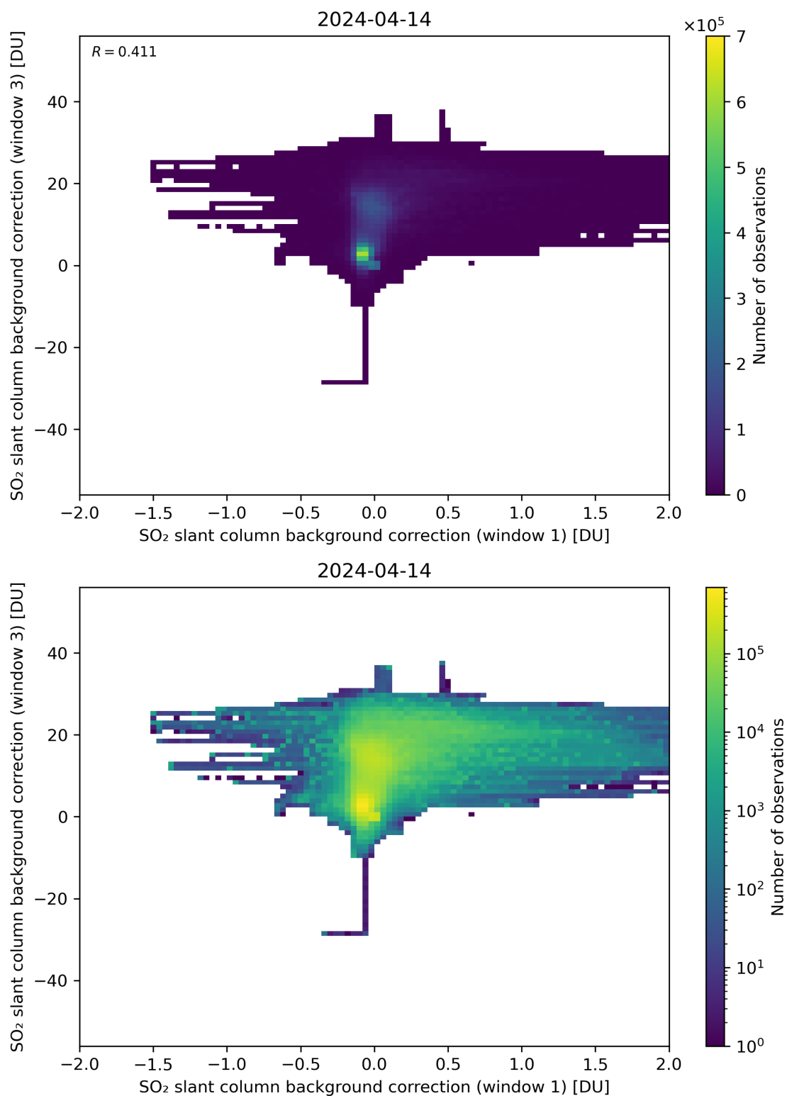
Figure 99: Scatter density plot of “SO 2 slant column background correction (window 1)” against “SO 2 slant column background correction (window 3)” for 2024-04-13 to 2024-04-15.
