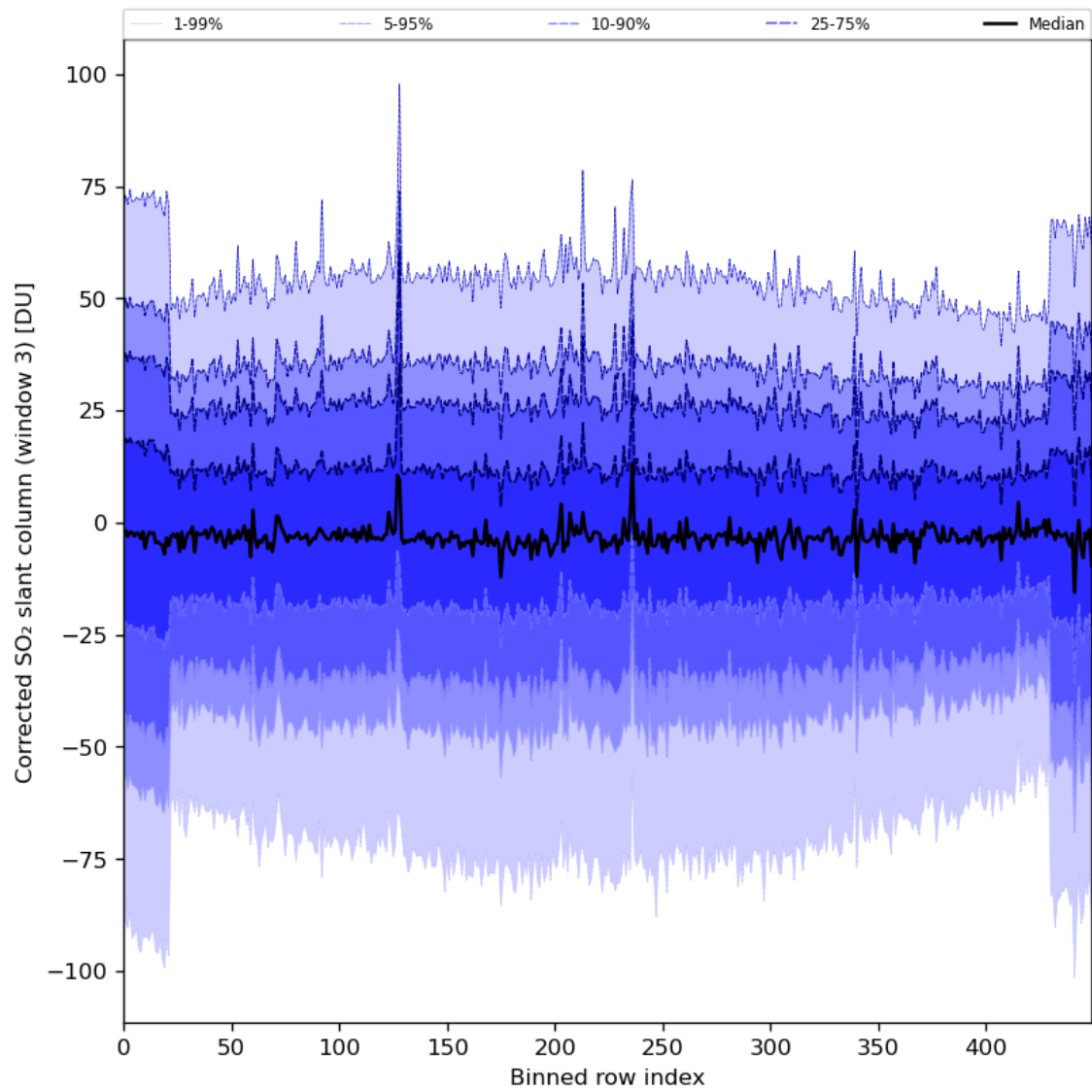
Figure 89: Along track statistics of “Corrected SO 2 slant column (window 3)” for 2024-04-13 to 2024-04-15
