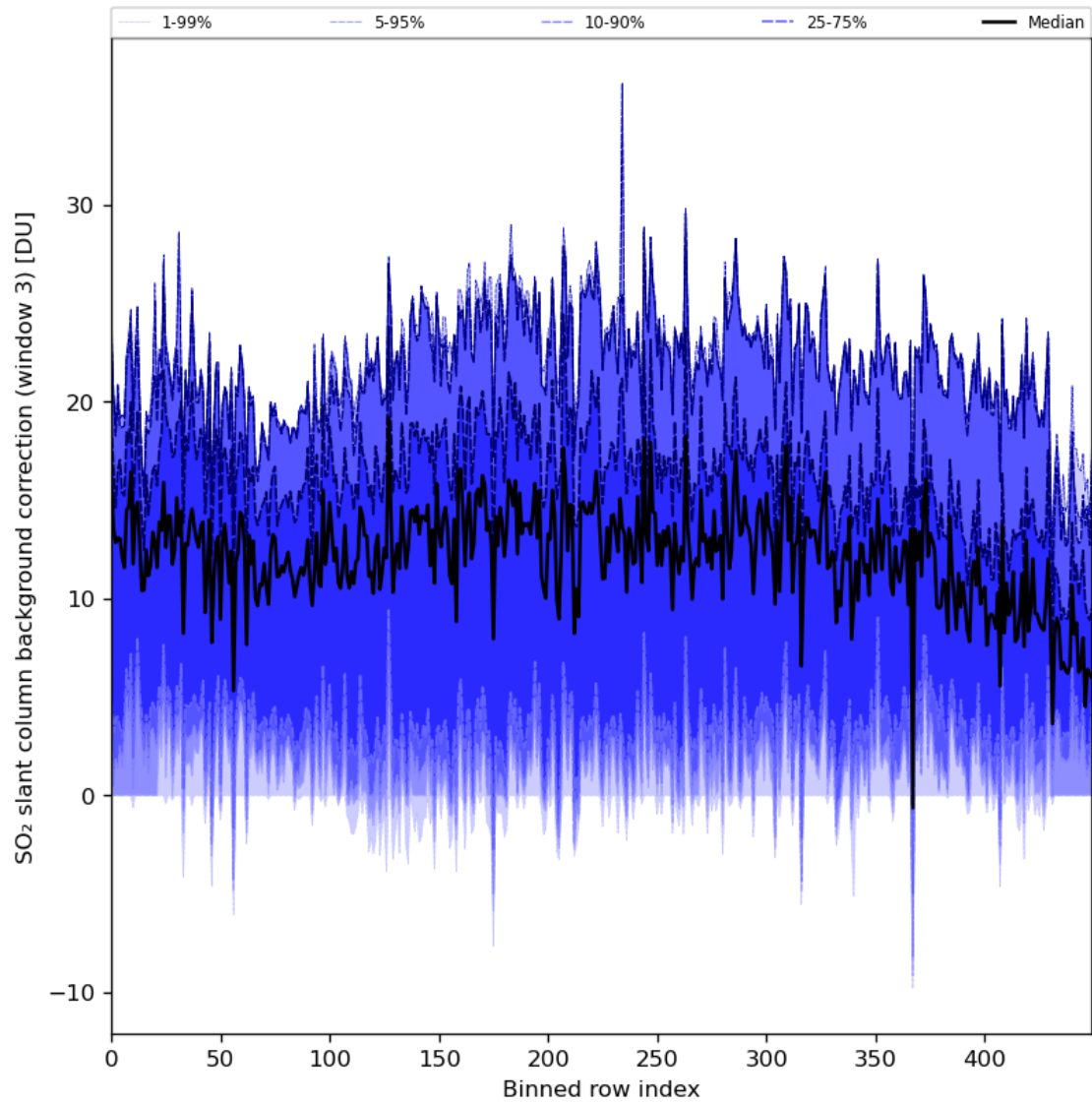
Figure 90: Along track statistics of “SO 2 slant column background correction (window 3)” for 2024-04-13 to 2024-04-15
