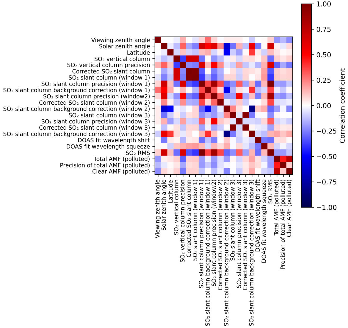
Figure 2: Map of correlation matrix for 2024-04-13 to 2024-04-15.
