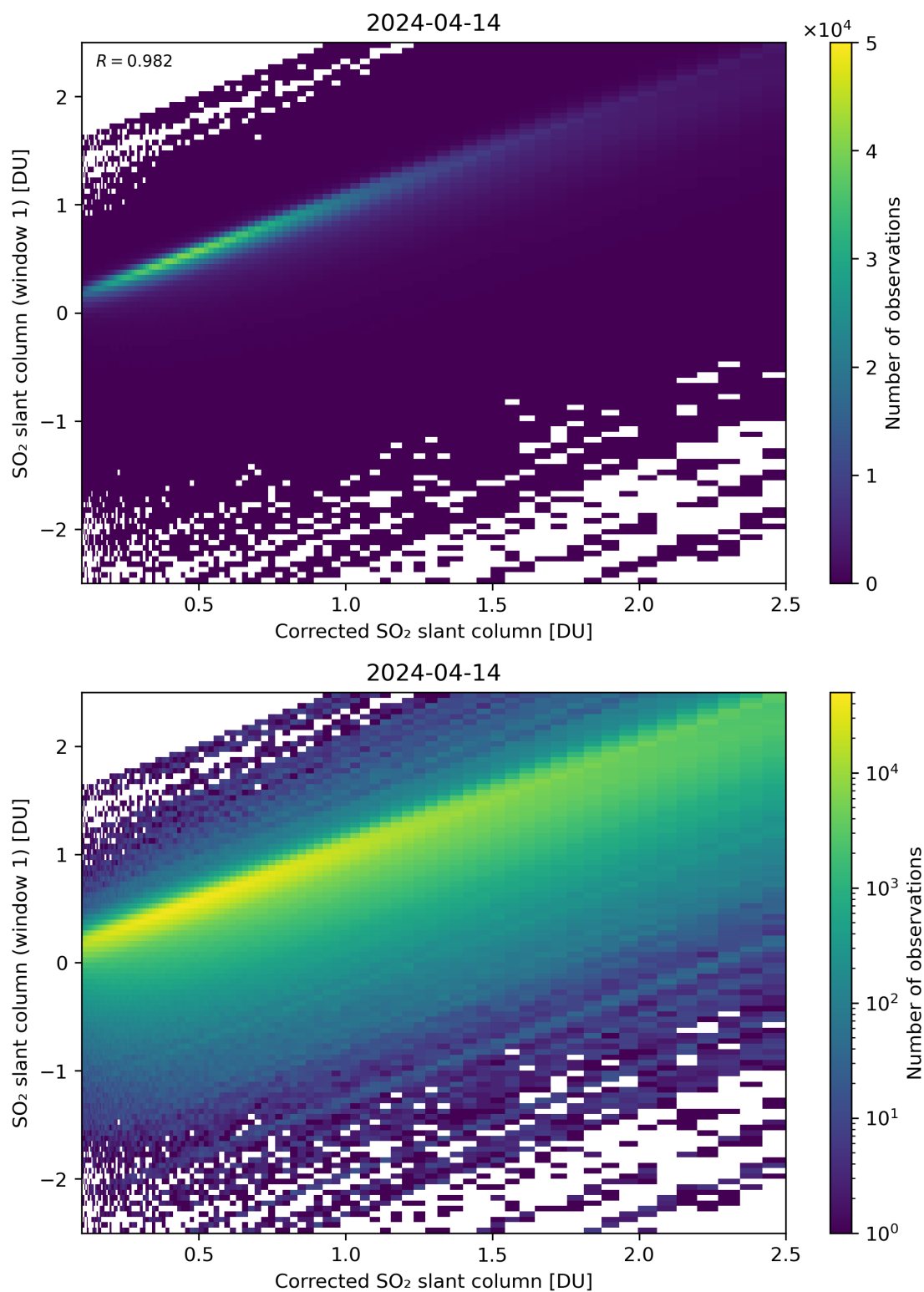
Figure 187: Scatter density plot of “Corrected SO 2 slant column” against “SO 2 slant column (window 1)” for 2024-04-13 to 2024-04-15.
