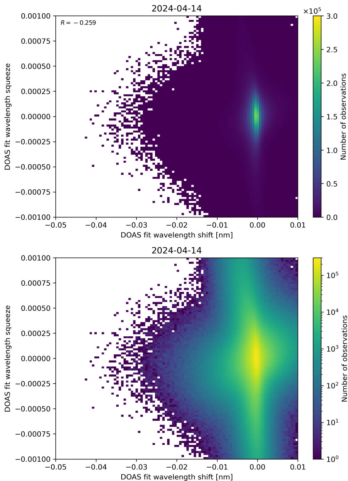
Figure 127: Scatter density plot of “DOAS fit wavelength shift” against “DOAS fit wavelength squeeze” for 2024-04-13 to 2024-04-15.
