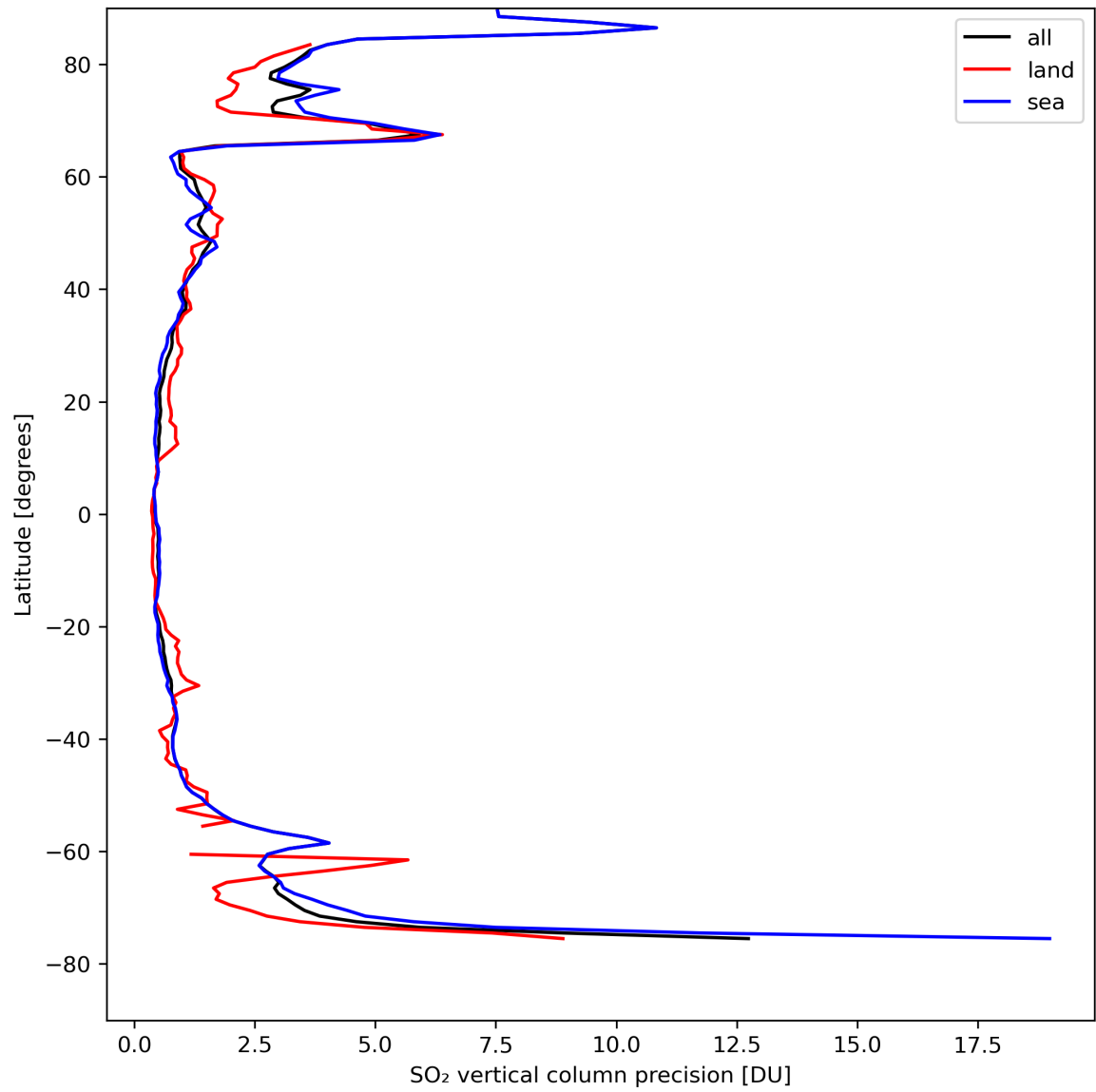
Figure 31: Zonal average of “SO 2 vertical column precision” for 2024-04-13 to 2024-04-15.
