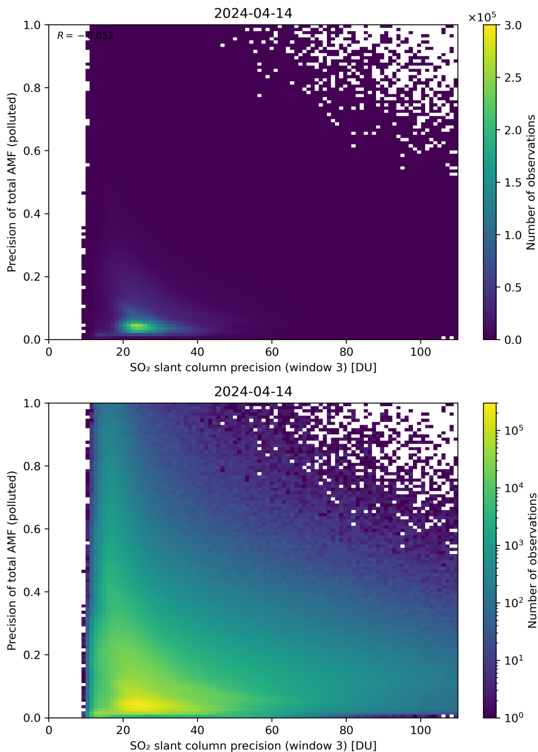
Figure 264: Scatter density plot of “SO 2 slant column precision (window 3)” against “Precision of total AMF (polluted)” for 2024-04-13 to 2024-04-15.
