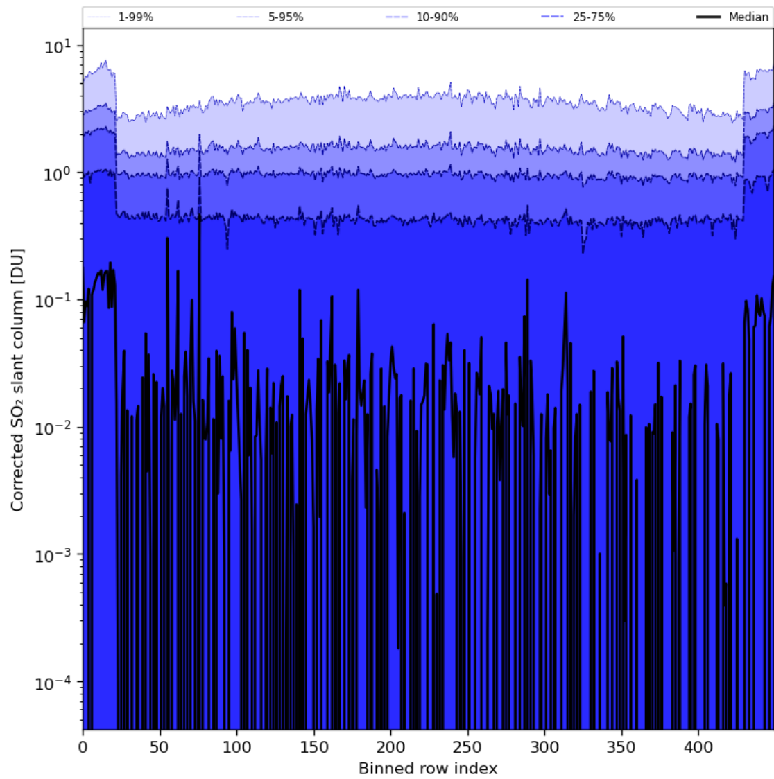
Figure 78: Along track statistics of “Corrected SO 2 slant column” for 2024-04-13 to 2024-04-15
