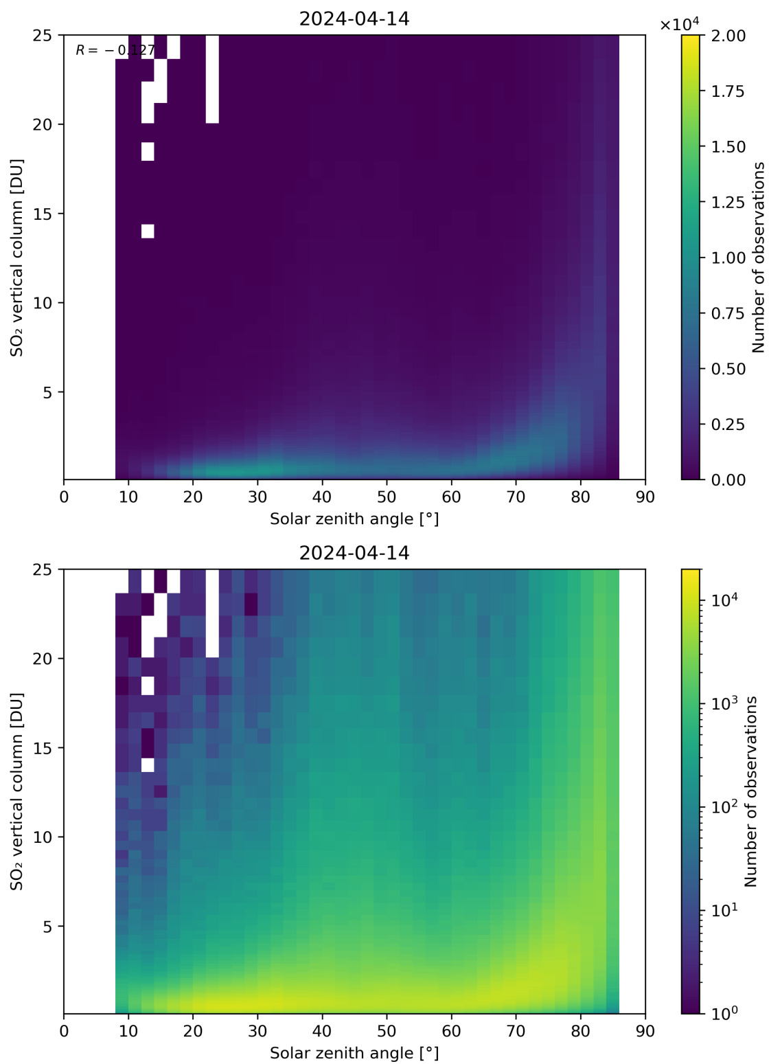
Figure 176: Scatter density plot of “Solar zenith angle” against “SO 2 vertical column” for 2024-04-13 to 2024-04-15.
