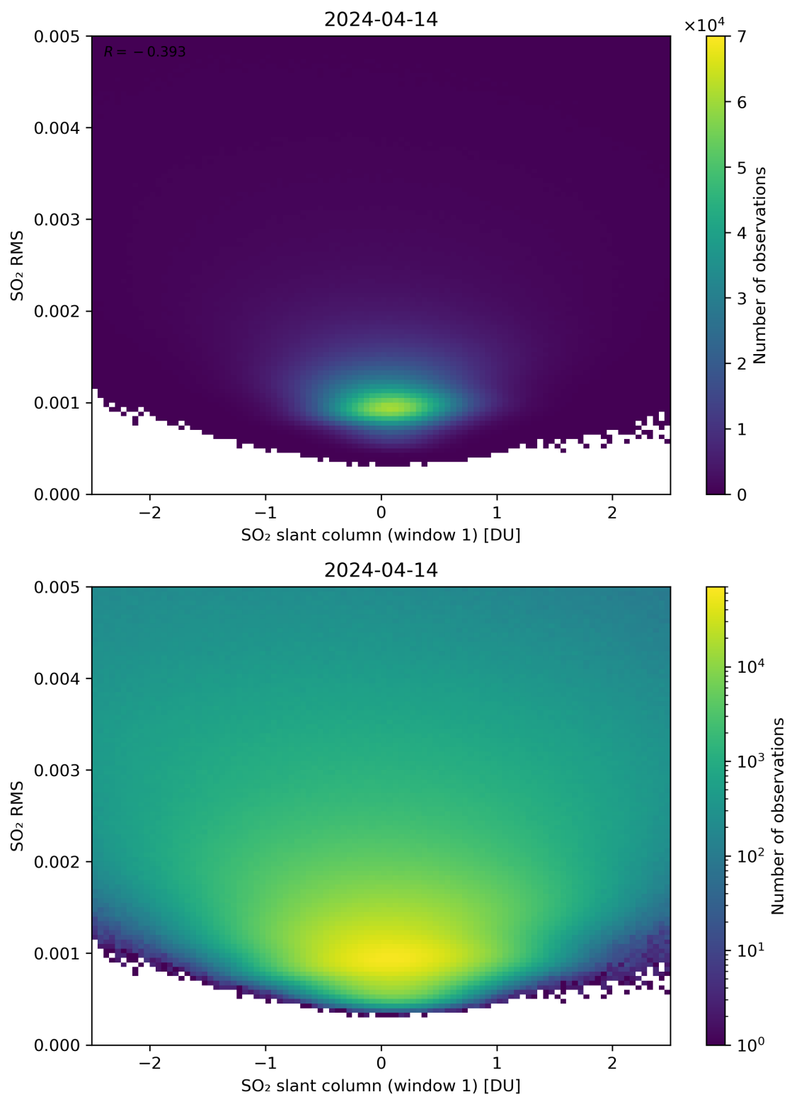
Figure 217: Scatter density plot of “SO 2 slant column (window 1)” against “SO 2 RMS” for 2024-04-13 to 2024-04-15.
