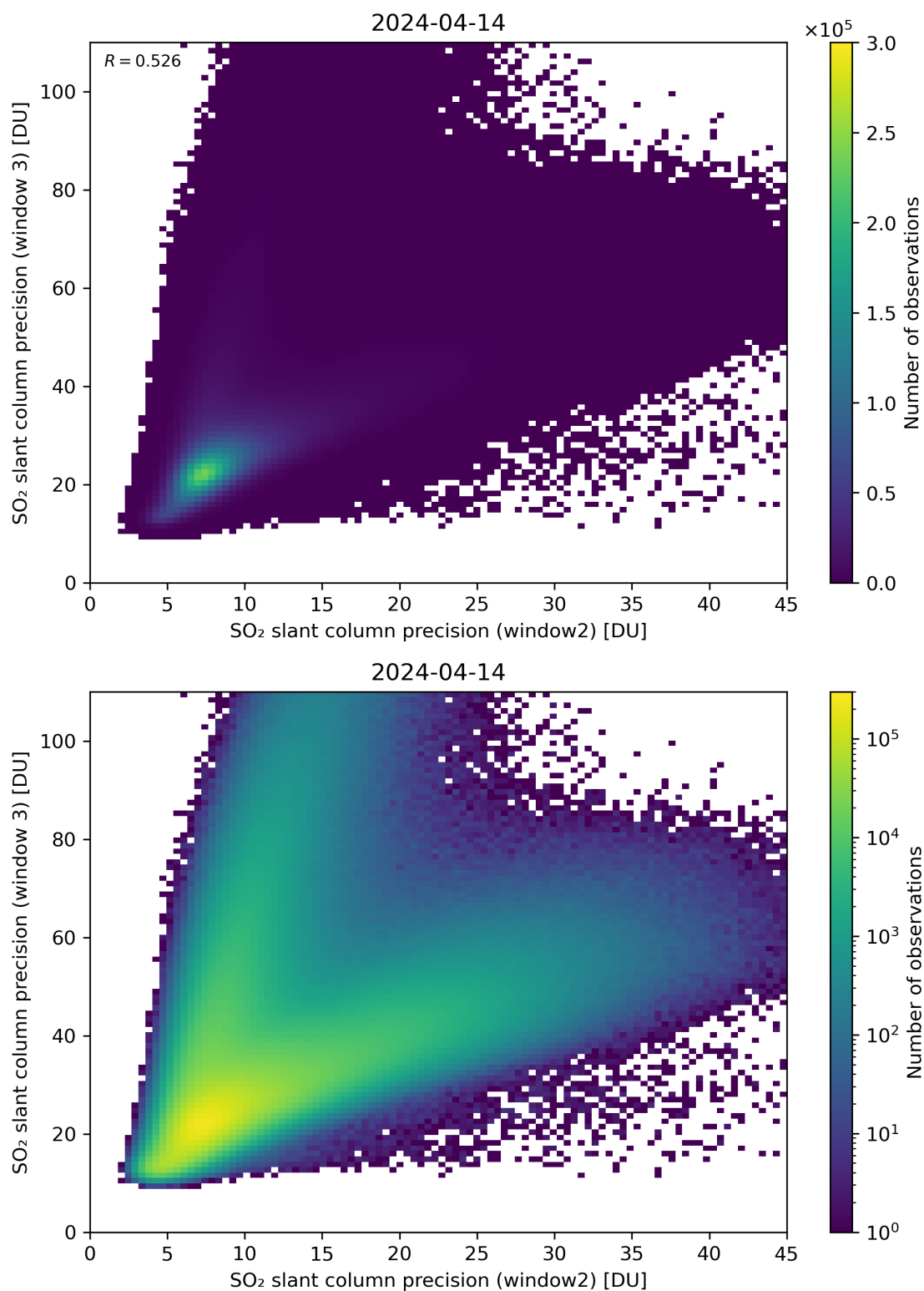
Figure 250: Scatter density plot of “SO 2 slant column precision (window2)” against “SO 2 slant column precision (window 3)” for 2024-04-13 to 2024-04-15.
