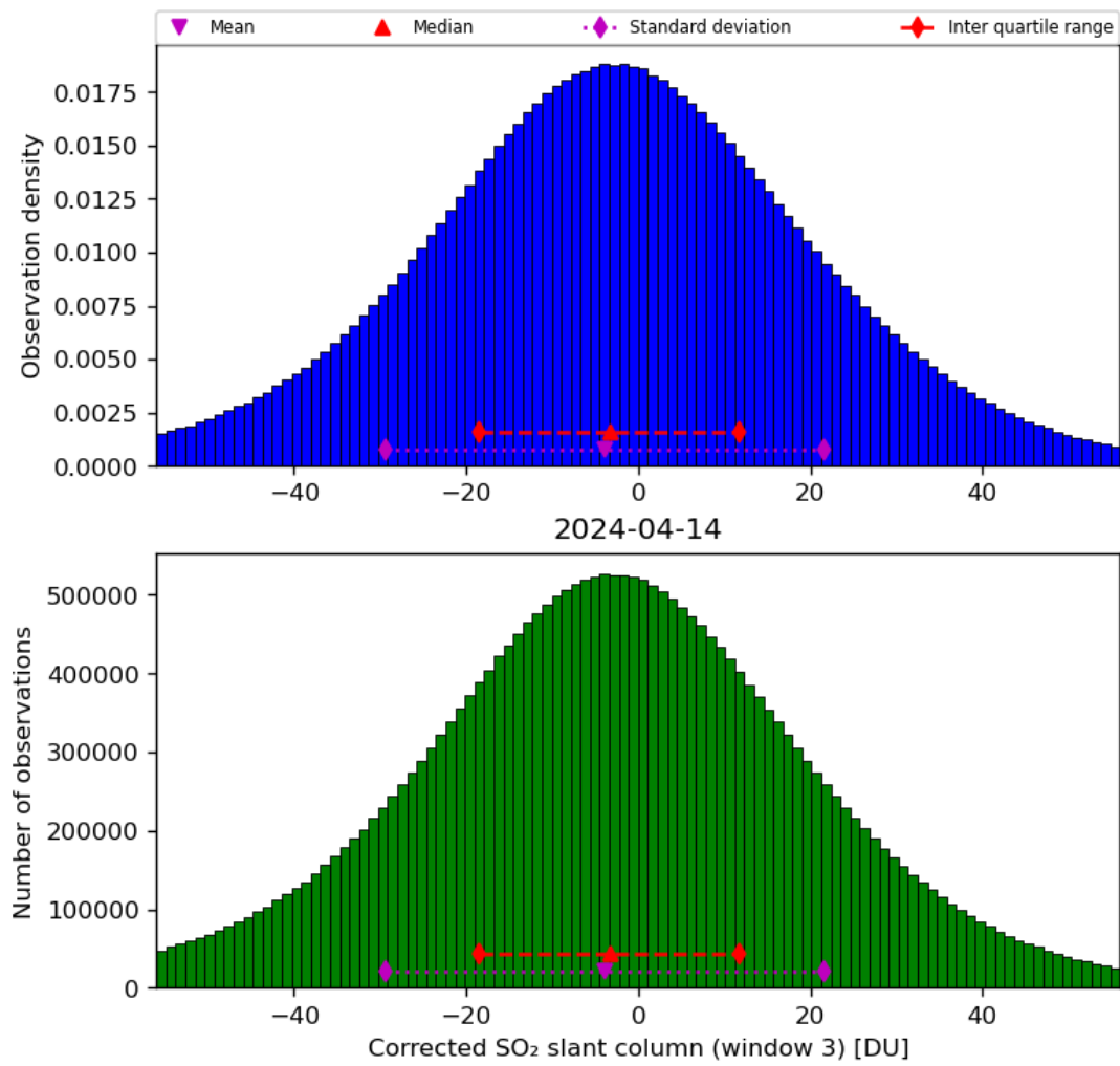
Figure 66: Histogram of “Corrected SO 2 slant column (window 3)” for 2024-04-13 to 2024-04-15
