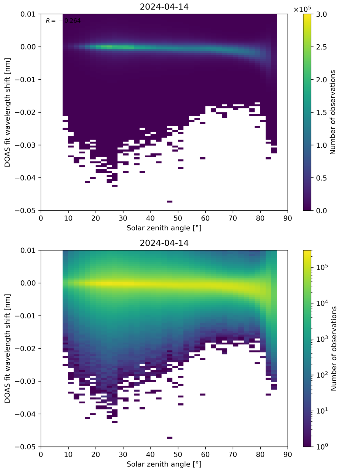
Figure 161: Scatter density plot of “Solar zenith angle” against “DOAS fit wavelength shift” for 2024-04-13 to 2024-04-15.
