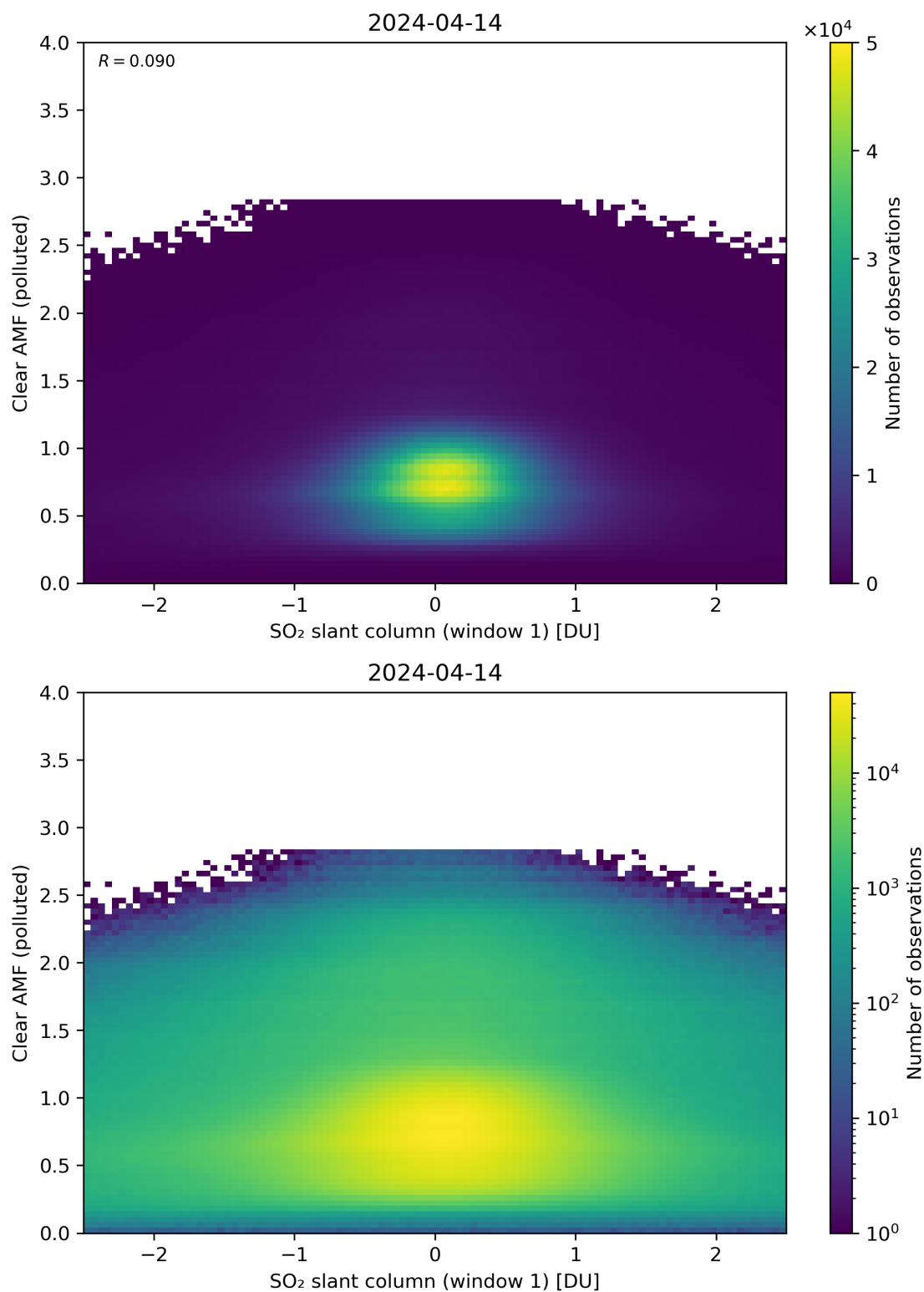
Figure 232: Scatter density plot of “SO 2 slant column (window 1)” against “Clear AMF (polluted)” for 2024-04-13 to 2024-04-15.
