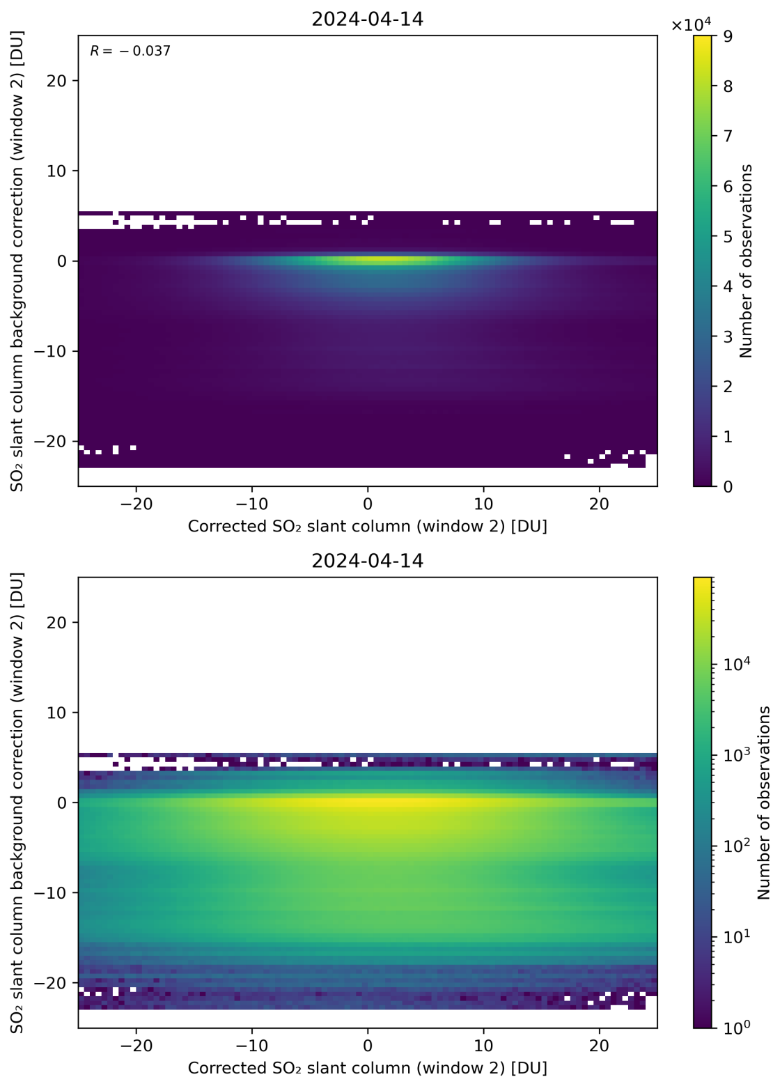
Figure 194: Scatter density plot of “Corrected SO 2 slant column (window 2)” against “SO 2 slant column background correction (window 2)” for 2024-04-13 to 2024-04-15.
