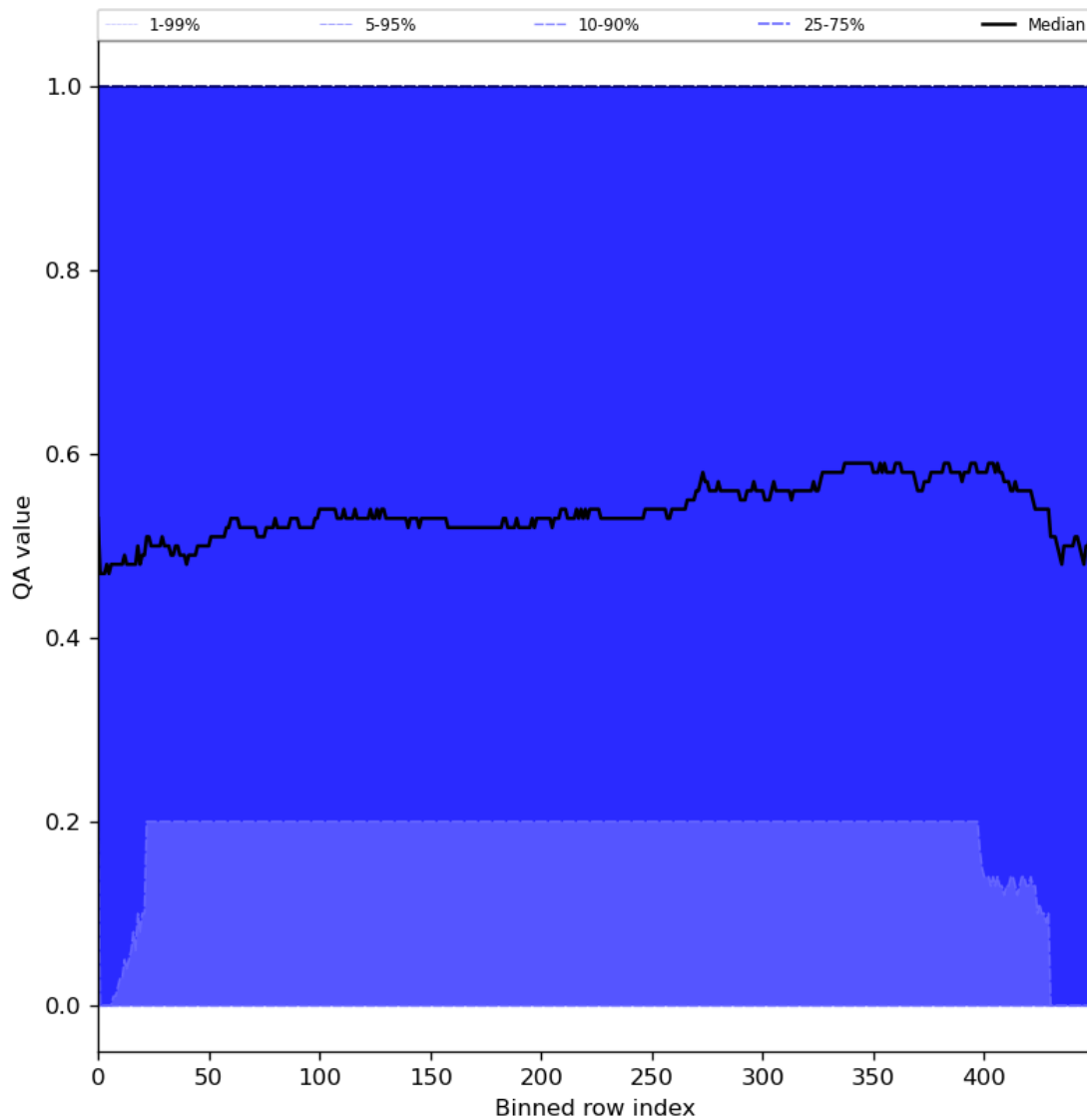
Figure 75: Along track statistics of “QA value” for 2024-04-13 to 2024-04-15
