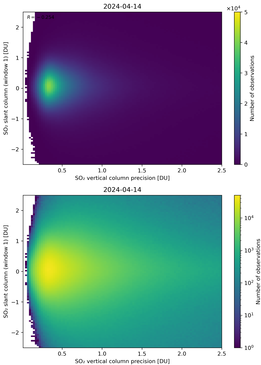
Figure 289: Scatter density plot of “SO 2 vertical column precision” against “SO 2 slant column (window 1)” for 2024-04-13 to 2024-04-15.
