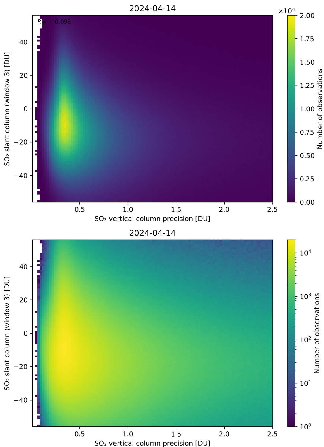
Figure 292: Scatter density plot of “SO 2 vertical column precision” against “SO 2 slant column (window 3)” for 2024-04-13 to 2024-04-15.
