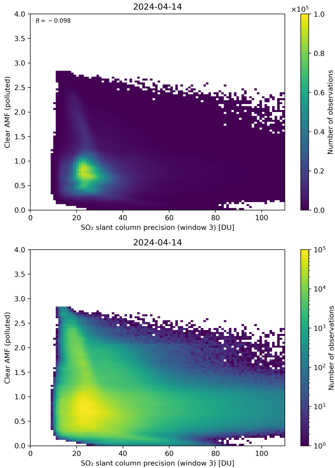
Figure 261: Scatter density plot of “SO 2 slant column precision (window 3)” against “Clear AMF (polluted)” for 2024-04-13 to 2024-04-15.
