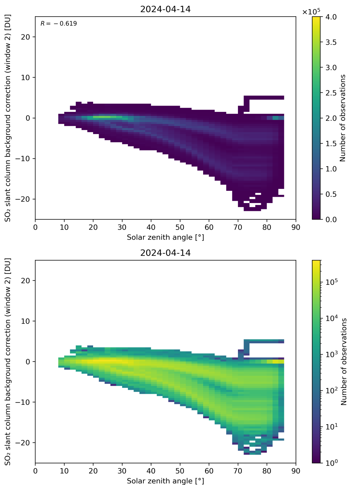
Figure 159: Scatter density plot of “Solar zenith angle” against “SO 2 slant column background correction (window 2)” for 2024-04-13 to 2024-04-15.
