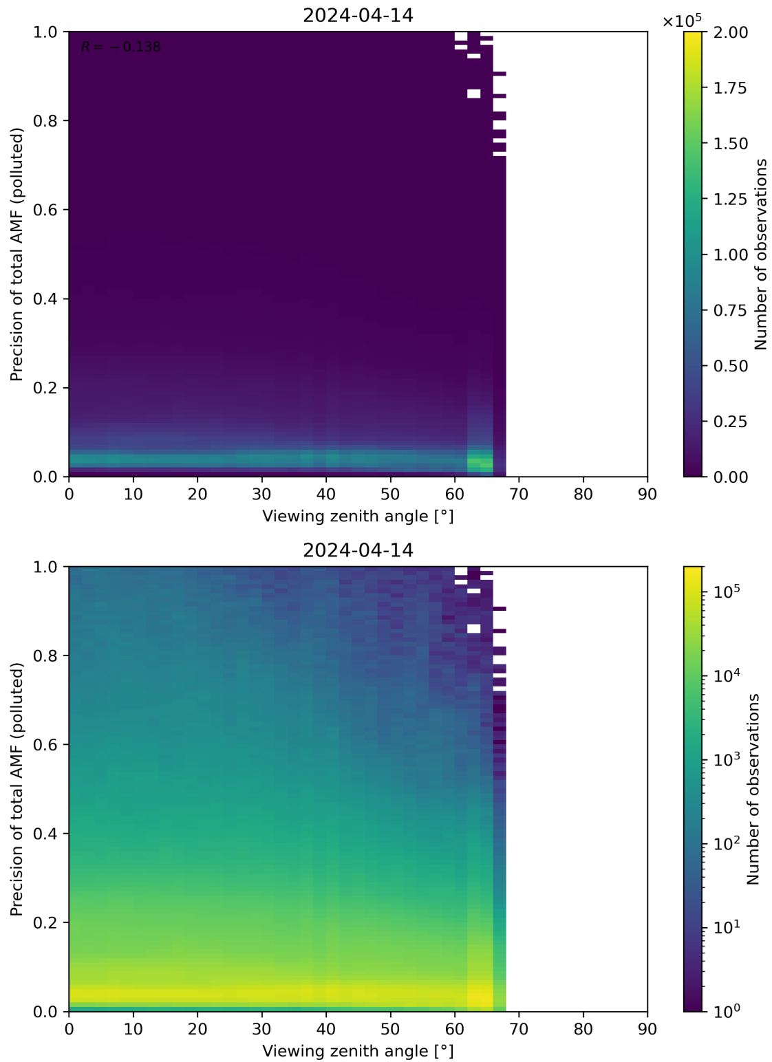
Figure 326: Scatter density plot of “Viewing zenith angle” against “Precision of total AMF (polluted)” for 2024-04-13 to 2024-04-15.
