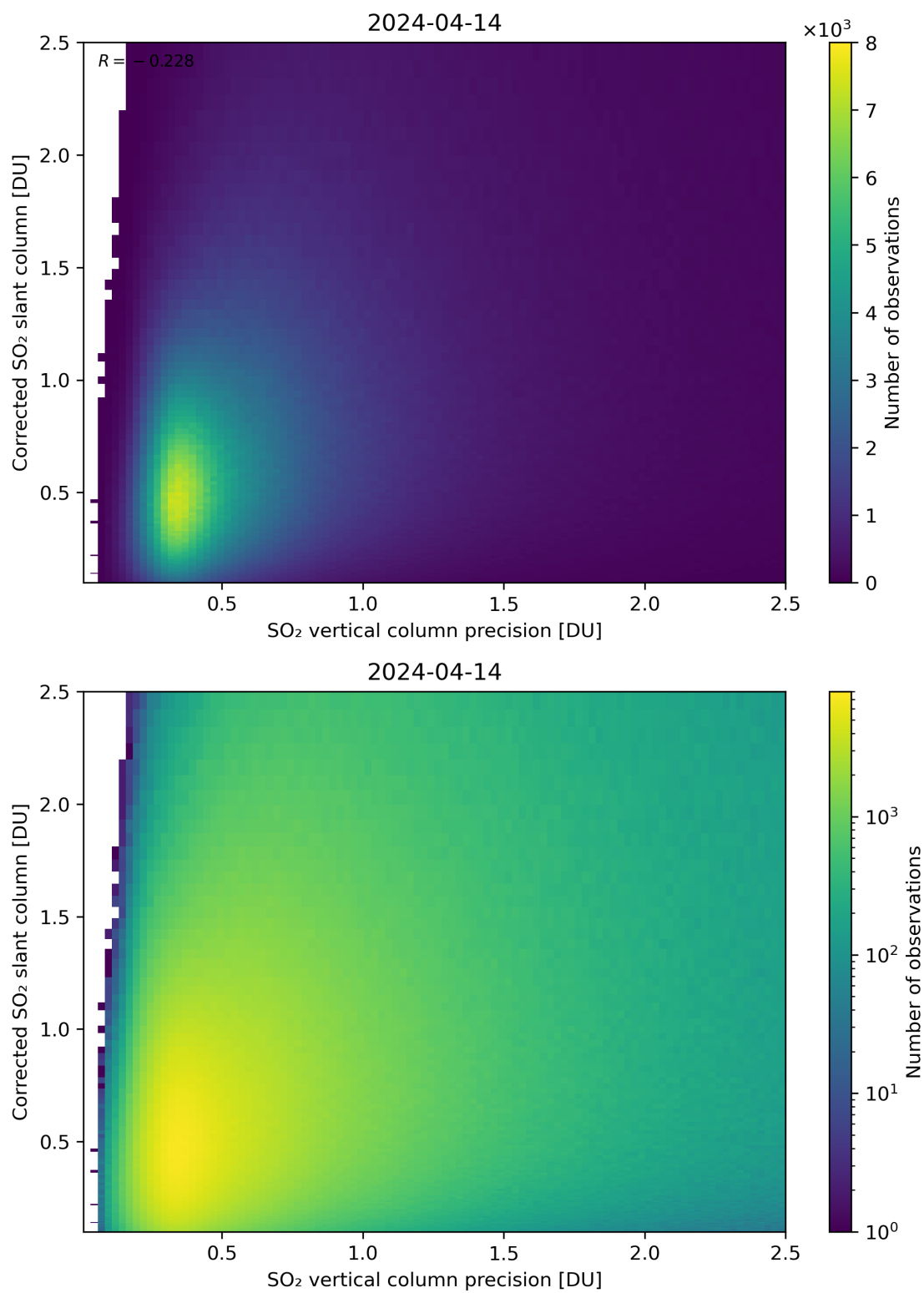
Figure 286: Scatter density plot of “SO 2 vertical column precision” against “Corrected SO 2 slant column” for 2024-04-13 to 2024-04-15.
