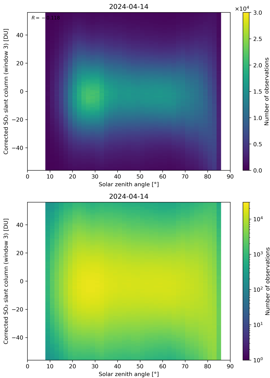
Figure 168: Scatter density plot of “Solar zenith angle” against “Corrected SO 2 slant column (window 3)” for 2024-04-13 to 2024-04-15.
