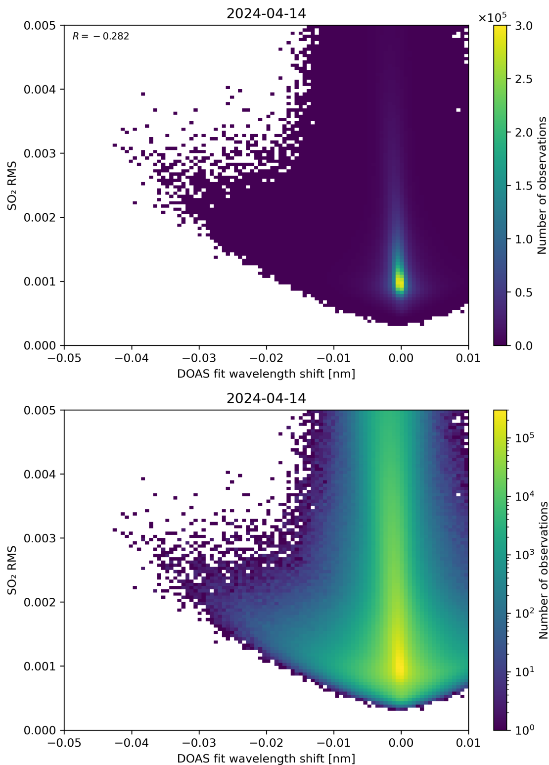
Figure 128: Scatter density plot of “DOAS fit wavelength shift” against “SO 2 RMS” for 2024-04-13 to 2024-04-15.
