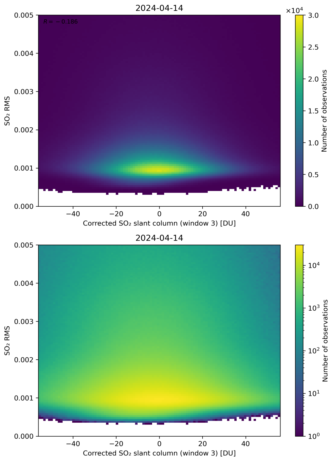
Figure 208: Scatter density plot of “Corrected SO 2 slant column (window 3)” against “SO 2 RMS” for 2024-04-13 to 2024-04-15.
