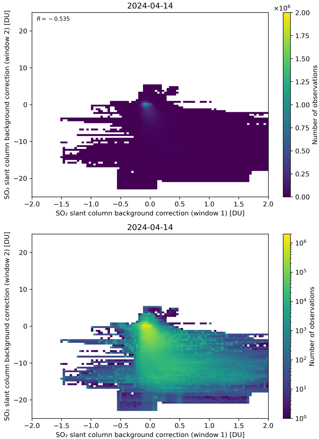
Figure 98: Scatter density plot of “SO 2 slant column background correction (window 1)” against “SO 2 slant column background correction (window 2)” for 2024-04-13 to 2024-04-15.
