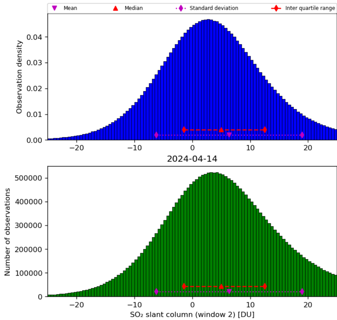
Figure 60: Histogram of “SO 2 slant column (window 2)” for 2024-04-13 to 2024-04-15
