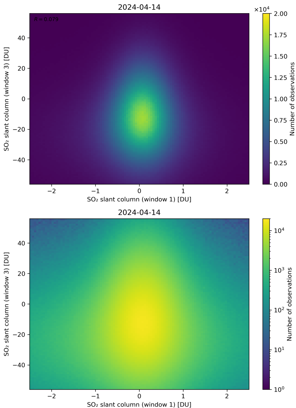
Figure 237: Scatter density plot of “SO 2 slant column (window 1)” against “SO 2 slant column (window 3)” for 2024-04-13 to 2024-04-15.
