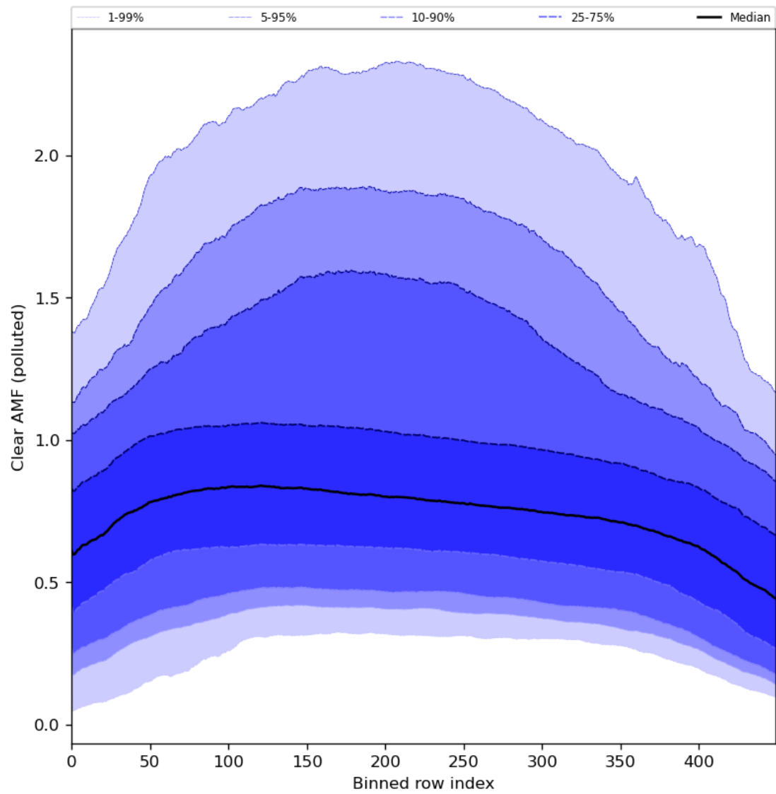
Figure 96: Along track statistics of “Clear AMF (polluted)” for 2024-04-13 to 2024-04-15
