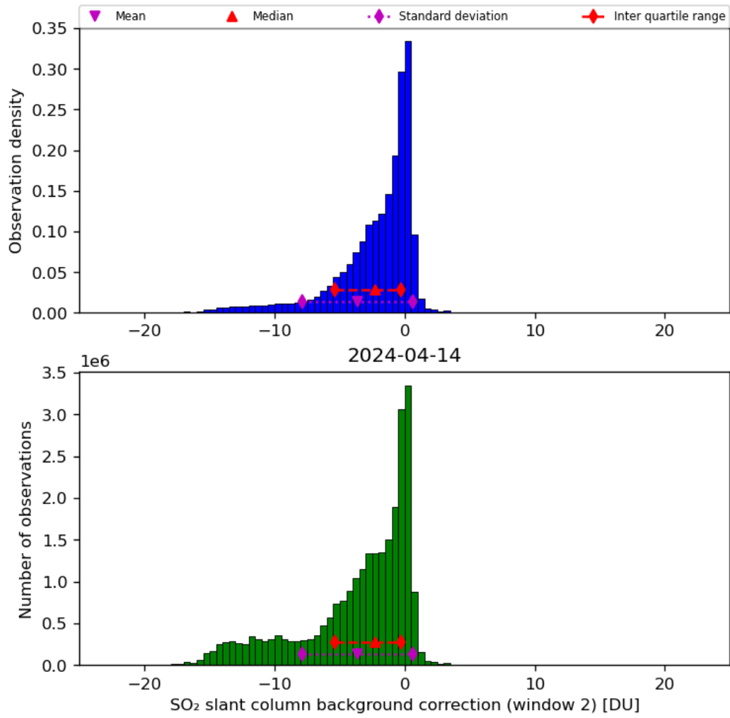
Figure 63: Histogram of “SO 2 slant column background correction (window 2)” for 2024-04-13 to 2024-04-15
