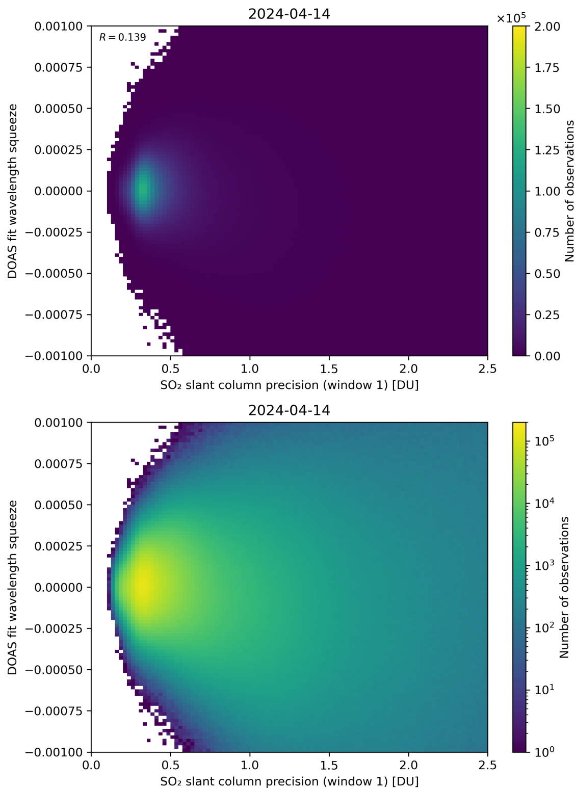
Figure 222: Scatter density plot of “SO 2 slant column precision (window 1)” against “DOAS fit wavelength squeeze” for 2024-04-13 to 2024-04-15.
