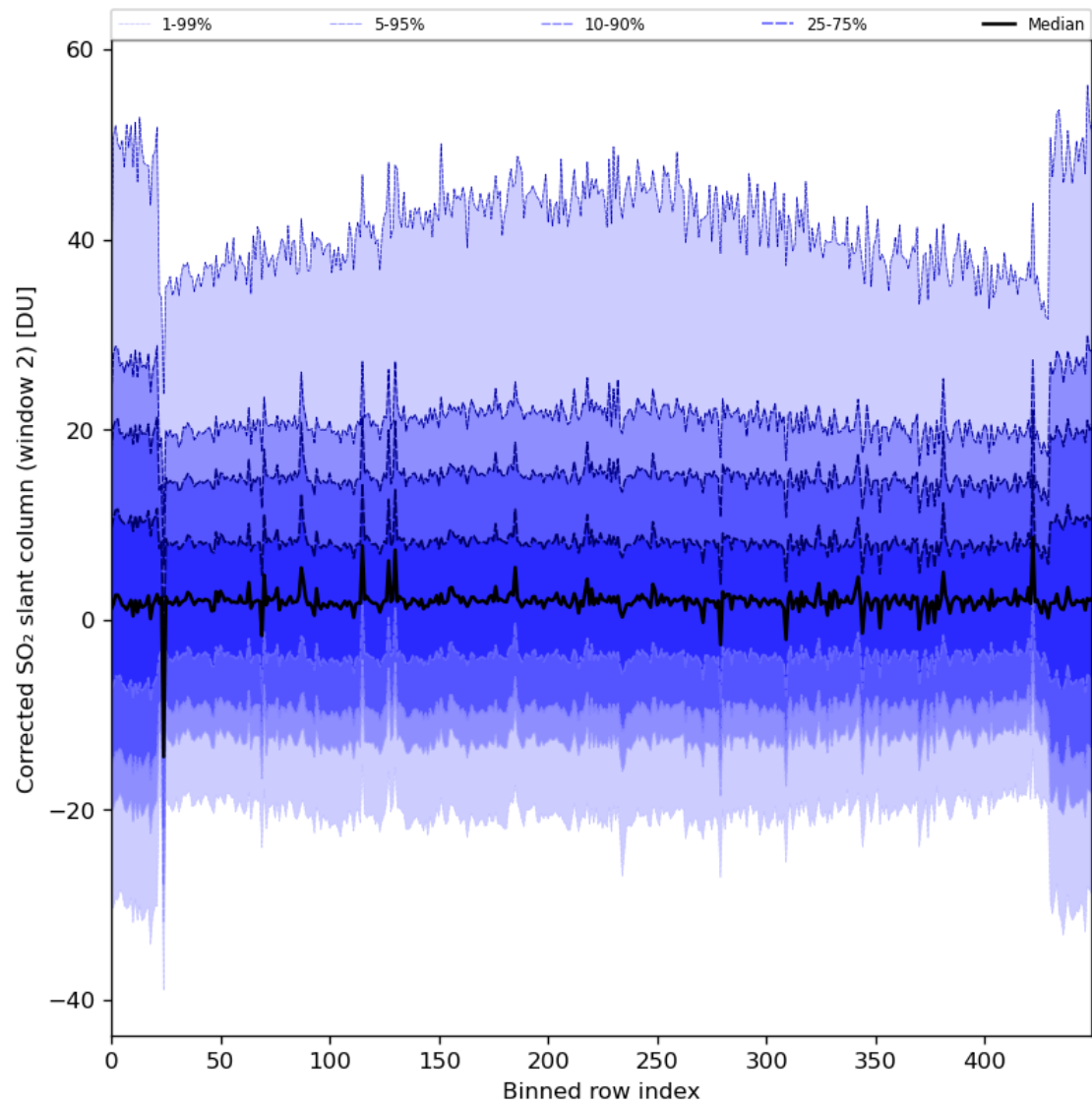
Figure 85: Along track statistics of “Corrected SO 2 slant column (window 2)” for 2024-04-13 to 2024-04-15
