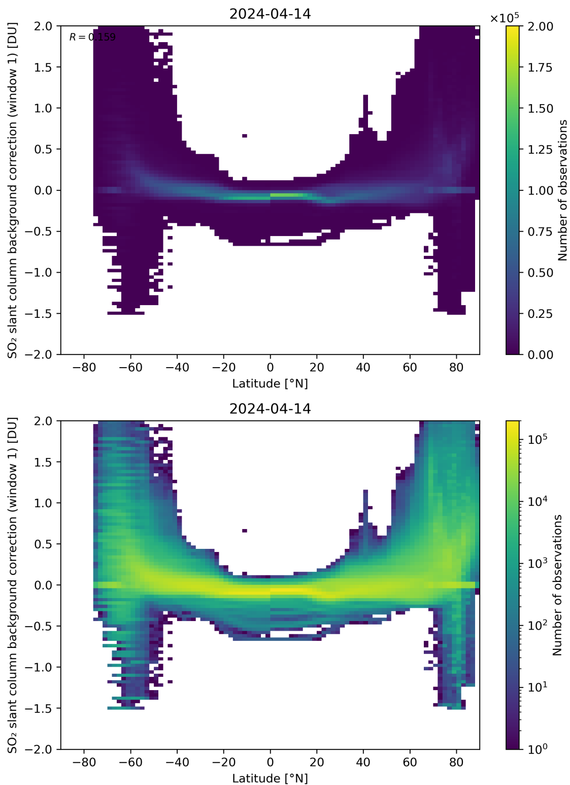
Figure 139: Scatter density plot of “Latitude” against “SO 2 slant column background correction (window 1)” for 2024-04-13 to 2024-04-15.
