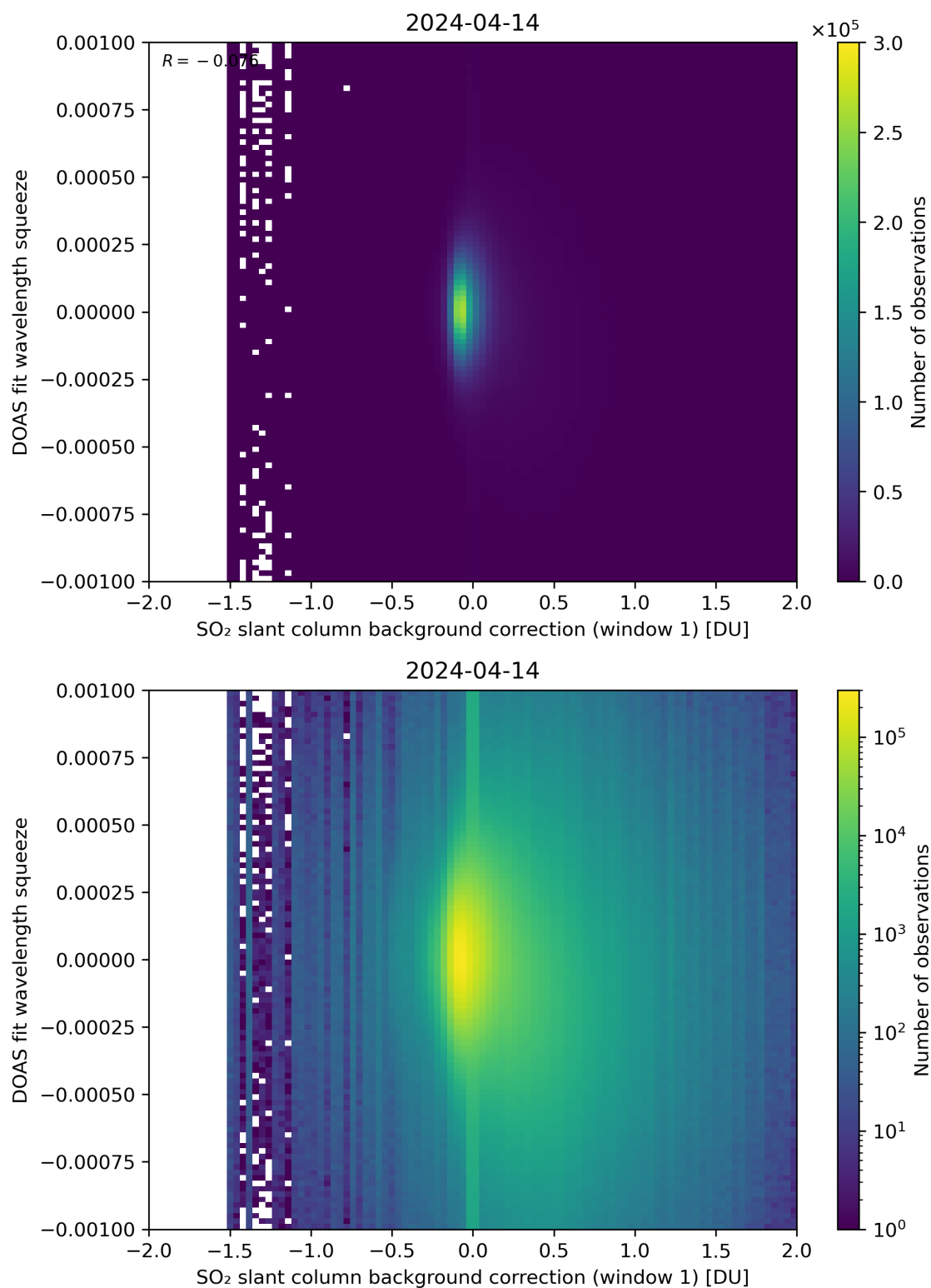
Figure 101: Scatter density plot of “SO 2 slant column background correction (window 1)” against “DOAS fit wavelength squeeze” for 2024-04-13 to 2024-04-15.
