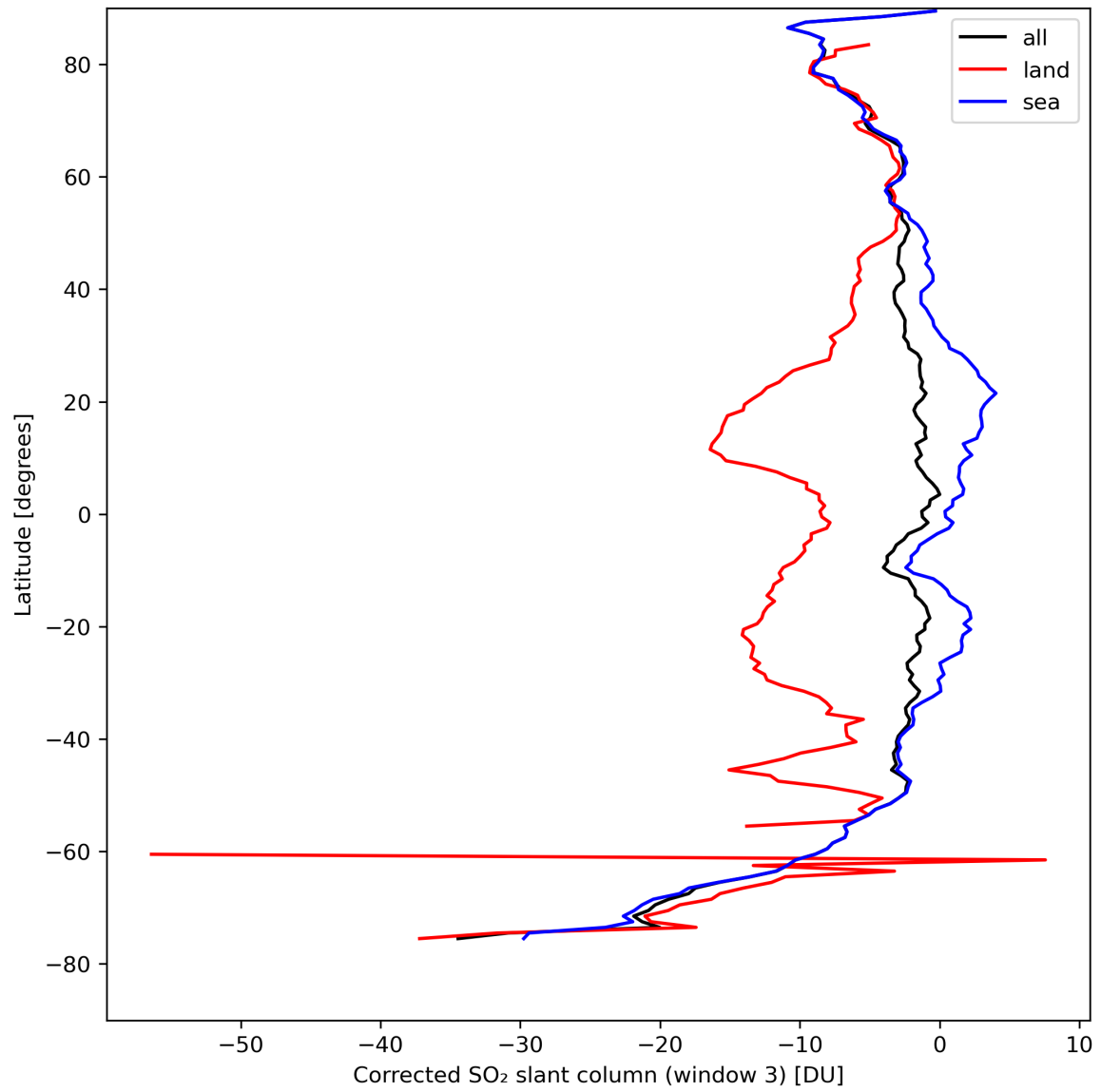
Figure 43: Zonal average of “Corrected SO 2 slant column (window 3)” for 2024-04-13 to 2024-04-15.
