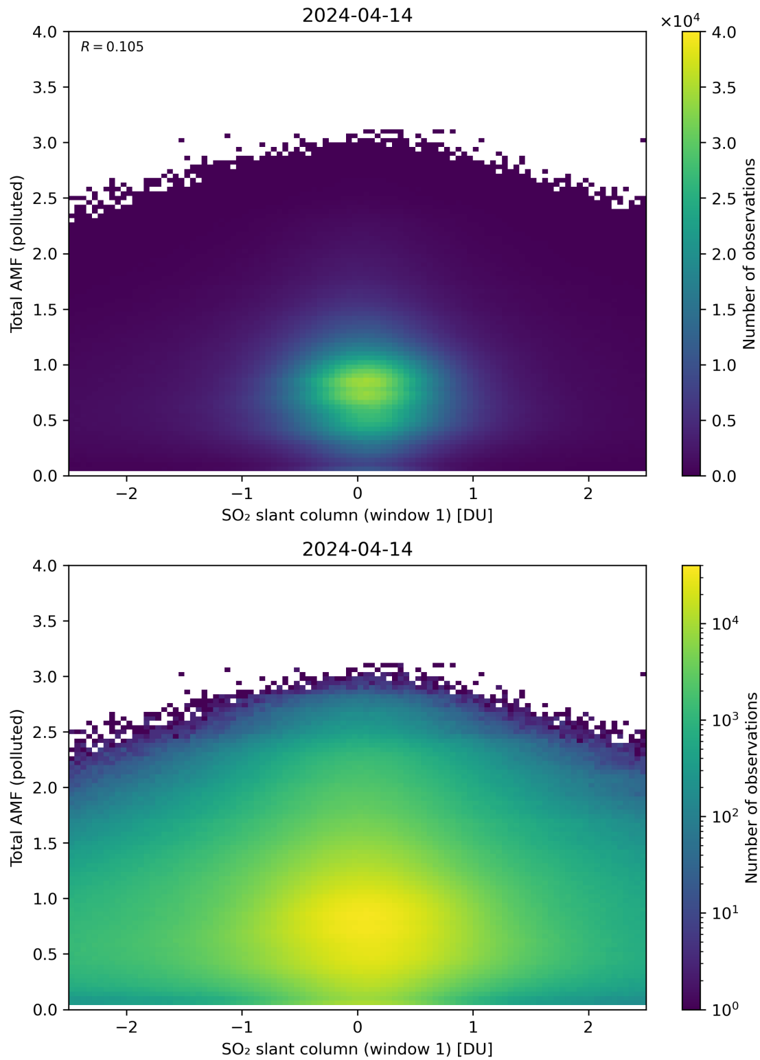
Figure 239: Scatter density plot of “SO 2 slant column (window 1)” against “Total AMF (polluted)” for 2024-04-13 to 2024-04-15.
