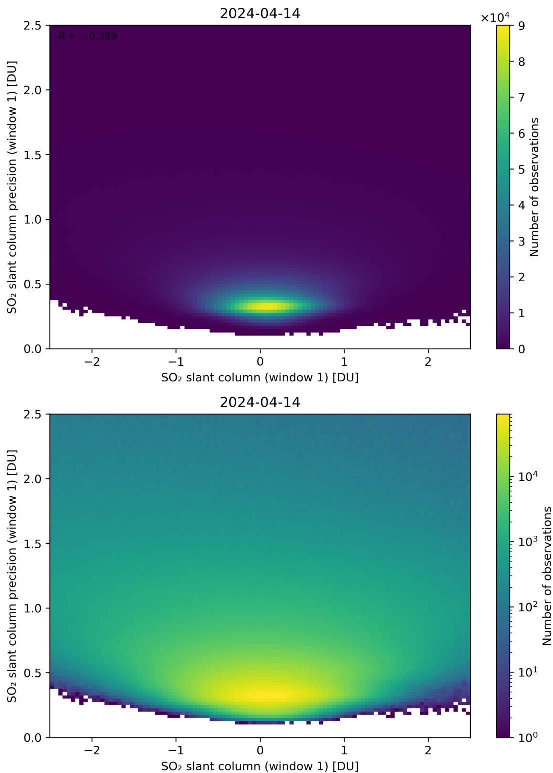
Figure 235: Scatter density plot of “SO 2 slant column (window 1)” against “SO 2 slant column precision (window 1)” for 2024-04-13 to 2024-04-15.
