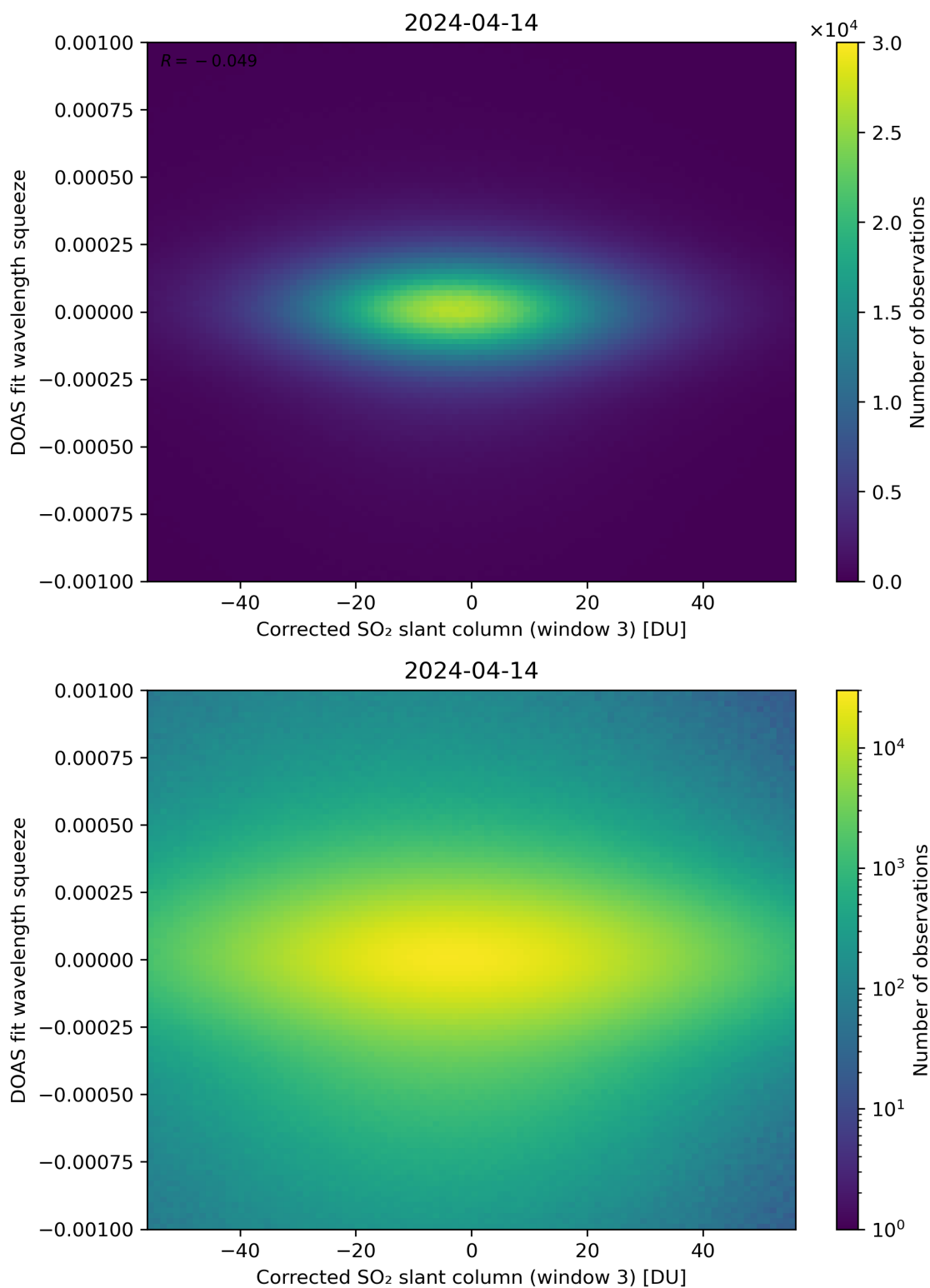
Figure 207: Scatter density plot of “Corrected SO 2 slant column (window 3)” against “DOAS fit wavelength squeeze” for 2024-04-13 to 2024-04-15.
