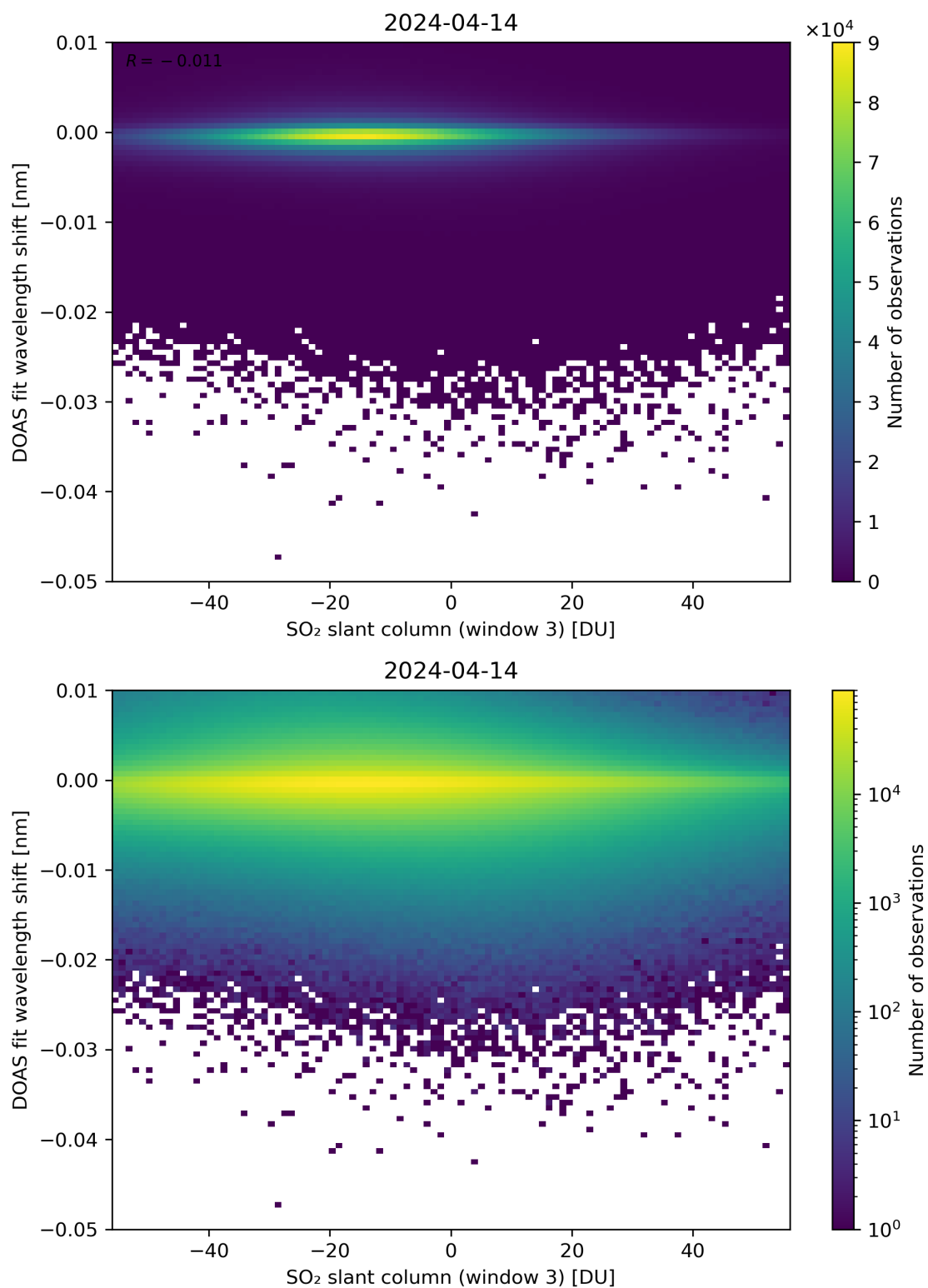
Figure 254: Scatter density plot of “SO 2 slant column (window 3)” against “DOAS fit wavelength shift” for 2024-04-13 to 2024-04-15.
