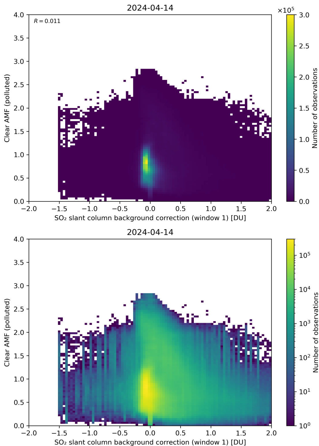
Figure 103: Scatter density plot of “SO 2 slant column background correction (window 1)” against “Clear AMF (polluted)” for 2024-04-13 to 2024-04-15.
