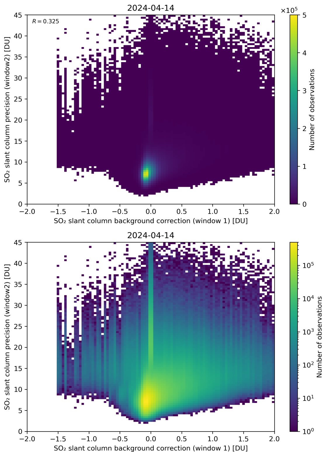
Figure 106: Scatter density plot of “SO 2 slant column background correction (window 1)” against “SO 2 slant column precision (window2)” for 2024-04-13 to 2024-04-15.
