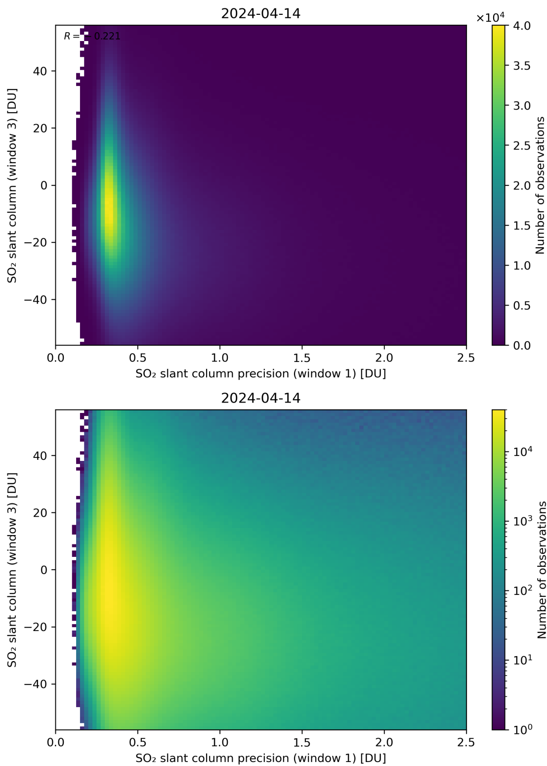
Figure 228: Scatter density plot of “SO 2 slant column precision (window 1)” against “SO 2 slant column (window 3)” for 2024-04-13 to 2024-04-15.
