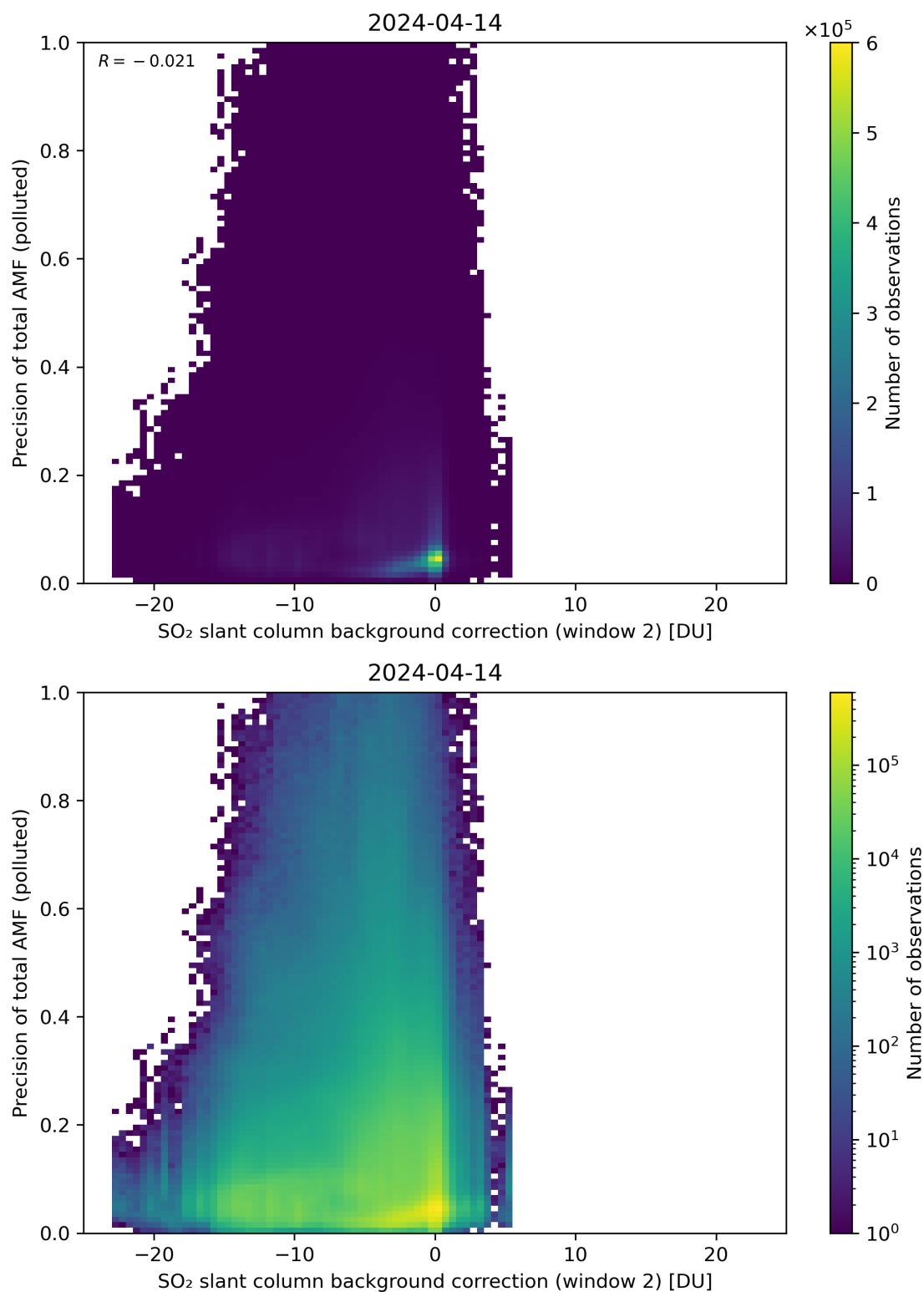
Figure 120: Scatter density plot of “SO 2 slant column background correction (window 2)” against “Precision of total AMF (polluted)” for 2024-04-13 to 2024-04-15.
