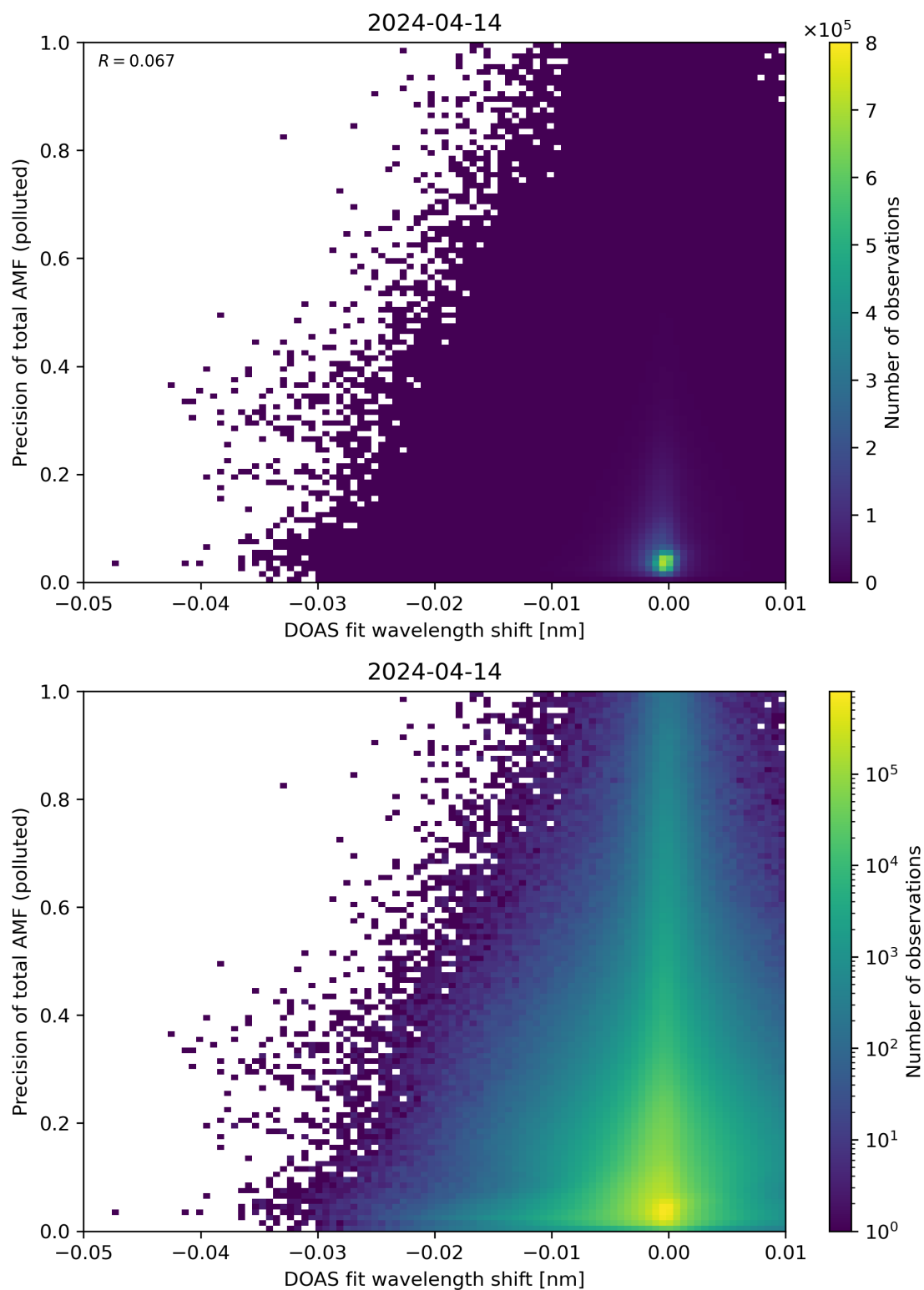
Figure 131: Scatter density plot of “DOAS fit wavelength shift” against “Precision of total AMF (polluted)” for 2024-04-13 to 2024-04-15.
