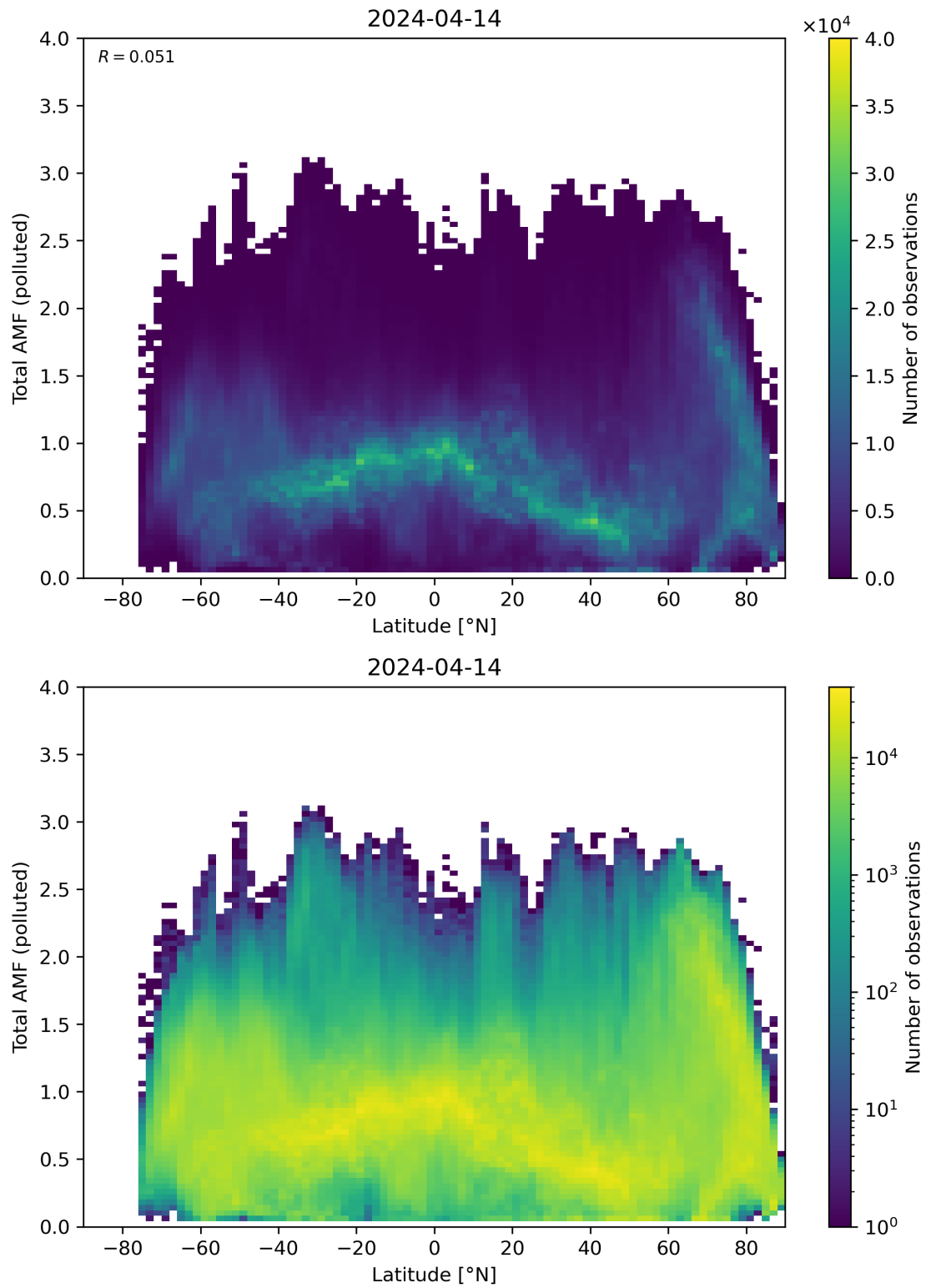
Figure 154: Scatter density plot of “Latitude” against “Total AMF (polluted)” for 2024-04-13 to 2024-04-15.
