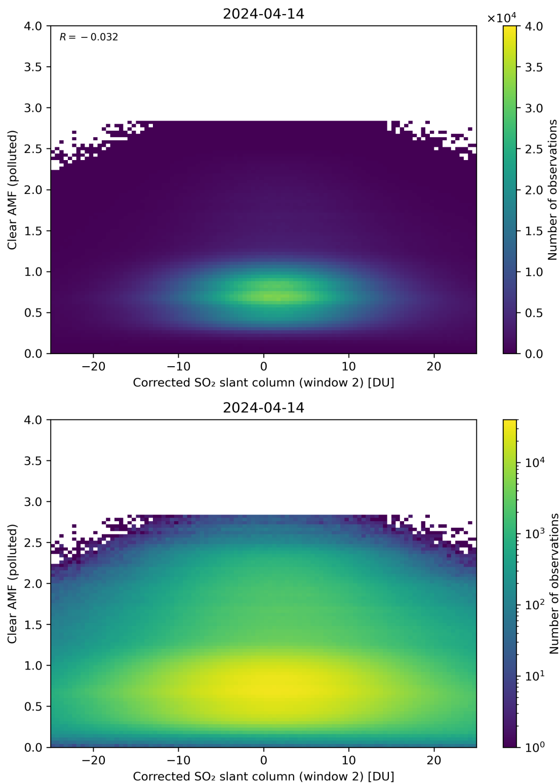
Figure 199: Scatter density plot of “Corrected SO 2 slant column (window 2)” against “Clear AMF (polluted)” for 2024-04-13 to 2024-04-15.
