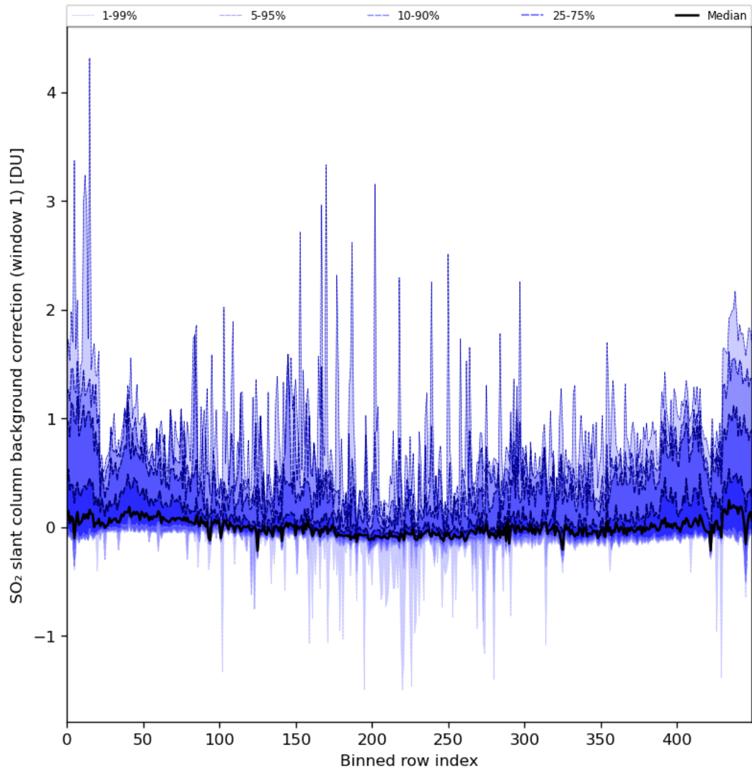
Figure 82: Along track statistics of “SO 2 slant column background correction (window 1)” for 2024-04-13 to 2024-04-15
