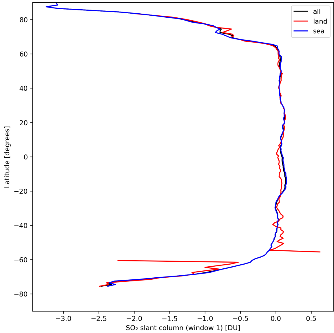
Figure 33: Zonal average of “SO 2 slant column (window 1)” for 2024-04-13 to 2024-04-15.
