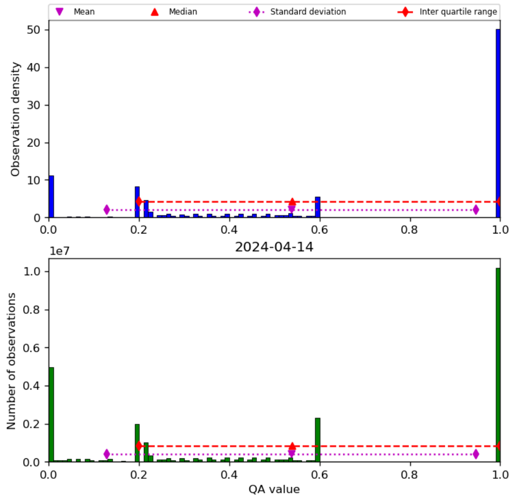
Figure 52: Histogram of “QA value” for 2024-04-13 to 2024-04-15
