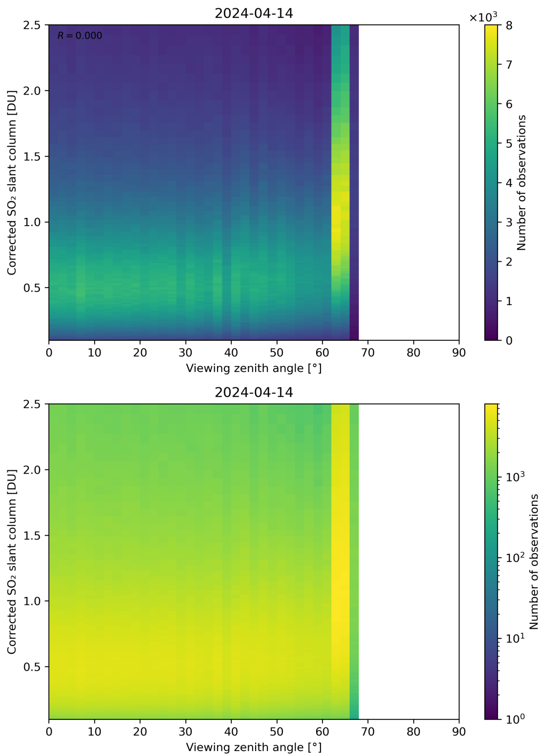
Figure 317: Scatter density plot of “Viewing zenith angle” against “Corrected SO 2 slant column” for 2024-04-13 to 2024-04-15.
