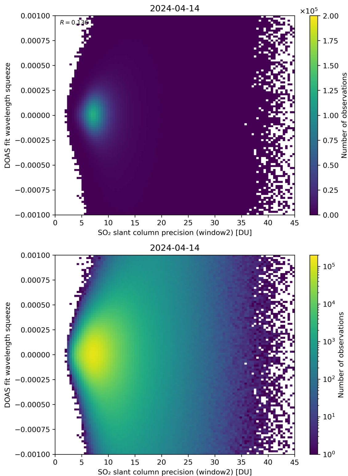
Figure 244: Scatter density plot of “SO 2 slant column precision (window2)” against “DOAS fit wavelength squeeze” for 2024-04-13 to 2024-04-15.
