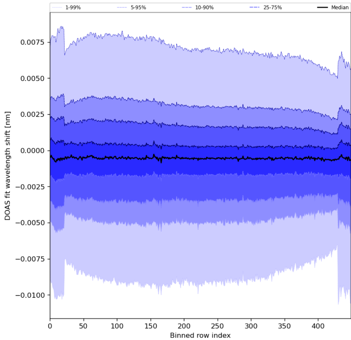
Figure 91: Along track statistics of “DOAS fit wavelength shift” for 2024-04-13 to 2024-04-15
