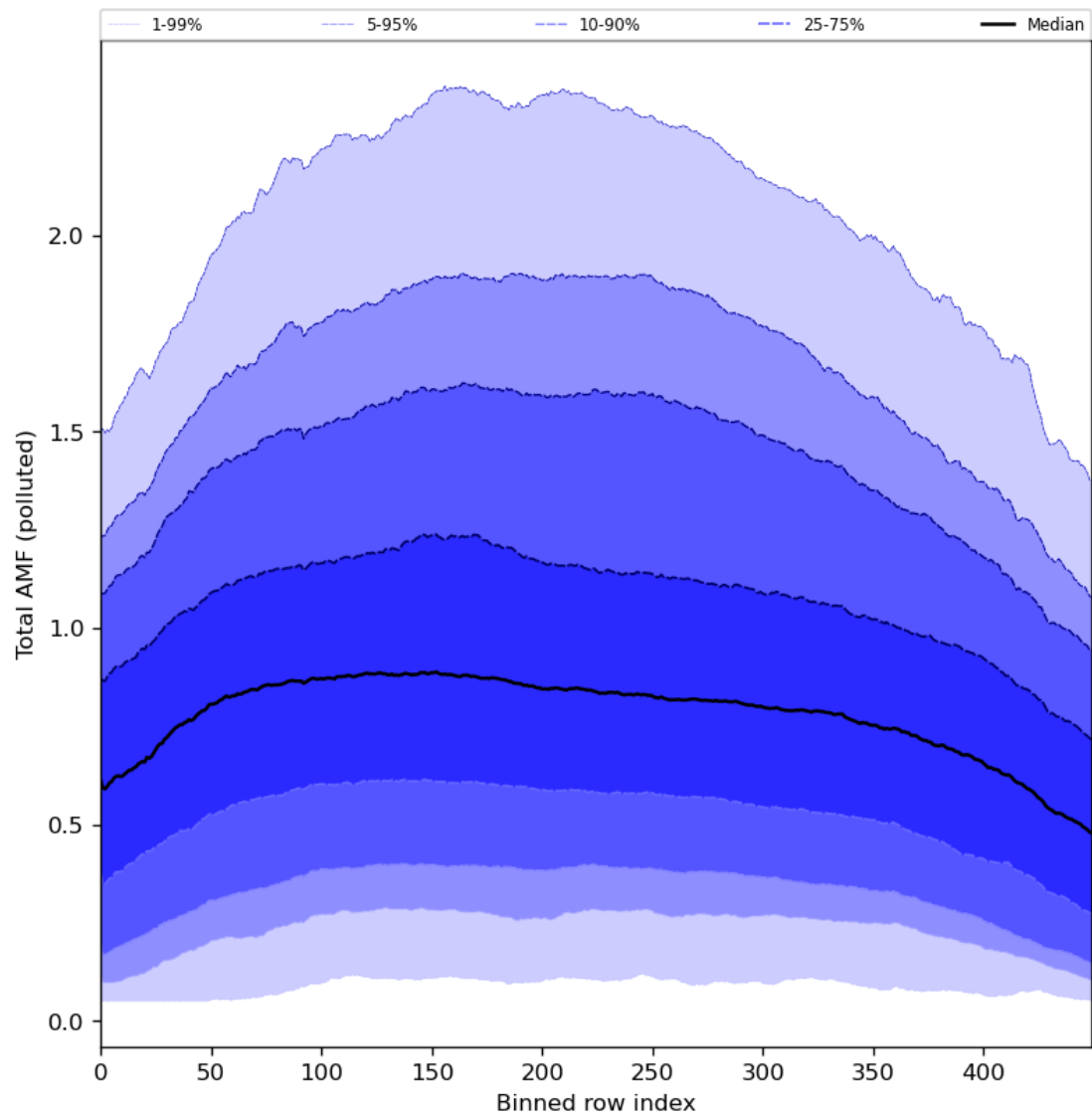
Figure 94: Along track statistics of “Total AMF (polluted)” for 2024-04-13 to 2024-04-15
