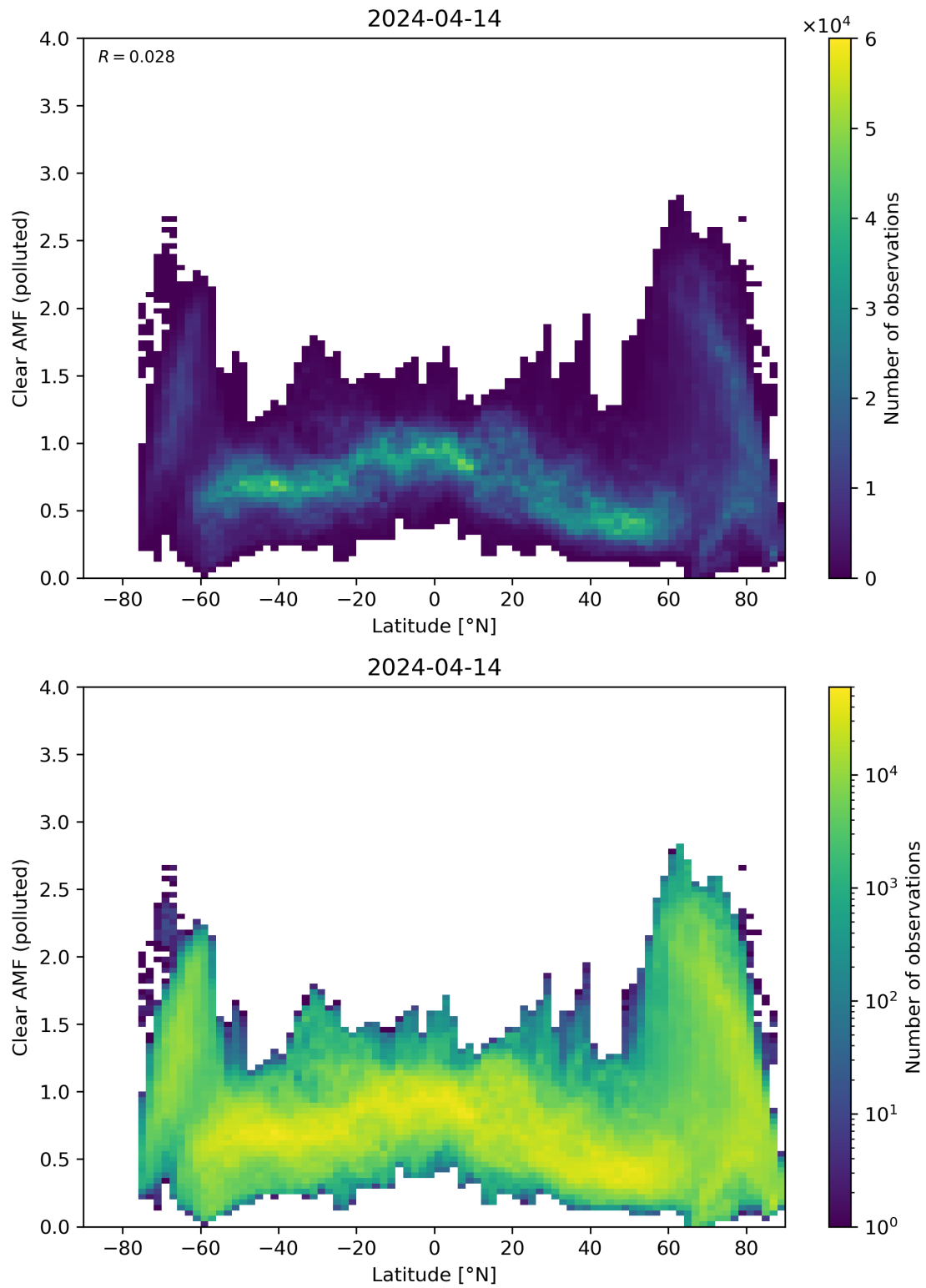
Figure 145: Scatter density plot of “Latitude” against “Clear AMF (polluted)” for 2024-04-13 to 2024-04-15.
