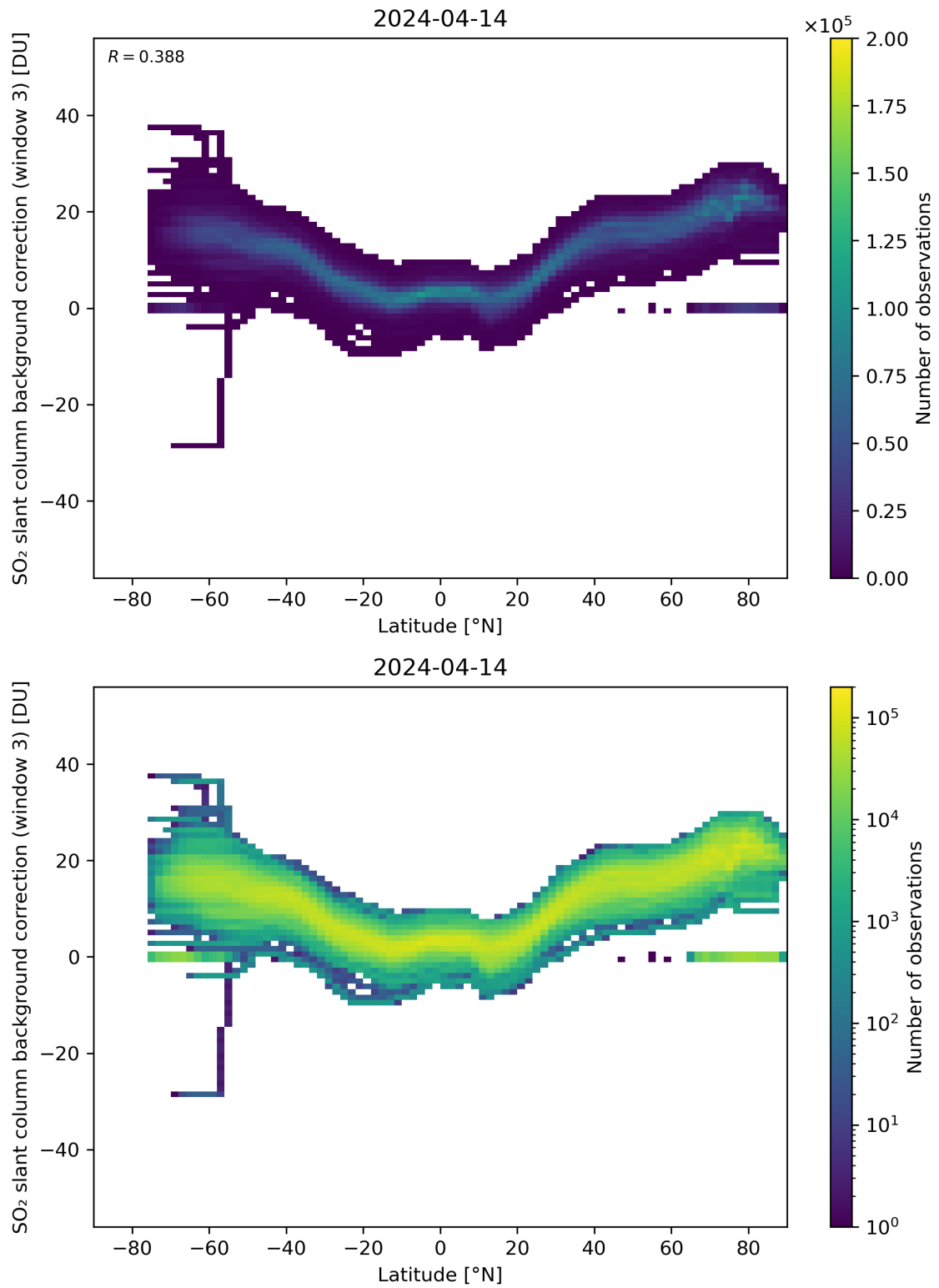
Figure 141: Scatter density plot of “Latitude” against “SO 2 slant column background correction (window 3)” for 2024-04-13 to 2024-04-15.
