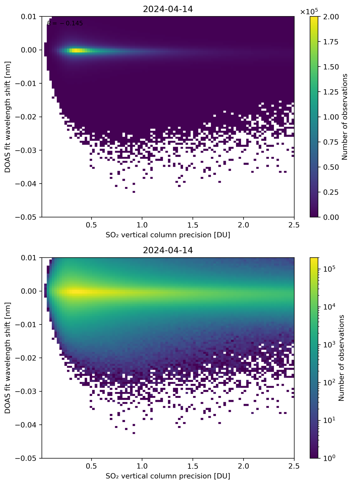
Figure 282: Scatter density plot of “SO 2 vertical column precision” against “DOAS fit wavelength shift” for 2024-04-13 to 2024-04-15.
