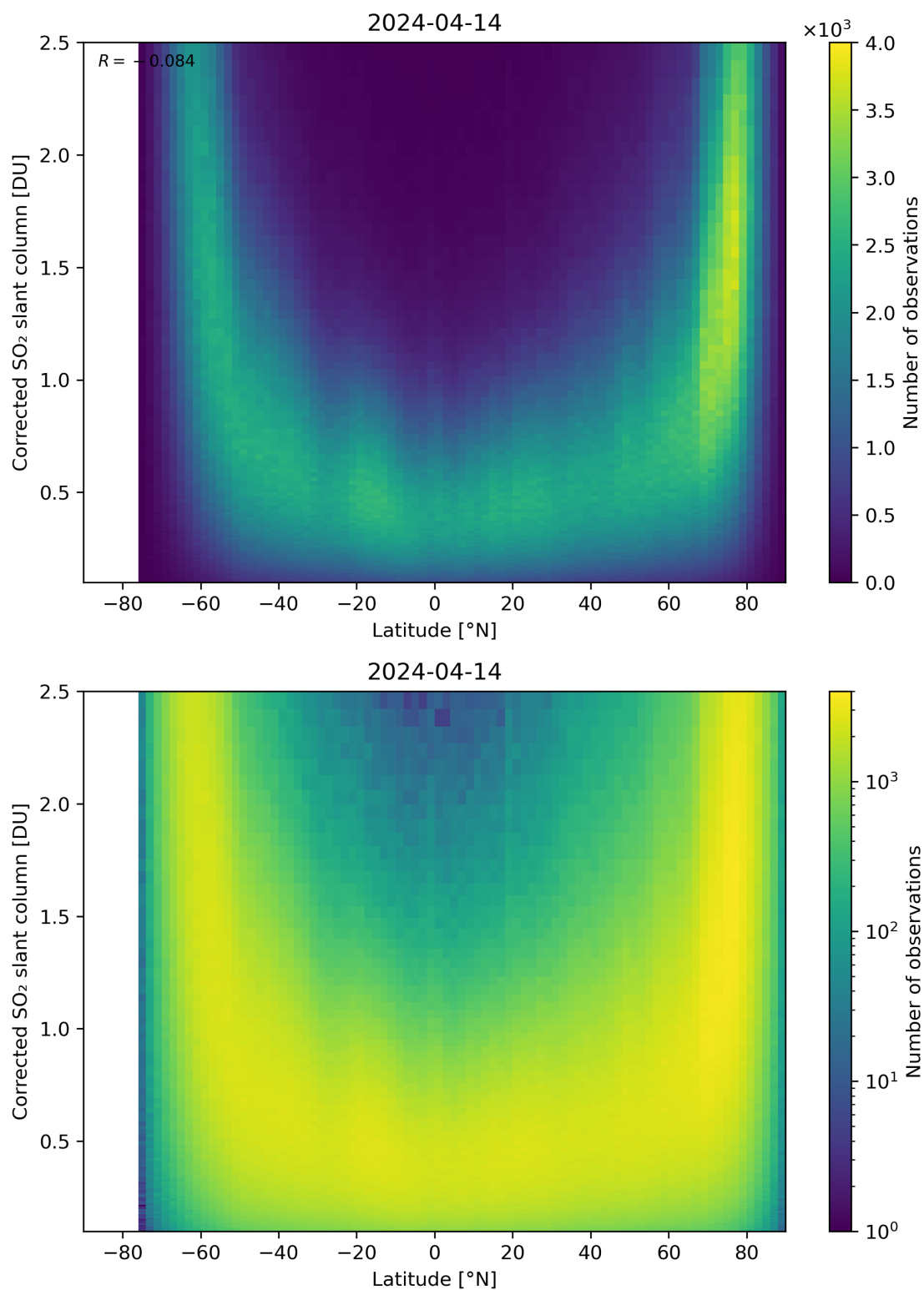
Figure 146: Scatter density plot of “Latitude” against “Corrected SO 2 slant column” for 2024-04-13 to 2024-04-15.
