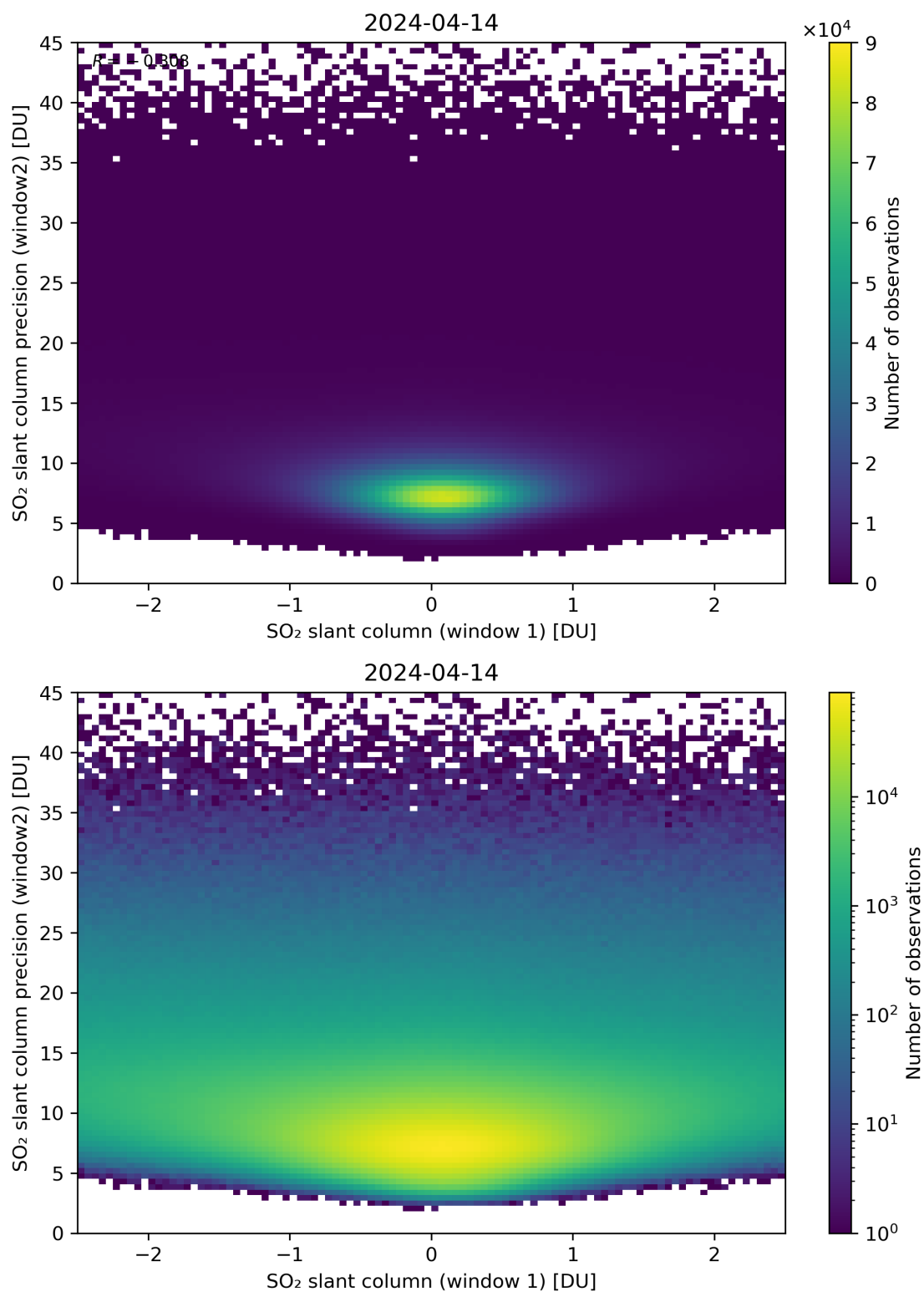
Figure 236: Scatter density plot of “SO 2 slant column (window 1)” against “SO 2 slant column precision (window2)” for 2024-04-13 to 2024-04-15.
