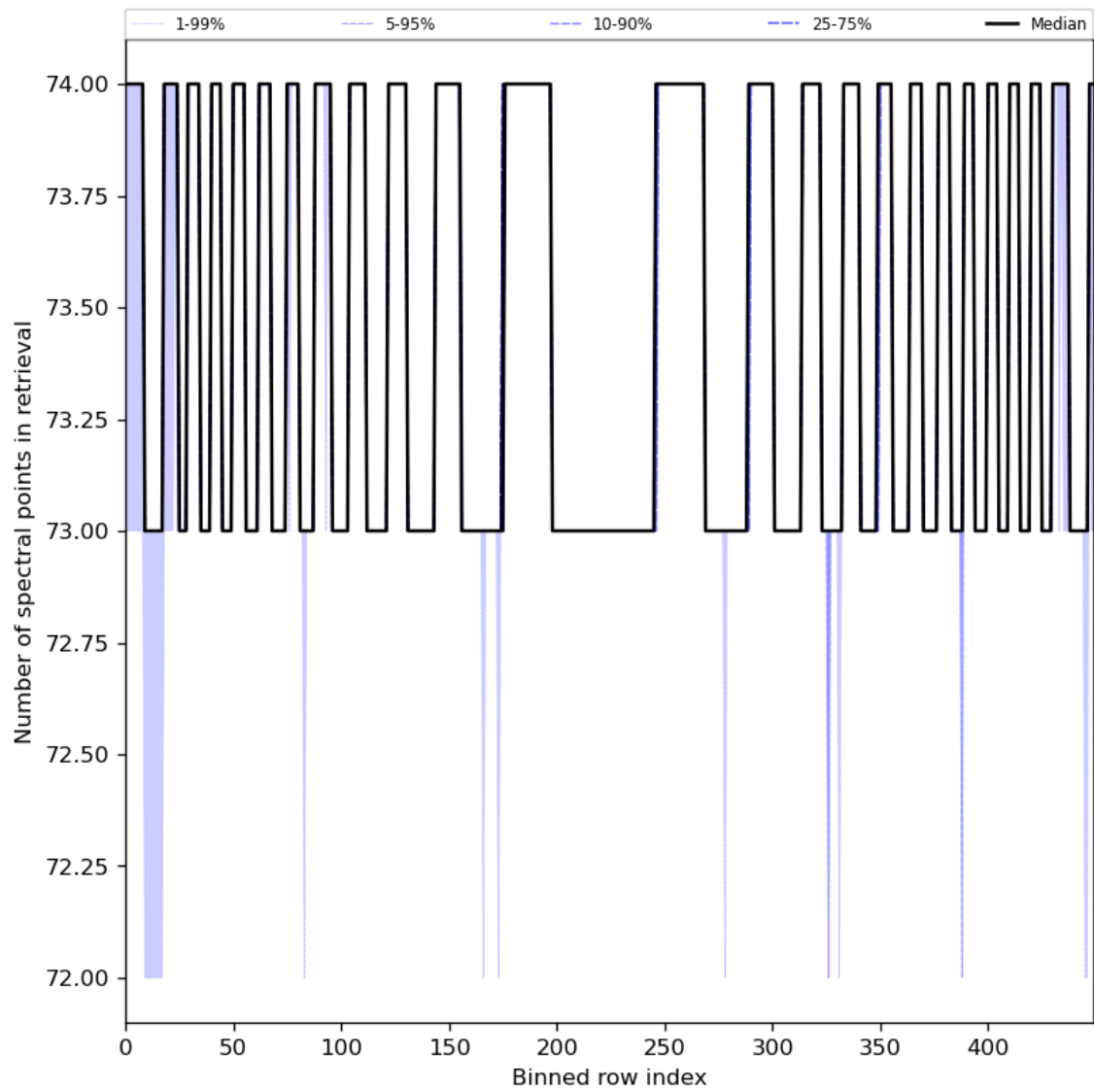
Figure 97: Along track statistics of “Number of spectral points in retrieval” for 2024-04-13 to 2024-04-15
