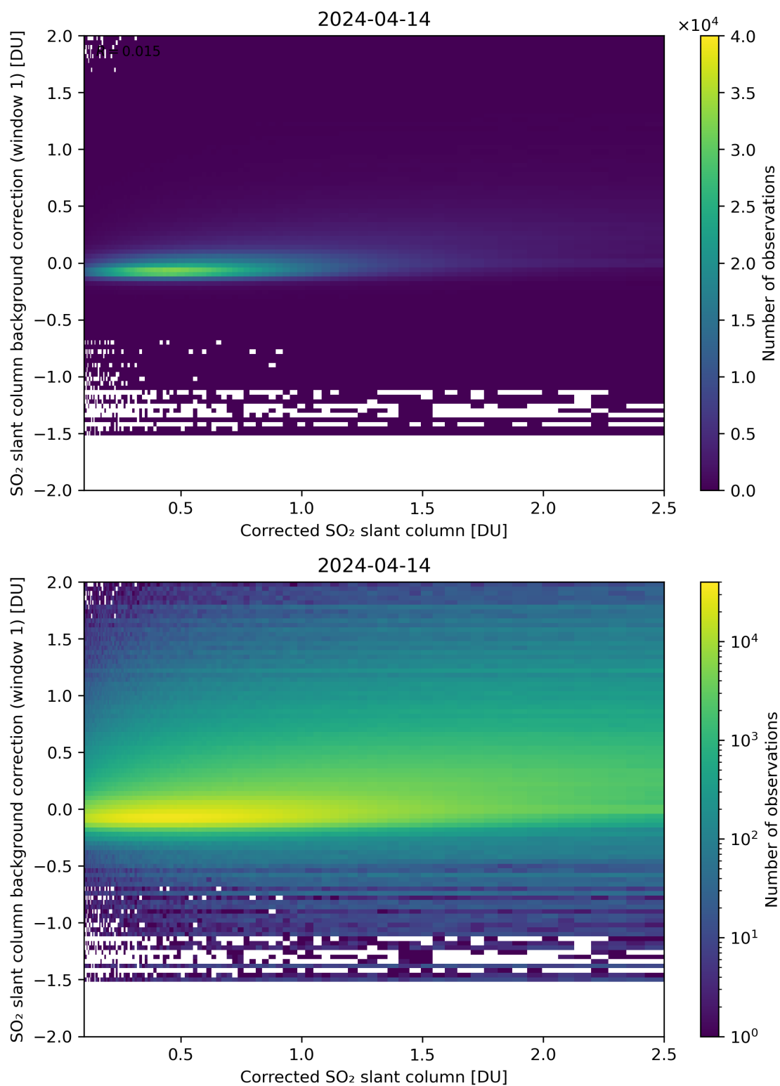
Figure 178: Scatter density plot of “Corrected SO 2 slant column” against “SO 2 slant column background correction (window 1)” for 2024-04-13 to 2024-04-15.
