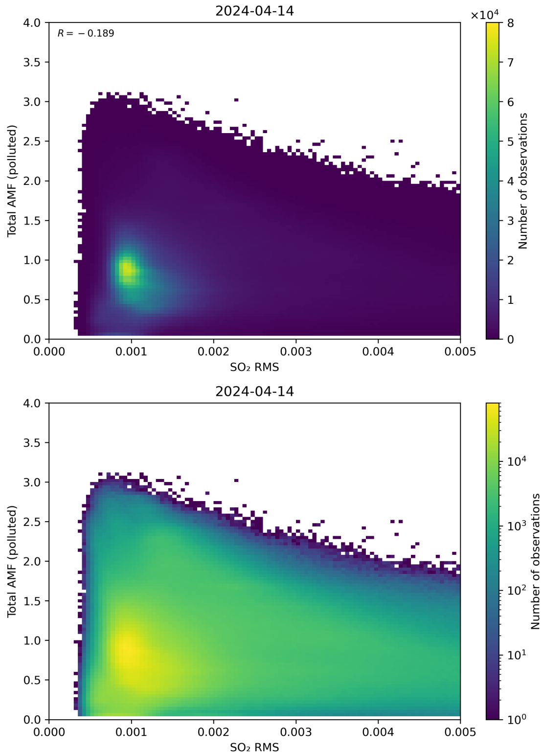
Figure 137: Scatter density plot of “SO 2 RMS” against “Total AMF (polluted)” for 2024-04-13 to 2024-04-15.
