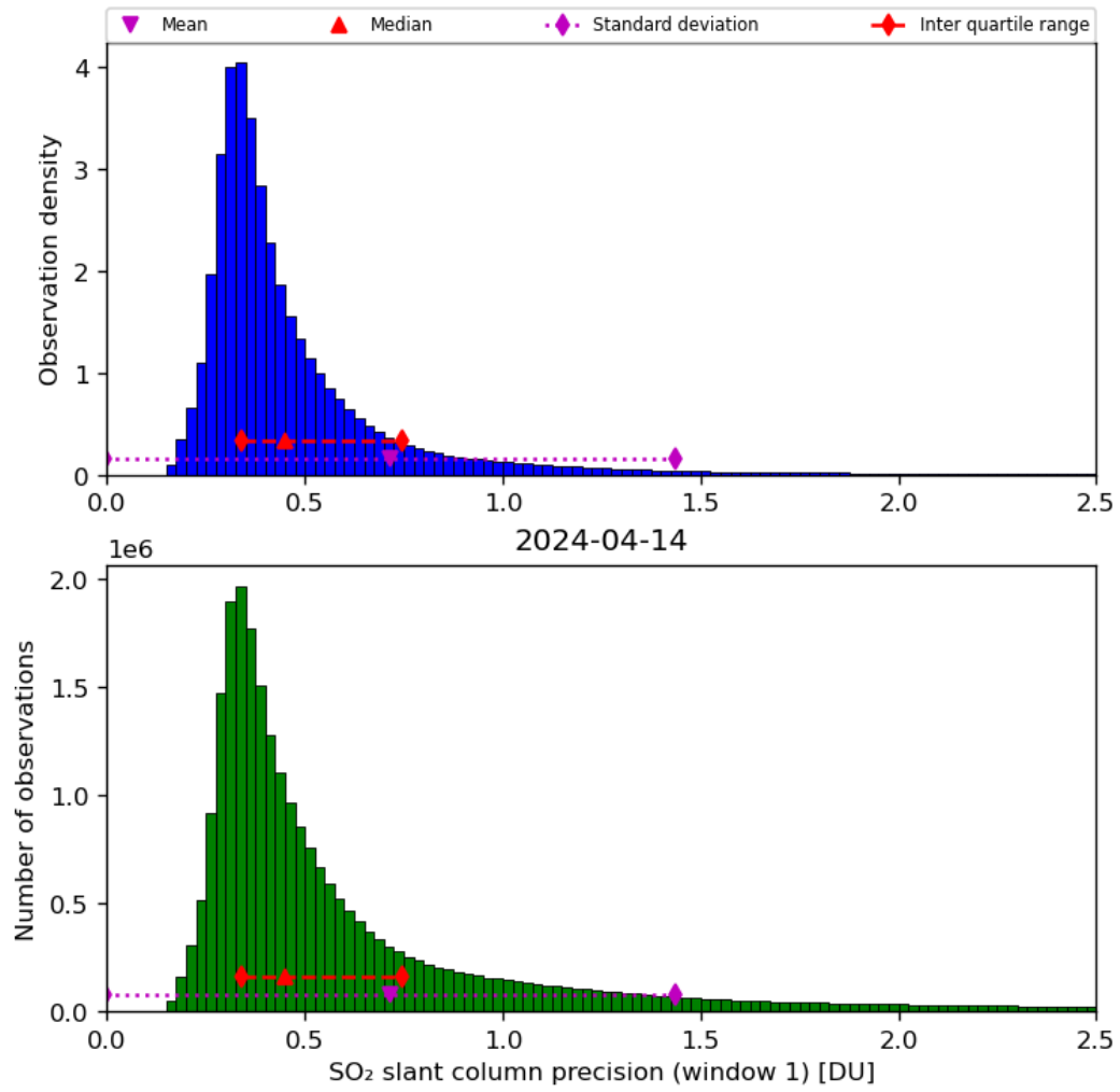
Figure 57: Histogram of “SO 2 slant column precision (window 1)” for 2024-04-13 to 2024-04-15
