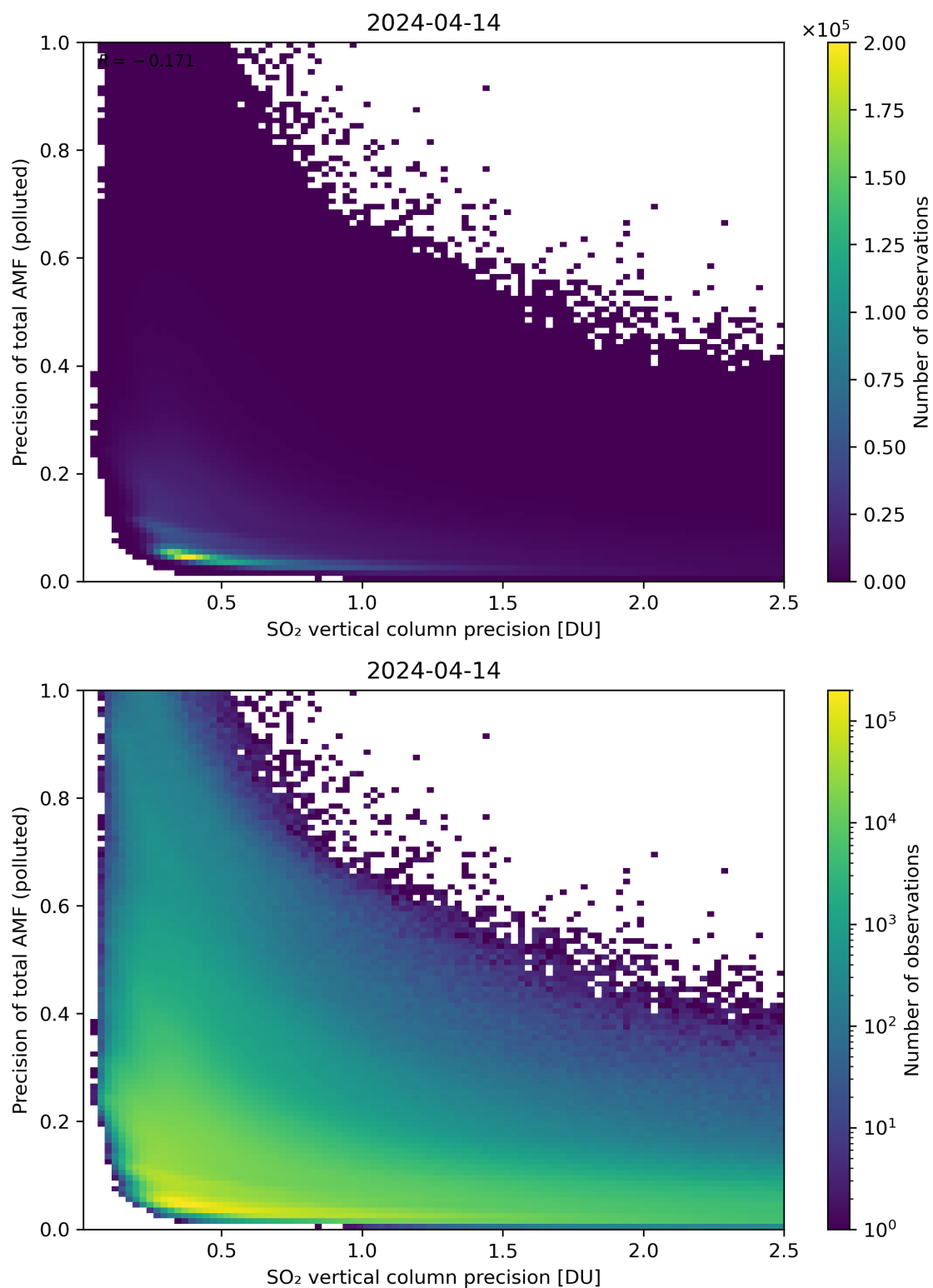
Figure 295: Scatter density plot of “SO 2 vertical column precision” against “Precision of total AMF (polluted)” for 2024-04-13 to 2024-04-15.
