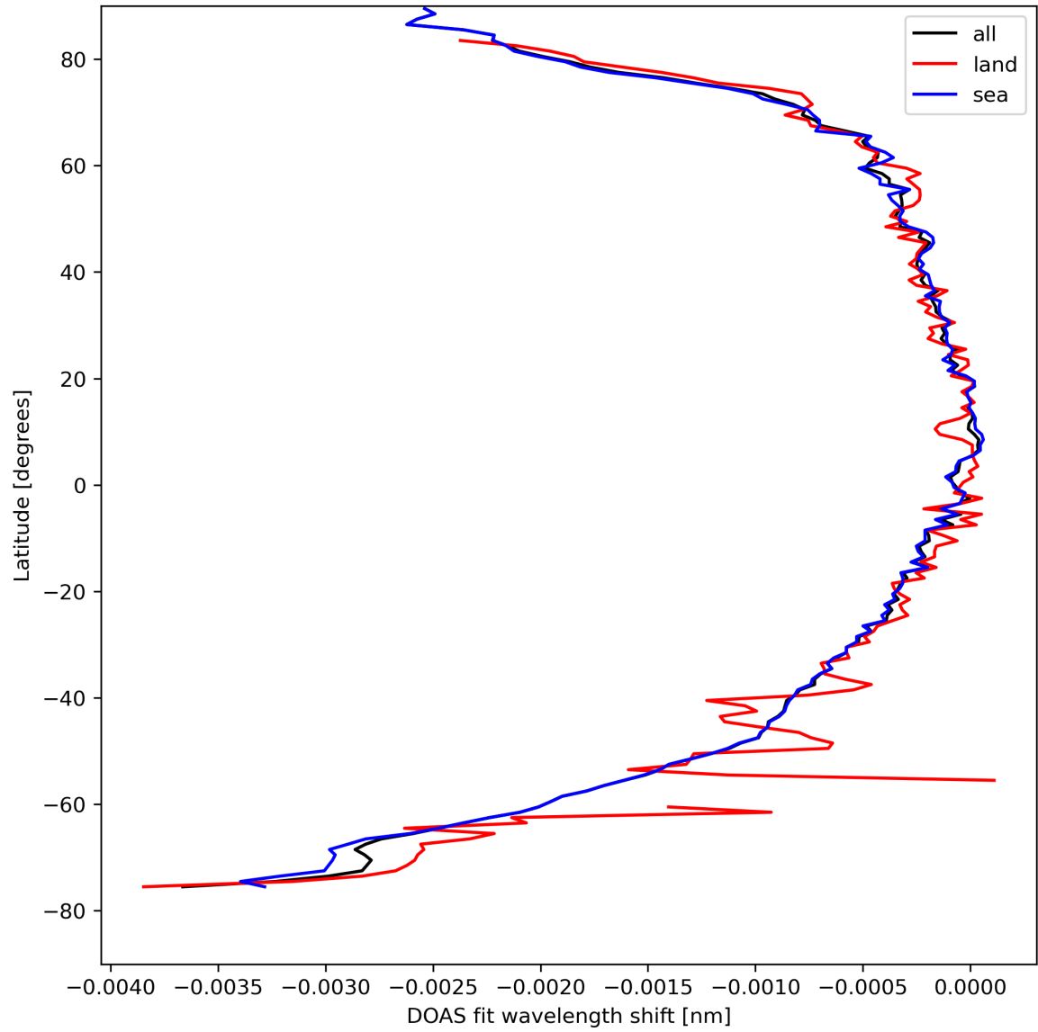
Figure 45: Zonal average of “DOAS fit wavelength shift” for 2024-04-13 to 2024-04-15.
