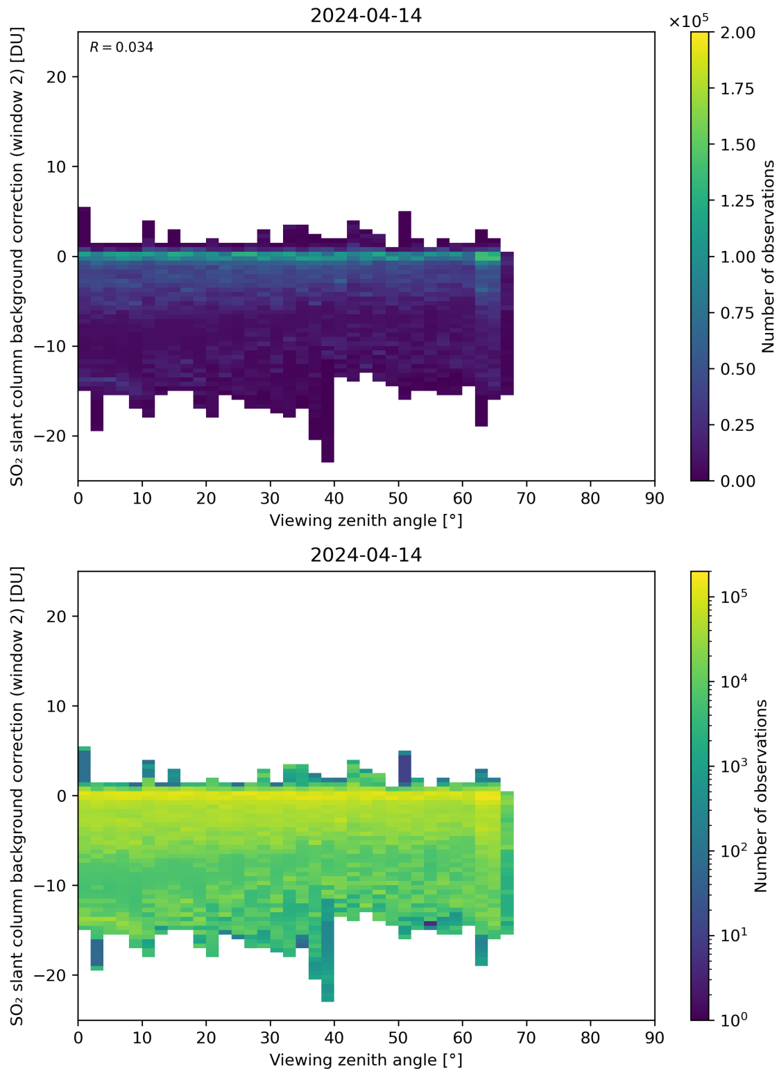
Figure 309: Scatter density plot of “Viewing zenith angle” against “SO 2 slant column background correction (window 2)” for 2024-04-13 to 2024-04-15.
