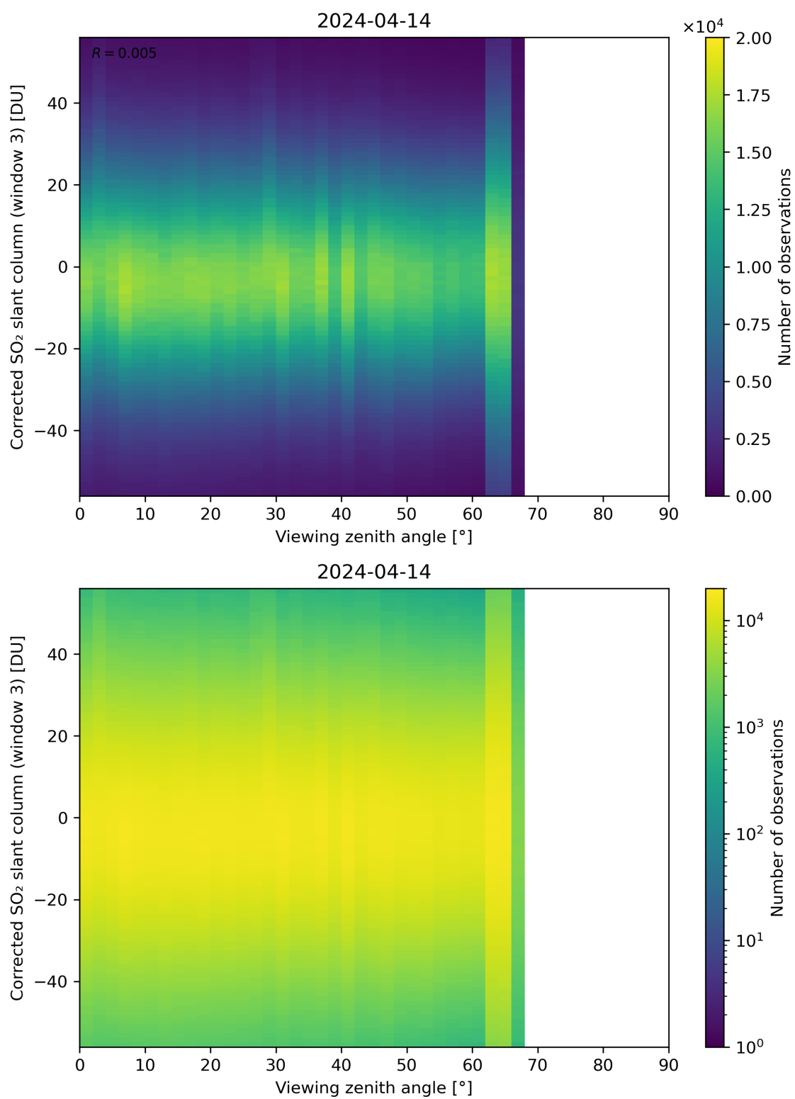
Figure 319: Scatter density plot of “Viewing zenith angle” against “Corrected SO 2 slant column (window 3)” for 2024-04-13 to 2024-04-15.
