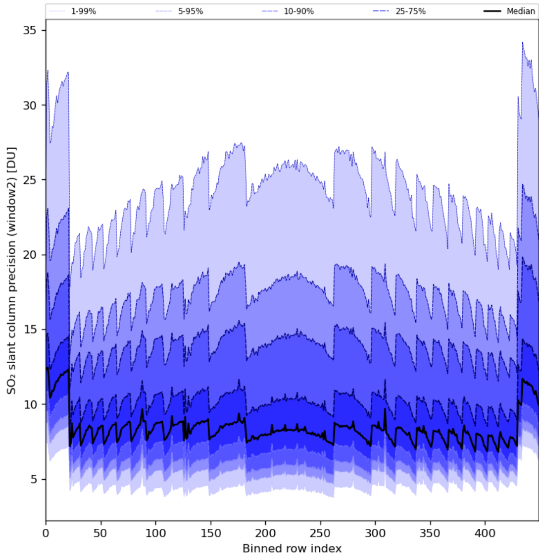
Figure 84: Along track statistics of “SO 2 slant column precision (window2)” for 2024-04-13 to 2024-04-15
