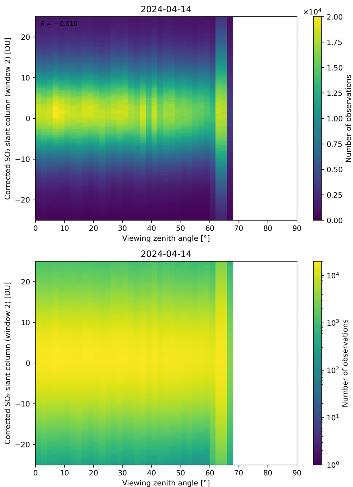
Figure 318: Scatter density plot of “Viewing zenith angle” against “Corrected SO 2 slant column (window 2)” for 2024-04-13 to 2024-04-15.
