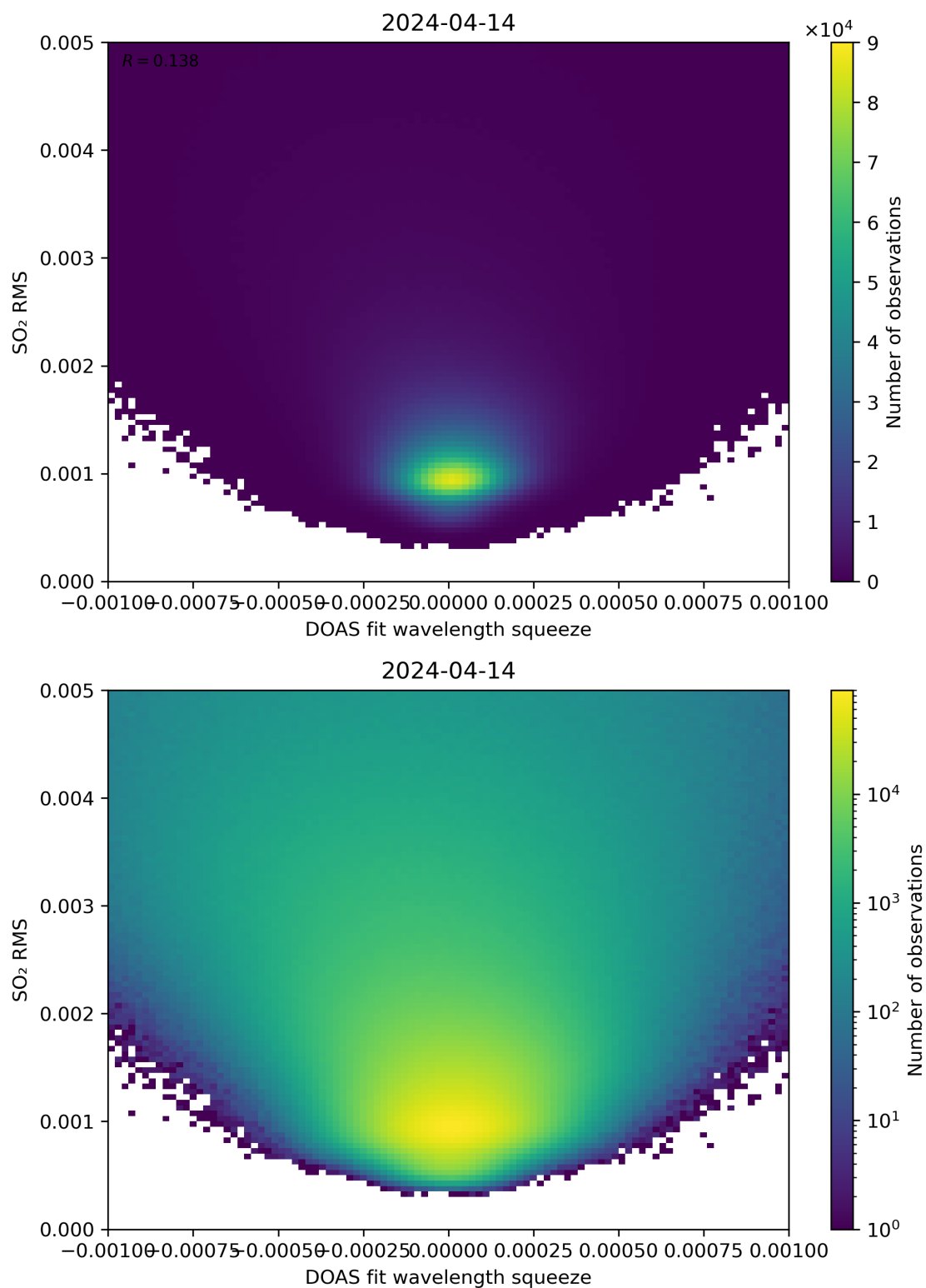
Figure 132: Scatter density plot of “DOAS fit wavelength squeeze” against “SO 2 RMS” for 2024-04-13 to 2024-04-15.
