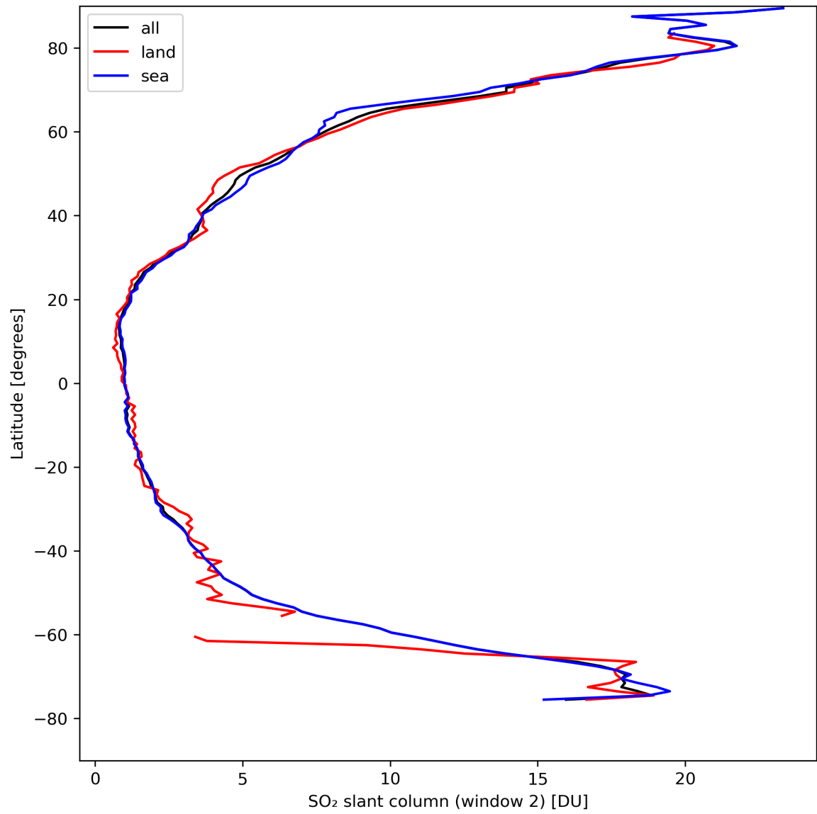
Figure 37: Zonal average of “SO 2 slant column (window 2)” for 2024-04-13 to 2024-04-15.
