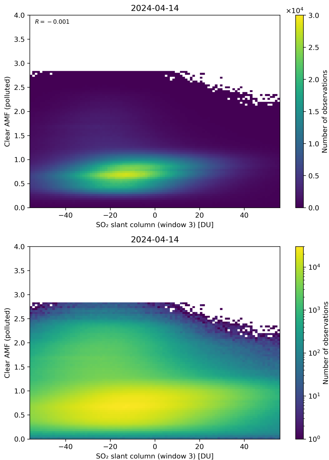
Figure 265: Scatter density plot of “SO 2 slant column (window 3)” against “Clear AMF (polluted)” for 2024-04-13 to 2024-04-15.
