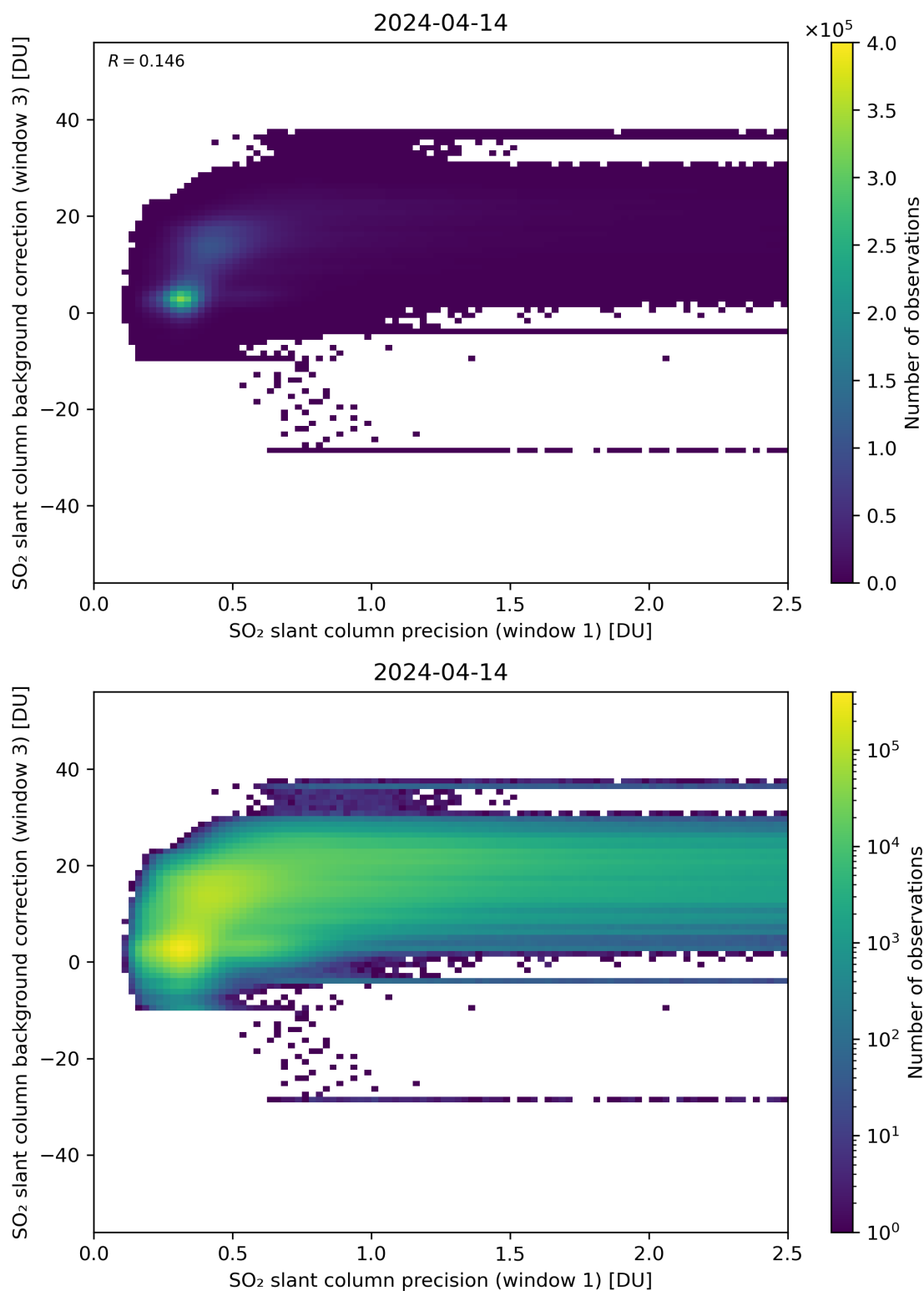
Figure 220: Scatter density plot of “SO 2 slant column precision (window 1)” against “SO 2 slant column background correction (window 3)” for 2024-04-13 to 2024-04-15.
