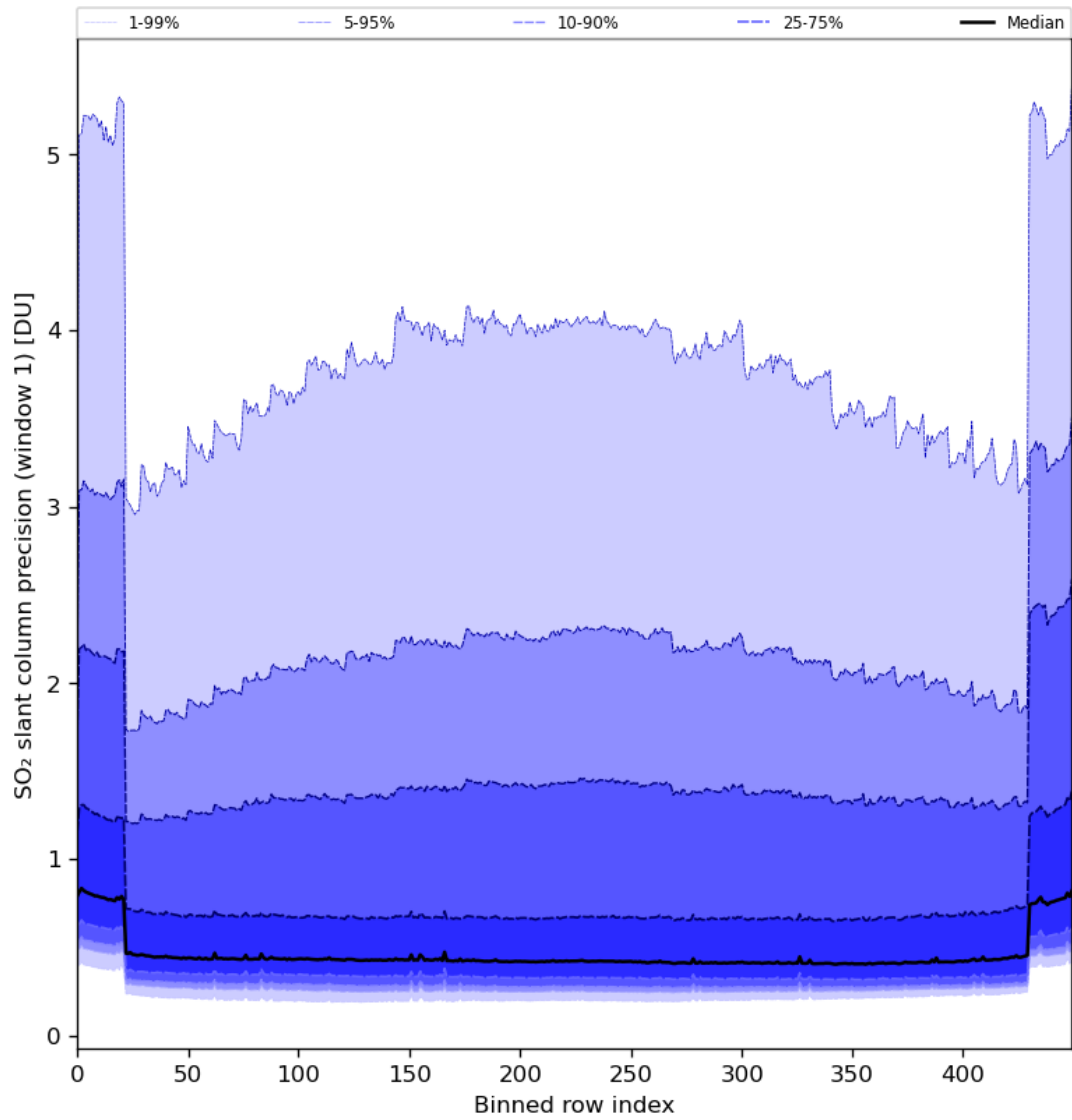
Figure 80: Along track statistics of “SO 2 slant column precision (window 1)” for 2024-04-13 to 2024-04-15
