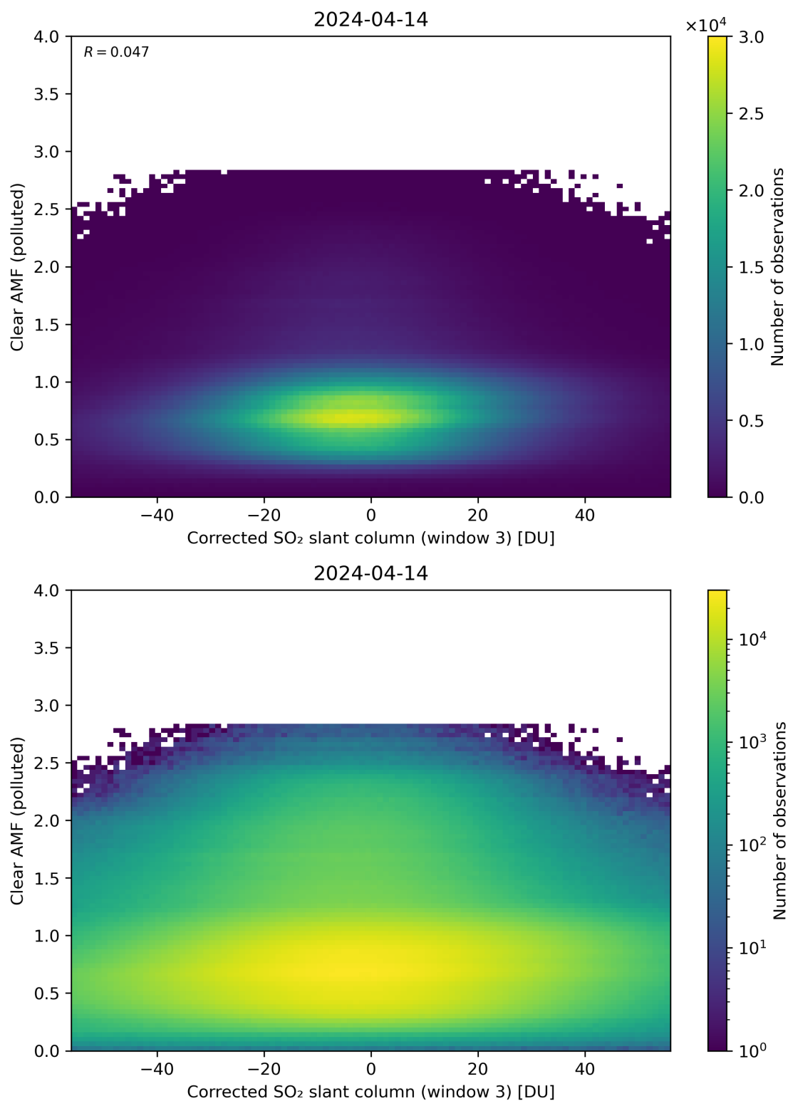
Figure 209: Scatter density plot of “Corrected SO 2 slant column (window 3)” against “Clear AMF (polluted)” for 2024-04-13 to 2024-04-15.
