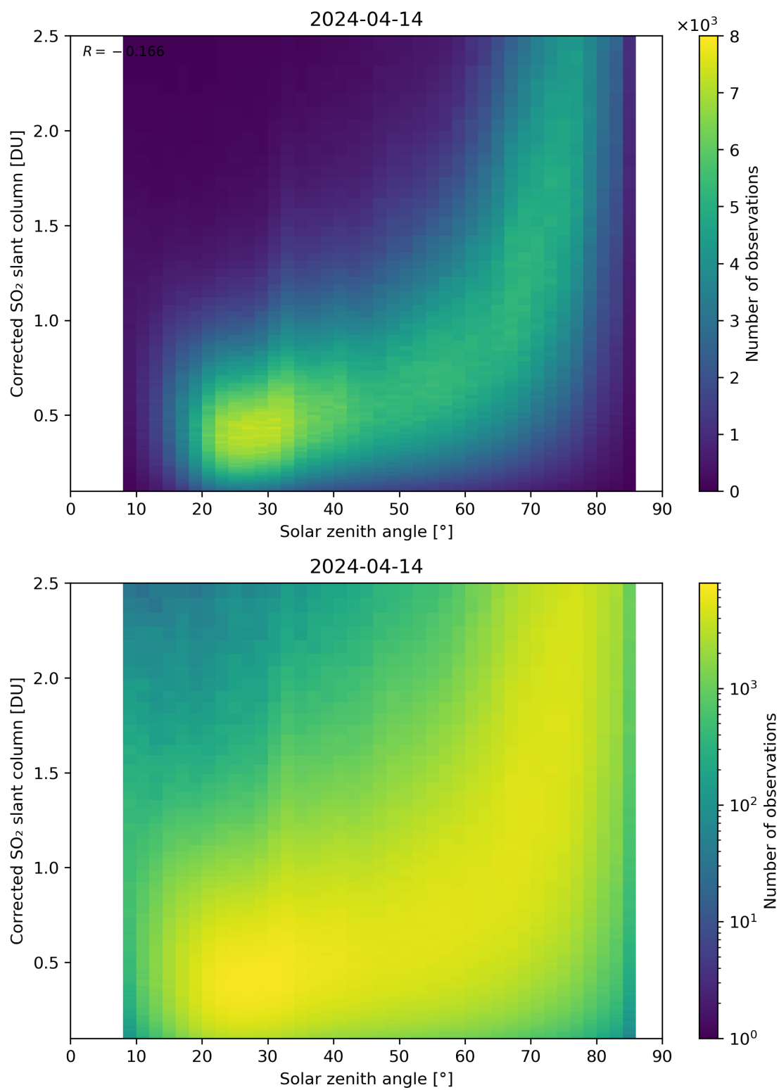
Figure 166: Scatter density plot of “Solar zenith angle” against “Corrected SO 2 slant column” for 2024-04-13 to 2024-04-15.
