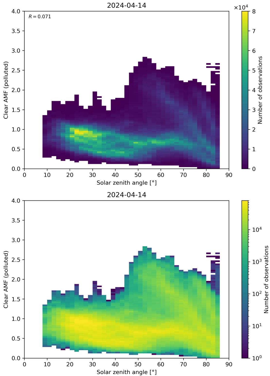
Figure 165: Scatter density plot of “Solar zenith angle” against “Clear AMF (polluted)” for 2024-04-13 to 2024-04-15.
