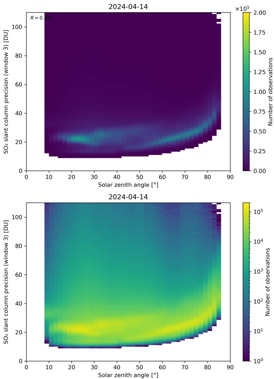
Figure 173: Scatter density plot of “Solar zenith angle” against “SO 2 slant column precision (window 3)” for 2024-04-13 to 2024-04-15.
