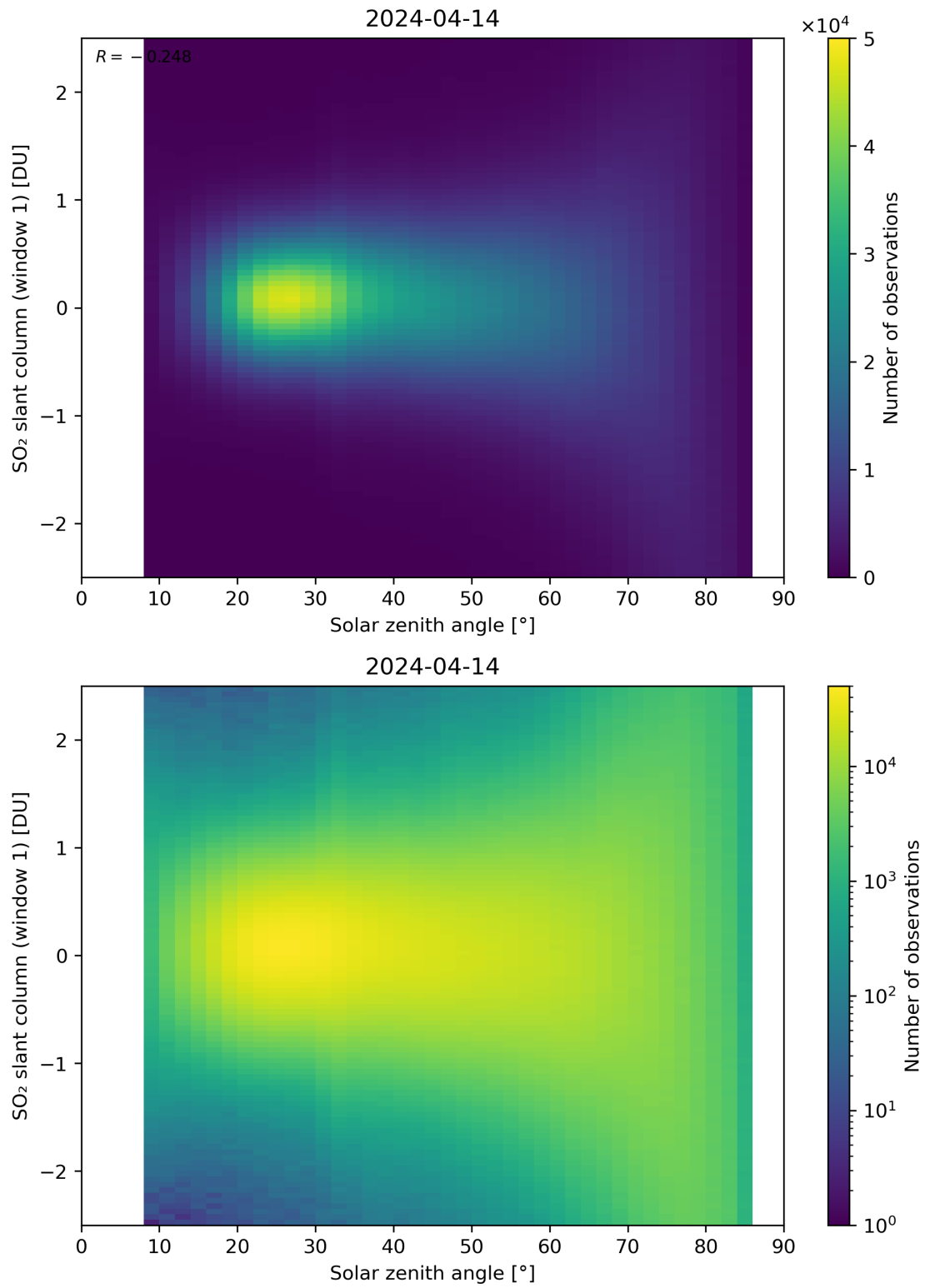
Figure 169: Scatter density plot of “Solar zenith angle” against “SO 2 slant column (window 1)” for 2024-04-13 to 2024-04-15.
