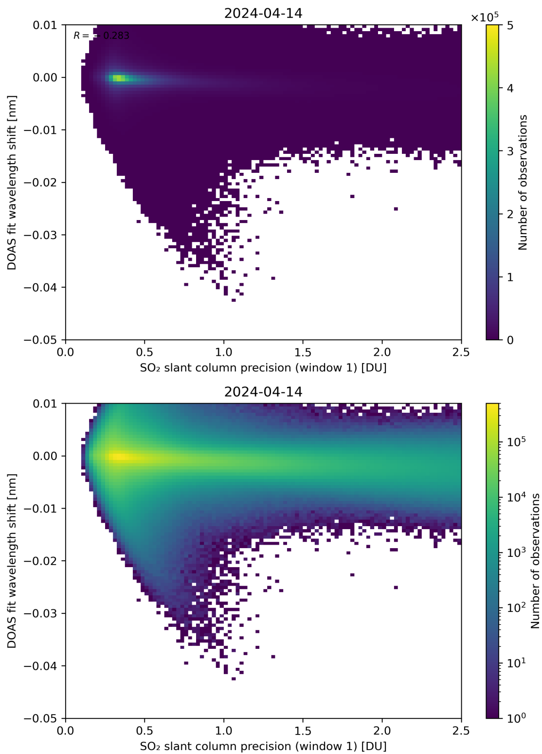
Figure 221: Scatter density plot of “SO 2 slant column precision (window 1)” against “DOAS fit wavelength shift” for 2024-04-13 to 2024-04-15.
