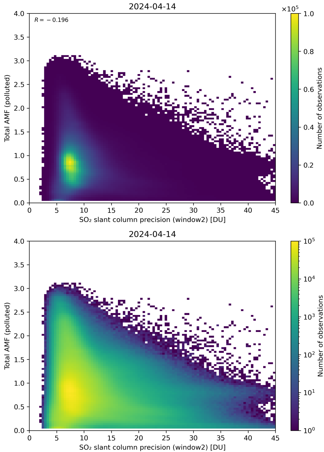
Figure 251: Scatter density plot of “SO 2 slant column precision (window2)” against “Total AMF (polluted)” for 2024-04-13 to 2024-04-15.
