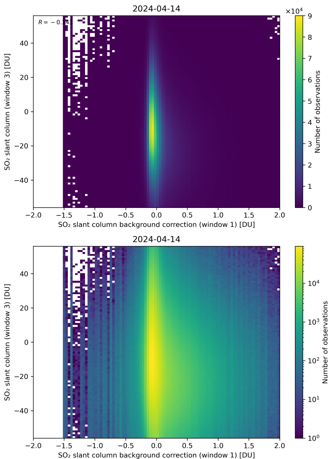
Figure 107: Scatter density plot of “SO 2 slant column background correction (window 1)” against “SO 2 slant column (window 3)” for 2024-04-13 to 2024-04-15.
