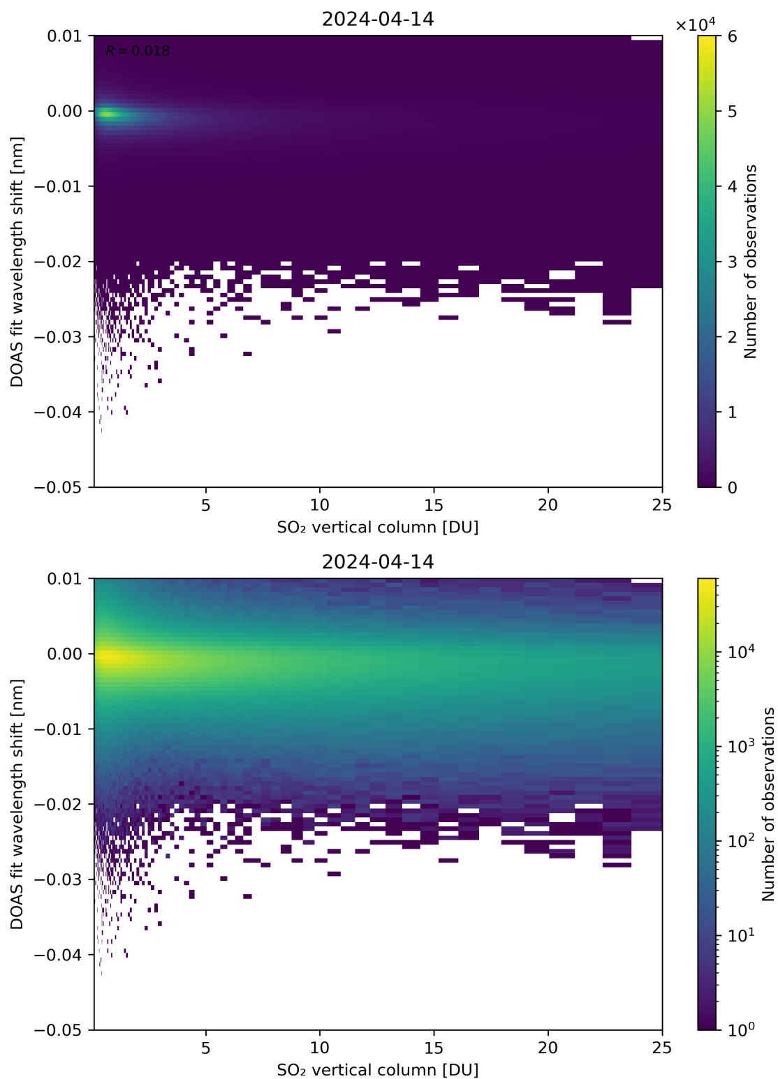
Figure 276: Scatter density plot of “SO 2 vertical column” against “DOAS fit wavelength shift” for 2024-04-13 to 2024-04-15.
