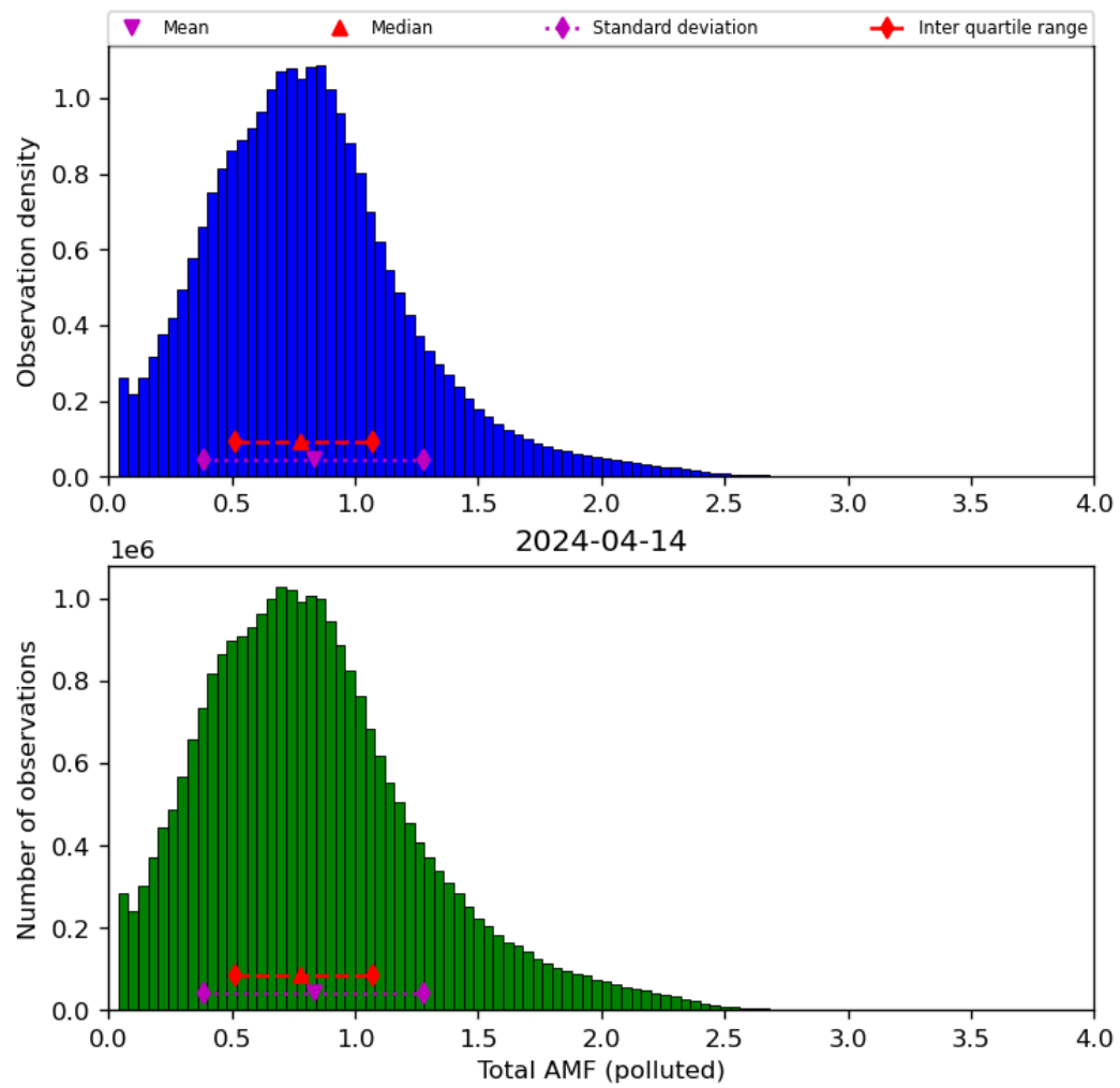
Figure 71: Histogram of “Total AMF (polluted)” for 2024-04-13 to 2024-04-15
