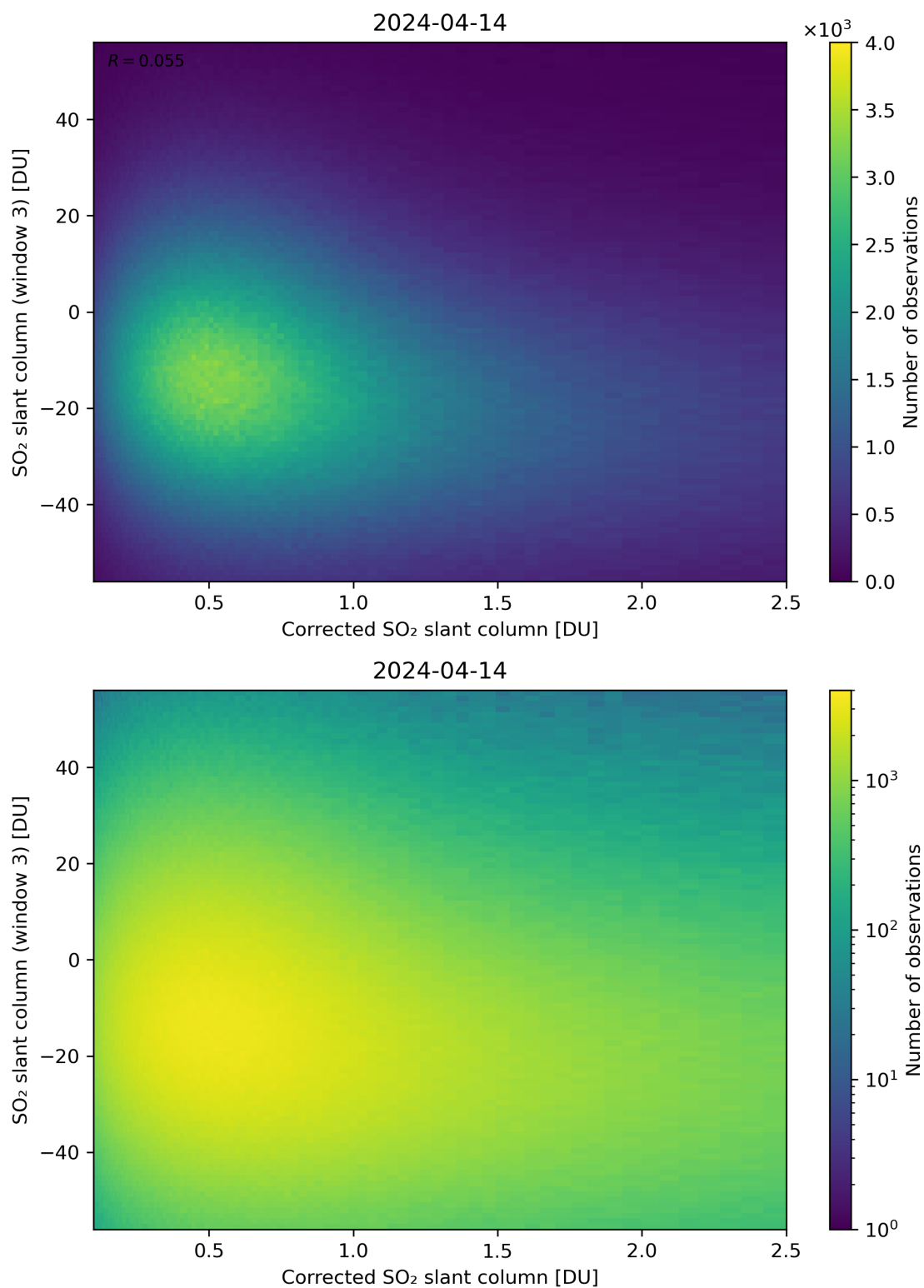
Figure 190: Scatter density plot of “Corrected SO 2 slant column” against “SO 2 slant column (window 3)” for 2024-04-13 to 2024-04-15.
