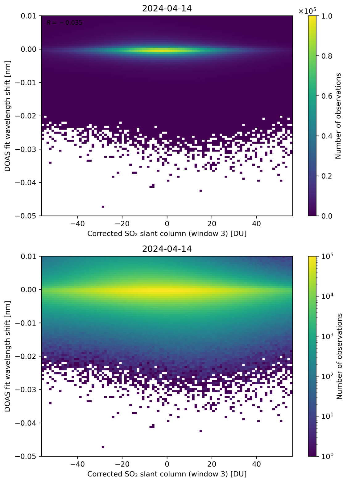
Figure 206: Scatter density plot of “Corrected SO 2 slant column (window 3)” against “DOAS fit wavelength shift” for 2024-04-13 to 2024-04-15.
