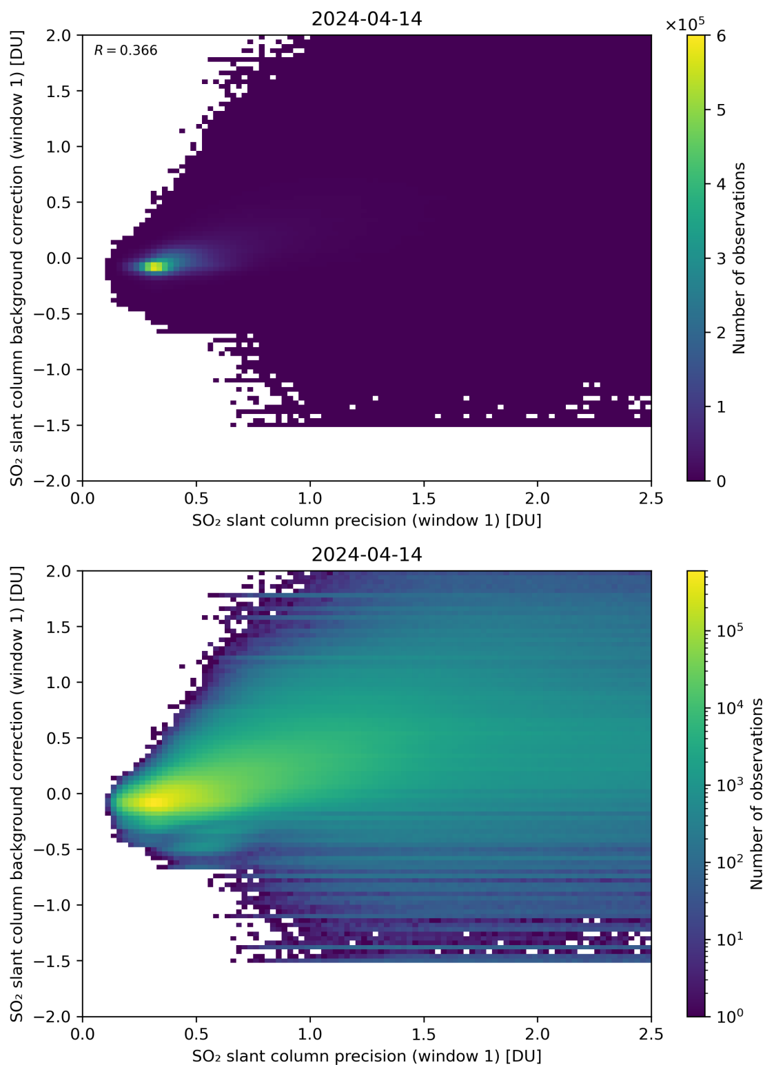
Figure 218: Scatter density plot of “SO 2 slant column precision (window 1)” against “SO 2 slant column background correction (window 1)” for 2024-04-13 to 2024-04-15.
