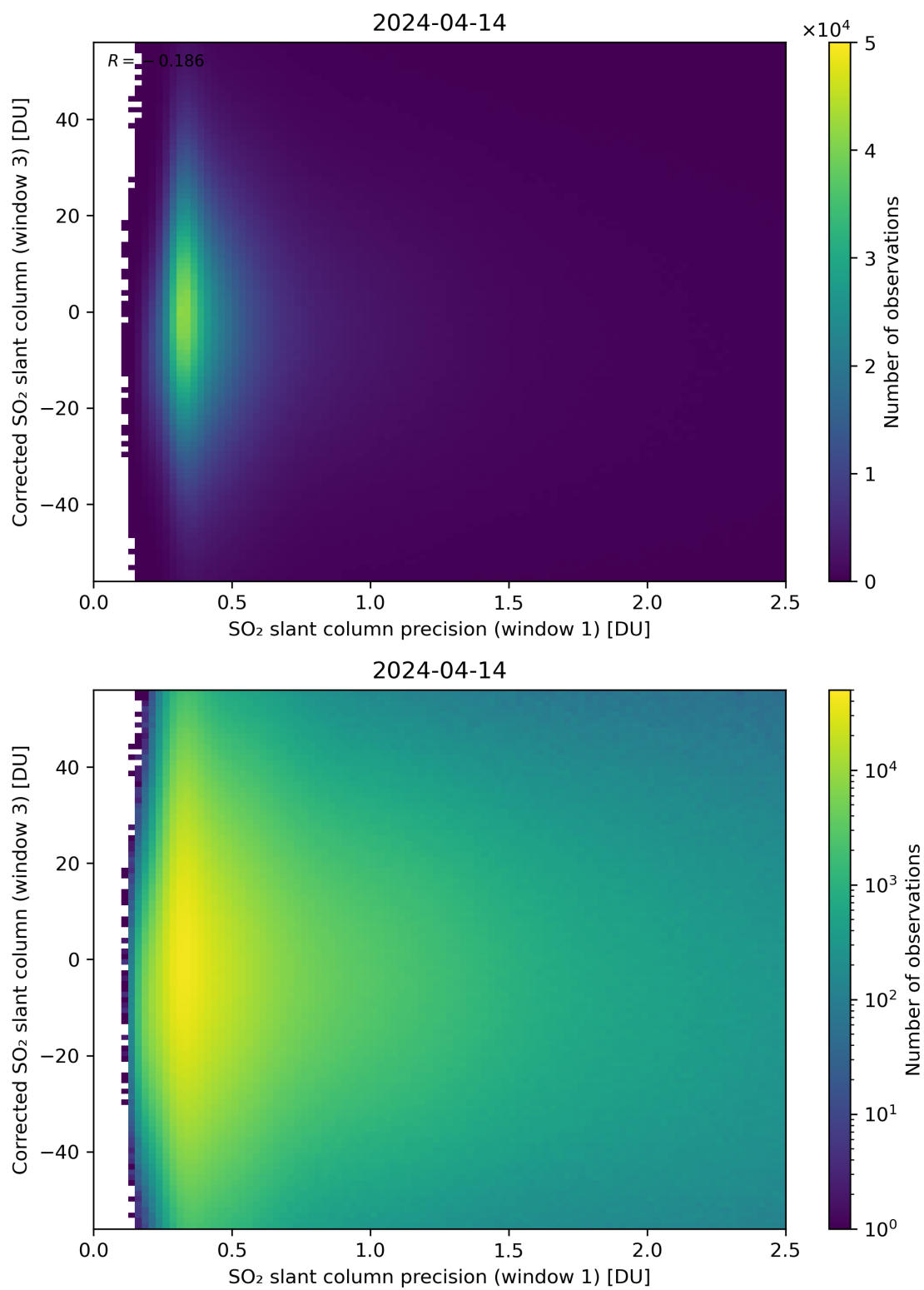
Figure 226: Scatter density plot of “SO 2 slant column precision (window 1)” against “Corrected SO 2 slant column (window 3)” for 2024-04-13 to 2024-04-15.
