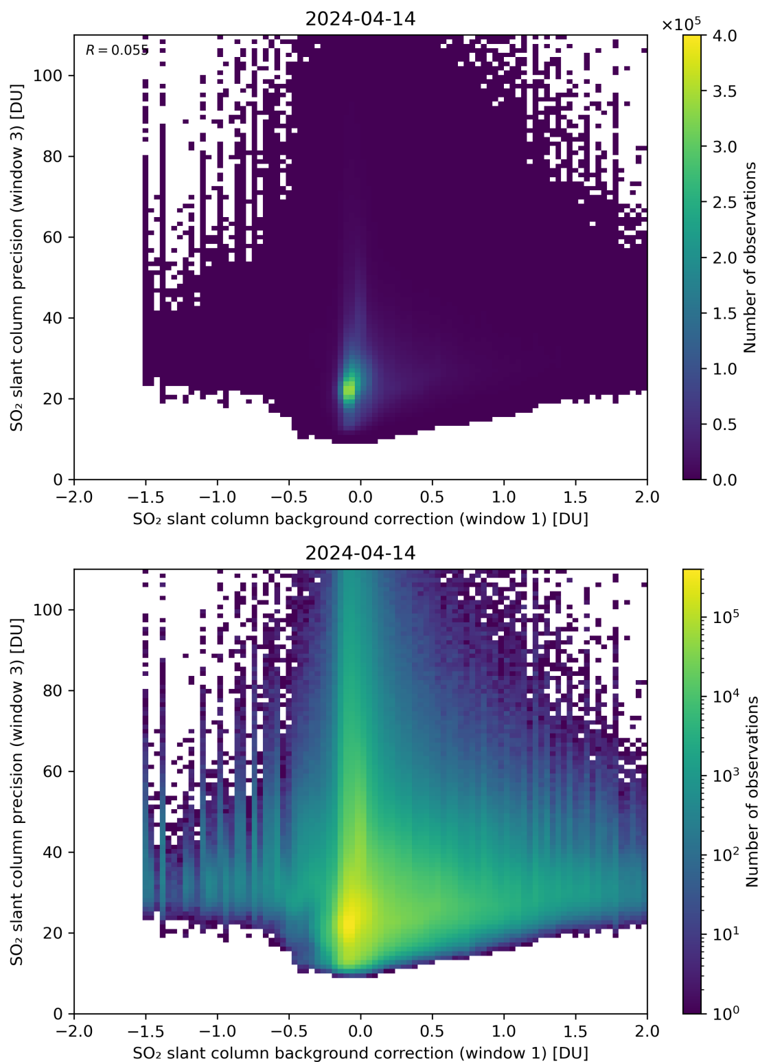
Figure 108: Scatter density plot of “SO 2 slant column background correction (window 1)” against “SO 2 slant column precision (window 3)” for 2024-04-13 to 2024-04-15.
