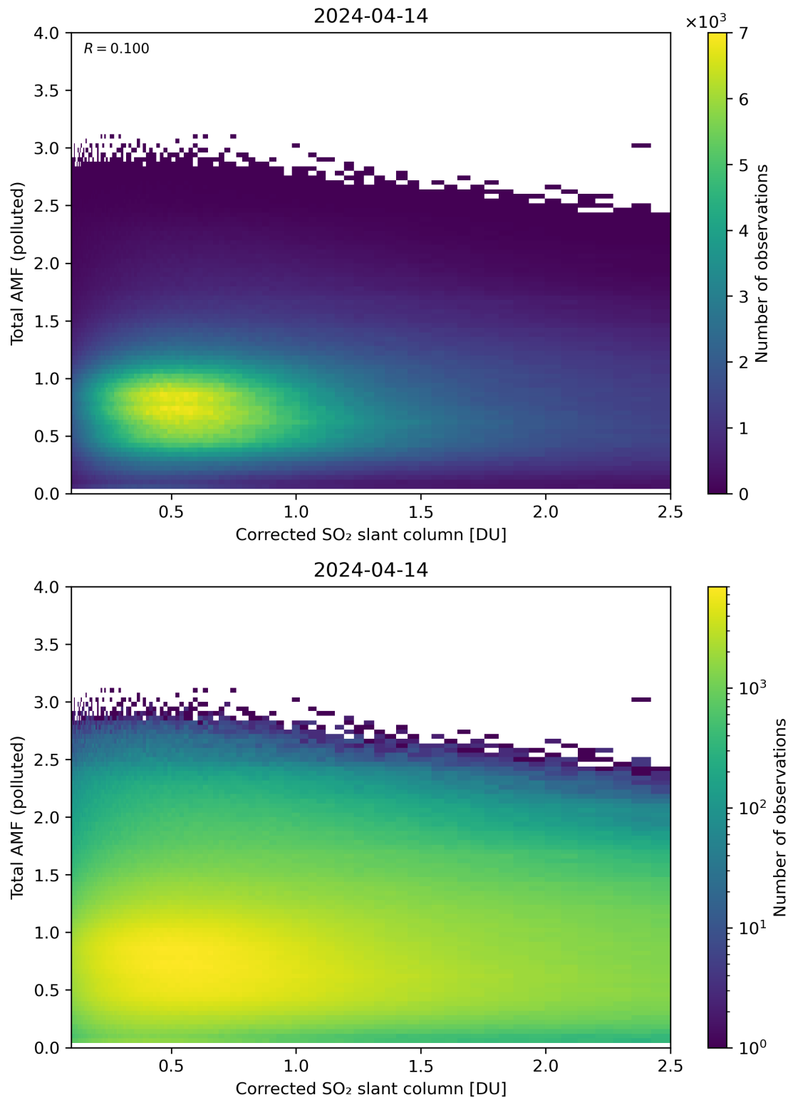
Figure 192: Scatter density plot of “Corrected SO 2 slant column” against “Total AMF (polluted)” for 2024-04-13 to 2024-04-15.
