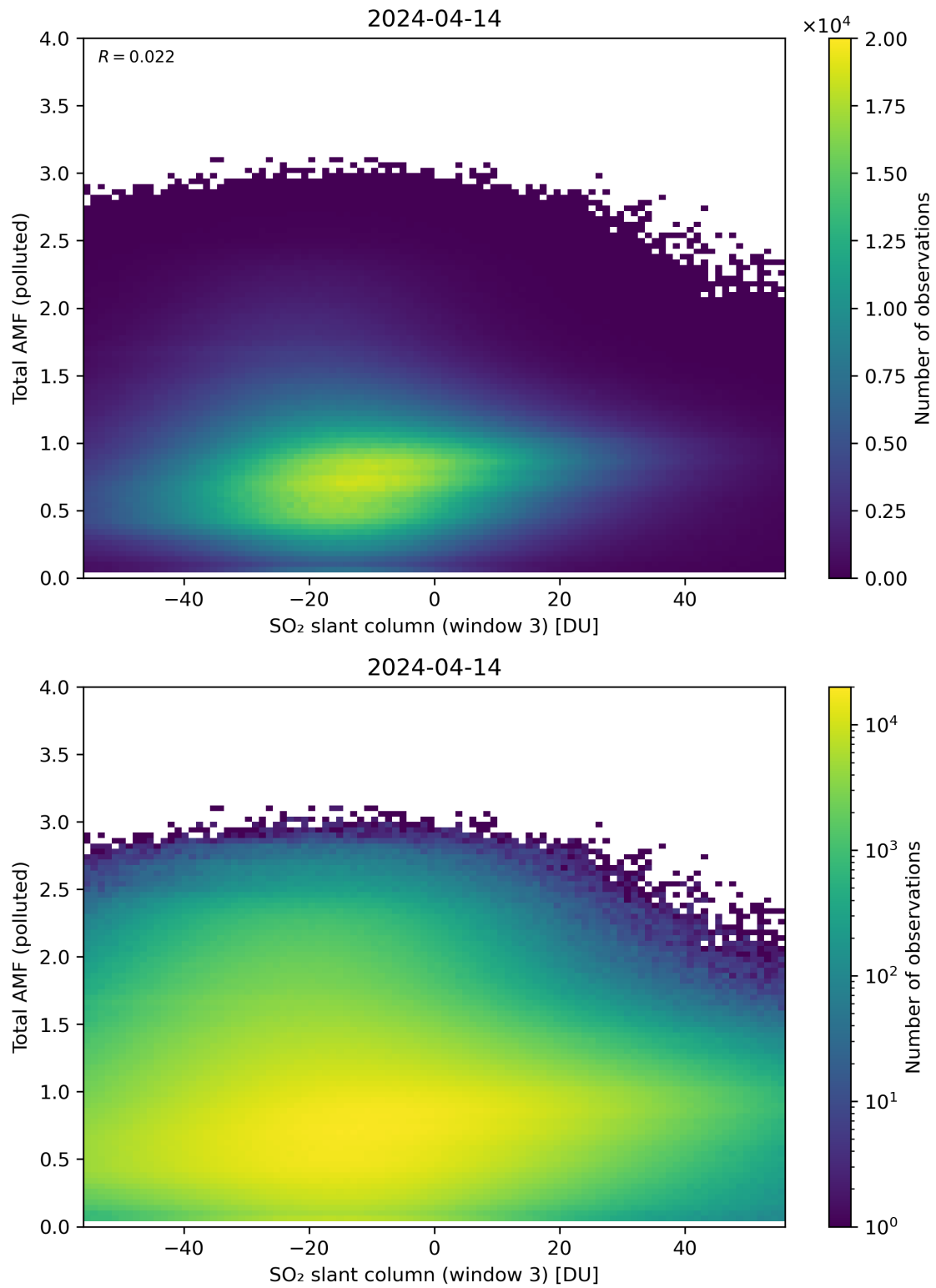
Figure 268: Scatter density plot of “SO 2 slant column (window 3)” against “Total AMF (polluted)” for 2024-04-13 to 2024-04-15.
