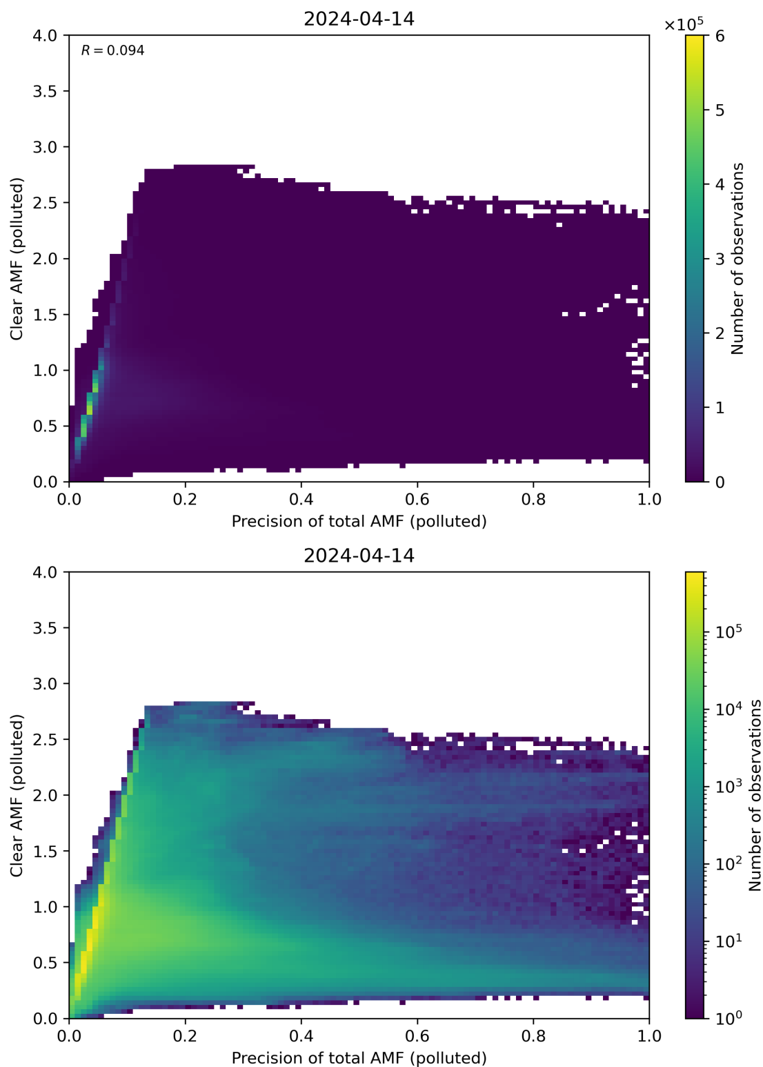
Figure 270: Scatter density plot of “Precision of total AMF (polluted)” against “Clear AMF (polluted)” for 2024-04-13 to 2024-04-15.
