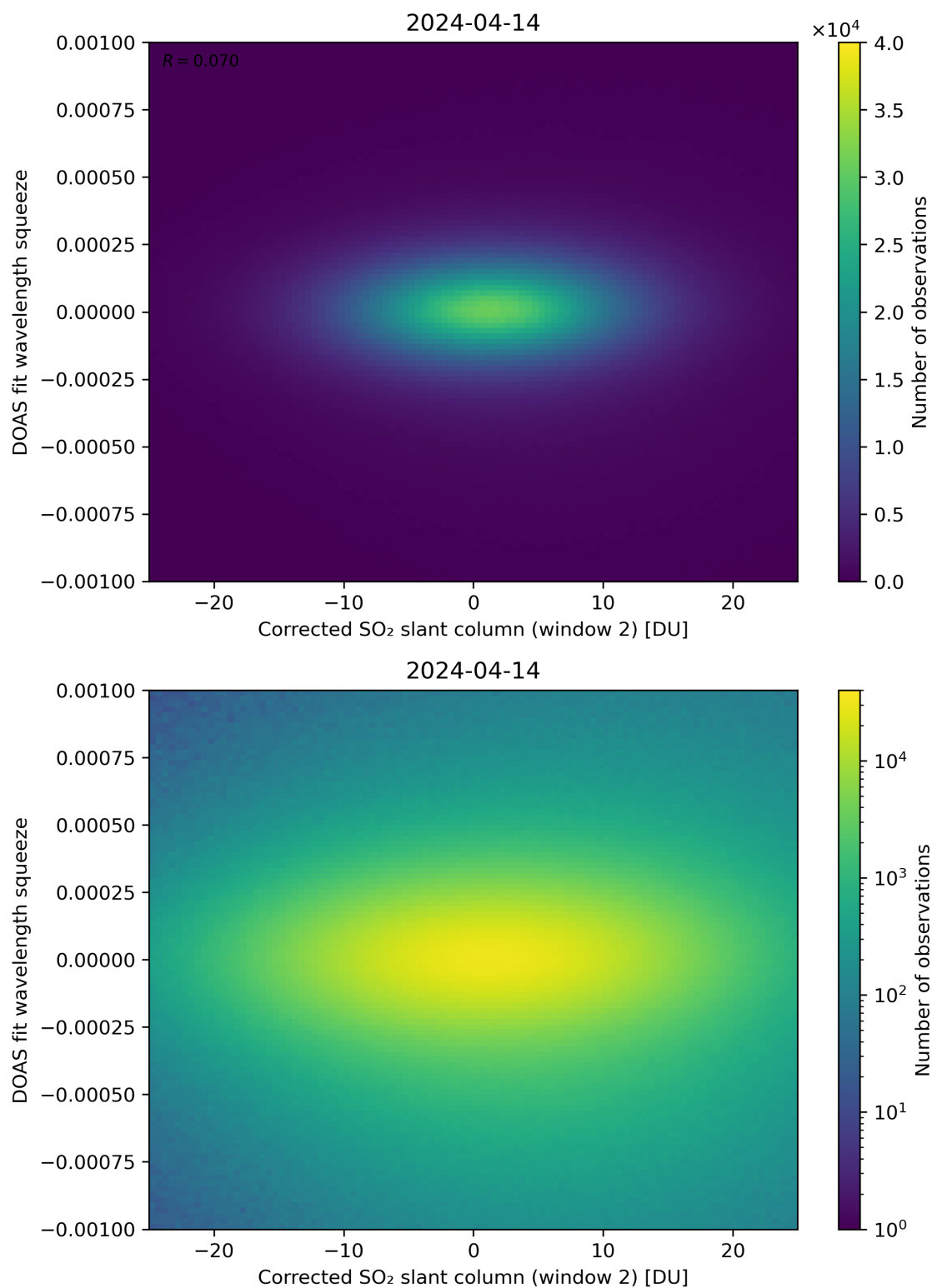
Figure 197: Scatter density plot of “Corrected SO 2 slant column (window 2)” against “DOAS fit wavelength squeeze” for 2024-04-13 to 2024-04-15.
