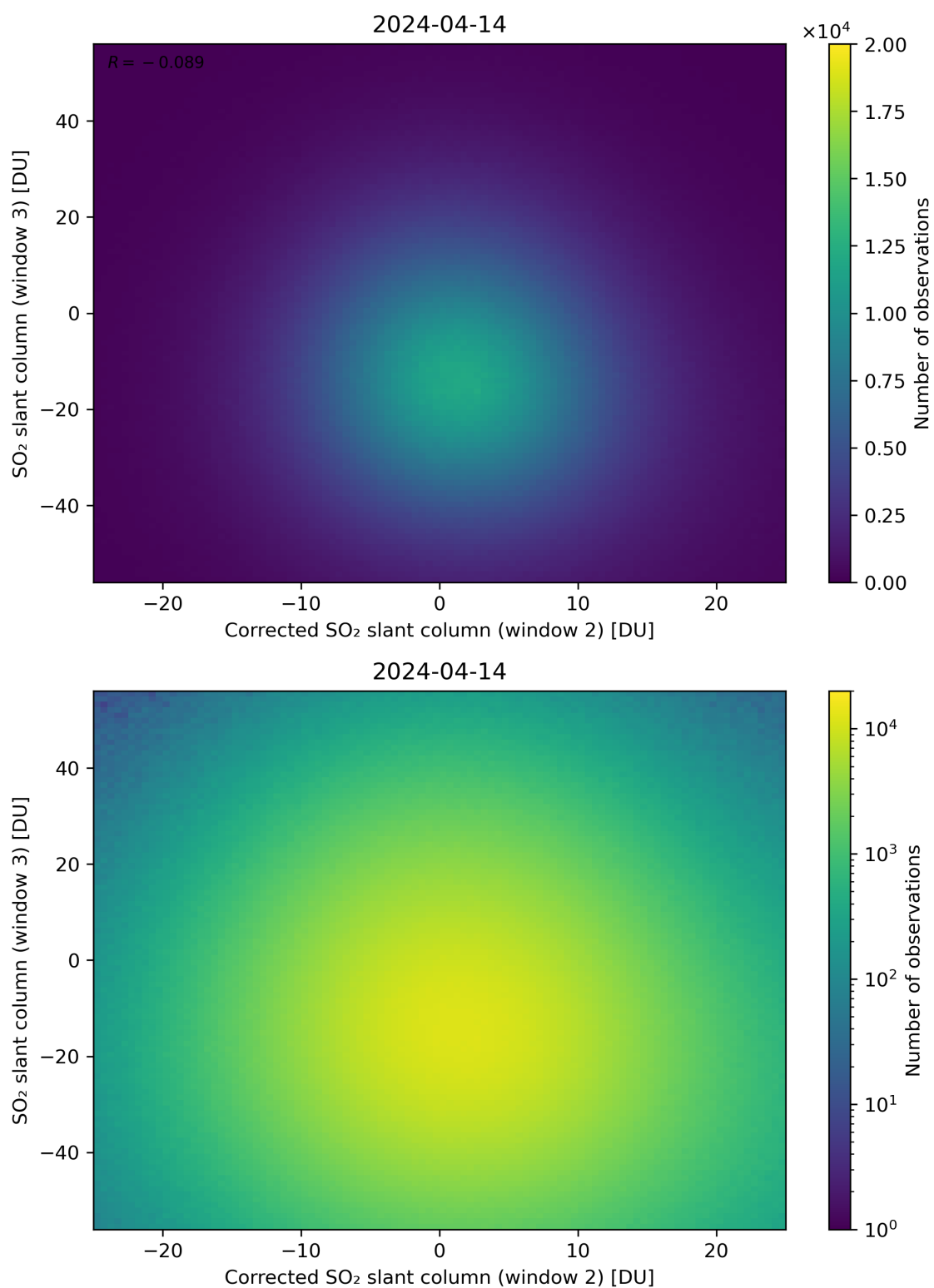
Figure 201: Scatter density plot of “Corrected SO 2 slant column (window 2)” against “SO 2 slant column (window 3)” for 2024-04-13 to 2024-04-15.
