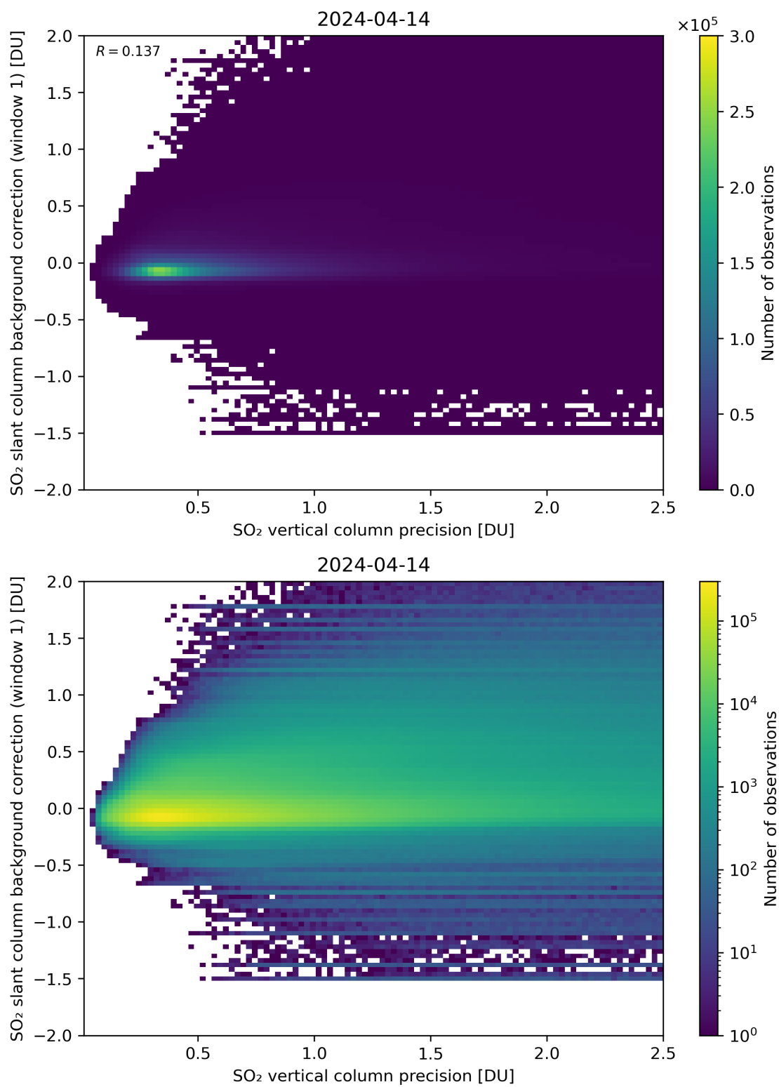
Figure 279: Scatter density plot of “SO 2 vertical column precision” against “SO 2 slant column background correction (window 1)” for 2024-04-13 to 2024-04-15.
