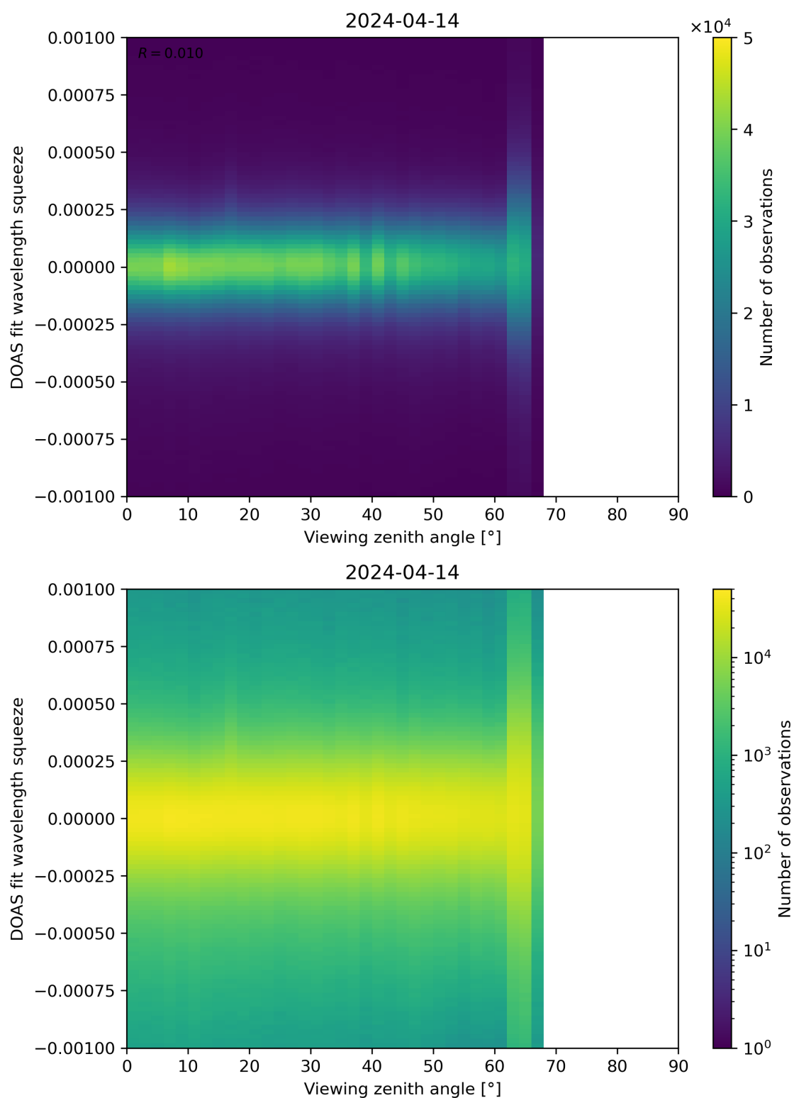
Figure 312: Scatter density plot of “Viewing zenith angle” against “DOAS fit wavelength squeeze” for 2024-04-13 to 2024-04-15.
