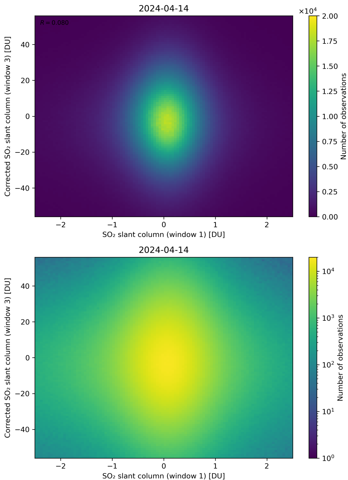
Figure 234: Scatter density plot of “SO 2 slant column (window 1)” against “Corrected SO 2 slant column (window 3)” for 2024-04-13 to 2024-04-15.
