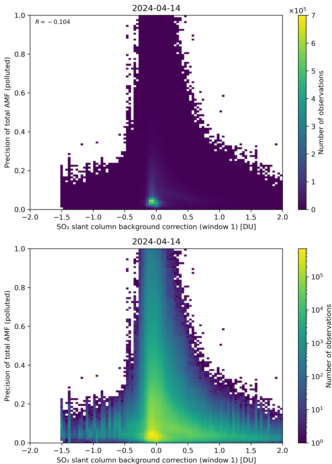
Figure 110: Scatter density plot of “SO 2 slant column background correction (window 1)” against “Precision of total AMF (polluted)” for 2024-04-13 to 2024-04-15.
