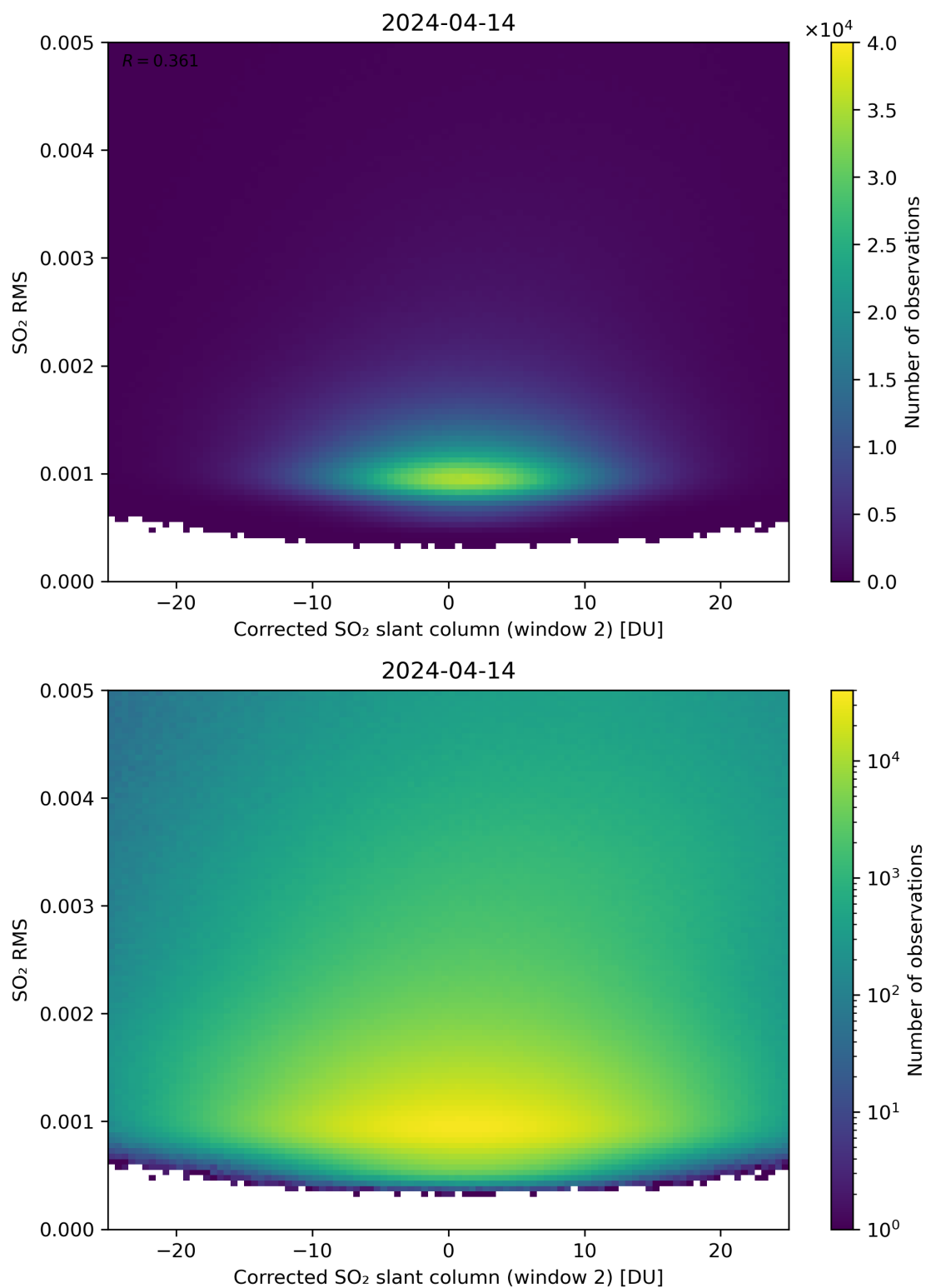
Figure 198: Scatter density plot of “Corrected SO 2 slant column (window 2)” against “SO 2 RMS” for 2024-04-13 to 2024-04-15.
