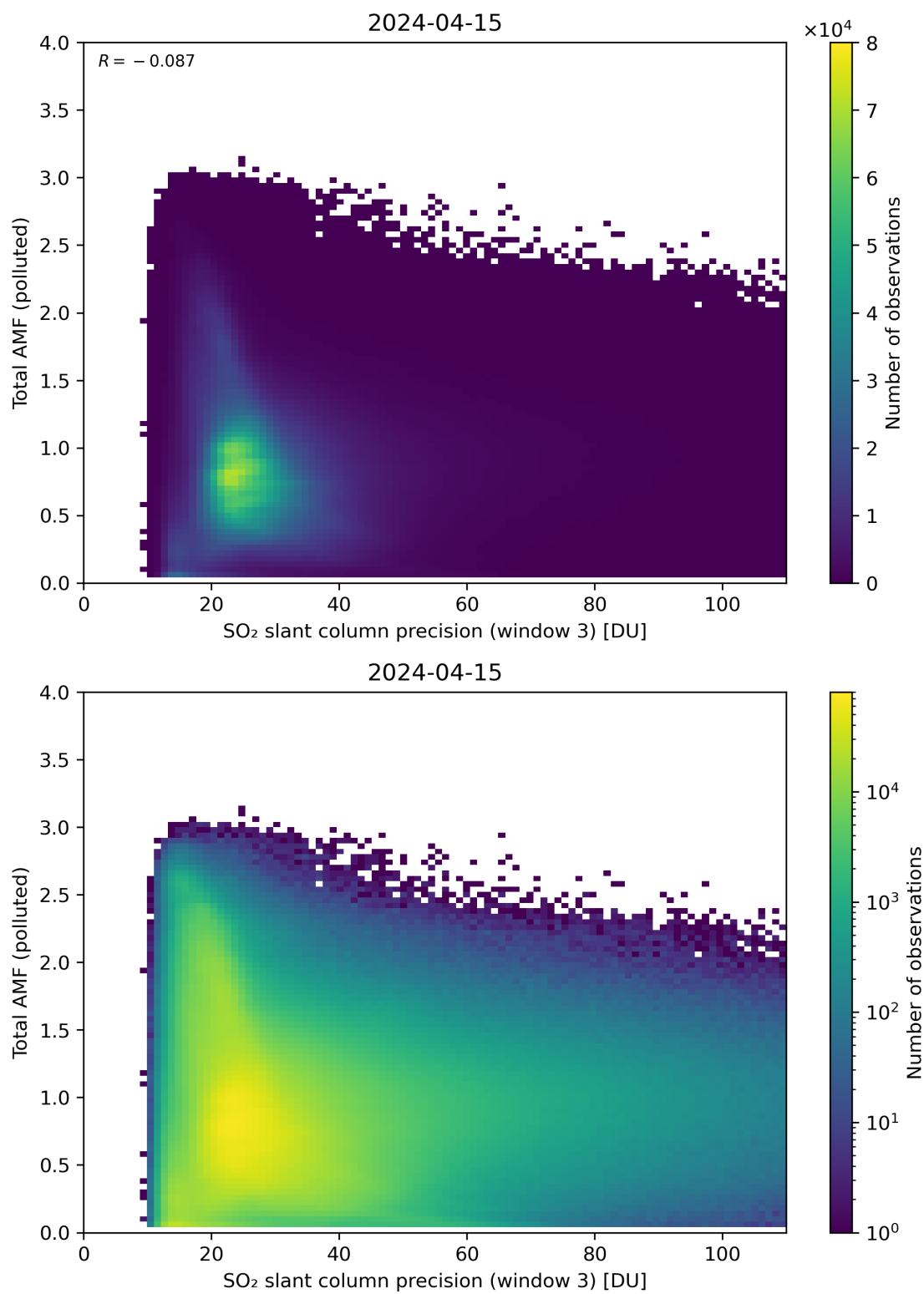
Figure 263: Scatter density plot of “SO 2 slant column precision (window 3)” against “Total AMF (polluted)” for 2024-04-15 to 2024-04-16.
