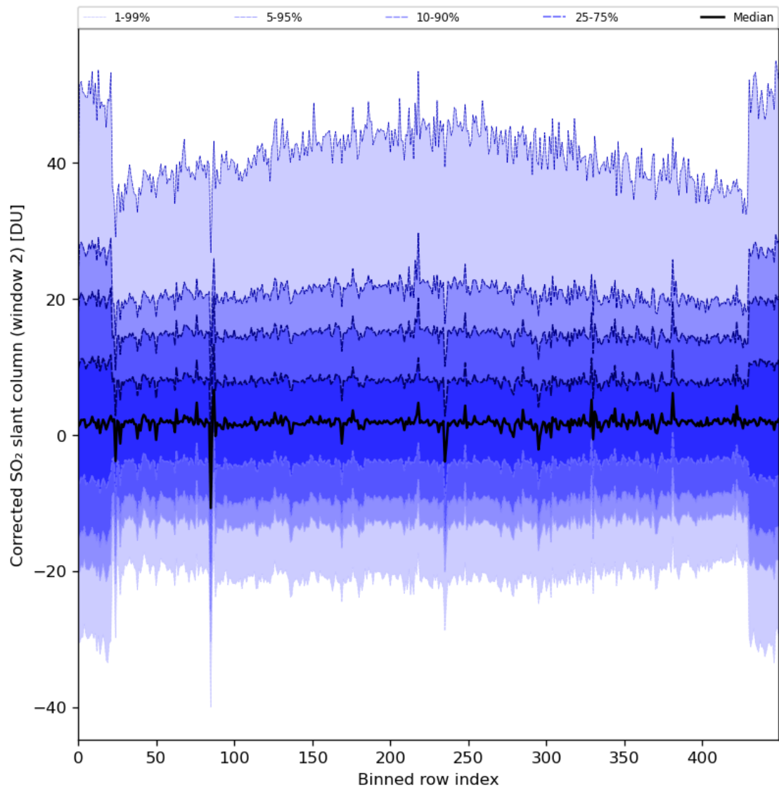
Figure 85: Along track statistics of “Corrected SO 2 slant column (window 2)” for 2024-04-15 to 2024-04-16
