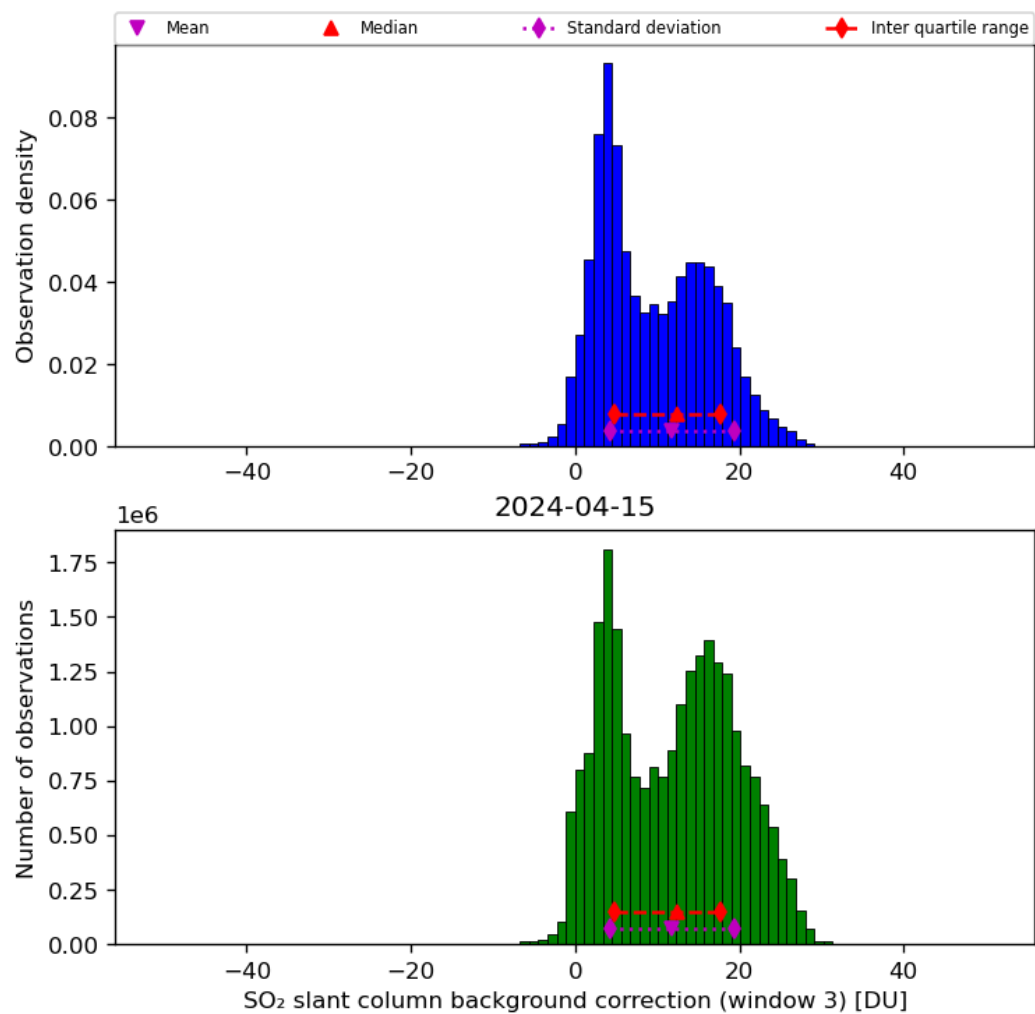
Figure 67: Histogram of “SO 2 slant column background correction (window 3)” for 2024-04-15 to 2024-04-16
