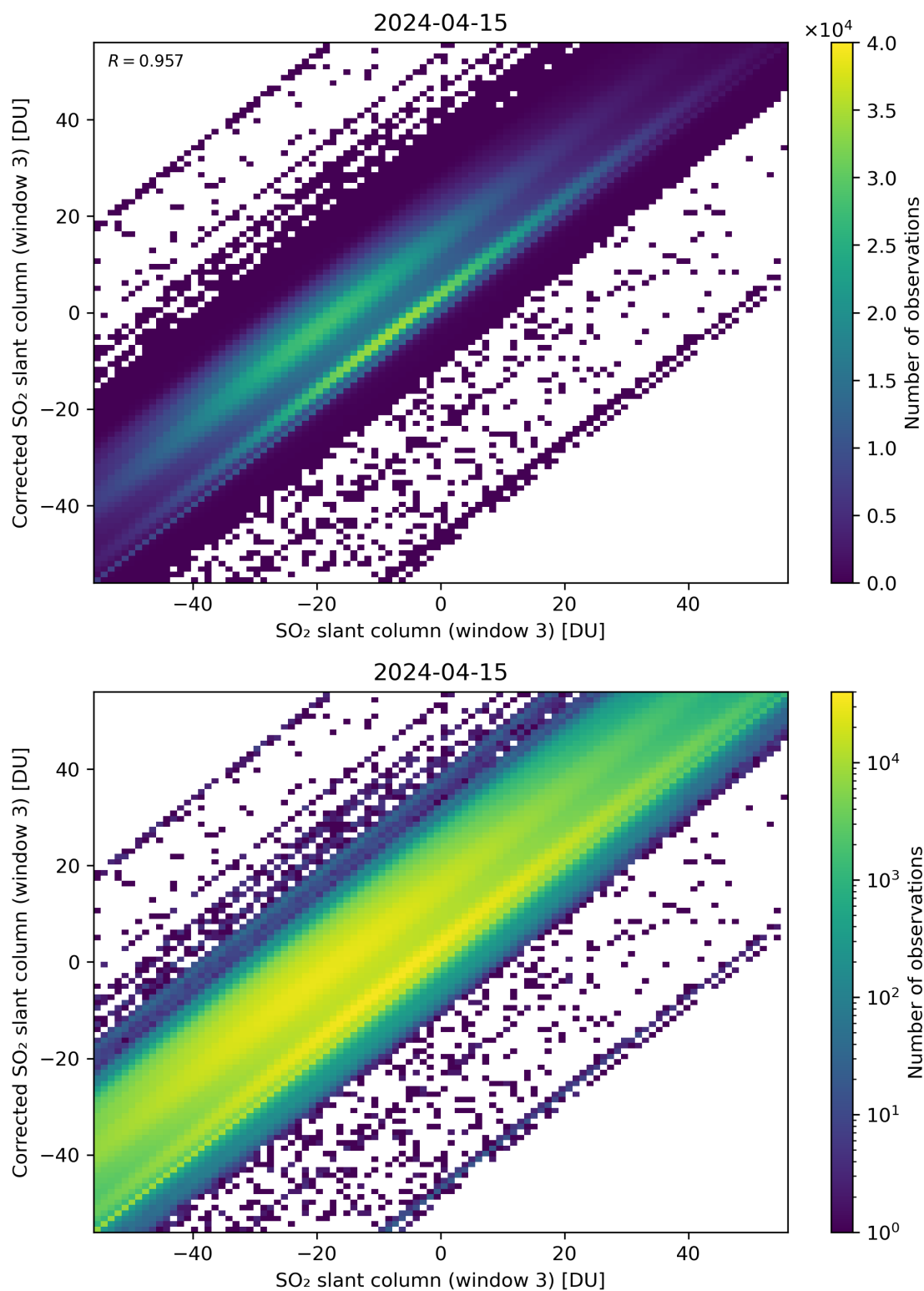
Figure 266: Scatter density plot of “SO 2 slant column (window 3)” against “Corrected SO 2 slant column (window 3)” for 2024-04-15 to 2024-04-16.
