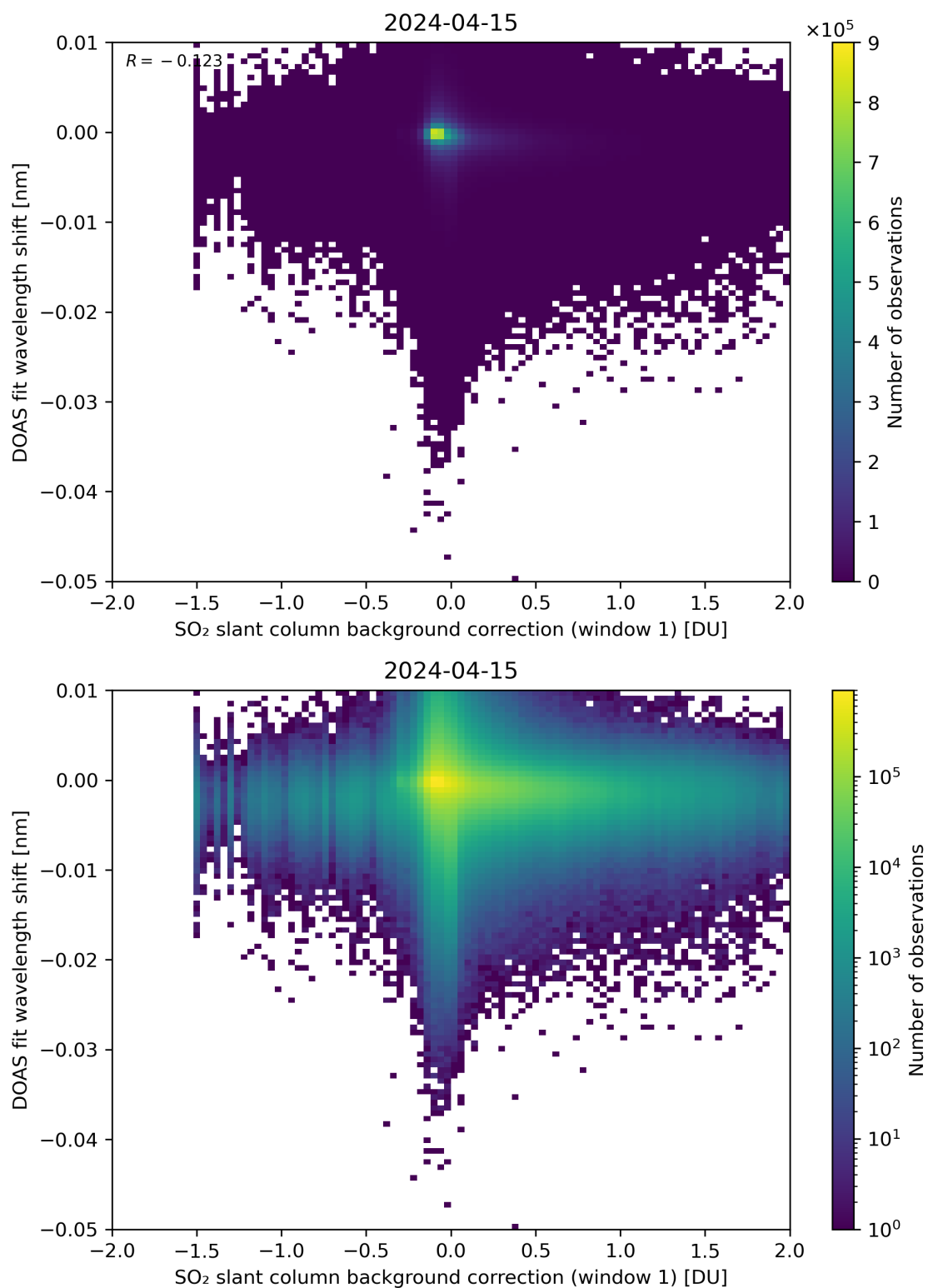
Figure 100: Scatter density plot of “SO 2 slant column background correction (window 1)” against “DOAS fit wavelength shift” for 2024-04-15 to 2024-04-16.
