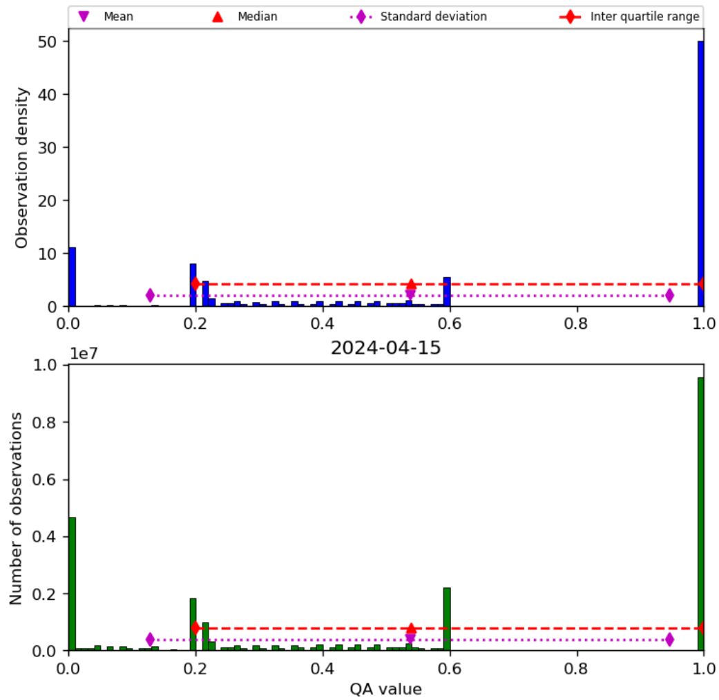
Figure 52: Histogram of “QA value” for 2024-04-15 to 2024-04-16
