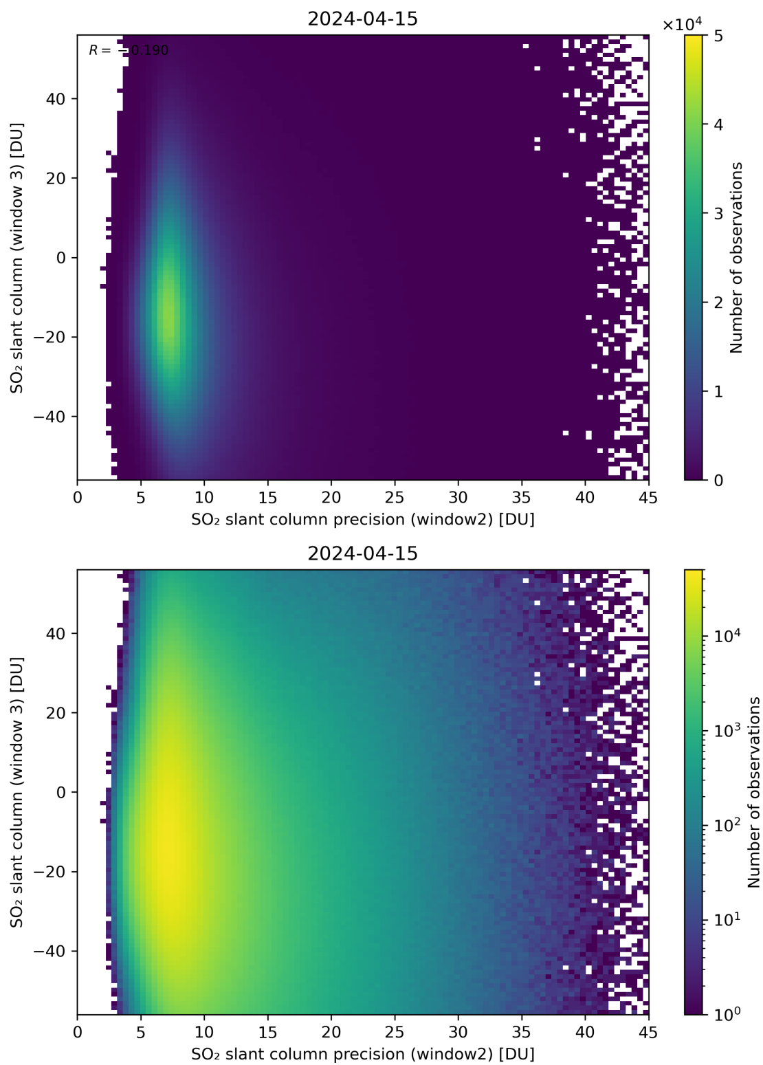
Figure 249: Scatter density plot of “SO 2 slant column precision (window2)” against “SO 2 slant column (window 3)” for 2024-04-15 to 2024-04-16.
