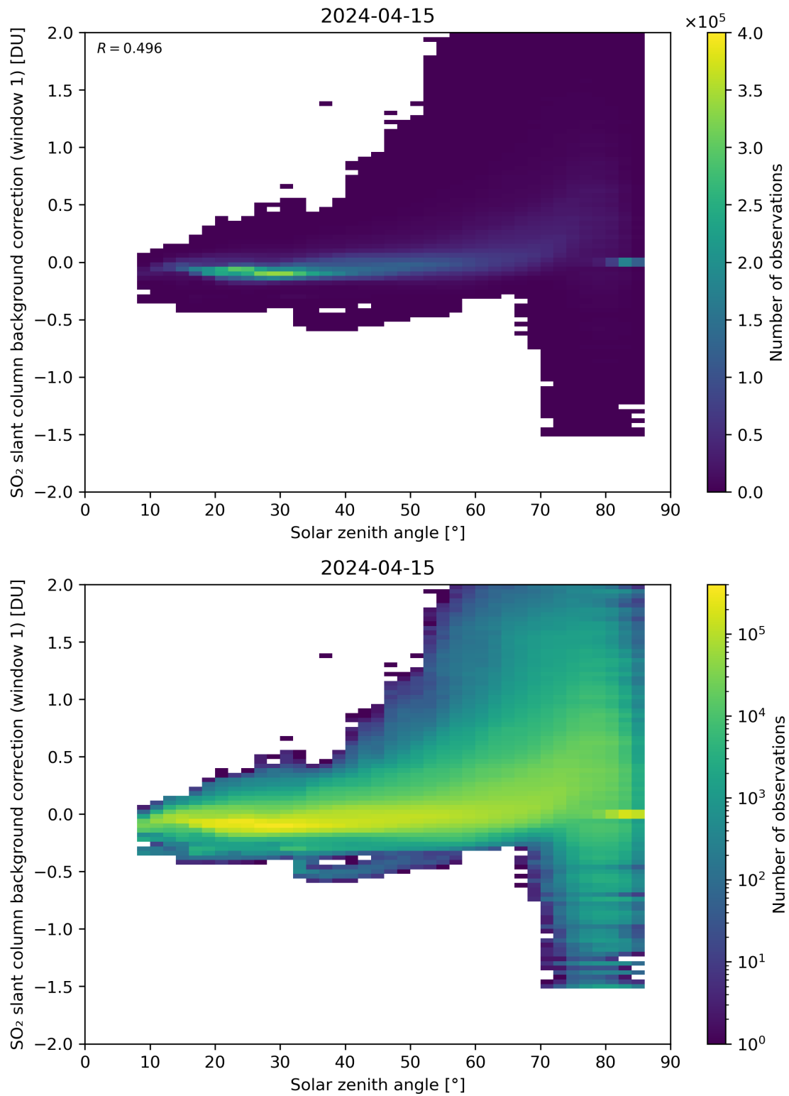
Figure 158: Scatter density plot of “Solar zenith angle” against “SO 2 slant column background correction (window 1)” for 2024-04-15 to 2024-04-16.
