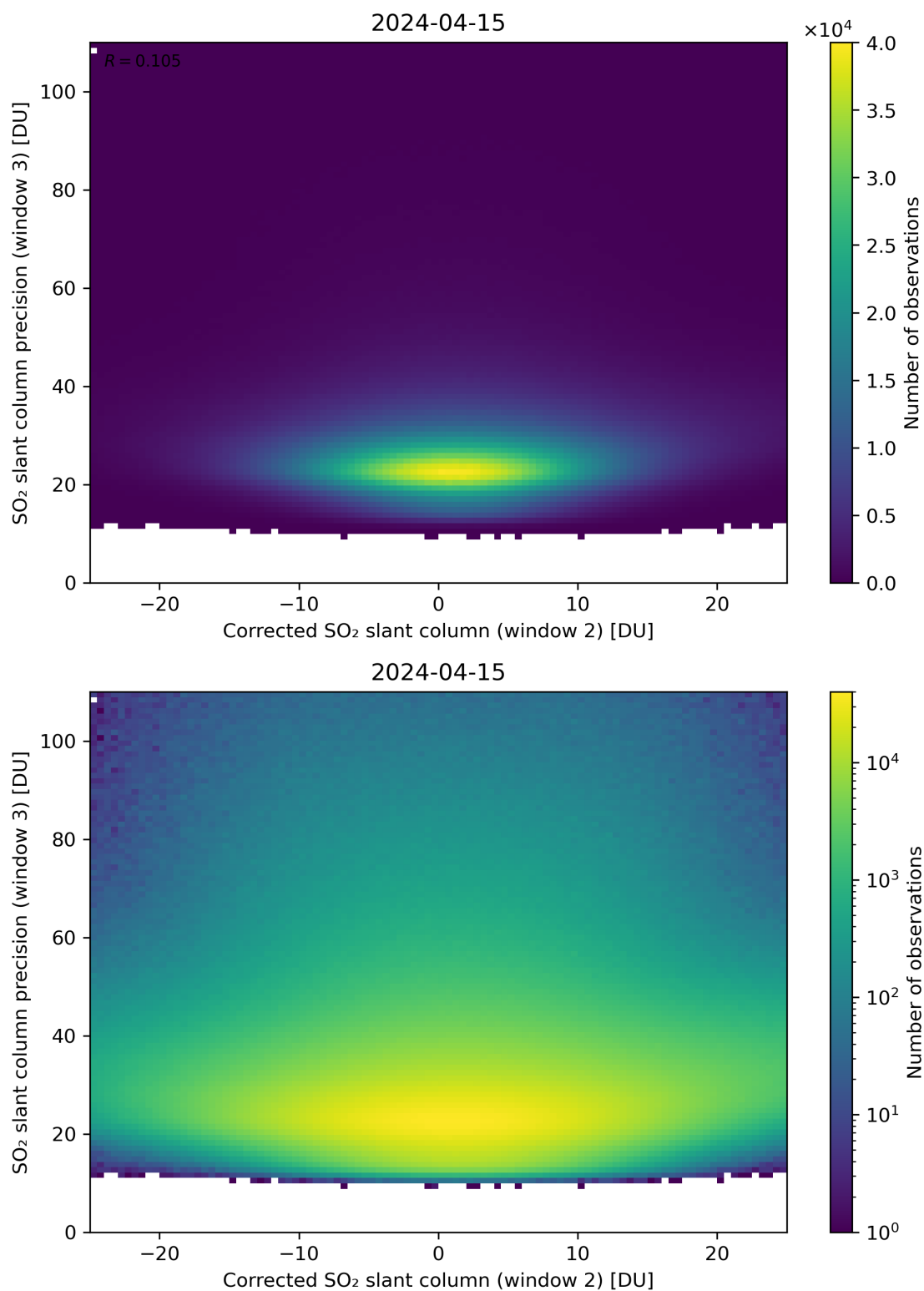
Figure 202: Scatter density plot of “Corrected SO 2 slant column (window 2)” against “SO 2 slant column precision (window 3)” for 2024-04-15 to 2024-04-16.
