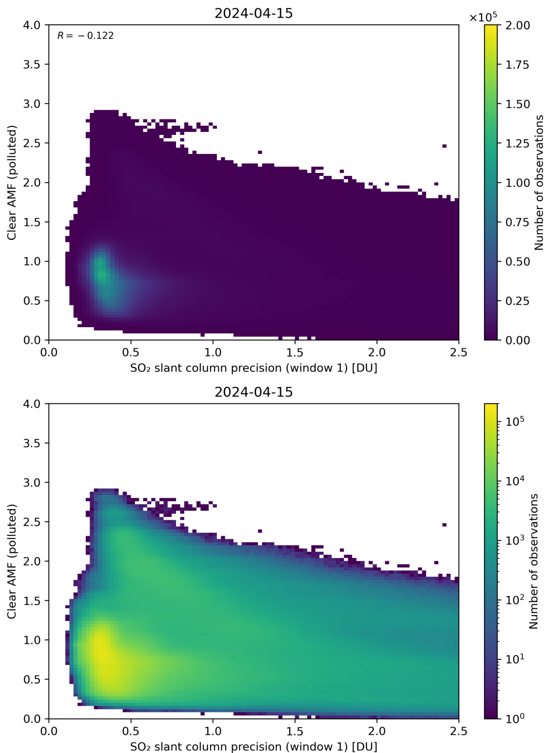
Figure 224: Scatter density plot of “SO 2 slant column precision (window 1)” against “Clear AMF (polluted)” for 2024-04-15 to 2024-04-16.
