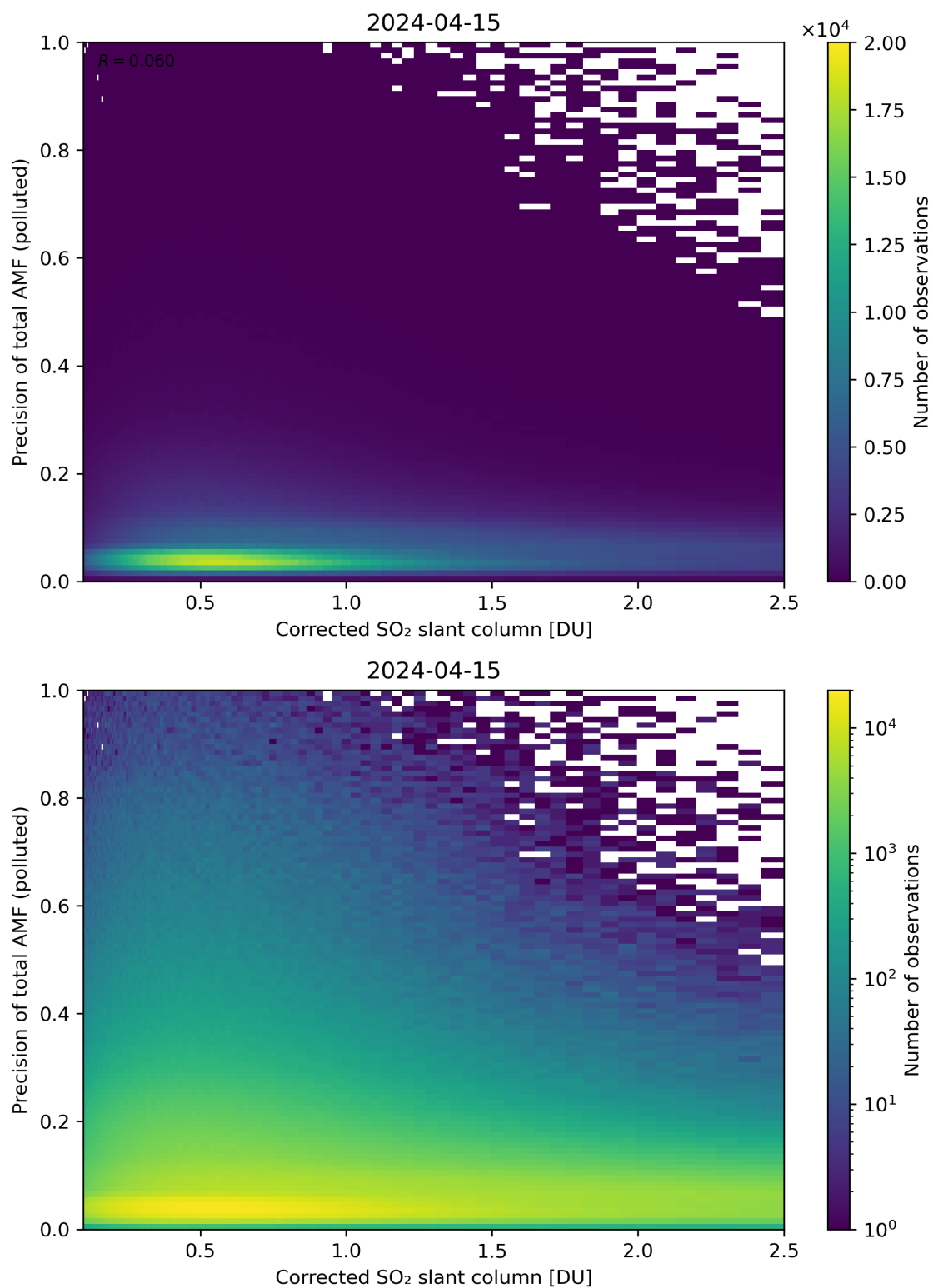
Figure 193: Scatter density plot of “Corrected SO 2 slant column” against “Precision of total AMF (polluted)” for 2024-04-15 to 2024-04-16.
