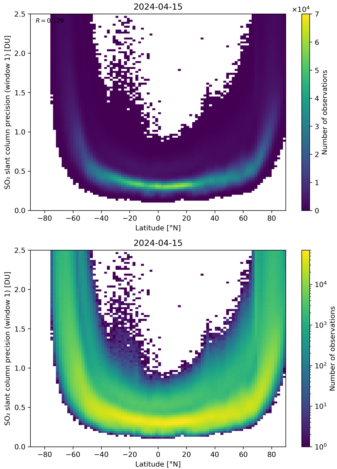
Figure 150: Scatter density plot of “Latitude” against “SO 2 slant column precision (window 1)” for 2024-04-15 to 2024-04-16.
