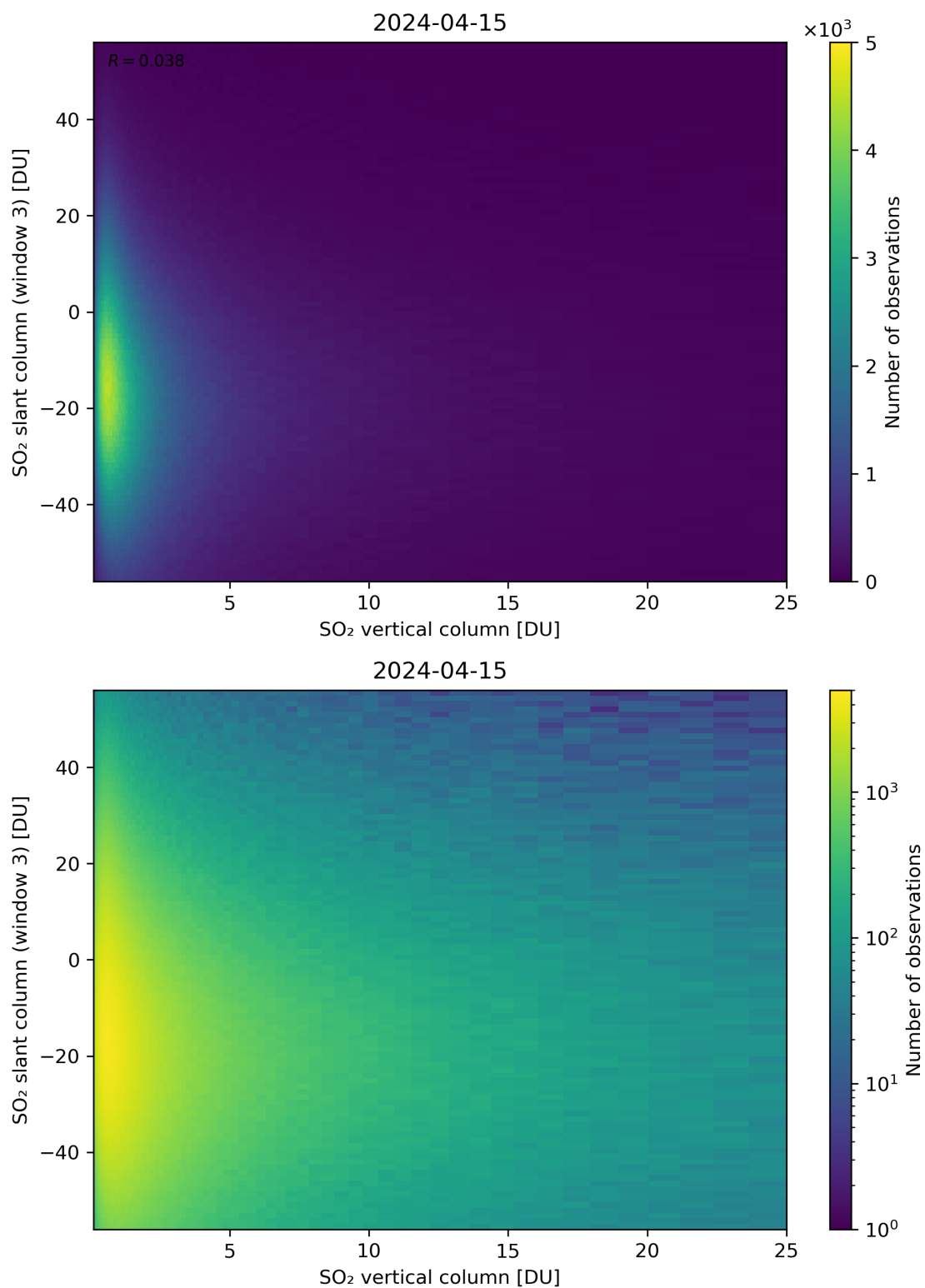
Figure 303: Scatter density plot of “SO 2 vertical column” against “SO 2 slant column (window 3)” for 2024-04-15 to 2024-04-16.
