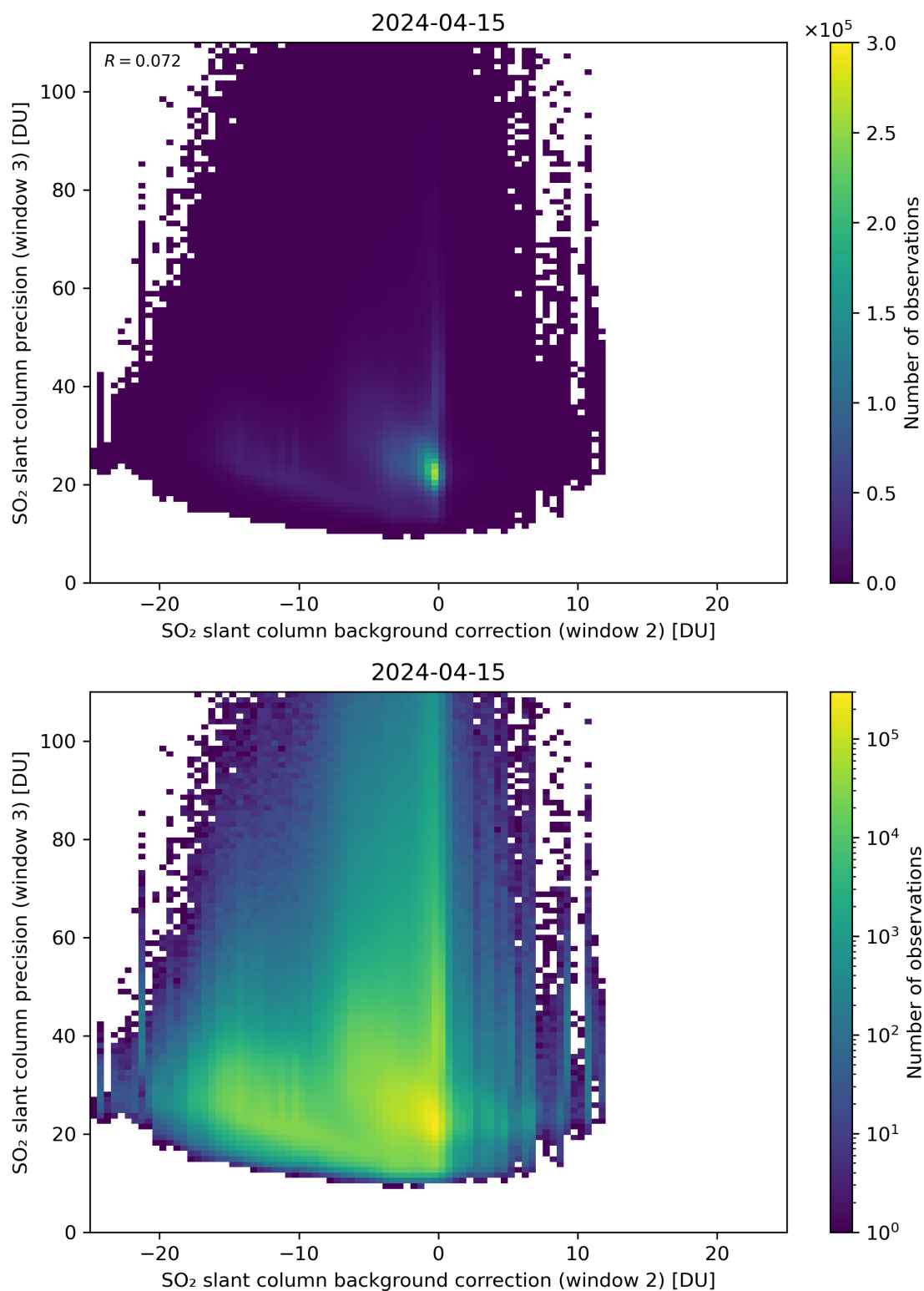
Figure 118: Scatter density plot of “SO 2 slant column background correction (window 2)” against “SO 2 slant column precision (window 3)” for 2024-04-15 to 2024-04-16.
