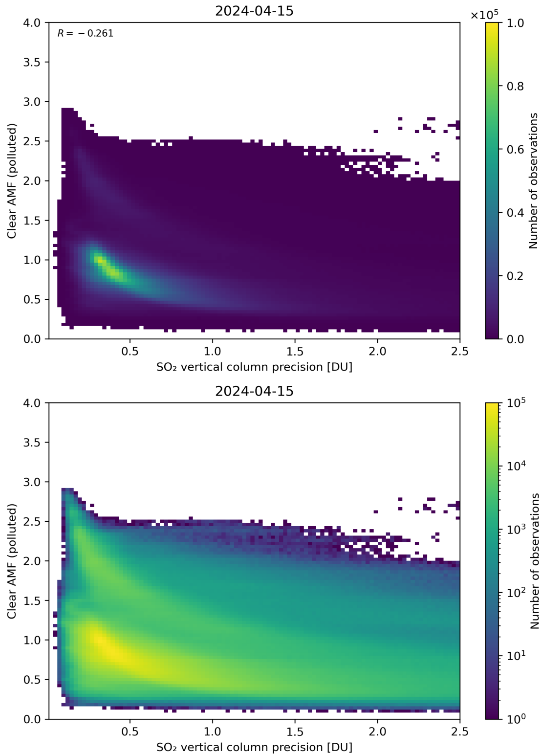
Figure 285: Scatter density plot of “SO 2 vertical column precision” against “Clear AMF (polluted)” for 2024-04-15 to 2024-04-16.
