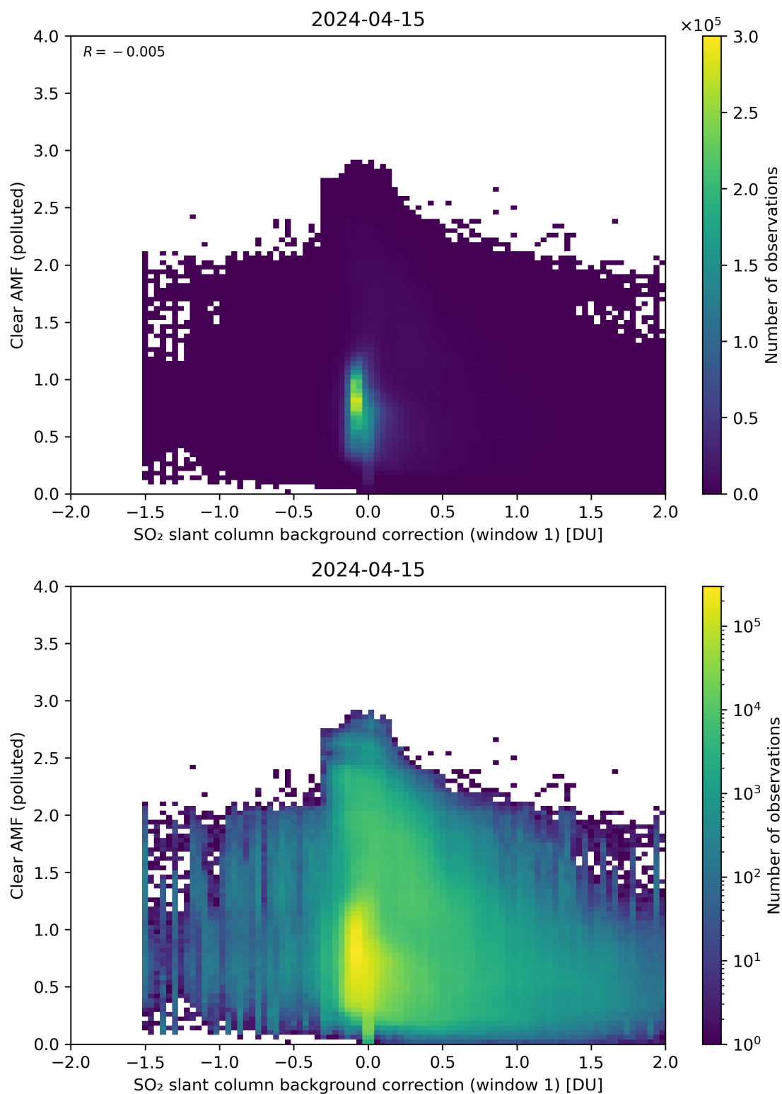
Figure 103: Scatter density plot of “SO 2 slant column background correction (window 1)” against “Clear AMF (polluted)” for 2024-04-15 to 2024-04-16.
