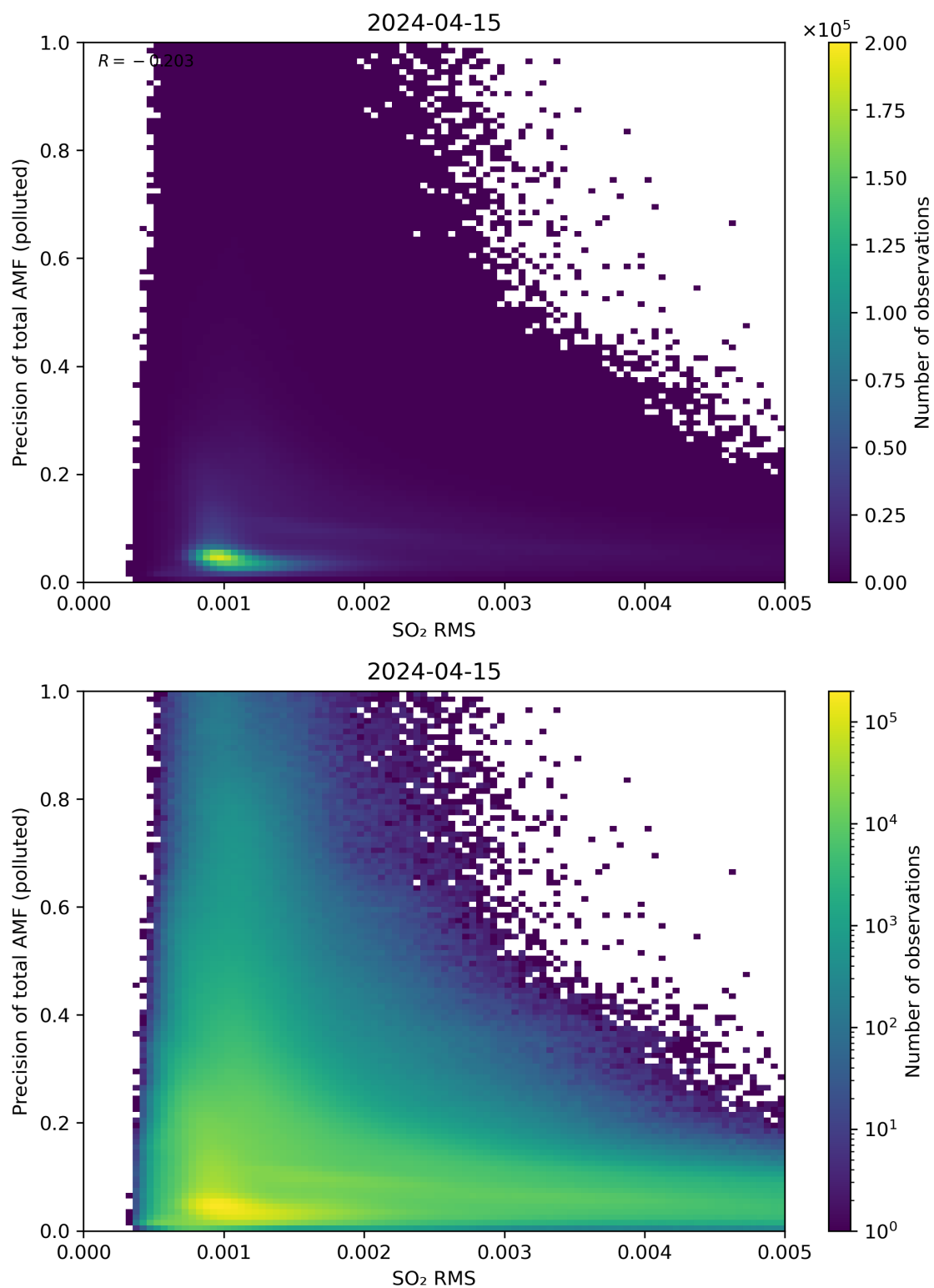
Figure 138: Scatter density plot of “SO 2 RMS” against “Precision of total AMF (polluted)” for 2024-04-15 to 2024-04-16.
