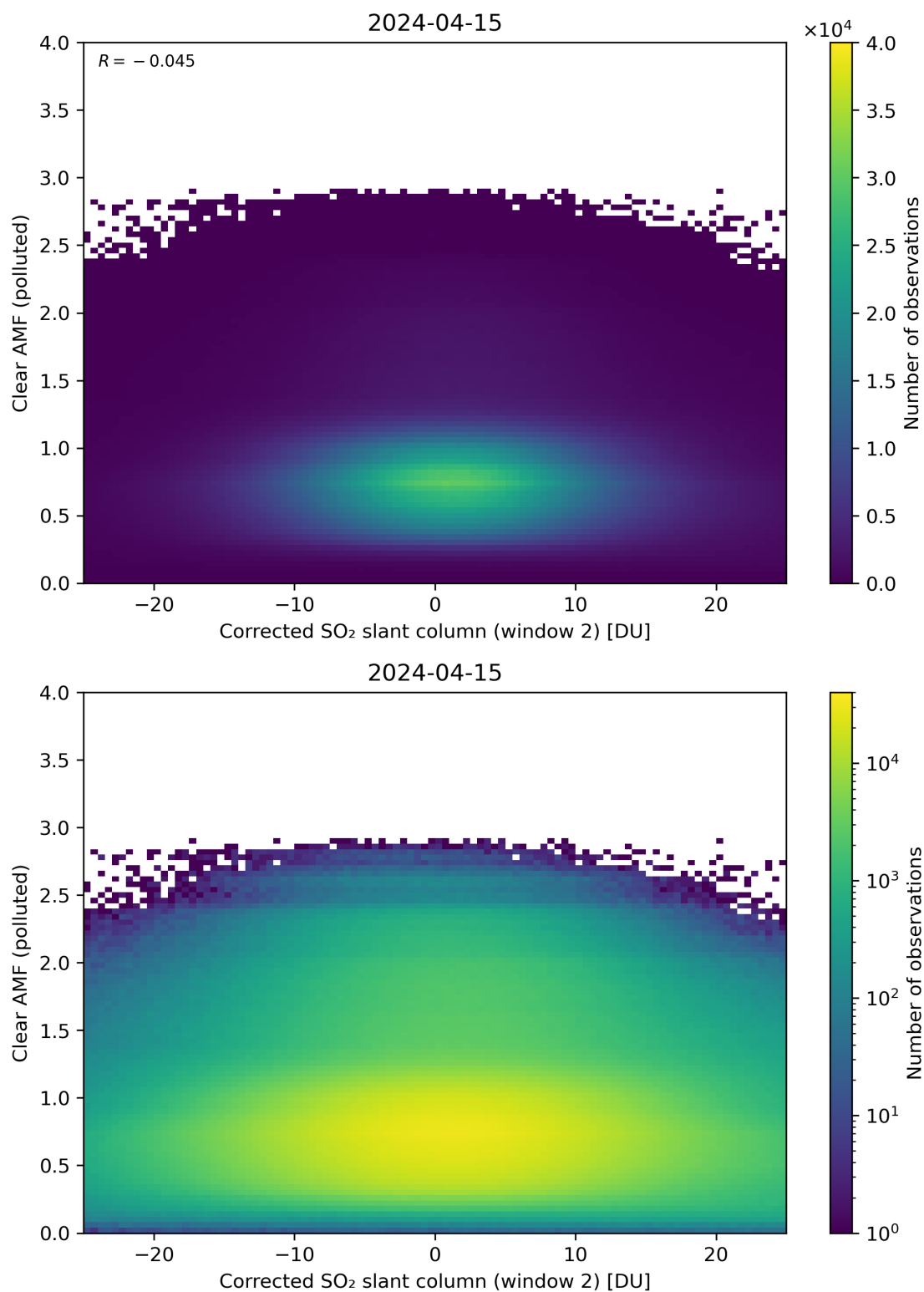
Figure 199: Scatter density plot of “Corrected SO 2 slant column (window 2)” against “Clear AMF (polluted)” for 2024-04-15 to 2024-04-16.
