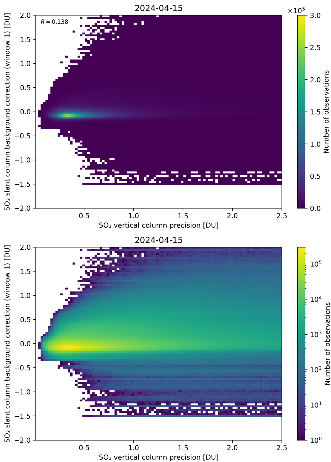
Figure 279: Scatter density plot of “SO 2 vertical column precision” against “SO 2 slant column background correction (window 1)” for 2024-04-15 to 2024-04-16.
