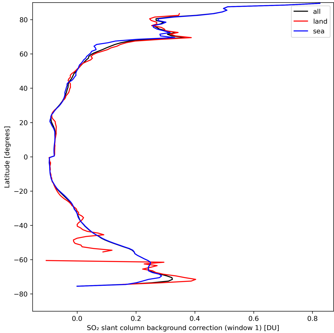
Figure 36: Zonal average of “SO 2 slant column background correction (window 1)” for 2024-04-15 to 2024-04-16.
