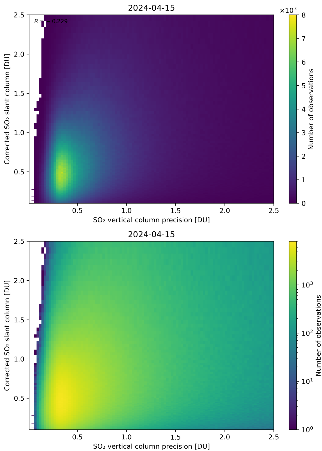
Figure 286: Scatter density plot of “SO 2 vertical column precision” against “Corrected SO 2 slant column” for 2024-04-15 to 2024-04-16.
