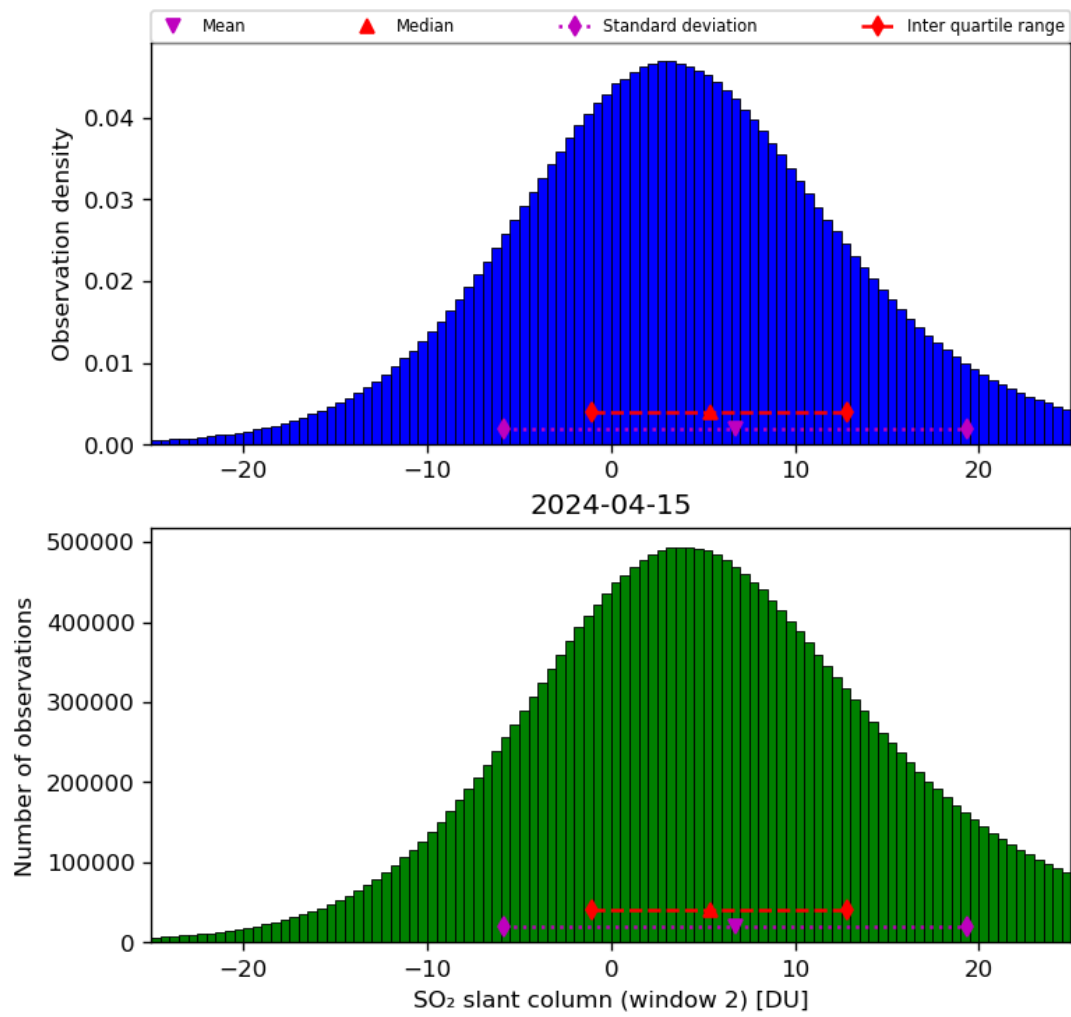
Figure 60: Histogram of “SO 2 slant column (window 2)” for 2024-04-15 to 2024-04-16
