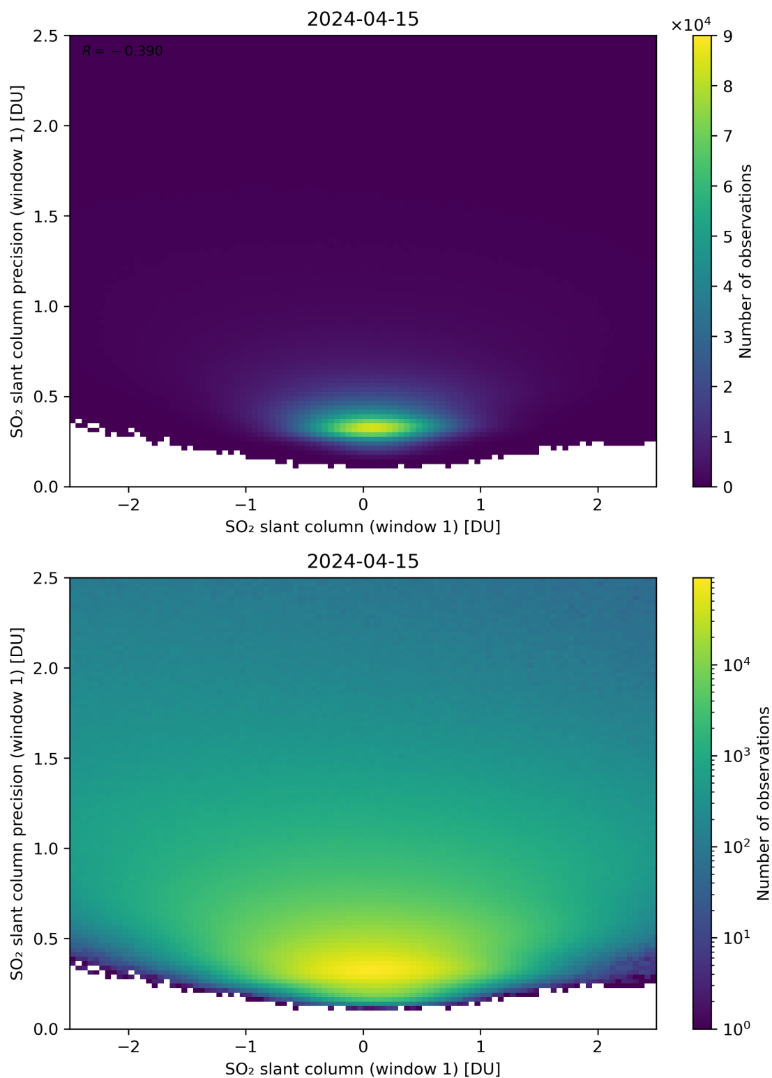
Figure 235: Scatter density plot of “SO 2 slant column (window 1)” against “SO 2 slant column precision (window 1)” for 2024-04-15 to 2024-04-16.
