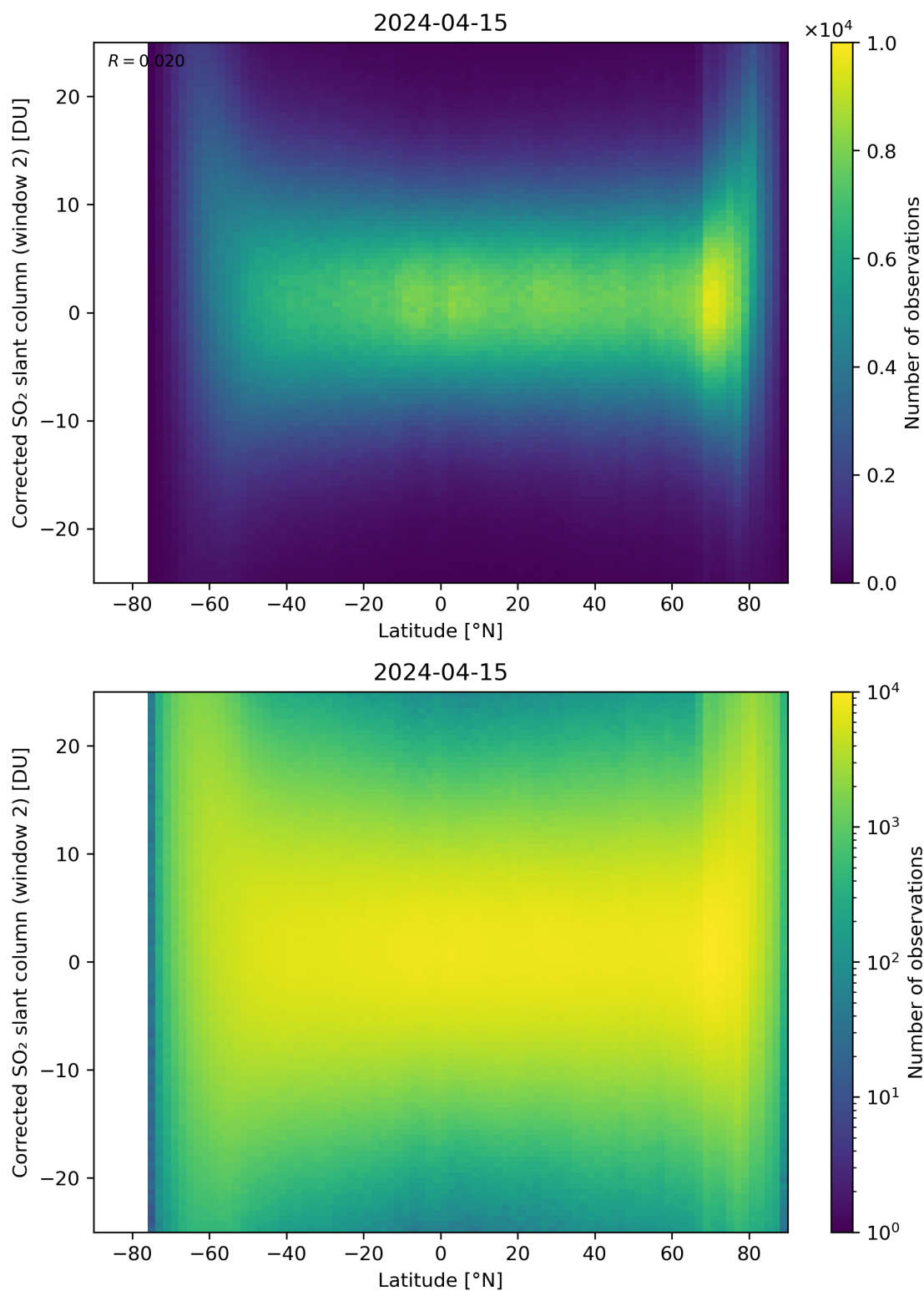
Figure 147: Scatter density plot of “Latitude” against “Corrected SO 2 slant column (window 2)” for 2024-04-15 to 2024-04-16.
