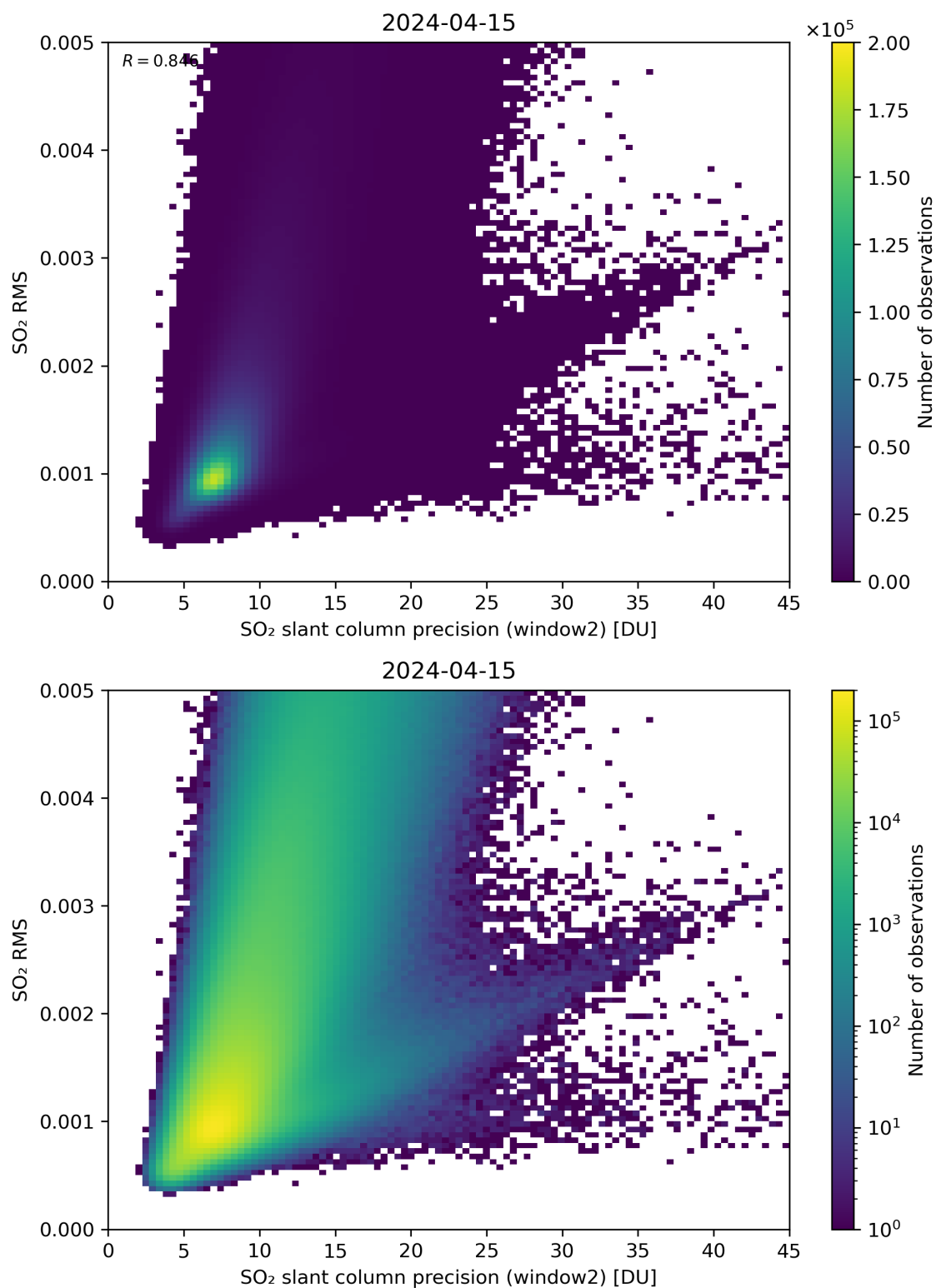
Figure 245: Scatter density plot of “SO 2 slant column precision (window2)” against “SO 2 RMS” for 2024-04-15 to 2024-04-16.
