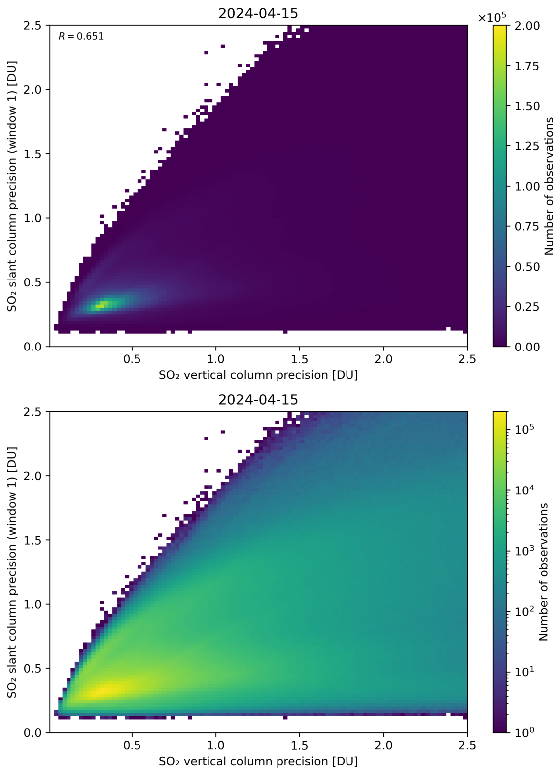
Figure 290: Scatter density plot of “SO 2 vertical column precision” against “SO 2 slant column precision (window 1)” for 2024-04-15 to 2024-04-16.
