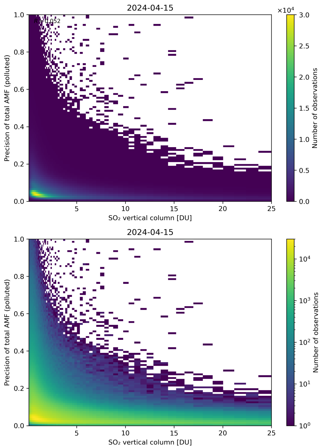
Figure 306: Scatter density plot of “SO 2 vertical column” against “Precision of total AMF (polluted)” for 2024-04-15 to 2024-04-16.
