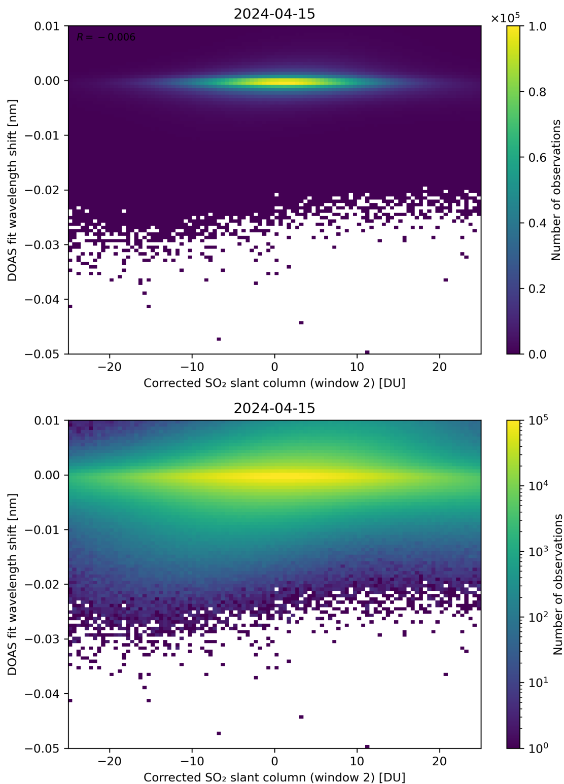
Figure 196: Scatter density plot of “Corrected SO 2 slant column (window 2)” against “DOAS fit wavelength shift” for 2024-04-15 to 2024-04-16.
