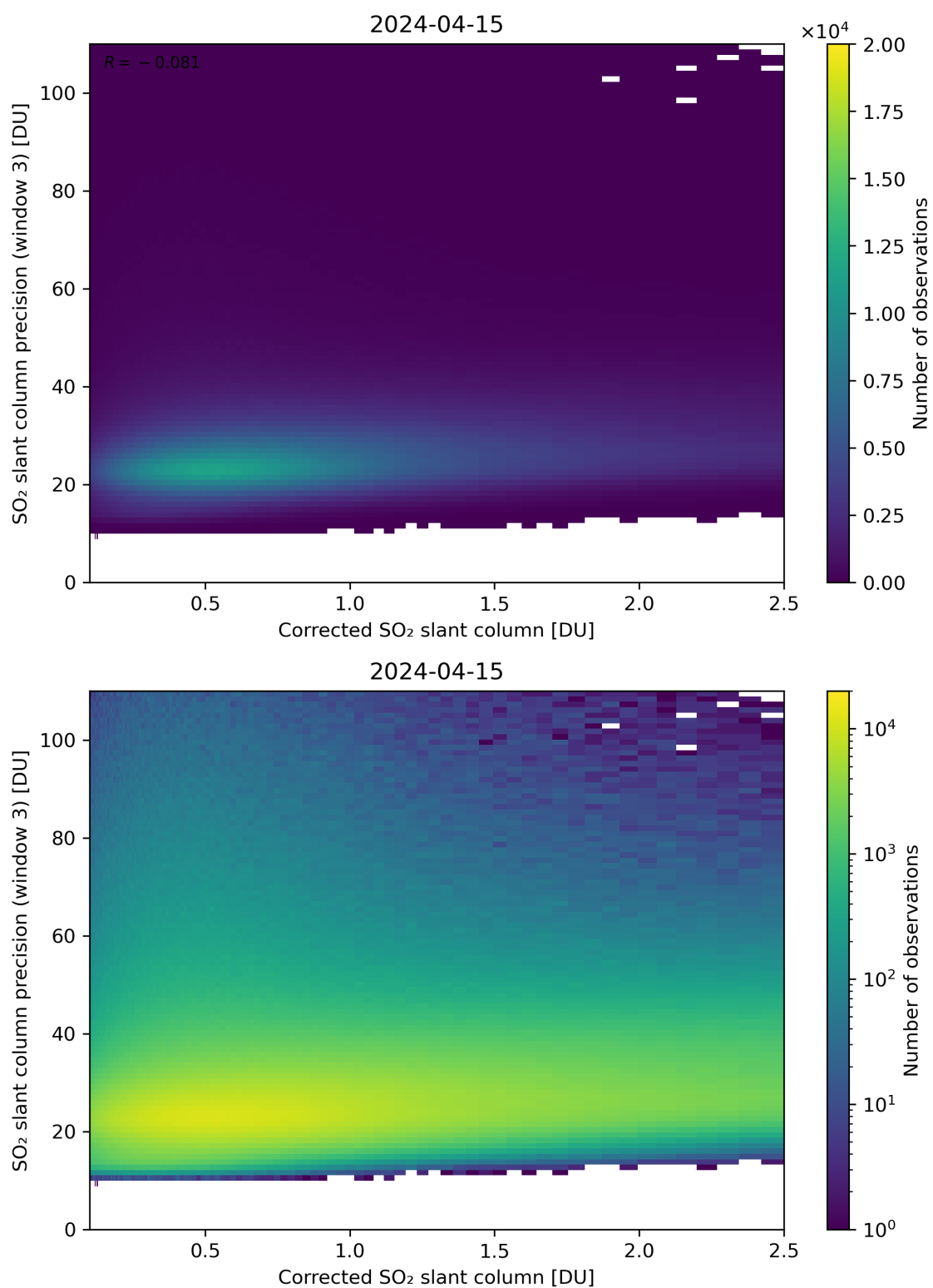
Figure 191: Scatter density plot of “Corrected SO 2 slant column” against “SO 2 slant column precision (window 3)” for 2024-04-15 to 2024-04-16.
