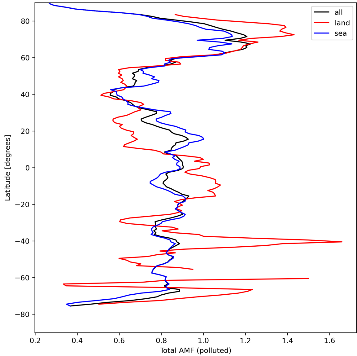
Figure 48: Zonal average of “Total AMF (polluted)” for 2024-04-15 to 2024-04-16.
