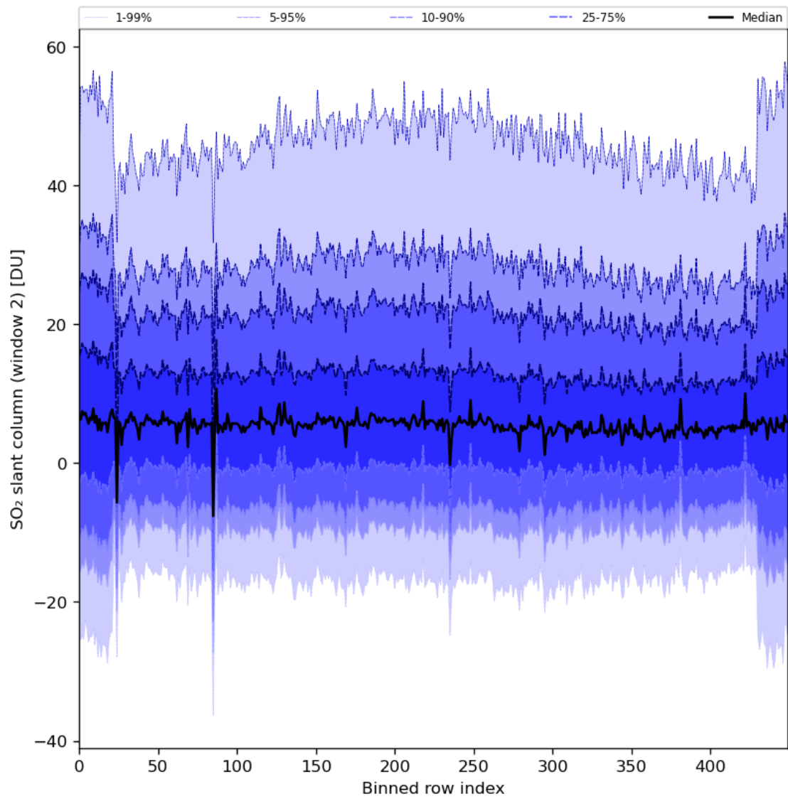
Figure 83: Along track statistics of “SO 2 slant column (window 2)” for 2024-04-15 to 2024-04-16
