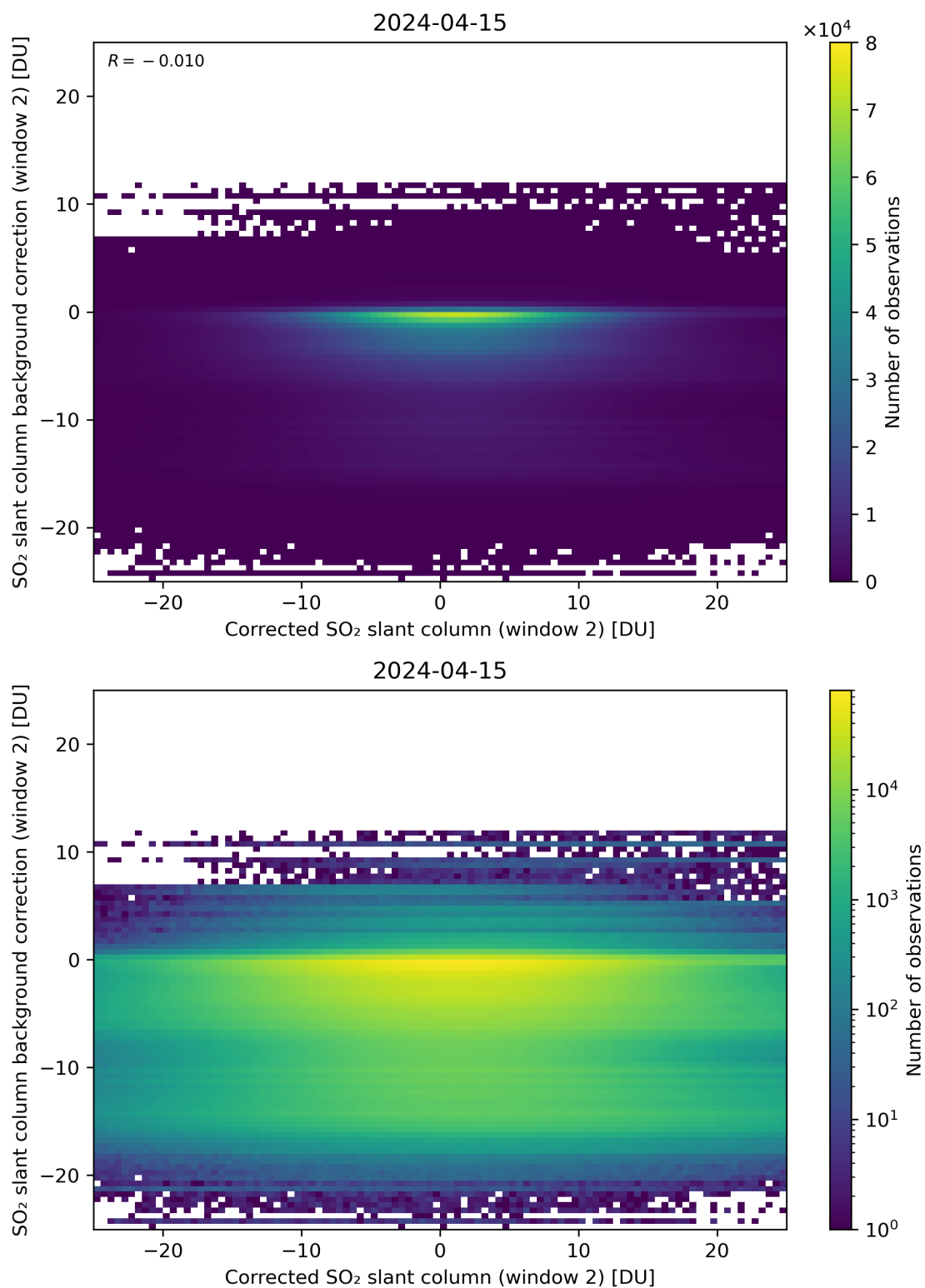
Figure 194: Scatter density plot of “Corrected SO 2 slant column (window 2)” against “SO 2 slant column background correction (window 2)” for 2024-04-15 to 2024-04-16.
