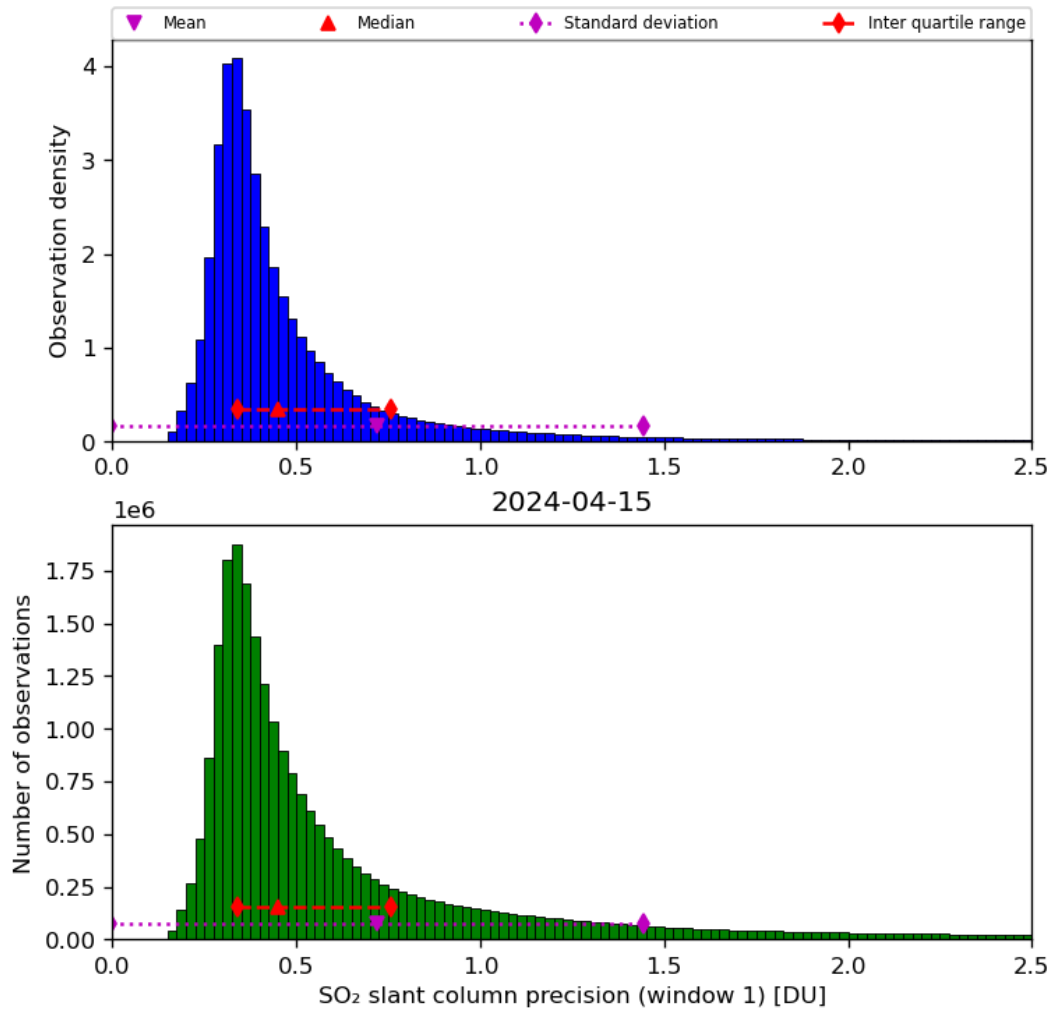
Figure 57: Histogram of “SO 2 slant column precision (window 1)” for 2024-04-15 to 2024-04-16
