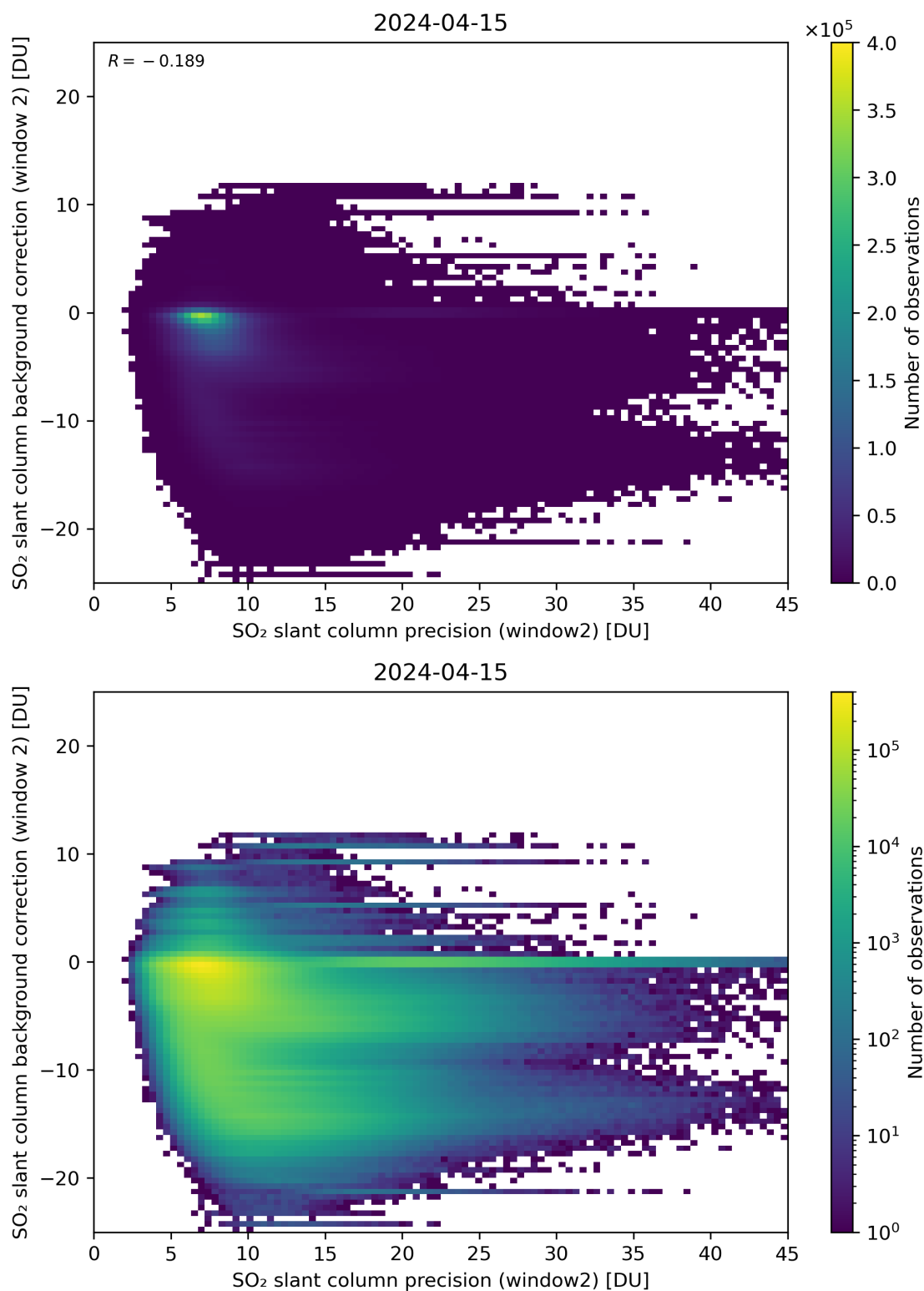
Figure 241: Scatter density plot of “SO 2 slant column precision (window2)” against “SO 2 slant column background correction (window 2)” for 2024-04-15 to 2024-04-16.
