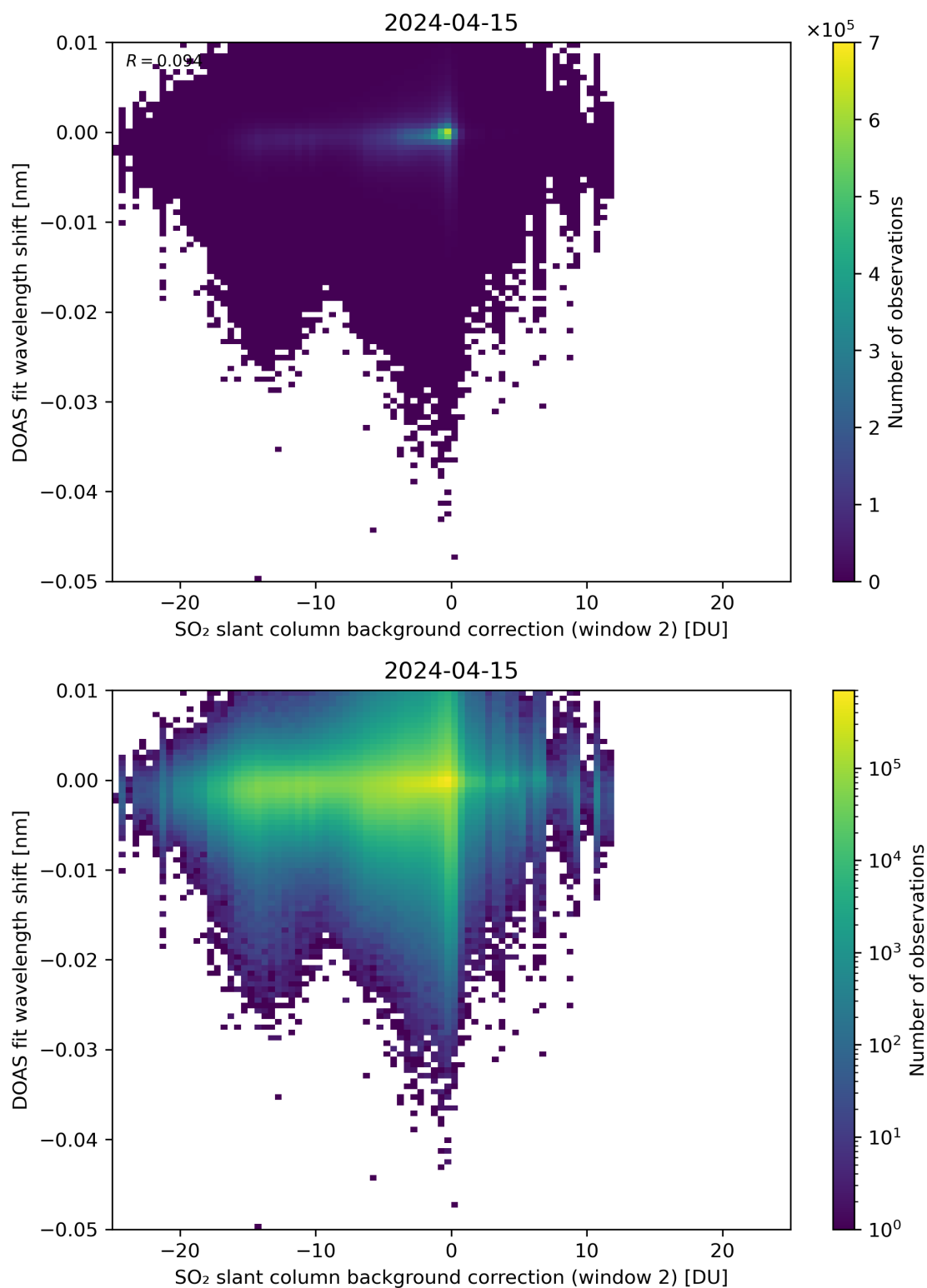
Figure 112: Scatter density plot of “SO 2 slant column background correction (window 2)” against “DOAS fit wavelength shift” for 2024-04-15 to 2024-04-16.
