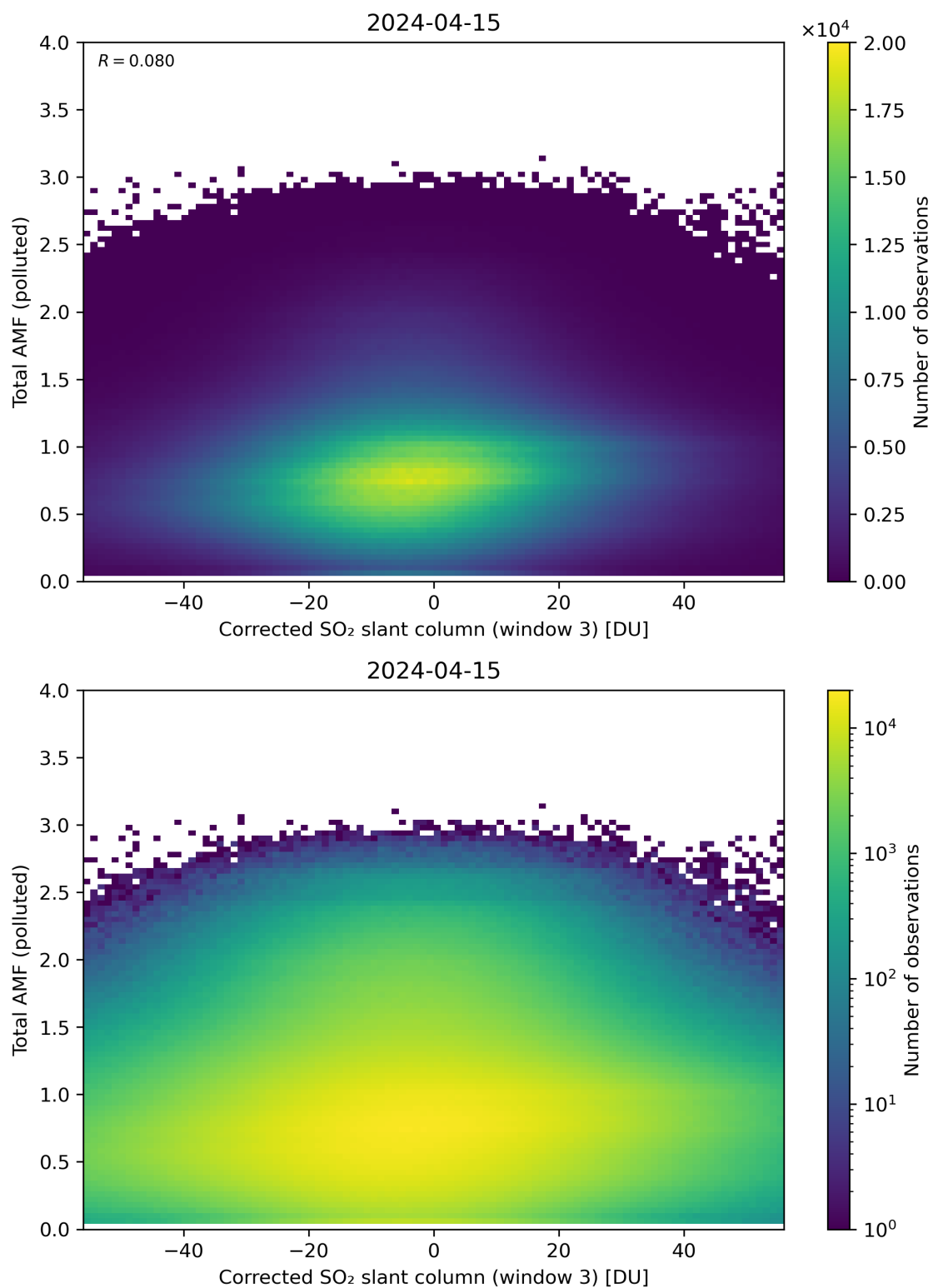
Figure 210: Scatter density plot of “Corrected SO 2 slant column (window 3)” against “Total AMF (polluted)” for 2024-04-15 to 2024-04-16.
