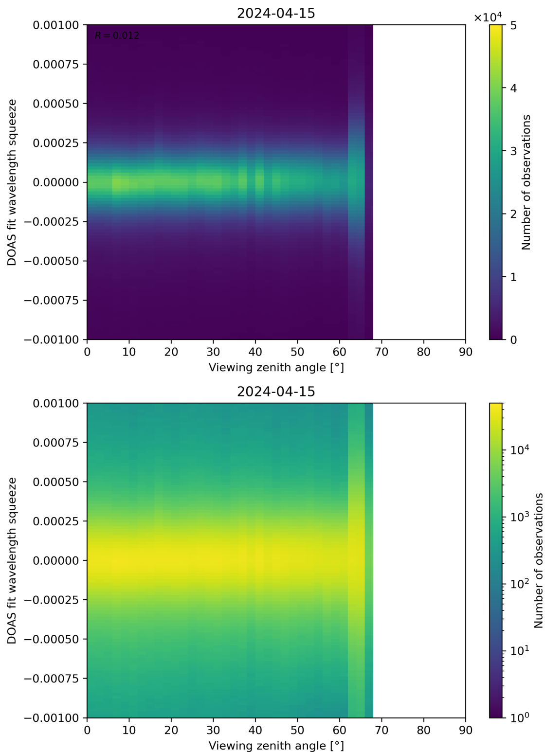
Figure 312: Scatter density plot of “Viewing zenith angle” against “DOAS fit wavelength squeeze” for 2024-04-15 to 2024-04-16.
