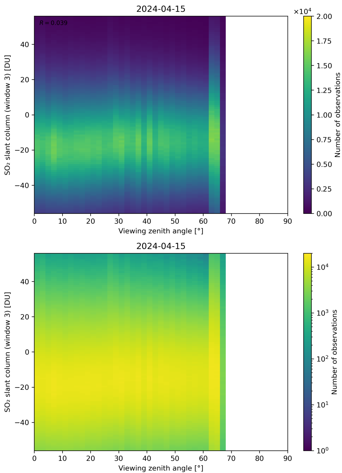
Figure 323: Scatter density plot of “Viewing zenith angle” against “SO 2 slant column (window 3)” for 2024-04-15 to 2024-04-16.
