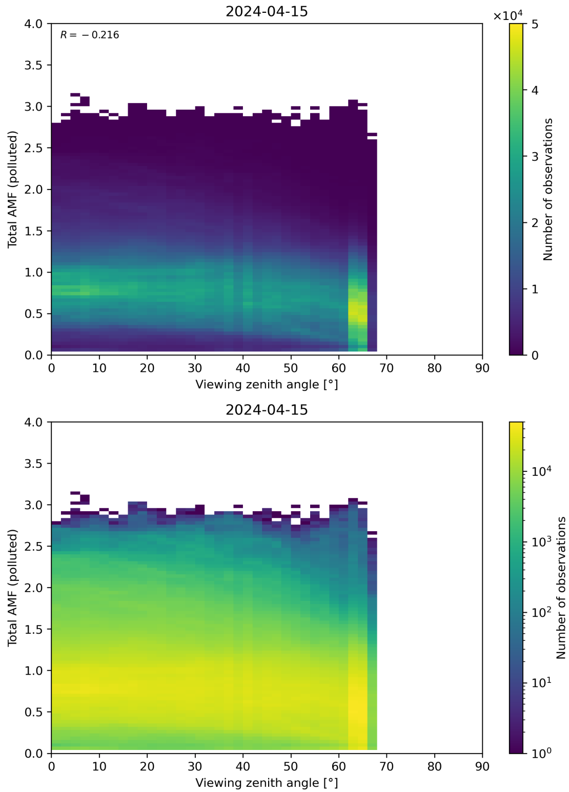
Figure 325: Scatter density plot of “Viewing zenith angle” against “Total AMF (polluted)” for 2024-04-15 to 2024-04-16.
