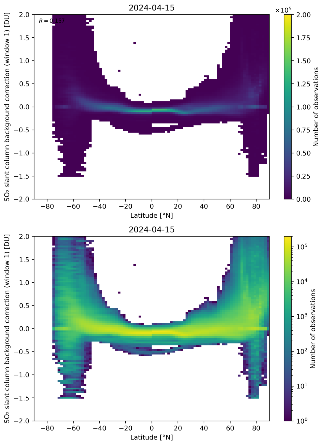
Figure 139: Scatter density plot of “Latitude” against “SO 2 slant column background correction (window 1)” for 2024-04-15 to 2024-04-16.
