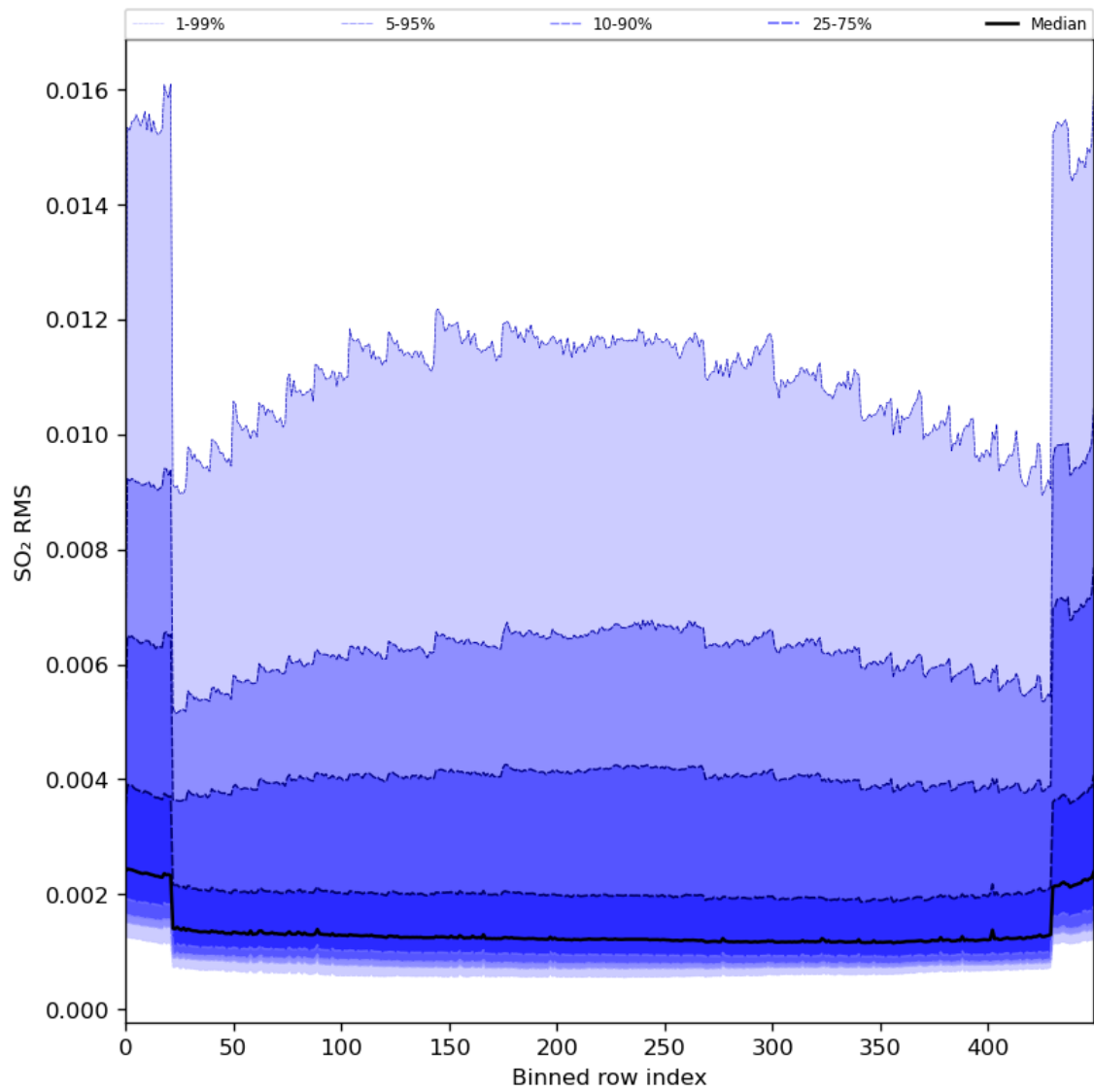
Figure 93: Along track statistics of “SO 2 RMS” for 2024-04-15 to 2024-04-16
