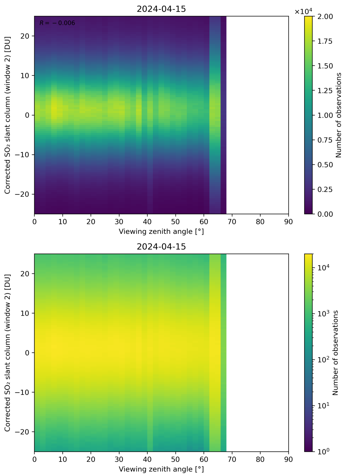
Figure 318: Scatter density plot of “Viewing zenith angle” against “Corrected SO 2 slant column (window 2)” for 2024-04-15 to 2024-04-16.
