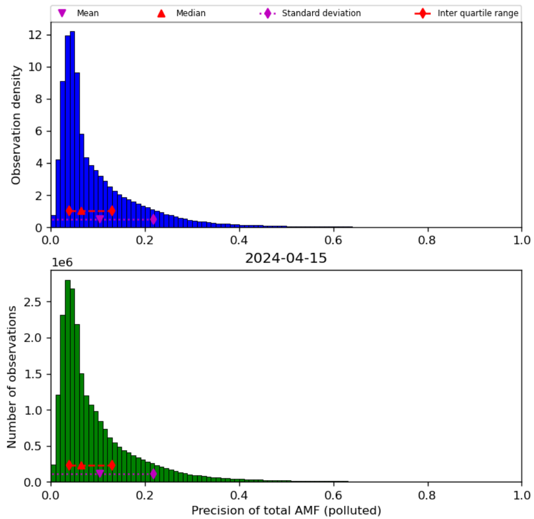
Figure 72: Histogram of “Precision of total AMF (polluted)” for 2024-04-15 to 2024-04-16
