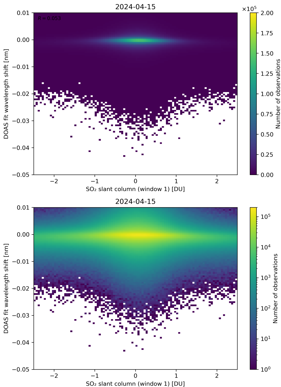
Figure 215: Scatter density plot of “SO 2 slant column (window 1)” against “DOAS fit wavelength shift” for 2024-04-15 to 2024-04-16.
