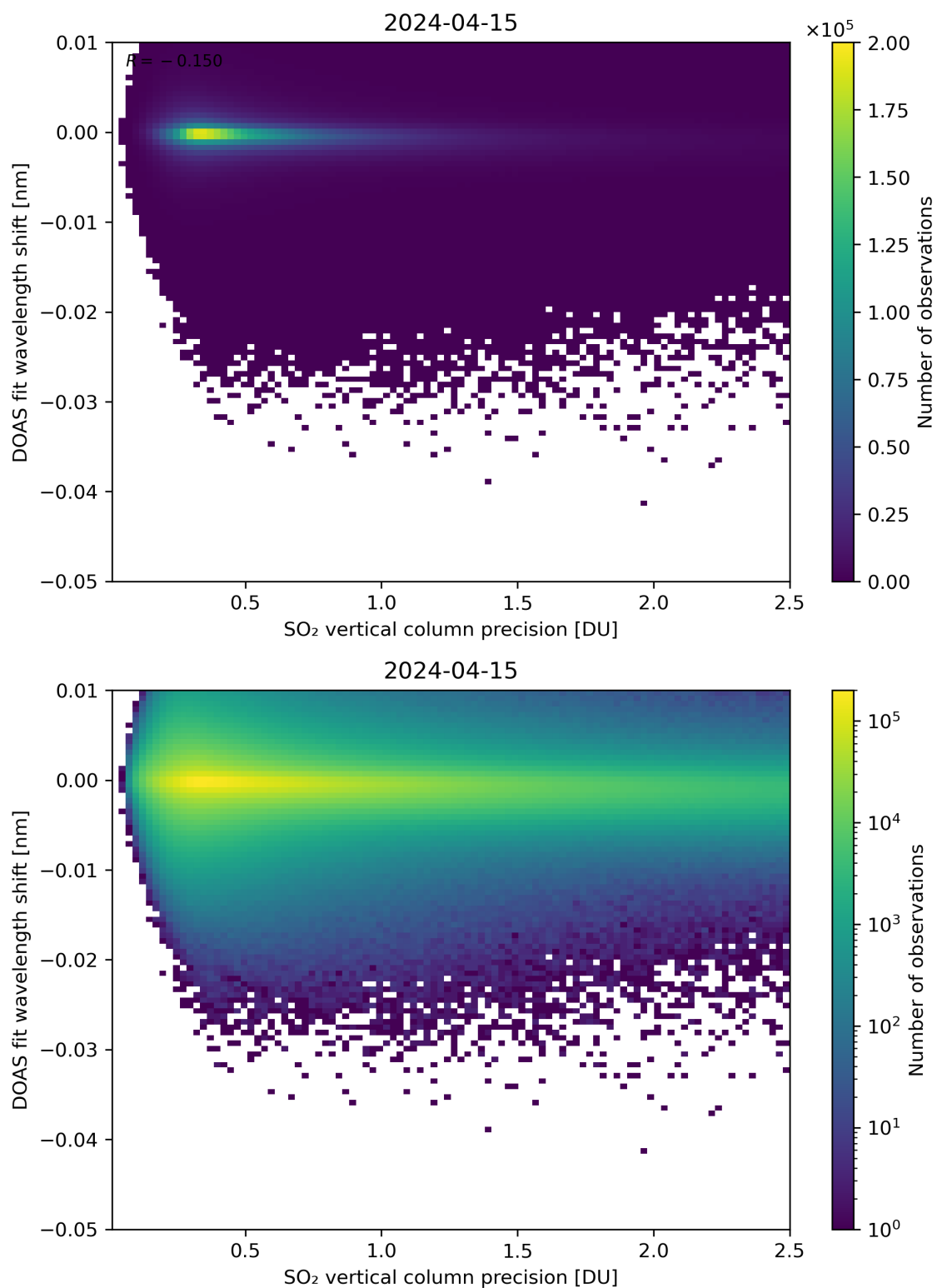
Figure 282: Scatter density plot of “SO 2 vertical column precision” against “DOAS fit wavelength shift” for 2024-04-15 to 2024-04-16.
