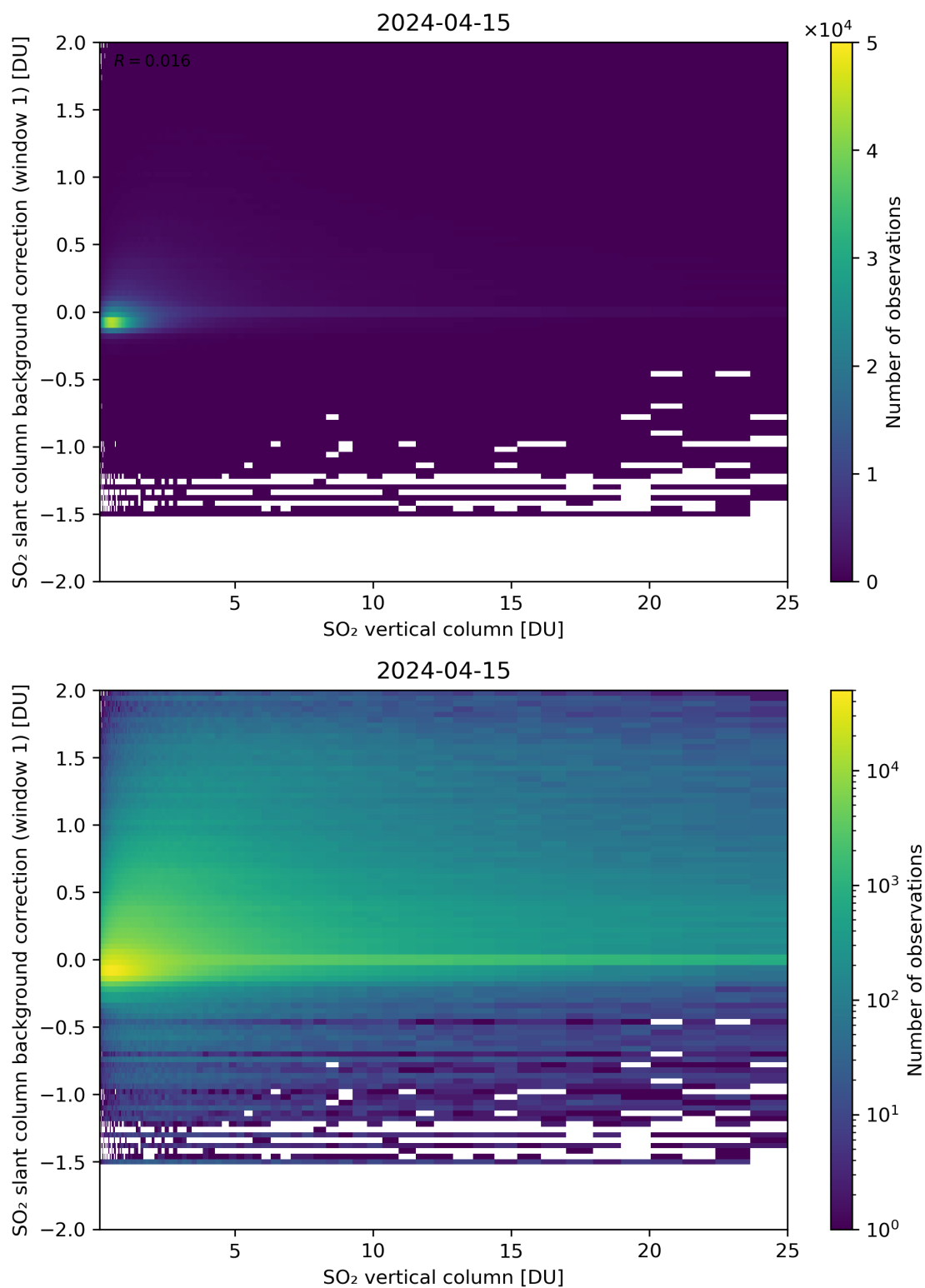
Figure 273: Scatter density plot of “SO 2 vertical column” against “SO 2 slant column background correction (window 1)” for 2024-04-15 to 2024-04-16.
