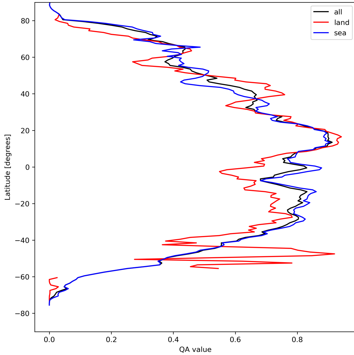
Figure 29: Zonal average of “QA value” for 2024-04-15 to 2024-04-16.
