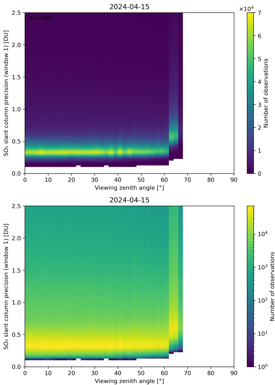
Figure 321: Scatter density plot of “Viewing zenith angle” against “SO 2 slant column precision (window 1)” for 2024-04-15 to 2024-04-16.
