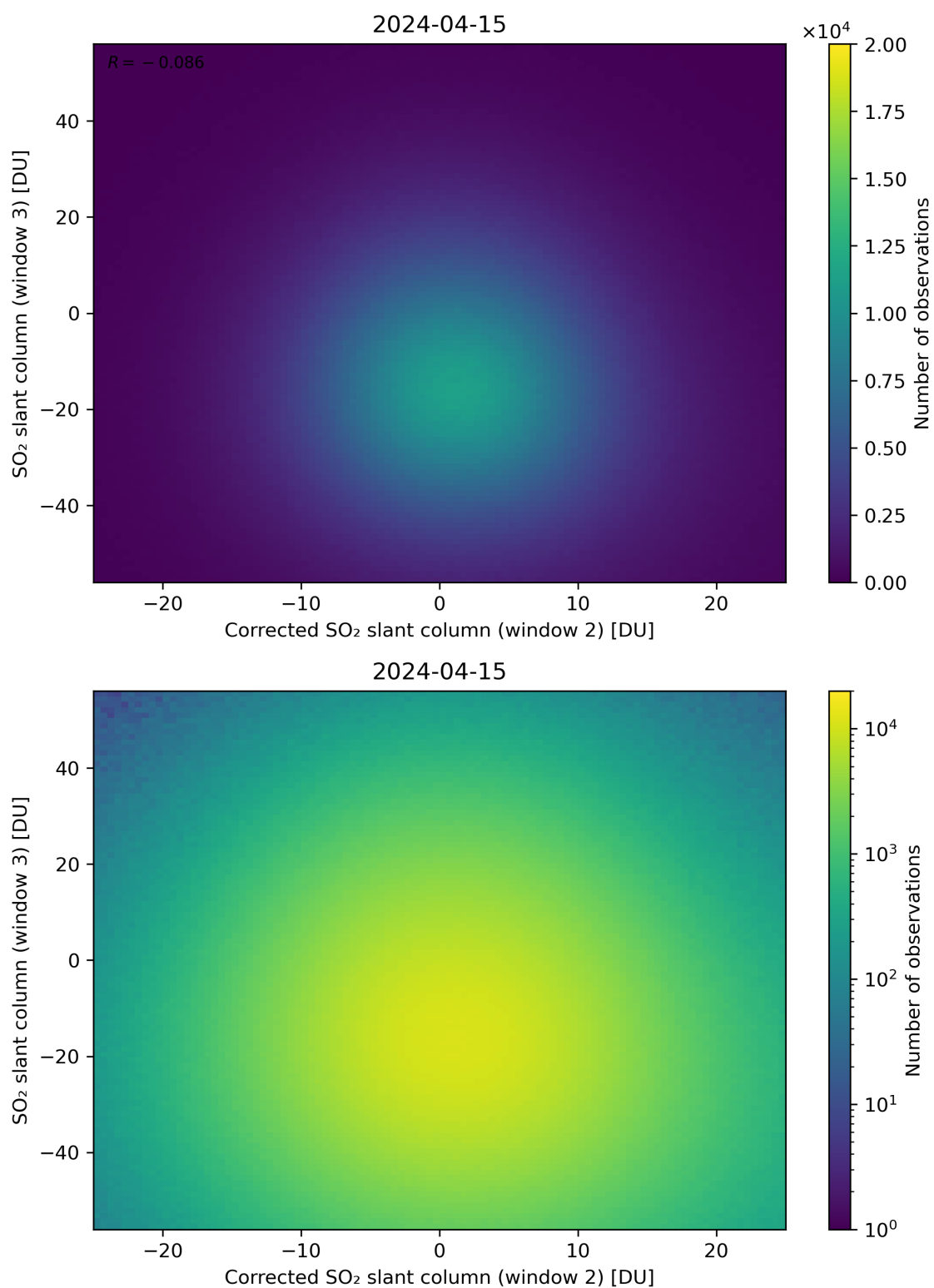
Figure 201: Scatter density plot of “Corrected SO 2 slant column (window 2)” against “SO 2 slant column (window 3)” for 2024-04-15 to 2024-04-16.
