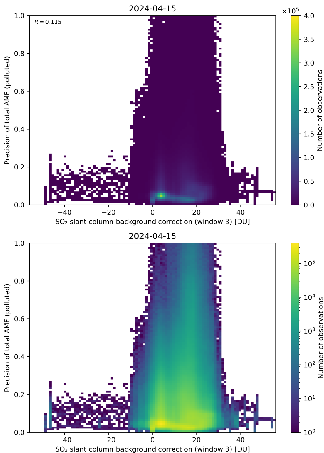
Figure 126: Scatter density plot of “SO 2 slant column background correction (window 3)” against “Precision of total AMF (polluted)” for 2024-04-15 to 2024-04-16.
