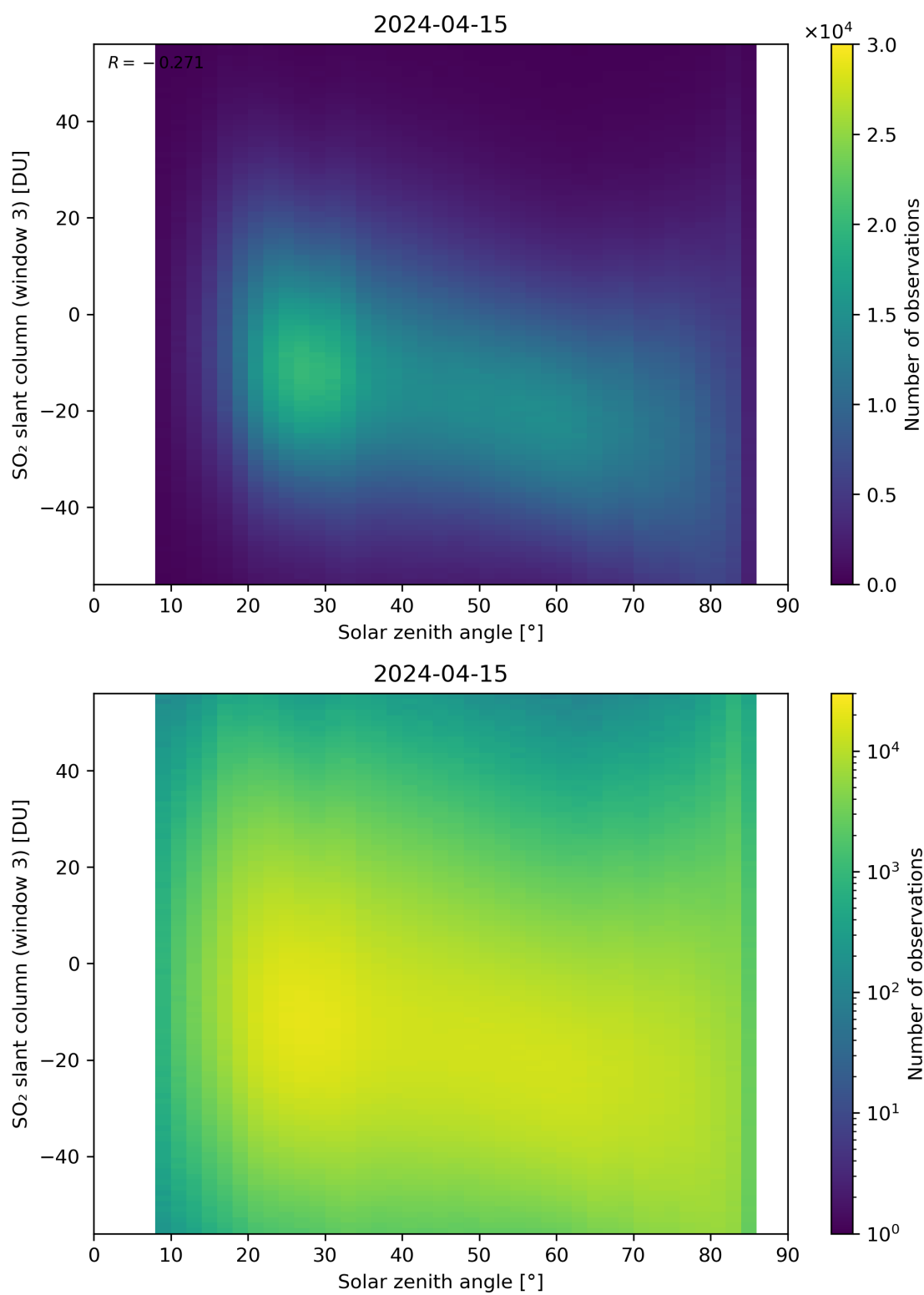
Figure 172: Scatter density plot of “Solar zenith angle” against “SO 2 slant column (window 3)” for 2024-04-15 to 2024-04-16.
