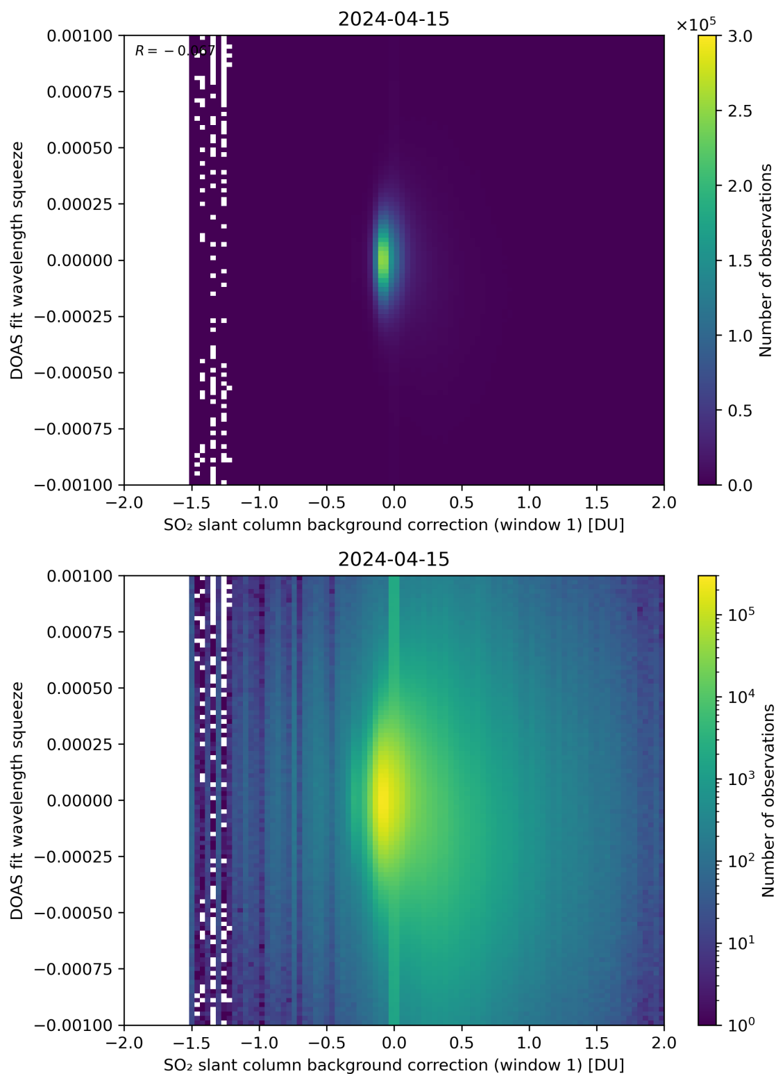
Figure 101: Scatter density plot of “SO 2 slant column background correction (window 1)” against “DOAS fit wavelength squeeze” for 2024-04-15 to 2024-04-16.
