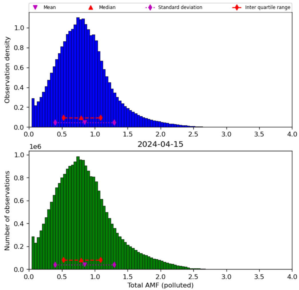
Figure 71: Histogram of “Total AMF (polluted)” for 2024-04-15 to 2024-04-16
