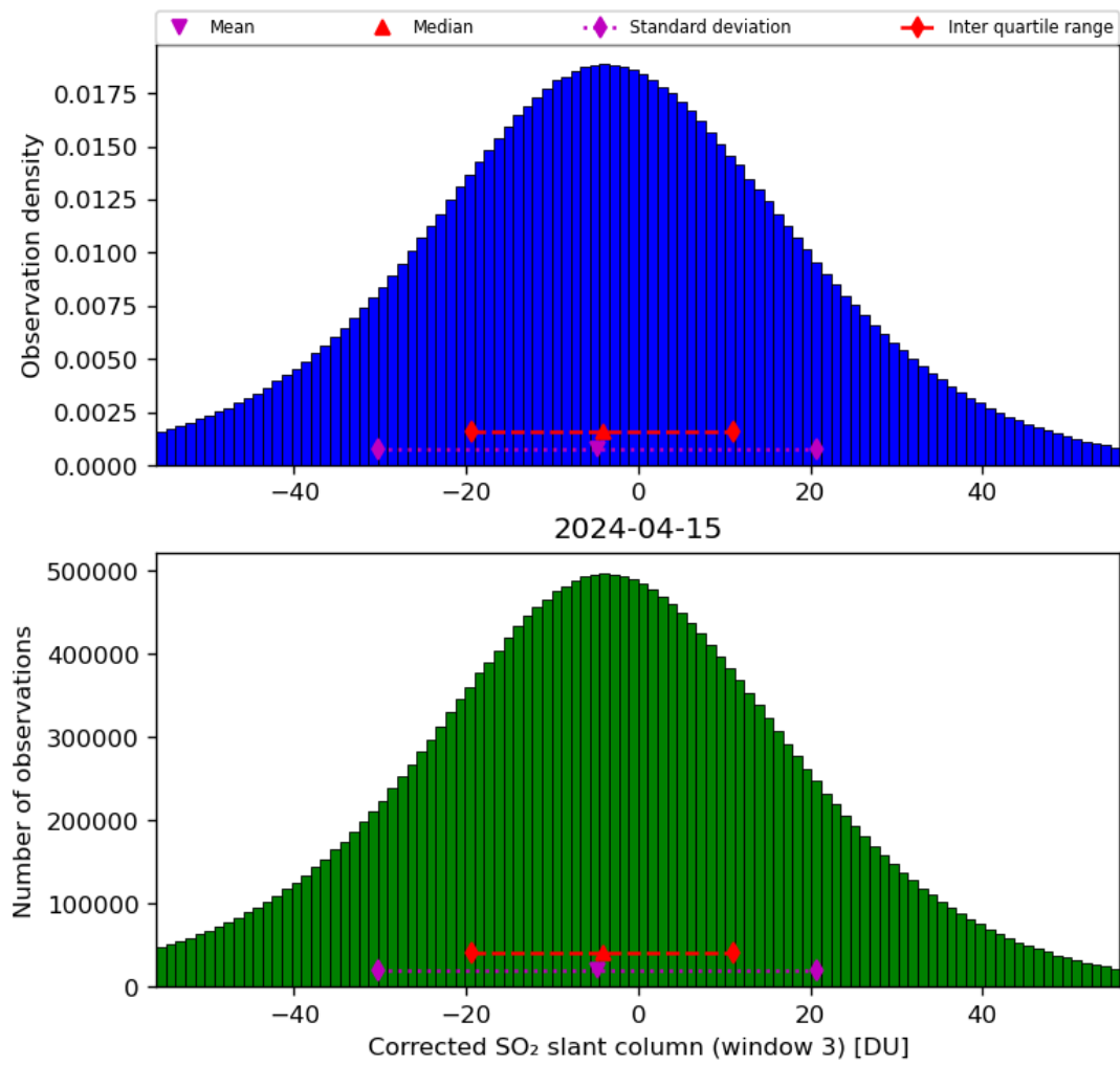
Figure 66: Histogram of “Corrected SO 2 slant column (window 3)” for 2024-04-15 to 2024-04-16
