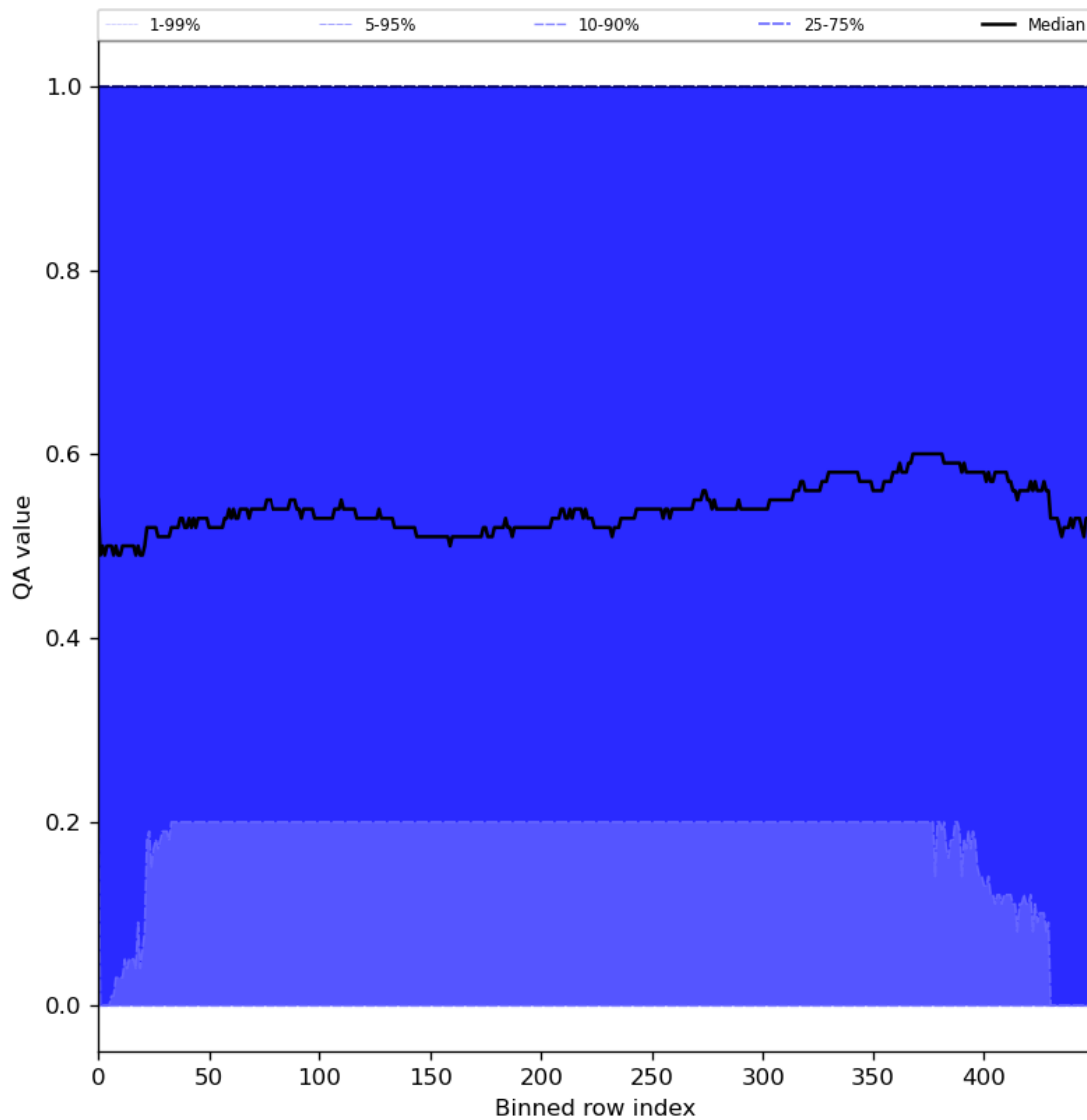
Figure 75: Along track statistics of “QA value” for 2024-04-15 to 2024-04-16
