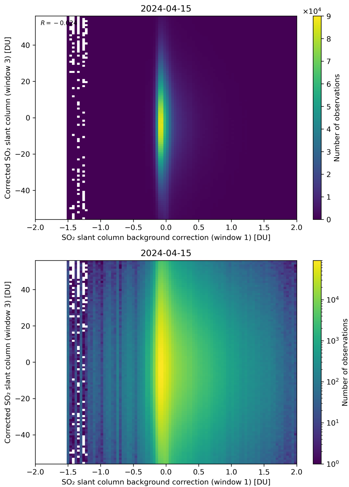
Figure 105: Scatter density plot of “SO 2 slant column background correction (window 1)” against “Corrected SO 2 slant column (window 3)” for 2024-04-15 to 2024-04-16.
