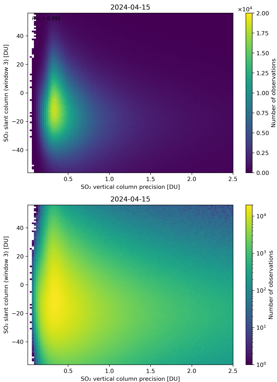
Figure 292: Scatter density plot of “SO 2 vertical column precision” against “SO 2 slant column (window 3)” for 2024-04-15 to 2024-04-16.
