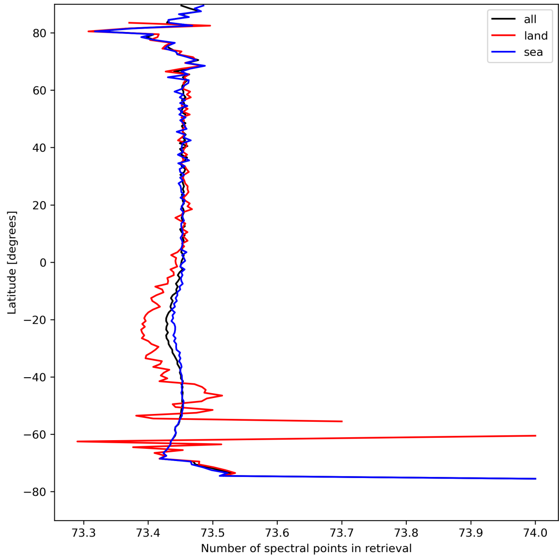
Figure 51: Zonal average of “Number of spectral points in retrieval” for 2024-04-15 to 2024-04-16.
