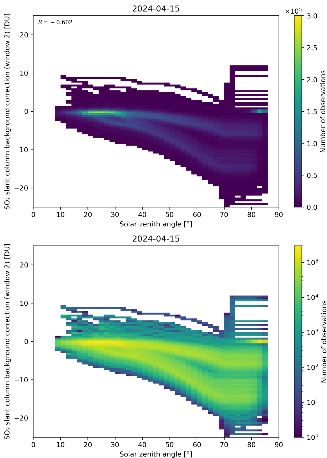
Figure 159: Scatter density plot of “Solar zenith angle” against “SO 2 slant column background correction (window 2)” for 2024-04-15 to 2024-04-16.
