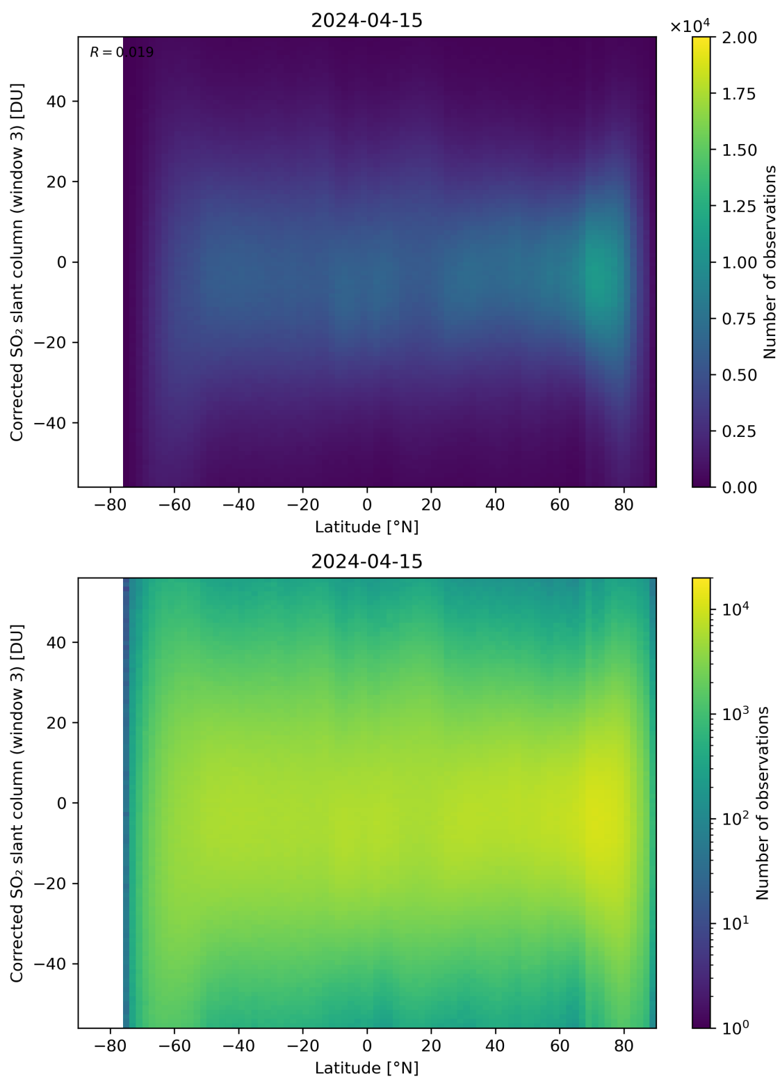
Figure 148: Scatter density plot of “Latitude” against “Corrected SO 2 slant column (window 3)” for 2024-04-15 to 2024-04-16.
