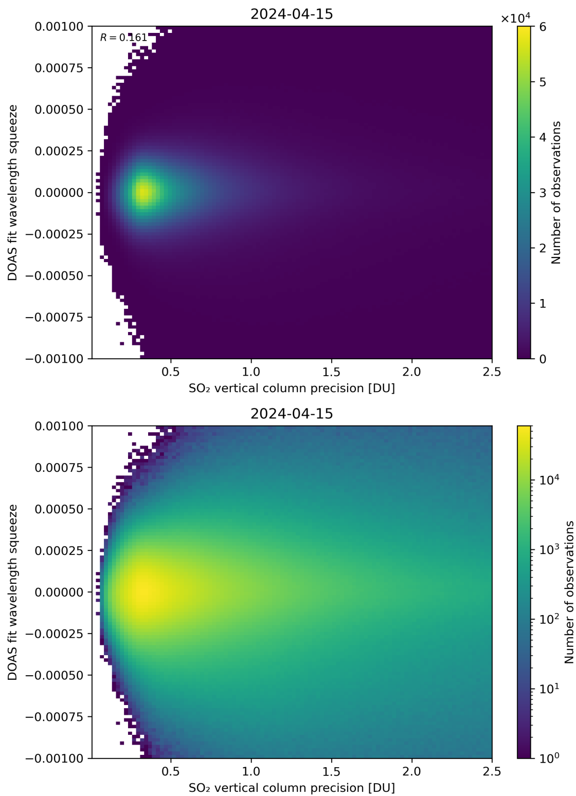
Figure 283: Scatter density plot of “SO 2 vertical column precision” against “DOAS fit wavelength squeeze” for 2024-04-15 to 2024-04-16.
