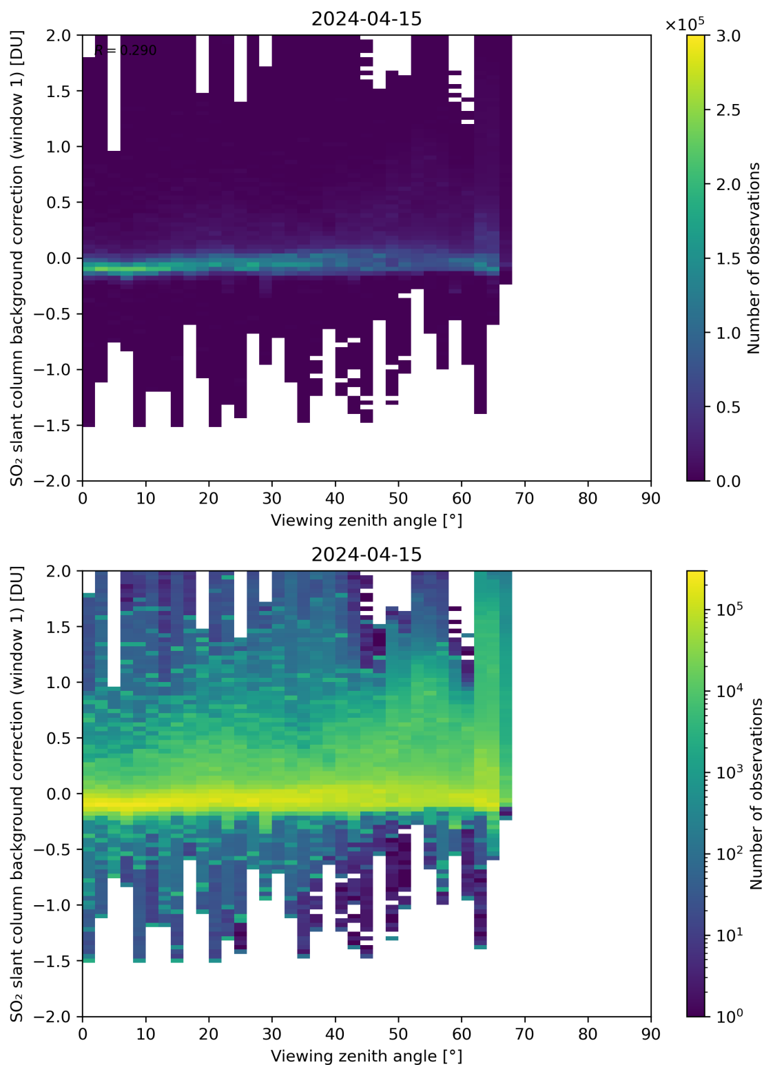
Figure 308: Scatter density plot of “Viewing zenith angle” against “SO 2 slant column background correction (window 1)” for 2024-04-15 to 2024-04-16.
