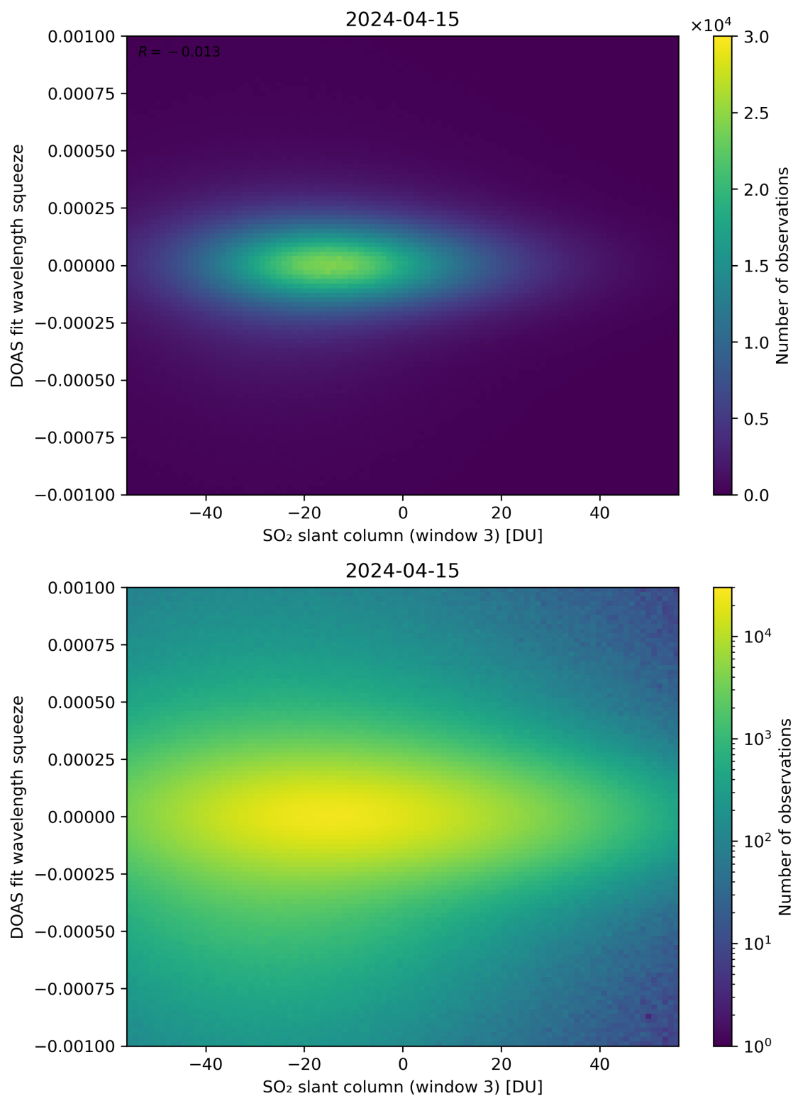
Figure 255: Scatter density plot of “SO 2 slant column (window 3)” against “DOAS fit wavelength squeeze” for 2024-04-15 to 2024-04-16.
