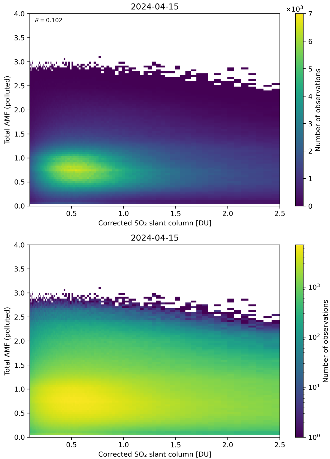
Figure 192: Scatter density plot of “Corrected SO 2 slant column” against “Total AMF (polluted)” for 2024-04-15 to 2024-04-16.
