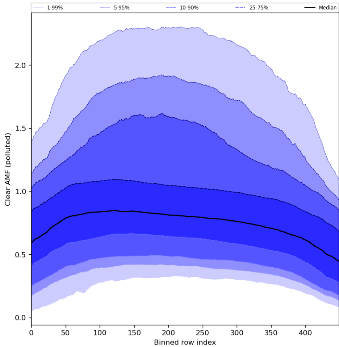
Figure 96: Along track statistics of “Clear AMF (polluted)” for 2024-04-15 to 2024-04-16
