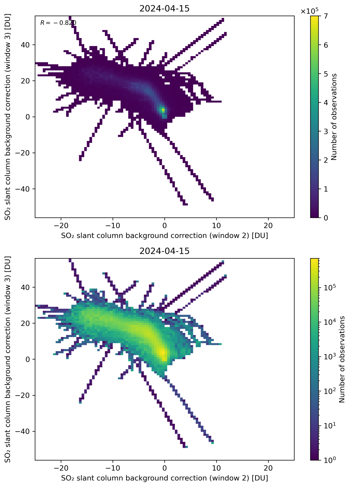
Figure 111: Scatter density plot of “SO 2 slant column background correction (window 2)” against “SO 2 slant column background correction (window 3)” for 2024-04-15 to 2024-04-16.
