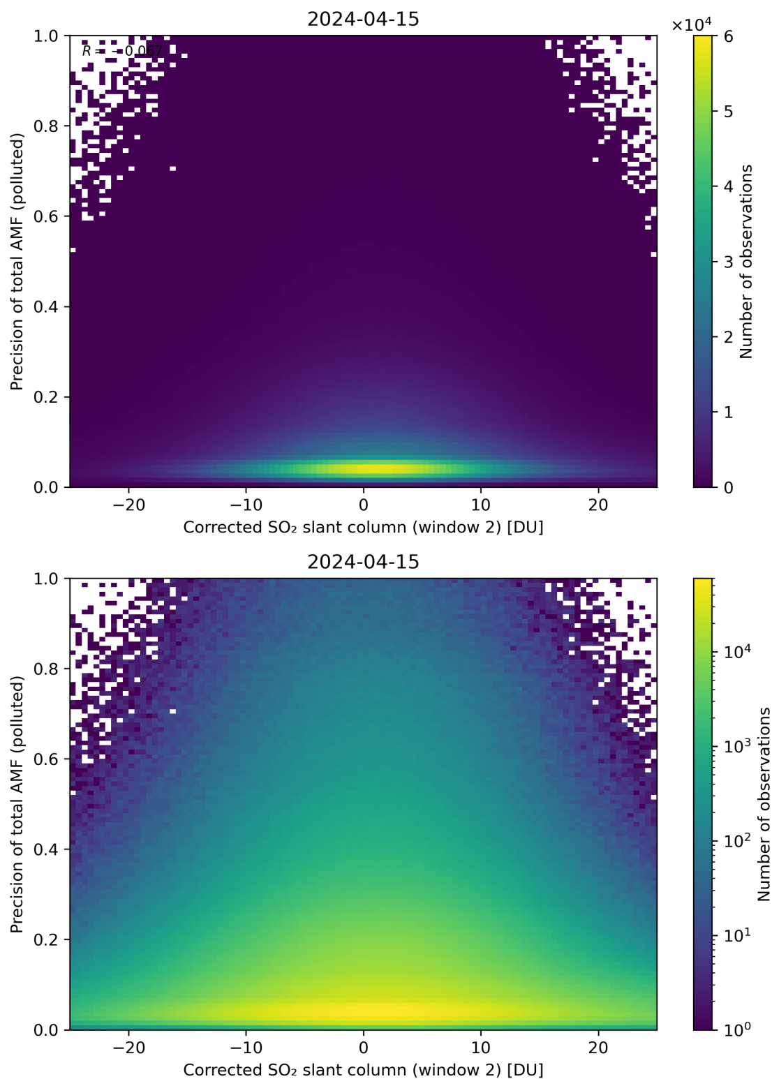
Figure 204: Scatter density plot of “Corrected SO 2 slant column (window 2)” against “Precision of total AMF (polluted)” for 2024-04-15 to 2024-04-16.
