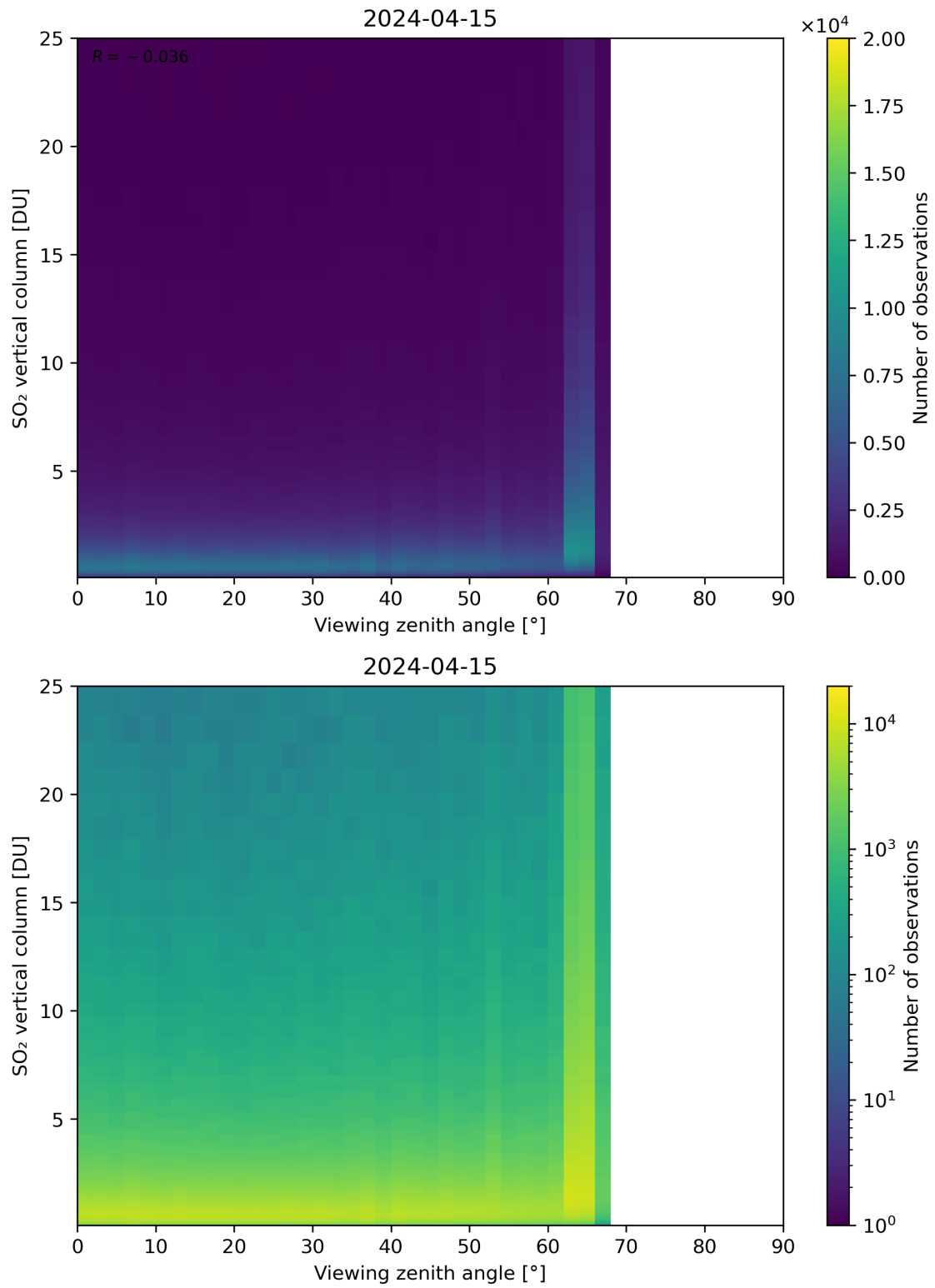
Figure 327: Scatter density plot of “Viewing zenith angle” against “SO 2 vertical column” for 2024-04-15 to 2024-04-16.
