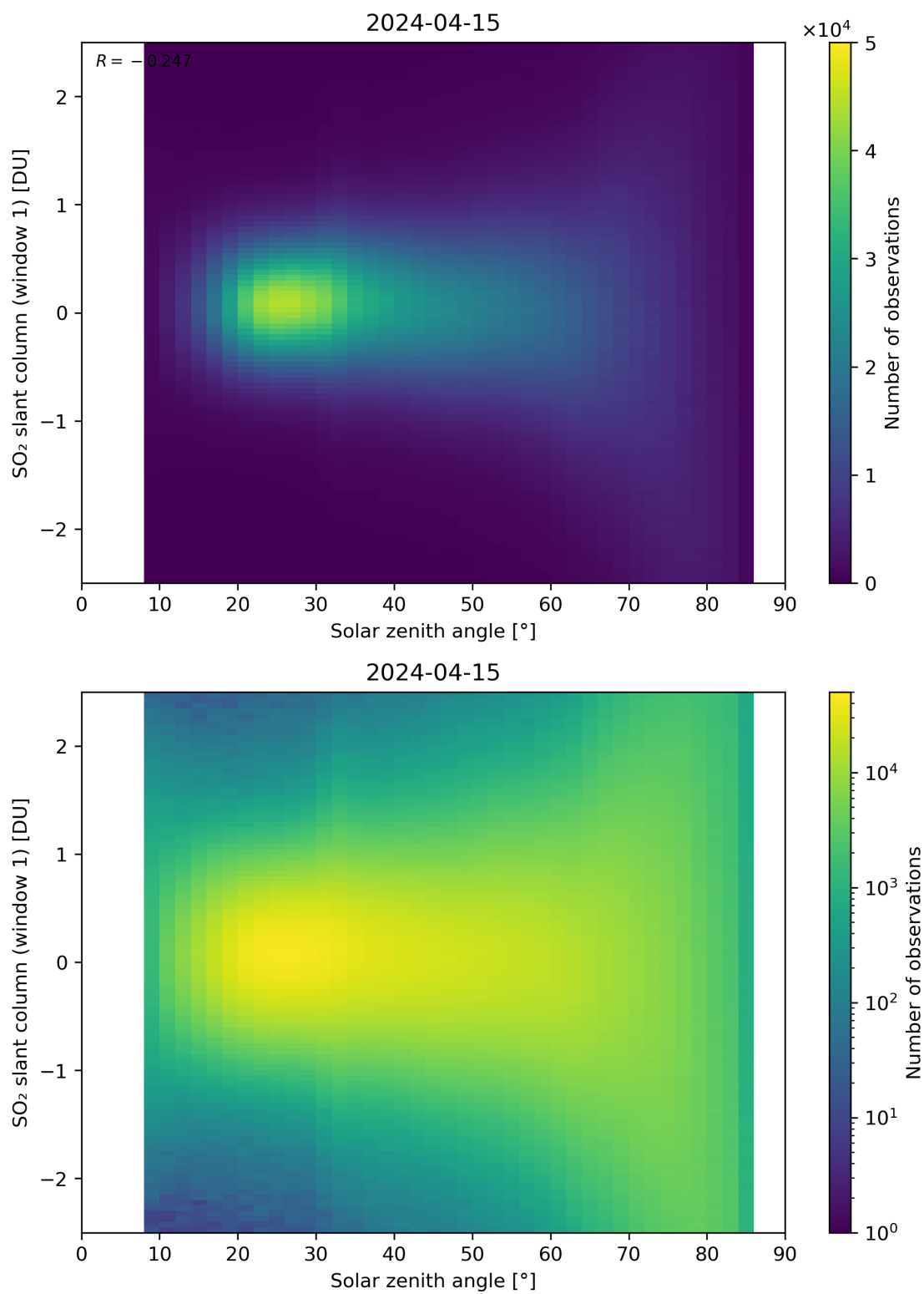
Figure 169: Scatter density plot of “Solar zenith angle” against “SO 2 slant column (window 1)” for 2024-04-15 to 2024-04-16.
