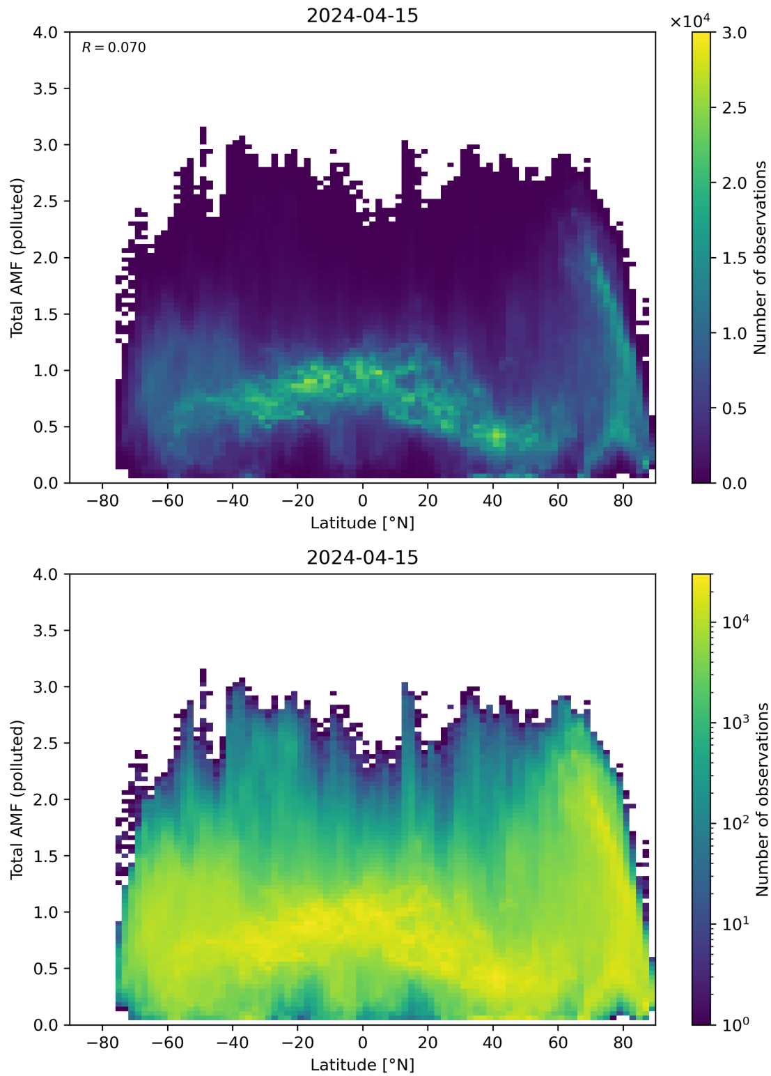
Figure 154: Scatter density plot of “Latitude” against “Total AMF (polluted)” for 2024-04-15 to 2024-04-16.
