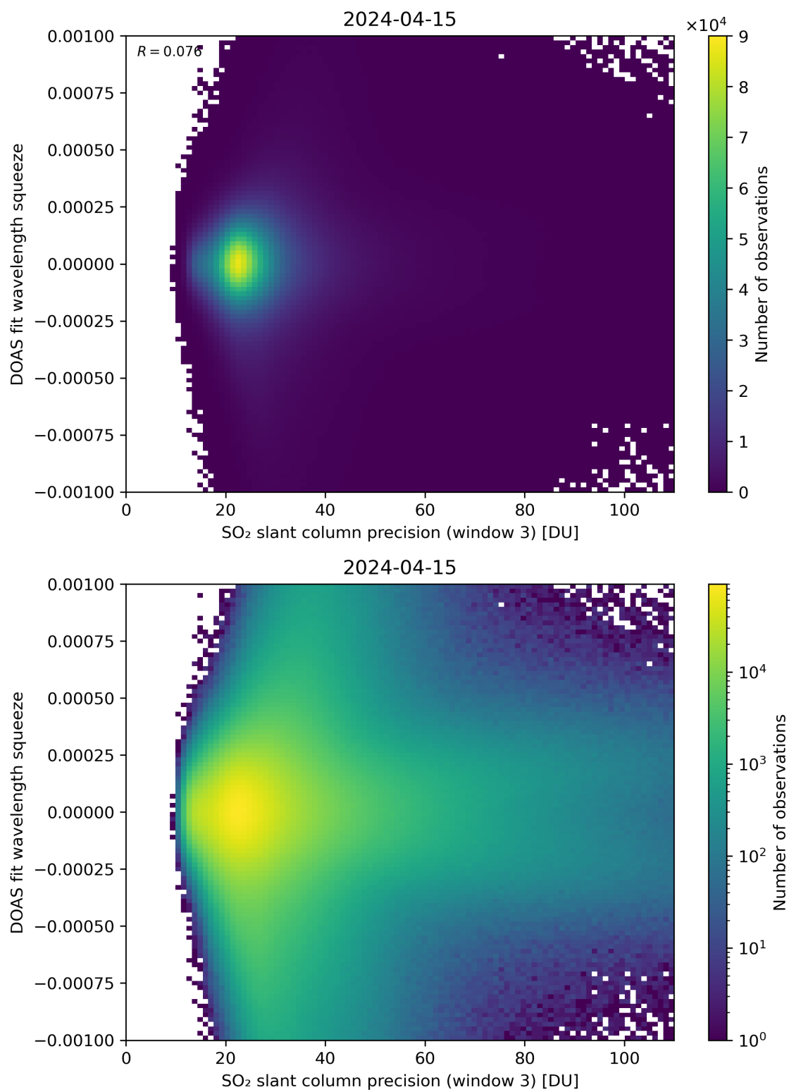
Figure 259: Scatter density plot of “SO 2 slant column precision (window 3)” against “DOAS fit wavelength squeeze” for 2024-04-15 to 2024-04-16.
