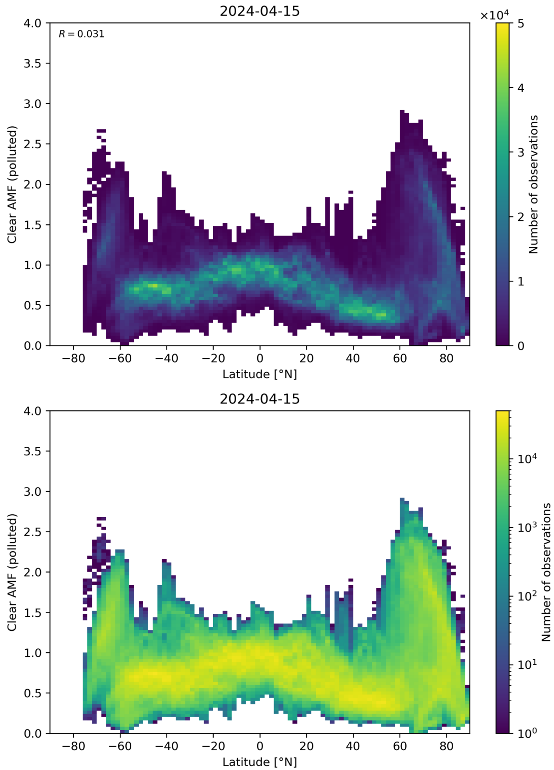
Figure 145: Scatter density plot of “Latitude” against “Clear AMF (polluted)” for 2024-04-15 to 2024-04-16.
