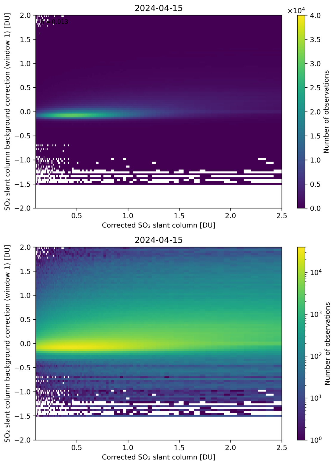
Figure 178: Scatter density plot of “Corrected SO 2 slant column” against “SO 2 slant column background correction (window 1)” for 2024-04-15 to 2024-04-16.
