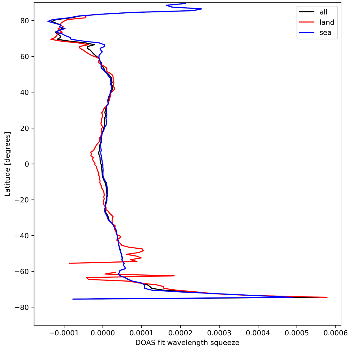
Figure 46: Zonal average of “DOAS fit wavelength squeeze” for 2024-04-15 to 2024-04-16.
