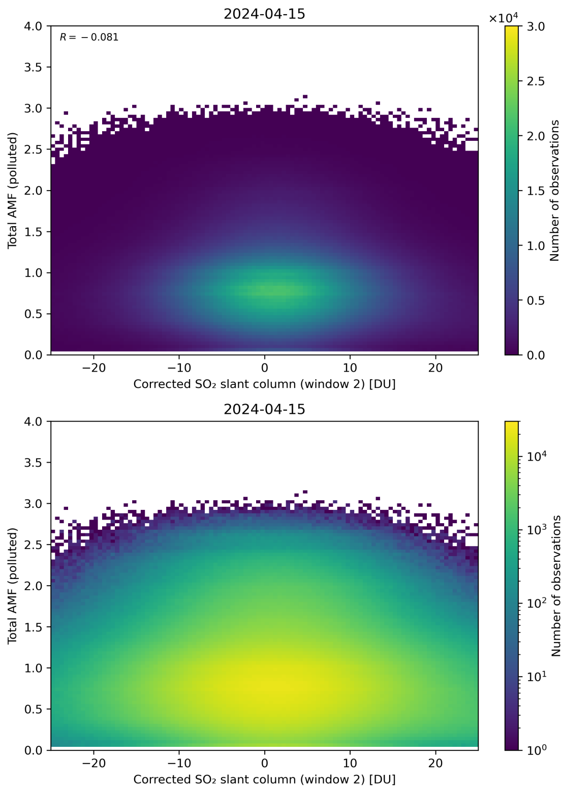
Figure 203: Scatter density plot of “Corrected SO 2 slant column (window 2)” against “Total AMF (polluted)” for 2024-04-15 to 2024-04-16.
