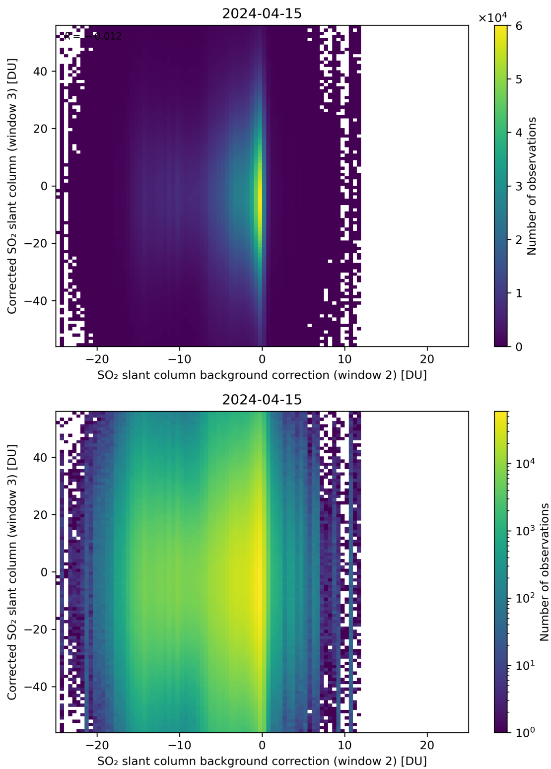
Figure 116: Scatter density plot of “SO 2 slant column background correction (window 2)” against “Corrected SO 2 slant column (window 3)” for 2024-04-15 to 2024-04-16.
