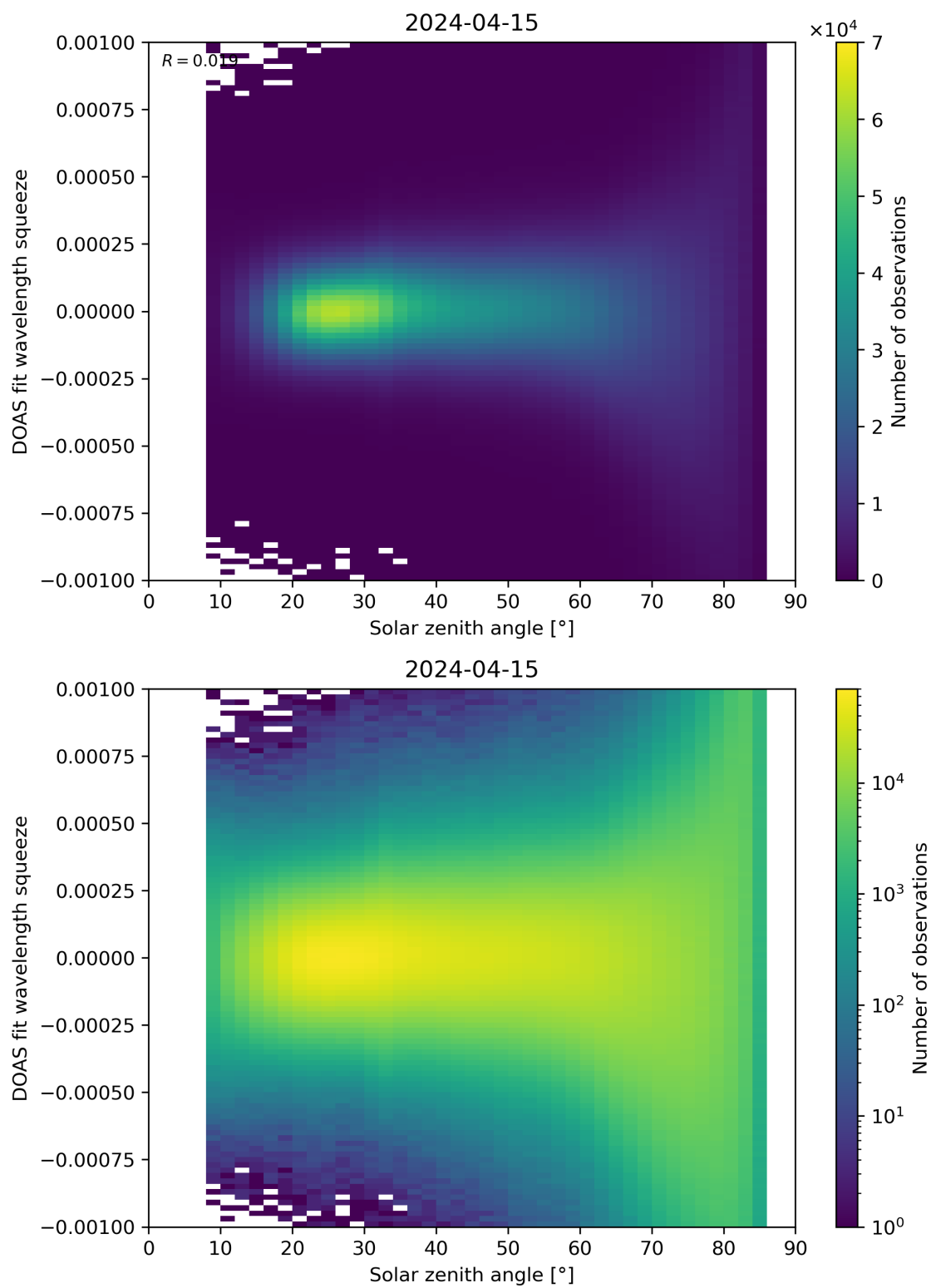
Figure 162: Scatter density plot of “Solar zenith angle” against “DOAS fit wavelength squeeze” for 2024-04-15 to 2024-04-16.
