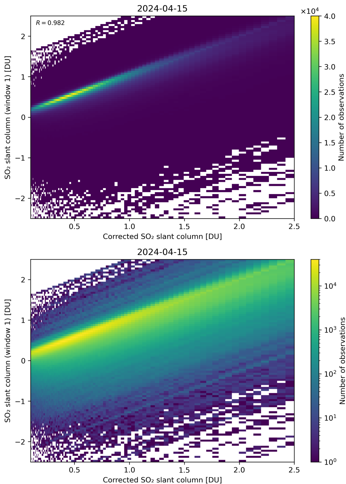
Figure 187: Scatter density plot of “Corrected SO 2 slant column” against “SO 2 slant column (window 1)” for 2024-04-15 to 2024-04-16.
