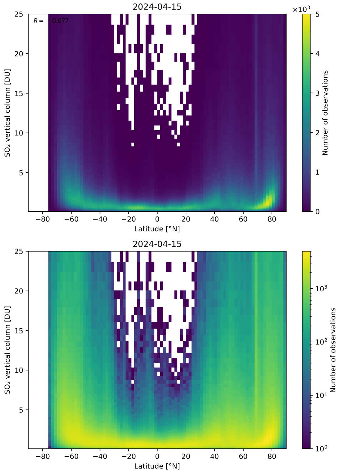
Figure 156: Scatter density plot of “Latitude” against “SO 2 vertical column” for 2024-04-15 to 2024-04-16.
