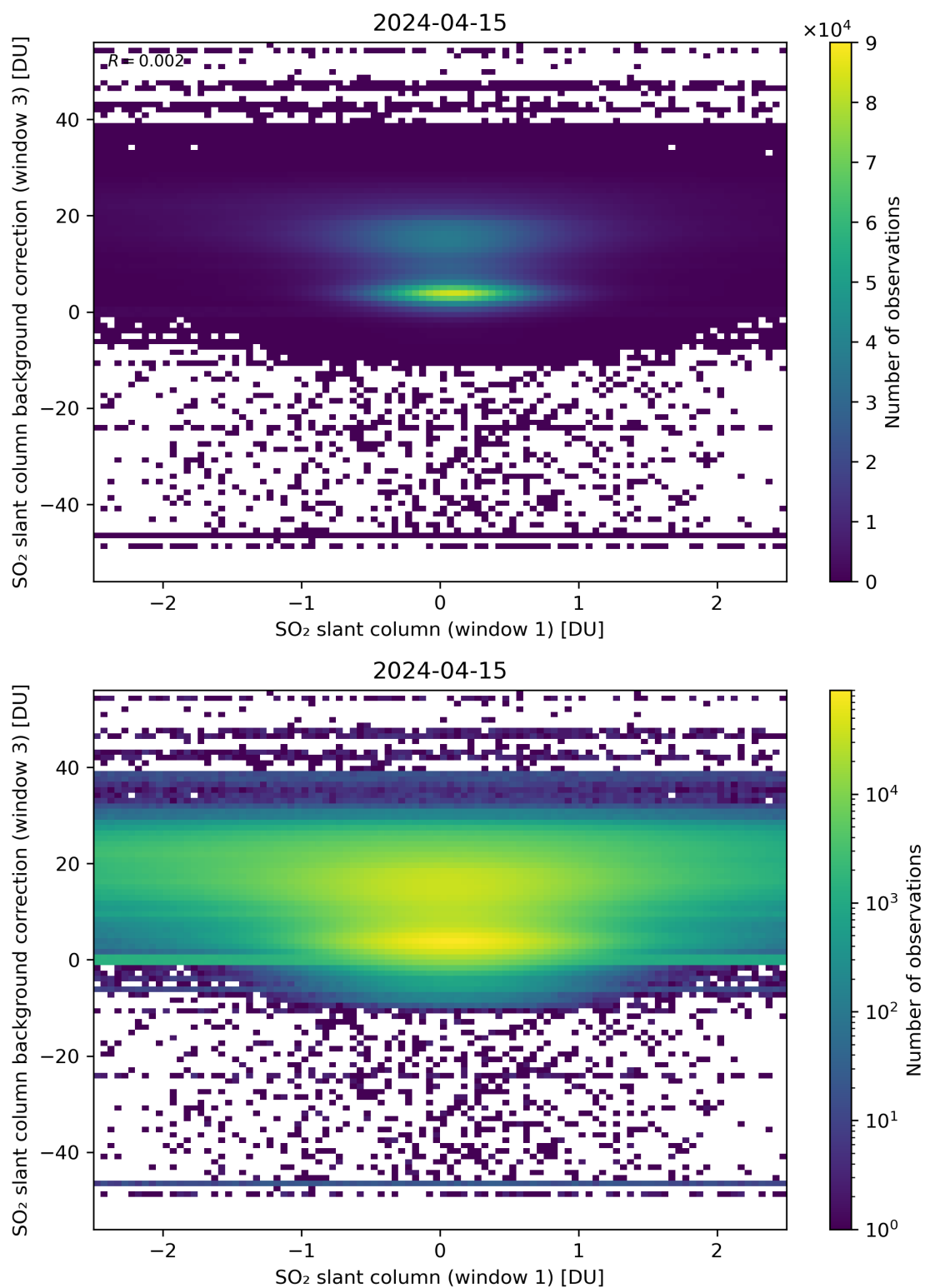
Figure 214: Scatter density plot of “SO 2 slant column (window 1)” against “SO 2 slant column background correction (window 3)” for 2024-04-15 to 2024-04-16.
