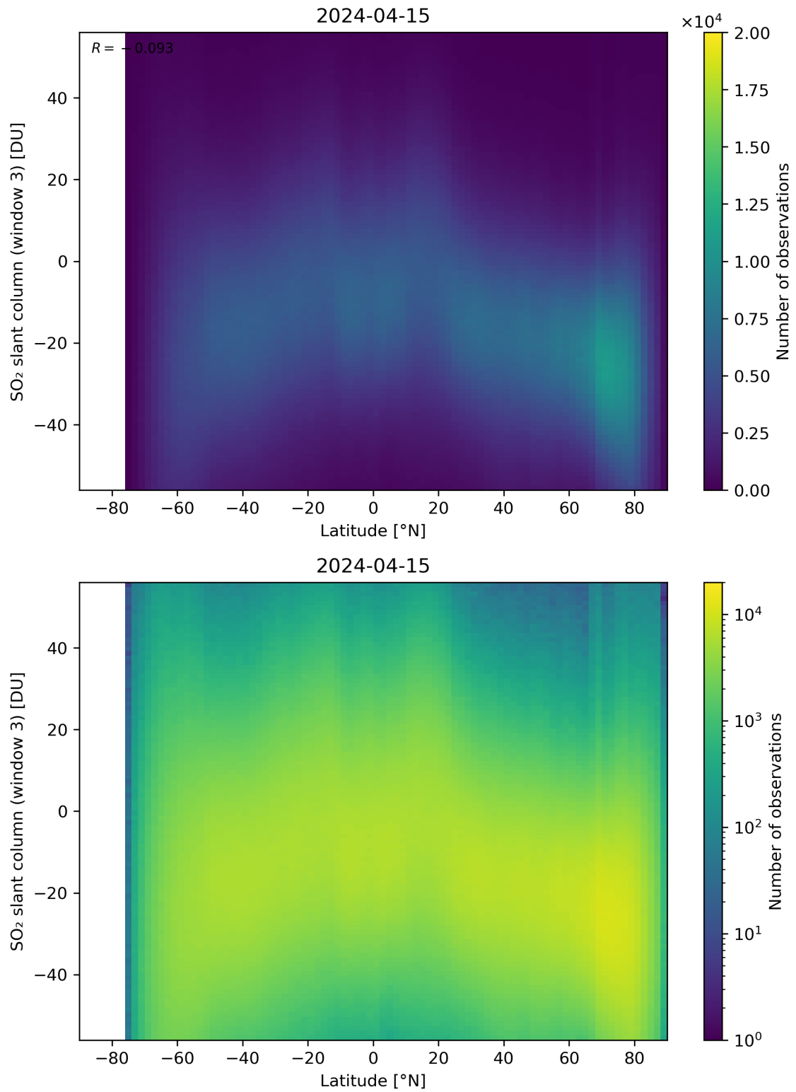
Figure 152: Scatter density plot of “Latitude” against “SO 2 slant column (window 3)” for 2024-04-15 to 2024-04-16.
