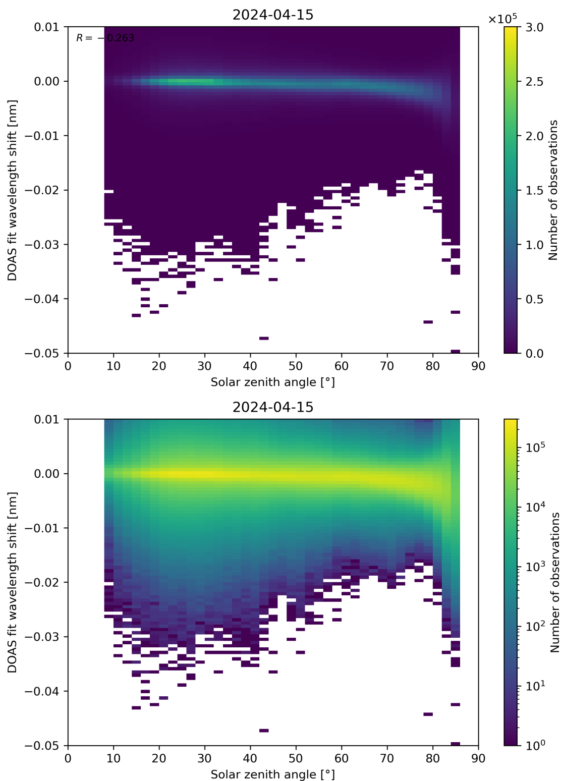
Figure 161: Scatter density plot of “Solar zenith angle” against “DOAS fit wavelength shift” for 2024-04-15 to 2024-04-16.
