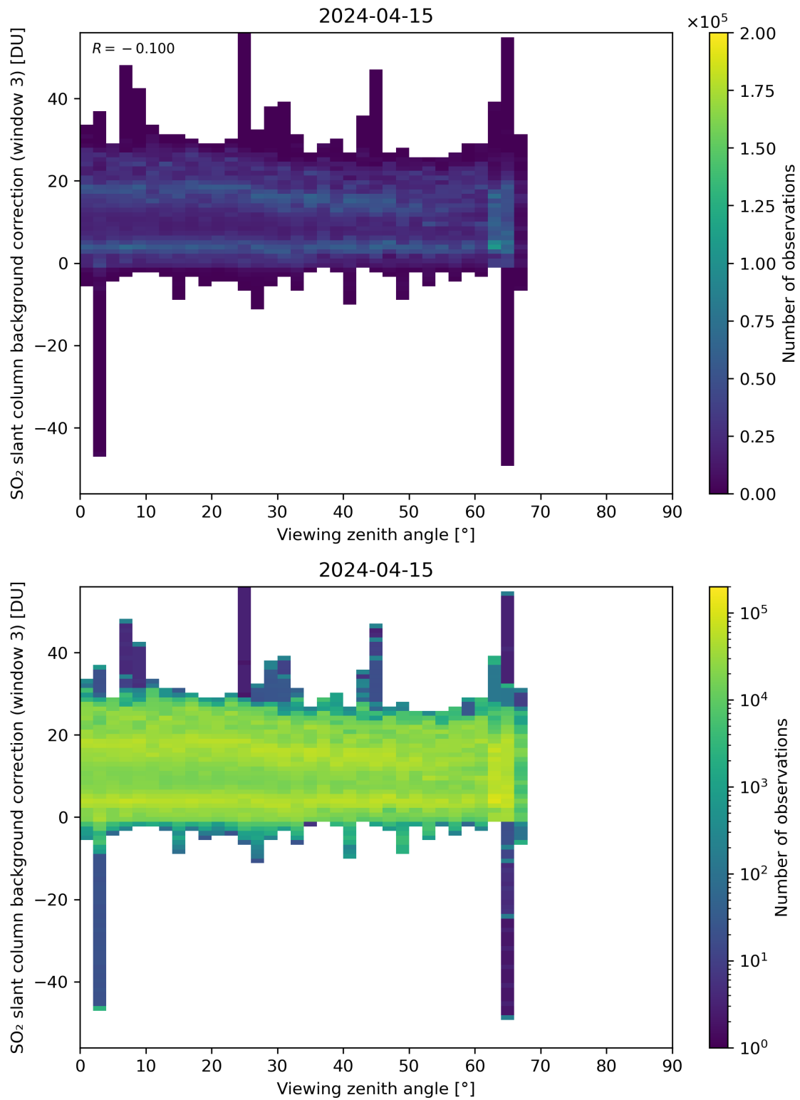
Figure 310: Scatter density plot of “Viewing zenith angle” against “SO 2 slant column background correction (window 3)” for 2024-04-15 to 2024-04-16.
