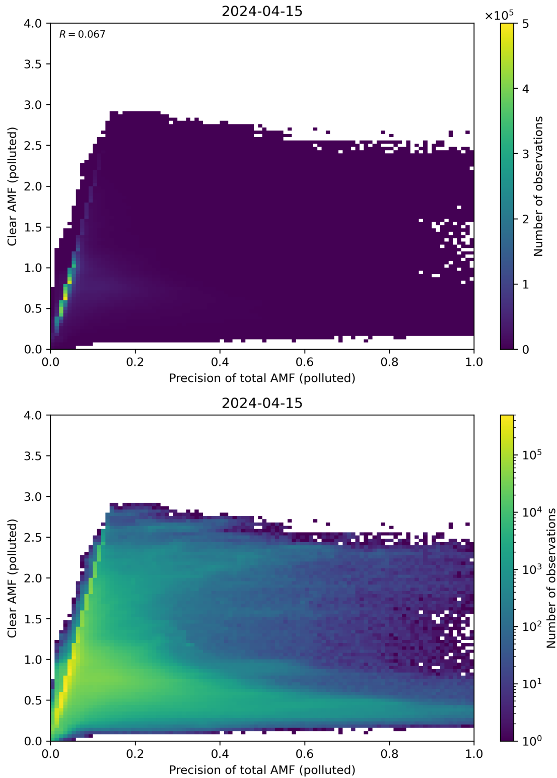
Figure 270: Scatter density plot of “Precision of total AMF (polluted)” against “Clear AMF (polluted)” for 2024-04-15 to 2024-04-16.
