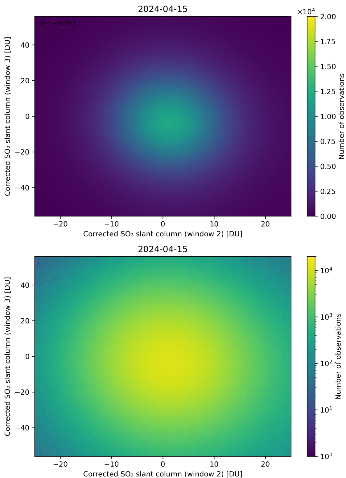
Figure 200: Scatter density plot of “Corrected SO 2 slant column (window 2)” against “Corrected SO 2 slant column (window 3)” for 2024-04-15 to 2024-04-16.
