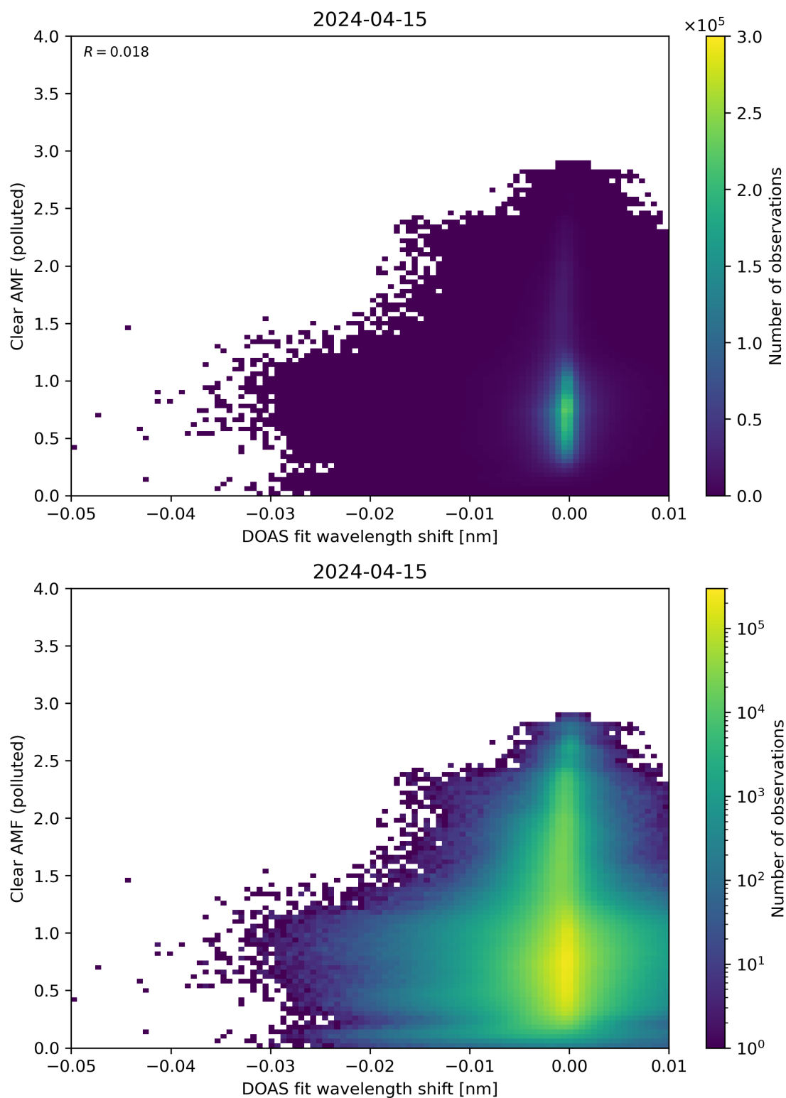
Figure 129: Scatter density plot of “DOAS fit wavelength shift” against “Clear AMF (polluted)” for 2024-04-15 to 2024-04-16.
