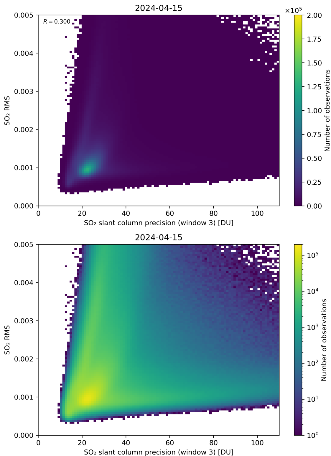
Figure 260: Scatter density plot of “SO 2 slant column precision (window 3)” against “SO 2 RMS” for 2024-04-15 to 2024-04-16.
