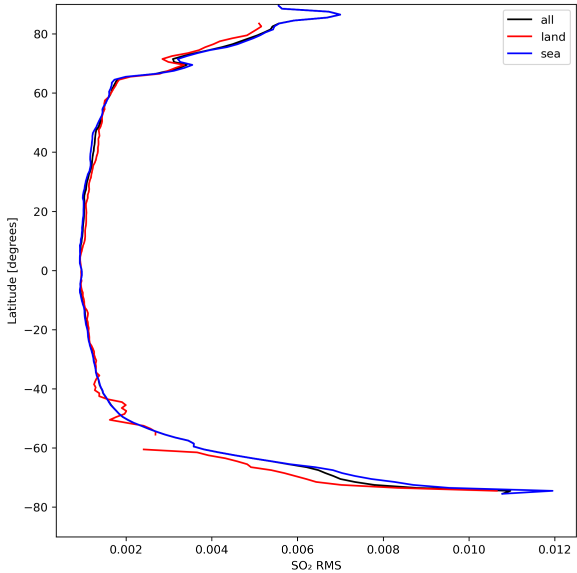
Figure 47: Zonal average of “SO 2 RMS” for 2024-04-15 to 2024-04-16.
