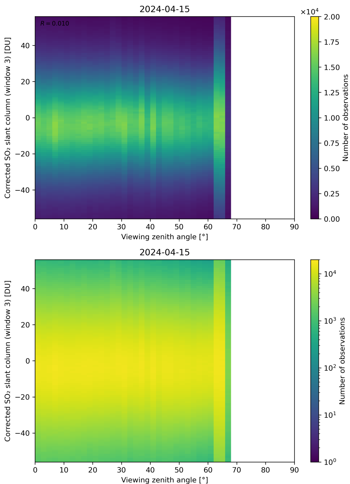
Figure 319: Scatter density plot of “Viewing zenith angle” against “Corrected SO 2 slant column (window 3)” for 2024-04-15 to 2024-04-16.
