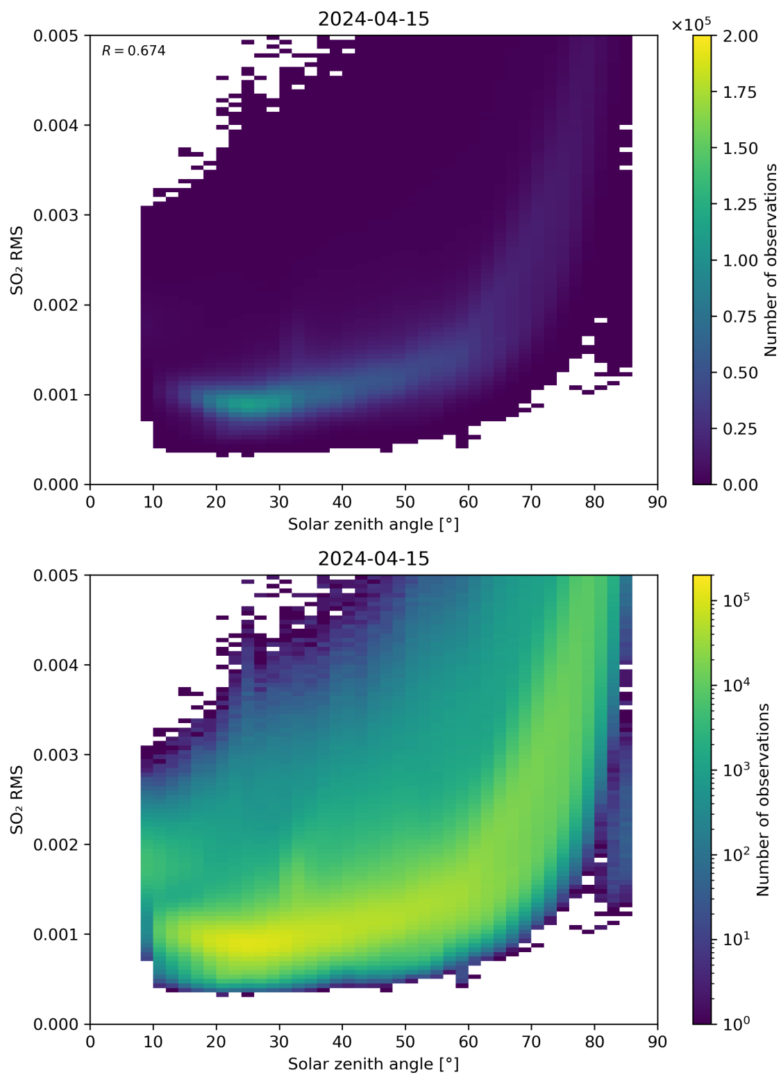
Figure 163: Scatter density plot of “Solar zenith angle” against “SO 2 RMS” for 2024-04-15 to 2024-04-16.
