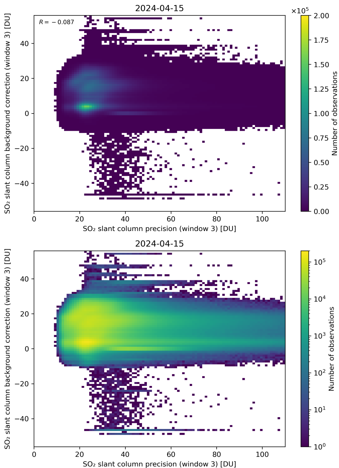
Figure 257: Scatter density plot of “SO 2 slant column precision (window 3)” against “SO 2 slant column background correction (window 3)” for 2024-04-15 to 2024-04-16.
