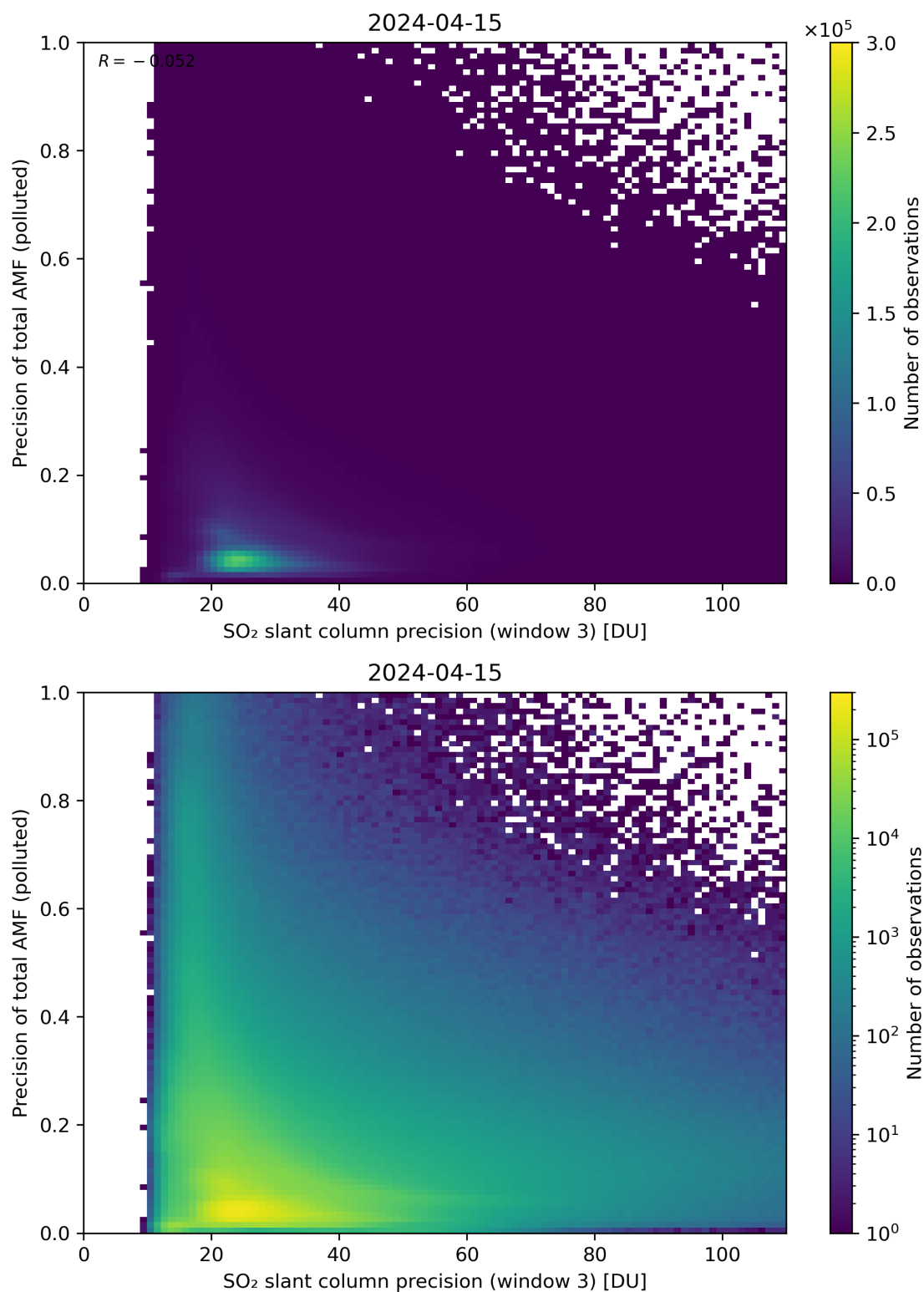
Figure 264: Scatter density plot of “SO 2 slant column precision (window 3)” against “Precision of total AMF (polluted)” for 2024-04-15 to 2024-04-16.
