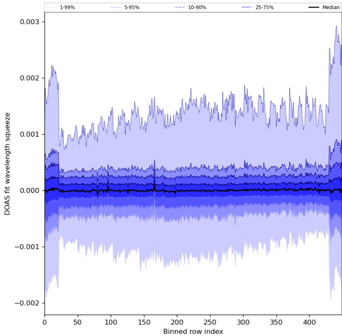
Figure 92: Along track statistics of “DOAS fit wavelength squeeze” for 2024-04-15 to 2024-04-16
