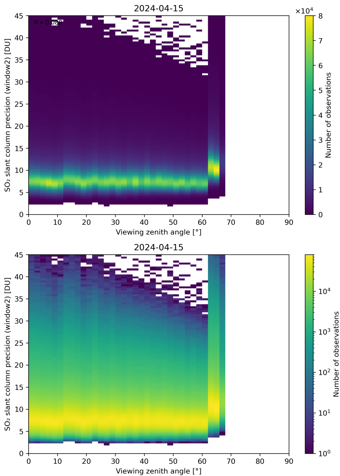
Figure 322: Scatter density plot of “Viewing zenith angle” against “SO 2 slant column precision (window2)” for 2024-04-15 to 2024-04-16.
