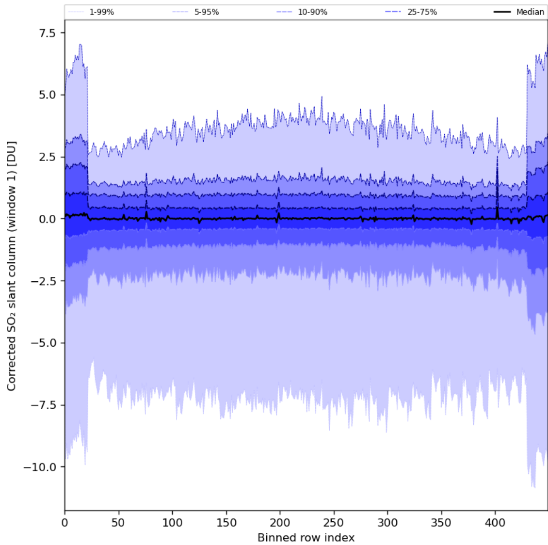
Figure 81: Along track statistics of “Corrected SO 2 slant column (window 1)” for 2024-04-15 to 2024-04-16
