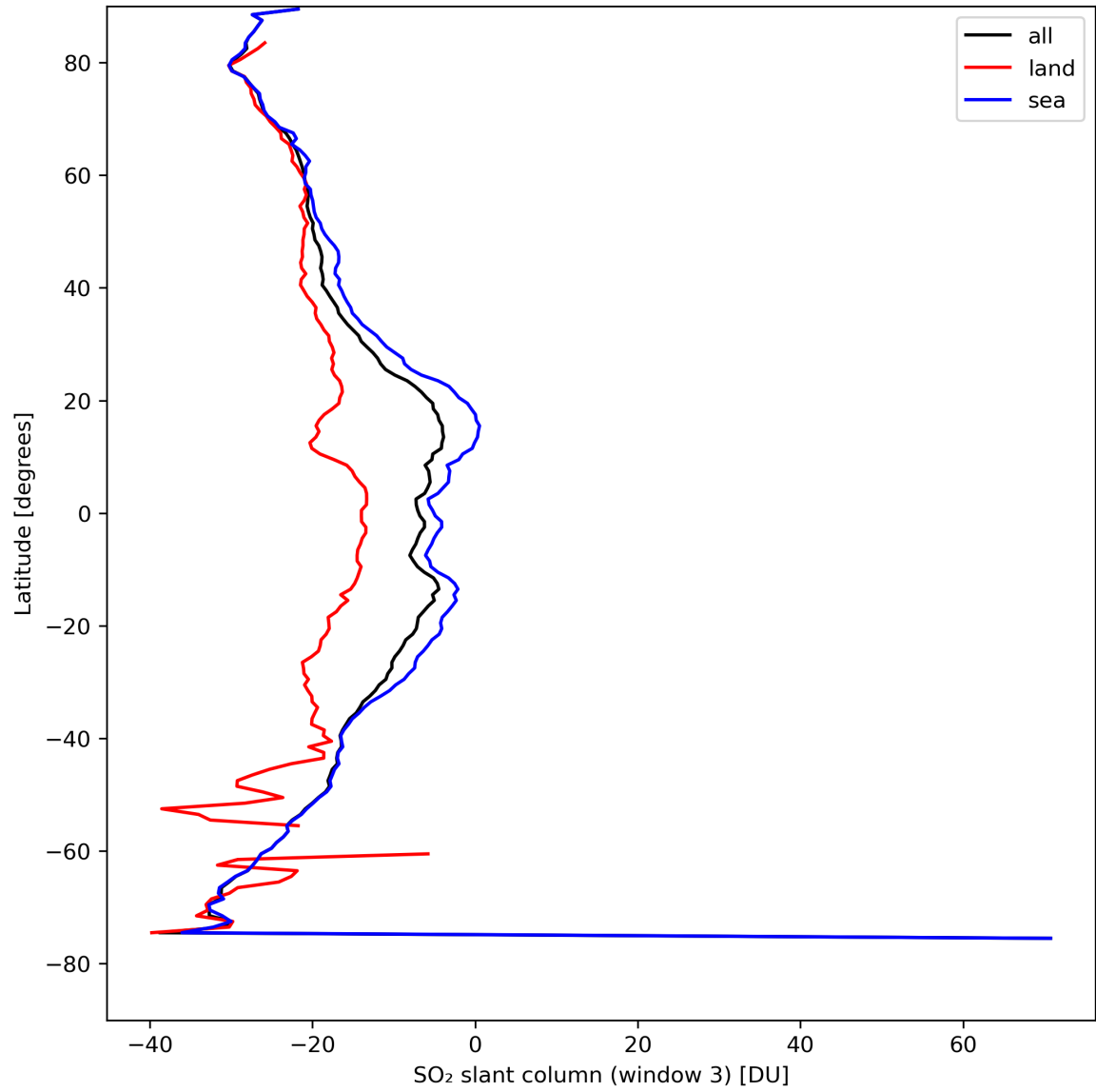
Figure 41: Zonal average of “SO 2 slant column (window 3)” for 2024-04-15 to 2024-04-16.
