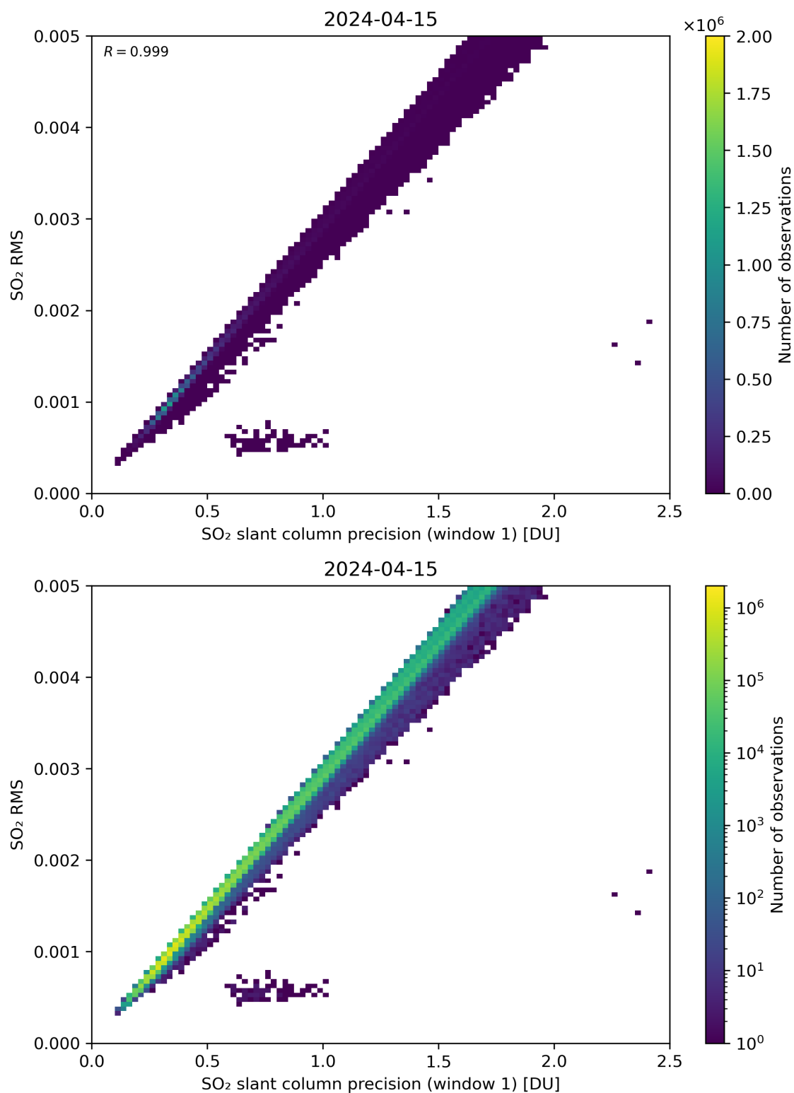
Figure 223: Scatter density plot of “SO 2 slant column precision (window 1)” against “SO 2 RMS” for 2024-04-15 to 2024-04-16.
