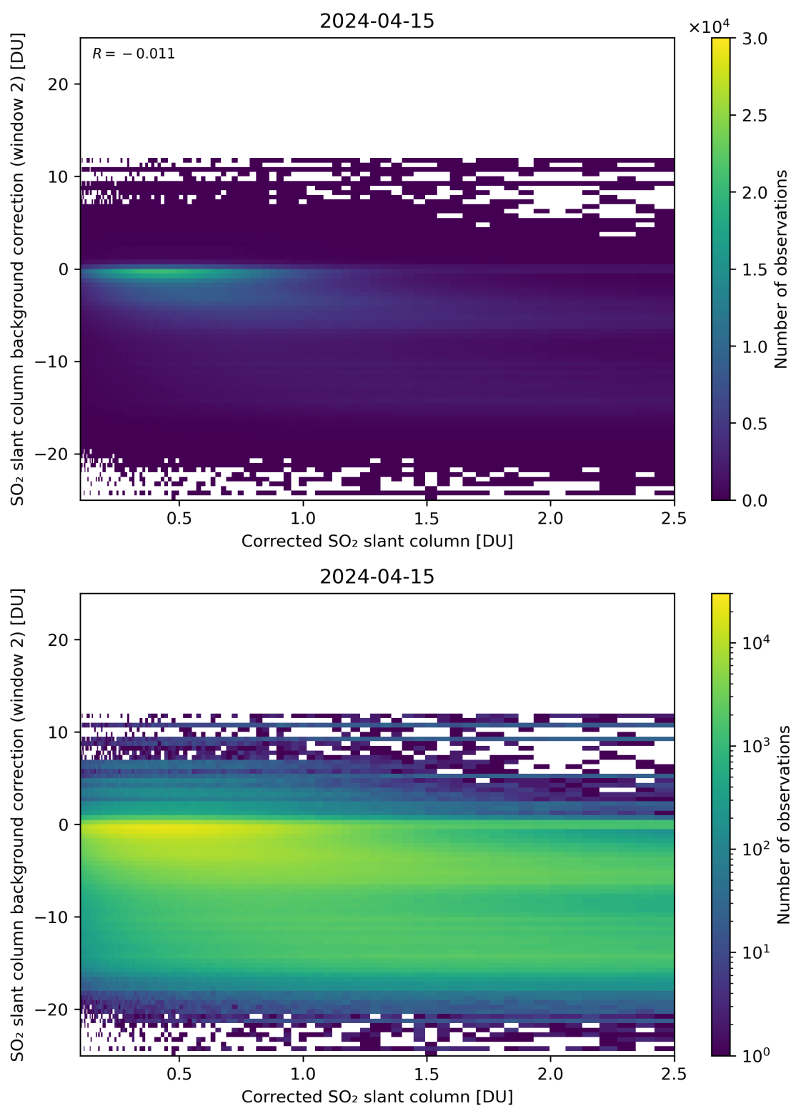
Figure 179: Scatter density plot of “Corrected SO 2 slant column” against “SO 2 slant column background correction (window 2)” for 2024-04-15 to 2024-04-16.
