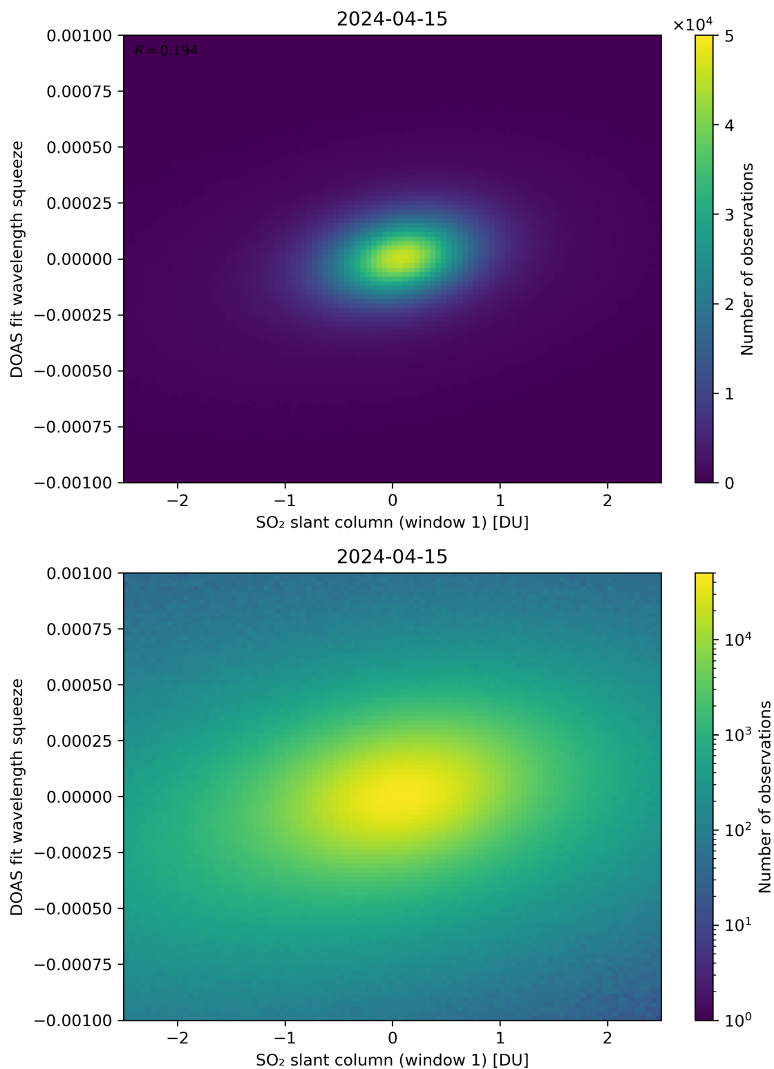
Figure 216: Scatter density plot of “SO 2 slant column (window 1)” against “DOAS fit wavelength squeeze” for 2024-04-15 to 2024-04-16.
