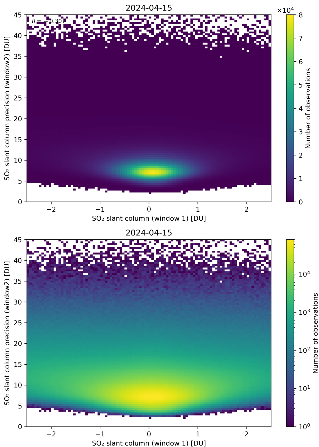
Figure 236: Scatter density plot of “SO 2 slant column (window 1)” against “SO 2 slant column precision (window2)” for 2024-04-15 to 2024-04-16.
