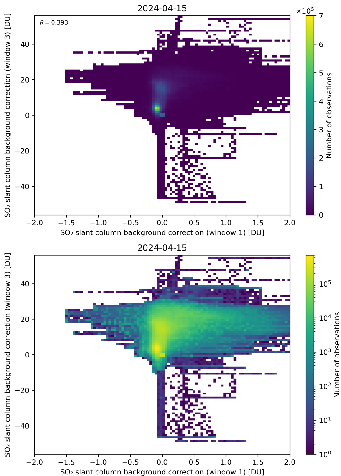
Figure 99: Scatter density plot of “SO 2 slant column background correction (window 1)” against “SO 2 slant column background correction (window 3)” for 2024-04-15 to 2024-04-16.
