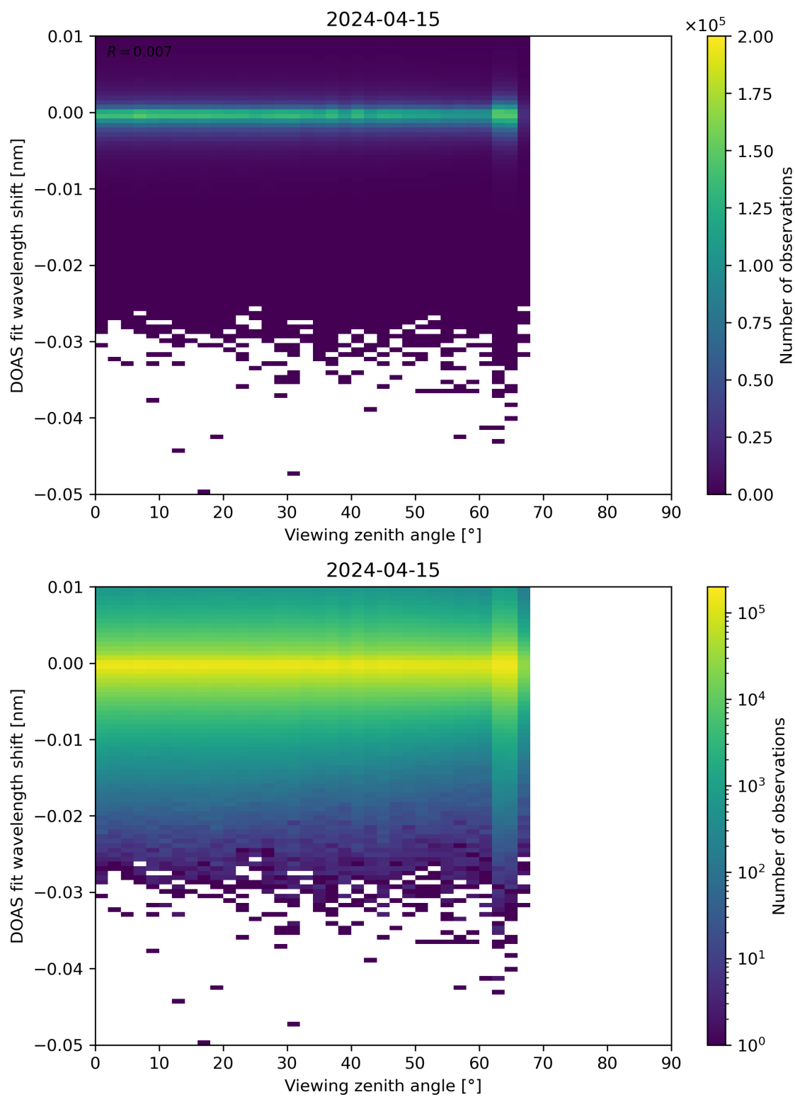
Figure 311: Scatter density plot of “Viewing zenith angle” against “DOAS fit wavelength shift” for 2024-04-15 to 2024-04-16.
