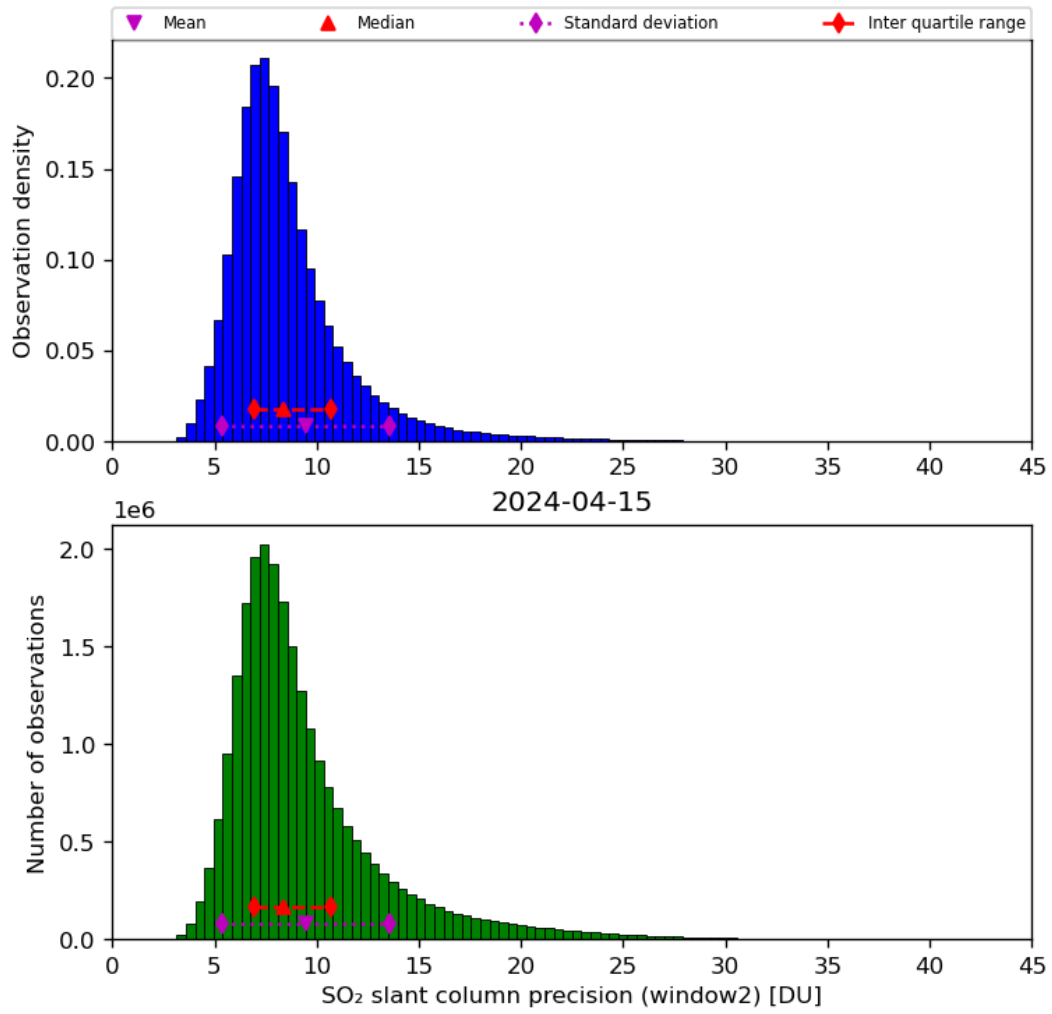
Figure 61: Histogram of “SO 2 slant column precision (window2)” for 2024-04-15 to 2024-04-16
