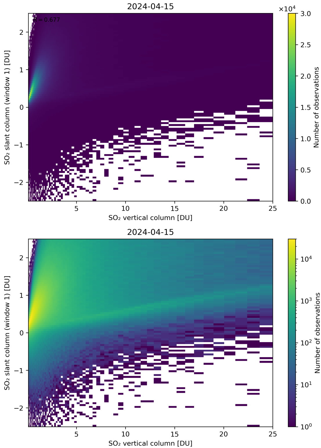
Figure 300: Scatter density plot of “SO 2 vertical column” against “SO 2 slant column (window 1)” for 2024-04-15 to 2024-04-16.
