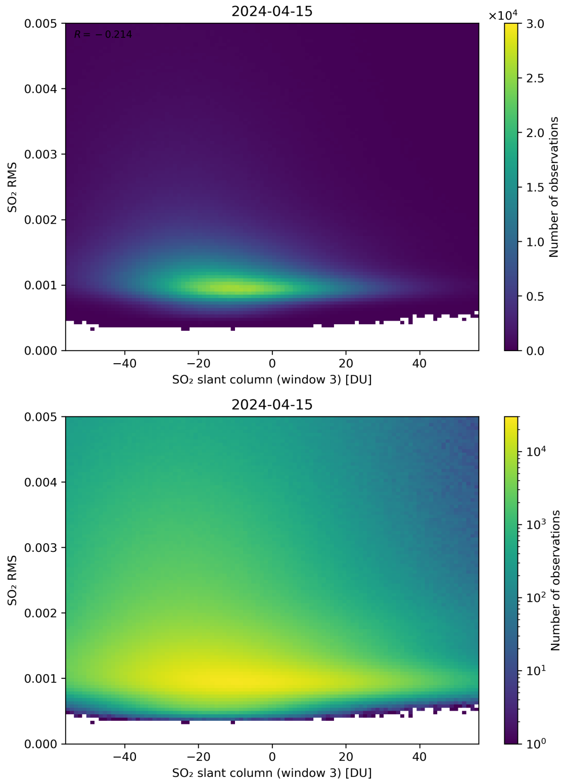
Figure 256: Scatter density plot of “SO 2 slant column (window 3)” against “SO 2 RMS” for 2024-04-15 to 2024-04-16.
