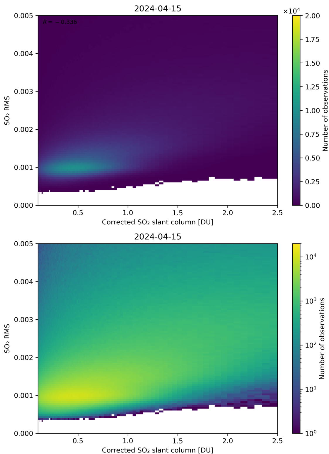
Figure 183: Scatter density plot of “Corrected SO 2 slant column” against “SO 2 RMS” for 2024-04-15 to 2024-04-16.
