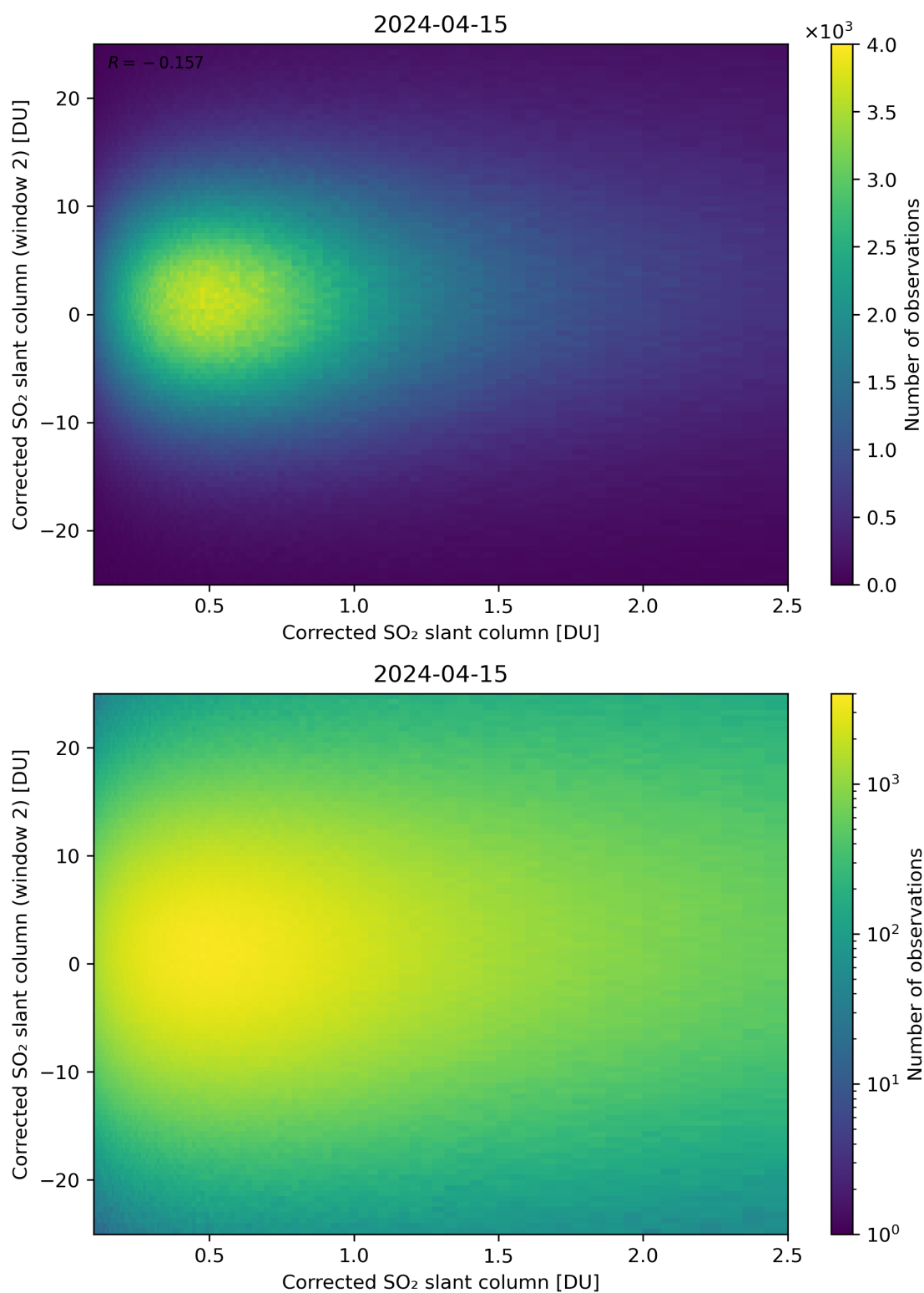
Figure 185: Scatter density plot of “Corrected SO 2 slant column” against “Corrected SO 2 slant column (window 2)” for 2024-04-15 to 2024-04-16.
