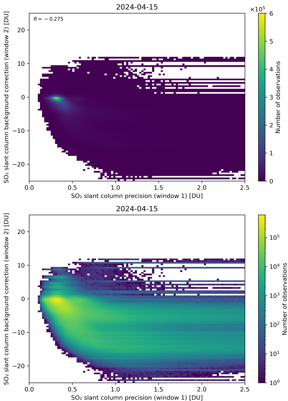
Figure 219: Scatter density plot of “SO 2 slant column precision (window 1)” against “SO 2 slant column background correction (window 2)” for 2024-04-15 to 2024-04-16.
