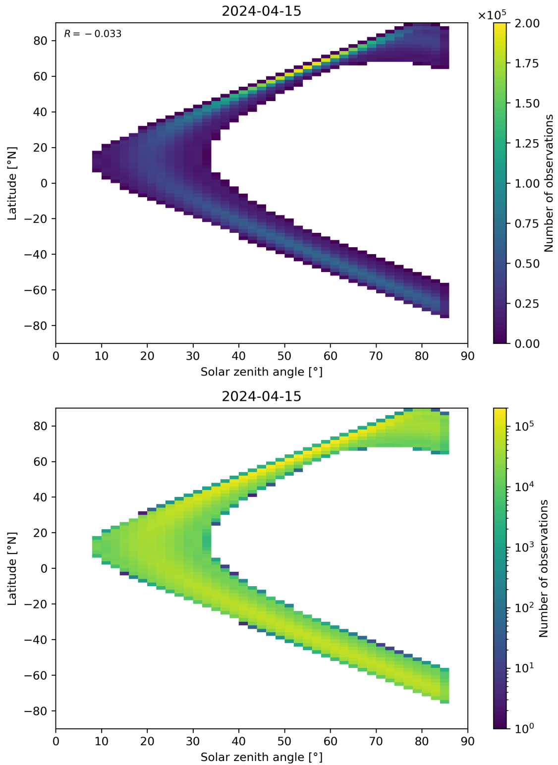
Figure 164: Scatter density plot of “Solar zenith angle” against “Latitude” for 2024-04-15 to 2024-04-16.
