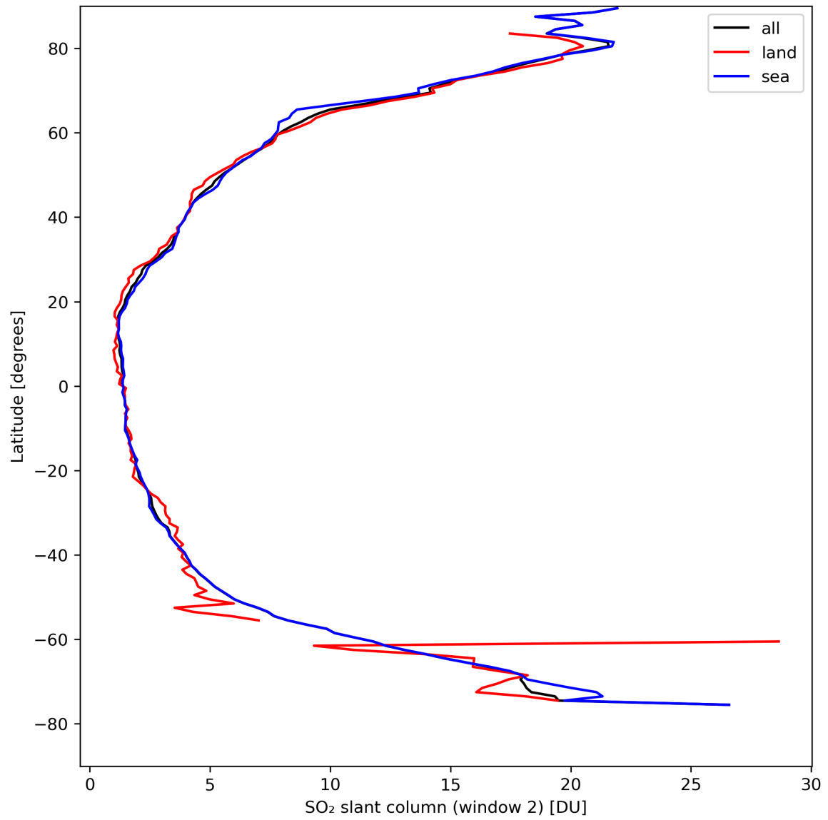
Figure 37: Zonal average of “SO 2 slant column (window 2)” for 2024-04-15 to 2024-04-16.
