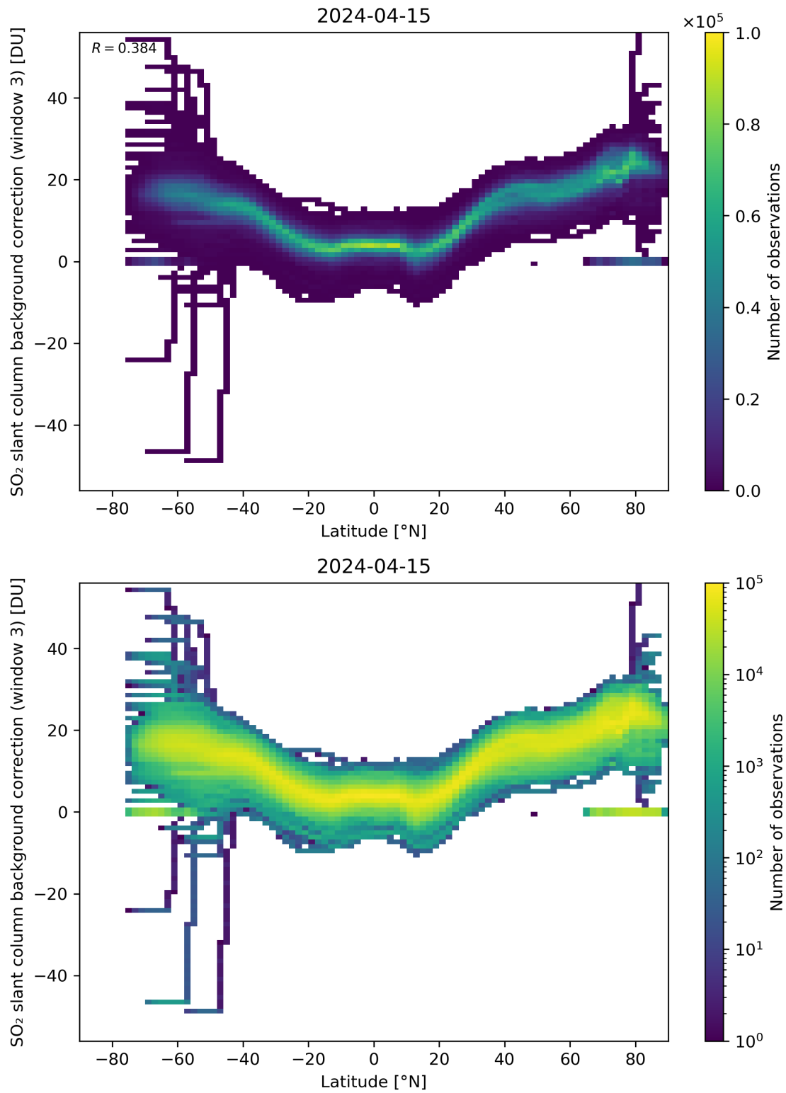
Figure 141: Scatter density plot of “Latitude” against “SO 2 slant column background correction (window 3)” for 2024-04-15 to 2024-04-16.
