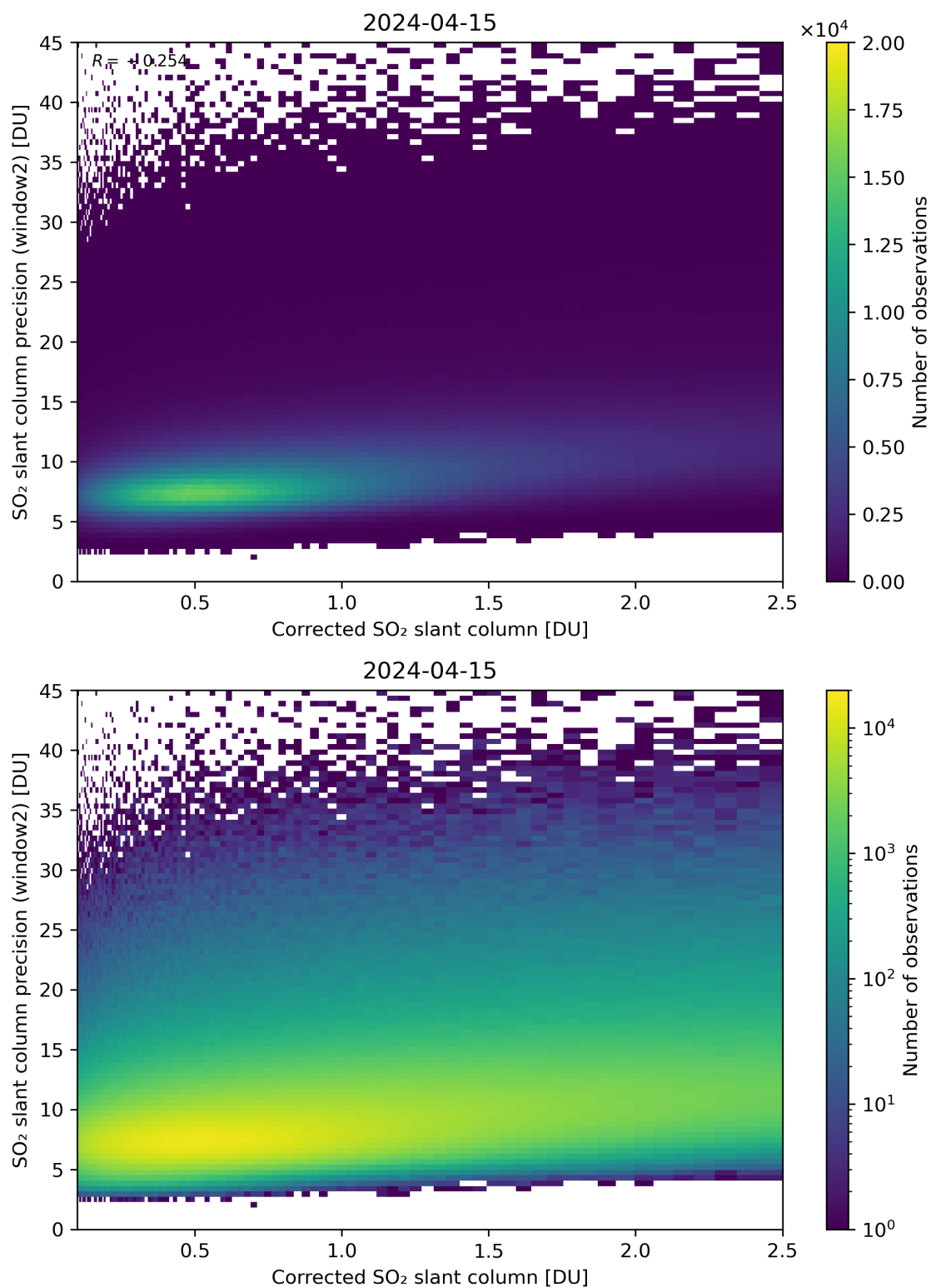
Figure 189: Scatter density plot of “Corrected SO 2 slant column” against “SO 2 slant column precision (window2)” for 2024-04-15 to 2024-04-16.
