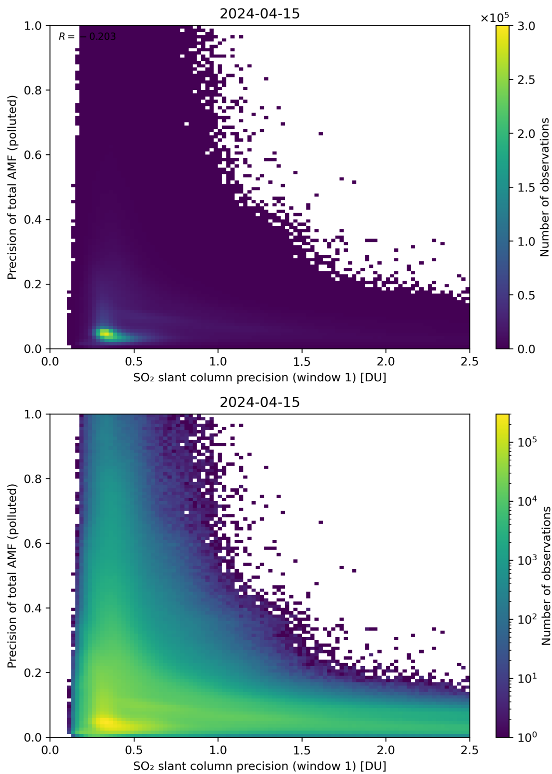
Figure 231: Scatter density plot of “SO 2 slant column precision (window 1)” against “Precision of total AMF (polluted)” for 2024-04-15 to 2024-04-16.
