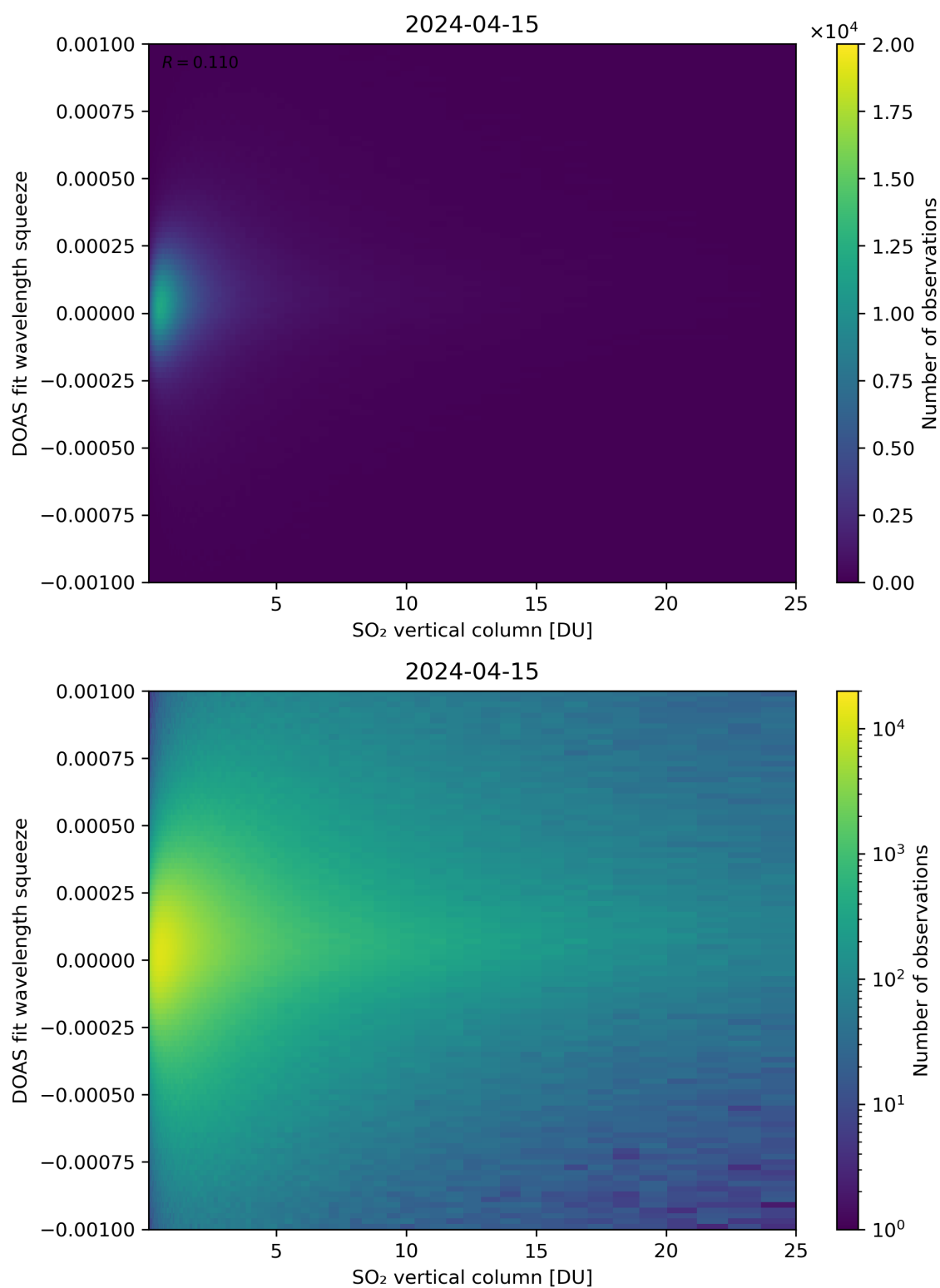
Figure 277: Scatter density plot of “SO 2 vertical column” against “DOAS fit wavelength squeeze” for 2024-04-15 to 2024-04-16.
