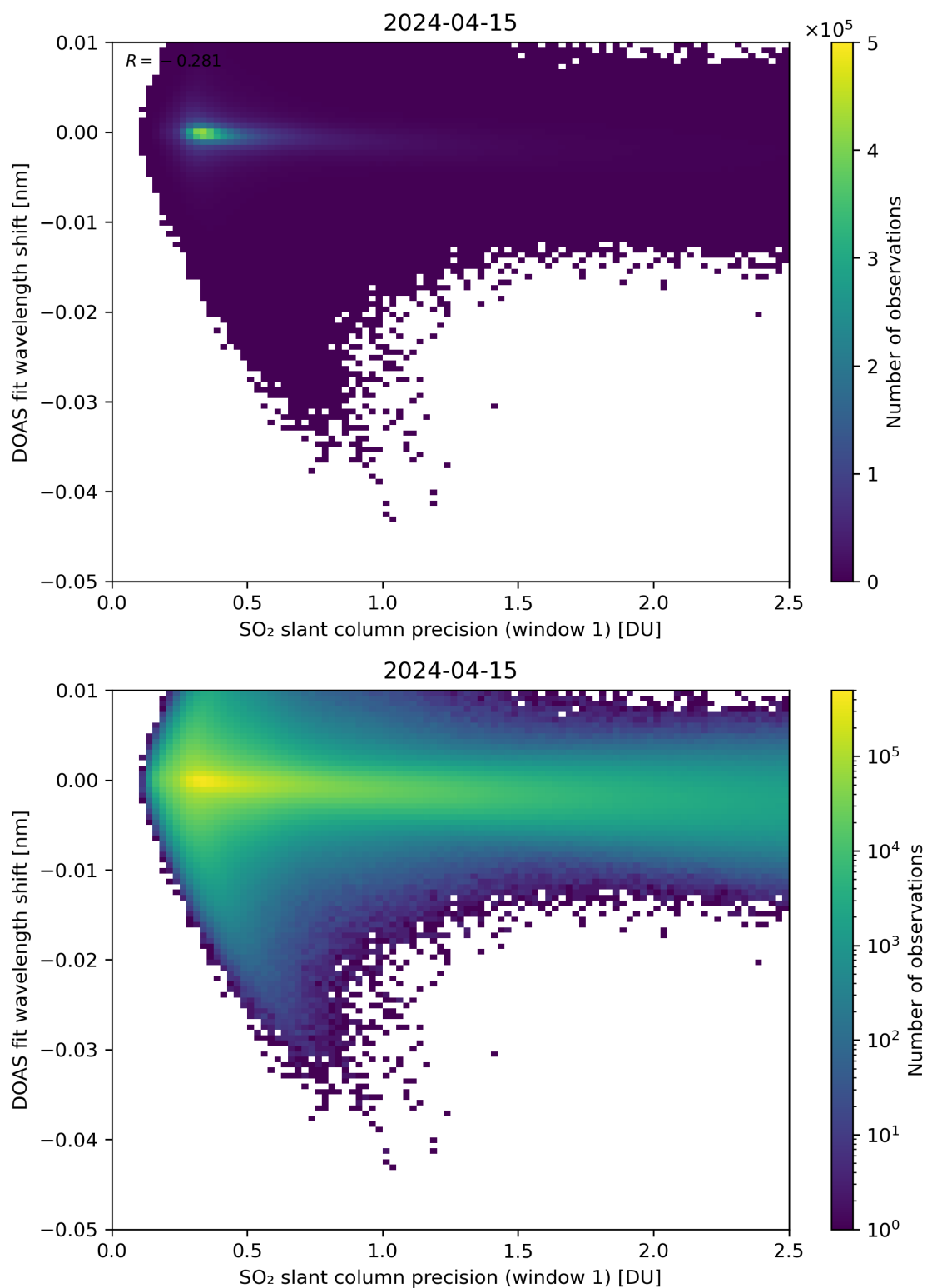
Figure 221: Scatter density plot of “SO 2 slant column precision (window 1)” against “DOAS fit wavelength shift” for 2024-04-15 to 2024-04-16.
