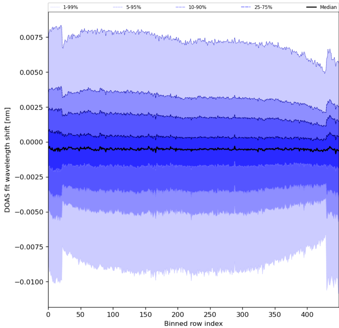
Figure 91: Along track statistics of “DOAS fit wavelength shift” for 2024-04-15 to 2024-04-16
