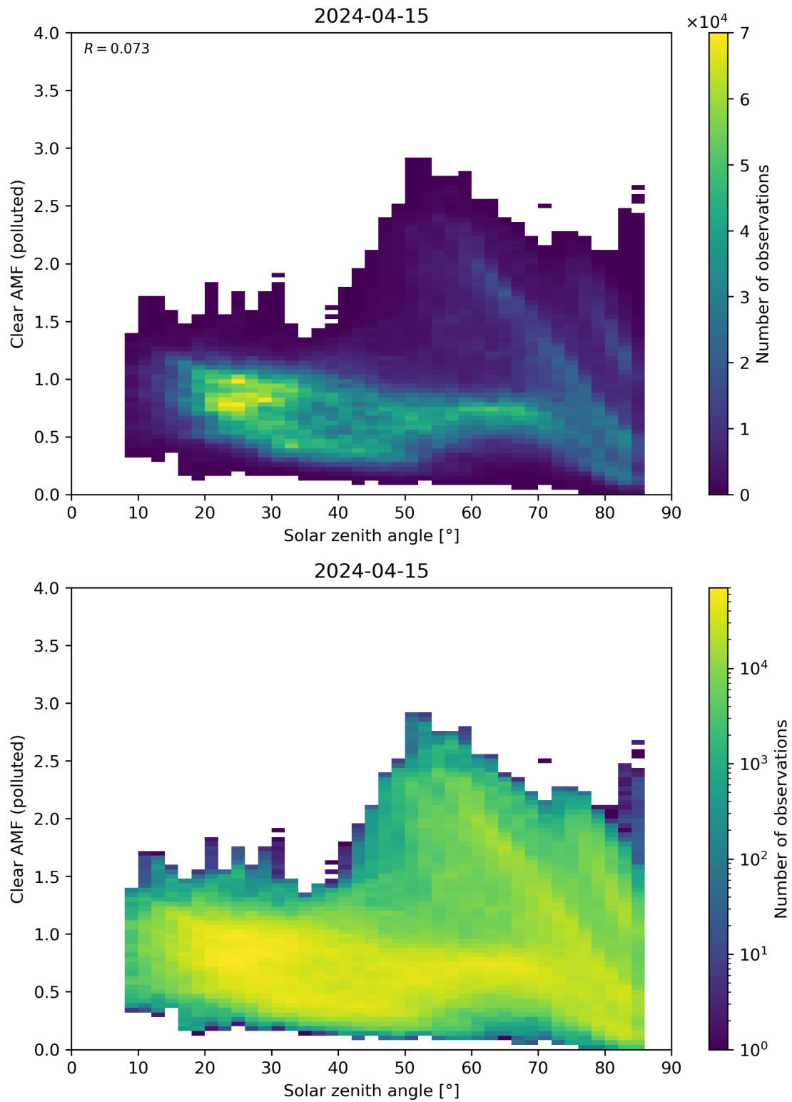
Figure 165: Scatter density plot of “Solar zenith angle” against “Clear AMF (polluted)” for 2024-04-15 to 2024-04-16.
