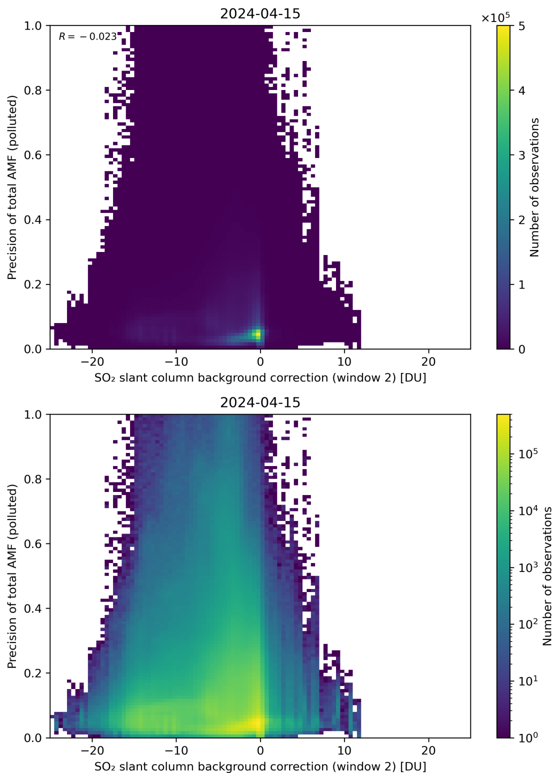
Figure 120: Scatter density plot of “SO 2 slant column background correction (window 2)” against “Precision of total AMF (polluted)” for 2024-04-15 to 2024-04-16.
