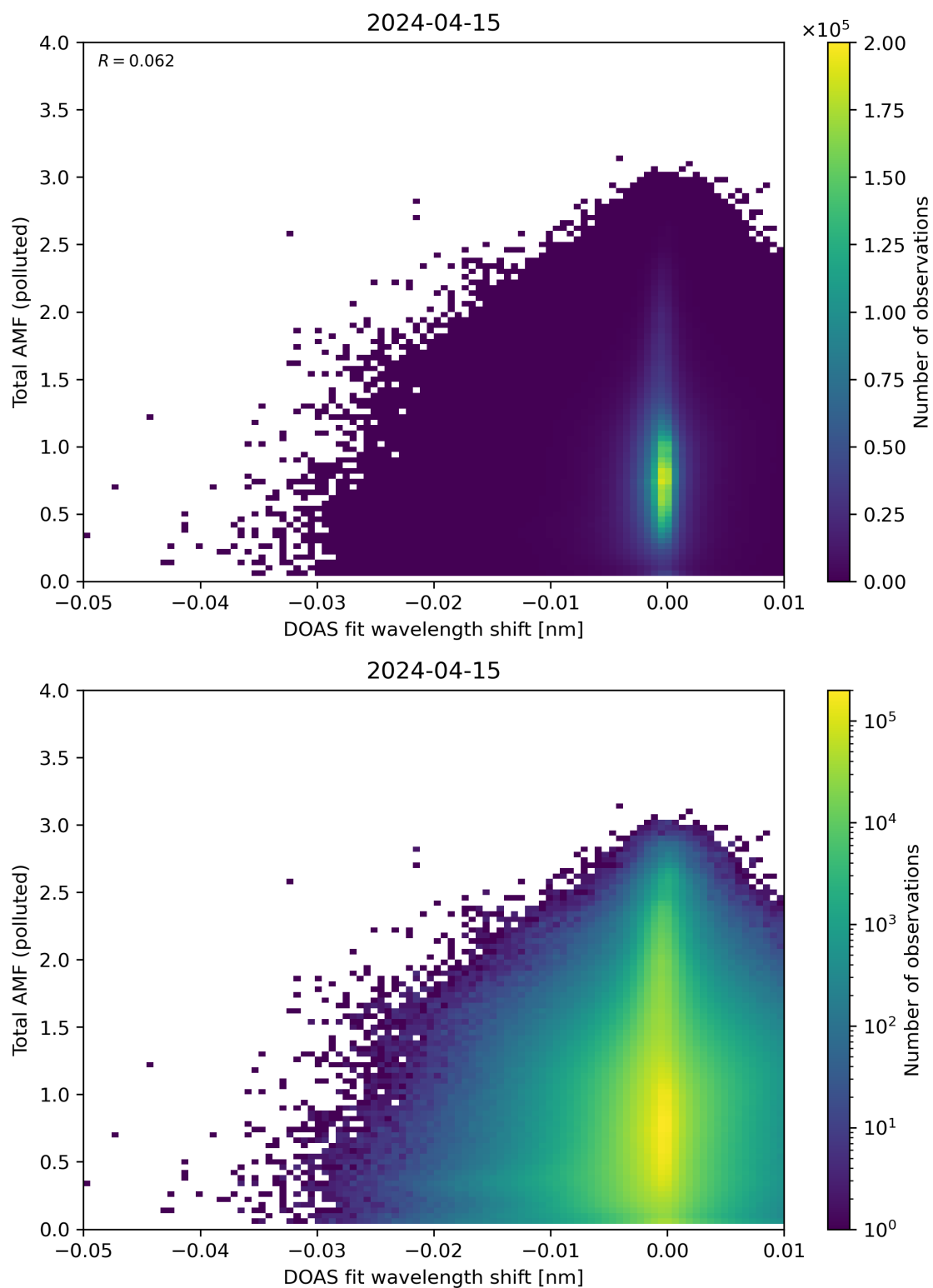
Figure 130: Scatter density plot of “DOAS fit wavelength shift” against “Total AMF (polluted)” for 2024-04-15 to 2024-04-16.
