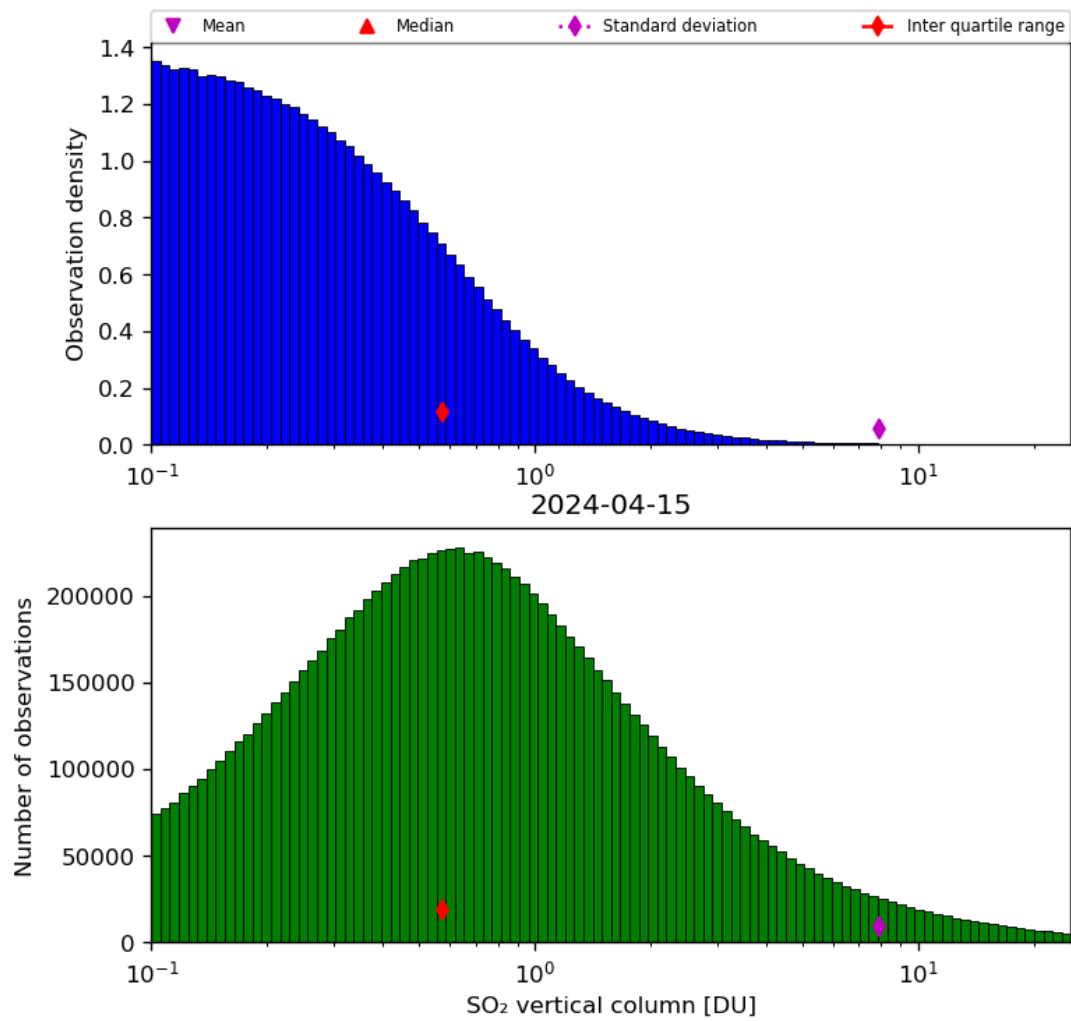
Figure 53: Histogram of “SO 2 vertical column” for 2024-04-15 to 2024-04-16
