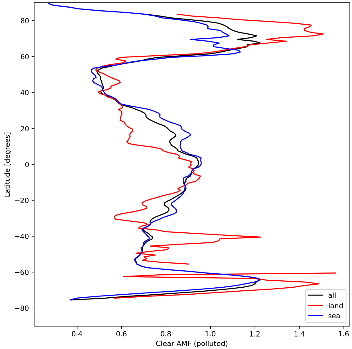
Figure 50: Zonal average of “Clear AMF (polluted)” for 2024-04-15 to 2024-04-16.
