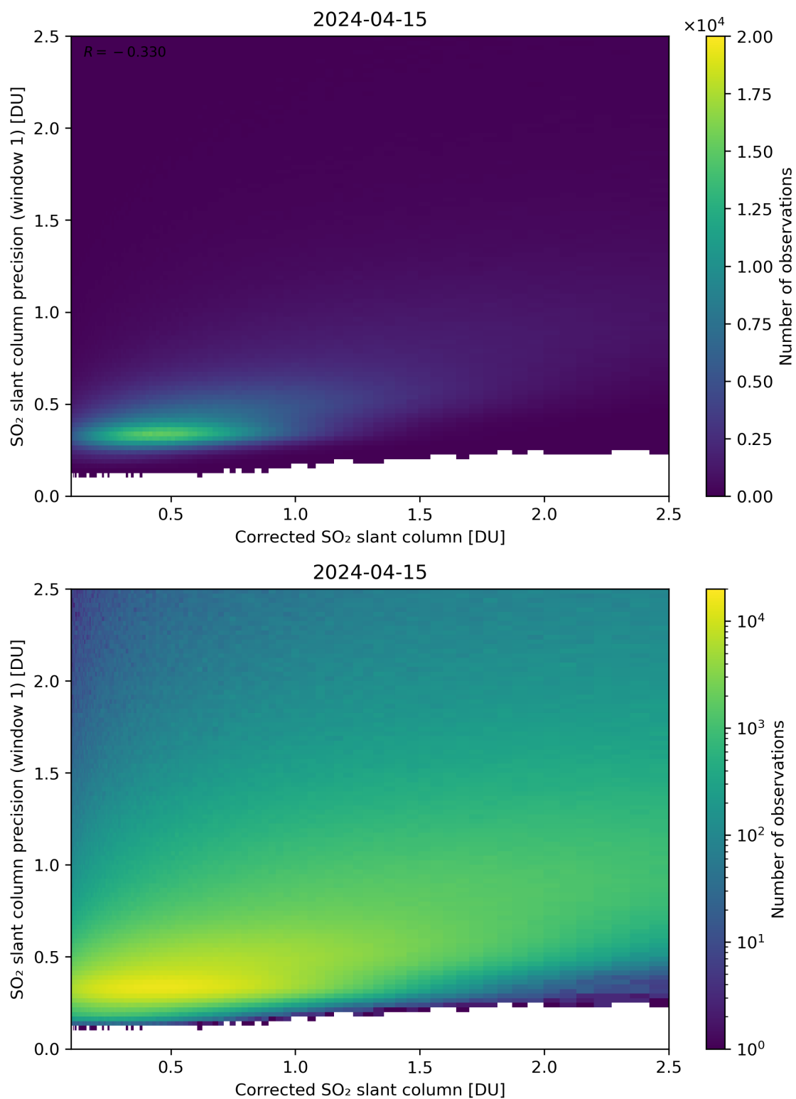
Figure 188: Scatter density plot of “Corrected SO 2 slant column” against “SO 2 slant column precision (window 1)” for 2024-04-15 to 2024-04-16.
