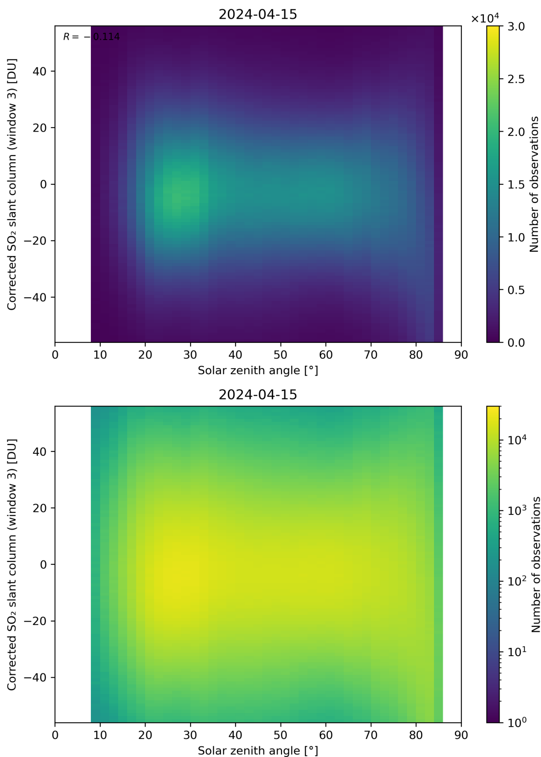
Figure 168: Scatter density plot of “Solar zenith angle” against “Corrected SO 2 slant column (window 3)” for 2024-04-15 to 2024-04-16.
