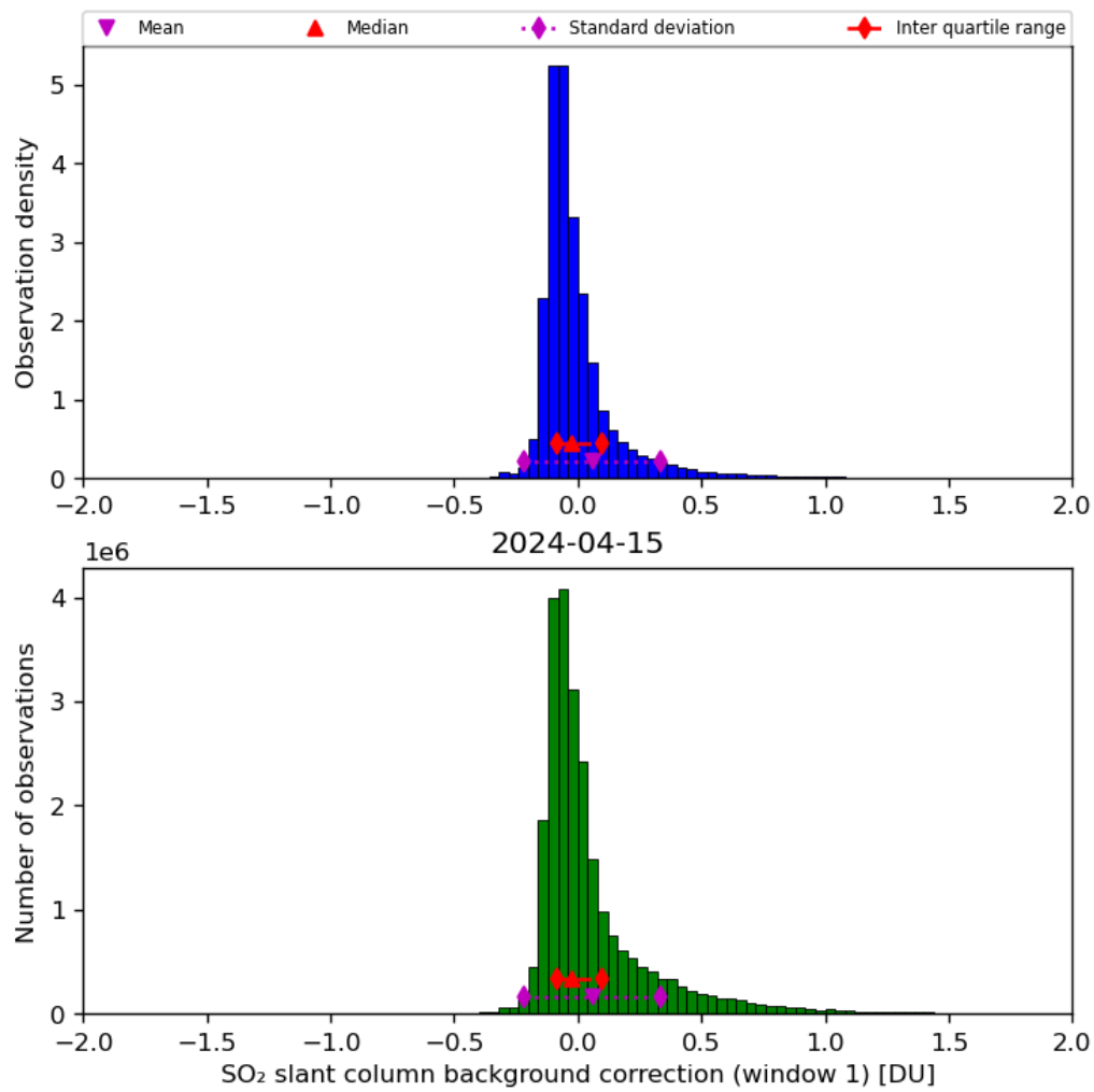
Figure 59: Histogram of “SO 2 slant column background correction (window 1)” for 2024-04-15 to 2024-04-16
