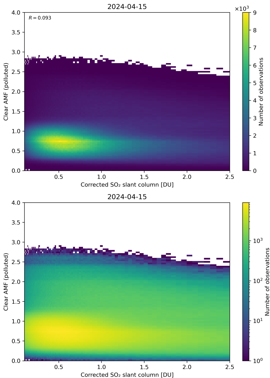
Figure 184: Scatter density plot of “Corrected SO 2 slant column” against “Clear AMF (polluted)” for 2024-04-15 to 2024-04-16.
