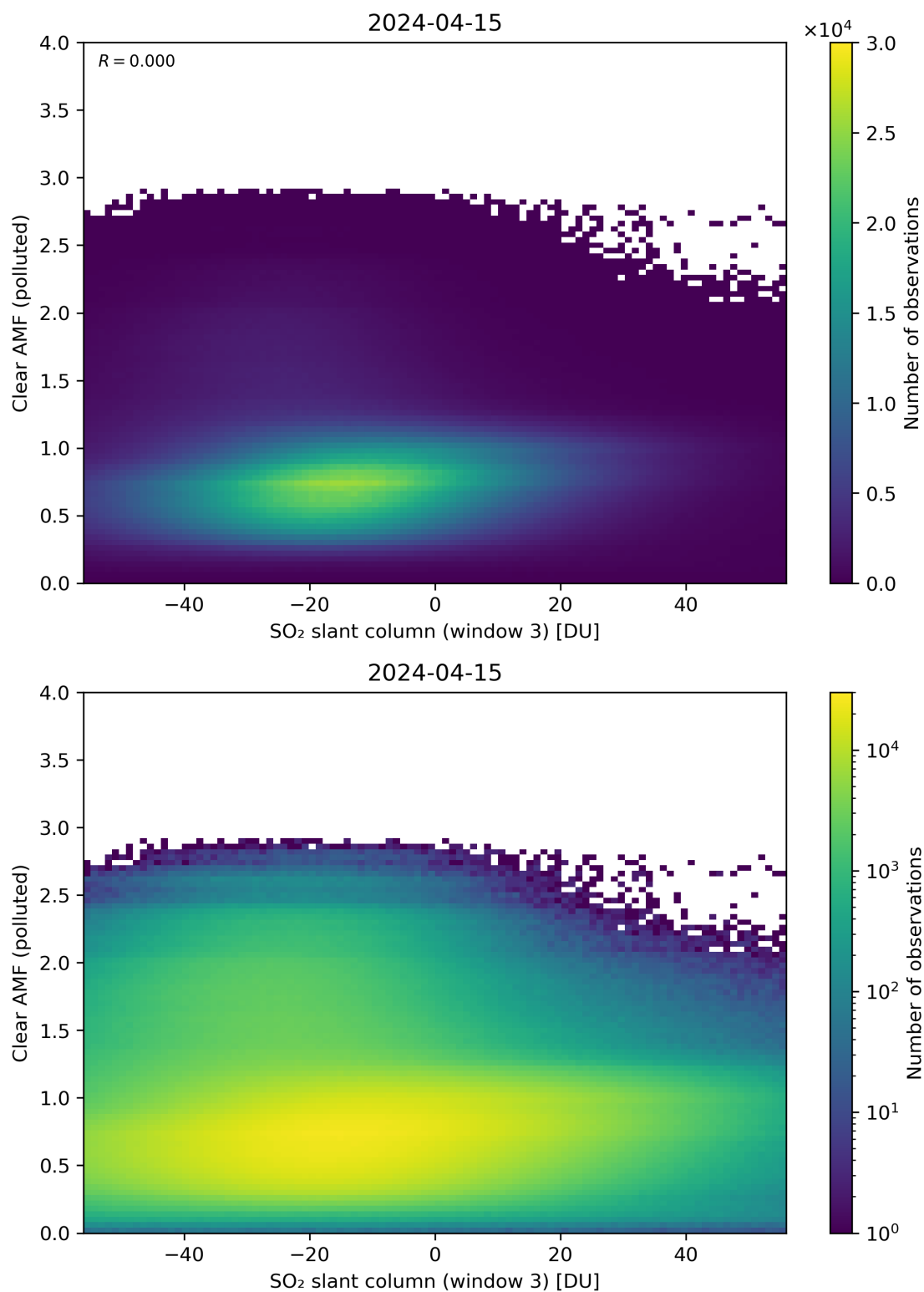
Figure 265: Scatter density plot of “SO 2 slant column (window 3)” against “Clear AMF (polluted)” for 2024-04-15 to 2024-04-16.
