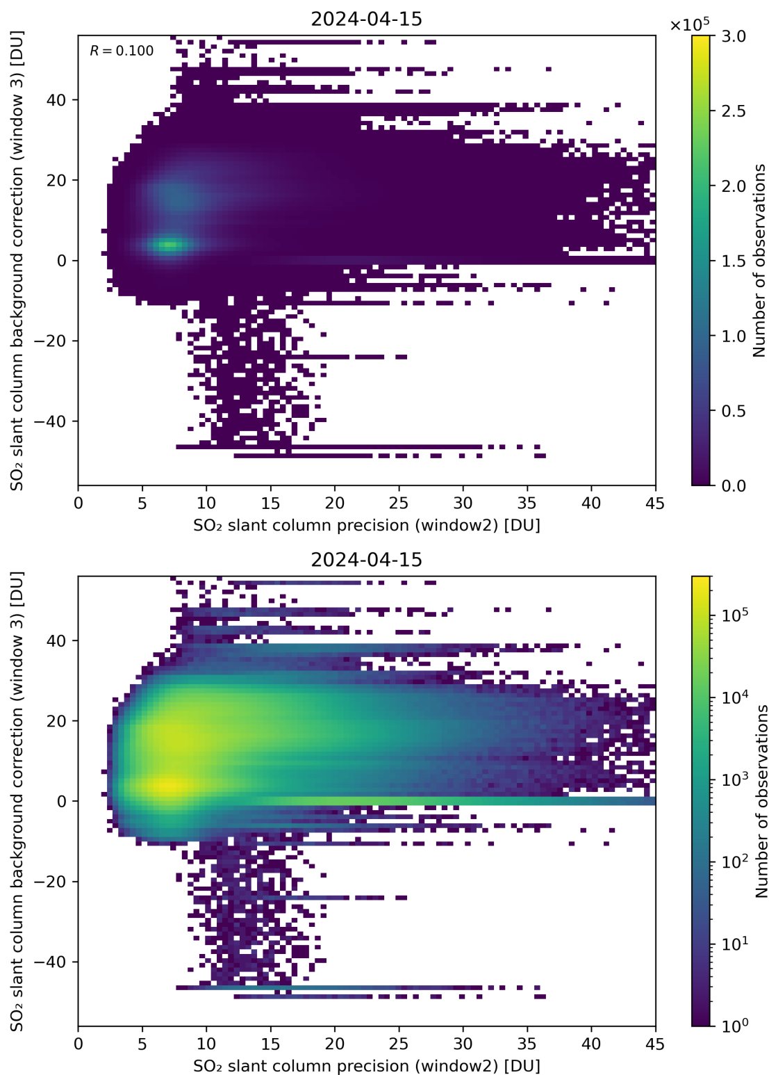
Figure 242: Scatter density plot of “SO 2 slant column precision (window2)” against “SO 2 slant column background correction (window 3)” for 2024-04-15 to 2024-04-16.
