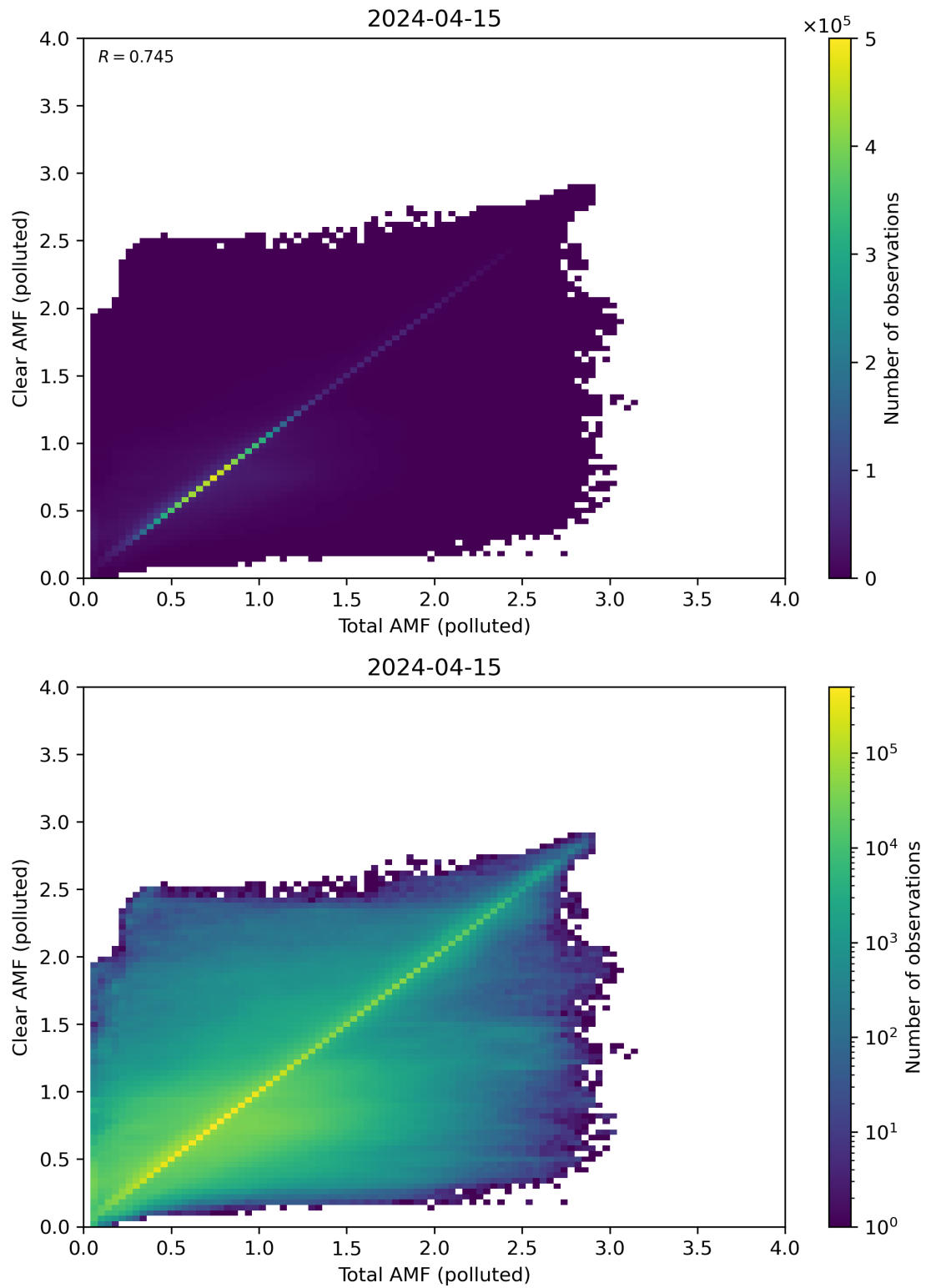
Figure 271: Scatter density plot of “Total AMF (polluted)” against “Clear AMF (polluted)” for 2024-04-15 to 2024-04-16.
