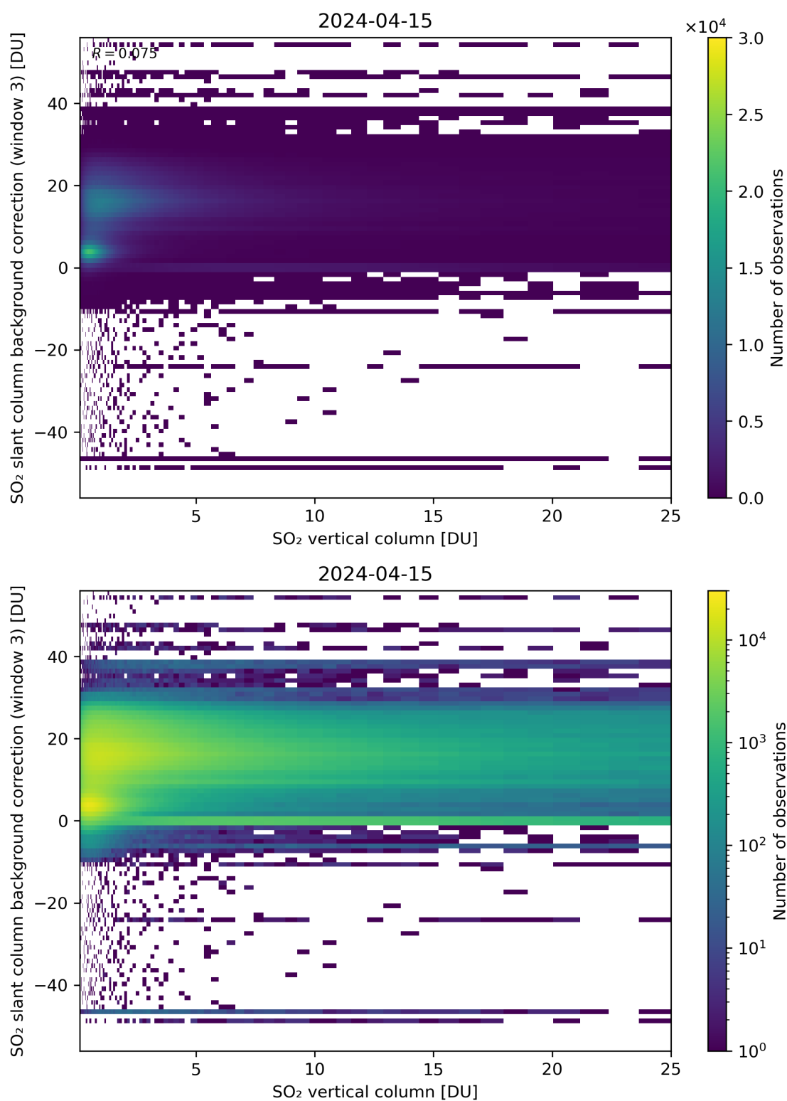
Figure 275: Scatter density plot of “SO 2 vertical column” against “SO 2 slant column background correction (window 3)” for 2024-04-15 to 2024-04-16.
