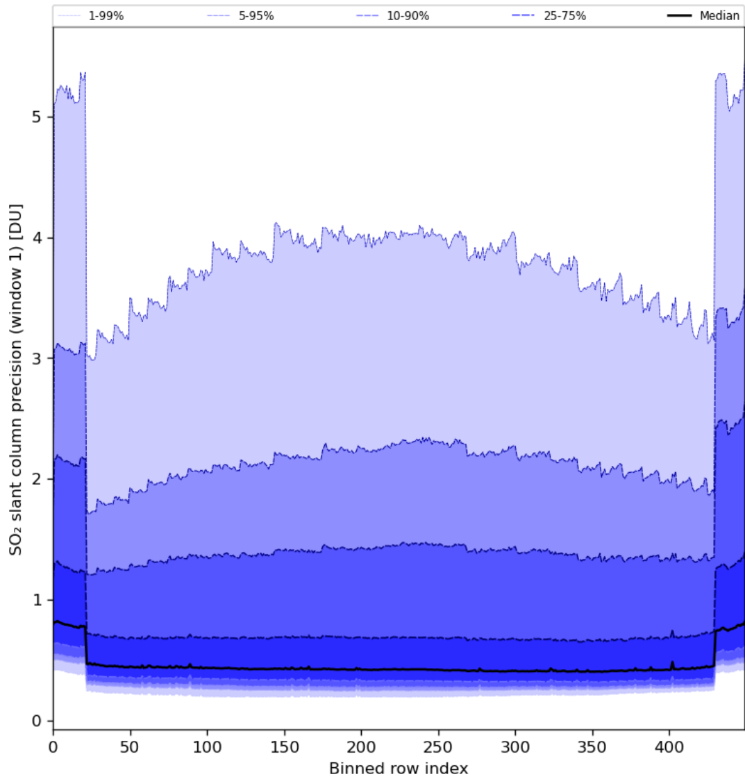
Figure 80: Along track statistics of “SO 2 slant column precision (window 1)” for 2024-04-15 to 2024-04-16
