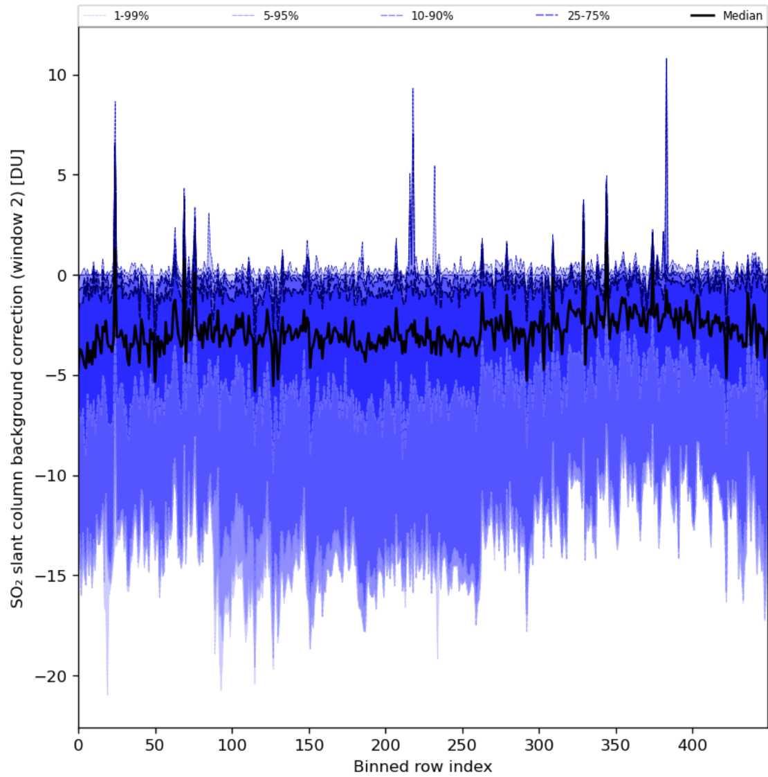
Figure 86: Along track statistics of “SO 2 slant column background correction (window 2)” for 2024-04-15 to 2024-04-16
