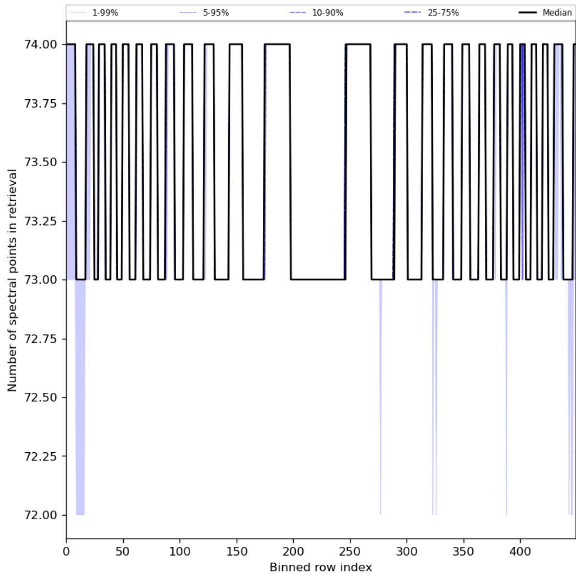
Figure 97: Along track statistics of “Number of spectral points in retrieval” for 2024-04-15 to 2024-04-16
