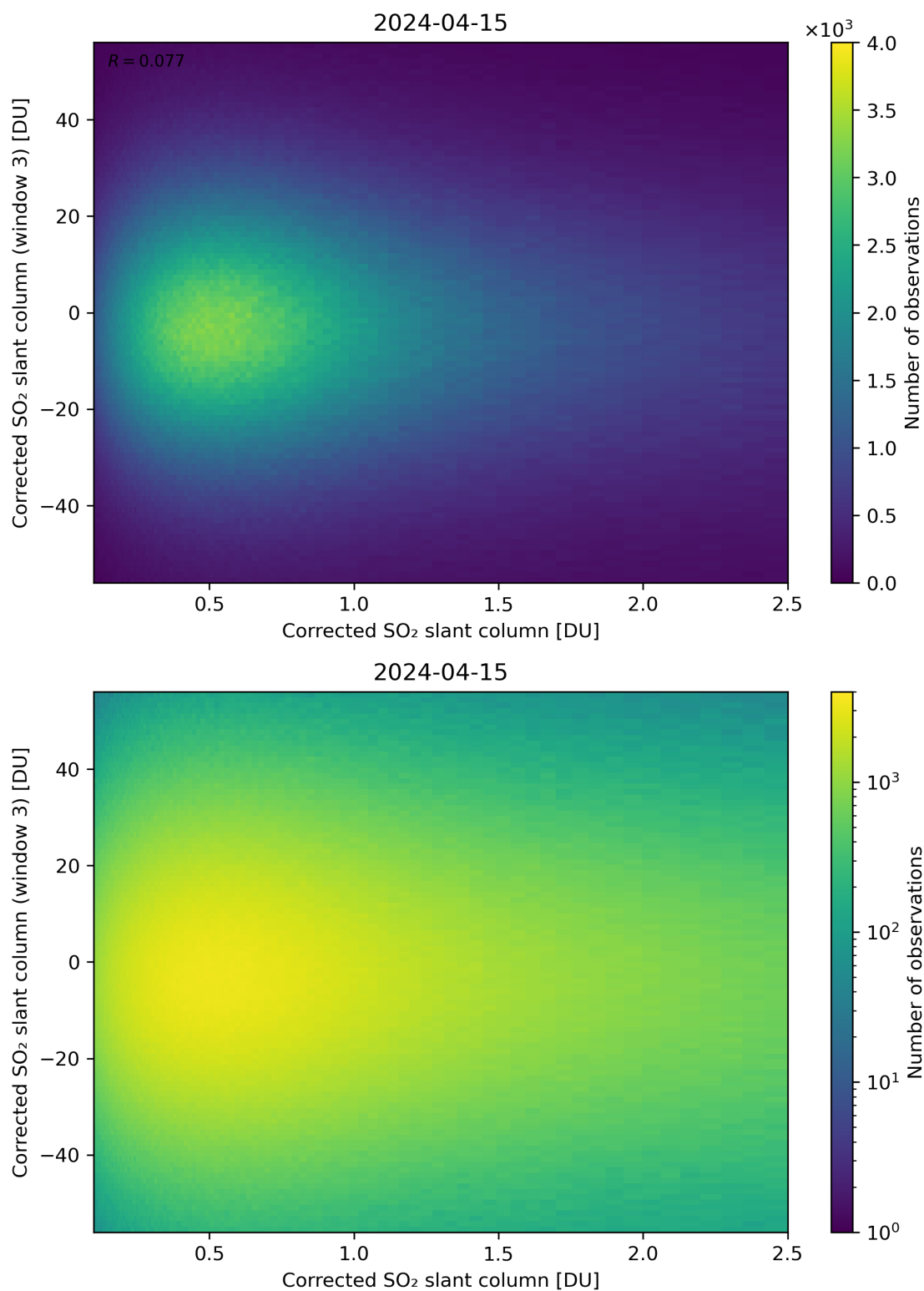
Figure 186: Scatter density plot of “Corrected SO 2 slant column” against “Corrected SO 2 slant column (window 3)” for 2024-04-15 to 2024-04-16.
