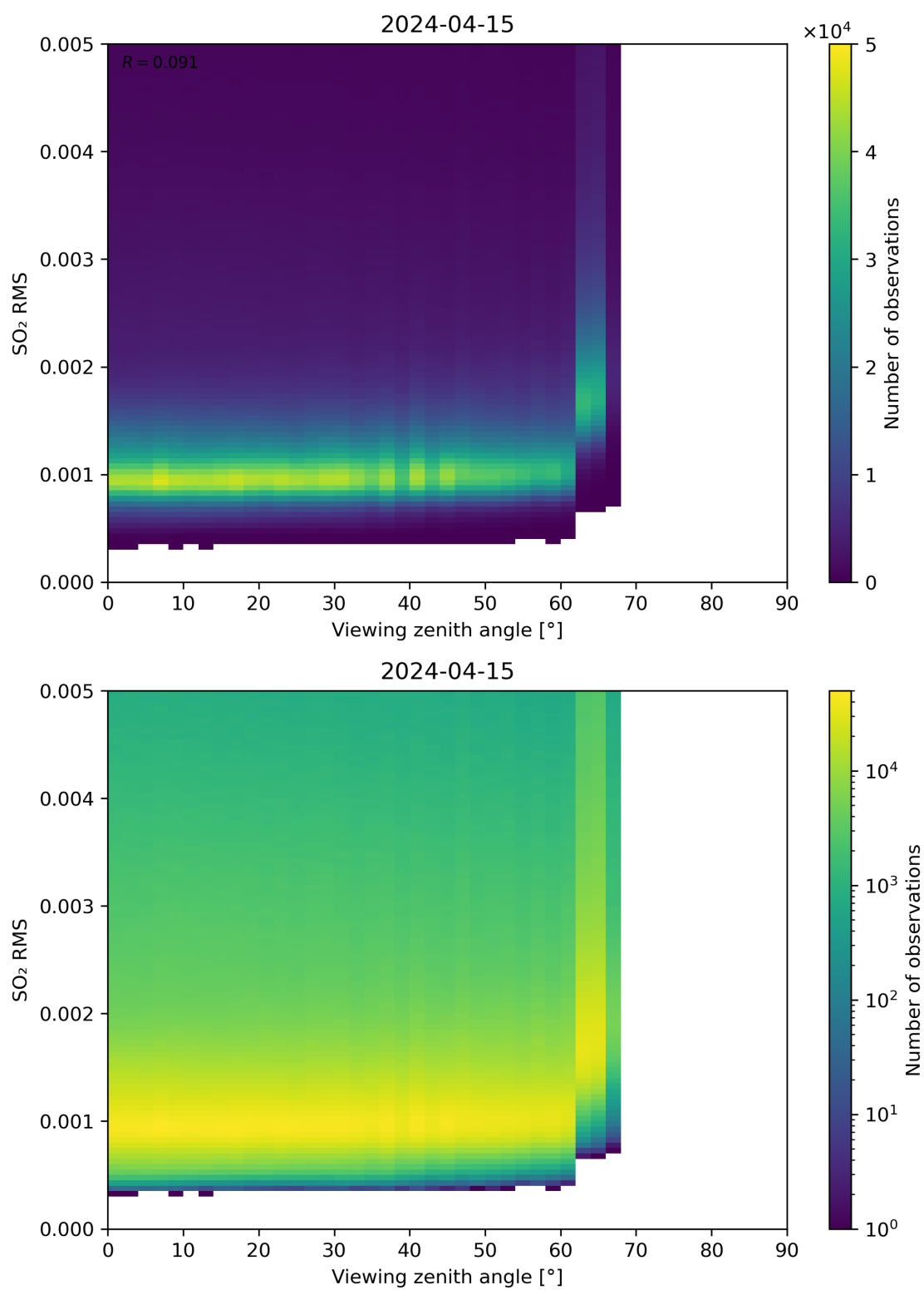
Figure 313: Scatter density plot of “Viewing zenith angle” against “SO 2 RMS” for 2024-04-15 to 2024-04-16.
