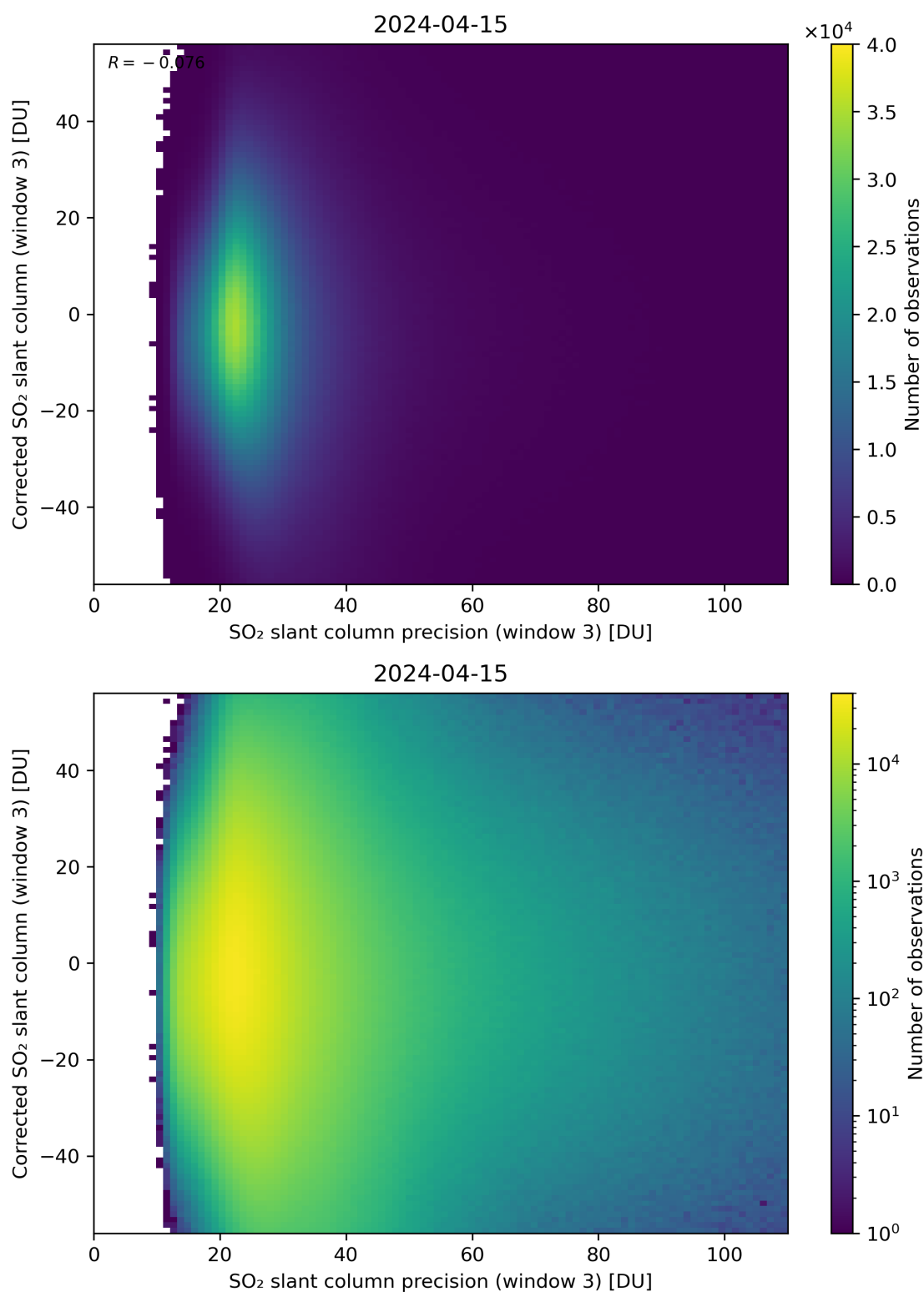
Figure 262: Scatter density plot of “SO 2 slant column precision (window 3)” against “Corrected SO 2 slant column (window 3)” for 2024-04-15 to 2024-04-16.
