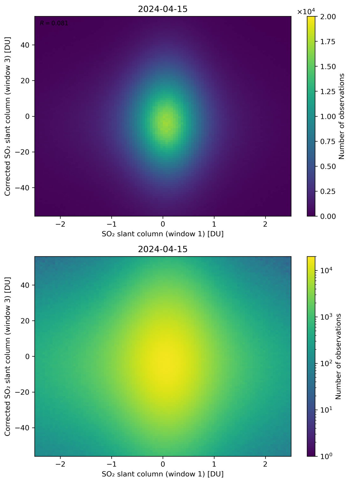
Figure 234: Scatter density plot of “SO 2 slant column (window 1)” against “Corrected SO 2 slant column (window 3)” for 2024-04-15 to 2024-04-16.
