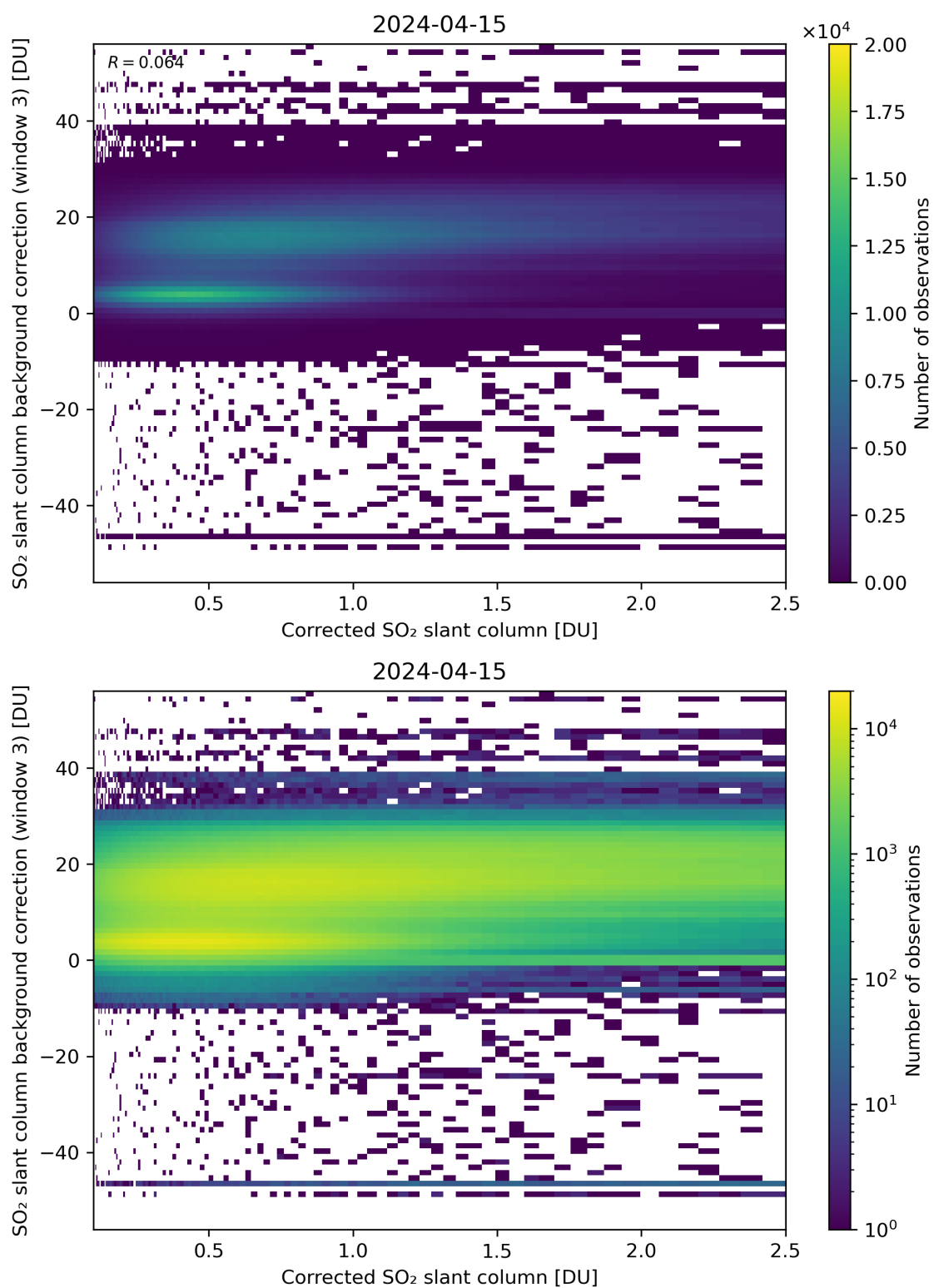
Figure 180: Scatter density plot of “Corrected SO 2 slant column” against “SO 2 slant column background correction (window 3)” for 2024-04-15 to 2024-04-16.
