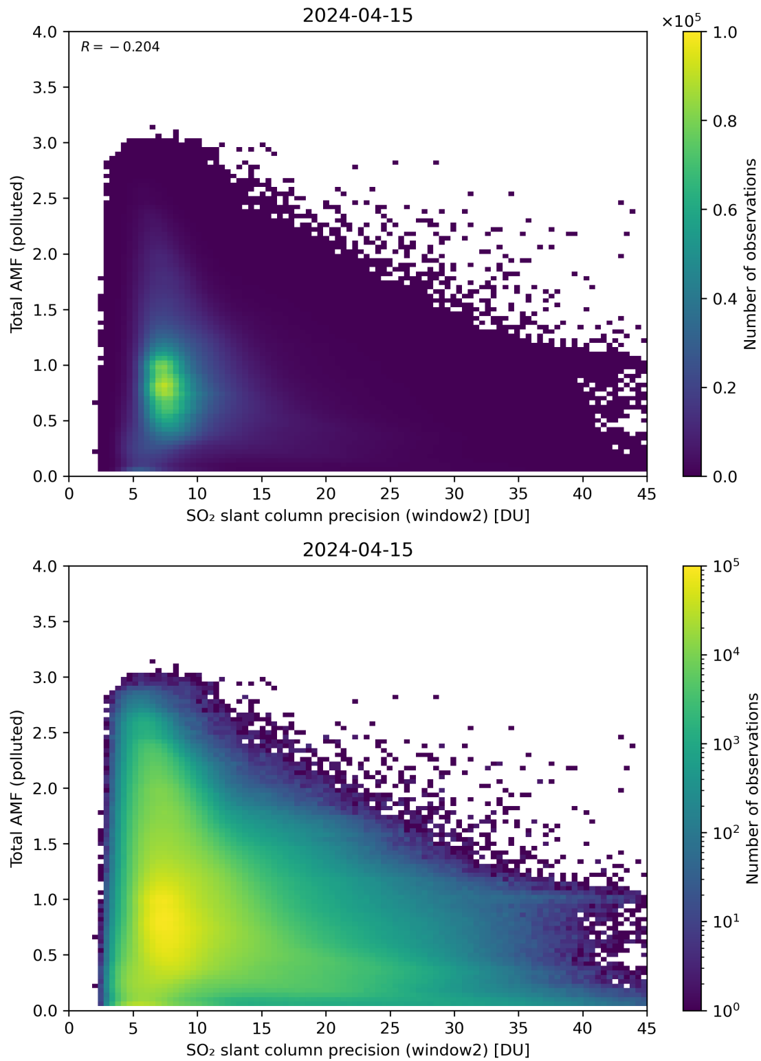
Figure 251: Scatter density plot of “SO 2 slant column precision (window2)” against “Total AMF (polluted)” for 2024-04-15 to 2024-04-16.
