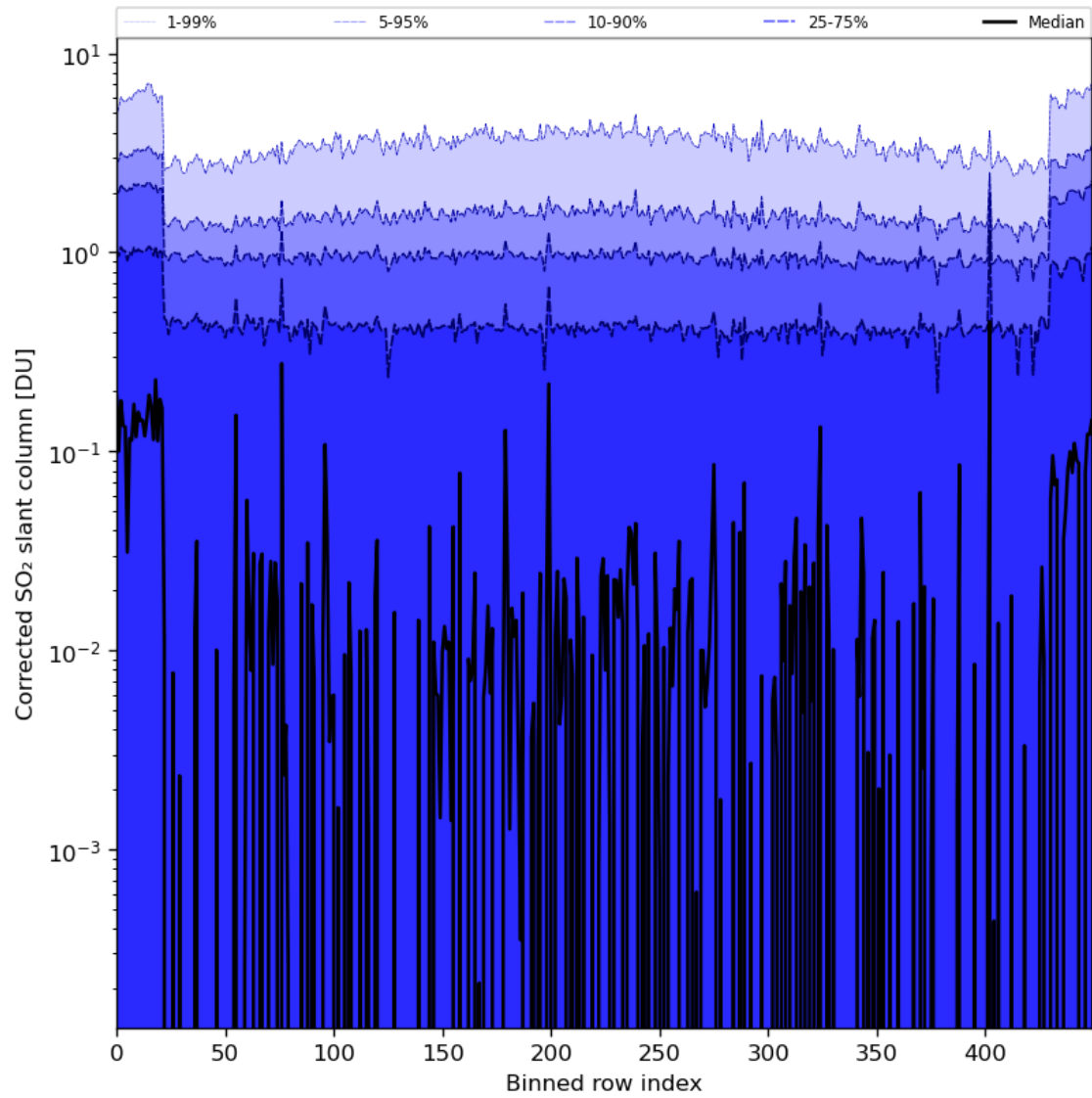
Figure 78: Along track statistics of “Corrected SO 2 slant column” for 2024-04-15 to 2024-04-16
