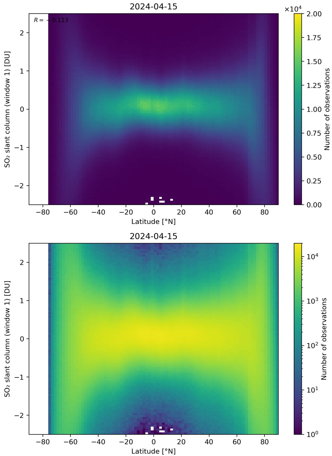
Figure 149: Scatter density plot of “Latitude” against “SO 2 slant column (window 1)” for 2024-04-15 to 2024-04-16.
