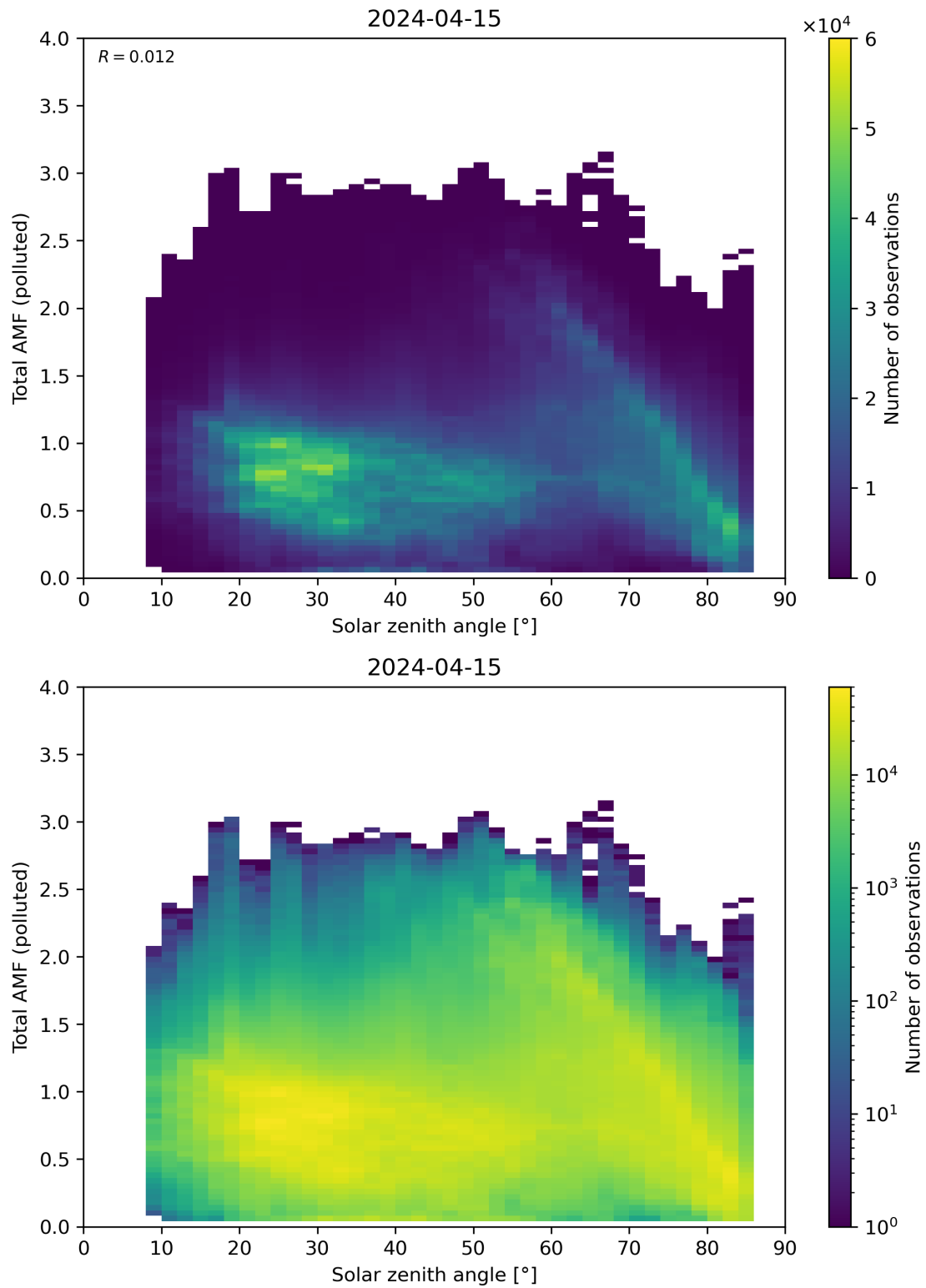
Figure 174: Scatter density plot of “Solar zenith angle” against “Total AMF (polluted)” for 2024-04-15 to 2024-04-16.
