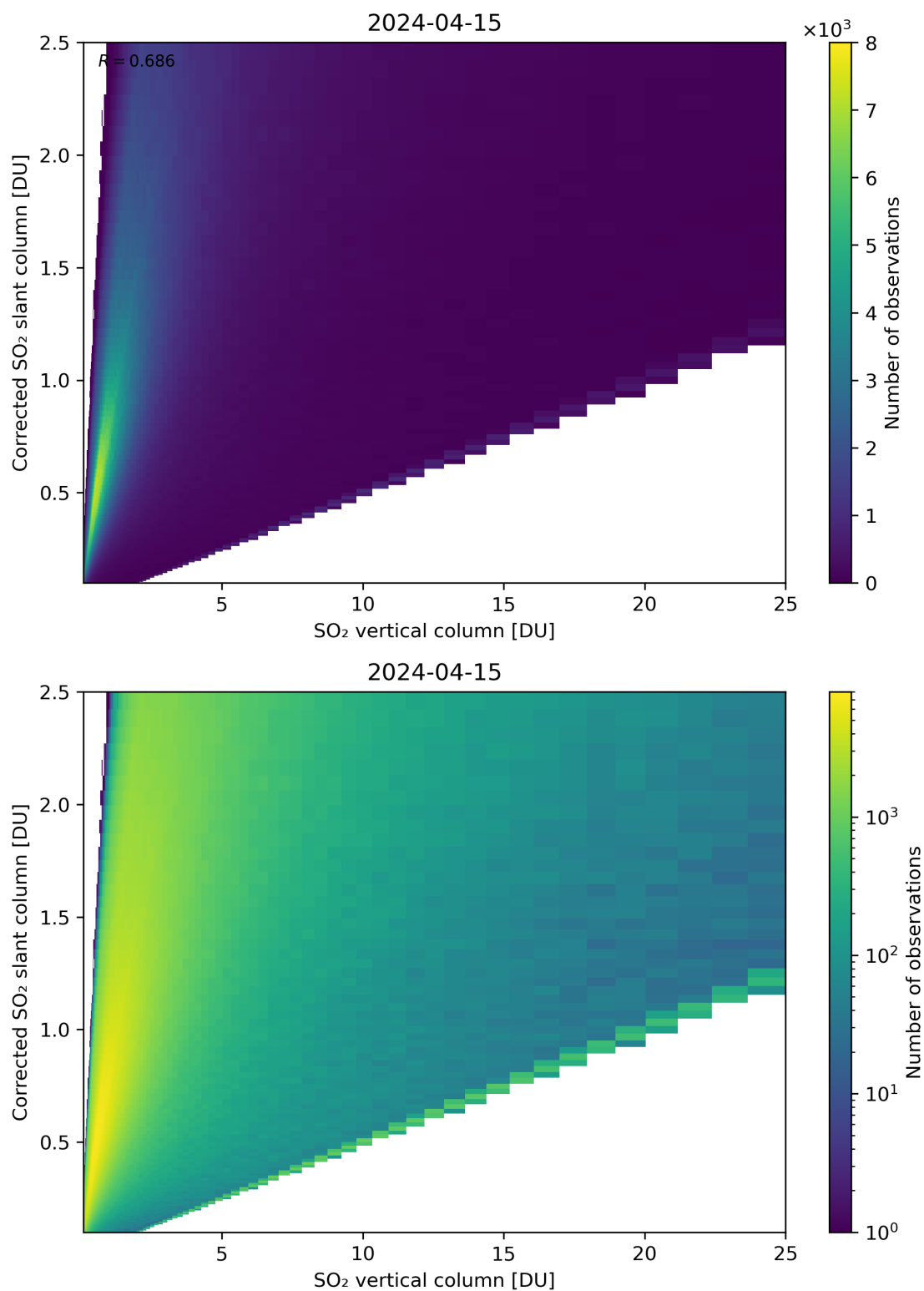
Figure 297: Scatter density plot of “SO 2 vertical column” against “Corrected SO 2 slant column” for 2024-04-15 to 2024-04-16.
