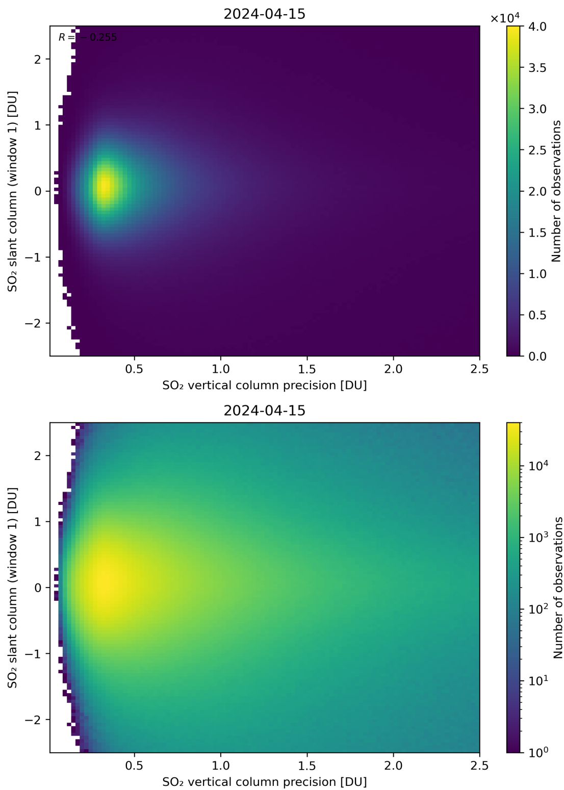
Figure 289: Scatter density plot of “SO 2 vertical column precision” against “SO 2 slant column (window 1)” for 2024-04-15 to 2024-04-16.
