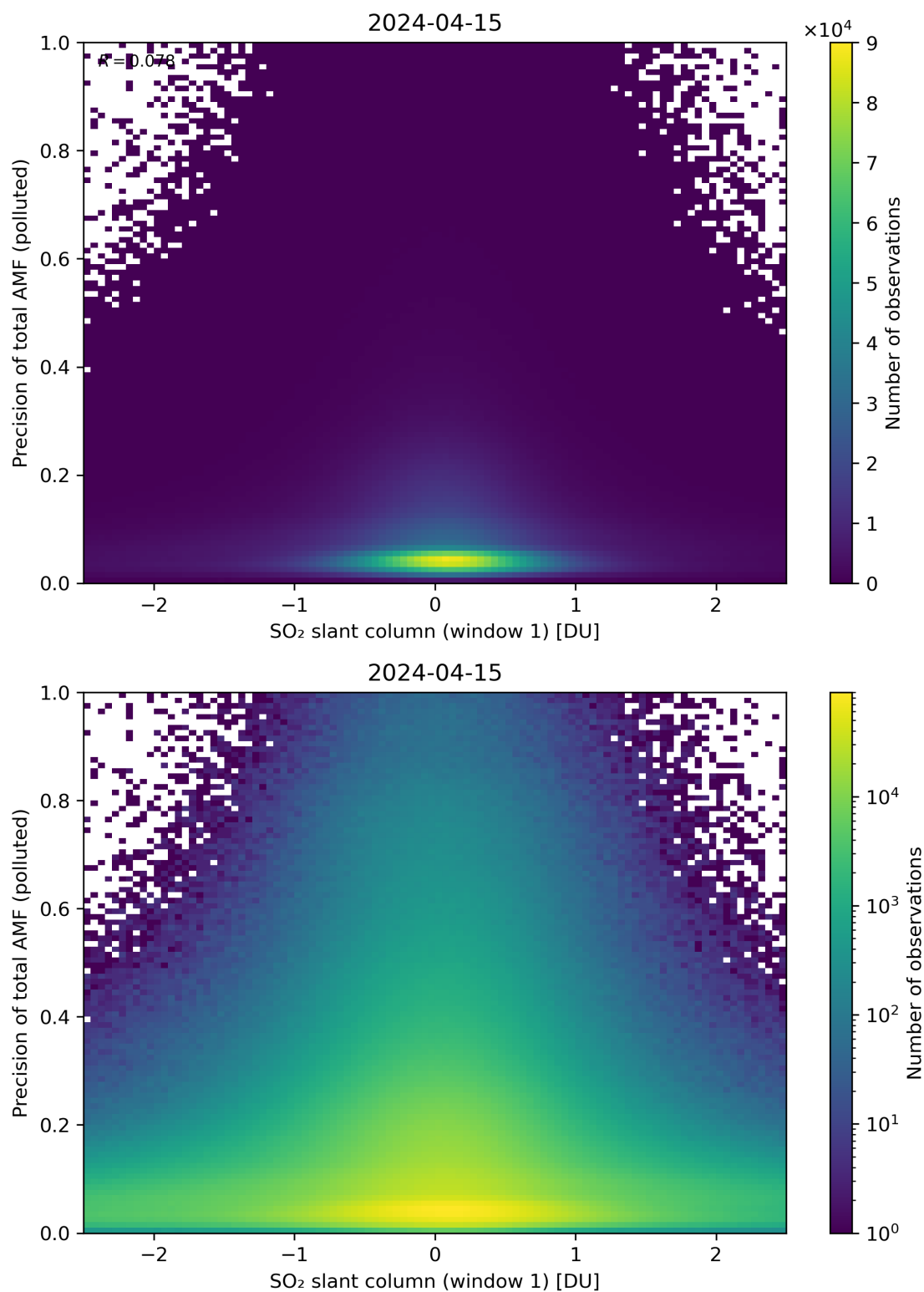
Figure 240: Scatter density plot of “SO 2 slant column (window 1)” against “Precision of total AMF (polluted)” for 2024-04-15 to 2024-04-16.
