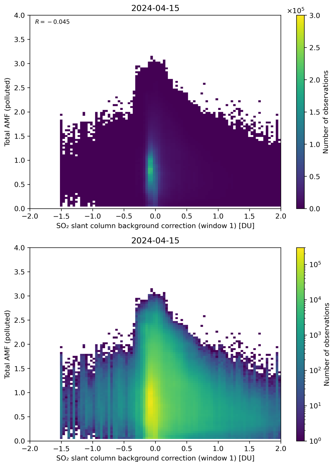
Figure 109: Scatter density plot of “SO 2 slant column background correction (window 1)” against “Total AMF (polluted)” for 2024-04-15 to 2024-04-16.
