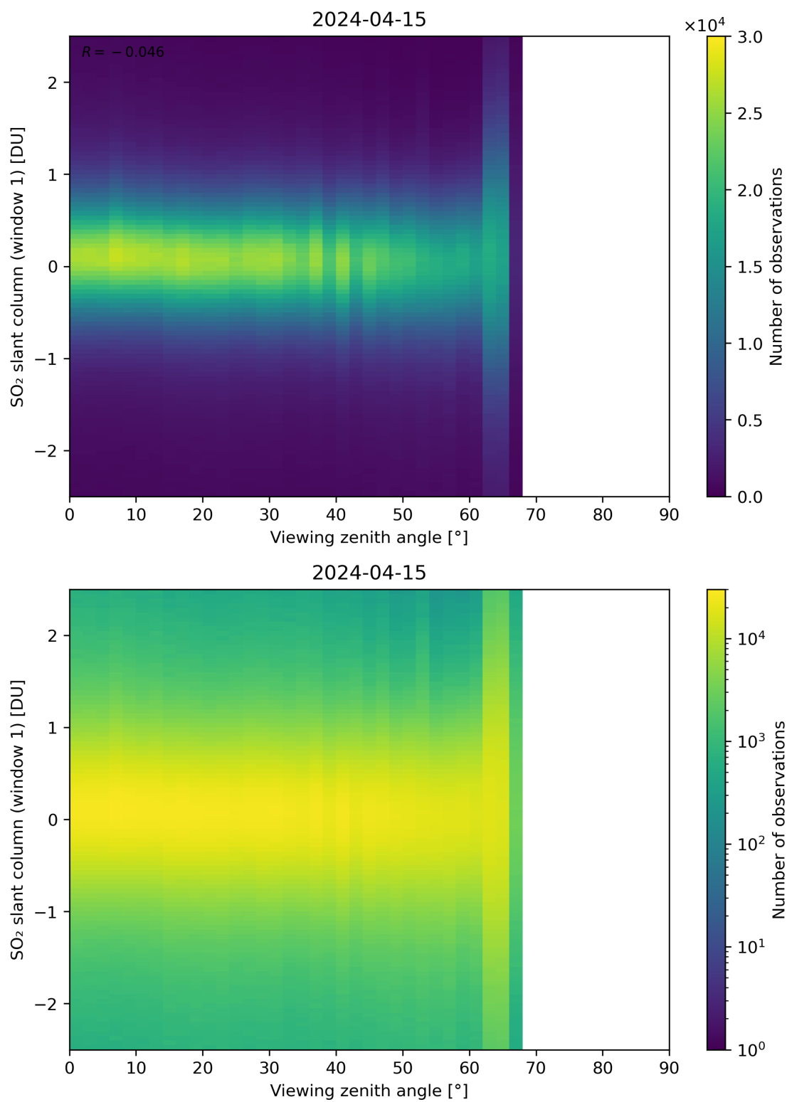
Figure 320: Scatter density plot of “Viewing zenith angle” against “SO 2 slant column (window 1)” for 2024-04-15 to 2024-04-16.
