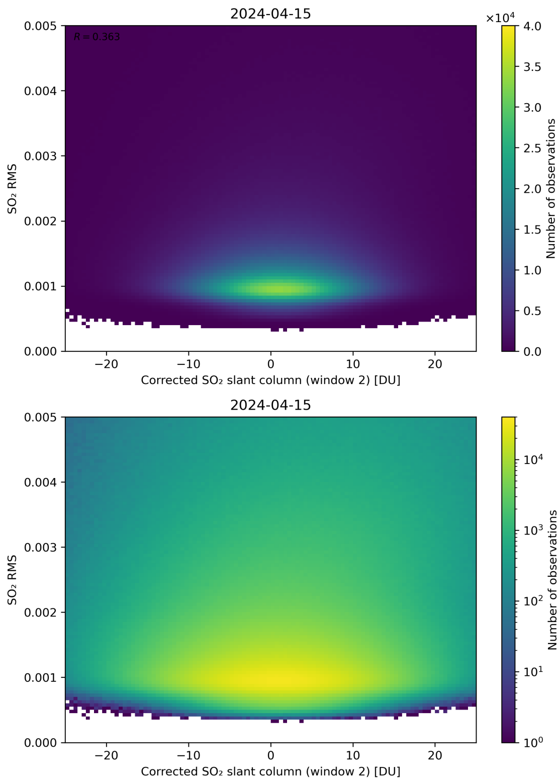
Figure 198: Scatter density plot of “Corrected SO 2 slant column (window 2)” against “SO 2 RMS” for 2024-04-15 to 2024-04-16.
