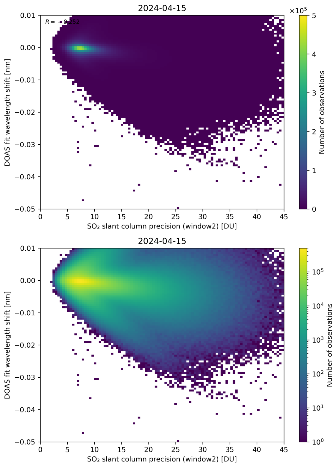
Figure 243: Scatter density plot of “SO 2 slant column precision (window2)” against “DOAS fit wavelength shift” for 2024-04-15 to 2024-04-16.
