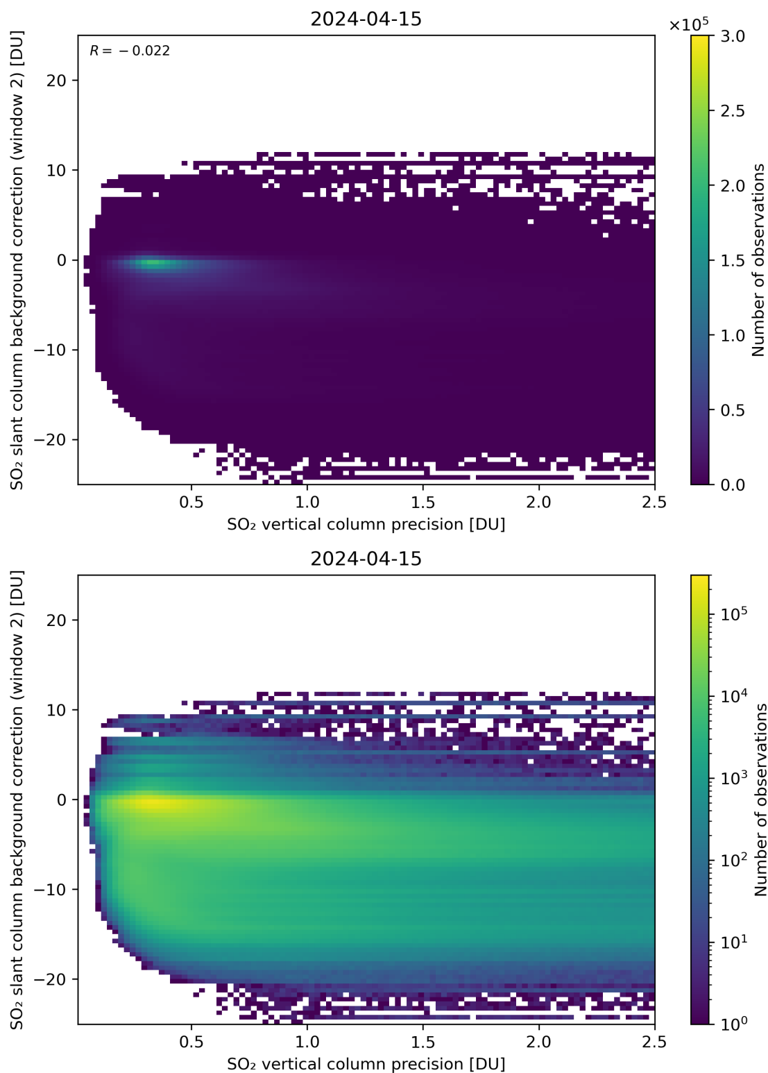
Figure 280: Scatter density plot of “SO 2 vertical column precision” against “SO 2 slant column background correction (window 2)” for 2024-04-15 to 2024-04-16.
