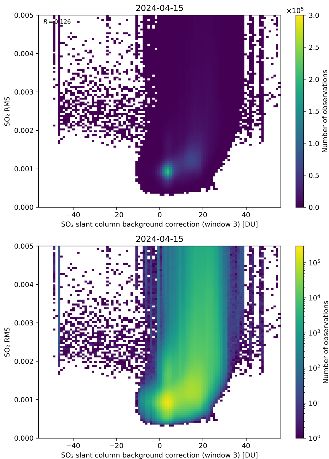
Figure 123: Scatter density plot of “SO 2 slant column background correction (window 3)” against “SO 2 RMS” for 2024-04-15 to 2024-04-16.
