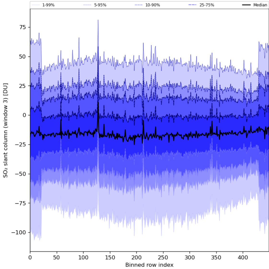
Figure 87: Along track statistics of “SO 2 slant column (window 3)” for 2024-04-15 to 2024-04-16
