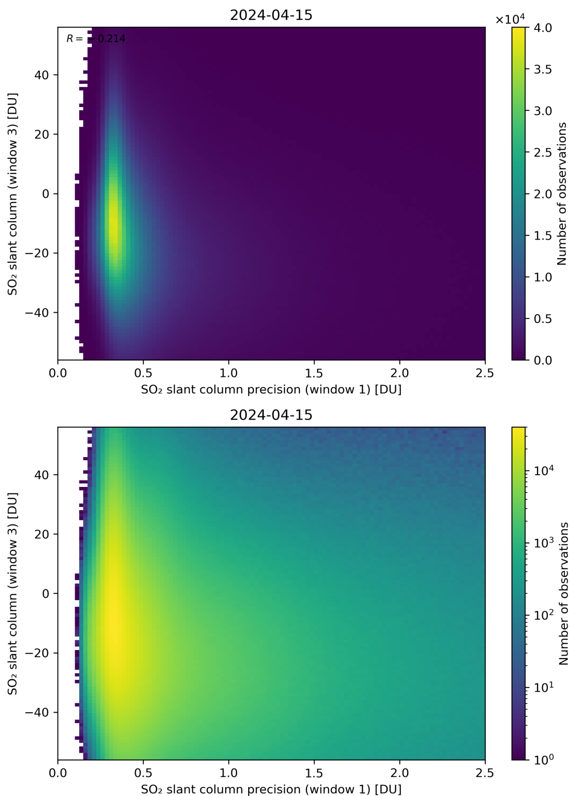
Figure 228: Scatter density plot of “SO 2 slant column precision (window 1)” against “SO 2 slant column (window 3)” for 2024-04-15 to 2024-04-16.
