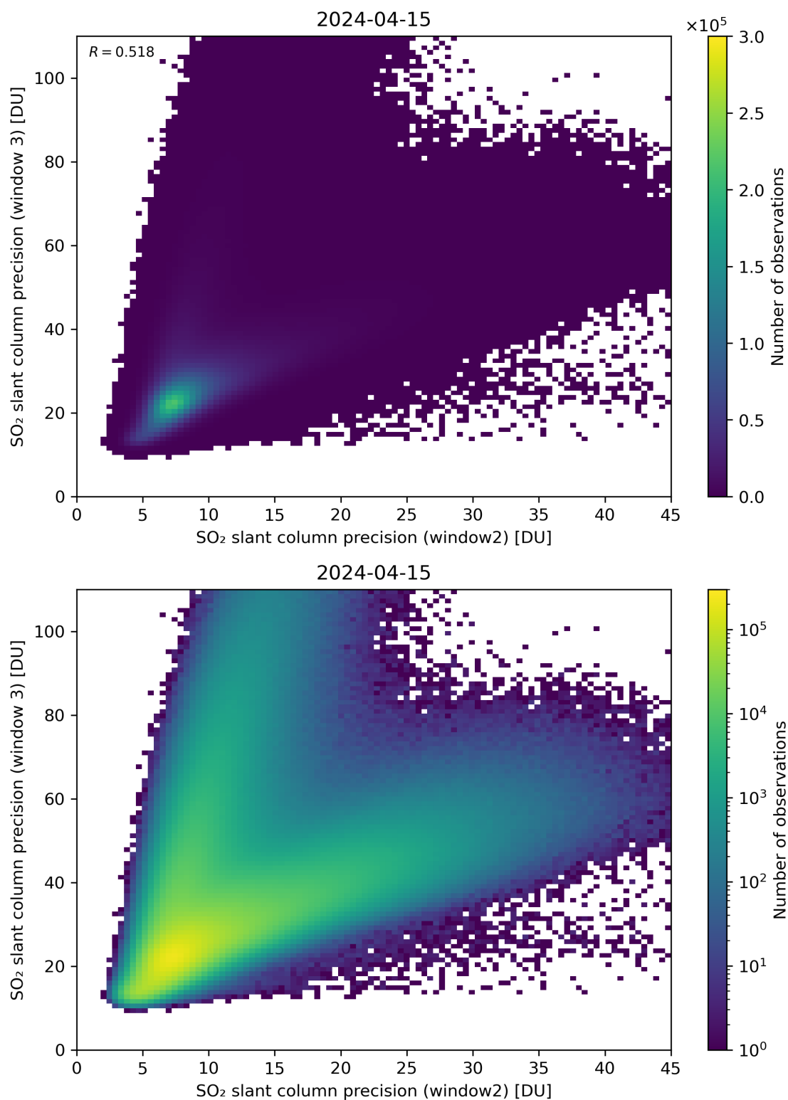
Figure 250: Scatter density plot of “SO 2 slant column precision (window2)” against “SO 2 slant column precision (window 3)” for 2024-04-15 to 2024-04-16.
