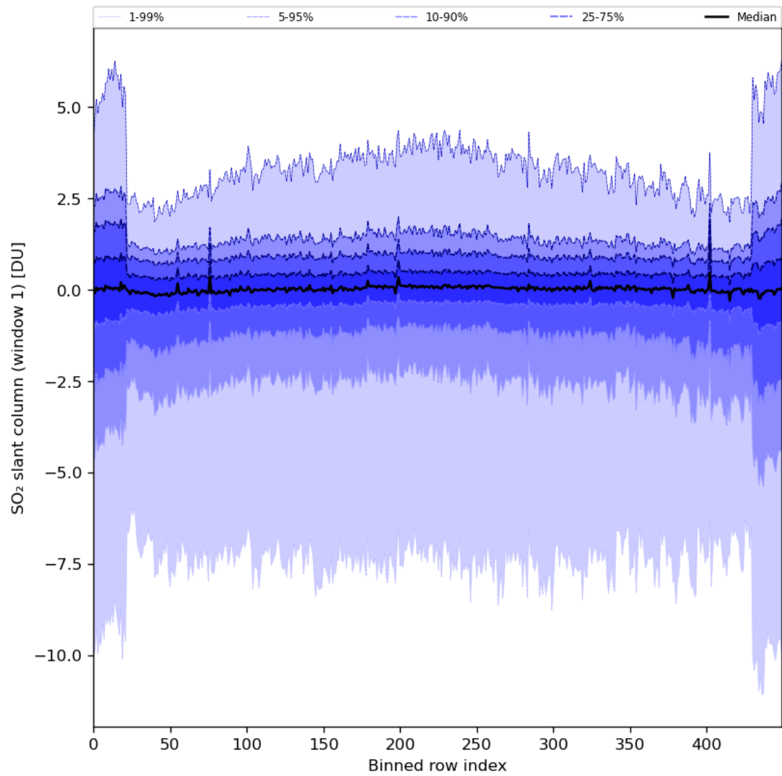
Figure 79: Along track statistics of “SO 2 slant column (window 1)” for 2024-04-15 to 2024-04-16
