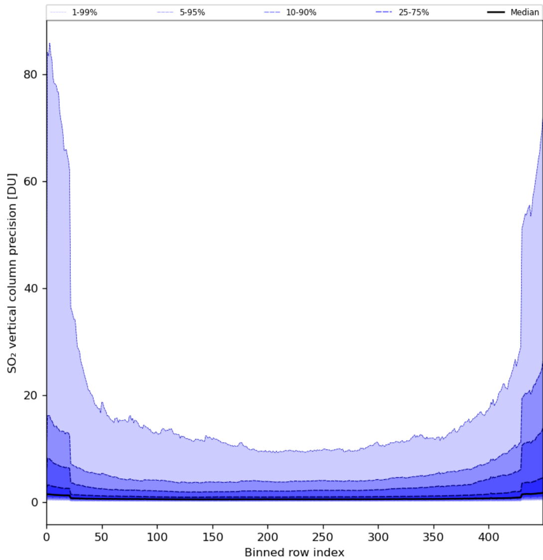
Figure 77: Along track statistics of “SO 2 vertical column precision” for 2024-04-15 to 2024-04-16
