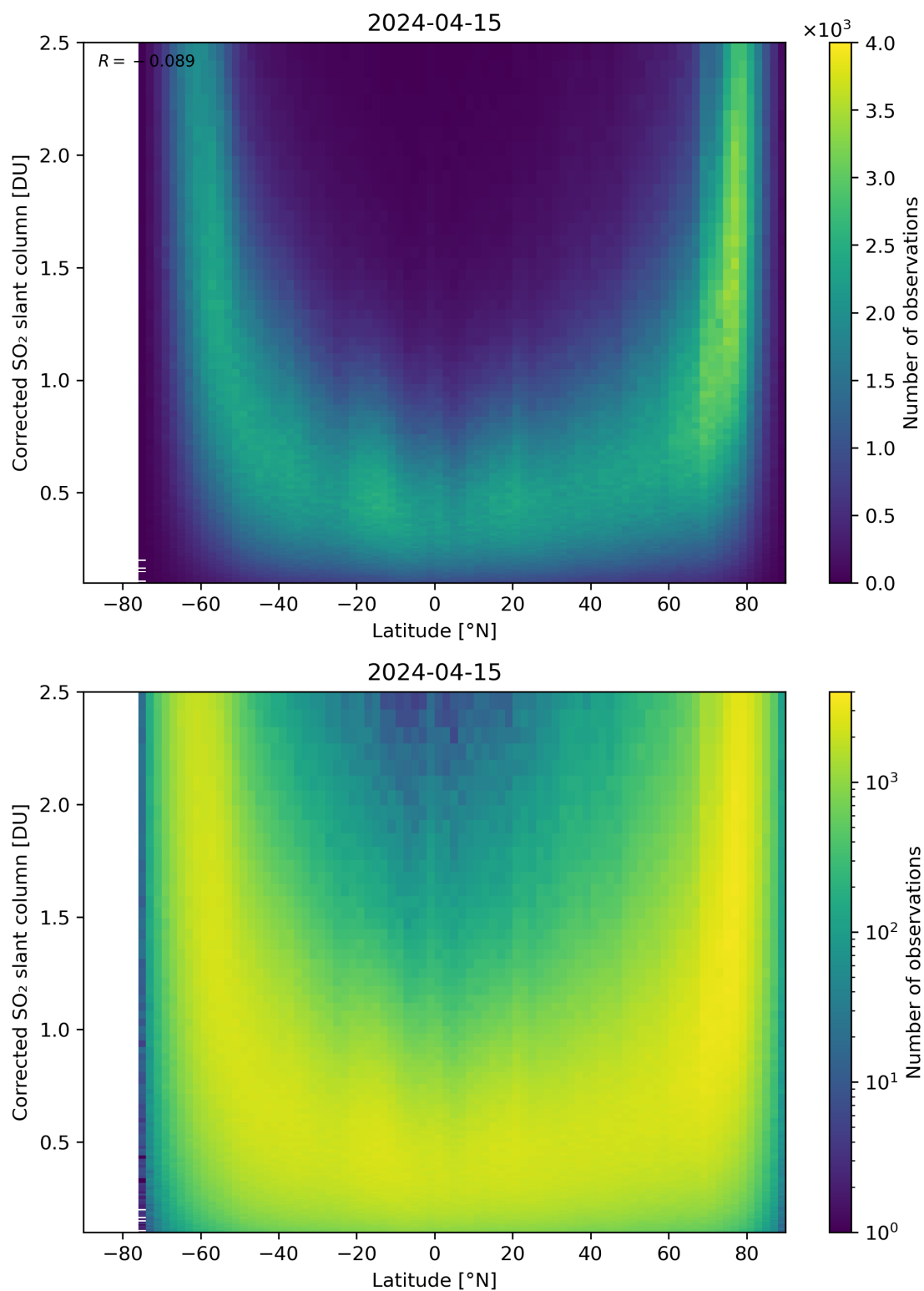
Figure 146: Scatter density plot of “Latitude” against “Corrected SO 2 slant column” for 2024-04-15 to 2024-04-16.
