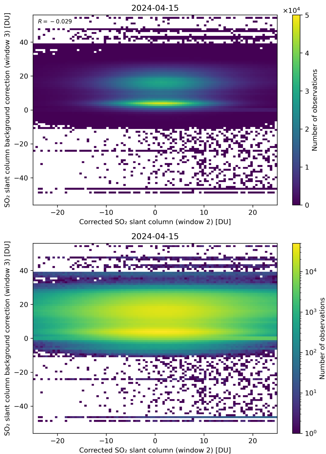
Figure 195: Scatter density plot of “Corrected SO 2 slant column (window 2)” against “SO 2 slant column background correction (window 3)” for 2024-04-15 to 2024-04-16.
