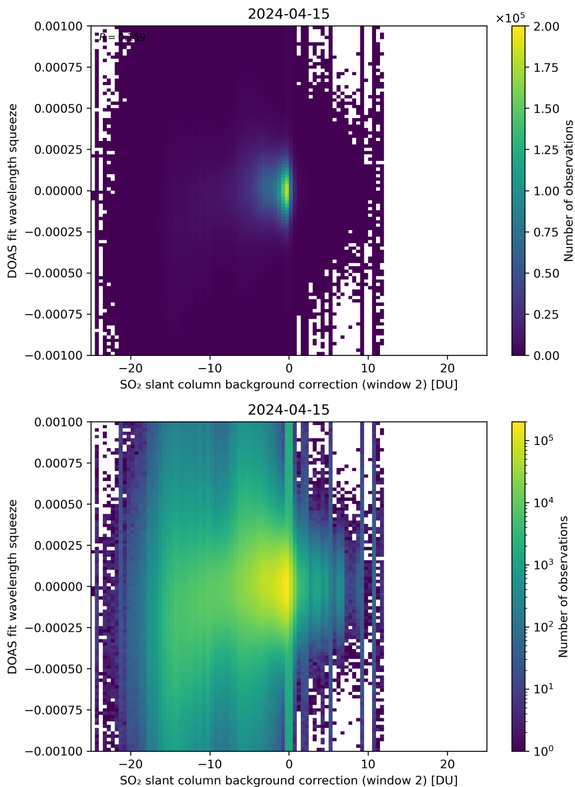
Figure 113: Scatter density plot of “SO 2 slant column background correction (window 2)” against “DOAS fit wavelength squeeze” for 2024-04-15 to 2024-04-16.
