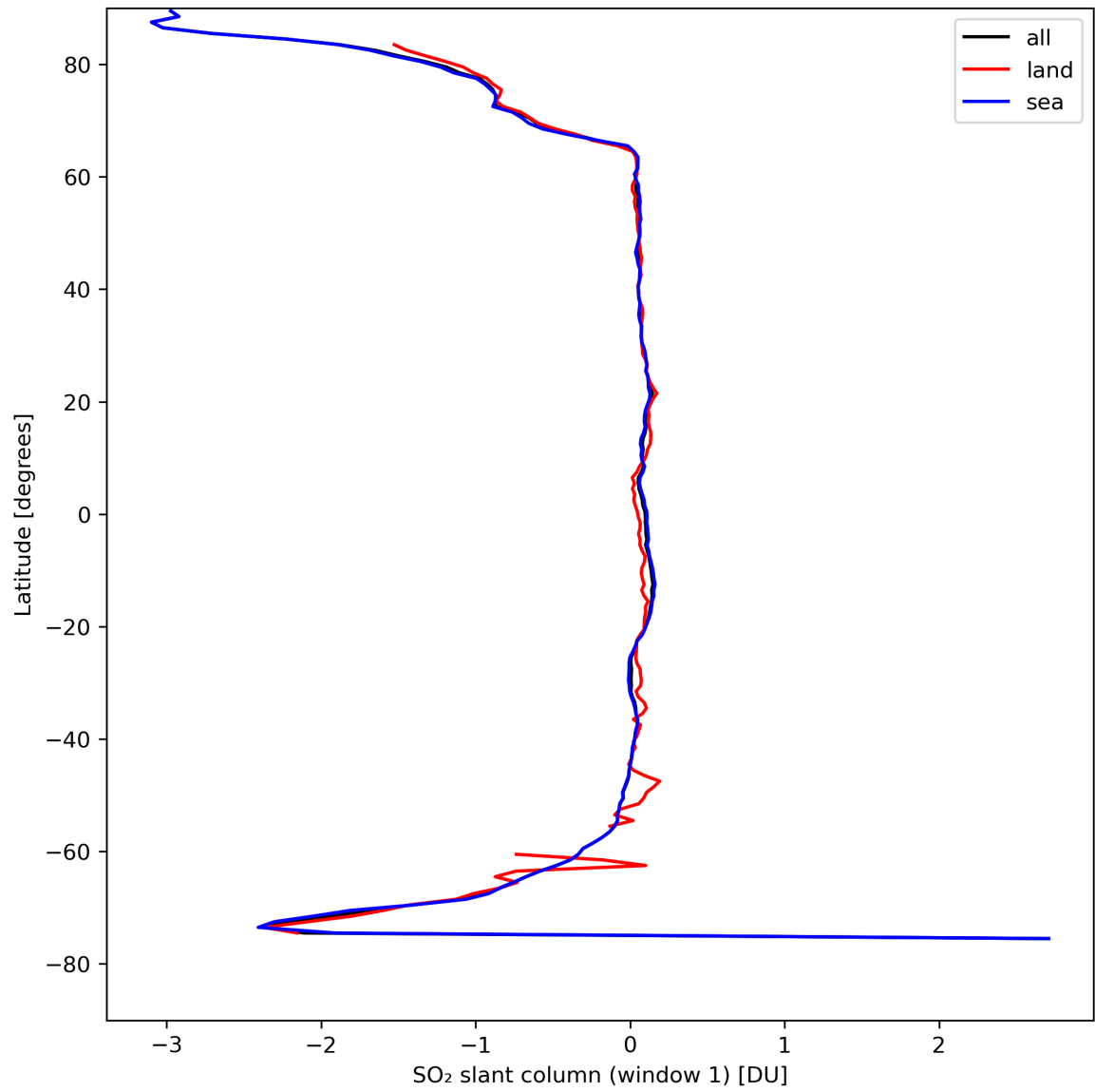
Figure 33: Zonal average of “SO 2 slant column (window 1)” for 2024-04-15 to 2024-04-16.
