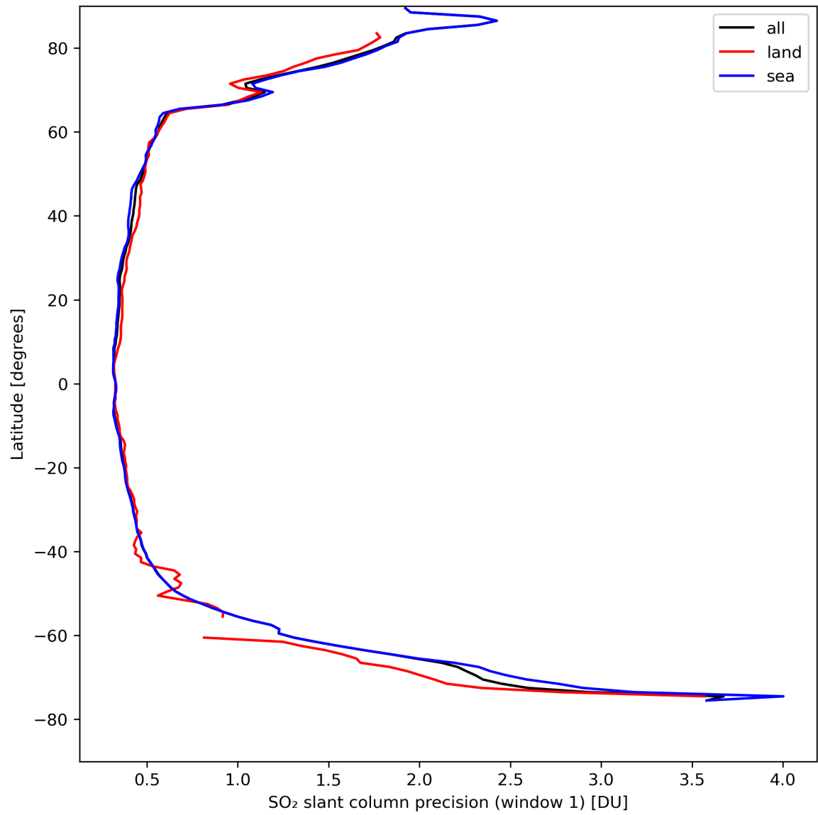
Figure 34: Zonal average of “SO 2 slant column precision (window 1)” for 2024-04-15 to 2024-04-16.
