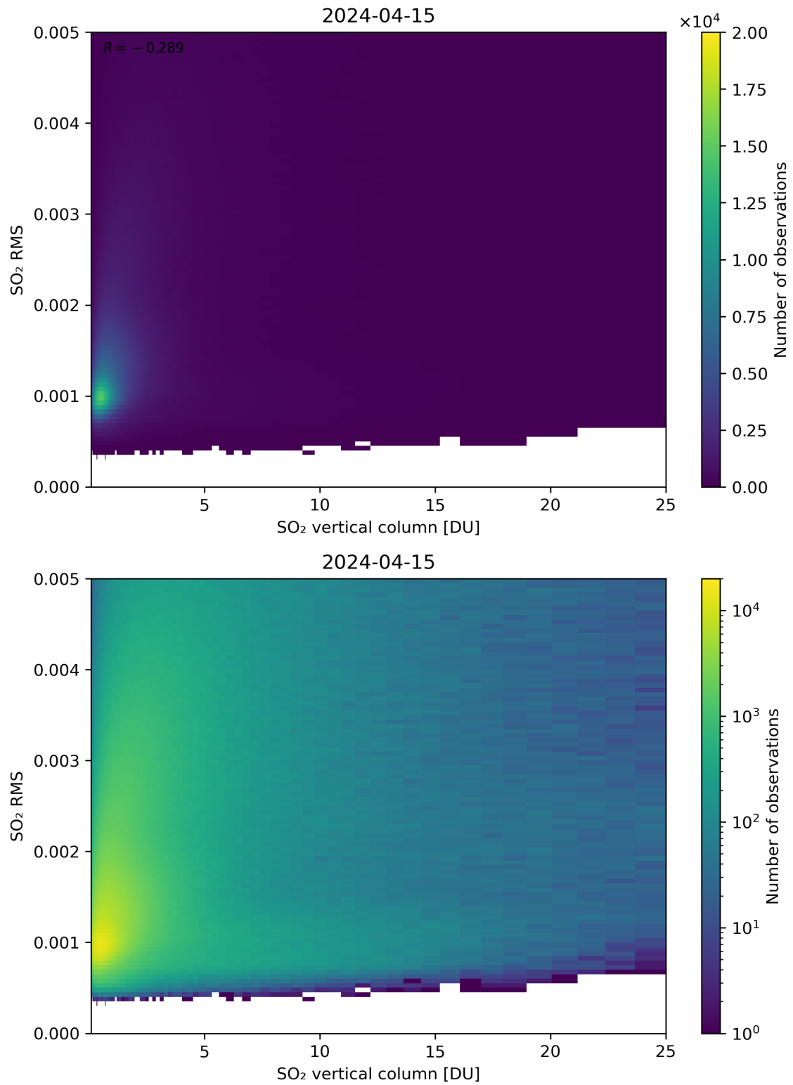
Figure 278: Scatter density plot of “SO 2 vertical column” against “SO 2 RMS” for 2024-04-15 to 2024-04-16.
