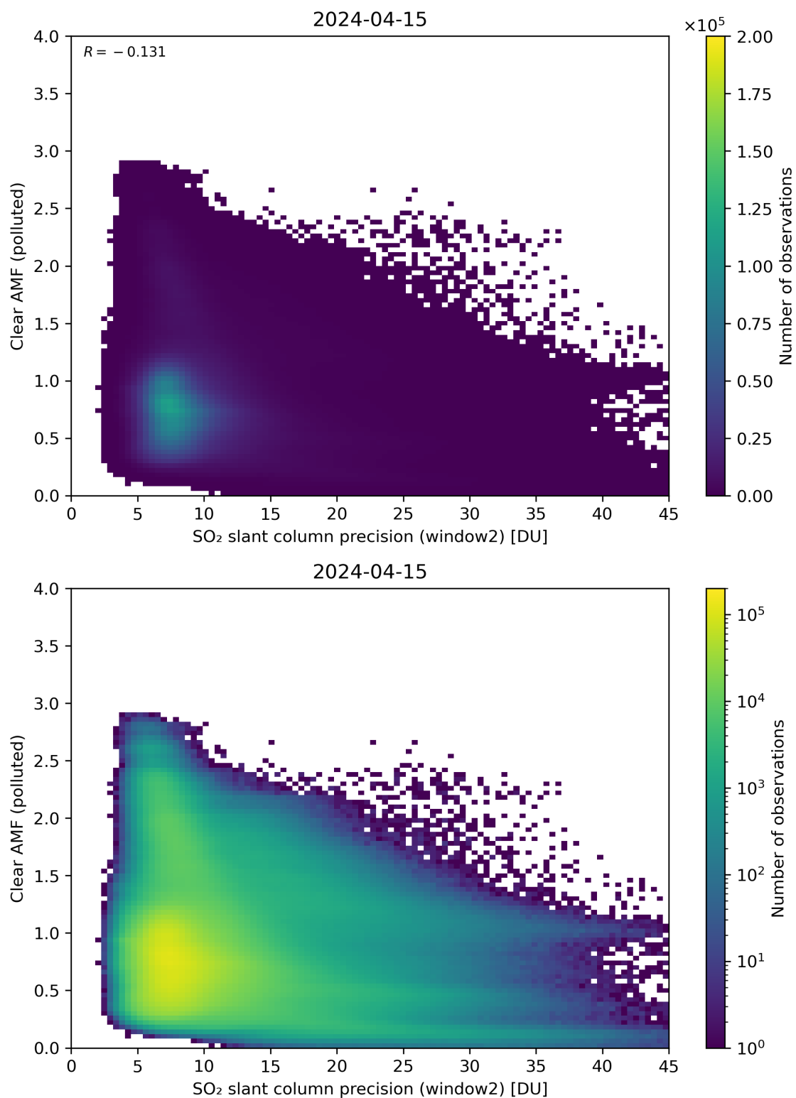
Figure 246: Scatter density plot of “SO 2 slant column precision (window2)” against “Clear AMF (polluted)” for 2024-04-15 to 2024-04-16.
