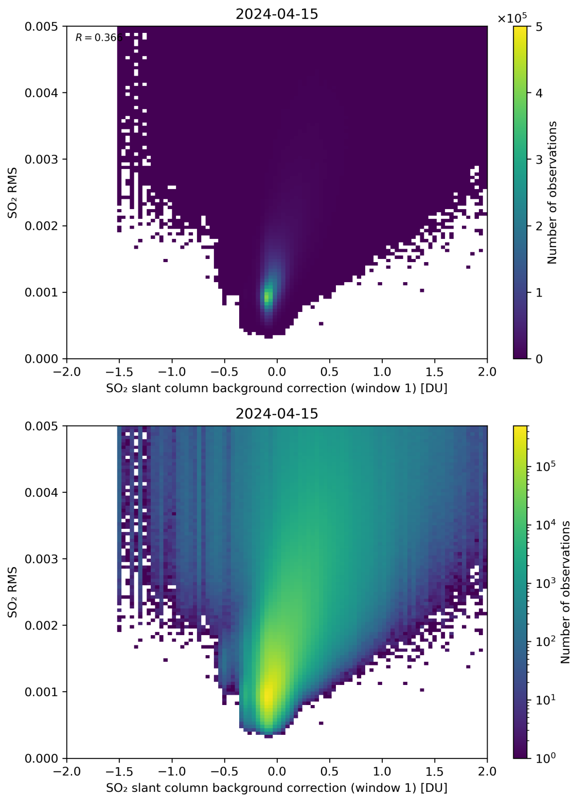
Figure 102: Scatter density plot of “SO 2 slant column background correction (window 1)” against “SO 2 RMS” for 2024-04-15 to 2024-04-16.
