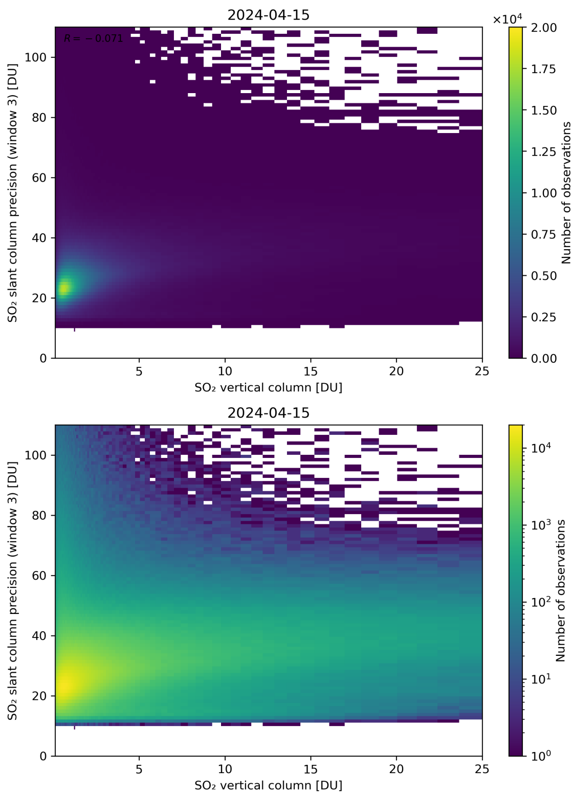
Figure 304: Scatter density plot of “SO 2 vertical column” against “SO 2 slant column precision (window 3)” for 2024-04-15 to 2024-04-16.
