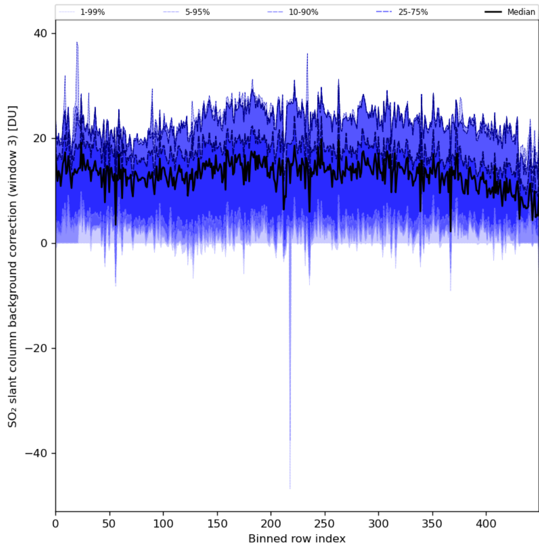
Figure 90: Along track statistics of “SO 2 slant column background correction (window 3)” for 2024-04-15 to 2024-04-16
