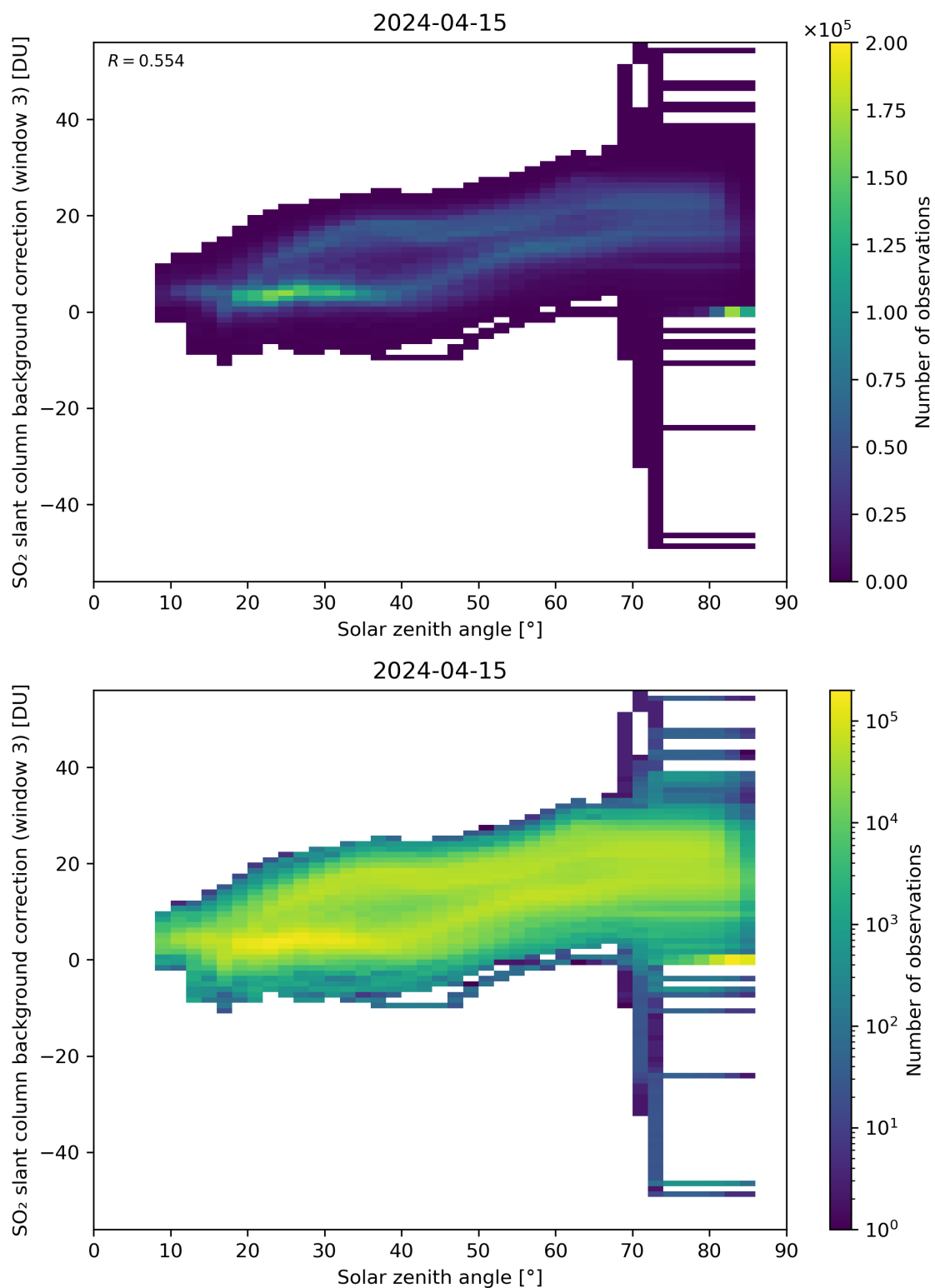
Figure 160: Scatter density plot of “Solar zenith angle” against “SO 2 slant column background correction (window 3)” for 2024-04-15 to 2024-04-16.
