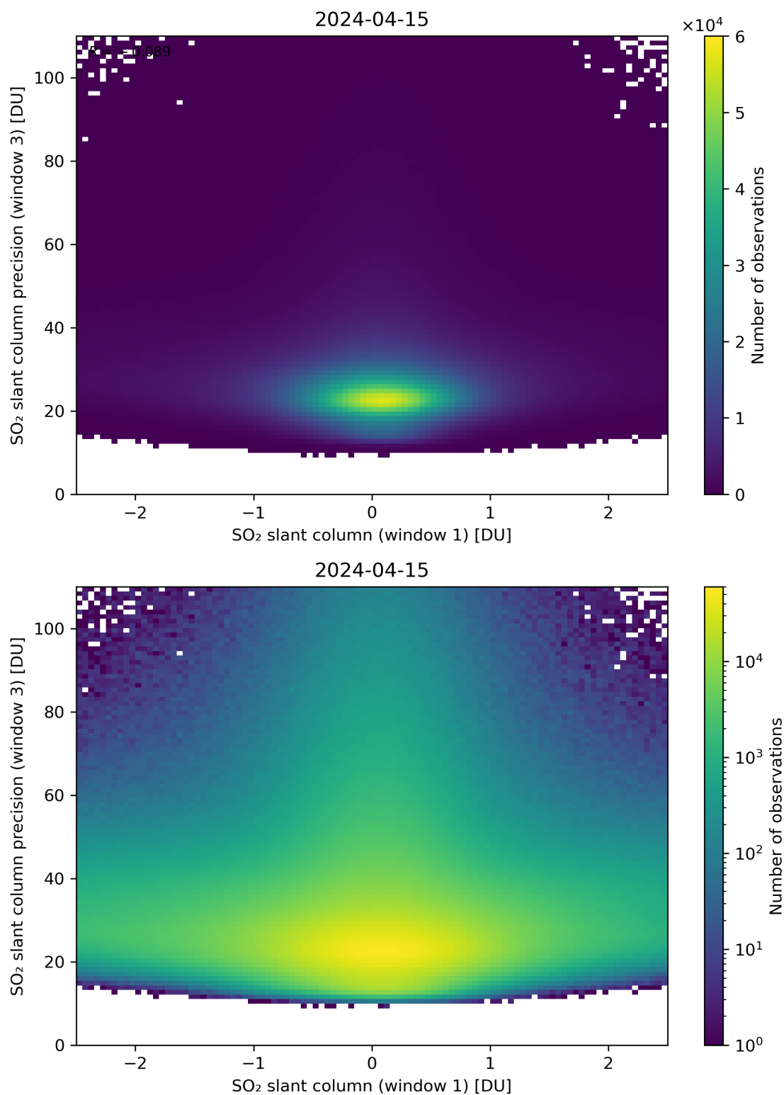
Figure 238: Scatter density plot of “SO 2 slant column (window 1)” against “SO 2 slant column precision (window 3)” for 2024-04-15 to 2024-04-16.
