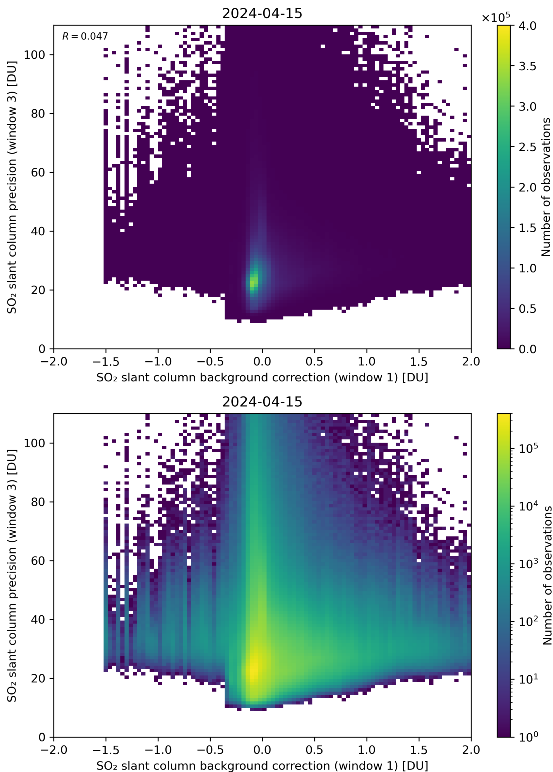
Figure 108: Scatter density plot of “SO 2 slant column background correction (window 1)” against “SO 2 slant column precision (window 3)” for 2024-04-15 to 2024-04-16.
