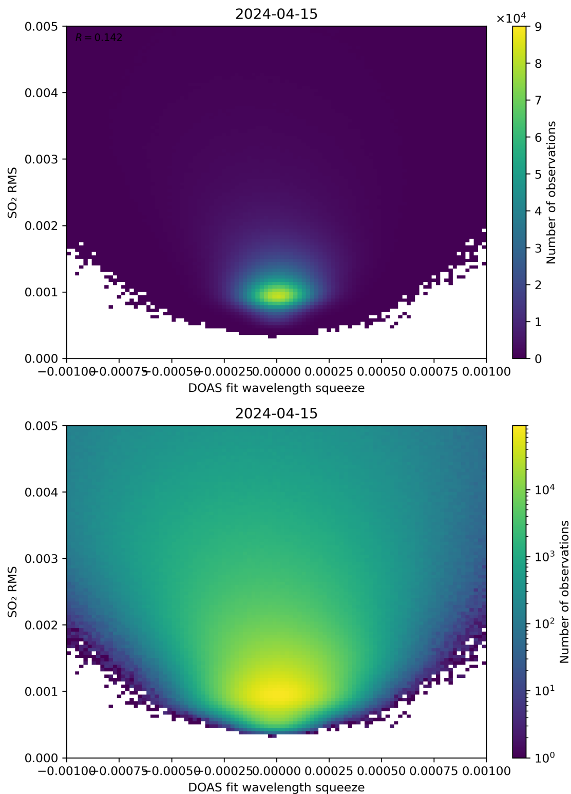
Figure 132: Scatter density plot of “DOAS fit wavelength squeeze” against “SO 2 RMS” for 2024-04-15 to 2024-04-16.
