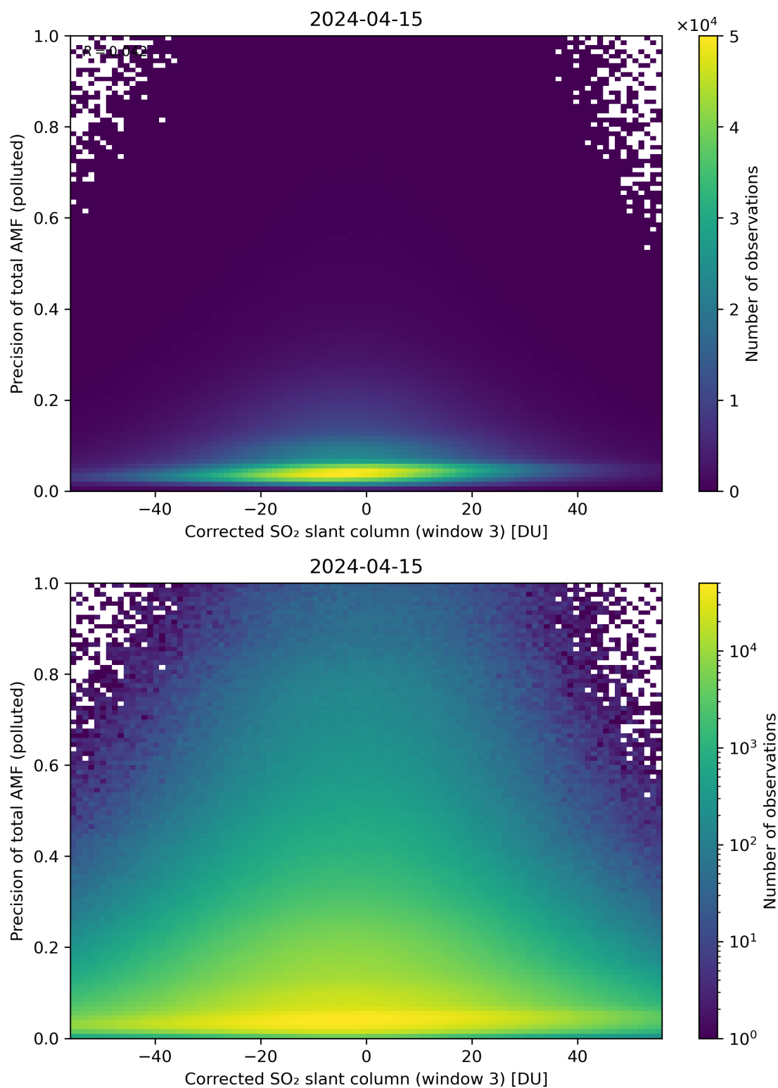
Figure 211: Scatter density plot of “Corrected SO 2 slant column (window 3)” against “Precision of total AMF (polluted)” for 2024-04-15 to 2024-04-16.
