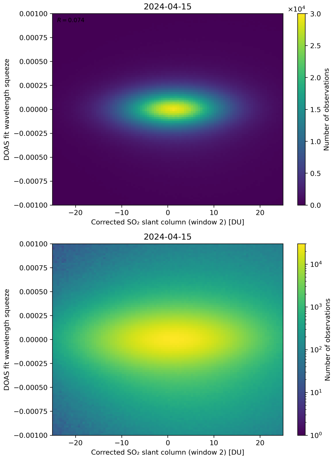
Figure 197: Scatter density plot of “Corrected SO 2 slant column (window 2)” against “DOAS fit wavelength squeeze” for 2024-04-15 to 2024-04-16.
