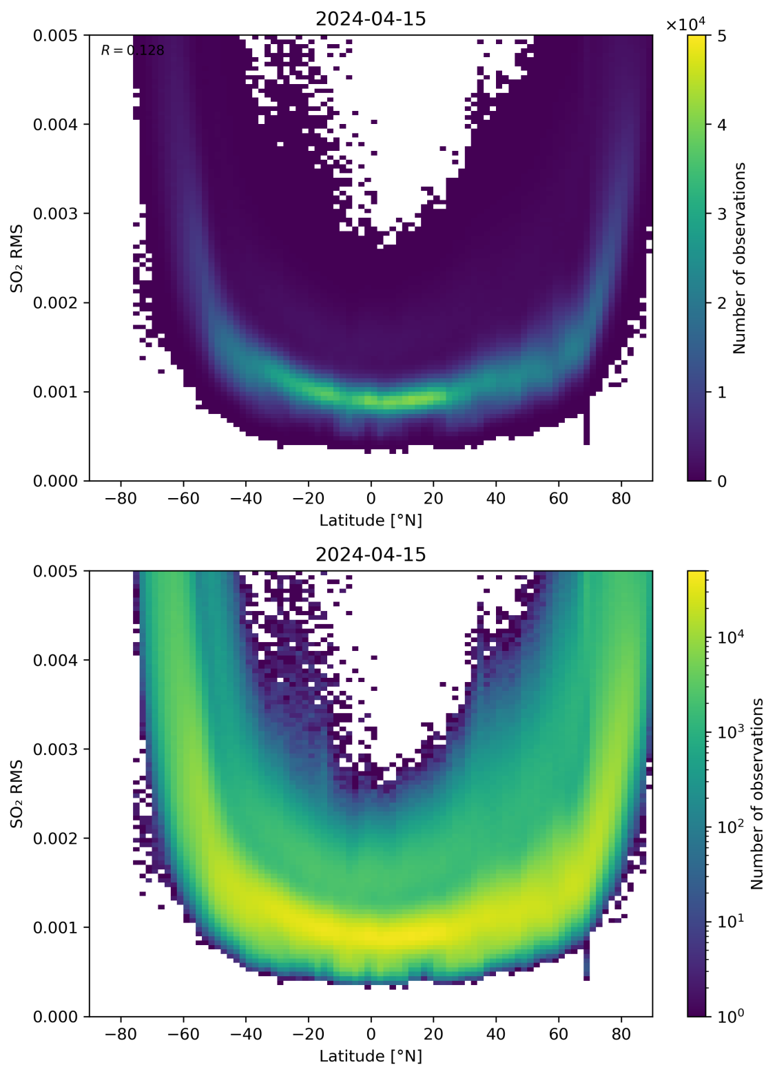
Figure 144: Scatter density plot of “Latitude” against “SO 2 RMS” for 2024-04-15 to 2024-04-16.
