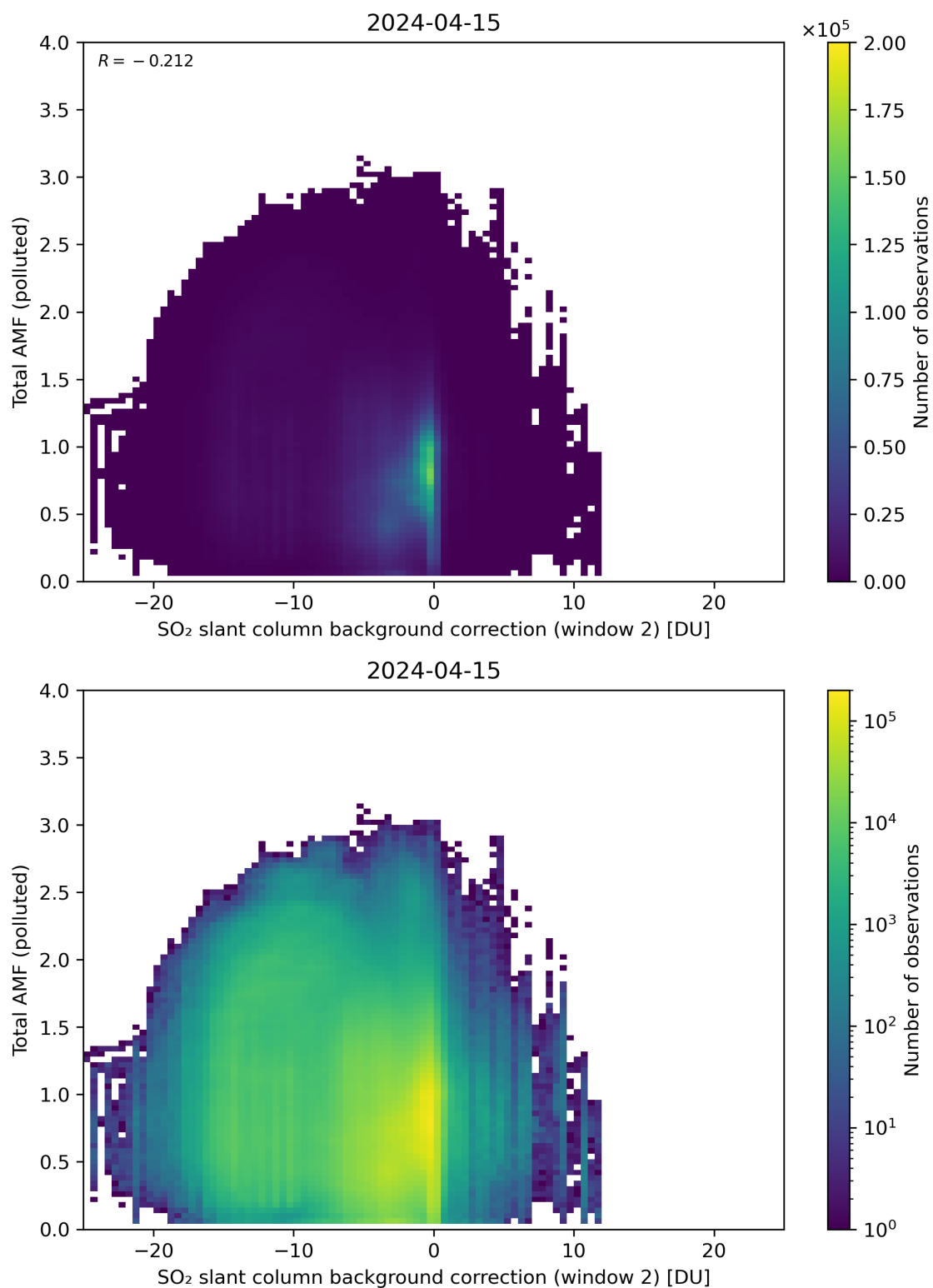
Figure 119: Scatter density plot of “SO 2 slant column background correction (window 2)” against “Total AMF (polluted)” for 2024-04-15 to 2024-04-16.
