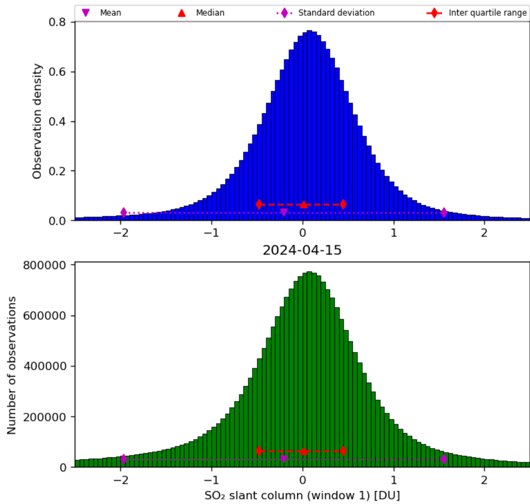
Figure 56: Histogram of “SO 2 slant column (window 1)” for 2024-04-15 to 2024-04-16
