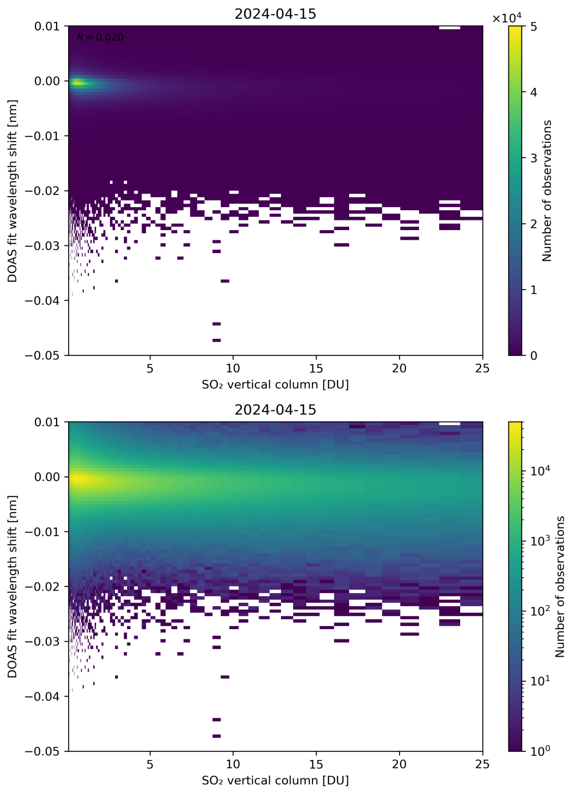
Figure 276: Scatter density plot of “SO 2 vertical column” against “DOAS fit wavelength shift” for 2024-04-15 to 2024-04-16.
