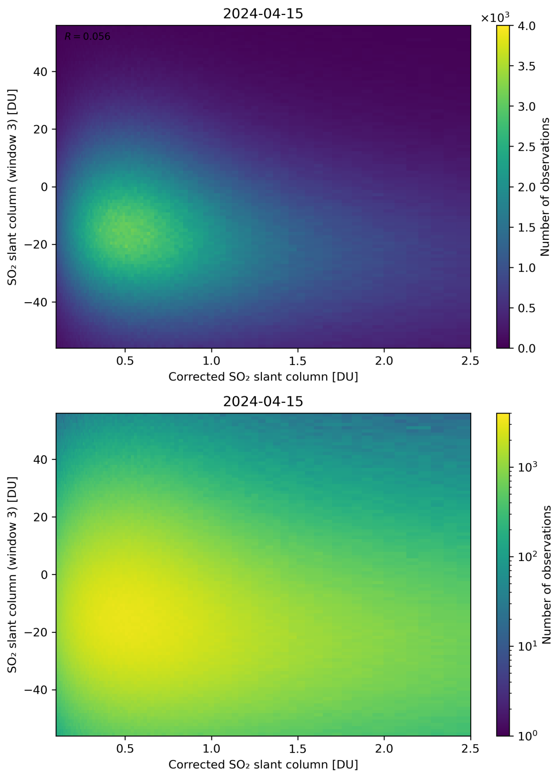
Figure 190: Scatter density plot of “Corrected SO 2 slant column” against “SO 2 slant column (window 3)” for 2024-04-15 to 2024-04-16.
