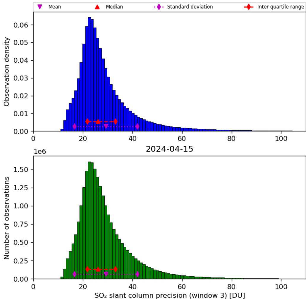
Figure 65: Histogram of “SO 2 slant column precision (window 3)” for 2024-04-15 to 2024-04-16
