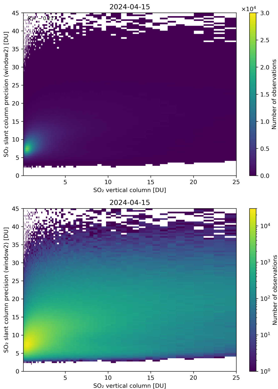
Figure 302: Scatter density plot of “SO 2 vertical column” against “SO 2 slant column precision (window2)” for 2024-04-15 to 2024-04-16.
