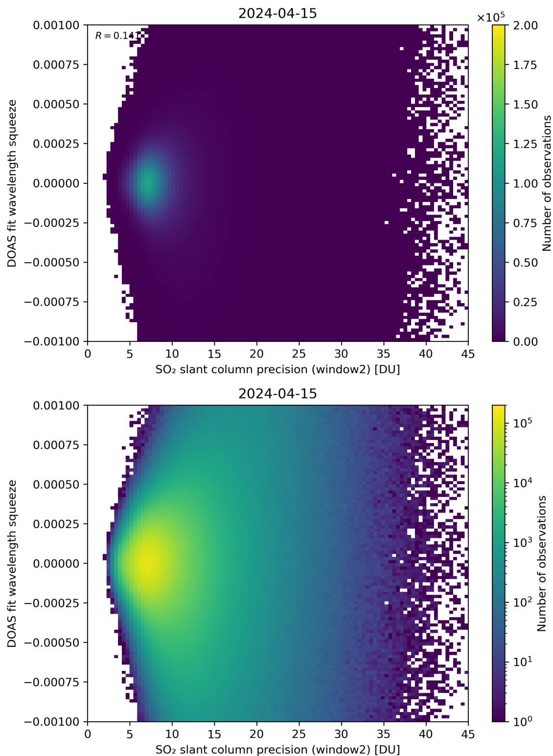
Figure 244: Scatter density plot of “SO 2 slant column precision (window2)” against “DOAS fit wavelength squeeze” for 2024-04-15 to 2024-04-16.
