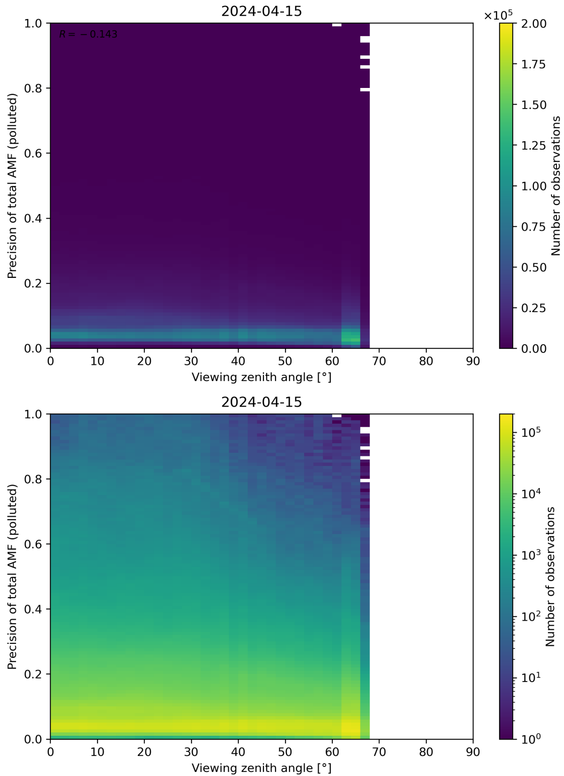
Figure 326: Scatter density plot of “Viewing zenith angle” against “Precision of total AMF (polluted)” for 2024-04-15 to 2024-04-16.
