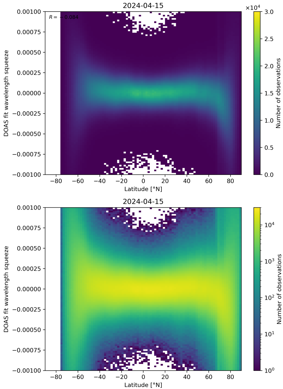
Figure 143: Scatter density plot of “Latitude” against “DOAS fit wavelength squeeze” for 2024-04-15 to 2024-04-16.
