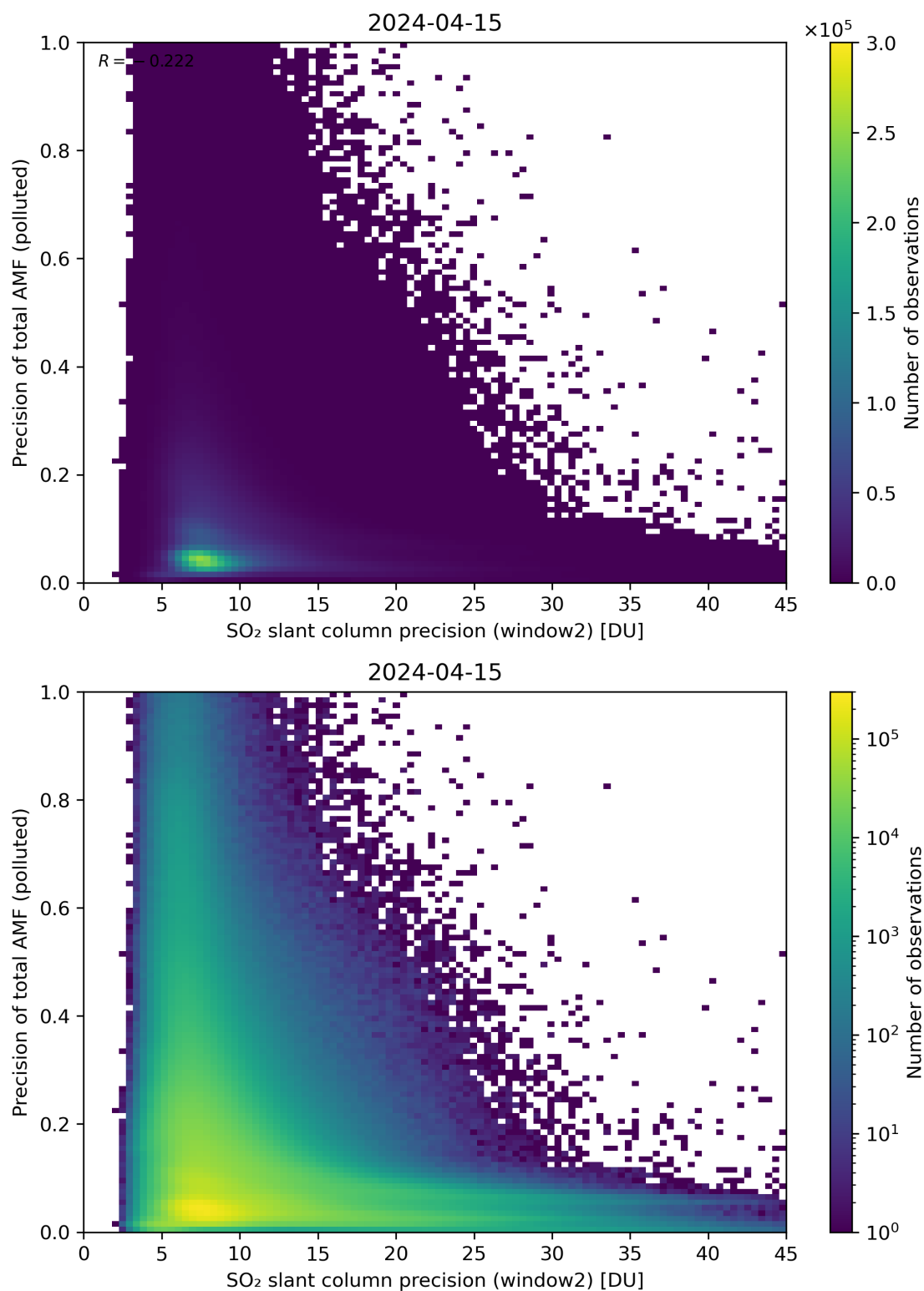
Figure 252: Scatter density plot of “SO 2 slant column precision (window2)” against “Precision of total AMF (polluted)” for 2024-04-15 to 2024-04-16.
