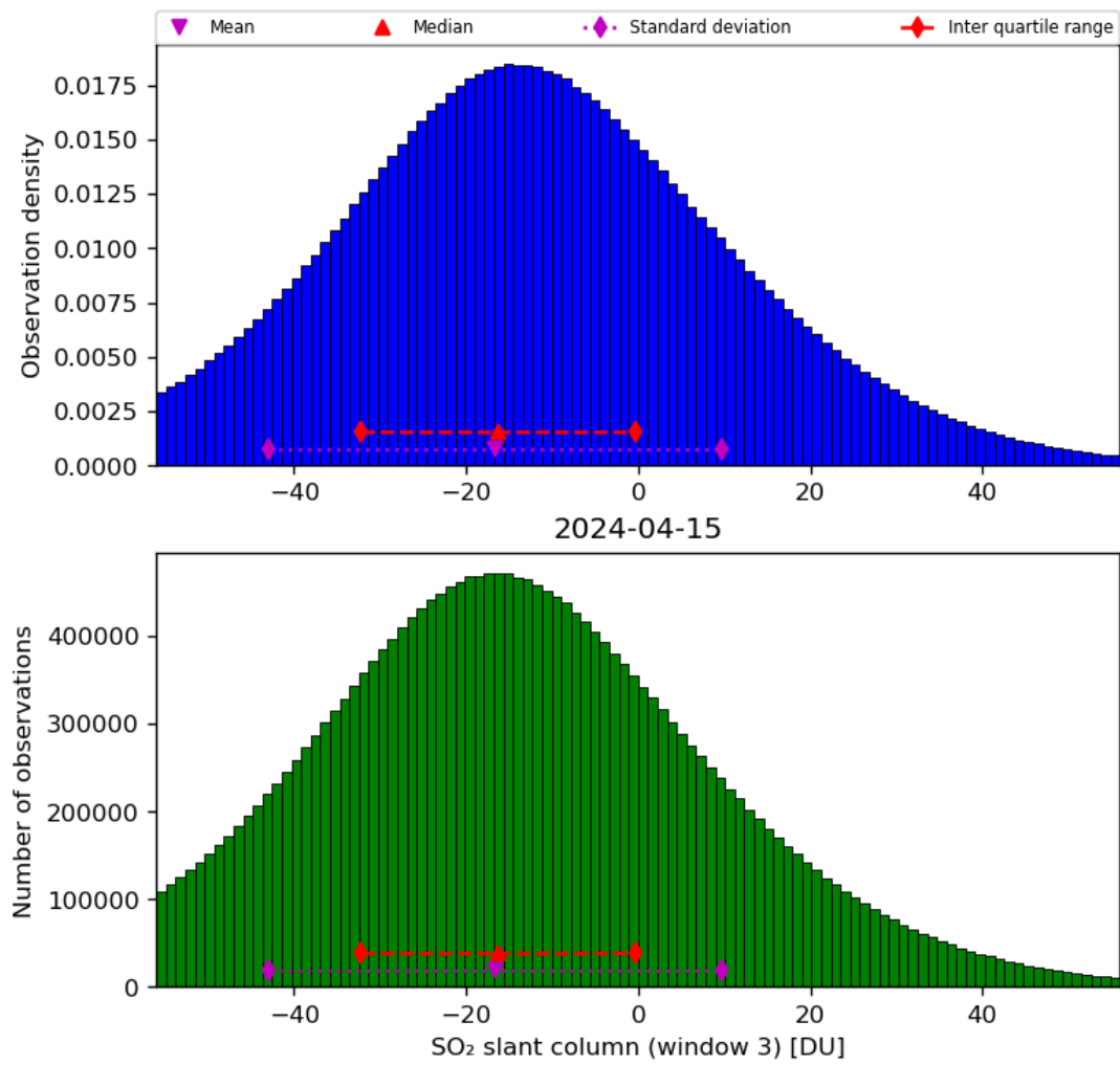
Figure 64: Histogram of “SO 2 slant column (window 3)” for 2024-04-15 to 2024-04-16
