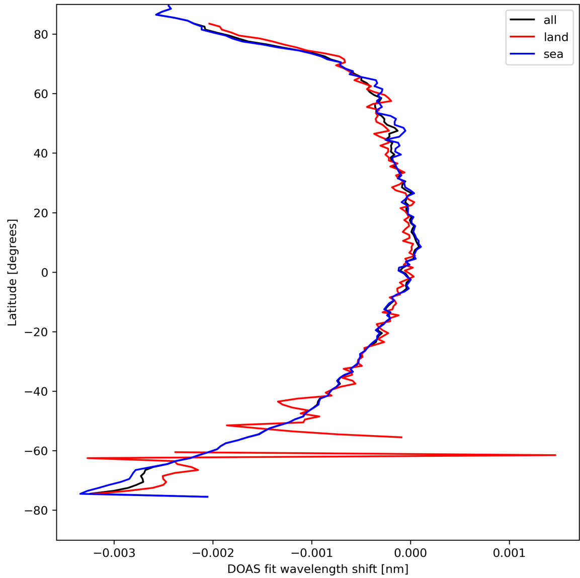
Figure 45: Zonal average of “DOAS fit wavelength shift” for 2024-04-15 to 2024-04-16.
