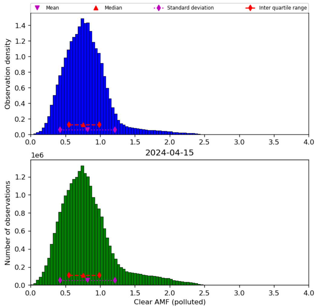
Figure 73: Histogram of “Clear AMF (polluted)” for 2024-04-15 to 2024-04-16
