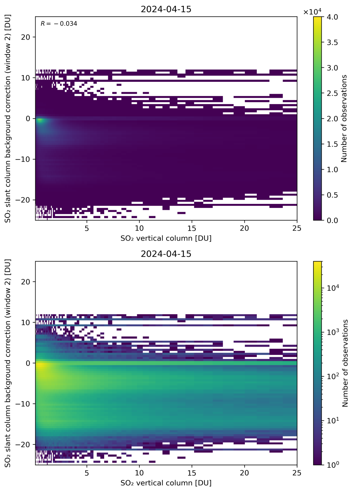
Figure 274: Scatter density plot of “SO 2 vertical column” against “SO 2 slant column background correction (window 2)” for 2024-04-15 to 2024-04-16.
