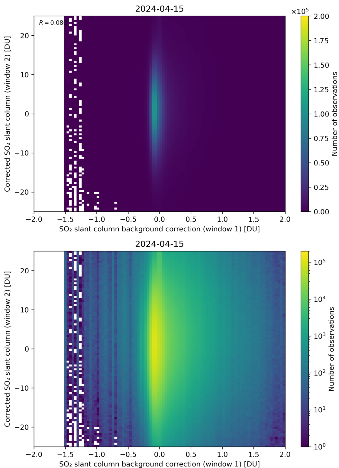
Figure 104: Scatter density plot of “SO 2 slant column background correction (window 1)” against “Corrected SO 2 slant column (window 2)” for 2024-04-15 to 2024-04-16.
