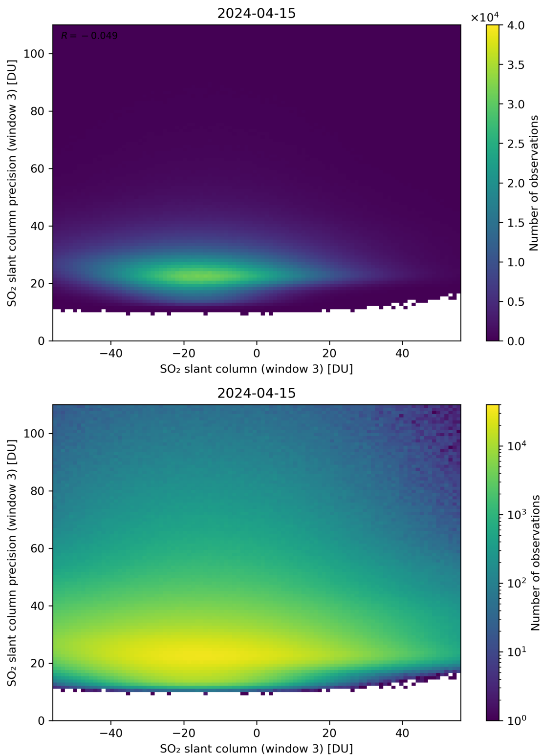
Figure 267: Scatter density plot of “SO 2 slant column (window 3)” against “SO 2 slant column precision (window 3)” for 2024-04-15 to 2024-04-16.
