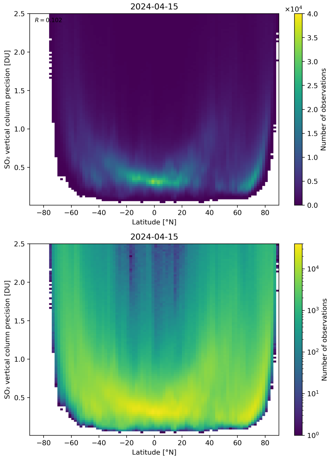
Figure 157: Scatter density plot of “Latitude” against “SO 2 vertical column precision” for 2024-04-15 to 2024-04-16.
