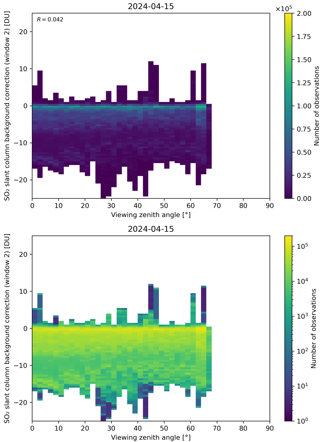
Figure 309: Scatter density plot of “Viewing zenith angle” against “SO 2 slant column background correction (window 2)” for 2024-04-15 to 2024-04-16.
