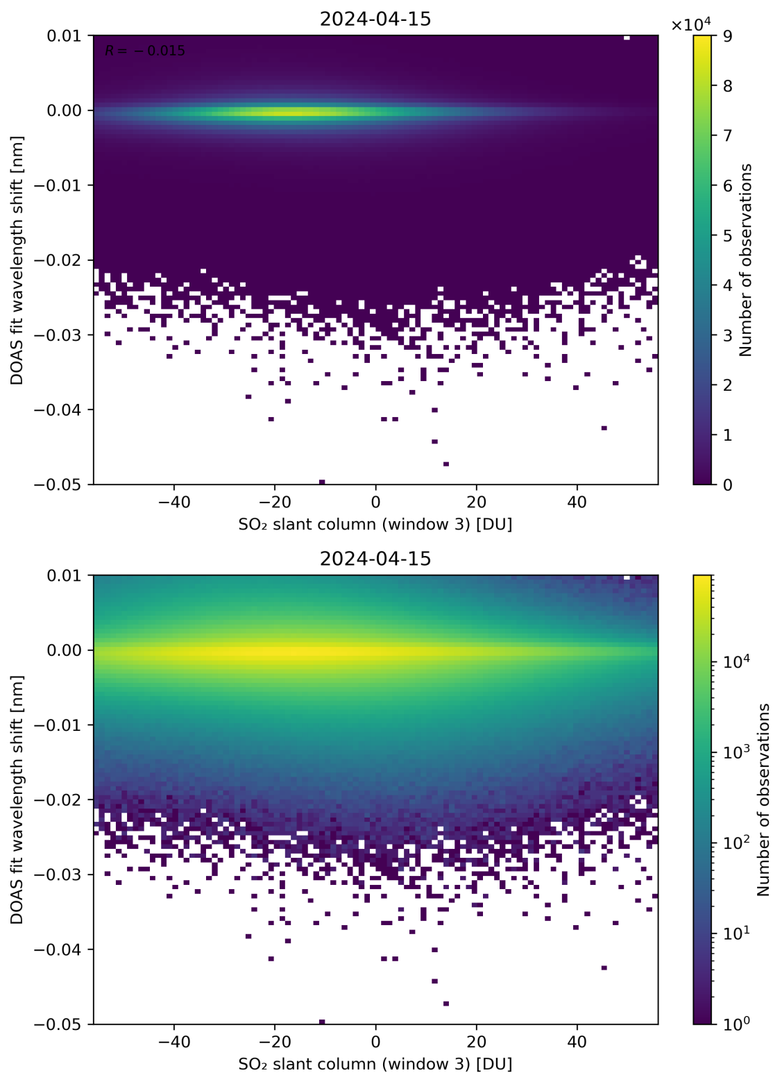
Figure 254: Scatter density plot of “SO 2 slant column (window 3)” against “DOAS fit wavelength shift” for 2024-04-15 to 2024-04-16.
