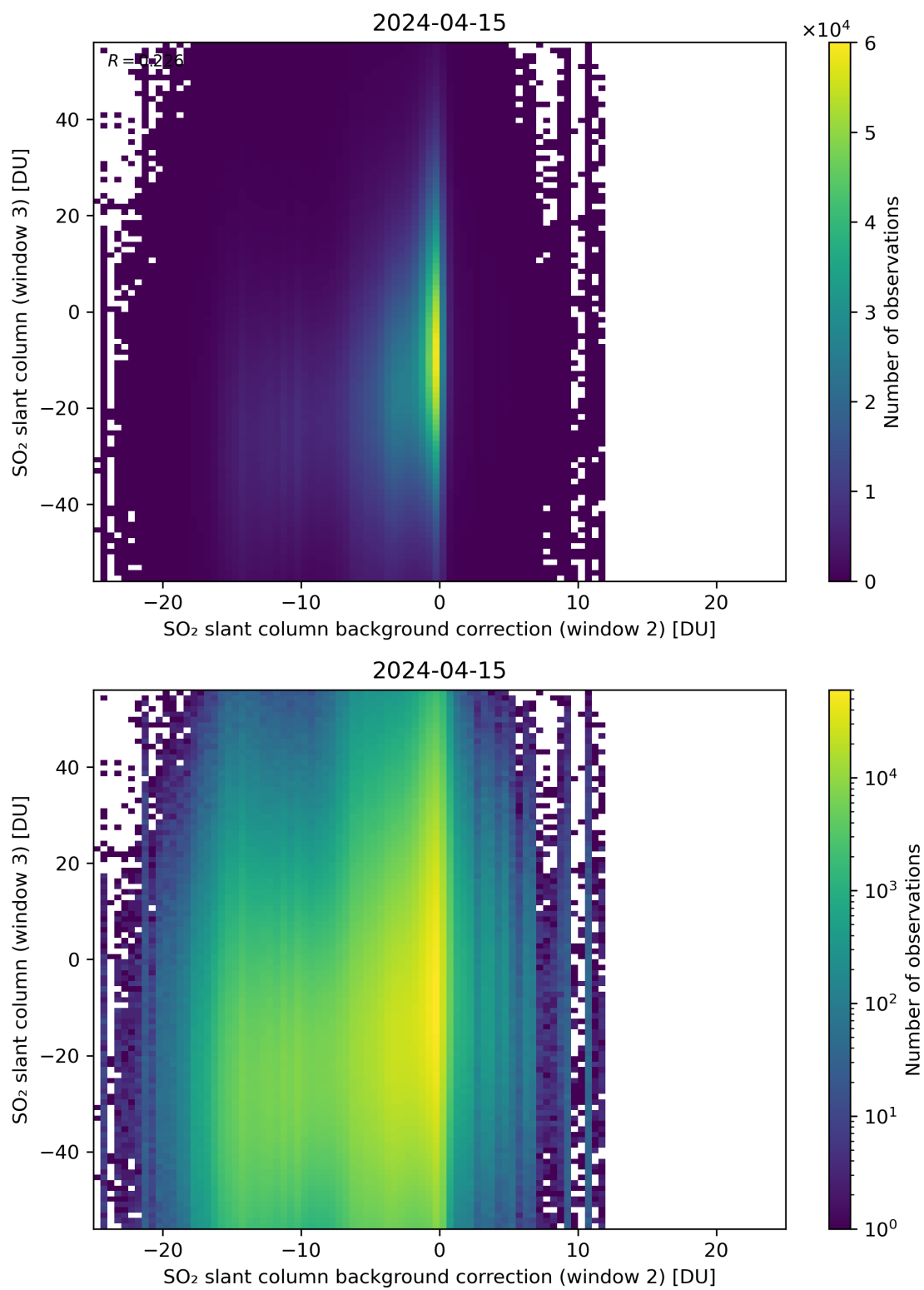
Figure 117: Scatter density plot of “SO 2 slant column background correction (window 2)” against “SO 2 slant column (window 3)” for 2024-04-15 to 2024-04-16.
