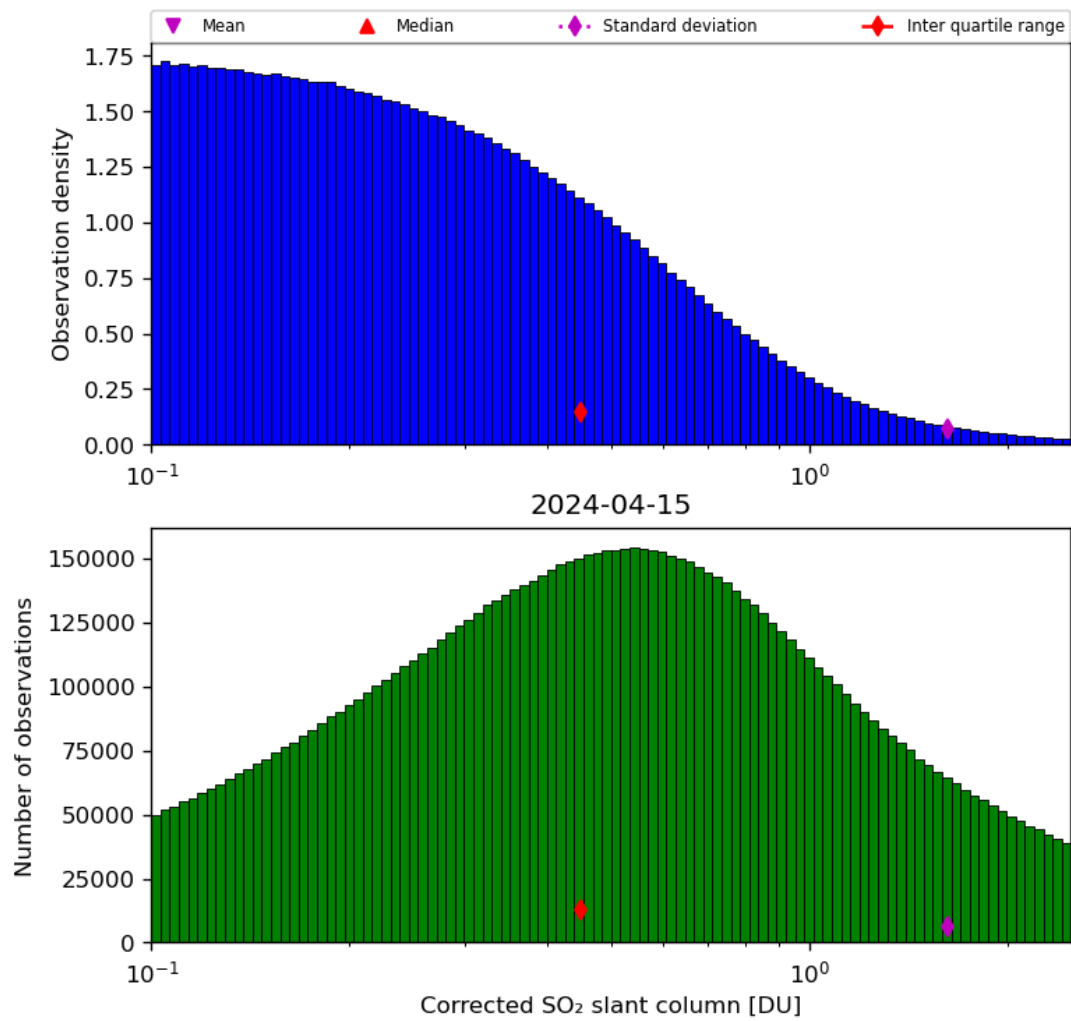
Figure 55: Histogram of “Corrected SO 2 slant column” for 2024-04-15 to 2024-04-16
