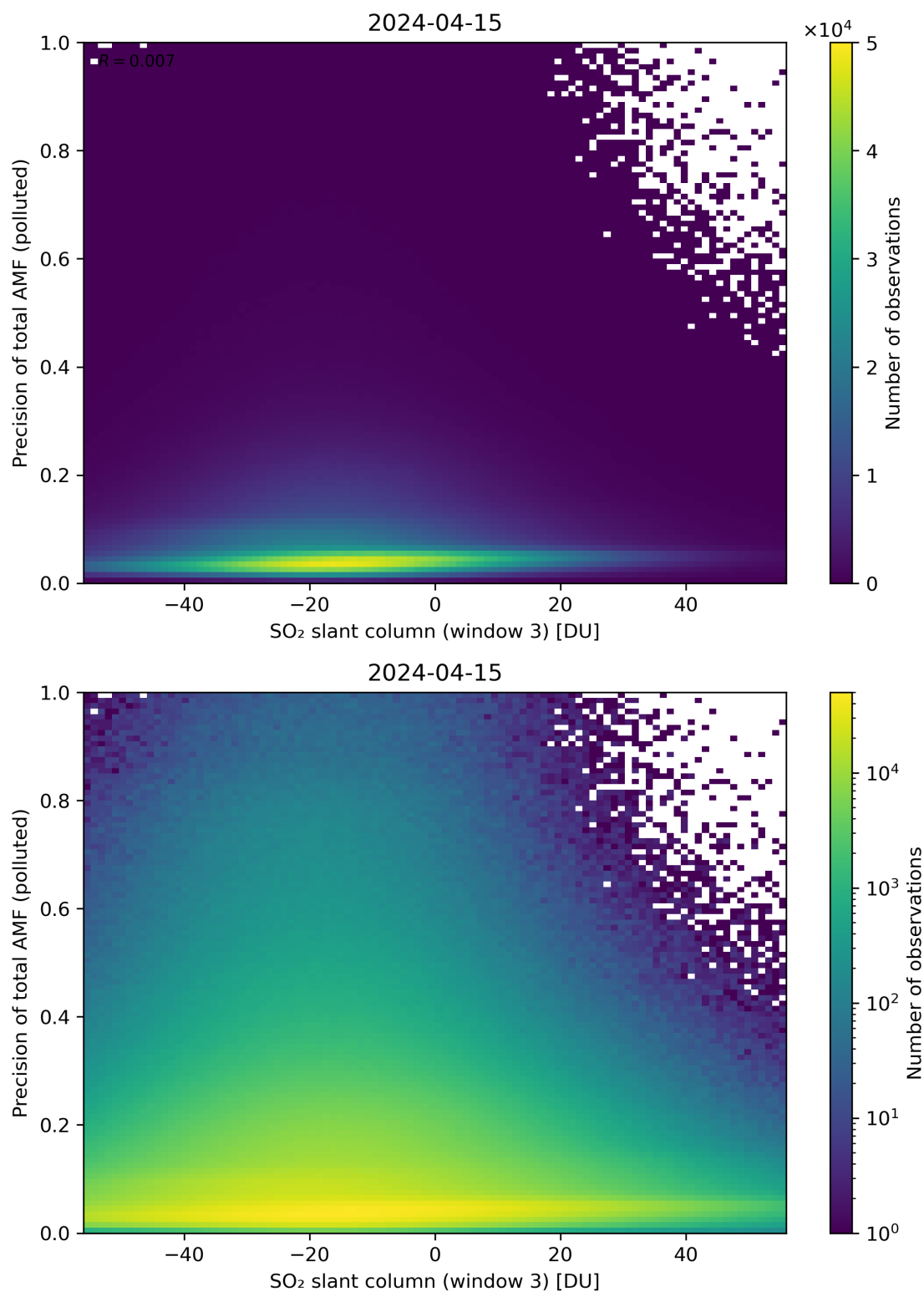
Figure 269: Scatter density plot of “SO 2 slant column (window 3)” against “Precision of total AMF (polluted)” for 2024-04-15 to 2024-04-16.
