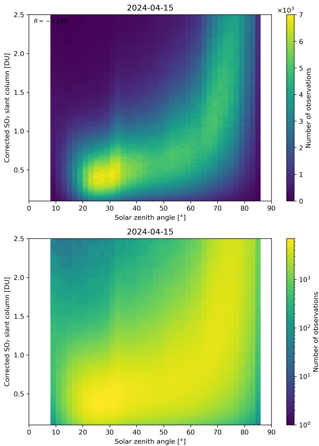
Figure 166: Scatter density plot of “Solar zenith angle” against “Corrected SO 2 slant column” for 2024-04-15 to 2024-04-16.
