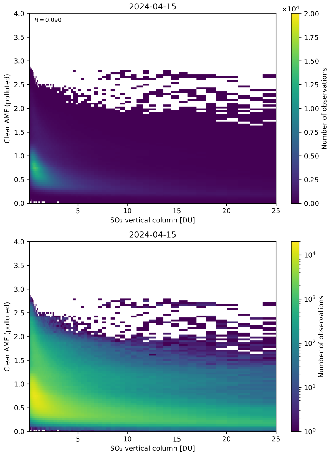
Figure 296: Scatter density plot of “SO 2 vertical column” against “Clear AMF (polluted)” for 2024-04-15 to 2024-04-16.
