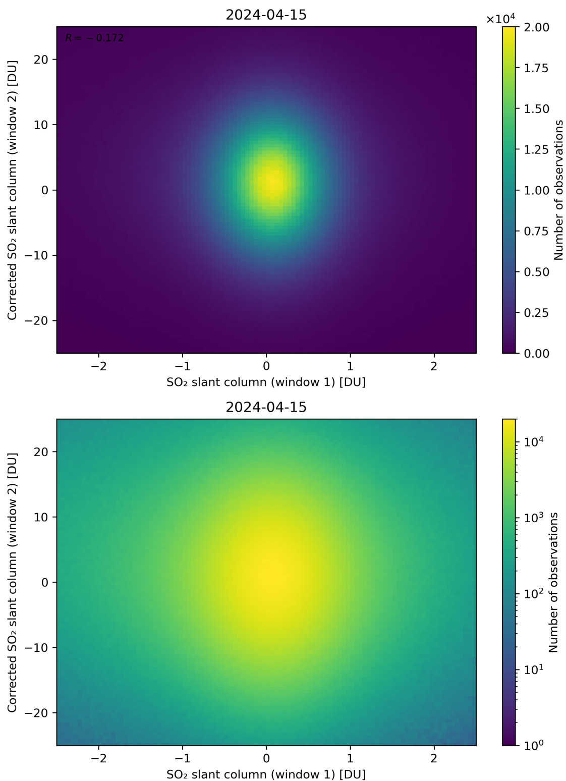
Figure 233: Scatter density plot of “SO 2 slant column (window 1)” against “Corrected SO 2 slant column (window 2)” for 2024-04-15 to 2024-04-16.
