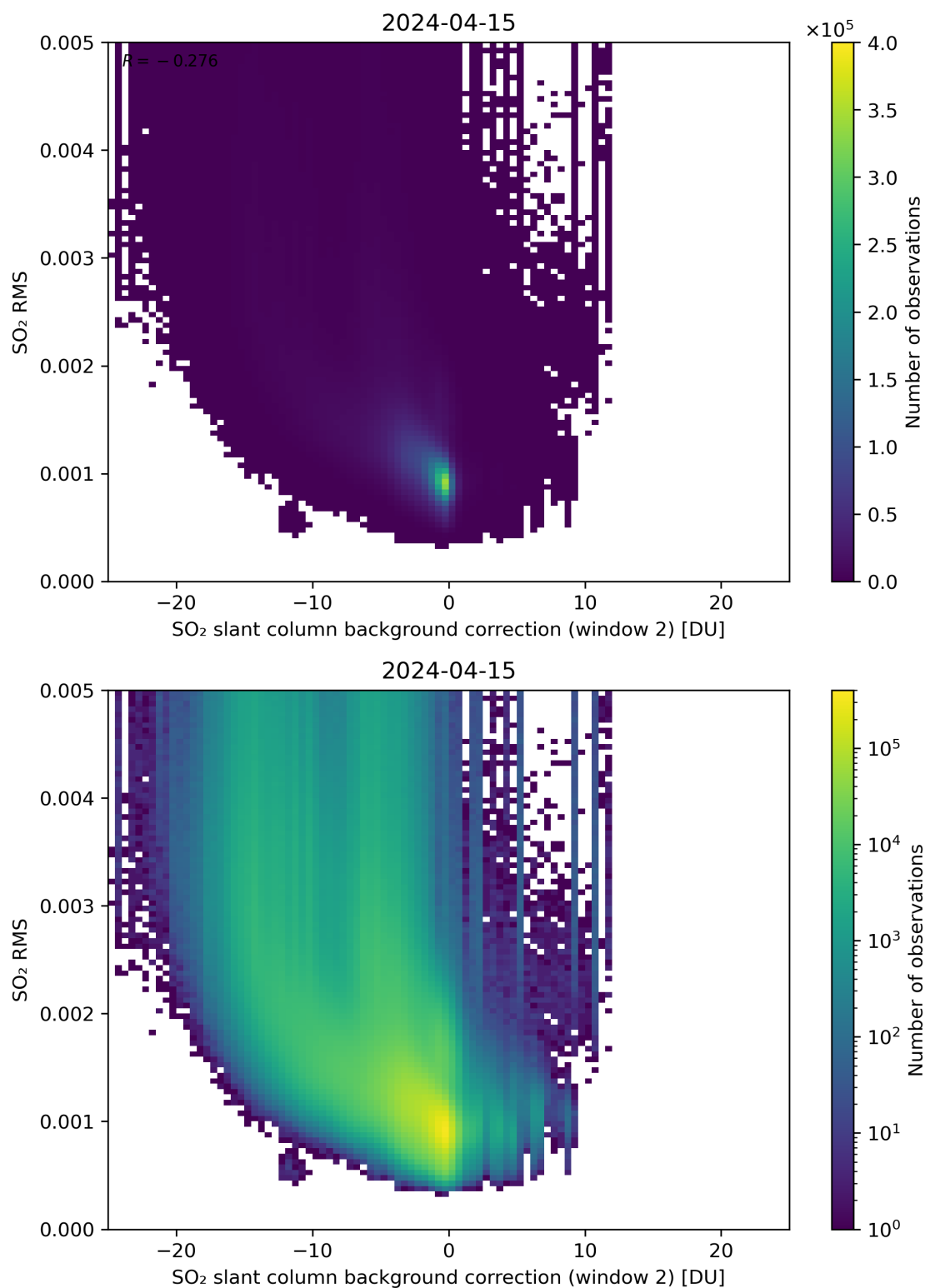
Figure 114: Scatter density plot of “SO 2 slant column background correction (window 2)” against “SO 2 RMS” for 2024-04-15 to 2024-04-16.
