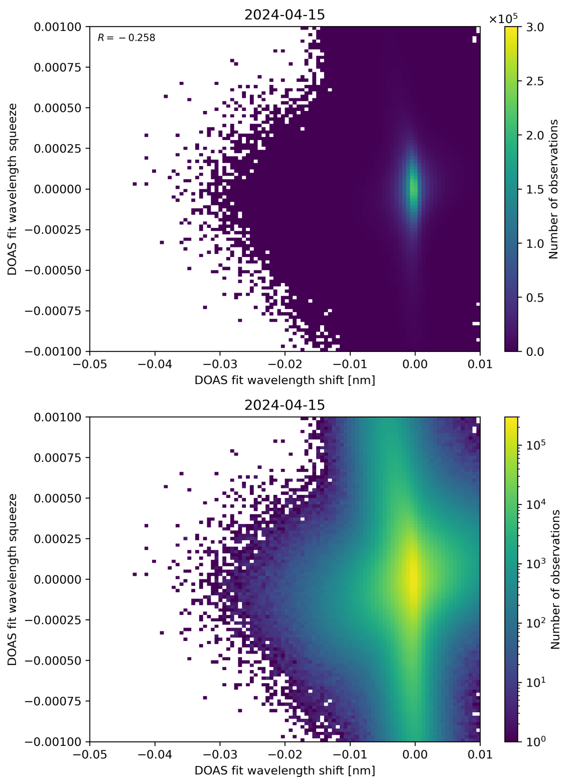
Figure 127: Scatter density plot of “DOAS fit wavelength shift” against “DOAS fit wavelength squeeze” for 2024-04-15 to 2024-04-16.
