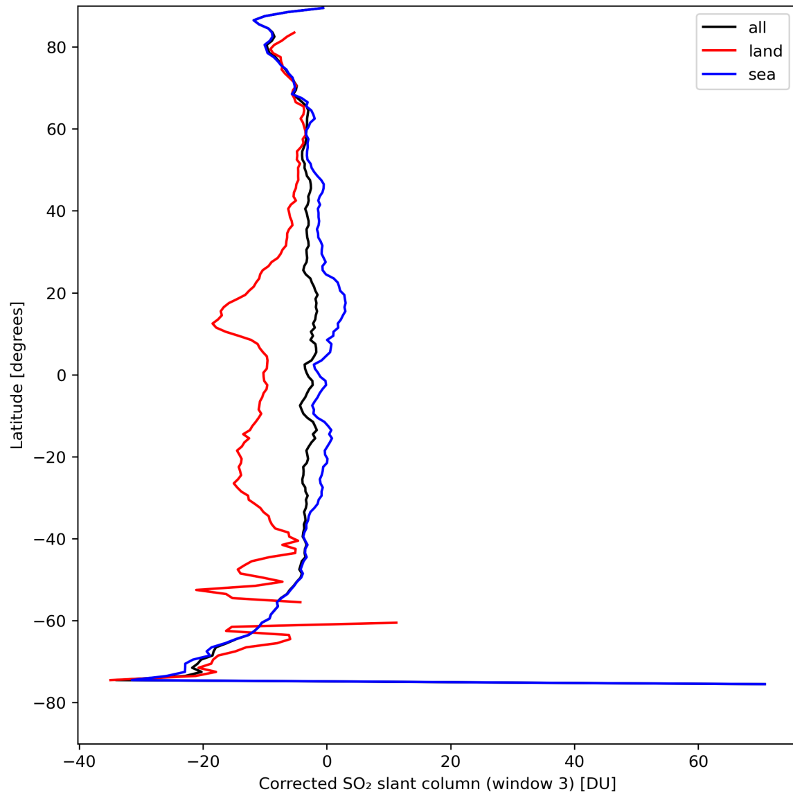
Figure 43: Zonal average of “Corrected SO 2 slant column (window 3)” for 2024-04-15 to 2024-04-16.
