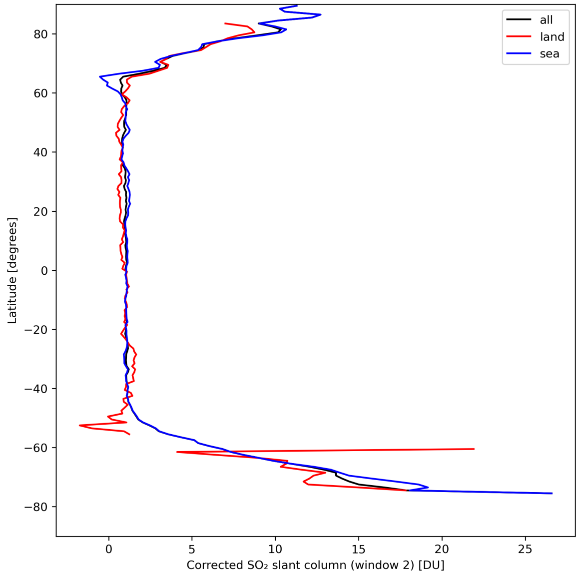
Figure 39: Zonal average of “Corrected SO 2 slant column (window 2)” for 2024-04-15 to 2024-04-16.
