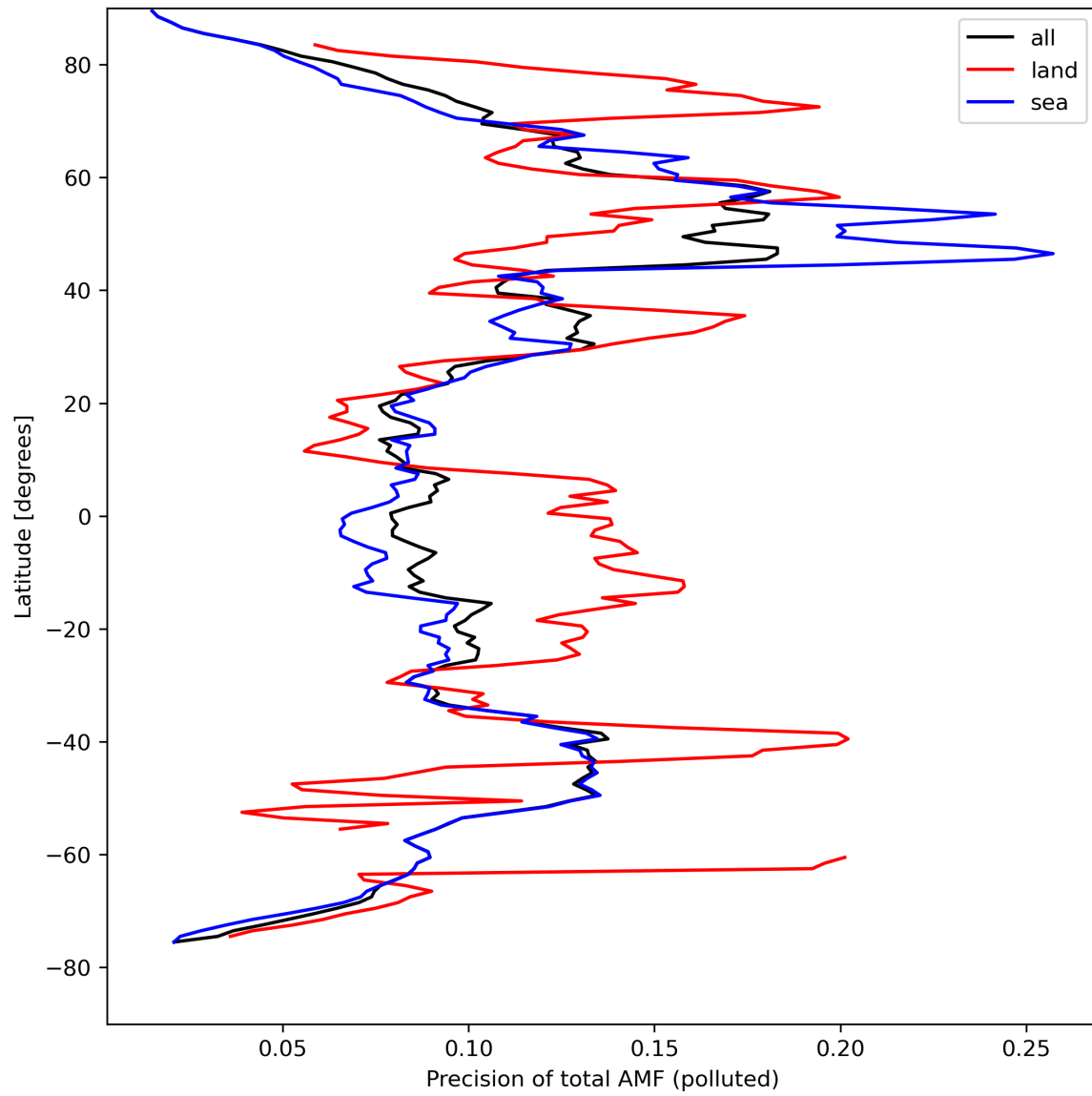
Figure 49: Zonal average of “Precision of total AMF (polluted)” for 2024-04-15 to 2024-04-16.
