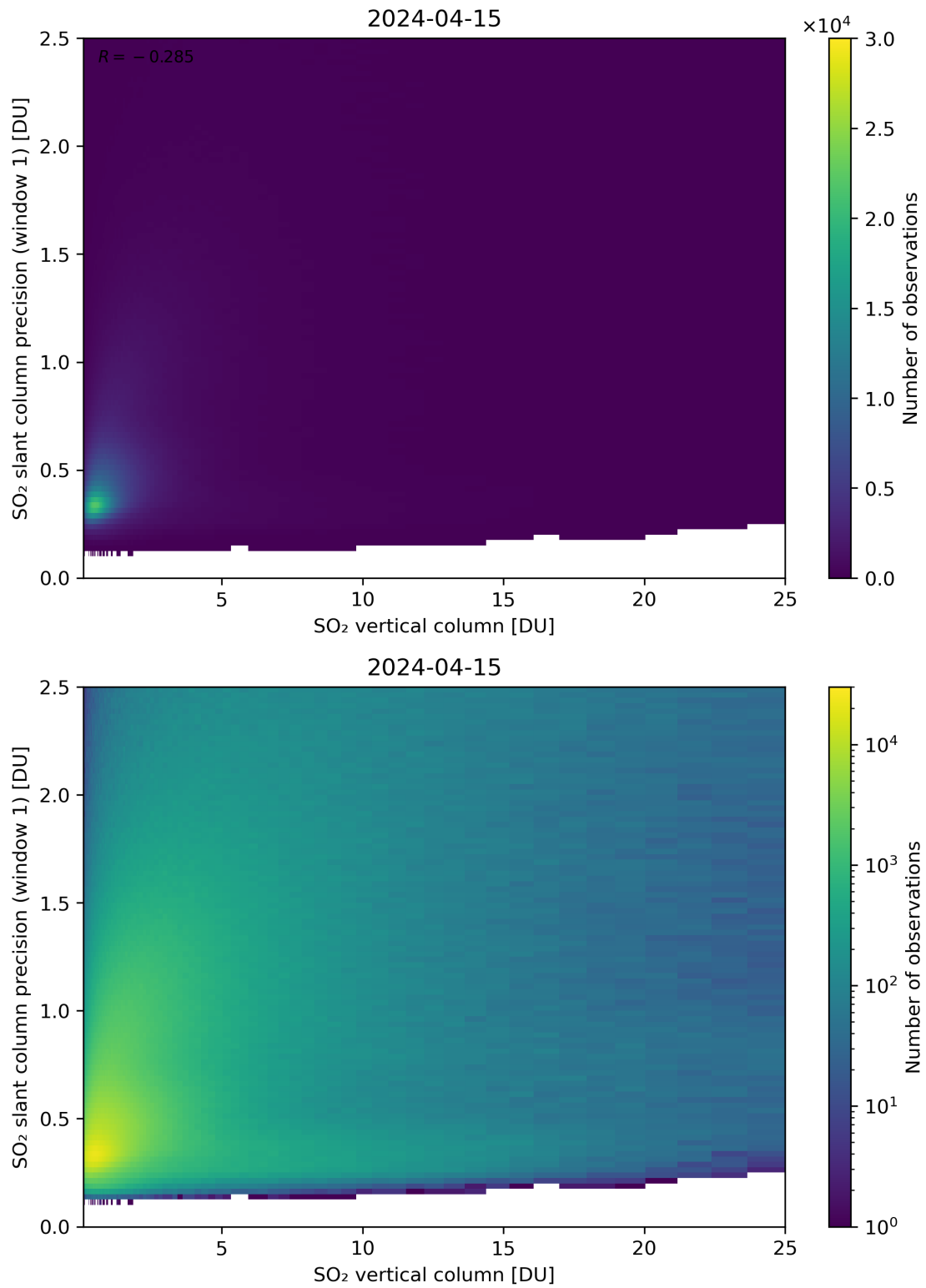
Figure 301: Scatter density plot of “SO 2 vertical column” against “SO 2 slant column precision (window 1)” for 2024-04-15 to 2024-04-16.
