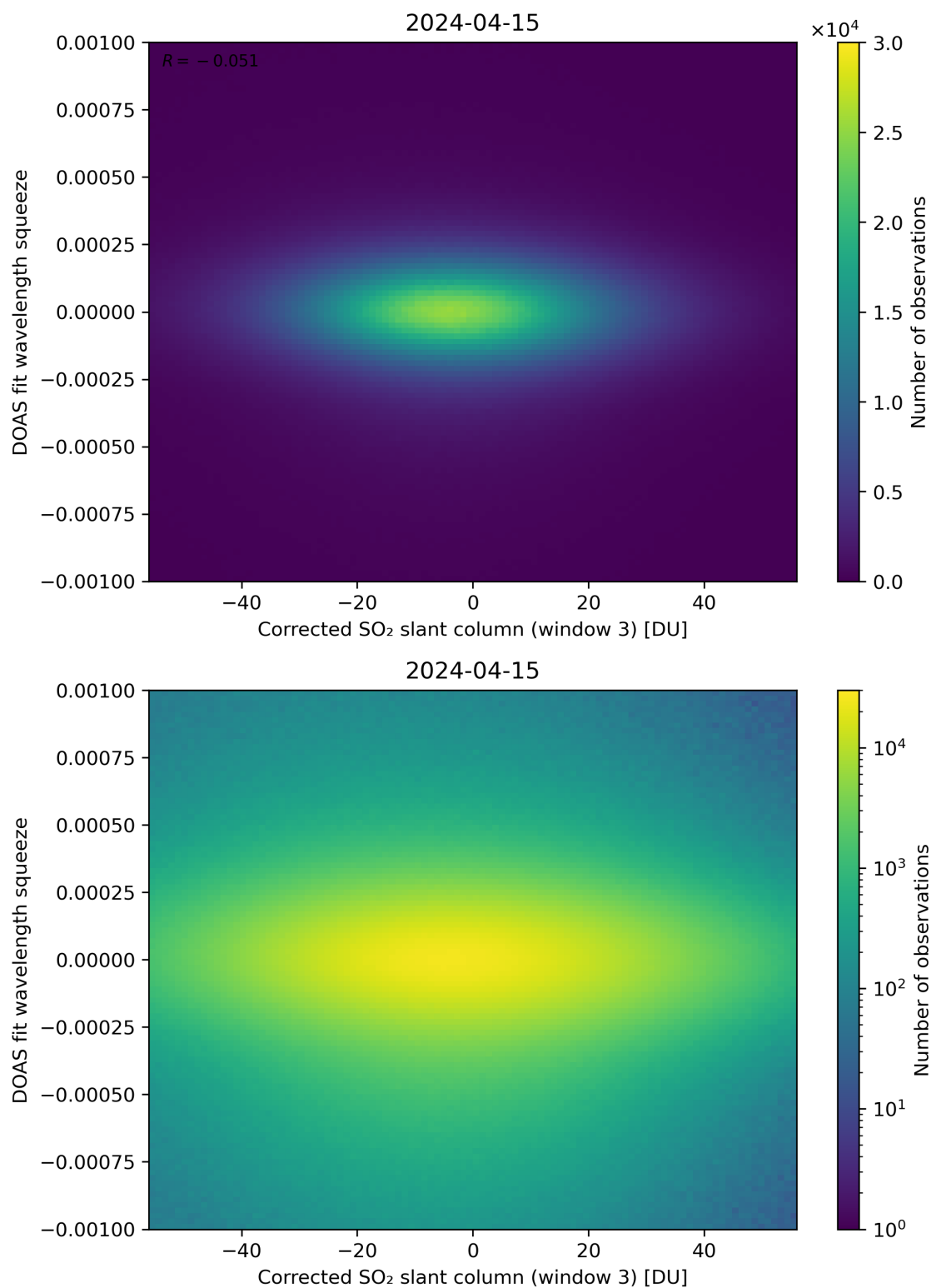
Figure 207: Scatter density plot of “Corrected SO 2 slant column (window 3)” against “DOAS fit wavelength squeeze” for 2024-04-15 to 2024-04-16.
