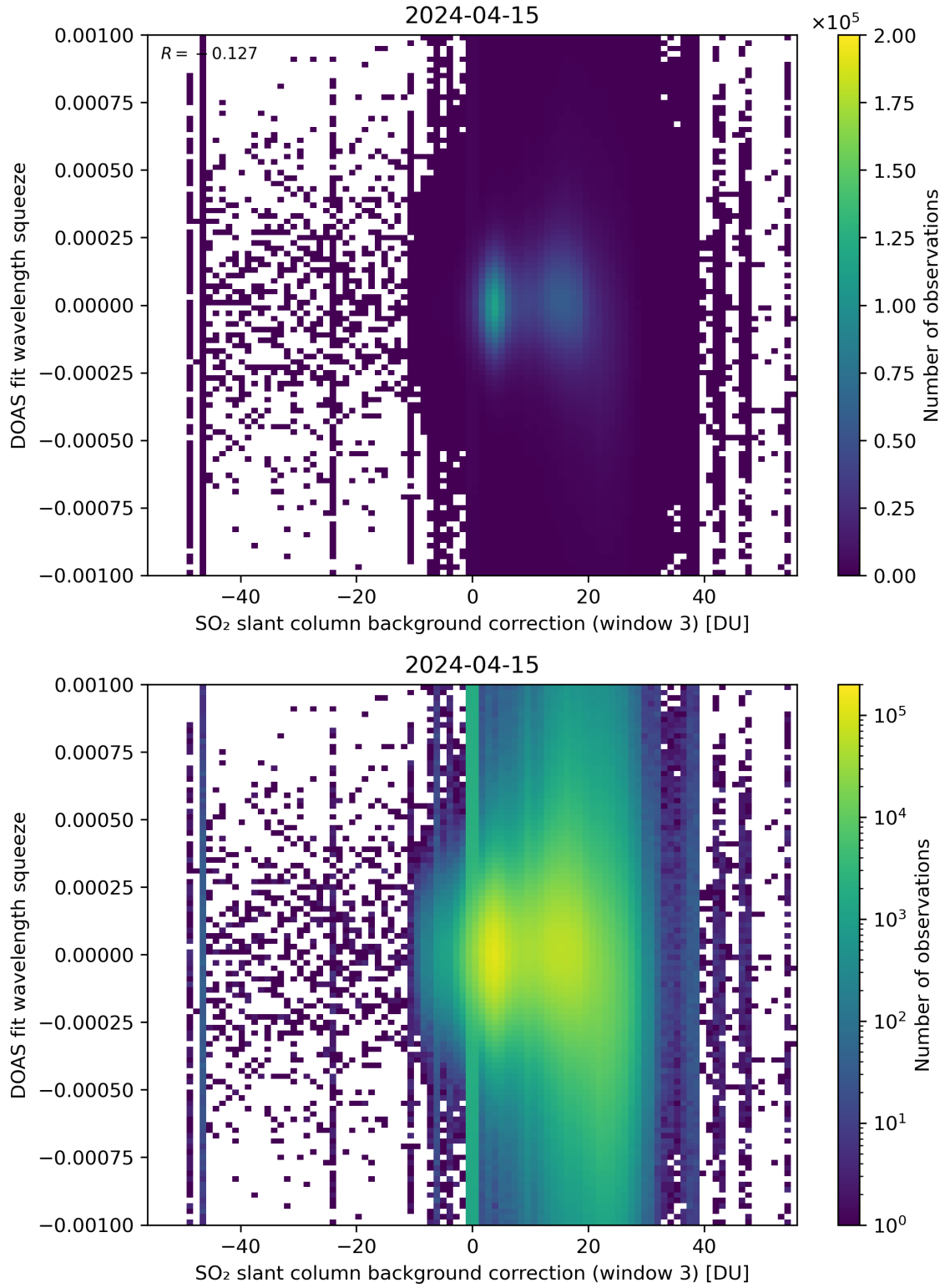
Figure 122: Scatter density plot of “SO 2 slant column background correction (window 3)” against “DOAS fit wavelength squeeze” for 2024-04-15 to 2024-04-16.
