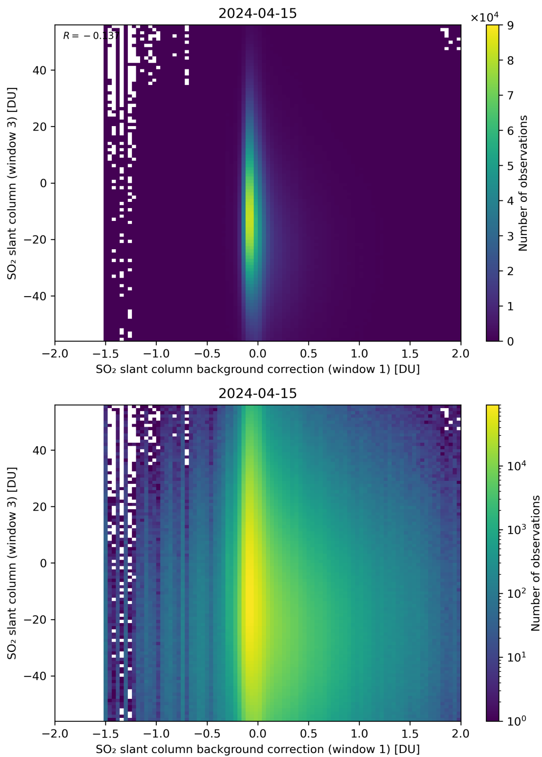
Figure 107: Scatter density plot of “SO 2 slant column background correction (window 1)” against “SO 2 slant column (window 3)” for 2024-04-15 to 2024-04-16.
