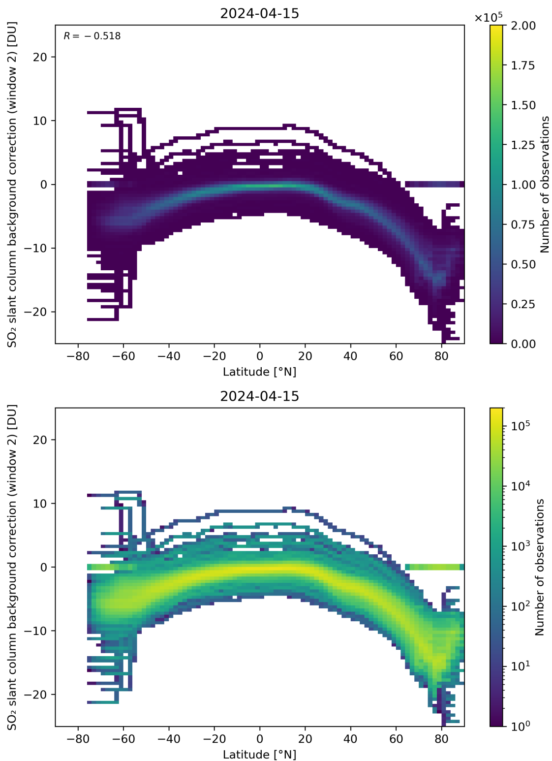
Figure 140: Scatter density plot of “Latitude” against “SO 2 slant column background correction (window 2)” for 2024-04-15 to 2024-04-16.
