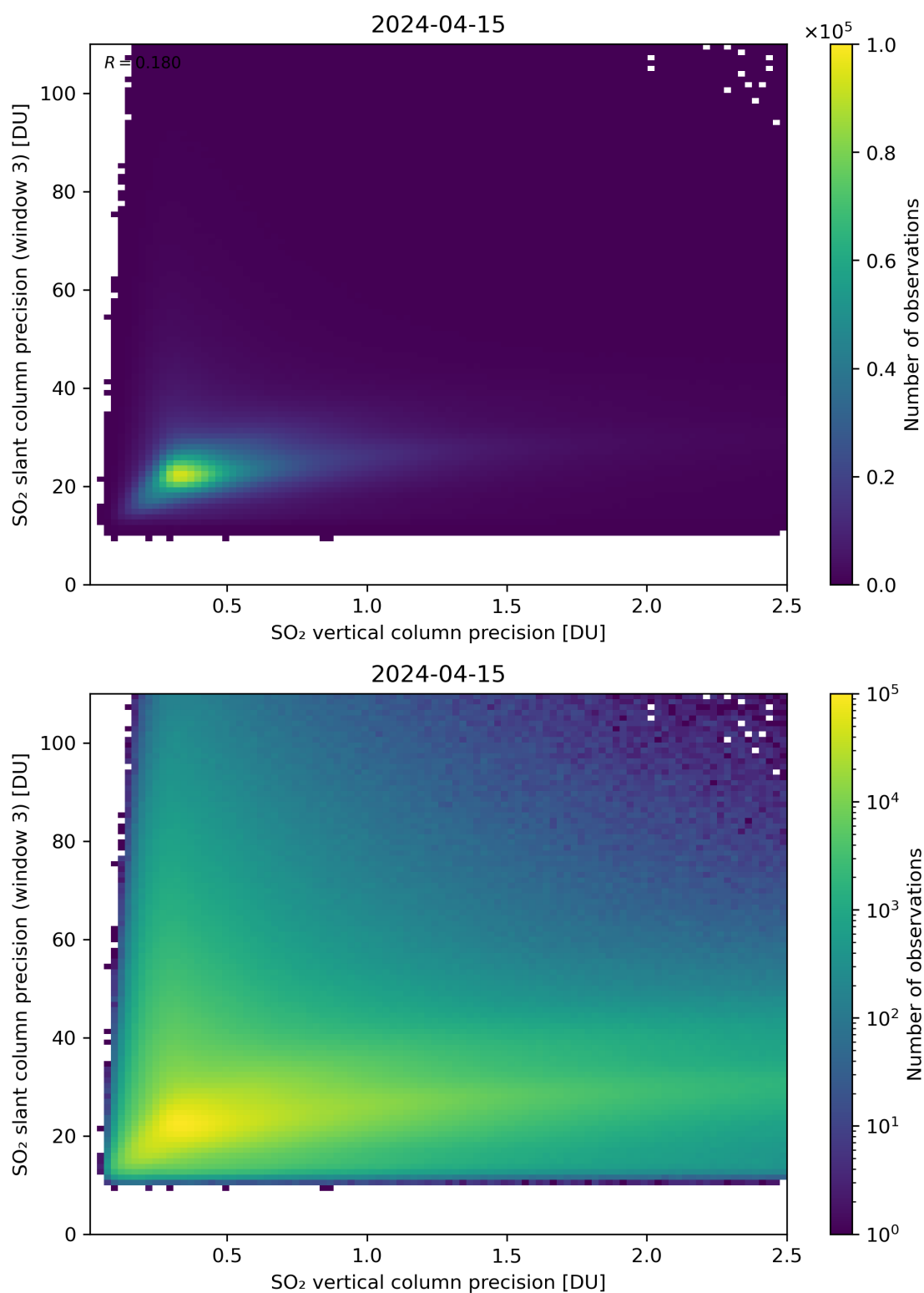
Figure 293: Scatter density plot of “SO 2 vertical column precision” against “SO 2 slant column precision (window 3)” for 2024-04-15 to 2024-04-16.
