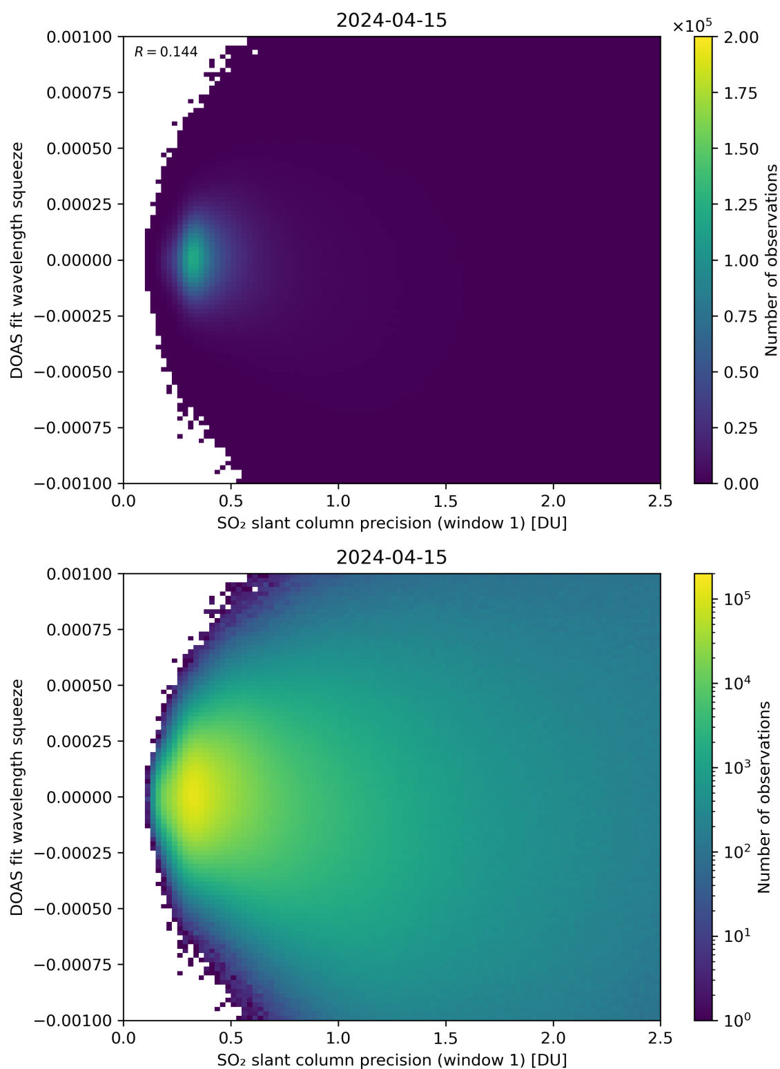
Figure 222: Scatter density plot of “SO 2 slant column precision (window 1)” against “DOAS fit wavelength squeeze” for 2024-04-15 to 2024-04-16.
