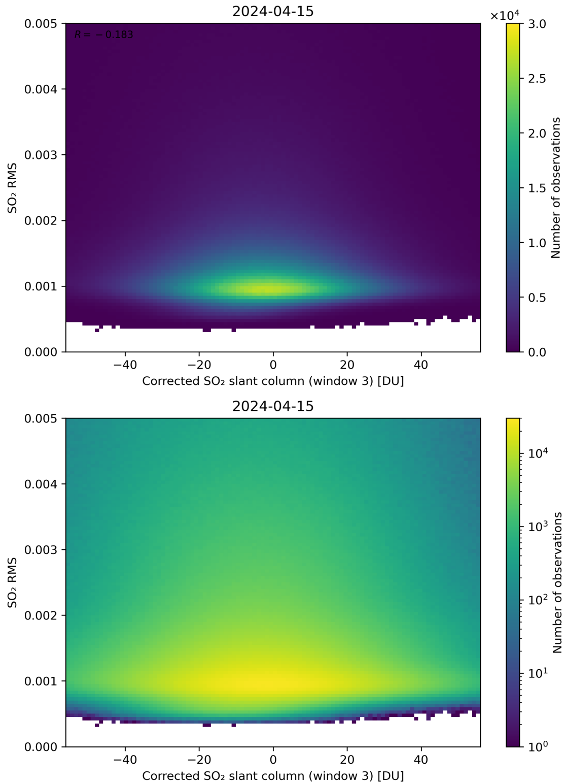
Figure 208: Scatter density plot of “Corrected SO 2 slant column (window 3)” against “SO 2 RMS” for 2024-04-15 to 2024-04-16.
