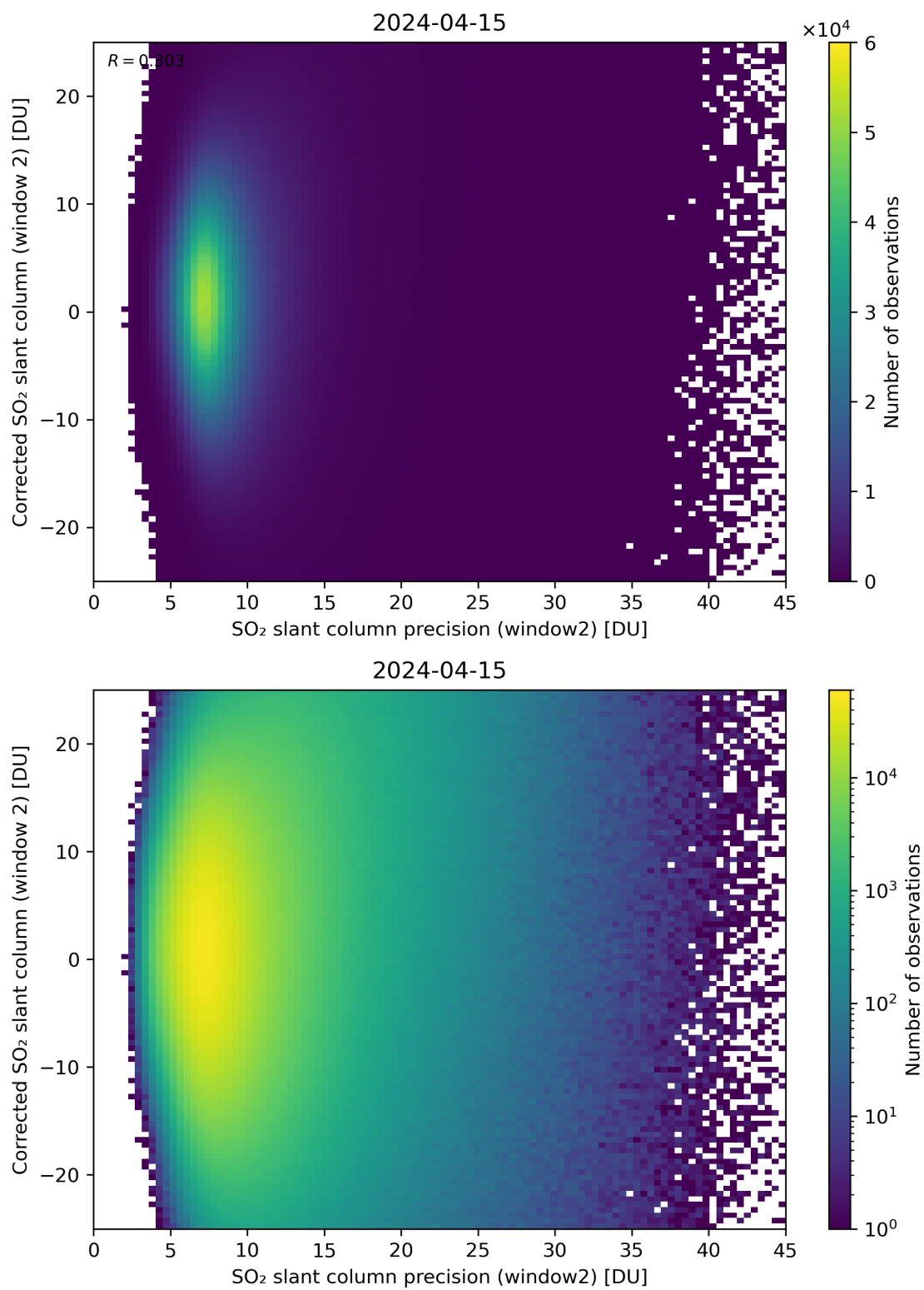
Figure 247: Scatter density plot of “SO 2 slant column precision (window2)” against “Corrected SO 2 slant column (window 2)” for 2024-04-15 to 2024-04-16.
