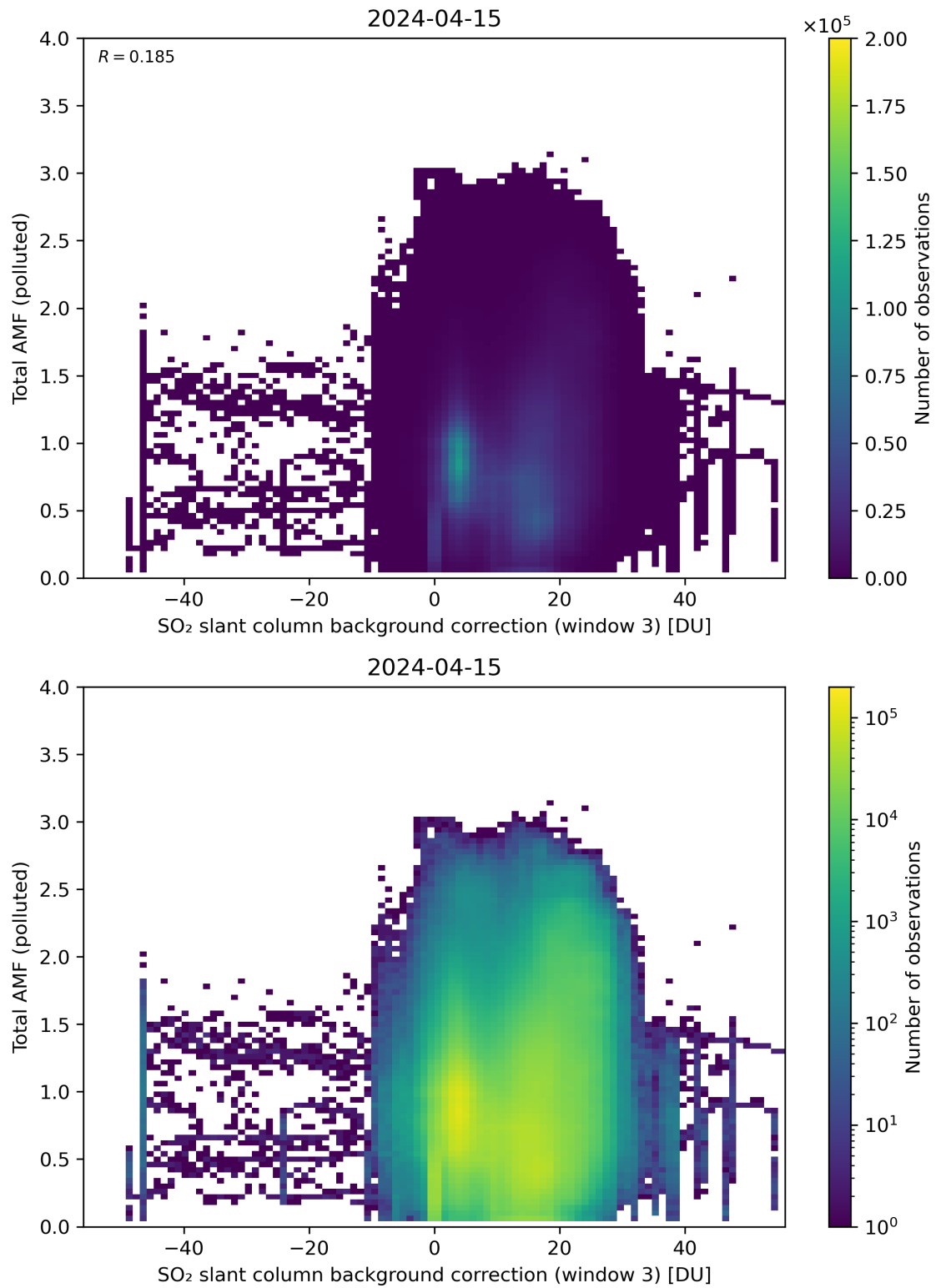
Figure 125: Scatter density plot of “SO 2 slant column background correction (window 3)” against “Total AMF (polluted)” for 2024-04-15 to 2024-04-16.
