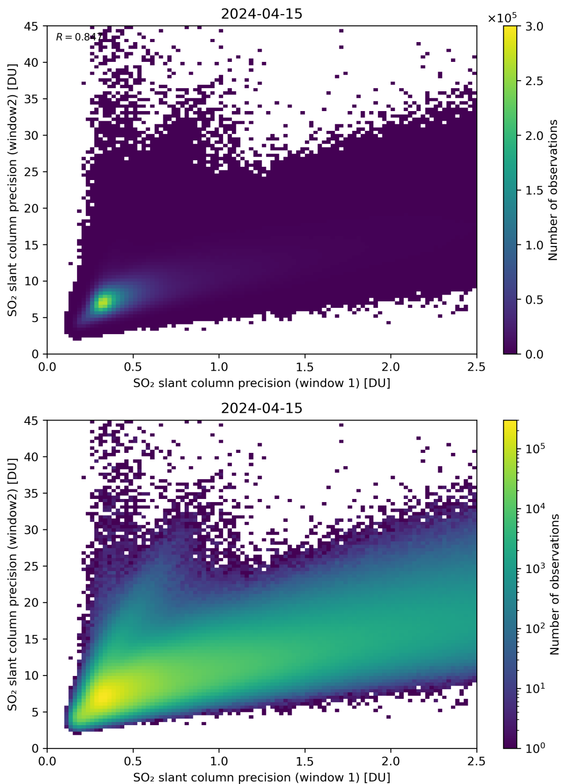
Figure 227: Scatter density plot of “SO 2 slant column precision (window 1)” against “SO 2 slant column precision (window2)” for 2024-04-15 to 2024-04-16.
