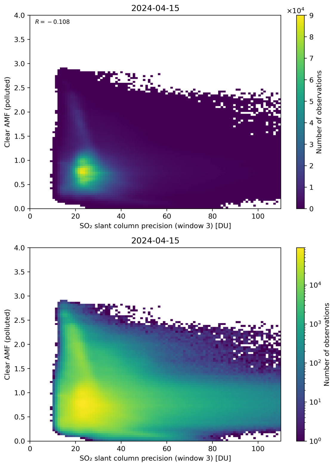
Figure 261: Scatter density plot of “SO 2 slant column precision (window 3)” against “Clear AMF (polluted)” for 2024-04-15 to 2024-04-16.
