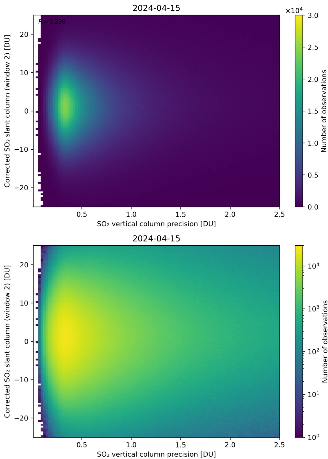
Figure 287: Scatter density plot of “SO 2 vertical column precision” against “Corrected SO 2 slant column (window 2)” for 2024-04-15 to 2024-04-16.
