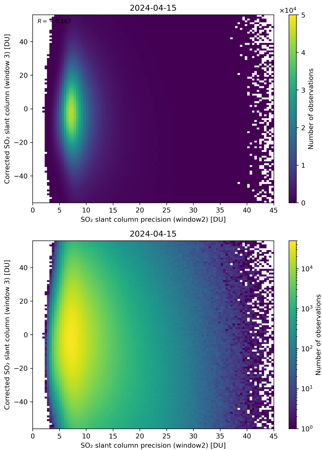
Figure 248: Scatter density plot of “SO 2 slant column precision (window2)” against “Corrected SO 2 slant column (window 3)” for 2024-04-15 to 2024-04-16.
