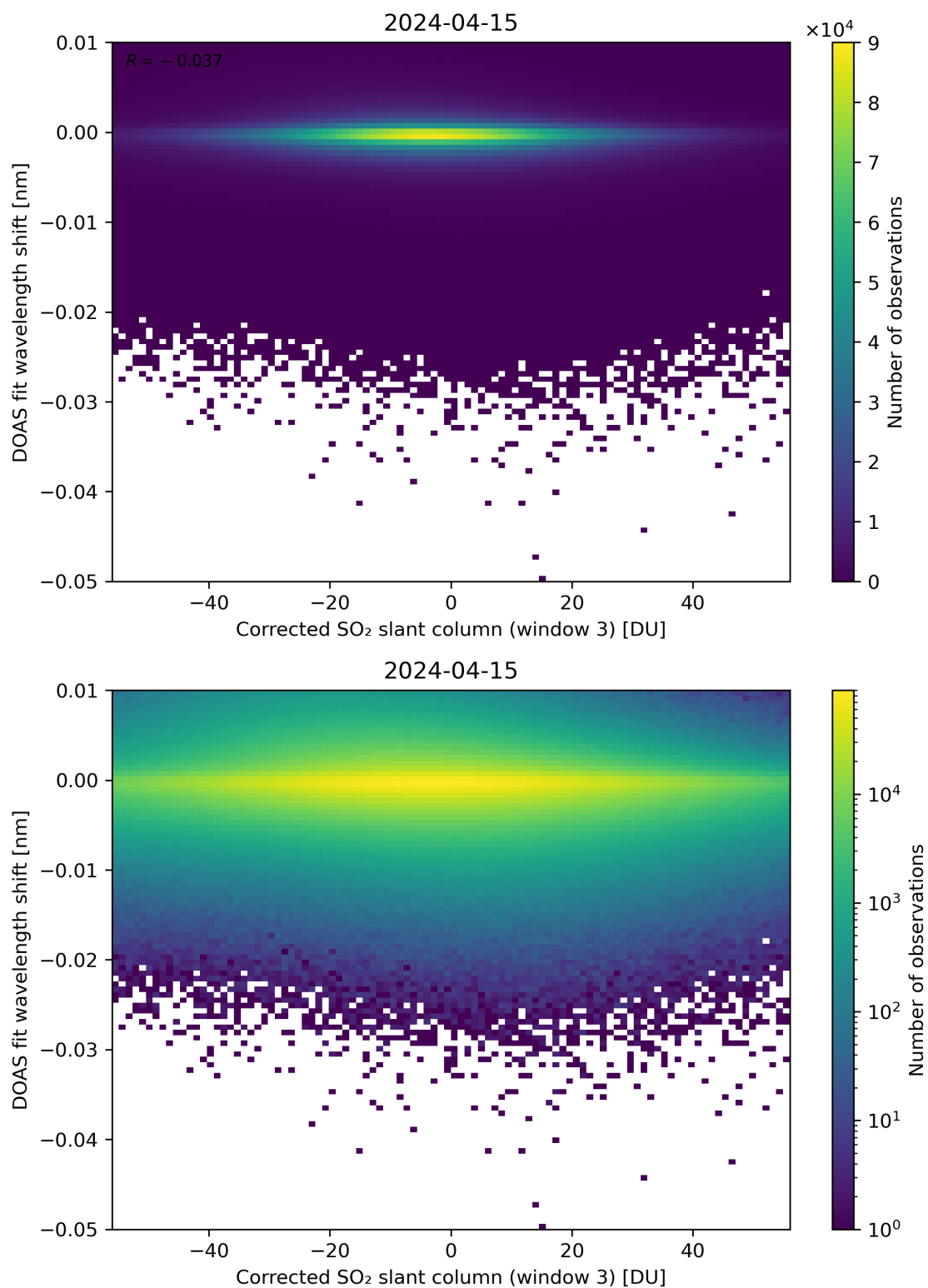
Figure 206: Scatter density plot of “Corrected SO 2 slant column (window 3)” against “DOAS fit wavelength shift” for 2024-04-15 to 2024-04-16.
