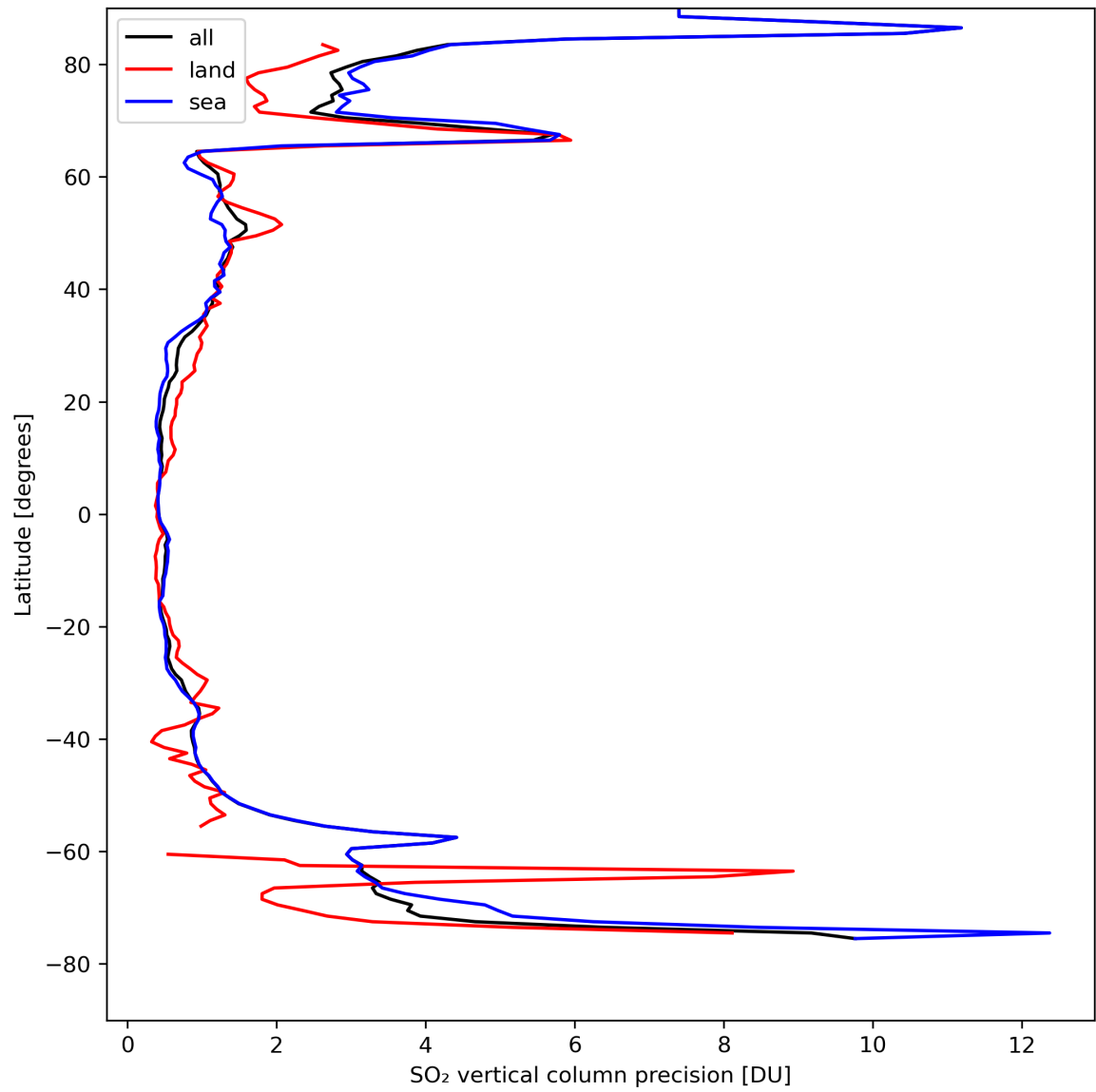
Figure 31: Zonal average of “SO 2 vertical column precision” for 2024-04-15 to 2024-04-16.
