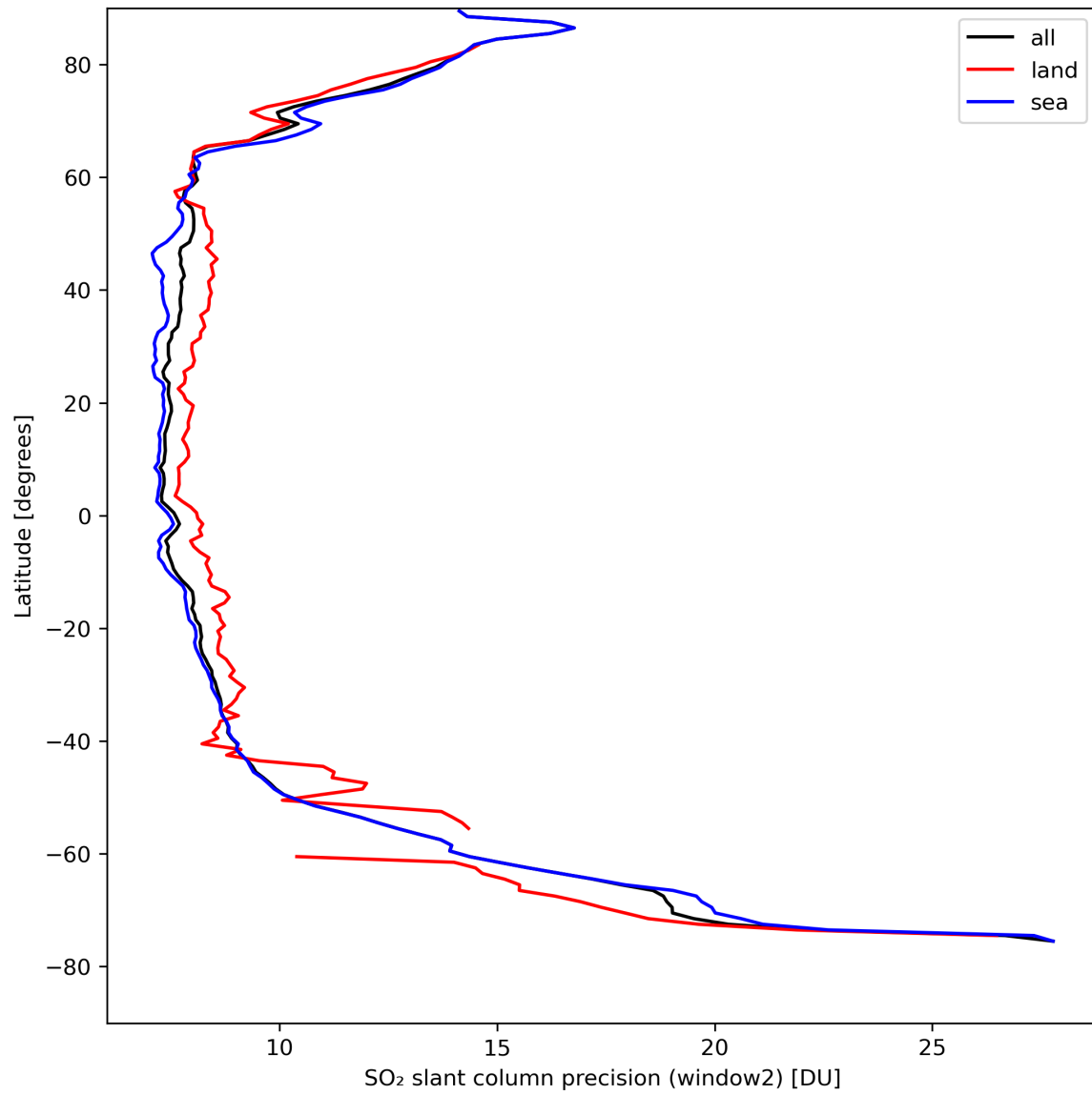
Figure 38: Zonal average of “SO 2 slant column precision (window2)” for 2024-04-15 to 2024-04-16.
