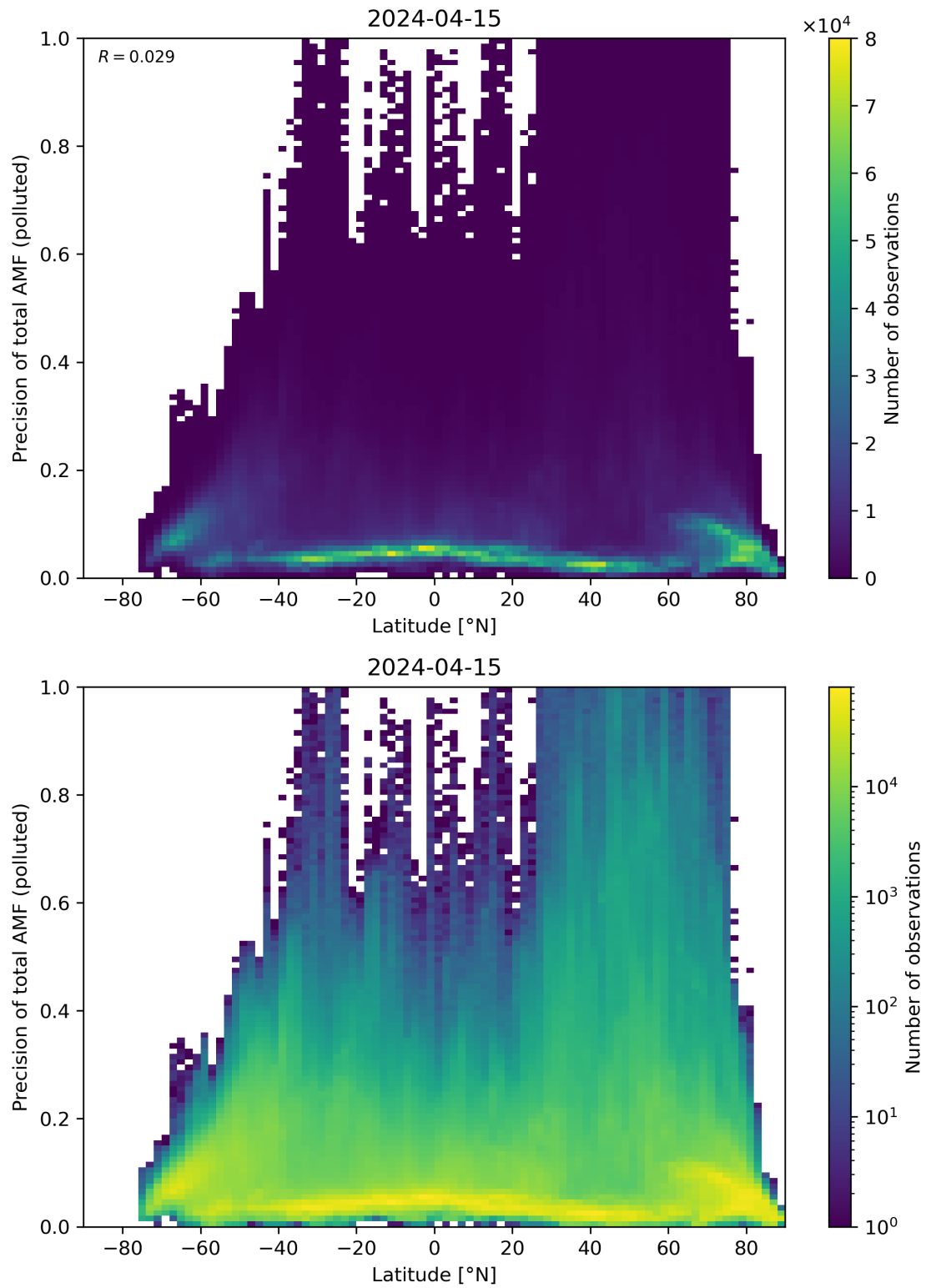
Figure 155: Scatter density plot of “Latitude” against “Precision of total AMF (polluted)” for 2024-04-15 to 2024-04-16.
