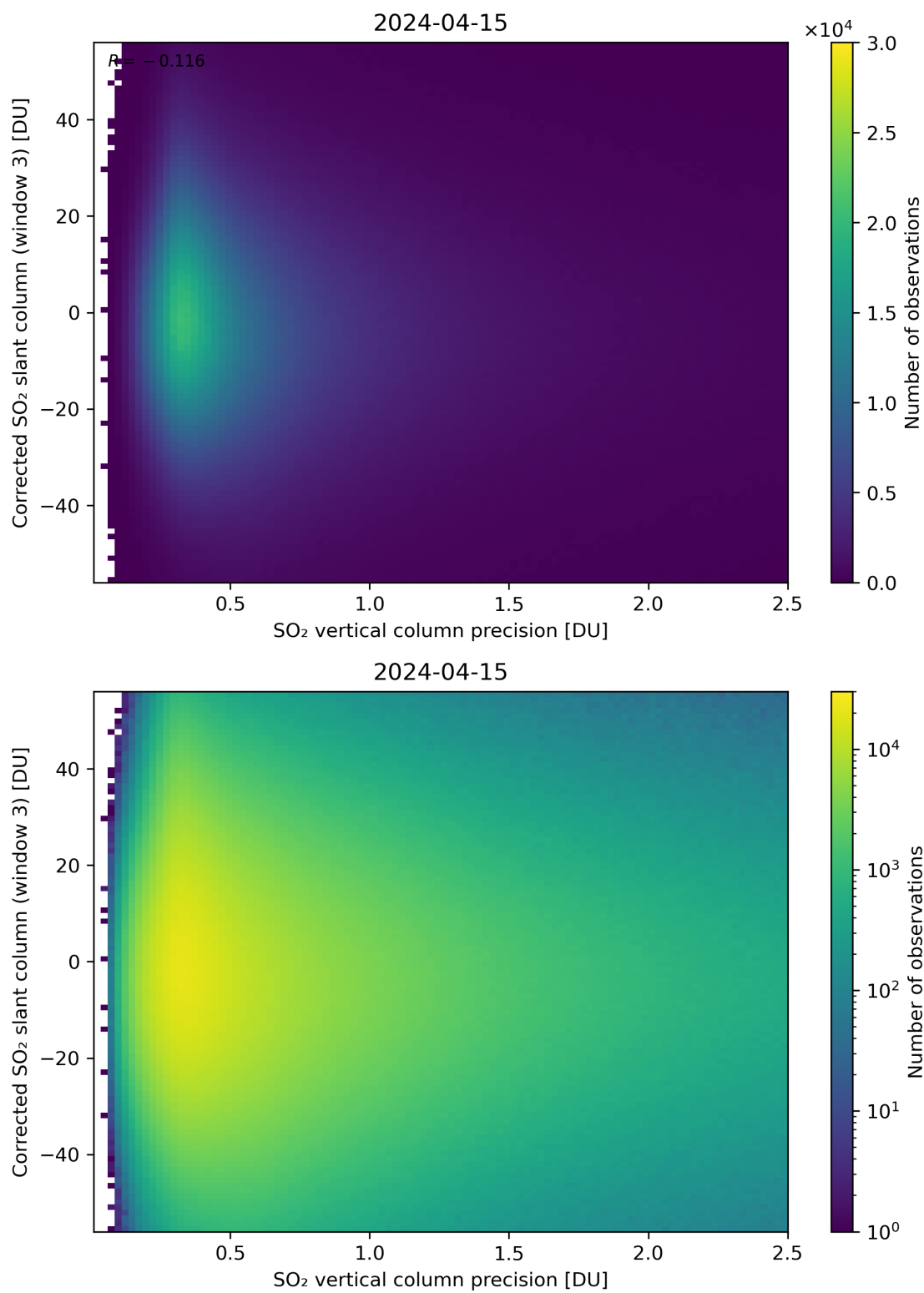
Figure 288: Scatter density plot of “SO 2 vertical column precision” against “Corrected SO 2 slant column (window 3)” for 2024-04-15 to 2024-04-16.
