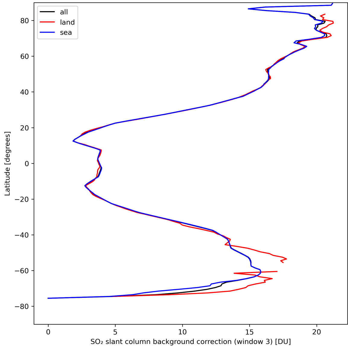
Figure 44: Zonal average of “SO 2 slant column background correction (window 3)” for 2024-04-15 to 2024-04-16.
