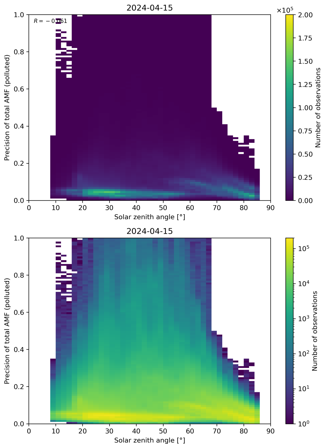
Figure 175: Scatter density plot of “Solar zenith angle” against “Precision of total AMF (polluted)” for 2024-04-15 to 2024-04-16.
