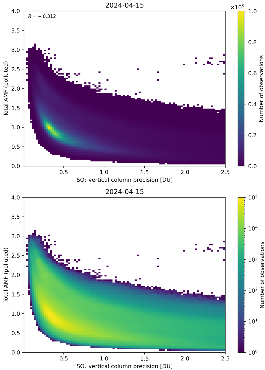
Figure 294: Scatter density plot of “SO 2 vertical column precision” against “Total AMF (polluted)” for 2024-04-15 to 2024-04-16.
