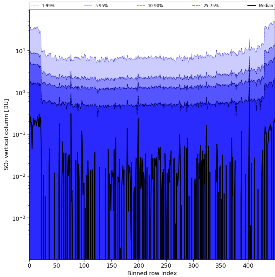
Figure 76: Along track statistics of “SO 2 vertical column” for 2024-04-15 to 2024-04-16
