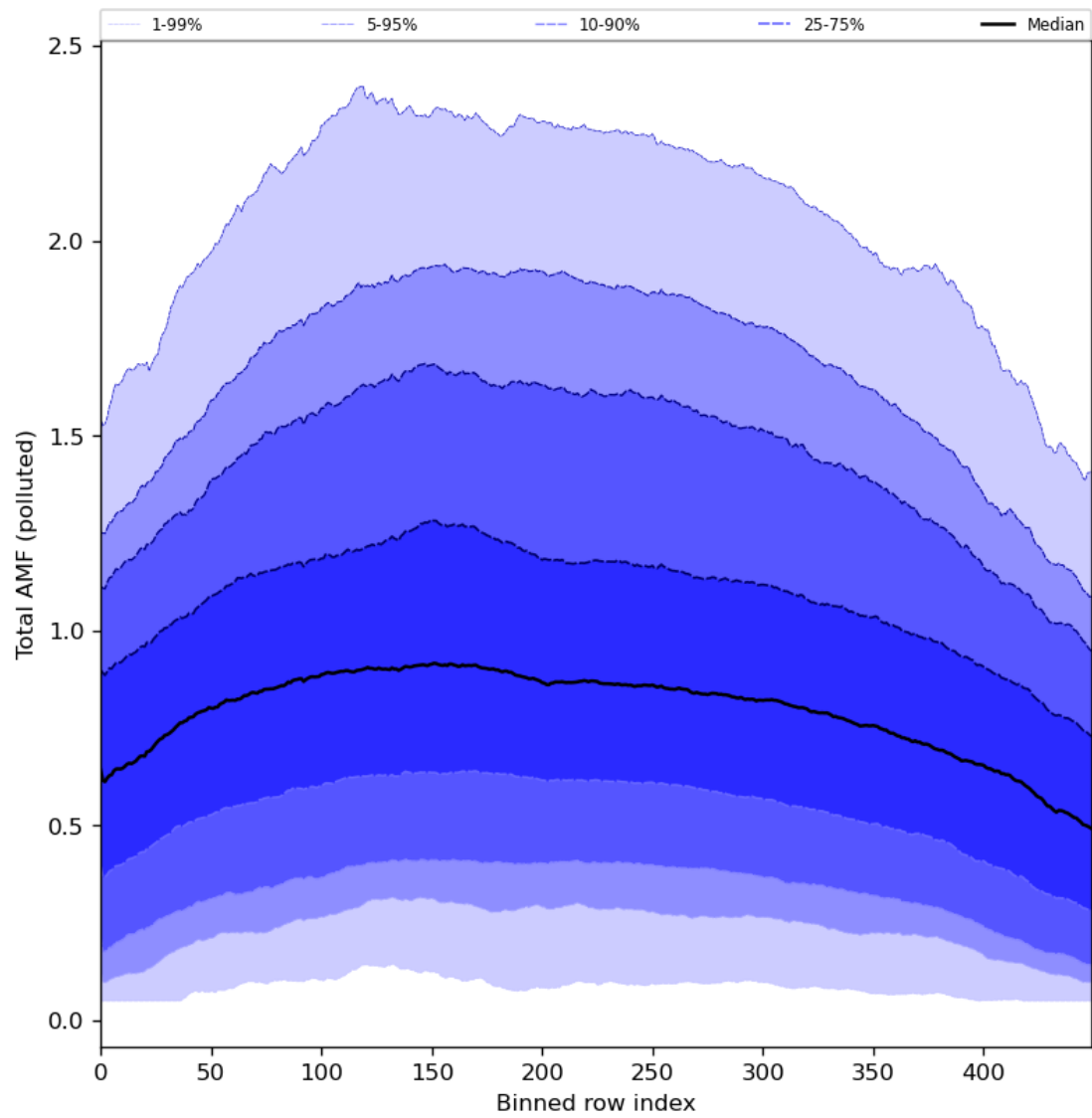
Figure 94: Along track statistics of “Total AMF (polluted)” for 2024-04-15 to 2024-04-16
