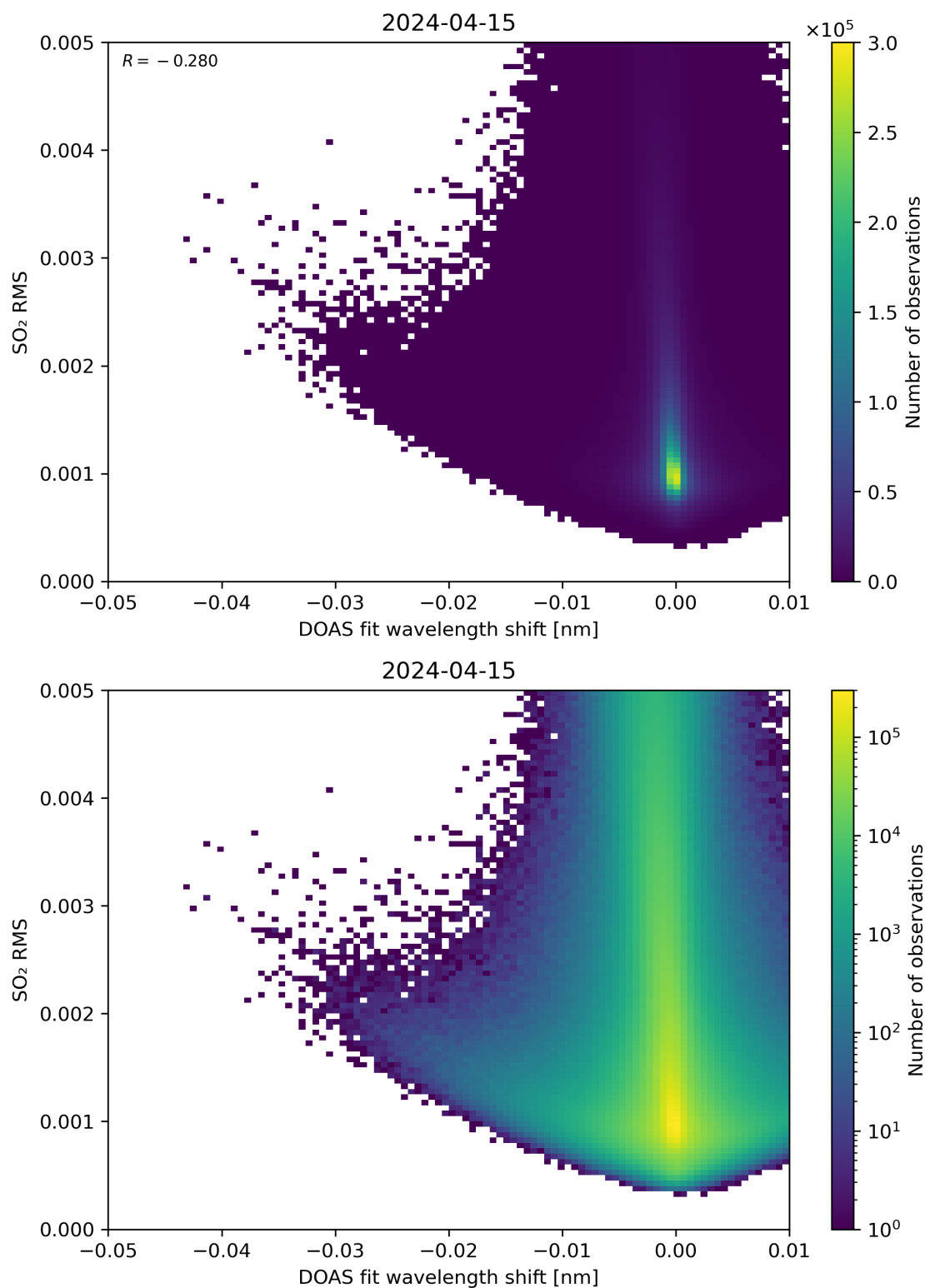
Figure 128: Scatter density plot of “DOAS fit wavelength shift” against “SO 2 RMS” for 2024-04-15 to 2024-04-16.
