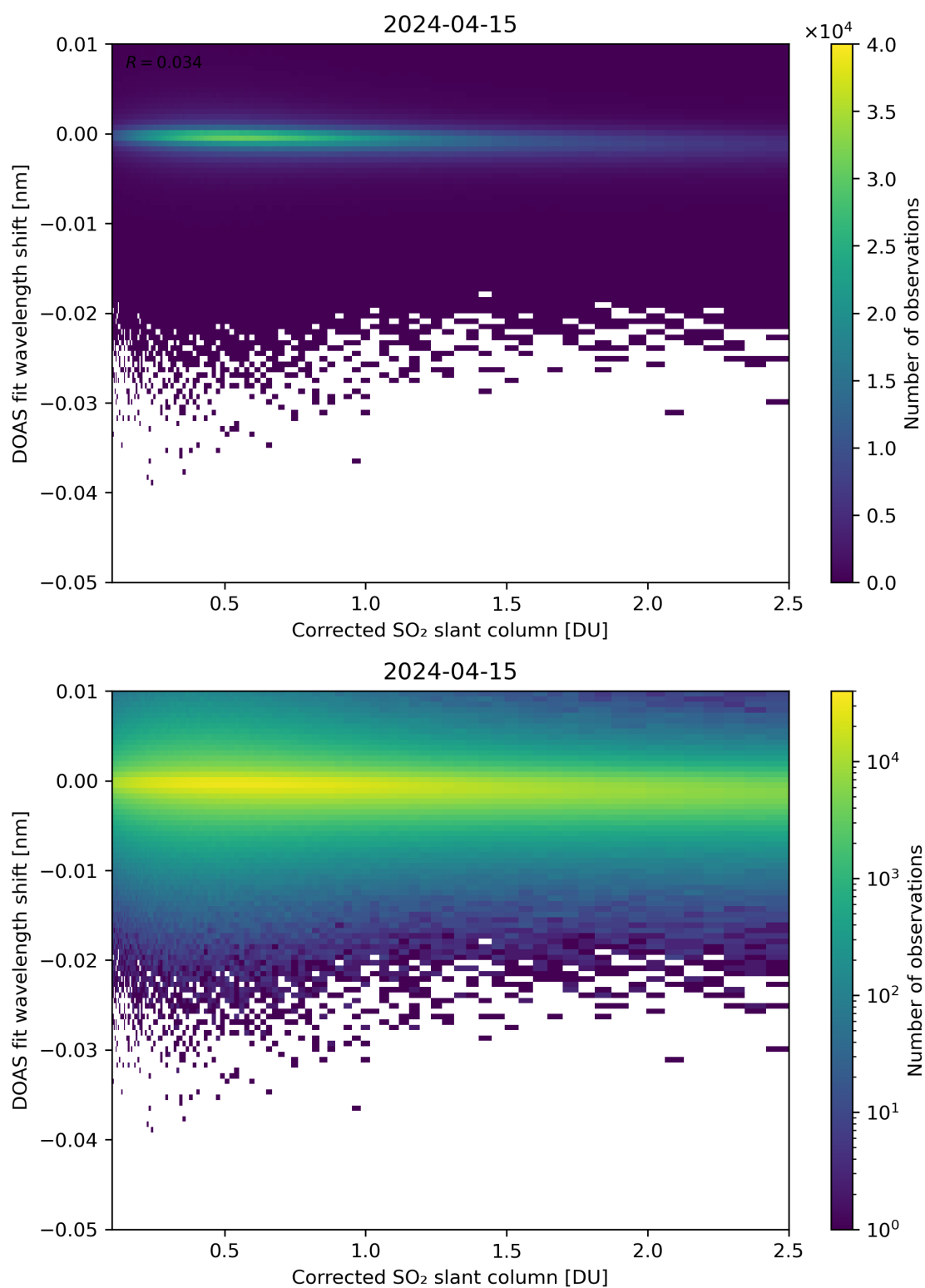
Figure 181: Scatter density plot of “Corrected SO 2 slant column” against “DOAS fit wavelength shift” for 2024-04-15 to 2024-04-16.
