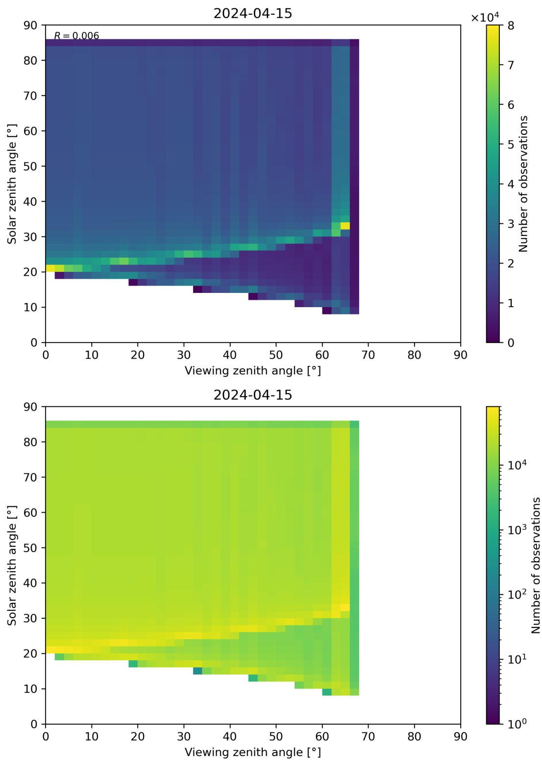
Figure 315: Scatter density plot of “Viewing zenith angle” against “Solar zenith angle” for 2024-04-15 to 2024-04-16.
