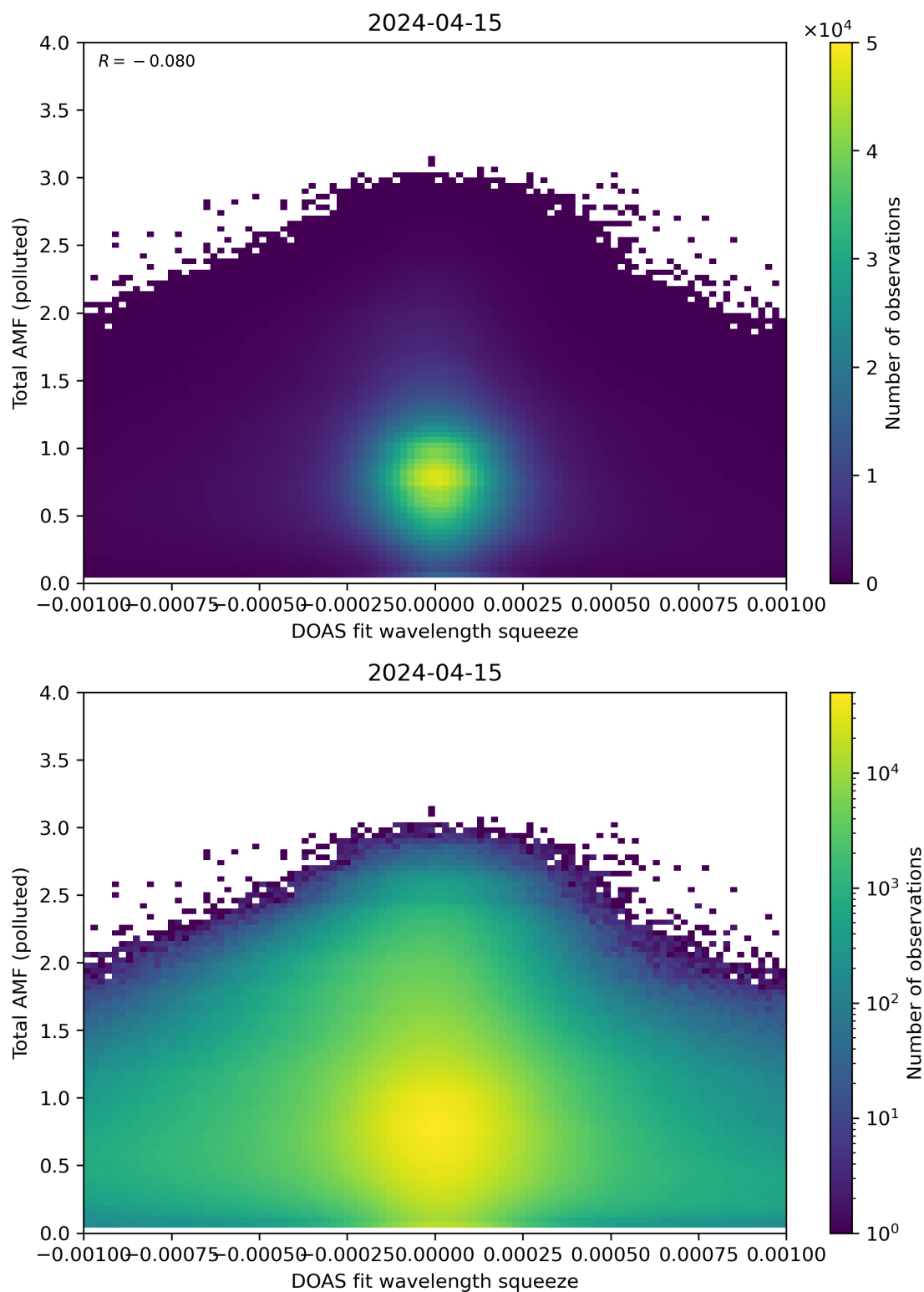
Figure 134: Scatter density plot of “DOAS fit wavelength squeeze” against “Total AMF (polluted)” for 2024-04-15 to 2024-04-16.
