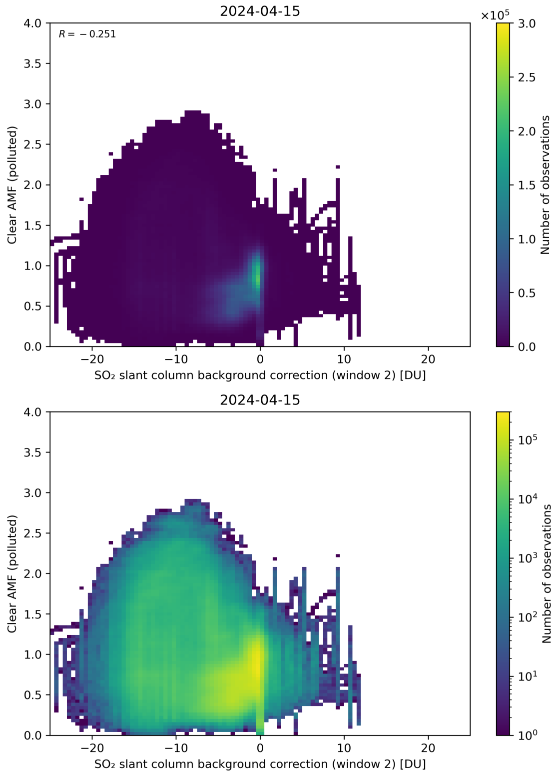
Figure 115: Scatter density plot of “SO 2 slant column background correction (window 2)” against “Clear AMF (polluted)” for 2024-04-15 to 2024-04-16.
