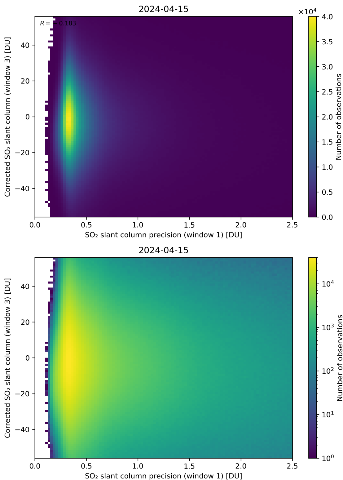
Figure 226: Scatter density plot of “SO 2 slant column precision (window 1)” against “Corrected SO 2 slant column (window 3)” for 2024-04-15 to 2024-04-16.
