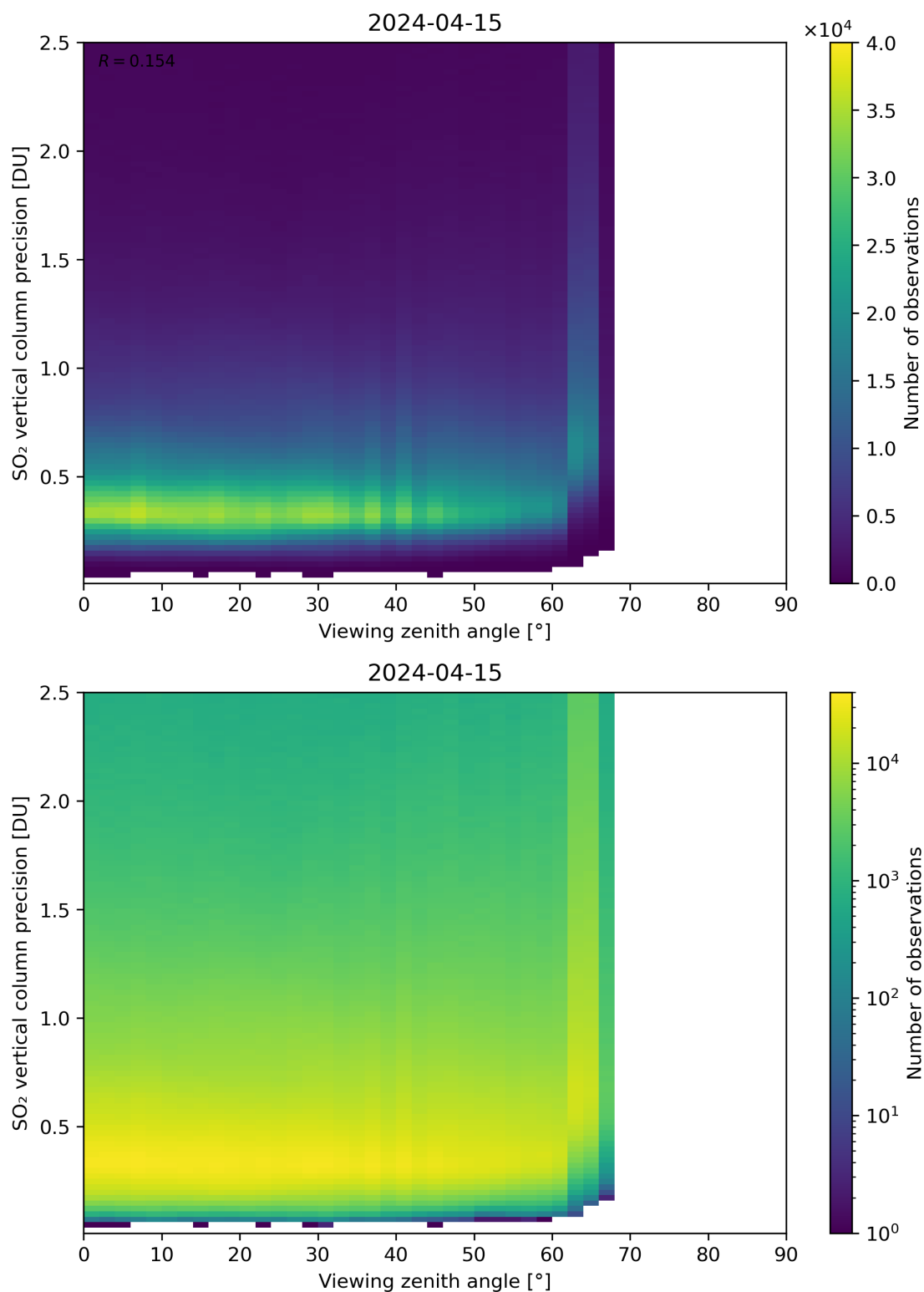
Figure 328: Scatter density plot of “Viewing zenith angle” against “SO 2 vertical column precision” for 2024-04-15 to 2024-04-16.
