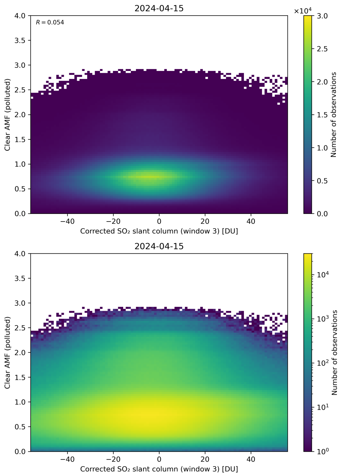
Figure 209: Scatter density plot of “Corrected SO 2 slant column (window 3)” against “Clear AMF (polluted)” for 2024-04-15 to 2024-04-16.
