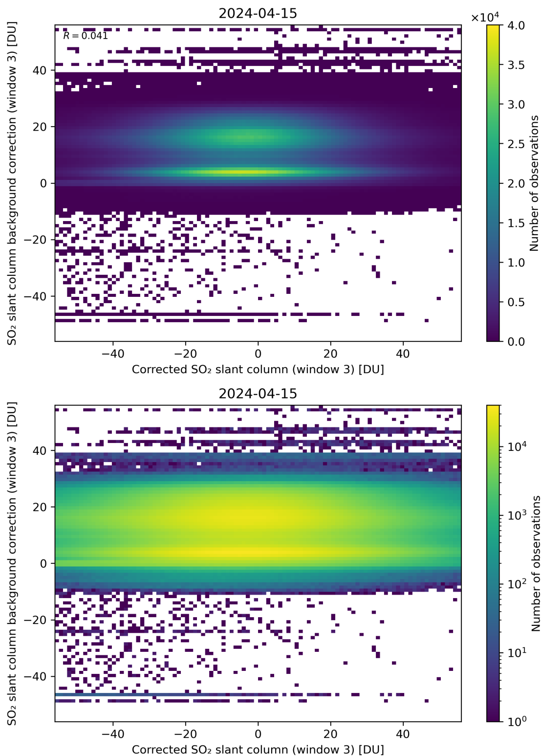
Figure 205: Scatter density plot of “Corrected SO 2 slant column (window 3)” against “SO 2 slant column background correction (window 3)” for 2024-04-15 to 2024-04-16.
