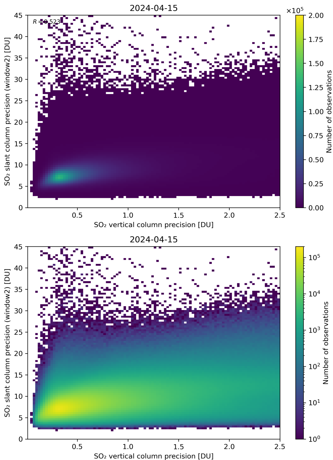
Figure 291: Scatter density plot of “SO 2 vertical column precision” against “SO 2 slant column precision (window2)” for 2024-04-15 to 2024-04-16.
