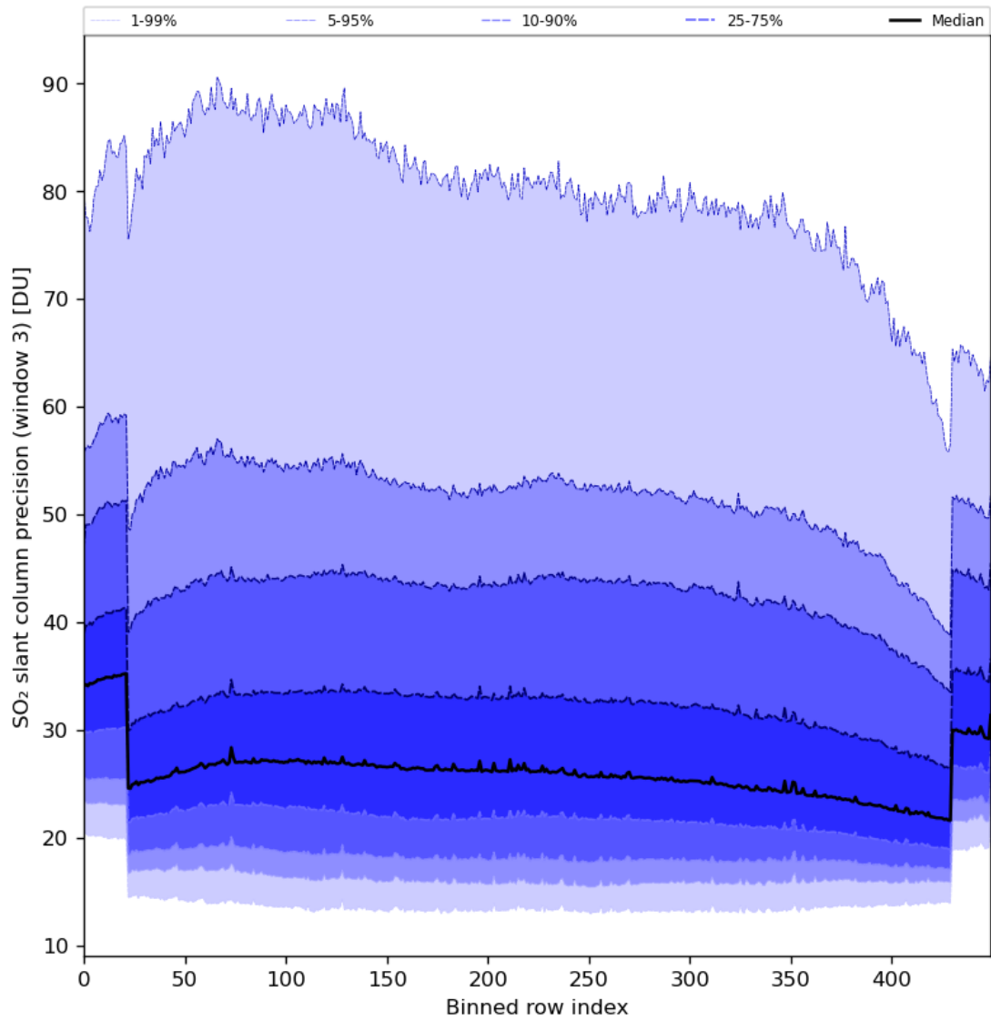
Figure 88: Along track statistics of “SO 2 slant column precision (window 3)” for 2024-04-15 to 2024-04-16
