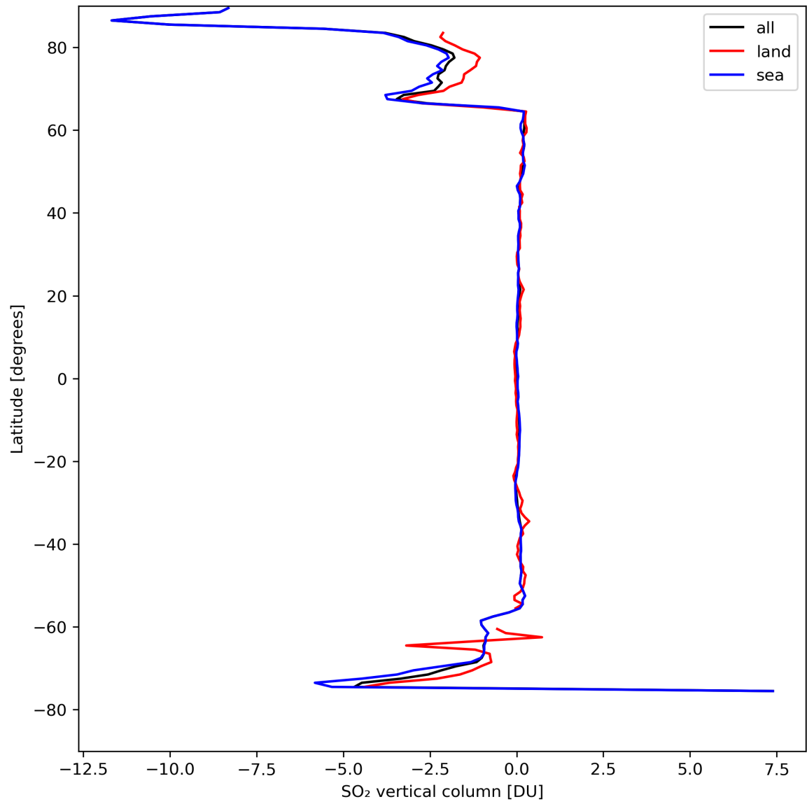
Figure 30: Zonal average of “SO 2 vertical column” for 2024-04-15 to 2024-04-16.
