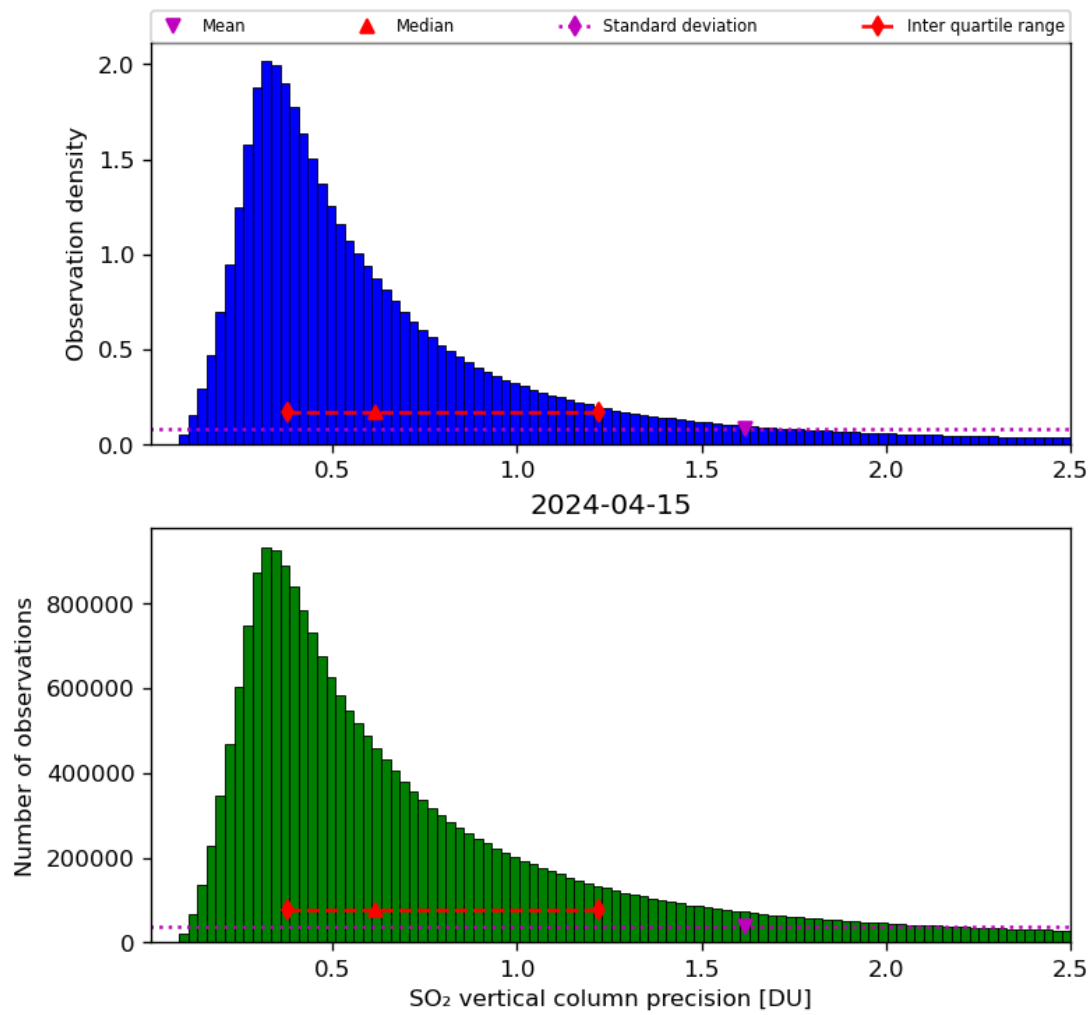
Figure 54: Histogram of “SO 2 vertical column precision” for 2024-04-15 to 2024-04-16
