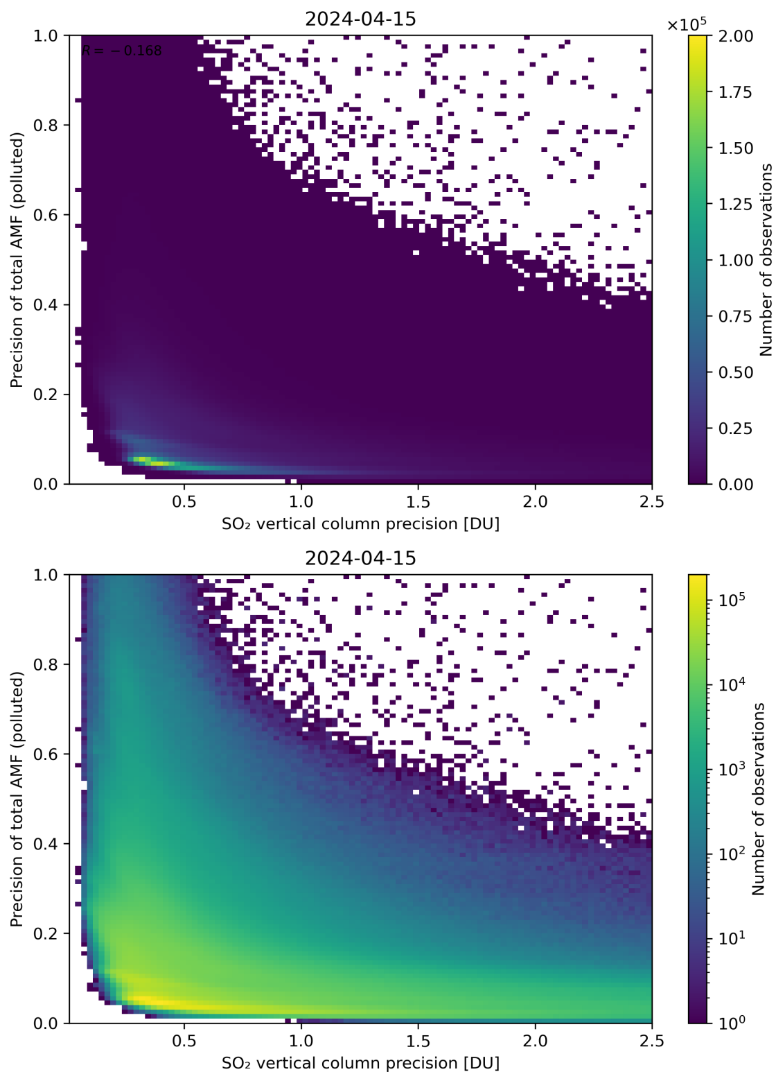
Figure 295: Scatter density plot of “SO 2 vertical column precision” against “Precision of total AMF (polluted)” for 2024-04-15 to 2024-04-16.
