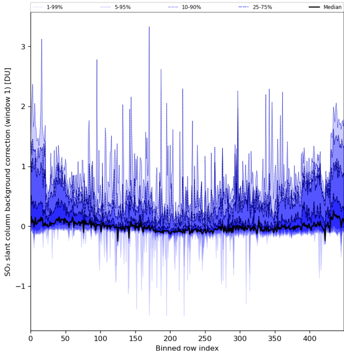
Figure 82: Along track statistics of “SO 2 slant column background correction (window 1)” for 2024-04-15 to 2024-04-16
