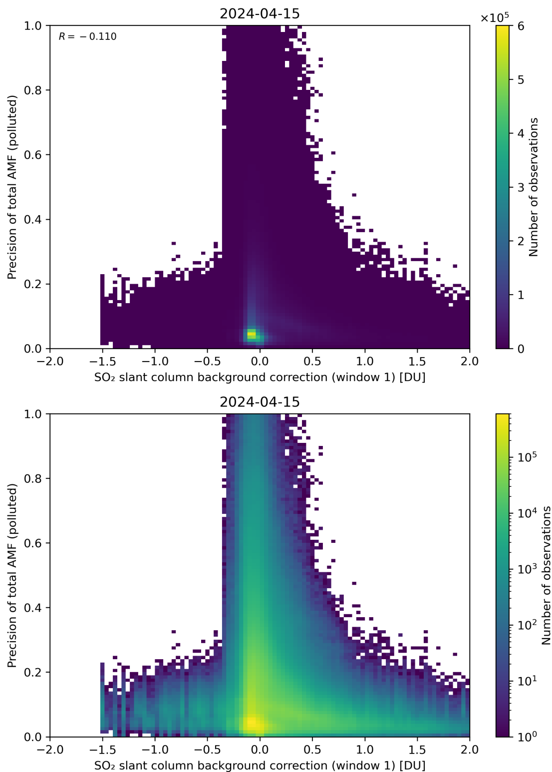
Figure 110: Scatter density plot of “SO 2 slant column background correction (window 1)” against “Precision of total AMF (polluted)” for 2024-04-15 to 2024-04-16.
