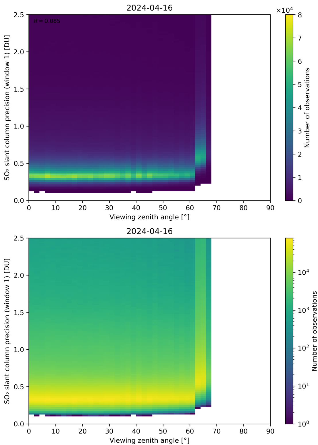
Figure 321: Scatter density plot of “Viewing zenith angle” against “SO 2 slant column precision (window 1)” for 2024-04-16 to 2024-04-17.
