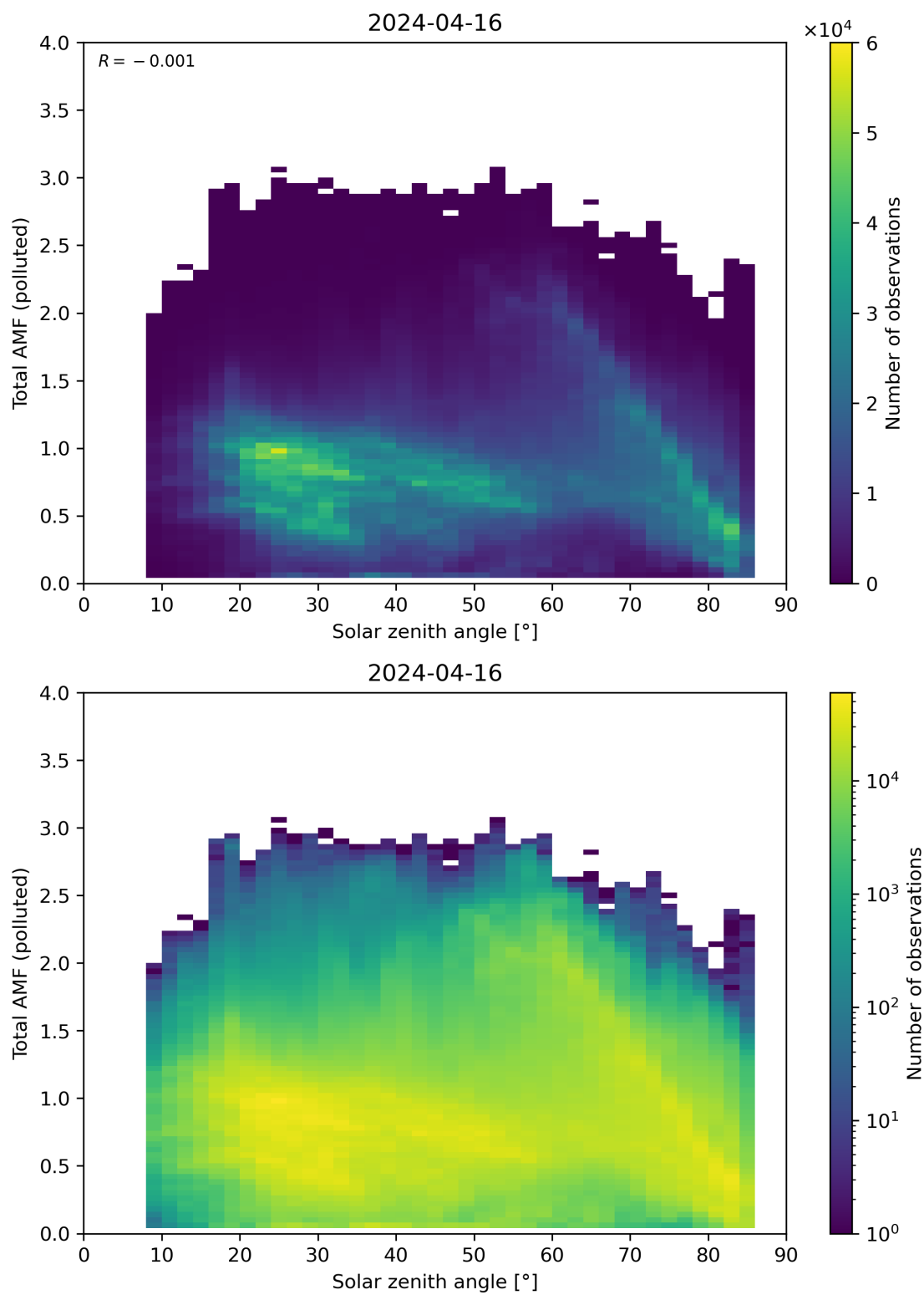
Figure 174: Scatter density plot of “Solar zenith angle” against “Total AMF (polluted)” for 2024-04-16 to 2024-04-17.
