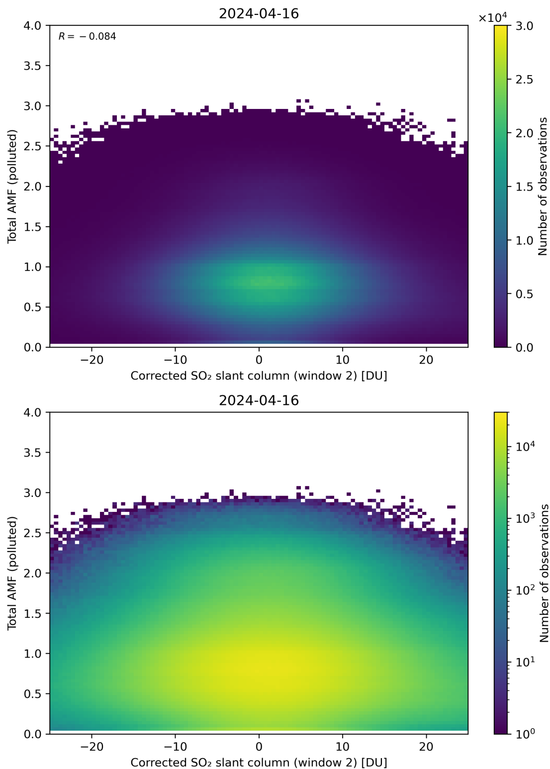
Figure 203: Scatter density plot of “Corrected SO 2 slant column (window 2)” against “Total AMF (polluted)” for 2024-04-16 to 2024-04-17.
