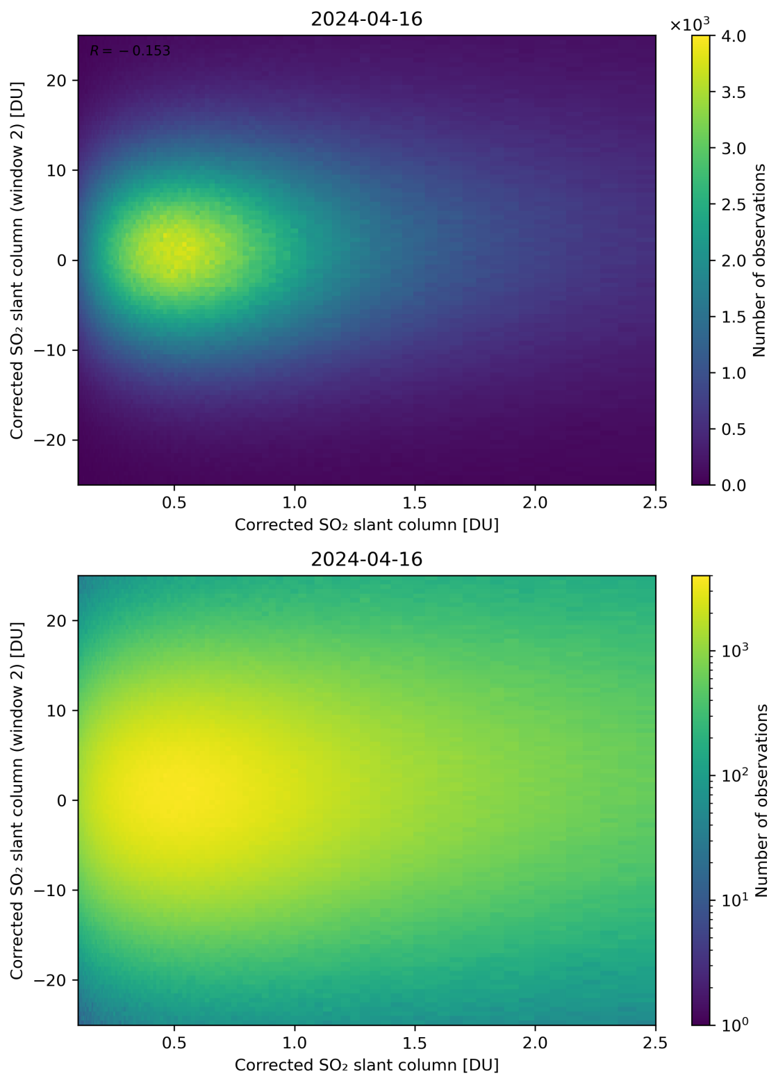
Figure 185: Scatter density plot of “Corrected SO 2 slant column” against “Corrected SO 2 slant column (window 2)” for 2024-04-16 to 2024-04-17.
