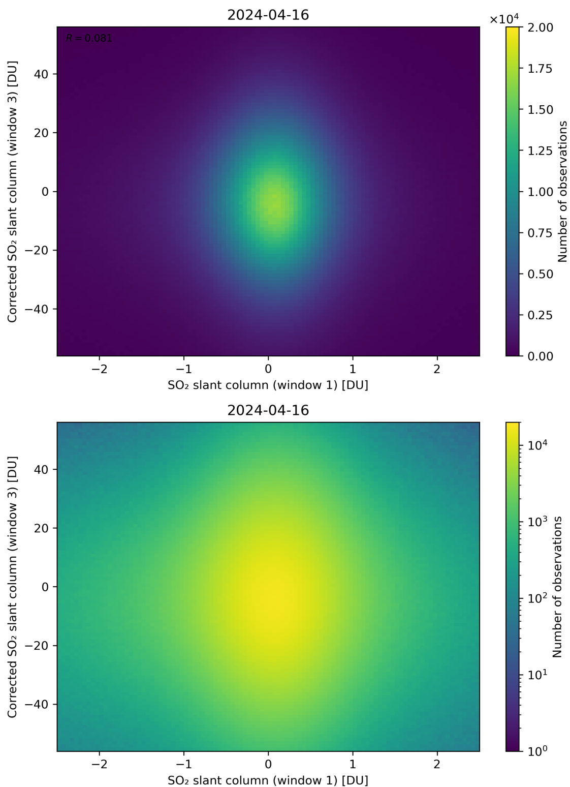
Figure 234: Scatter density plot of “SO 2 slant column (window 1)” against “Corrected SO 2 slant column (window 3)” for 2024-04-16 to 2024-04-17.
