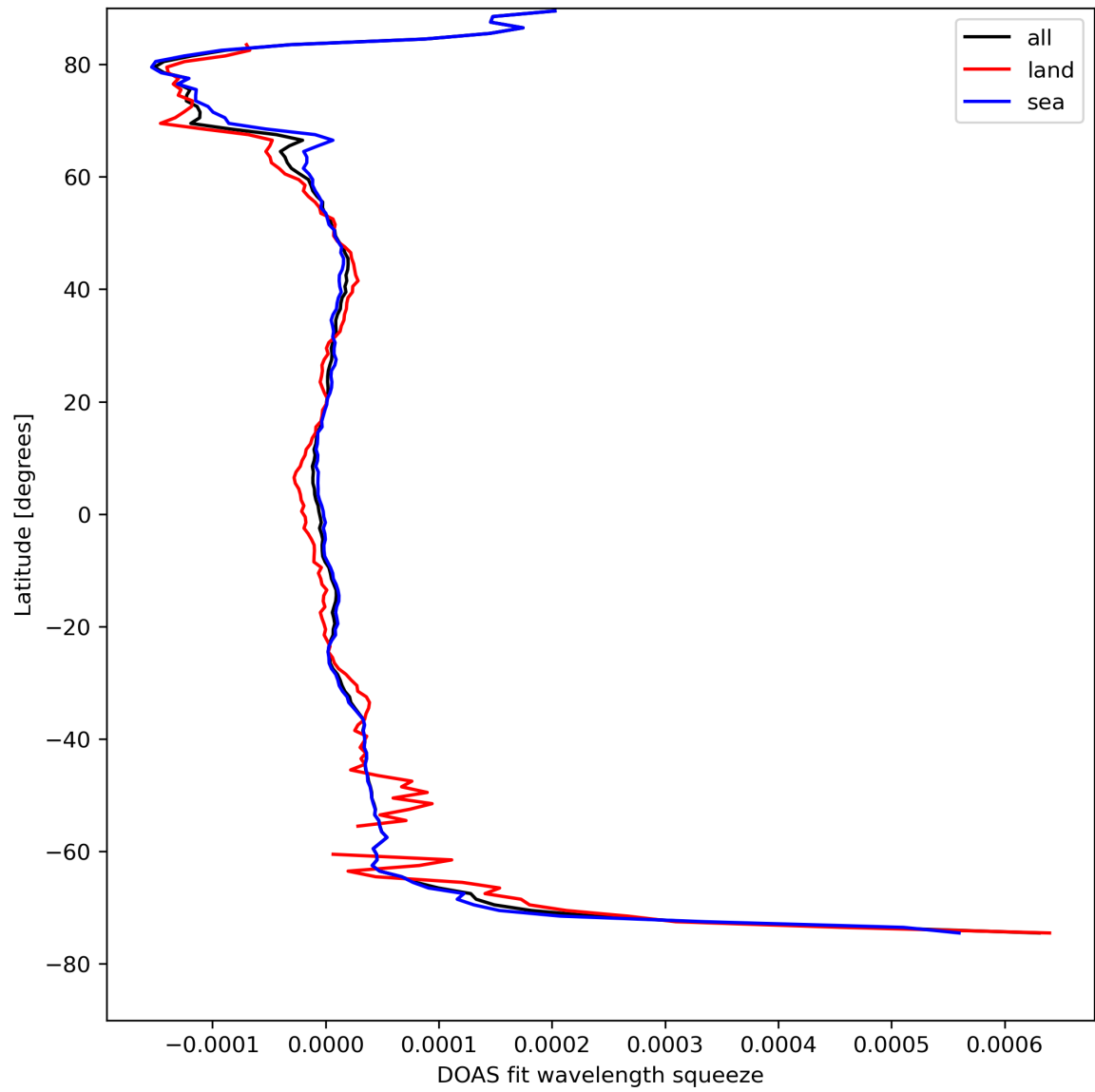
Figure 46: Zonal average of “DOAS fit wavelength squeeze” for 2024-04-16 to 2024-04-17.
