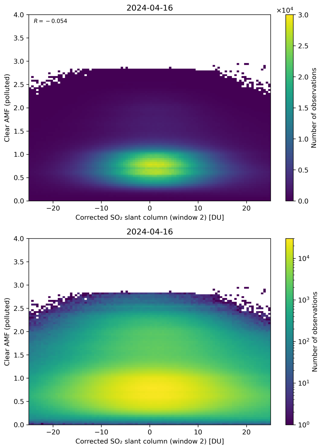
Figure 199: Scatter density plot of “Corrected SO 2 slant column (window 2)” against “Clear AMF (polluted)” for 2024-04-16 to 2024-04-17.
