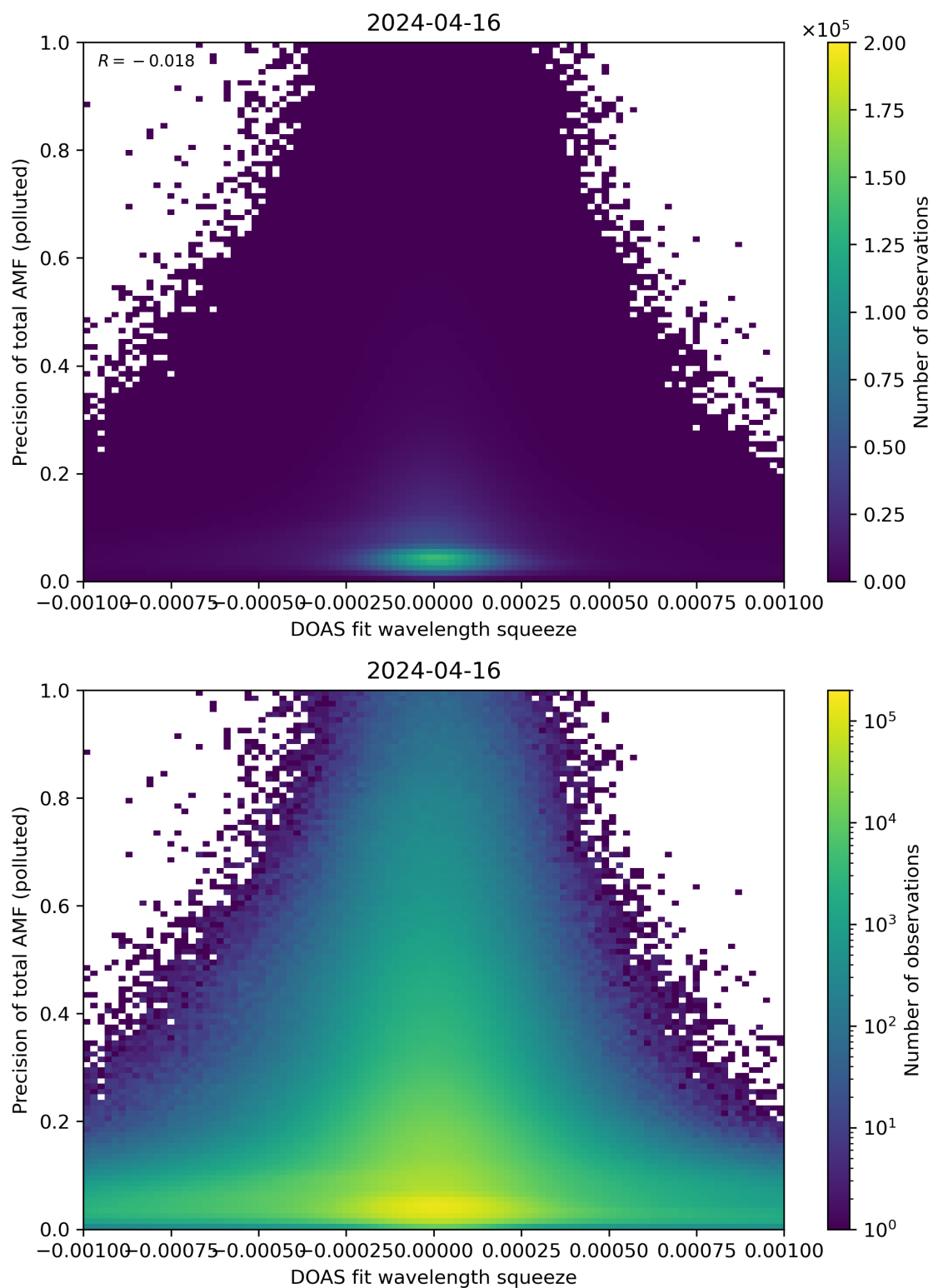
Figure 135: Scatter density plot of “DOAS fit wavelength squeeze” against “Precision of total AMF (polluted)” for 2024-04-16 to 2024-04-17.
