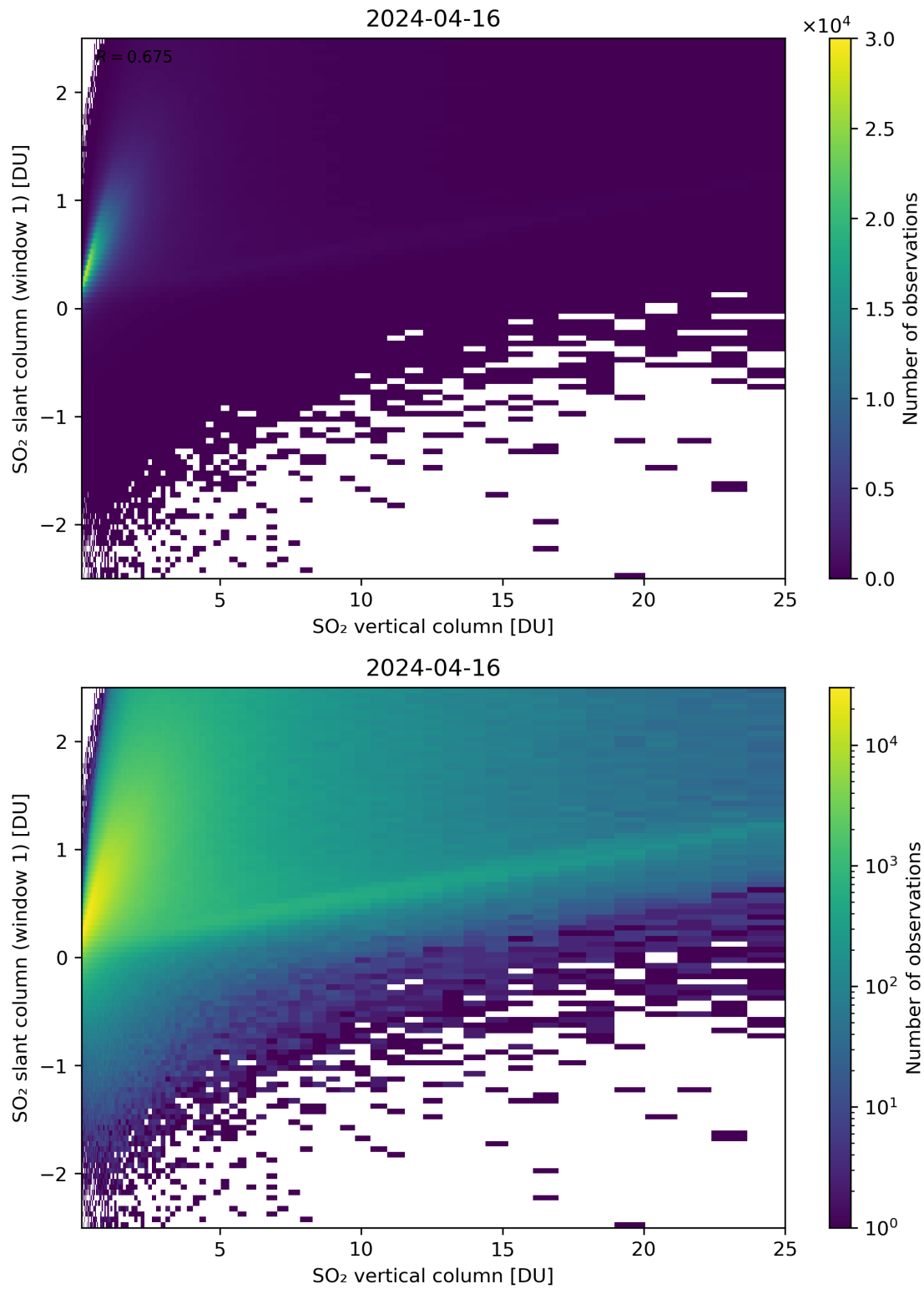
Figure 300: Scatter density plot of “SO 2 vertical column” against “SO 2 slant column (window 1)” for 2024-04-16 to 2024-04-17.
