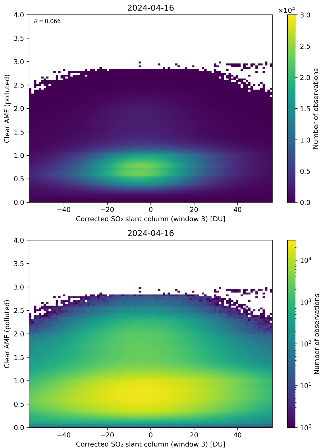
Figure 209: Scatter density plot of “Corrected SO 2 slant column (window 3)” against “Clear AMF (polluted)” for 2024-04-16 to 2024-04-17.
