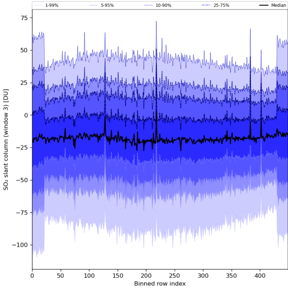
Figure 87: Along track statistics of “SO 2 slant column (window 3)” for 2024-04-16 to 2024-04-17
