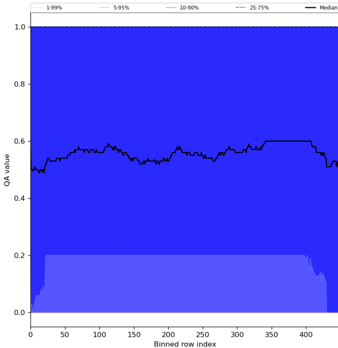
Figure 75: Along track statistics of “QA value” for 2024-04-16 to 2024-04-17
