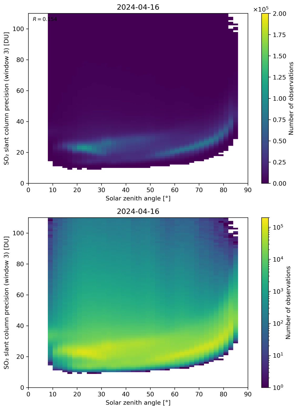
Figure 173: Scatter density plot of “Solar zenith angle” against “SO 2 slant column precision (window 3)” for 2024-04-16 to 2024-04-17.
