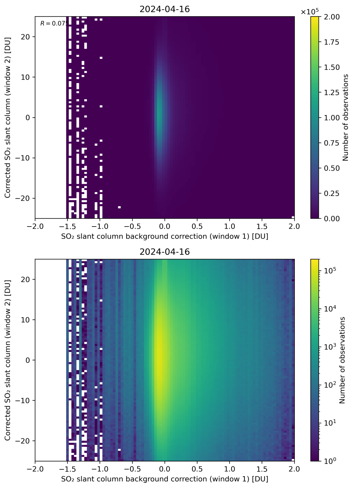
Figure 104: Scatter density plot of “SO 2 slant column background correction (window 1)” against “Corrected SO 2 slant column (window 2)” for 2024-04-16 to 2024-04-17.
