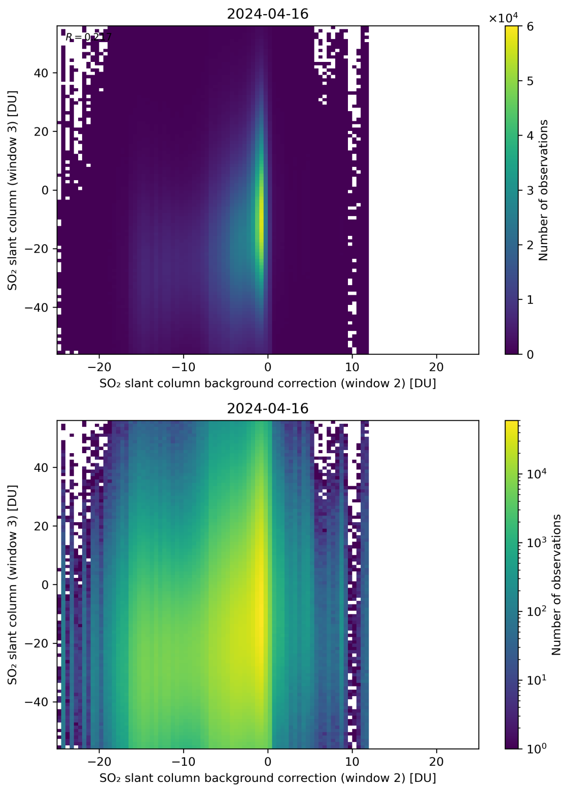
Figure 117: Scatter density plot of “SO 2 slant column background correction (window 2)” against “SO 2 slant column (window 3)” for 2024-04-16 to 2024-04-17.
