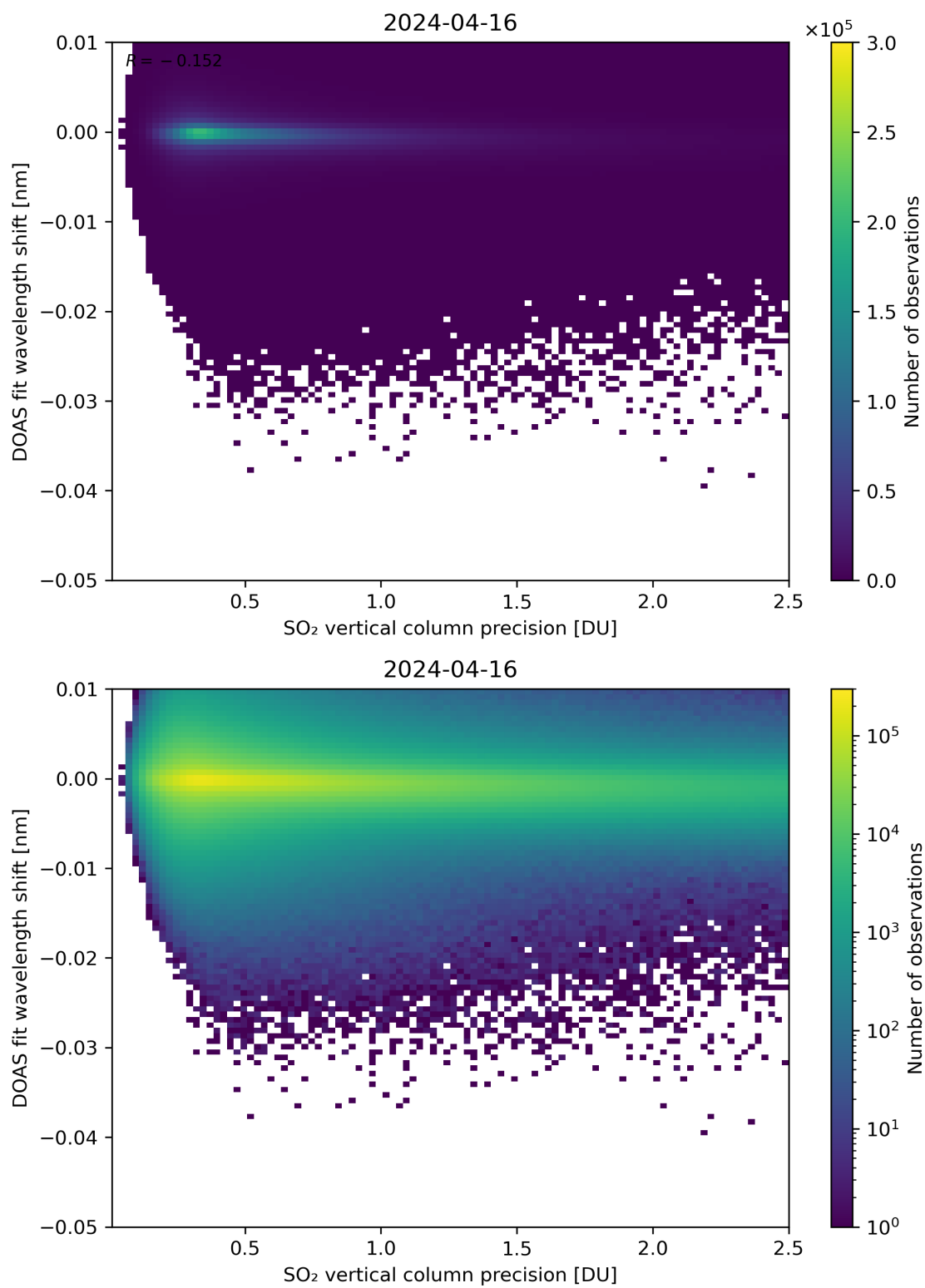
Figure 282: Scatter density plot of “SO 2 vertical column precision” against “DOAS fit wavelength shift” for 2024-04-16 to 2024-04-17.
