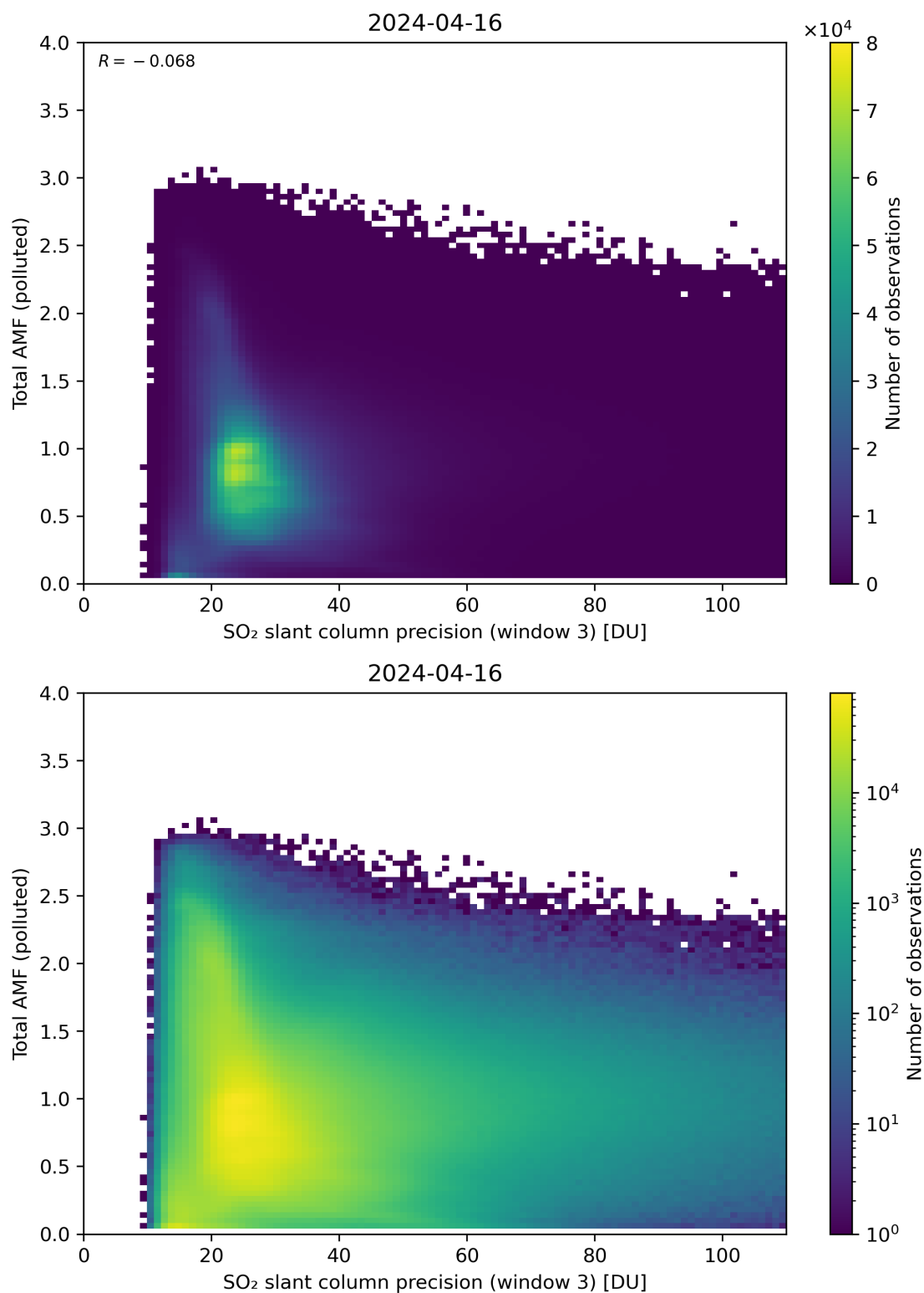
Figure 263: Scatter density plot of “SO 2 slant column precision (window 3)” against “Total AMF (polluted)” for 2024-04-16 to 2024-04-17.
