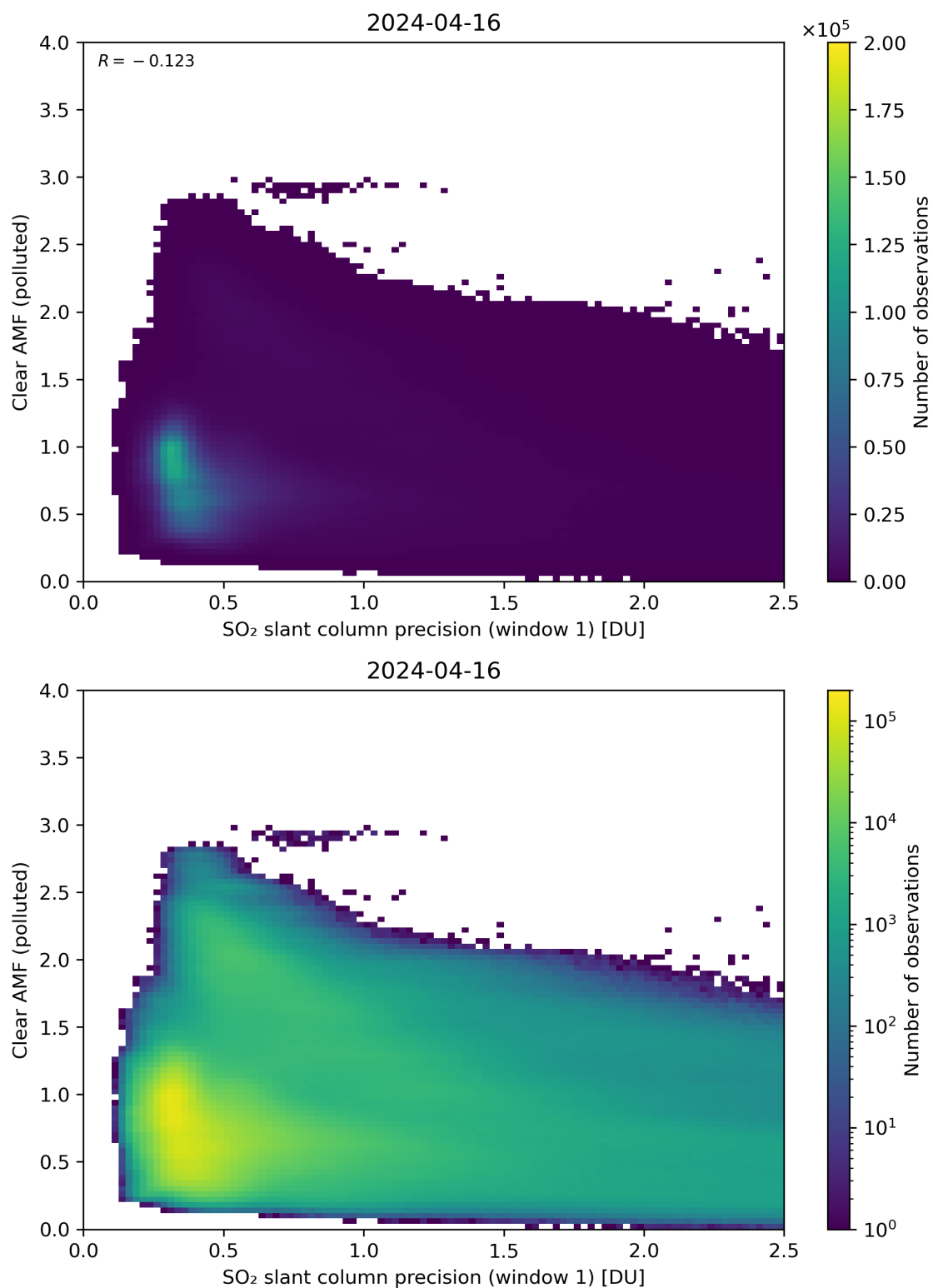
Figure 224: Scatter density plot of “SO 2 slant column precision (window 1)” against “Clear AMF (polluted)” for 2024-04-16 to 2024-04-17.
