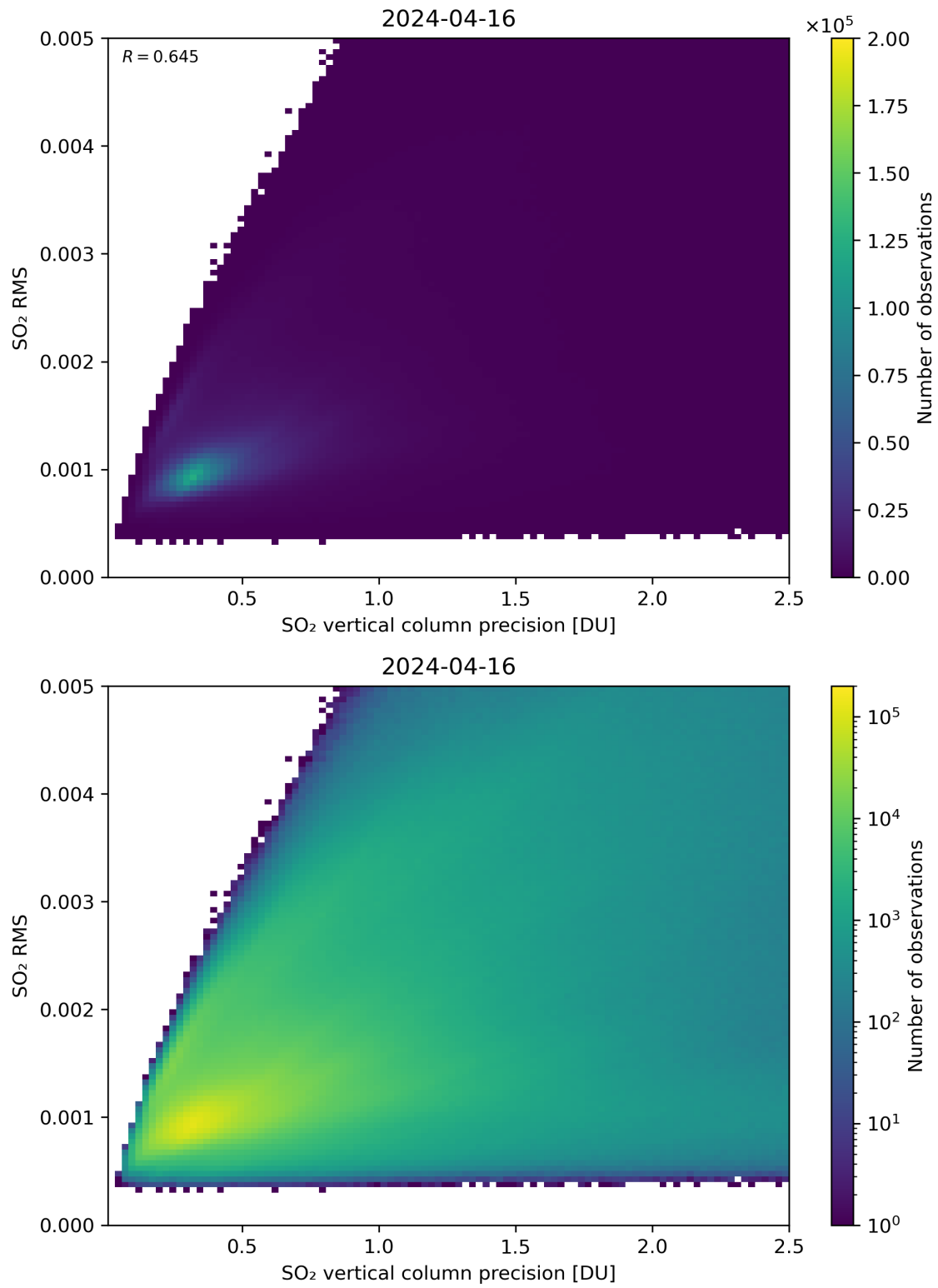
Figure 284: Scatter density plot of “SO 2 vertical column precision” against “SO 2 RMS” for 2024-04-16 to 2024-04-17.
