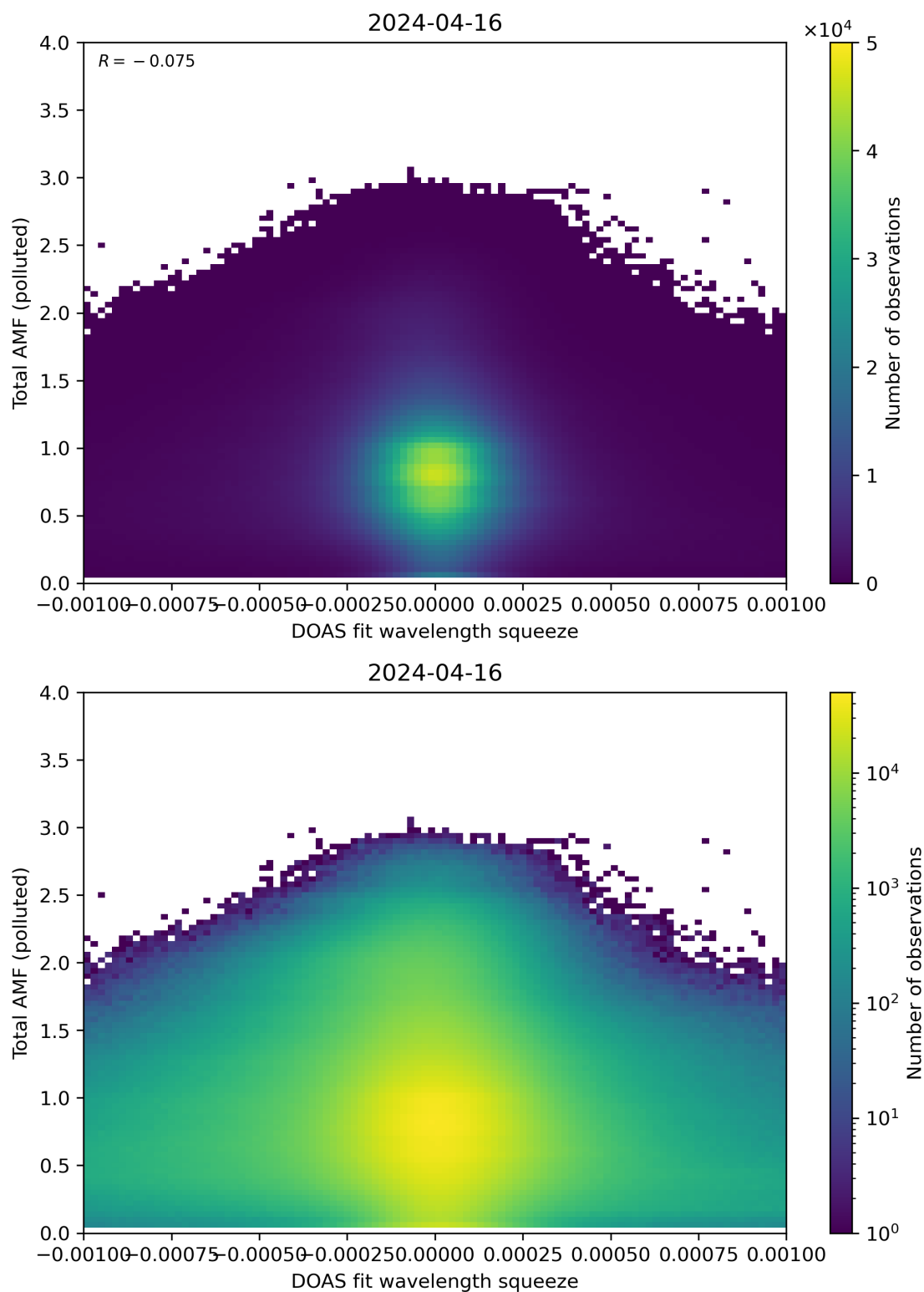
Figure 134: Scatter density plot of “DOAS fit wavelength squeeze” against “Total AMF (polluted)” for 2024-04-16 to 2024-04-17.
