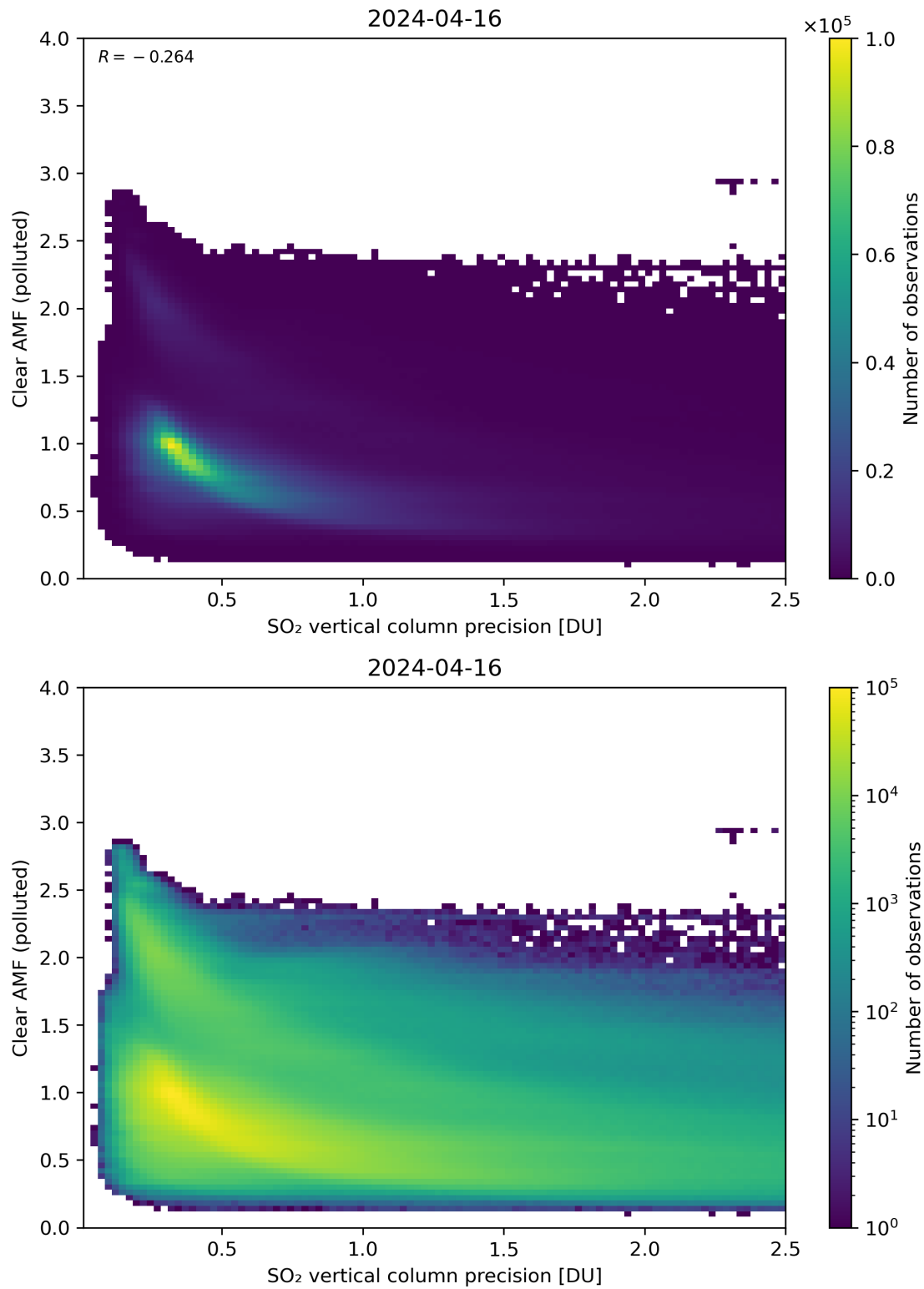
Figure 285: Scatter density plot of “SO 2 vertical column precision” against “Clear AMF (polluted)” for 2024-04-16 to 2024-04-17.
