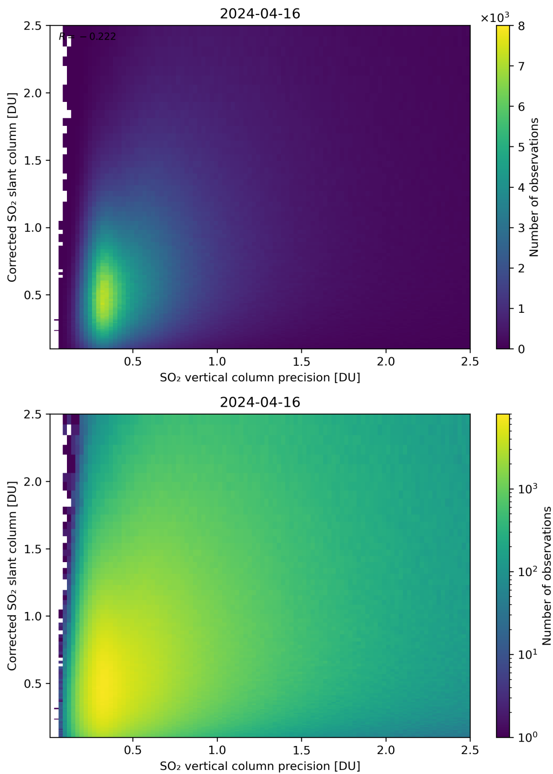
Figure 286: Scatter density plot of “SO 2 vertical column precision” against “Corrected SO 2 slant column” for 2024-04-16 to 2024-04-17.
