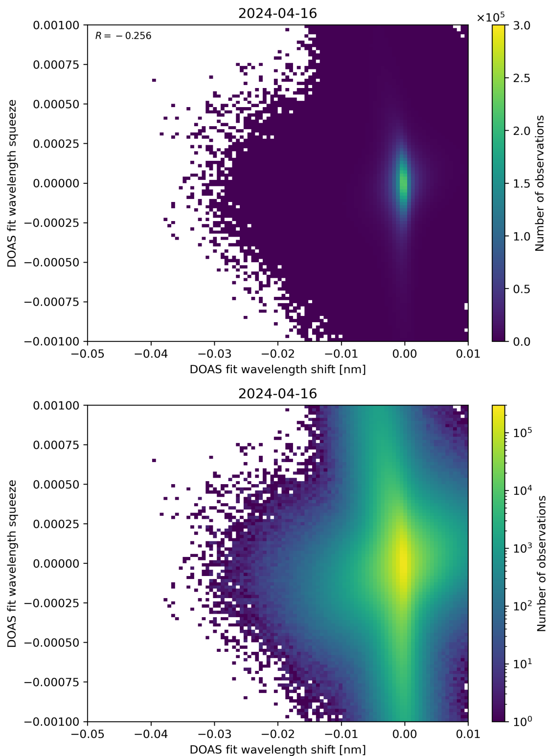
Figure 127: Scatter density plot of “DOAS fit wavelength shift” against “DOAS fit wavelength squeeze” for 2024-04-16 to 2024-04-17.
