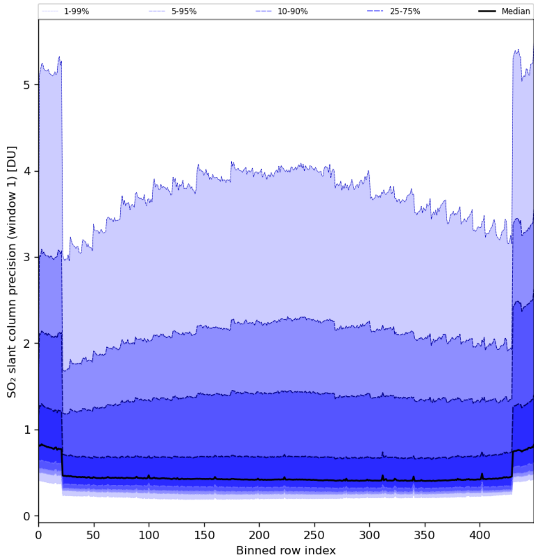
Figure 80: Along track statistics of “SO 2 slant column precision (window 1)” for 2024-04-16 to 2024-04-17
