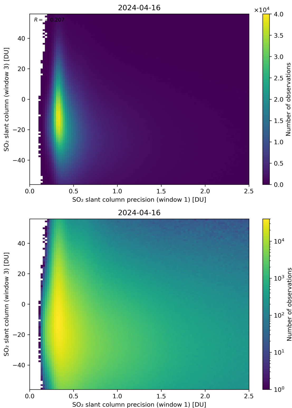
Figure 228: Scatter density plot of “SO 2 slant column precision (window 1)” against “SO 2 slant column (window 3)” for 2024-04-16 to 2024-04-17.
