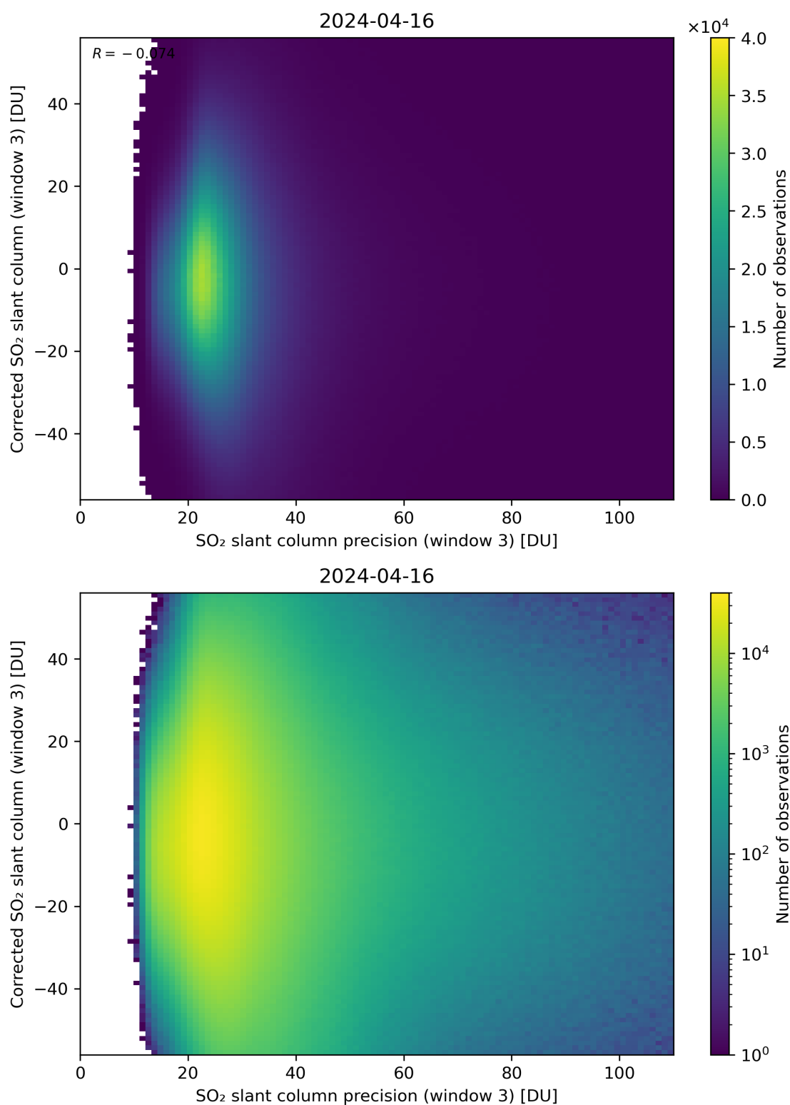
Figure 262: Scatter density plot of “SO 2 slant column precision (window 3)” against “Corrected SO 2 slant column (window 3)” for 2024-04-16 to 2024-04-17.
