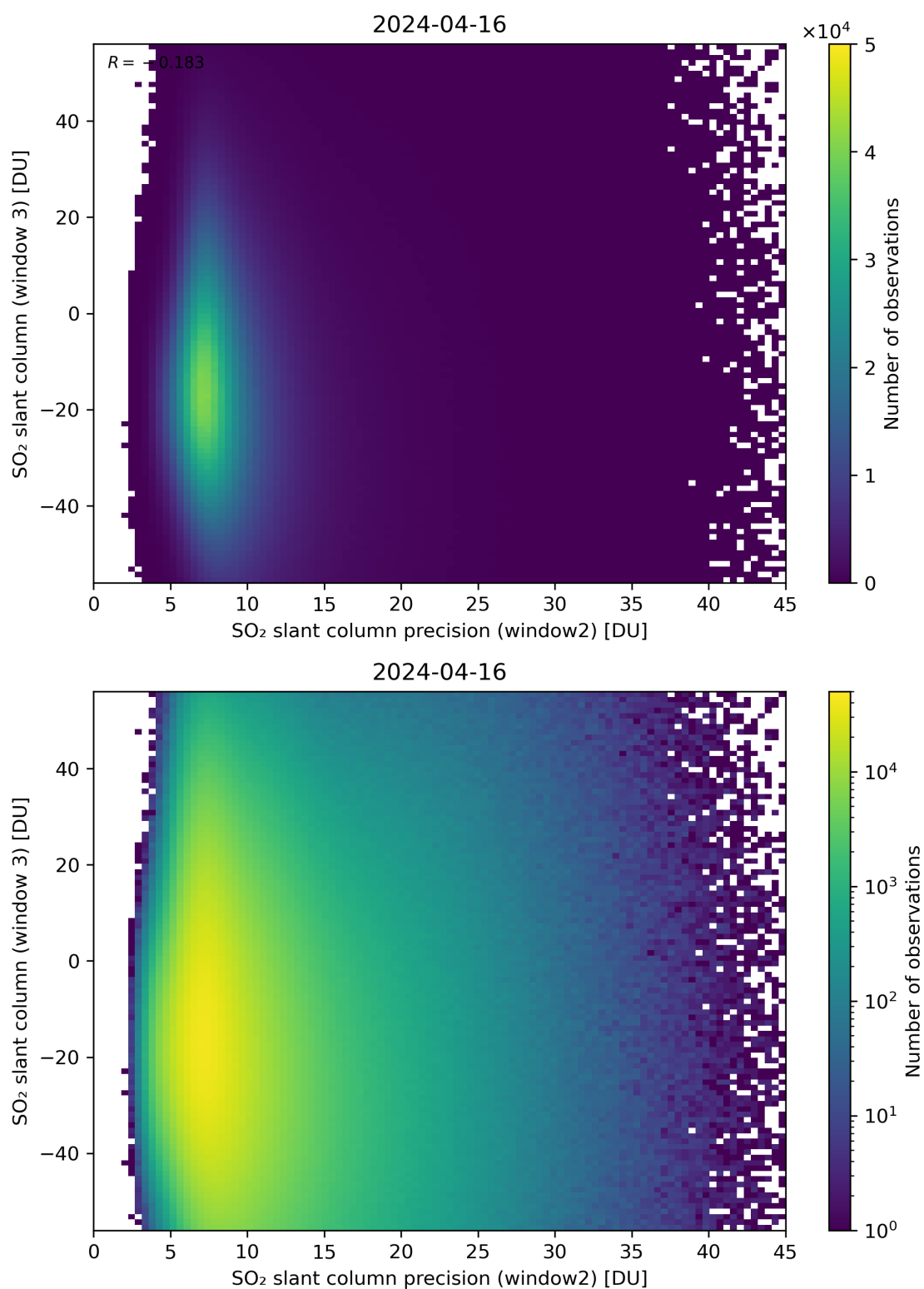
Figure 249: Scatter density plot of “SO 2 slant column precision (window2)” against “SO 2 slant column (window 3)” for 2024-04-16 to 2024-04-17.
