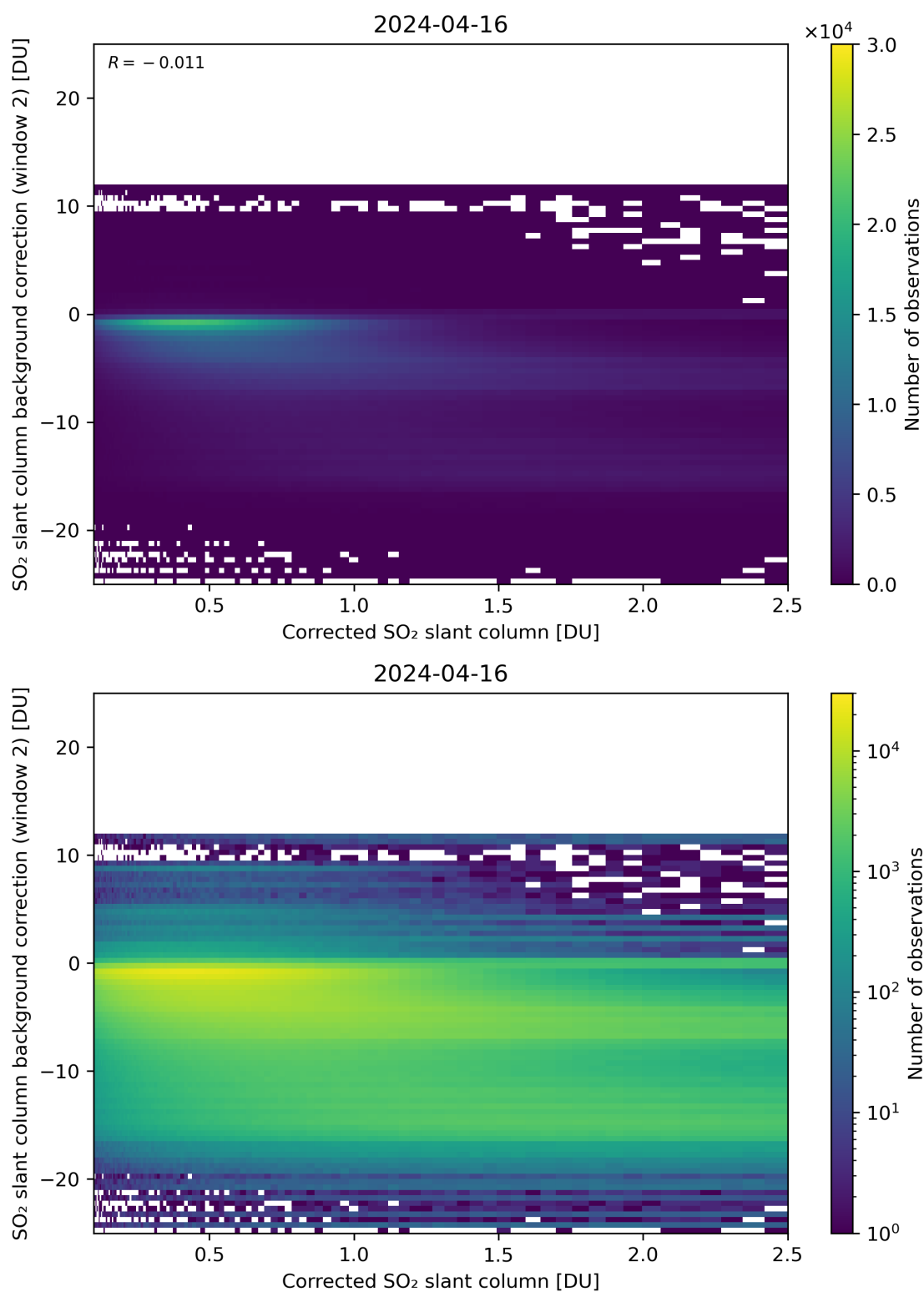
Figure 179: Scatter density plot of “Corrected SO 2 slant column” against “SO 2 slant column background correction (window 2)” for 2024-04-16 to 2024-04-17.
