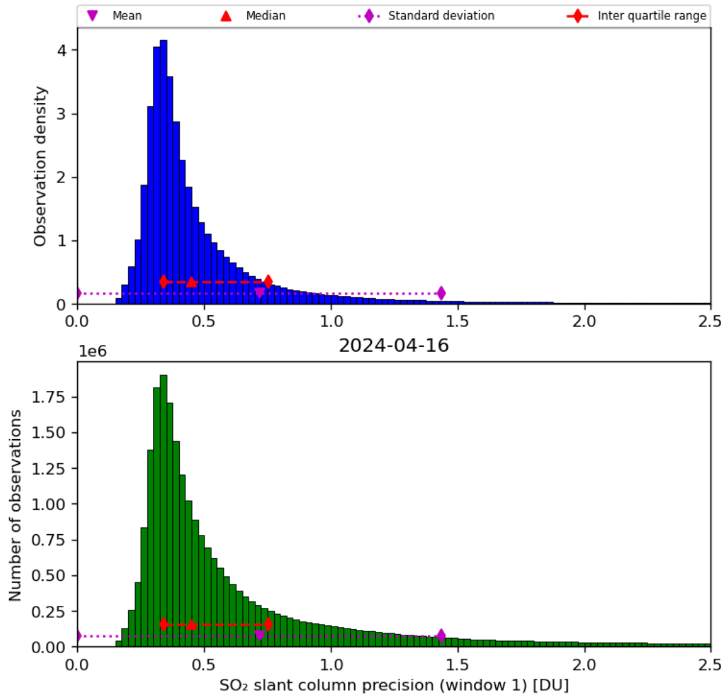
Figure 57: Histogram of “SO 2 slant column precision (window 1)” for 2024-04-16 to 2024-04-17
