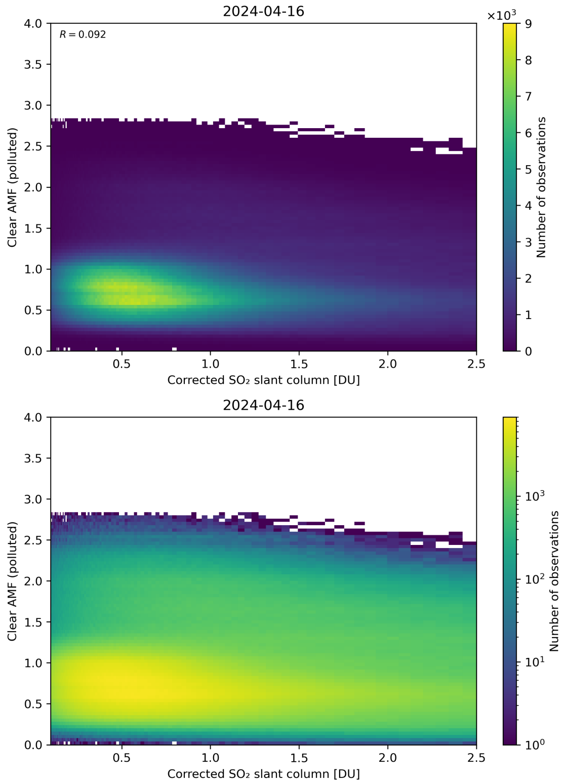
Figure 184: Scatter density plot of “Corrected SO 2 slant column” against “Clear AMF (polluted)” for 2024-04-16 to 2024-04-17.
