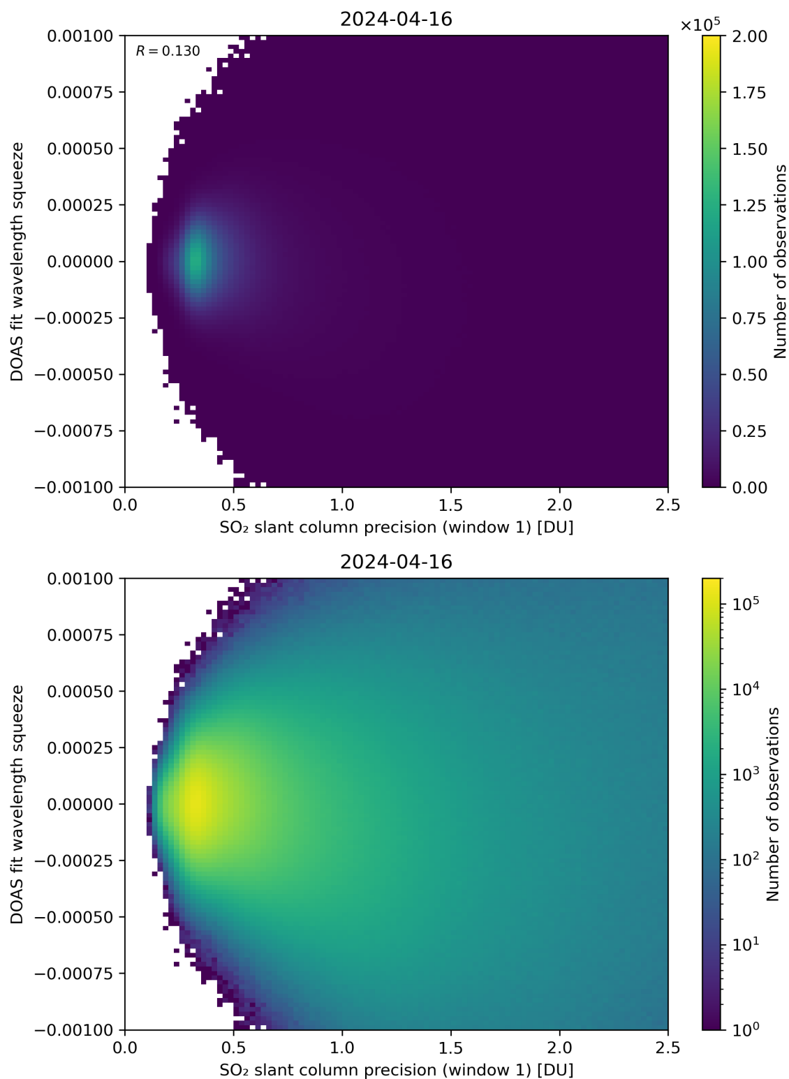
Figure 222: Scatter density plot of “SO 2 slant column precision (window 1)” against “DOAS fit wavelength squeeze” for 2024-04-16 to 2024-04-17.
