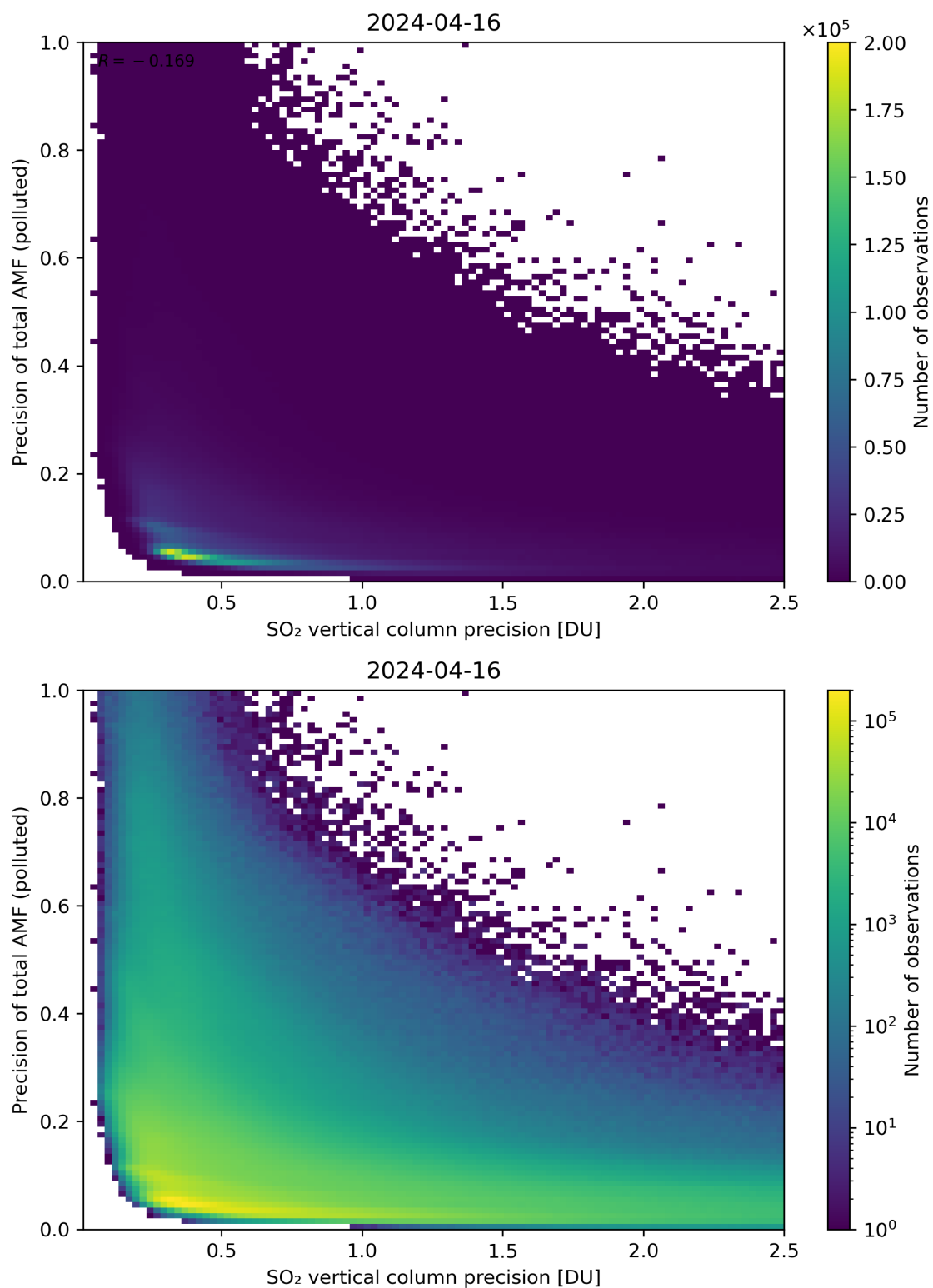
Figure 295: Scatter density plot of “SO 2 vertical column precision” against “Precision of total AMF (polluted)” for 2024-04-16 to 2024-04-17.
