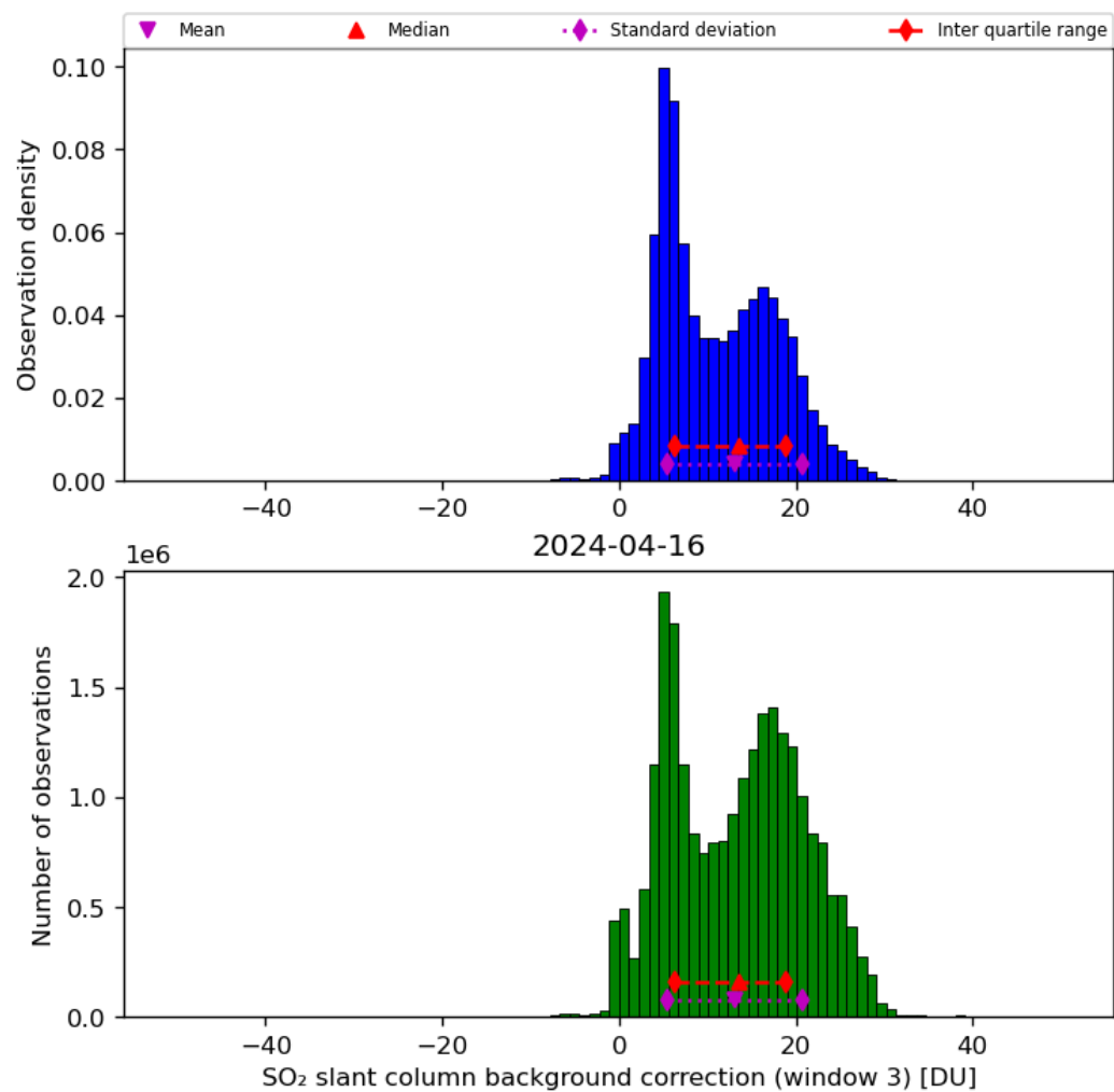
Figure 67: Histogram of “SO 2 slant column background correction (window 3)” for 2024-04-16 to 2024-04-17
