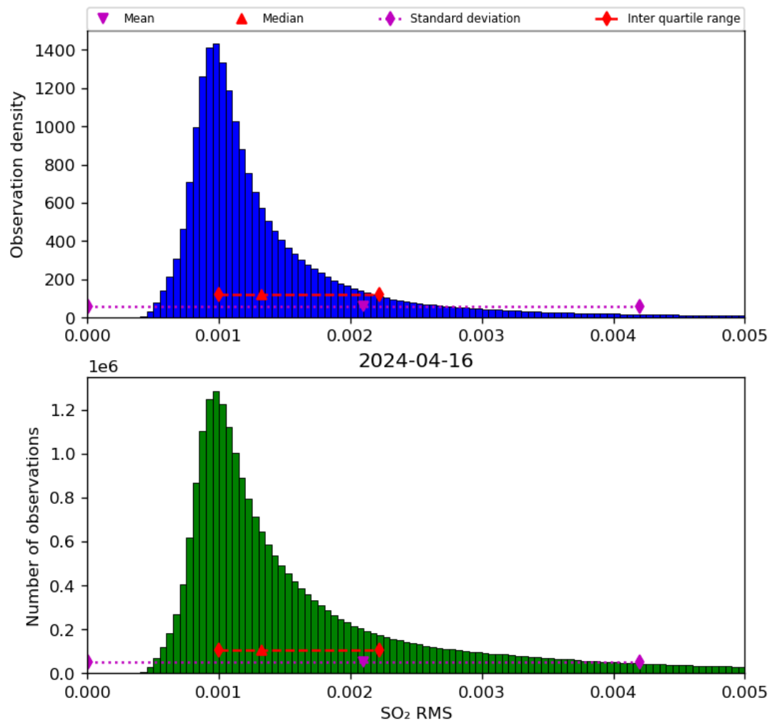
Figure 70: Histogram of “SO 2 RMS” for 2024-04-16 to 2024-04-17
