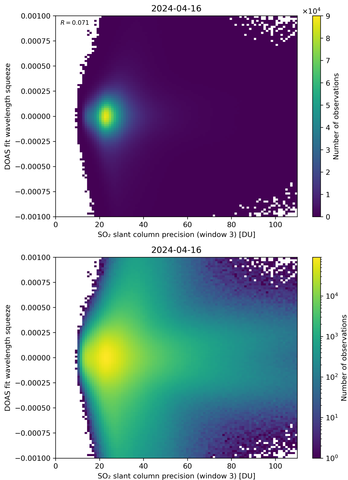
Figure 259: Scatter density plot of “SO 2 slant column precision (window 3)” against “DOAS fit wavelength squeeze” for 2024-04-16 to 2024-04-17.
