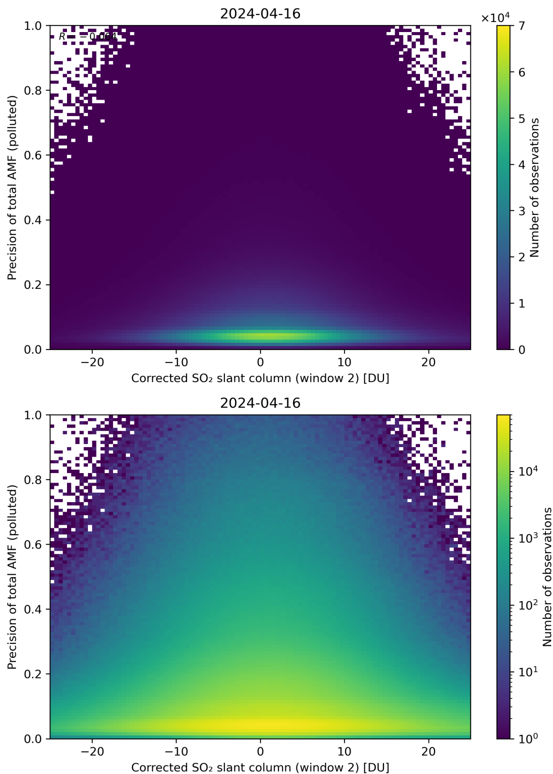
Figure 204: Scatter density plot of “Corrected SO 2 slant column (window 2)” against “Precision of total AMF (polluted)” for 2024-04-16 to 2024-04-17.
