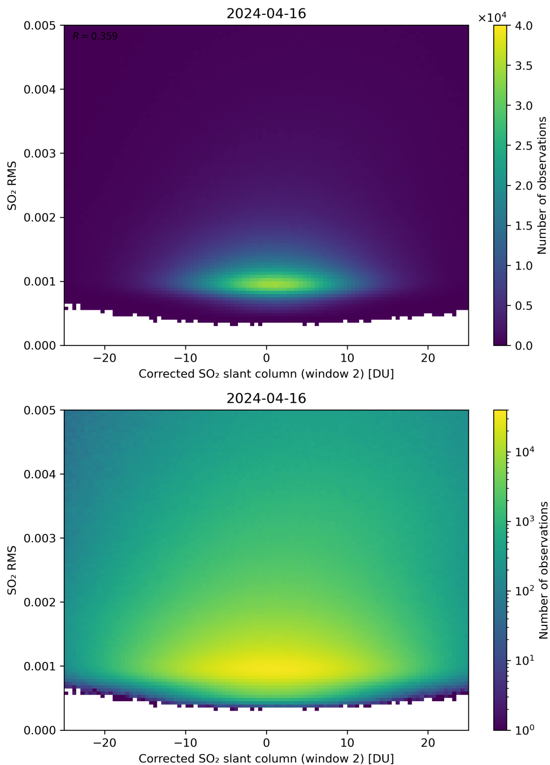
Figure 198: Scatter density plot of “Corrected SO 2 slant column (window 2)” against “SO 2 RMS” for 2024-04-16 to 2024-04-17.
