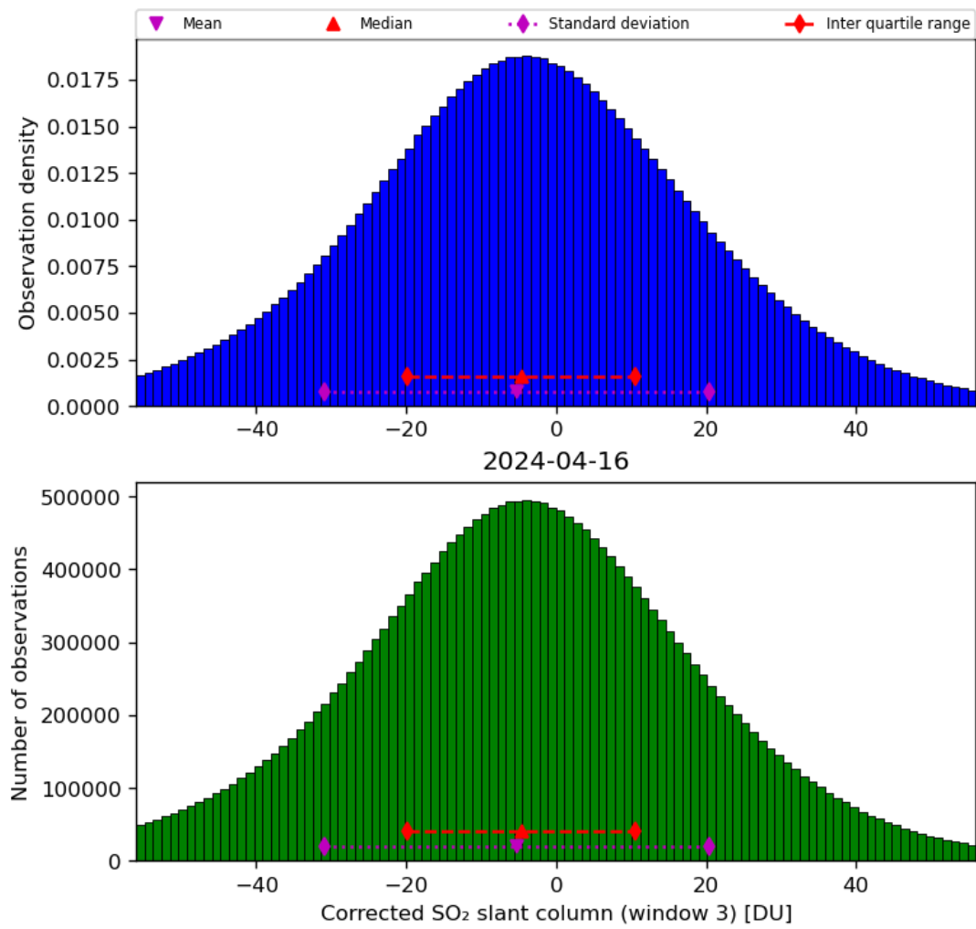
Figure 66: Histogram of “Corrected SO 2 slant column (window 3)” for 2024-04-16 to 2024-04-17
