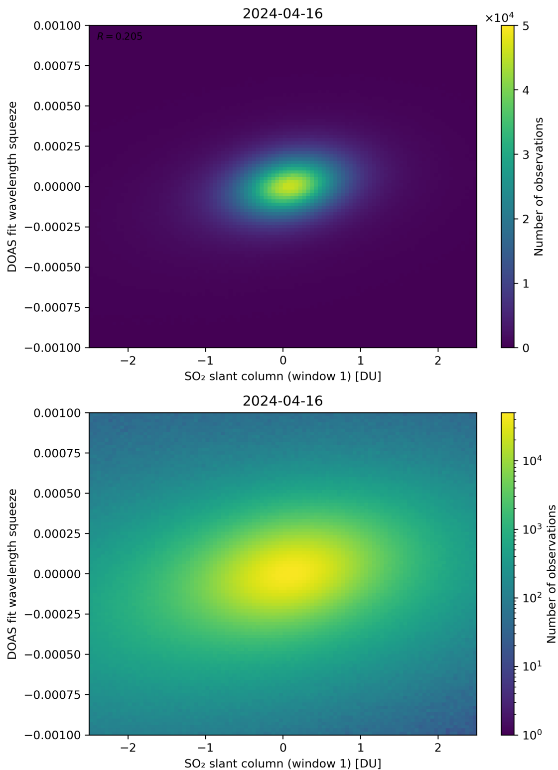
Figure 216: Scatter density plot of “SO 2 slant column (window 1)” against “DOAS fit wavelength squeeze” for 2024-04-16 to 2024-04-17.
