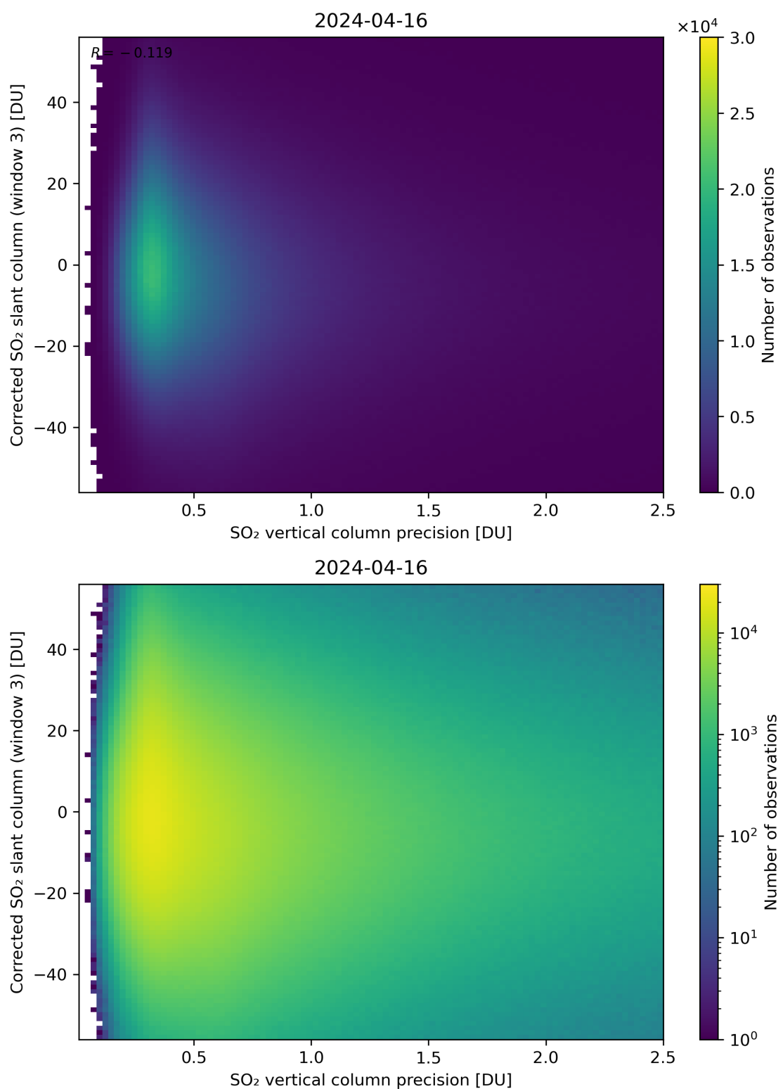
Figure 288: Scatter density plot of “SO 2 vertical column precision” against “Corrected SO 2 slant column (window 3)” for 2024-04-16 to 2024-04-17.
