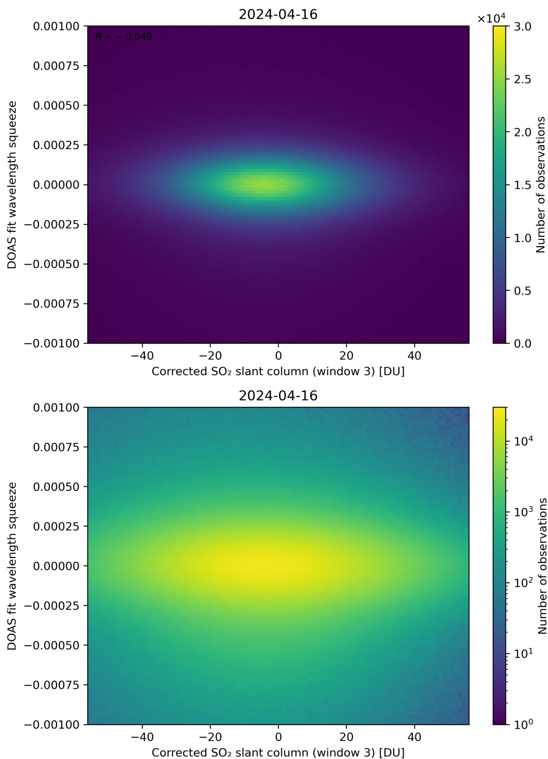
Figure 207: Scatter density plot of “Corrected SO 2 slant column (window 3)” against “DOAS fit wavelength squeeze” for 2024-04-16 to 2024-04-17.
