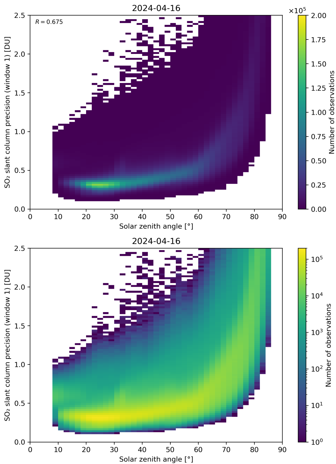
Figure 170: Scatter density plot of “Solar zenith angle” against “SO 2 slant column precision (window 1)” for 2024-04-16 to 2024-04-17.
