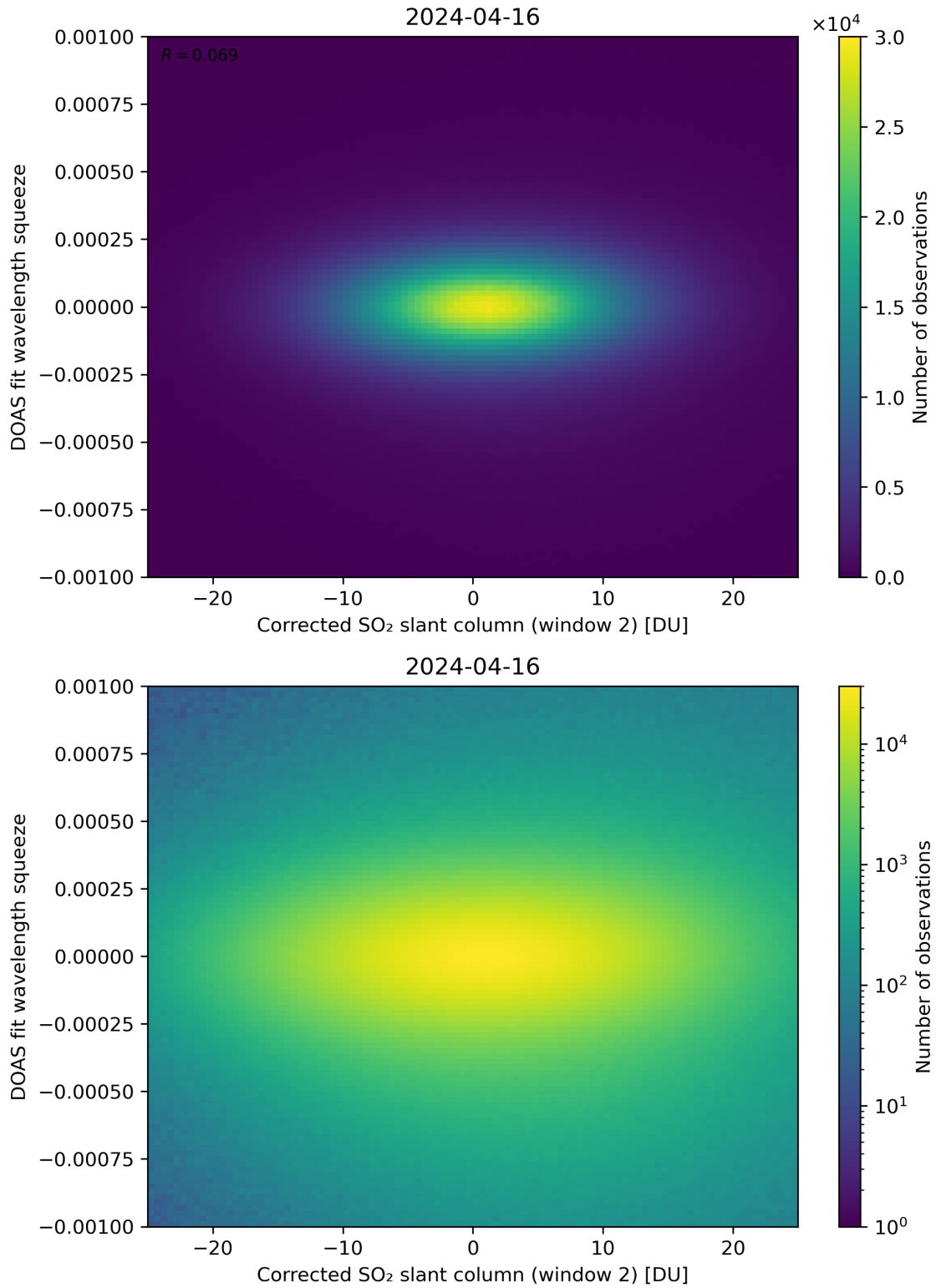
Figure 197: Scatter density plot of “Corrected SO 2 slant column (window 2)” against “DOAS fit wavelength squeeze” for 2024-04-16 to 2024-04-17.
