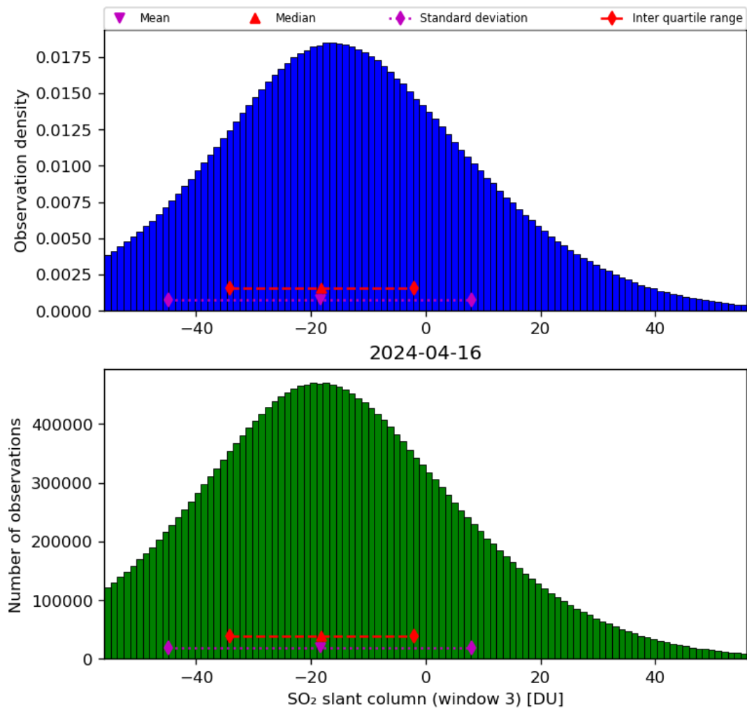
Figure 64: Histogram of “SO 2 slant column (window 3)” for 2024-04-16 to 2024-04-17
