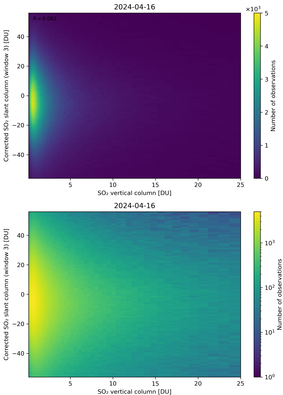
Figure 299: Scatter density plot of “SO 2 vertical column” against “Corrected SO 2 slant column (window 3)” for 2024-04-16 to 2024-04-17.
