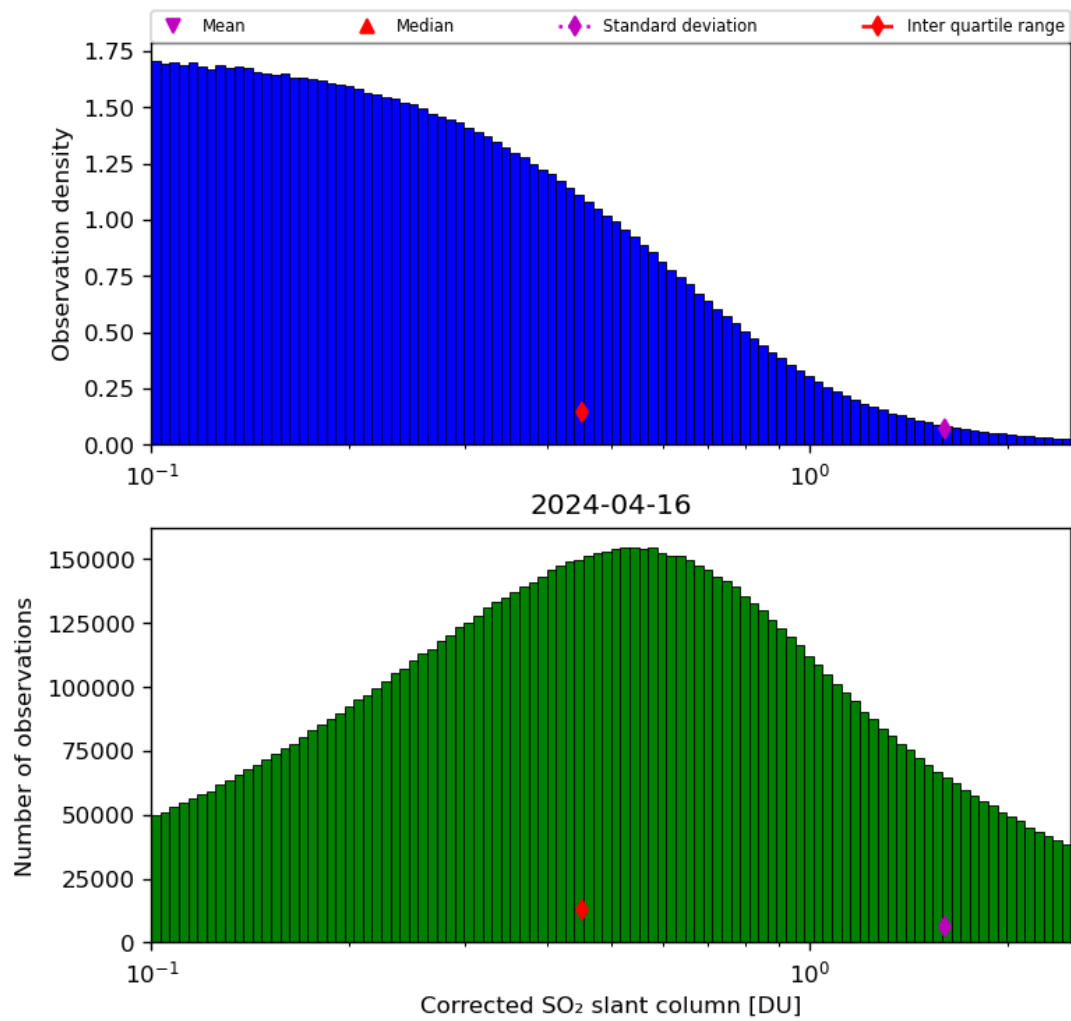
Figure 55: Histogram of “Corrected SO 2 slant column” for 2024-04-16 to 2024-04-17
