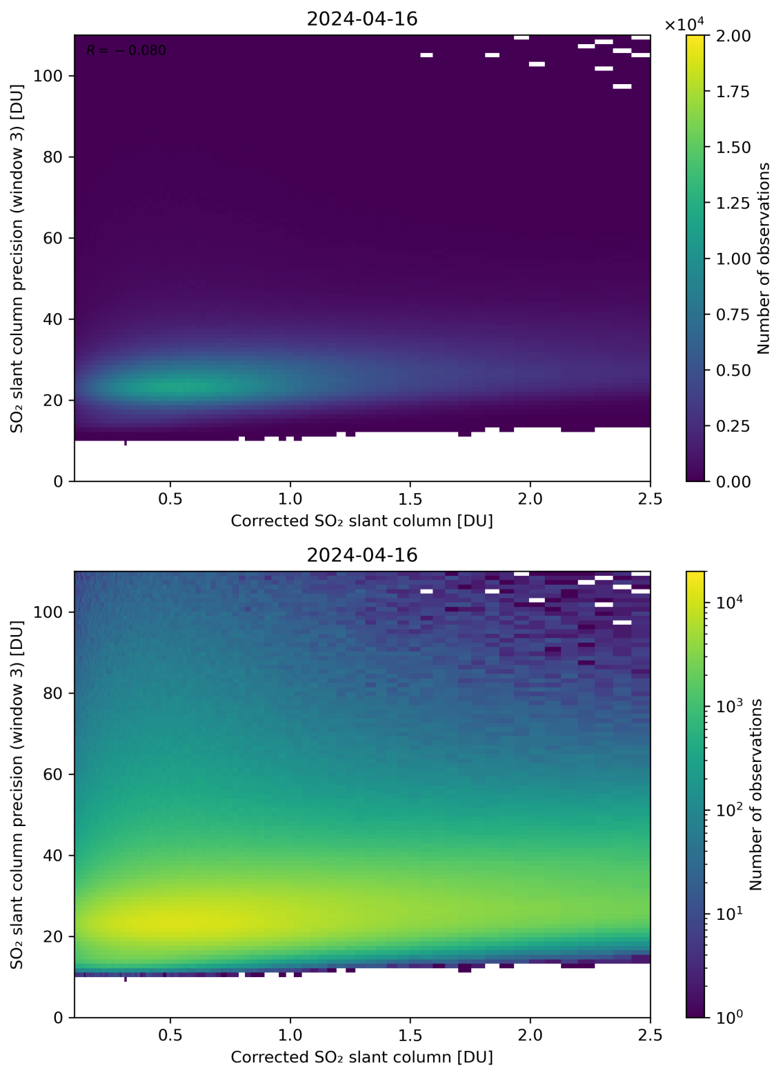
Figure 191: Scatter density plot of “Corrected SO 2 slant column” against “SO 2 slant column precision (window 3)” for 2024-04-16 to 2024-04-17.
