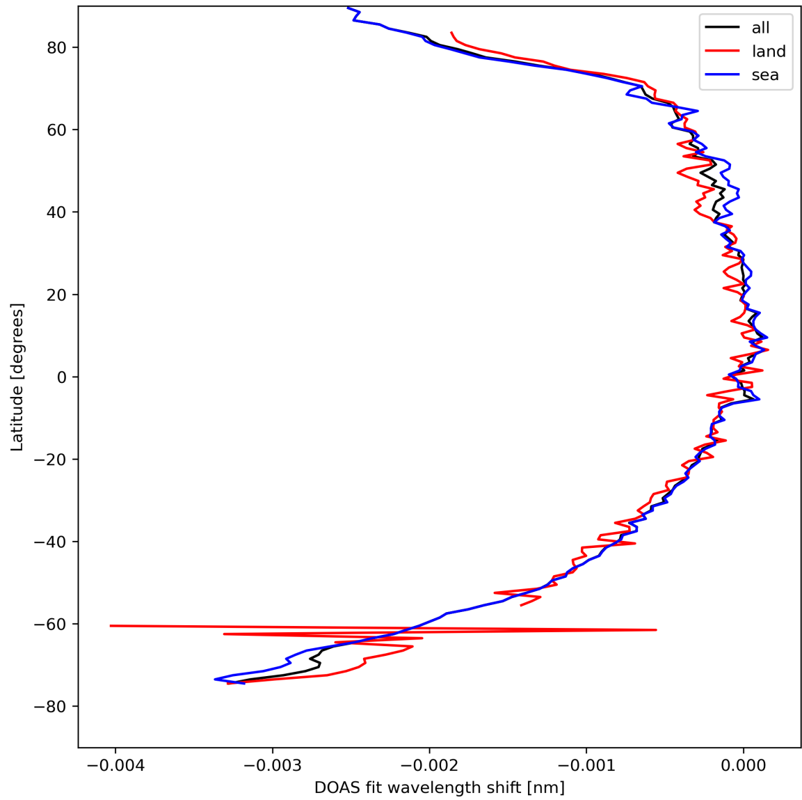
Figure 45: Zonal average of "DOAS fit wavelength shift" for 2024-04-16 to 2024-04-17.
