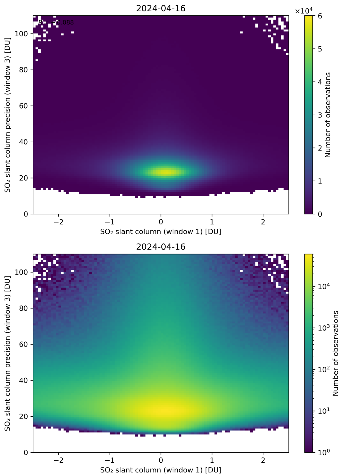
Figure 238: Scatter density plot of “SO 2 slant column (window 1)” against “SO 2 slant column precision (window 3)” for 2024-04-16 to 2024-04-17.
