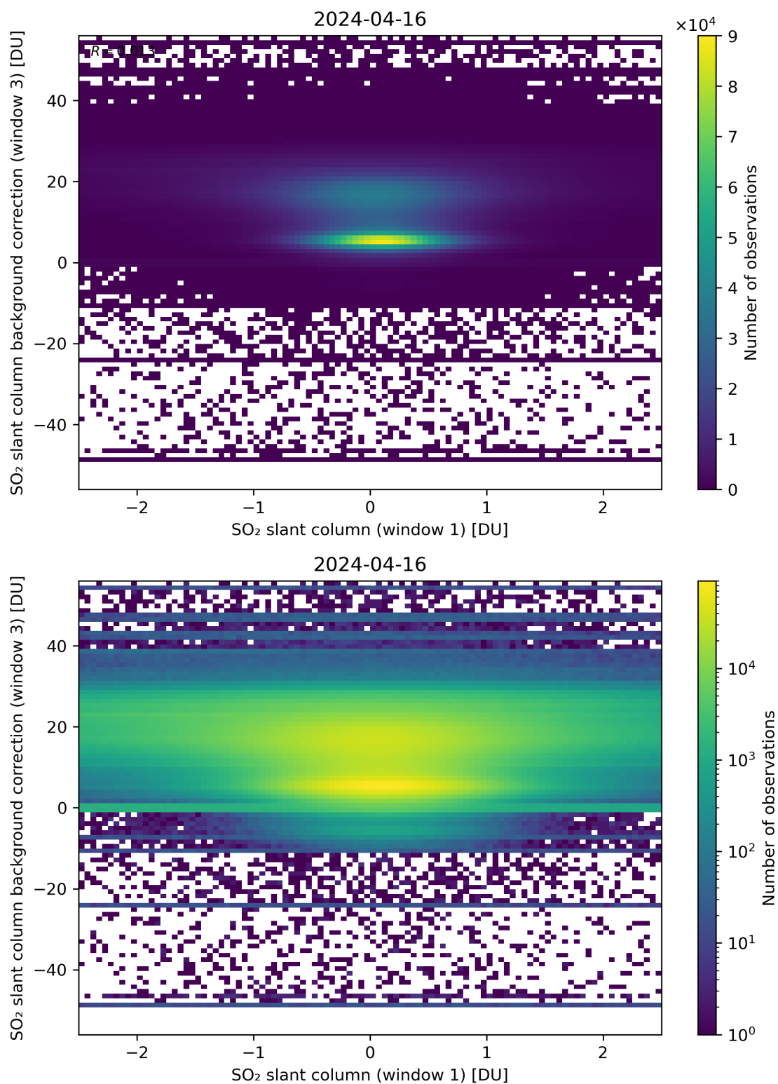
Figure 214: Scatter density plot of “SO 2 slant column (window 1)” against “SO 2 slant column background correction (window 3)” for 2024-04-16 to 2024-04-17.
