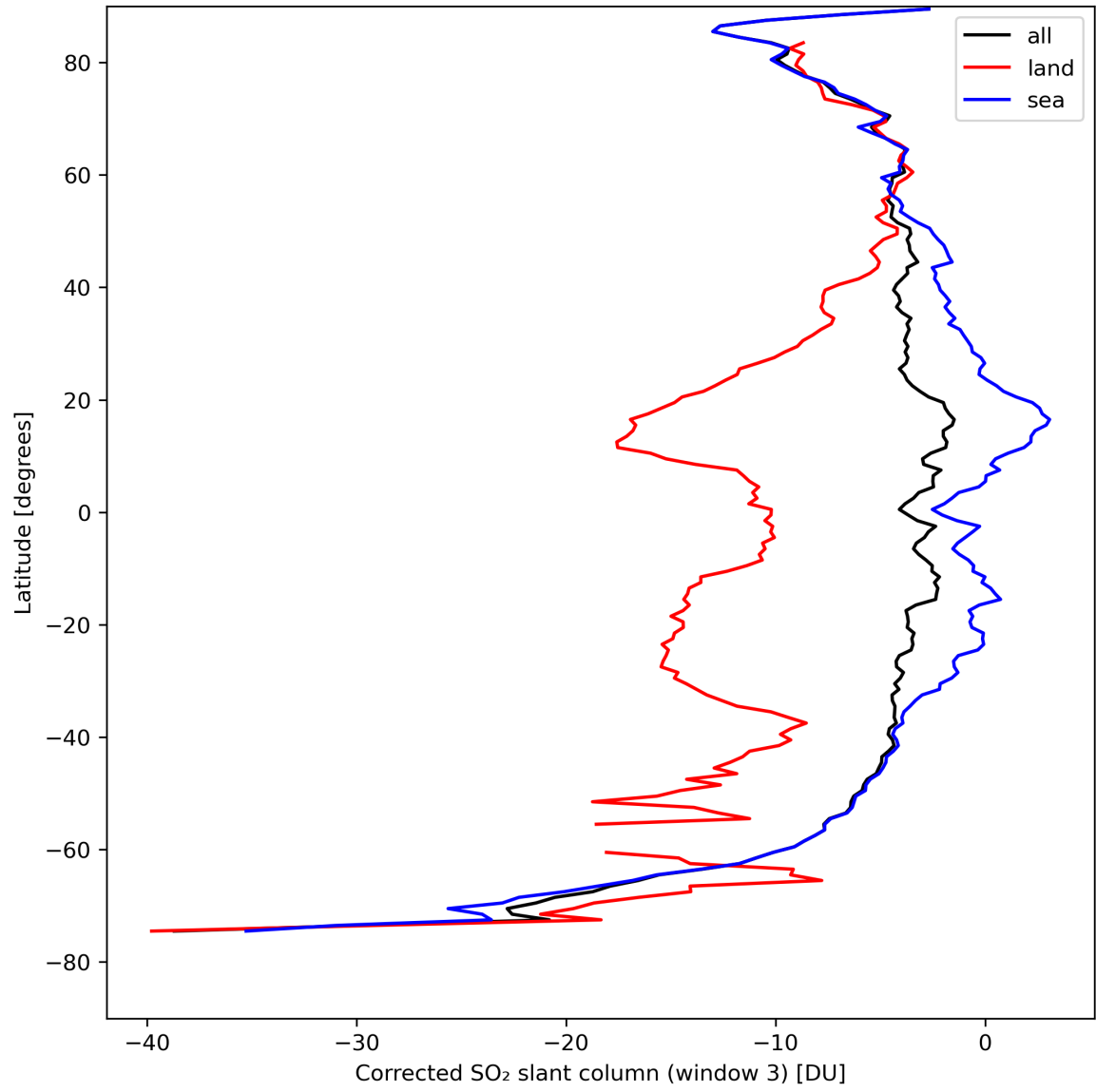
Figure 43: Zonal average of “Corrected SO 2 slant column (window 3)” for 2024-04-16 to 2024-04-17.
