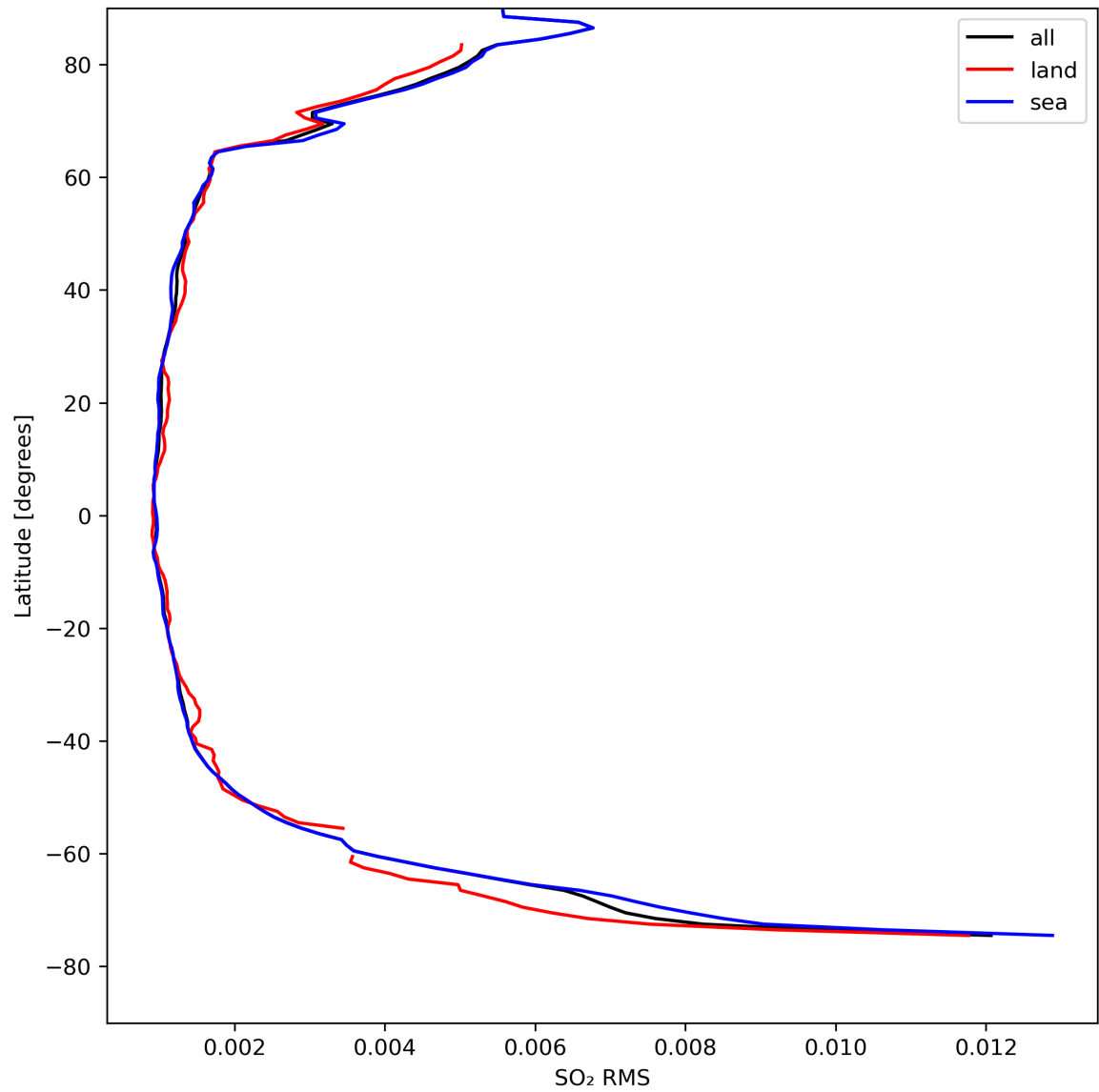
Figure 47: Zonal average of “SO 2 RMS” for 2024-04-16 to 2024-04-17.
