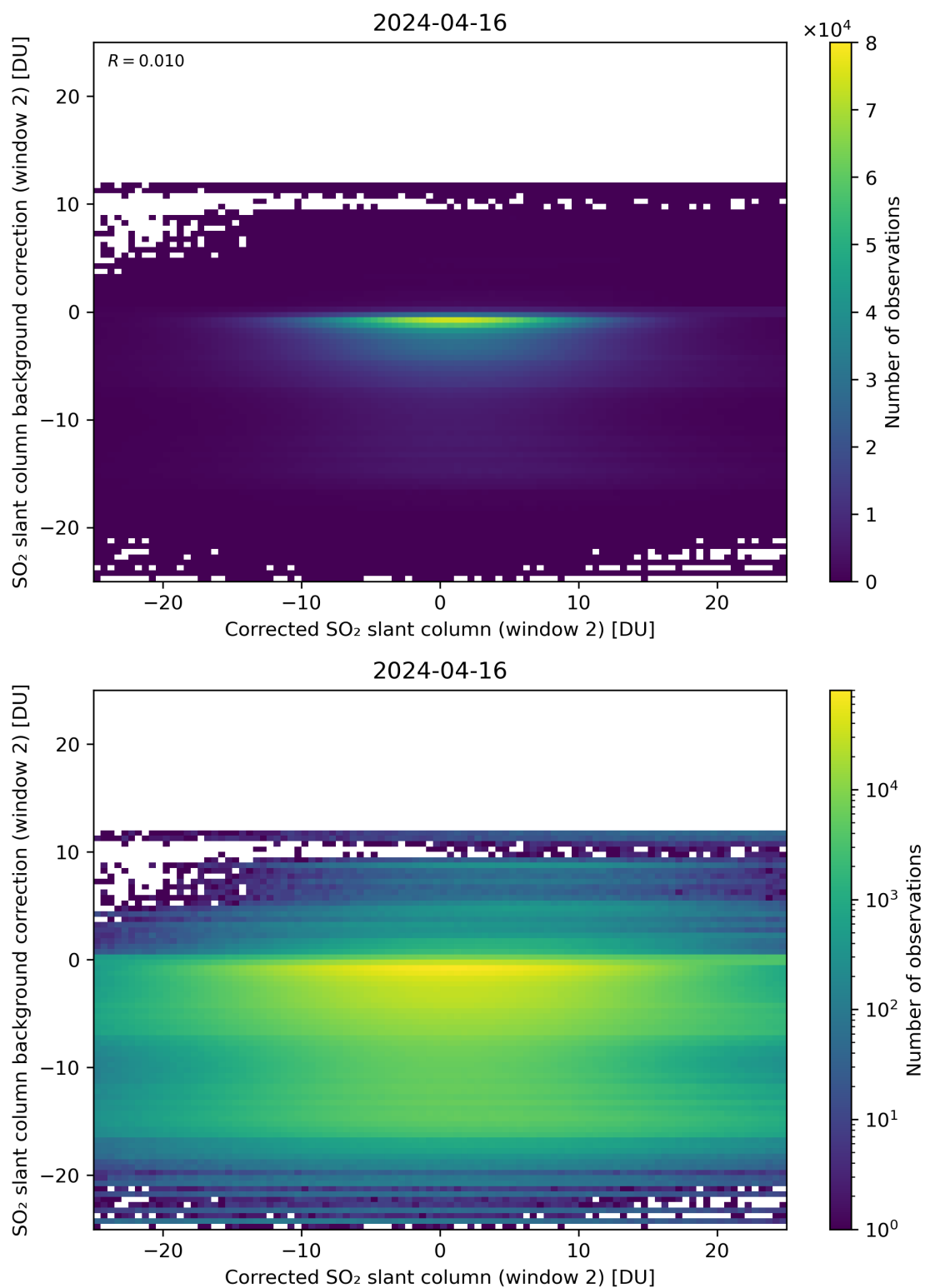
Figure 194: Scatter density plot of “Corrected SO 2 slant column (window 2)” against “SO 2 slant column background correction (window 2)” for 2024-04-16 to 2024-04-17.
