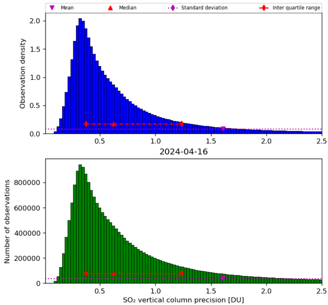
Figure 54: Histogram of “SO 2 vertical column precision” for 2024-04-16 to 2024-04-17
