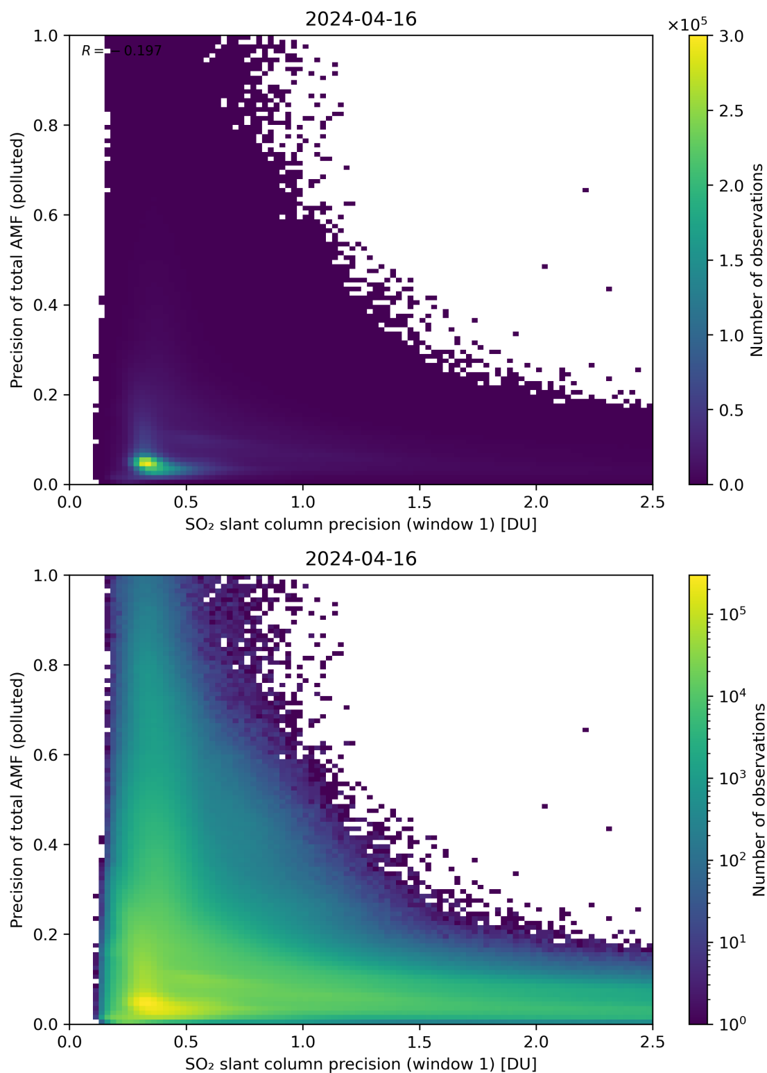
Figure 231: Scatter density plot of “SO 2 slant column precision (window 1)” against “Precision of total AMF (polluted)” for 2024-04-16 to 2024-04-17.
