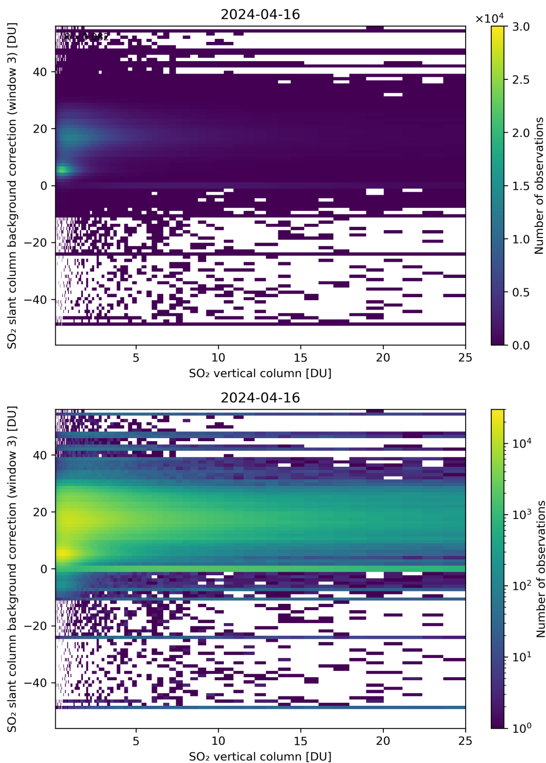
Figure 275: Scatter density plot of “SO 2 vertical column” against “SO 2 slant column background correction (window 3)” for 2024-04-16 to 2024-04-17.
