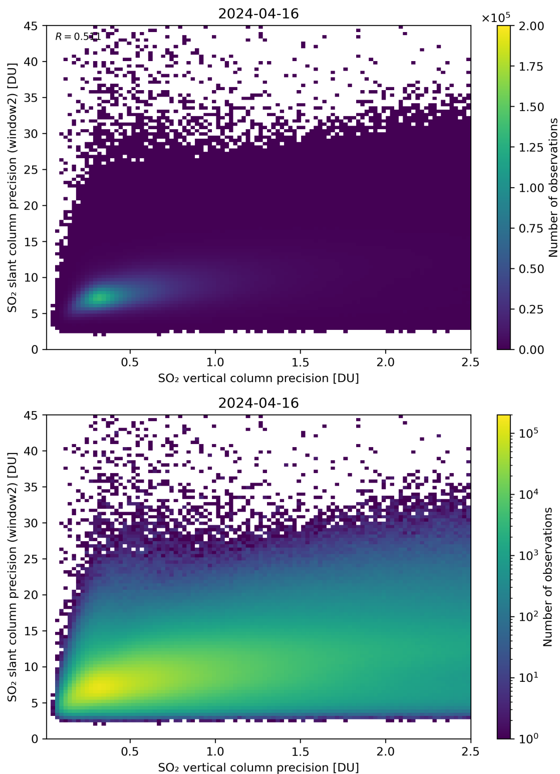
Figure 291: Scatter density plot of “SO 2 vertical column precision” against “SO 2 slant column precision (window2)” for 2024-04-16 to 2024-04-17.
