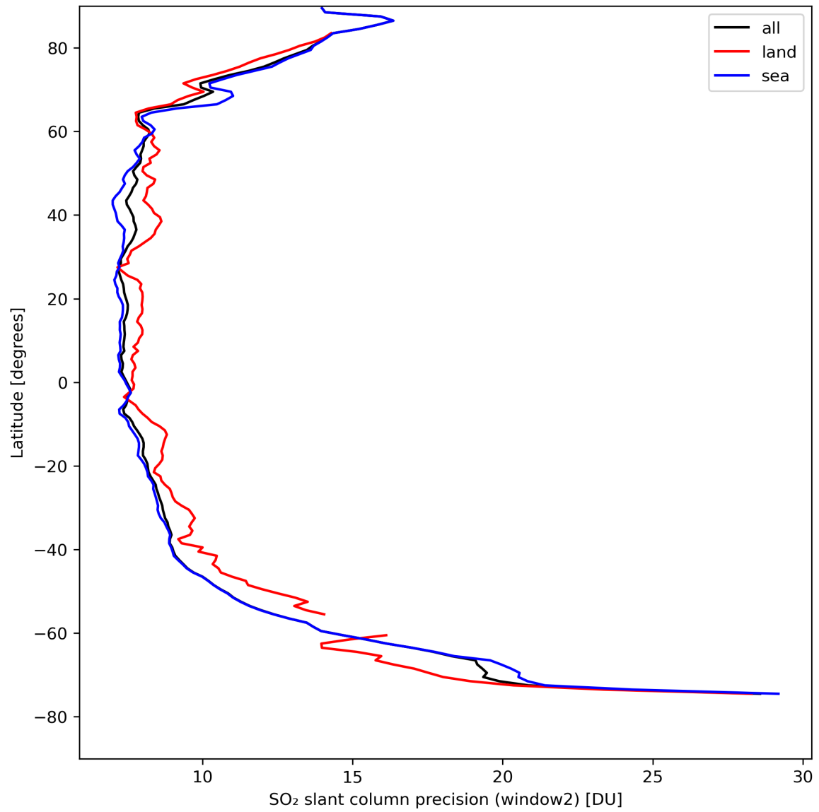
Figure 38: Zonal average of “SO 2 slant column precision (window2)” for 2024-04-16 to 2024-04-17.
