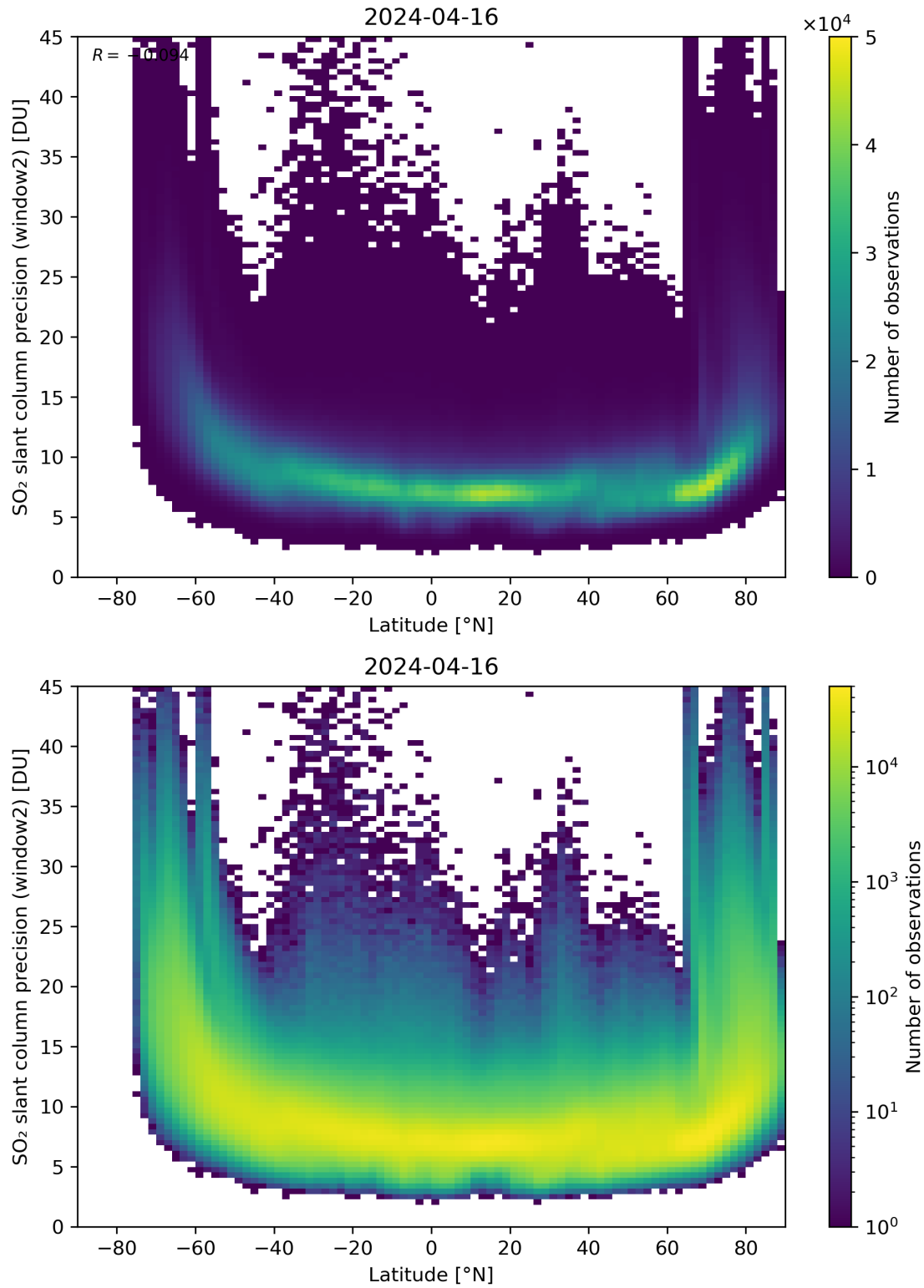
Figure 151: Scatter density plot of “Latitude” against “SO 2 slant column precision (window2)” for 2024-04-16 to 2024-04-17.
