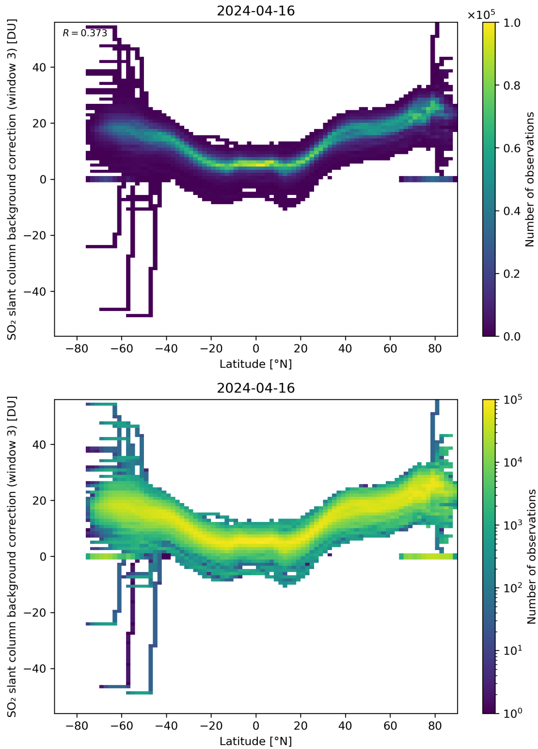
Figure 141: Scatter density plot of “Latitude” against “SO 2 slant column background correction (window 3)” for 2024-04-16 to 2024-04-17.
