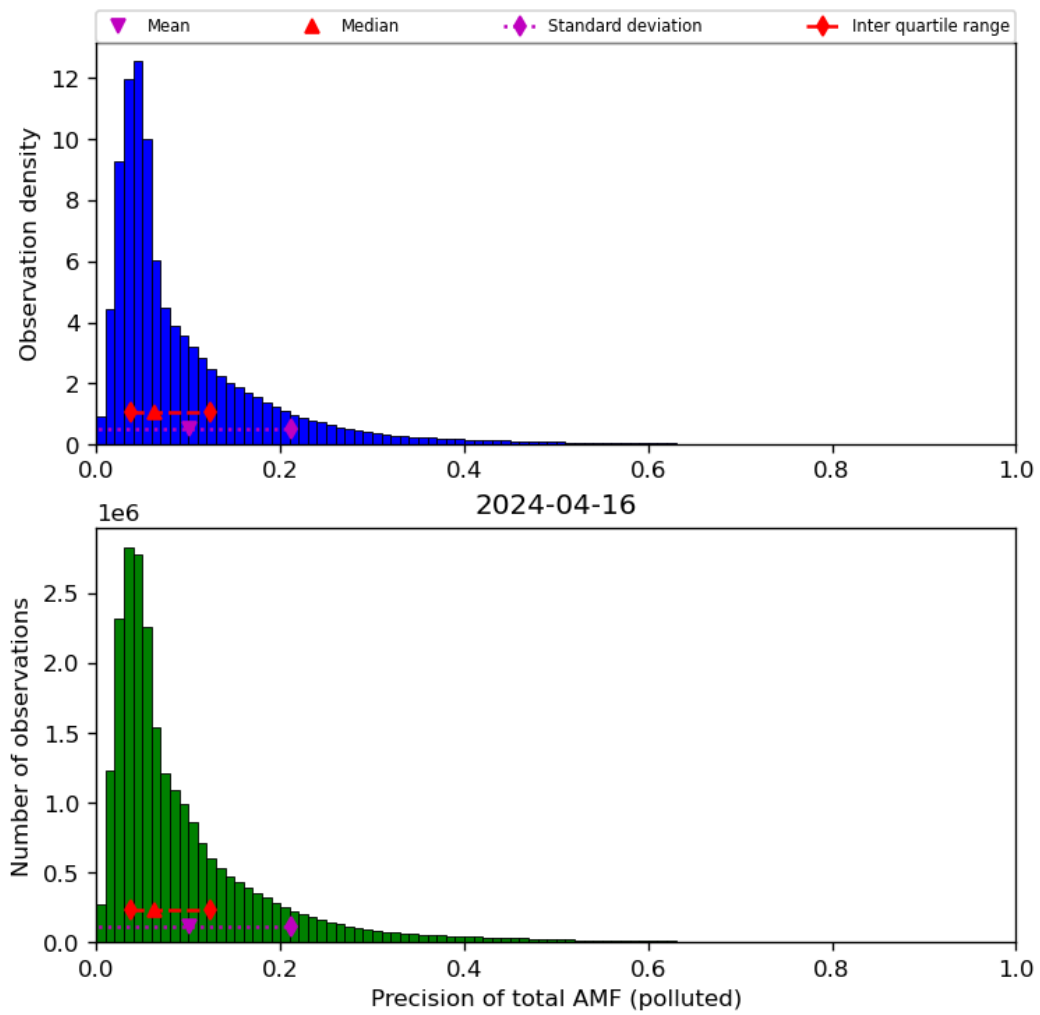
Figure 72: Histogram of “Precision of total AMF (polluted)” for 2024-04-16 to 2024-04-17
