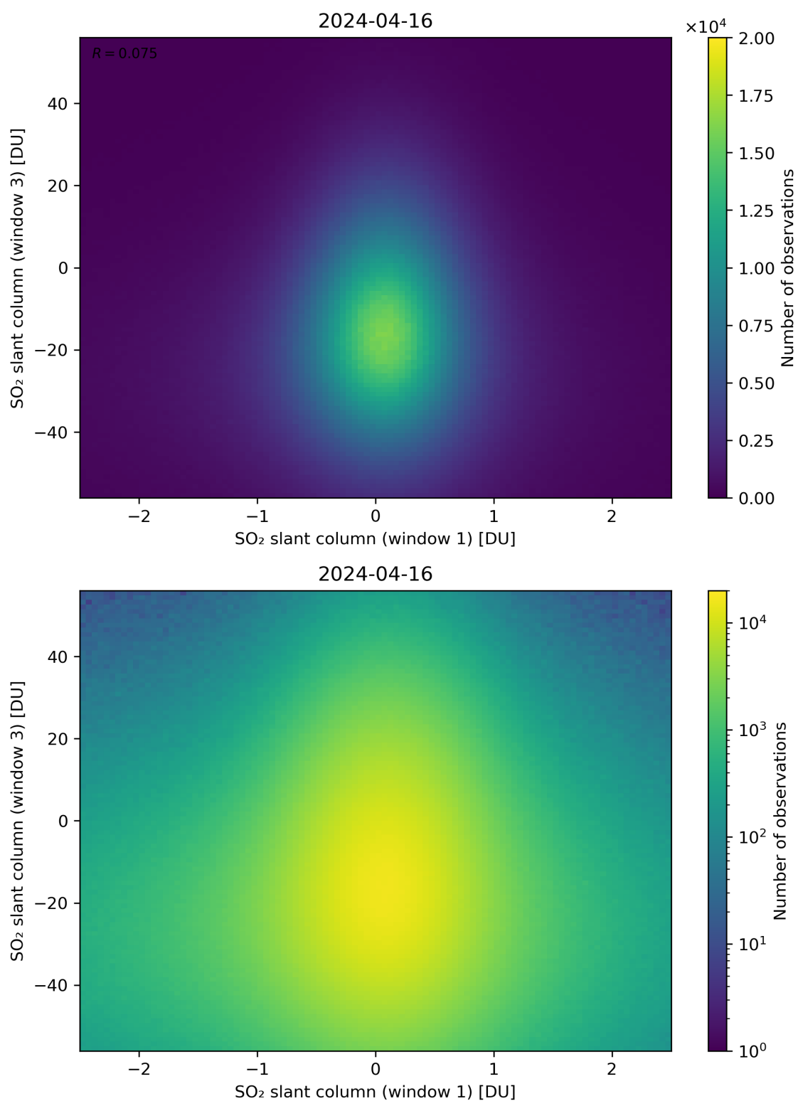
Figure 237: Scatter density plot of “SO 2 slant column (window 1)” against “SO 2 slant column (window 3)” for 2024-04-16 to 2024-04-17.
