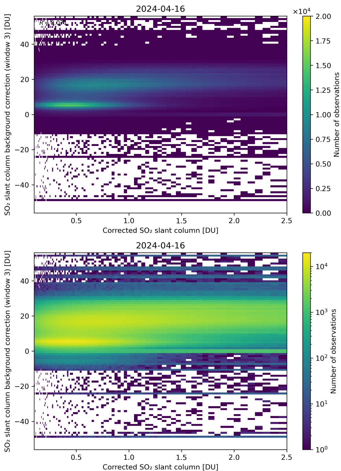
Figure 180: Scatter density plot of “Corrected SO 2 slant column” against “SO 2 slant column background correction (window 3)” for 2024-04-16 to 2024-04-17.
