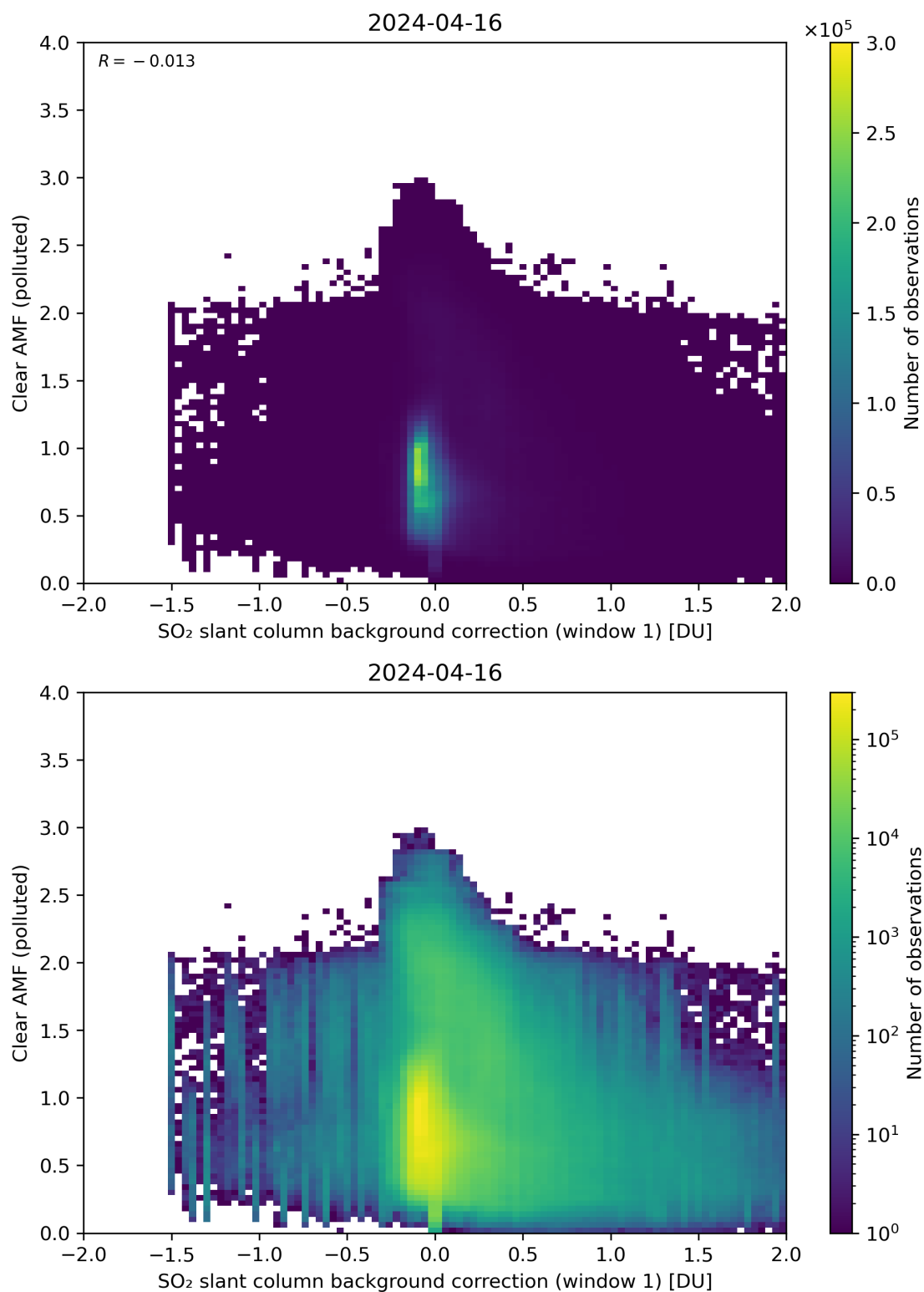
Figure 103: Scatter density plot of “SO 2 slant column background correction (window 1)” against “Clear AMF (polluted)” for 2024-04-16 to 2024-04-17.
