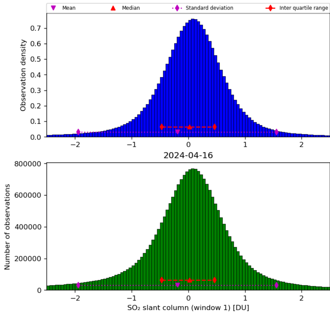
Figure 56: Histogram of “SO 2 slant column (window 1)” for 2024-04-16 to 2024-04-17
