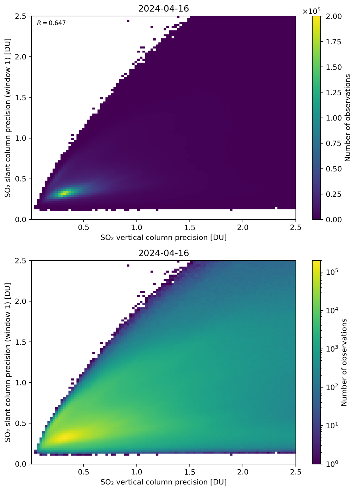
Figure 290: Scatter density plot of “SO 2 vertical column precision” against “SO 2 slant column precision (window 1)” for 2024-04-16 to 2024-04-17.
