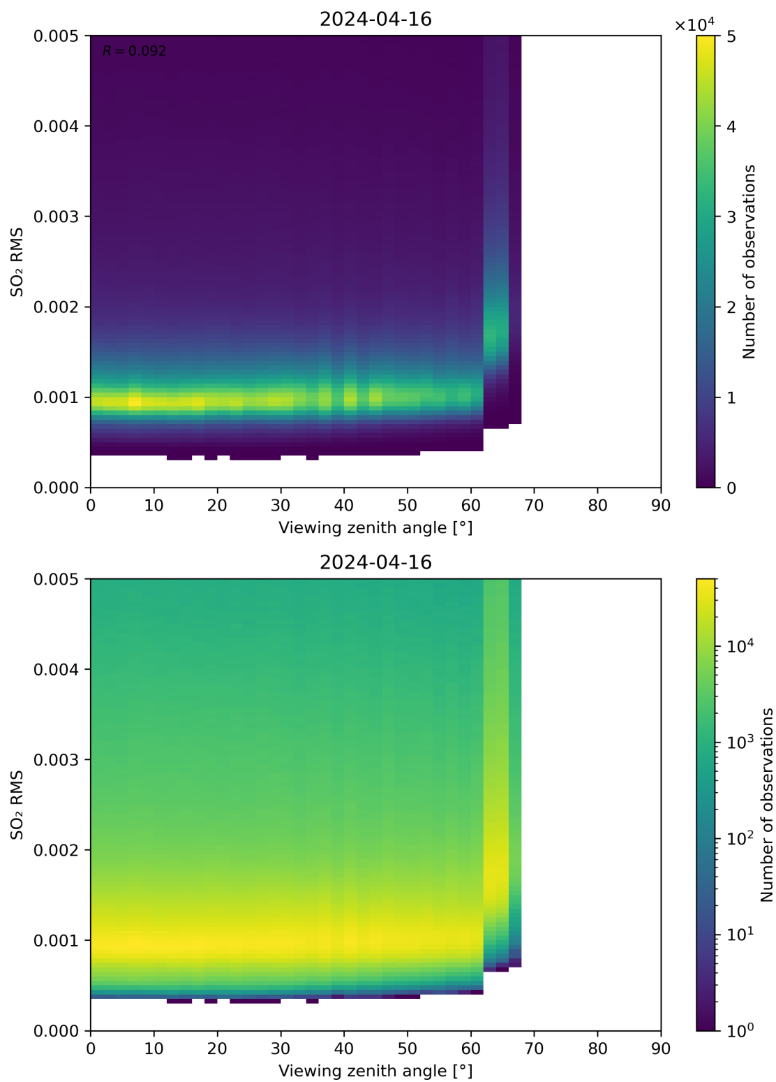
Figure 313: Scatter density plot of “Viewing zenith angle” against “SO 2 RMS” for 2024-04-16 to 2024-04-17.
