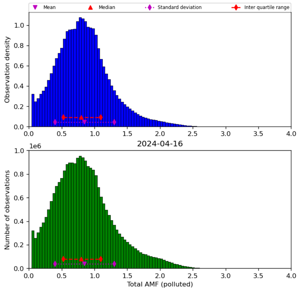
Figure 71: Histogram of “Total AMF (polluted)” for 2024-04-16 to 2024-04-17
