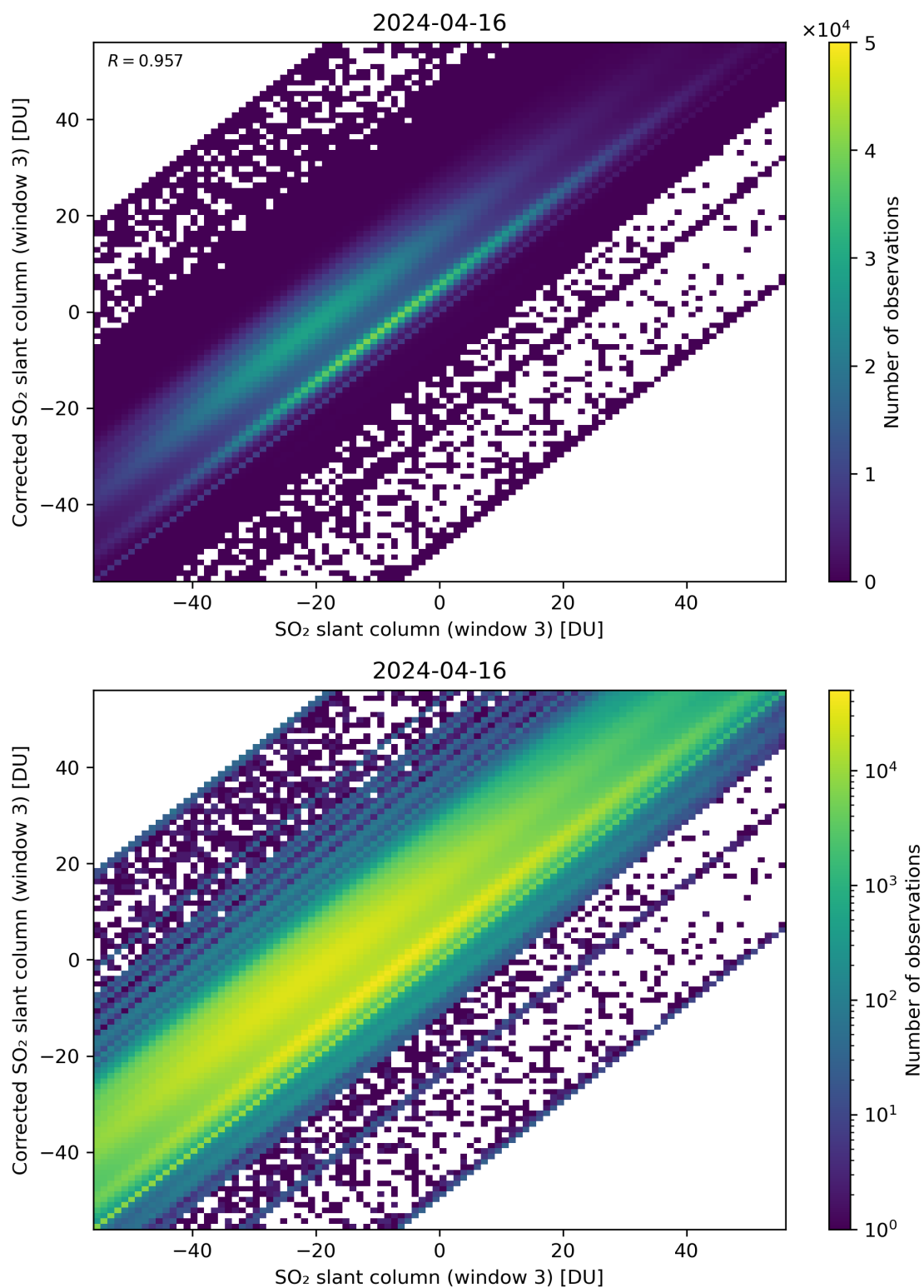
Figure 266: Scatter density plot of “SO 2 slant column (window 3)” against “Corrected SO 2 slant column (window 3)” for 2024-04-16 to 2024-04-17.
