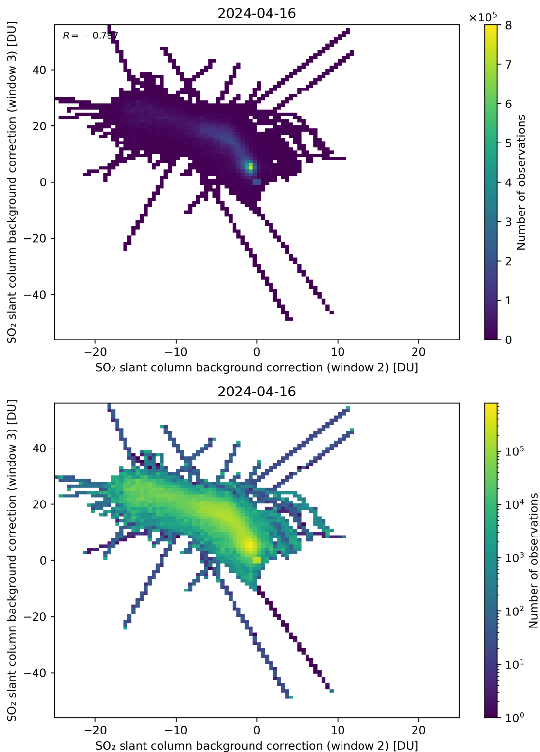
Figure 111: Scatter density plot of “SO 2 slant column background correction (window 2)” against “SO 2 slant column background correction (window 3)” for 2024-04-16 to 2024-04-17.
