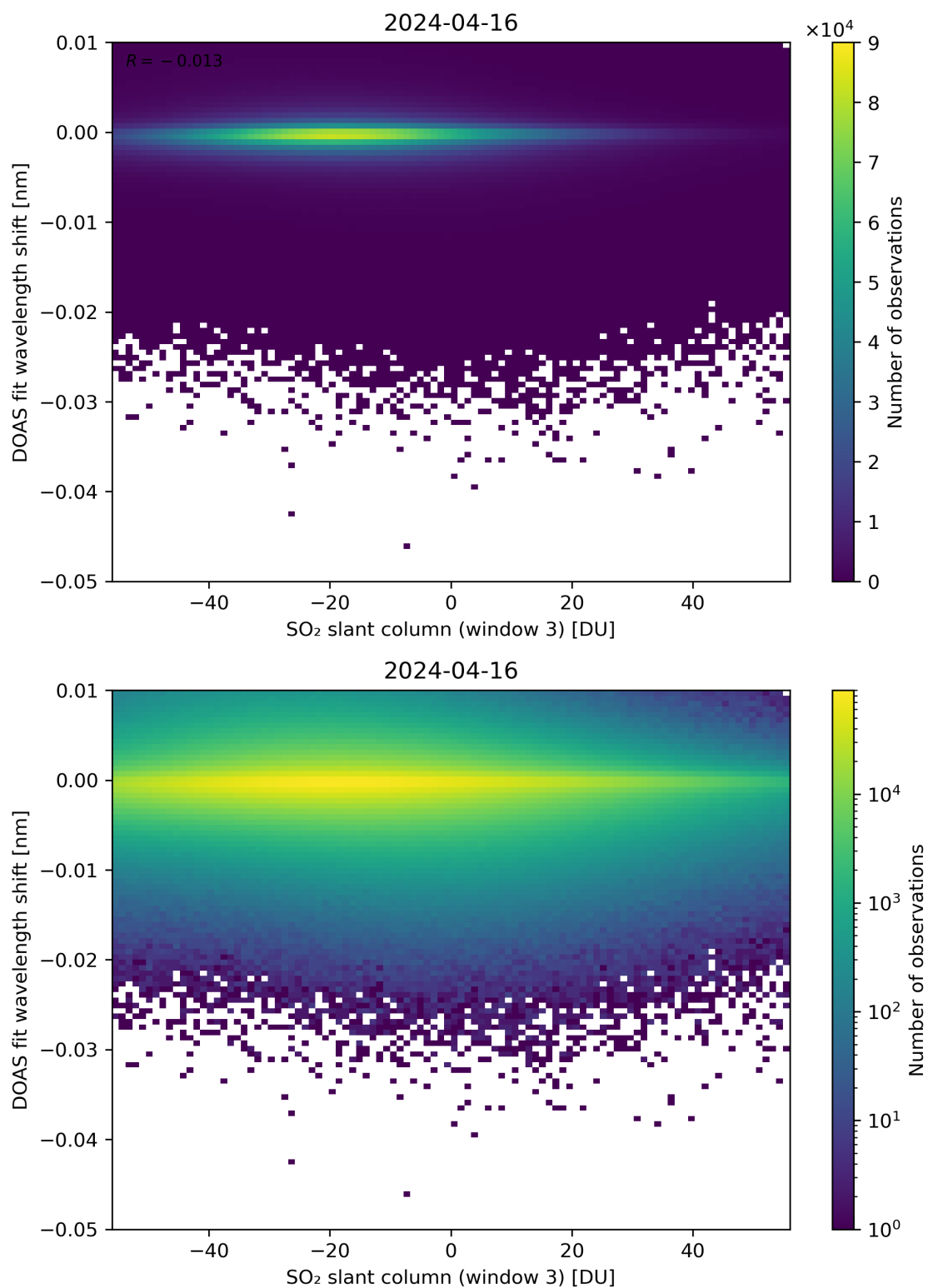
Figure 254: Scatter density plot of “SO 2 slant column (window 3)” against “DOAS fit wavelength shift” for 2024-04-16 to 2024-04-17.
