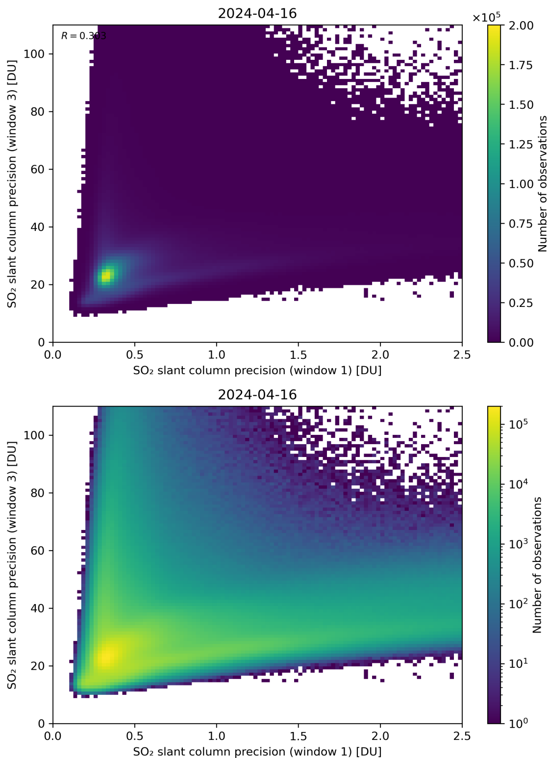
Figure 229: Scatter density plot of “SO 2 slant column precision (window 1)” against “SO 2 slant column precision (window 3)” for 2024-04-16 to 2024-04-17.
