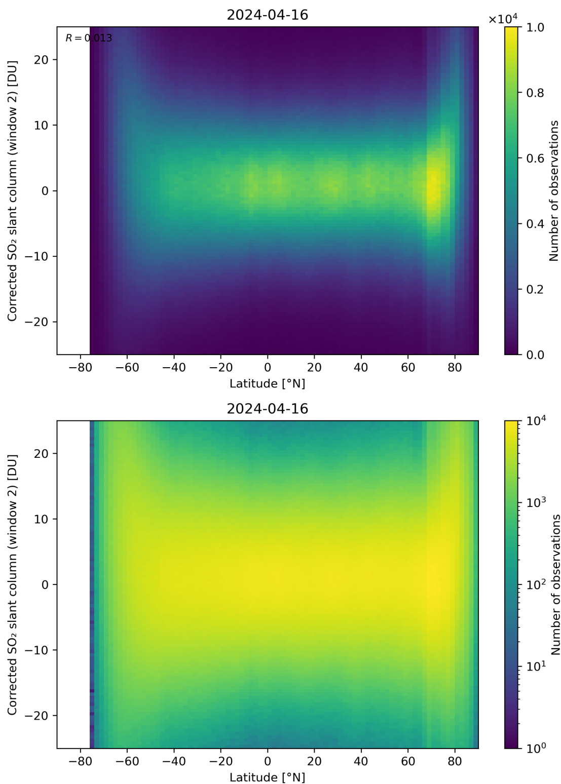
Figure 147: Scatter density plot of “Latitude” against “Corrected SO 2 slant column (window 2)” for 2024-04-16 to 2024-04-17.
