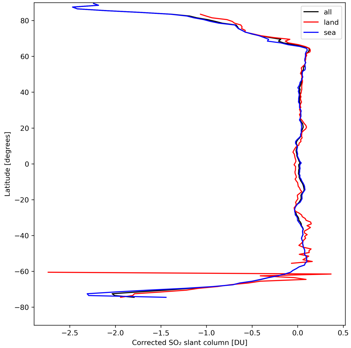
Figure 32: Zonal average of "Corrected SO 2 slant column" for 2024-04-16 to 2024-04-17.
