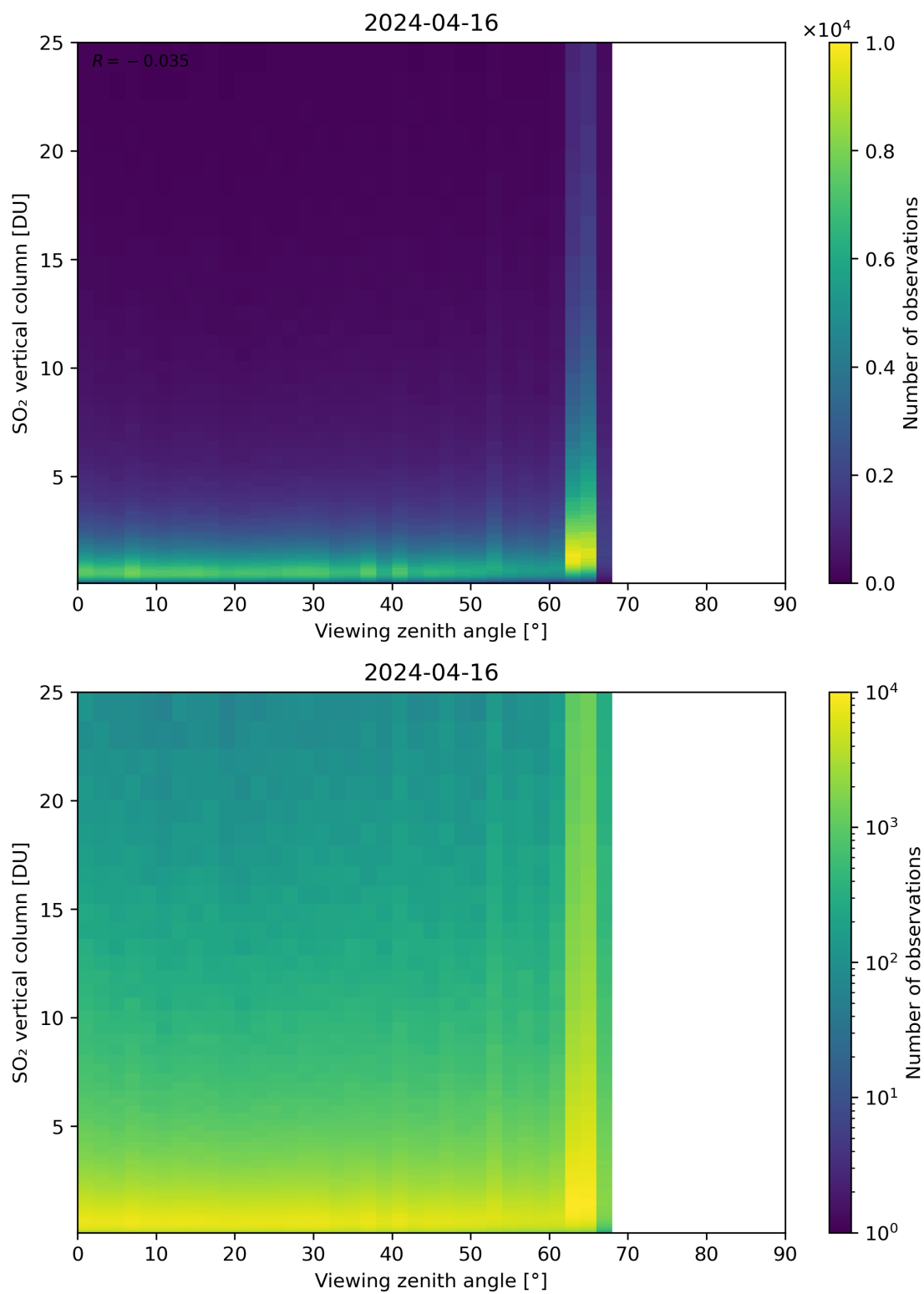
Figure 327: Scatter density plot of “Viewing zenith angle” against “SO 2 vertical column” for 2024-04-16 to 2024-04-17.
