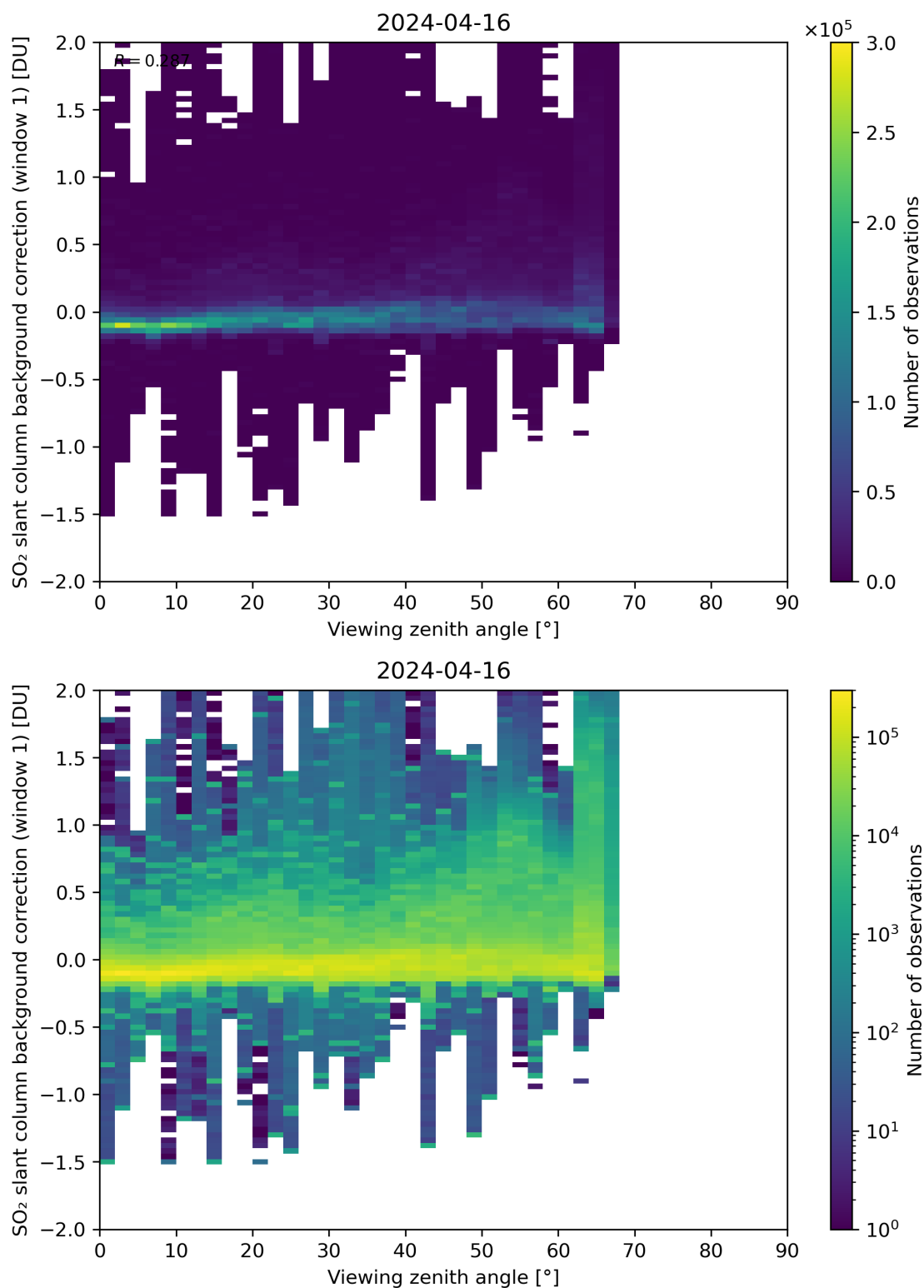
Figure 308: Scatter density plot of “Viewing zenith angle” against “SO 2 slant column background correction (window 1)” for 2024-04-16 to 2024-04-17.
