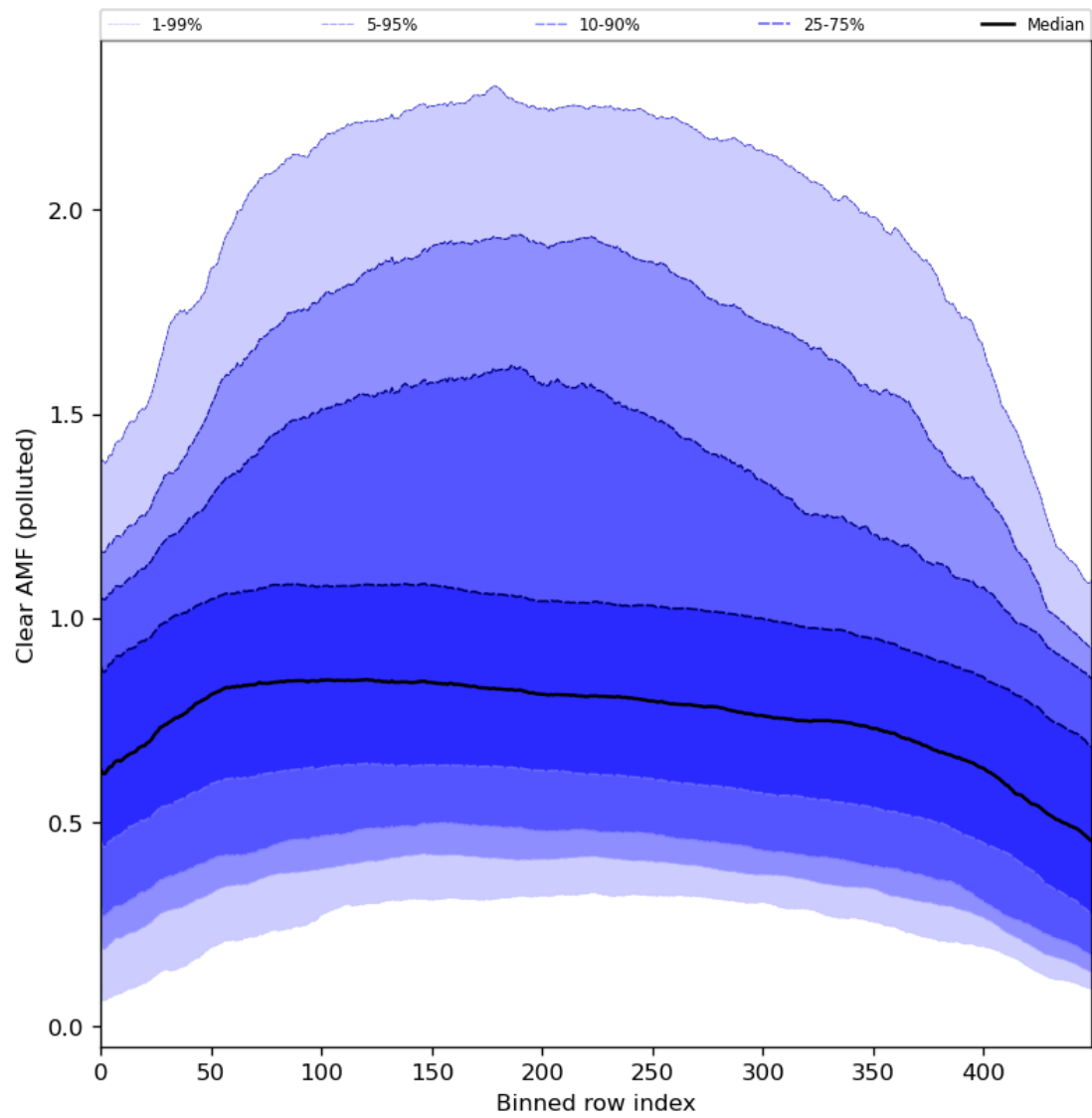
Figure 96: Along track statistics of “Clear AMF (polluted)” for 2024-04-16 to 2024-04-17
