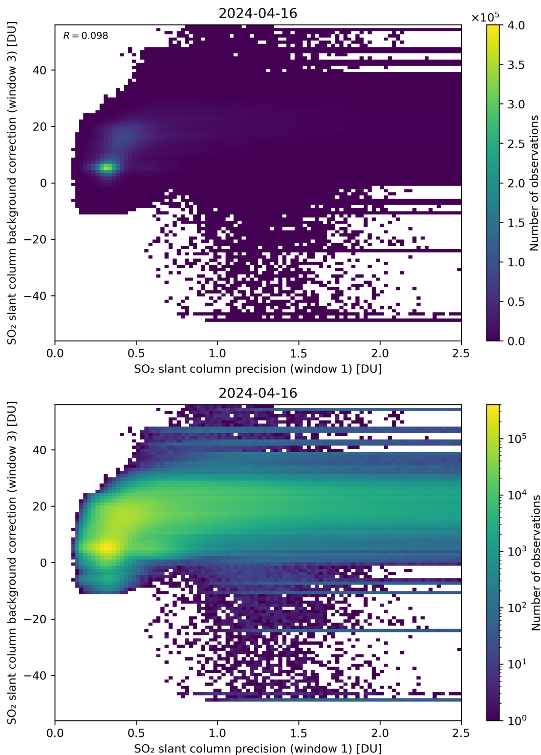
Figure 220: Scatter density plot of “SO 2 slant column precision (window 1)” against “SO 2 slant column background correction (window 3)” for 2024-04-16 to 2024-04-17.
