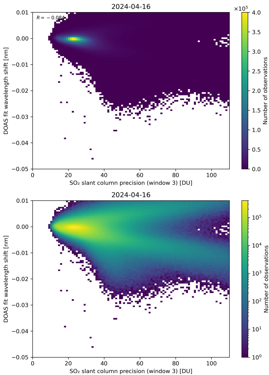
Figure 258: Scatter density plot of “SO 2 slant column precision (window 3)” against “DOAS fit wavelength shift” for 2024-04-16 to 2024-04-17.
