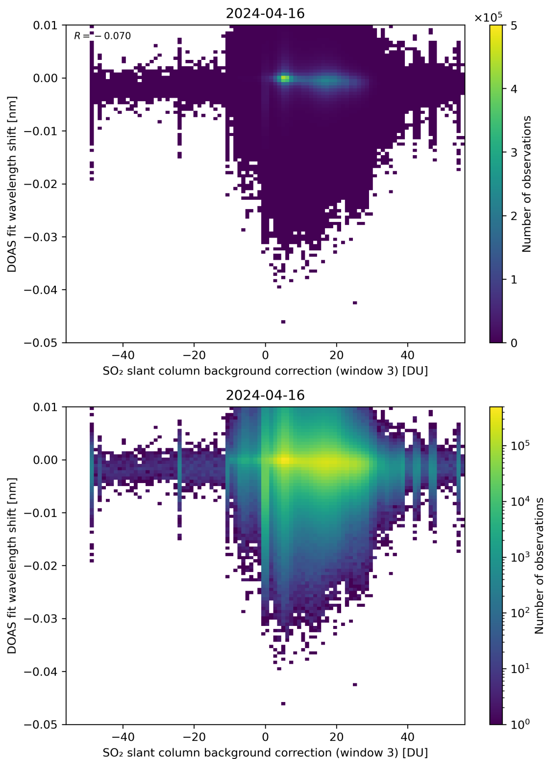
Figure 121: Scatter density plot of “SO 2 slant column background correction (window 3)” against “DOAS fit wavelength shift” for 2024-04-16 to 2024-04-17.
