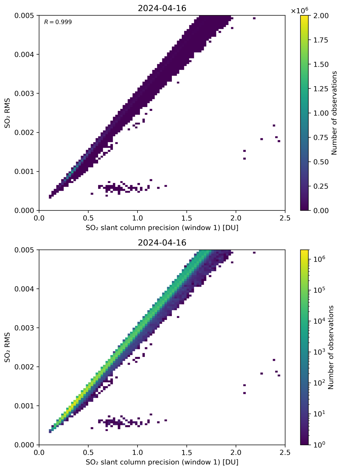
Figure 223: Scatter density plot of “SO 2 slant column precision (window 1)” against “SO 2 RMS” for 2024-04-16 to 2024-04-17.
