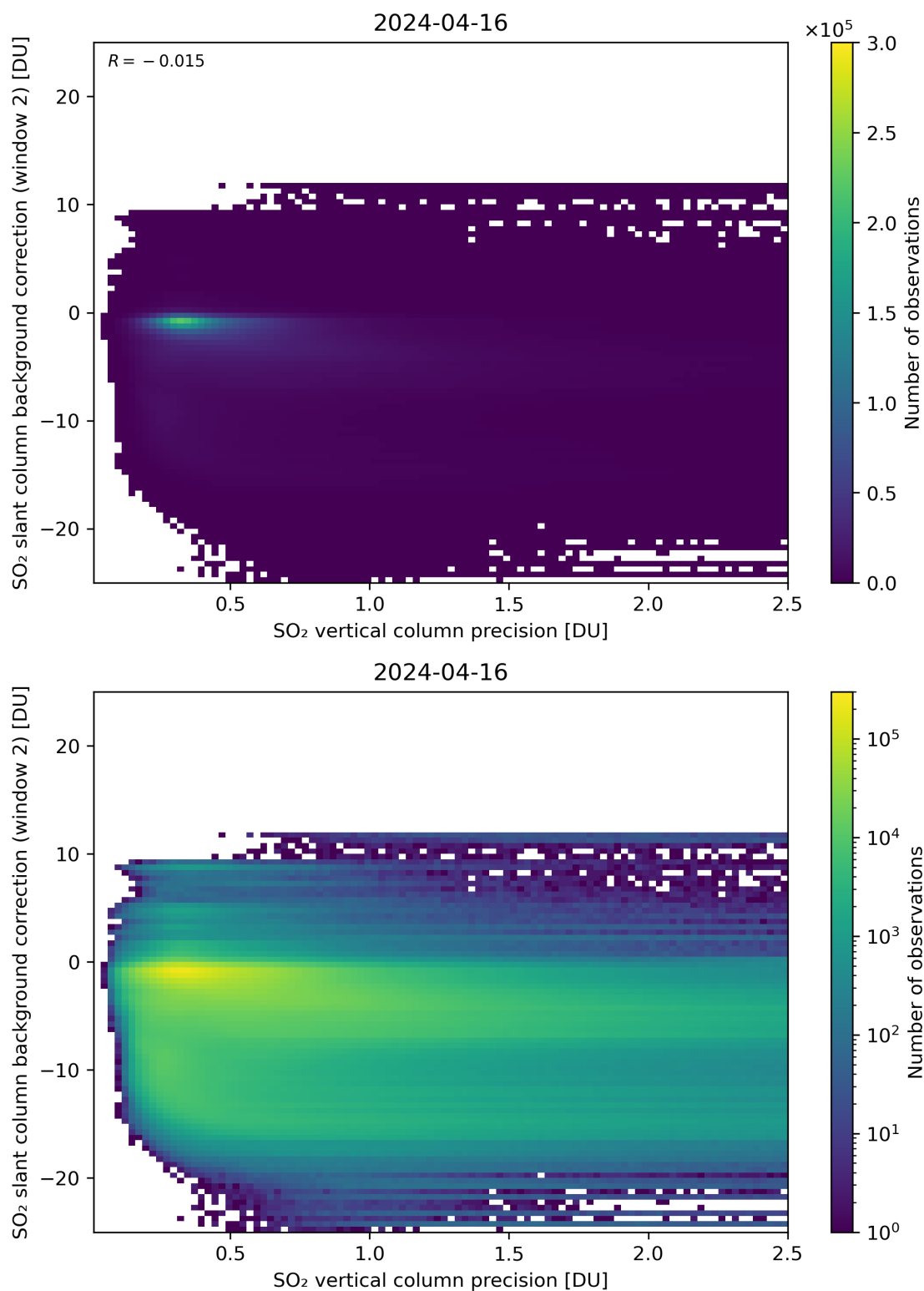
Figure 280: Scatter density plot of “SO 2 vertical column precision” against “SO 2 slant column background correction (window 2)” for 2024-04-16 to 2024-04-17.
