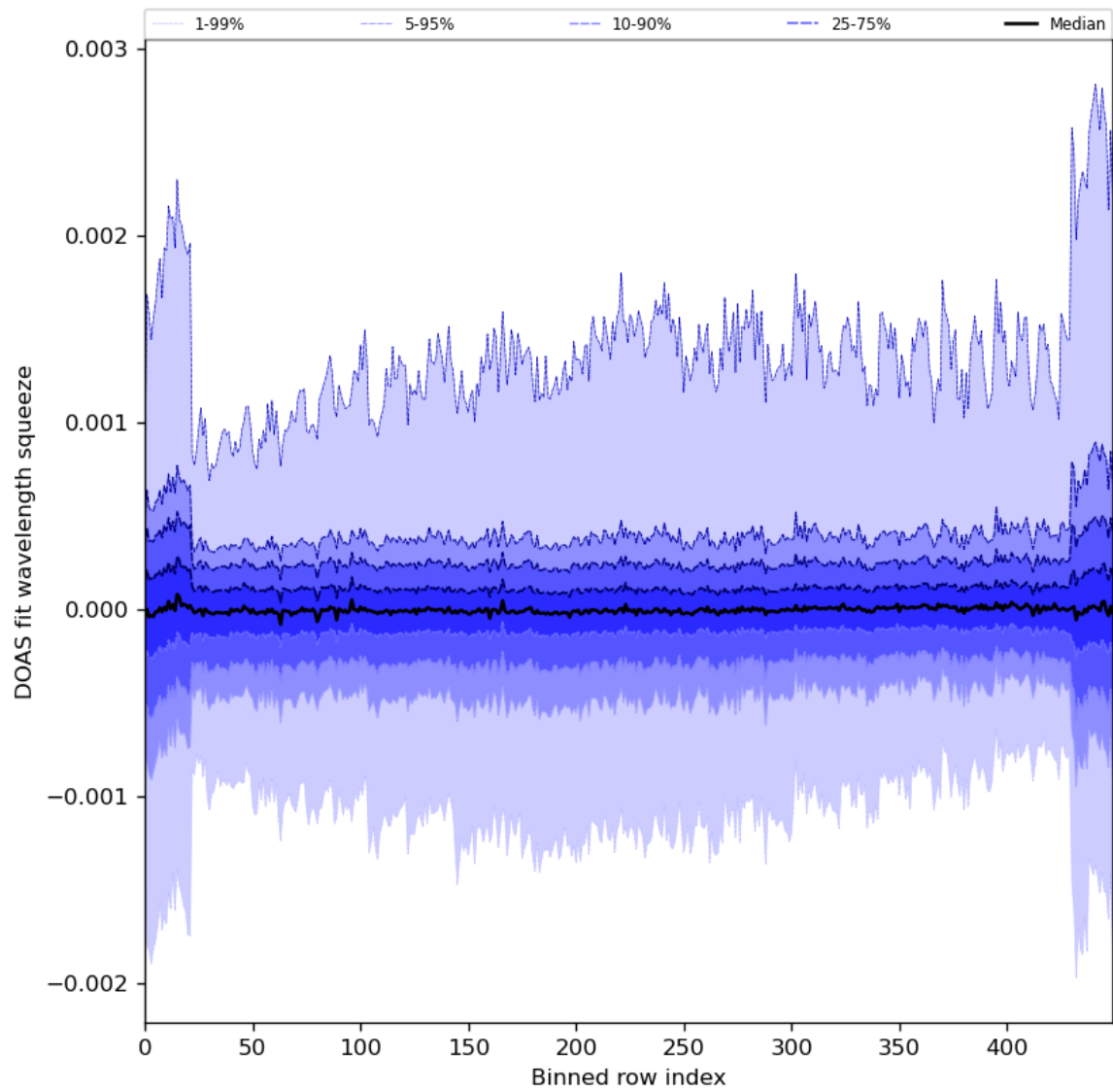
Figure 92: Along track statistics of “DOAS fit wavelength squeeze” for 2024-04-16 to 2024-04-17
