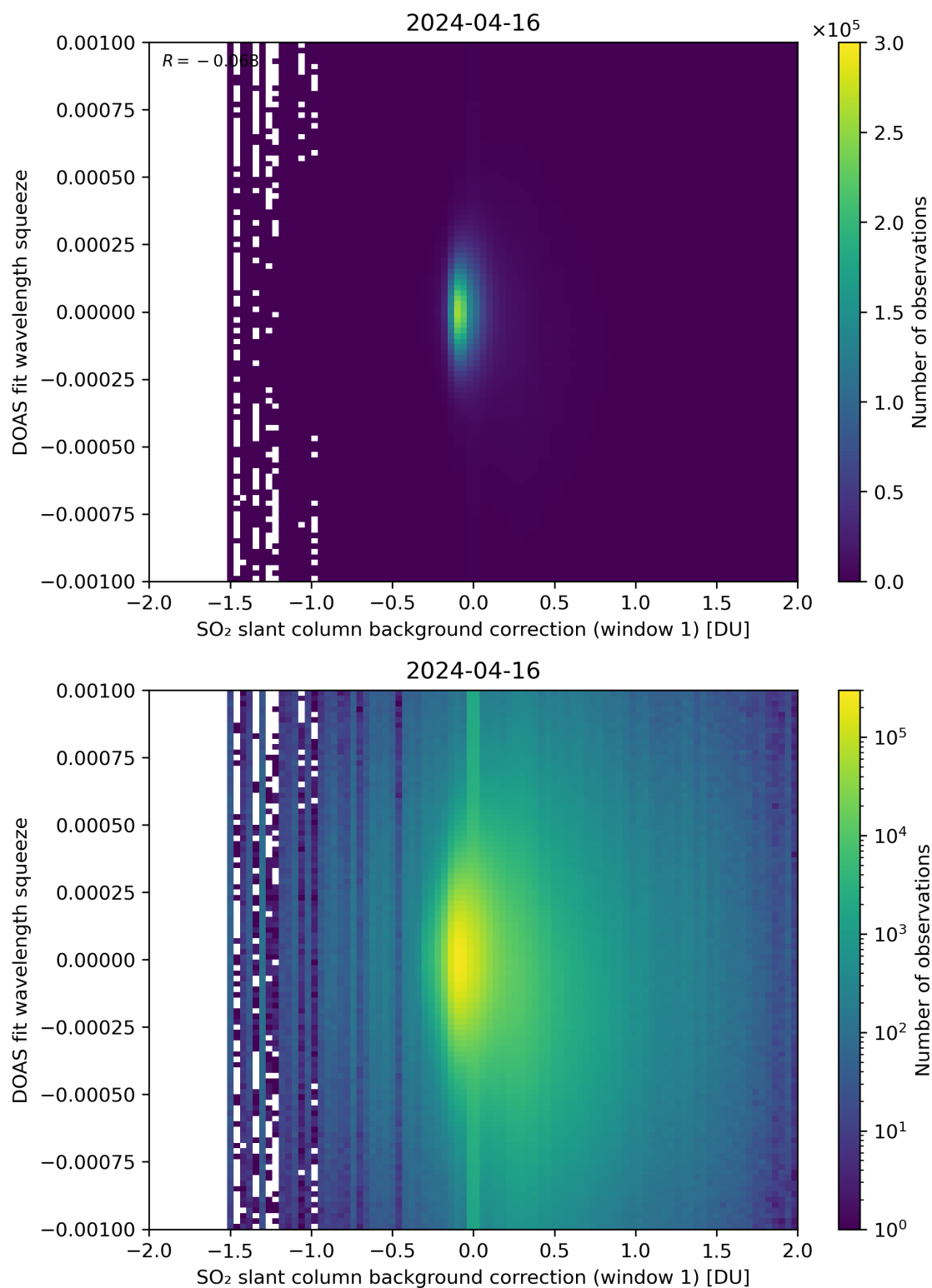
Figure 101: Scatter density plot of “SO 2 slant column background correction (window 1)” against “DOAS fit wavelength squeeze” for 2024-04-16 to 2024-04-17.
