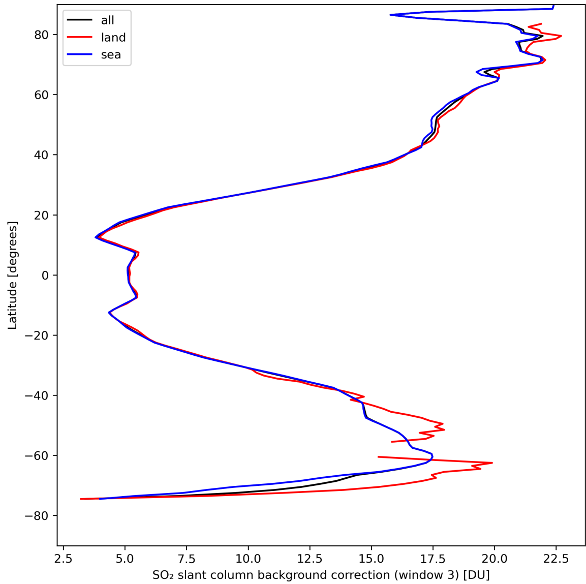
Figure 44: Zonal average of “SO 2 slant column background correction (window 3)” for 2024-04-16 to 2024-04-17.
