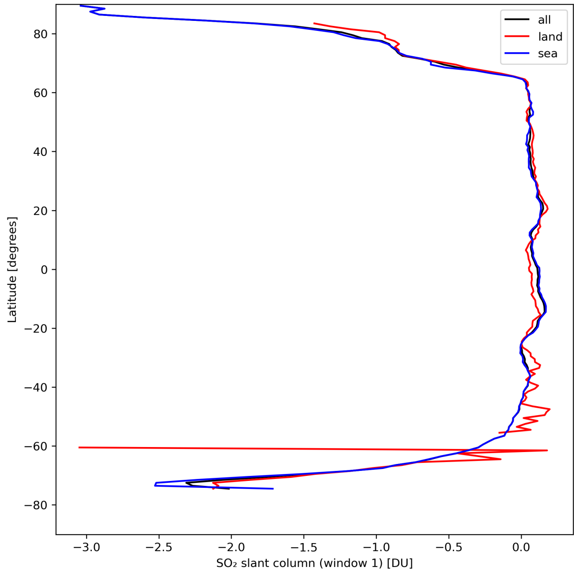
Figure 33: Zonal average of “SO 2 slant column (window 1)” for 2024-04-16 to 2024-04-17.
