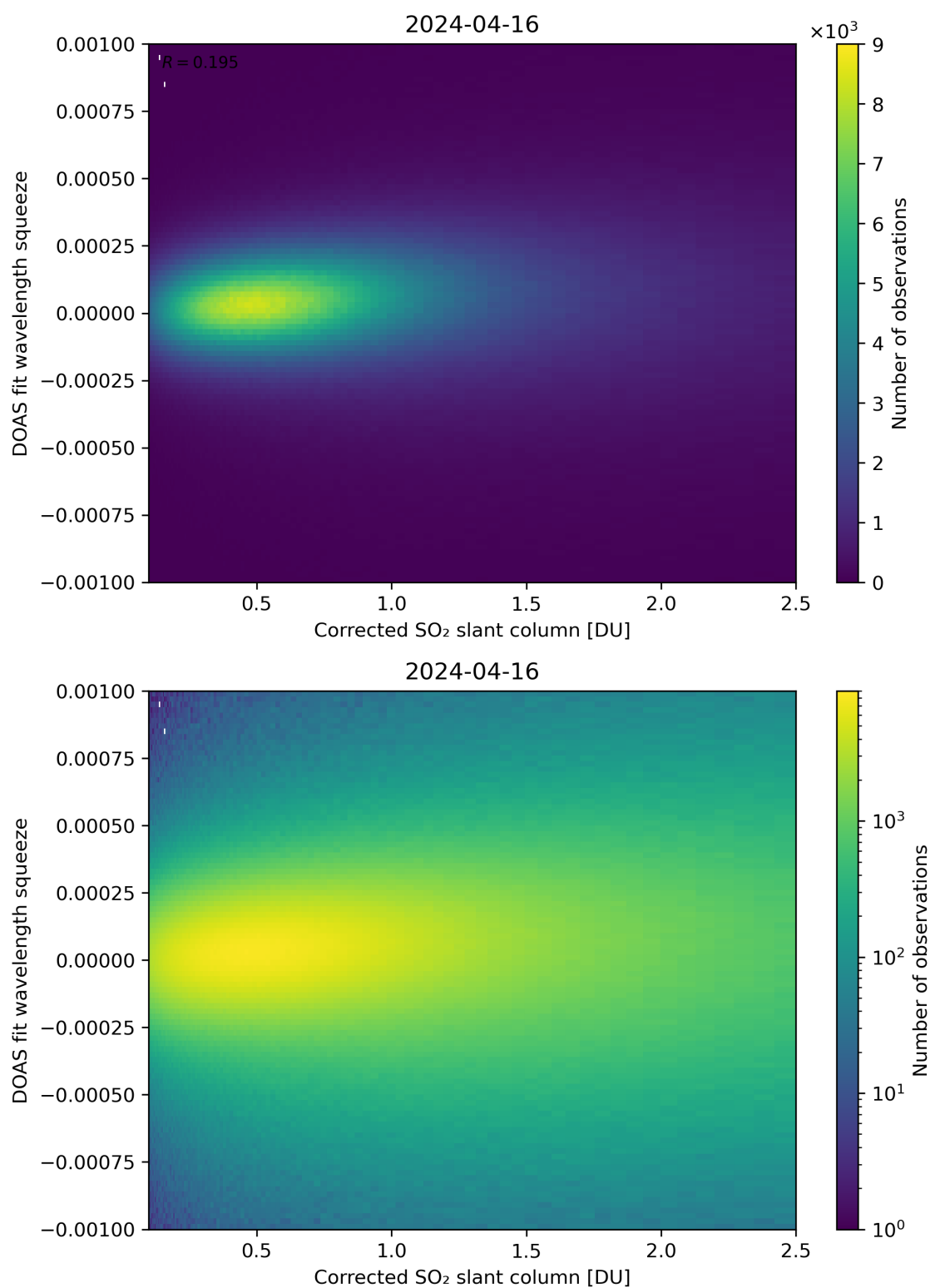
Figure 182: Scatter density plot of “Corrected SO 2 slant column” against “DOAS fit wavelength squeeze” for 2024-04-16 to 2024-04-17.
