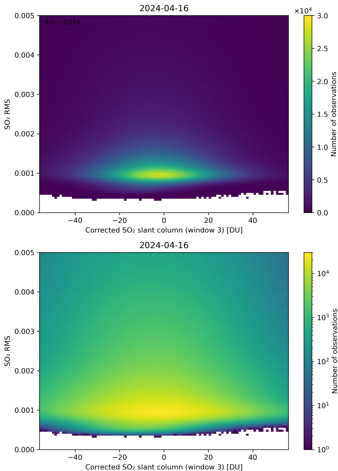
Figure 208: Scatter density plot of “Corrected SO 2 slant column (window 3)” against “SO 2 RMS” for 2024-04-16 to 2024-04-17.
