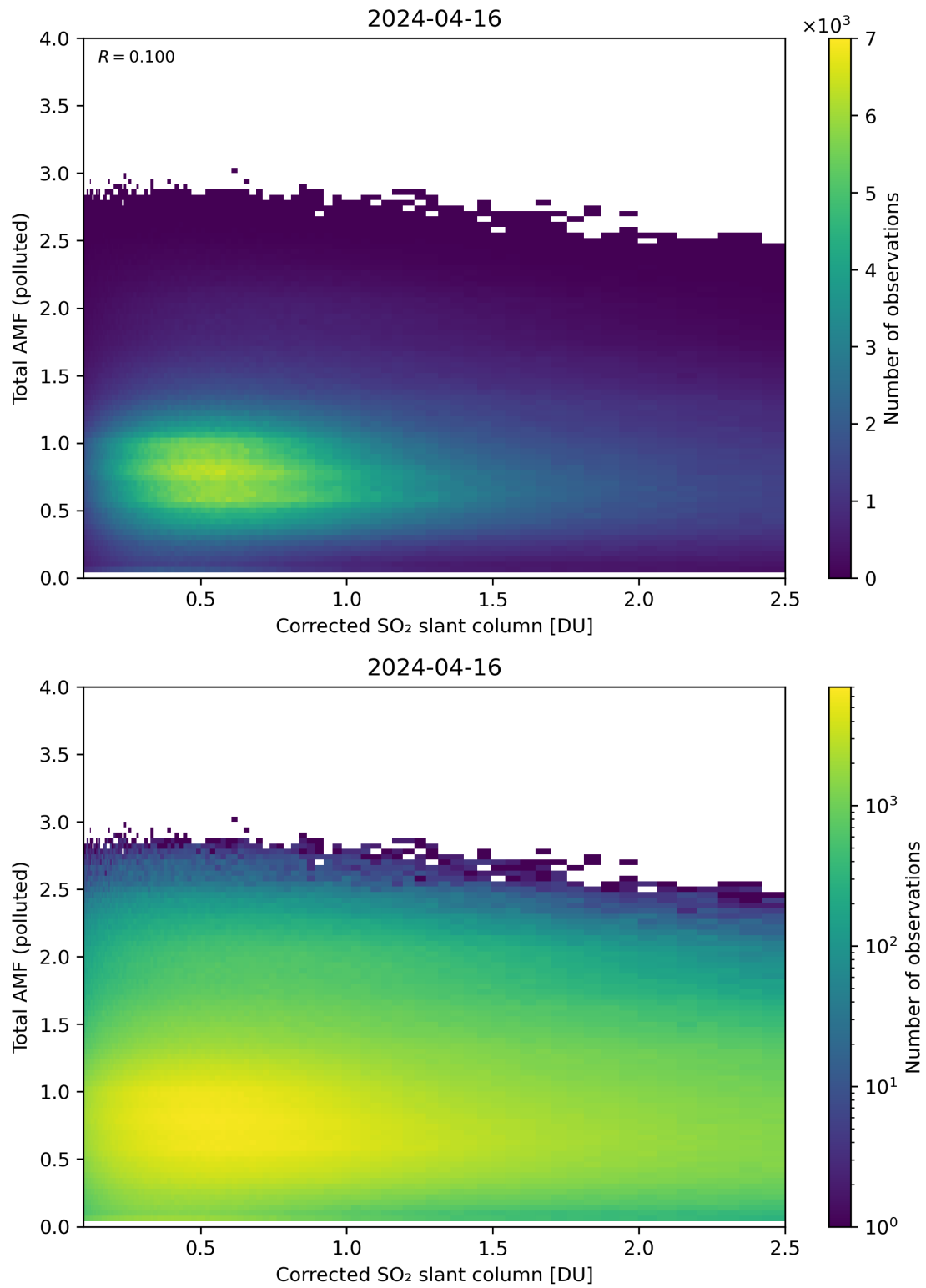
Figure 192: Scatter density plot of “Corrected SO 2 slant column” against “Total AMF (polluted)” for 2024-04-16 to 2024-04-17.
