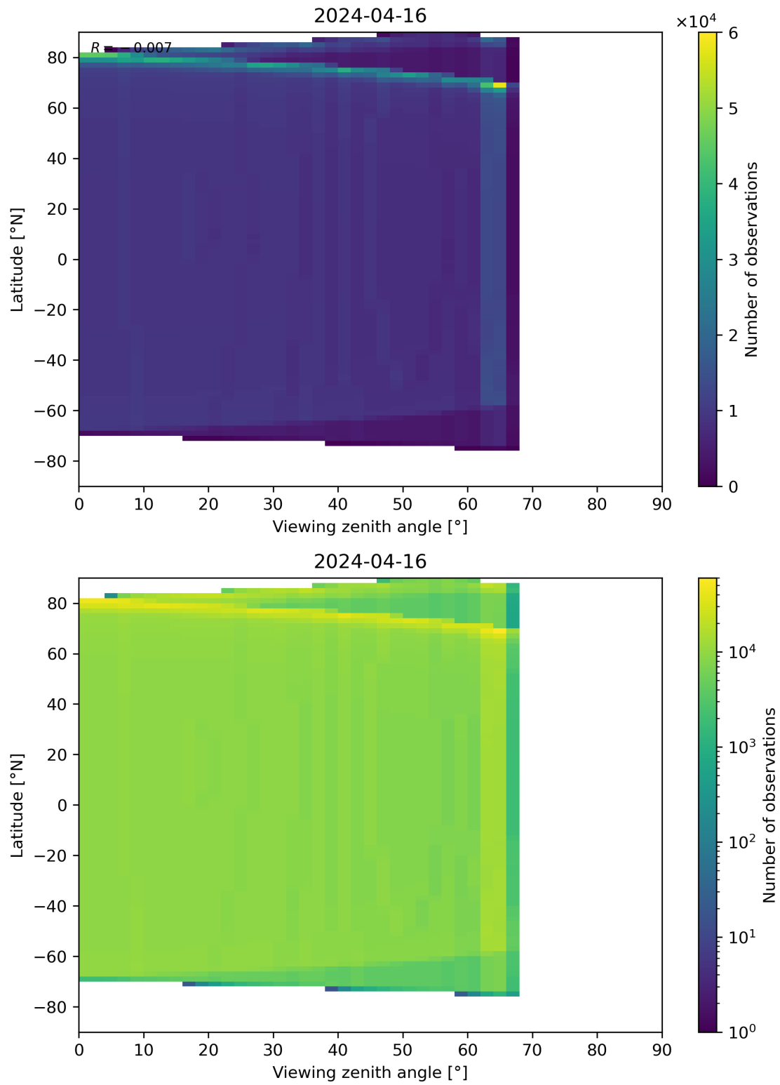
Figure 314: Scatter density plot of “Viewing zenith angle” against “Latitude” for 2024-04-16 to 2024-04-17.
