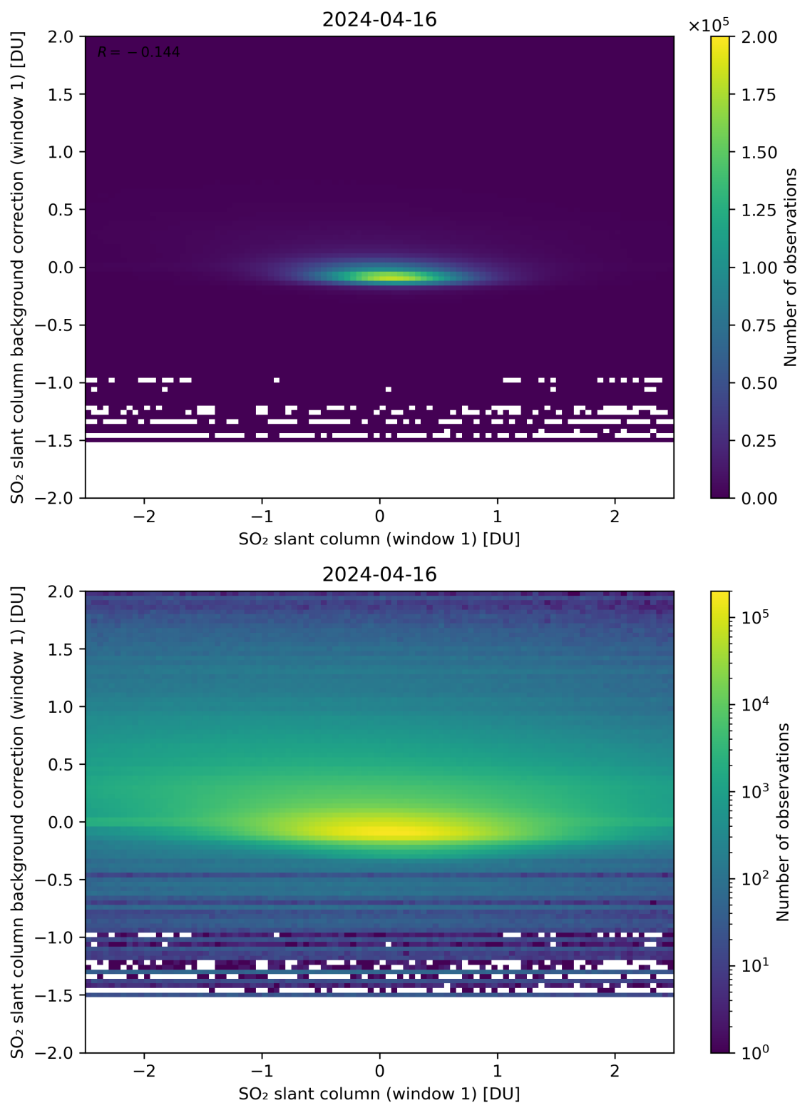
Figure 212: Scatter density plot of “SO 2 slant column (window 1)” against “SO 2 slant column background correction (window 1)” for 2024-04-16 to 2024-04-17.
