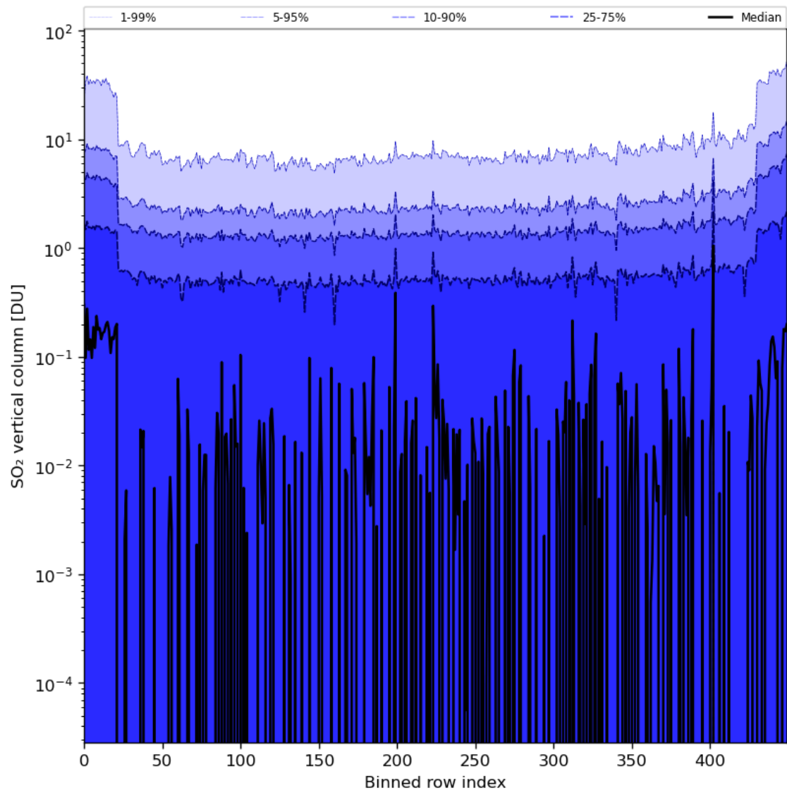
Figure 76: Along track statistics of “SO 2 vertical column” for 2024-04-16 to 2024-04-17
