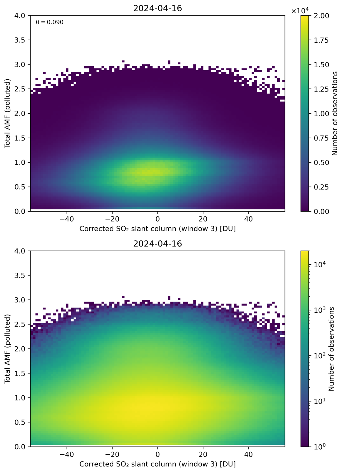
Figure 210: Scatter density plot of “Corrected SO 2 slant column (window 3)” against “Total AMF (polluted)” for 2024-04-16 to 2024-04-17.
