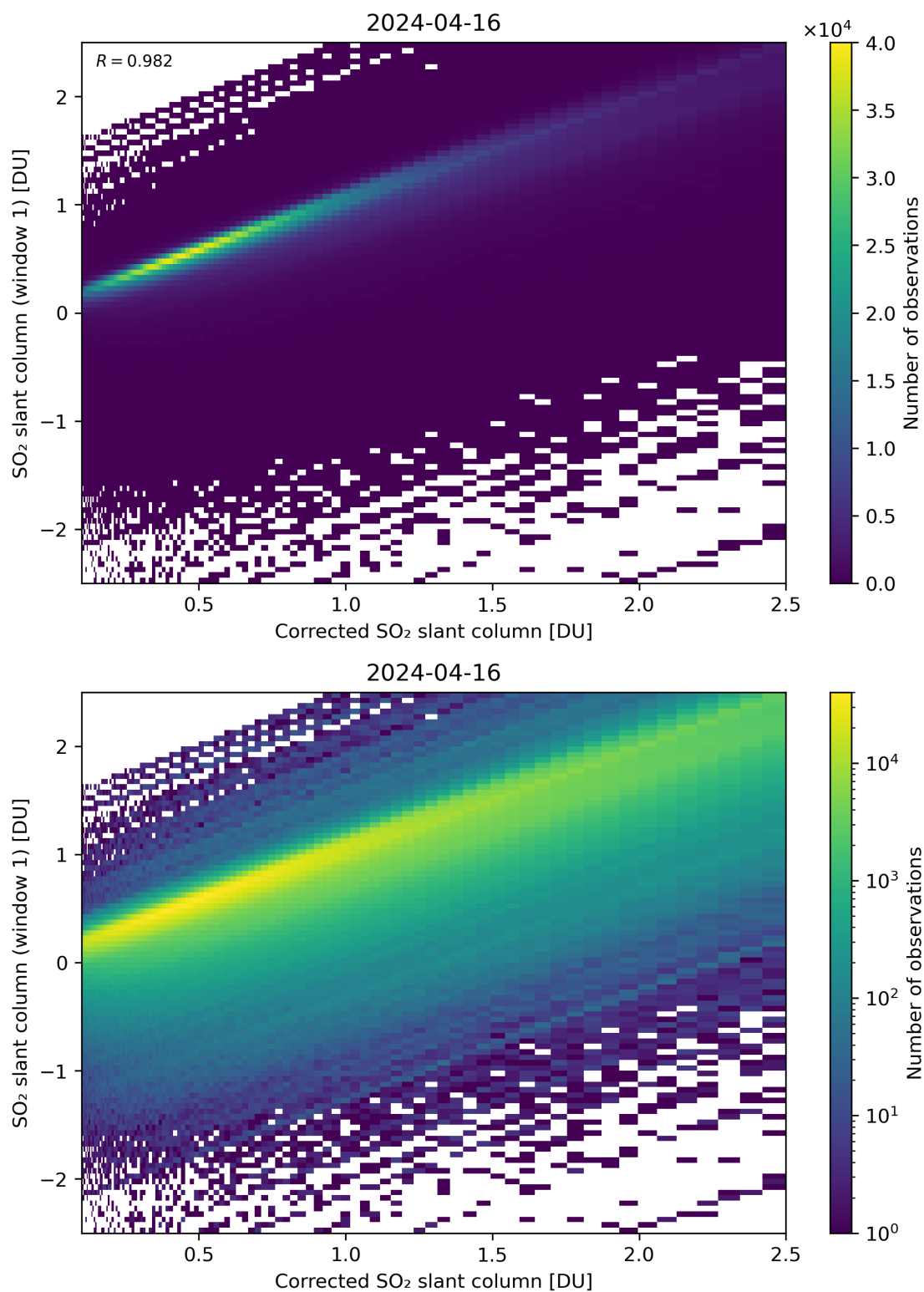
Figure 187: Scatter density plot of “Corrected SO 2 slant column” against “SO 2 slant column (window 1)” for 2024-04-16 to 2024-04-17.
