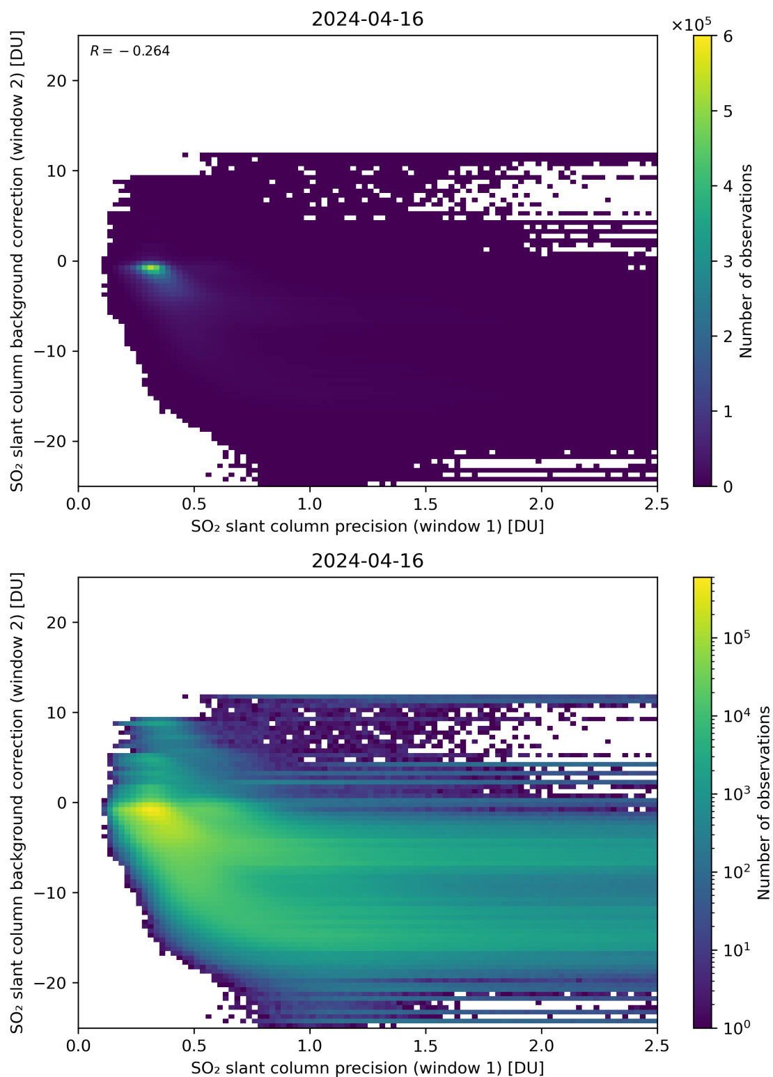
Figure 219: Scatter density plot of “SO 2 slant column precision (window 1)” against “SO 2 slant column background correction (window 2)” for 2024-04-16 to 2024-04-17.
