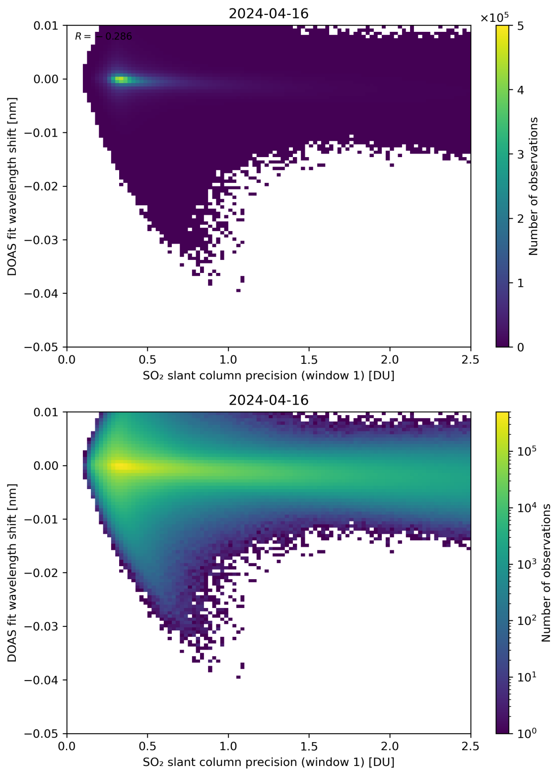
Figure 221: Scatter density plot of “SO 2 slant column precision (window 1)” against “DOAS fit wavelength shift” for 2024-04-16 to 2024-04-17.
