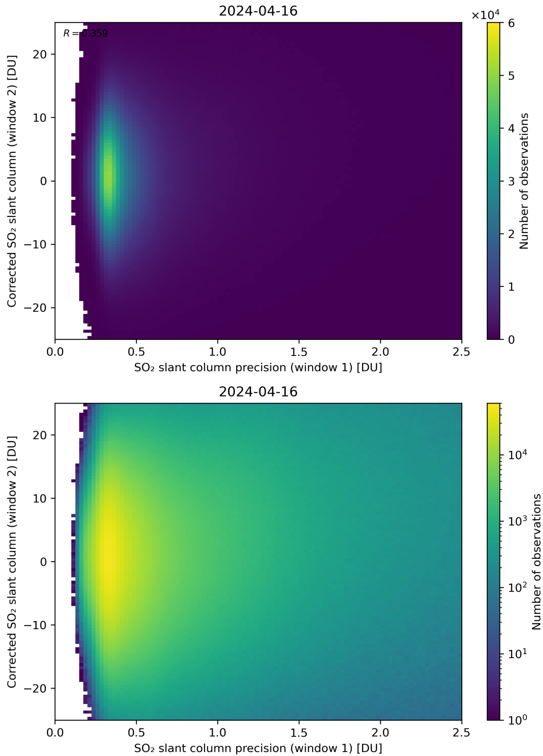
Figure 225: Scatter density plot of “SO 2 slant column precision (window 1)” against “Corrected SO 2 slant column (window 2)” for 2024-04-16 to 2024-04-17.
