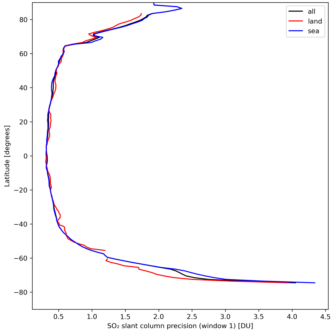
Figure 34: Zonal average of “SO 2 slant column precision (window 1)” for 2024-04-16 to 2024-04-17.
