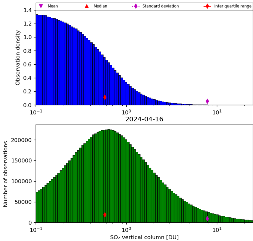
Figure 53: Histogram of “SO 2 vertical column” for 2024-04-16 to 2024-04-17
