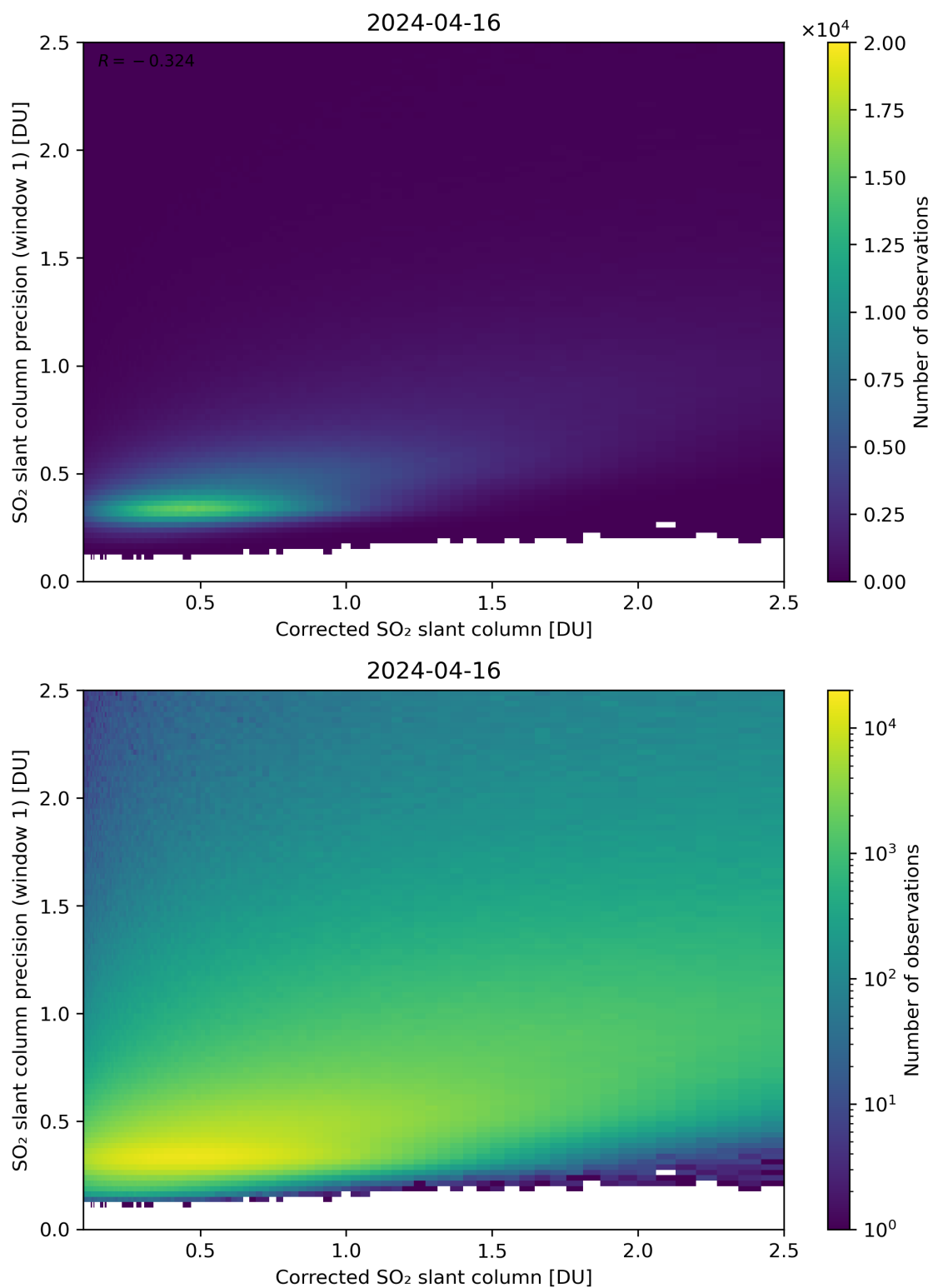
Figure 188: Scatter density plot of “Corrected SO 2 slant column” against “SO 2 slant column precision (window 1)” for 2024-04-16 to 2024-04-17.
