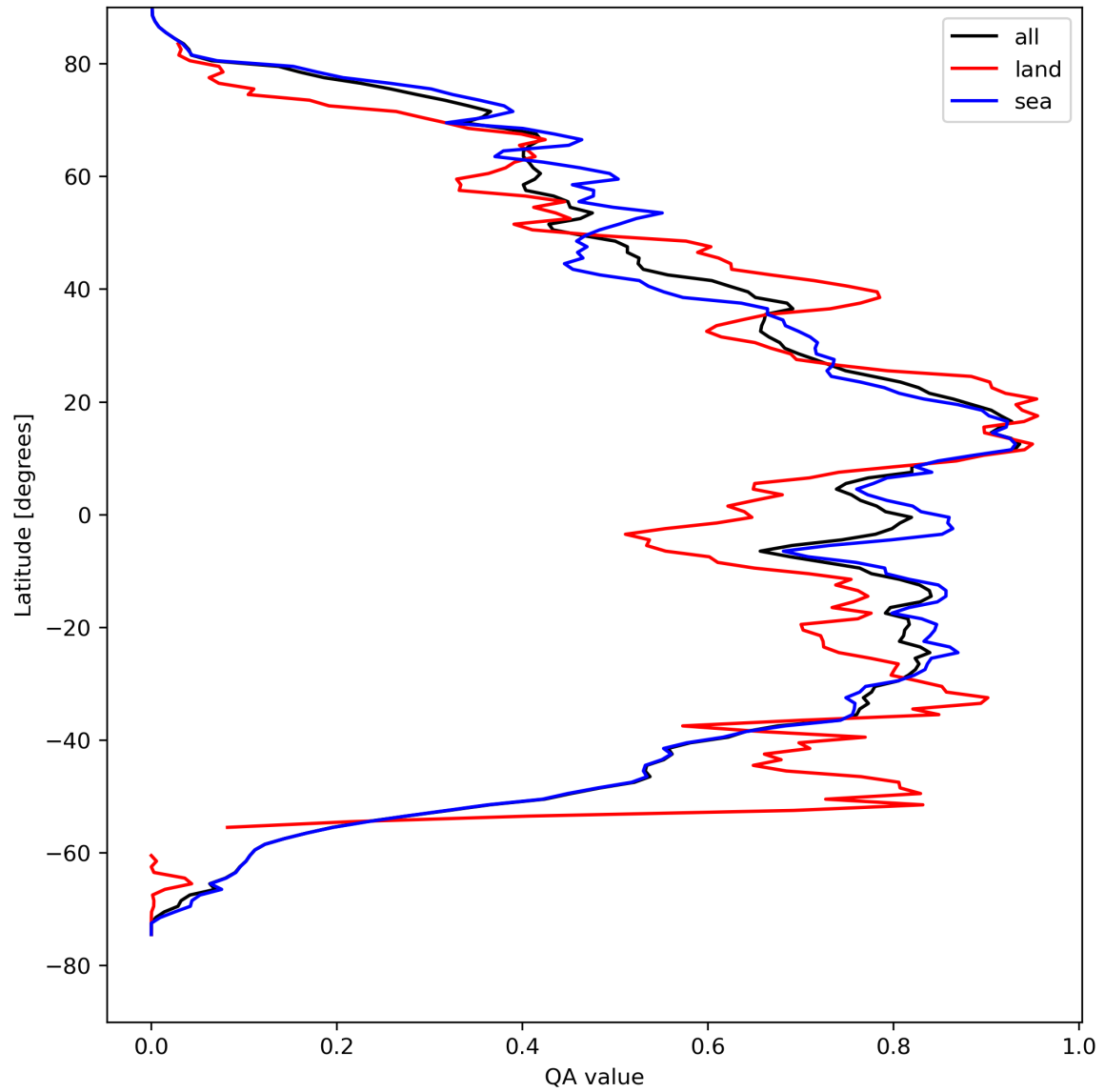
Figure 29: Zonal average of “QA value” for 2024-04-16 to 2024-04-17.
