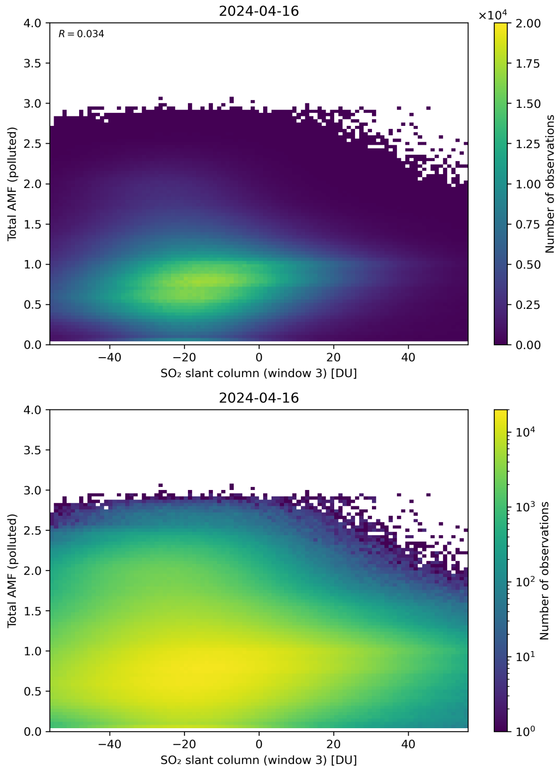
Figure 268: Scatter density plot of “SO 2 slant column (window 3)” against “Total AMF (polluted)” for 2024-04-16 to 2024-04-17.
