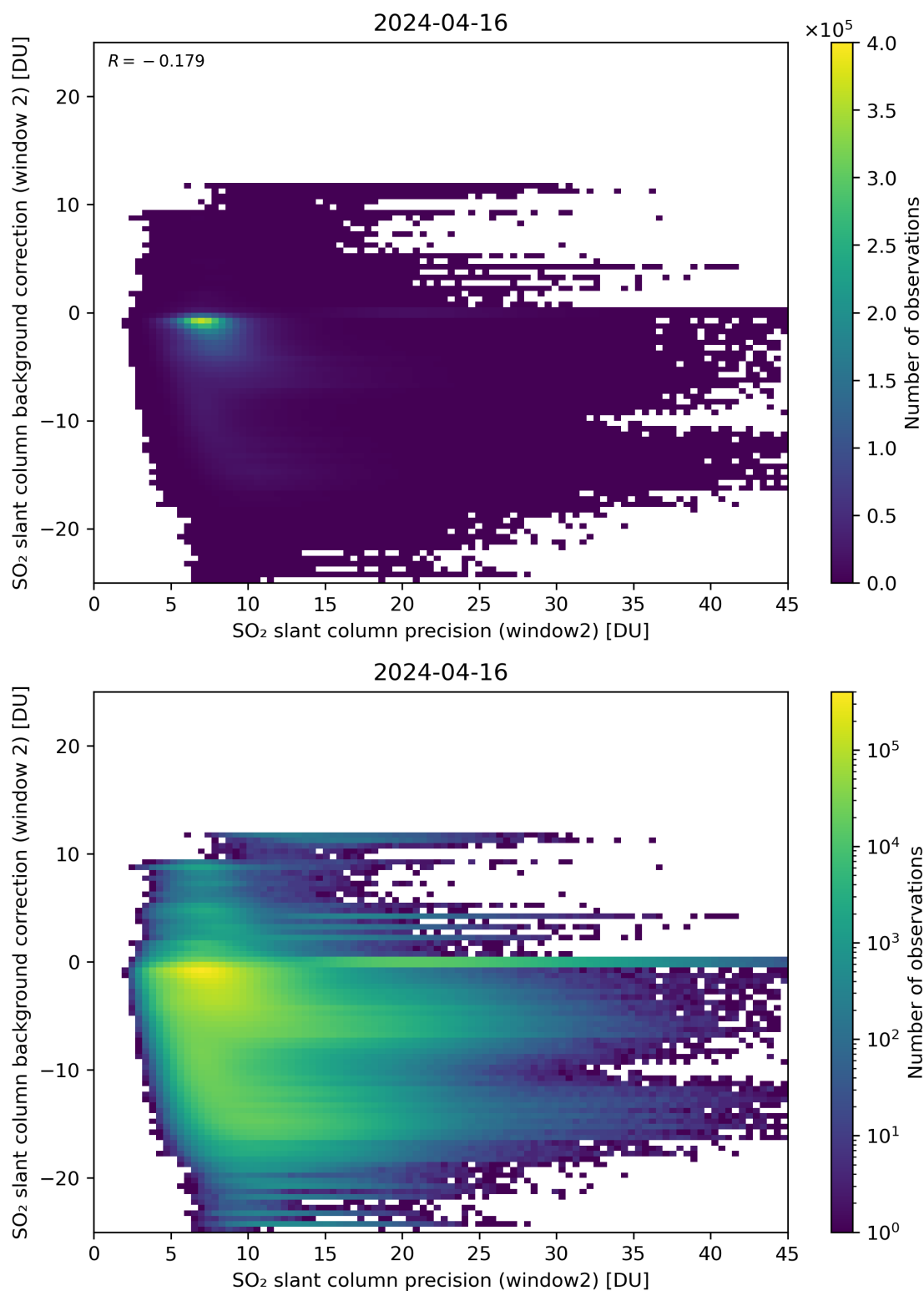
Figure 241: Scatter density plot of “SO 2 slant column precision (window2)” against “SO 2 slant column background correction (window 2)” for 2024-04-16 to 2024-04-17.
