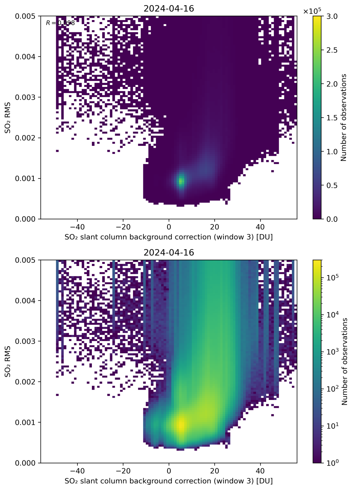
Figure 123: Scatter density plot of “SO 2 slant column background correction (window 3)” against “SO 2 RMS” for 2024-04-16 to 2024-04-17.
