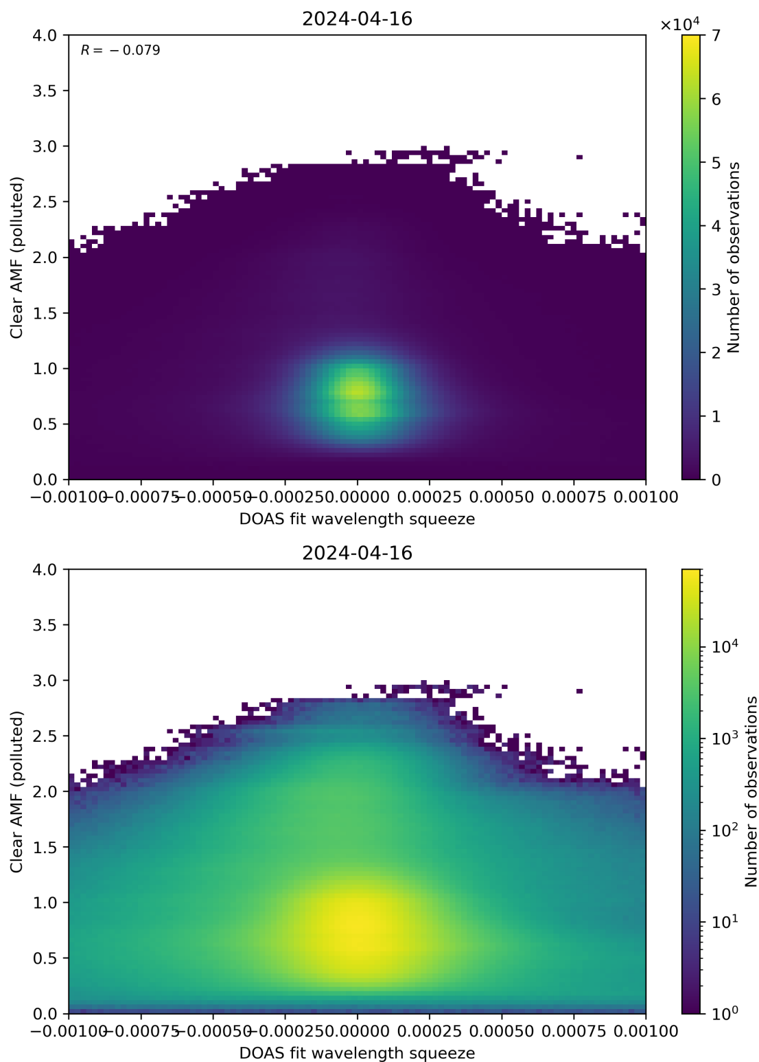
Figure 133: Scatter density plot of “DOAS fit wavelength squeeze” against “Clear AMF (polluted)” for 2024-04-16 to 2024-04-17.
