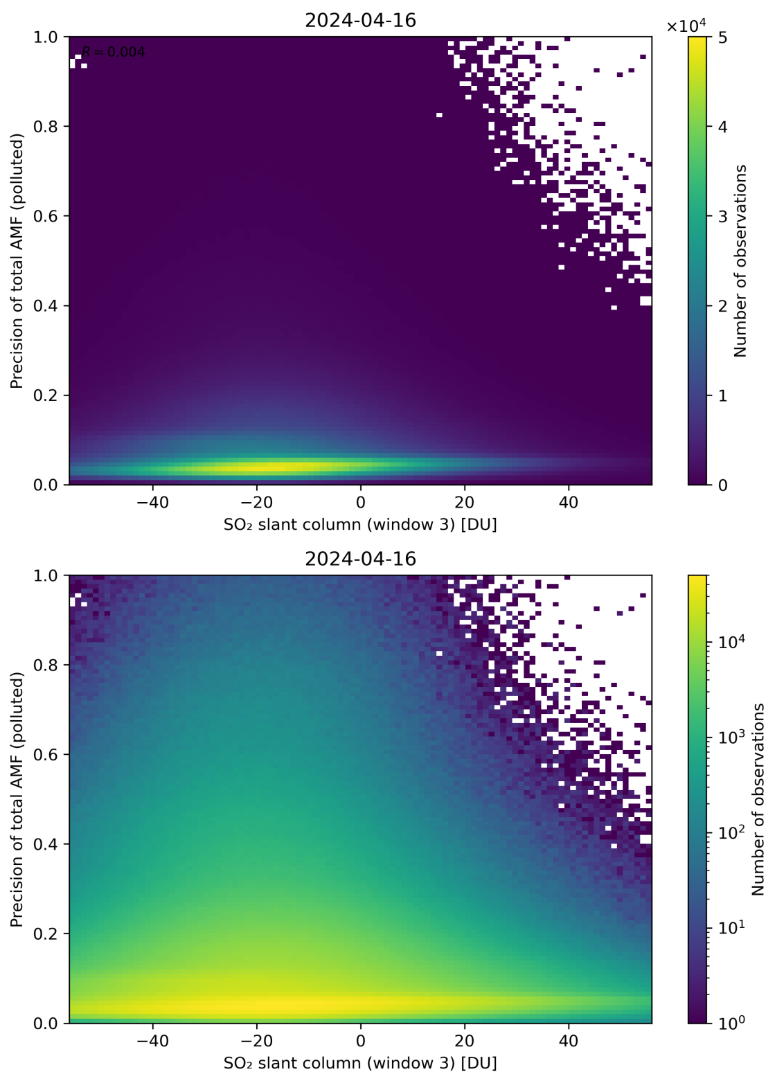
Figure 269: Scatter density plot of “SO 2 slant column (window 3)” against “Precision of total AMF (polluted)” for 2024-04-16 to 2024-04-17.
