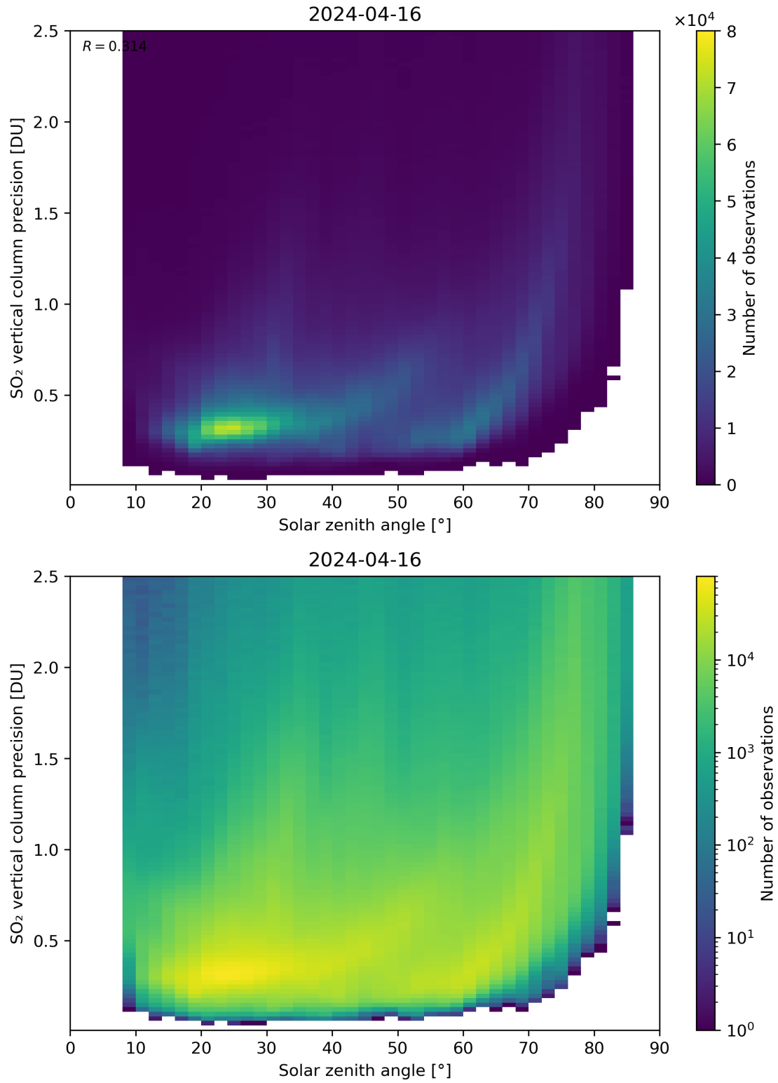
Figure 177: Scatter density plot of “Solar zenith angle” against “SO 2 vertical column precision” for 2024-04-16 to 2024-04-17.
