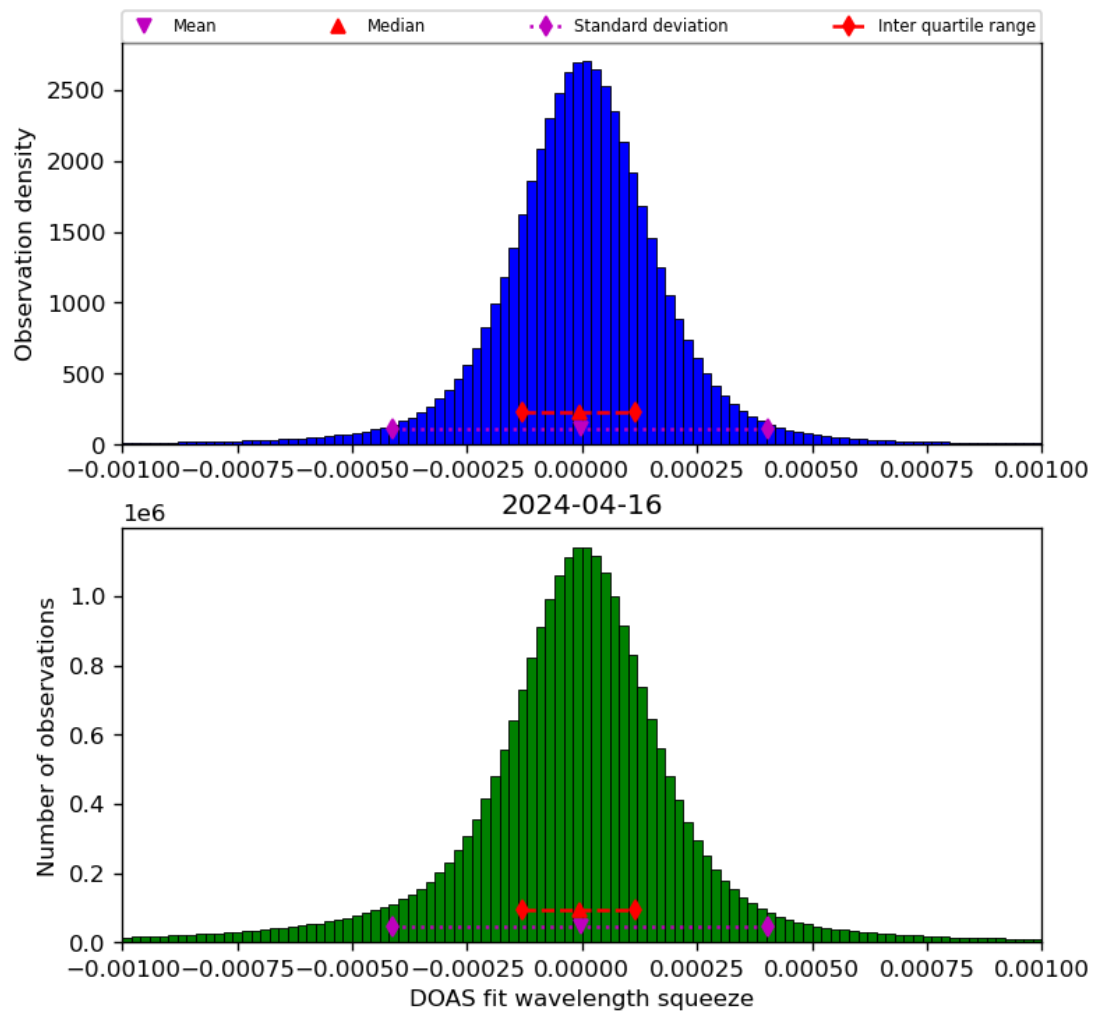
Figure 69: Histogram of “DOAS fit wavelength squeeze” for 2024-04-16 to 2024-04-17
