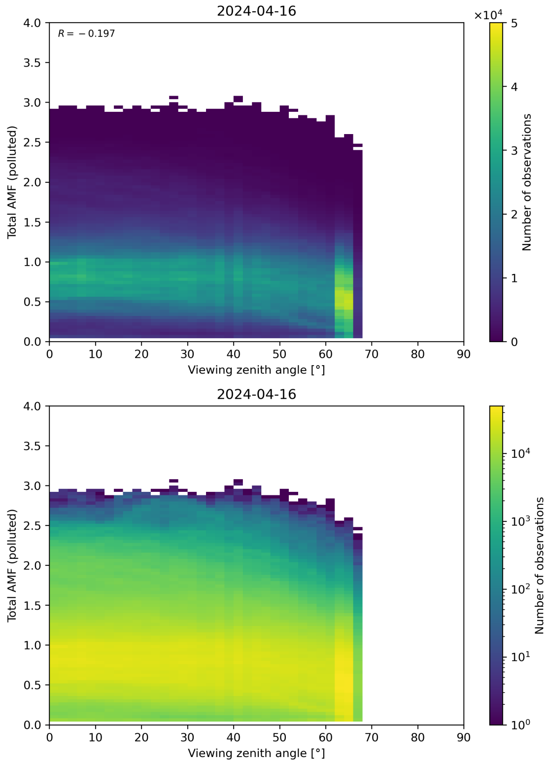
Figure 325: Scatter density plot of “Viewing zenith angle” against “Total AMF (polluted)” for 2024-04-16 to 2024-04-17.
