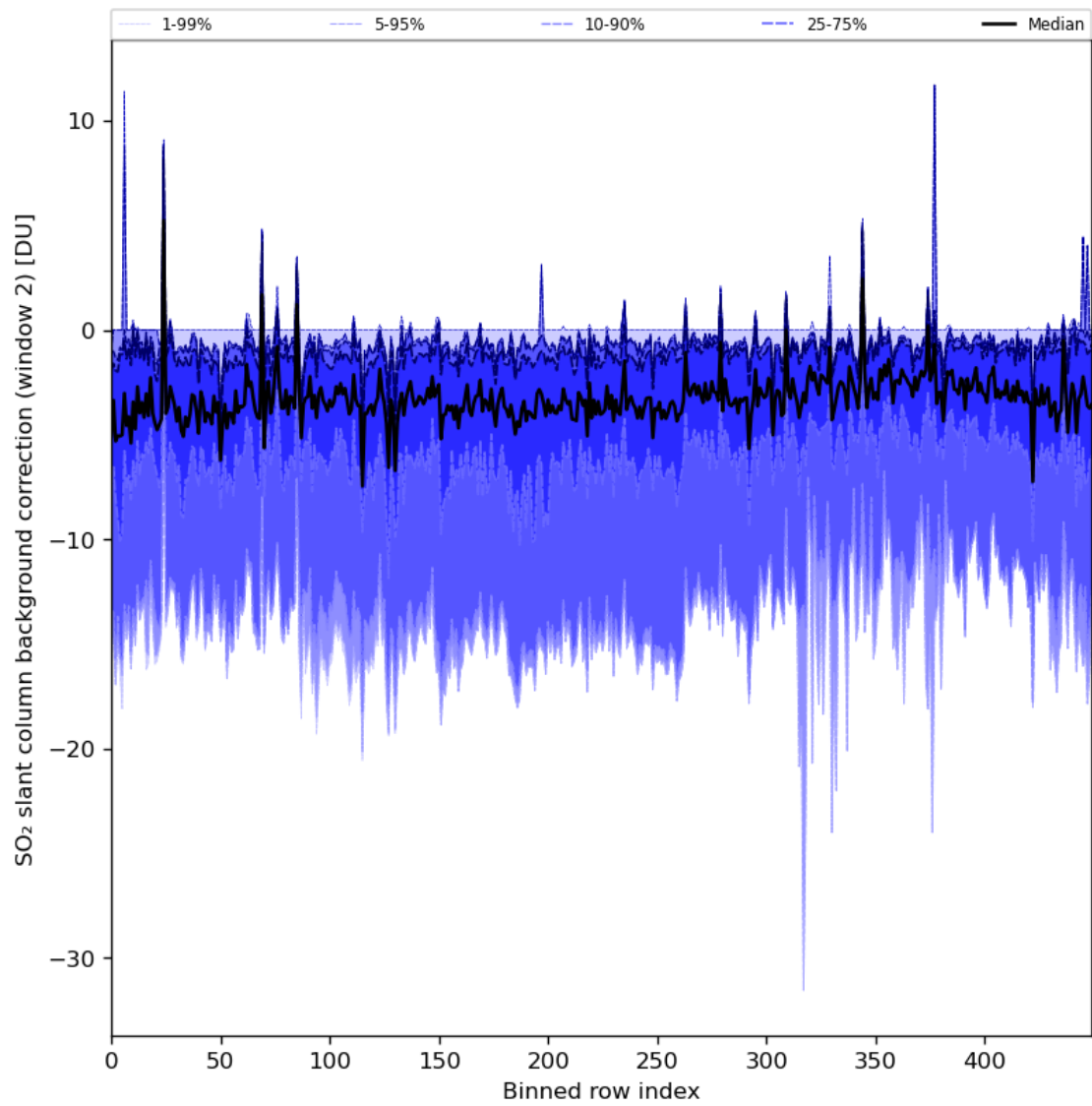
Figure 86: Along track statistics of “SO 2 slant column background correction (window 2)” for 2024-04-16 to 2024-04-17
