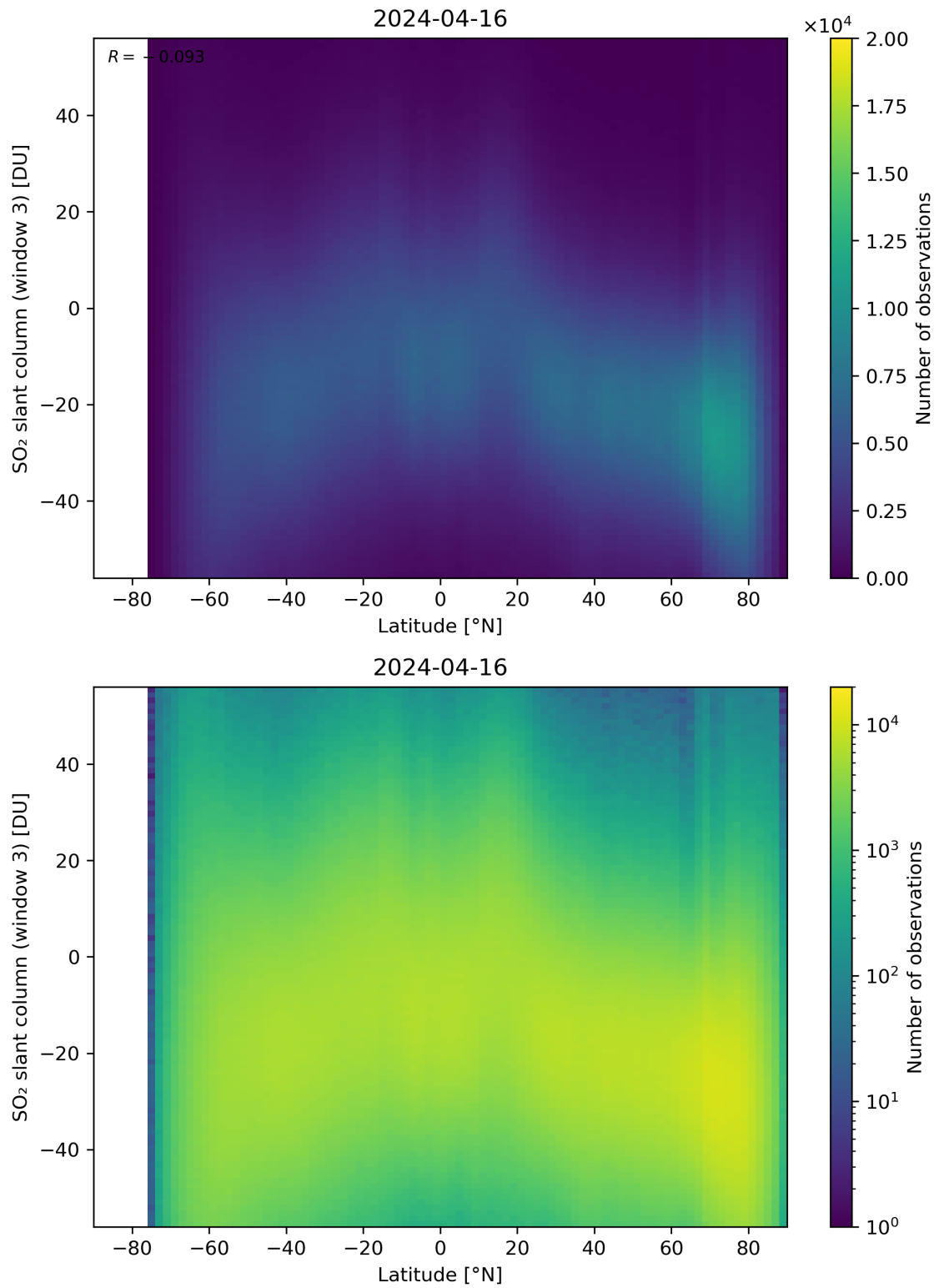
Figure 152: Scatter density plot of “Latitude” against “SO 2 slant column (window 3)” for 2024-04-16 to 2024-04-17.
