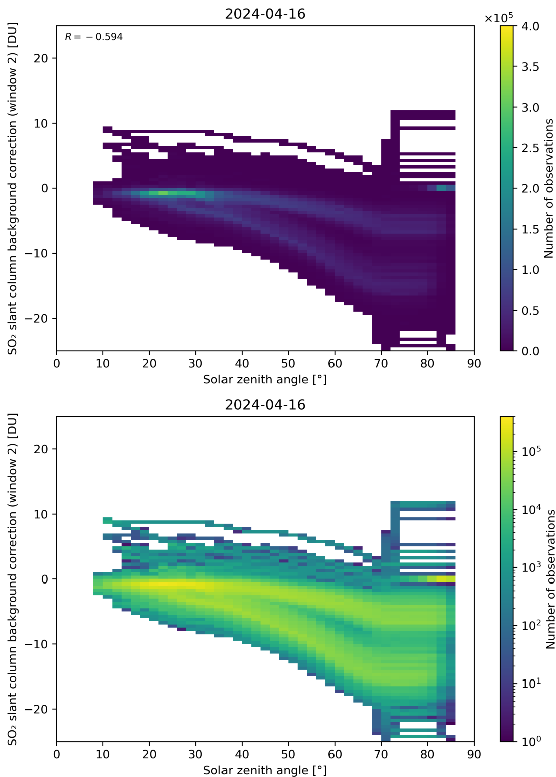
Figure 159: Scatter density plot of “Solar zenith angle” against “SO 2 slant column background correction (window 2)” for 2024-04-16 to 2024-04-17.
