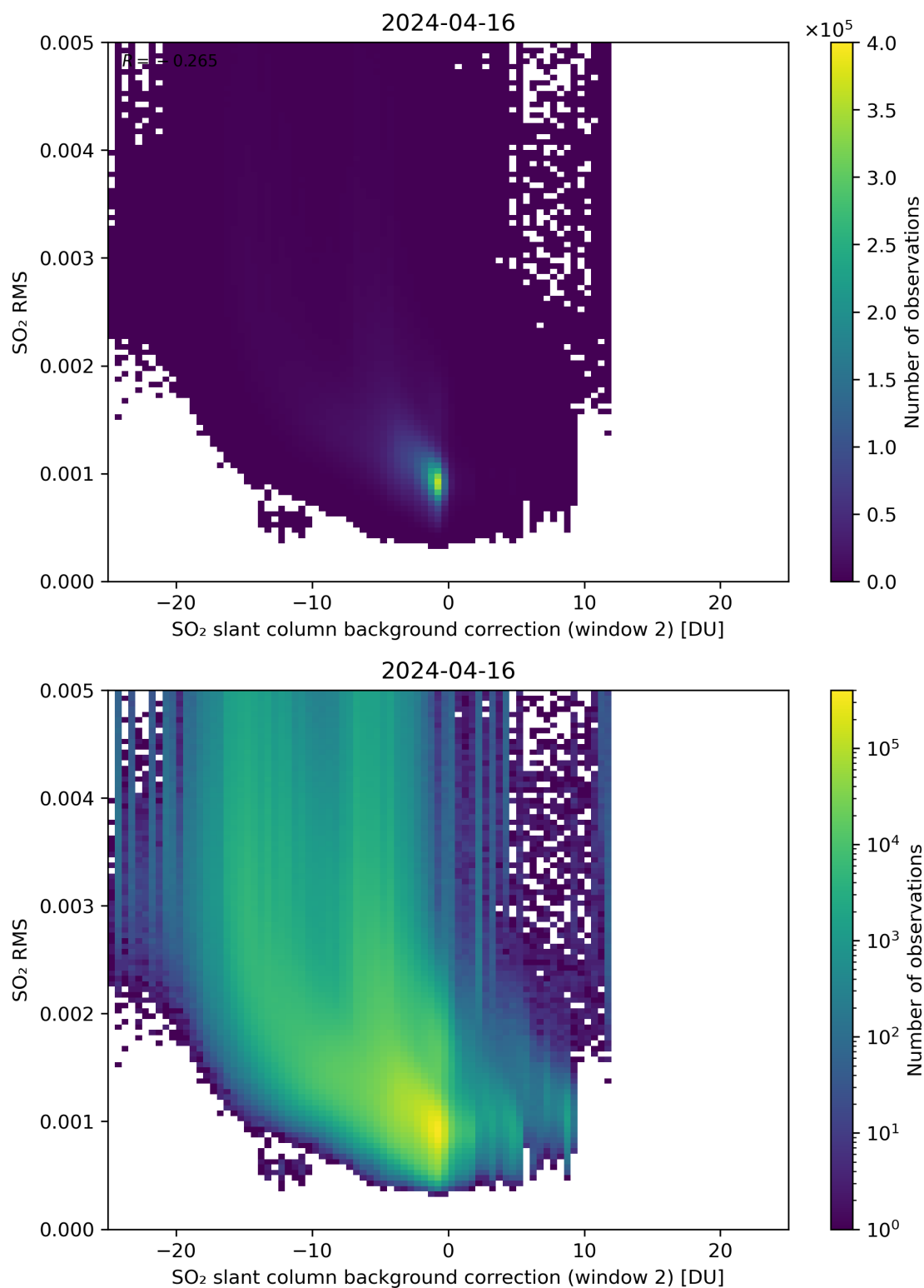
Figure 114: Scatter density plot of “SO 2 slant column background correction (window 2)” against “SO 2 RMS” for 2024-04-16 to 2024-04-17.
