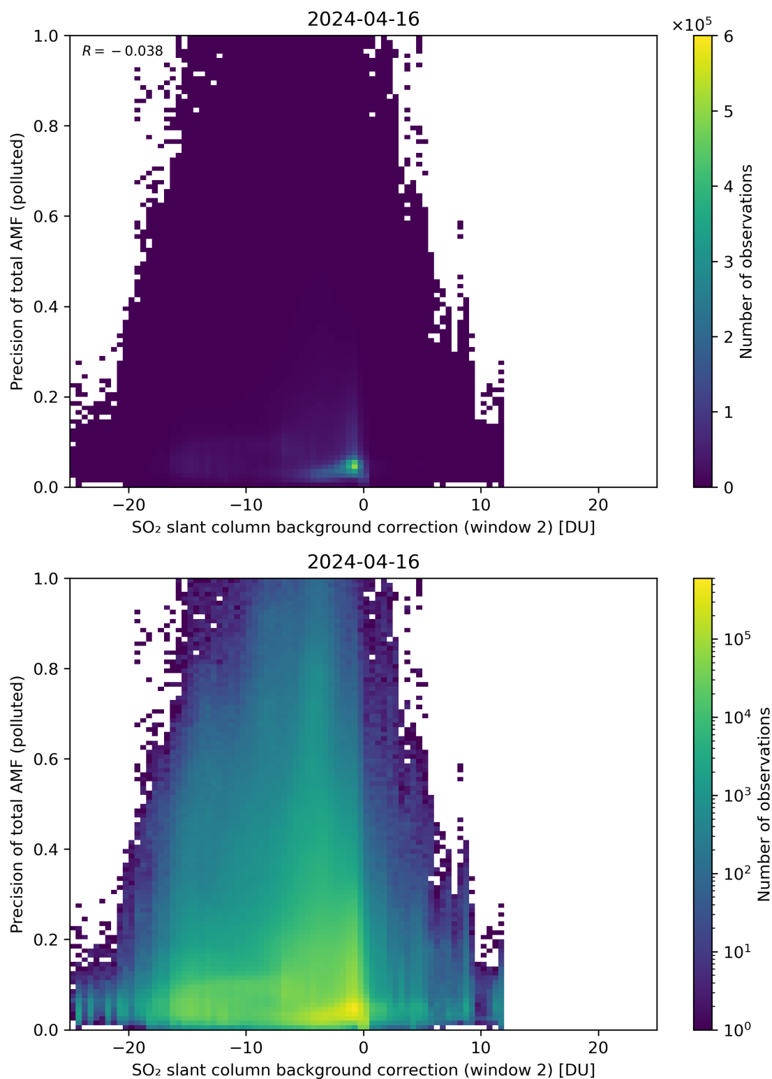
Figure 120: Scatter density plot of “SO 2 slant column background correction (window 2)” against “Precision of total AMF (polluted)” for 2024-04-16 to 2024-04-17.
