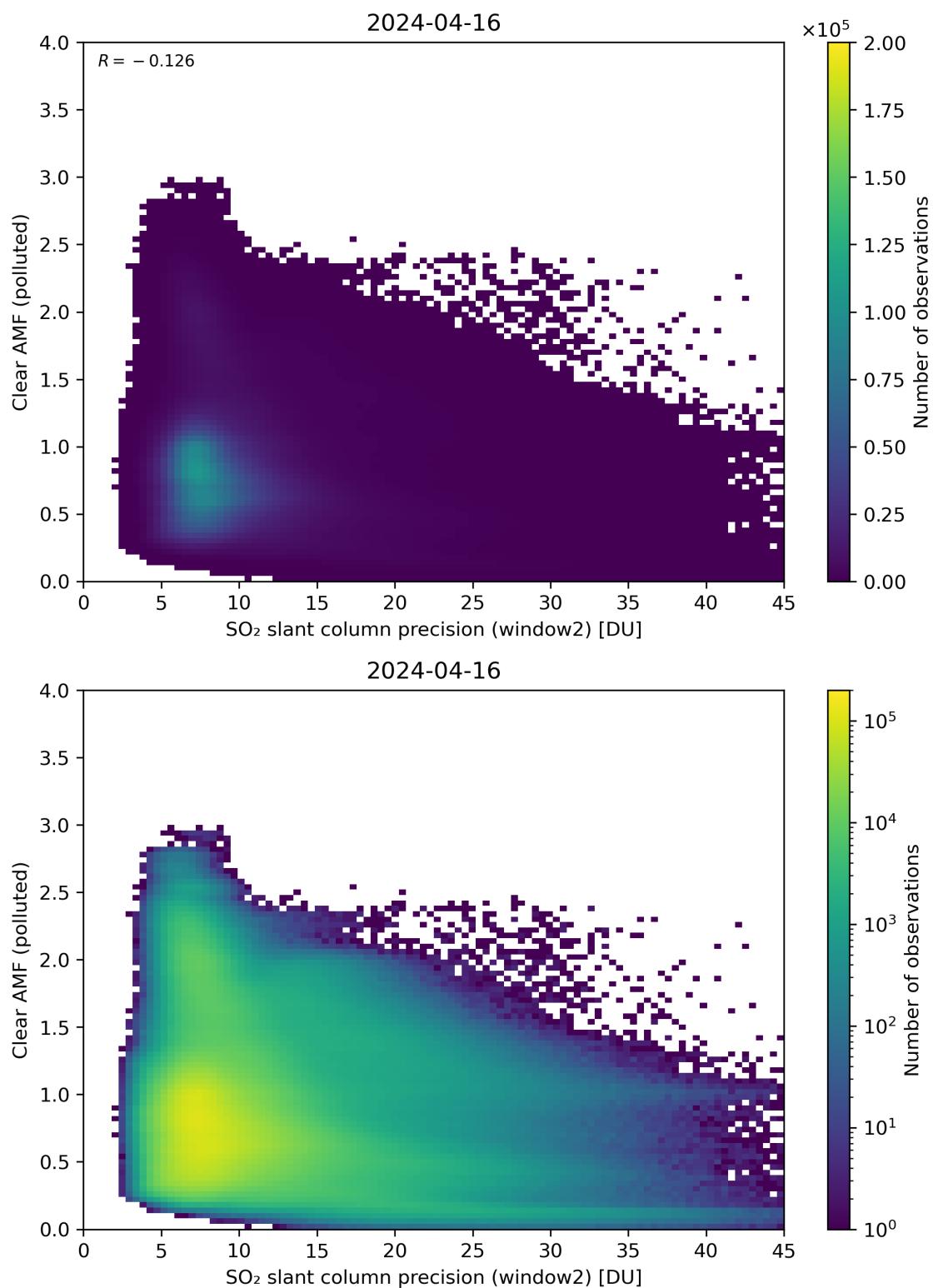
Figure 246: Scatter density plot of “SO 2 slant column precision (window2)” against “Clear AMF (polluted)” for 2024-04-16 to 2024-04-17.
