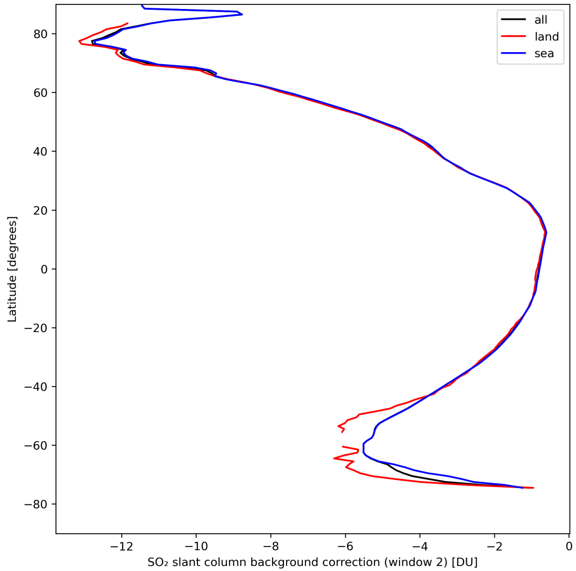
Figure 40: Zonal average of "SO 2 slant column background correction (window 2)" for 2024-04-16 to 2024-04-17.
