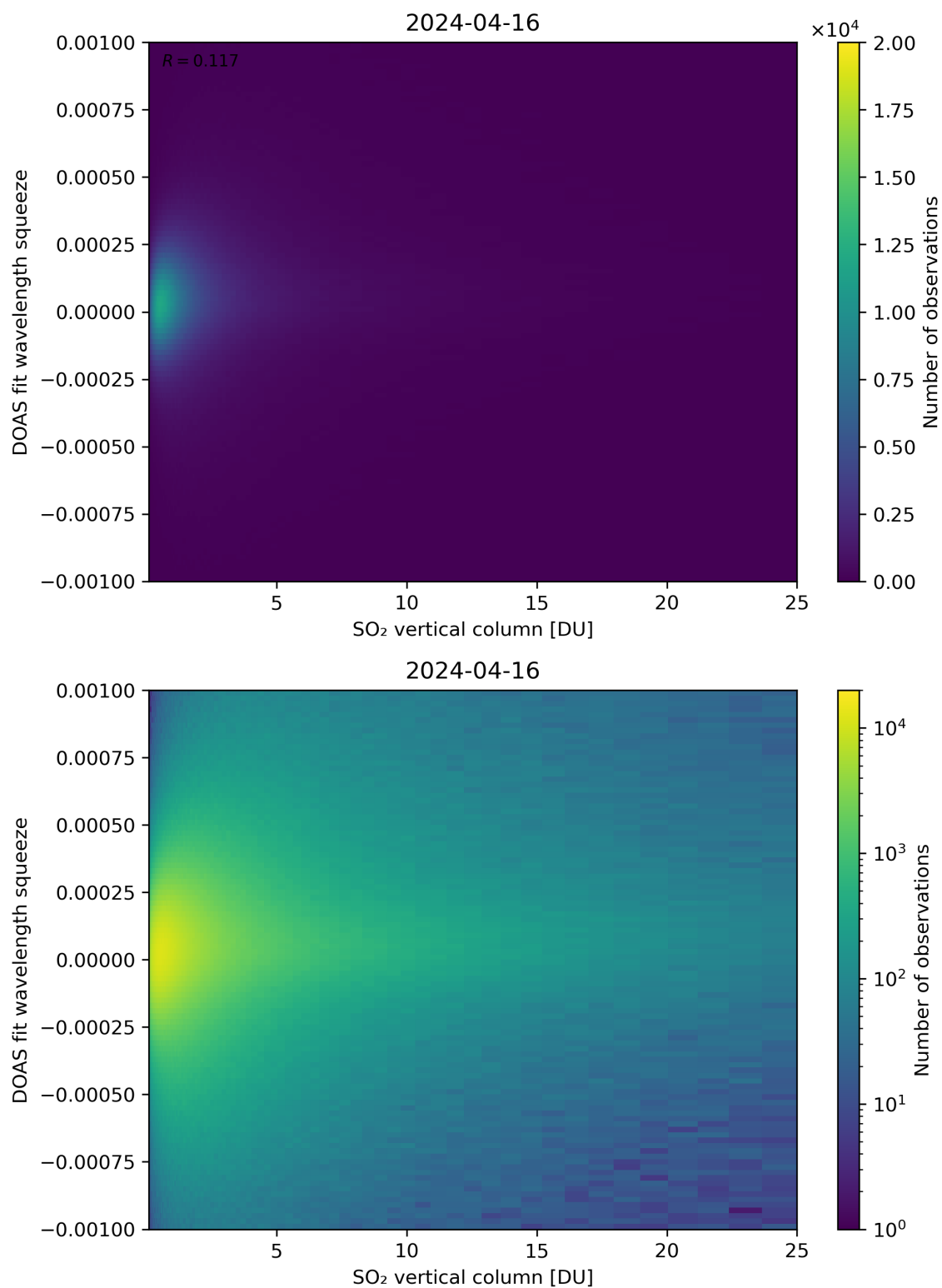
Figure 277: Scatter density plot of “SO 2 vertical column” against “DOAS fit wavelength squeeze” for 2024-04-16 to 2024-04-17.
