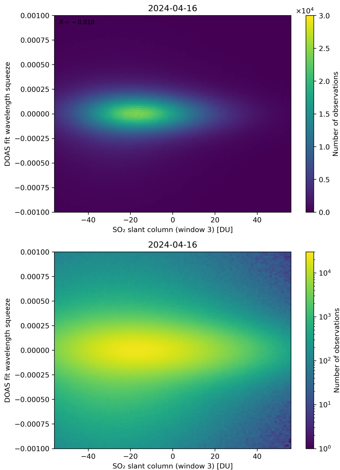
Figure 255: Scatter density plot of “SO 2 slant column (window 3)” against “DOAS fit wavelength squeeze” for 2024-04-16 to 2024-04-17.
