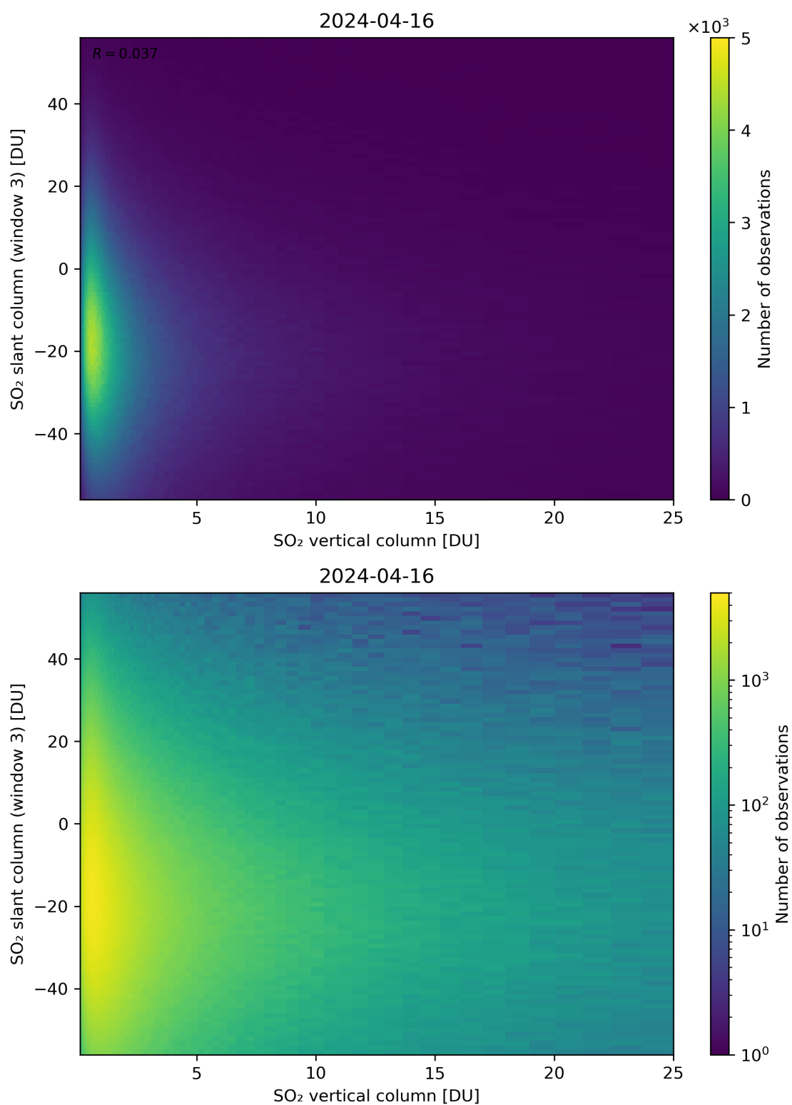
Figure 303: Scatter density plot of “SO 2 vertical column” against “SO 2 slant column (window 3)” for 2024-04-16 to 2024-04-17.
