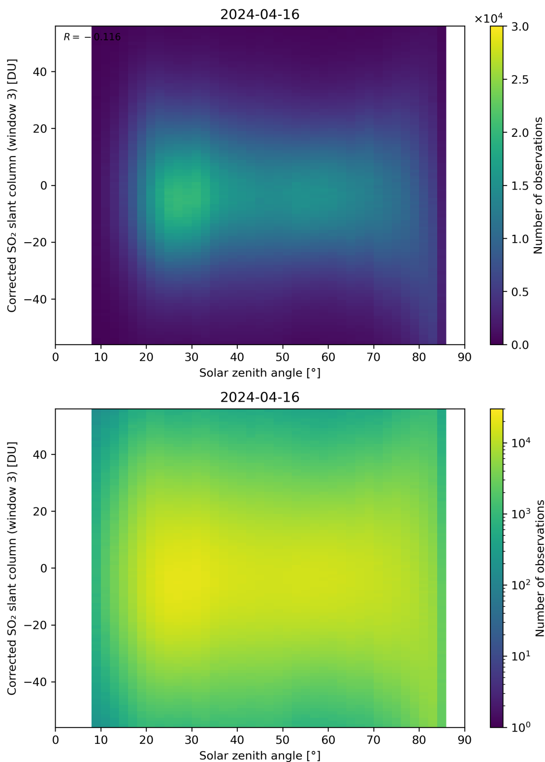
Figure 168: Scatter density plot of “Solar zenith angle” against “Corrected SO 2 slant column (window 3)” for 2024-04-16 to 2024-04-17.
