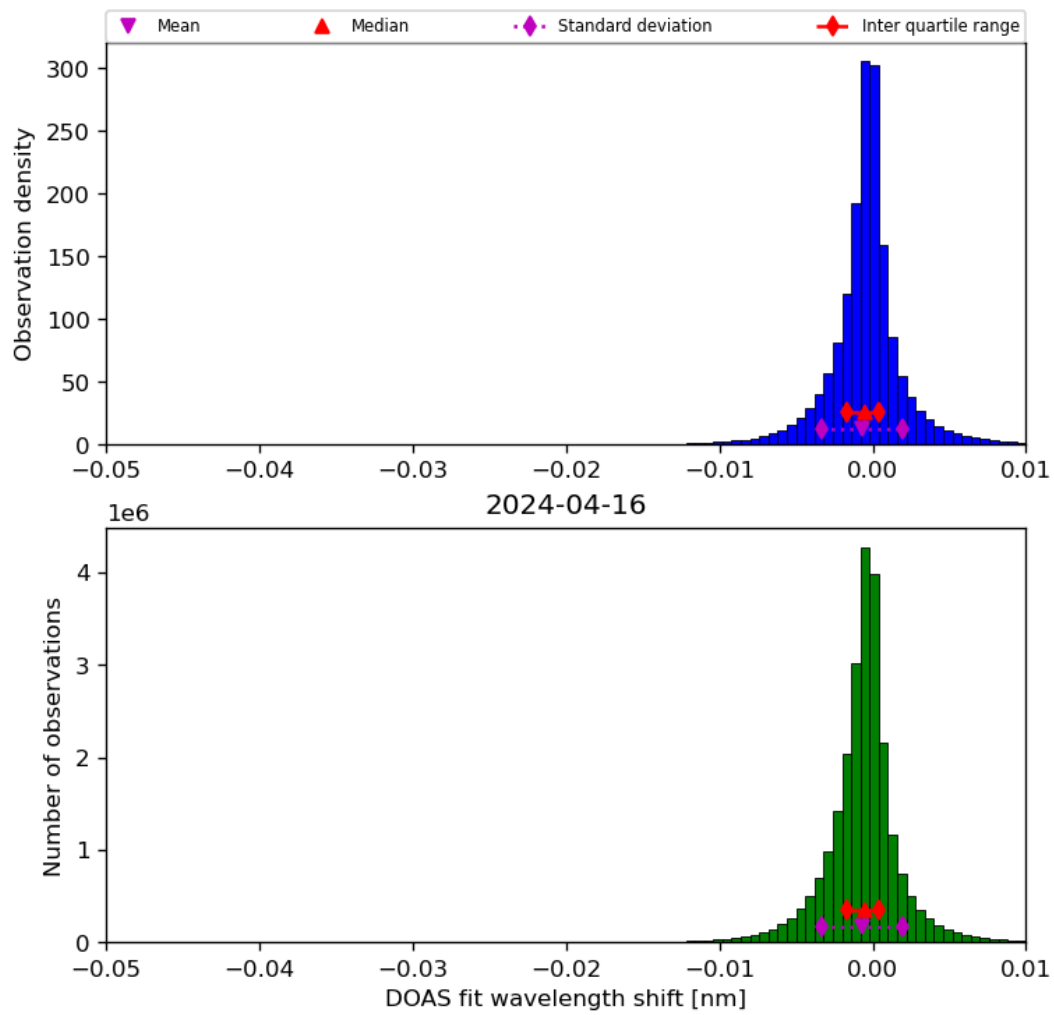
Figure 68: Histogram of “DOAS fit wavelength shift” for 2024-04-16 to 2024-04-17
