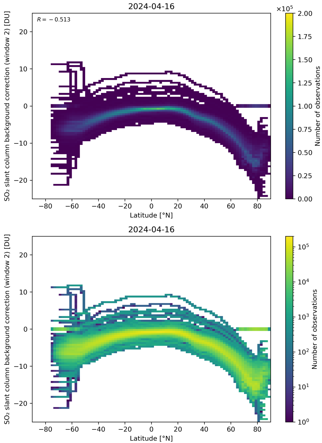
Figure 140: Scatter density plot of “Latitude” against “SO 2 slant column background correction (window 2)” for 2024-04-16 to 2024-04-17.
