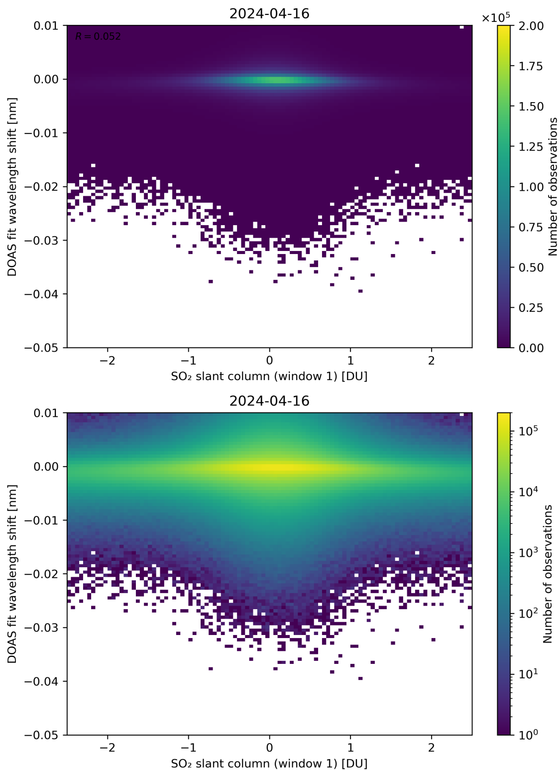
Figure 215: Scatter density plot of “SO 2 slant column (window 1)” against “DOAS fit wavelength shift” for 2024-04-16 to 2024-04-17.
