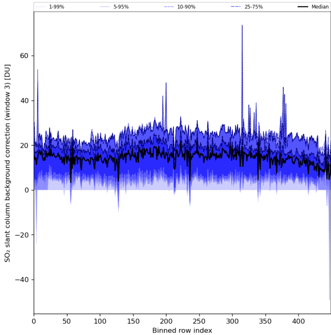
Figure 90: Along track statistics of “SO 2 slant column background correction (window 3)” for 2024-04-16 to 2024-04-17
