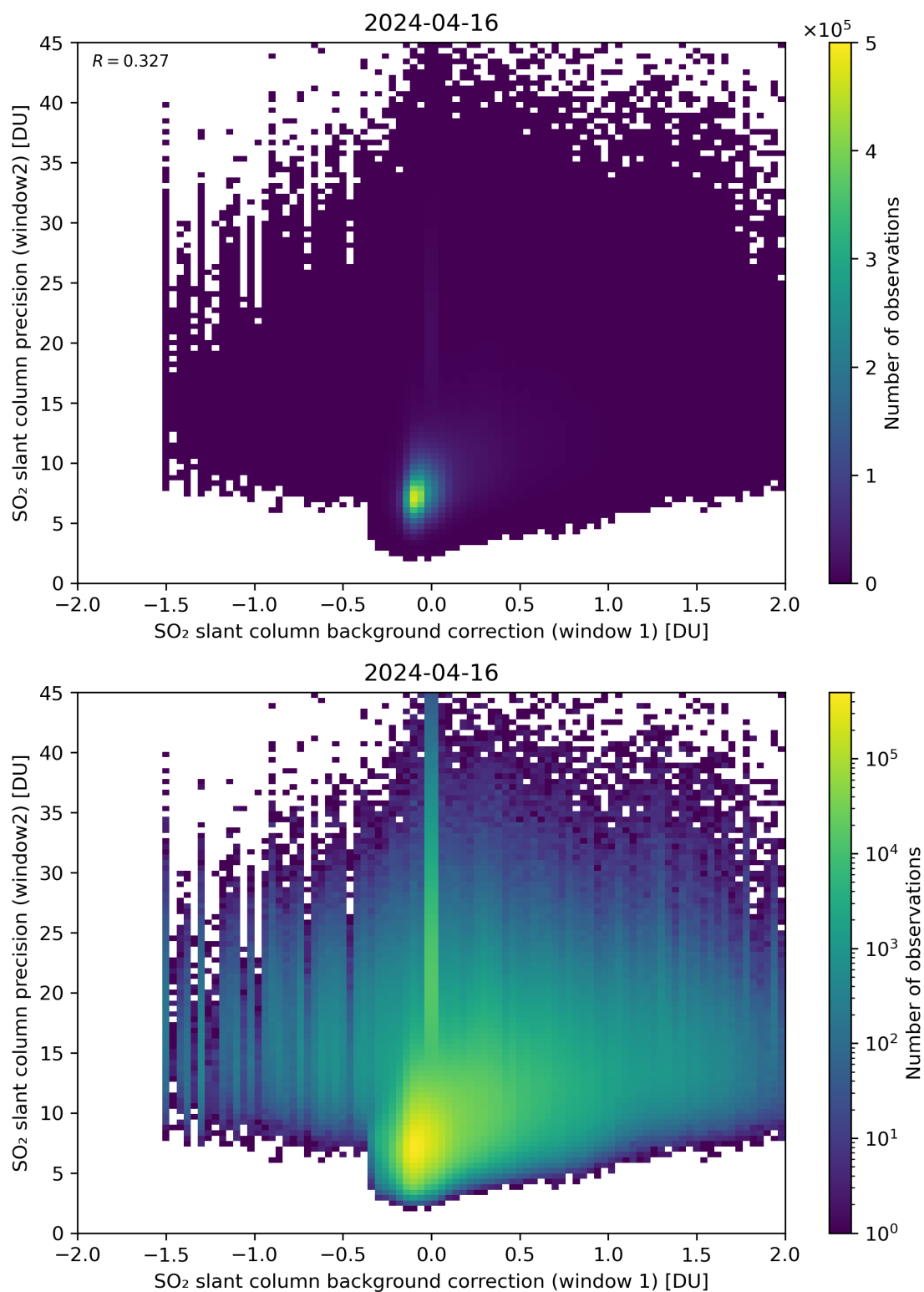
Figure 106: Scatter density plot of “SO 2 slant column background correction (window 1)” against “SO 2 slant column precision (window2)” for 2024-04-16 to 2024-04-17.
