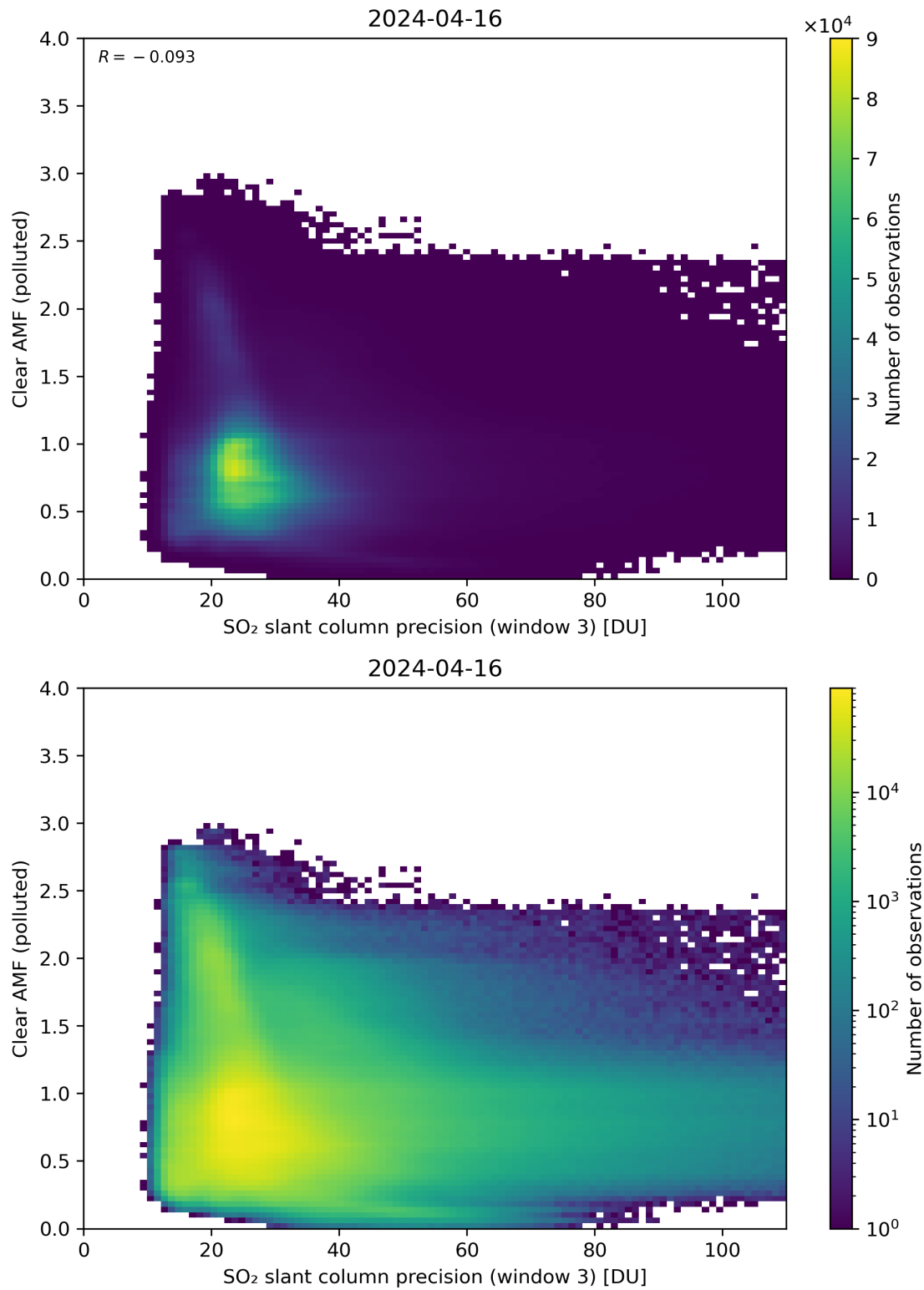
Figure 261: Scatter density plot of “SO 2 slant column precision (window 3)” against “Clear AMF (polluted)” for 2024-04-16 to 2024-04-17.
