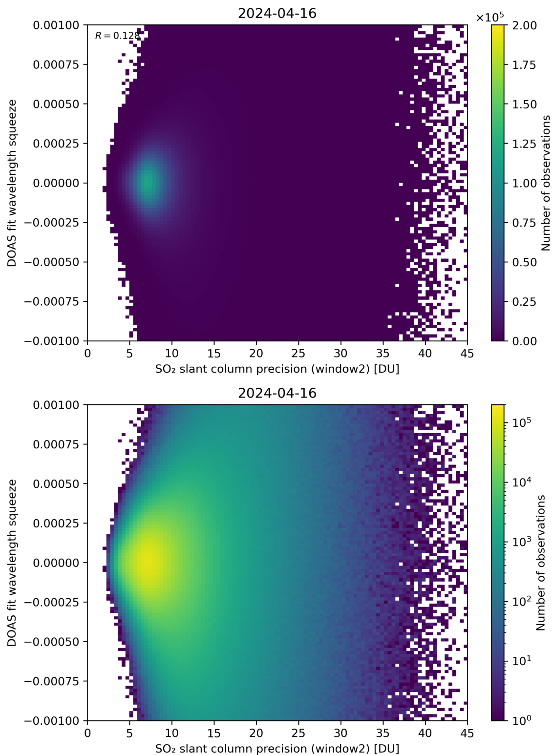
Figure 244: Scatter density plot of “SO 2 slant column precision (window2)” against “DOAS fit wavelength squeeze” for 2024-04-16 to 2024-04-17.
