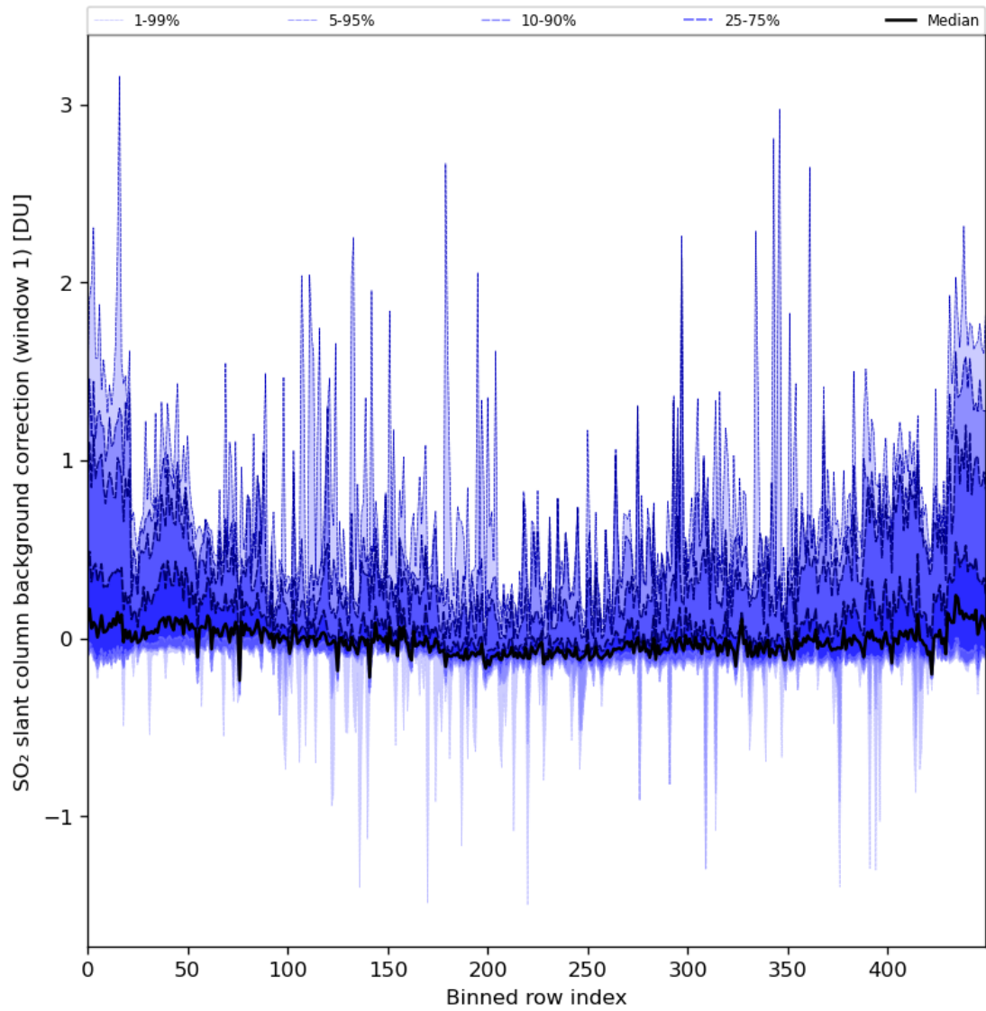
Figure 82: Along track statistics of “SO 2 slant column background correction (window 1)” for 2024-04-16 to 2024-04-17
