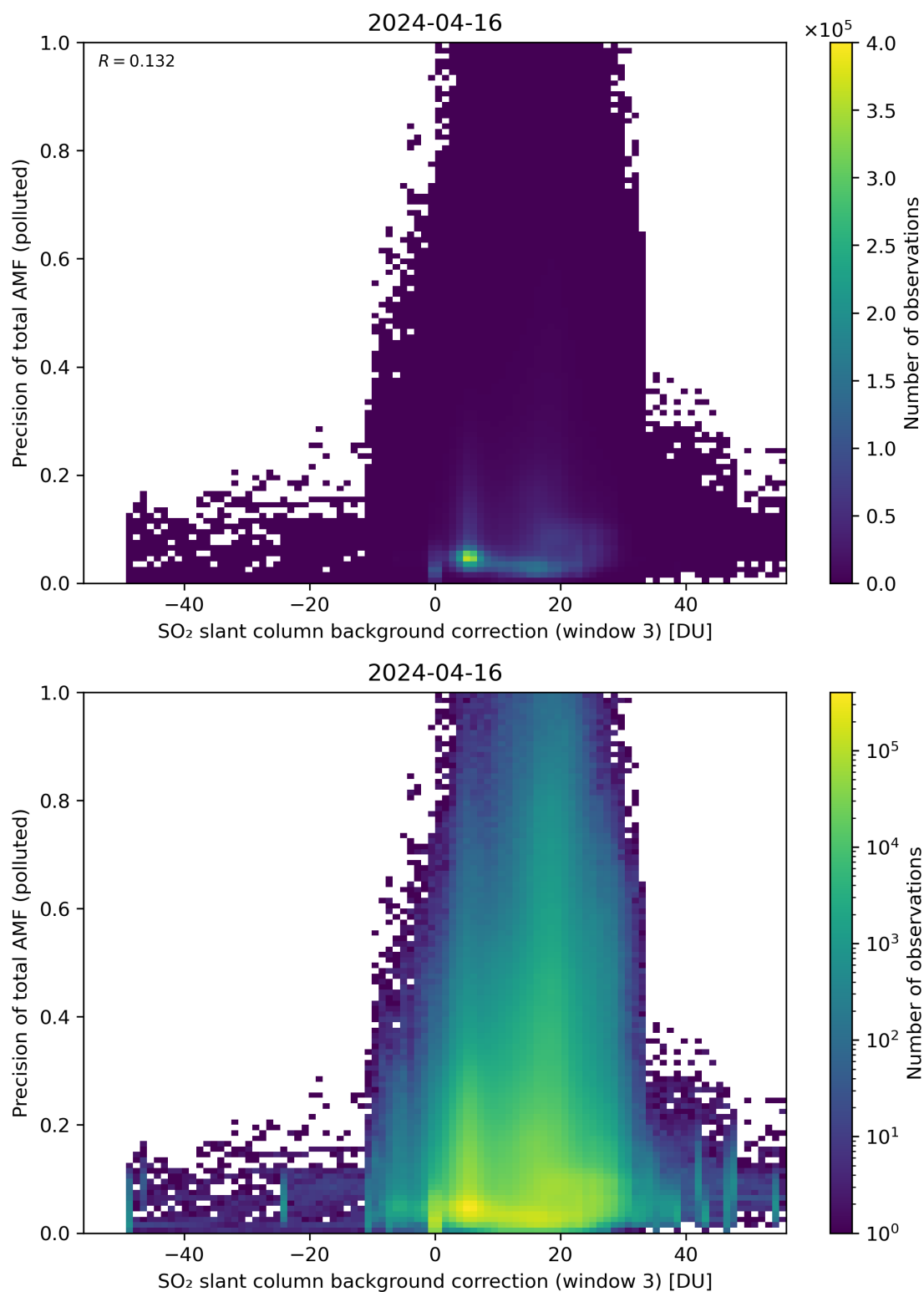
Figure 126: Scatter density plot of “SO 2 slant column background correction (window 3)” against “Precision of total AMF (polluted)” for 2024-04-16 to 2024-04-17.
