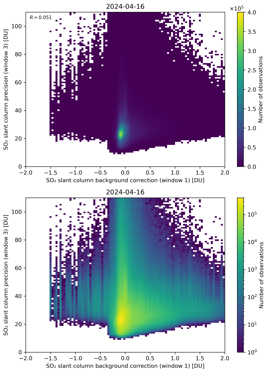
Figure 108: Scatter density plot of “SO 2 slant column background correction (window 1)” against “SO 2 slant column precision (window 3)” for 2024-04-16 to 2024-04-17.
