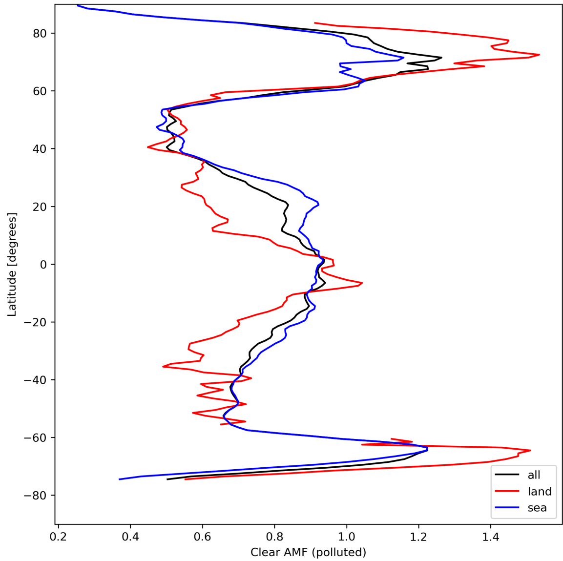
Figure 50: Zonal average of “Clear AMF (polluted)” for 2024-04-16 to 2024-04-17.
