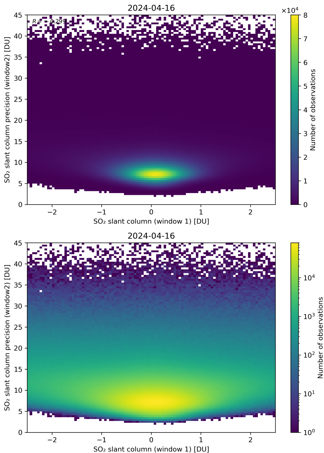
Figure 236: Scatter density plot of “SO 2 slant column (window 1)” against “SO 2 slant column precision (window2)” for 2024-04-16 to 2024-04-17.
