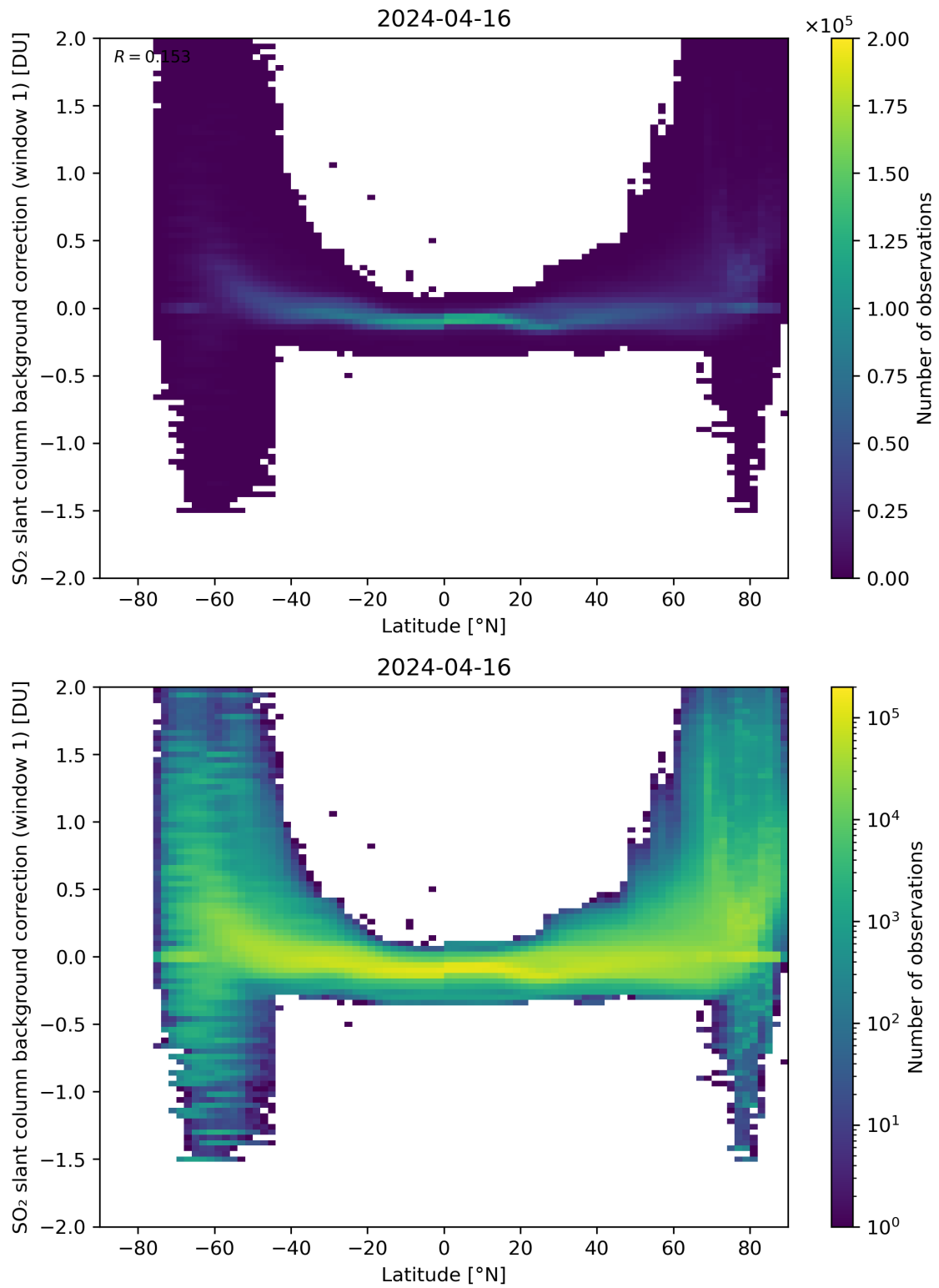
Figure 139: Scatter density plot of “Latitude” against “SO 2 slant column background correction (window 1)” for 2024-04-16 to 2024-04-17.
