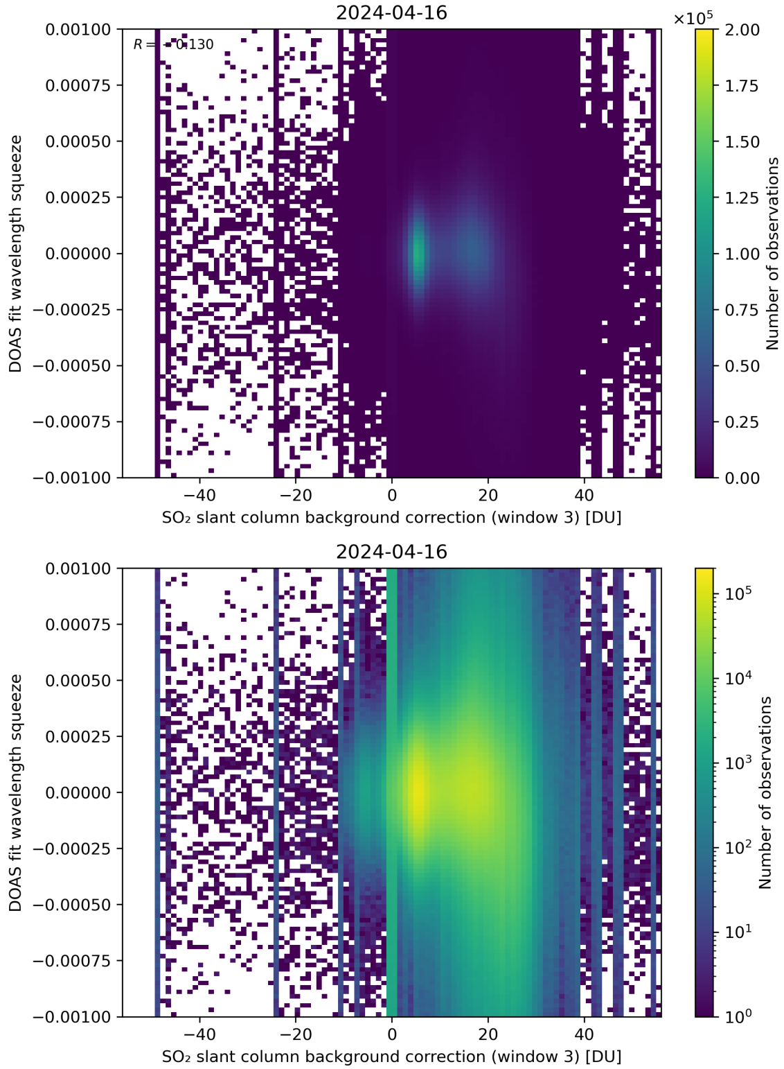
Figure 122: Scatter density plot of “SO 2 slant column background correction (window 3)” against “DOAS fit wavelength squeeze” for 2024-04-16 to 2024-04-17.
