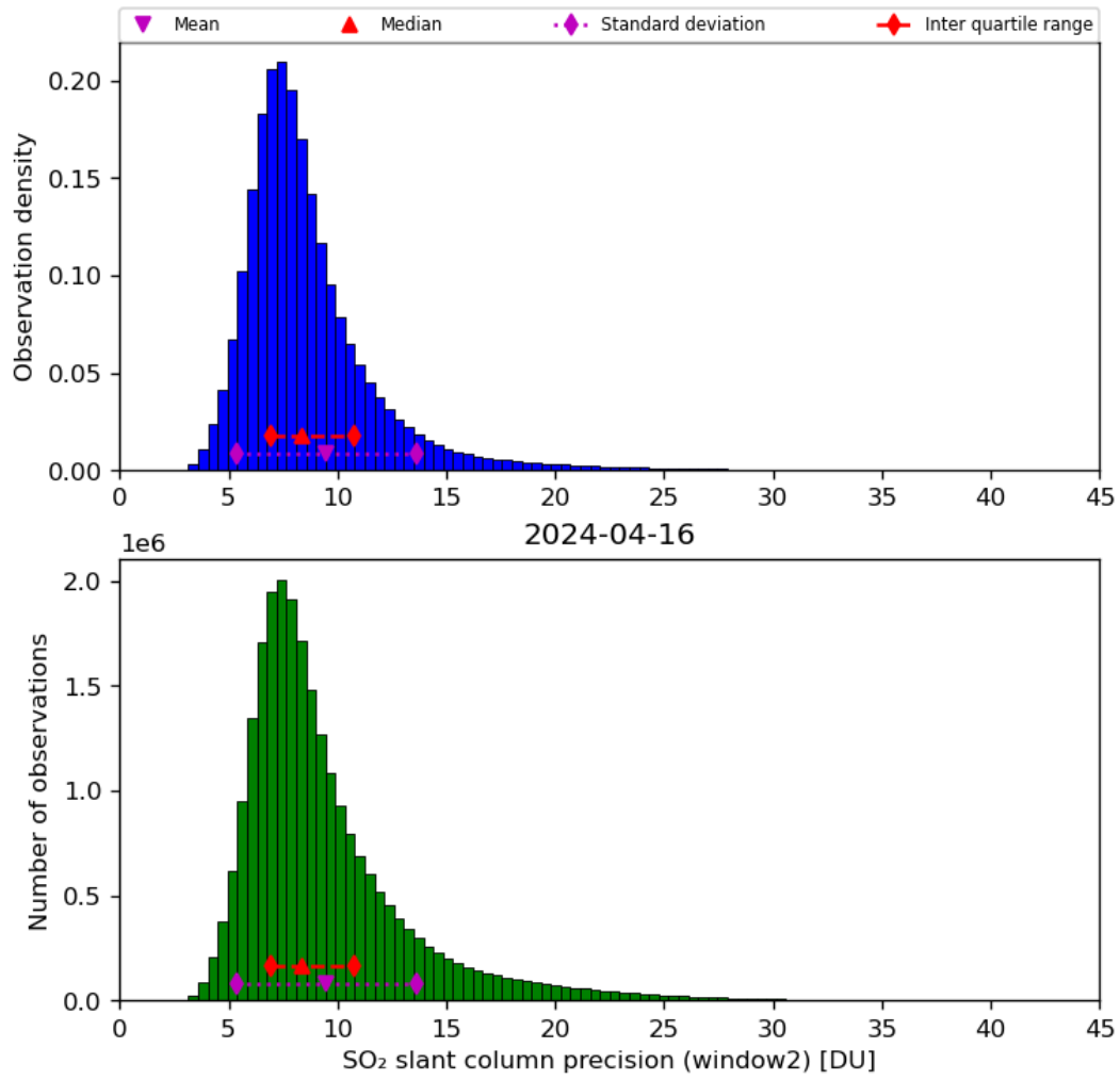
Figure 61: Histogram of “SO 2 slant column precision (window2)” for 2024-04-16 to 2024-04-17
