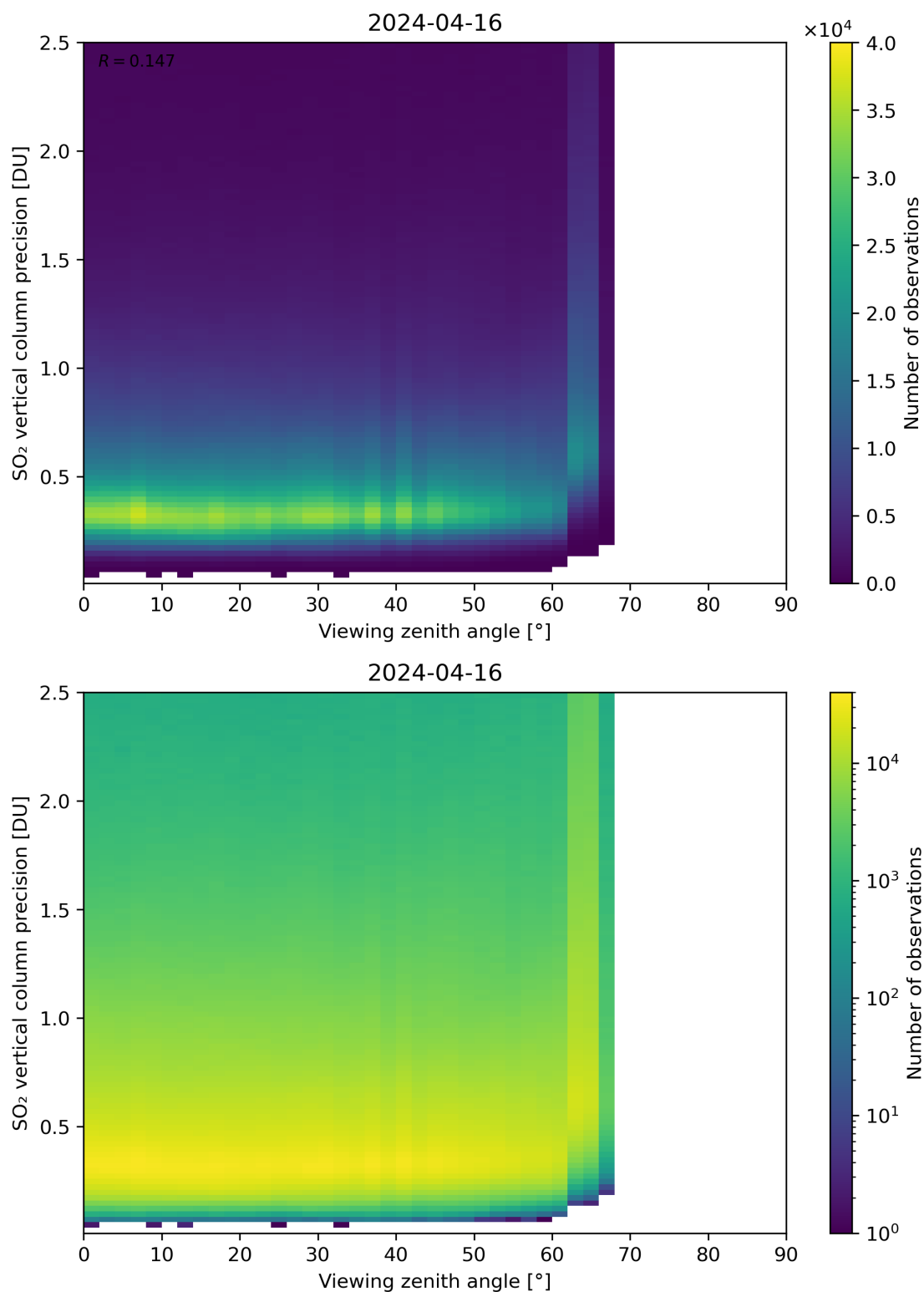
Figure 328: Scatter density plot of “Viewing zenith angle” against “SO 2 vertical column precision” for 2024-04-16 to 2024-04-17.
