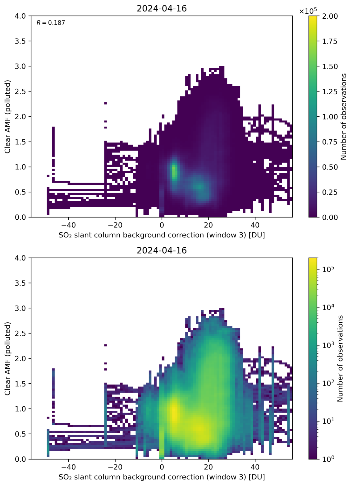
Figure 124: Scatter density plot of “SO 2 slant column background correction (window 3)” against “Clear AMF (polluted)” for 2024-04-16 to 2024-04-17.
