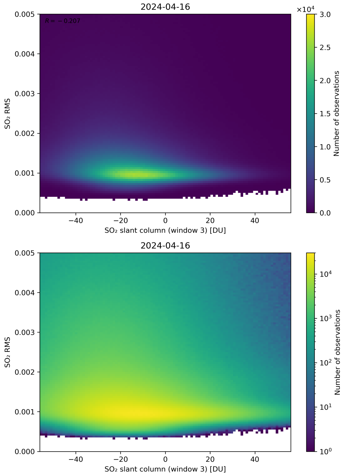
Figure 256: Scatter density plot of “SO 2 slant column (window 3)” against “SO 2 RMS” for 2024-04-16 to 2024-04-17.
