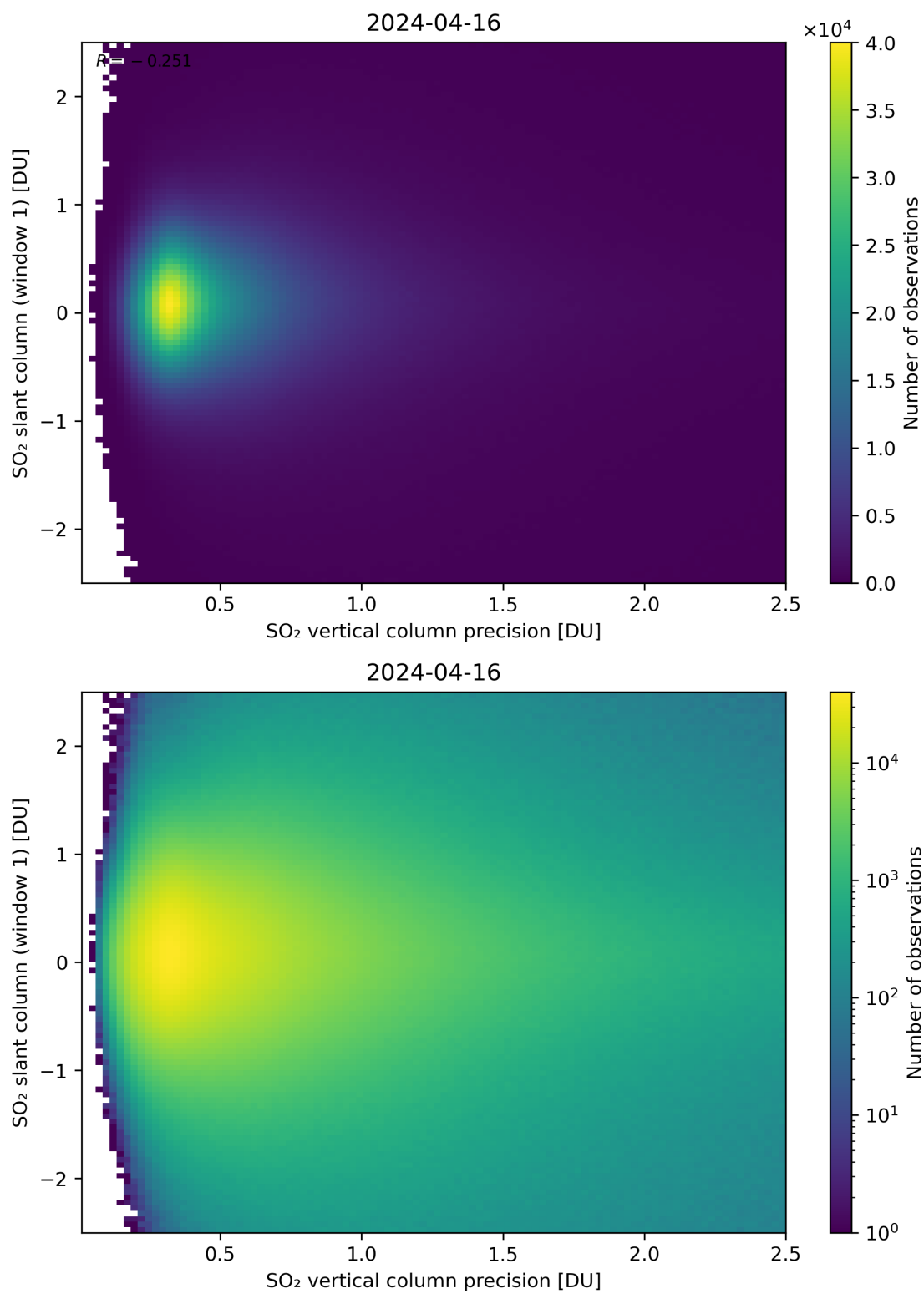
Figure 289: Scatter density plot of “SO 2 vertical column precision” against “SO 2 slant column (window 1)” for 2024-04-16 to 2024-04-17.
