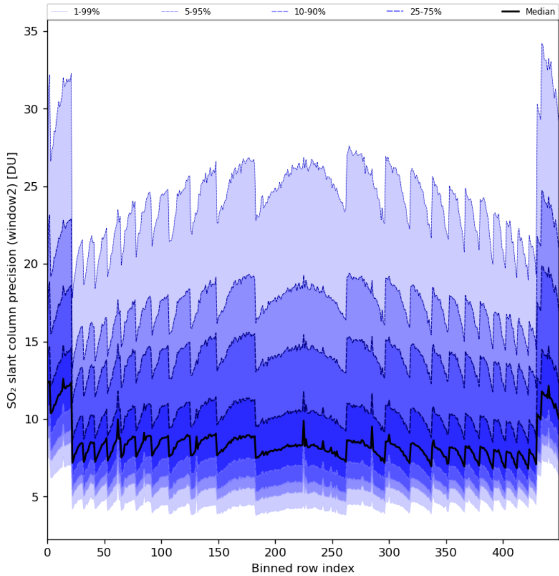
Figure 84: Along track statistics of “SO 2 slant column precision (window2)” for 2024-04-16 to 2024-04-17
