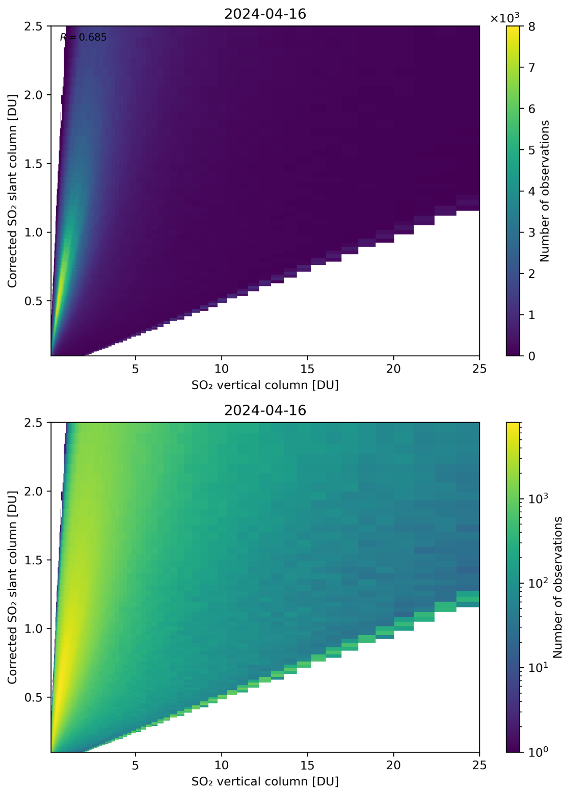
Figure 297: Scatter density plot of “SO 2 vertical column” against “Corrected SO 2 slant column” for 2024-04-16 to 2024-04-17.
