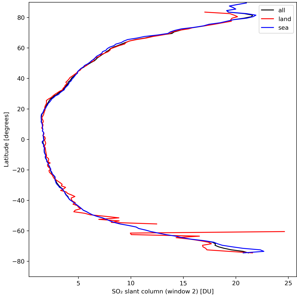
Figure 37: Zonal average of “SO 2 slant column (window 2)” for 2024-04-16 to 2024-04-17.
