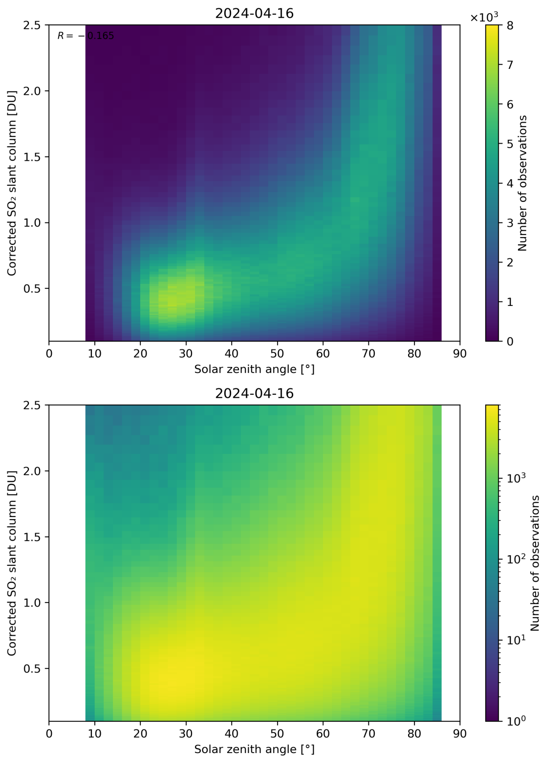
Figure 166: Scatter density plot of “Solar zenith angle” against “Corrected SO 2 slant column” for 2024-04-16 to 2024-04-17.
