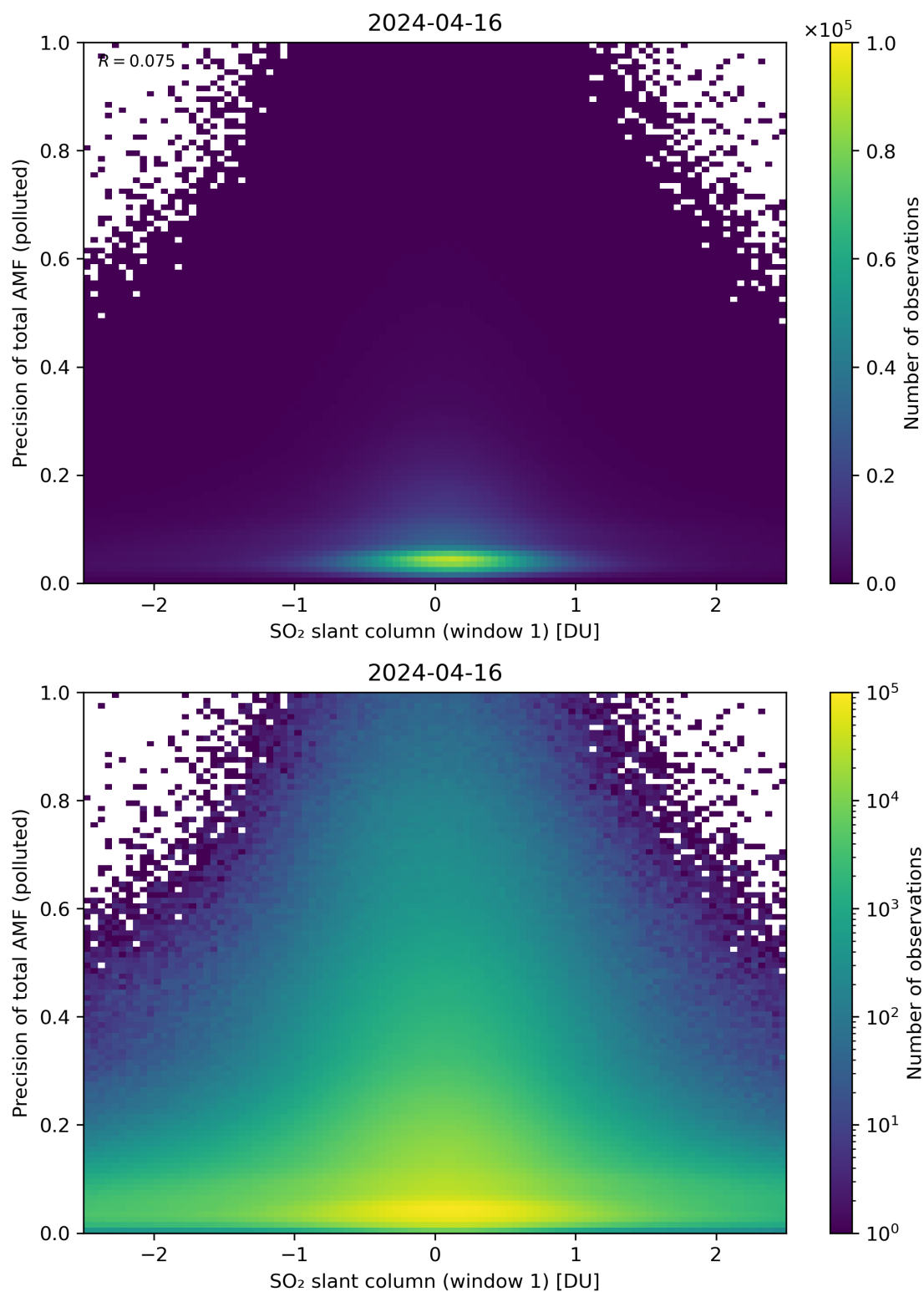
Figure 240: Scatter density plot of “SO 2 slant column (window 1)” against “Precision of total AMF (polluted)” for 2024-04-16 to 2024-04-17.
