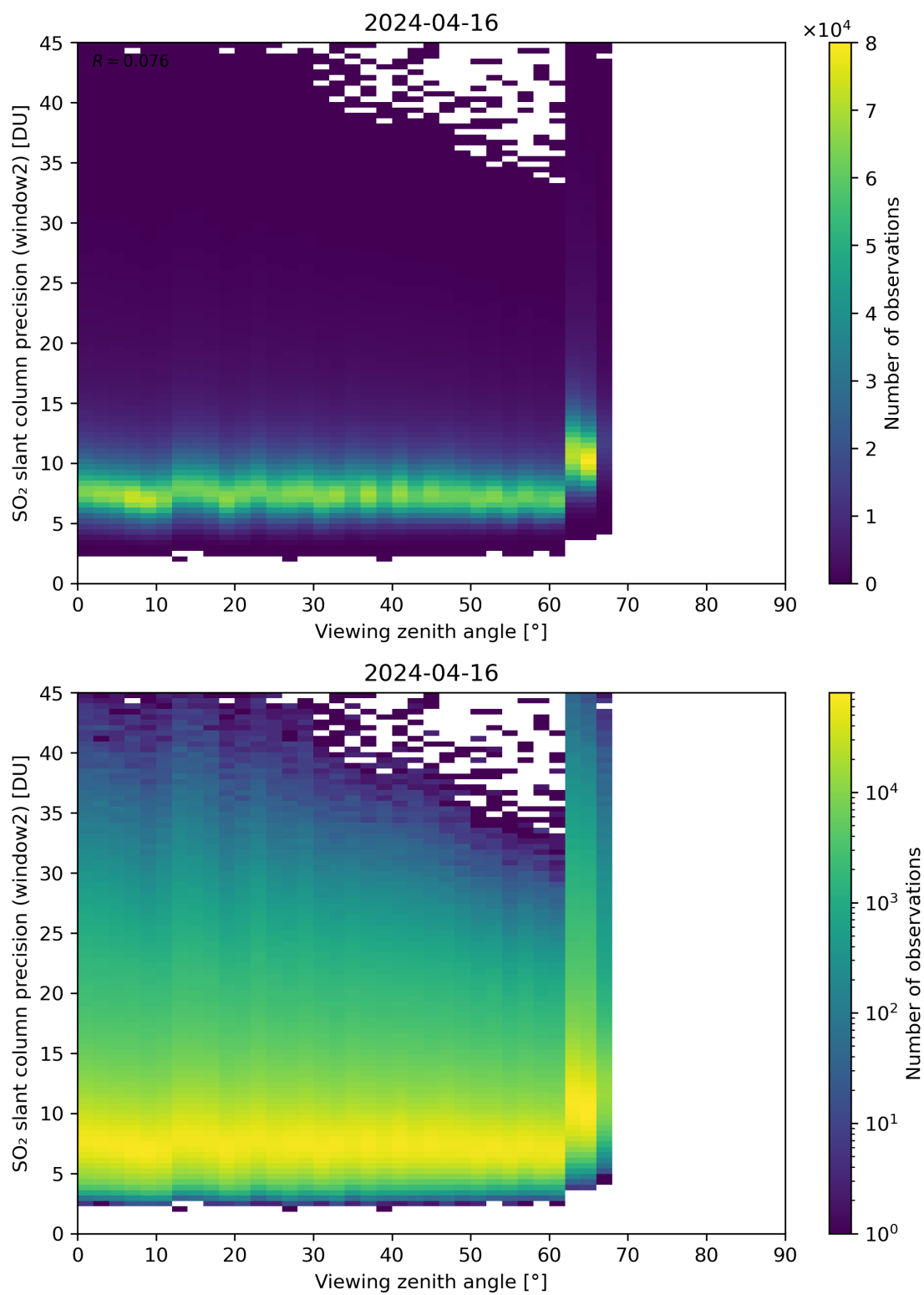
Figure 322: Scatter density plot of “Viewing zenith angle” against “SO 2 slant column precision (window2)” for 2024-04-16 to 2024-04-17.
