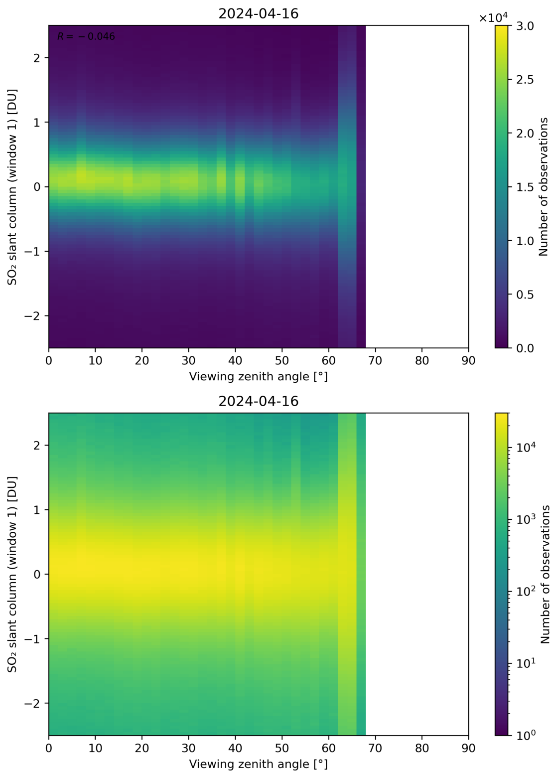
Figure 320: Scatter density plot of “Viewing zenith angle” against “SO 2 slant column (window 1)” for 2024-04-16 to 2024-04-17.
