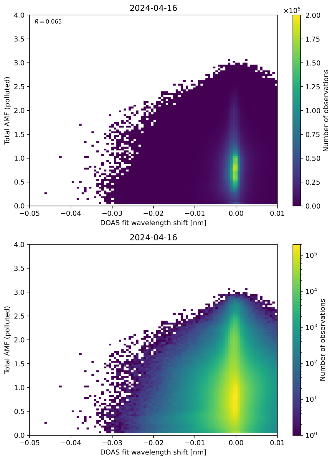
Figure 130: Scatter density plot of “DOAS fit wavelength shift” against “Total AMF (polluted)” for 2024-04-16 to 2024-04-17.
