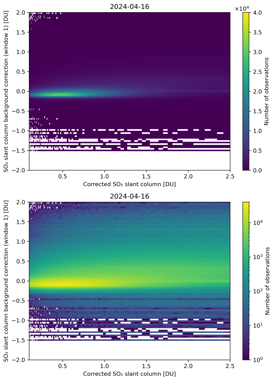
Figure 178: Scatter density plot of “Corrected SO 2 slant column” against “SO 2 slant column background correction (window 1)” for 2024-04-16 to 2024-04-17.
