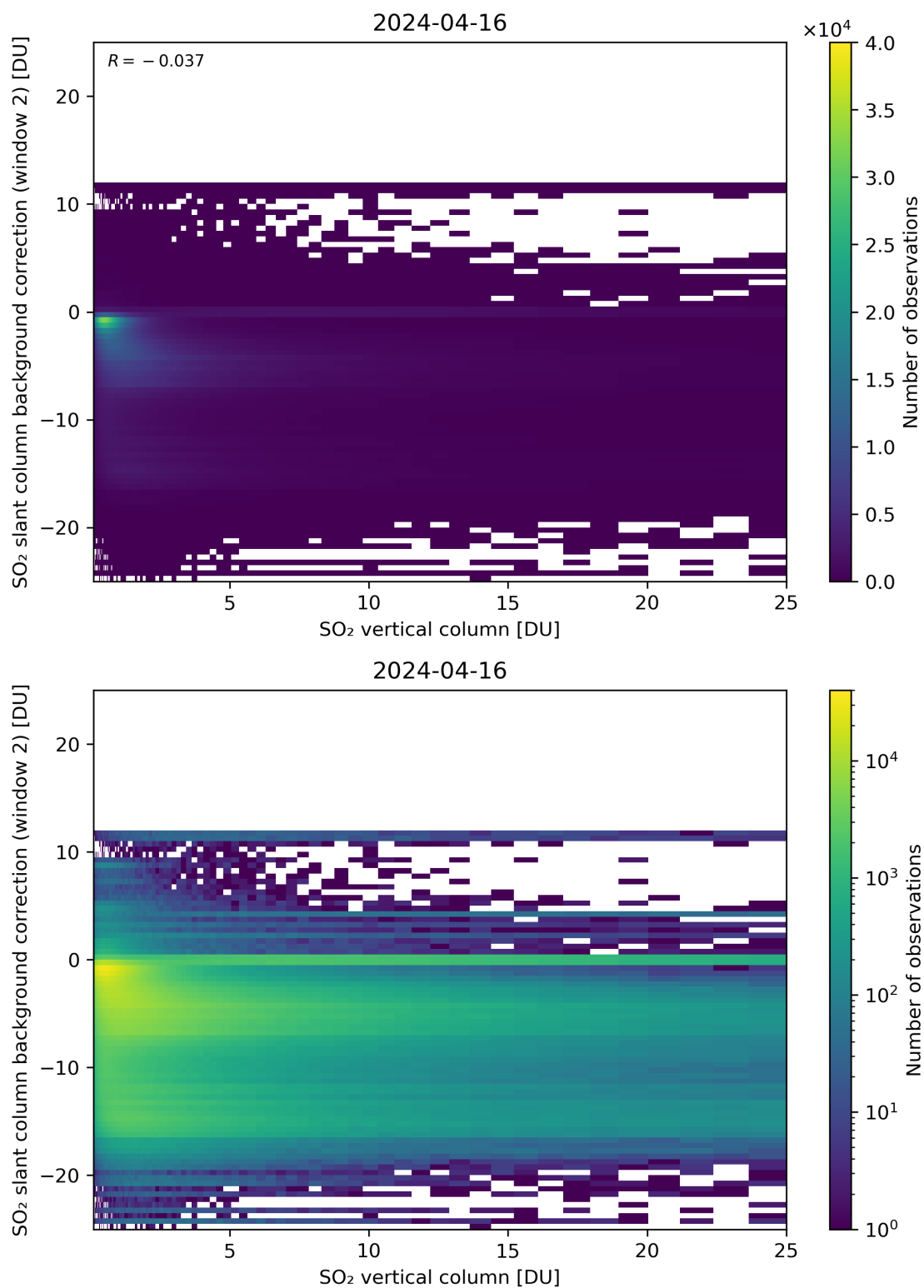
Figure 274: Scatter density plot of “SO 2 vertical column” against “SO 2 slant column background correction (window 2)” for 2024-04-16 to 2024-04-17.
