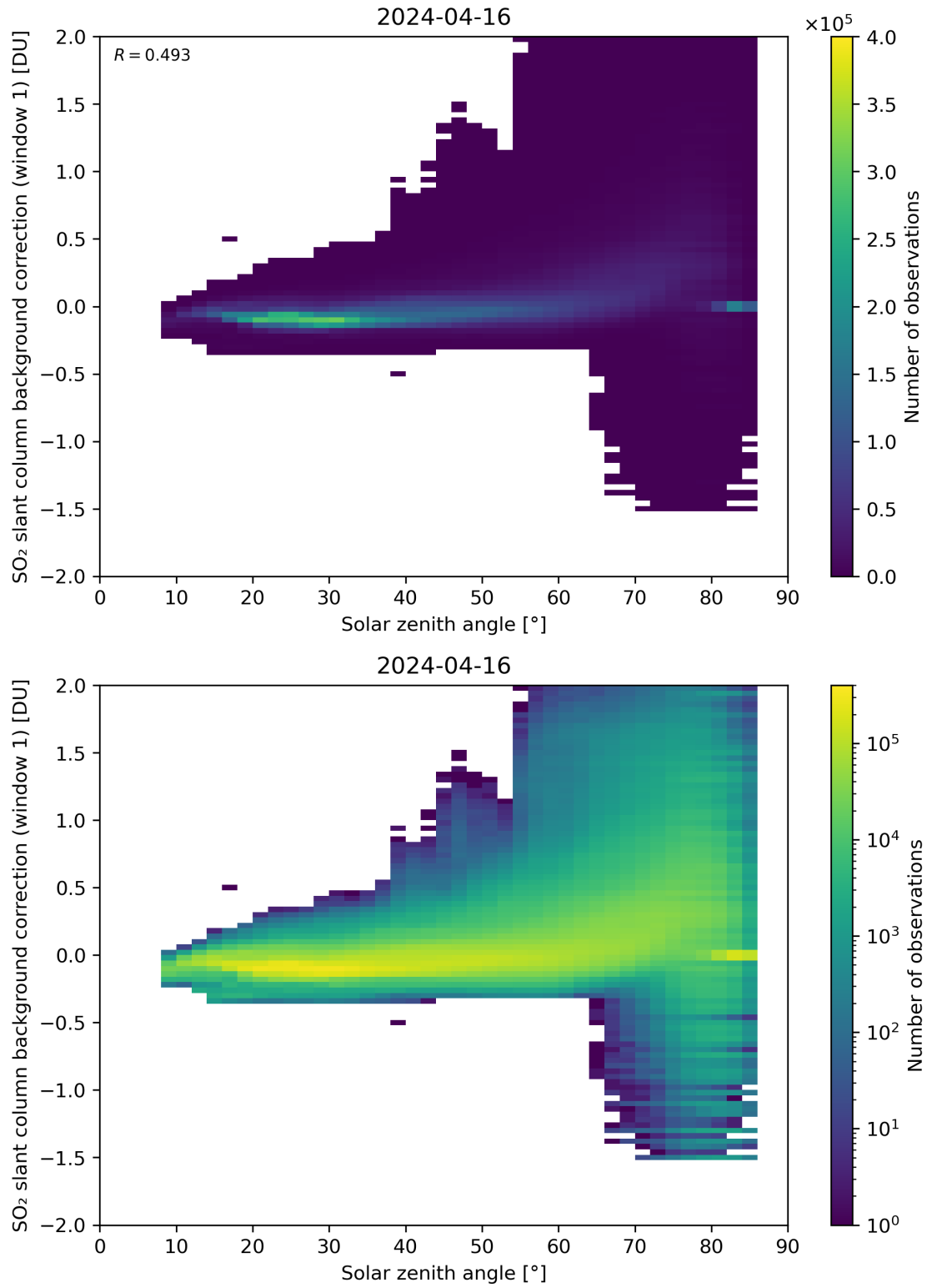
Figure 158: Scatter density plot of “Solar zenith angle” against “SO 2 slant column background correction (window 1)” for 2024-04-16 to 2024-04-17.
