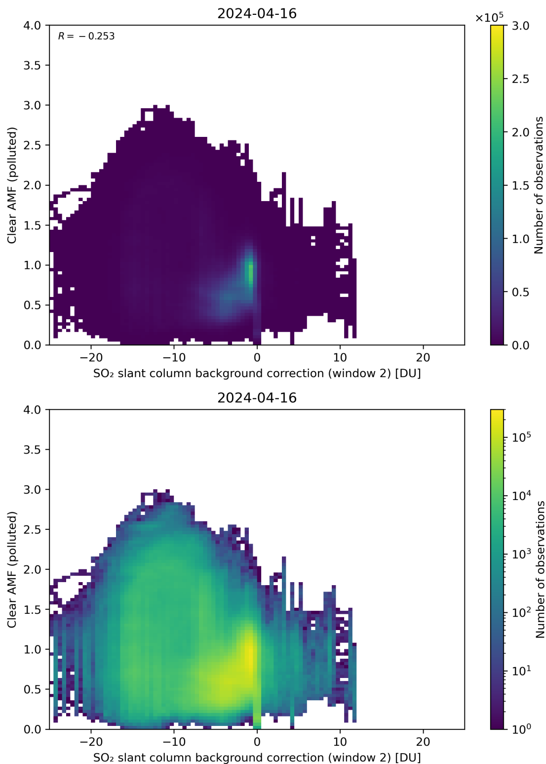
Figure 115: Scatter density plot of “SO 2 slant column background correction (window 2)” against “Clear AMF (polluted)” for 2024-04-16 to 2024-04-17.
