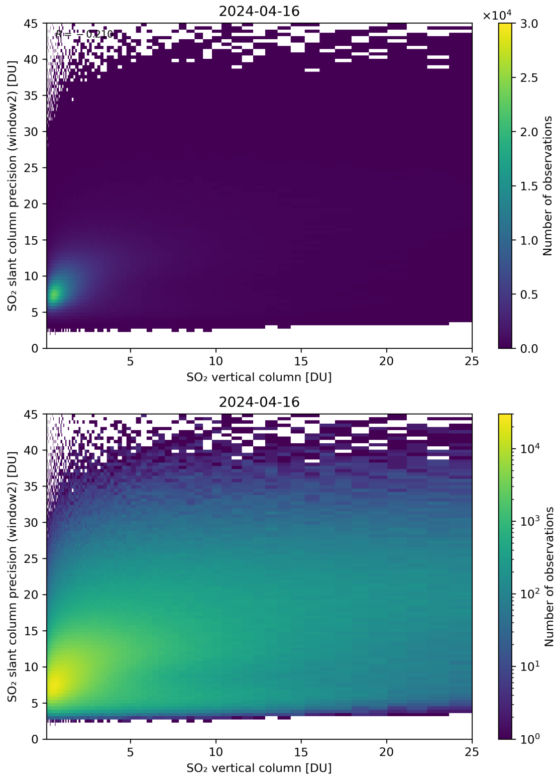
Figure 302: Scatter density plot of “SO 2 vertical column” against “SO 2 slant column precision (window2)” for 2024-04-16 to 2024-04-17.
