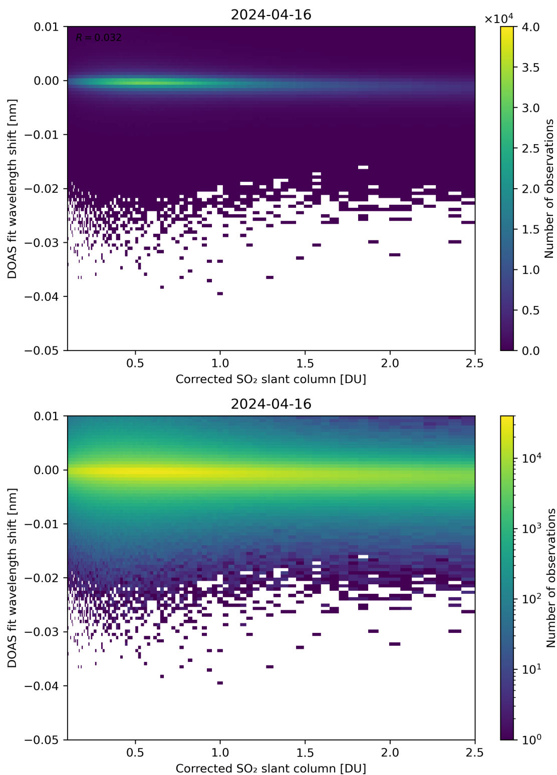
Figure 181: Scatter density plot of “Corrected SO 2 slant column” against “DOAS fit wavelength shift” for 2024-04-16 to 2024-04-17.
