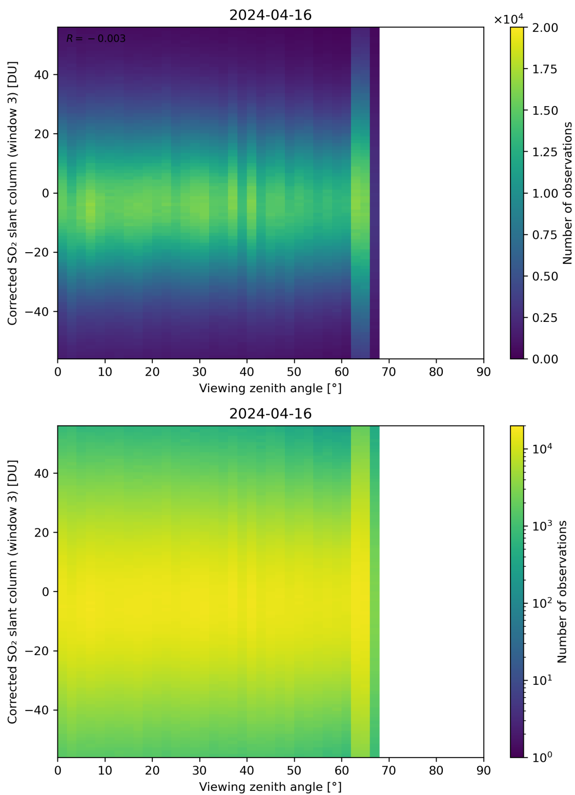
Figure 319: Scatter density plot of “Viewing zenith angle” against “Corrected SO 2 slant column (window 3)” for 2024-04-16 to 2024-04-17.
