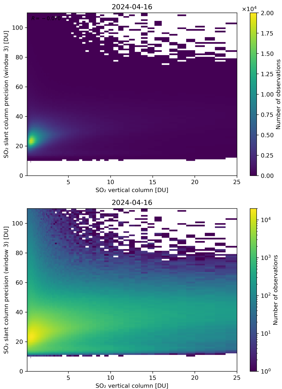
Figure 304: Scatter density plot of “SO 2 vertical column” against “SO 2 slant column precision (window 3)” for 2024-04-16 to 2024-04-17.
