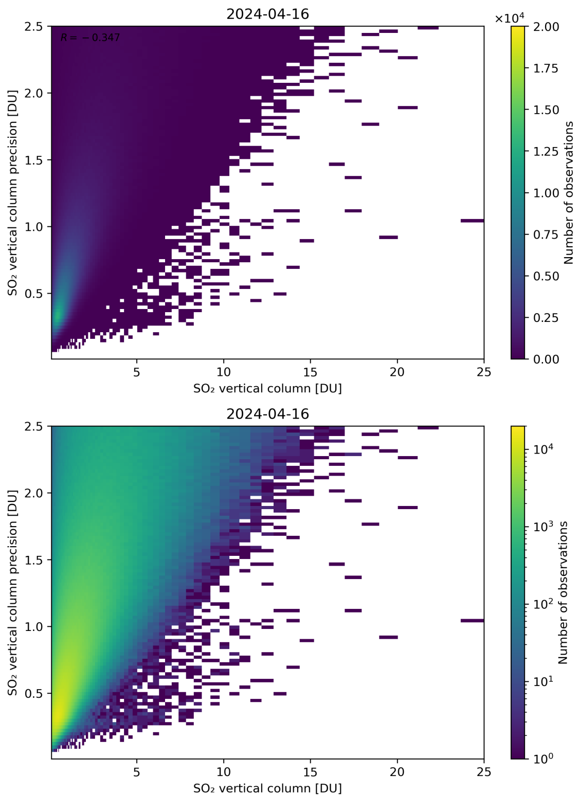
Figure 307: Scatter density plot of “SO 2 vertical column” against “SO 2 vertical column precision” for 2024-04-16 to 2024-04-17.
