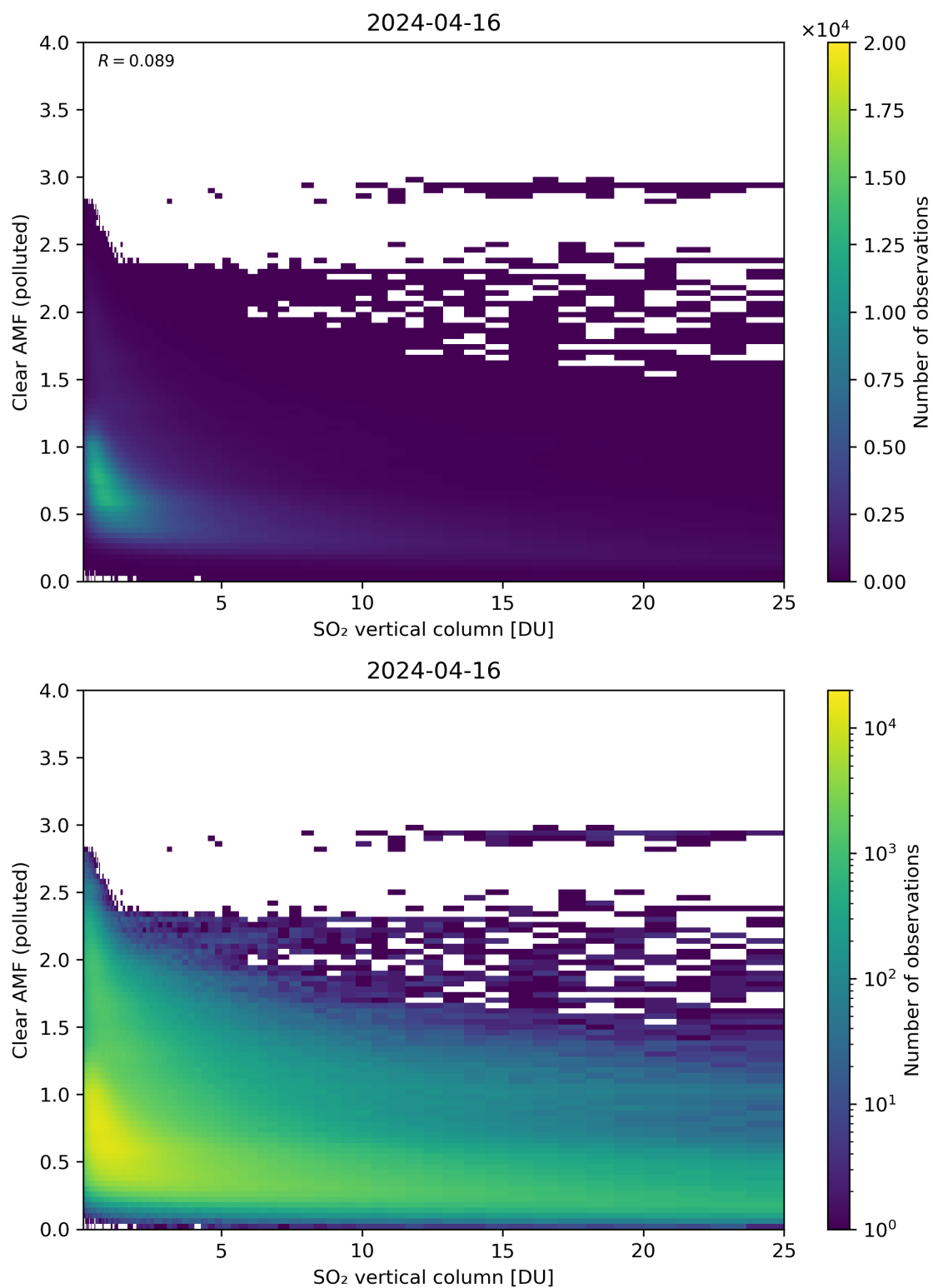
Figure 296: Scatter density plot of “SO 2 vertical column” against “Clear AMF (polluted)” for 2024-04-16 to 2024-04-17.
