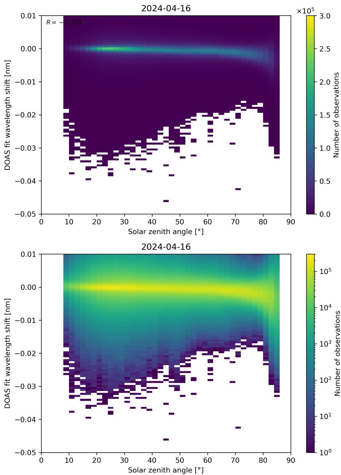
Figure 161: Scatter density plot of “Solar zenith angle” against “DOAS fit wavelength shift” for 2024-04-16 to 2024-04-17.
