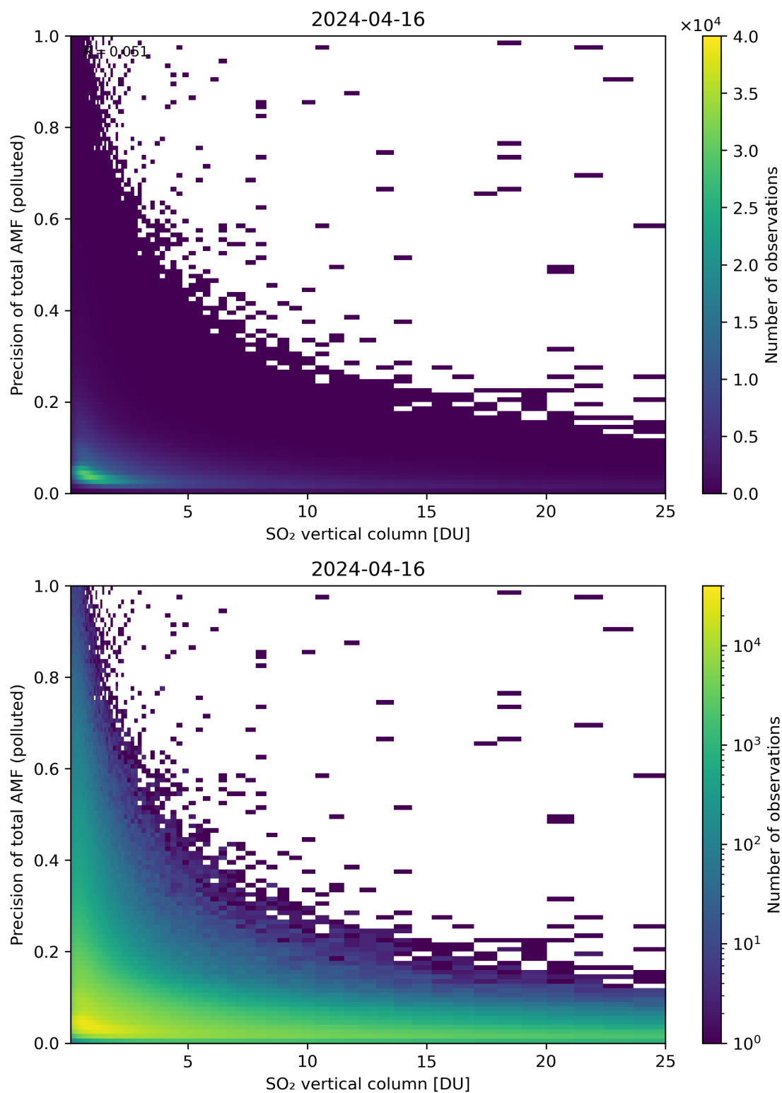
Figure 306: Scatter density plot of “SO 2 vertical column” against “Precision of total AMF (polluted)” for 2024-04-16 to 2024-04-17.
