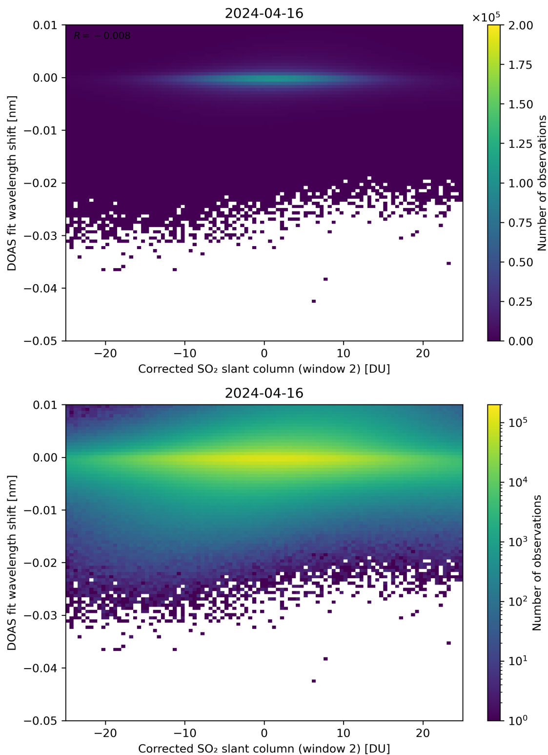
Figure 196: Scatter density plot of “Corrected SO 2 slant column (window 2)” against “DOAS fit wavelength shift” for 2024-04-16 to 2024-04-17.
