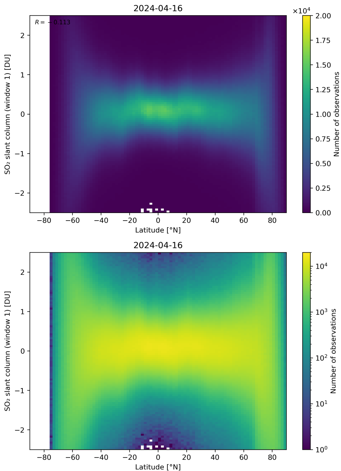
Figure 149: Scatter density plot of “Latitude” against “SO 2 slant column (window 1)” for 2024-04-16 to 2024-04-17.
