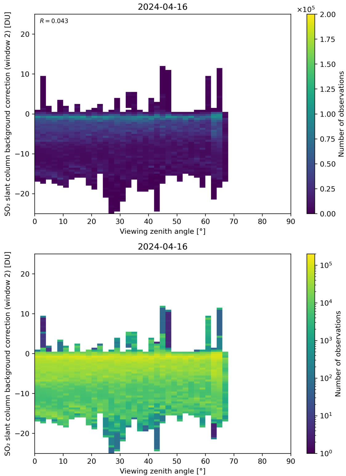
Figure 309: Scatter density plot of “Viewing zenith angle” against “SO 2 slant column background correction (window 2)” for 2024-04-16 to 2024-04-17.
