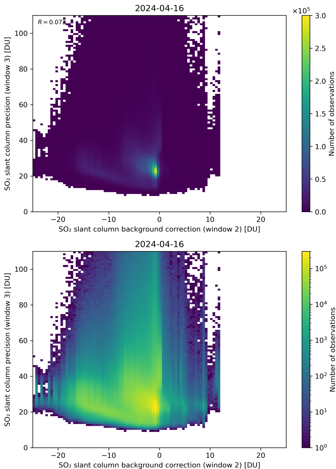
Figure 118: Scatter density plot of “SO 2 slant column background correction (window 2)” against “SO 2 slant column precision (window 3)” for 2024-04-16 to 2024-04-17.
