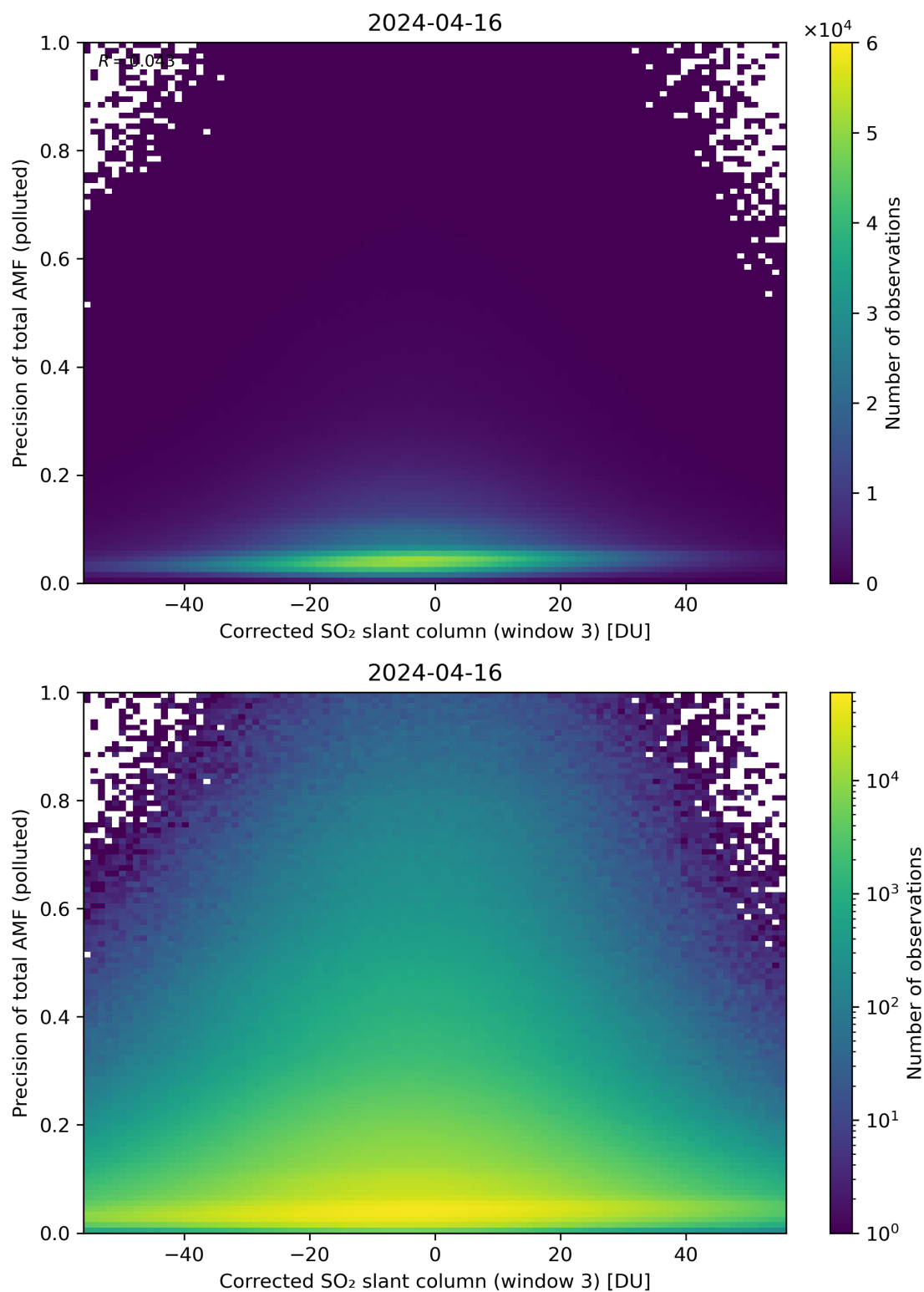
Figure 211: Scatter density plot of “Corrected SO 2 slant column (window 3)” against “Precision of total AMF (polluted)” for 2024-04-16 to 2024-04-17.
