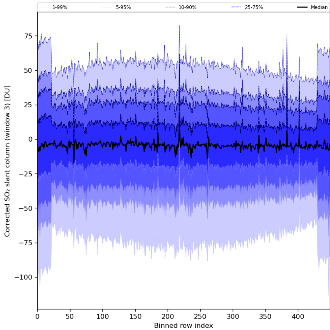
Figure 89: Along track statistics of “Corrected SO 2 slant column (window 3)” for 2024-04-16 to 2024-04-17
