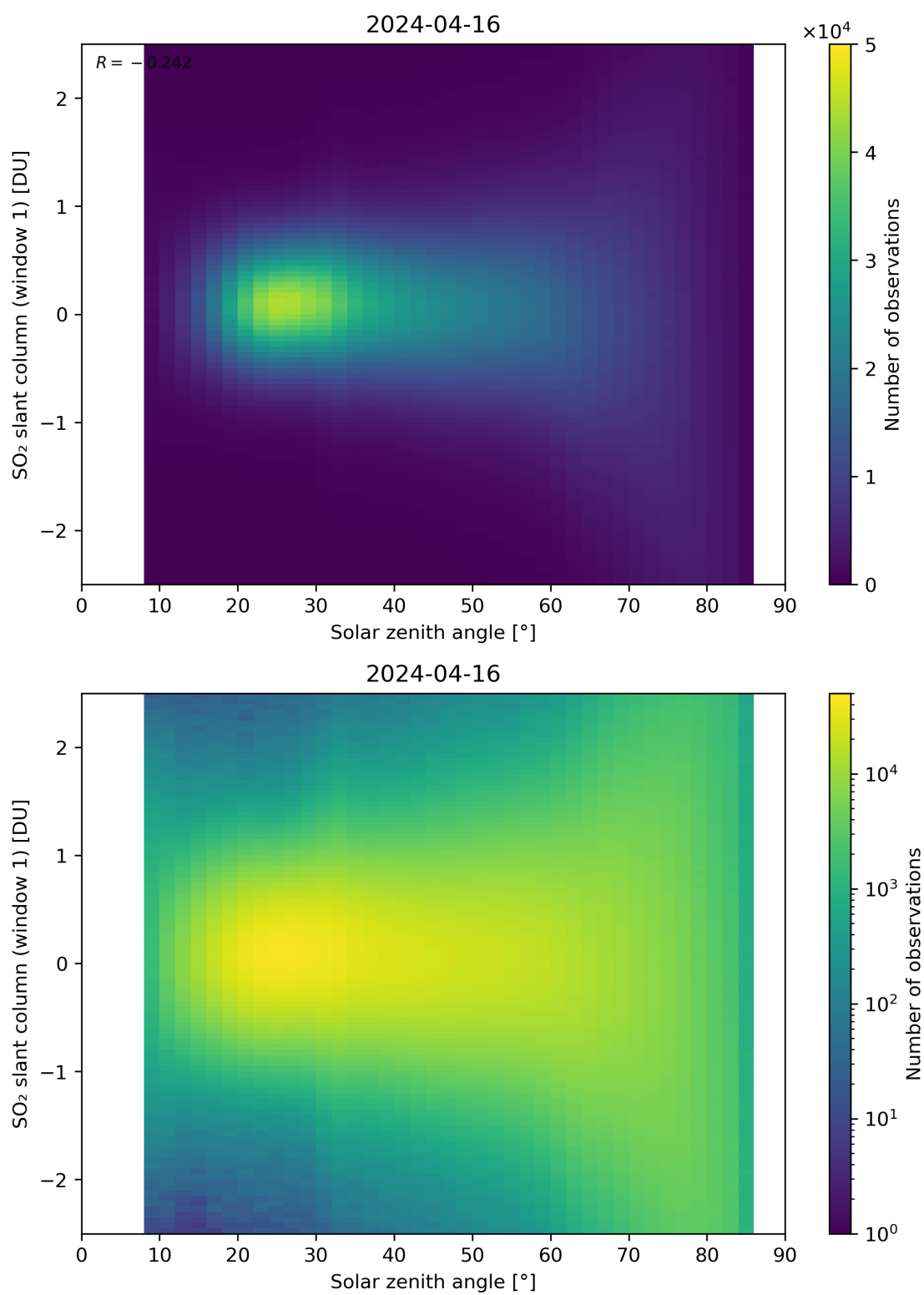
Figure 169: Scatter density plot of “Solar zenith angle” against “SO 2 slant column (window 1)” for 2024-04-16 to 2024-04-17.
