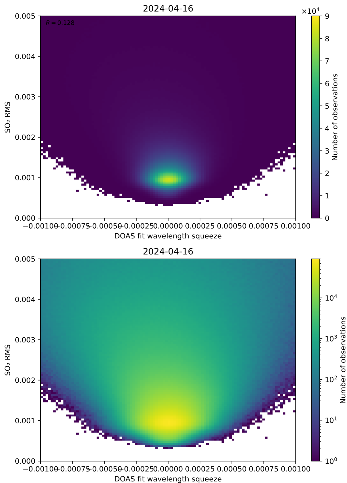
Figure 132: Scatter density plot of “DOAS fit wavelength squeeze” against “SO 2 RMS” for 2024-04-16 to 2024-04-17.
