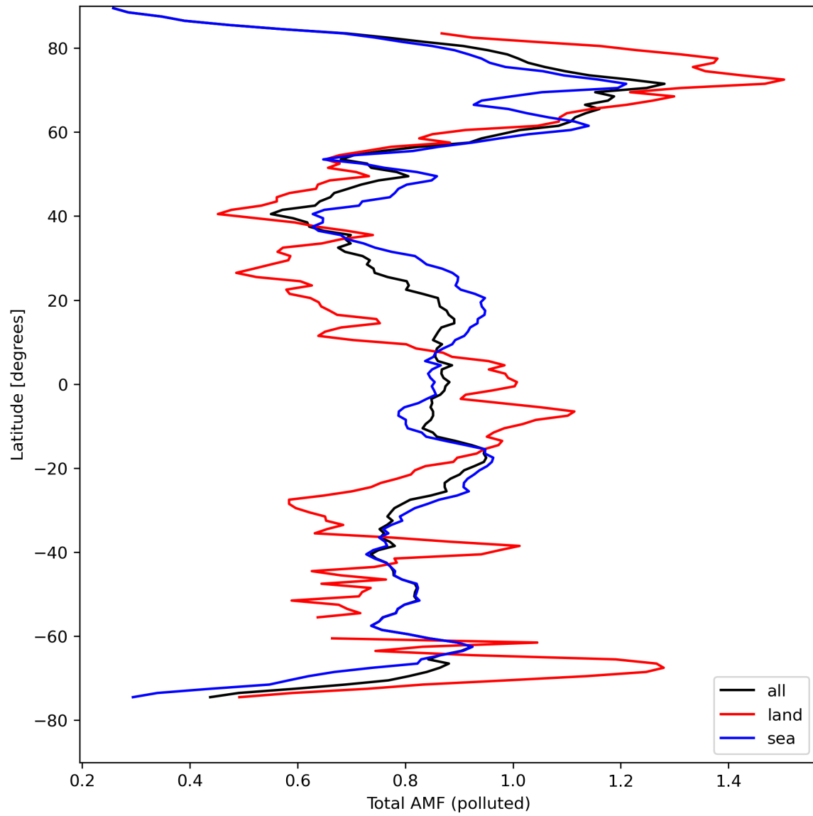
Figure 48: Zonal average of “Total AMF (polluted)” for 2024-04-16 to 2024-04-17.
