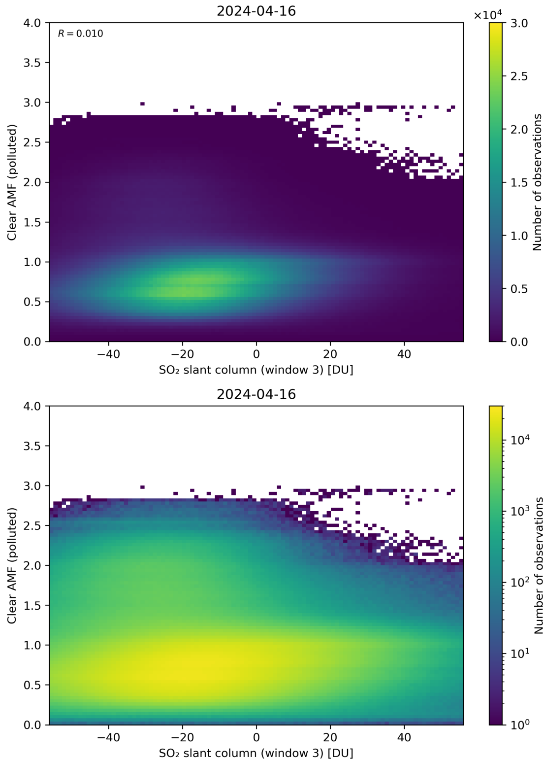
Figure 265: Scatter density plot of “SO 2 slant column (window 3)” against “Clear AMF (polluted)” for 2024-04-16 to 2024-04-17.
