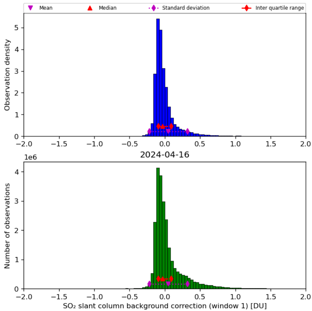
Figure 59: Histogram of “SO 2 slant column background correction (window 1)” for 2024-04-16 to 2024-04-17
