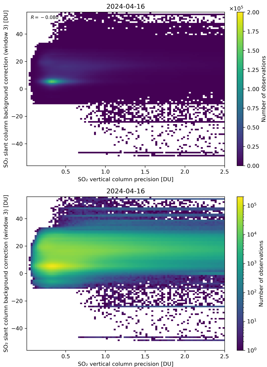
Figure 281: Scatter density plot of “SO 2 vertical column precision” against “SO 2 slant column background correction (window 3)” for 2024-04-16 to 2024-04-17.
