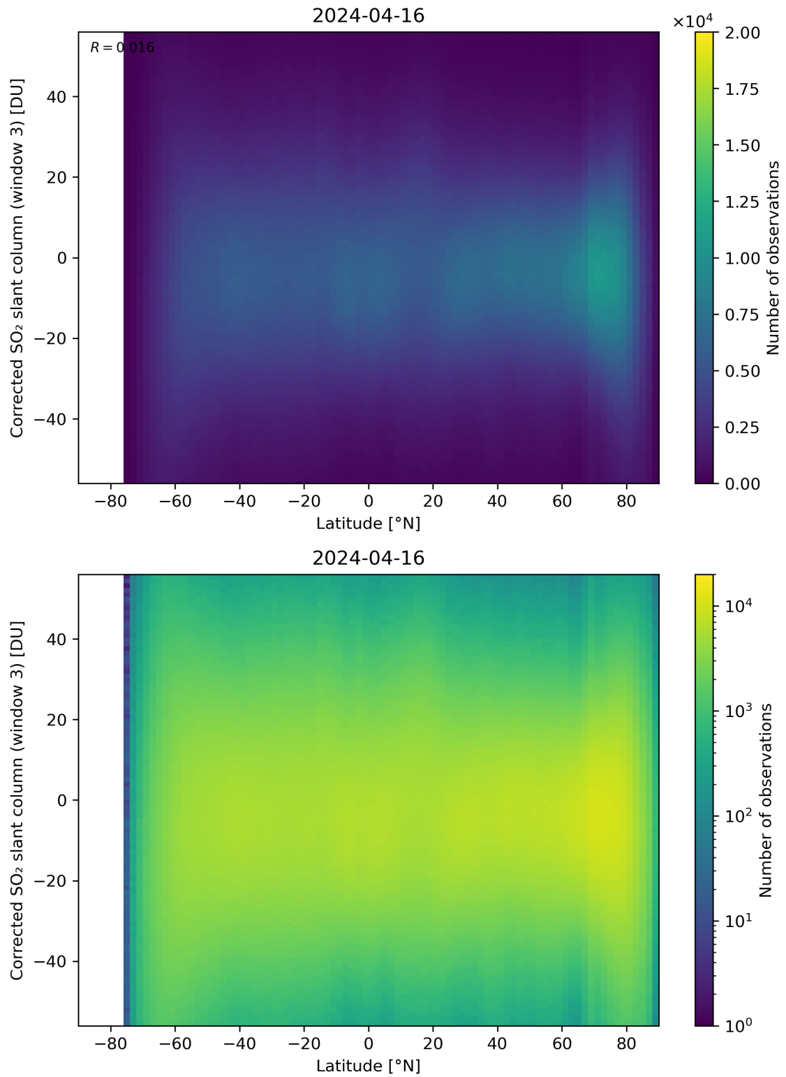
Figure 148: Scatter density plot of “Latitude” against “Corrected SO 2 slant column (window 3)” for 2024-04-16 to 2024-04-17.
