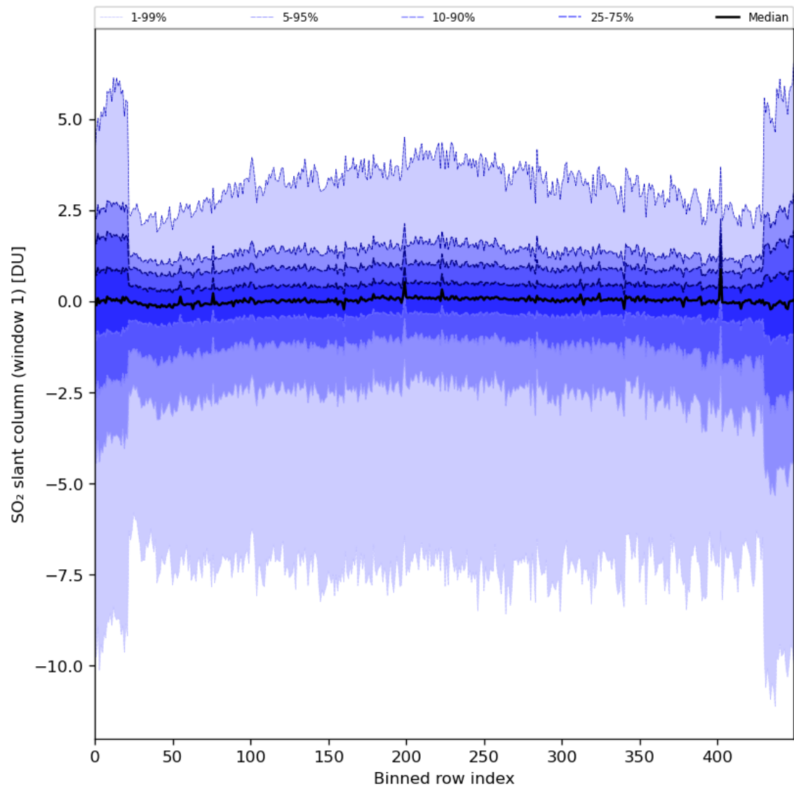
Figure 79: Along track statistics of “SO 2 slant column (window 1)” for 2024-04-16 to 2024-04-17
