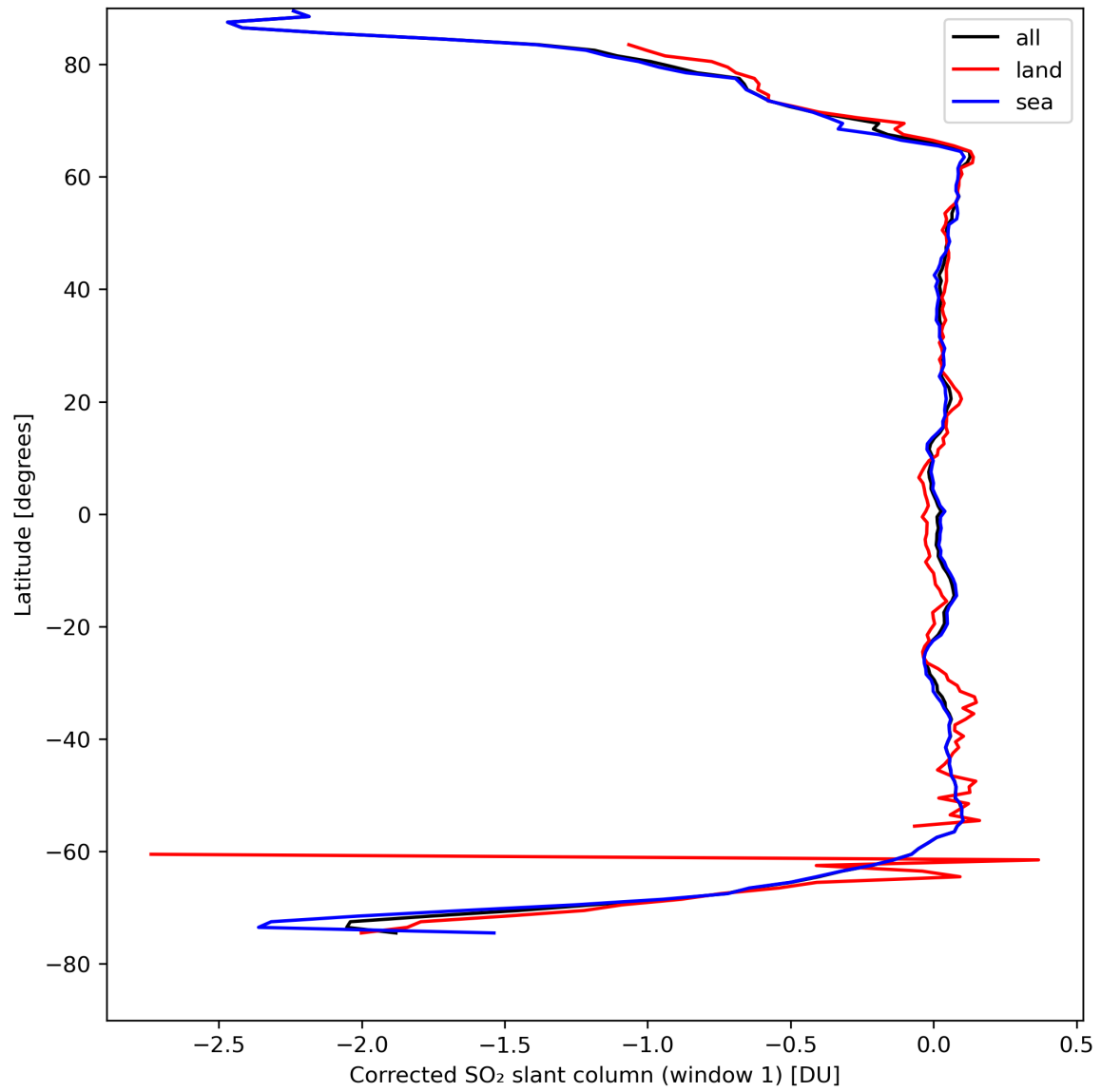
Figure 35: Zonal average of “Corrected SO 2 slant column (window 1)” for 2024-04-16 to 2024-04-17.
