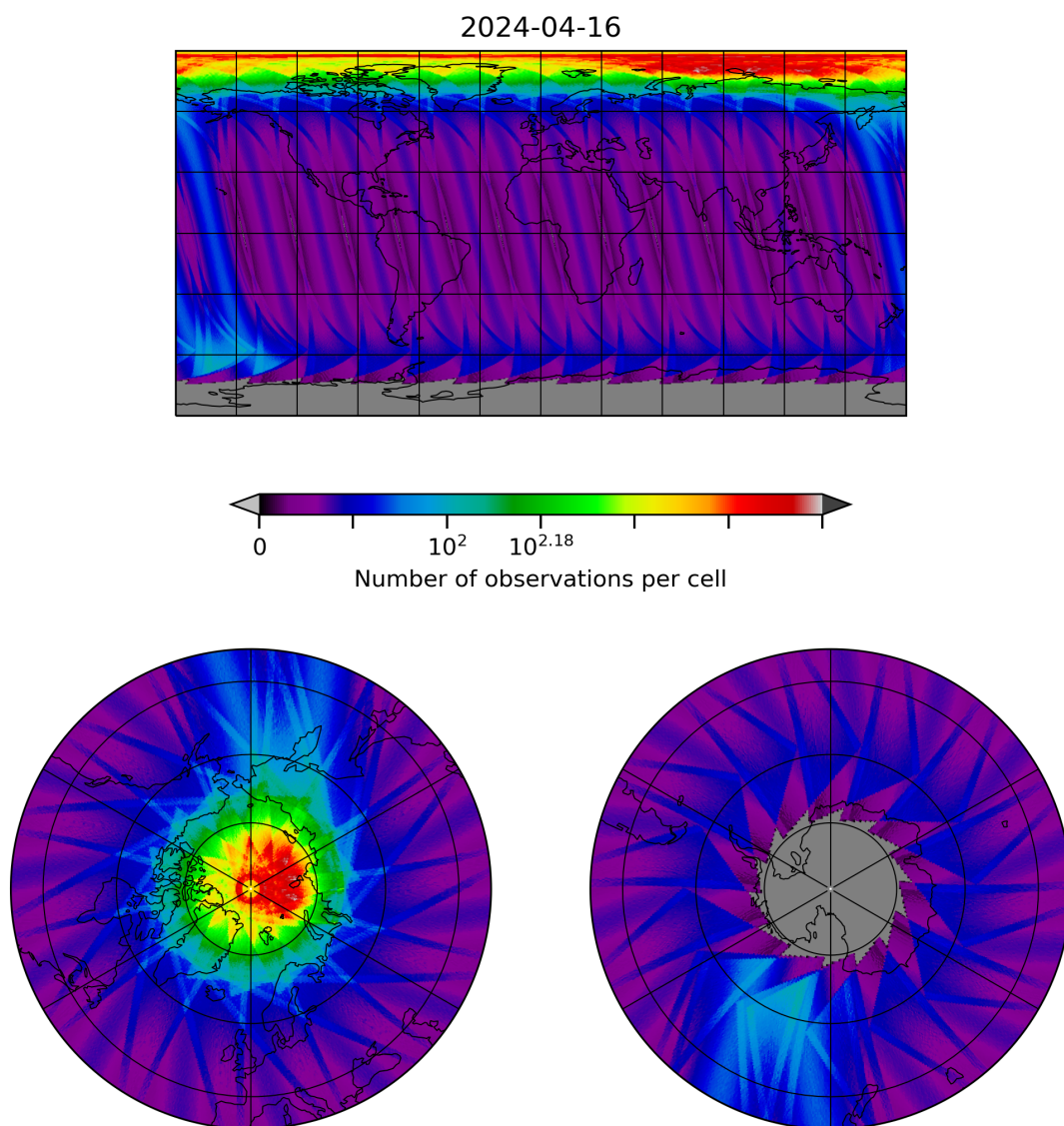
Figure 28: Map of the number of observations for 2024-04-16 to 2024-04-17
