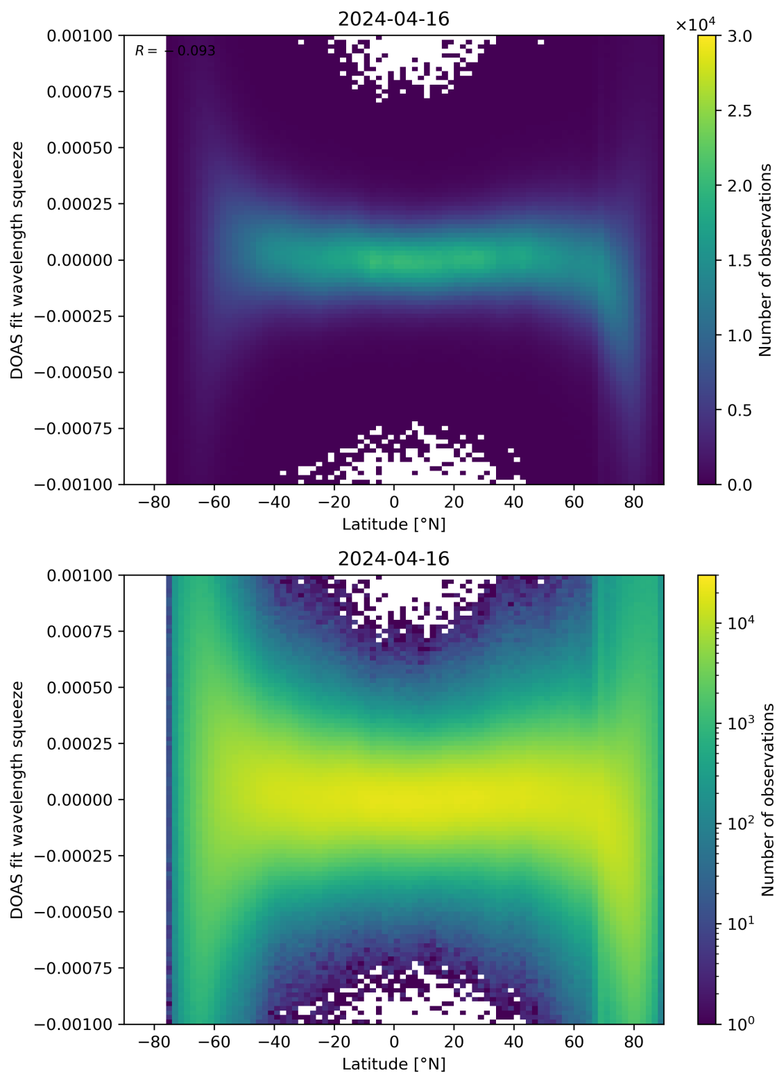
Figure 143: Scatter density plot of “Latitude” against “DOAS fit wavelength squeeze” for 2024-04-16 to 2024-04-17.
