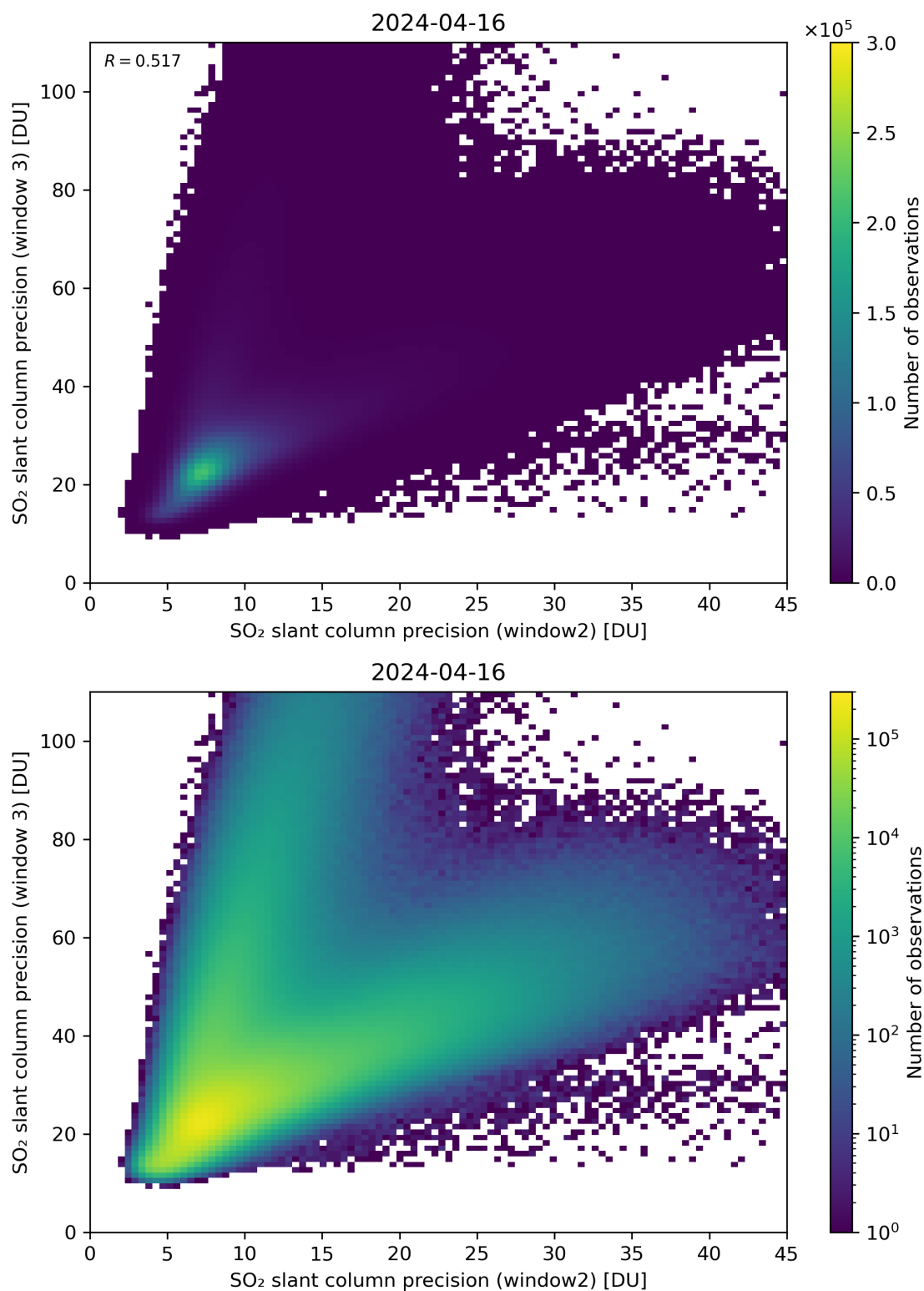
Figure 250: Scatter density plot of “SO 2 slant column precision (window2)” against “SO 2 slant column precision (window 3)” for 2024-04-16 to 2024-04-17.
