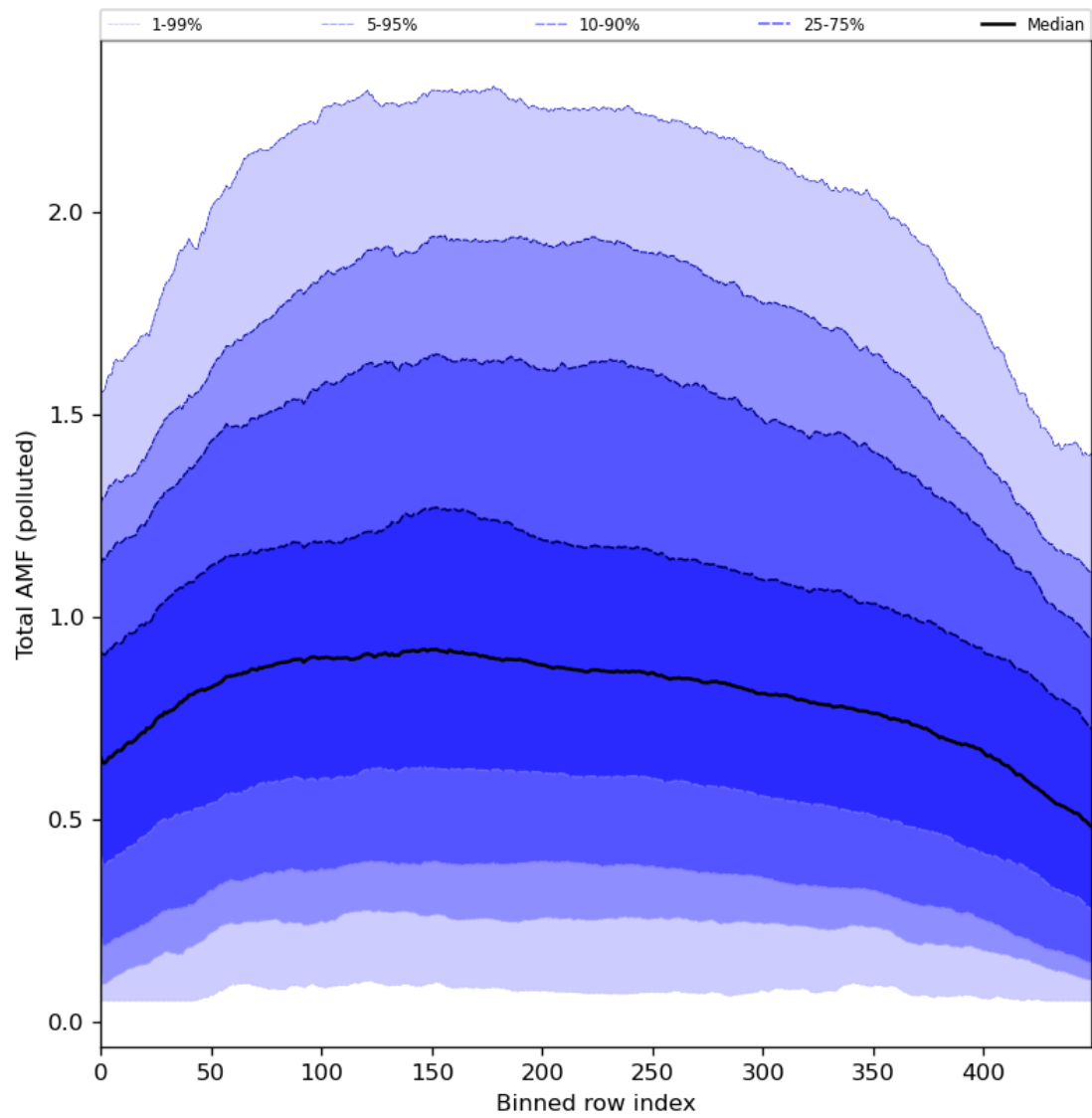
Figure 94: Along track statistics of “Total AMF (polluted)” for 2024-04-16 to 2024-04-17
