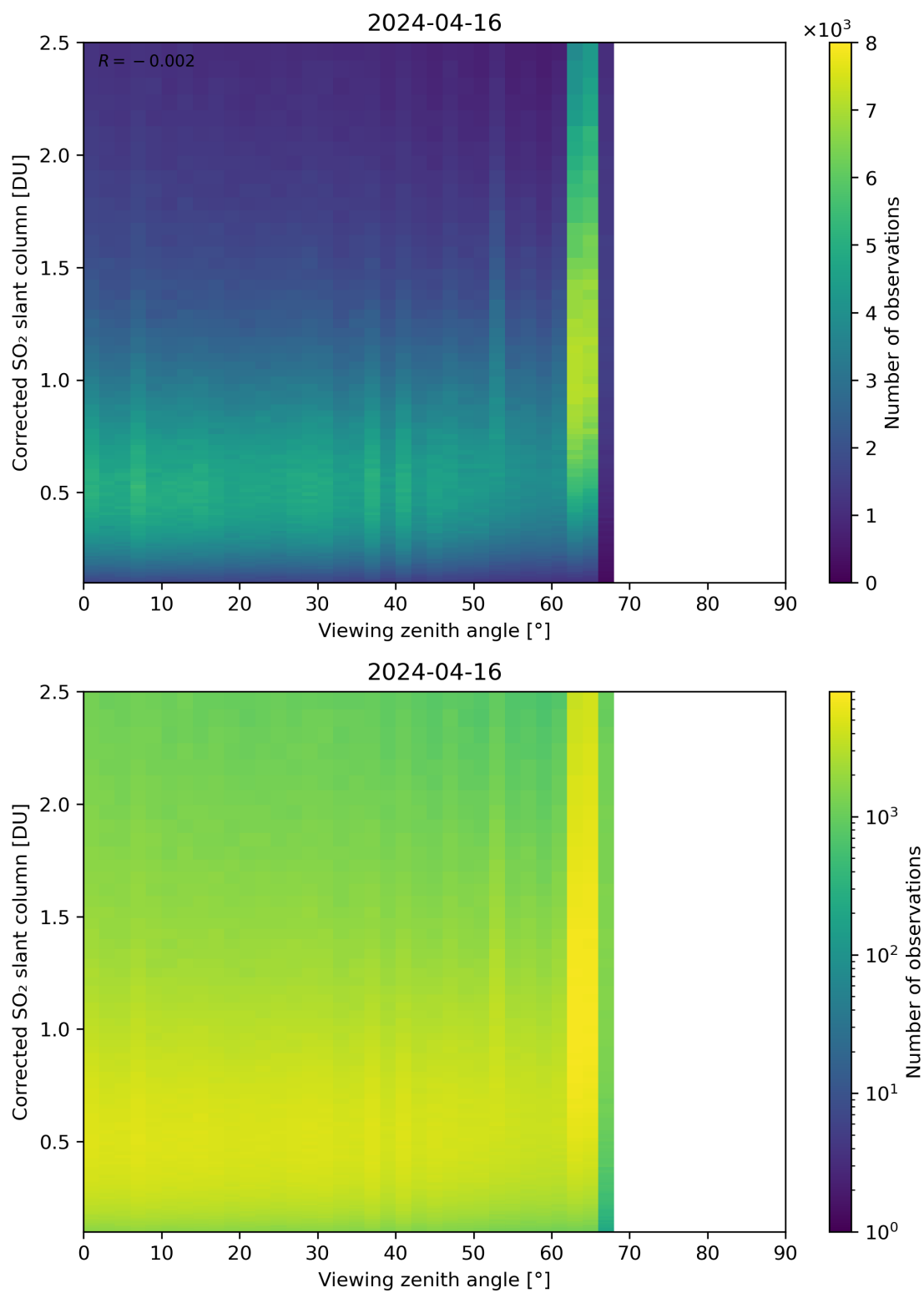
Figure 317: Scatter density plot of “Viewing zenith angle” against “Corrected SO 2 slant column” for 2024-04-16 to 2024-04-17.
