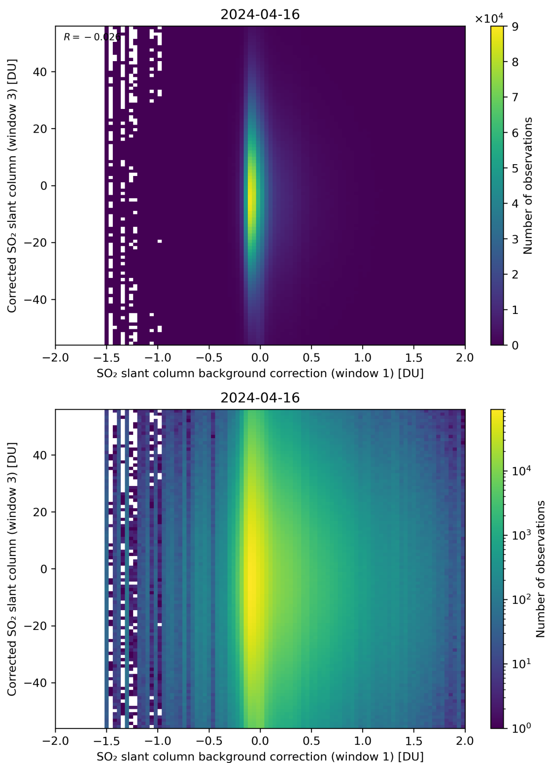
Figure 105: Scatter density plot of “SO 2 slant column background correction (window 1)” against “Corrected SO 2 slant column (window 3)” for 2024-04-16 to 2024-04-17.
