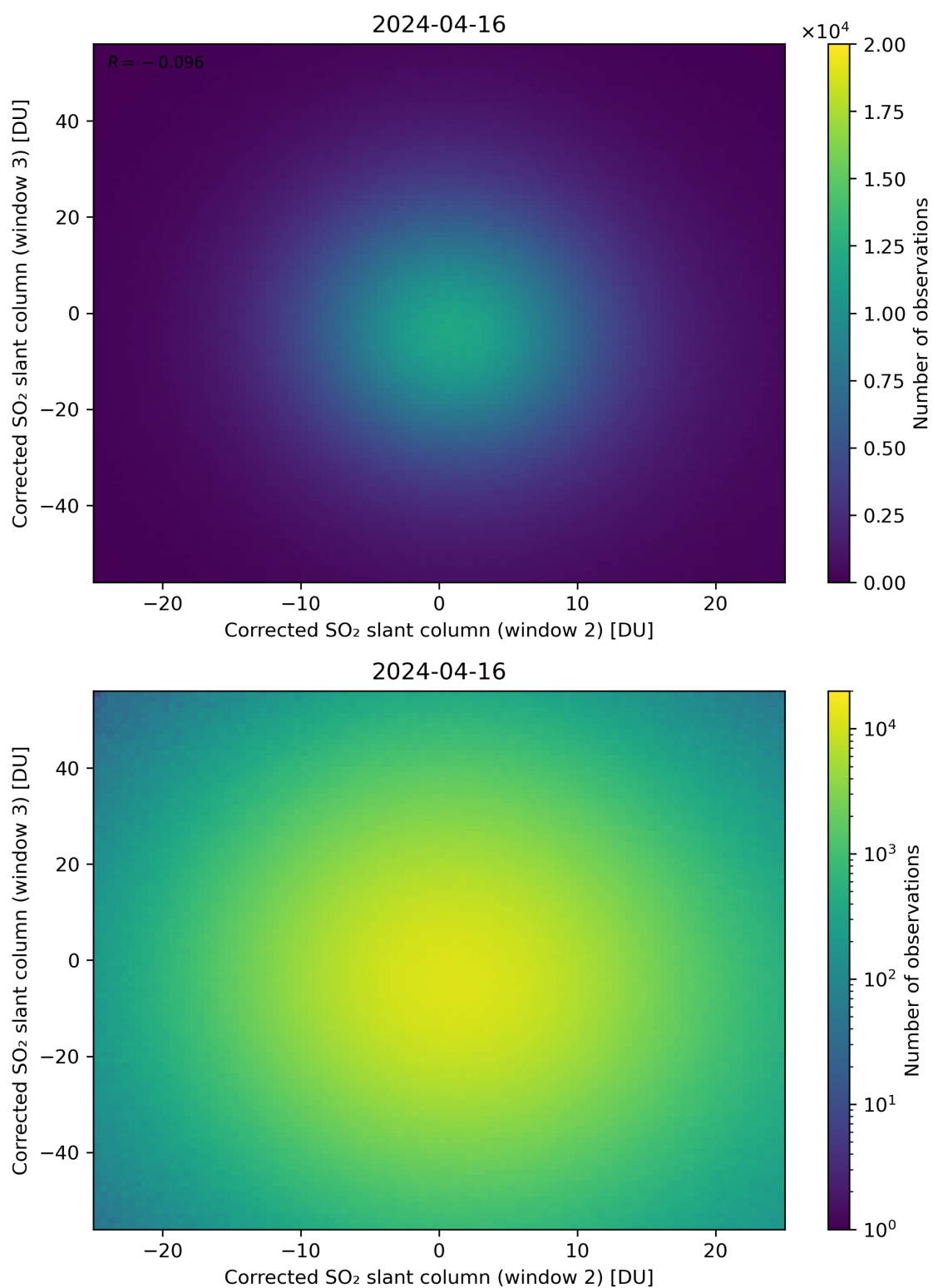
Figure 200: Scatter density plot of “Corrected SO 2 slant column (window 2)” against “Corrected SO 2 slant column (window 3)” for 2024-04-16 to 2024-04-17.
