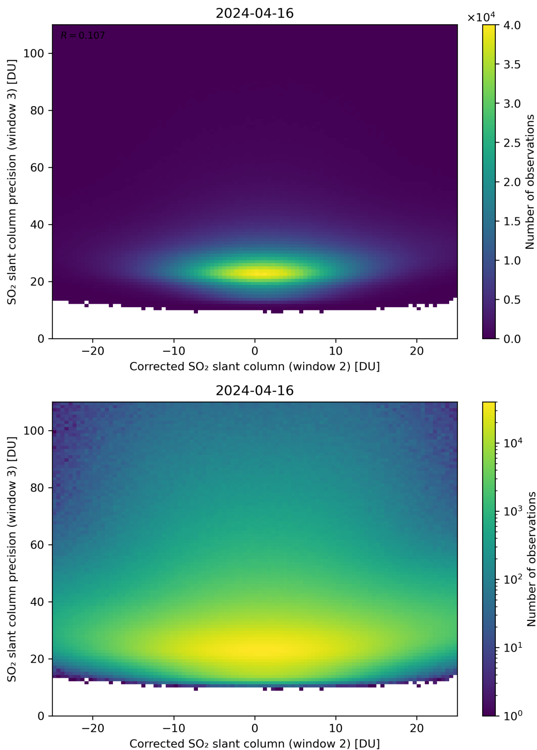
Figure 202: Scatter density plot of “Corrected SO 2 slant column (window 2)” against “SO 2 slant column precision (window 3)” for 2024-04-16 to 2024-04-17.
