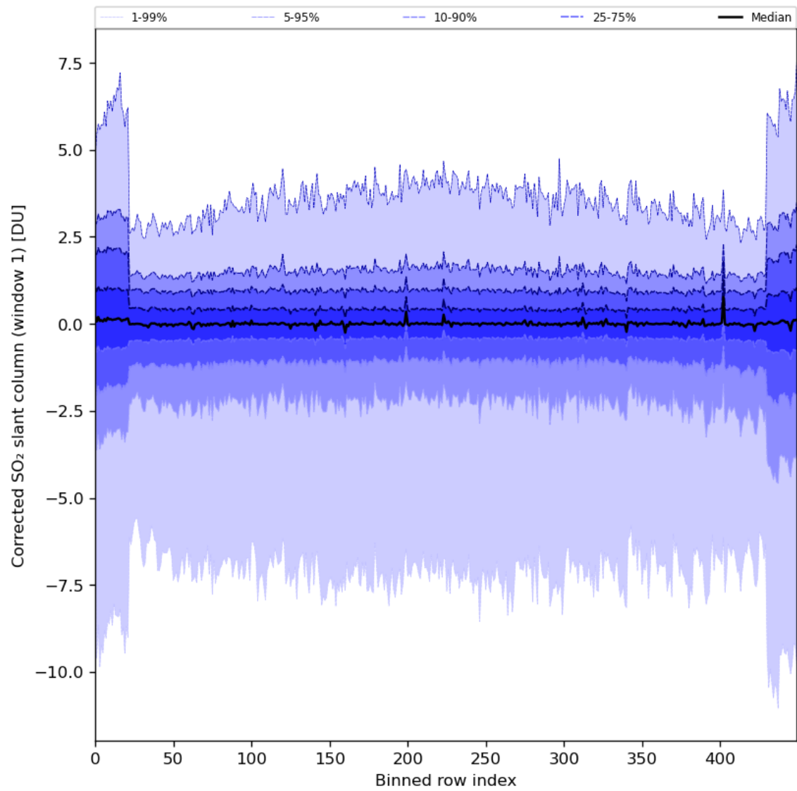
Figure 81: Along track statistics of “Corrected SO 2 slant column (window 1)” for 2024-04-16 to 2024-04-17
