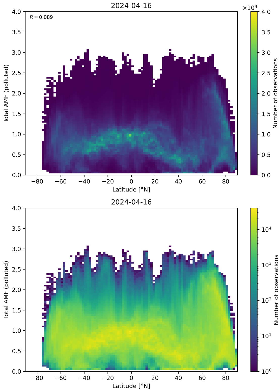
Figure 154: Scatter density plot of “Latitude” against “Total AMF (polluted)” for 2024-04-16 to 2024-04-17.
