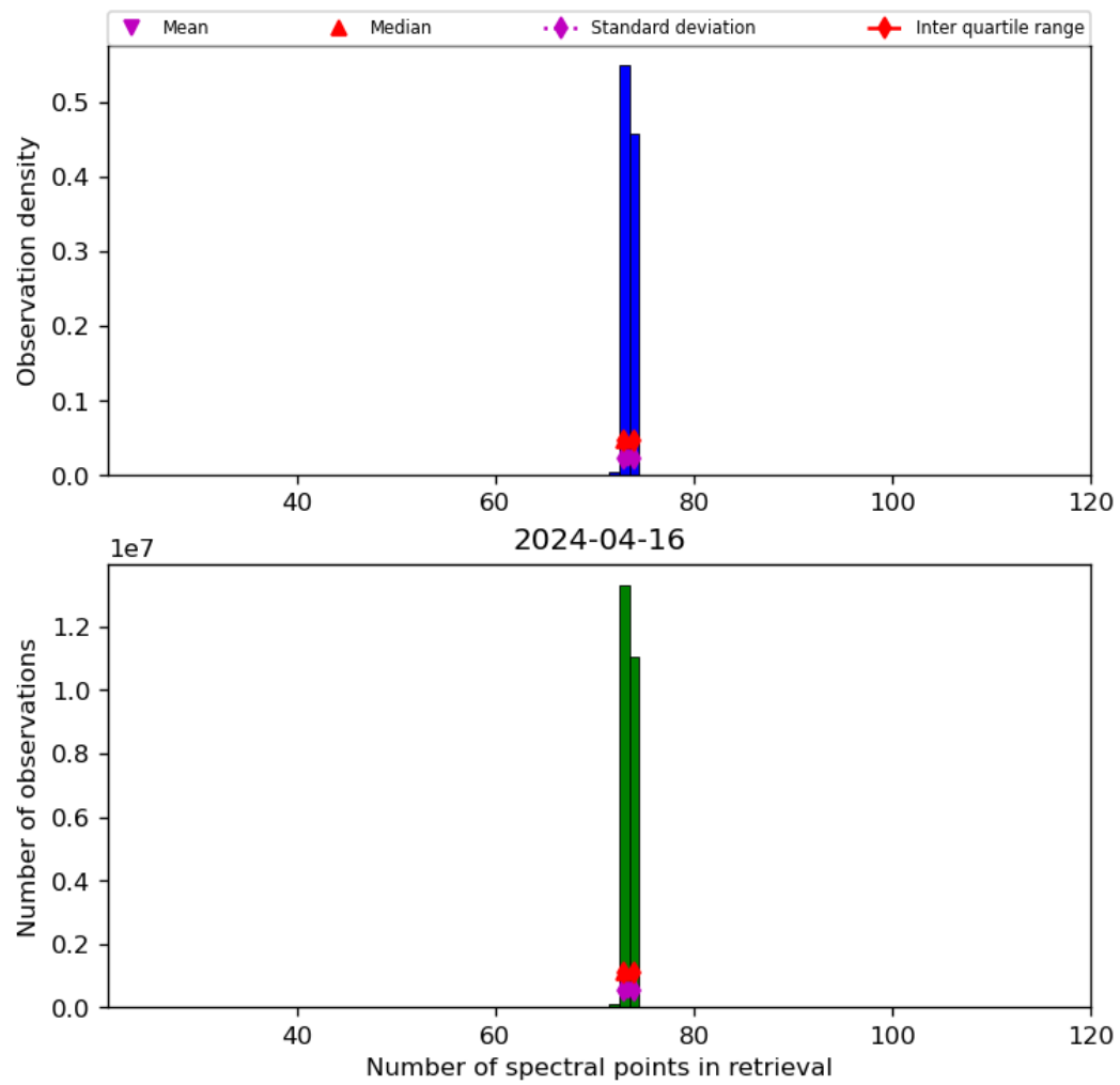
Figure 74: Histogram of “Number of spectral points in retrieval” for 2024-04-16 to 2024-04-17
