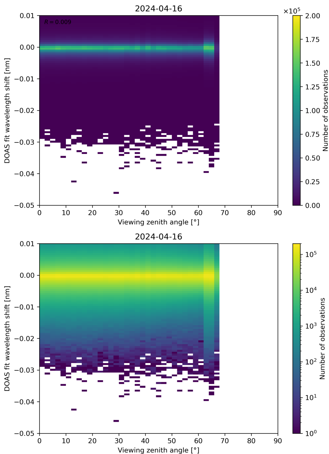
Figure 311: Scatter density plot of “Viewing zenith angle” against “DOAS fit wavelength shift” for 2024-04-16 to 2024-04-17.
