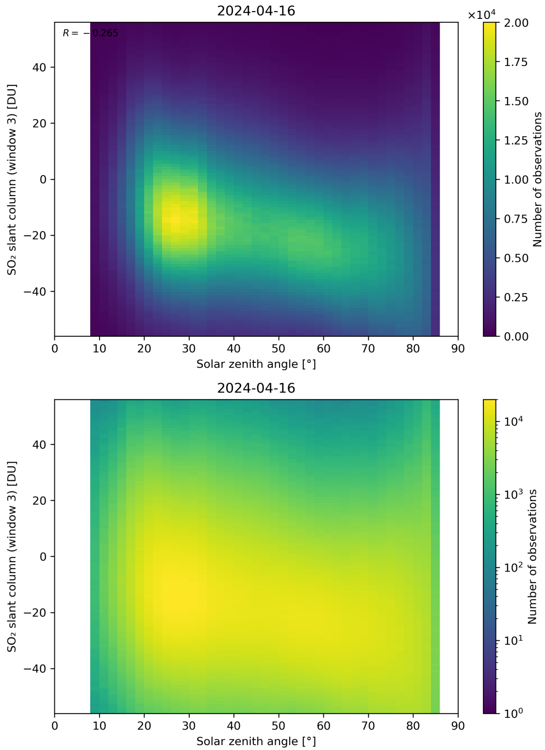
Figure 172: Scatter density plot of “Solar zenith angle” against “SO 2 slant column (window 3)” for 2024-04-16 to 2024-04-17.
