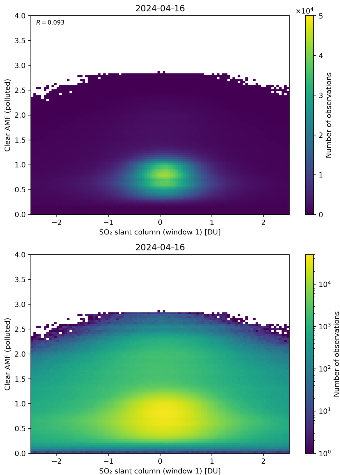
Figure 232: Scatter density plot of “SO 2 slant column (window 1)” against “Clear AMF (polluted)” for 2024-04-16 to 2024-04-17.
