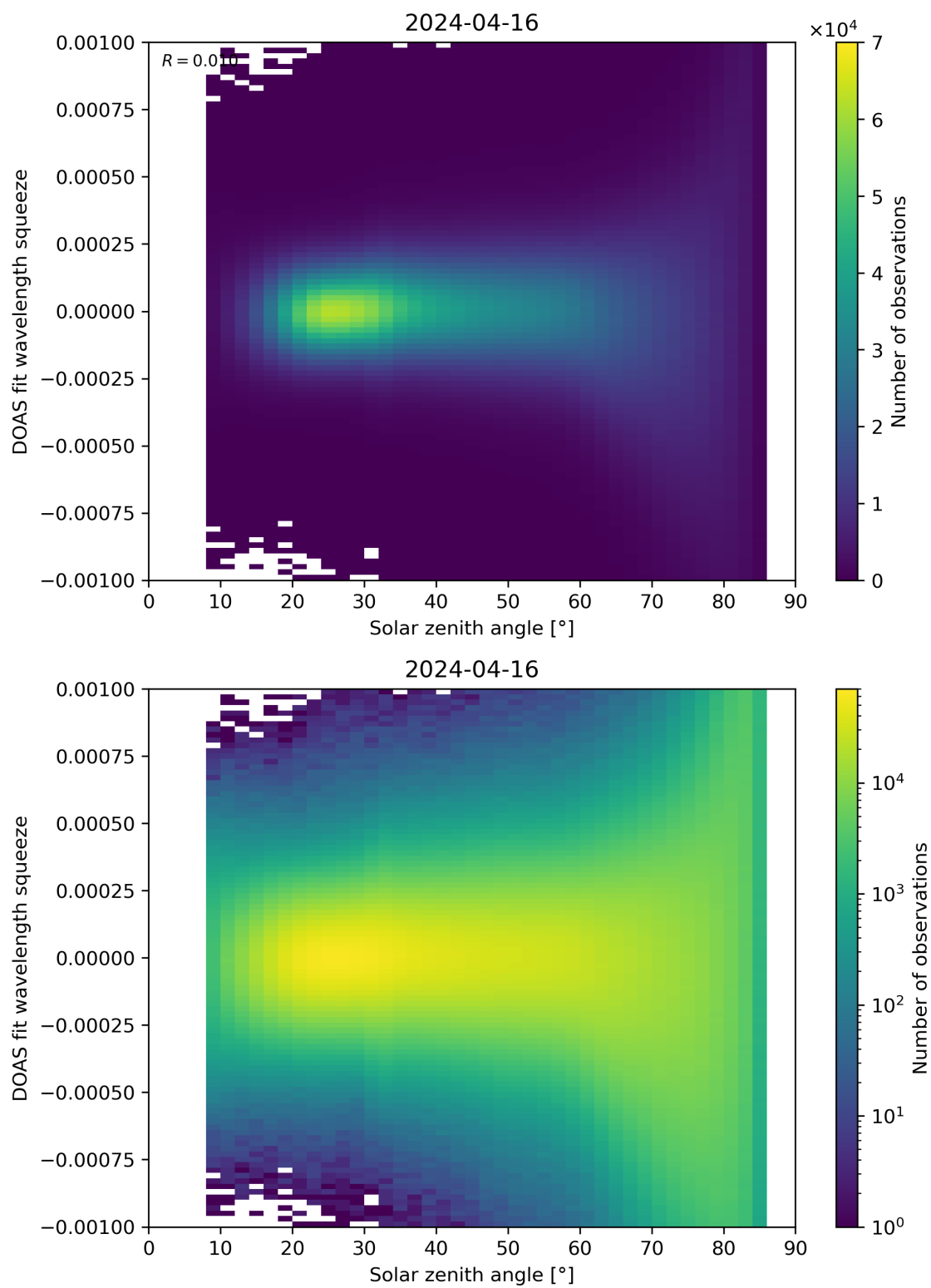
Figure 162: Scatter density plot of “Solar zenith angle” against “DOAS fit wavelength squeeze” for 2024-04-16 to 2024-04-17.
