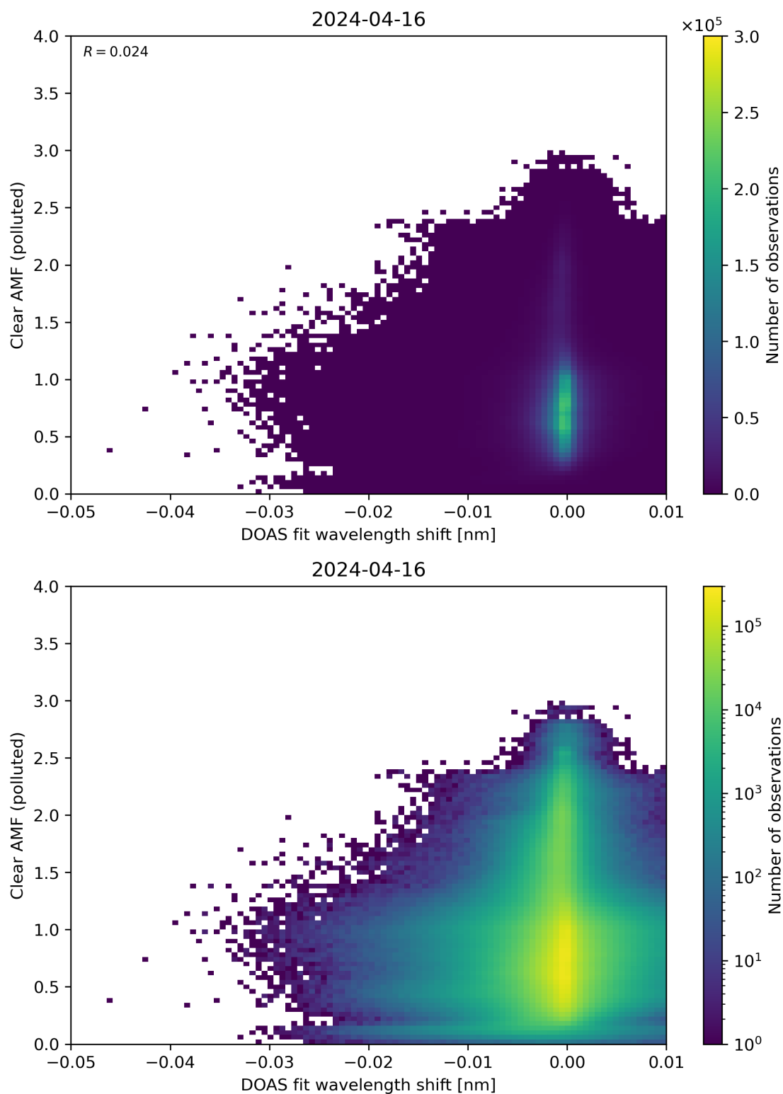
Figure 129: Scatter density plot of “DOAS fit wavelength shift” against “Clear AMF (polluted)” for 2024-04-16 to 2024-04-17.
