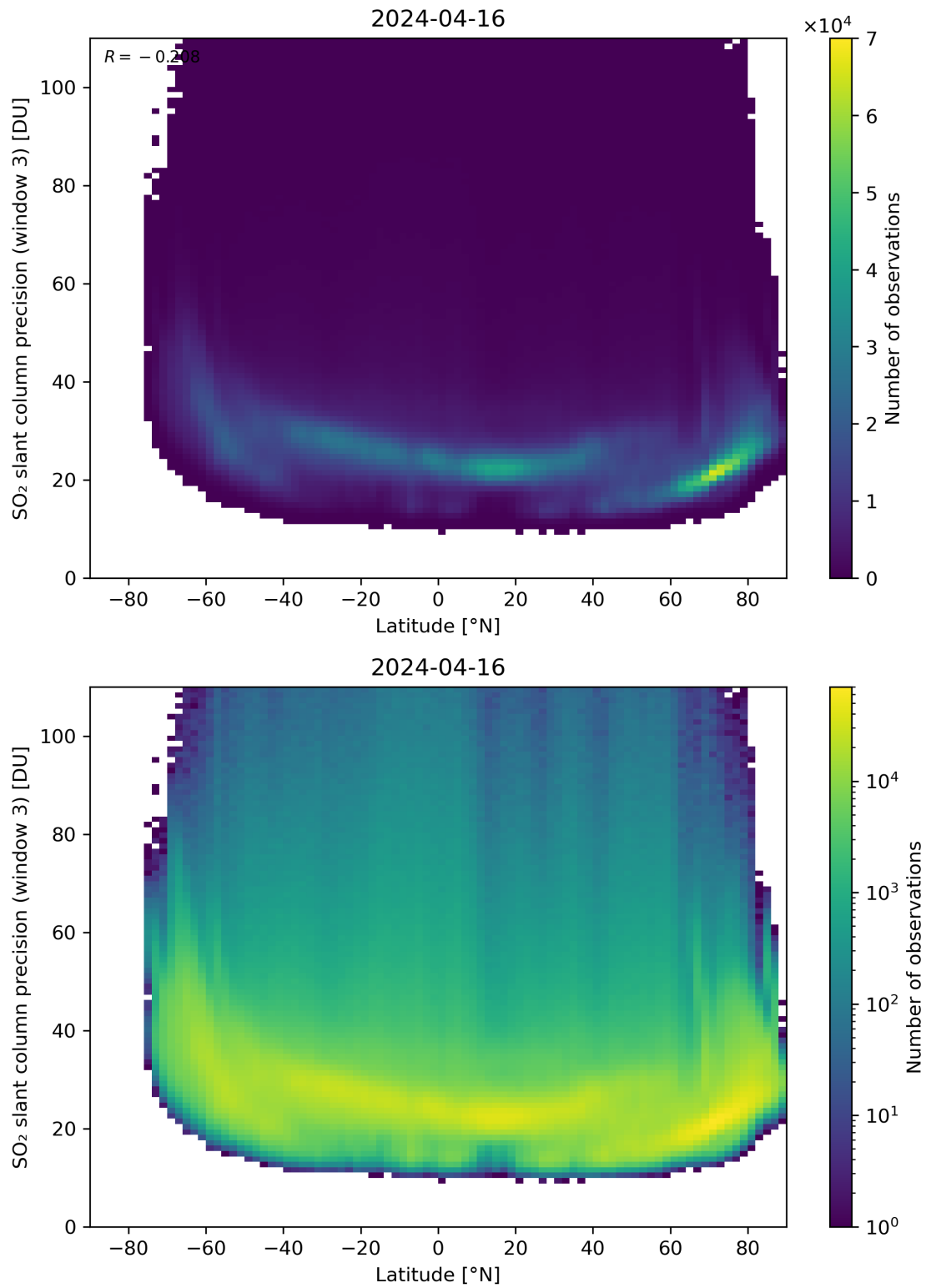
Figure 153: Scatter density plot of “Latitude” against “SO 2 slant column precision (window 3)” for 2024-04-16 to 2024-04-17.
