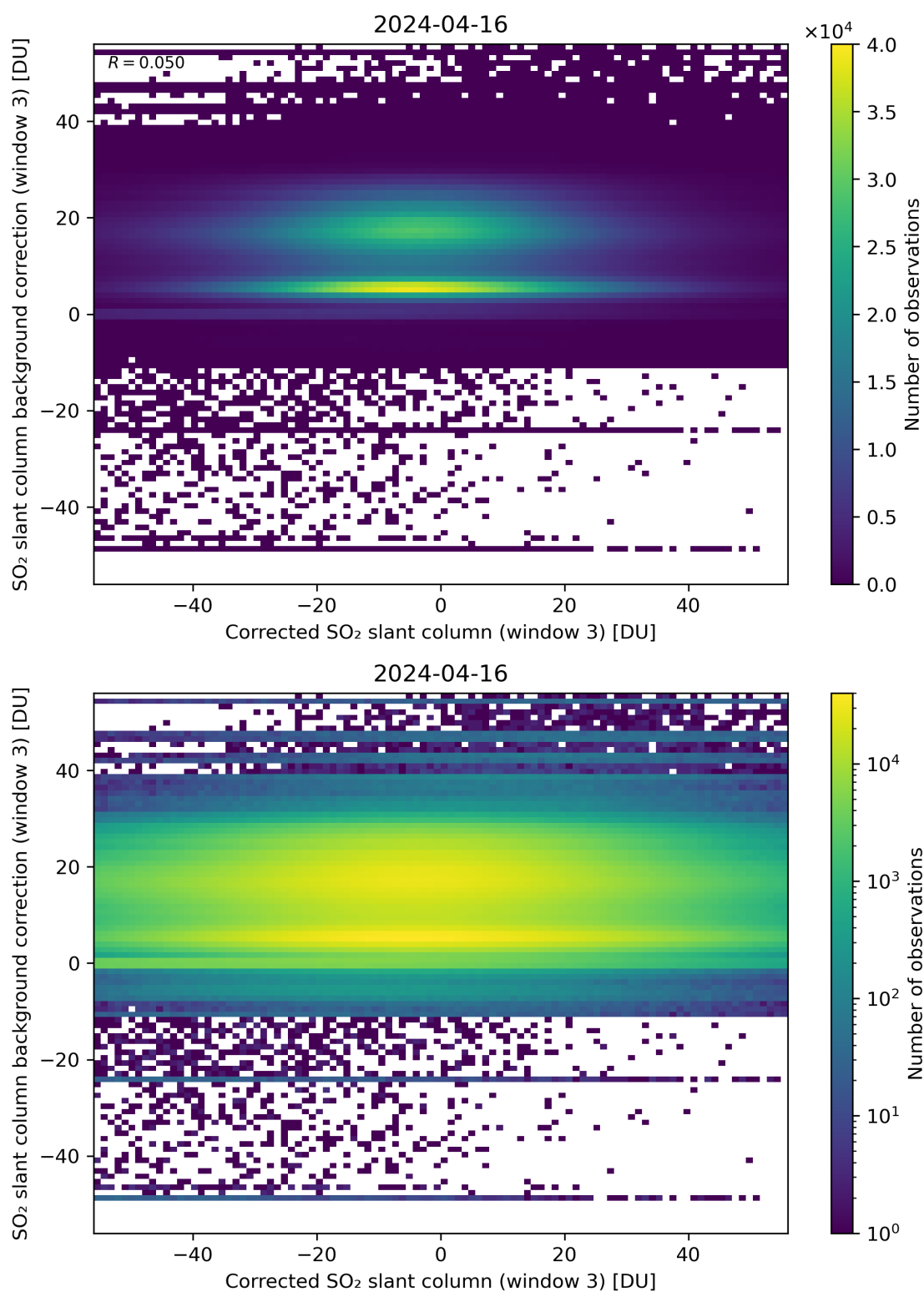
Figure 205: Scatter density plot of “Corrected SO 2 slant column (window 3)” against “SO 2 slant column background correction (window 3)” for 2024-04-16 to 2024-04-17.
