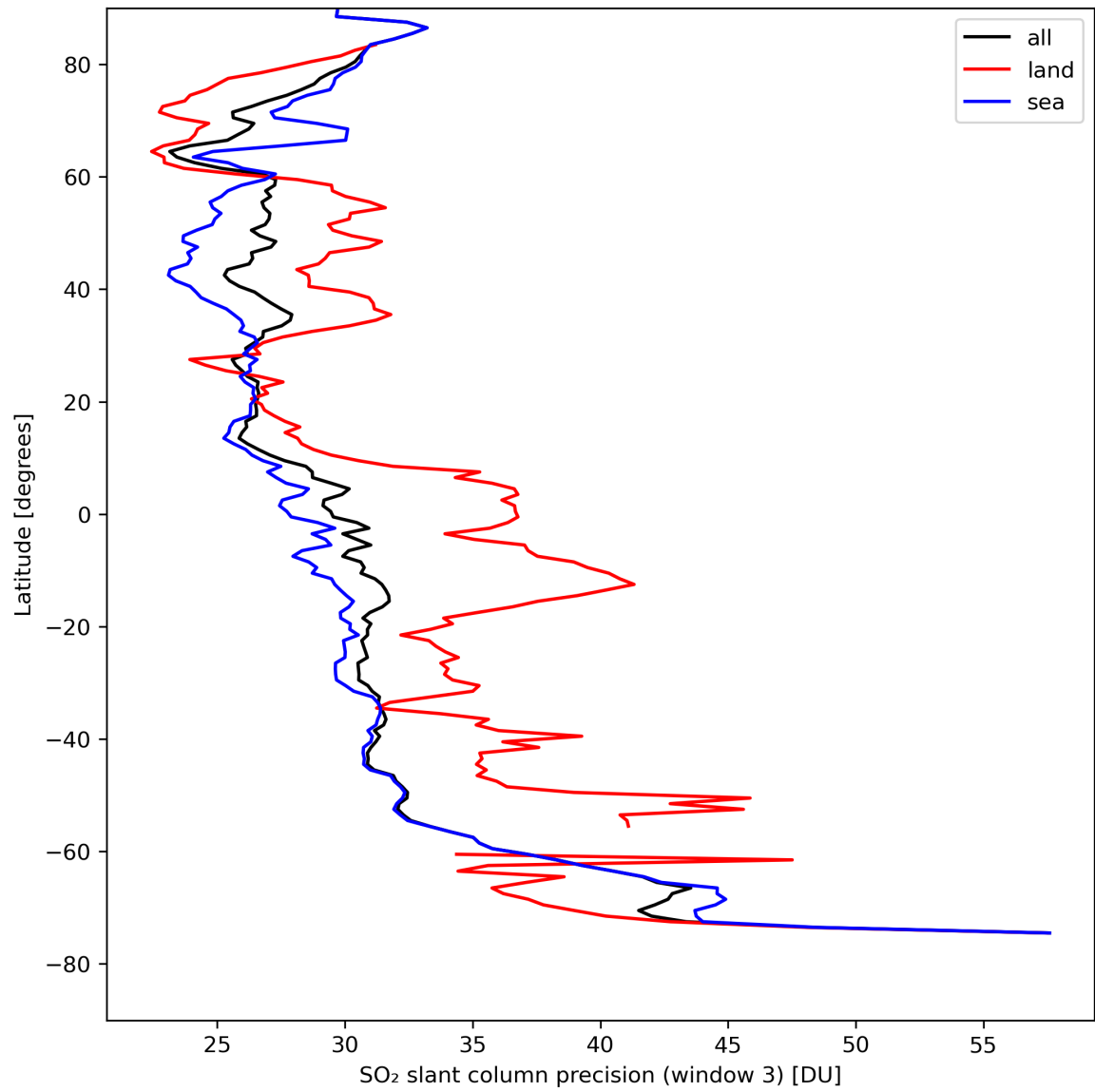
Figure 42: Zonal average of “SO 2 slant column precision (window 3)” for 2024-04-16 to 2024-04-17.
