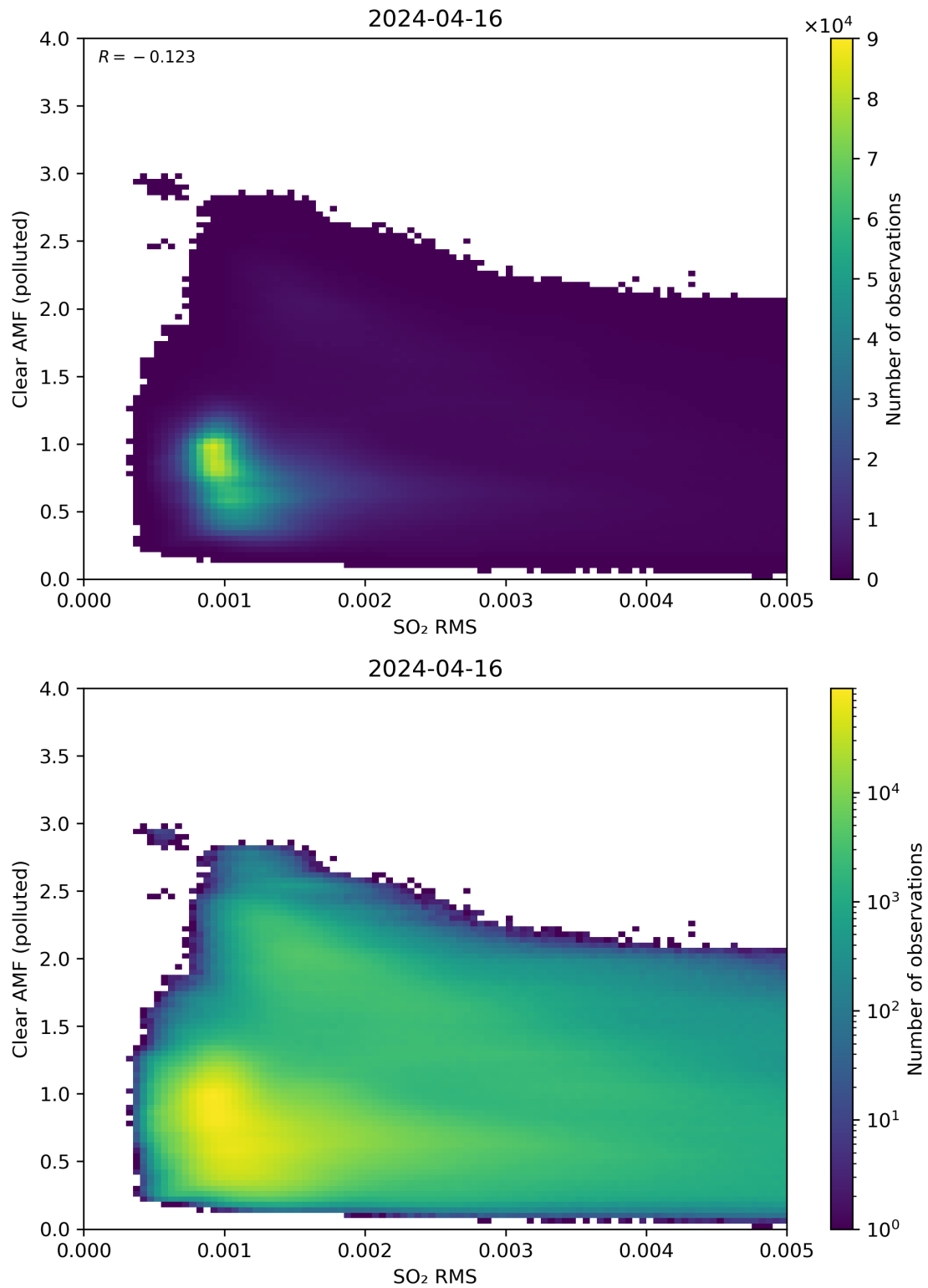
Figure 136: Scatter density plot of “SO 2 RMS” against “Clear AMF (polluted)” for 2024-04-16 to 2024-04-17.
