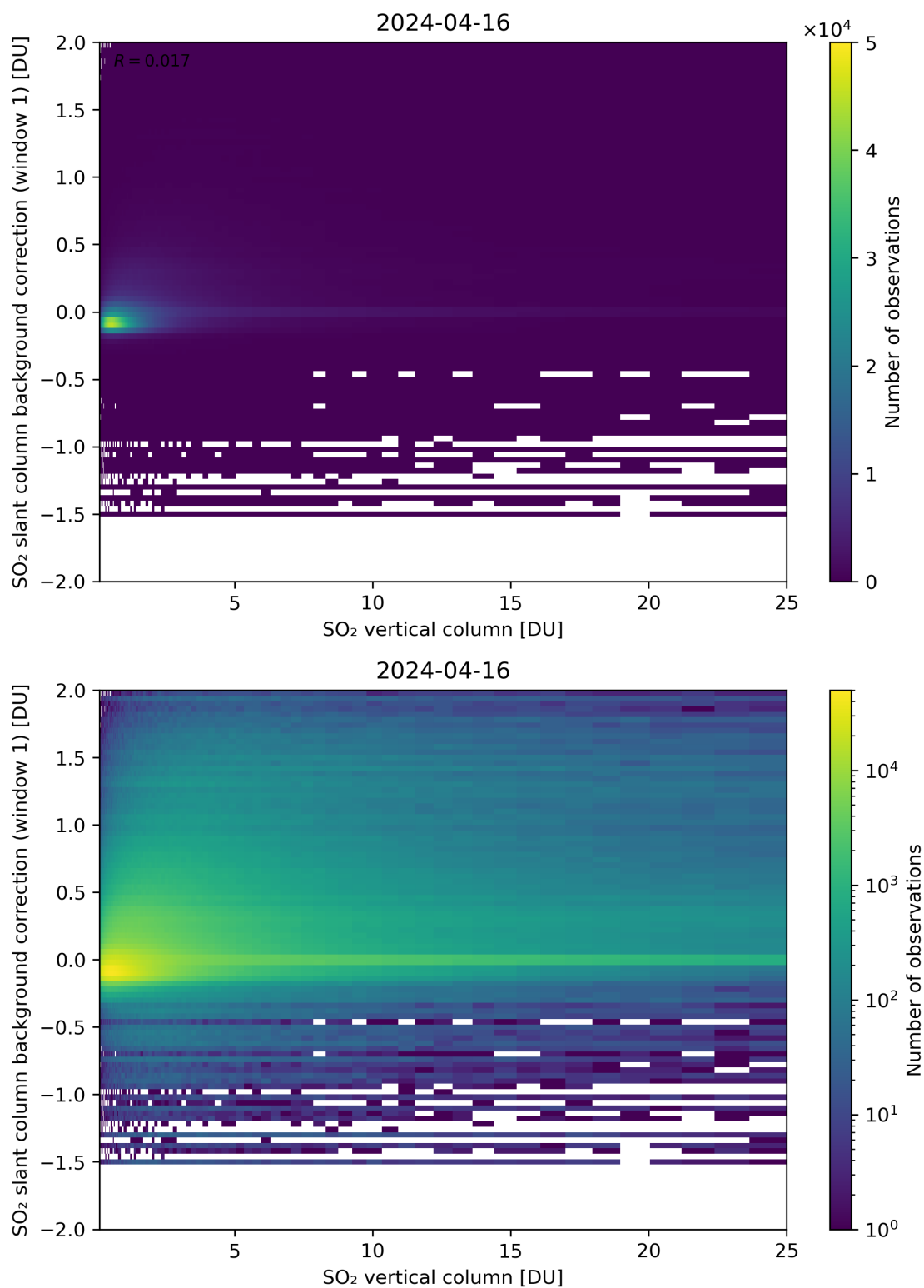
Figure 273: Scatter density plot of “SO 2 vertical column” against “SO 2 slant column background correction (window 1)” for 2024-04-16 to 2024-04-17.
