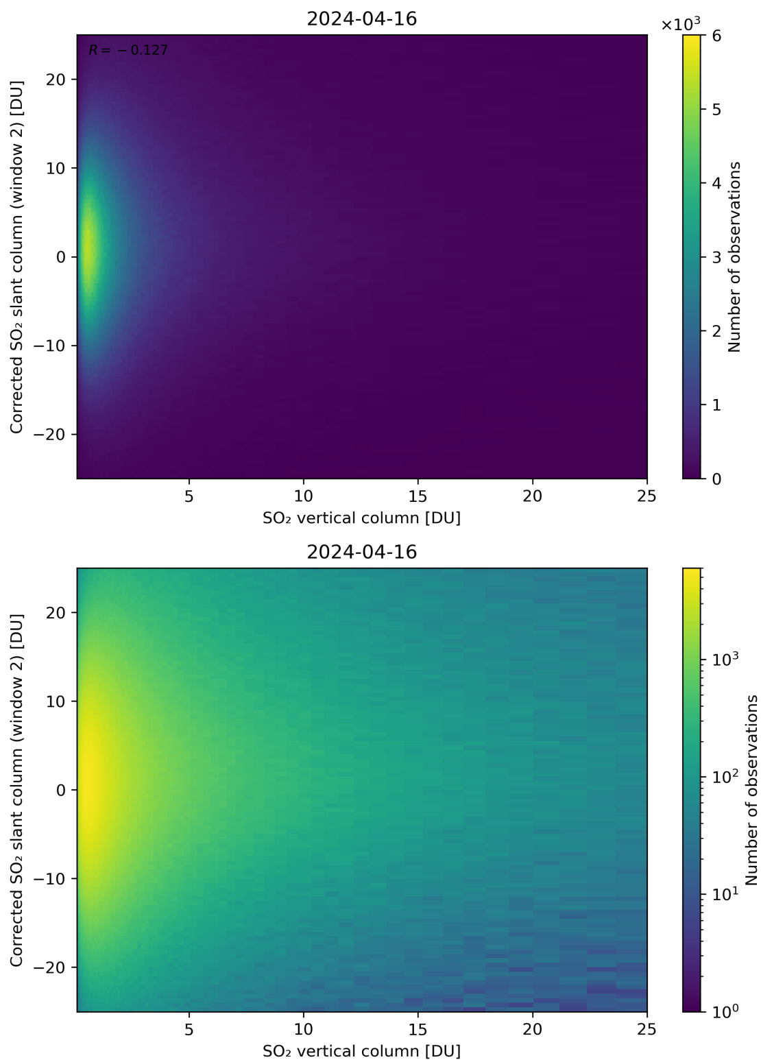
Figure 298: Scatter density plot of “SO 2 vertical column” against “Corrected SO 2 slant column (window 2)” for 2024-04-16 to 2024-04-17.
