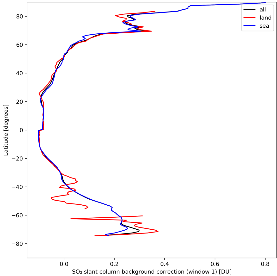
Figure 36: Zonal average of “SO 2 slant column background correction (window 1)” for 2024-04-16 to 2024-04-17.
