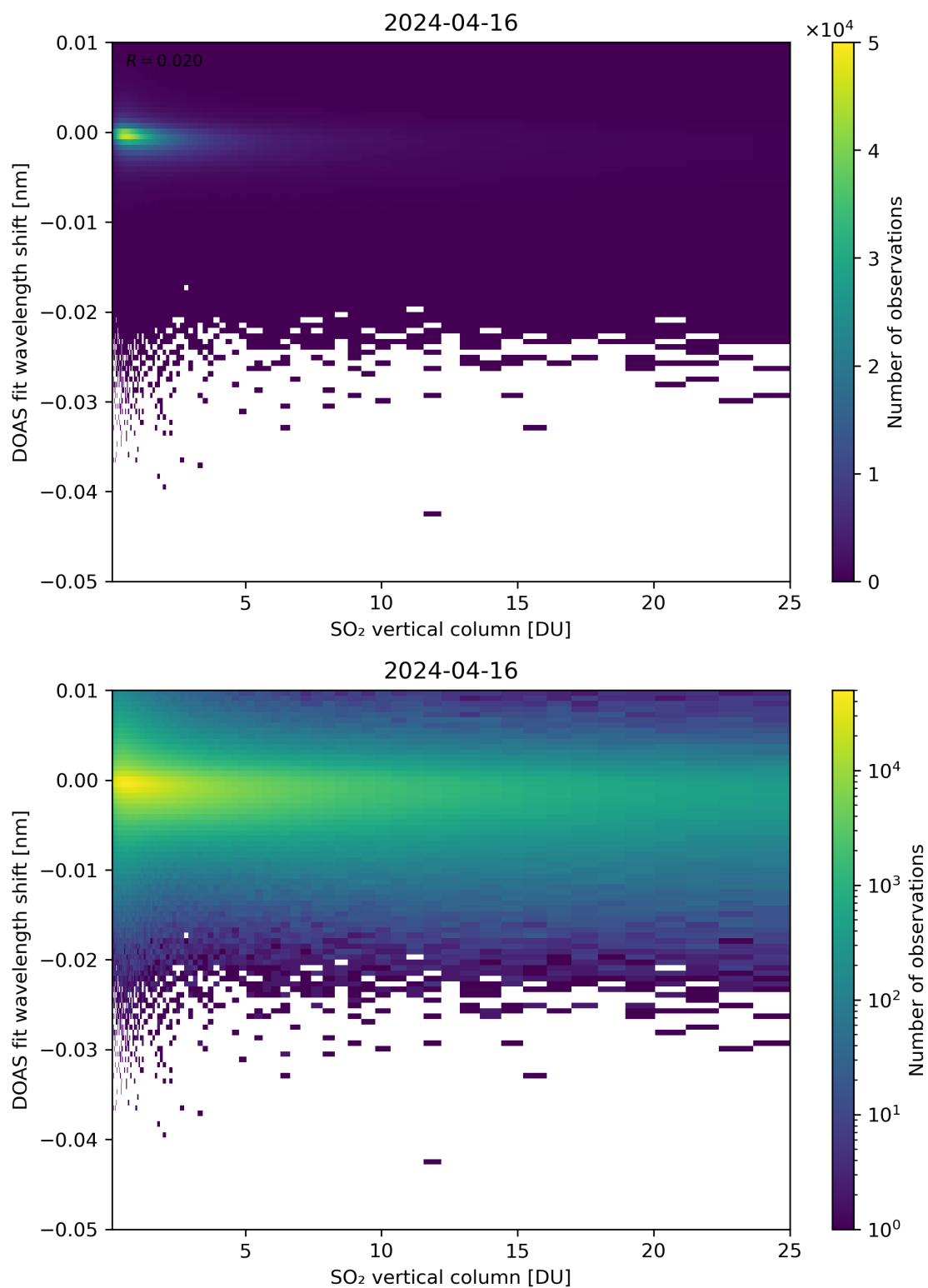
Figure 276: Scatter density plot of “SO 2 vertical column” against “DOAS fit wavelength shift” for 2024-04-16 to 2024-04-17.
