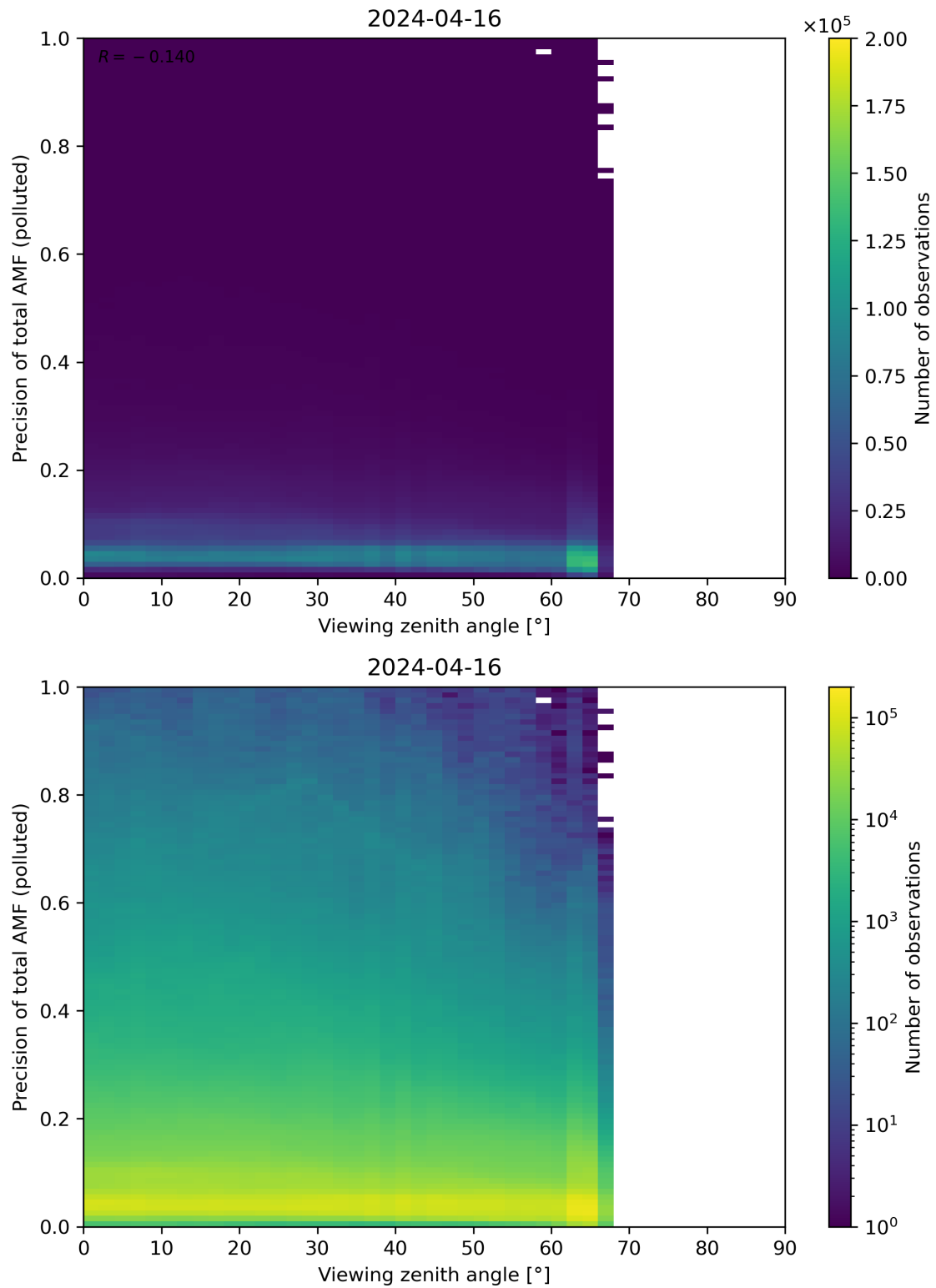
Figure 326: Scatter density plot of “Viewing zenith angle” against “Precision of total AMF (polluted)” for 2024-04-16 to 2024-04-17.
