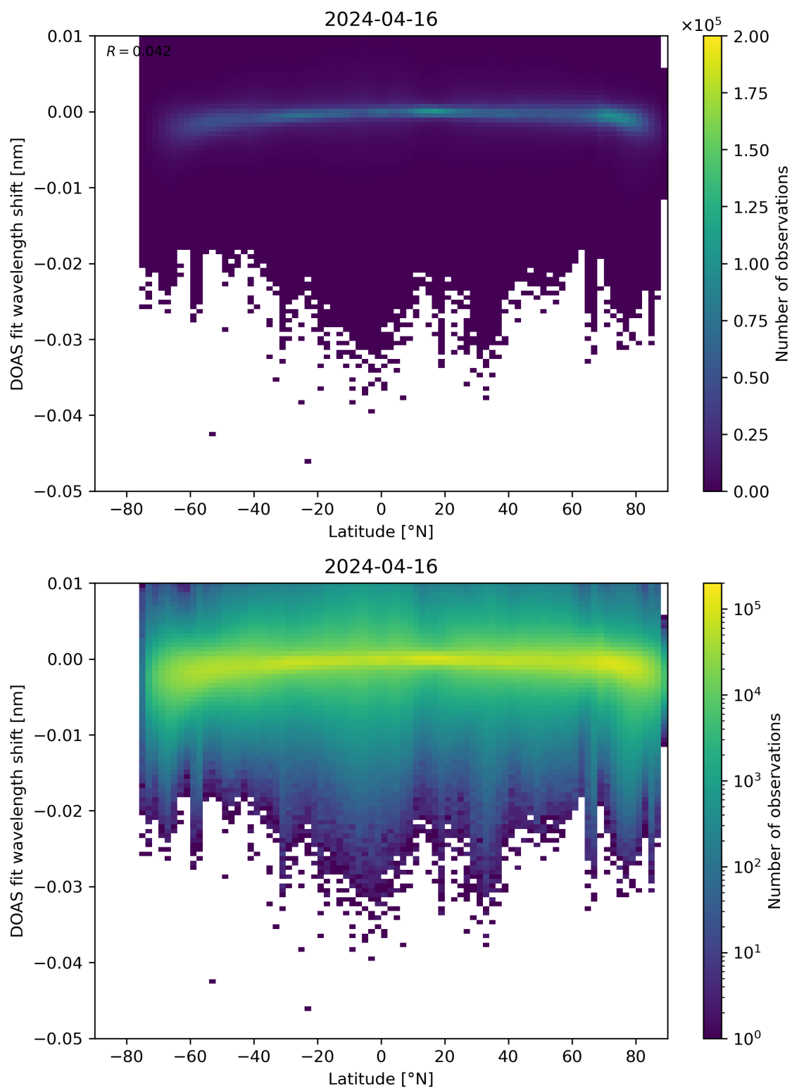
Figure 142: Scatter density plot of “Latitude” against “DOAS fit wavelength shift” for 2024-04-16 to 2024-04-17.
