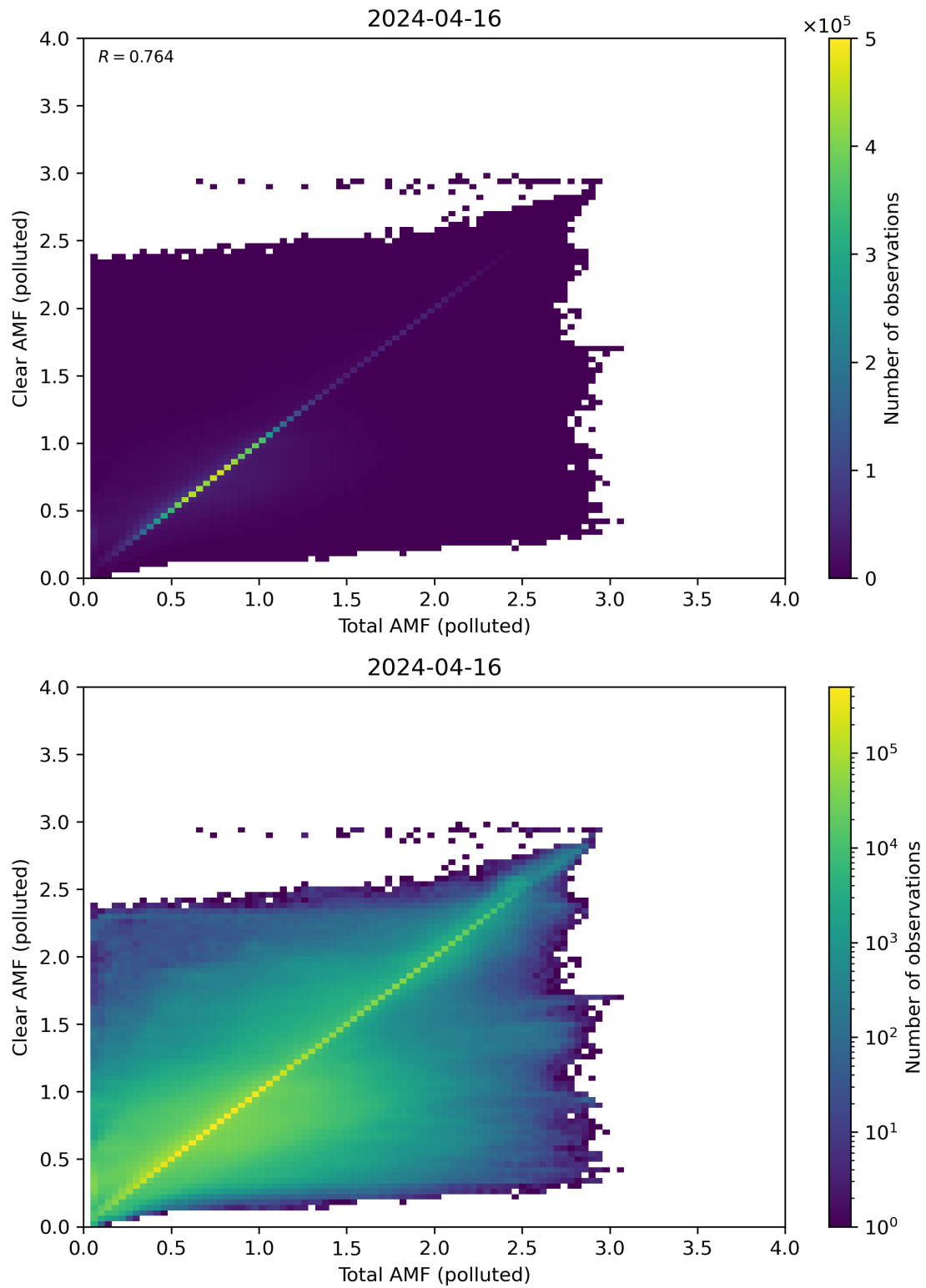
Figure 271: Scatter density plot of “Total AMF (polluted)” against “Clear AMF (polluted)” for 2024-04-16 to 2024-04-17.
