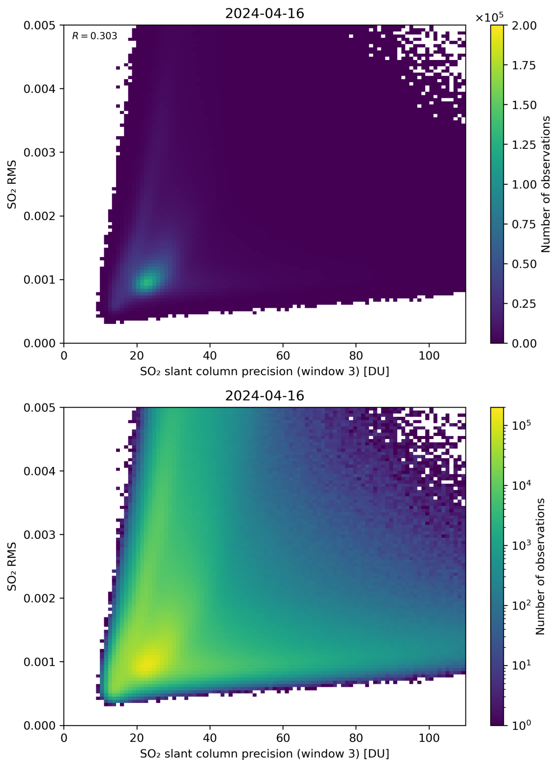
Figure 260: Scatter density plot of “SO 2 slant column precision (window 3)” against “SO 2 RMS” for 2024-04-16 to 2024-04-17.
