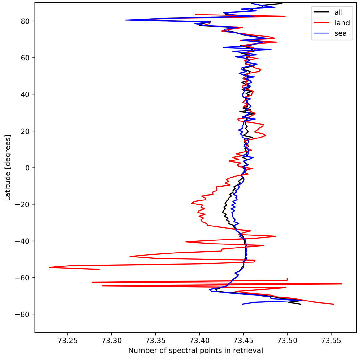
Figure 51: Zonal average of “Number of spectral points in retrieval” for 2024-04-16 to 2024-04-17.
