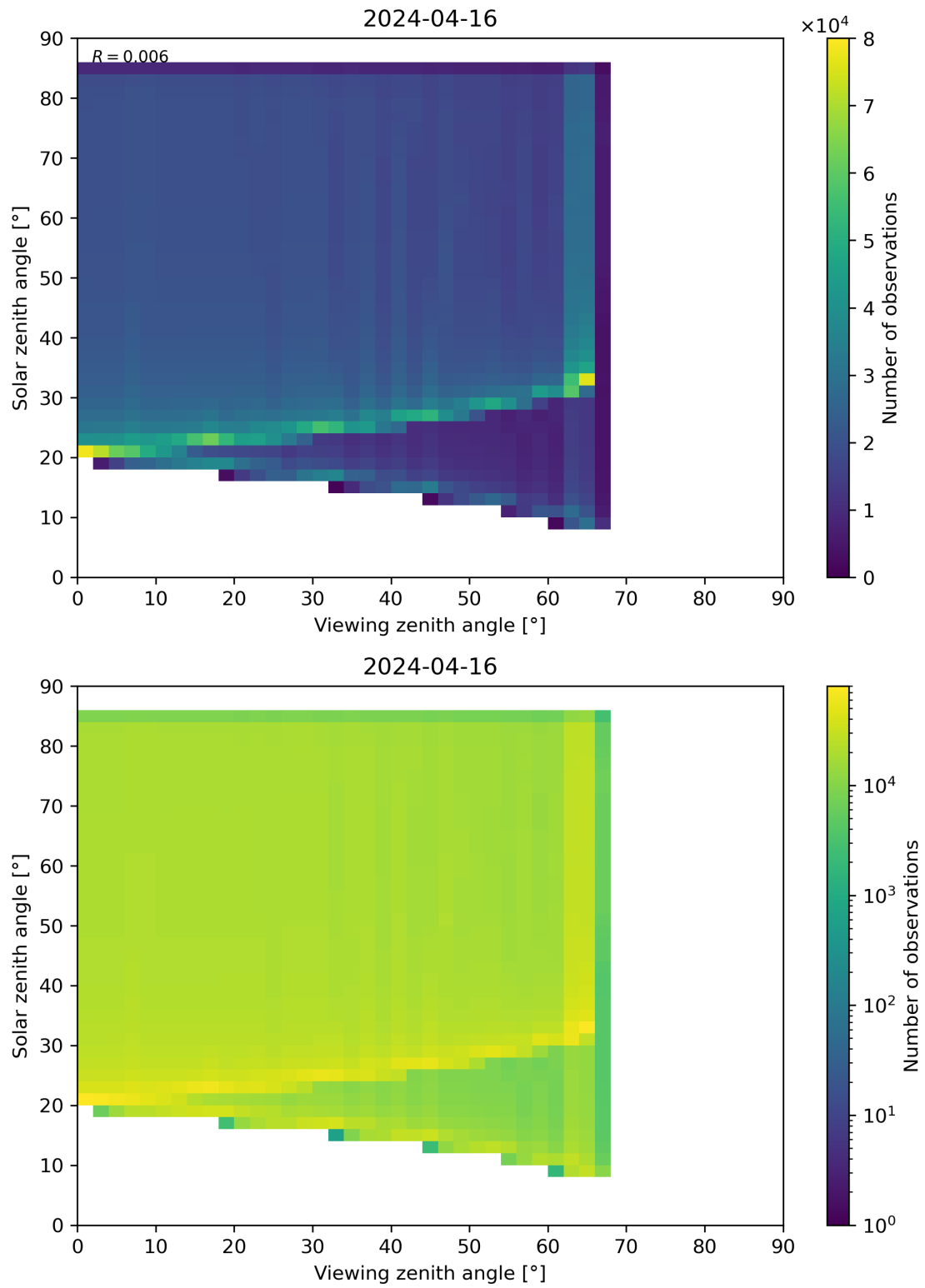
Figure 315: Scatter density plot of “Viewing zenith angle” against “Solar zenith angle” for 2024-04-16 to 2024-04-17.
