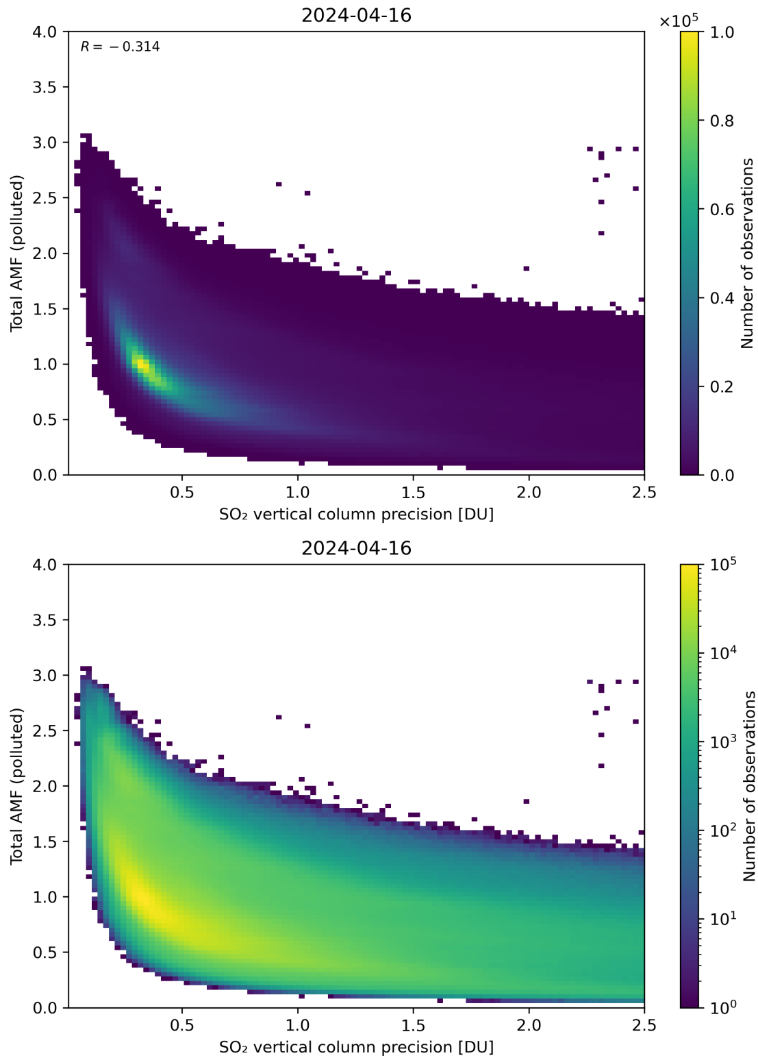
Figure 294: Scatter density plot of “SO 2 vertical column precision” against “Total AMF (polluted)” for 2024-04-16 to 2024-04-17.
