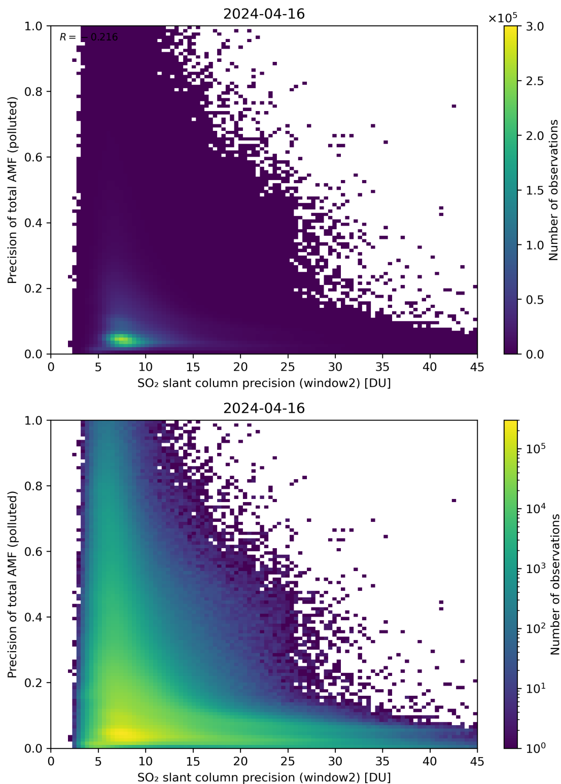
Figure 252: Scatter density plot of “SO 2 slant column precision (window2)” against “Precision of total AMF (polluted)” for 2024-04-16 to 2024-04-17.
