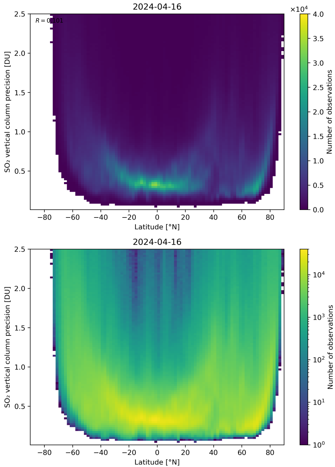
Figure 157: Scatter density plot of “Latitude” against “SO 2 vertical column precision” for 2024-04-16 to 2024-04-17.
