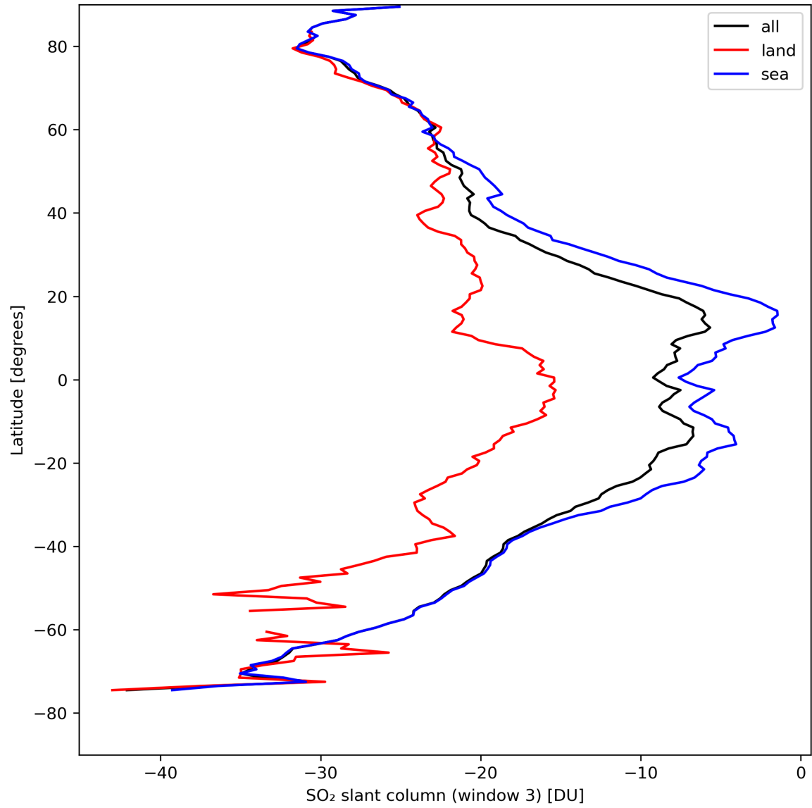
Figure 41: Zonal average of “SO 2 slant column (window 3)” for 2024-04-16 to 2024-04-17.
