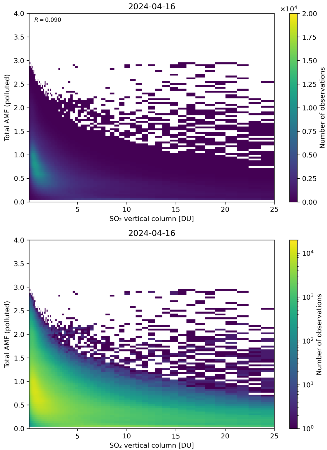
Figure 305: Scatter density plot of “SO 2 vertical column” against “Total AMF (polluted)” for 2024-04-16 to 2024-04-17.
