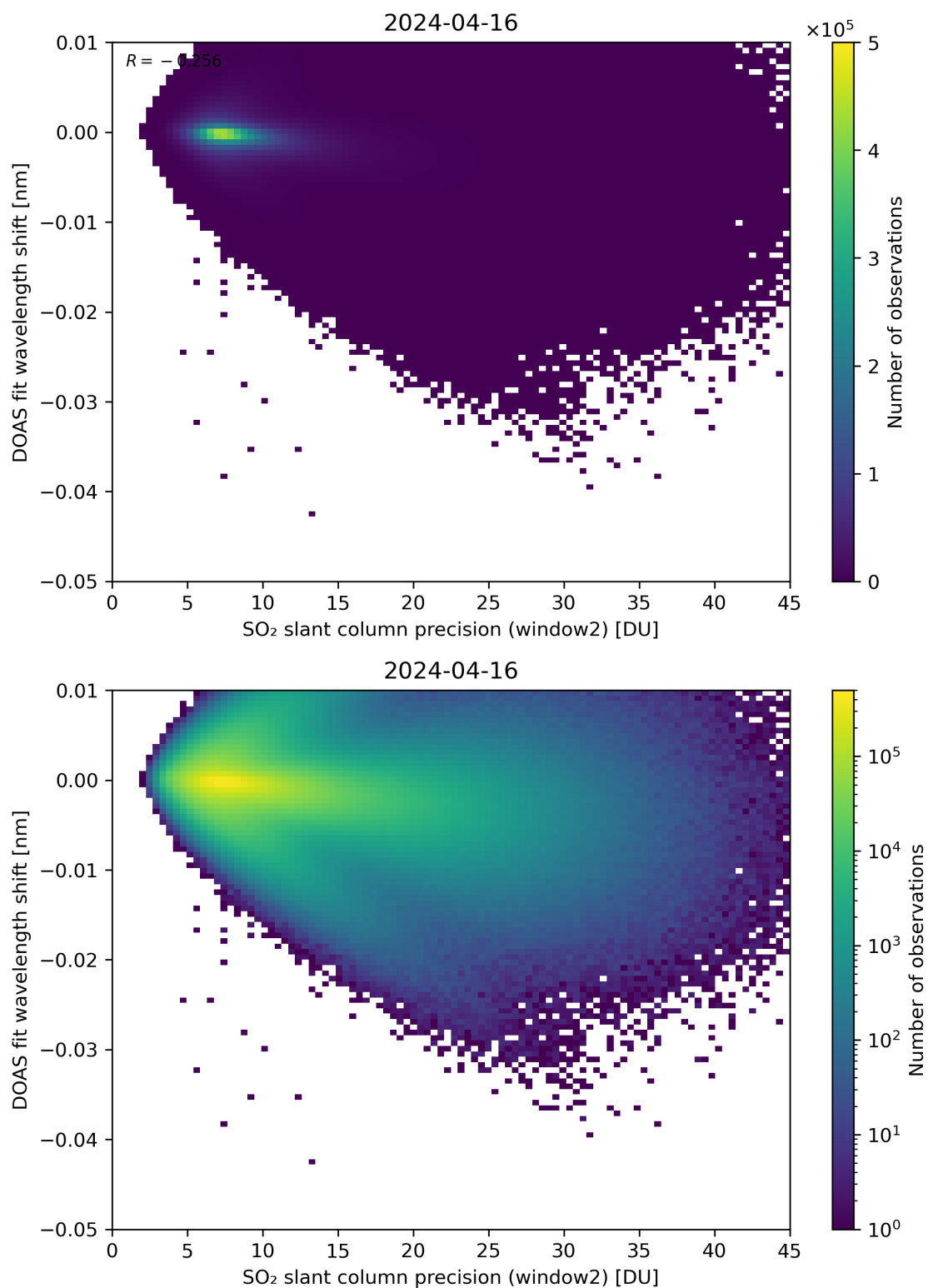
Figure 243: Scatter density plot of “SO 2 slant column precision (window2)” against “DOAS fit wavelength shift” for 2024-04-16 to 2024-04-17.
