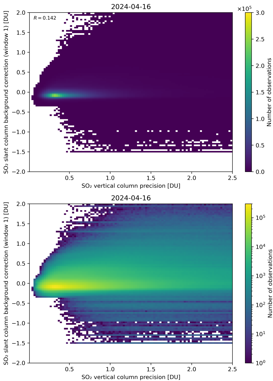
Figure 279: Scatter density plot of “SO 2 vertical column precision” against “SO 2 slant column background correction (window 1)” for 2024-04-16 to 2024-04-17.
