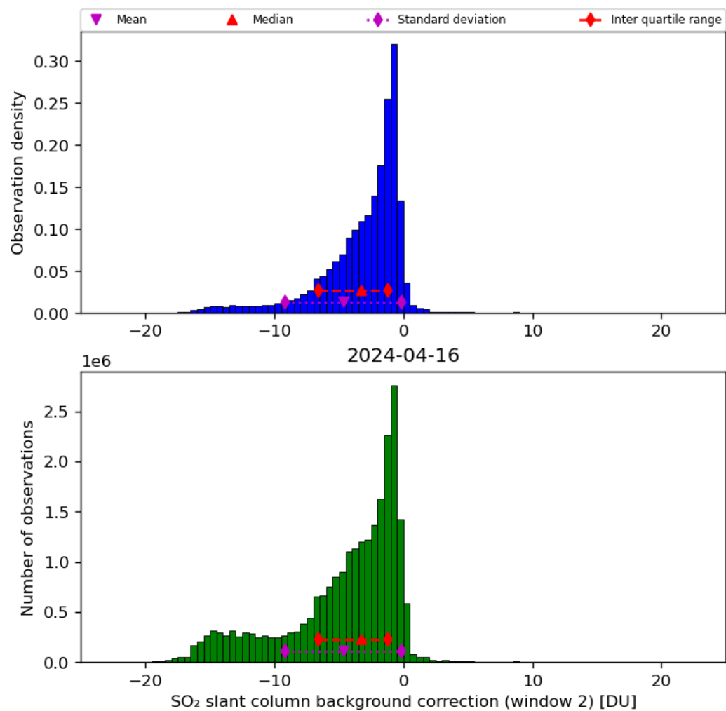
Figure 63: Histogram of “SO 2 slant column background correction (window 2)” for 2024-04-16 to 2024-04-17
