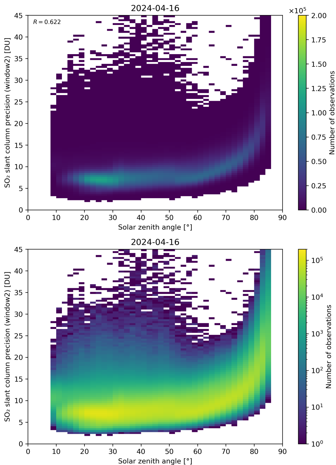
Figure 171: Scatter density plot of “Solar zenith angle” against “SO 2 slant column precision (window2)” for 2024-04-16 to 2024-04-17.
