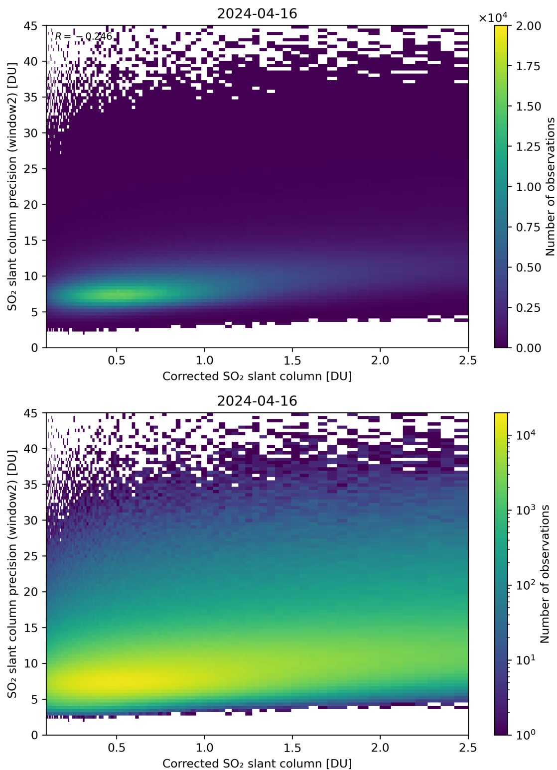
Figure 189: Scatter density plot of “Corrected SO 2 slant column” against “SO 2 slant column precision (window2)” for 2024-04-16 to 2024-04-17.
