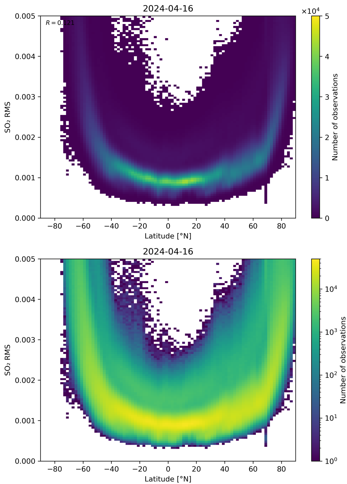
Figure 144: Scatter density plot of “Latitude” against “SO 2 RMS” for 2024-04-16 to 2024-04-17.
