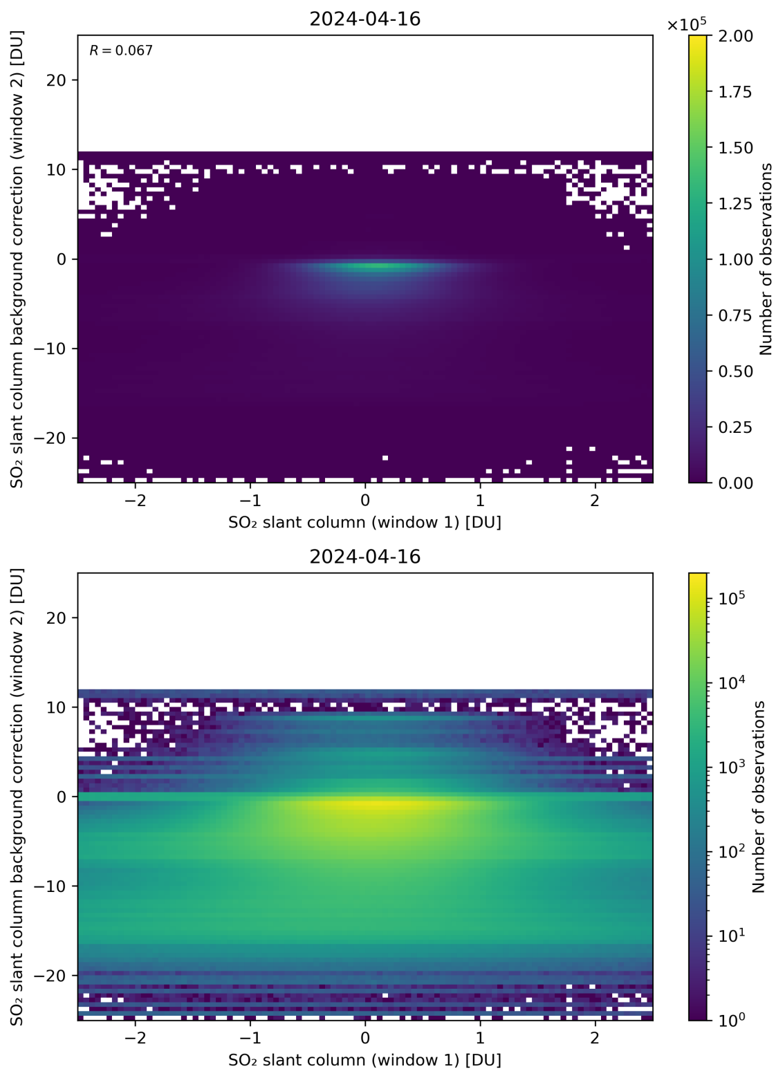
Figure 213: Scatter density plot of “SO 2 slant column (window 1)” against “SO 2 slant column background correction (window 2)” for 2024-04-16 to 2024-04-17.
