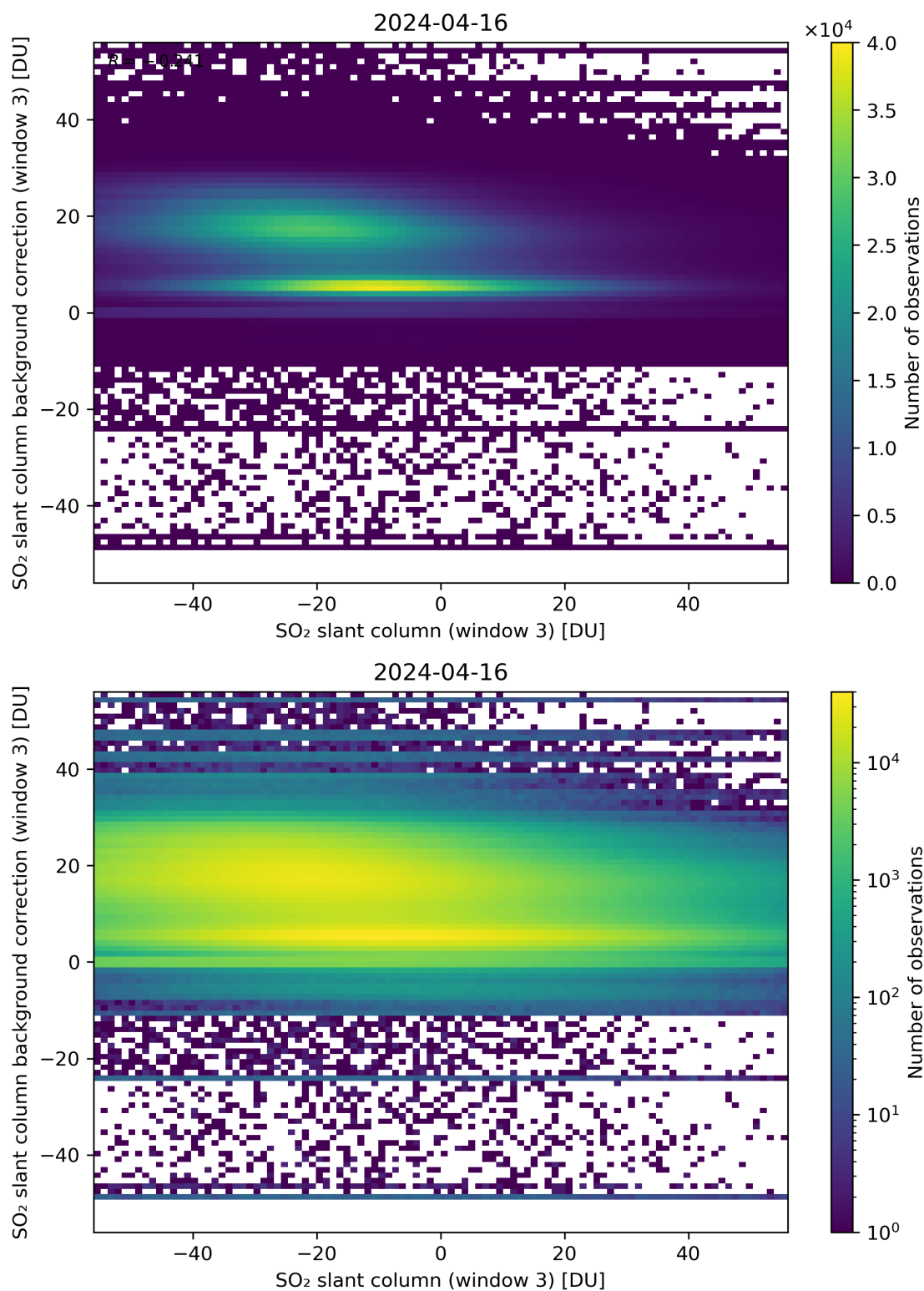
Figure 253: Scatter density plot of “SO 2 slant column (window 3)” against “SO 2 slant column background correction (window 3)” for 2024-04-16 to 2024-04-17.
