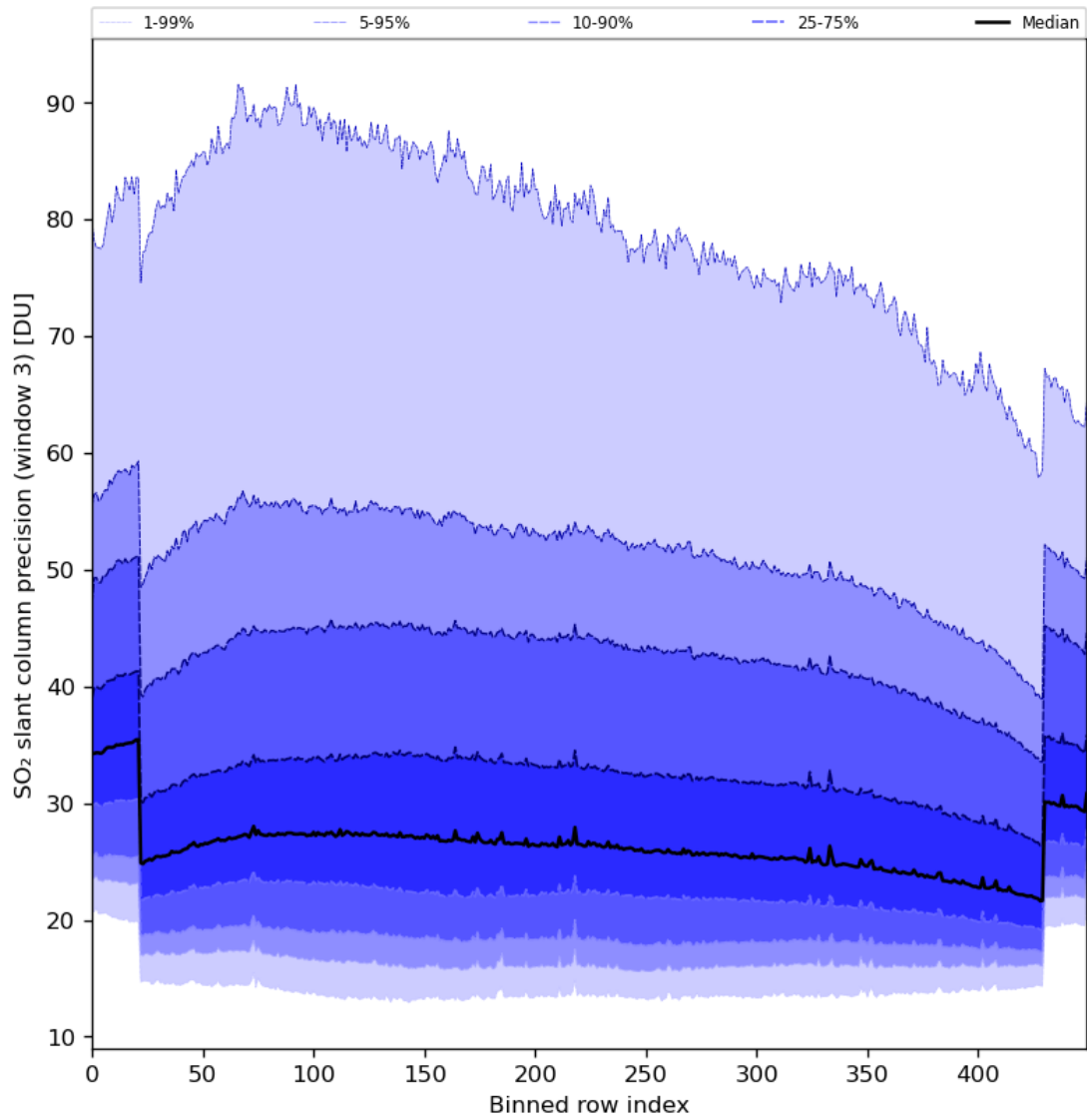
Figure 88: Along track statistics of “SO 2 slant column precision (window 3)” for 2024-04-16 to 2024-04-17
