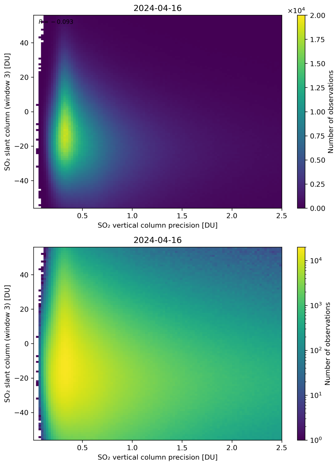
Figure 292: Scatter density plot of “SO 2 vertical column precision” against “SO 2 slant column (window 3)” for 2024-04-16 to 2024-04-17.
