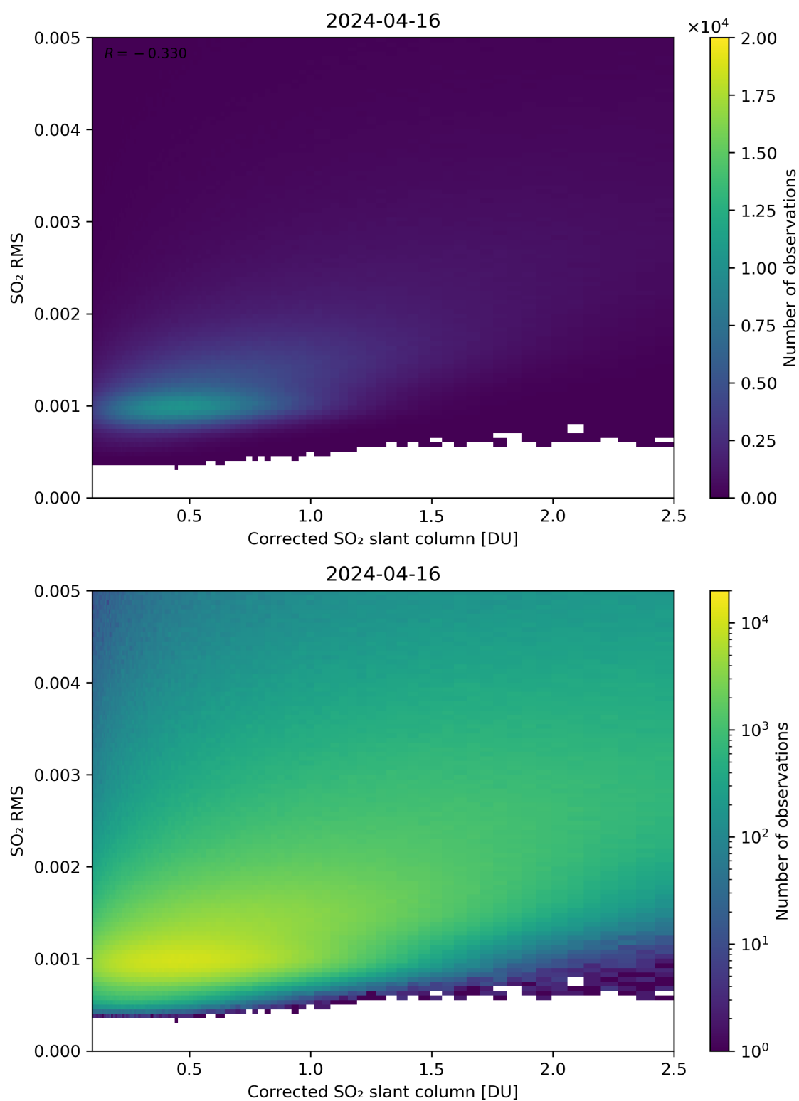
Figure 183: Scatter density plot of “Corrected SO 2 slant column” against “SO 2 RMS” for 2024-04-16 to 2024-04-17.
