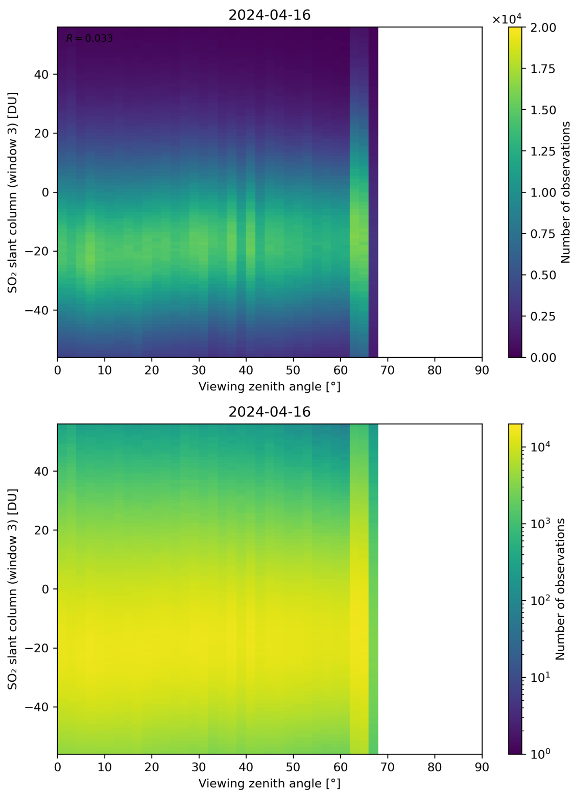
Figure 323: Scatter density plot of “Viewing zenith angle” against “SO 2 slant column (window 3)” for 2024-04-16 to 2024-04-17.
