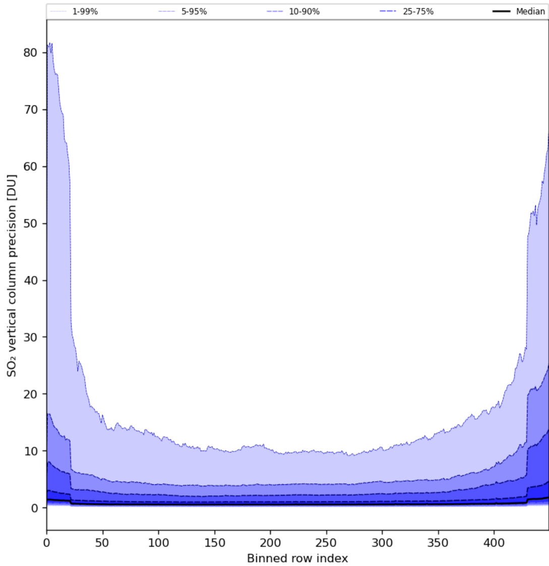
Figure 77: Along track statistics of “SO 2 vertical column precision” for 2024-04-16 to 2024-04-17
