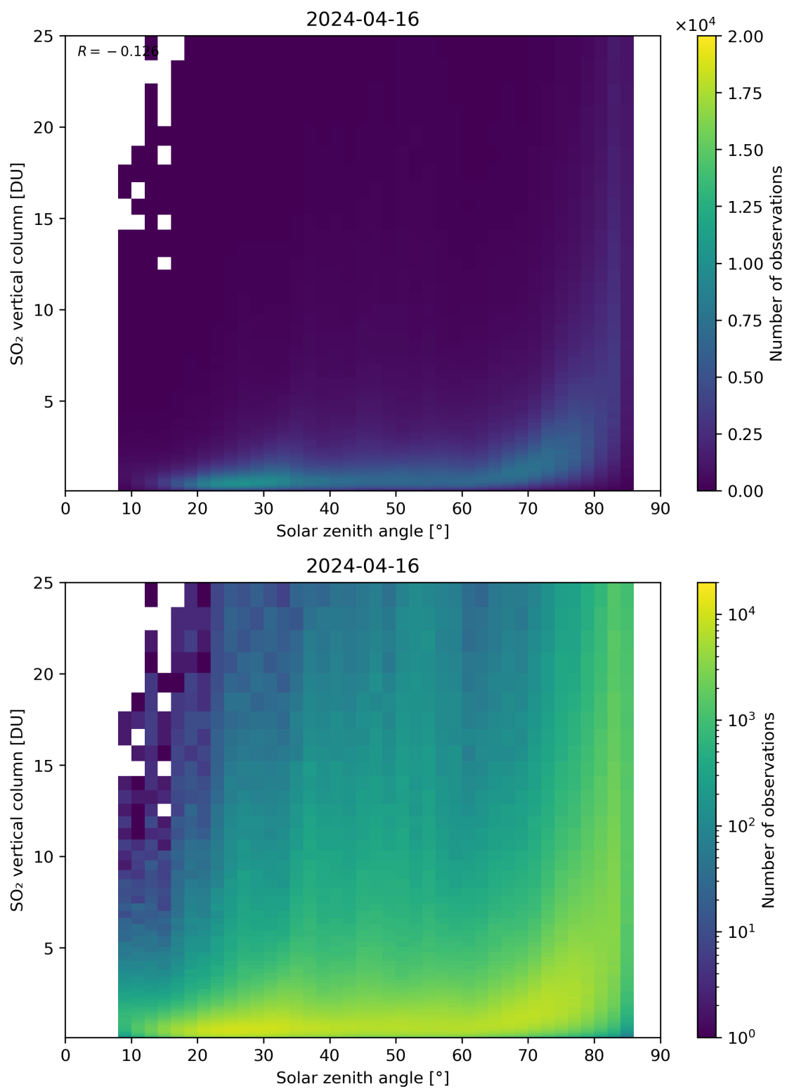
Figure 176: Scatter density plot of “Solar zenith angle” against “SO 2 vertical column” for 2024-04-16 to 2024-04-17.
