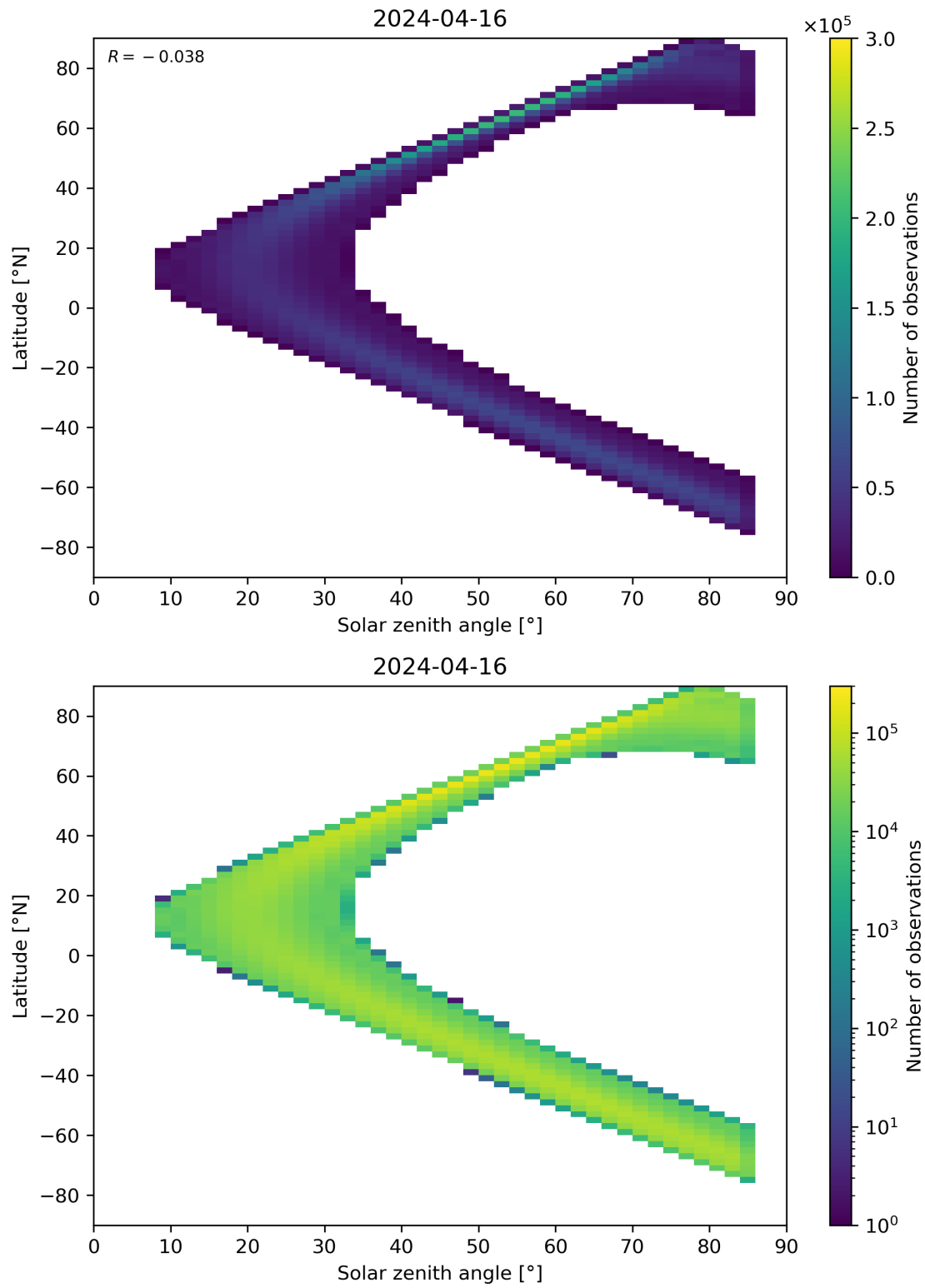
Figure 164: Scatter density plot of “Solar zenith angle” against “Latitude” for 2024-04-16 to 2024-04-17.
