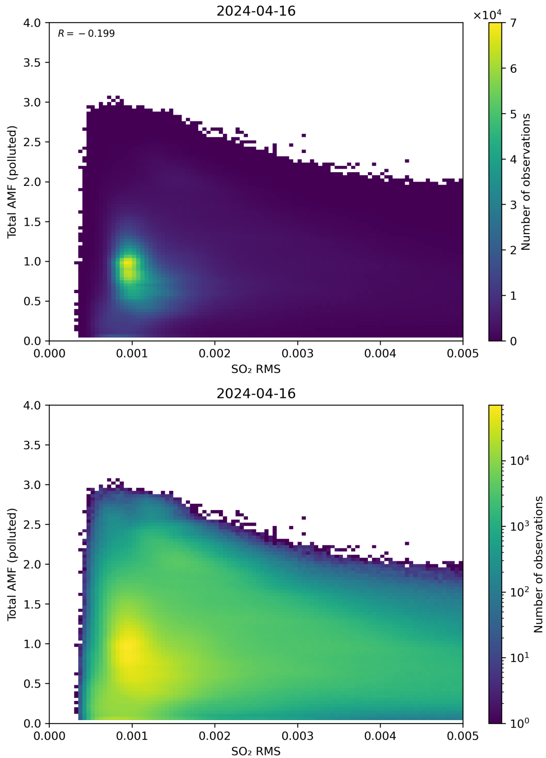
Figure 137: Scatter density plot of “SO 2 RMS” against “Total AMF (polluted)” for 2024-04-16 to 2024-04-17.
