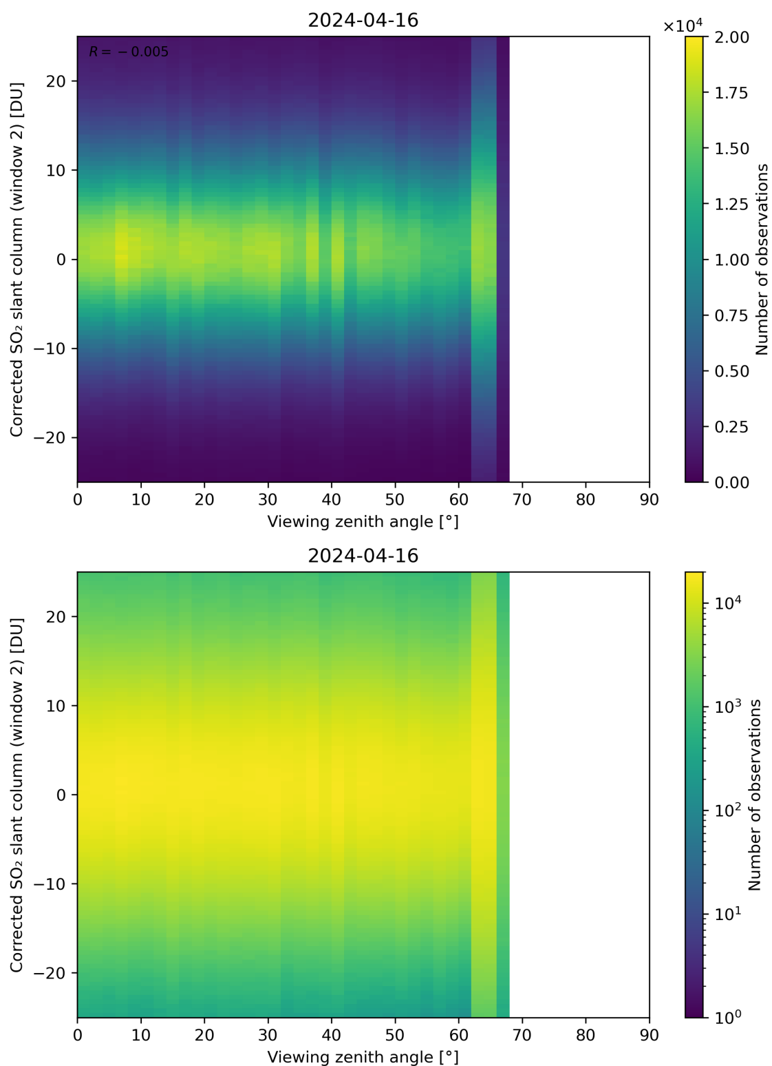
Figure 318: Scatter density plot of “Viewing zenith angle” against “Corrected SO 2 slant column (window 2)” for 2024-04-16 to 2024-04-17.
