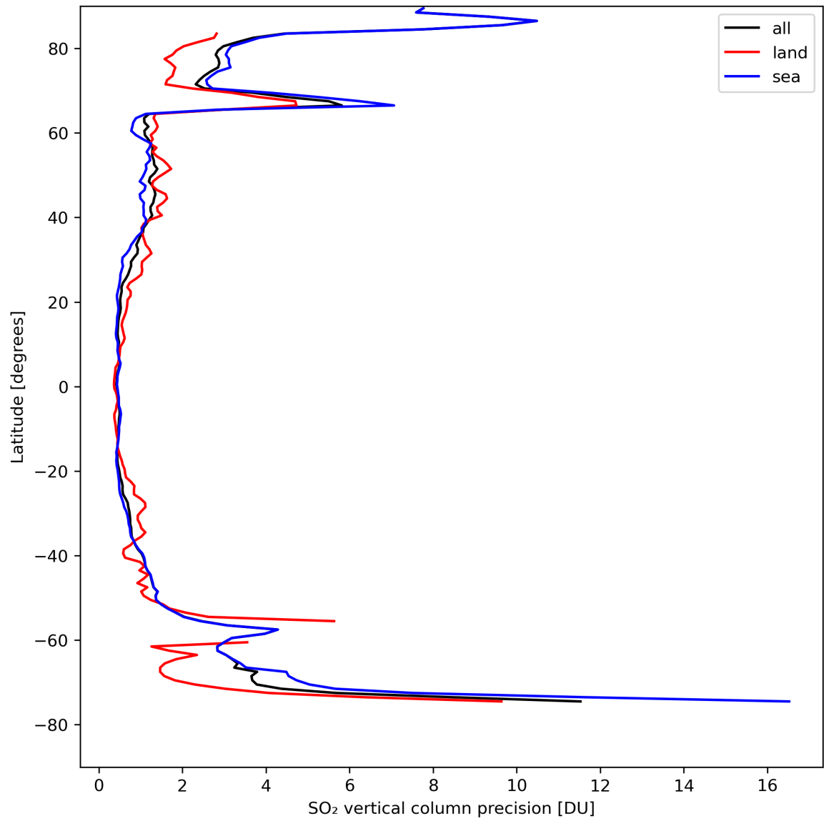
Figure 31: Zonal average of “SO 2 vertical column precision” for 2024-04-16 to 2024-04-17.
