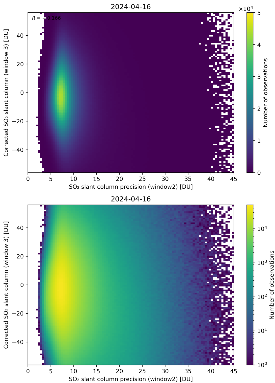
Figure 248: Scatter density plot of “SO 2 slant column precision (window2)” against “Corrected SO 2 slant column (window 3)” for 2024-04-16 to 2024-04-17.
