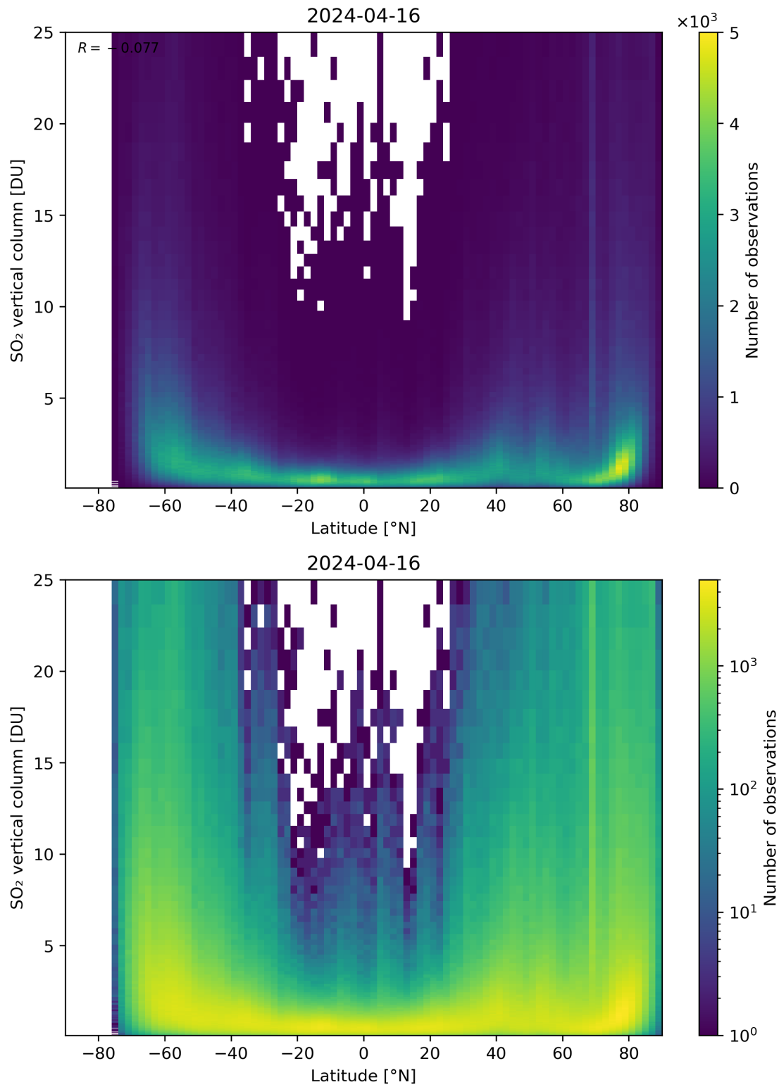
Figure 156: Scatter density plot of “Latitude” against “SO 2 vertical column” for 2024-04-16 to 2024-04-17.
