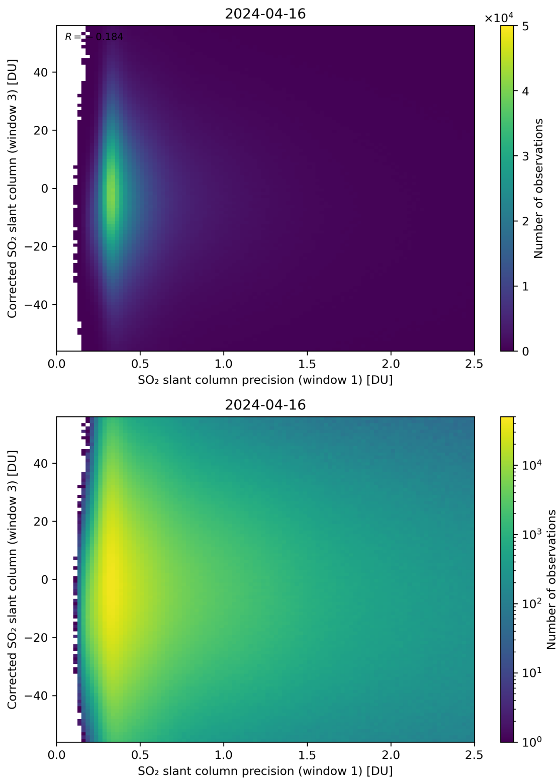
Figure 226: Scatter density plot of “SO 2 slant column precision (window 1)” against “Corrected SO 2 slant column (window 3)” for 2024-04-16 to 2024-04-17.
