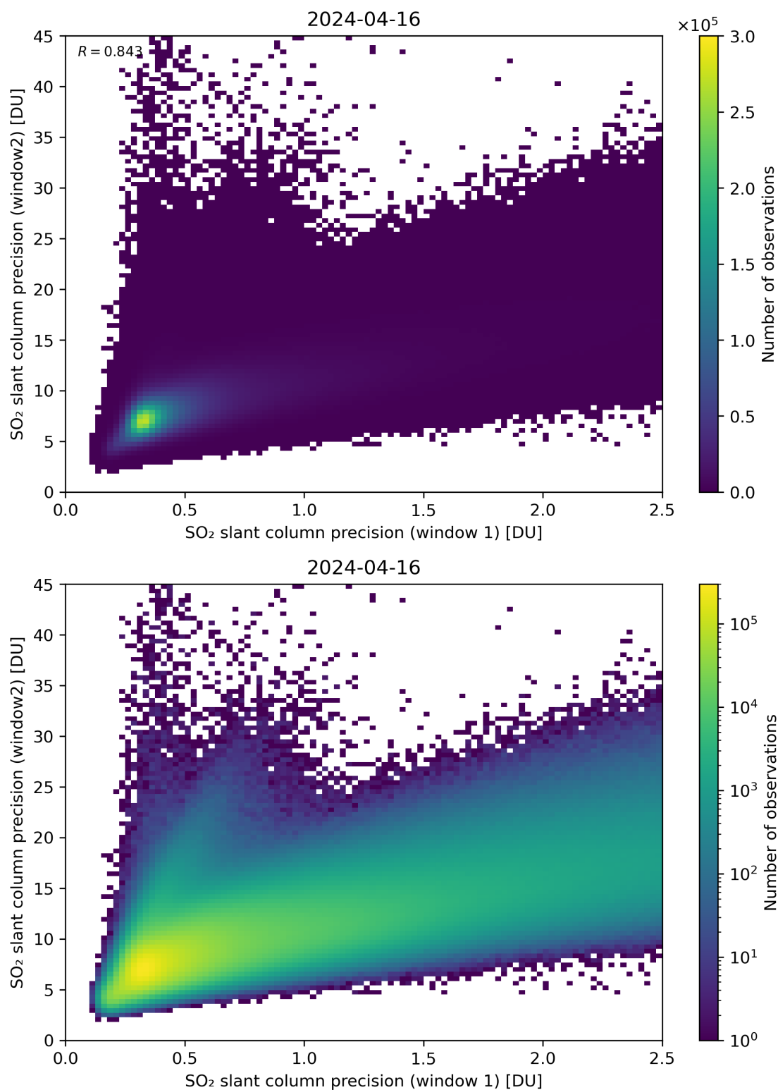
Figure 227: Scatter density plot of “SO 2 slant column precision (window 1)” against “SO 2 slant column precision (window 2)” for 2024-04-16 to 2024-04-17.
