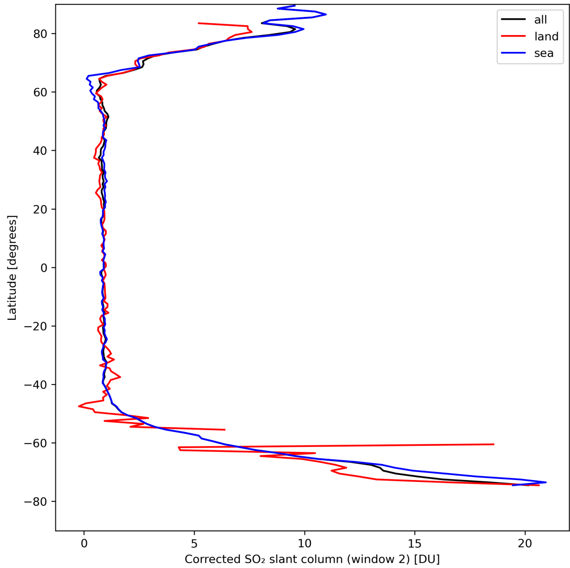
Figure 39: Zonal average of “Corrected SO 2 slant column (window 2)” for 2024-04-16 to 2024-04-17.
