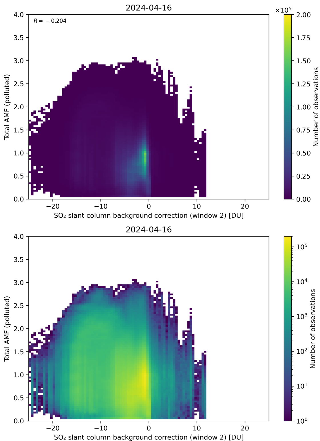
Figure 119: Scatter density plot of “SO 2 slant column background correction (window 2)” against “Total AMF (polluted)” for 2024-04-16 to 2024-04-17.
