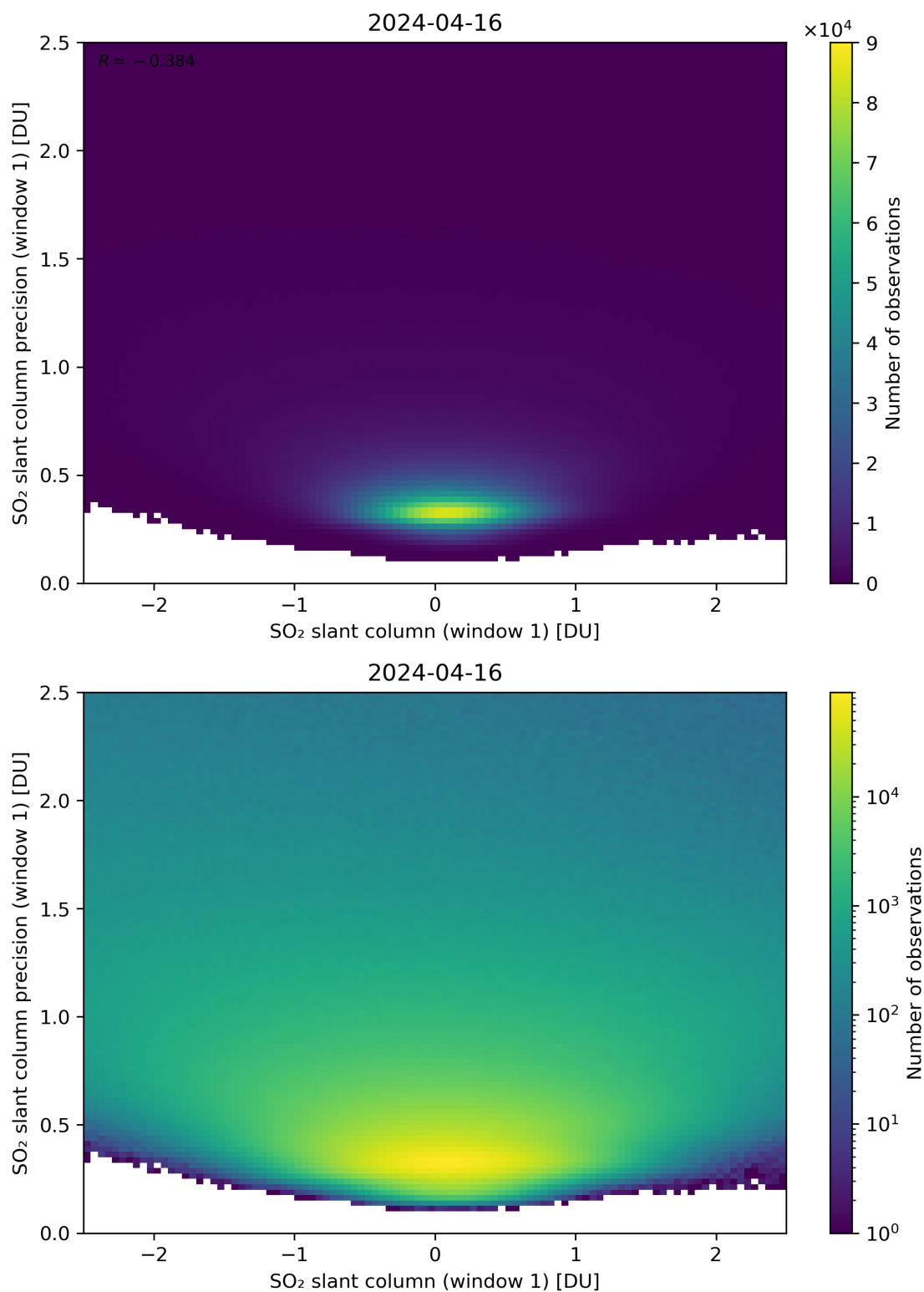
Figure 235: Scatter density plot of “SO 2 slant column (window 1)” against “SO 2 slant column precision (window 1)” for 2024-04-16 to 2024-04-17.
