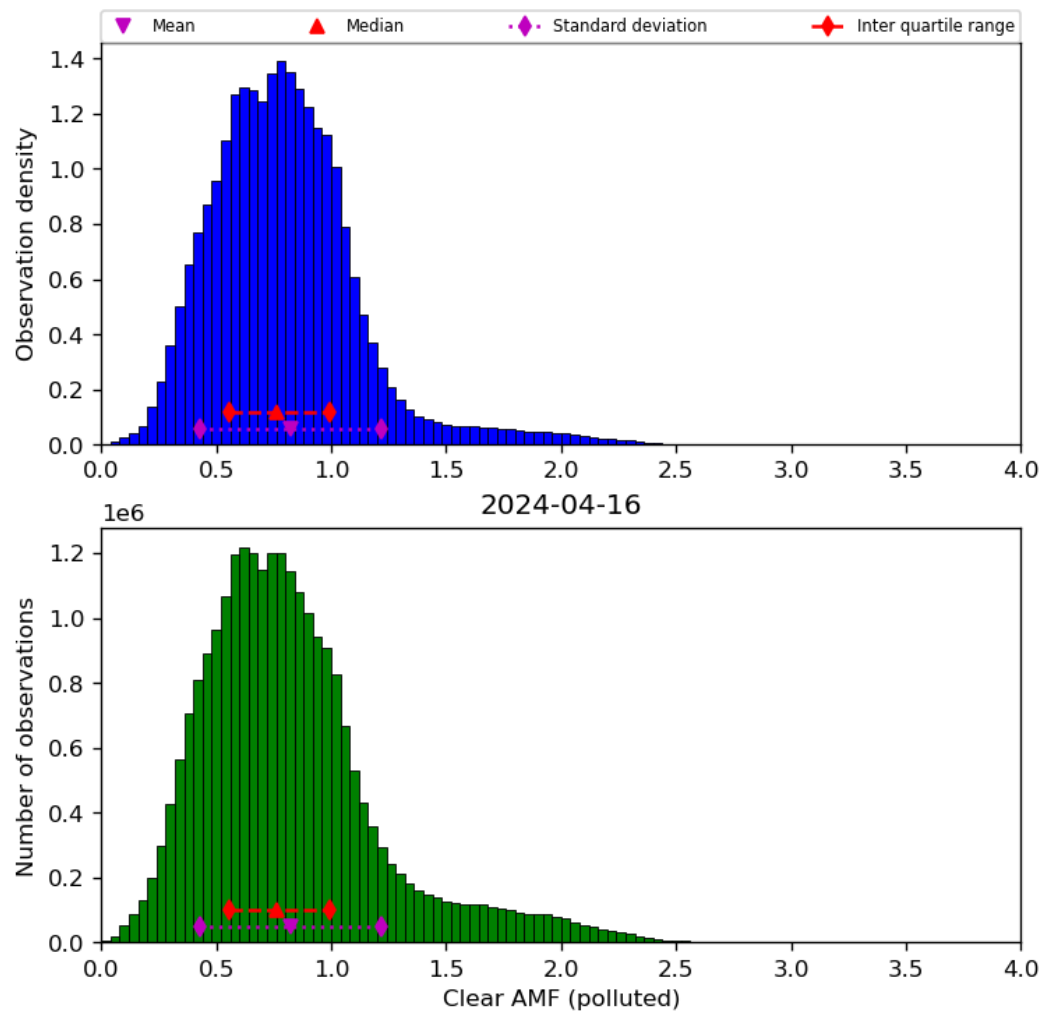
Figure 73: Histogram of “Clear AMF (polluted)” for 2024-04-16 to 2024-04-17
