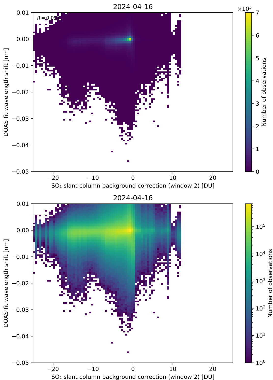
Figure 112: Scatter density plot of “SO 2 slant column background correction (window 2)” against “DOAS fit wavelength shift” for 2024-04-16 to 2024-04-17.
