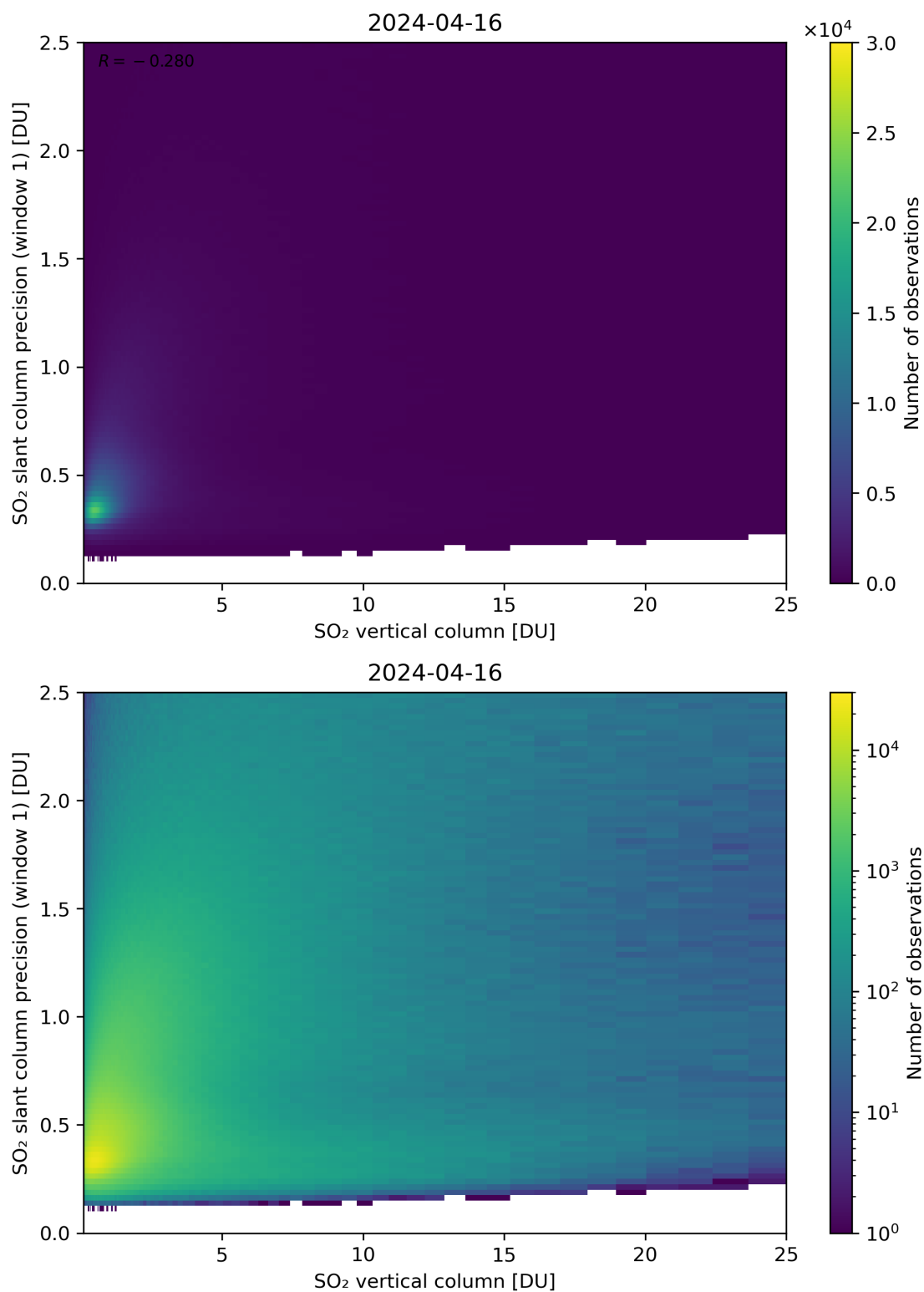
Figure 301: Scatter density plot of “SO 2 vertical column” against “SO 2 slant column precision (window 1)” for 2024-04-16 to 2024-04-17.
