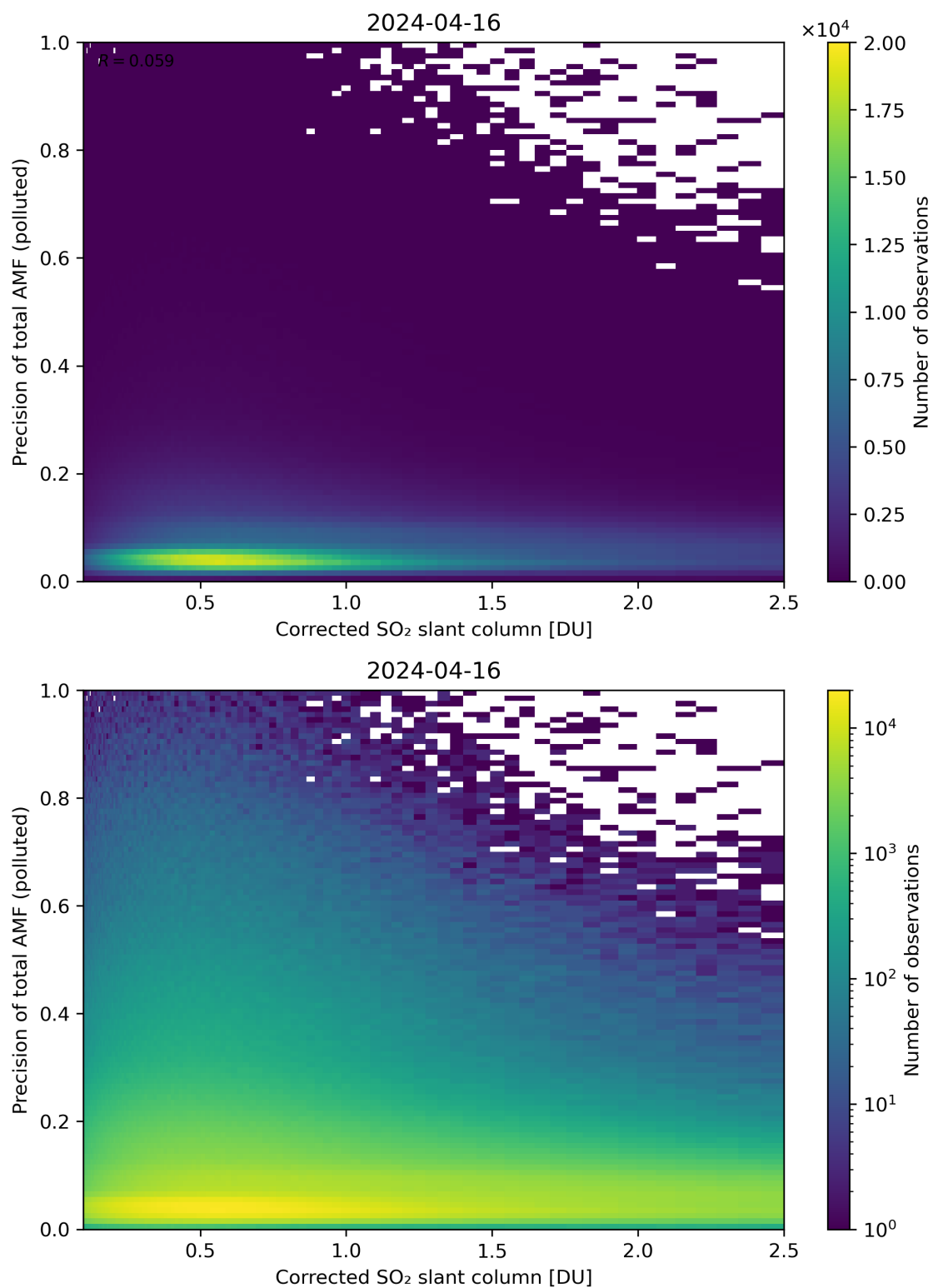
Figure 193: Scatter density plot of “Corrected SO 2 slant column” against “Precision of total AMF (polluted)” for 2024-04-16 to 2024-04-17.
