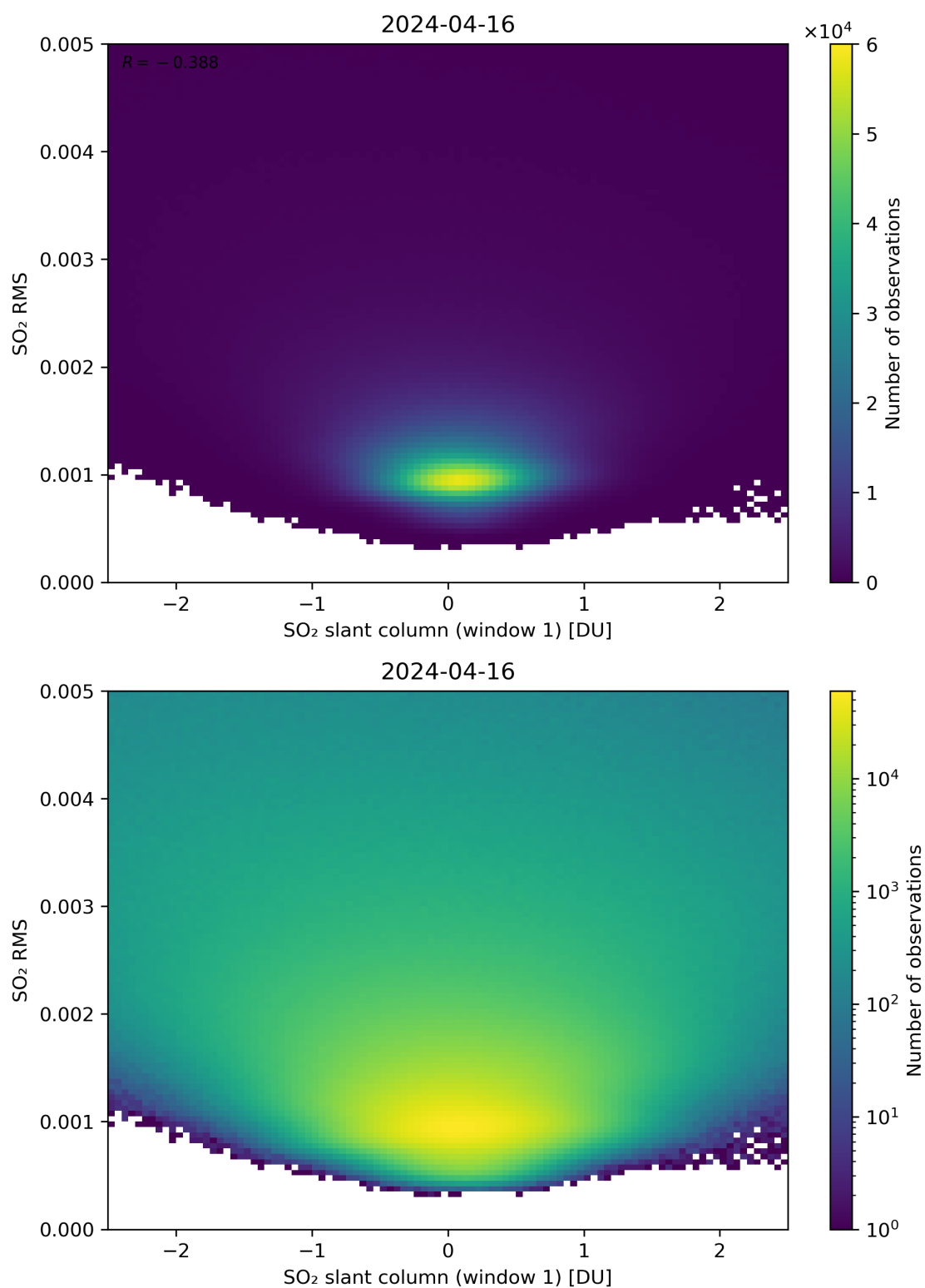
Figure 217: Scatter density plot of “SO 2 slant column (window 1)” against “SO 2 RMS” for 2024-04-16 to 2024-04-17.
