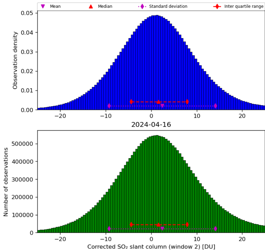
Figure 62: Histogram of “Corrected SO 2 slant column (window 2)” for 2024-04-16 to 2024-04-17
