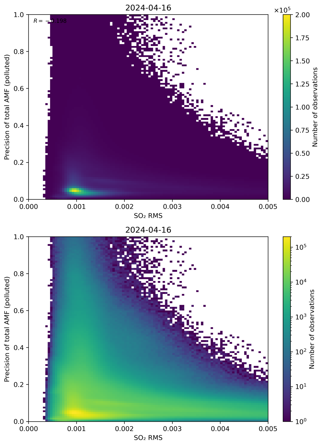
Figure 138: Scatter density plot of “SO 2 RMS” against “Precision of total AMF (polluted)” for 2024-04-16 to 2024-04-17.
