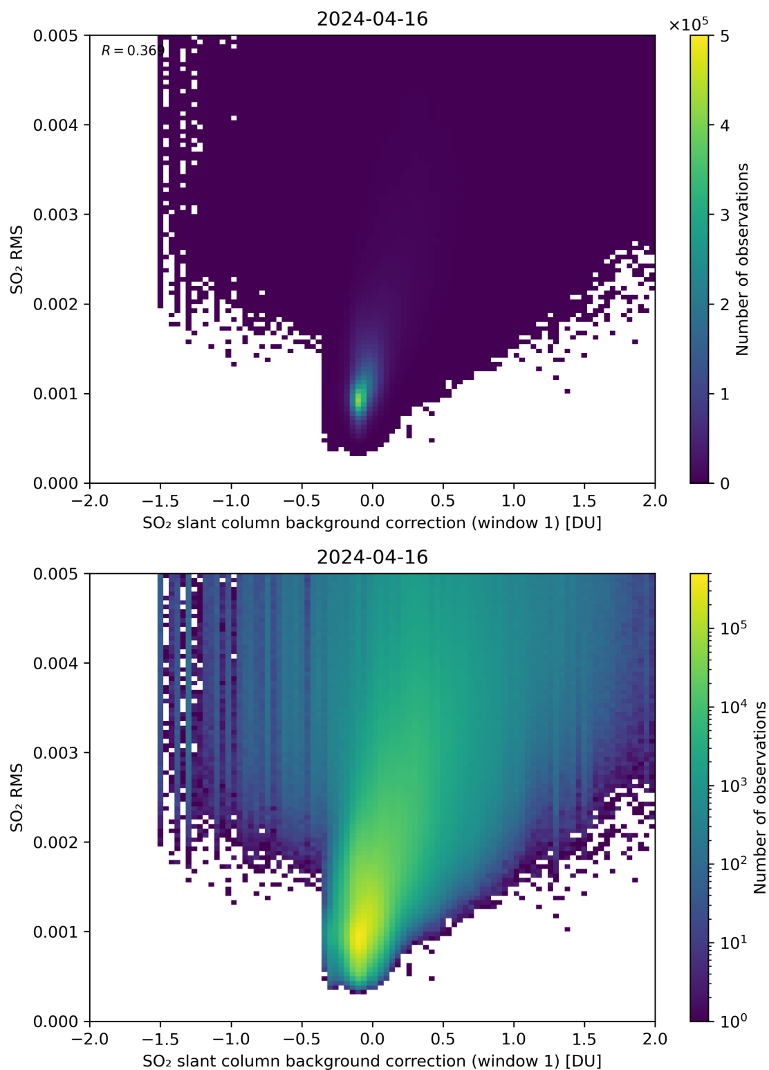
Figure 102: Scatter density plot of “SO 2 slant column background correction (window 1)” against “SO 2 RMS” for 2024-04-16 to 2024-04-17.
