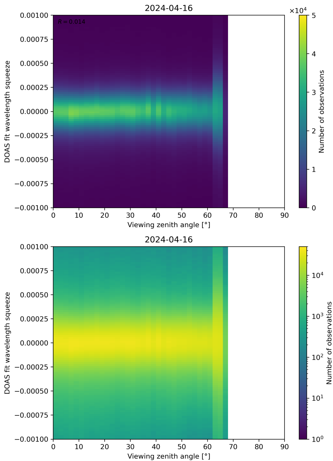
Figure 312: Scatter density plot of “Viewing zenith angle” against “DOAS fit wavelength squeeze” for 2024-04-16 to 2024-04-17.
