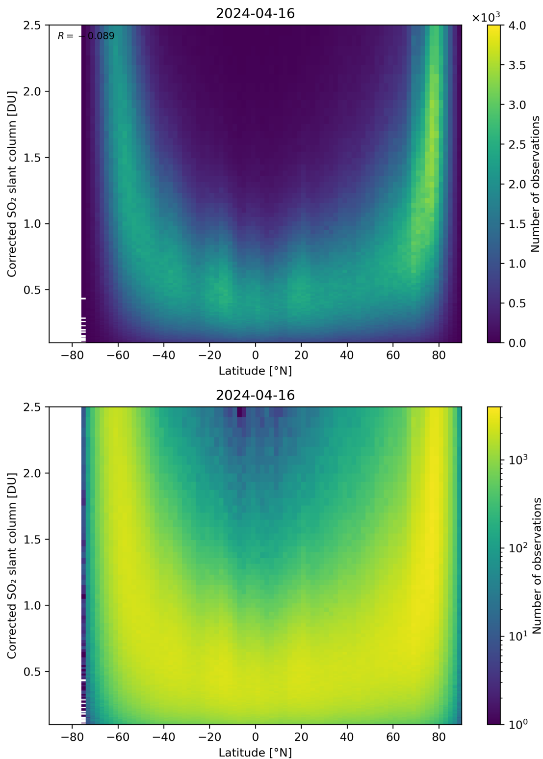
Figure 146: Scatter density plot of “Latitude” against “Corrected SO 2 slant column” for 2024-04-16 to 2024-04-17.
