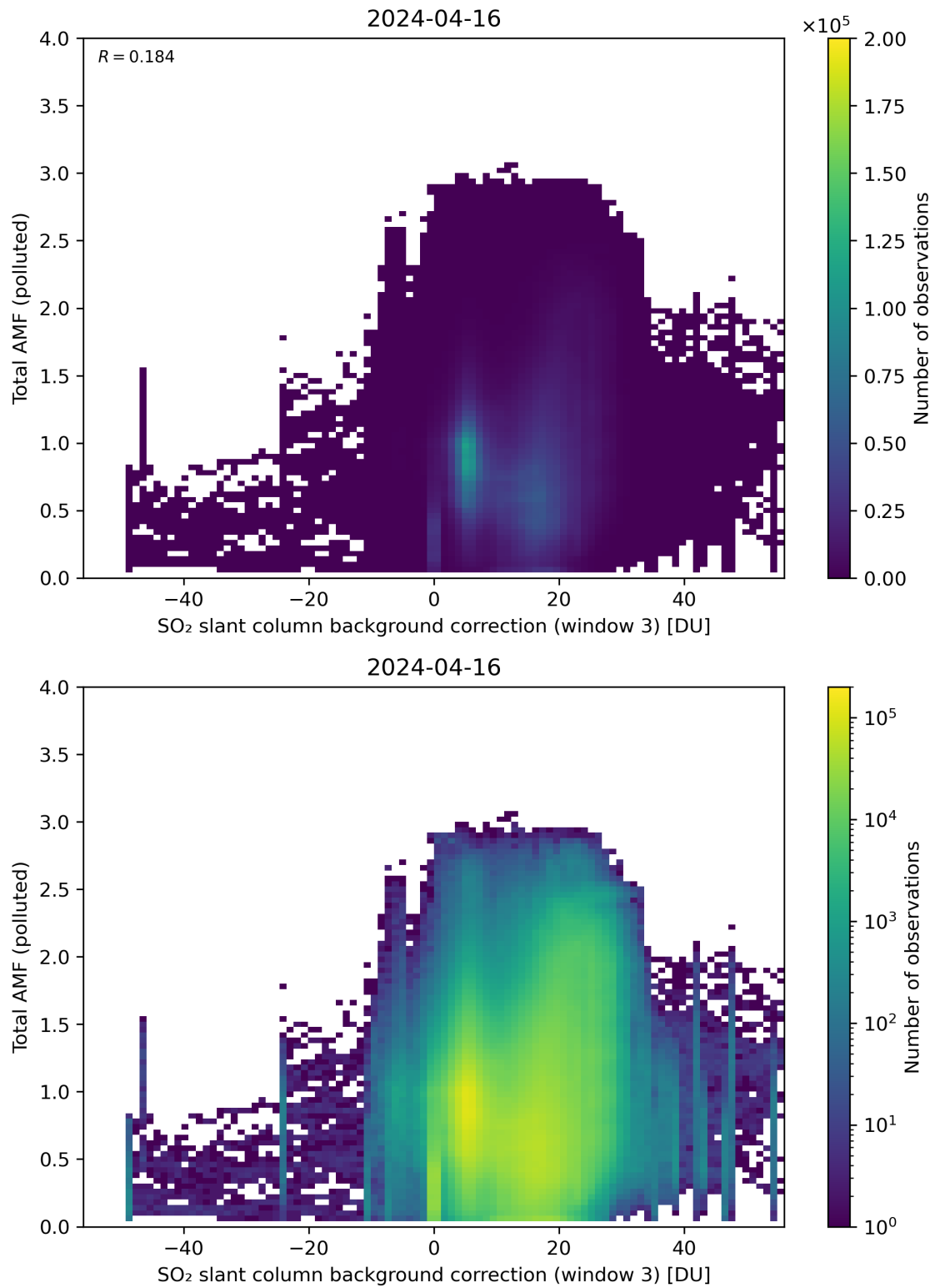
Figure 125: Scatter density plot of “SO 2 slant column background correction (window 3)” against “Total AMF (polluted)” for 2024-04-16 to 2024-04-17.
