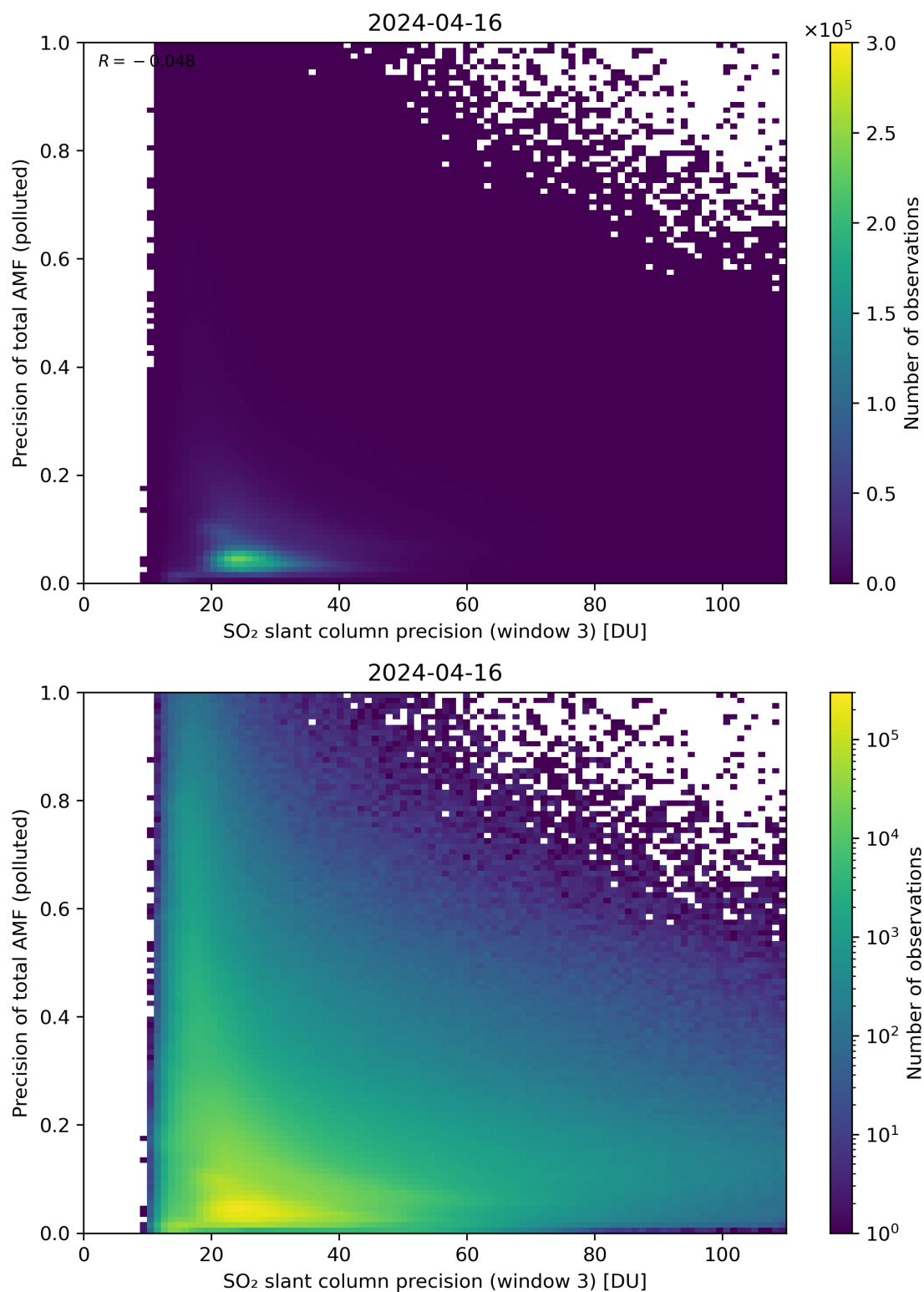
Figure 264: Scatter density plot of “SO 2 slant column precision (window 3)” against “Precision of total AMF (polluted)” for 2024-04-16 to 2024-04-17.
