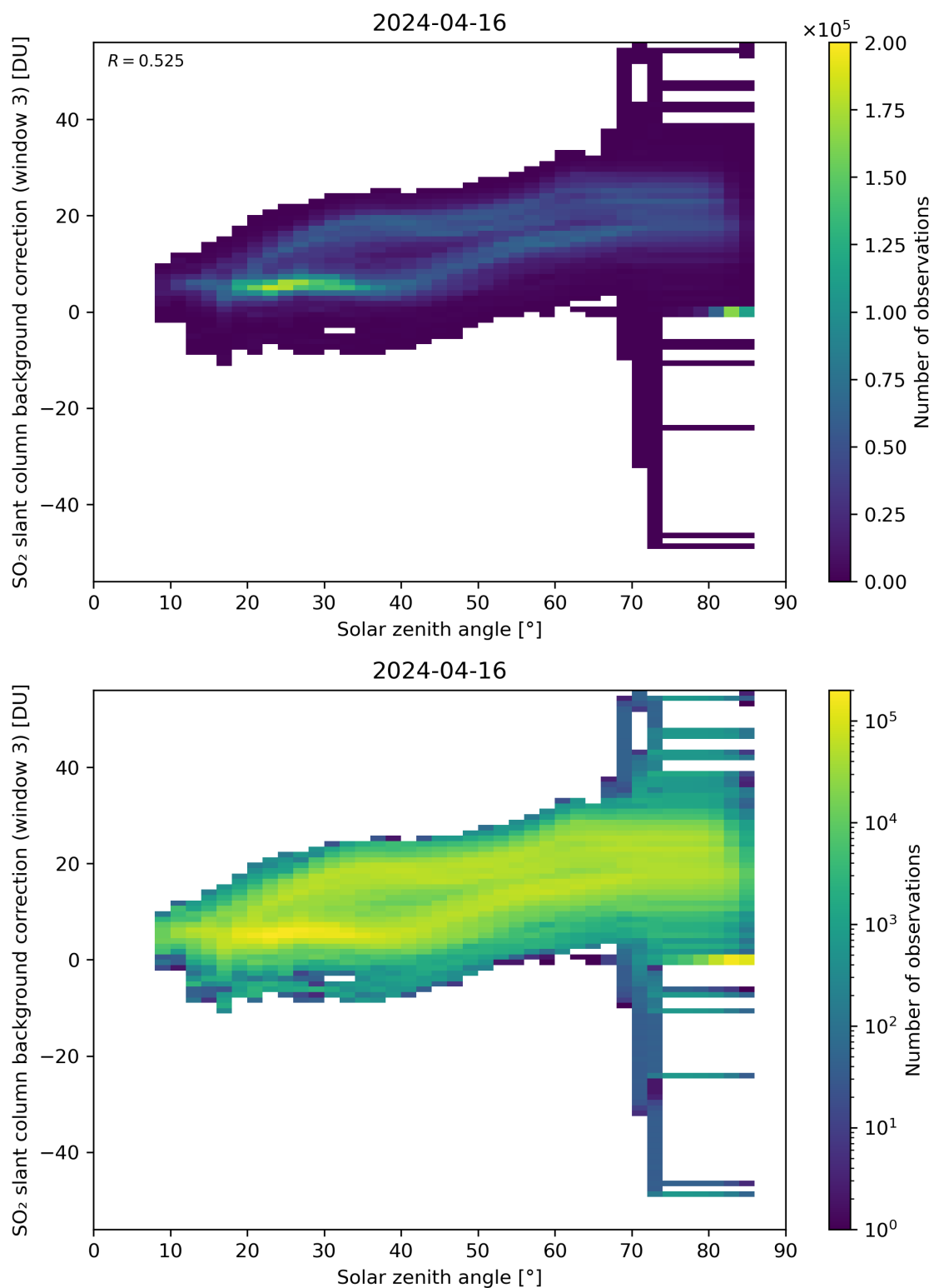
Figure 160: Scatter density plot of “Solar zenith angle” against “SO 2 slant column background correction (window 3)” for 2024-04-16 to 2024-04-17.
