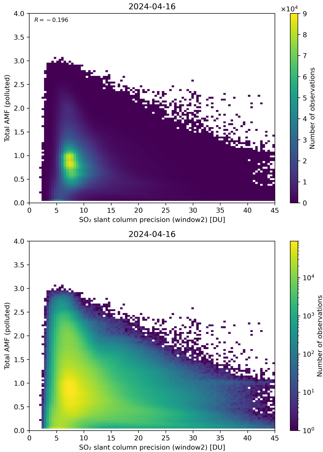
Figure 251: Scatter density plot of “SO 2 slant column precision (window2)” against “Total AMF (polluted)” for 2024-04-16 to 2024-04-17.
