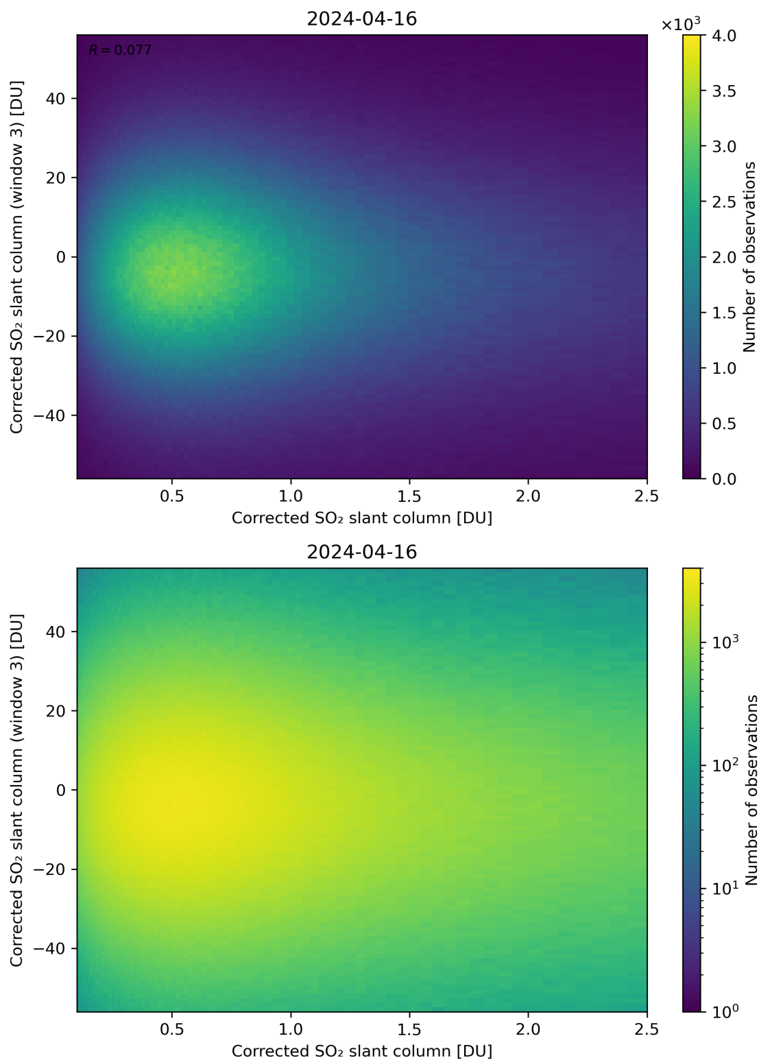
Figure 186: Scatter density plot of “Corrected SO 2 slant column” against “Corrected SO 2 slant column (window 3)” for 2024-04-16 to 2024-04-17.
