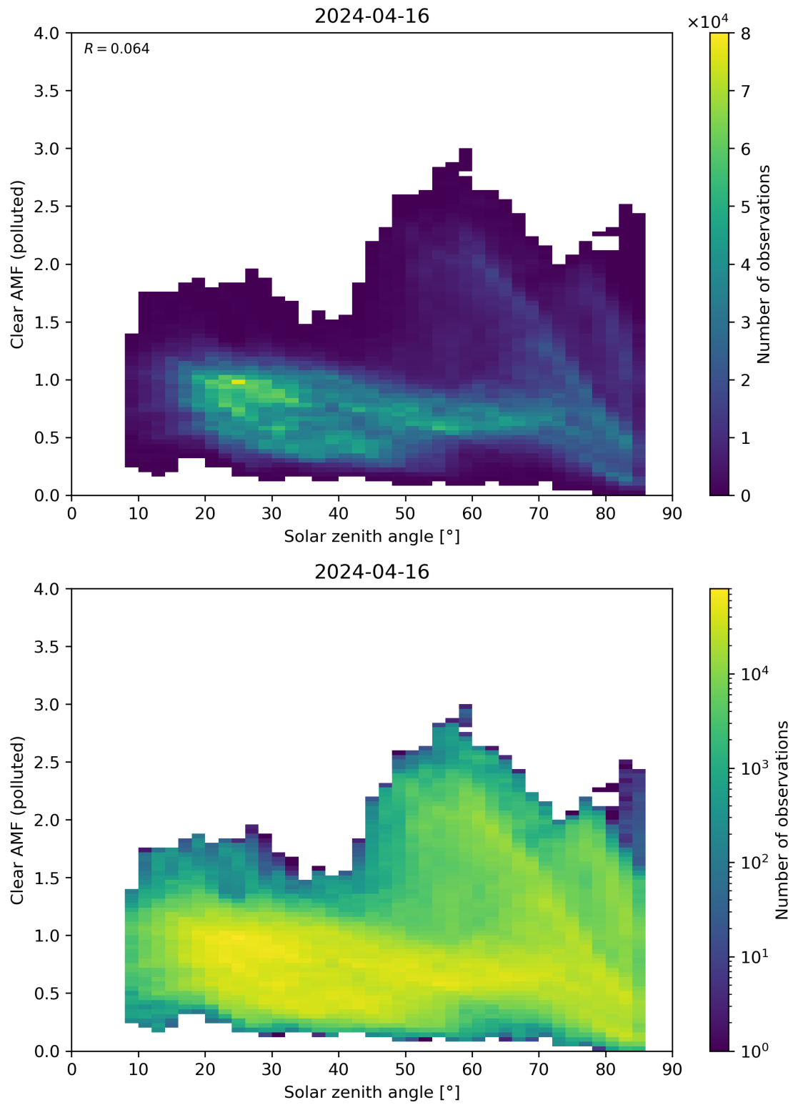
Figure 165: Scatter density plot of “Solar zenith angle” against “Clear AMF (polluted)” for 2024-04-16 to 2024-04-17.
