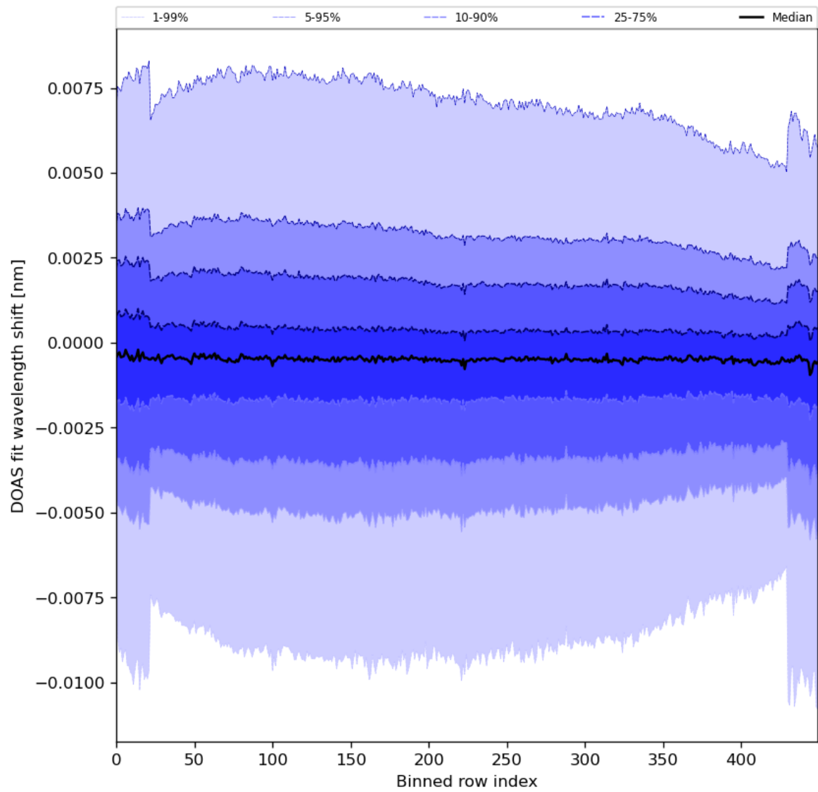
Figure 91: Along track statistics of “DOAS fit wavelength shift” for 2024-04-16 to 2024-04-17
