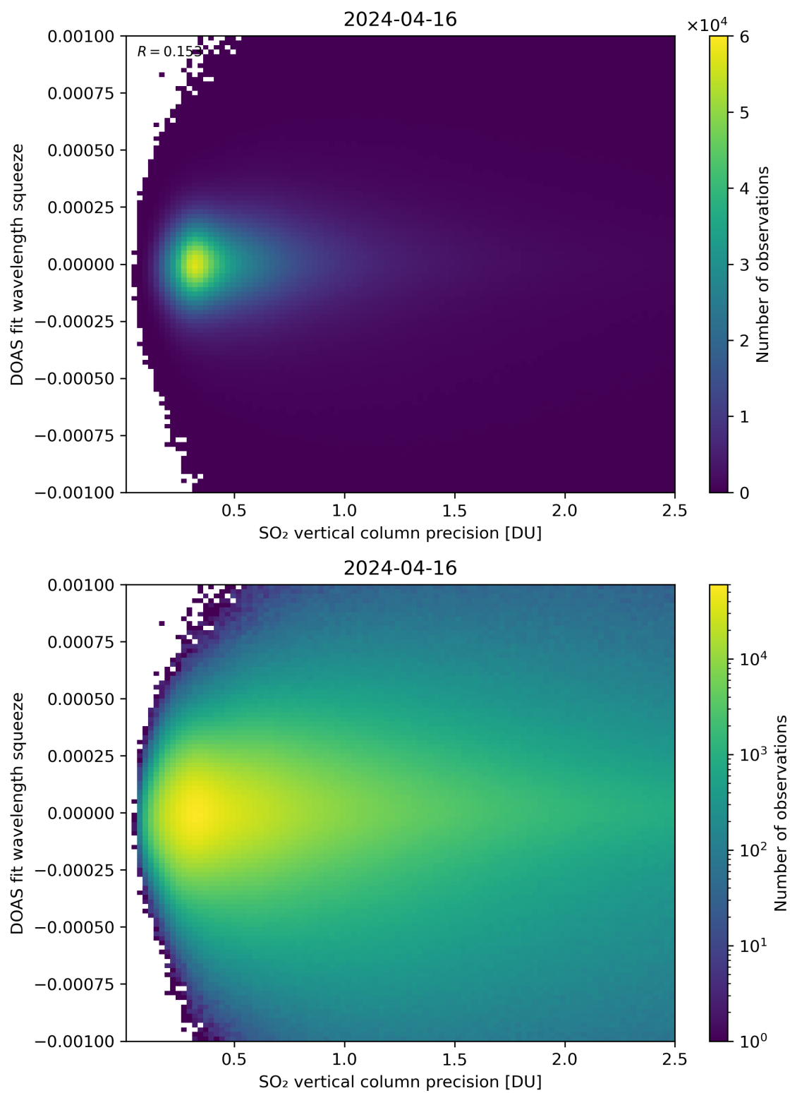
Figure 283: Scatter density plot of “SO 2 vertical column precision” against “DOAS fit wavelength squeeze” for 2024-04-16 to 2024-04-17.
