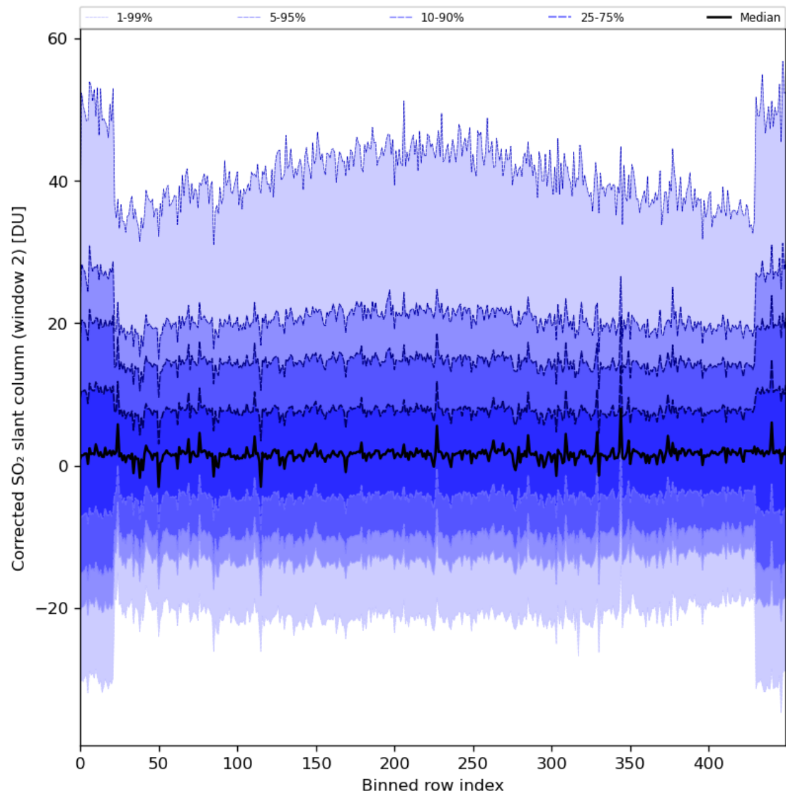
Figure 85: Along track statistics of “Corrected SO 2 slant column (window 2)” for 2024-04-16 to 2024-04-17
