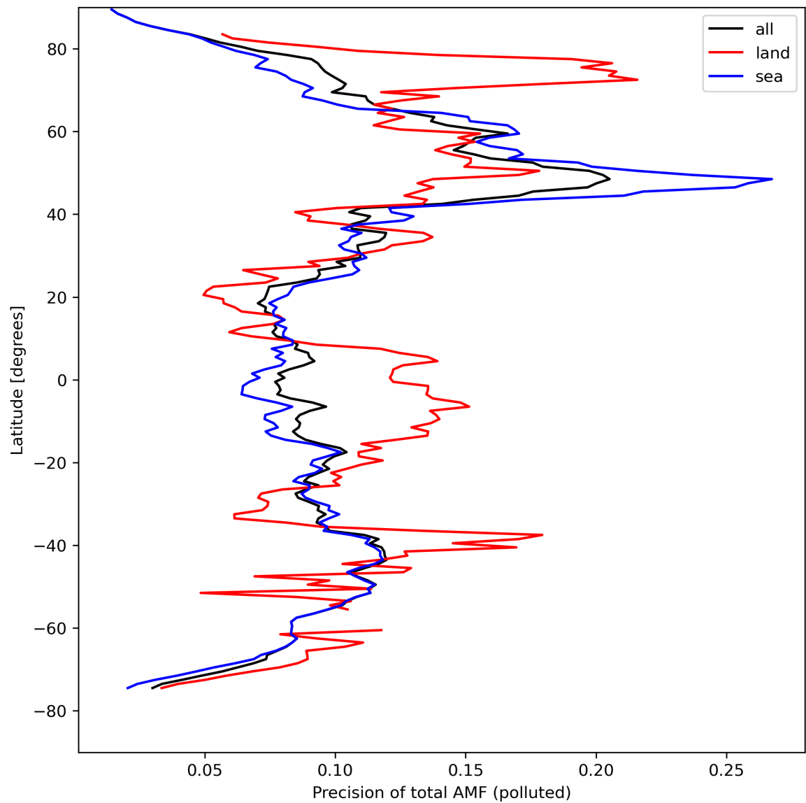
Figure 49: Zonal average of “Precision of total AMF (polluted)” for 2024-04-16 to 2024-04-17.
