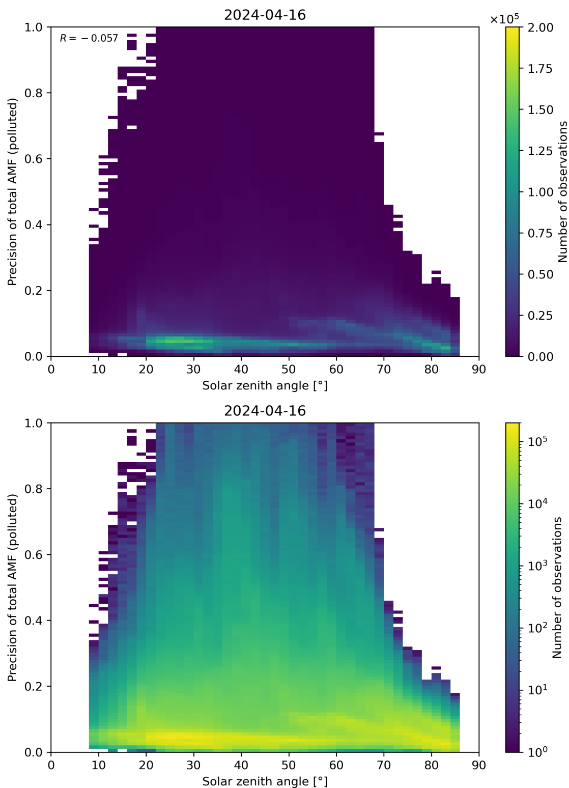
Figure 175: Scatter density plot of “Solar zenith angle” against “Precision of total AMF (polluted)” for 2024-04-16 to 2024-04-17.
