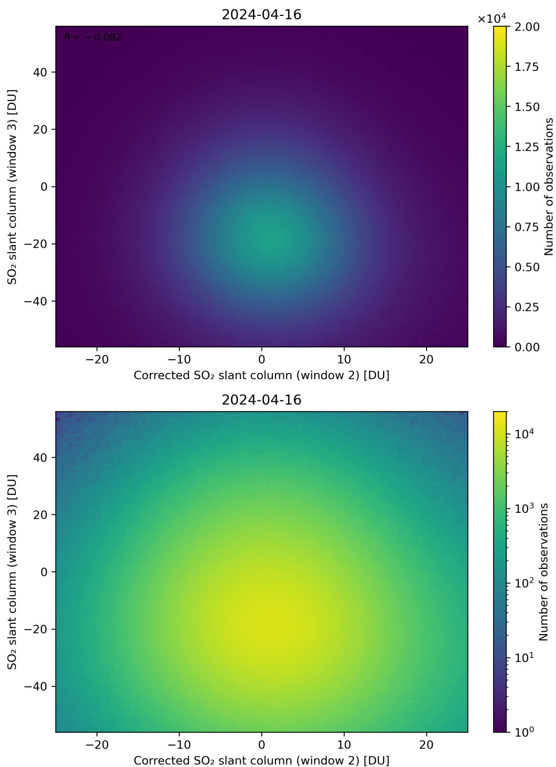
Figure 201: Scatter density plot of “Corrected SO 2 slant column (window 2)” against “SO 2 slant column (window 3)” for 2024-04-16 to 2024-04-17.
