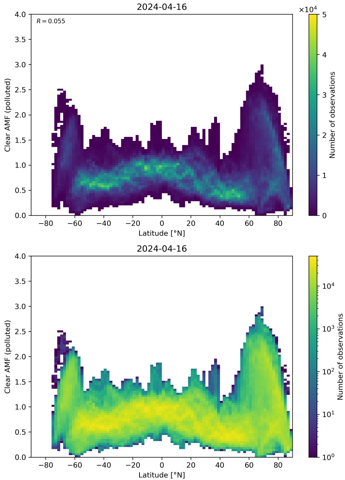
Figure 145: Scatter density plot of “Latitude” against “Clear AMF (polluted)” for 2024-04-16 to 2024-04-17.
