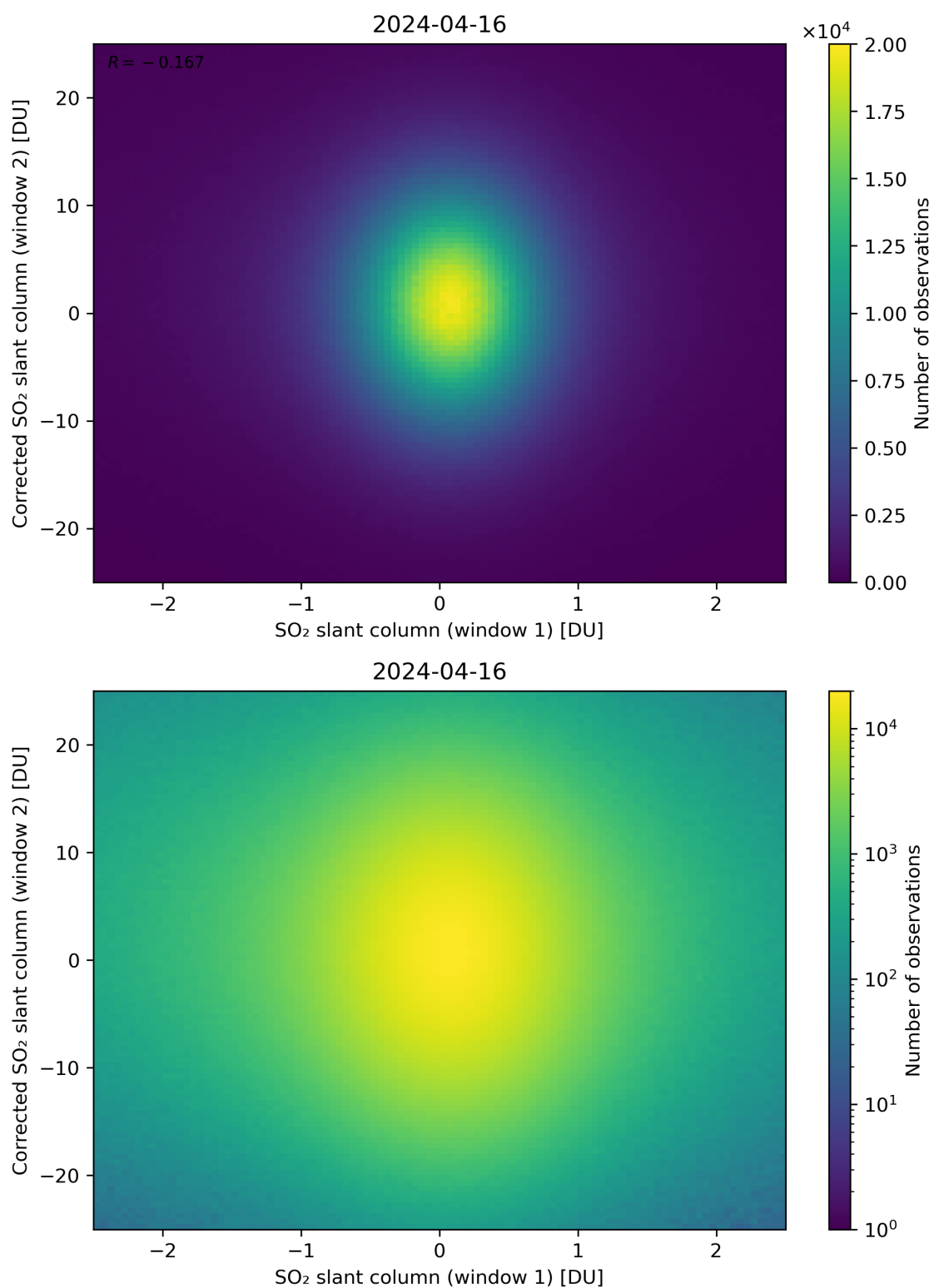
Figure 233: Scatter density plot of “SO 2 slant column (window 1)” against “Corrected SO 2 slant column (window 2)” for 2024-04-16 to 2024-04-17.
