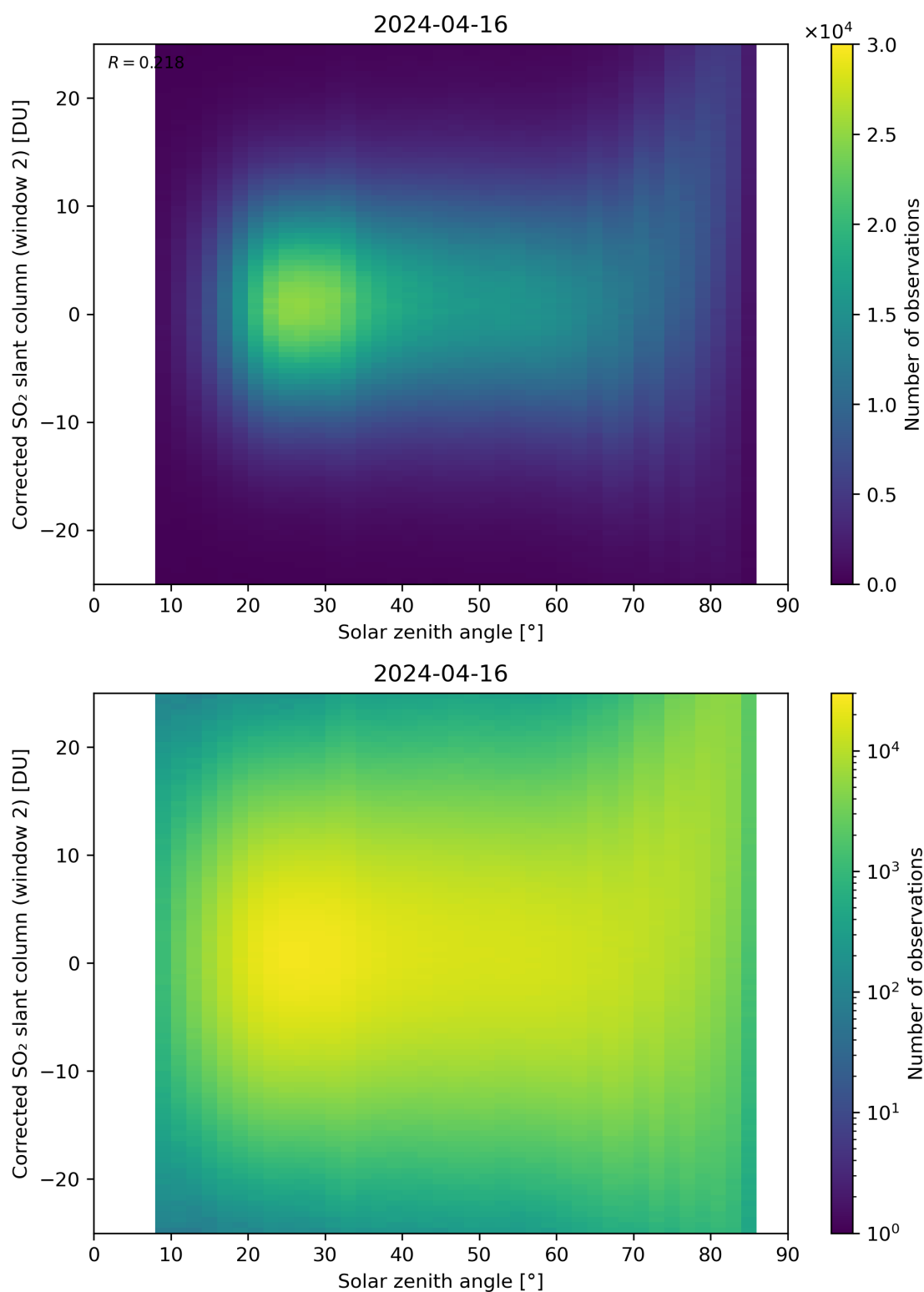
Figure 167: Scatter density plot of “Solar zenith angle” against “Corrected SO 2 slant column (window 2)” for 2024-04-16 to 2024-04-17.
