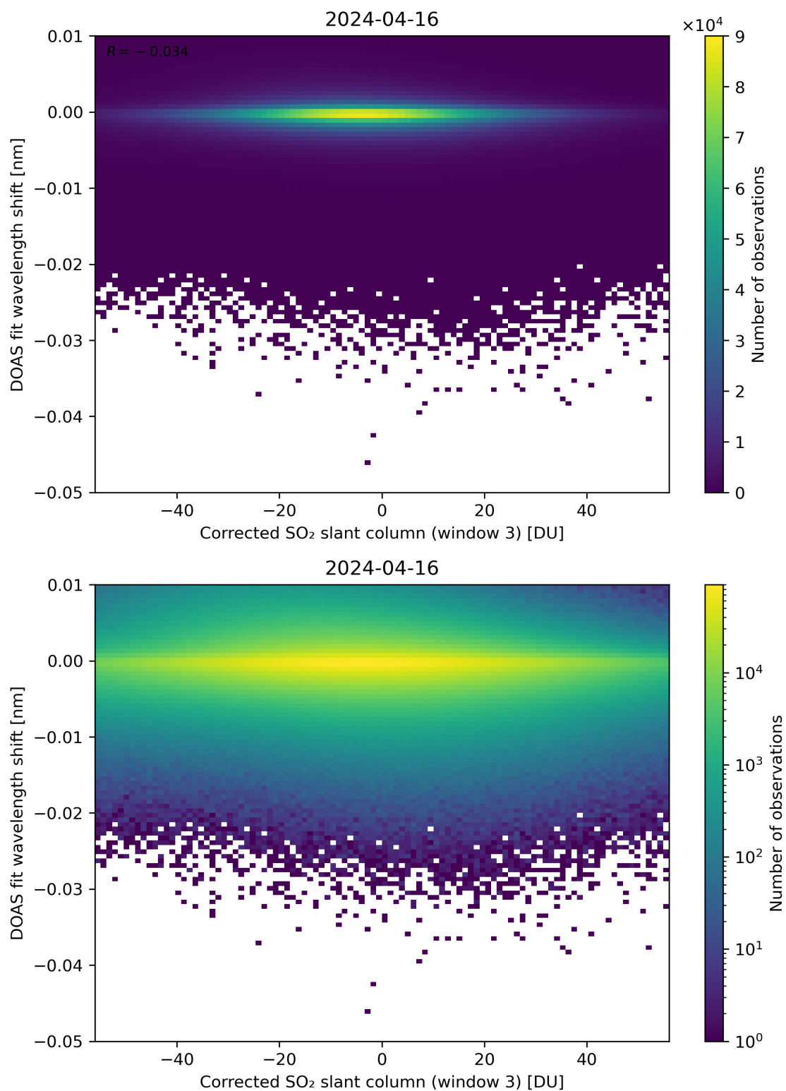
Figure 206: Scatter density plot of “Corrected SO 2 slant column (window 3)” against “DOAS fit wavelength shift” for 2024-04-16 to 2024-04-17.
