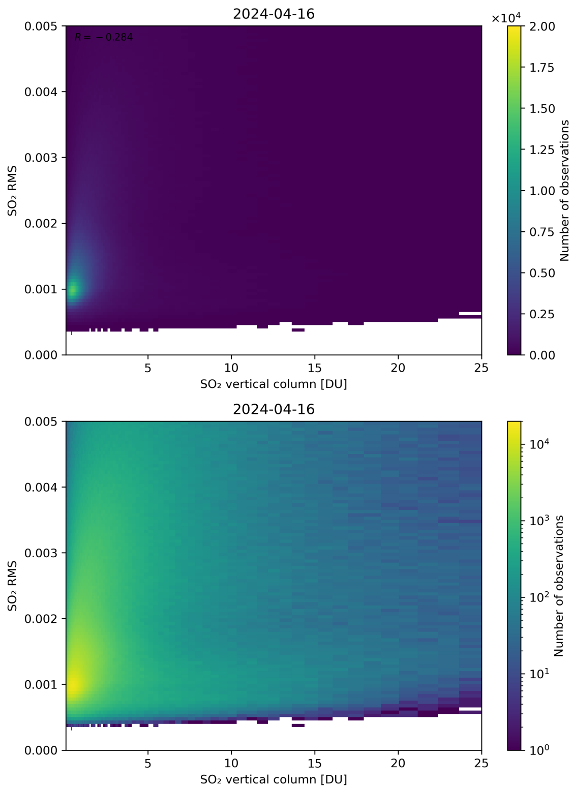
Figure 278: Scatter density plot of “SO 2 vertical column” against “SO 2 RMS” for 2024-04-16 to 2024-04-17.
