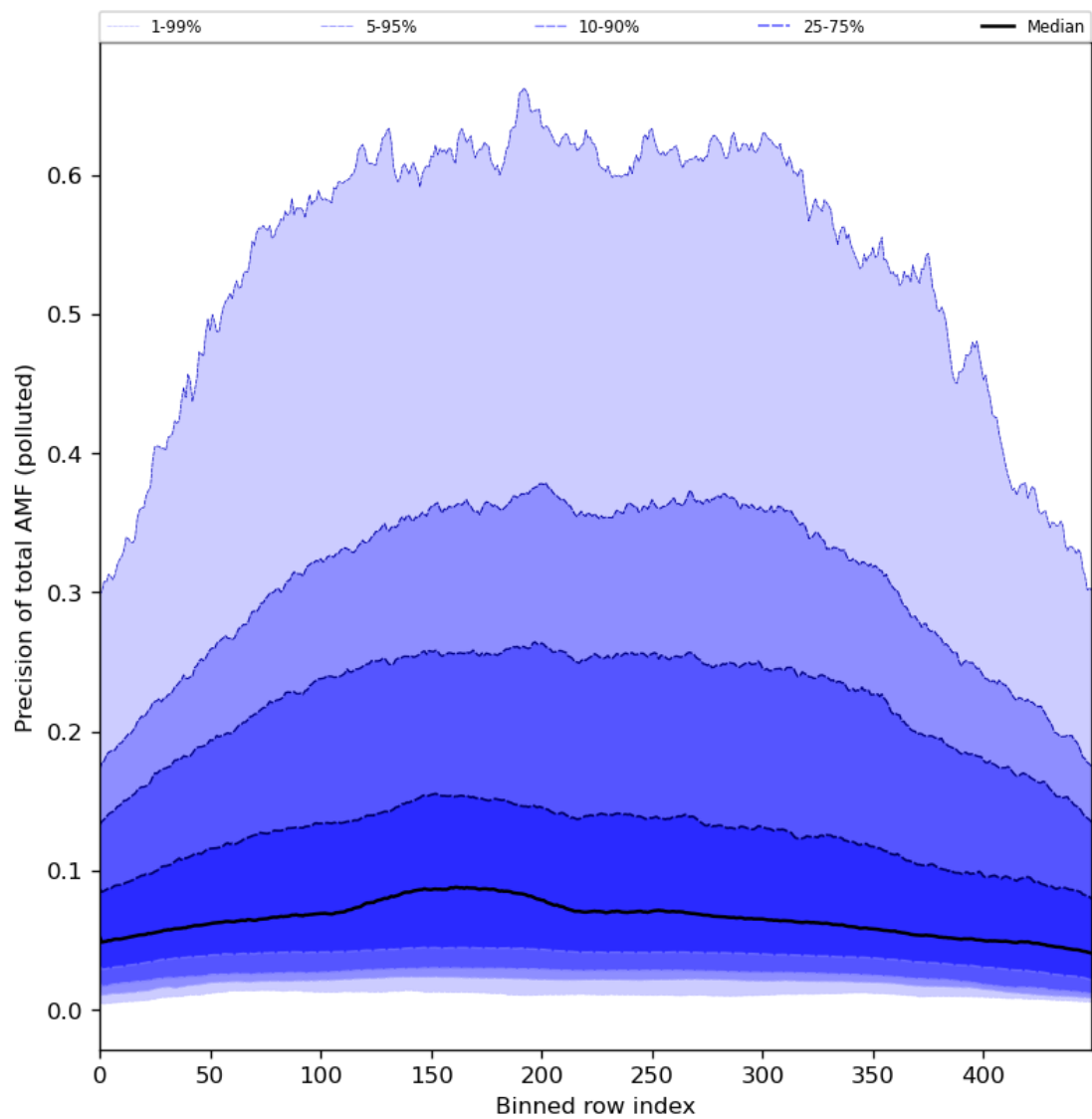
Figure 95: Along track statistics of “Precision of total AMF (polluted)” for 2024-04-16 to 2024-04-17
