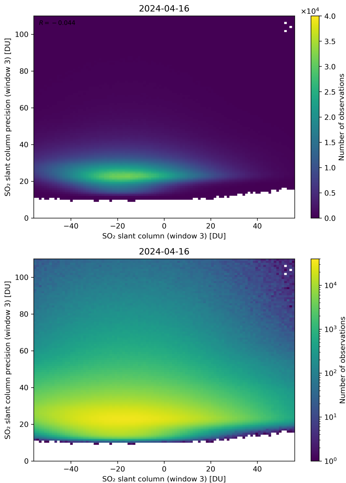
Figure 267: Scatter density plot of “SO 2 slant column (window 3)” against “SO 2 slant column precision (window 3)” for 2024-04-16 to 2024-04-17.
