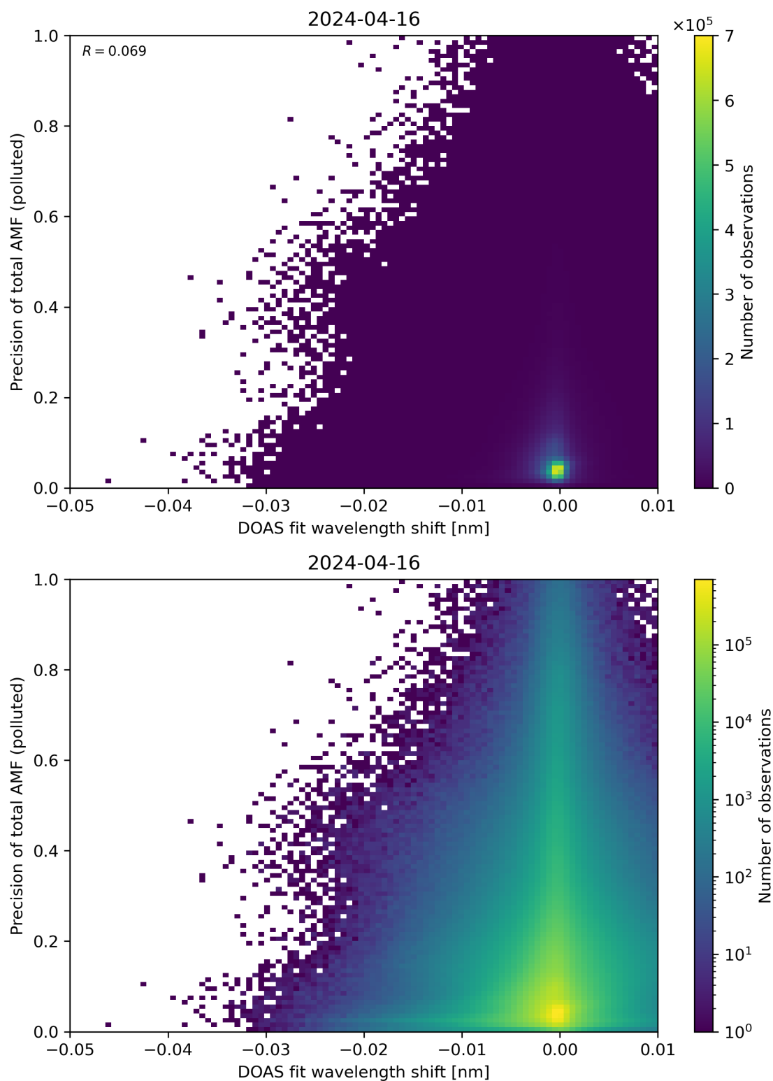
Figure 131: Scatter density plot of “DOAS fit wavelength shift” against “Precision of total AMF (polluted)” for 2024-04-16 to 2024-04-17.
