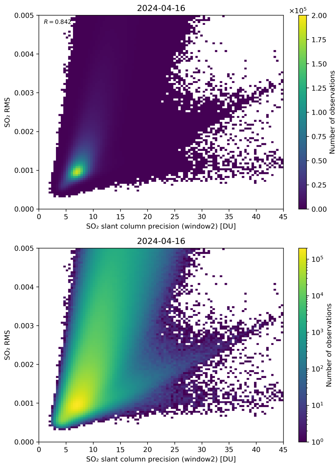
Figure 245: Scatter density plot of “SO 2 slant column precision (window2)” against “SO 2 RMS” for 2024-04-16 to 2024-04-17.
