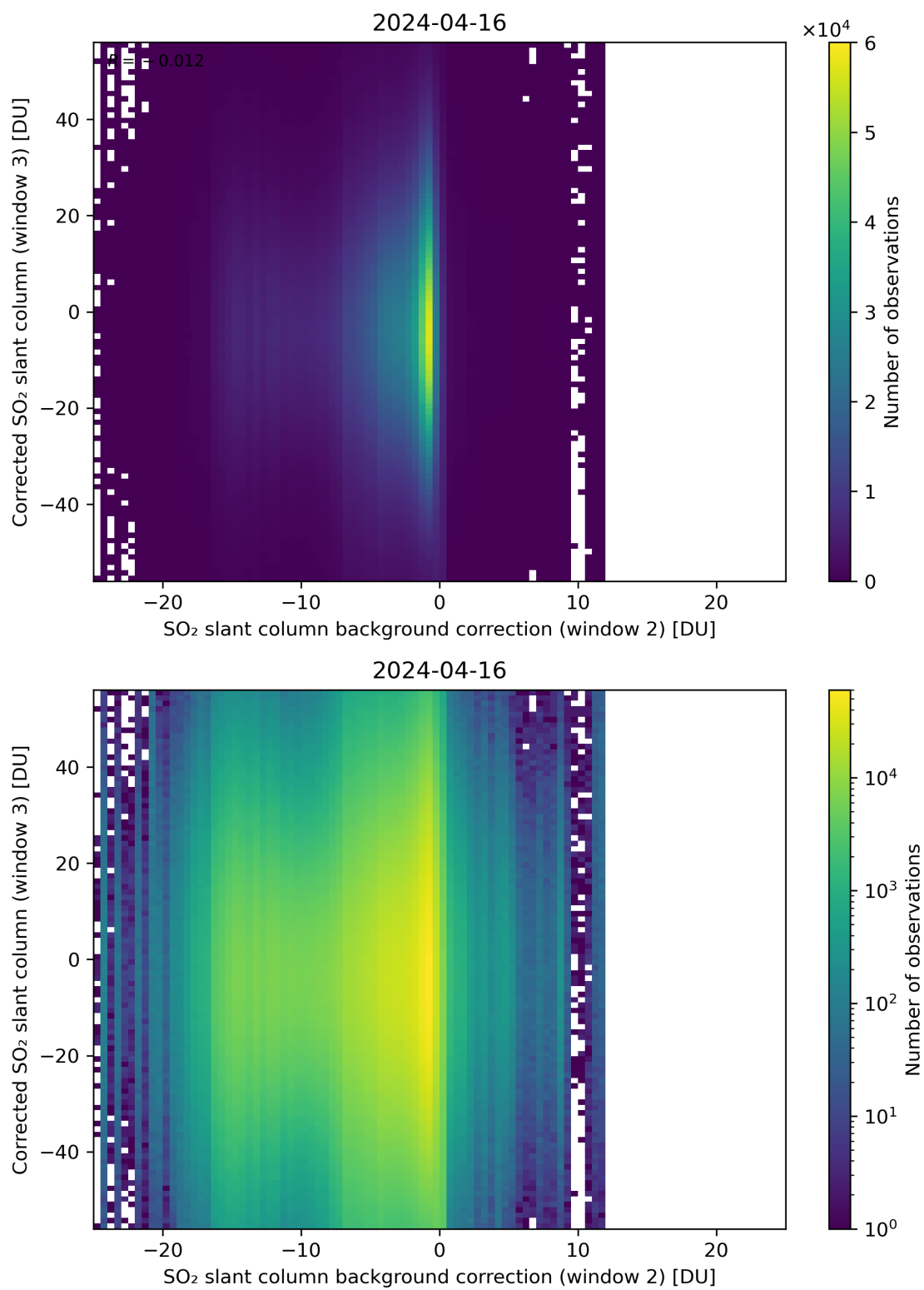
Figure 116: Scatter density plot of “SO 2 slant column background correction (window 2)” against “Corrected SO 2 slant column (window 3)” for 2024-04-16 to 2024-04-17.
