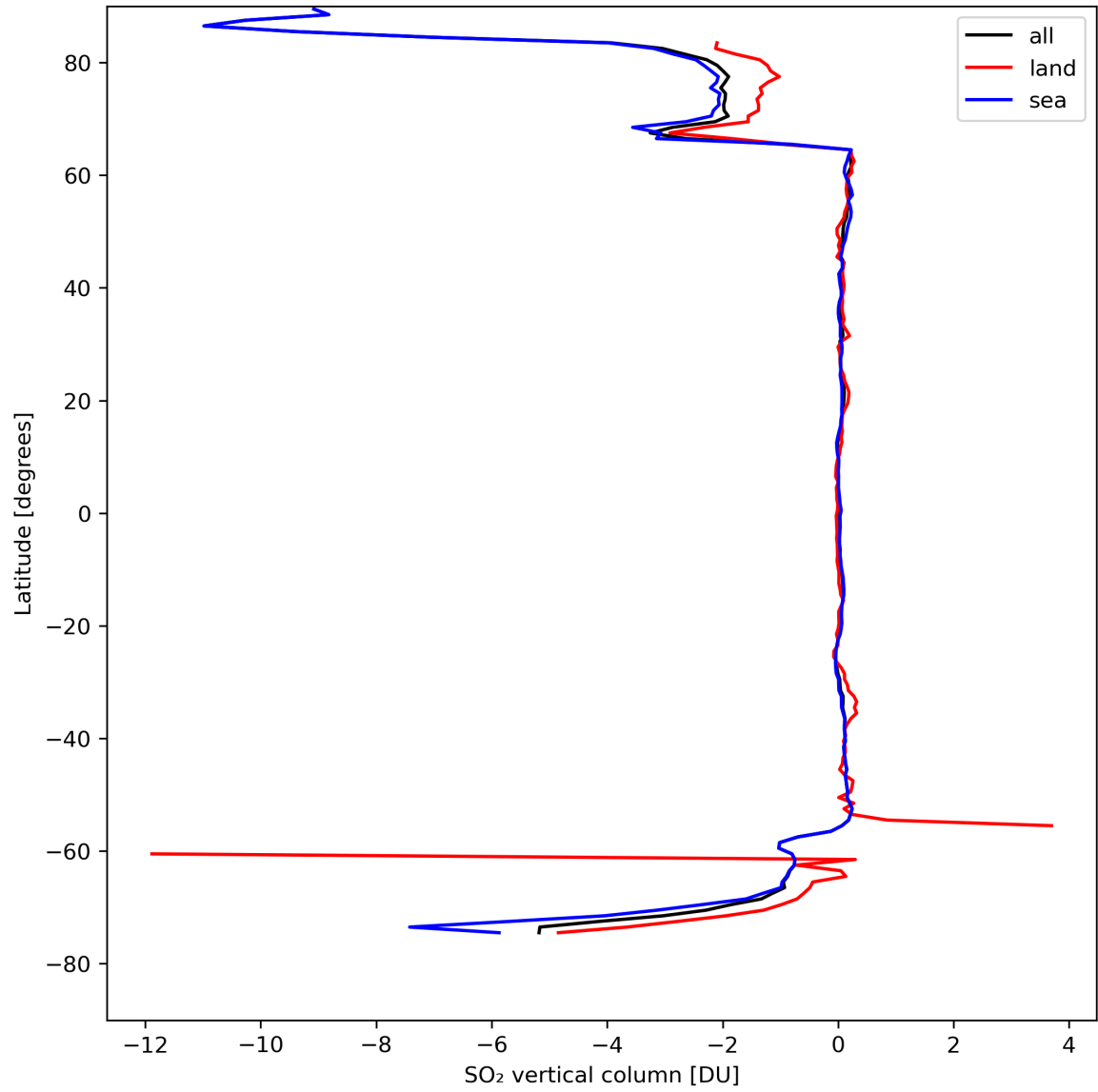
Figure 30: Zonal average of “SO 2 vertical column” for 2024-04-16 to 2024-04-17.
