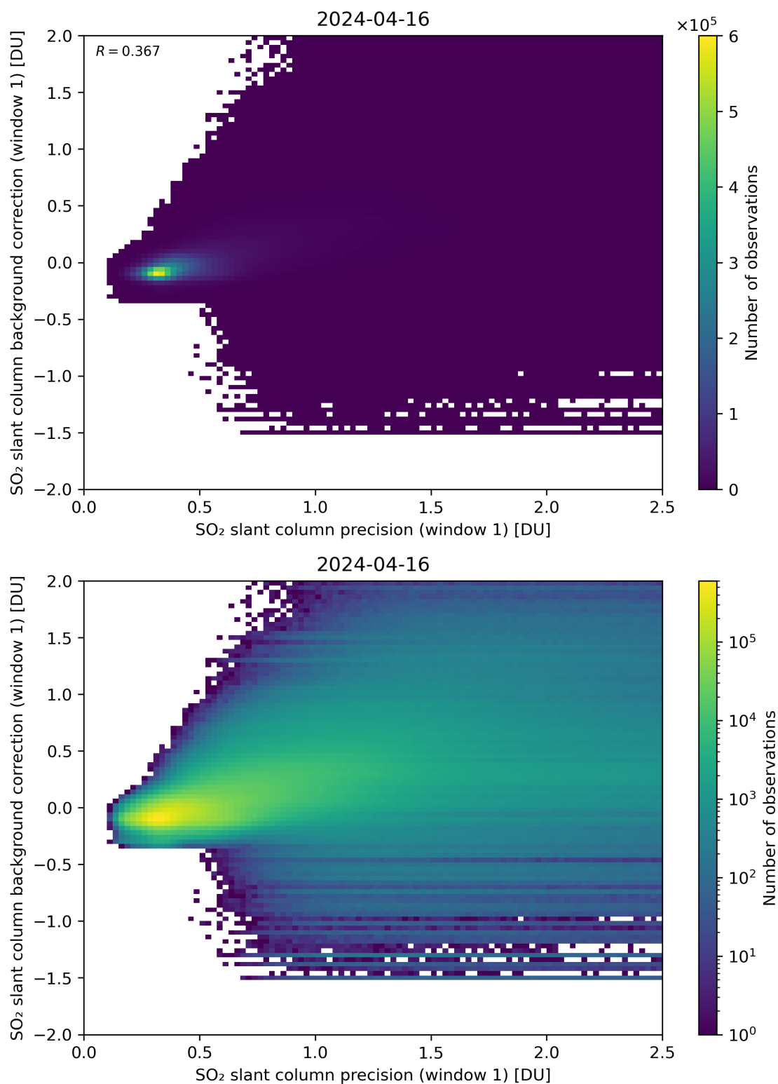
Figure 218: Scatter density plot of “SO 2 slant column precision (window 1)” against “SO 2 slant column background correction (window 1)” for 2024-04-16 to 2024-04-17.
