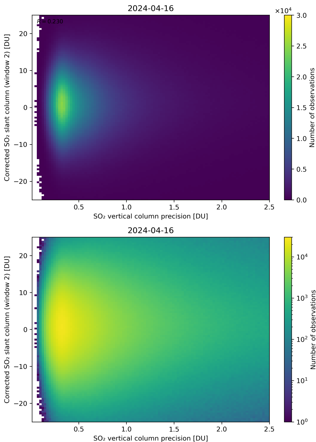
Figure 287: Scatter density plot of “SO 2 vertical column precision” against “Corrected SO 2 slant column (window 2)” for 2024-04-16 to 2024-04-17.
