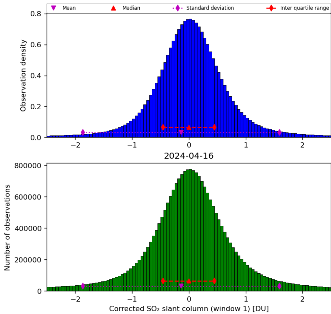
Figure 58: Histogram of “Corrected SO 2 slant column (window 1)” for 2024-04-16 to 2024-04-17
