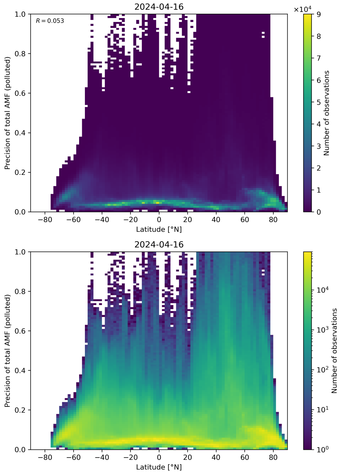
Figure 155: Scatter density plot of “Latitude” against “Precision of total AMF (polluted)” for 2024-04-16 to 2024-04-17.
