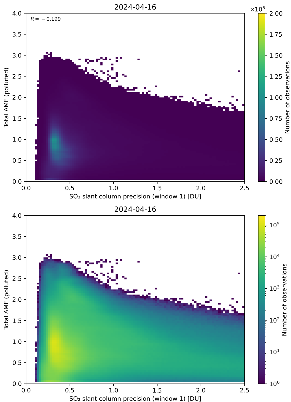
Figure 230: Scatter density plot of “SO 2 slant column precision (window 1)” against “Total AMF (polluted)” for 2024-04-16 to 2024-04-17.
