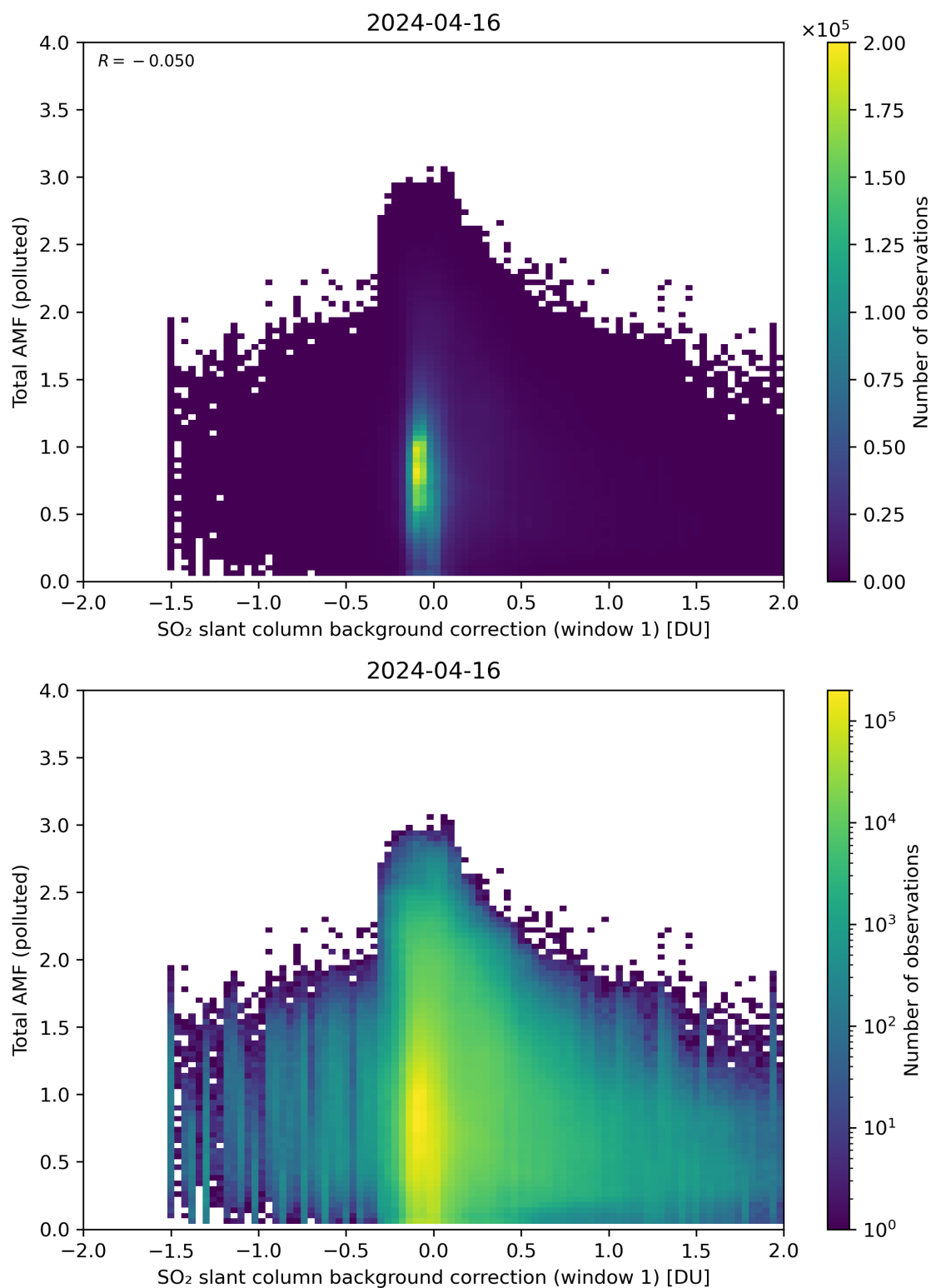
Figure 109: Scatter density plot of “SO 2 slant column background correction (window 1)” against “Total AMF (polluted)” for 2024-04-16 to 2024-04-17.
