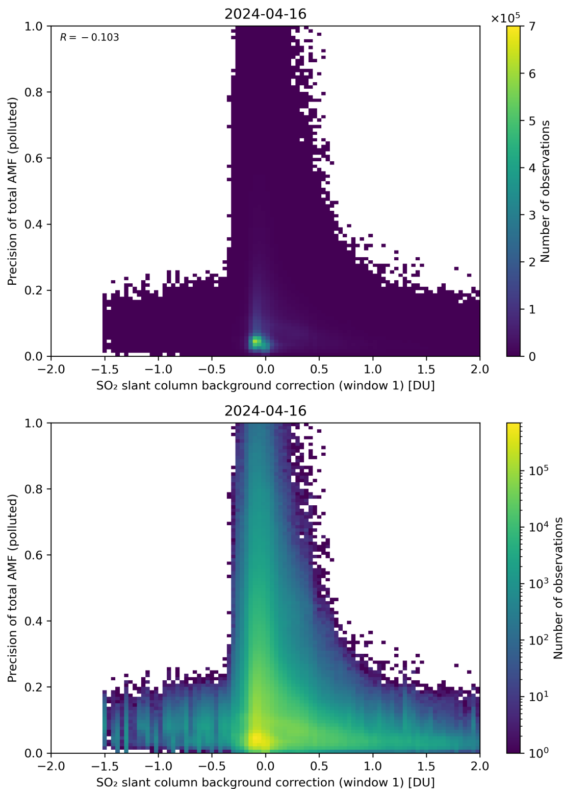
Figure 110: Scatter density plot of “SO 2 slant column background correction (window 1)” against “Precision of total AMF (polluted)” for 2024-04-16 to 2024-04-17.
