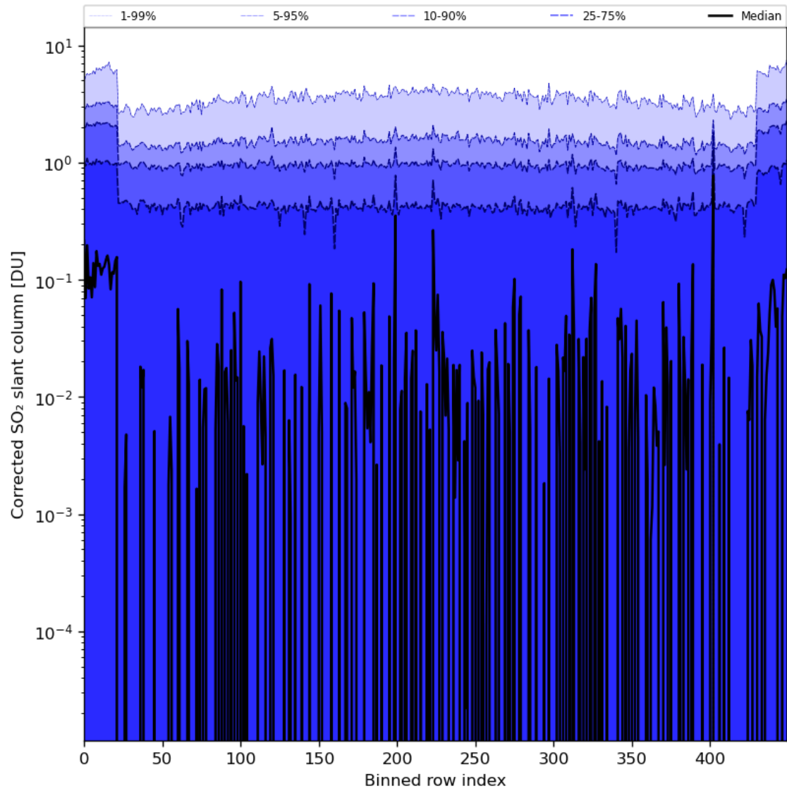
Figure 78: Along track statistics of “Corrected SO 2 slant column” for 2024-04-16 to 2024-04-17
