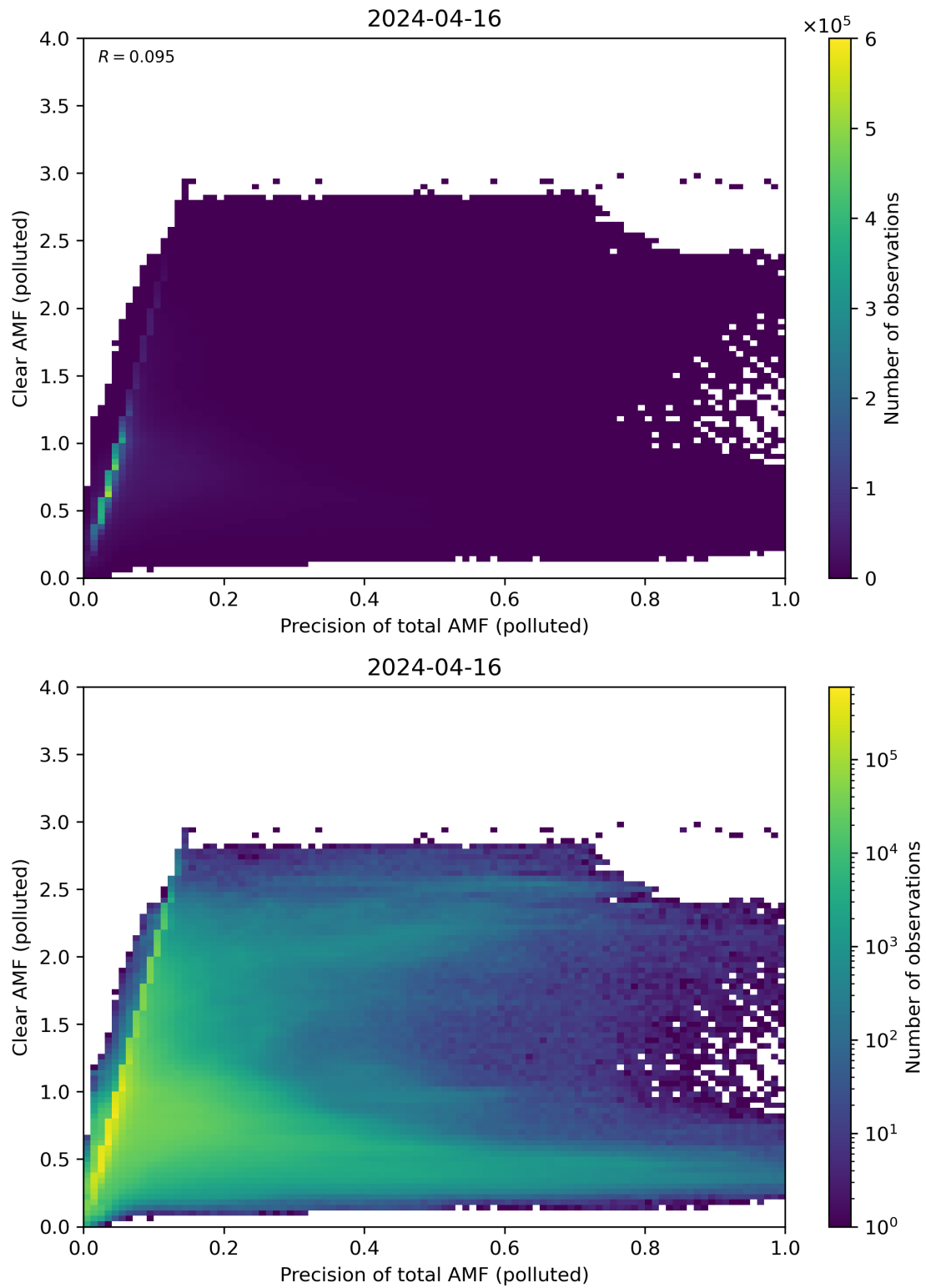
Figure 270: Scatter density plot of “Precision of total AMF (polluted)” against “Clear AMF (polluted)” for 2024-04-16 to 2024-04-17.
