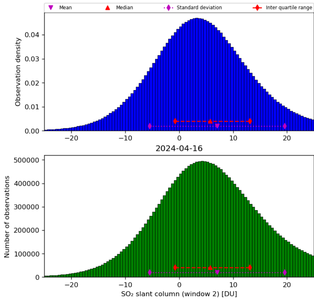
Figure 60: Histogram of “SO 2 slant column (window 2)” for 2024-04-16 to 2024-04-17
