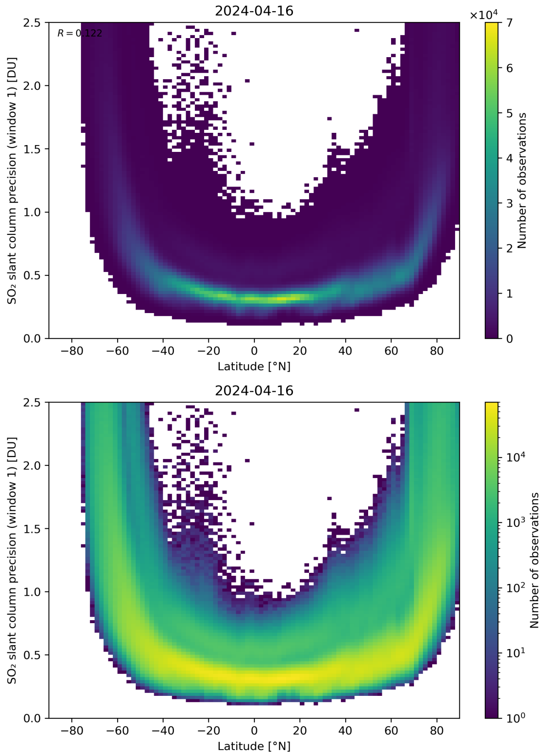
Figure 150: Scatter density plot of “Latitude” against “SO 2 slant column precision (window 1)” for 2024-04-16 to 2024-04-17.
