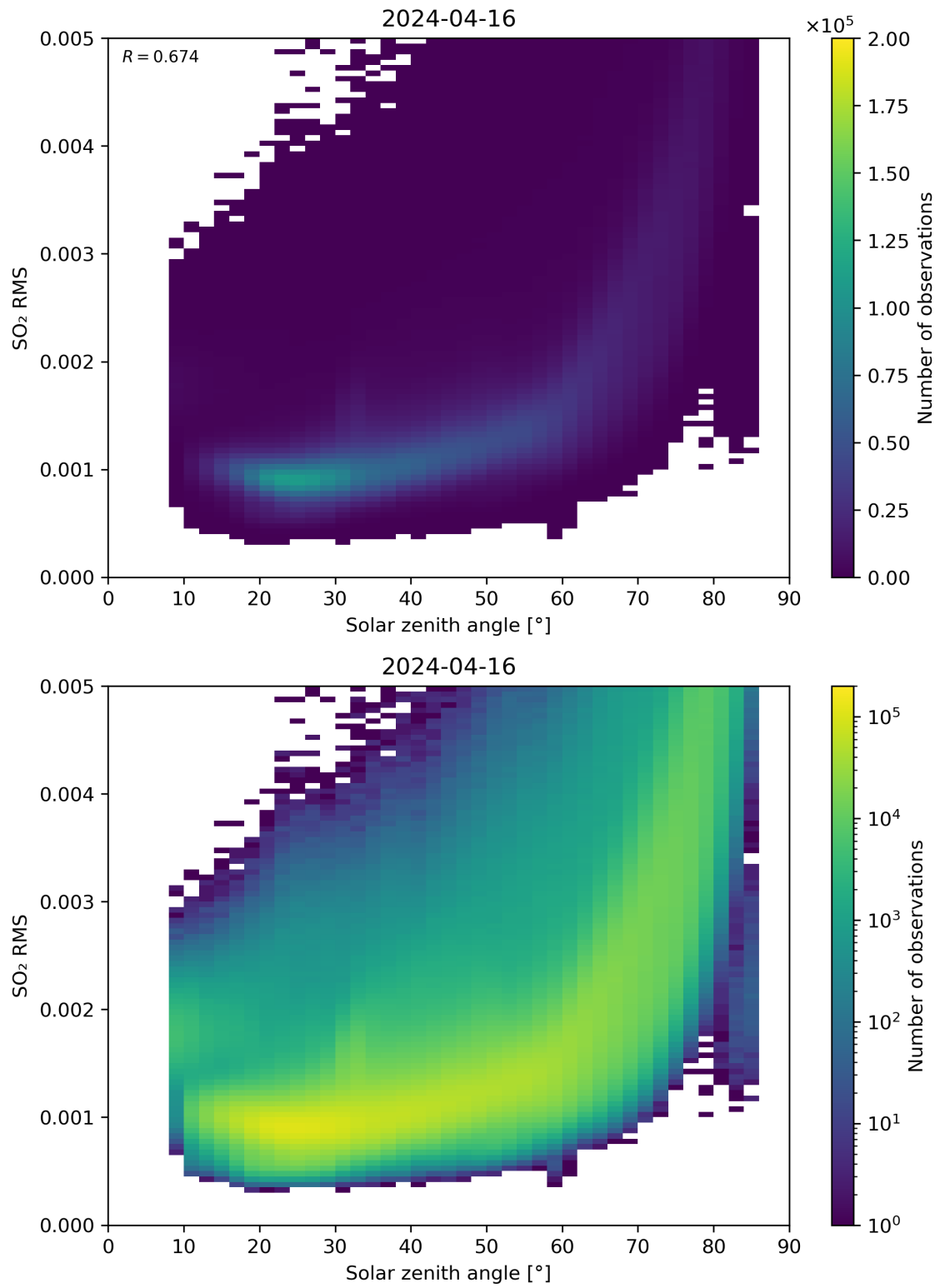
Figure 163: Scatter density plot of “Solar zenith angle” against “SO 2 RMS” for 2024-04-16 to 2024-04-17.
