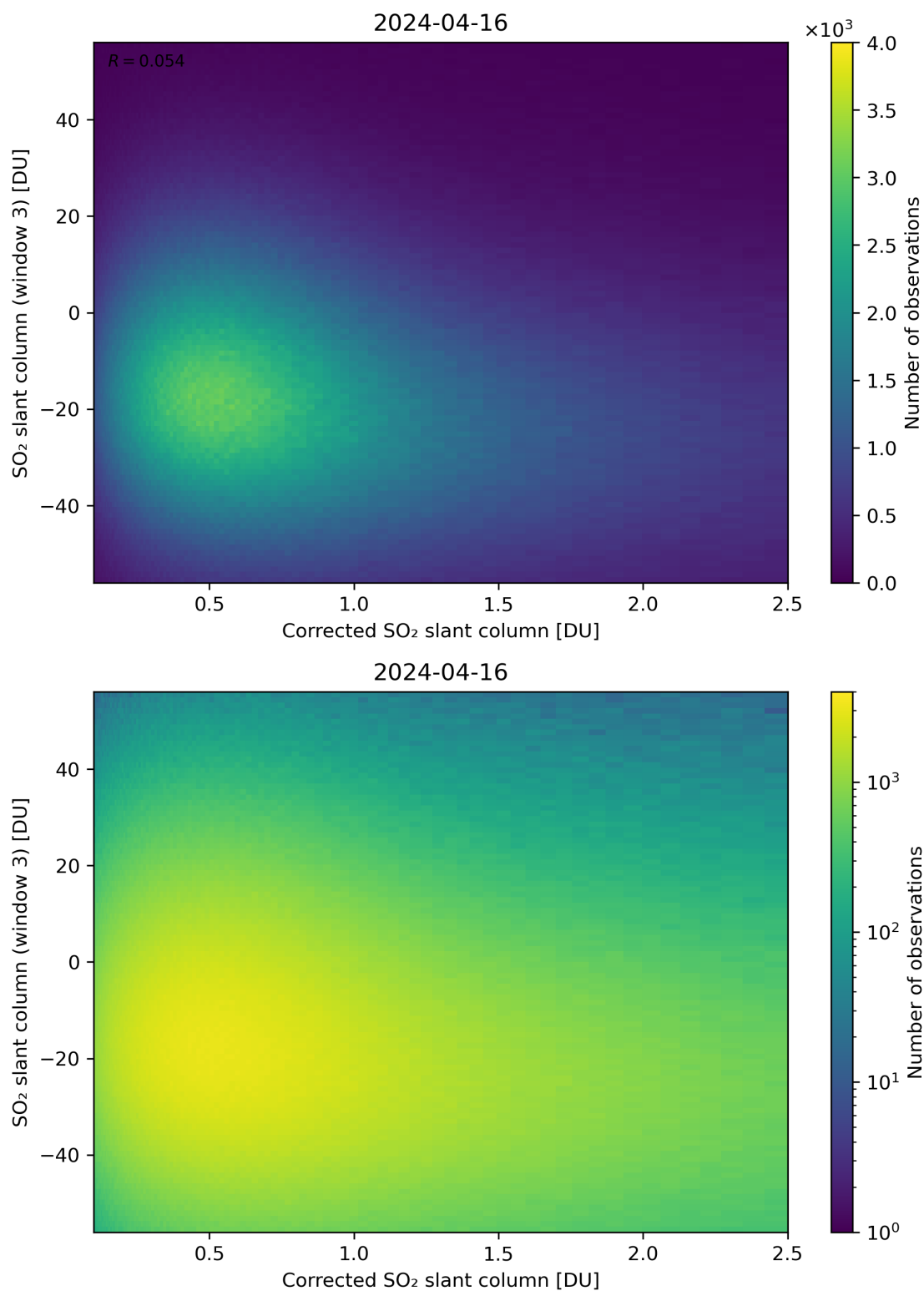
Figure 190: Scatter density plot of “Corrected SO 2 slant column” against “SO 2 slant column (window 3)” for 2024-04-16 to 2024-04-17.
