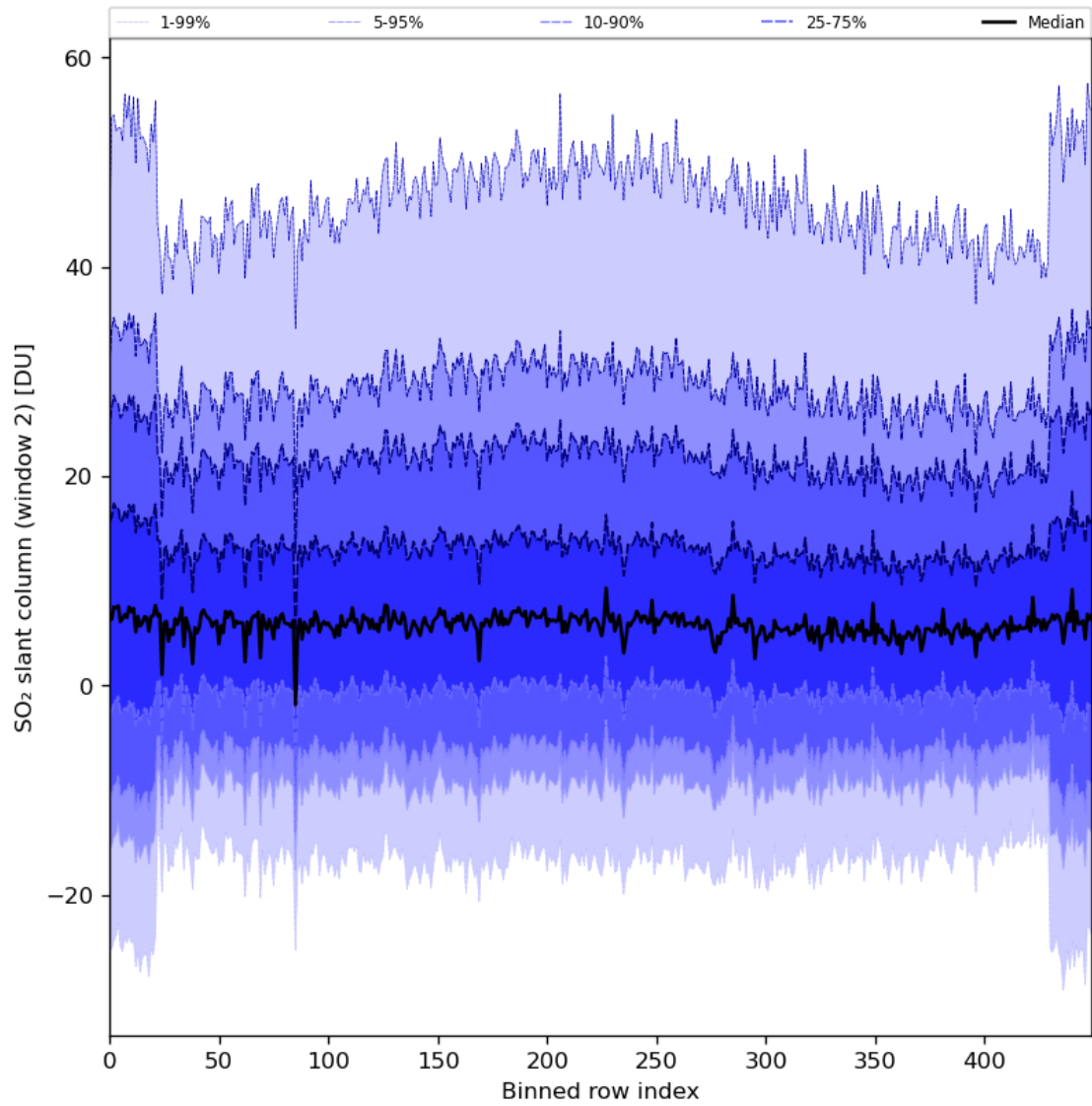
Figure 83: Along track statistics of “SO 2 slant column (window 2)” for 2024-04-16 to 2024-04-17
