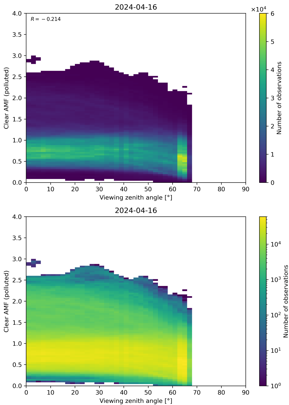
Figure 316: Scatter density plot of “Viewing zenith angle” against “Clear AMF (polluted)” for 2024-04-16 to 2024-04-17.
