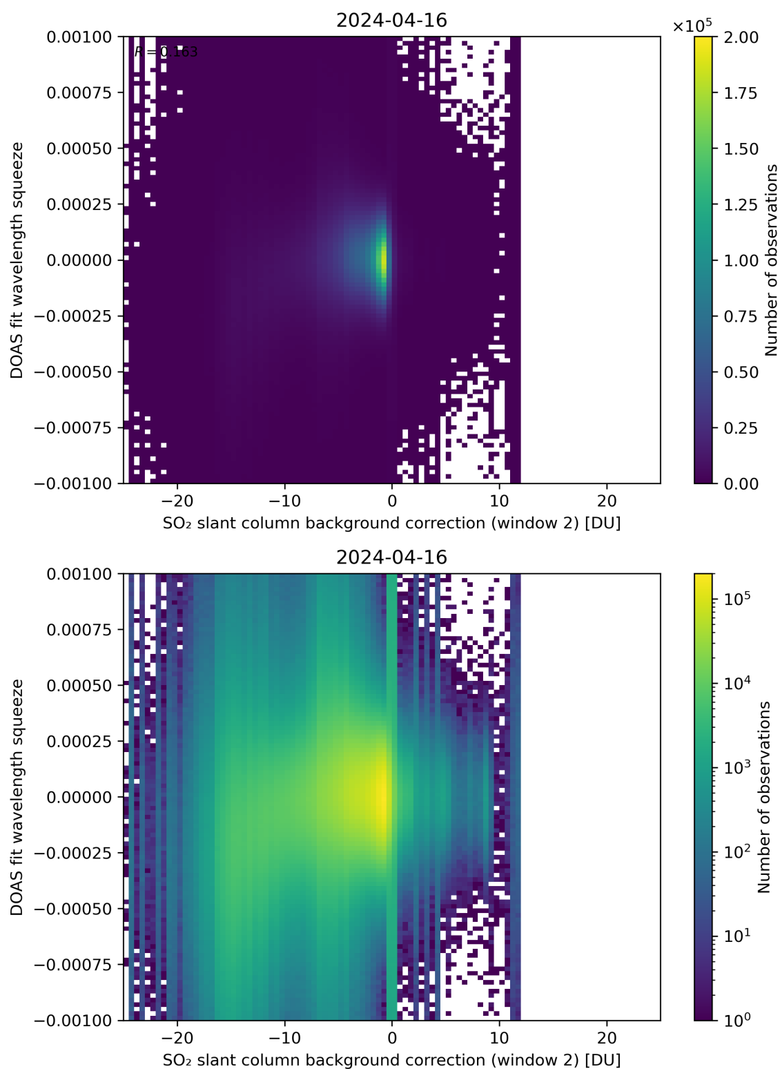
Figure 113: Scatter density plot of “SO 2 slant column background correction (window 2)” against “DOAS fit wavelength squeeze” for 2024-04-16 to 2024-04-17.
