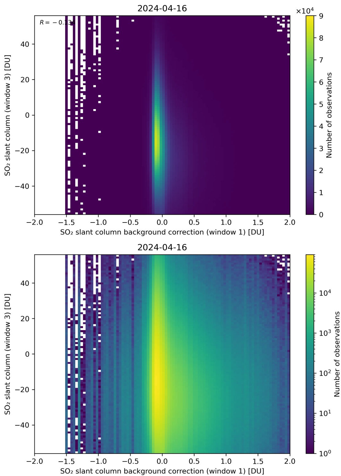
Figure 107: Scatter density plot of “SO 2 slant column background correction (window 1)” against “SO 2 slant column (window 3)” for 2024-04-16 to 2024-04-17.
