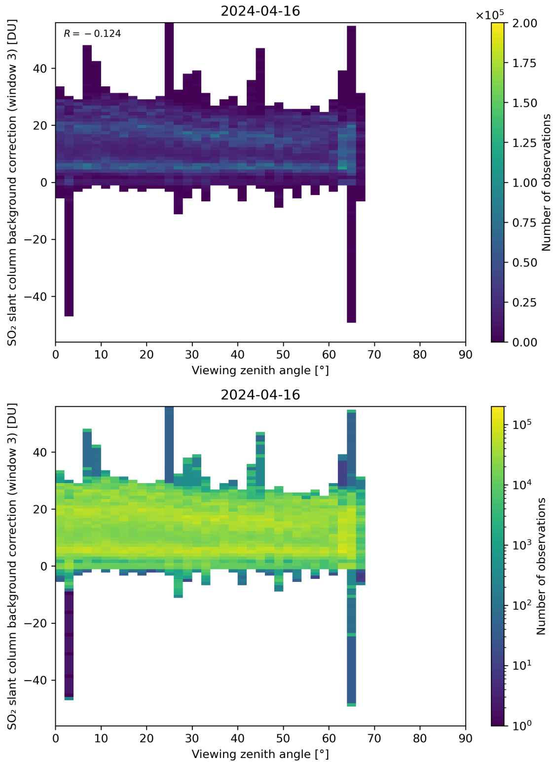
Figure 310: Scatter density plot of “Viewing zenith angle” against “SO 2 slant column background correction (window 3)” for 2024-04-16 to 2024-04-17.
