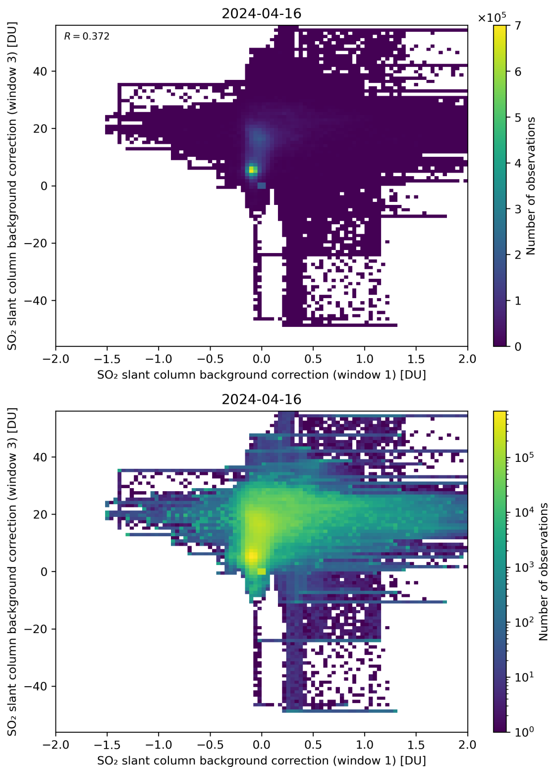
Figure 99: Scatter density plot of “SO 2 slant column background correction (window 1)” against “SO 2 slant column background correction (window 3)” for 2024-04-16 to 2024-04-17.
