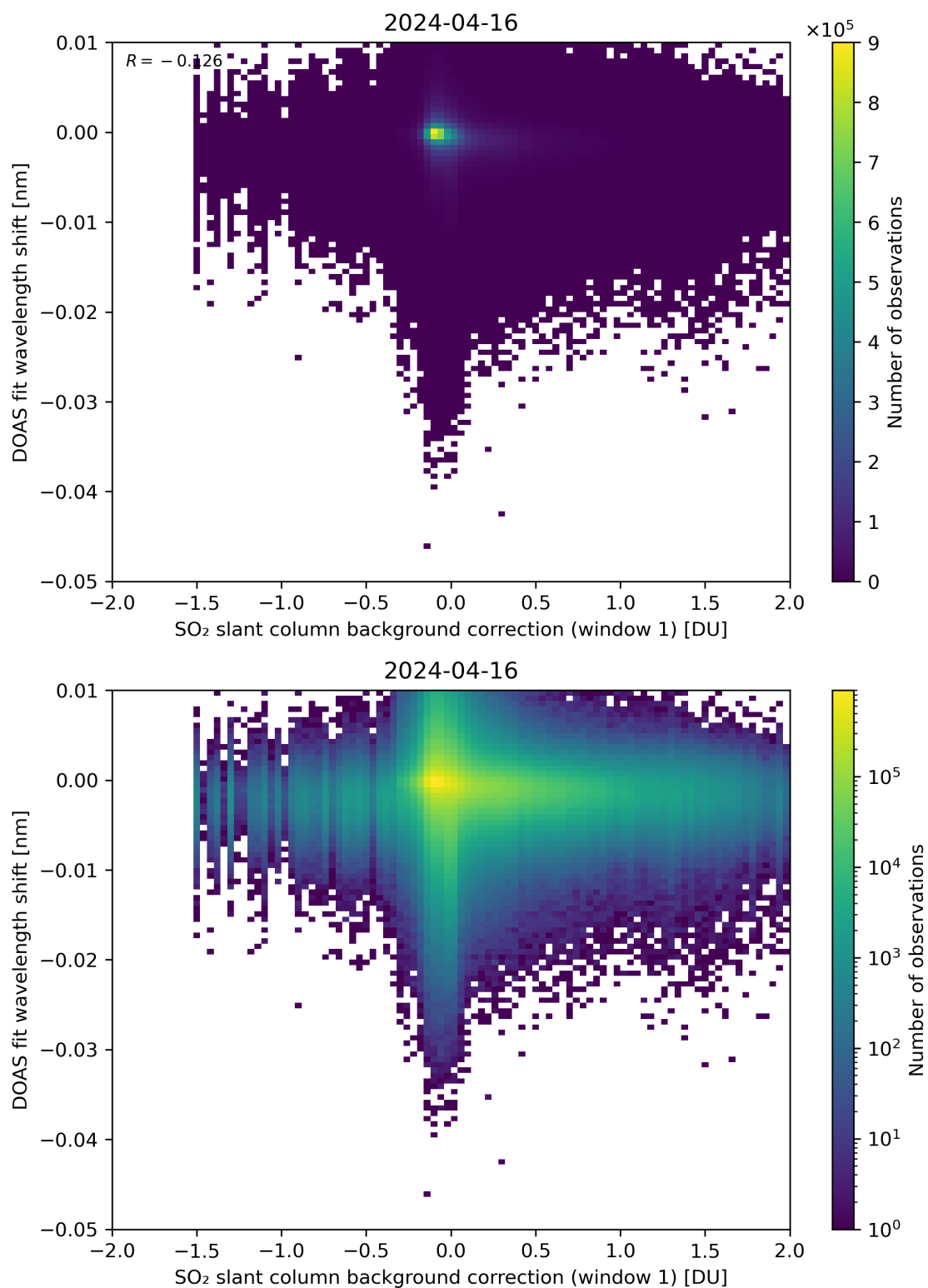
Figure 100: Scatter density plot of “SO 2 slant column background correction (window 1)” against “DOAS fit wavelength shift” for 2024-04-16 to 2024-04-17.
