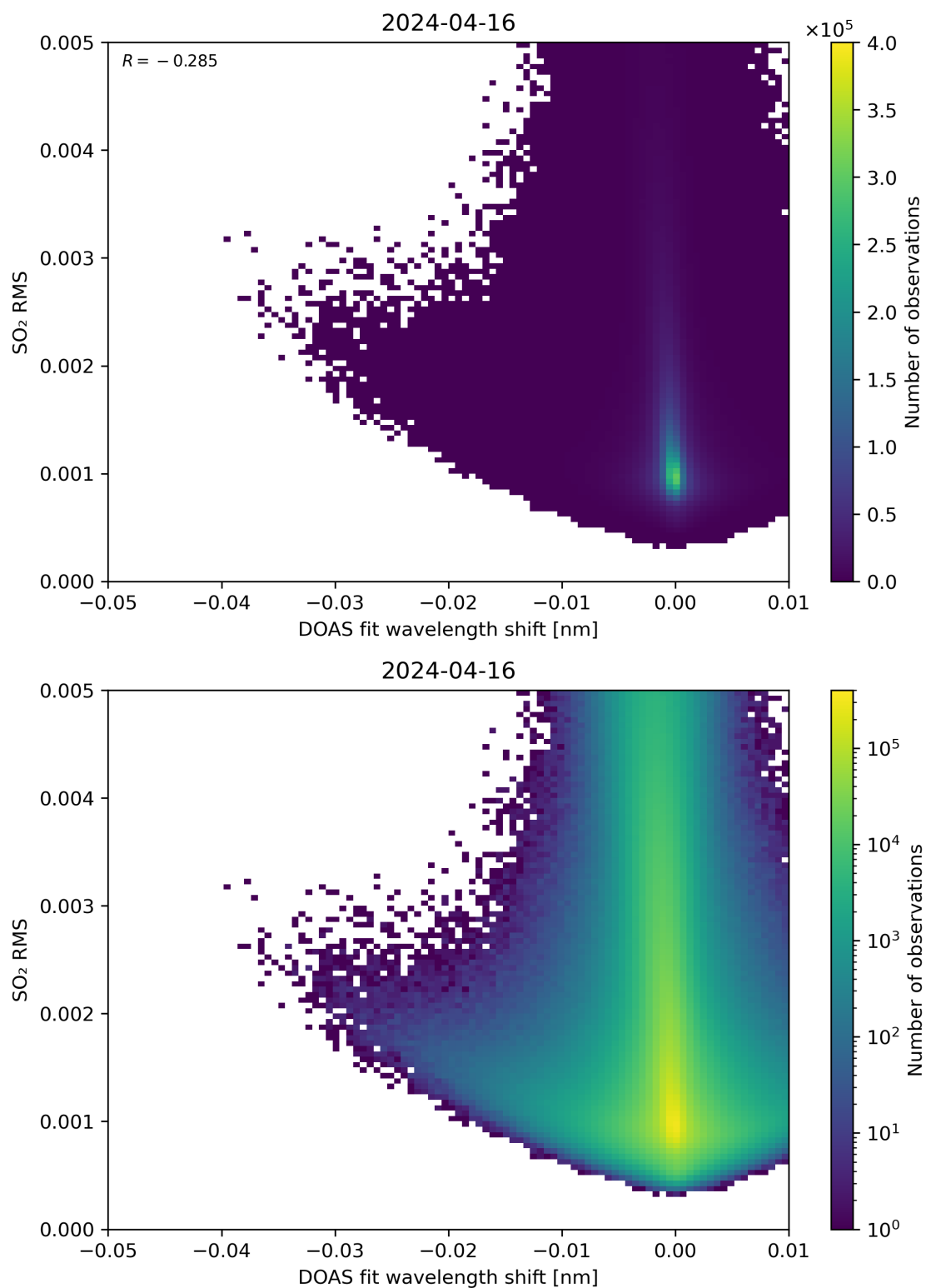
Figure 128: Scatter density plot of “DOAS fit wavelength shift” against “SO 2 RMS” for 2024-04-16 to 2024-04-17.
