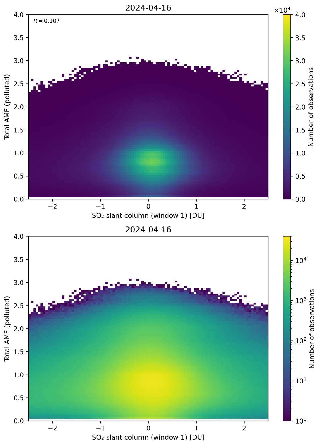
Figure 239: Scatter density plot of “SO 2 slant column (window 1)” against “Total AMF (polluted)” for 2024-04-16 to 2024-04-17.
