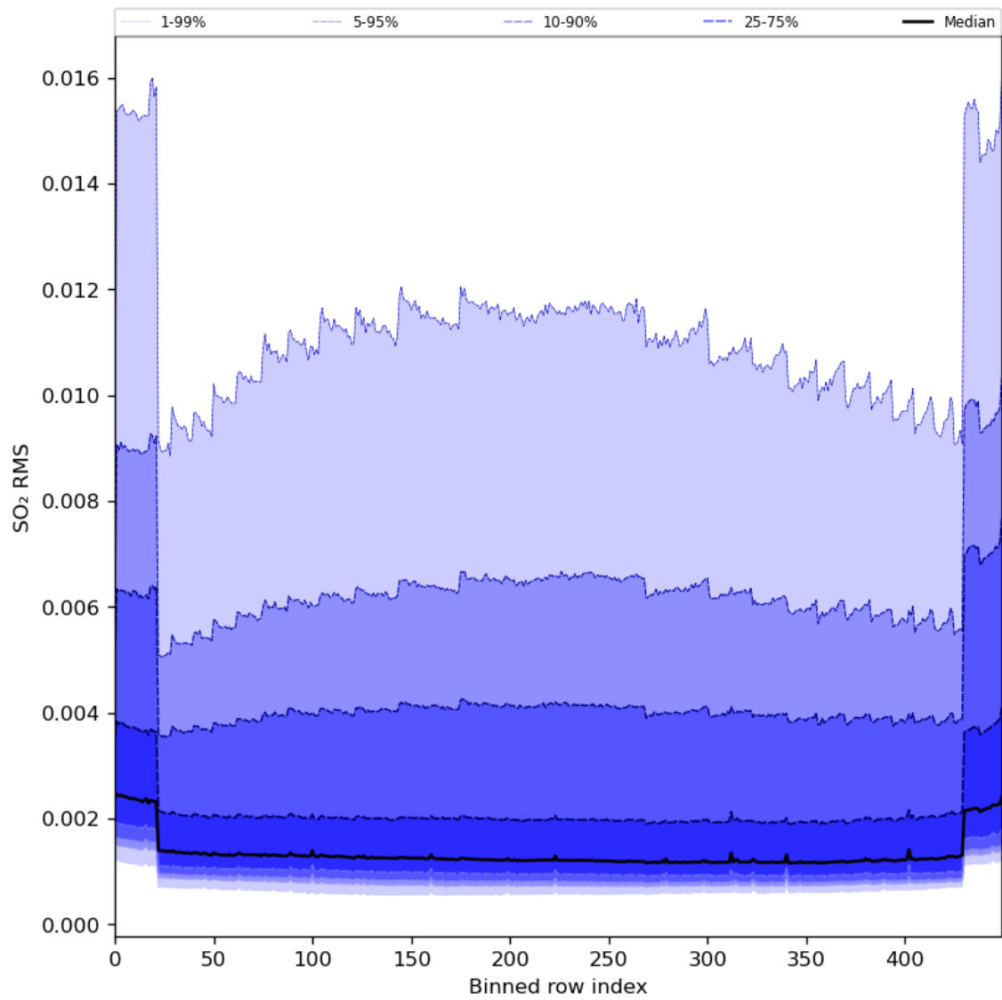
Figure 93: Along track statistics of “SO 2 RMS” for 2024-04-16 to 2024-04-17
