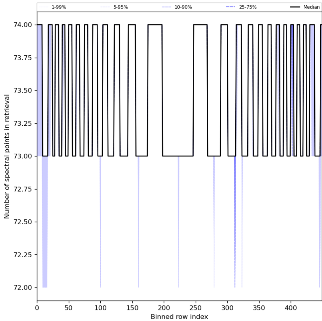
Figure 97: Along track statistics of “Number of spectral points in retrieval” for 2024-04-16 to 2024-04-17
