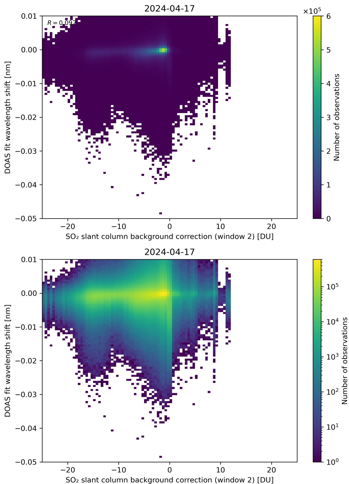
Figure 112: Scatter density plot of “SO 2 slant column background correction (window 2)” against “DOAS fit wavelength shift” for 2024-04-16 to 2024-04-18.
