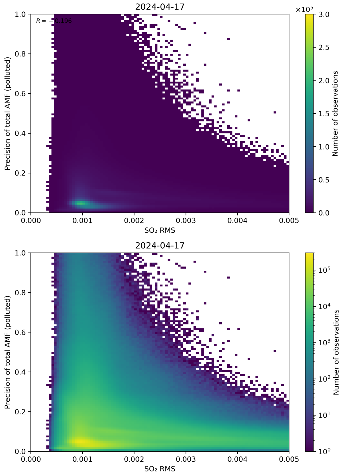
Figure 138: Scatter density plot of “SO 2 RMS” against “Precision of total AMF (polluted)” for 2024-04-16 to 2024-04-18.
