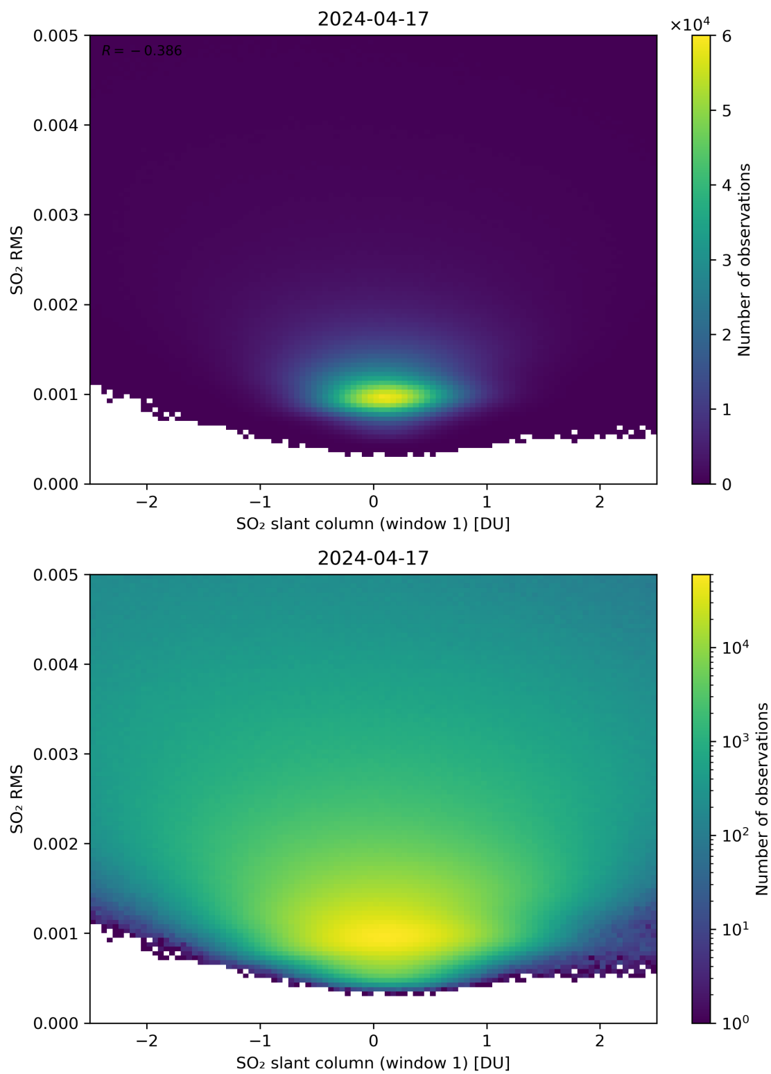
Figure 217: Scatter density plot of “SO 2 slant column (window 1)” against “SO 2 RMS” for 2024-04-16 to 2024-04-18.
