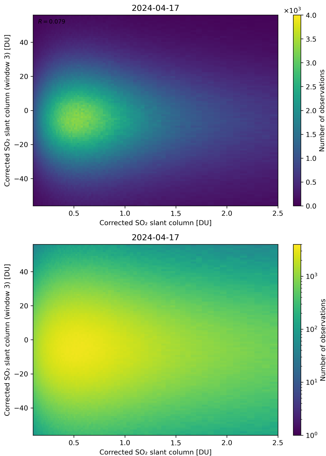
Figure 186: Scatter density plot of “Corrected SO 2 slant column” against “Corrected SO 2 slant column (window 3)” for 2024-04-16 to 2024-04-18.
