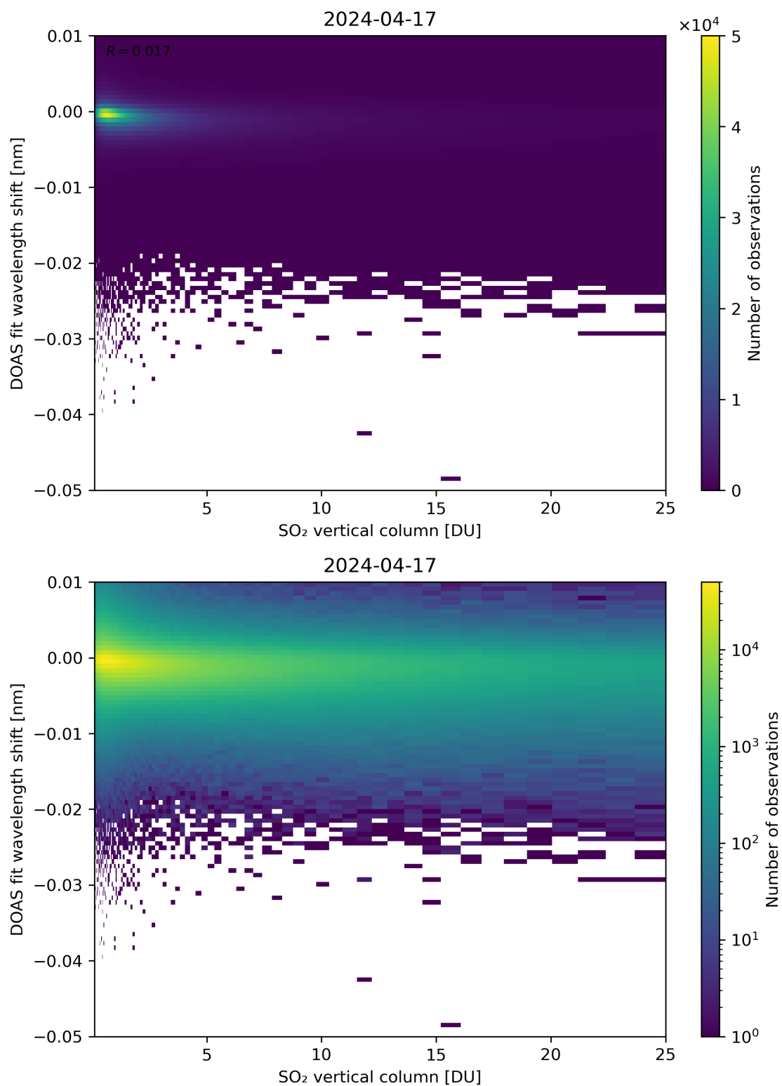
Figure 276: Scatter density plot of “SO 2 vertical column” against “DOAS fit wavelength shift” for 2024-04-16 to 2024-04-18.
