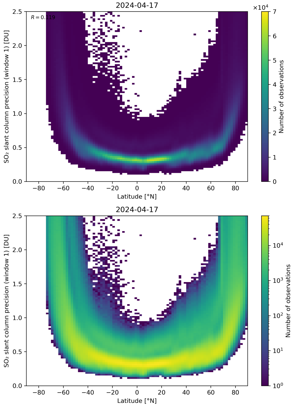
Figure 150: Scatter density plot of “Latitude” against “SO 2 slant column precision (window 1)” for 2024-04-16 to 2024-04-18.
