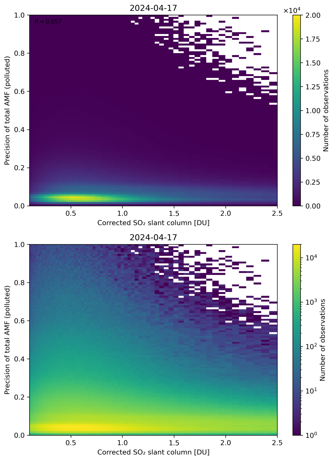
Figure 193: Scatter density plot of “Corrected SO 2 slant column” against “Precision of total AMF (polluted)” for 2024-04-16 to 2024-04-18.
