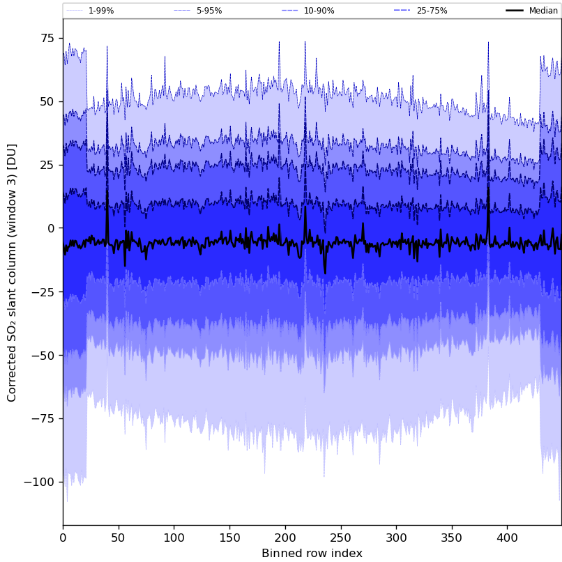
Figure 89: Along track statistics of “Corrected SO 2 slant column (window 3)” for 2024-04-16 to 2024-04-18
