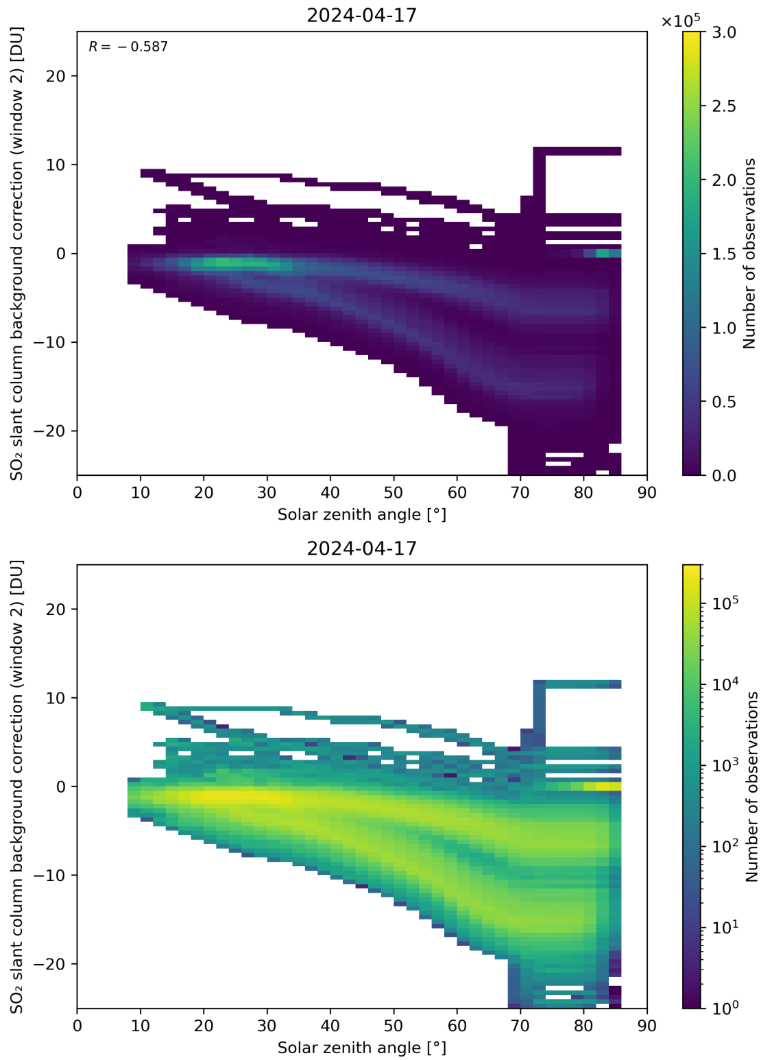
Figure 159: Scatter density plot of “Solar zenith angle” against “SO 2 slant column background correction (window 2)” for 2024-04-16 to 2024-04-18.
