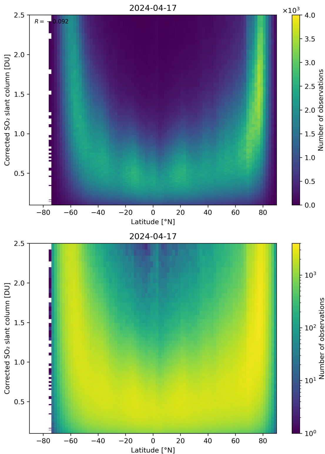
Figure 146: Scatter density plot of “Latitude” against “Corrected SO 2 slant column” for 2024-04-16 to 2024-04-18.
