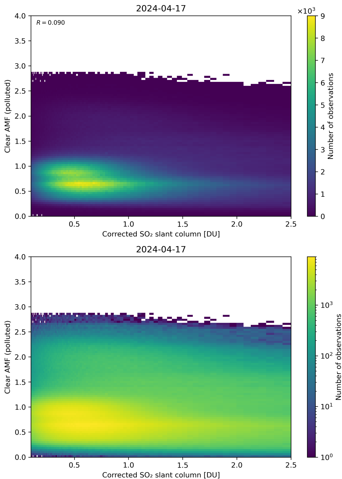
Figure 184: Scatter density plot of “Corrected SO 2 slant column” against “Clear AMF (polluted)” for 2024-04-16 to 2024-04-18.
