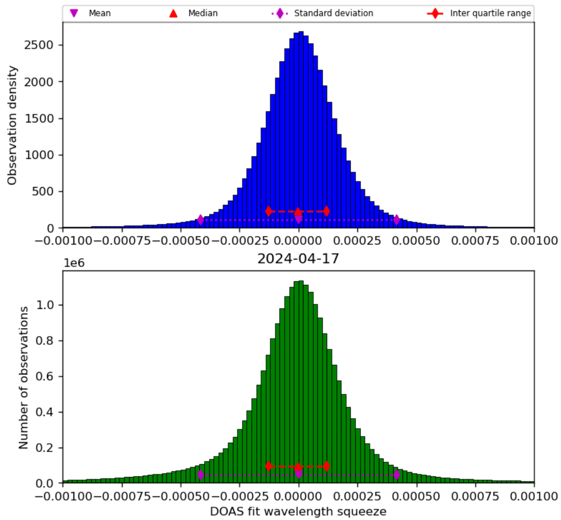
Figure 69: Histogram of “DOAS fit wavelength squeeze” for 2024-04-16 to 2024-04-18
