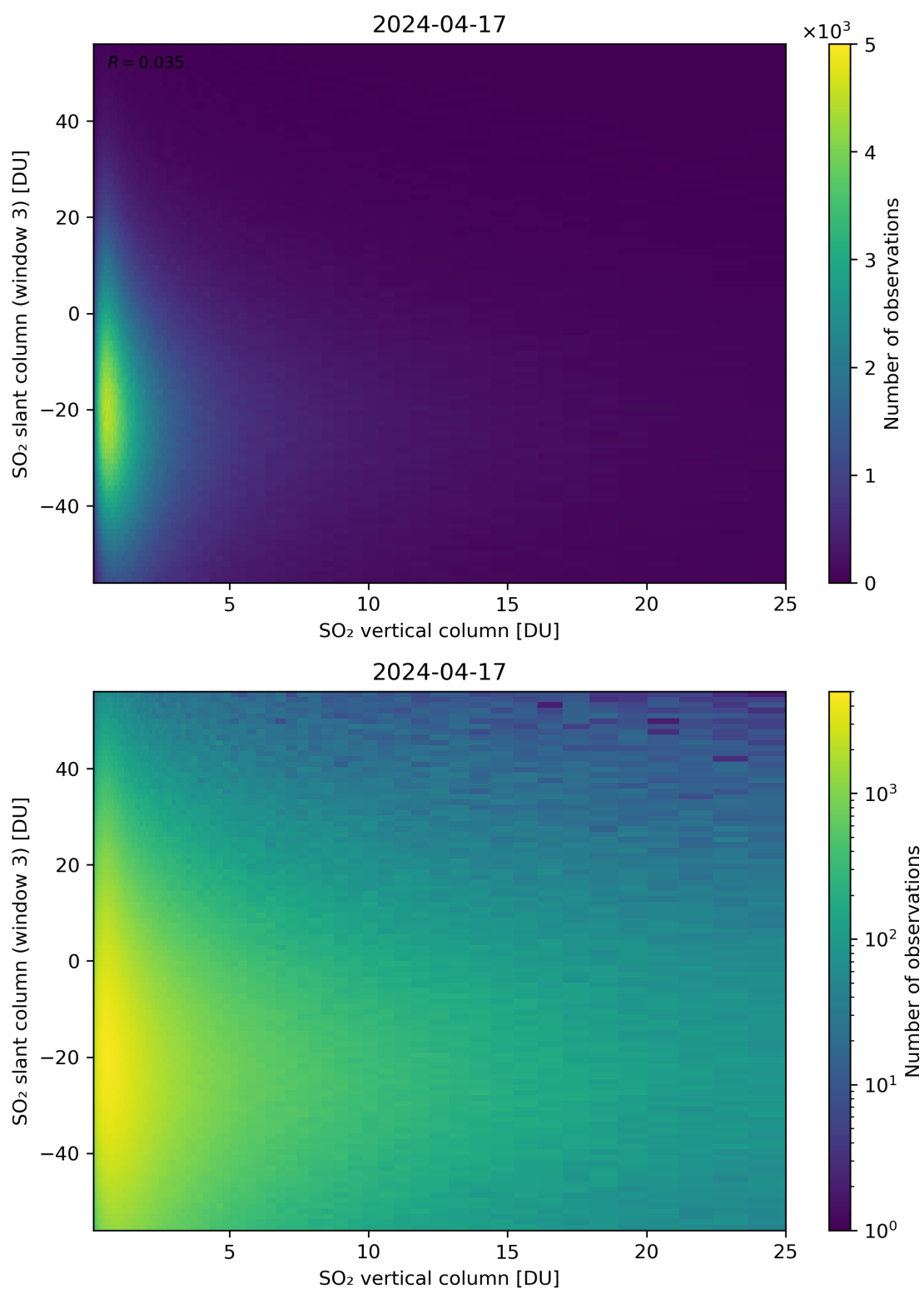
Figure 303: Scatter density plot of “SO 2 vertical column” against “SO 2 slant column (window 3)” for 2024-04-16 to 2024-04-18.
