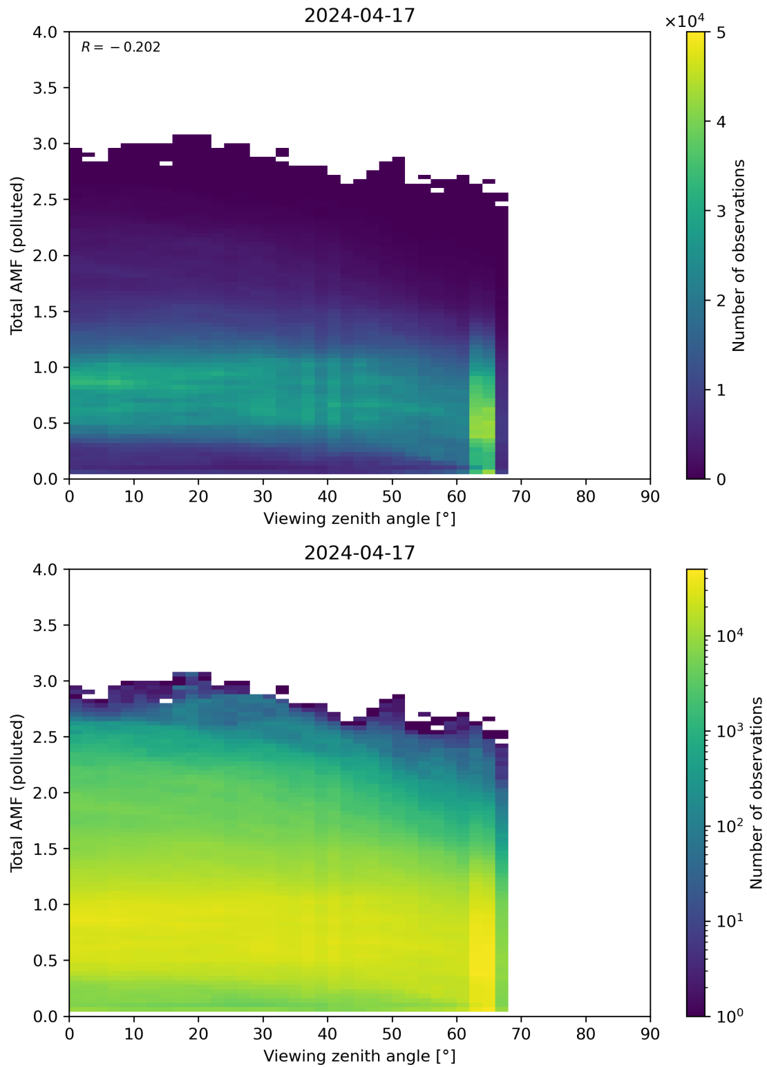
Figure 325: Scatter density plot of “Viewing zenith angle” against “Total AMF (polluted)” for 2024-04-16 to 2024-04-18.
