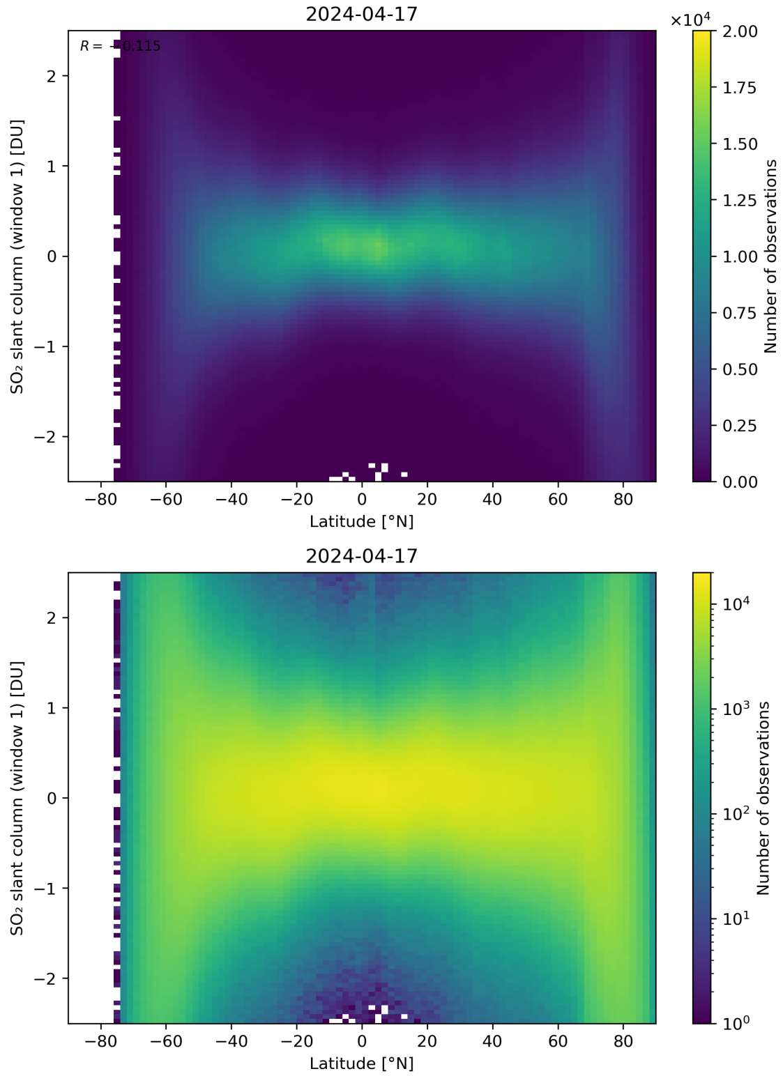
Figure 149: Scatter density plot of “Latitude” against “SO 2 slant column (window 1)” for 2024-04-16 to 2024-04-18.
