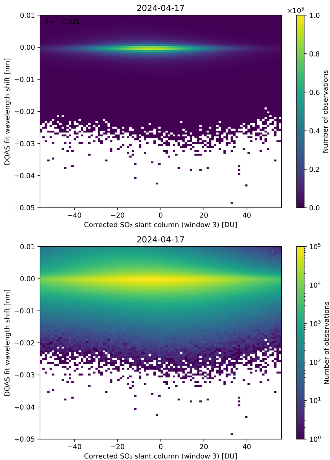
Figure 206: Scatter density plot of “Corrected SO 2 slant column (window 3)” against “DOAS fit wavelength shift” for 2024-04-16 to 2024-04-18.
