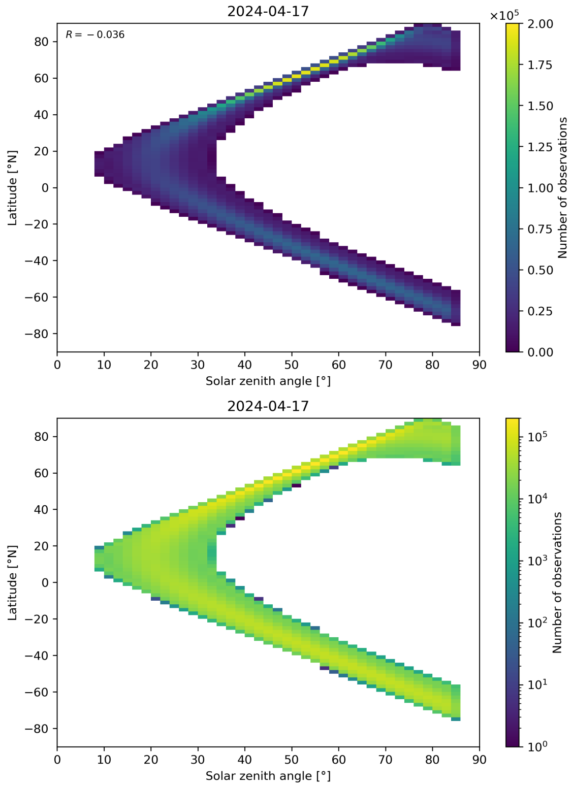
Figure 164: Scatter density plot of “Solar zenith angle” against “Latitude” for 2024-04-16 to 2024-04-18.
