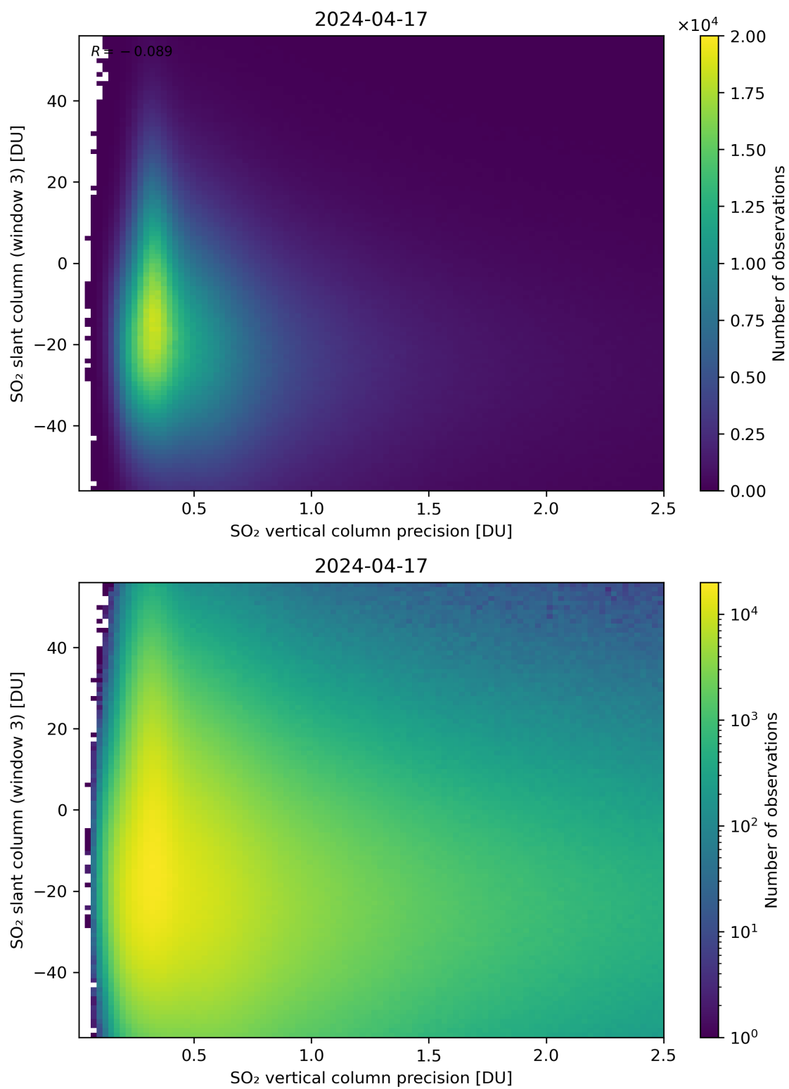
Figure 292: Scatter density plot of “SO 2 vertical column precision” against “SO 2 slant column (window 3)” for 2024-04-16 to 2024-04-18.
