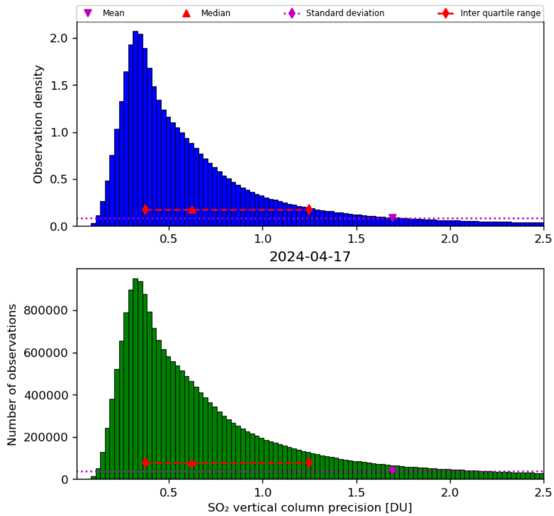
Figure 54: Histogram of “SO 2 vertical column precision” for 2024-04-16 to 2024-04-18
