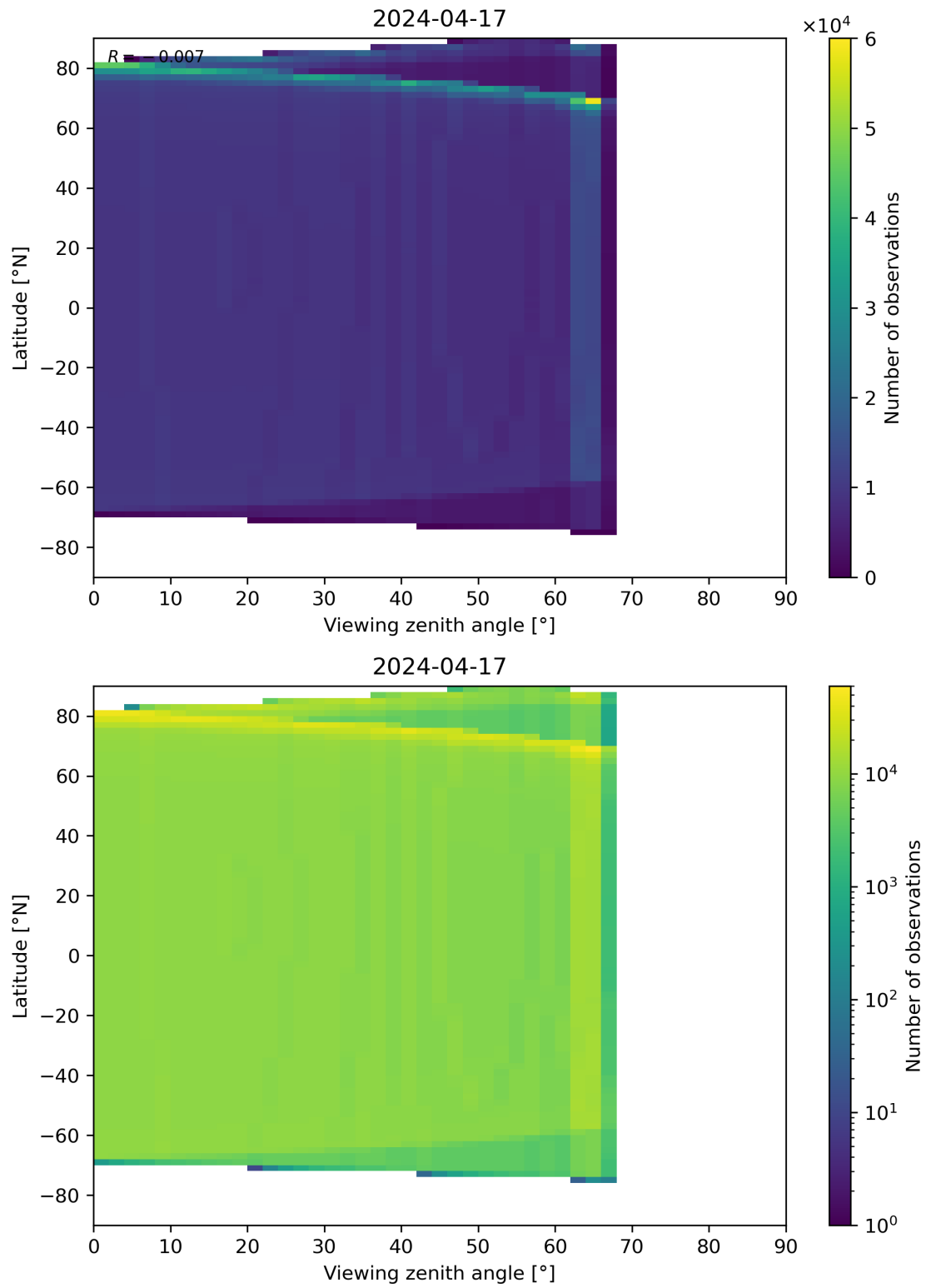
Figure 314: Scatter density plot of “Viewing zenith angle” against “Latitude” for 2024-04-16 to 2024-04-18.
