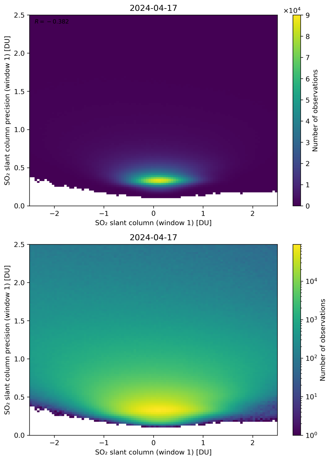
Figure 235: Scatter density plot of “SO 2 slant column (window 1)” against “SO 2 slant column precision (window 1)” for 2024-04-16 to 2024-04-18.
