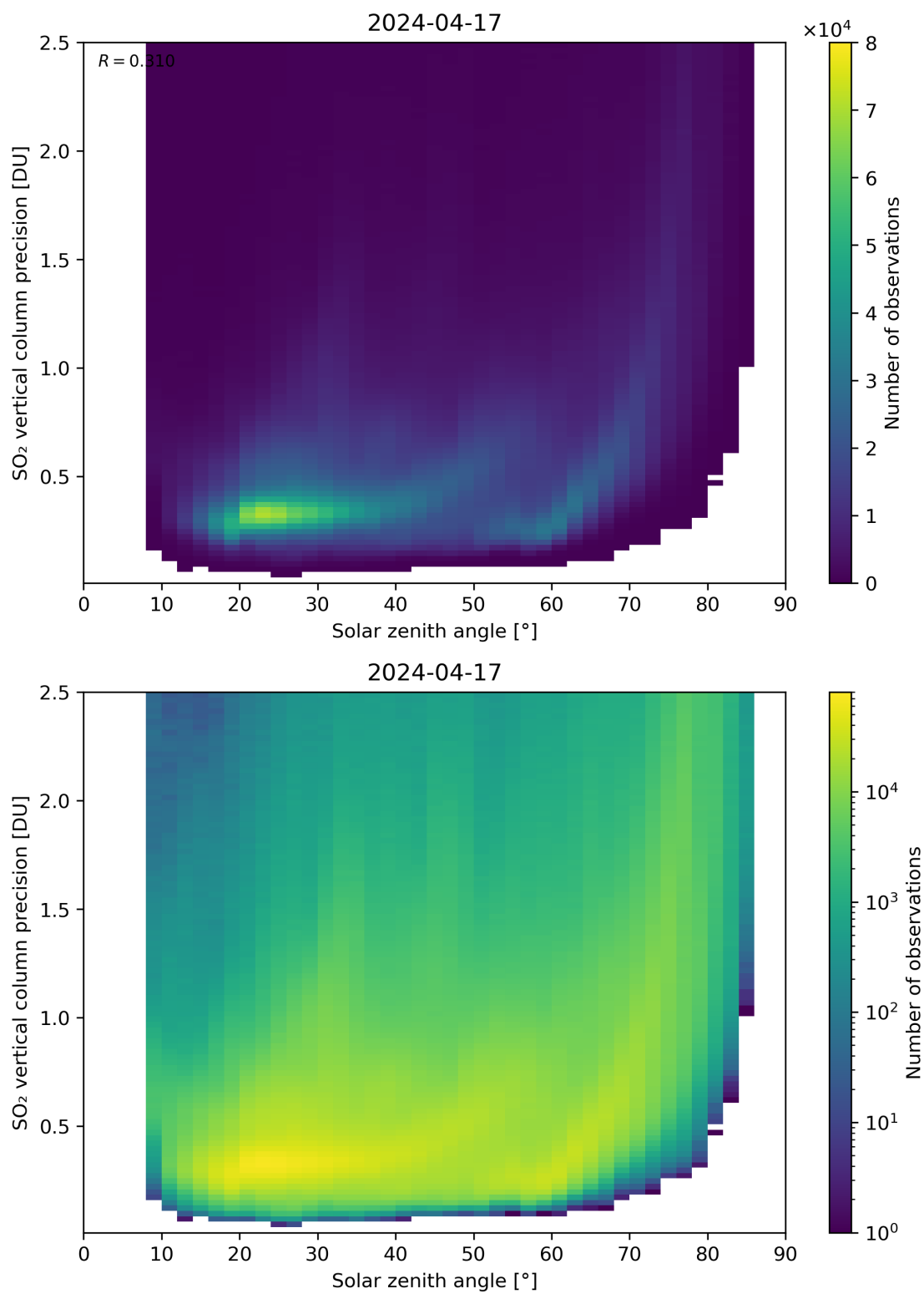
Figure 177: Scatter density plot of “Solar zenith angle” against “SO 2 vertical column precision” for 2024-04-16 to 2024-04-18.
