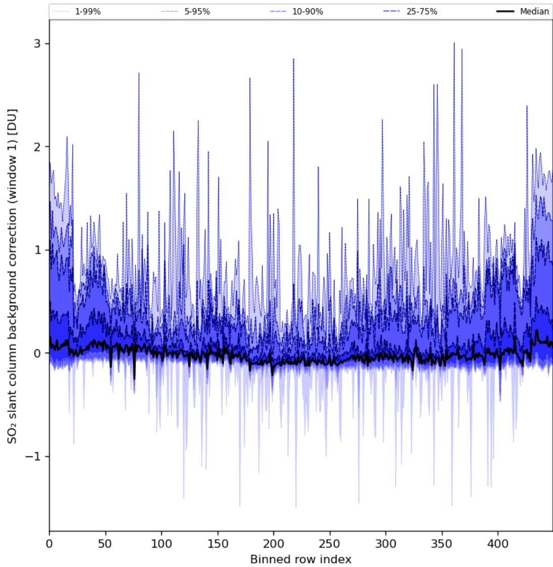
Figure 82: Along track statistics of “SO 2 slant column background correction (window 1)” for 2024-04-16 to 2024-04-18
