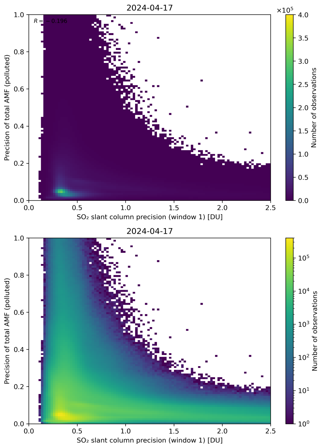
Figure 231: Scatter density plot of “SO 2 slant column precision (window 1)” against “Precision of total AMF (polluted)” for 2024-04-16 to 2024-04-18.
