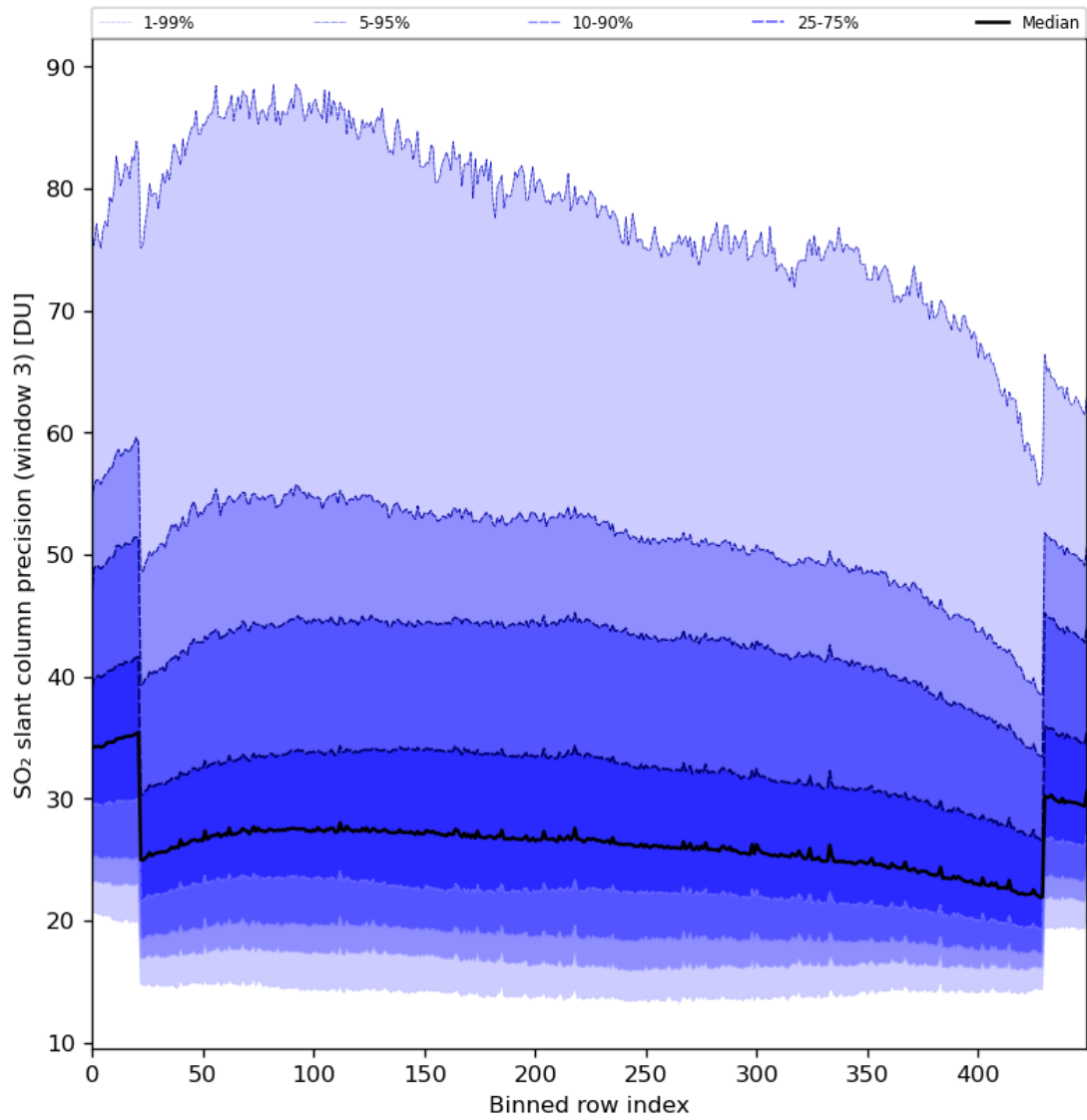
Figure 88: Along track statistics of “SO 2 slant column precision (window 3)” for 2024-04-16 to 2024-04-18
