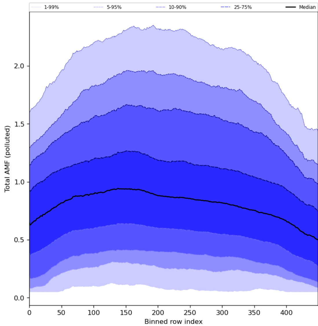
Figure 94: Along track statistics of “Total AMF (polluted)” for 2024-04-16 to 2024-04-18
