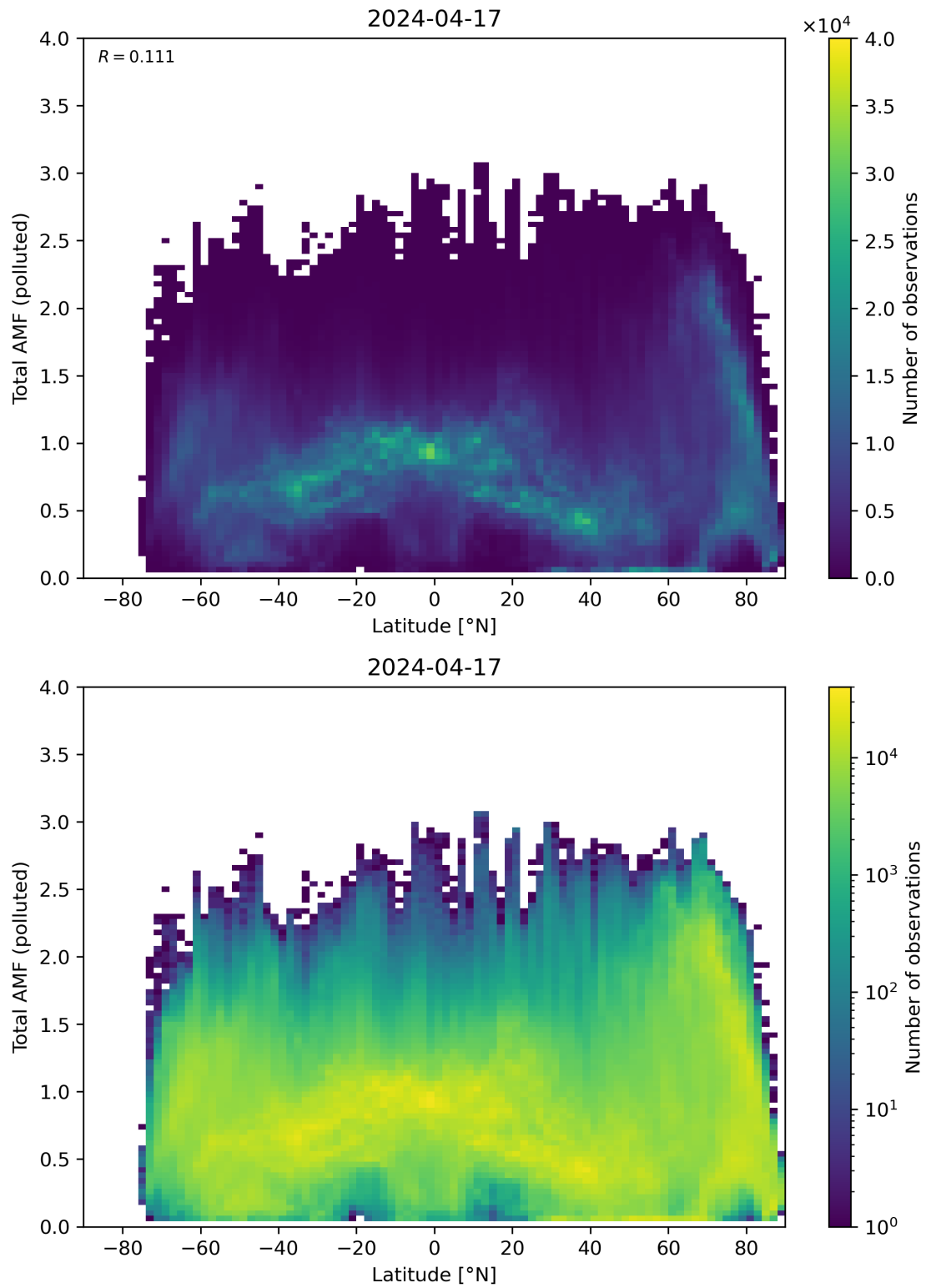
Figure 154: Scatter density plot of “Latitude” against “Total AMF (polluted)” for 2024-04-16 to 2024-04-18.
