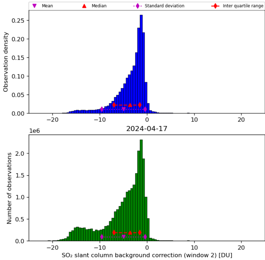
Figure 63: Histogram of “SO 2 slant column background correction (window 2)” for 2024-04-16 to 2024-04-18
