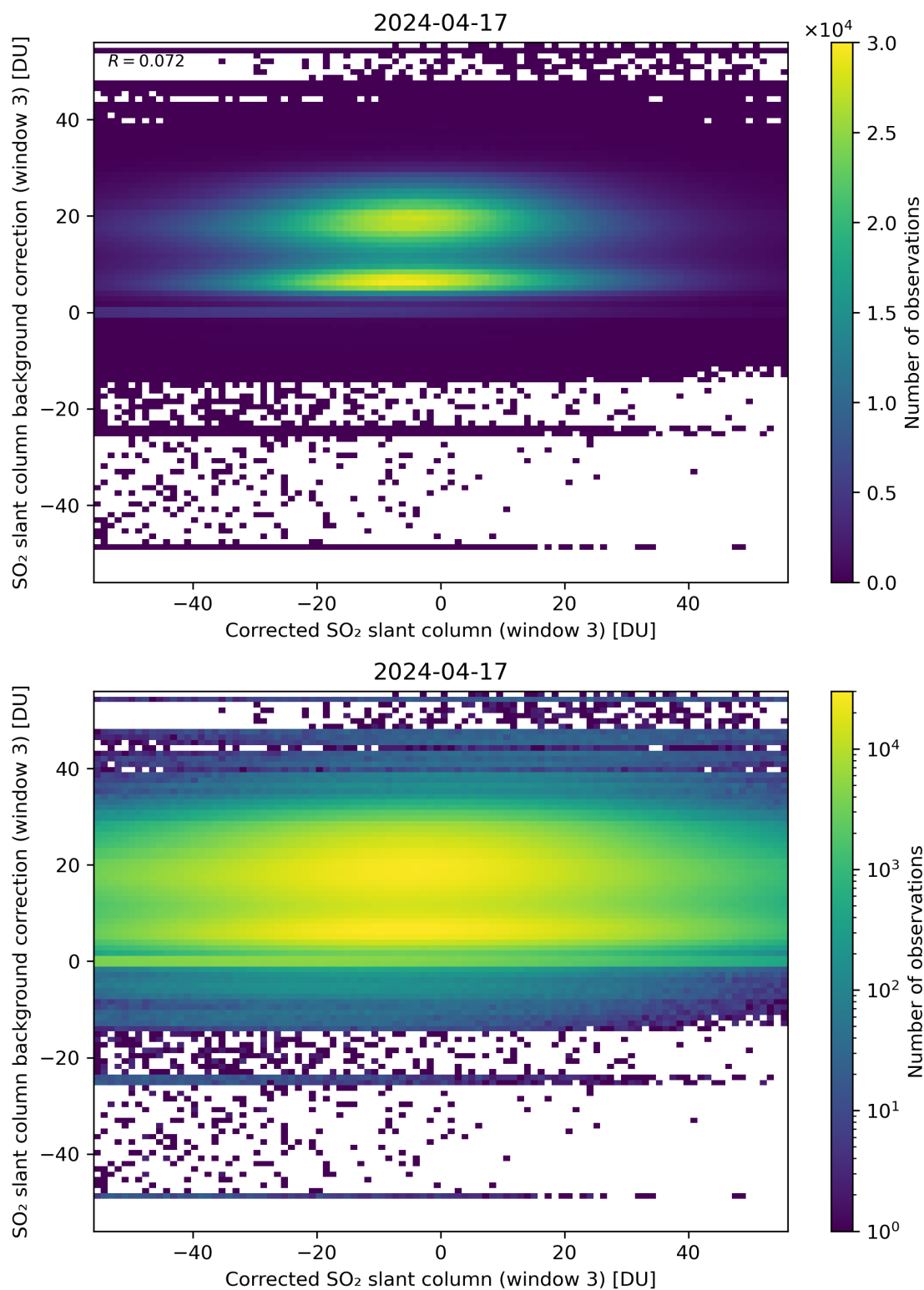
Figure 205: Scatter density plot of “Corrected SO 2 slant column (window 3)” against “SO 2 slant column background correction (window 3)” for 2024-04-16 to 2024-04-18.
