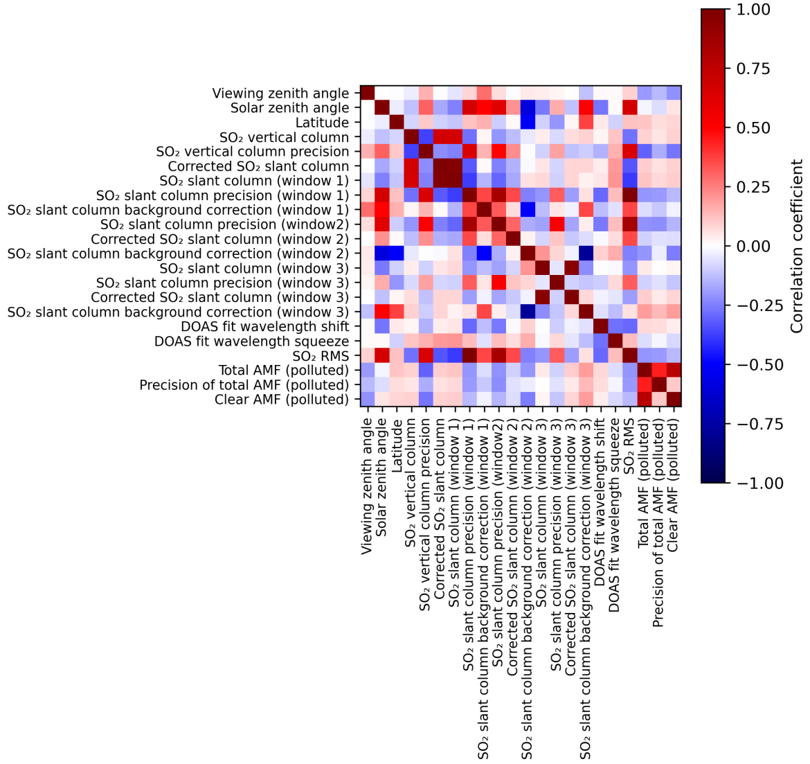
Figure 2: Map of correlation matrix for 2024-04-16 to 2024-04-18.
