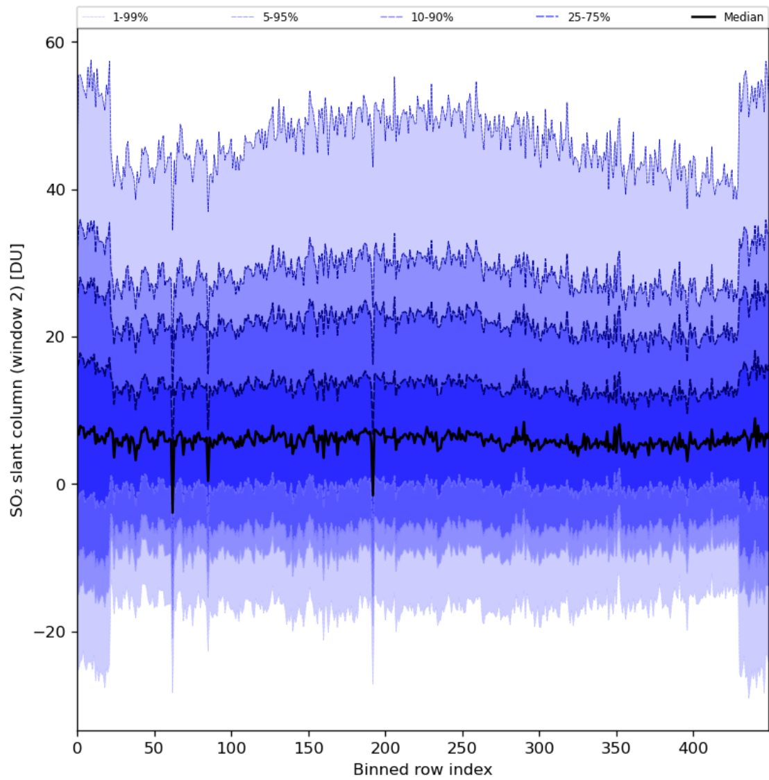
Figure 83: Along track statistics of “SO 2 slant column (window 2)” for 2024-04-16 to 2024-04-18
