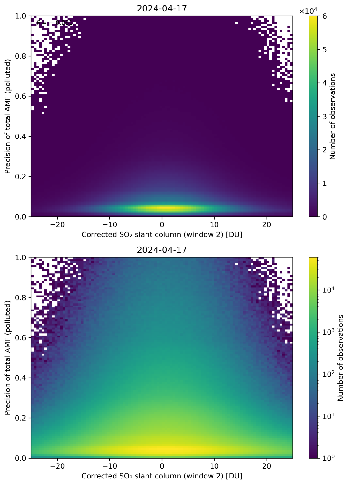
Figure 204: Scatter density plot of “Corrected SO 2 slant column (window 2)” against “Precision of total AMF (polluted)” for 2024-04-16 to 2024-04-18.
