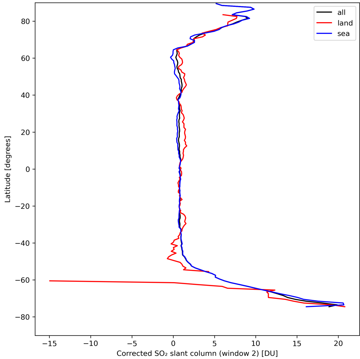
Figure 39: Zonal average of “Corrected SO 2 slant column (window 2)” for 2024-04-16 to 2024-04-18.
