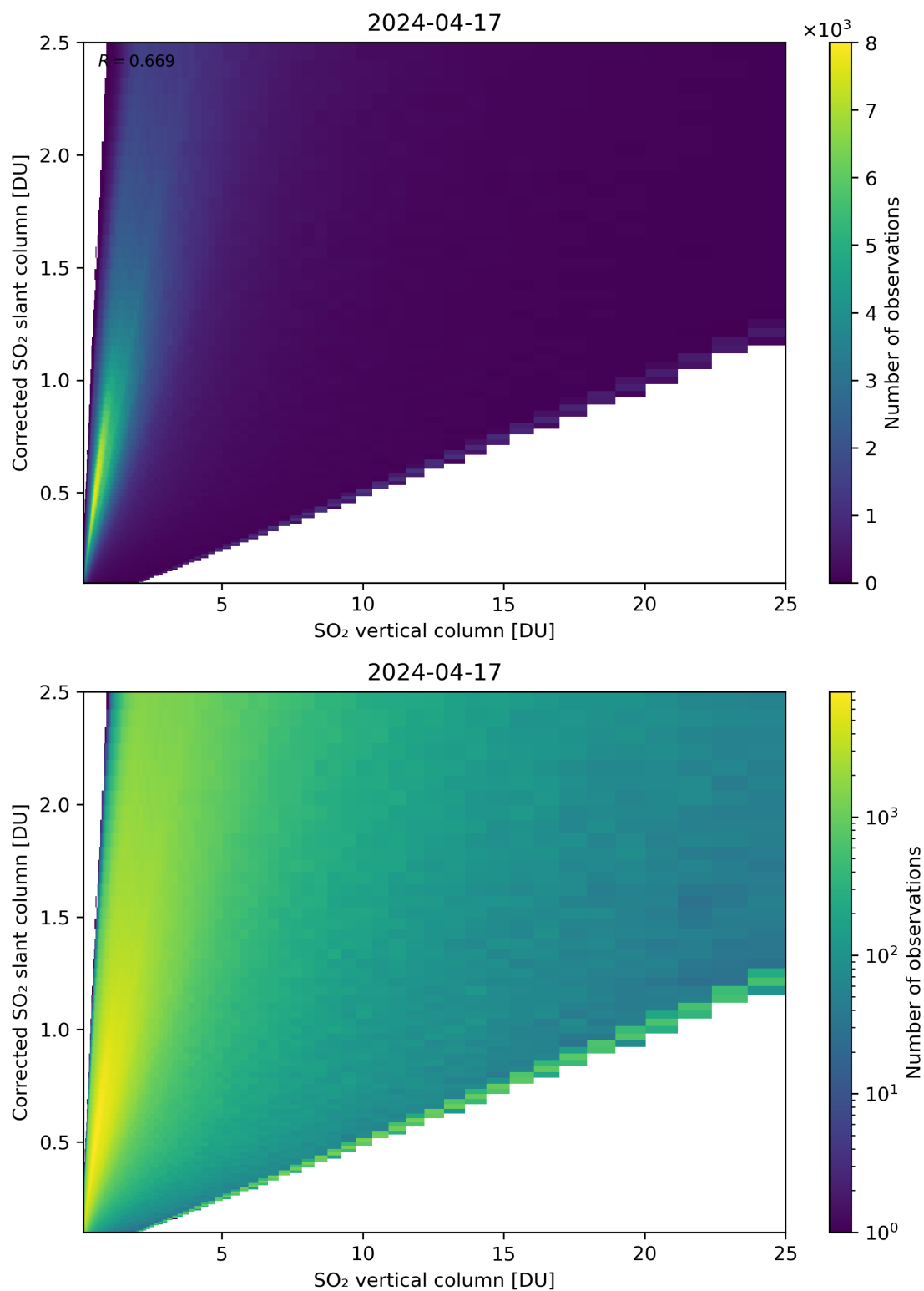
Figure 297: Scatter density plot of “SO 2 vertical column” against “Corrected SO 2 slant column” for 2024-04-16 to 2024-04-18.
