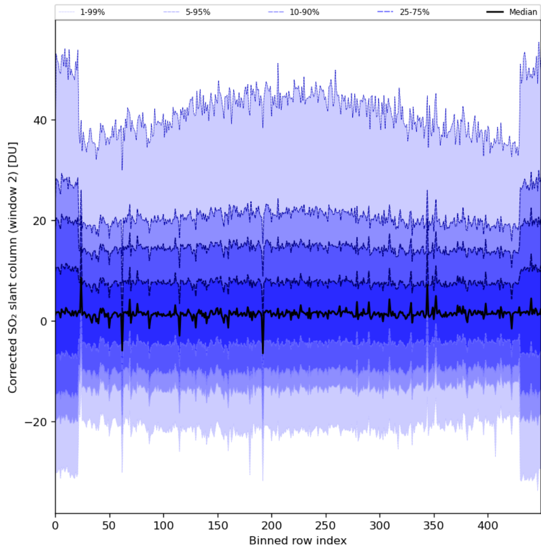
Figure 85: Along track statistics of “Corrected SO 2 slant column (window 2)” for 2024-04-16 to 2024-04-18
