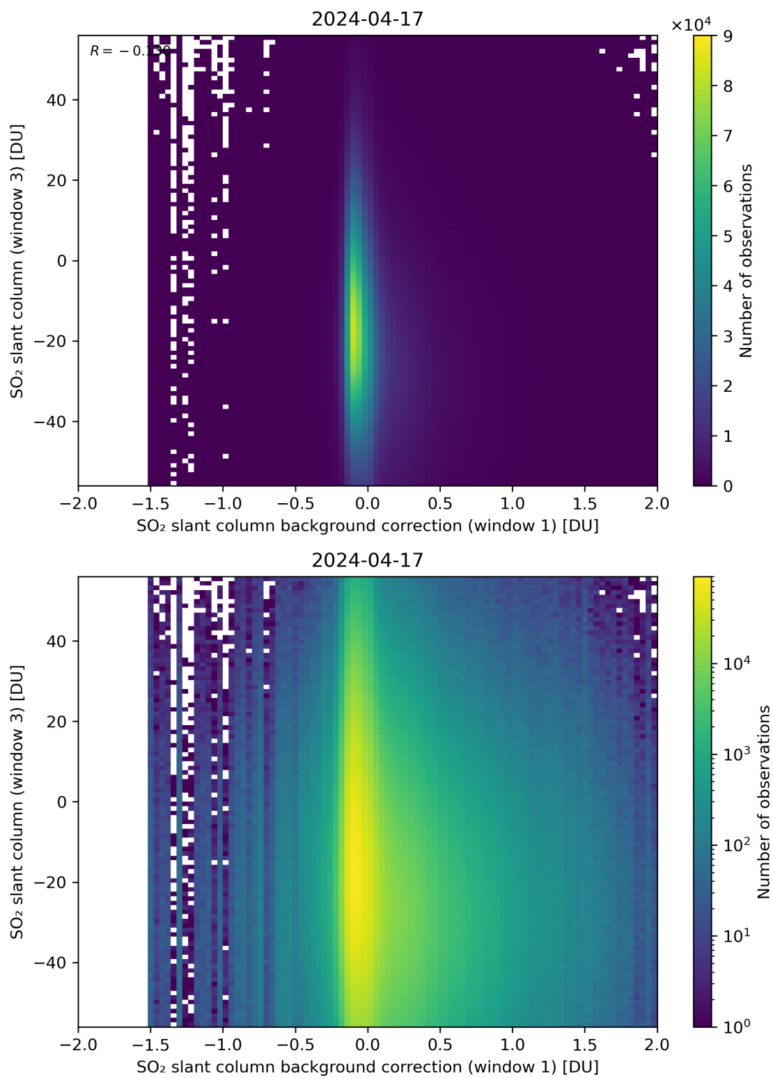
Figure 107: Scatter density plot of “SO 2 slant column background correction (window 1)” against “SO 2 slant column (window 3)” for 2024-04-16 to 2024-04-18.
