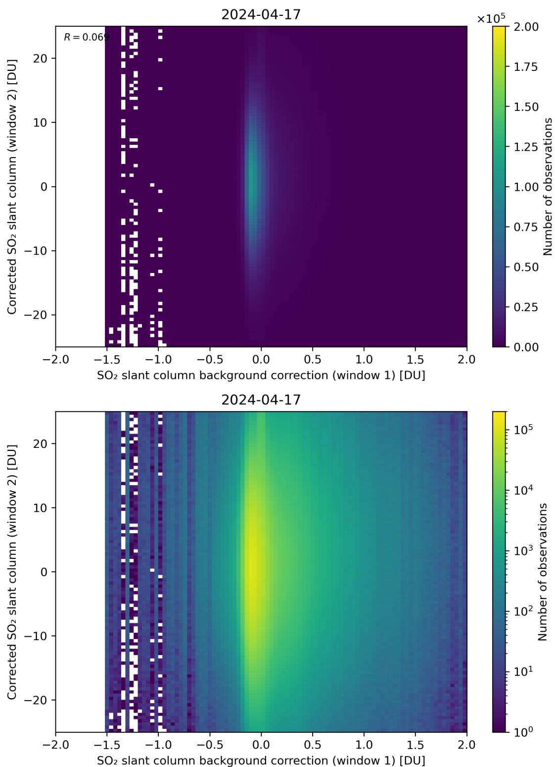
Figure 104: Scatter density plot of “SO 2 slant column background correction (window 1)” against “Corrected SO 2 slant column (window 2)” for 2024-04-16 to 2024-04-18.
