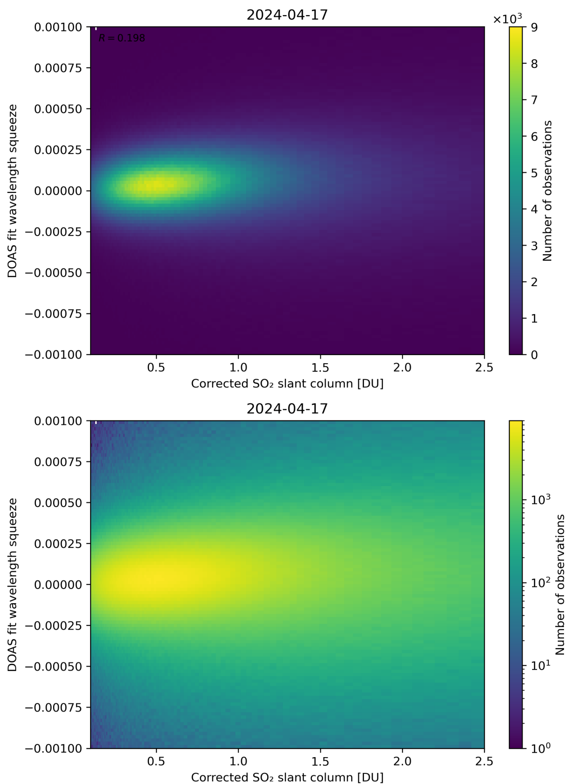
Figure 182: Scatter density plot of “Corrected SO 2 slant column” against “DOAS fit wavelength squeeze” for 2024-04-16 to 2024-04-18.
