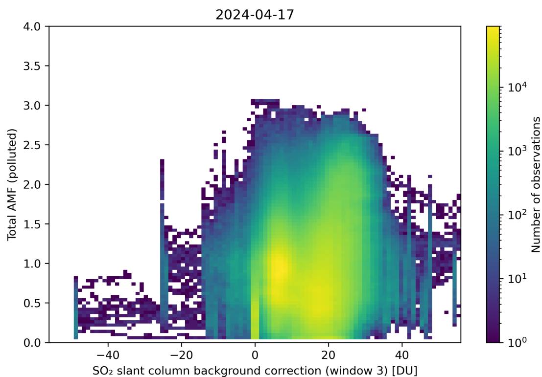
Figure 125: Scatter density plot of “SO 2 slant column background correction (window 3)” against “Total AMF (polluted)” for 2024-04-16 to 2024-04-18.
