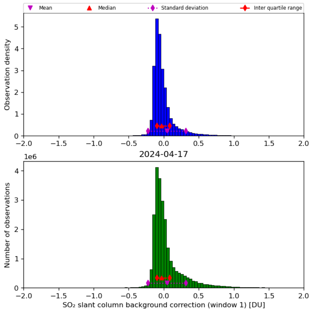
Figure 59: Histogram of “SO 2 slant column background correction (window 1)” for 2024-04-16 to 2024-04-18
