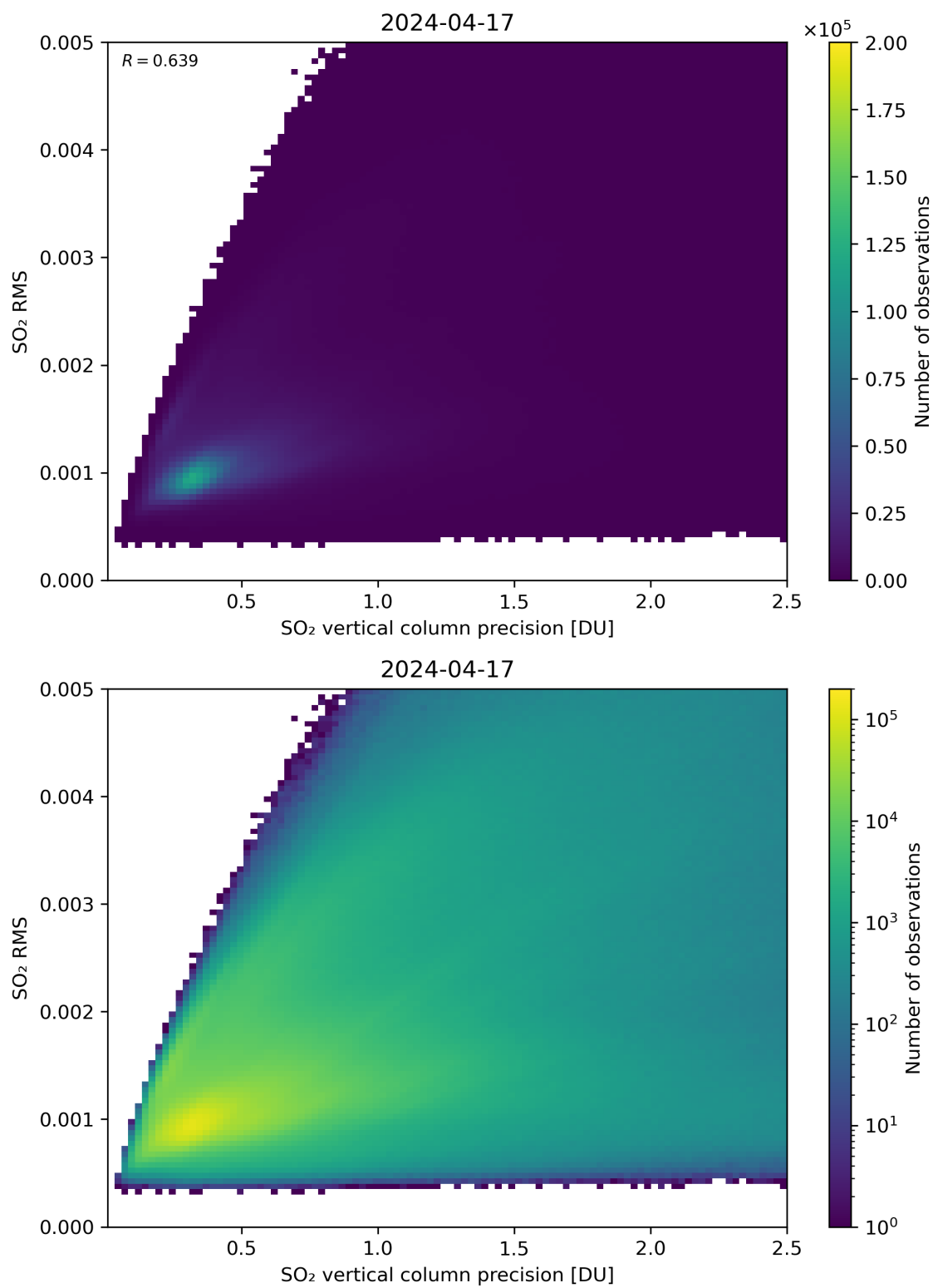
Figure 284: Scatter density plot of “SO 2 vertical column precision” against “SO 2 RMS” for 2024-04-16 to 2024-04-18.
