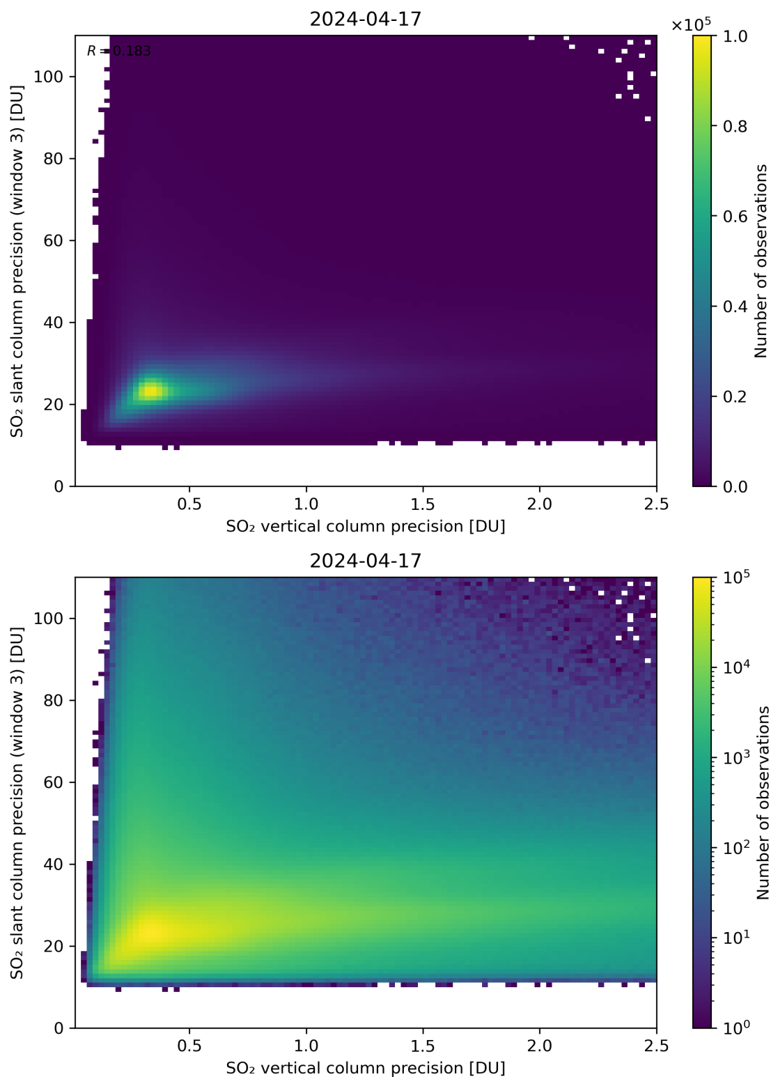
Figure 293: Scatter density plot of “SO 2 vertical column precision” against “SO 2 slant column precision (window 3)” for 2024-04-16 to 2024-04-18.
