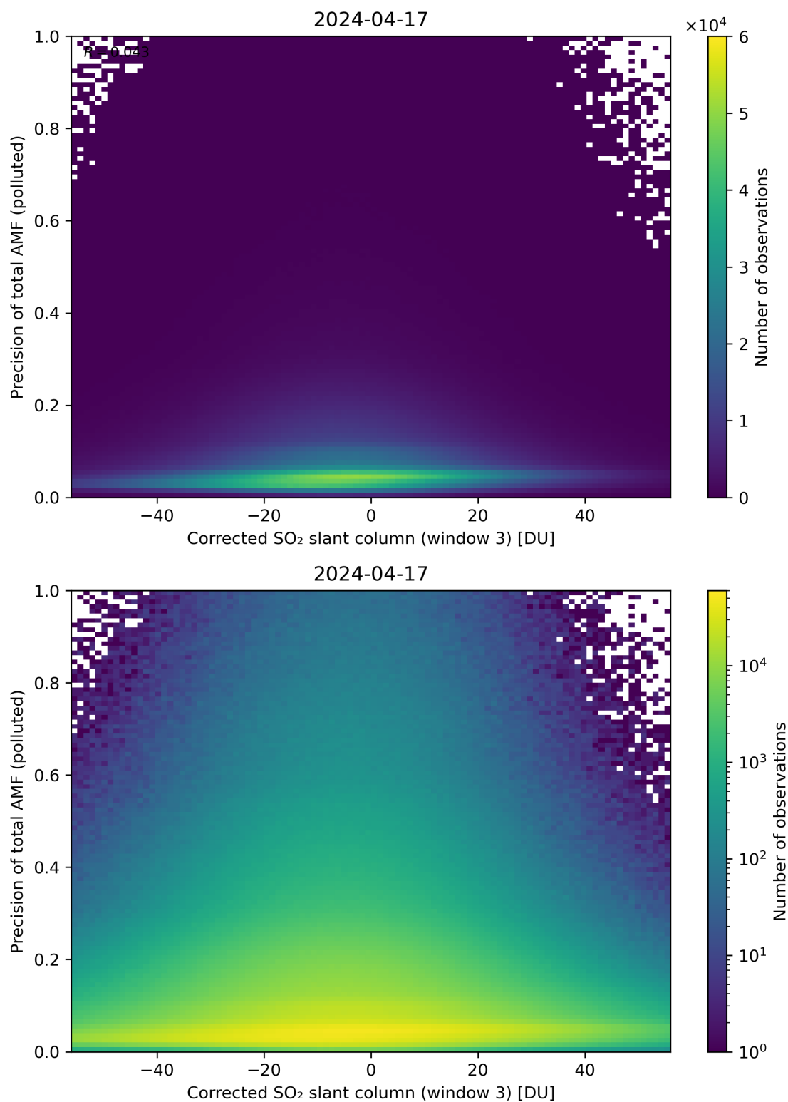
Figure 211: Scatter density plot of “Corrected SO 2 slant column (window 3)” against “Precision of total AMF (polluted)” for 2024-04-16 to 2024-04-18.
