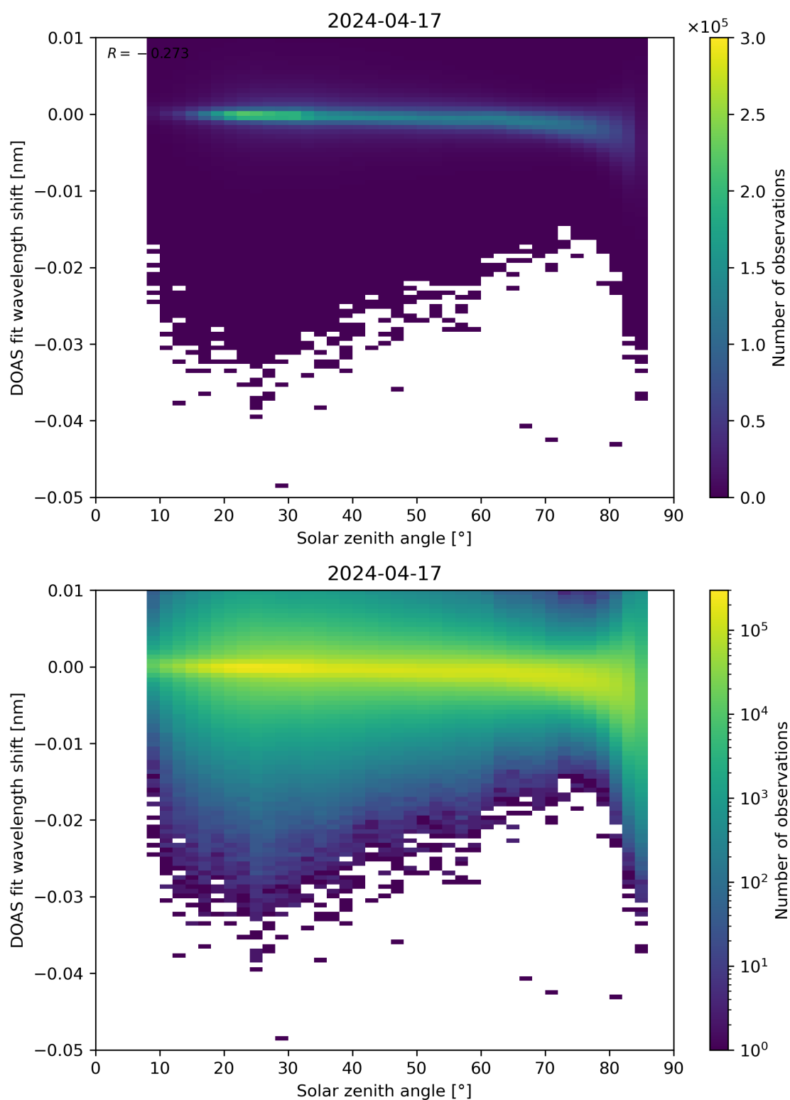
Figure 161: Scatter density plot of “Solar zenith angle” against “DOAS fit wavelength shift” for 2024-04-16 to 2024-04-18.
