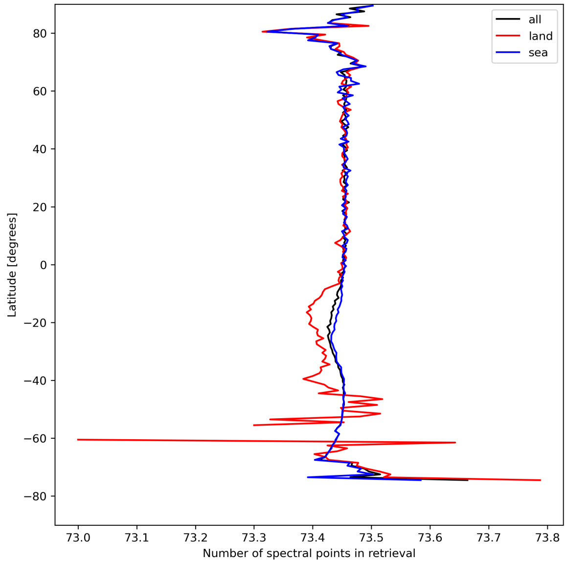
Figure 51: Zonal average of “Number of spectral points in retrieval” for 2024-04-16 to 2024-04-18.
