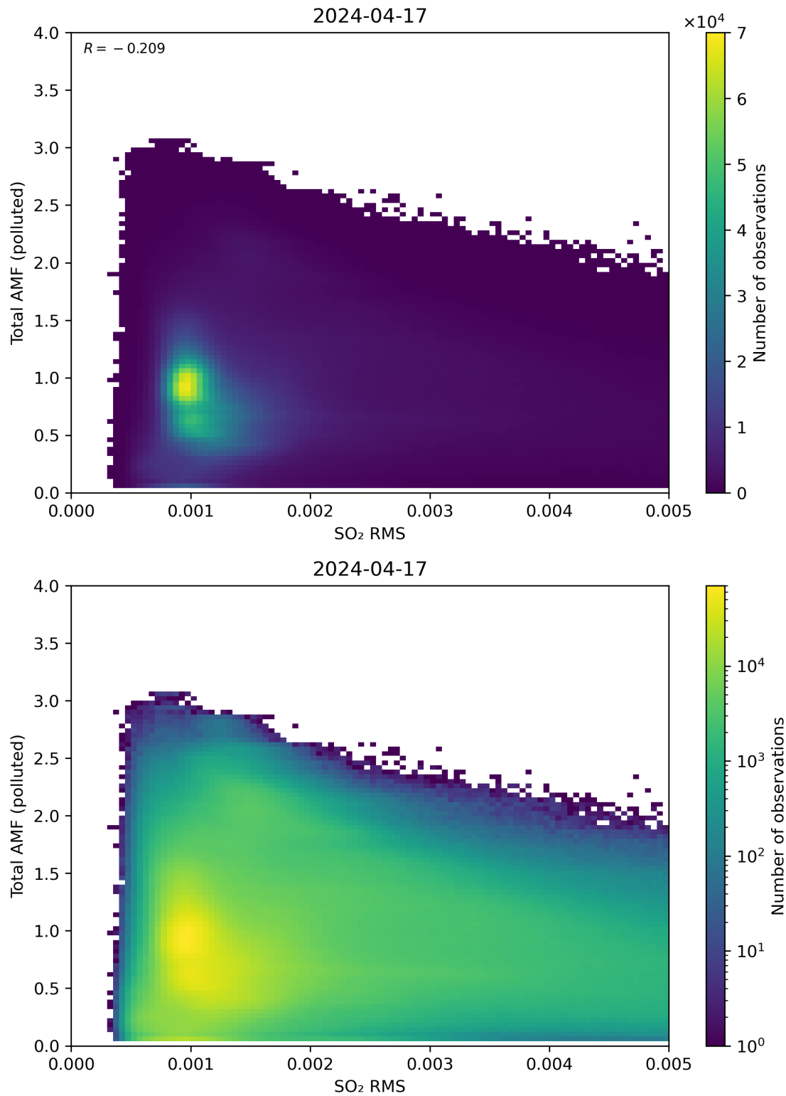
Figure 137: Scatter density plot of “SO 2 RMS” against “Total AMF (polluted)” for 2024-04-16 to 2024-04-18.
