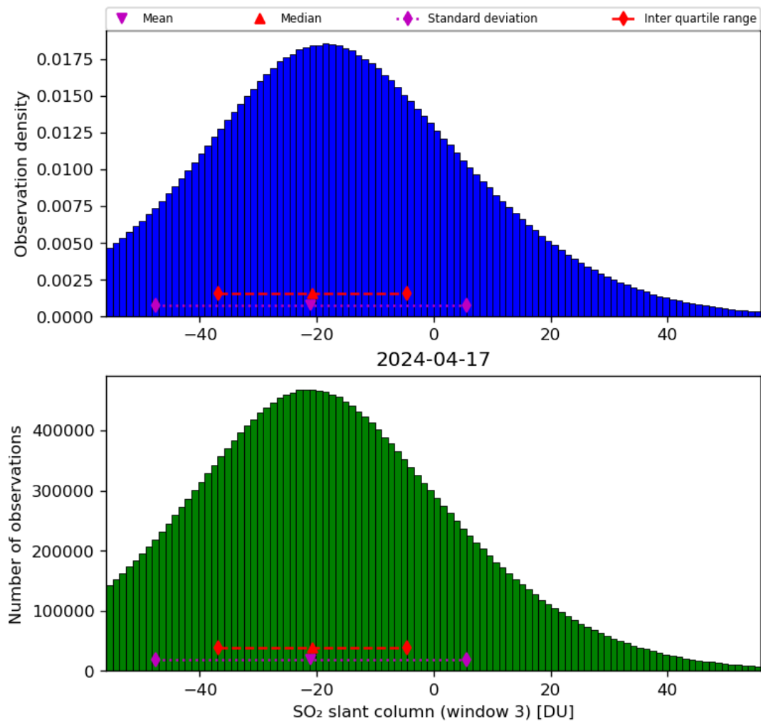
Figure 64: Histogram of “SO 2 slant column (window 3)” for 2024-04-16 to 2024-04-18
