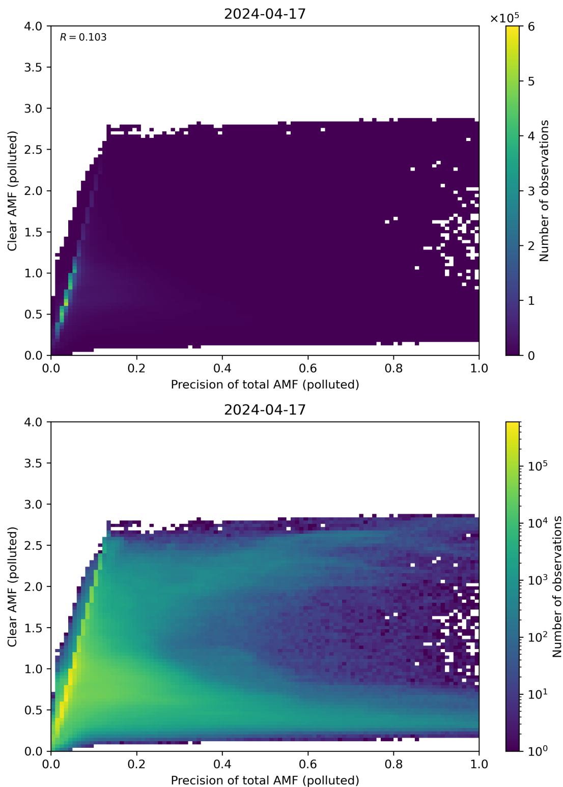
Figure 270: Scatter density plot of “Precision of total AMF (polluted)” against “Clear AMF (polluted)” for 2024-04-16 to 2024-04-18.
