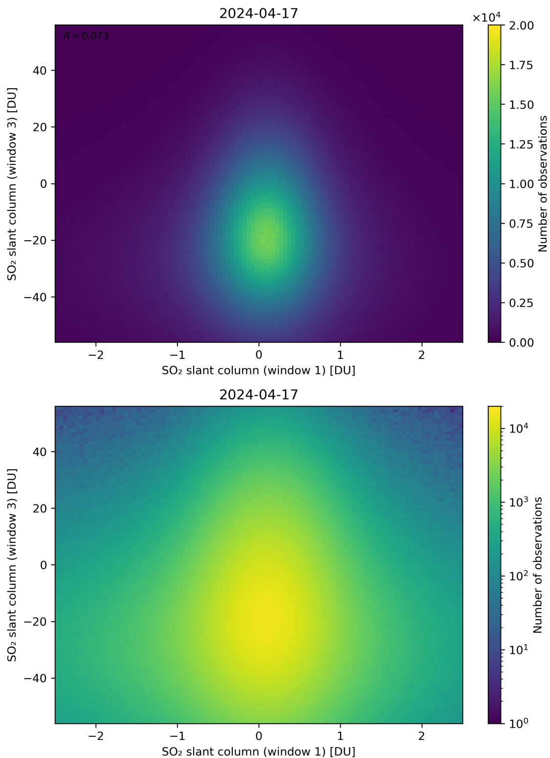
Figure 237: Scatter density plot of “SO 2 slant column (window 1)” against “SO 2 slant column (window 3)” for 2024-04-16 to 2024-04-18.
