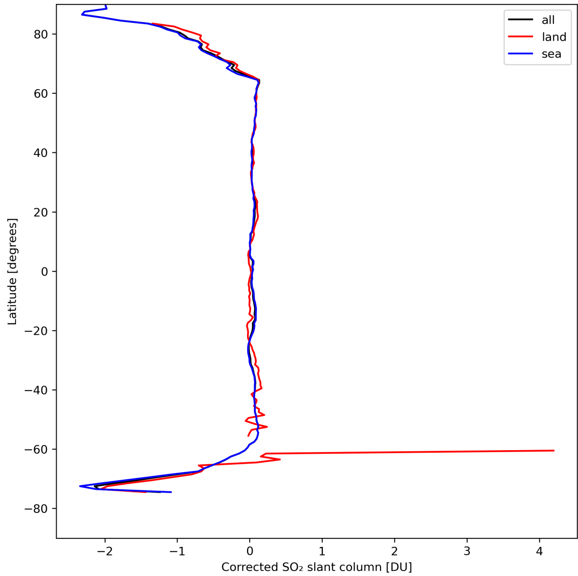
Figure 32: Zonal average of “Corrected SO 2 slant column” for 2024-04-16 to 2024-04-18.
