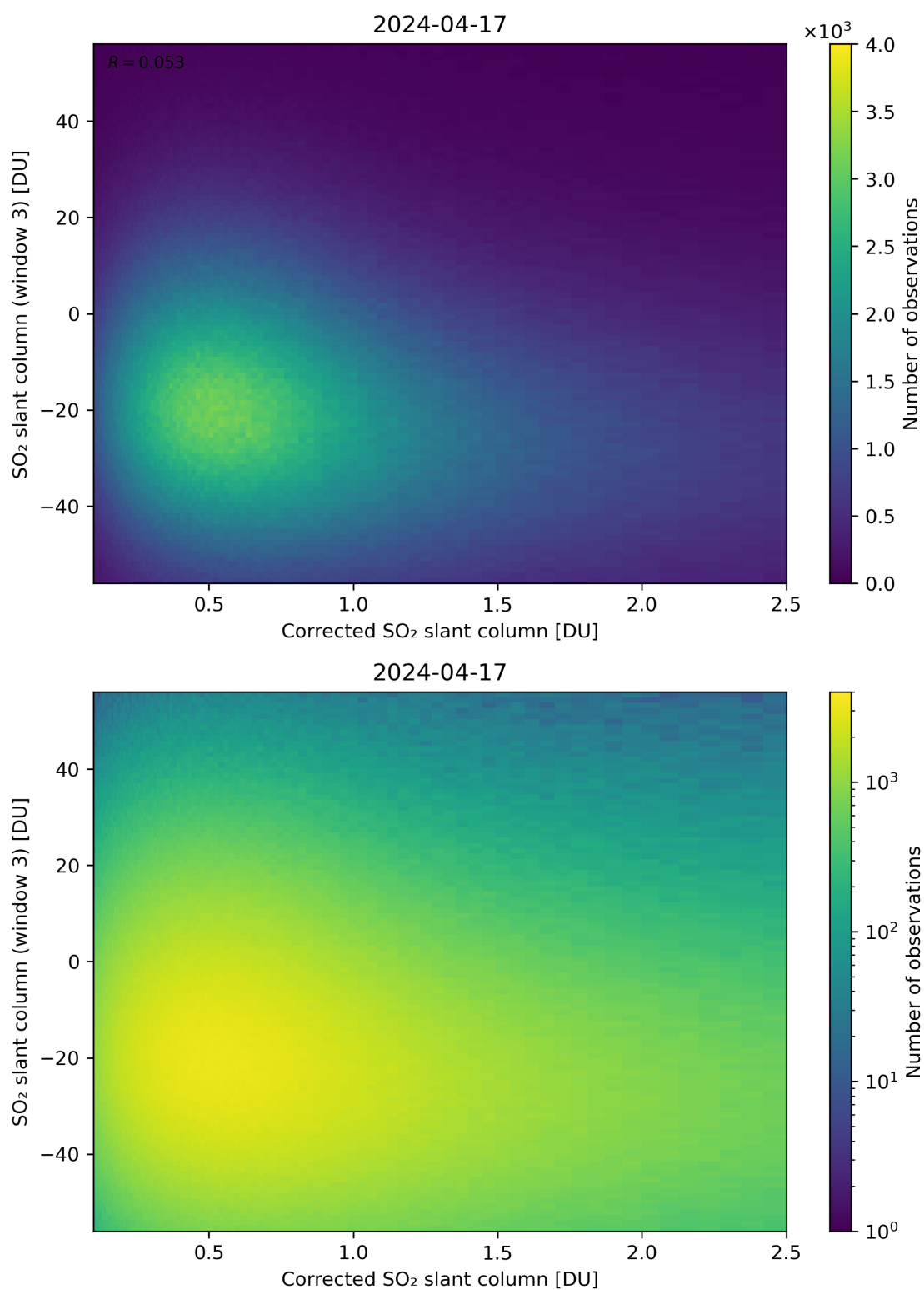
Figure 190: Scatter density plot of “Corrected SO 2 slant column” against “SO 2 slant column (window 3)” for 2024-04-16 to 2024-04-18.
