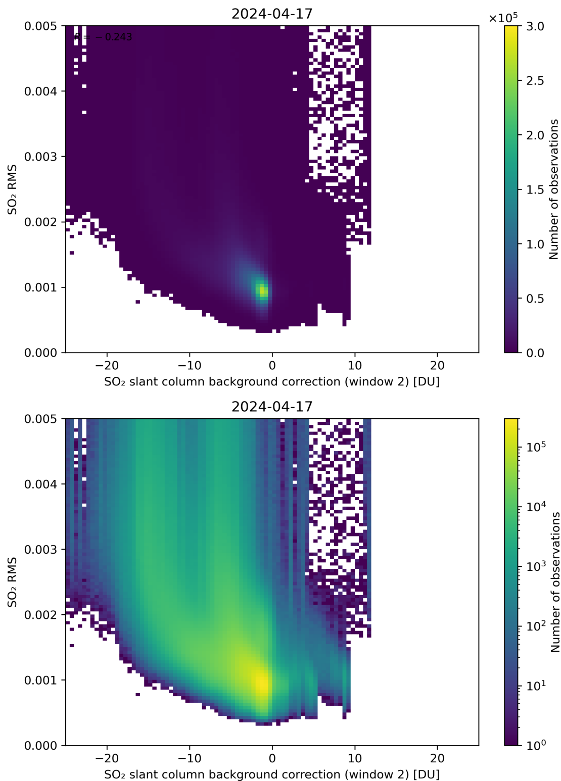
Figure 114: Scatter density plot of “SO 2 slant column background correction (window 2)” against “SO 2 RMS” for 2024-04-16 to 2024-04-18.
