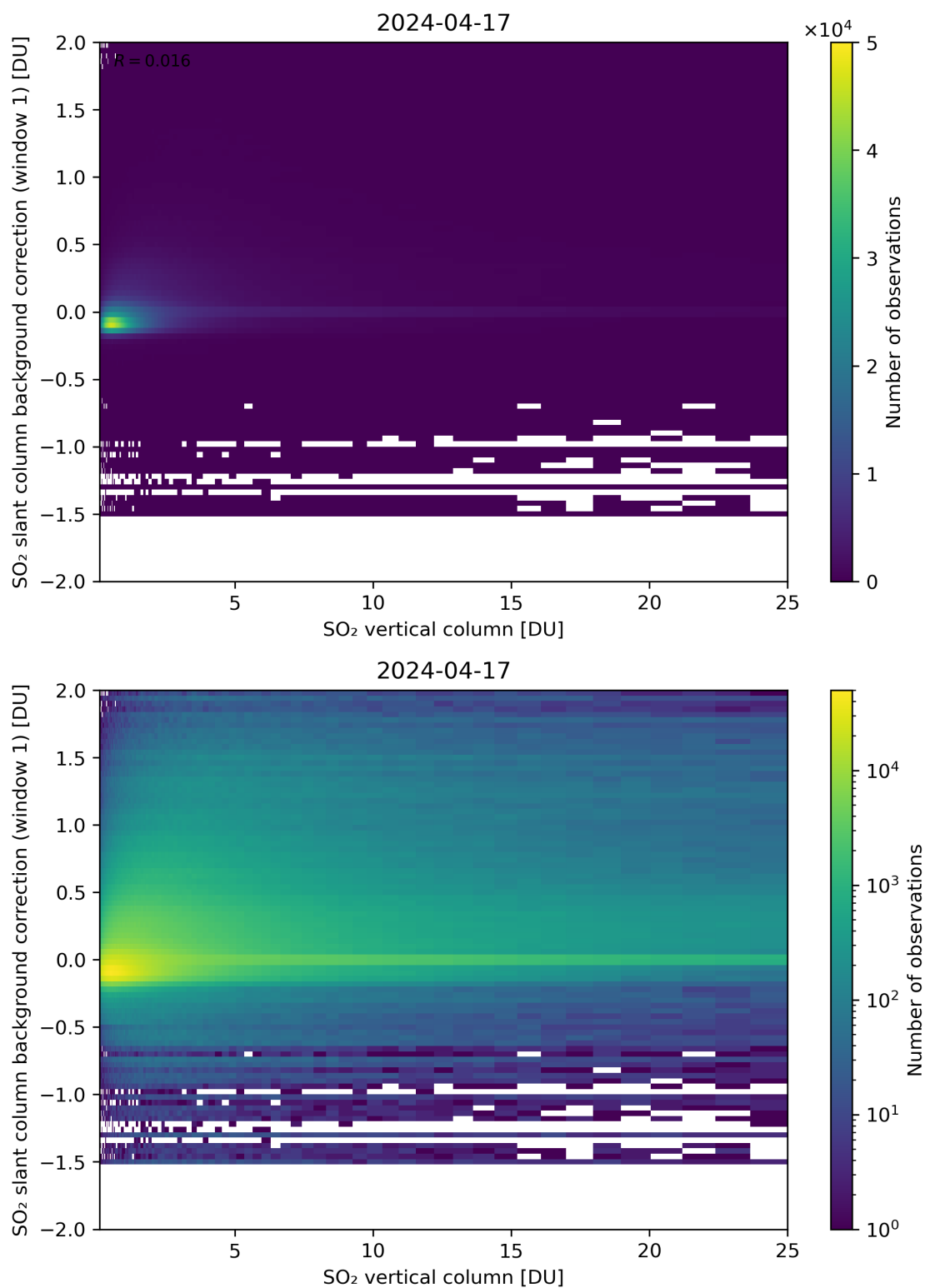
Figure 273: Scatter density plot of “SO 2 vertical column” against “SO 2 slant column background correction (window 1)” for 2024-04-16 to 2024-04-18.
