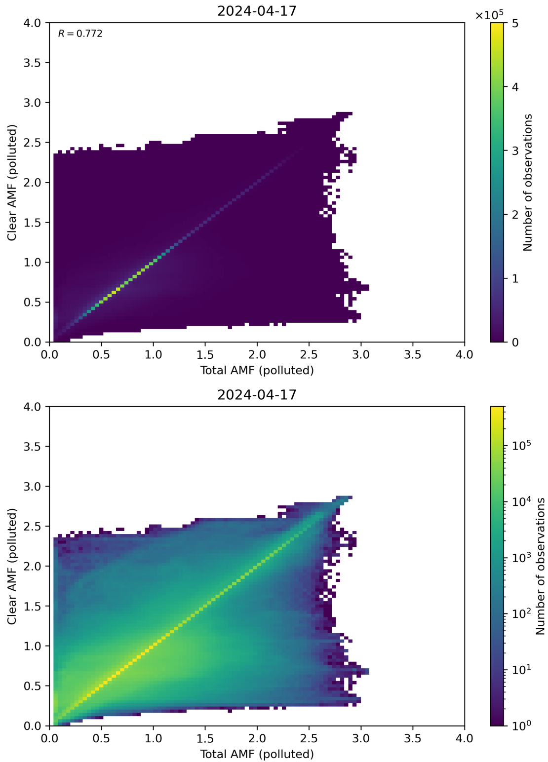
Figure 271: Scatter density plot of “Total AMF (polluted)” against “Clear AMF (polluted)” for 2024-04-16 to 2024-04-18.
