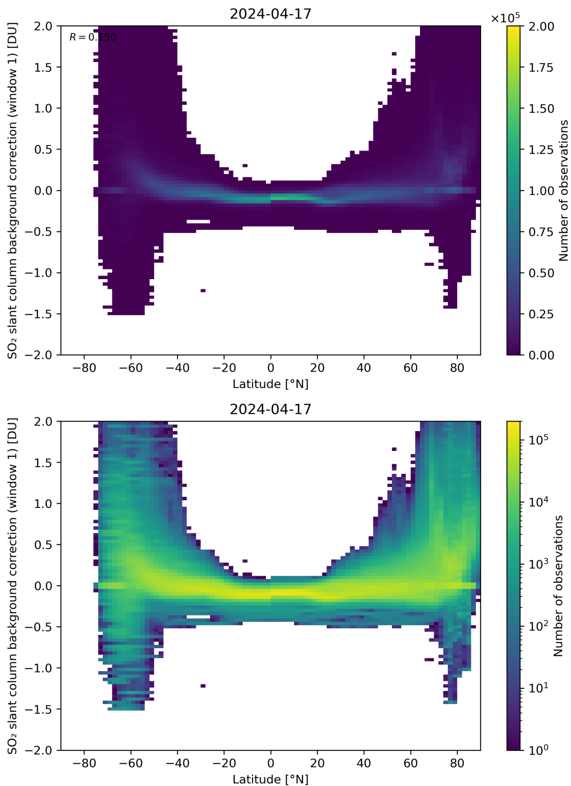
Figure 139: Scatter density plot of “Latitude” against “SO 2 slant column background correction (window 1)” for 2024-04-16 to 2024-04-18.
