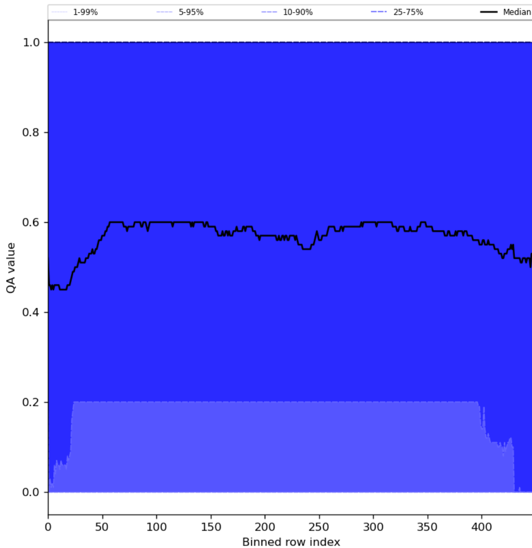
Figure 75: Along track statistics of “QA value” for 2024-04-16 to 2024-04-18
