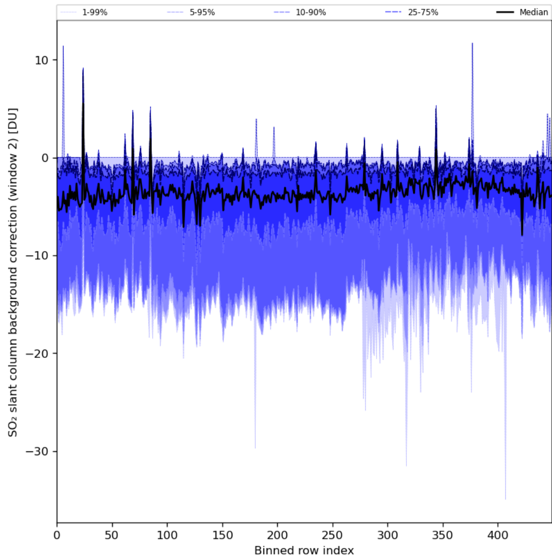
Figure 86: Along track statistics of “SO 2 slant column background correction (window 2)” for 2024-04-16 to 2024-04-18
