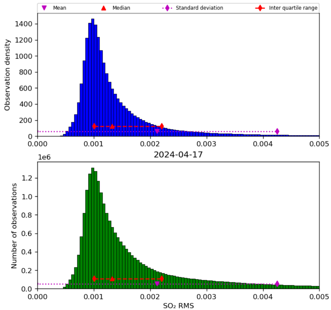
Figure 70: Histogram of “SO 2 RMS” for 2024-04-16 to 2024-04-18
