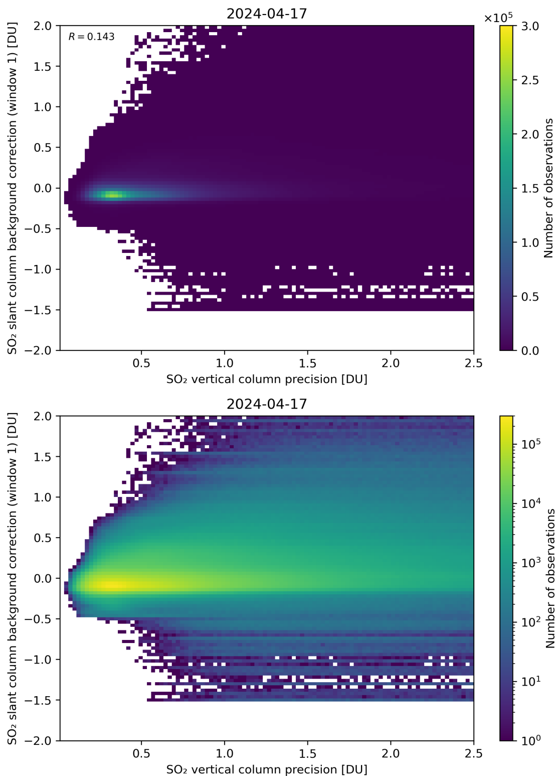
Figure 279: Scatter density plot of “SO 2 vertical column precision” against “SO 2 slant column background correction (window 1)” for 2024-04-16 to 2024-04-18.
