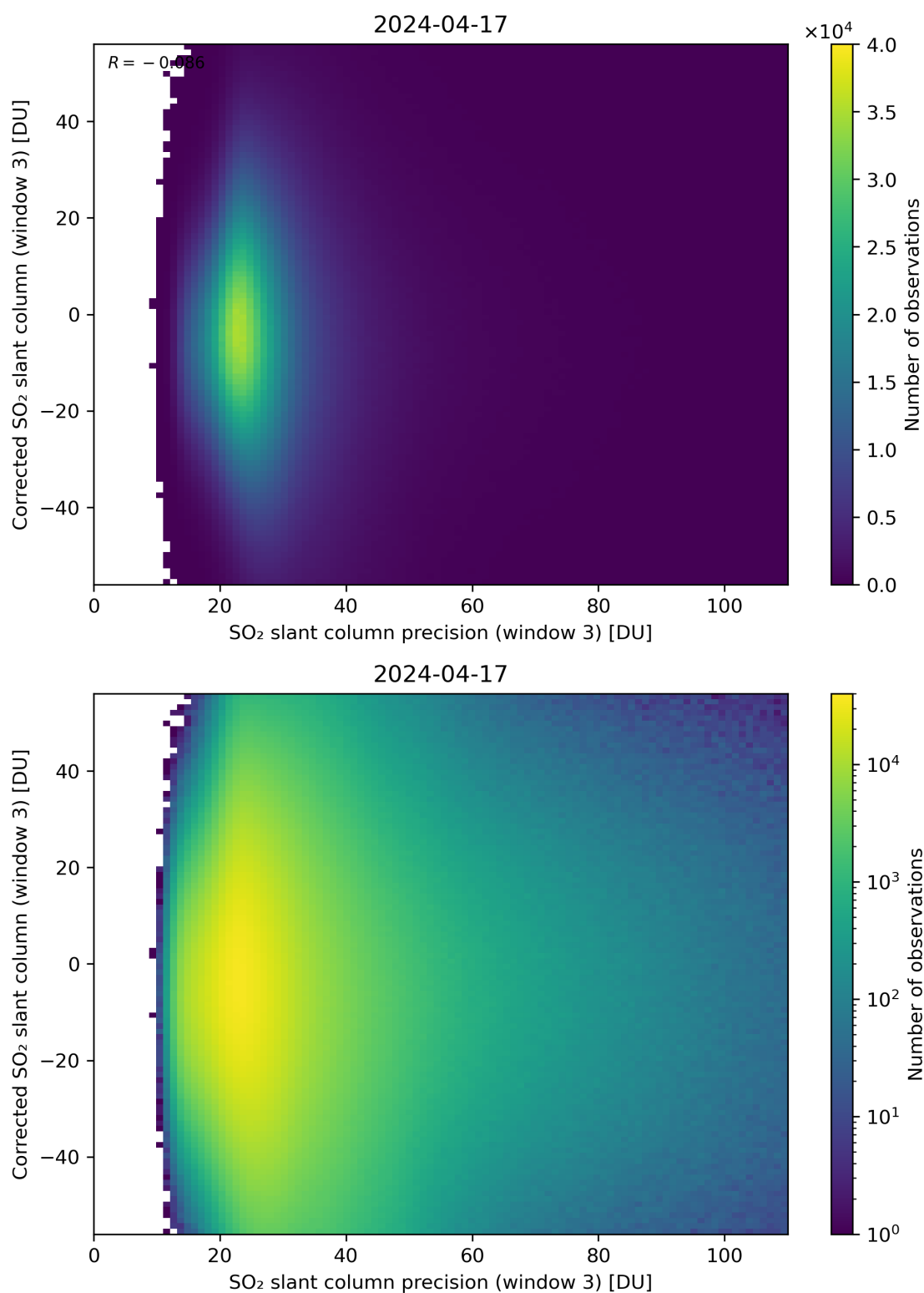
Figure 262: Scatter density plot of “SO 2 slant column precision (window 3)” against “Corrected SO 2 slant column (window 3)” for 2024-04-16 to 2024-04-18.
