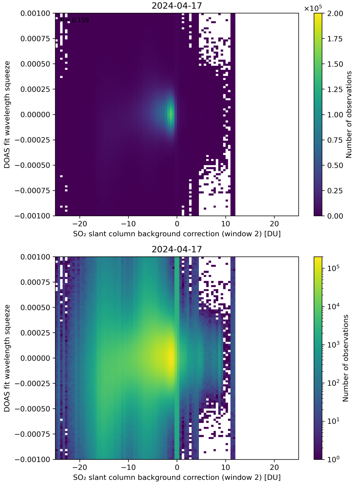
Figure 113: Scatter density plot of “SO 2 slant column background correction (window 2)” against “DOAS fit wavelength squeeze” for 2024-04-16 to 2024-04-18.
