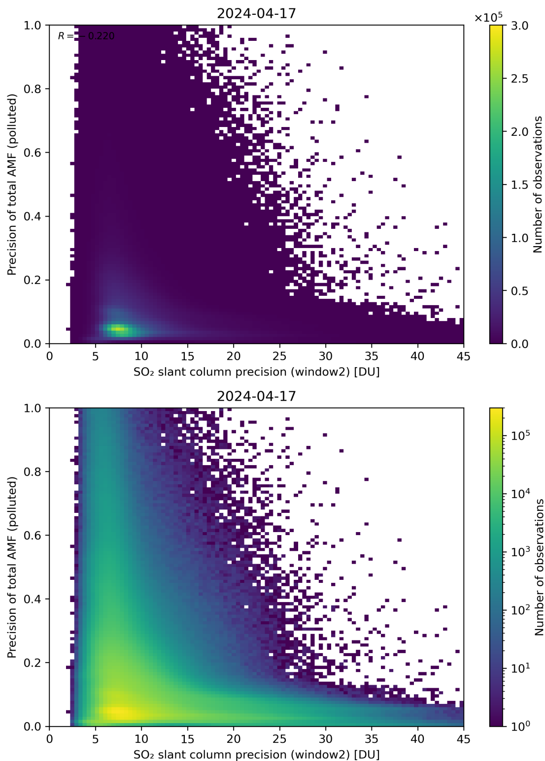
Figure 252: Scatter density plot of “SO 2 slant column precision (window2)” against “Precision of total AMF (polluted)” for 2024-04-16 to 2024-04-18.
