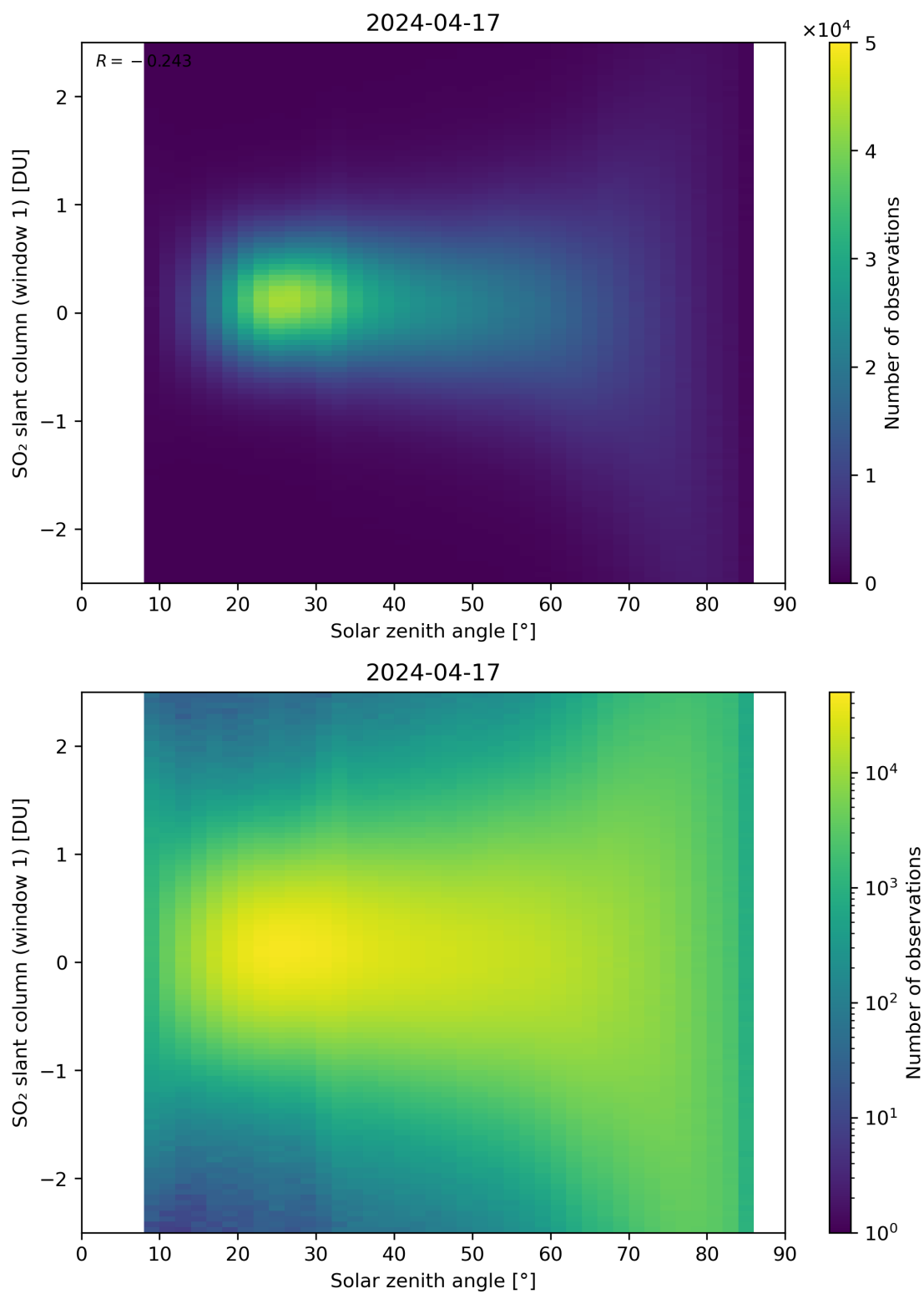
Figure 169: Scatter density plot of “Solar zenith angle” against “SO 2 slant column (window 1)” for 2024-04-16 to 2024-04-18.
