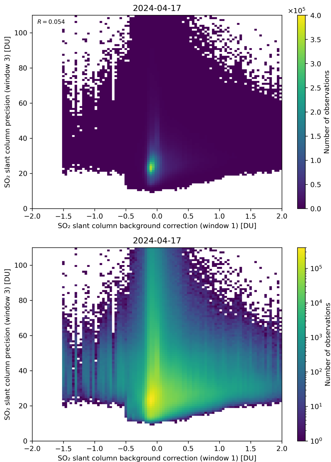
Figure 108: Scatter density plot of “SO 2 slant column background correction (window 1)” against “SO 2 slant column precision (window 3)” for 2024-04-16 to 2024-04-18.
