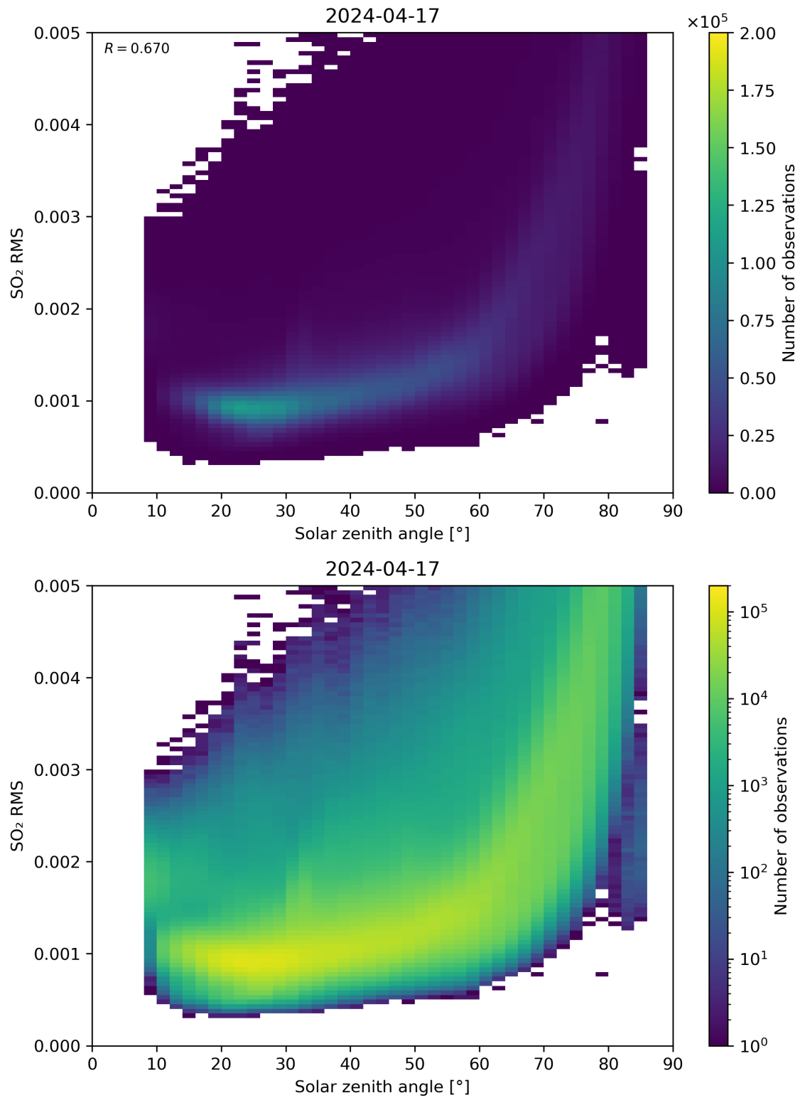
Figure 163: Scatter density plot of “Solar zenith angle” against “SO 2 RMS” for 2024-04-16 to 2024-04-18.
