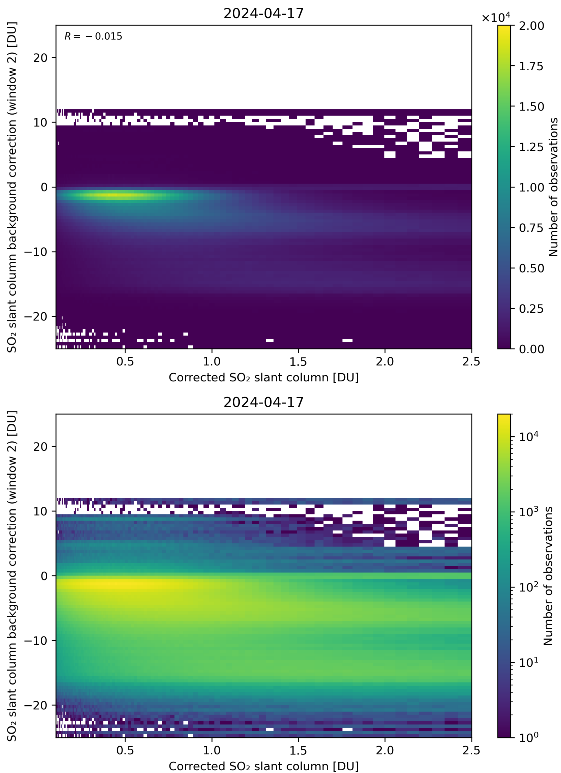
Figure 179: Scatter density plot of “Corrected SO 2 slant column” against “SO 2 slant column background correction (window 2)” for 2024-04-16 to 2024-04-18.
