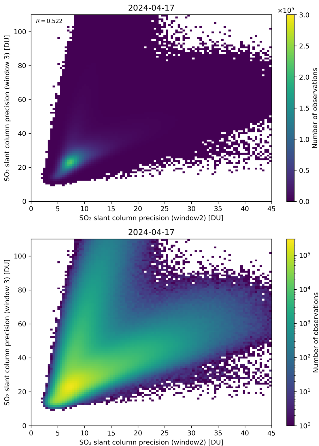
Figure 250: Scatter density plot of “SO 2 slant column precision (window2)” against “SO 2 slant column precision (window 3)” for 2024-04-16 to 2024-04-18.
