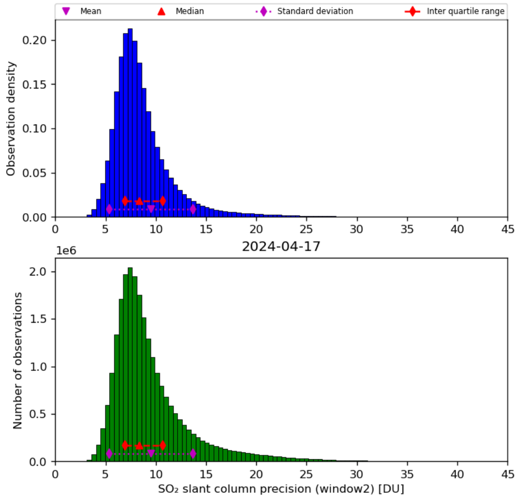
Figure 61: Histogram of “SO 2 slant column precision (window2)” for 2024-04-16 to 2024-04-18
