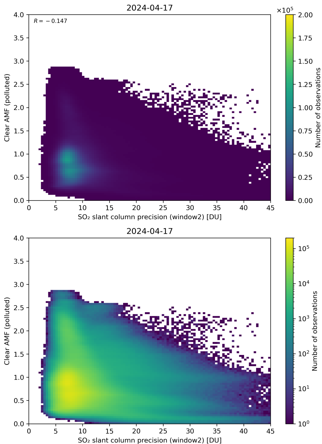
Figure 246: Scatter density plot of “SO 2 slant column precision (window2)” against “Clear AMF (polluted)” for 2024-04-16 to 2024-04-18.
