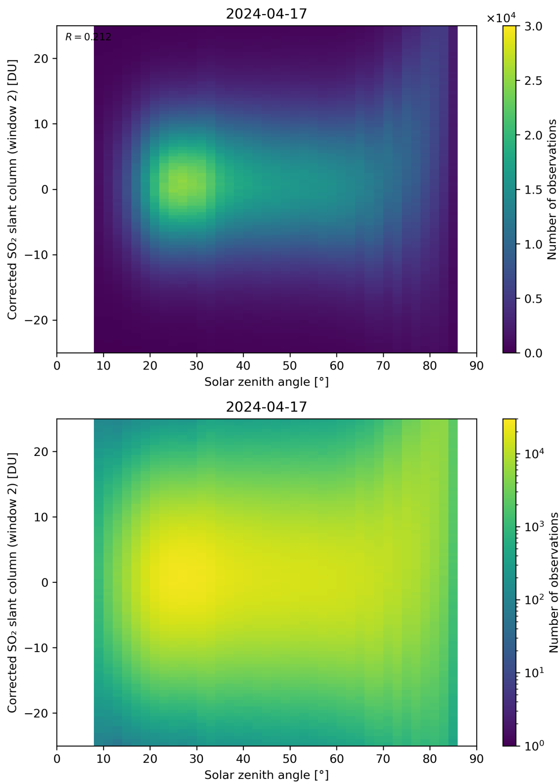
Figure 167: Scatter density plot of “Solar zenith angle” against “Corrected SO 2 slant column (window 2)” for 2024-04-16 to 2024-04-18.
