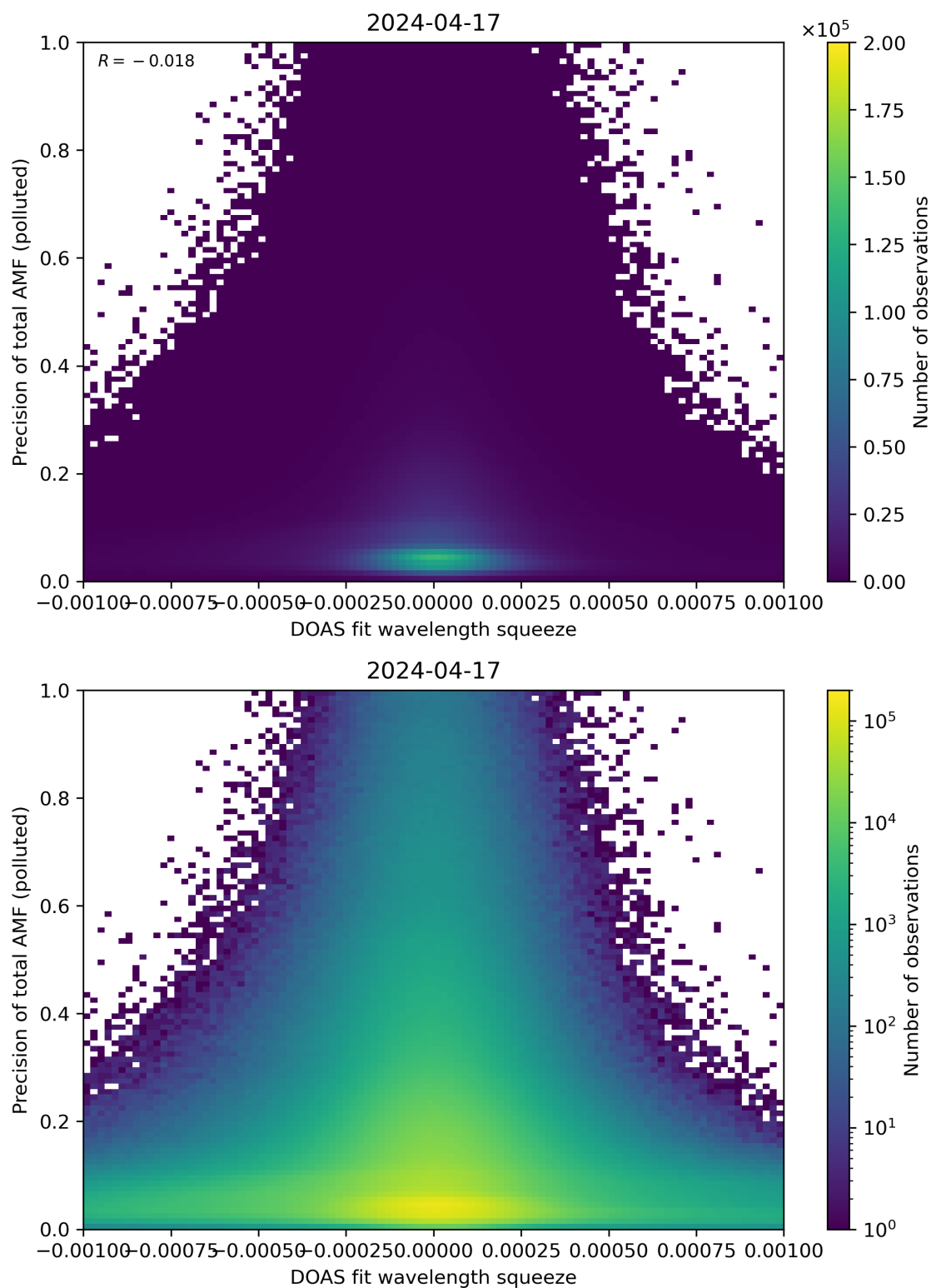
Figure 135: Scatter density plot of “DOAS fit wavelength squeeze” against “Precision of total AMF (polluted)” for 2024-04-16 to 2024-04-18.
