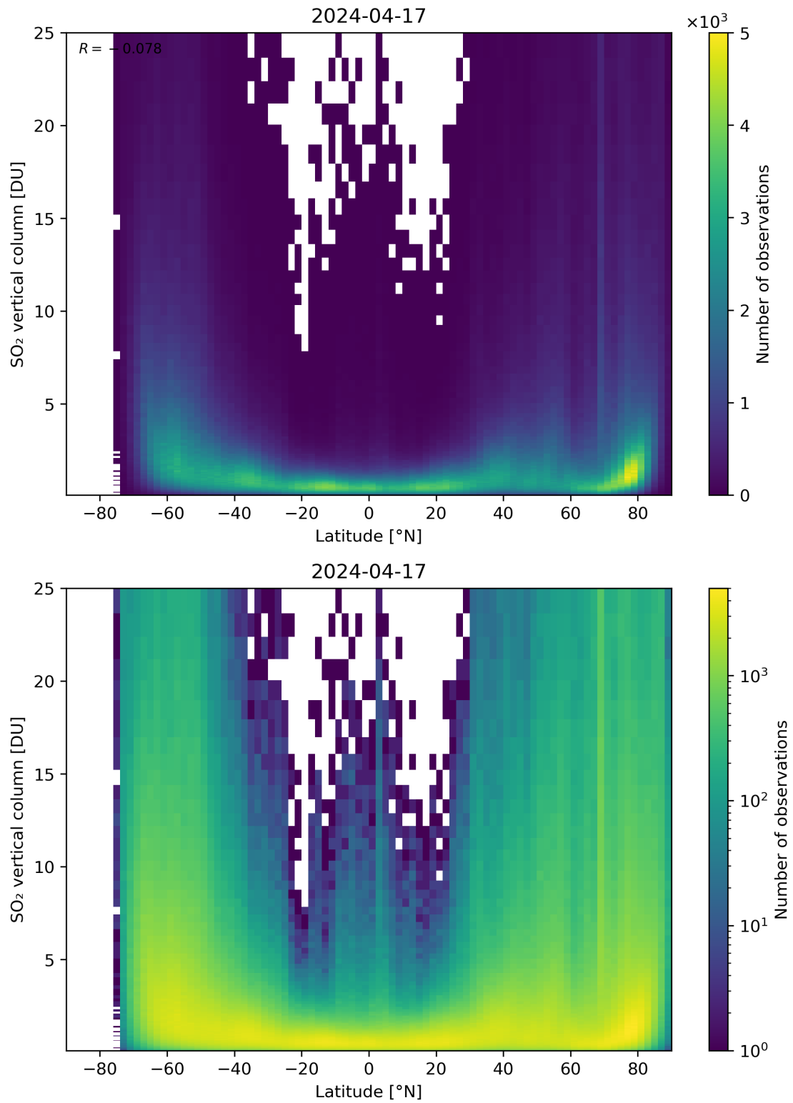
Figure 156: Scatter density plot of “Latitude” against “SO 2 vertical column” for 2024-04-16 to 2024-04-18.
