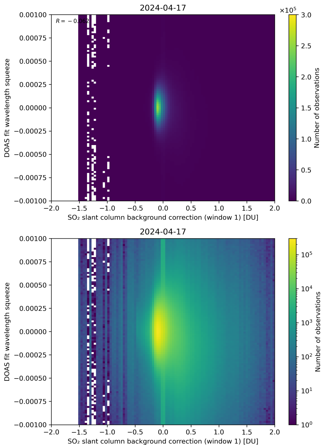
Figure 101: Scatter density plot of “SO 2 slant column background correction (window 1)” against “DOAS fit wavelength squeeze” for 2024-04-16 to 2024-04-18.
