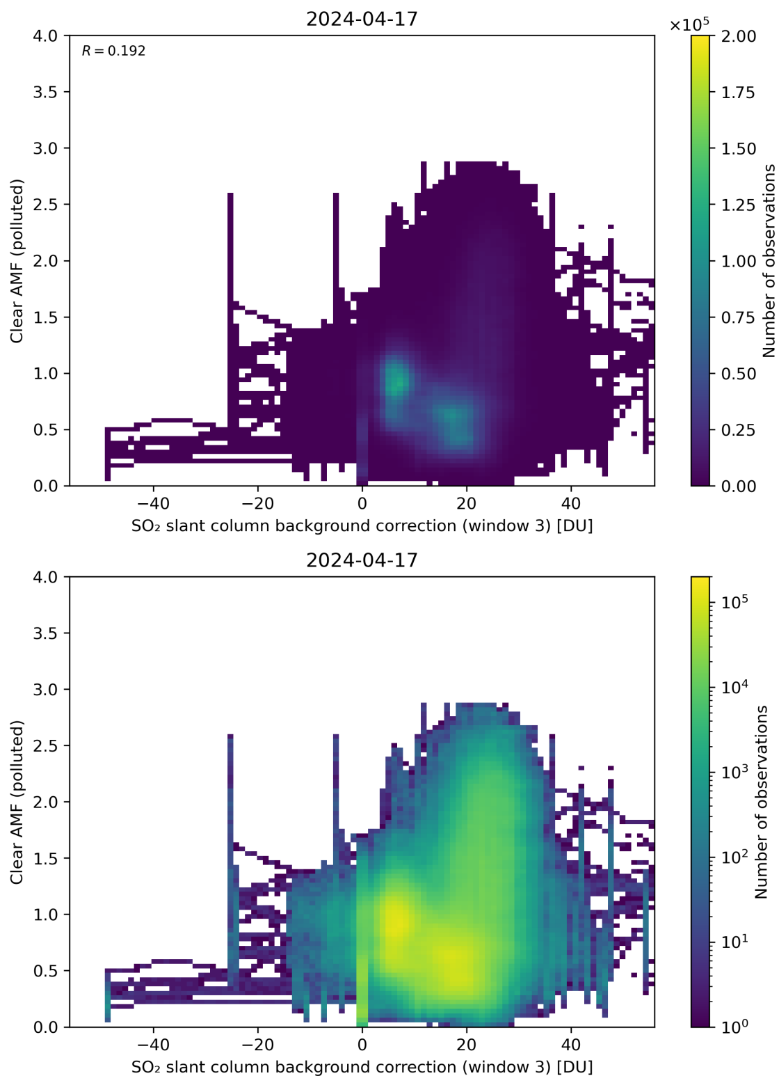
Figure 124: Scatter density plot of “SO 2 slant column background correction (window 3)” against “Clear AMF (polluted)” for 2024-04-16 to 2024-04-18.
