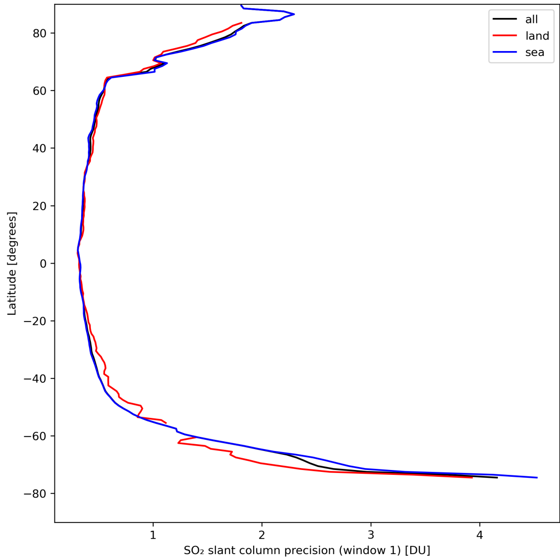
Figure 34: Zonal average of “SO 2 slant column precision (window 1)” for 2024-04-16 to 2024-04-18.
