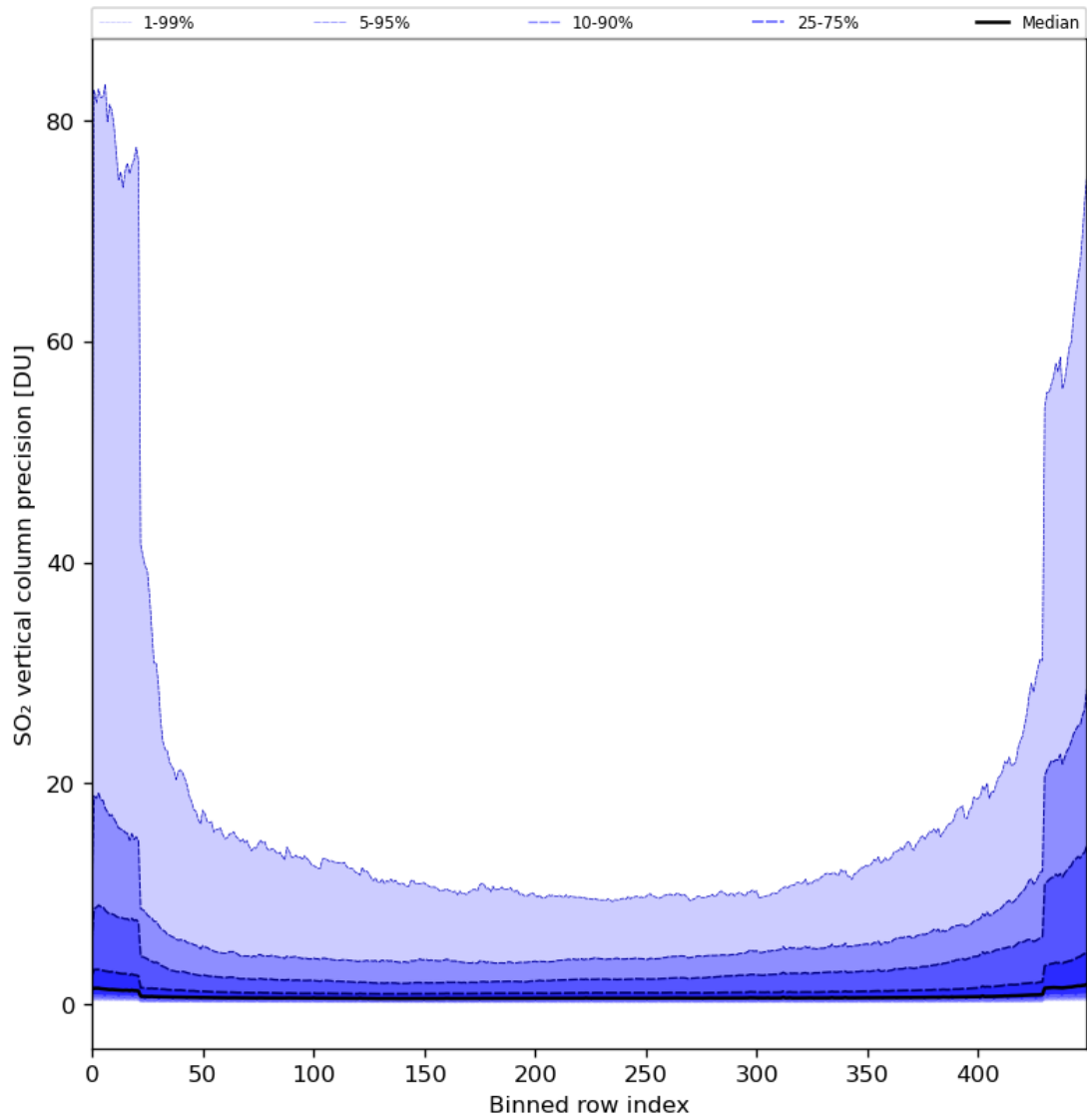
Figure 77: Along track statistics of “SO 2 vertical column precision” for 2024-04-16 to 2024-04-18
