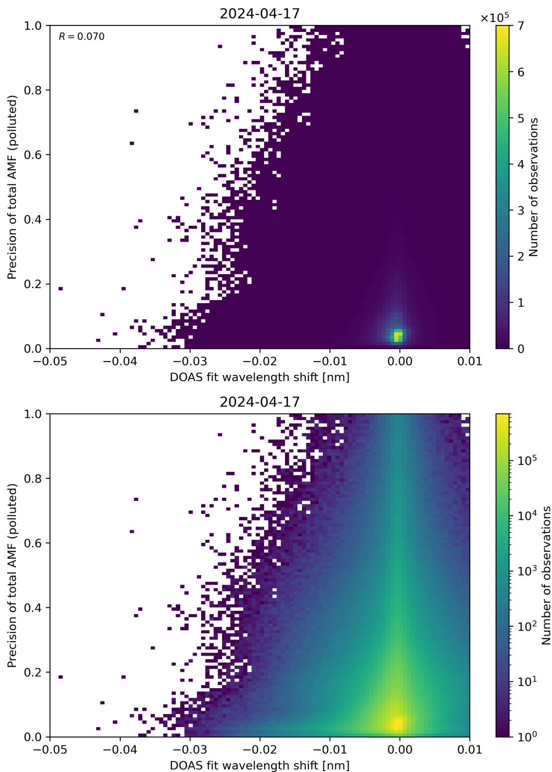
Figure 131: Scatter density plot of “DOAS fit wavelength shift” against “Precision of total AMF (polluted)” for 2024-04-16 to 2024-04-18.
