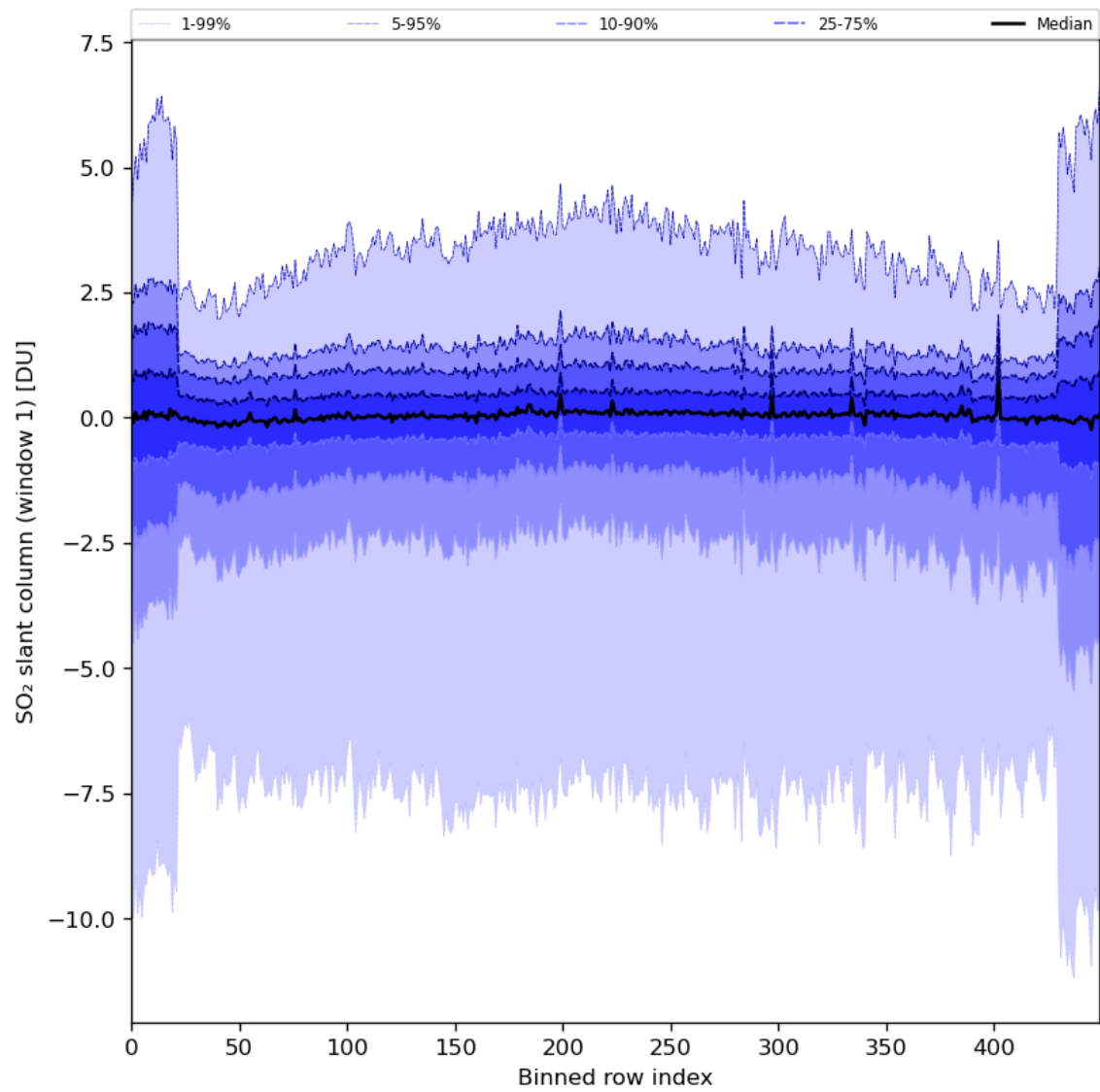
Figure 79: Along track statistics of “SO 2 slant column (window 1)” for 2024-04-16 to 2024-04-18
