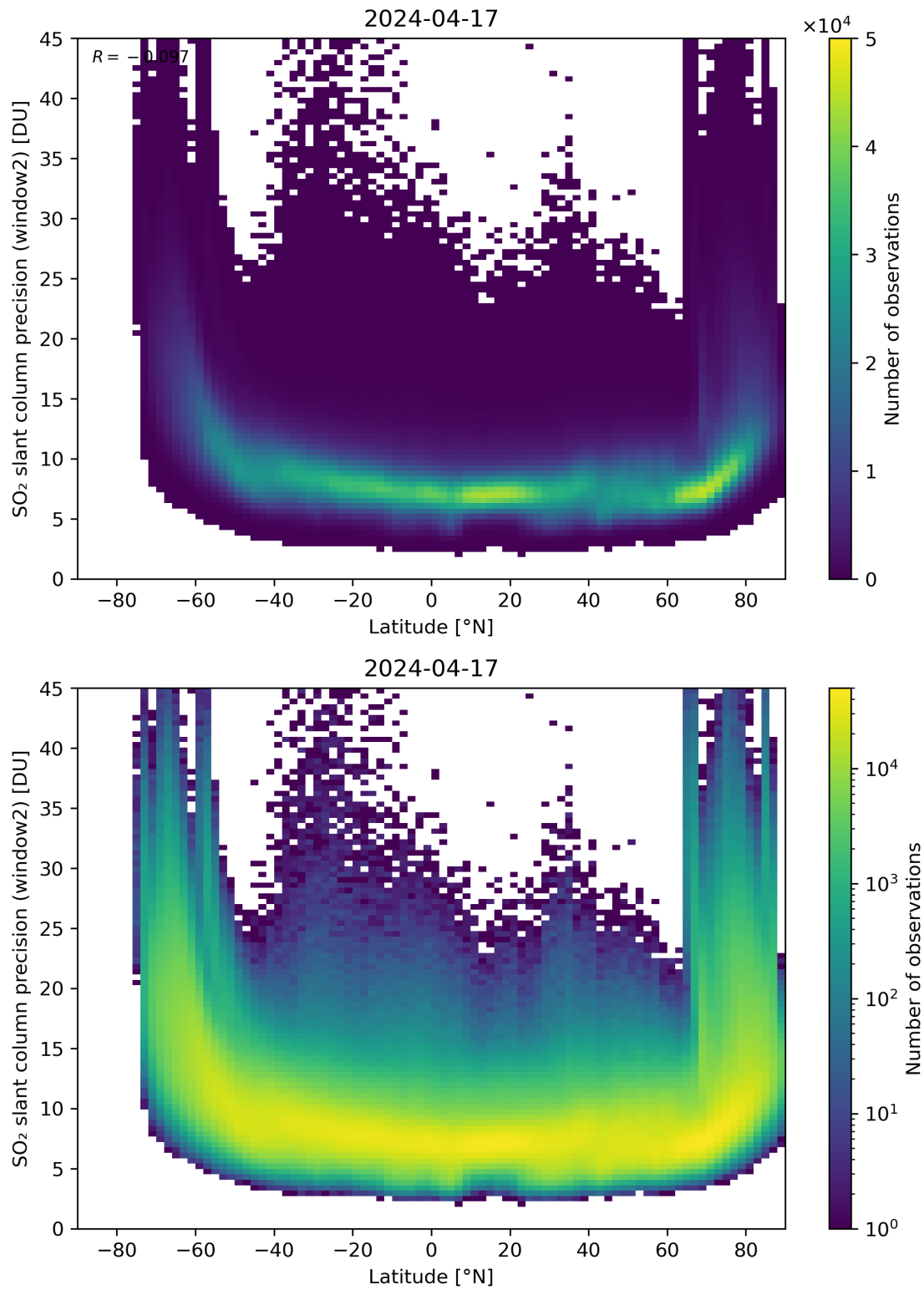
Figure 151: Scatter density plot of “Latitude” against “SO 2 slant column precision (window2)” for 2024-04-16 to 2024-04-18.
