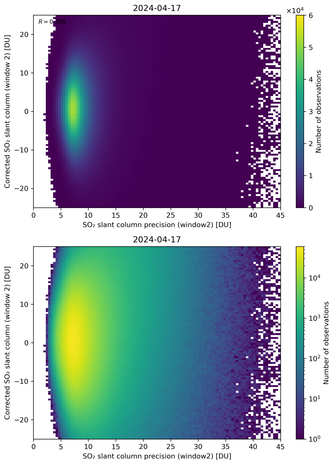
Figure 247: Scatter density plot of “SO 2 slant column precision (window2)” against “Corrected SO 2 slant column (window 2)” for 2024-04-16 to 2024-04-18.
