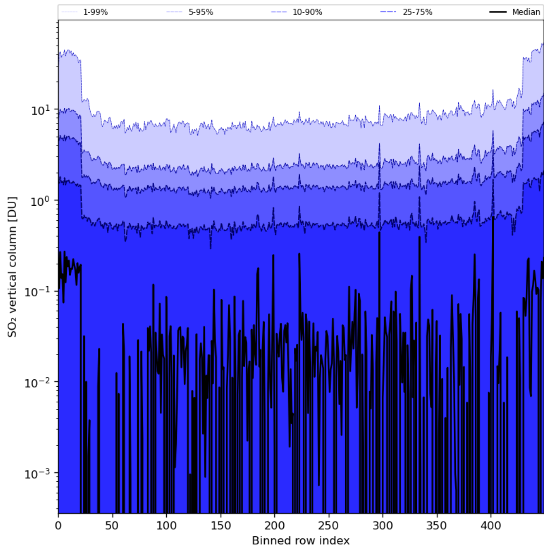
Figure 76: Along track statistics of “SO 2 vertical column” for 2024-04-16 to 2024-04-18
