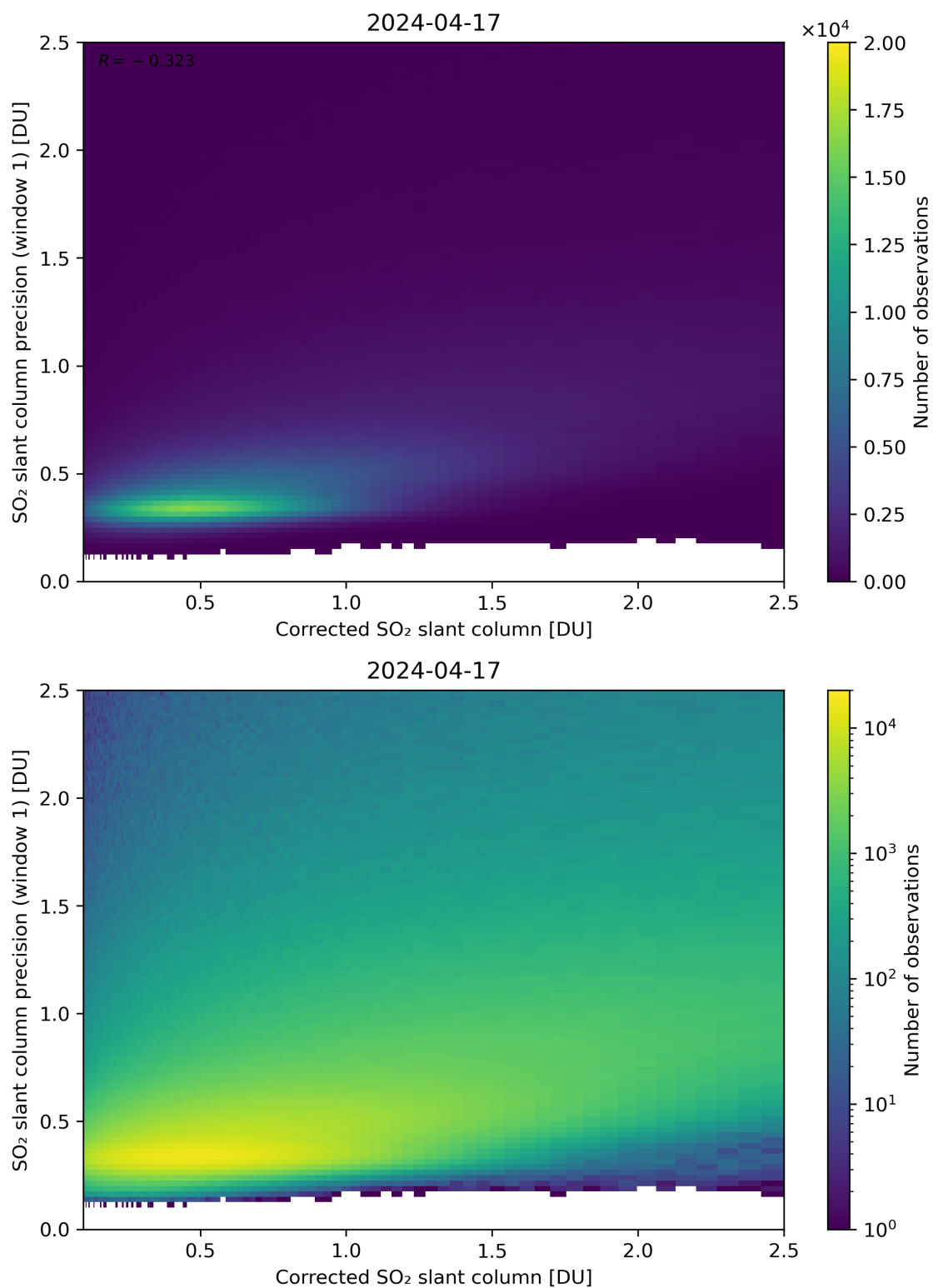
Figure 188: Scatter density plot of “Corrected SO 2 slant column” against “SO 2 slant column precision (window 1)” for 2024-04-16 to 2024-04-18.
