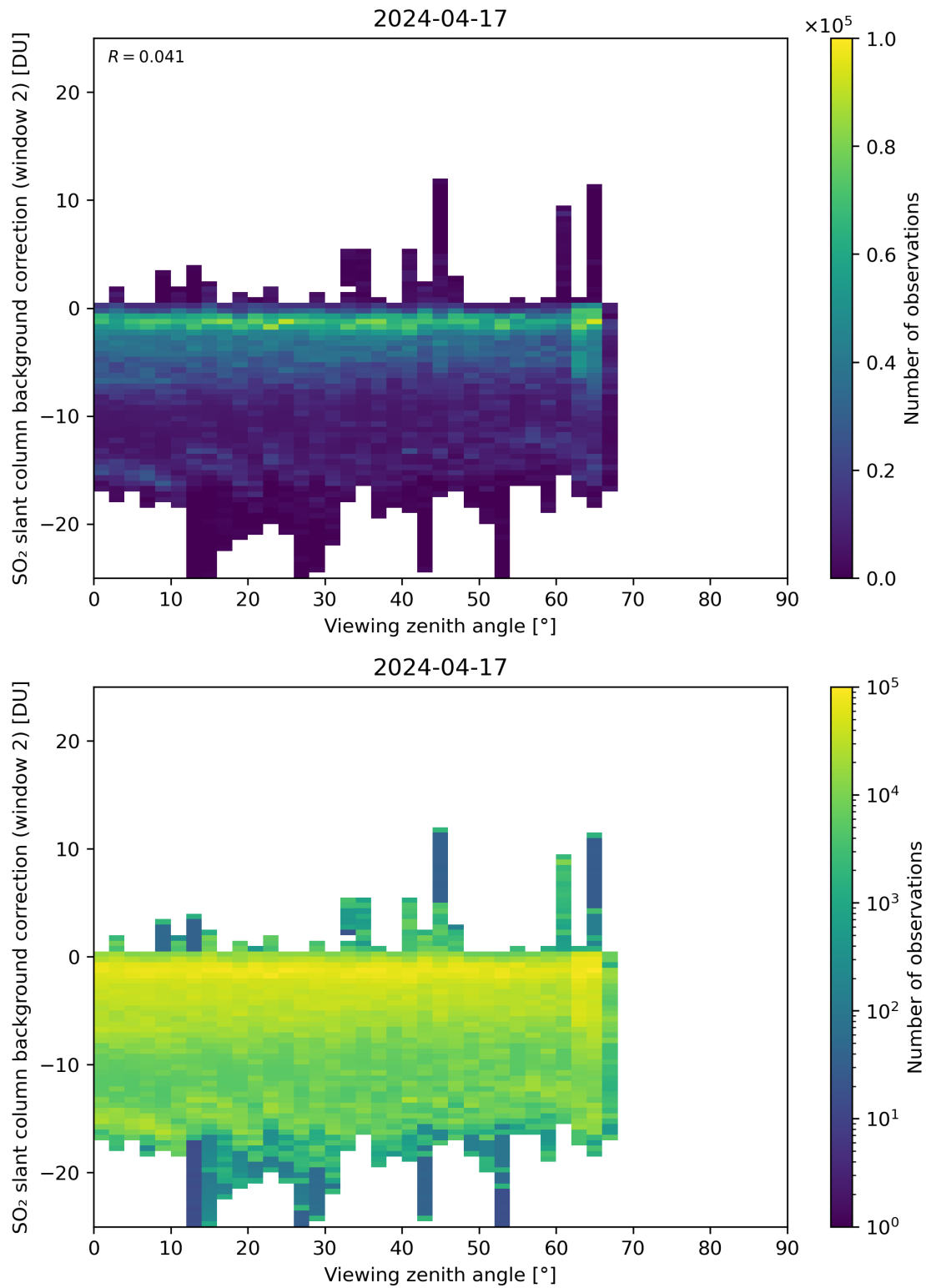
Figure 309: Scatter density plot of “Viewing zenith angle” against “SO 2 slant column background correction (window 2)” for 2024-04-16 to 2024-04-18.
