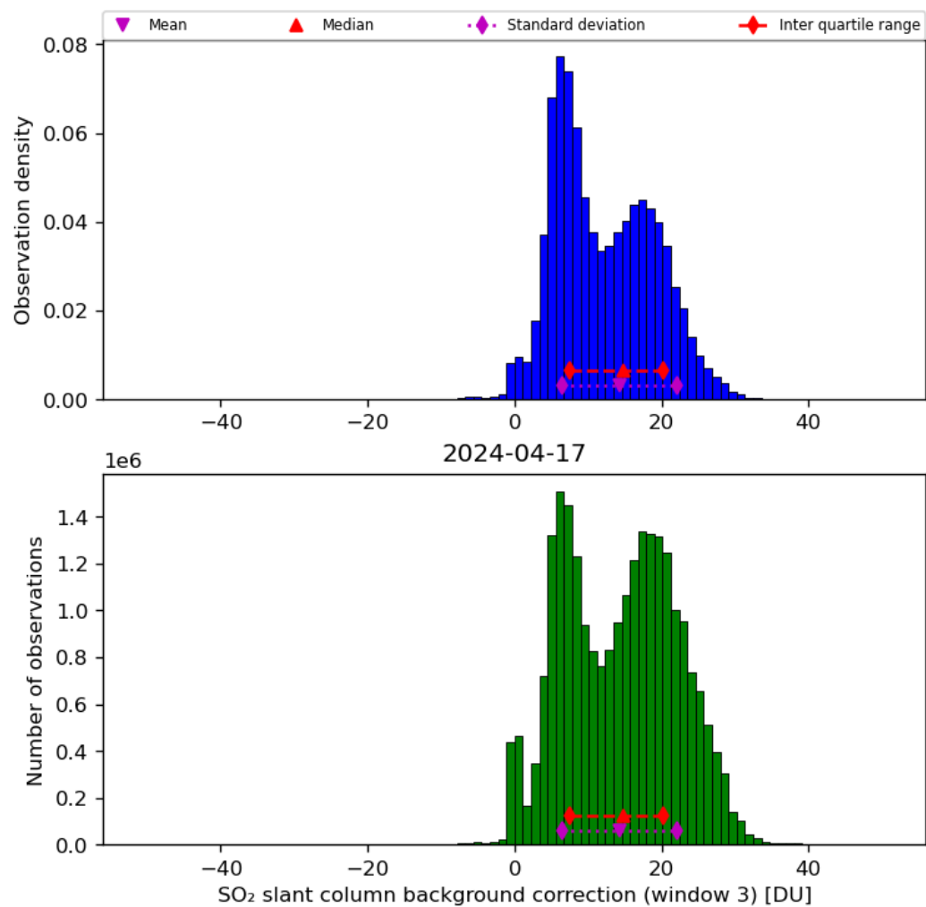
Figure 67: Histogram of “SO 2 slant column background correction (window 3)” for 2024-04-16 to 2024-04-18
