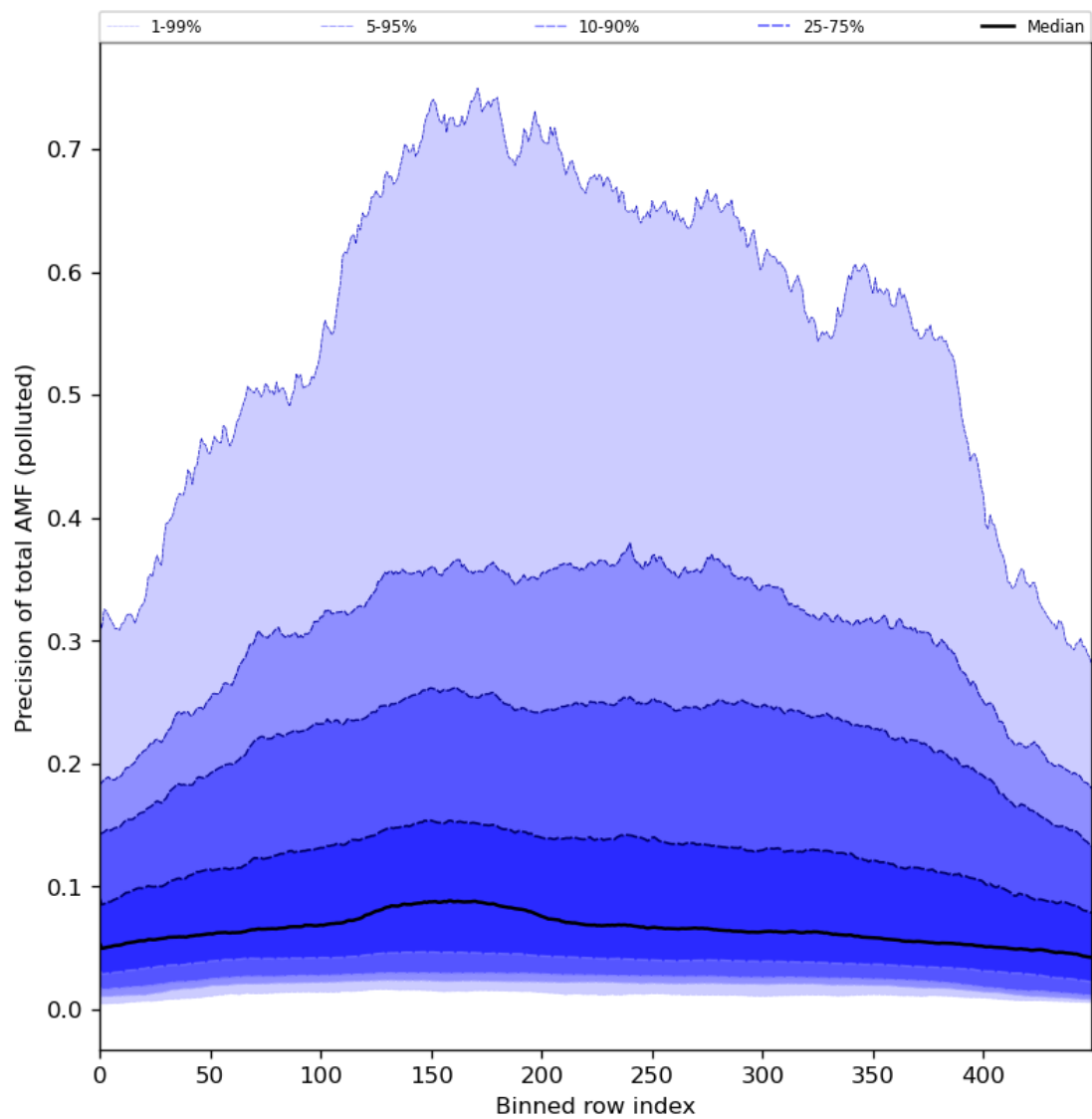
Figure 95: Along track statistics of “Precision of total AMF (polluted)” for 2024-04-16 to 2024-04-18
