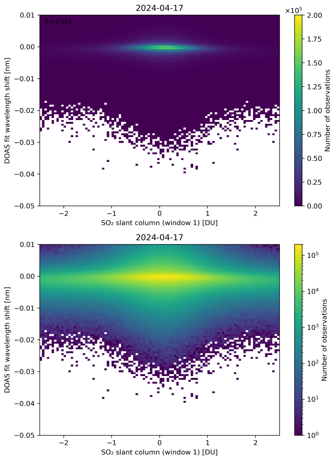
Figure 215: Scatter density plot of “SO 2 slant column (window 1)” against “DOAS fit wavelength shift” for 2024-04-16 to 2024-04-18.
