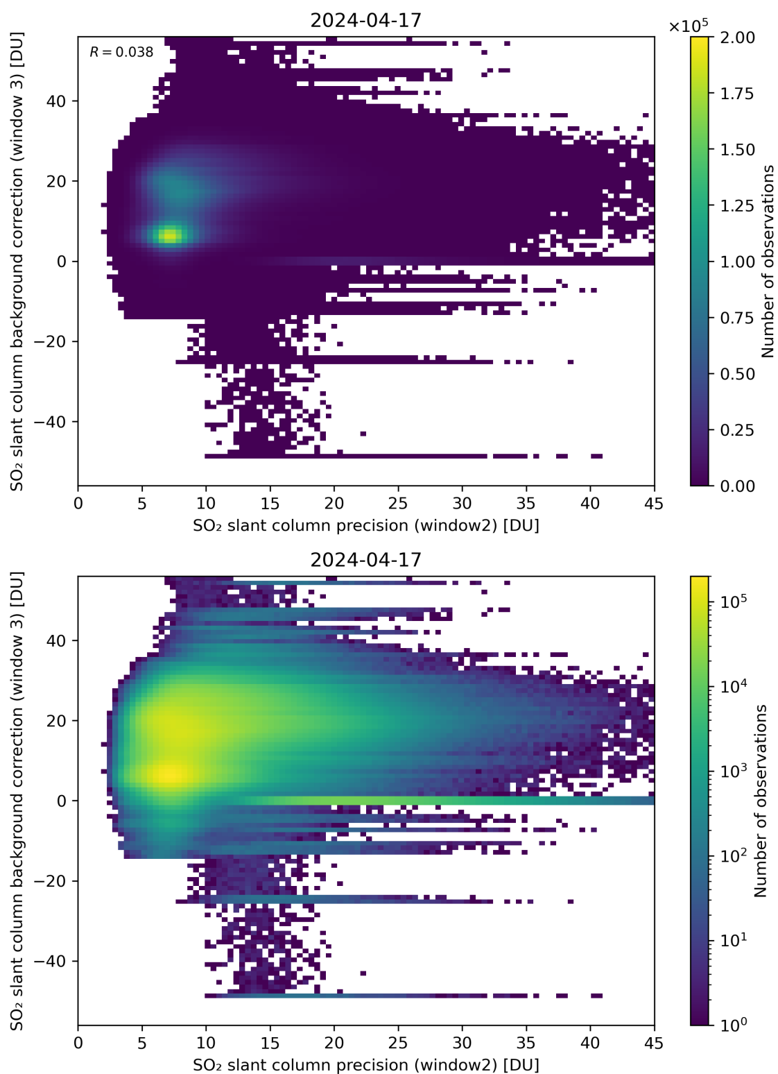
Figure 242: Scatter density plot of “SO 2 slant column precision (window2)” against “SO 2 slant column background correction (window 3)” for 2024-04-16 to 2024-04-18.
