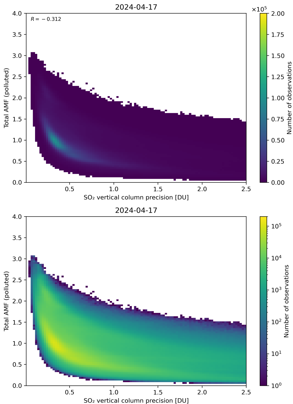
Figure 294: Scatter density plot of “SO 2 vertical column precision” against “Total AMF (polluted)” for 2024-04-16 to 2024-04-18.
