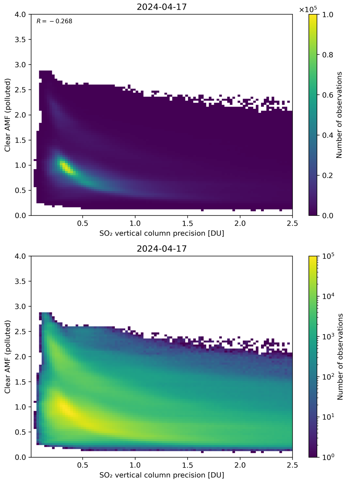
Figure 285: Scatter density plot of “SO 2 vertical column precision” against “Clear AMF (polluted)” for 2024-04-16 to 2024-04-18.
