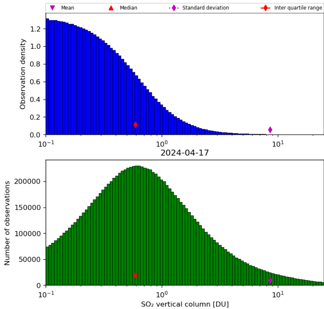
Figure 53: Histogram of “SO 2 vertical column” for 2024-04-16 to 2024-04-18
