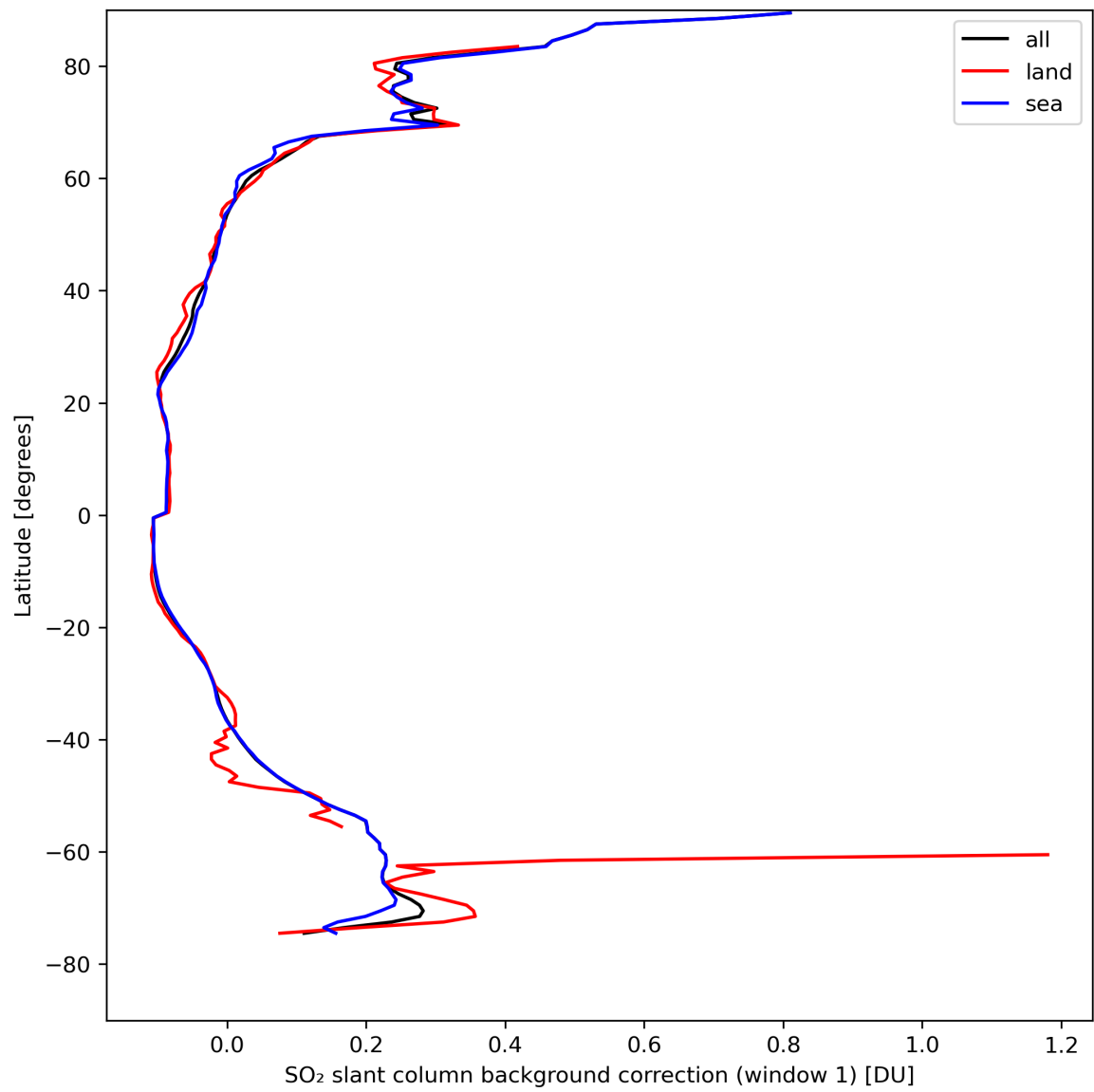
Figure 36: Zonal average of “SO 2 slant column background correction (window 1)” for 2024-04-16 to 2024-04-18.
