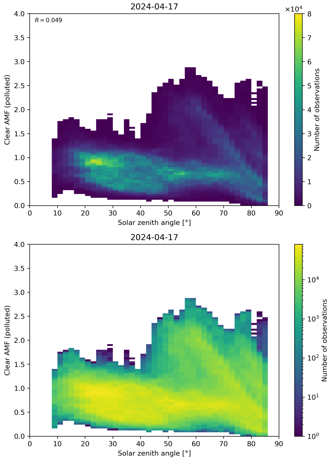
Figure 165: Scatter density plot of “Solar zenith angle” against “Clear AMF (polluted)” for 2024-04-16 to 2024-04-18.
