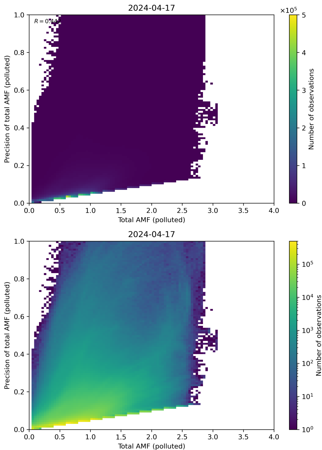
Figure 272: Scatter density plot of “Total AMF (polluted)” against “Precision of total AMF (polluted)” for 2024-04-16 to 2024-04-18.
