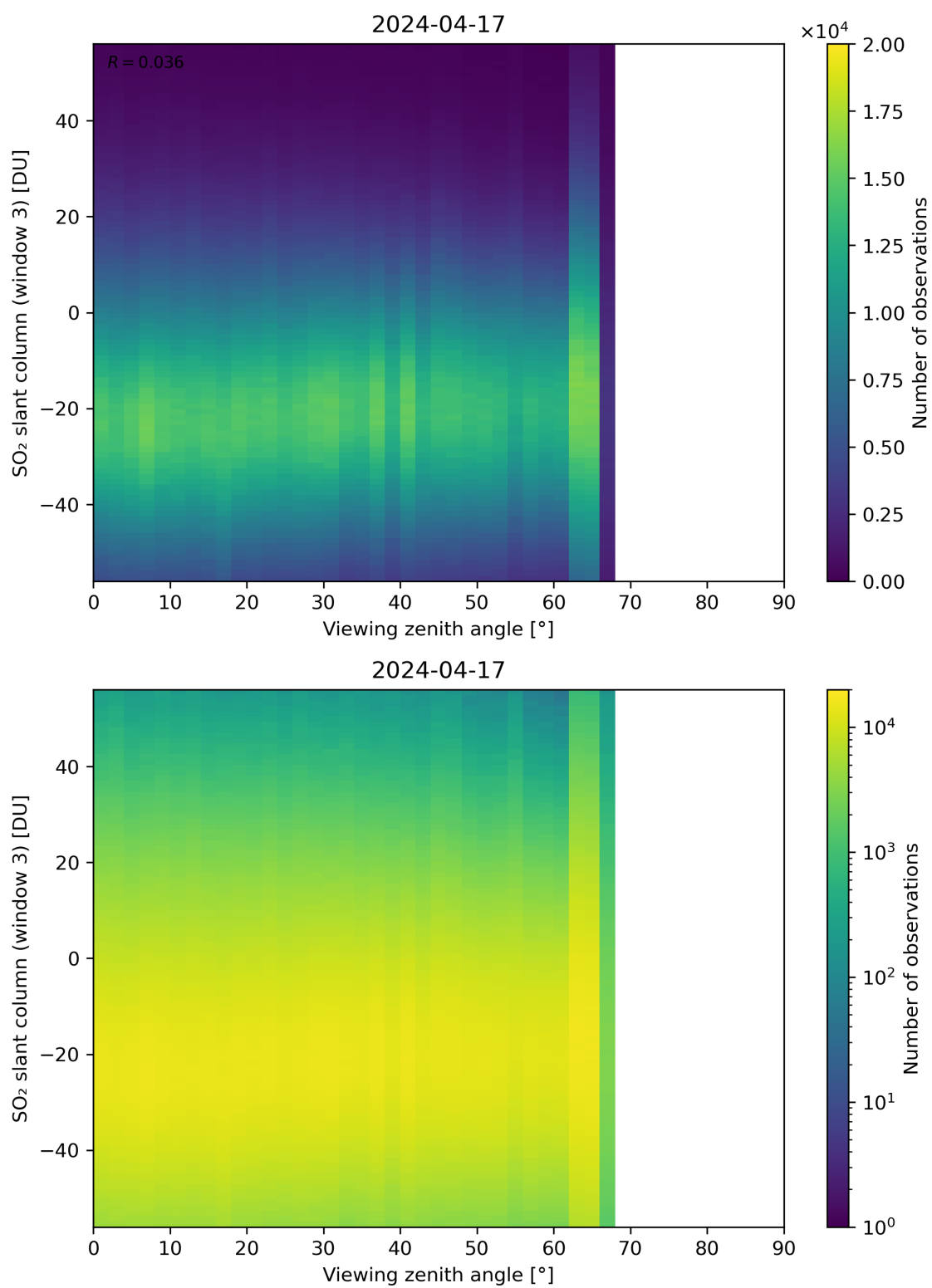
Figure 323: Scatter density plot of “Viewing zenith angle” against “SO 2 slant column (window 3)” for 2024-04-16 to 2024-04-18.
