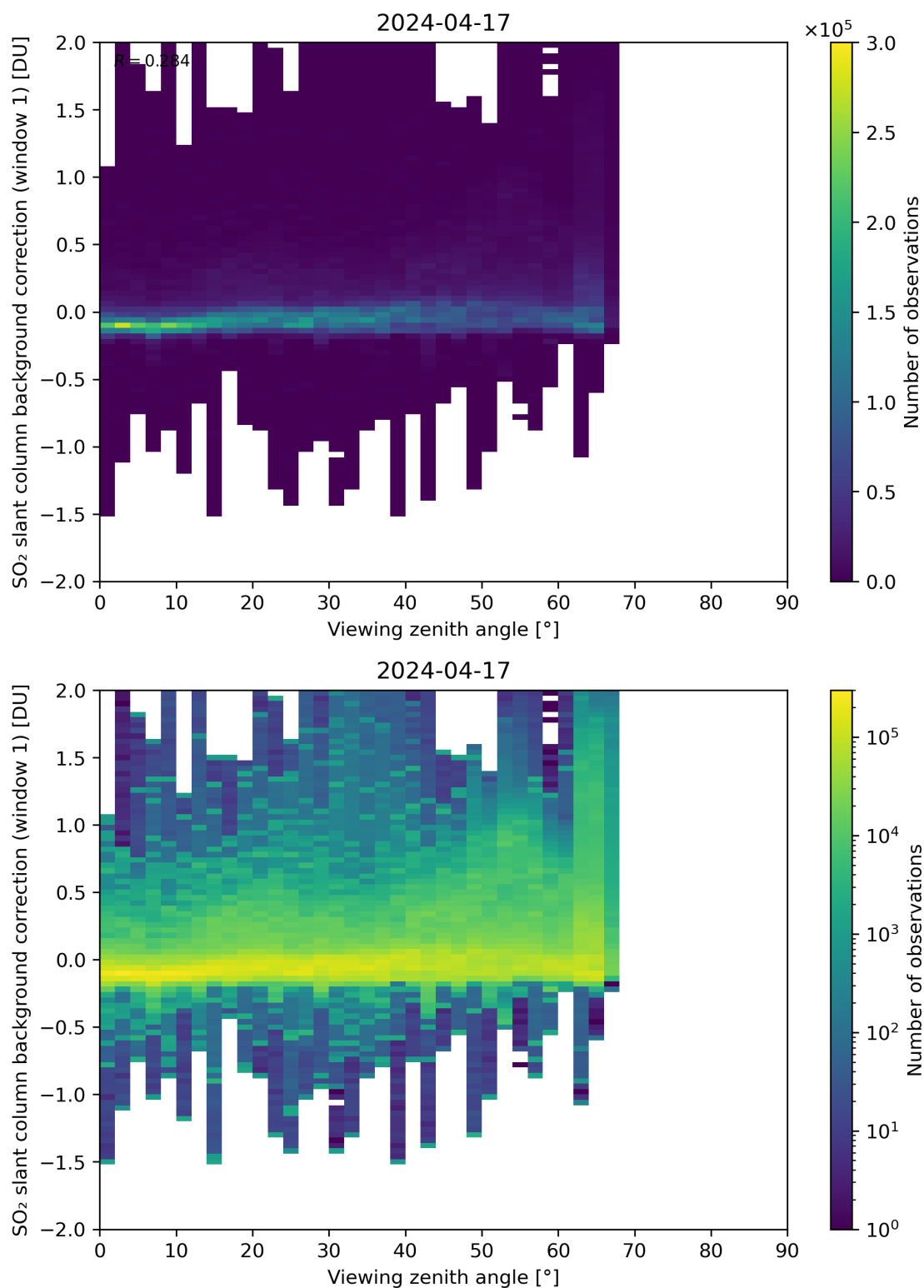
Figure 308: Scatter density plot of “Viewing zenith angle” against “SO 2 slant column background correction (window 1)” for 2024-04-16 to 2024-04-18.
