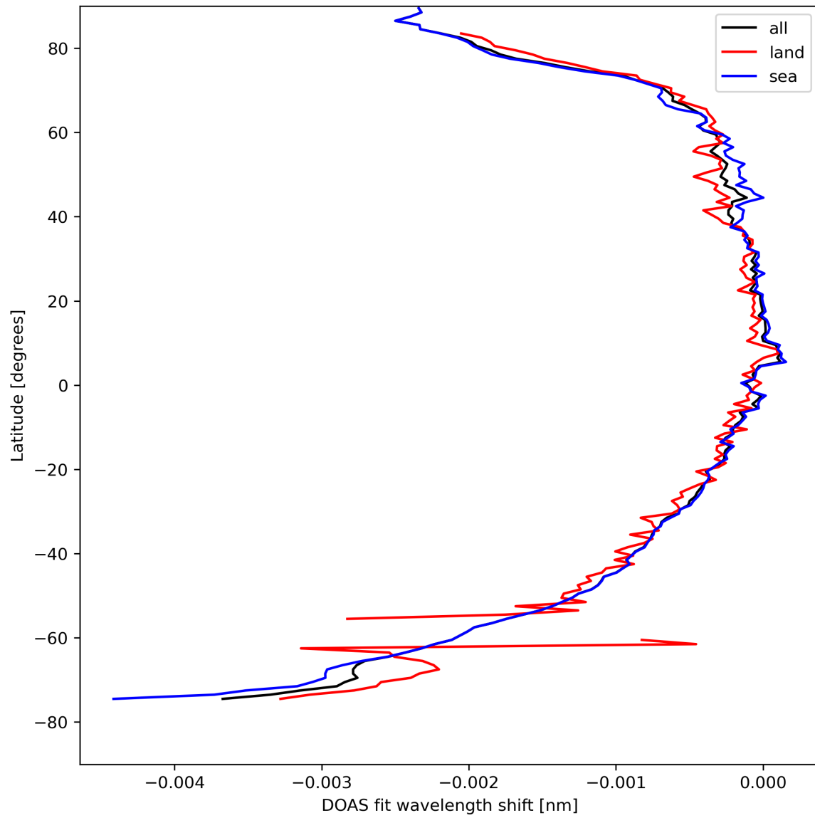
Figure 45: Zonal average of “DOAS fit wavelength shift” for 2024-04-16 to 2024-04-18.
