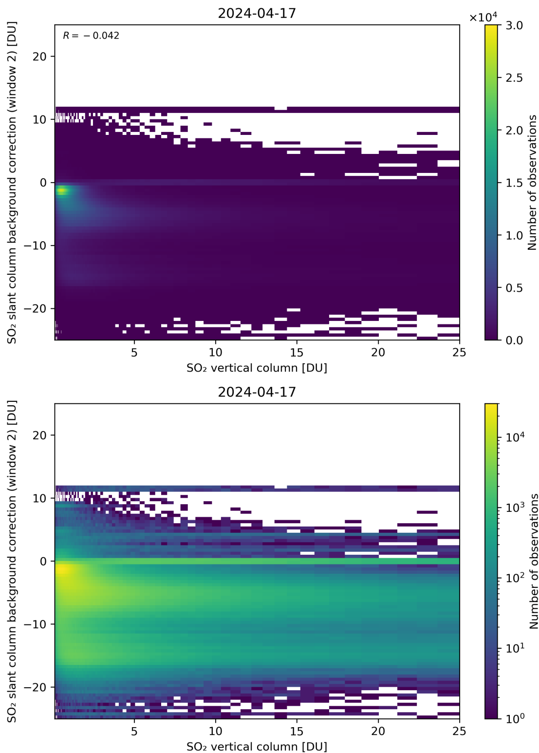
Figure 274: Scatter density plot of “SO 2 vertical column” against “SO 2 slant column background correction (window 2)” for 2024-04-16 to 2024-04-18.
