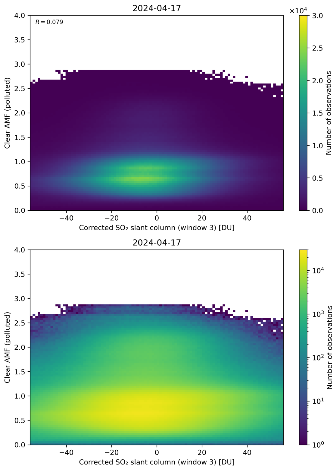
Figure 209: Scatter density plot of “Corrected SO 2 slant column (window 3)” against “Clear AMF (polluted)” for 2024-04-16 to 2024-04-18.
