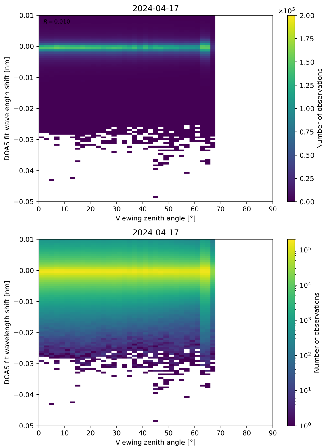
Figure 311: Scatter density plot of “Viewing zenith angle” against “DOAS fit wavelength shift” for 2024-04-16 to 2024-04-18.
