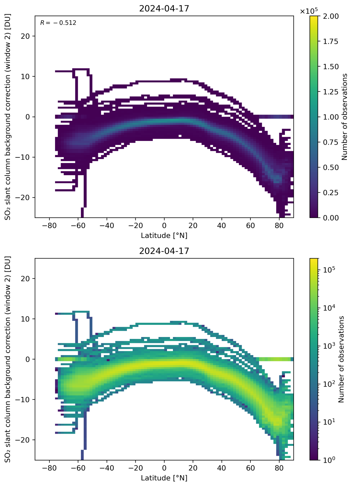
Figure 140: Scatter density plot of “Latitude” against “SO 2 slant column background correction (window 2)” for 2024-04-16 to 2024-04-18.
