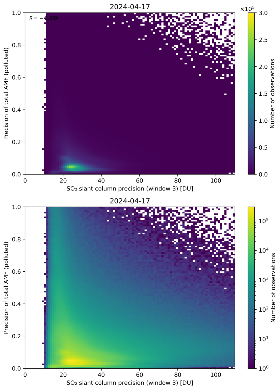
Figure 264: Scatter density plot of “SO 2 slant column precision (window 3)” against “Precision of total AMF (polluted)” for 2024-04-16 to 2024-04-18.
