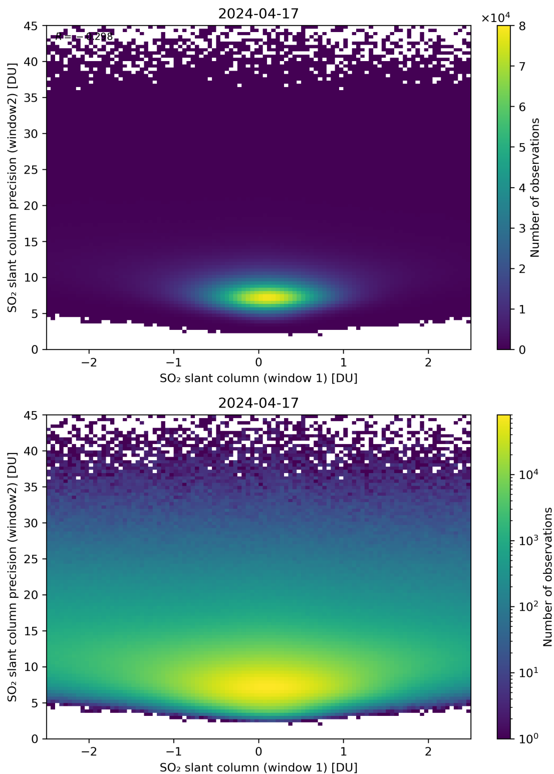
Figure 236: Scatter density plot of “SO 2 slant column (window 1)” against “SO 2 slant column precision (window2)” for 2024-04-16 to 2024-04-18.
