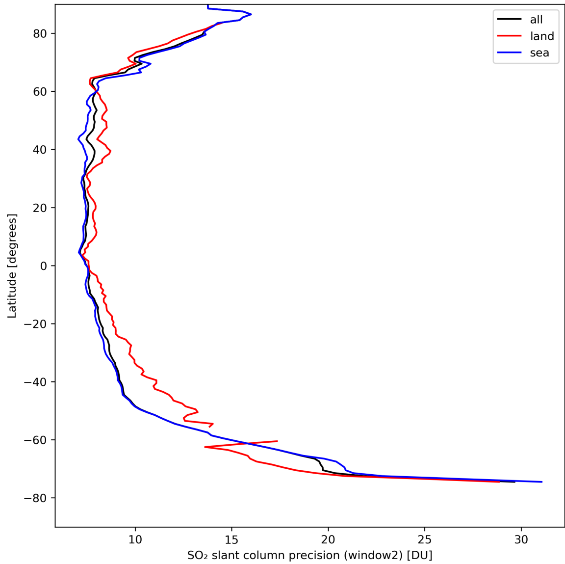
Figure 38: Zonal average of “SO 2 slant column precision (window2)” for 2024-04-16 to 2024-04-18.
