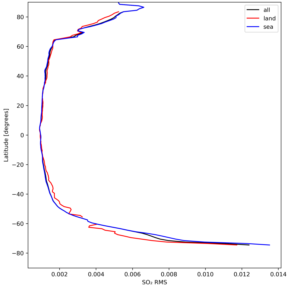
Figure 47: Zonal average of “SO 2 RMS” for 2024-04-16 to 2024-04-18.
