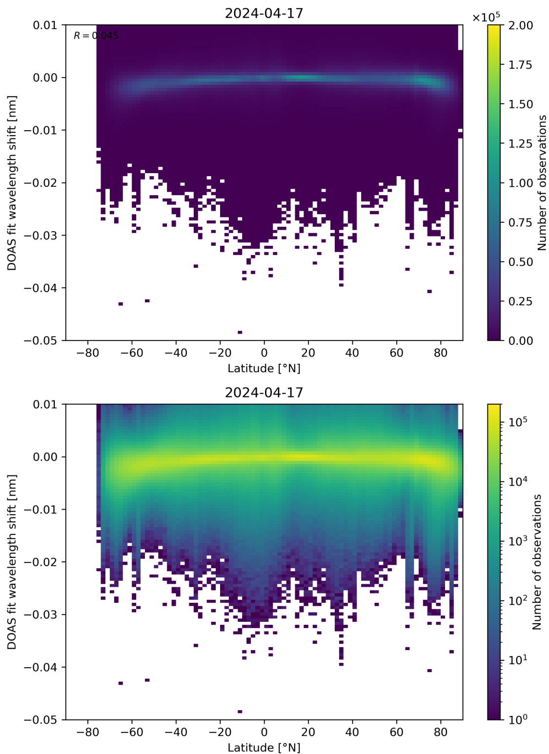
Figure 142: Scatter density plot of “Latitude” against “DOAS fit wavelength shift” for 2024-04-16 to 2024-04-18.
