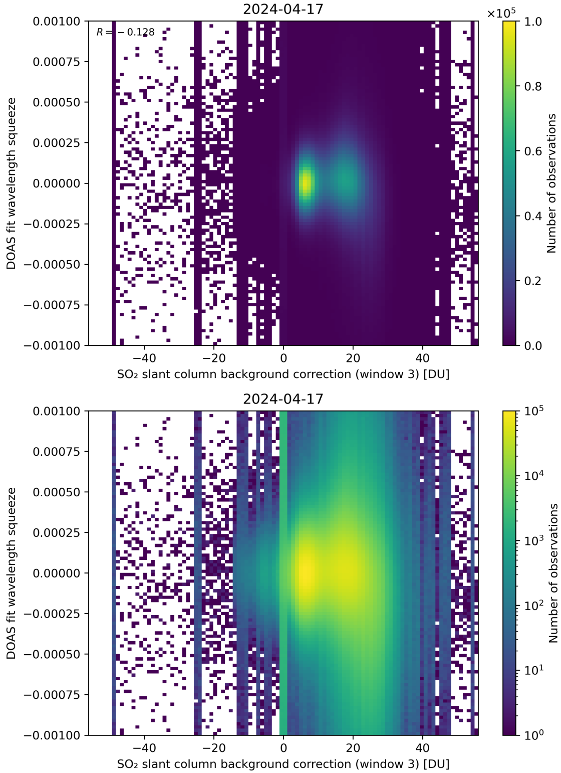
Figure 122: Scatter density plot of “SO 2 slant column background correction (window 3)” against “DOAS fit wavelength squeeze” for 2024-04-16 to 2024-04-18.
