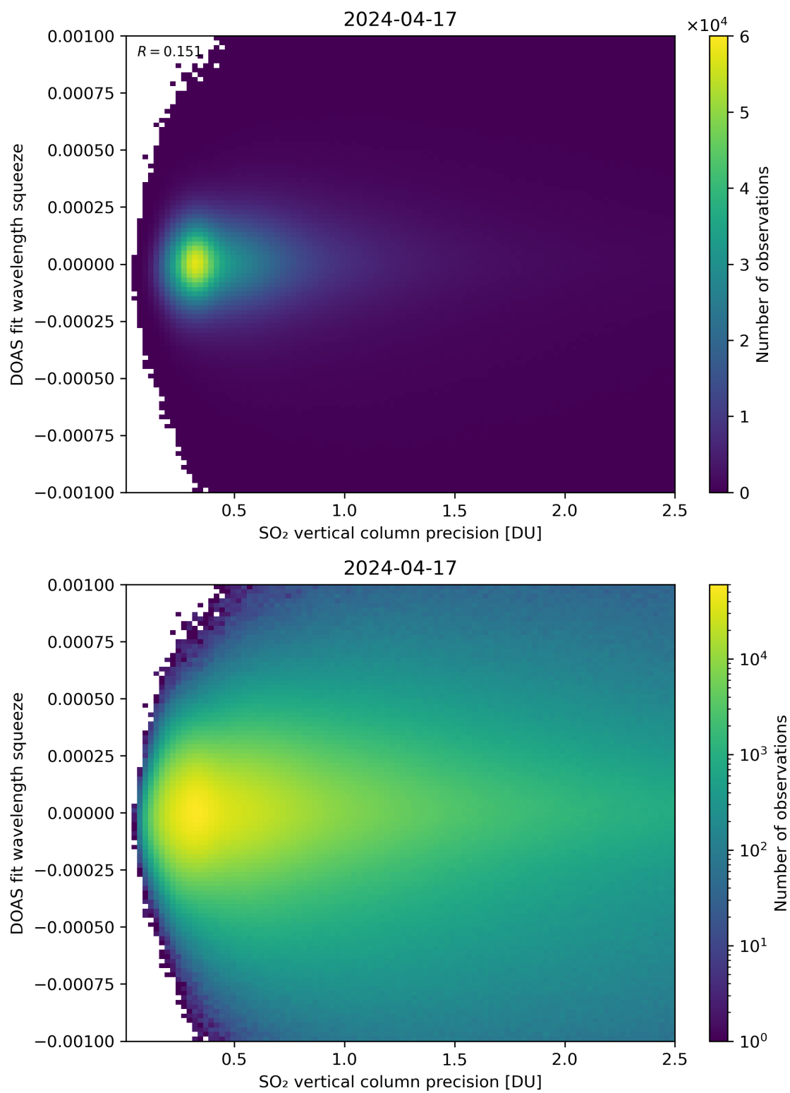
Figure 283: Scatter density plot of “SO 2 vertical column precision” against “DOAS fit wavelength squeeze” for 2024-04-16 to 2024-04-18.
