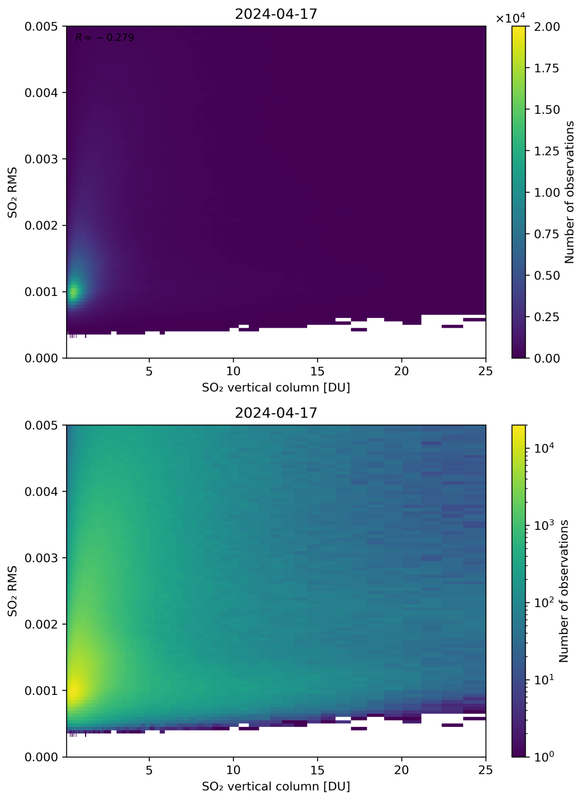
Figure 278: Scatter density plot of “SO 2 vertical column” against “SO 2 RMS” for 2024-04-16 to 2024-04-18.
