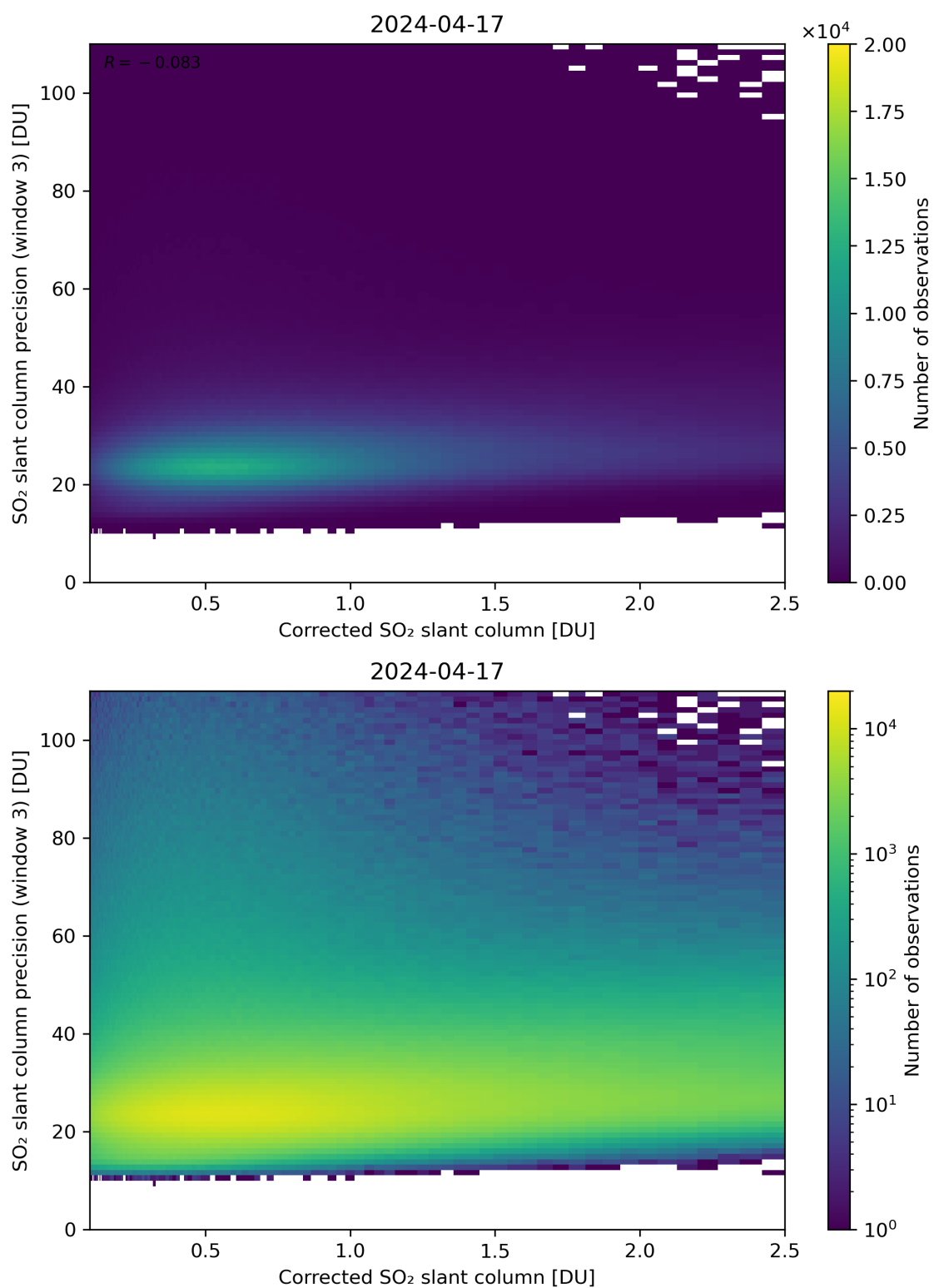
Figure 191: Scatter density plot of “Corrected SO 2 slant column” against “SO 2 slant column precision (window 3)” for 2024-04-16 to 2024-04-18.
