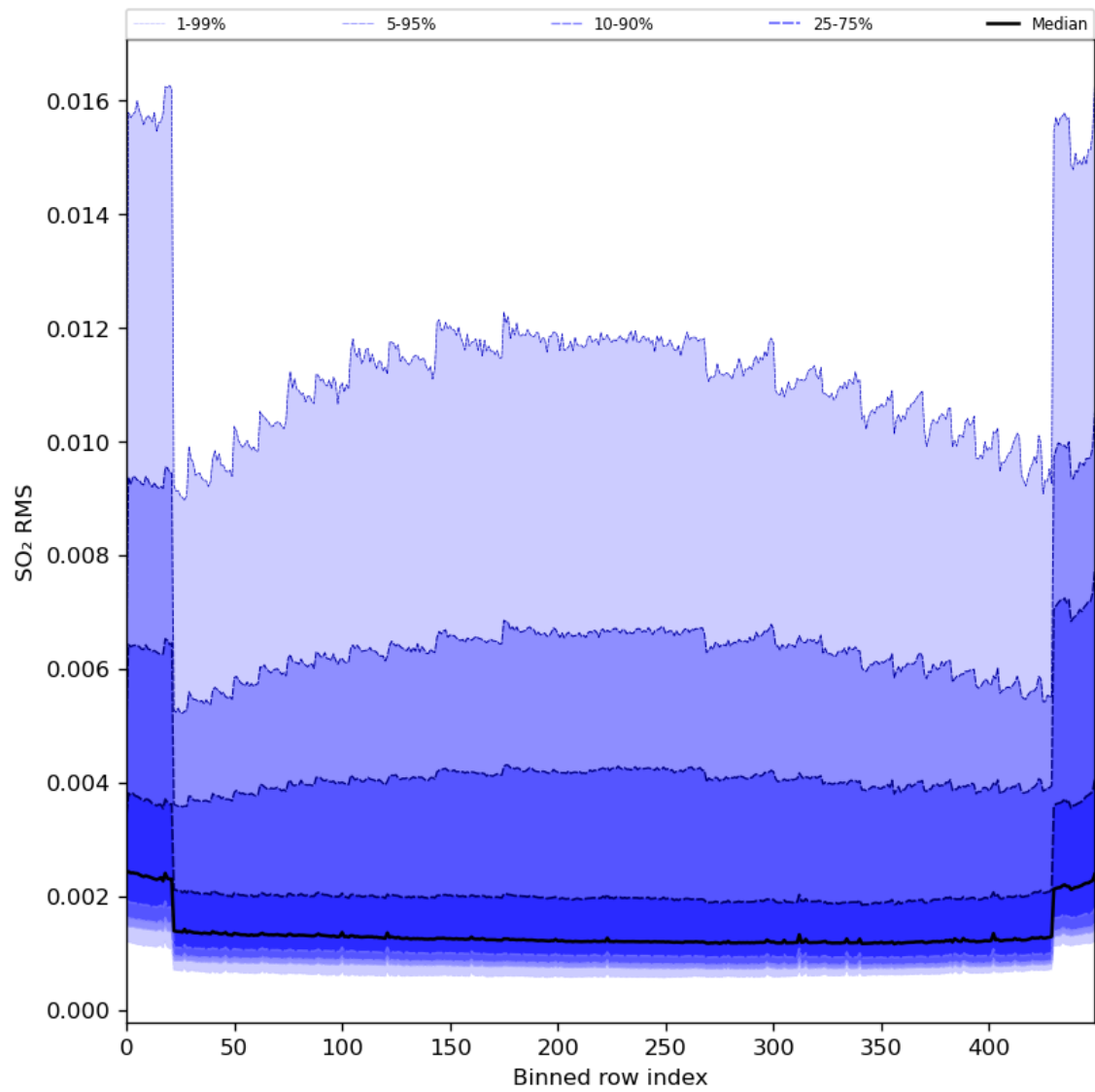
Figure 93: Along track statistics of “SO 2 RMS” for 2024-04-16 to 2024-04-18
