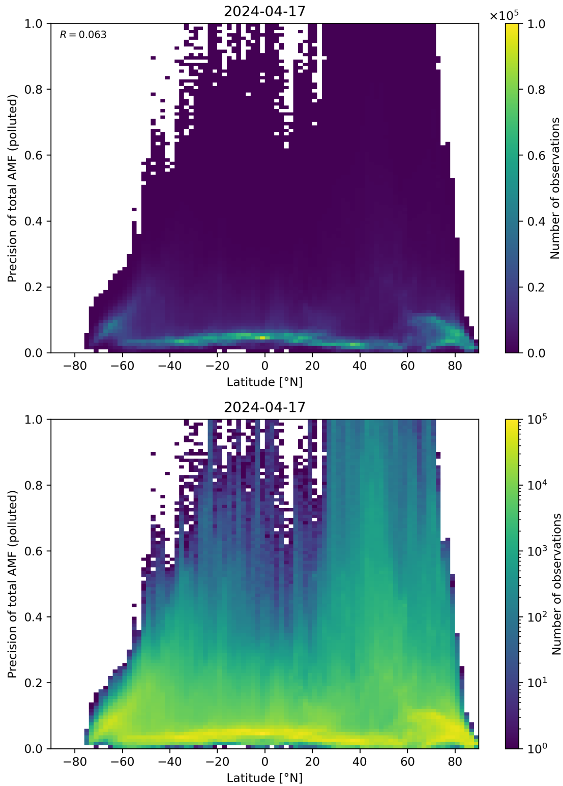
Figure 155: Scatter density plot of “Latitude” against “Precision of total AMF (polluted)” for 2024-04-16 to 2024-04-18.
