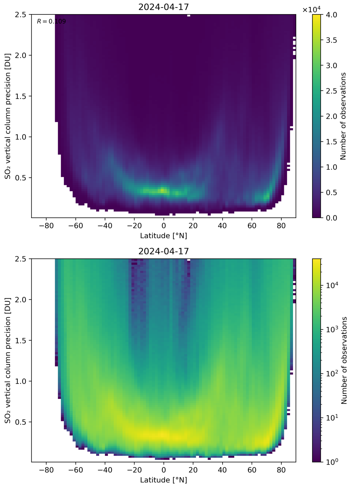
Figure 157: Scatter density plot of “Latitude” against “SO 2 vertical column precision” for 2024-04-16 to 2024-04-18.
