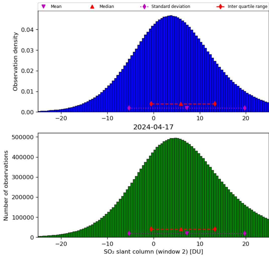
Figure 60: Histogram of “SO 2 slant column (window 2)” for 2024-04-16 to 2024-04-18
