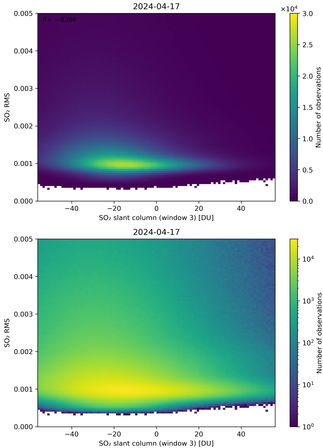
Figure 256: Scatter density plot of “SO 2 slant column (window 3)” against “SO 2 RMS” for 2024-04-16 to 2024-04-18.
