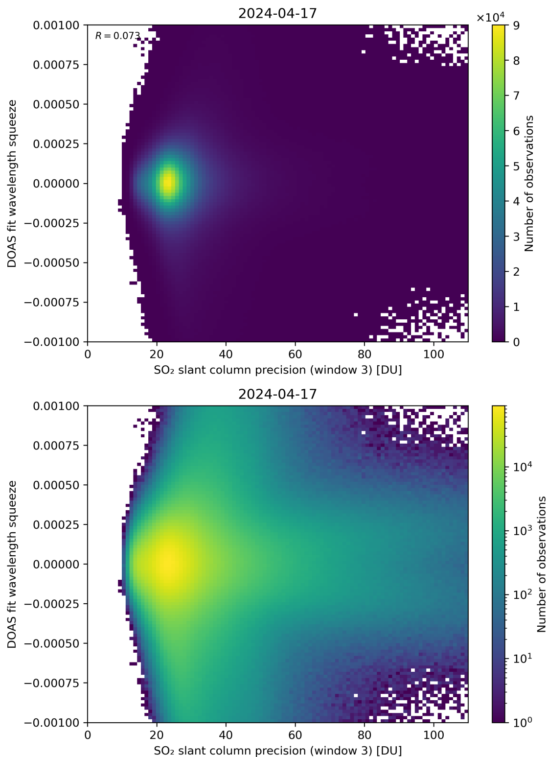
Figure 259: Scatter density plot of “SO 2 slant column precision (window 3)” against “DOAS fit wavelength squeeze” for 2024-04-16 to 2024-04-18.
