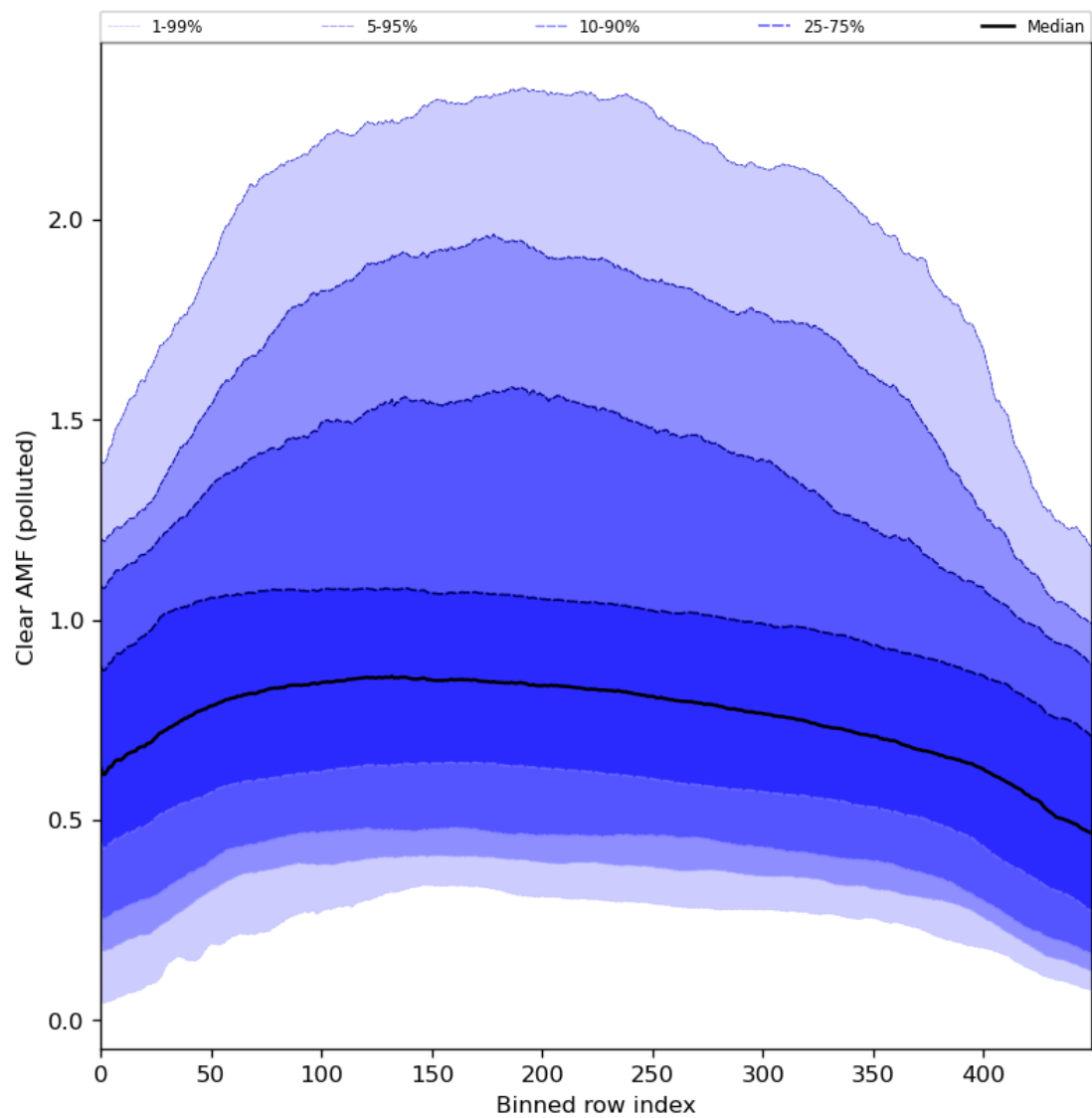
Figure 96: Along track statistics of “Clear AMF (polluted)” for 2024-04-16 to 2024-04-18
