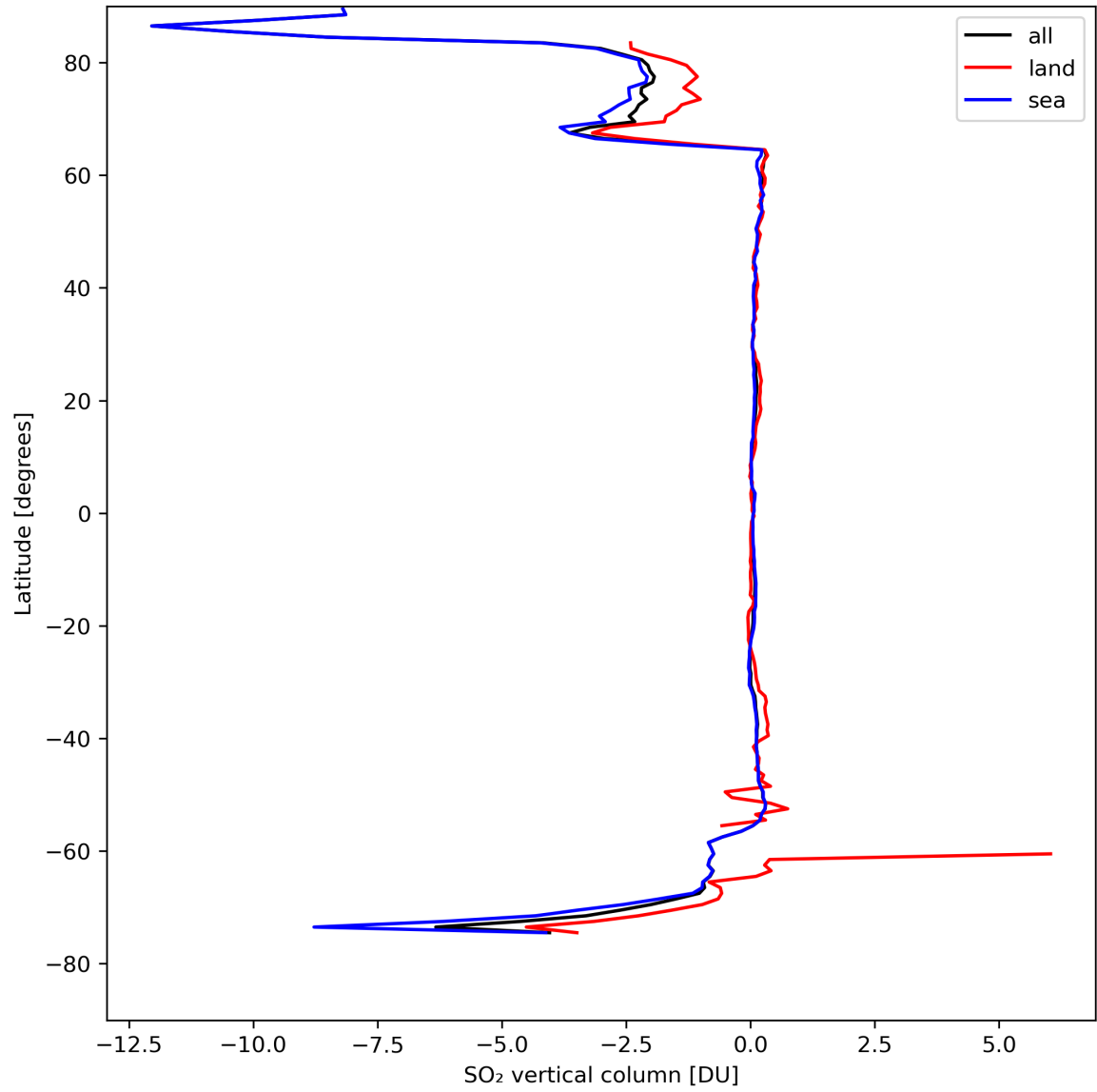
Figure 30: Zonal average of “SO 2 vertical column” for 2024-04-16 to 2024-04-18.
