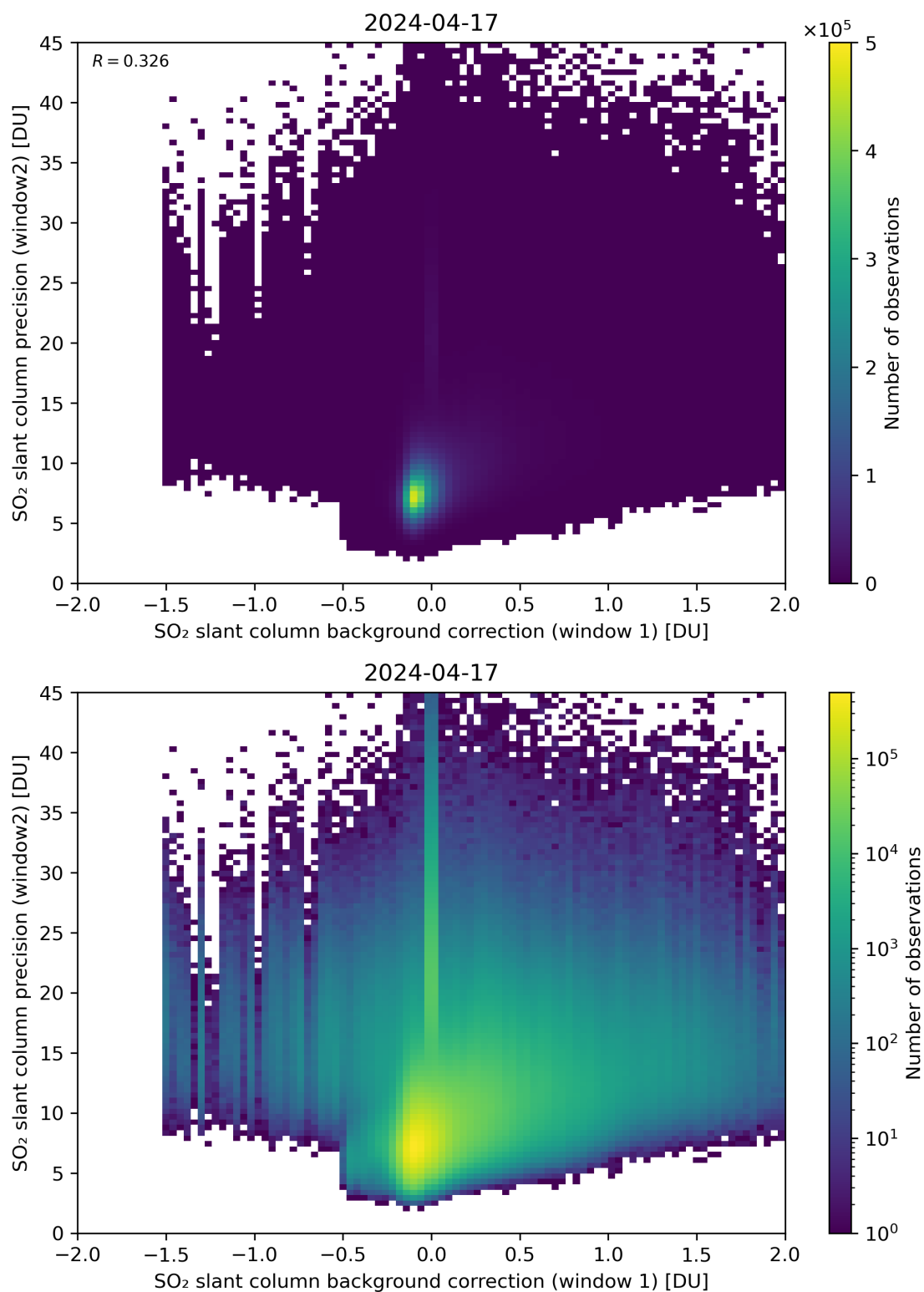
Figure 106: Scatter density plot of “SO 2 slant column background correction (window 1)” against “SO 2 slant column precision (window2)” for 2024-04-16 to 2024-04-18.
