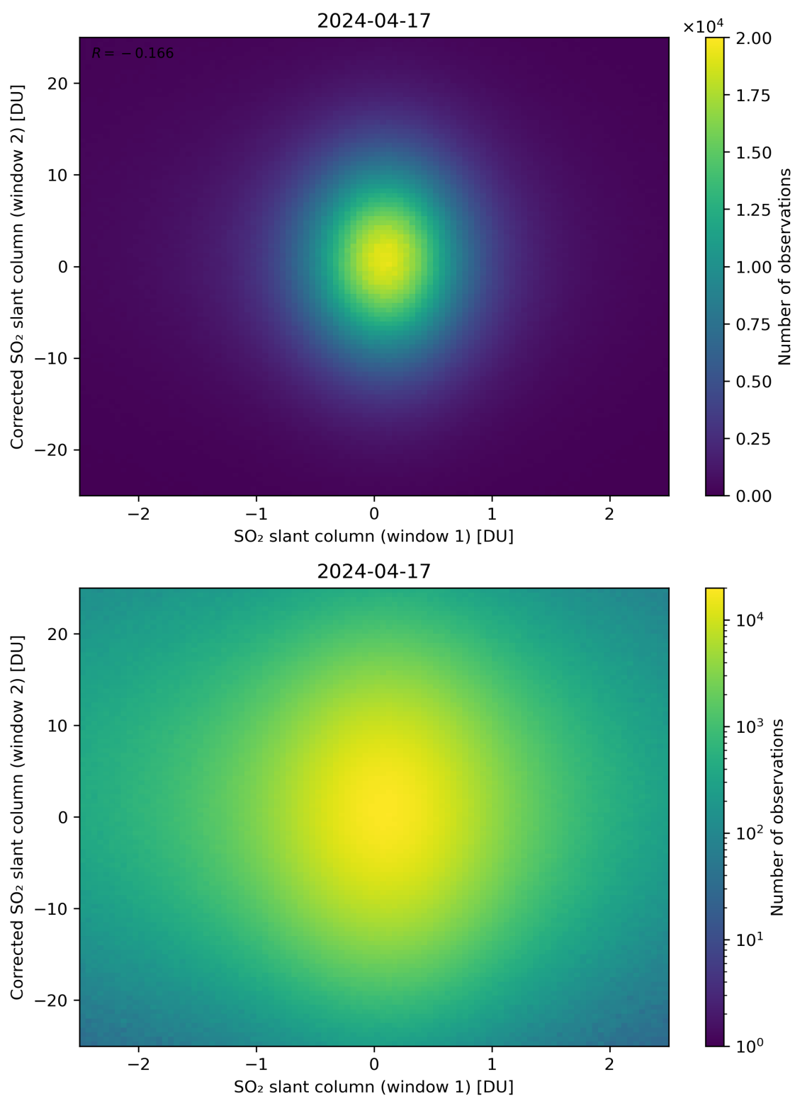
Figure 233: Scatter density plot of “SO 2 slant column (window 1)” against “Corrected SO 2 slant column (window 2)” for 2024-04-16 to 2024-04-18.
