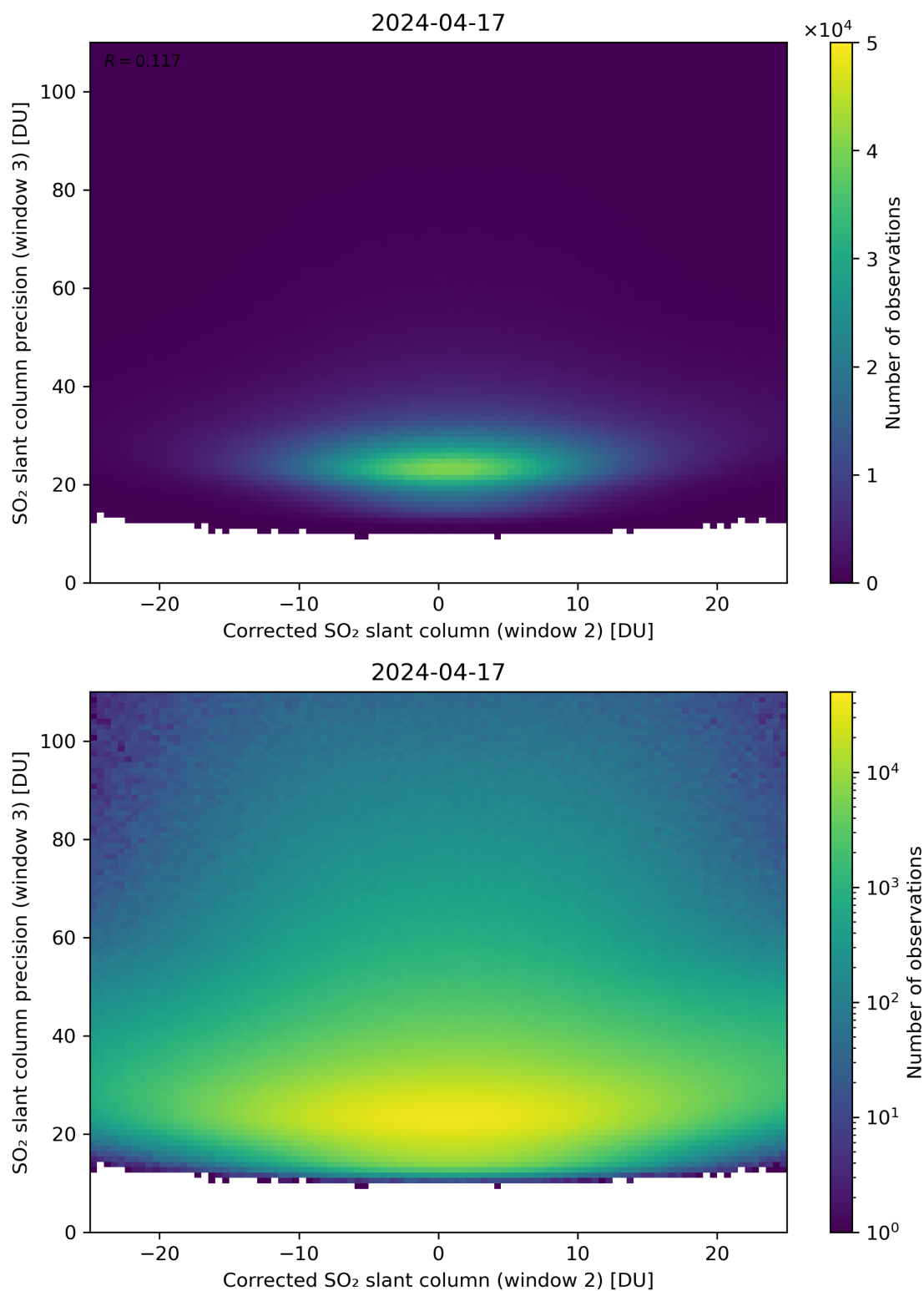
Figure 202: Scatter density plot of “Corrected SO 2 slant column (window 2)” against “SO 2 slant column precision (window 3)” for 2024-04-16 to 2024-04-18.
