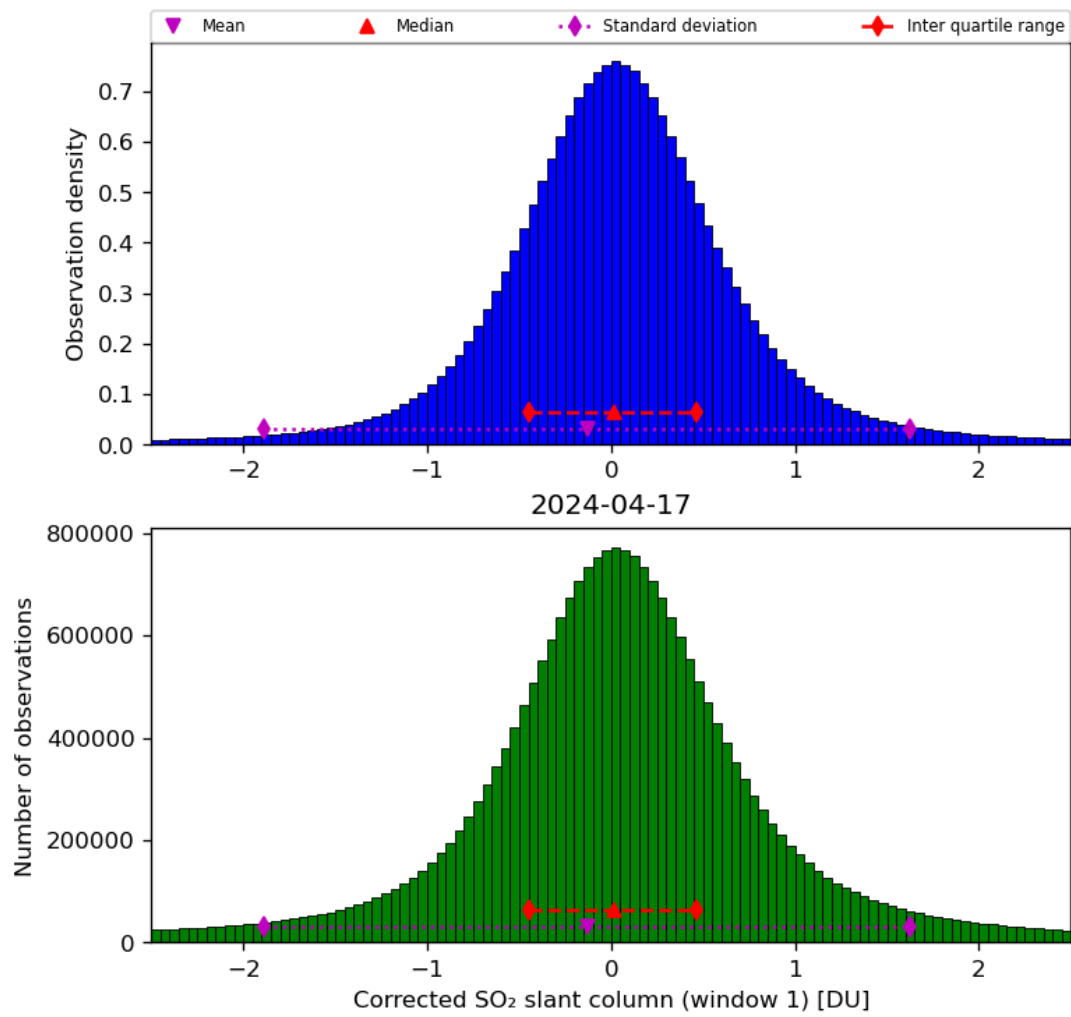
Figure 58: Histogram of “Corrected SO 2 slant column (window 1)” for 2024-04-16 to 2024-04-18
