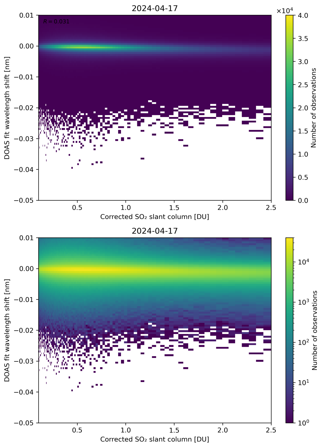
Figure 181: Scatter density plot of “Corrected SO 2 slant column” against “DOAS fit wavelength shift” for 2024-04-16 to 2024-04-18.
