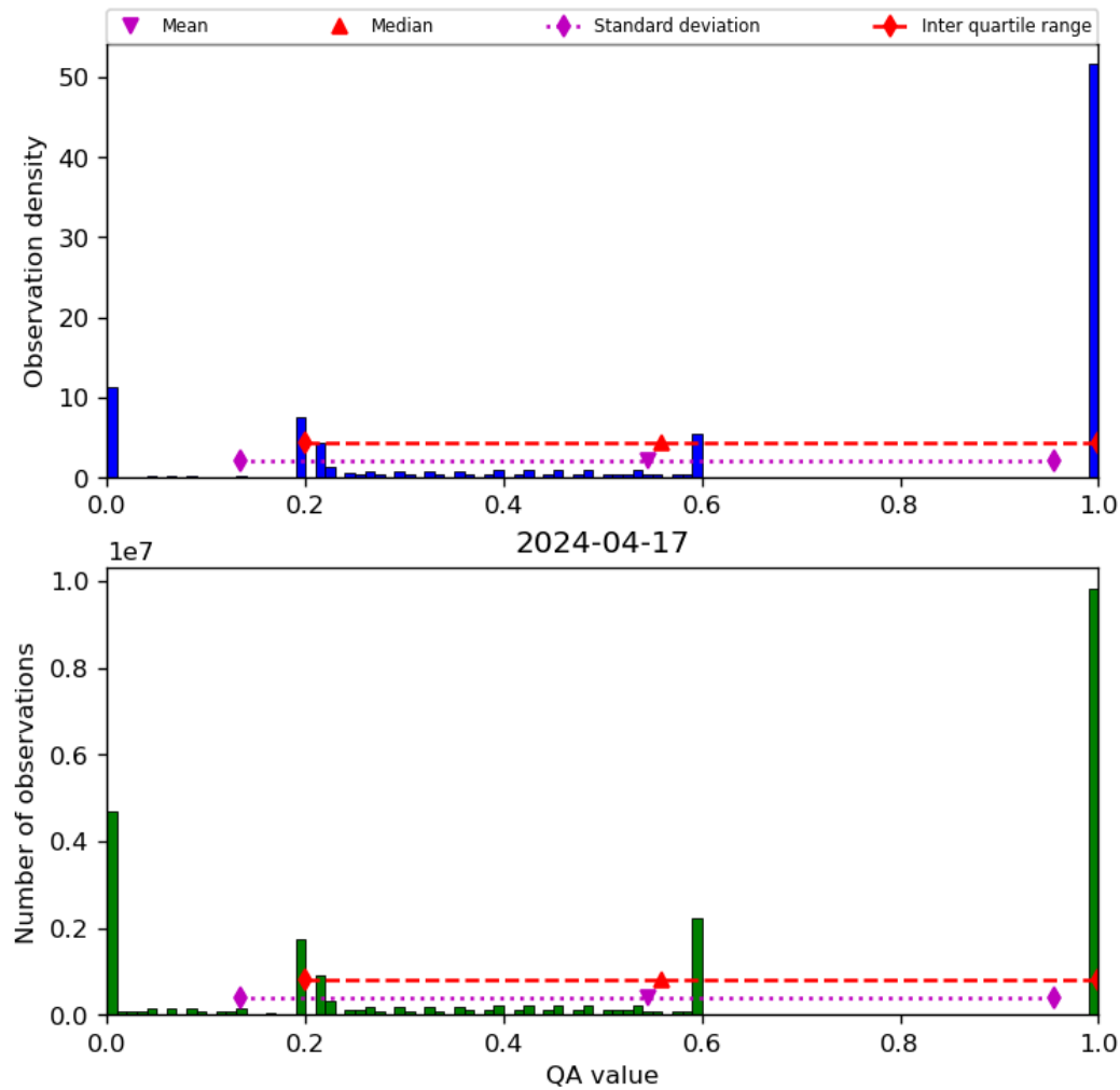
Figure 52: Histogram of “QA value” for 2024-04-16 to 2024-04-18
