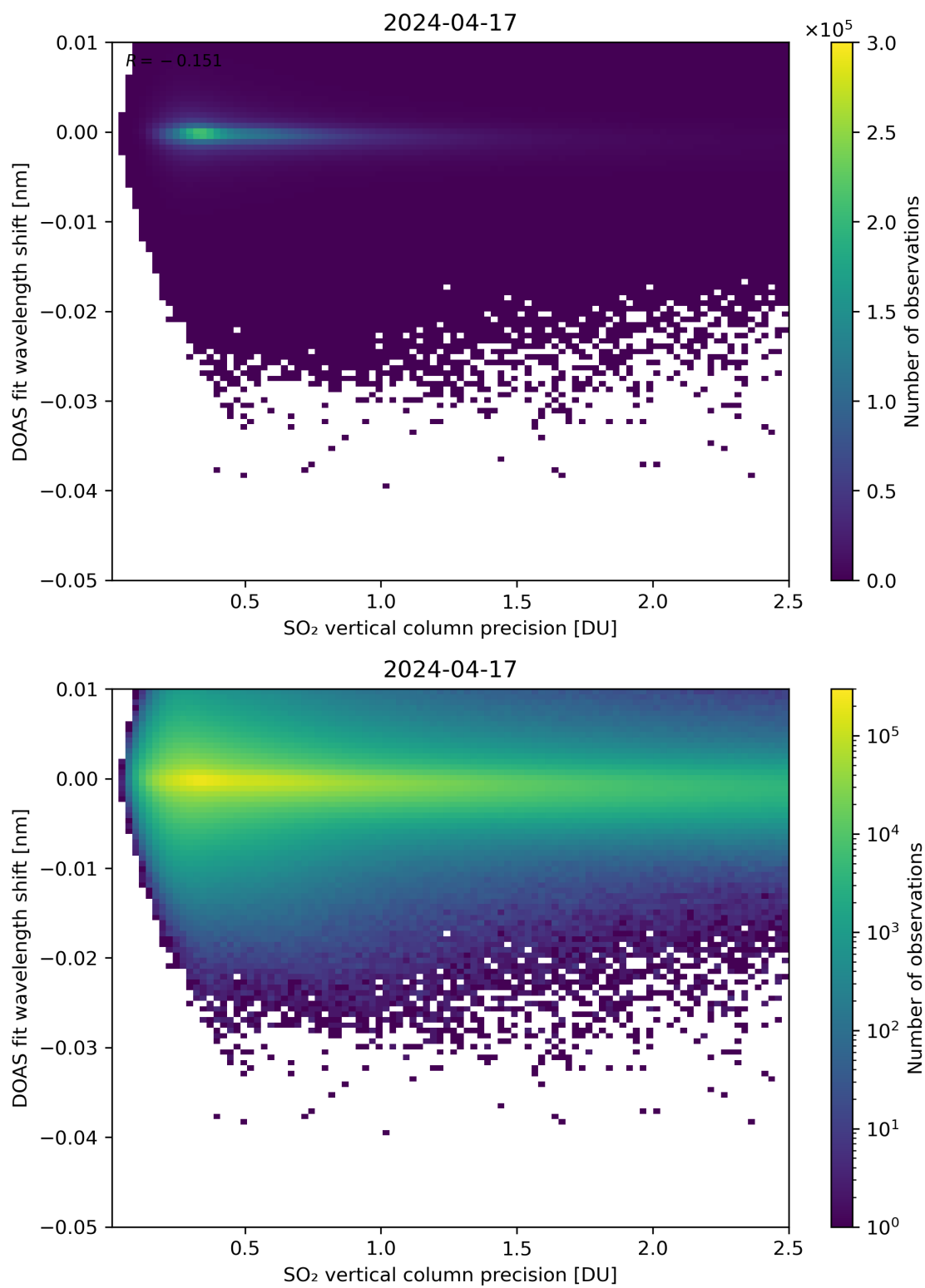
Figure 282: Scatter density plot of “SO 2 vertical column precision” against “DOAS fit wavelength shift” for 2024-04-16 to 2024-04-18.
