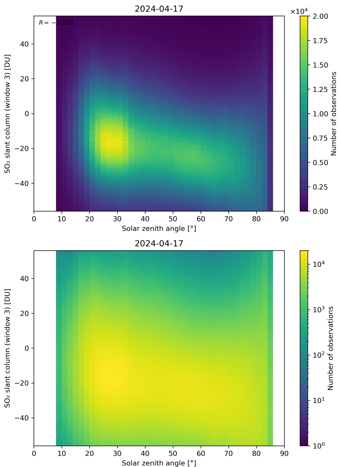
Figure 172: Scatter density plot of “Solar zenith angle” against “SO 2 slant column (window 3)” for 2024-04-16 to 2024-04-18.
