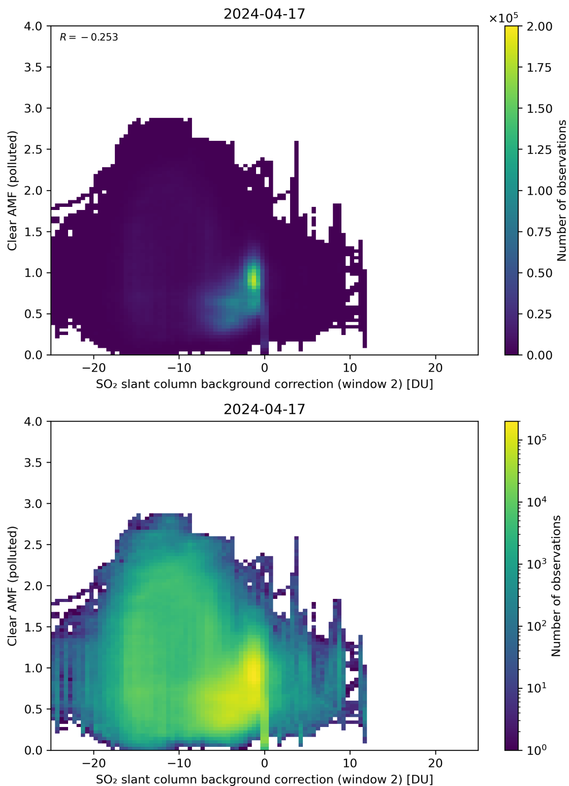
Figure 115: Scatter density plot of “SO 2 slant column background correction (window 2)” against “Clear AMF (polluted)” for 2024-04-16 to 2024-04-18.
