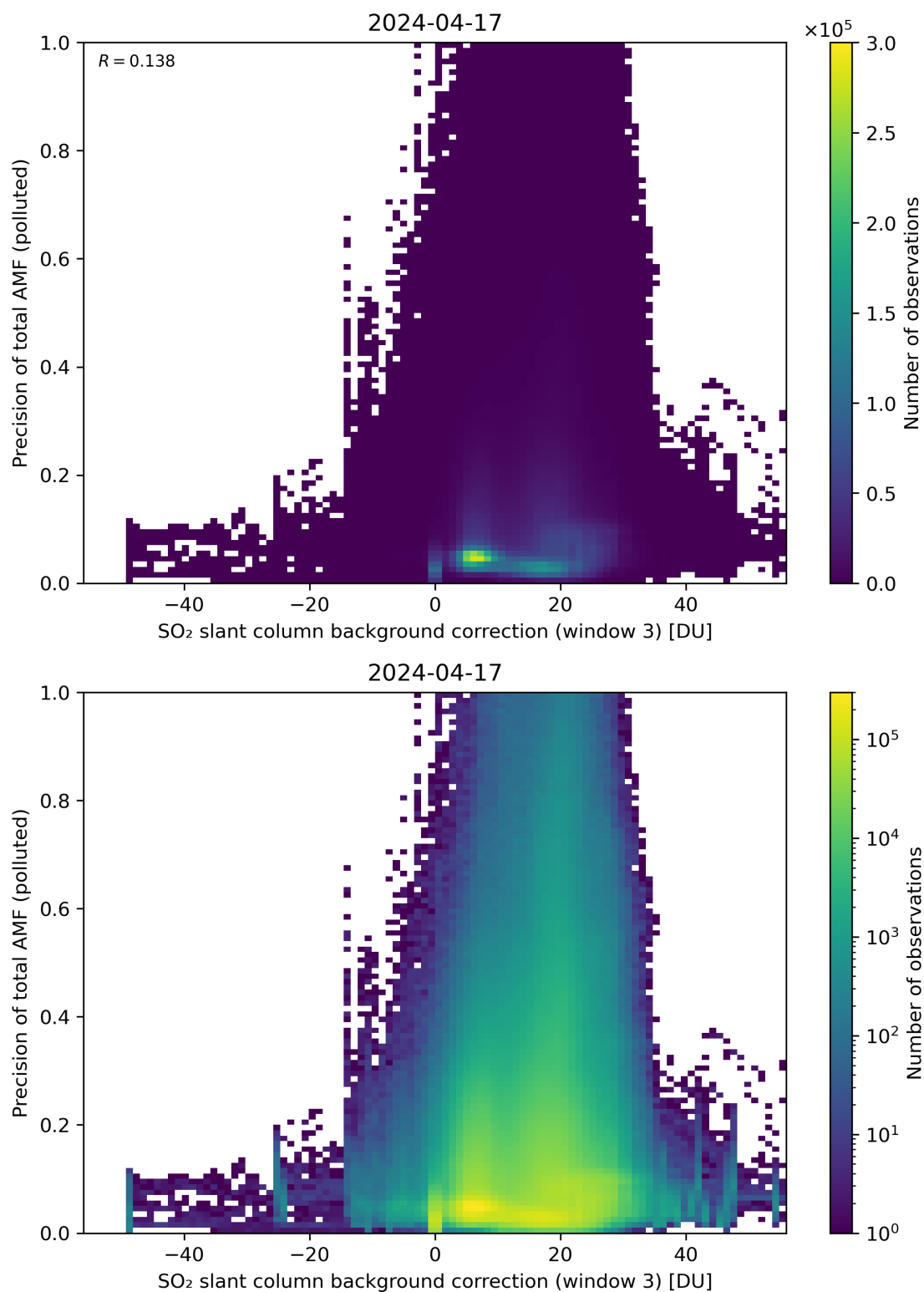
Figure 126: Scatter density plot of “SO 2 slant column background correction (window 3)” against “Precision of total AMF (polluted)” for 2024-04-16 to 2024-04-18.
