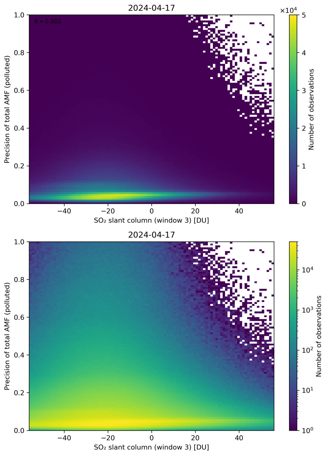
Figure 269: Scatter density plot of “SO 2 slant column (window 3)” against “Precision of total AMF (polluted)” for 2024-04-16 to 2024-04-18.
