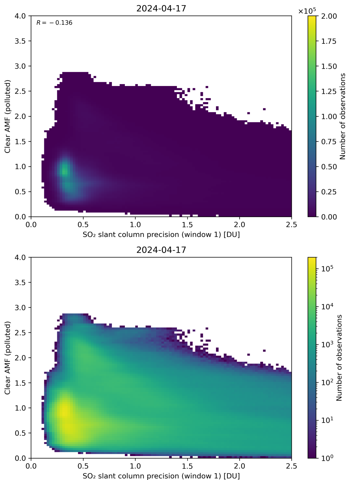
Figure 224: Scatter density plot of “SO 2 slant column precision (window 1)” against “Clear AMF (polluted)” for 2024-04-16 to 2024-04-18.
