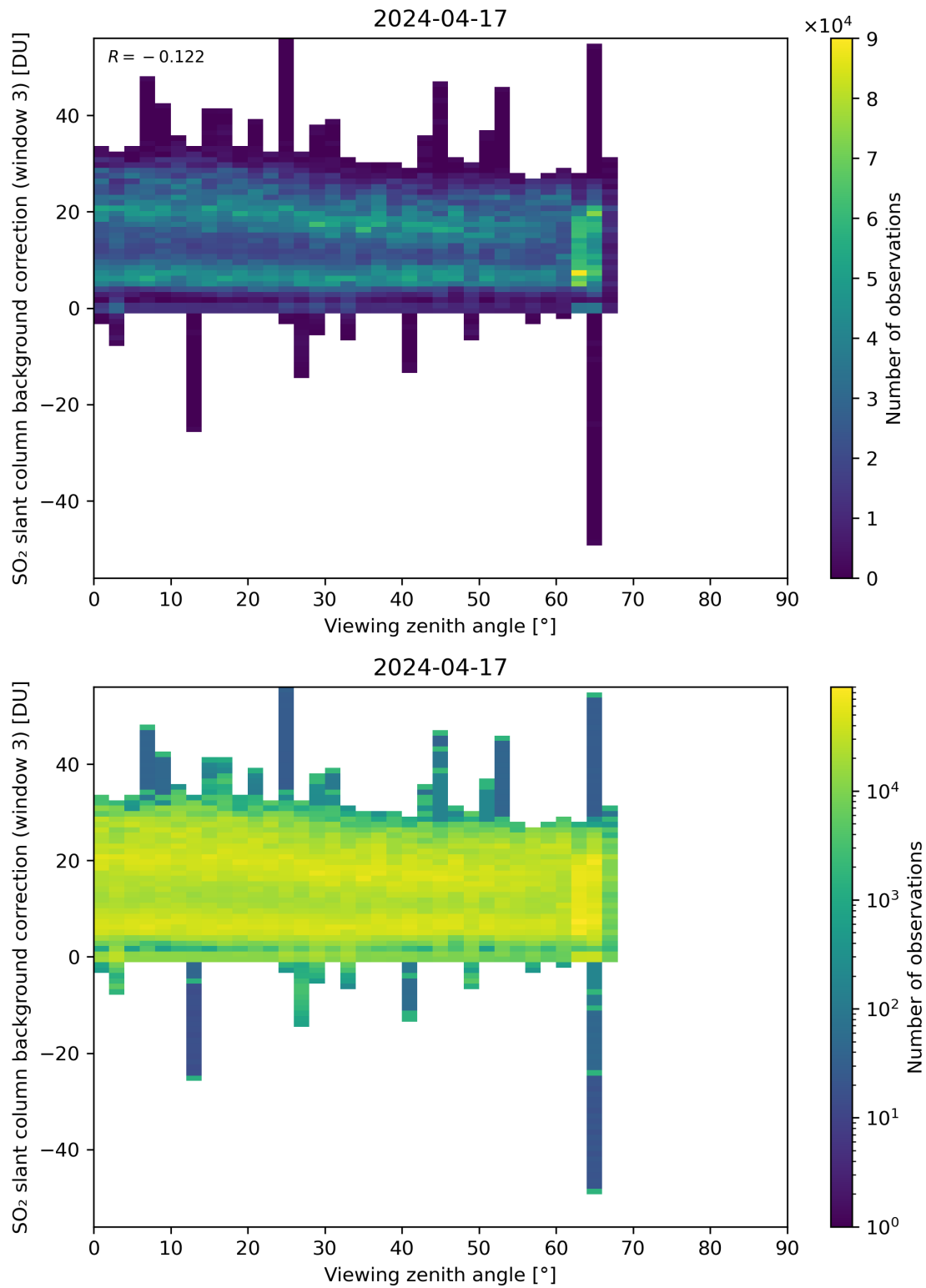
Figure 310: Scatter density plot of “Viewing zenith angle” against “SO 2 slant column background correction (window 3)” for 2024-04-16 to 2024-04-18.
