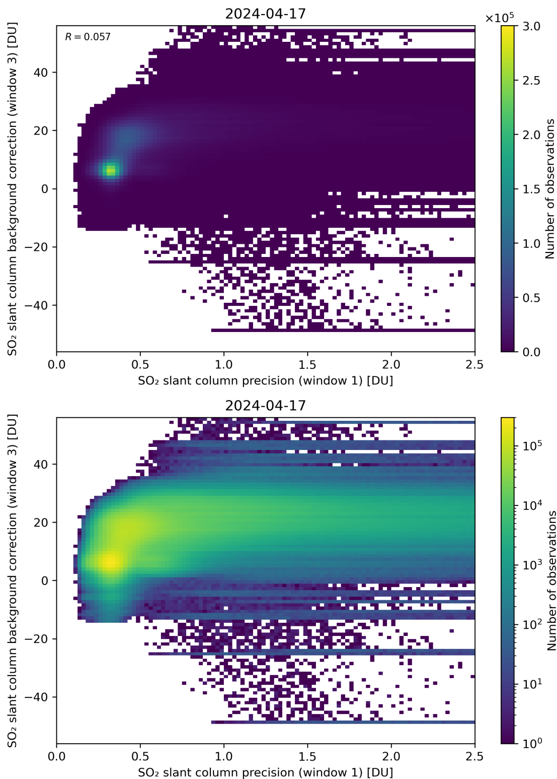
Figure 220: Scatter density plot of “SO 2 slant column precision (window 1)” against “SO 2 slant column background correction (window 3)” for 2024-04-16 to 2024-04-18.
