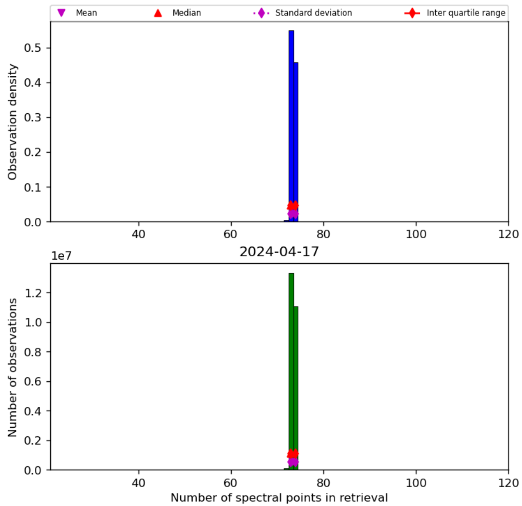
Figure 74: Histogram of “Number of spectral points in retrieval” for 2024-04-16 to 2024-04-18
