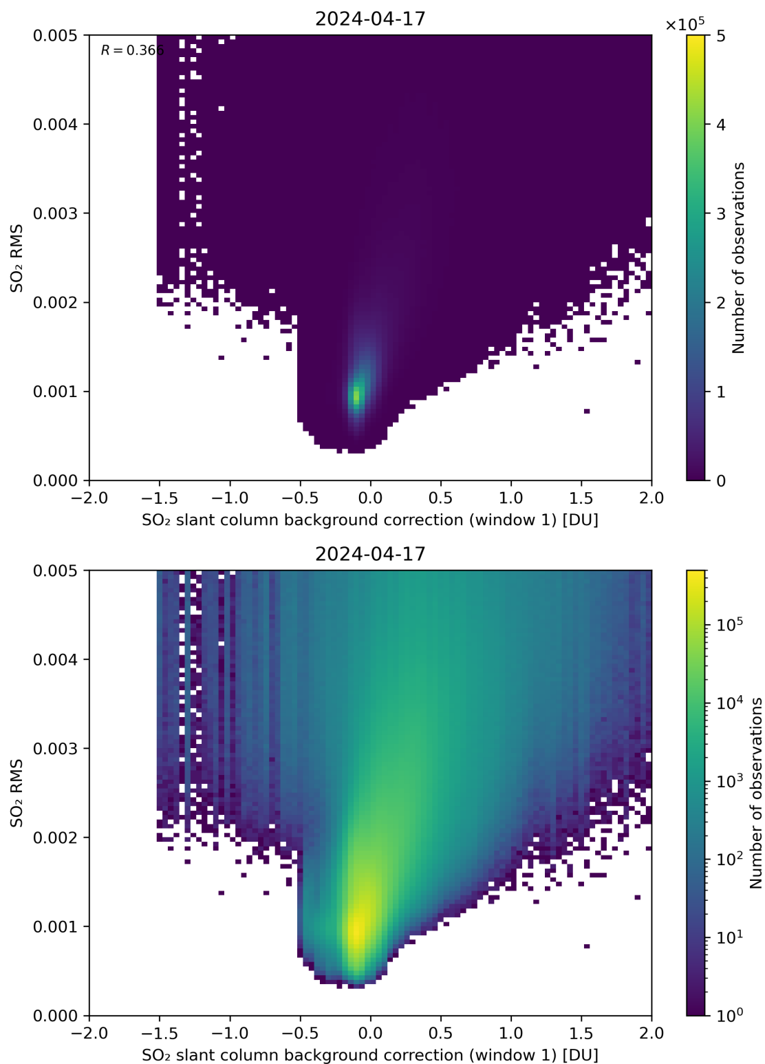
Figure 102: Scatter density plot of “SO 2 slant column background correction (window 1)” against “SO 2 RMS” for 2024-04-16 to 2024-04-18.
