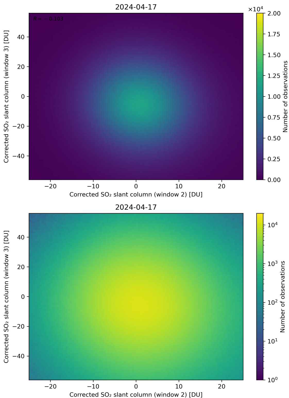
Figure 200: Scatter density plot of “Corrected SO 2 slant column (window 2)” against “Corrected SO 2 slant column (window 3)” for 2024-04-16 to 2024-04-18.
