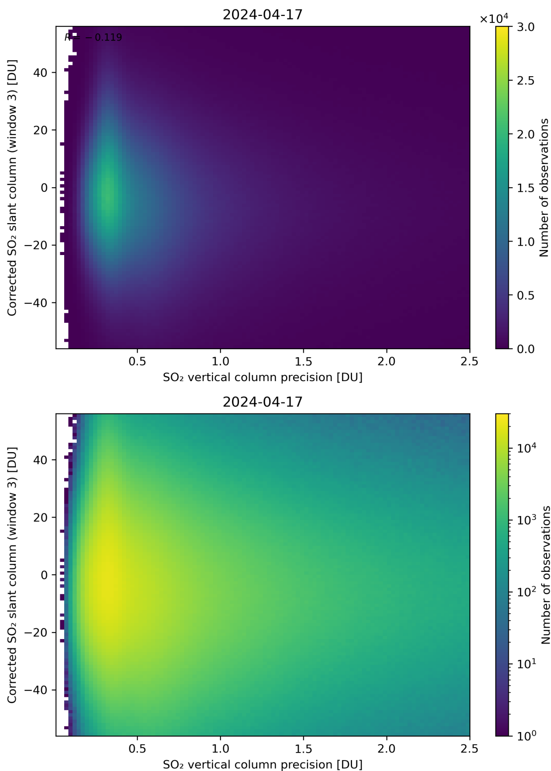
Figure 288: Scatter density plot of “SO 2 vertical column precision” against “Corrected SO 2 slant column (window 3)” for 2024-04-16 to 2024-04-18.
