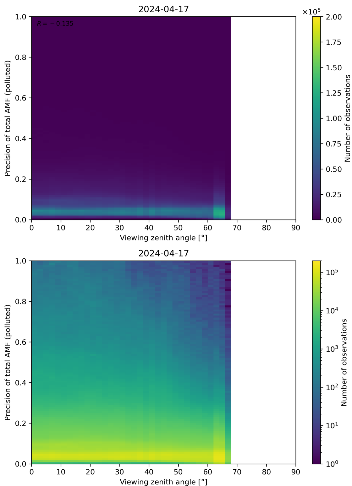
Figure 326: Scatter density plot of “Viewing zenith angle” against “Precision of total AMF (polluted)” for 2024-04-16 to 2024-04-18.
