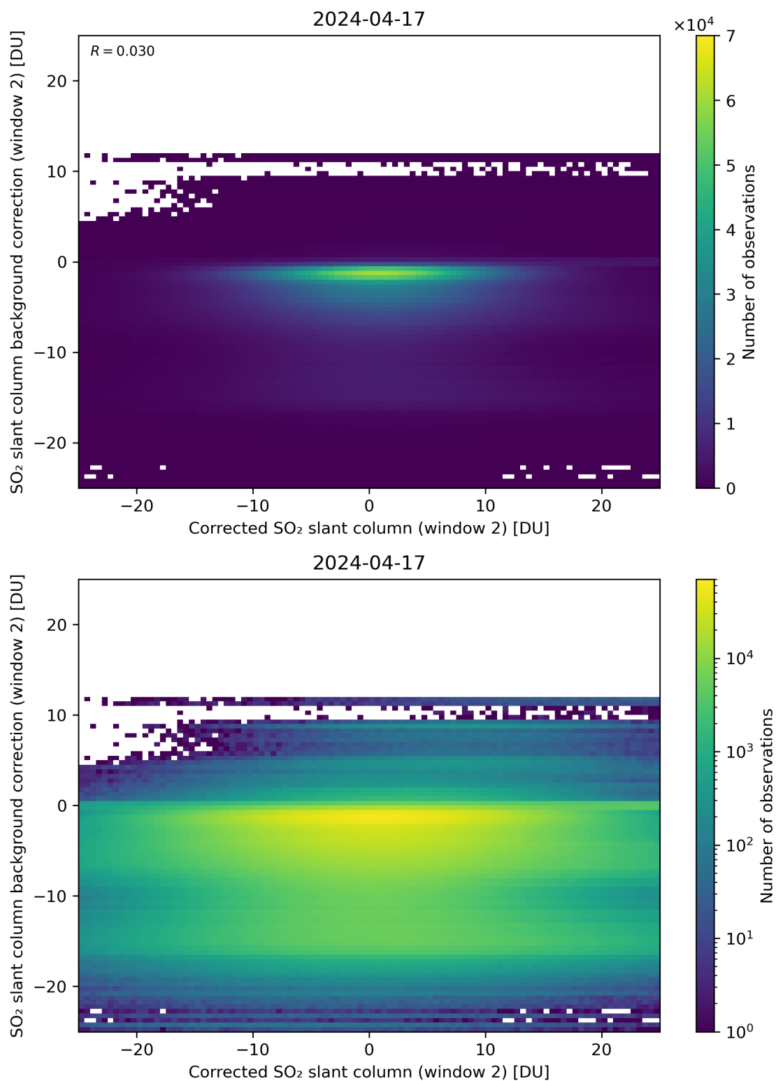
Figure 194: Scatter density plot of “Corrected SO 2 slant column (window 2)” against “SO 2 slant column background correction (window 2)” for 2024-04-16 to 2024-04-18.
