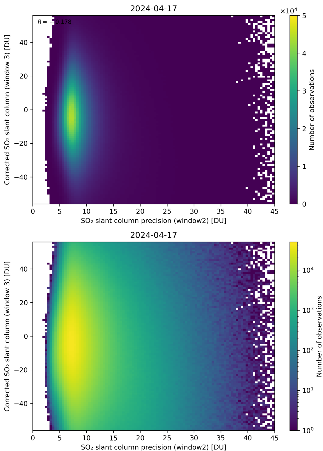
Figure 248: Scatter density plot of “SO 2 slant column precision (window2)” against “Corrected SO 2 slant column (window 3)” for 2024-04-16 to 2024-04-18.
