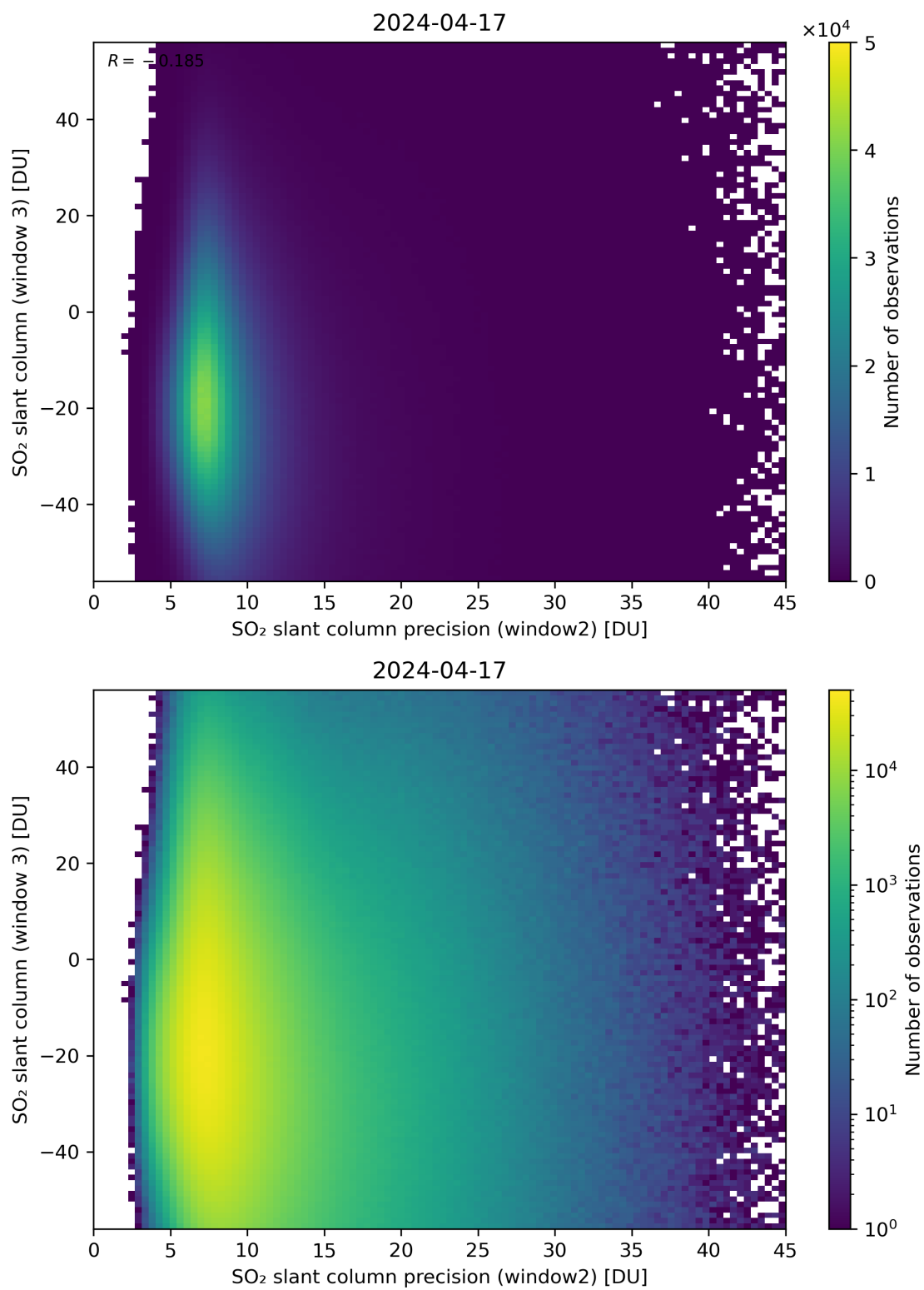
Figure 249: Scatter density plot of “SO 2 slant column precision (window2)” against “SO 2 slant column (window 3)” for 2024-04-16 to 2024-04-18.
