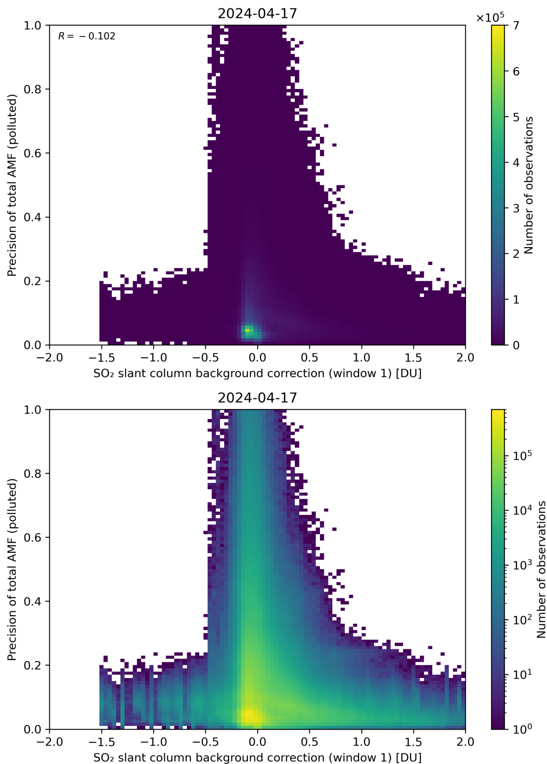
Figure 110: Scatter density plot of “SO 2 slant column background correction (window 1)” against “Precision of total AMF (polluted)” for 2024-04-16 to 2024-04-18.
