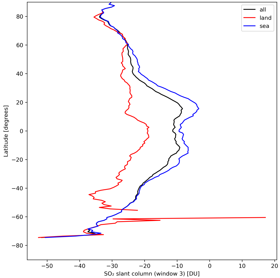
Figure 41: Zonal average of “SO 2 slant column (window 3)” for 2024-04-16 to 2024-04-18.
