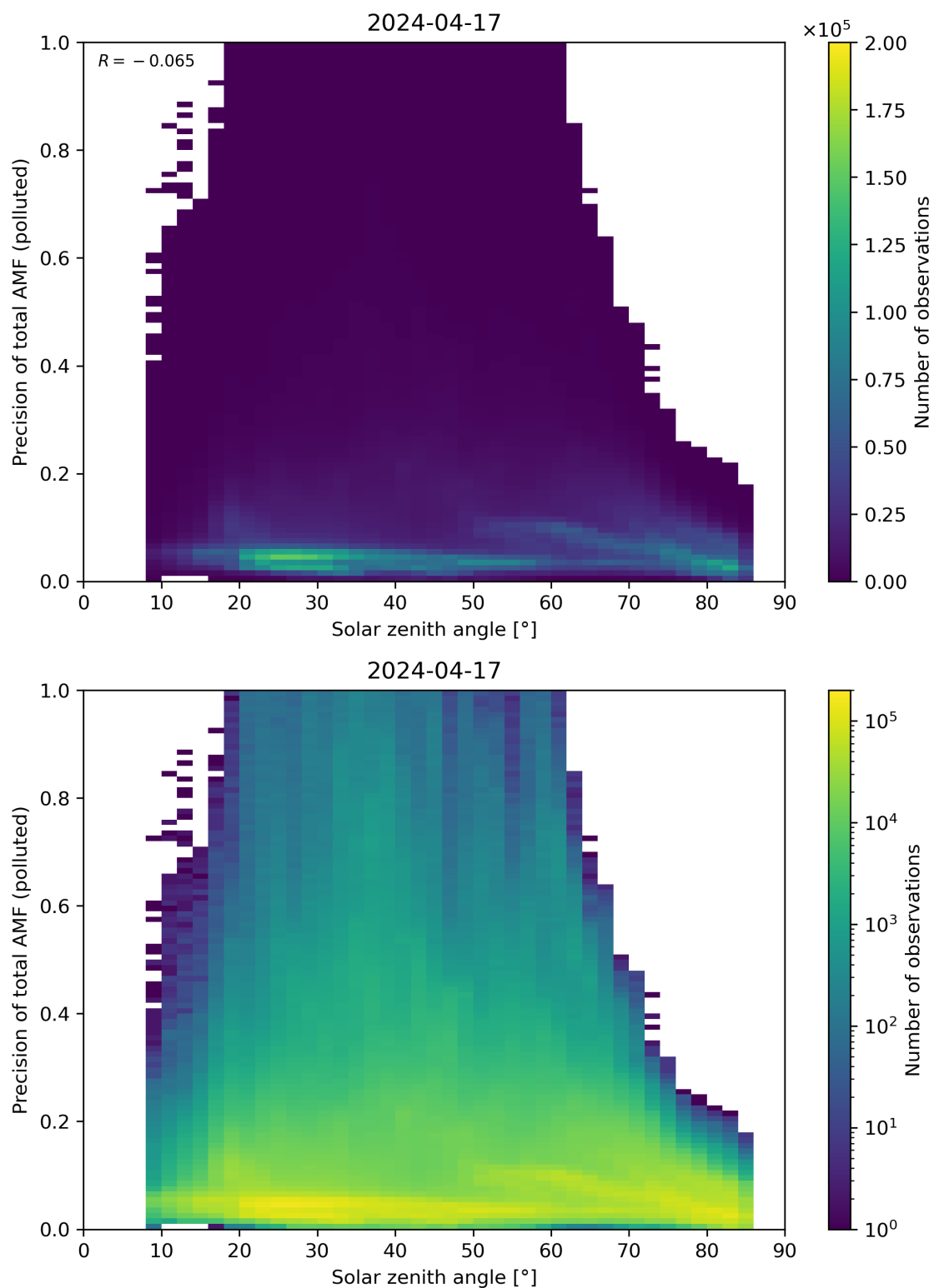
Figure 175: Scatter density plot of “Solar zenith angle” against “Precision of total AMF (polluted)” for 2024-04-16 to 2024-04-18.
