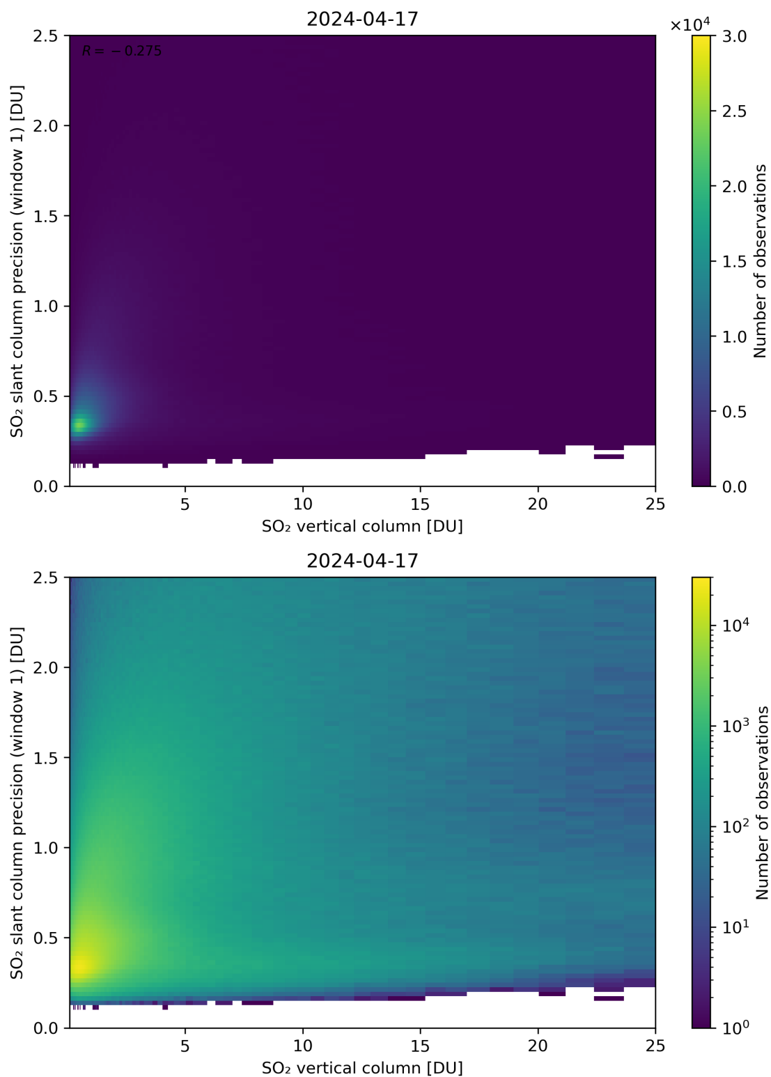
Figure 301: Scatter density plot of “SO 2 vertical column” against “SO 2 slant column precision (window 1)” for 2024-04-16 to 2024-04-18.
