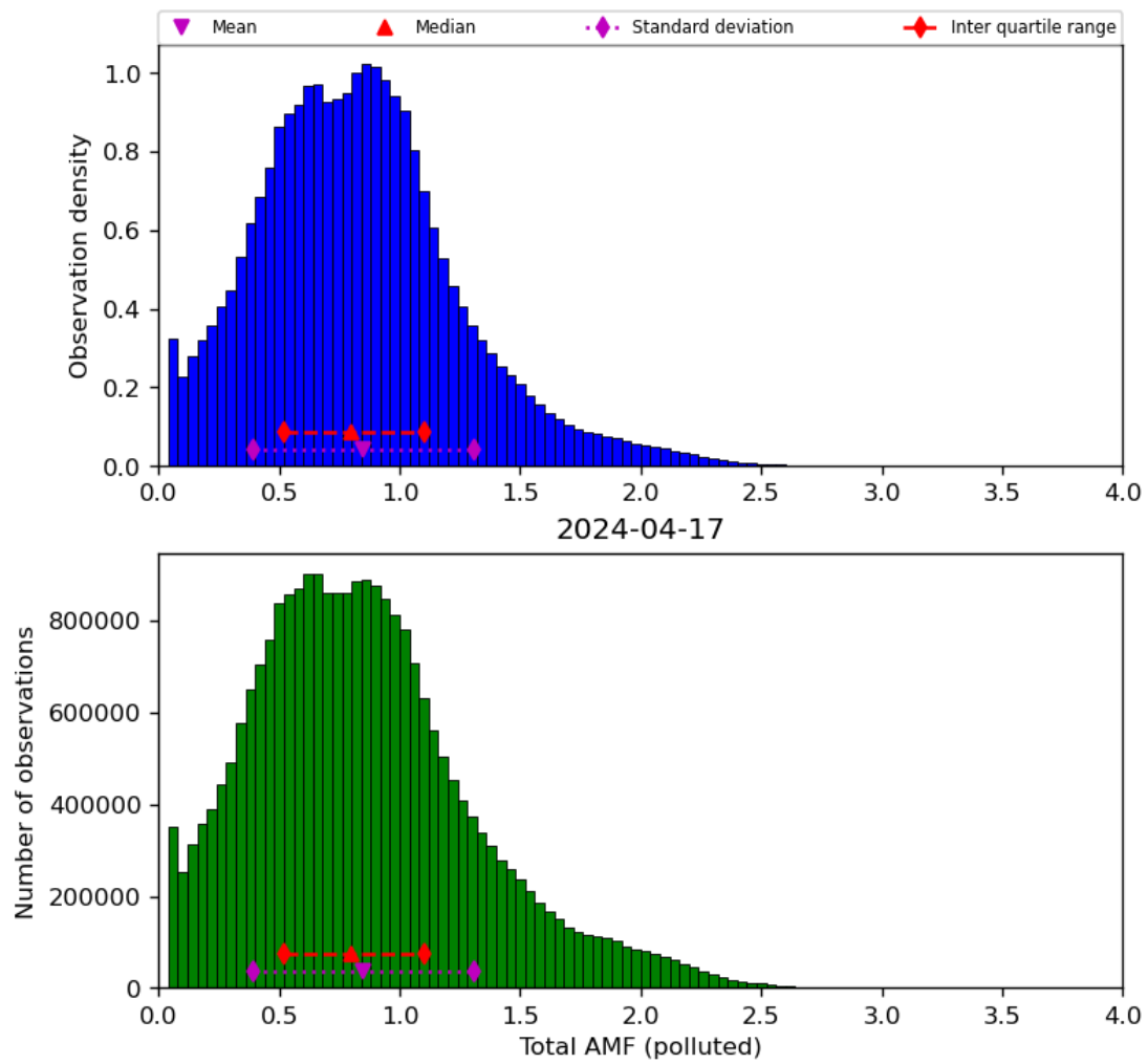
Figure 71: Histogram of “Total AMF (polluted)” for 2024-04-16 to 2024-04-18
