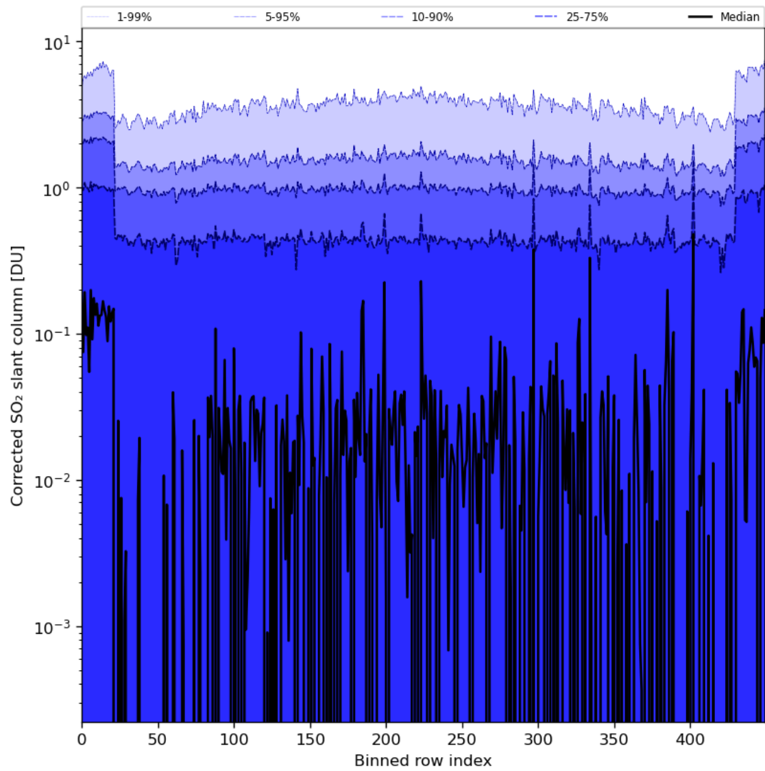
Figure 78: Along track statistics of “Corrected SO 2 slant column” for 2024-04-16 to 2024-04-18
