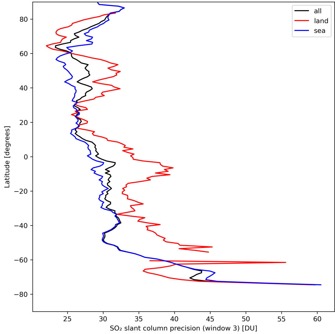
Figure 42: Zonal average of “SO 2 slant column precision (window 3)” for 2024-04-16 to 2024-04-18.
