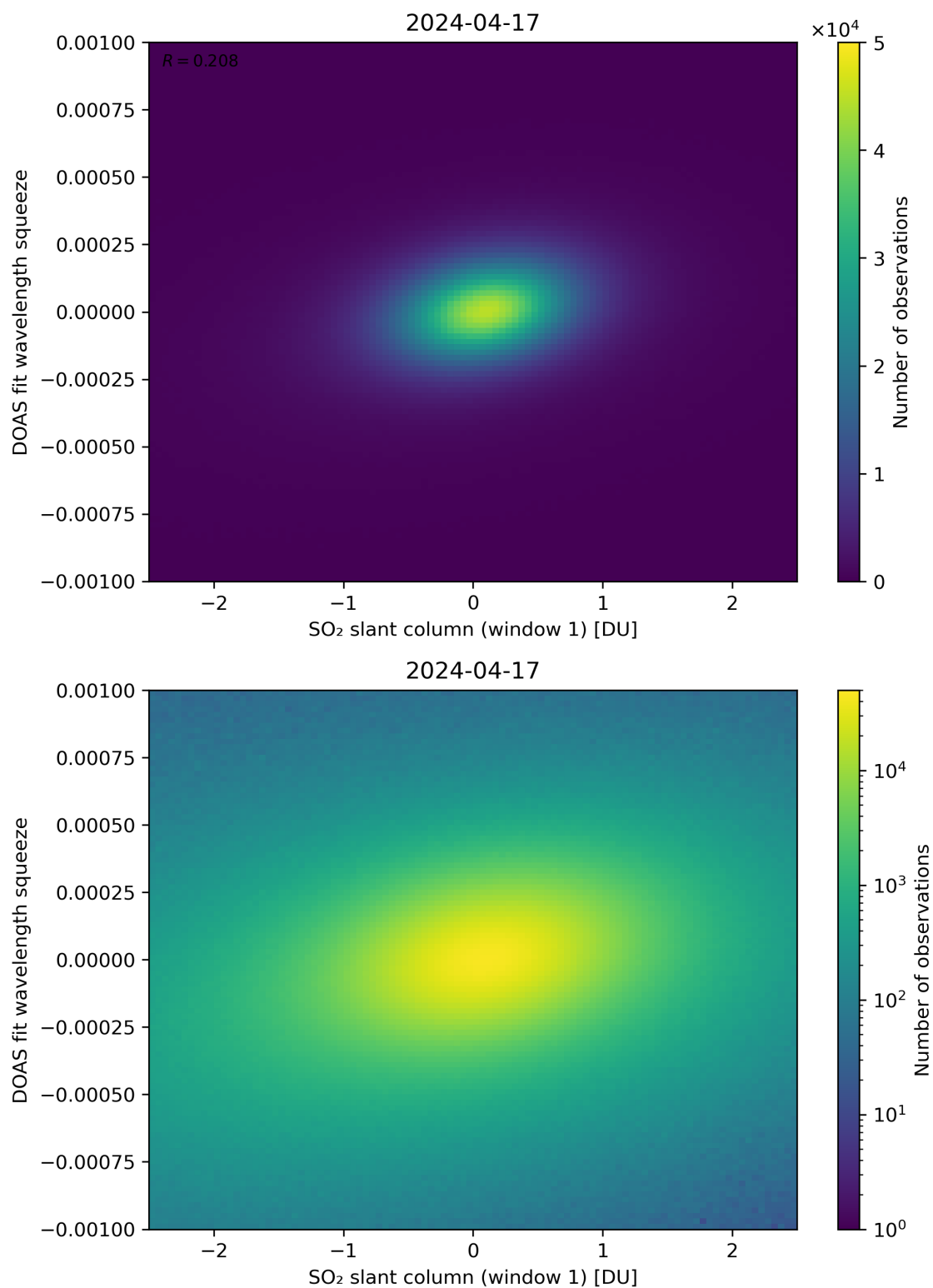
Figure 216: Scatter density plot of “SO 2 slant column (window 1)” against “DOAS fit wavelength squeeze” for 2024-04-16 to 2024-04-18.
