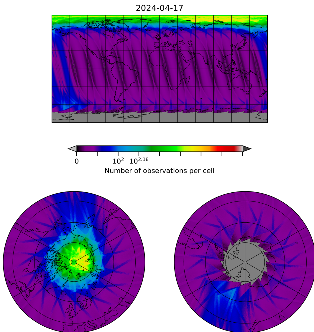
Figure 28: Map of the number of observations for 2024-04-16 to 2024-04-18
