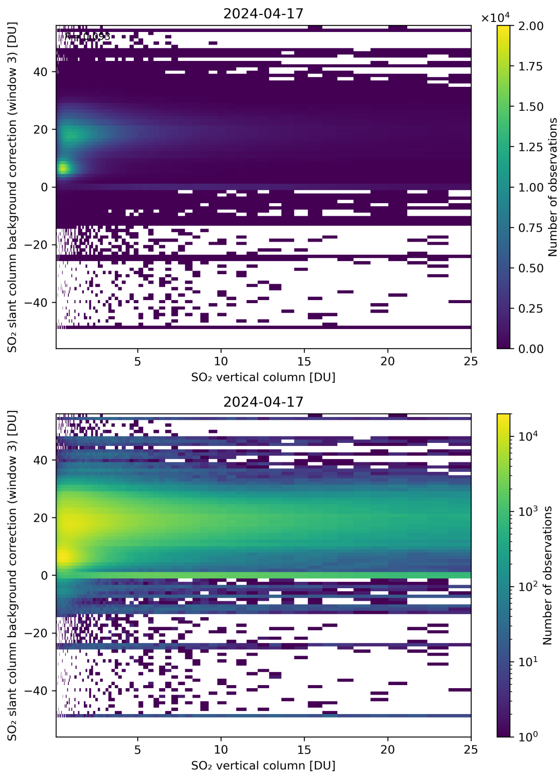
Figure 275: Scatter density plot of “SO 2 vertical column” against “SO 2 slant column background correction (window 3)” for 2024-04-16 to 2024-04-18.
