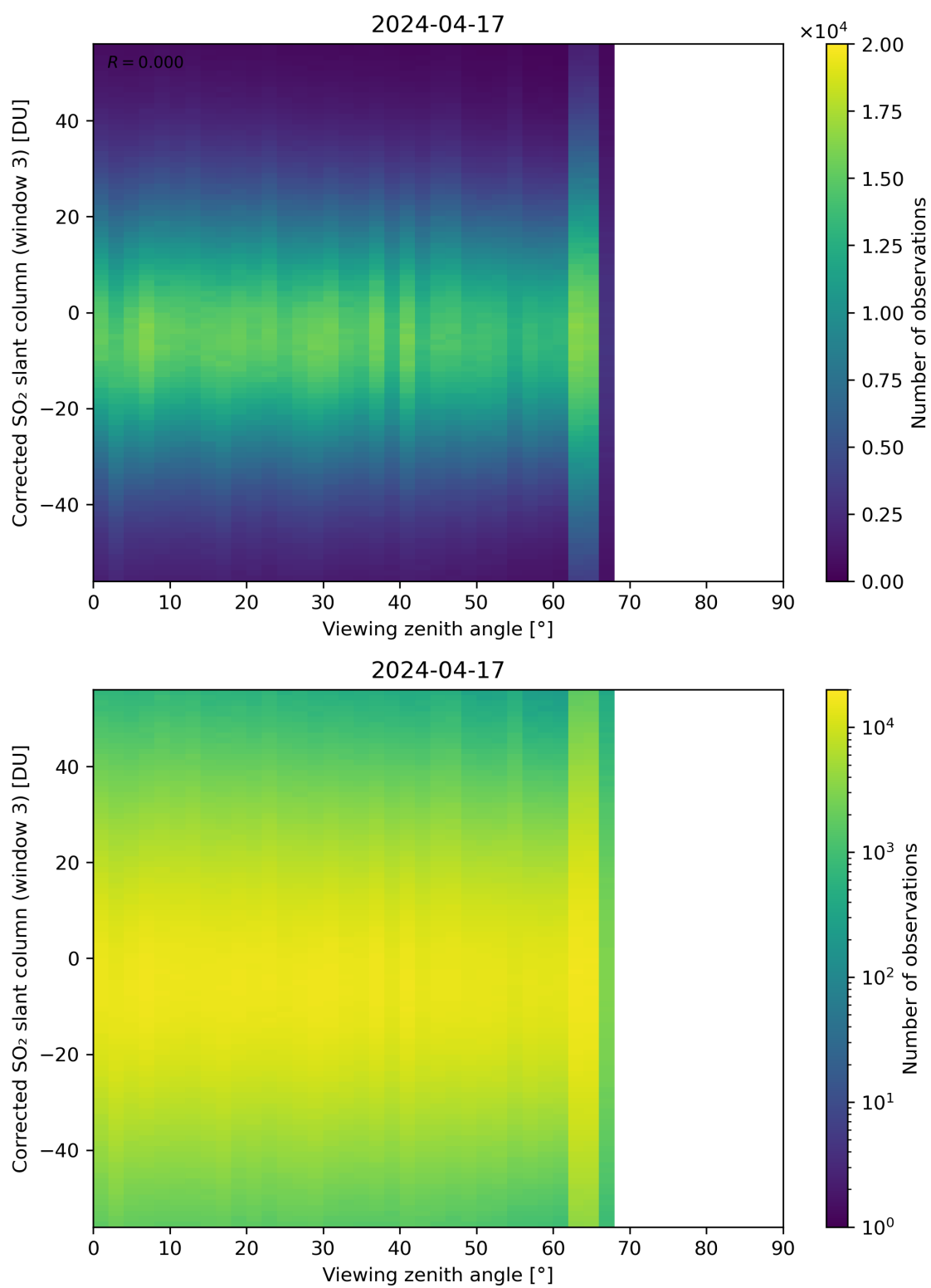
Figure 319: Scatter density plot of “Viewing zenith angle” against “Corrected SO 2 slant column (window 3)” for 2024-04-16 to 2024-04-18.
