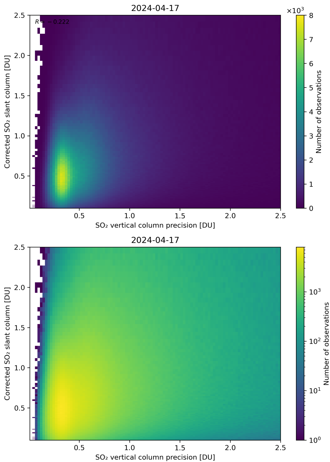
Figure 286: Scatter density plot of “SO 2 vertical column precision” against “Corrected SO 2 slant column” for 2024-04-16 to 2024-04-18.
