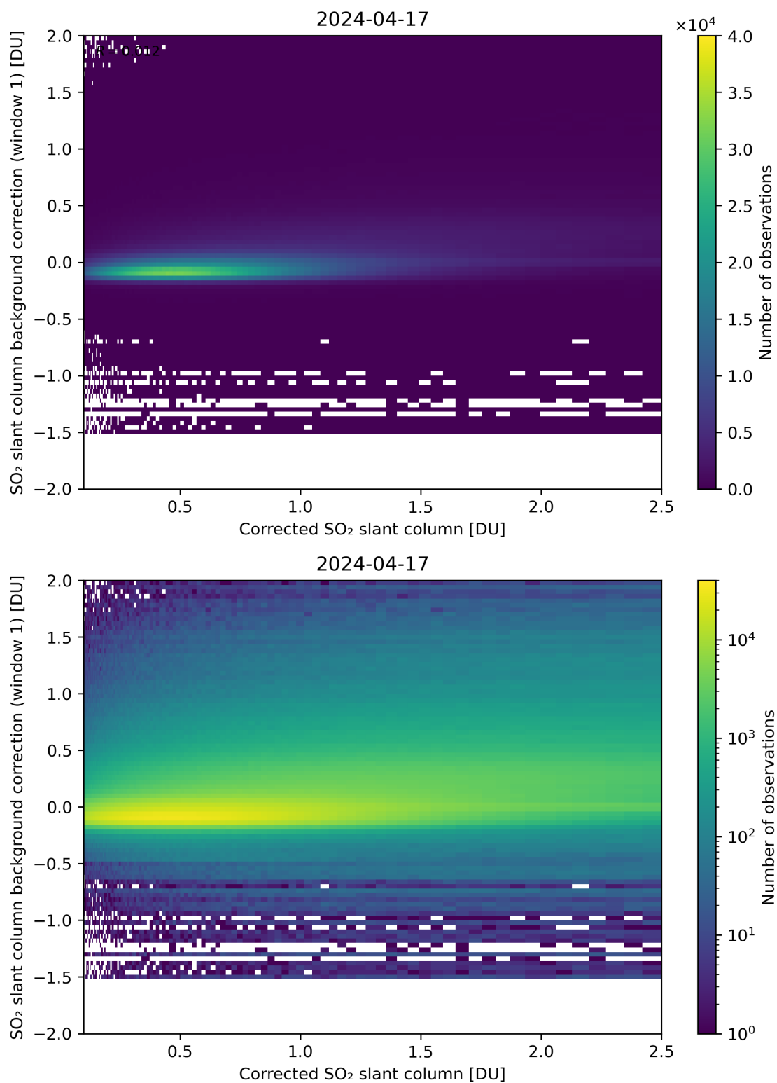
Figure 178: Scatter density plot of “Corrected SO 2 slant column” against “SO 2 slant column background correction (window 1)” for 2024-04-16 to 2024-04-18.
