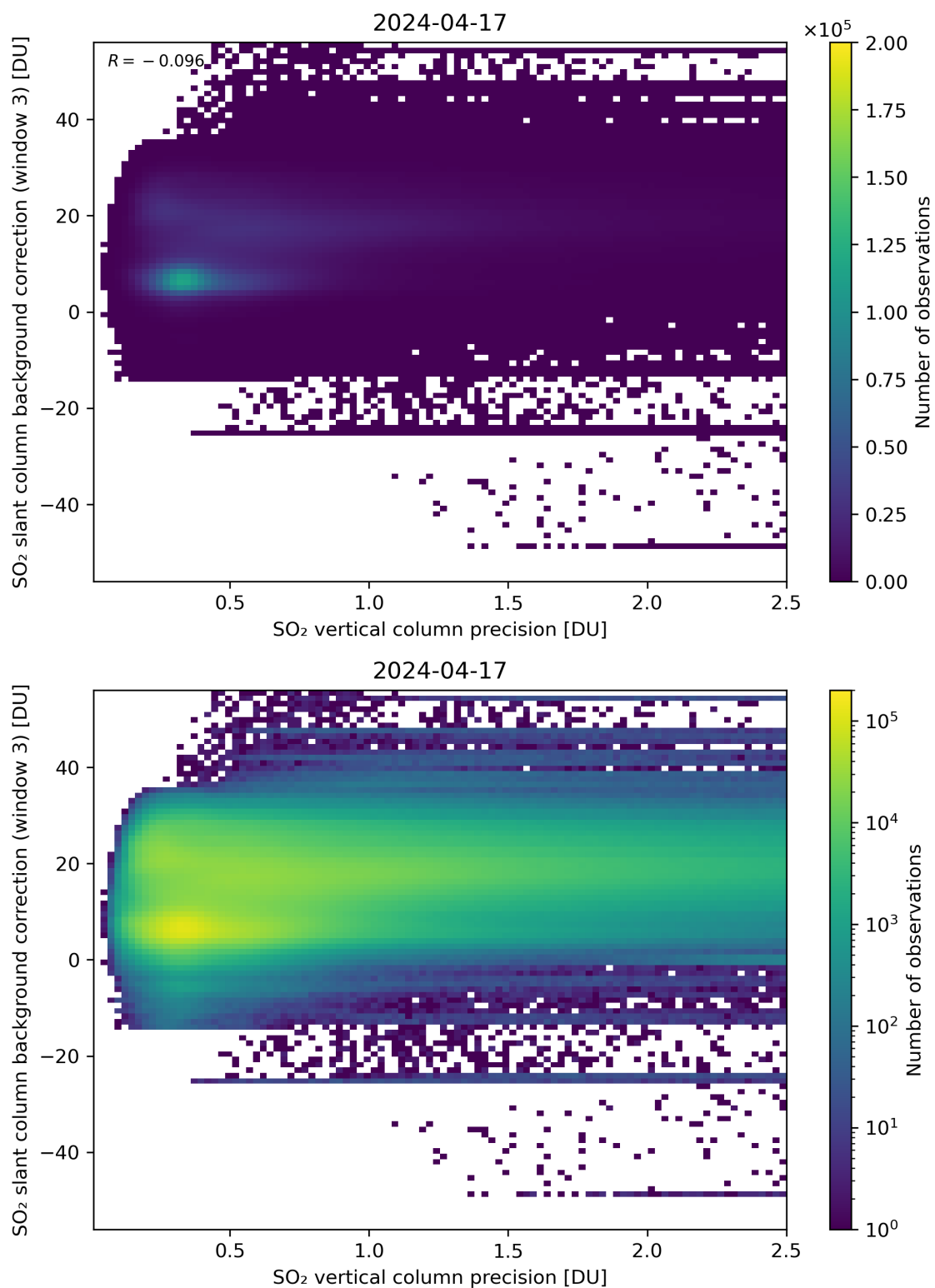
Figure 281: Scatter density plot of “SO 2 vertical column precision” against “SO 2 slant column background correction (window 3)” for 2024-04-16 to 2024-04-18.
