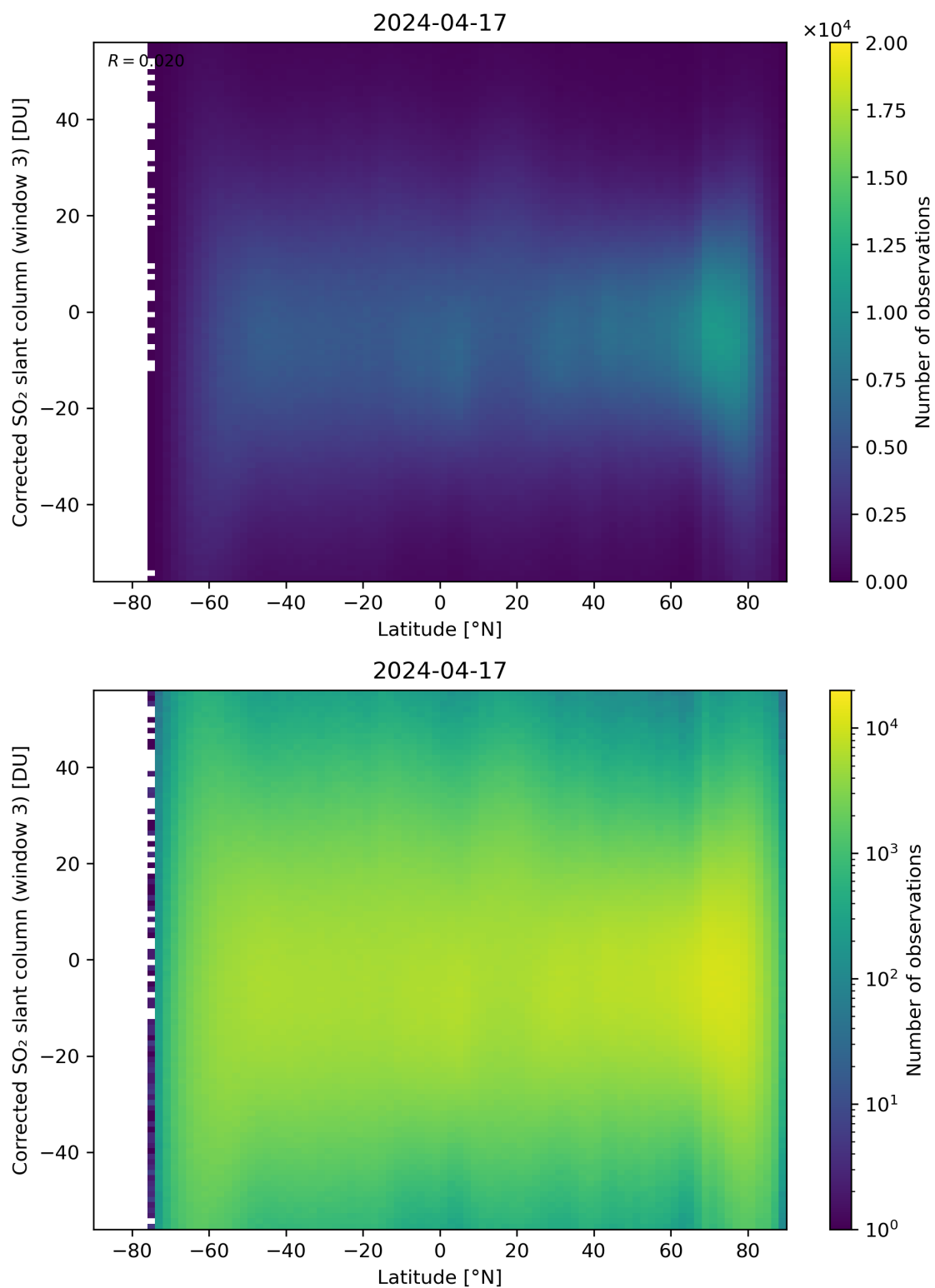
Figure 148: Scatter density plot of “Latitude” against “Corrected SO 2 slant column (window 3)” for 2024-04-16 to 2024-04-18.
