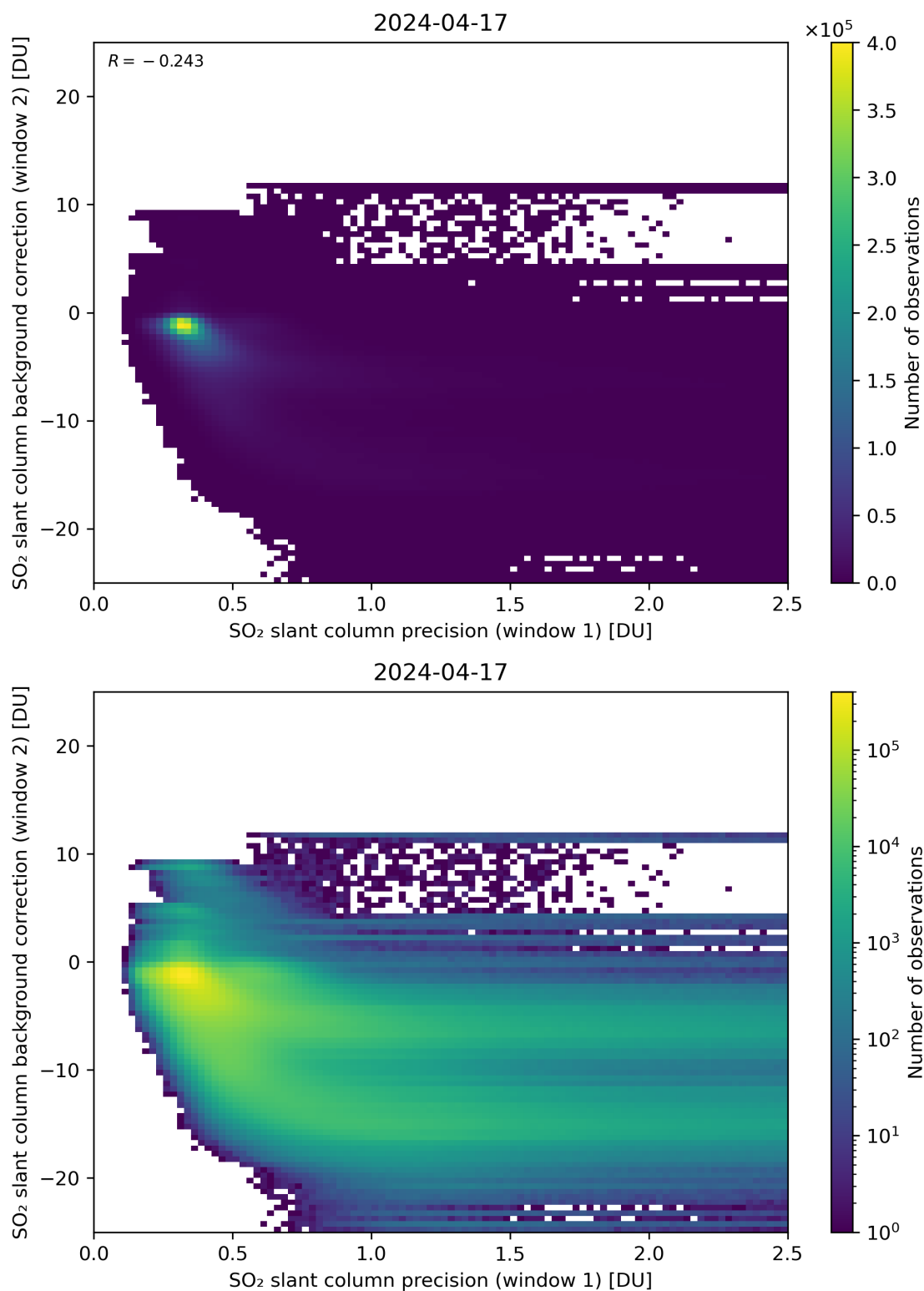
Figure 219: Scatter density plot of “SO 2 slant column precision (window 1)” against “SO 2 slant column background correction (window 2)” for 2024-04-16 to 2024-04-18.
