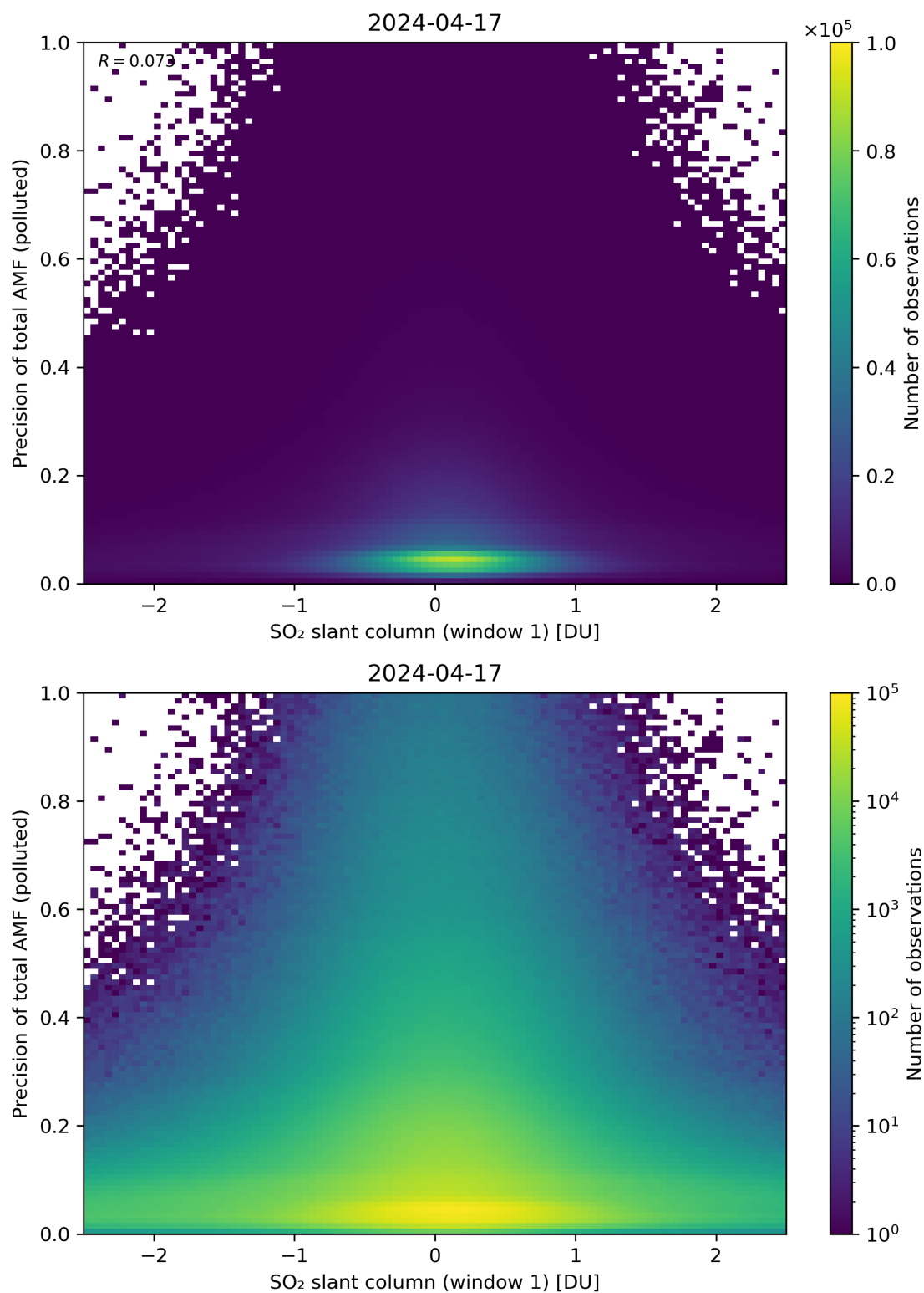
Figure 240: Scatter density plot of “SO 2 slant column (window 1)” against “Precision of total AMF (polluted)” for 2024-04-16 to 2024-04-18.
