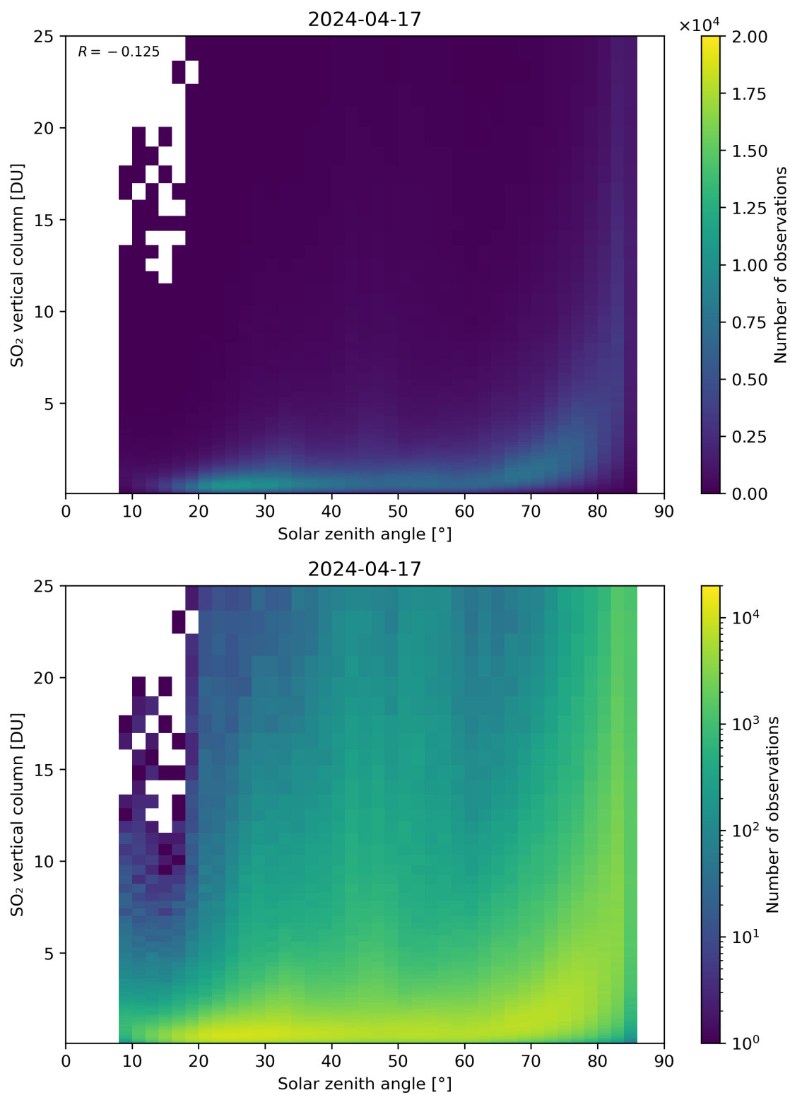
Figure 176: Scatter density plot of “Solar zenith angle” against “SO 2 vertical column” for 2024-04-16 to 2024-04-18.
