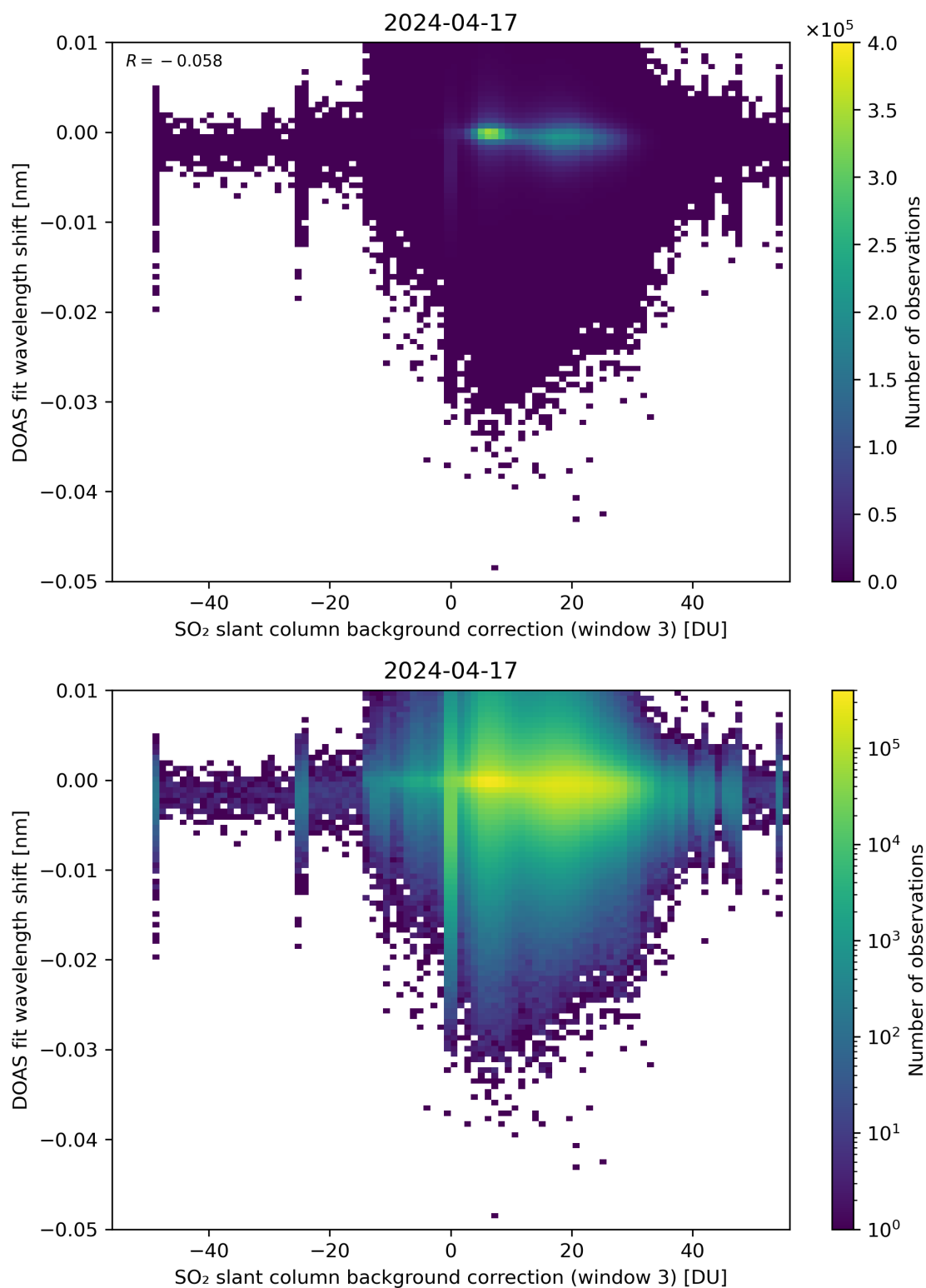
Figure 121: Scatter density plot of “SO 2 slant column background correction (window 3)” against “DOAS fit wavelength shift” for 2024-04-16 to 2024-04-18.
