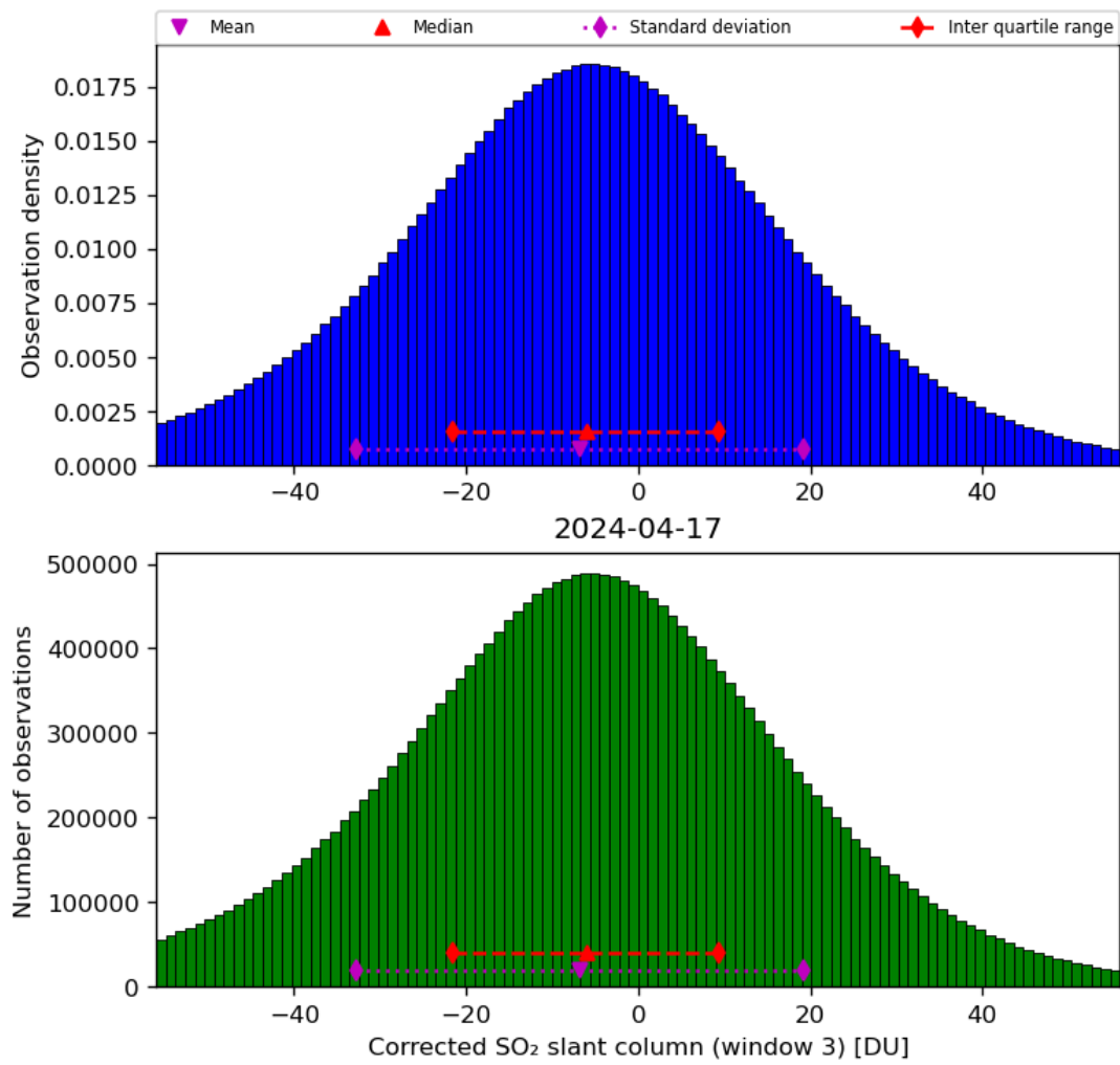
Figure 66: Histogram of “Corrected SO 2 slant column (window 3)” for 2024-04-16 to 2024-04-18
