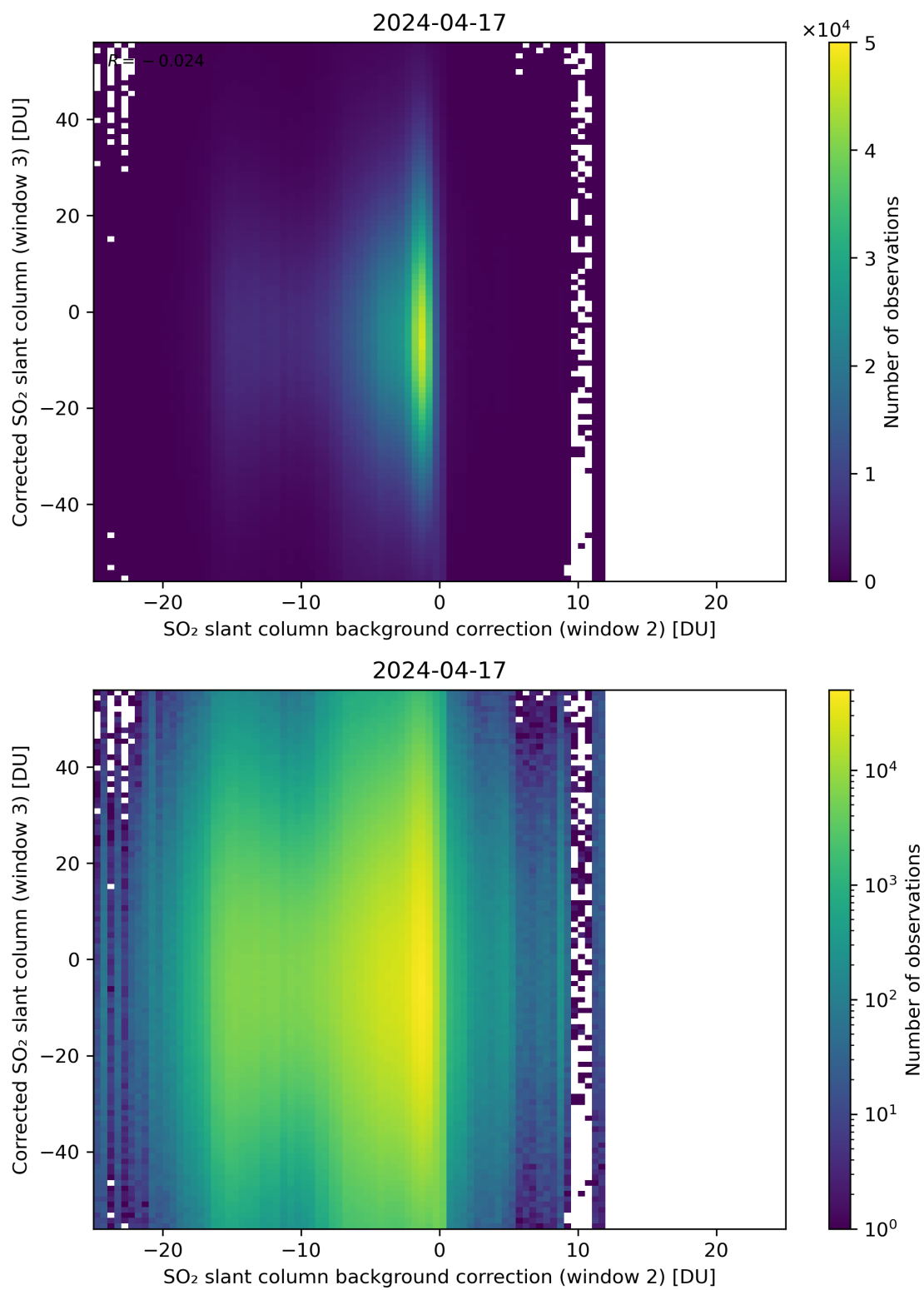
Figure 116: Scatter density plot of “SO 2 slant column background correction (window 2)” against “Corrected SO 2 slant column (window 3)” for 2024-04-16 to 2024-04-18.
