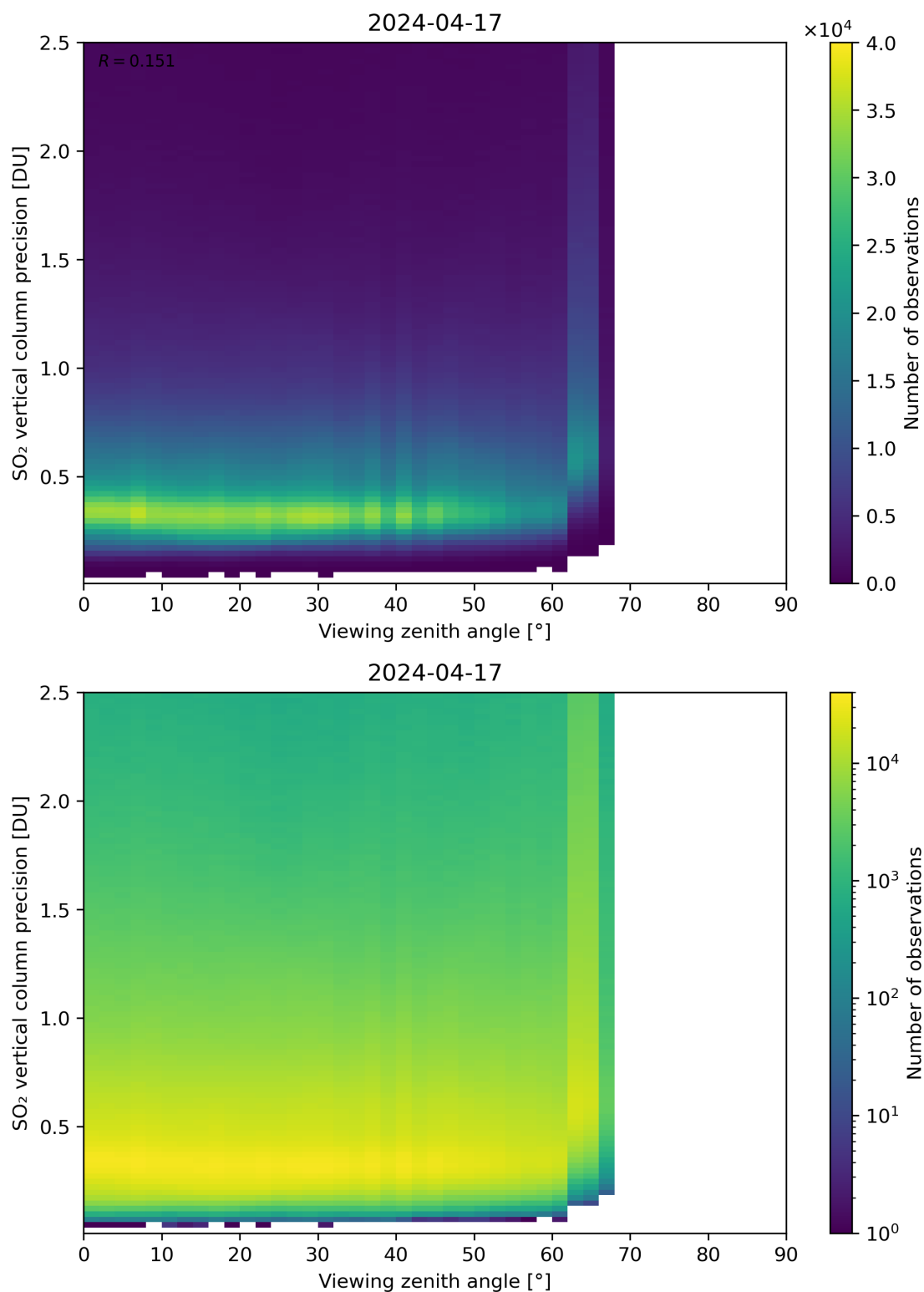
Figure 328: Scatter density plot of “Viewing zenith angle” against “SO 2 vertical column precision” for 2024-04-16 to 2024-04-18.
