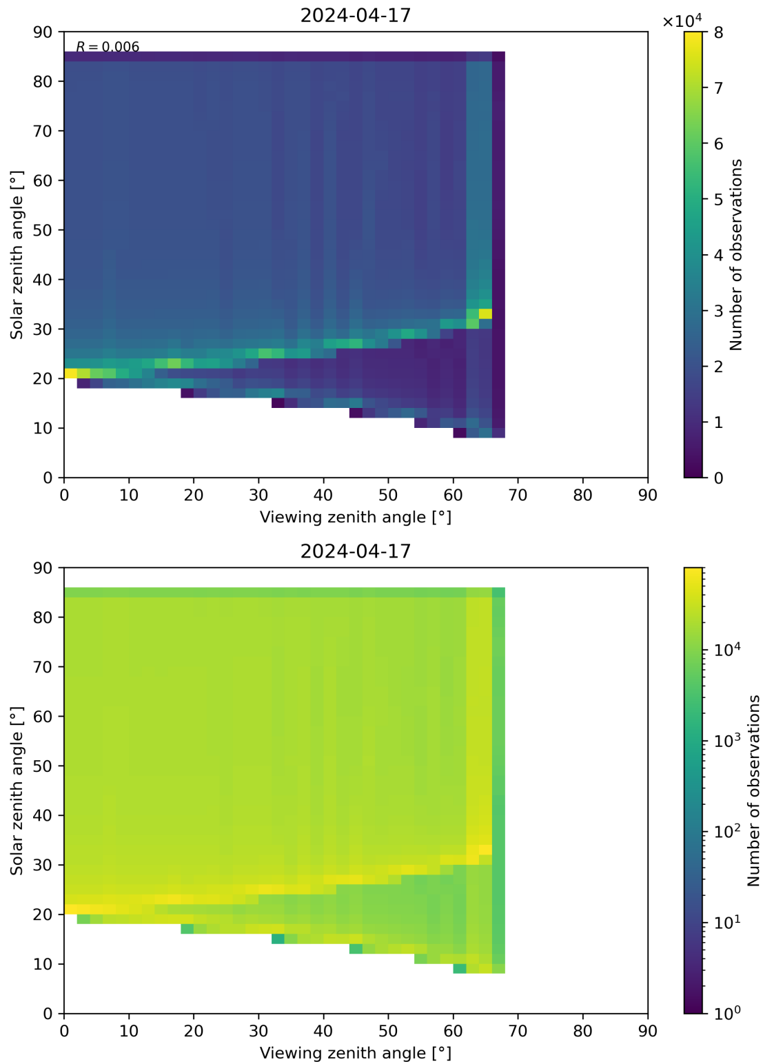
Figure 315: Scatter density plot of “Viewing zenith angle” against “Solar zenith angle” for 2024-04-16 to 2024-04-18.
