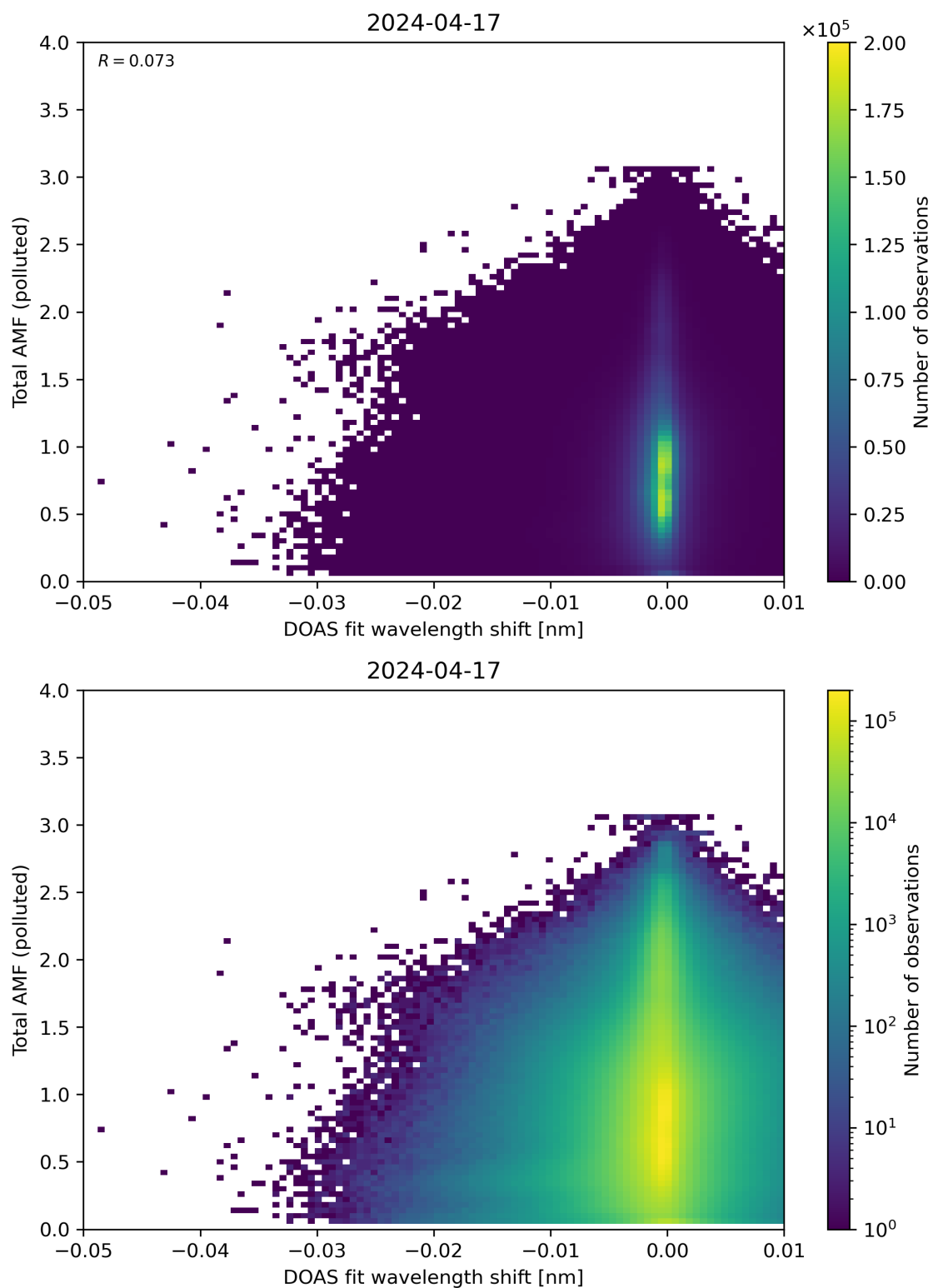
Figure 130: Scatter density plot of “DOAS fit wavelength shift” against “Total AMF (polluted)” for 2024-04-16 to 2024-04-18.
