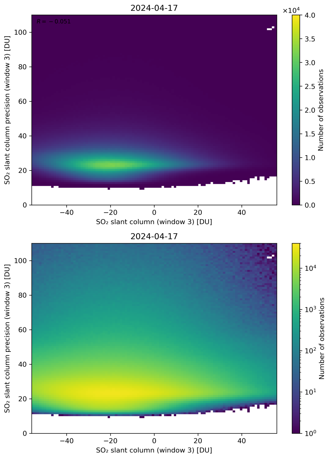
Figure 267: Scatter density plot of “SO 2 slant column (window 3)” against “SO 2 slant column precision (window 3)” for 2024-04-16 to 2024-04-18.
