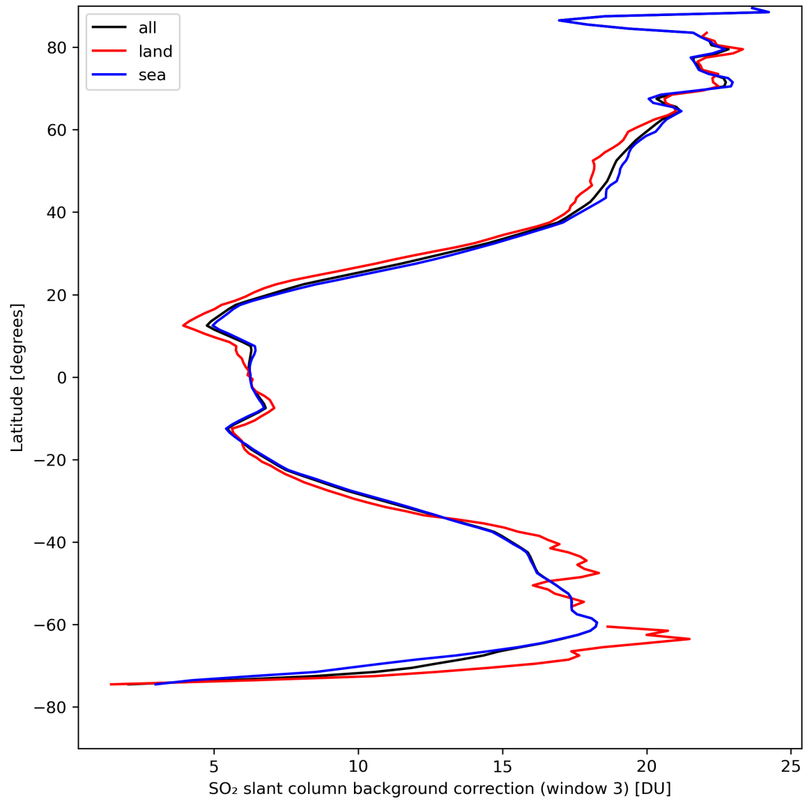
Figure 44: Zonal average of “SO 2 slant column background correction (window 3)” for 2024-04-16 to 2024-04-18.
