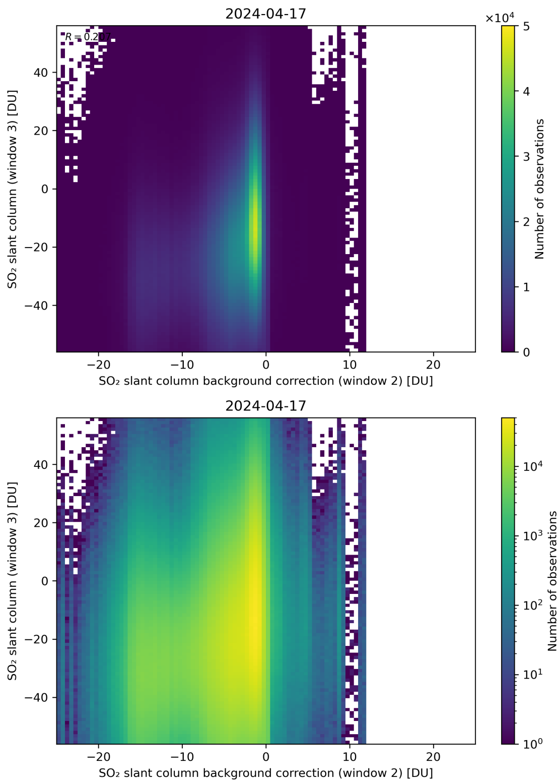
Figure 117: Scatter density plot of “SO 2 slant column background correction (window 2)” against “SO 2 slant column (window 3)” for 2024-04-16 to 2024-04-18.
