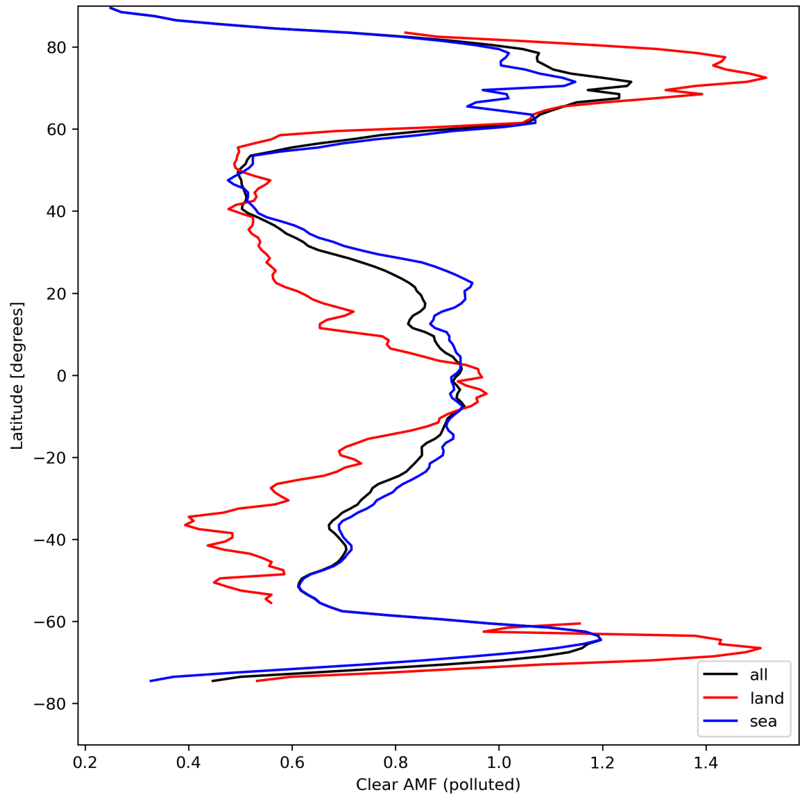
Figure 50: Zonal average of “Clear AMF (polluted)” for 2024-04-16 to 2024-04-18.
