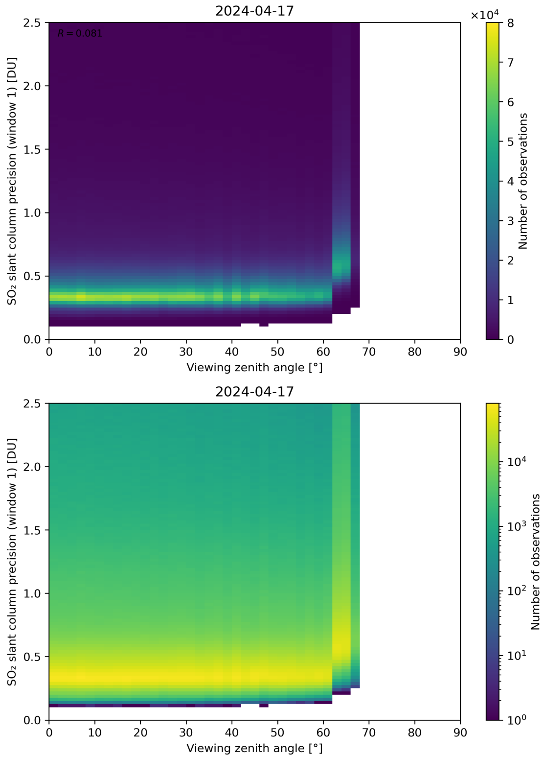
Figure 321: Scatter density plot of “Viewing zenith angle” against “SO 2 slant column precision (window 1)” for 2024-04-16 to 2024-04-18.
