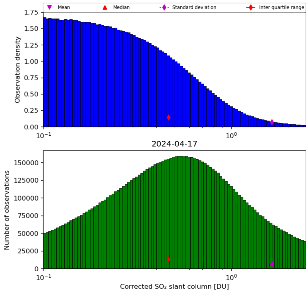
Figure 55: Histogram of “Corrected SO 2 slant column” for 2024-04-16 to 2024-04-18
