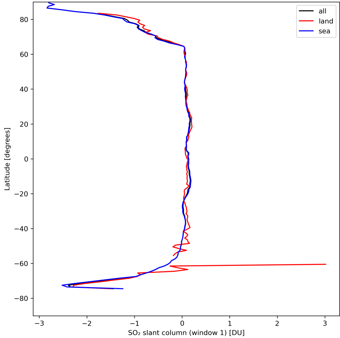
Figure 33: Zonal average of “SO 2 slant column (window 1)” for 2024-04-16 to 2024-04-18.
