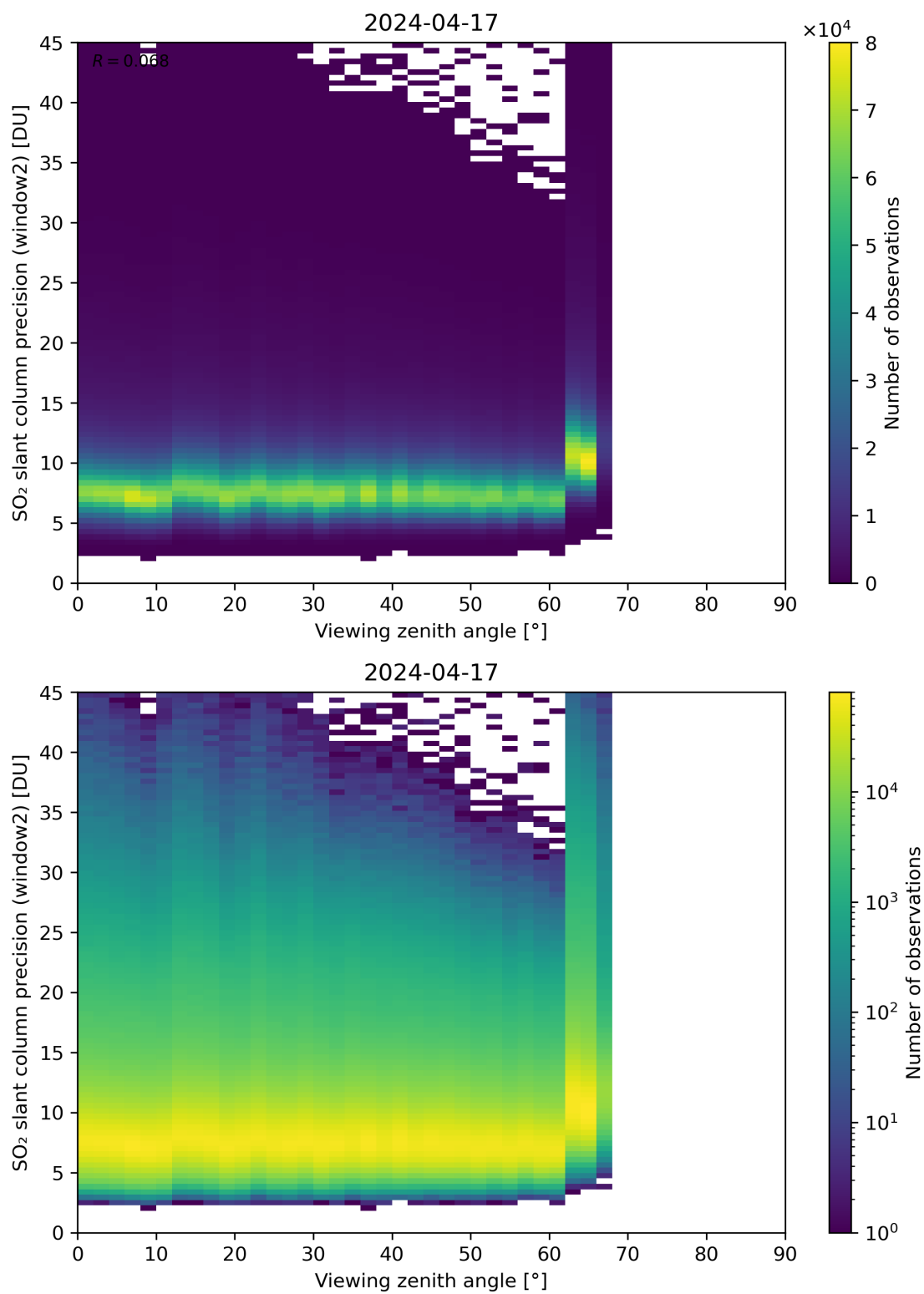
Figure 322: Scatter density plot of “Viewing zenith angle” against “SO 2 slant column precision (window2)” for 2024-04-16 to 2024-04-18.
