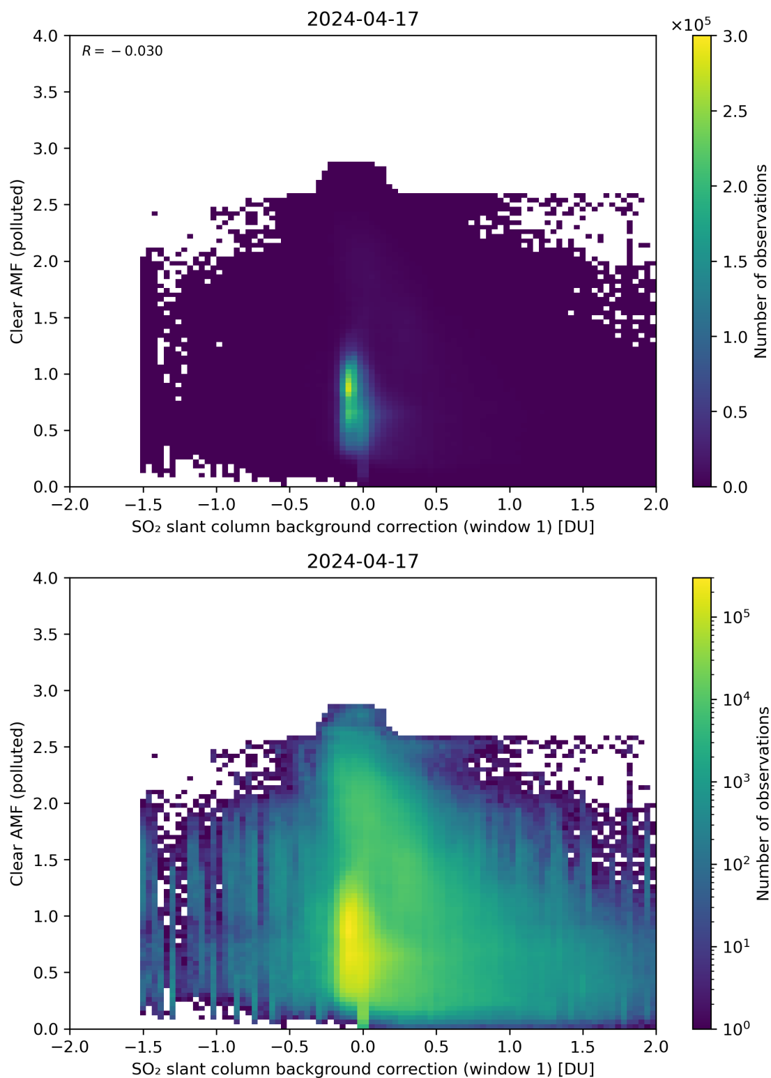
Figure 103: Scatter density plot of “SO 2 slant column background correction (window 1)” against “Clear AMF (polluted)” for 2024-04-16 to 2024-04-18.
