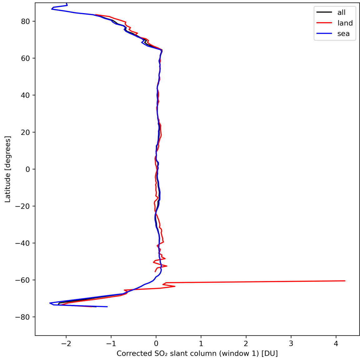
Figure 35: Zonal average of “Corrected SO 2 slant column (window 1)” for 2024-04-16 to 2024-04-18.
