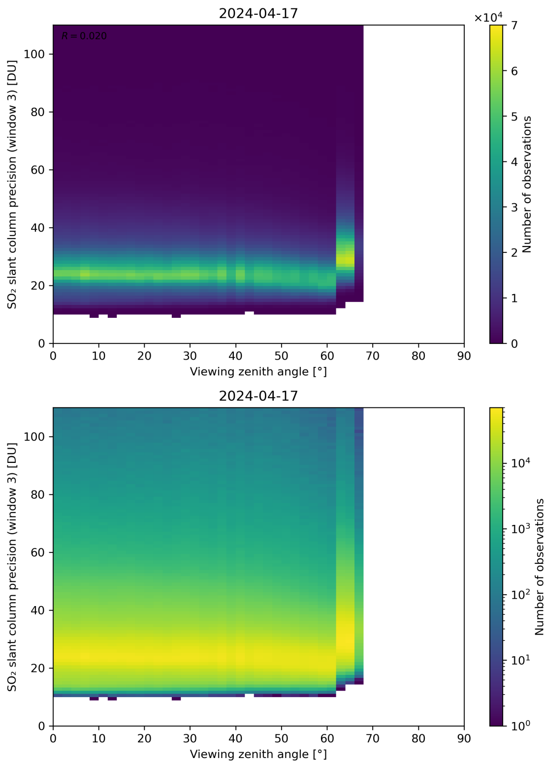
Figure 324: Scatter density plot of “Viewing zenith angle” against “SO 2 slant column precision (window 3)” for 2024-04-16 to 2024-04-18.
