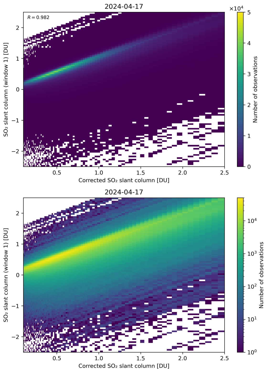
Figure 187: Scatter density plot of “Corrected SO 2 slant column” against “SO 2 slant column (window 1)” for 2024-04-16 to 2024-04-18.
