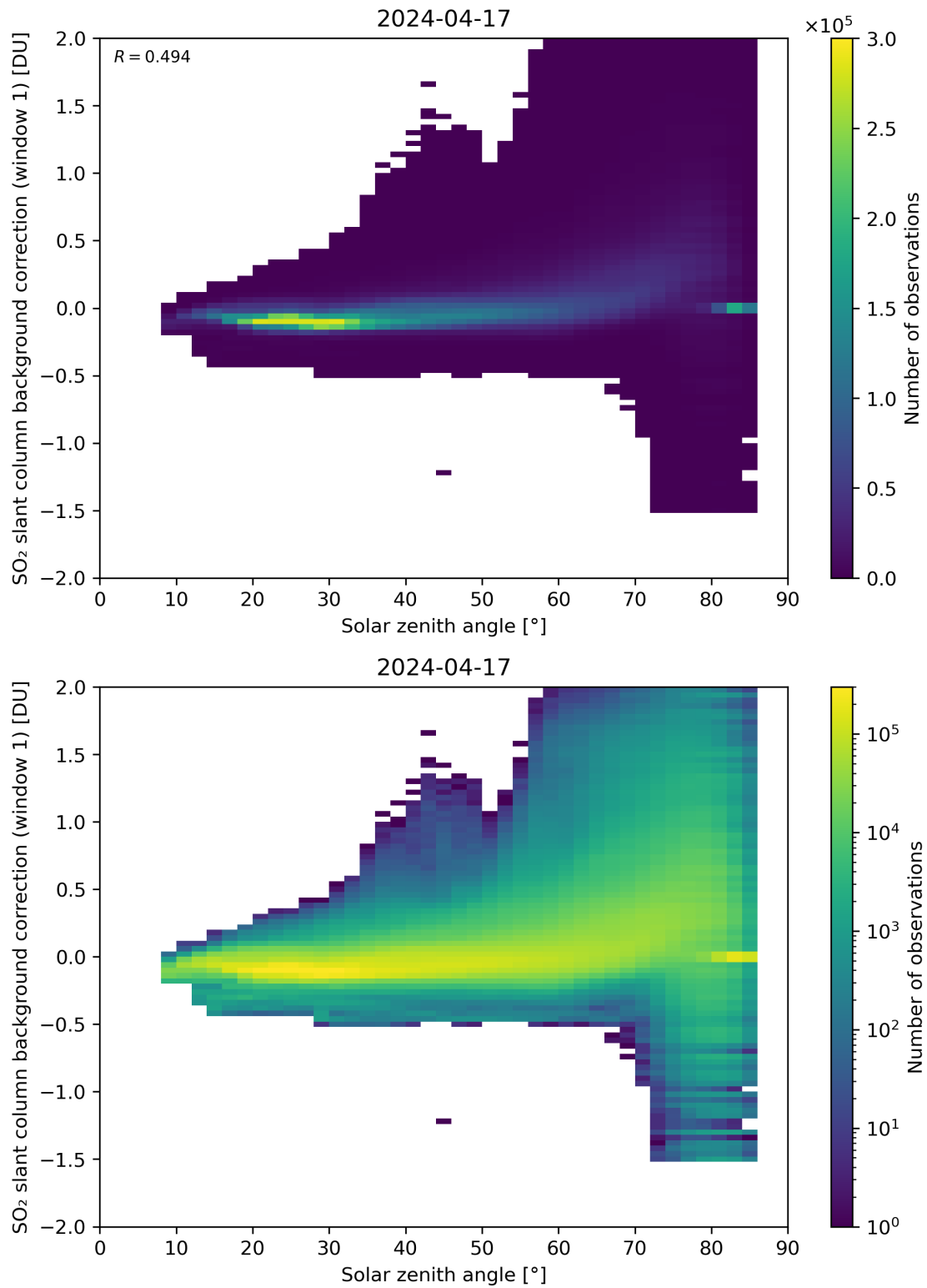
Figure 158: Scatter density plot of “Solar zenith angle” against “SO 2 slant column background correction (window 1)” for 2024-04-16 to 2024-04-18.
