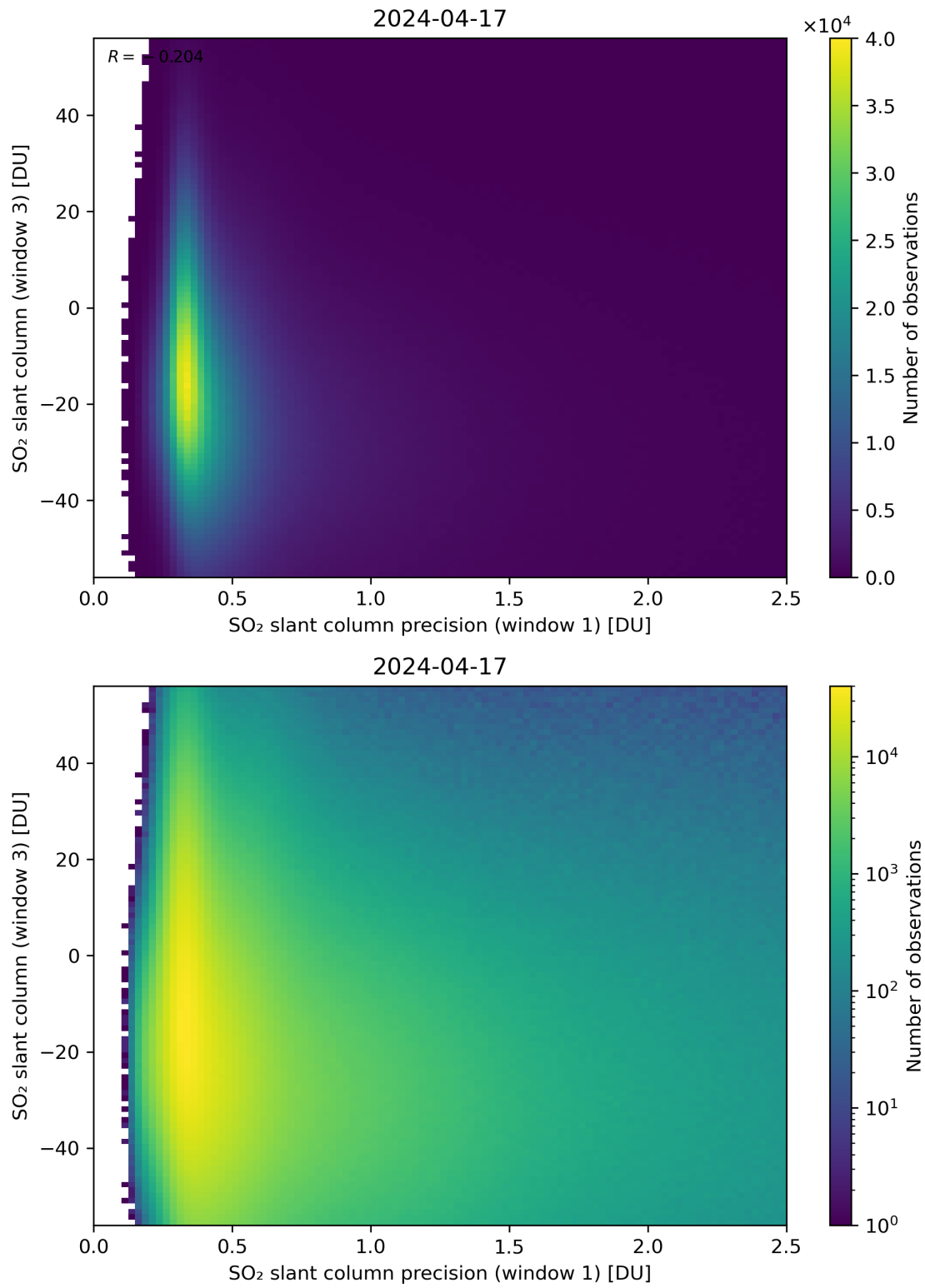
Figure 228: Scatter density plot of “SO 2 slant column precision (window 1)” against “SO 2 slant column (window 3)” for 2024-04-16 to 2024-04-18.
