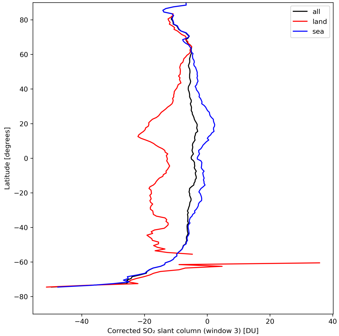
Figure 43: Zonal average of “Corrected SO 2 slant column (window 3)” for 2024-04-16 to 2024-04-18.
