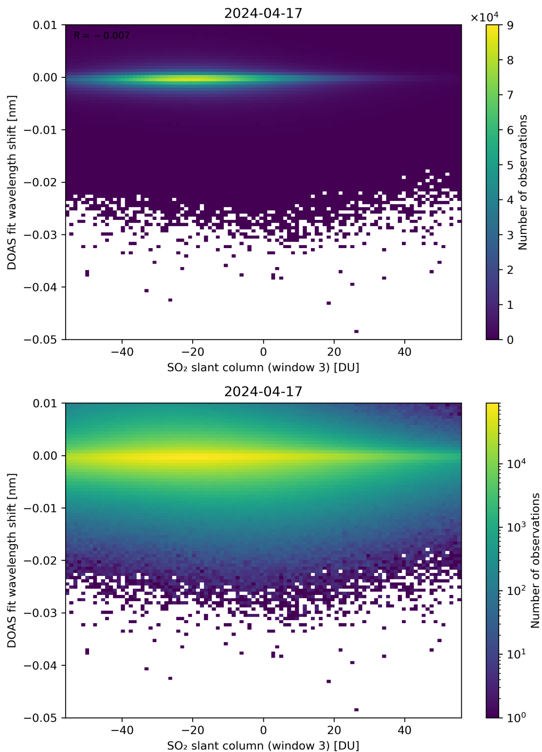
Figure 254: Scatter density plot of “SO 2 slant column (window 3)” against “DOAS fit wavelength shift” for 2024-04-16 to 2024-04-18.
