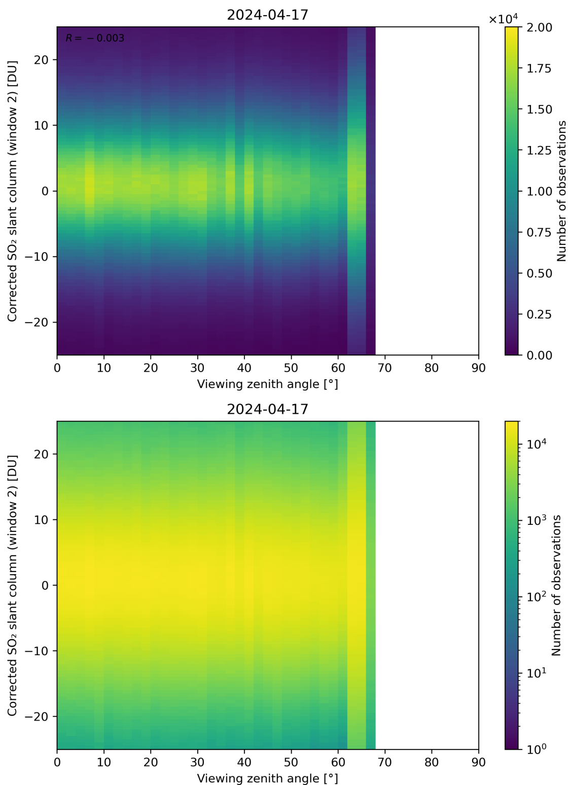
Figure 318: Scatter density plot of “Viewing zenith angle” against “Corrected SO 2 slant column (window 2)” for 2024-04-16 to 2024-04-18.
