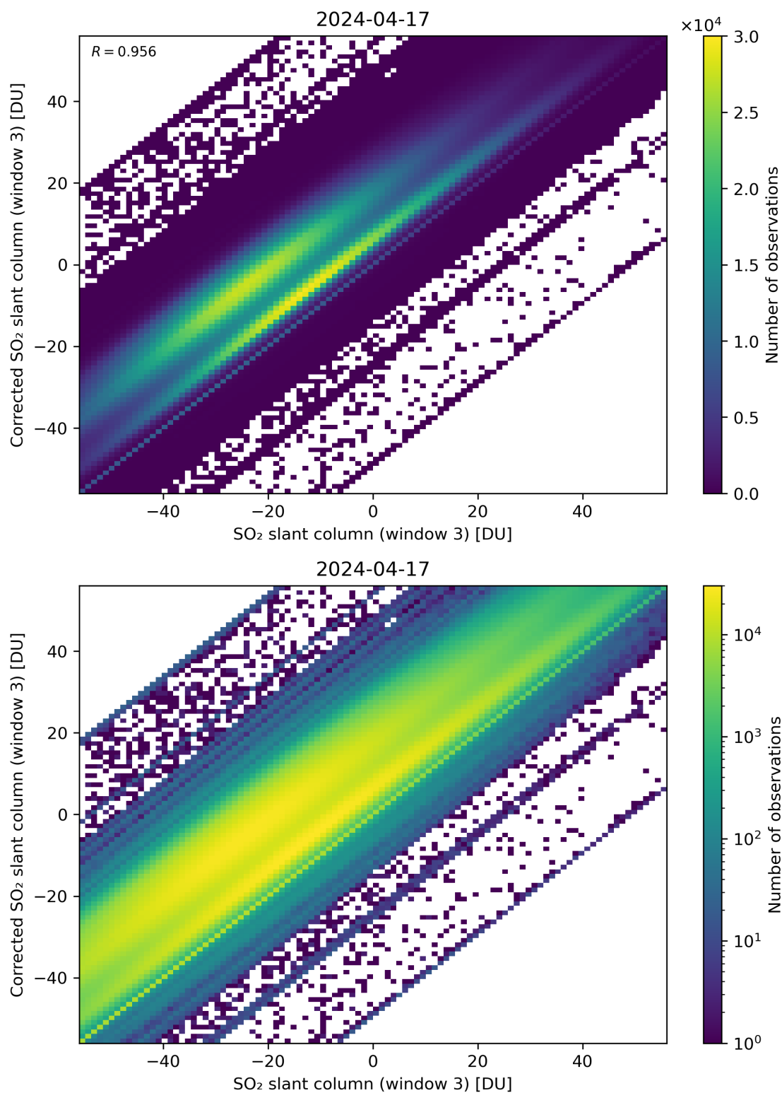
Figure 266: Scatter density plot of “SO 2 slant column (window 3)” against “Corrected SO 2 slant column (window 3)” for 2024-04-16 to 2024-04-18.
