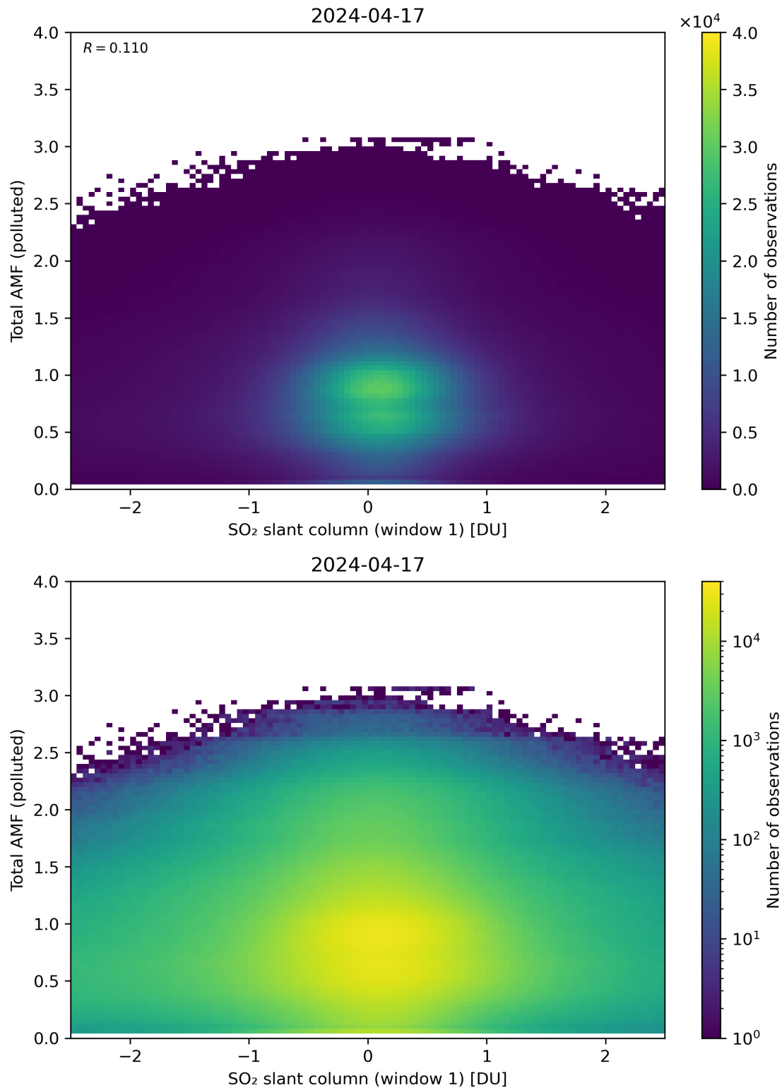
Figure 239: Scatter density plot of “SO 2 slant column (window 1)” against “Total AMF (polluted)” for 2024-04-16 to 2024-04-18.
