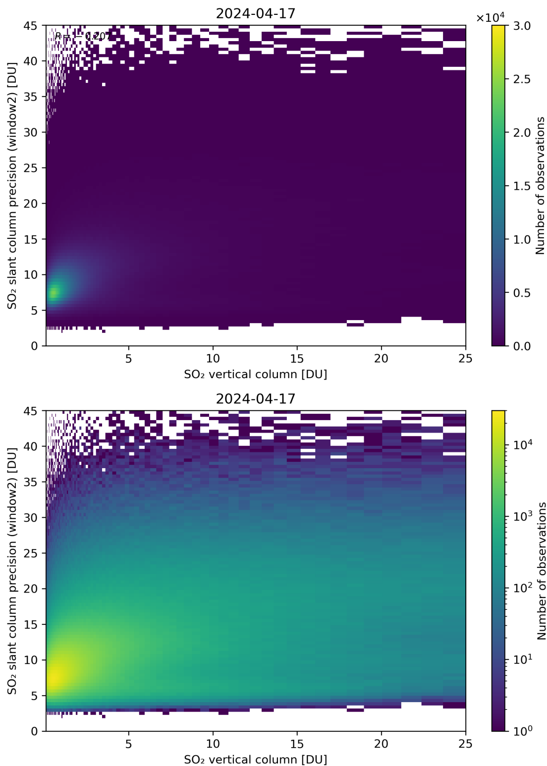
Figure 302: Scatter density plot of “SO 2 vertical column” against “SO 2 slant column precision (window2)” for 2024-04-16 to 2024-04-18.
