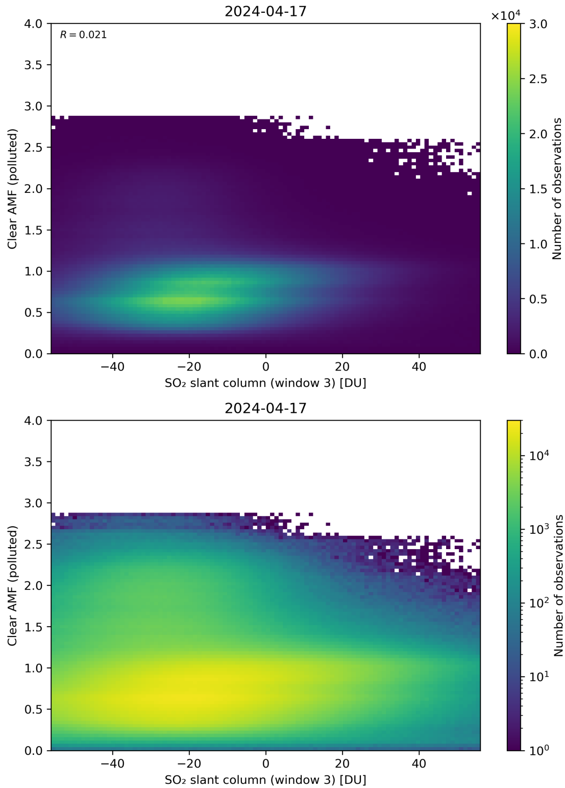
Figure 265: Scatter density plot of “SO 2 slant column (window 3)” against “Clear AMF (polluted)” for 2024-04-16 to 2024-04-18.
