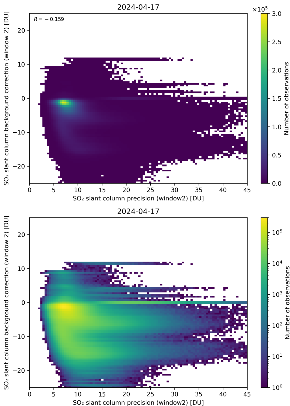
Figure 241: Scatter density plot of “SO 2 slant column precision (window2)” against “SO 2 slant column background correction (window 2)” for 2024-04-16 to 2024-04-18.
