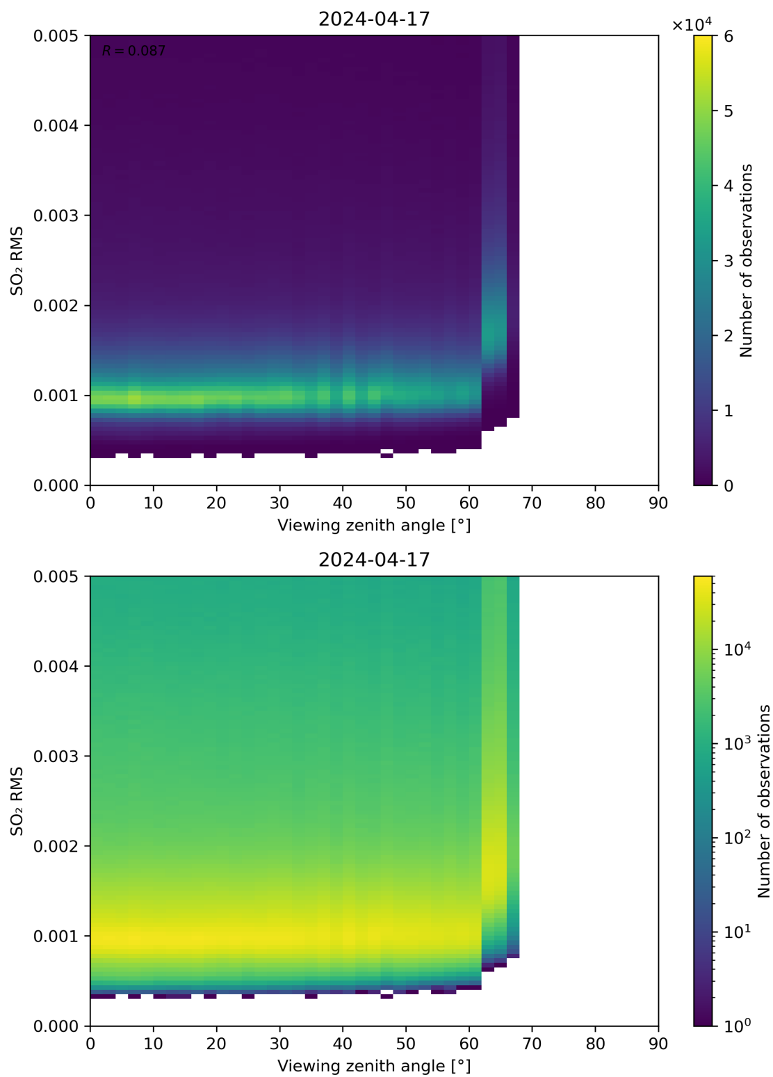
Figure 313: Scatter density plot of “Viewing zenith angle” against “SO 2 RMS” for 2024-04-16 to 2024-04-18.
