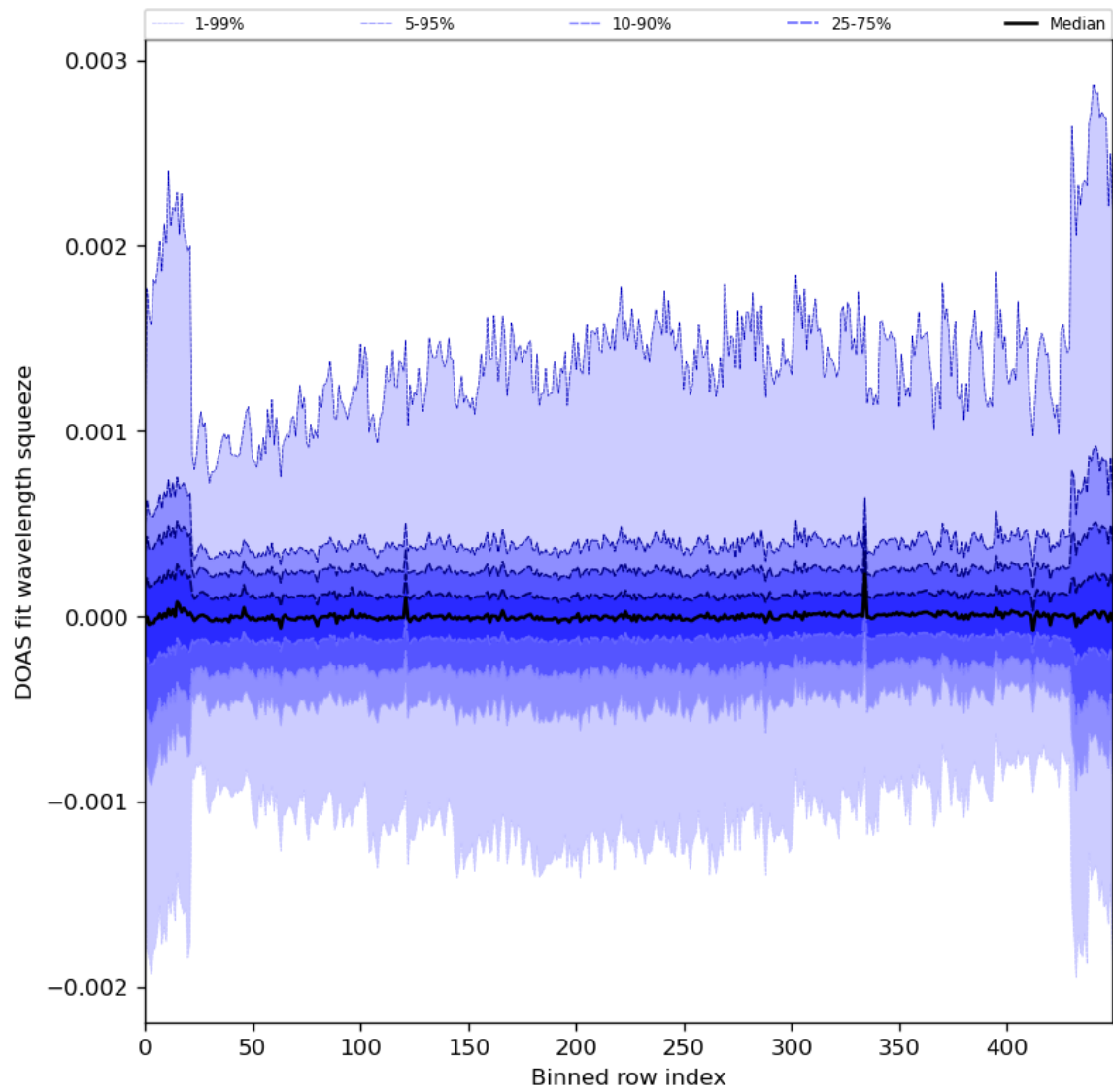
Figure 92: Along track statistics of “DOAS fit wavelength squeeze” for 2024-04-16 to 2024-04-18
