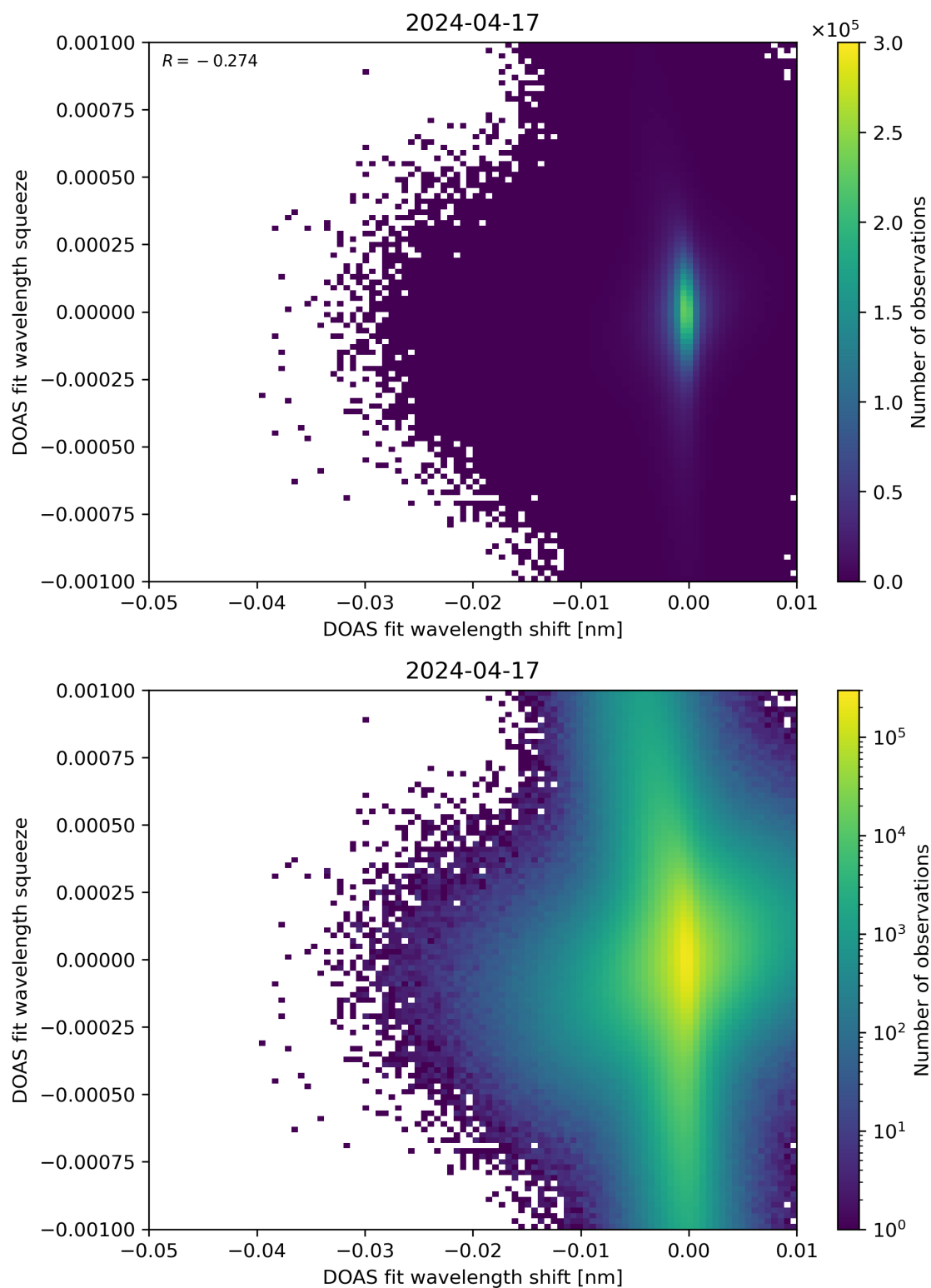
Figure 127: Scatter density plot of “DOAS fit wavelength shift” against “DOAS fit wavelength squeeze” for 2024-04-16 to 2024-04-18.
