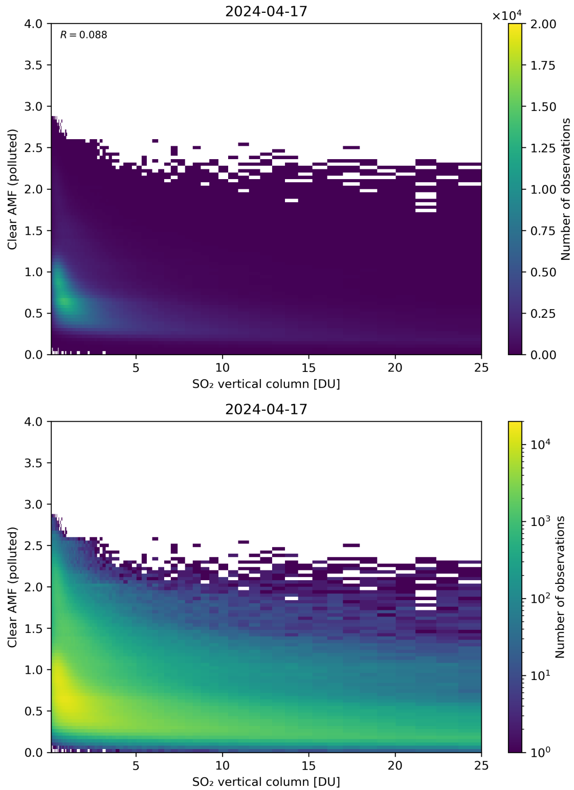
Figure 296: Scatter density plot of “SO 2 vertical column” against “Clear AMF (polluted)” for 2024-04-16 to 2024-04-18.
