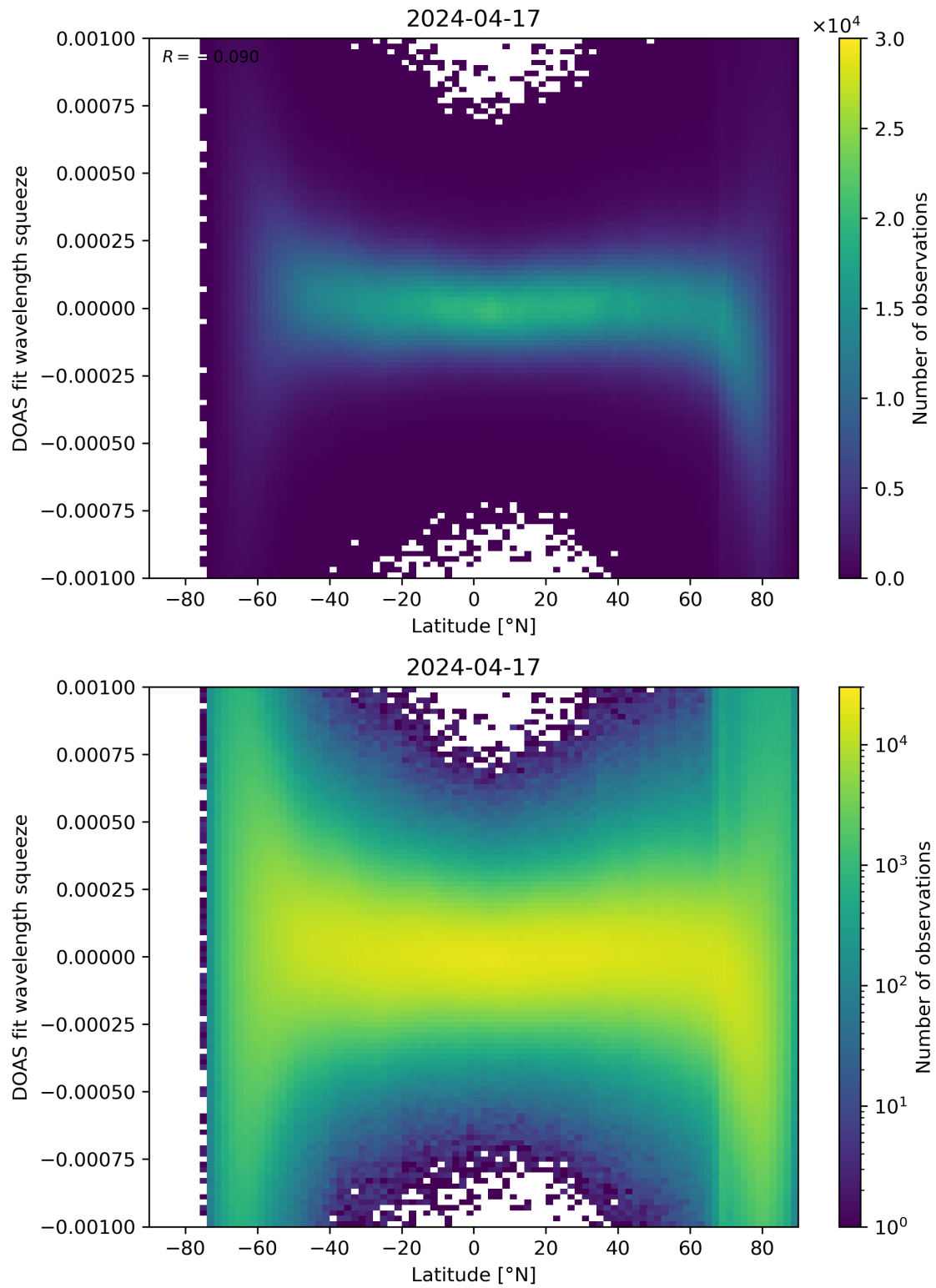
Figure 143: Scatter density plot of “Latitude” against “DOAS fit wavelength squeeze” for 2024-04-16 to 2024-04-18.
