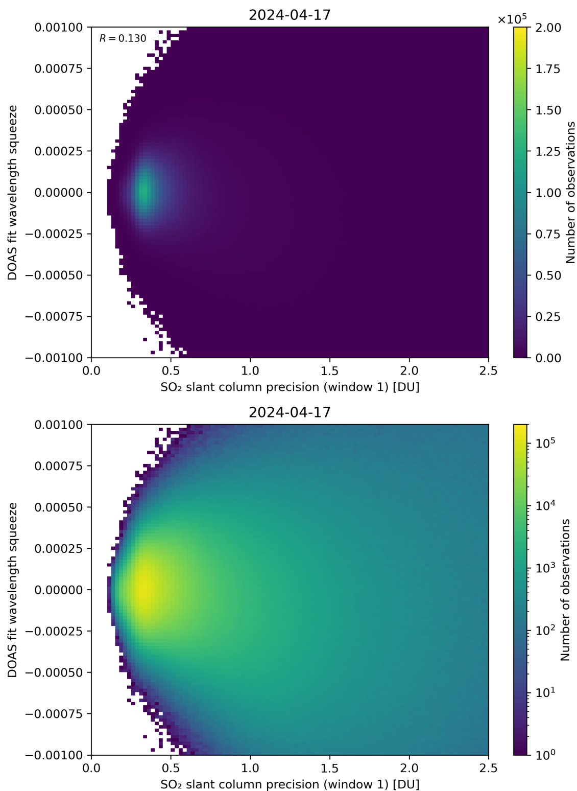
Figure 222: Scatter density plot of “SO 2 slant column precision (window 1)” against “DOAS fit wavelength squeeze” for 2024-04-16 to 2024-04-18.
