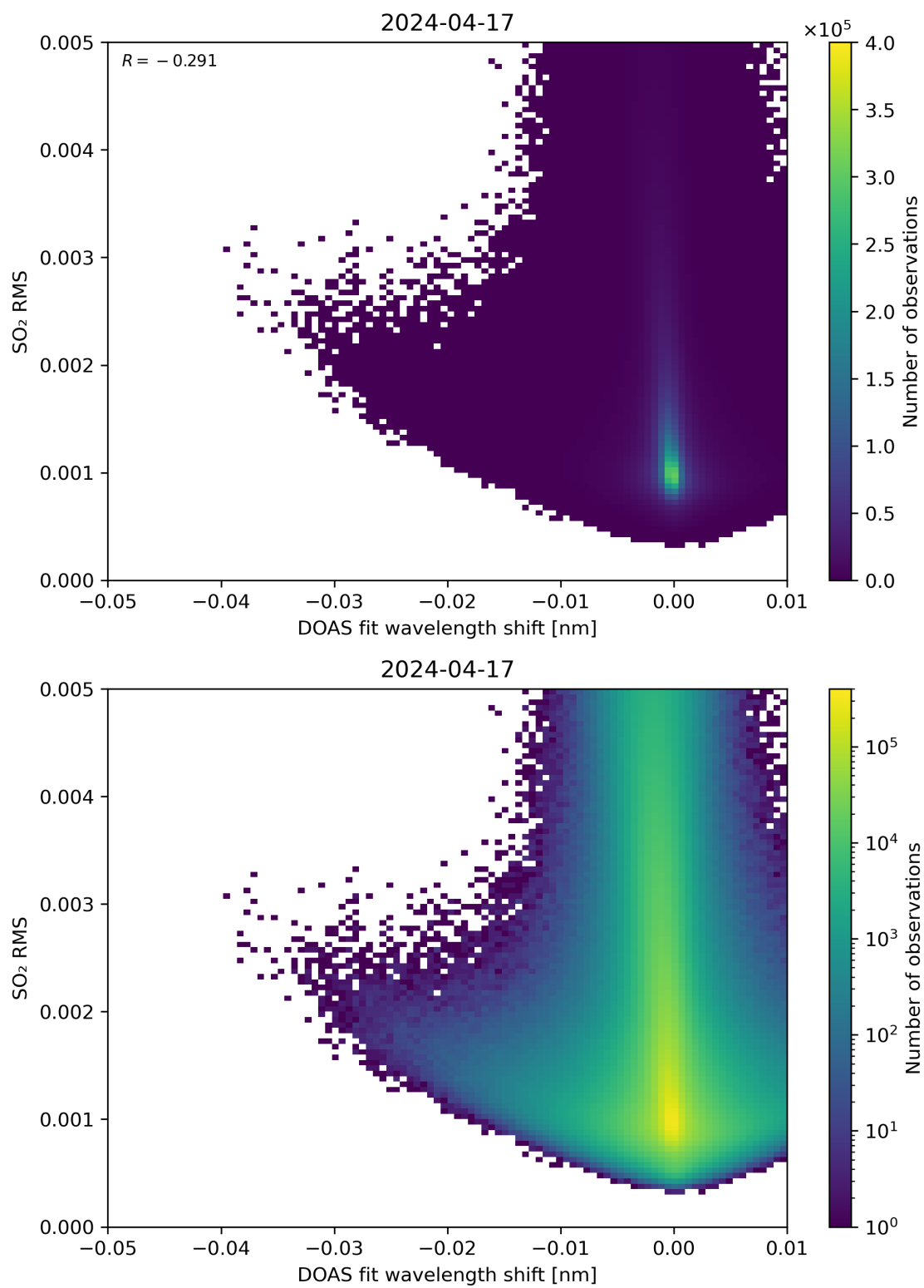
Figure 128: Scatter density plot of “DOAS fit wavelength shift” against “SO 2 RMS” for 2024-04-16 to 2024-04-18.
