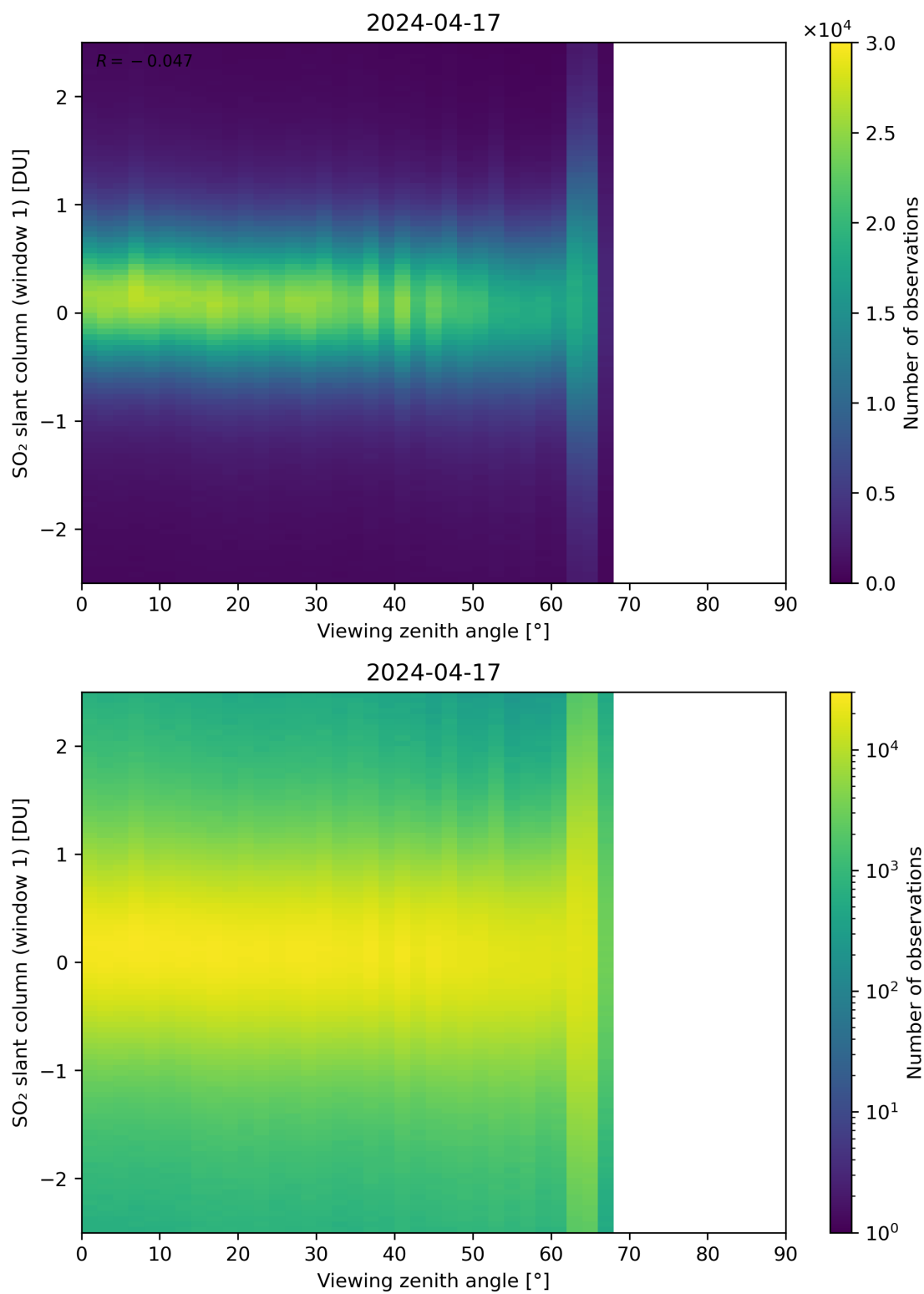
Figure 320: Scatter density plot of “Viewing zenith angle” against “SO 2 slant column (window 1)” for 2024-04-16 to 2024-04-18.
