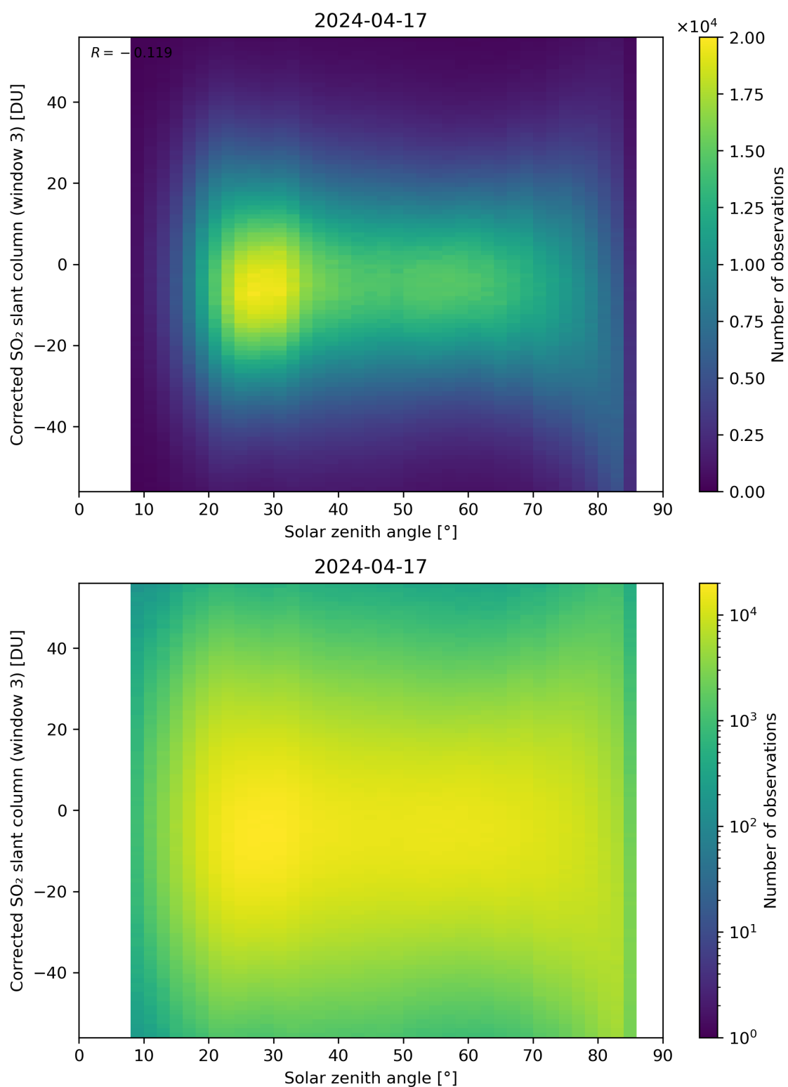
Figure 168: Scatter density plot of “Solar zenith angle” against “Corrected SO 2 slant column (window 3)” for 2024-04-16 to 2024-04-18.
