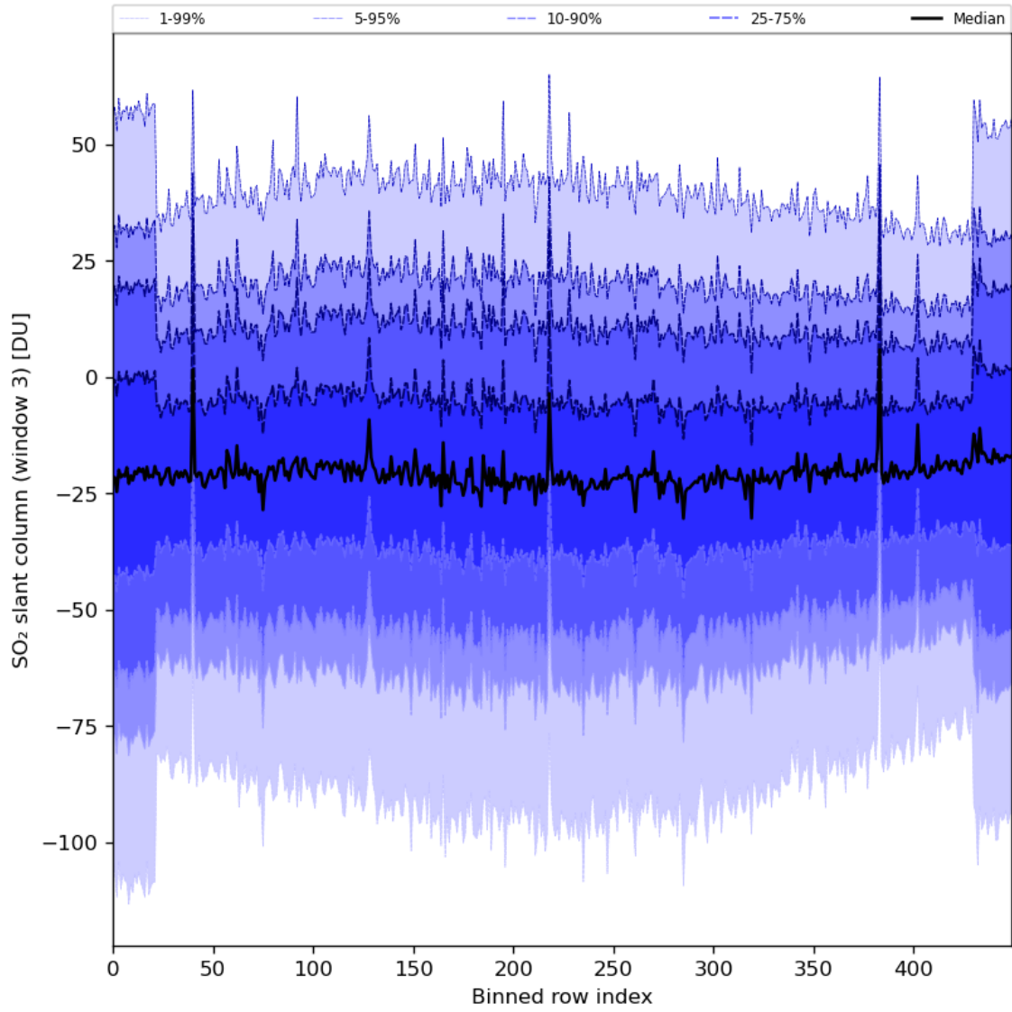
Figure 87: Along track statistics of “SO 2 slant column (window 3)” for 2024-04-16 to 2024-04-18
