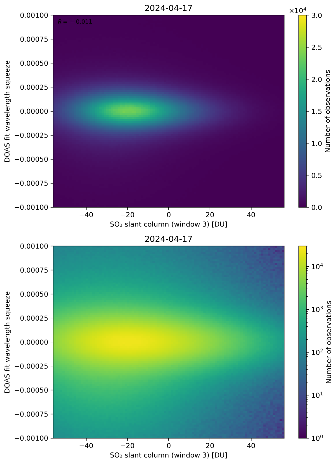
Figure 255: Scatter density plot of “SO 2 slant column (window 3)” against “DOAS fit wavelength squeeze” for 2024-04-16 to 2024-04-18.
