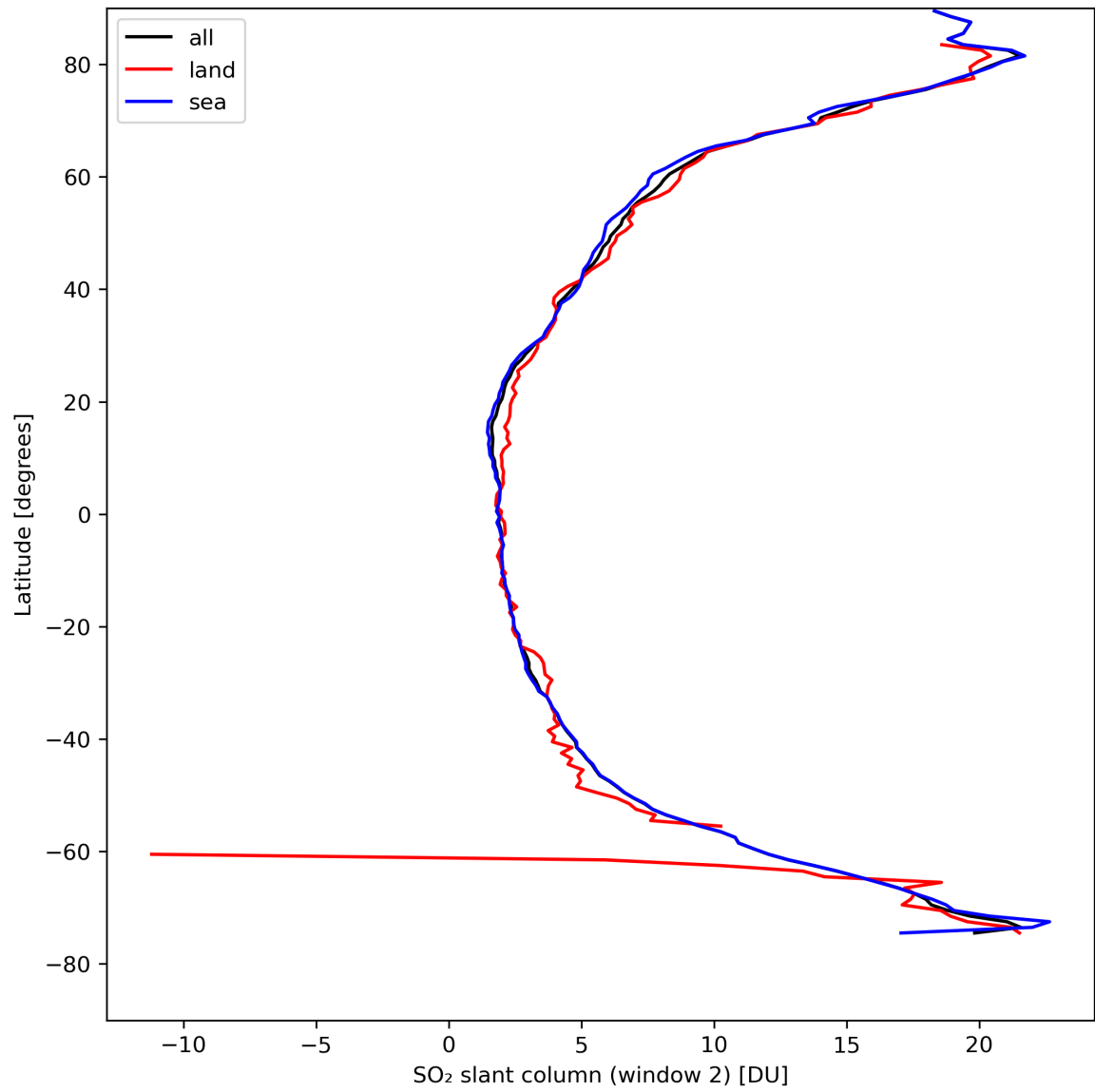
Figure 37: Zonal average of “SO 2 slant column (window 2)” for 2024-04-16 to 2024-04-18.
