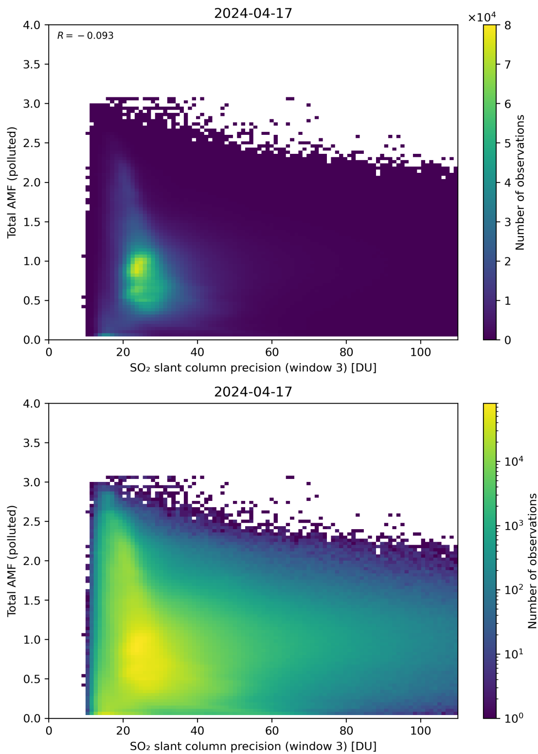
Figure 263: Scatter density plot of “SO 2 slant column precision (window 3)” against “Total AMF (polluted)” for 2024-04-16 to 2024-04-18.
