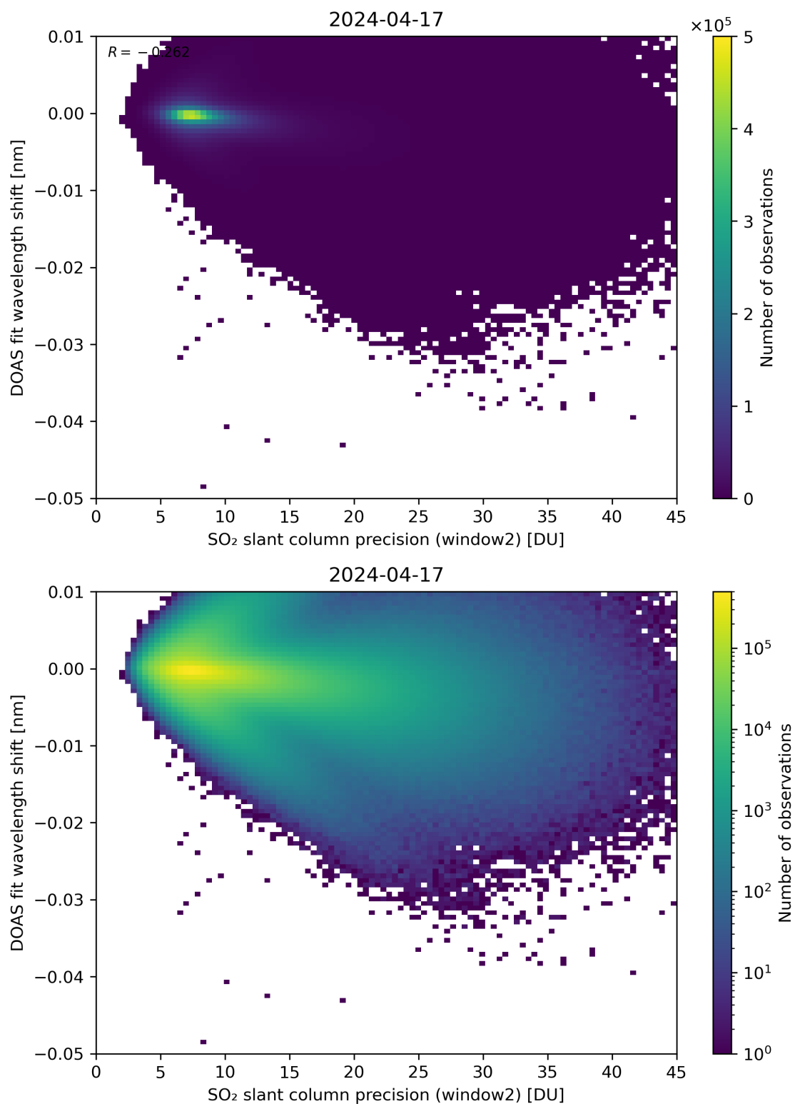
Figure 243: Scatter density plot of “SO 2 slant column precision (window2)” against “DOAS fit wavelength shift” for 2024-04-16 to 2024-04-18.
