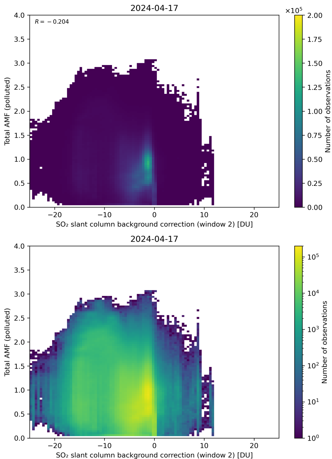
Figure 119: Scatter density plot of “SO 2 slant column background correction (window 2)” against “Total AMF (polluted)” for 2024-04-16 to 2024-04-18.
