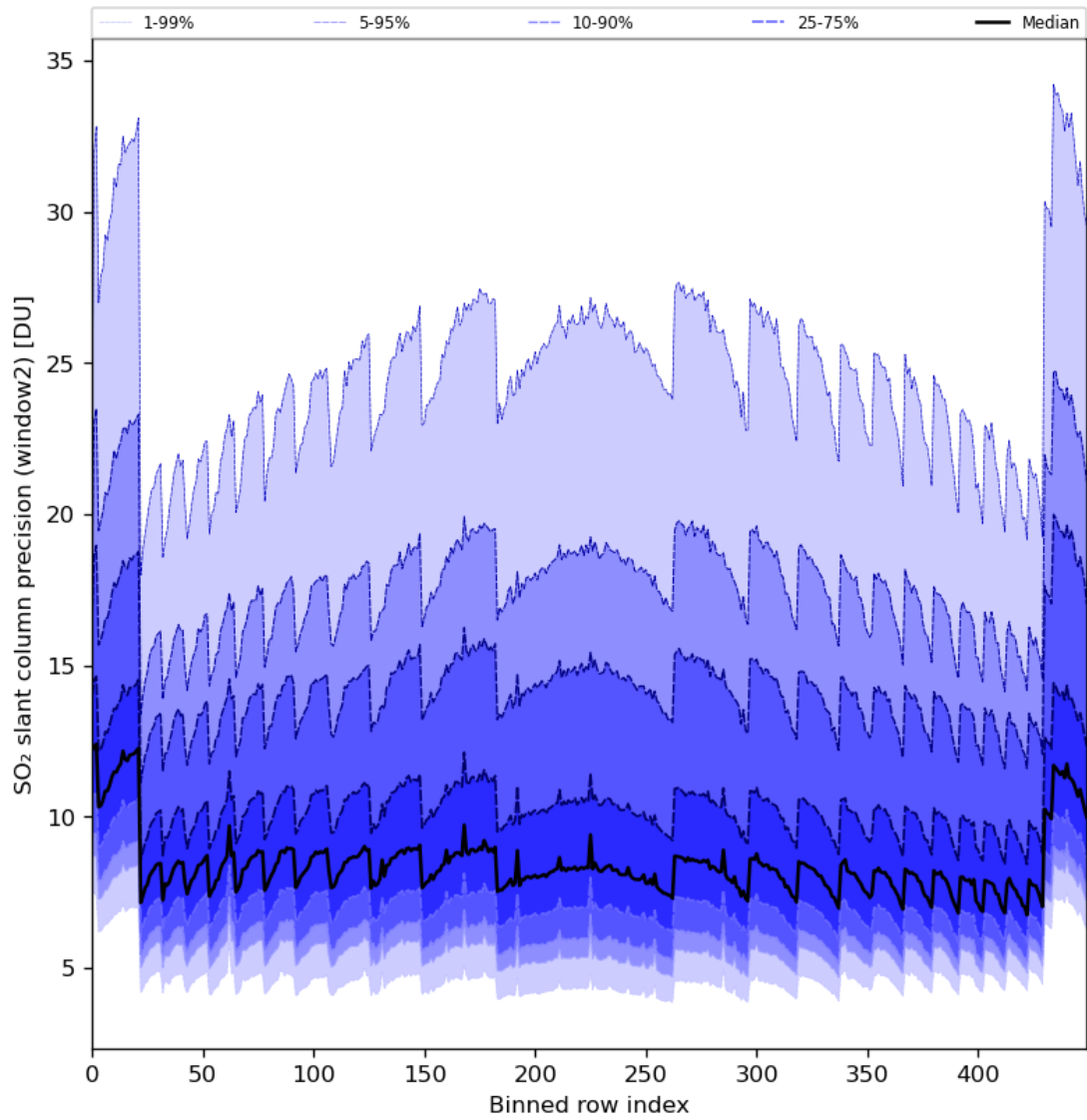
Figure 84: Along track statistics of “SO 2 slant column precision (window2)” for 2024-04-16 to 2024-04-18
