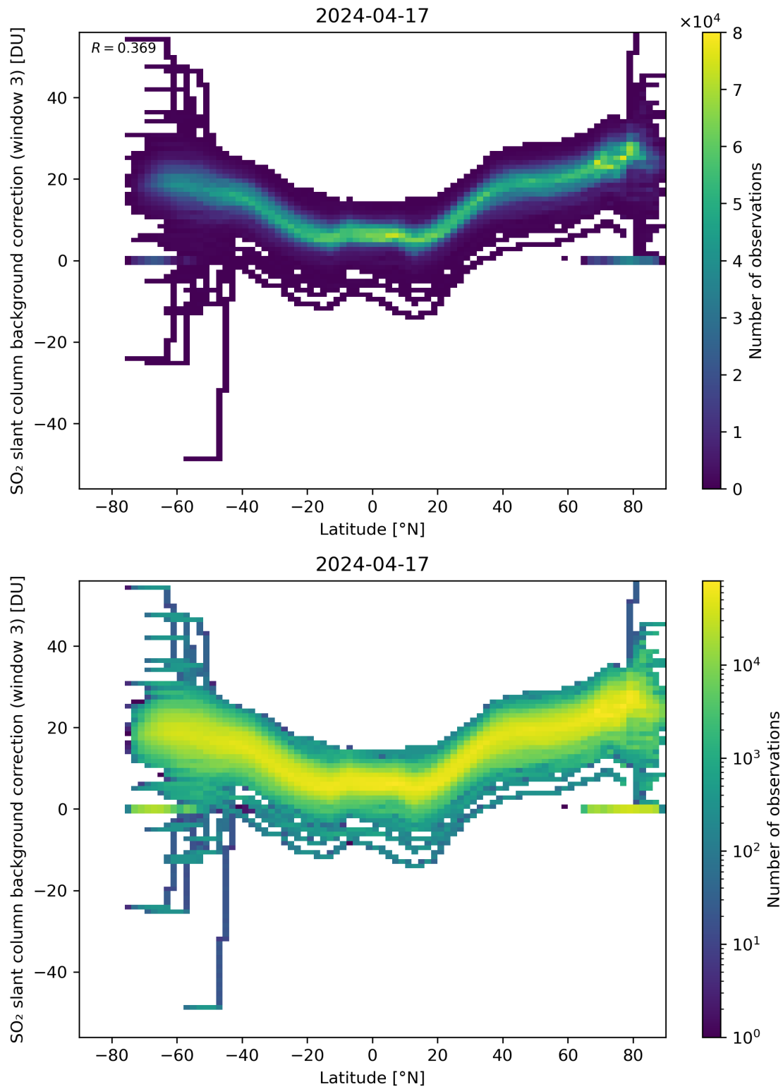
Figure 141: Scatter density plot of “Latitude” against “SO 2 slant column background correction (window 3)” for 2024-04-16 to 2024-04-18.
