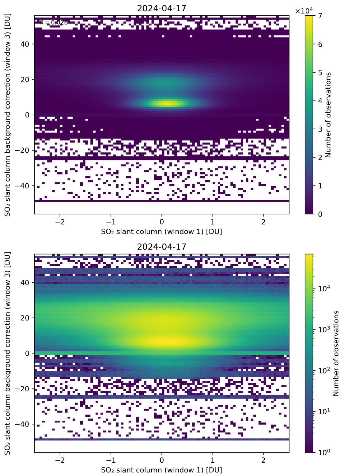
Figure 214: Scatter density plot of “SO 2 slant column (window 1)” against “SO 2 slant column background correction (window 3)” for 2024-04-16 to 2024-04-18.
