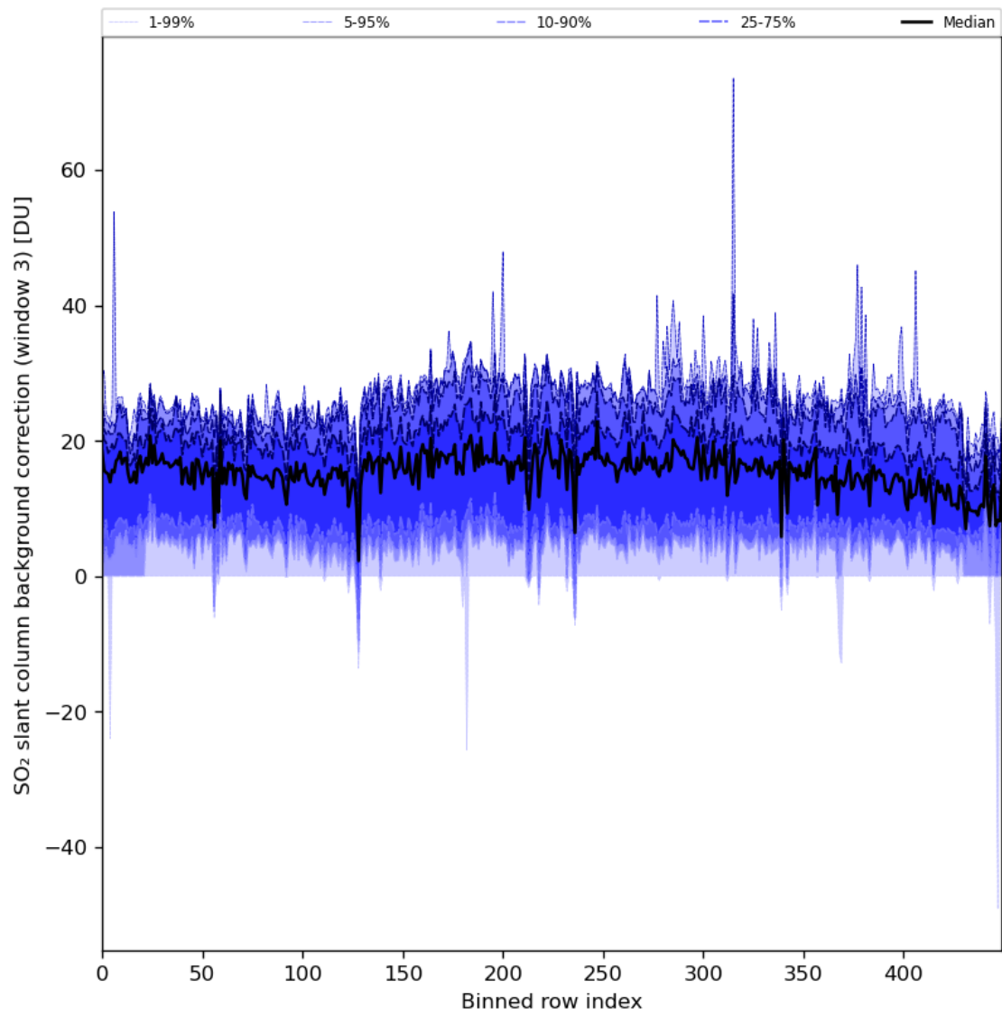
Figure 90: Along track statistics of “SO 2 slant column background correction (window 3)” for 2024-04-16 to 2024-04-18
