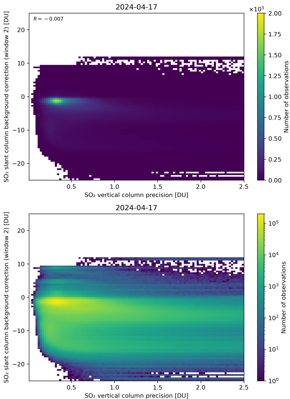
Figure 280: Scatter density plot of “SO 2 vertical column precision” against “SO 2 slant column background correction (window 2)” for 2024-04-16 to 2024-04-18.
