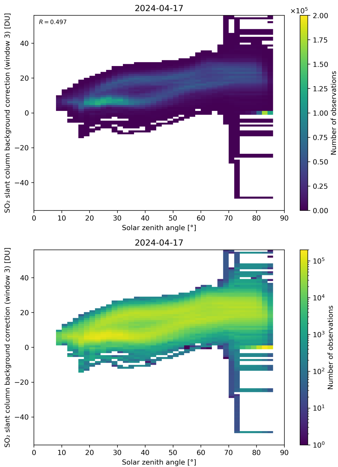
Figure 160: Scatter density plot of “Solar zenith angle” against “SO 2 slant column background correction (window 3)” for 2024-04-16 to 2024-04-18.
