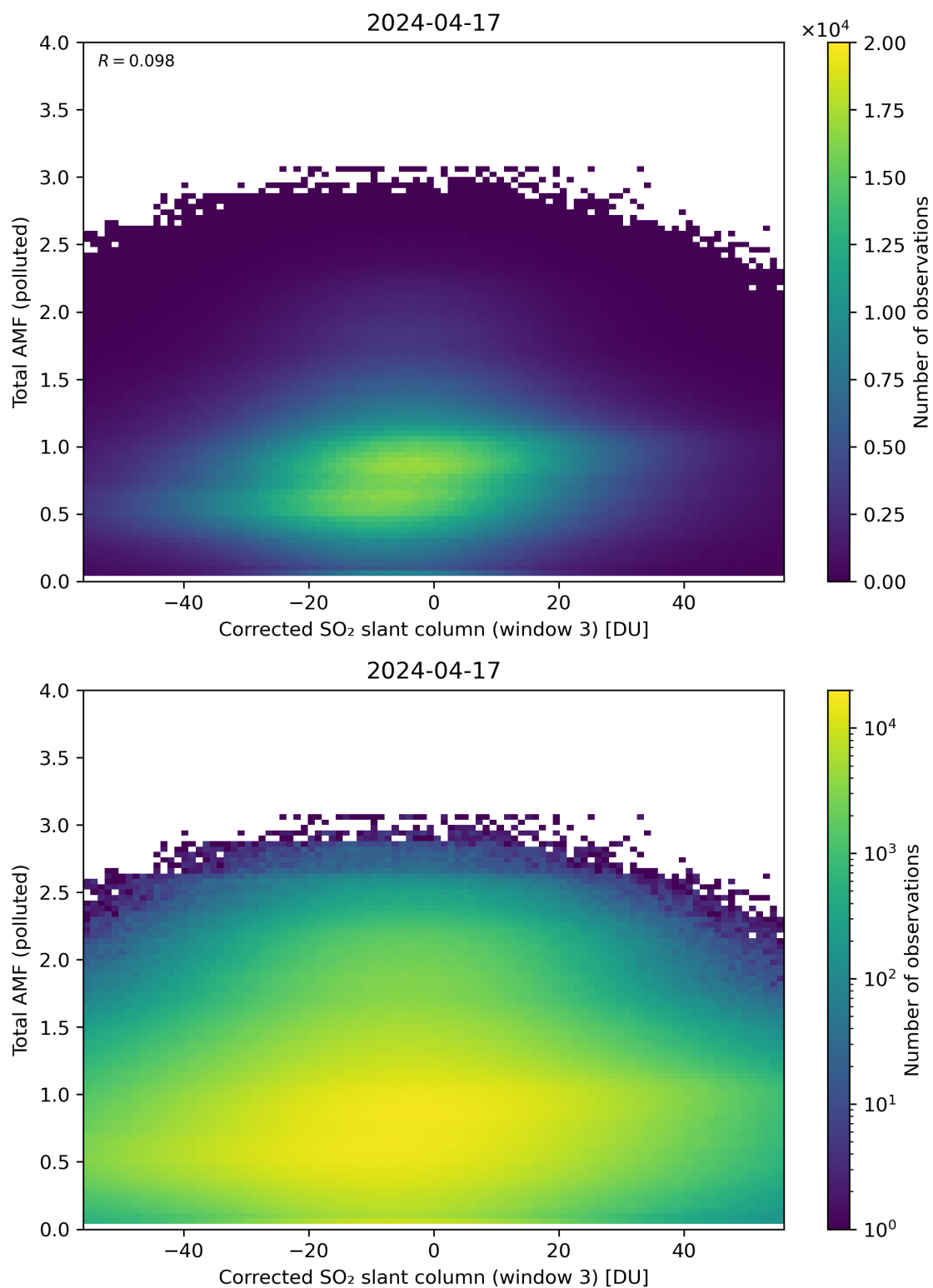
Figure 210: Scatter density plot of “Corrected SO 2 slant column (window 3)” against “Total AMF (polluted)” for 2024-04-16 to 2024-04-18.
