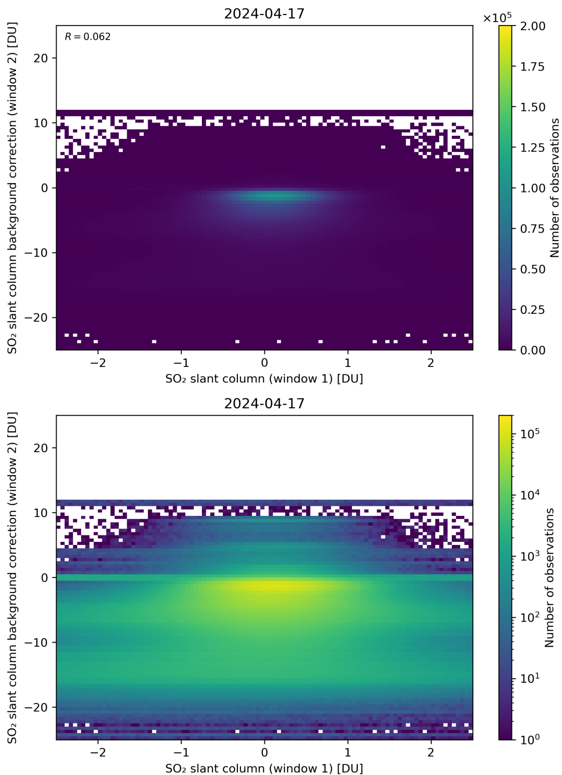
Figure 213: Scatter density plot of “SO 2 slant column (window 1)” against “SO 2 slant column background correction (window 2)” for 2024-04-16 to 2024-04-18.
