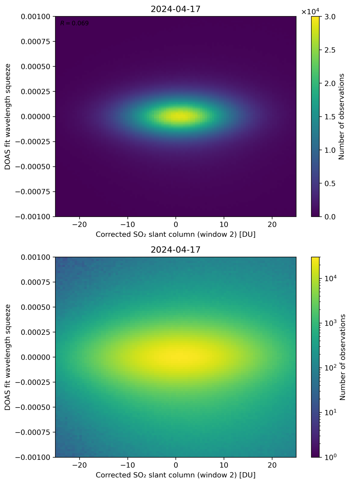
Figure 197: Scatter density plot of “Corrected SO 2 slant column (window 2)” against “DOAS fit wavelength squeeze” for 2024-04-16 to 2024-04-18.
