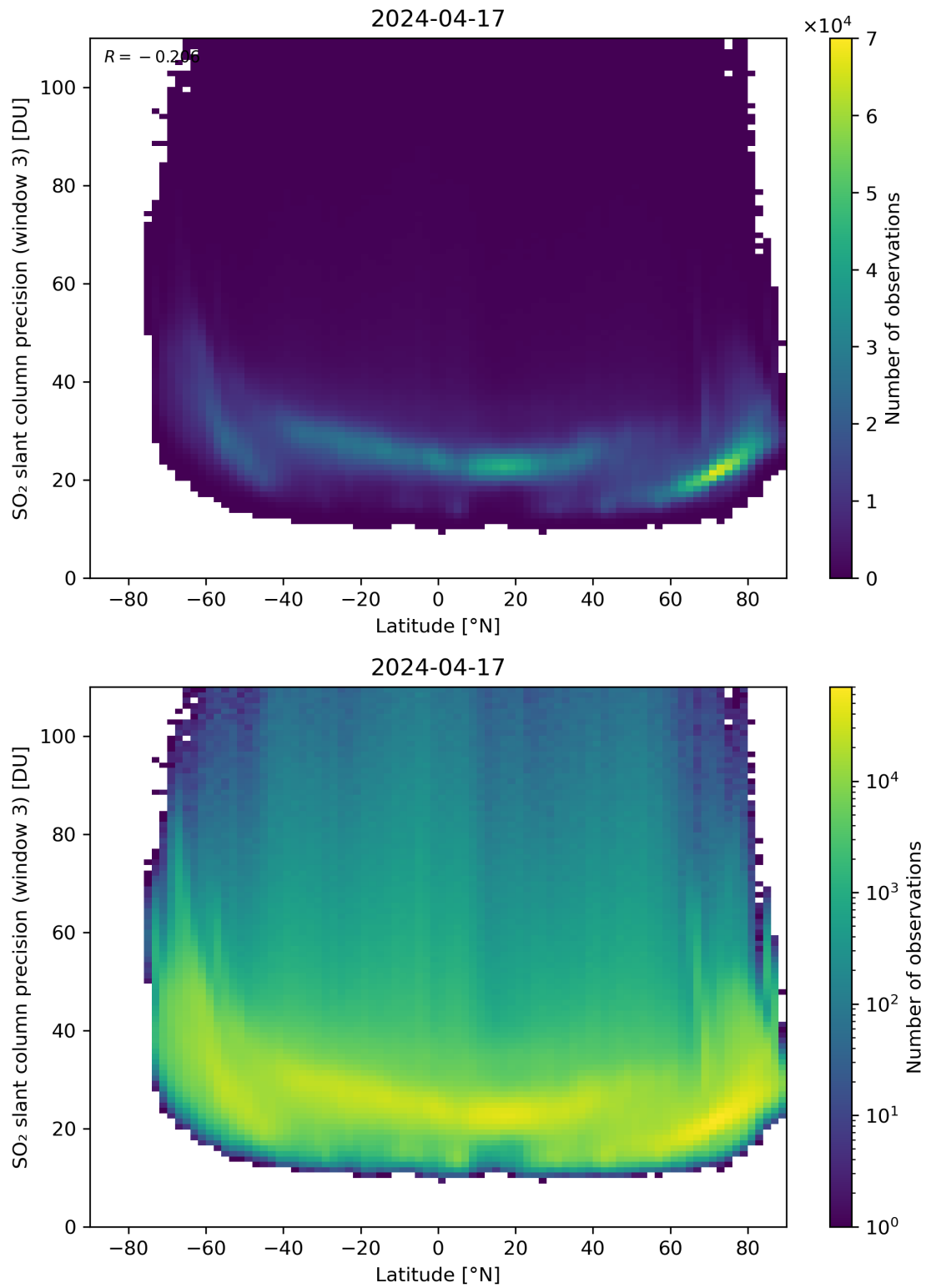
Figure 153: Scatter density plot of “Latitude” against “SO 2 slant column precision (window 3)” for 2024-04-16 to 2024-04-18.
