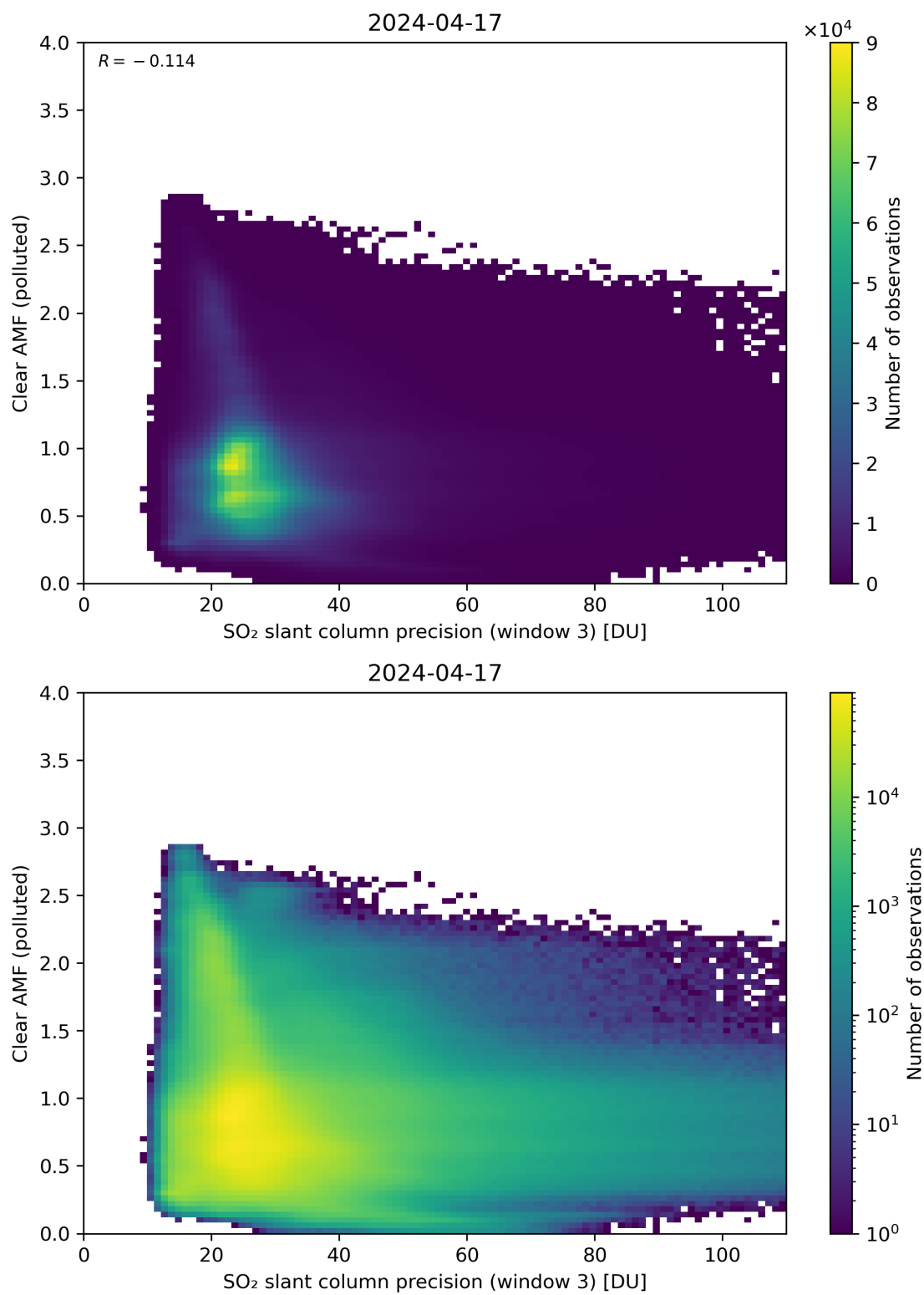
Figure 261: Scatter density plot of “SO 2 slant column precision (window 3)” against “Clear AMF (polluted)” for 2024-04-16 to 2024-04-18.
