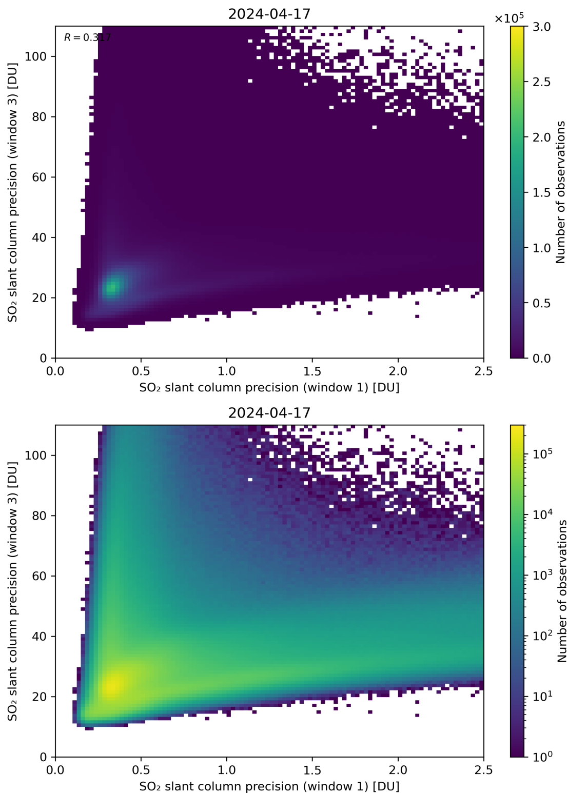
Figure 229: Scatter density plot of “SO 2 slant column precision (window 1)” against “SO 2 slant column precision (window 3)” for 2024-04-16 to 2024-04-18.
