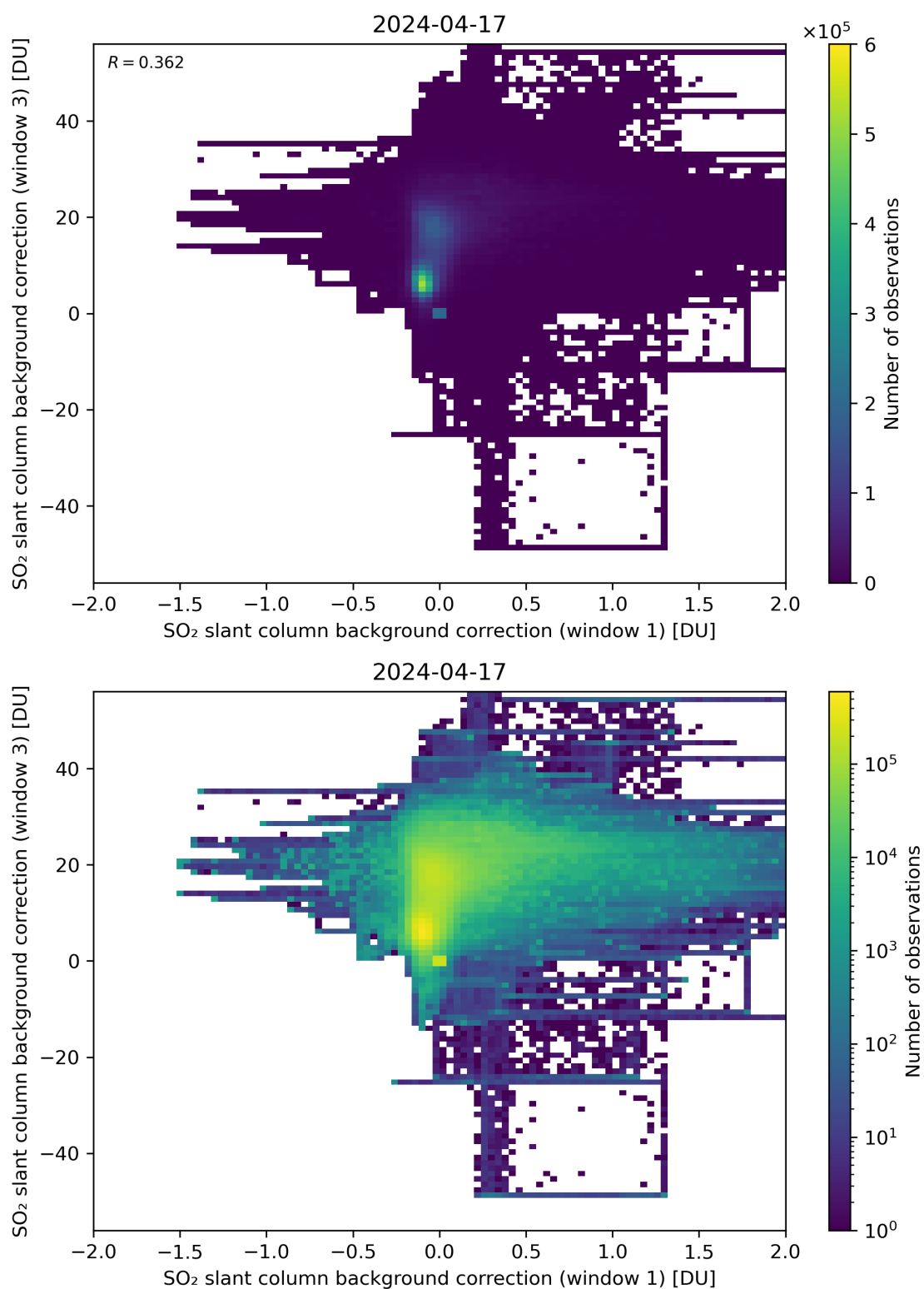
Figure 99: Scatter density plot of “SO 2 slant column background correction (window 1)” against “SO 2 slant column background correction (window 3)” for 2024-04-16 to 2024-04-18.
