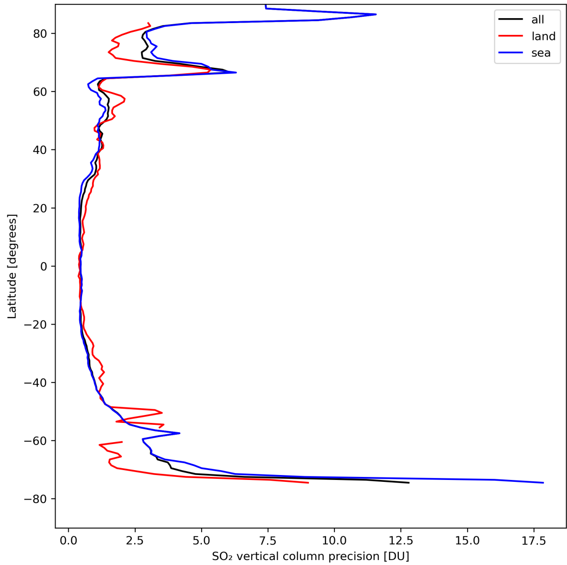
Figure 31: Zonal average of “SO 2 vertical column precision” for 2024-04-16 to 2024-04-18.
