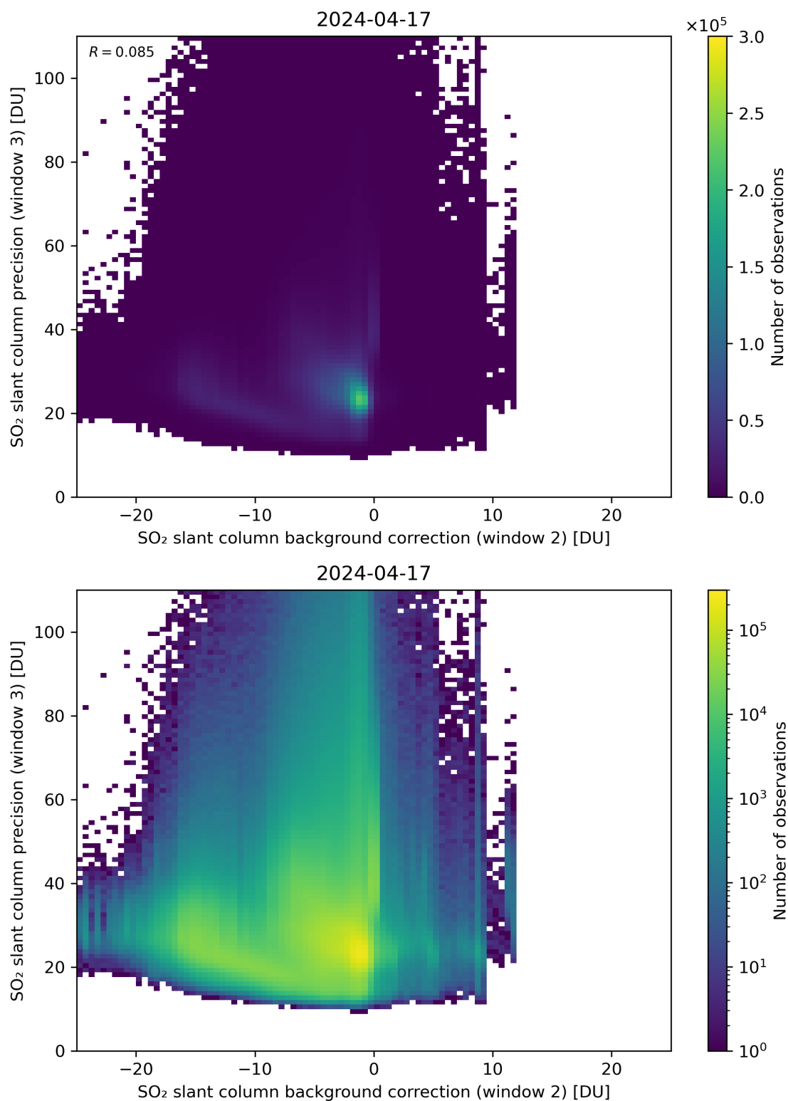
Figure 118: Scatter density plot of “SO 2 slant column background correction (window 2)” against “SO 2 slant column precision (window 3)” for 2024-04-16 to 2024-04-18.
