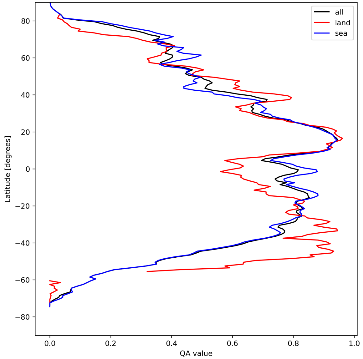
Figure 29: Zonal average of “QA value” for 2024-04-16 to 2024-04-18.
