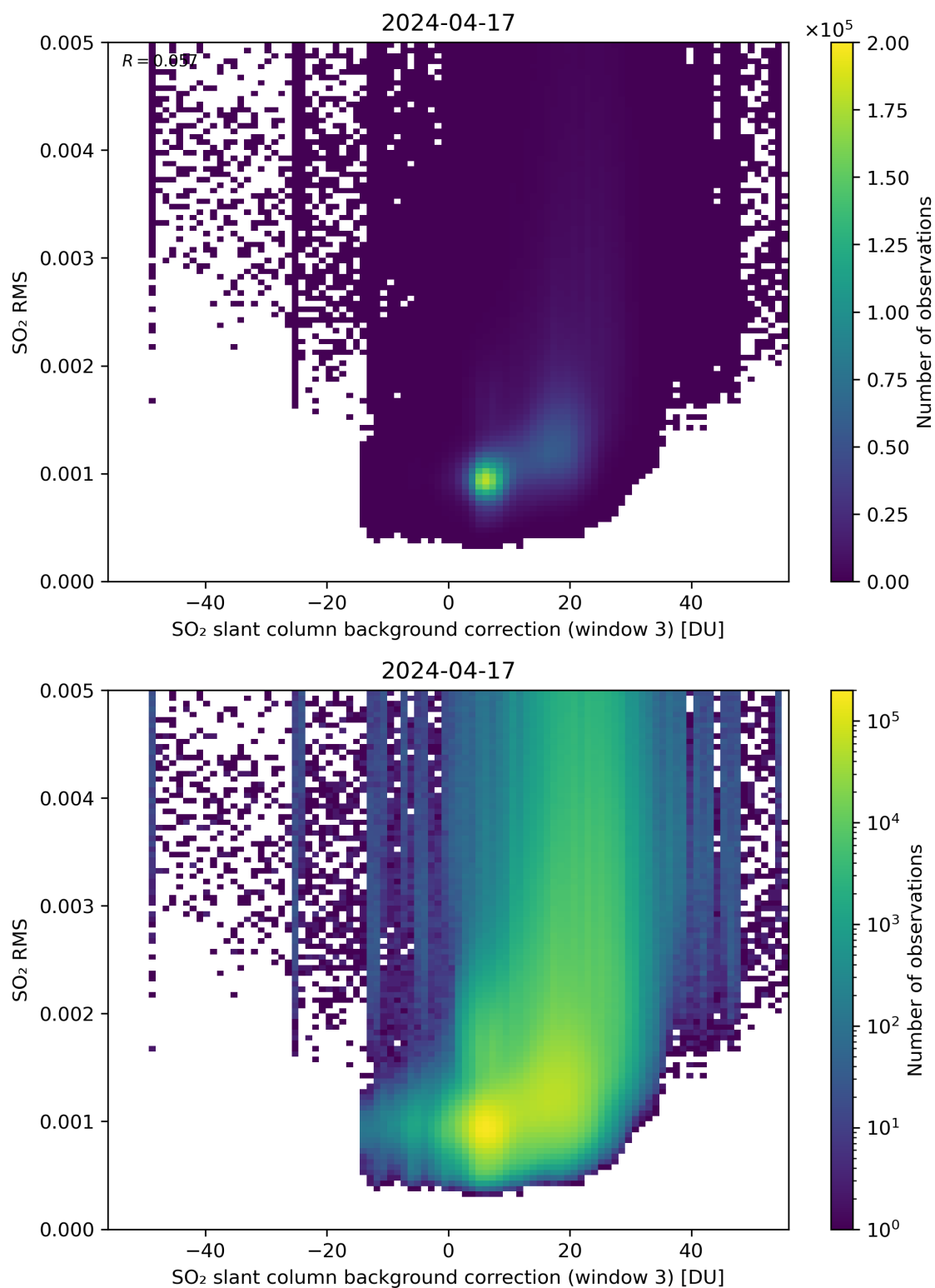
Figure 123: Scatter density plot of “SO 2 slant column background correction (window 3)” against “SO 2 RMS” for 2024-04-16 to 2024-04-18.
