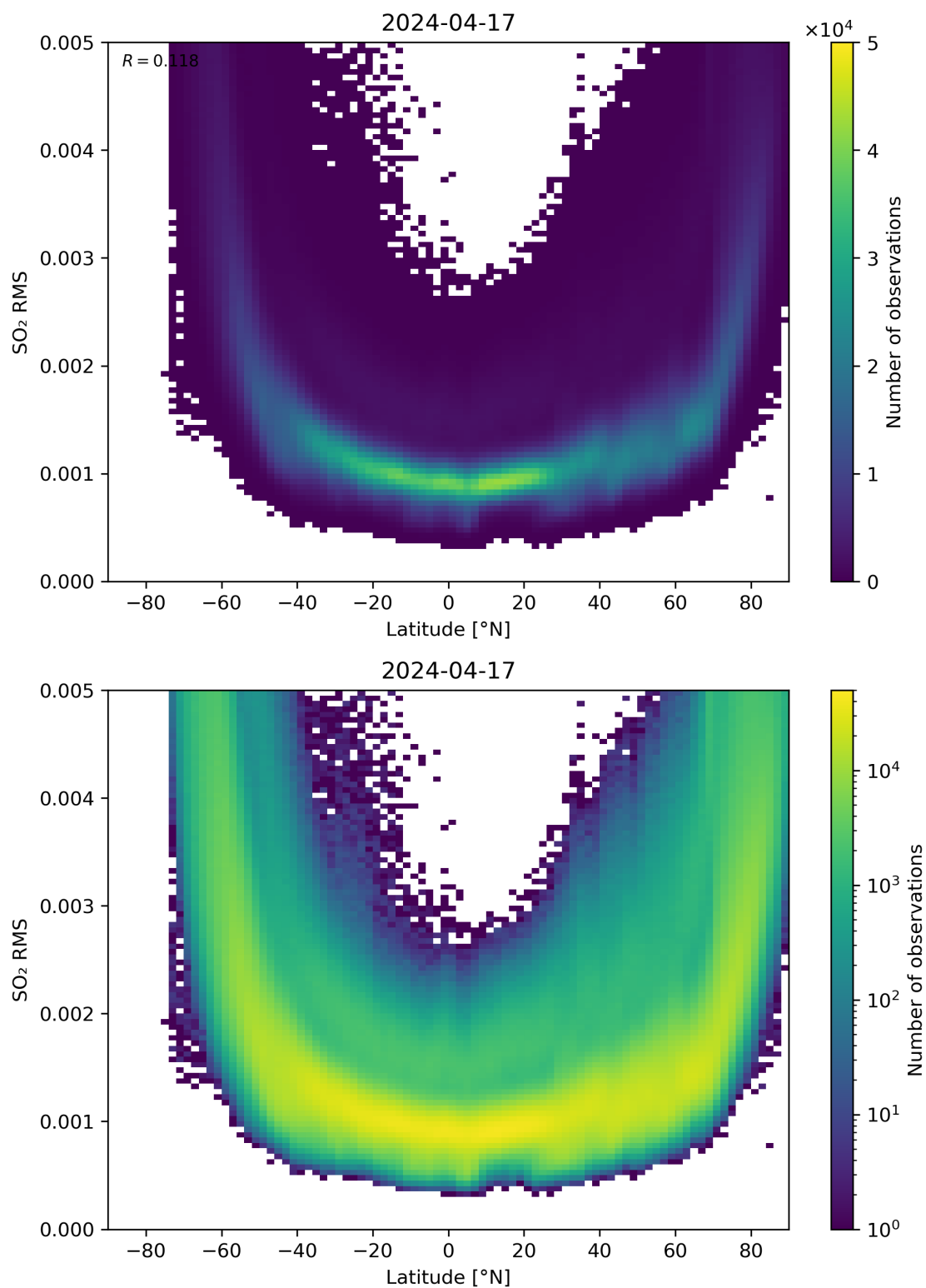
Figure 144: Scatter density plot of “Latitude” against “SO 2 RMS” for 2024-04-16 to 2024-04-18.
