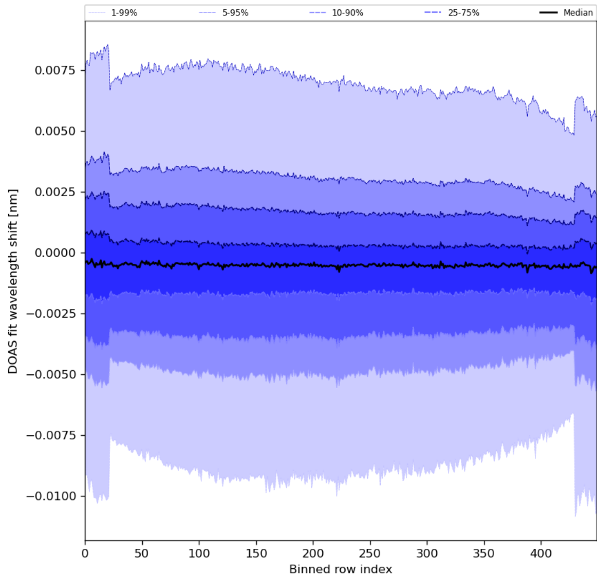
Figure 91: Along track statistics of “DOAS fit wavelength shift” for 2024-04-16 to 2024-04-18
