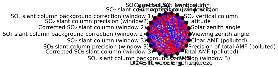
Figure 1: Map of correlation graph for 2024-04-16 to 2024-04-18.
