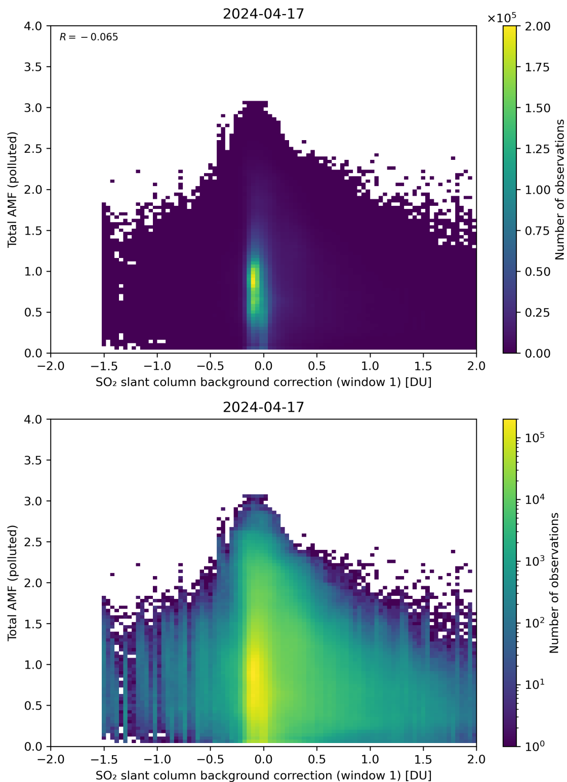
Figure 109: Scatter density plot of “SO 2 slant column background correction (window 1)” against “Total AMF (polluted)” for 2024-04-16 to 2024-04-18.
