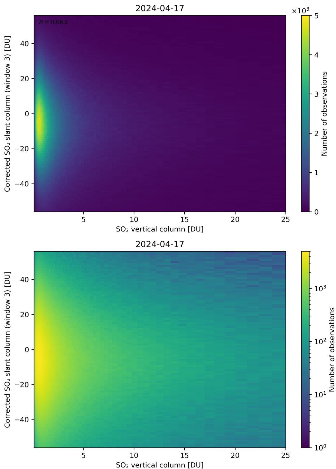
Figure 299: Scatter density plot of “SO 2 vertical column” against “Corrected SO 2 slant column (window 3)” for 2024-04-16 to 2024-04-18.
