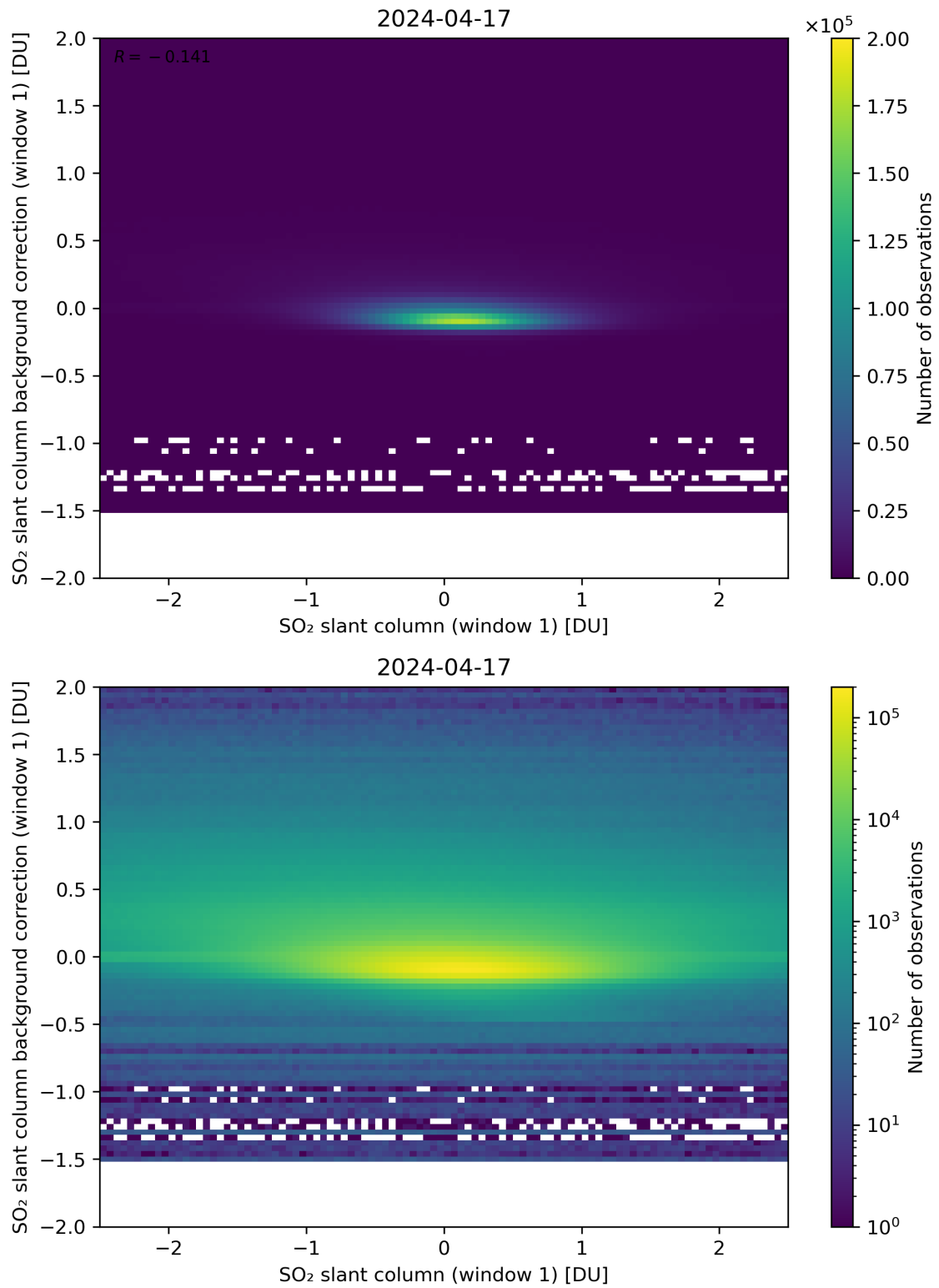
Figure 212: Scatter density plot of “SO 2 slant column (window 1)” against “SO 2 slant column background correction (window 1)” for 2024-04-16 to 2024-04-18.
