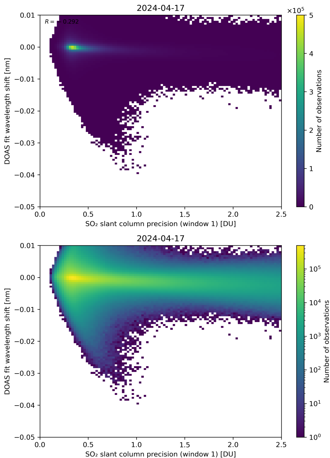
Figure 221: Scatter density plot of “SO 2 slant column precision (window 1)” against “DOAS fit wavelength shift” for 2024-04-16 to 2024-04-18.
