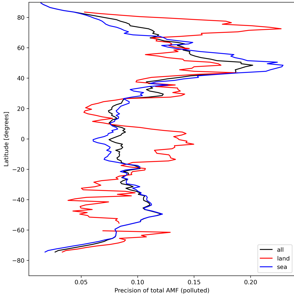
Figure 49: Zonal average of “Precision of total AMF (polluted)” for 2024-04-16 to 2024-04-18.
