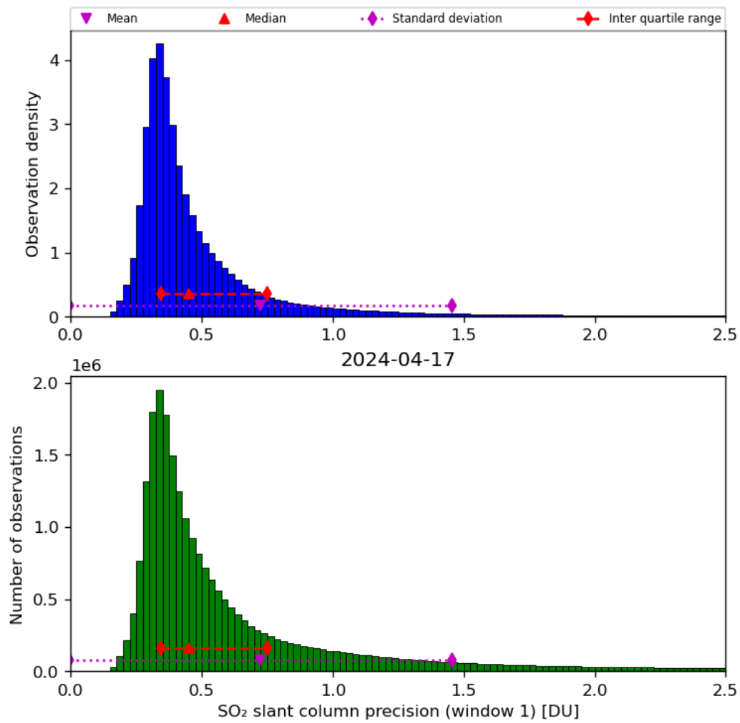
Figure 57: Histogram of “SO 2 slant column precision (window 1)” for 2024-04-16 to 2024-04-18
