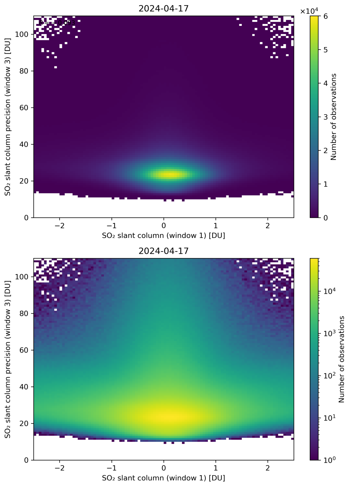
Figure 238: Scatter density plot of “SO 2 slant column (window 1)” against “SO 2 slant column precision (window 3)” for 2024-04-16 to 2024-04-18.
