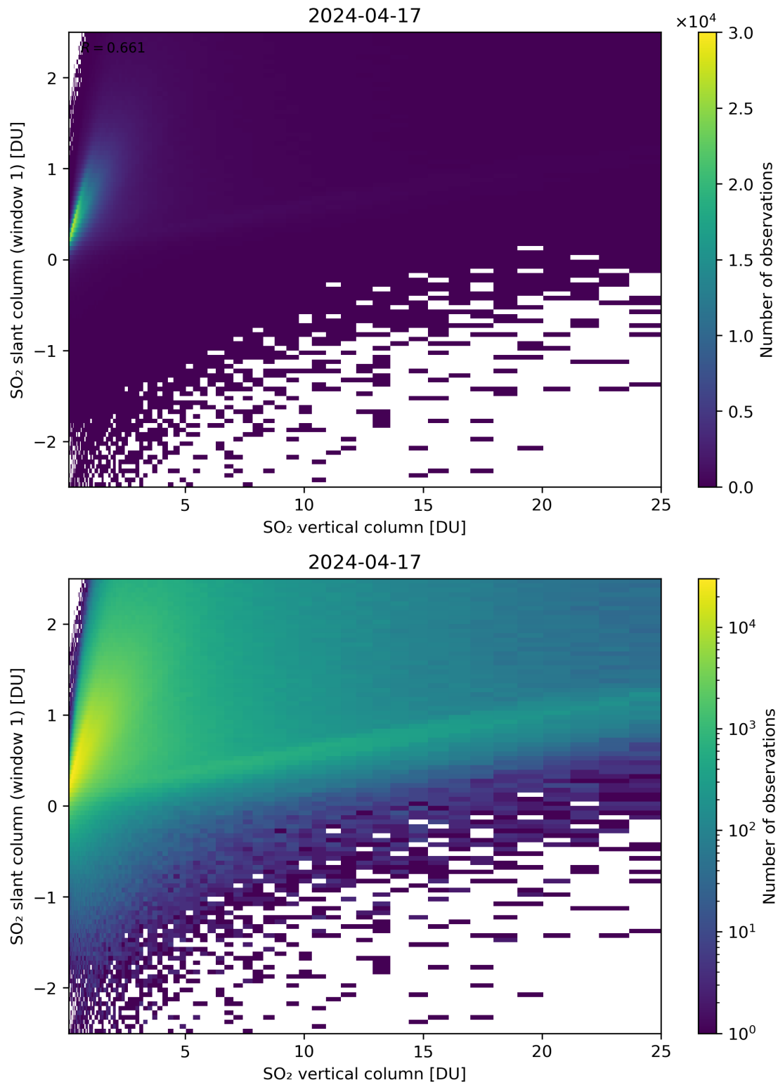
Figure 300: Scatter density plot of “SO 2 vertical column” against “SO 2 slant column (window 1)” for 2024-04-16 to 2024-04-18.
