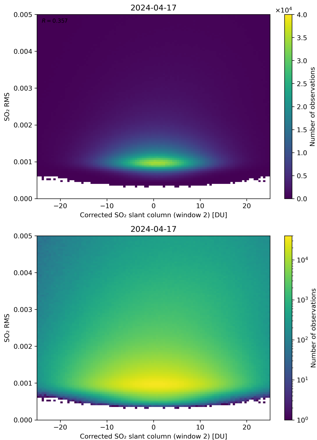
Figure 198: Scatter density plot of “Corrected SO 2 slant column (window 2)” against “SO 2 RMS” for 2024-04-16 to 2024-04-18.
