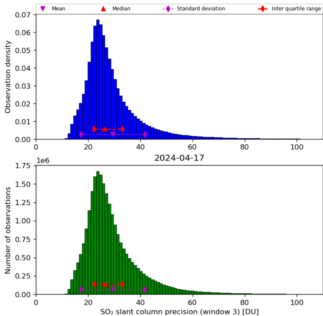
Figure 65: Histogram of “SO 2 slant column precision (window 3)” for 2024-04-16 to 2024-04-18
