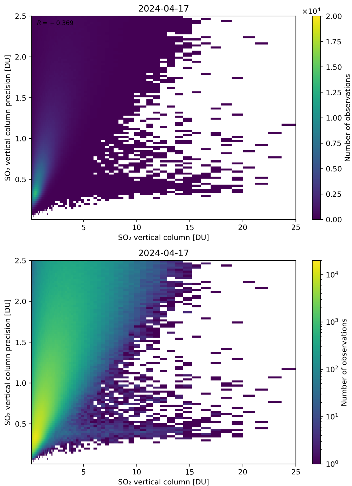
Figure 307: Scatter density plot of “SO 2 vertical column” against “SO 2 vertical column precision” for 2024-04-16 to 2024-04-18.
