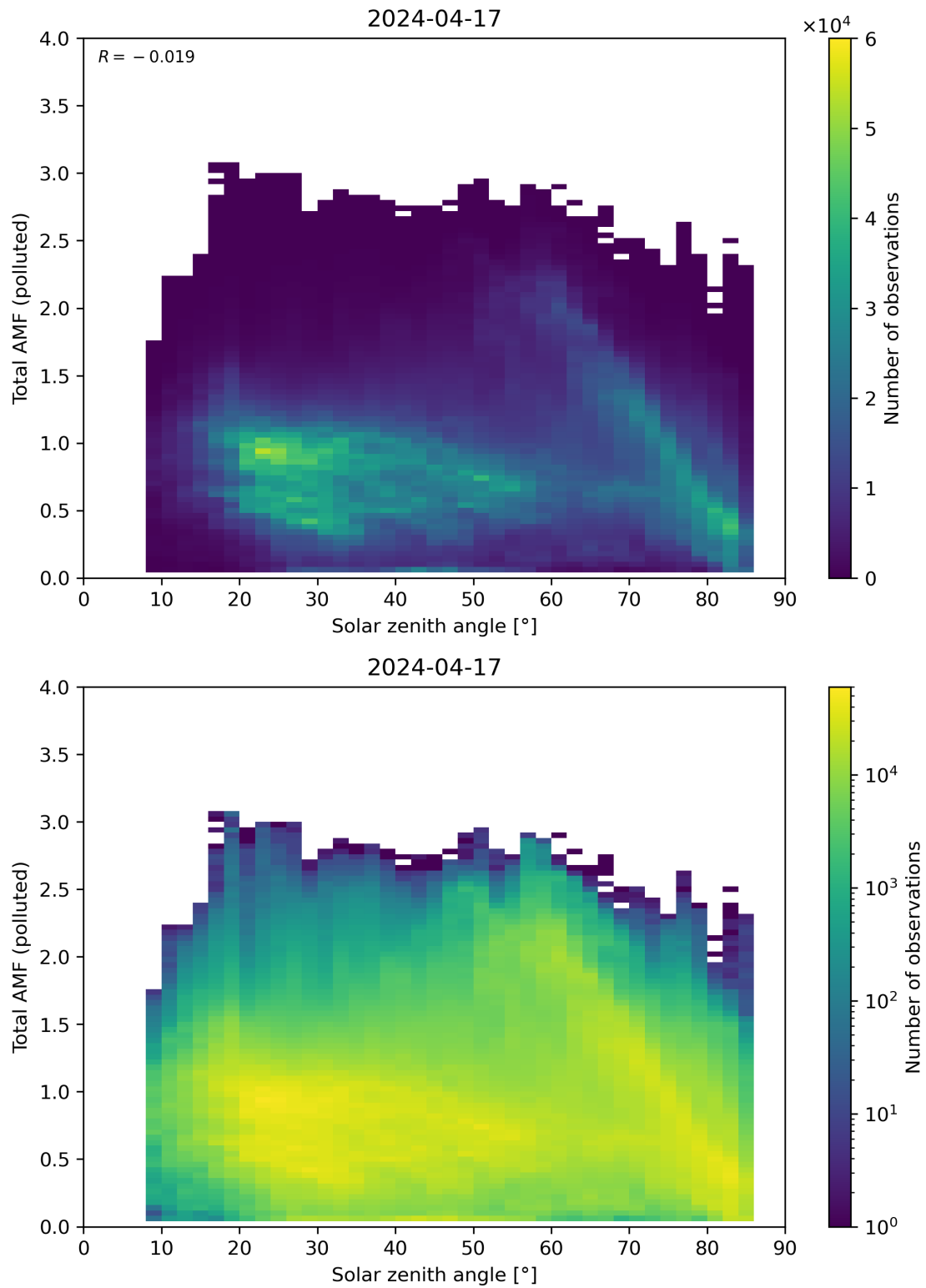
Figure 174: Scatter density plot of “Solar zenith angle” against “Total AMF (polluted)” for 2024-04-16 to 2024-04-18.
