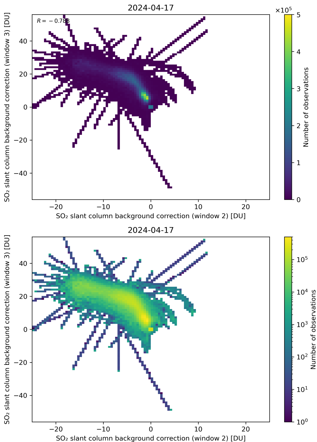
Figure 111: Scatter density plot of “SO 2 slant column background correction (window 2)” against “SO 2 slant column background correction (window 3)” for 2024-04-16 to 2024-04-18.
