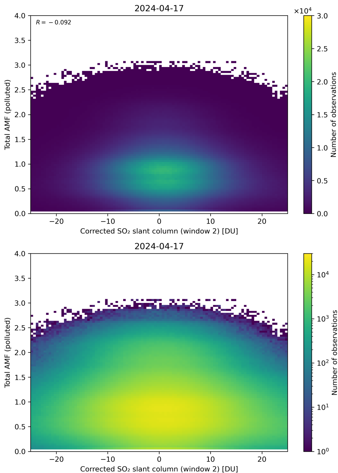
Figure 203: Scatter density plot of “Corrected SO 2 slant column (window 2)” against “Total AMF (polluted)” for 2024-04-16 to 2024-04-18.
