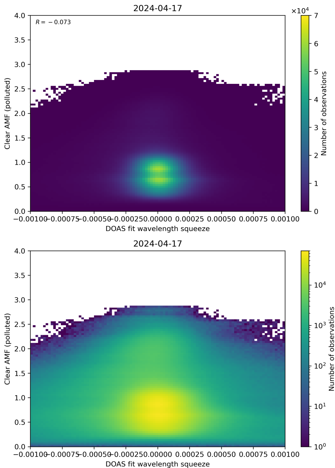
Figure 133: Scatter density plot of “DOAS fit wavelength squeeze” against “Clear AMF (polluted)” for 2024-04-16 to 2024-04-18.
