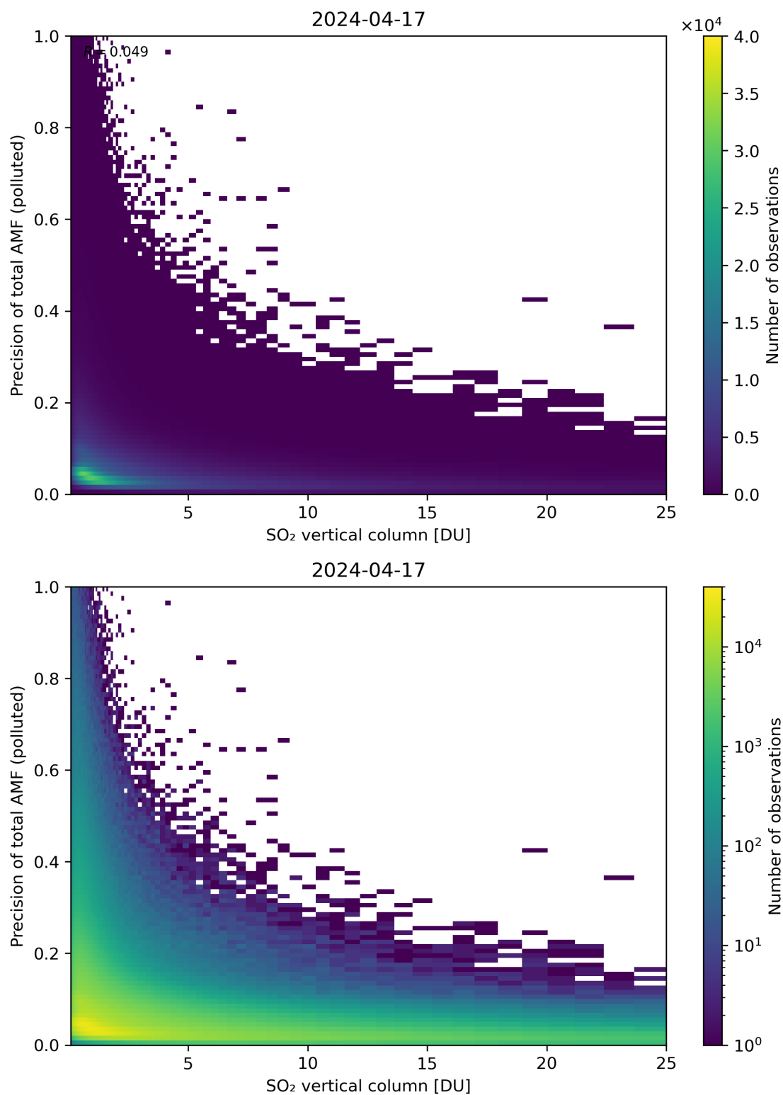
Figure 306: Scatter density plot of “SO 2 vertical column” against “Precision of total AMF (polluted)” for 2024-04-16 to 2024-04-18.
