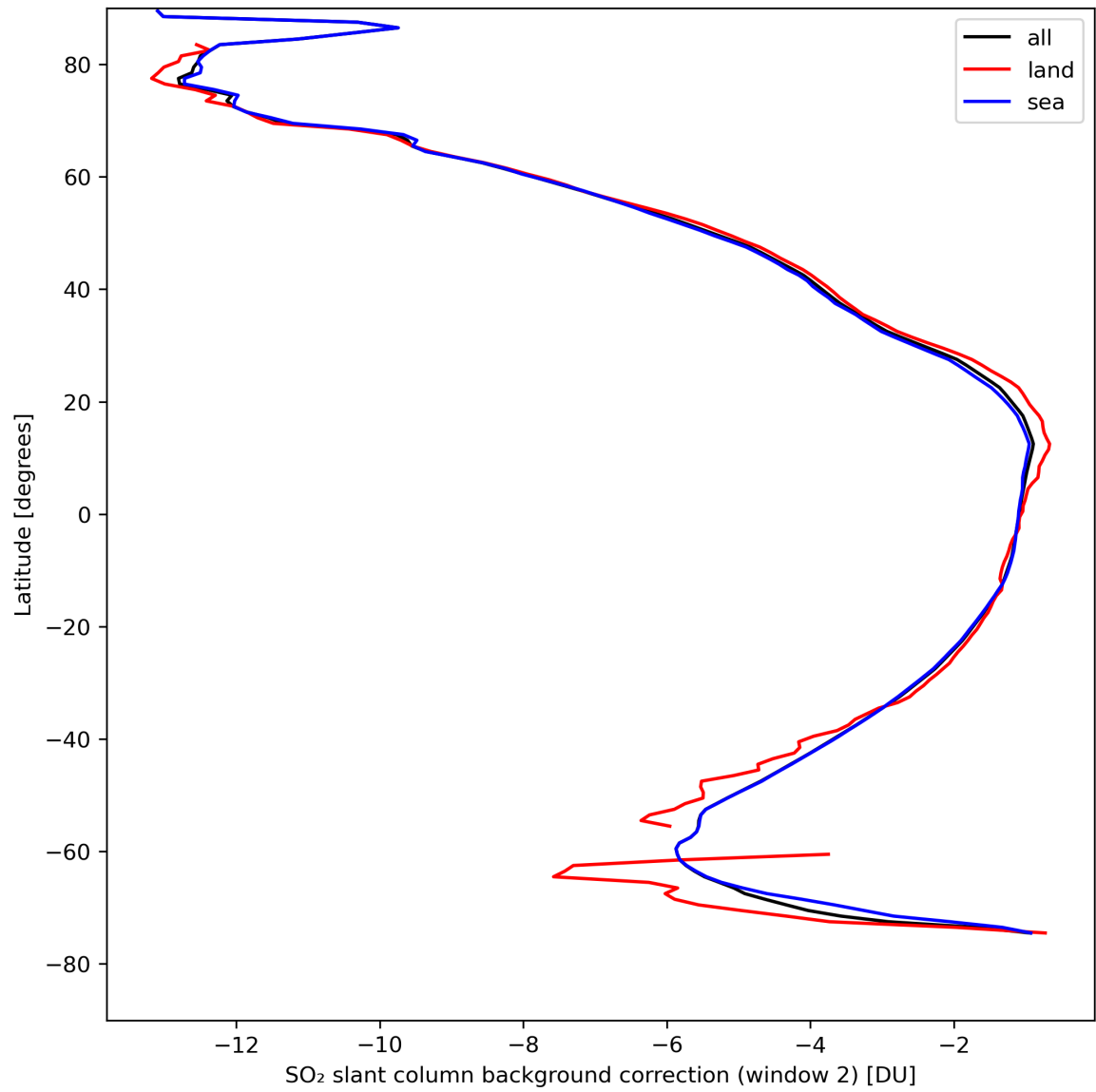
Figure 40: Zonal average of “SO 2 slant column background correction (window 2)” for 2024-04-16 to 2024-04-18.
