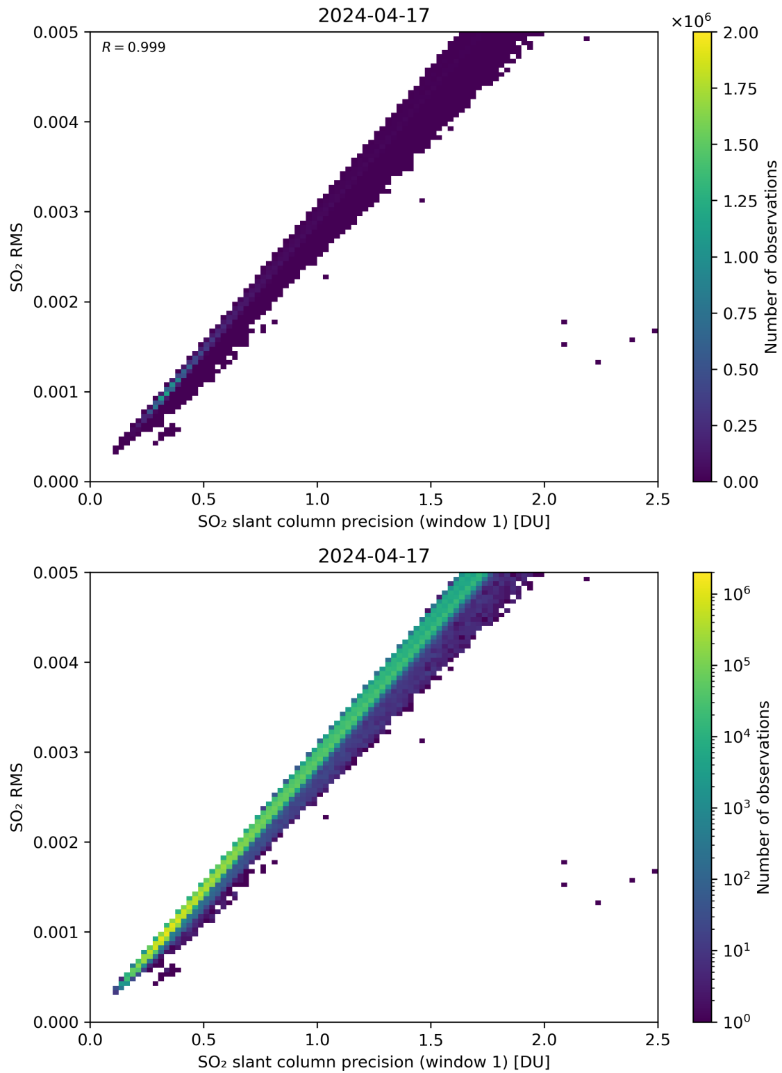
Figure 223: Scatter density plot of “SO 2 slant column precision (window 1)” against “SO 2 RMS” for 2024-04-16 to 2024-04-18.
