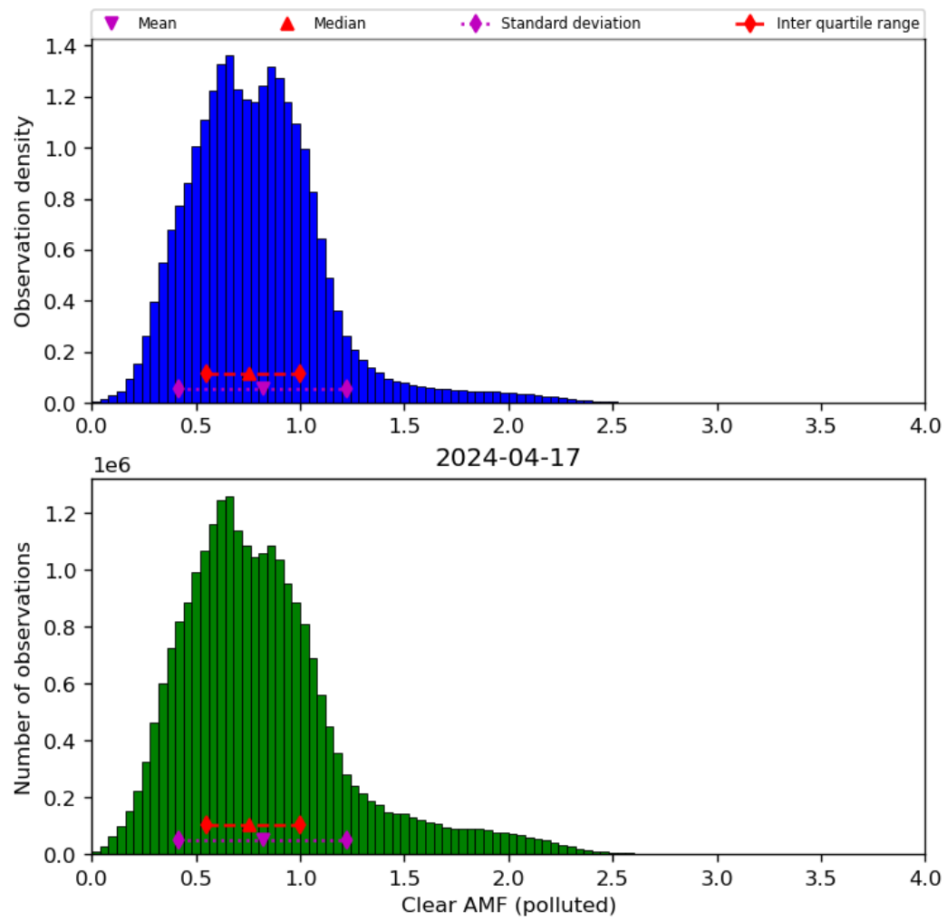
Figure 73: Histogram of “Clear AMF (polluted)” for 2024-04-16 to 2024-04-18
