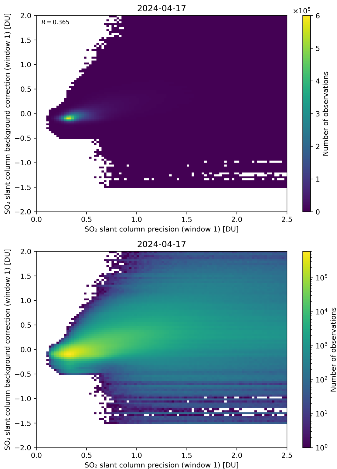
Figure 218: Scatter density plot of “SO 2 slant column precision (window 1)” against “SO 2 slant column background correction (window 1)” for 2024-04-16 to 2024-04-18.
