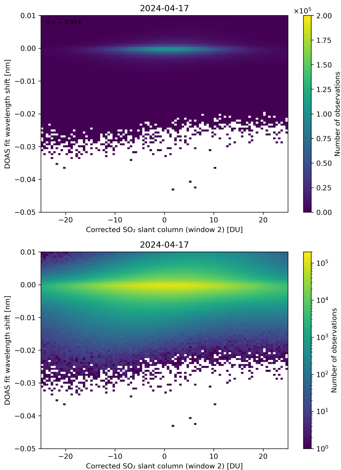
Figure 196: Scatter density plot of “Corrected SO 2 slant column (window 2)” against “DOAS fit wavelength shift” for 2024-04-16 to 2024-04-18.
