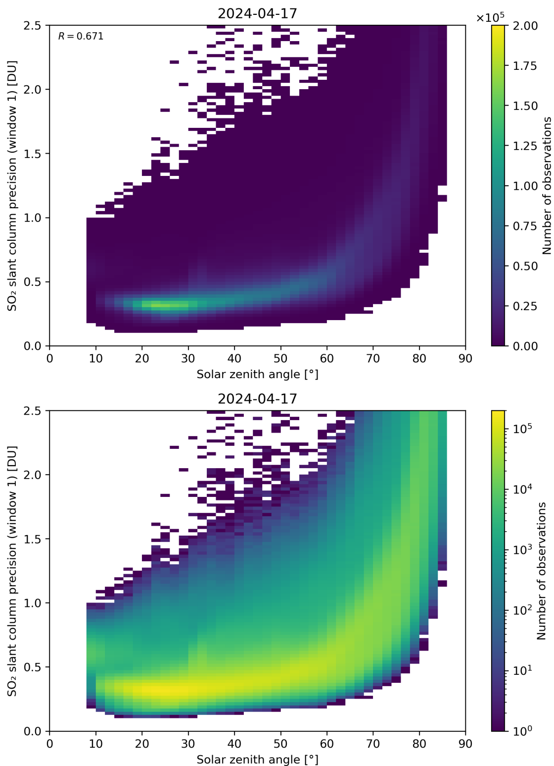
Figure 170: Scatter density plot of “Solar zenith angle” against “SO 2 slant column precision (window 1)” for 2024-04-16 to 2024-04-18.
