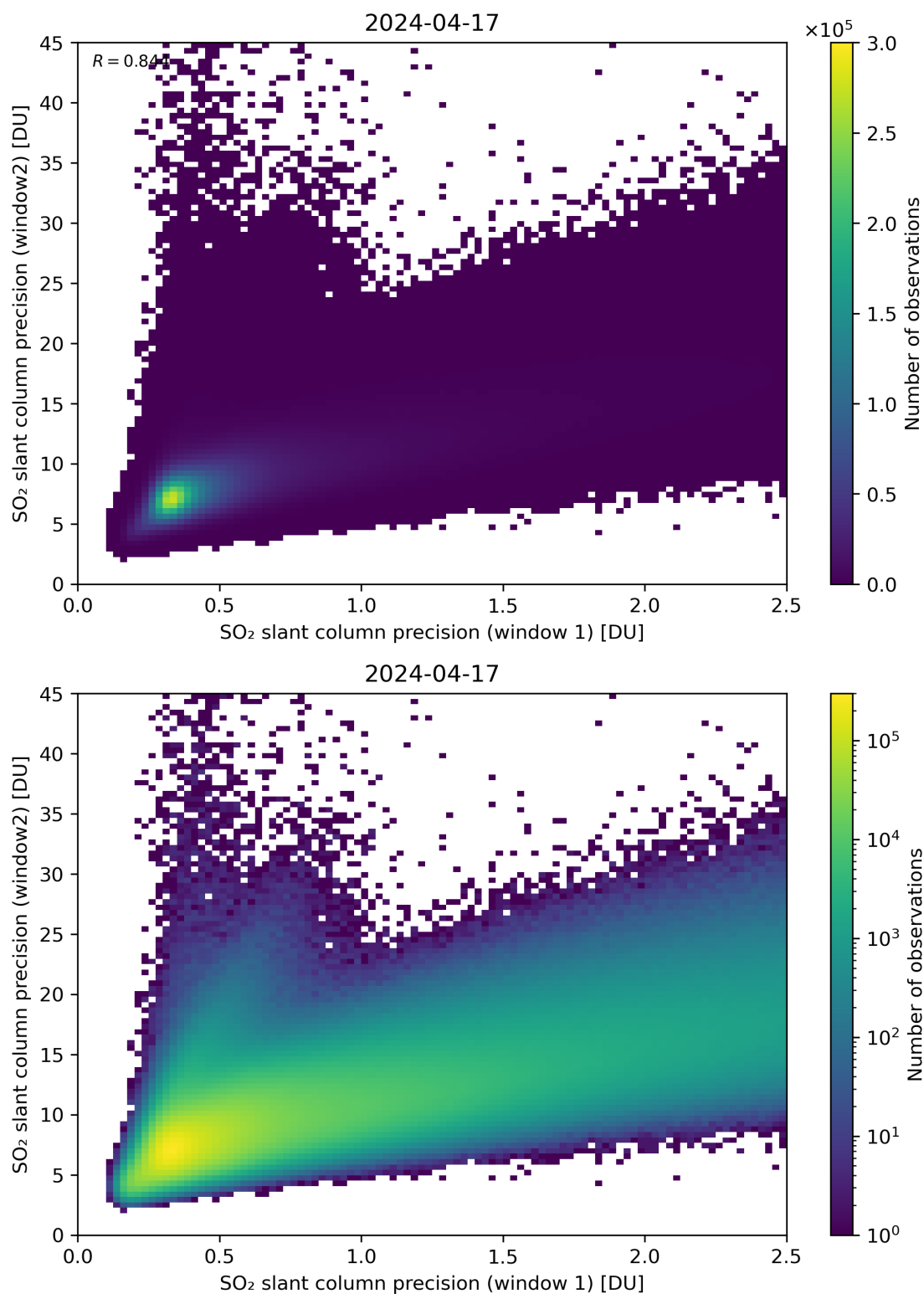
Figure 227: Scatter density plot of “SO 2 slant column precision (window 1)” against “SO 2 slant column precision (window2)” for 2024-04-16 to 2024-04-18.
