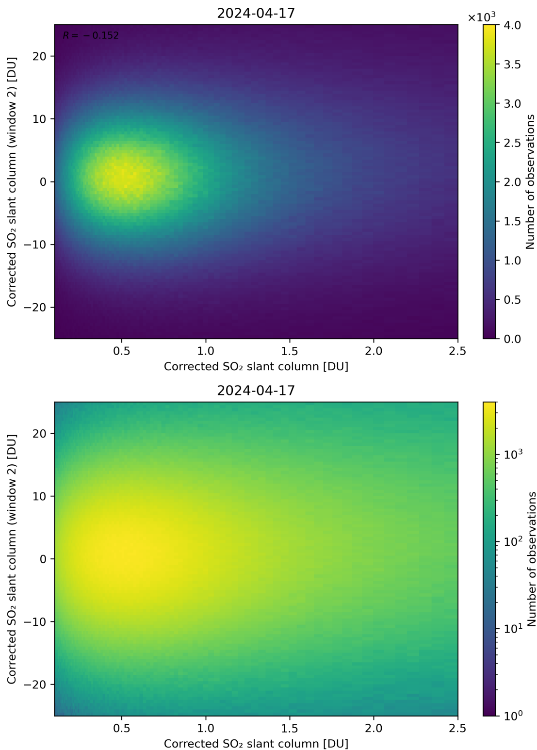
Figure 185: Scatter density plot of “Corrected SO 2 slant column” against “Corrected SO 2 slant column (window 2)” for 2024-04-16 to 2024-04-18.
