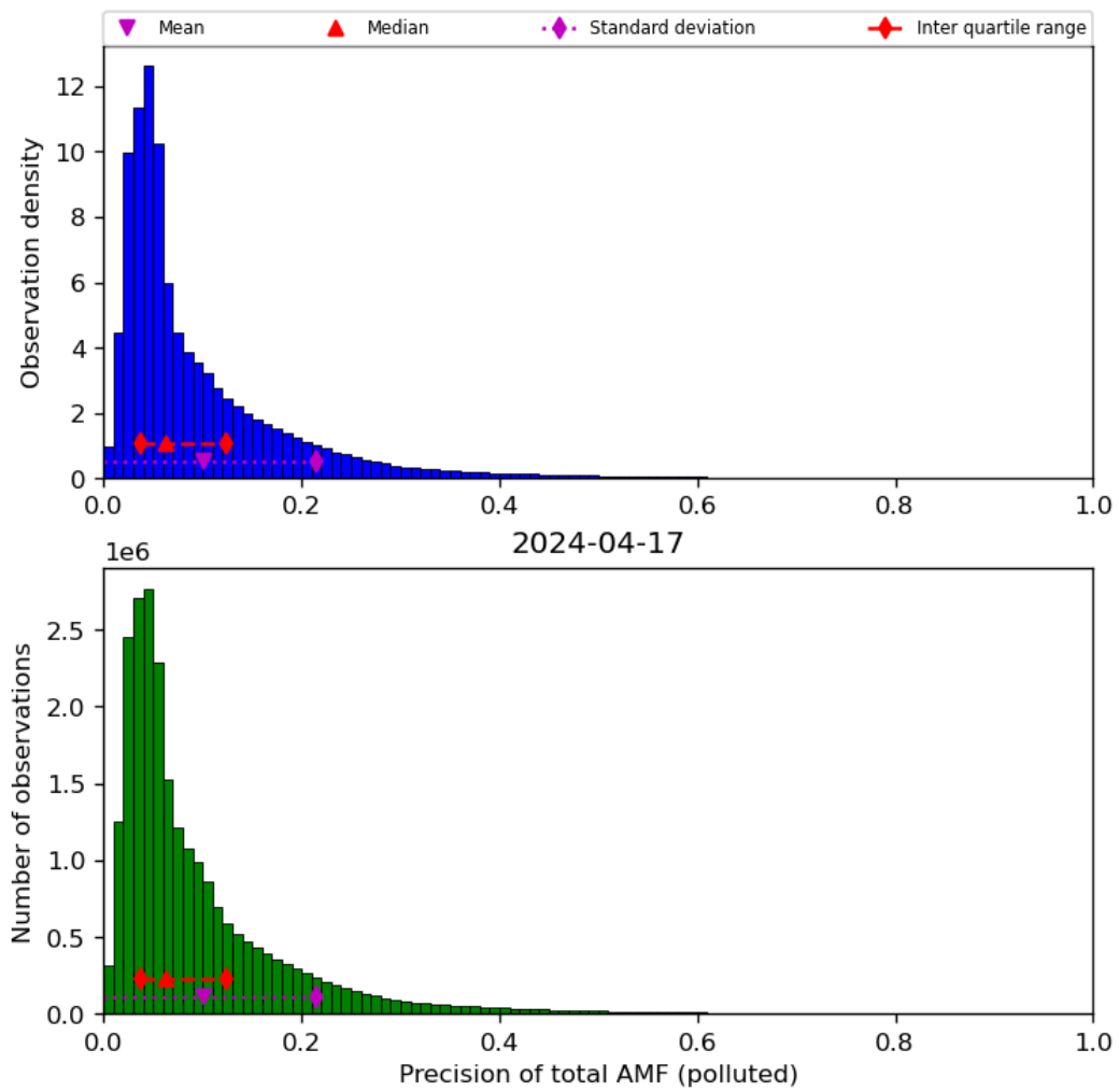
Figure 72: Histogram of “Precision of total AMF (polluted)” for 2024-04-16 to 2024-04-18
