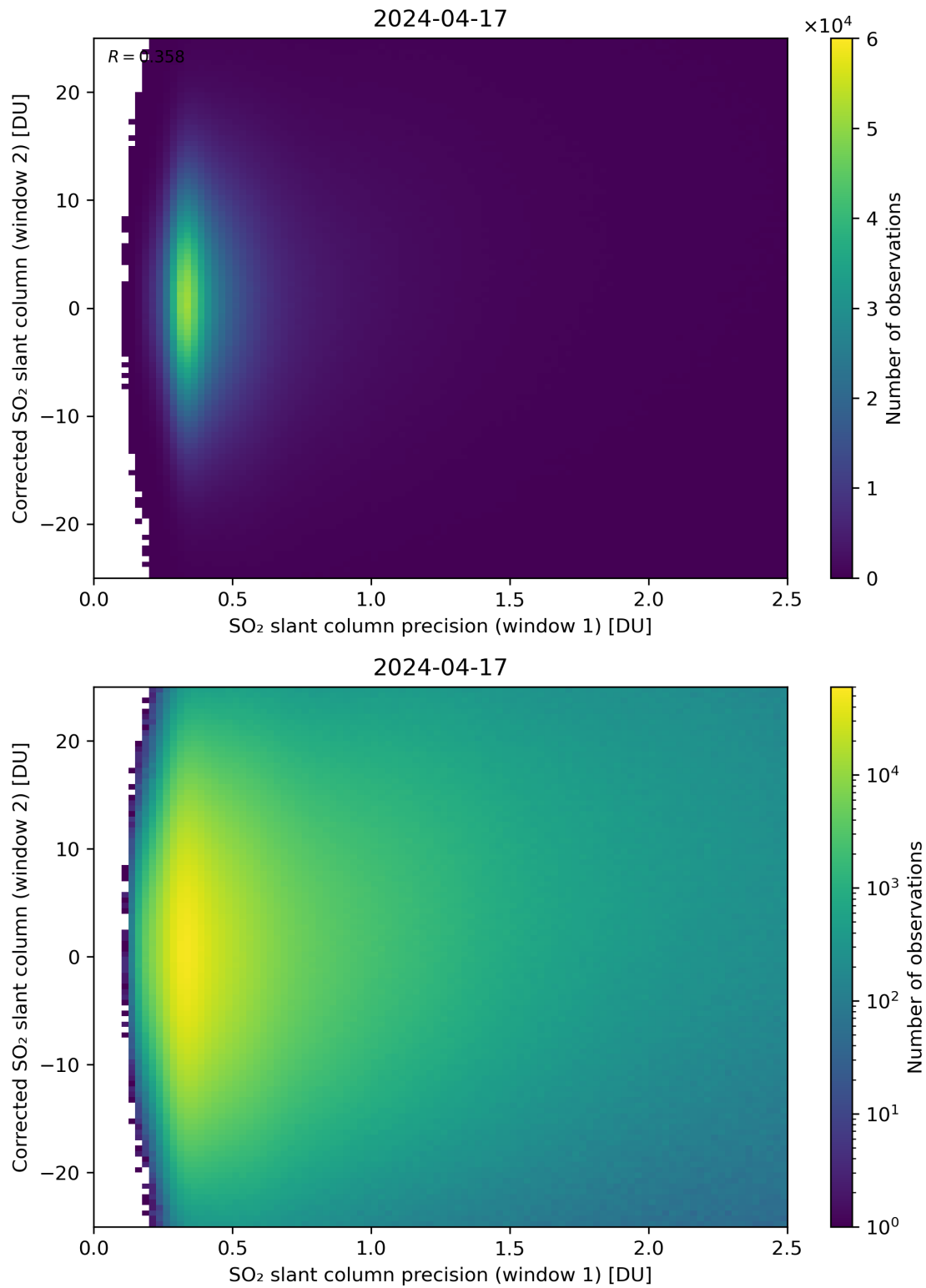
Figure 225: Scatter density plot of “SO 2 slant column precision (window 1)” against “Corrected SO 2 slant column (window 2)” for 2024-04-16 to 2024-04-18.
