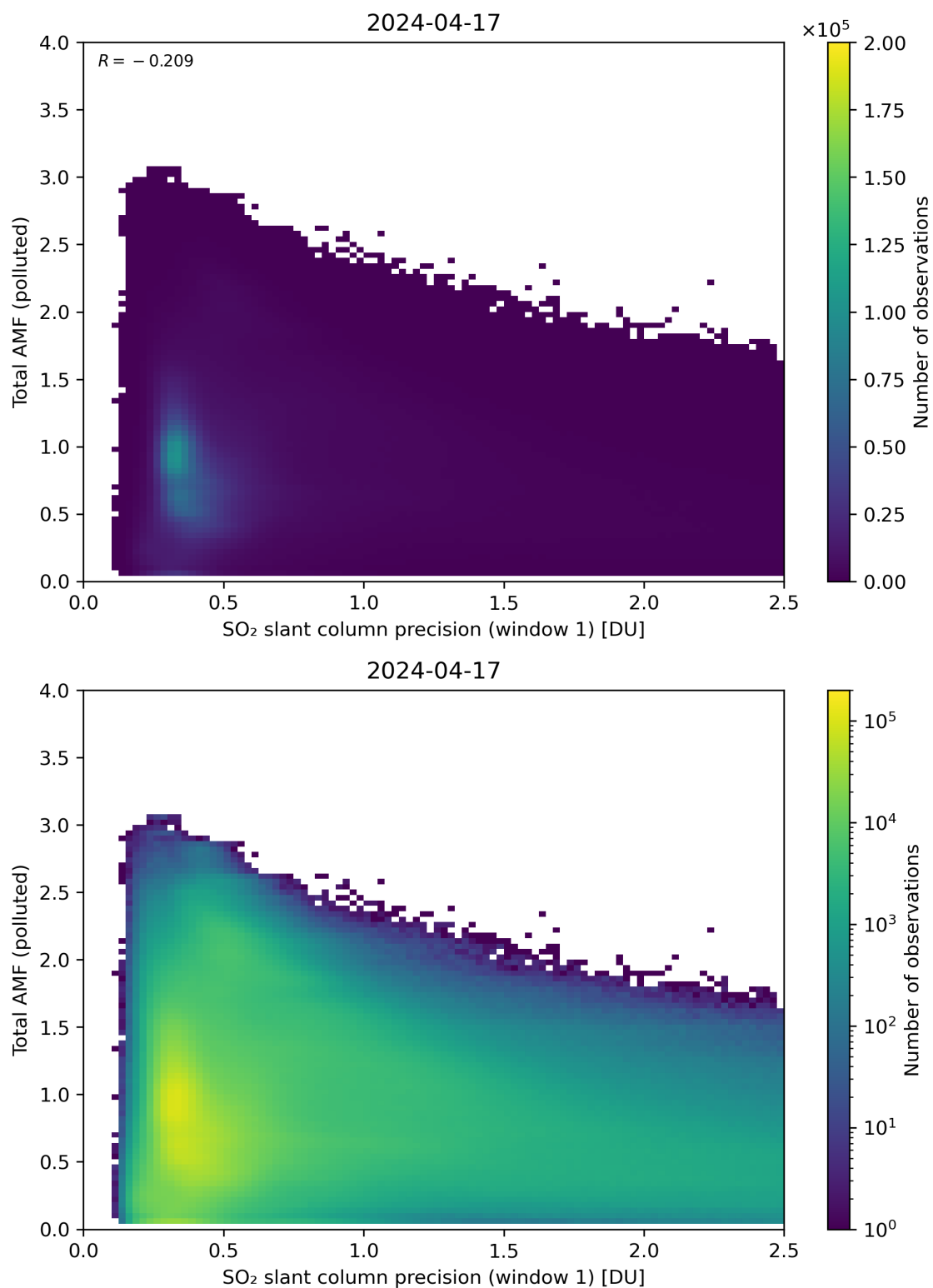
Figure 230: Scatter density plot of “SO 2 slant column precision (window 1)” against “Total AMF (polluted)” for 2024-04-16 to 2024-04-18.
