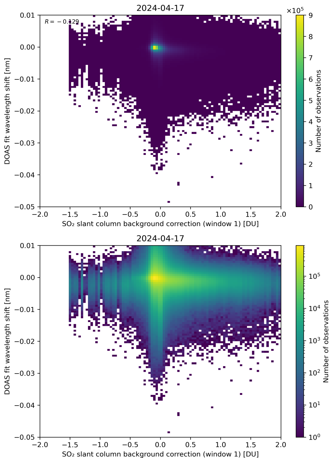
Figure 100: Scatter density plot of “SO 2 slant column background correction (window 1)” against “DOAS fit wavelength shift” for 2024-04-16 to 2024-04-18.
