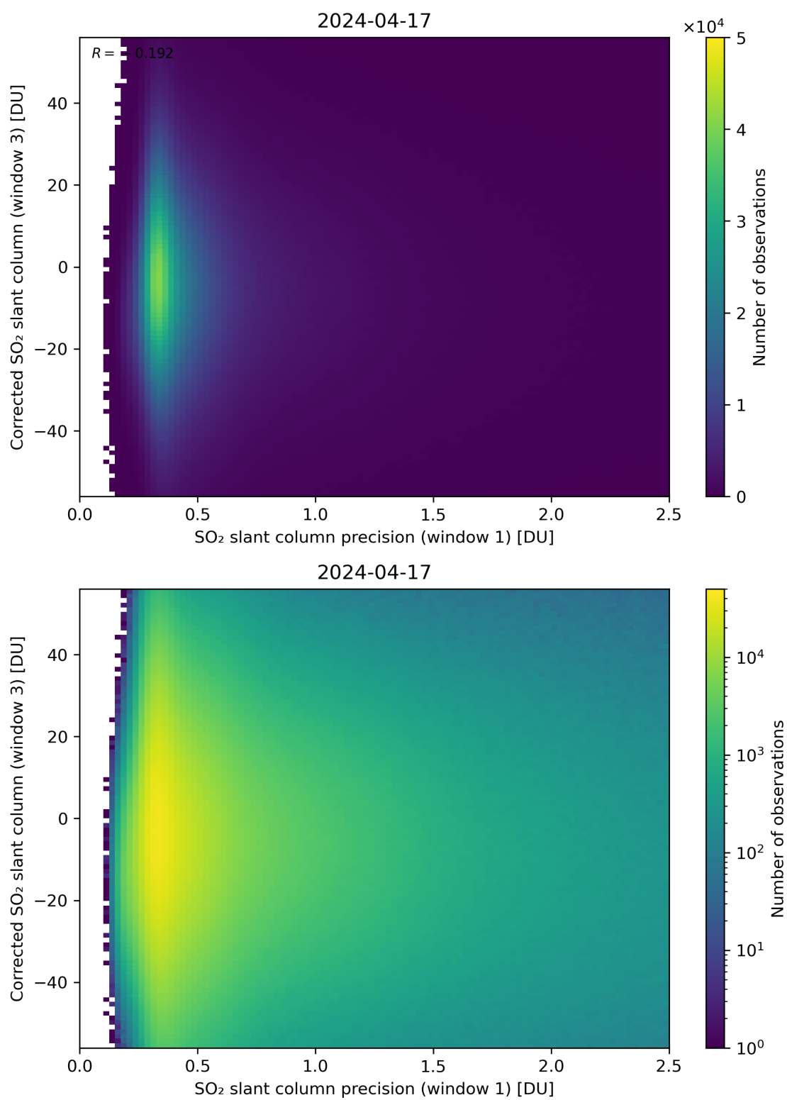
Figure 226: Scatter density plot of “SO 2 slant column precision (window 1)” against “Corrected SO 2 slant column (window 3)” for 2024-04-16 to 2024-04-18.
