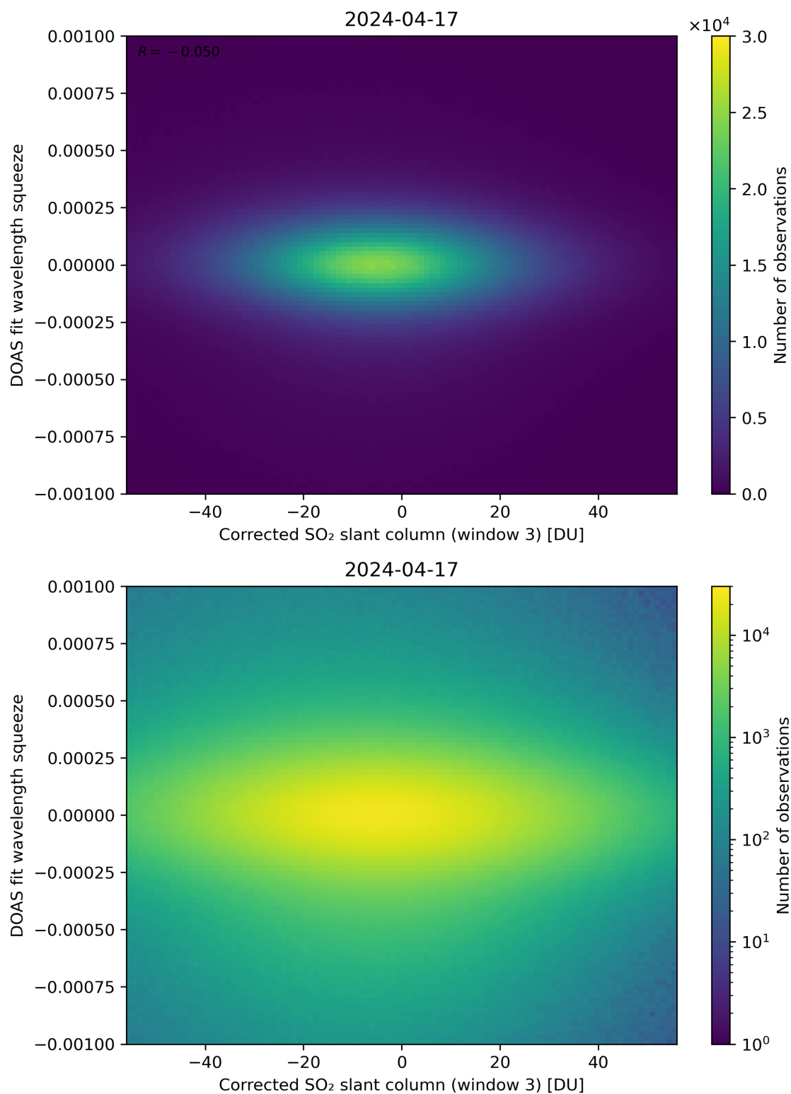
Figure 207: Scatter density plot of “Corrected SO 2 slant column (window 3)” against “DOAS fit wavelength squeeze” for 2024-04-16 to 2024-04-18.
