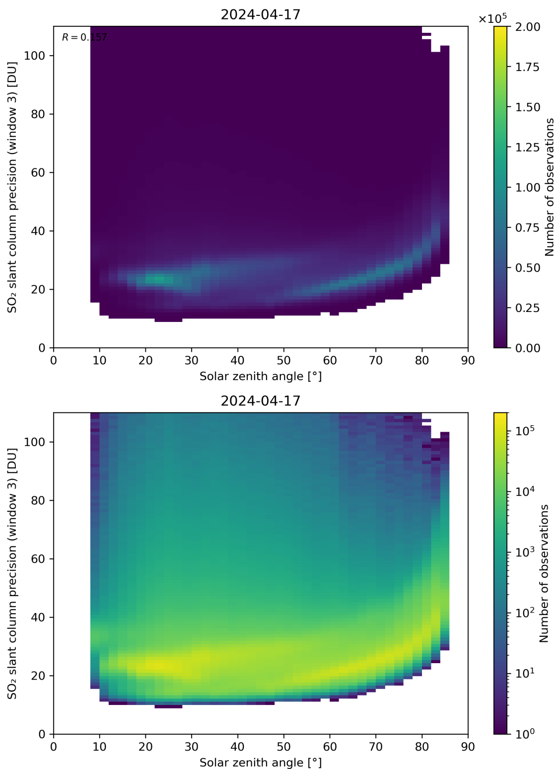
Figure 173: Scatter density plot of “Solar zenith angle” against “SO 2 slant column precision (window 3)” for 2024-04-16 to 2024-04-18.
