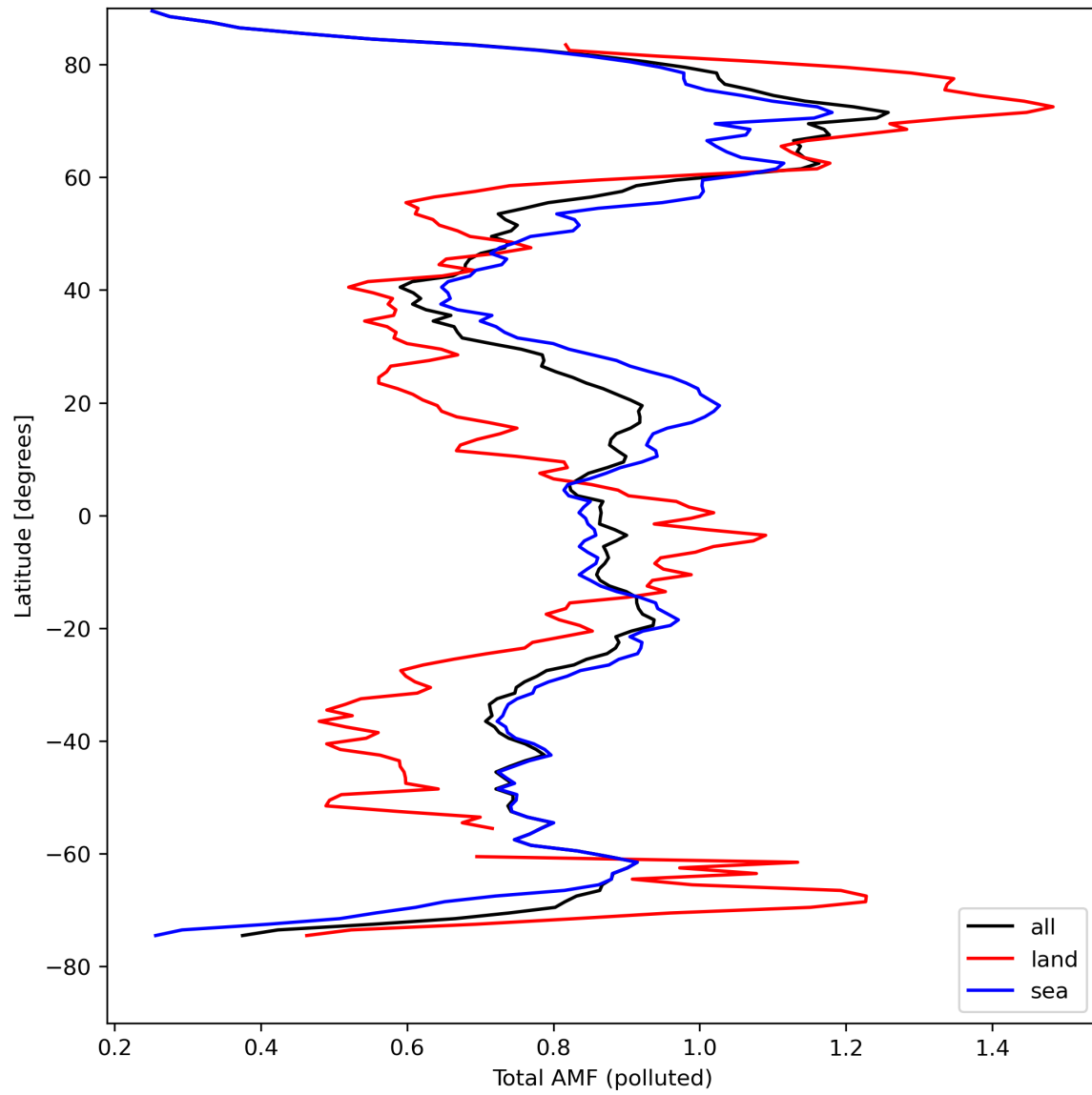
Figure 48: Zonal average of “Total AMF (polluted)” for 2024-04-16 to 2024-04-18.
