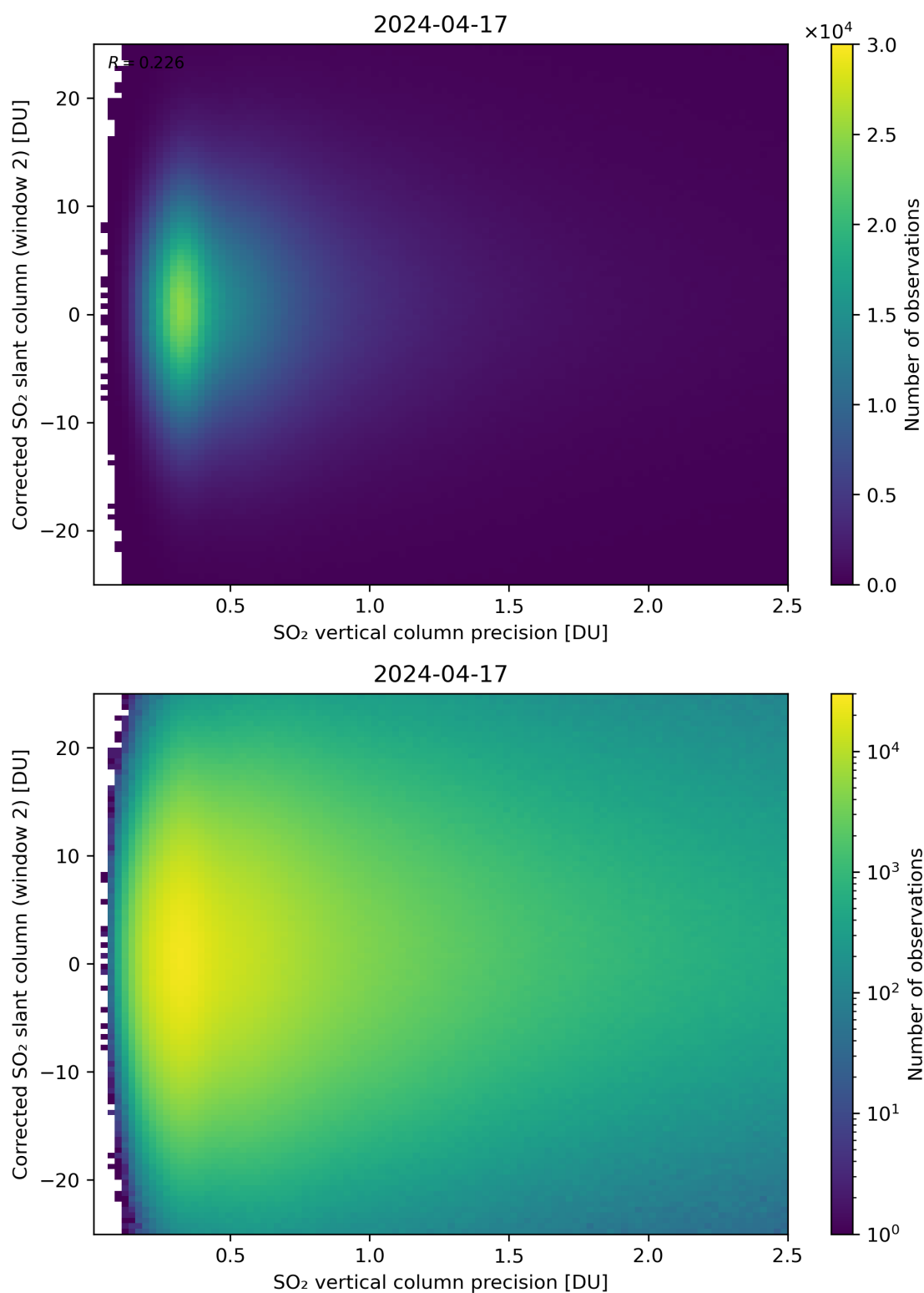
Figure 287: Scatter density plot of “SO 2 vertical column precision” against “Corrected SO 2 slant column (window 2)” for 2024-04-16 to 2024-04-18.
