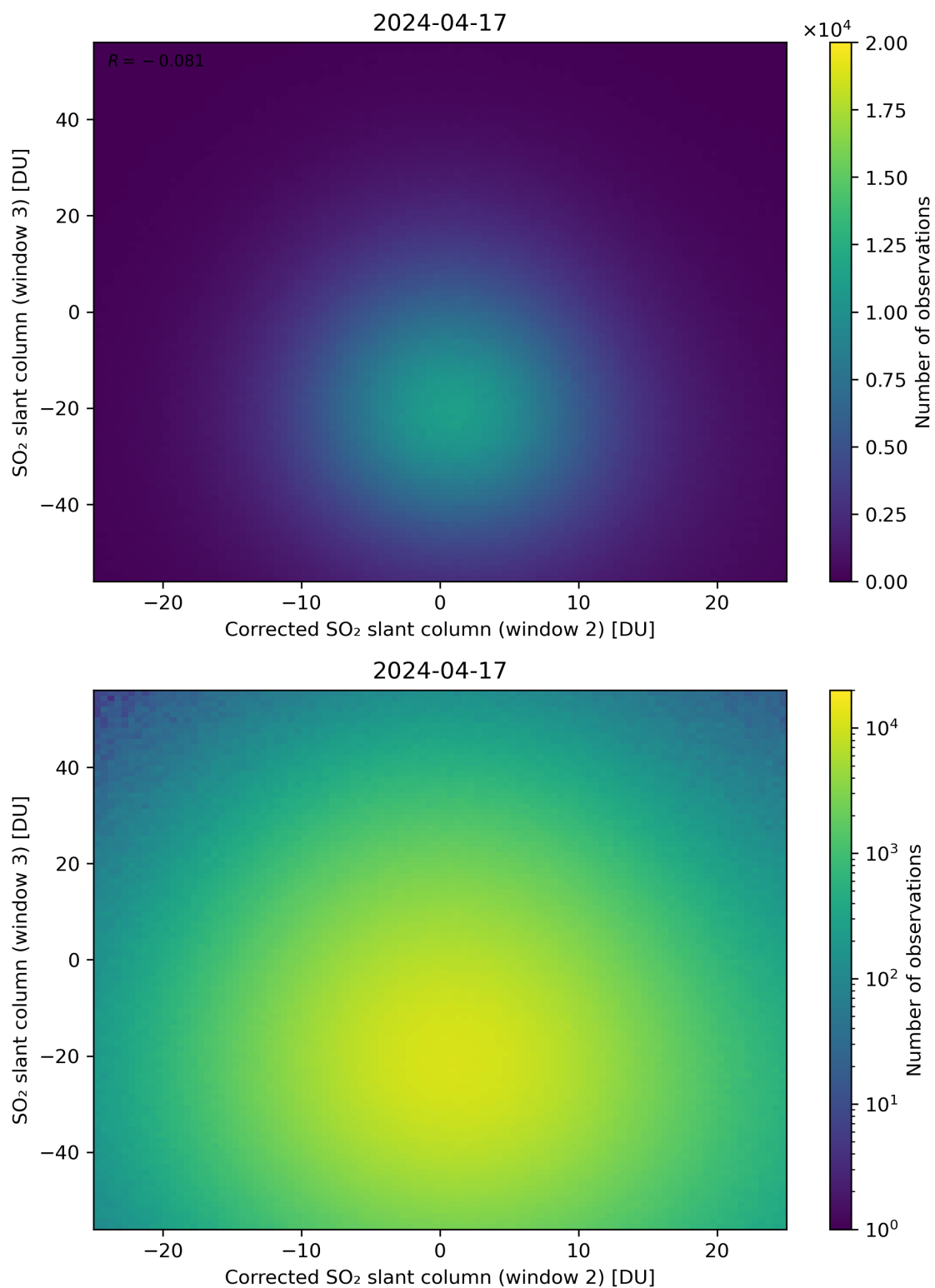
Figure 201: Scatter density plot of “Corrected SO 2 slant column (window 2)” against “SO 2 slant column (window 3)” for 2024-04-16 to 2024-04-18.
