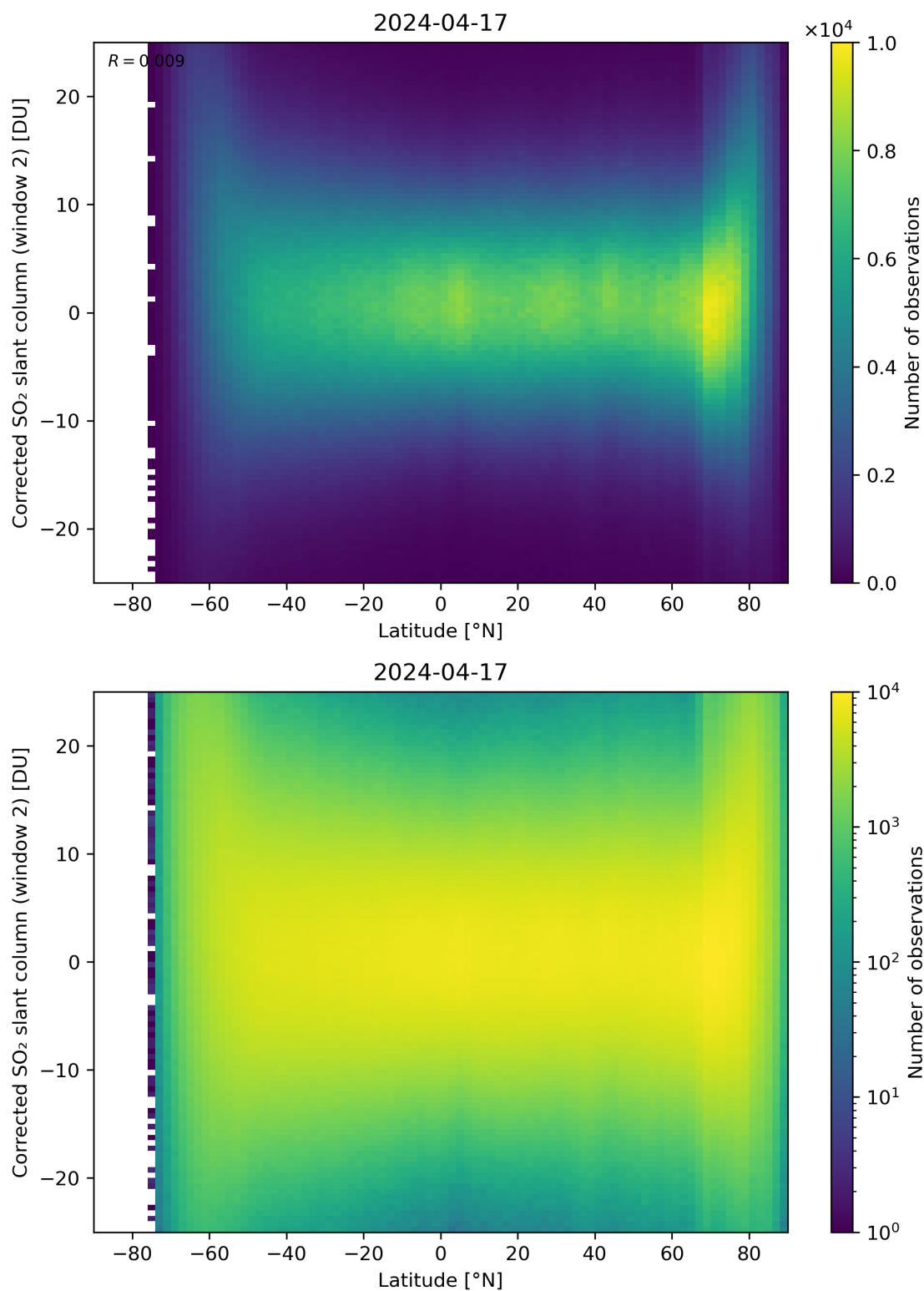
Figure 147: Scatter density plot of “Latitude” against “Corrected SO 2 slant column (window 2)” for 2024-04-16 to 2024-04-18.
