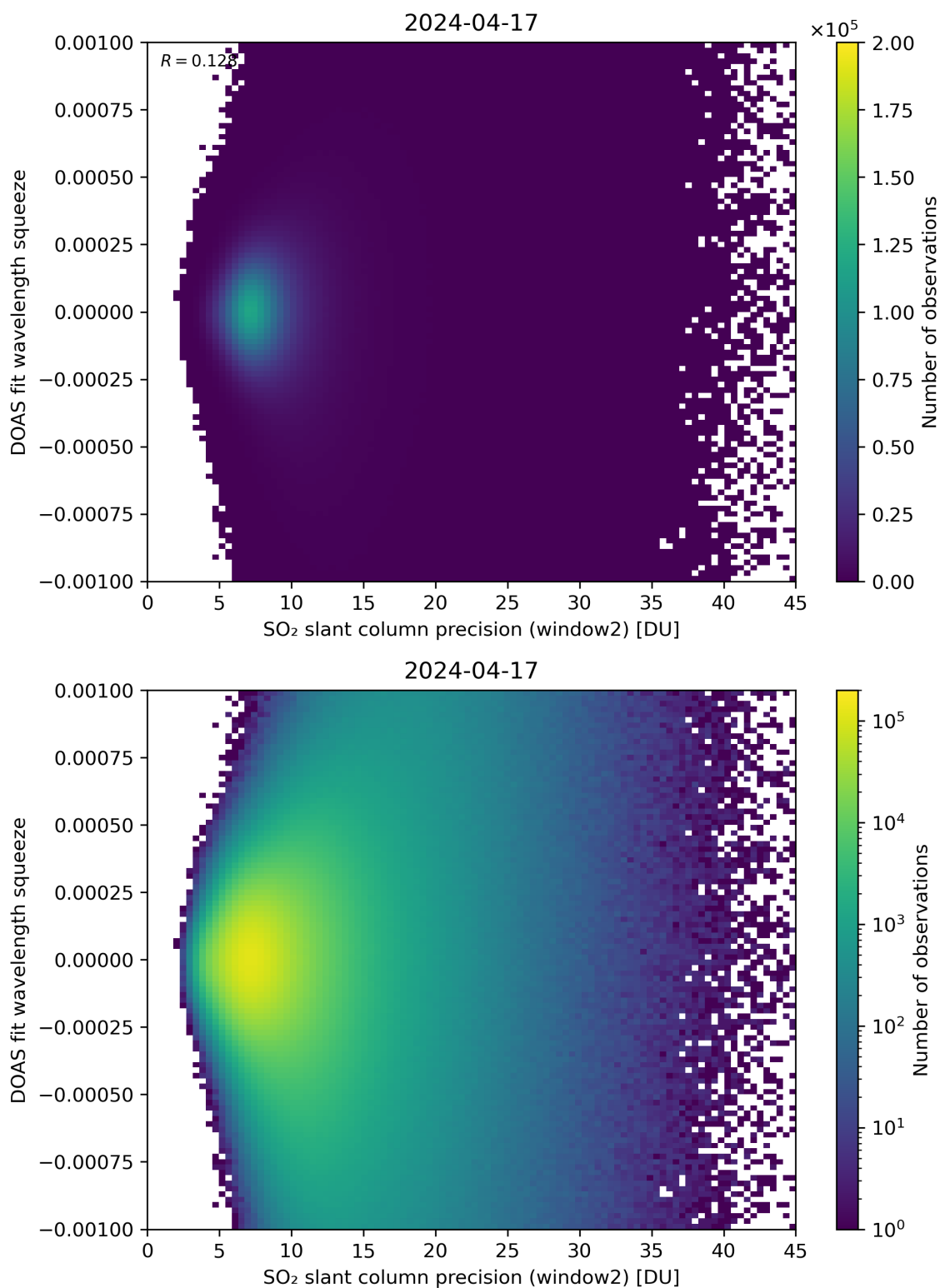
Figure 244: Scatter density plot of “SO 2 slant column precision (window2)” against “DOAS fit wavelength squeeze” for 2024-04-16 to 2024-04-18.
