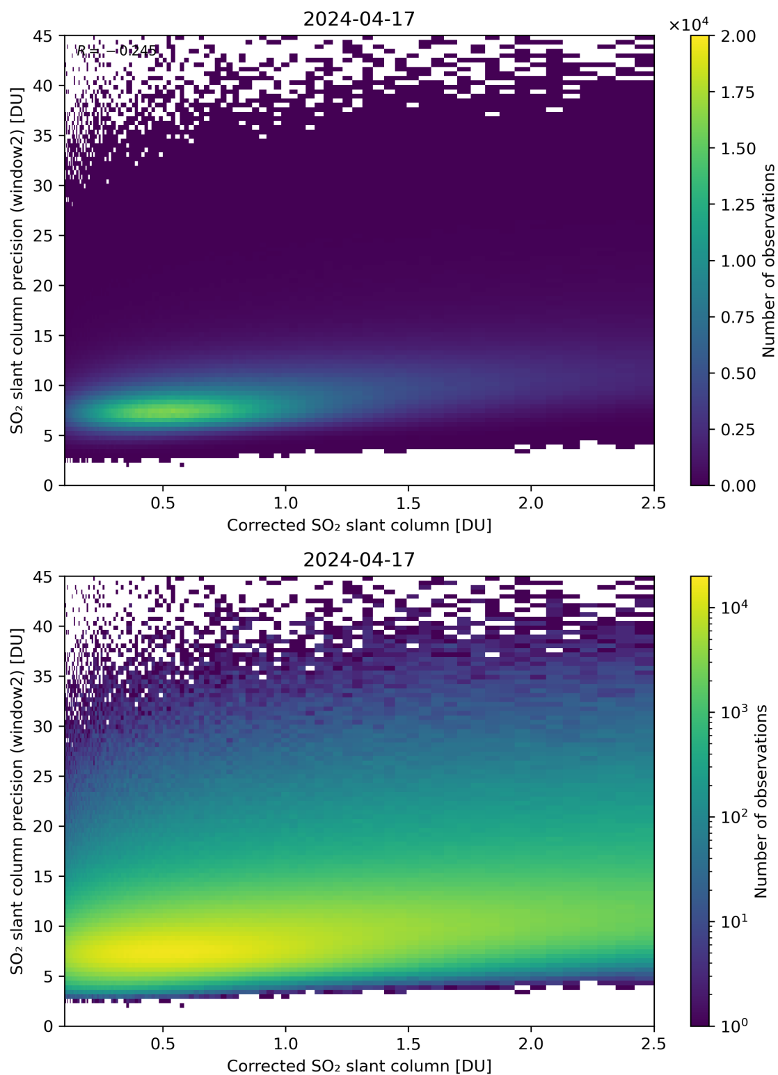
Figure 189: Scatter density plot of “Corrected SO 2 slant column” against “SO 2 slant column precision (window2)” for 2024-04-16 to 2024-04-18.
