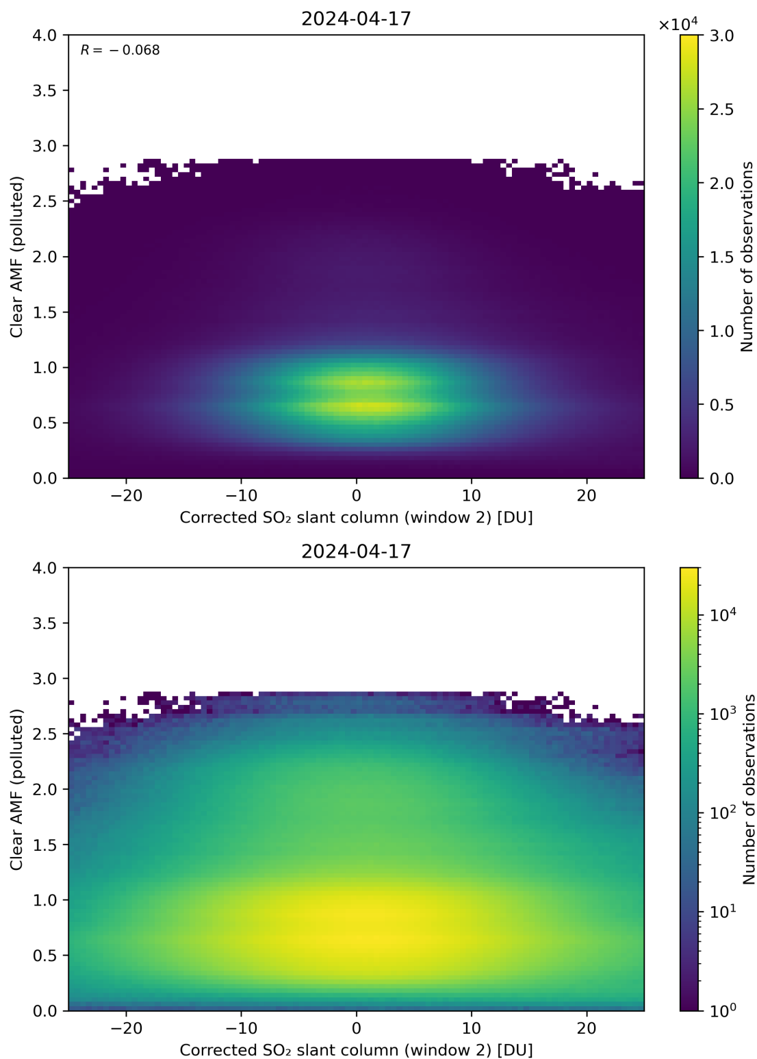
Figure 199: Scatter density plot of “Corrected SO 2 slant column (window 2)” against “Clear AMF (polluted)” for 2024-04-16 to 2024-04-18.
