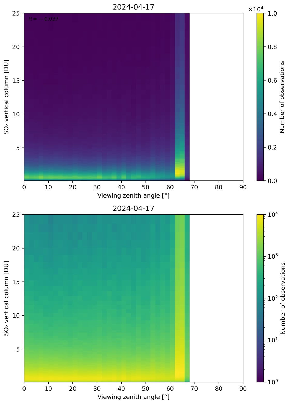
Figure 327: Scatter density plot of “Viewing zenith angle” against “SO 2 vertical column” for 2024-04-16 to 2024-04-18.
