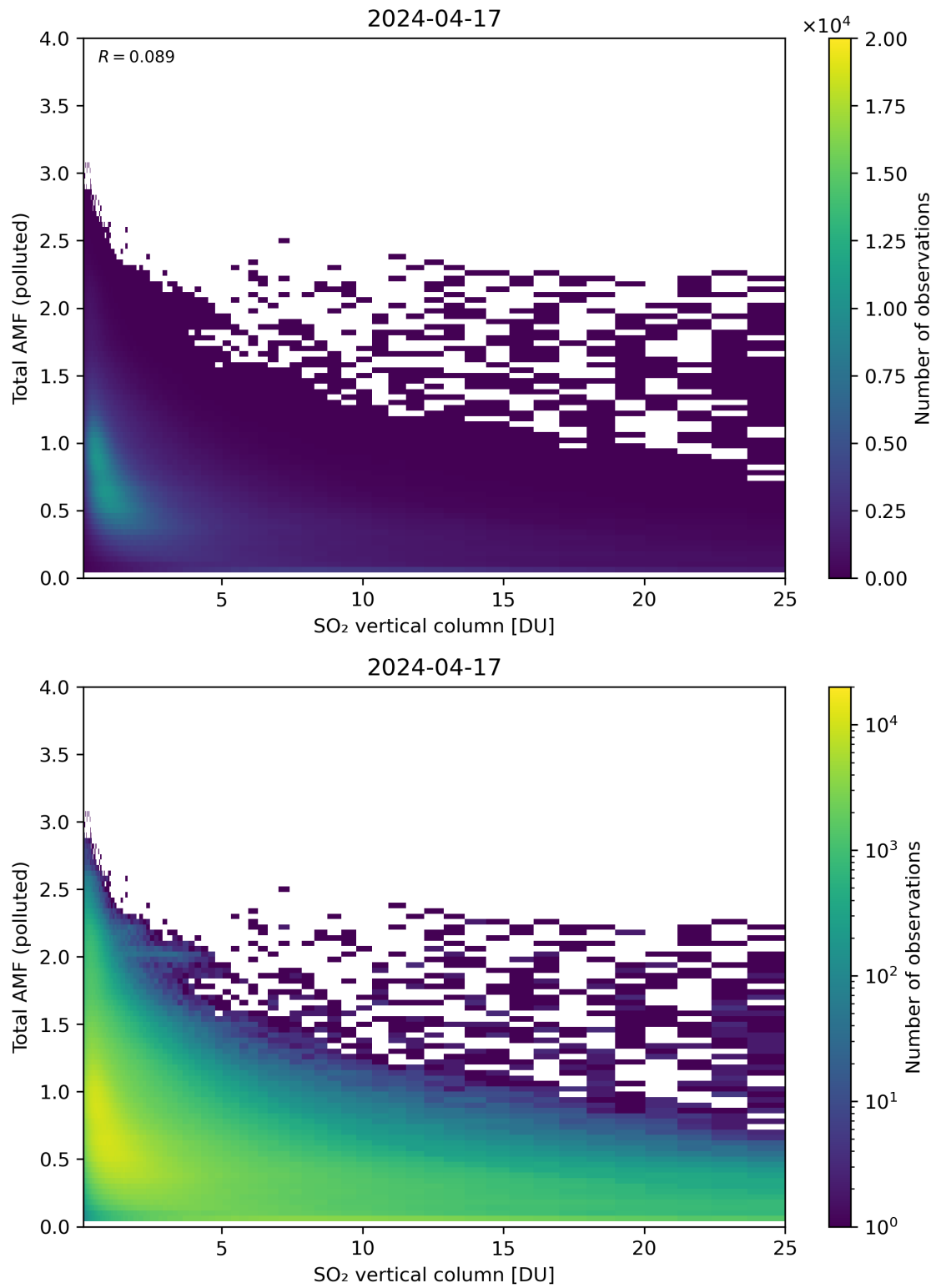
Figure 305: Scatter density plot of “SO 2 vertical column” against “Total AMF (polluted)” for 2024-04-16 to 2024-04-18.
