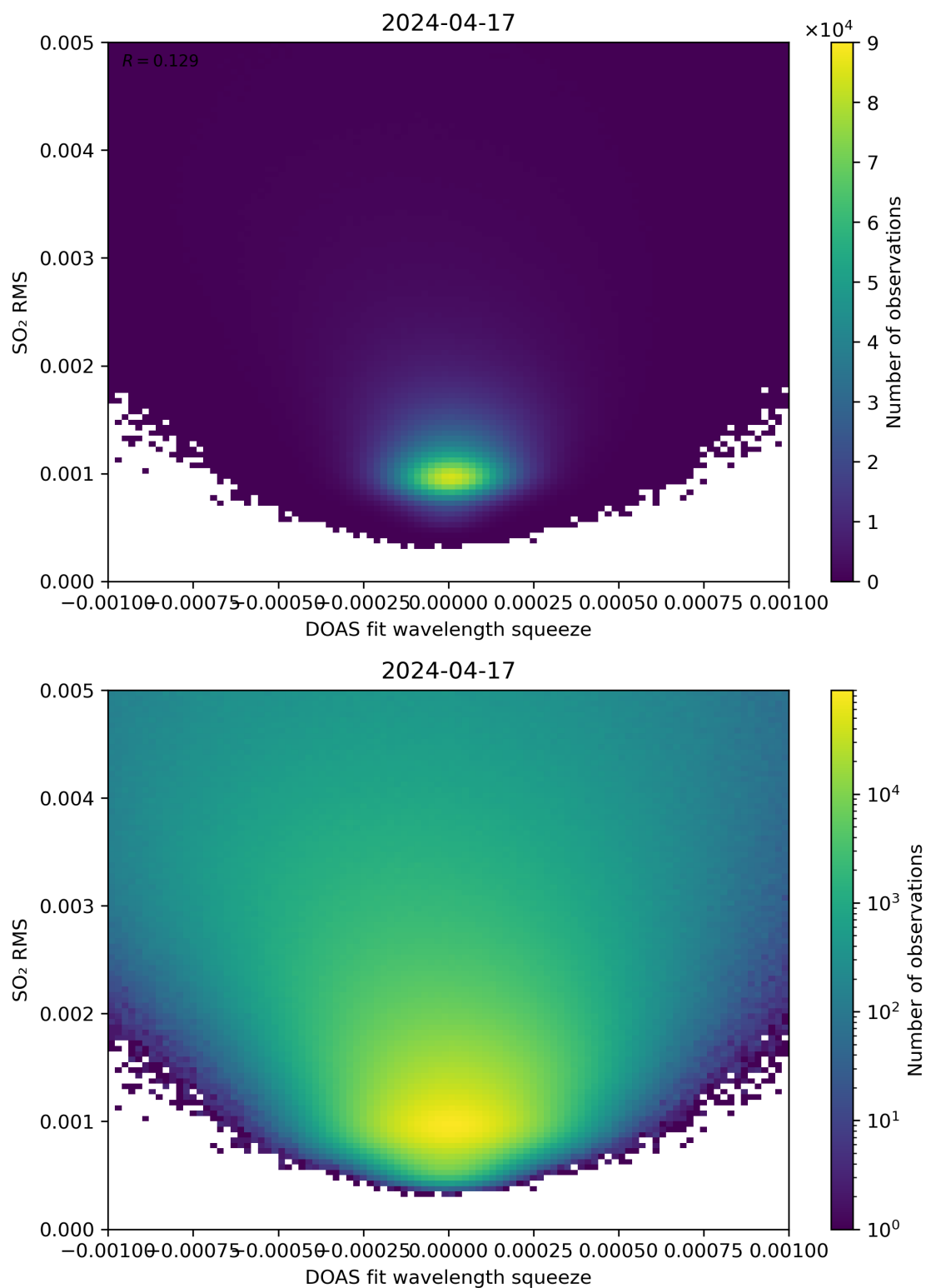
Figure 132: Scatter density plot of “DOAS fit wavelength squeeze” against “SO 2 RMS” for 2024-04-16 to 2024-04-18.
