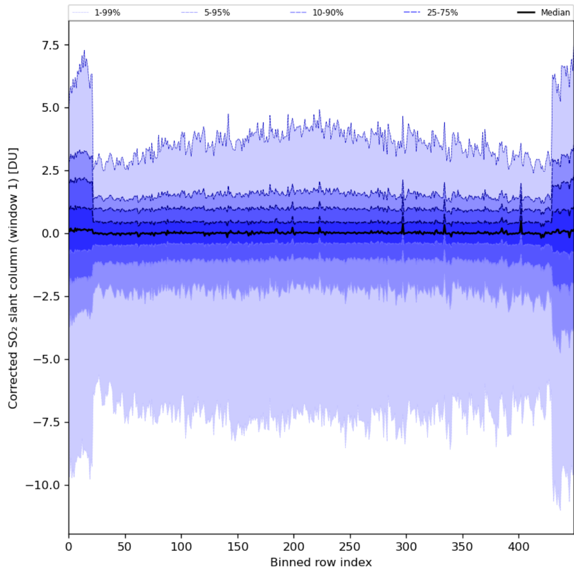
Figure 81: Along track statistics of “Corrected SO 2 slant column (window 1)” for 2024-04-16 to 2024-04-18
