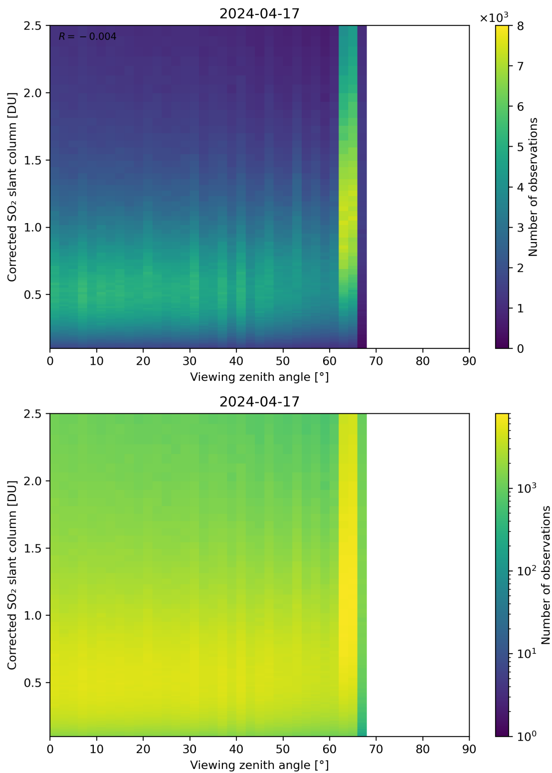
Figure 317: Scatter density plot of “Viewing zenith angle” against “Corrected SO 2 slant column” for 2024-04-16 to 2024-04-18.
