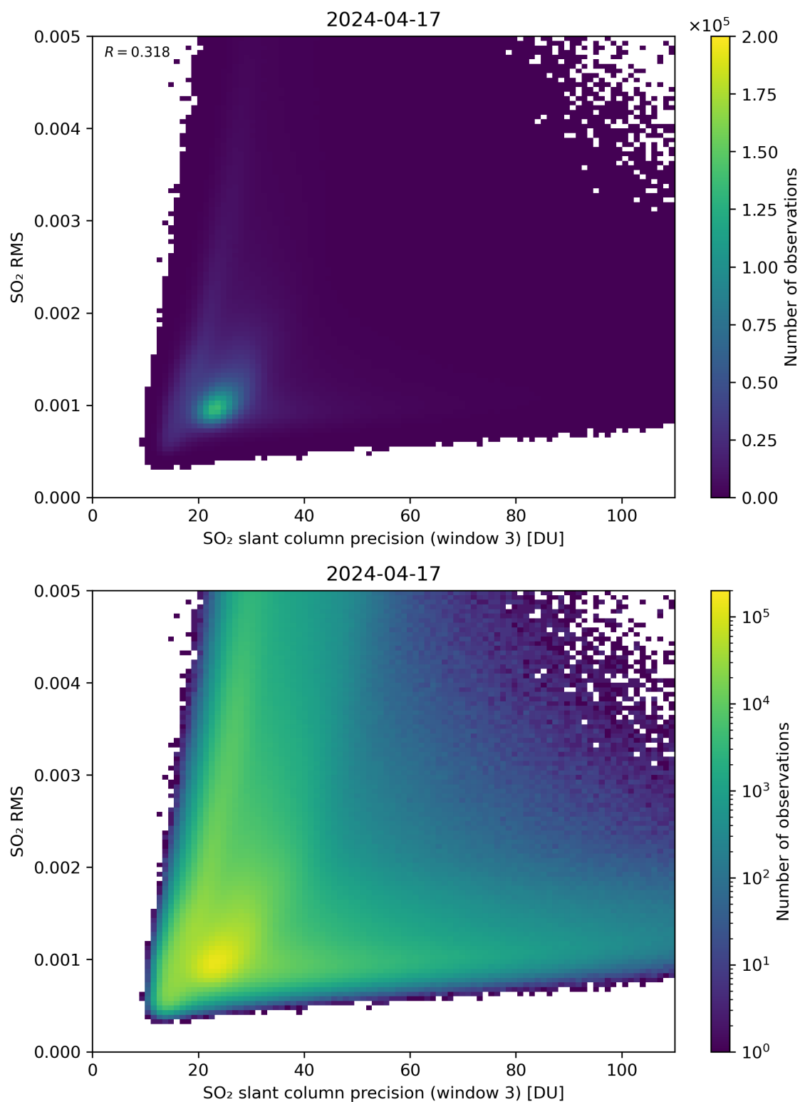
Figure 260: Scatter density plot of “SO 2 slant column precision (window 3)” against “SO 2 RMS” for 2024-04-16 to 2024-04-18.
