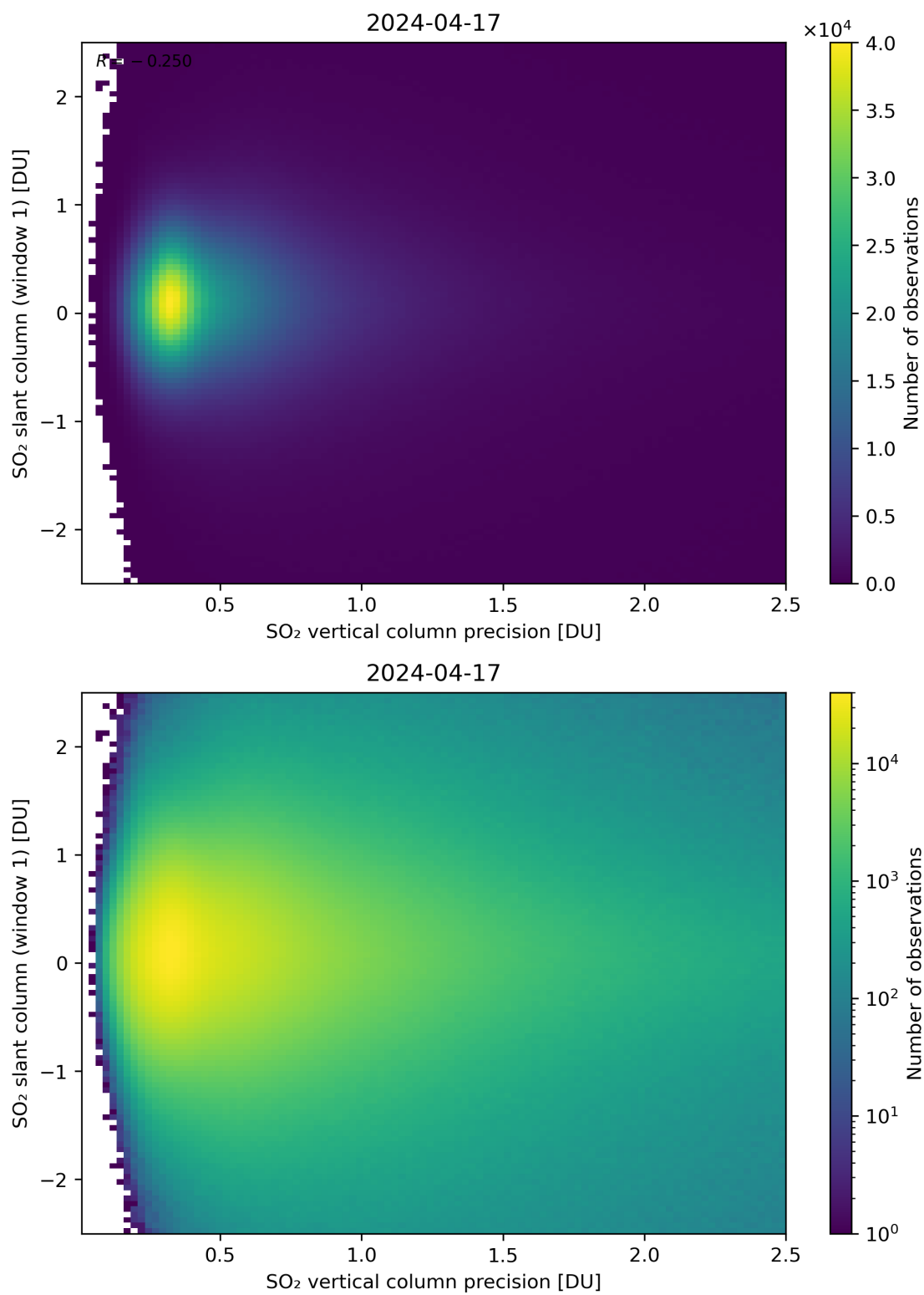
Figure 289: Scatter density plot of “SO 2 vertical column precision” against “SO 2 slant column (window 1)” for 2024-04-16 to 2024-04-18.
