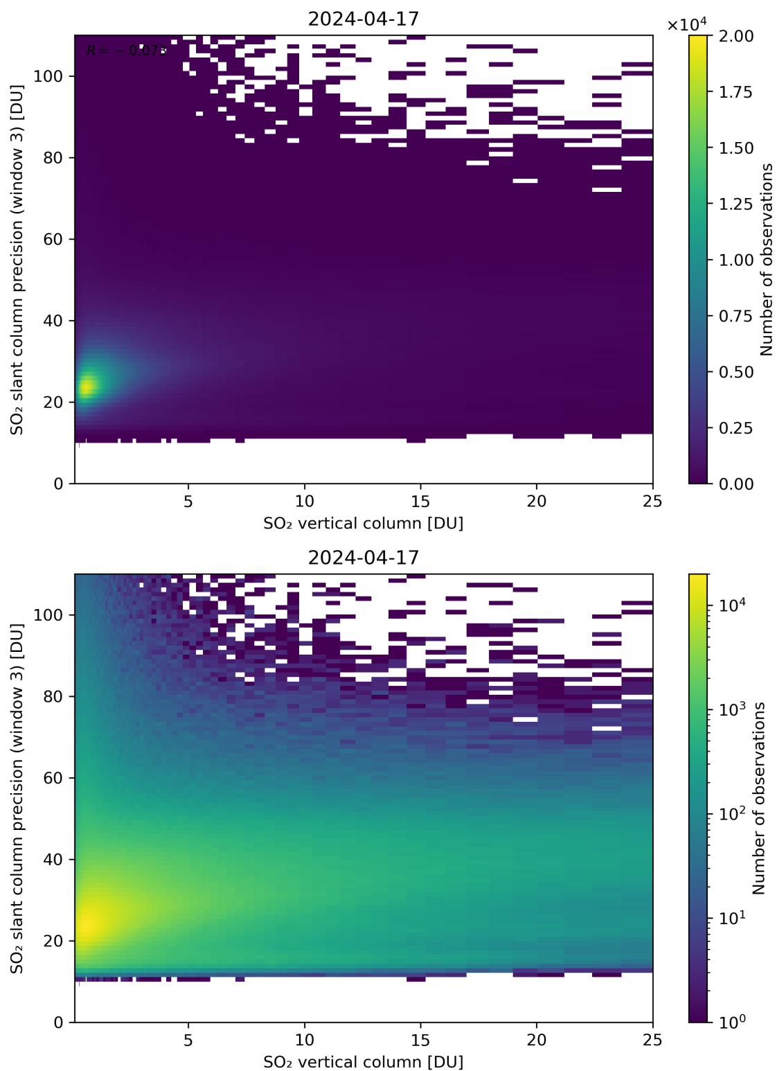
Figure 304: Scatter density plot of “SO 2 vertical column” against “SO 2 slant column precision (window 3)” for 2024-04-16 to 2024-04-18.
