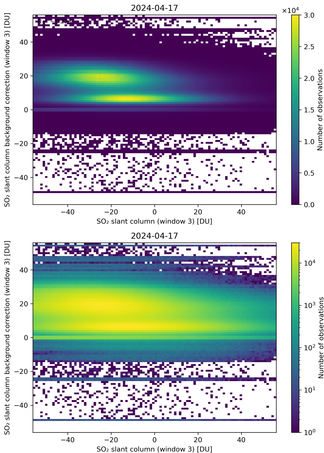
Figure 253: Scatter density plot of “SO 2 slant column (window 3)” against “SO 2 slant column background correction (window 3)” for 2024-04-16 to 2024-04-18.
