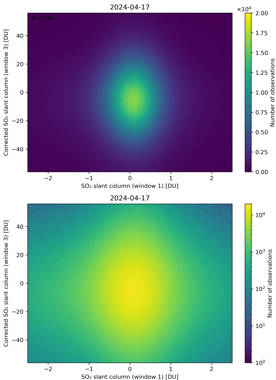
Figure 234: Scatter density plot of “SO 2 slant column (window 1)” against “Corrected SO 2 slant column (window 3)” for 2024-04-16 to 2024-04-18.
