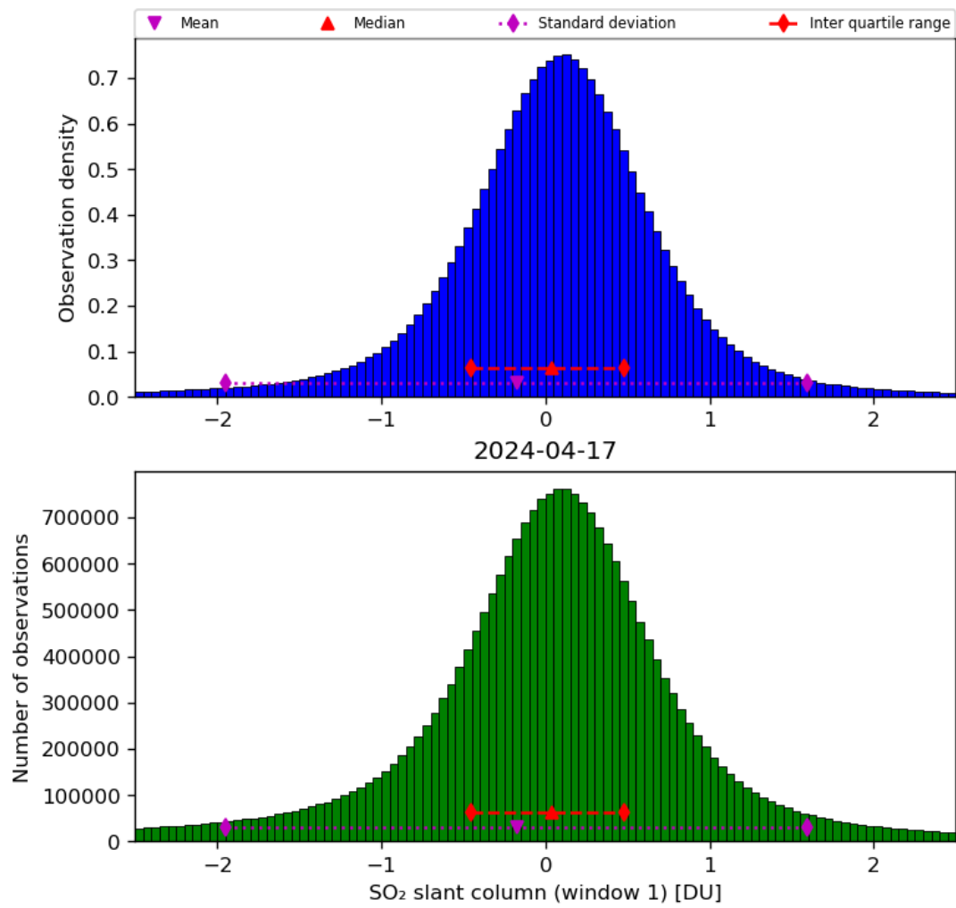
Figure 56: Histogram of “SO 2 slant column (window 1)” for 2024-04-16 to 2024-04-18
