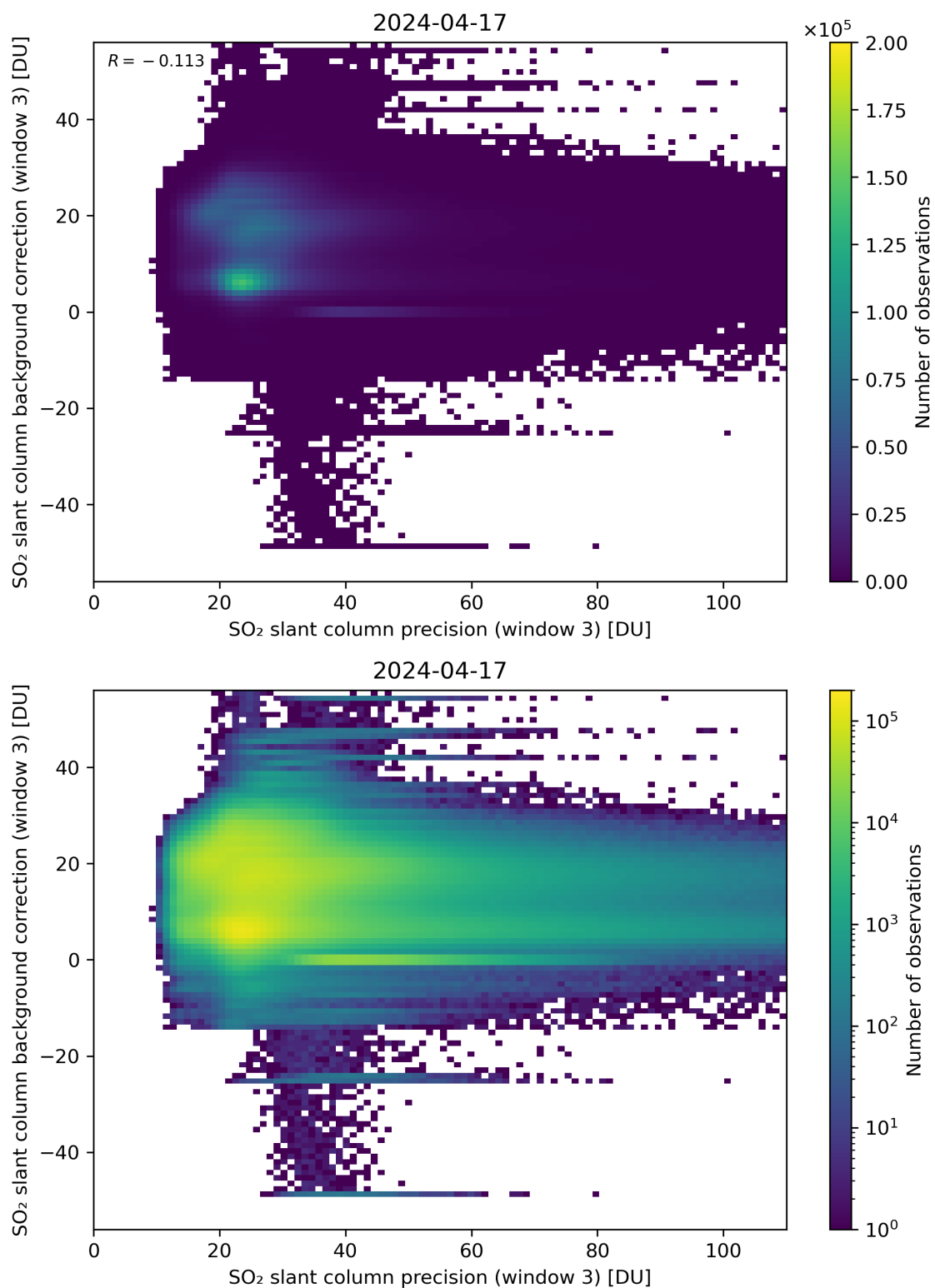
Figure 257: Scatter density plot of “SO 2 slant column precision (window 3)” against “SO 2 slant column background correction (window 3)” for 2024-04-16 to 2024-04-18.
