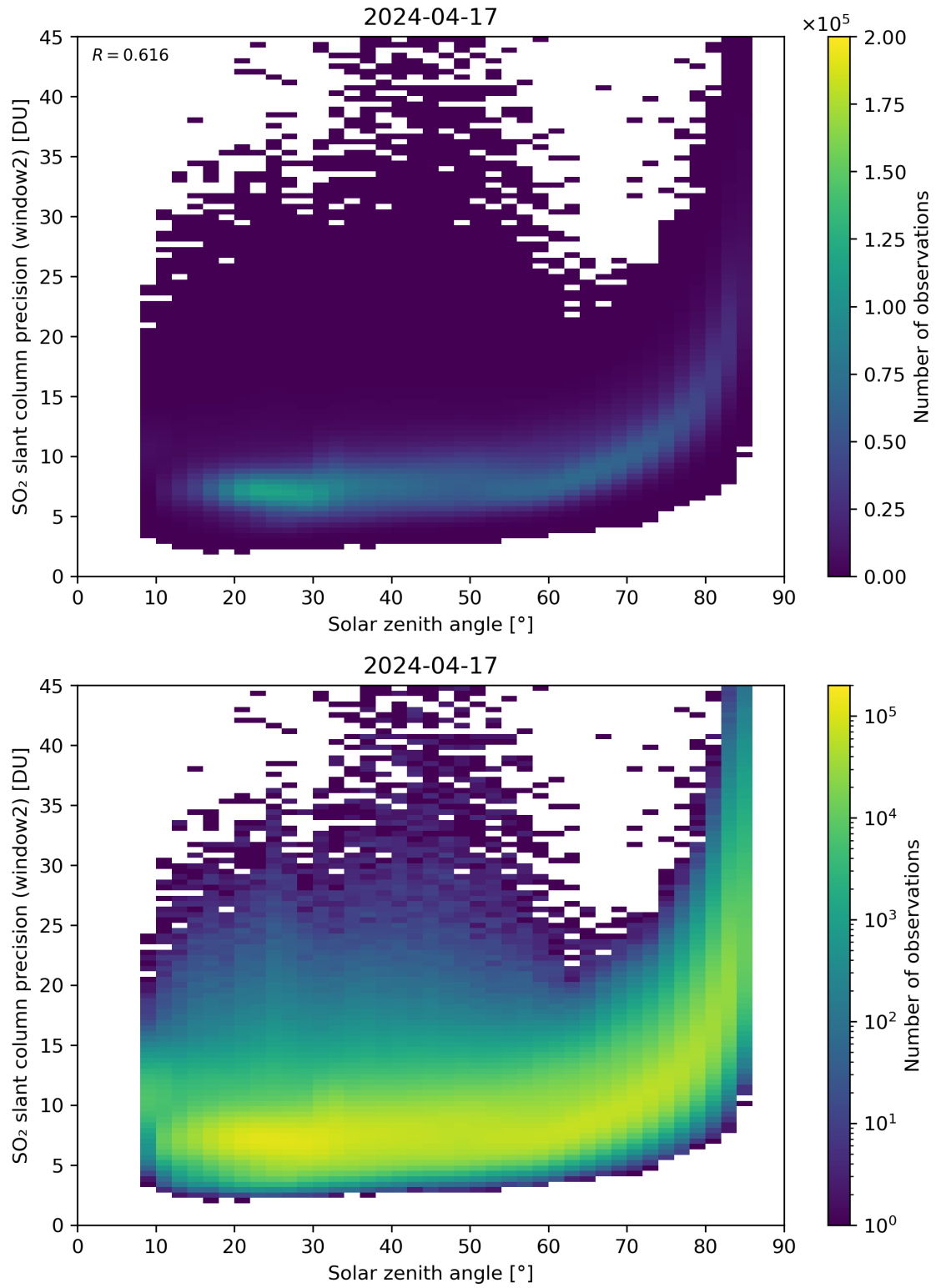
Figure 171: Scatter density plot of “Solar zenith angle” against “SO 2 slant column precision (window2)” for 2024-04-16 to 2024-04-18.
