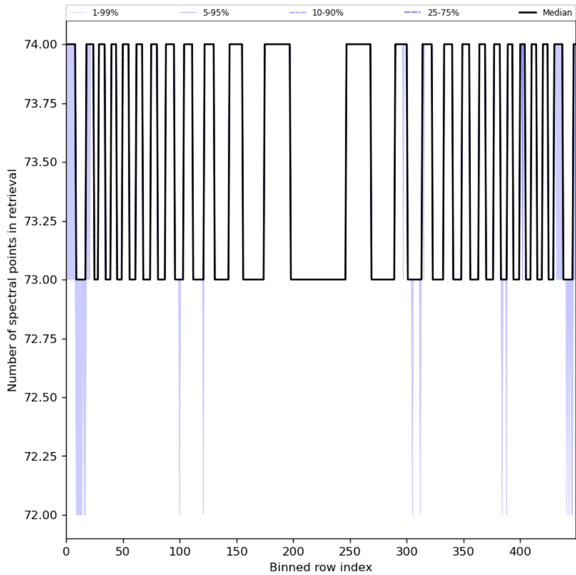
Figure 97: Along track statistics of “Number of spectral points in retrieval” for 2024-04-16 to 2024-04-18
