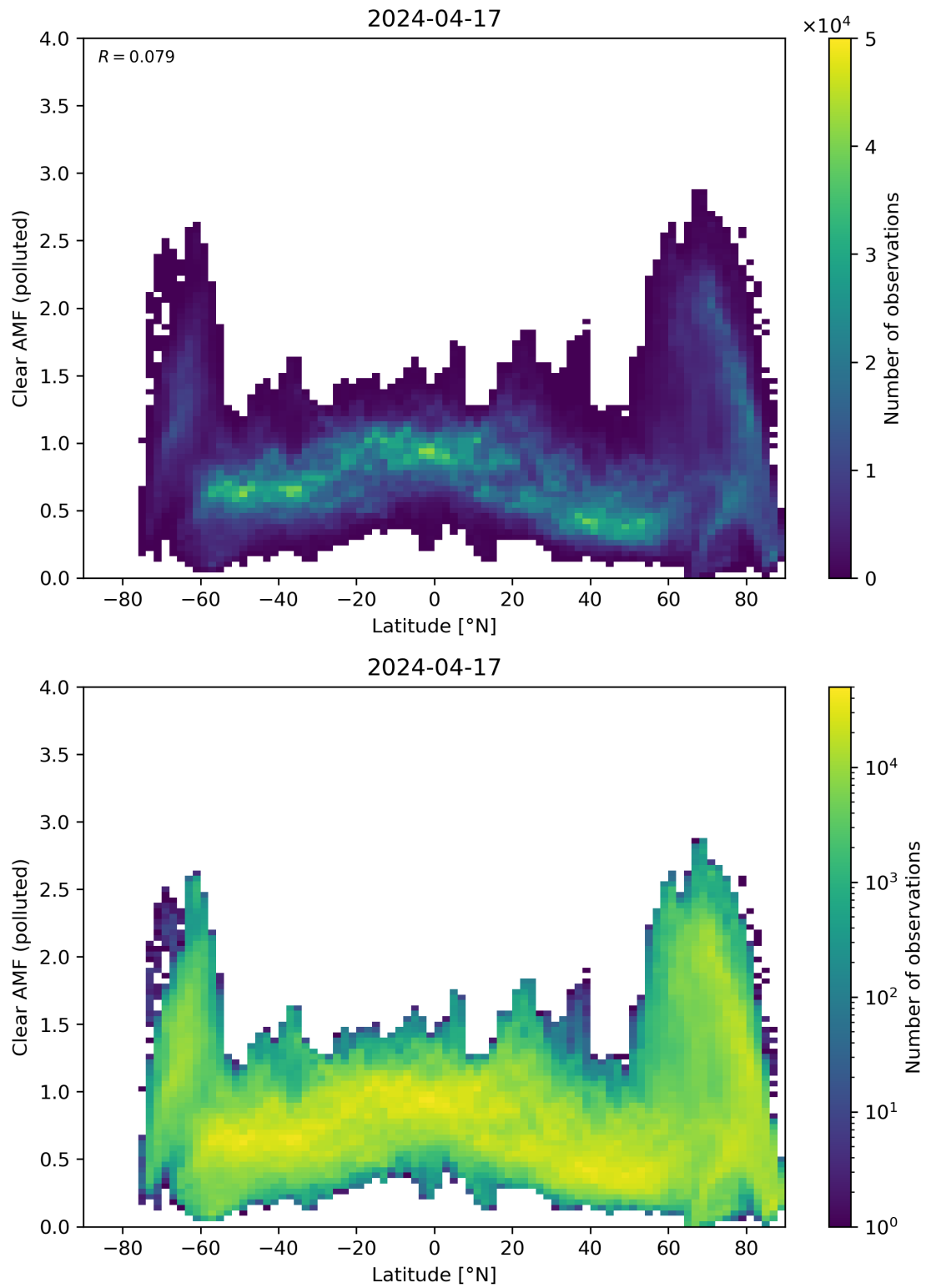
Figure 145: Scatter density plot of “Latitude” against “Clear AMF (polluted)” for 2024-04-16 to 2024-04-18.
