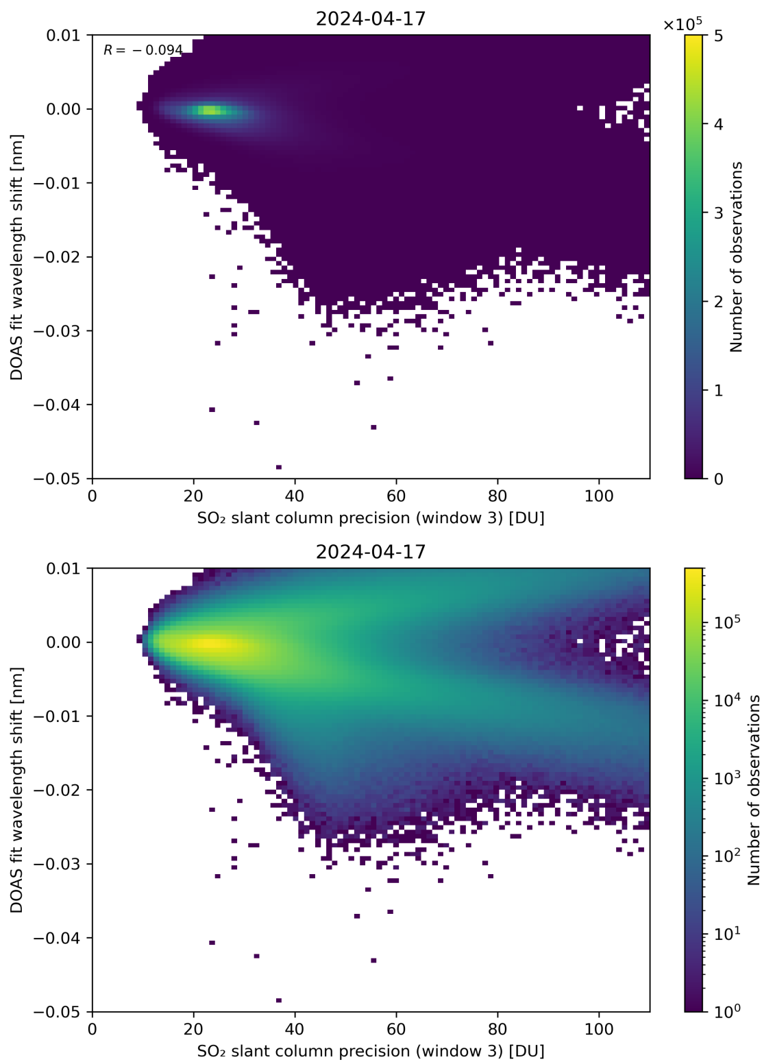
Figure 258: Scatter density plot of “SO 2 slant column precision (window 3)” against “DOAS fit wavelength shift” for 2024-04-16 to 2024-04-18.
