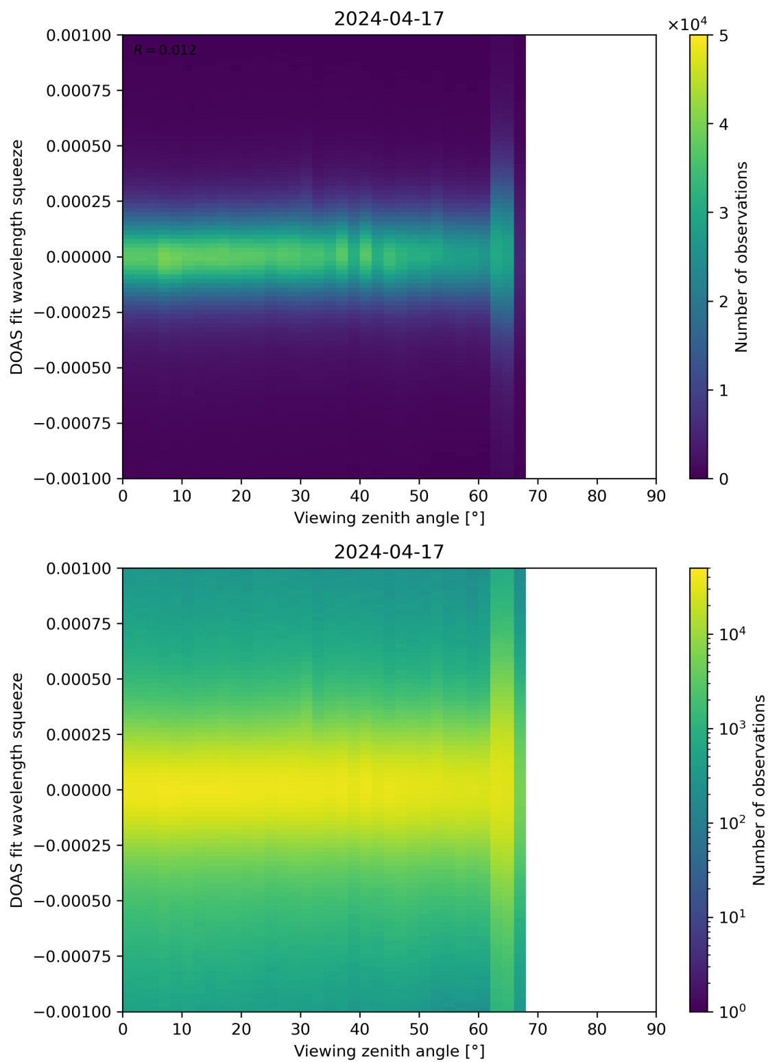
Figure 312: Scatter density plot of “Viewing zenith angle” against “DOAS fit wavelength squeeze” for 2024-04-16 to 2024-04-18.
