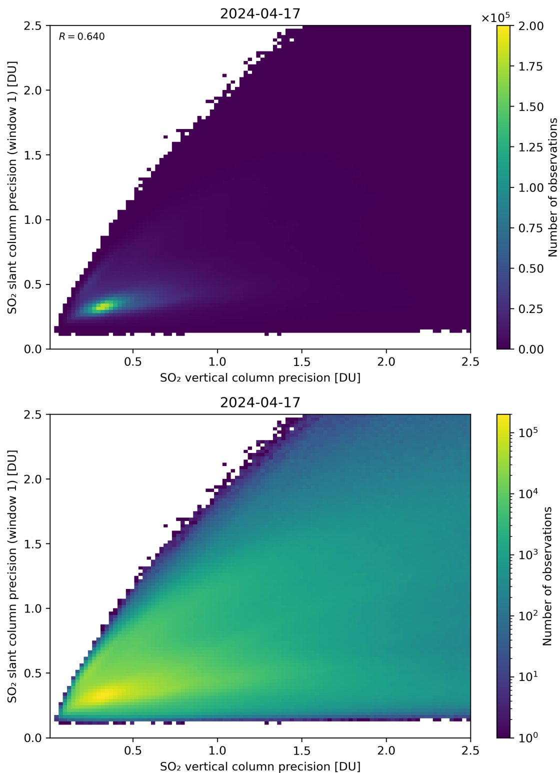
Figure 290: Scatter density plot of “SO 2 vertical column precision” against “SO 2 slant column precision (window 1)” for 2024-04-16 to 2024-04-18.
