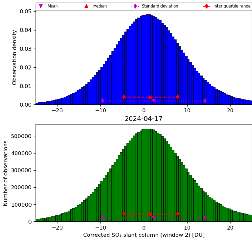
Figure 62: Histogram of “Corrected SO 2 slant column (window 2)” for 2024-04-16 to 2024-04-18
