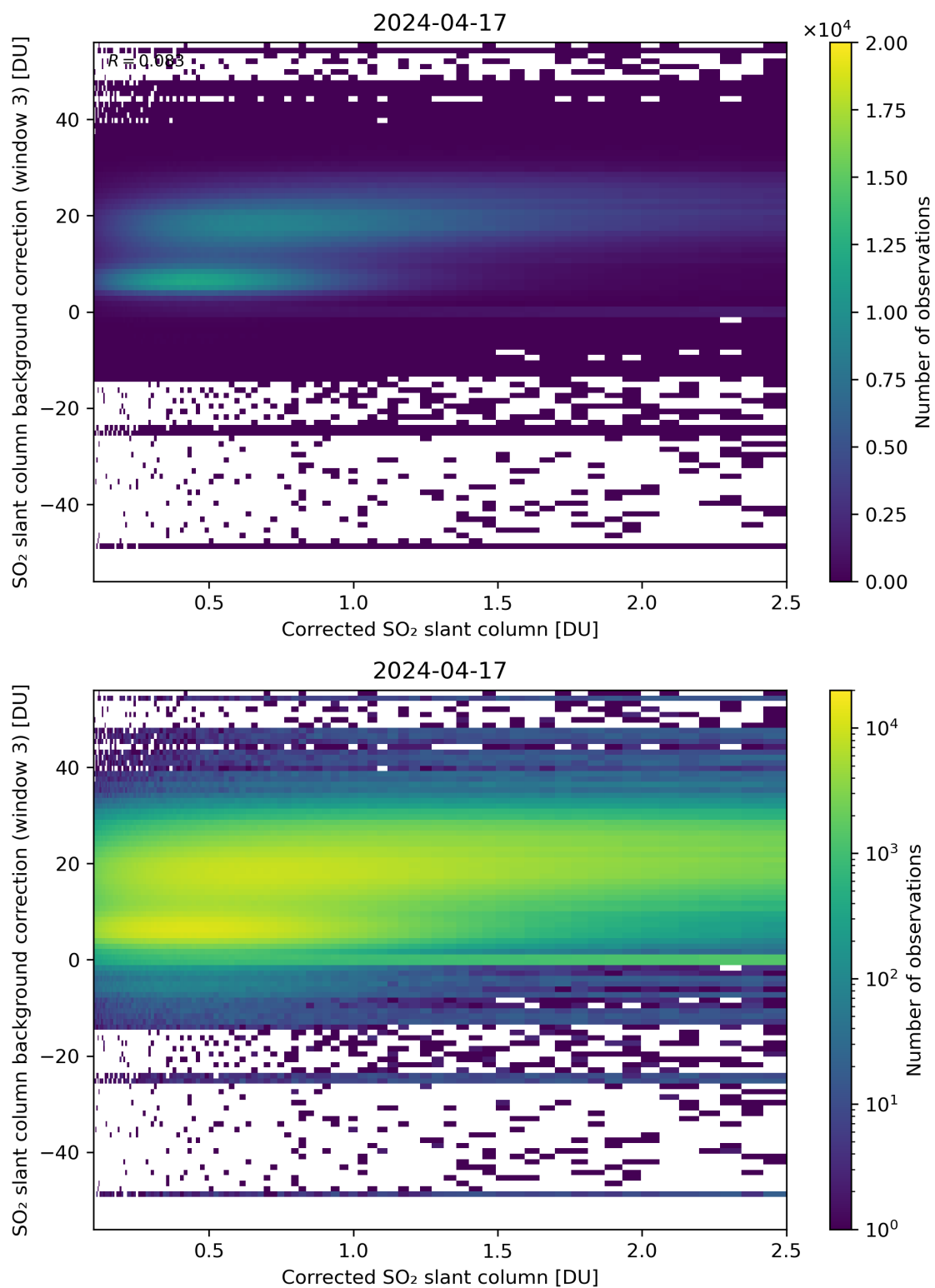
Figure 180: Scatter density plot of “Corrected SO 2 slant column” against “SO 2 slant column background correction (window 3)” for 2024-04-16 to 2024-04-18.
