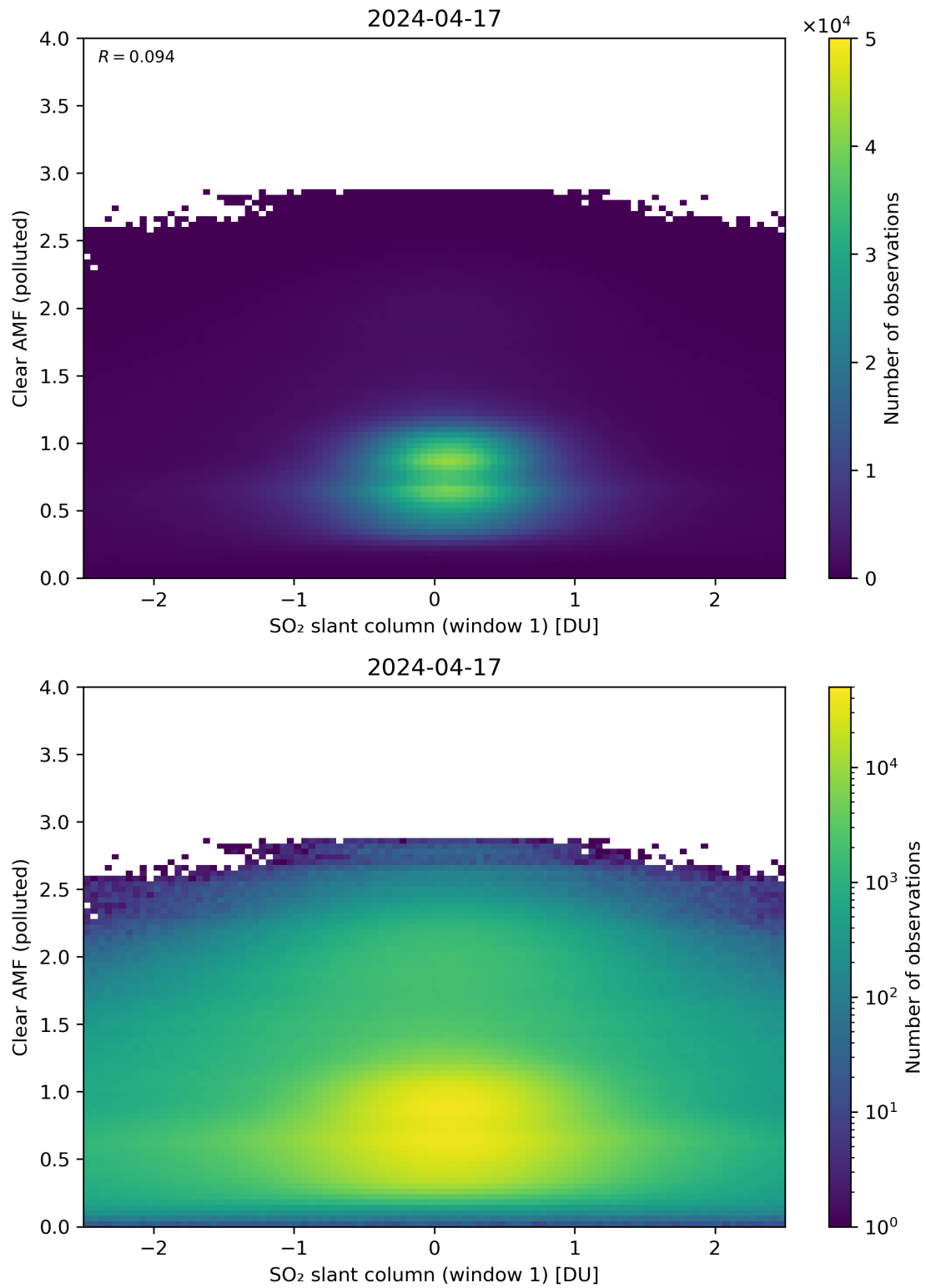
Figure 232: Scatter density plot of “SO 2 slant column (window 1)” against “Clear AMF (polluted)” for 2024-04-16 to 2024-04-18.
