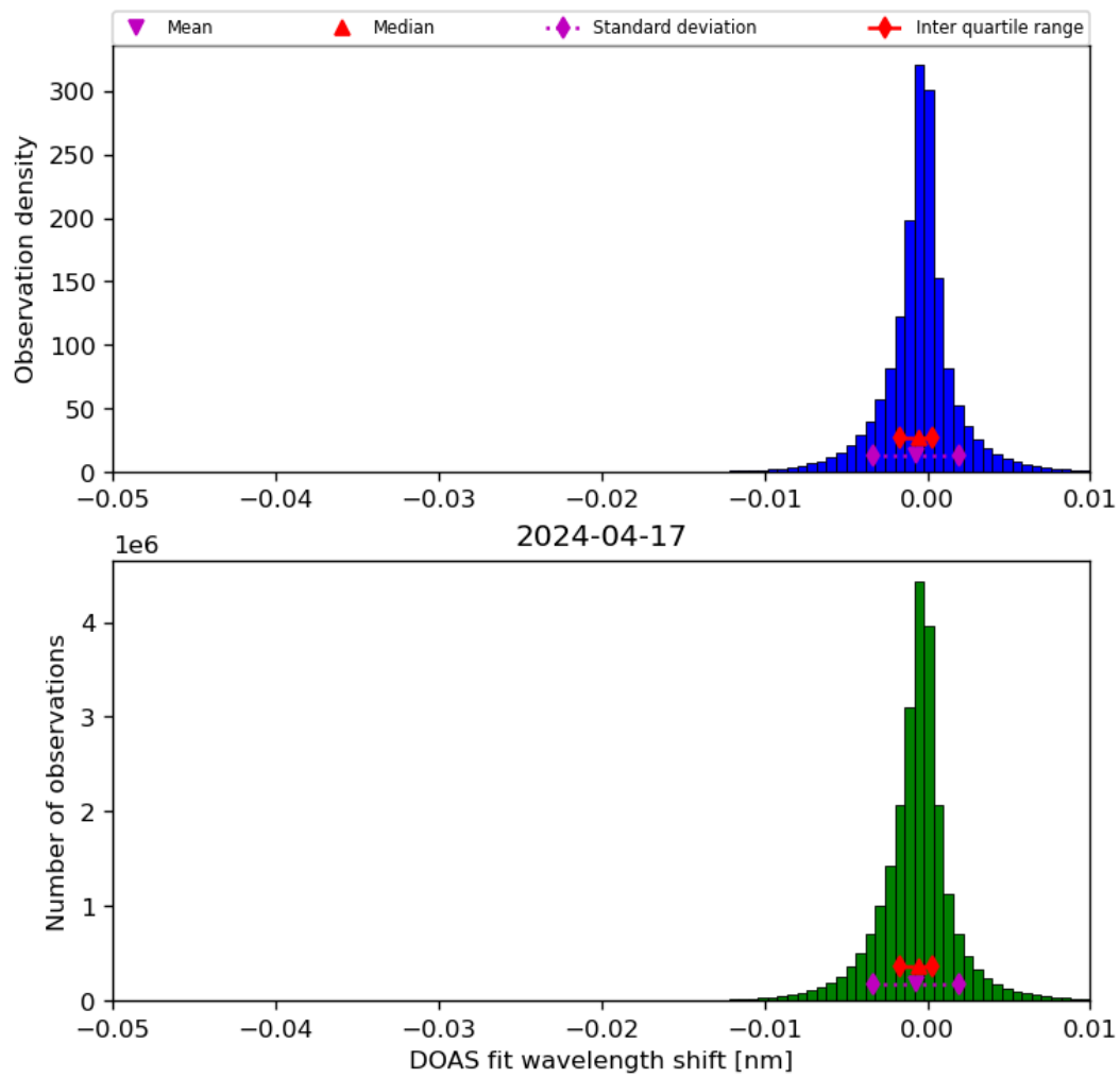
Figure 68: Histogram of “DOAS fit wavelength shift” for 2024-04-16 to 2024-04-18
