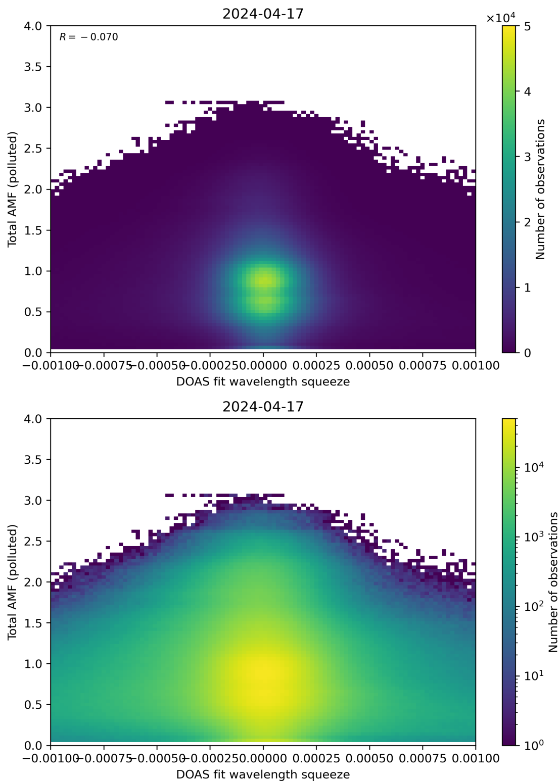
Figure 134: Scatter density plot of “DOAS fit wavelength squeeze” against “Total AMF (polluted)” for 2024-04-16 to 2024-04-18.
