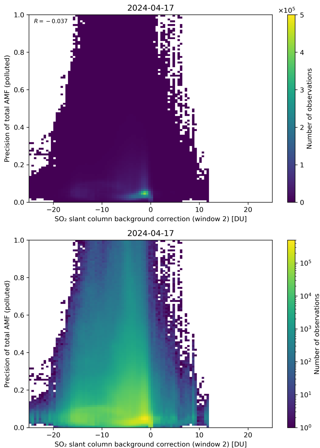
Figure 120: Scatter density plot of “SO 2 slant column background correction (window 2)” against “Precision of total AMF (polluted)” for 2024-04-16 to 2024-04-18.
