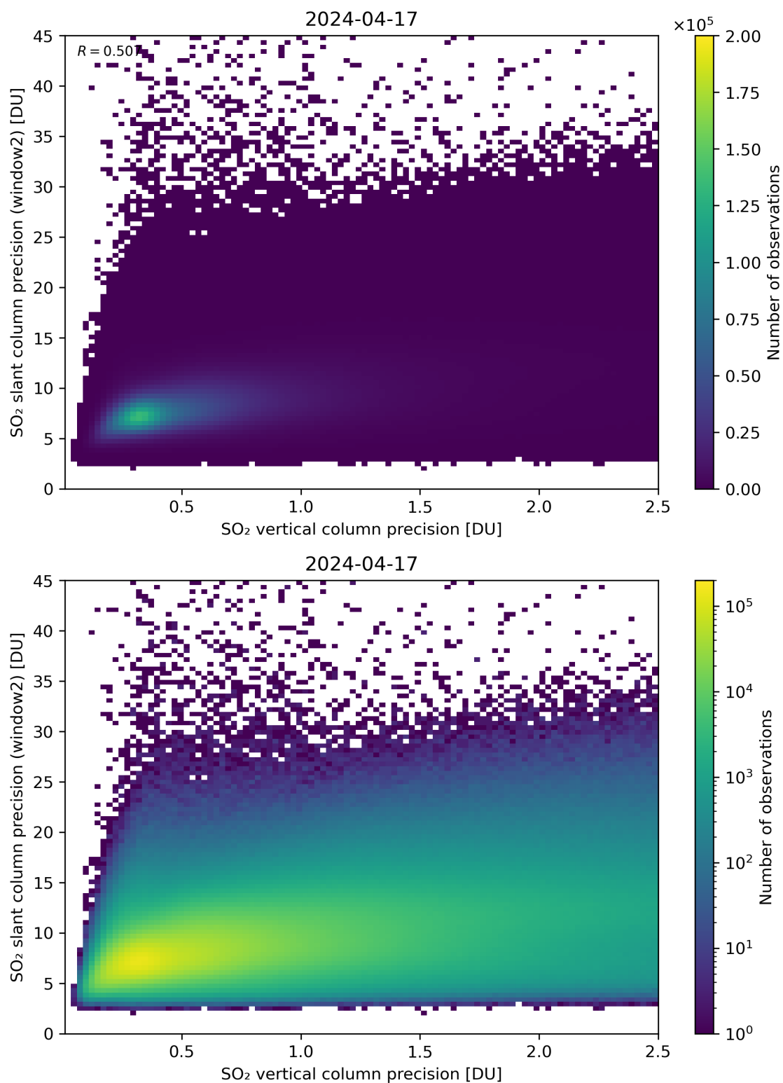
Figure 291: Scatter density plot of “SO 2 vertical column precision” against “SO 2 slant column precision (window2)” for 2024-04-16 to 2024-04-18.
