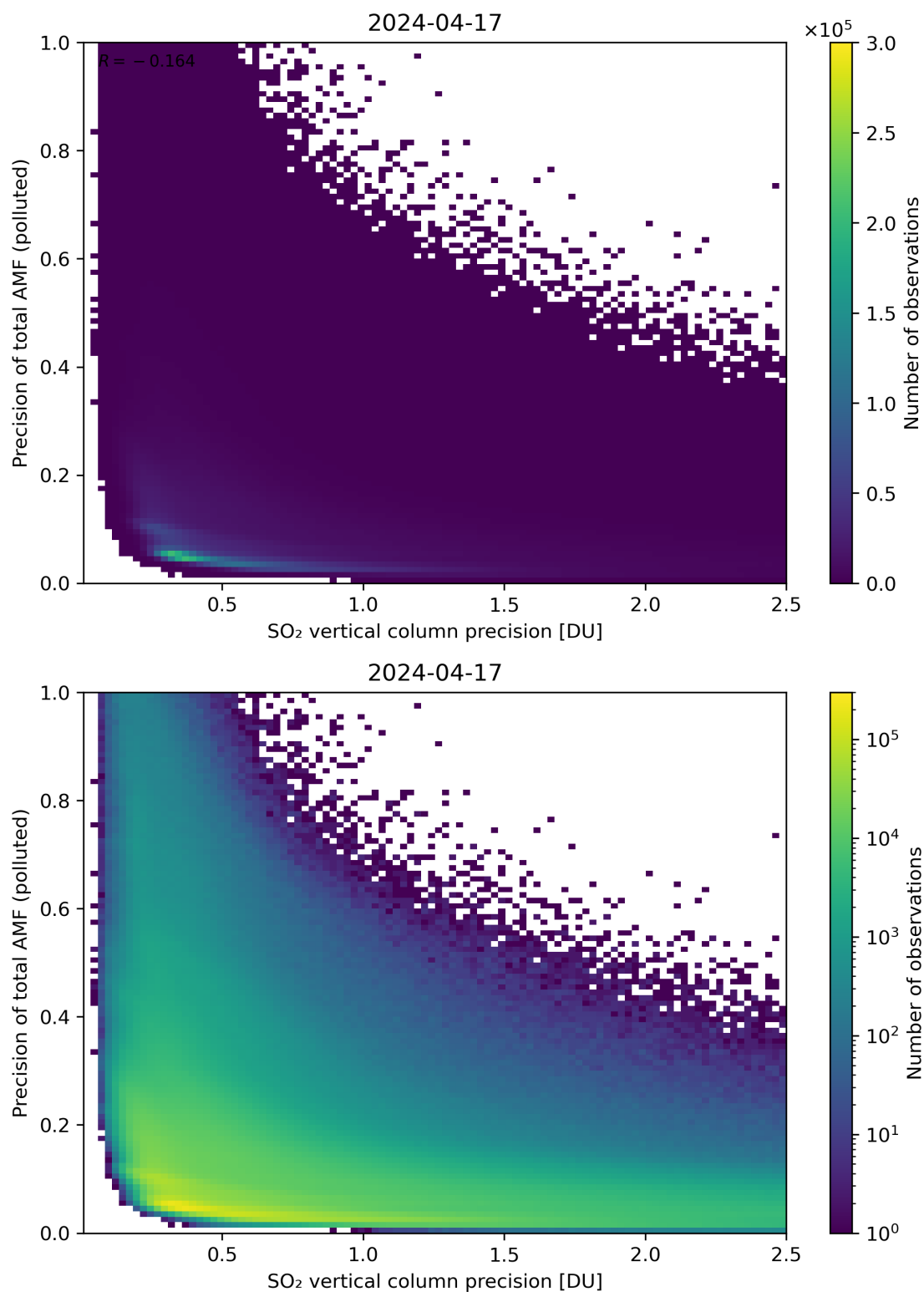
Figure 295: Scatter density plot of “SO 2 vertical column precision” against “Precision of total AMF (polluted)” for 2024-04-16 to 2024-04-18.
