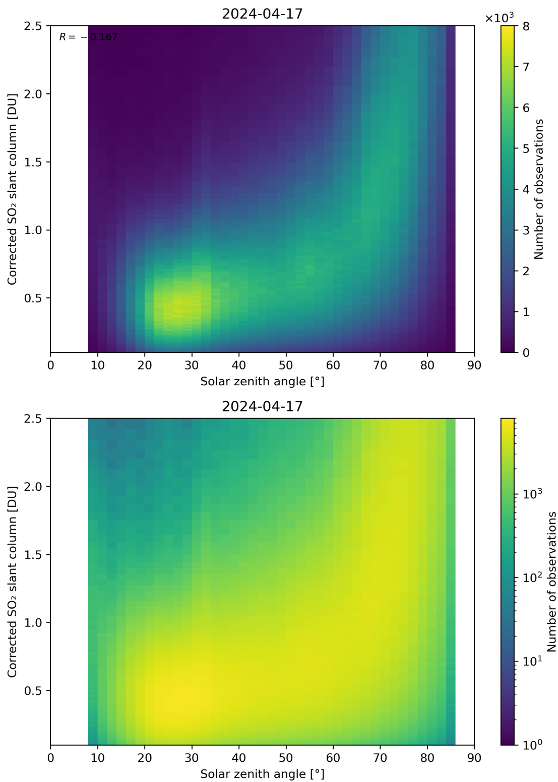
Figure 166: Scatter density plot of “Solar zenith angle” against “Corrected SO 2 slant column” for 2024-04-16 to 2024-04-18.
