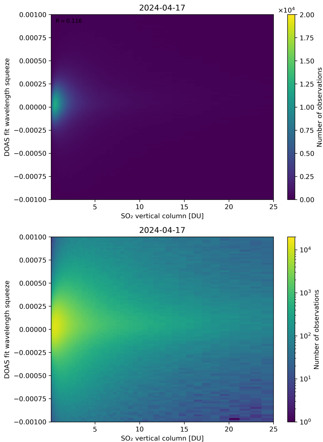
Figure 277: Scatter density plot of “SO 2 vertical column” against “DOAS fit wavelength squeeze” for 2024-04-16 to 2024-04-18.
