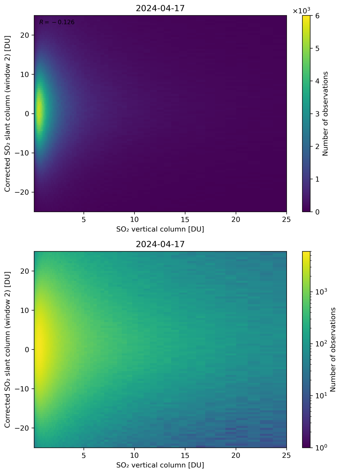
Figure 298: Scatter density plot of “SO 2 vertical column” against “Corrected SO 2 slant column (window 2)” for 2024-04-16 to 2024-04-18.
