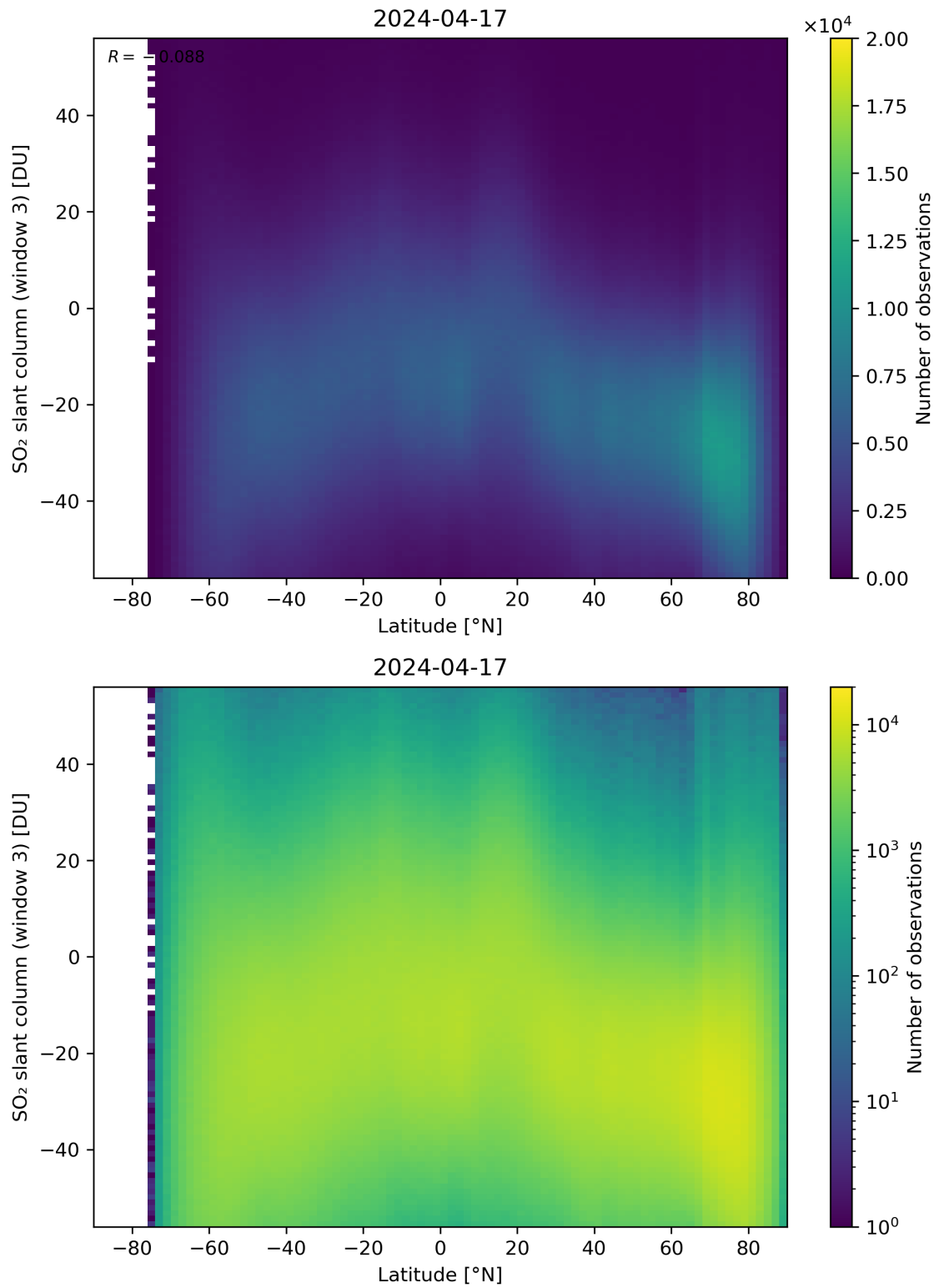
Figure 152: Scatter density plot of “Latitude” against “SO 2 slant column (window 3)” for 2024-04-16 to 2024-04-18.
