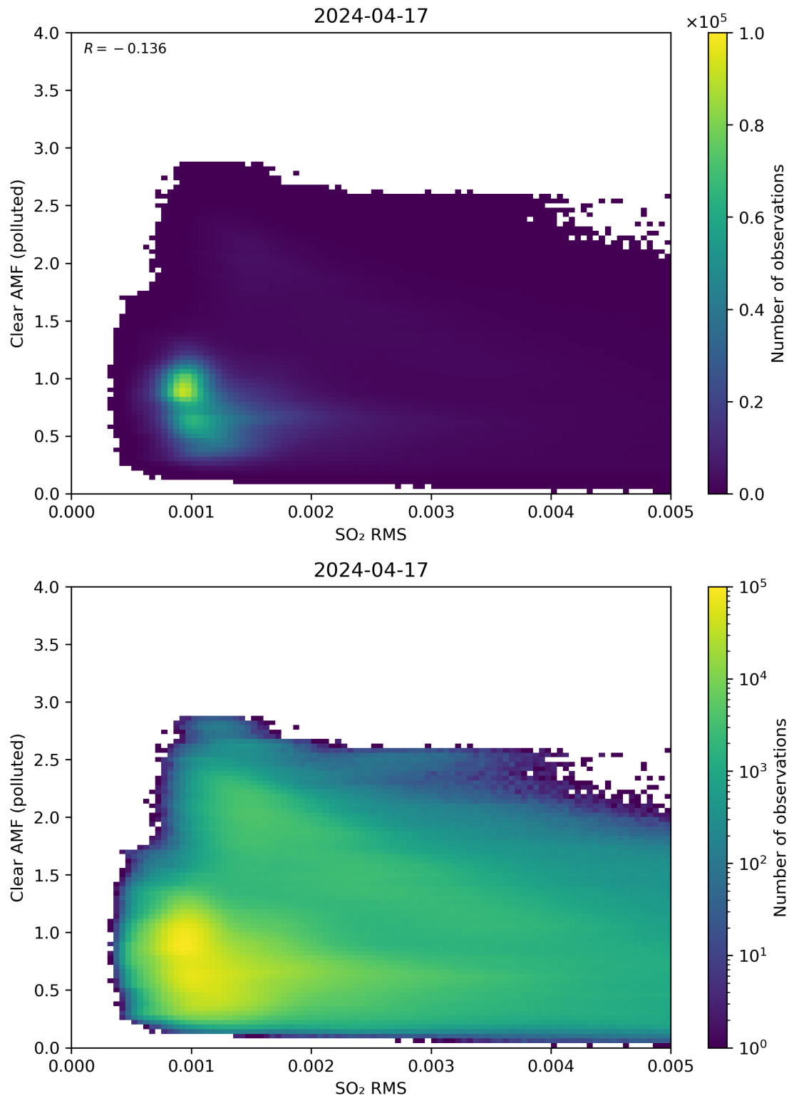
Figure 136: Scatter density plot of “SO 2 RMS” against “Clear AMF (polluted)” for 2024-04-16 to 2024-04-18.
