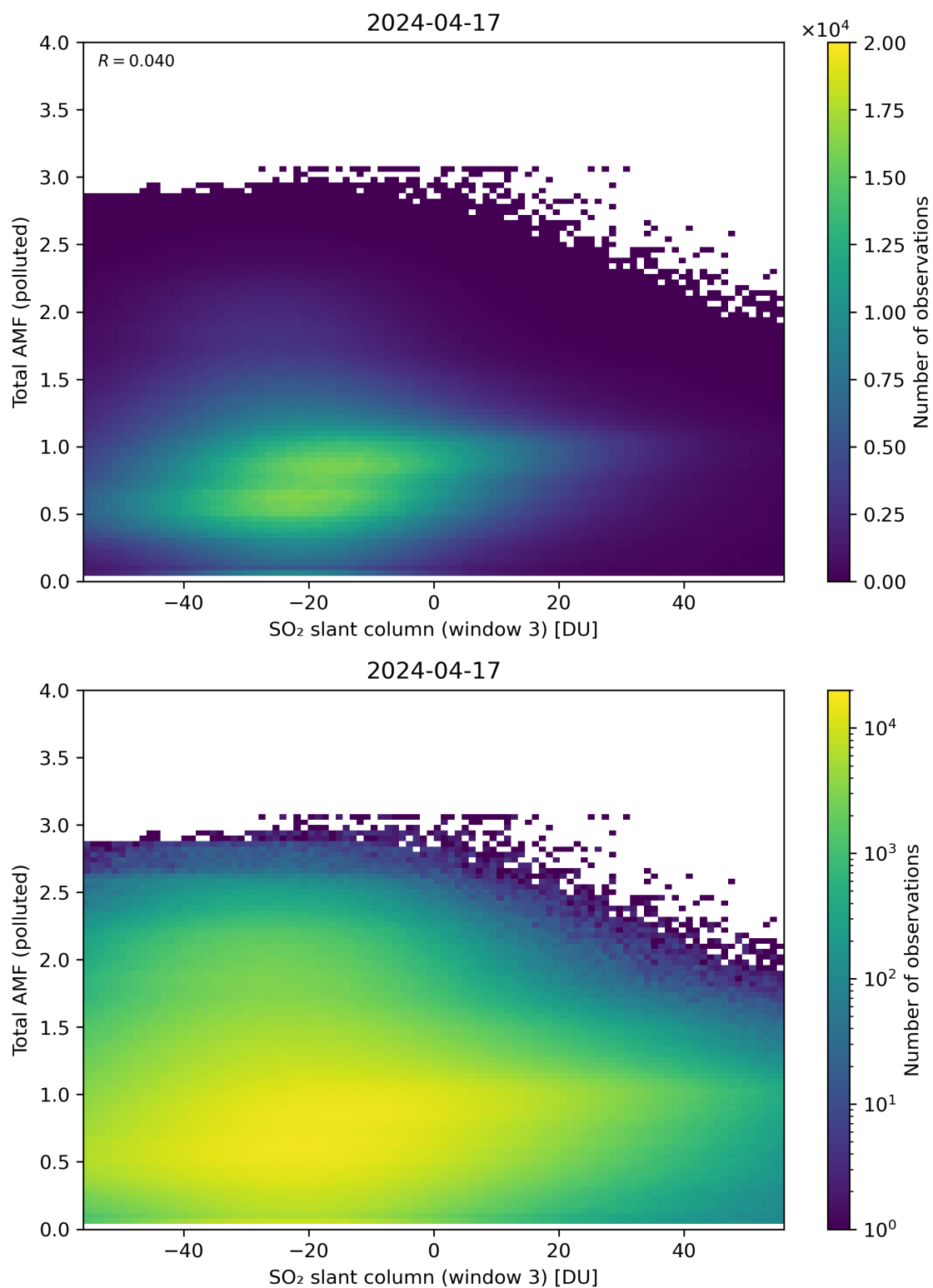
Figure 268: Scatter density plot of “SO 2 slant column (window 3)” against “Total AMF (polluted)” for 2024-04-16 to 2024-04-18.
