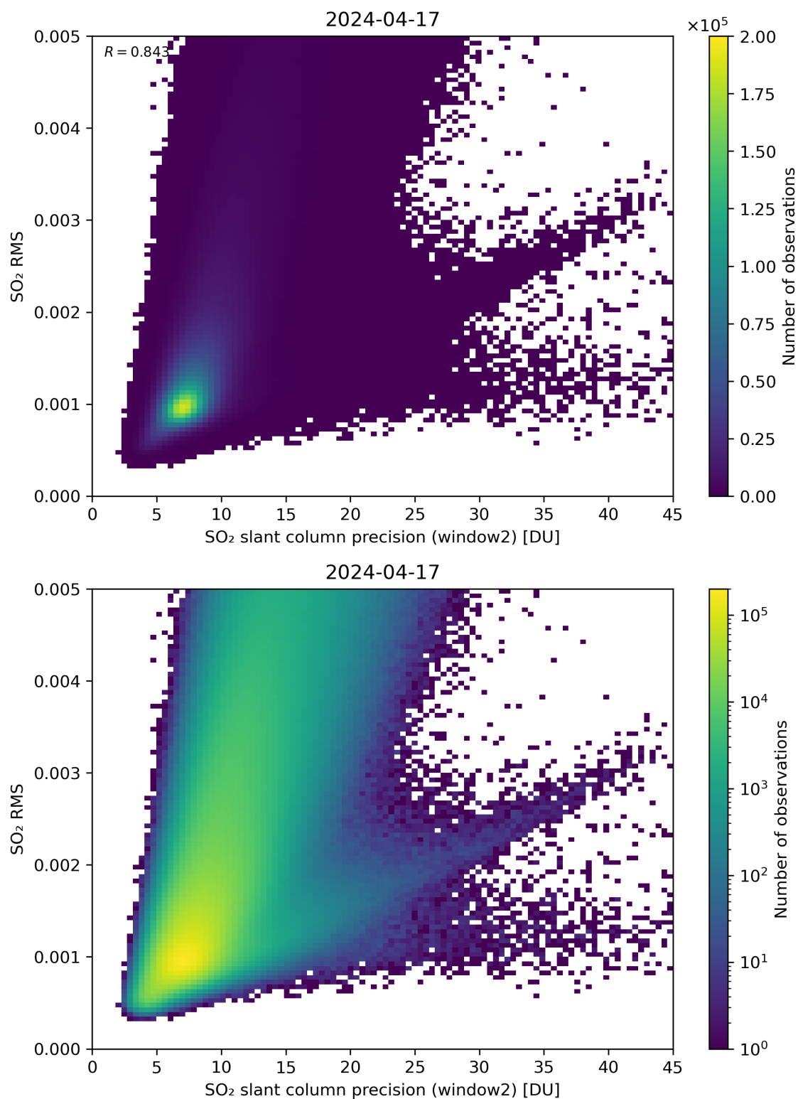
Figure 245: Scatter density plot of “SO 2 slant column precision (window2)” against “SO 2 RMS” for 2024-04-16 to 2024-04-18.
