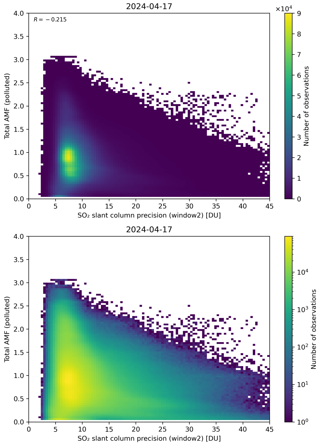
Figure 251: Scatter density plot of “SO 2 slant column precision (window2)” against “Total AMF (polluted)” for 2024-04-16 to 2024-04-18.
