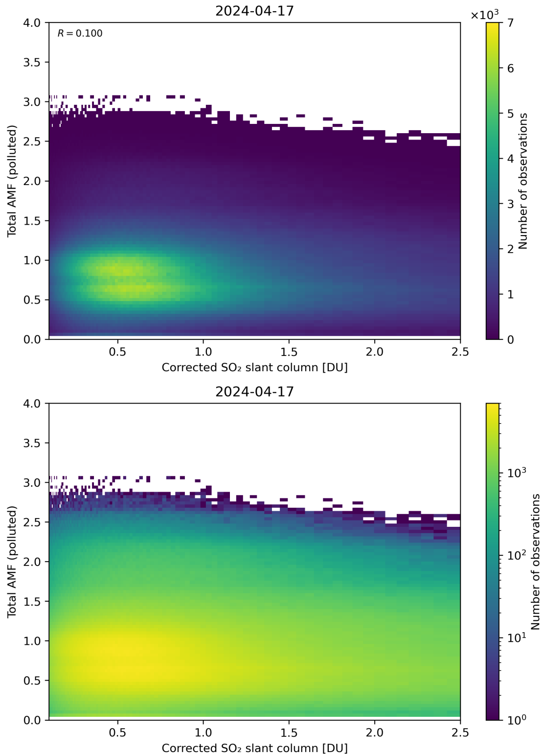
Figure 192: Scatter density plot of “Corrected SO 2 slant column” against “Total AMF (polluted)” for 2024-04-16 to 2024-04-18.
