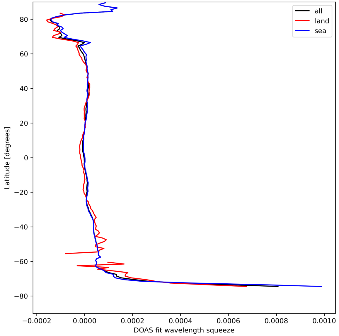
Figure 46: Zonal average of “DOAS fit wavelength squeeze” for 2024-04-16 to 2024-04-18.
