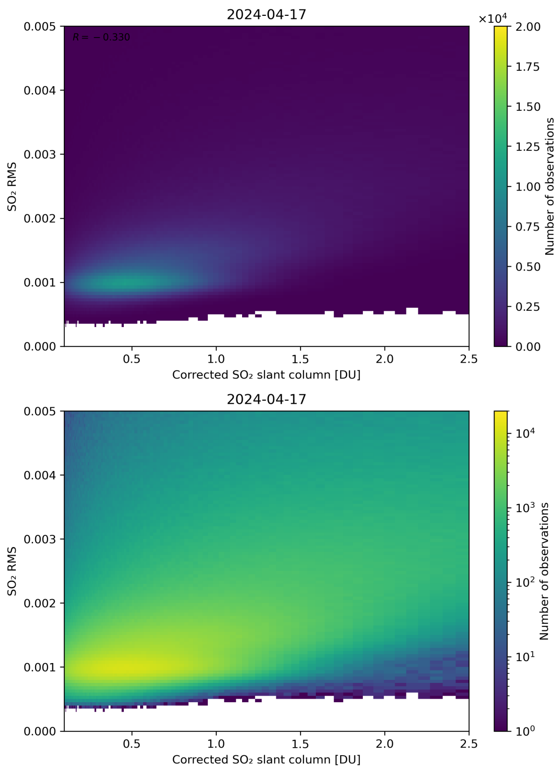
Figure 183: Scatter density plot of “Corrected SO 2 slant column” against “SO 2 RMS” for 2024-04-16 to 2024-04-18.
