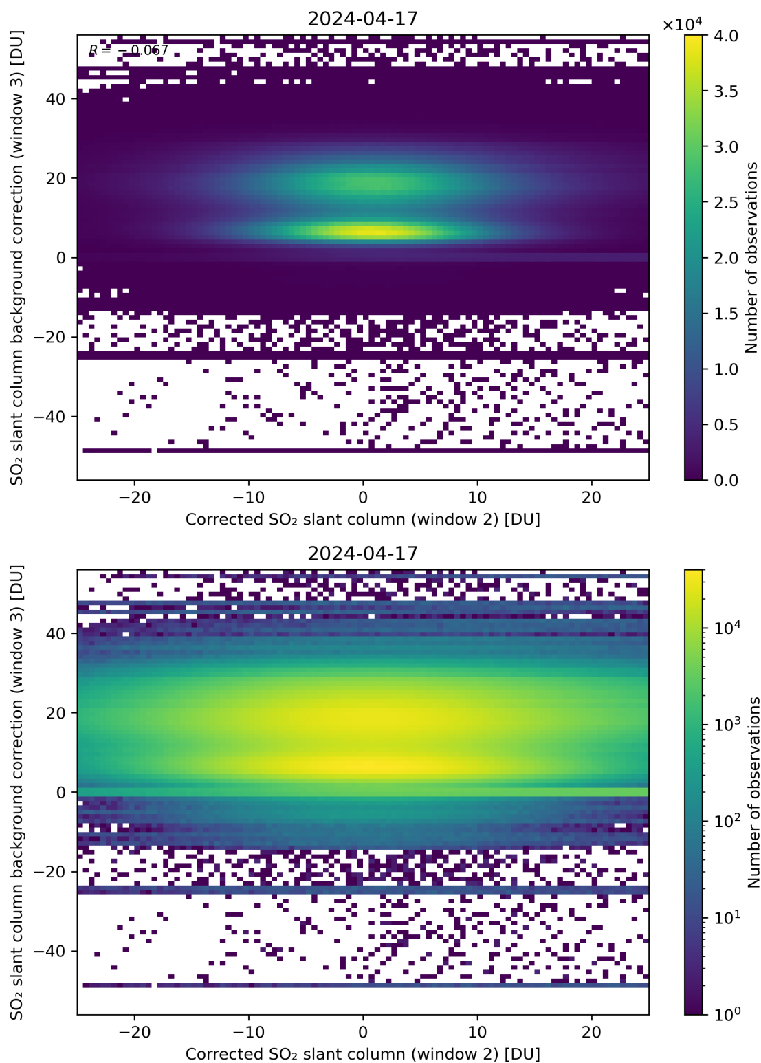
Figure 195: Scatter density plot of “Corrected SO 2 slant column (window 2)” against “SO 2 slant column background correction (window 3)” for 2024-04-16 to 2024-04-18.
