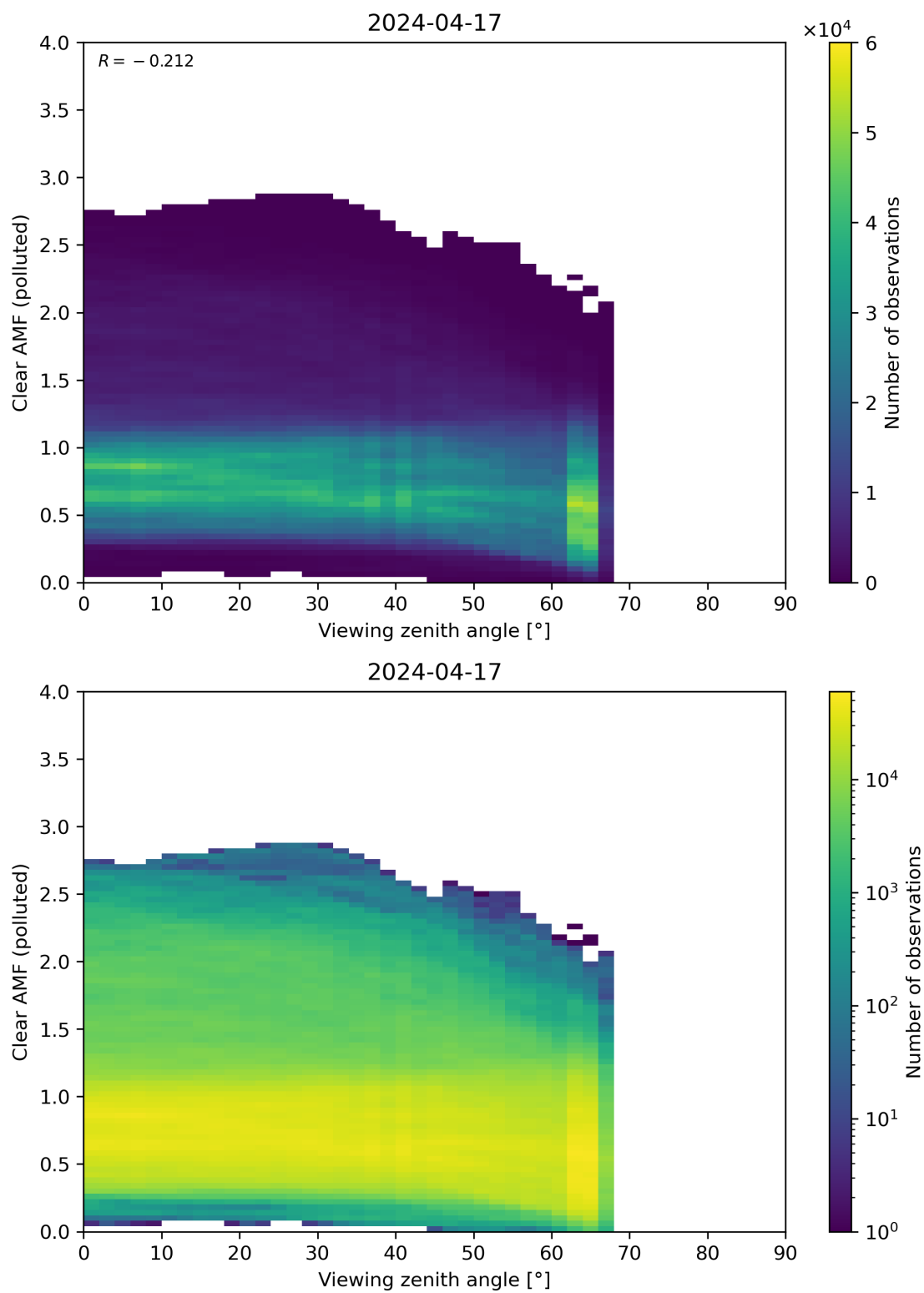
Figure 316: Scatter density plot of “Viewing zenith angle” against “Clear AMF (polluted)” for 2024-04-16 to 2024-04-18.
