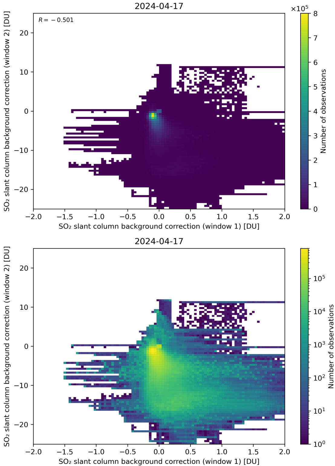
Figure 98: Scatter density plot of “SO 2 slant column background correction (window 1)” against “SO 2 slant column background correction (window 2)” for 2024-04-16 to 2024-04-18.
