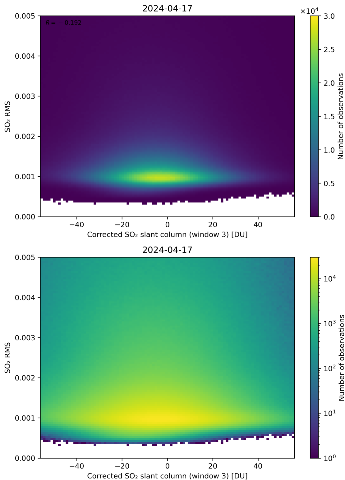
Figure 208: Scatter density plot of “Corrected SO 2 slant column (window 3)” against “SO 2 RMS” for 2024-04-16 to 2024-04-18.
