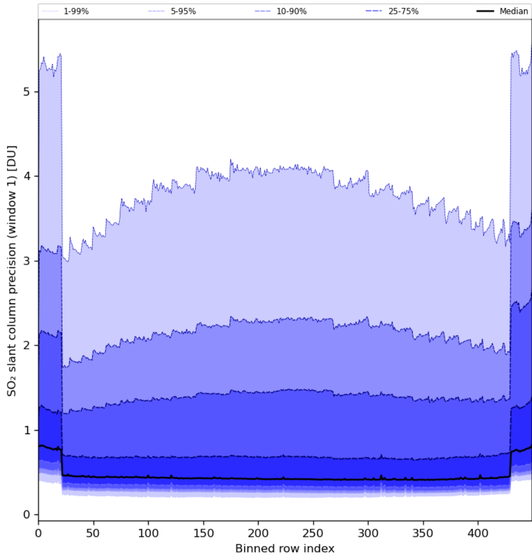
Figure 80: Along track statistics of “SO 2 slant column precision (window 1)” for 2024-04-16 to 2024-04-18
