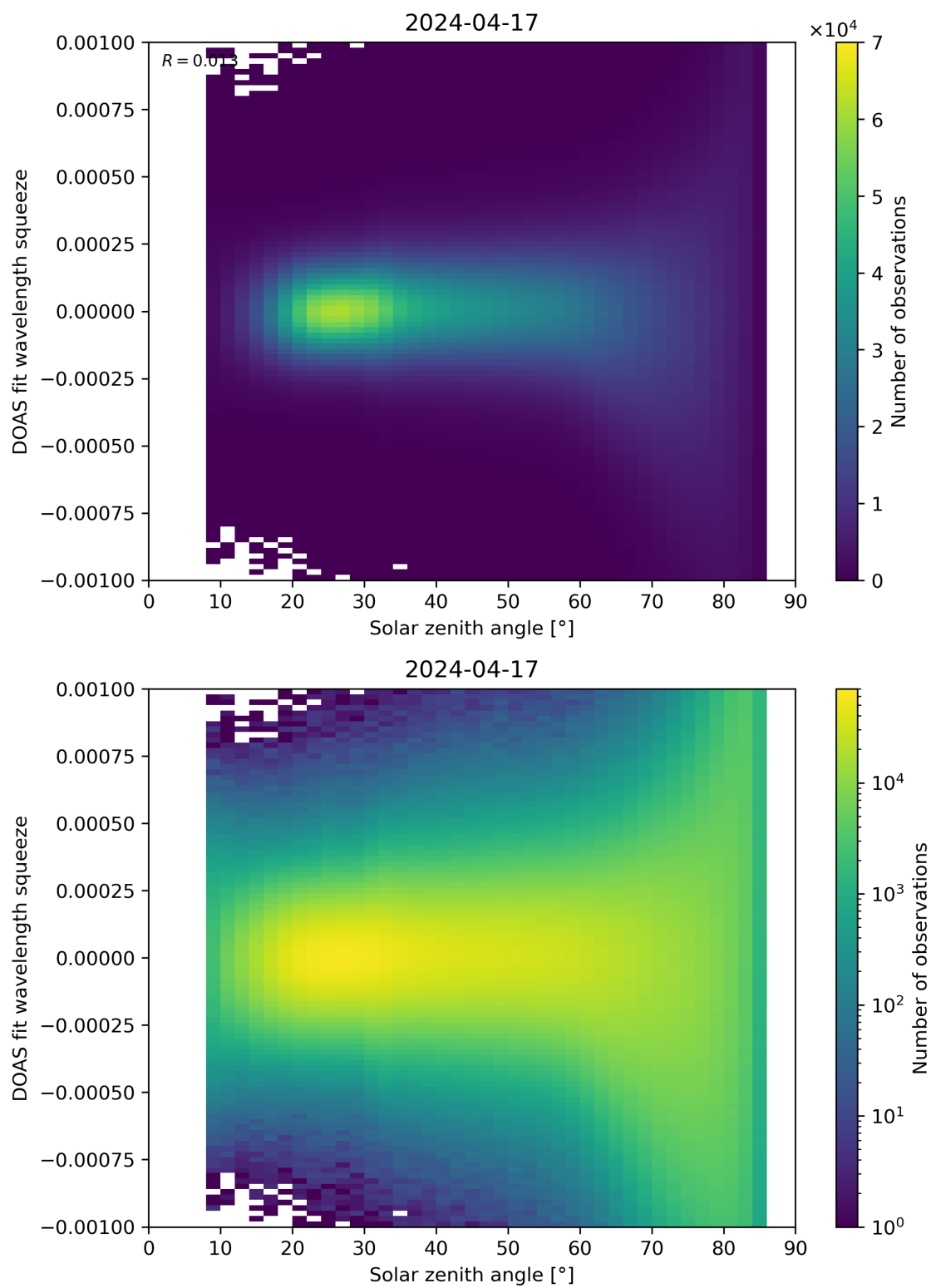
Figure 162: Scatter density plot of “Solar zenith angle” against “DOAS fit wavelength squeeze” for 2024-04-16 to 2024-04-18.
