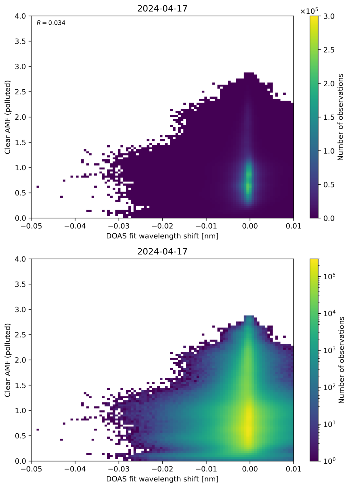
Figure 129: Scatter density plot of “DOAS fit wavelength shift” against “Clear AMF (polluted)” for 2024-04-16 to 2024-04-18.
