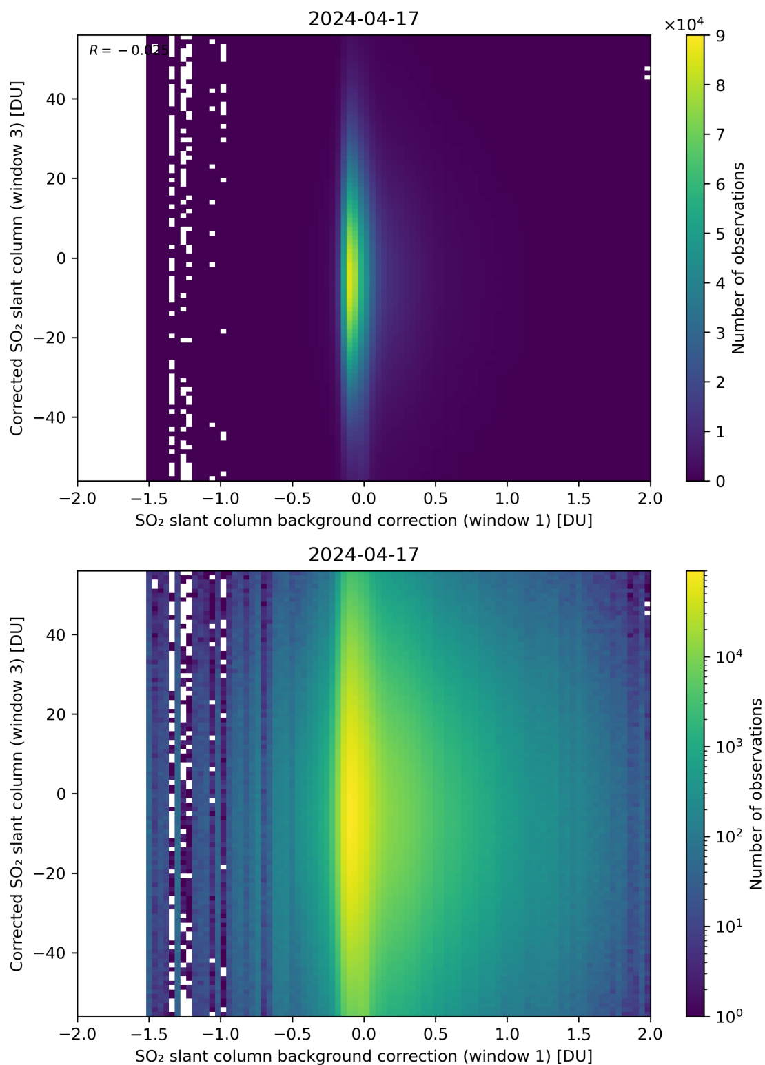
Figure 105: Scatter density plot of “SO 2 slant column background correction (window 1)” against “Corrected SO 2 slant column (window 3)” for 2024-04-16 to 2024-04-18.
