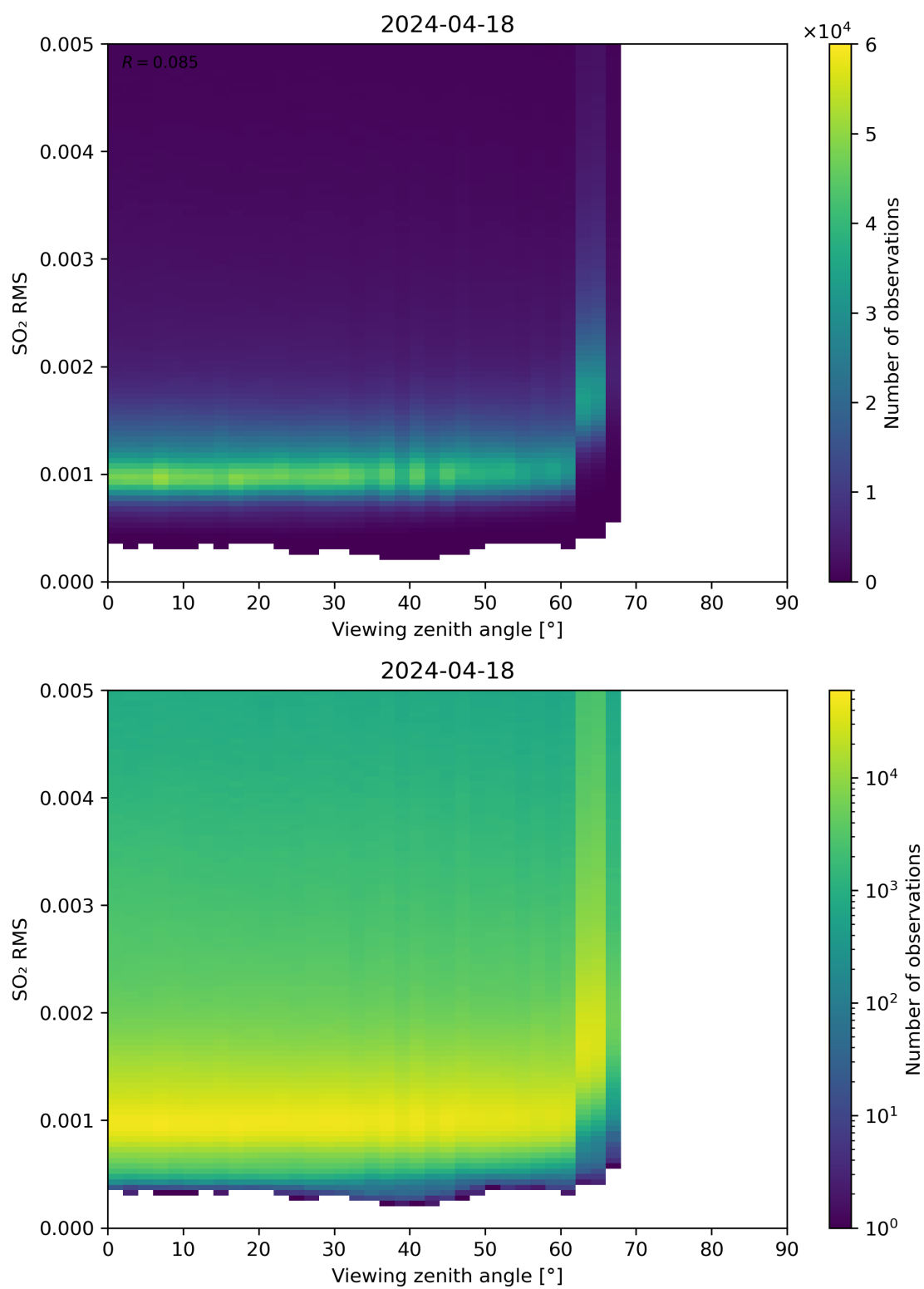
Figure 313: Scatter density plot of “Viewing zenith angle” against “SO 2 RMS” for 2024-04-17 to 2024-04-19.
