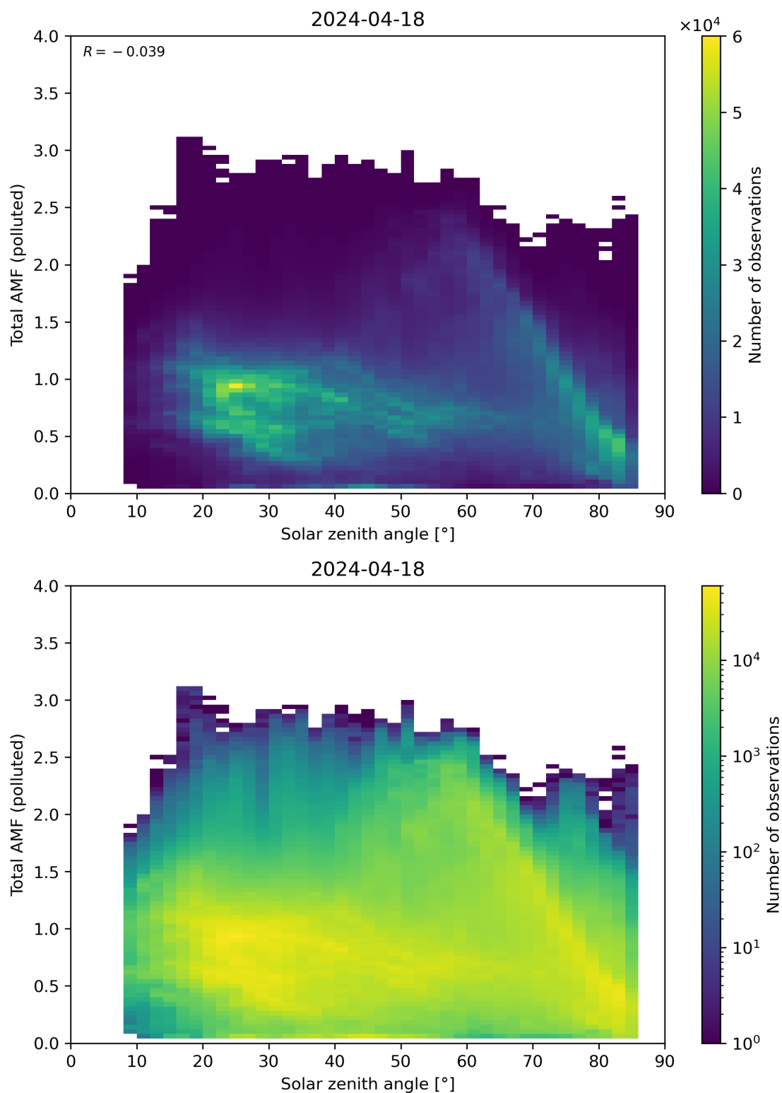
Figure 174: Scatter density plot of “Solar zenith angle” against “Total AMF (polluted)” for 2024-04-17 to 2024-04-19.
