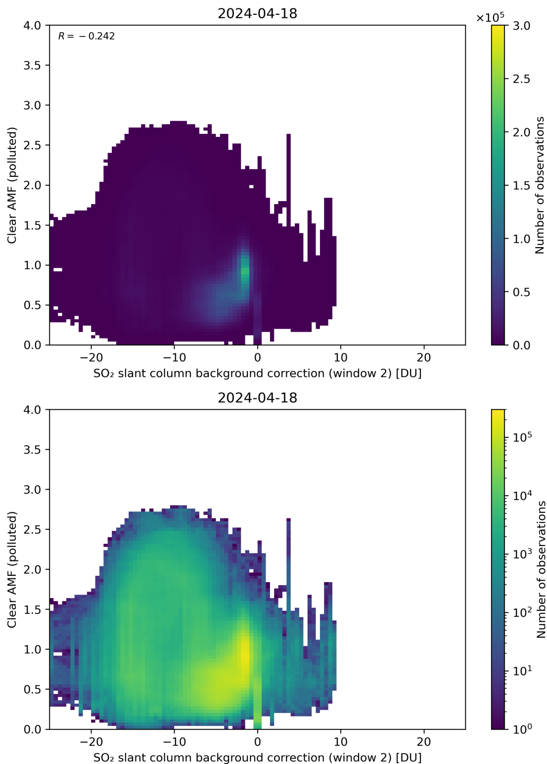
Figure 115: Scatter density plot of “SO 2 slant column background correction (window 2)” against “Clear AMF (polluted)” for 2024-04-17 to 2024-04-19.
