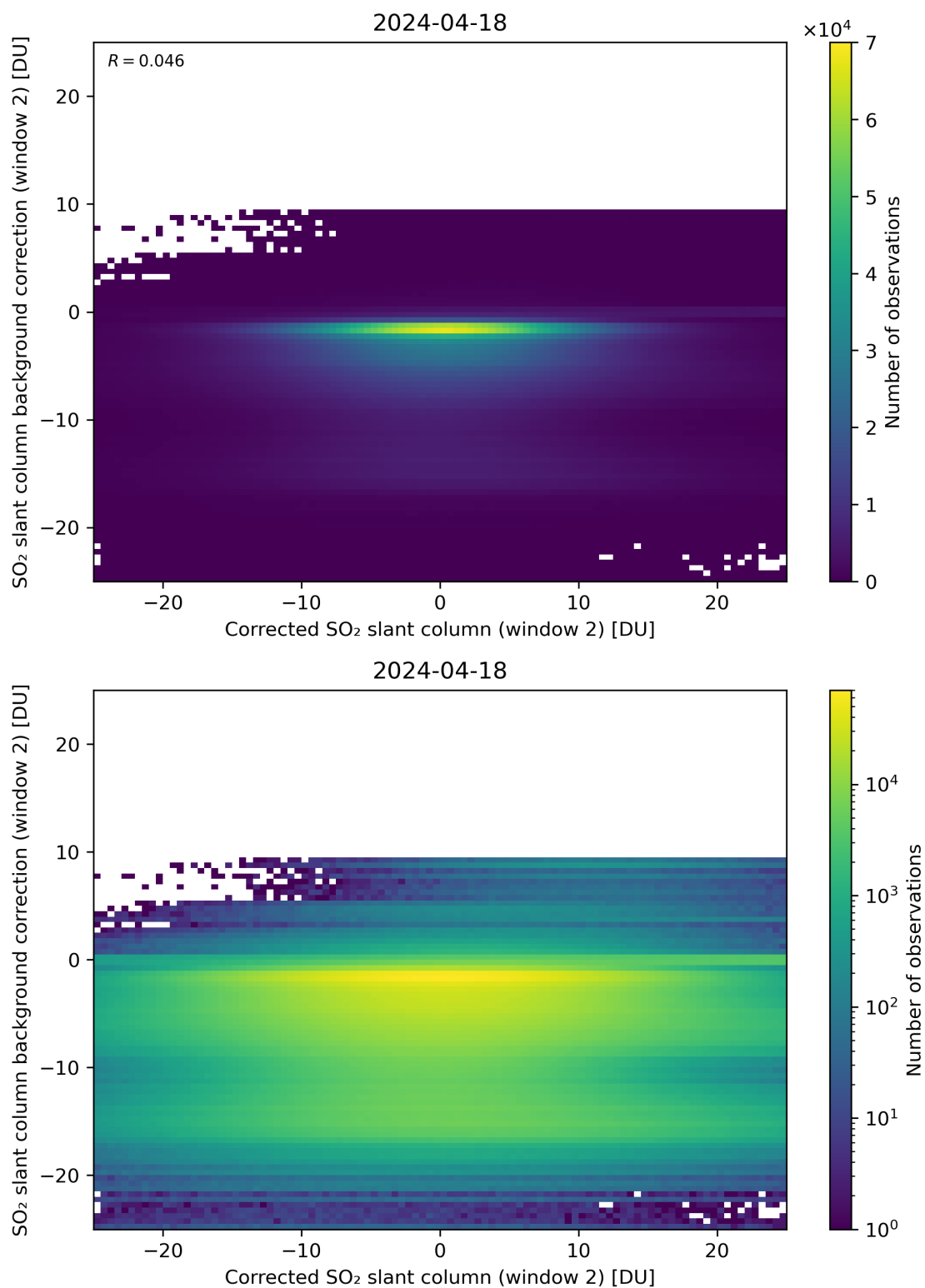
Figure 194: Scatter density plot of “Corrected SO 2 slant column (window 2)” against “SO 2 slant column background correction (window 2)” for 2024-04-17 to 2024-04-19.
