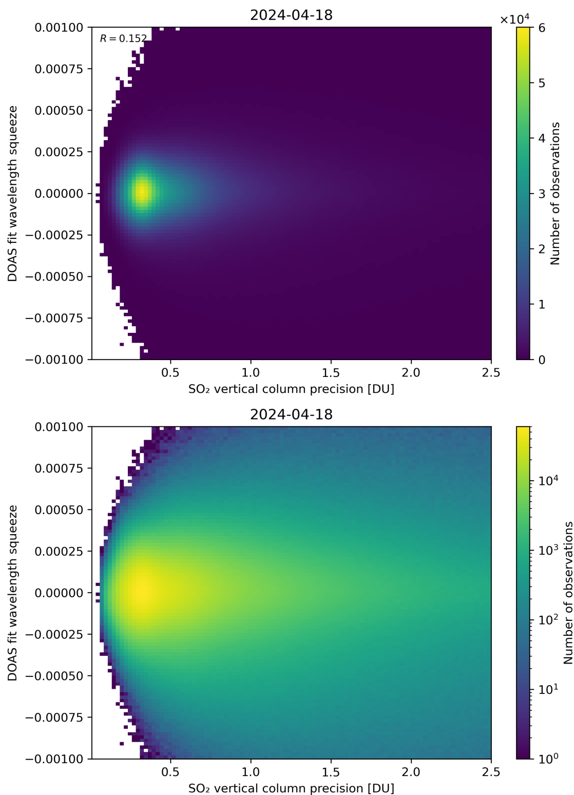
Figure 283: Scatter density plot of “SO 2 vertical column precision” against “DOAS fit wavelength squeeze” for 2024-04-17 to 2024-04-19.
