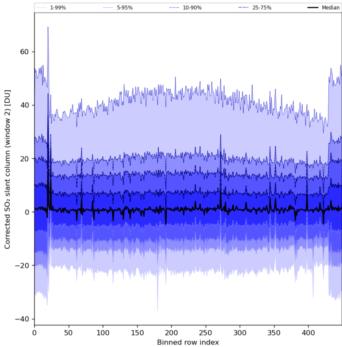
Figure 85: Along track statistics of “Corrected SO 2 slant column (window 2)” for 2024-04-17 to 2024-04-19
