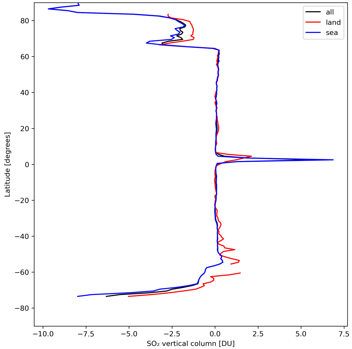
Figure 30: Zonal average of “SO 2 vertical column” for 2024-04-17 to 2024-04-19.
