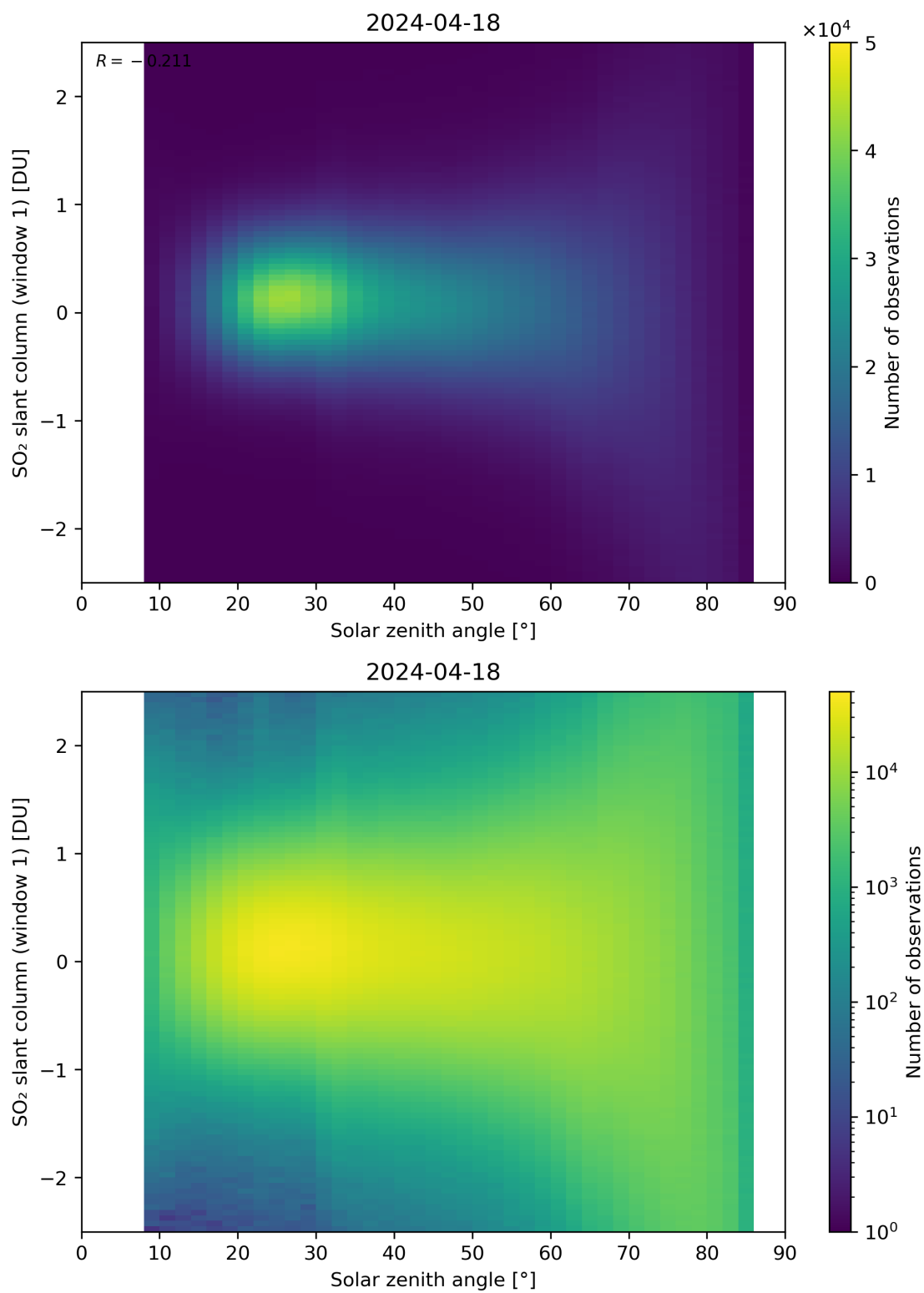
Figure 169: Scatter density plot of “Solar zenith angle” against “SO 2 slant column (window 1)” for 2024-04-17 to 2024-04-19.
