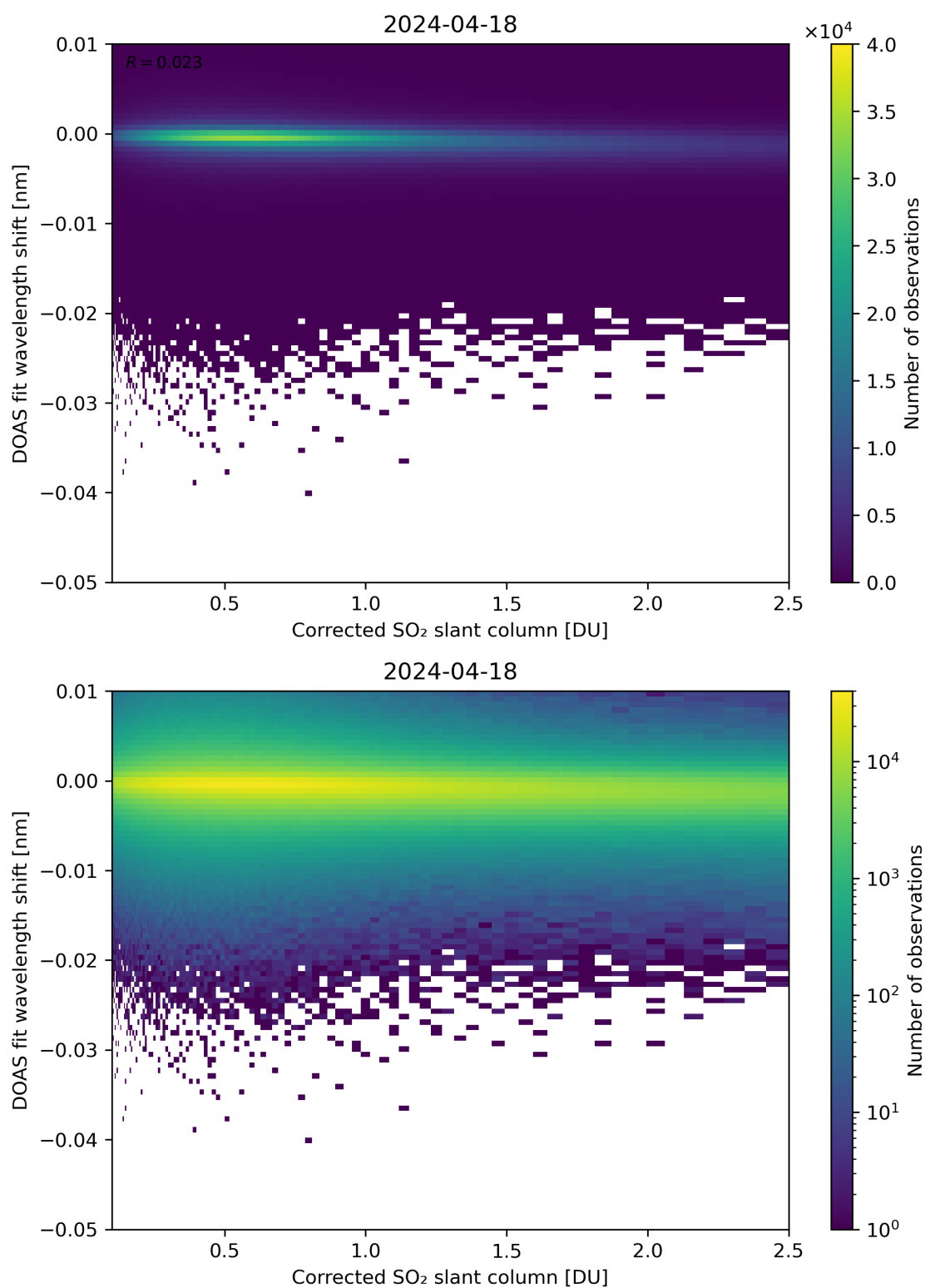
Figure 181: Scatter density plot of “Corrected SO 2 slant column” against “DOAS fit wavelength shift” for 2024-04-17 to 2024-04-19.
