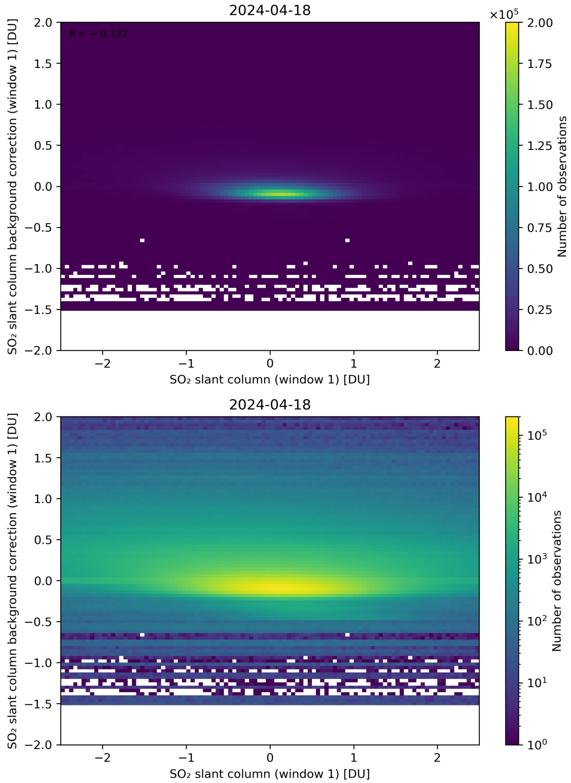
Figure 212: Scatter density plot of “SO 2 slant column (window 1)” against “SO 2 slant column background correction (window 1)” for 2024-04-17 to 2024-04-19.
