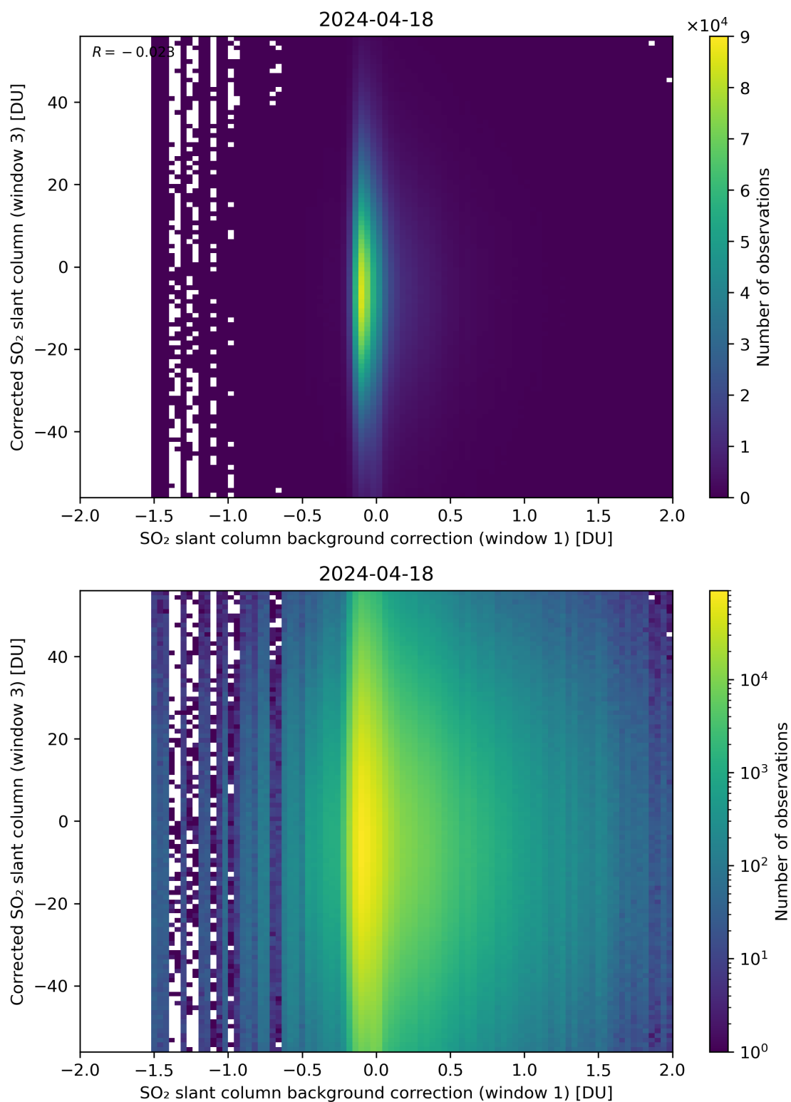
Figure 105: Scatter density plot of “SO 2 slant column background correction (window 1)” against “Corrected SO 2 slant column (window 3)” for 2024-04-17 to 2024-04-19.
