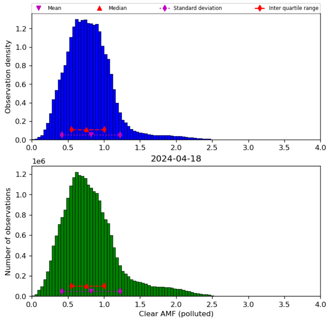
Figure 73: Histogram of “Clear AMF (polluted)” for 2024-04-17 to 2024-04-19
