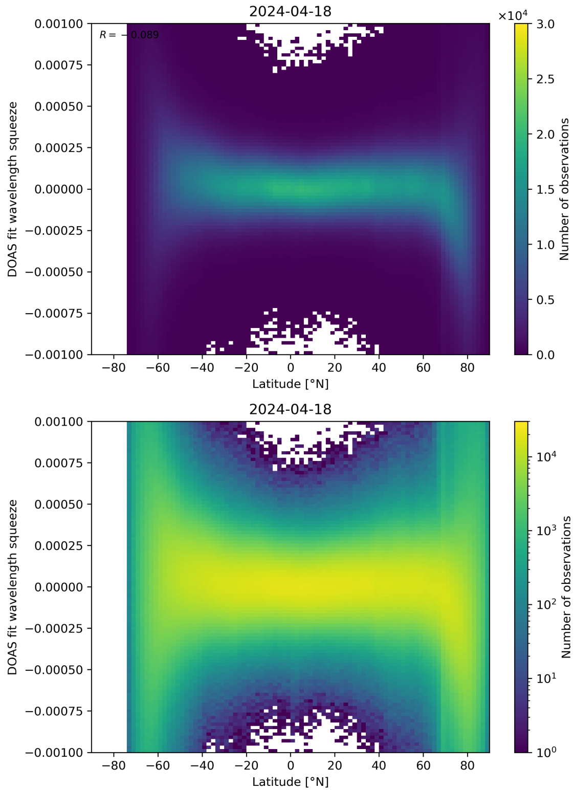
Figure 143: Scatter density plot of “Latitude” against “DOAS fit wavelength squeeze” for 2024-04-17 to 2024-04-19.
