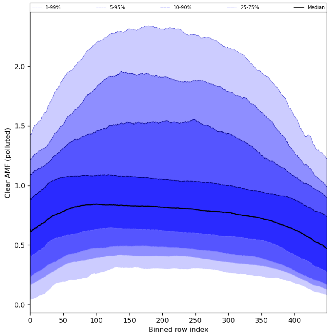
Figure 96: Along track statistics of “Clear AMF (polluted)” for 2024-04-17 to 2024-04-19
