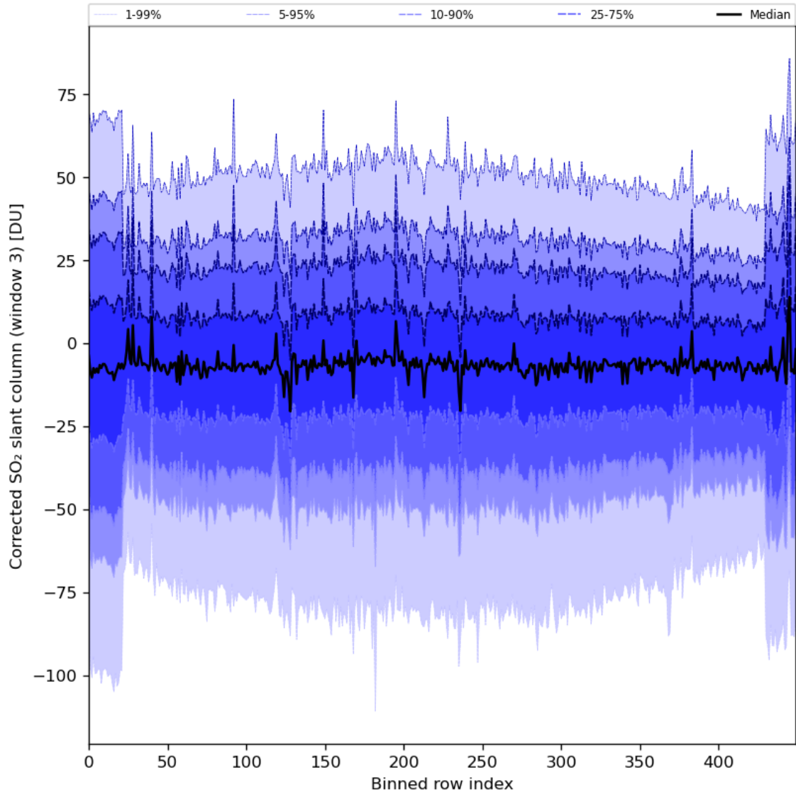
Figure 89: Along track statistics of “Corrected SO 2 slant column (window 3)” for 2024-04-17 to 2024-04-19
