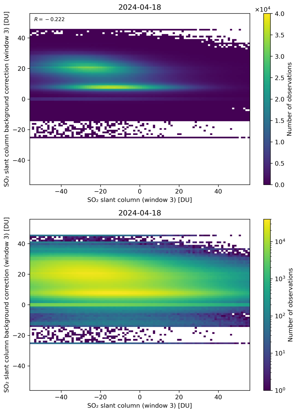
Figure 253: Scatter density plot of “SO 2 slant column (window 3)” against “SO 2 slant column background correction (window 3)” for 2024-04-17 to 2024-04-19.
