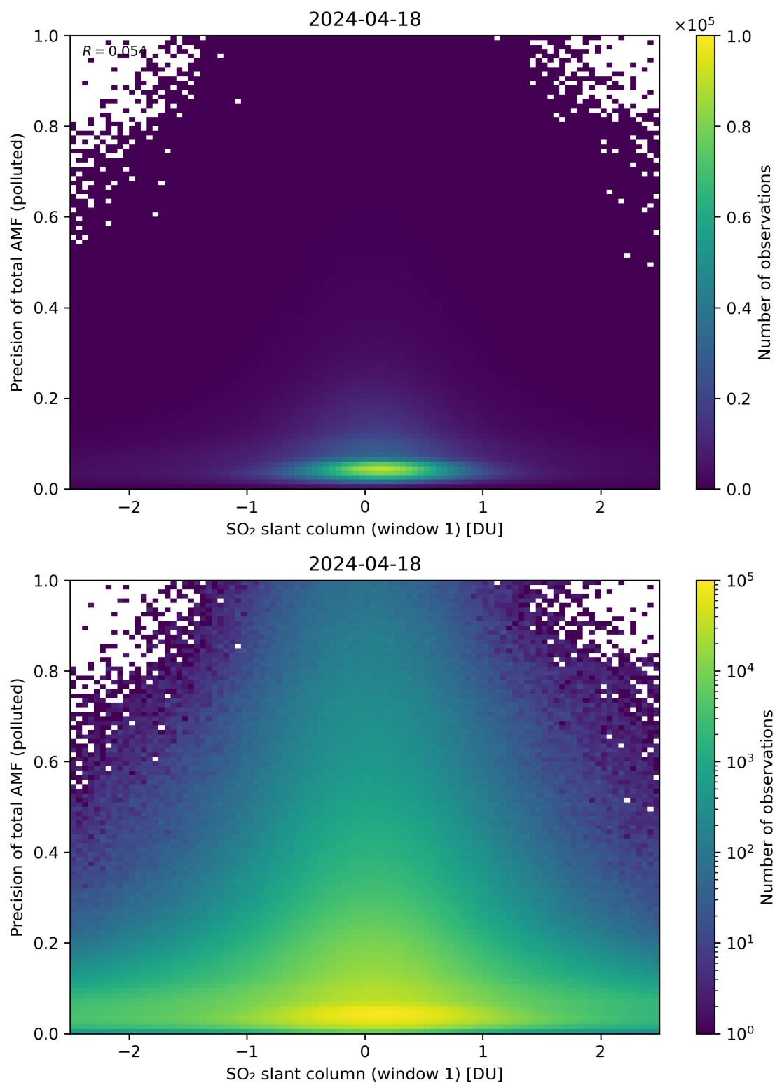
Figure 240: Scatter density plot of “SO 2 slant column (window 1)” against “Precision of total AMF (polluted)” for 2024-04-17 to 2024-04-19.
