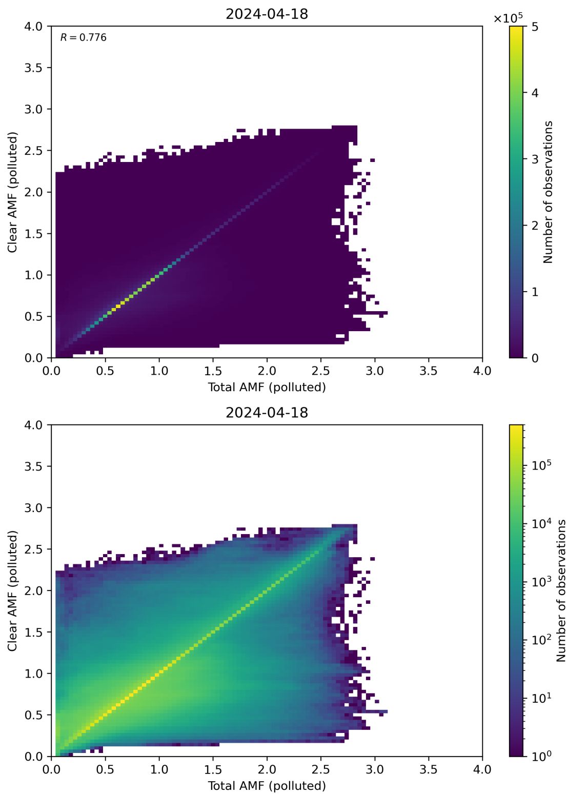
Figure 271: Scatter density plot of “Total AMF (polluted)” against “Clear AMF (polluted)” for 2024-04-17 to 2024-04-19.
