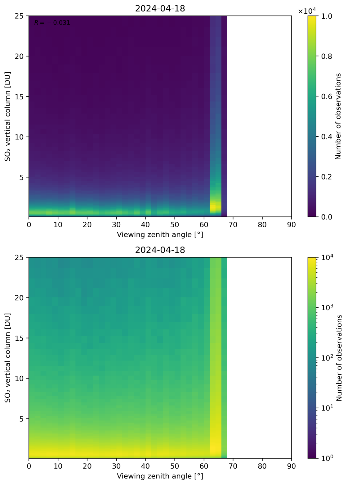
Figure 327: Scatter density plot of “Viewing zenith angle” against “SO 2 vertical column” for 2024-04-17 to 2024-04-19.
