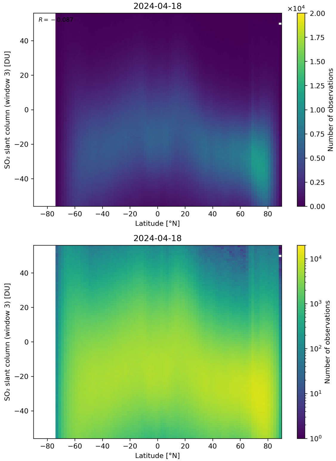
Figure 152: Scatter density plot of “Latitude” against “SO 2 slant column (window 3)” for 2024-04-17 to 2024-04-19.
