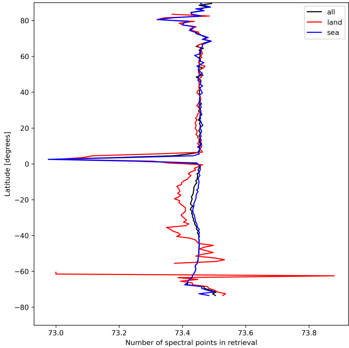
Figure 51: Zonal average of “Number of spectral points in retrieval” for 2024-04-17 to 2024-04-19.
