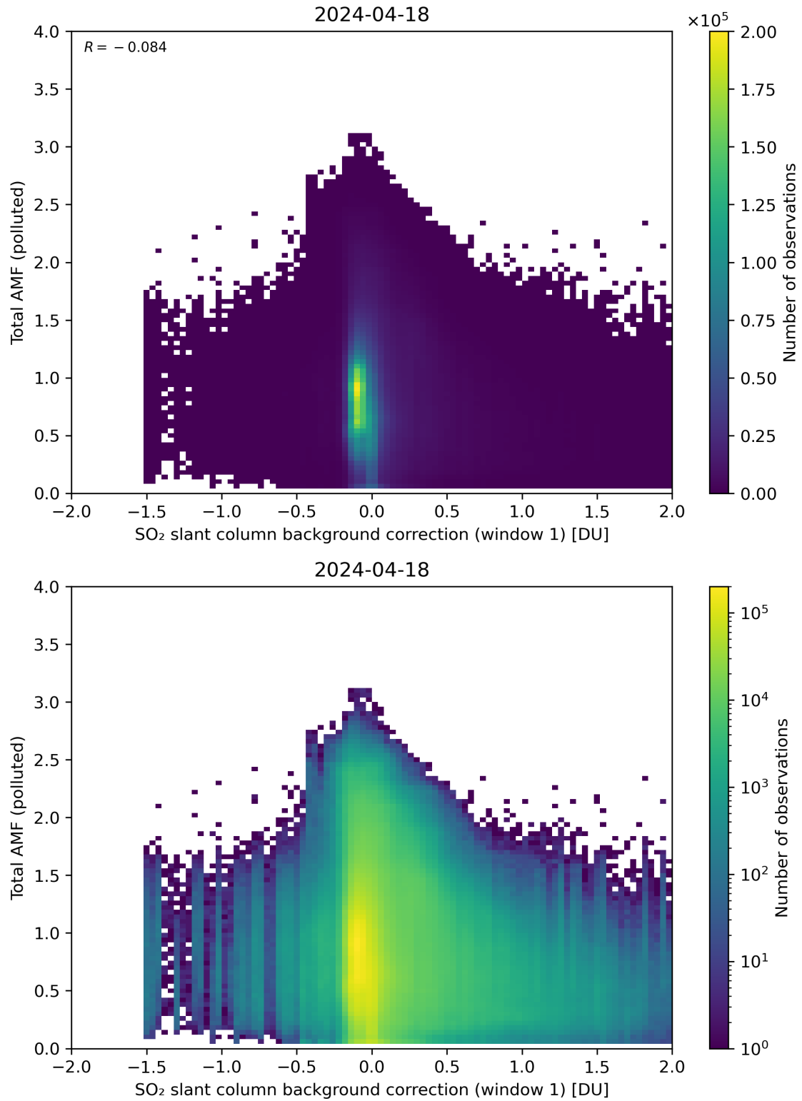
Figure 109: Scatter density plot of “SO 2 slant column background correction (window 1)” against “Total AMF (polluted)” for 2024-04-17 to 2024-04-19.
