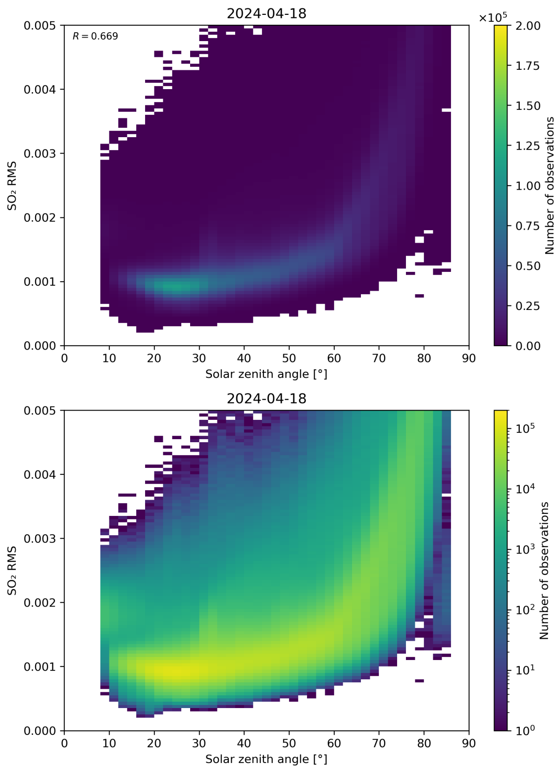
Figure 163: Scatter density plot of “Solar zenith angle” against “SO 2 RMS” for 2024-04-17 to 2024-04-19.
