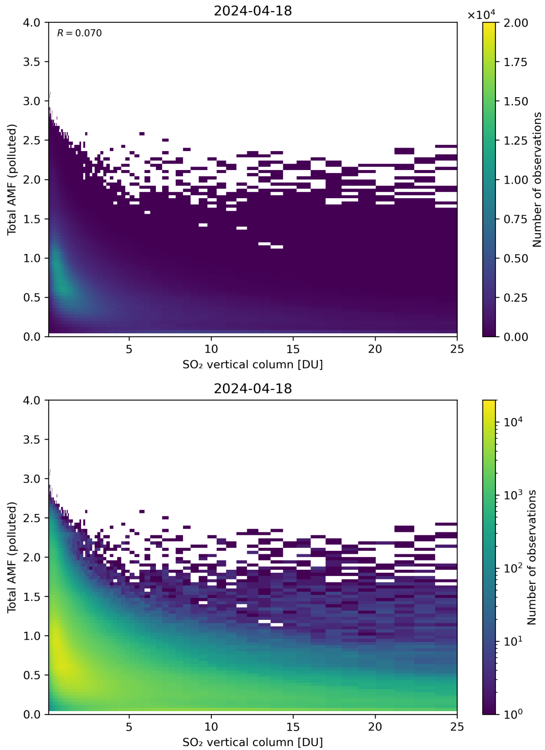
Figure 305: Scatter density plot of “SO 2 vertical column” against “Total AMF (polluted)” for 2024-04-17 to 2024-04-19.
