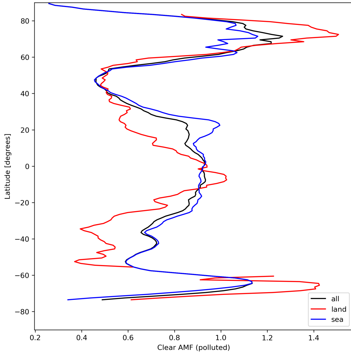
Figure 50: Zonal average of “Clear AMF (polluted)” for 2024-04-17 to 2024-04-19.
