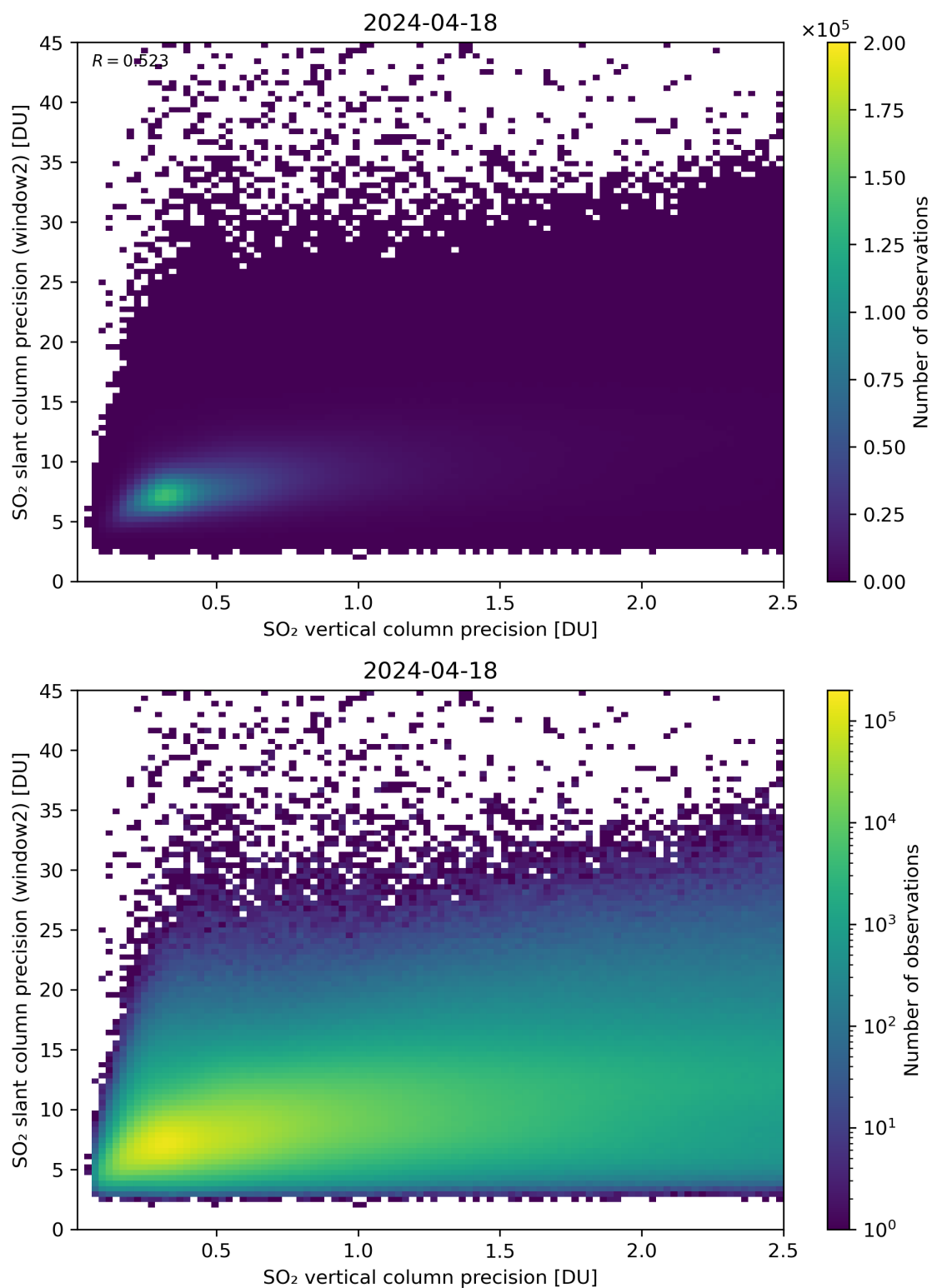
Figure 291: Scatter density plot of “SO 2 vertical column precision” against “SO 2 slant column precision (window2)” for 2024-04-17 to 2024-04-19.
