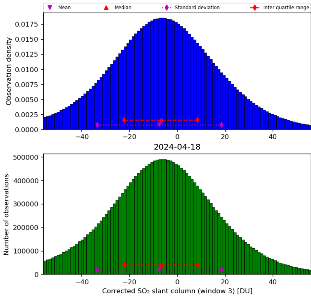
Figure 66: Histogram of “Corrected SO 2 slant column (window 3)” for 2024-04-17 to 2024-04-19
