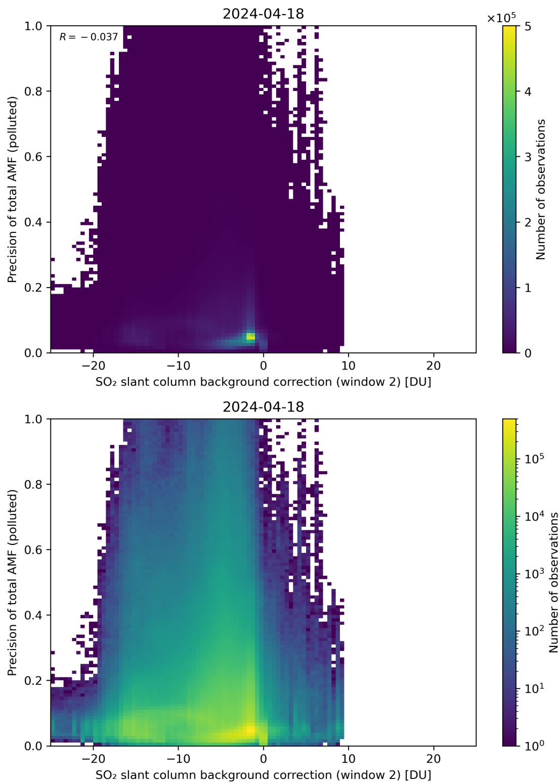
Figure 120: Scatter density plot of “SO 2 slant column background correction (window 2)” against “Precision of total AMF (polluted)” for 2024-04-17 to 2024-04-19.
