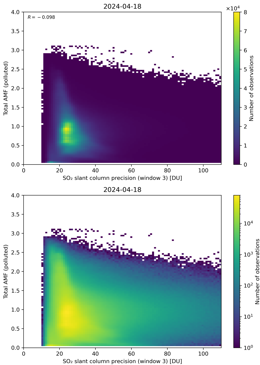
Figure 263: Scatter density plot of “SO 2 slant column precision (window 3)” against “Total AMF (polluted)” for 2024-04-17 to 2024-04-19.
