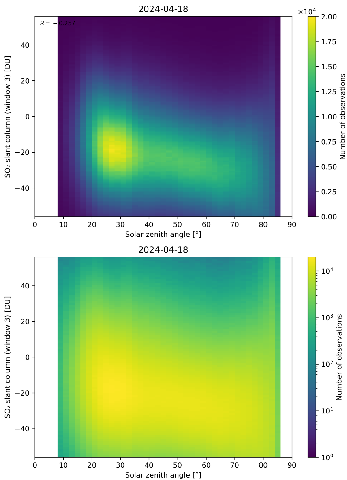
Figure 172: Scatter density plot of “Solar zenith angle” against “SO 2 slant column (window 3)” for 2024-04-17 to 2024-04-19.
