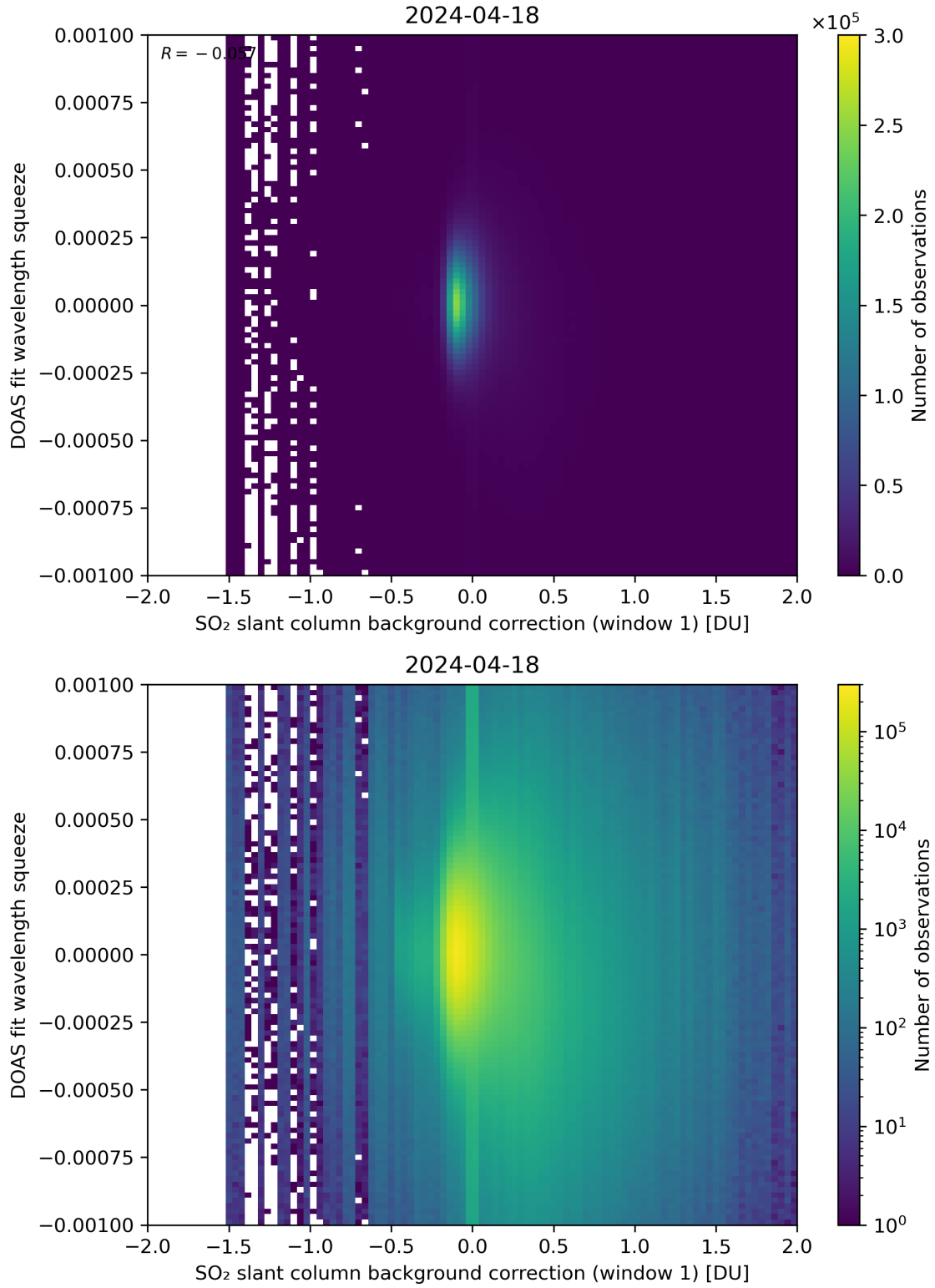
Figure 101: Scatter density plot of “SO 2 slant column background correction (window 1)” against “DOAS fit wavelength squeeze” for 2024-04-17 to 2024-04-19.
