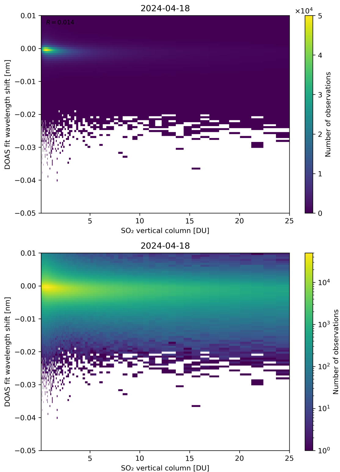
Figure 276: Scatter density plot of “SO 2 vertical column” against “DOAS fit wavelength shift” for 2024-04-17 to 2024-04-19.
