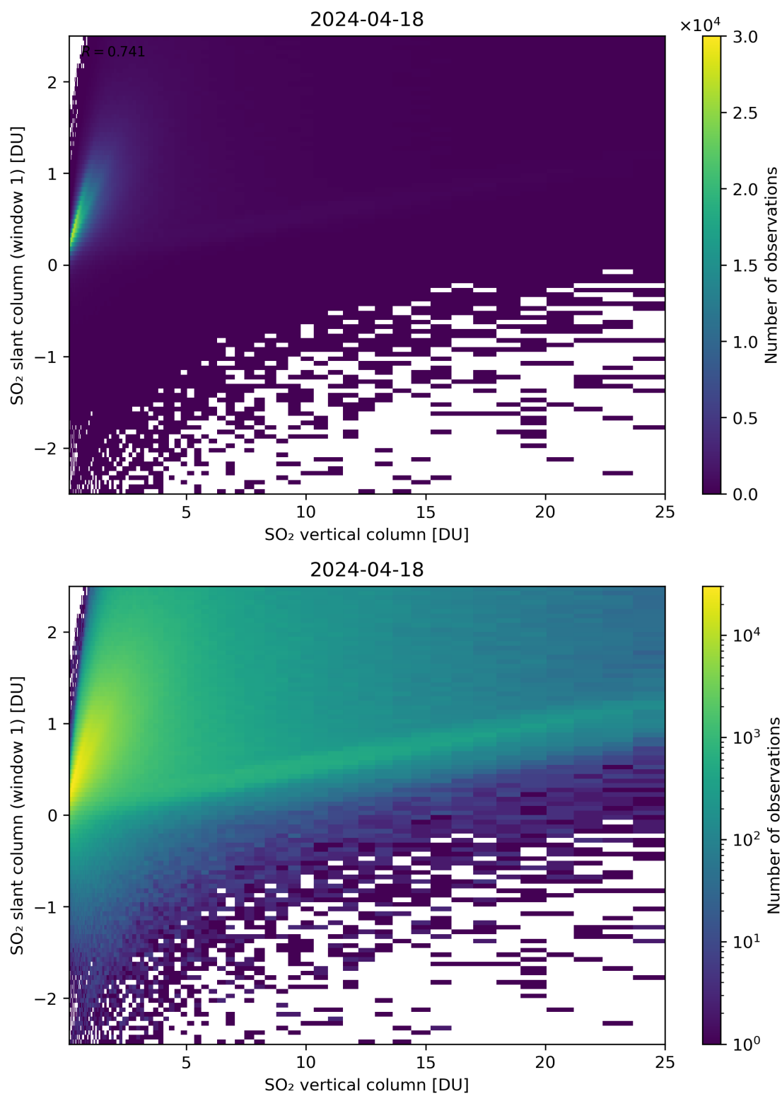
Figure 300: Scatter density plot of “SO 2 vertical column” against “SO 2 slant column (window 1)” for 2024-04-17 to 2024-04-19.
