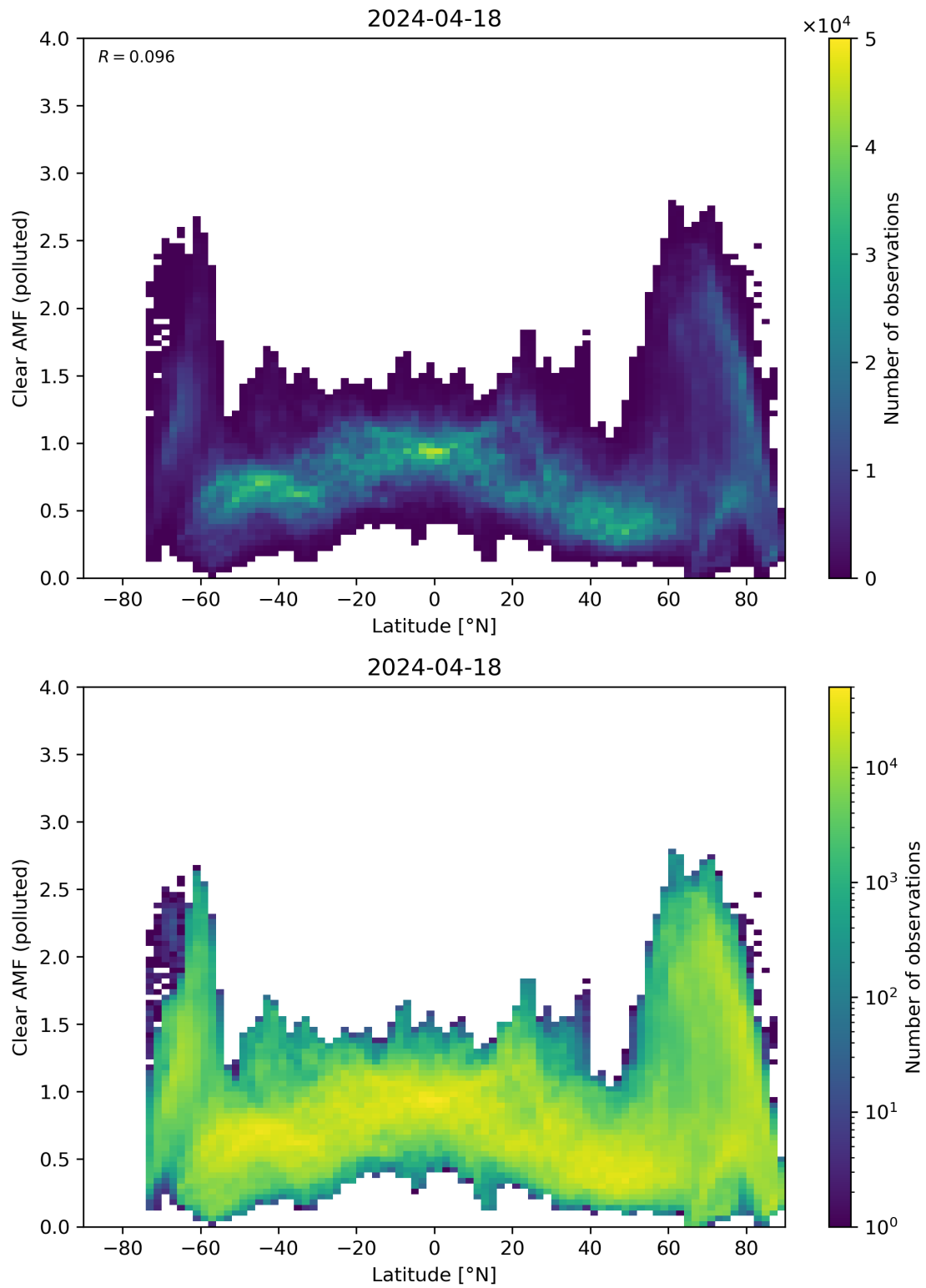
Figure 145: Scatter density plot of “Latitude” against “Clear AMF (polluted)” for 2024-04-17 to 2024-04-19.
