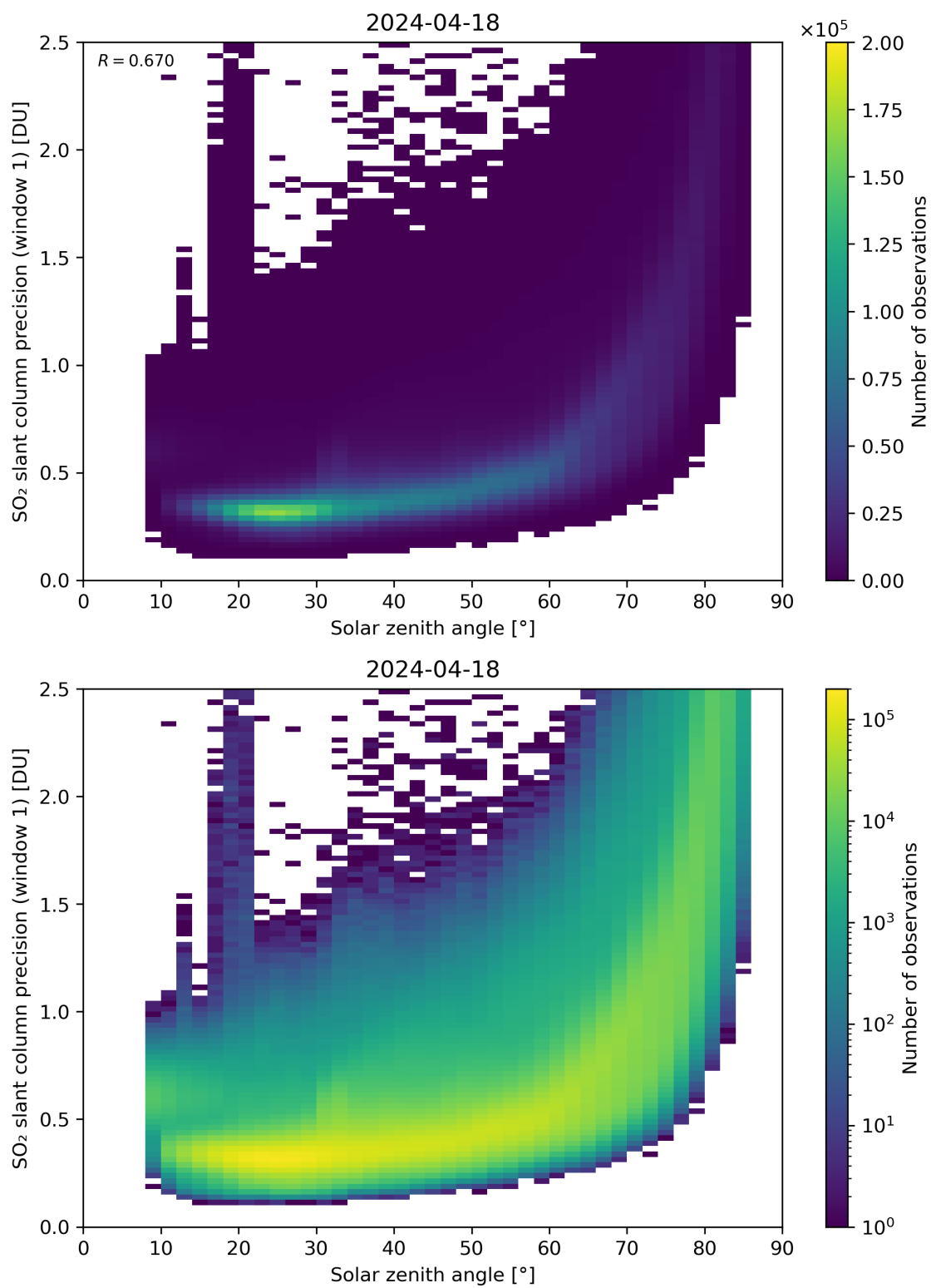
Figure 170: Scatter density plot of “Solar zenith angle” against “SO 2 slant column precision (window 1)” for 2024-04-17 to 2024-04-19.
