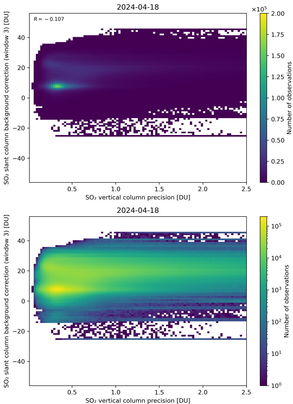
Figure 281: Scatter density plot of “SO 2 vertical column precision” against “SO 2 slant column background correction (window 3)” for 2024-04-17 to 2024-04-19.
