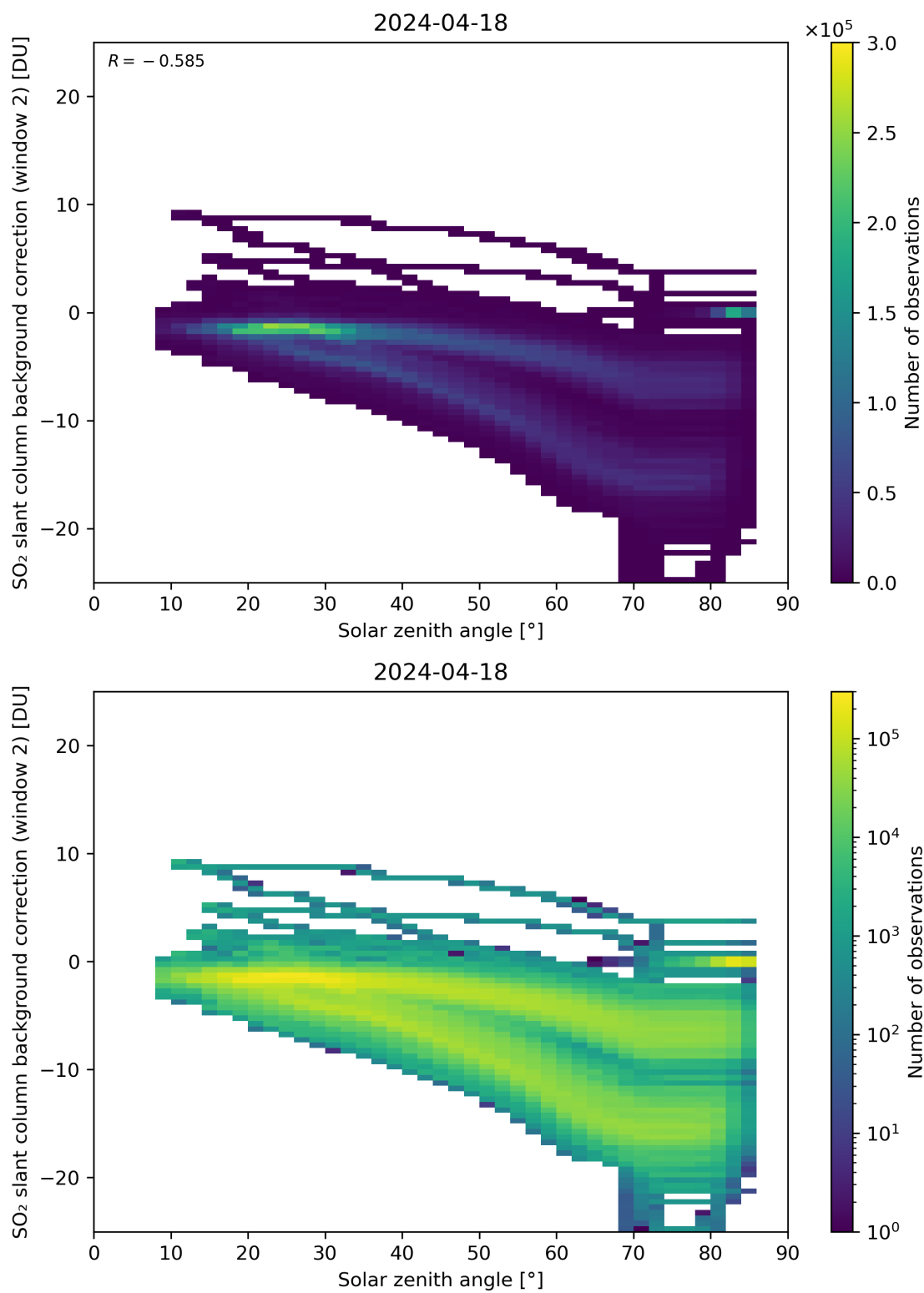
Figure 159: Scatter density plot of “Solar zenith angle” against “SO 2 slant column background correction (window 2)” for 2024-04-17 to 2024-04-19.
