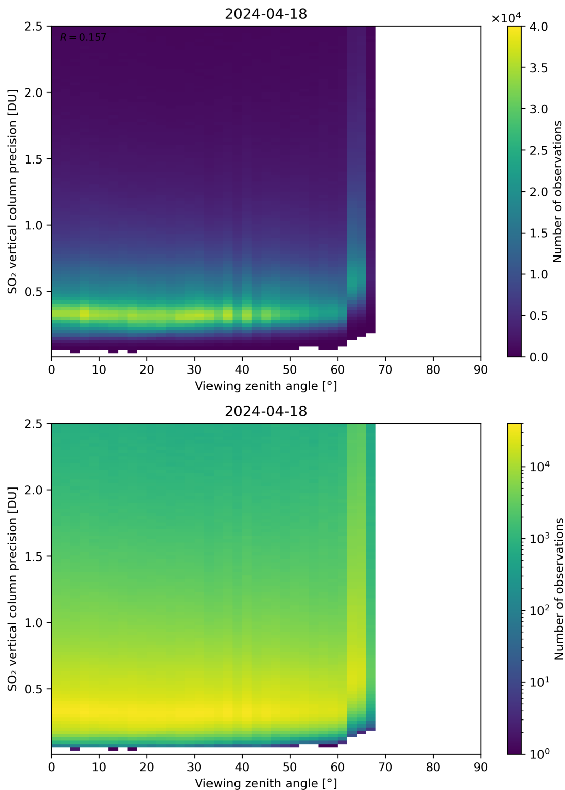
Figure 328: Scatter density plot of “Viewing zenith angle” against “SO 2 vertical column precision” for 2024-04-17 to 2024-04-19.
