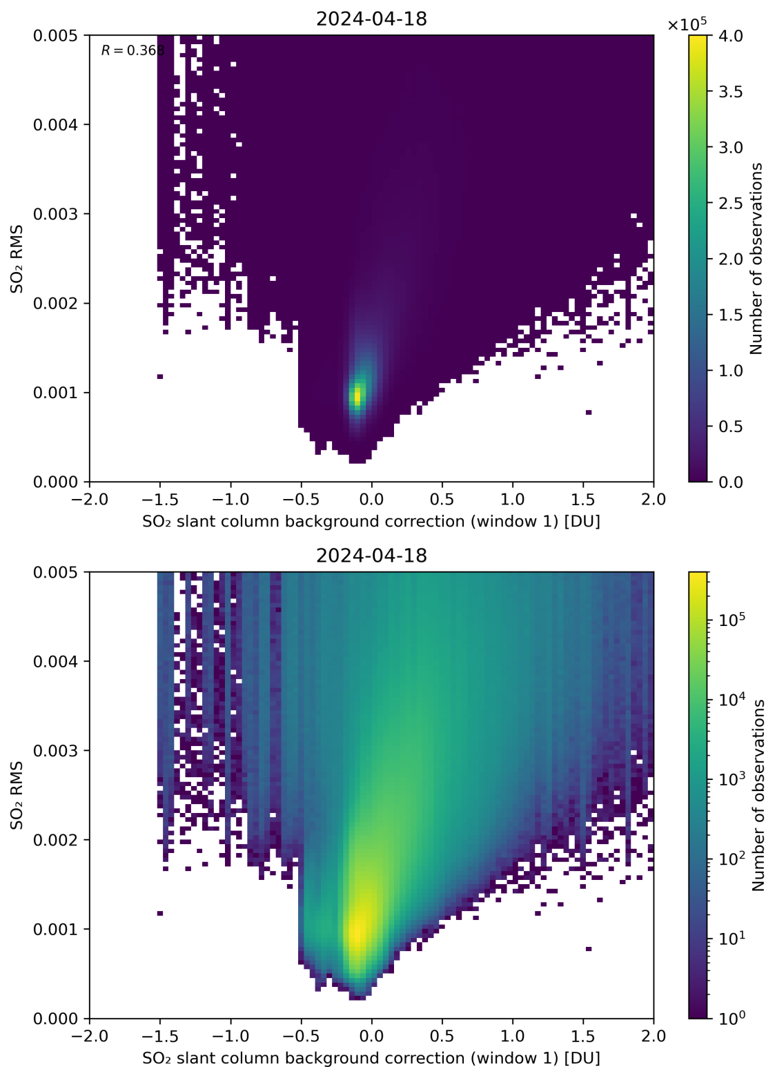
Figure 102: Scatter density plot of “SO 2 slant column background correction (window 1)” against “SO 2 RMS” for 2024-04-17 to 2024-04-19.
