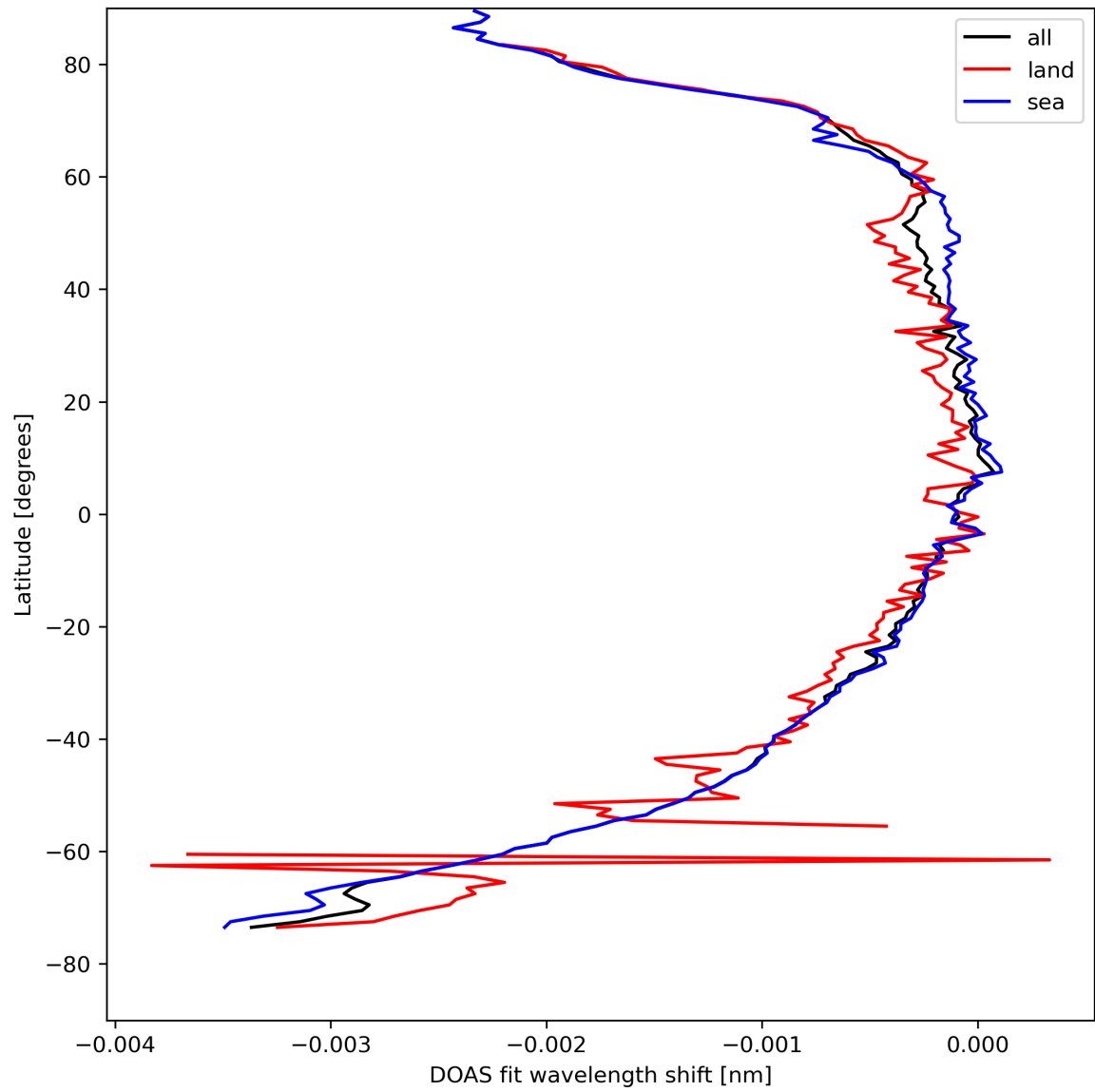
Figure 45: Zonal average of “DOAS fit wavelength shift” for 2024-04-17 to 2024-04-19.
