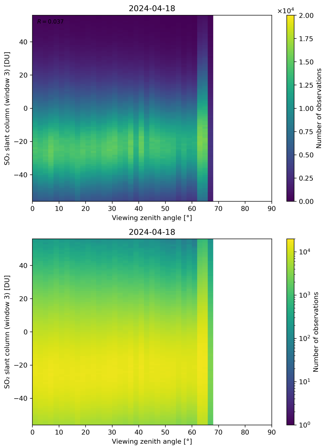
Figure 323: Scatter density plot of “Viewing zenith angle” against “SO 2 slant column (window 3)” for 2024-04-17 to 2024-04-19.
