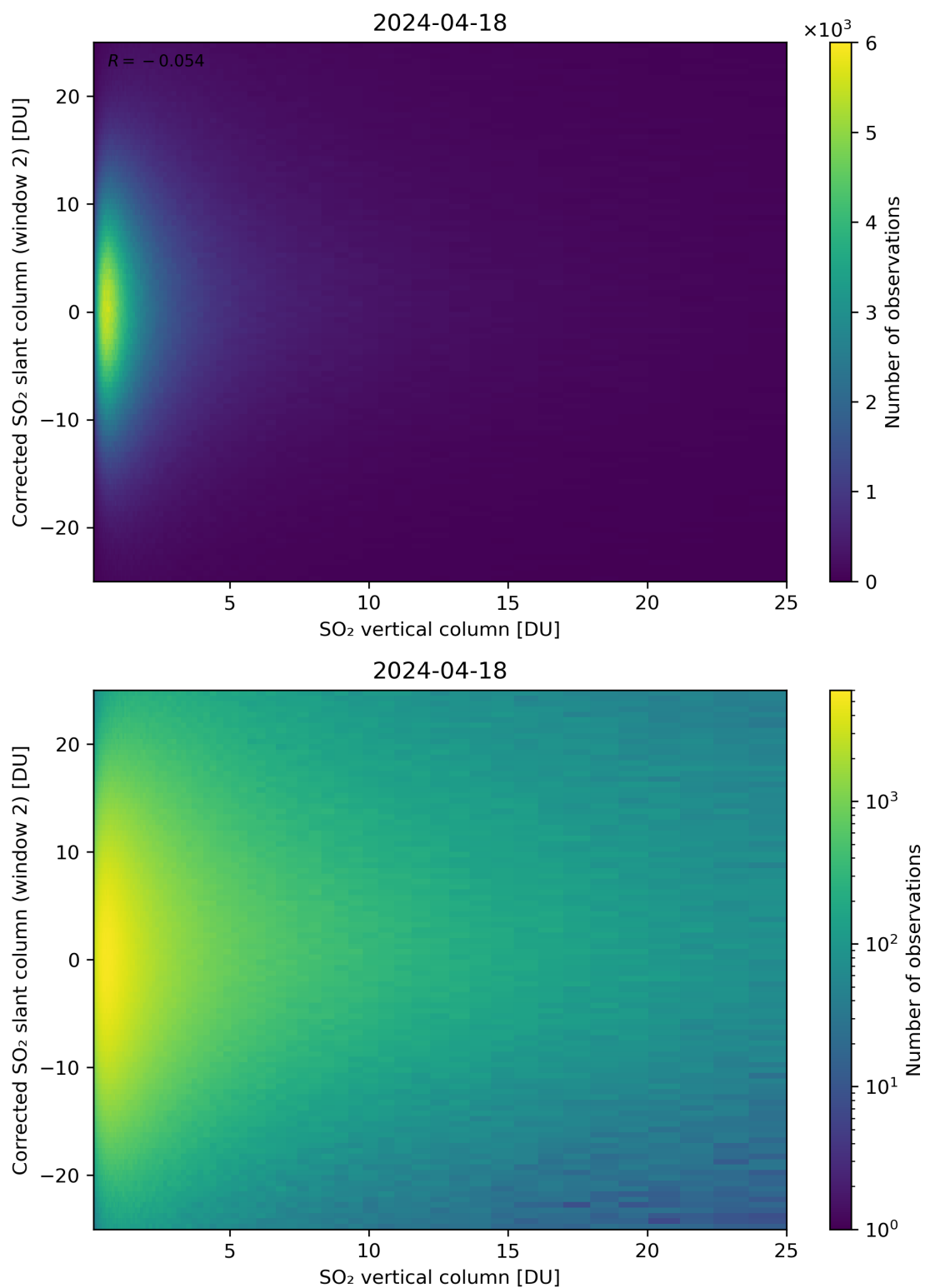
Figure 298: Scatter density plot of “SO 2 vertical column” against “Corrected SO 2 slant column (window 2)” for 2024-04-17 to 2024-04-19.
