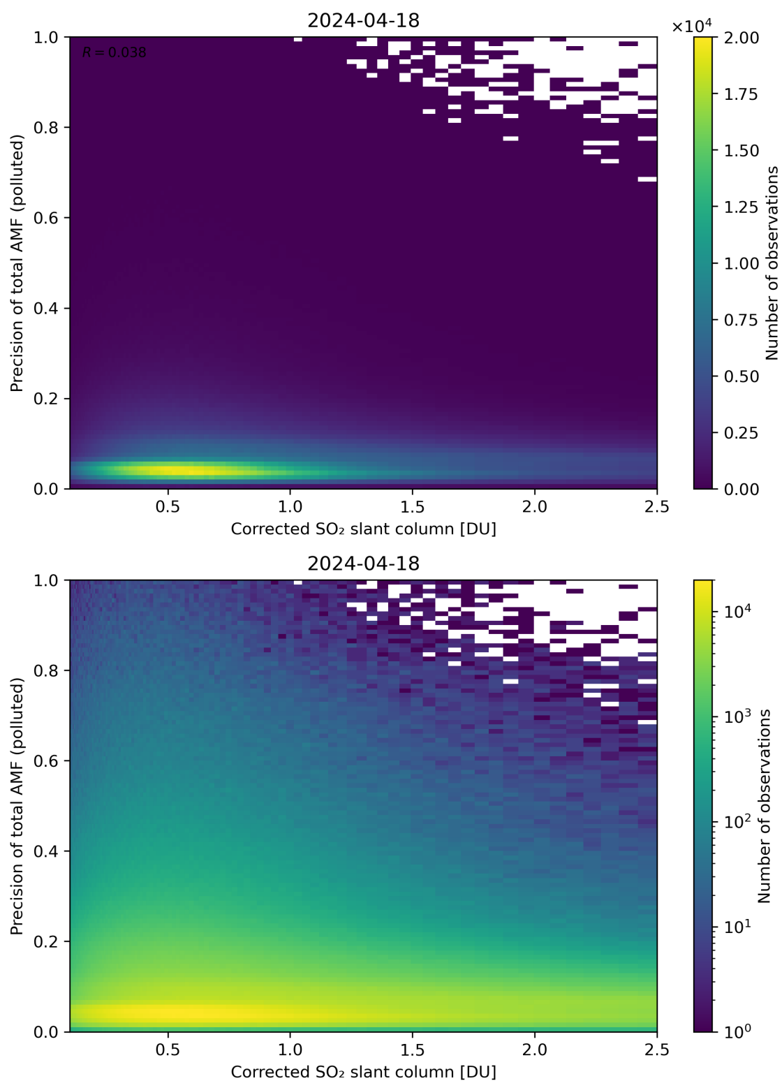
Figure 193: Scatter density plot of “Corrected SO 2 slant column” against “Precision of total AMF (polluted)” for 2024-04-17 to 2024-04-19.
