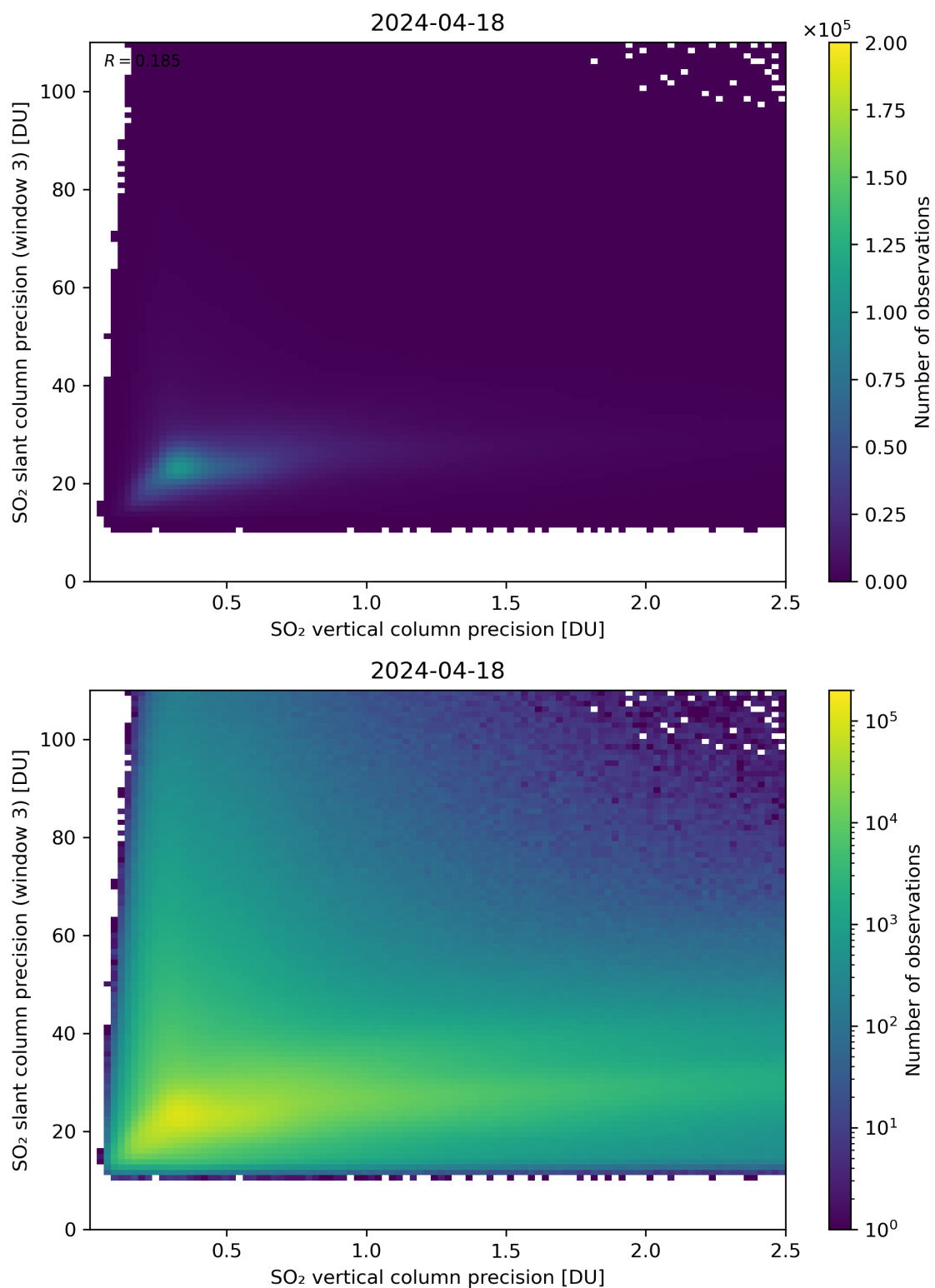
Figure 293: Scatter density plot of “SO 2 vertical column precision” against “SO 2 slant column precision (window 3)” for 2024-04-17 to 2024-04-19.
