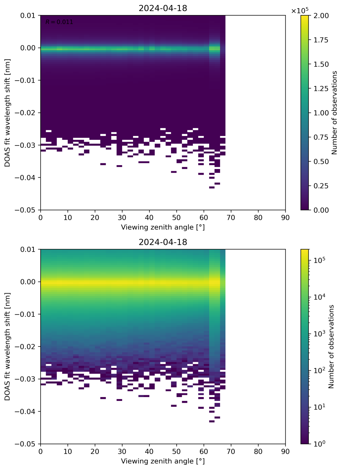
Figure 311: Scatter density plot of “Viewing zenith angle” against “DOAS fit wavelength shift” for 2024-04-17 to 2024-04-19.
