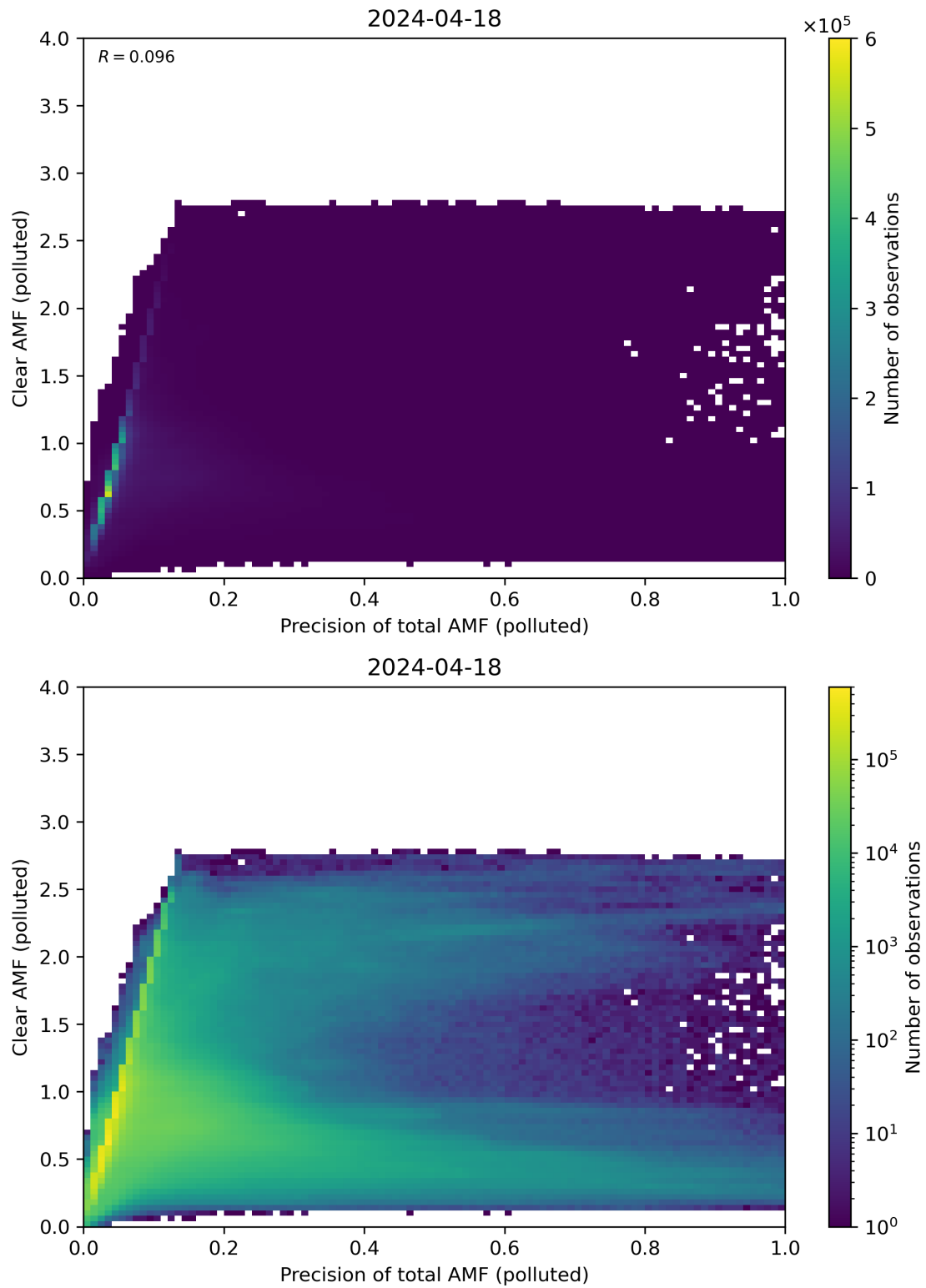
Figure 270: Scatter density plot of “Precision of total AMF (polluted)” against “Clear AMF (polluted)” for 2024-04-17 to 2024-04-19.
