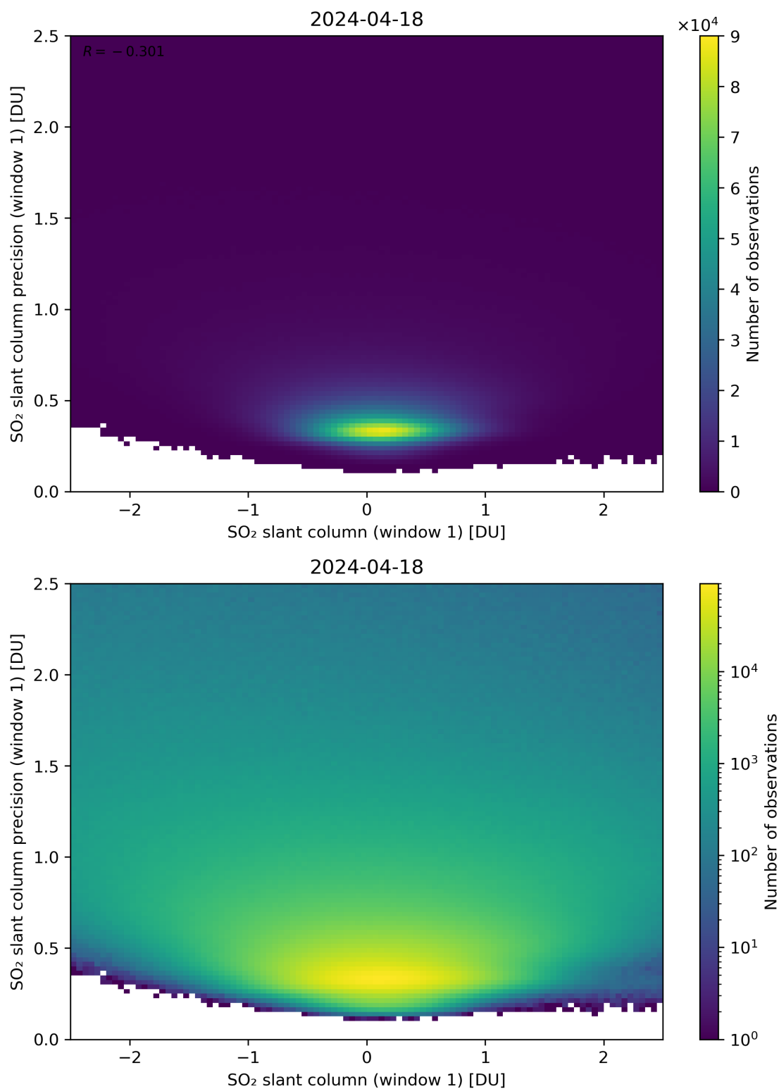
Figure 235: Scatter density plot of “SO 2 slant column (window 1)” against “SO 2 slant column precision (window 1)” for 2024-04-17 to 2024-04-19.
