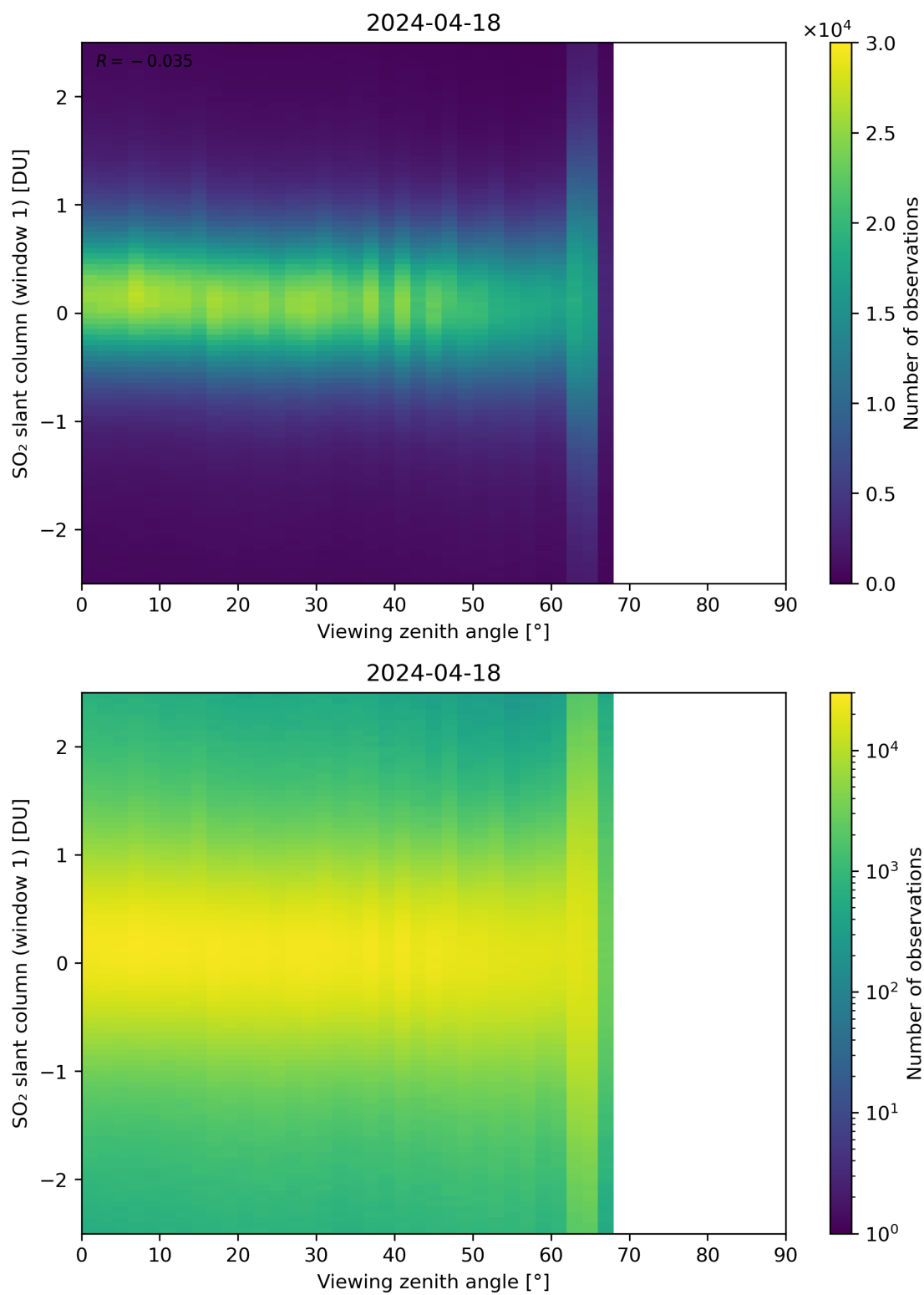
Figure 320: Scatter density plot of “Viewing zenith angle” against “SO 2 slant column (window 1)” for 2024-04-17 to 2024-04-19.
