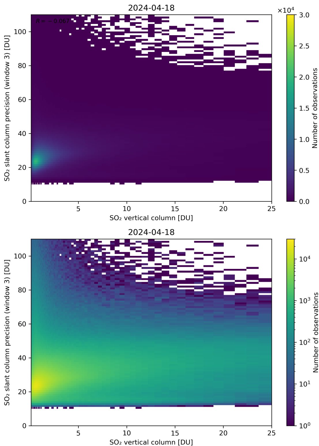
Figure 304: Scatter density plot of “SO 2 vertical column” against “SO 2 slant column precision (window 3)” for 2024-04-17 to 2024-04-19.
