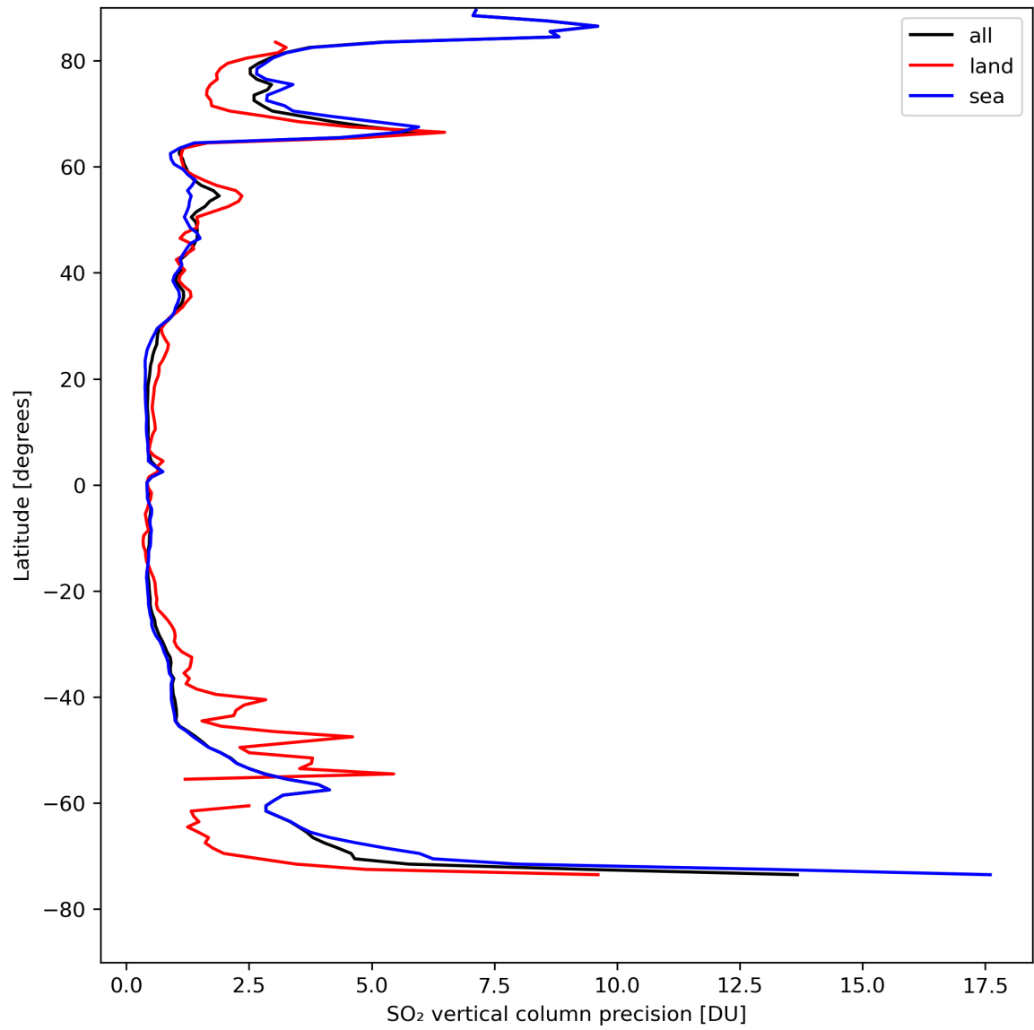
Figure 31: Zonal average of “SO 2 vertical column precision” for 2024-04-17 to 2024-04-19.
