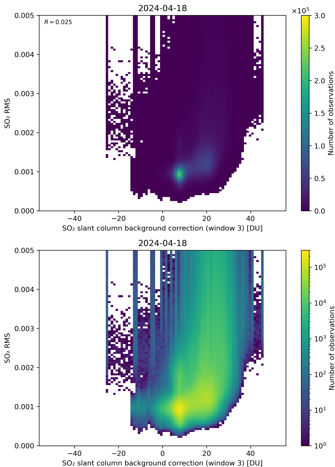
Figure 123: Scatter density plot of “SO 2 slant column background correction (window 3)” against “SO 2 RMS” for 2024-04-17 to 2024-04-19.
