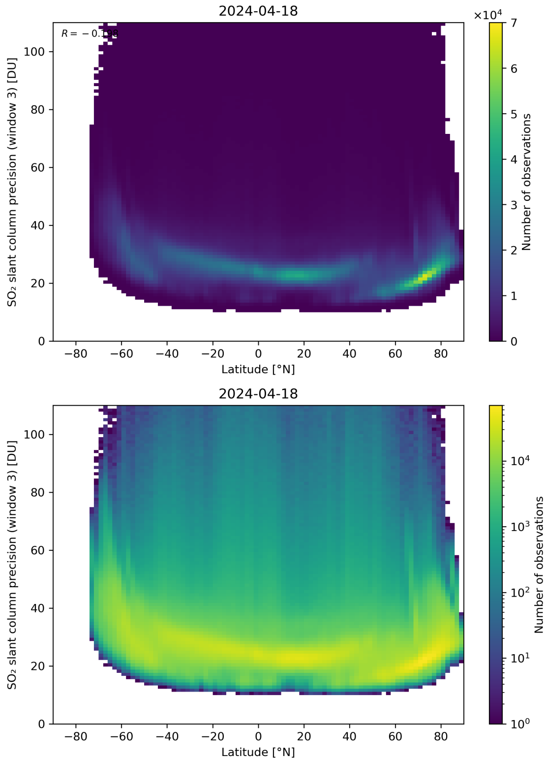
Figure 153: Scatter density plot of “Latitude” against “SO 2 slant column precision (window 3)” for 2024-04-17 to 2024-04-19.
