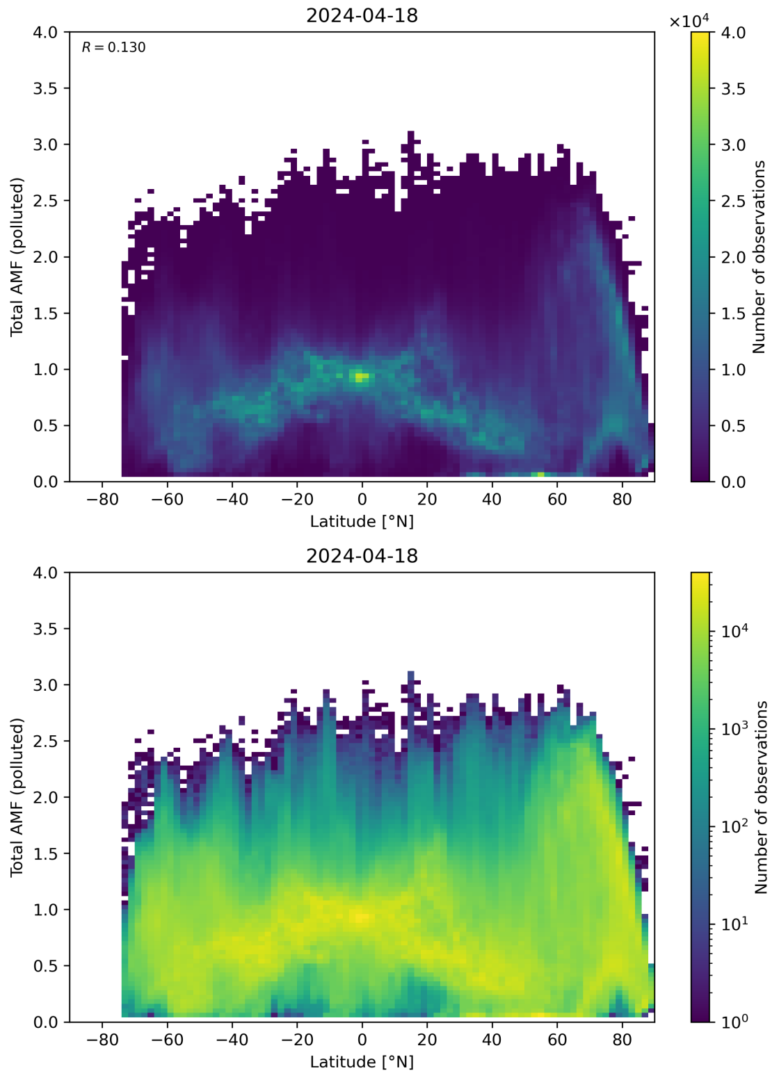
Figure 154: Scatter density plot of “Latitude” against “Total AMF (polluted)” for 2024-04-17 to 2024-04-19.
