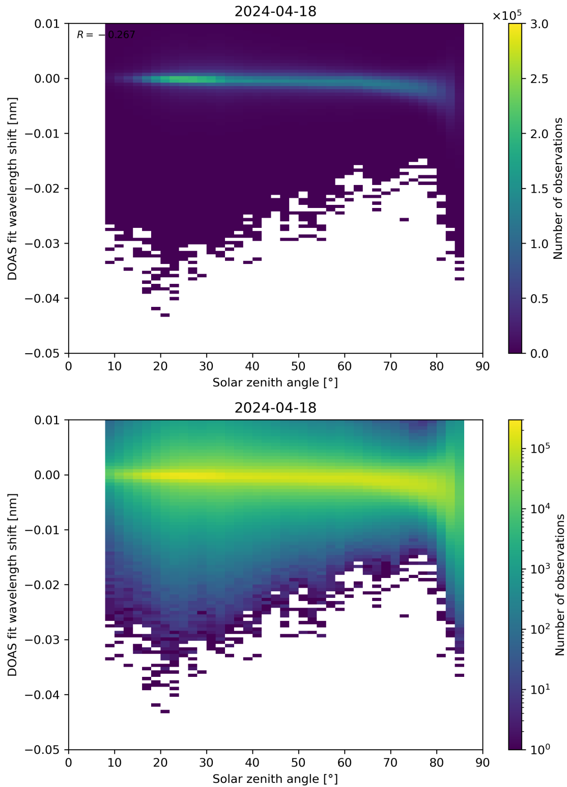
Figure 161: Scatter density plot of “Solar zenith angle” against “DOAS fit wavelength shift” for 2024-04-17 to 2024-04-19.
