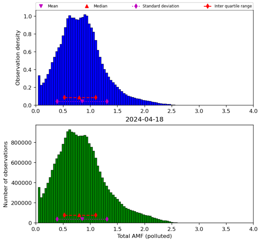
Figure 71: Histogram of “Total AMF (polluted)” for 2024-04-17 to 2024-04-19
