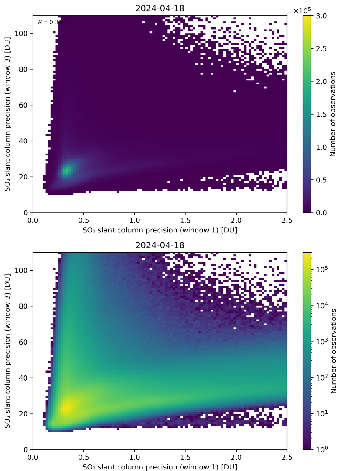
Figure 229: Scatter density plot of “SO 2 slant column precision (window 1)” against “SO 2 slant column precision (window 3)” for 2024-04-17 to 2024-04-19.
