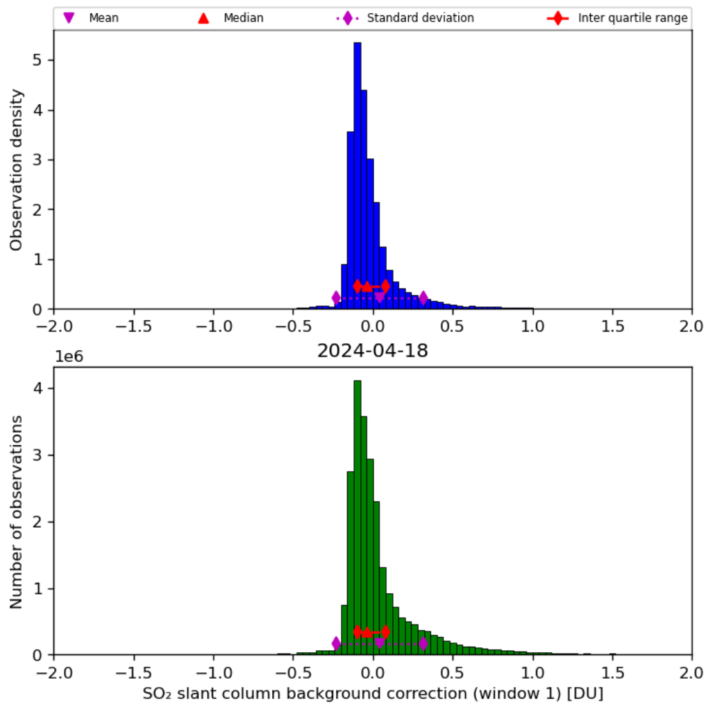
Figure 59: Histogram of “SO 2 slant column background correction (window 1)” for 2024-04-17 to 2024-04-19
