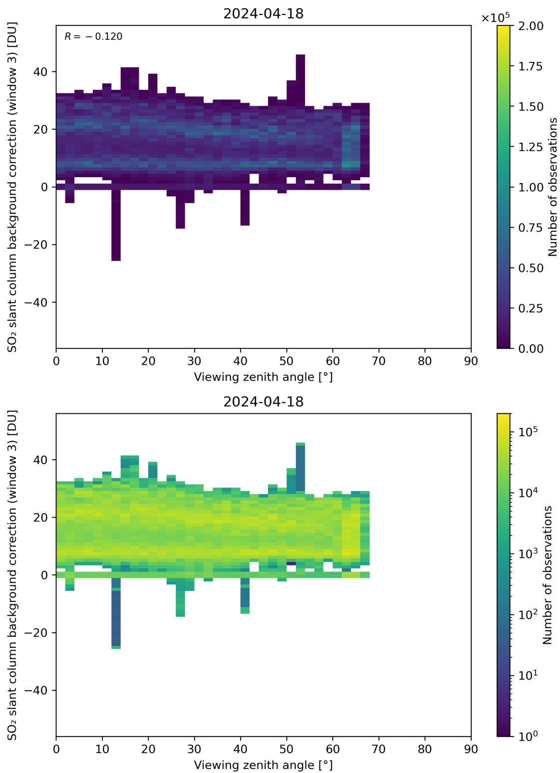
Figure 310: Scatter density plot of “Viewing zenith angle” against “SO 2 slant column background correction (window 3)” for 2024-04-17 to 2024-04-19.
