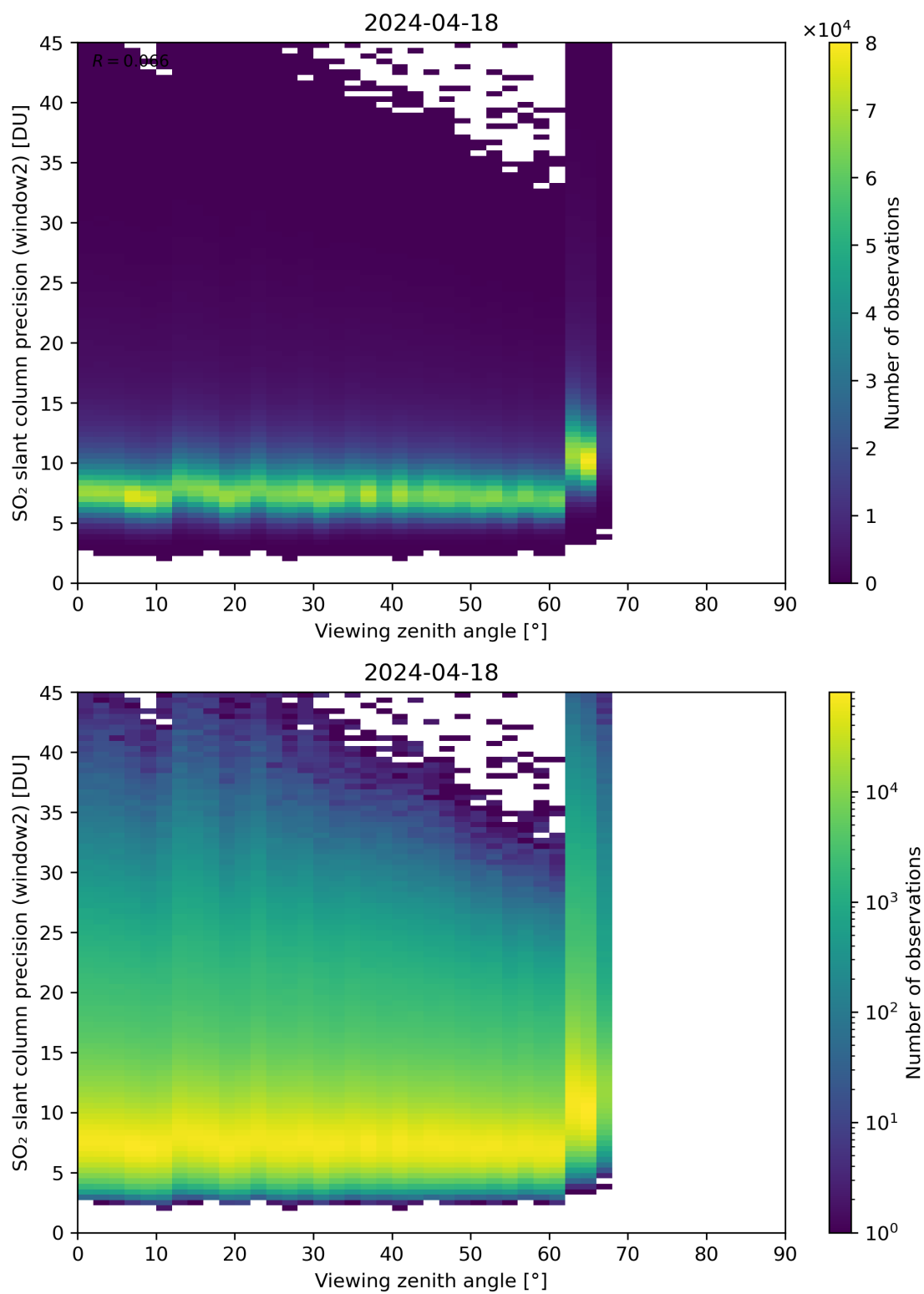
Figure 322: Scatter density plot of “Viewing zenith angle” against “SO 2 slant column precision (window2)” for 2024-04-17 to 2024-04-19.
