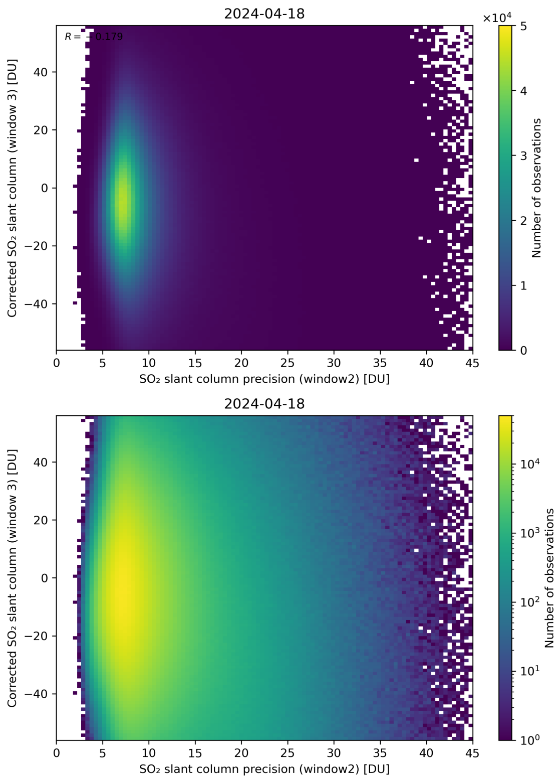
Figure 248: Scatter density plot of “SO 2 slant column precision (window2)” against “Corrected SO 2 slant column (window 3)” for 2024-04-17 to 2024-04-19.
