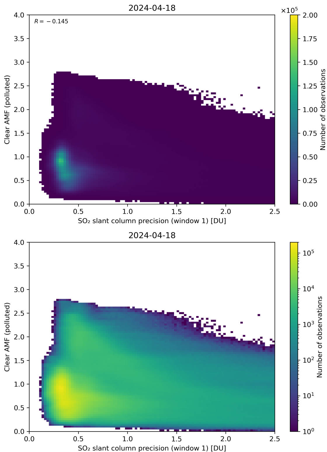
Figure 224: Scatter density plot of “SO 2 slant column precision (window 1)” against “Clear AMF (polluted)” for 2024-04-17 to 2024-04-19.
