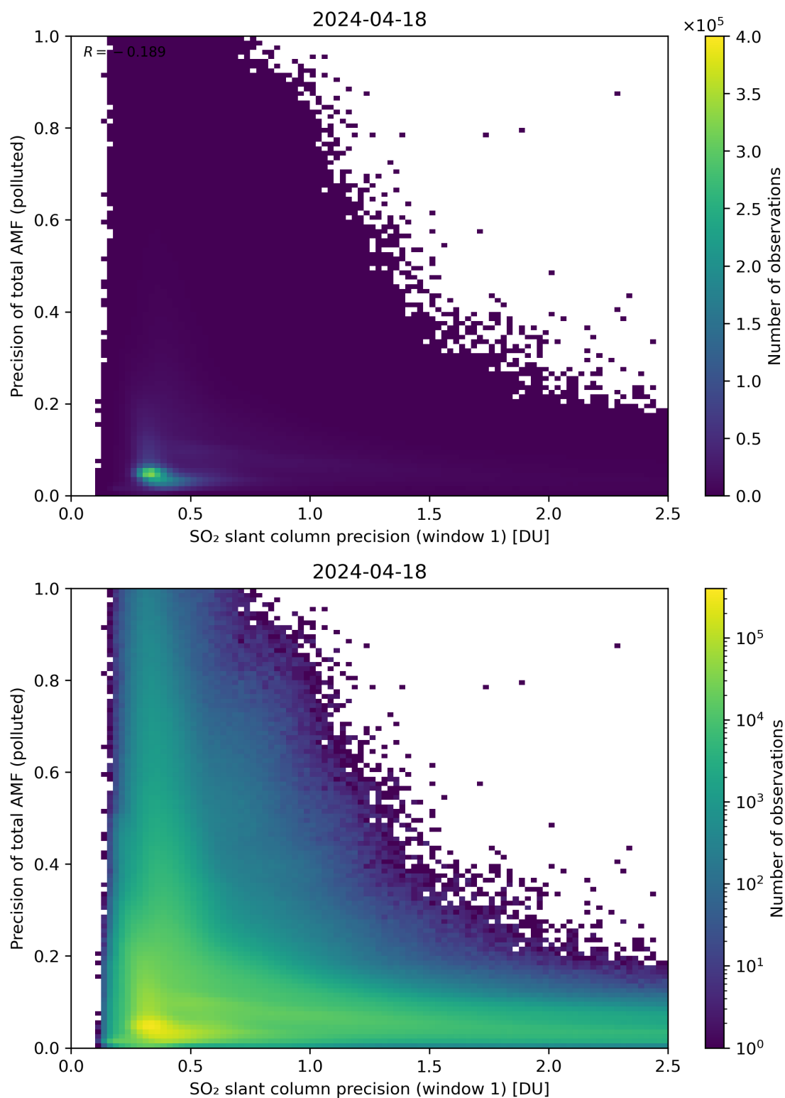
Figure 231: Scatter density plot of “SO 2 slant column precision (window 1)” against “Precision of total AMF (polluted)” for 2024-04-17 to 2024-04-19.
