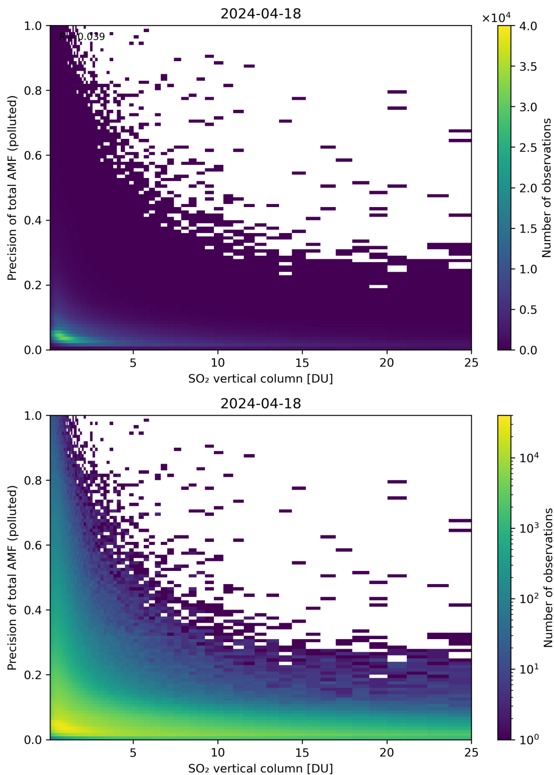
Figure 306: Scatter density plot of “SO 2 vertical column” against “Precision of total AMF (polluted)” for 2024-04-17 to 2024-04-19.
