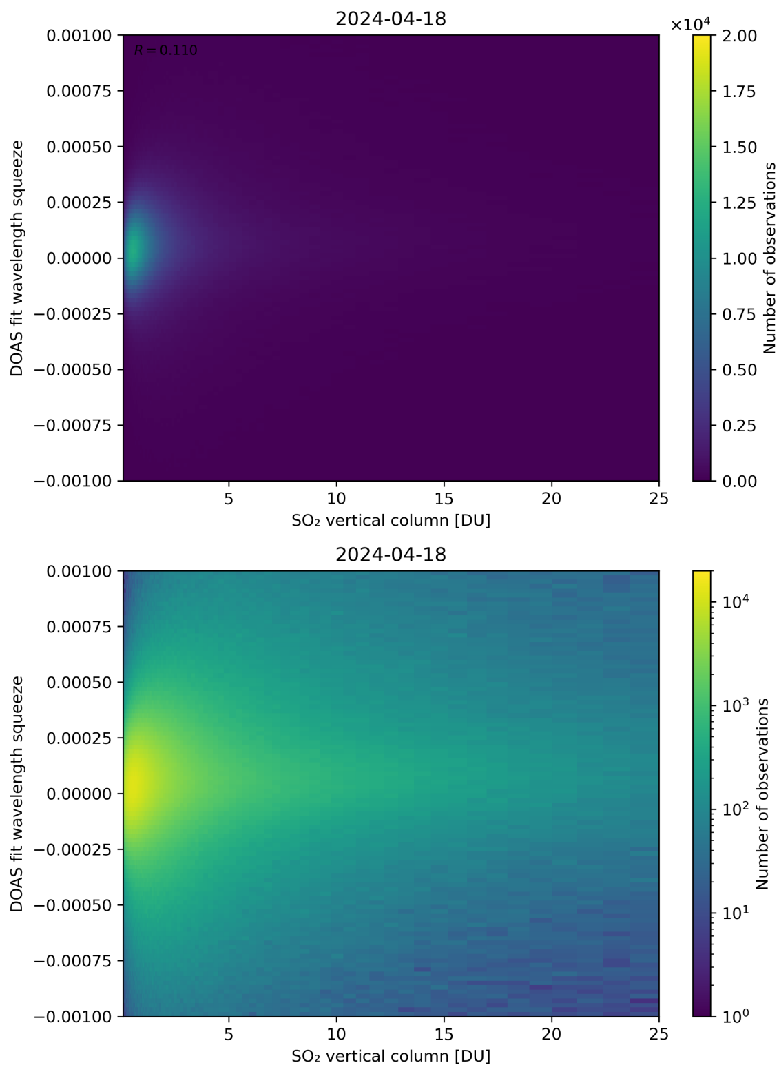
Figure 277: Scatter density plot of “SO 2 vertical column” against “DOAS fit wavelength squeeze” for 2024-04-17 to 2024-04-19.
