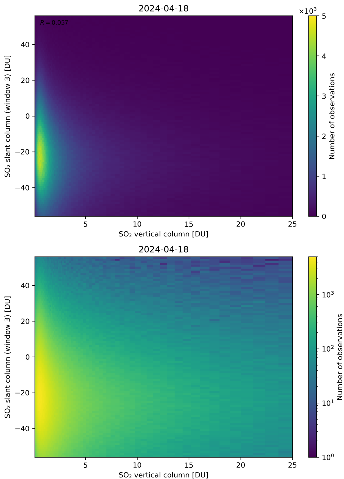
Figure 303: Scatter density plot of “SO 2 vertical column” against “SO 2 slant column (window 3)” for 2024-04-17 to 2024-04-19.
