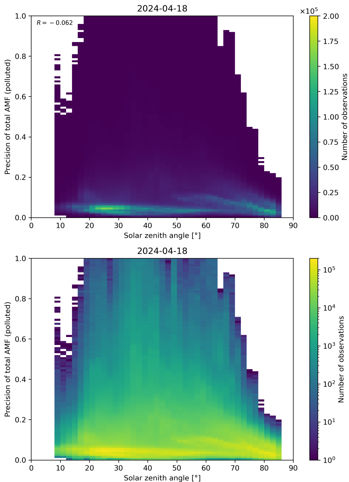
Figure 175: Scatter density plot of “Solar zenith angle” against “Precision of total AMF (polluted)” for 2024-04-17 to 2024-04-19.
