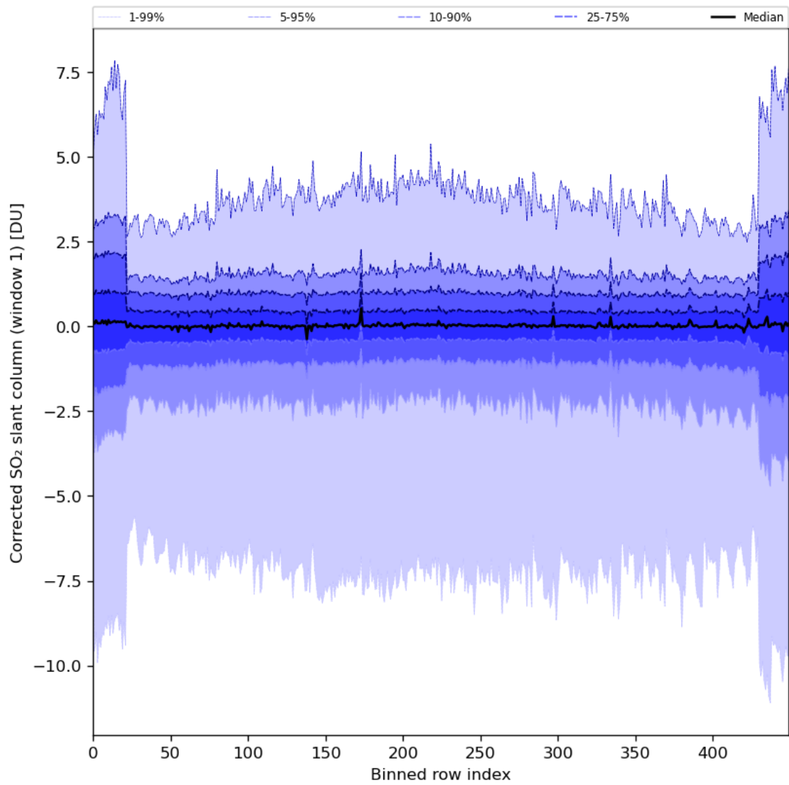
Figure 81: Along track statistics of “Corrected SO 2 slant column (window 1)” for 2024-04-17 to 2024-04-19
