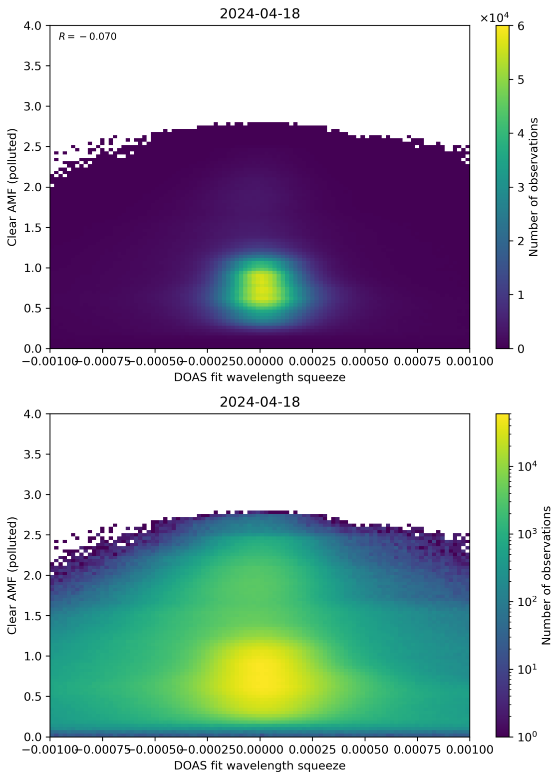
Figure 133: Scatter density plot of “DOAS fit wavelength squeeze” against “Clear AMF (polluted)” for 2024-04-17 to 2024-04-19.
