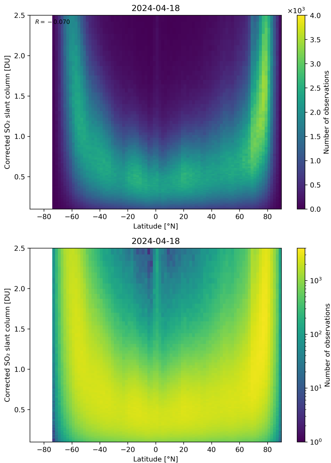
Figure 146: Scatter density plot of “Latitude” against “Corrected SO 2 slant column” for 2024-04-17 to 2024-04-19.
