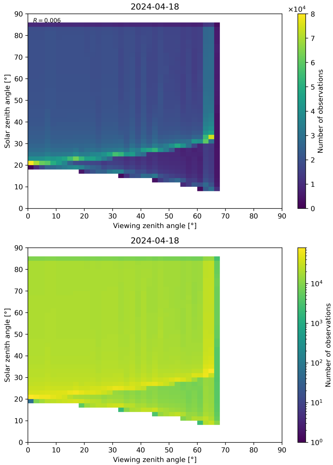
Figure 315: Scatter density plot of “Viewing zenith angle” against “Solar zenith angle” for 2024-04-17 to 2024-04-19.
