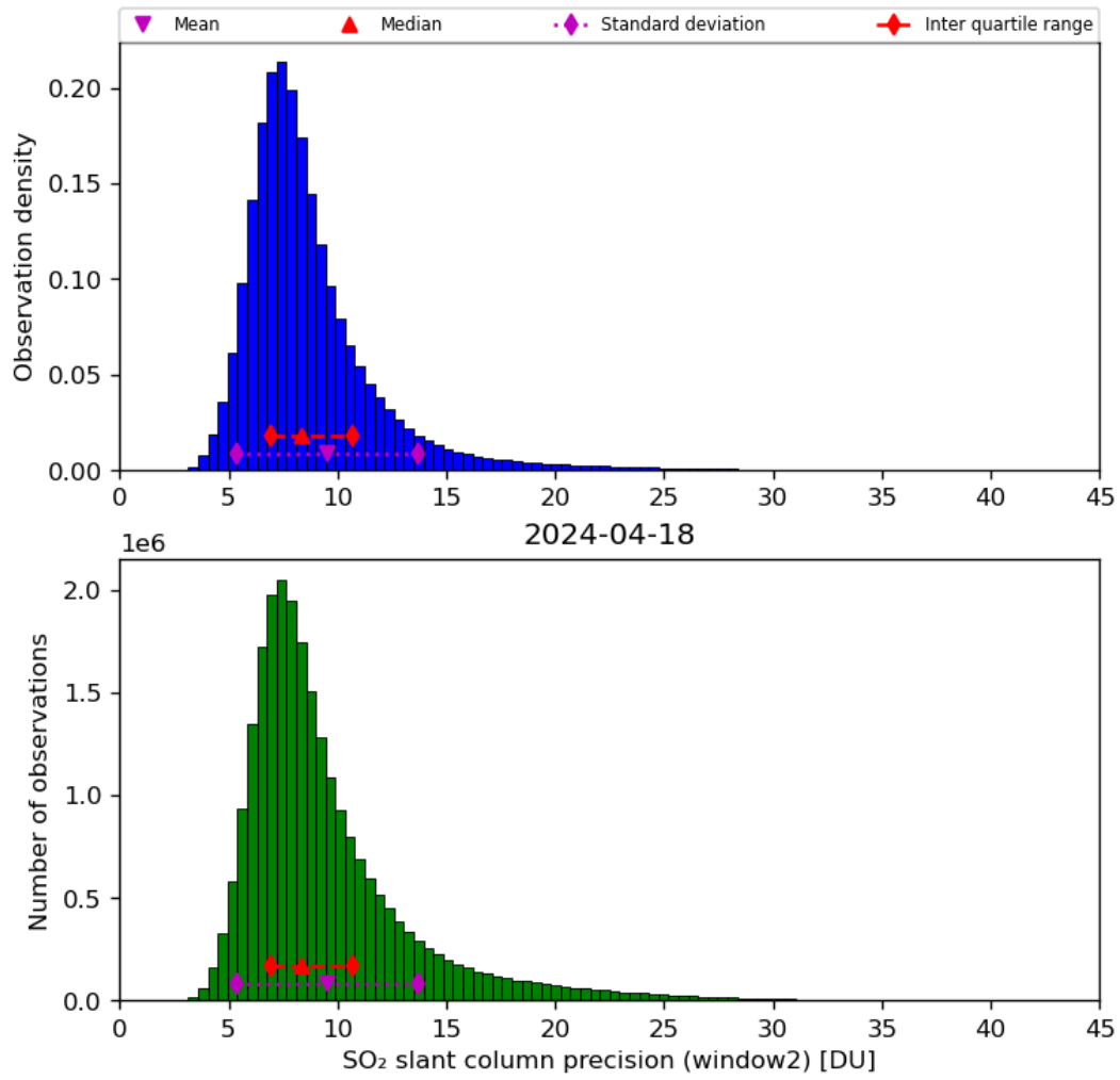
Figure 61: Histogram of “SO 2 slant column precision (window2)” for 2024-04-17 to 2024-04-19
