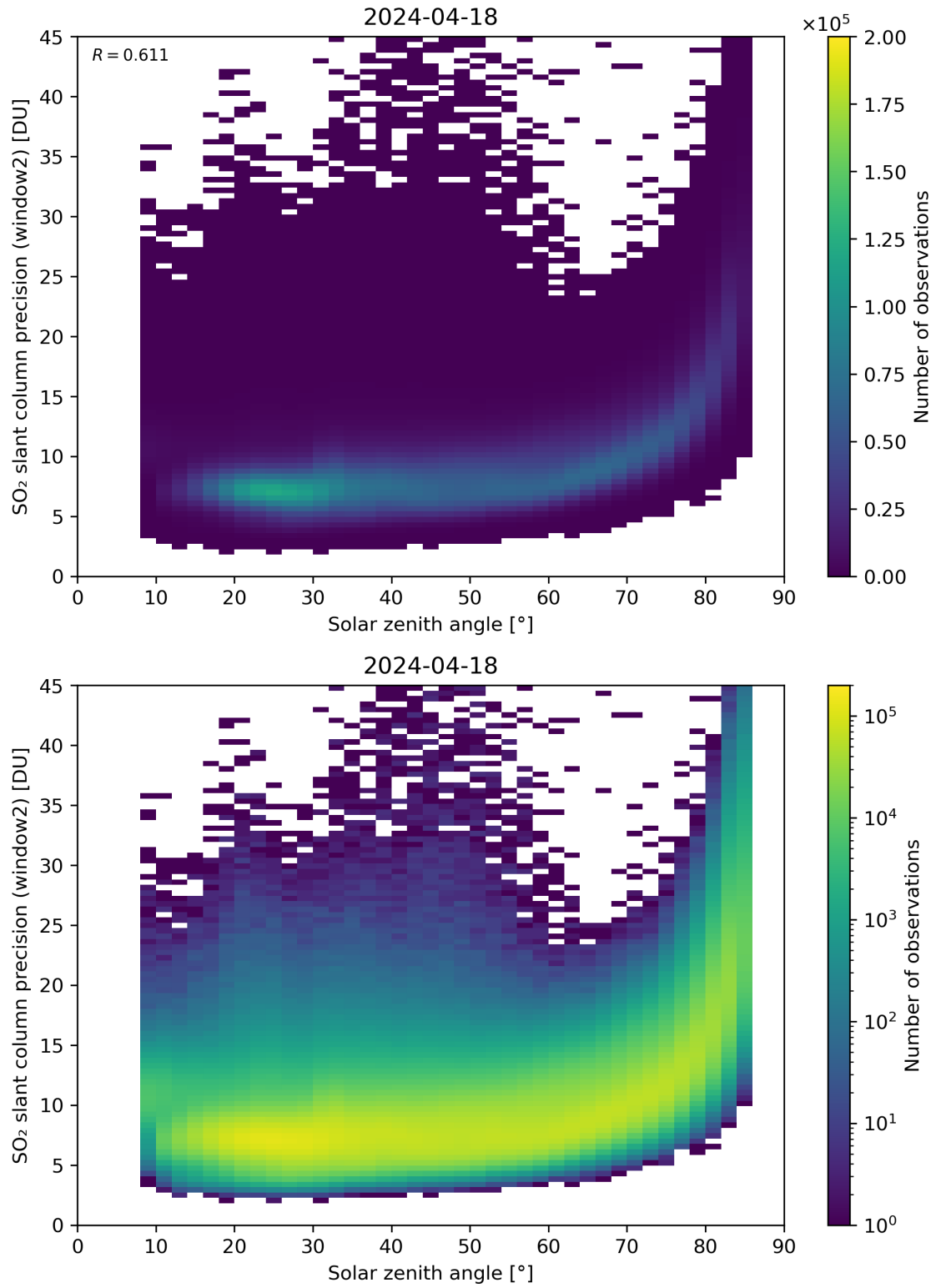
Figure 171: Scatter density plot of “Solar zenith angle” against “SO 2 slant column precision (window2)” for 2024-04-17 to 2024-04-19.
