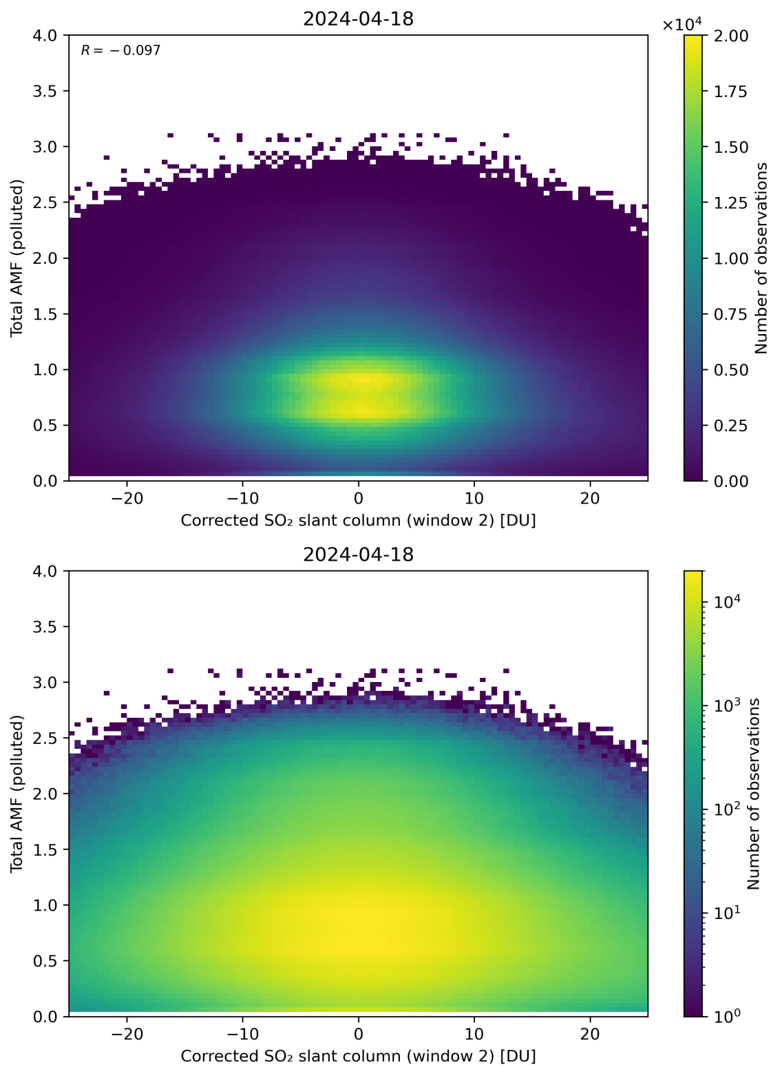
Figure 203: Scatter density plot of “Corrected SO 2 slant column (window 2)” against “Total AMF (polluted)” for 2024-04-17 to 2024-04-19.
