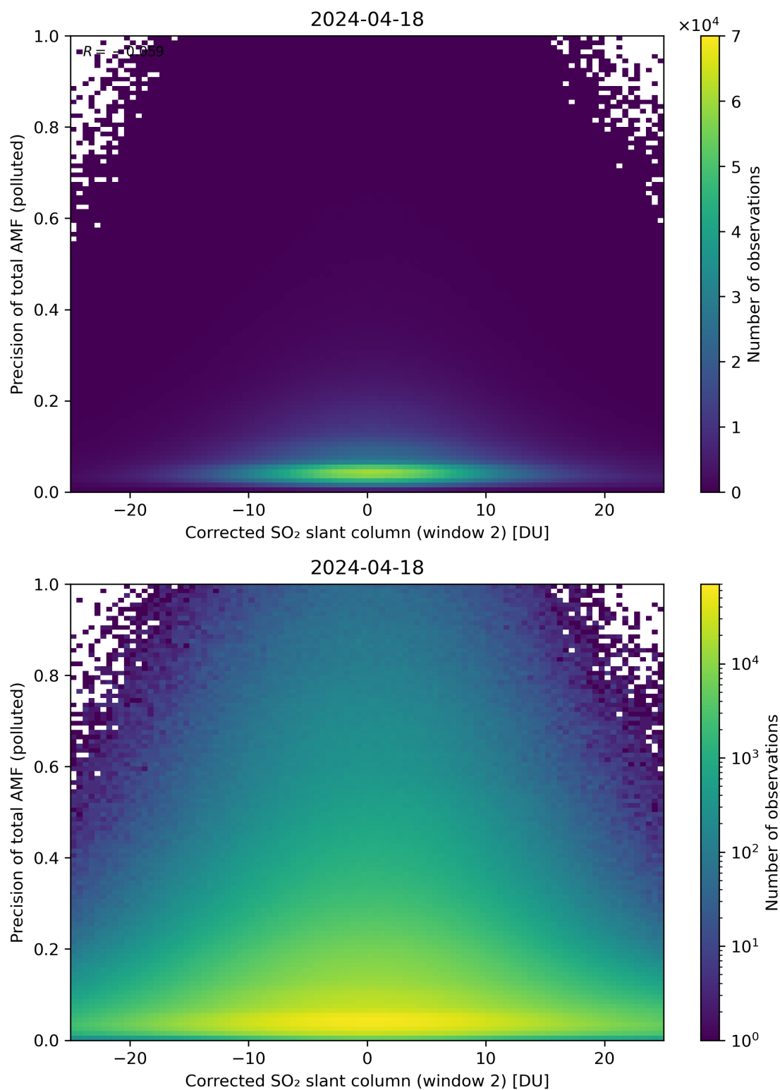
Figure 204: Scatter density plot of “Corrected SO 2 slant column (window 2)” against “Precision of total AMF (polluted)” for 2024-04-17 to 2024-04-19.
