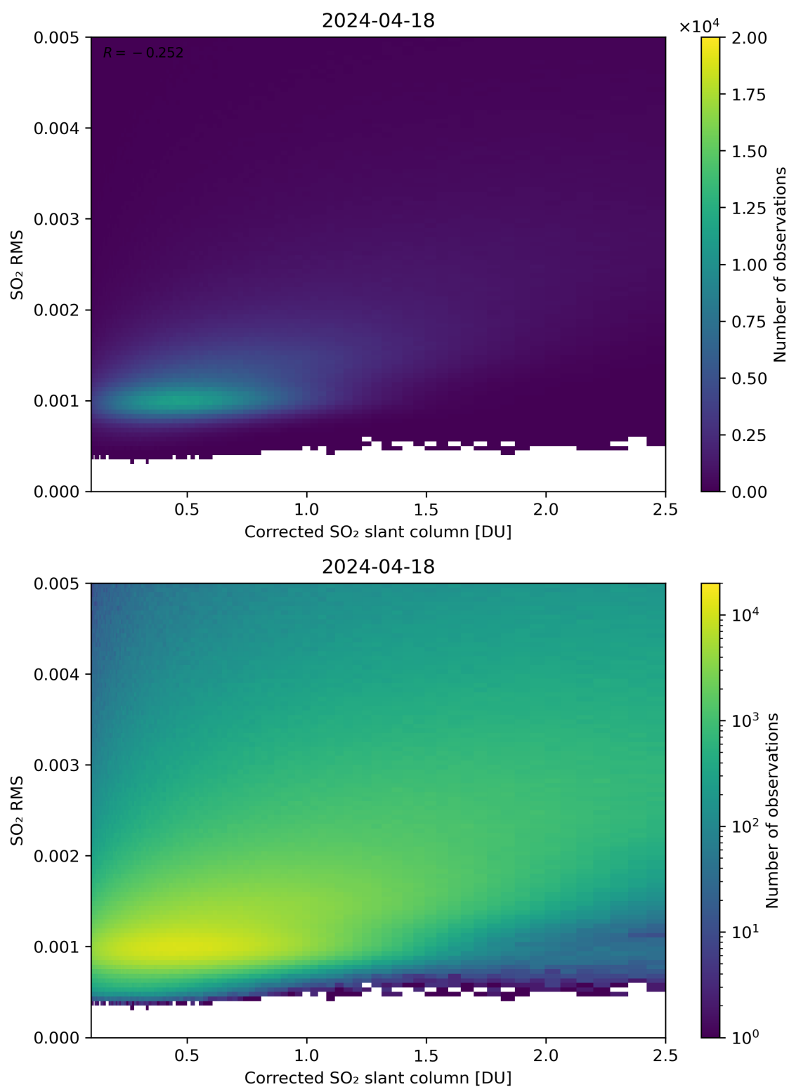
Figure 183: Scatter density plot of “Corrected SO 2 slant column” against “SO 2 RMS” for 2024-04-17 to 2024-04-19.
