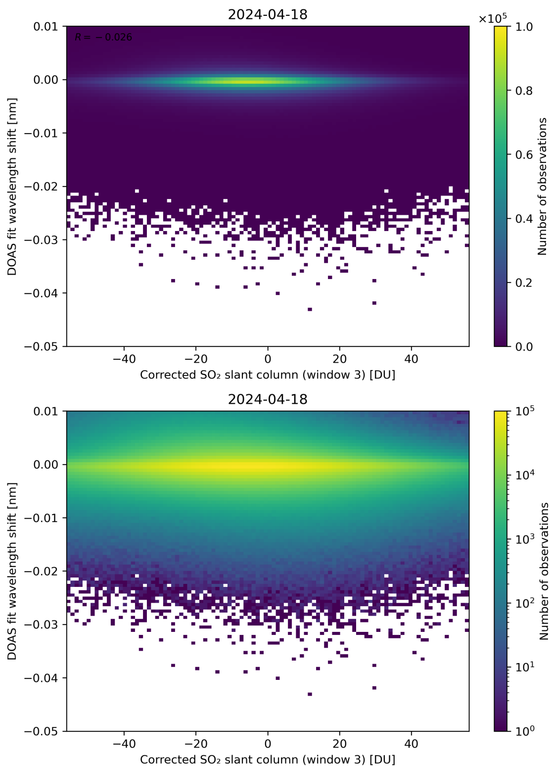
Figure 206: Scatter density plot of “Corrected SO 2 slant column (window 3)” against “DOAS fit wavelength shift” for 2024-04-17 to 2024-04-19.
