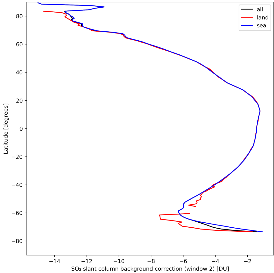
Figure 40: Zonal average of “SO 2 slant column background correction (window 2)” for 2024-04-17 to 2024-04-19.
