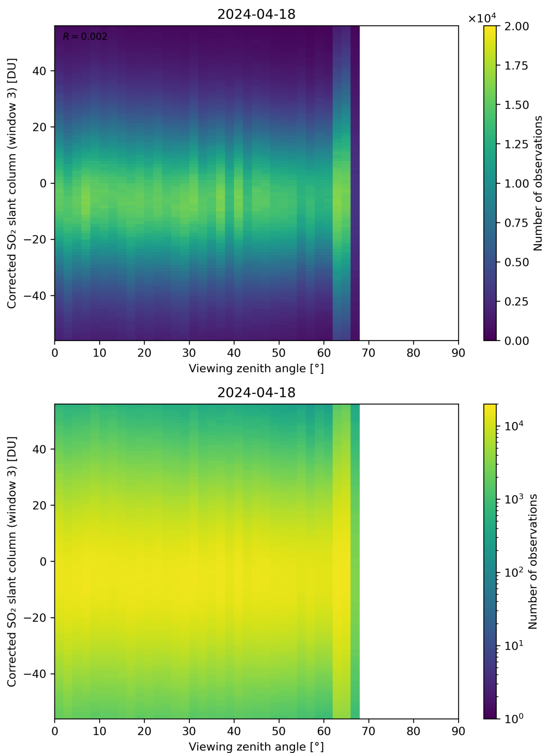
Figure 319: Scatter density plot of “Viewing zenith angle” against “Corrected SO 2 slant column (window 3)” for 2024-04-17 to 2024-04-19.
