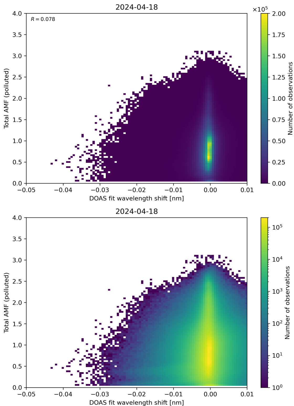
Figure 130: Scatter density plot of “DOAS fit wavelength shift” against “Total AMF (polluted)” for 2024-04-17 to 2024-04-19.
