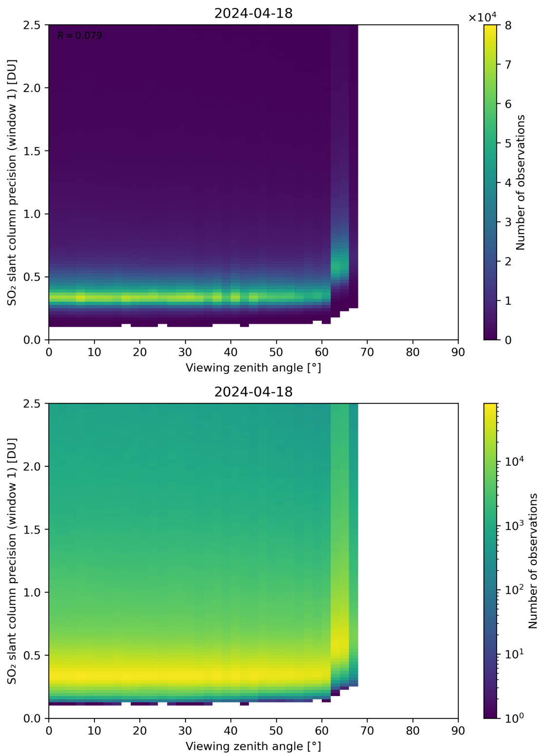
Figure 321: Scatter density plot of “Viewing zenith angle” against “SO 2 slant column precision (window 1)” for 2024-04-17 to 2024-04-19.
