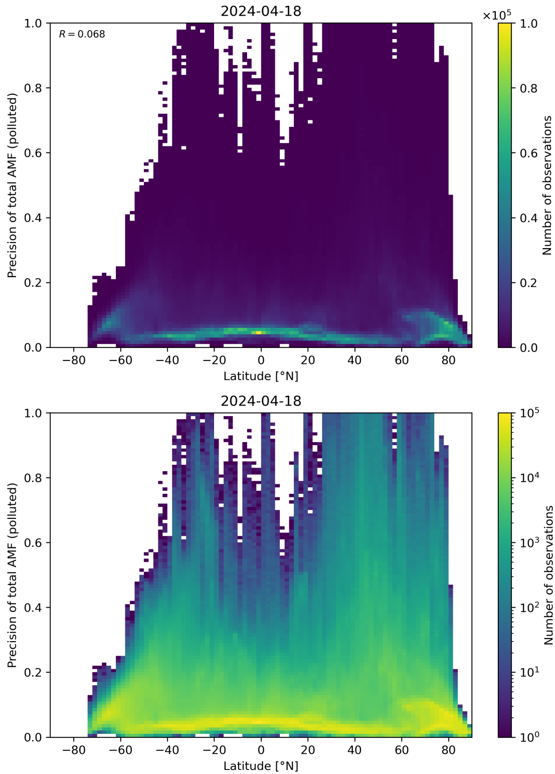
Figure 155: Scatter density plot of “Latitude” against “Precision of total AMF (polluted)” for 2024-04-17 to 2024-04-19.
