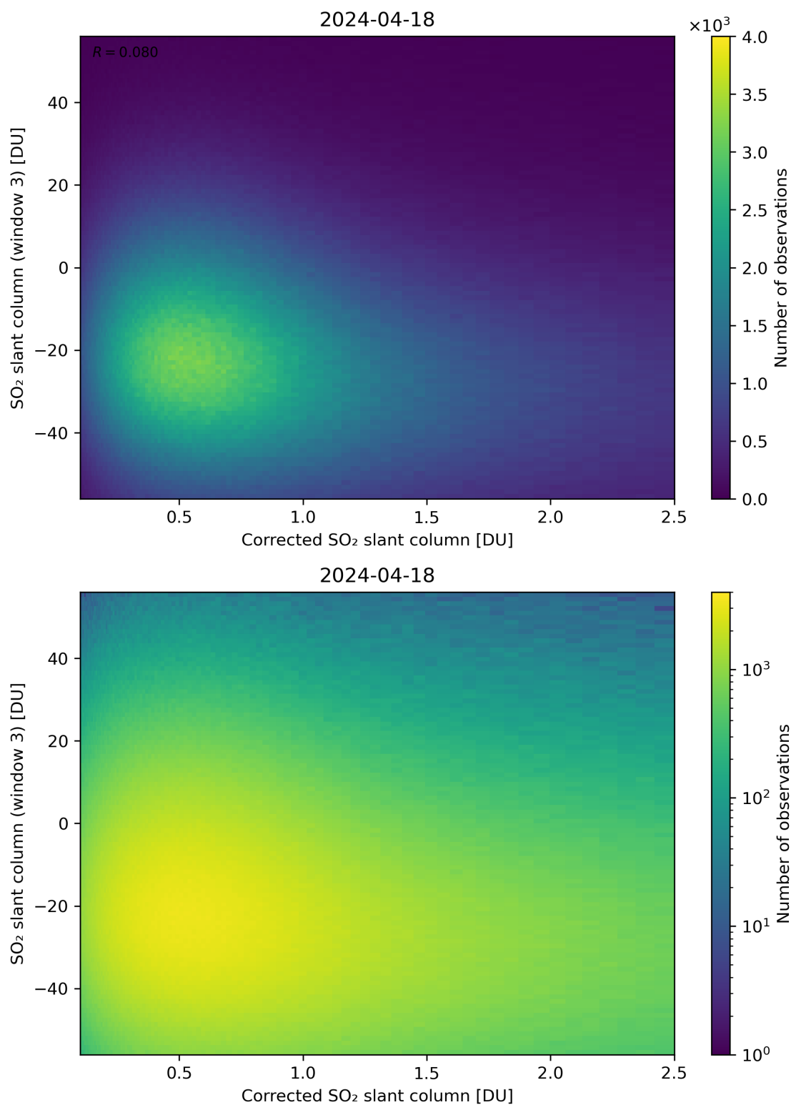
Figure 190: Scatter density plot of “Corrected SO 2 slant column” against “SO 2 slant column (window 3)” for 2024-04-17 to 2024-04-19.
