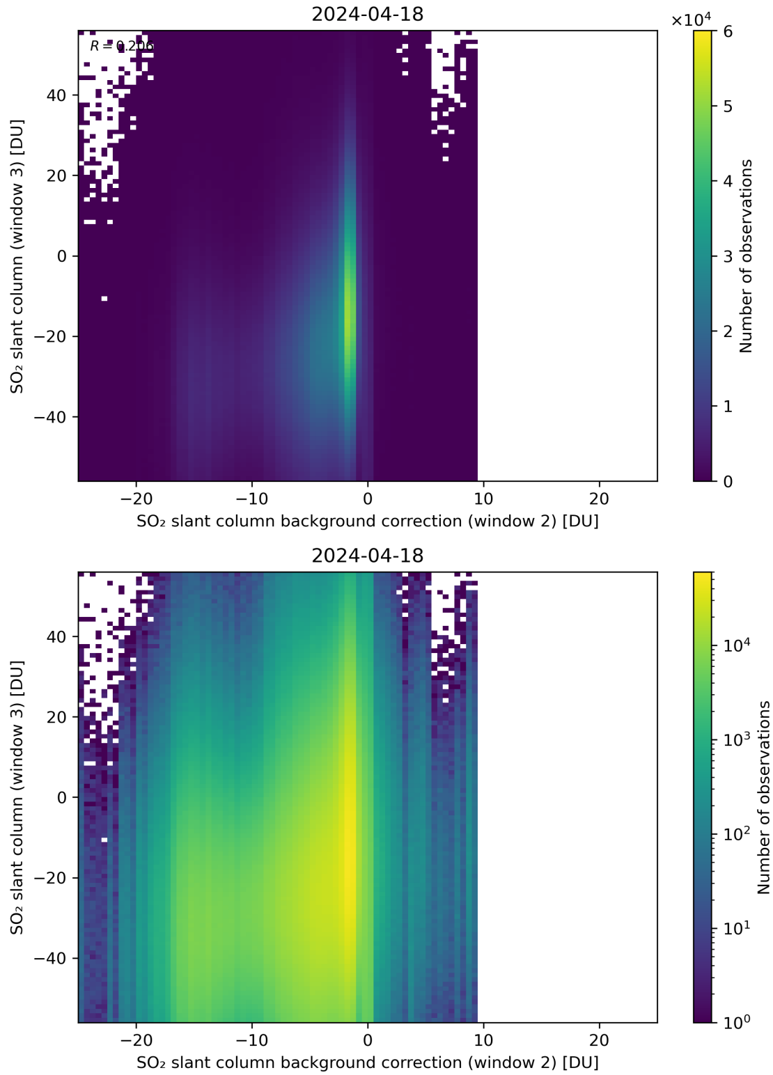
Figure 117: Scatter density plot of “SO 2 slant column background correction (window 2)” against “SO 2 slant column (window 3)” for 2024-04-17 to 2024-04-19.
