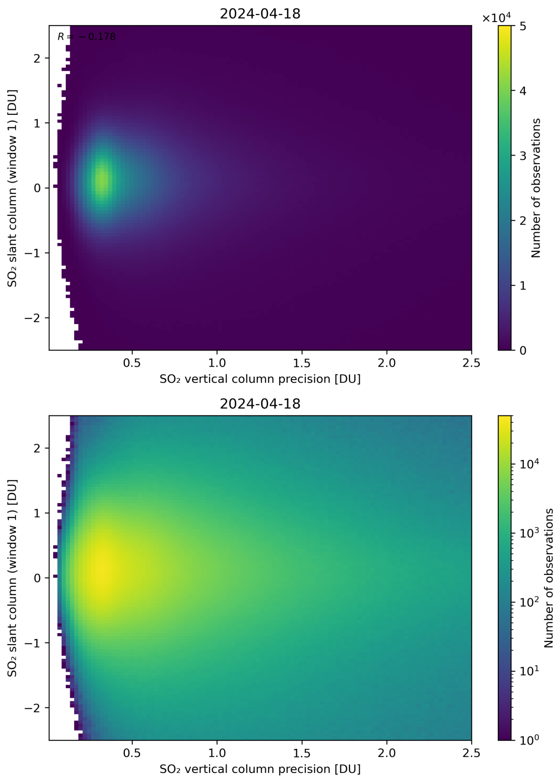
Figure 289: Scatter density plot of “SO 2 vertical column precision” against “SO 2 slant column (window 1)” for 2024-04-17 to 2024-04-19.
