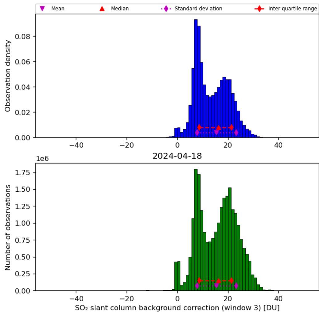
Figure 67: Histogram of “SO 2 slant column background correction (window 3)” for 2024-04-17 to 2024-04-19
