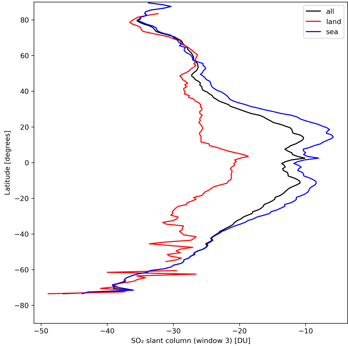
Figure 41: Zonal average of “SO 2 slant column (window 3)” for 2024-04-17 to 2024-04-19.
