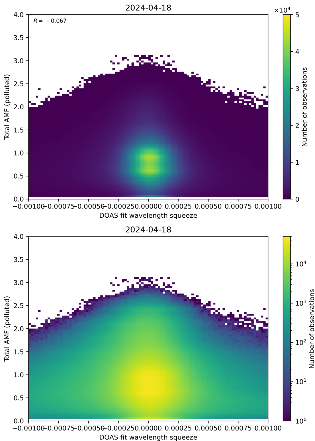
Figure 134: Scatter density plot of “DOAS fit wavelength squeeze” against “Total AMF (polluted)” for 2024-04-17 to 2024-04-19.
