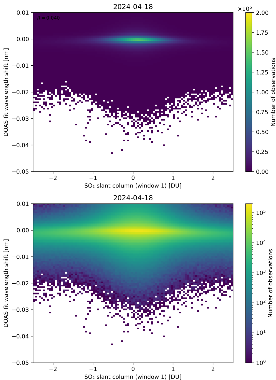
Figure 215: Scatter density plot of “SO 2 slant column (window 1)” against “DOAS fit wavelength shift” for 2024-04-17 to 2024-04-19.
