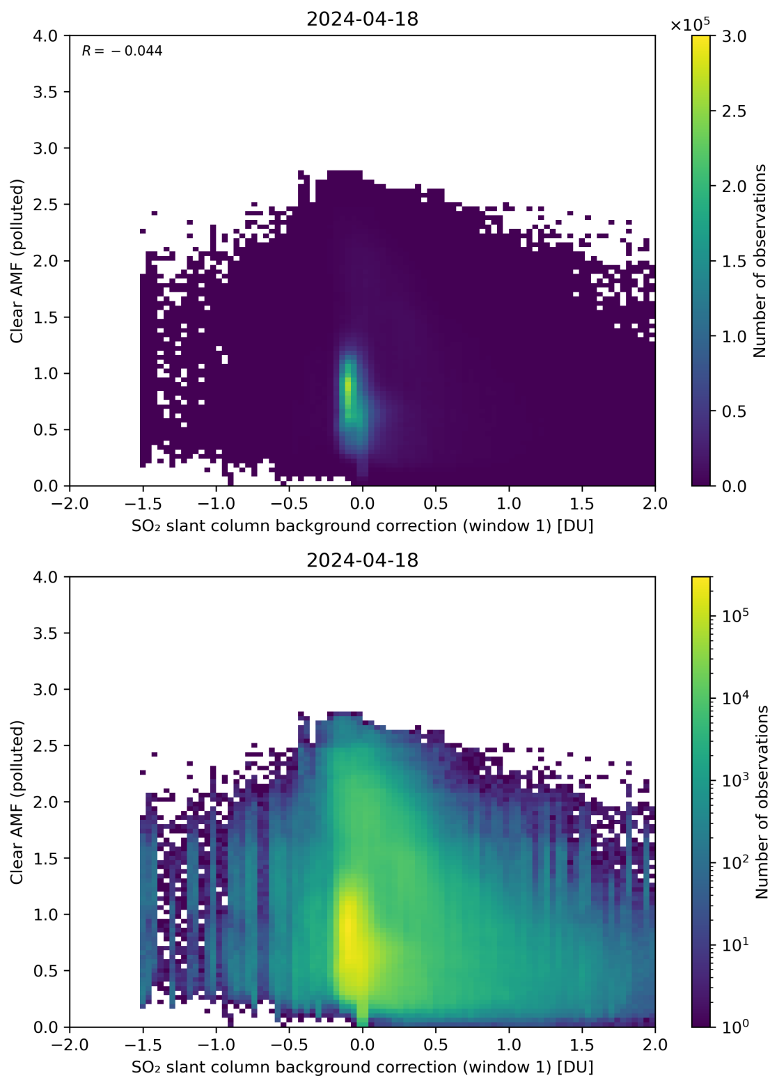
Figure 103: Scatter density plot of “SO 2 slant column background correction (window 1)” against “Clear AMF (polluted)” for 2024-04-17 to 2024-04-19.
