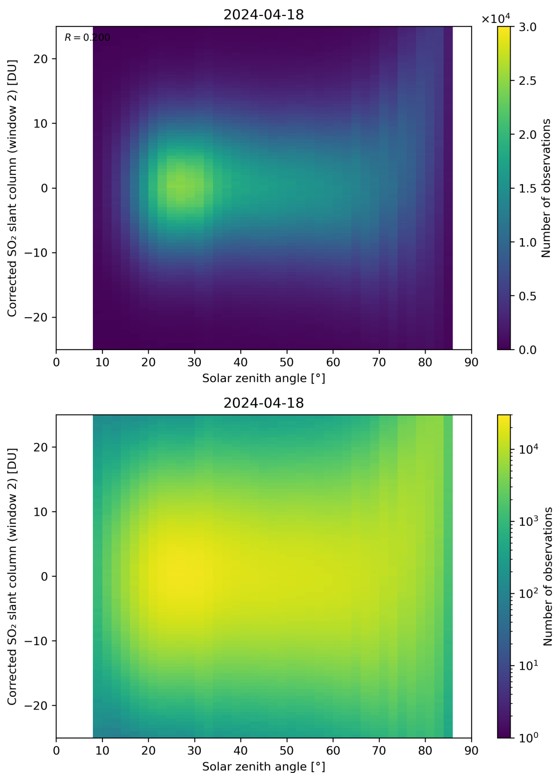
Figure 167: Scatter density plot of “Solar zenith angle” against “Corrected SO 2 slant column (window 2)” for 2024-04-17 to 2024-04-19.
