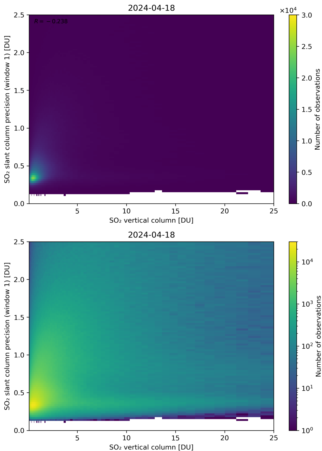
Figure 301: Scatter density plot of “SO 2 vertical column” against “SO 2 slant column precision (window 1)” for 2024-04-17 to 2024-04-19.
