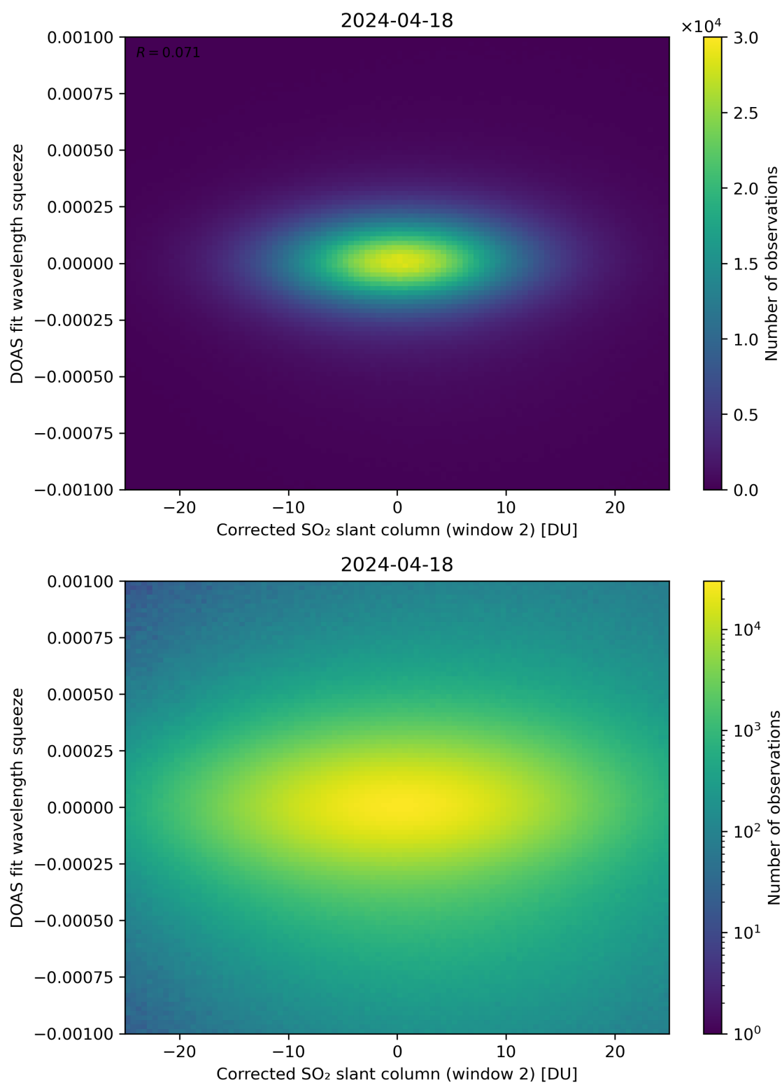
Figure 197: Scatter density plot of “Corrected SO 2 slant column (window 2)” against “DOAS fit wavelength squeeze” for 2024-04-17 to 2024-04-19.
