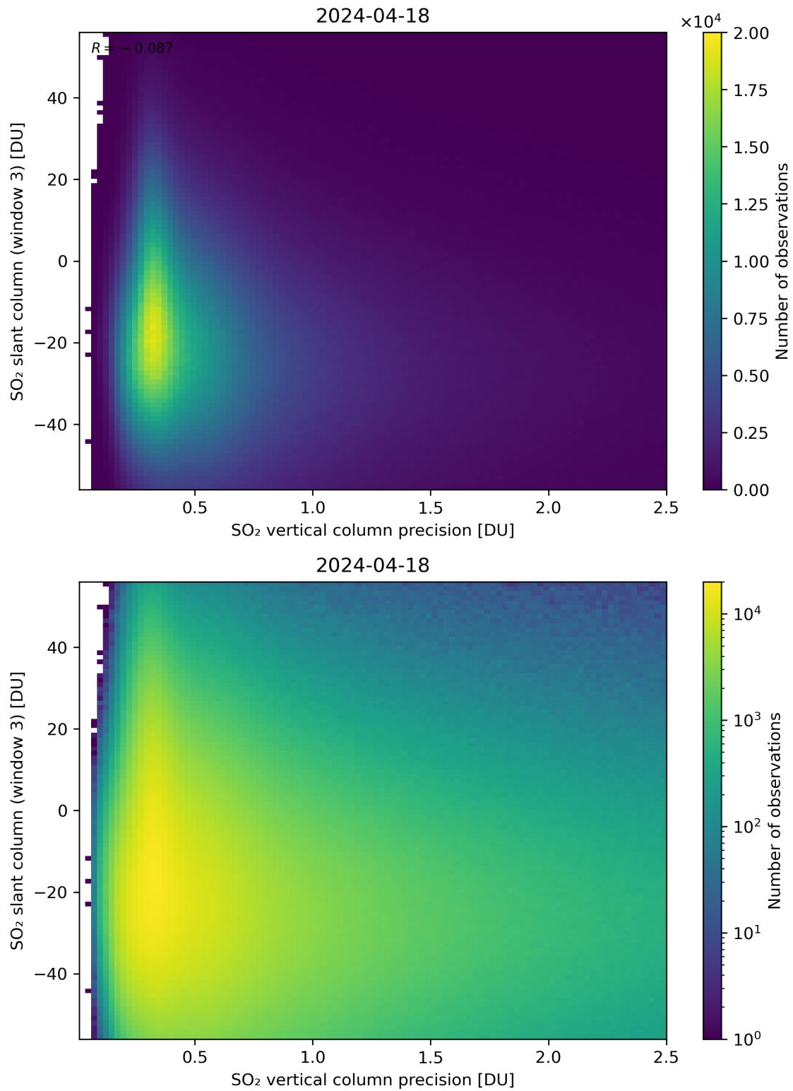
Figure 292: Scatter density plot of “SO 2 vertical column precision” against “SO 2 slant column (window 3)” for 2024-04-17 to 2024-04-19.
