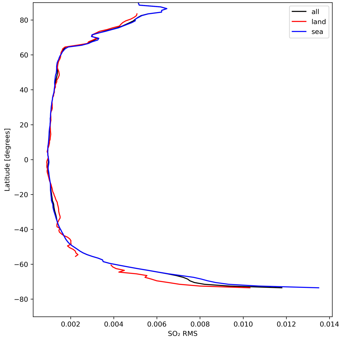
Figure 47: Zonal average of “SO 2 RMS” for 2024-04-17 to 2024-04-19.
