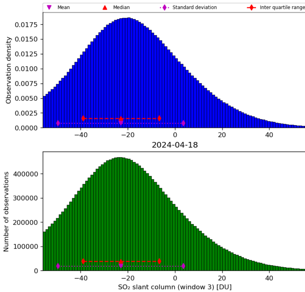
Figure 64: Histogram of “SO 2 slant column (window 3)” for 2024-04-17 to 2024-04-19
