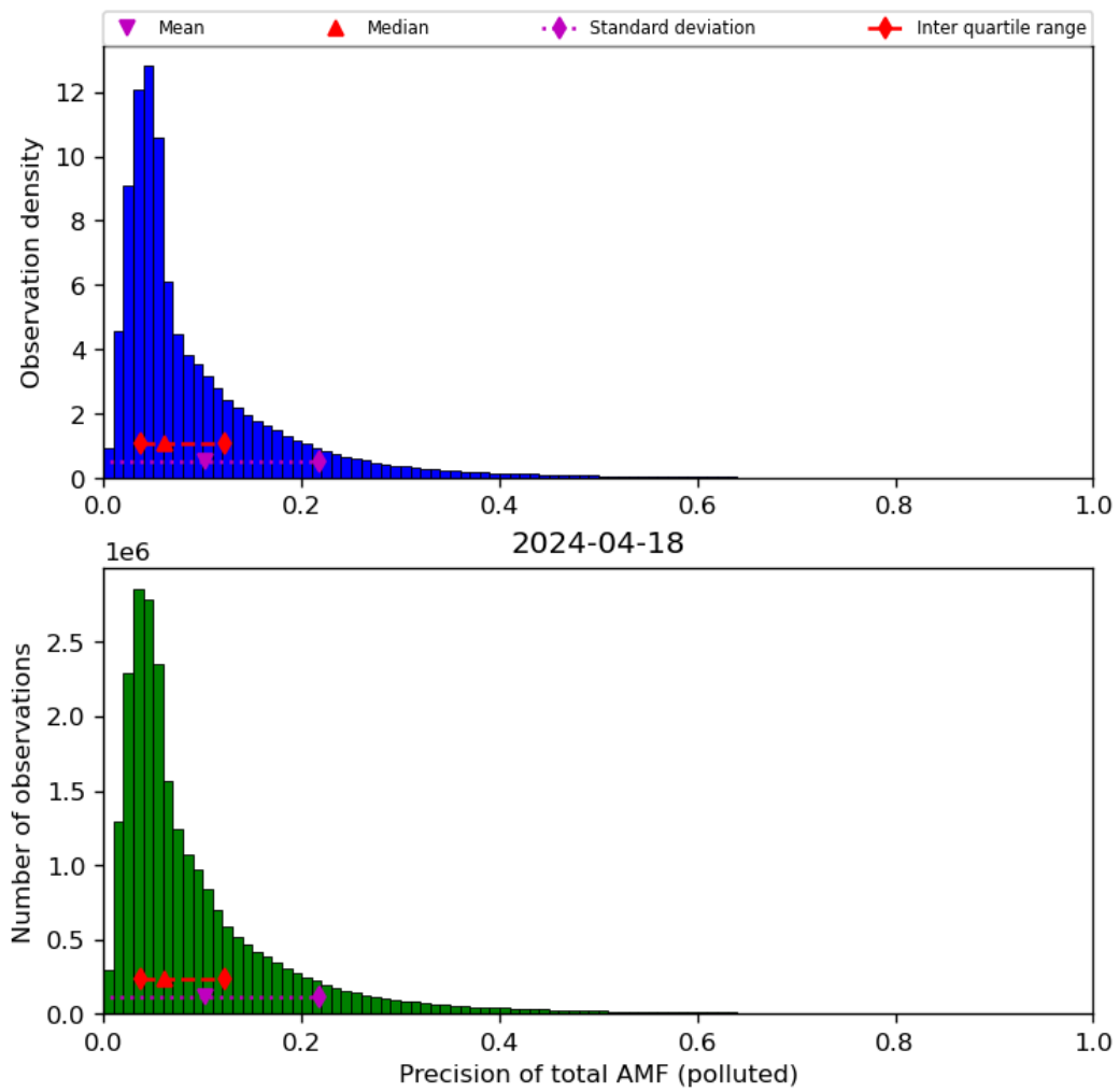
Figure 72: Histogram of “Precision of total AMF (polluted)” for 2024-04-17 to 2024-04-19
