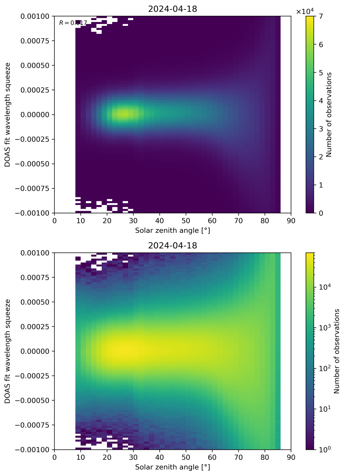
Figure 162: Scatter density plot of “Solar zenith angle” against “DOAS fit wavelength squeeze” for 2024-04-17 to 2024-04-19.
