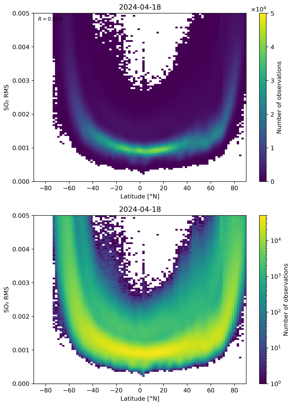
Figure 144: Scatter density plot of “Latitude” against “SO 2 RMS” for 2024-04-17 to 2024-04-19.
