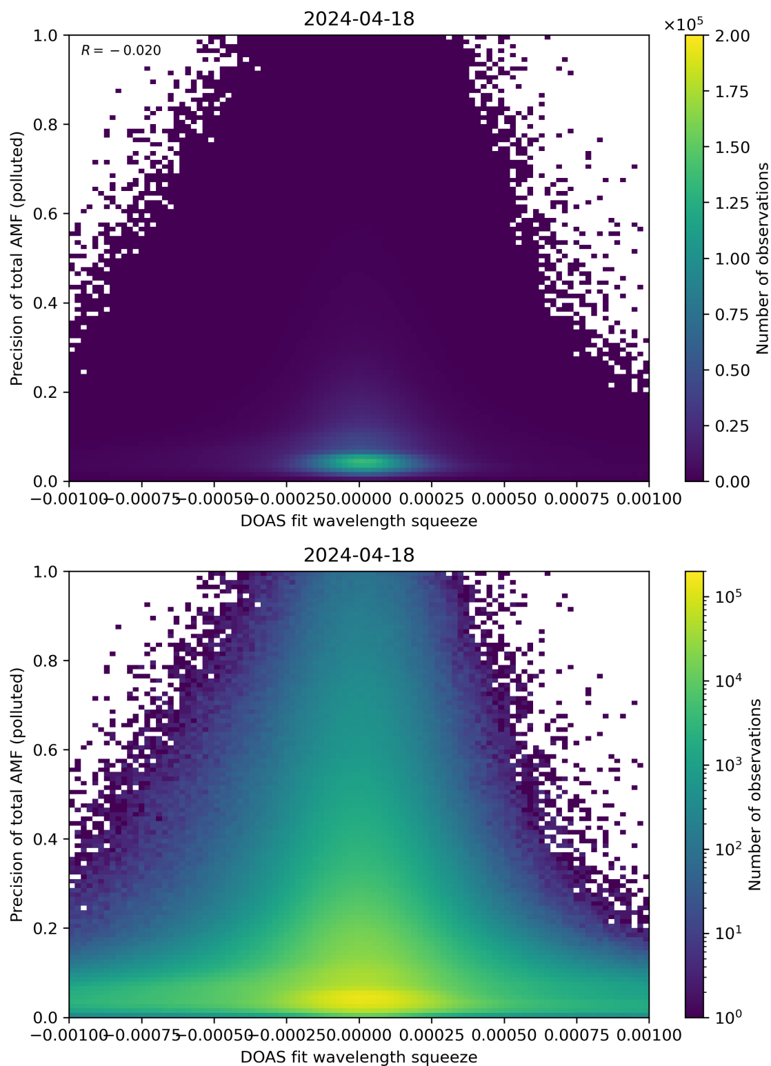
Figure 135: Scatter density plot of “DOAS fit wavelength squeeze” against “Precision of total AMF (polluted)” for 2024-04-17 to 2024-04-19.
