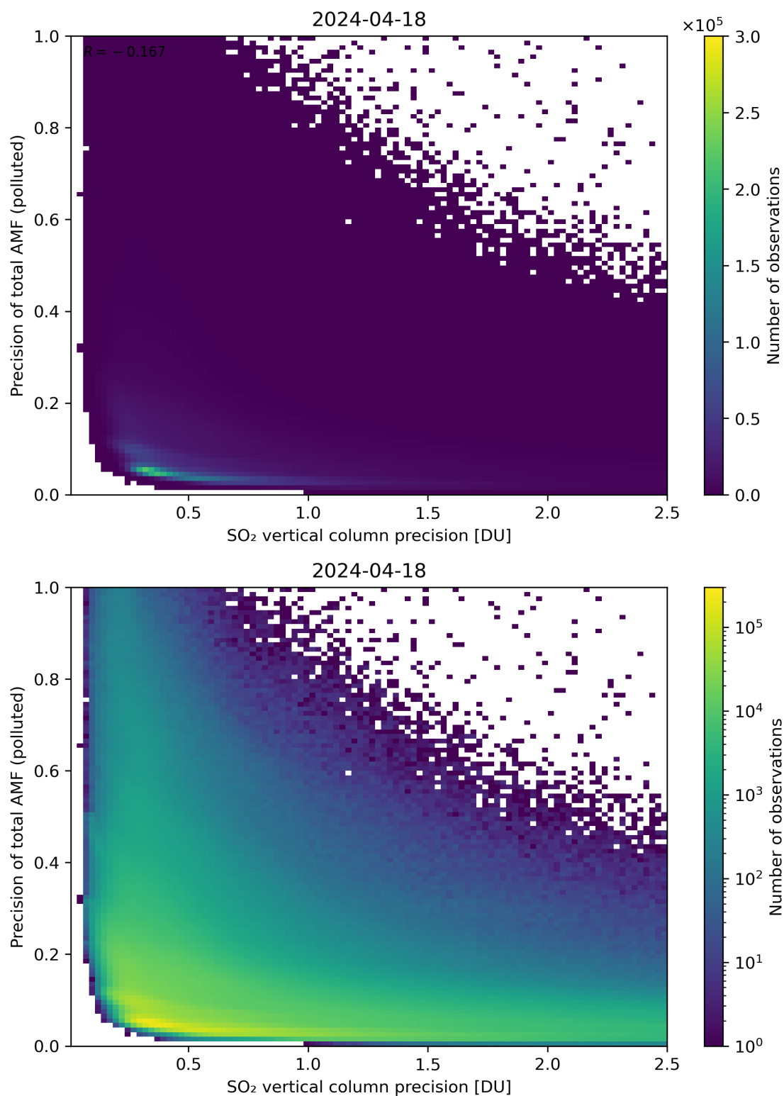
Figure 295: Scatter density plot of “SO 2 vertical column precision” against “Precision of total AMF (polluted)” for 2024-04-17 to 2024-04-19.
