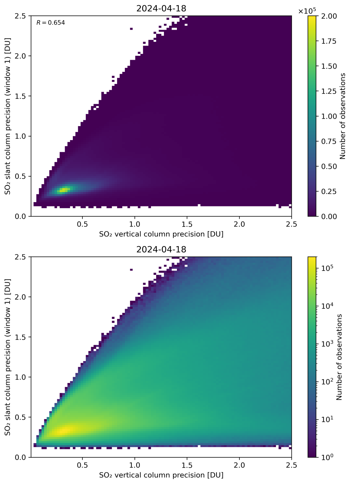
Figure 290: Scatter density plot of “SO 2 vertical column precision” against “SO 2 slant column precision (window 1)” for 2024-04-17 to 2024-04-19.
