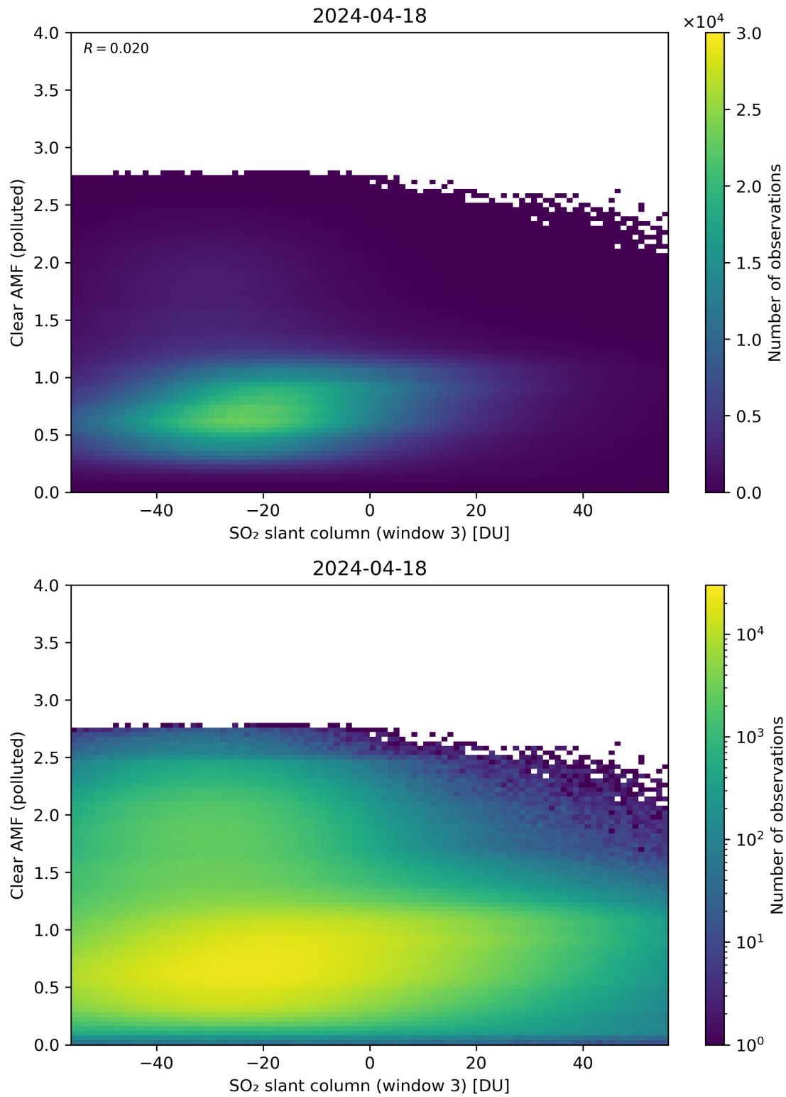
Figure 265: Scatter density plot of “SO 2 slant column (window 3)” against “Clear AMF (polluted)” for 2024-04-17 to 2024-04-19.
