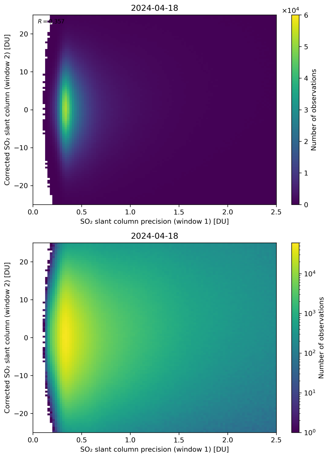
Figure 225: Scatter density plot of “SO 2 slant column precision (window 1)” against “Corrected SO 2 slant column (window 2)” for 2024-04-17 to 2024-04-19.
