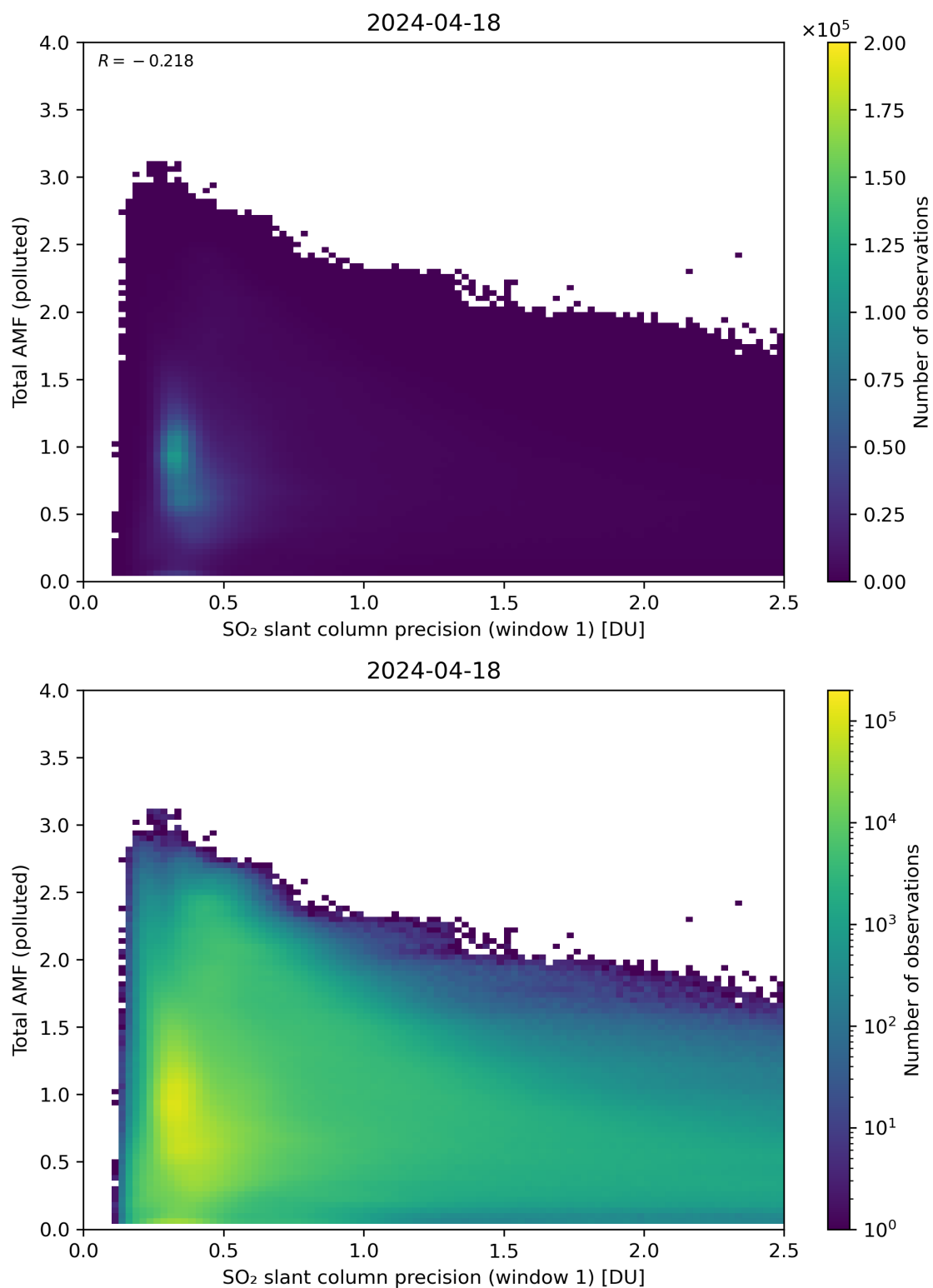
Figure 230: Scatter density plot of “SO 2 slant column precision (window 1)” against “Total AMF (polluted)” for 2024-04-17 to 2024-04-19.
