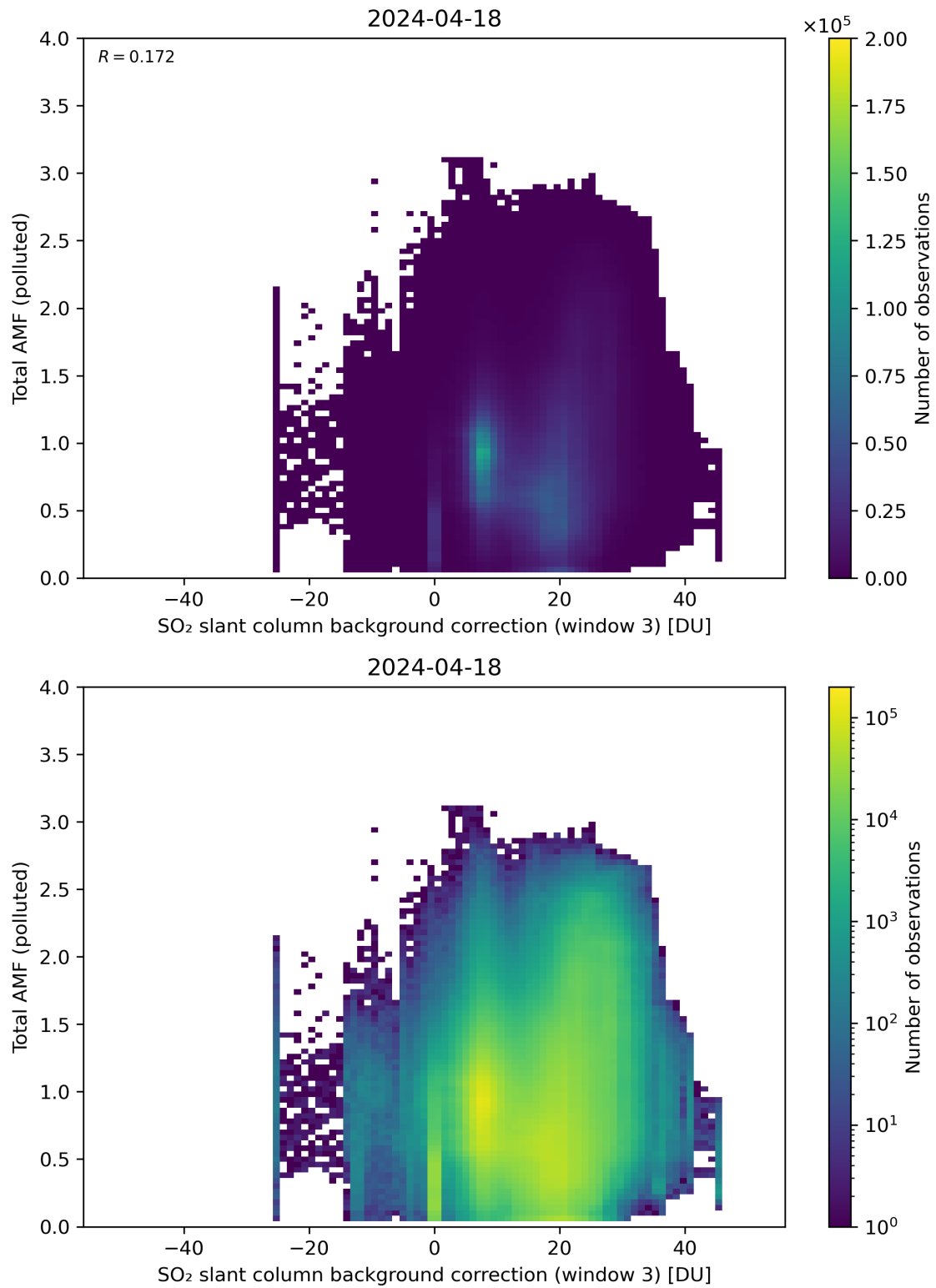
Figure 125: Scatter density plot of “SO 2 slant column background correction (window 3)” against “Total AMF (polluted)” for 2024-04-17 to 2024-04-19.
