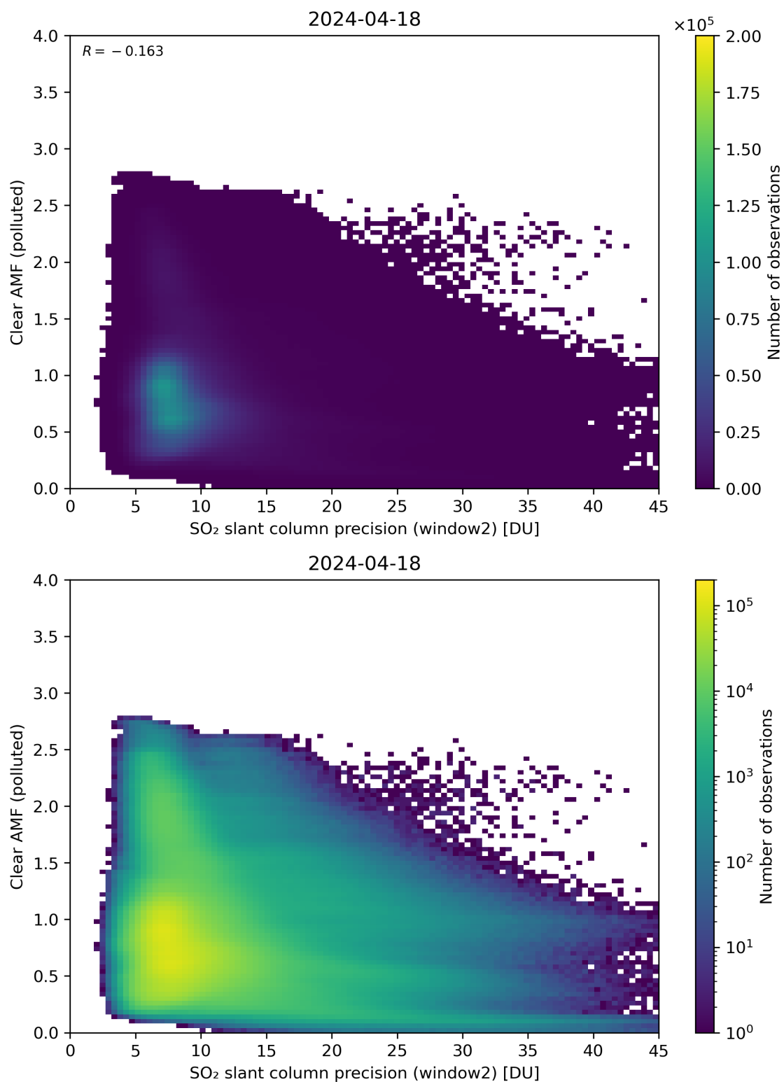
Figure 246: Scatter density plot of “SO 2 slant column precision (window2)” against “Clear AMF (polluted)” for 2024-04-17 to 2024-04-19.
