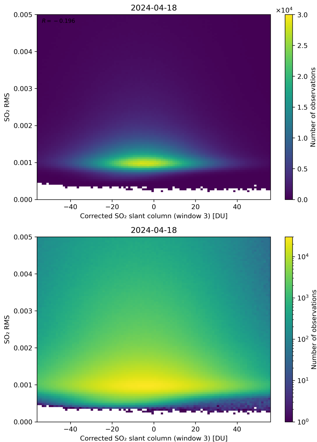
Figure 208: Scatter density plot of “Corrected SO 2 slant column (window 3)” against “SO 2 RMS” for 2024-04-17 to 2024-04-19.
