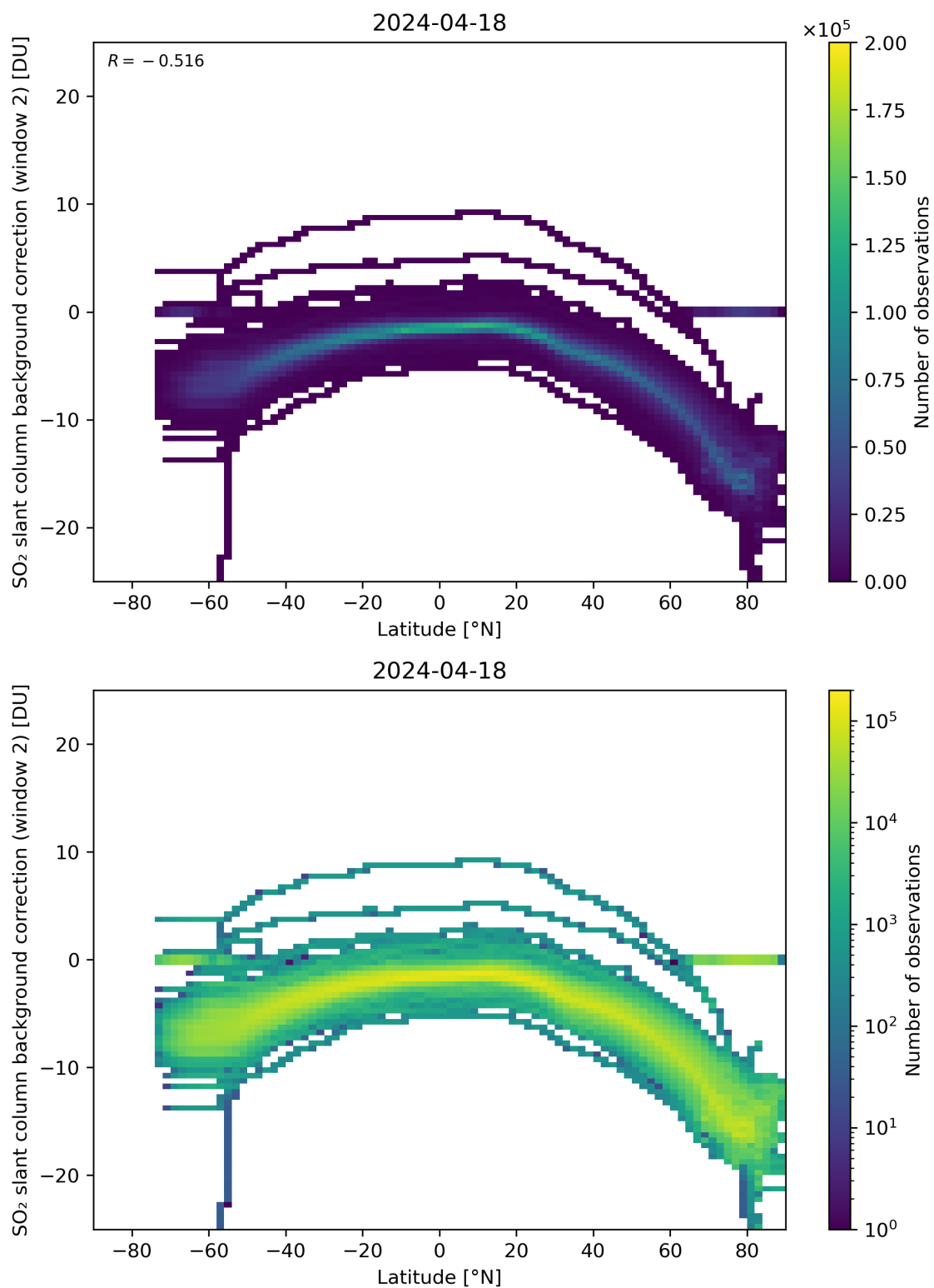
Figure 140: Scatter density plot of “Latitude” against “SO 2 slant column background correction (window 2)” for 2024-04-17 to 2024-04-19.
