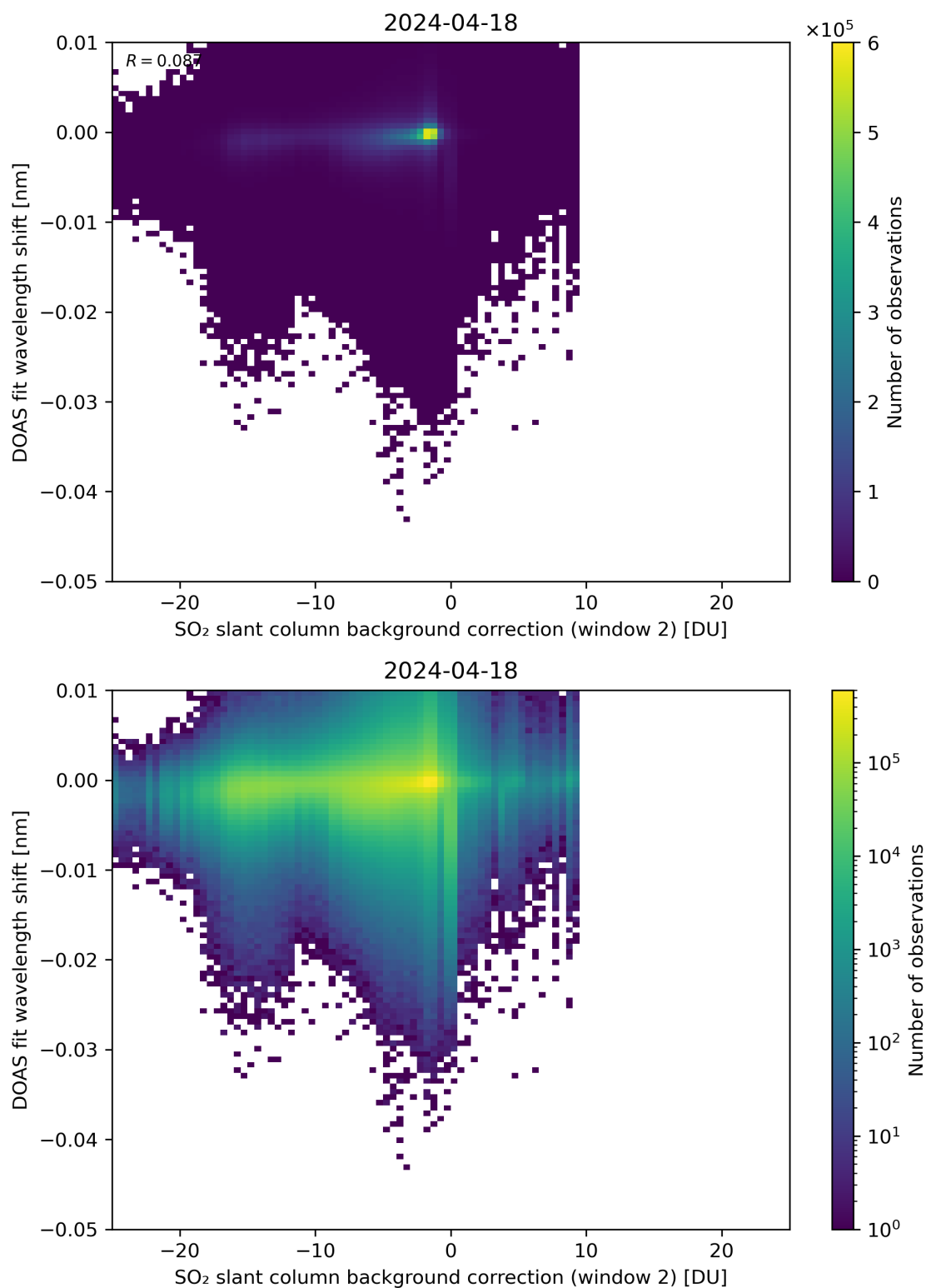
Figure 112: Scatter density plot of “SO 2 slant column background correction (window 2)” against “DOAS fit wavelength shift” for 2024-04-17 to 2024-04-19.
