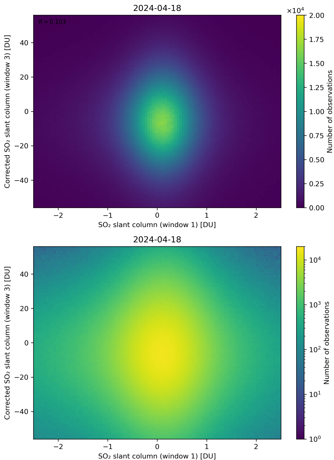
Figure 234: Scatter density plot of “SO 2 slant column (window 1)” against “Corrected SO 2 slant column (window 3)” for 2024-04-17 to 2024-04-19.
