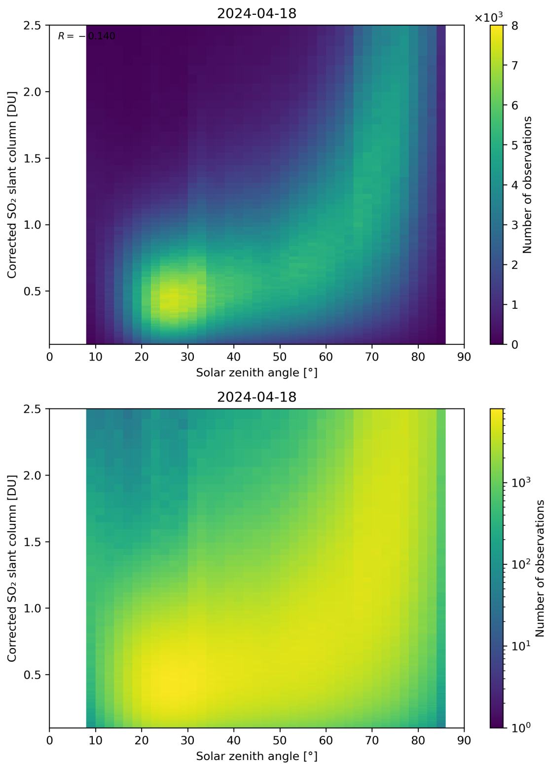
Figure 166: Scatter density plot of “Solar zenith angle” against “Corrected SO 2 slant column” for 2024-04-17 to 2024-04-19.
