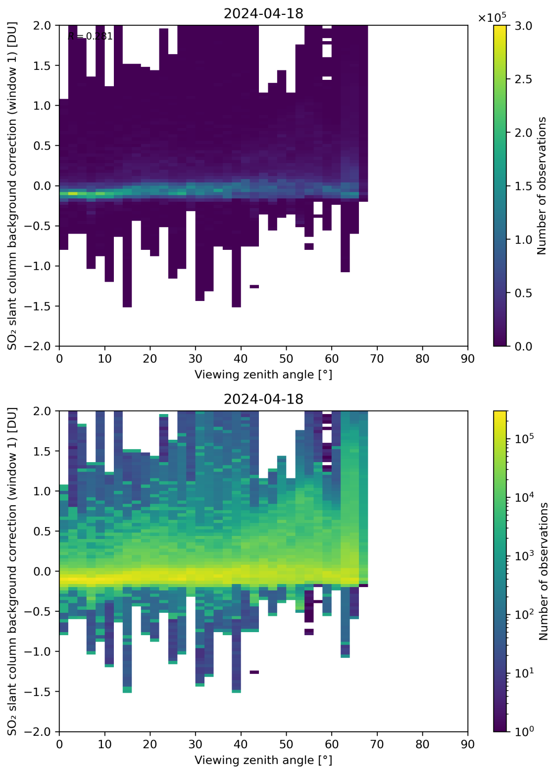
Figure 308: Scatter density plot of “Viewing zenith angle” against “SO 2 slant column background correction (window 1)” for 2024-04-17 to 2024-04-19.
