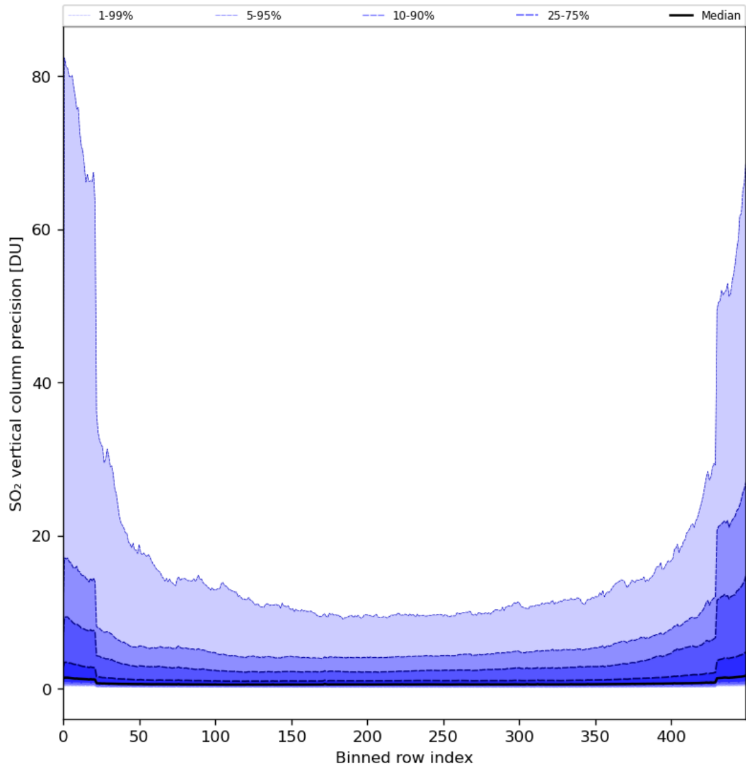
Figure 77: Along track statistics of “SO 2 vertical column precision” for 2024-04-17 to 2024-04-19
