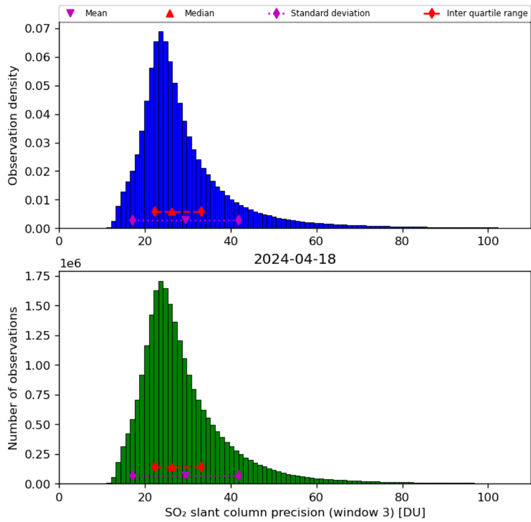
Figure 65: Histogram of “SO 2 slant column precision (window 3)” for 2024-04-17 to 2024-04-19
