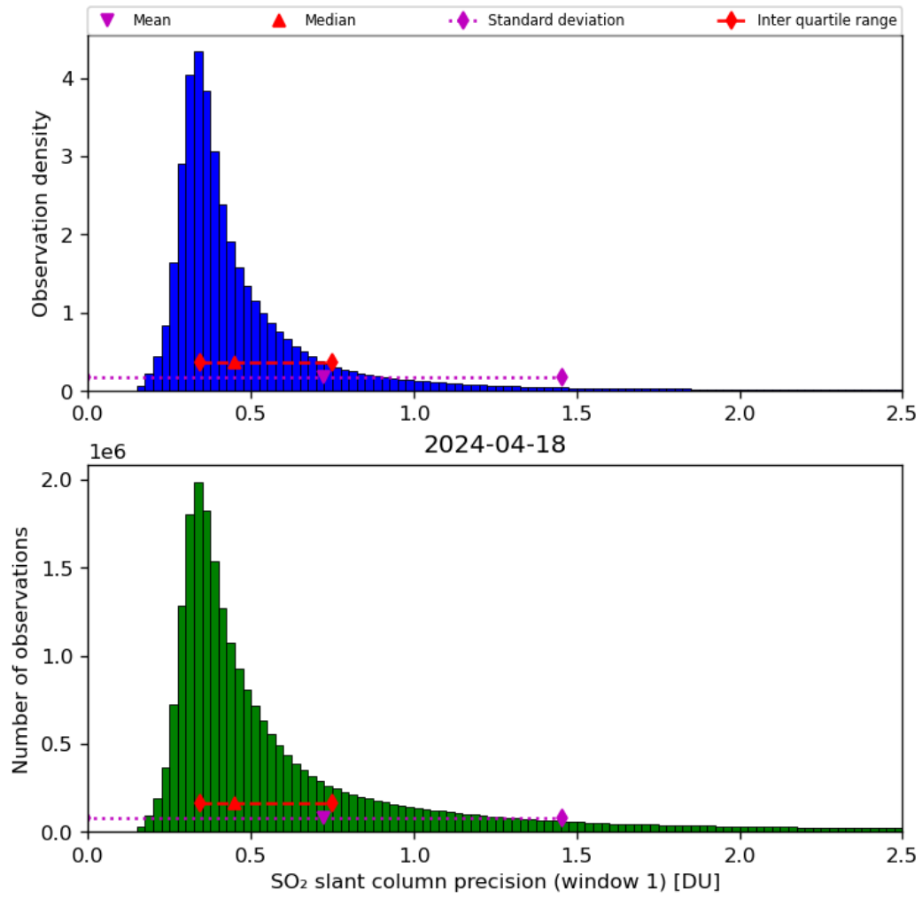
Figure 57: Histogram of “SO 2 slant column precision (window 1)” for 2024-04-17 to 2024-04-19
