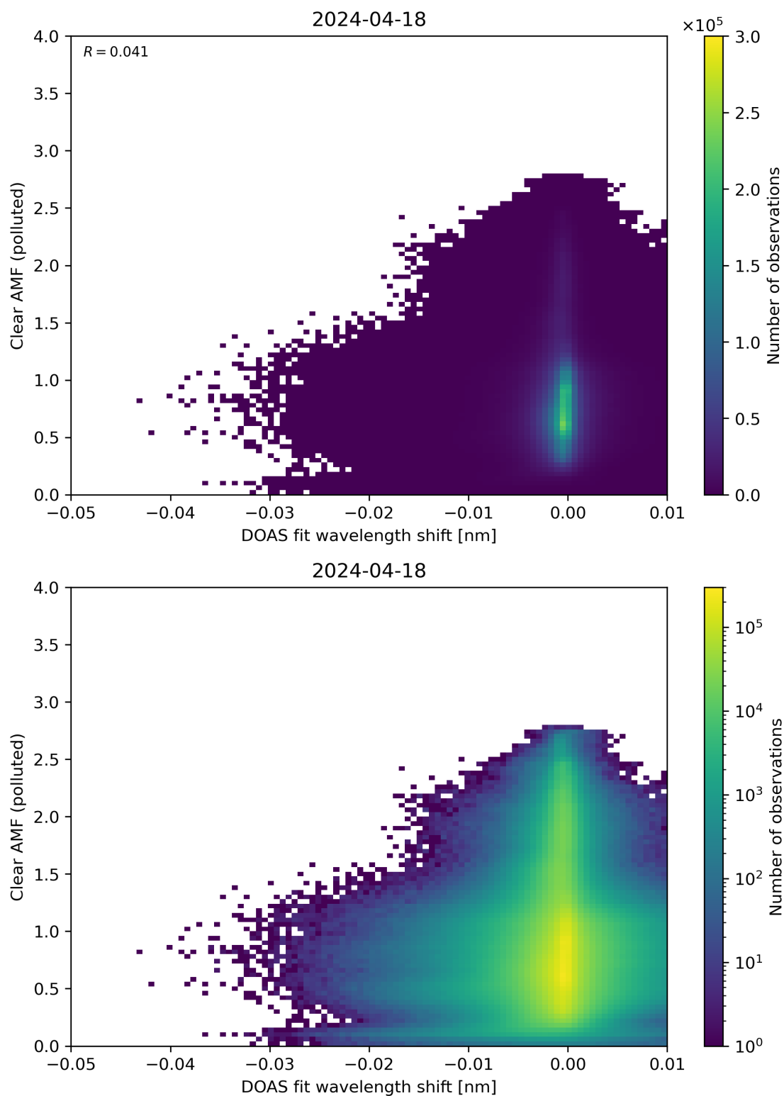
Figure 129: Scatter density plot of “DOAS fit wavelength shift” against “Clear AMF (polluted)” for 2024-04-17 to 2024-04-19.
