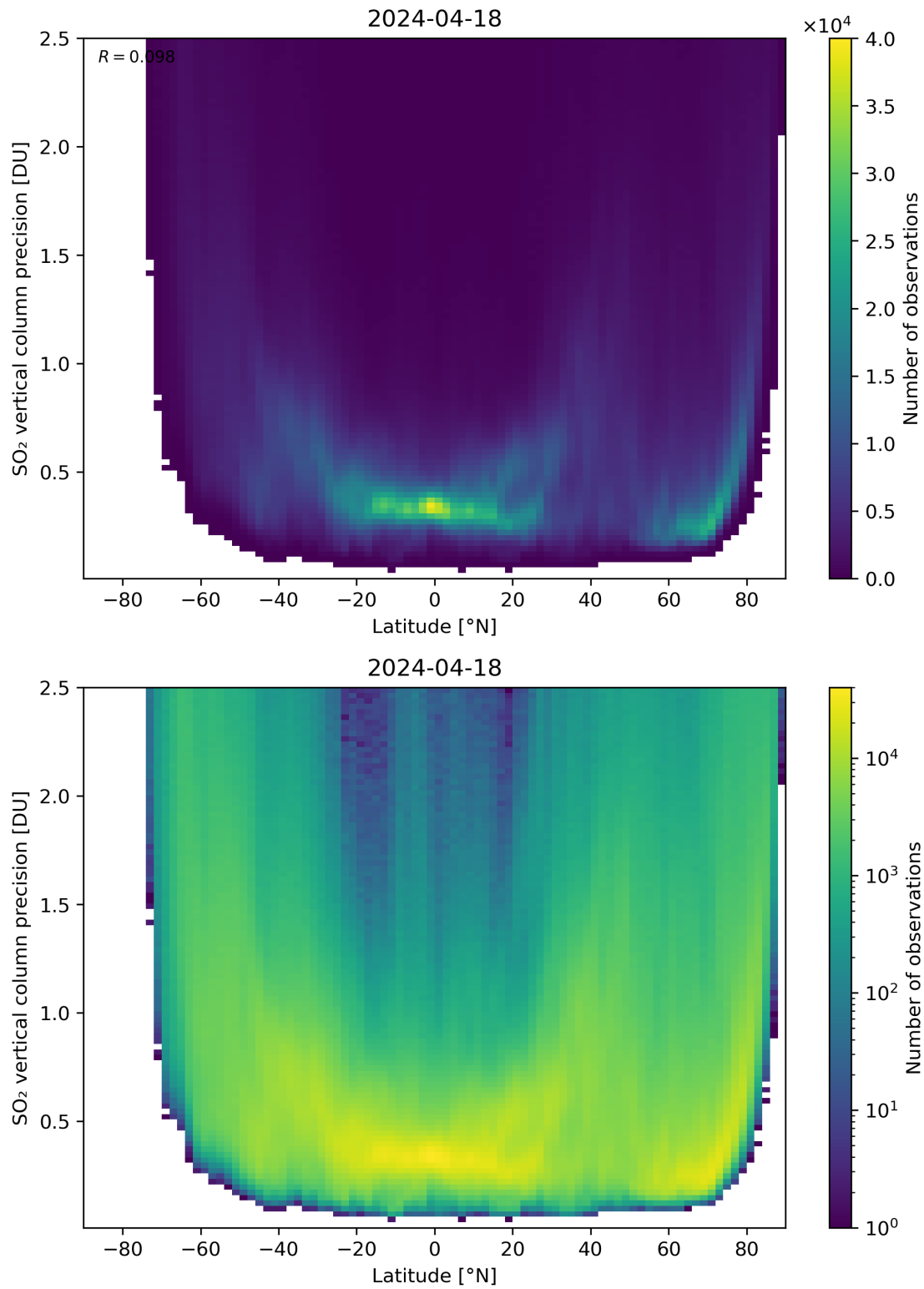
Figure 157: Scatter density plot of “Latitude” against “SO 2 vertical column precision” for 2024-04-17 to 2024-04-19.
