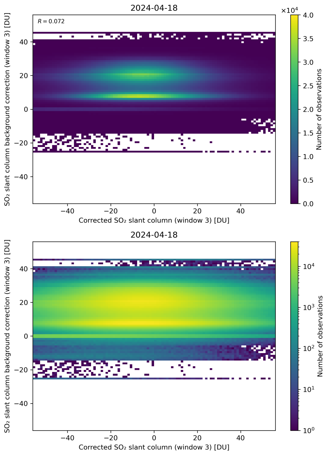
Figure 205: Scatter density plot of “Corrected SO 2 slant column (window 3)” against “SO 2 slant column background correction (window 3)” for 2024-04-17 to 2024-04-19.
