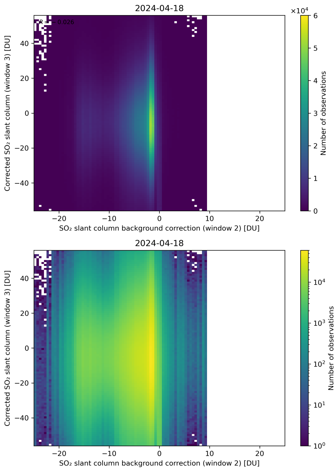
Figure 116: Scatter density plot of “SO 2 slant column background correction (window 2)” against “Corrected SO 2 slant column (window 3)” for 2024-04-17 to 2024-04-19.
