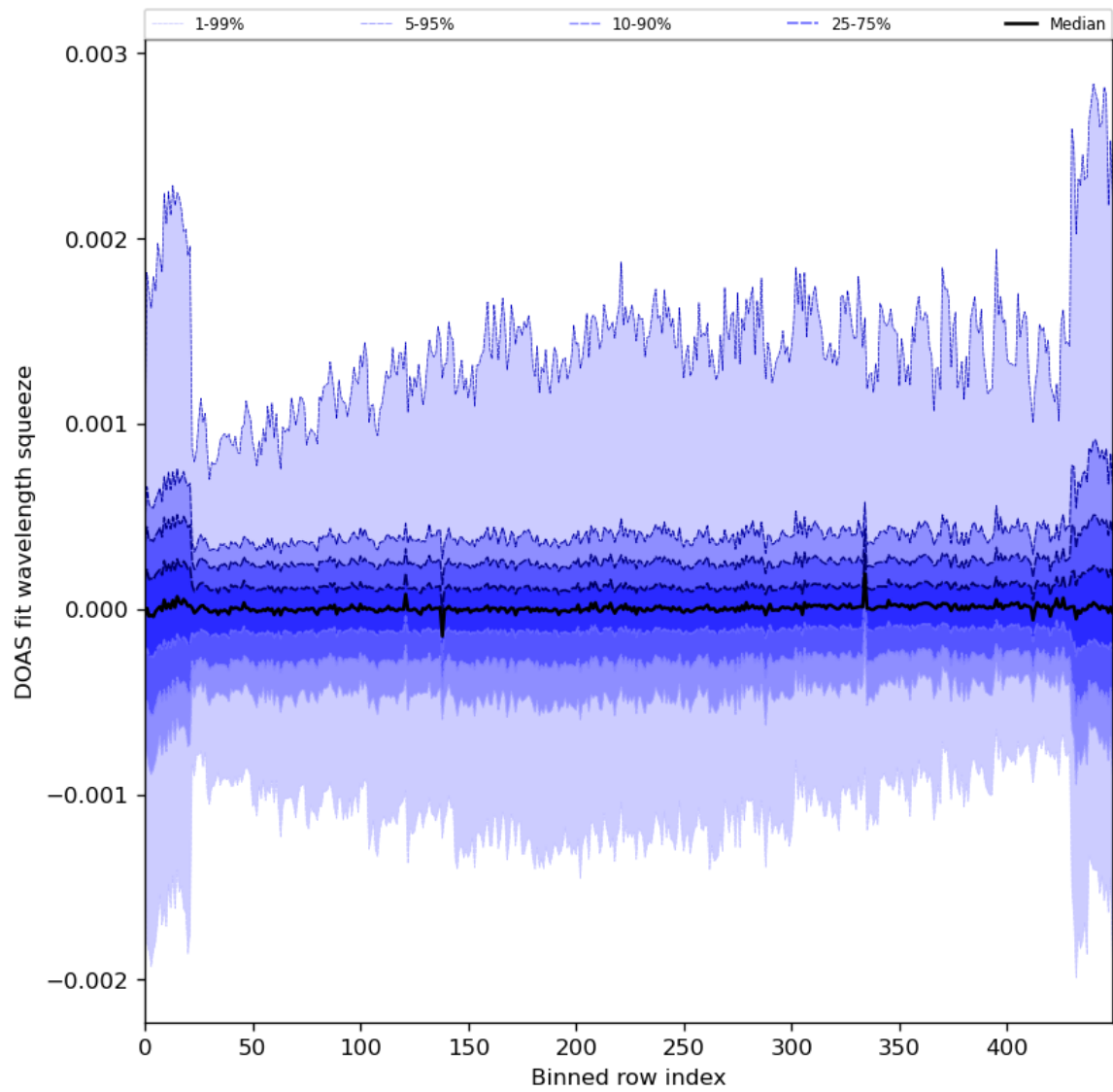
Figure 92: Along track statistics of “DOAS fit wavelength squeeze” for 2024-04-17 to 2024-04-19
