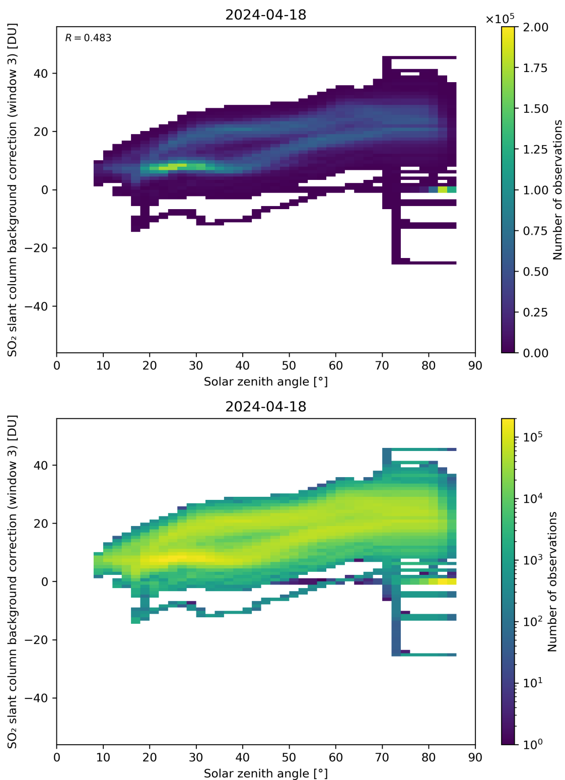
Figure 160: Scatter density plot of “Solar zenith angle” against “SO 2 slant column background correction (window 3)” for 2024-04-17 to 2024-04-19.
