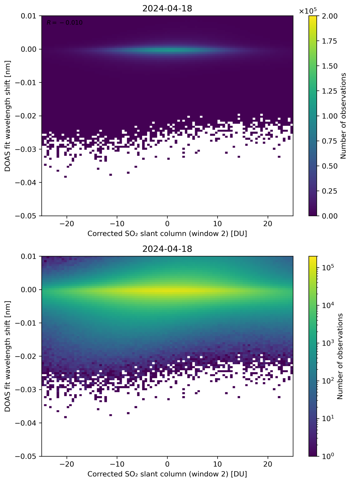
Figure 196: Scatter density plot of “Corrected SO 2 slant column (window 2)” against “DOAS fit wavelength shift” for 2024-04-17 to 2024-04-19.
