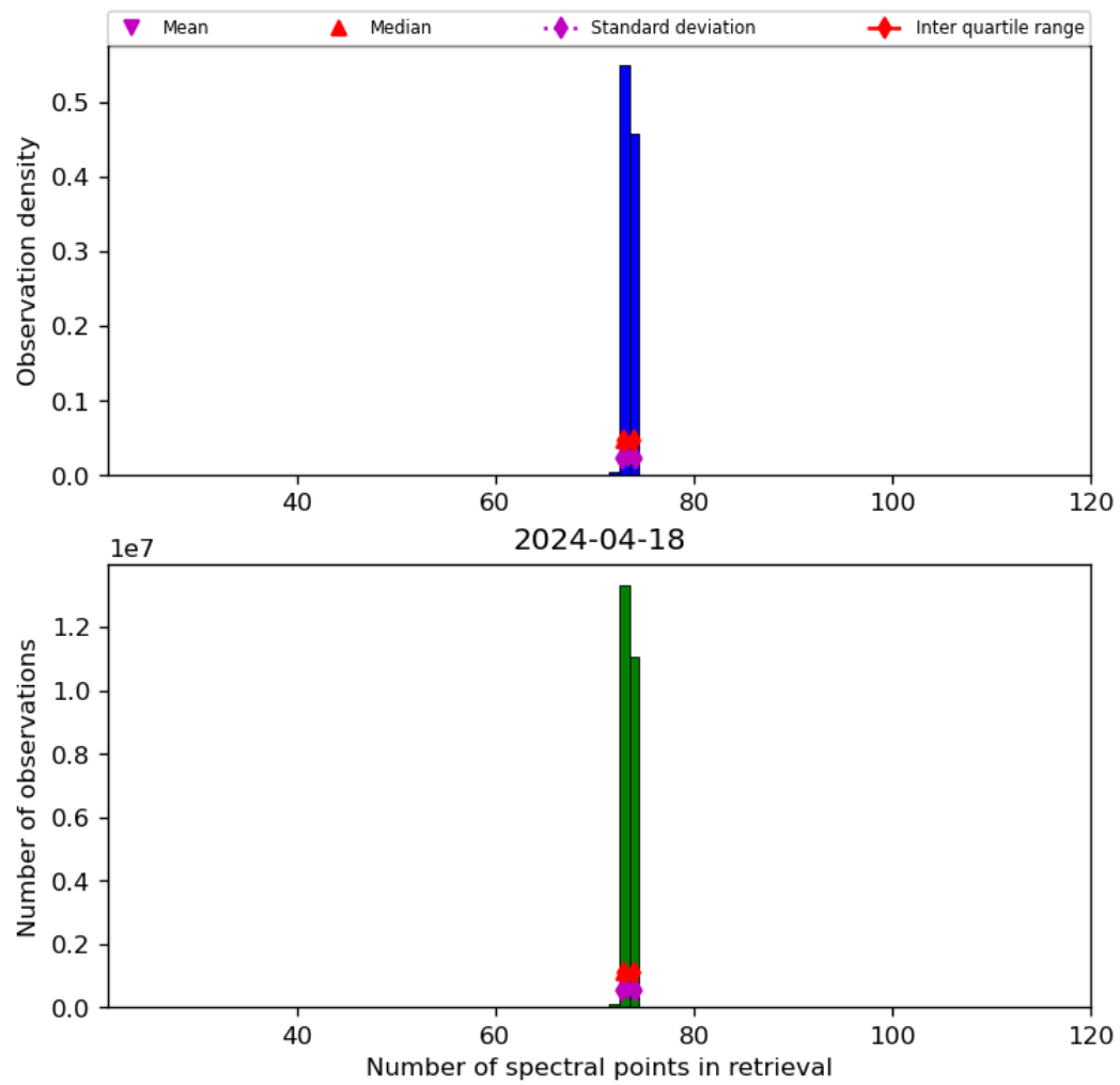
Figure 74: Histogram of “Number of spectral points in retrieval” for 2024-04-17 to 2024-04-19
