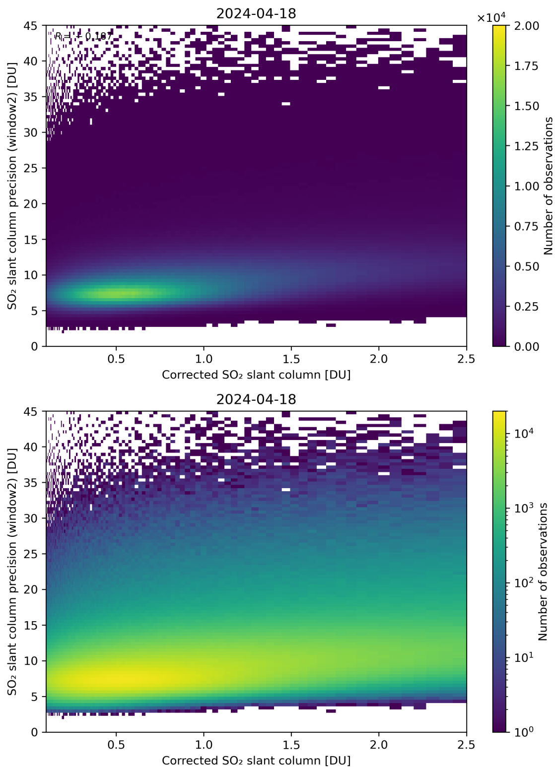
Figure 189: Scatter density plot of “Corrected SO 2 slant column” against “SO 2 slant column precision (window2)” for 2024-04-17 to 2024-04-19.
