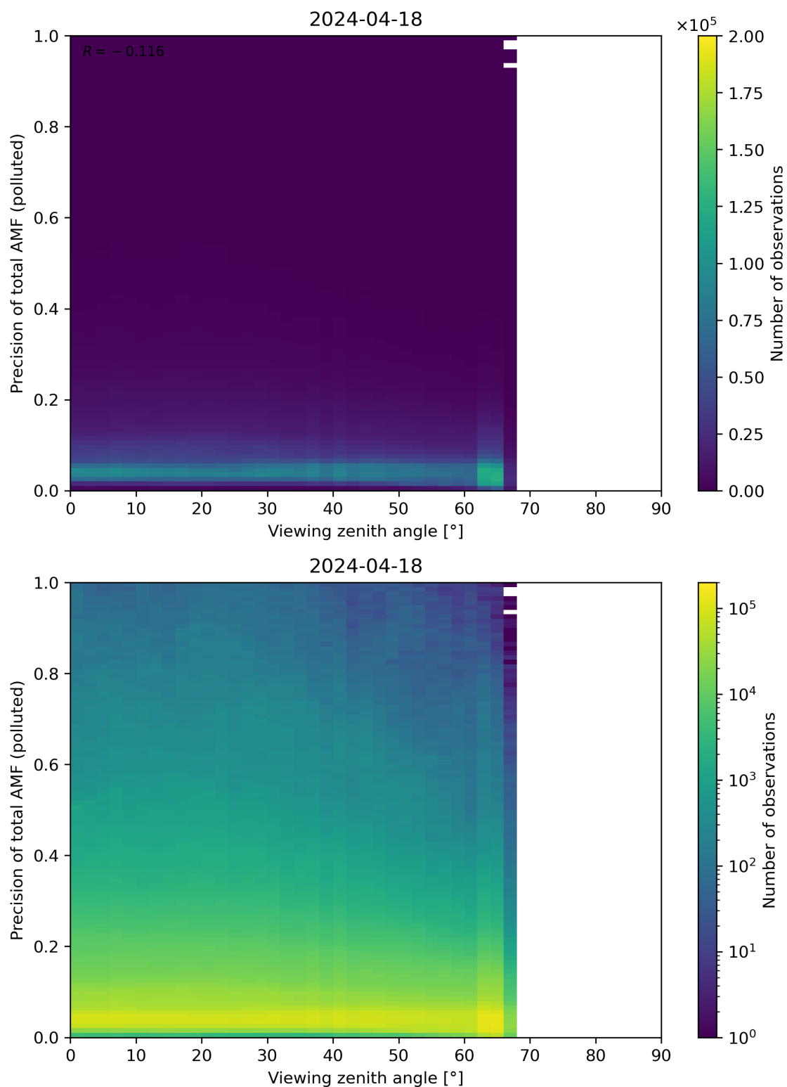
Figure 326: Scatter density plot of “Viewing zenith angle” against “Precision of total AMF (polluted)” for 2024-04-17 to 2024-04-19.
