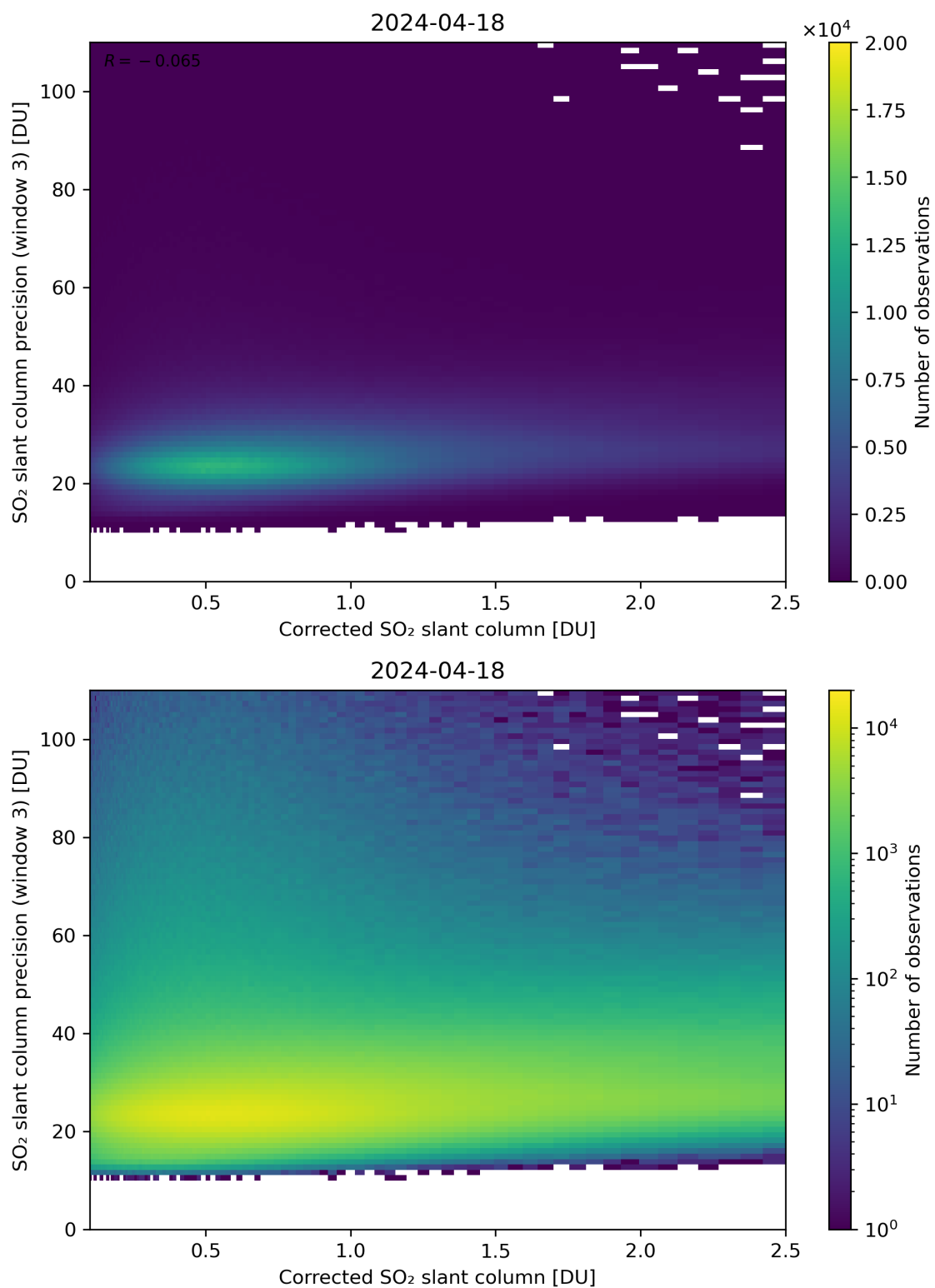
Figure 191: Scatter density plot of “Corrected SO 2 slant column” against “SO 2 slant column precision (window 3)” for 2024-04-17 to 2024-04-19.
