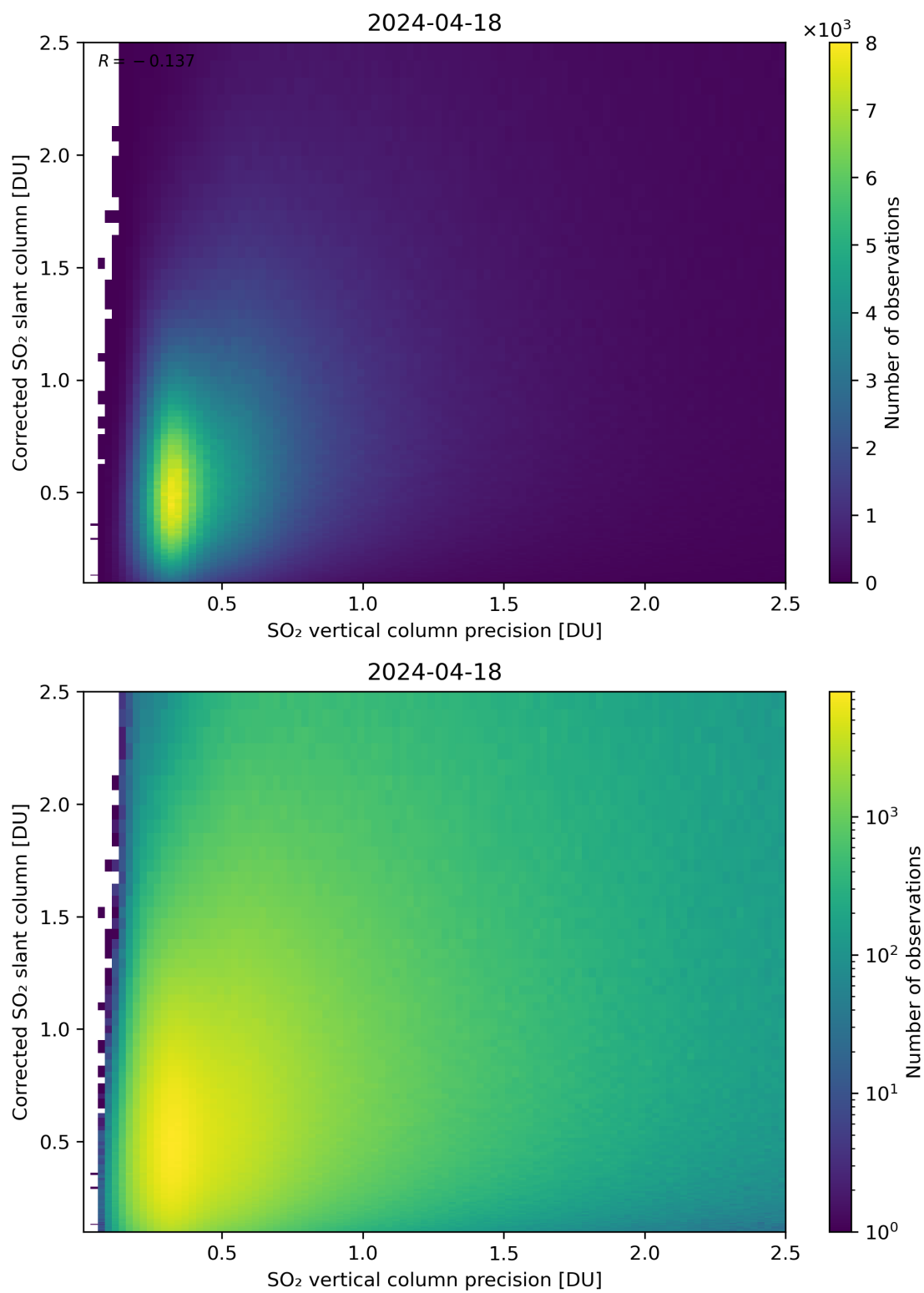
Figure 286: Scatter density plot of “SO 2 vertical column precision” against “Corrected SO 2 slant column” for 2024-04-17 to 2024-04-19.
