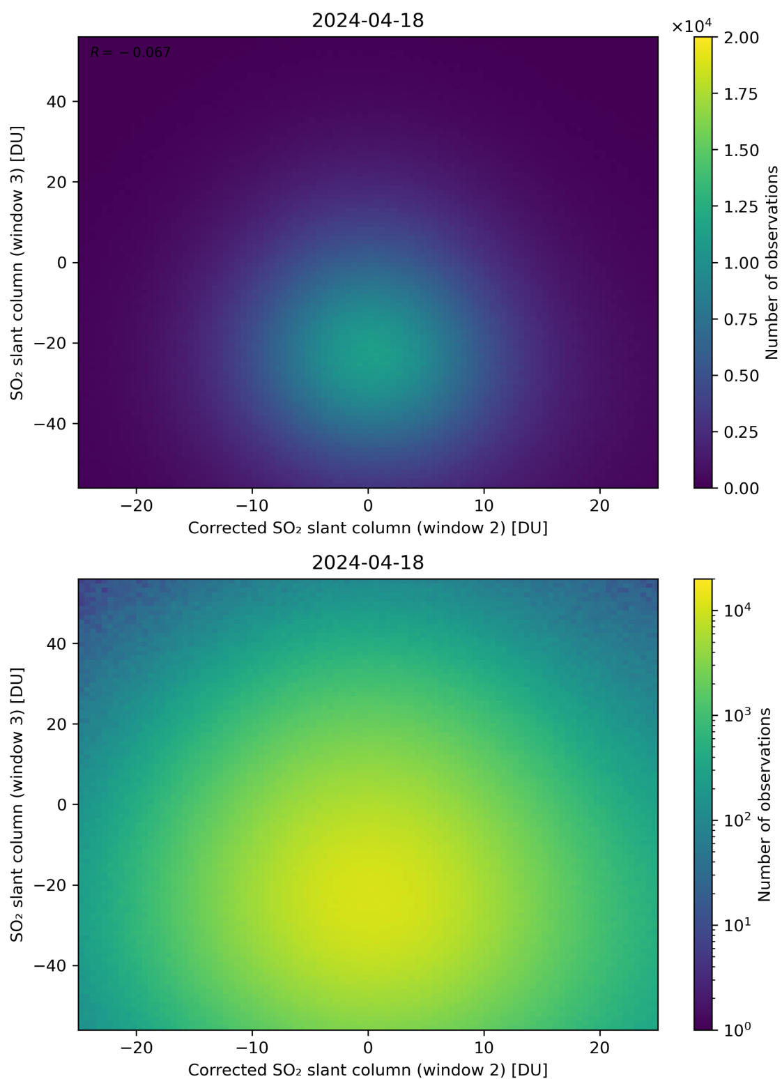
Figure 201: Scatter density plot of “Corrected SO 2 slant column (window 2)” against “SO 2 slant column (window 3)” for 2024-04-17 to 2024-04-19.
