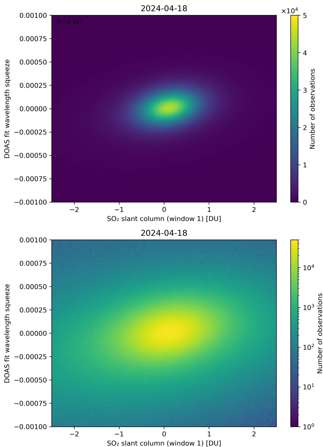
Figure 216: Scatter density plot of “SO 2 slant column (window 1)” against “DOAS fit wavelength squeeze” for 2024-04-17 to 2024-04-19.
