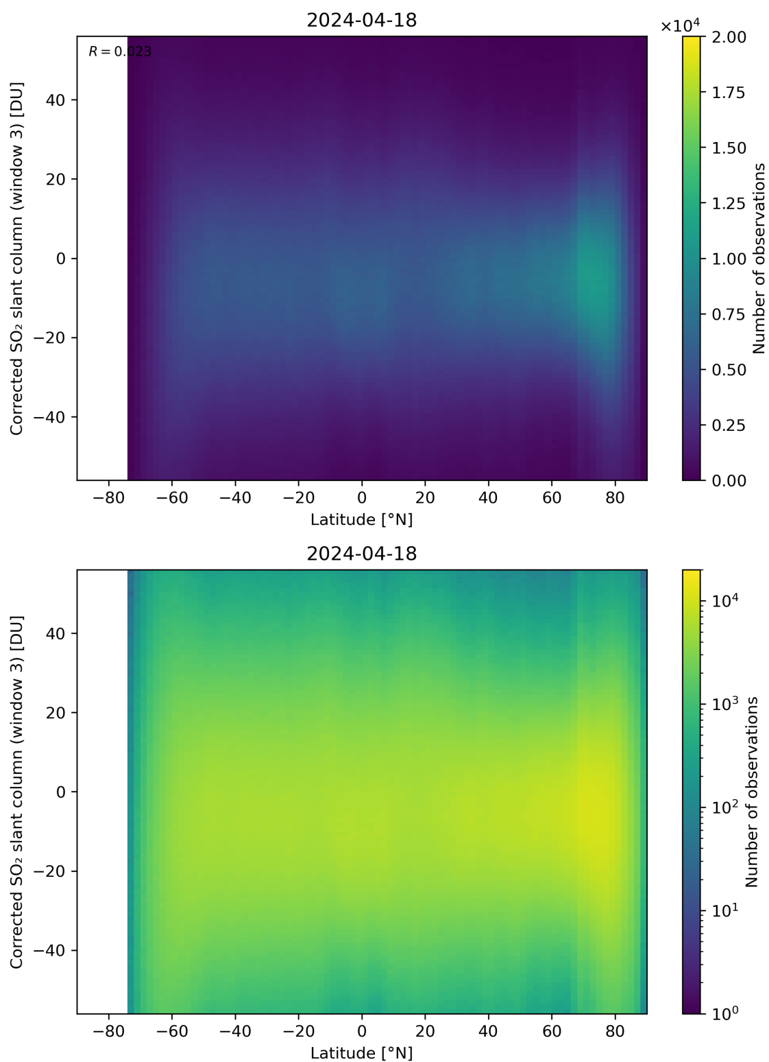
Figure 148: Scatter density plot of “Latitude” against “Corrected SO 2 slant column (window 3)” for 2024-04-17 to 2024-04-19.
