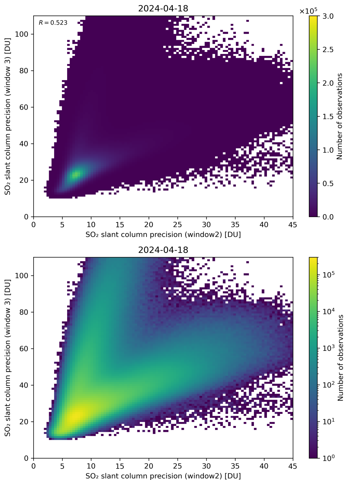
Figure 250: Scatter density plot of “SO 2 slant column precision (window2)” against “SO 2 slant column precision (window 3)” for 2024-04-17 to 2024-04-19.
