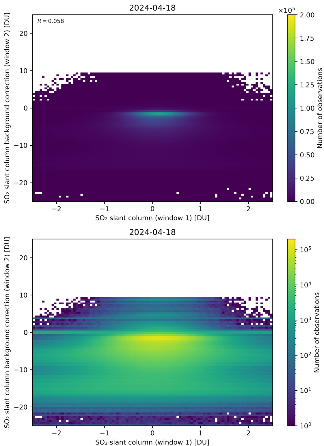
Figure 213: Scatter density plot of “SO 2 slant column (window 1)” against “SO 2 slant column background correction (window 2)” for 2024-04-17 to 2024-04-19.
