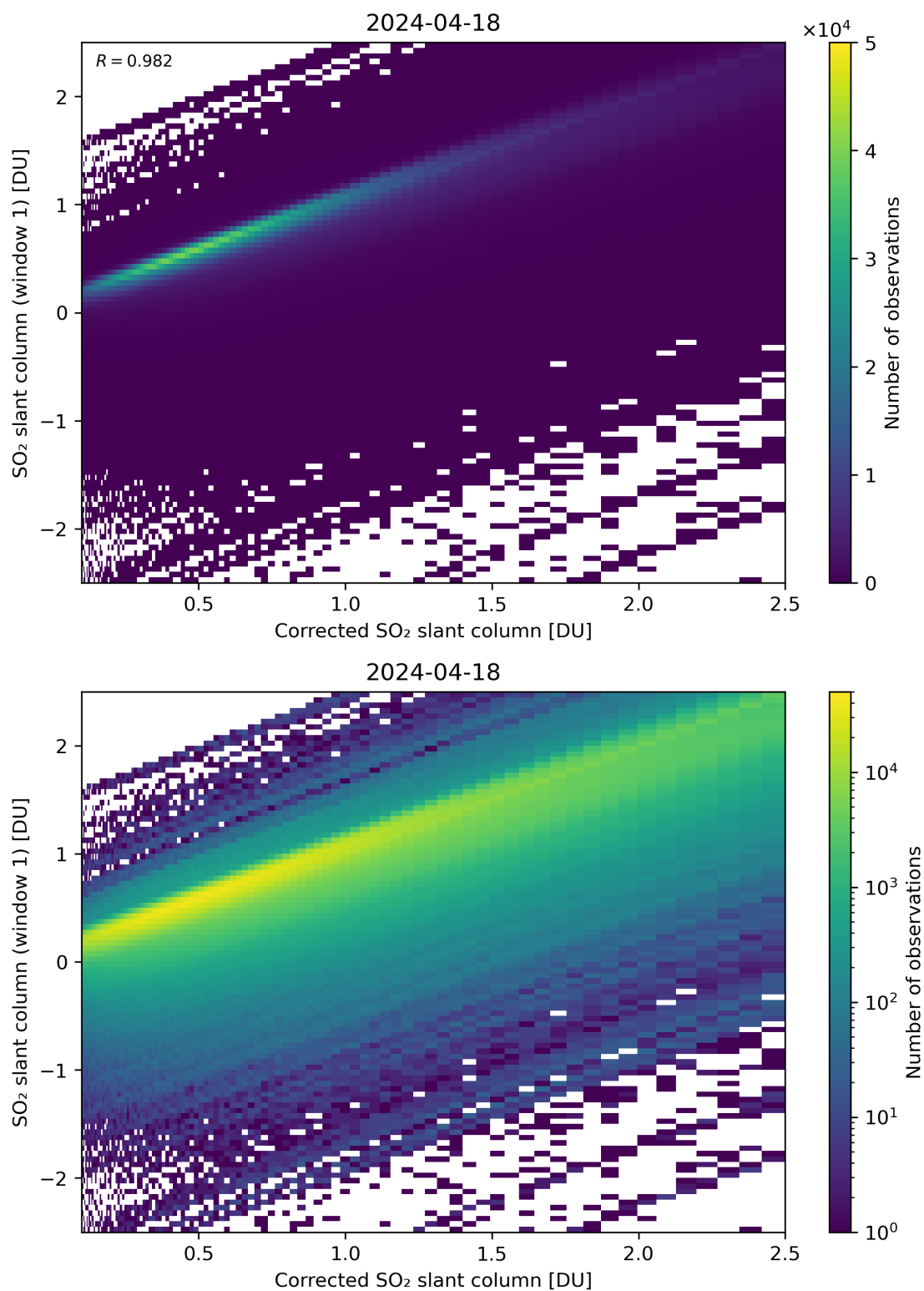
Figure 187: Scatter density plot of “Corrected SO 2 slant column” against “SO 2 slant column (window 1)” for 2024-04-17 to 2024-04-19.
