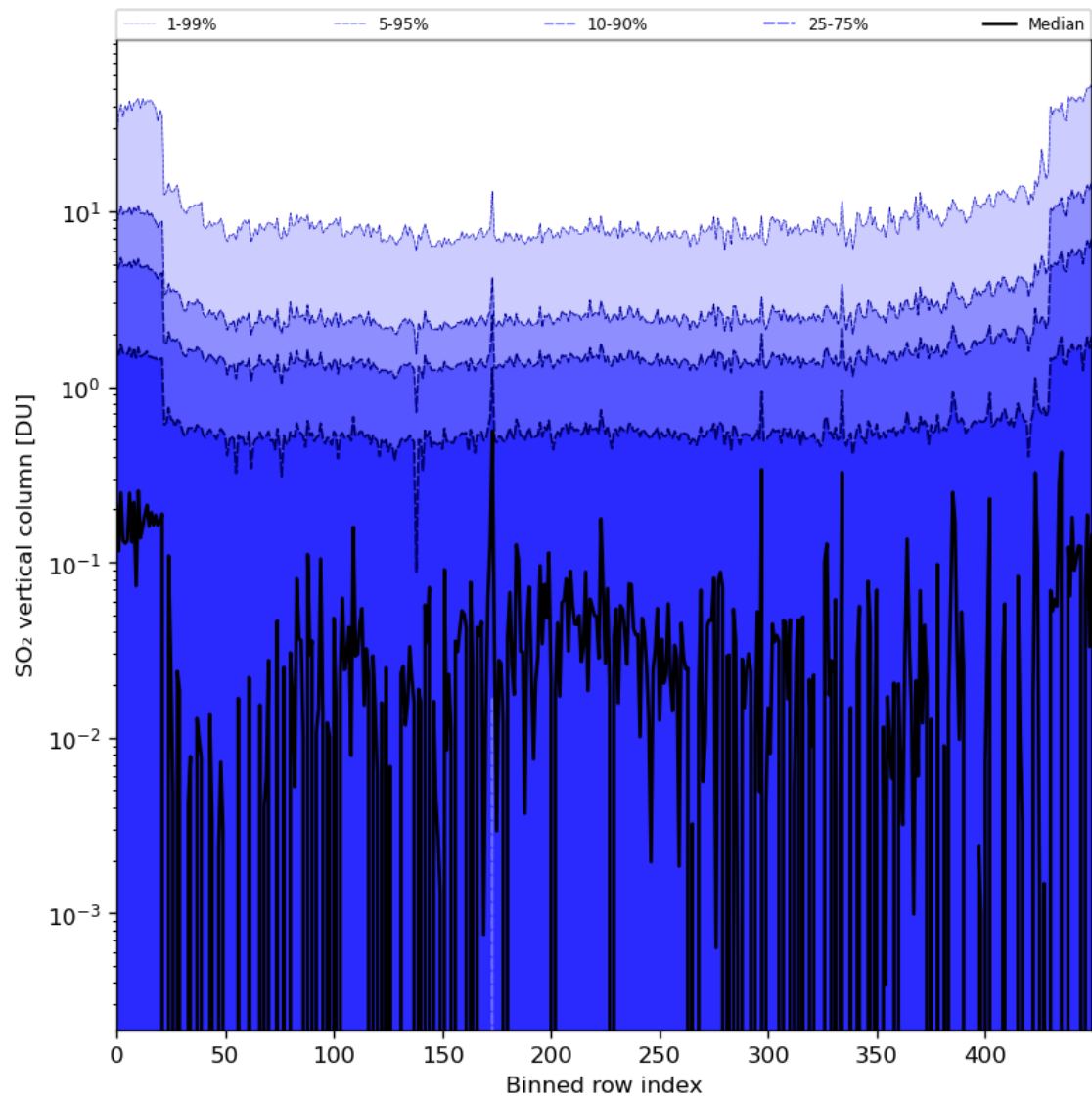
Figure 76: Along track statistics of “SO 2 vertical column” for 2024-04-17 to 2024-04-19
