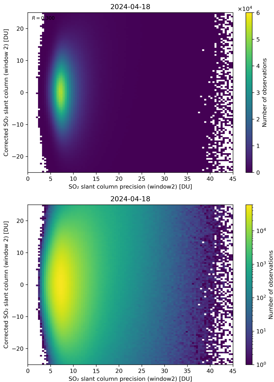
Figure 247: Scatter density plot of “SO 2 slant column precision (window2)” against “Corrected SO 2 slant column (window 2)” for 2024-04-17 to 2024-04-19.
