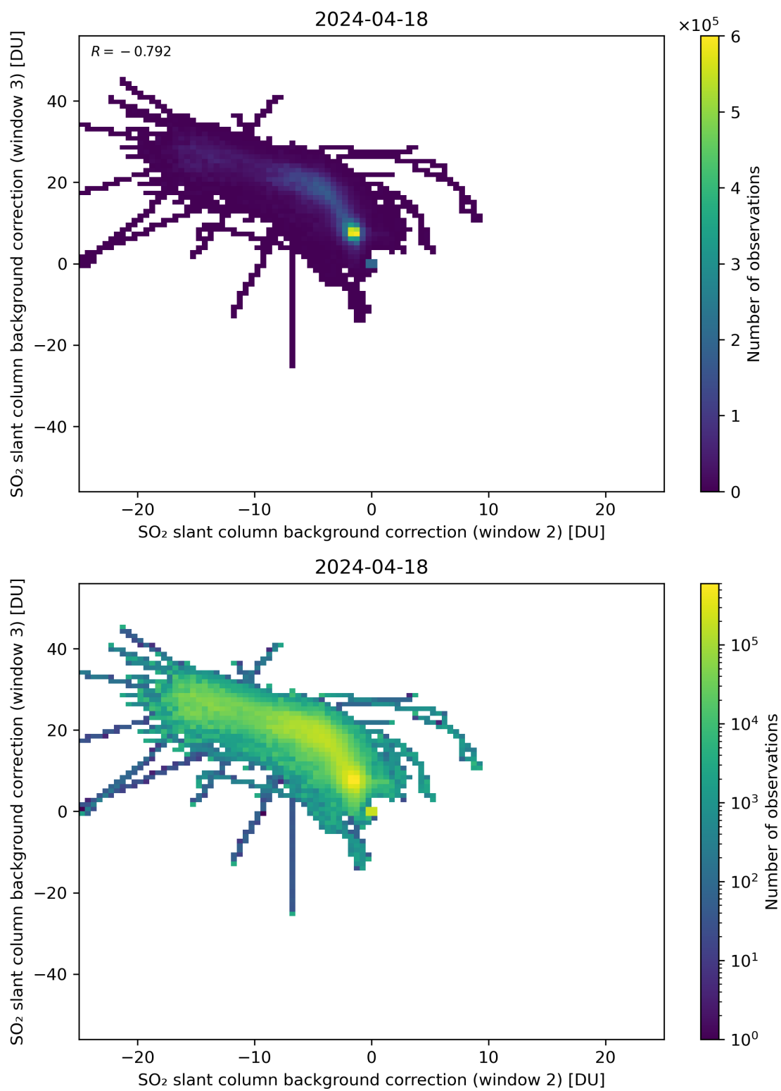
Figure 111: Scatter density plot of “SO 2 slant column background correction (window 2)” against “SO 2 slant column background correction (window 3)” for 2024-04-17 to 2024-04-19.
