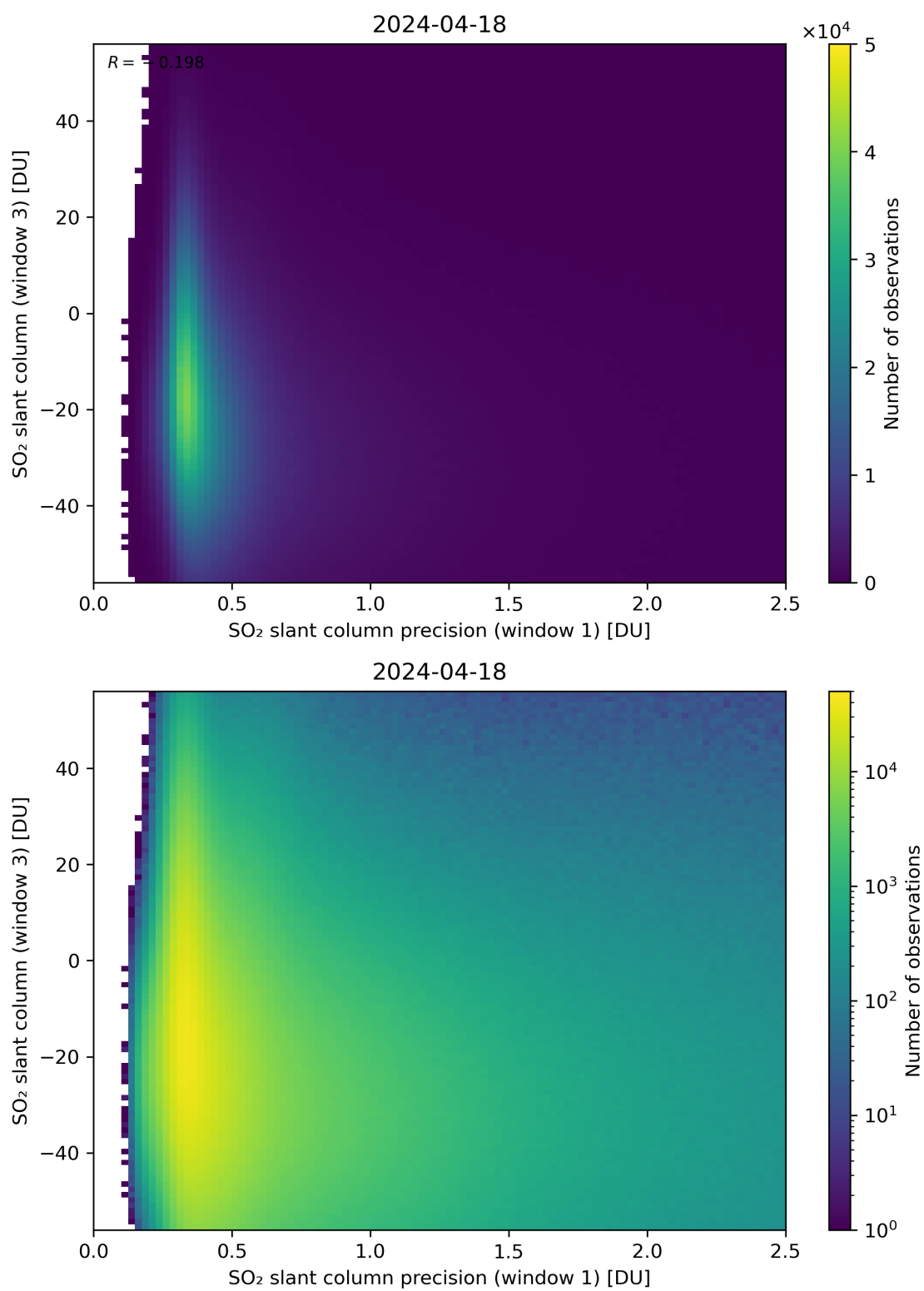
Figure 228: Scatter density plot of “SO 2 slant column precision (window 1)” against “SO 2 slant column (window 3)” for 2024-04-17 to 2024-04-19.
