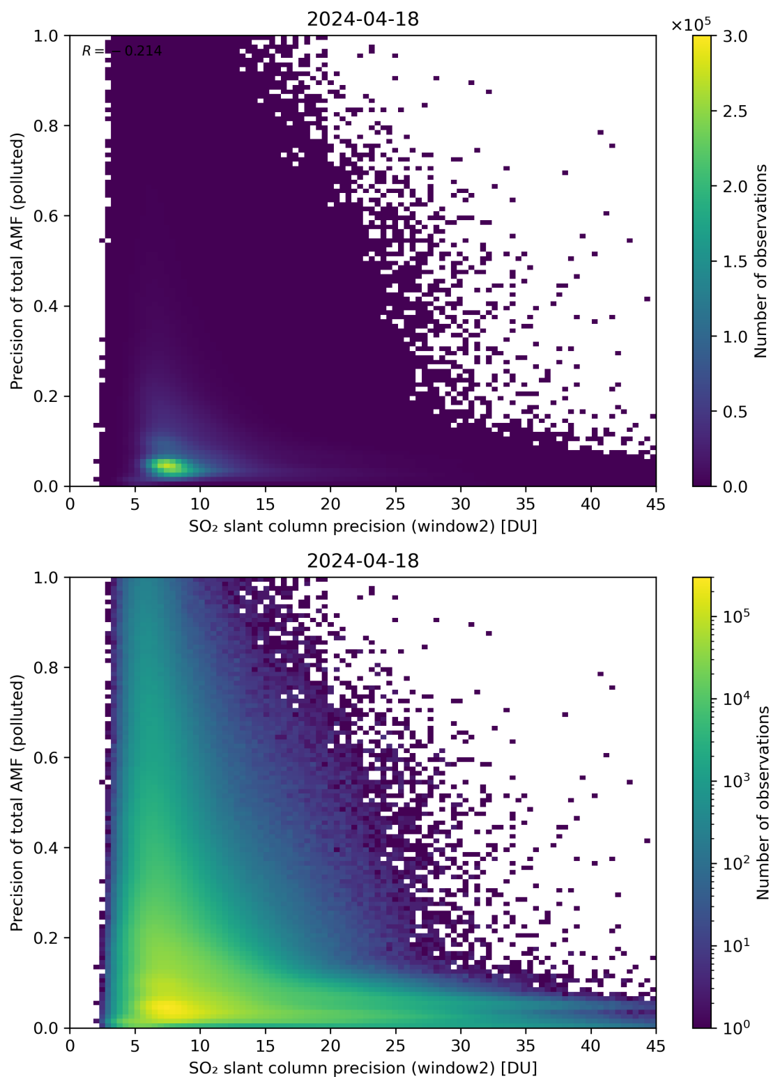
Figure 252: Scatter density plot of “SO 2 slant column precision (window2)” against “Precision of total AMF (polluted)” for 2024-04-17 to 2024-04-19.
