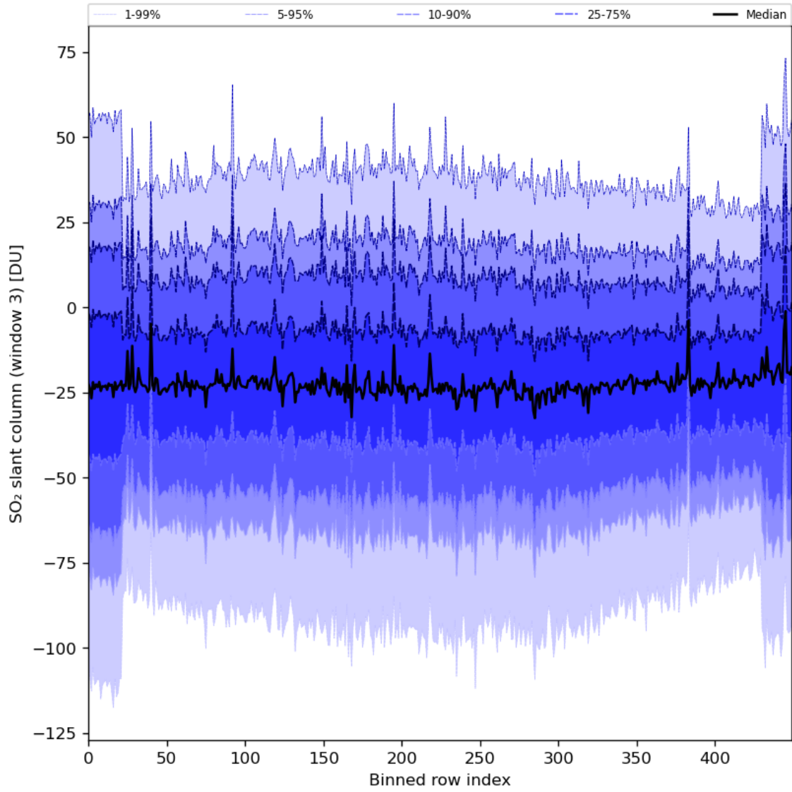
Figure 87: Along track statistics of “SO 2 slant column (window 3)” for 2024-04-17 to 2024-04-19
