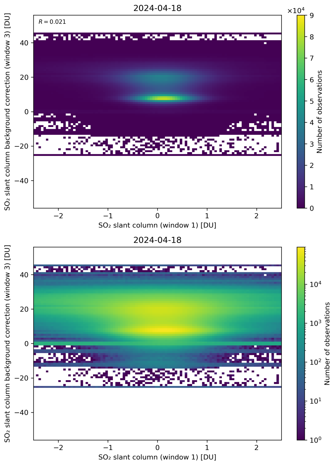
Figure 214: Scatter density plot of “SO 2 slant column (window 1)” against “SO 2 slant column background correction (window 3)” for 2024-04-17 to 2024-04-19.
