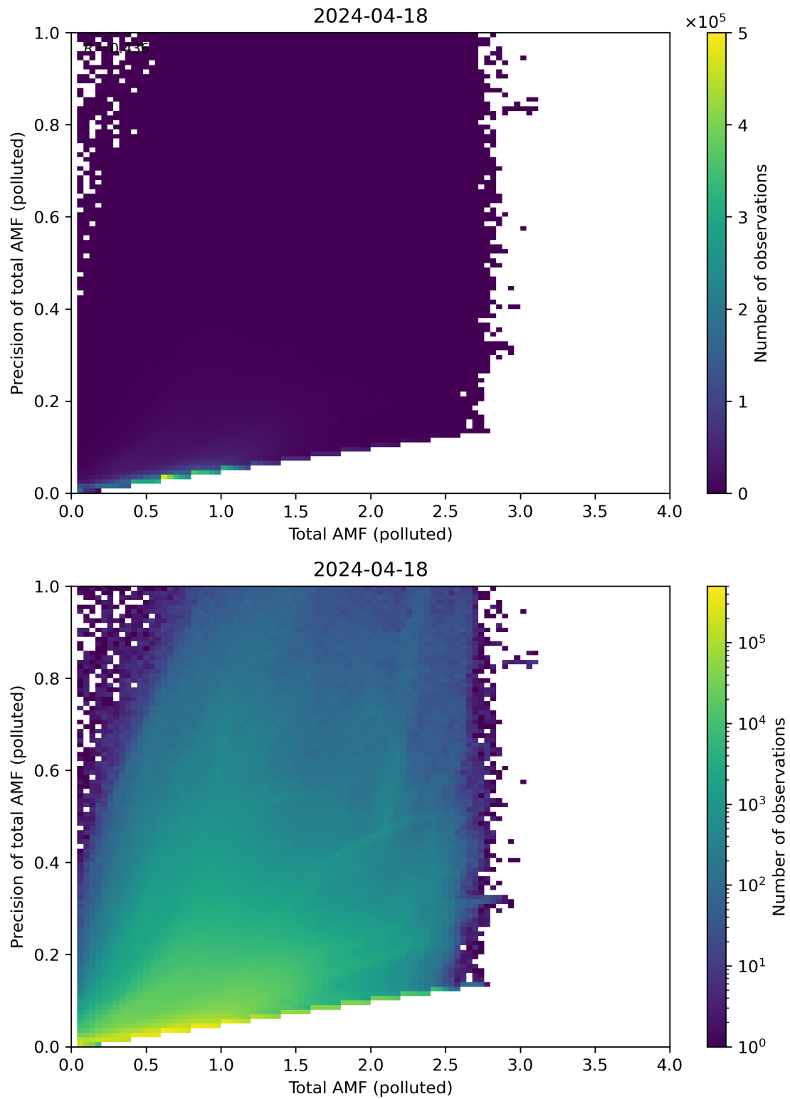
Figure 272: Scatter density plot of “Total AMF (polluted)” against “Precision of total AMF (polluted)” for 2024-04-17 to 2024-04-19.
