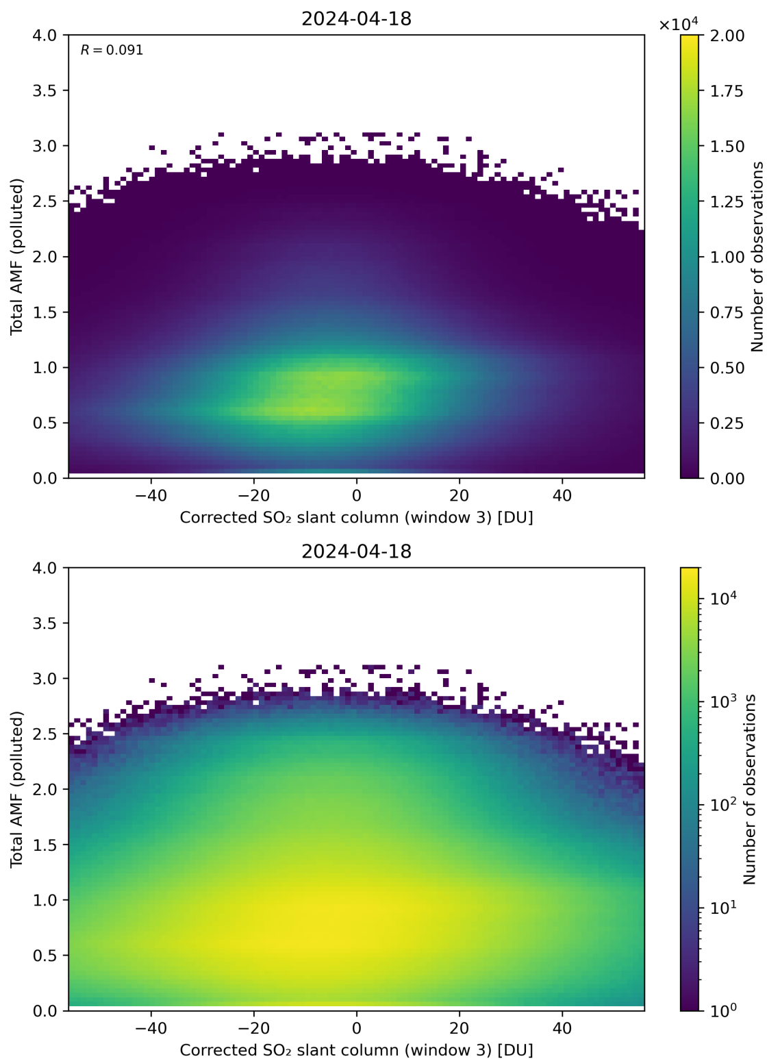
Figure 210: Scatter density plot of “Corrected SO 2 slant column (window 3)” against “Total AMF (polluted)” for 2024-04-17 to 2024-04-19.
