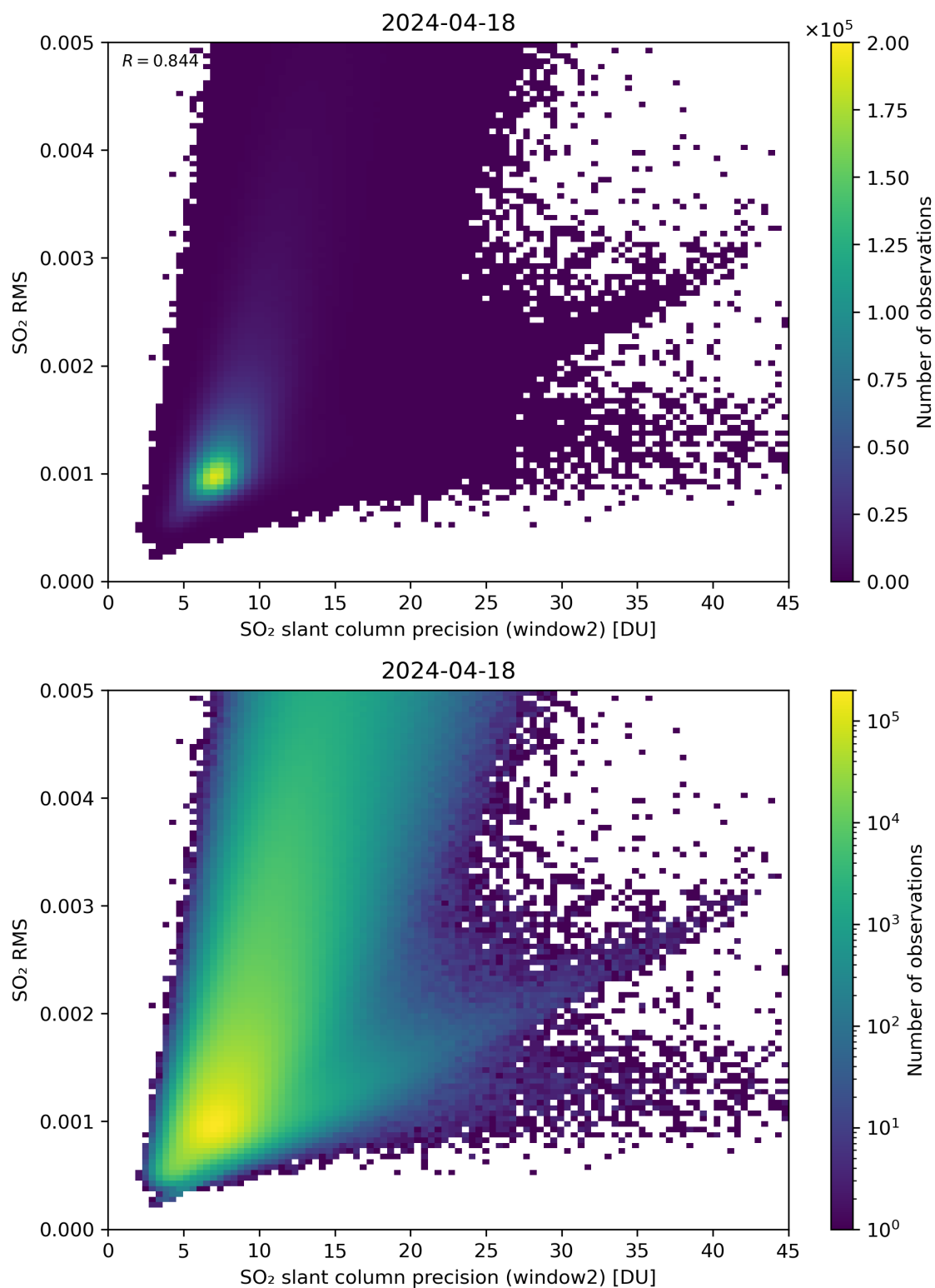
Figure 245: Scatter density plot of “SO 2 slant column precision (window2)” against “SO 2 RMS” for 2024-04-17 to 2024-04-19.
