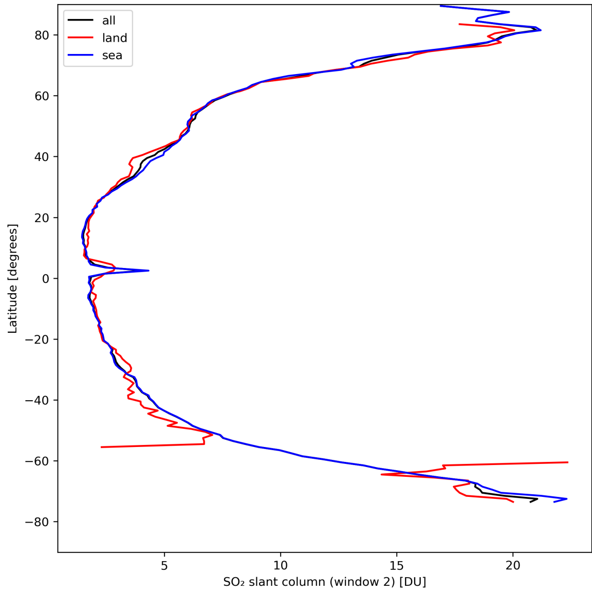
Figure 37: Zonal average of “SO 2 slant column (window 2)” for 2024-04-17 to 2024-04-19.
