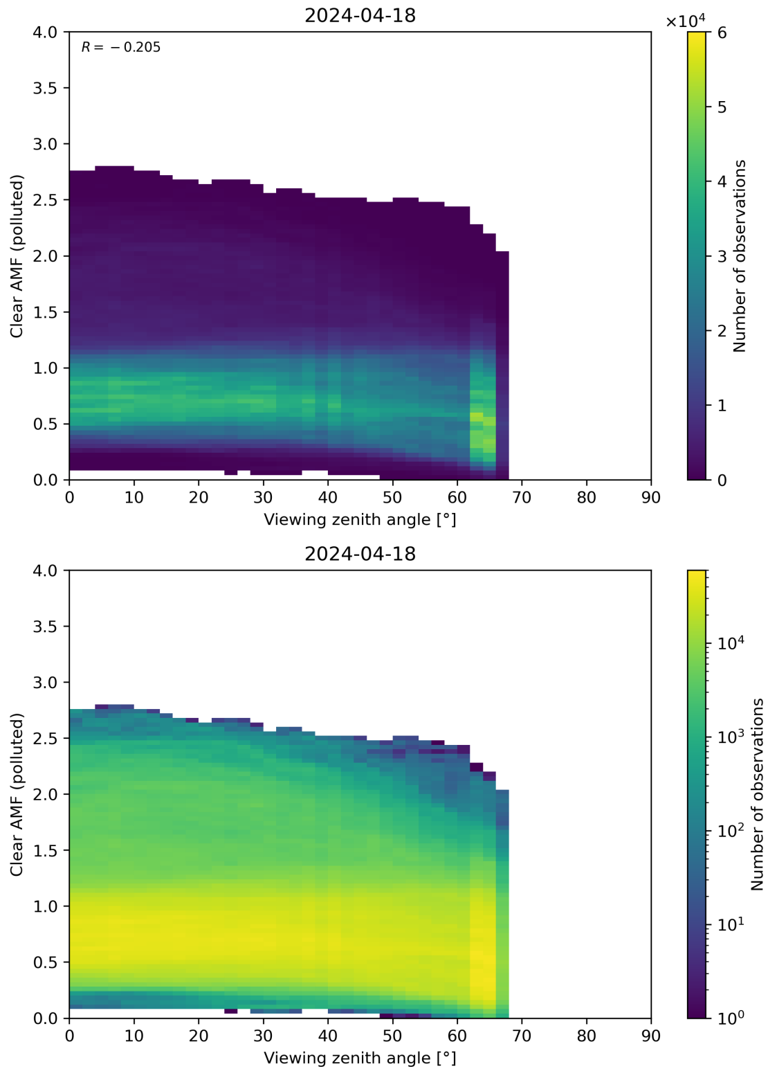
Figure 316: Scatter density plot of “Viewing zenith angle” against “Clear AMF (polluted)” for 2024-04-17 to 2024-04-19.
