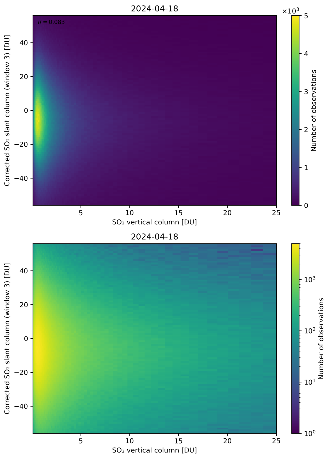
Figure 299: Scatter density plot of “SO 2 vertical column” against “Corrected SO 2 slant column (window 3)” for 2024-04-17 to 2024-04-19.
