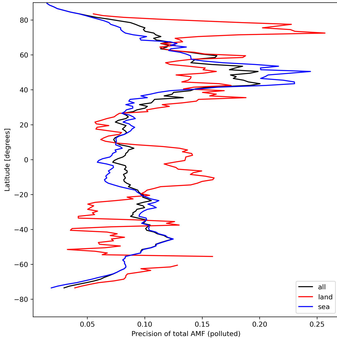
Figure 49: Zonal average of “Precision of total AMF (polluted)” for 2024-04-17 to 2024-04-19.
