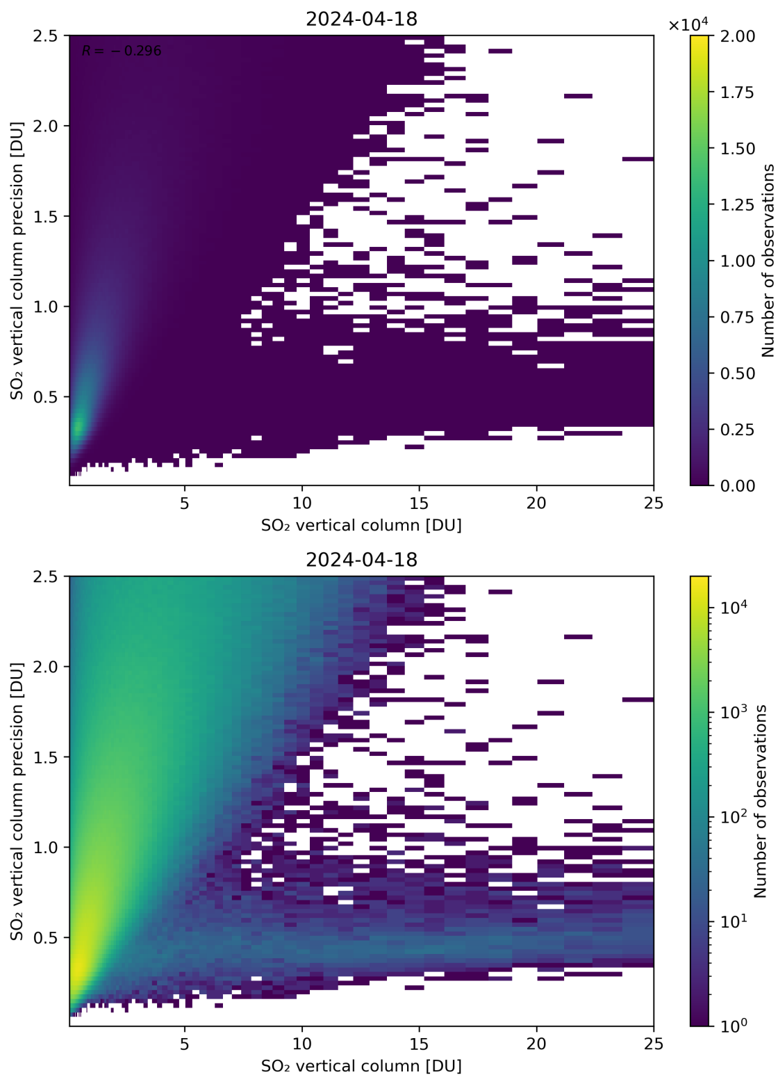
Figure 307: Scatter density plot of “SO 2 vertical column” against “SO 2 vertical column precision” for 2024-04-17 to 2024-04-19.
