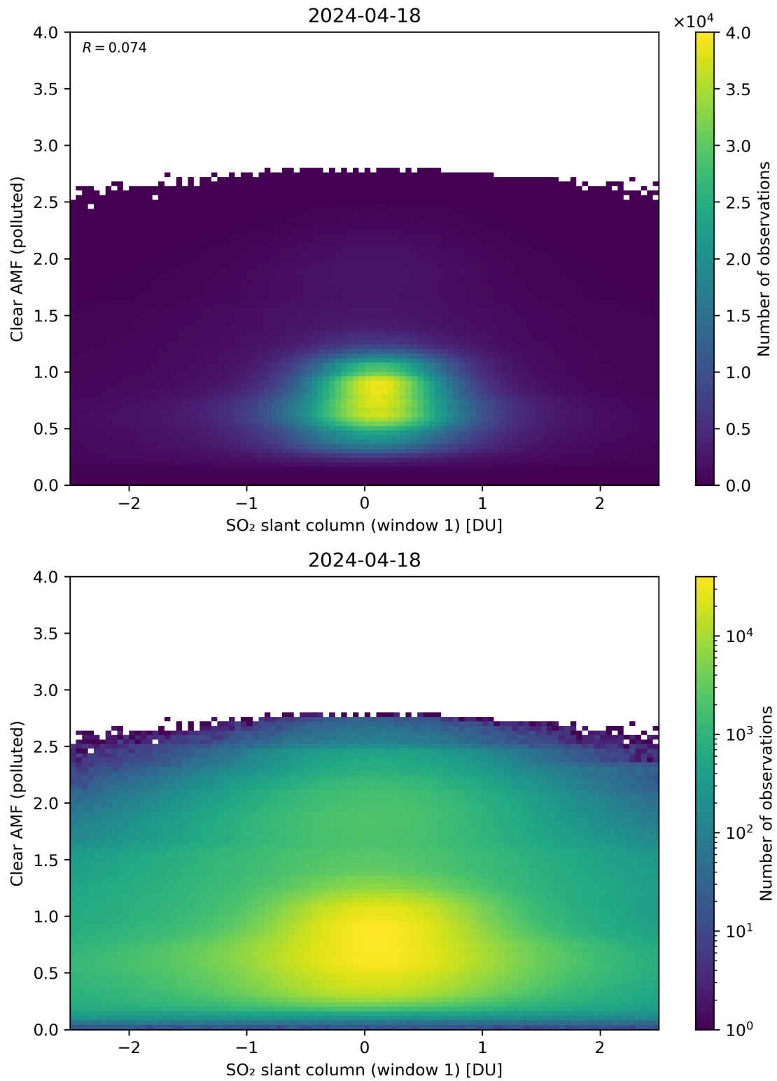
Figure 232: Scatter density plot of “SO 2 slant column (window 1)” against “Clear AMF (polluted)” for 2024-04-17 to 2024-04-19.
