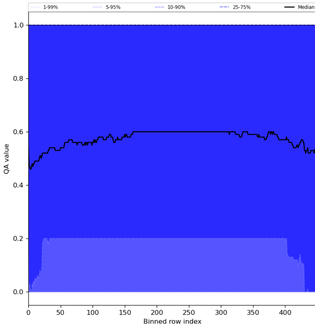
Figure 75: Along track statistics of “QA value” for 2024-04-17 to 2024-04-19
