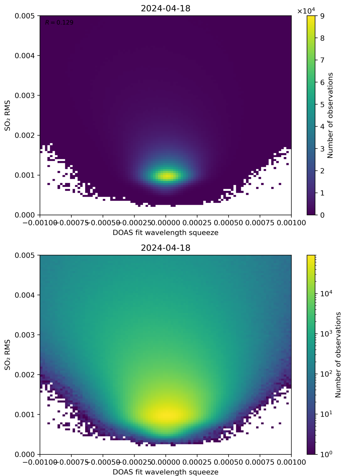
Figure 132: Scatter density plot of “DOAS fit wavelength squeeze” against “SO 2 RMS” for 2024-04-17 to 2024-04-19.
