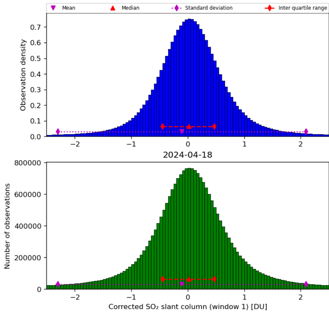
Figure 58: Histogram of “Corrected SO 2 slant column (window 1)” for 2024-04-17 to 2024-04-19
