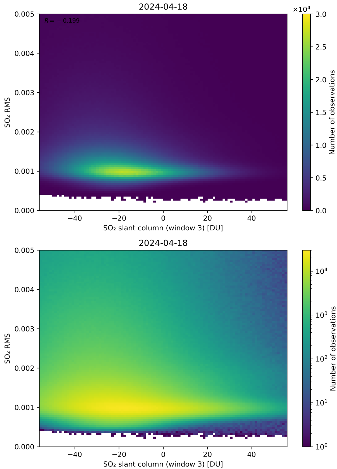
Figure 256: Scatter density plot of “SO 2 slant column (window 3)” against “SO 2 RMS” for 2024-04-17 to 2024-04-19.
