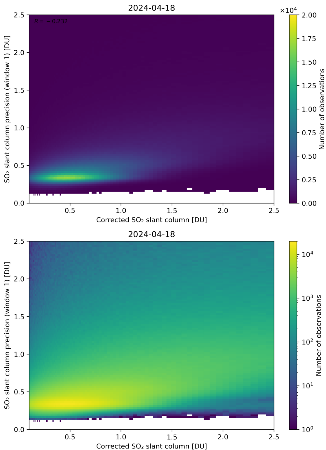
Figure 188: Scatter density plot of “Corrected SO 2 slant column” against “SO 2 slant column precision (window 1)” for 2024-04-17 to 2024-04-19.
