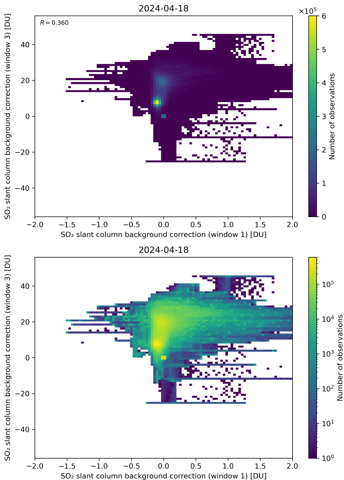
Figure 99: Scatter density plot of “SO 2 slant column background correction (window 1)” against “SO 2 slant column background correction (window 3)” for 2024-04-17 to 2024-04-19.
