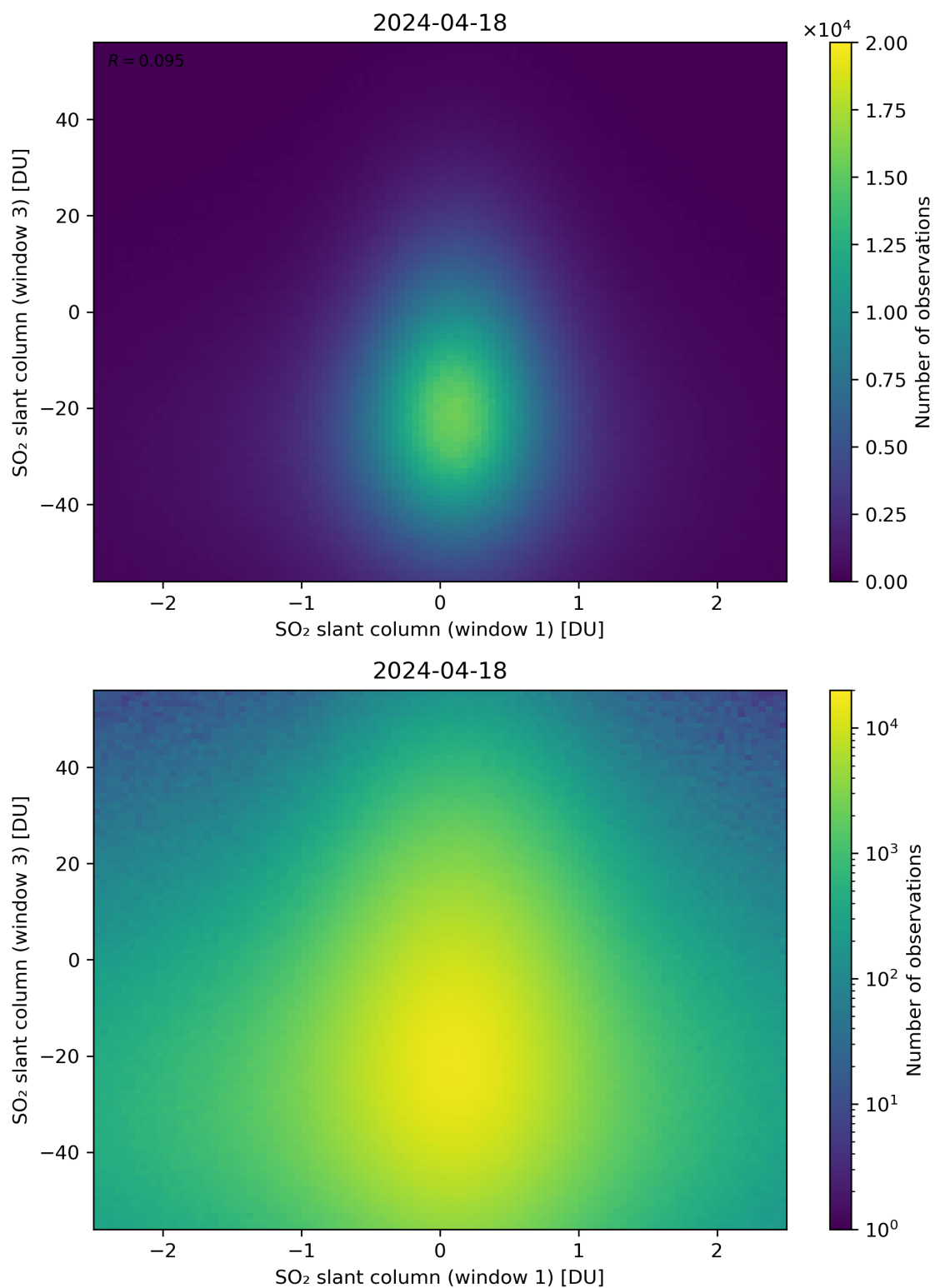
Figure 237: Scatter density plot of “SO 2 slant column (window 1)” against “SO 2 slant column (window 3)” for 2024-04-17 to 2024-04-19.
