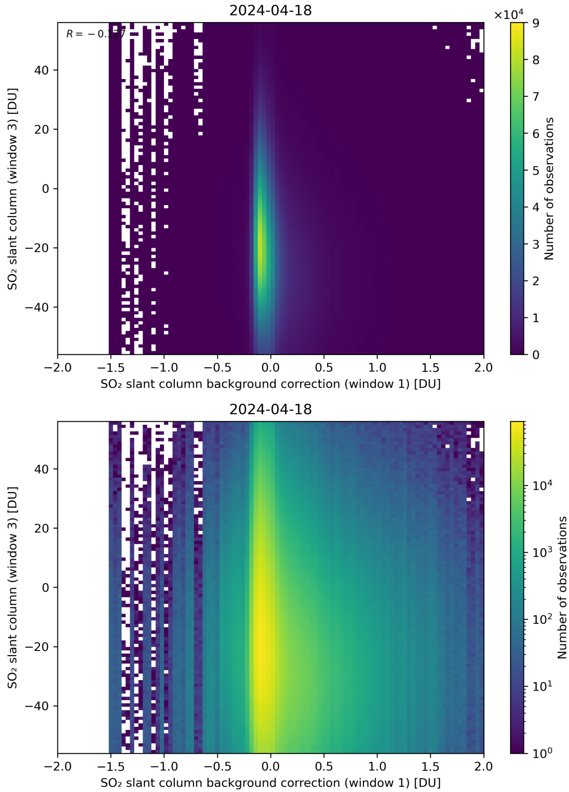
Figure 107: Scatter density plot of “SO 2 slant column background correction (window 1)” against “SO 2 slant column (window 3)” for 2024-04-17 to 2024-04-19.
