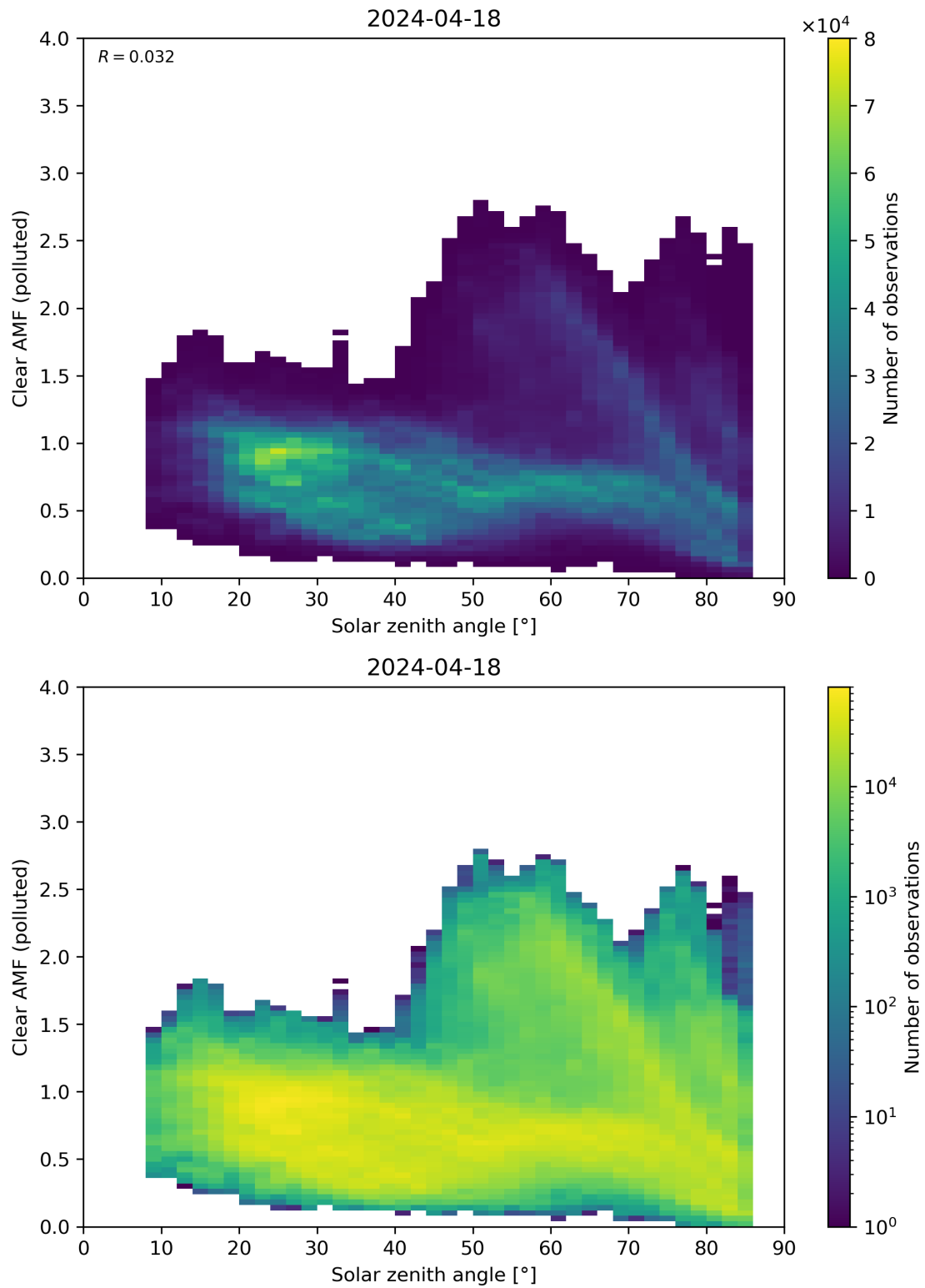
Figure 165: Scatter density plot of “Solar zenith angle” against “Clear AMF (polluted)” for 2024-04-17 to 2024-04-19.
