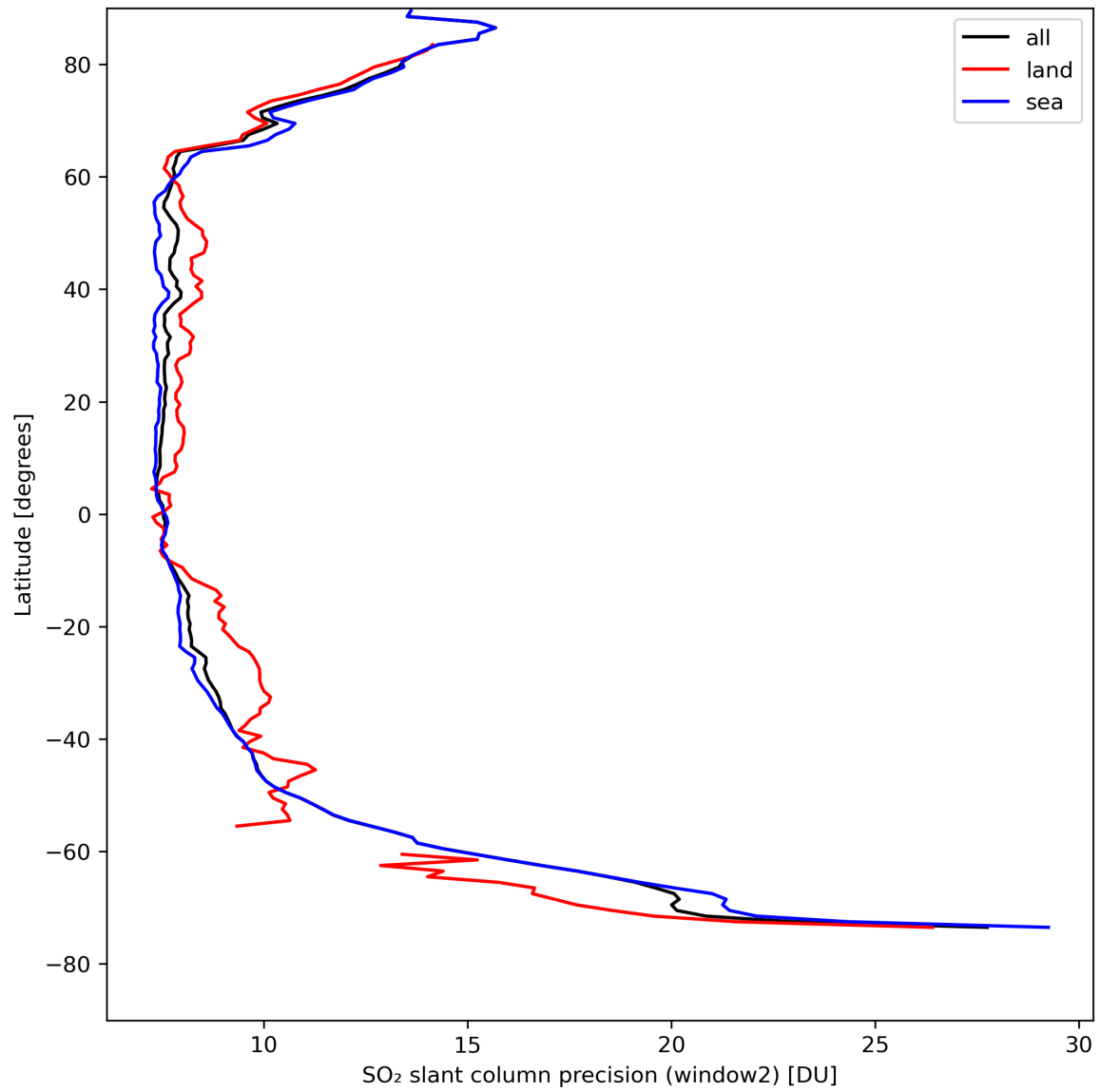
Figure 38: Zonal average of “SO 2 slant column precision (window2)” for 2024-04-17 to 2024-04-19.
