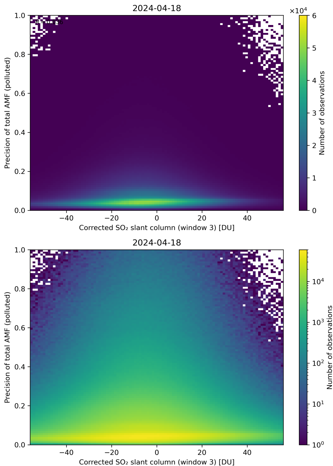
Figure 211: Scatter density plot of “Corrected SO 2 slant column (window 3)” against “Precision of total AMF (polluted)” for 2024-04-17 to 2024-04-19.
