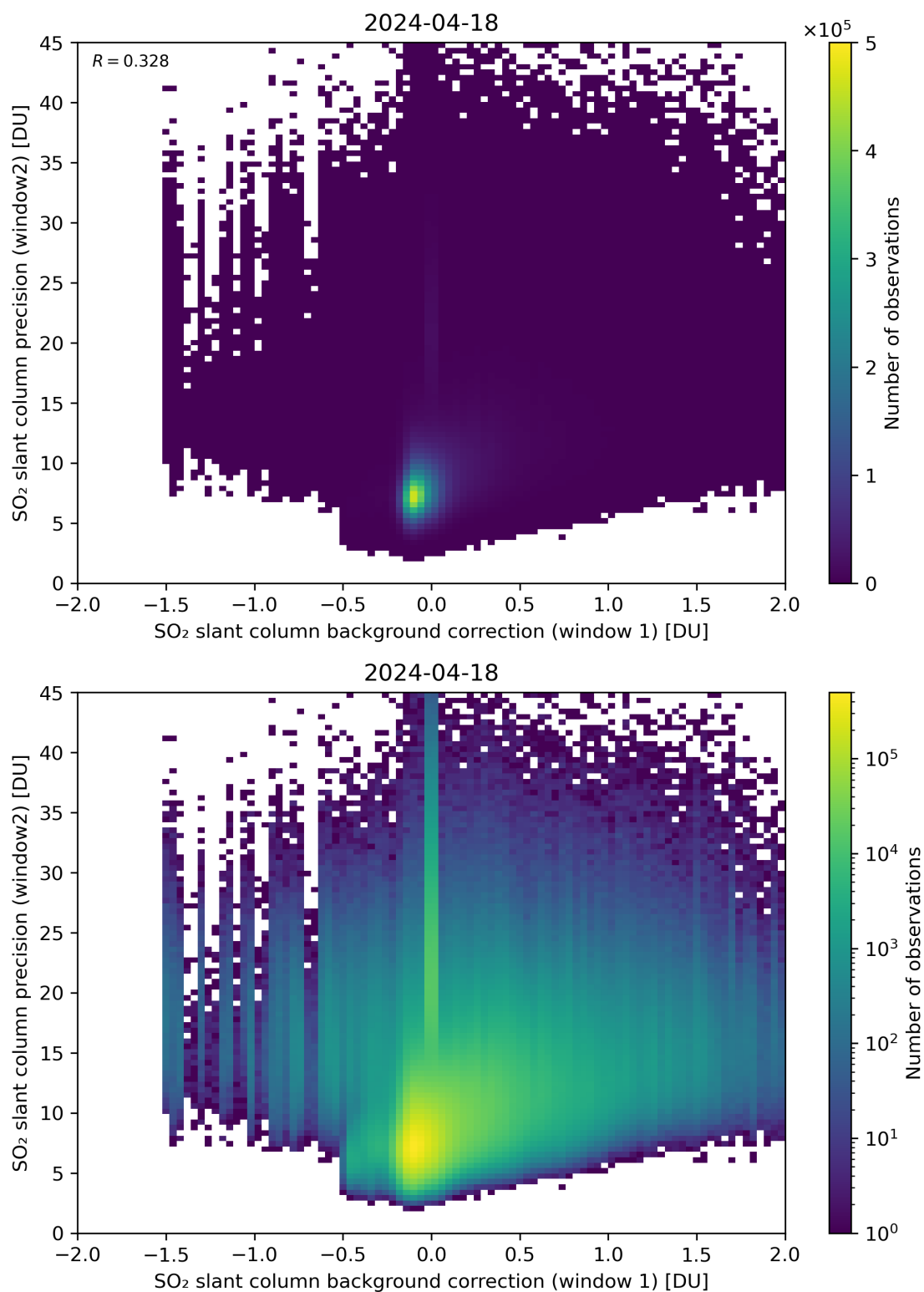
Figure 106: Scatter density plot of “SO 2 slant column background correction (window 1)” against “SO 2 slant column precision (window2)” for 2024-04-17 to 2024-04-19.
