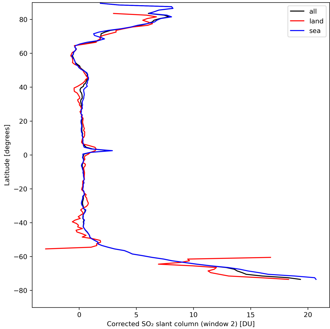
Figure 39: Zonal average of “Corrected SO 2 slant column (window 2)” for 2024-04-17 to 2024-04-19.
