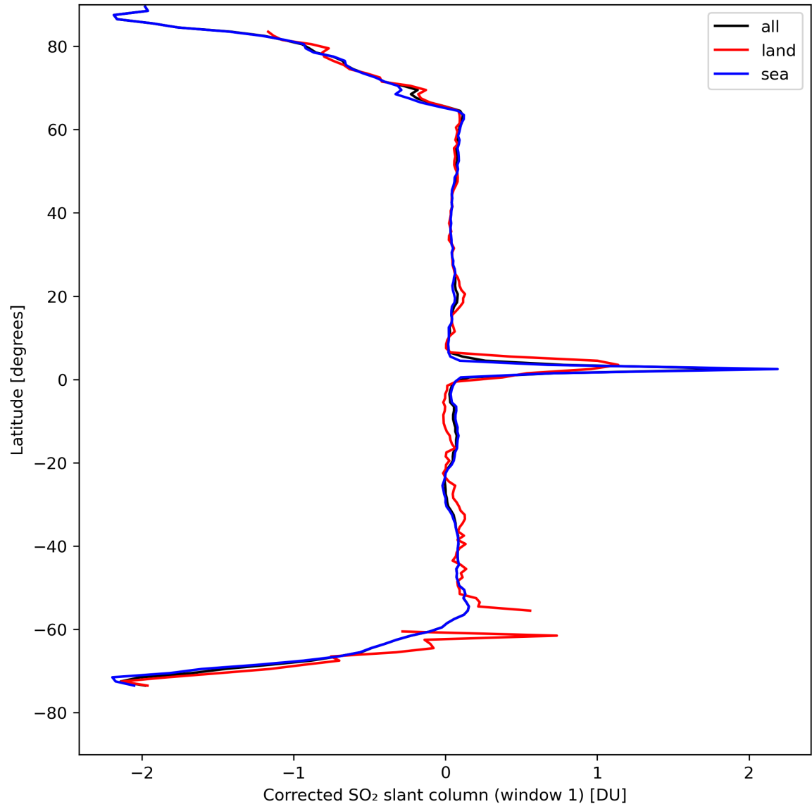
Figure 35: Zonal average of “Corrected SO 2 slant column (window 1)” for 2024-04-17 to 2024-04-19.
