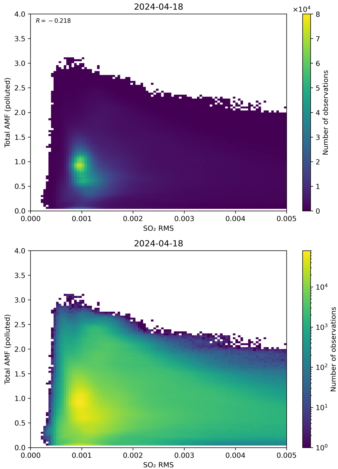
Figure 137: Scatter density plot of “SO 2 RMS” against “Total AMF (polluted)” for 2024-04-17 to 2024-04-19.
