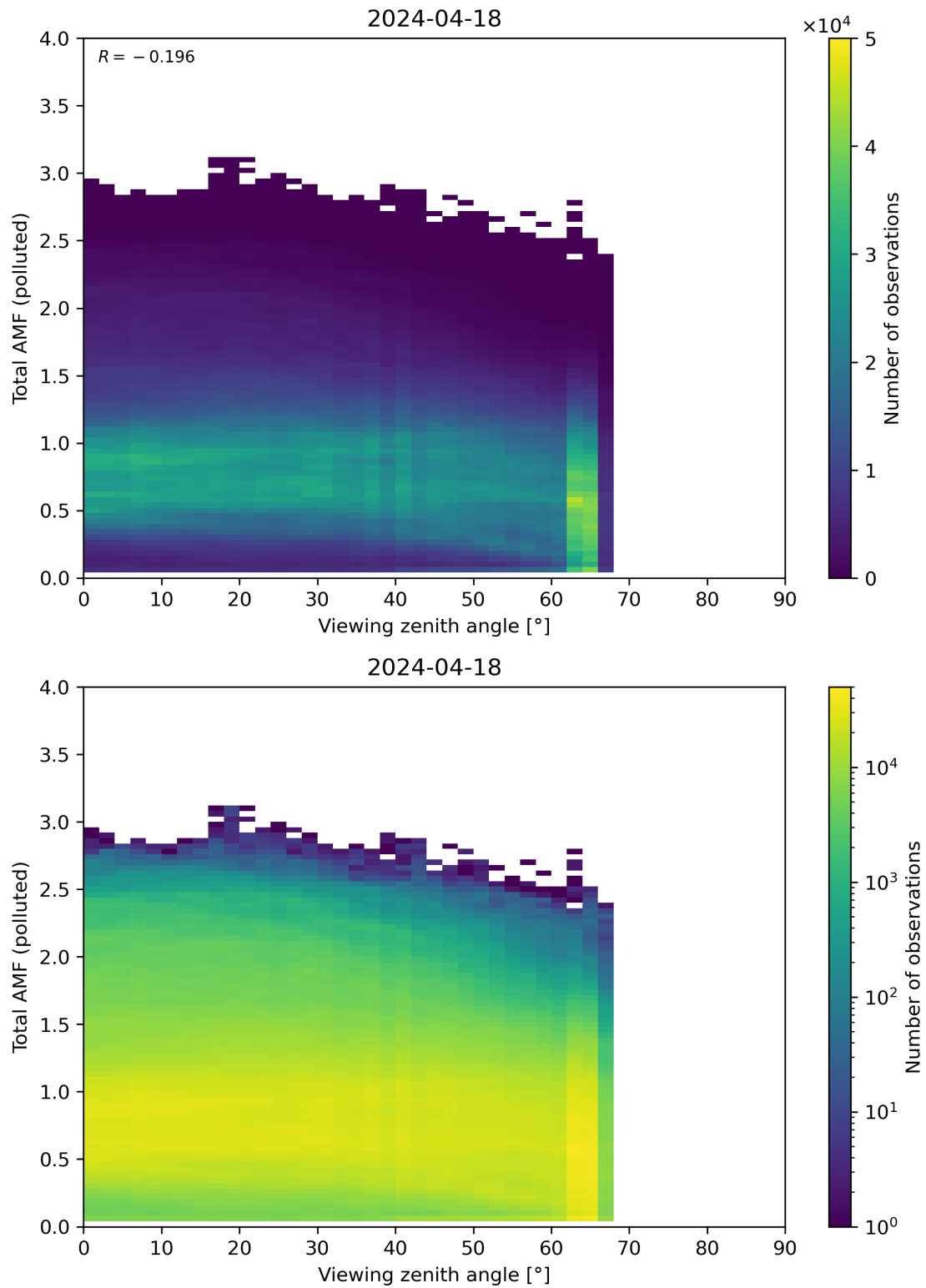
Figure 325: Scatter density plot of “Viewing zenith angle” against “Total AMF (polluted)” for 2024-04-17 to 2024-04-19.
