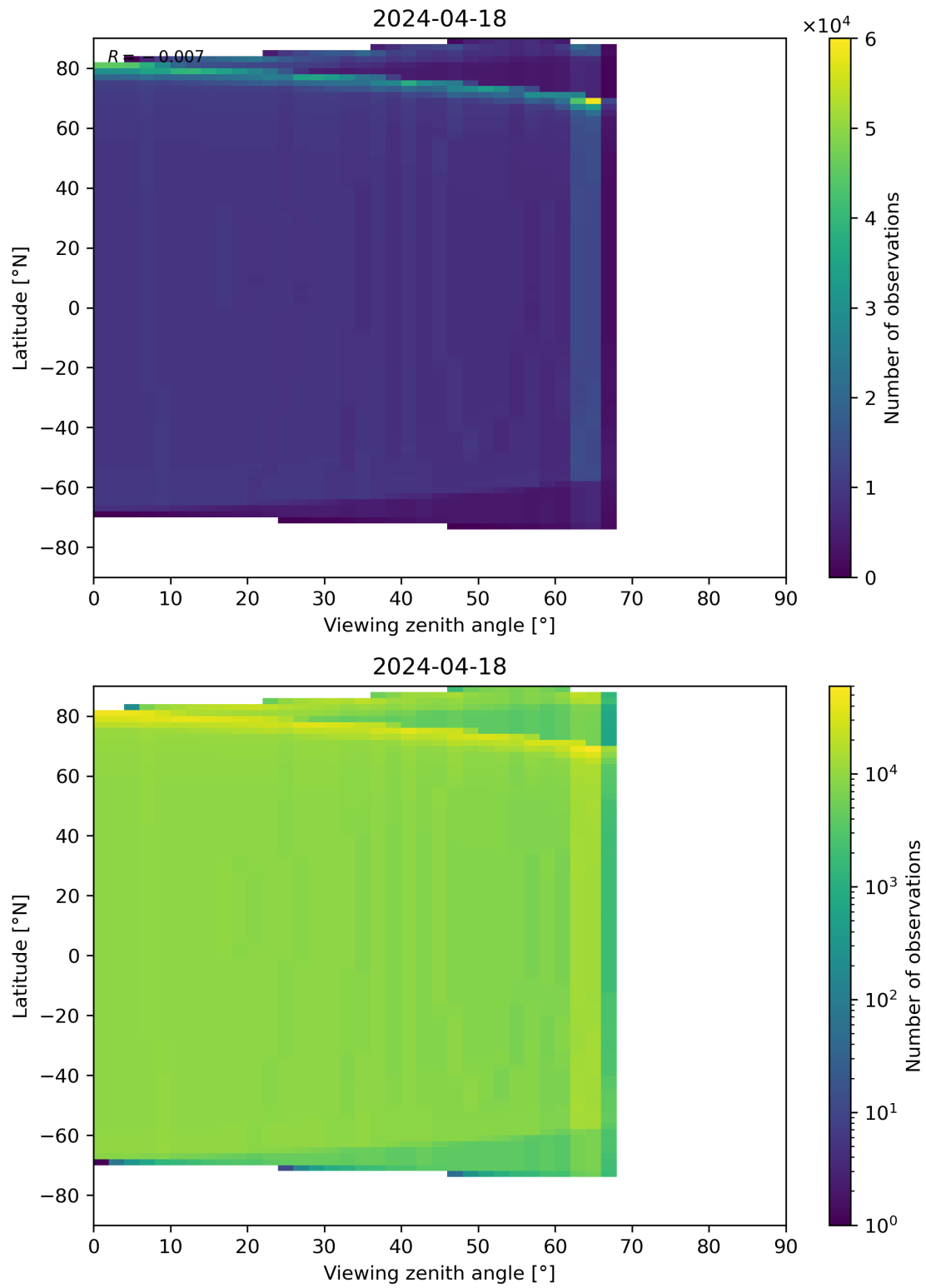
Figure 314: Scatter density plot of “Viewing zenith angle” against “Latitude” for 2024-04-17 to 2024-04-19.
