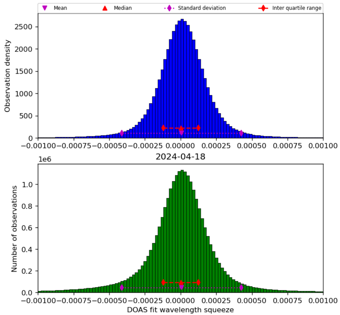
Figure 69: Histogram of “DOAS fit wavelength squeeze” for 2024-04-17 to 2024-04-19
