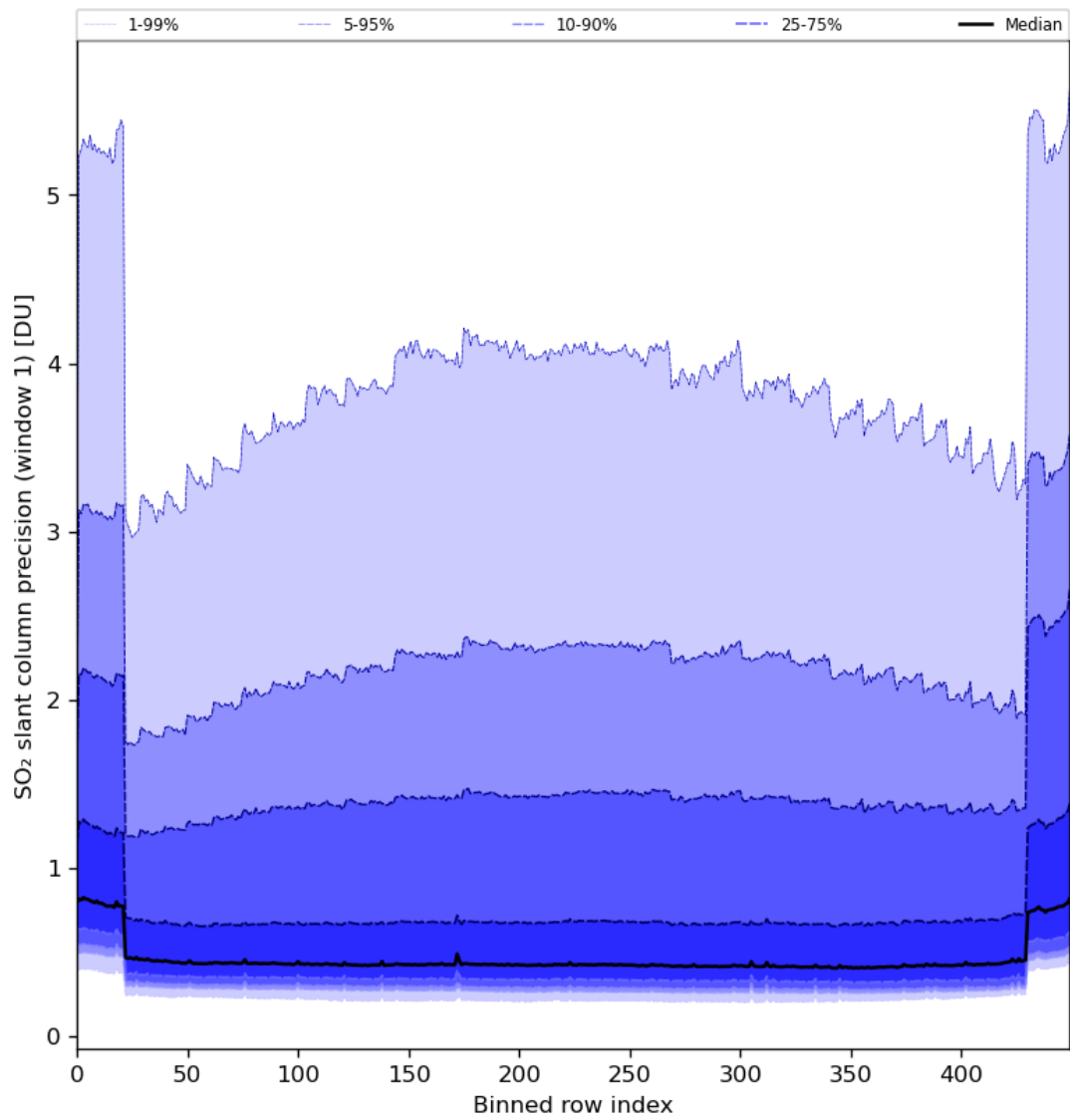
Figure 80: Along track statistics of “SO 2 slant column precision (window 1)” for 2024-04-17 to 2024-04-19
