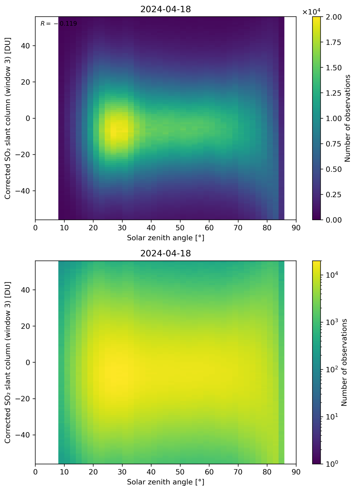
Figure 168: Scatter density plot of “Solar zenith angle” against “Corrected SO 2 slant column (window 3)” for 2024-04-17 to 2024-04-19.
