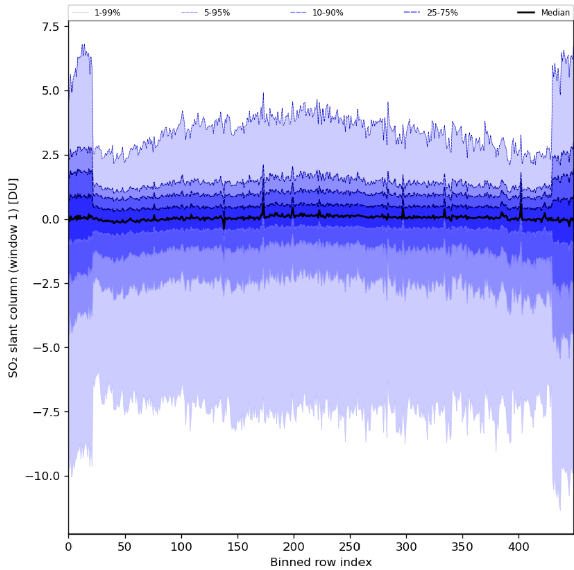
Figure 79: Along track statistics of “SO 2 slant column (window 1)” for 2024-04-17 to 2024-04-19
