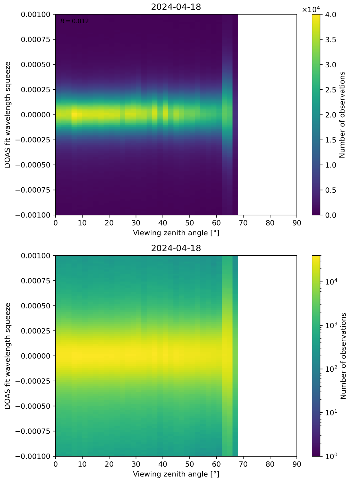
Figure 312: Scatter density plot of “Viewing zenith angle” against “DOAS fit wavelength squeeze” for 2024-04-17 to 2024-04-19.
