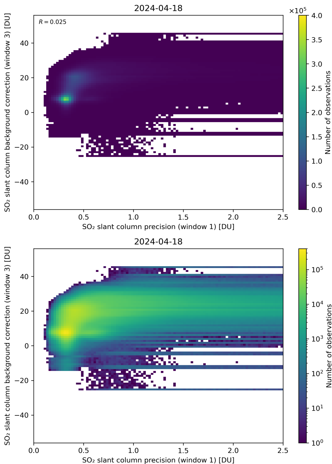
Figure 220: Scatter density plot of “SO 2 slant column precision (window 1)” against “SO 2 slant column background correction (window 3)” for 2024-04-17 to 2024-04-19.
