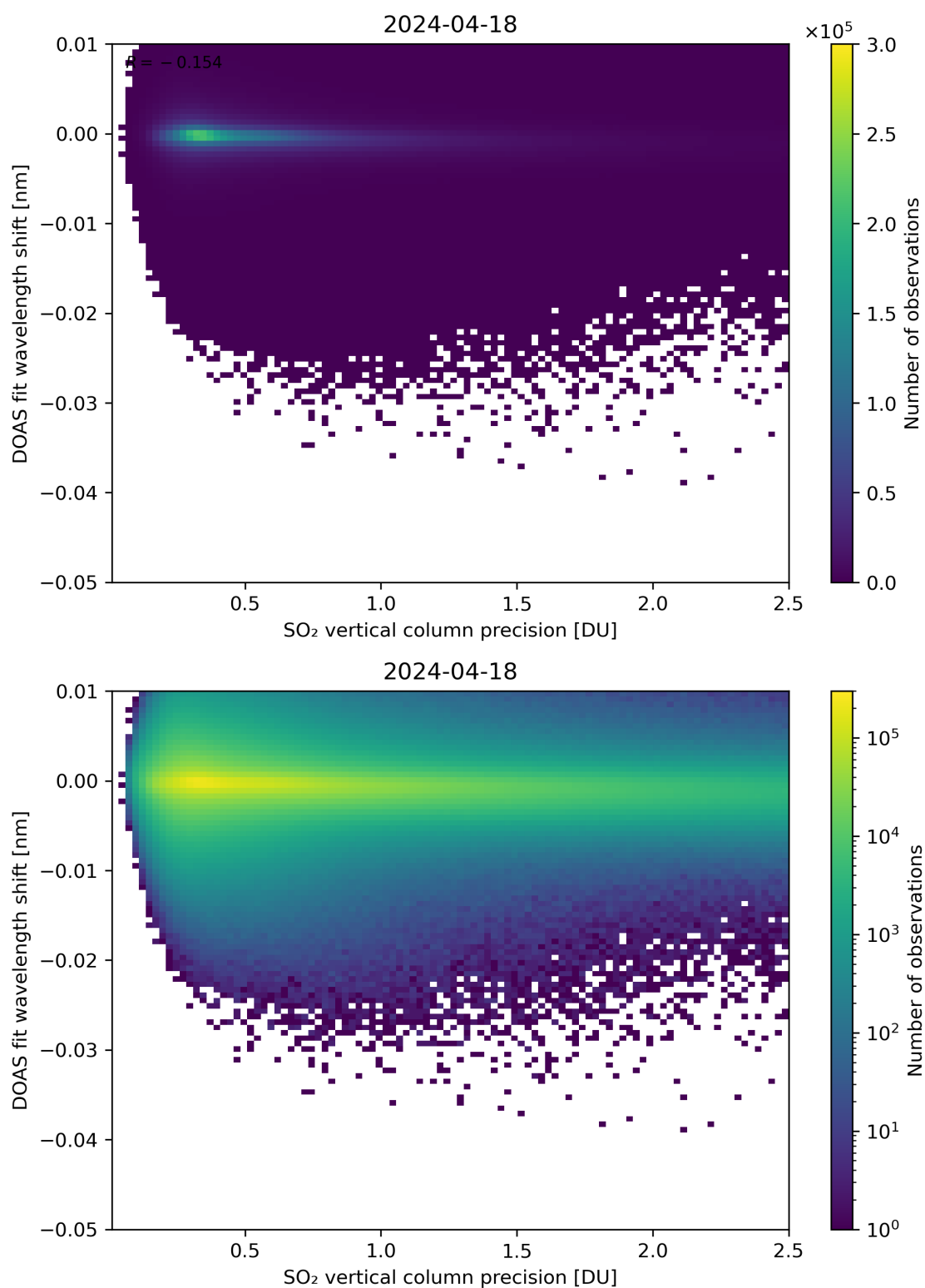
Figure 282: Scatter density plot of “SO 2 vertical column precision” against “DOAS fit wavelength shift” for 2024-04-17 to 2024-04-19.
