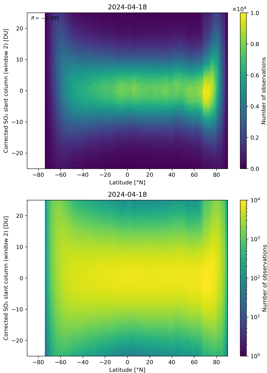
Figure 147: Scatter density plot of “Latitude” against “Corrected SO 2 slant column (window 2)” for 2024-04-17 to 2024-04-19.
