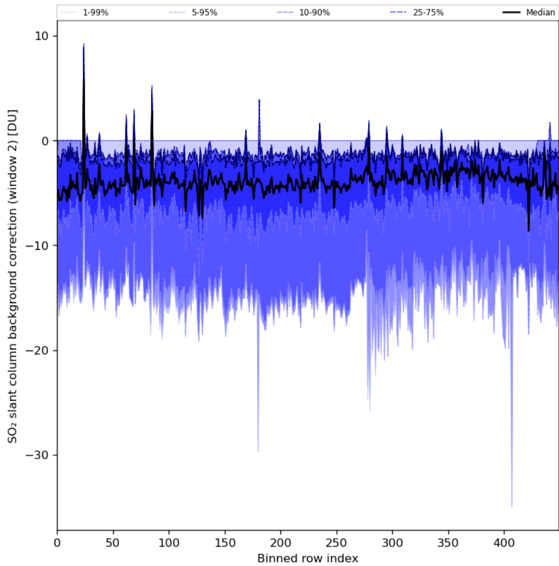
Figure 86: Along track statistics of “SO 2 slant column background correction (window 2)” for 2024-04-17 to 2024-04-19
