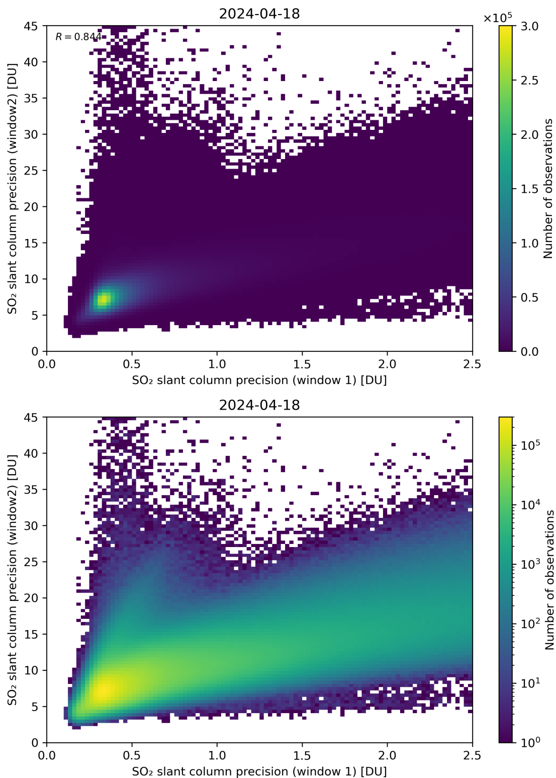
Figure 227: Scatter density plot of “SO 2 slant column precision (window 1)” against “SO 2 slant column precision (window 2)” for 2024-04-17 to 2024-04-19.
