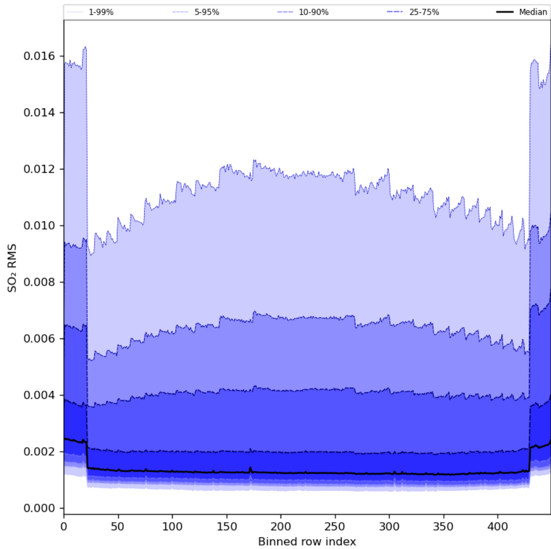
Figure 93: Along track statistics of “SO 2 RMS” for 2024-04-17 to 2024-04-19
