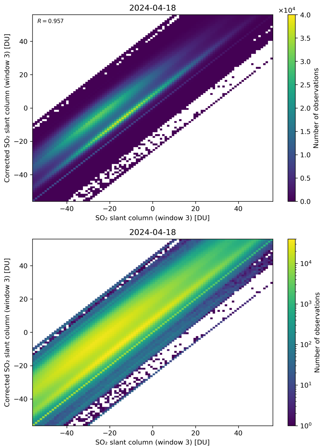
Figure 266: Scatter density plot of “SO 2 slant column (window 3)” against “Corrected SO 2 slant column (window 3)” for 2024-04-17 to 2024-04-19.
