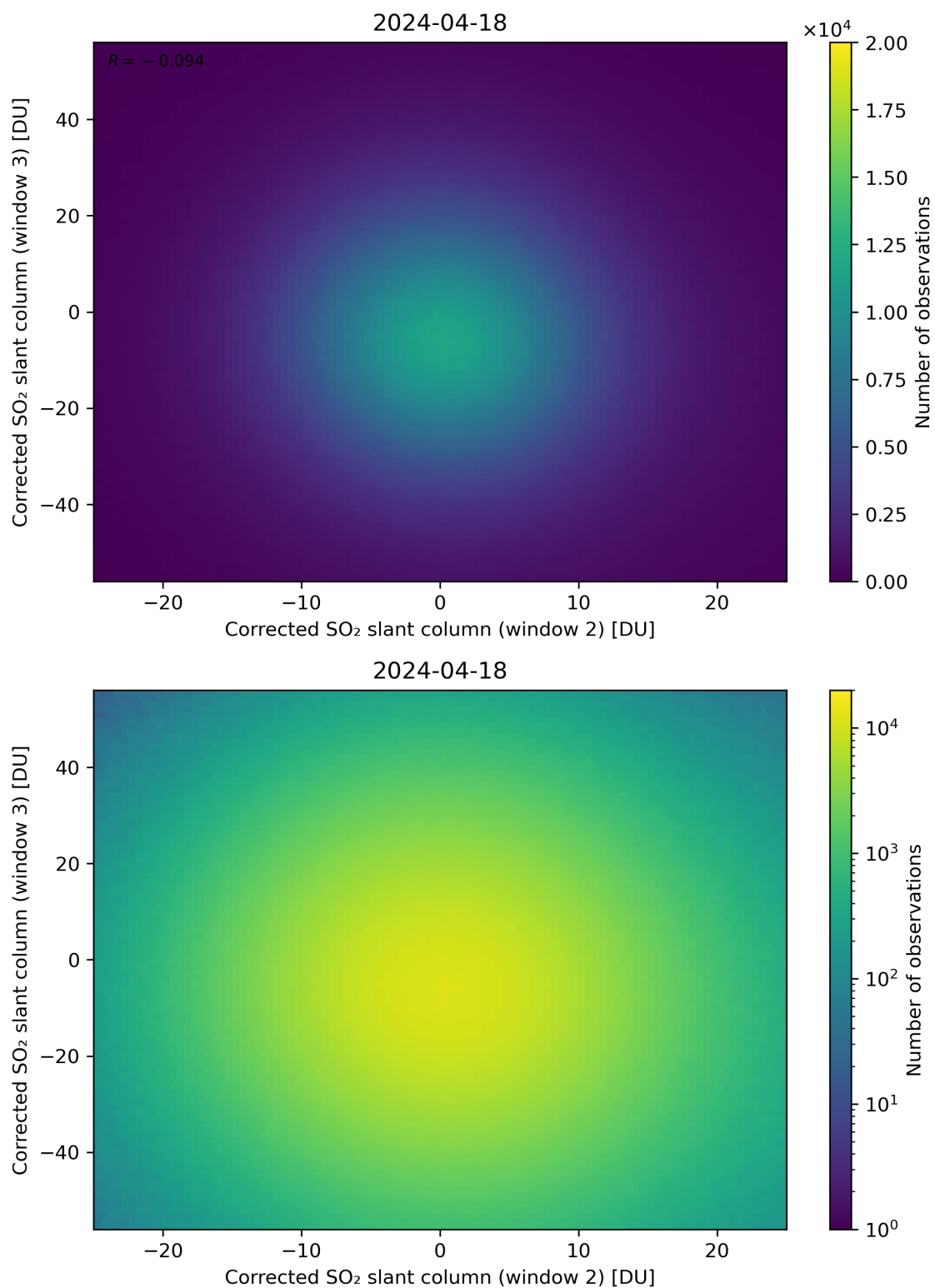
Figure 200: Scatter density plot of “Corrected SO 2 slant column (window 2)” against “Corrected SO 2 slant column (window 3)” for 2024-04-17 to 2024-04-19.
