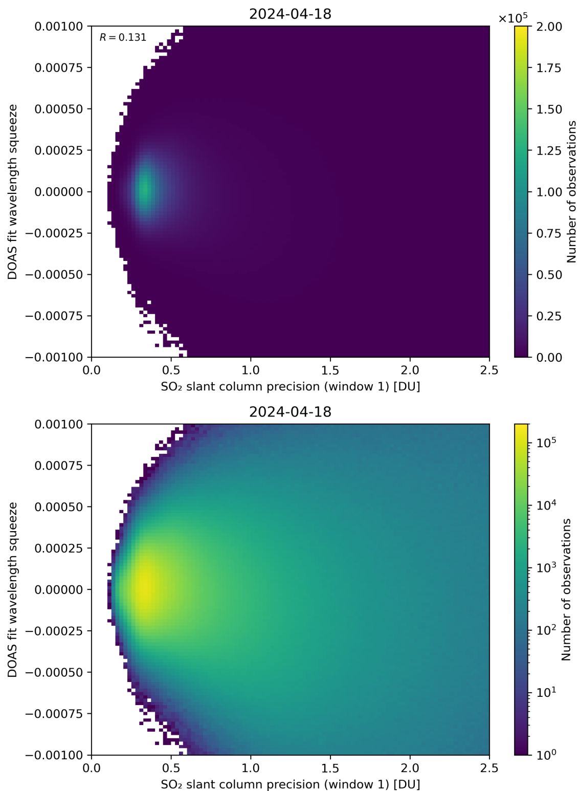
Figure 222: Scatter density plot of “SO 2 slant column precision (window 1)” against “DOAS fit wavelength squeeze” for 2024-04-17 to 2024-04-19.
