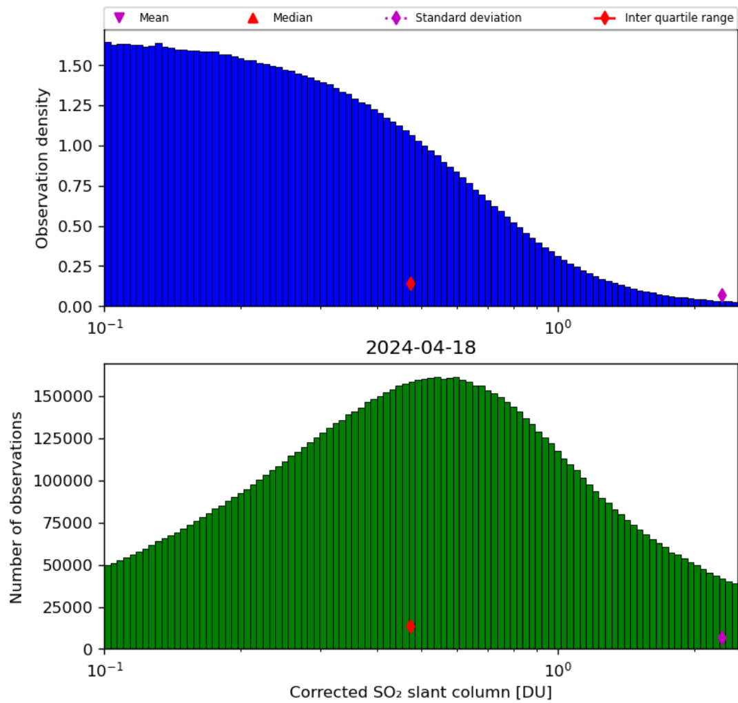
Figure 55: Histogram of “Corrected SO 2 slant column” for 2024-04-17 to 2024-04-19
