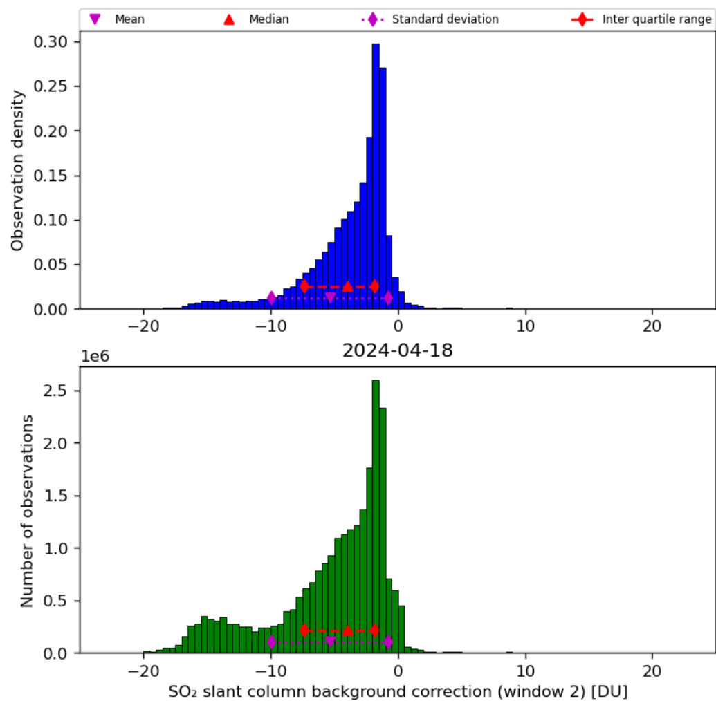
Figure 63: Histogram of “SO 2 slant column background correction (window 2)” for 2024-04-17 to 2024-04-19
