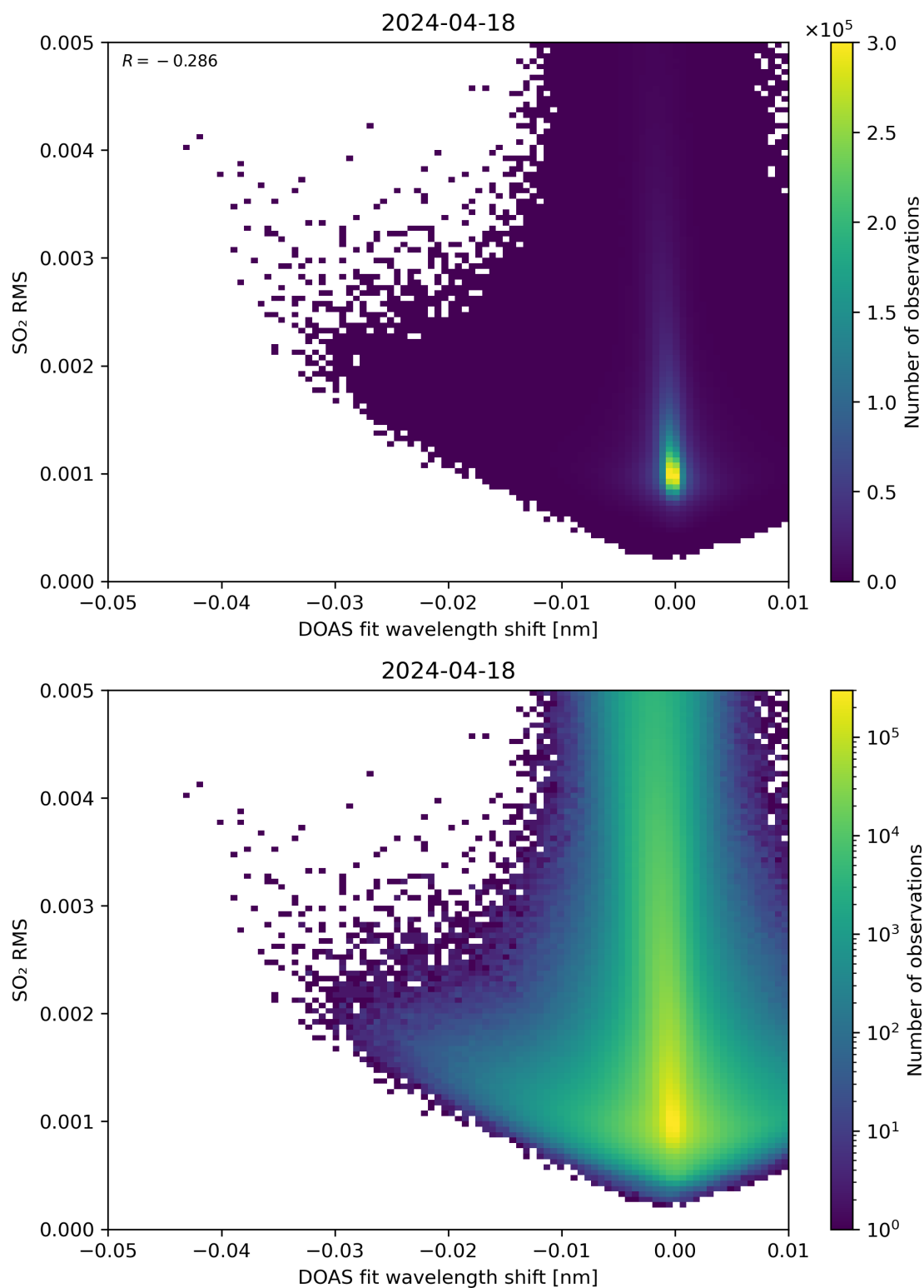
Figure 128: Scatter density plot of “DOAS fit wavelength shift” against “SO 2 RMS” for 2024-04-17 to 2024-04-19.
