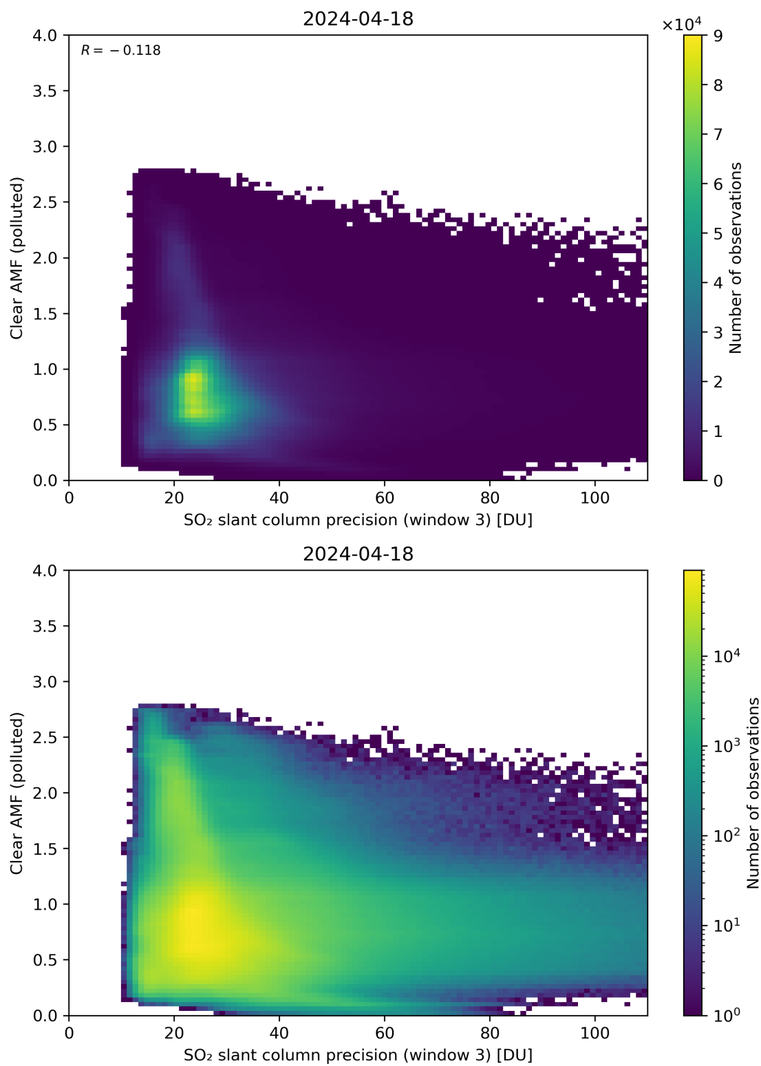
Figure 261: Scatter density plot of “SO 2 slant column precision (window 3)” against “Clear AMF (polluted)” for 2024-04-17 to 2024-04-19.
