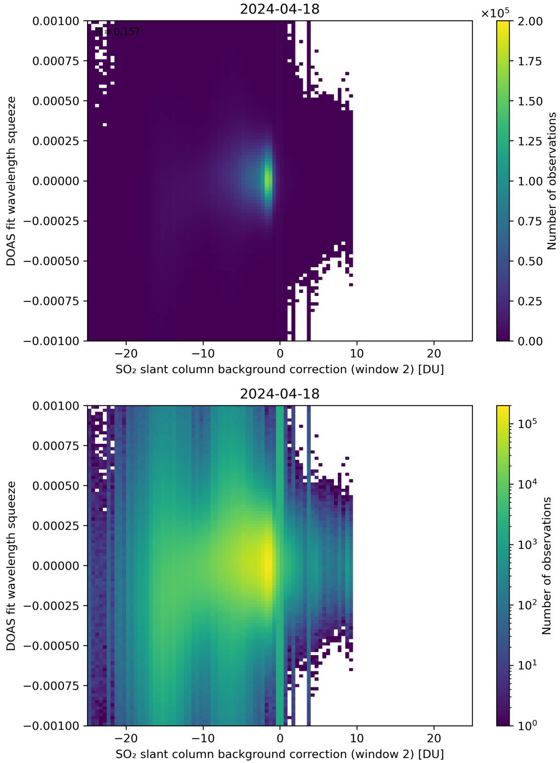
Figure 113: Scatter density plot of “SO 2 slant column background correction (window 2)” against “DOAS fit wavelength squeeze” for 2024-04-17 to 2024-04-19.
