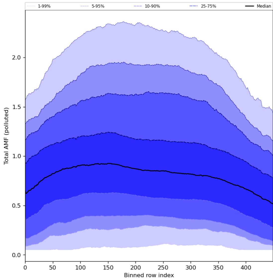
Figure 94: Along track statistics of “Total AMF (polluted)” for 2024-04-17 to 2024-04-19
