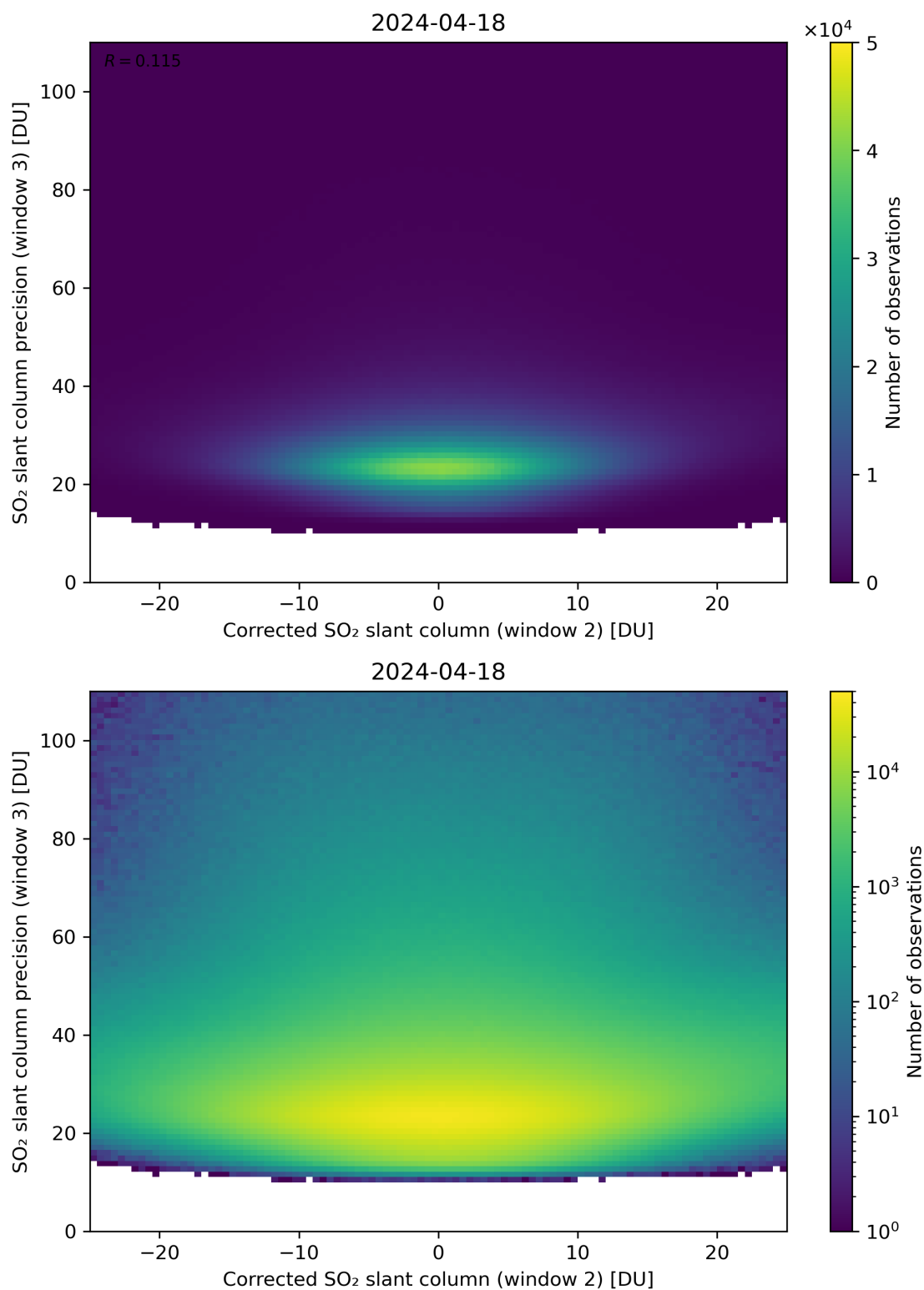
Figure 202: Scatter density plot of “Corrected SO 2 slant column (window 2)” against “SO 2 slant column precision (window 3)” for 2024-04-17 to 2024-04-19.
