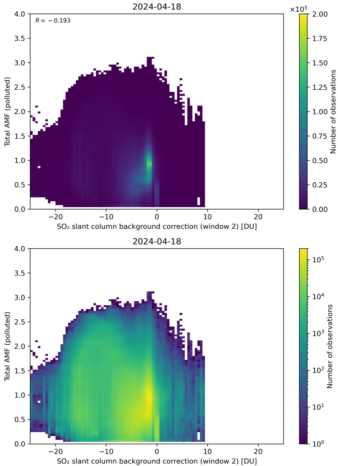
Figure 119: Scatter density plot of “SO 2 slant column background correction (window 2)” against “Total AMF (polluted)” for 2024-04-17 to 2024-04-19.
