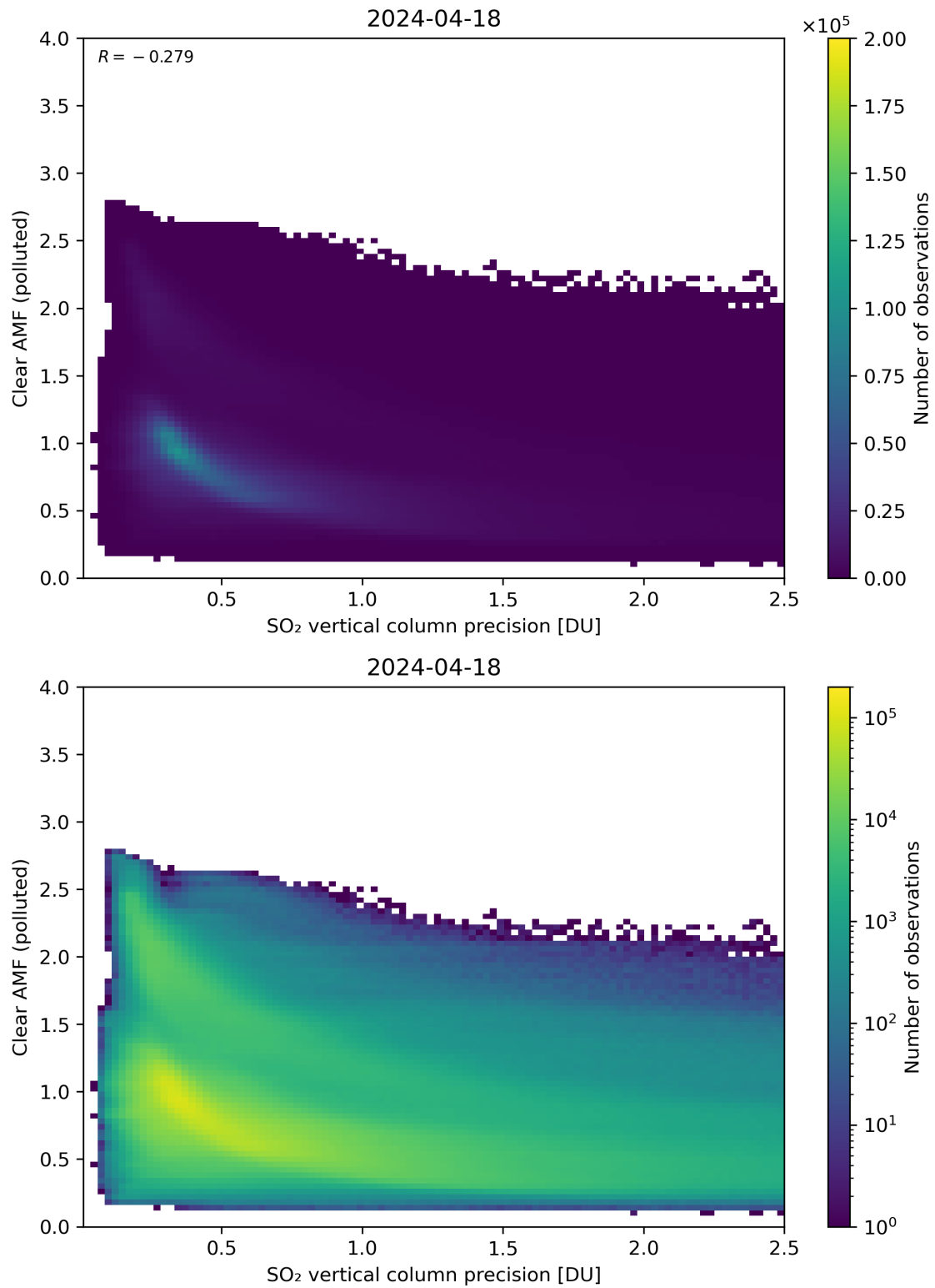
Figure 285: Scatter density plot of “SO 2 vertical column precision” against “Clear AMF (polluted)” for 2024-04-17 to 2024-04-19.
