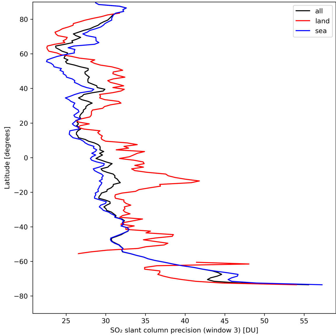
Figure 42: Zonal average of “SO 2 slant column precision (window 3)” for 2024-04-17 to 2024-04-19.
