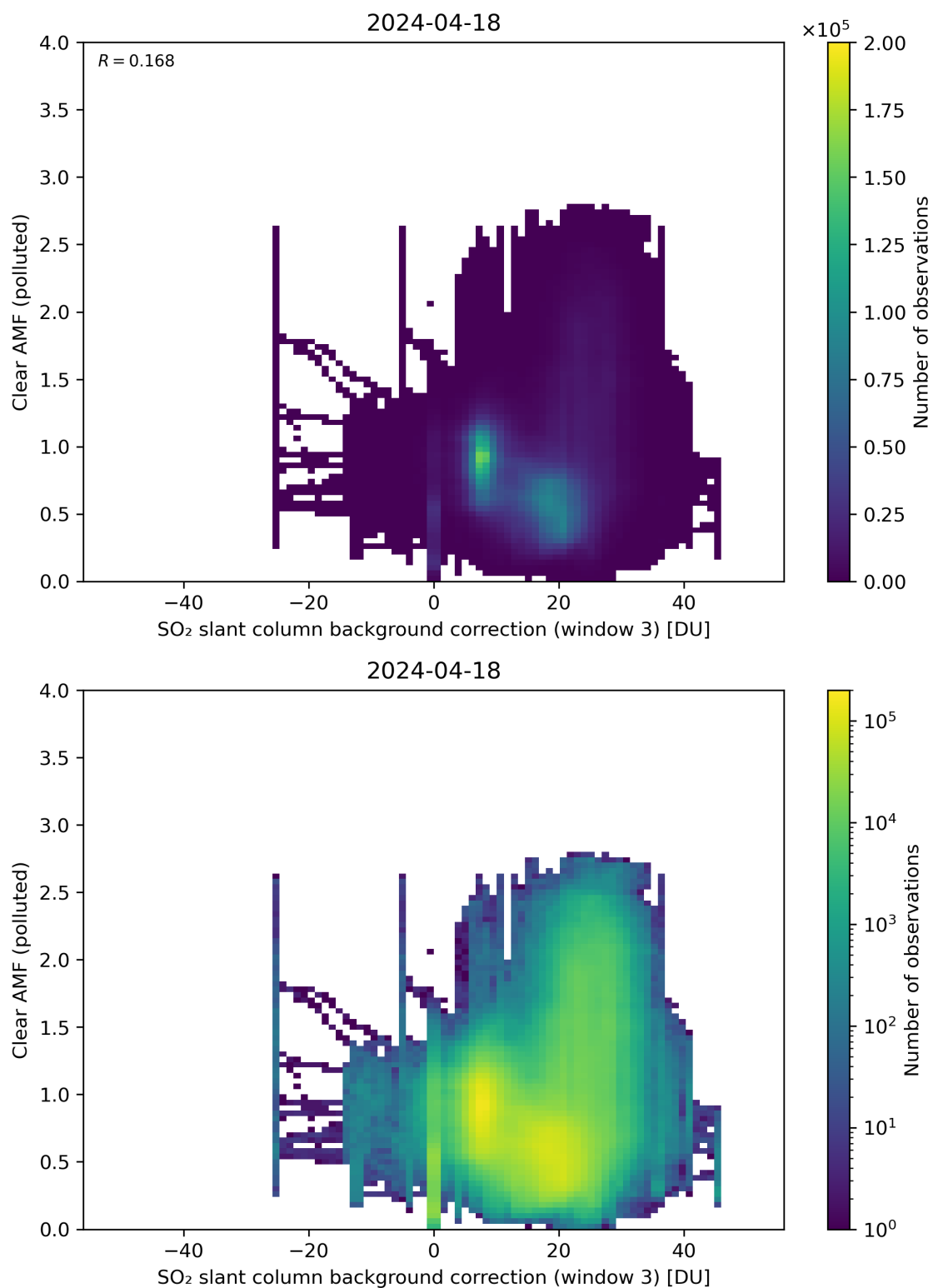
Figure 124: Scatter density plot of “SO 2 slant column background correction (window 3)” against “Clear AMF (polluted)” for 2024-04-17 to 2024-04-19.
