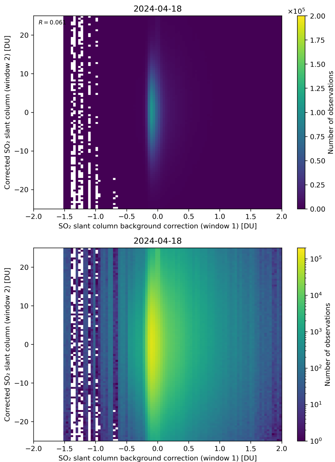
Figure 104: Scatter density plot of “SO 2 slant column background correction (window 1)” against “Corrected SO 2 slant column (window 2)” for 2024-04-17 to 2024-04-19.
