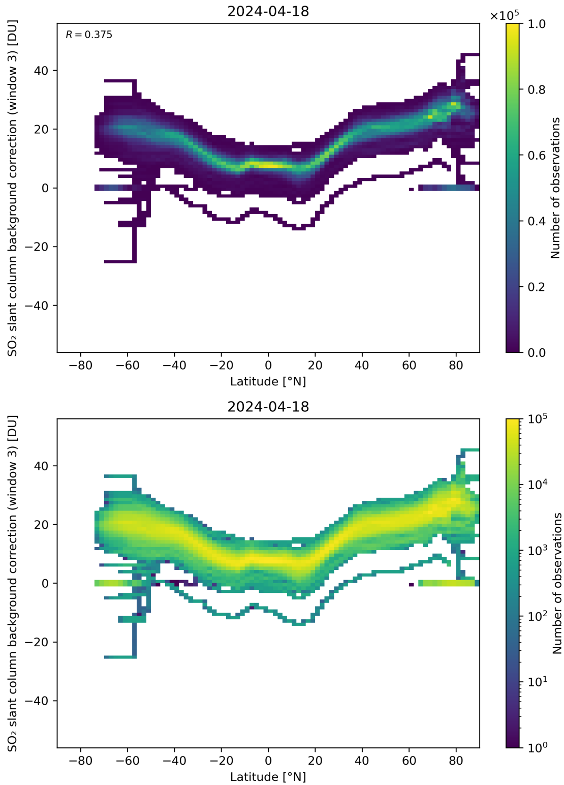
Figure 141: Scatter density plot of “Latitude” against “SO 2 slant column background correction (window 3)” for 2024-04-17 to 2024-04-19.
