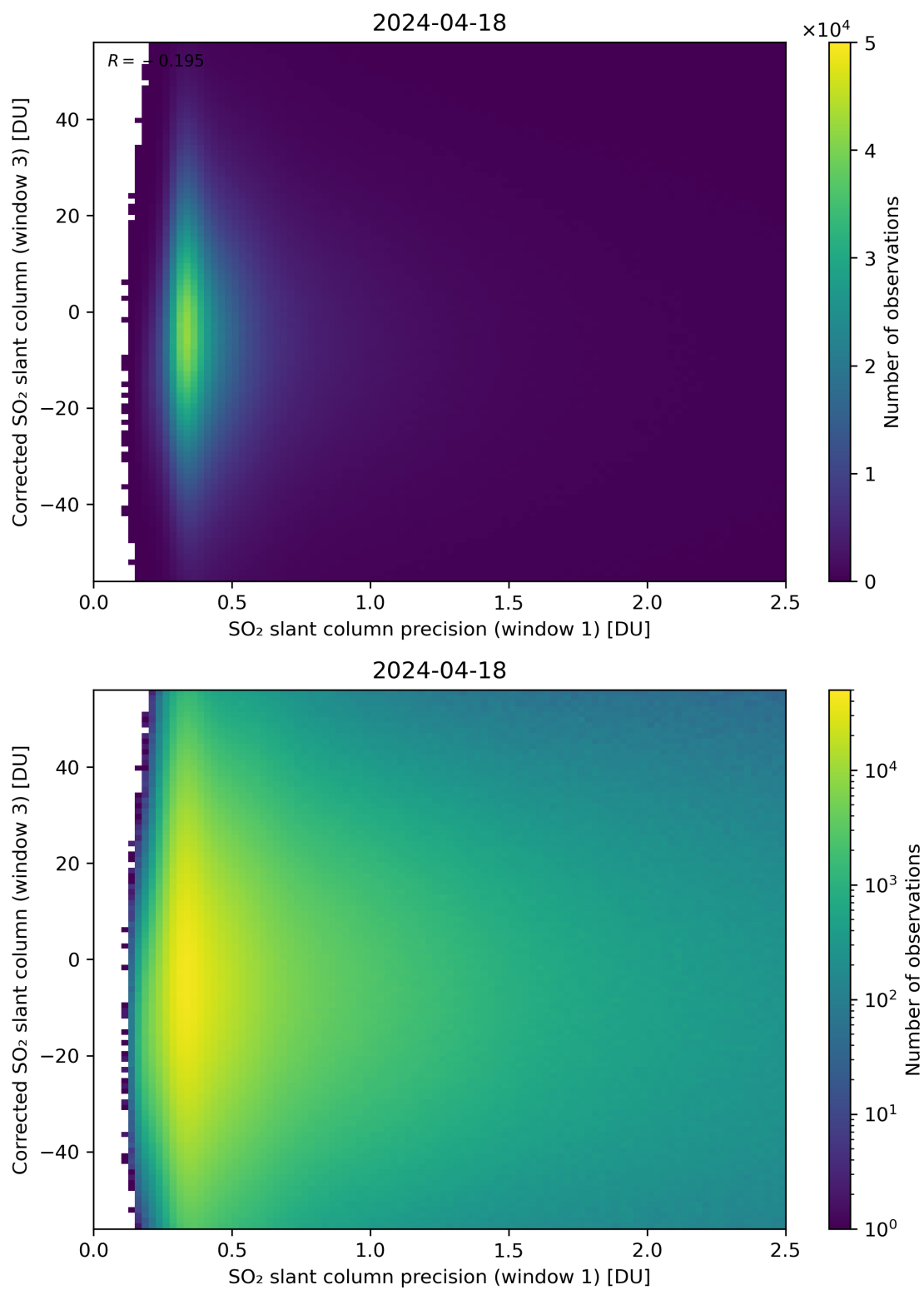
Figure 226: Scatter density plot of “SO 2 slant column precision (window 1)” against “Corrected SO 2 slant column (window 3)” for 2024-04-17 to 2024-04-19.
