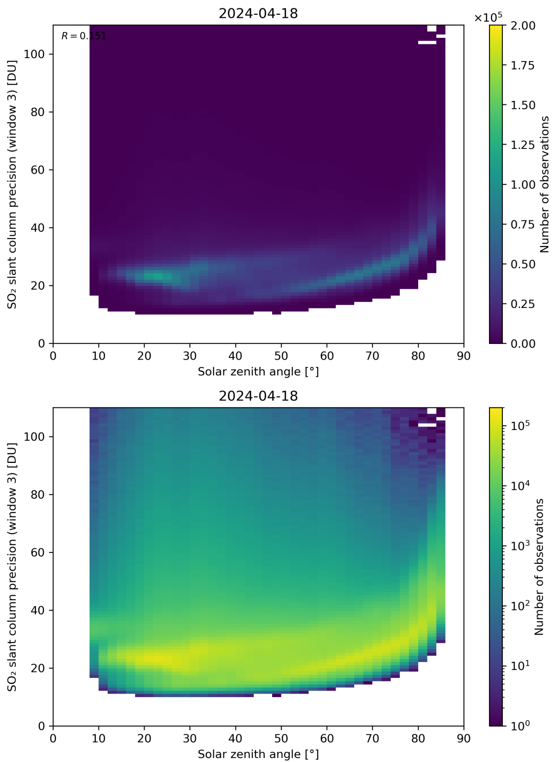
Figure 173: Scatter density plot of “Solar zenith angle” against “SO 2 slant column precision (window 3)” for 2024-04-17 to 2024-04-19.
