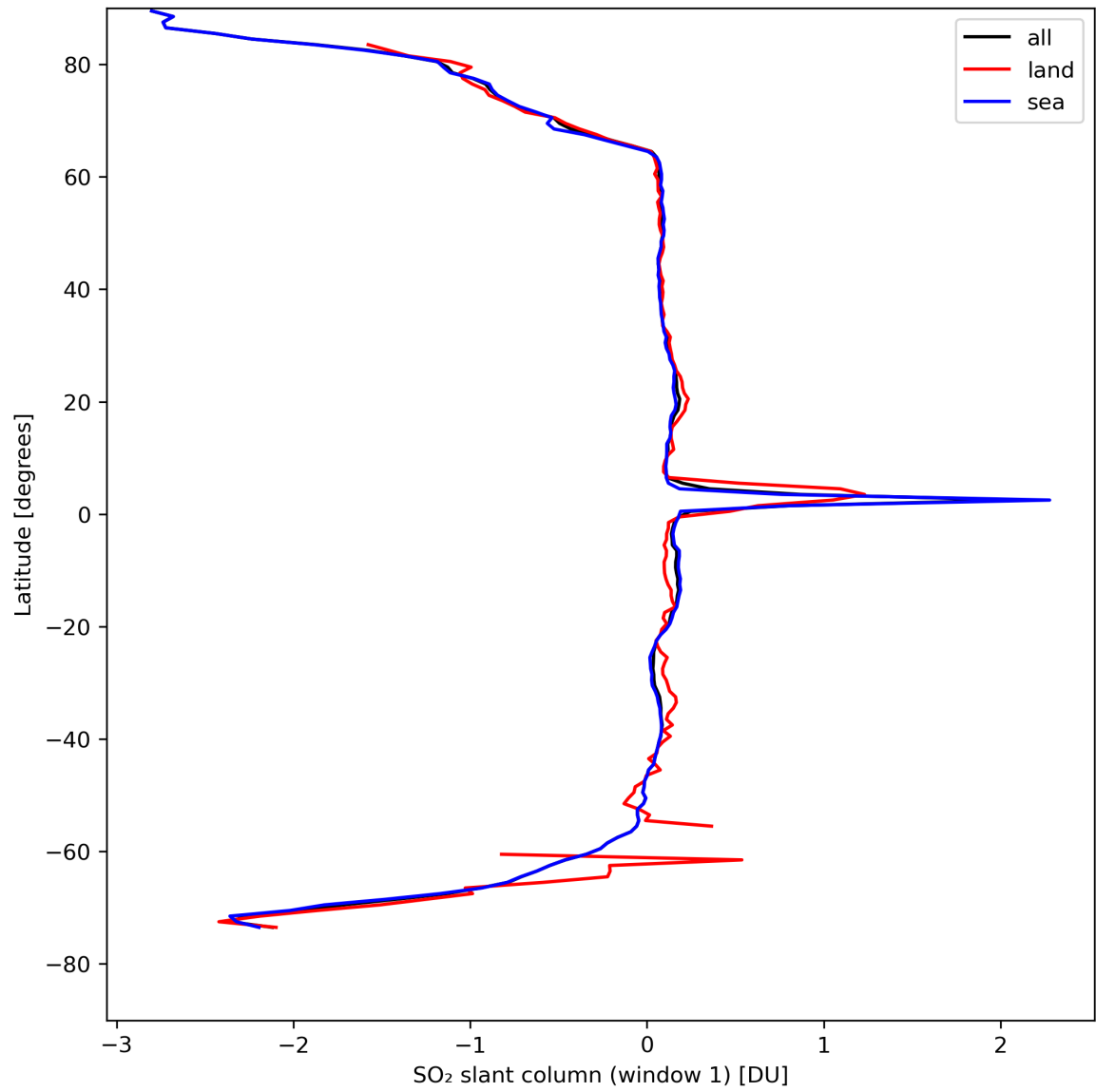
Figure 33: Zonal average of “SO 2 slant column (window 1)” for 2024-04-17 to 2024-04-19.
