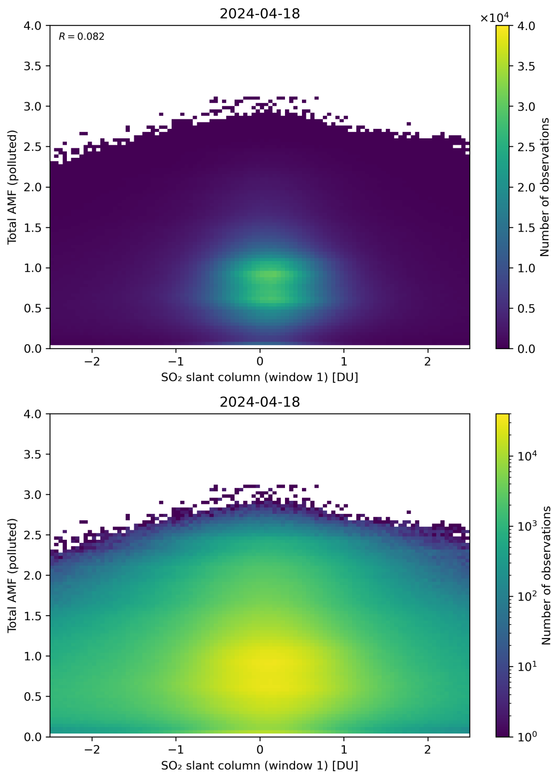
Figure 239: Scatter density plot of “SO 2 slant column (window 1)” against “Total AMF (polluted)” for 2024-04-17 to 2024-04-19.
