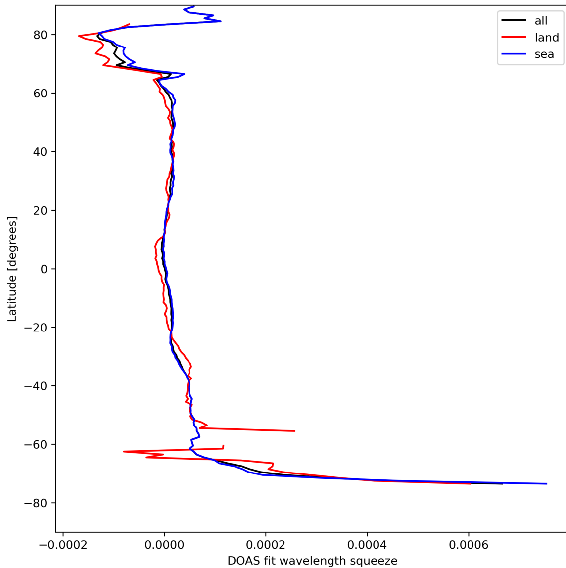
Figure 46: Zonal average of “DOAS fit wavelength squeeze” for 2024-04-17 to 2024-04-19.
