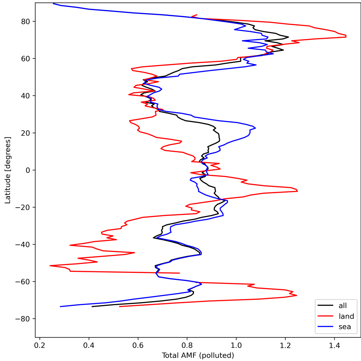
Figure 48: Zonal average of “Total AMF (polluted)” for 2024-04-17 to 2024-04-19.
