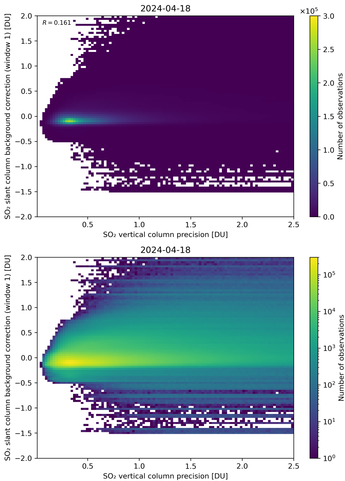
Figure 279: Scatter density plot of “SO 2 vertical column precision” against “SO 2 slant column background correction (window 1)” for 2024-04-17 to 2024-04-19.
