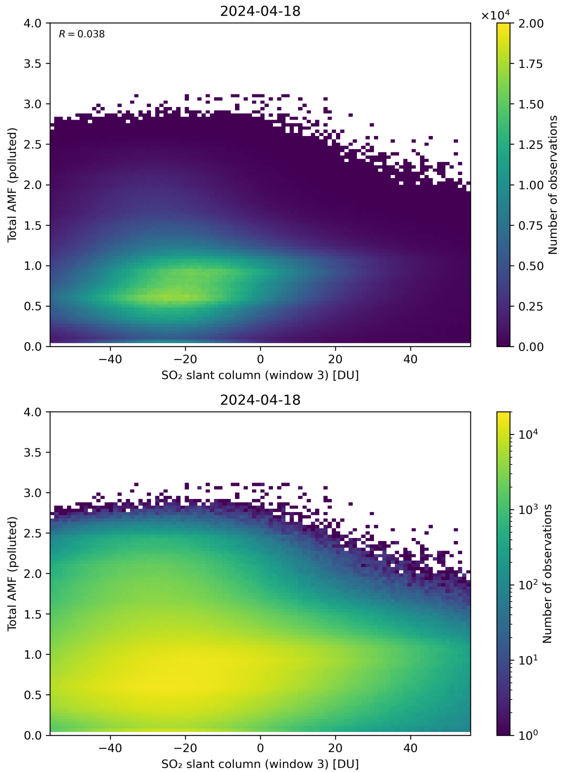
Figure 268: Scatter density plot of “SO 2 slant column (window 3)” against “Total AMF (polluted)” for 2024-04-17 to 2024-04-19.
