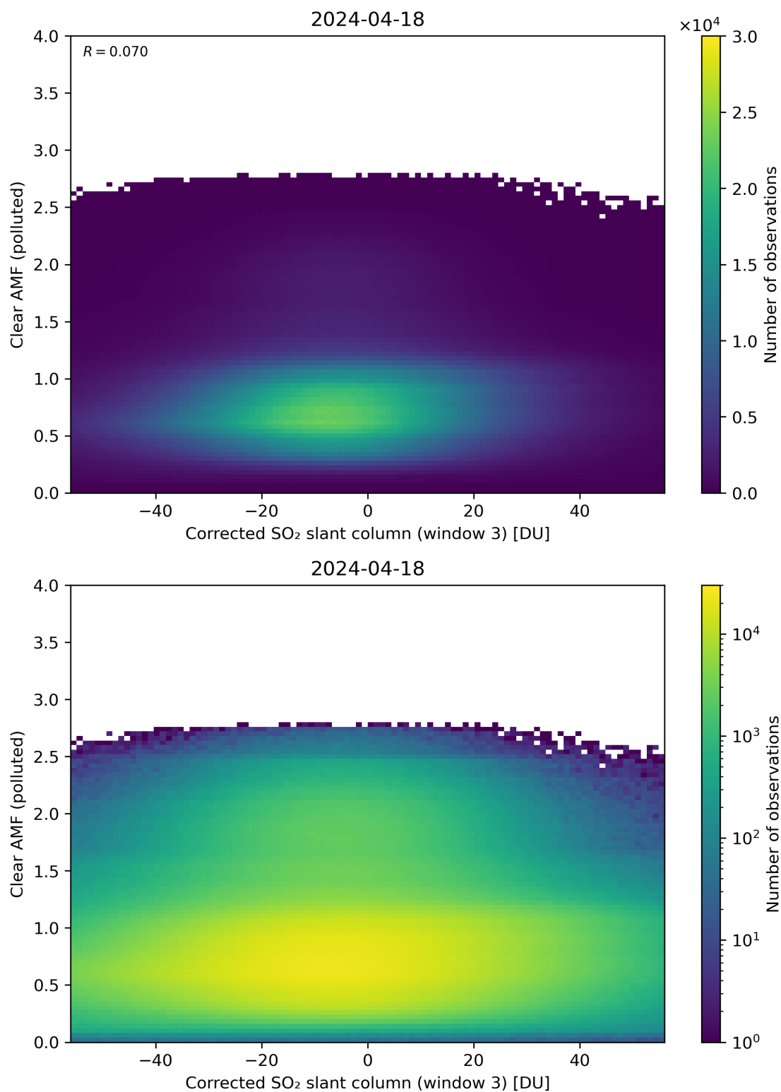
Figure 209: Scatter density plot of “Corrected SO 2 slant column (window 3)” against “Clear AMF (polluted)” for 2024-04-17 to 2024-04-19.
