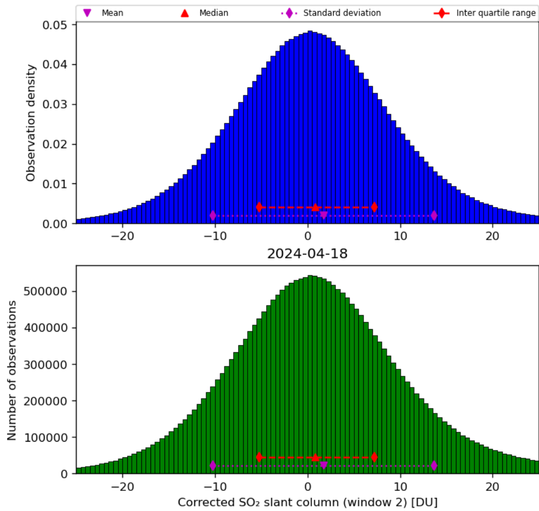
Figure 62: Histogram of “Corrected SO 2 slant column (window 2)” for 2024-04-17 to 2024-04-19
