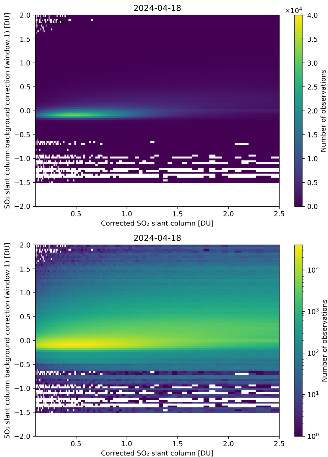
Figure 178: Scatter density plot of “Corrected SO 2 slant column” against “SO 2 slant column background correction (window 1)” for 2024-04-17 to 2024-04-19.
