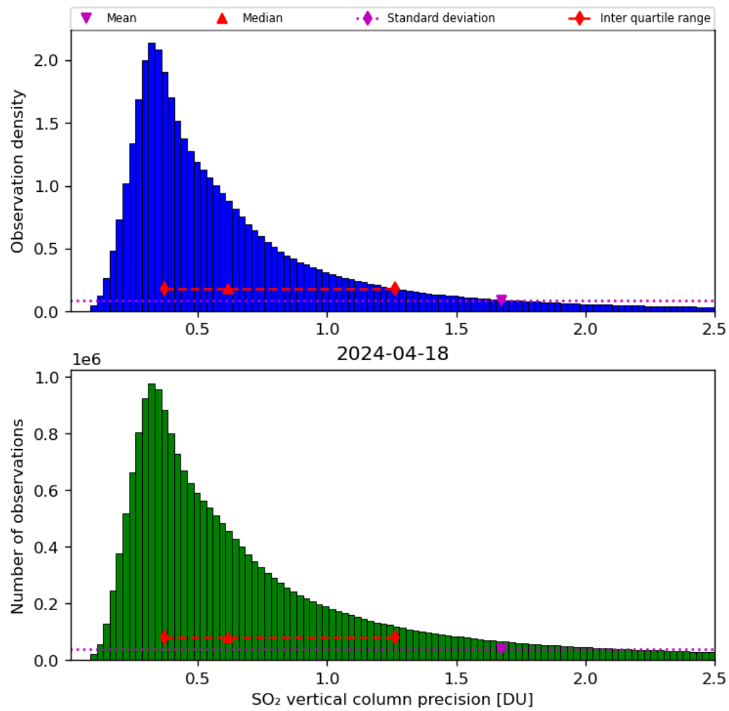
Figure 54: Histogram of “SO 2 vertical column precision” for 2024-04-17 to 2024-04-19
