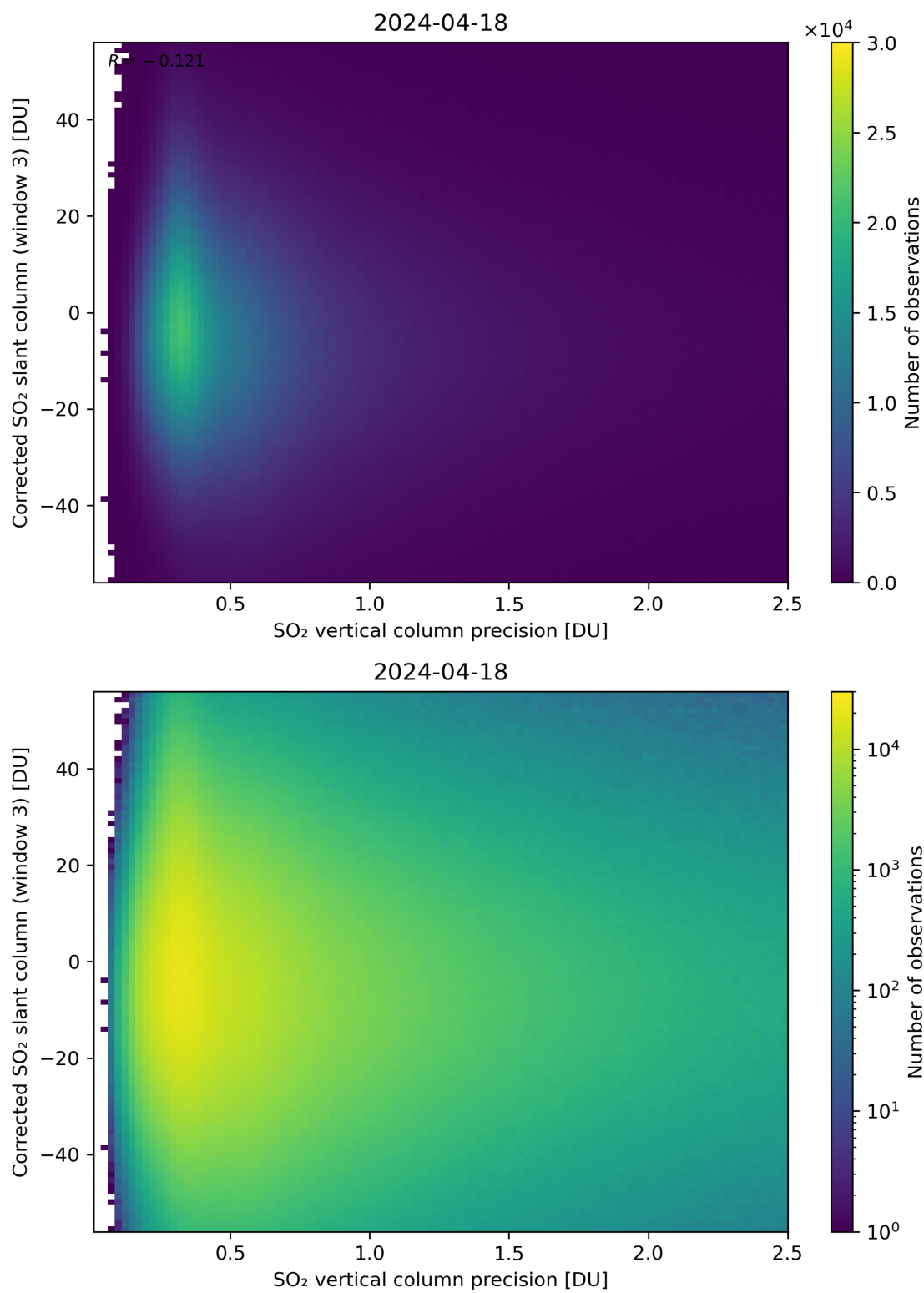
Figure 288: Scatter density plot of “SO 2 vertical column precision” against “Corrected SO 2 slant column (window 3)” for 2024-04-17 to 2024-04-19.
