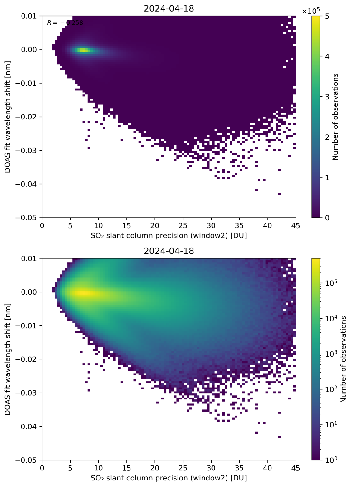
Figure 243: Scatter density plot of “SO 2 slant column precision (window2)” against “DOAS fit wavelength shift” for 2024-04-17 to 2024-04-19.
