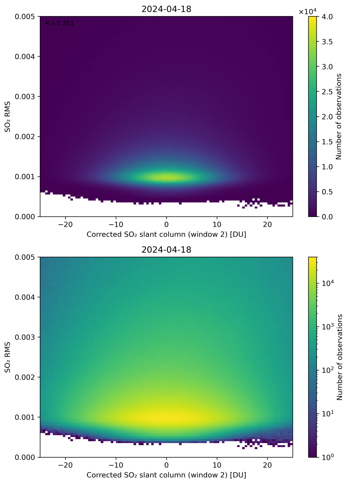
Figure 198: Scatter density plot of “Corrected SO 2 slant column (window 2)” against “SO 2 RMS” for 2024-04-17 to 2024-04-19.
