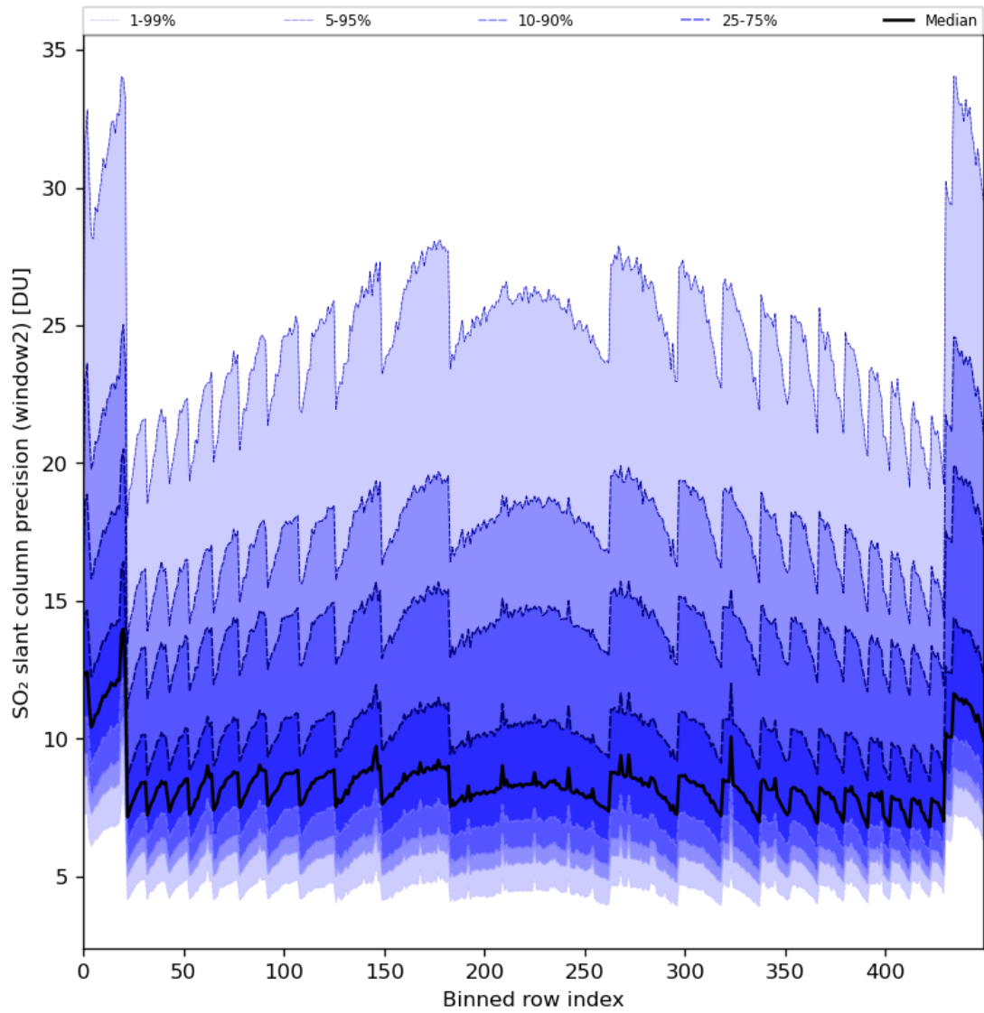
Figure 84: Along track statistics of “SO 2 slant column precision (window2)” for 2024-04-17 to 2024-04-19
