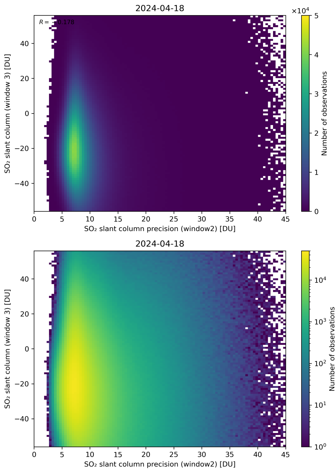
Figure 249: Scatter density plot of “SO 2 slant column precision (window2)” against “SO 2 slant column (window 3)” for 2024-04-17 to 2024-04-19.
