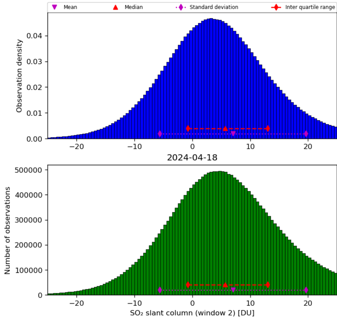
Figure 60: Histogram of “SO 2 slant column (window 2)” for 2024-04-17 to 2024-04-19
