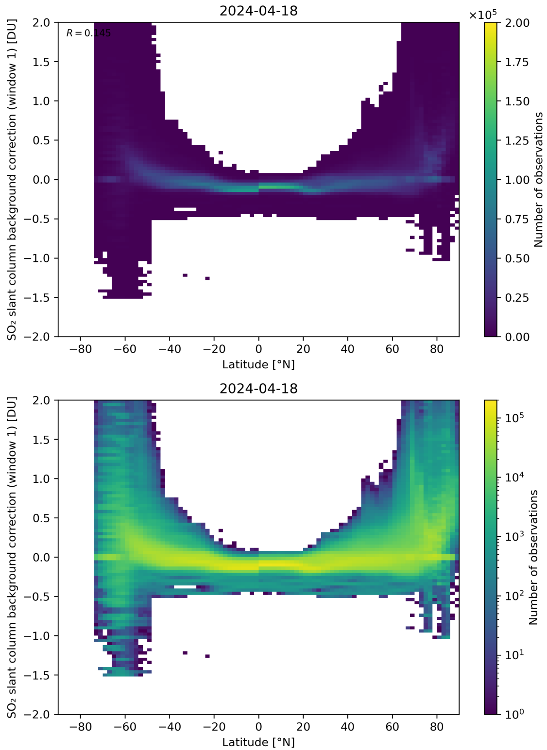
Figure 139: Scatter density plot of “Latitude” against “SO 2 slant column background correction (window 1)” for 2024-04-17 to 2024-04-19.
