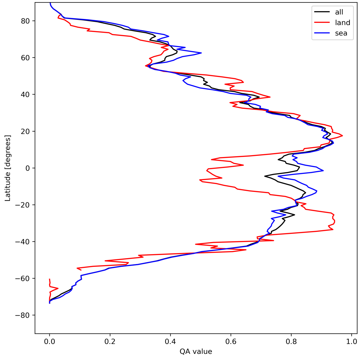
Figure 29: Zonal average of “QA value” for 2024-04-17 to 2024-04-19.
