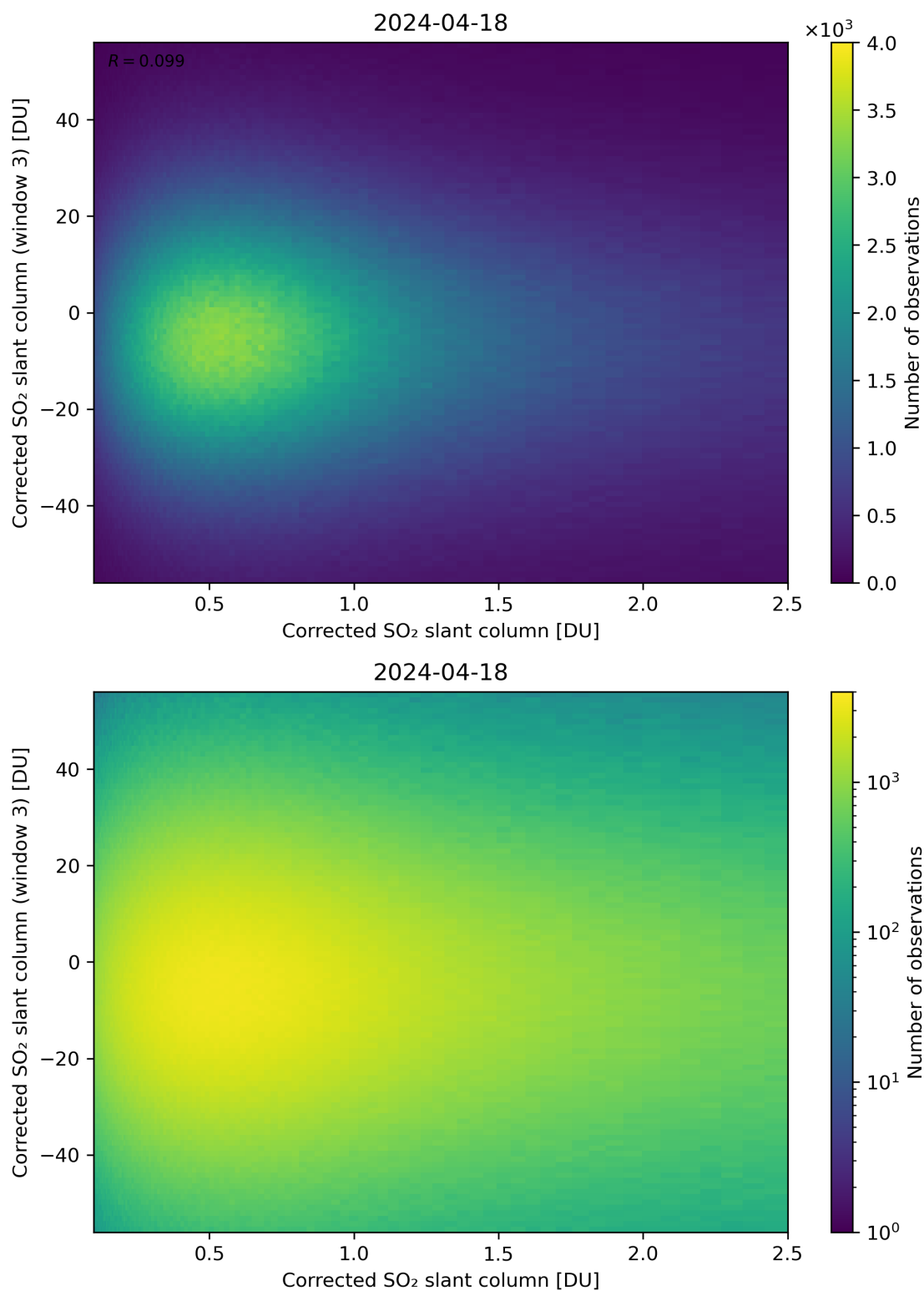
Figure 186: Scatter density plot of “Corrected SO 2 slant column” against “Corrected SO 2 slant column (window 3)” for 2024-04-17 to 2024-04-19.
