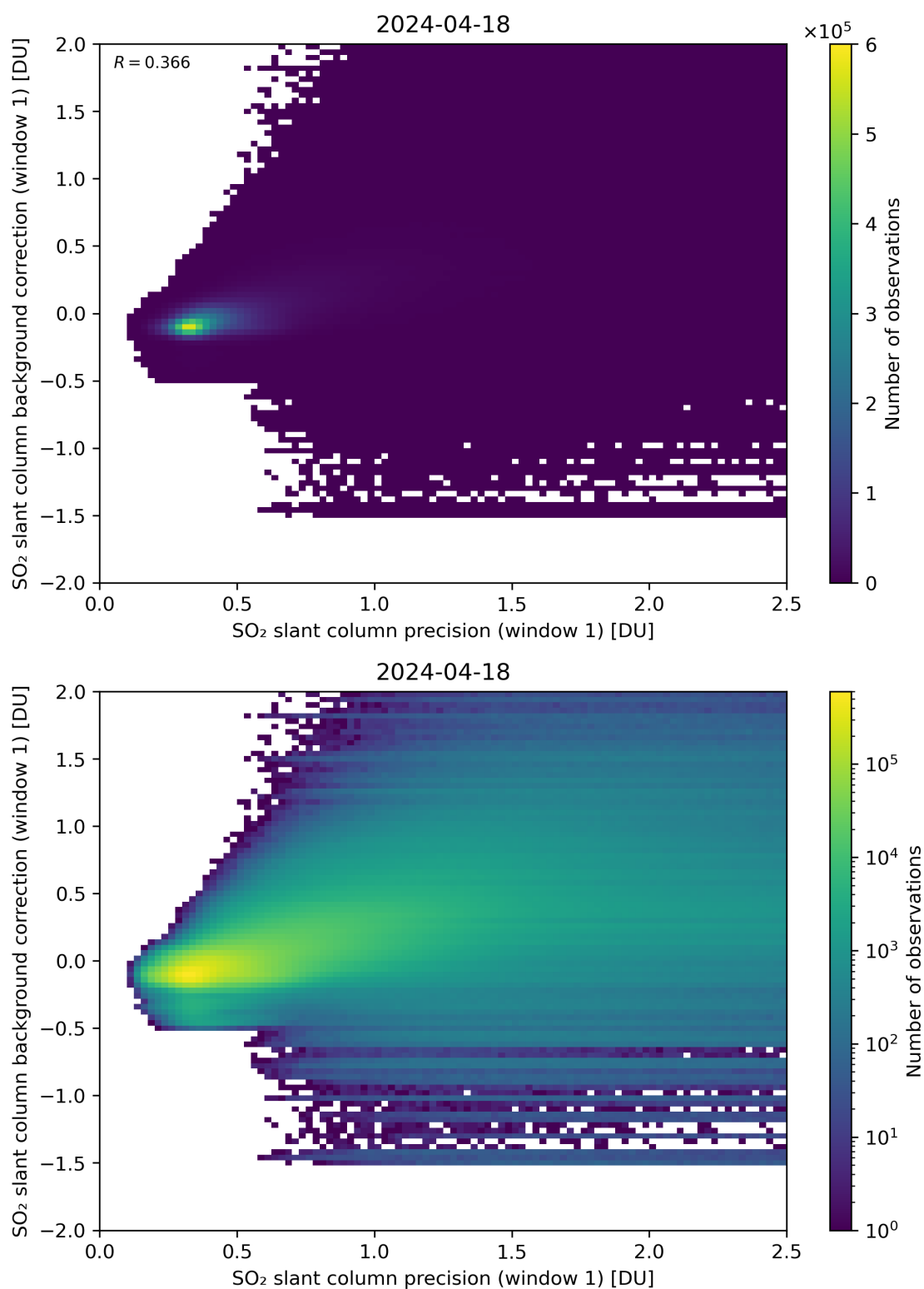
Figure 218: Scatter density plot of “SO 2 slant column precision (window 1)” against “SO 2 slant column background correction (window 1)” for 2024-04-17 to 2024-04-19.
