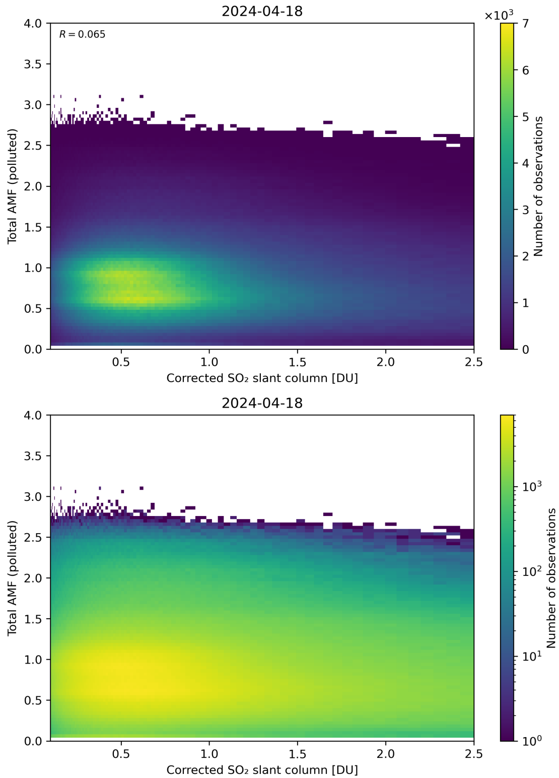
Figure 192: Scatter density plot of “Corrected SO 2 slant column” against “Total AMF (polluted)” for 2024-04-17 to 2024-04-19.
