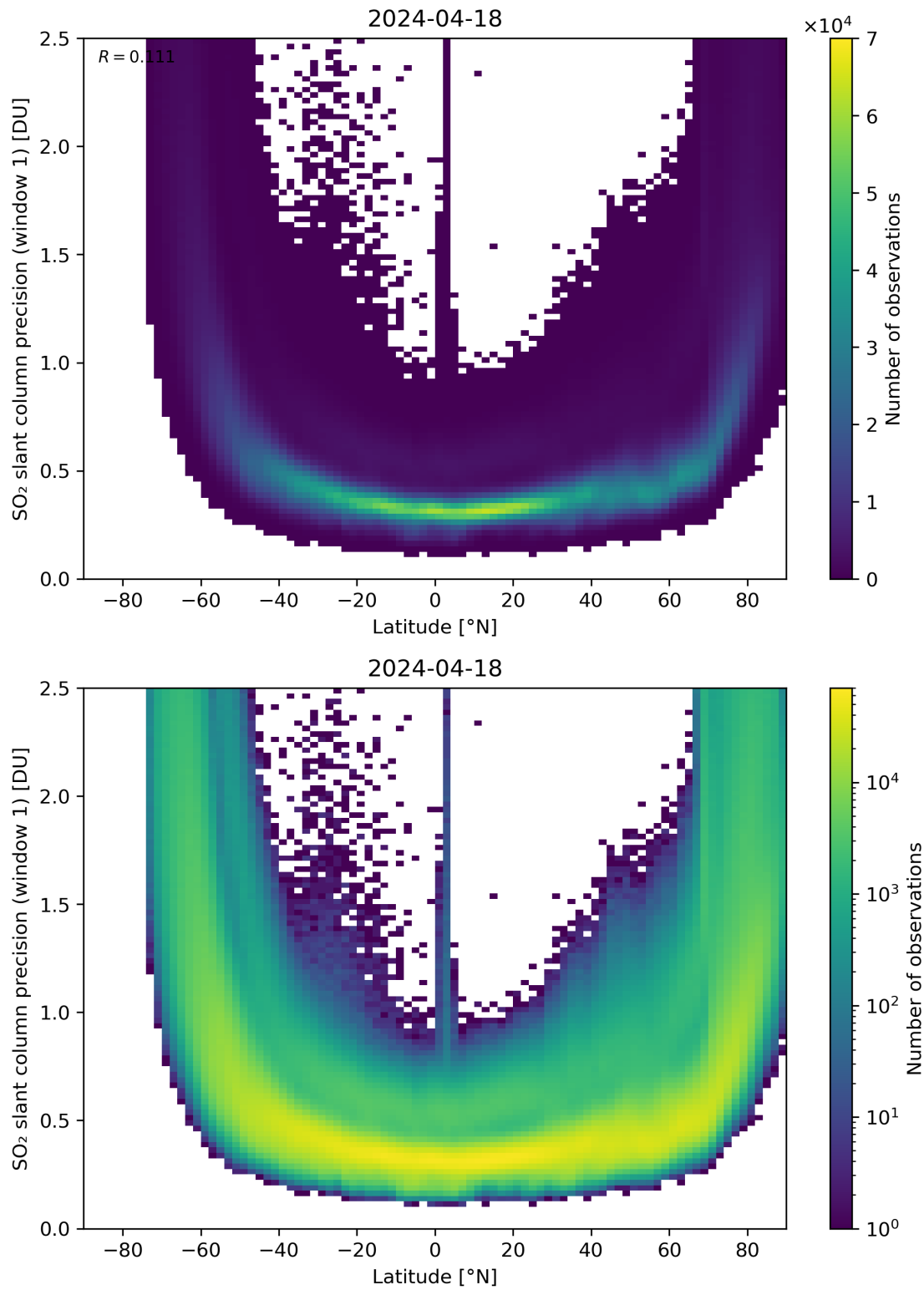
Figure 150: Scatter density plot of “Latitude” against “SO 2 slant column precision (window 1)” for 2024-04-17 to 2024-04-19.
