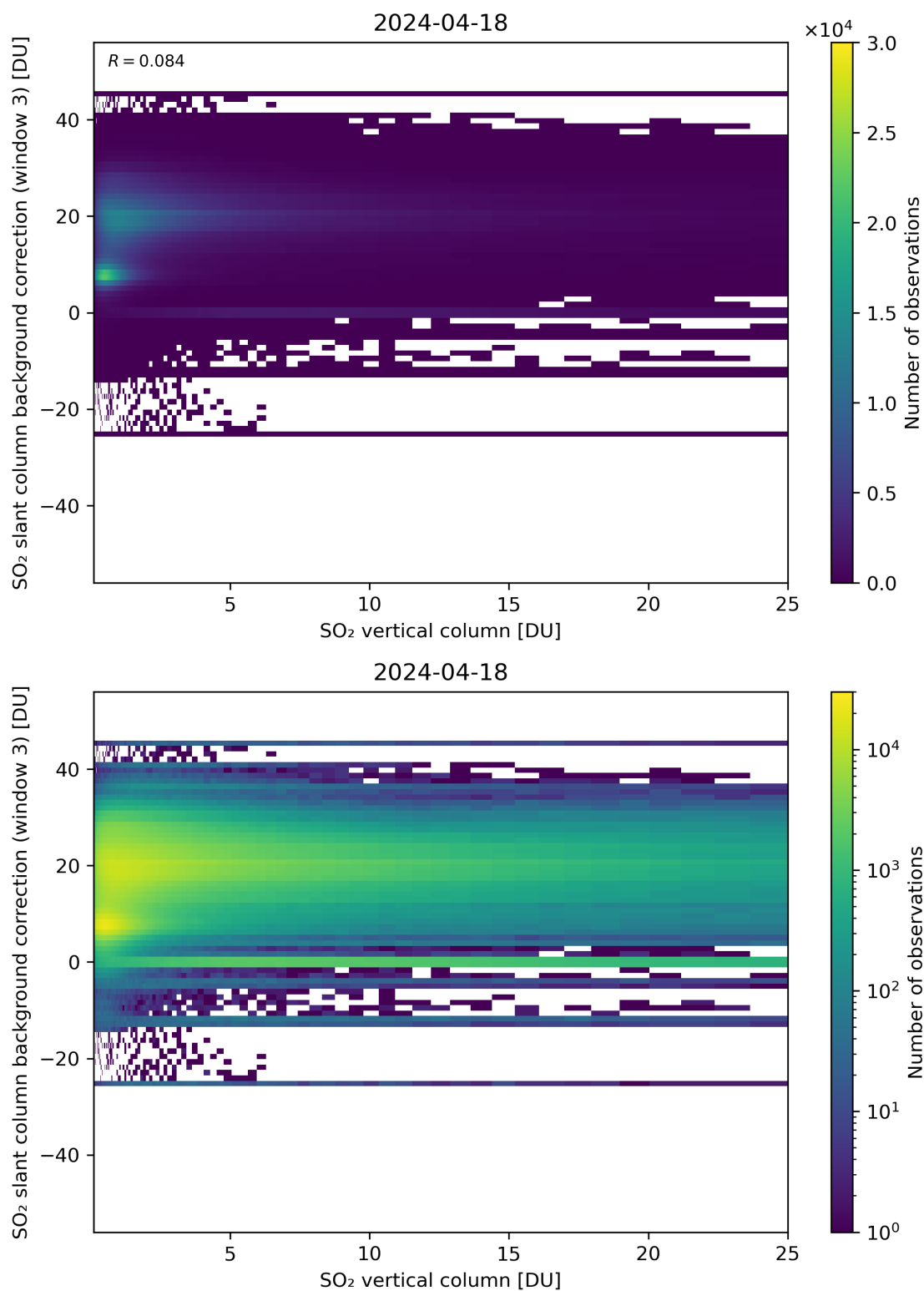
Figure 275: Scatter density plot of “SO 2 vertical column” against “SO 2 slant column background correction (window 3)” for 2024-04-17 to 2024-04-19.
