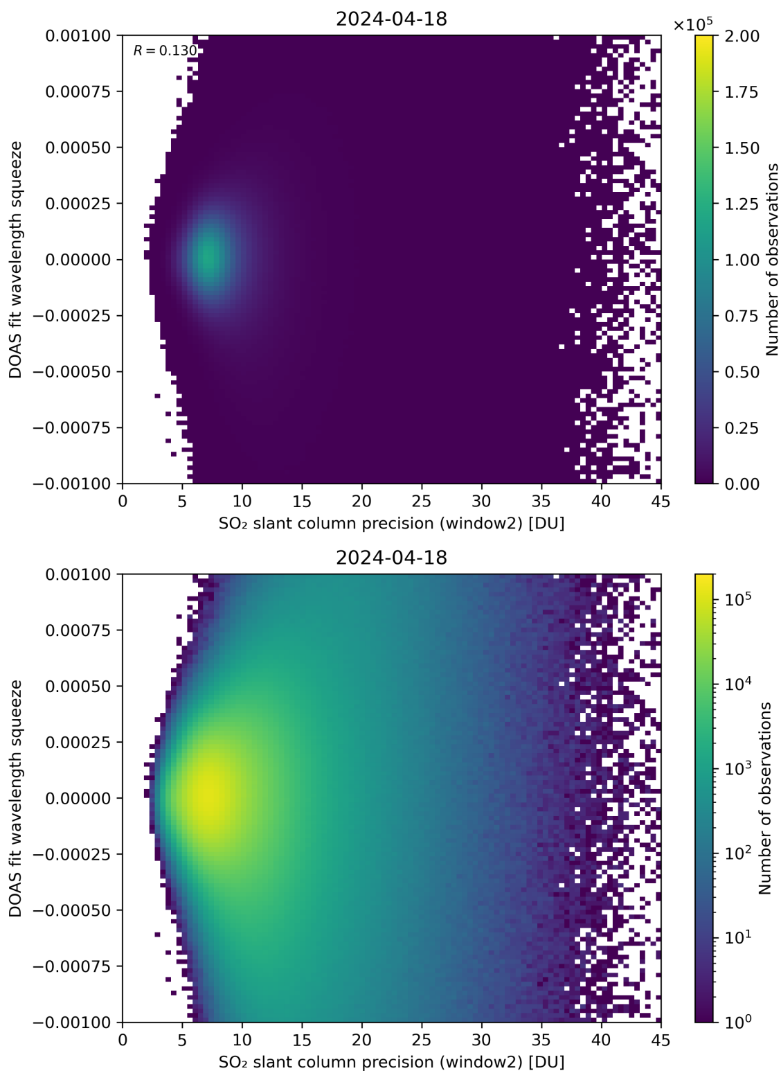
Figure 244: Scatter density plot of “SO 2 slant column precision (window2)” against “DOAS fit wavelength squeeze” for 2024-04-17 to 2024-04-19.
