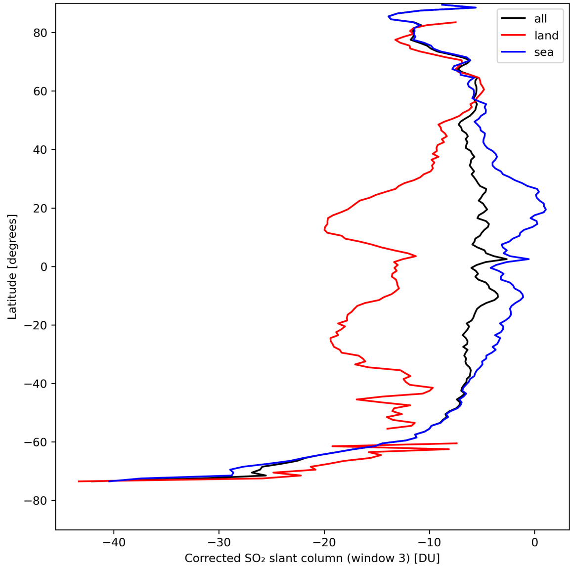
Figure 43: Zonal average of “Corrected SO 2 slant column (window 3)” for 2024-04-17 to 2024-04-19.
