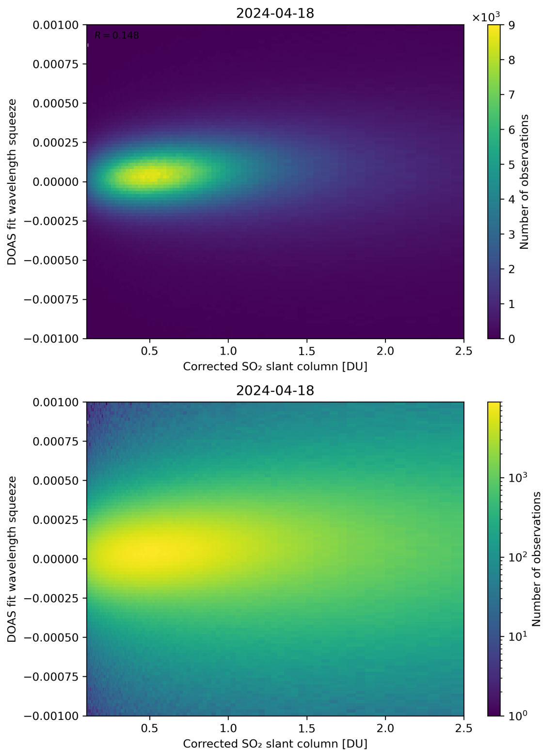
Figure 182: Scatter density plot of “Corrected SO 2 slant column” against “DOAS fit wavelength squeeze” for 2024-04-17 to 2024-04-19.
