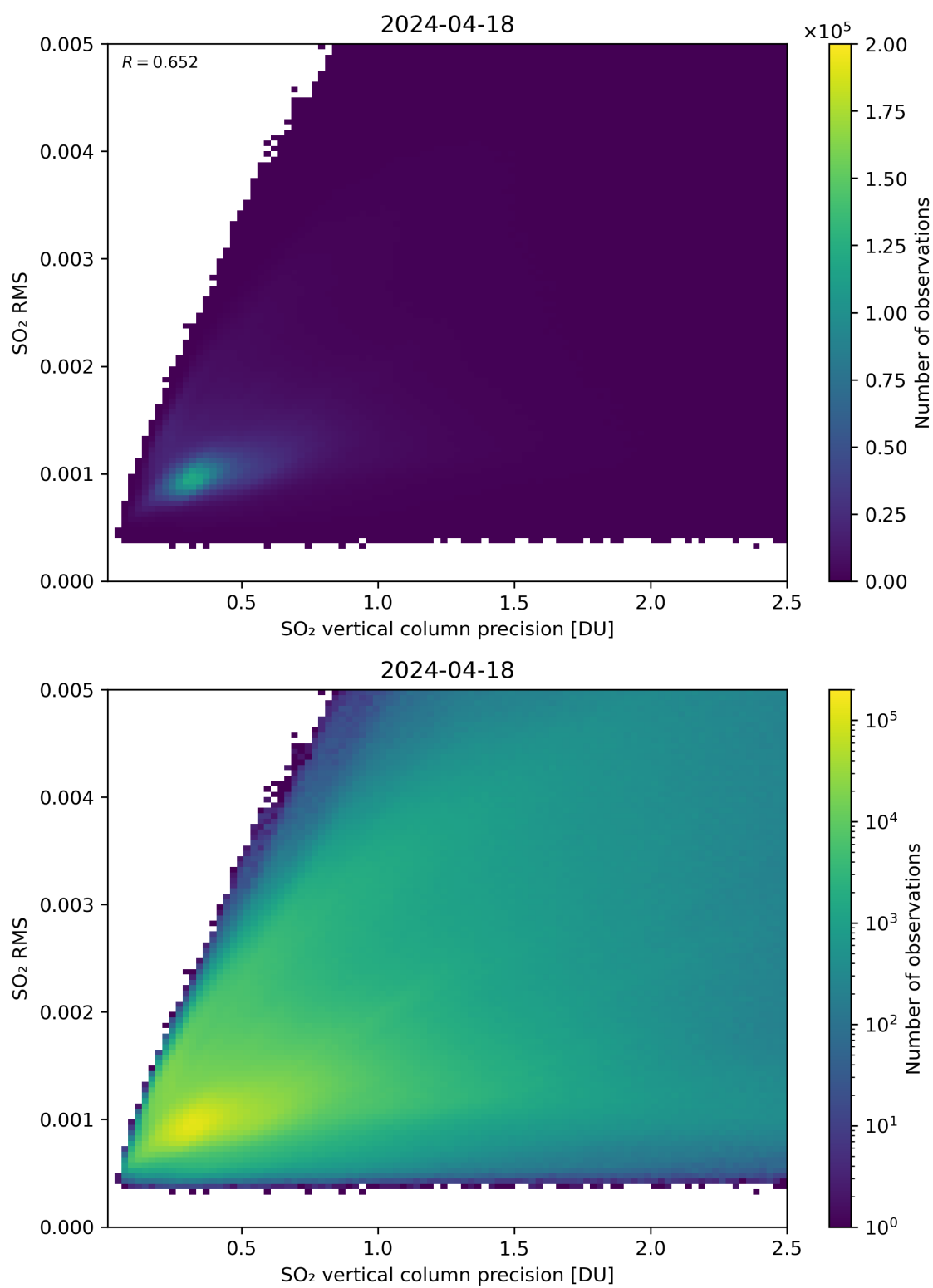
Figure 284: Scatter density plot of “SO 2 vertical column precision” against “SO 2 RMS” for 2024-04-17 to 2024-04-19.
