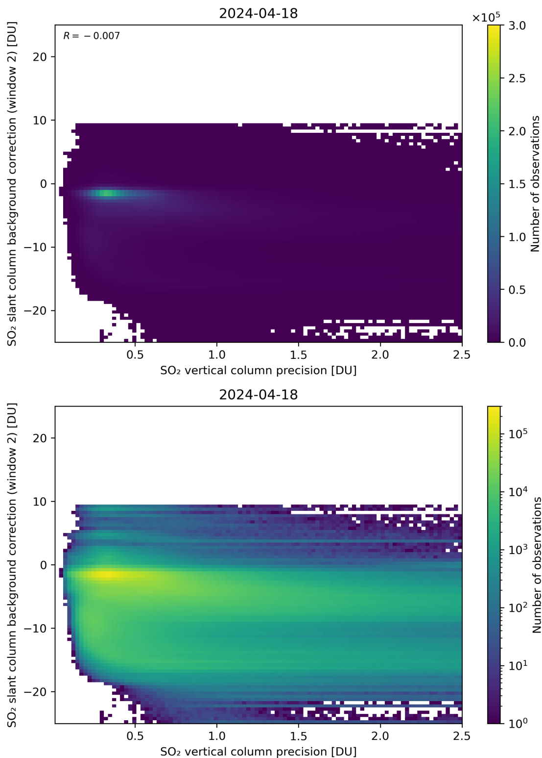
Figure 280: Scatter density plot of “SO 2 vertical column precision” against “SO 2 slant column background correction (window 2)” for 2024-04-17 to 2024-04-19.
