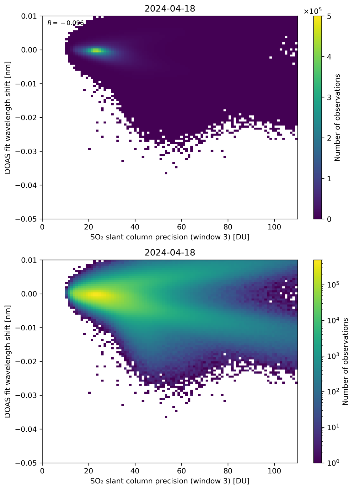
Figure 258: Scatter density plot of “SO 2 slant column precision (window 3)” against “DOAS fit wavelength shift” for 2024-04-17 to 2024-04-19.
