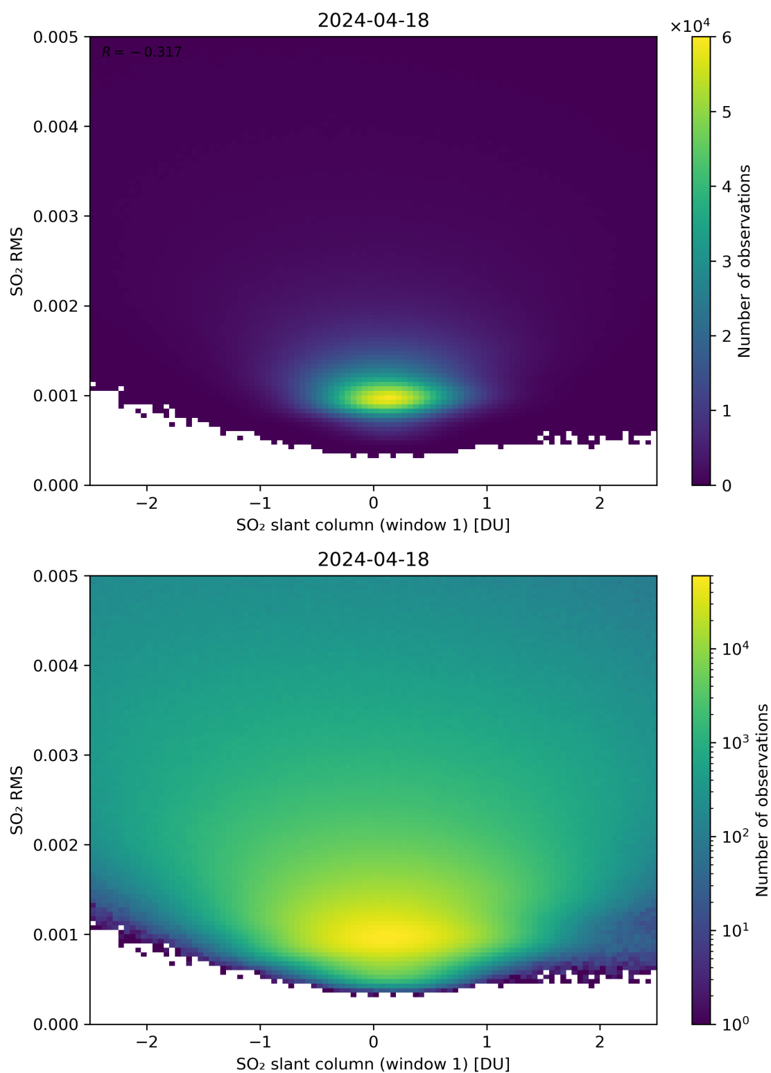
Figure 217: Scatter density plot of “SO 2 slant column (window 1)” against “SO 2 RMS” for 2024-04-17 to 2024-04-19.
