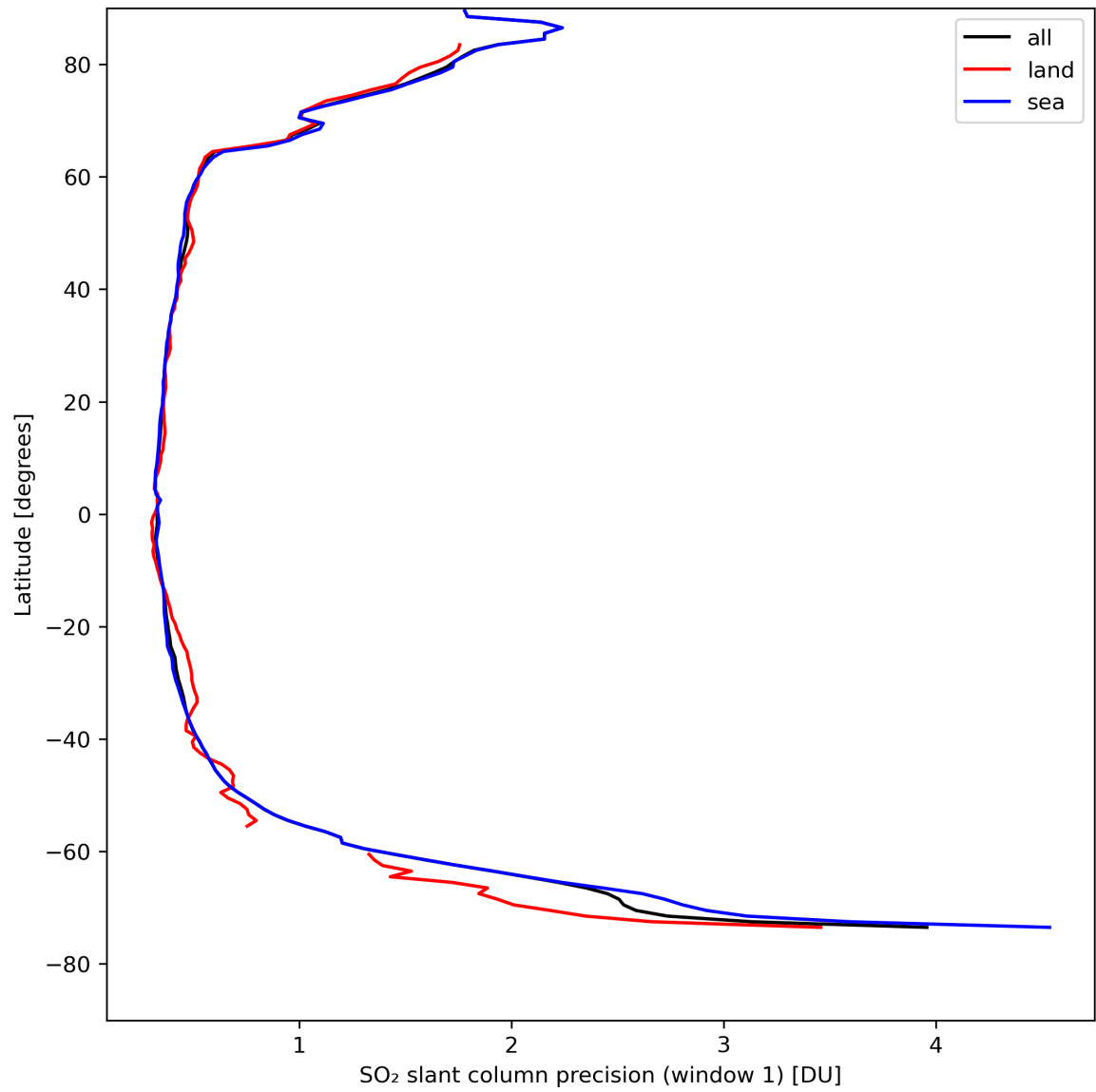
Figure 34: Zonal average of “SO 2 slant column precision (window 1)” for 2024-04-17 to 2024-04-19.
