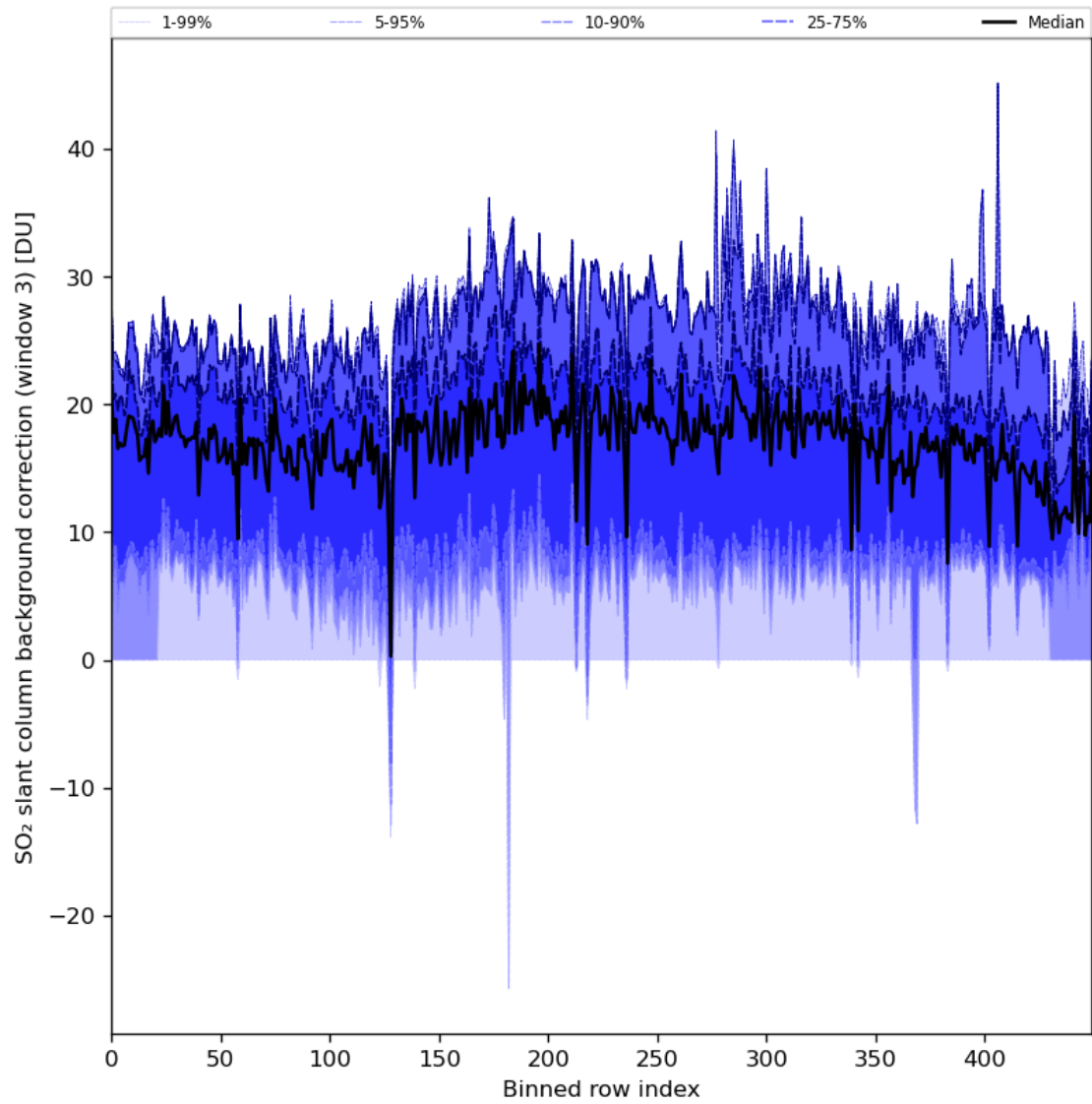
Figure 90: Along track statistics of “SO 2 slant column background correction (window 3)” for 2024-04-17 to 2024-04-19
