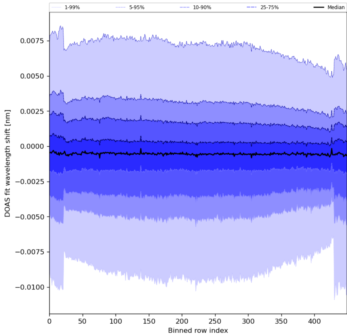
Figure 91: Along track statistics of “DOAS fit wavelength shift” for 2024-04-17 to 2024-04-19
