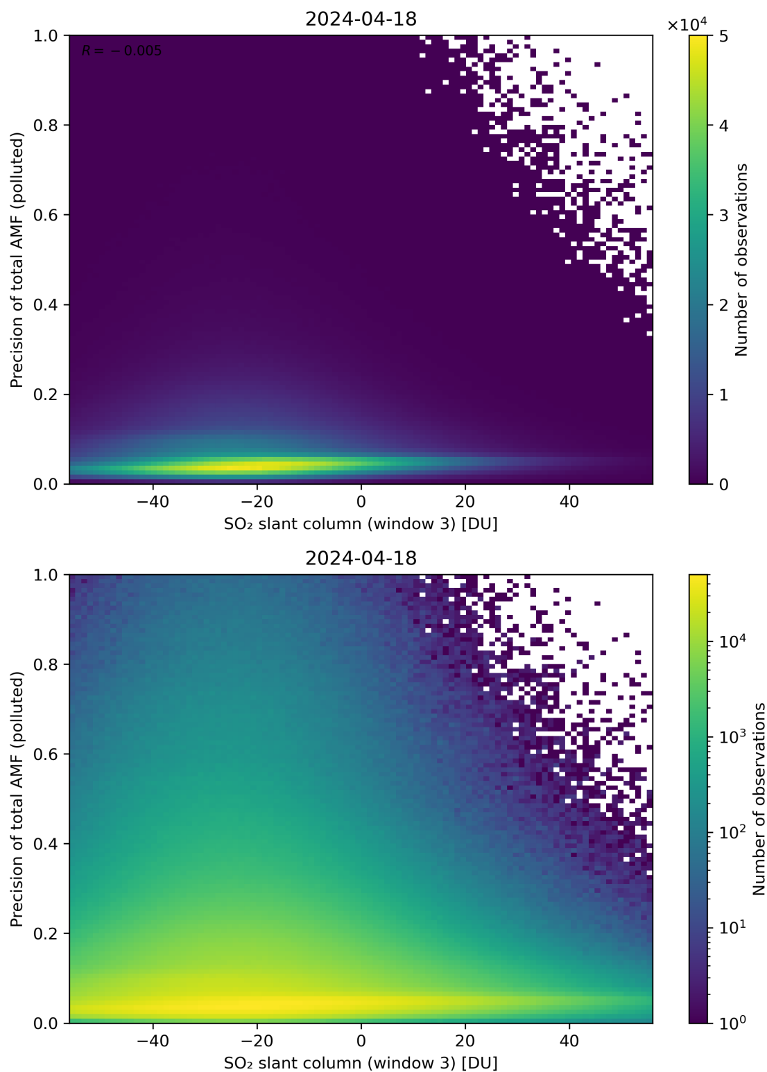
Figure 269: Scatter density plot of “SO 2 slant column (window 3)” against “Precision of total AMF (polluted)” for 2024-04-17 to 2024-04-19.
