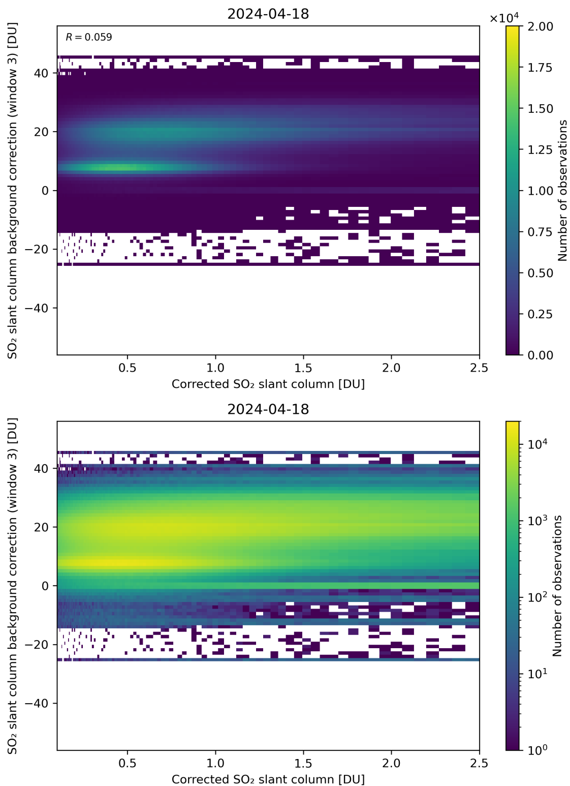
Figure 180: Scatter density plot of “Corrected SO 2 slant column” against “SO 2 slant column background correction (window 3)” for 2024-04-17 to 2024-04-19.
