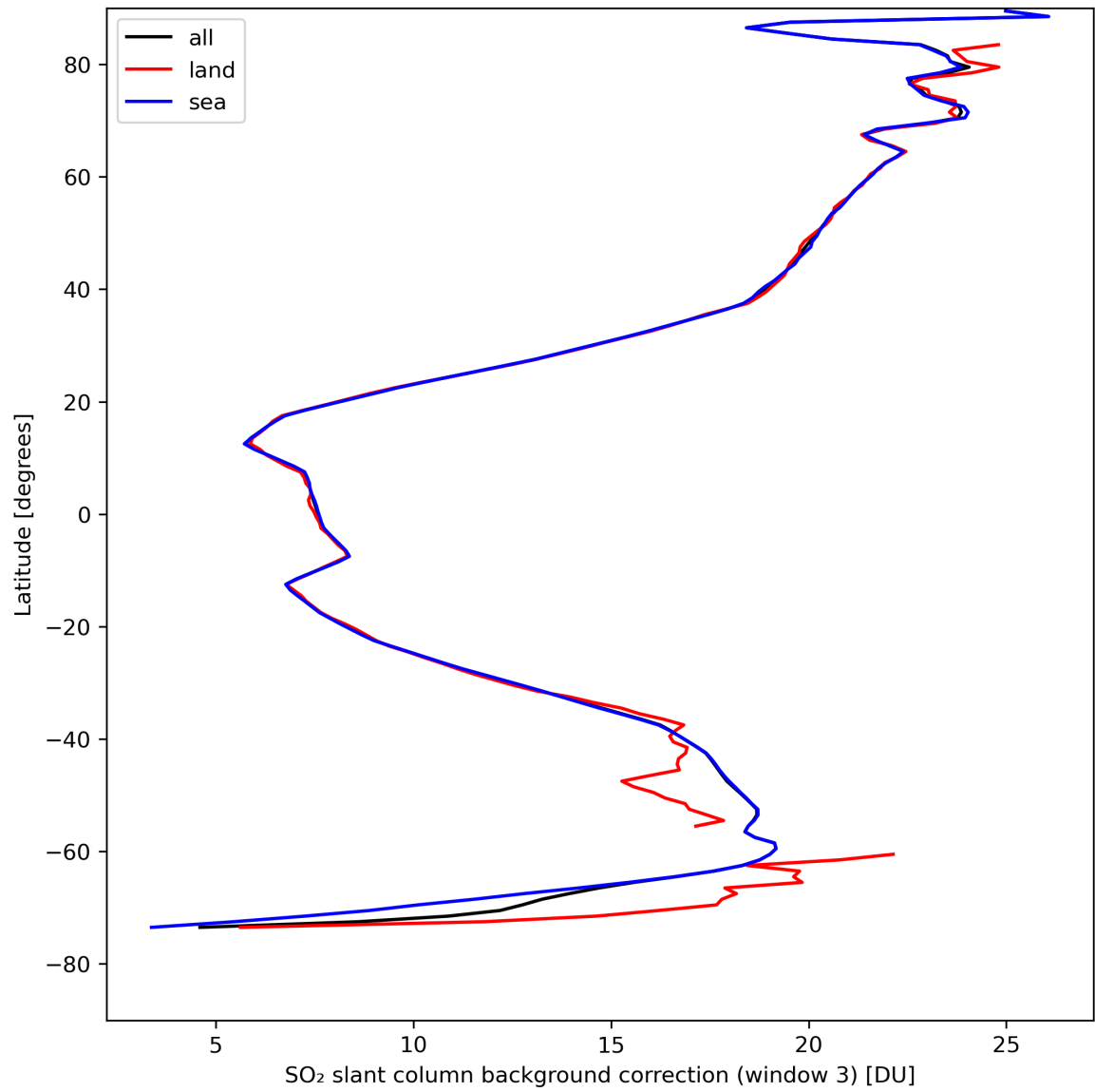
Figure 44: Zonal average of “SO 2 slant column background correction (window 3)” for 2024-04-17 to 2024-04-19.
