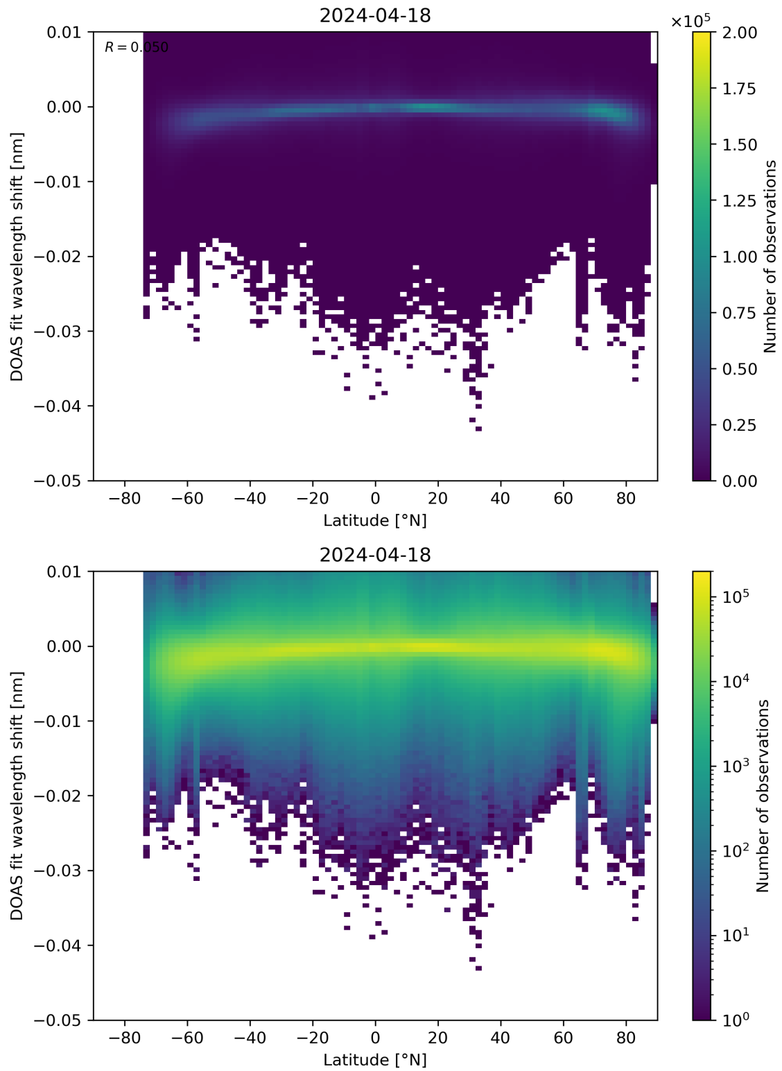
Figure 142: Scatter density plot of “Latitude” against “DOAS fit wavelength shift” for 2024-04-17 to 2024-04-19.
