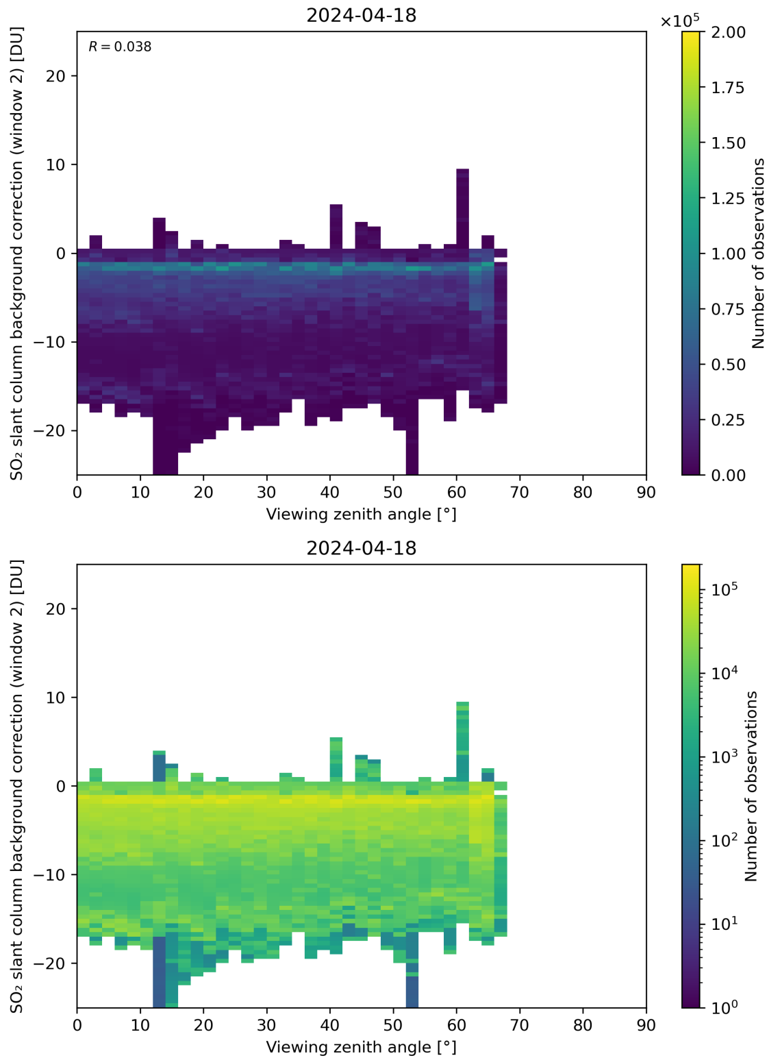
Figure 309: Scatter density plot of “Viewing zenith angle” against “SO 2 slant column background correction (window 2)” for 2024-04-17 to 2024-04-19.
