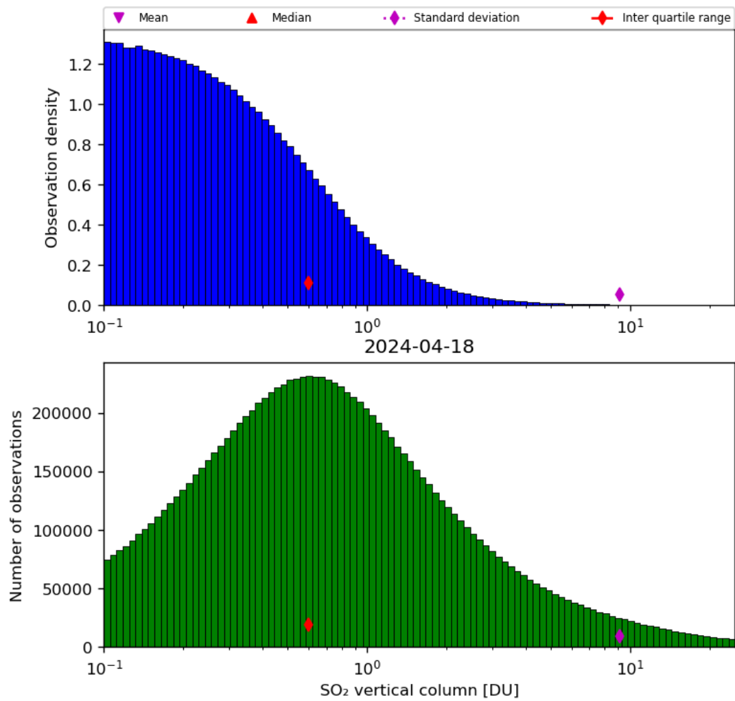
Figure 53: Histogram of “SO 2 vertical column” for 2024-04-17 to 2024-04-19
