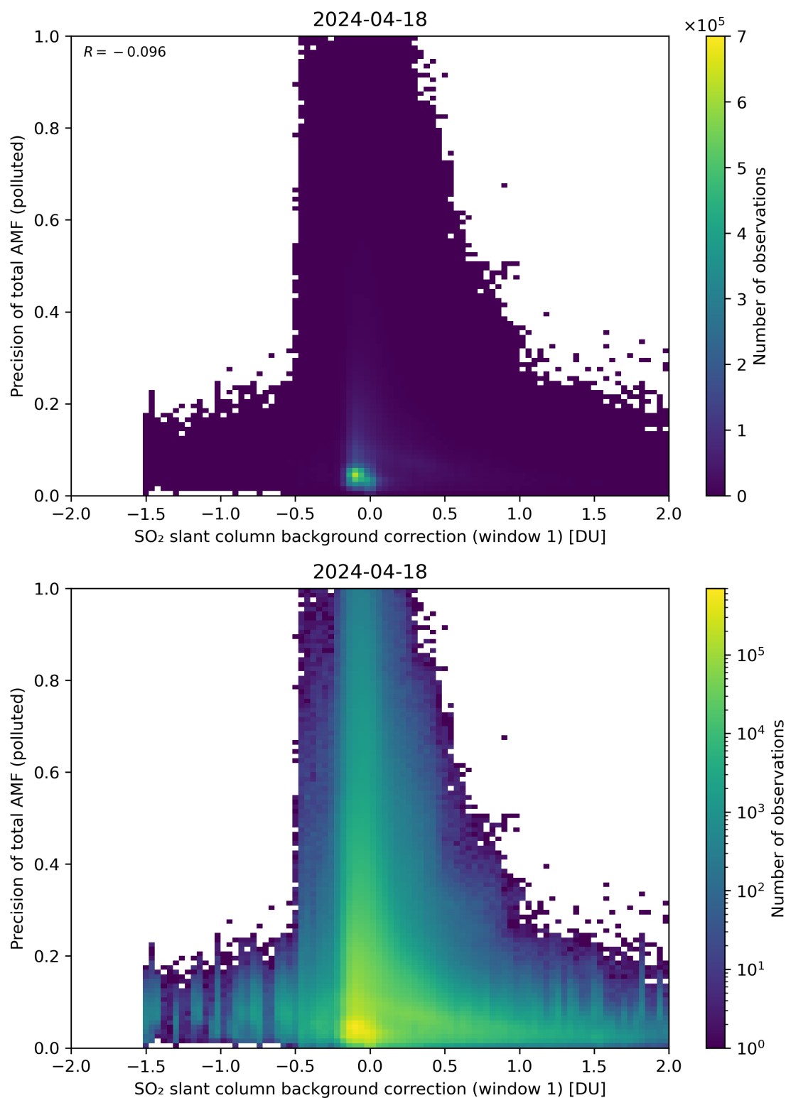
Figure 110: Scatter density plot of “SO 2 slant column background correction (window 1)” against “Precision of total AMF (polluted)” for 2024-04-17 to 2024-04-19.
