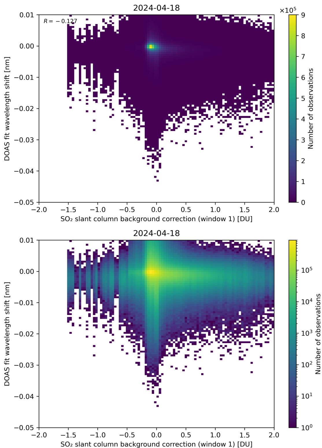
Figure 100: Scatter density plot of “SO 2 slant column background correction (window 1)” against “DOAS fit wavelength shift” for 2024-04-17 to 2024-04-19.
