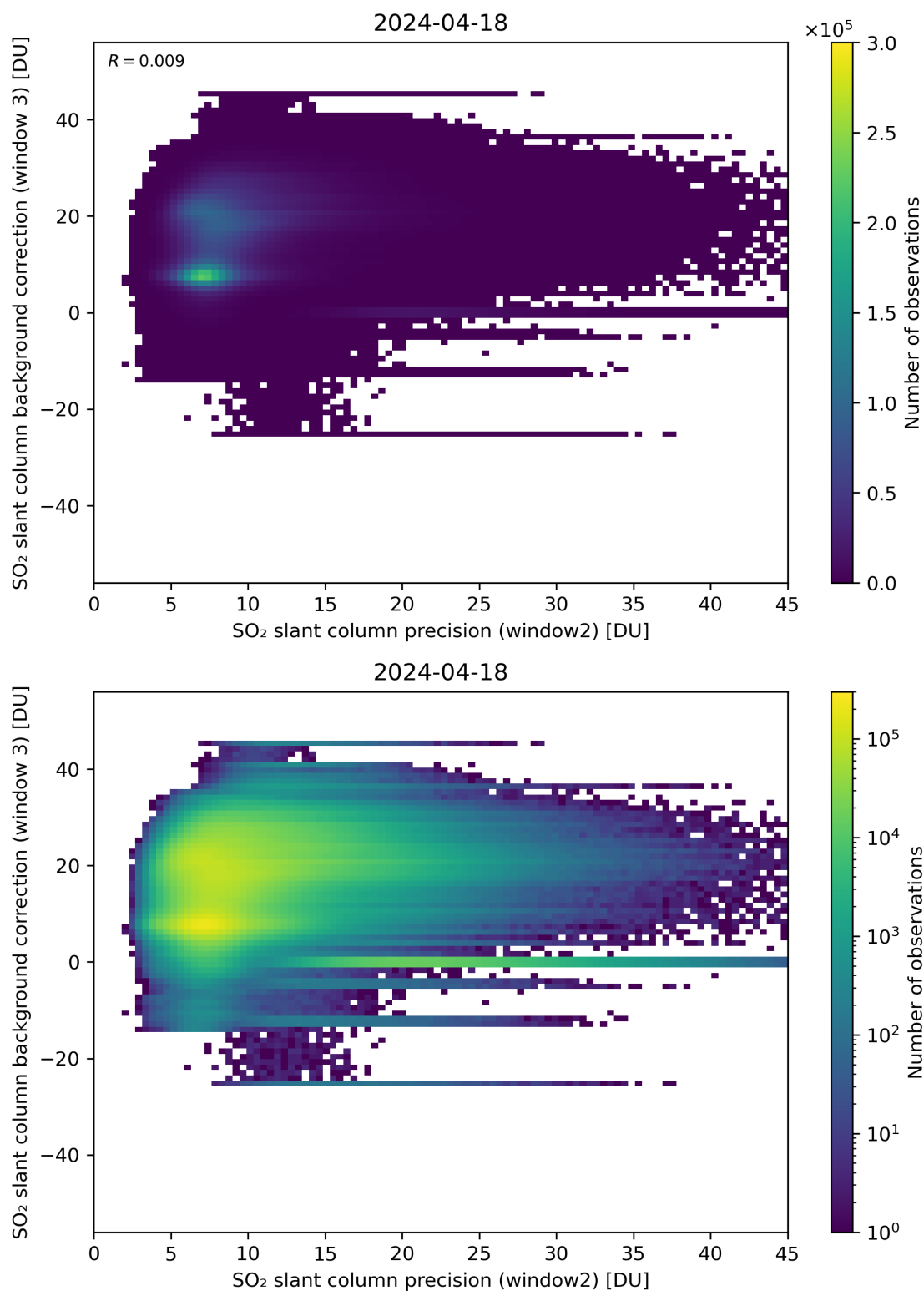
Figure 242: Scatter density plot of “SO 2 slant column precision (window2)” against “SO 2 slant column background correction (window 3)” for 2024-04-17 to 2024-04-19.
