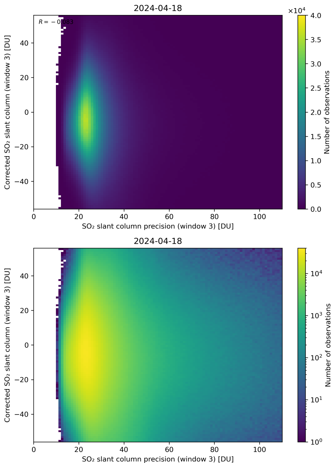
Figure 262: Scatter density plot of “SO 2 slant column precision (window 3)” against “Corrected SO 2 slant column (window 3)” for 2024-04-17 to 2024-04-19.
