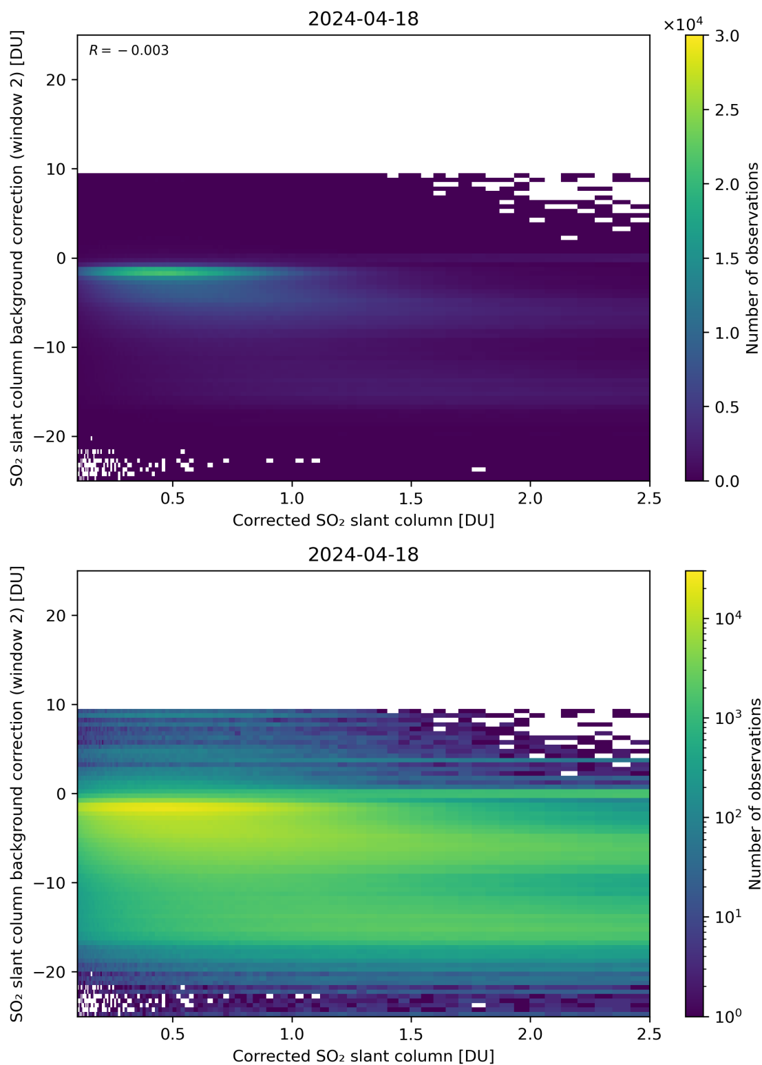
Figure 179: Scatter density plot of “Corrected SO 2 slant column” against “SO 2 slant column background correction (window 2)” for 2024-04-17 to 2024-04-19.
