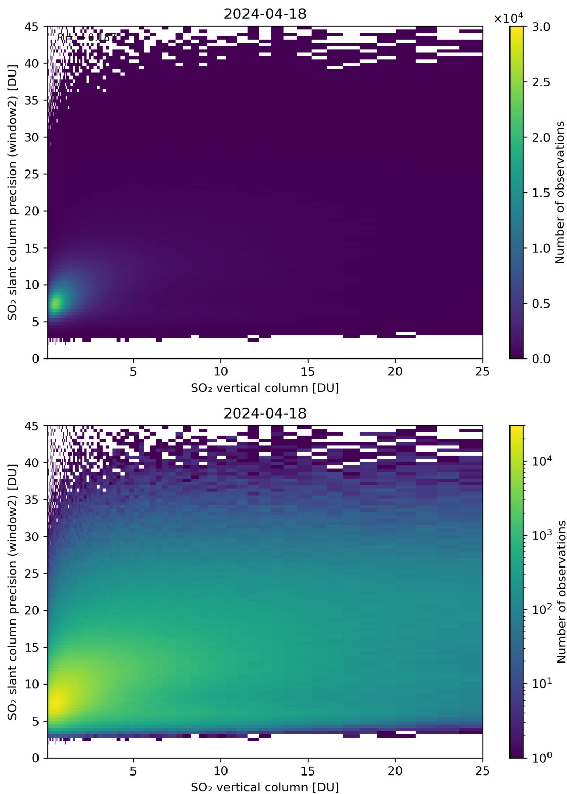
Figure 302: Scatter density plot of “SO 2 vertical column” against “SO 2 slant column precision (window2)” for 2024-04-17 to 2024-04-19.
