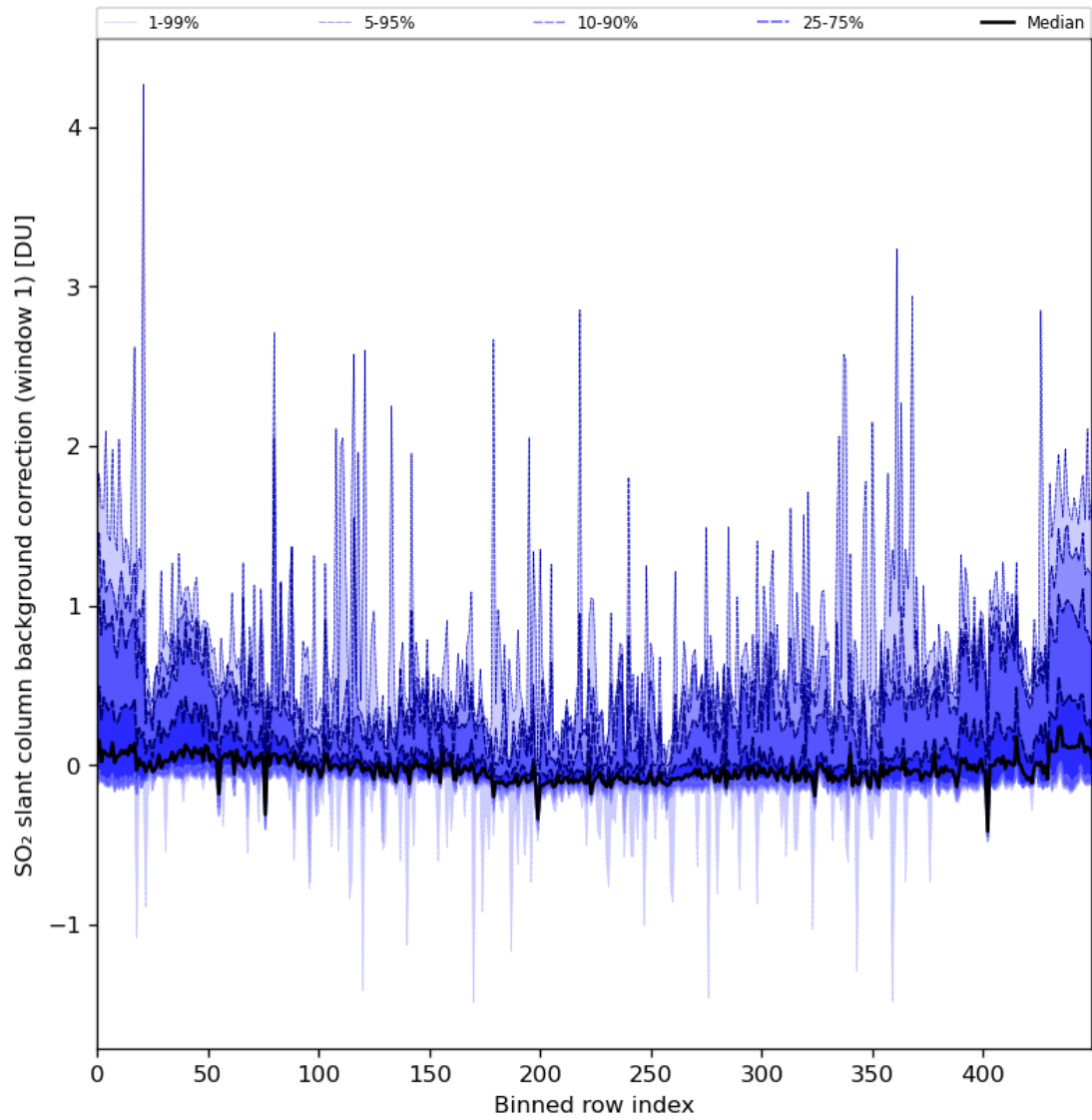
Figure 82: Along track statistics of "SO 2 slant column background correction (window 1)" for 2024-04-17 to 2024-04-19
