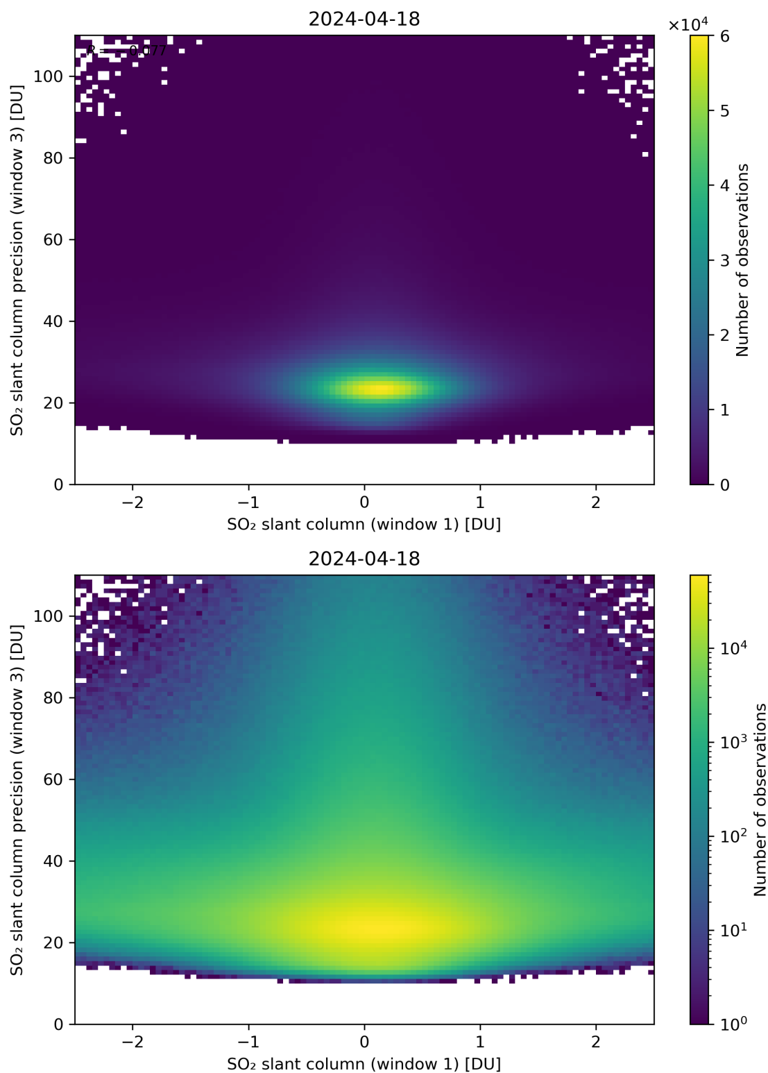
Figure 238: Scatter density plot of “SO 2 slant column (window 1)” against “SO 2 slant column precision (window 3)” for 2024-04-17 to 2024-04-19.
