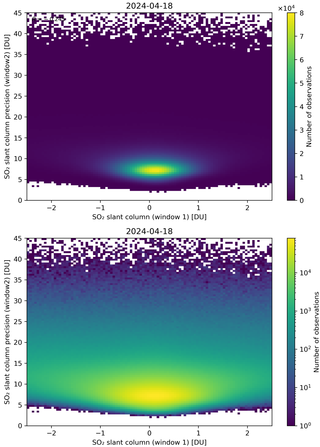
Figure 236: Scatter density plot of “SO 2 slant column (window 1)” against “SO 2 slant column precision (window2)” for 2024-04-17 to 2024-04-19.
