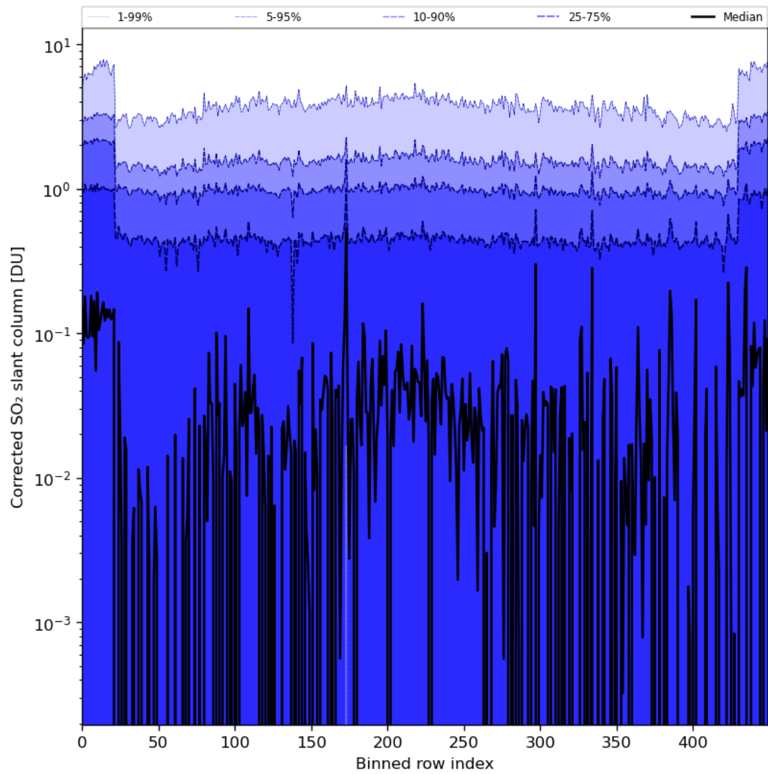
Figure 78: Along track statistics of “Corrected SO 2 slant column” for 2024-04-17 to 2024-04-19
