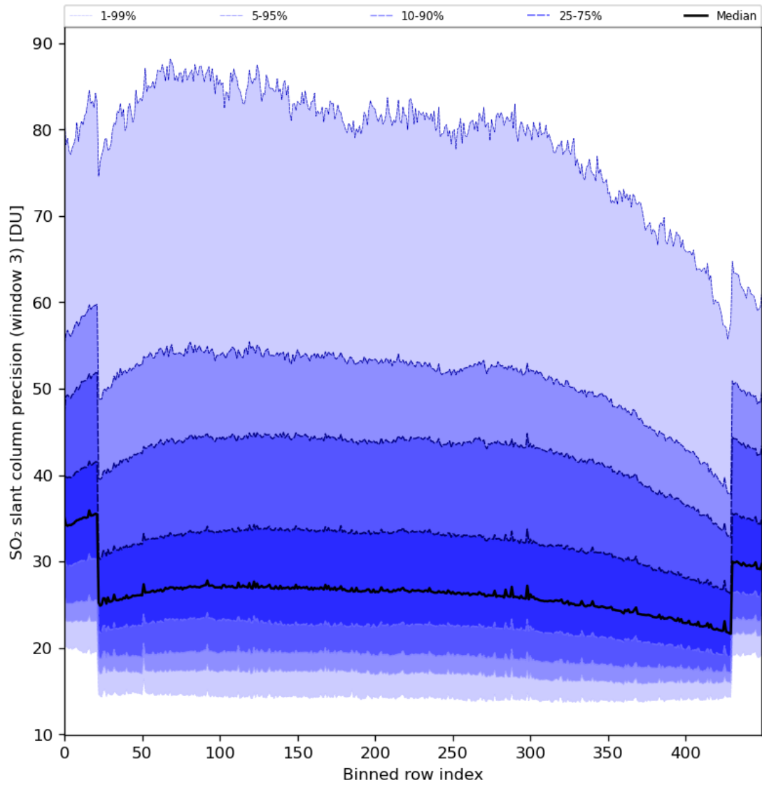
Figure 88: Along track statistics of “SO 2 slant column precision (window 3)” for 2024-04-17 to 2024-04-19
