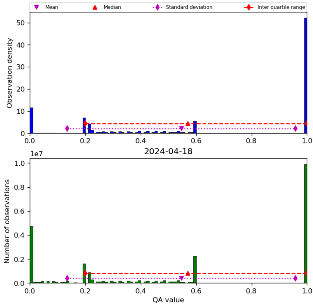
Figure 52: Histogram of “QA value” for 2024-04-17 to 2024-04-19
