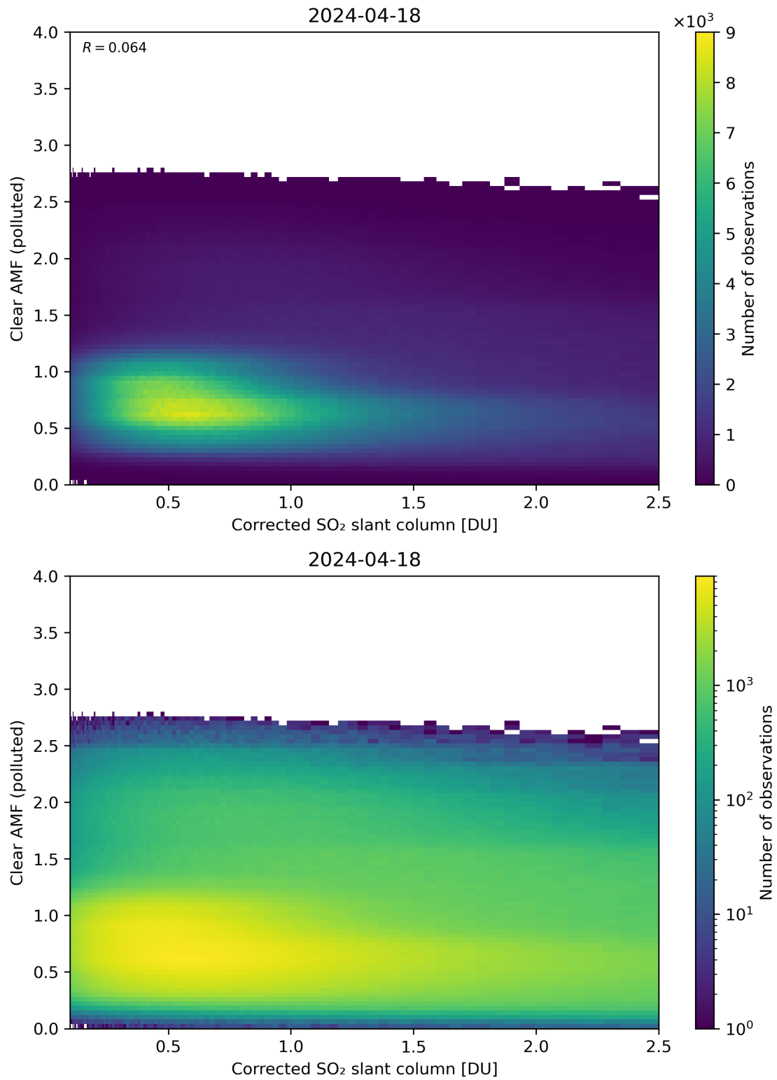
Figure 184: Scatter density plot of “Corrected SO 2 slant column” against “Clear AMF (polluted)” for 2024-04-17 to 2024-04-19.
