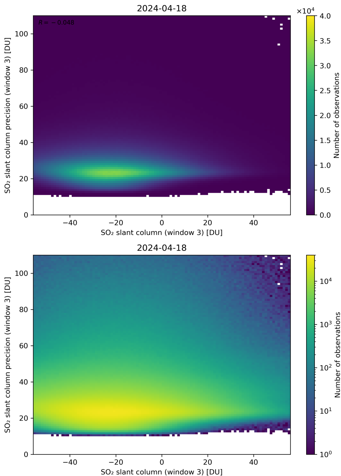
Figure 267: Scatter density plot of “SO 2 slant column (window 3)” against “SO 2 slant column precision (window 3)” for 2024-04-17 to 2024-04-19.
