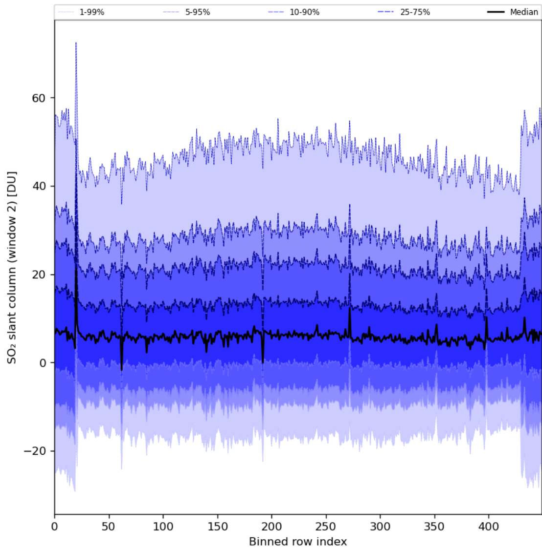
Figure 83: Along track statistics of “SO 2 slant column (window 2)” for 2024-04-17 to 2024-04-19
