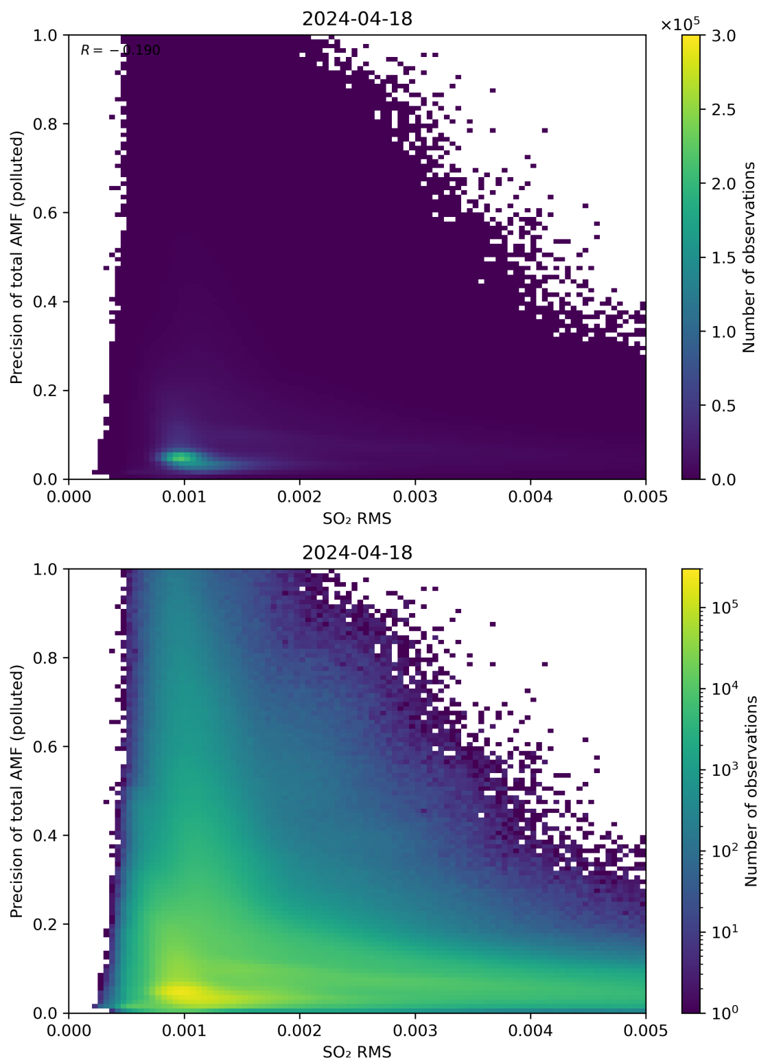
Figure 138: Scatter density plot of “SO 2 RMS” against “Precision of total AMF (polluted)” for 2024-04-17 to 2024-04-19.
