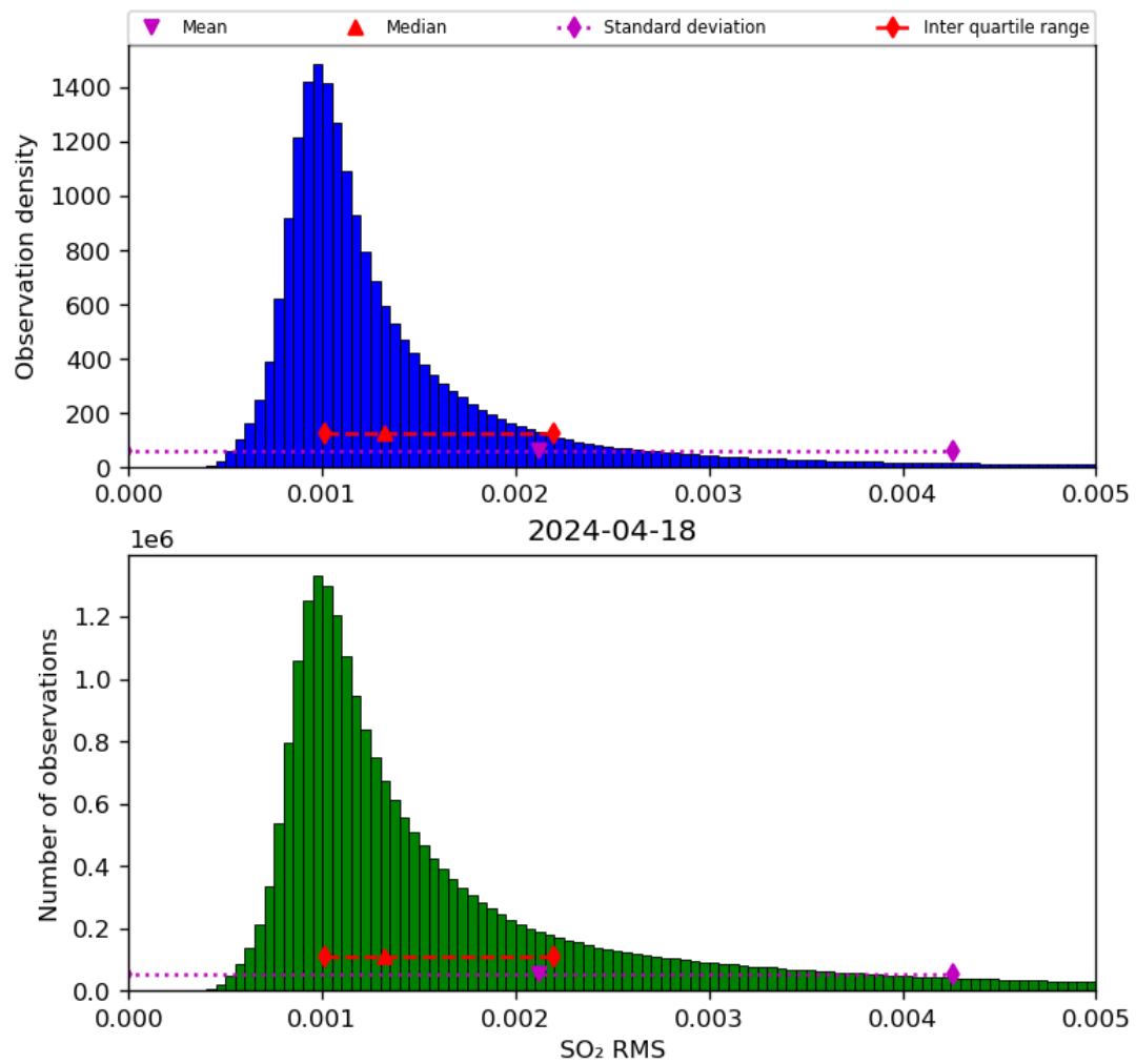
Figure 70: Histogram of “SO 2 RMS” for 2024-04-17 to 2024-04-19
