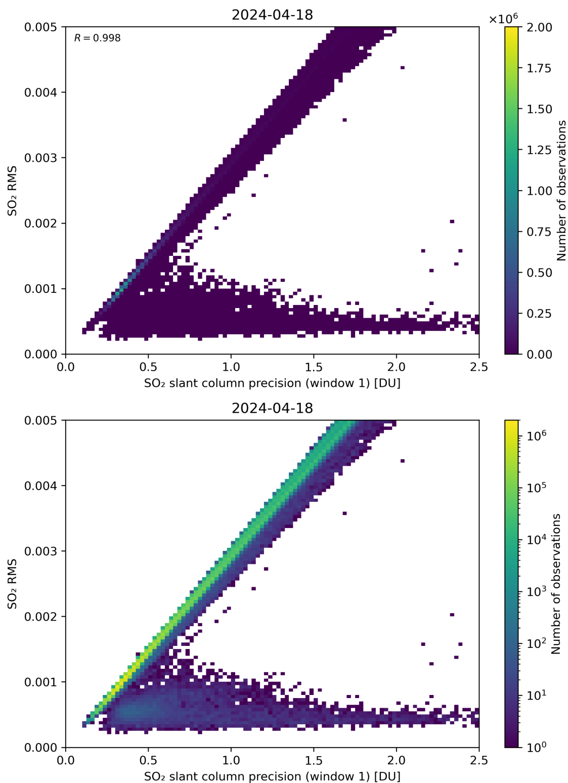
Figure 223: Scatter density plot of “SO 2 slant column precision (window 1)” against “SO 2 RMS” for 2024-04-17 to 2024-04-19.
