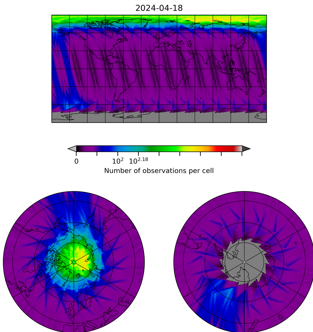
Figure 28: Map of the number of observations for 2024-04-17 to 2024-04-19
