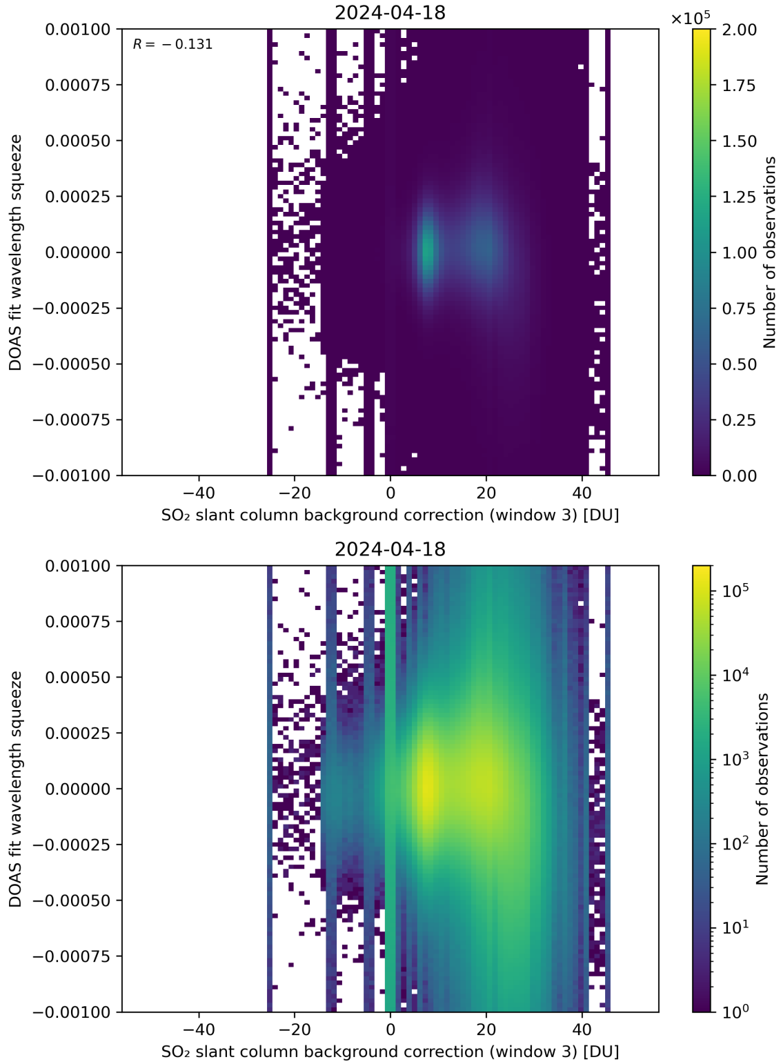
Figure 122: Scatter density plot of “SO 2 slant column background correction (window 3)” against “DOAS fit wavelength squeeze” for 2024-04-17 to 2024-04-19.
