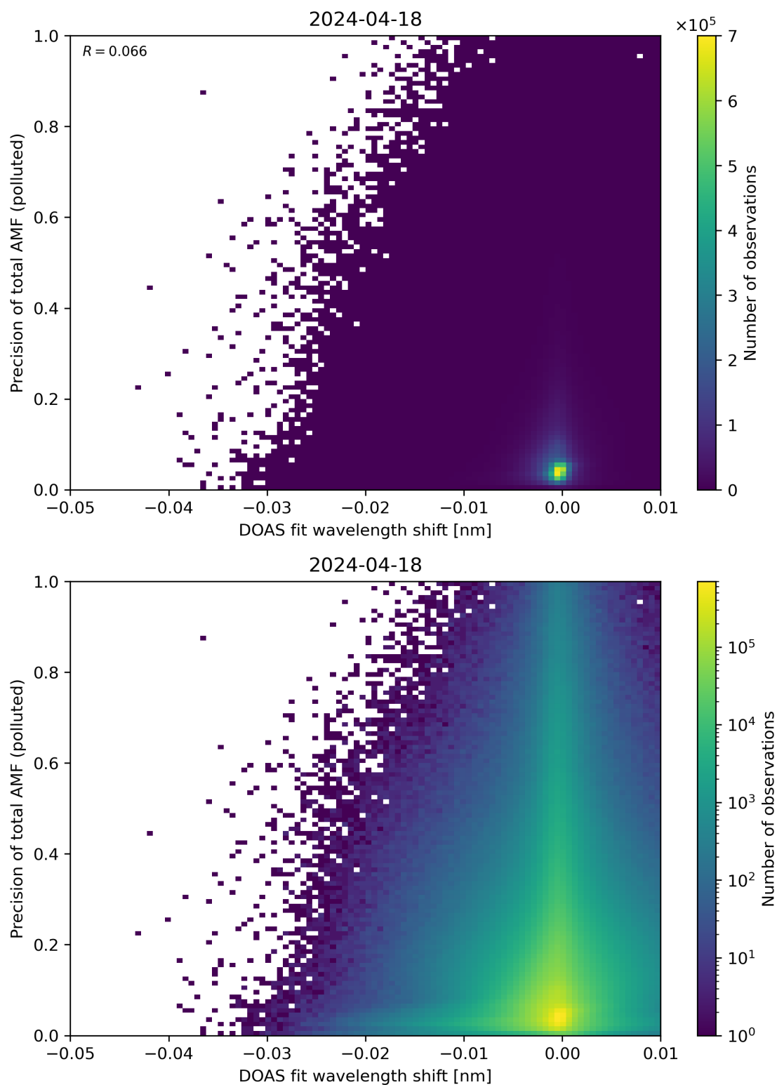
Figure 131: Scatter density plot of “DOAS fit wavelength shift” against “Precision of total AMF (polluted)” for 2024-04-17 to 2024-04-19.
