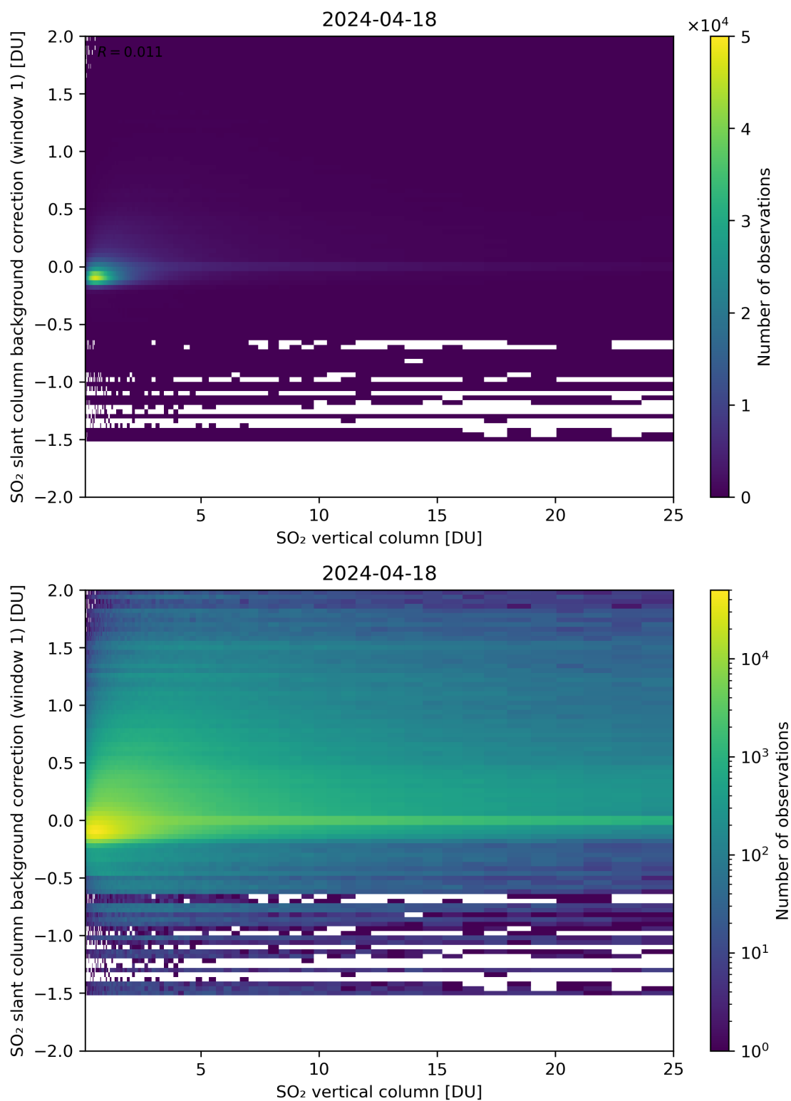
Figure 273: Scatter density plot of “SO 2 vertical column” against “SO 2 slant column background correction (window 1)” for 2024-04-17 to 2024-04-19.
