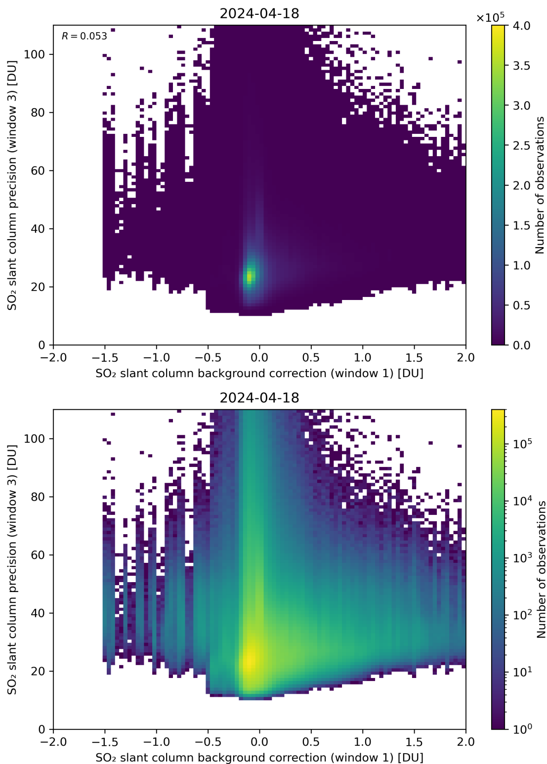
Figure 108: Scatter density plot of “SO 2 slant column background correction (window 1)” against “SO 2 slant column precision (window 3)” for 2024-04-17 to 2024-04-19.
