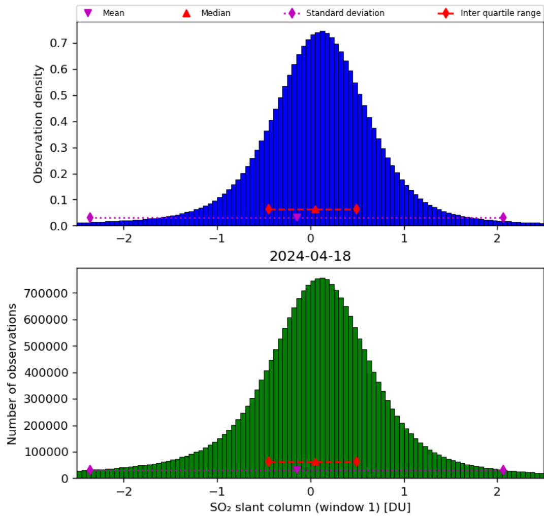
Figure 56: Histogram of “SO 2 slant column (window 1)” for 2024-04-17 to 2024-04-19
