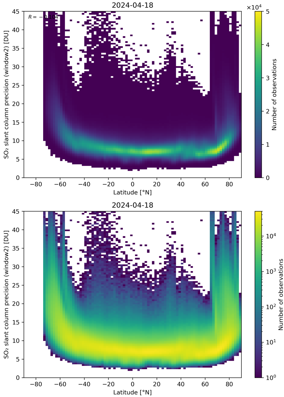
Figure 151: Scatter density plot of “Latitude” against “SO 2 slant column precision (window2)” for 2024-04-17 to 2024-04-19.
