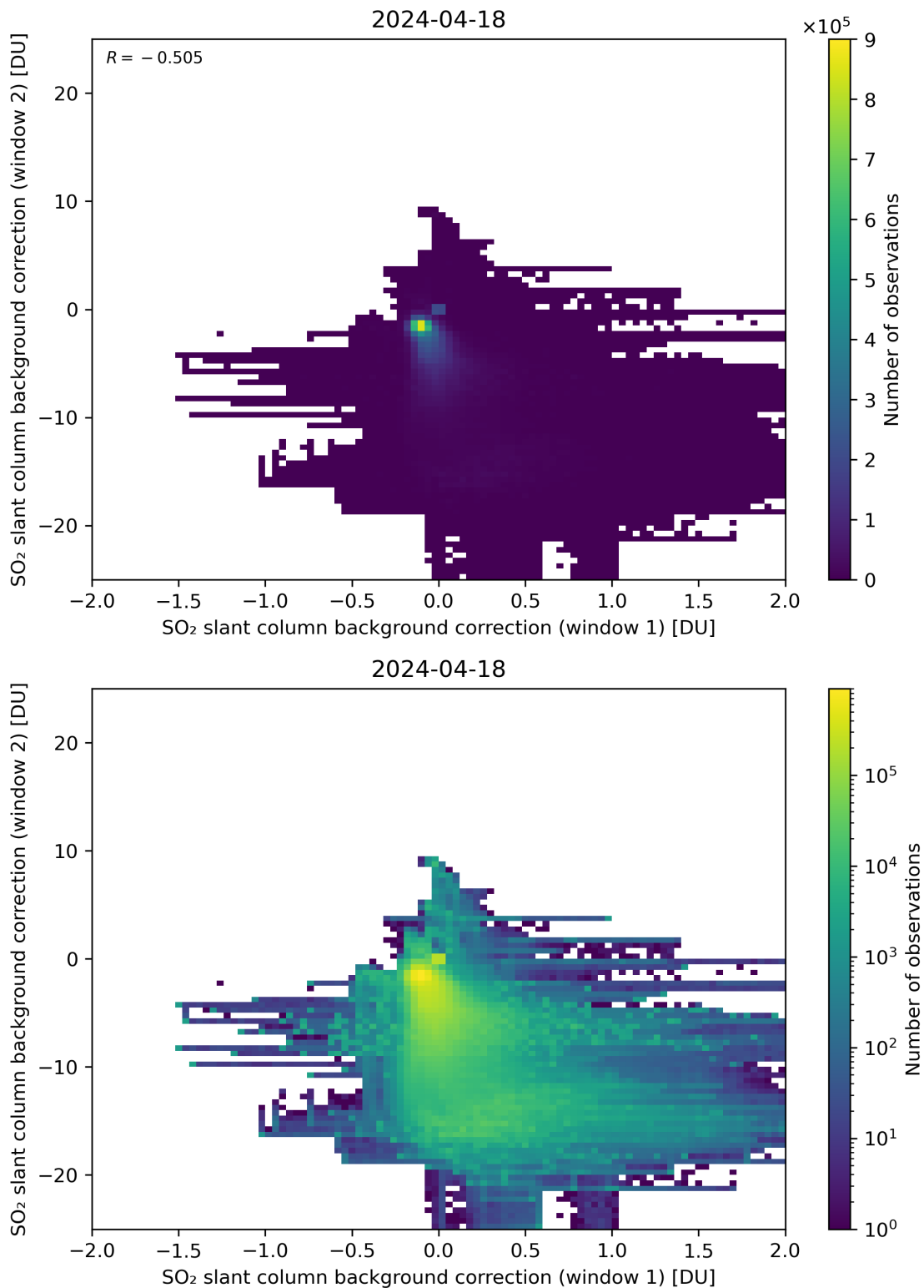
Figure 98: Scatter density plot of “SO 2 slant column background correction (window 1)” against “SO 2 slant column background correction (window 2)” for 2024-04-17 to 2024-04-19.
