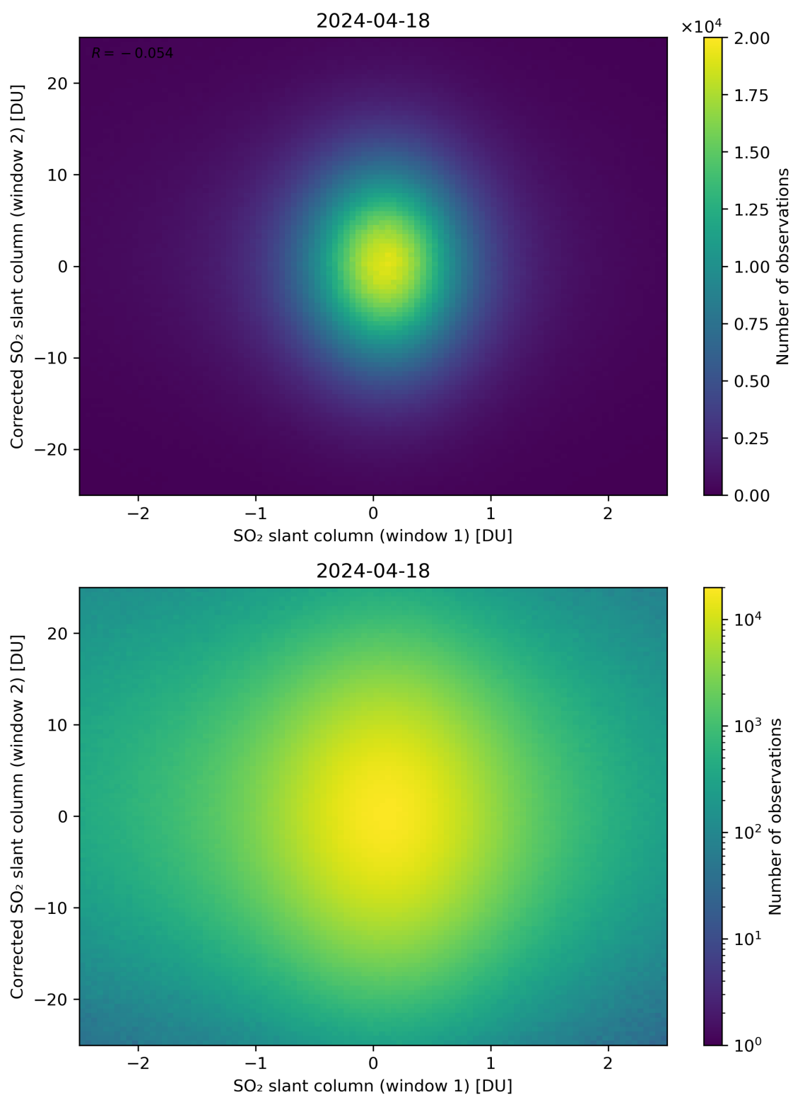
Figure 233: Scatter density plot of “SO 2 slant column (window 1)” against “Corrected SO 2 slant column (window 2)” for 2024-04-17 to 2024-04-19.
