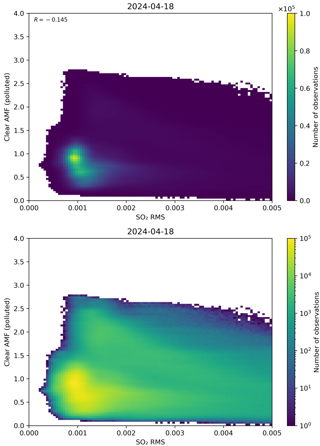
Figure 136: Scatter density plot of “SO 2 RMS” against “Clear AMF (polluted)” for 2024-04-17 to 2024-04-19.
