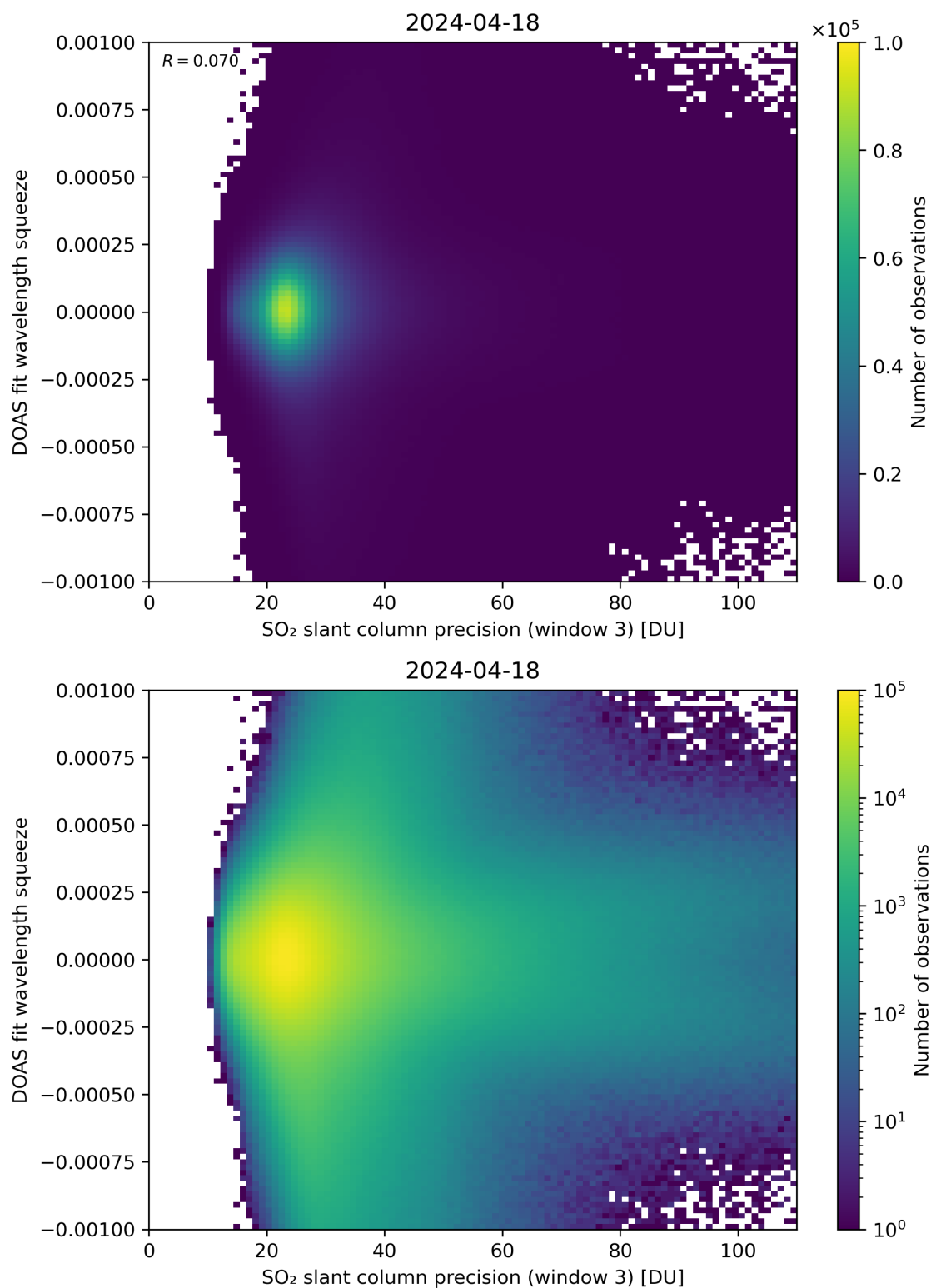
Figure 259: Scatter density plot of “SO 2 slant column precision (window 3)” against “DOAS fit wavelength squeeze” for 2024-04-17 to 2024-04-19.
