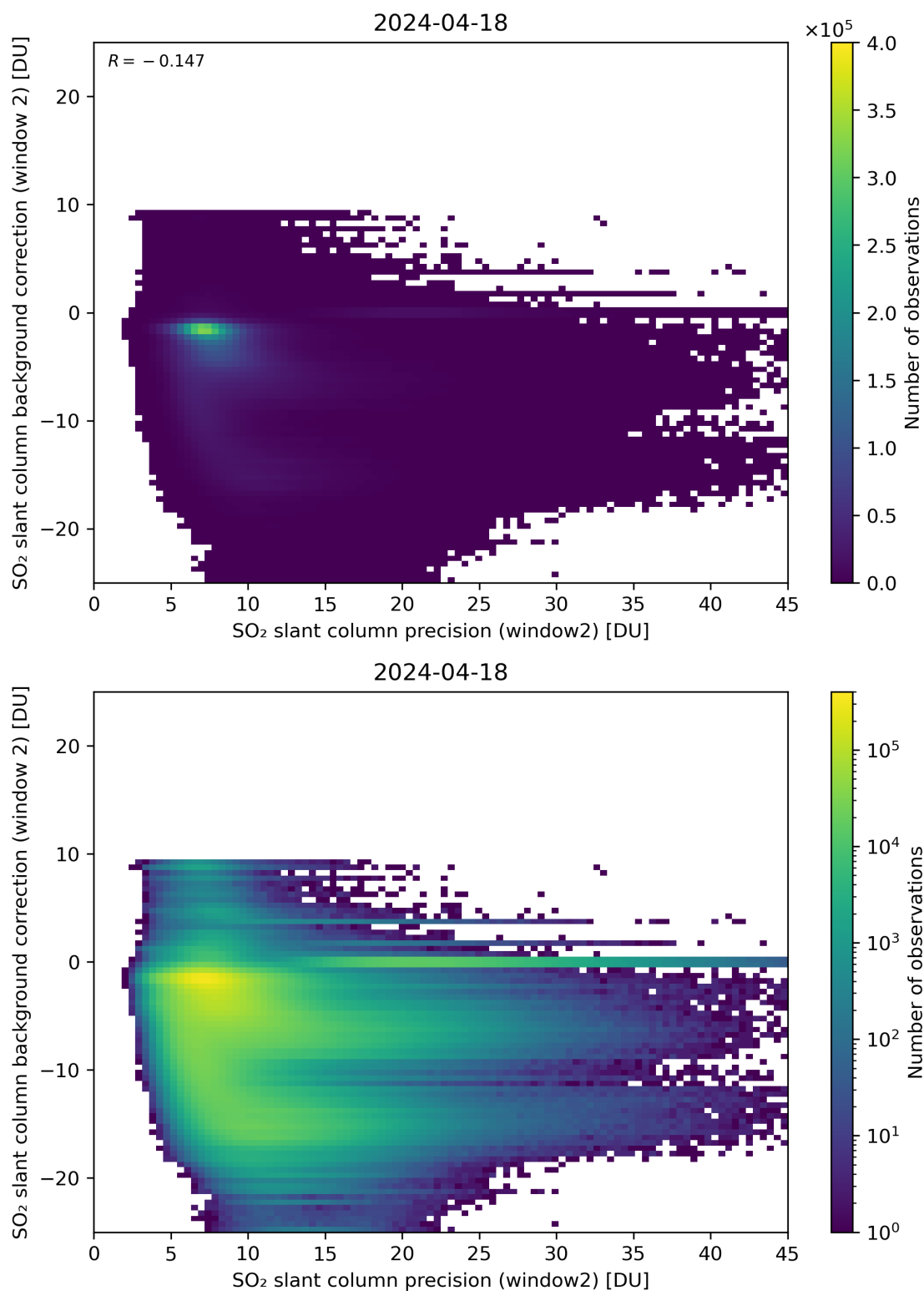
Figure 241: Scatter density plot of “SO 2 slant column precision (window2)” against “SO 2 slant column background correction (window 2)” for 2024-04-17 to 2024-04-19.
