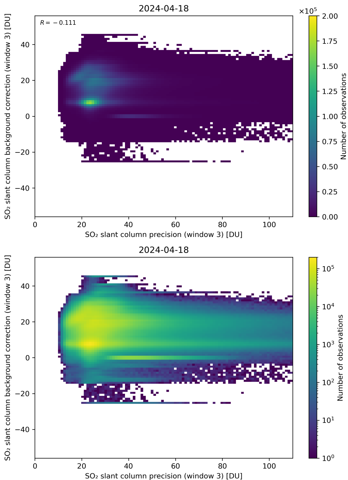
Figure 257: Scatter density plot of “SO 2 slant column precision (window 3)” against “SO 2 slant column background correction (window 3)” for 2024-04-17 to 2024-04-19.
