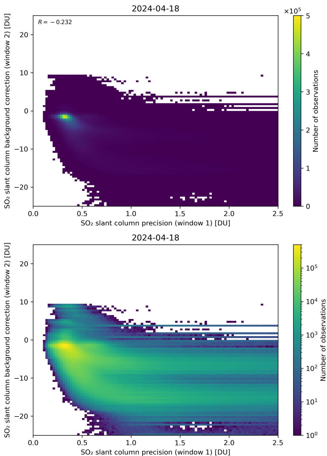
Figure 219: Scatter density plot of “SO 2 slant column precision (window 1)” against “SO 2 slant column background correction (window 2)” for 2024-04-17 to 2024-04-19.
