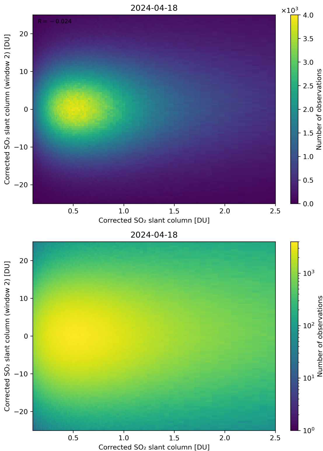
Figure 185: Scatter density plot of “Corrected SO 2 slant column” against “Corrected SO 2 slant column (window 2)” for 2024-04-17 to 2024-04-19.
