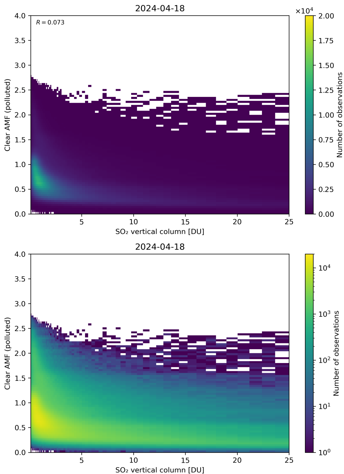
Figure 296: Scatter density plot of “SO 2 vertical column” against “Clear AMF (polluted)” for 2024-04-17 to 2024-04-19.
