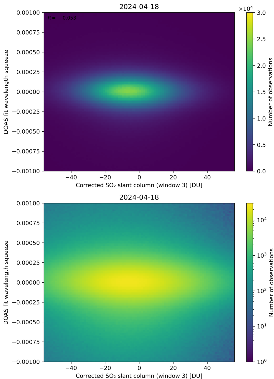
Figure 207: Scatter density plot of “Corrected SO 2 slant column (window 3)” against “DOAS fit wavelength squeeze” for 2024-04-17 to 2024-04-19.
