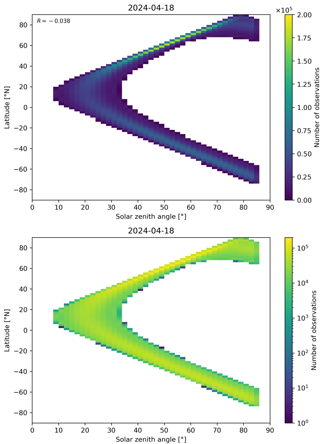
Figure 164: Scatter density plot of “Solar zenith angle” against “Latitude” for 2024-04-17 to 2024-04-19.
