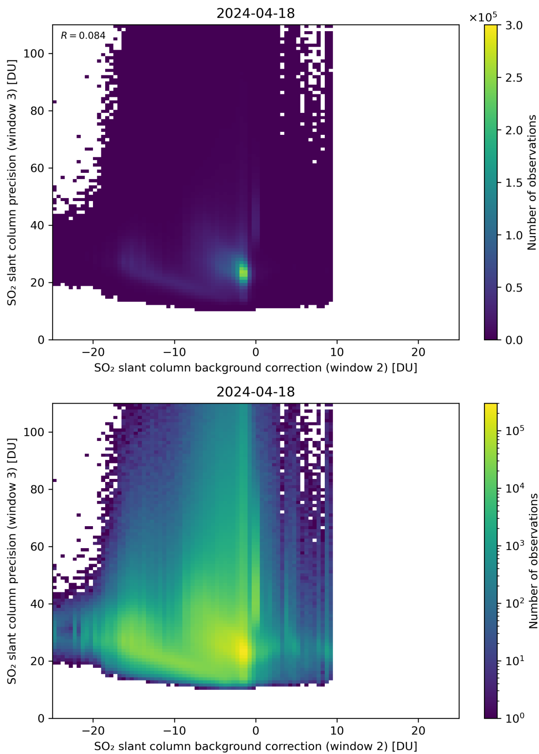
Figure 118: Scatter density plot of “SO 2 slant column background correction (window 2)” against “SO 2 slant column precision (window 3)” for 2024-04-17 to 2024-04-19.
