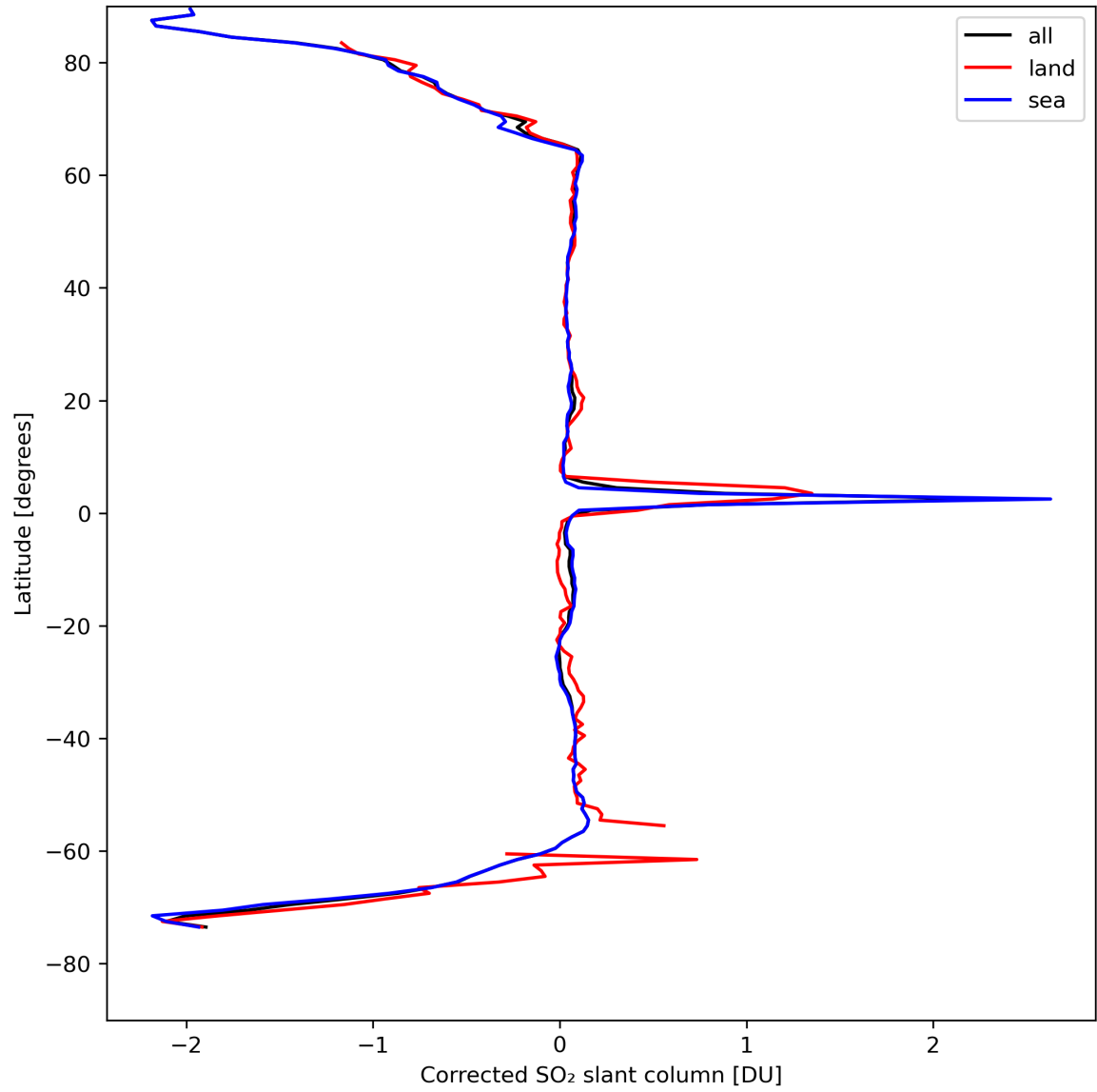
Figure 32: Zonal average of “Corrected SO 2 slant column” for 2024-04-17 to 2024-04-19.
