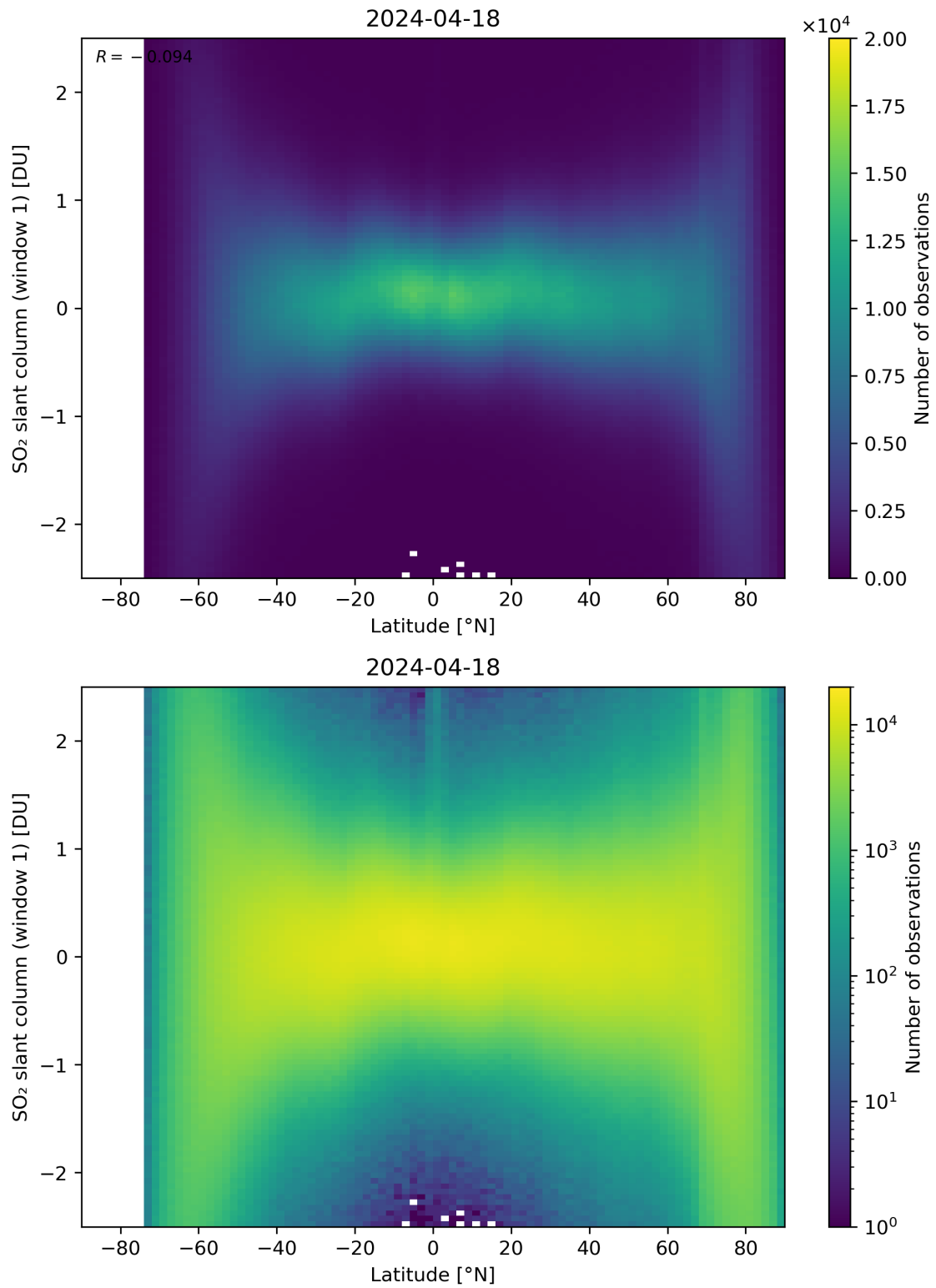
Figure 149: Scatter density plot of “Latitude” against “SO 2 slant column (window 1)” for 2024-04-17 to 2024-04-19.
