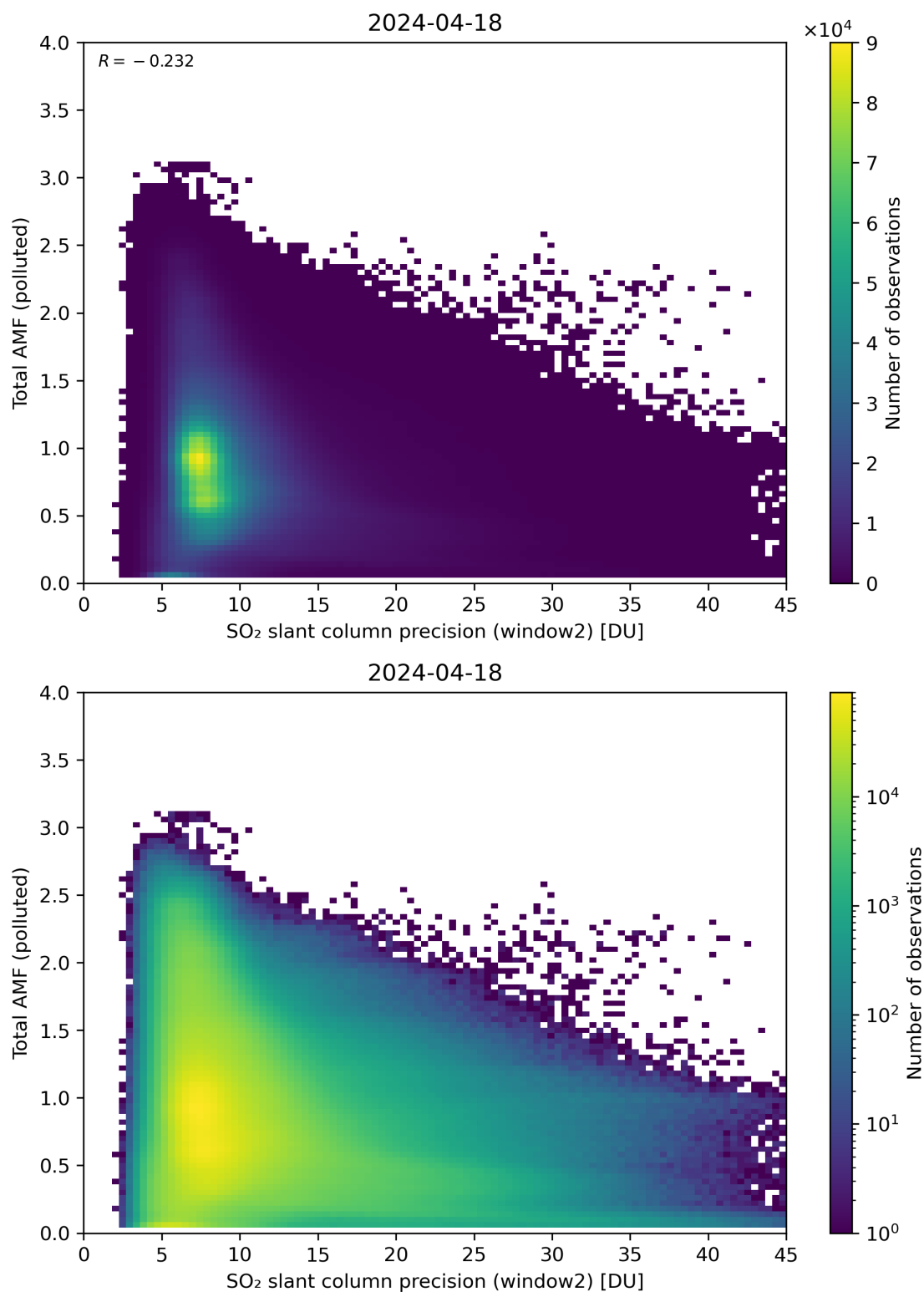
Figure 251: Scatter density plot of “SO 2 slant column precision (window2)” against “Total AMF (polluted)” for 2024-04-17 to 2024-04-19.
