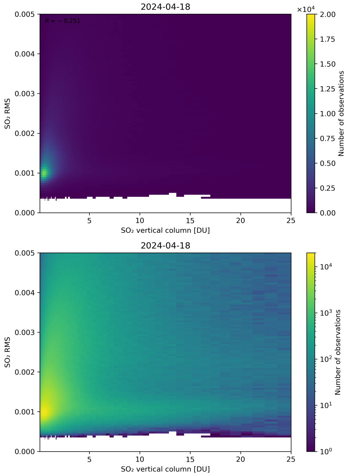
Figure 278: Scatter density plot of “SO 2 vertical column” against “SO 2 RMS” for 2024-04-17 to 2024-04-19.
