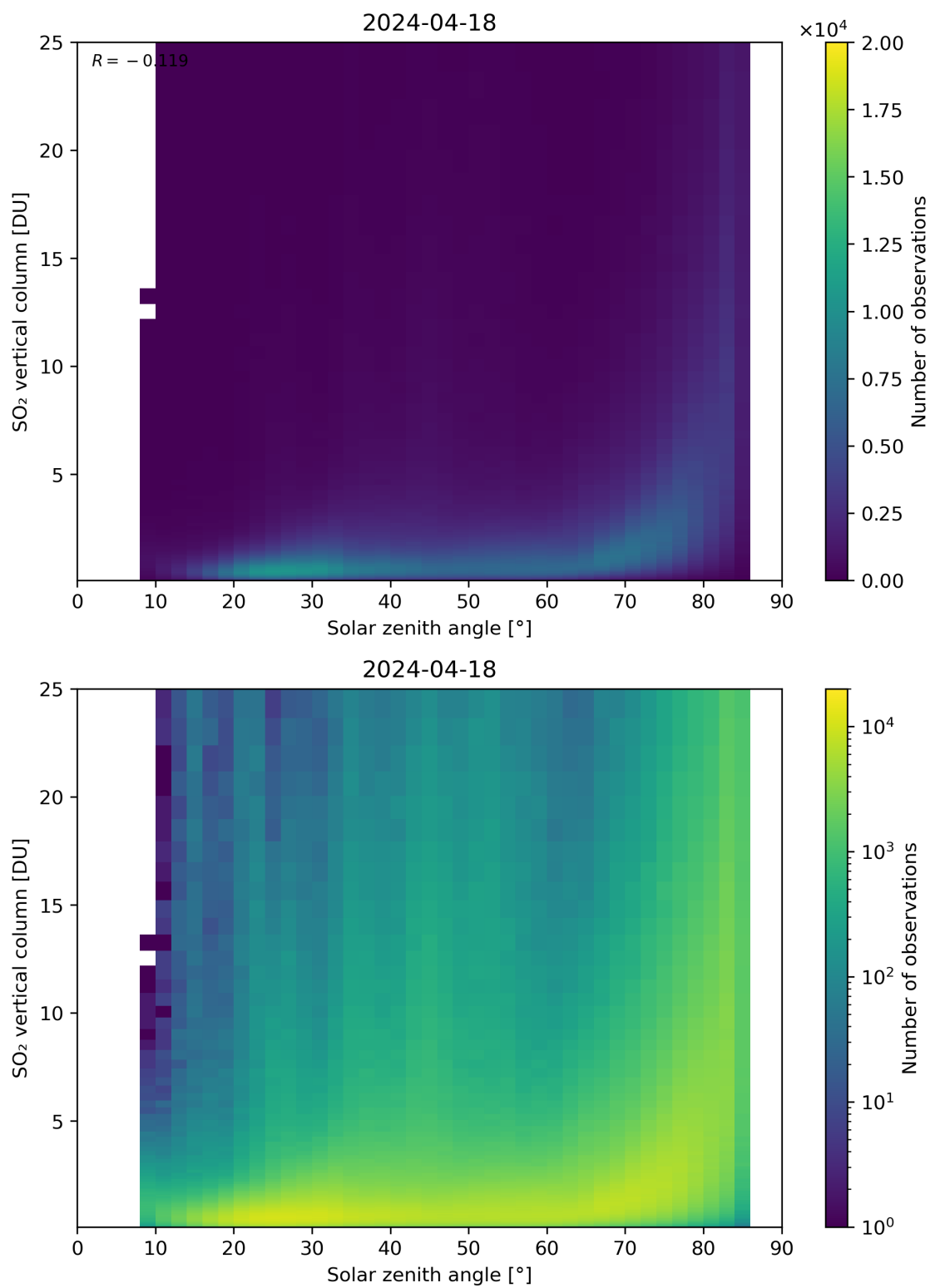
Figure 176: Scatter density plot of “Solar zenith angle” against “SO 2 vertical column” for 2024-04-17 to 2024-04-19.
