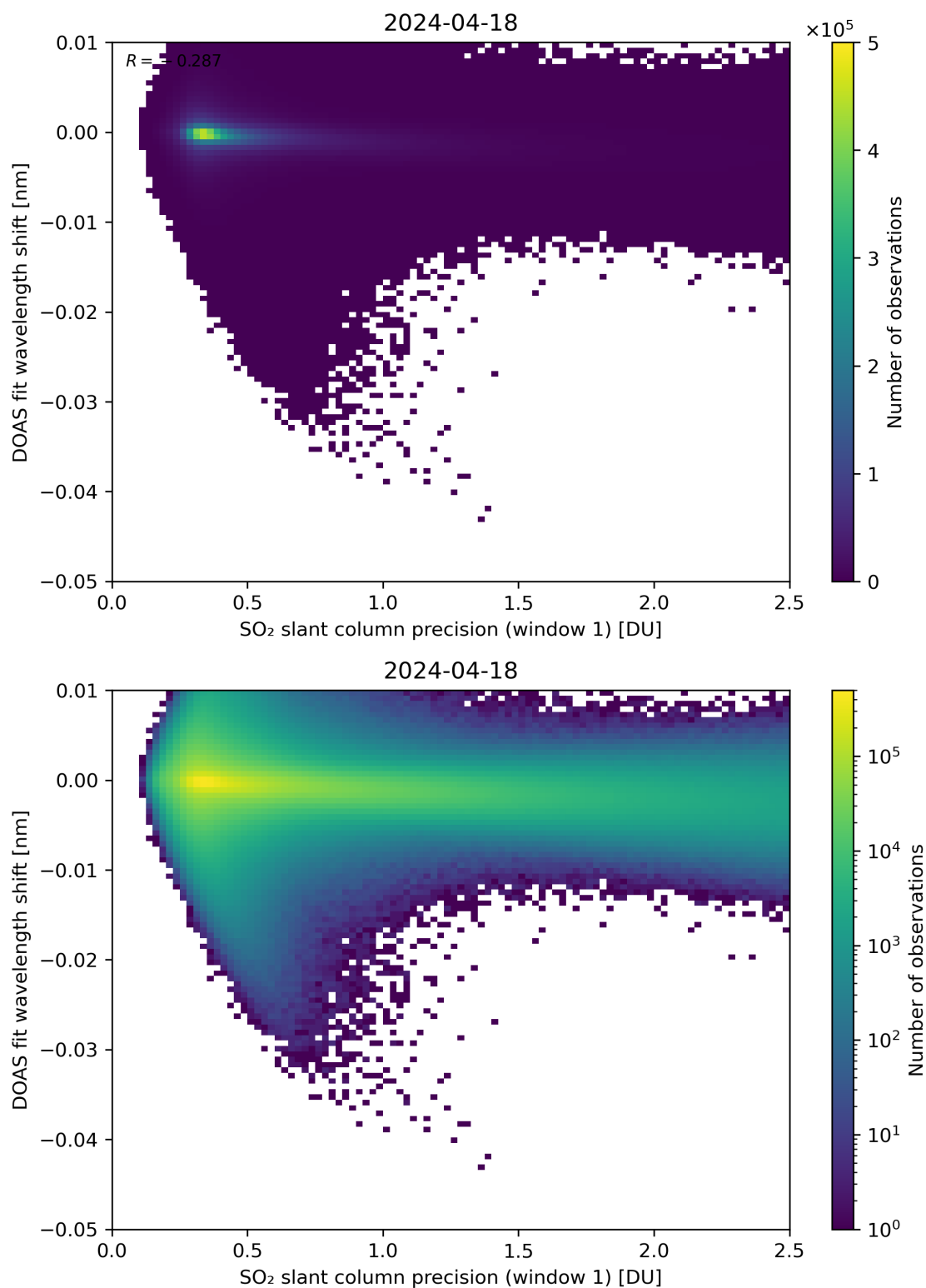
Figure 221: Scatter density plot of “SO 2 slant column precision (window 1)” against “DOAS fit wavelength shift” for 2024-04-17 to 2024-04-19.
