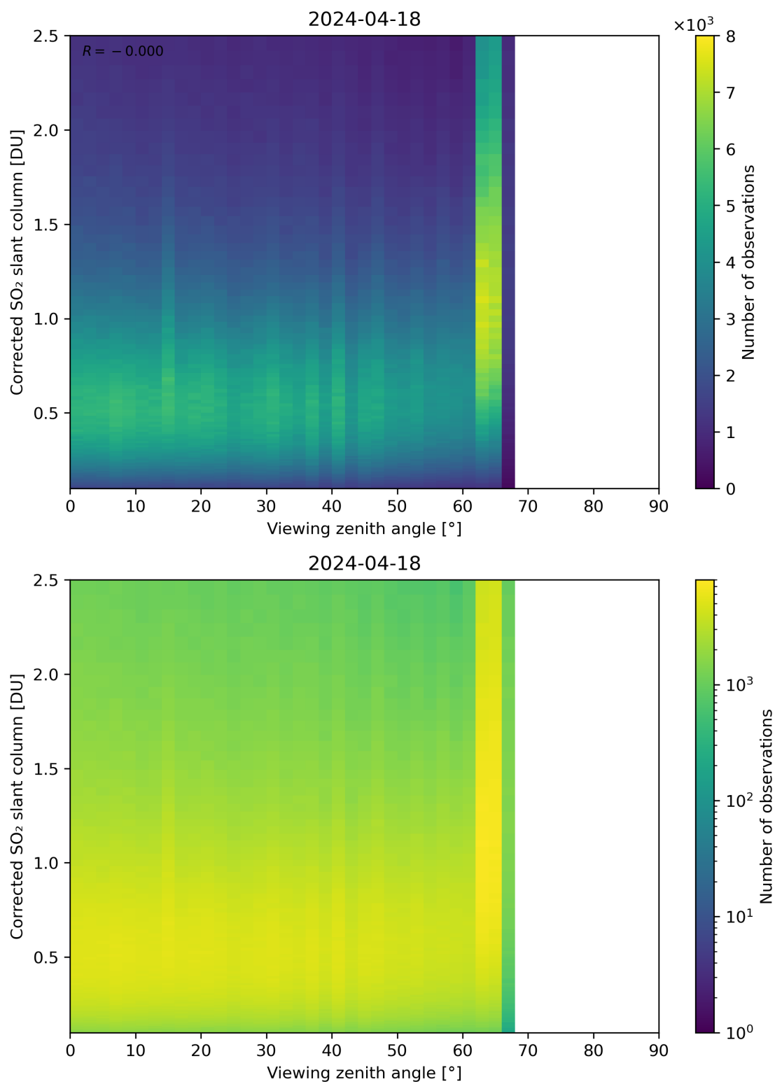
Figure 317: Scatter density plot of “Viewing zenith angle” against “Corrected SO 2 slant column” for 2024-04-17 to 2024-04-19.
