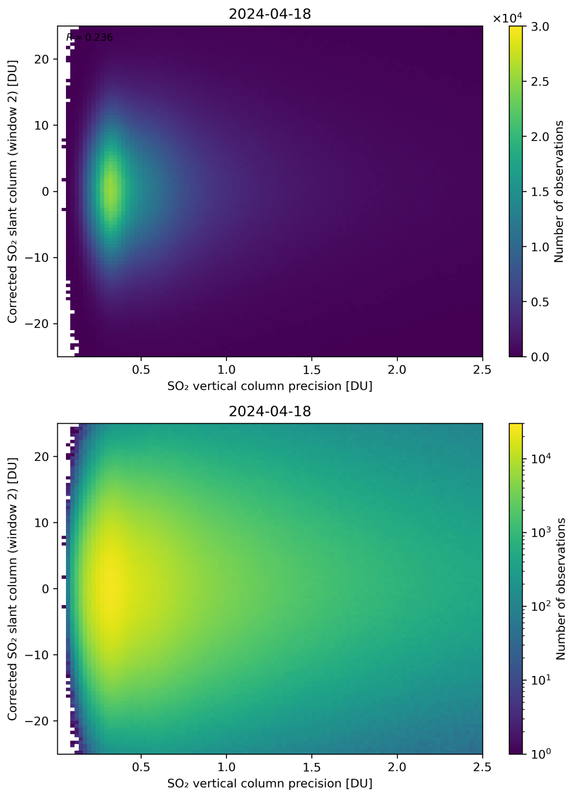
Figure 287: Scatter density plot of “SO 2 vertical column precision” against “Corrected SO 2 slant column (window 2)” for 2024-04-17 to 2024-04-19.
