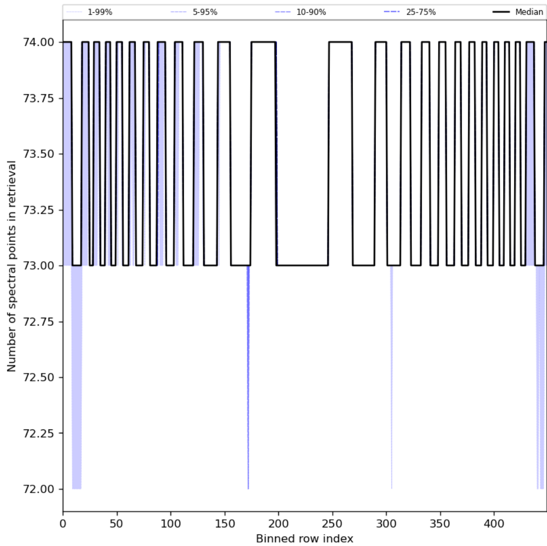
Figure 97: Along track statistics of “Number of spectral points in retrieval” for 2024-04-17 to 2024-04-19
