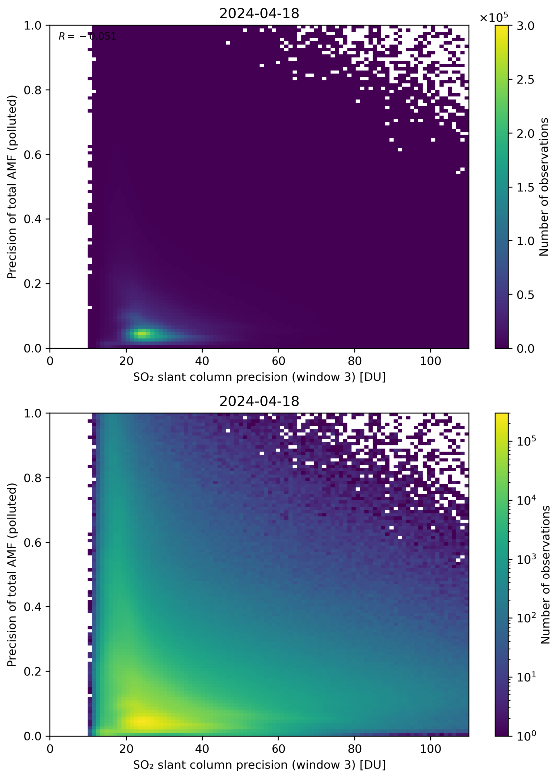
Figure 264: Scatter density plot of “SO 2 slant column precision (window 3)” against “Precision of total AMF (polluted)” for 2024-04-17 to 2024-04-19.
