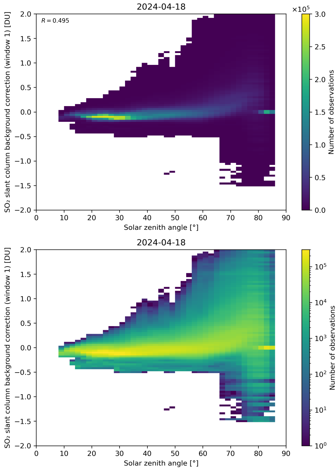
Figure 158: Scatter density plot of “Solar zenith angle” against “SO 2 slant column background correction (window 1)” for 2024-04-17 to 2024-04-19.
