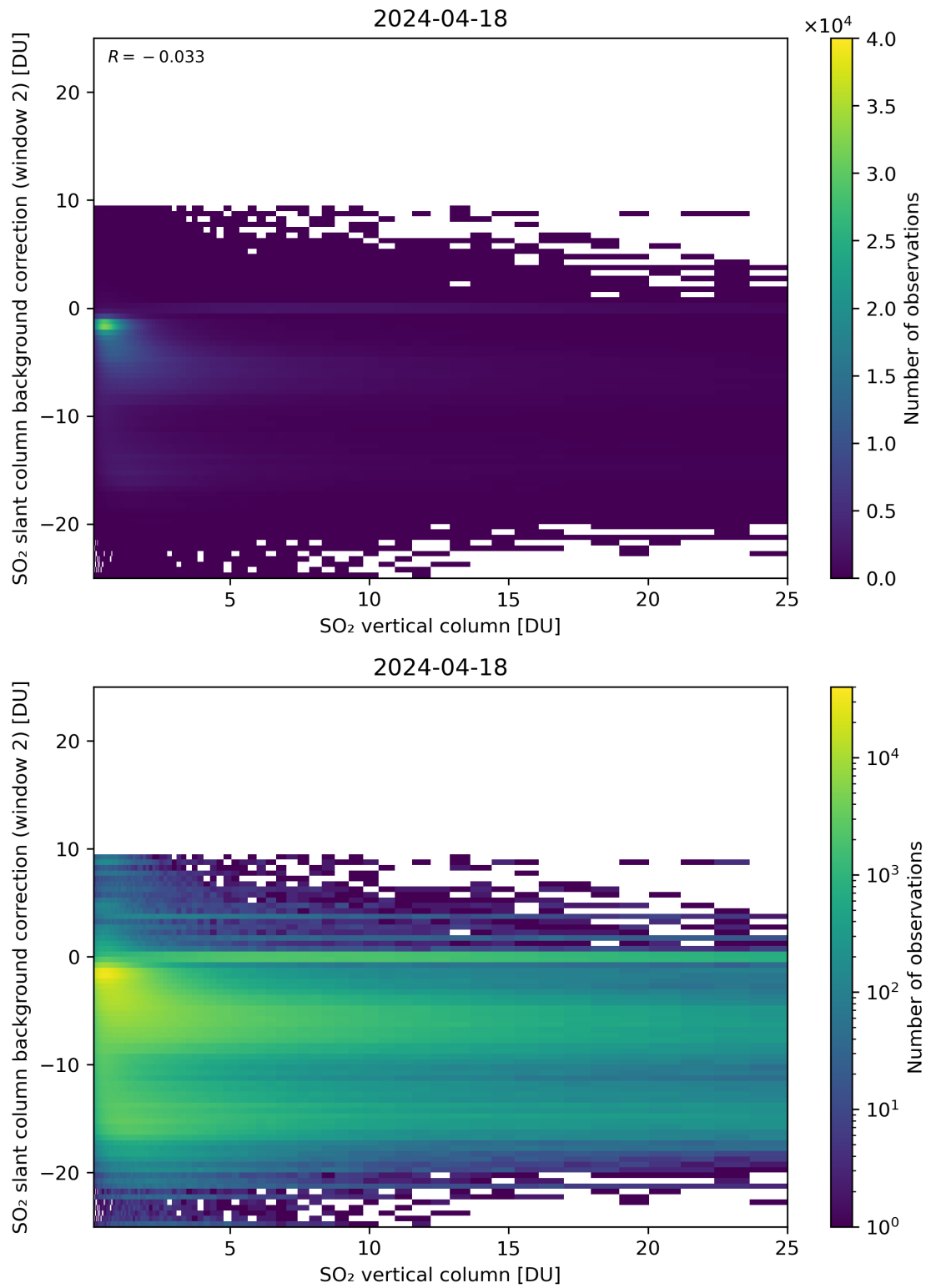
Figure 274: Scatter density plot of “SO 2 vertical column” against “SO 2 slant column background correction (window 2)” for 2024-04-17 to 2024-04-19.
