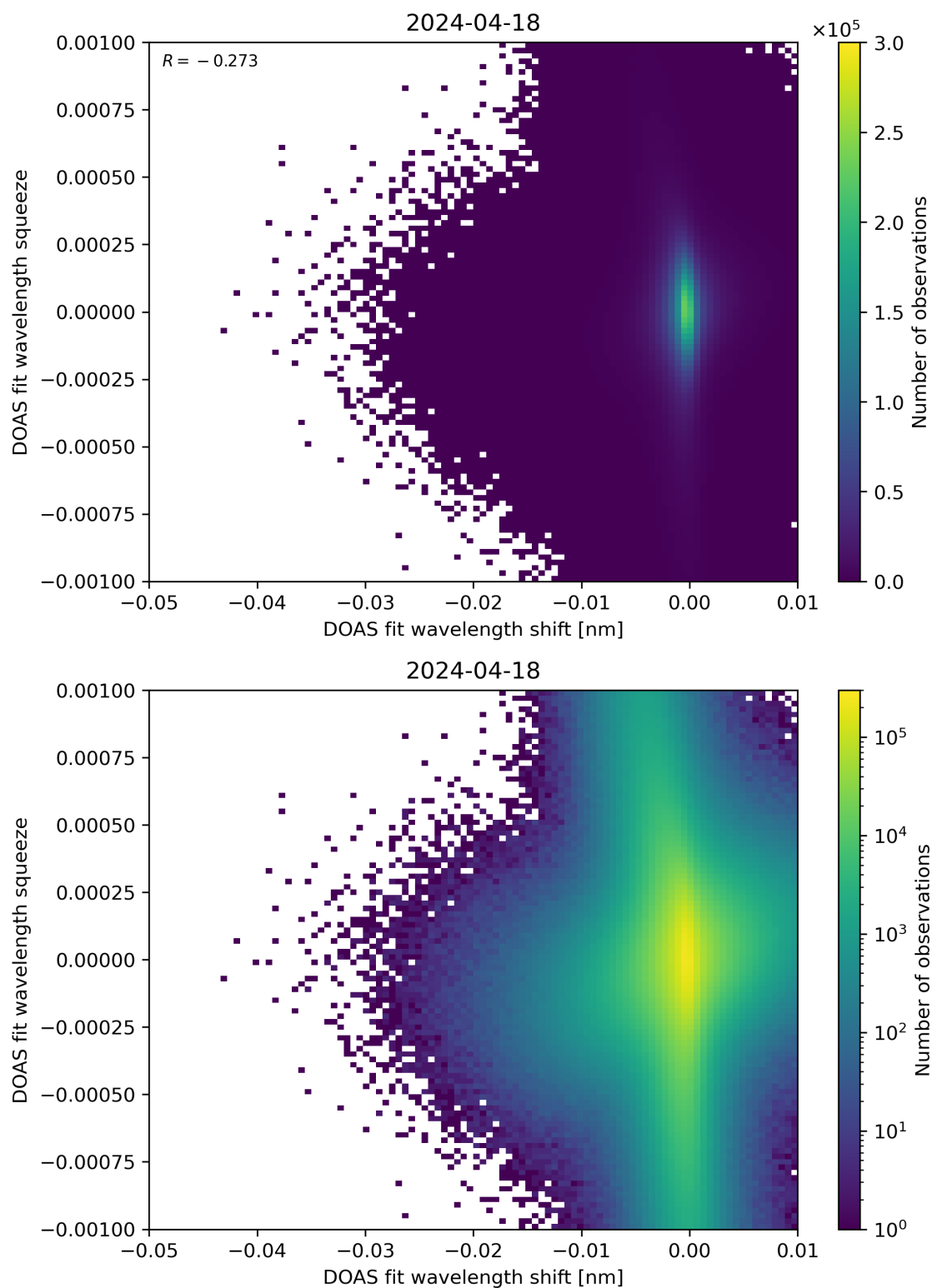
Figure 127: Scatter density plot of “DOAS fit wavelength shift” against “DOAS fit wavelength squeeze” for 2024-04-17 to 2024-04-19.
