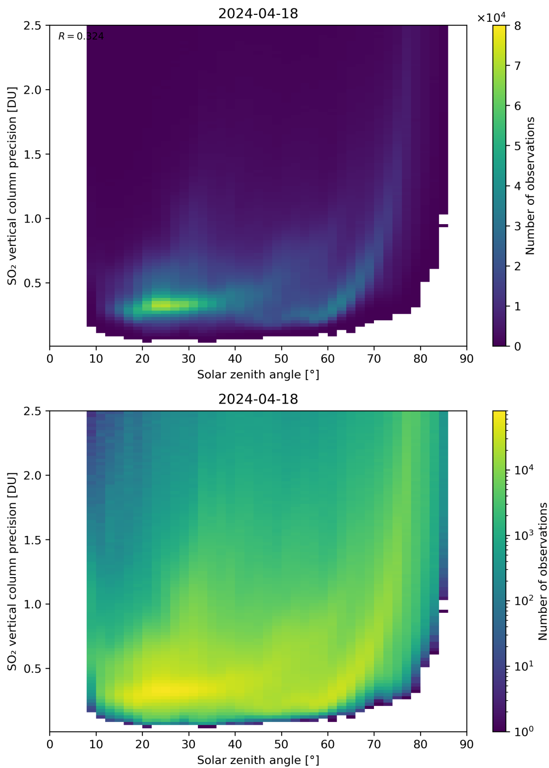
Figure 177: Scatter density plot of “Solar zenith angle” against “SO 2 vertical column precision” for 2024-04-17 to 2024-04-19.
