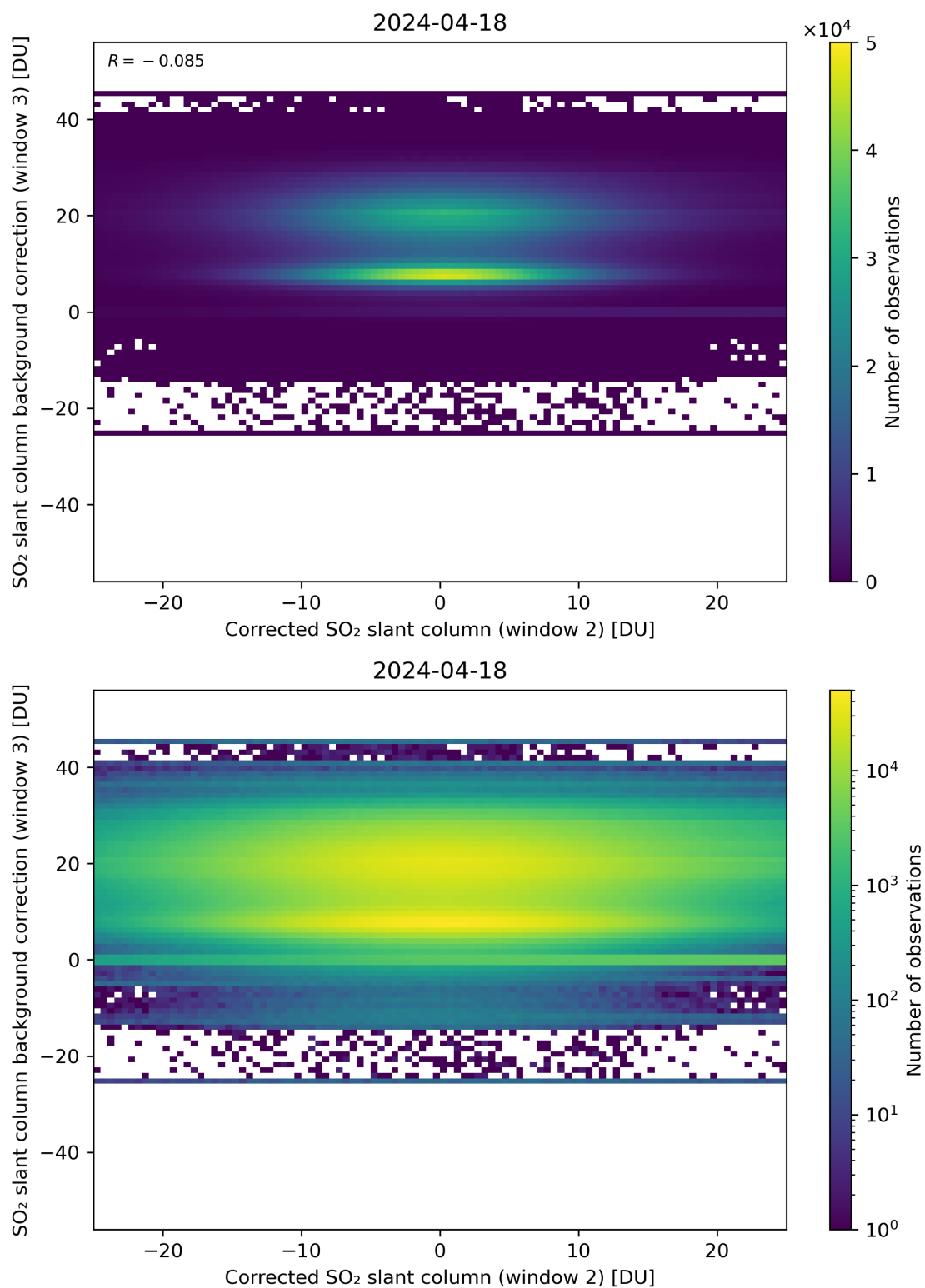
Figure 195: Scatter density plot of “Corrected SO 2 slant column (window 2)” against “SO 2 slant column background correction (window 3)” for 2024-04-17 to 2024-04-19.
