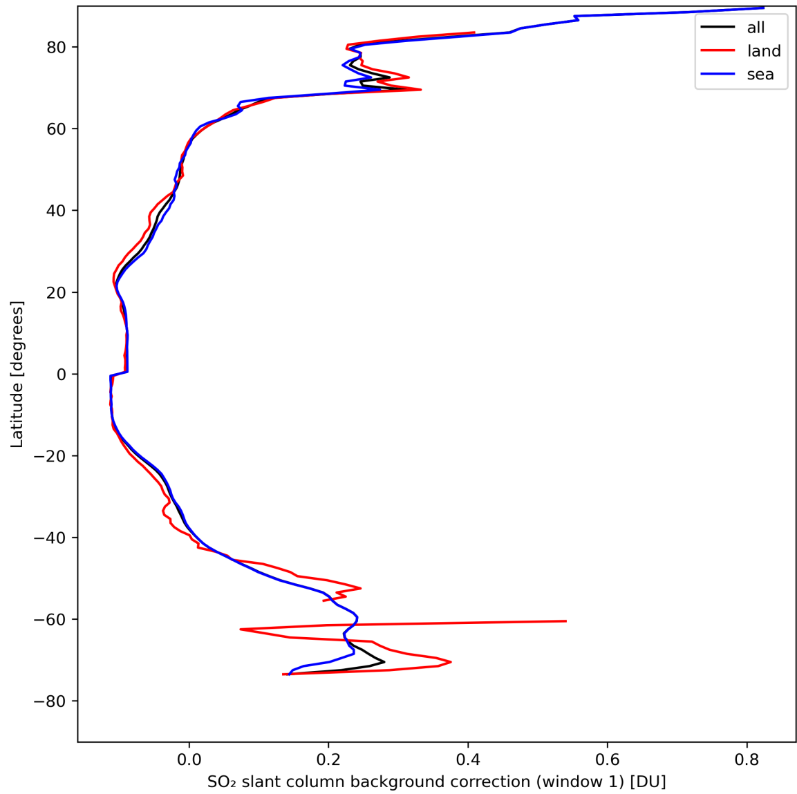
Figure 36: Zonal average of "SO 2 slant column background correction (window 1)" for 2024-04-17 to 2024-04-19.
