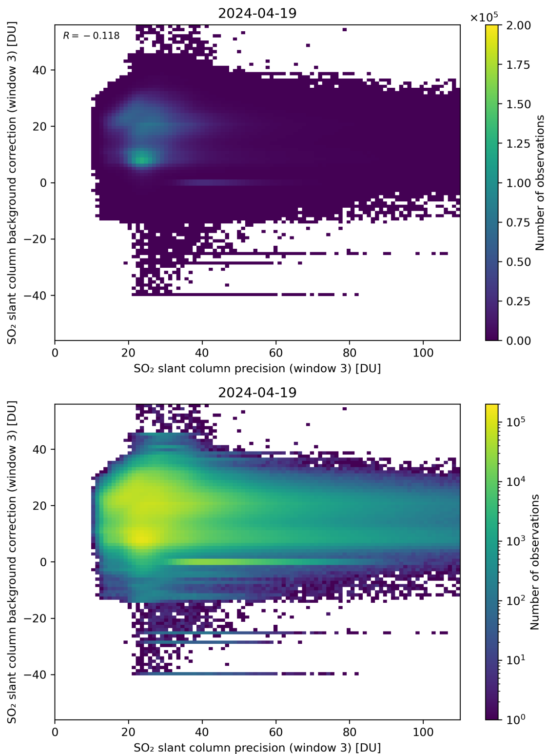
Figure 257: Scatter density plot of “SO 2 slant column precision (window 3)” against “SO 2 slant column background correction (window 3)” for 2024-04-18 to 2024-04-20.
