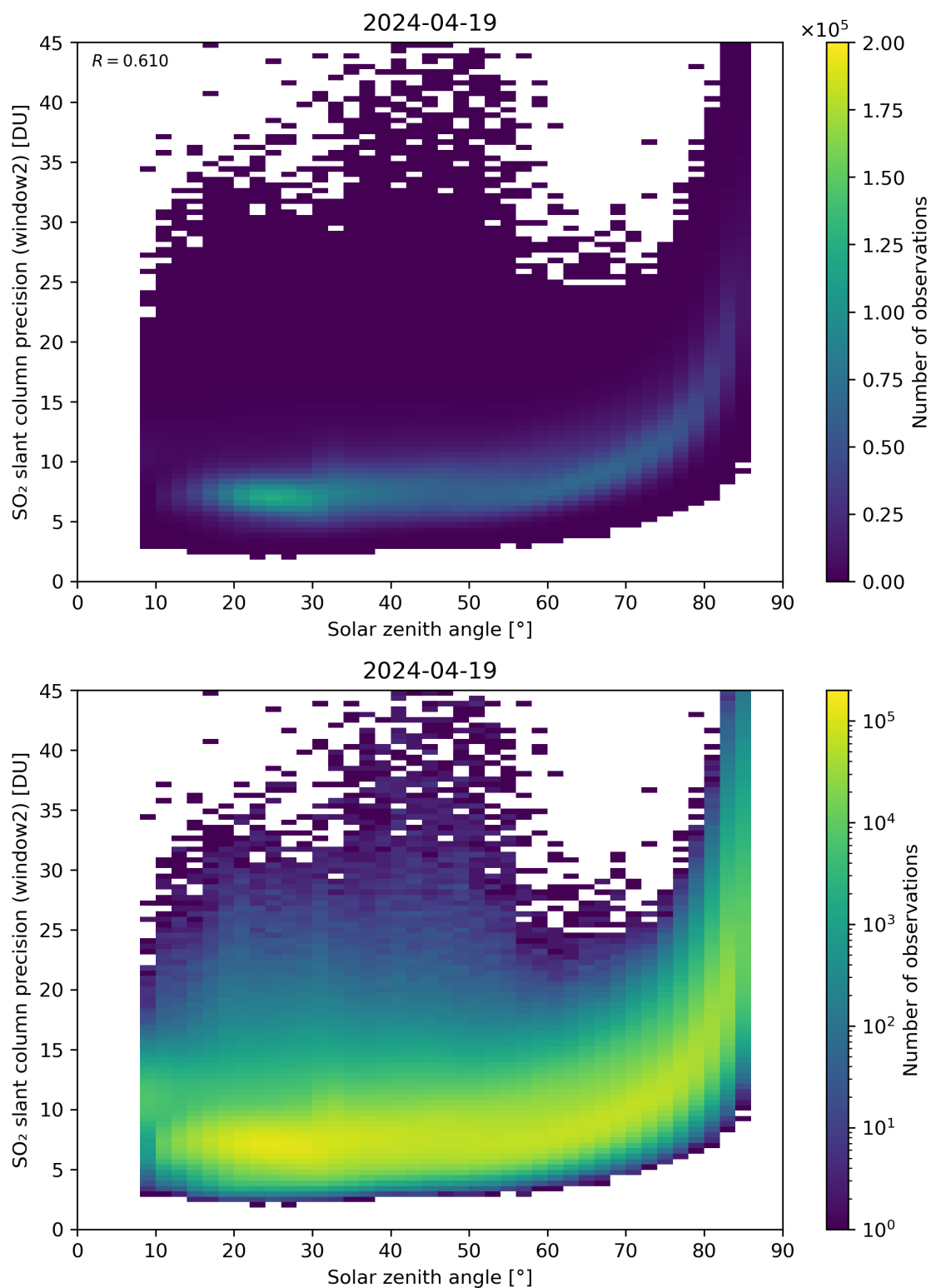
Figure 171: Scatter density plot of “Solar zenith angle” against “SO 2 slant column precision (window2)” for 2024-04-18 to 2024-04-20.
