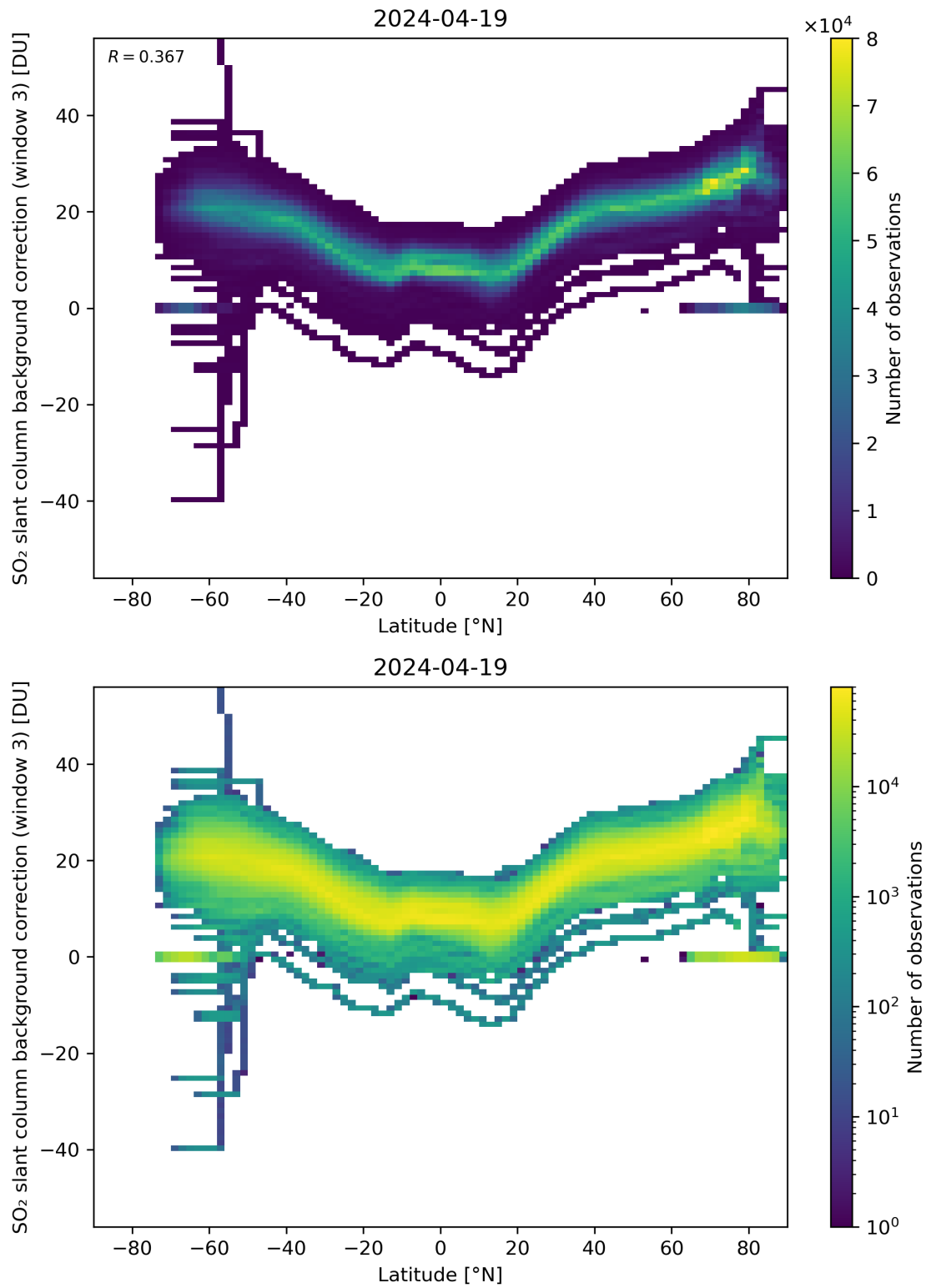
Figure 141: Scatter density plot of “Latitude” against “SO 2 slant column background correction (window 3)” for 2024-04-18 to 2024-04-20.
