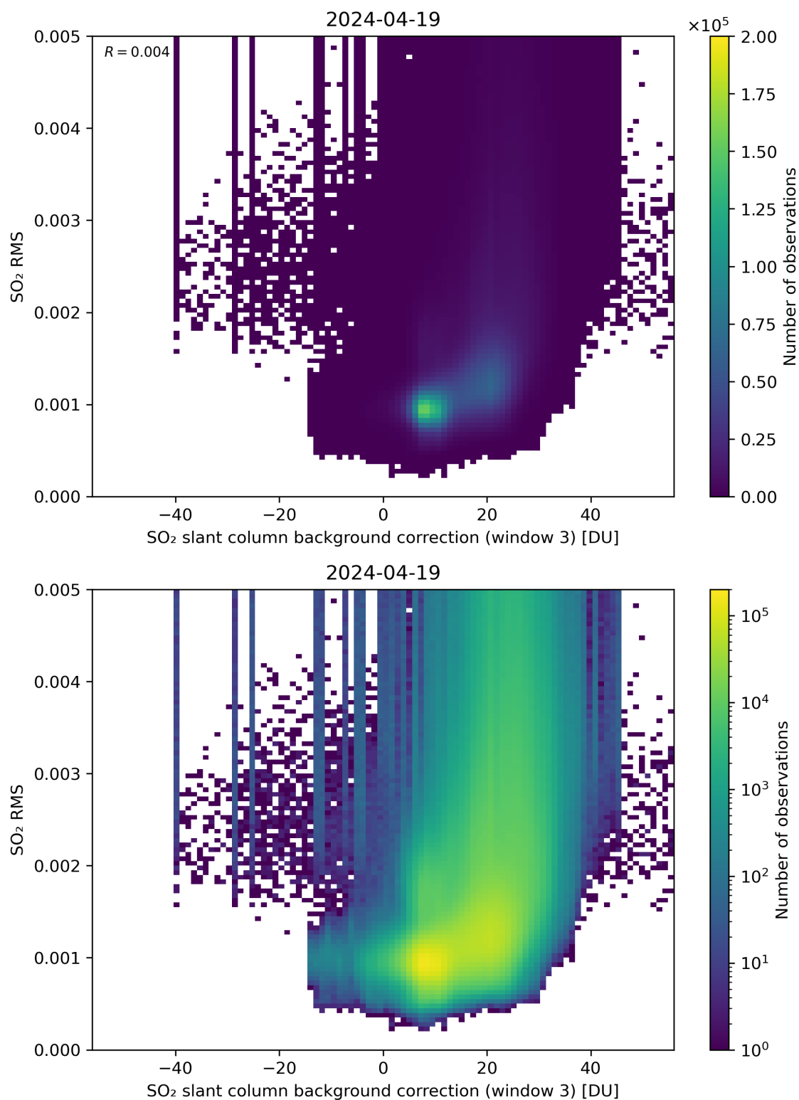
Figure 123: Scatter density plot of “SO 2 slant column background correction (window 3)” against “SO 2 RMS” for 2024-04-18 to 2024-04-20.
