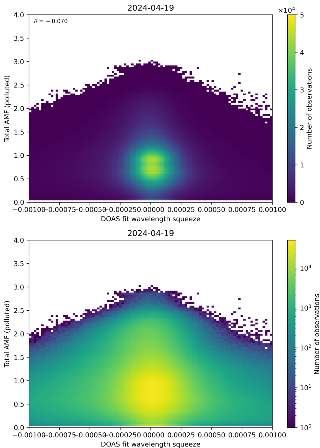
Figure 134: Scatter density plot of “DOAS fit wavelength squeeze” against “Total AMF (polluted)” for 2024-04-18 to 2024-04-20.
