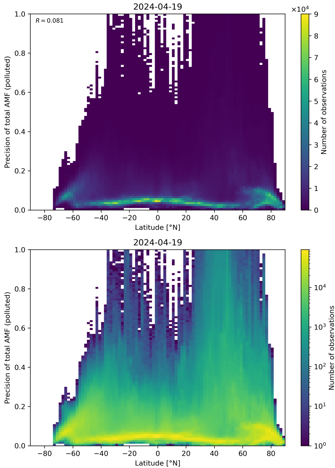
Figure 155: Scatter density plot of “Latitude” against “Precision of total AMF (polluted)” for 2024-04-18 to 2024-04-20.
