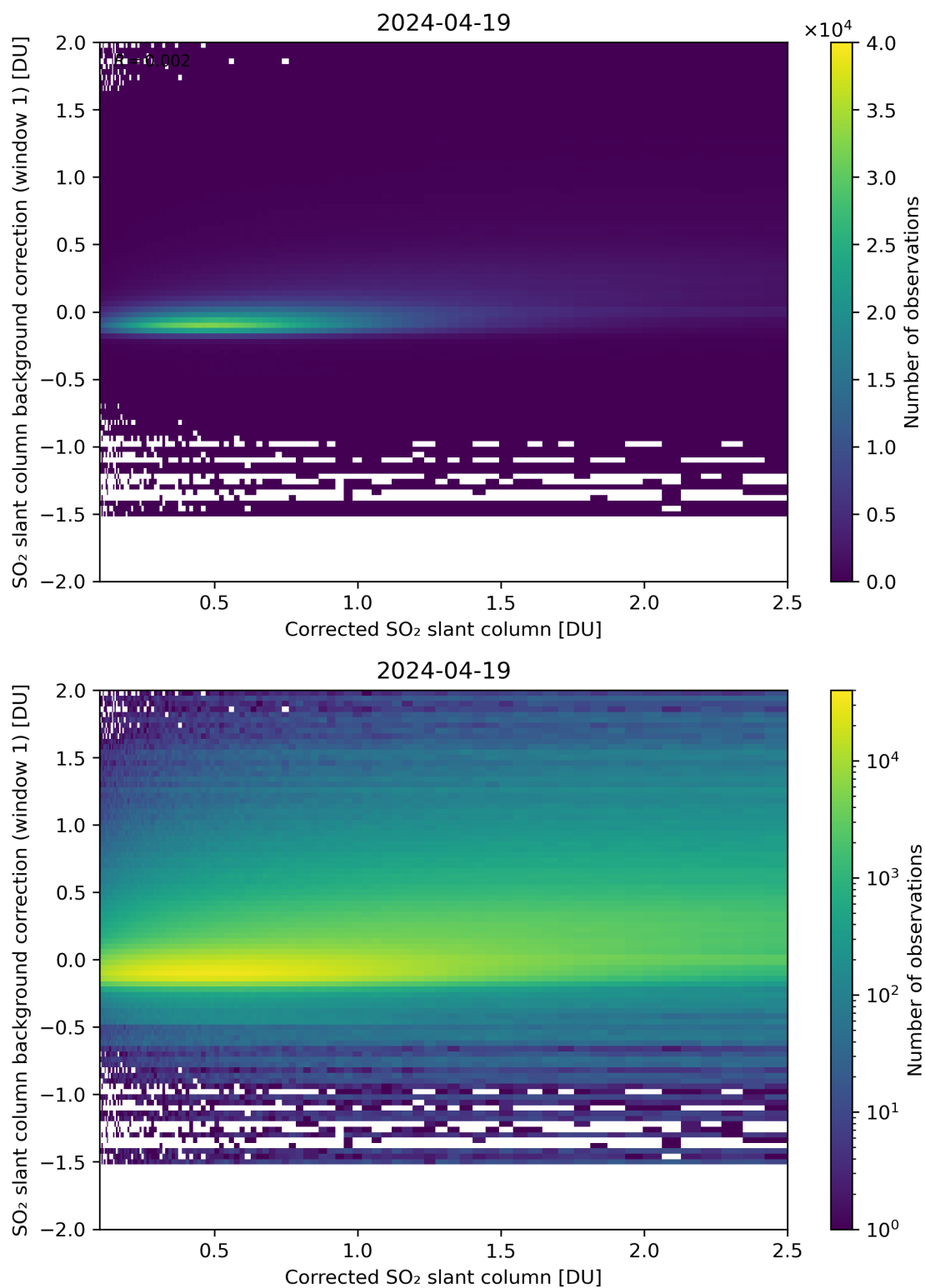
Figure 178: Scatter density plot of “Corrected SO 2 slant column” against “SO 2 slant column background correction (window 1)” for 2024-04-18 to 2024-04-20.
