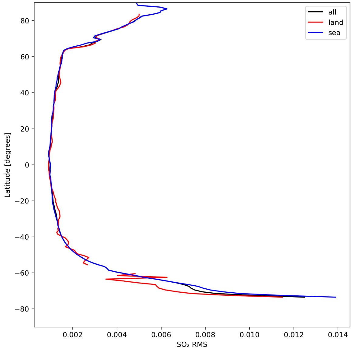
Figure 47: Zonal average of “SO 2 RMS” for 2024-04-18 to 2024-04-20.
