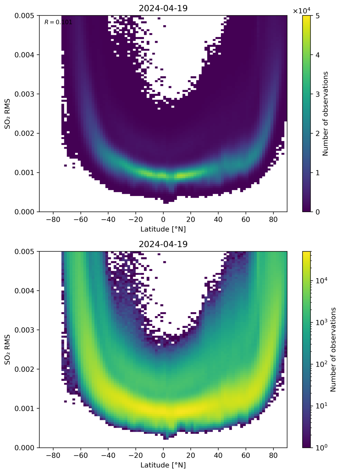
Figure 144: Scatter density plot of “Latitude” against “SO 2 RMS” for 2024-04-18 to 2024-04-20.
