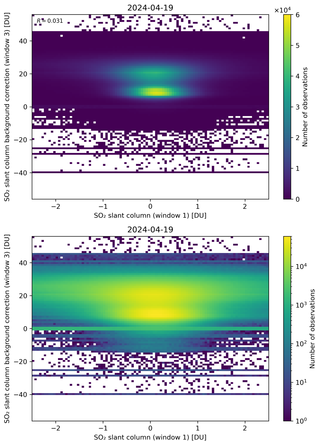
Figure 214: Scatter density plot of “SO 2 slant column (window 1)” against “SO 2 slant column background correction (window 3)” for 2024-04-18 to 2024-04-20.
