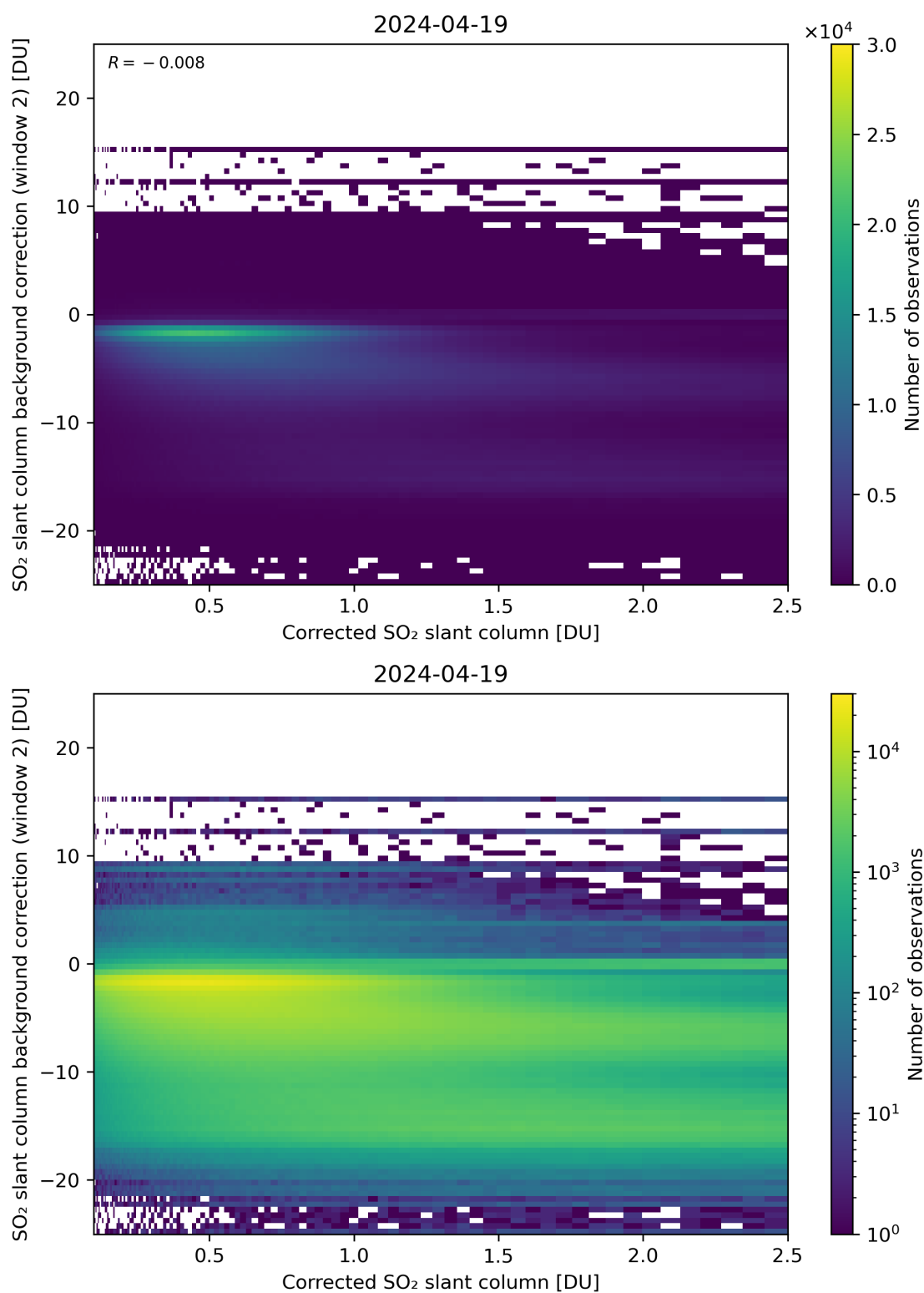
Figure 179: Scatter density plot of “Corrected SO 2 slant column” against “SO 2 slant column background correction (window 2)” for 2024-04-18 to 2024-04-20.
