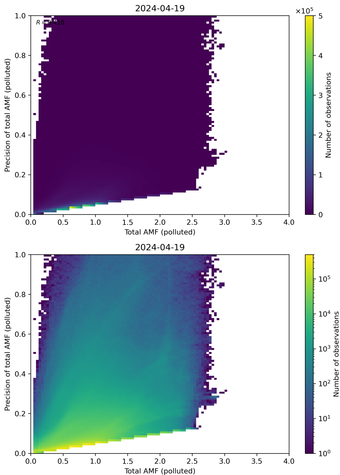
Figure 272: Scatter density plot of “Total AMF (polluted)” against “Precision of total AMF (polluted)” for 2024-04-18 to 2024-04-20.
