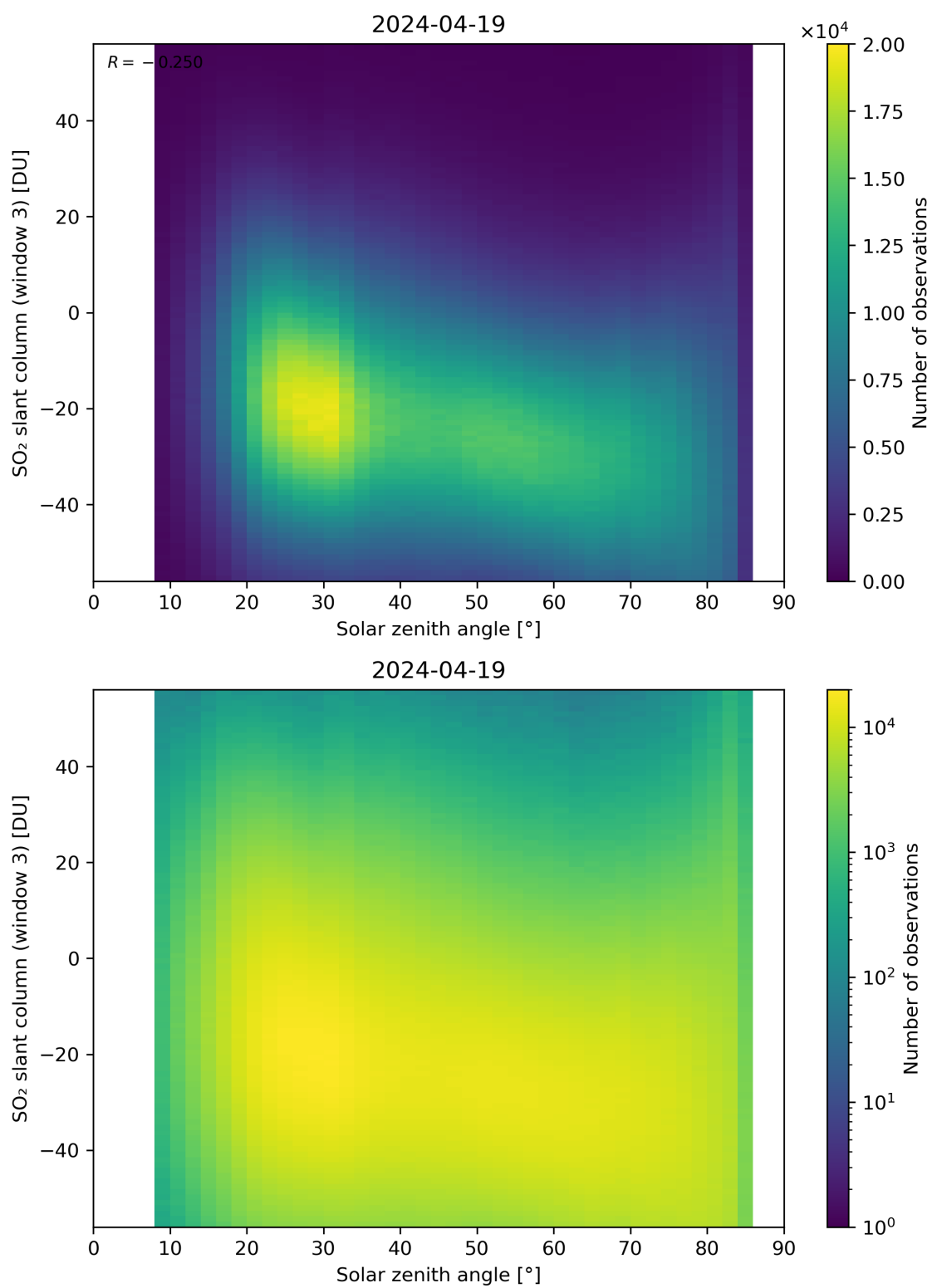
Figure 172: Scatter density plot of “Solar zenith angle” against “SO 2 slant column (window 3)” for 2024-04-18 to 2024-04-20.
