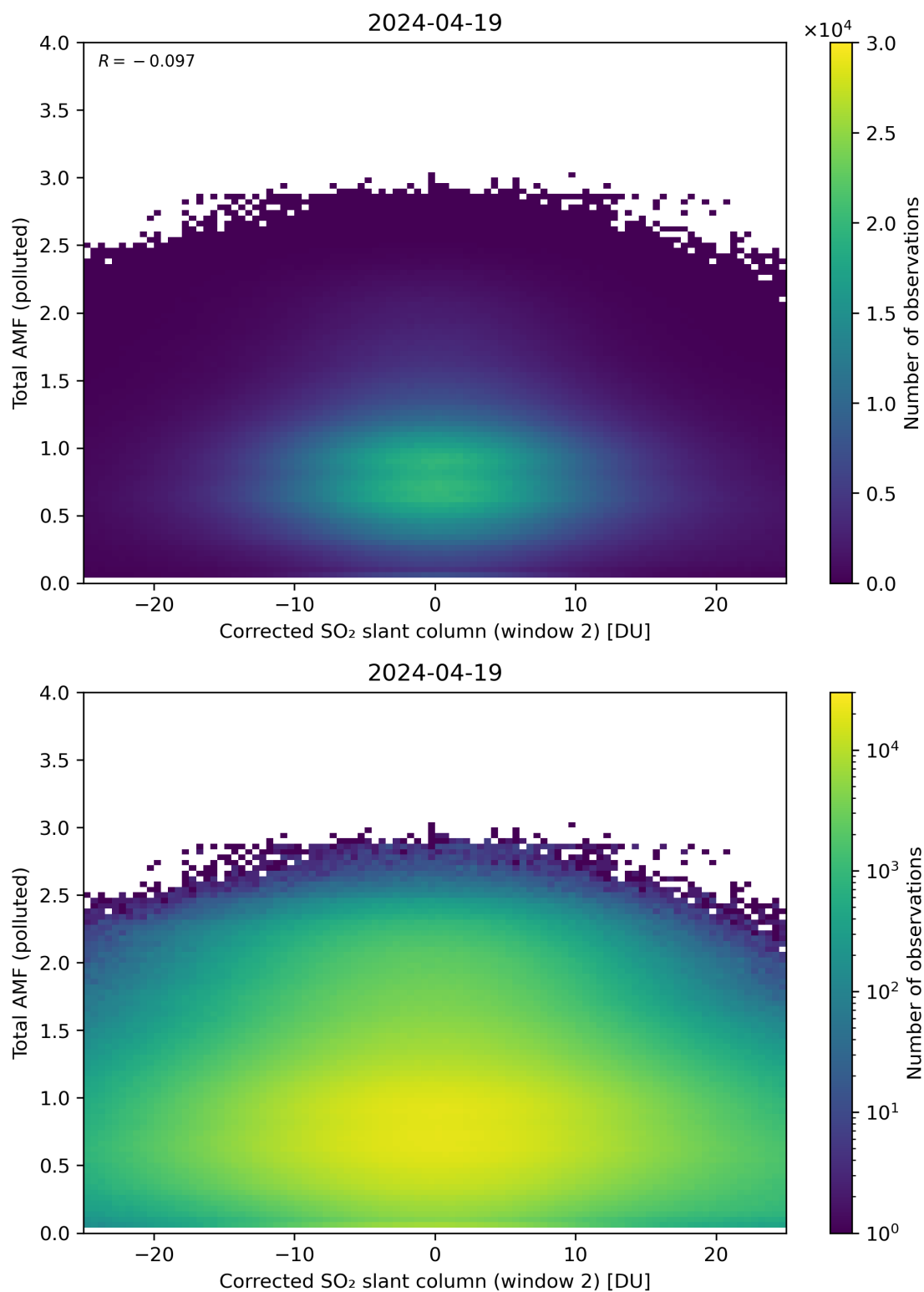
Figure 203: Scatter density plot of “Corrected SO 2 slant column (window 2)” against “Total AMF (polluted)” for 2024-04-18 to 2024-04-20.
