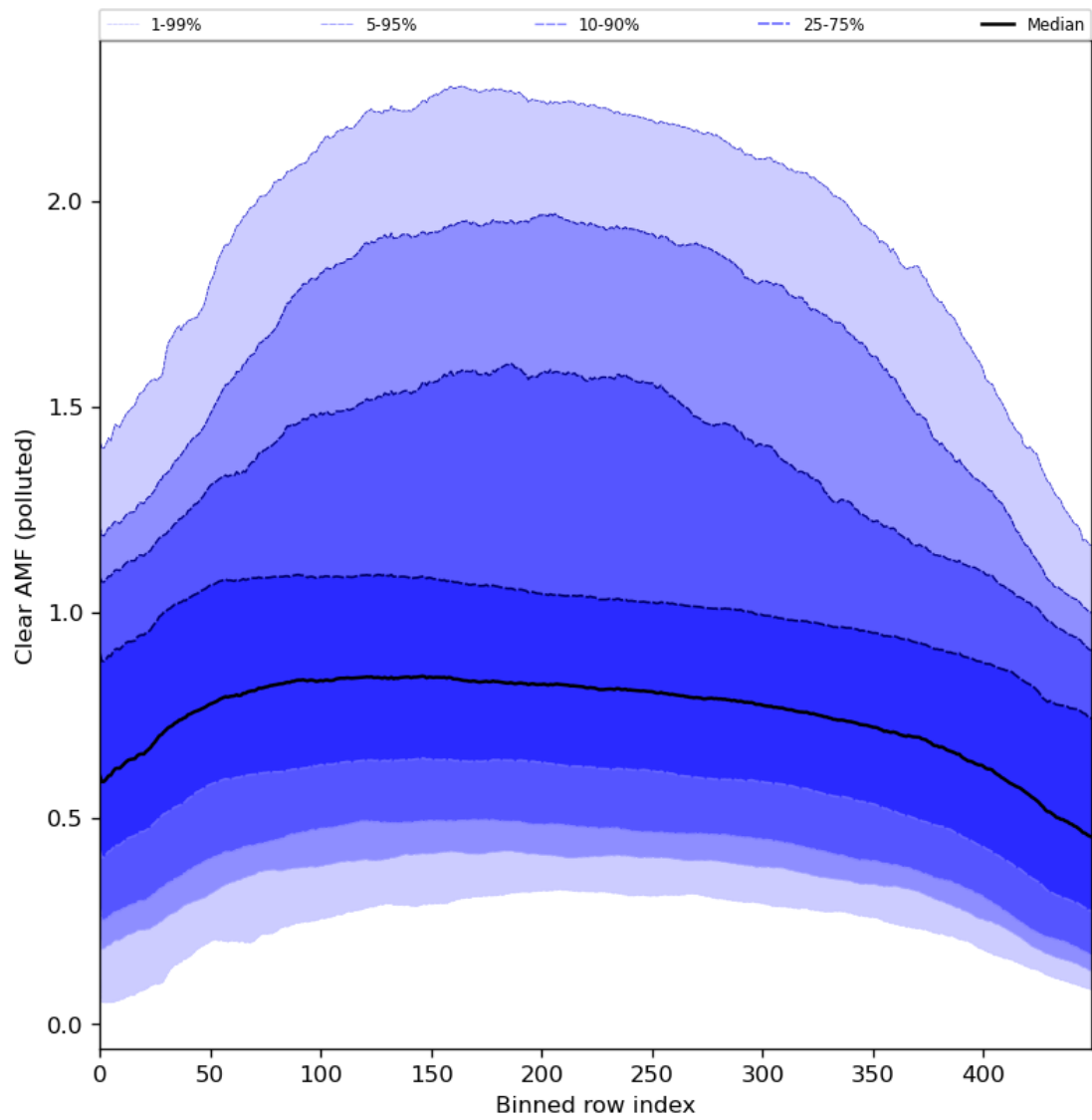
Figure 96: Along track statistics of “Clear AMF (polluted)” for 2024-04-18 to 2024-04-20
