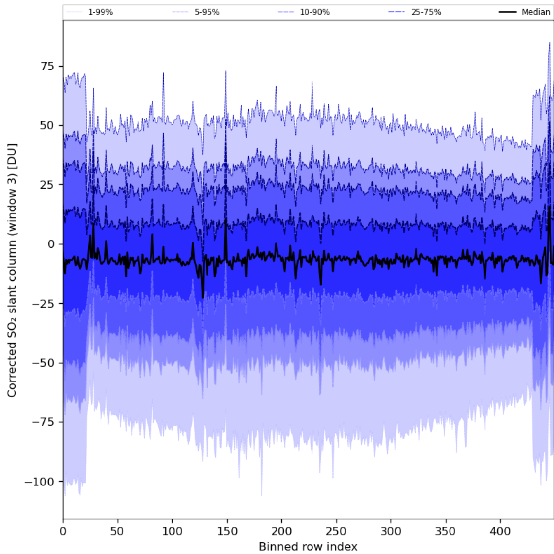
Figure 89: Along track statistics of “Corrected SO 2 slant column (window 3)” for 2024-04-18 to 2024-04-20
