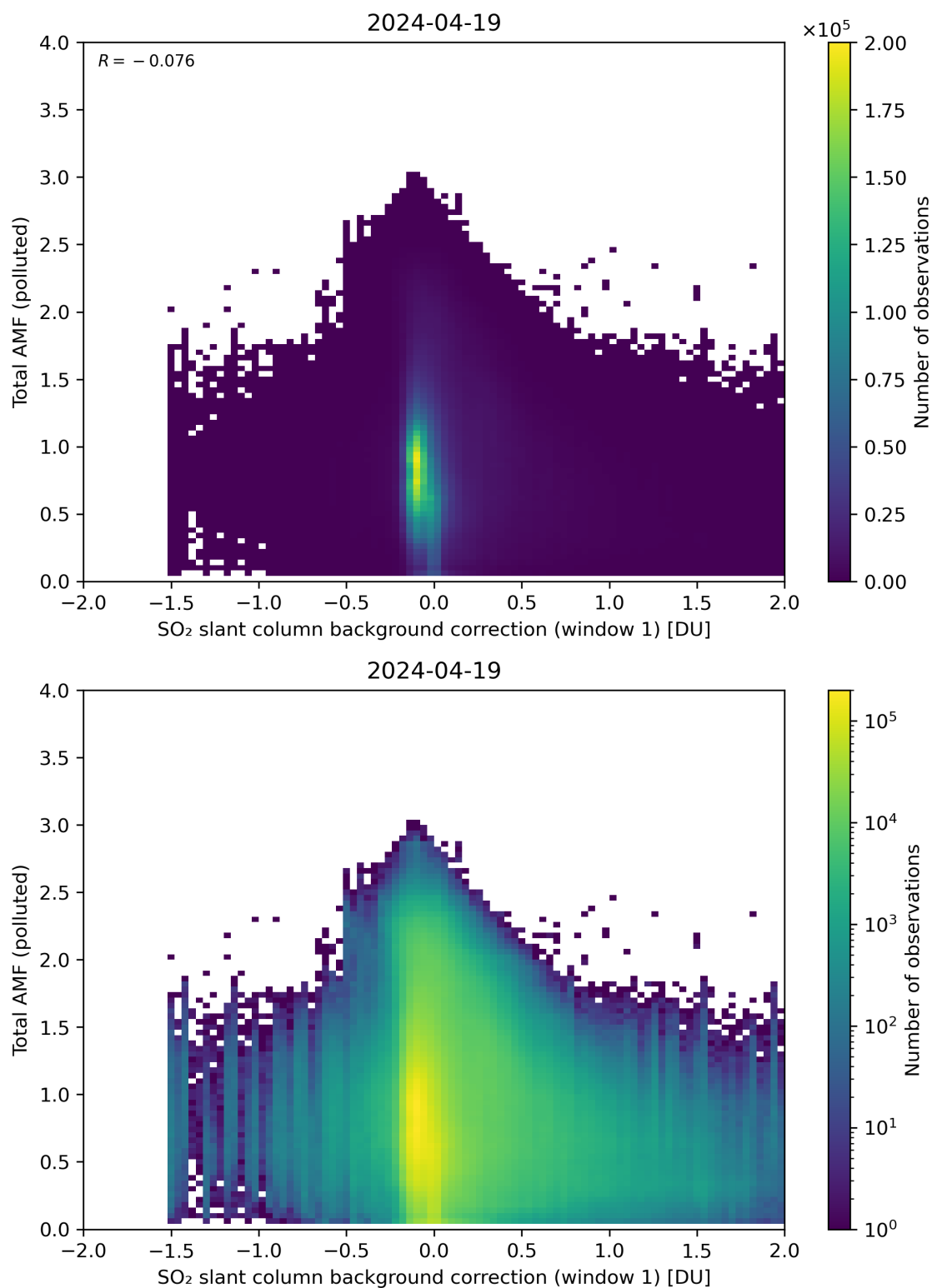
Figure 109: Scatter density plot of “SO 2 slant column background correction (window 1)” against “Total AMF (polluted)” for 2024-04-18 to 2024-04-20.
