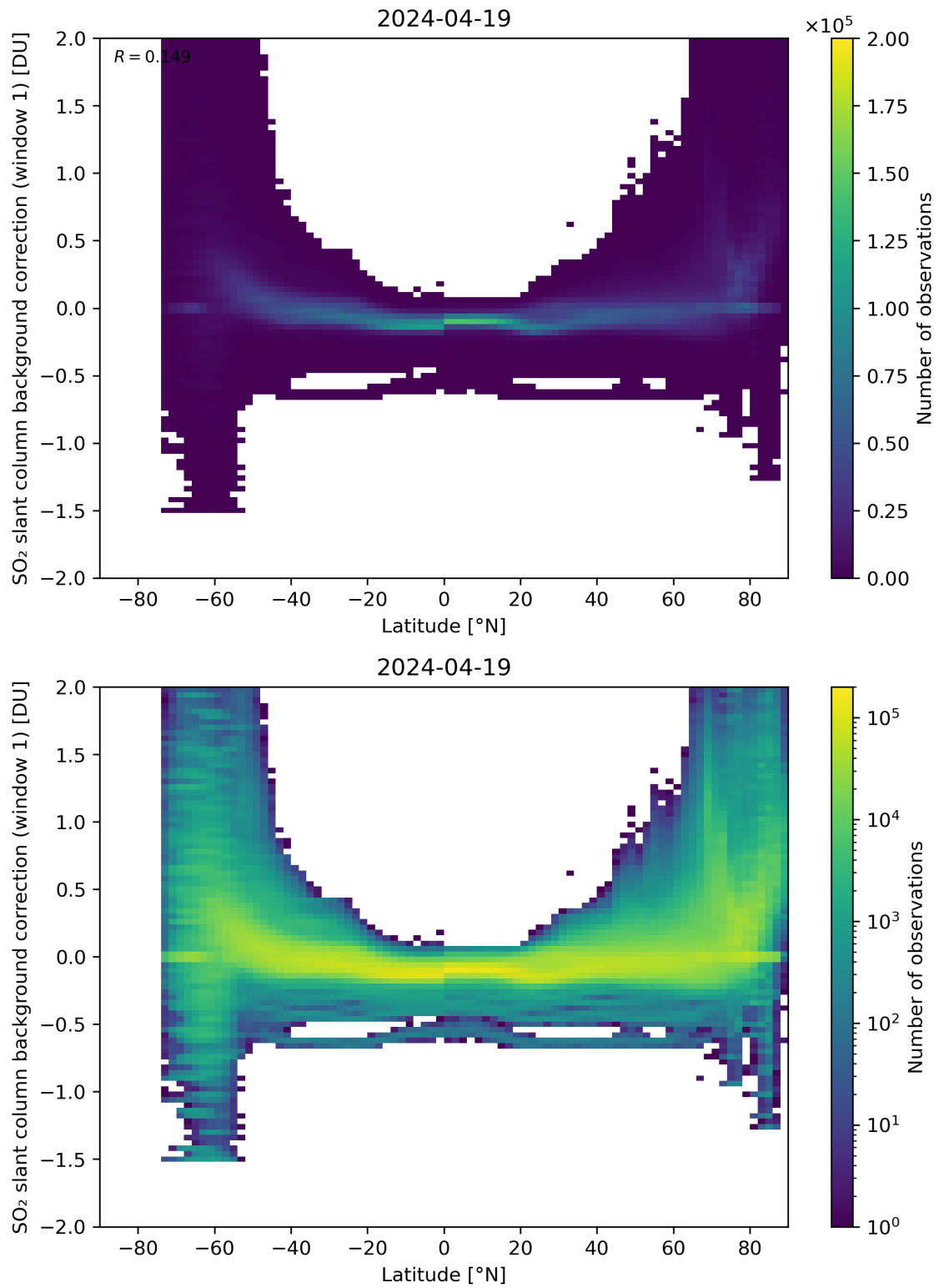
Figure 139: Scatter density plot of “Latitude” against “SO 2 slant column background correction (window 1)” for 2024-04-18 to 2024-04-20.
