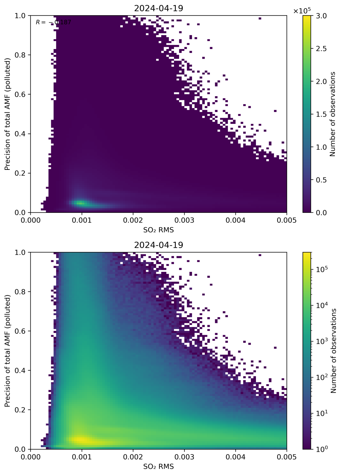
Figure 138: Scatter density plot of “SO 2 RMS” against “Precision of total AMF (polluted)” for 2024-04-18 to 2024-04-20.
