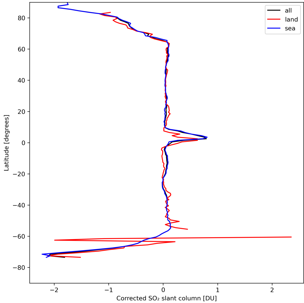
Figure 32: Zonal average of “Corrected SO 2 slant column” for 2024-04-18 to 2024-04-20.
