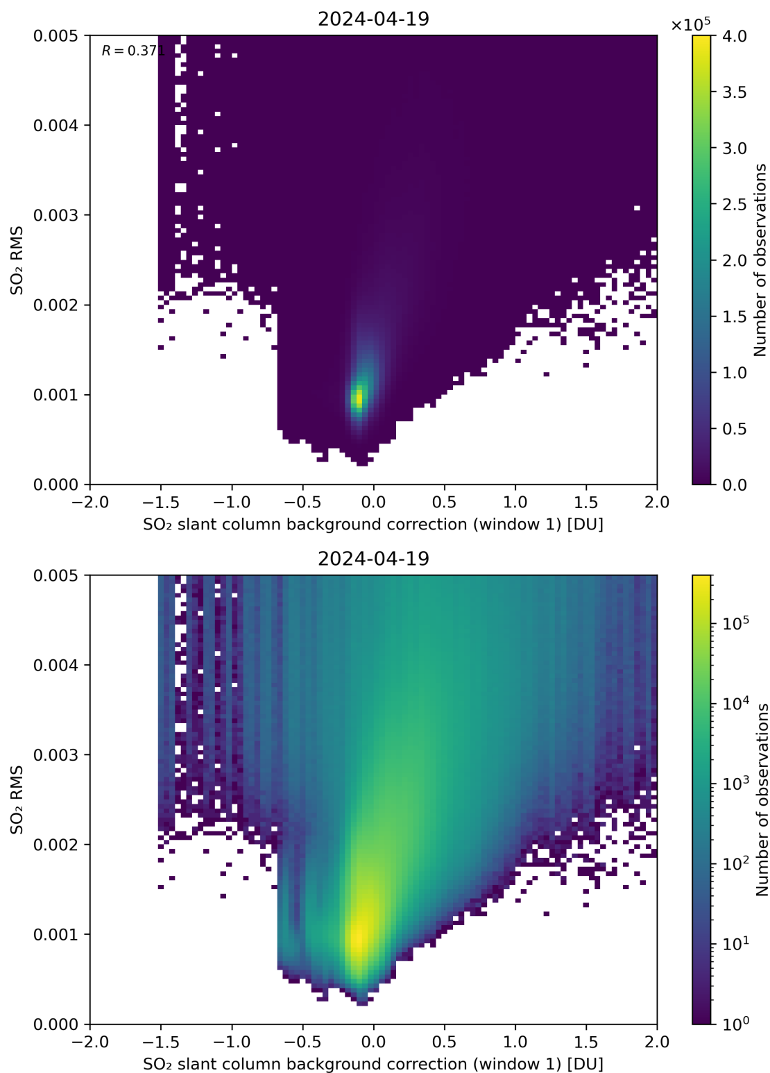
Figure 102: Scatter density plot of “SO 2 slant column background correction (window 1)” against “SO 2 RMS” for 2024-04-18 to 2024-04-20.
