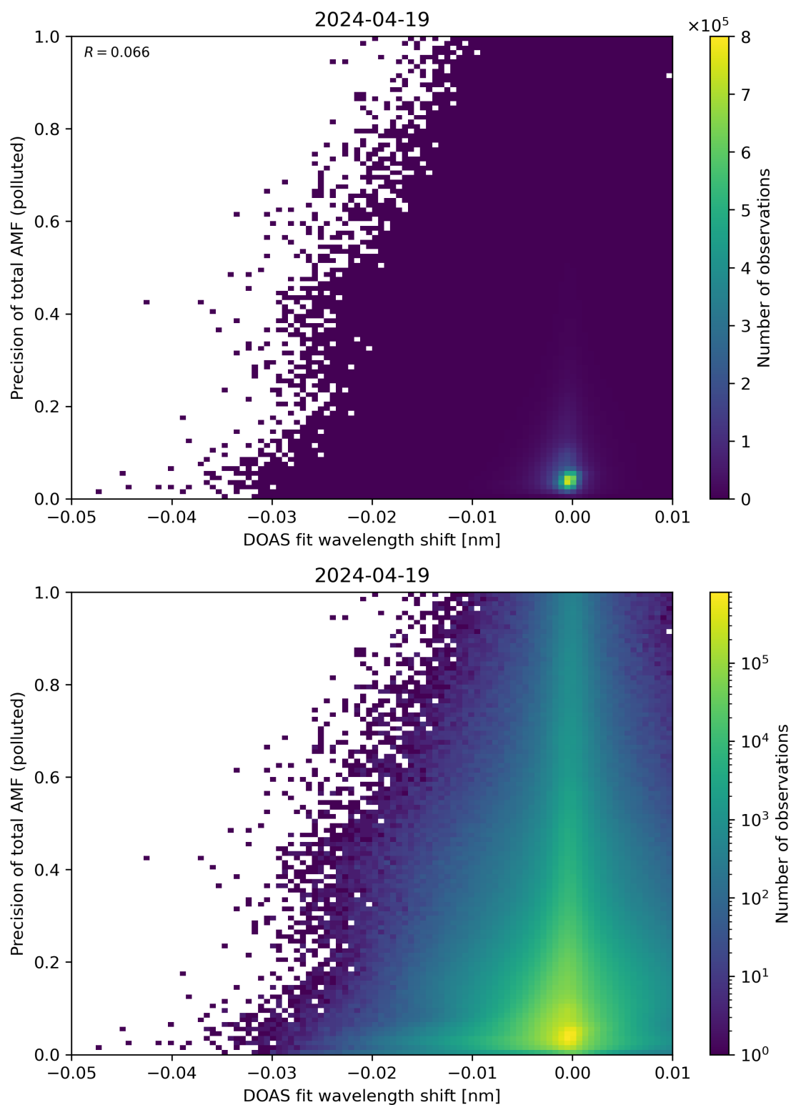
Figure 131: Scatter density plot of “DOAS fit wavelength shift” against “Precision of total AMF (polluted)” for 2024-04-18 to 2024-04-20.
