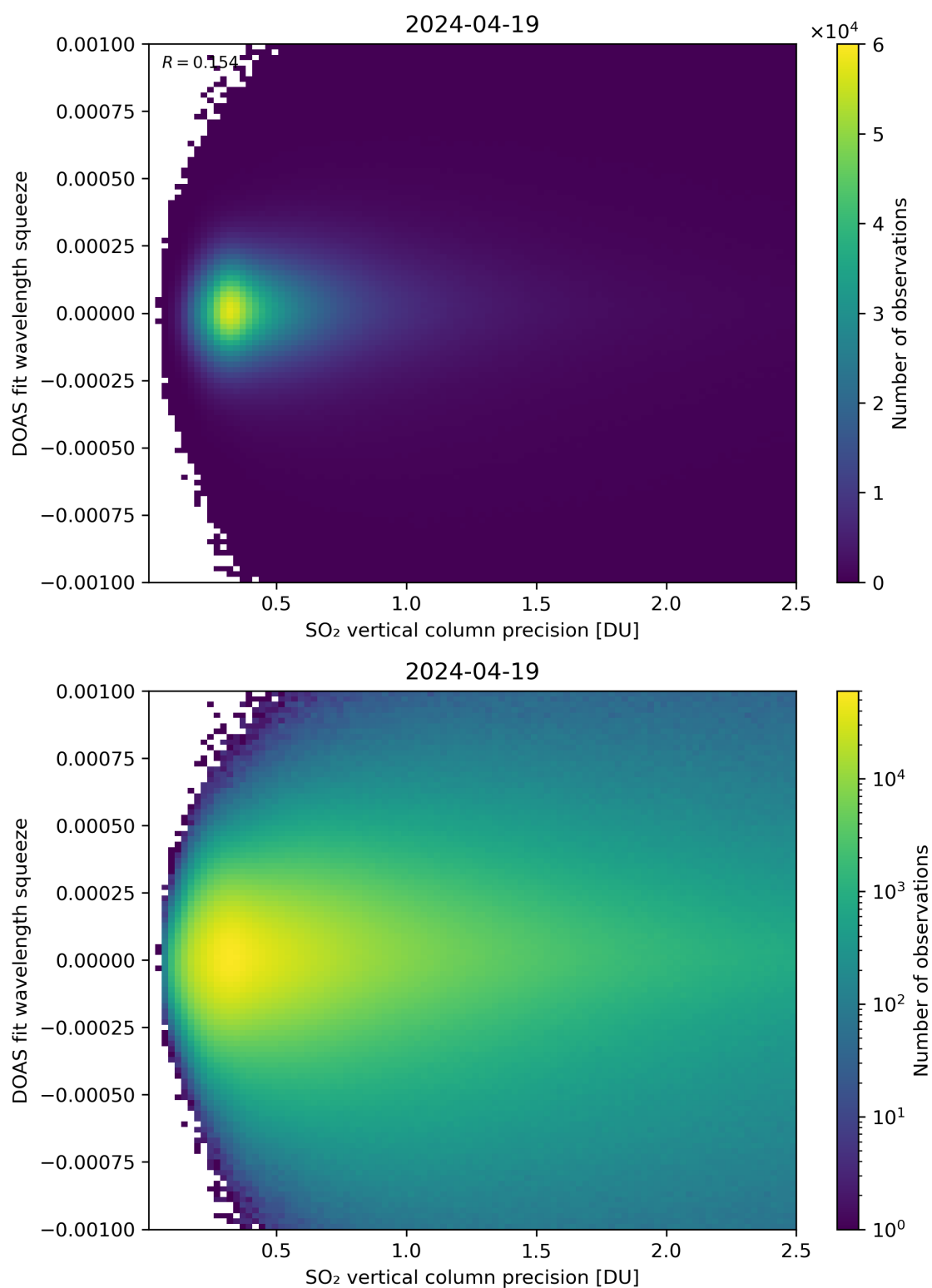
Figure 283: Scatter density plot of “SO 2 vertical column precision” against “DOAS fit wavelength squeeze” for 2024-04-18 to 2024-04-20.
