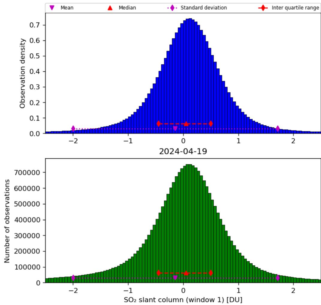
Figure 56: Histogram of “SO 2 slant column (window 1)” for 2024-04-18 to 2024-04-20
