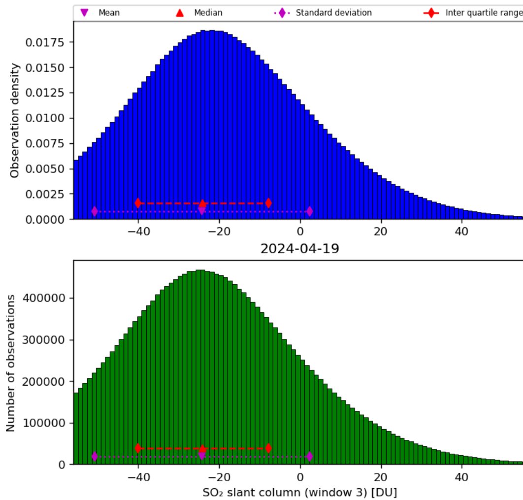
Figure 64: Histogram of “SO 2 slant column (window 3)” for 2024-04-18 to 2024-04-20
