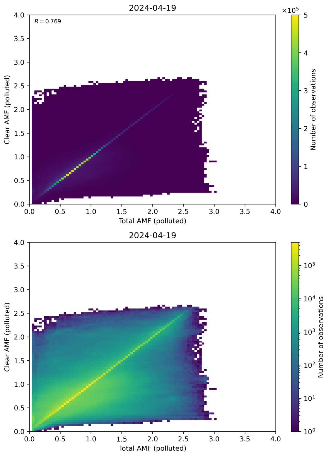
Figure 271: Scatter density plot of “Total AMF (polluted)” against “Clear AMF (polluted)” for 2024-04-18 to 2024-04-20.
