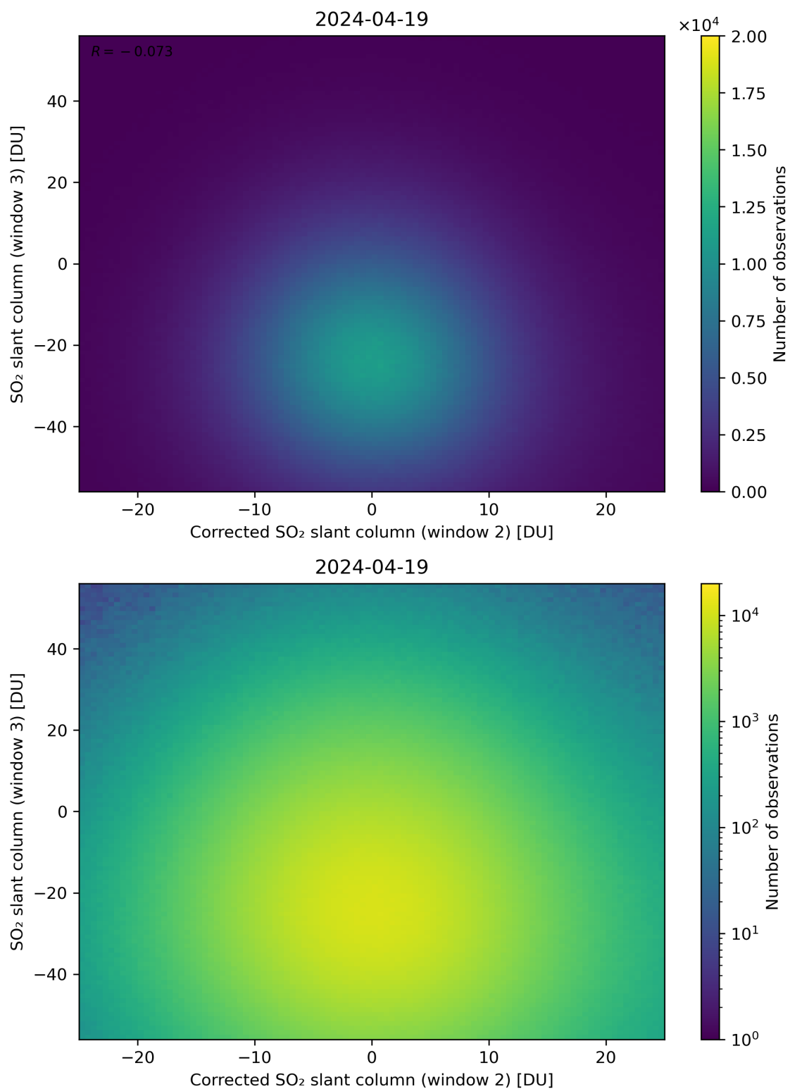
Figure 201: Scatter density plot of “Corrected SO 2 slant column (window 2)” against “SO 2 slant column (window 3)” for 2024-04-18 to 2024-04-20.
