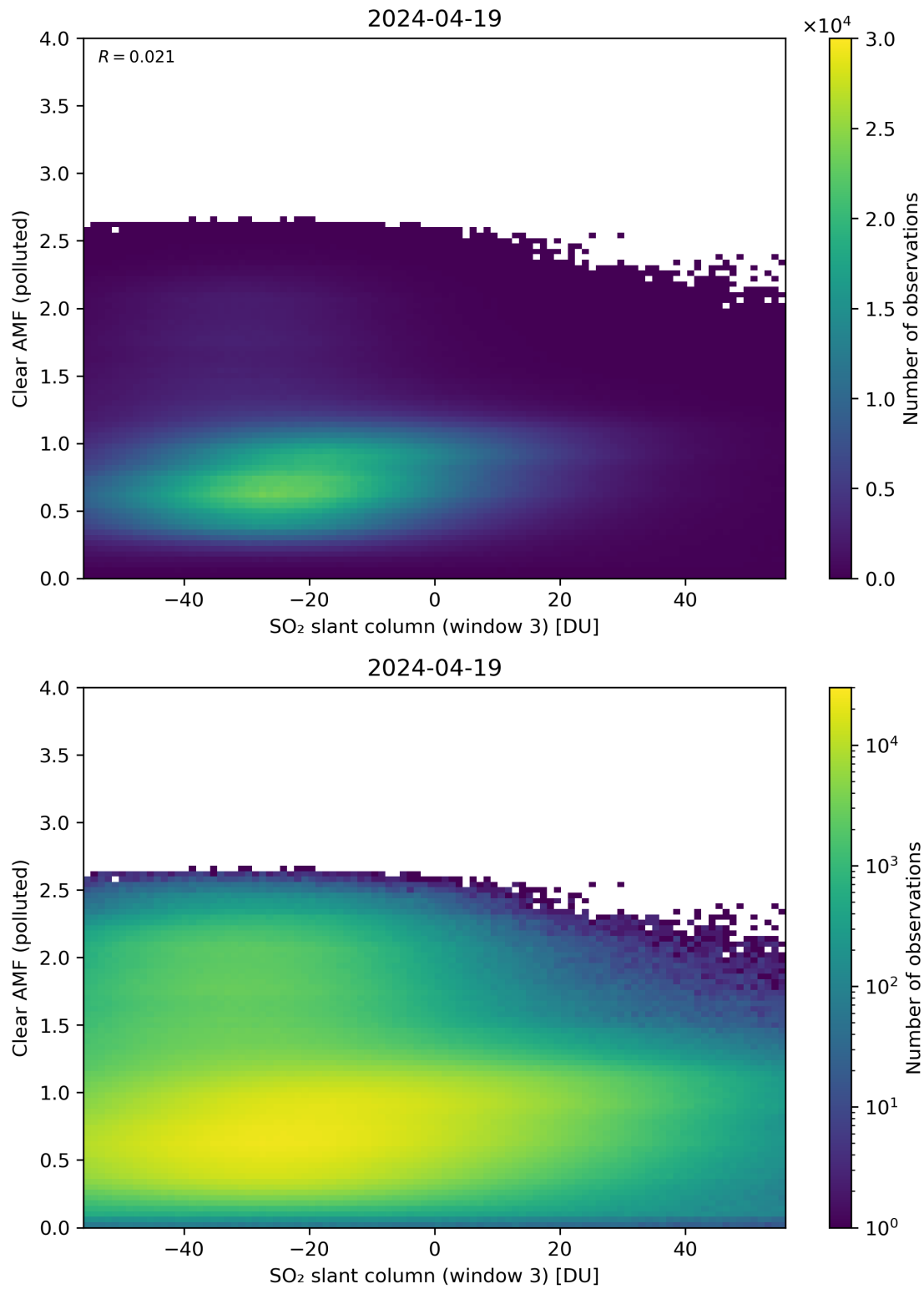
Figure 265: Scatter density plot of “SO 2 slant column (window 3)” against “Clear AMF (polluted)” for 2024-04-18 to 2024-04-20.
