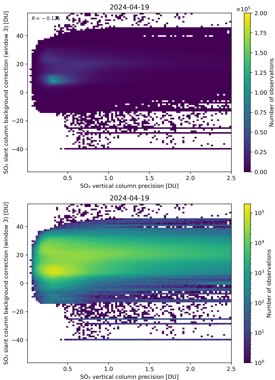
Figure 281: Scatter density plot of “SO 2 vertical column precision” against “SO 2 slant column background correction (window 3)” for 2024-04-18 to 2024-04-20.
