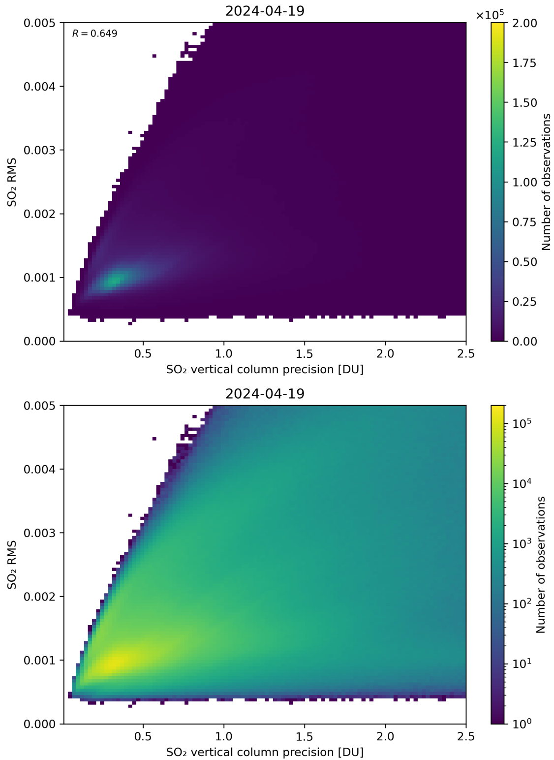
Figure 284: Scatter density plot of “SO 2 vertical column precision” against “SO 2 RMS” for 2024-04-18 to 2024-04-20.
