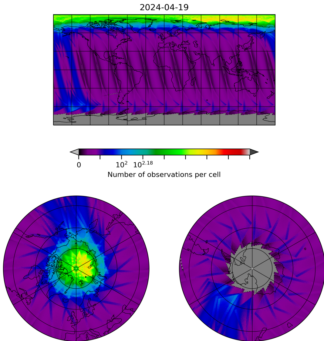
Figure 28: Map of the number of observations for 2024-04-18 to 2024-04-20
