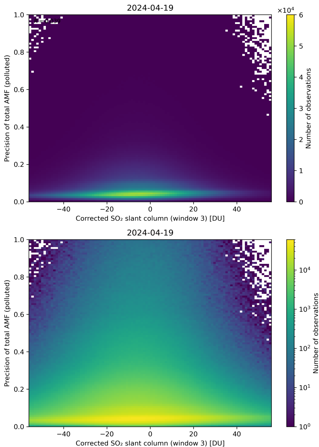
Figure 211: Scatter density plot of “Corrected SO 2 slant column (window 3)” against “Precision of total AMF (polluted)” for 2024-04-18 to 2024-04-20.
