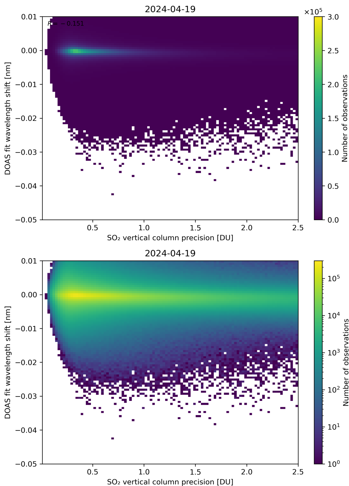
Figure 282: Scatter density plot of “SO 2 vertical column precision” against “DOAS fit wavelength shift” for 2024-04-18 to 2024-04-20.
