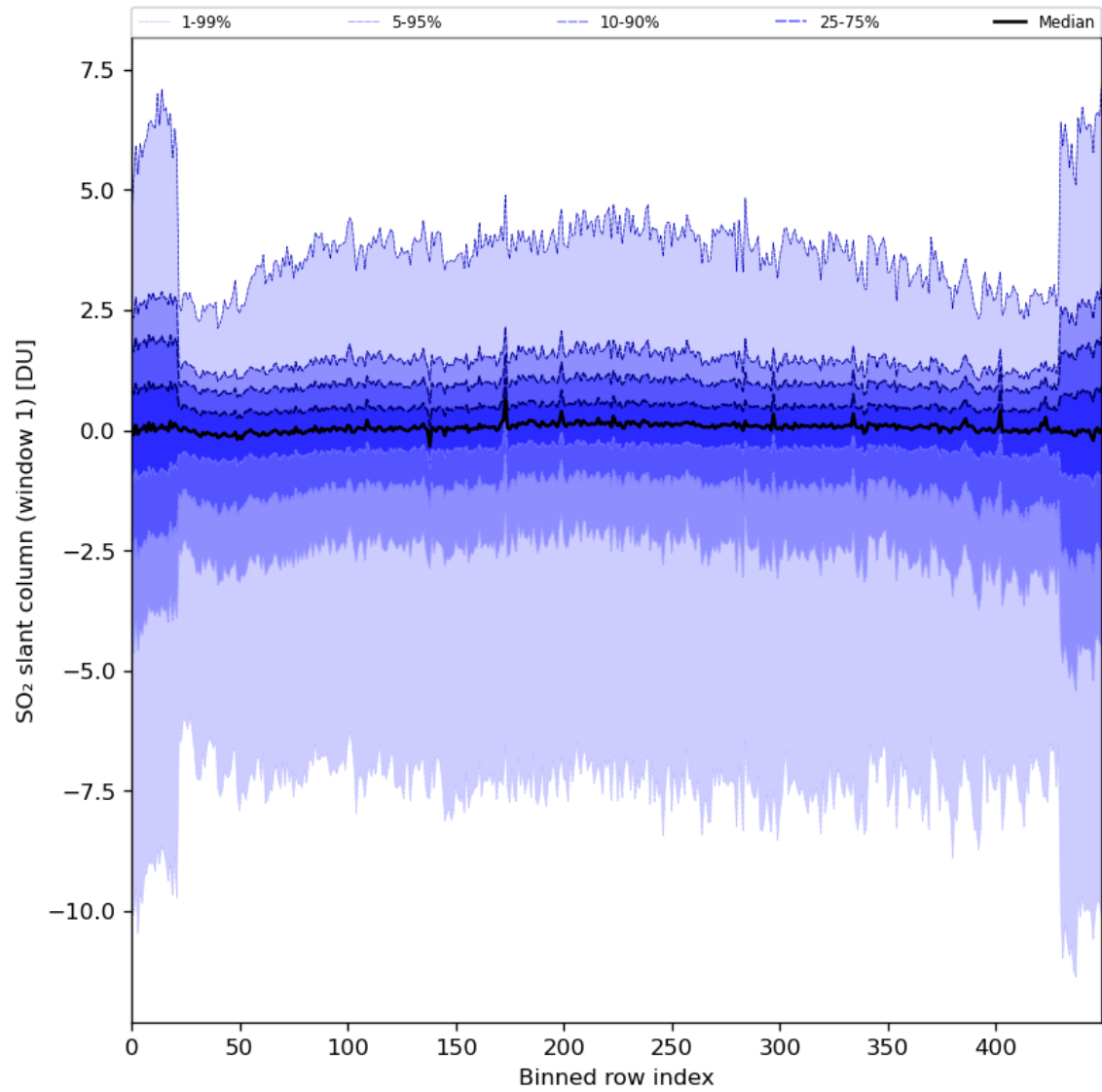
Figure 79: Along track statistics of “SO 2 slant column (window 1)” for 2024-04-18 to 2024-04-20
