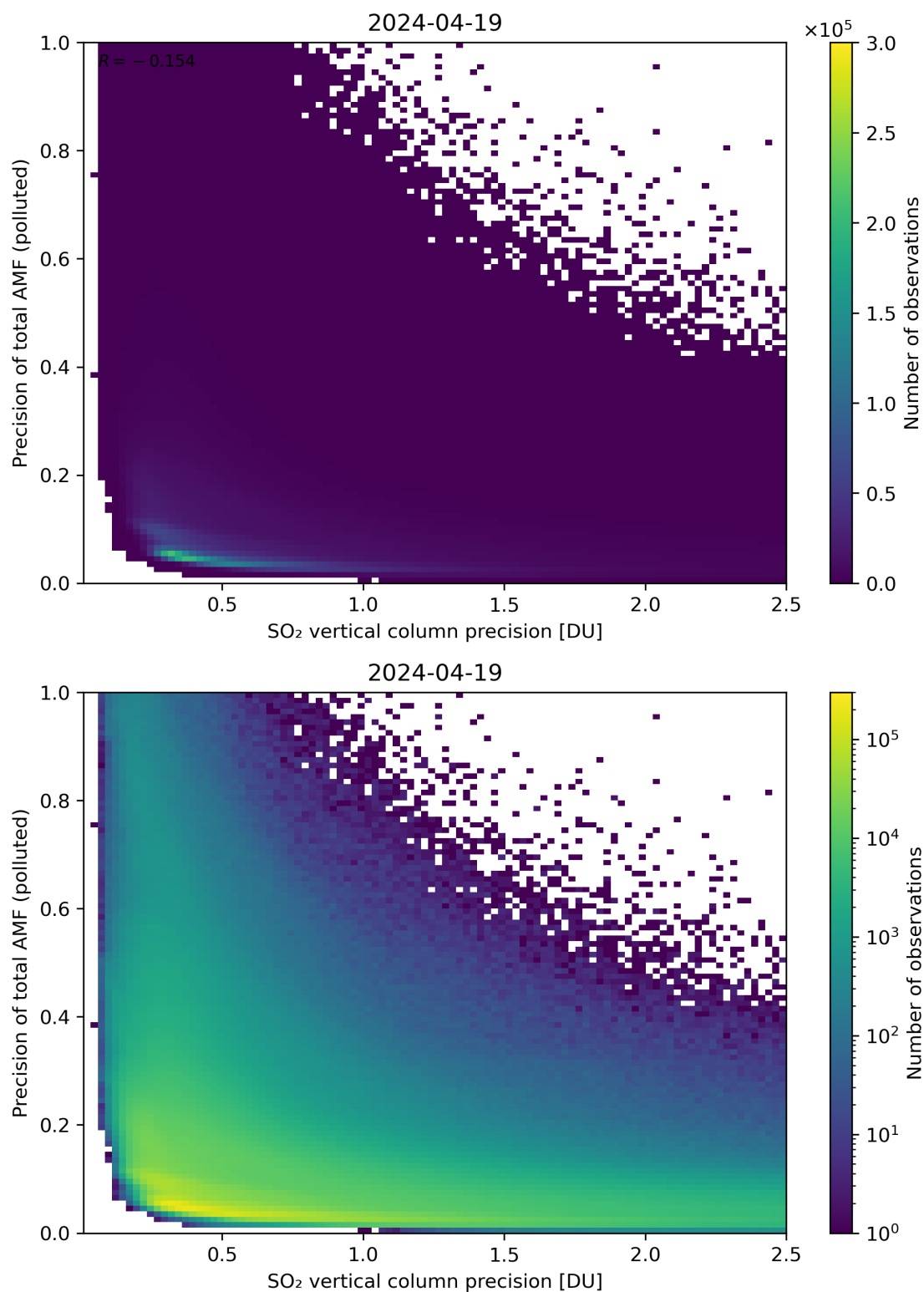
Figure 295: Scatter density plot of “SO 2 vertical column precision” against “Precision of total AMF (polluted)” for 2024-04-18 to 2024-04-20.
