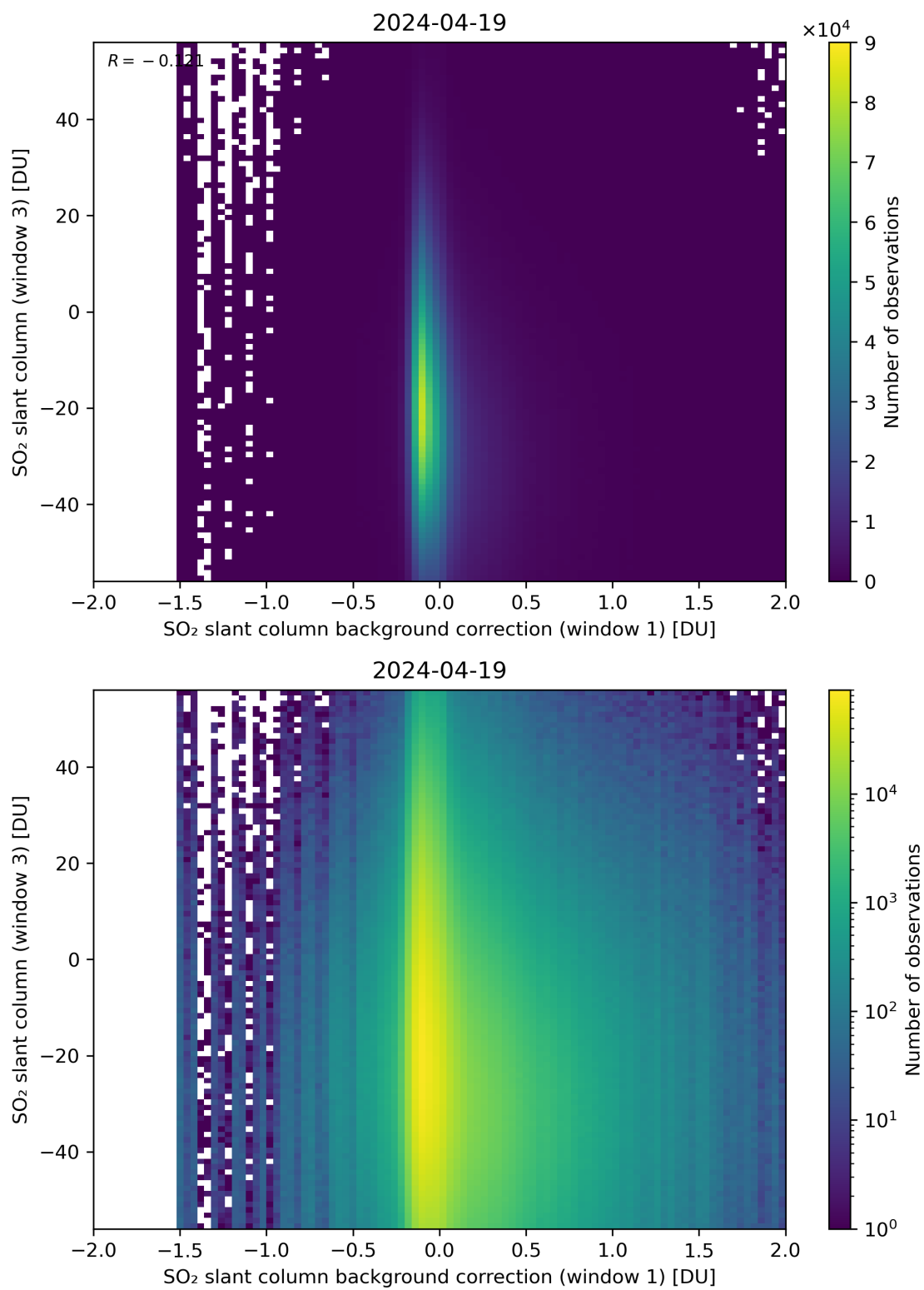
Figure 107: Scatter density plot of “SO 2 slant column background correction (window 1)” against “SO 2 slant column (window 3)” for 2024-04-18 to 2024-04-20.
