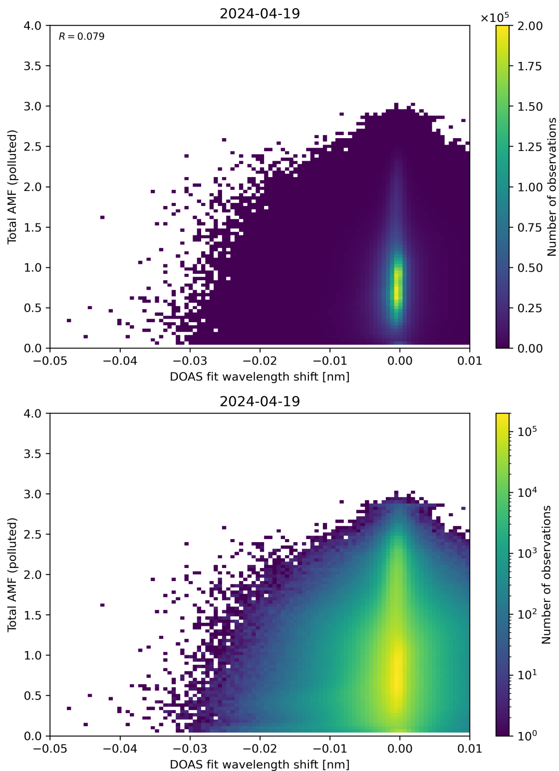
Figure 130: Scatter density plot of “DOAS fit wavelength shift” against “Total AMF (polluted)” for 2024-04-18 to 2024-04-20.
