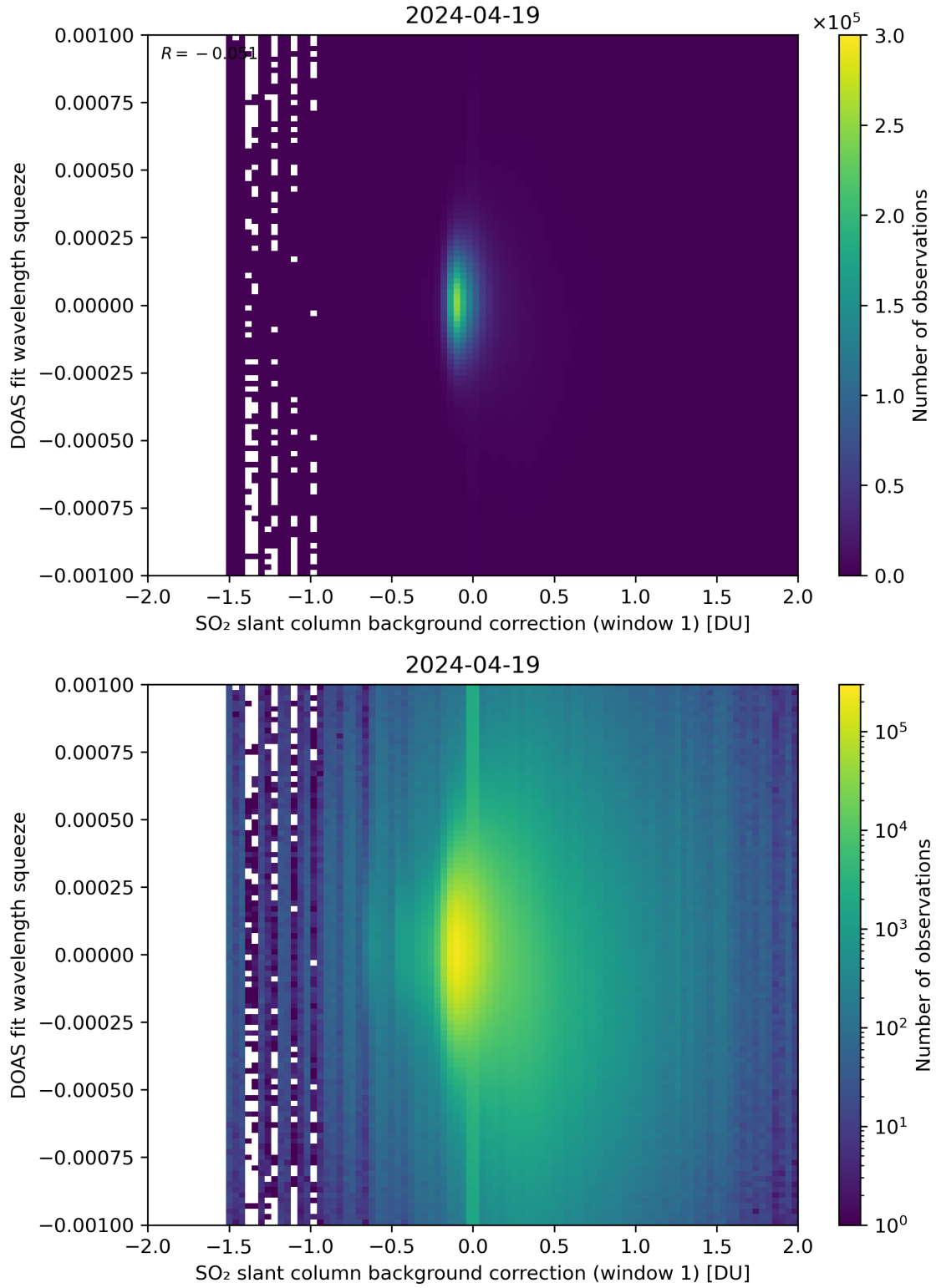
Figure 101: Scatter density plot of “SO 2 slant column background correction (window 1)” against “DOAS fit wavelength squeeze” for 2024-04-18 to 2024-04-20.
