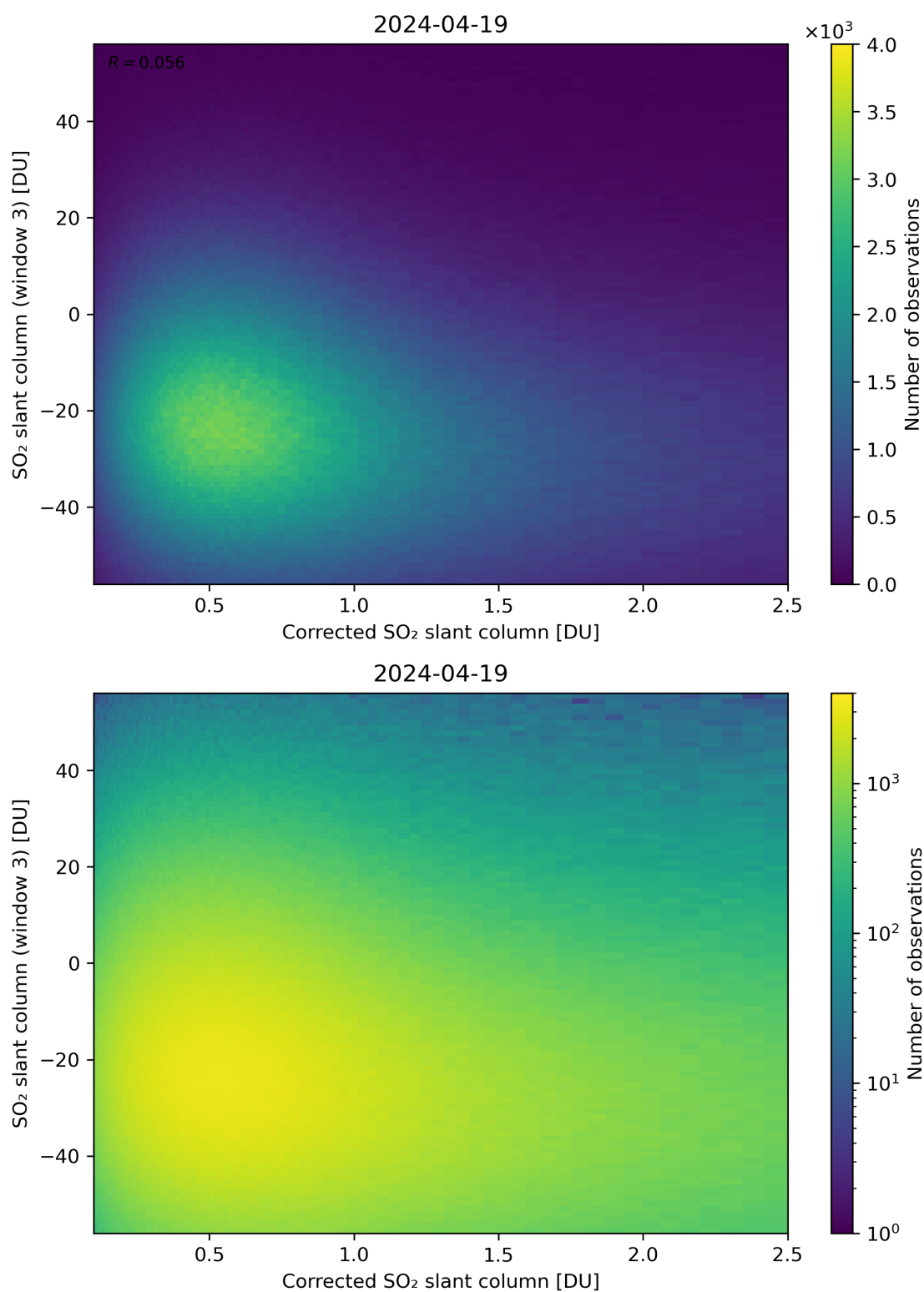
Figure 190: Scatter density plot of “Corrected SO 2 slant column” against “SO 2 slant column (window 3)” for 2024-04-18 to 2024-04-20.
