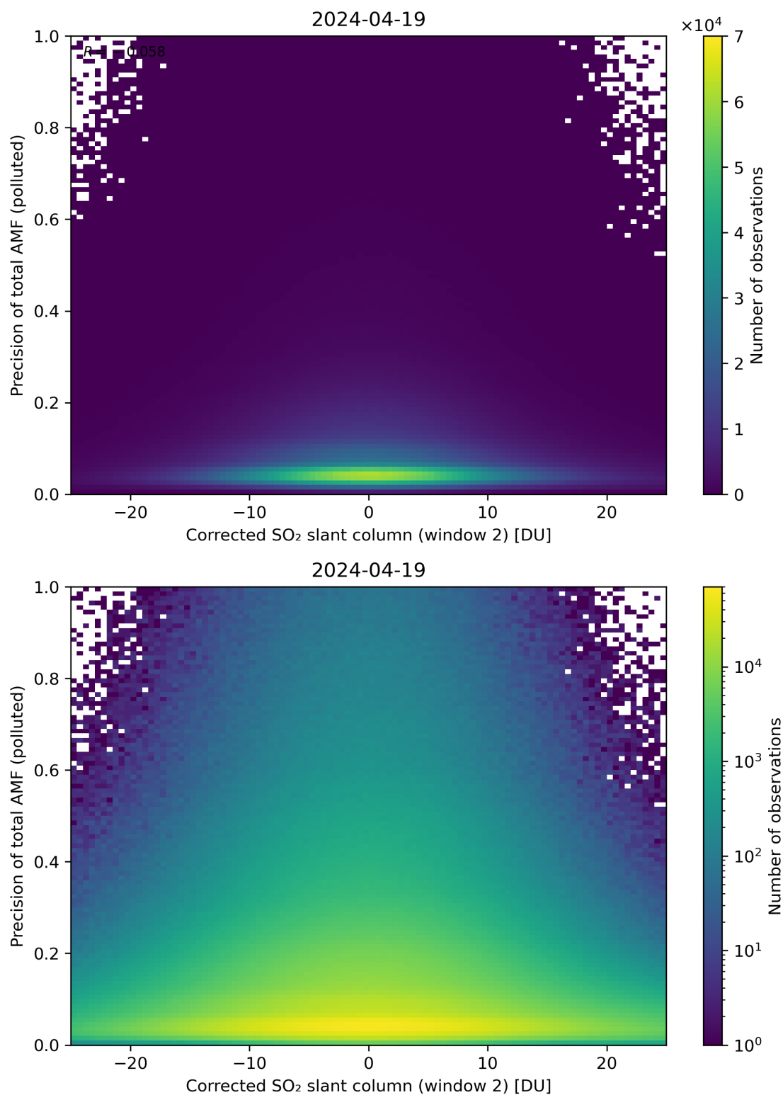
Figure 204: Scatter density plot of “Corrected SO 2 slant column (window 2)” against “Precision of total AMF (polluted)” for 2024-04-18 to 2024-04-20.
