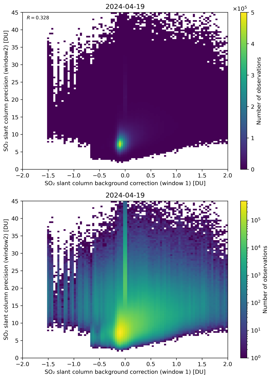
Figure 106: Scatter density plot of “SO 2 slant column background correction (window 1)” against “SO 2 slant column precision (window2)” for 2024-04-18 to 2024-04-20.
