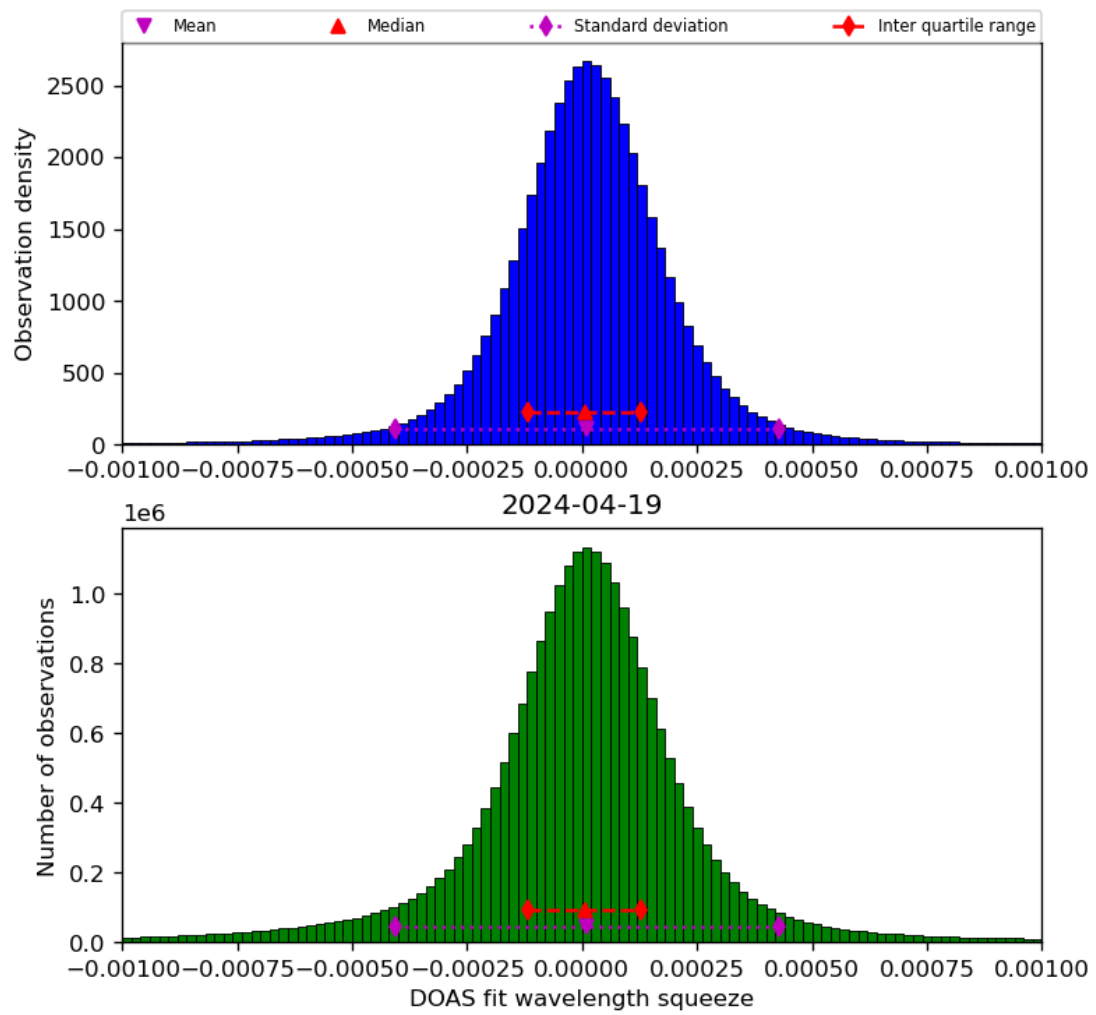
Figure 69: Histogram of “DOAS fit wavelength squeeze” for 2024-04-18 to 2024-04-20
