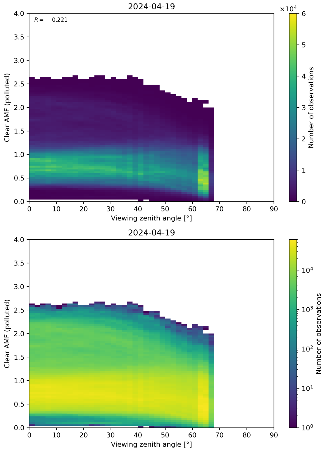
Figure 316: Scatter density plot of “Viewing zenith angle” against “Clear AMF (polluted)” for 2024-04-18 to 2024-04-20.
