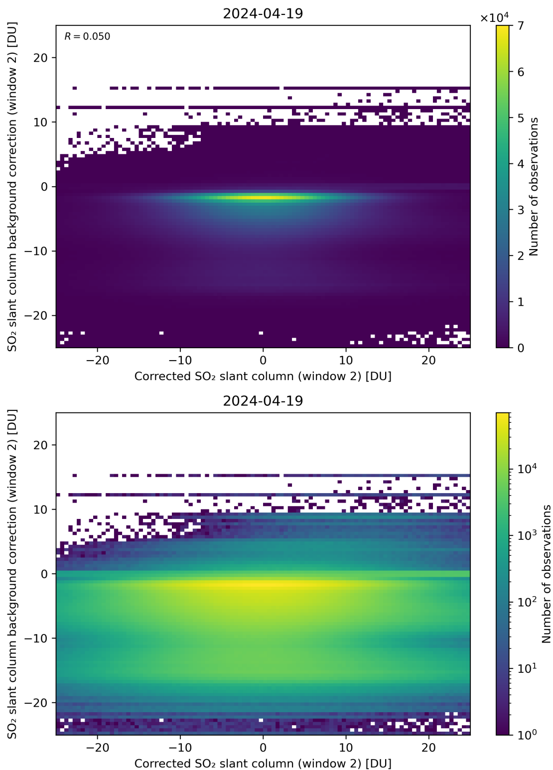
Figure 194: Scatter density plot of “Corrected SO 2 slant column (window 2)” against “SO 2 slant column background correction (window 2)” for 2024-04-18 to 2024-04-20.
