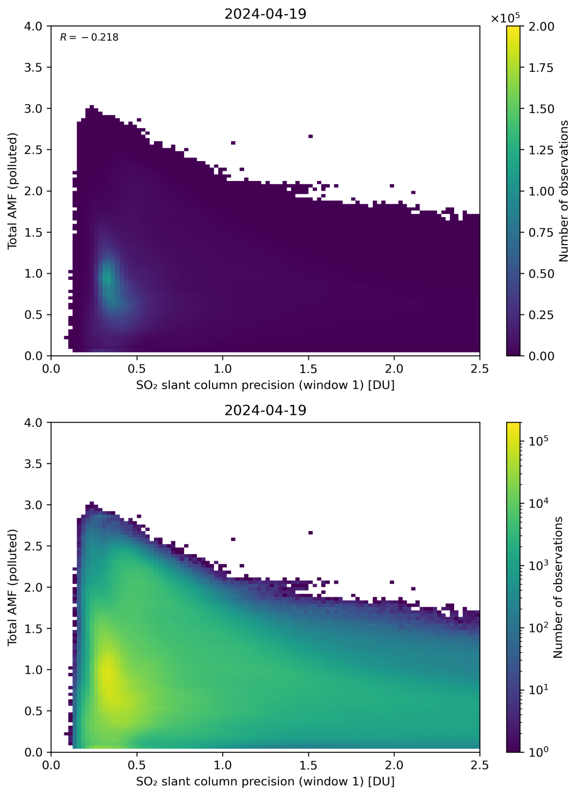
Figure 230: Scatter density plot of “SO 2 slant column precision (window 1)” against “Total AMF (polluted)” for 2024-04-18 to 2024-04-20.
