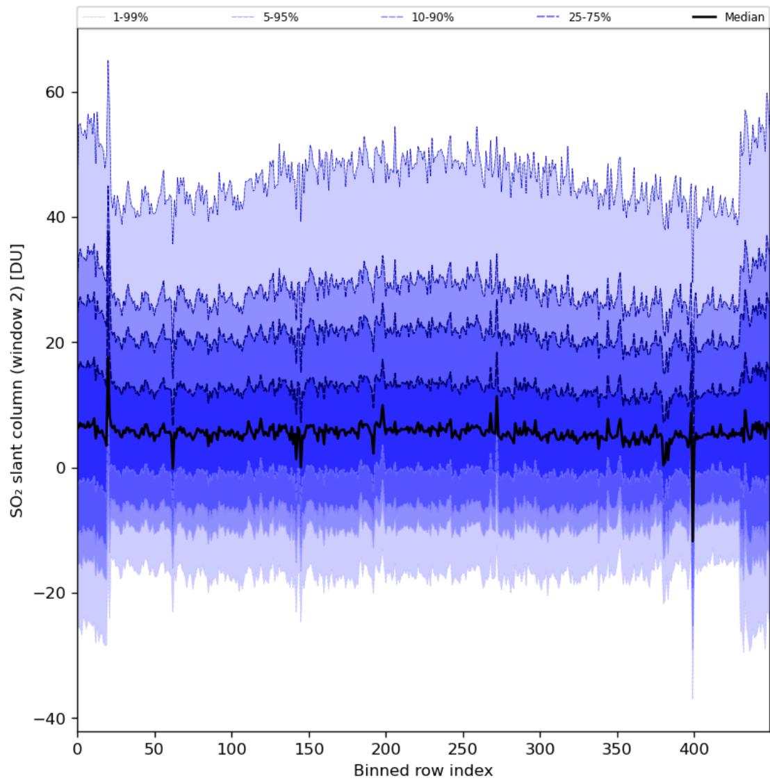
Figure 83: Along track statistics of “SO 2 slant column (window 2)” for 2024-04-18 to 2024-04-20
