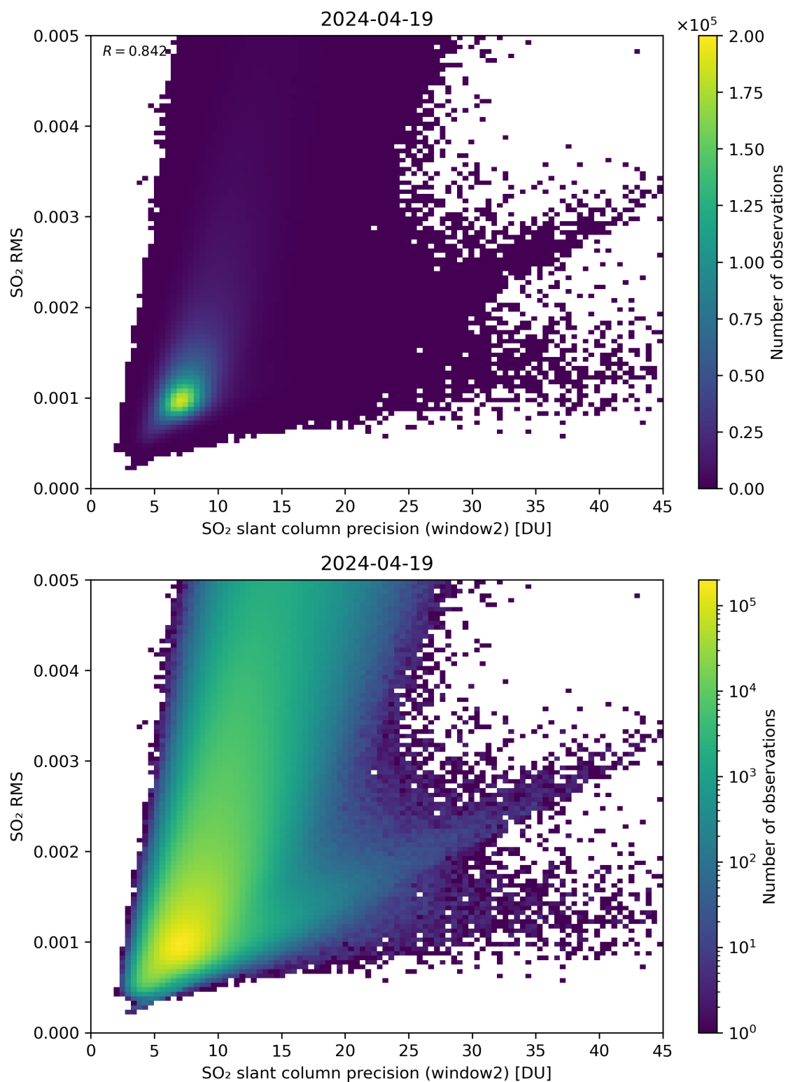
Figure 245: Scatter density plot of “SO 2 slant column precision (window2)” against “SO 2 RMS” for 2024-04-18 to 2024-04-20.
