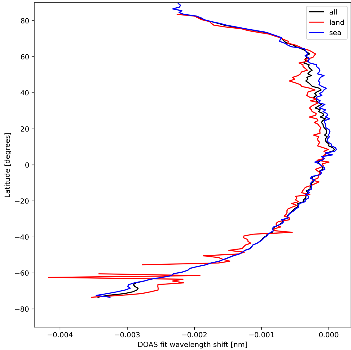
Figure 45: Zonal average of “DOAS fit wavelength shift” for 2024-04-18 to 2024-04-20.
