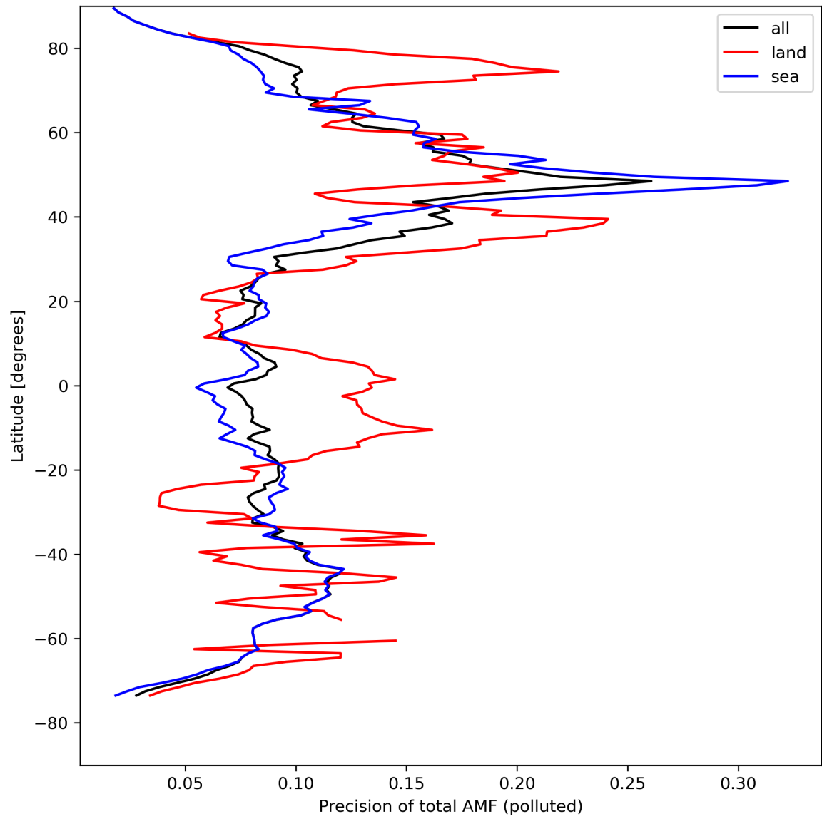
Figure 49: Zonal average of “Precision of total AMF (polluted)” for 2024-04-18 to 2024-04-20.
