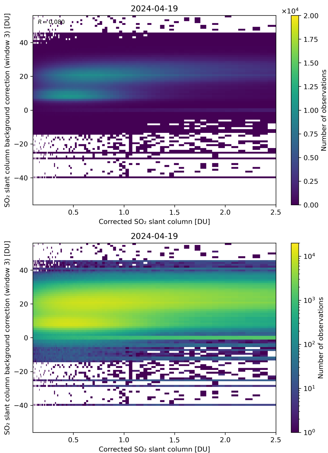
Figure 180: Scatter density plot of “Corrected SO 2 slant column” against “SO 2 slant column background correction (window 3)” for 2024-04-18 to 2024-04-20.
