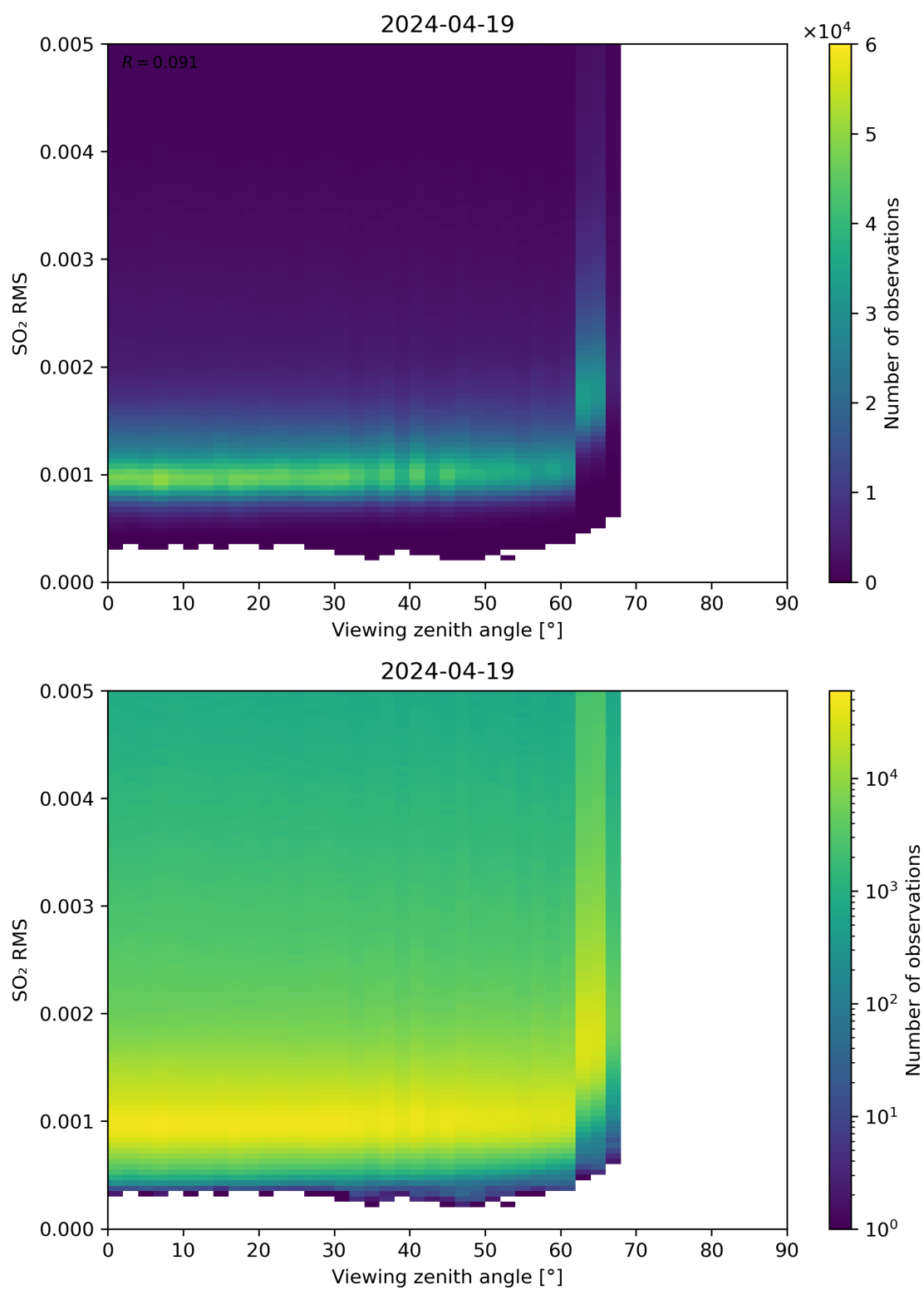
Figure 313: Scatter density plot of “Viewing zenith angle” against “SO 2 RMS” for 2024-04-18 to 2024-04-20.
