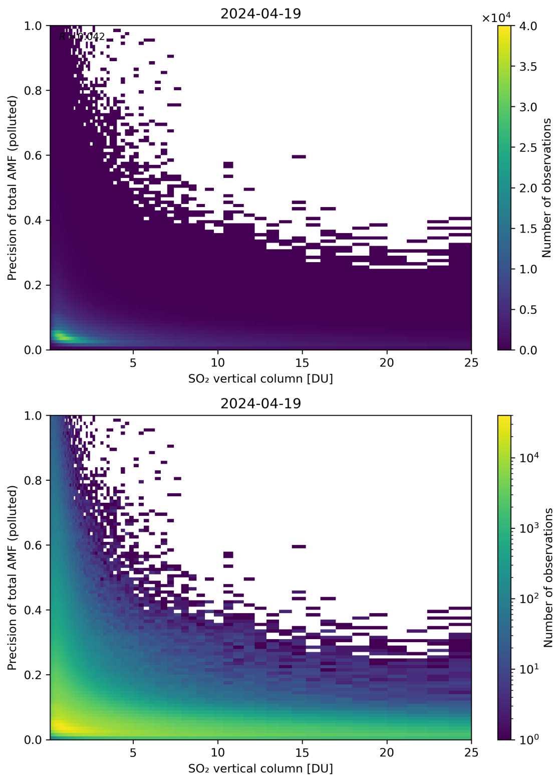
Figure 306: Scatter density plot of “SO 2 vertical column” against “Precision of total AMF (polluted)” for 2024-04-18 to 2024-04-20.
