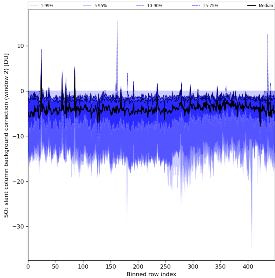
Figure 86: Along track statistics of “SO 2 slant column background correction (window 2)” for 2024-04-18 to 2024-04-20
