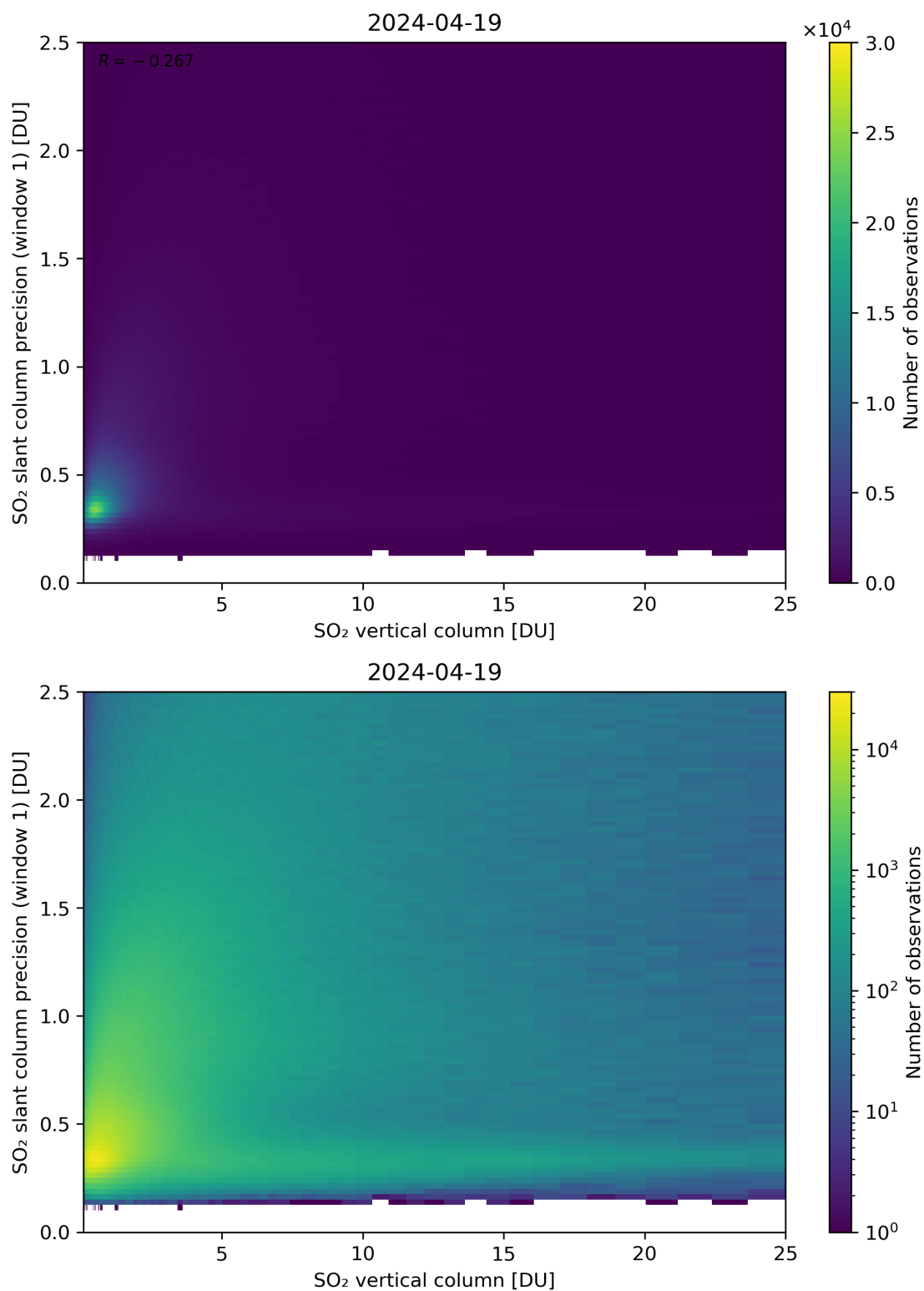
Figure 301: Scatter density plot of “SO 2 vertical column” against “SO 2 slant column precision (window 1)” for 2024-04-18 to 2024-04-20.
