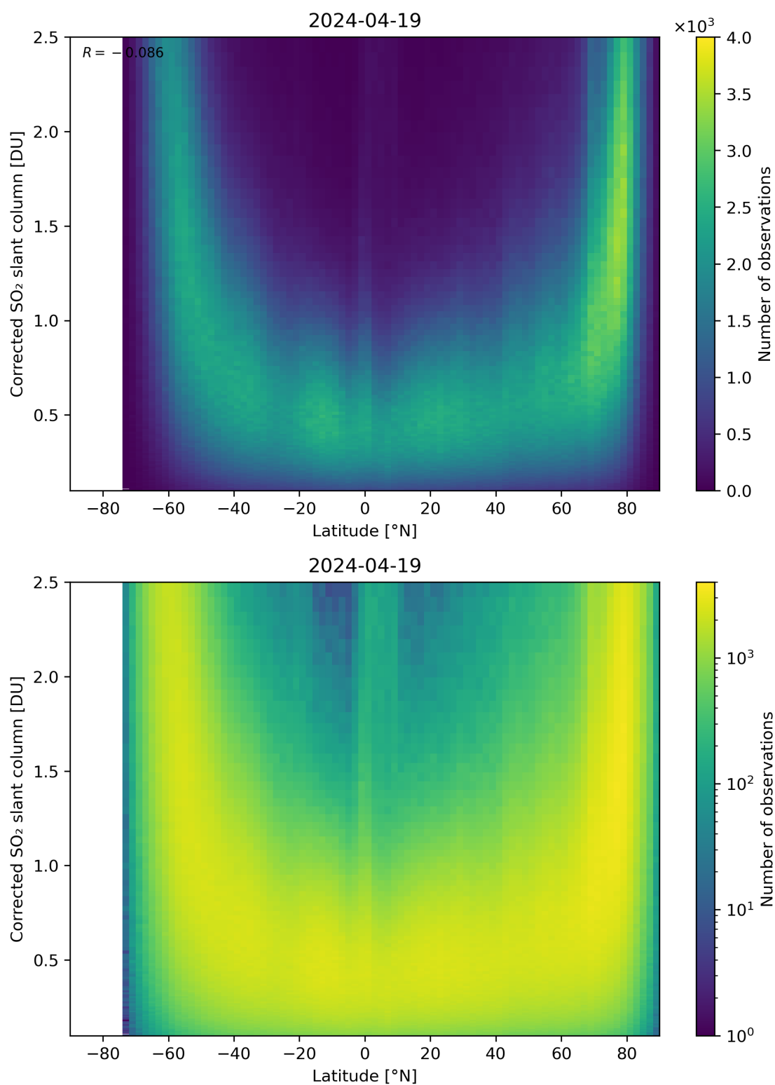
Figure 146: Scatter density plot of “Latitude” against “Corrected SO 2 slant column” for 2024-04-18 to 2024-04-20.
