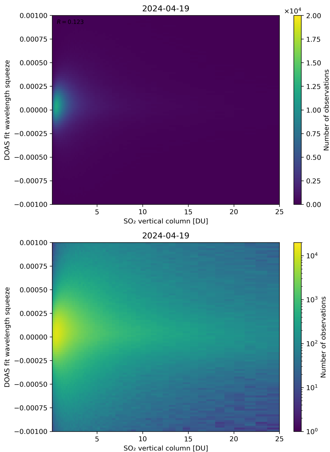
Figure 277: Scatter density plot of “SO 2 vertical column” against “DOAS fit wavelength squeeze” for 2024-04-18 to 2024-04-20.
