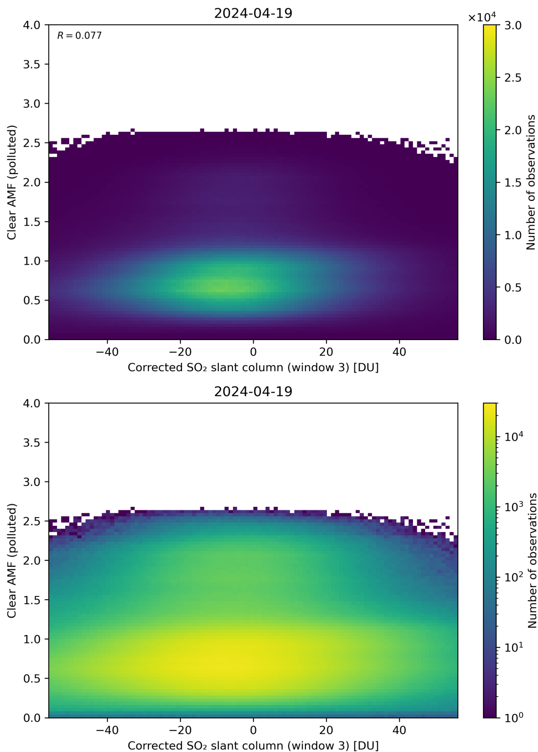
Figure 209: Scatter density plot of “Corrected SO 2 slant column (window 3)” against “Clear AMF (polluted)” for 2024-04-18 to 2024-04-20.
