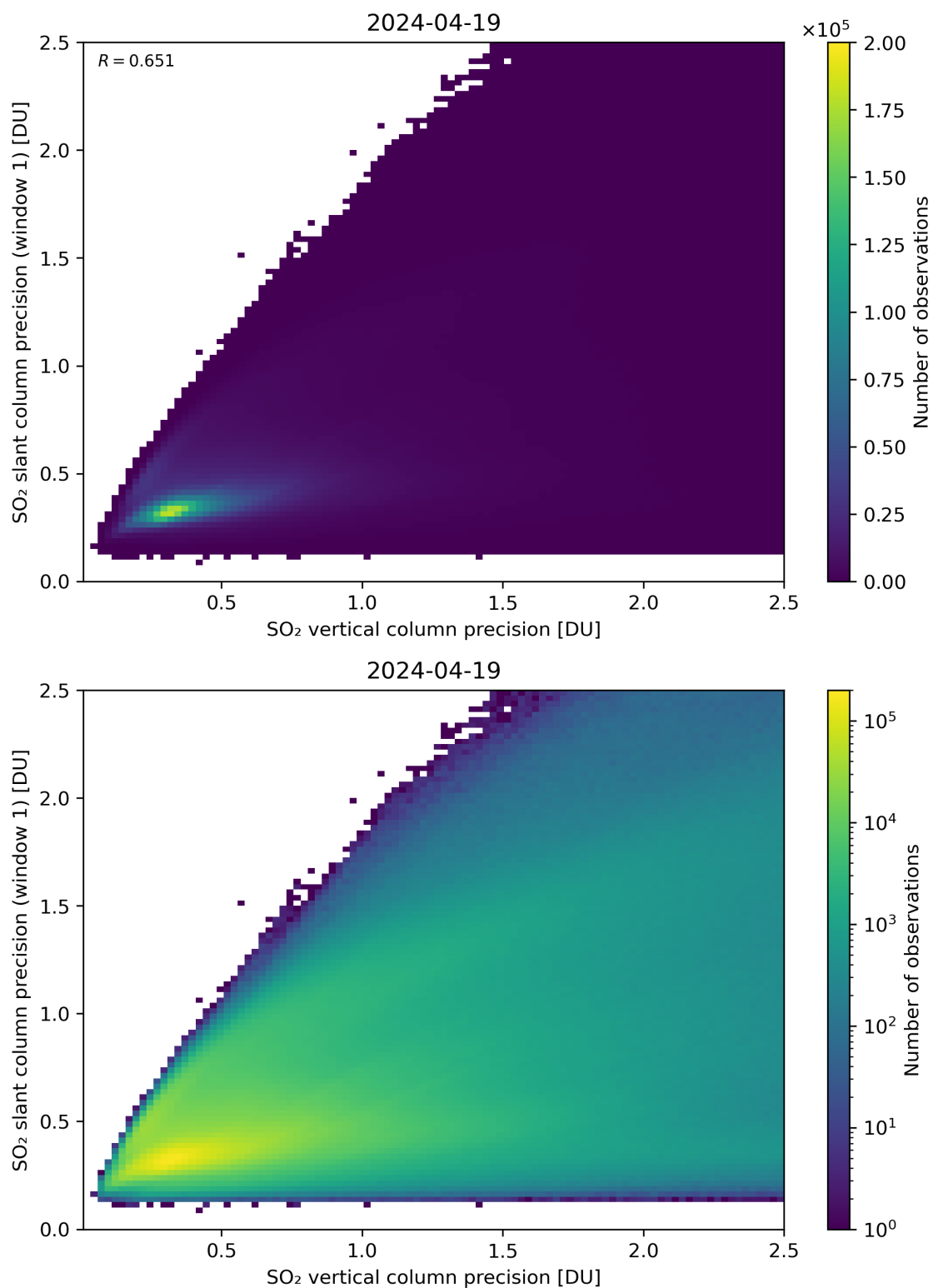
Figure 290: Scatter density plot of “SO 2 vertical column precision” against “SO 2 slant column precision (window 1)” for 2024-04-18 to 2024-04-20.
