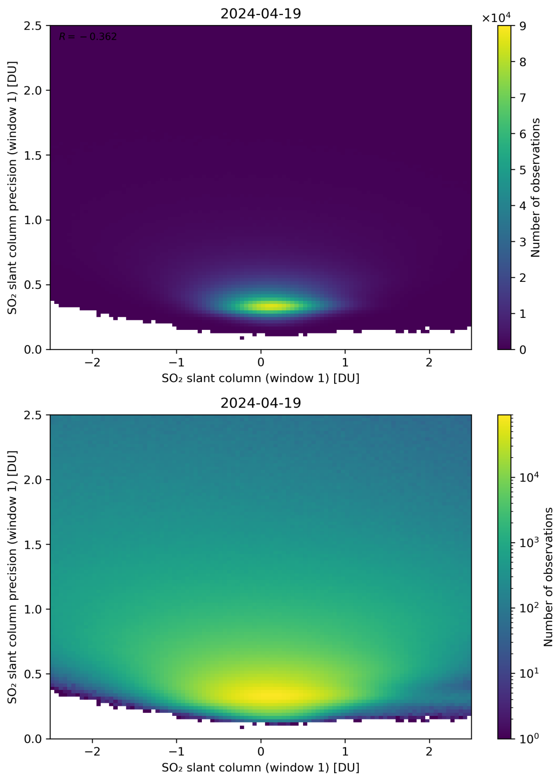
Figure 235: Scatter density plot of “SO 2 slant column (window 1)” against “SO 2 slant column precision (window 1)” for 2024-04-18 to 2024-04-20.
