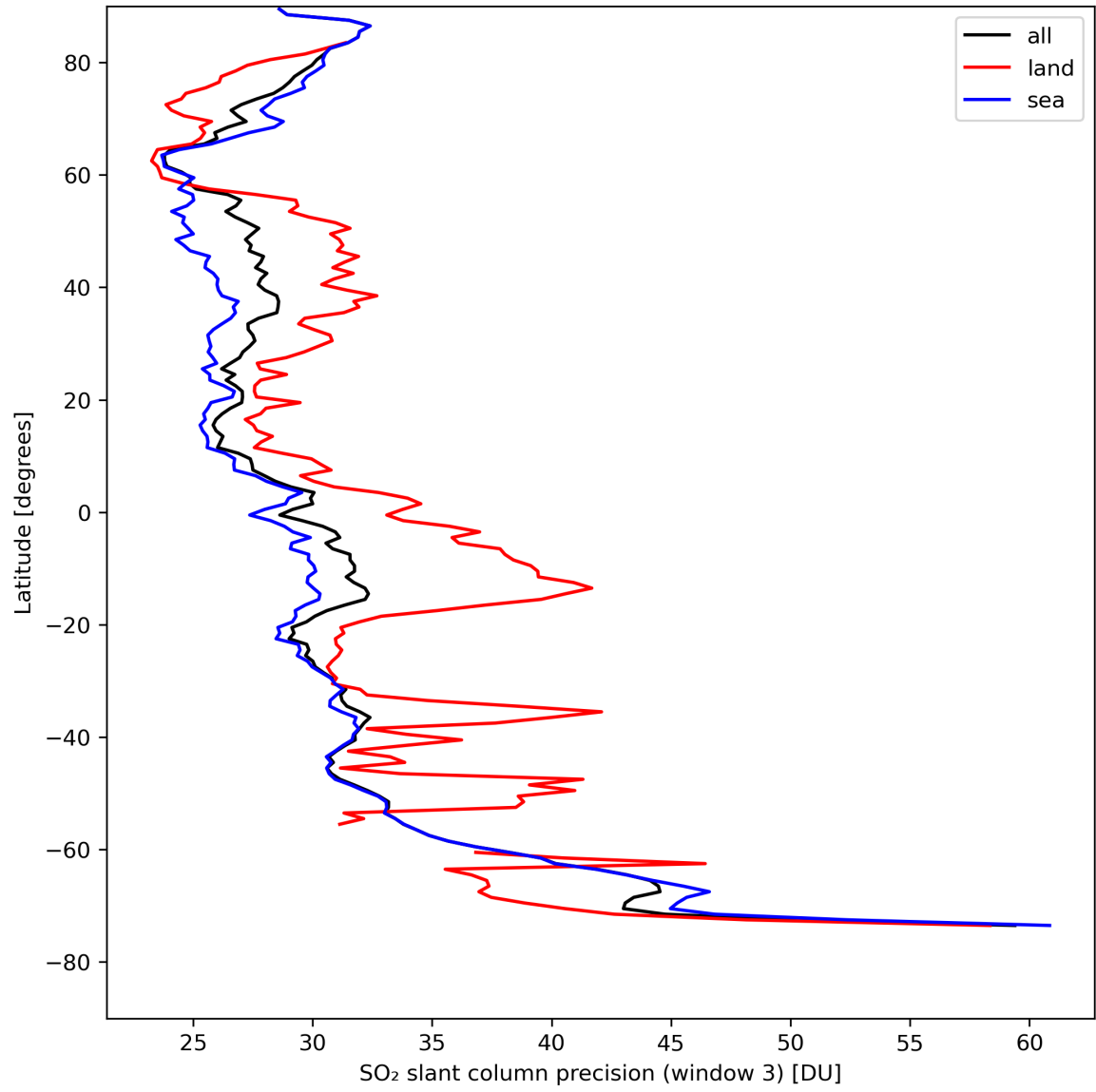
Figure 42: Zonal average of “SO 2 slant column precision (window 3)” for 2024-04-18 to 2024-04-20.
