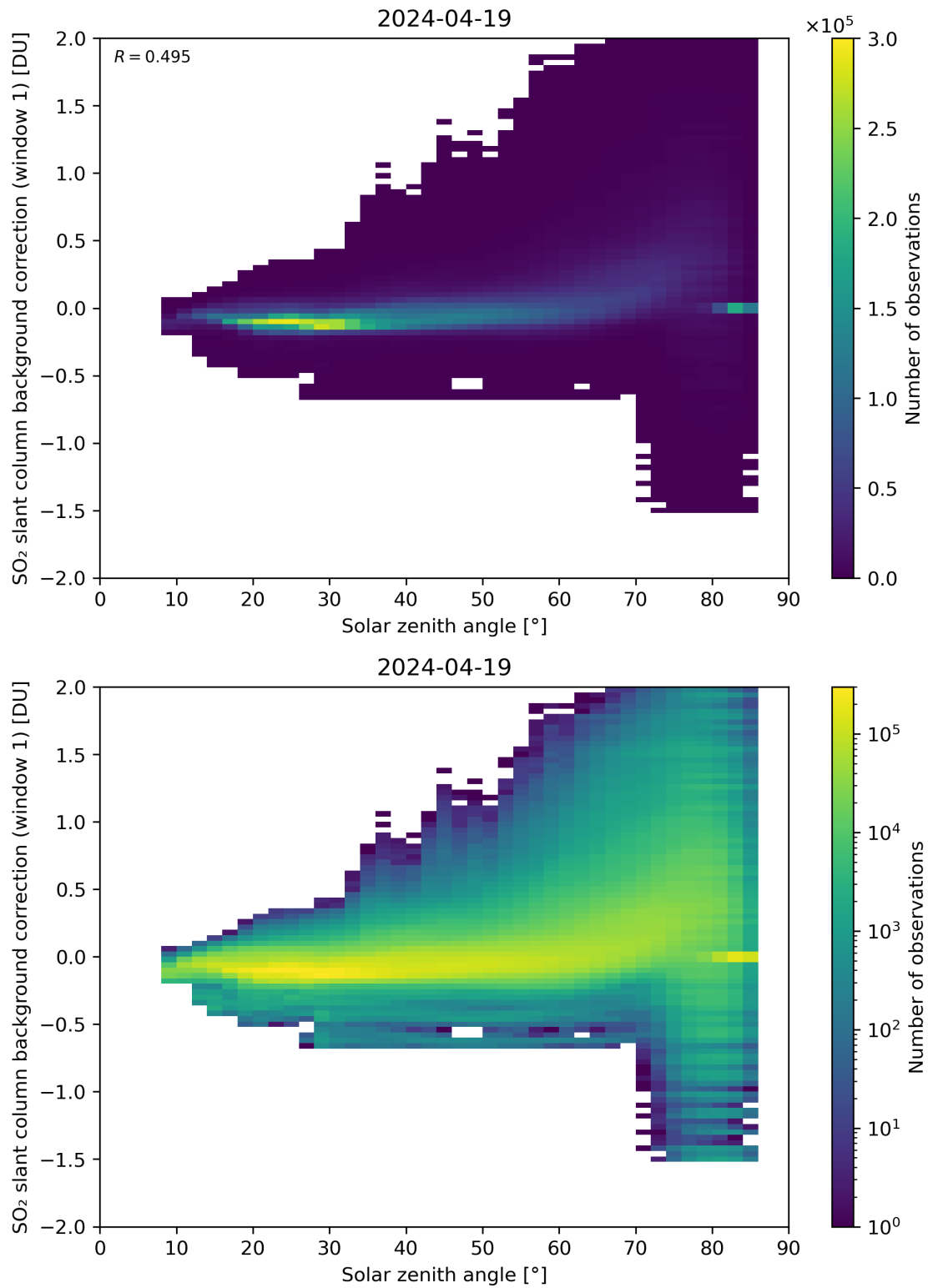
Figure 158: Scatter density plot of “Solar zenith angle” against “SO 2 slant column background correction (window 1)” for 2024-04-18 to 2024-04-20.
