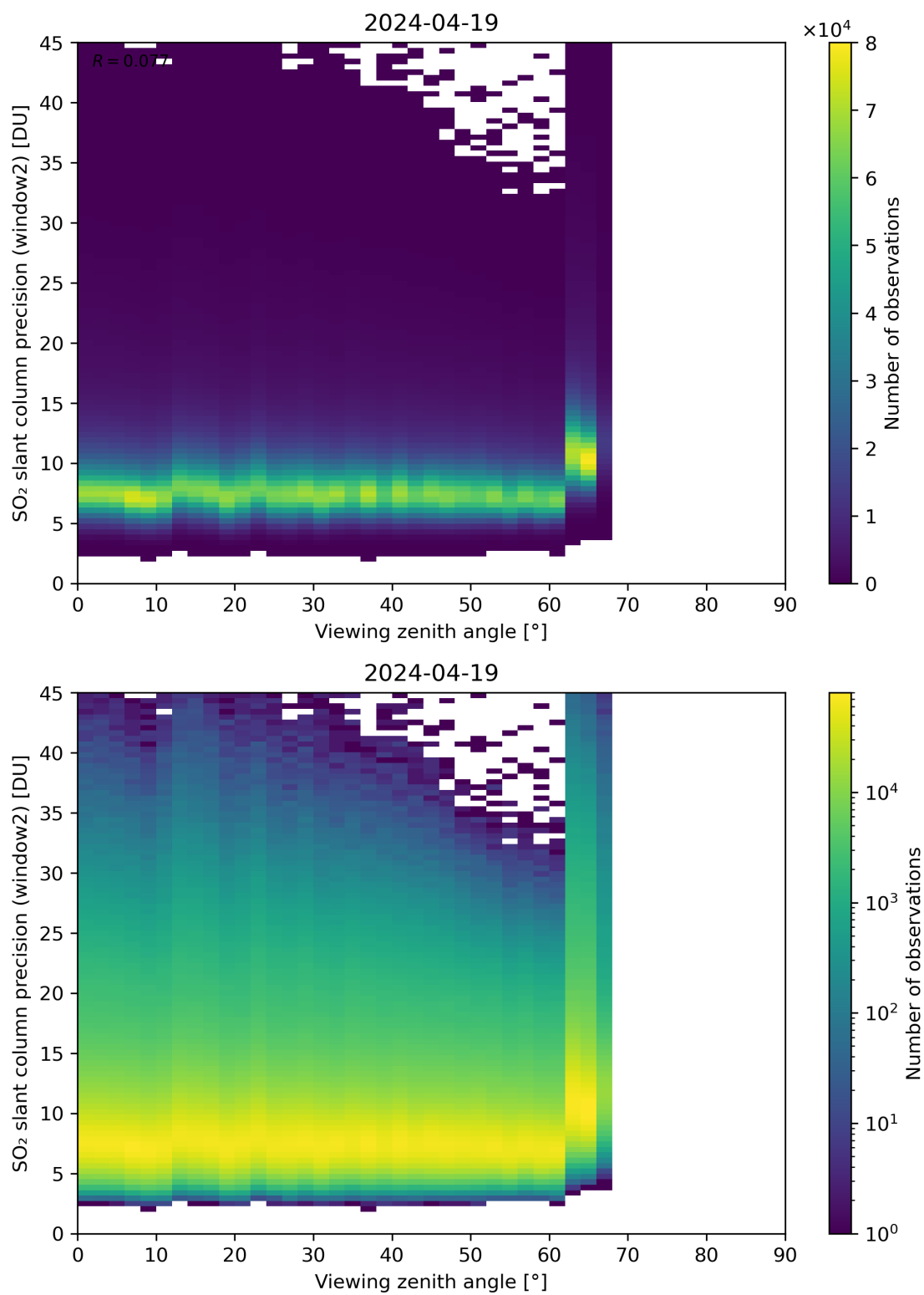
Figure 322: Scatter density plot of “Viewing zenith angle” against “SO 2 slant column precision (window2)” for 2024-04-18 to 2024-04-20.
