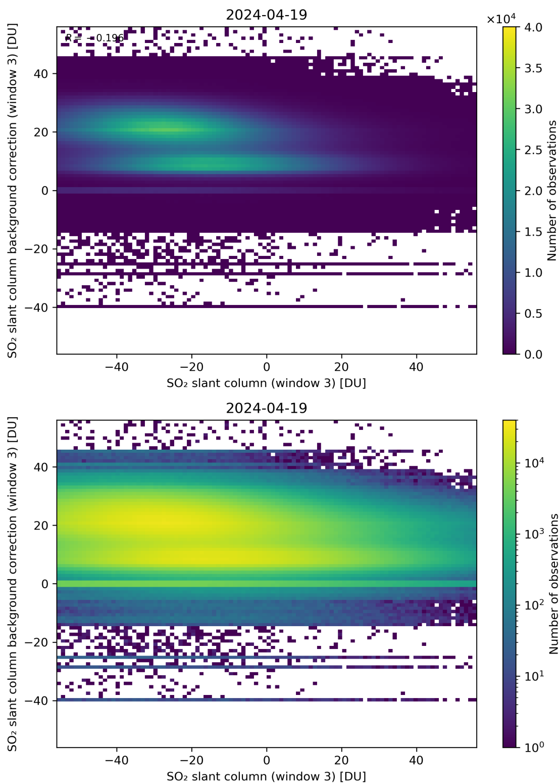
Figure 253: Scatter density plot of “SO 2 slant column (window 3)” against “SO 2 slant column background correction (window 3)” for 2024-04-18 to 2024-04-20.
