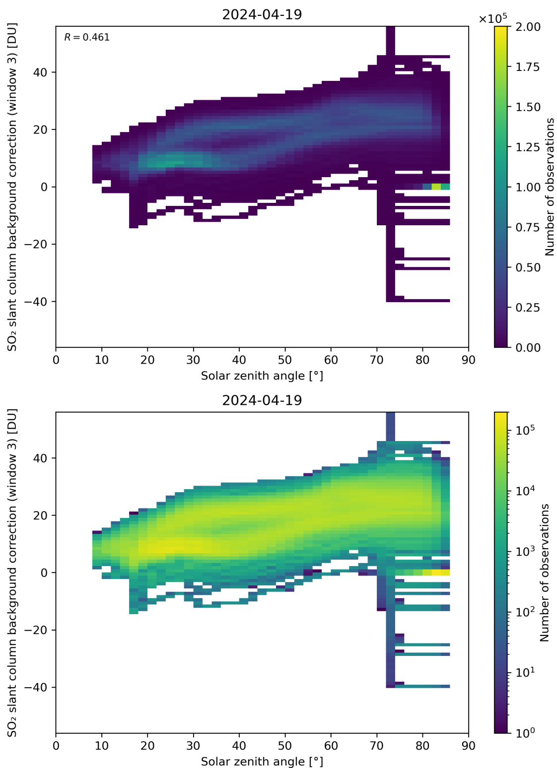
Figure 160: Scatter density plot of “Solar zenith angle” against “SO 2 slant column background correction (window 3)” for 2024-04-18 to 2024-04-20.
