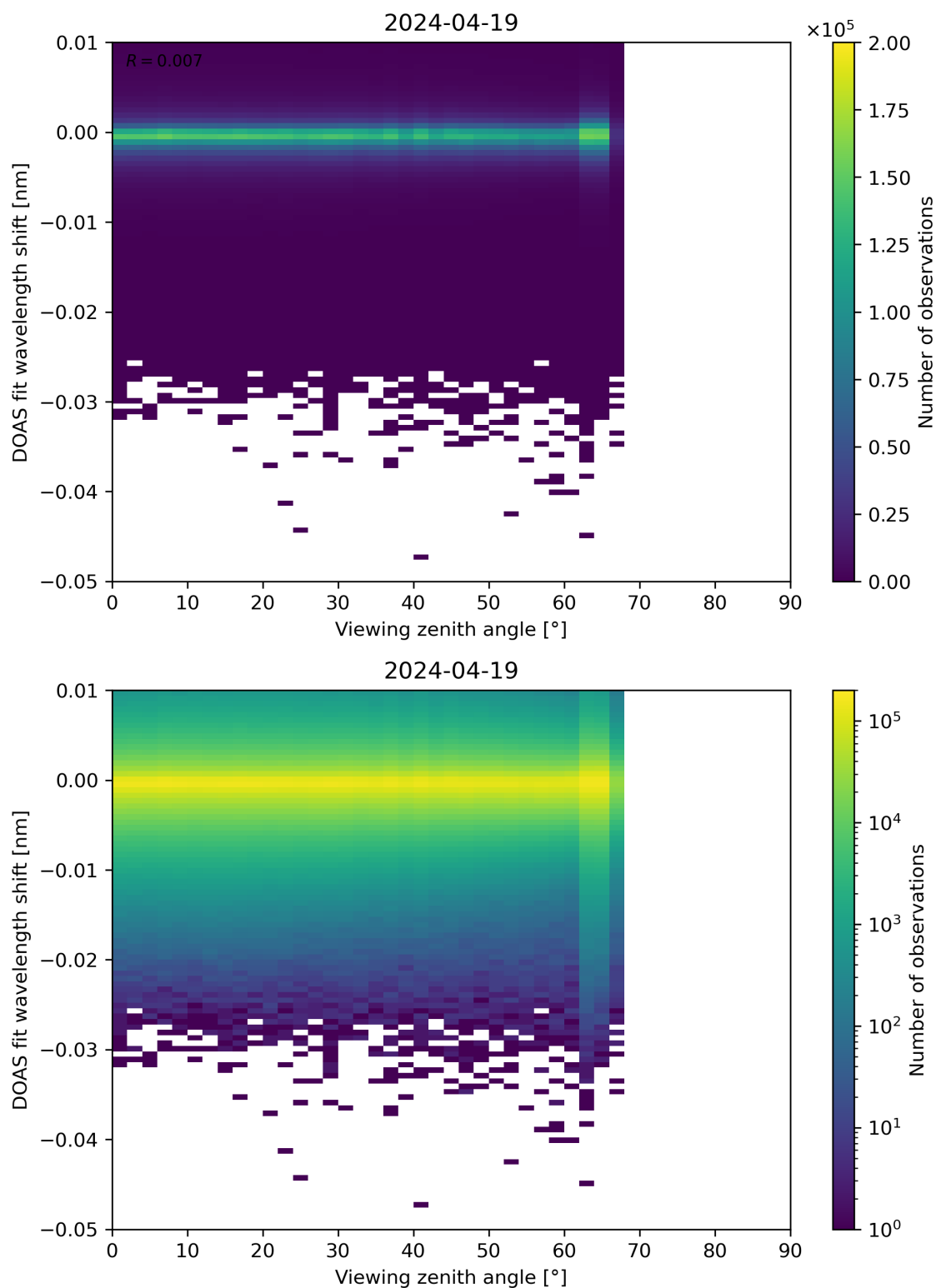
Figure 311: Scatter density plot of “Viewing zenith angle” against “DOAS fit wavelength shift” for 2024-04-18 to 2024-04-20.
