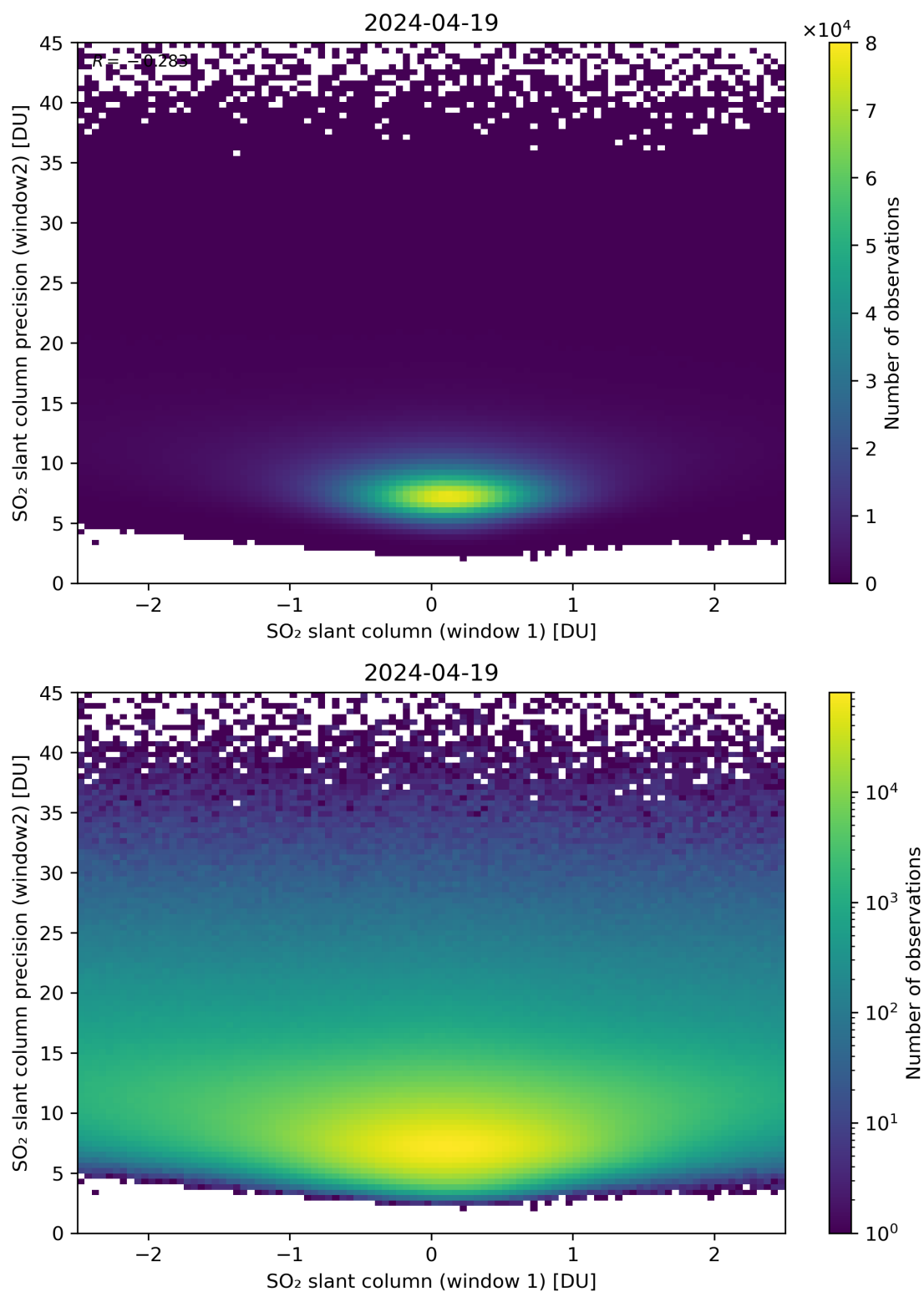
Figure 236: Scatter density plot of “SO 2 slant column (window 1)” against “SO 2 slant column precision (window2)” for 2024-04-18 to 2024-04-20.
