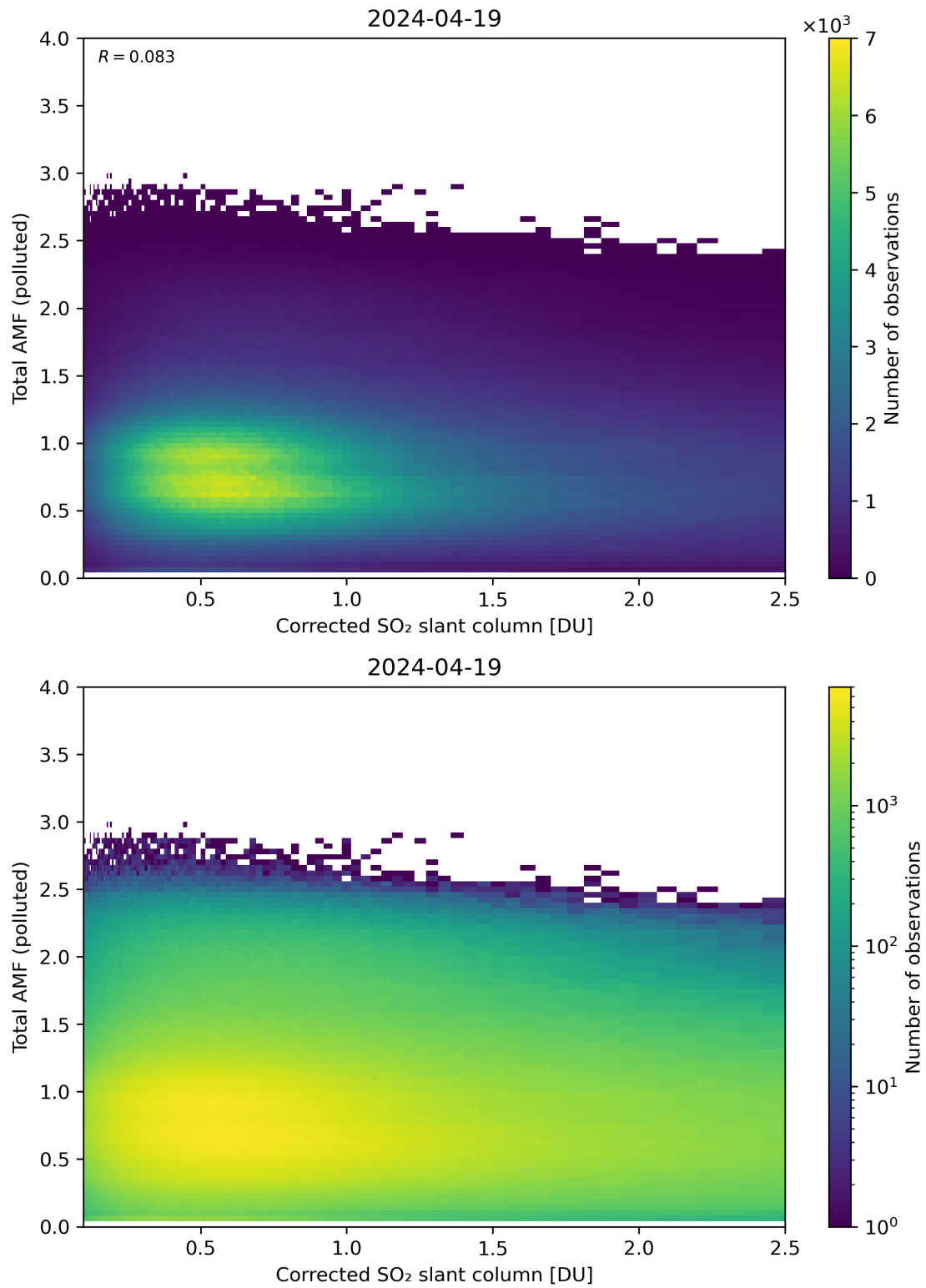
Figure 192: Scatter density plot of “Corrected SO 2 slant column” against “Total AMF (polluted)” for 2024-04-18 to 2024-04-20.
