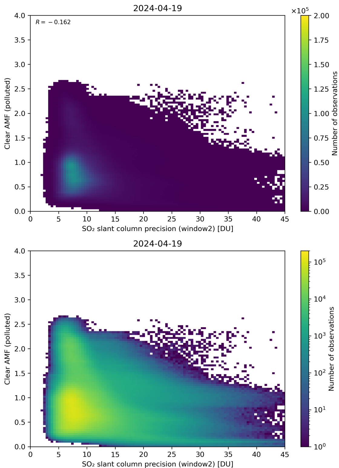
Figure 246: Scatter density plot of “SO 2 slant column precision (window2)” against “Clear AMF (polluted)” for 2024-04-18 to 2024-04-20.
