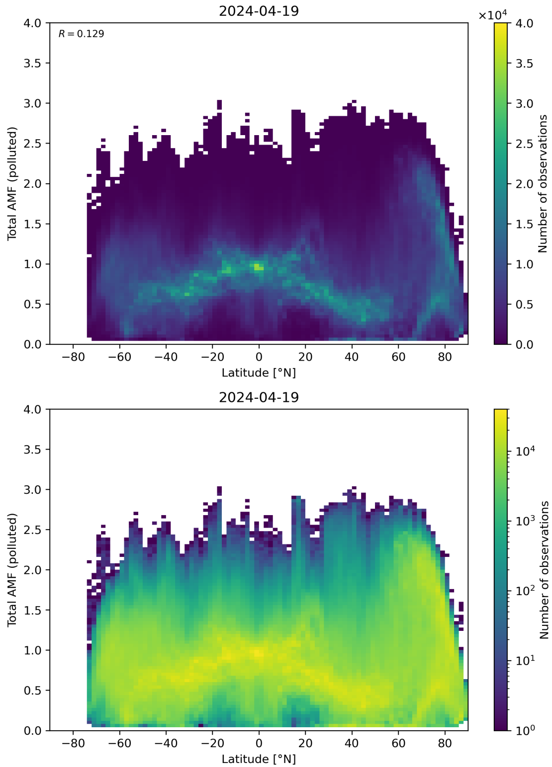
Figure 154: Scatter density plot of “Latitude” against “Total AMF (polluted)” for 2024-04-18 to 2024-04-20.
