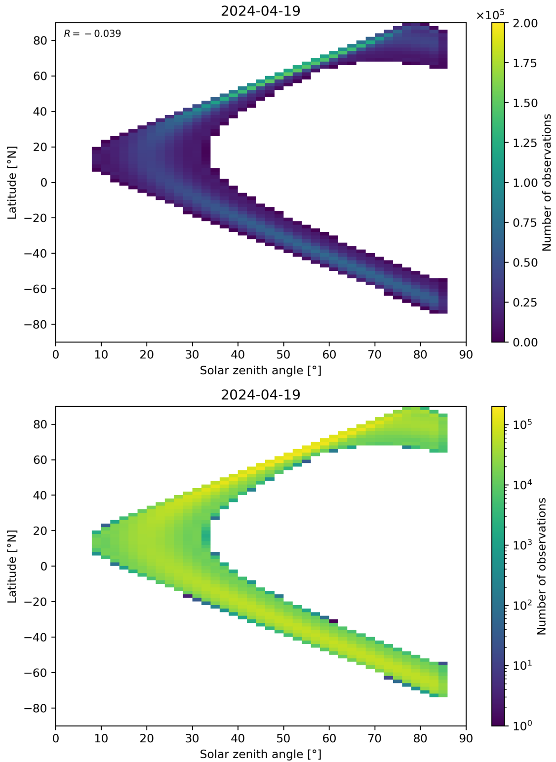
Figure 164: Scatter density plot of “Solar zenith angle” against “Latitude” for 2024-04-18 to 2024-04-20.
