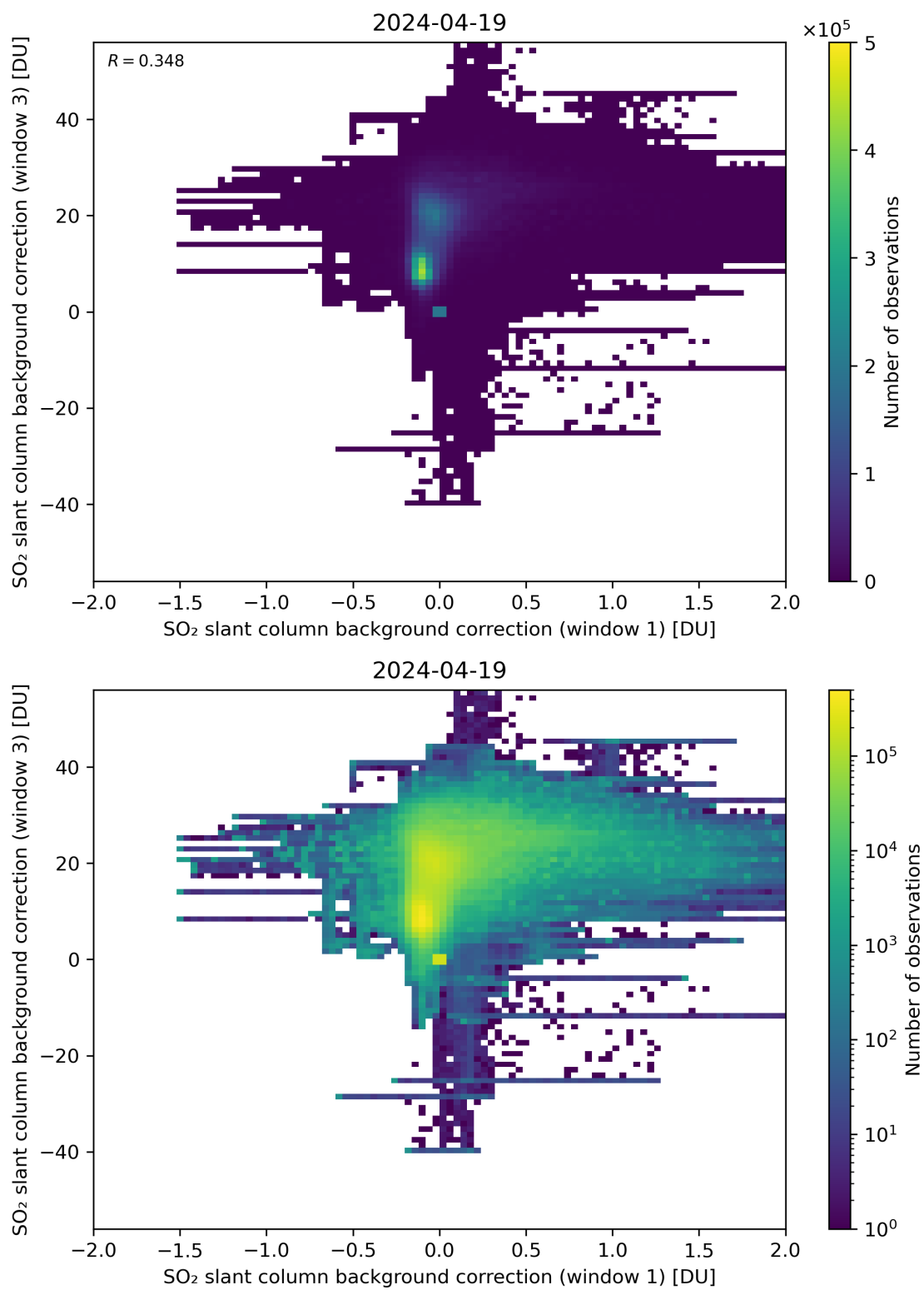
Figure 99: Scatter density plot of “SO 2 slant column background correction (window 1)” against “SO 2 slant column background correction (window 3)” for 2024-04-18 to 2024-04-20.
