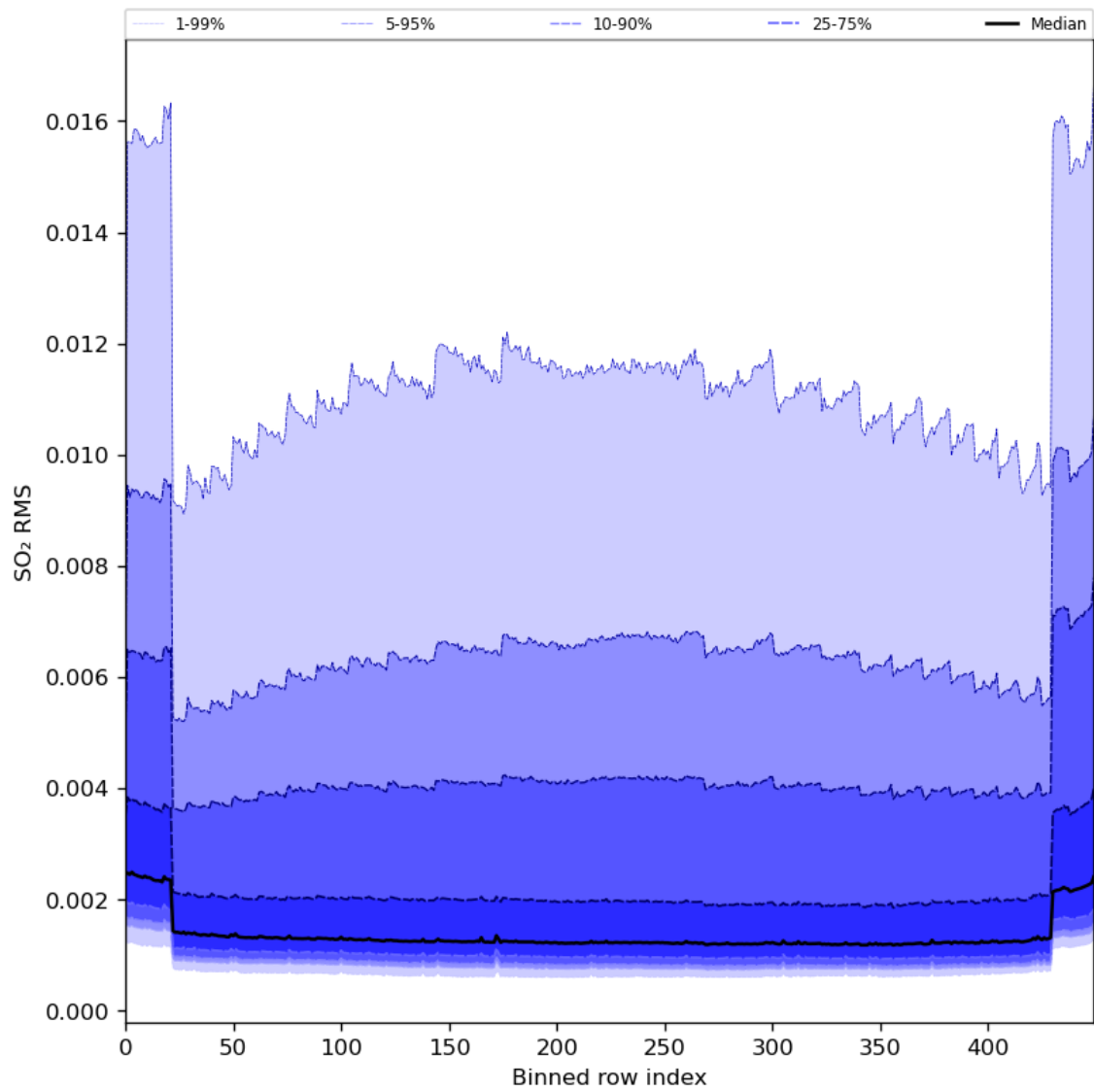
Figure 93: Along track statistics of “SO 2 RMS” for 2024-04-18 to 2024-04-20
