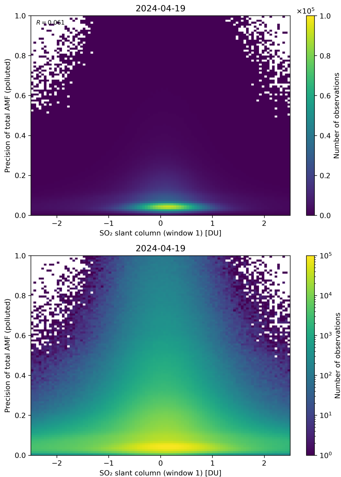
Figure 240: Scatter density plot of “SO 2 slant column (window 1)” against “Precision of total AMF (polluted)” for 2024-04-18 to 2024-04-20.
