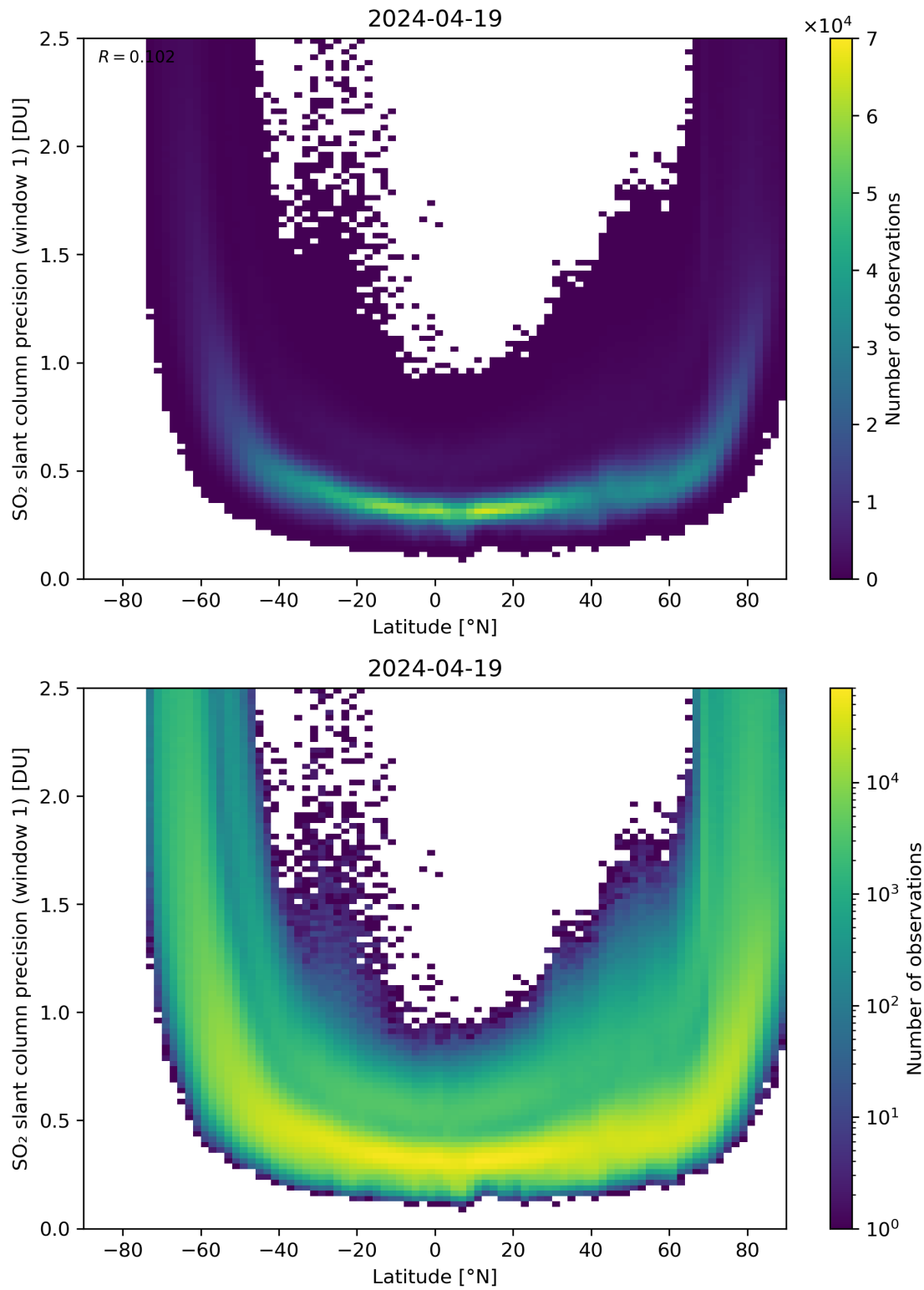
Figure 150: Scatter density plot of “Latitude” against “SO 2 slant column precision (window 1)” for 2024-04-18 to 2024-04-20.
