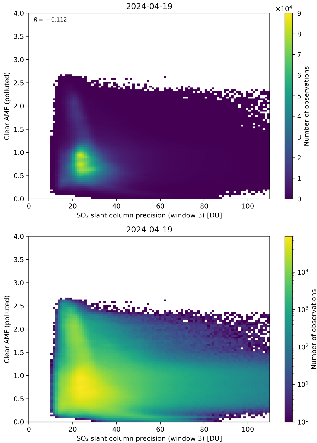
Figure 261: Scatter density plot of “SO 2 slant column precision (window 3)” against “Clear AMF (polluted)” for 2024-04-18 to 2024-04-20.
