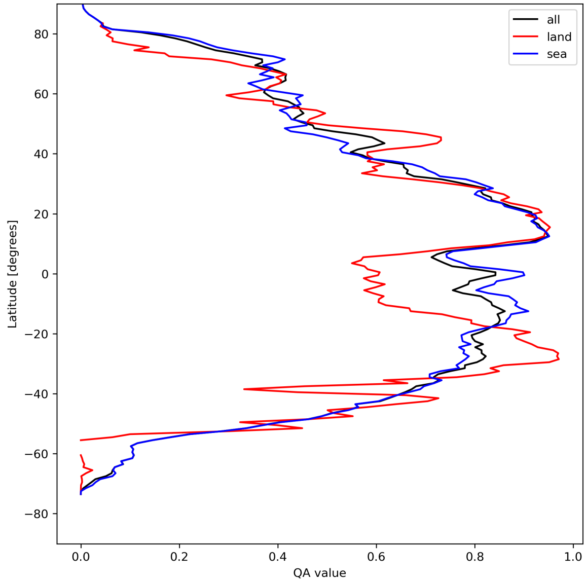
Figure 29: Zonal average of “QA value” for 2024-04-18 to 2024-04-20.
