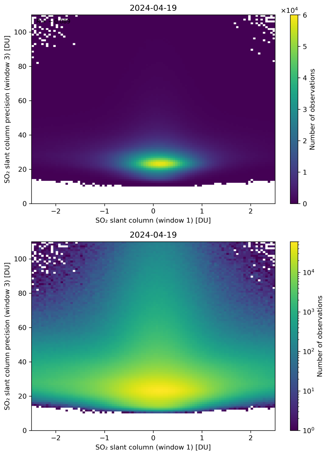
Figure 238: Scatter density plot of “SO 2 slant column (window 1)” against “SO 2 slant column precision (window 3)” for 2024-04-18 to 2024-04-20.
