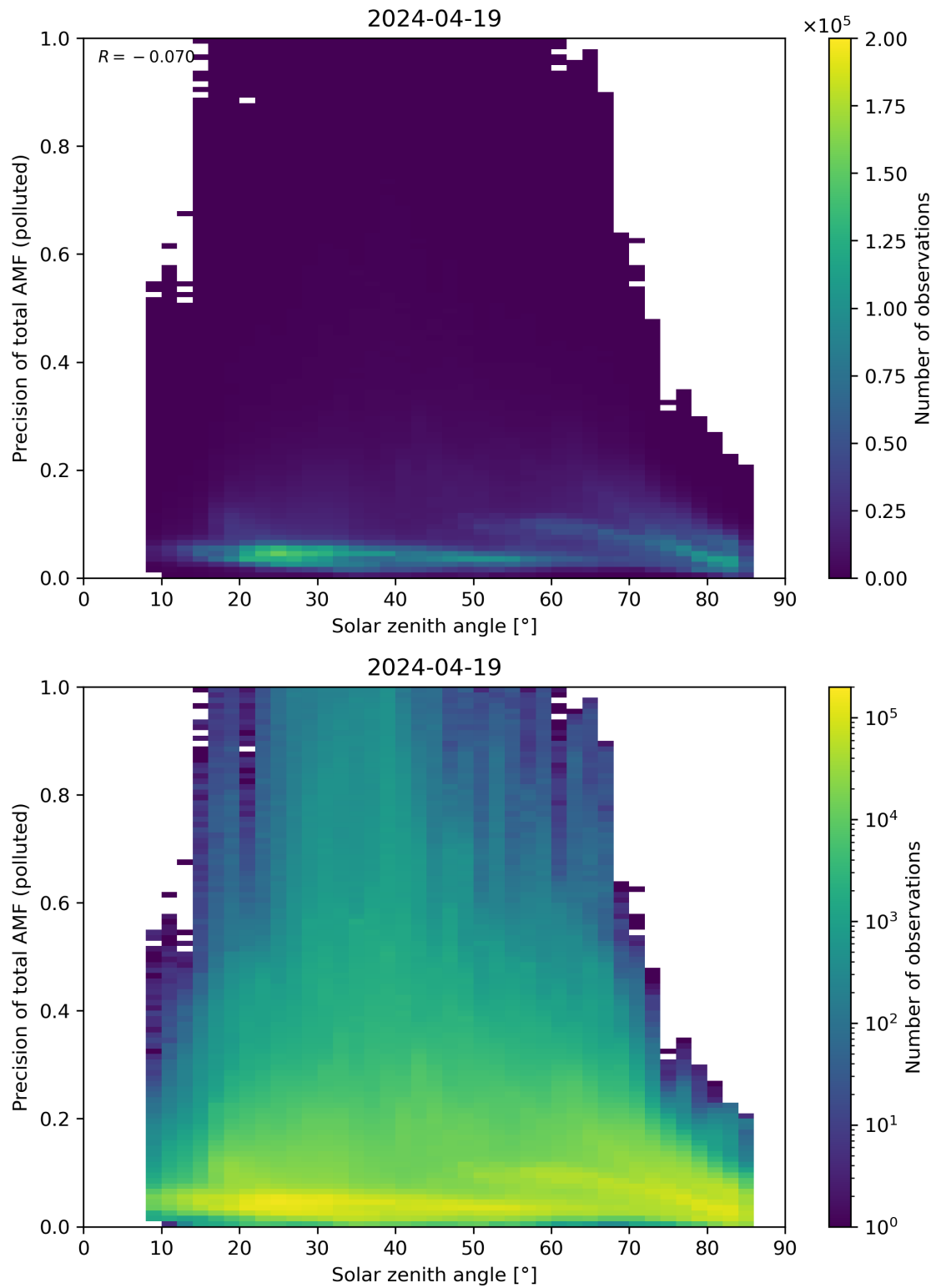
Figure 175: Scatter density plot of “Solar zenith angle” against “Precision of total AMF (polluted)” for 2024-04-18 to 2024-04-20.
