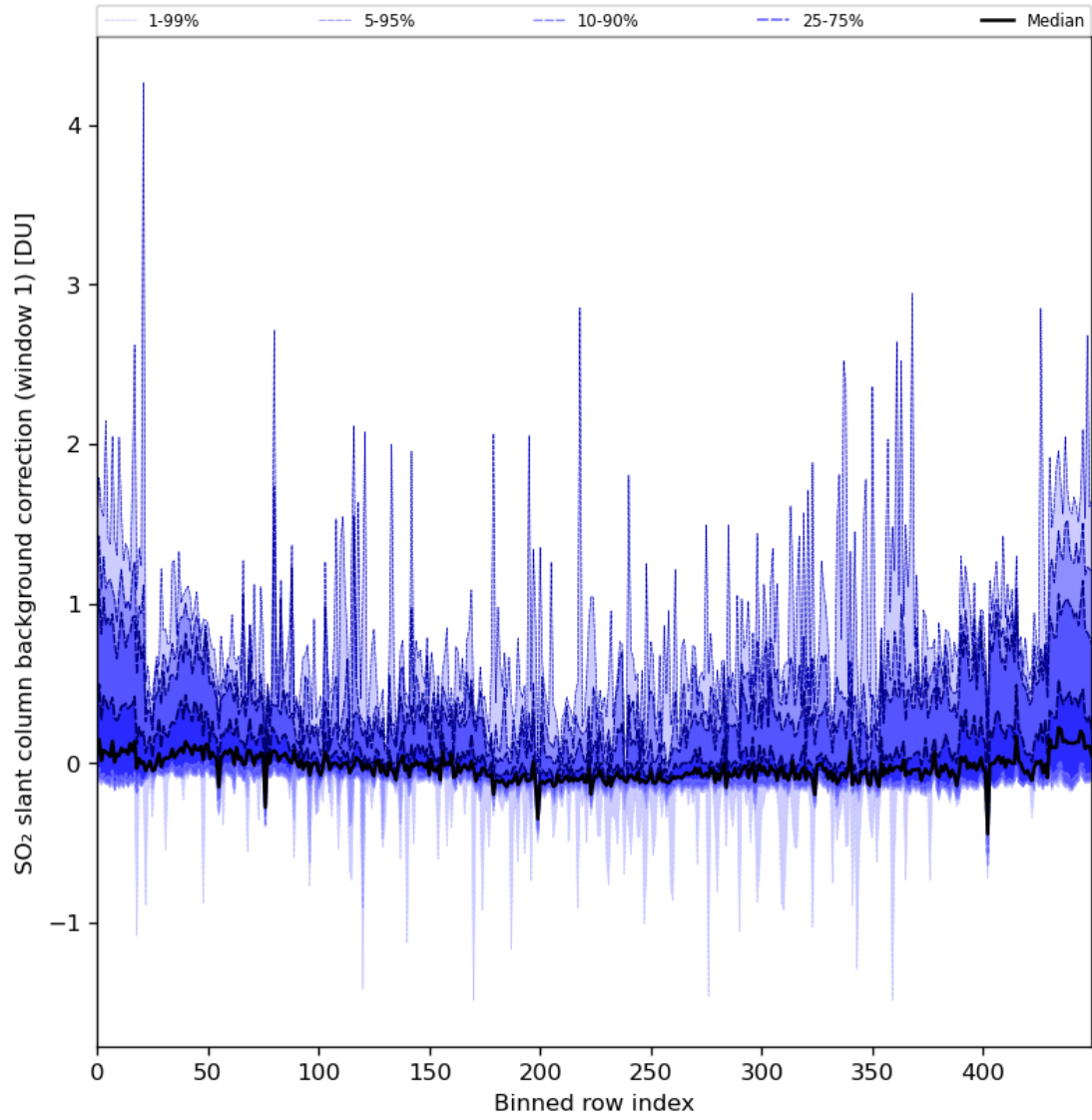
Figure 82: Along track statistics of “SO 2 slant column background correction (window 1)” for 2024-04-18 to 2024-04-20
