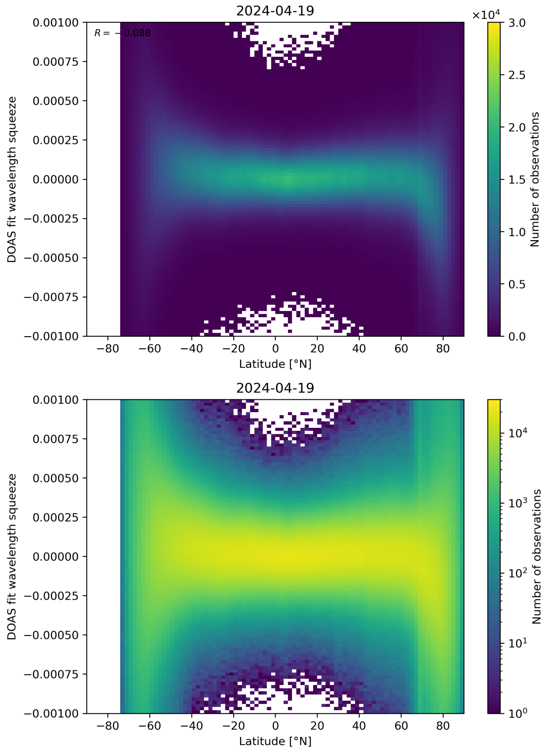
Figure 143: Scatter density plot of “Latitude” against “DOAS fit wavelength squeeze” for 2024-04-18 to 2024-04-20.
