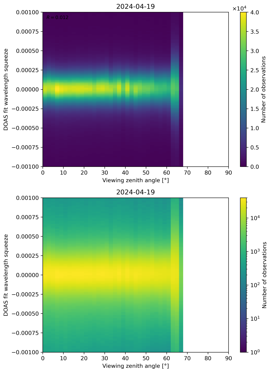
Figure 312: Scatter density plot of “Viewing zenith angle” against “DOAS fit wavelength squeeze” for 2024-04-18 to 2024-04-20.
