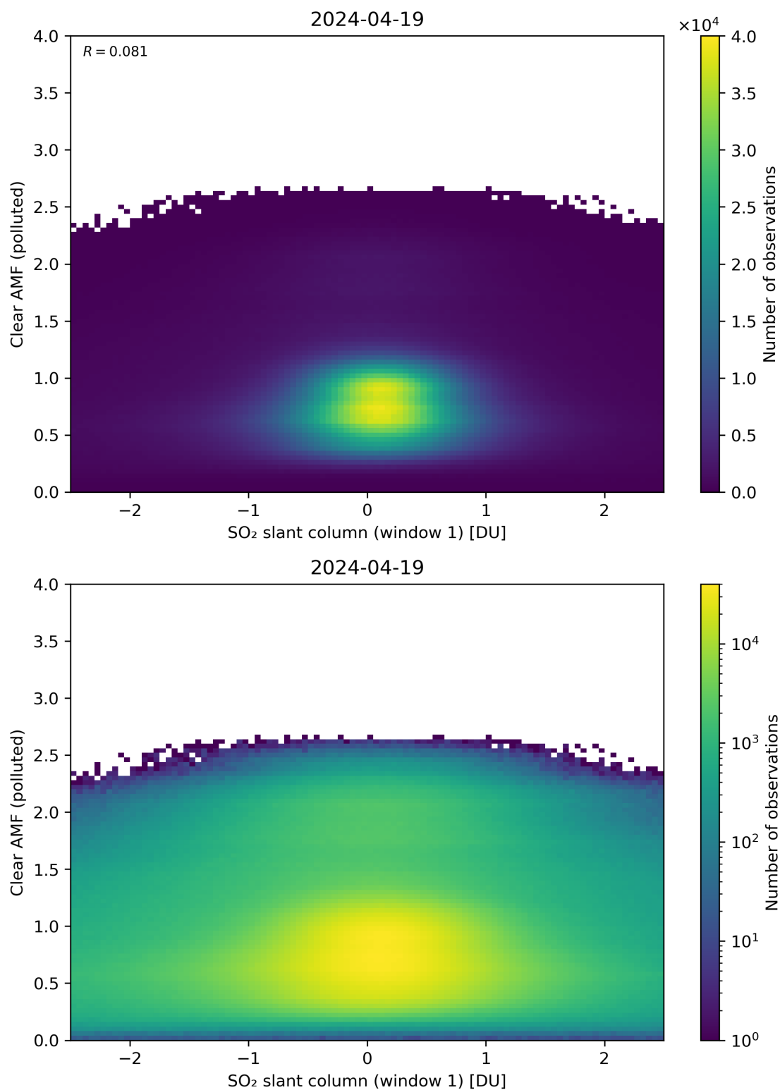
Figure 232: Scatter density plot of “SO 2 slant column (window 1)” against “Clear AMF (polluted)” for 2024-04-18 to 2024-04-20.
