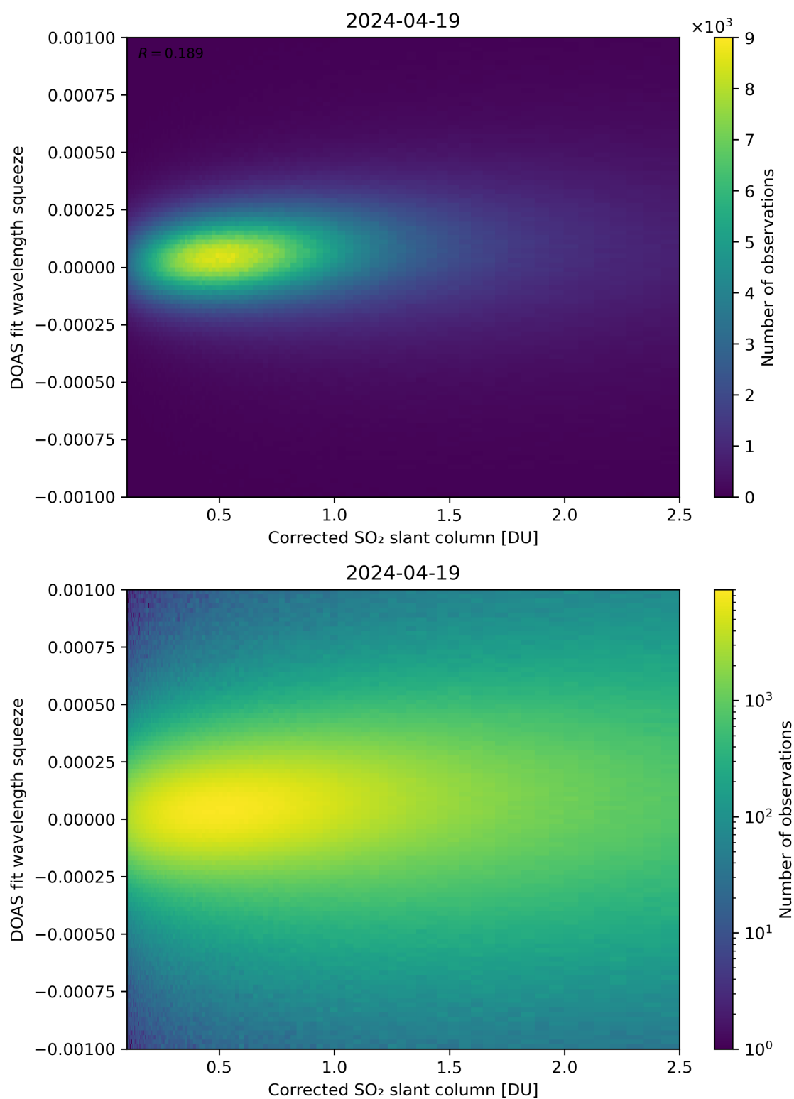
Figure 182: Scatter density plot of “Corrected SO 2 slant column” against “DOAS fit wavelength squeeze” for 2024-04-18 to 2024-04-20.
