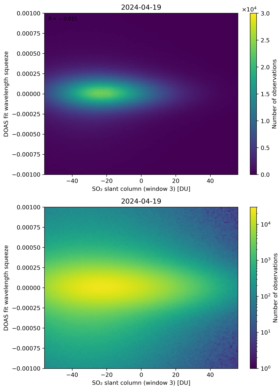
Figure 255: Scatter density plot of “SO 2 slant column (window 3)” against “DOAS fit wavelength squeeze” for 2024-04-18 to 2024-04-20.
