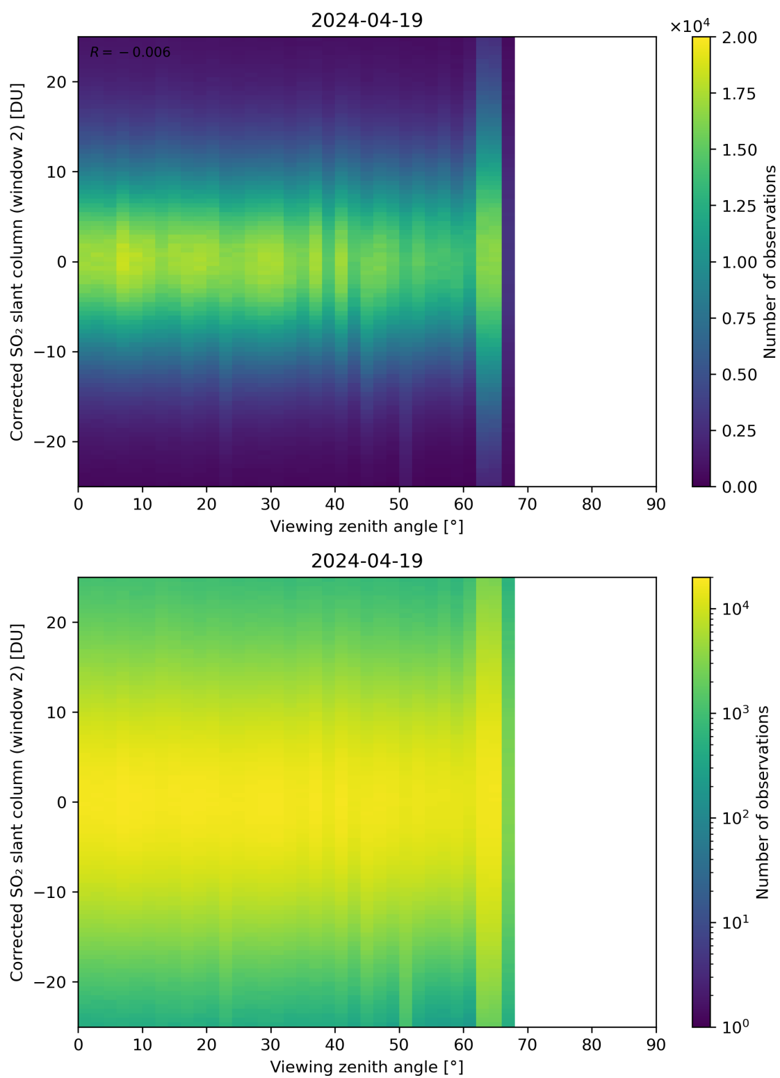
Figure 318: Scatter density plot of “Viewing zenith angle” against “Corrected SO 2 slant column (window 2)” for 2024-04-18 to 2024-04-20.
