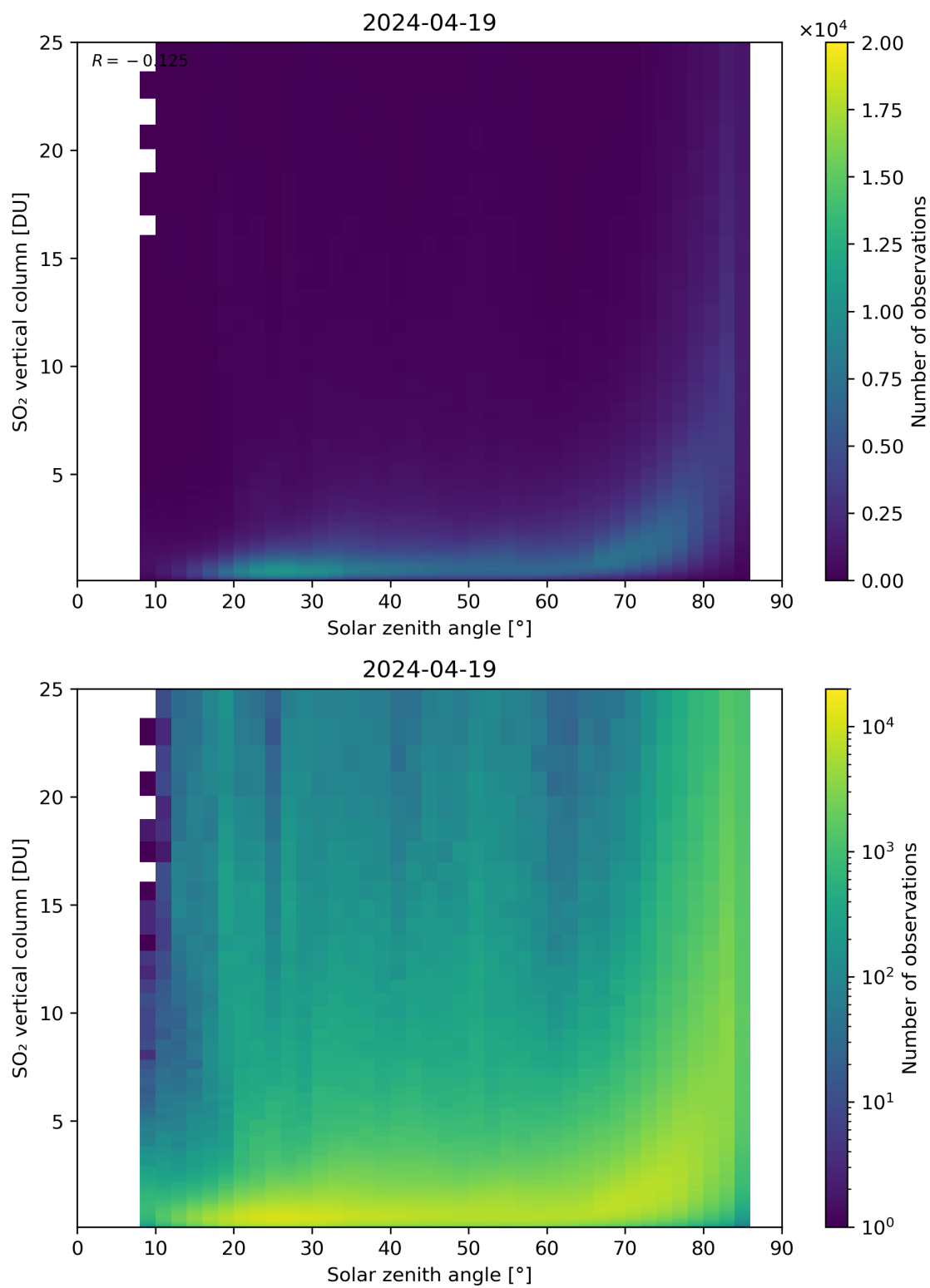
Figure 176: Scatter density plot of “Solar zenith angle” against “SO 2 vertical column” for 2024-04-18 to 2024-04-20.
