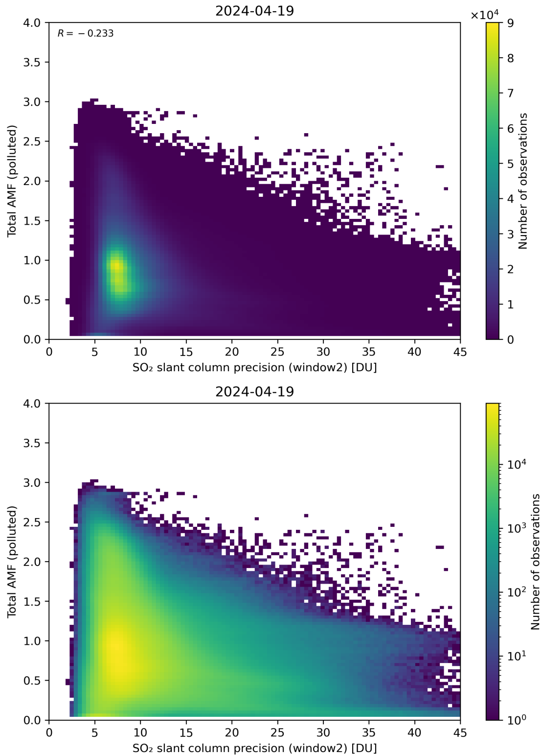
Figure 251: Scatter density plot of “SO 2 slant column precision (window2)” against “Total AMF (polluted)” for 2024-04-18 to 2024-04-20.
