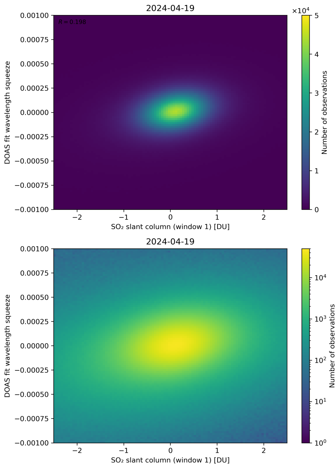
Figure 216: Scatter density plot of “SO 2 slant column (window 1)” against “DOAS fit wavelength squeeze” for 2024-04-18 to 2024-04-20.
