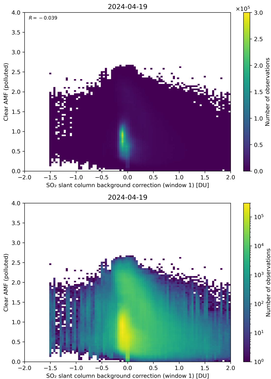
Figure 103: Scatter density plot of “SO 2 slant column background correction (window 1)” against “Clear AMF (polluted)” for 2024-04-18 to 2024-04-20.
