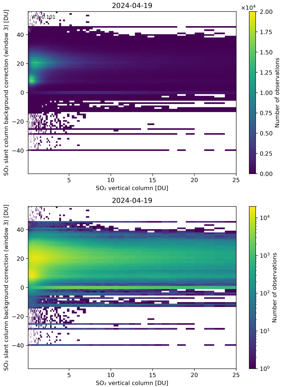
Figure 275: Scatter density plot of “SO 2 vertical column” against “SO 2 slant column background correction (window 3)” for 2024-04-18 to 2024-04-20.
