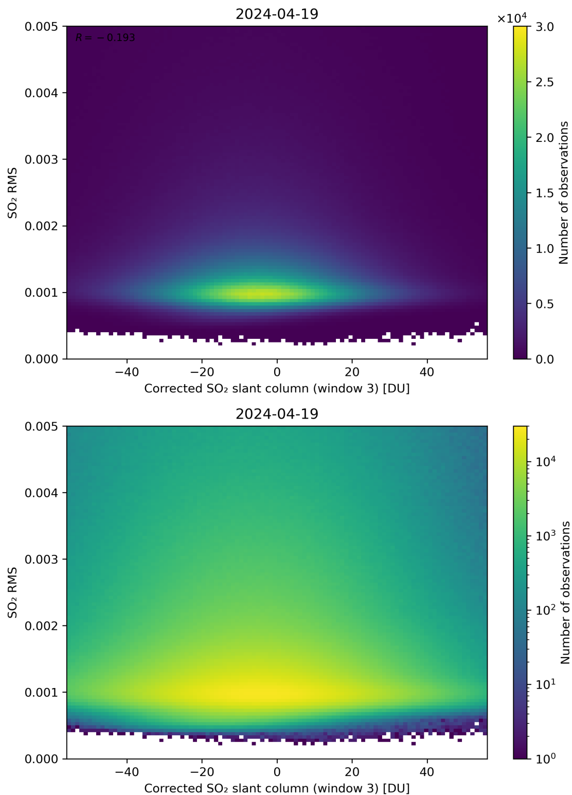
Figure 208: Scatter density plot of “Corrected SO 2 slant column (window 3)” against “SO 2 RMS” for 2024-04-18 to 2024-04-20.
