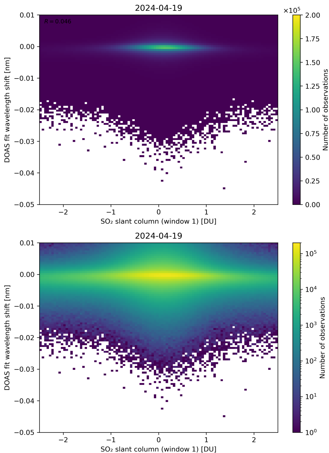
Figure 215: Scatter density plot of “SO 2 slant column (window 1)” against “DOAS fit wavelength shift” for 2024-04-18 to 2024-04-20.
