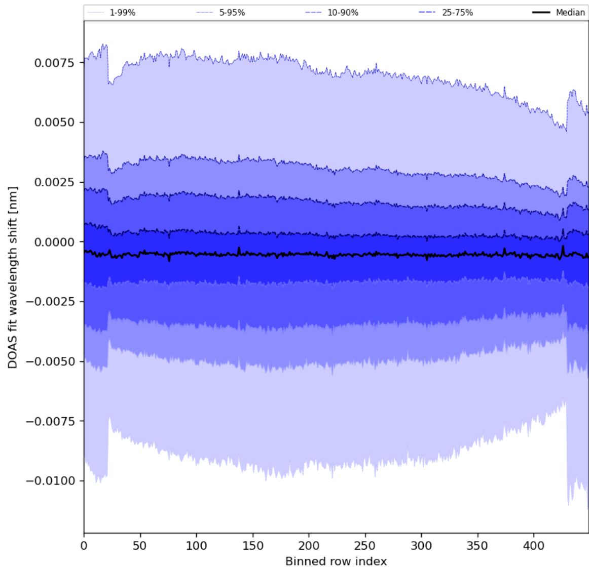
Figure 91: Along track statistics of “DOAS fit wavelength shift” for 2024-04-18 to 2024-04-20
