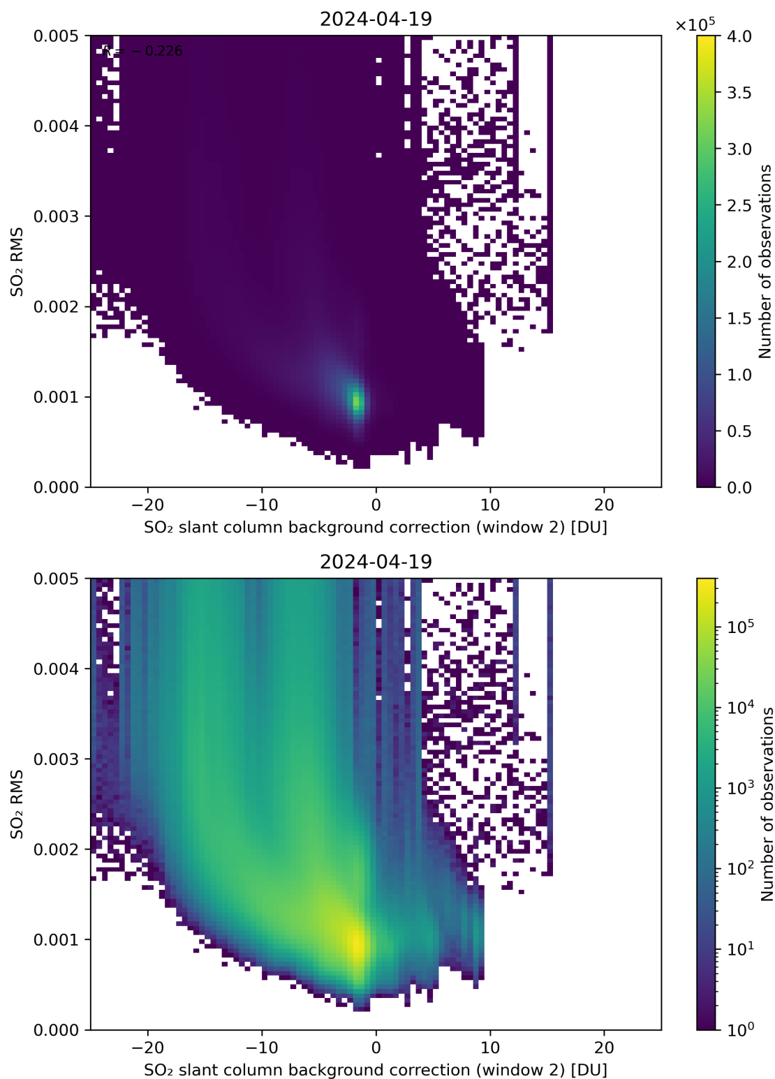
Figure 114: Scatter density plot of “SO 2 slant column background correction (window 2)” against “SO 2 RMS” for 2024-04-18 to 2024-04-20.
