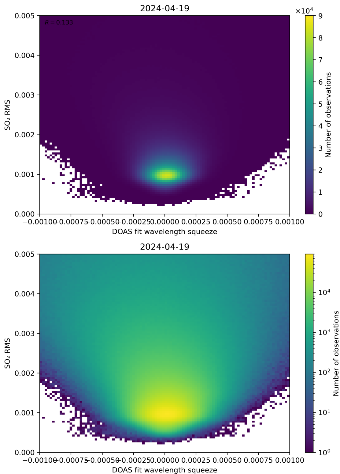
Figure 132: Scatter density plot of “DOAS fit wavelength squeeze” against “SO 2 RMS” for 2024-04-18 to 2024-04-20.
