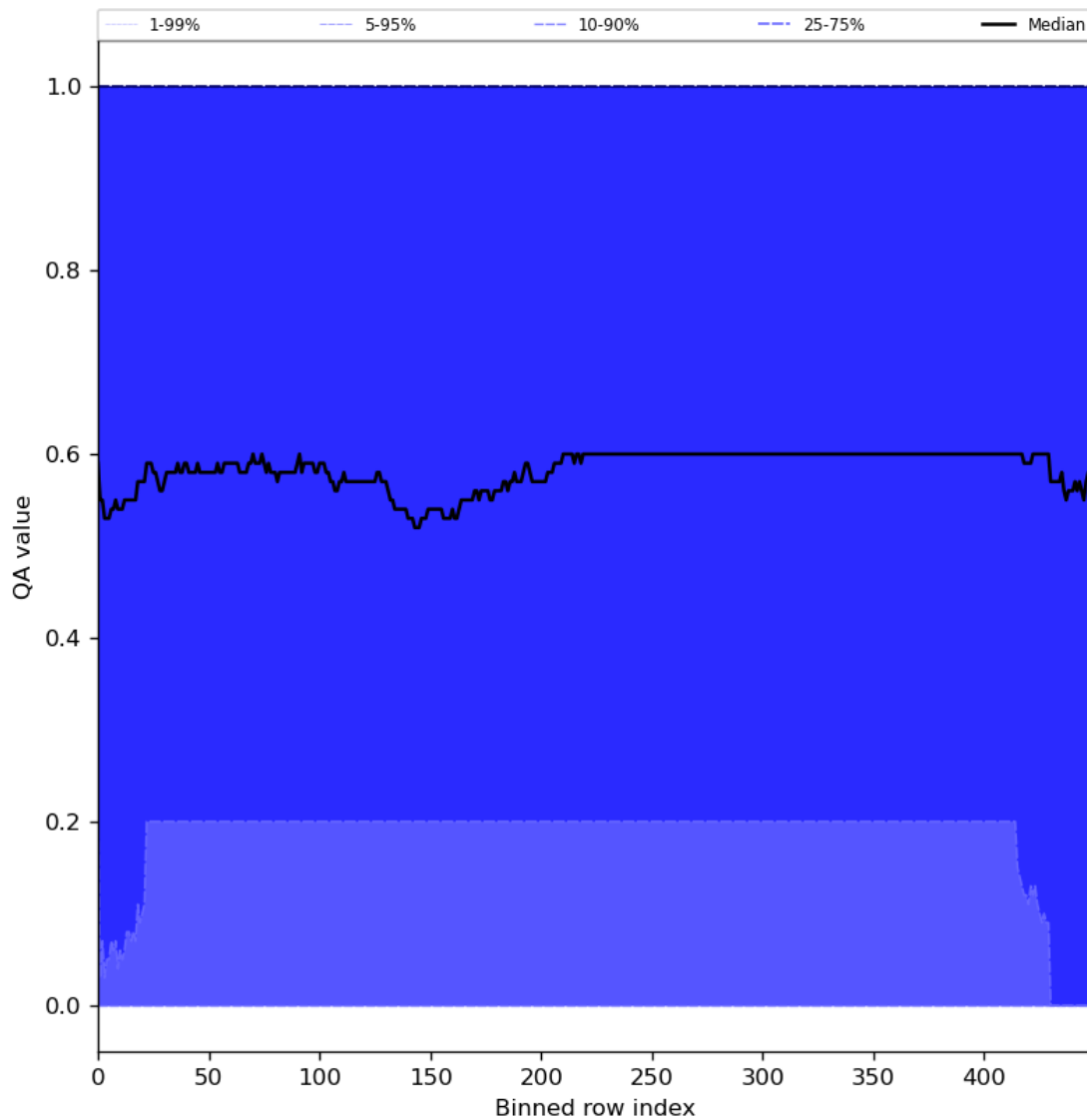
Figure 75: Along track statistics of “QA value” for 2024-04-18 to 2024-04-20
