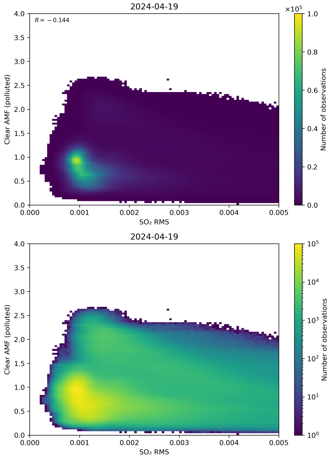
Figure 136: Scatter density plot of “SO 2 RMS” against “Clear AMF (polluted)” for 2024-04-18 to 2024-04-20.
