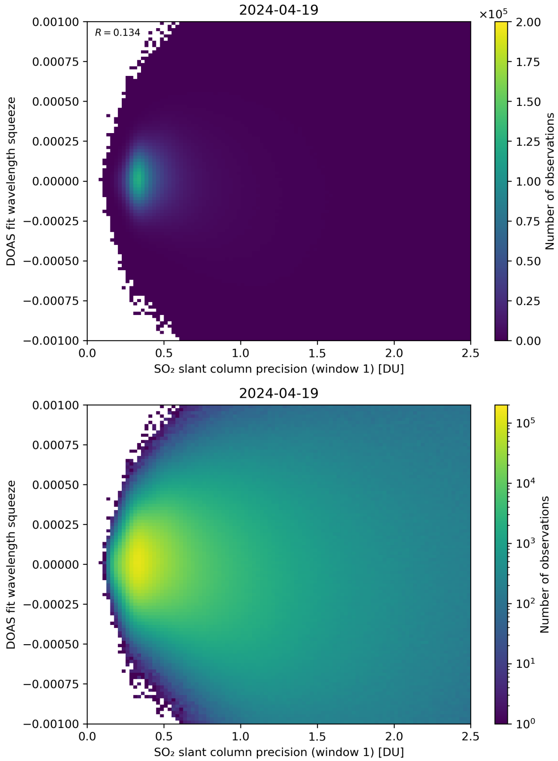
Figure 222: Scatter density plot of “SO 2 slant column precision (window 1)” against “DOAS fit wavelength squeeze” for 2024-04-18 to 2024-04-20.
