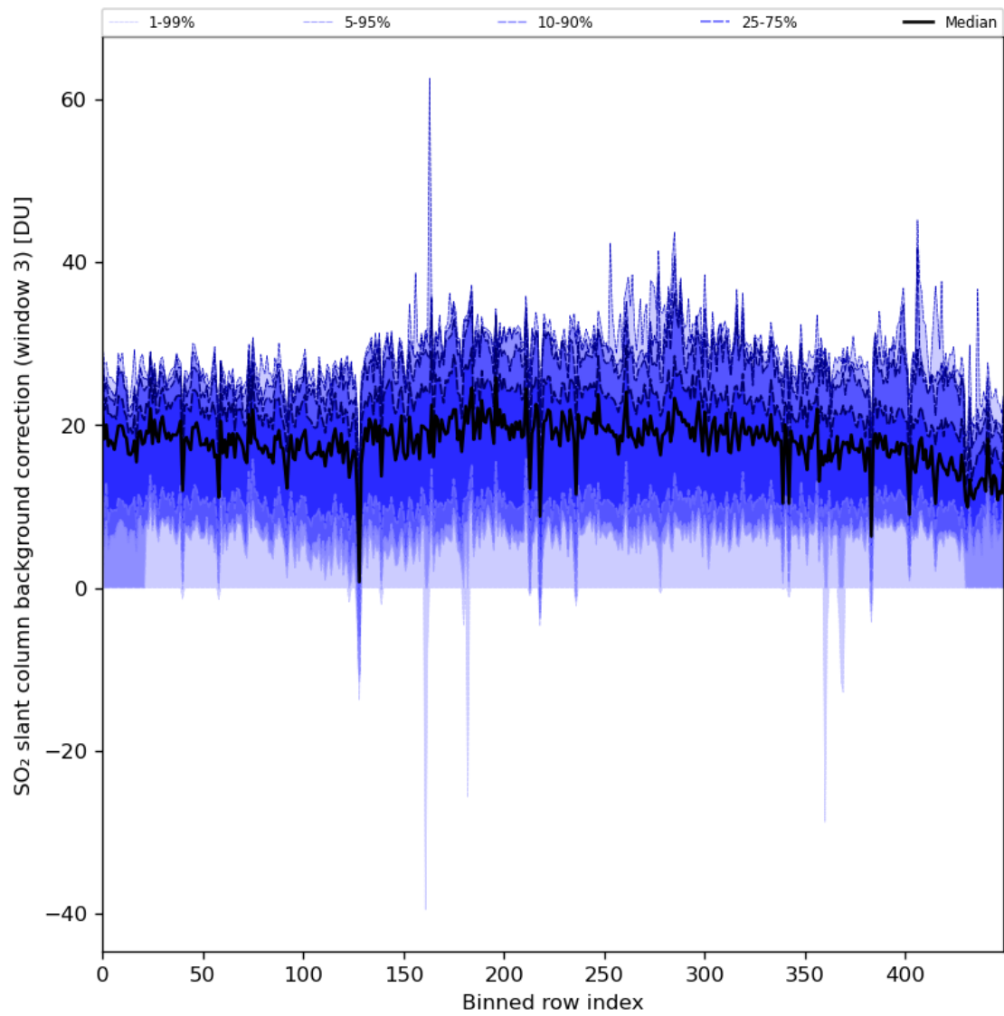
Figure 90: Along track statistics of “SO 2 slant column background correction (window 3)” for 2024-04-18 to 2024-04-20
