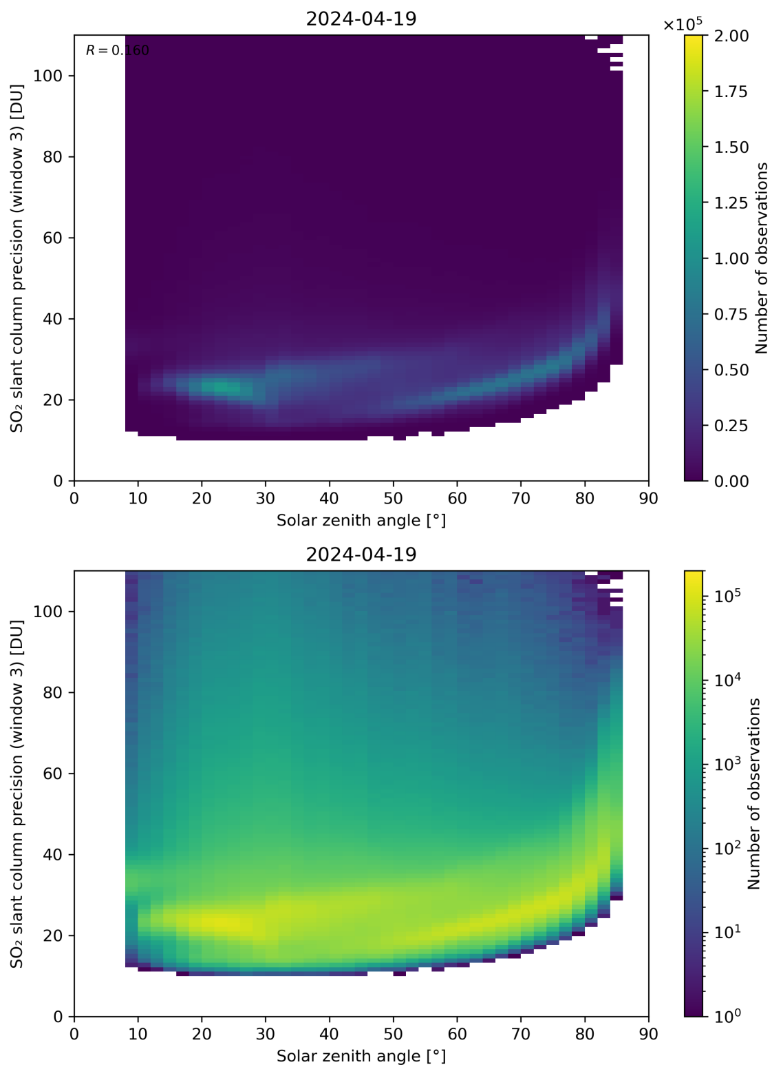
Figure 173: Scatter density plot of “Solar zenith angle” against “SO 2 slant column precision (window 3)” for 2024-04-18 to 2024-04-20.
