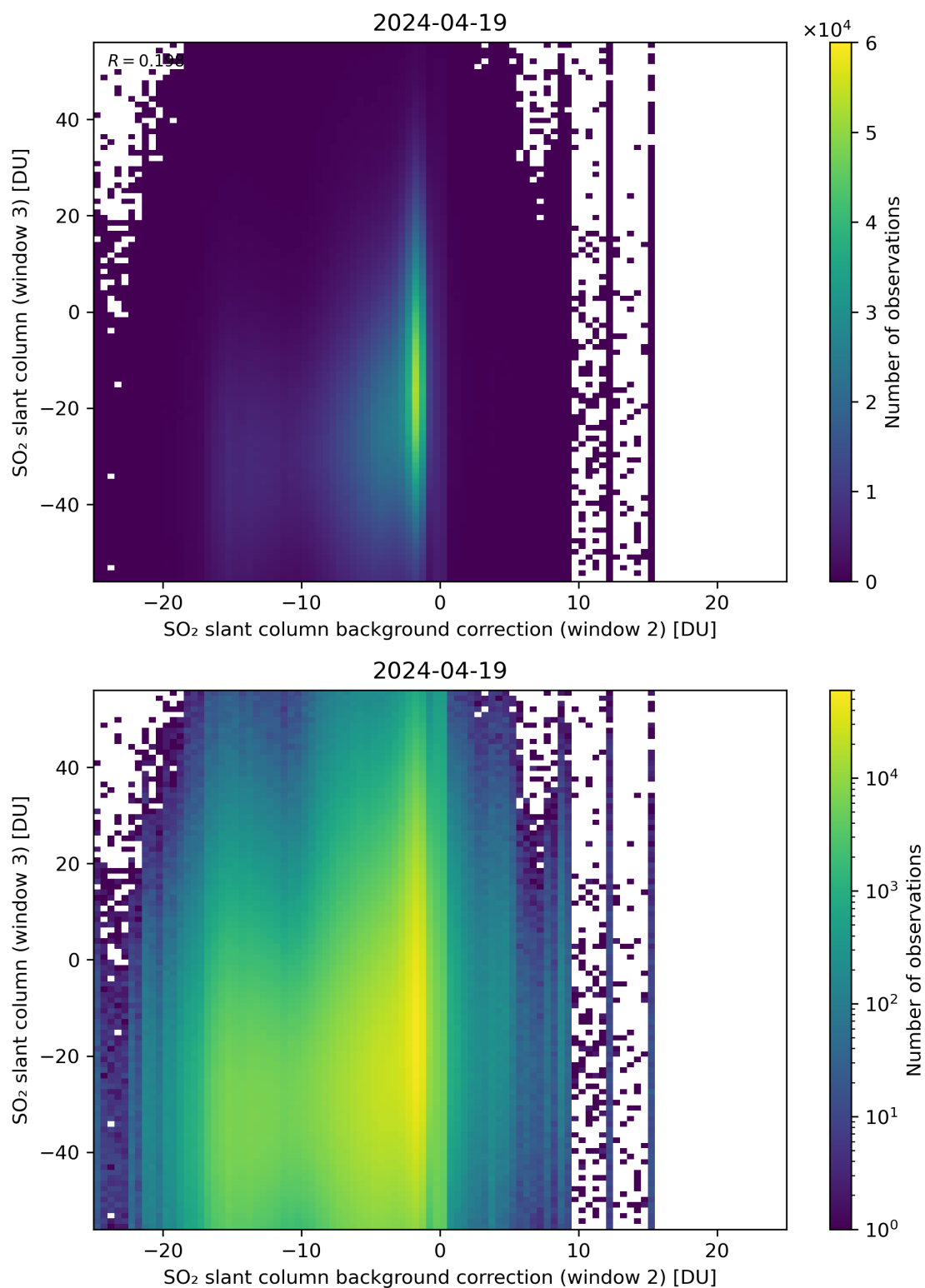
Figure 117: Scatter density plot of “SO 2 slant column background correction (window 2)” against “SO 2 slant column (window 3)” for 2024-04-18 to 2024-04-20.
