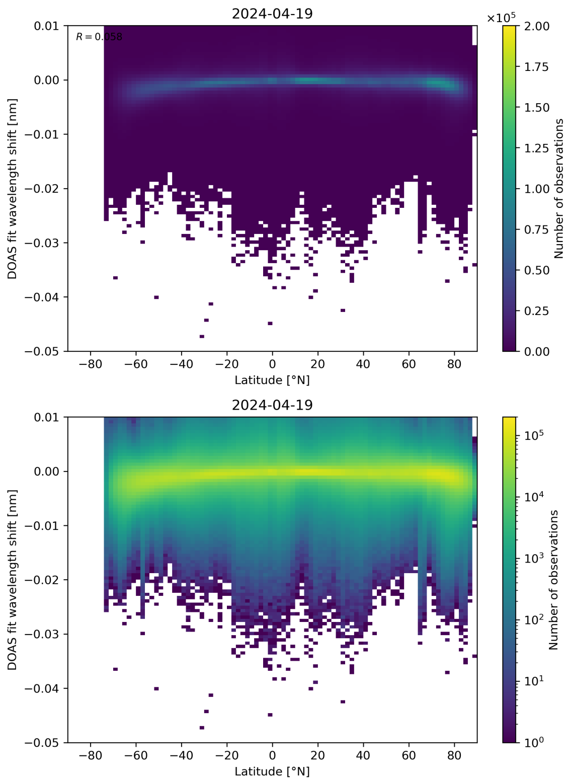
Figure 142: Scatter density plot of “Latitude” against “DOAS fit wavelength shift” for 2024-04-18 to 2024-04-20.
