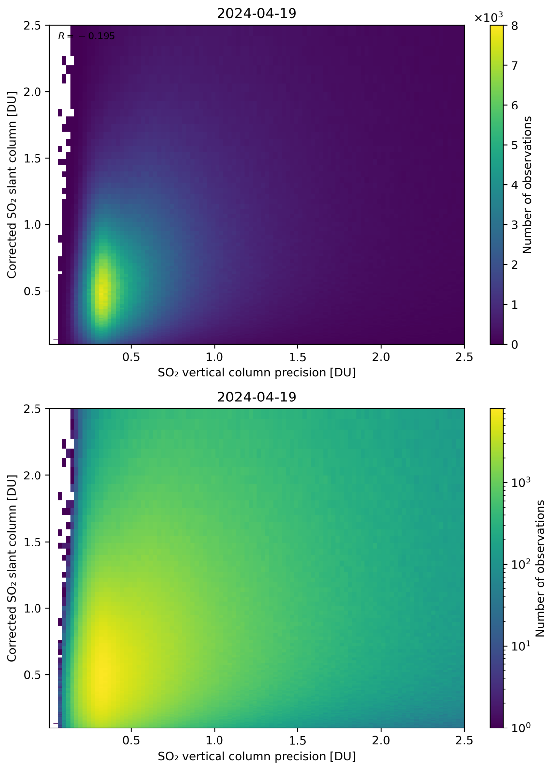
Figure 286: Scatter density plot of “SO 2 vertical column precision” against “Corrected SO 2 slant column” for 2024-04-18 to 2024-04-20.
