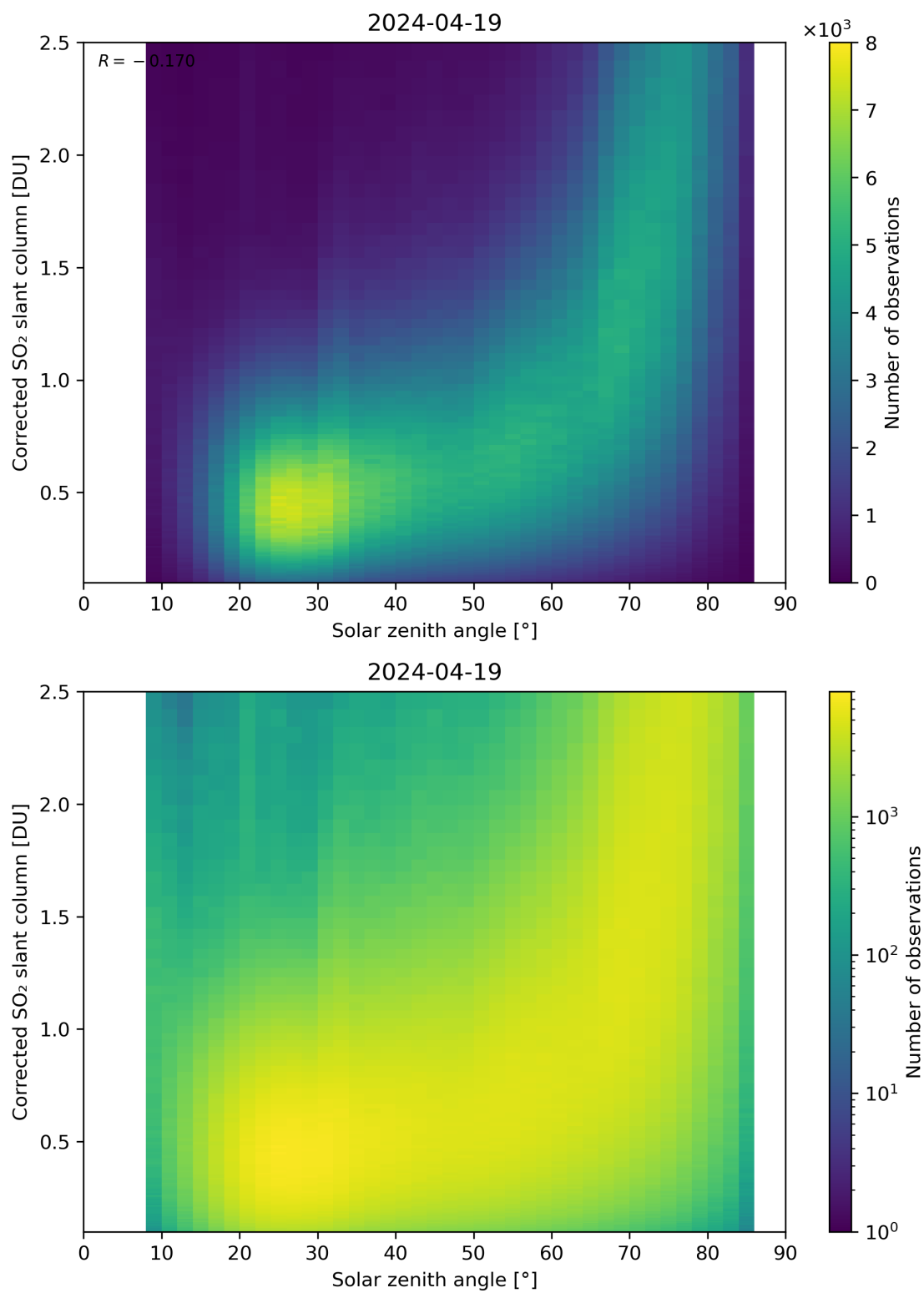
Figure 166: Scatter density plot of “Solar zenith angle” against “Corrected SO 2 slant column” for 2024-04-18 to 2024-04-20.
