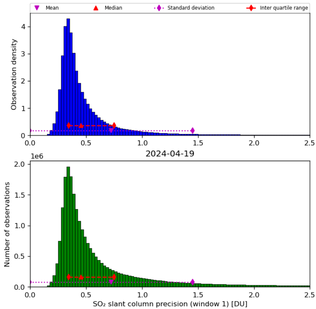
Figure 57: Histogram of “SO 2 slant column precision (window 1)” for 2024-04-18 to 2024-04-20
