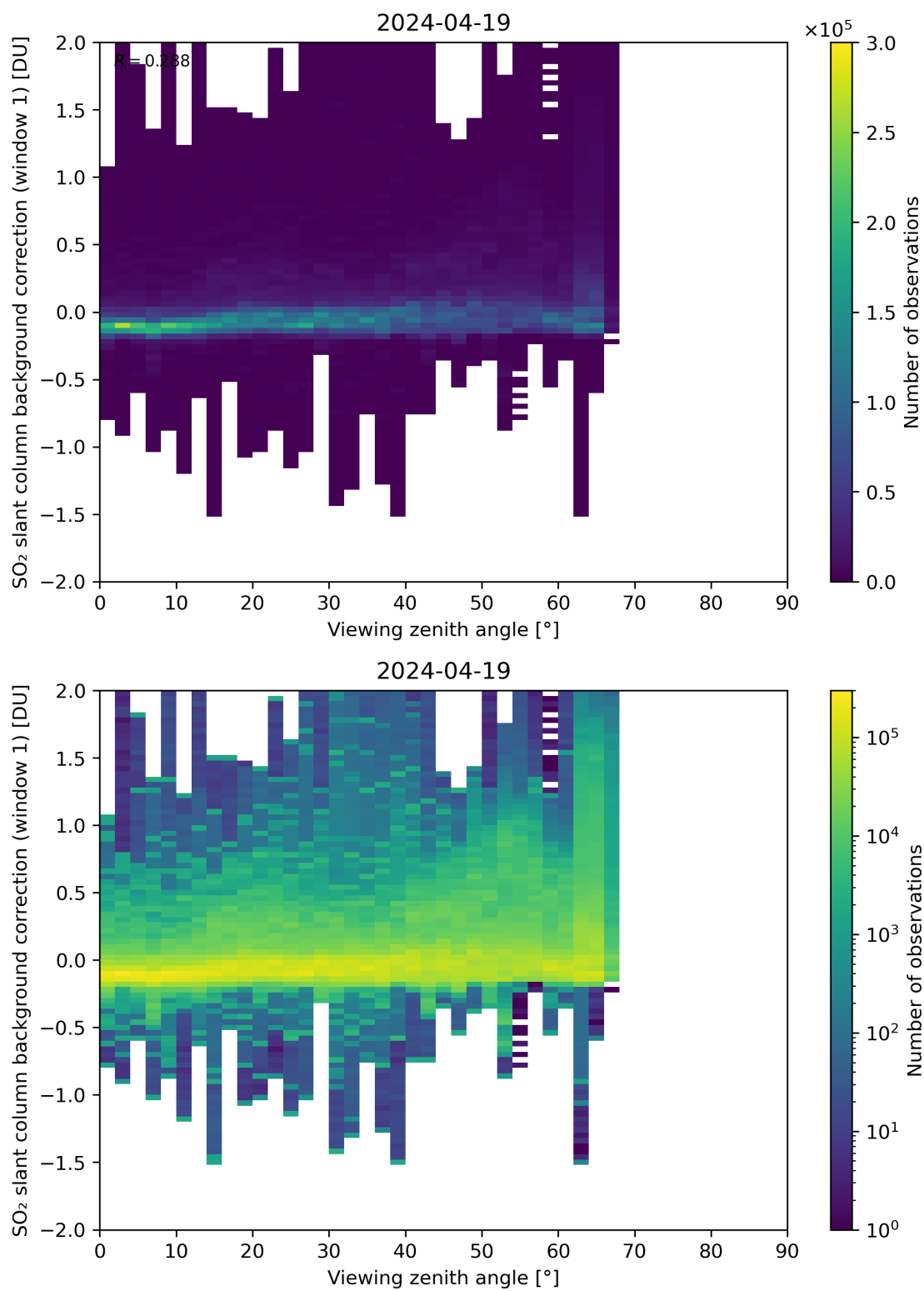
Figure 308: Scatter density plot of “Viewing zenith angle” against “SO 2 slant column background correction (window 1)” for 2024-04-18 to 2024-04-20.
