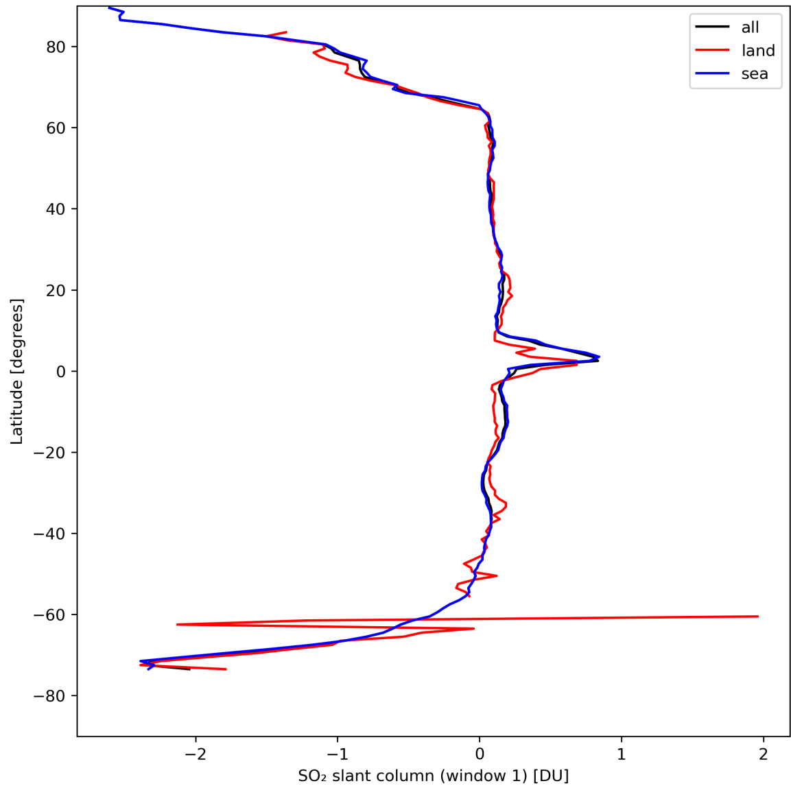
Figure 33: Zonal average of “SO 2 slant column (window 1)” for 2024-04-18 to 2024-04-20.
