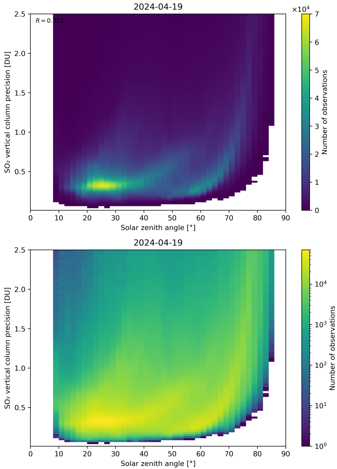
Figure 177: Scatter density plot of “Solar zenith angle” against “SO 2 vertical column precision” for 2024-04-18 to 2024-04-20.
