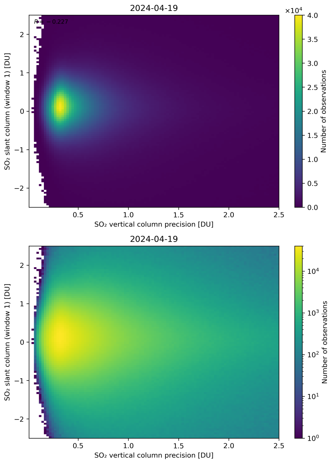
Figure 289: Scatter density plot of “SO 2 vertical column precision” against “SO 2 slant column (window 1)” for 2024-04-18 to 2024-04-20.
