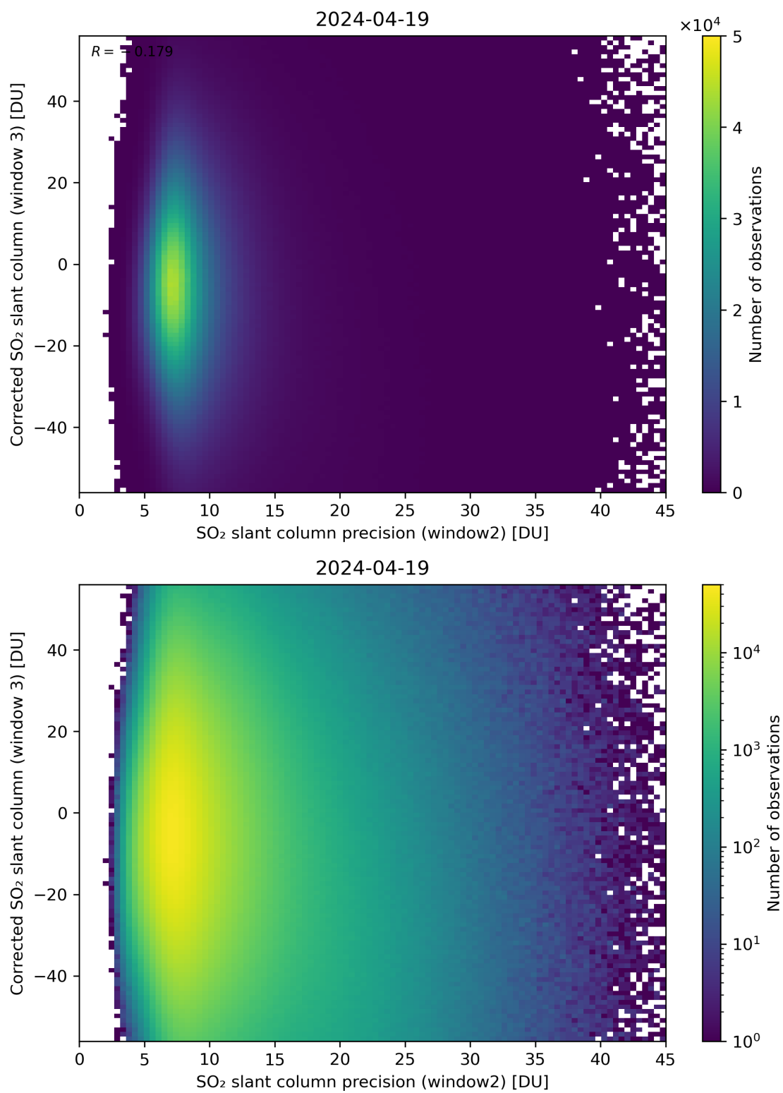
Figure 248: Scatter density plot of “SO 2 slant column precision (window2)” against “Corrected SO 2 slant column (window 3)” for 2024-04-18 to 2024-04-20.
