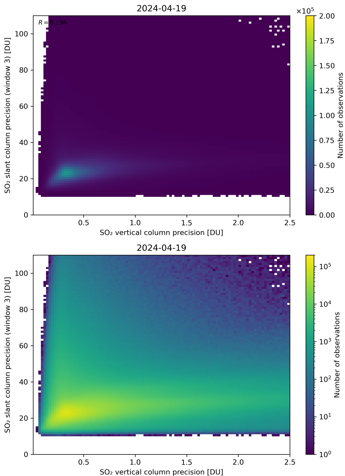
Figure 293: Scatter density plot of “SO 2 vertical column precision” against “SO 2 slant column precision (window 3)” for 2024-04-18 to 2024-04-20.
