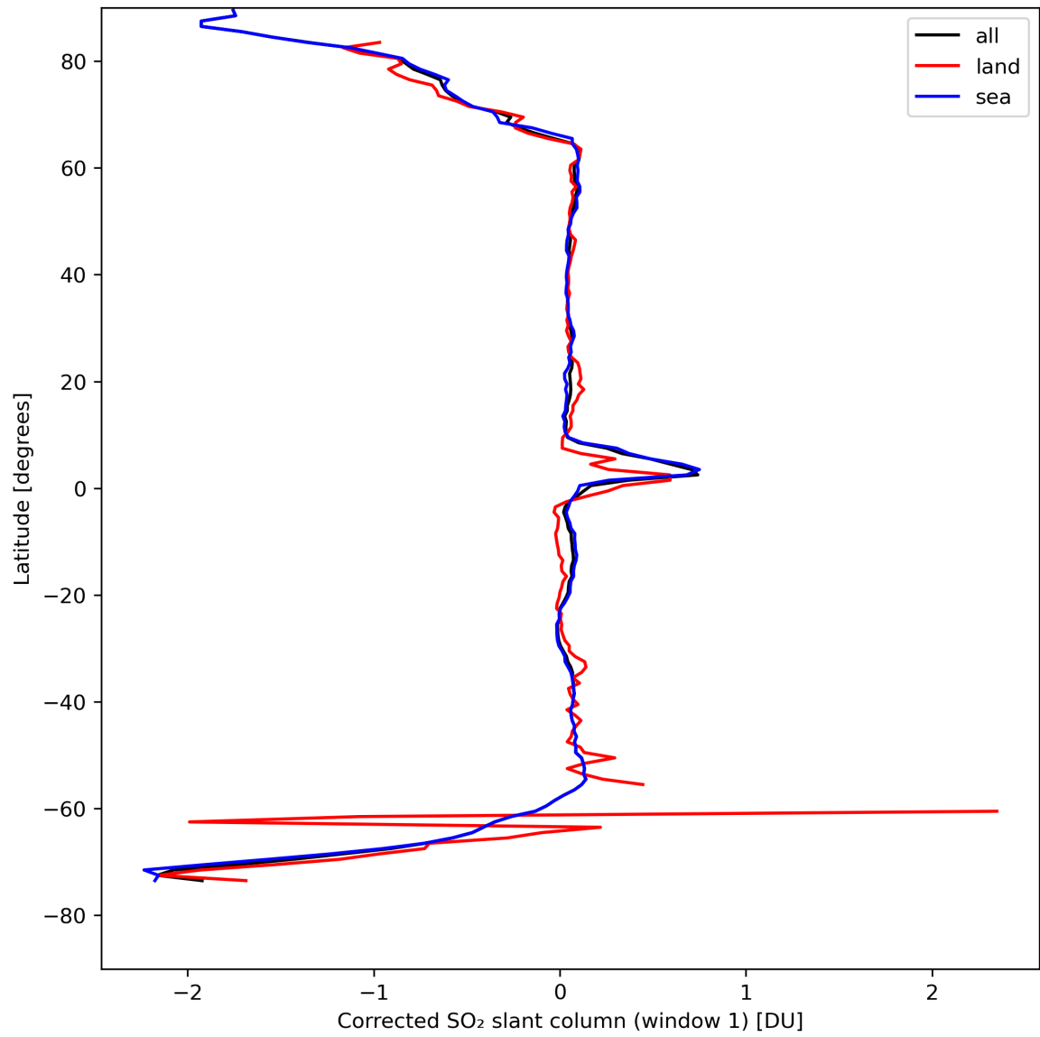
Figure 35: Zonal average of “Corrected SO 2 slant column (window 1)” for 2024-04-18 to 2024-04-20.
