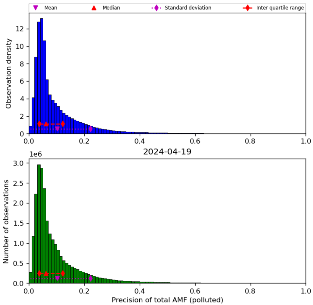
Figure 72: Histogram of “Precision of total AMF (polluted)” for 2024-04-18 to 2024-04-20
