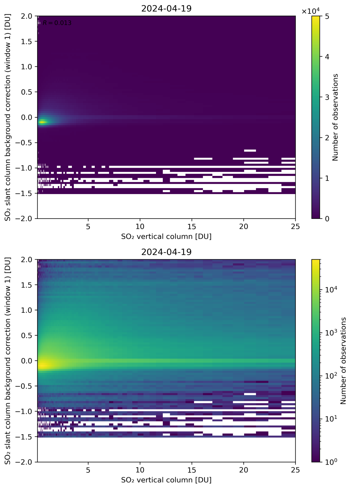
Figure 273: Scatter density plot of “SO 2 vertical column” against “SO 2 slant column background correction (window 1)” for 2024-04-18 to 2024-04-20.
