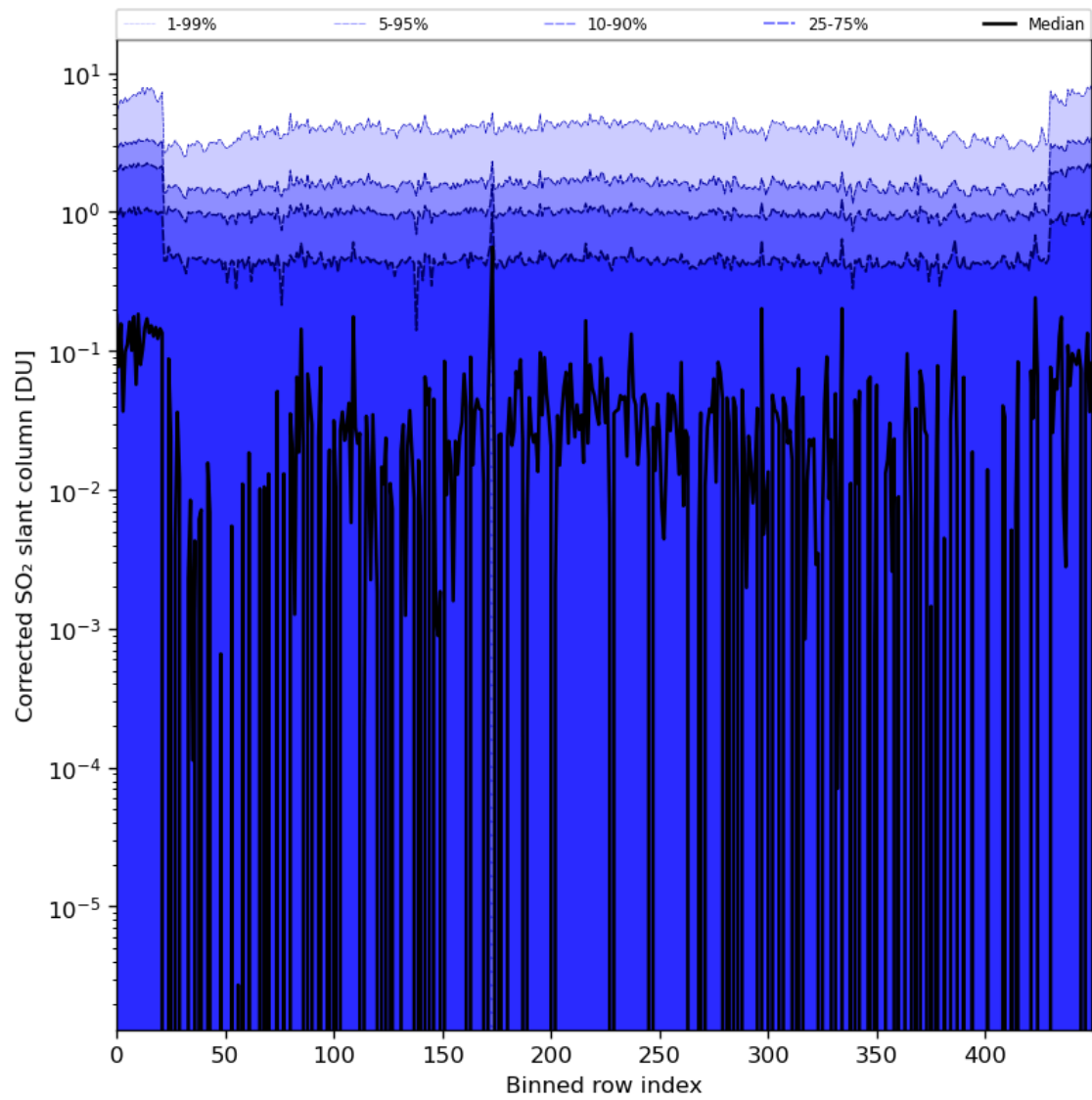
Figure 78: Along track statistics of “Corrected SO 2 slant column” for 2024-04-18 to 2024-04-20
