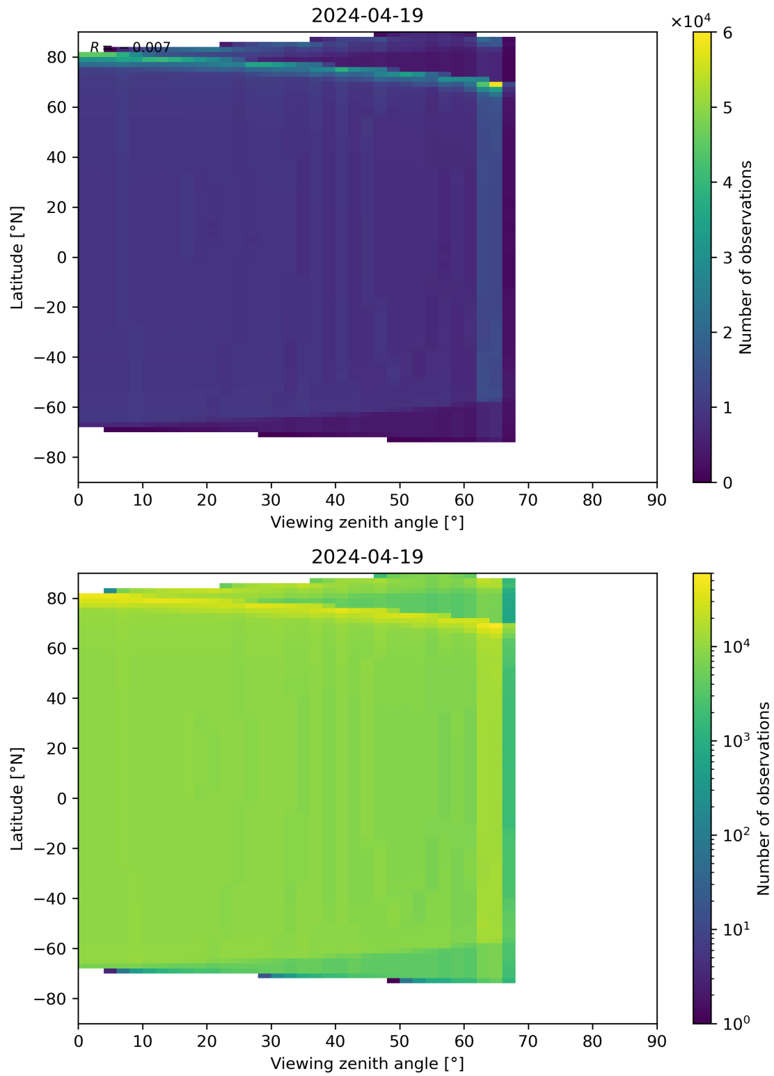
Figure 314: Scatter density plot of “Viewing zenith angle” against “Latitude” for 2024-04-18 to 2024-04-20.
