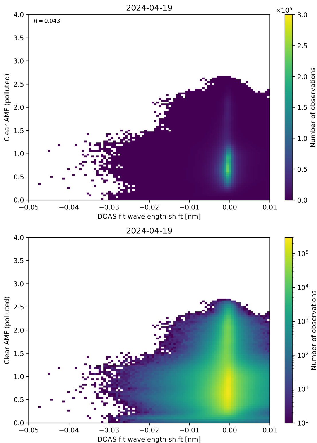
Figure 129: Scatter density plot of “DOAS fit wavelength shift” against “Clear AMF (polluted)” for 2024-04-18 to 2024-04-20.
