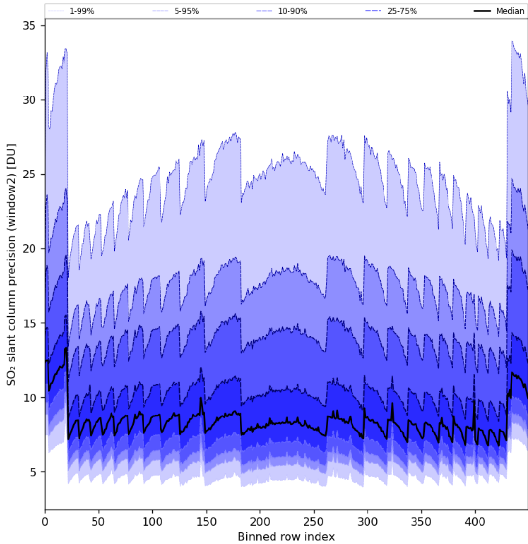
Figure 84: Along track statistics of "SO 2 slant column precision (window2)" for 2024-04-18 to 2024-04-20
