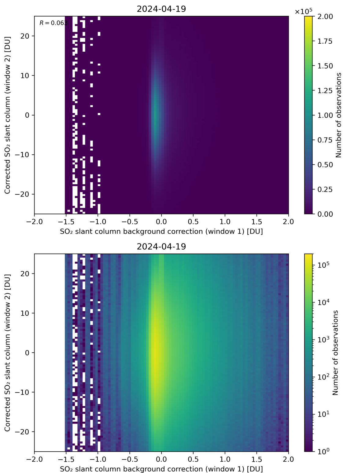
Figure 104: Scatter density plot of “SO 2 slant column background correction (window 1)” against “Corrected SO 2 slant column (window 2)” for 2024-04-18 to 2024-04-20.
