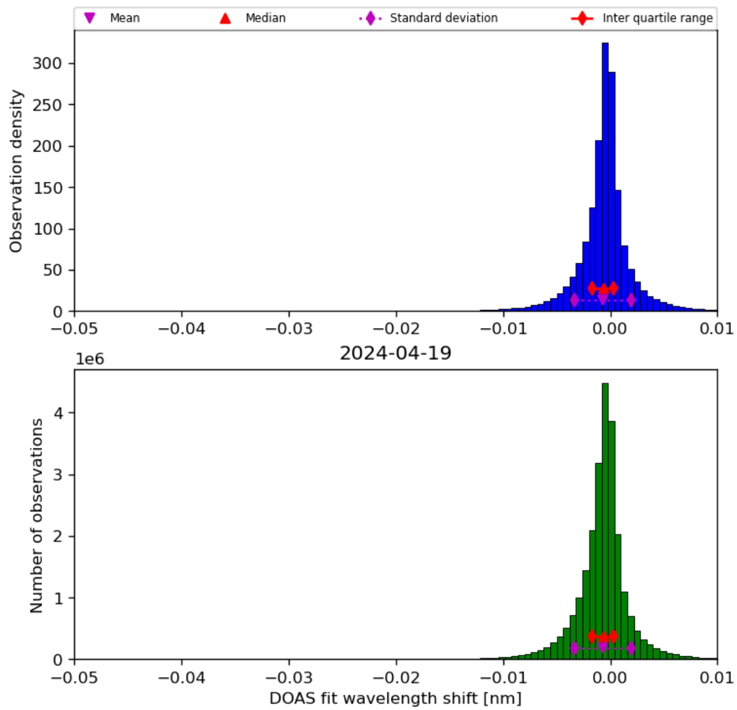
Figure 68: Histogram of “DOAS fit wavelength shift” for 2024-04-18 to 2024-04-20
