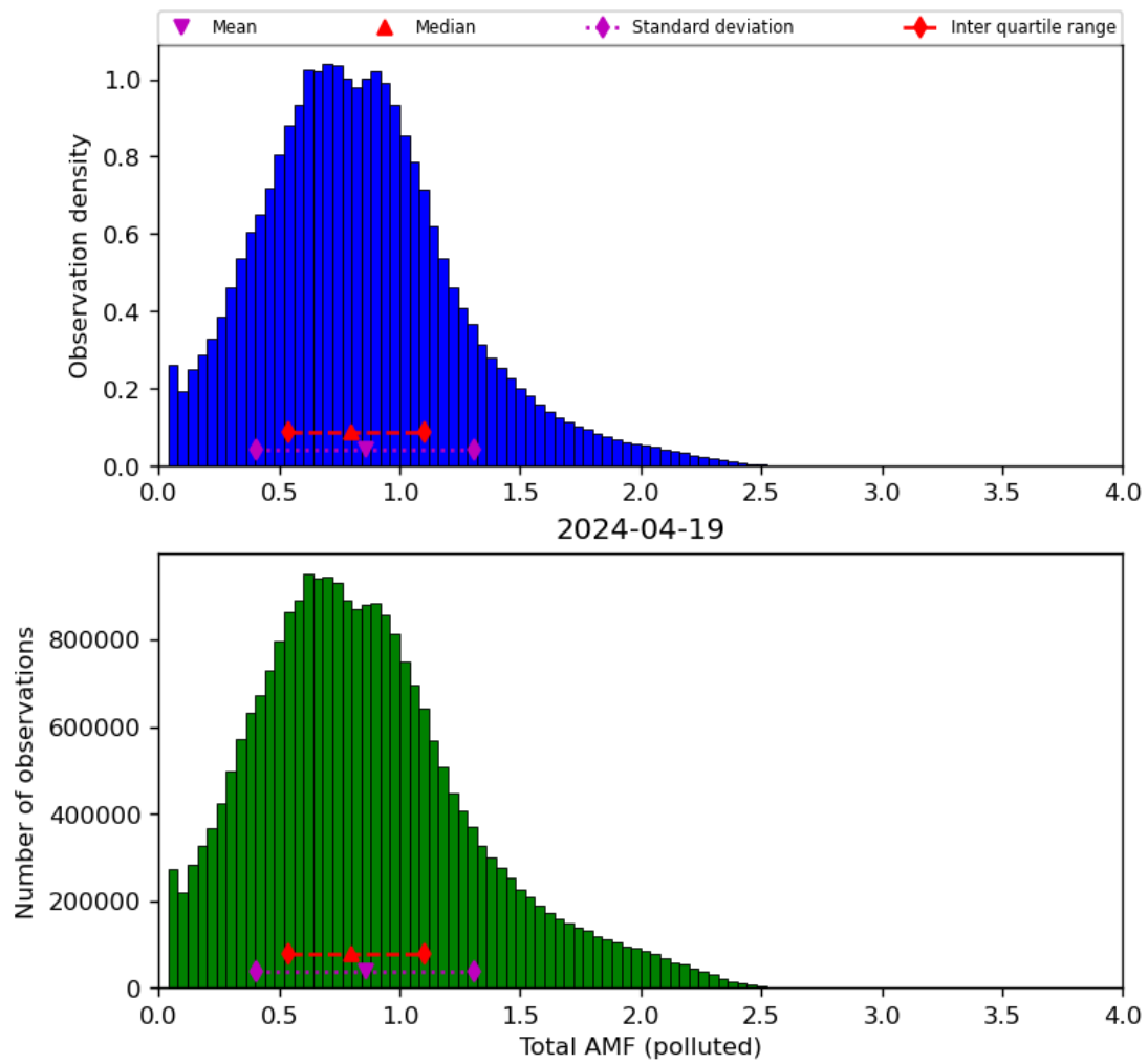
Figure 71: Histogram of “Total AMF (polluted)” for 2024-04-18 to 2024-04-20
