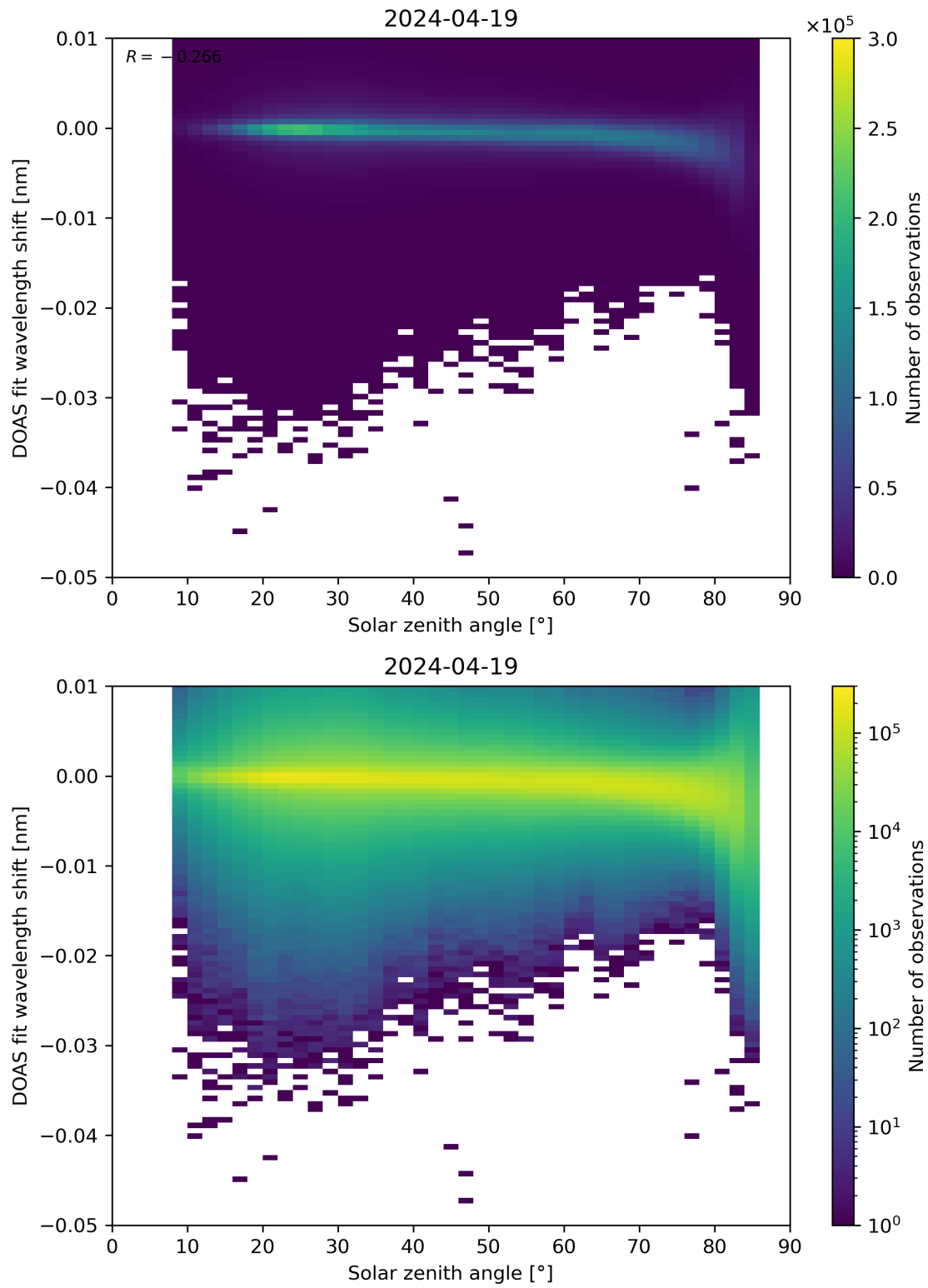
Figure 161: Scatter density plot of “Solar zenith angle” against “DOAS fit wavelength shift” for 2024-04-18 to 2024-04-20.
