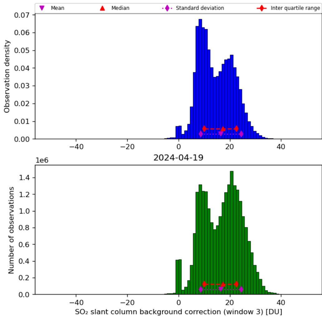
Figure 67: Histogram of “SO 2 slant column background correction (window 3)” for 2024-04-18 to 2024-04-20
