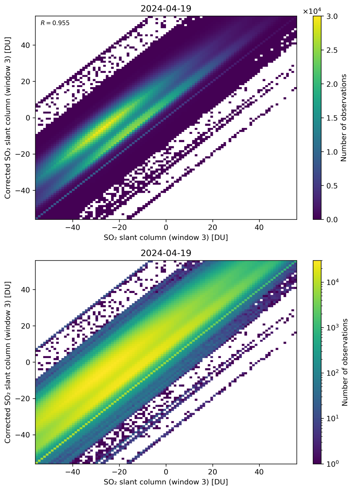
Figure 266: Scatter density plot of “SO 2 slant column (window 3)” against “Corrected SO 2 slant column (window 3)” for 2024-04-18 to 2024-04-20.
