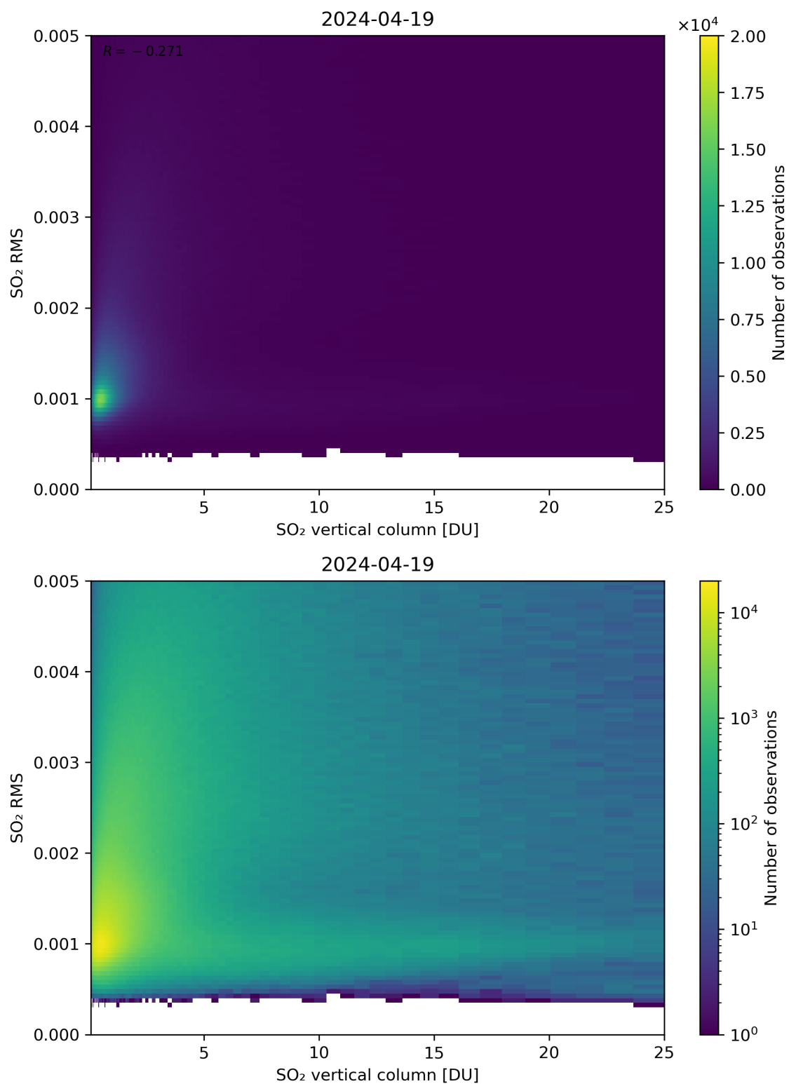
Figure 278: Scatter density plot of “SO 2 vertical column” against “SO 2 RMS” for 2024-04-18 to 2024-04-20.
