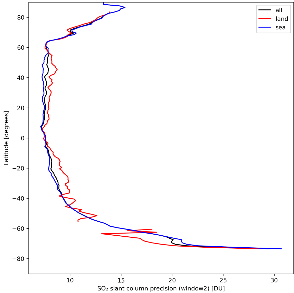
Figure 38: Zonal average of “SO 2 slant column precision (window2)” for 2024-04-18 to 2024-04-20.
