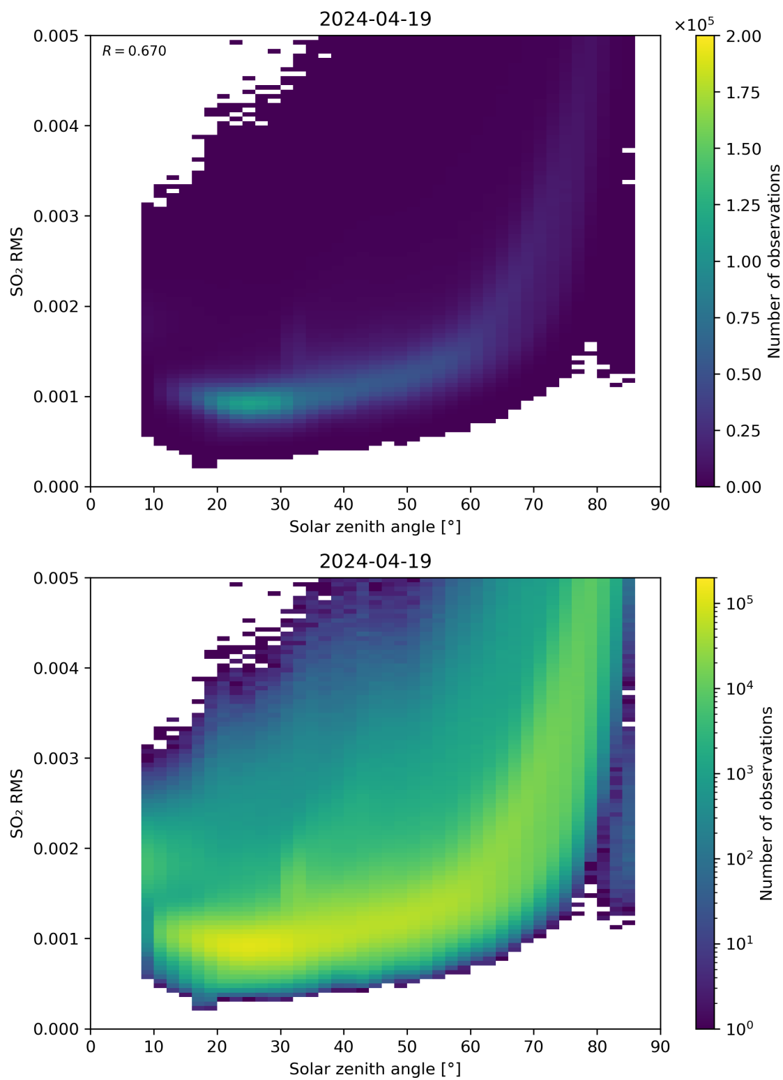
Figure 163: Scatter density plot of “Solar zenith angle” against “SO 2 RMS” for 2024-04-18 to 2024-04-20.
