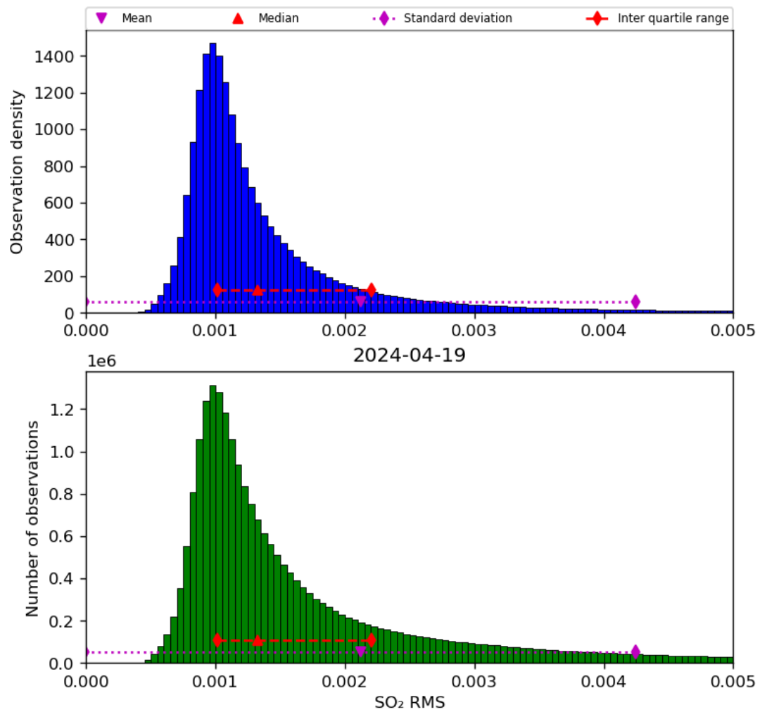
Figure 70: Histogram of “SO 2 RMS” for 2024-04-18 to 2024-04-20
