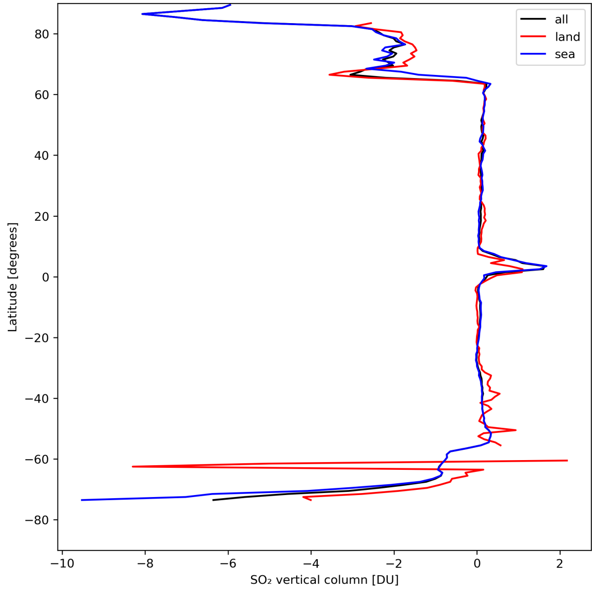
Figure 30: Zonal average of “SO 2 vertical column” for 2024-04-18 to 2024-04-20.
