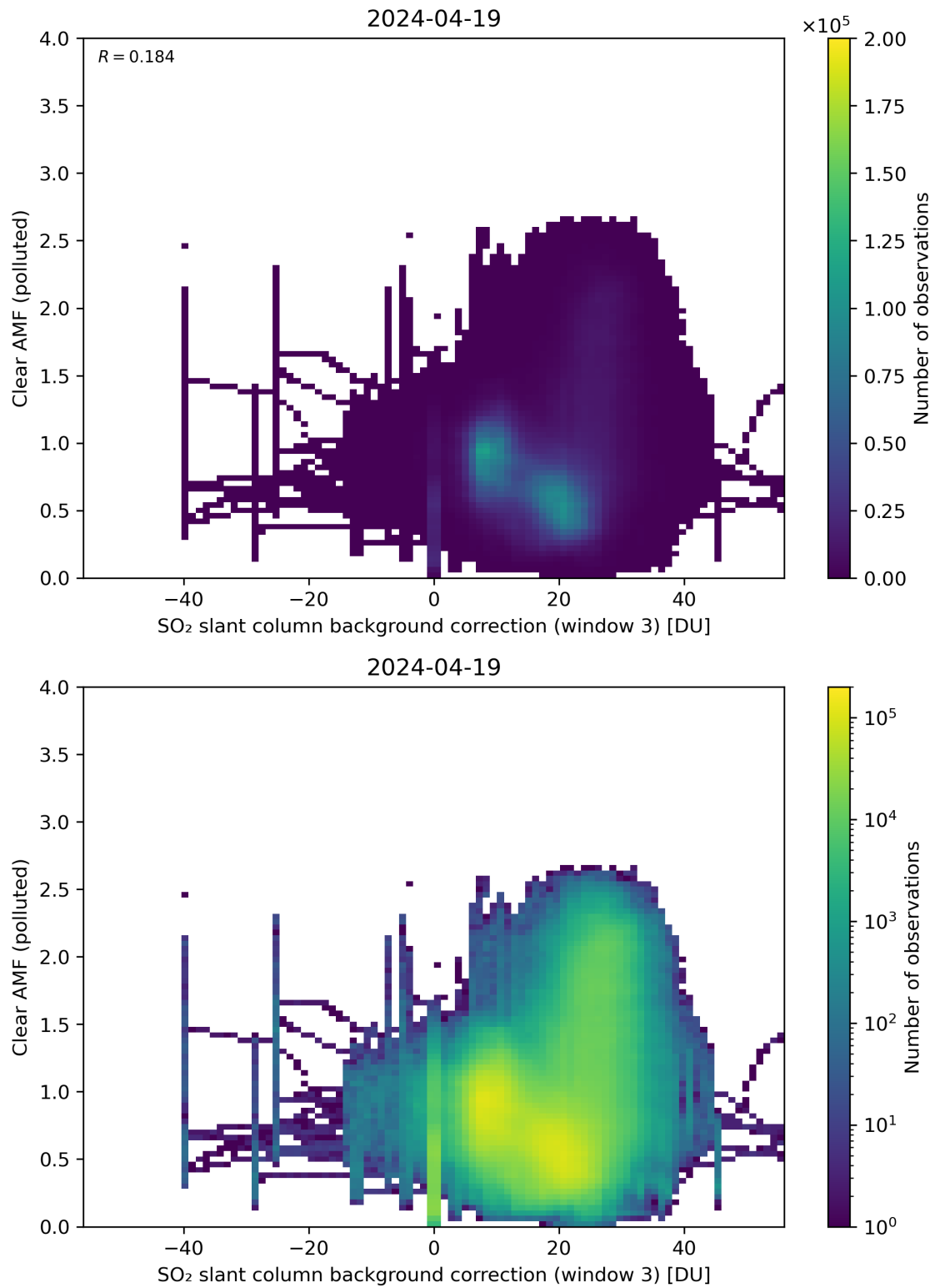
Figure 124: Scatter density plot of “SO 2 slant column background correction (window 3)” against “Clear AMF (polluted)” for 2024-04-18 to 2024-04-20.
