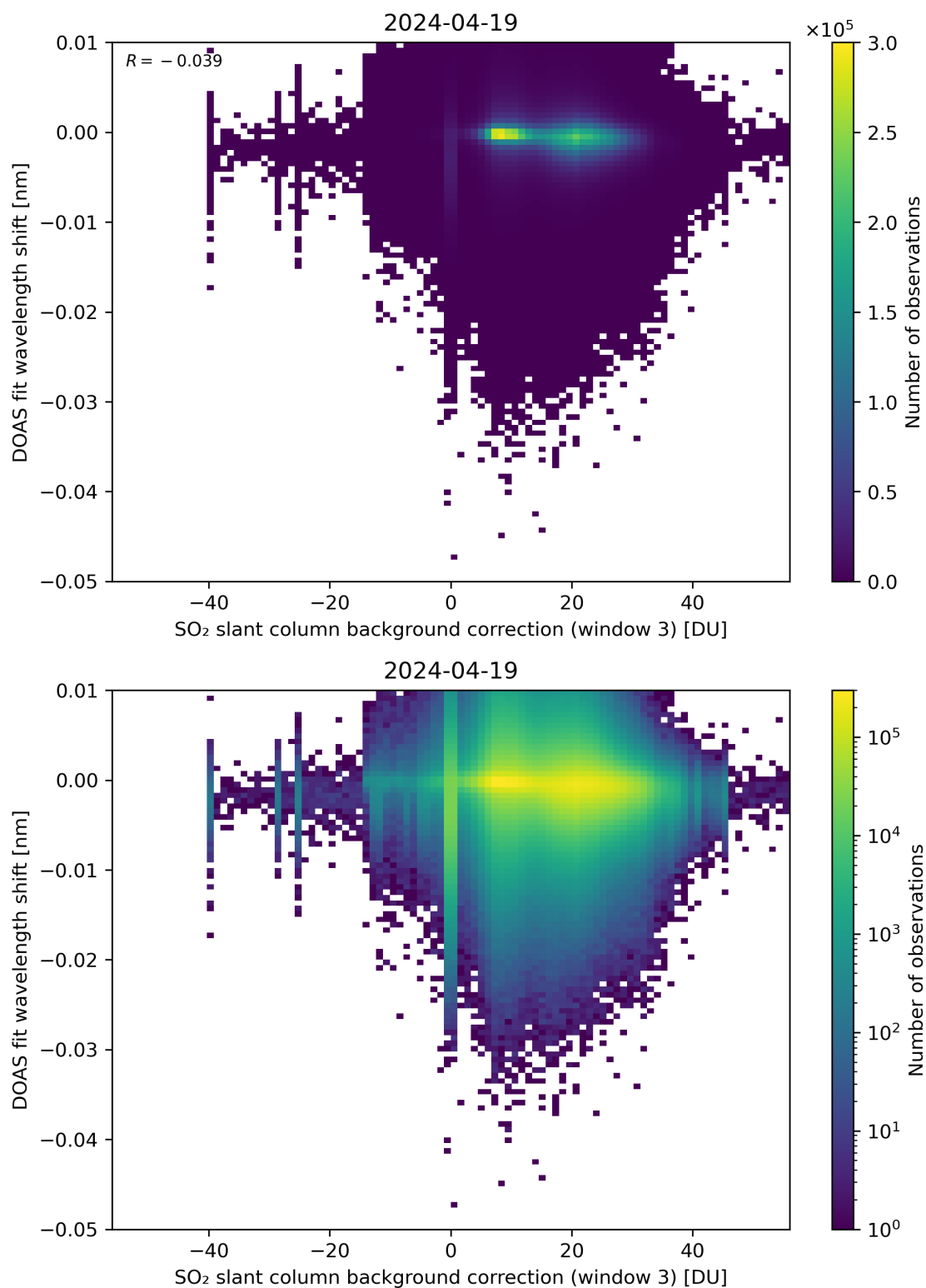
Figure 121: Scatter density plot of “SO 2 slant column background correction (window 3)” against “DOAS fit wavelength shift” for 2024-04-18 to 2024-04-20.
