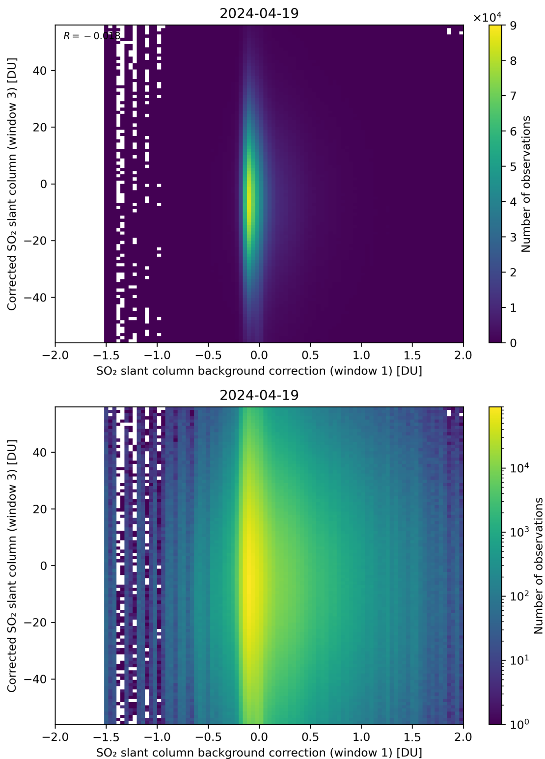
Figure 105: Scatter density plot of “SO 2 slant column background correction (window 1)” against “Corrected SO 2 slant column (window 3)” for 2024-04-18 to 2024-04-20.
