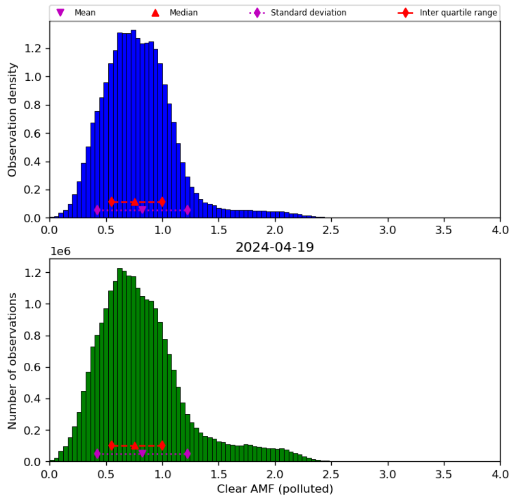
Figure 73: Histogram of “Clear AMF (polluted)” for 2024-04-18 to 2024-04-20
