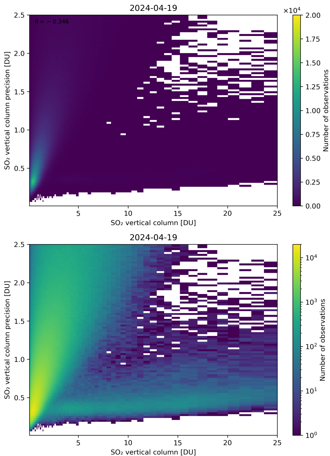
Figure 307: Scatter density plot of “SO 2 vertical column” against “SO 2 vertical column precision” for 2024-04-18 to 2024-04-20.
