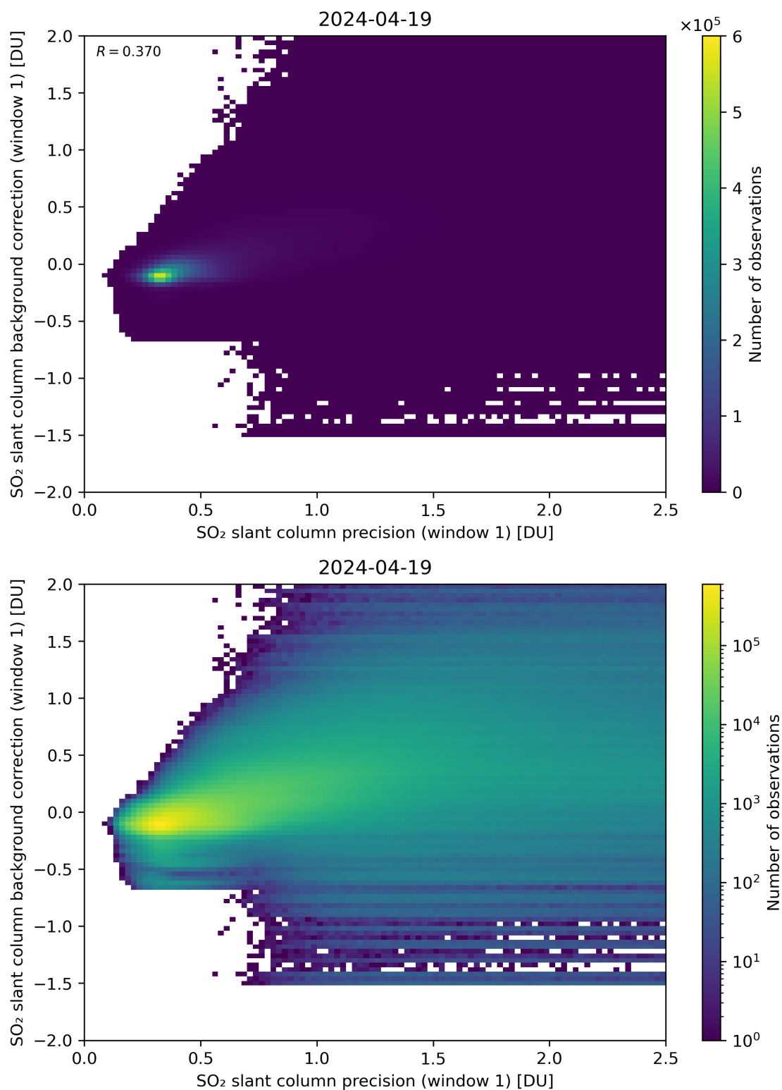
Figure 218: Scatter density plot of “SO 2 slant column precision (window 1)” against “SO 2 slant column background correction (window 1)” for 2024-04-18 to 2024-04-20.
