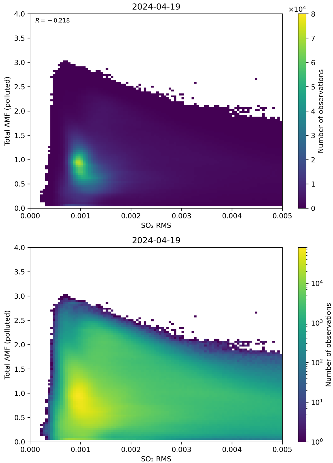
Figure 137: Scatter density plot of “SO 2 RMS” against “Total AMF (polluted)” for 2024-04-18 to 2024-04-20.
