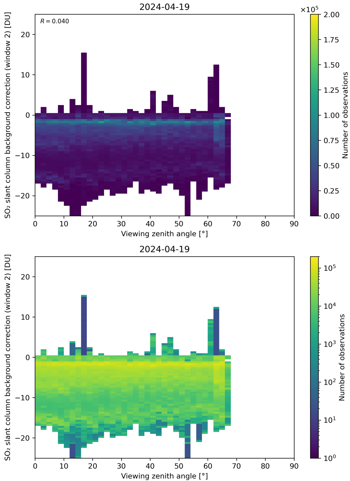
Figure 309: Scatter density plot of “Viewing zenith angle” against “SO 2 slant column background correction (window 2)” for 2024-04-18 to 2024-04-20.
