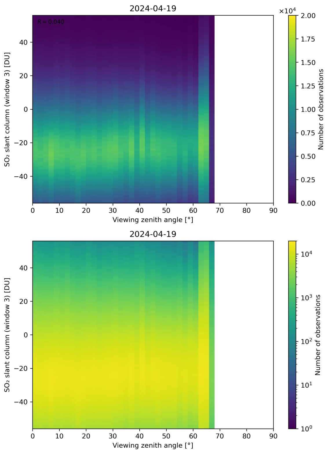
Figure 323: Scatter density plot of “Viewing zenith angle” against “SO 2 slant column (window 3)” for 2024-04-18 to 2024-04-20.
