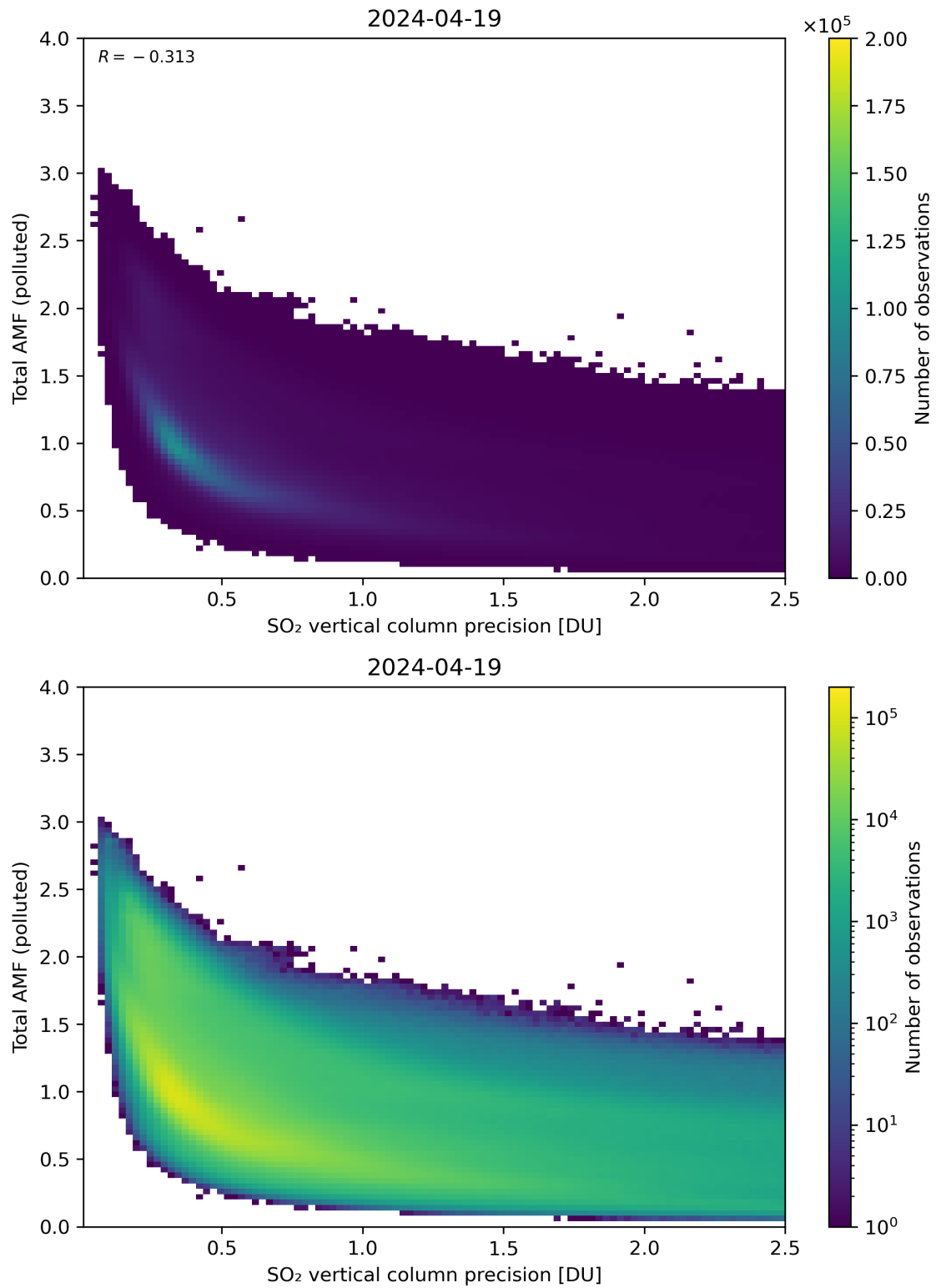
Figure 294: Scatter density plot of “SO 2 vertical column precision” against “Total AMF (polluted)” for 2024-04-18 to 2024-04-20.
