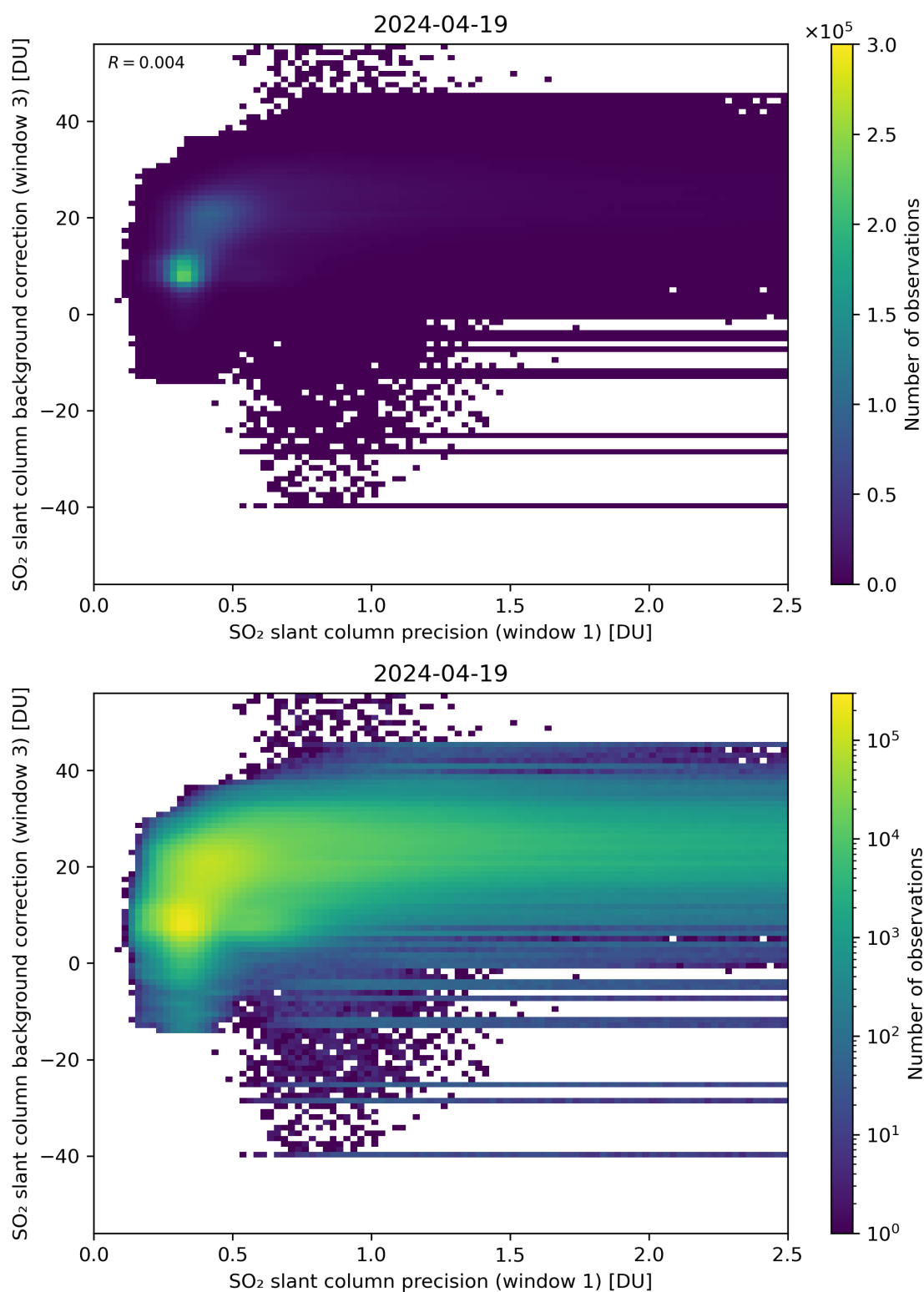
Figure 220: Scatter density plot of “SO 2 slant column precision (window 1)” against “SO 2 slant column background correction (window 3)” for 2024-04-18 to 2024-04-20.
