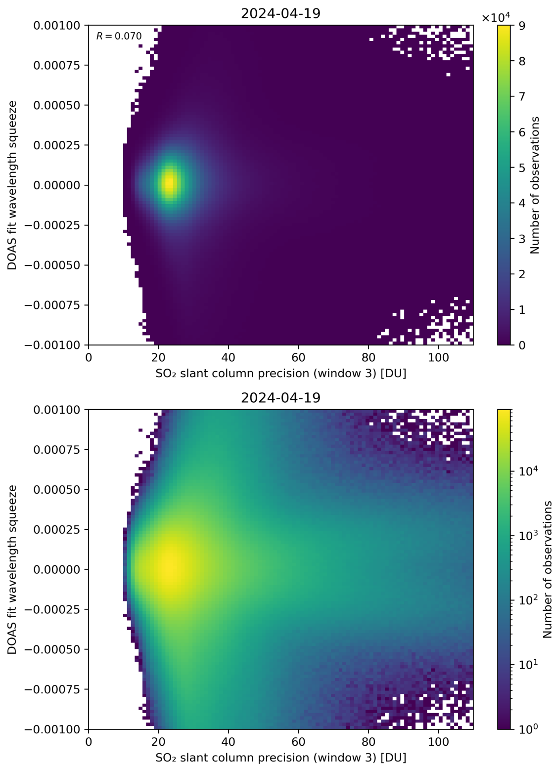
Figure 259: Scatter density plot of “SO 2 slant column precision (window 3)” against “DOAS fit wavelength squeeze” for 2024-04-18 to 2024-04-20.
