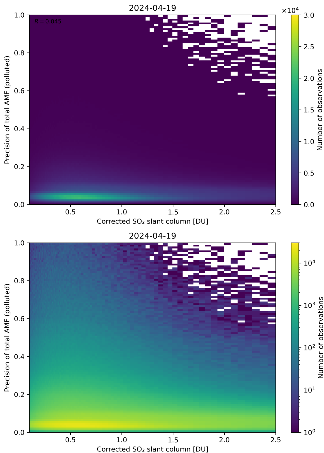
Figure 193: Scatter density plot of “Corrected SO 2 slant column” against “Precision of total AMF (polluted)” for 2024-04-18 to 2024-04-20.
