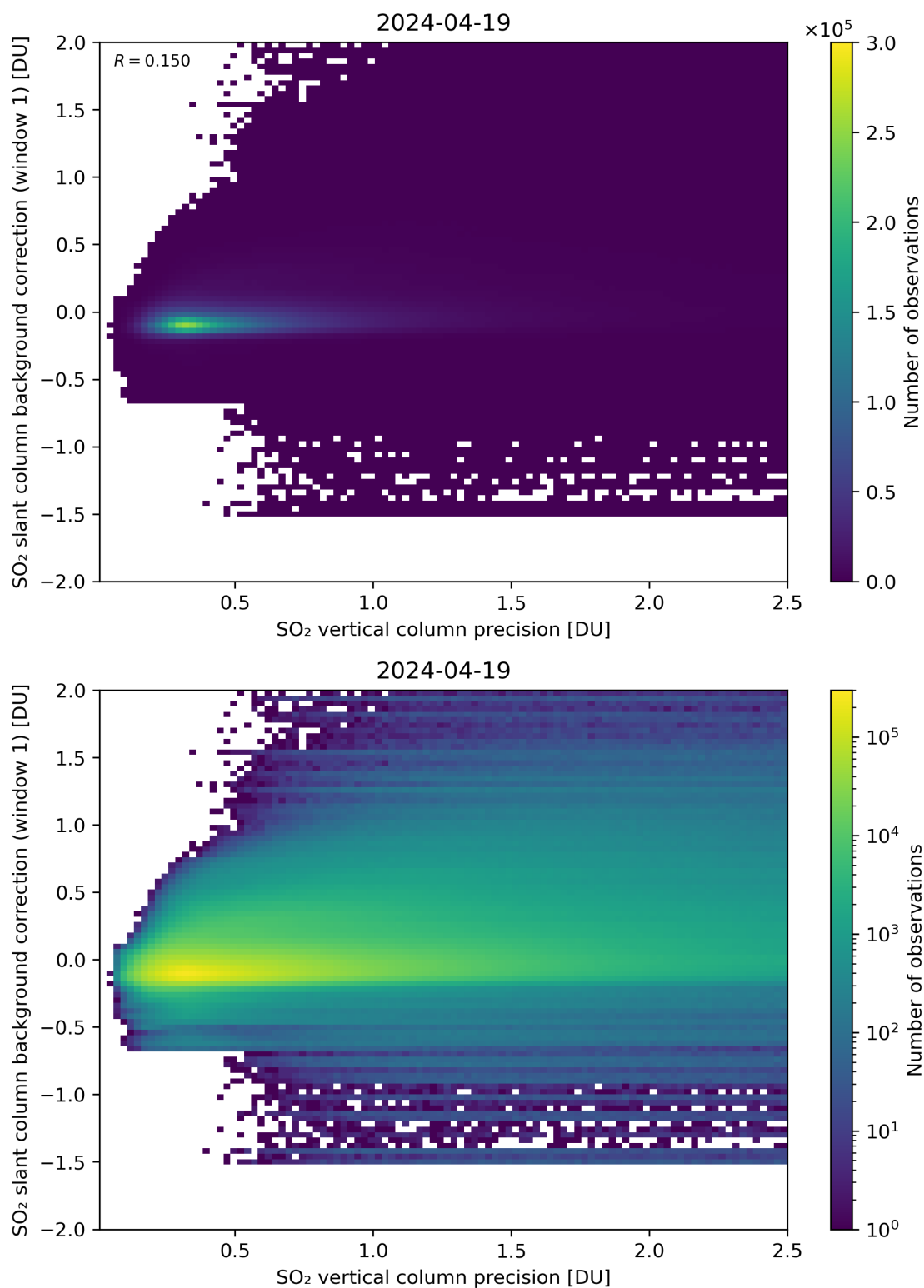
Figure 279: Scatter density plot of “SO 2 vertical column precision” against “SO 2 slant column background correction (window 1)” for 2024-04-18 to 2024-04-20.
