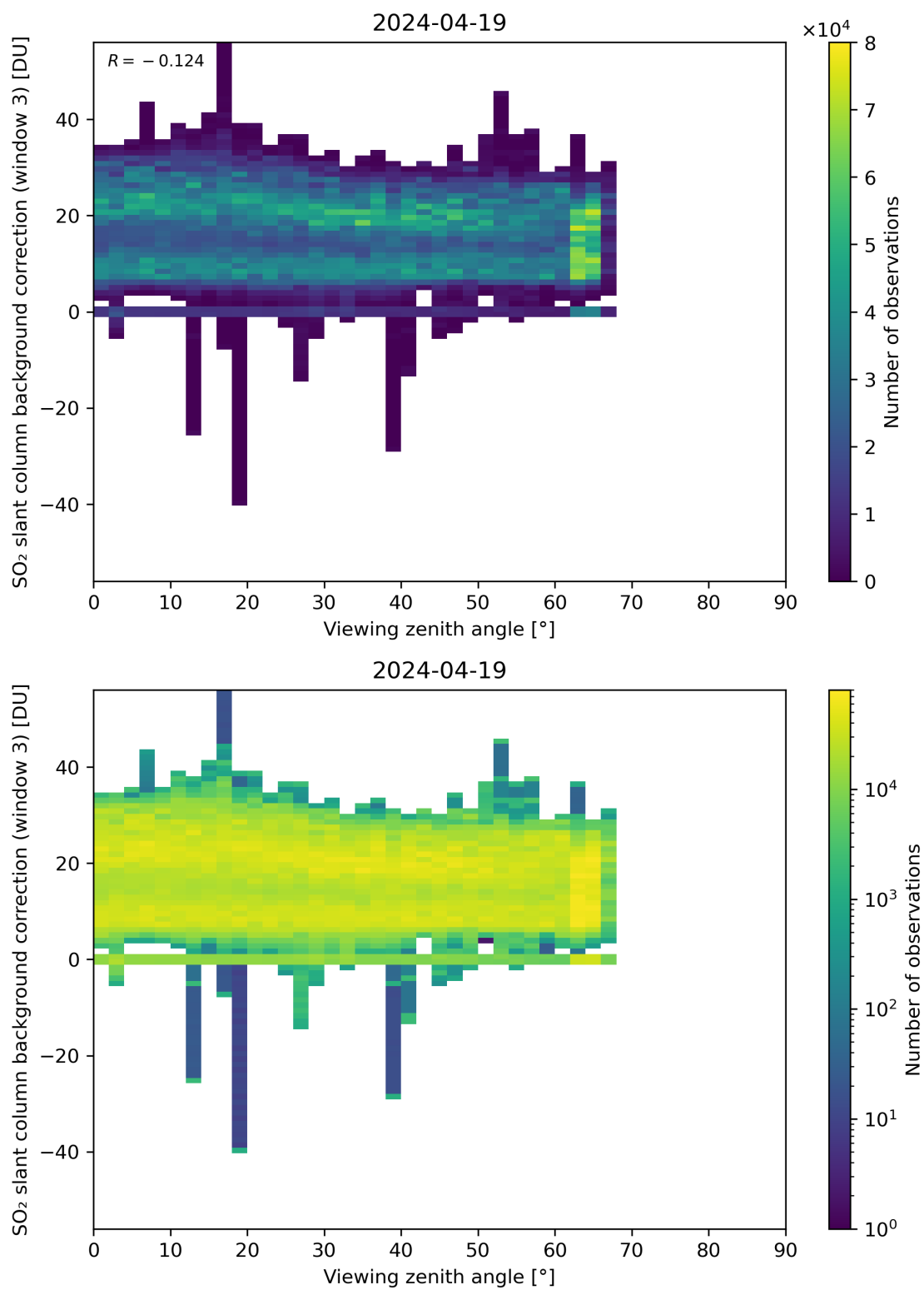
Figure 310: Scatter density plot of “Viewing zenith angle” against “SO 2 slant column background correction (window 3)” for 2024-04-18 to 2024-04-20.
