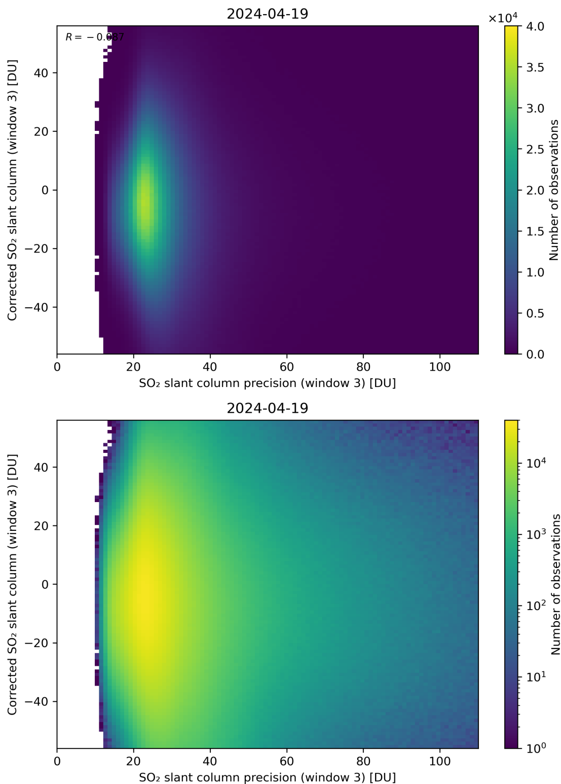
Figure 262: Scatter density plot of “SO 2 slant column precision (window 3)” against “Corrected SO 2 slant column (window 3)” for 2024-04-18 to 2024-04-20.
