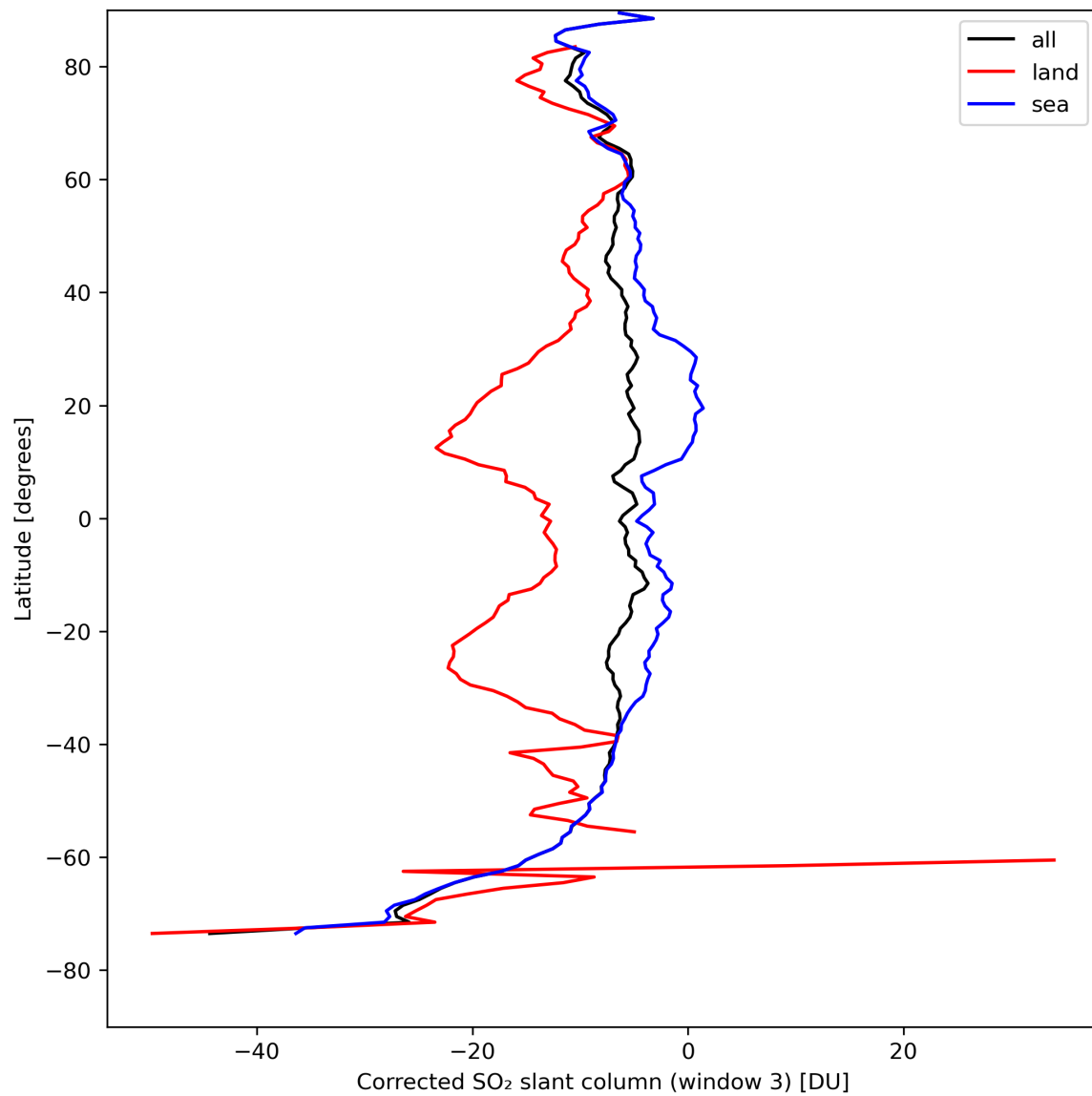
Figure 43: Zonal average of “Corrected SO 2 slant column (window 3)” for 2024-04-18 to 2024-04-20.
