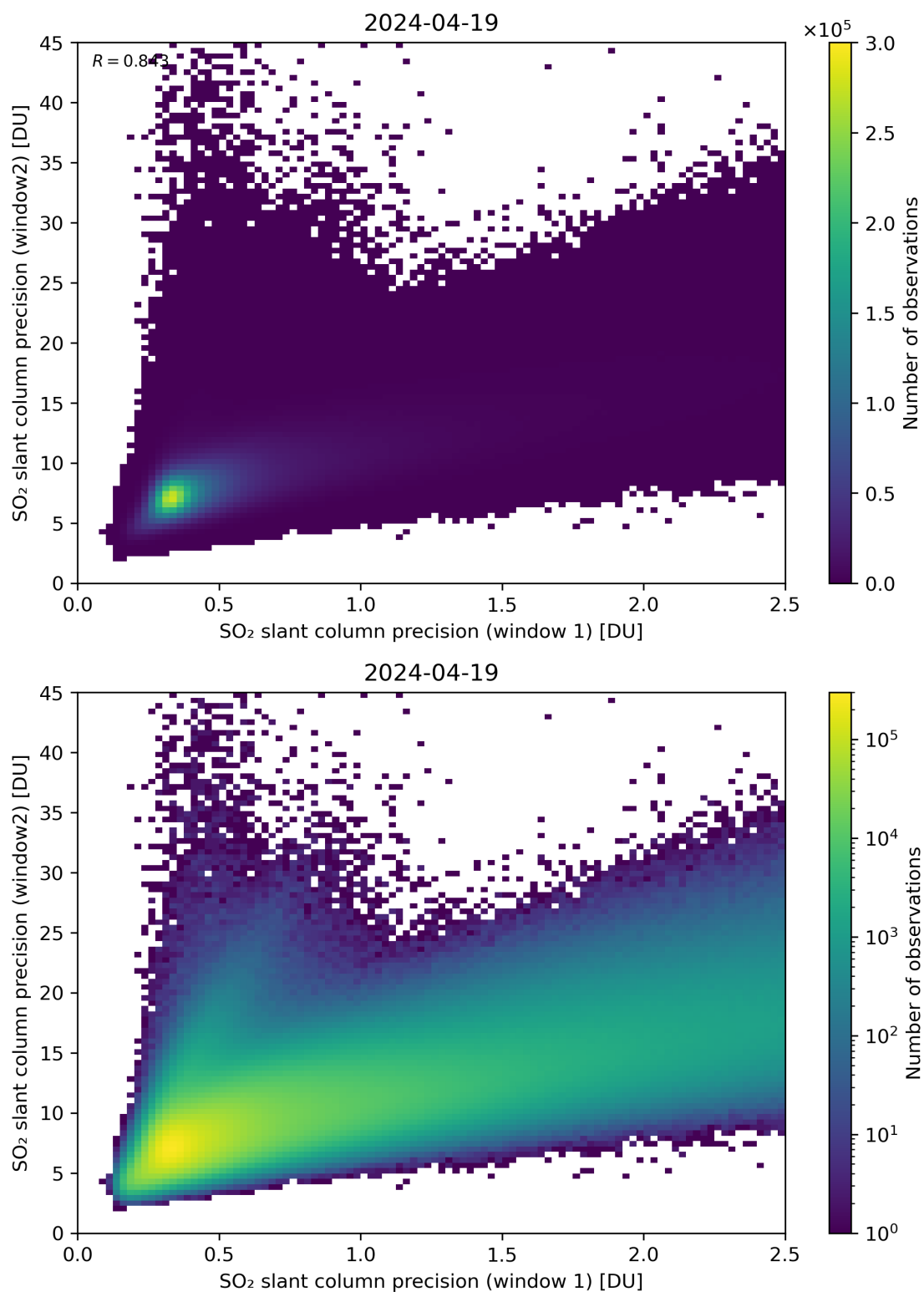
Figure 227: Scatter density plot of “SO 2 slant column precision (window 1)” against “SO 2 slant column precision (window2)” for 2024-04-18 to 2024-04-20.
