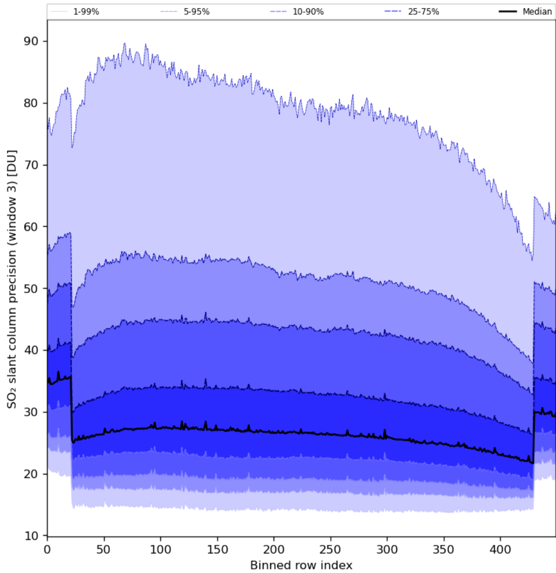
Figure 88: Along track statistics of “SO 2 slant column precision (window 3)” for 2024-04-18 to 2024-04-20
