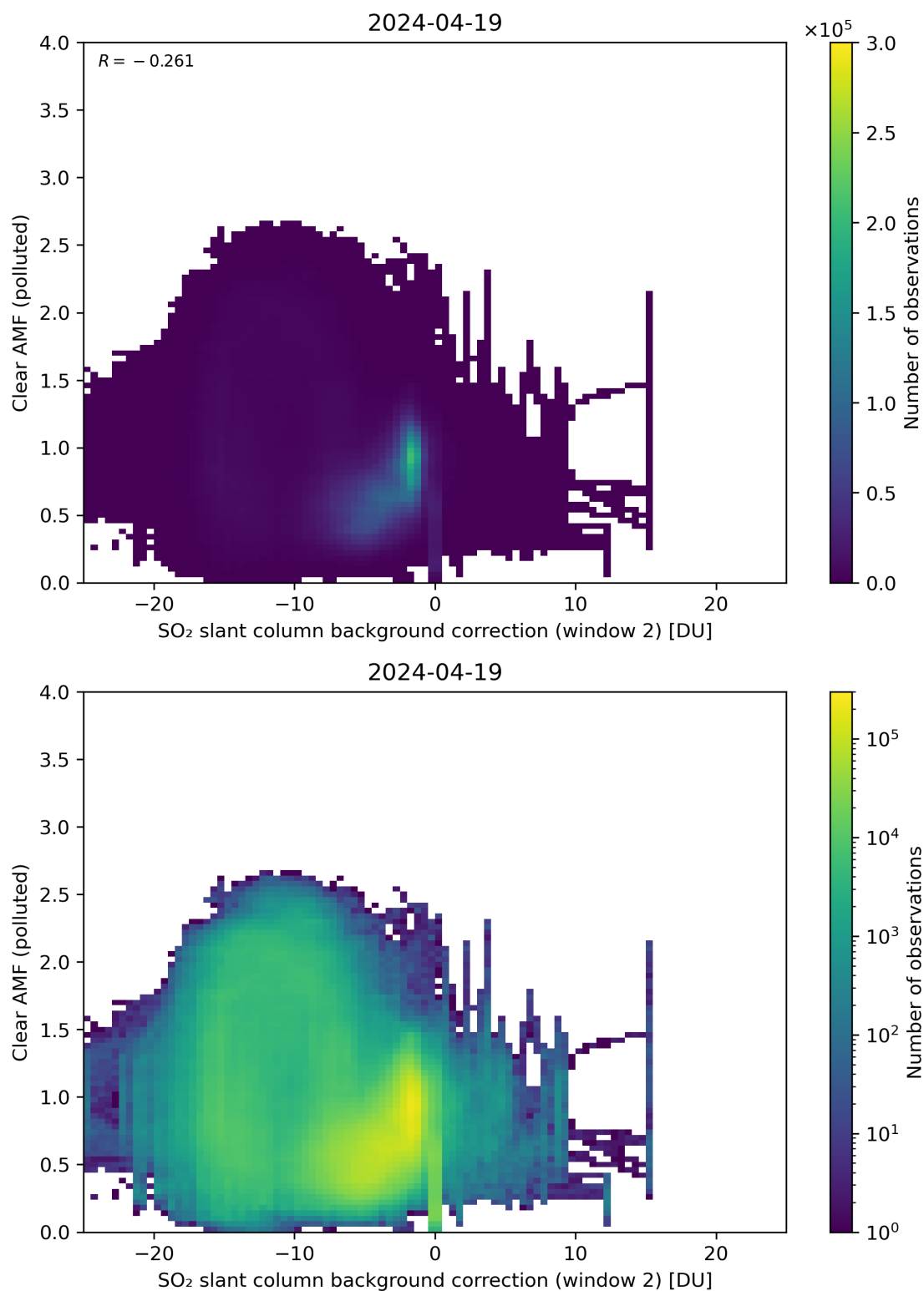
Figure 115: Scatter density plot of “SO 2 slant column background correction (window 2)” against “Clear AMF (polluted)” for 2024-04-18 to 2024-04-20.
