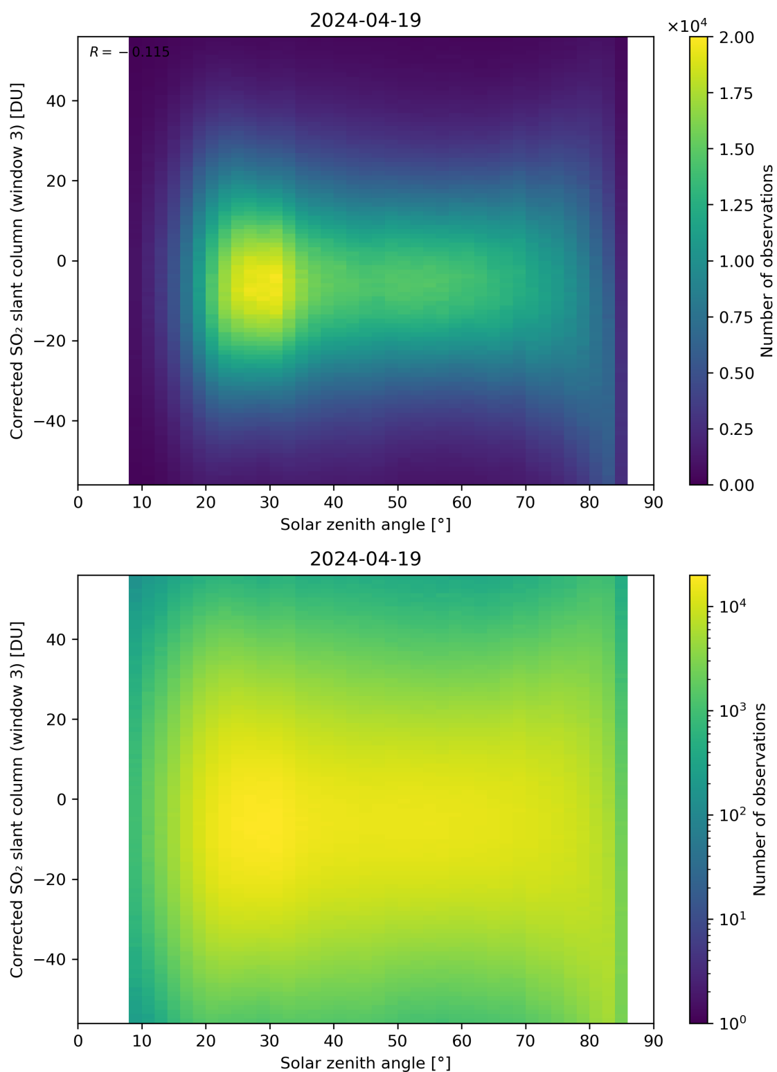
Figure 168: Scatter density plot of “Solar zenith angle” against “Corrected SO 2 slant column (window 3)” for 2024-04-18 to 2024-04-20.
