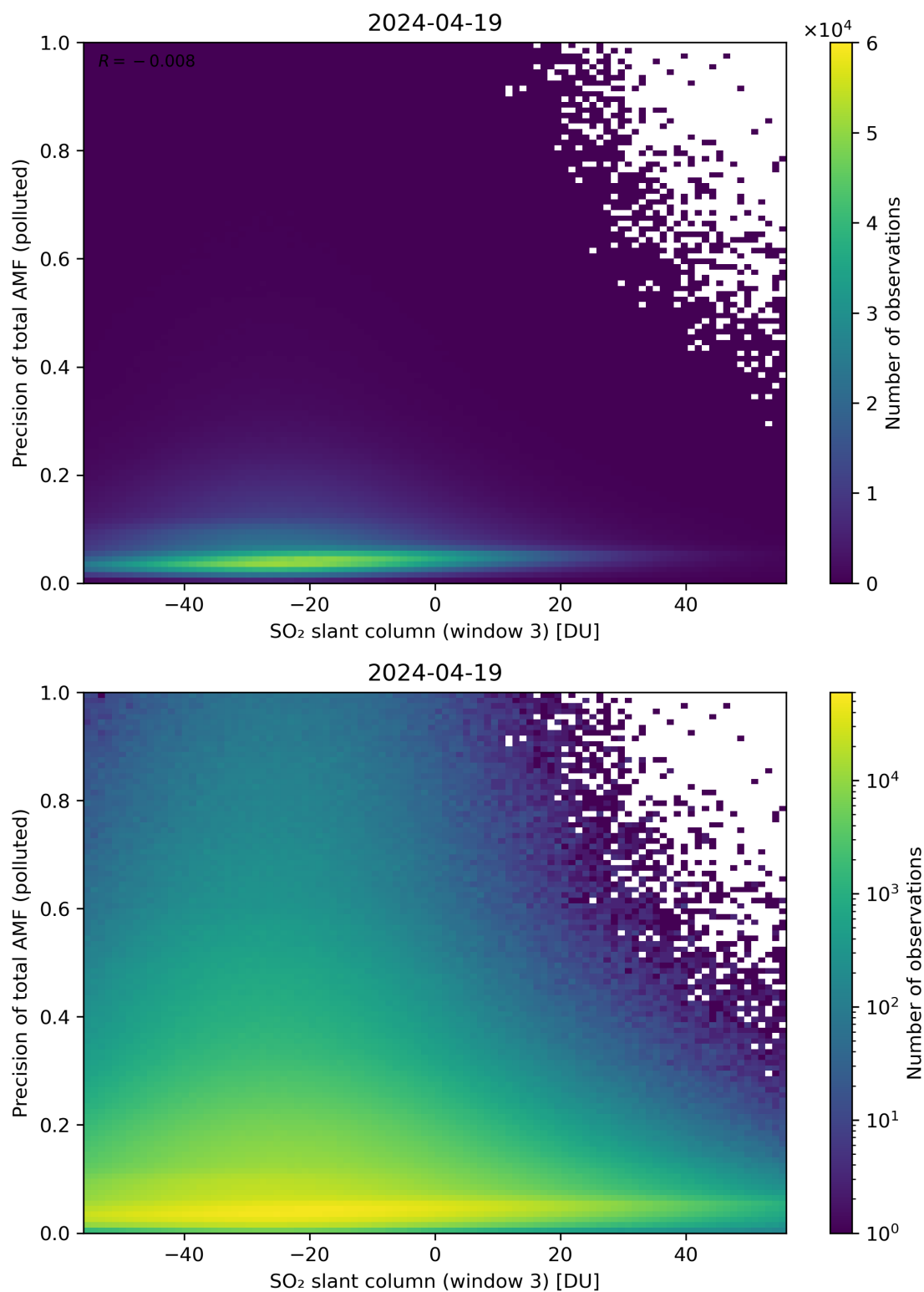
Figure 269: Scatter density plot of “SO 2 slant column (window 3)” against “Precision of total AMF (polluted)” for 2024-04-18 to 2024-04-20.
