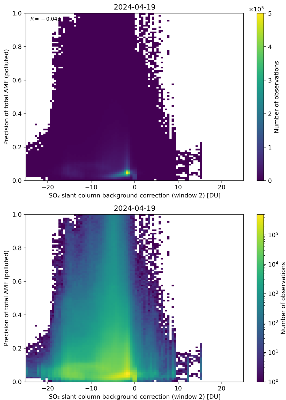
Figure 120: Scatter density plot of “SO 2 slant column background correction (window 2)” against “Precision of total AMF (polluted)” for 2024-04-18 to 2024-04-20.
