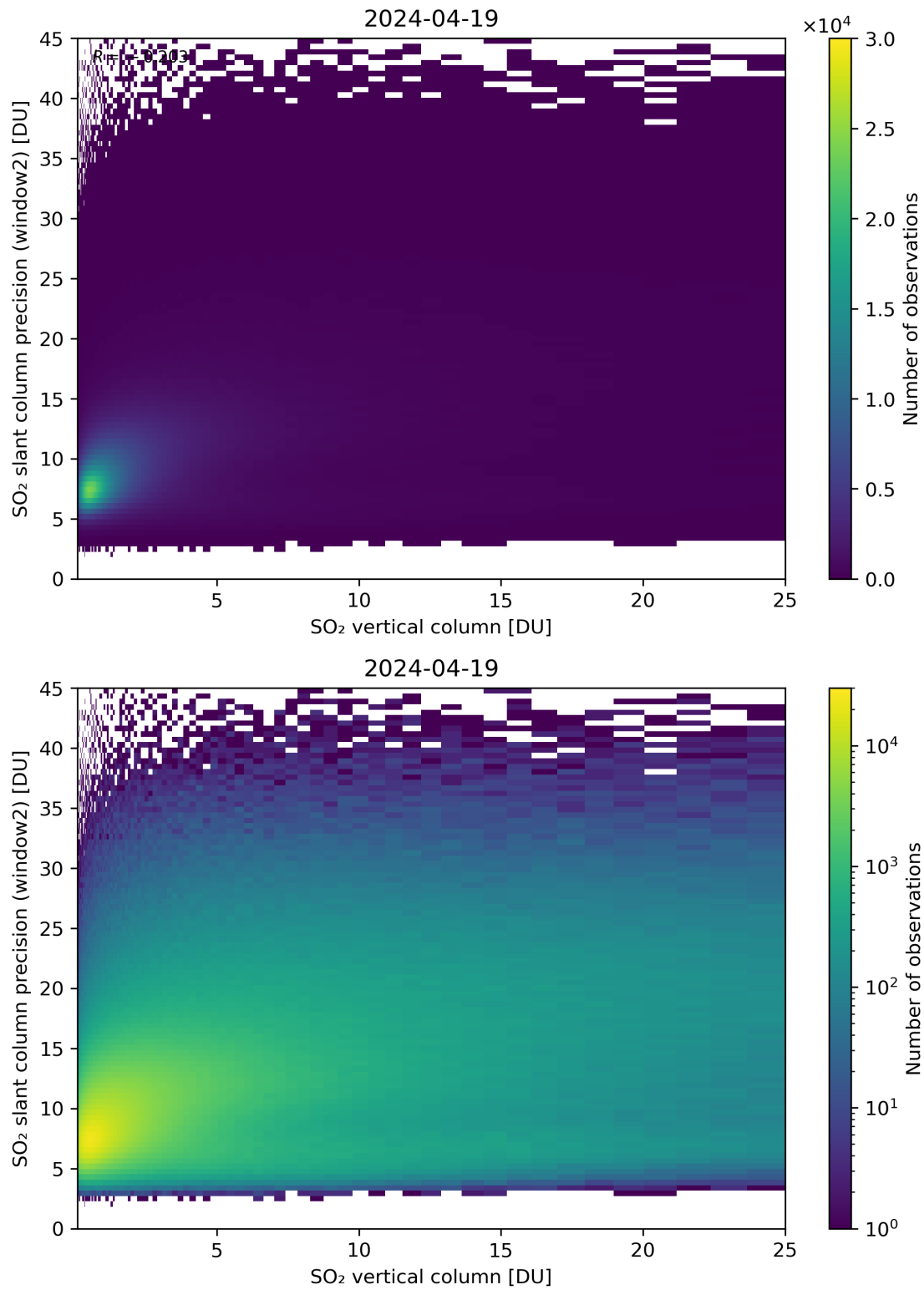
Figure 302: Scatter density plot of “SO 2 vertical column” against “SO 2 slant column precision (window2)” for 2024-04-18 to 2024-04-20.
