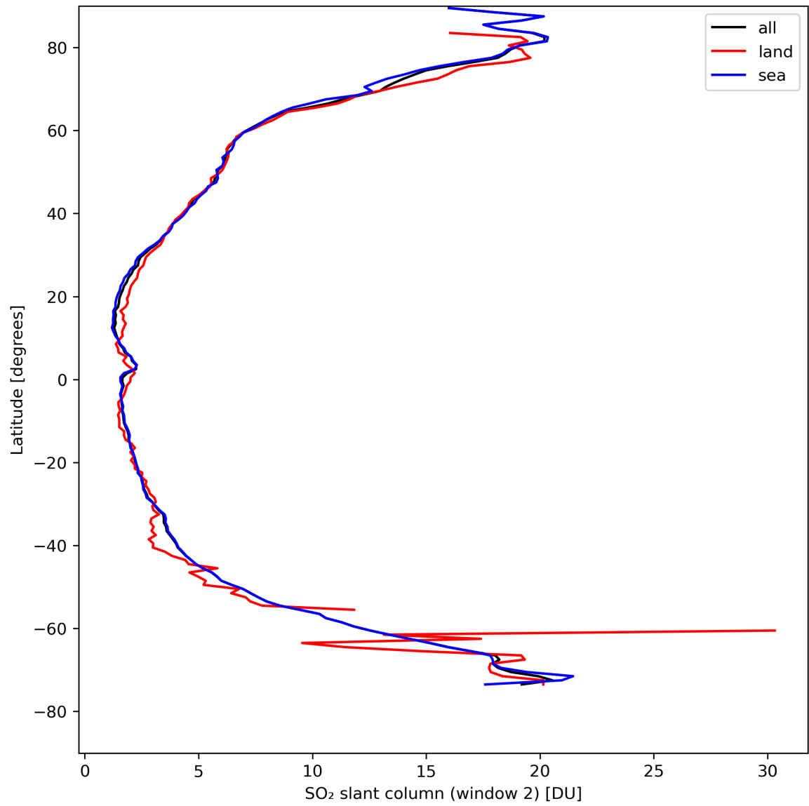
Figure 37: Zonal average of “SO 2 slant column (window 2)” for 2024-04-18 to 2024-04-20.
