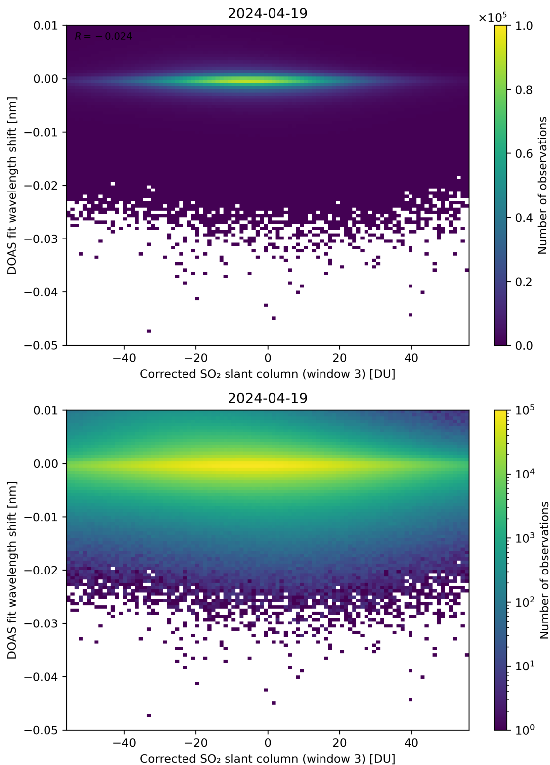
Figure 206: Scatter density plot of “Corrected SO 2 slant column (window 3)” against “DOAS fit wavelength shift” for 2024-04-18 to 2024-04-20.
