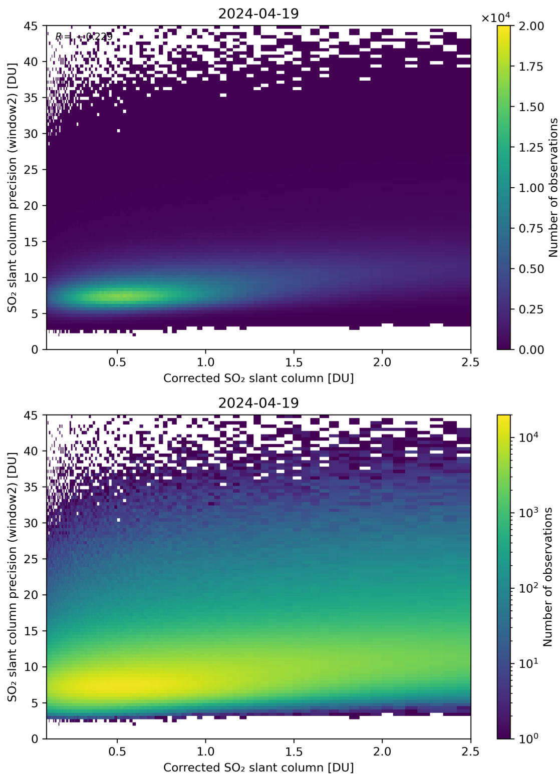
Figure 189: Scatter density plot of “Corrected SO 2 slant column” against “SO 2 slant column precision (window2)” for 2024-04-18 to 2024-04-20.
