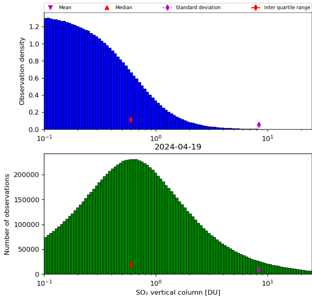
Figure 53: Histogram of “SO 2 vertical column” for 2024-04-18 to 2024-04-20
