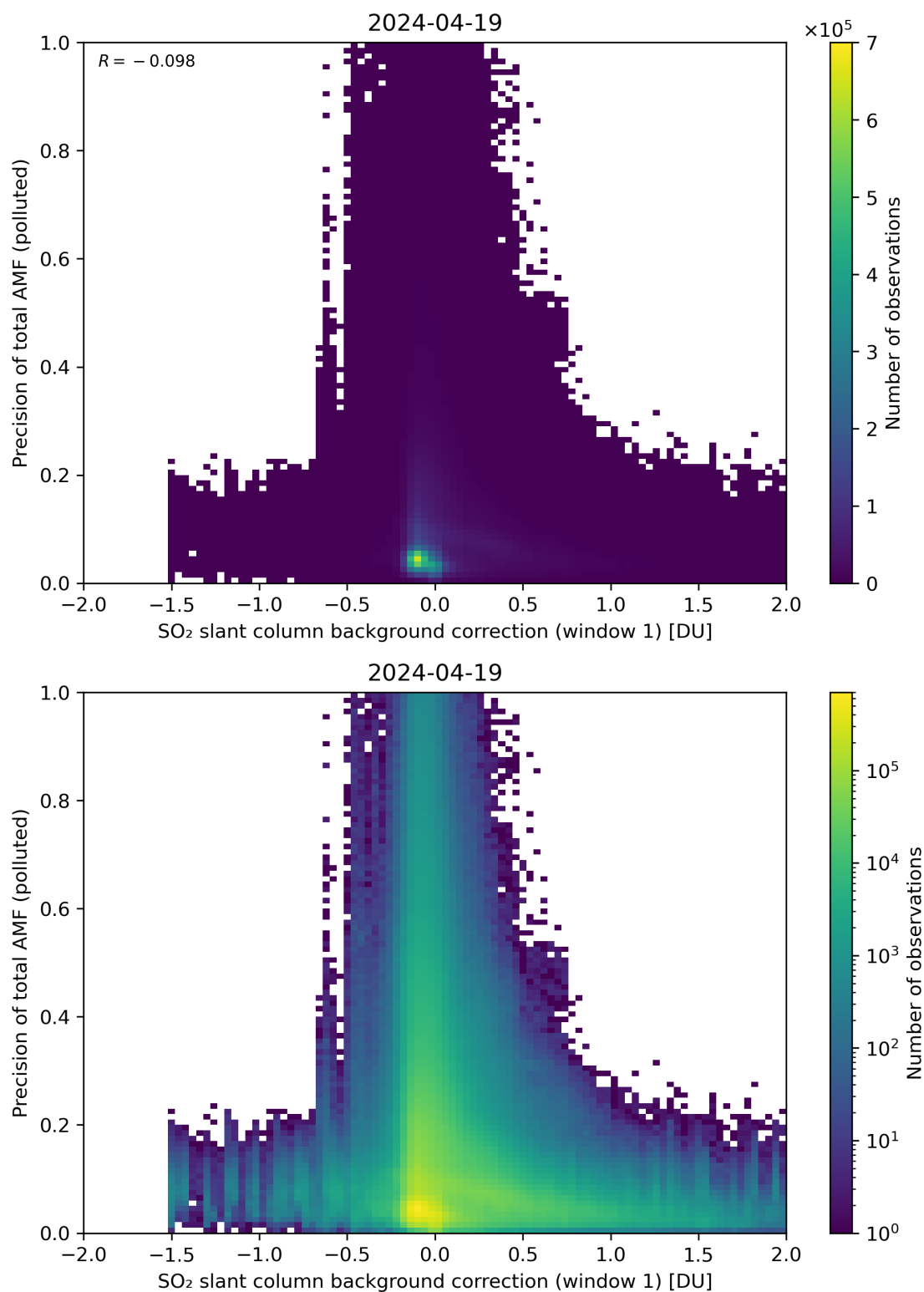
Figure 110: Scatter density plot of “SO 2 slant column background correction (window 1)” against “Precision of total AMF (polluted)” for 2024-04-18 to 2024-04-20.
