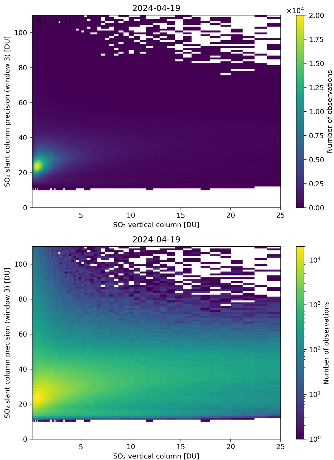
Figure 304: Scatter density plot of “SO 2 vertical column” against “SO 2 slant column precision (window 3)” for 2024-04-18 to 2024-04-20.
