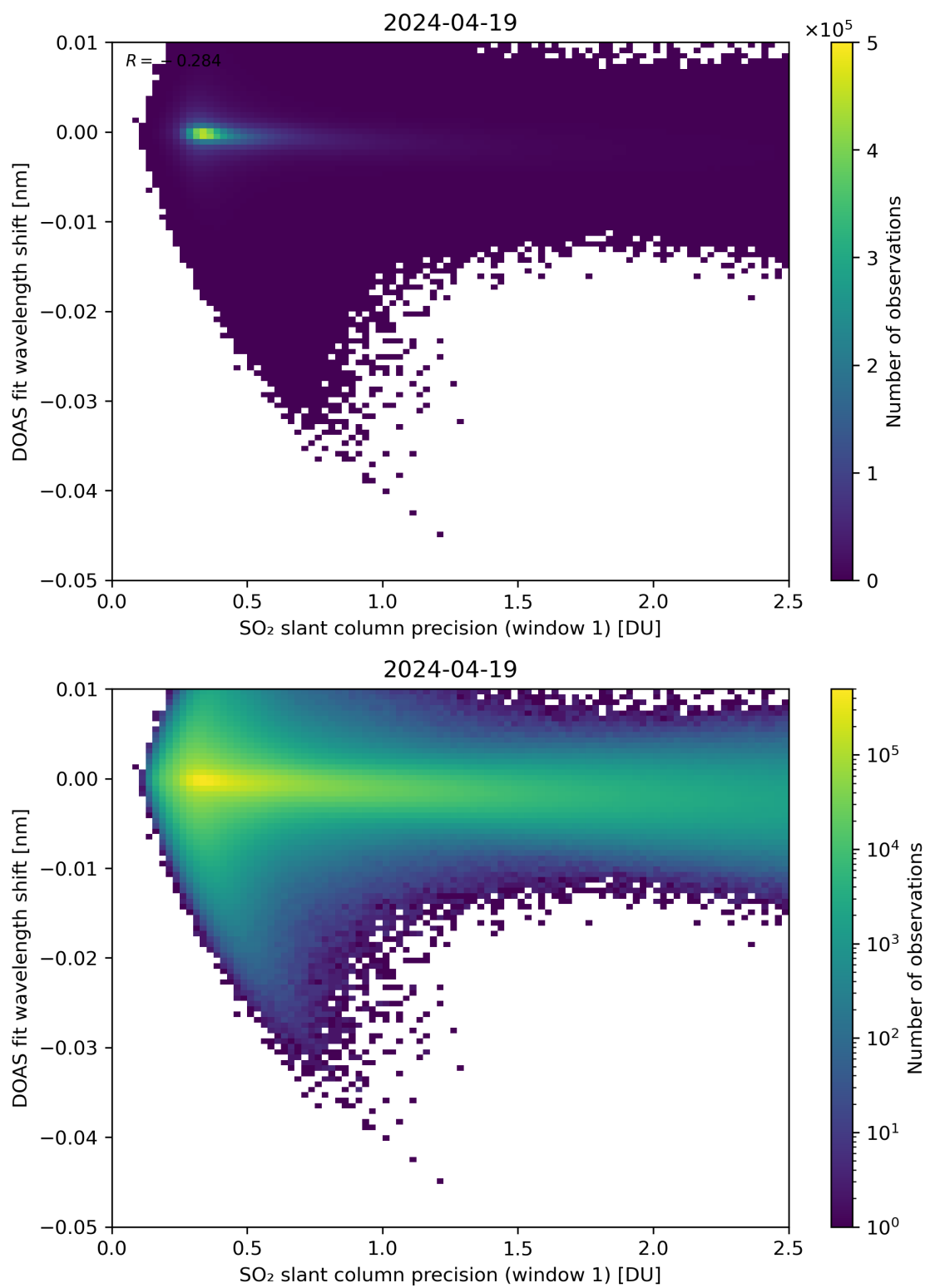
Figure 221: Scatter density plot of “SO 2 slant column precision (window 1)” against “DOAS fit wavelength shift” for 2024-04-18 to 2024-04-20.
