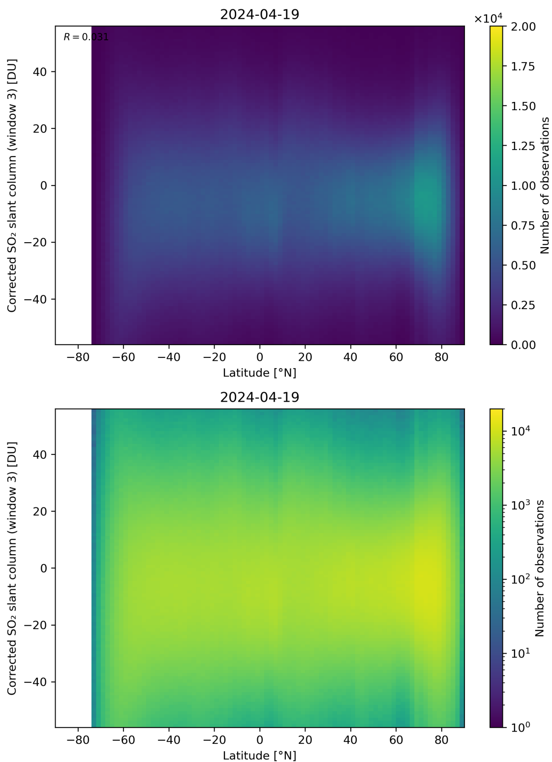
Figure 148: Scatter density plot of “Latitude” against “Corrected SO 2 slant column (window 3)” for 2024-04-18 to 2024-04-20.
