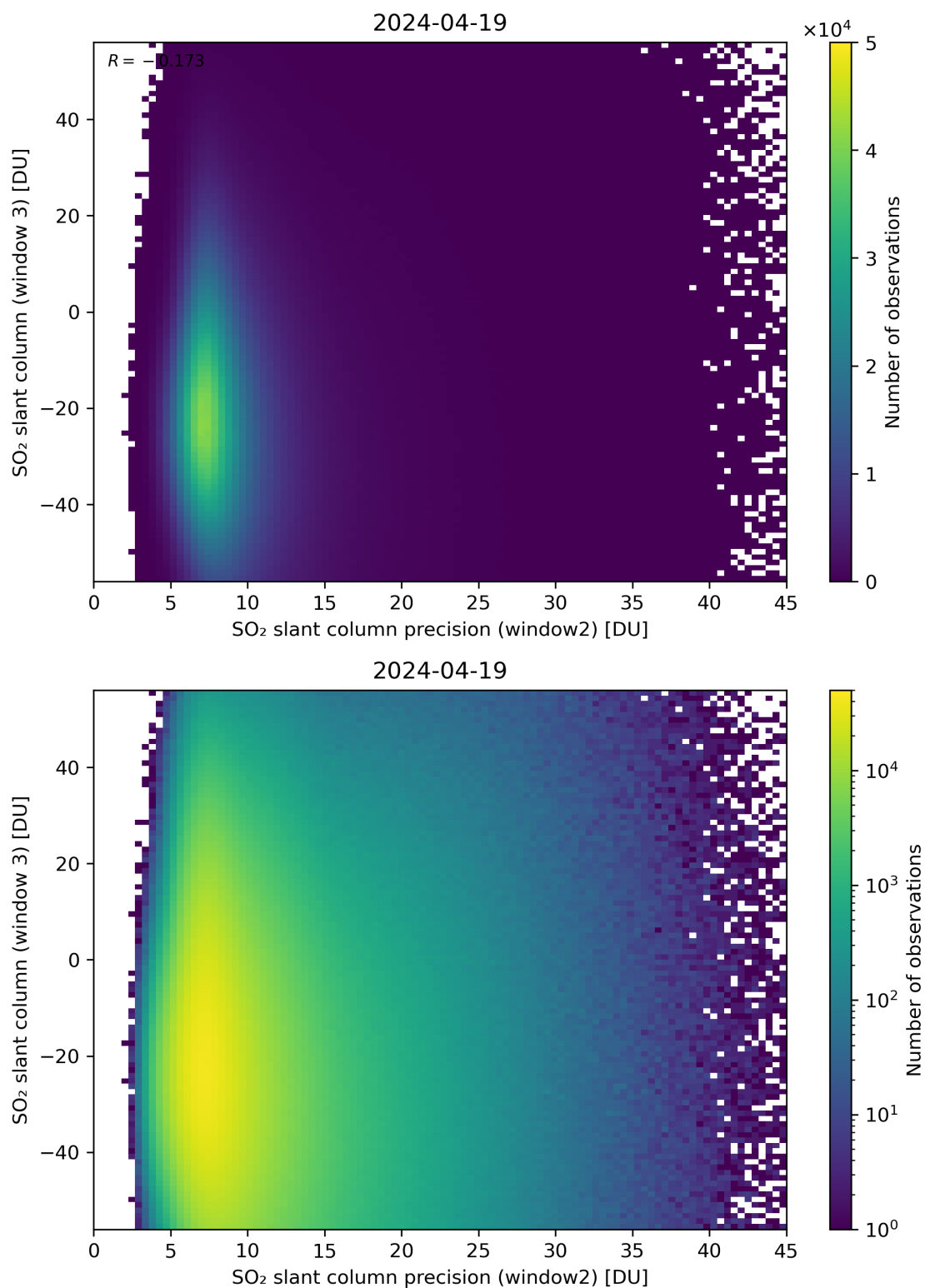
Figure 249: Scatter density plot of “SO 2 slant column precision (window2)” against “SO 2 slant column (window 3)” for 2024-04-18 to 2024-04-20.
