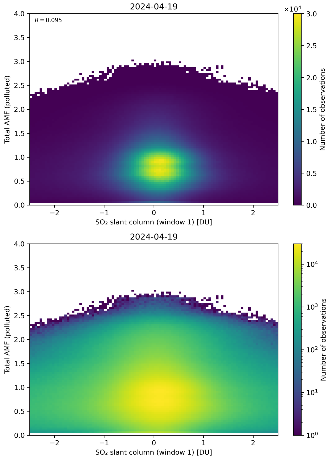
Figure 239: Scatter density plot of “SO 2 slant column (window 1)” against “Total AMF (polluted)” for 2024-04-18 to 2024-04-20.
