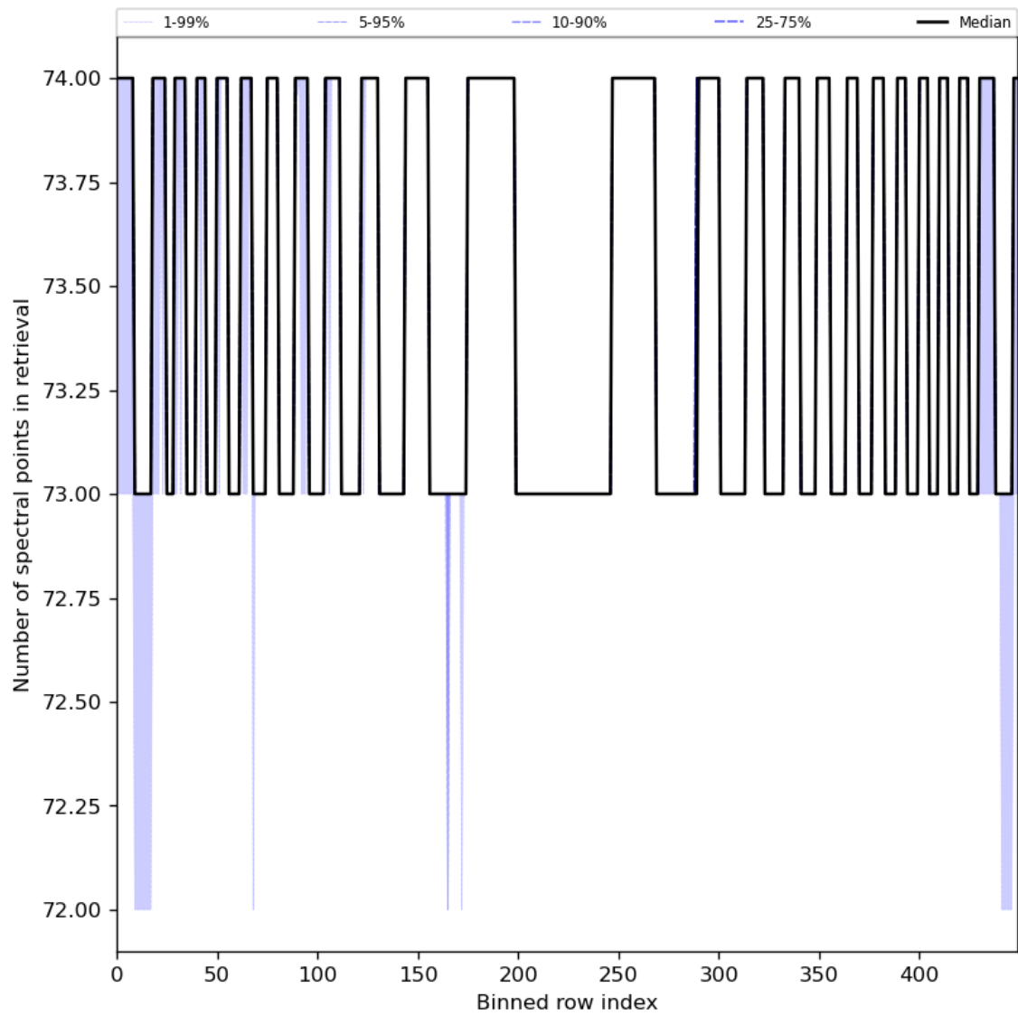
Figure 97: Along track statistics of “Number of spectral points in retrieval” for 2024-04-18 to 2024-04-20
