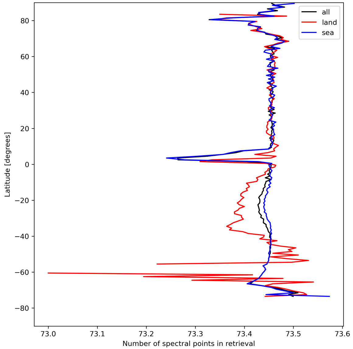
Figure 51: Zonal average of “Number of spectral points in retrieval” for 2024-04-18 to 2024-04-20.
