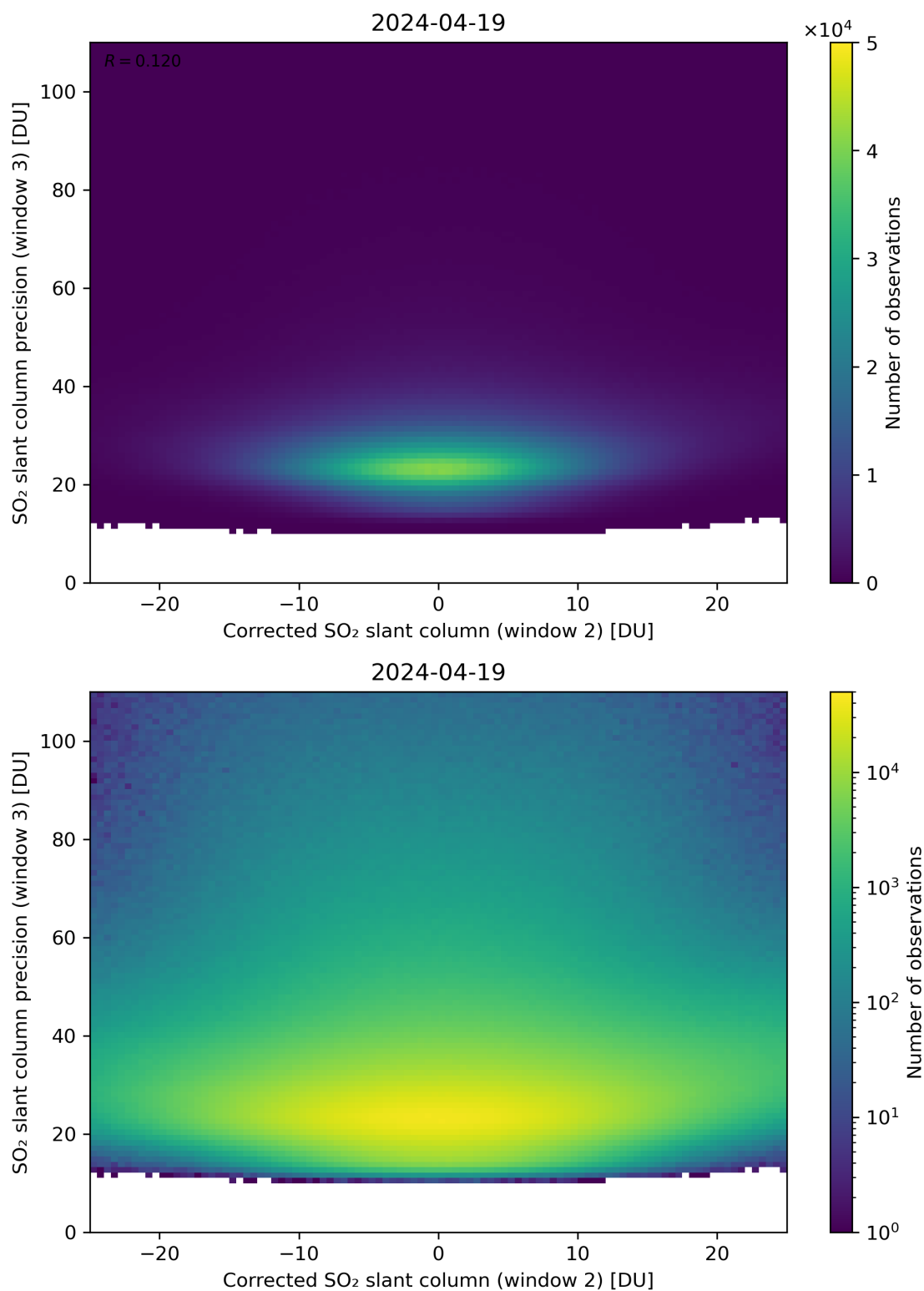
Figure 202: Scatter density plot of “Corrected SO 2 slant column (window 2)” against “SO 2 slant column precision (window 3)” for 2024-04-18 to 2024-04-20.
