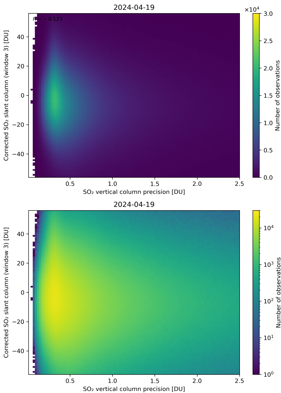
Figure 288: Scatter density plot of “SO 2 vertical column precision” against “Corrected SO 2 slant column (window 3)” for 2024-04-18 to 2024-04-20.
