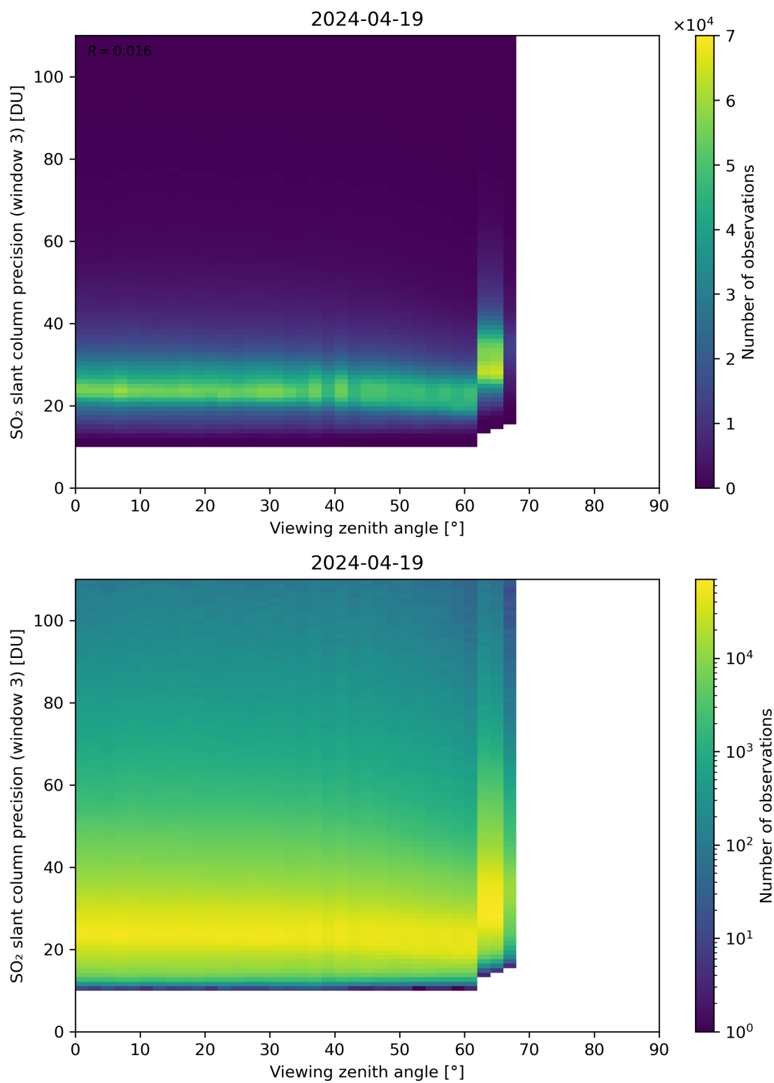
Figure 324: Scatter density plot of “Viewing zenith angle” against “SO 2 slant column precision (window 3)” for 2024-04-18 to 2024-04-20.
