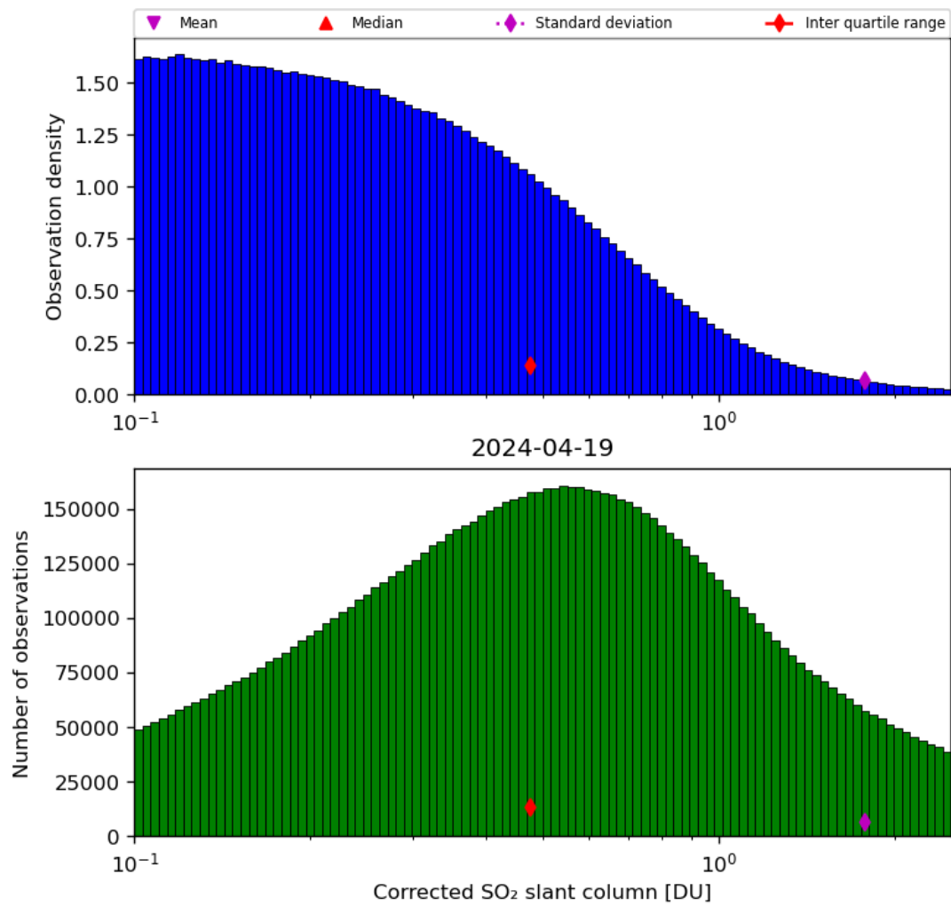
Figure 55: Histogram of “Corrected SO 2 slant column” for 2024-04-18 to 2024-04-20
