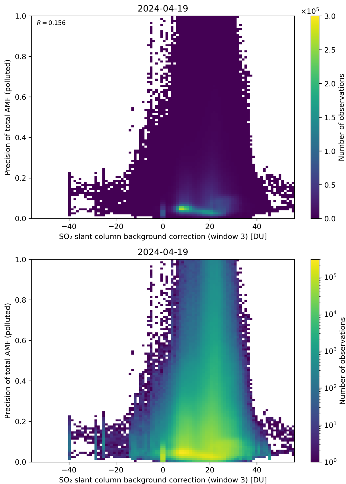
Figure 126: Scatter density plot of “SO 2 slant column background correction (window 3)” against “Precision of total AMF (polluted)” for 2024-04-18 to 2024-04-20.
