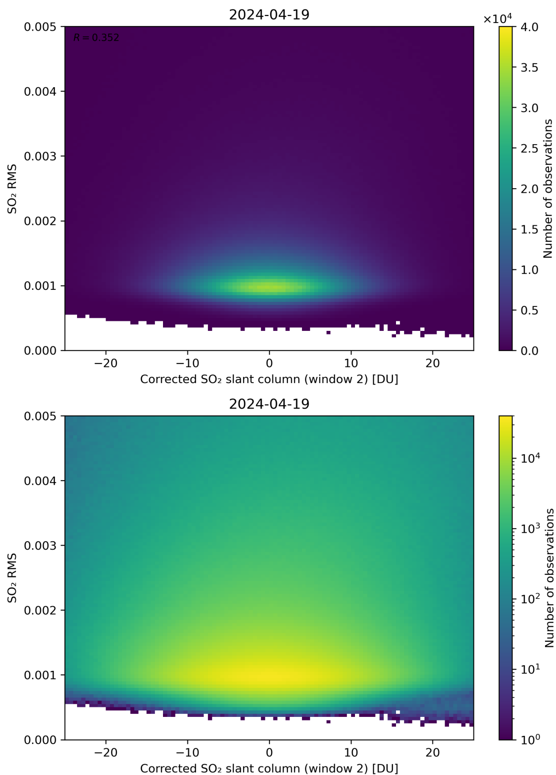
Figure 198: Scatter density plot of “Corrected SO 2 slant column (window 2)” against “SO 2 RMS” for 2024-04-18 to 2024-04-20.
