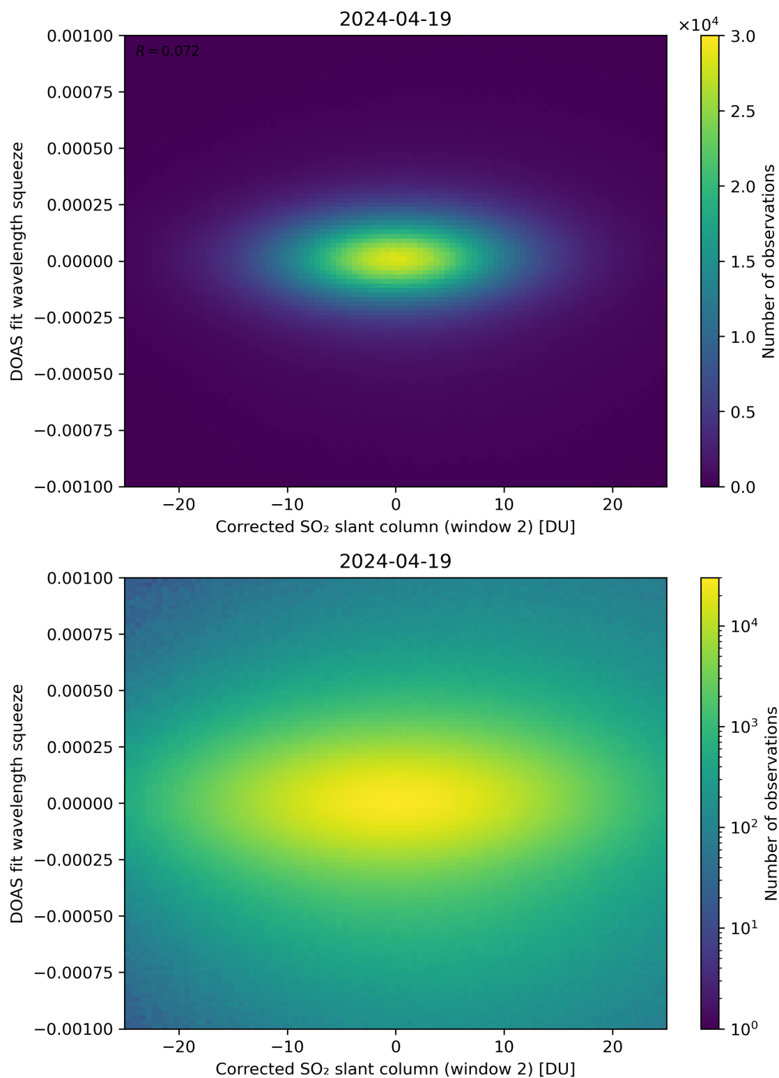
Figure 197: Scatter density plot of “Corrected SO 2 slant column (window 2)” against “DOAS fit wavelength squeeze” for 2024-04-18 to 2024-04-20.
