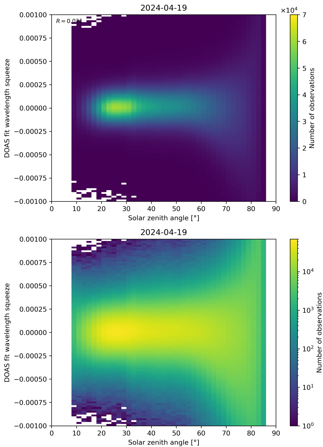
Figure 162: Scatter density plot of “Solar zenith angle” against “DOAS fit wavelength squeeze” for 2024-04-18 to 2024-04-20.
