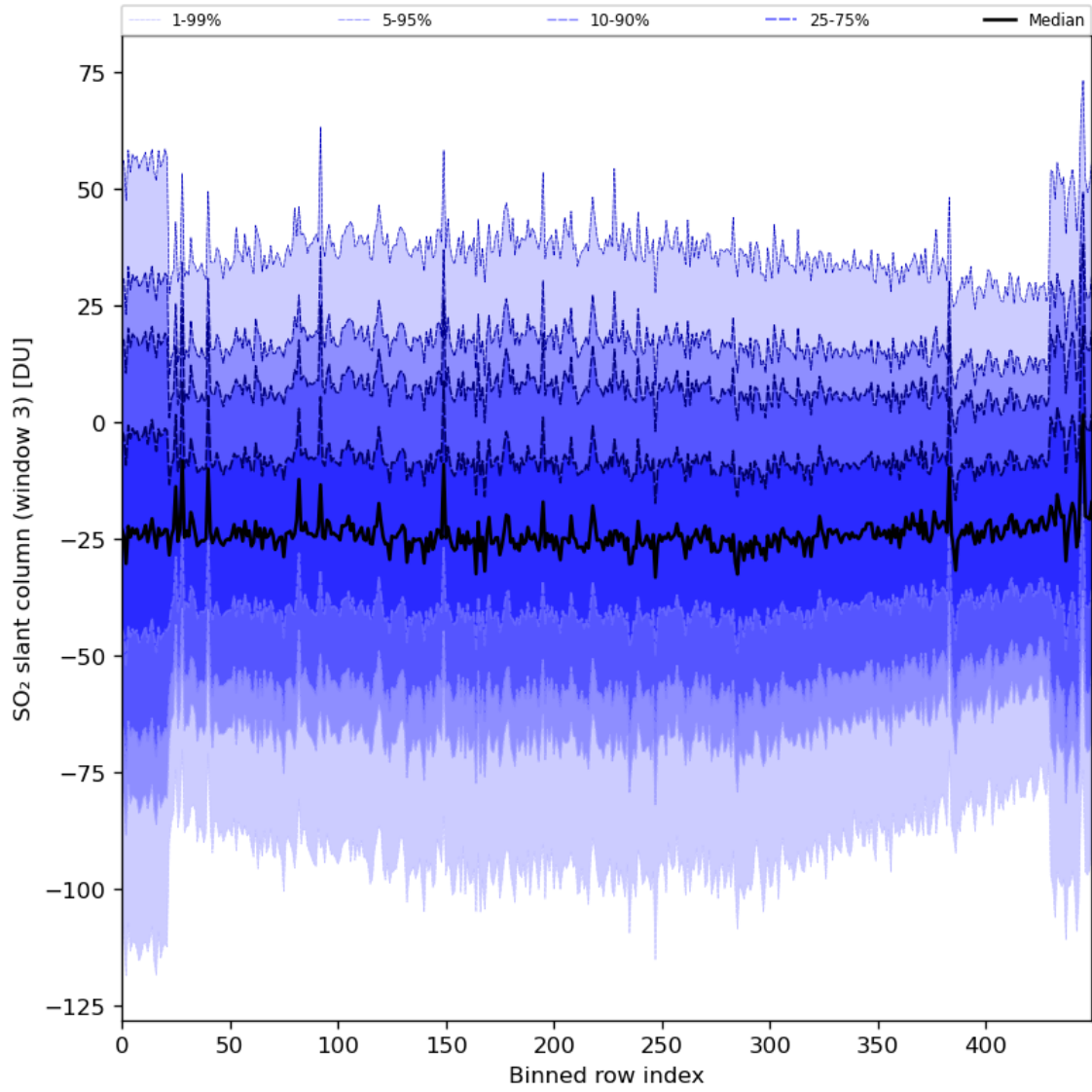
Figure 87: Along track statistics of “SO 2 slant column (window 3)” for 2024-04-18 to 2024-04-20
