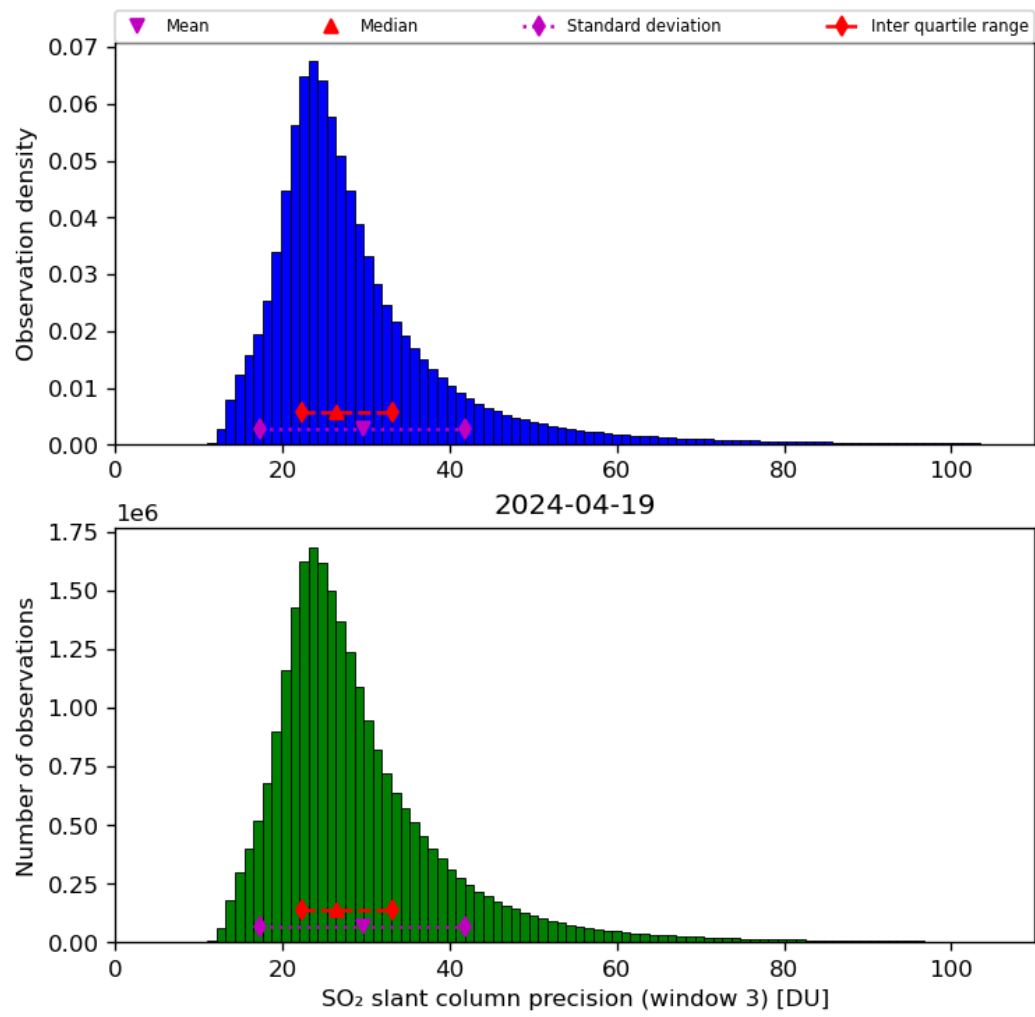
Figure 65: Histogram of “SO 2 slant column precision (window 3)” for 2024-04-18 to 2024-04-20
