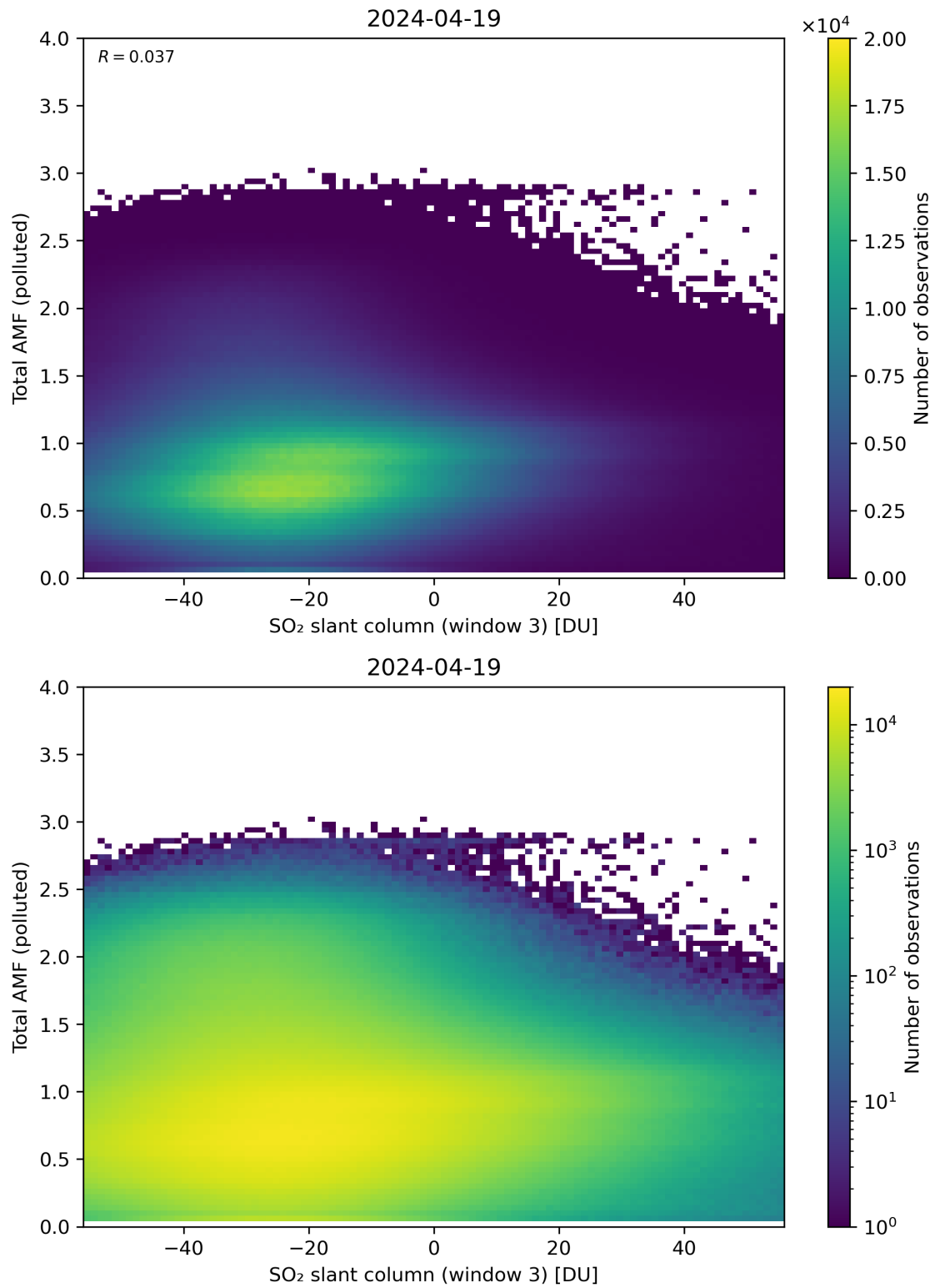
Figure 268: Scatter density plot of “SO 2 slant column (window 3)” against “Total AMF (polluted)” for 2024-04-18 to 2024-04-20.
