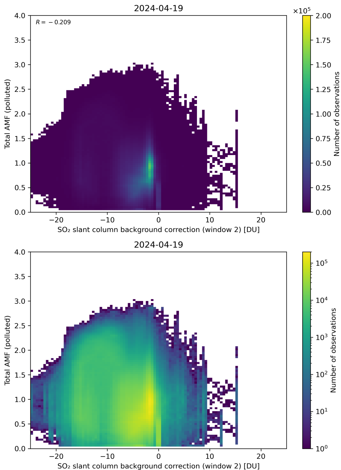
Figure 119: Scatter density plot of “SO 2 slant column background correction (window 2)” against “Total AMF (polluted)” for 2024-04-18 to 2024-04-20.
