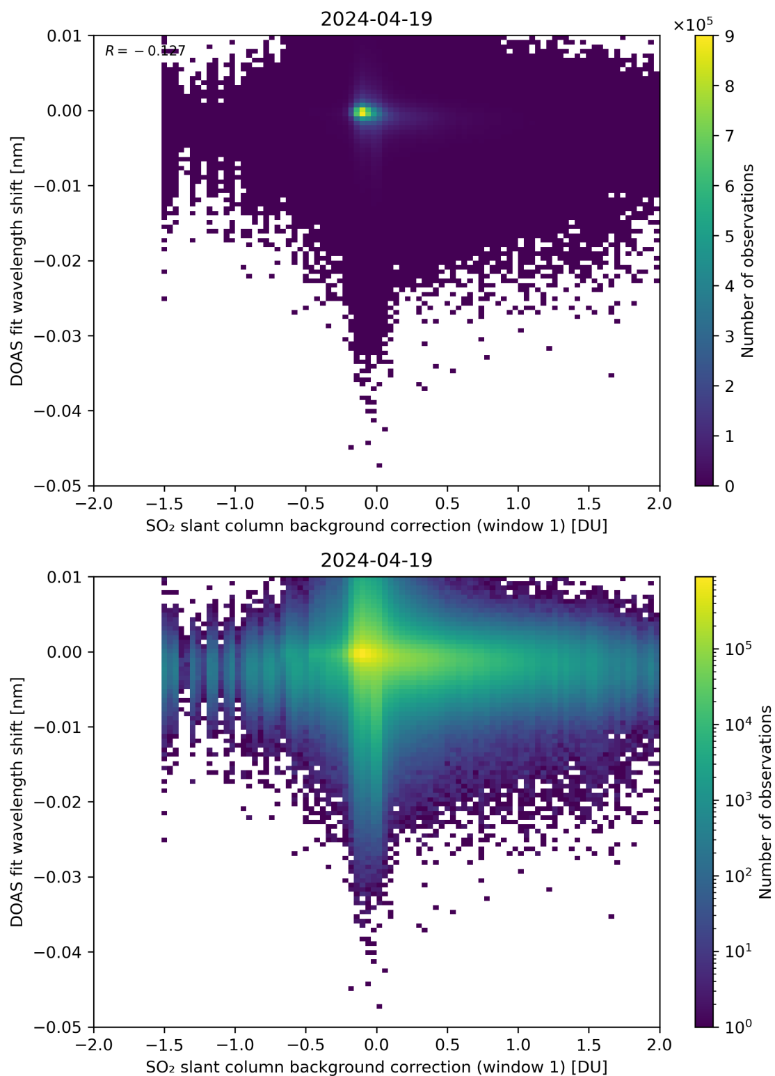
Figure 100: Scatter density plot of “SO 2 slant column background correction (window 1)” against “DOAS fit wavelength shift” for 2024-04-18 to 2024-04-20.
