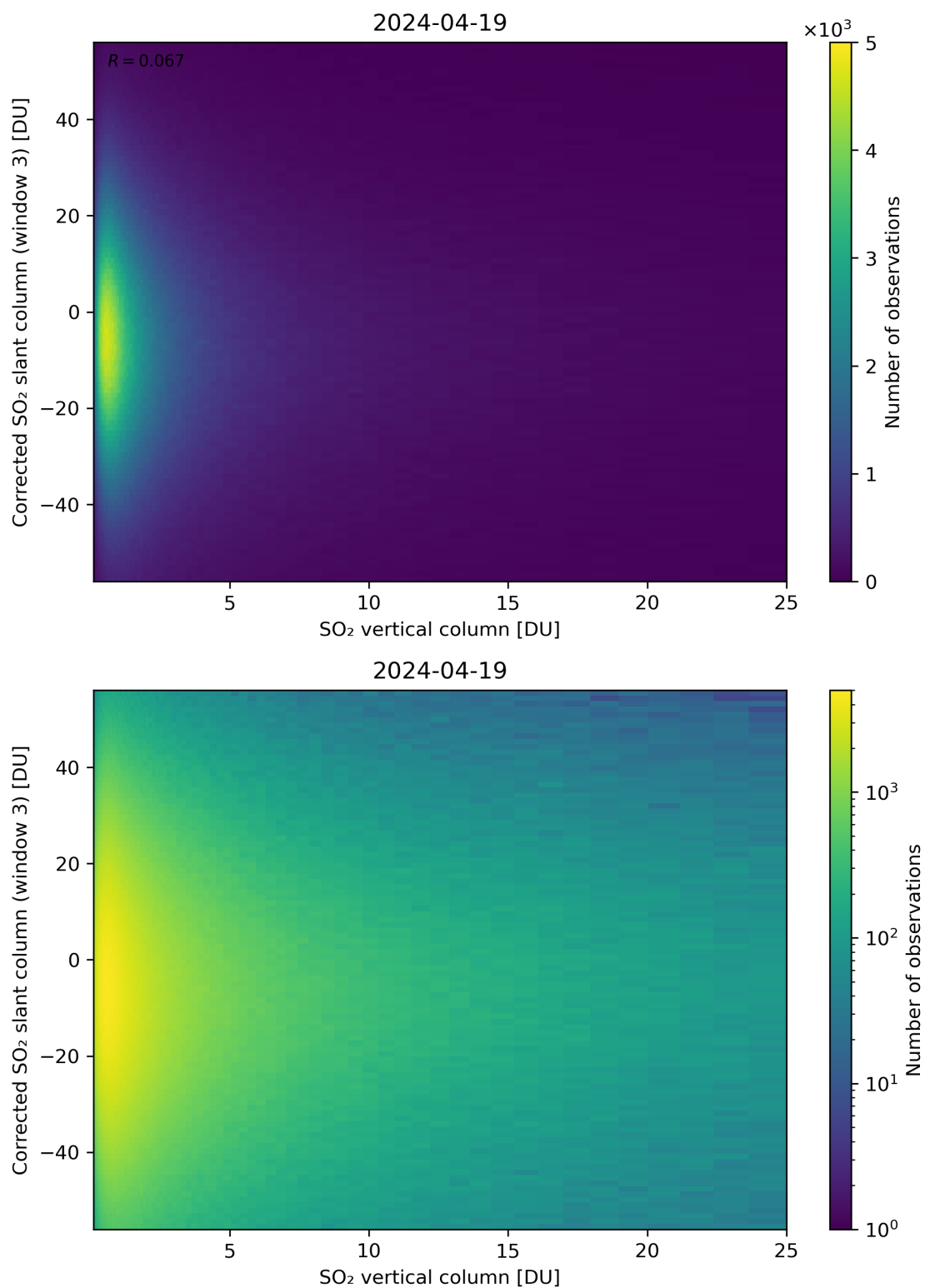
Figure 299: Scatter density plot of “SO 2 vertical column” against “Corrected SO 2 slant column (window 3)” for 2024-04-18 to 2024-04-20.
