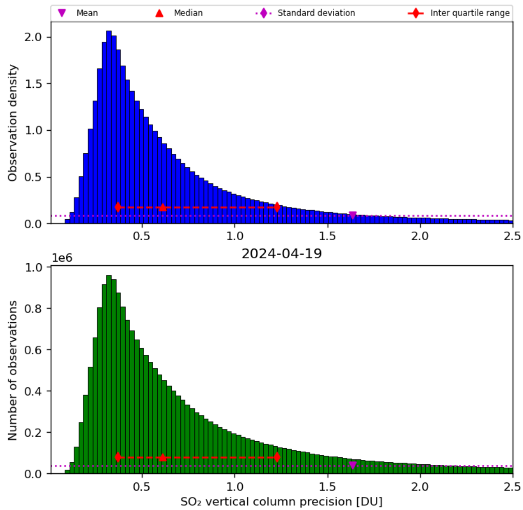
Figure 54: Histogram of “SO 2 vertical column precision” for 2024-04-18 to 2024-04-20
