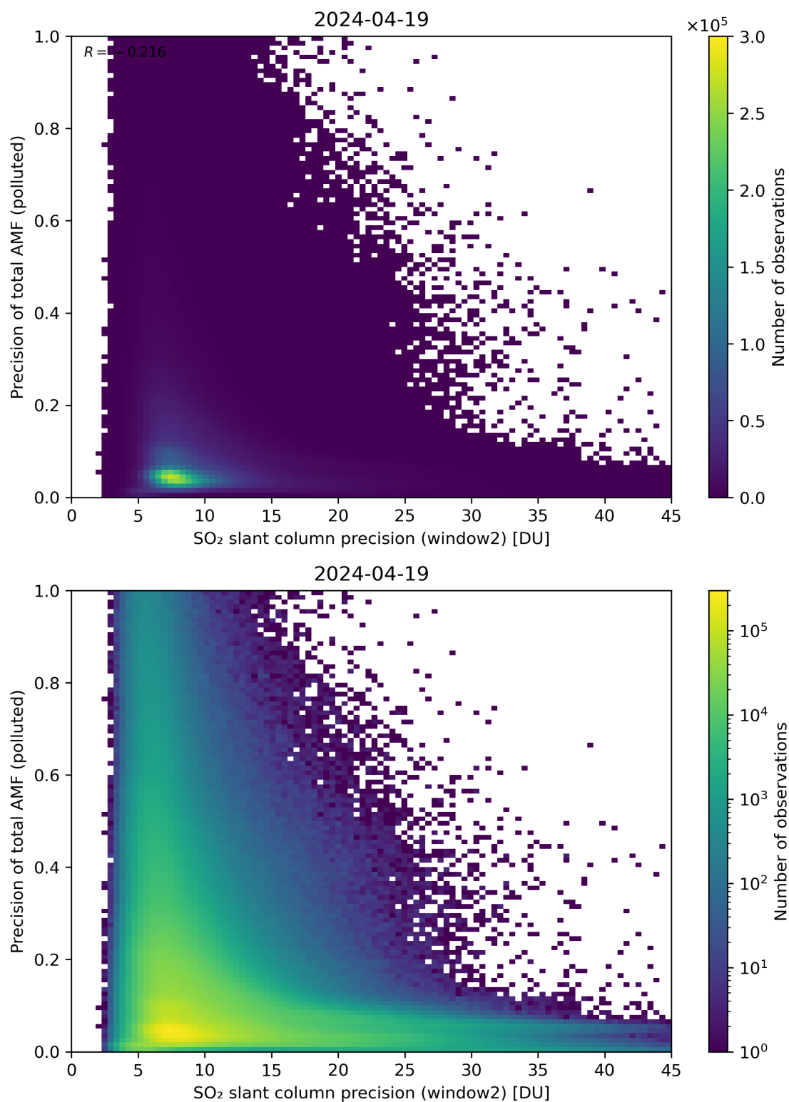
Figure 252: Scatter density plot of “SO 2 slant column precision (window2)” against “Precision of total AMF (polluted)” for 2024-04-18 to 2024-04-20.
