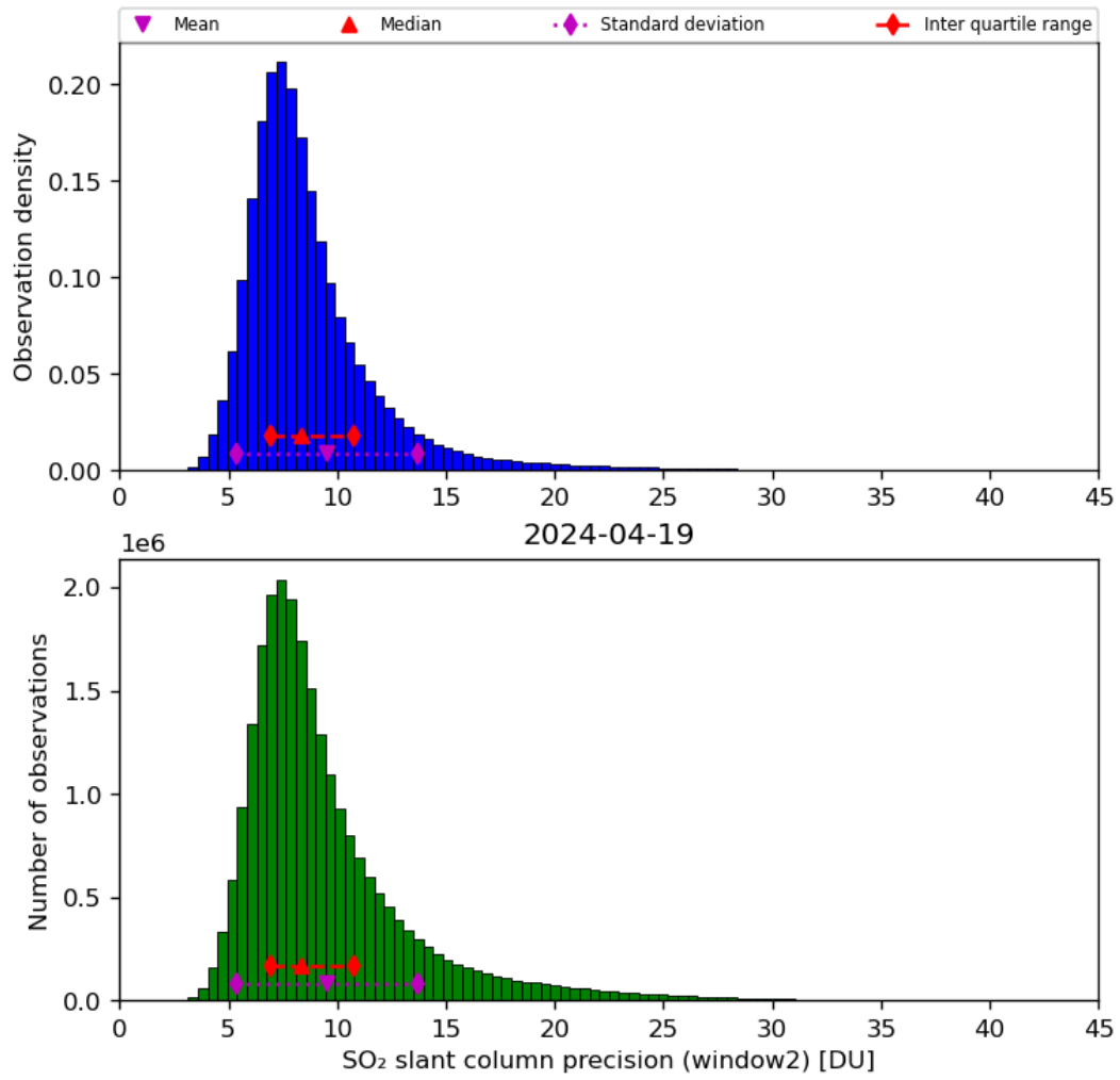
Figure 61: Histogram of “SO 2 slant column precision (window2)” for 2024-04-18 to 2024-04-20
