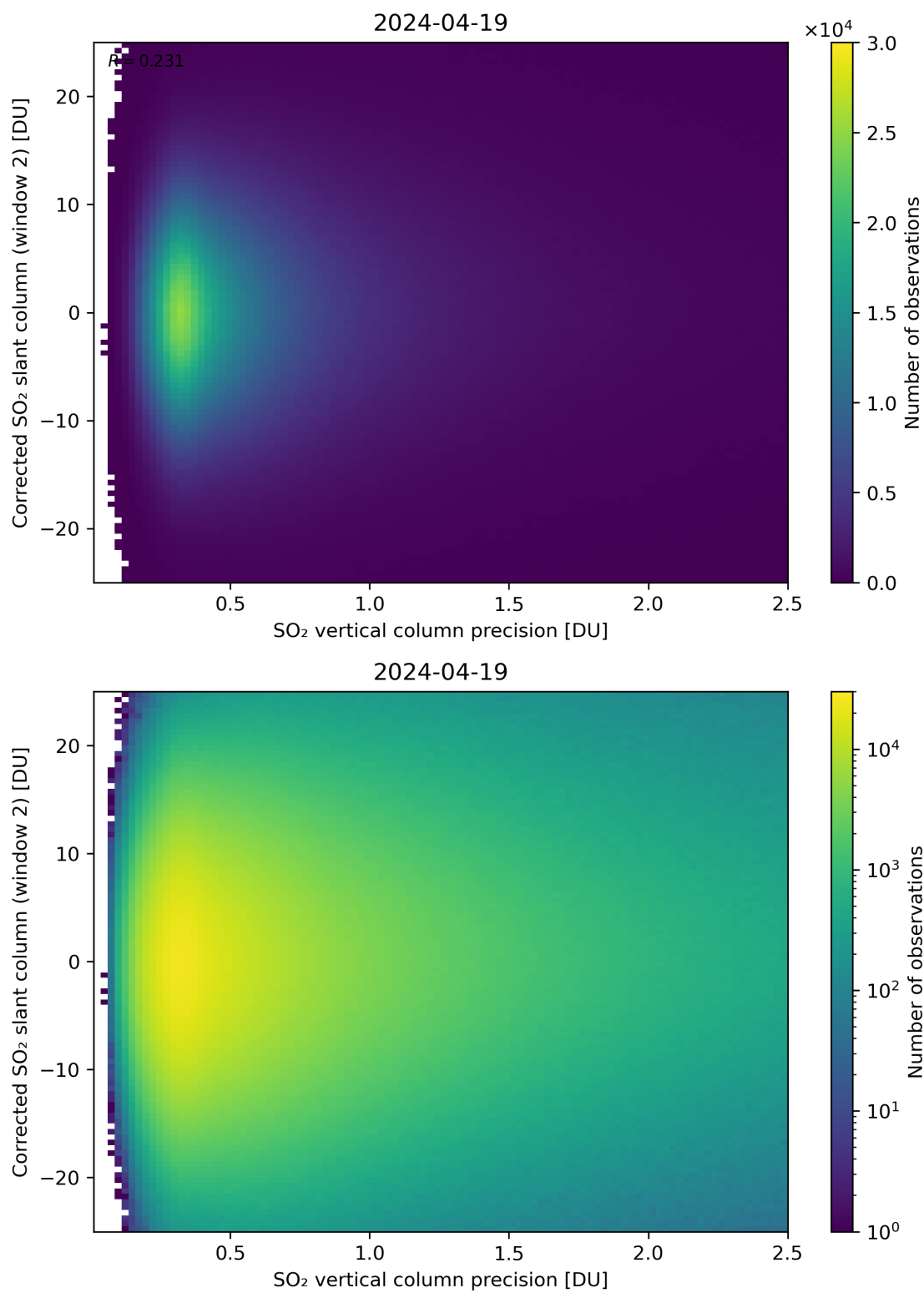
Figure 287: Scatter density plot of “SO 2 vertical column precision” against “Corrected SO 2 slant column (window 2)” for 2024-04-18 to 2024-04-20.
