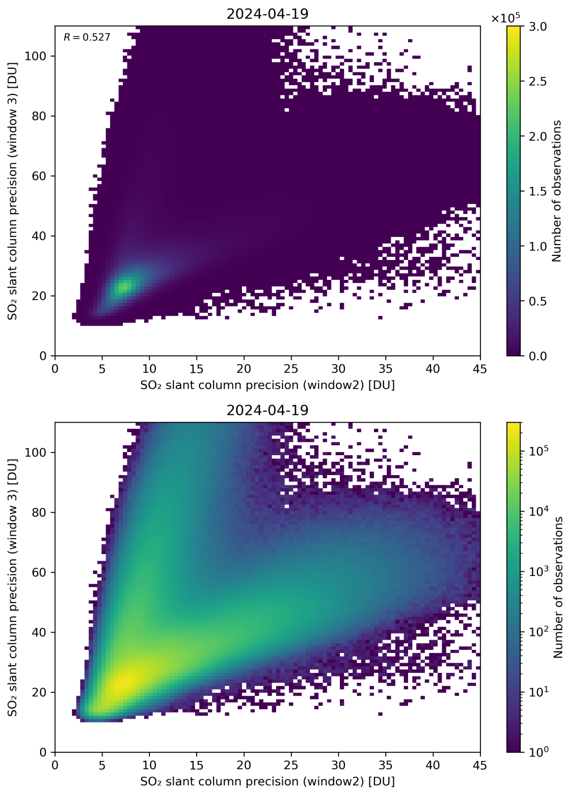
Figure 250: Scatter density plot of “SO 2 slant column precision (window2)” against “SO 2 slant column precision (window 3)” for 2024-04-18 to 2024-04-20.
