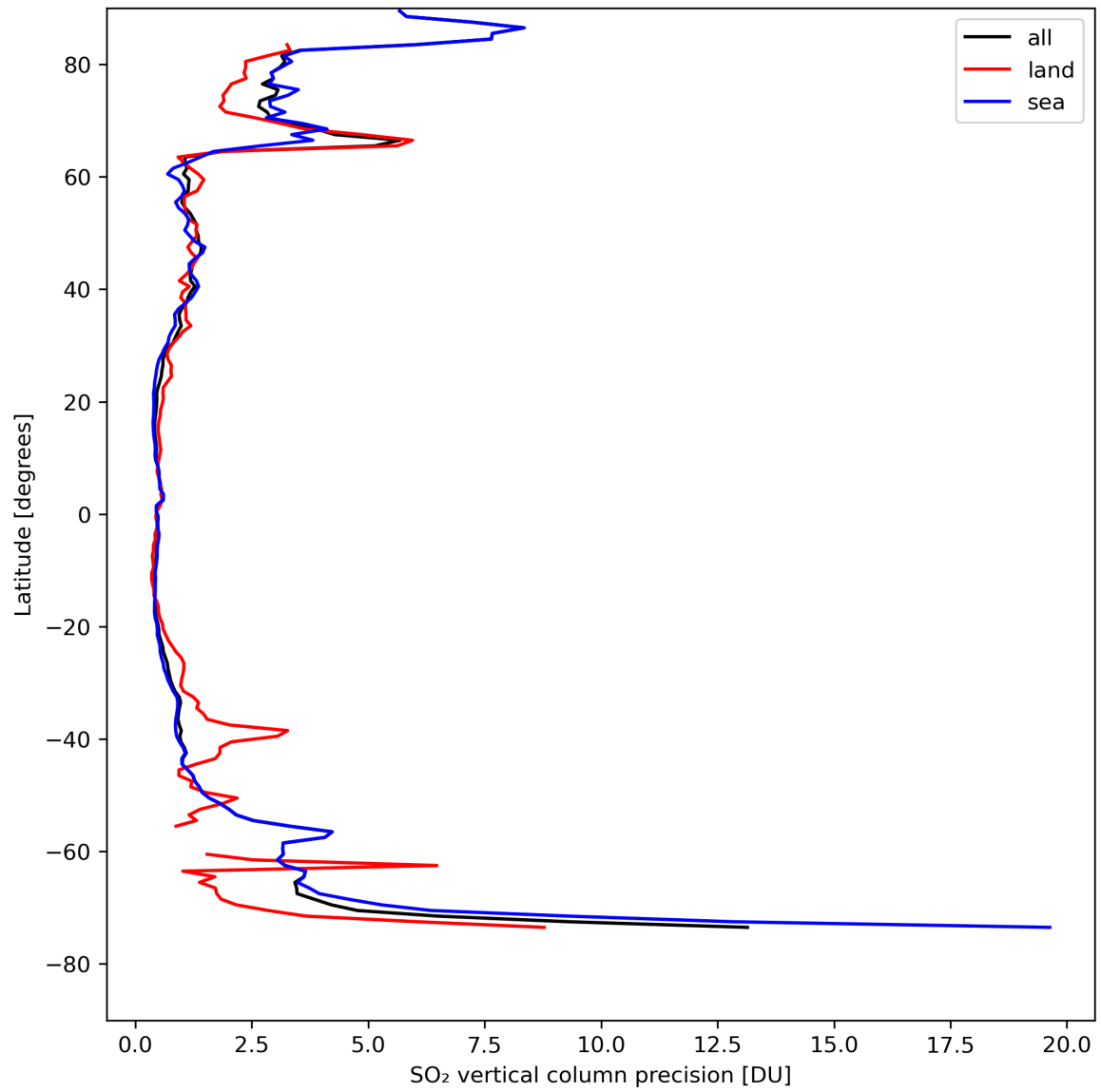
Figure 31: Zonal average of “SO 2 vertical column precision” for 2024-04-18 to 2024-04-20.
