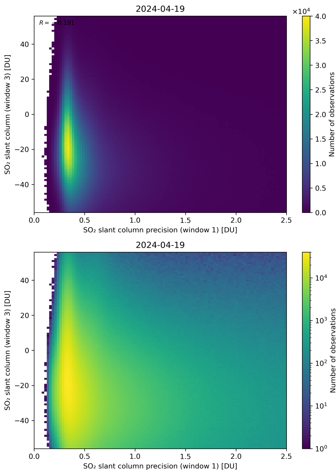
Figure 228: Scatter density plot of “SO 2 slant column precision (window 1)” against “SO 2 slant column (window 3)” for 2024-04-18 to 2024-04-20.
