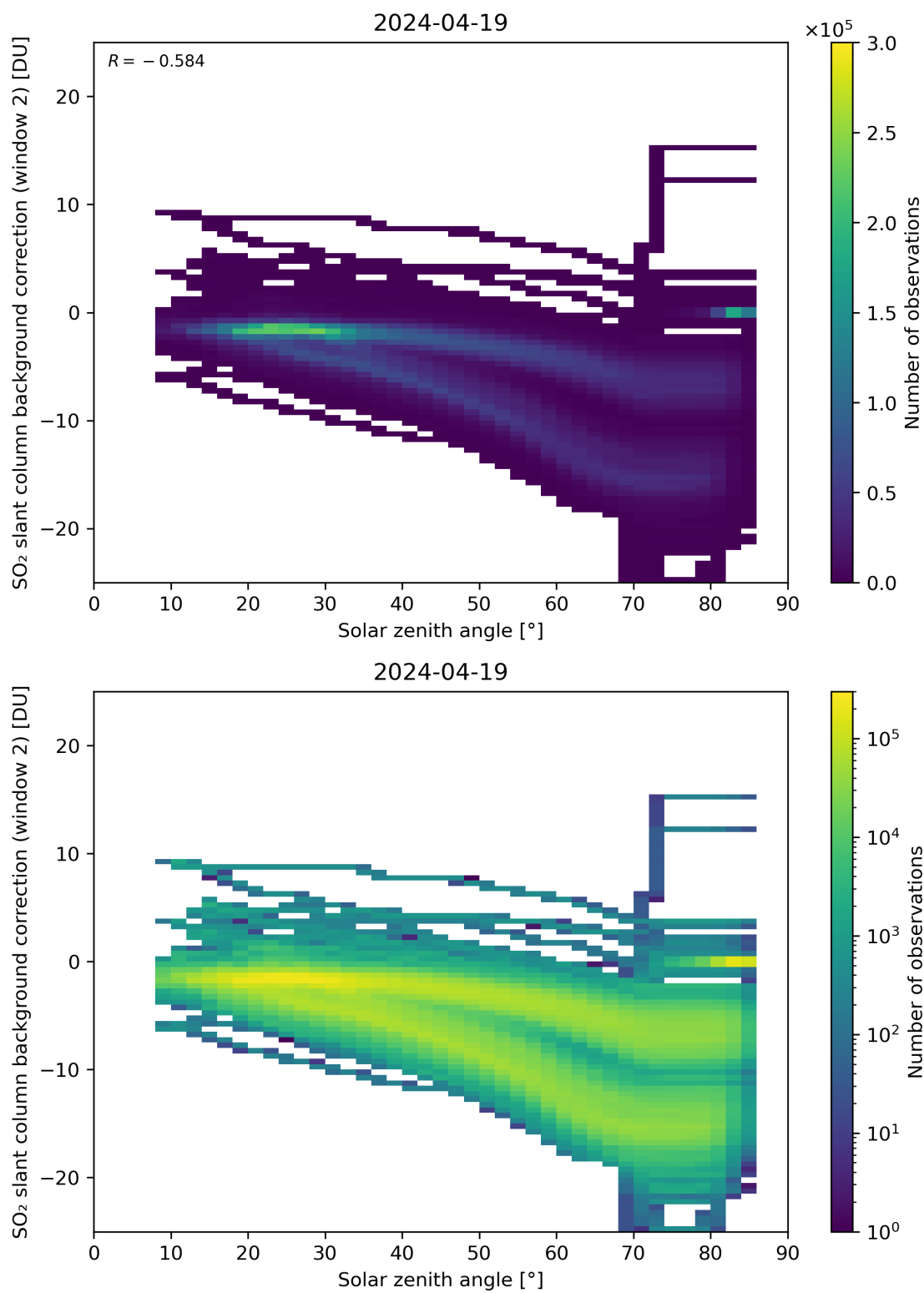
Figure 159: Scatter density plot of “Solar zenith angle” against “SO 2 slant column background correction (window 2)” for 2024-04-18 to 2024-04-20.
