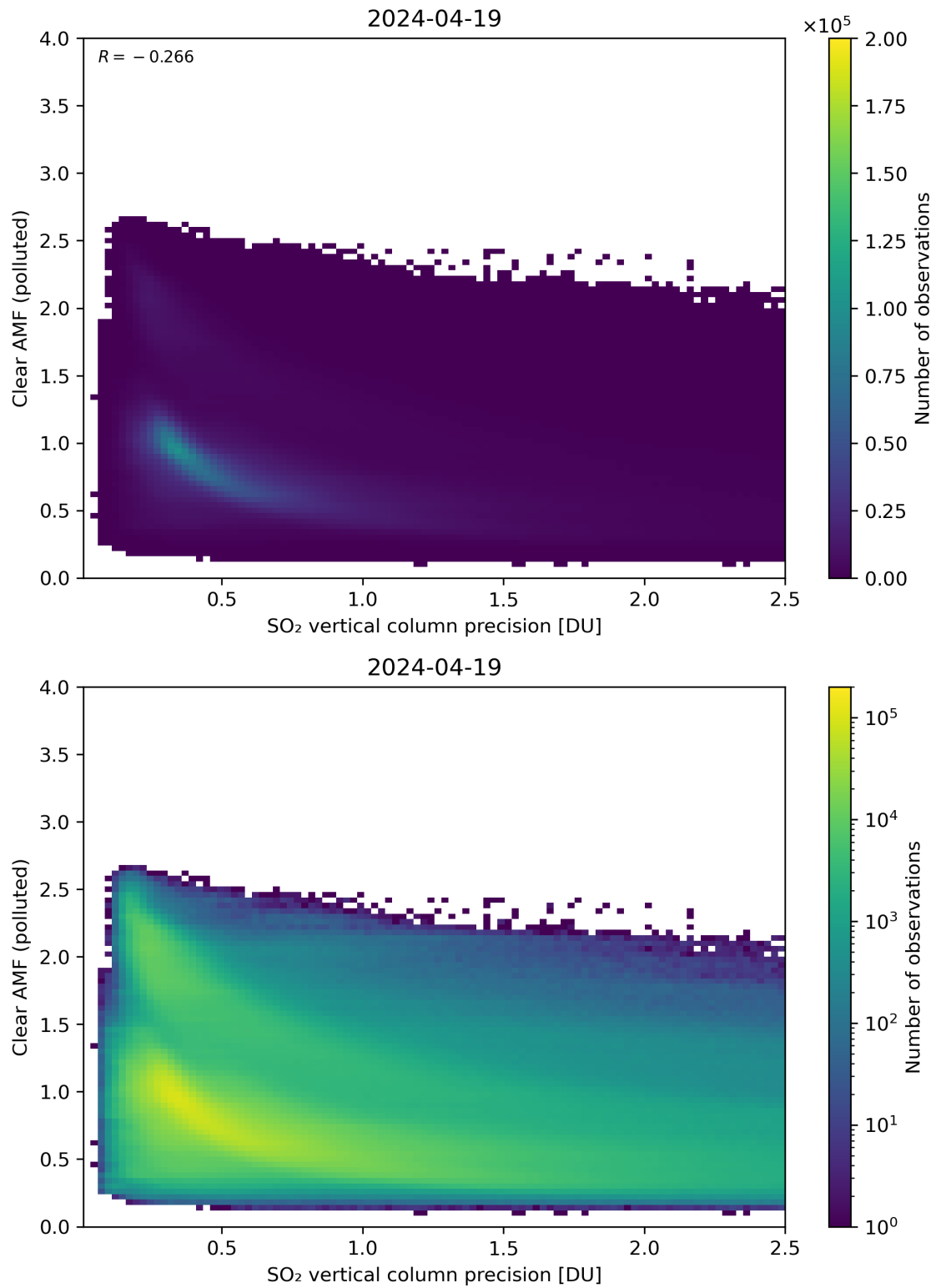
Figure 285: Scatter density plot of “SO 2 vertical column precision” against “Clear AMF (polluted)” for 2024-04-18 to 2024-04-20.
