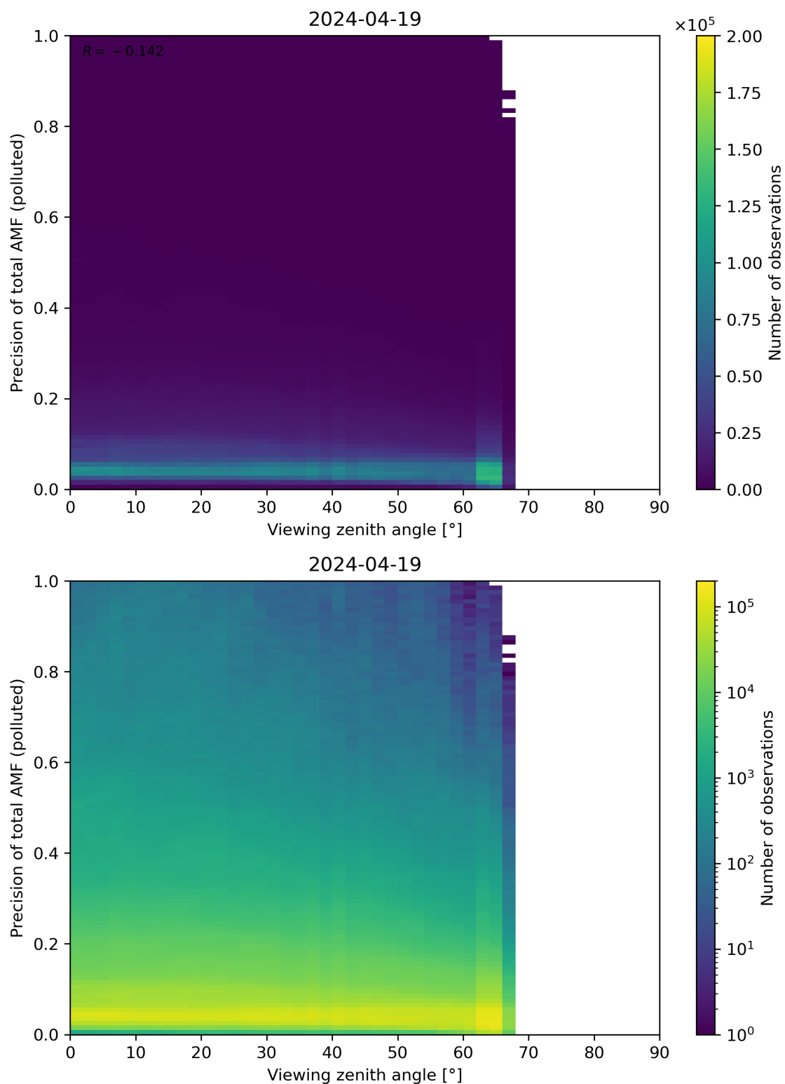
Figure 326: Scatter density plot of “Viewing zenith angle” against “Precision of total AMF (polluted)” for 2024-04-18 to 2024-04-20.
