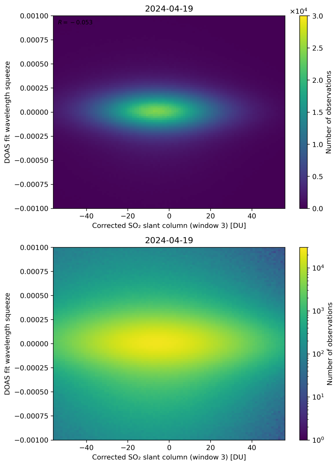
Figure 207: Scatter density plot of “Corrected SO 2 slant column (window 3)” against “DOAS fit wavelength squeeze” for 2024-04-18 to 2024-04-20.
