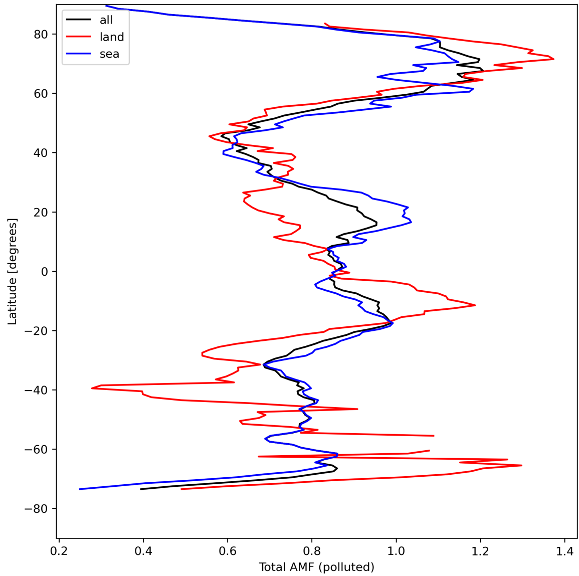
Figure 48: Zonal average of “Total AMF (polluted)” for 2024-04-18 to 2024-04-20.
