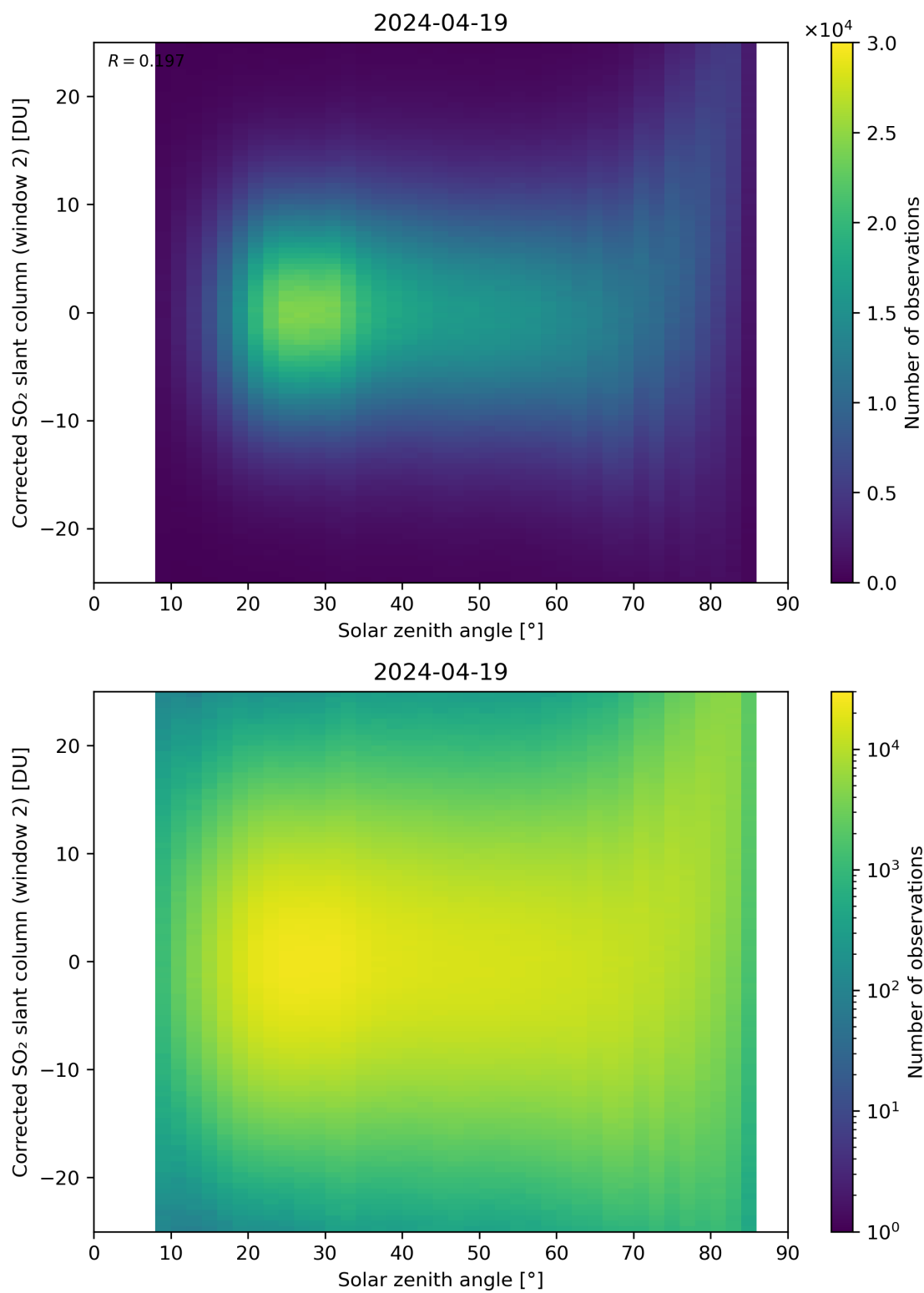
Figure 167: Scatter density plot of “Solar zenith angle” against “Corrected SO 2 slant column (window 2)” for 2024-04-18 to 2024-04-20.
