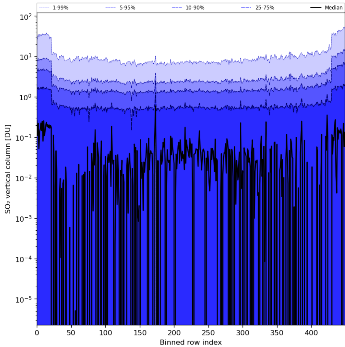
Figure 76: Along track statistics of “SO 2 vertical column” for 2024-04-18 to 2024-04-20
