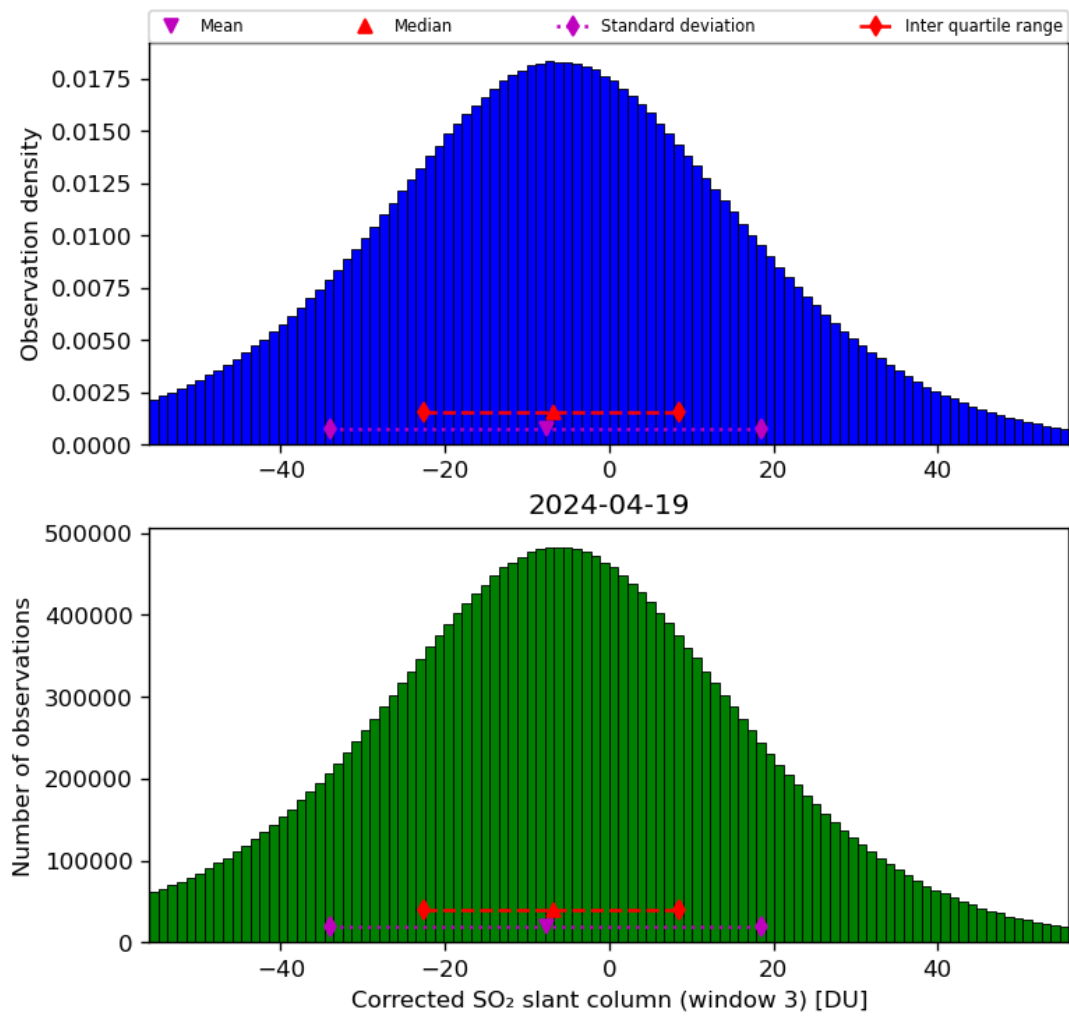
Figure 66: Histogram of “Corrected SO 2 slant column (window 3)” for 2024-04-18 to 2024-04-20
