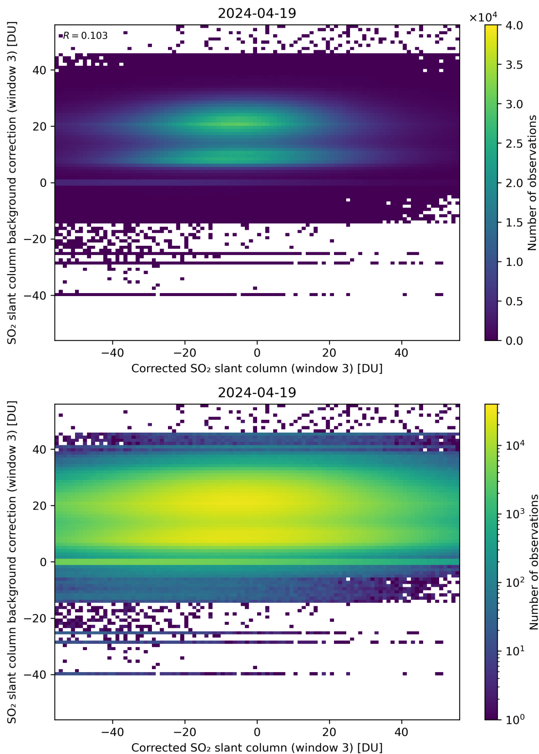
Figure 205: Scatter density plot of “Corrected SO 2 slant column (window 3)” against “SO 2 slant column background correction (window 3)” for 2024-04-18 to 2024-04-20.
