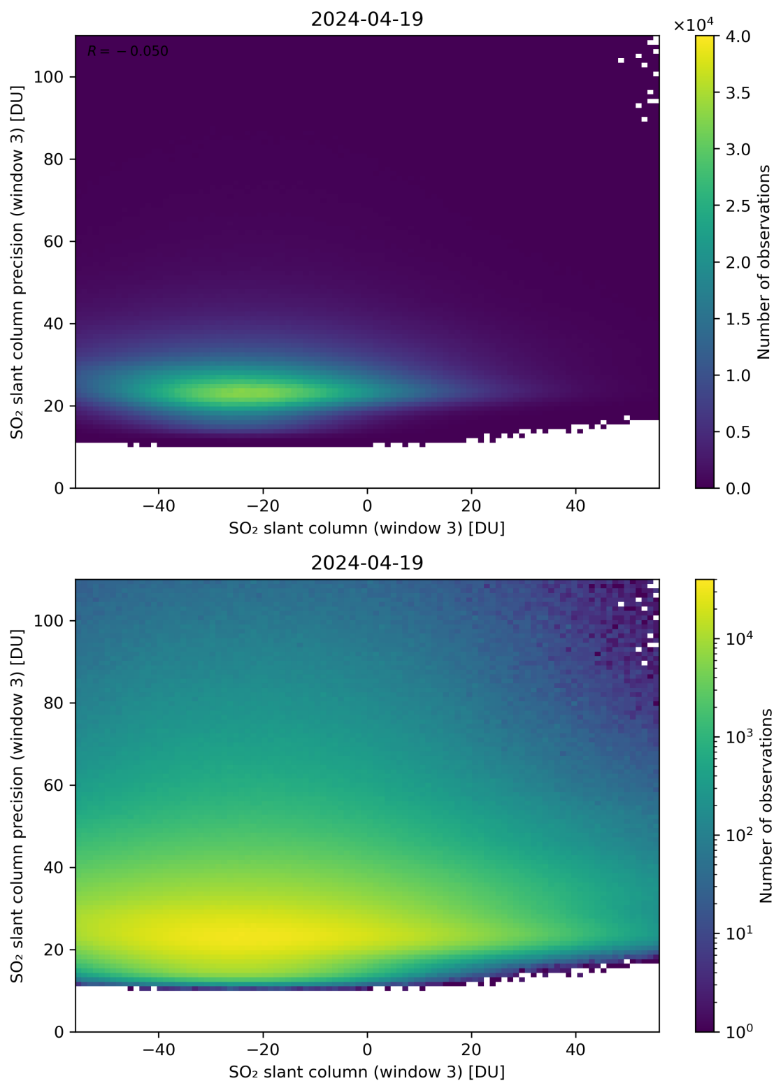
Figure 267: Scatter density plot of “SO 2 slant column (window 3)” against “SO 2 slant column precision (window 3)” for 2024-04-18 to 2024-04-20.
