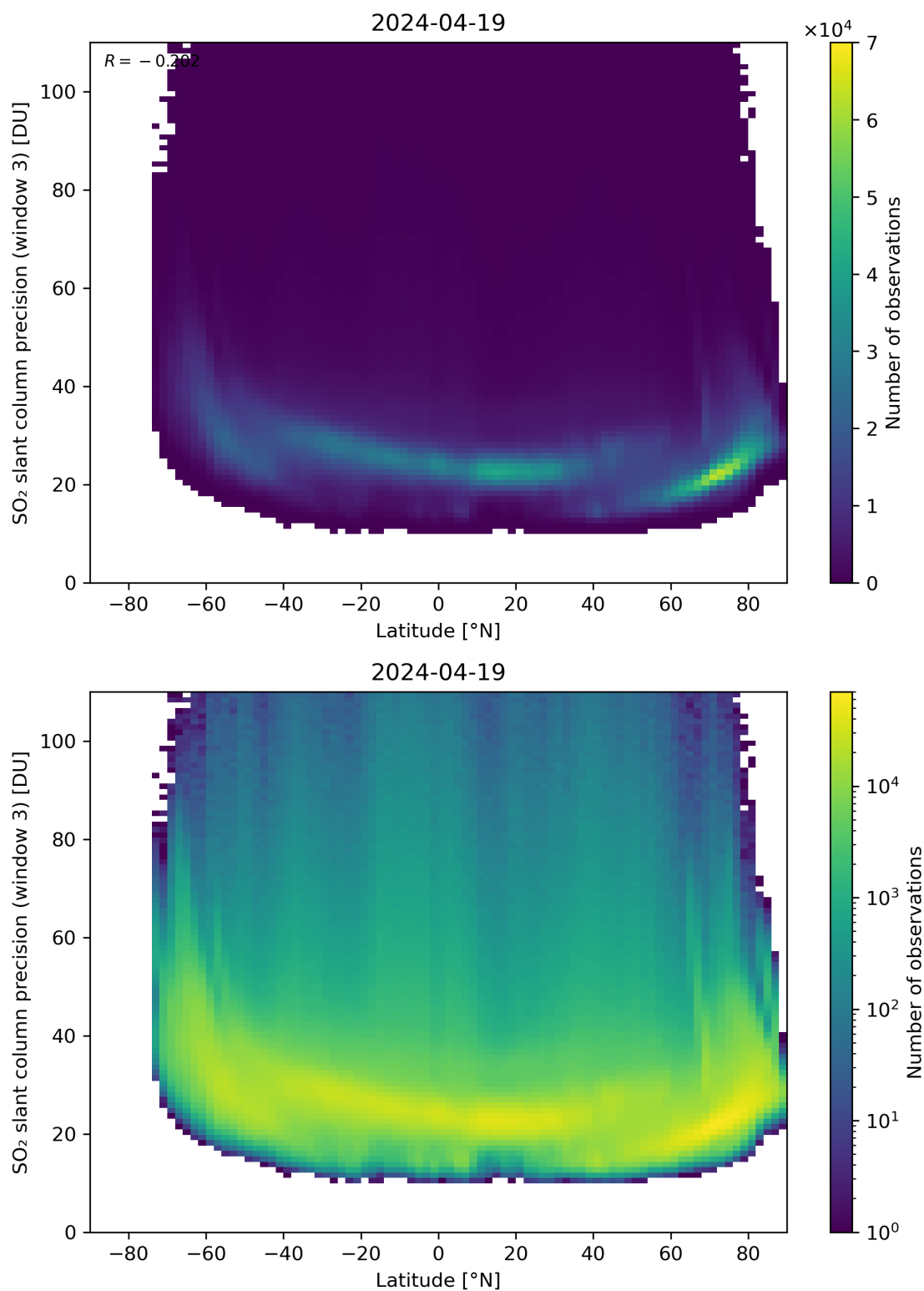
Figure 153: Scatter density plot of “Latitude” against “SO 2 slant column precision (window 3)” for 2024-04-18 to 2024-04-20.
