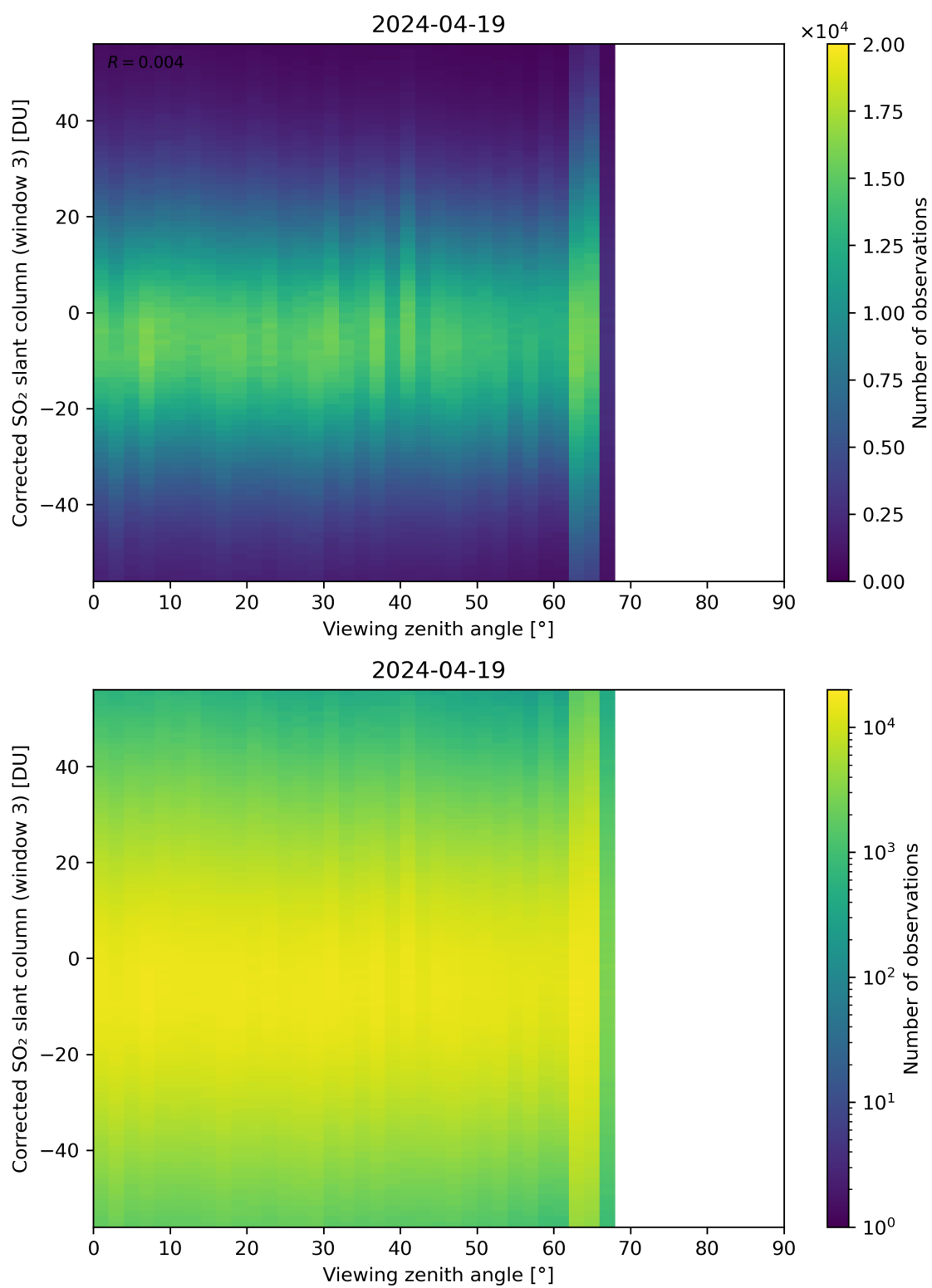
Figure 319: Scatter density plot of “Viewing zenith angle” against “Corrected SO 2 slant column (window 3)” for 2024-04-18 to 2024-04-20.
