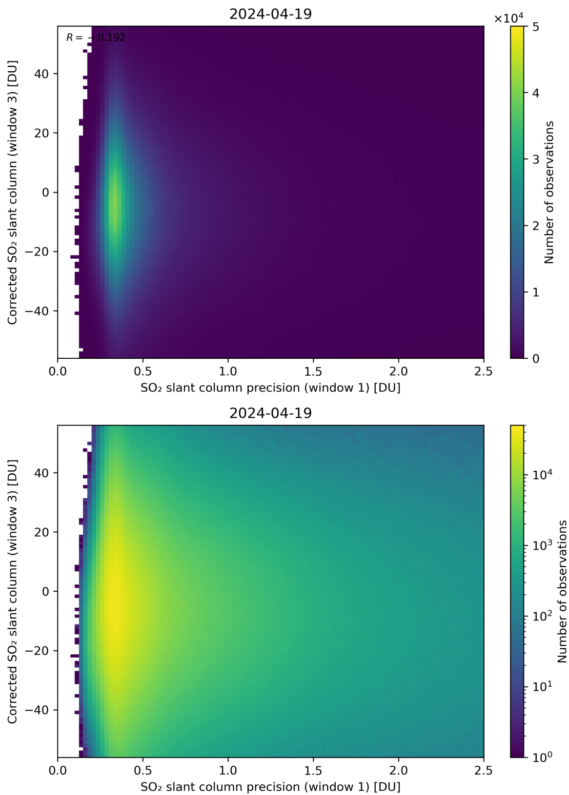
Figure 226: Scatter density plot of “SO 2 slant column precision (window 1)” against “Corrected SO 2 slant column (window 3)” for 2024-04-18 to 2024-04-20.
