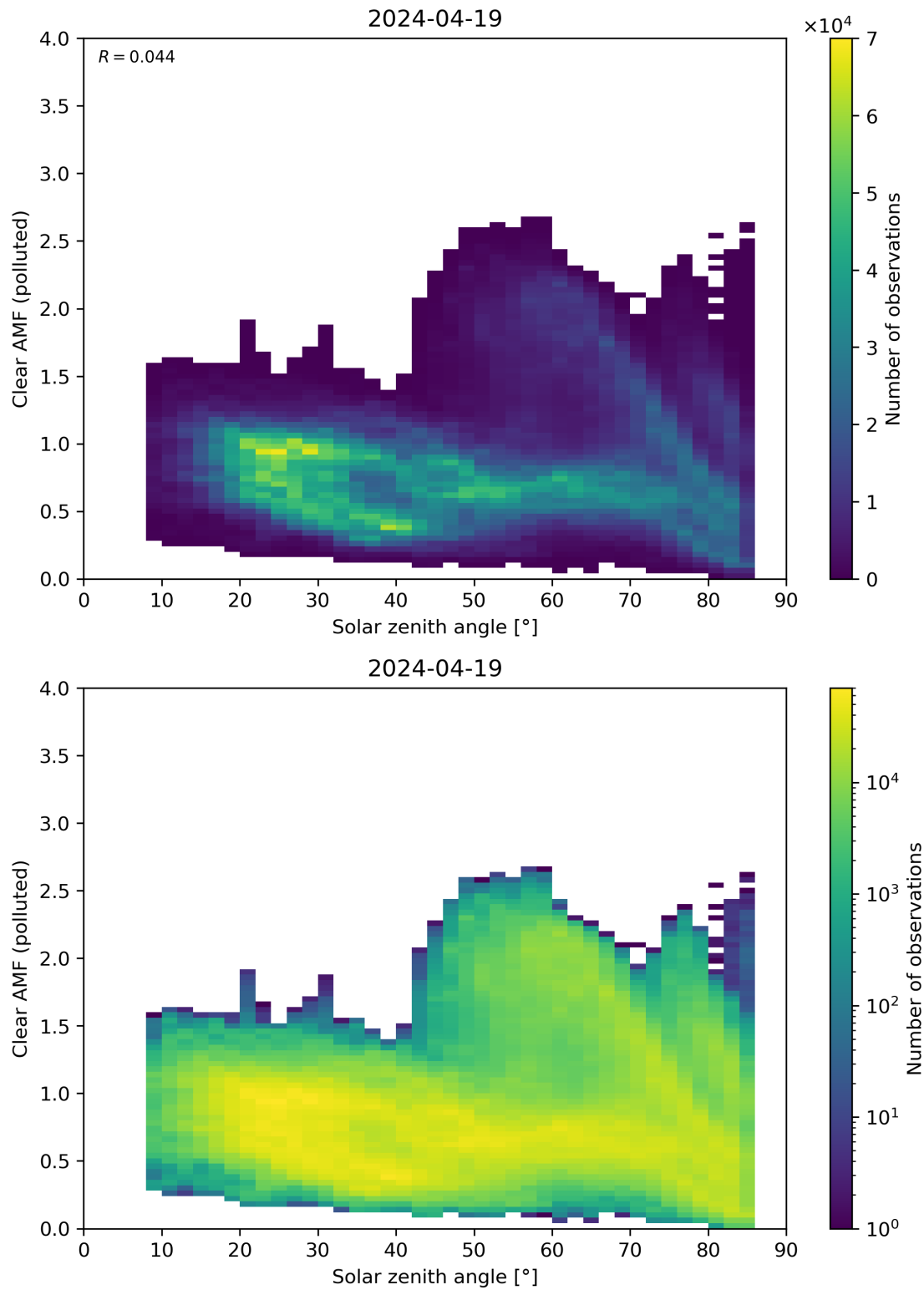
Figure 165: Scatter density plot of “Solar zenith angle” against “Clear AMF (polluted)” for 2024-04-18 to 2024-04-20.
