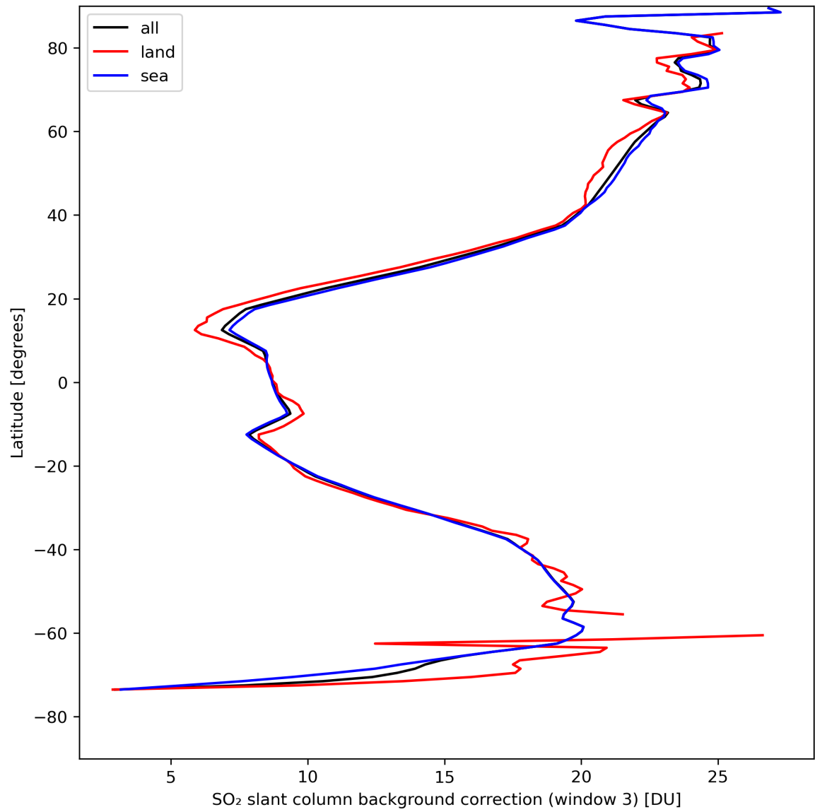
Figure 44: Zonal average of “SO 2 slant column background correction (window 3)” for 2024-04-18 to 2024-04-20.
