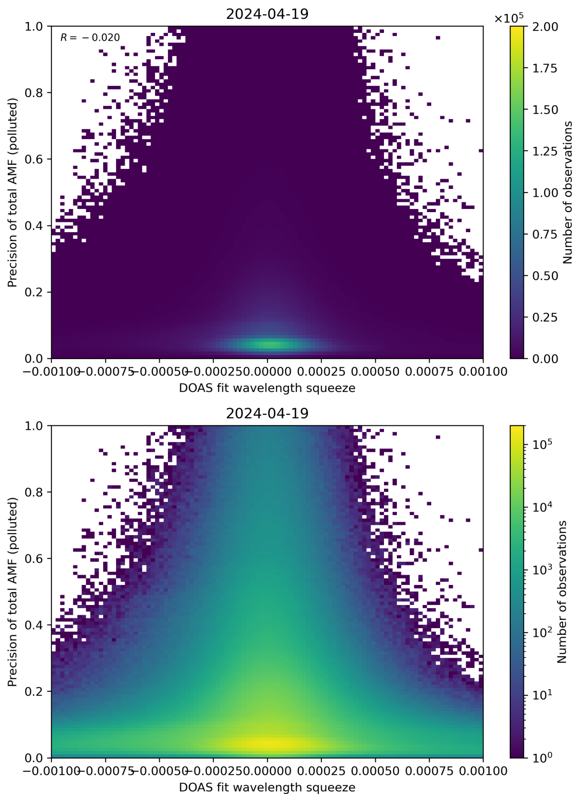
Figure 135: Scatter density plot of “DOAS fit wavelength squeeze” against “Precision of total AMF (polluted)” for 2024-04-18 to 2024-04-20.
