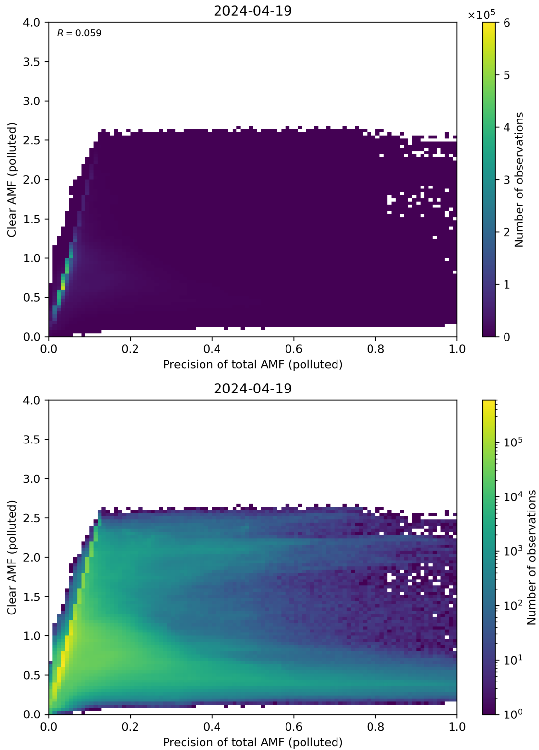
Figure 270: Scatter density plot of “Precision of total AMF (polluted)” against “Clear AMF (polluted)” for 2024-04-18 to 2024-04-20.
