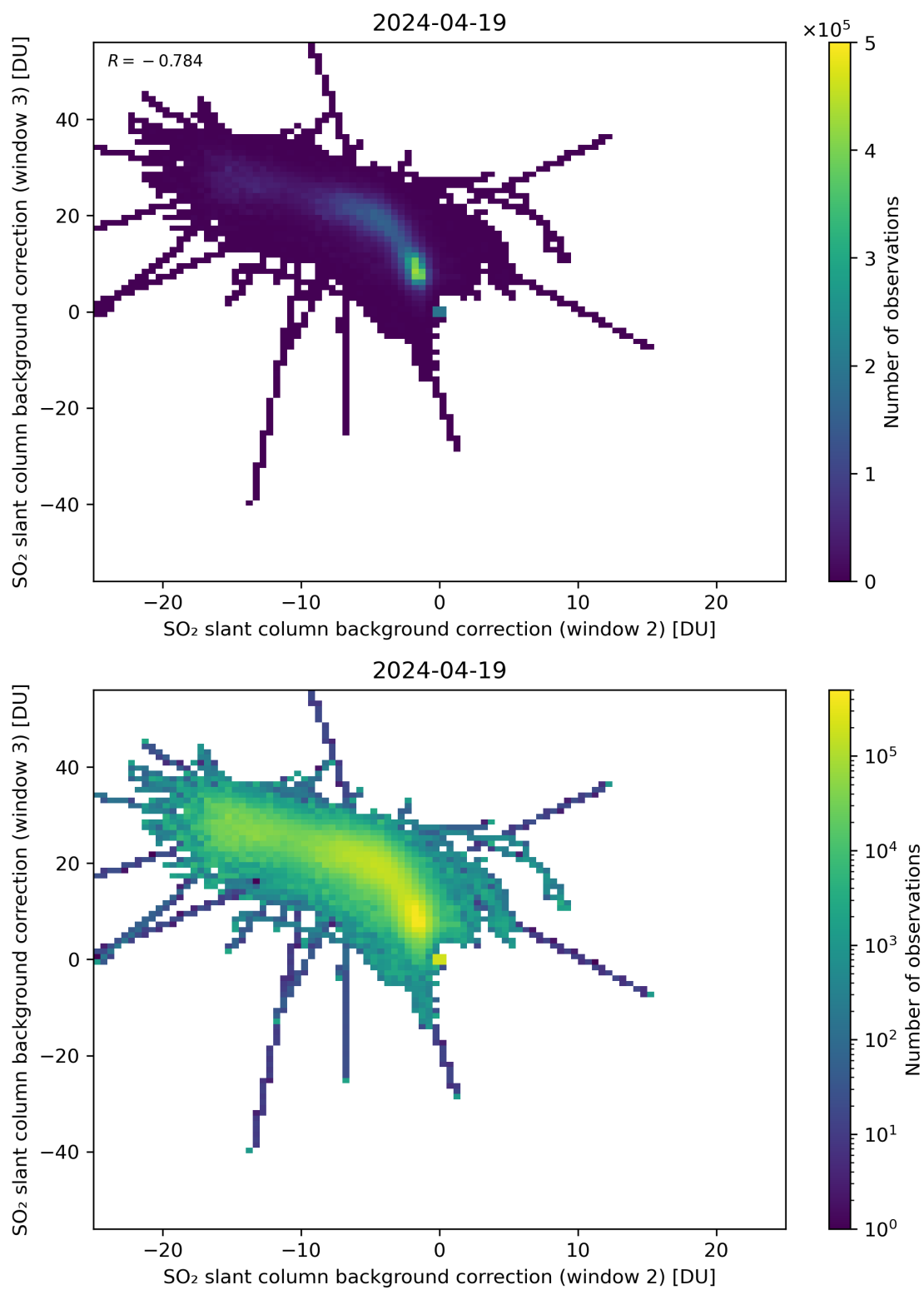
Figure 111: Scatter density plot of “SO 2 slant column background correction (window 2)” against “SO 2 slant column background correction (window 3)” for 2024-04-18 to 2024-04-20.
