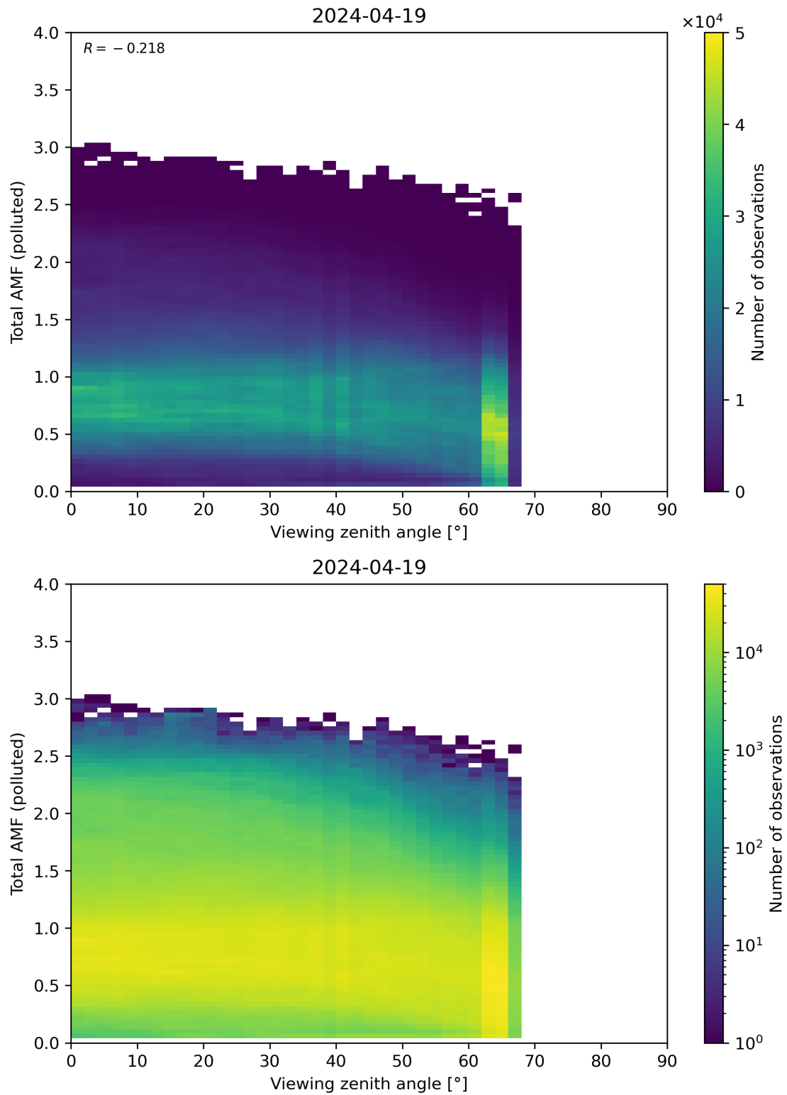
Figure 325: Scatter density plot of “Viewing zenith angle” against “Total AMF (polluted)” for 2024-04-18 to 2024-04-20.
