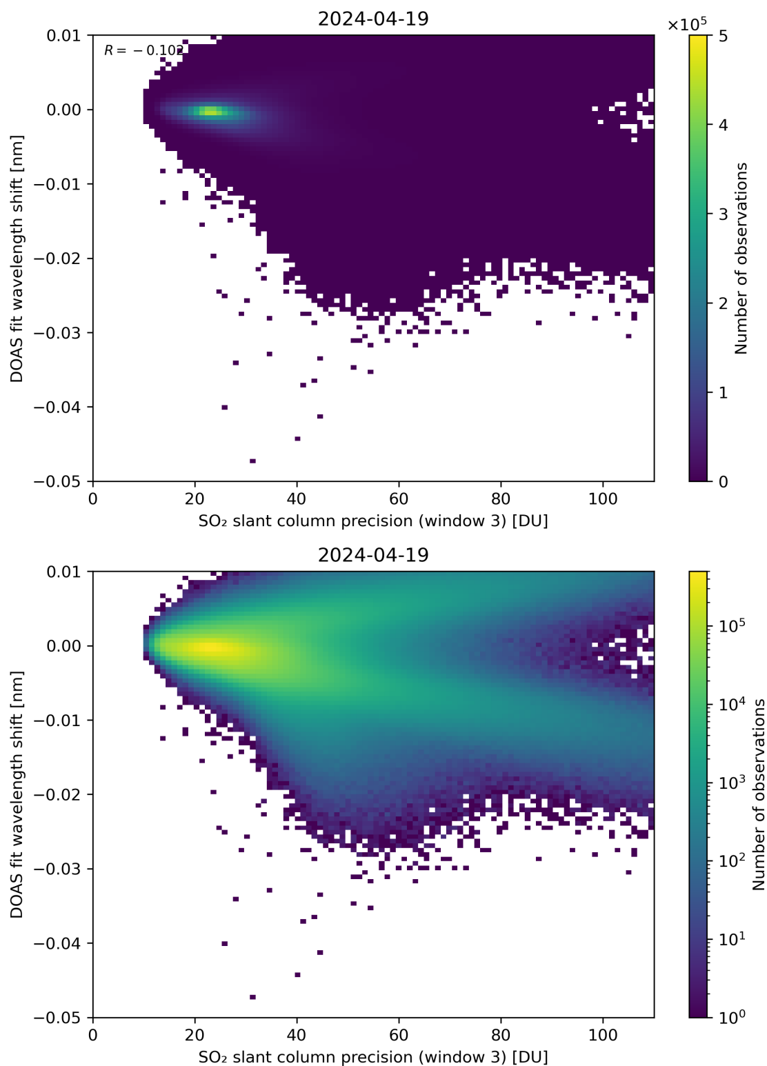
Figure 258: Scatter density plot of “SO 2 slant column precision (window 3)” against “DOAS fit wavelength shift” for 2024-04-18 to 2024-04-20.
