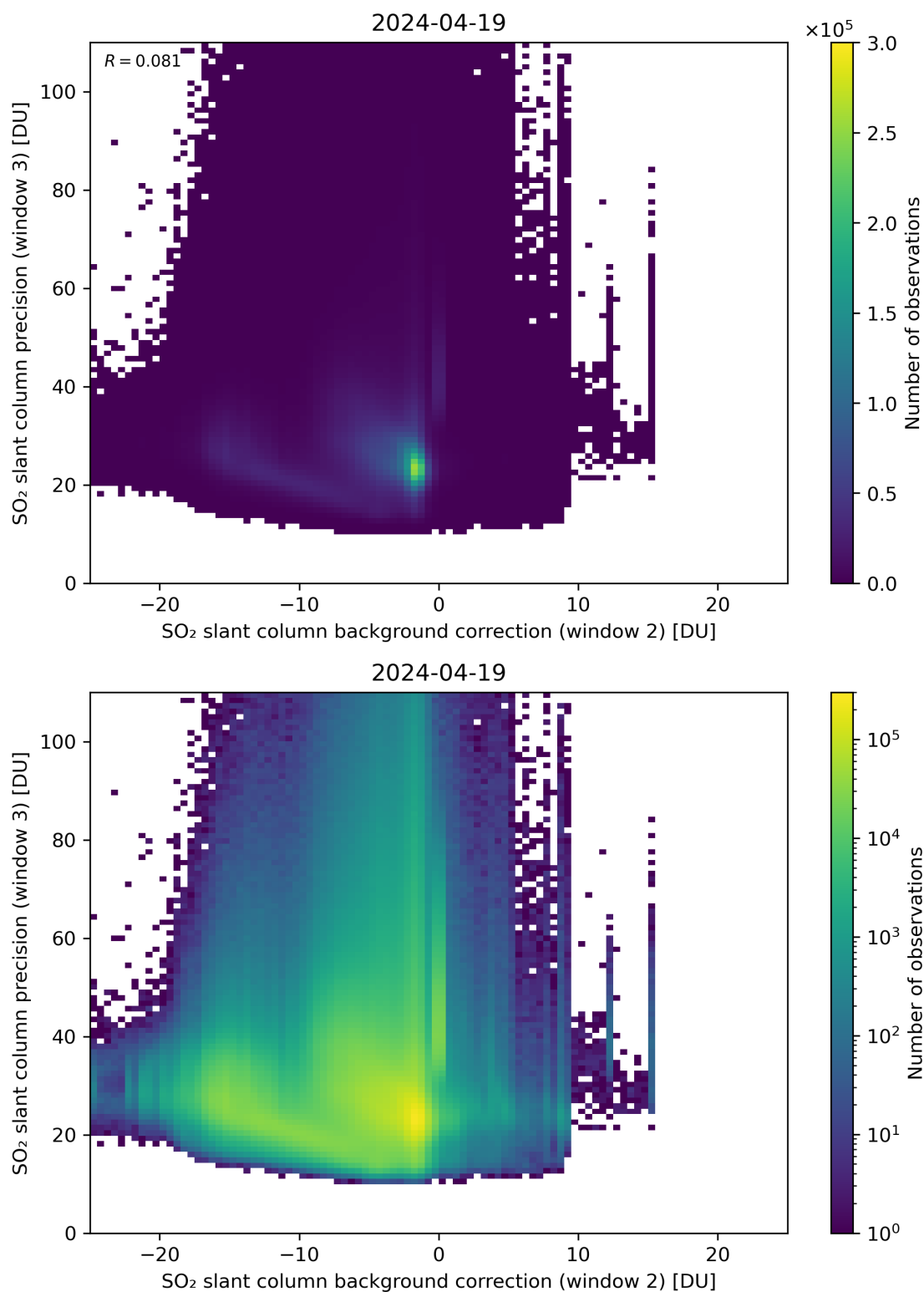
Figure 118: Scatter density plot of “SO 2 slant column background correction (window 2)” against “SO 2 slant column precision (window 3)” for 2024-04-18 to 2024-04-20.
