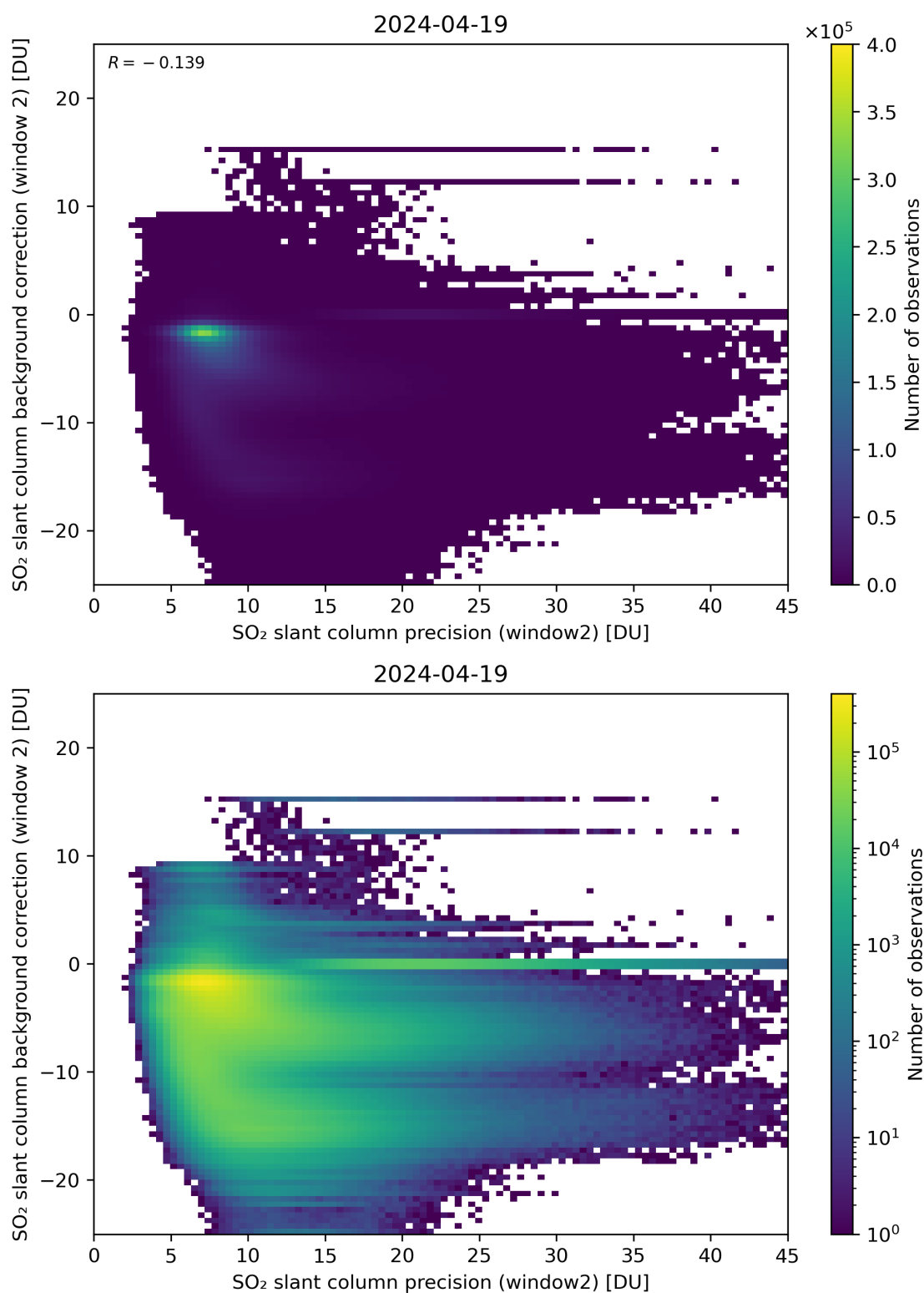
Figure 241: Scatter density plot of “SO 2 slant column precision (window2)” against “SO 2 slant column background correction (window 2)” for 2024-04-18 to 2024-04-20.
