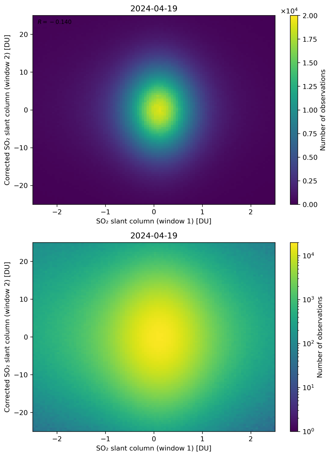
Figure 233: Scatter density plot of “SO 2 slant column (window 1)” against “Corrected SO 2 slant column (window 2)” for 2024-04-18 to 2024-04-20.
