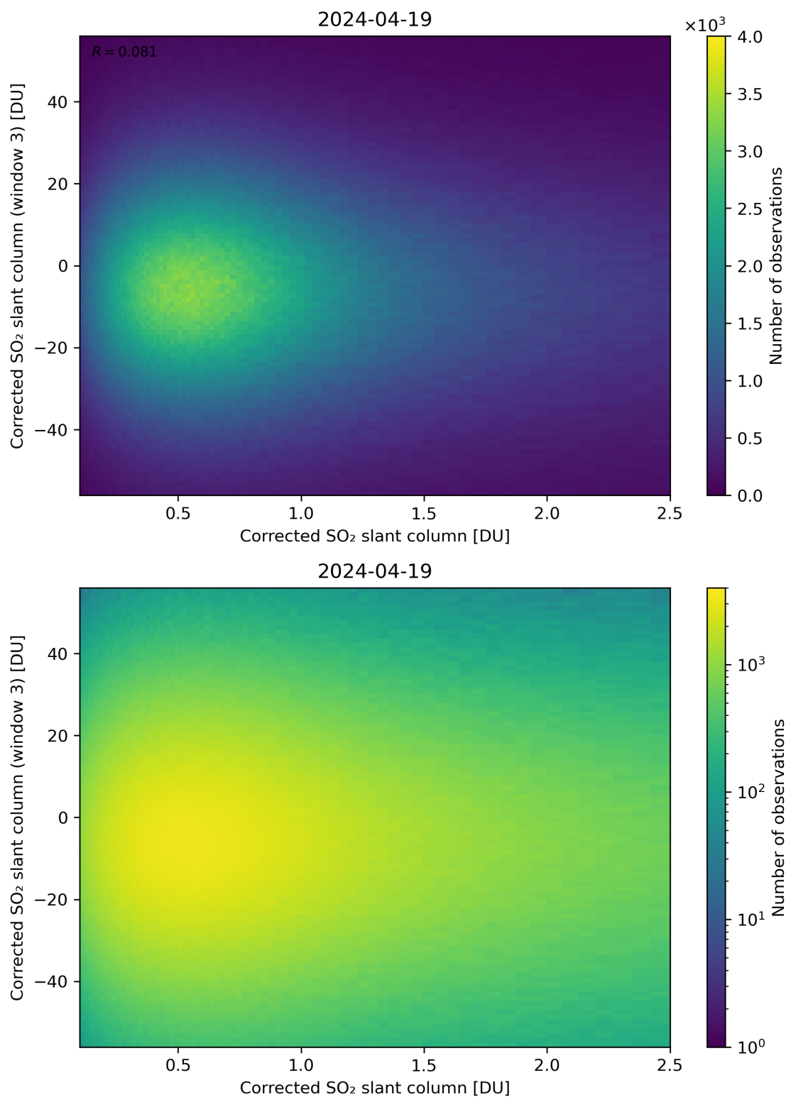
Figure 186: Scatter density plot of “Corrected SO 2 slant column” against “Corrected SO 2 slant column (window 3)” for 2024-04-18 to 2024-04-20.
