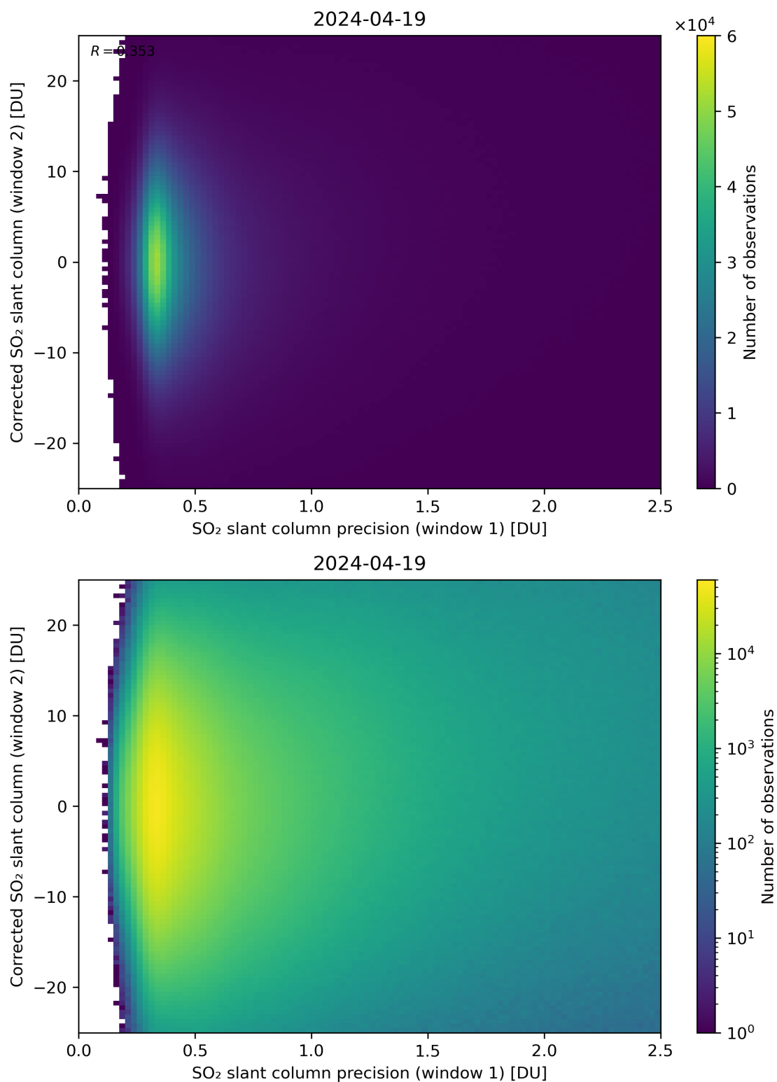
Figure 225: Scatter density plot of “SO 2 slant column precision (window 1)” against “Corrected SO 2 slant column (window 2)” for 2024-04-18 to 2024-04-20.
