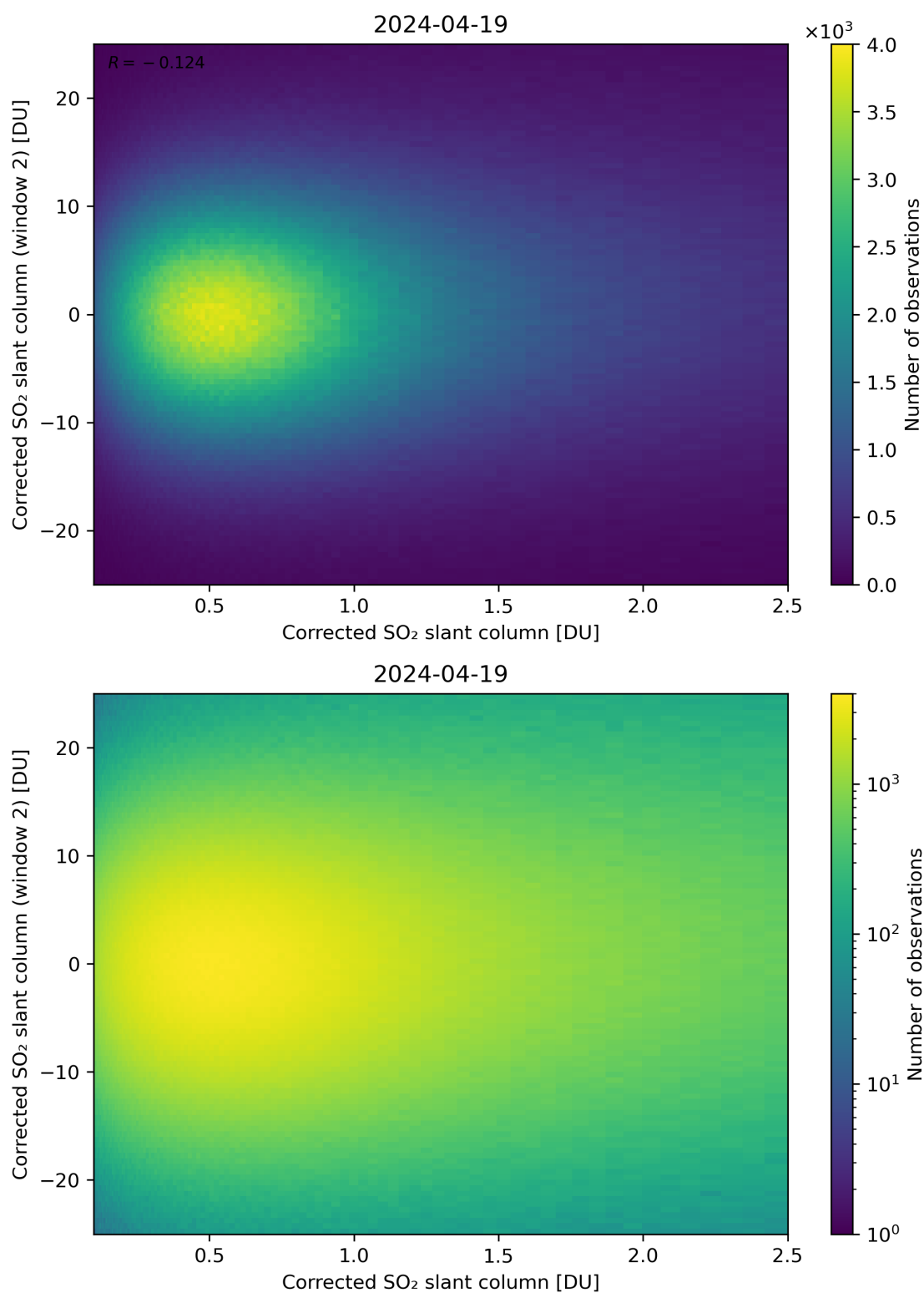
Figure 185: Scatter density plot of “Corrected SO 2 slant column” against “Corrected SO 2 slant column (window 2)” for 2024-04-18 to 2024-04-20.
