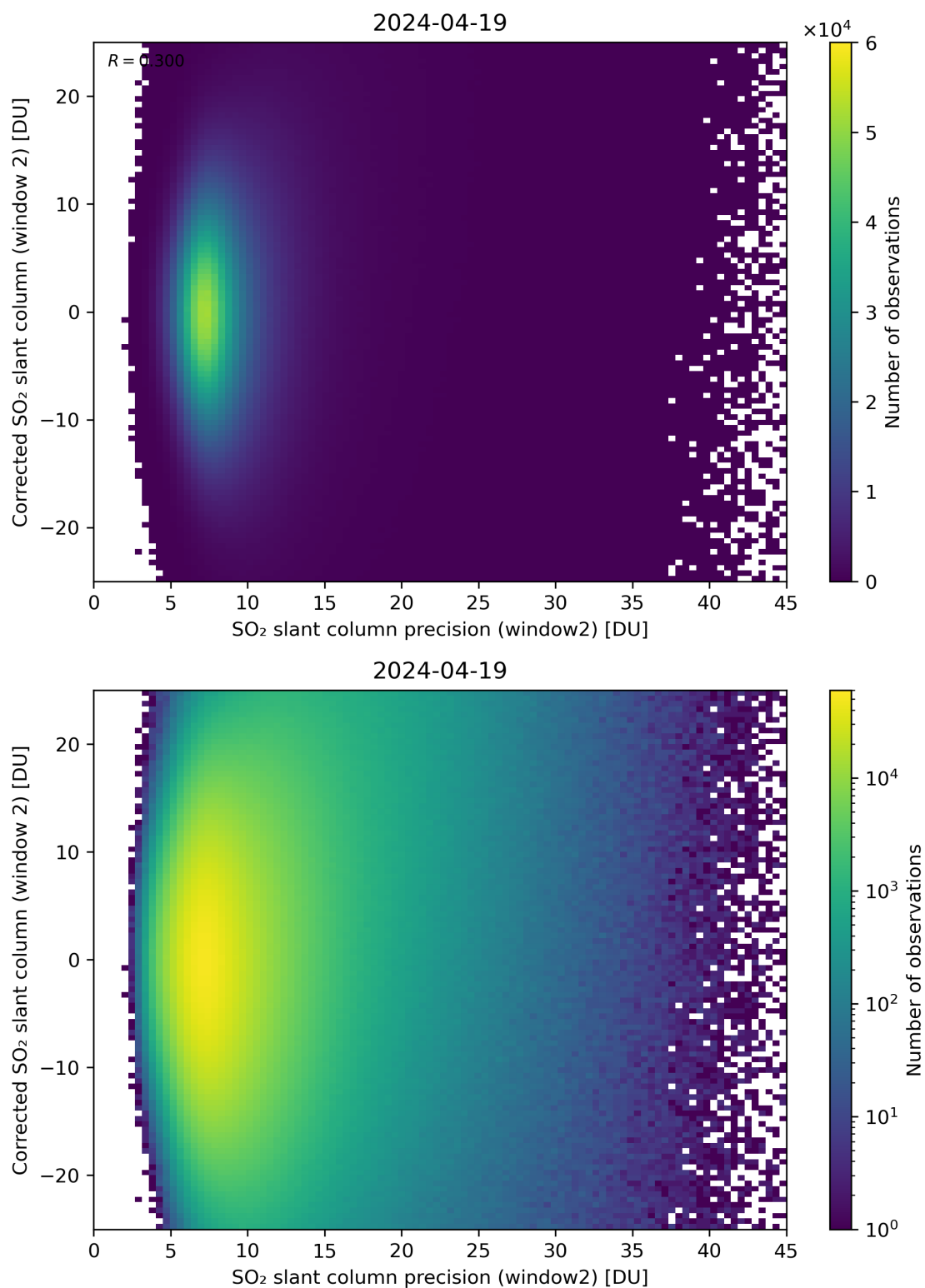
Figure 247: Scatter density plot of “SO 2 slant column precision (window2)” against “Corrected SO 2 slant column (window 2)” for 2024-04-18 to 2024-04-20.
