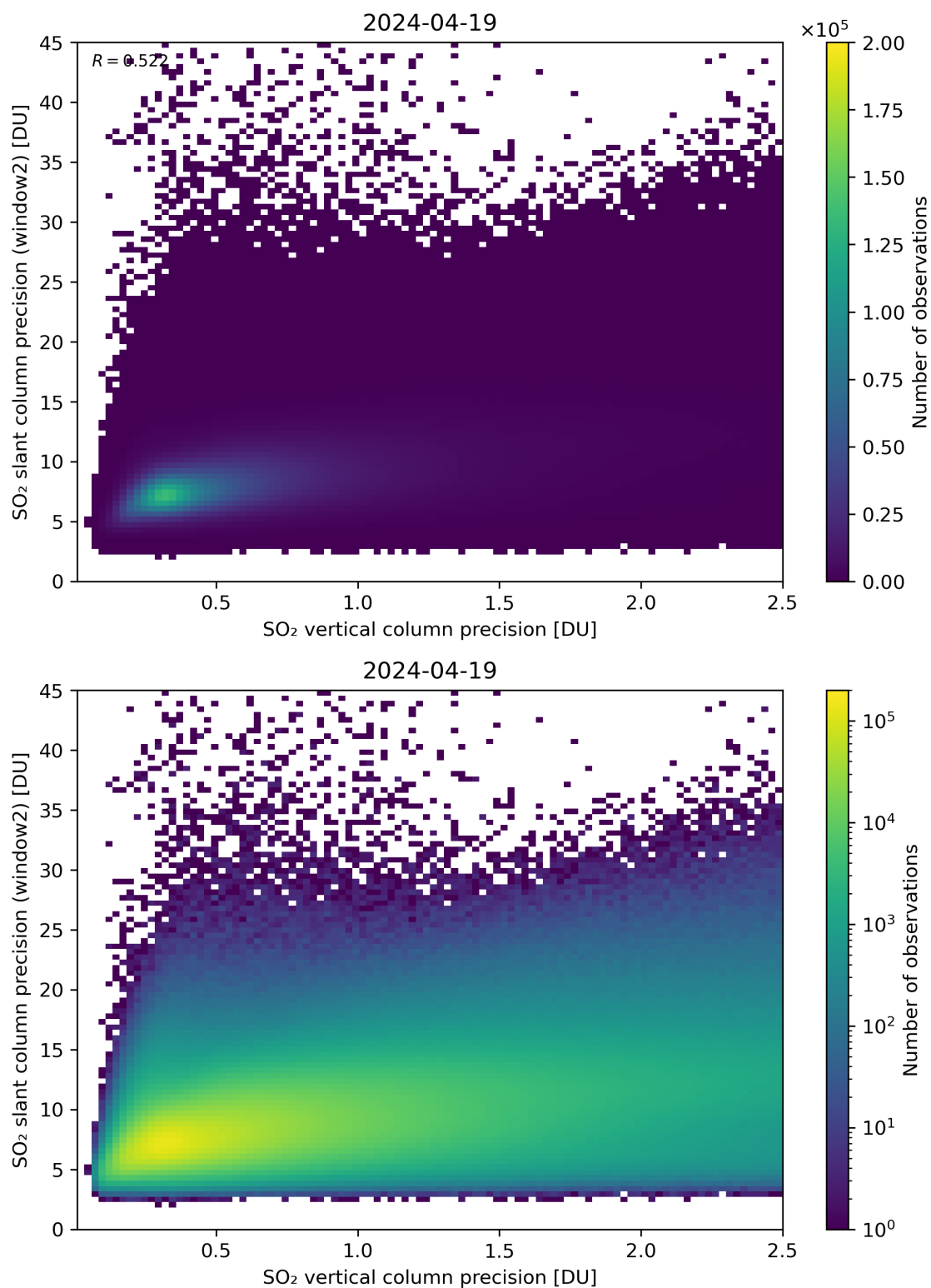
Figure 291: Scatter density plot of “SO 2 vertical column precision” against “SO 2 slant column precision (window2)” for 2024-04-18 to 2024-04-20.
