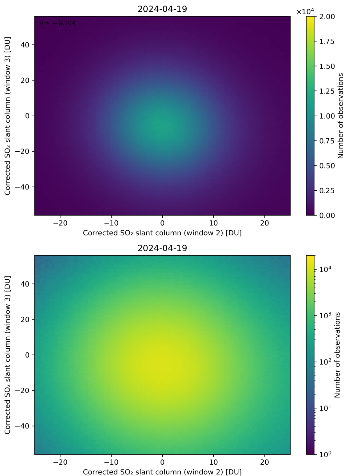
Figure 200: Scatter density plot of “Corrected SO 2 slant column (window 2)” against “Corrected SO 2 slant column (window 3)” for 2024-04-18 to 2024-04-20.
