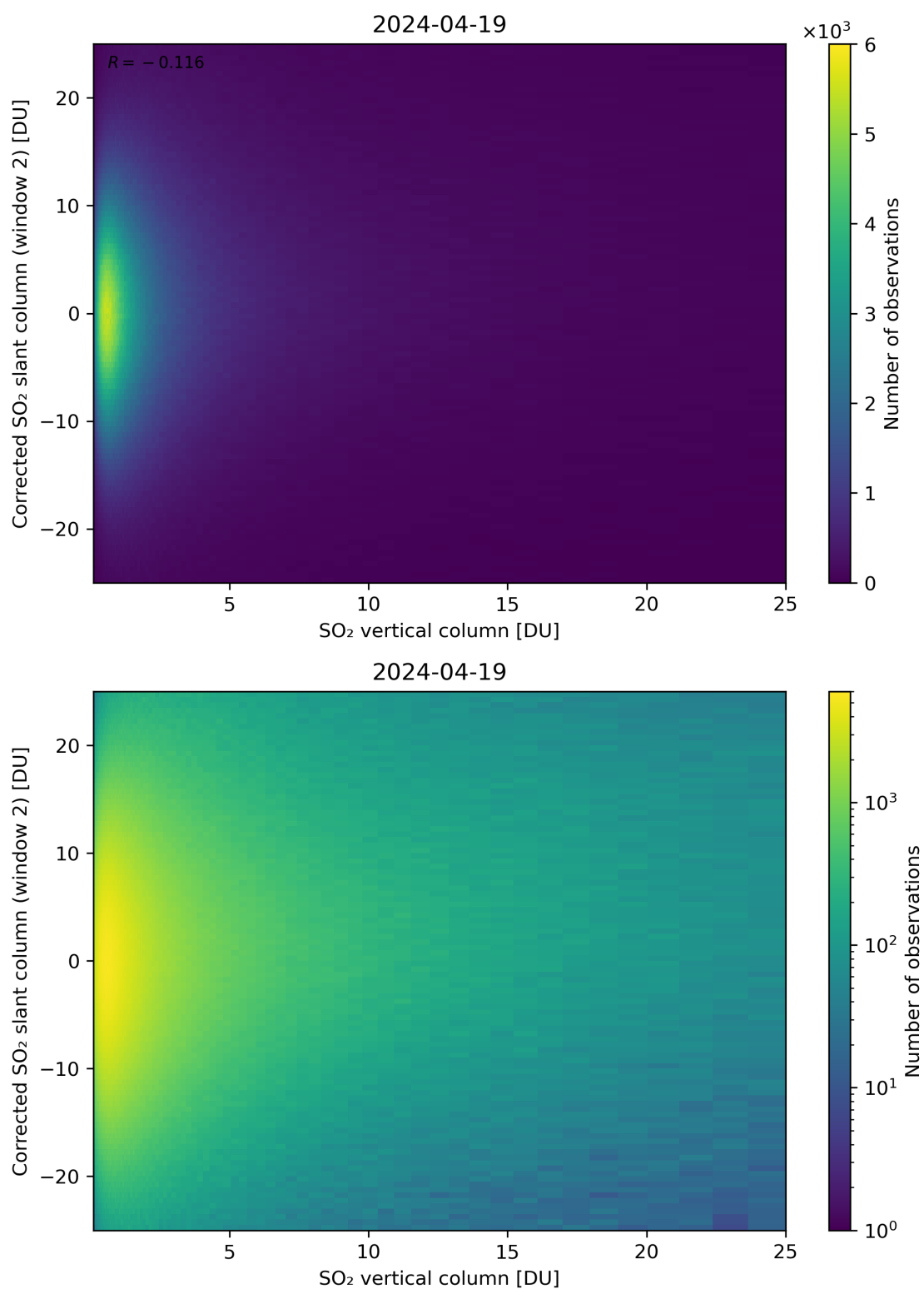
Figure 298: Scatter density plot of “SO 2 vertical column” against “Corrected SO 2 slant column (window 2)” for 2024-04-18 to 2024-04-20.
