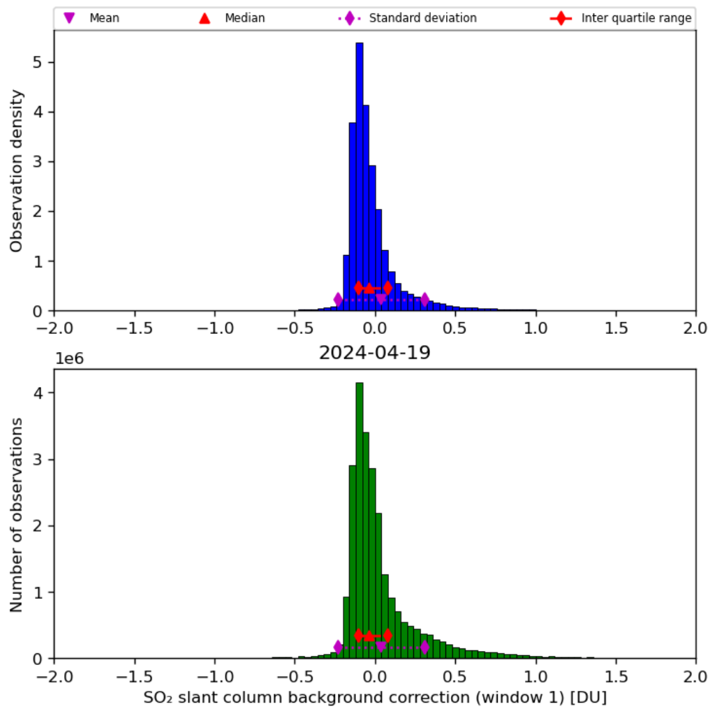
Figure 59: Histogram of “SO 2 slant column background correction (window 1)” for 2024-04-18 to 2024-04-20
