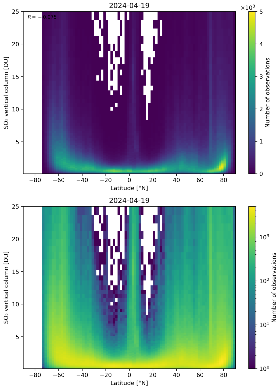
Figure 156: Scatter density plot of “Latitude” against “SO 2 vertical column” for 2024-04-18 to 2024-04-20.
