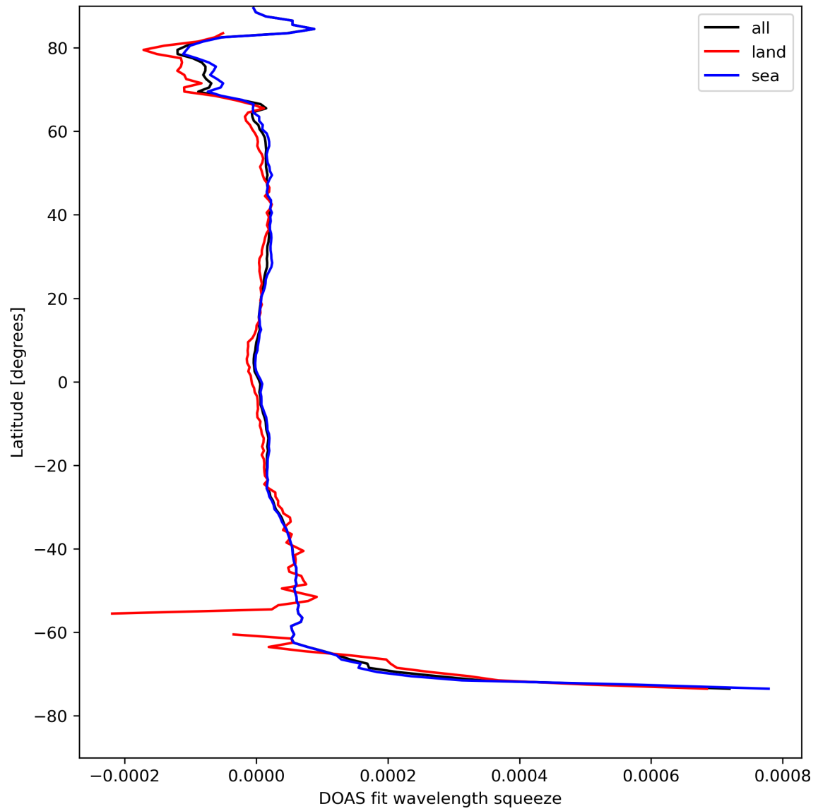
Figure 46: Zonal average of “DOAS fit wavelength squeeze” for 2024-04-18 to 2024-04-20.
