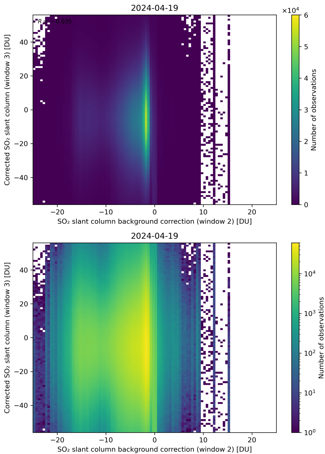
Figure 116: Scatter density plot of “SO 2 slant column background correction (window 2)” against “Corrected SO 2 slant column (window 3)” for 2024-04-18 to 2024-04-20.
