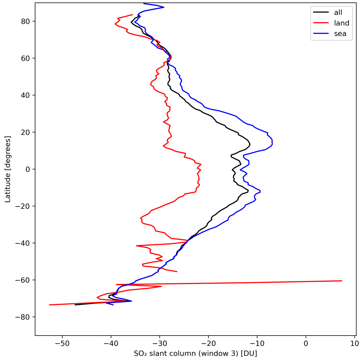
Figure 41: Zonal average of “SO 2 slant column (window 3)” for 2024-04-18 to 2024-04-20.
