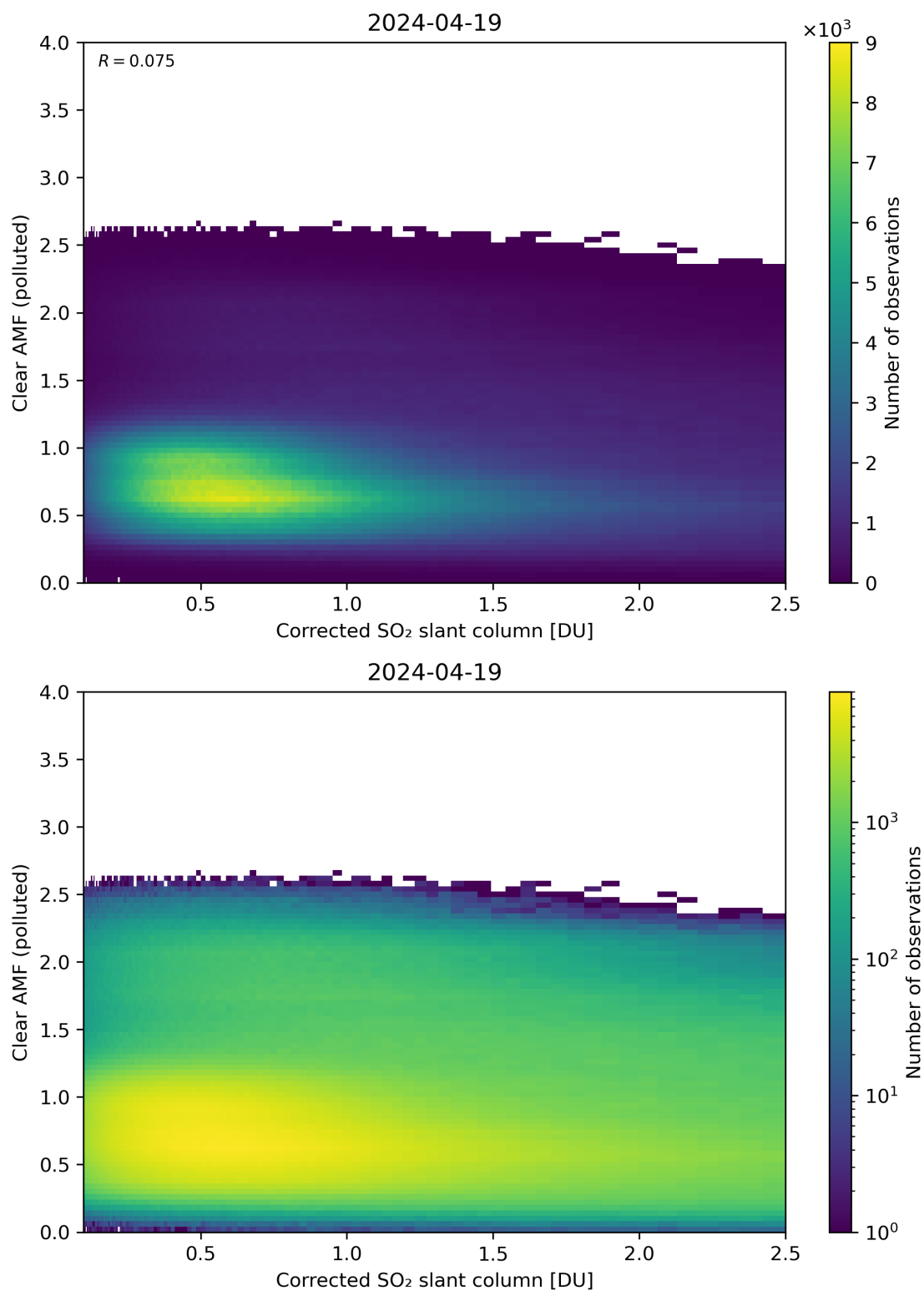
Figure 184: Scatter density plot of “Corrected SO 2 slant column” against “Clear AMF (polluted)” for 2024-04-18 to 2024-04-20.
