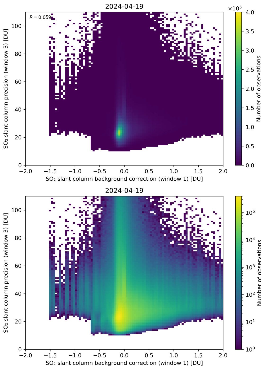
Figure 108: Scatter density plot of “SO 2 slant column background correction (window 1)” against “SO 2 slant column precision (window 3)” for 2024-04-18 to 2024-04-20.
