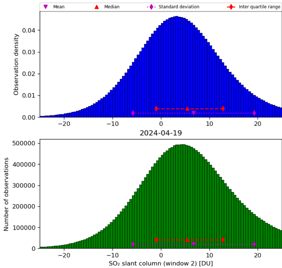
Figure 60: Histogram of “SO 2 slant column (window 2)” for 2024-04-18 to 2024-04-20
