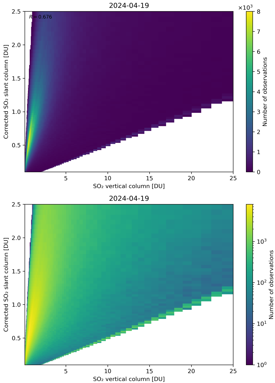
Figure 297: Scatter density plot of “SO 2 vertical column” against “Corrected SO 2 slant column” for 2024-04-18 to 2024-04-20.
