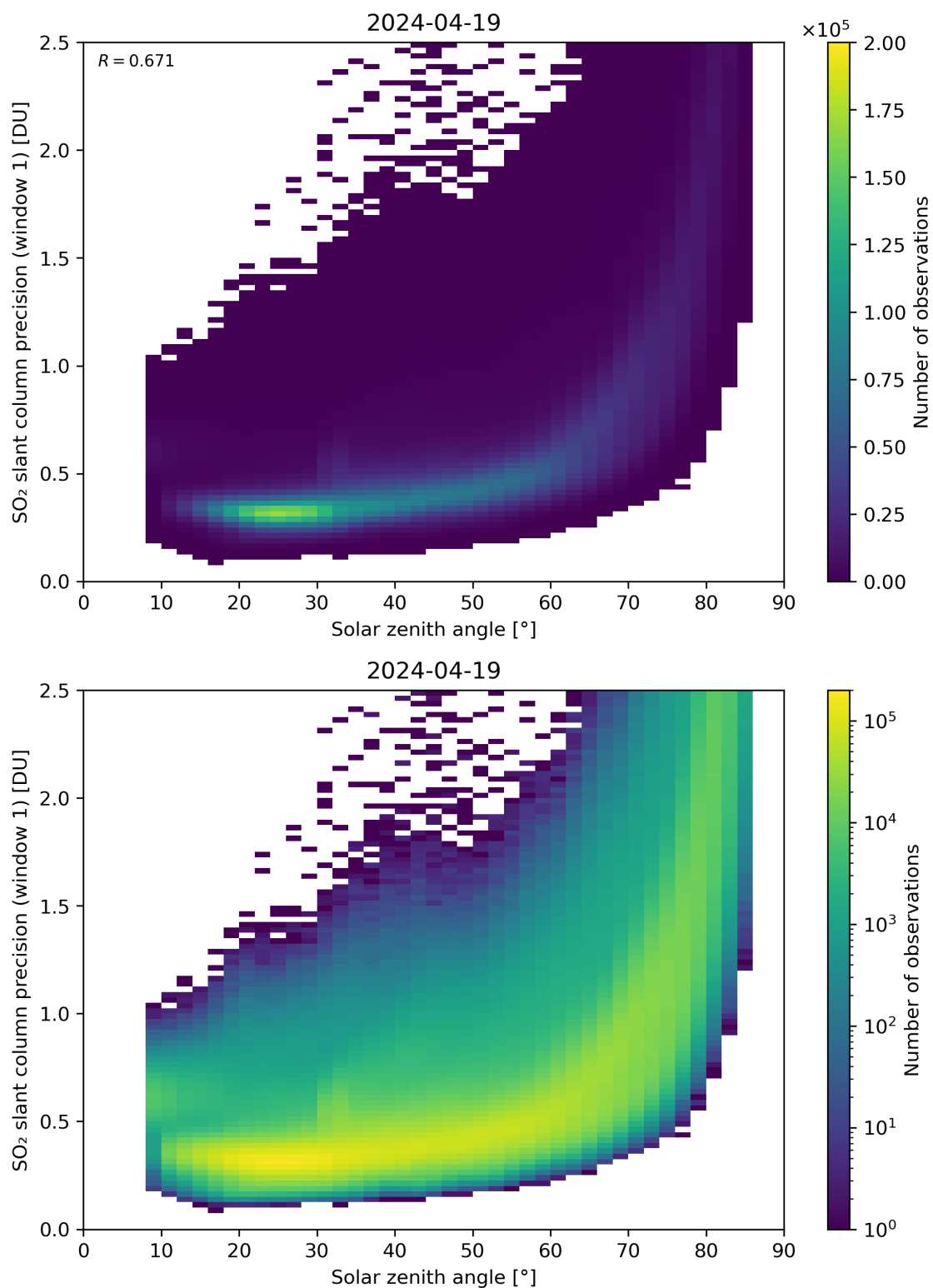
Figure 170: Scatter density plot of “Solar zenith angle” against “SO 2 slant column precision (window 1)” for 2024-04-18 to 2024-04-20.
