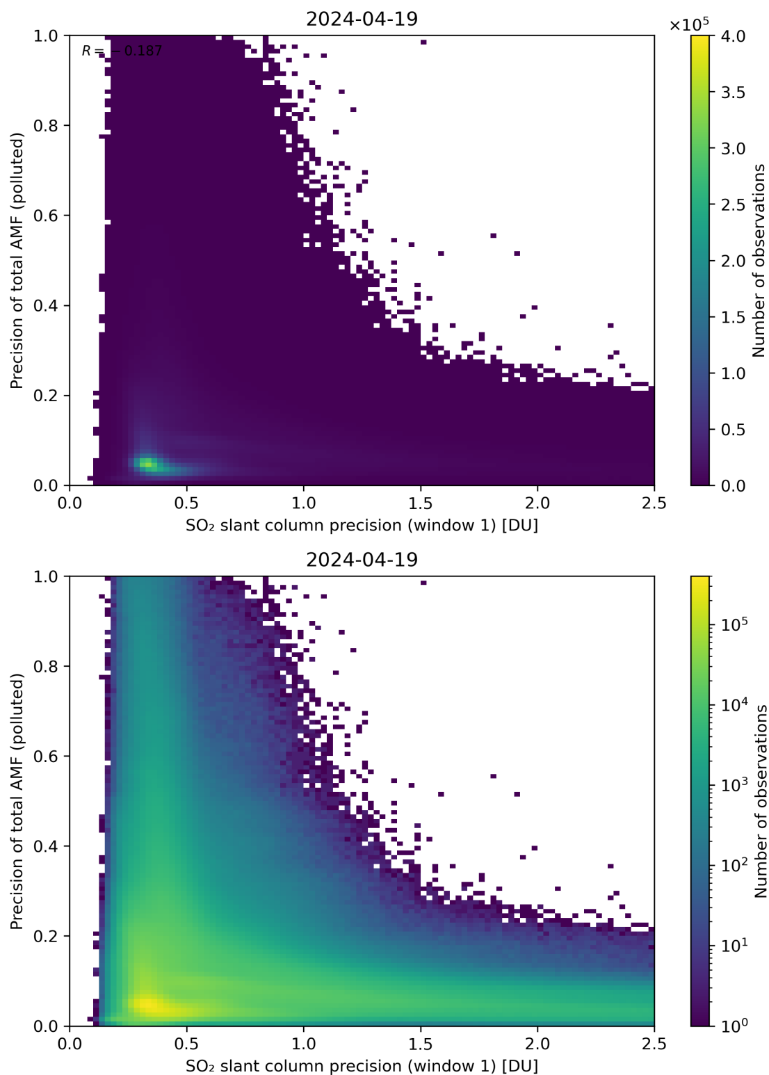
Figure 231: Scatter density plot of “SO 2 slant column precision (window 1)” against “Precision of total AMF (polluted)” for 2024-04-18 to 2024-04-20.
