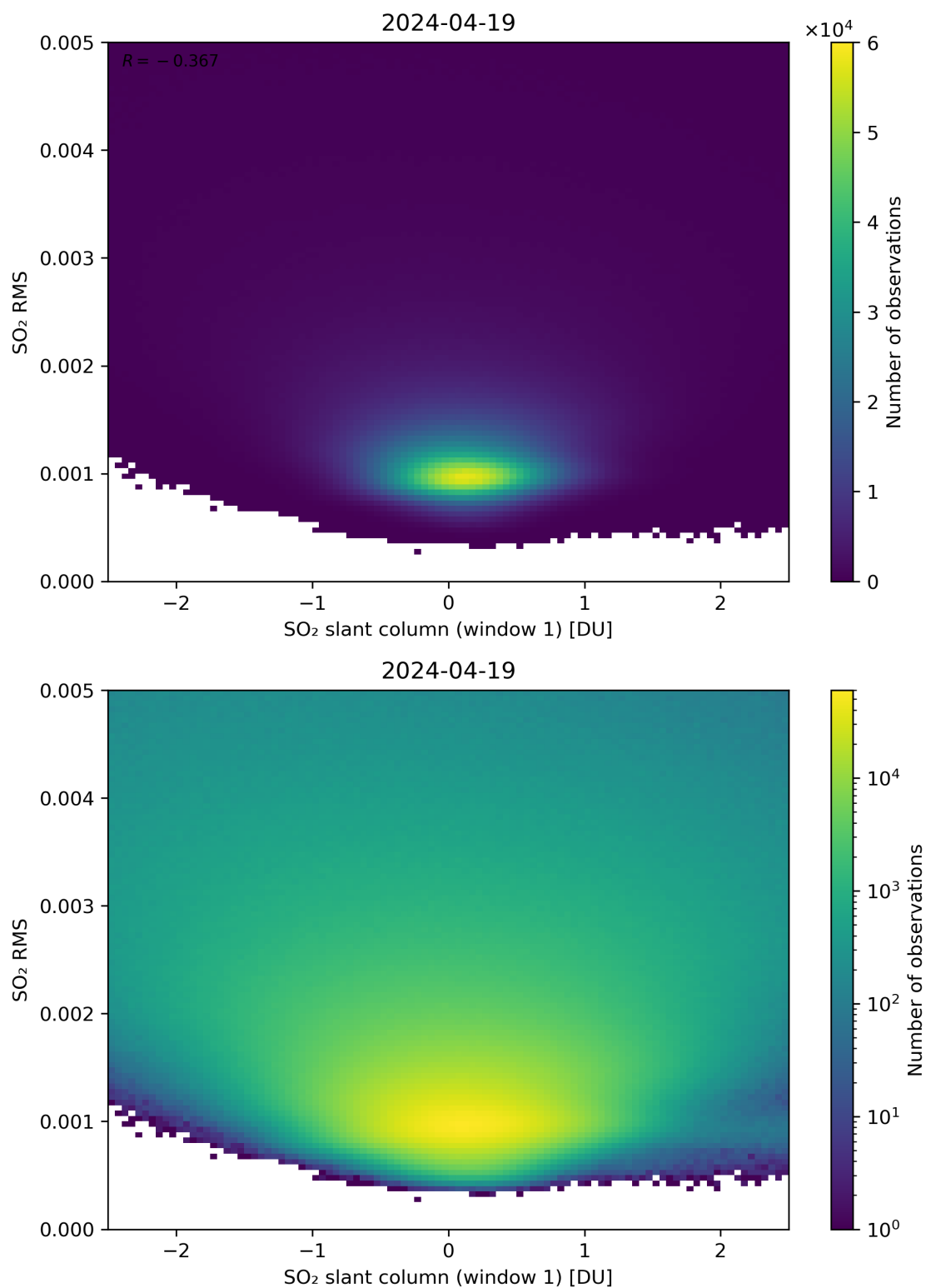
Figure 217: Scatter density plot of “SO 2 slant column (window 1)” against “SO 2 RMS” for 2024-04-18 to 2024-04-20.
