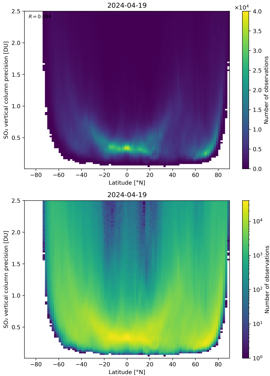
Figure 157: Scatter density plot of “Latitude” against “SO 2 vertical column precision” for 2024-04-18 to 2024-04-20.
