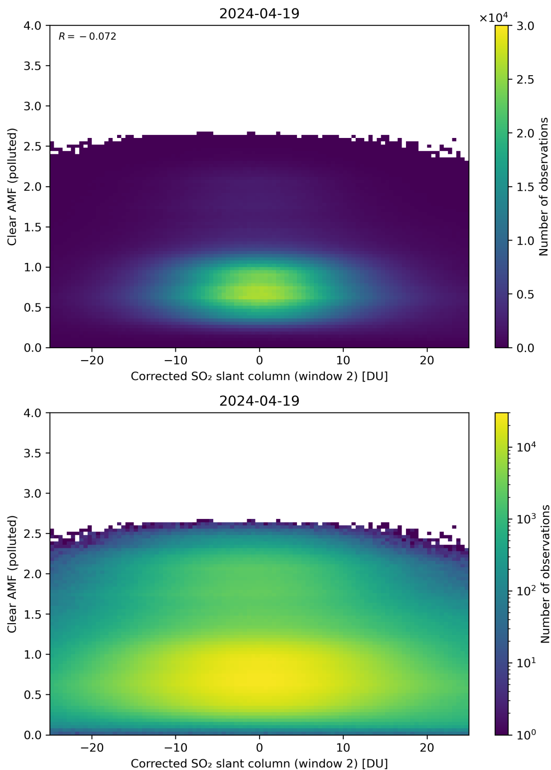
Figure 199: Scatter density plot of “Corrected SO 2 slant column (window 2)” against “Clear AMF (polluted)” for 2024-04-18 to 2024-04-20.
