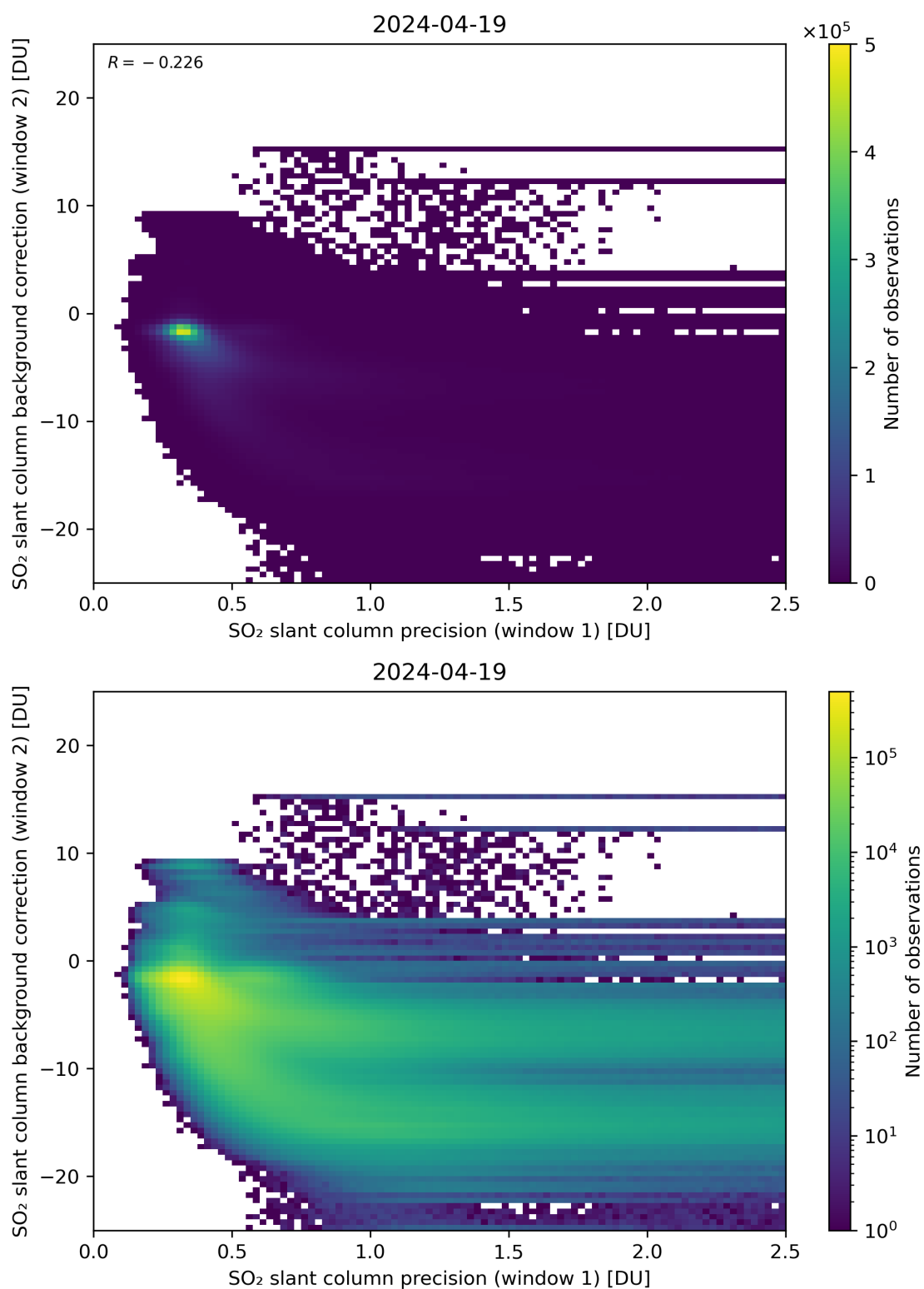
Figure 219: Scatter density plot of “SO 2 slant column precision (window 1)” against “SO 2 slant column background correction (window 2)” for 2024-04-18 to 2024-04-20.
