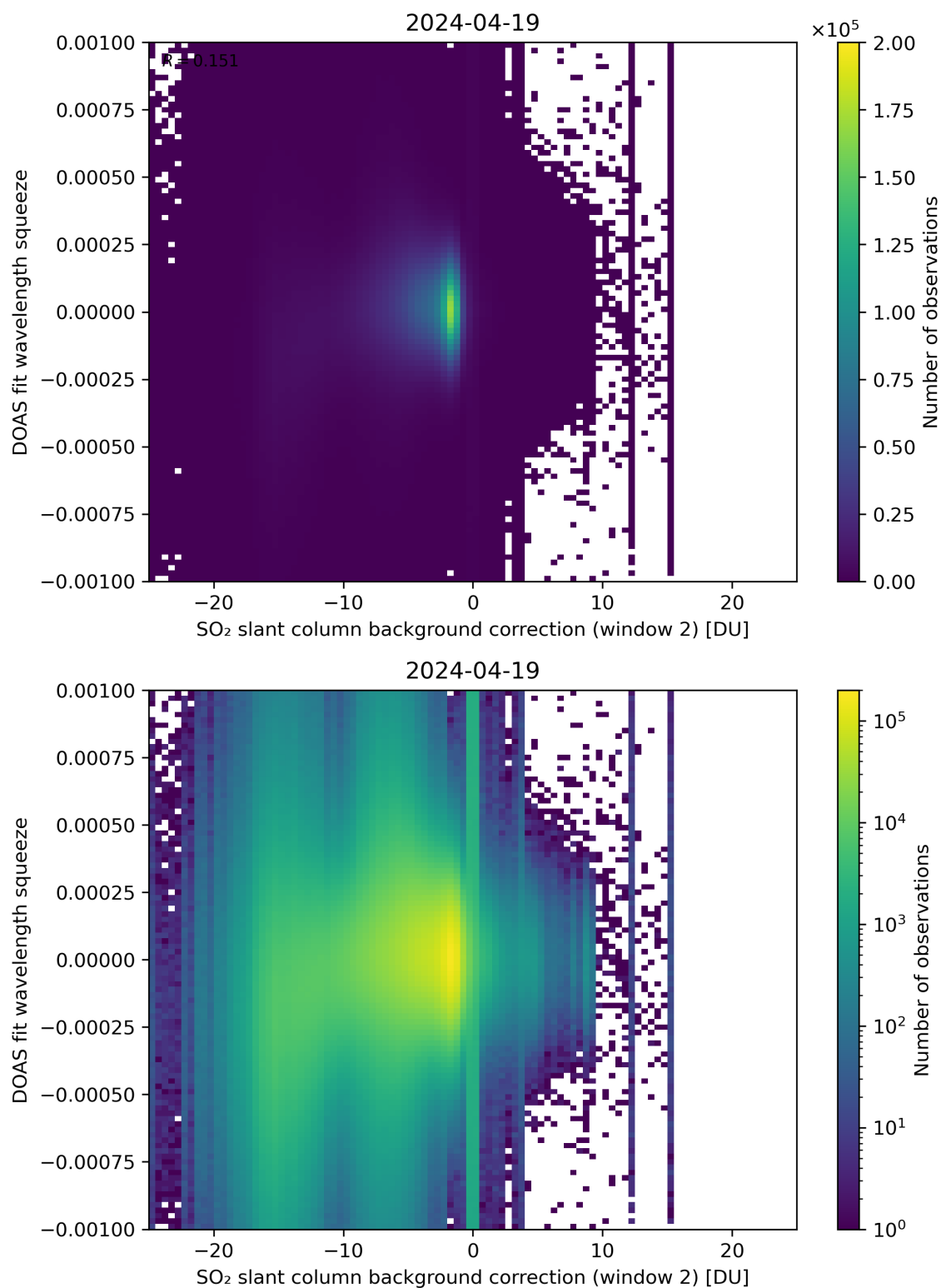
Figure 113: Scatter density plot of “SO 2 slant column background correction (window 2)” against “DOAS fit wavelength squeeze” for 2024-04-18 to 2024-04-20.
