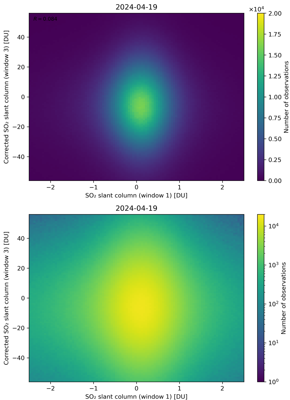
Figure 234: Scatter density plot of “SO 2 slant column (window 1)” against “Corrected SO 2 slant column (window 3)” for 2024-04-18 to 2024-04-20.
