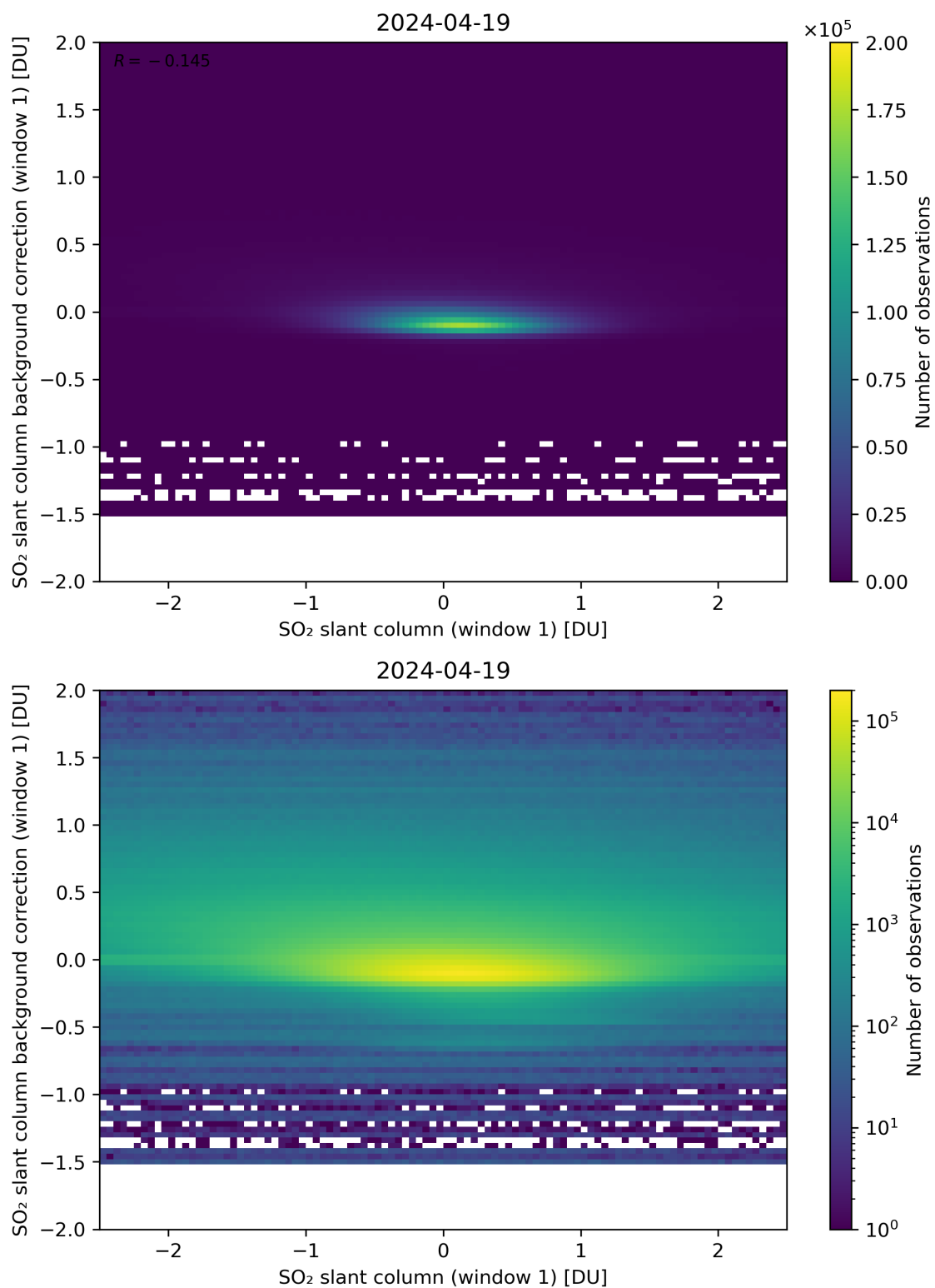
Figure 212: Scatter density plot of “SO 2 slant column (window 1)” against “SO 2 slant column background correction (window 1)” for 2024-04-18 to 2024-04-20.
