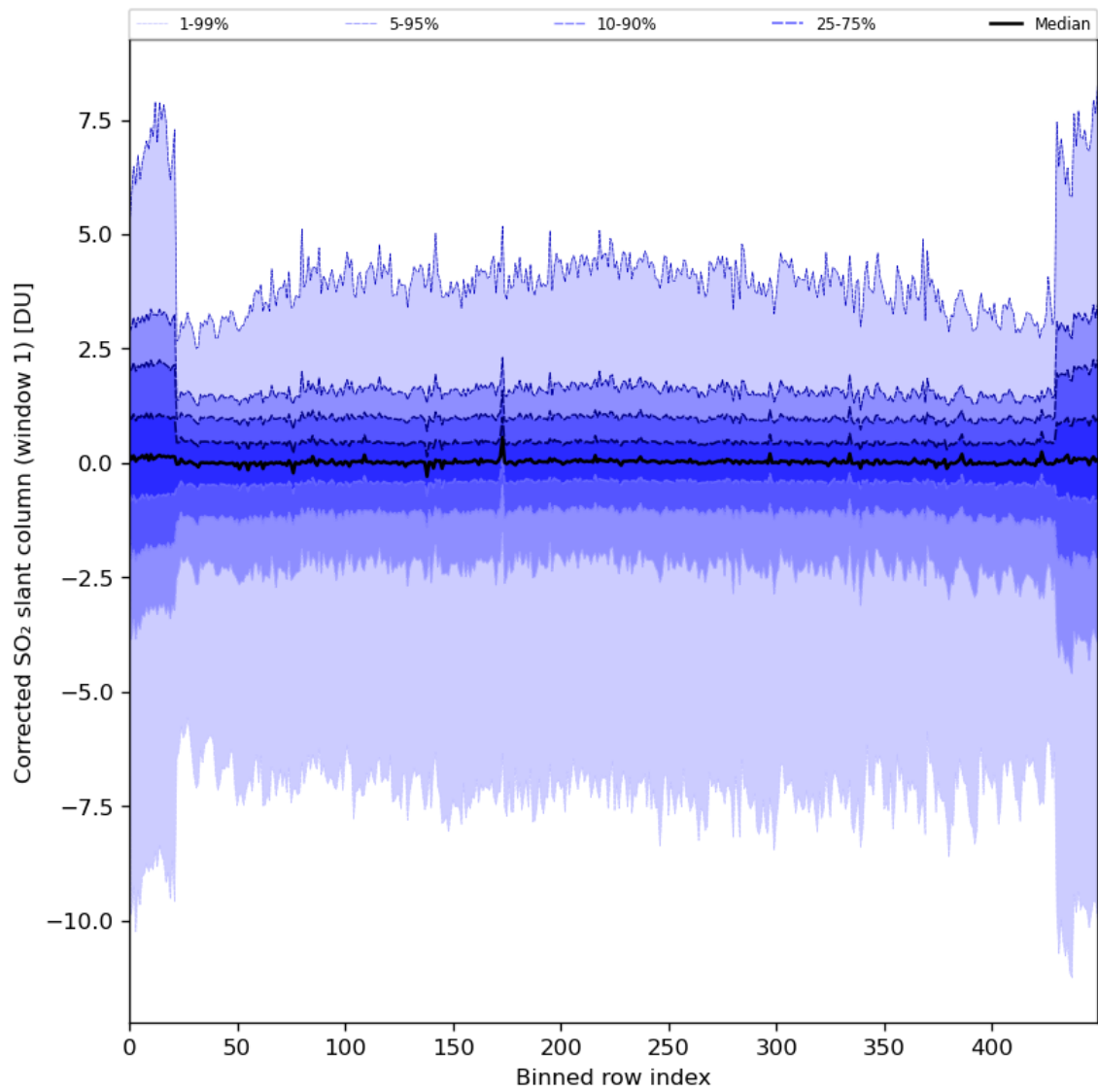
Figure 81: Along track statistics of “Corrected SO 2 slant column (window 1)” for 2024-04-18 to 2024-04-20
