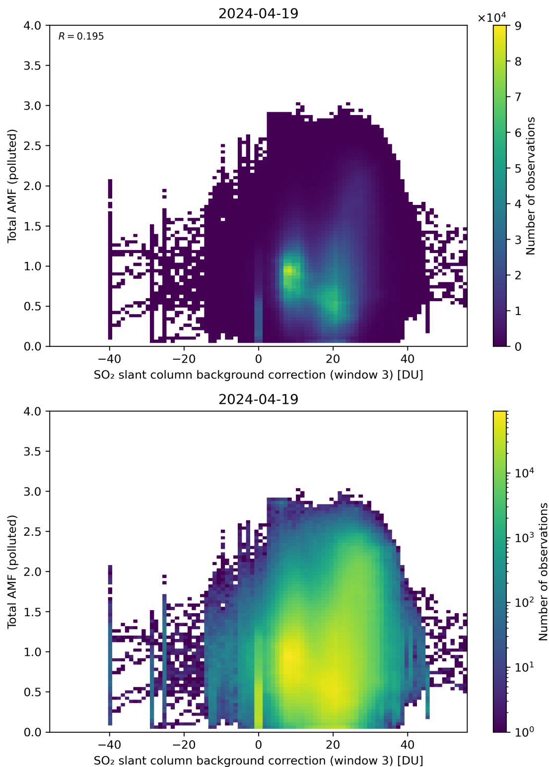
Figure 125: Scatter density plot of “SO 2 slant column background correction (window 3)” against “Total AMF (polluted)” for 2024-04-18 to 2024-04-20.
