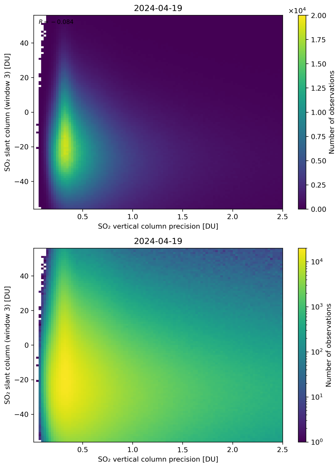
Figure 292: Scatter density plot of “SO 2 vertical column precision” against “SO 2 slant column (window 3)” for 2024-04-18 to 2024-04-20.
