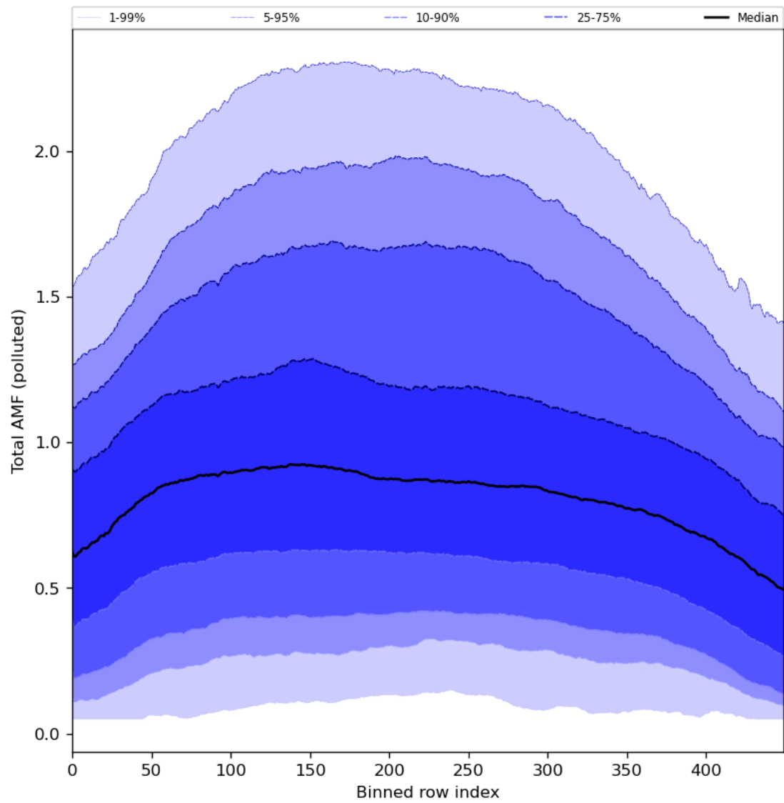
Figure 94: Along track statistics of “Total AMF (polluted)” for 2024-04-18 to 2024-04-20
