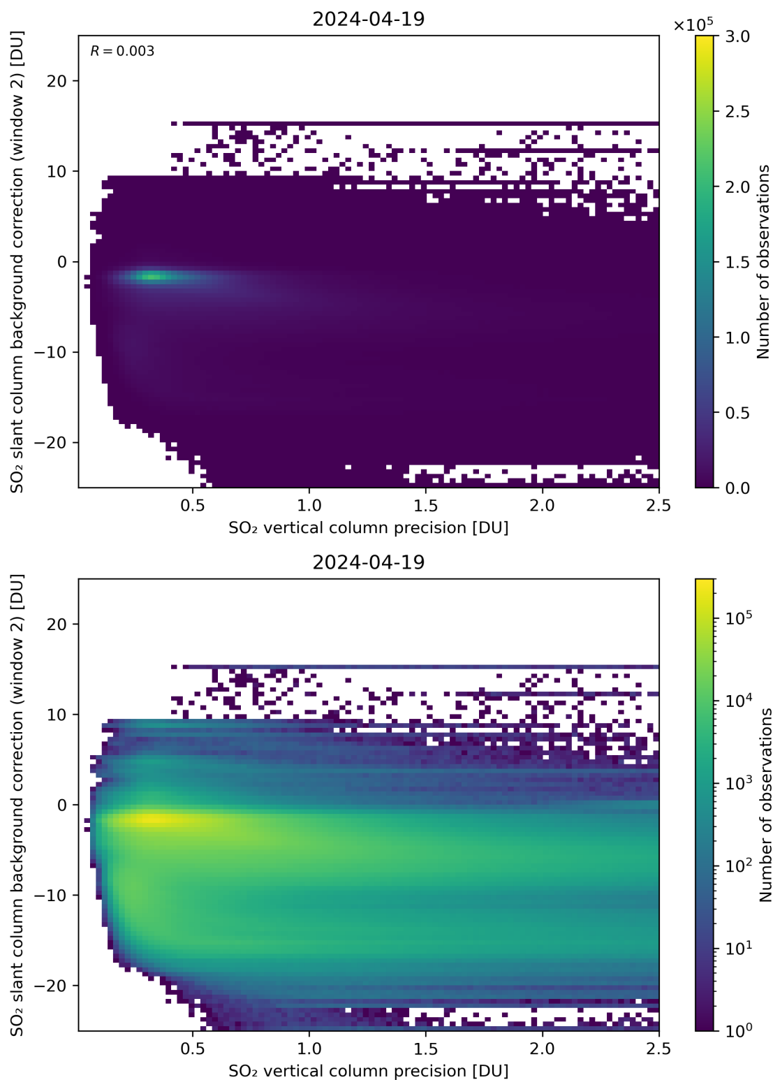
Figure 280: Scatter density plot of “SO 2 vertical column precision” against “SO 2 slant column background correction (window 2)” for 2024-04-18 to 2024-04-20.
