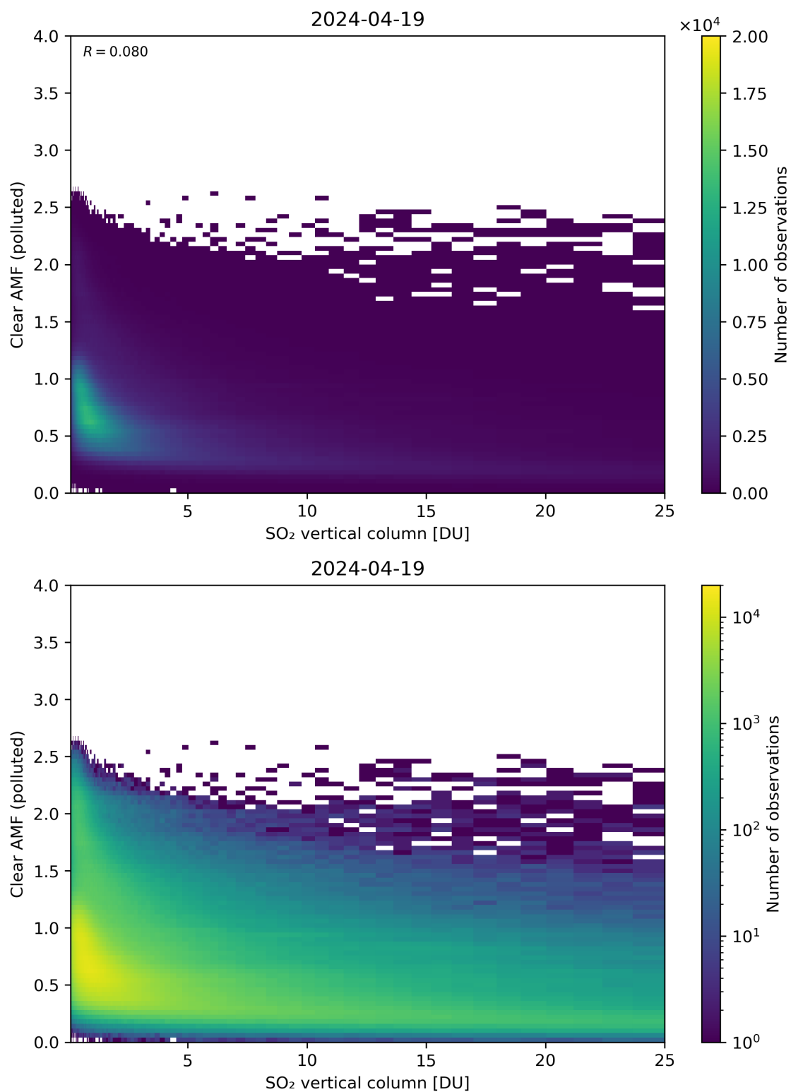
Figure 296: Scatter density plot of “SO 2 vertical column” against “Clear AMF (polluted)” for 2024-04-18 to 2024-04-20.
