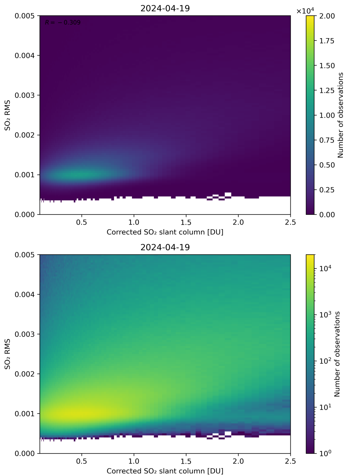
Figure 183: Scatter density plot of “Corrected SO 2 slant column” against “SO 2 RMS” for 2024-04-18 to 2024-04-20.
