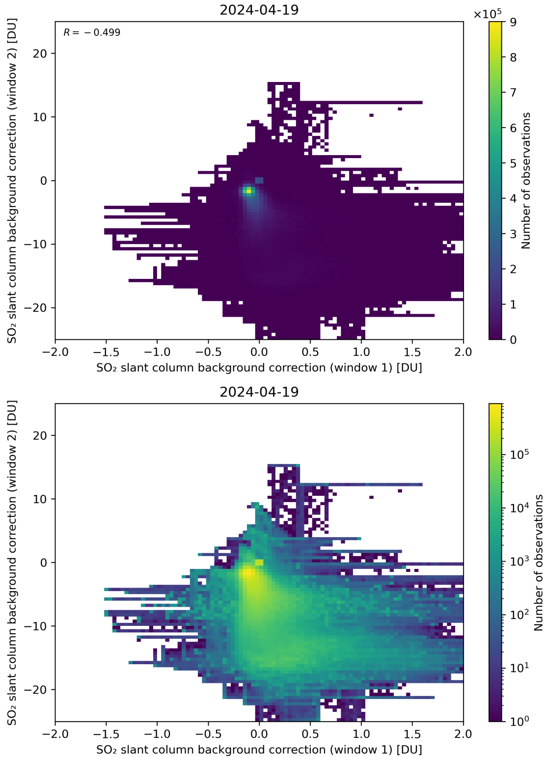
Figure 98: Scatter density plot of “SO 2 slant column background correction (window 1)” against “SO 2 slant column background correction (window 2)” for 2024-04-18 to 2024-04-20.
