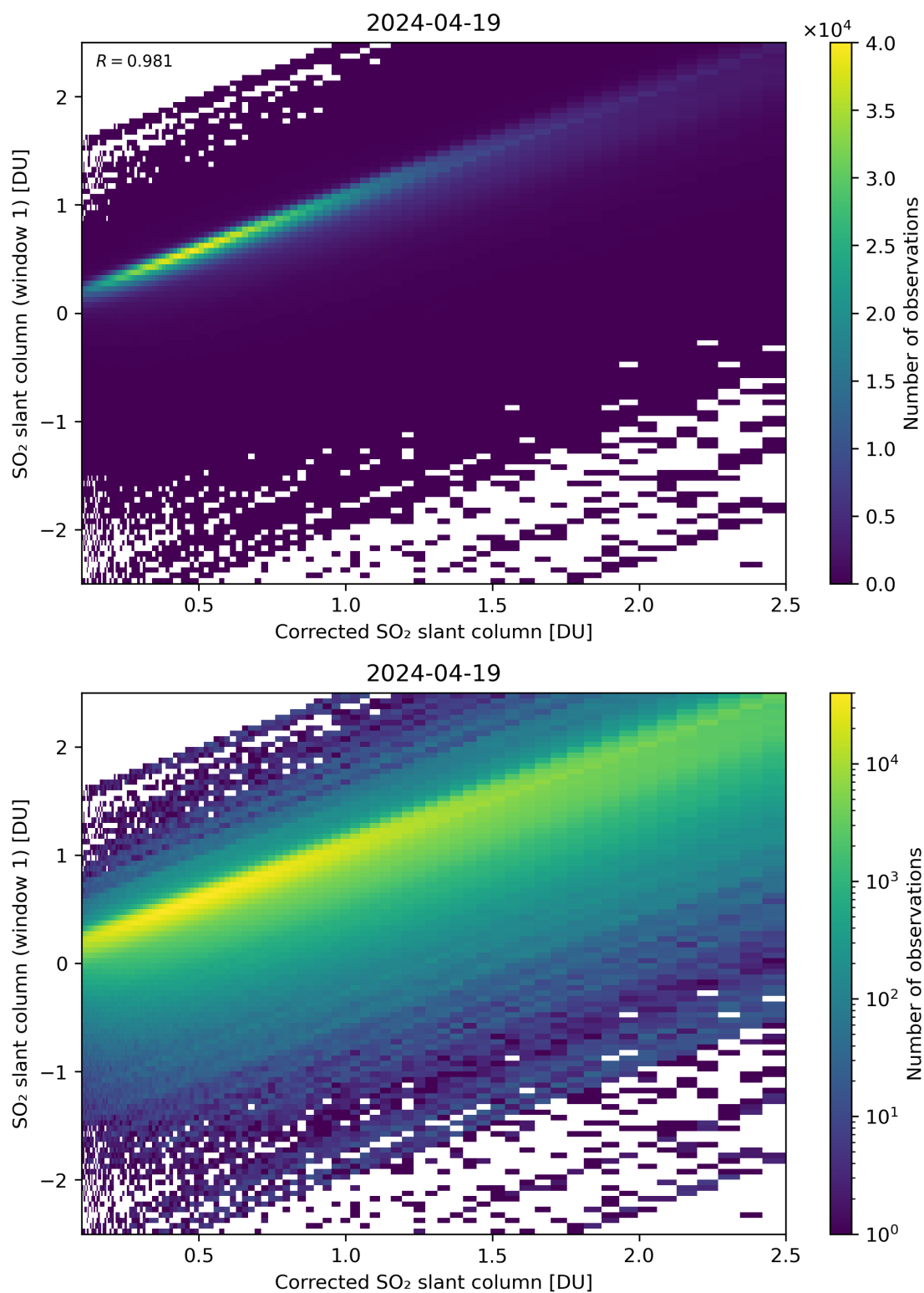
Figure 187: Scatter density plot of “Corrected SO 2 slant column” against “SO 2 slant column (window 1)” for 2024-04-18 to 2024-04-20.
