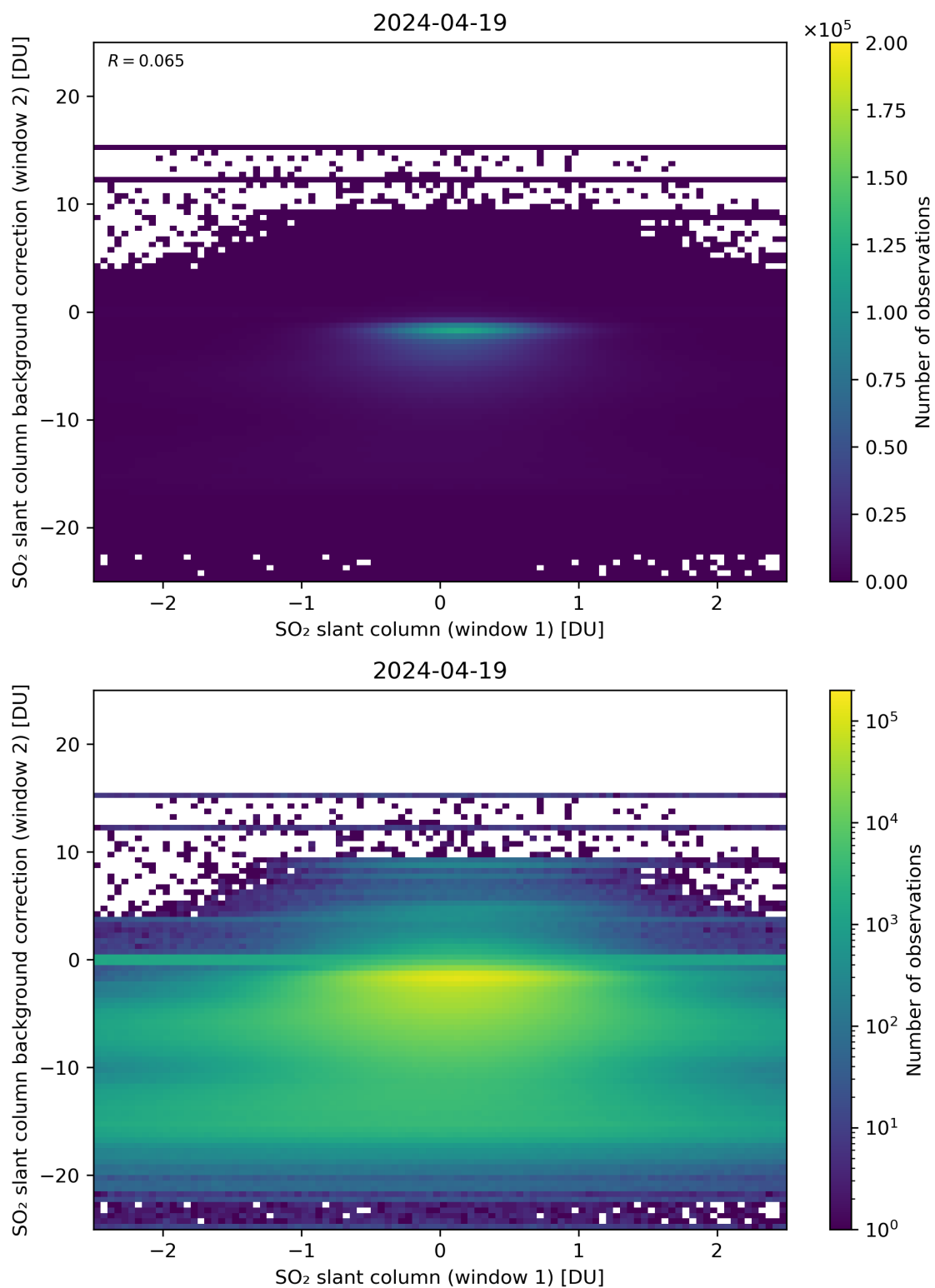
Figure 213: Scatter density plot of “SO 2 slant column (window 1)” against “SO 2 slant column background correction (window 2)” for 2024-04-18 to 2024-04-20.
