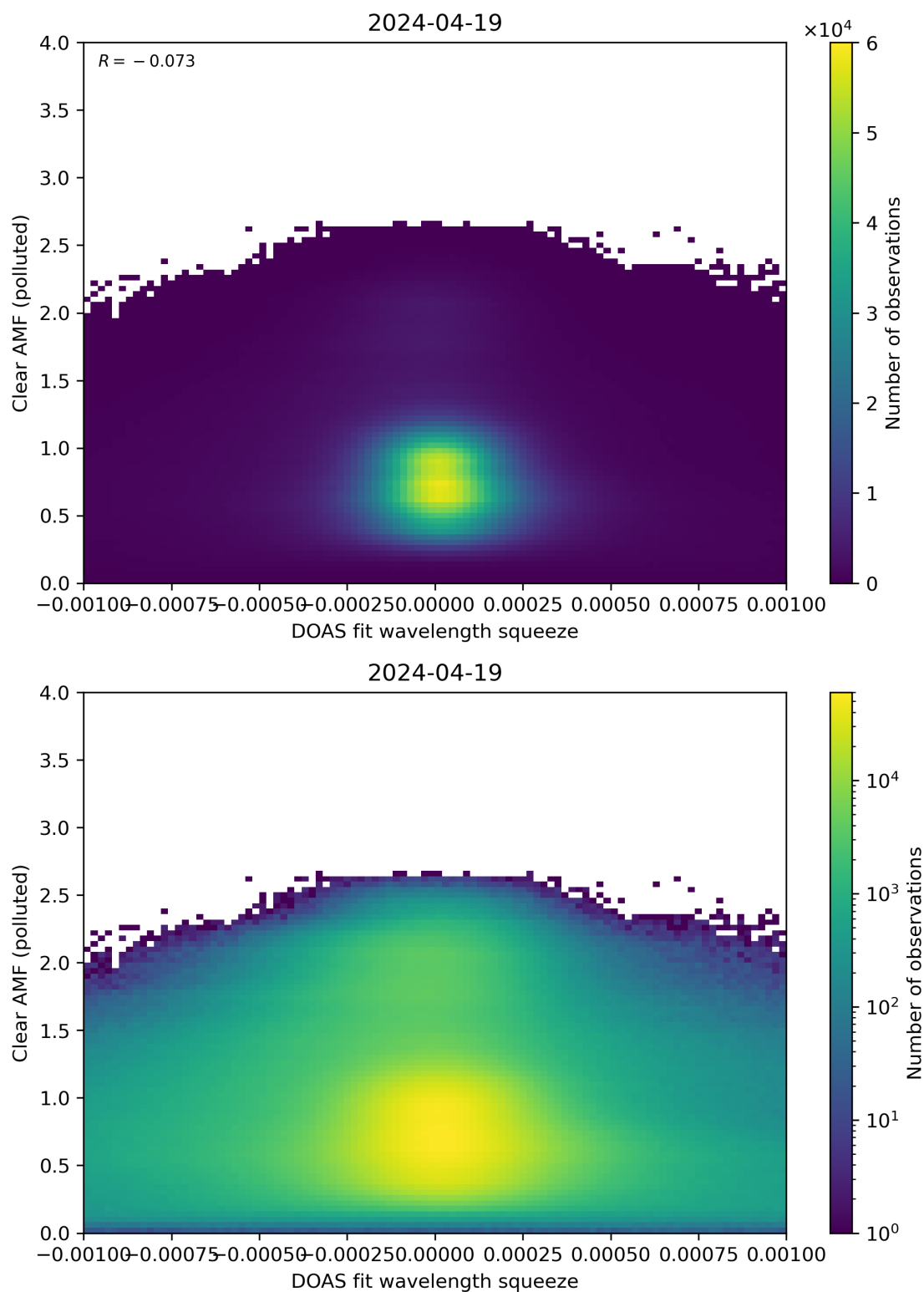
Figure 133: Scatter density plot of “DOAS fit wavelength squeeze” against “Clear AMF (polluted)” for 2024-04-18 to 2024-04-20.
