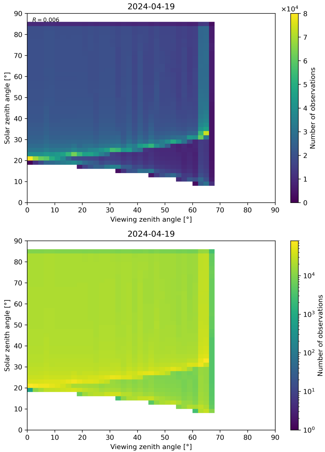
Figure 315: Scatter density plot of “Viewing zenith angle” against “Solar zenith angle” for 2024-04-18 to 2024-04-20.
