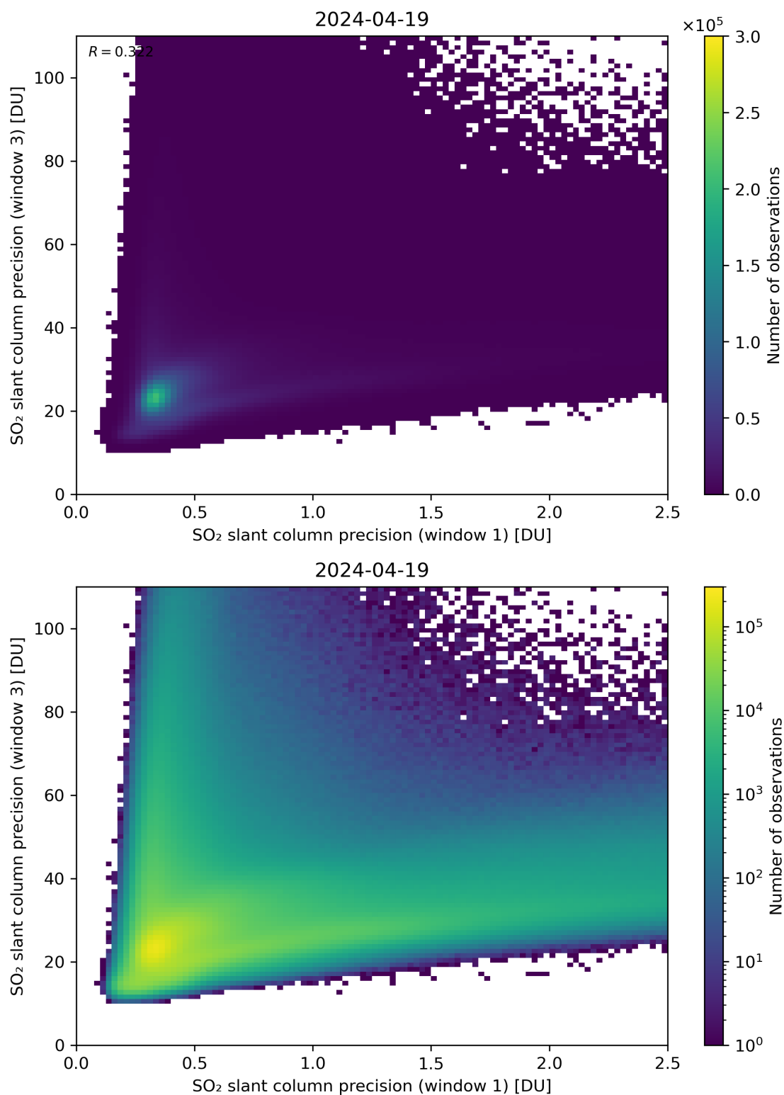
Figure 229: Scatter density plot of “SO 2 slant column precision (window 1)” against “SO 2 slant column precision (window 3)” for 2024-04-18 to 2024-04-20.
