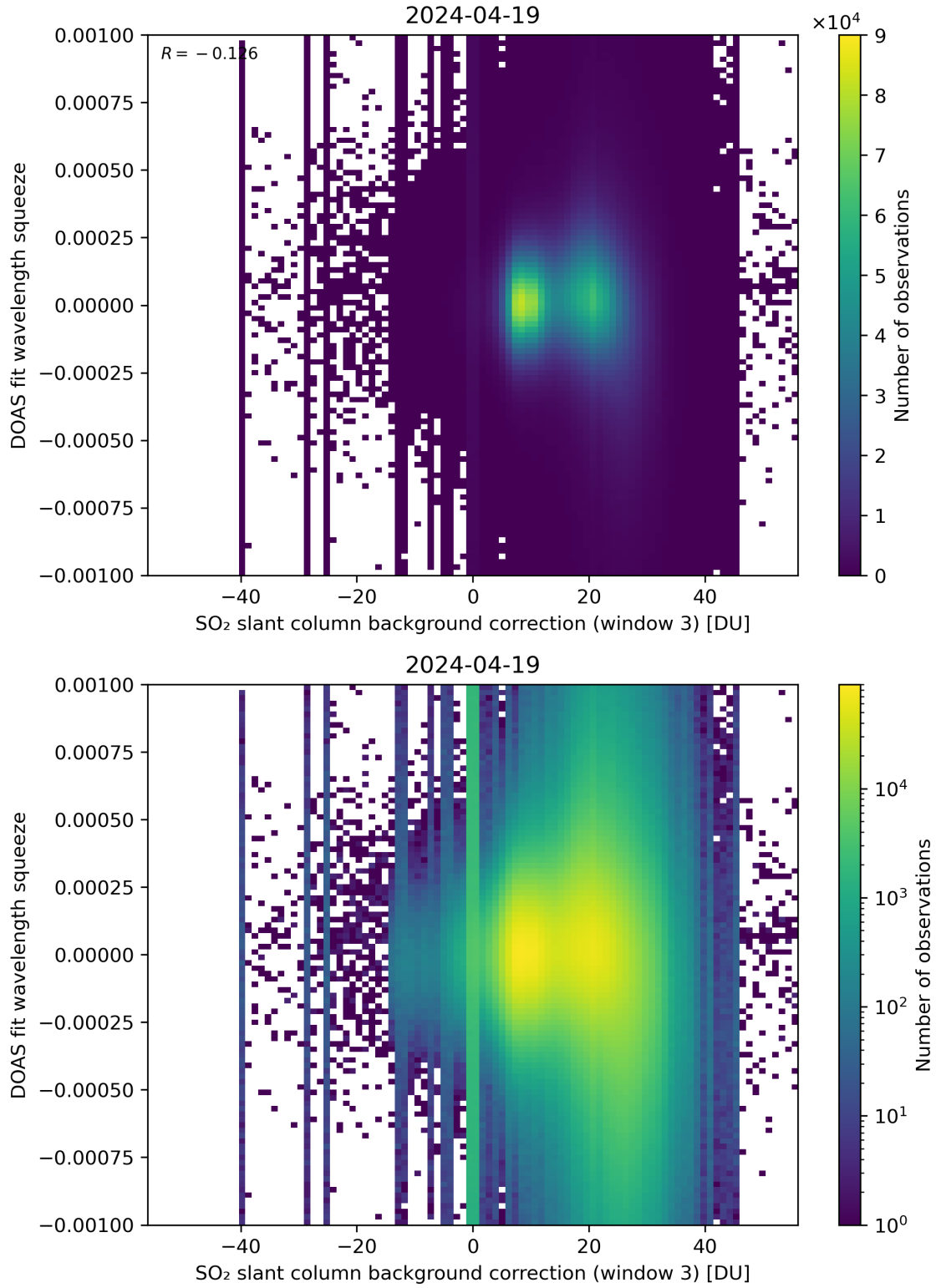
Figure 122: Scatter density plot of “SO 2 slant column background correction (window 3)” against “DOAS fit wavelength squeeze” for 2024-04-18 to 2024-04-20.
