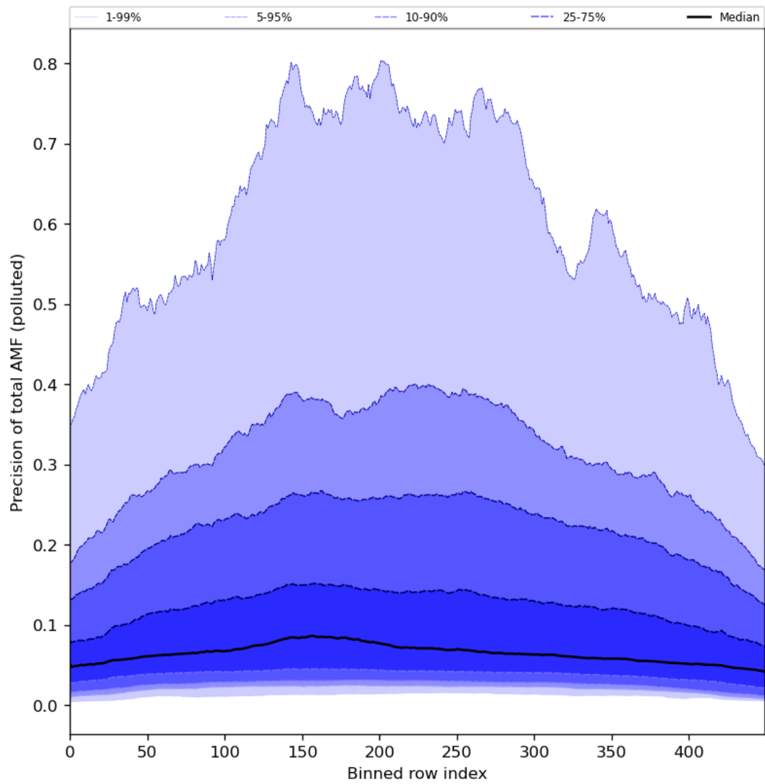
Figure 95: Along track statistics of “Precision of total AMF (polluted)” for 2024-04-18 to 2024-04-20
