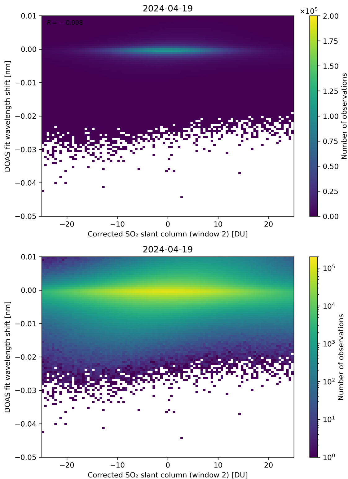
Figure 196: Scatter density plot of “Corrected SO 2 slant column (window 2)” against “DOAS fit wavelength shift” for 2024-04-18 to 2024-04-20.
