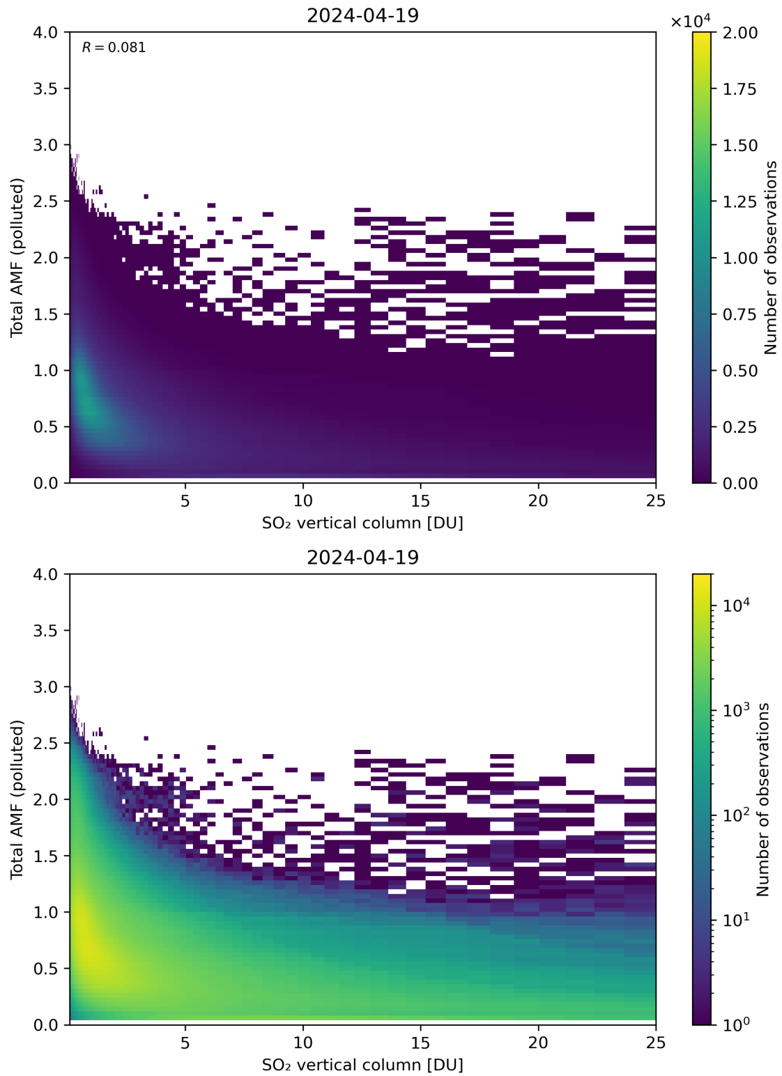
Figure 305: Scatter density plot of “SO 2 vertical column” against “Total AMF (polluted)” for 2024-04-18 to 2024-04-20.
