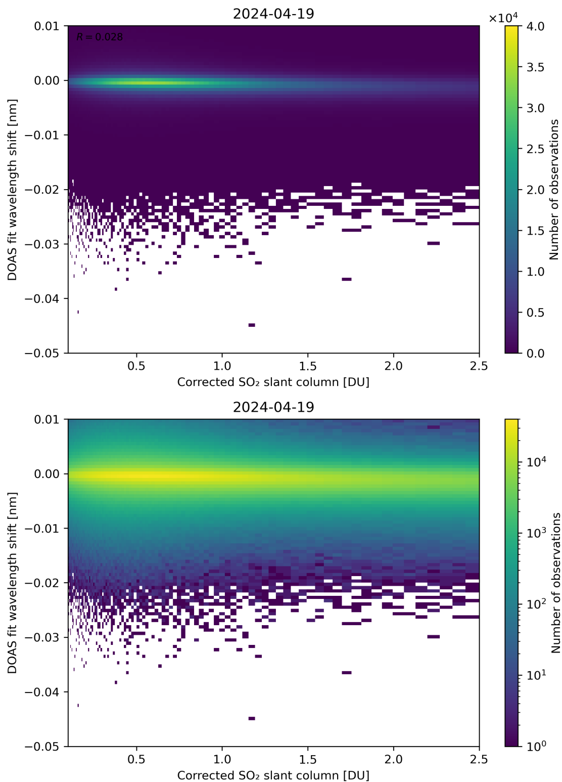
Figure 181: Scatter density plot of “Corrected SO 2 slant column” against “DOAS fit wavelength shift” for 2024-04-18 to 2024-04-20.
