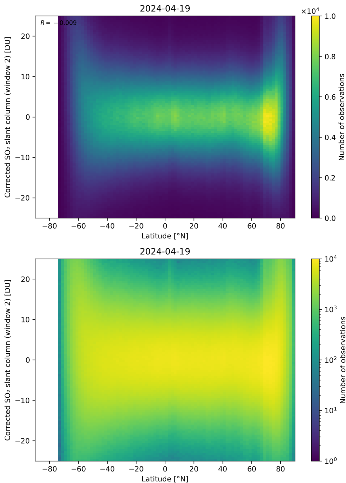
Figure 147: Scatter density plot of “Latitude” against “Corrected SO 2 slant column (window 2)” for 2024-04-18 to 2024-04-20.
