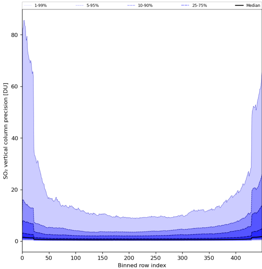
Figure 77: Along track statistics of “SO 2 vertical column precision” for 2024-04-18 to 2024-04-20
