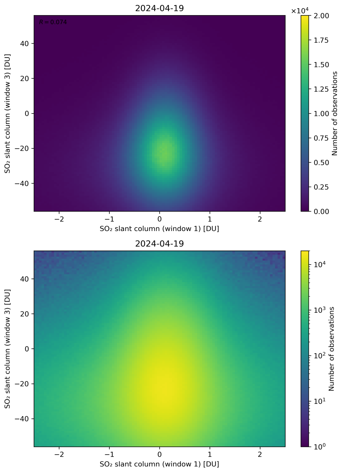
Figure 237: Scatter density plot of “SO 2 slant column (window 1)” against “SO 2 slant column (window 3)” for 2024-04-18 to 2024-04-20.
