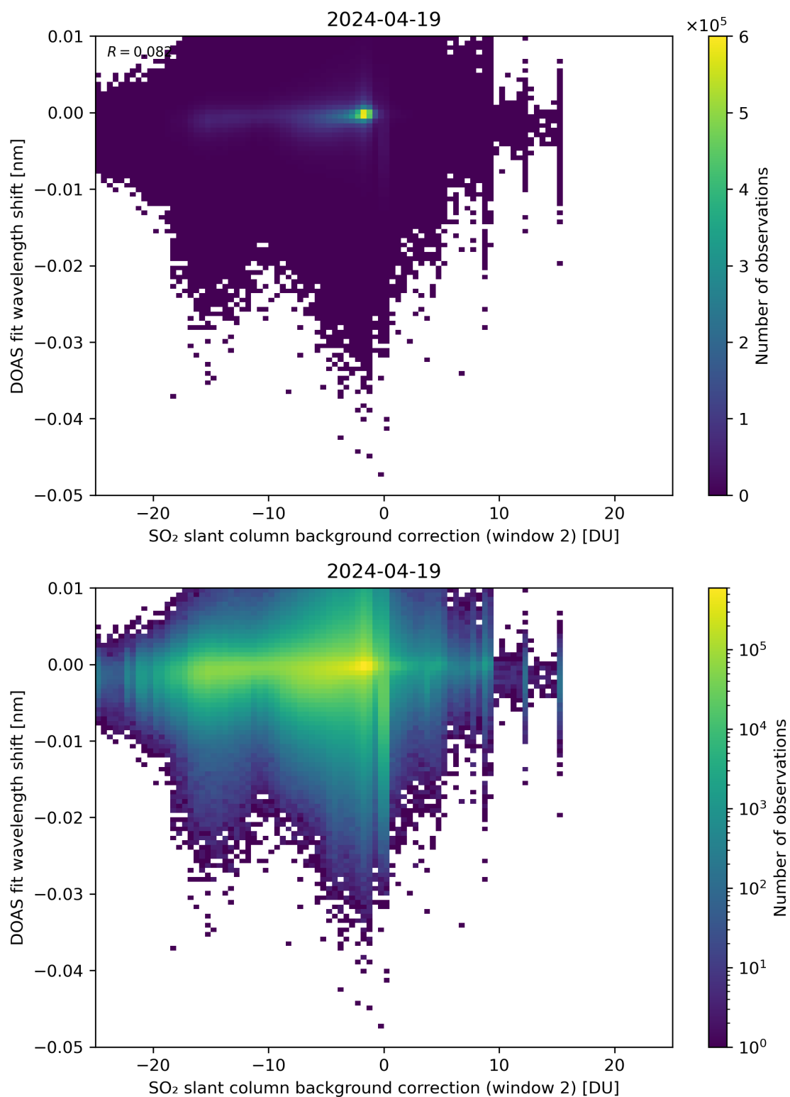
Figure 112: Scatter density plot of “SO 2 slant column background correction (window 2)” against “DOAS fit wavelength shift” for 2024-04-18 to 2024-04-20.
