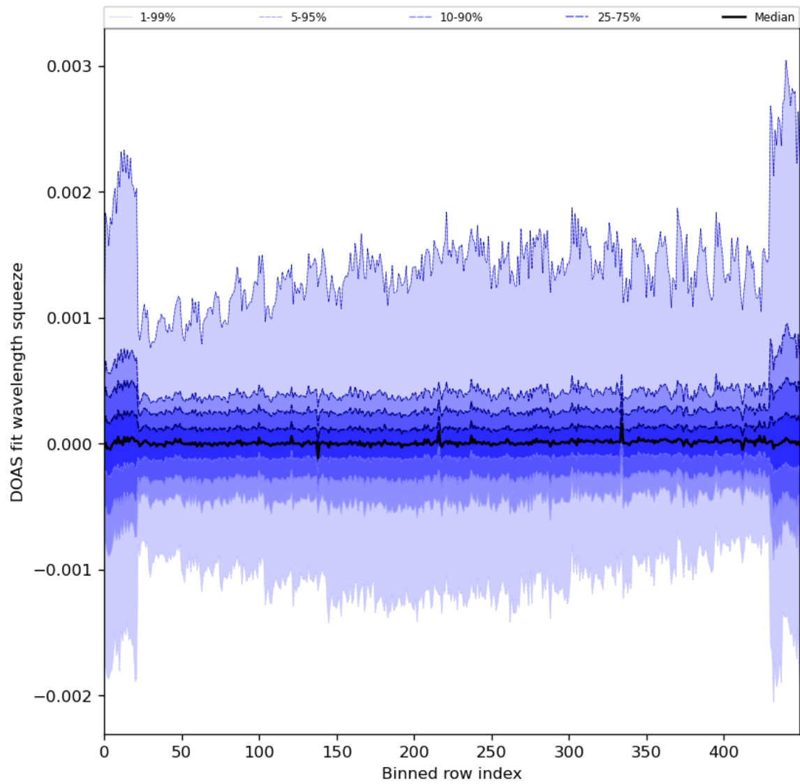
Figure 92: Along track statistics of “DOAS fit wavelength squeeze” for 2024-04-18 to 2024-04-20
