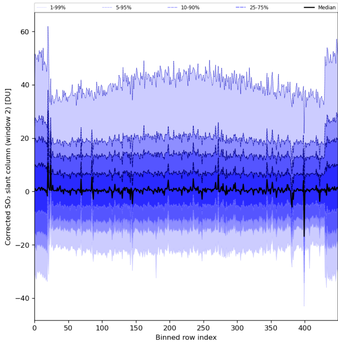
Figure 85: Along track statistics of “Corrected SO 2 slant column (window 2)” for 2024-04-18 to 2024-04-20
