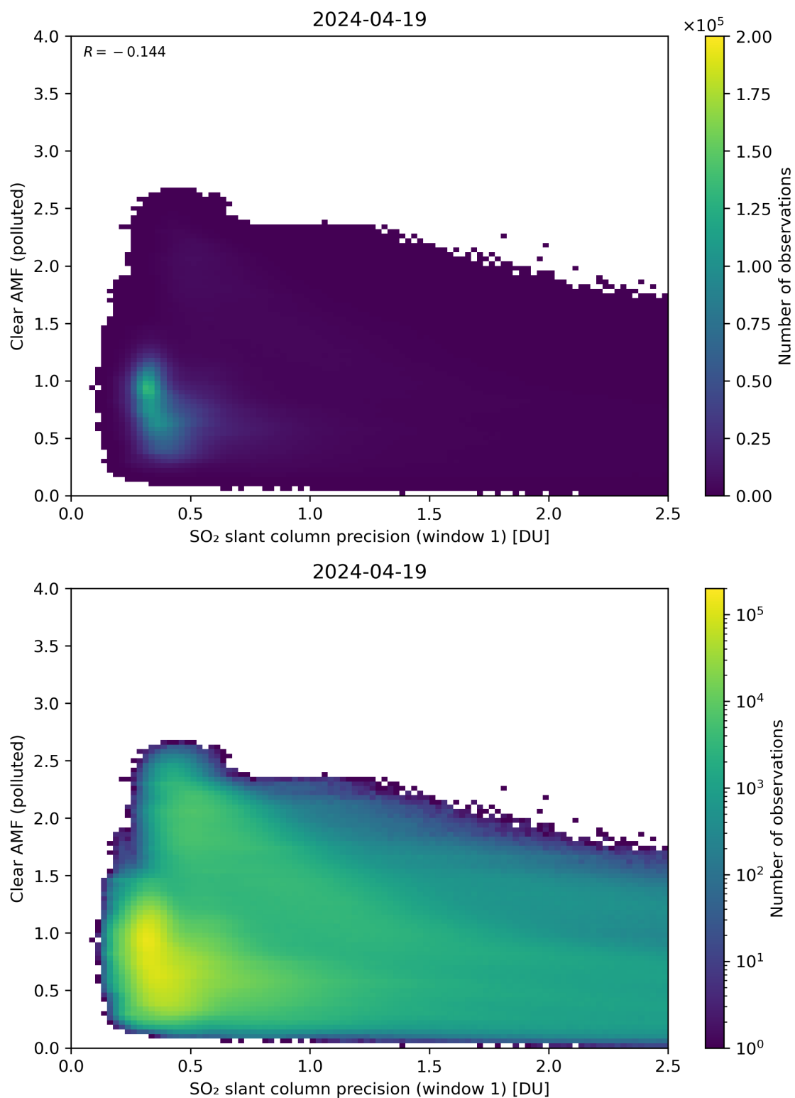
Figure 224: Scatter density plot of “SO 2 slant column precision (window 1)” against “Clear AMF (polluted)” for 2024-04-18 to 2024-04-20.
