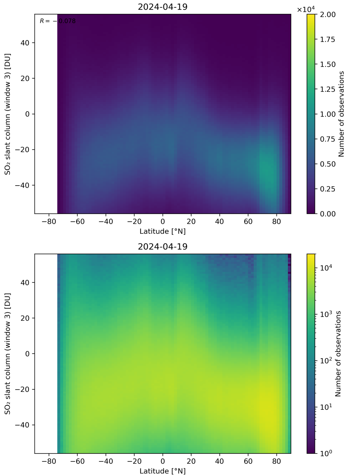
Figure 152: Scatter density plot of “Latitude” against “SO 2 slant column (window 3)” for 2024-04-18 to 2024-04-20.
