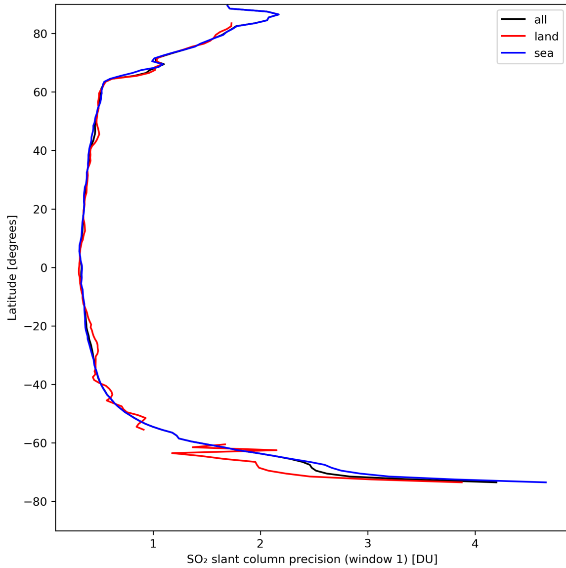
Figure 34: Zonal average of “SO 2 slant column precision (window 1)” for 2024-04-18 to 2024-04-20.
