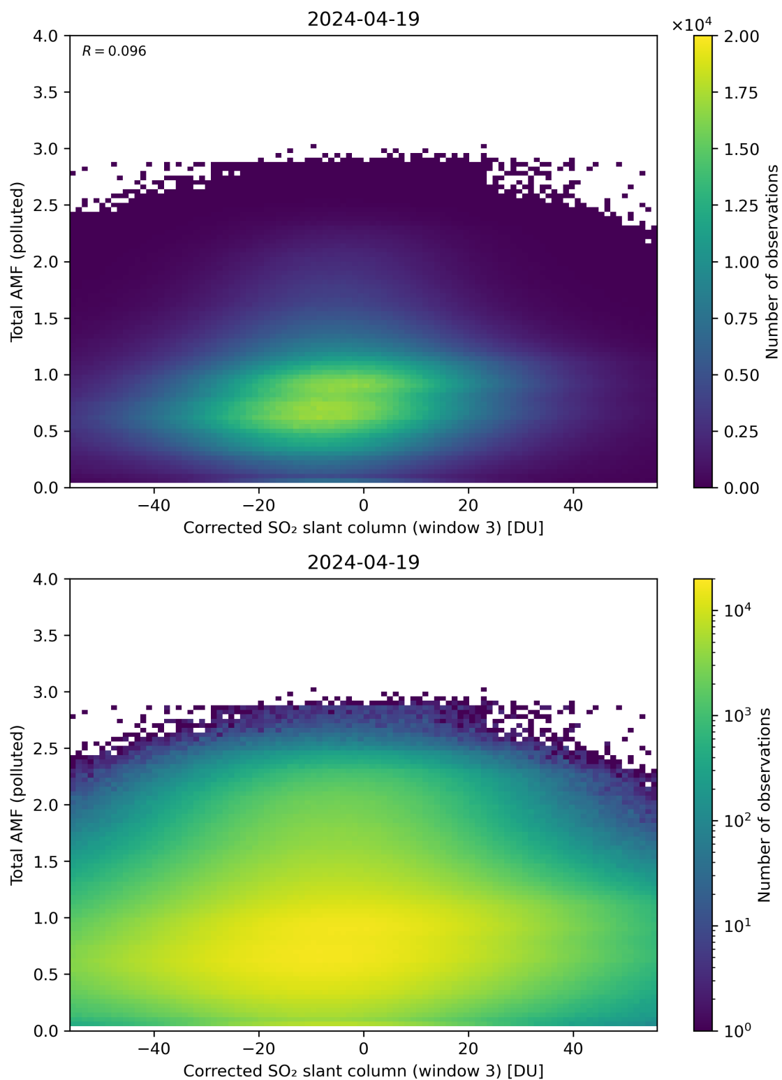
Figure 210: Scatter density plot of “Corrected SO 2 slant column (window 3)” against “Total AMF (polluted)” for 2024-04-18 to 2024-04-20.
