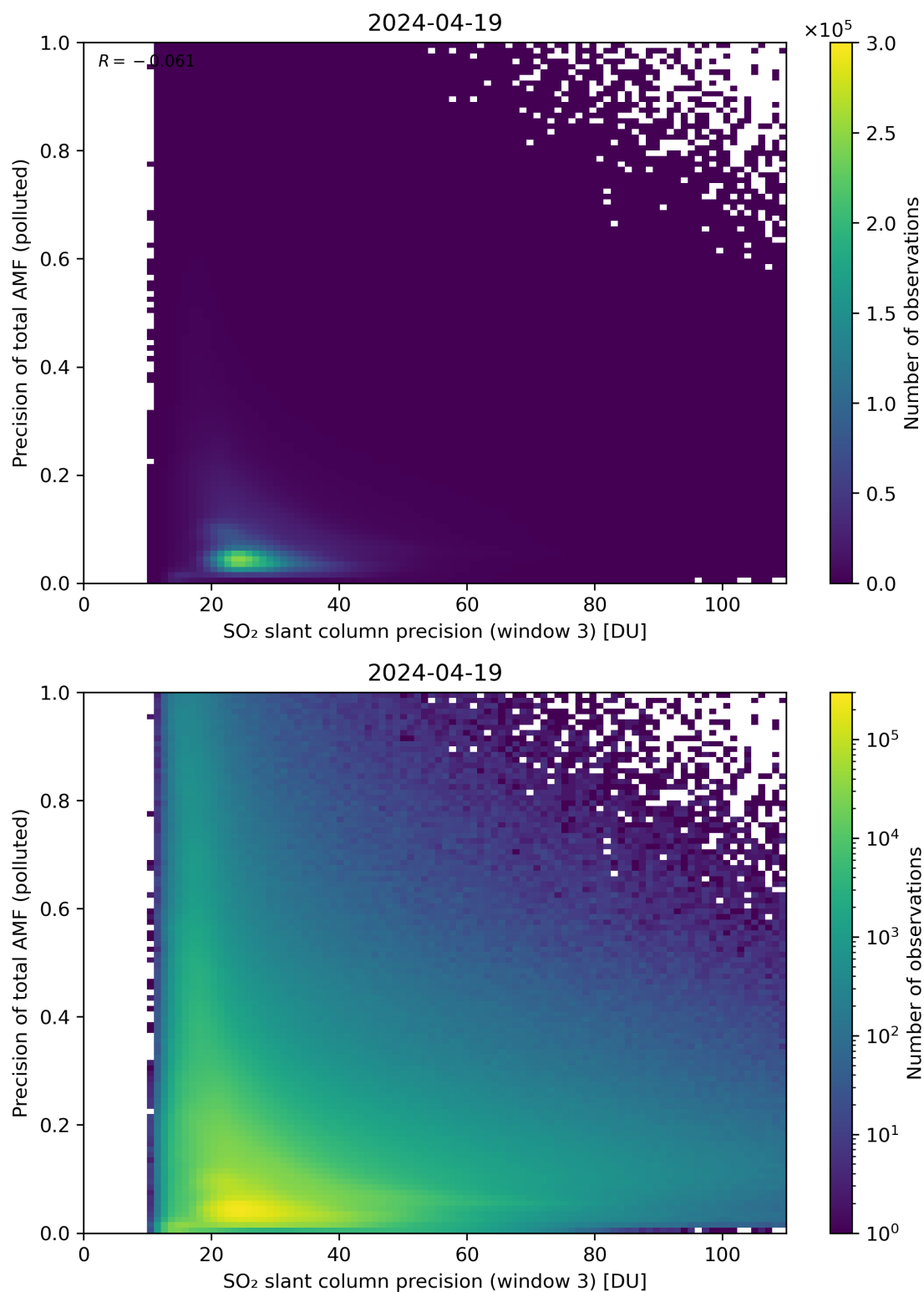
Figure 264: Scatter density plot of “SO 2 slant column precision (window 3)” against “Precision of total AMF (polluted)” for 2024-04-18 to 2024-04-20.
