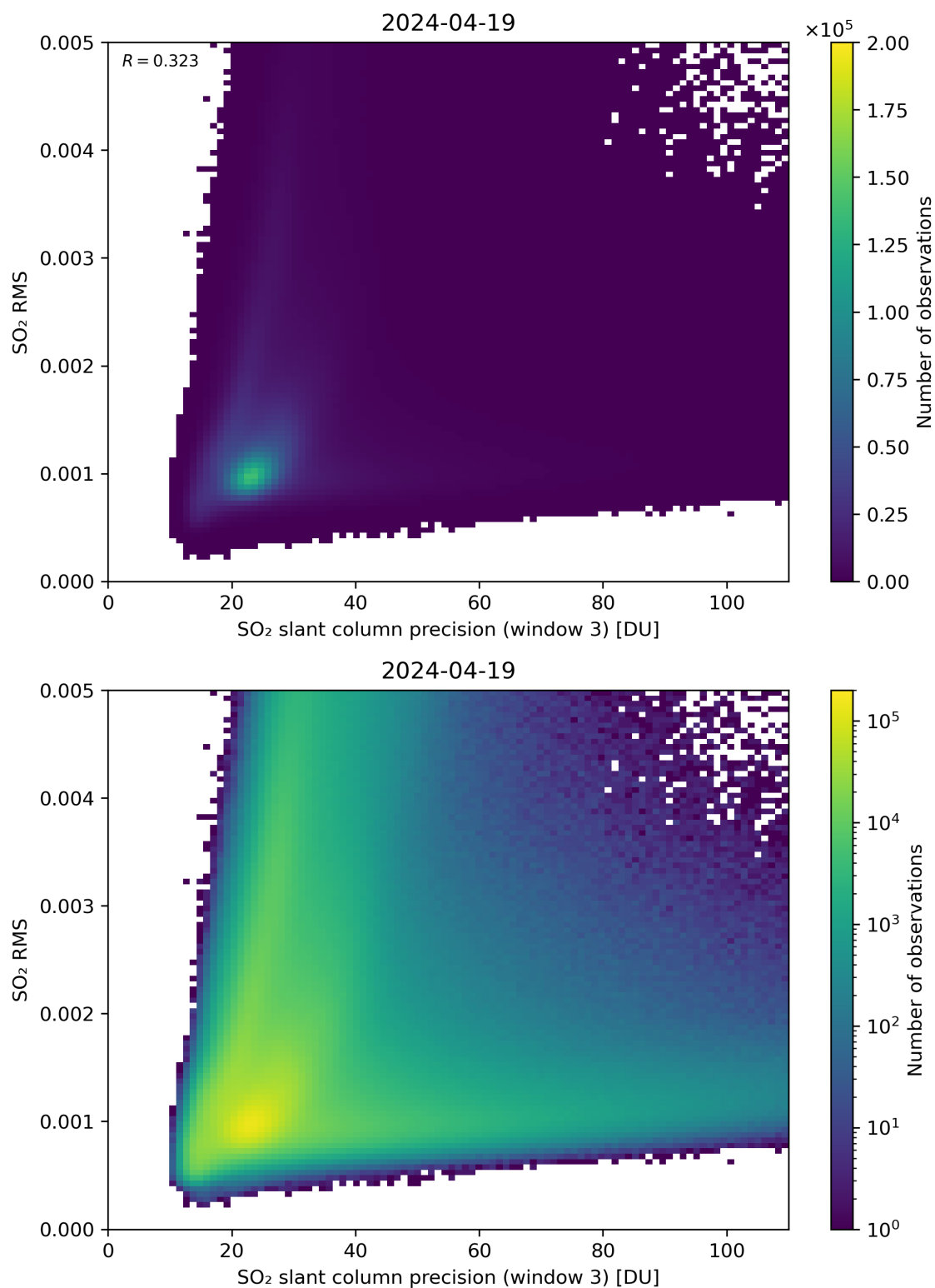
Figure 260: Scatter density plot of “SO 2 slant column precision (window 3)” against “SO 2 RMS” for 2024-04-18 to 2024-04-20.
