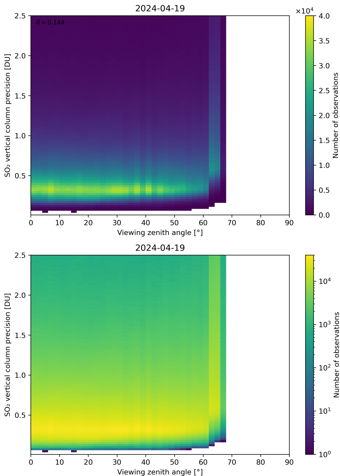
Figure 328: Scatter density plot of “Viewing zenith angle” against “SO 2 vertical column precision” for 2024-04-18 to 2024-04-20.
