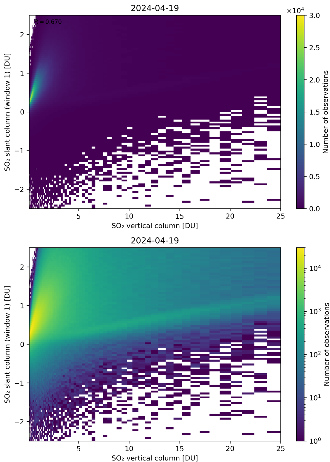
Figure 300: Scatter density plot of “SO 2 vertical column” against “SO 2 slant column (window 1)” for 2024-04-18 to 2024-04-20.
