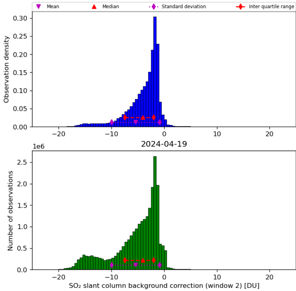
Figure 63: Histogram of “SO 2 slant column background correction (window 2)” for 2024-04-18 to 2024-04-20
