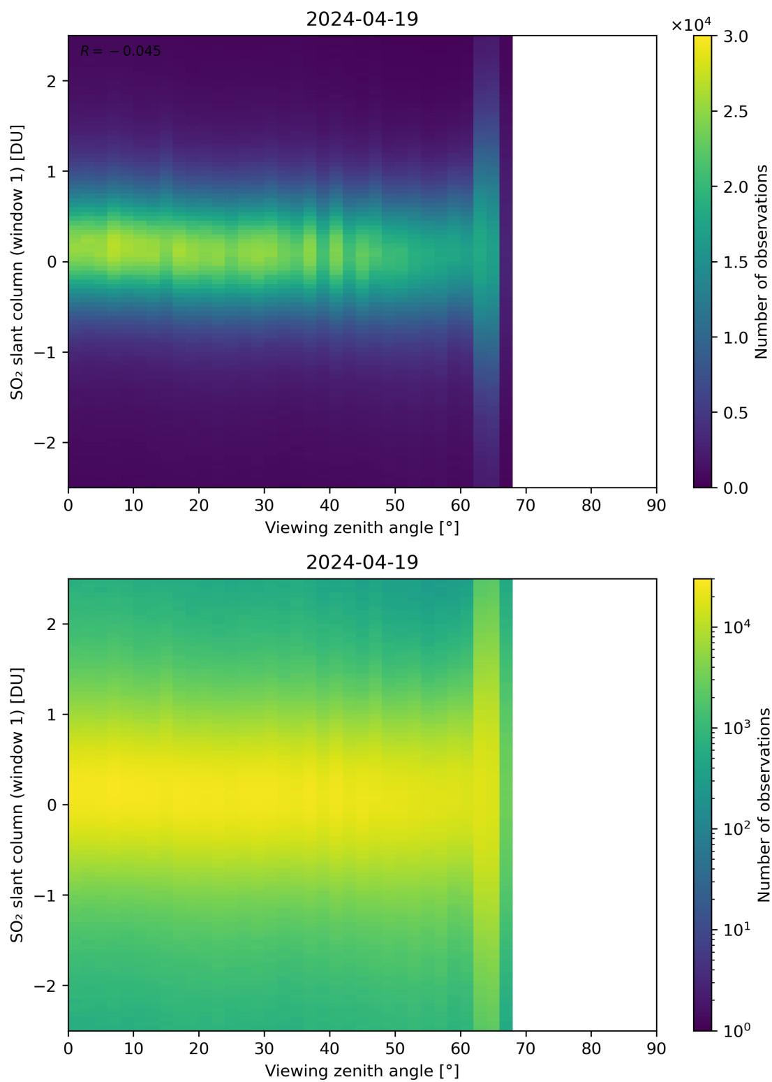
Figure 320: Scatter density plot of “Viewing zenith angle” against “SO 2 slant column (window 1)” for 2024-04-18 to 2024-04-20.
