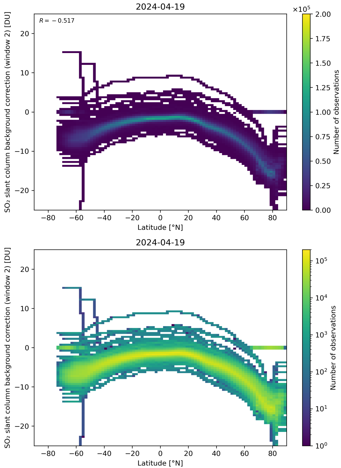
Figure 140: Scatter density plot of “Latitude” against “SO 2 slant column background correction (window 2)” for 2024-04-18 to 2024-04-20.
