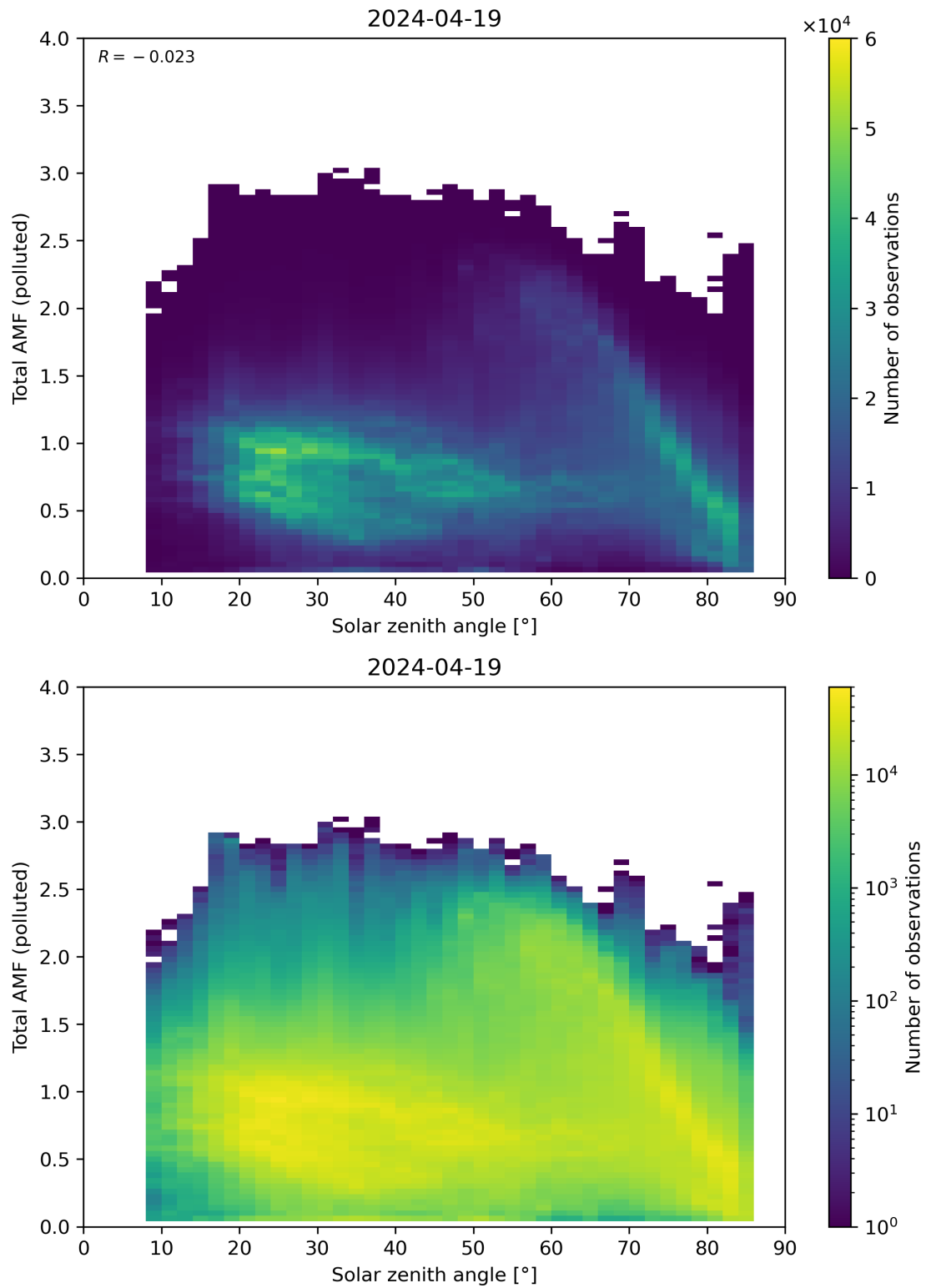
Figure 174: Scatter density plot of “Solar zenith angle” against “Total AMF (polluted)” for 2024-04-18 to 2024-04-20.
