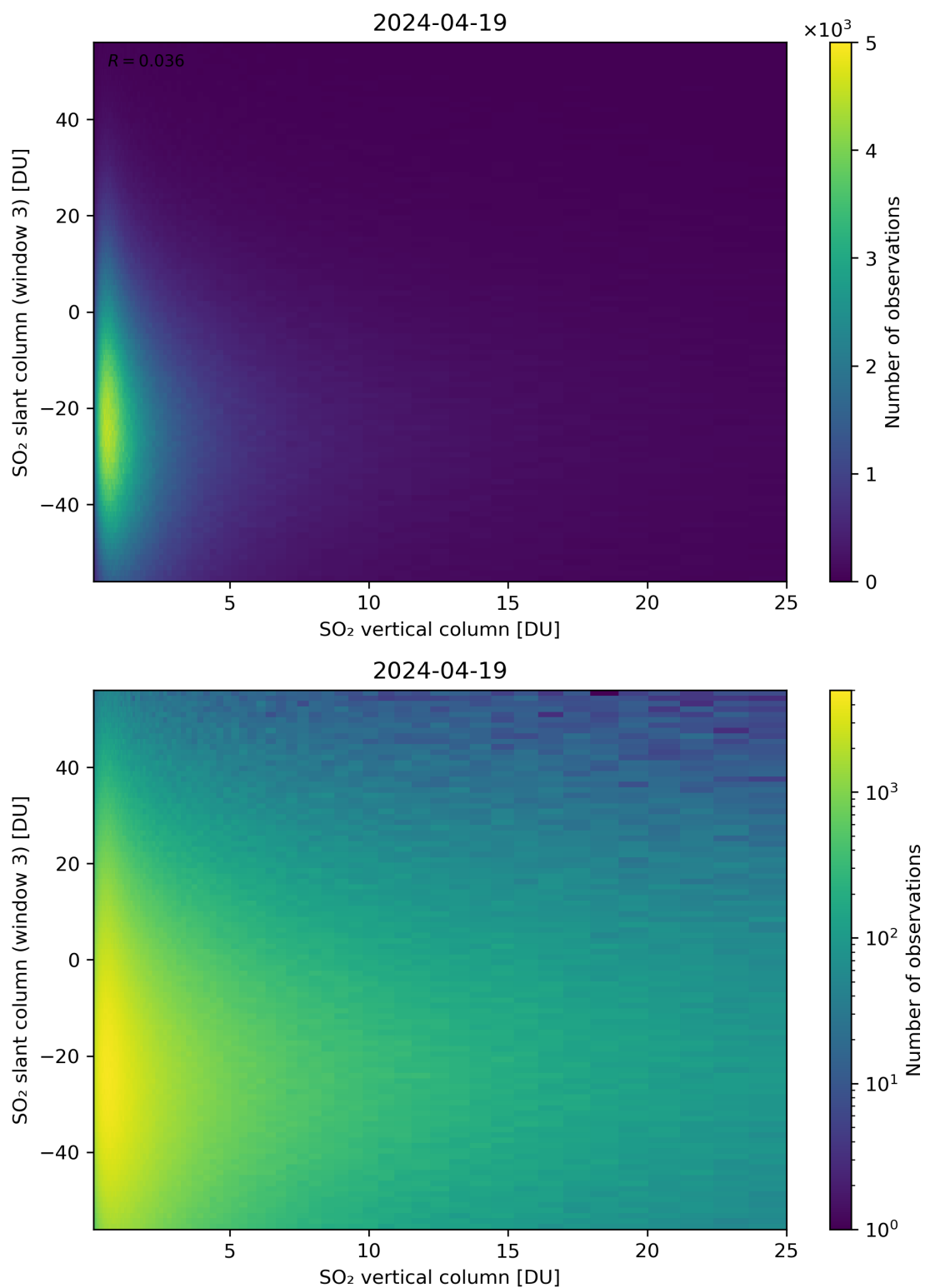
Figure 303: Scatter density plot of “SO 2 vertical column” against “SO 2 slant column (window 3)” for 2024-04-18 to 2024-04-20.
