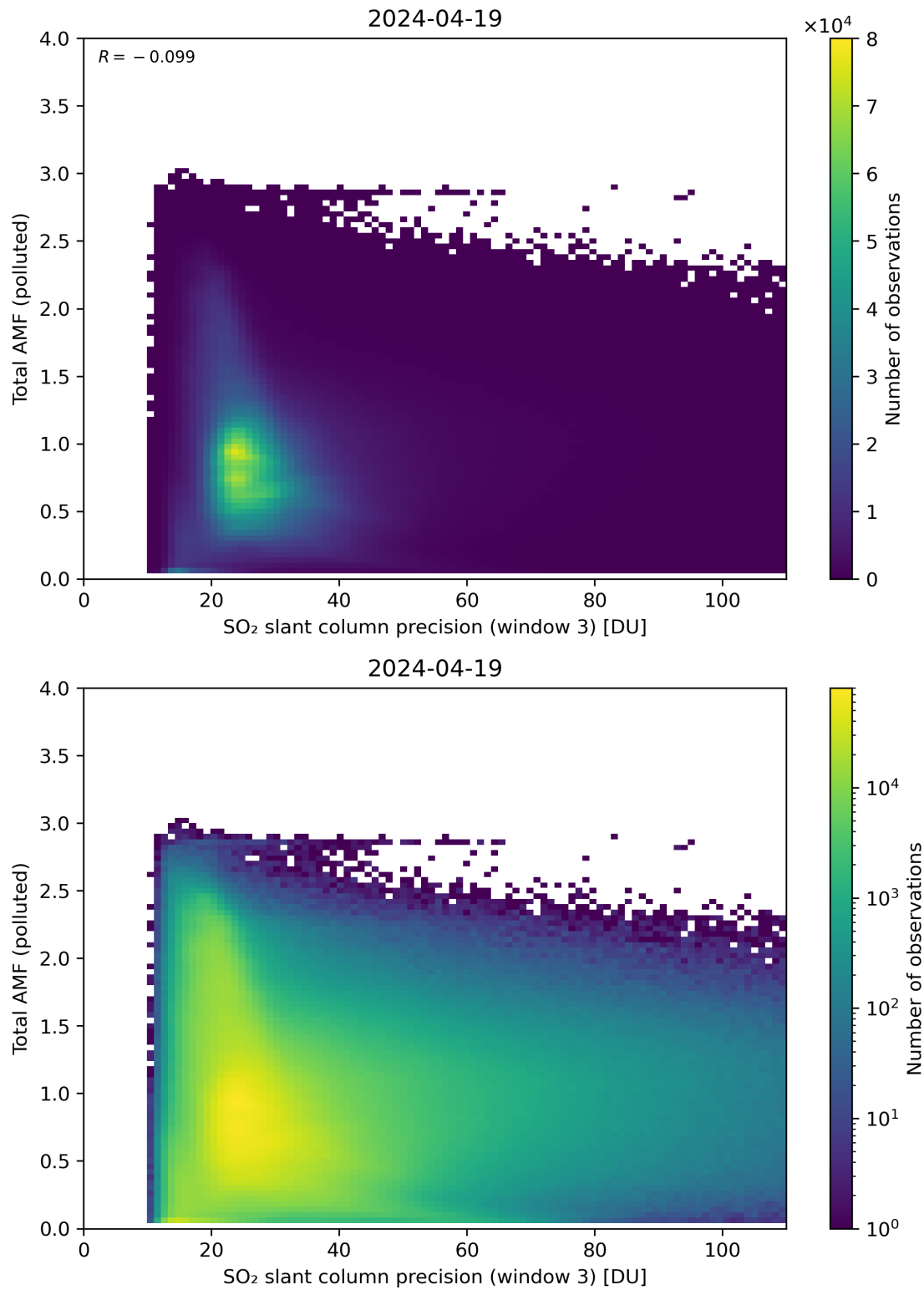
Figure 263: Scatter density plot of “SO 2 slant column precision (window 3)” against “Total AMF (polluted)” for 2024-04-18 to 2024-04-20.
