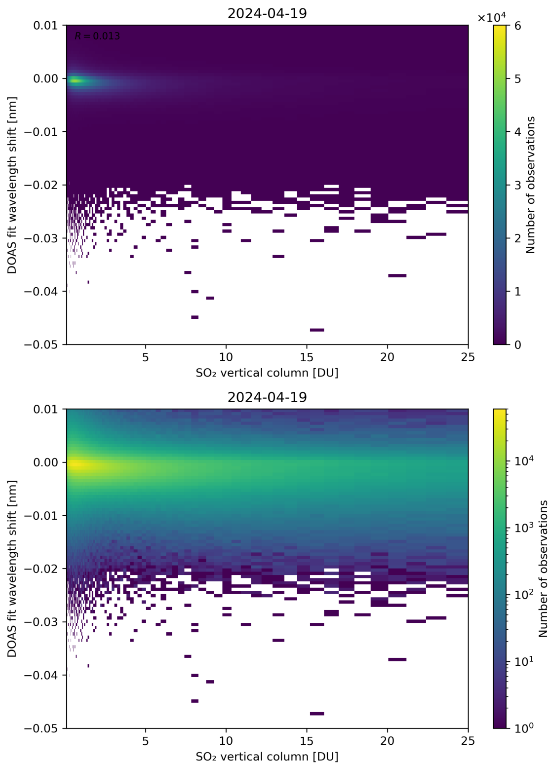
Figure 276: Scatter density plot of “SO 2 vertical column” against “DOAS fit wavelength shift” for 2024-04-18 to 2024-04-20.
