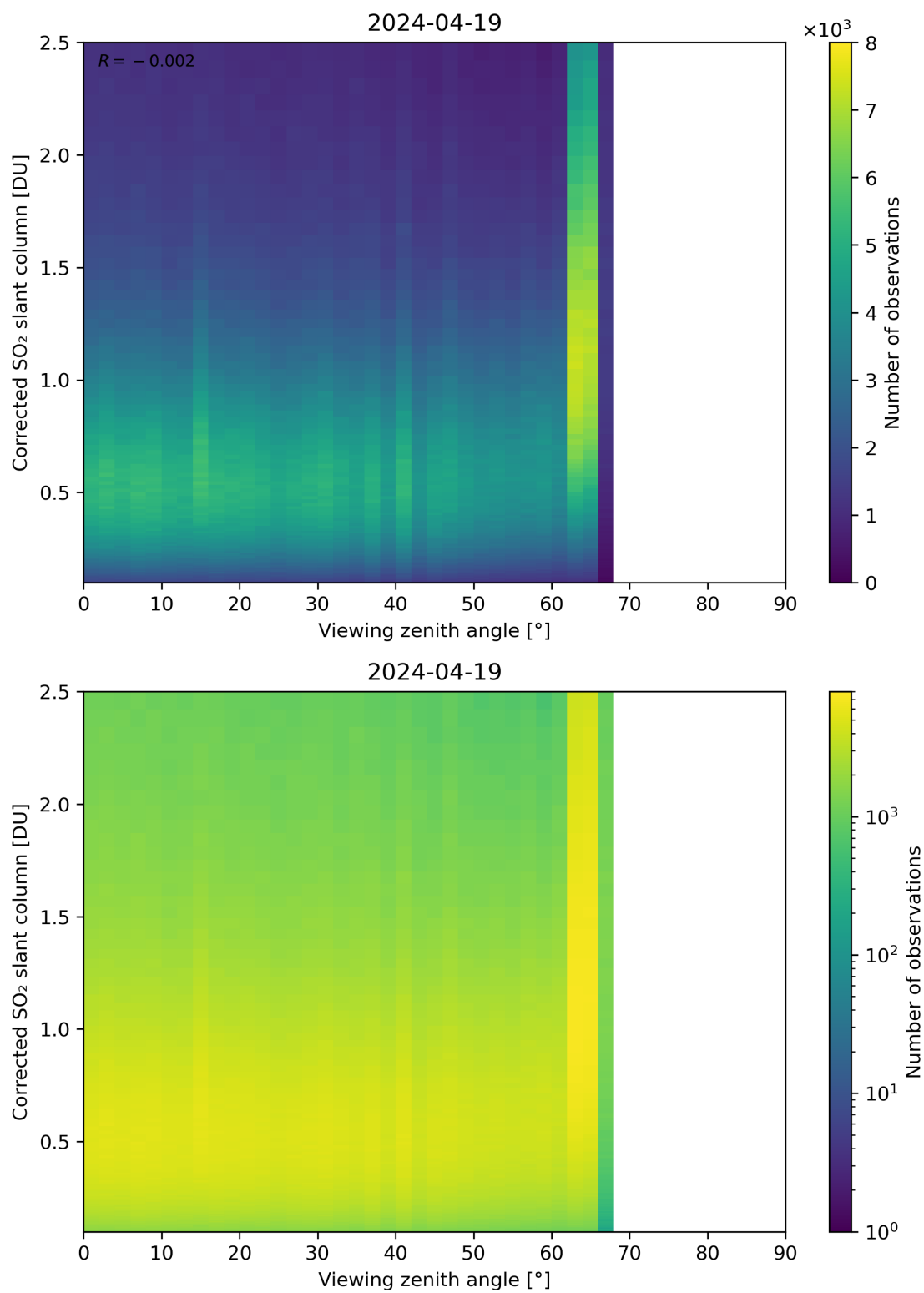
Figure 317: Scatter density plot of “Viewing zenith angle” against “Corrected SO 2 slant column” for 2024-04-18 to 2024-04-20.
