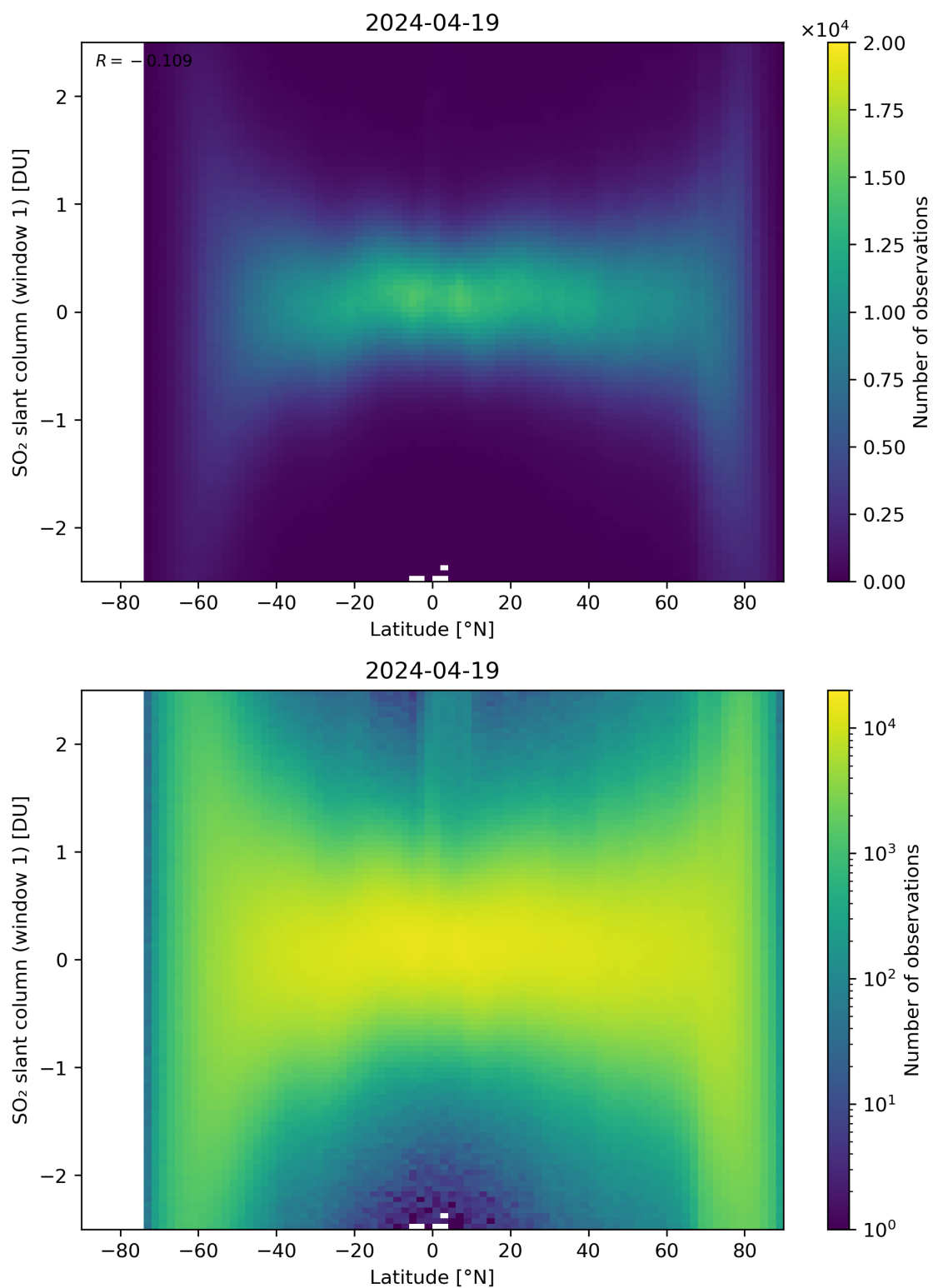
Figure 149: Scatter density plot of “Latitude” against “SO 2 slant column (window 1)” for 2024-04-18 to 2024-04-20.
