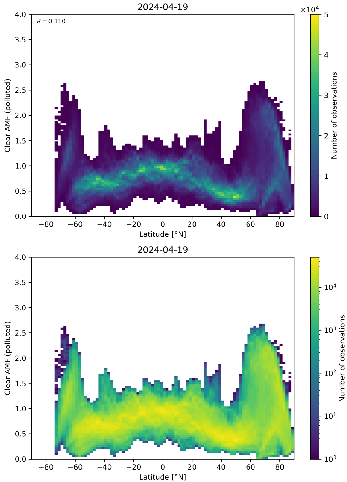
Figure 145: Scatter density plot of “Latitude” against “Clear AMF (polluted)” for 2024-04-18 to 2024-04-20.
