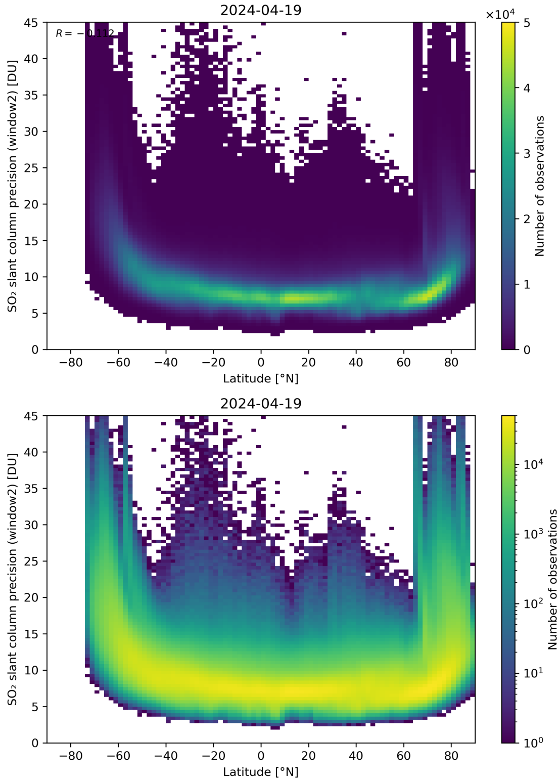
Figure 151: Scatter density plot of “Latitude” against “SO 2 slant column precision (window2)” for 2024-04-18 to 2024-04-20.
