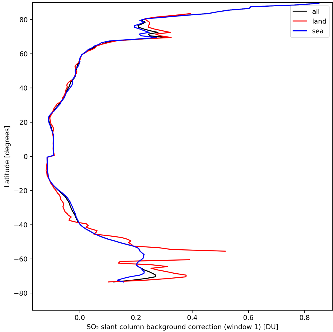
Figure 36: Zonal average of "SO 2 slant column background correction (window 1)" for 2024-04-18 to 2024-04-20.
