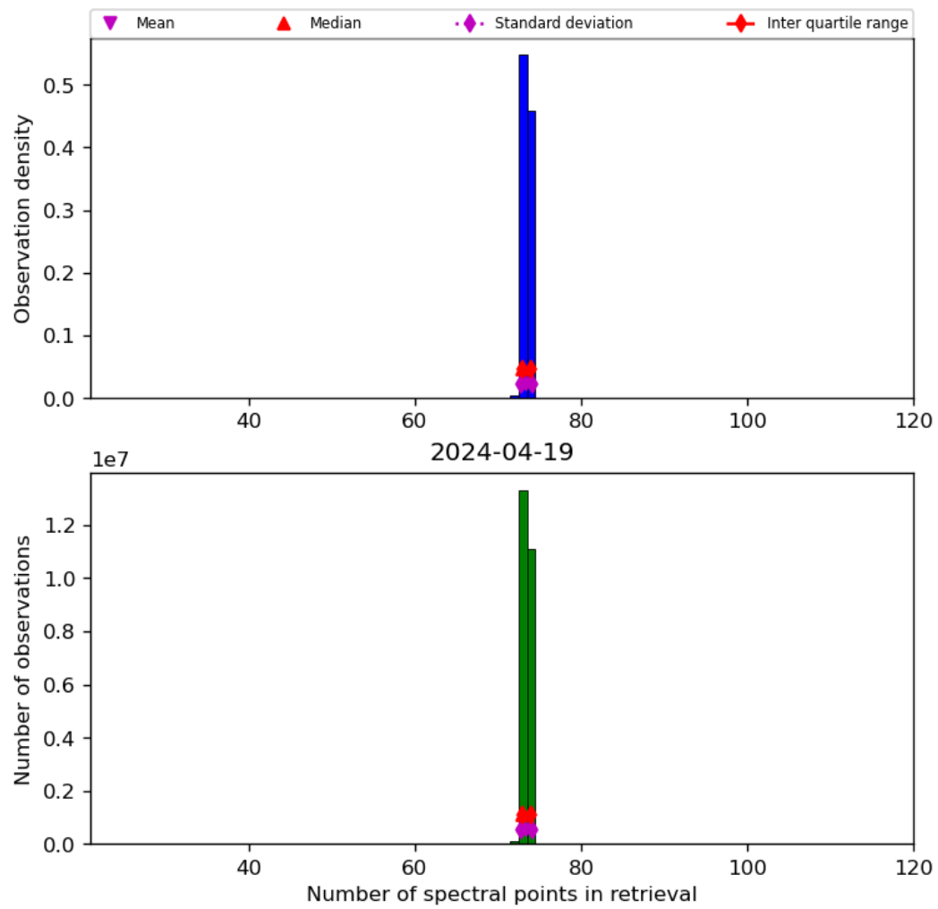
Figure 74: Histogram of “Number of spectral points in retrieval” for 2024-04-18 to 2024-04-20
