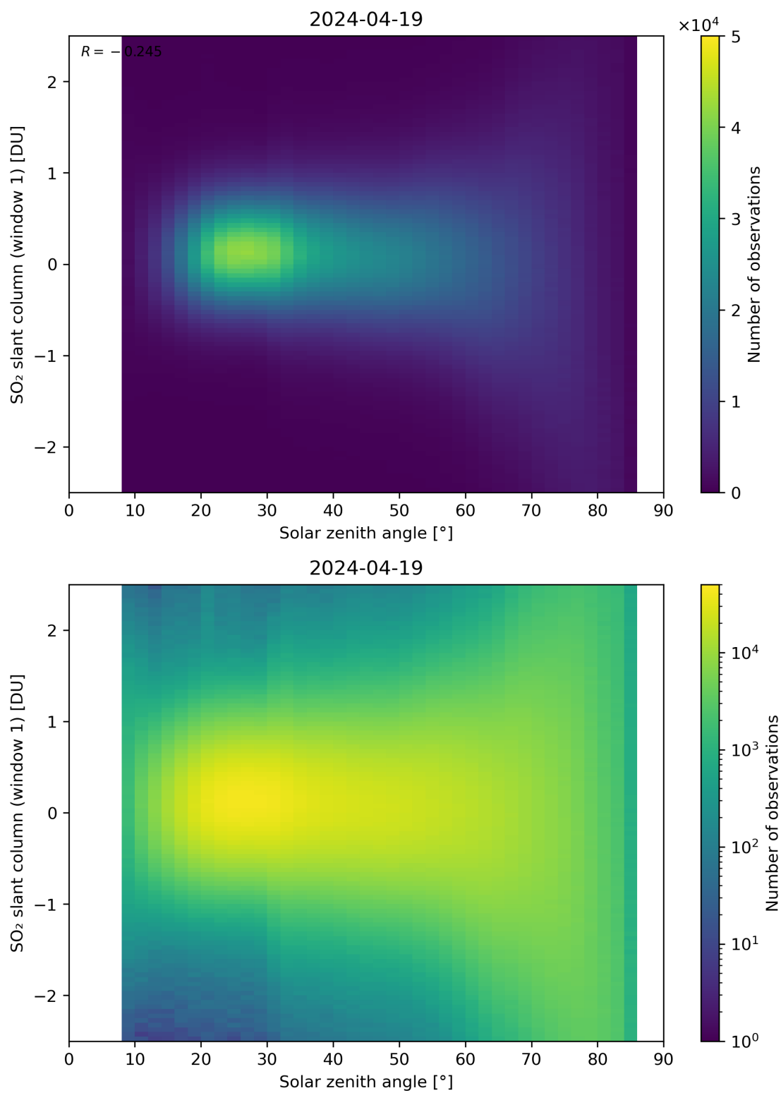
Figure 169: Scatter density plot of “Solar zenith angle” against “SO 2 slant column (window 1)” for 2024-04-18 to 2024-04-20.
