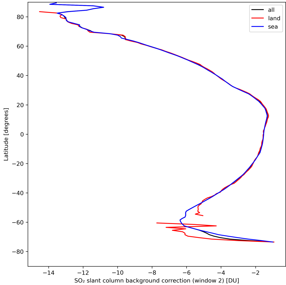
Figure 40: Zonal average of “SO 2 slant column background correction (window 2)” for 2024-04-18 to 2024-04-20.
