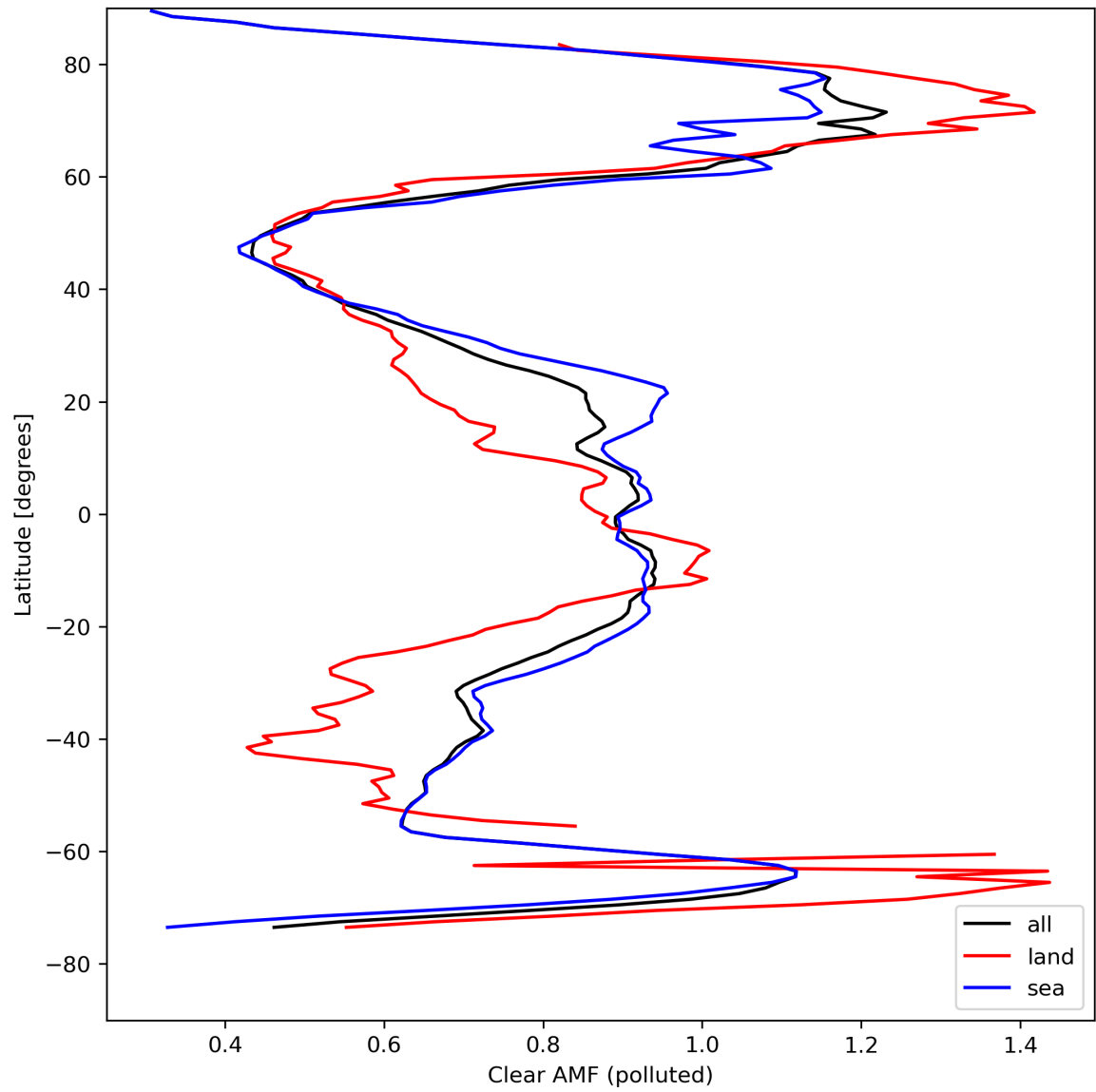
Figure 50: Zonal average of “Clear AMF (polluted)” for 2024-04-18 to 2024-04-20.
