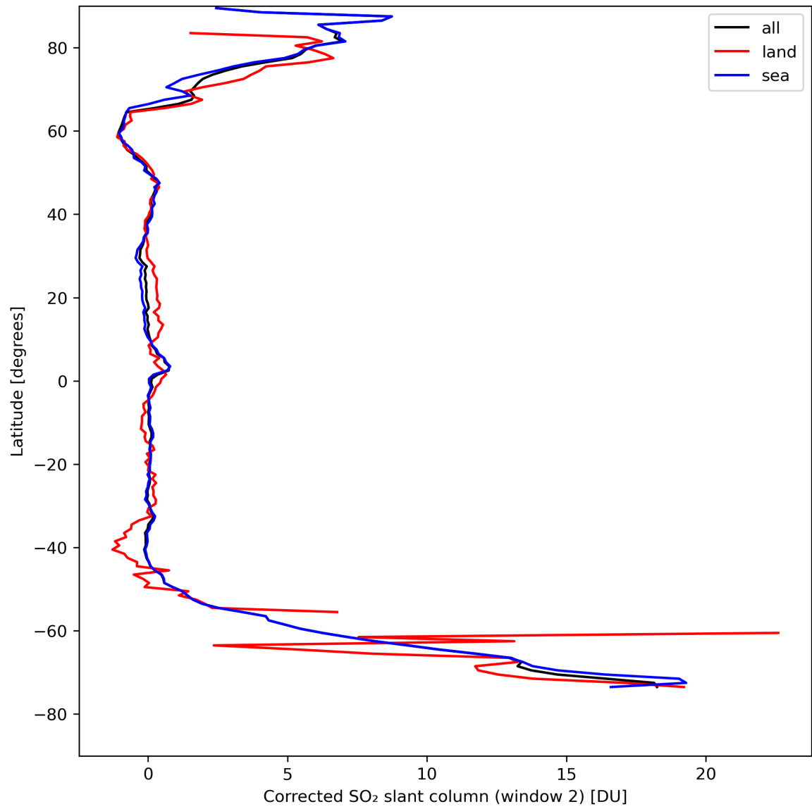
Figure 39: Zonal average of “Corrected SO 2 slant column (window 2)” for 2024-04-18 to 2024-04-20.
