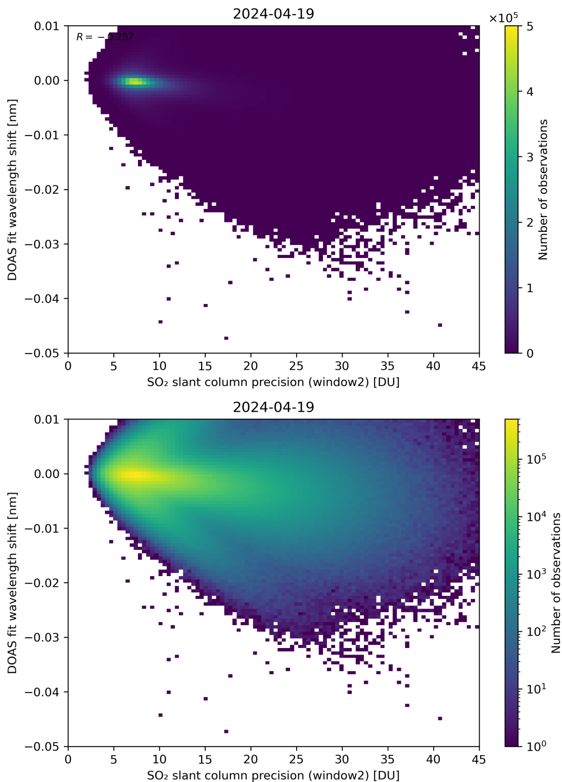
Figure 243: Scatter density plot of “SO 2 slant column precision (window2)” against “DOAS fit wavelength shift” for 2024-04-18 to 2024-04-20.
