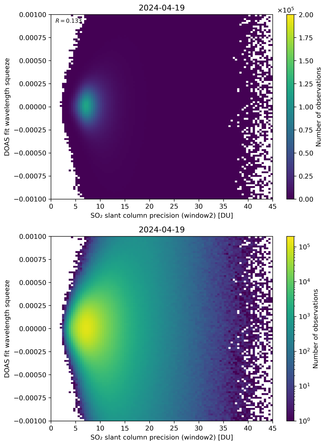
Figure 244: Scatter density plot of “SO 2 slant column precision (window2)” against “DOAS fit wavelength squeeze” for 2024-04-18 to 2024-04-20.
