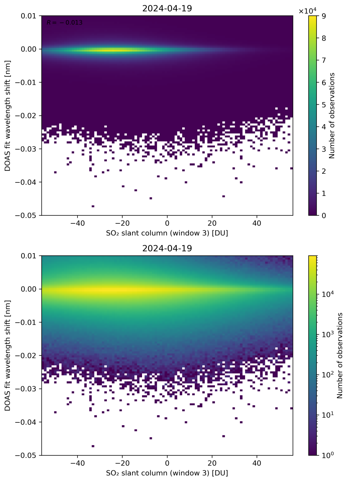
Figure 254: Scatter density plot of “SO 2 slant column (window 3)” against “DOAS fit wavelength shift” for 2024-04-18 to 2024-04-20.
