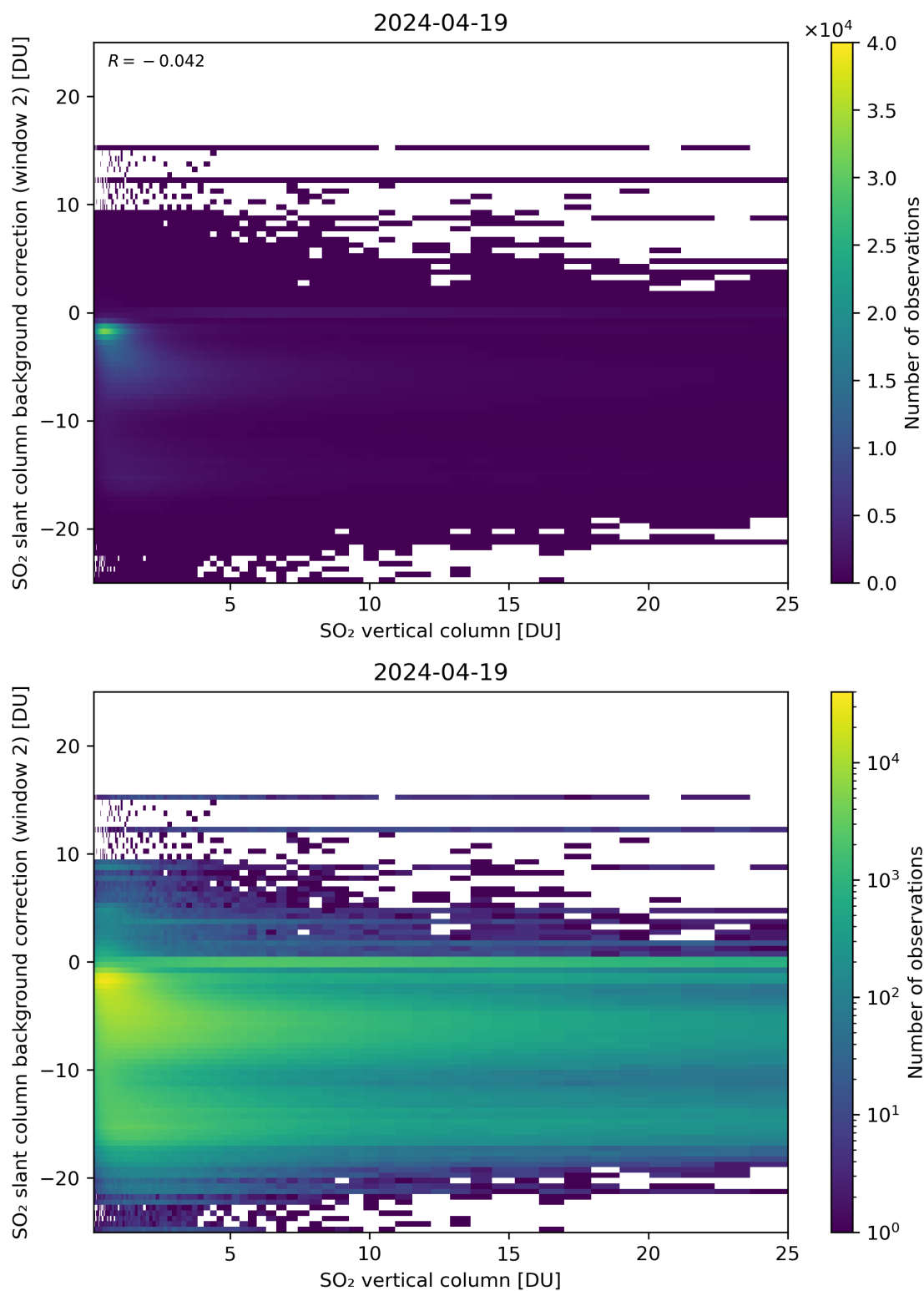
Figure 274: Scatter density plot of “SO 2 vertical column” against “SO 2 slant column background correction (window 2)” for 2024-04-18 to 2024-04-20.
