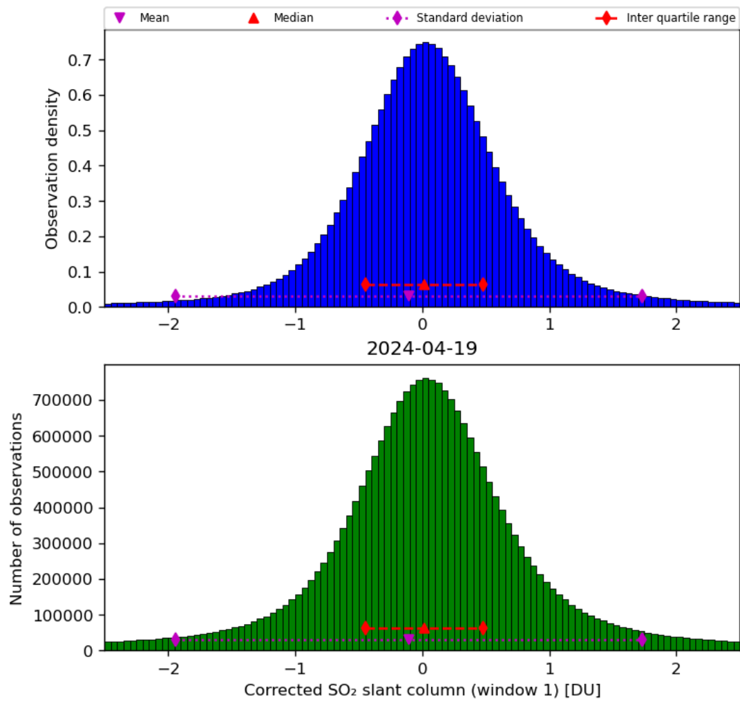
Figure 58: Histogram of “Corrected SO 2 slant column (window 1)” for 2024-04-18 to 2024-04-20
