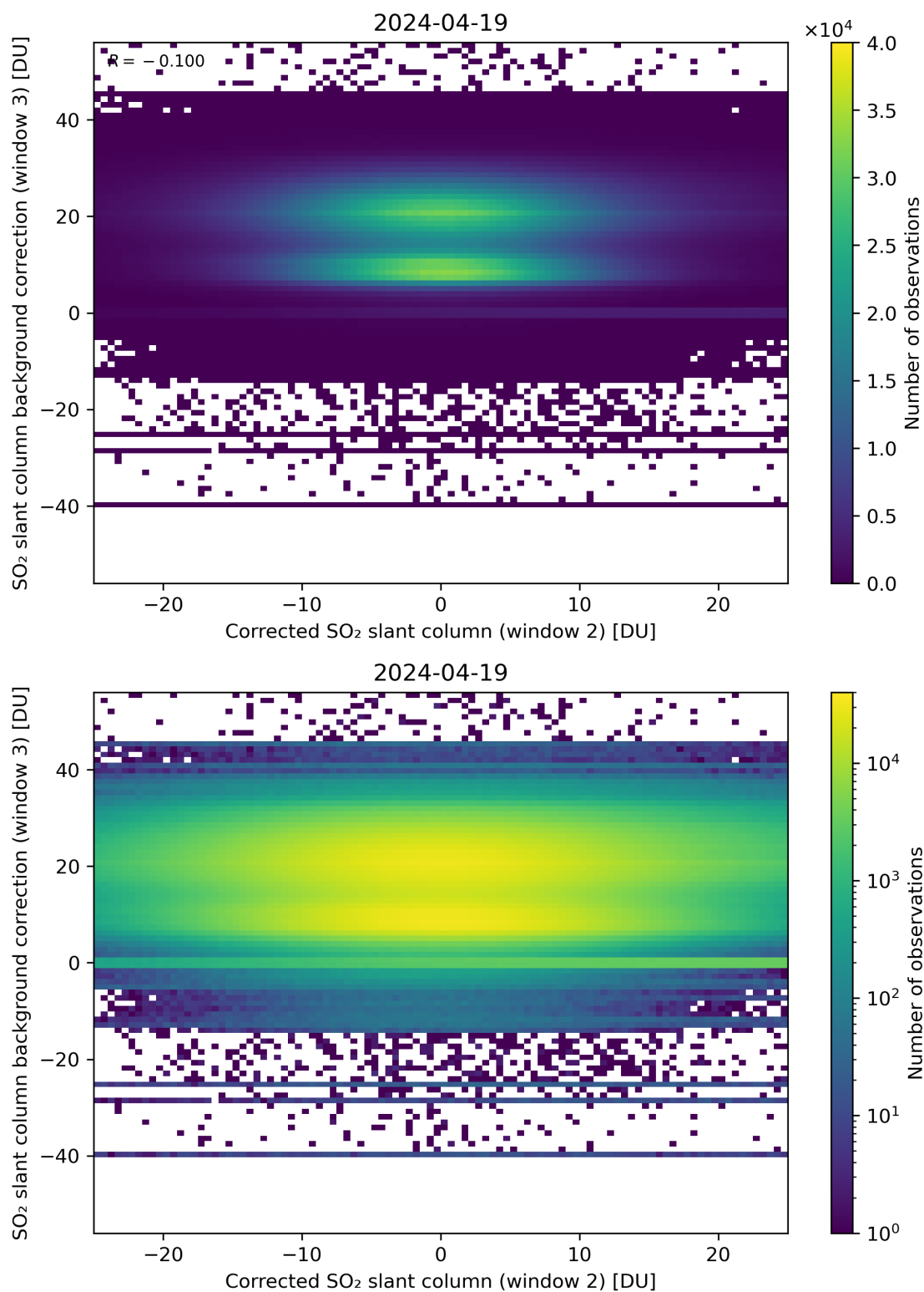
Figure 195: Scatter density plot of “Corrected SO 2 slant column (window 2)” against “SO 2 slant column background correction (window 3)” for 2024-04-18 to 2024-04-20.
