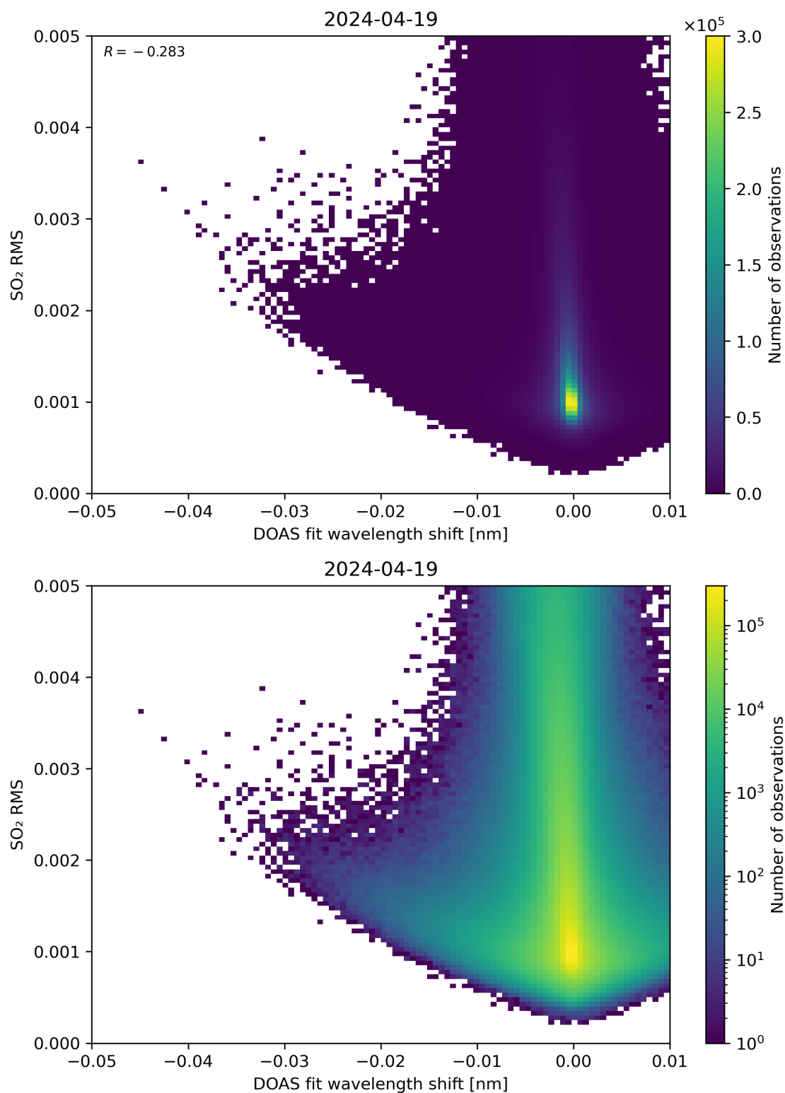
Figure 128: Scatter density plot of “DOAS fit wavelength shift” against “SO 2 RMS” for 2024-04-18 to 2024-04-20.
