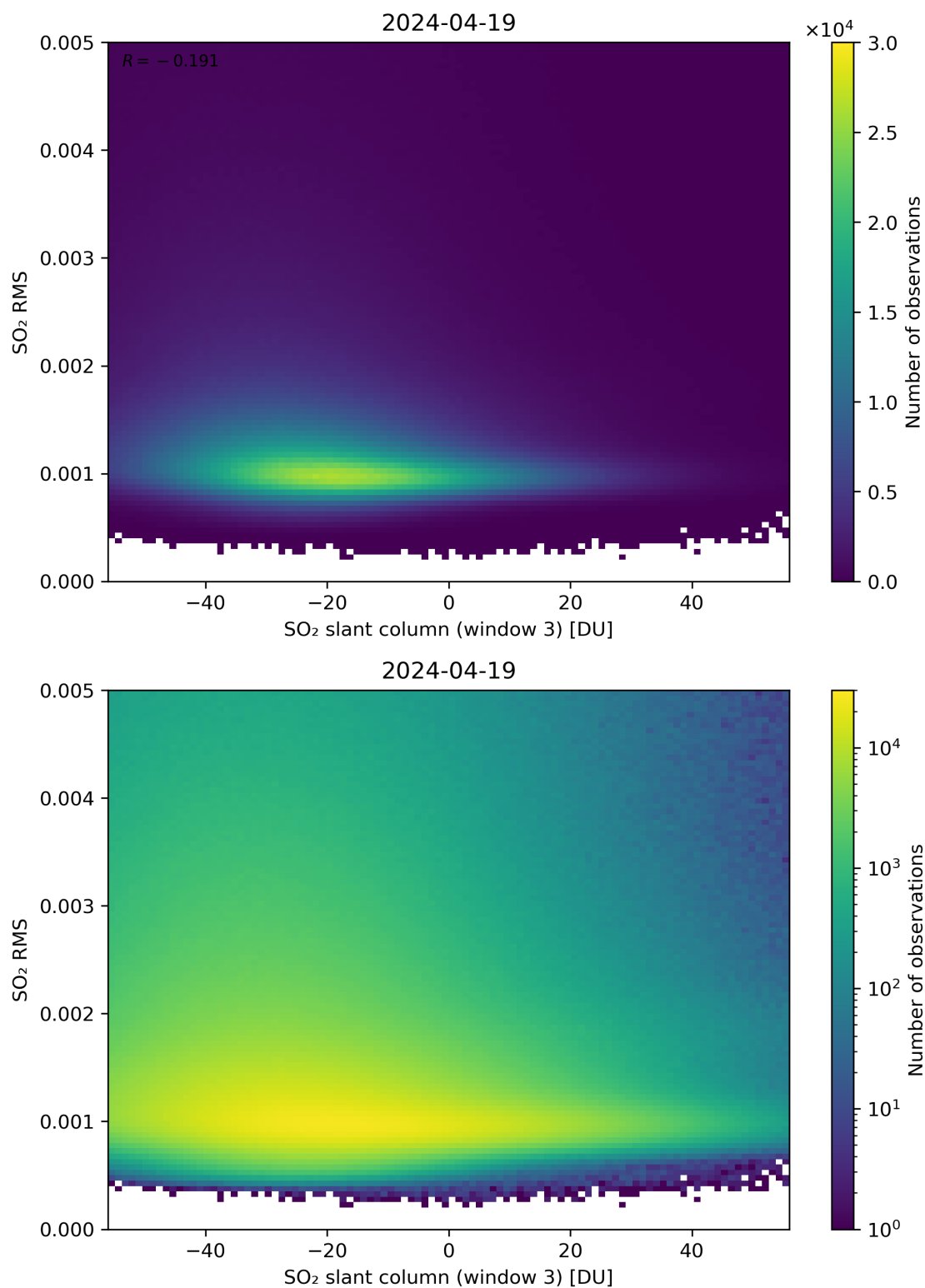
Figure 256: Scatter density plot of “SO 2 slant column (window 3)” against “SO 2 RMS” for 2024-04-18 to 2024-04-20.
