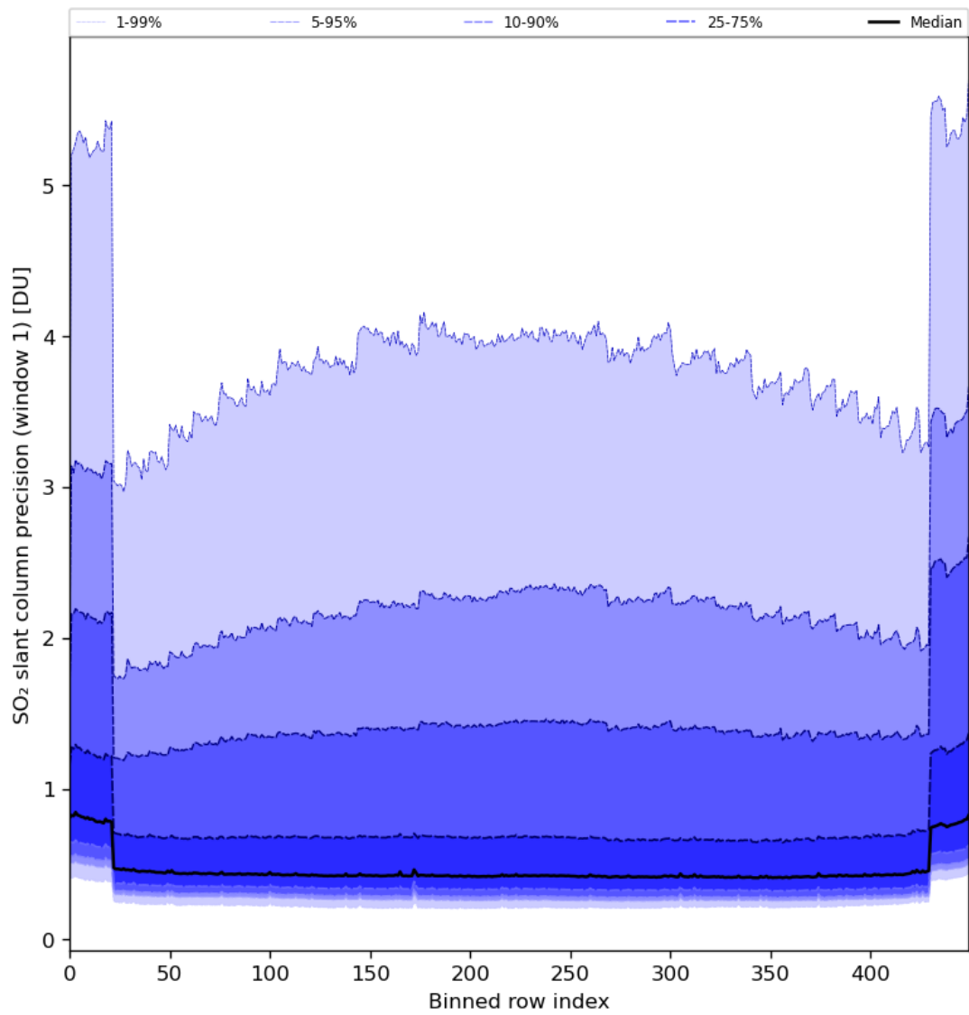
Figure 80: Along track statistics of “SO 2 slant column precision (window 1)” for 2024-04-18 to 2024-04-20
