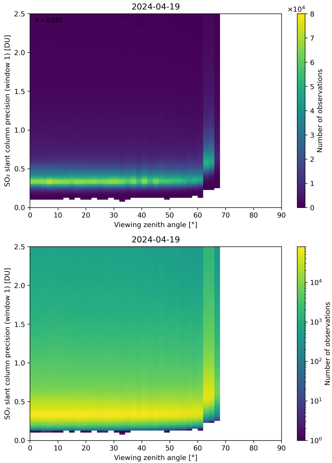
Figure 321: Scatter density plot of “Viewing zenith angle” against “SO 2 slant column precision (window 1)” for 2024-04-18 to 2024-04-20.
