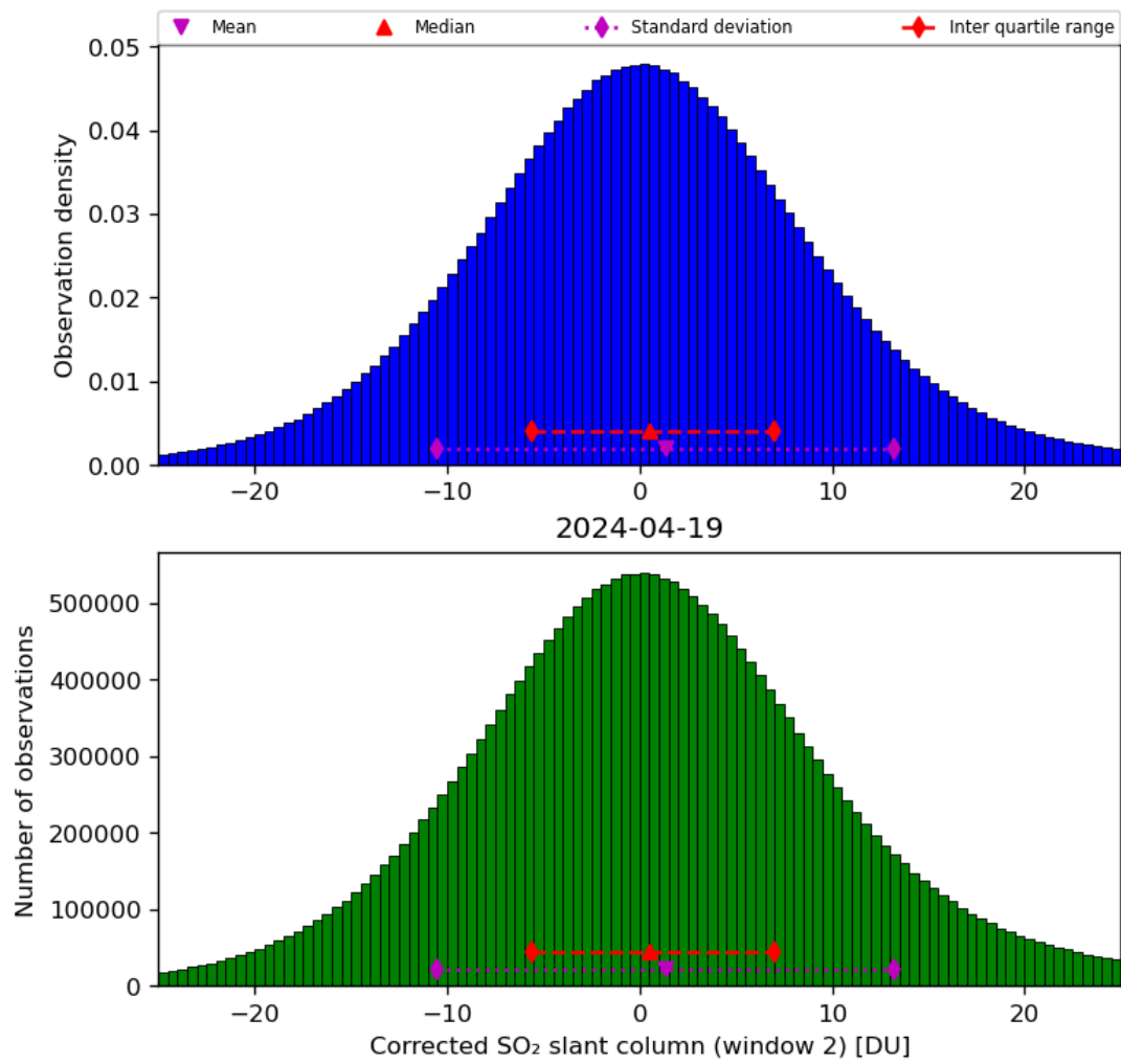
Figure 62: Histogram of “Corrected SO 2 slant column (window 2)” for 2024-04-18 to 2024-04-20
