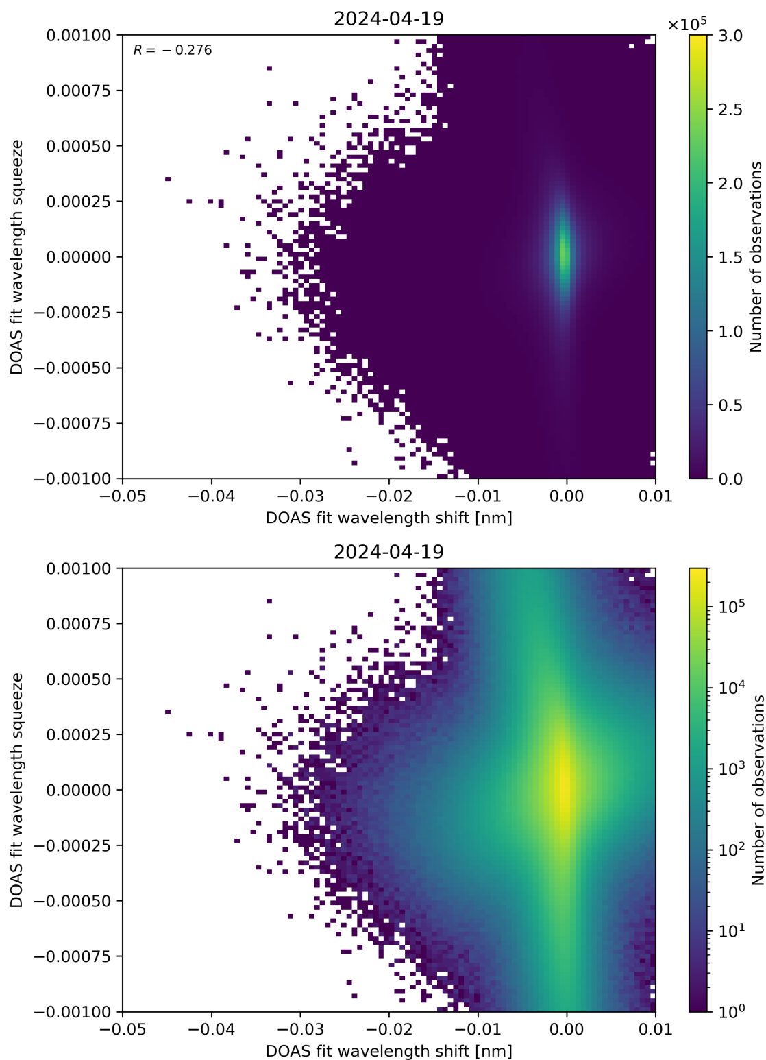
Figure 127: Scatter density plot of “DOAS fit wavelength shift” against “DOAS fit wavelength squeeze” for 2024-04-18 to 2024-04-20.
