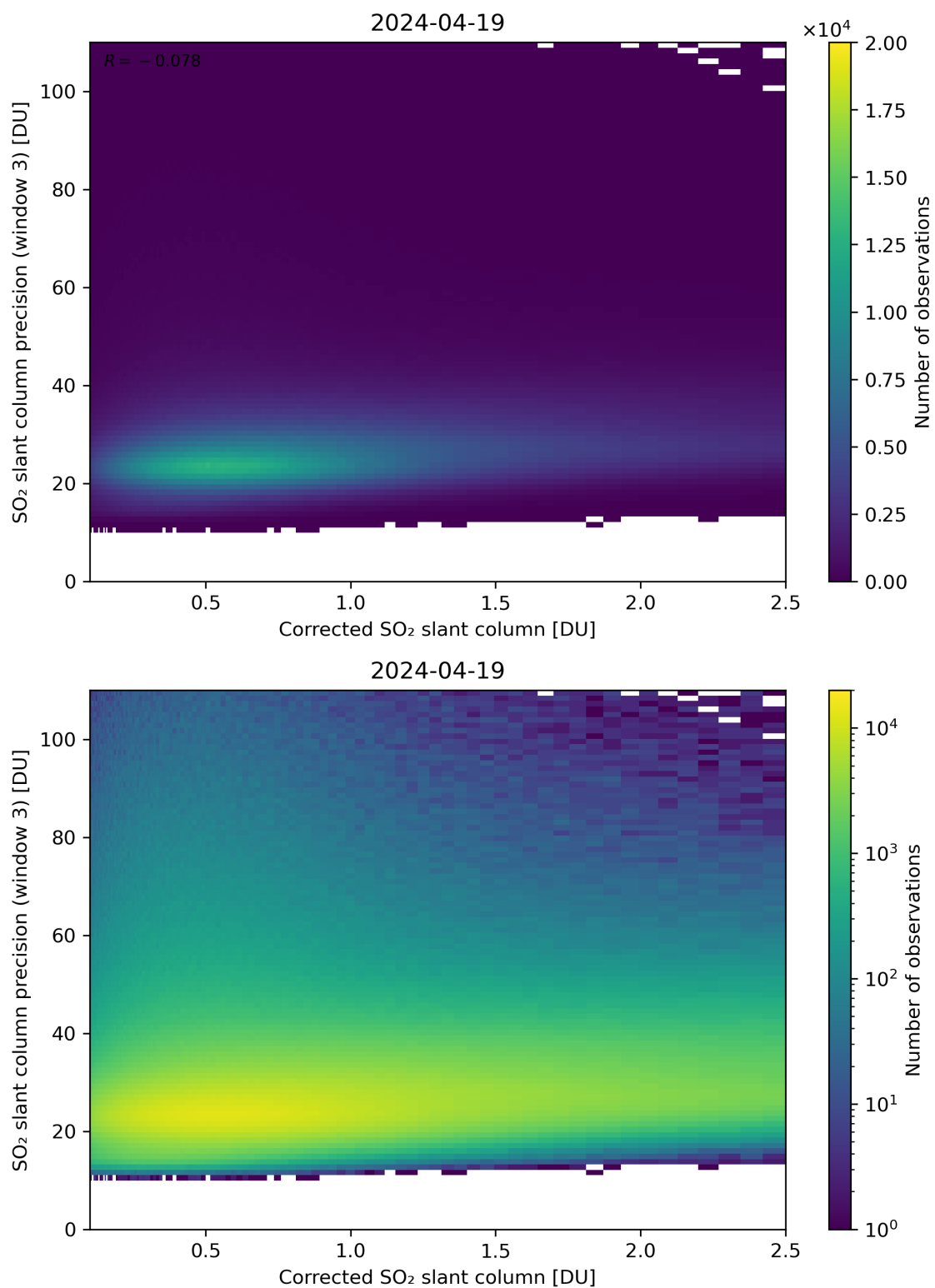
Figure 191: Scatter density plot of “Corrected SO 2 slant column” against “SO 2 slant column precision (window 3)” for 2024-04-18 to 2024-04-20.
