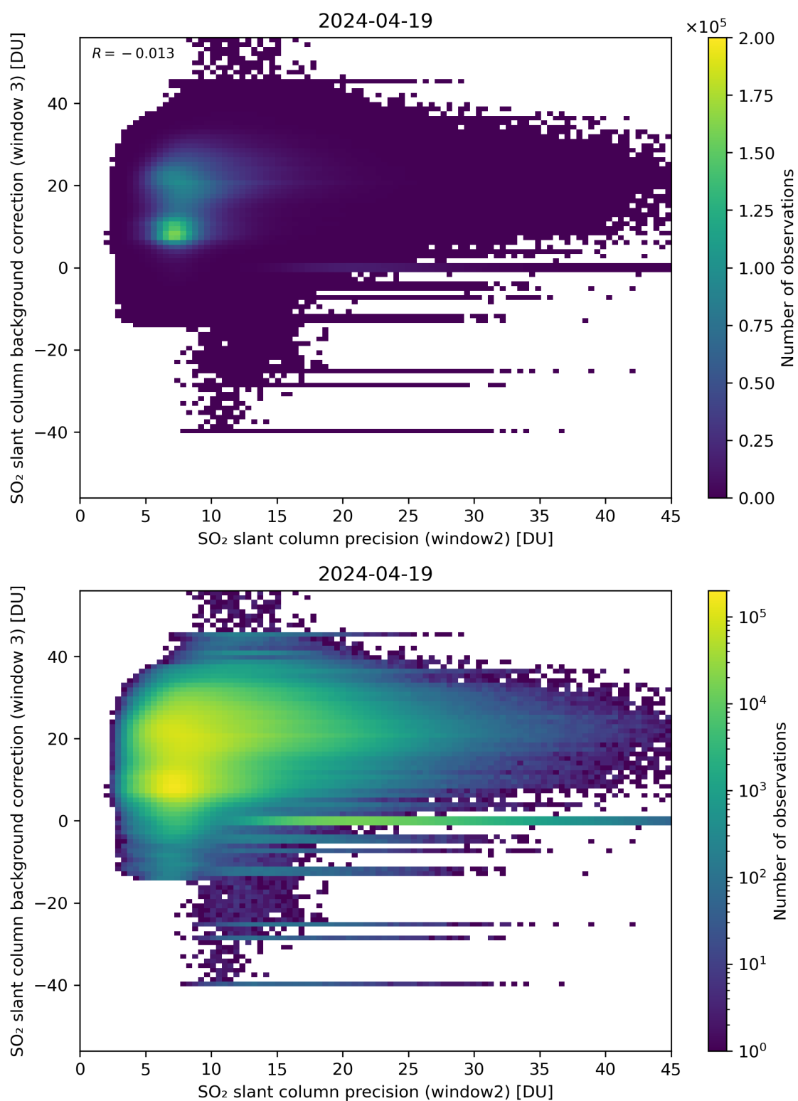
Figure 242: Scatter density plot of “SO 2 slant column precision (window2)” against “SO 2 slant column background correction (window 3)” for 2024-04-18 to 2024-04-20.
