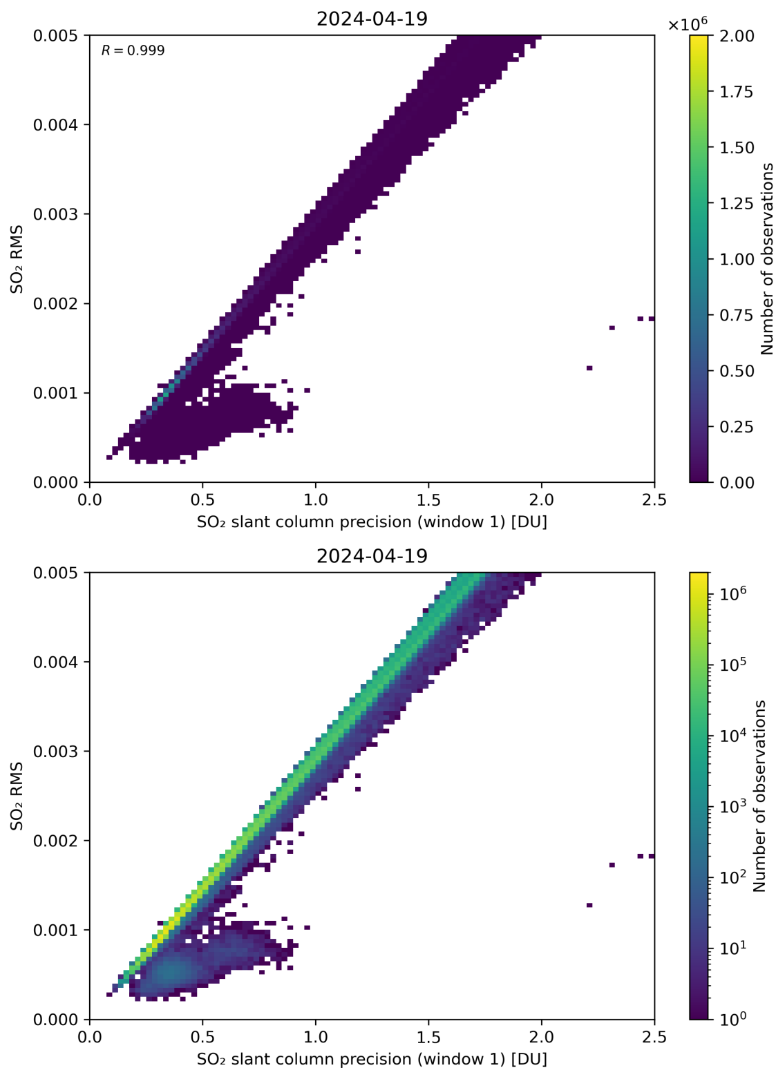
Figure 223: Scatter density plot of “SO 2 slant column precision (window 1)” against “SO 2 RMS” for 2024-04-18 to 2024-04-20.
