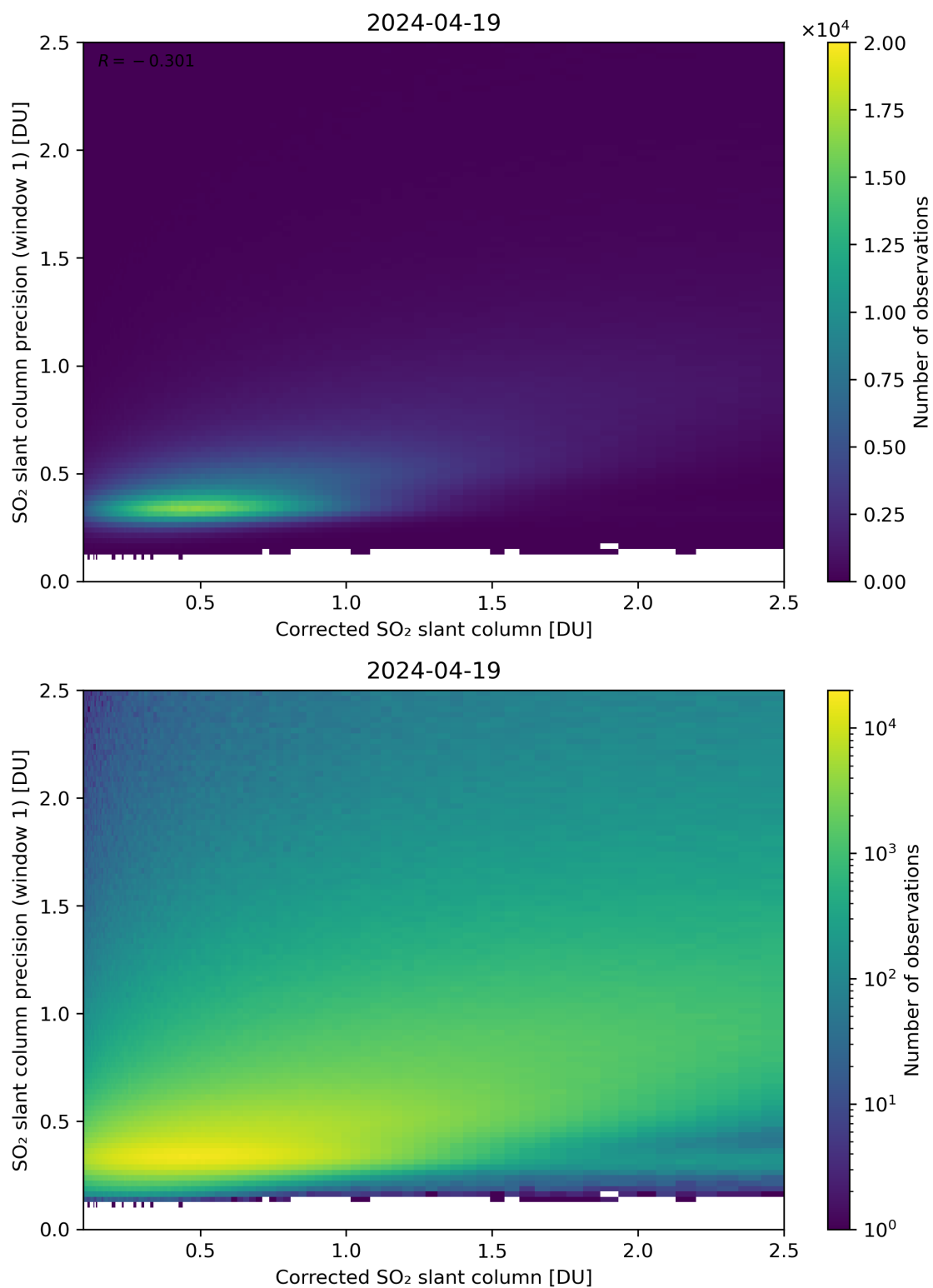
Figure 188: Scatter density plot of “Corrected SO 2 slant column” against “SO 2 slant column precision (window 1)” for 2024-04-18 to 2024-04-20.
