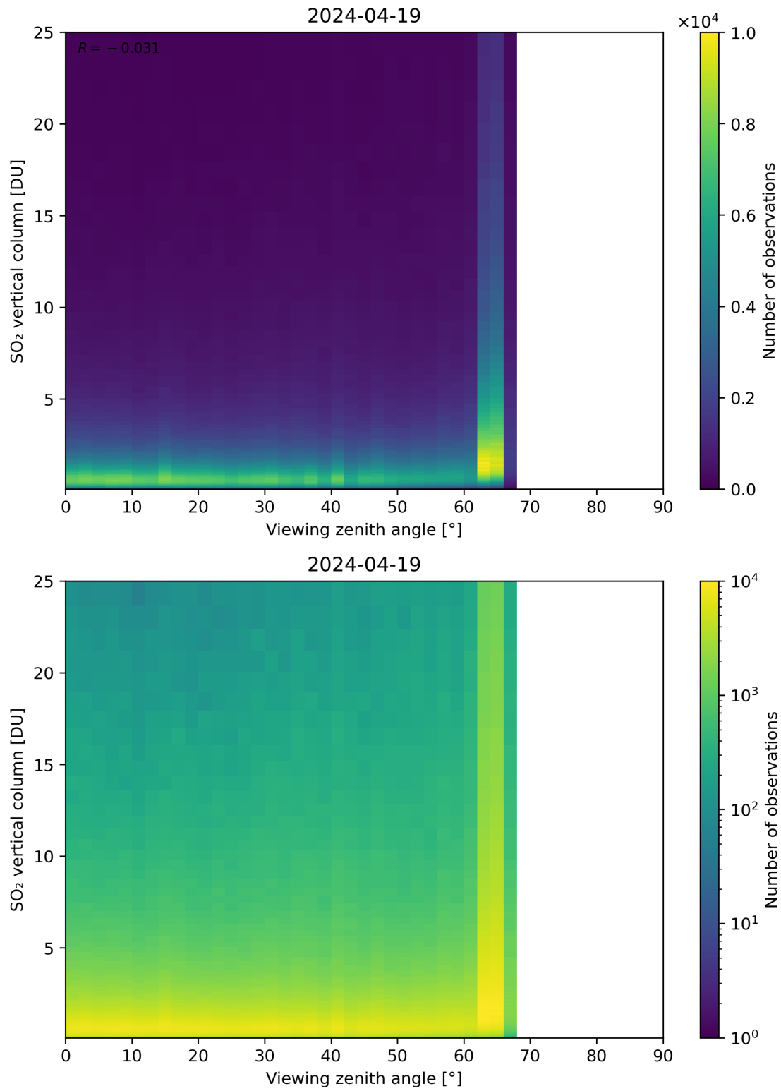
Figure 327: Scatter density plot of “Viewing zenith angle” against “SO 2 vertical column” for 2024-04-18 to 2024-04-20.
