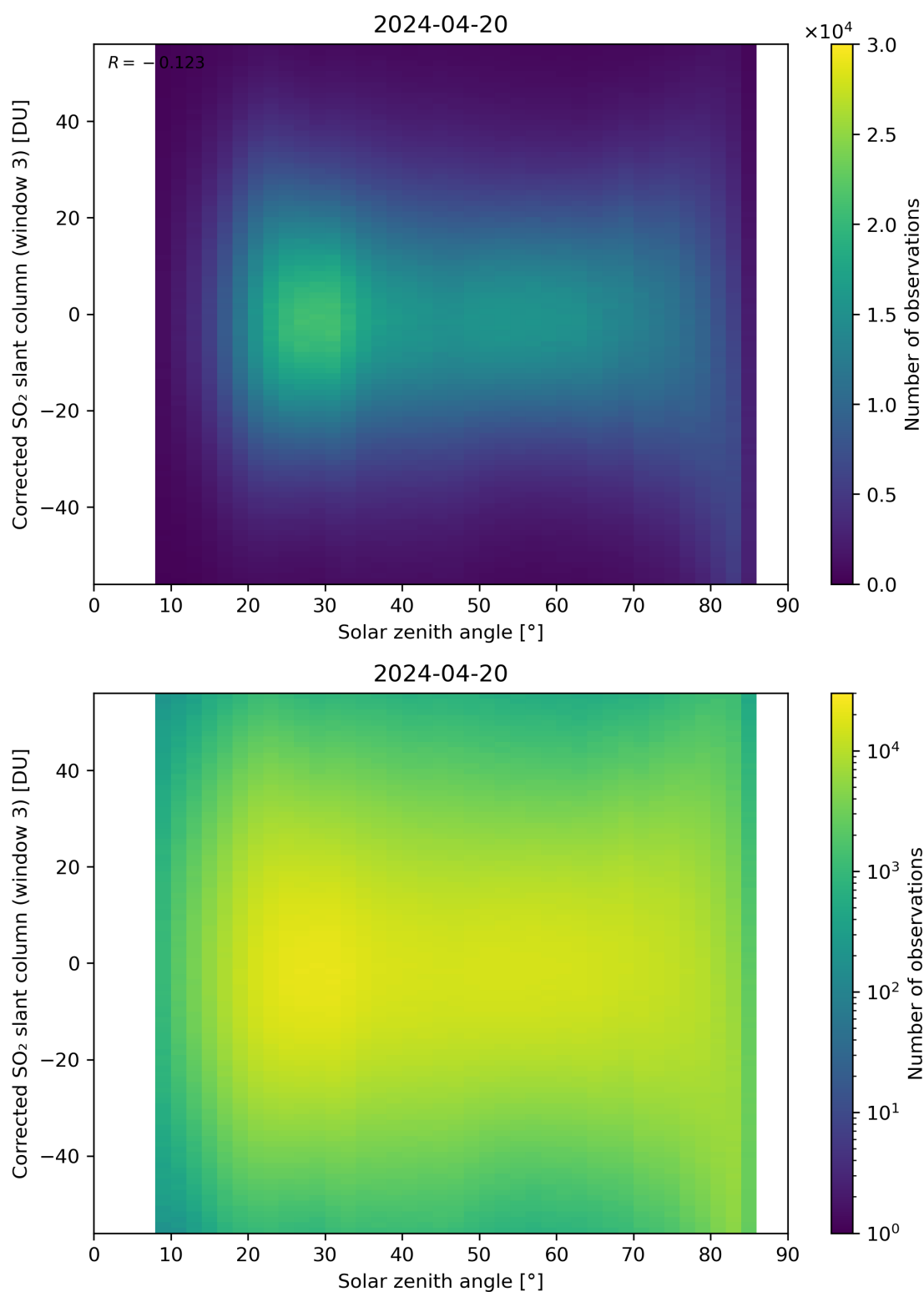
Figure 168: Scatter density plot of “Solar zenith angle” against “Corrected SO 2 slant column (window 3)” for 2024-04-19 to 2024-04-21.
