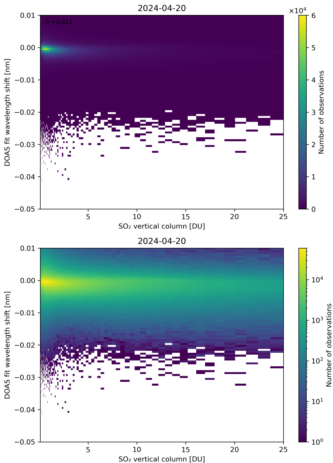
Figure 276: Scatter density plot of “SO 2 vertical column” against “DOAS fit wavelength shift” for 2024-04-19 to 2024-04-21.
