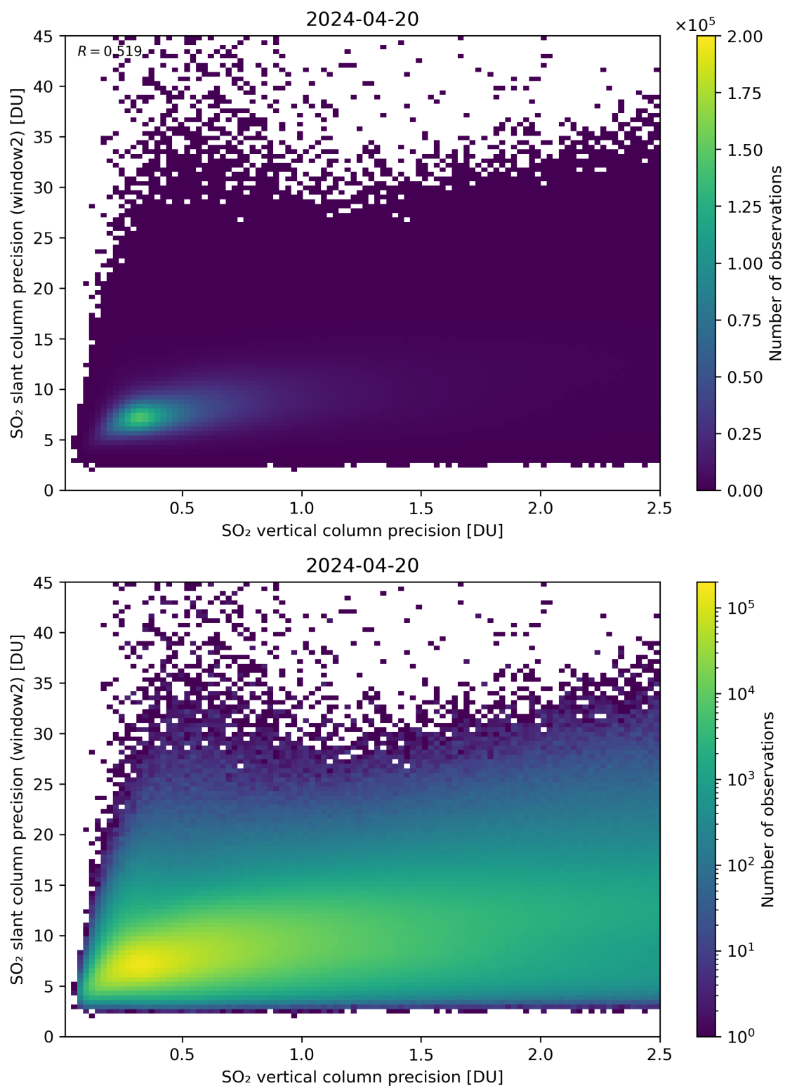
Figure 291: Scatter density plot of “SO 2 vertical column precision” against “SO 2 slant column precision (window2)” for 2024-04-19 to 2024-04-21.
