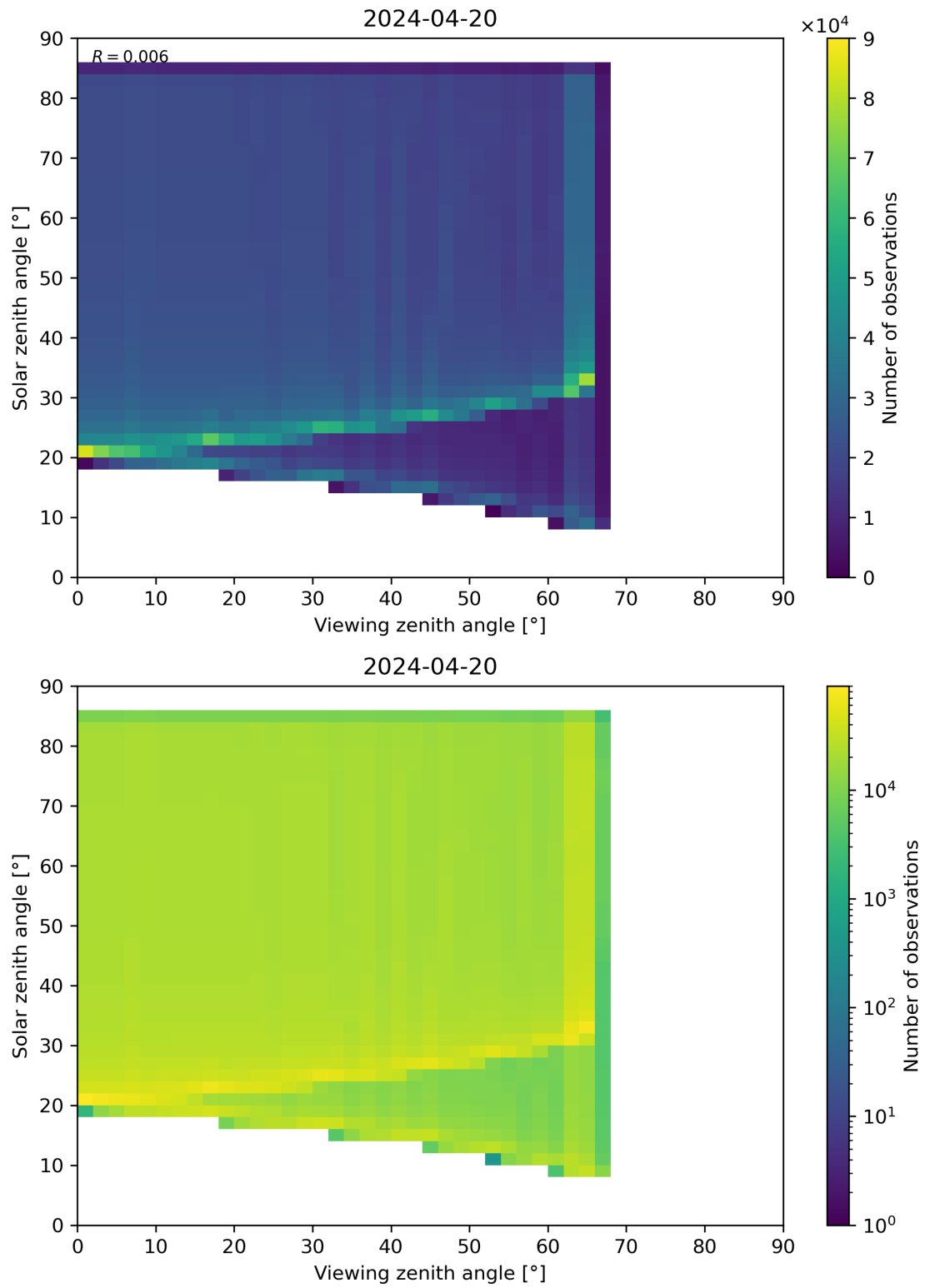
Figure 315: Scatter density plot of “Viewing zenith angle” against “Solar zenith angle” for 2024-04-19 to 2024-04-21.
