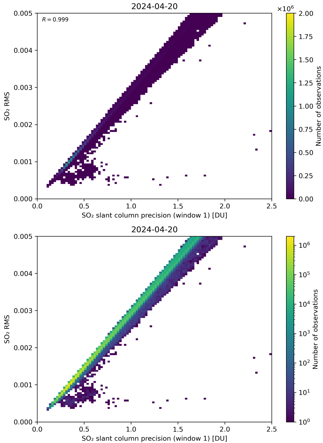
Figure 223: Scatter density plot of “SO 2 slant column precision (window 1)” against “SO 2 RMS” for 2024-04-19 to 2024-04-21.
