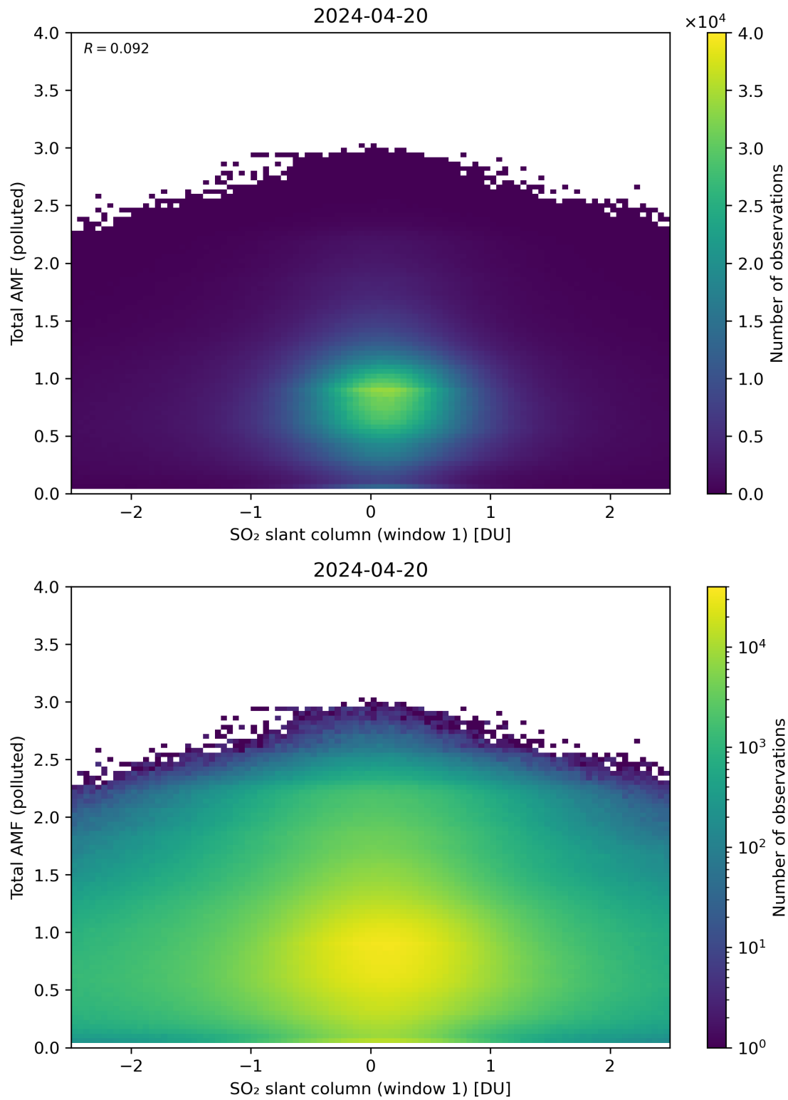
Figure 239: Scatter density plot of “SO 2 slant column (window 1)” against “Total AMF (polluted)” for 2024-04-19 to 2024-04-21.
