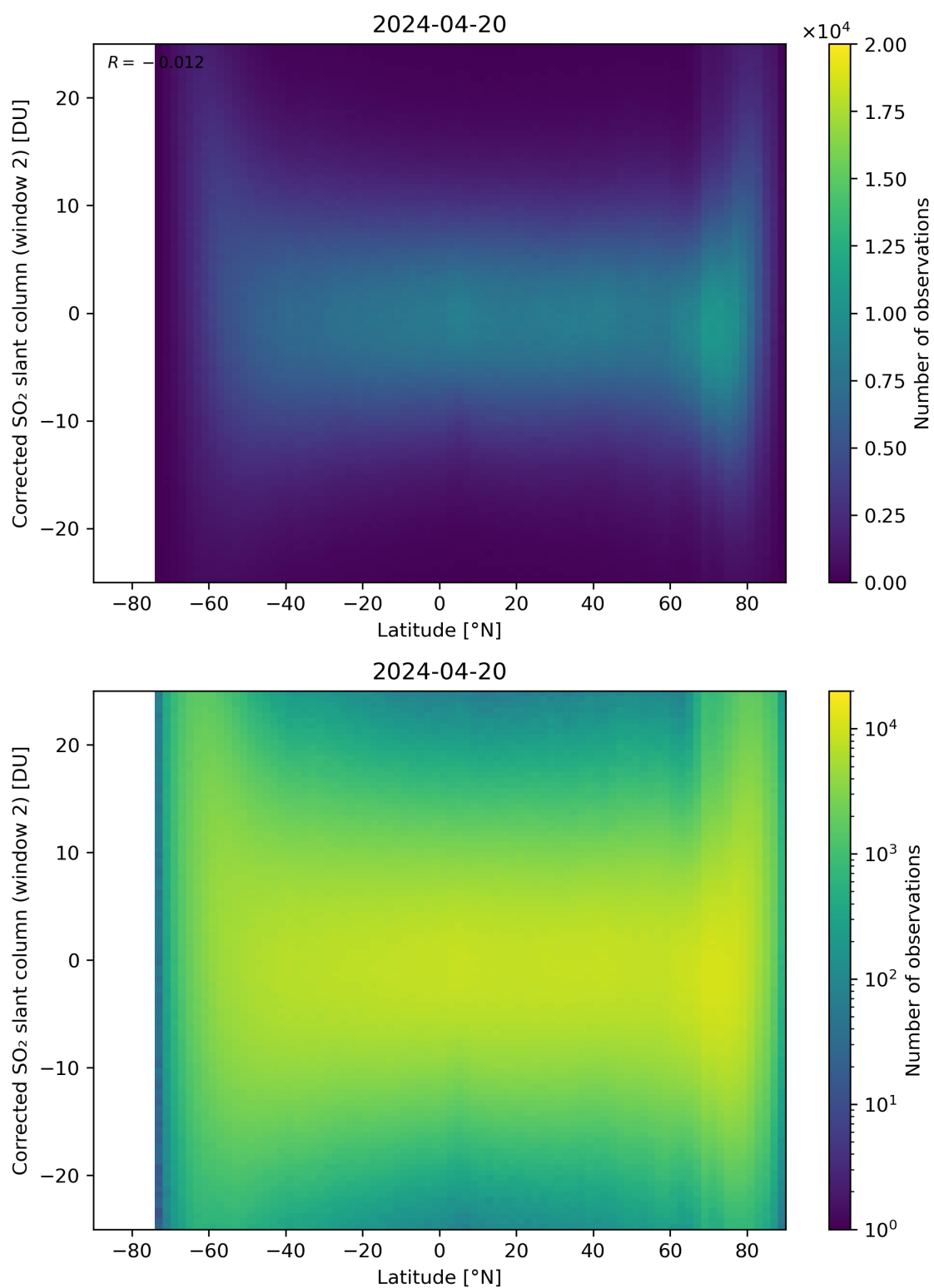
Figure 147: Scatter density plot of “Latitude” against “Corrected SO 2 slant column (window 2)” for 2024-04-19 to 2024-04-21.
