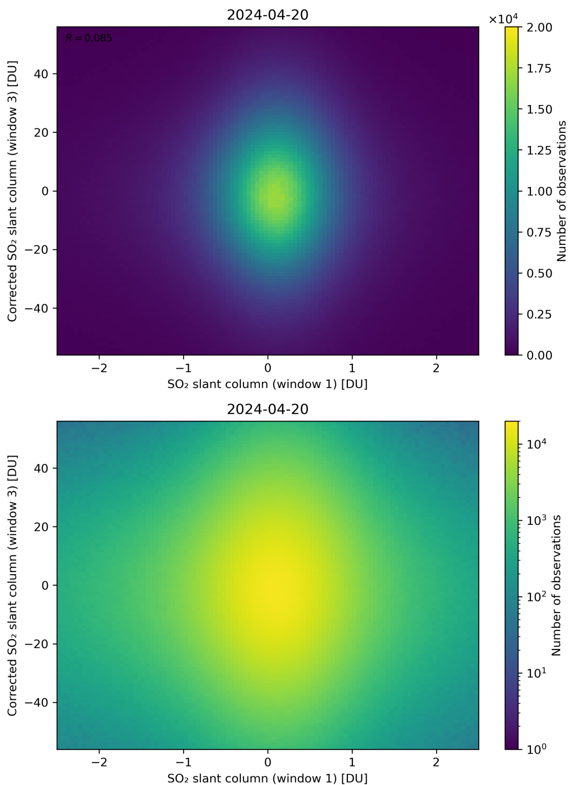
Figure 234: Scatter density plot of “SO 2 slant column (window 1)” against “Corrected SO 2 slant column (window 3)” for 2024-04-19 to 2024-04-21.
