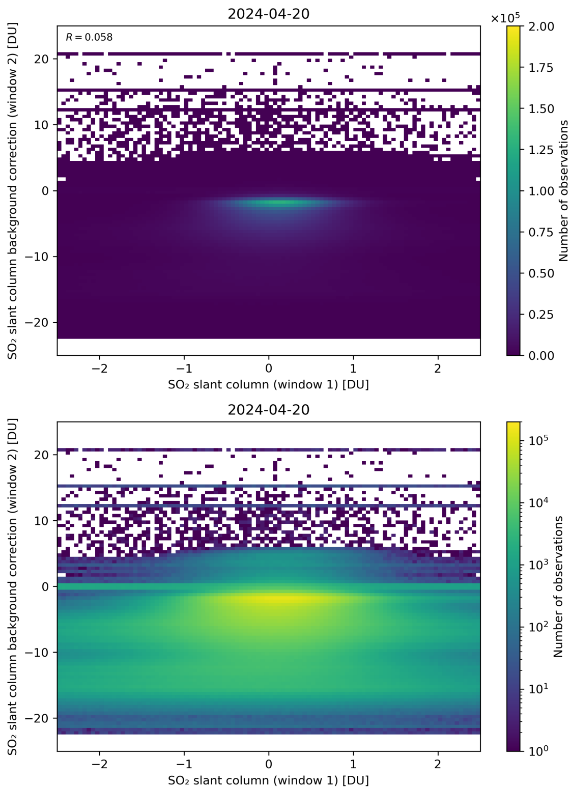
Figure 213: Scatter density plot of “SO 2 slant column (window 1)” against “SO 2 slant column background correction (window 2)” for 2024-04-19 to 2024-04-21.
