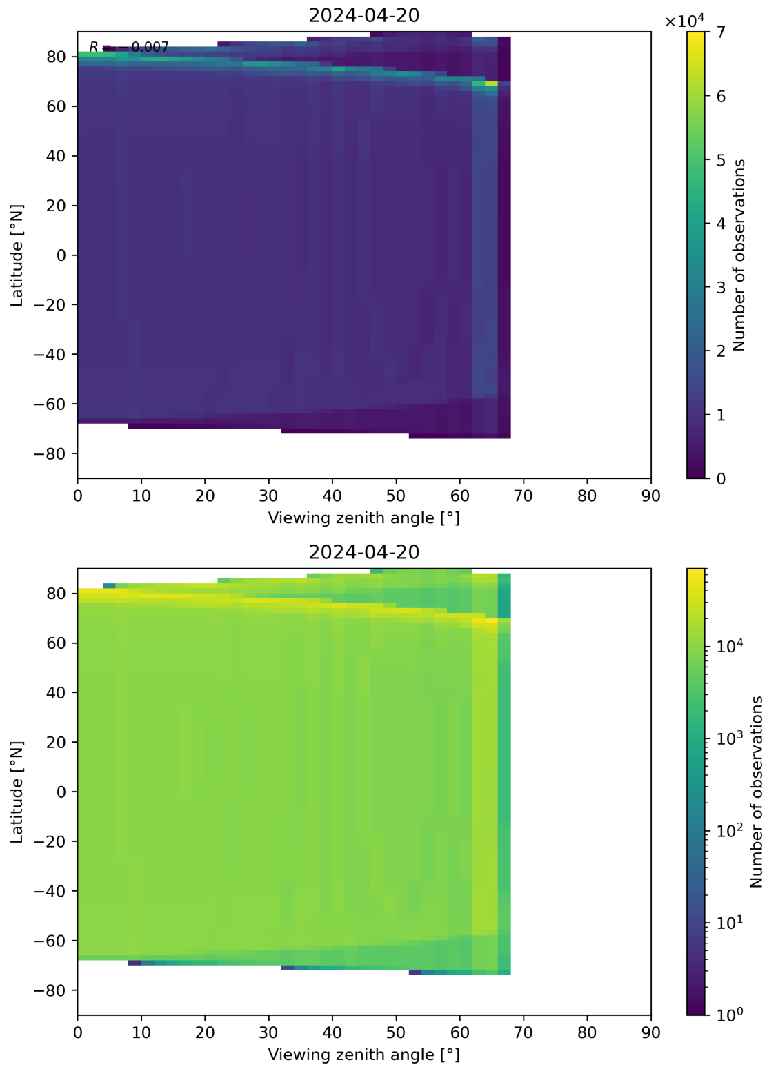
Figure 314: Scatter density plot of “Viewing zenith angle” against “Latitude” for 2024-04-19 to 2024-04-21.
