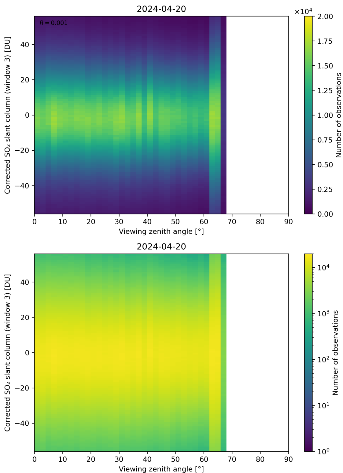
Figure 319: Scatter density plot of “Viewing zenith angle” against “Corrected SO 2 slant column (window 3)” for 2024-04-19 to 2024-04-21.
