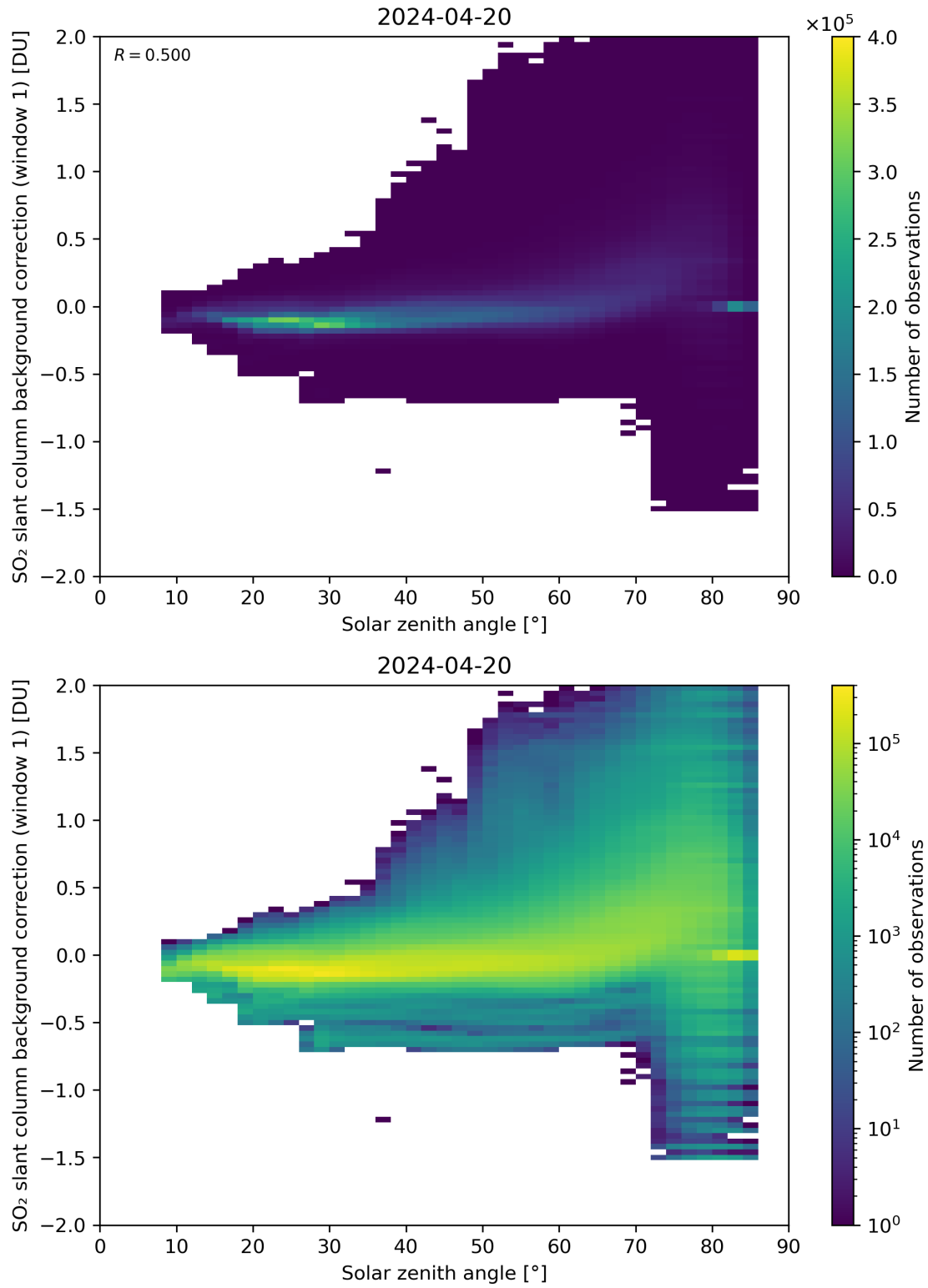
Figure 158: Scatter density plot of “Solar zenith angle” against “SO 2 slant column background correction (window 1)” for 2024-04-19 to 2024-04-21.
