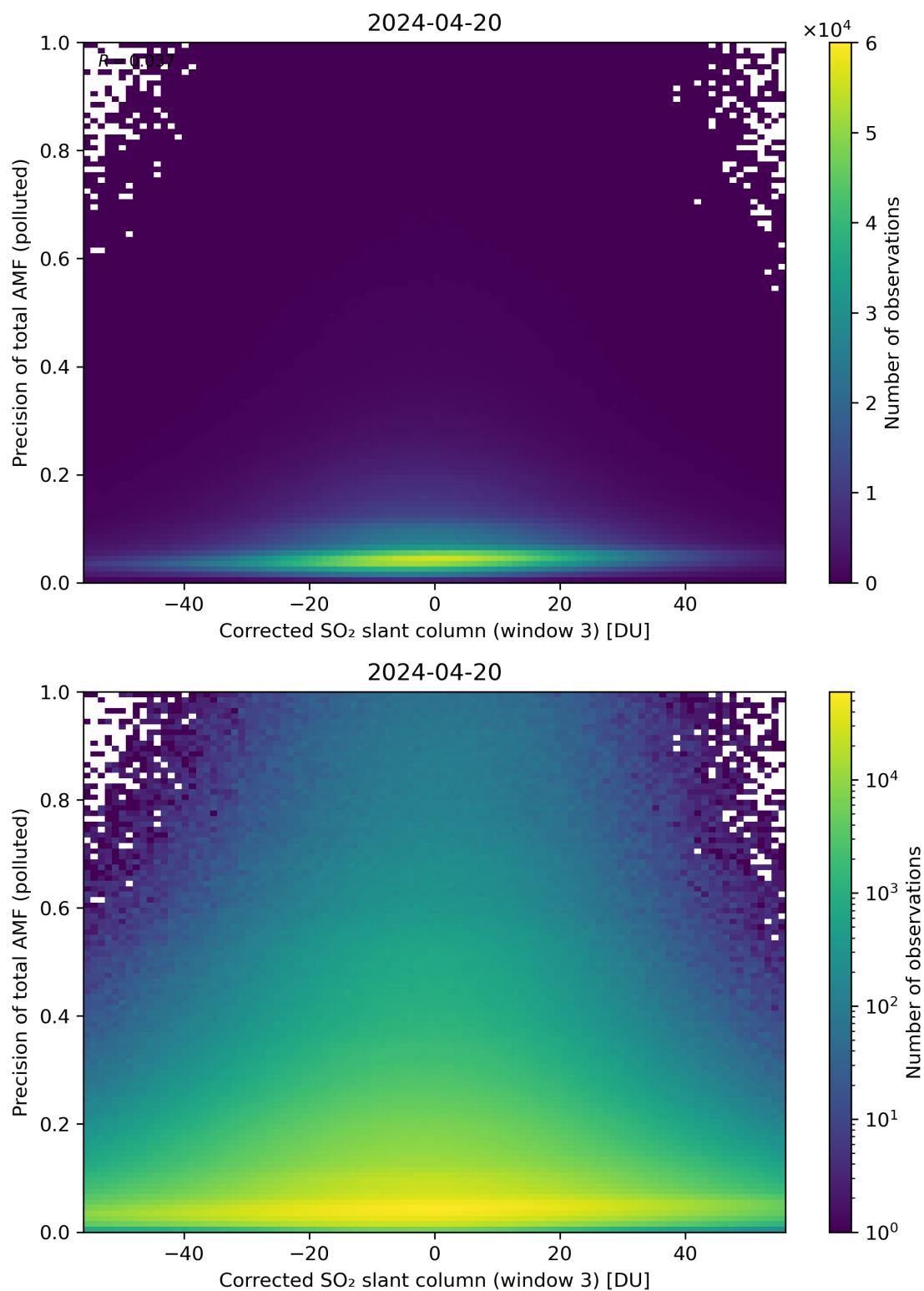
Figure 211: Scatter density plot of “Corrected SO 2 slant column (window 3)” against “Precision of total AMF (polluted)” for 2024-04-19 to 2024-04-21.
