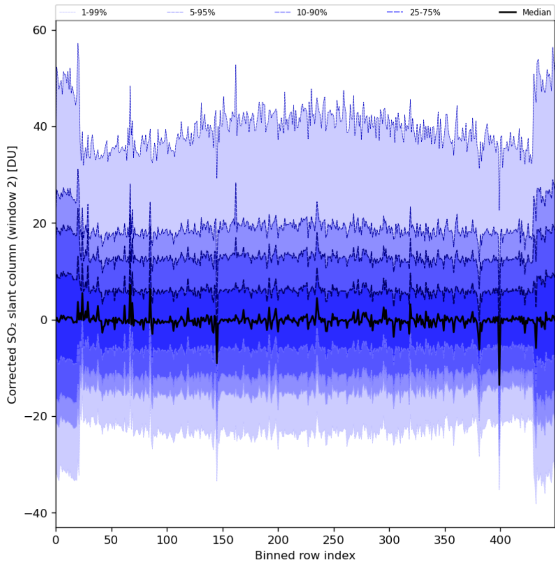
Figure 85: Along track statistics of “Corrected SO 2 slant column (window 2)” for 2024-04-19 to 2024-04-21
