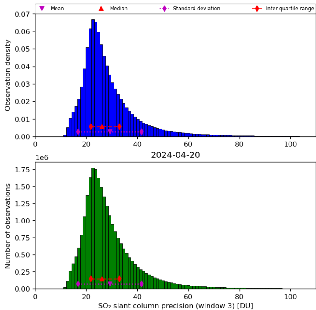
Figure 65: Histogram of “SO 2 slant column precision (window 3)” for 2024-04-19 to 2024-04-21
