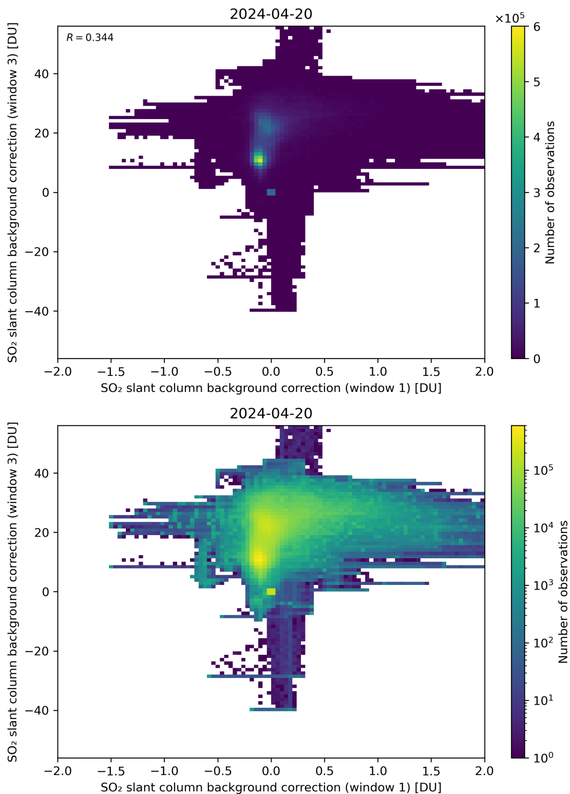
Figure 99: Scatter density plot of “SO 2 slant column background correction (window 1)” against “SO 2 slant column background correction (window 3)” for 2024-04-19 to 2024-04-21.
