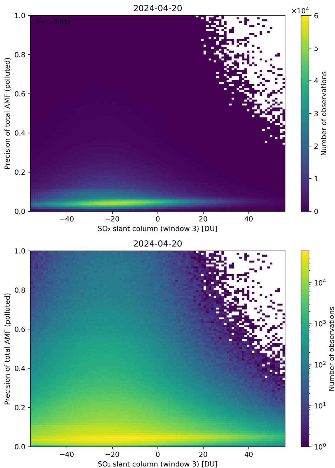
Figure 269: Scatter density plot of “SO 2 slant column (window 3)” against “Precision of total AMF (polluted)” for 2024-04-19 to 2024-04-21.
