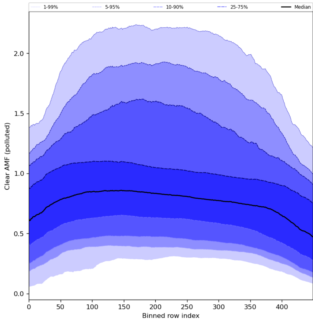
Figure 96: Along track statistics of “Clear AMF (polluted)” for 2024-04-19 to 2024-04-21
