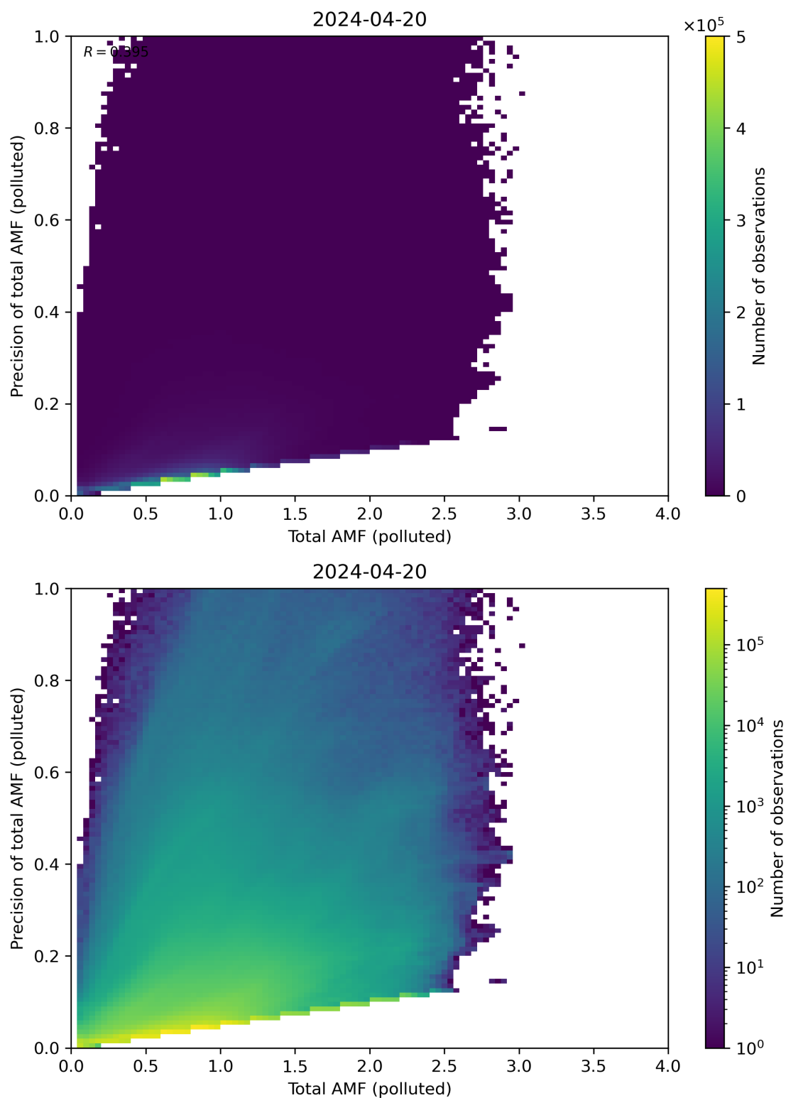
Figure 272: Scatter density plot of “Total AMF (polluted)” against “Precision of total AMF (polluted)” for 2024-04-19 to 2024-04-21.
