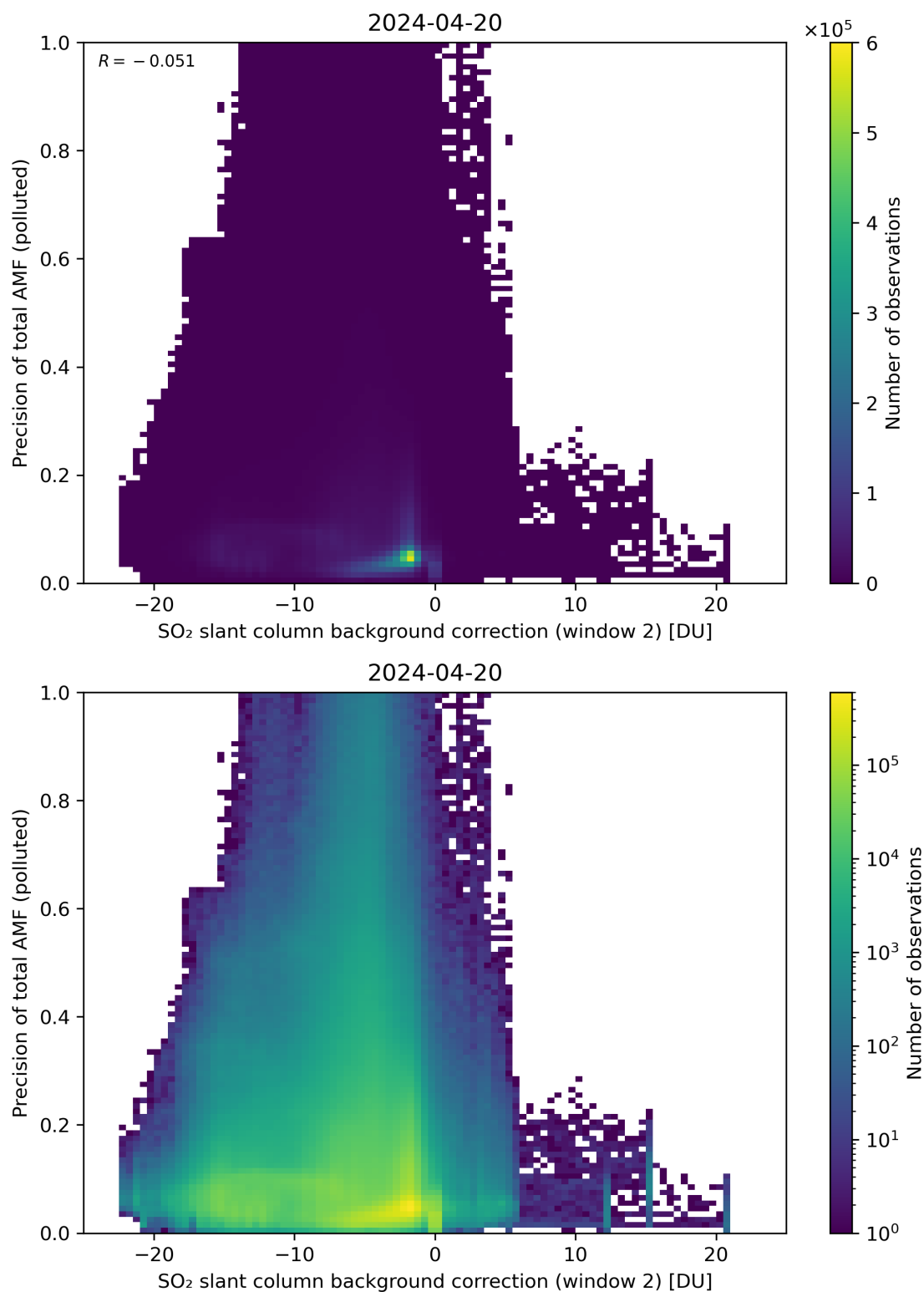
Figure 120: Scatter density plot of “SO 2 slant column background correction (window 2)” against “Precision of total AMF (polluted)” for 2024-04-19 to 2024-04-21.
