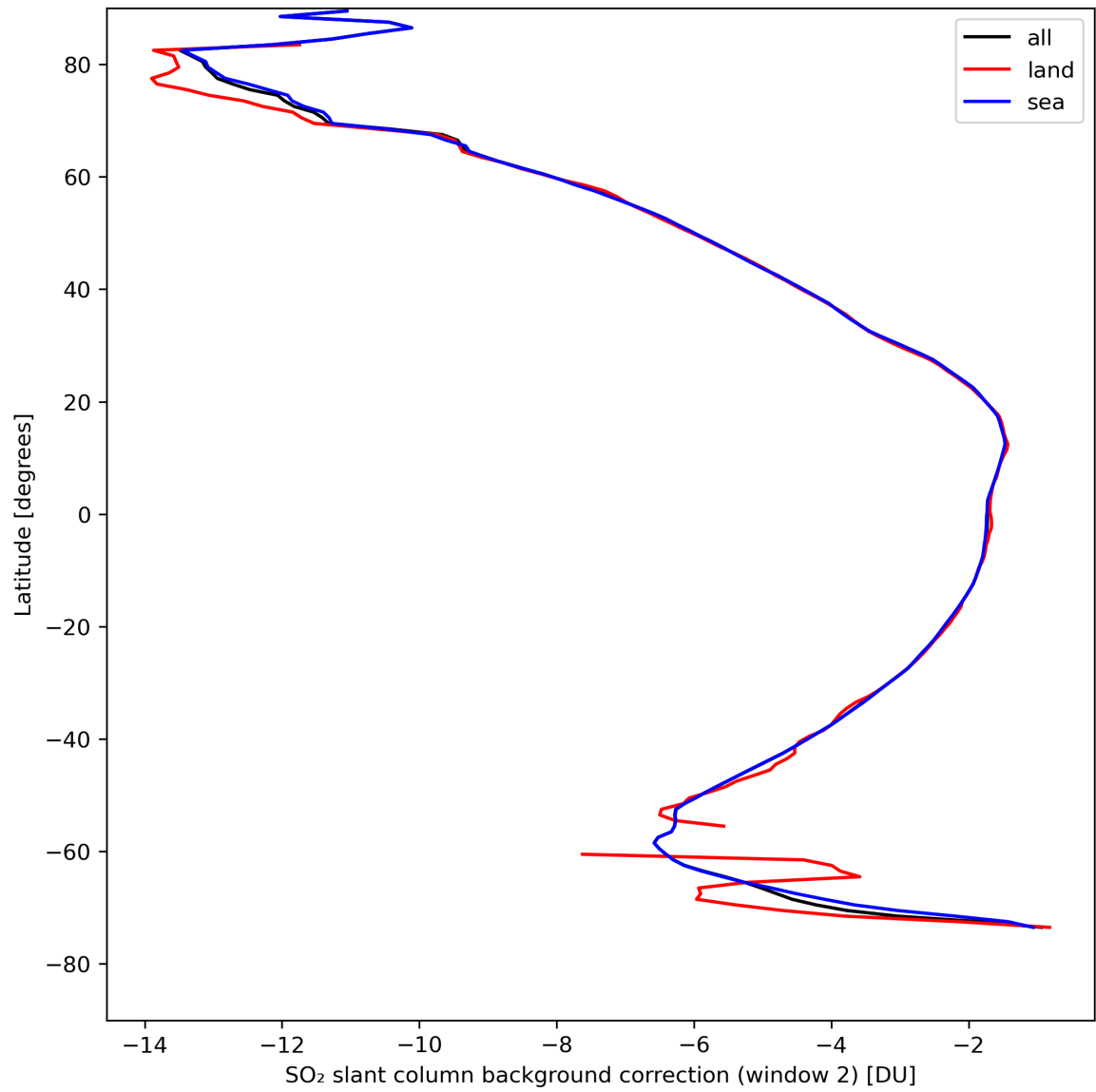
Figure 40: Zonal average of “SO 2 slant column background correction (window 2)” for 2024-04-19 to 2024-04-21.
