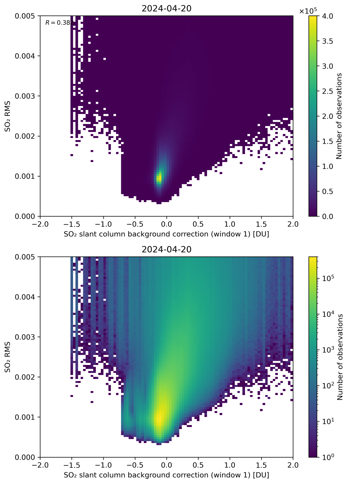
Figure 102: Scatter density plot of “SO 2 slant column background correction (window 1)” against “SO 2 RMS” for 2024-04-19 to 2024-04-21.
