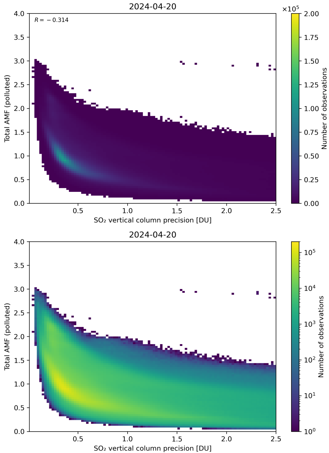
Figure 294: Scatter density plot of “SO 2 vertical column precision” against “Total AMF (polluted)” for 2024-04-19 to 2024-04-21.
