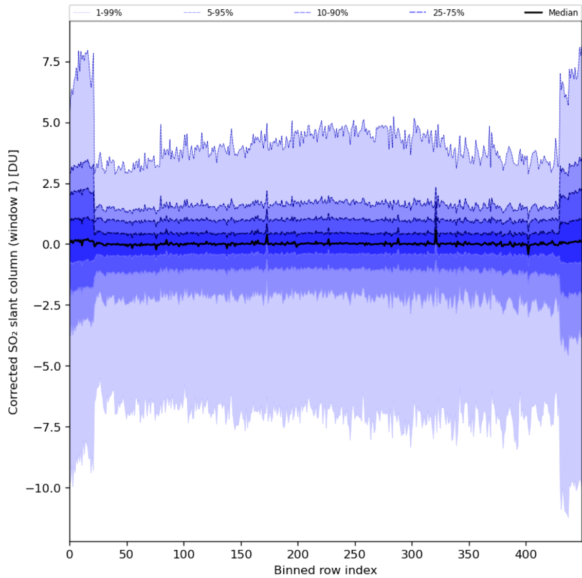
Figure 81: Along track statistics of “Corrected SO 2 slant column (window 1)” for 2024-04-19 to 2024-04-21
