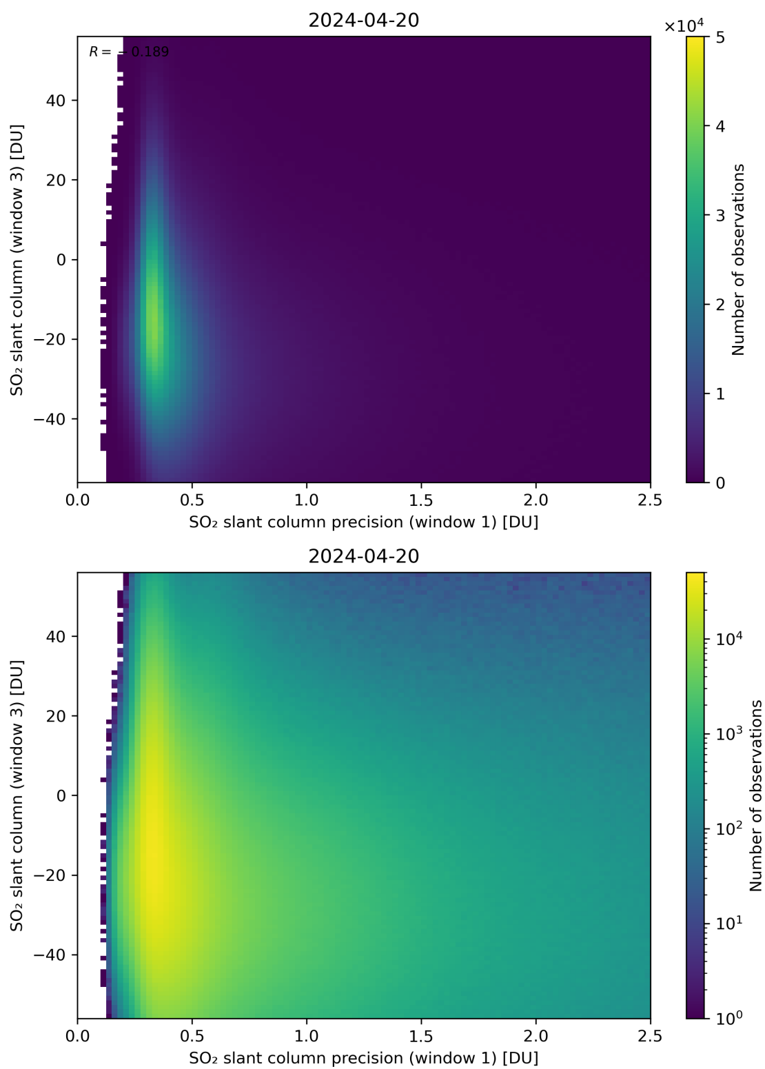
Figure 228: Scatter density plot of “SO 2 slant column precision (window 1)” against “SO 2 slant column (window 3)” for 2024-04-19 to 2024-04-21.
