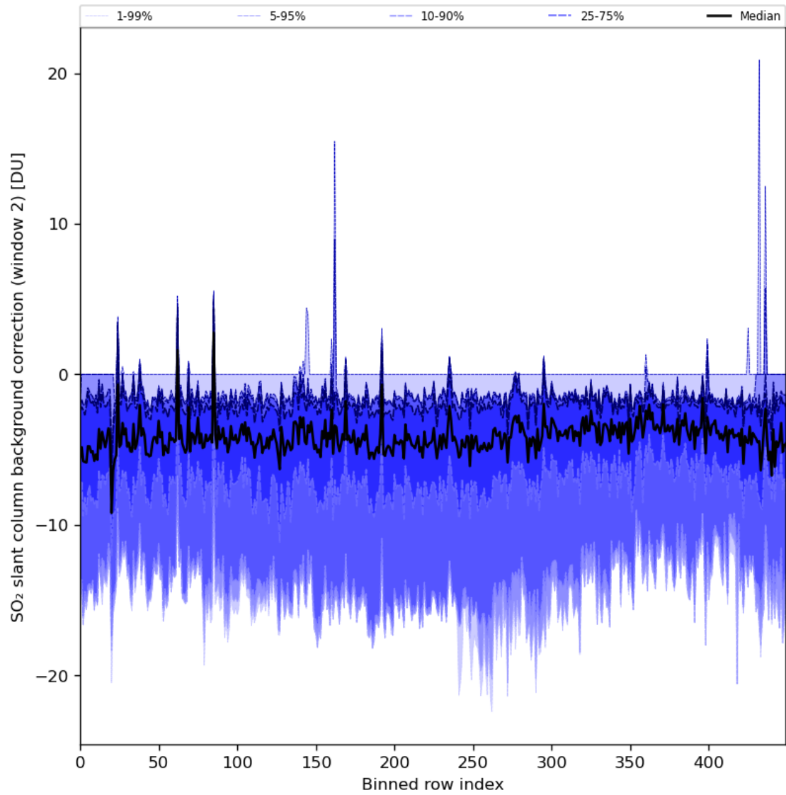
Figure 86: Along track statistics of “SO 2 slant column background correction (window 2)” for 2024-04-19 to 2024-04-21
