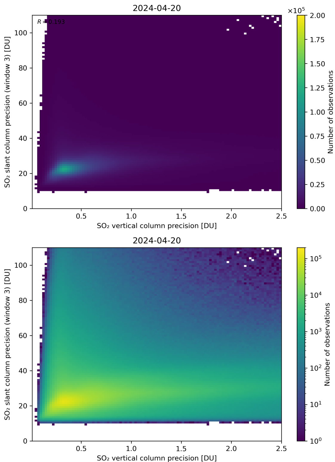
Figure 293: Scatter density plot of “SO 2 vertical column precision” against “SO 2 slant column precision (window 3)” for 2024-04-19 to 2024-04-21.
