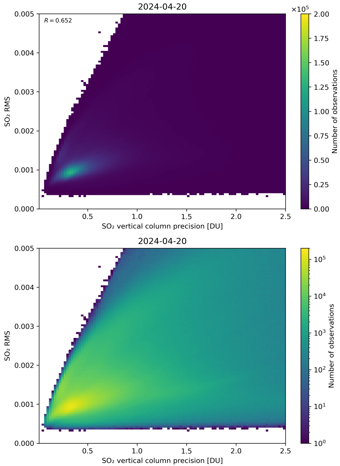
Figure 284: Scatter density plot of “SO 2 vertical column precision” against “SO 2 RMS” for 2024-04-19 to 2024-04-21.
