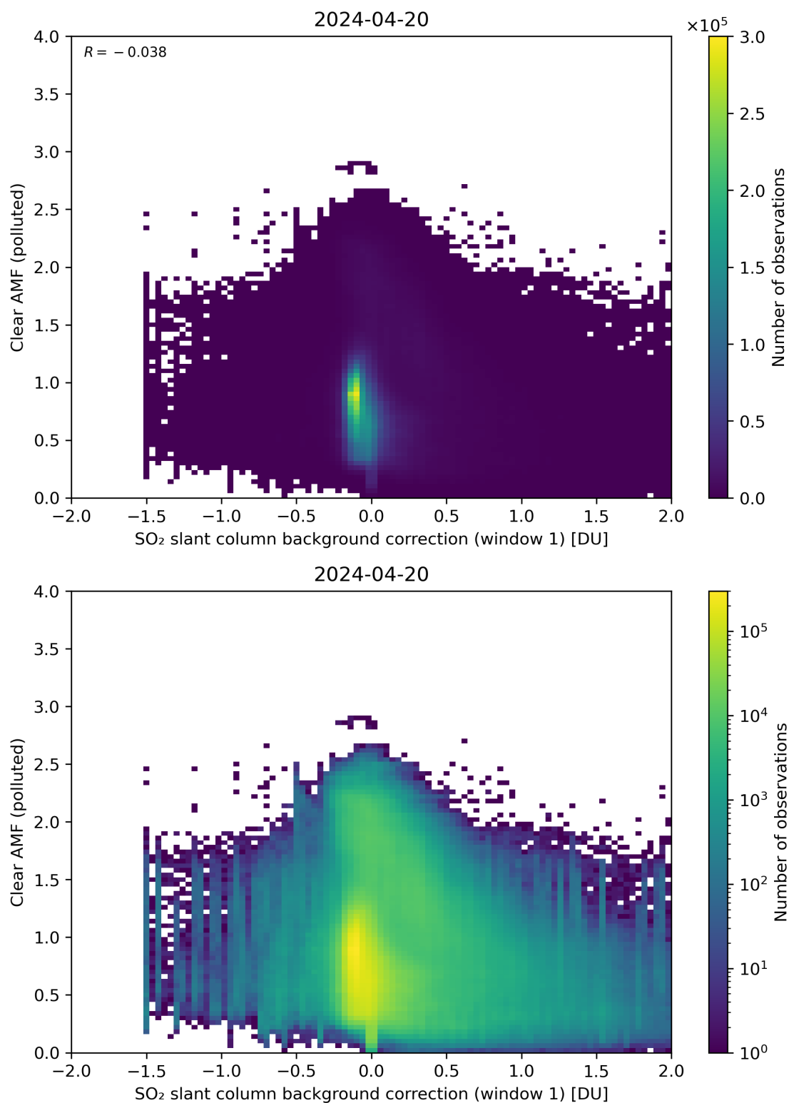
Figure 103: Scatter density plot of “SO 2 slant column background correction (window 1)” against “Clear AMF (polluted)” for 2024-04-19 to 2024-04-21.
