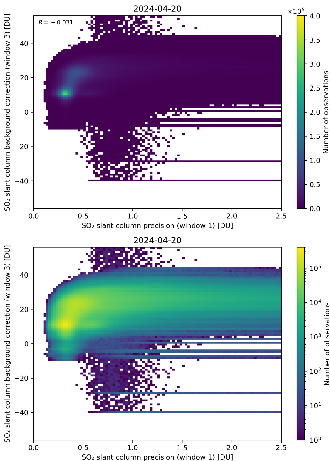
Figure 220: Scatter density plot of “SO 2 slant column precision (window 1)” against “SO 2 slant column background correction (window 3)” for 2024-04-19 to 2024-04-21.
