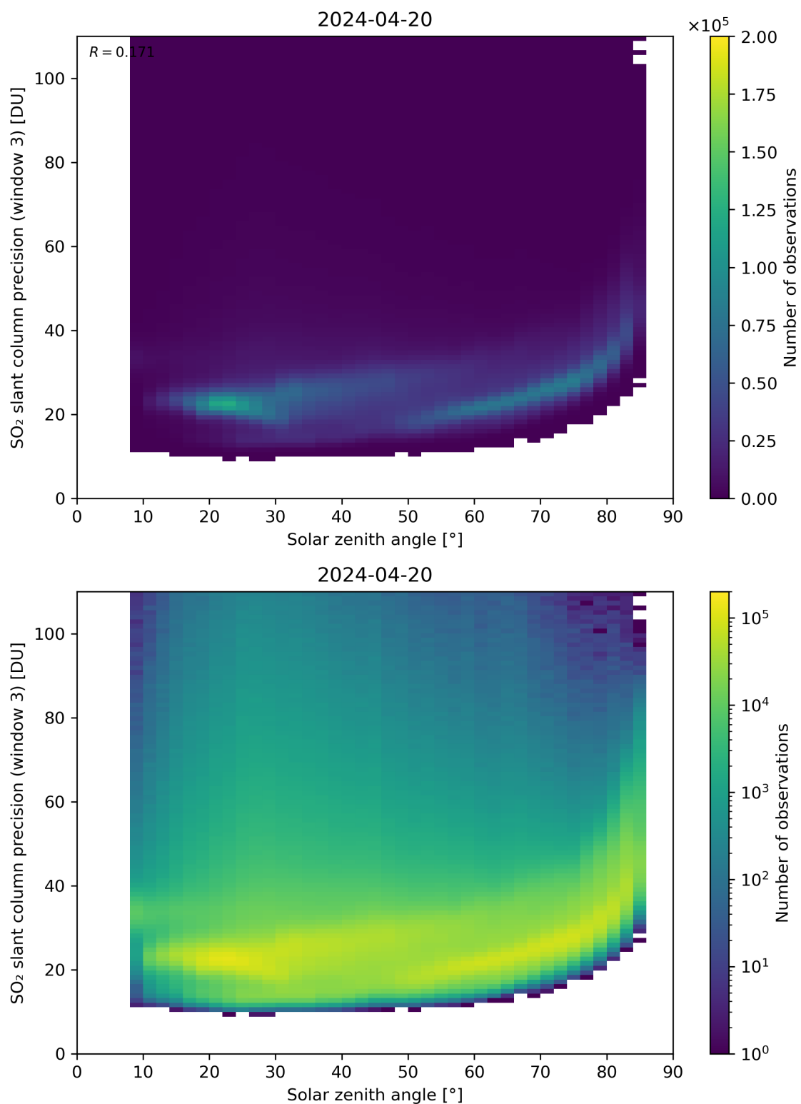
Figure 173: Scatter density plot of “Solar zenith angle” against “SO 2 slant column precision (window 3)” for 2024-04-19 to 2024-04-21.
