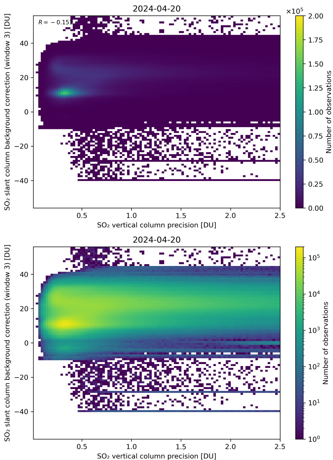
Figure 281: Scatter density plot of “SO 2 vertical column precision” against “SO 2 slant column background correction (window 3)” for 2024-04-19 to 2024-04-21.
