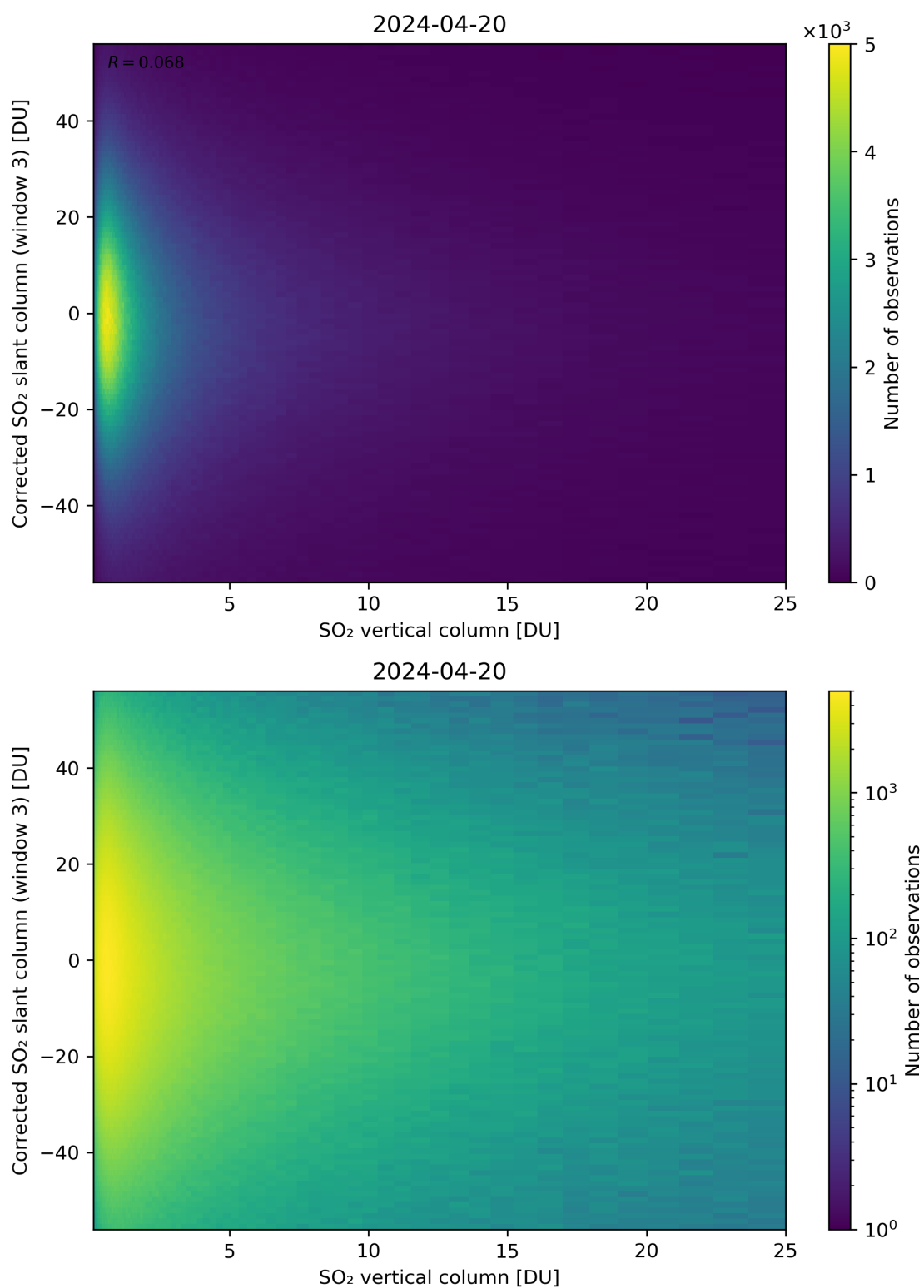
Figure 299: Scatter density plot of “SO 2 vertical column” against “Corrected SO 2 slant column (window 3)” for 2024-04-19 to 2024-04-21.
