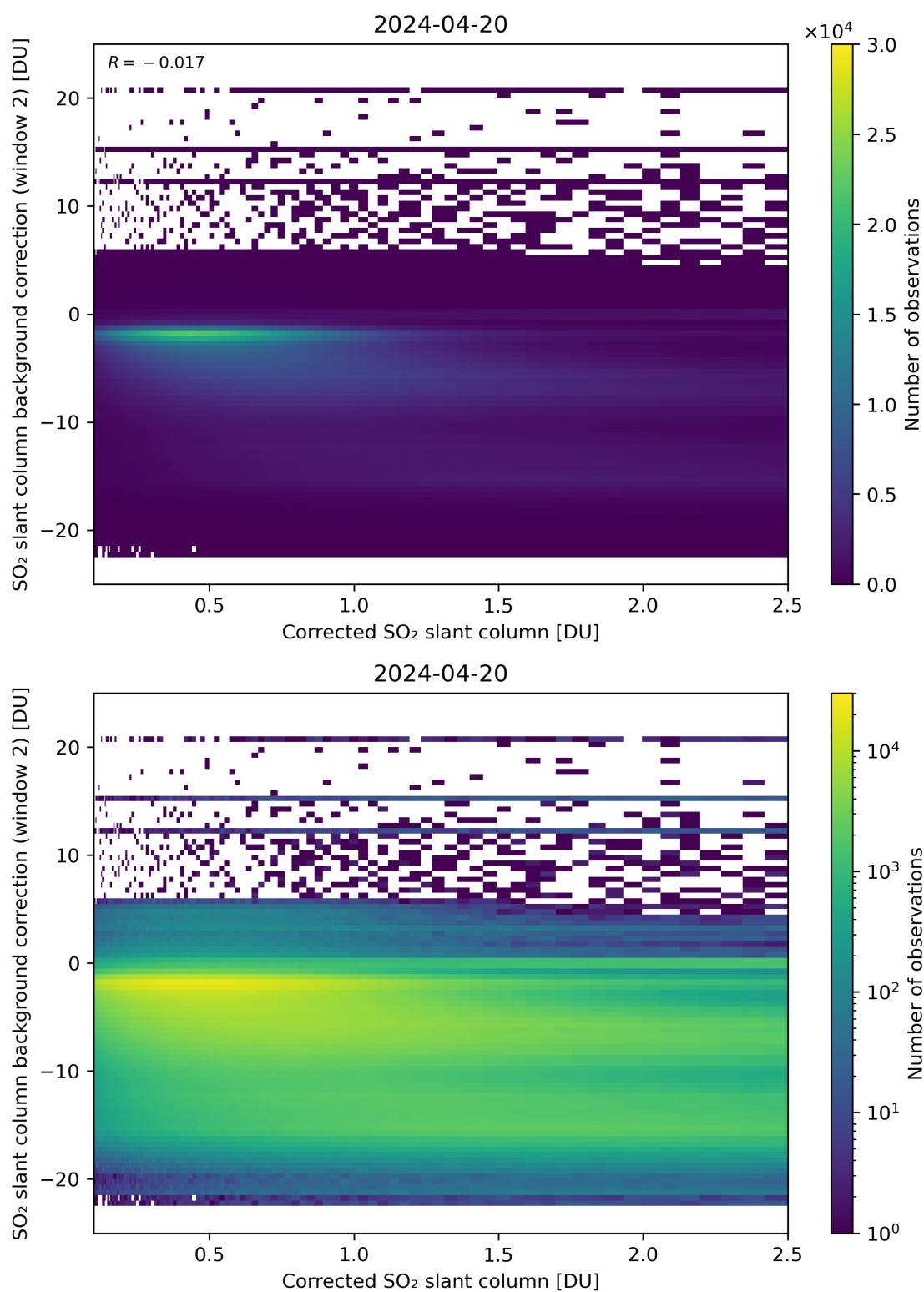
Figure 179: Scatter density plot of “Corrected SO 2 slant column” against “SO 2 slant column background correction (window 2)” for 2024-04-19 to 2024-04-21.
