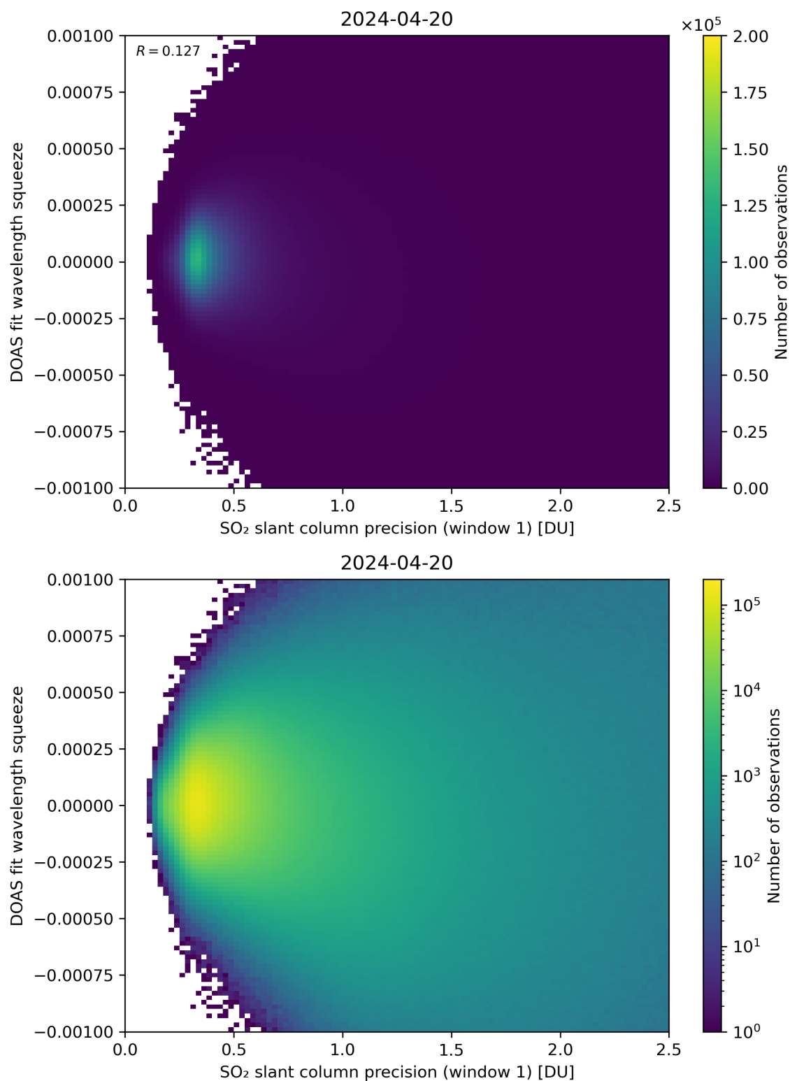
Figure 222: Scatter density plot of “SO 2 slant column precision (window 1)” against “DOAS fit wavelength squeeze” for 2024-04-19 to 2024-04-21.
