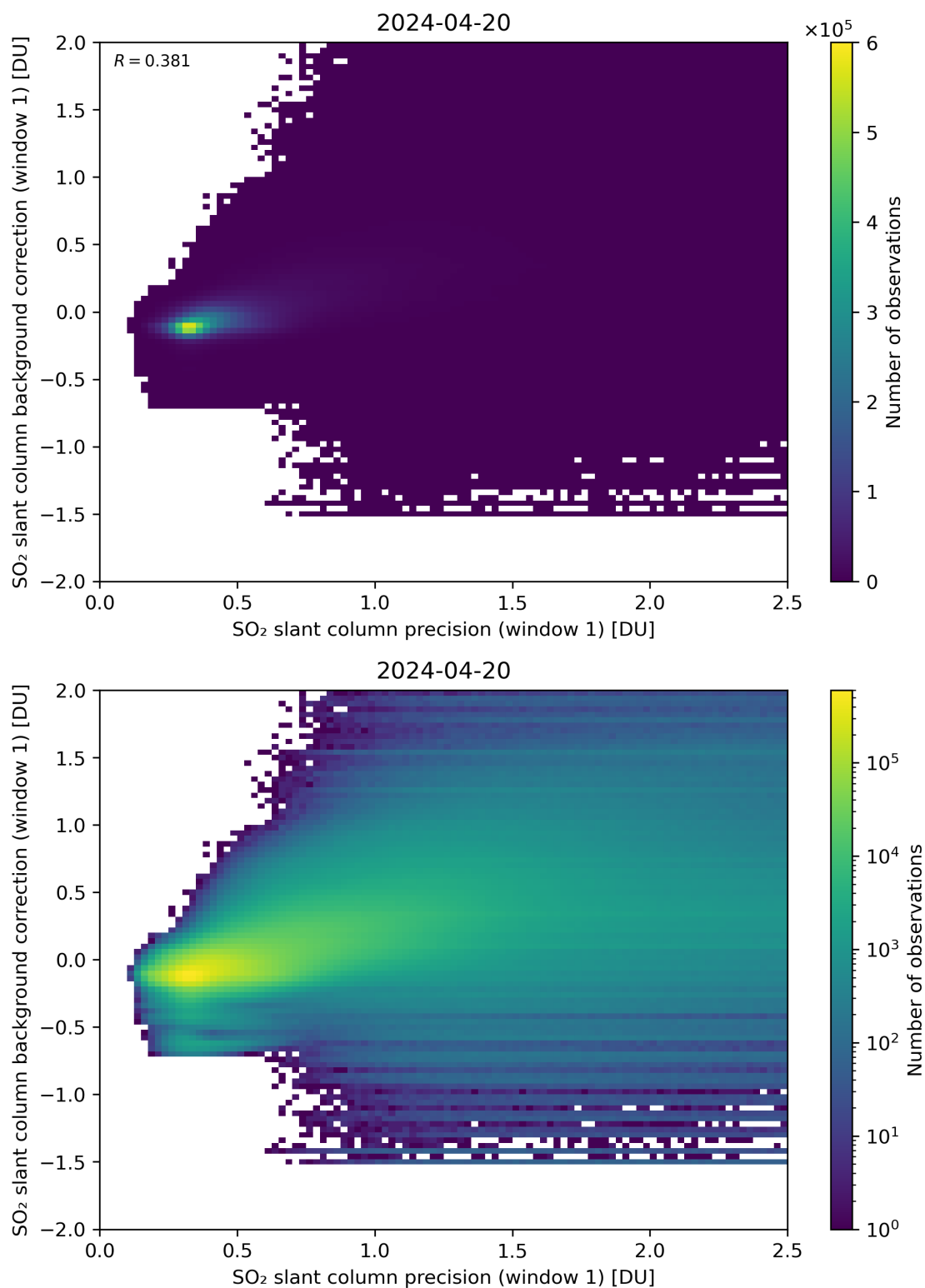
Figure 218: Scatter density plot of “SO 2 slant column precision (window 1)” against “SO 2 slant column background correction (window 1)” for 2024-04-19 to 2024-04-21.
