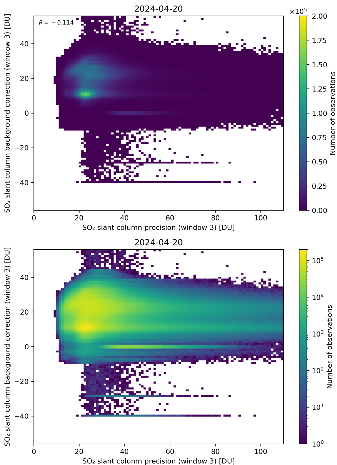
Figure 257: Scatter density plot of “SO 2 slant column precision (window 3)” against “SO 2 slant column background correction (window 3)” for 2024-04-19 to 2024-04-21.
