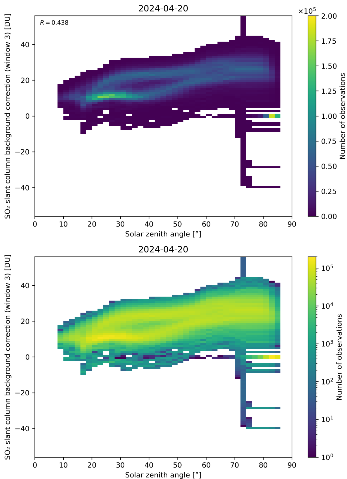
Figure 160: Scatter density plot of “Solar zenith angle” against “SO 2 slant column background correction (window 3)” for 2024-04-19 to 2024-04-21.
