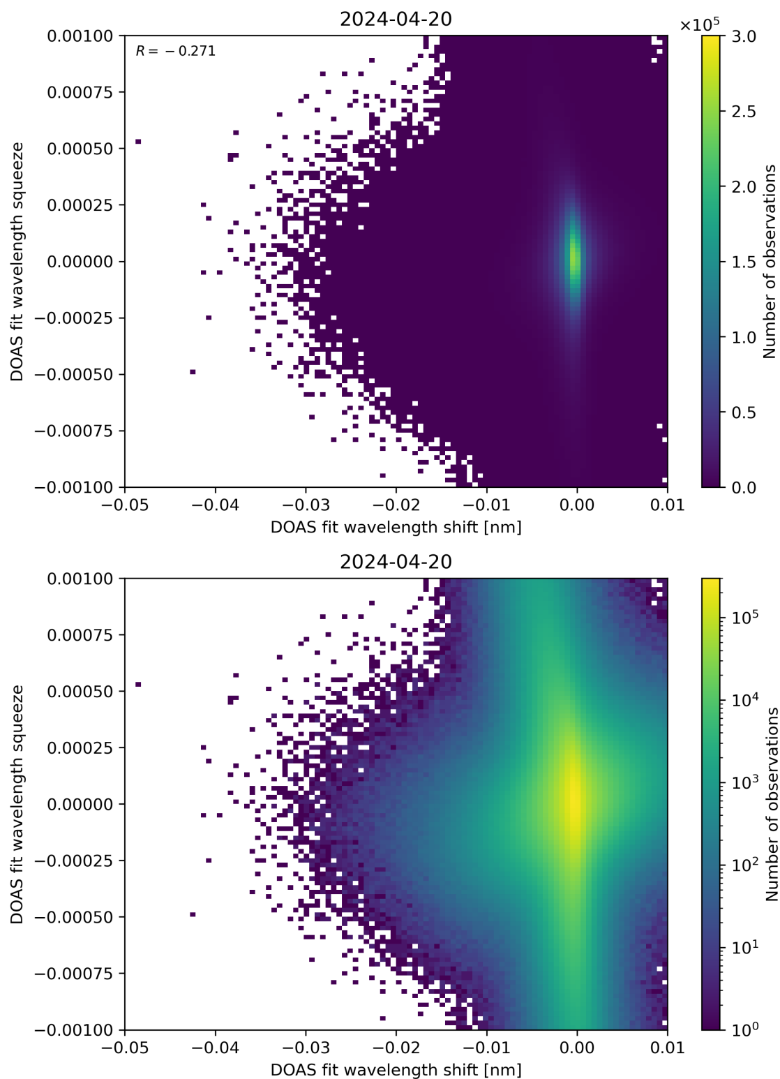
Figure 127: Scatter density plot of “DOAS fit wavelength shift” against “DOAS fit wavelength squeeze” for 2024-04-19 to 2024-04-21.
