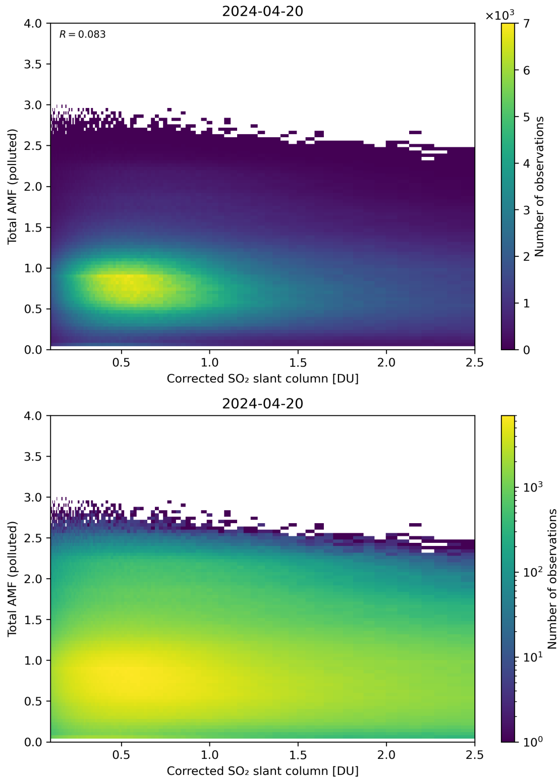
Figure 192: Scatter density plot of “Corrected SO 2 slant column” against “Total AMF (polluted)” for 2024-04-19 to 2024-04-21.
