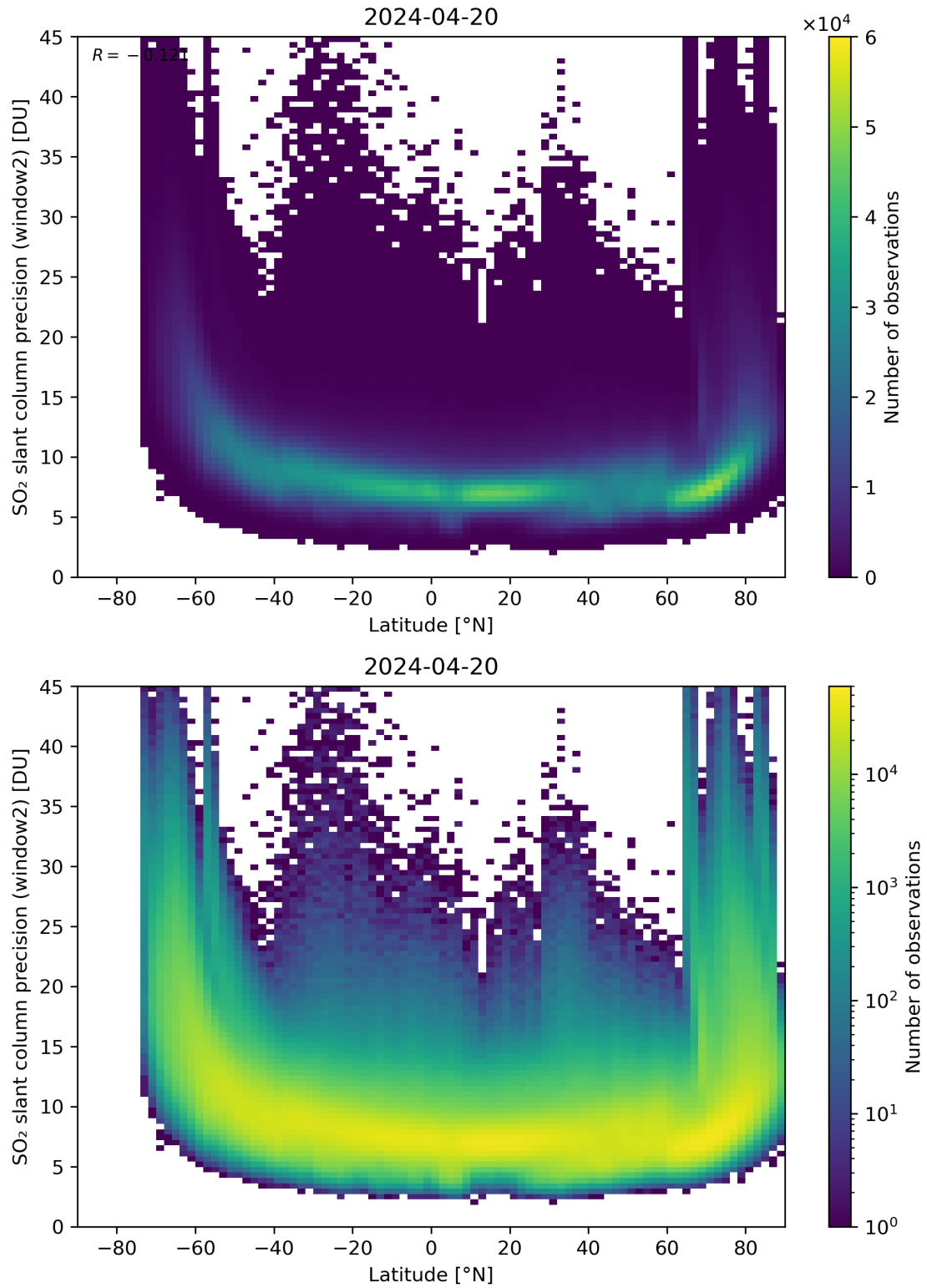
Figure 151: Scatter density plot of “Latitude” against “SO 2 slant column precision (window2)” for 2024-04-19 to 2024-04-21.
