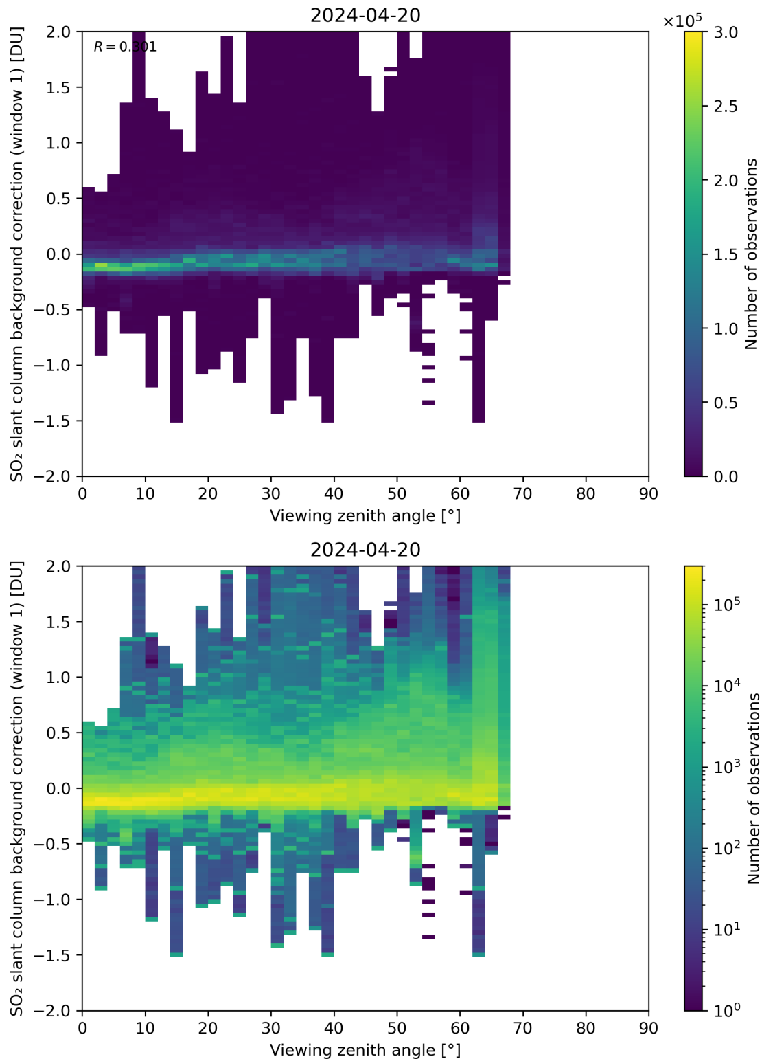
Figure 308: Scatter density plot of “Viewing zenith angle” against “SO 2 slant column background correction (window 1)” for 2024-04-19 to 2024-04-21.
