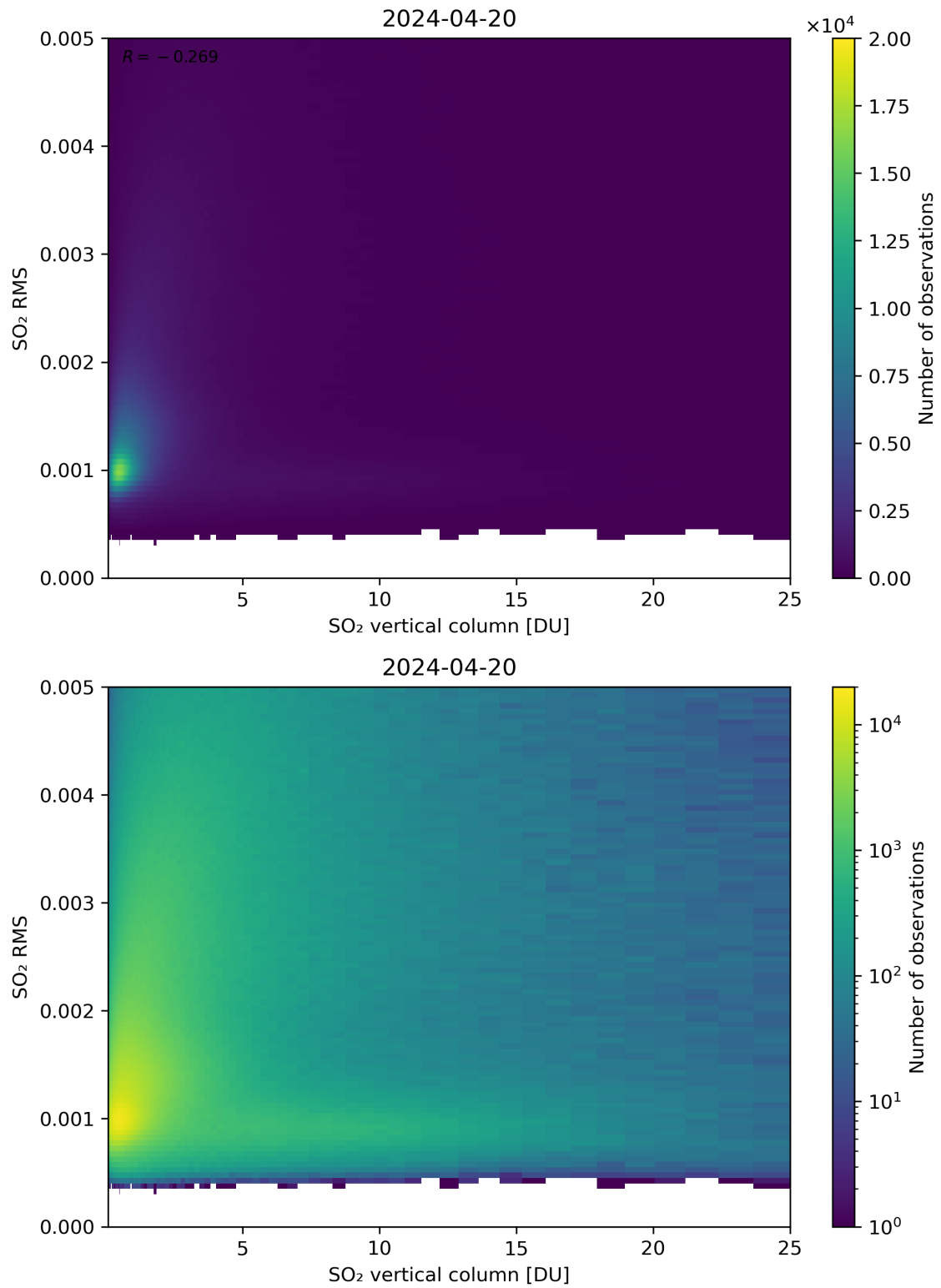
Figure 278: Scatter density plot of “SO 2 vertical column” against “SO 2 RMS” for 2024-04-19 to 2024-04-21.
