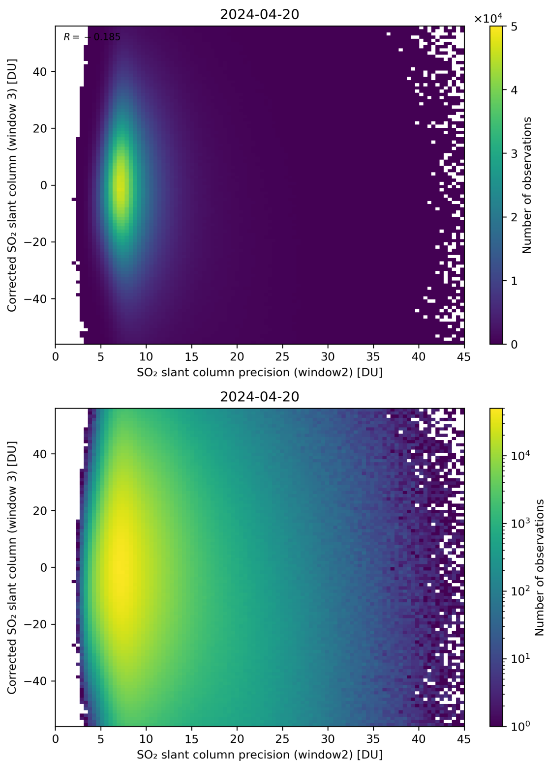
Figure 248: Scatter density plot of “SO 2 slant column precision (window2)” against “Corrected SO 2 slant column (window 3)” for 2024-04-19 to 2024-04-21.
