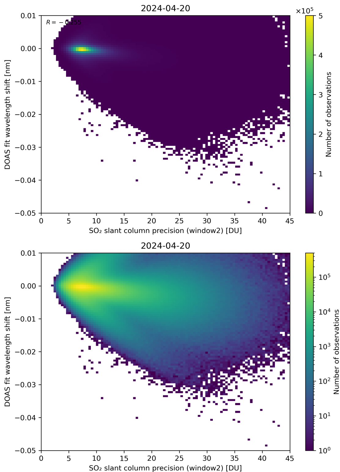
Figure 243: Scatter density plot of “SO 2 slant column precision (window2)” against “DOAS fit wavelength shift” for 2024-04-19 to 2024-04-21.
