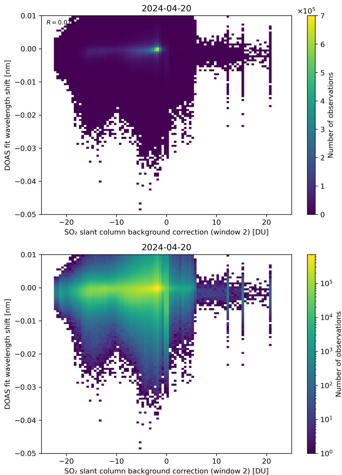
Figure 112: Scatter density plot of “SO 2 slant column background correction (window 2)” against “DOAS fit wavelength shift” for 2024-04-19 to 2024-04-21.
