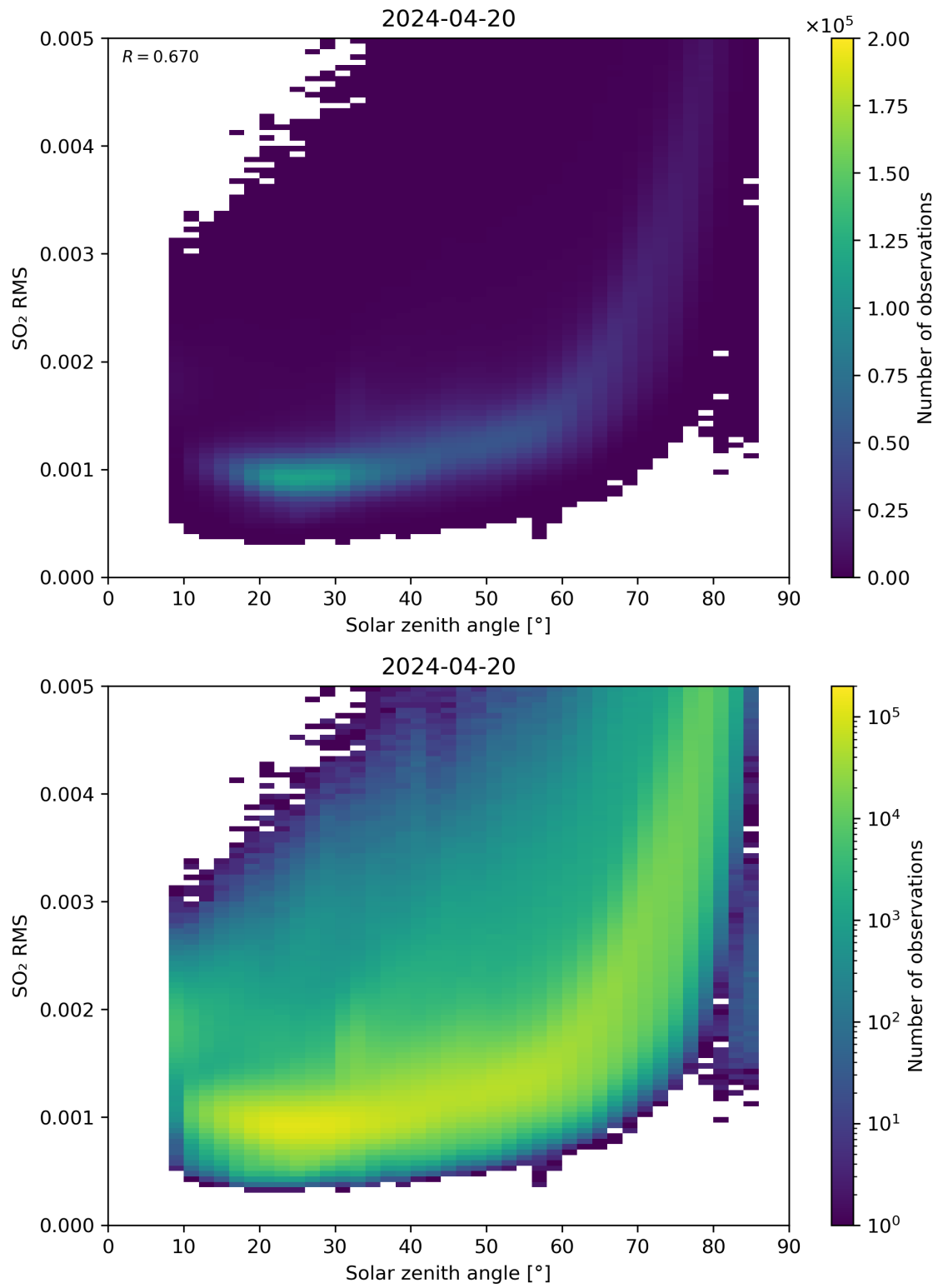
Figure 163: Scatter density plot of “Solar zenith angle” against “SO 2 RMS” for 2024-04-19 to 2024-04-21.
