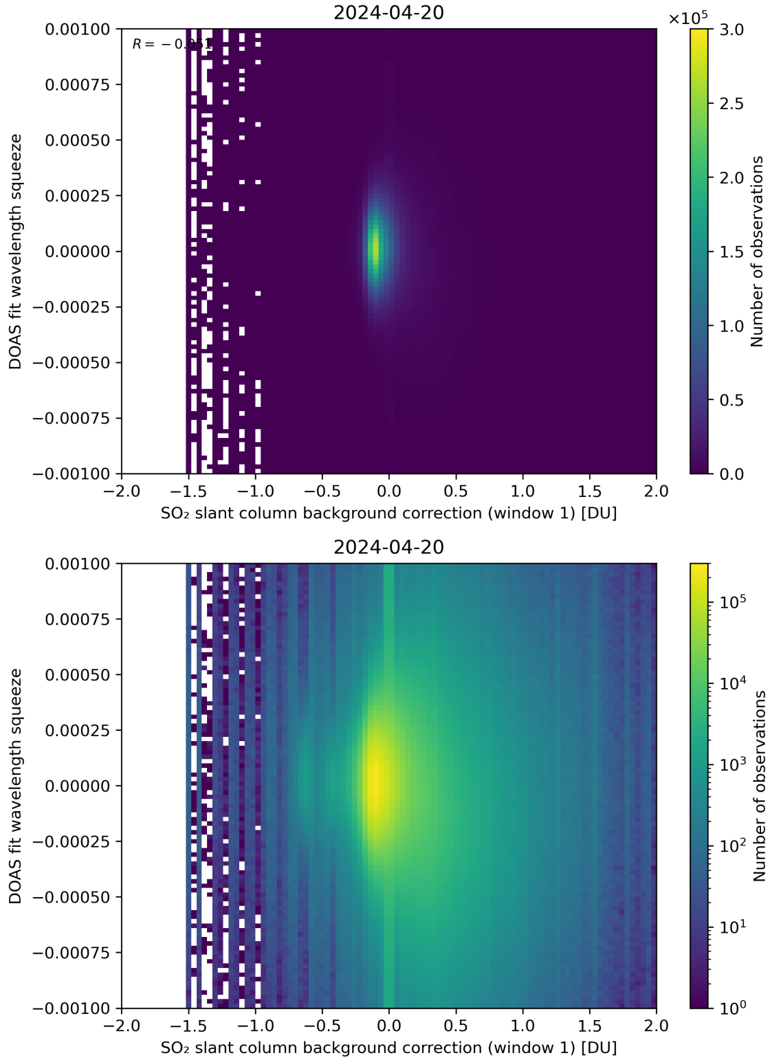
Figure 101: Scatter density plot of “SO 2 slant column background correction (window 1)” against “DOAS fit wavelength squeeze” for 2024-04-19 to 2024-04-21.
