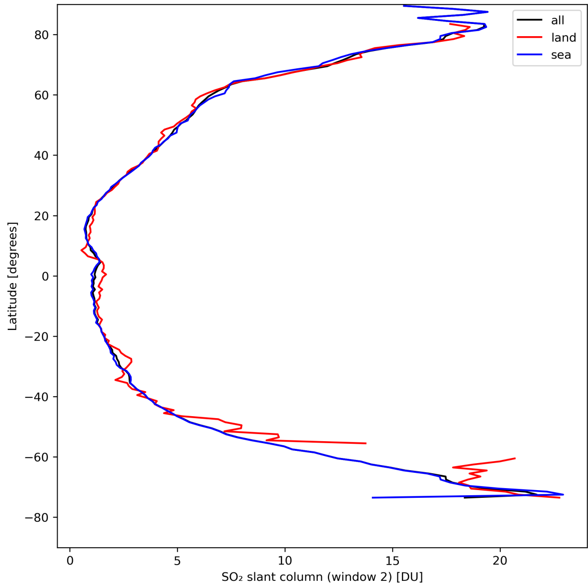
Figure 37: Zonal average of “SO 2 slant column (window 2)” for 2024-04-19 to 2024-04-21.
