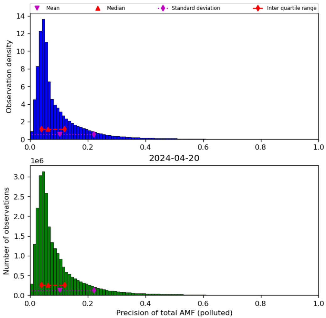
Figure 72: Histogram of “Precision of total AMF (polluted)” for 2024-04-19 to 2024-04-21
