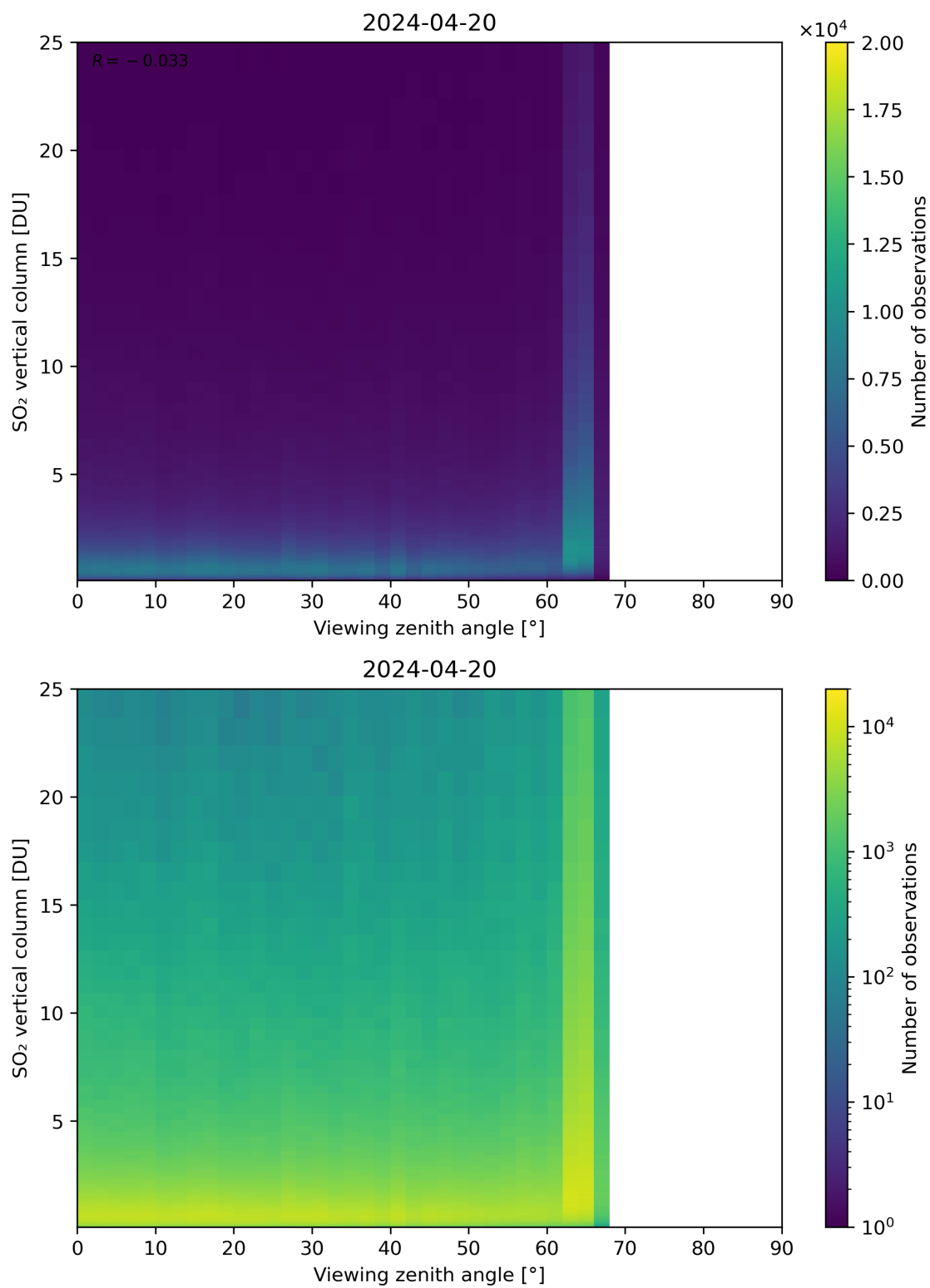
Figure 327: Scatter density plot of “Viewing zenith angle” against “SO 2 vertical column” for 2024-04-19 to 2024-04-21.
