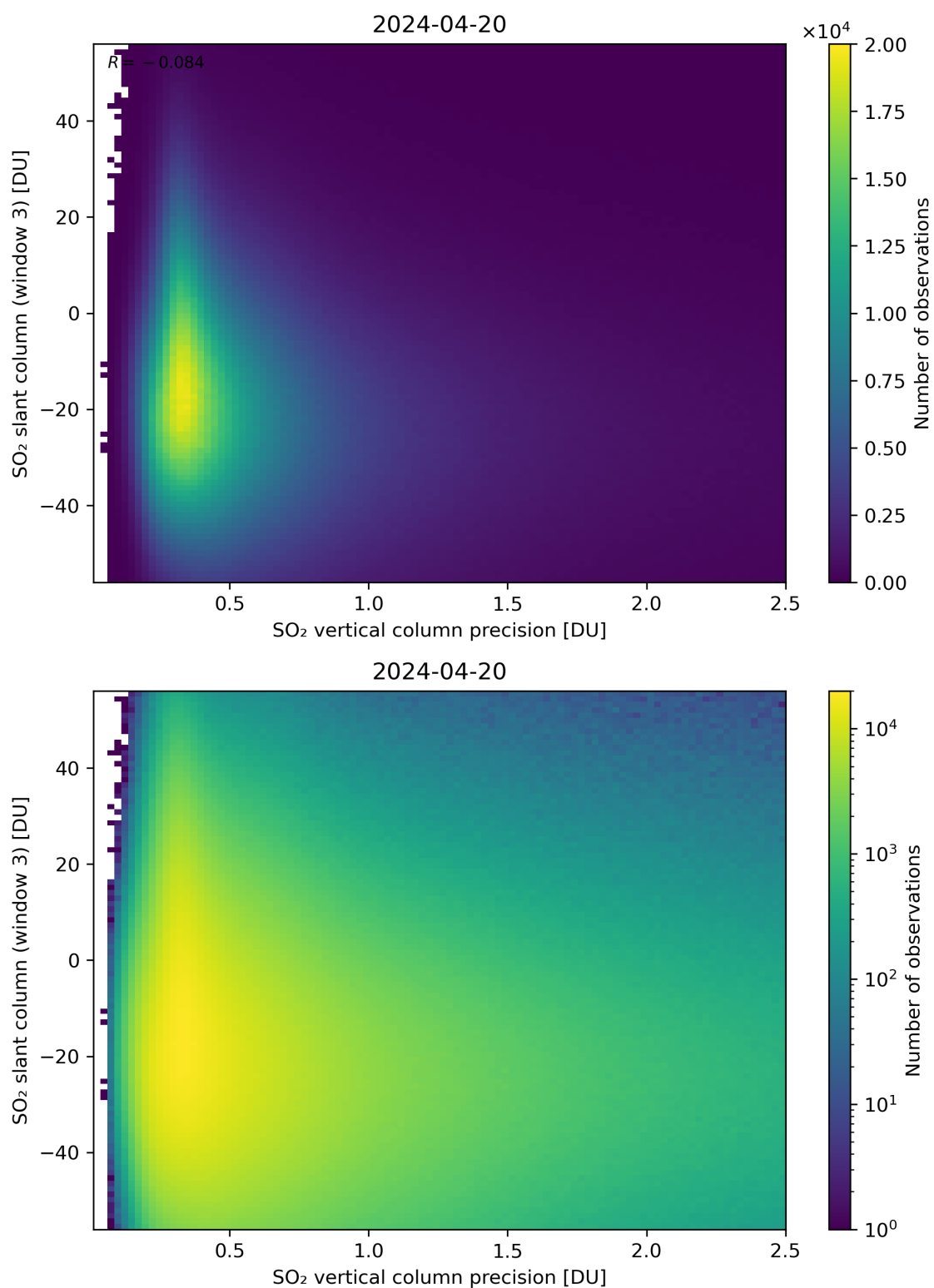
Figure 292: Scatter density plot of “SO 2 vertical column precision” against “SO 2 slant column (window 3)” for 2024-04-19 to 2024-04-21.
