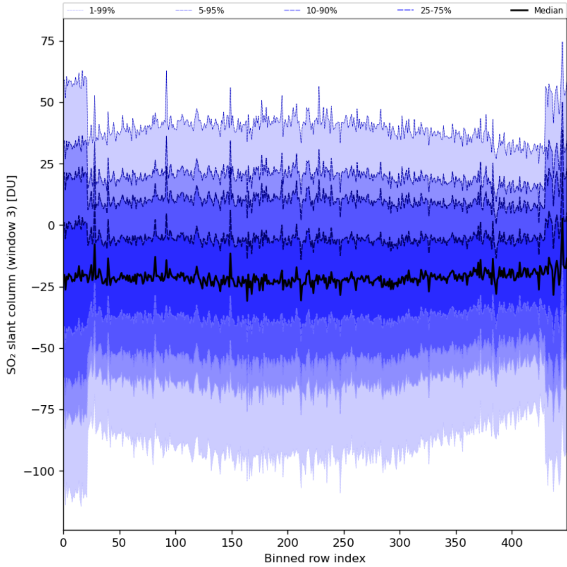
Figure 87: Along track statistics of “SO 2 slant column (window 3)” for 2024-04-19 to 2024-04-21
