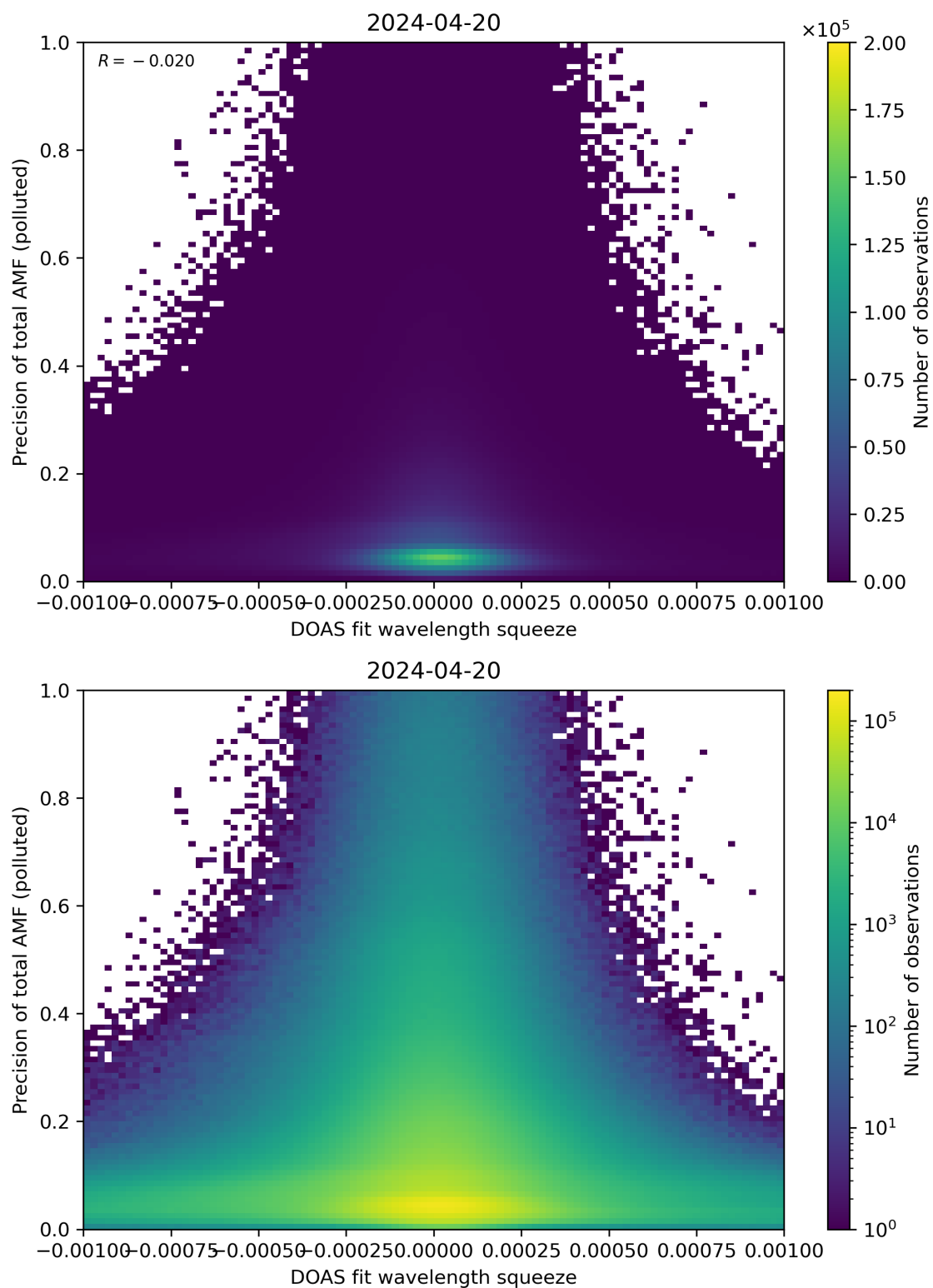
Figure 135: Scatter density plot of “DOAS fit wavelength squeeze” against “Precision of total AMF (polluted)” for 2024-04-19 to 2024-04-21.
