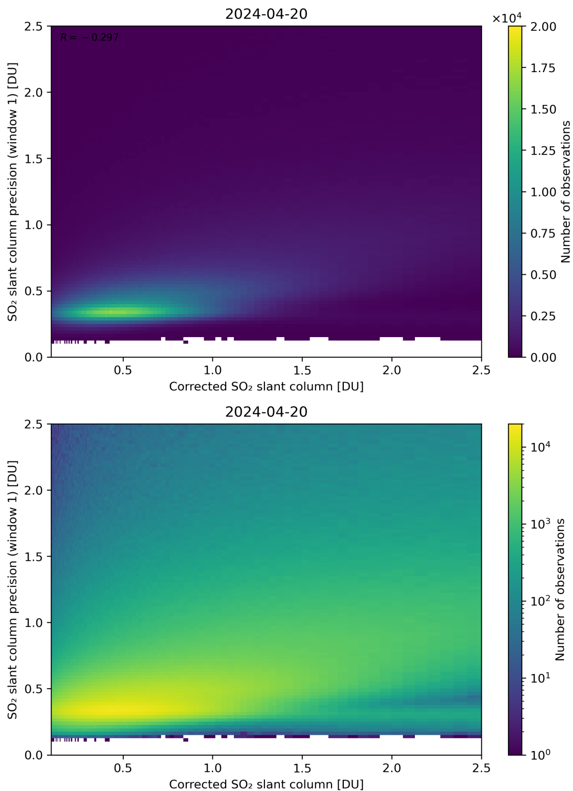
Figure 188: Scatter density plot of “Corrected SO 2 slant column” against “SO 2 slant column precision (window 1)” for 2024-04-19 to 2024-04-21.
