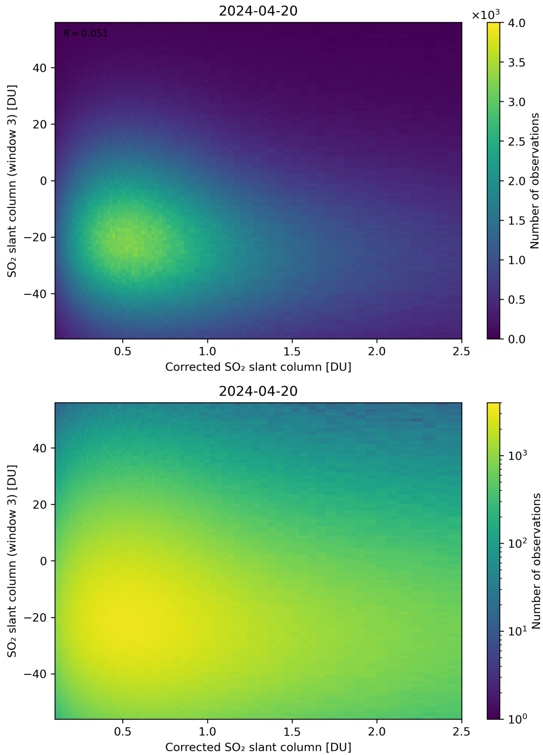
Figure 190: Scatter density plot of “Corrected SO 2 slant column” against “SO 2 slant column (window 3)” for 2024-04-19 to 2024-04-21.
