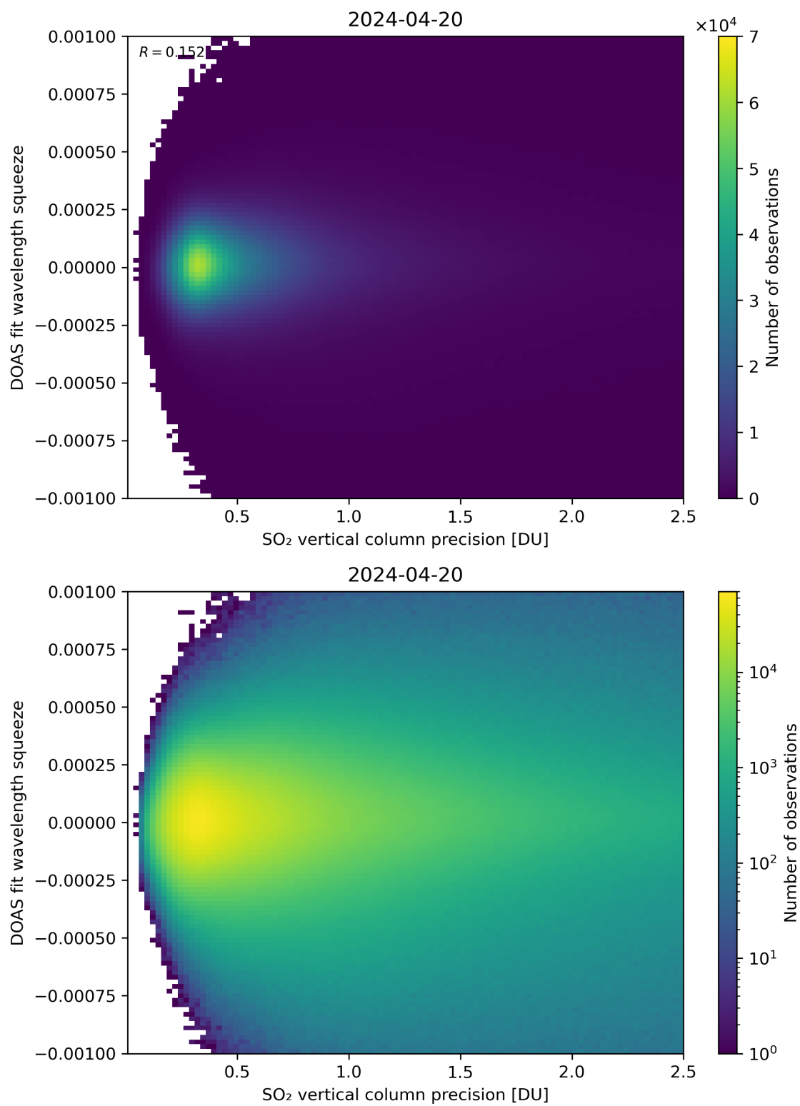
Figure 283: Scatter density plot of “SO 2 vertical column precision” against “DOAS fit wavelength squeeze” for 2024-04-19 to 2024-04-21.
