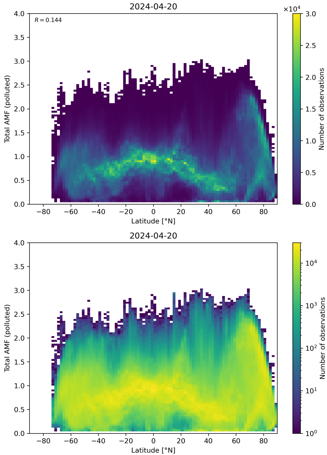
Figure 154: Scatter density plot of “Latitude” against “Total AMF (polluted)” for 2024-04-19 to 2024-04-21.
