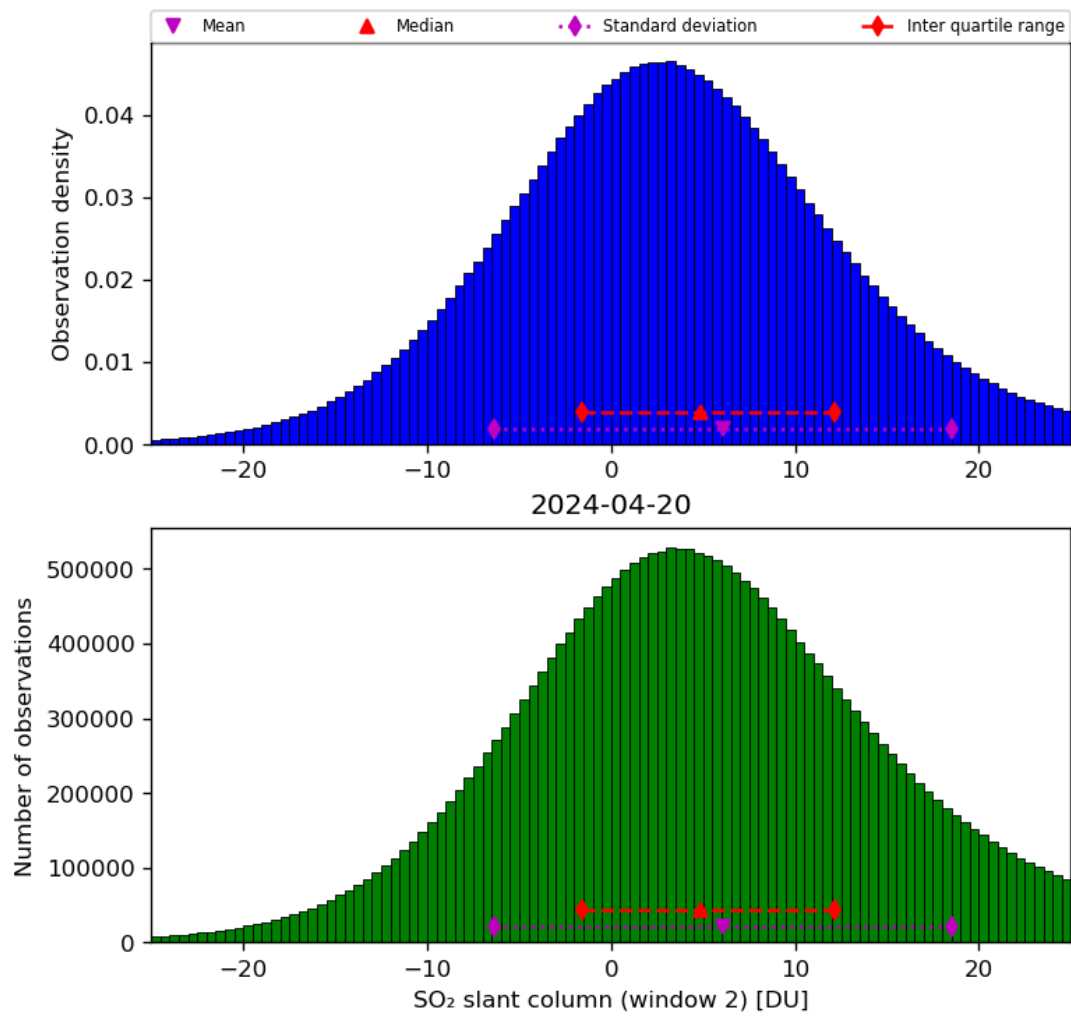
Figure 60: Histogram of “SO 2 slant column (window 2)” for 2024-04-19 to 2024-04-21
