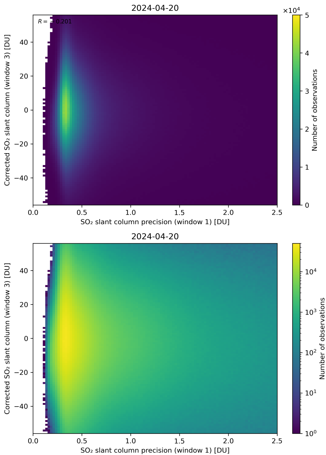
Figure 226: Scatter density plot of “SO 2 slant column precision (window 1)” against “Corrected SO 2 slant column (window 3)” for 2024-04-19 to 2024-04-21.
