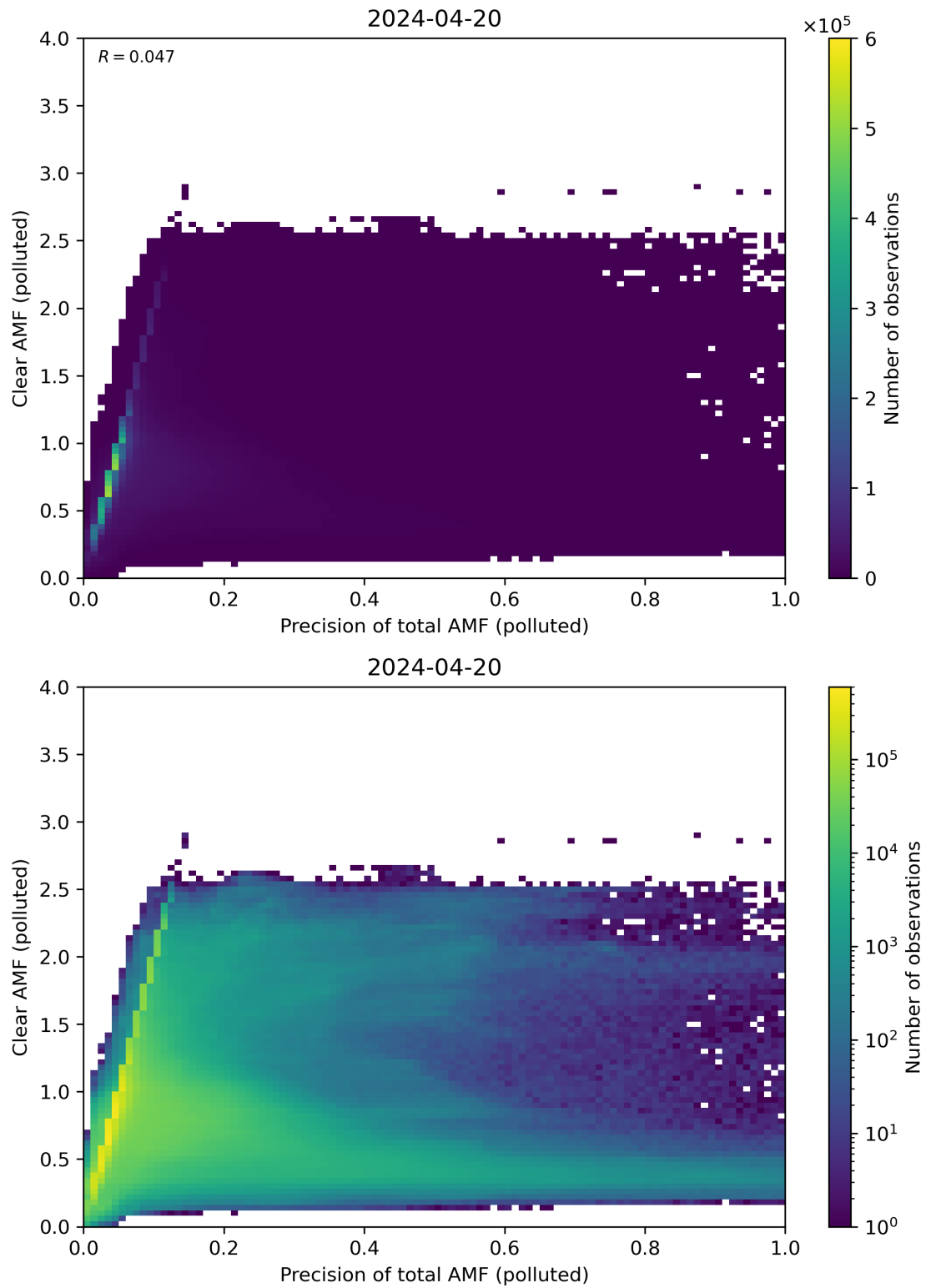
Figure 270: Scatter density plot of “Precision of total AMF (polluted)” against “Clear AMF (polluted)” for 2024-04-19 to 2024-04-21.
