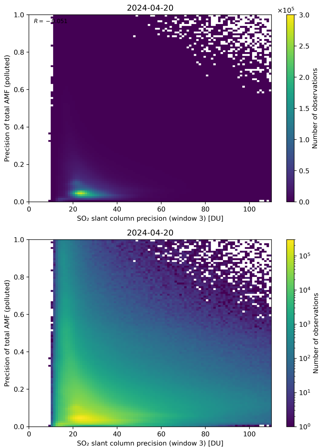
Figure 264: Scatter density plot of “SO 2 slant column precision (window 3)” against “Precision of total AMF (polluted)” for 2024-04-19 to 2024-04-21.
