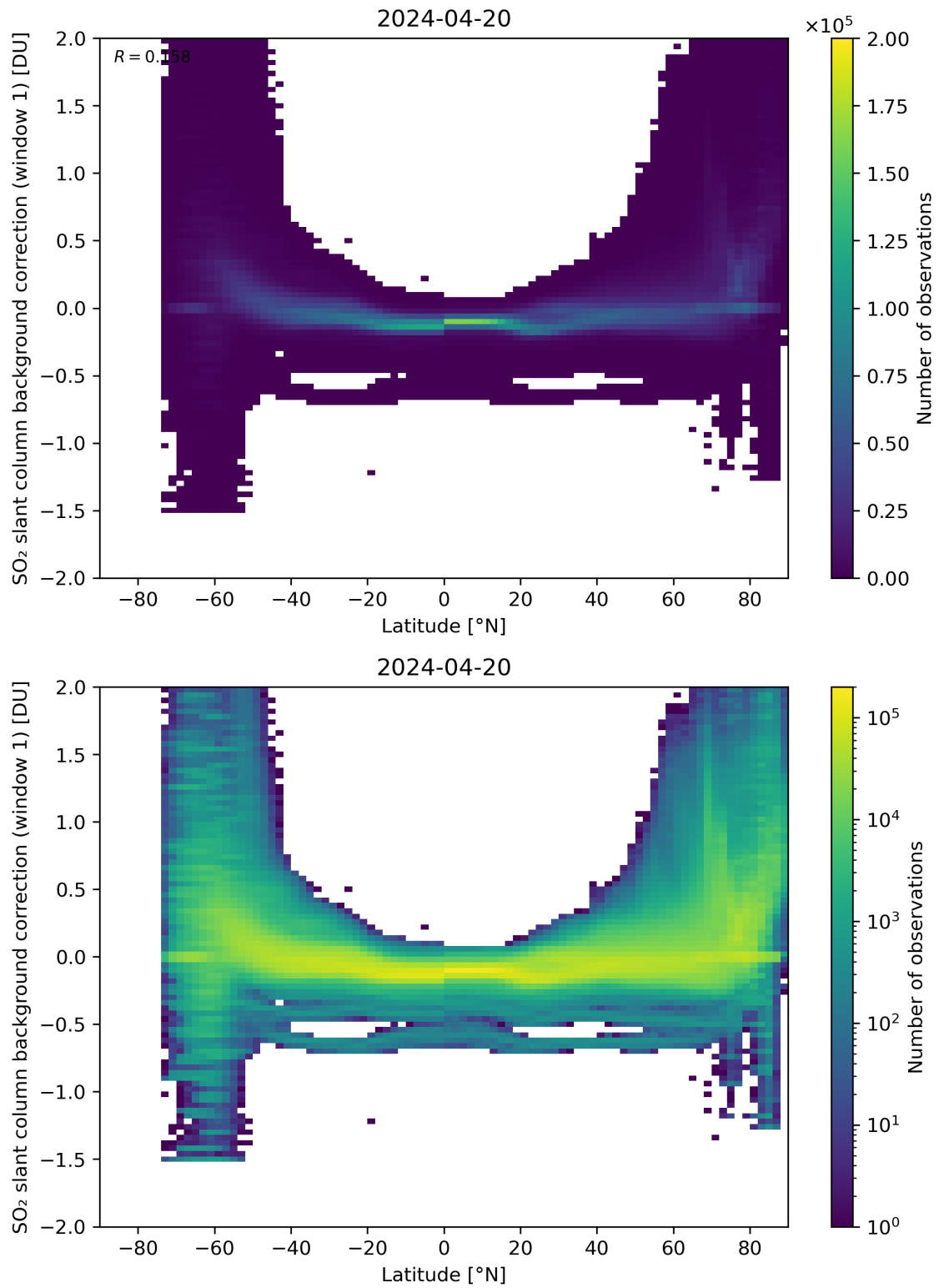
Figure 139: Scatter density plot of “Latitude” against “SO 2 slant column background correction (window 1)” for 2024-04-19 to 2024-04-21.
