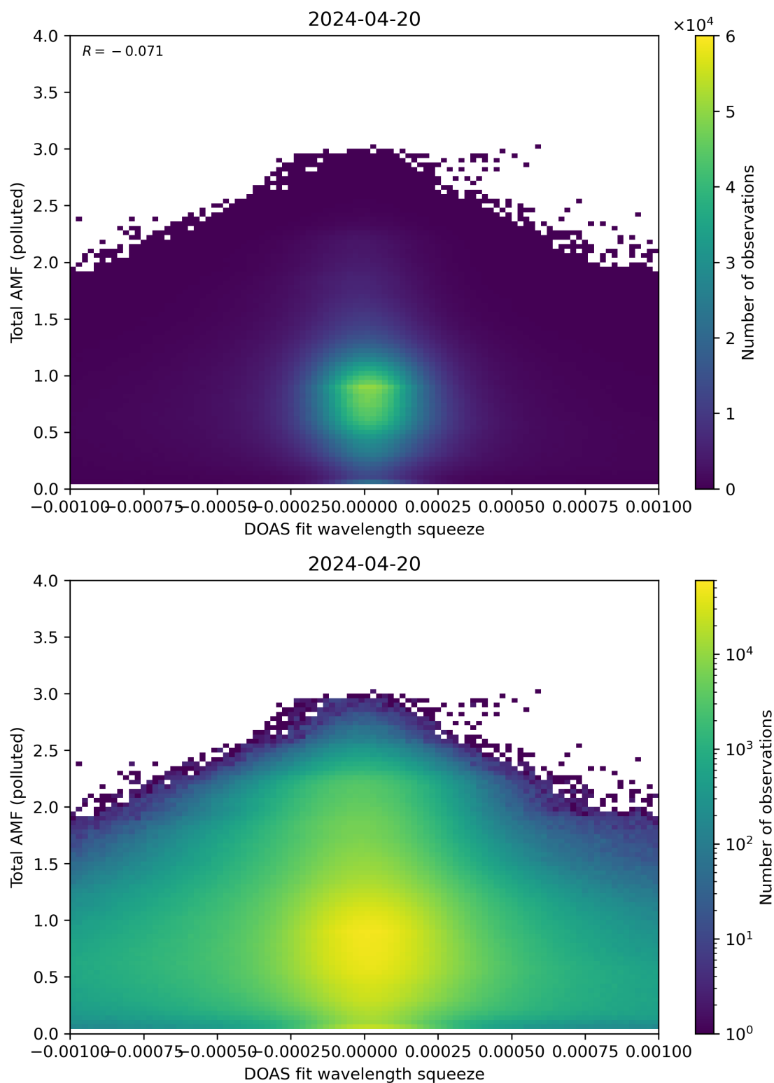
Figure 134: Scatter density plot of “DOAS fit wavelength squeeze” against “Total AMF (polluted)” for 2024-04-19 to 2024-04-21.
