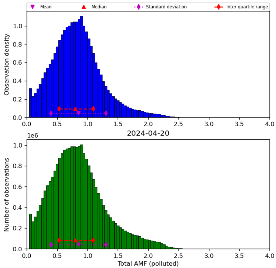
Figure 71: Histogram of “Total AMF (polluted)” for 2024-04-19 to 2024-04-21
