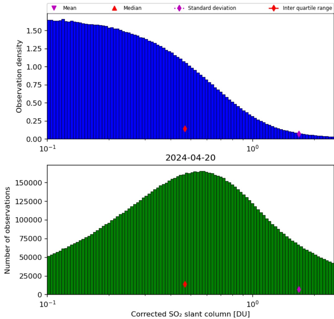
Figure 55: Histogram of “Corrected SO 2 slant column” for 2024-04-19 to 2024-04-21
