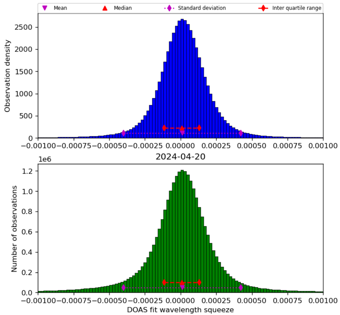
Figure 69: Histogram of “DOAS fit wavelength squeeze” for 2024-04-19 to 2024-04-21
