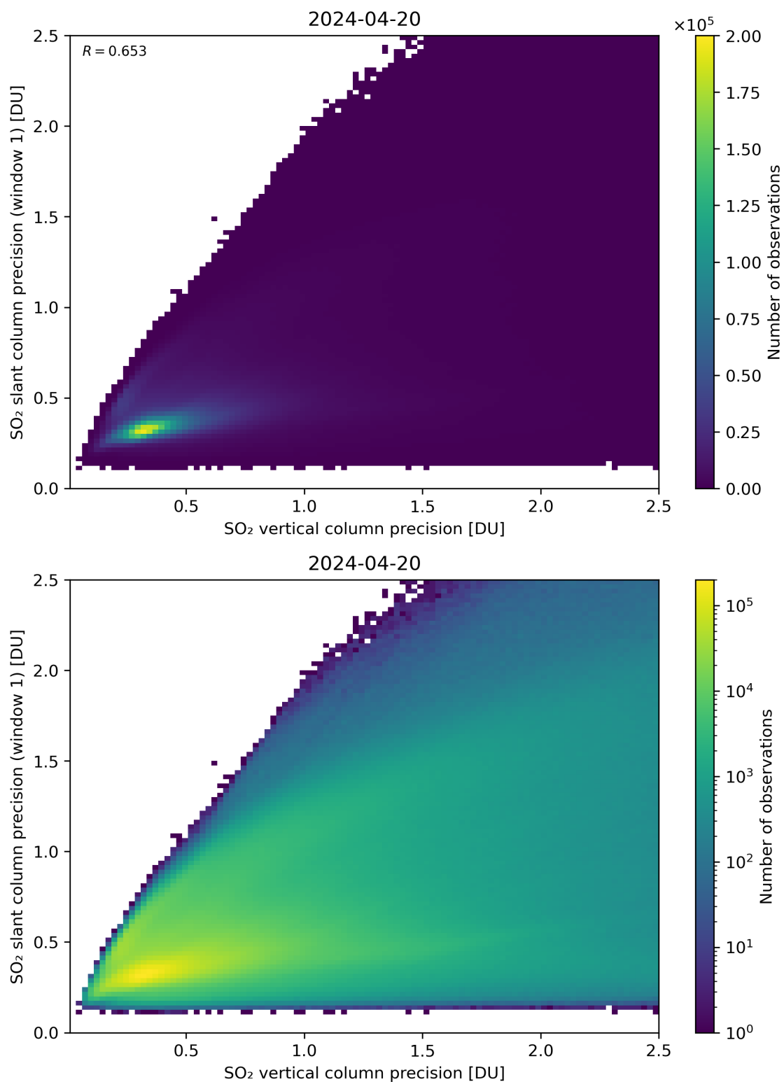
Figure 290: Scatter density plot of “SO 2 vertical column precision” against “SO 2 slant column precision (window 1)” for 2024-04-19 to 2024-04-21.
