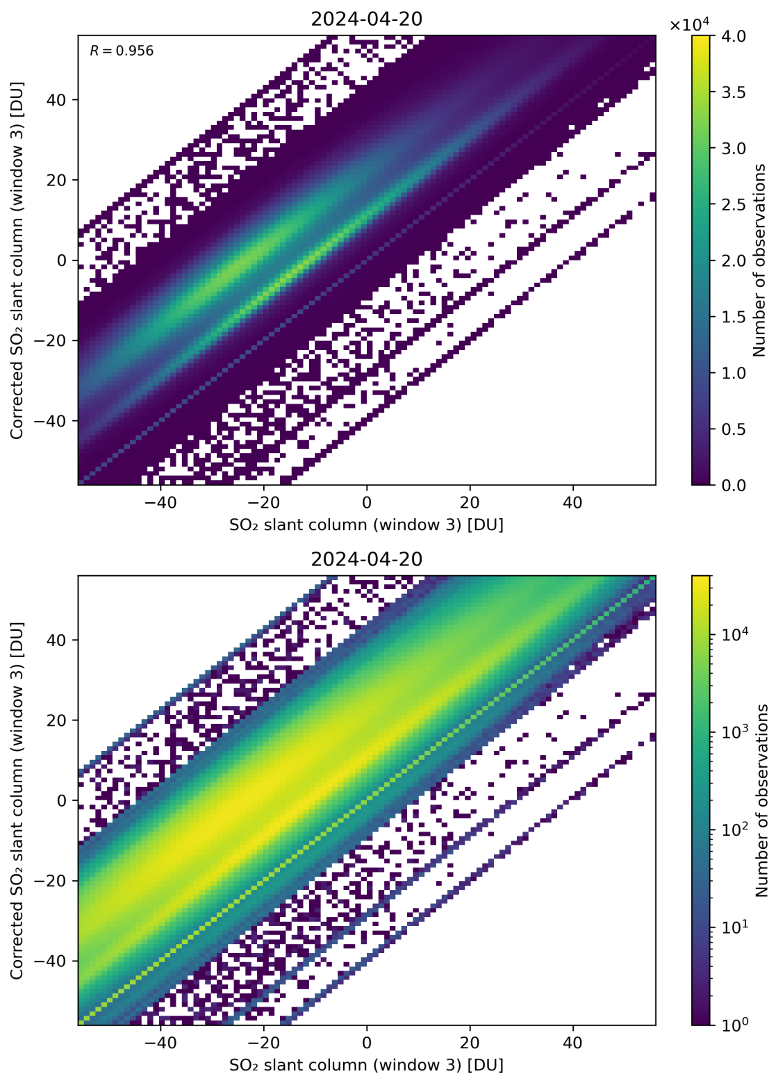
Figure 266: Scatter density plot of “SO 2 slant column (window 3)” against “Corrected SO 2 slant column (window 3)” for 2024-04-19 to 2024-04-21.
