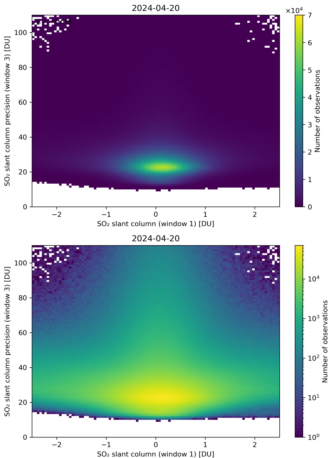
Figure 238: Scatter density plot of “SO 2 slant column (window 1)” against “SO 2 slant column precision (window 3)” for 2024-04-19 to 2024-04-21.
