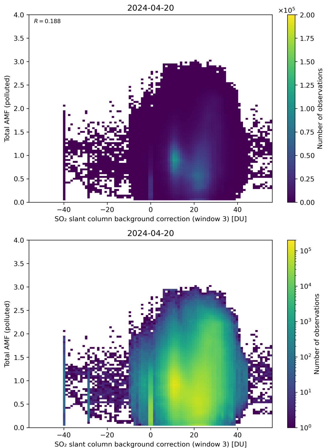
Figure 125: Scatter density plot of “SO 2 slant column background correction (window 3)” against “Total AMF (polluted)” for 2024-04-19 to 2024-04-21.
