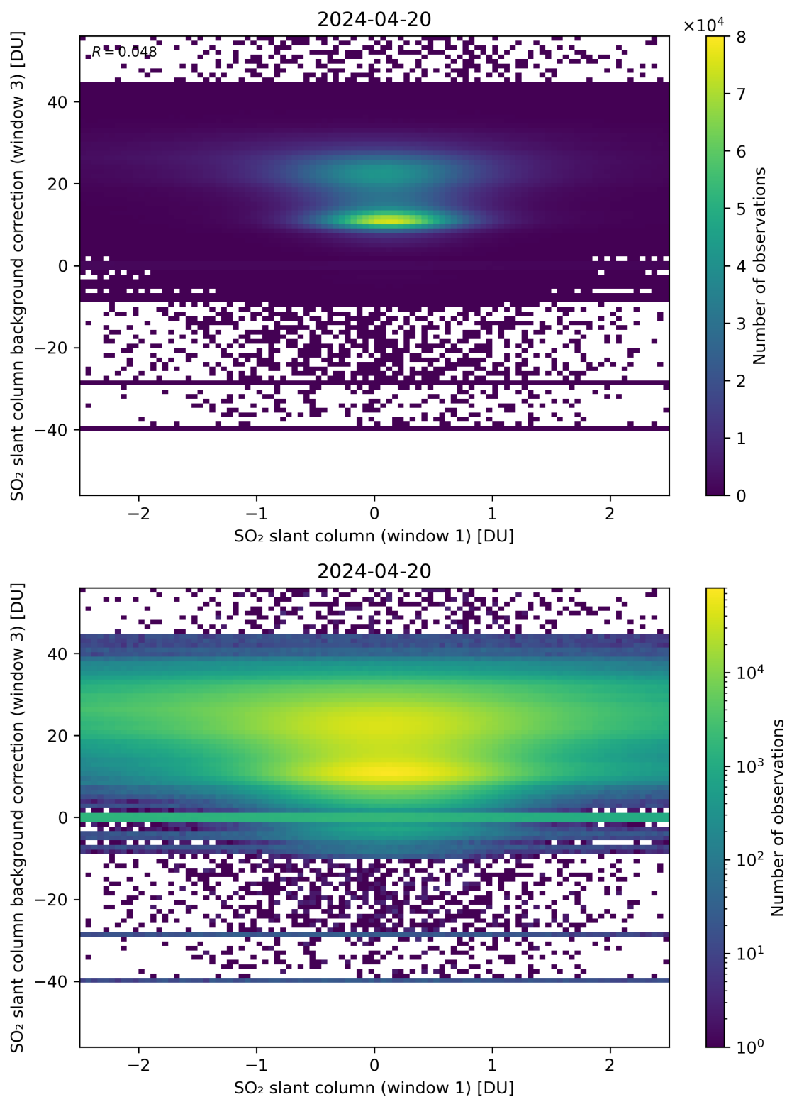
Figure 214: Scatter density plot of “SO 2 slant column (window 1)” against “SO 2 slant column background correction (window 3)” for 2024-04-19 to 2024-04-21.
