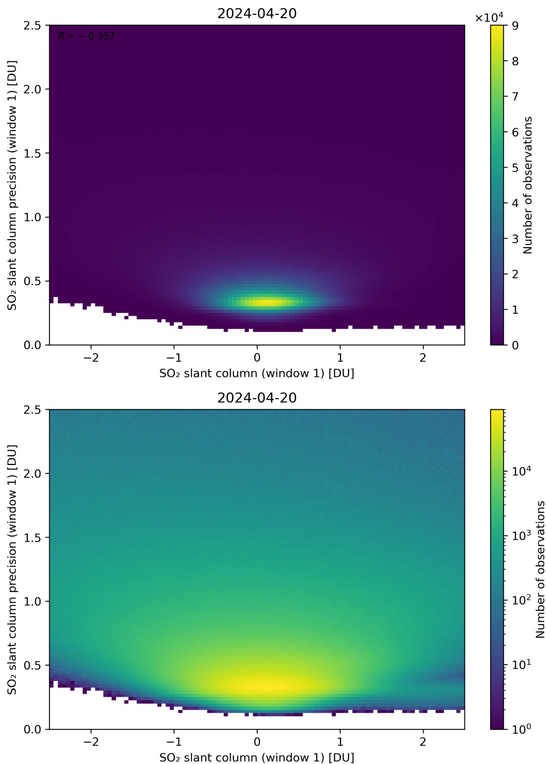
Figure 235: Scatter density plot of “SO 2 slant column (window 1)” against “SO 2 slant column precision (window 1)” for 2024-04-19 to 2024-04-21.
