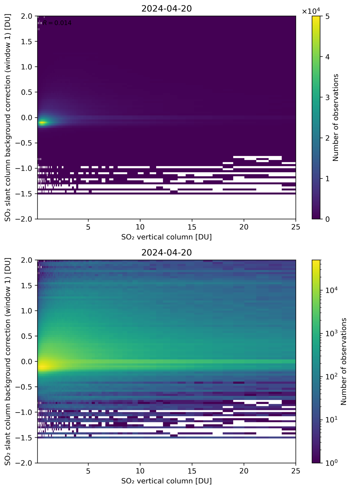
Figure 273: Scatter density plot of “SO 2 vertical column” against “SO 2 slant column background correction (window 1)” for 2024-04-19 to 2024-04-21.
