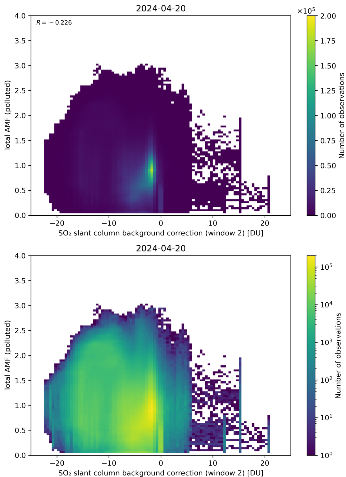
Figure 119: Scatter density plot of “SO 2 slant column background correction (window 2)” against “Total AMF (polluted)” for 2024-04-19 to 2024-04-21.
