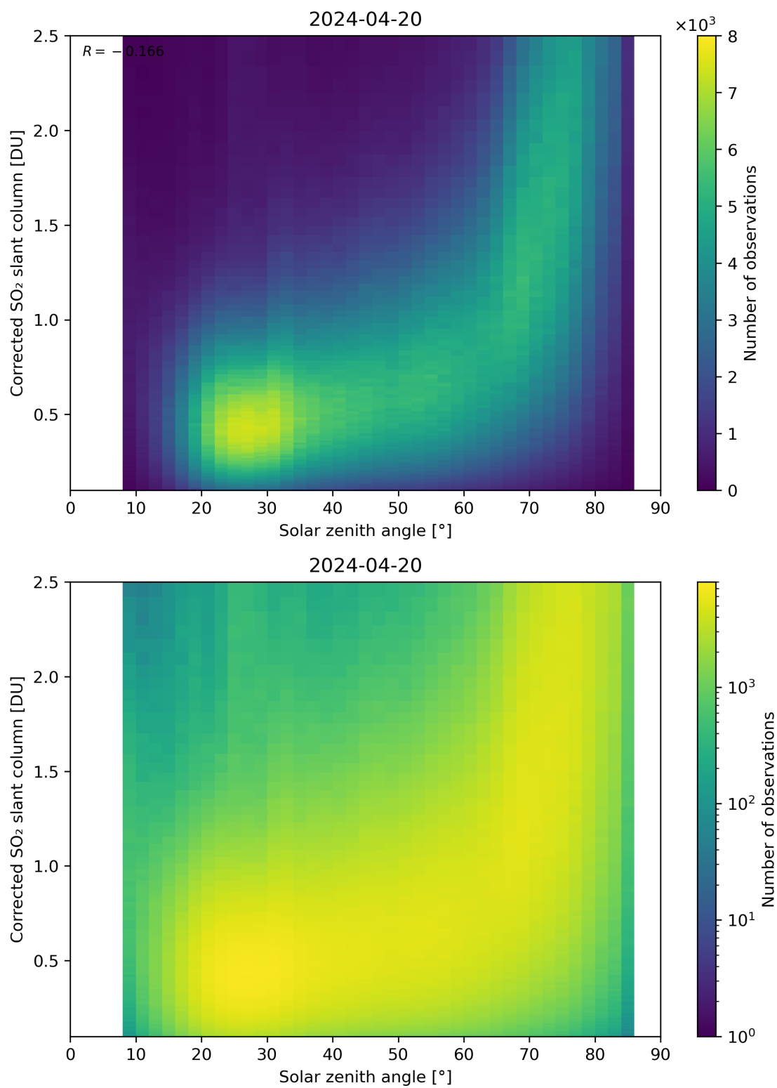
Figure 166: Scatter density plot of “Solar zenith angle” against “Corrected SO 2 slant column” for 2024-04-19 to 2024-04-21.
