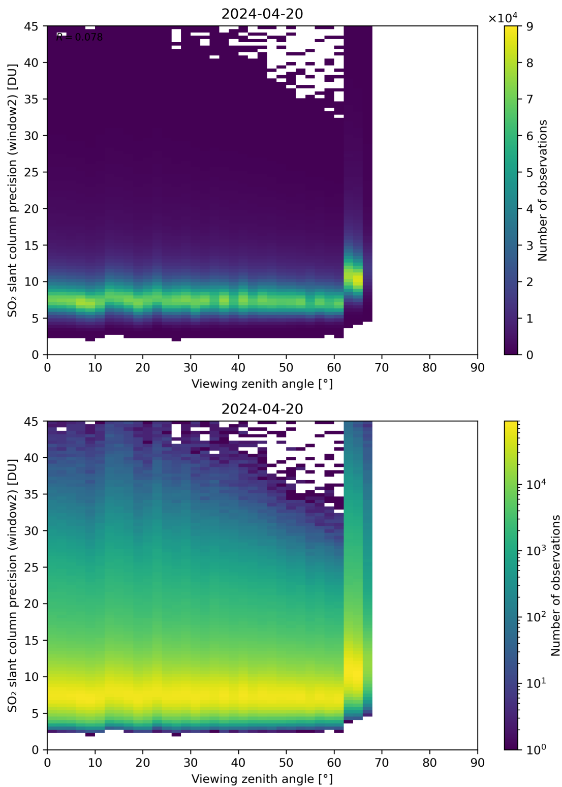
Figure 322: Scatter density plot of “Viewing zenith angle” against “SO 2 slant column precision (window2)” for 2024-04-19 to 2024-04-21.
