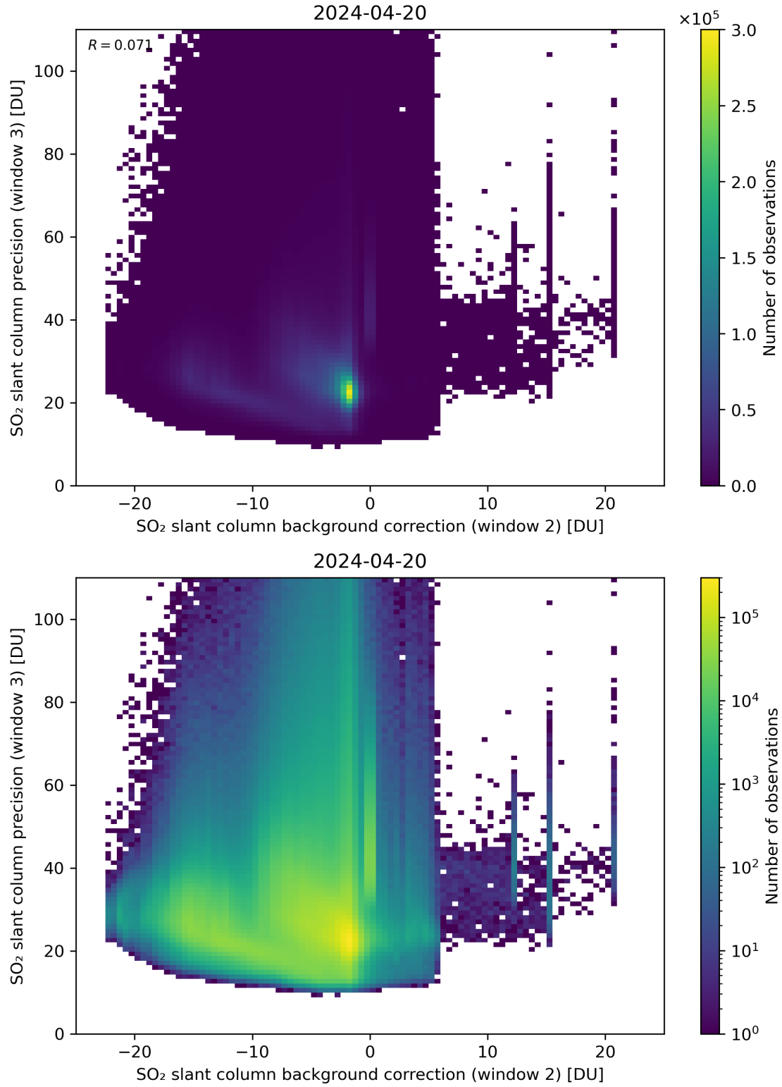
Figure 118: Scatter density plot of “SO 2 slant column background correction (window 2)” against “SO 2 slant column precision (window 3)” for 2024-04-19 to 2024-04-21.
