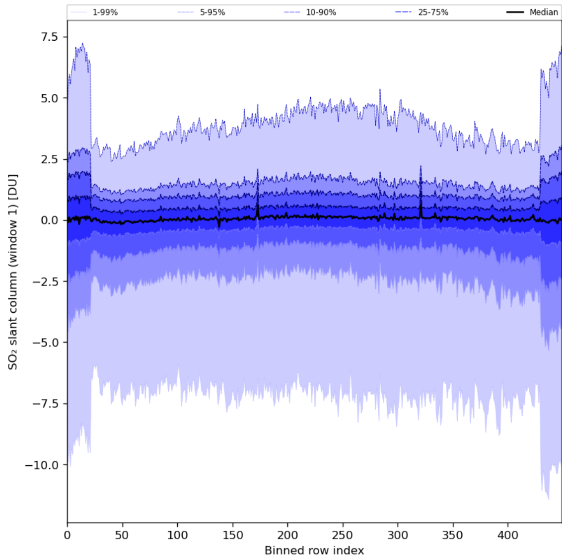
Figure 79: Along track statistics of “SO 2 slant column (window 1)” for 2024-04-19 to 2024-04-21
