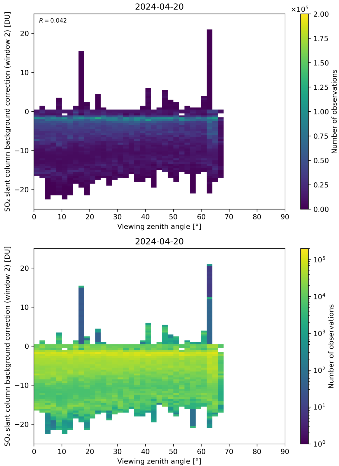
Figure 309: Scatter density plot of “Viewing zenith angle” against “SO 2 slant column background correction (window 2)” for 2024-04-19 to 2024-04-21.
