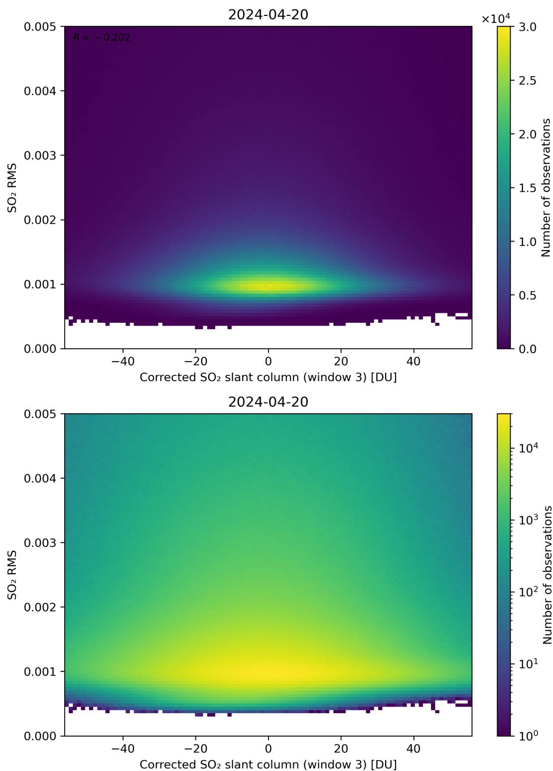
Figure 208: Scatter density plot of “Corrected SO 2 slant column (window 3)” against “SO 2 RMS” for 2024-04-19 to 2024-04-21.
