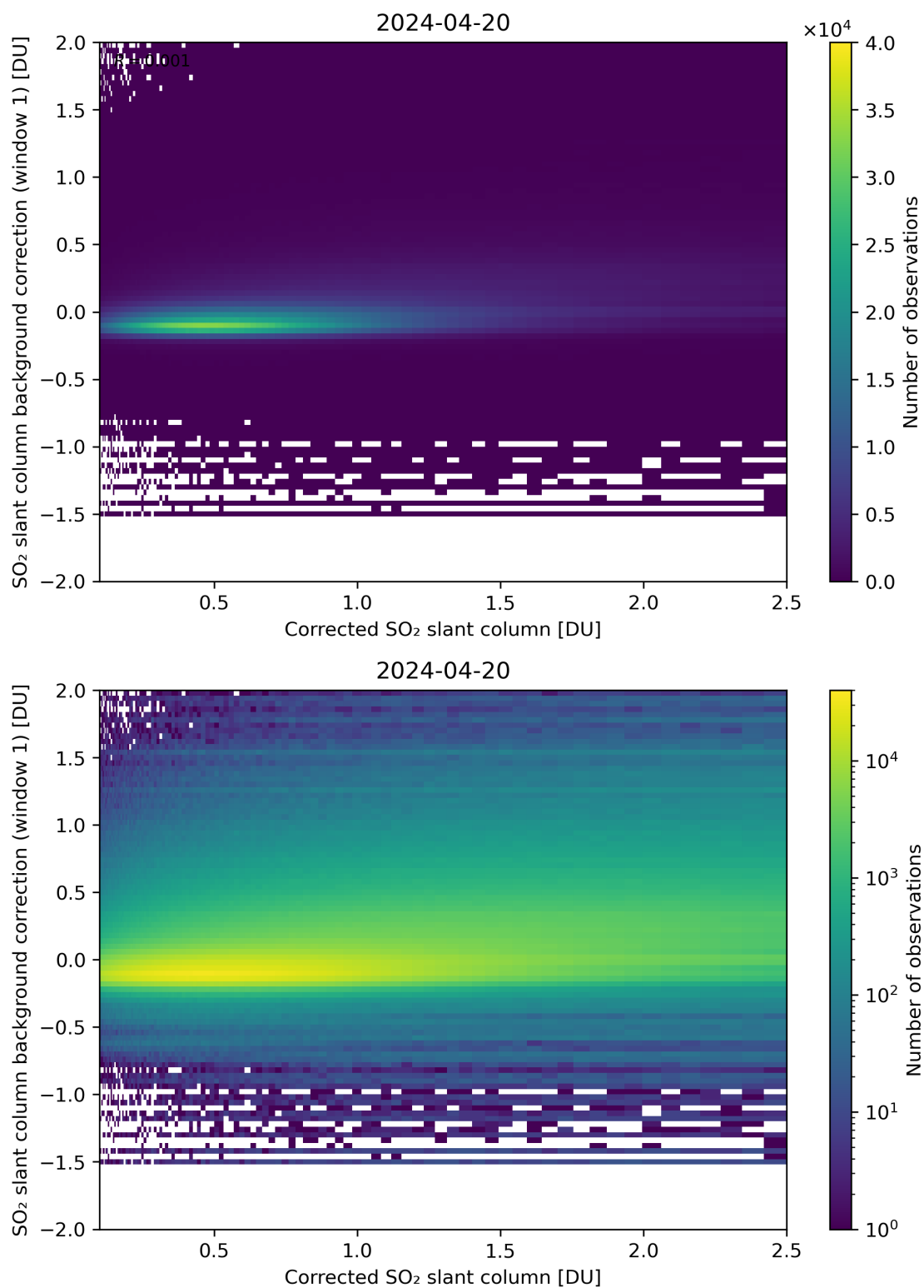
Figure 178: Scatter density plot of “Corrected SO 2 slant column” against “SO 2 slant column background correction (window 1)” for 2024-04-19 to 2024-04-21.
