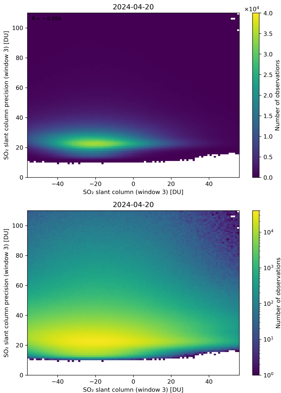
Figure 267: Scatter density plot of “SO 2 slant column (window 3)” against “SO 2 slant column precision (window 3)” for 2024-04-19 to 2024-04-21.
