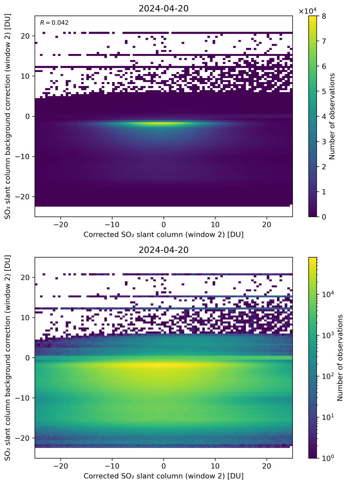
Figure 194: Scatter density plot of “Corrected SO 2 slant column (window 2)” against “SO 2 slant column background correction (window 2)” for 2024-04-19 to 2024-04-21.
