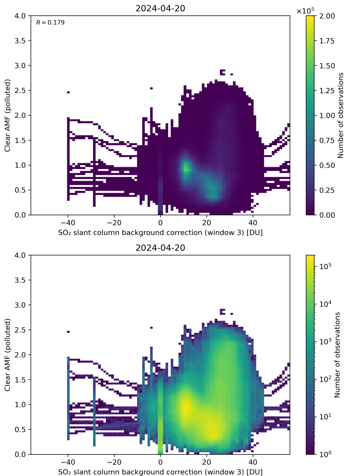
Figure 124: Scatter density plot of “SO 2 slant column background correction (window 3)” against “Clear AMF (polluted)” for 2024-04-19 to 2024-04-21.
