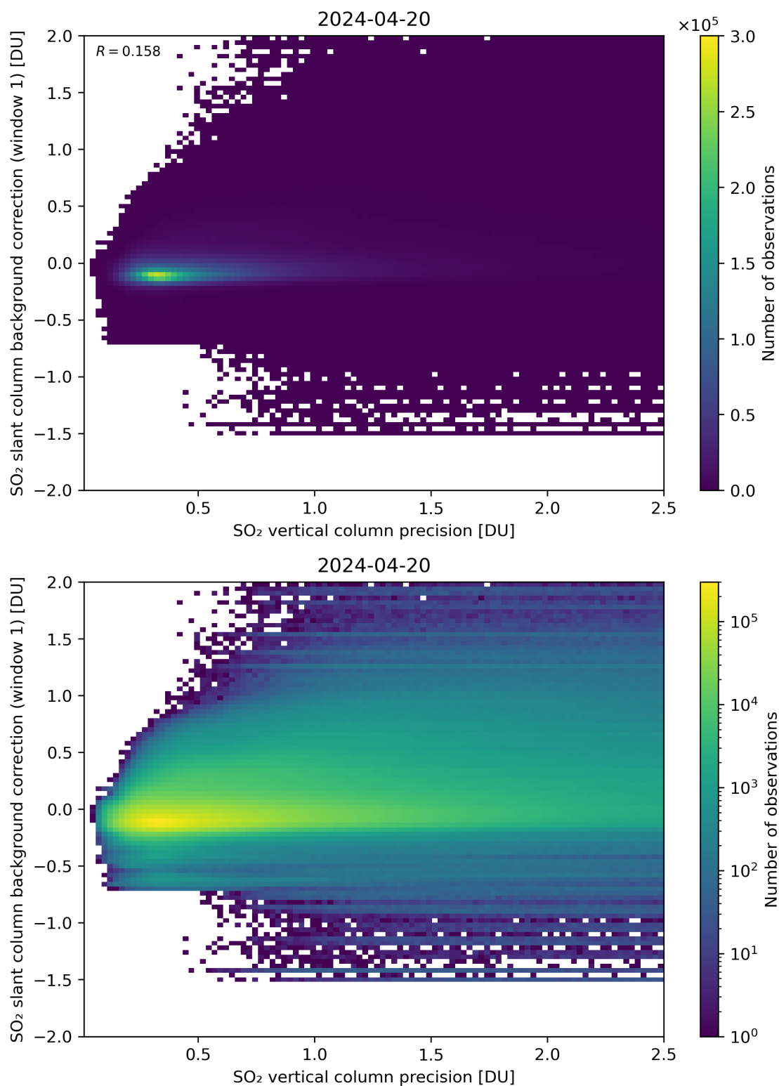
Figure 279: Scatter density plot of “SO 2 vertical column precision” against “SO 2 slant column background correction (window 1)” for 2024-04-19 to 2024-04-21.
