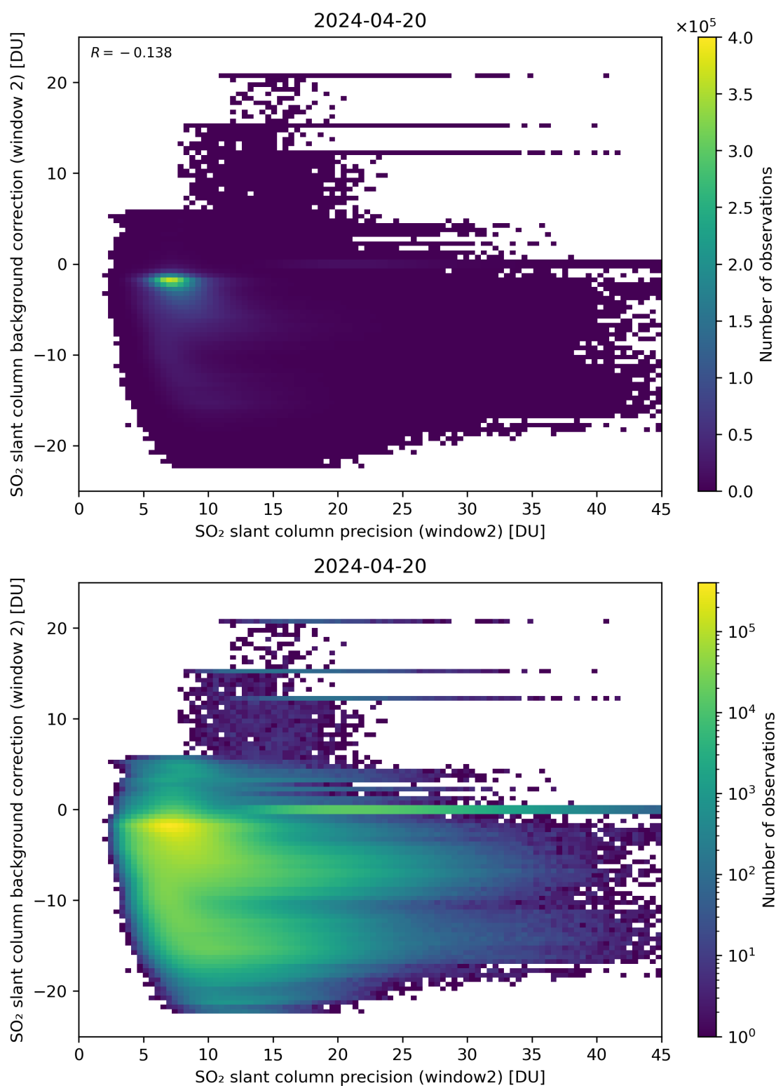
Figure 241: Scatter density plot of “SO 2 slant column precision (window2)” against “SO 2 slant column background correction (window 2)” for 2024-04-19 to 2024-04-21.
