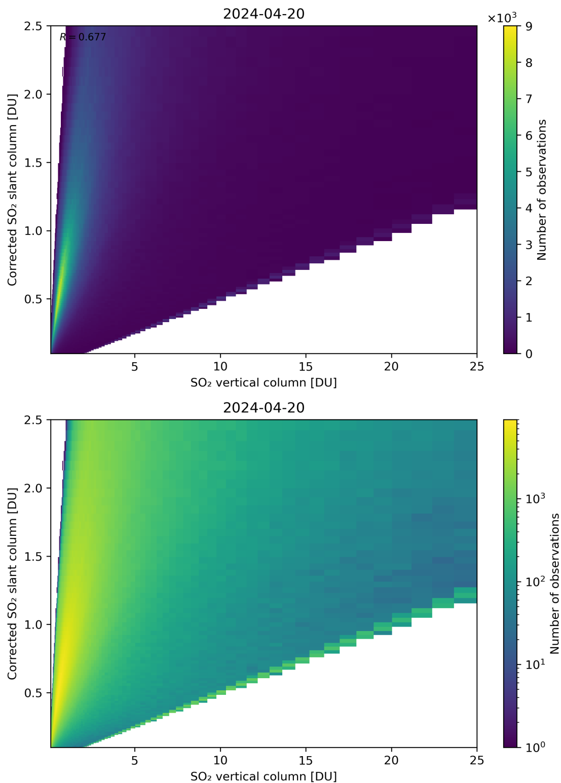
Figure 297: Scatter density plot of “SO 2 vertical column” against “Corrected SO 2 slant column” for 2024-04-19 to 2024-04-21.
