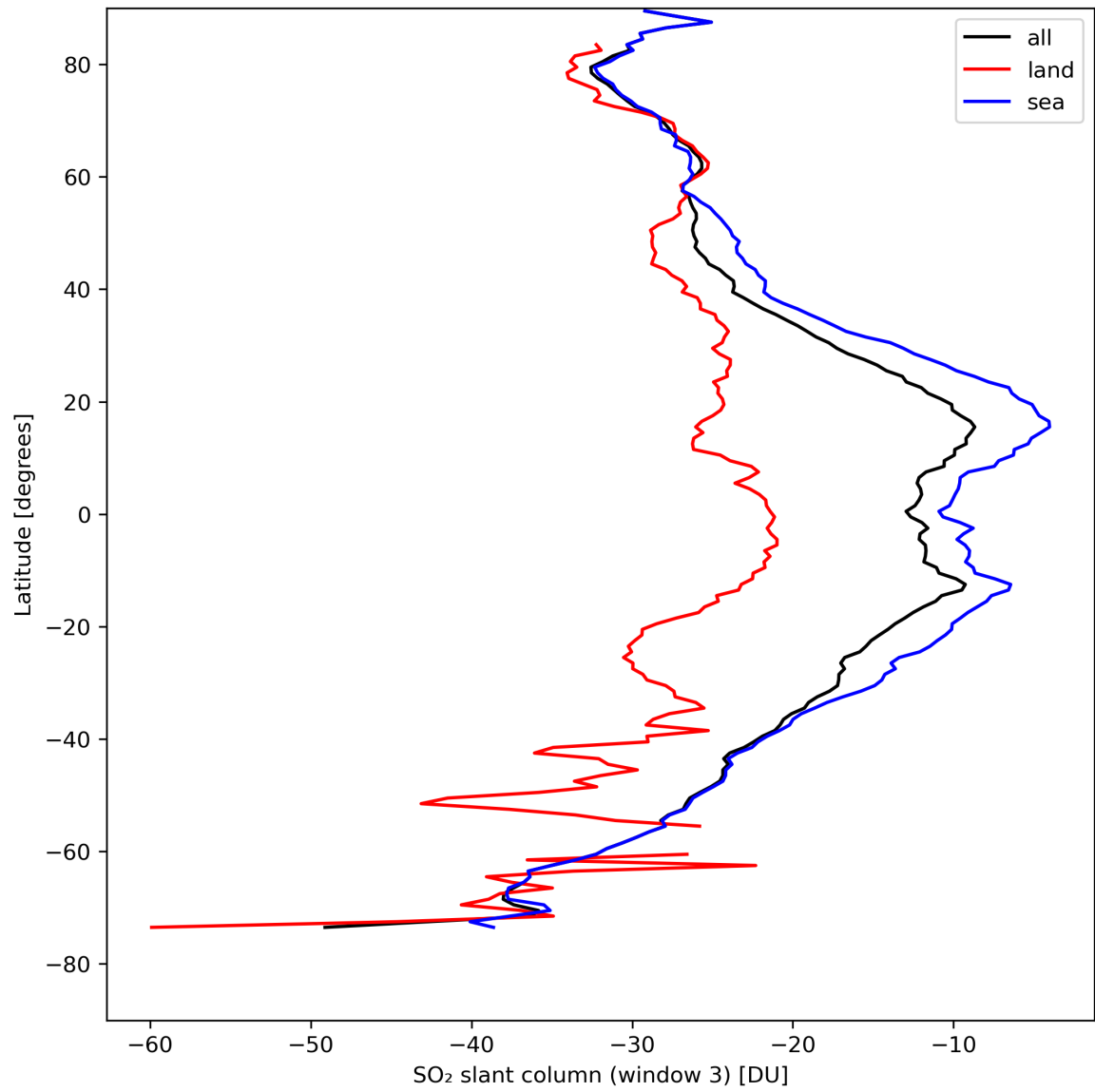
Figure 41: Zonal average of “SO 2 slant column (window 3)” for 2024-04-19 to 2024-04-21.
