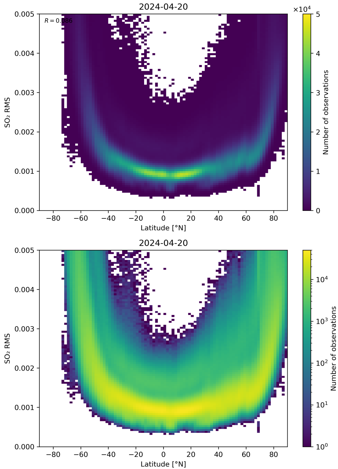
Figure 144: Scatter density plot of “Latitude” against “SO 2 RMS” for 2024-04-19 to 2024-04-21.
