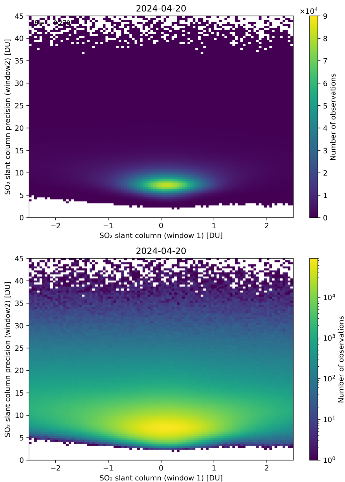
Figure 236: Scatter density plot of “SO 2 slant column (window 1)” against “SO 2 slant column precision (window2)” for 2024-04-19 to 2024-04-21.
