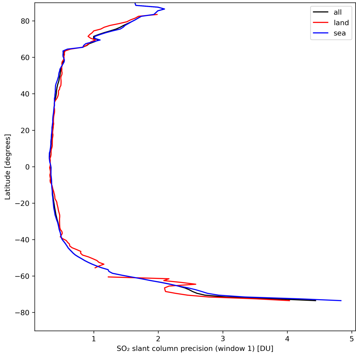
Figure 34: Zonal average of “SO 2 slant column precision (window 1)” for 2024-04-19 to 2024-04-21.
