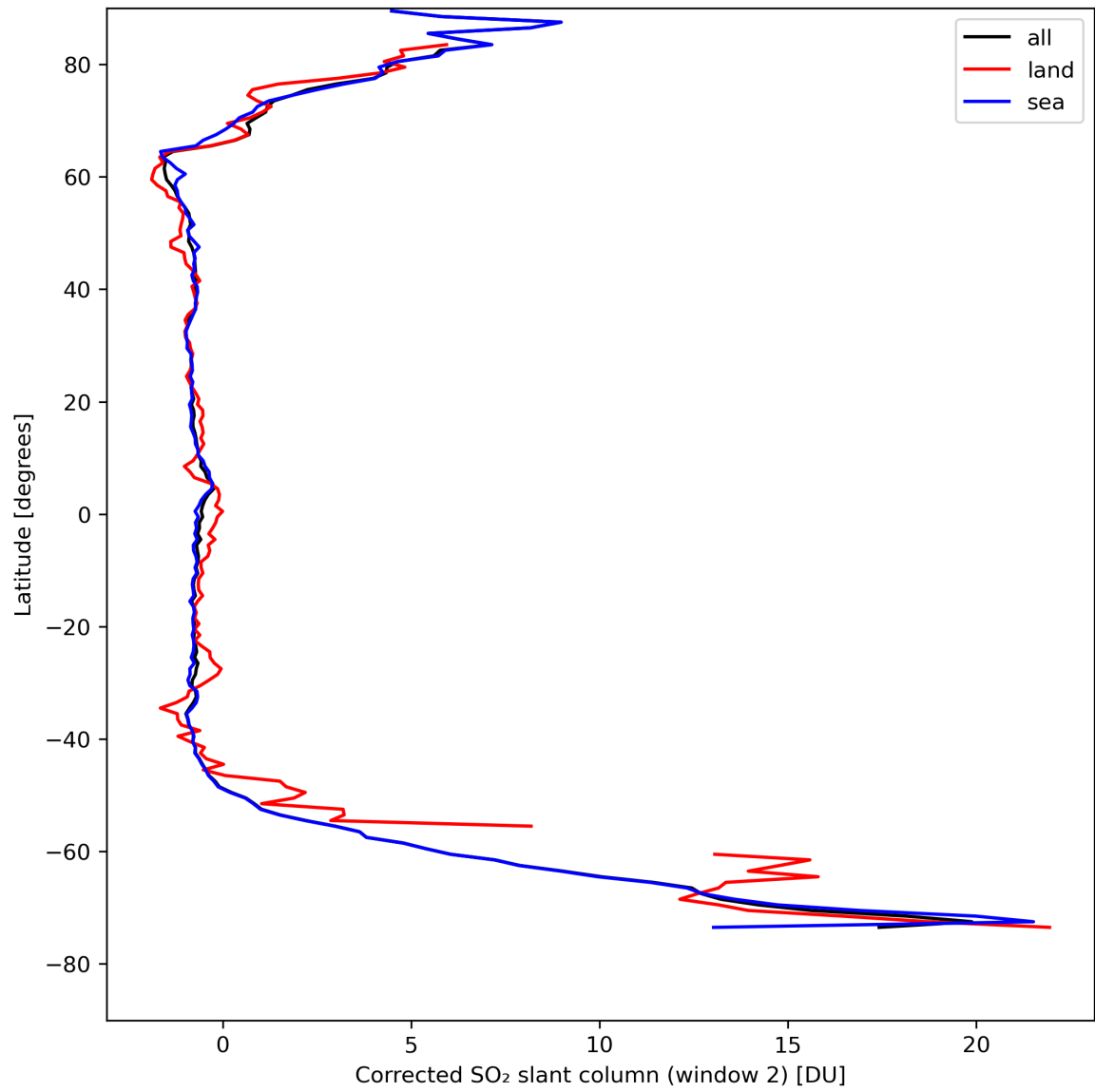
Figure 39: Zonal average of “Corrected SO 2 slant column (window 2)” for 2024-04-19 to 2024-04-21.
