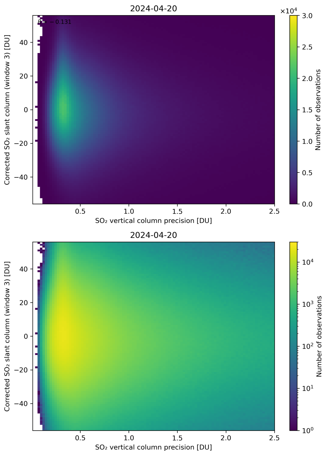
Figure 288: Scatter density plot of “SO 2 vertical column precision” against “Corrected SO 2 slant column (window 3)” for 2024-04-19 to 2024-04-21.
