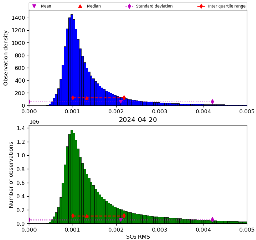
Figure 70: Histogram of “SO 2 RMS” for 2024-04-19 to 2024-04-21
