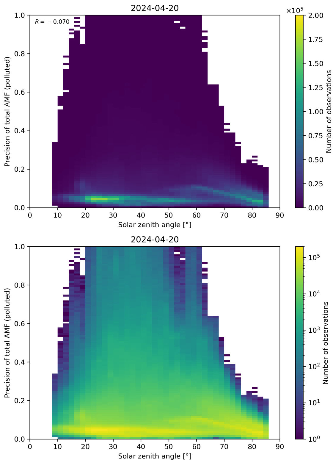
Figure 175: Scatter density plot of “Solar zenith angle” against “Precision of total AMF (polluted)” for 2024-04-19 to 2024-04-21.
