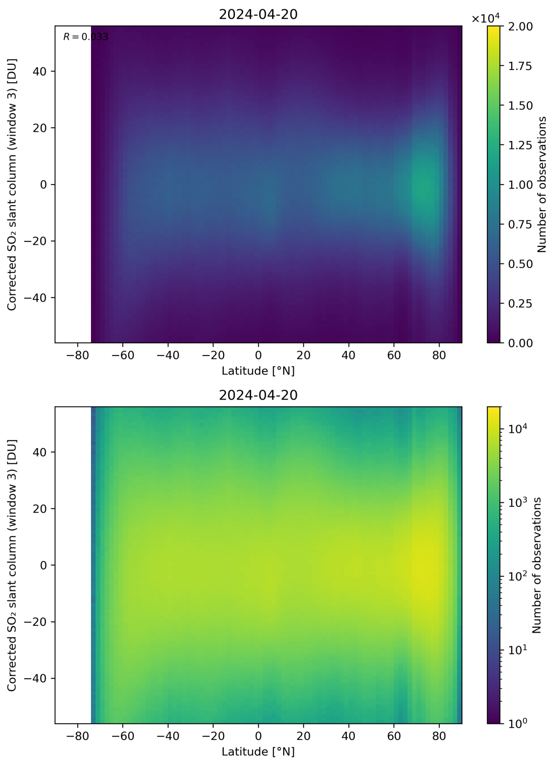
Figure 148: Scatter density plot of “Latitude” against “Corrected SO 2 slant column (window 3)” for 2024-04-19 to 2024-04-21.
