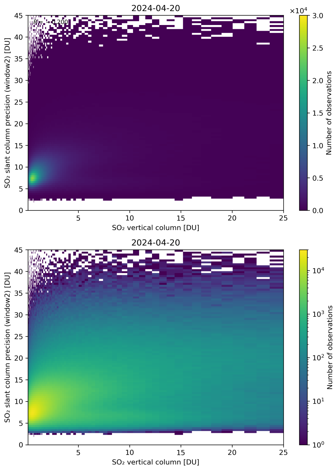
Figure 302: Scatter density plot of “SO 2 vertical column” against “SO 2 slant column precision (window2)” for 2024-04-19 to 2024-04-21.
