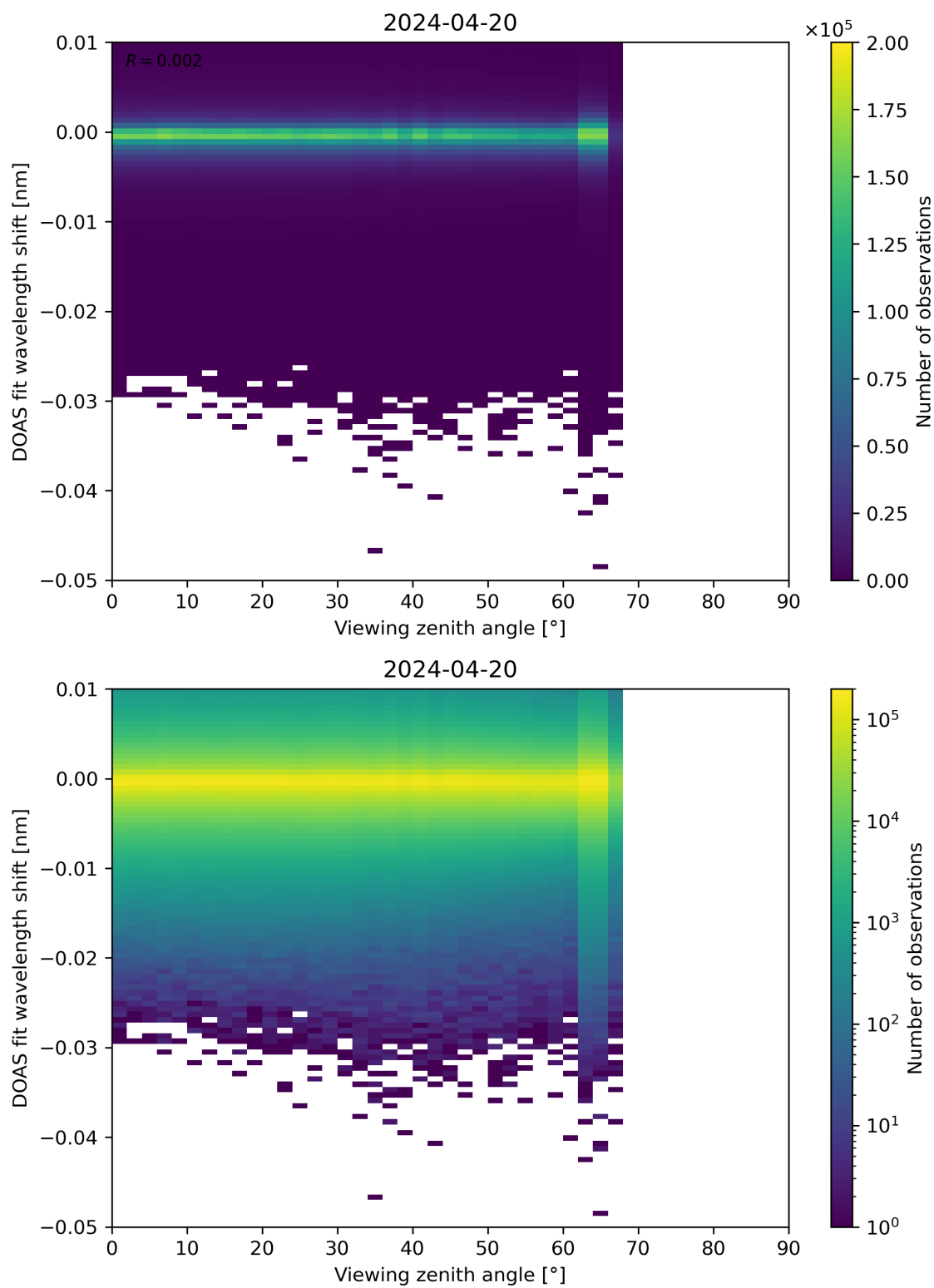
Figure 311: Scatter density plot of “Viewing zenith angle” against “DOAS fit wavelength shift” for 2024-04-19 to 2024-04-21.
