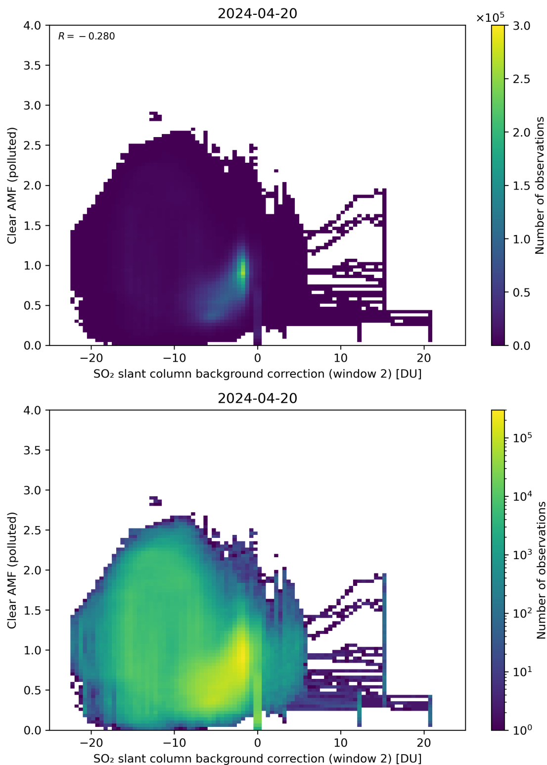
Figure 115: Scatter density plot of “SO 2 slant column background correction (window 2)” against “Clear AMF (polluted)” for 2024-04-19 to 2024-04-21.
