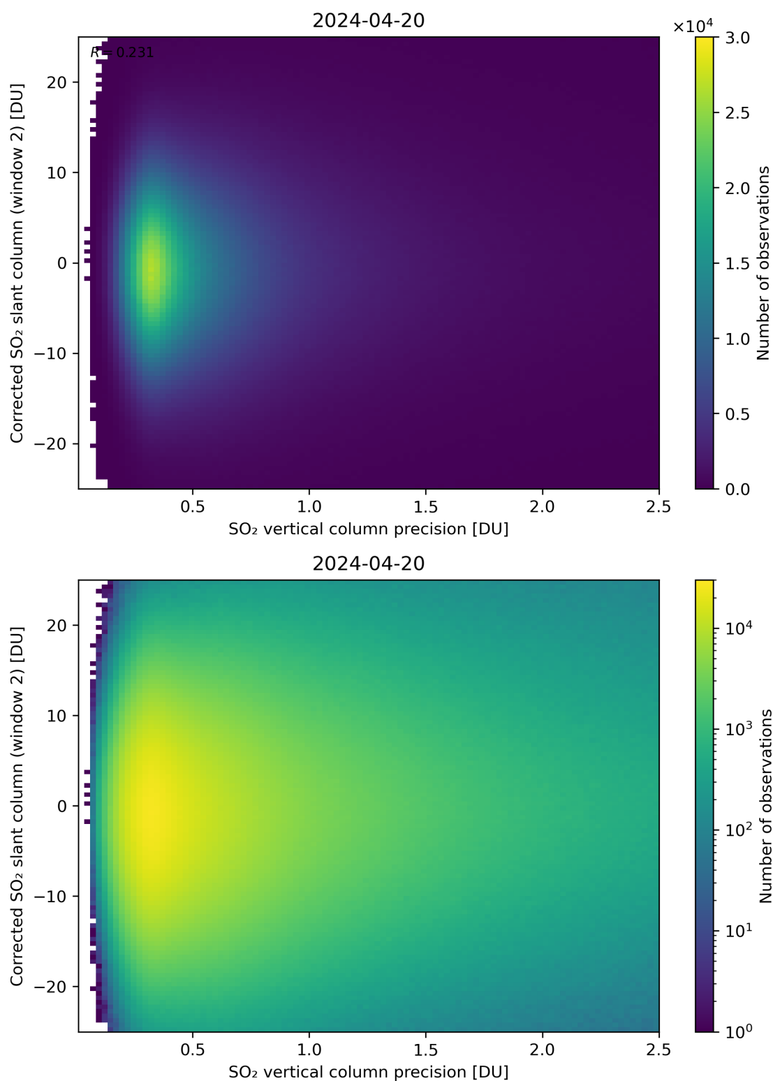
Figure 287: Scatter density plot of “SO 2 vertical column precision” against “Corrected SO 2 slant column (window 2)” for 2024-04-19 to 2024-04-21.
