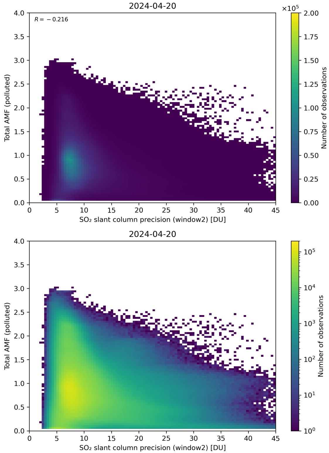
Figure 251: Scatter density plot of “SO 2 slant column precision (window2)” against “Total AMF (polluted)” for 2024-04-19 to 2024-04-21.
