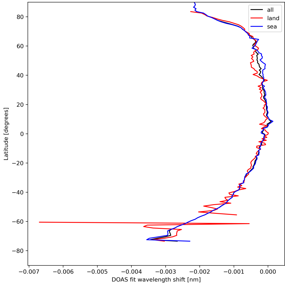
Figure 45: Zonal average of “DOAS fit wavelength shift” for 2024-04-19 to 2024-04-21.
