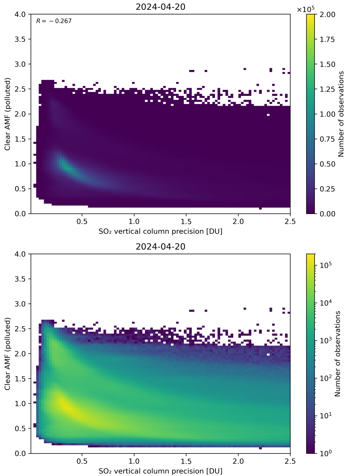
Figure 285: Scatter density plot of “SO 2 vertical column precision” against “Clear AMF (polluted)” for 2024-04-19 to 2024-04-21.
