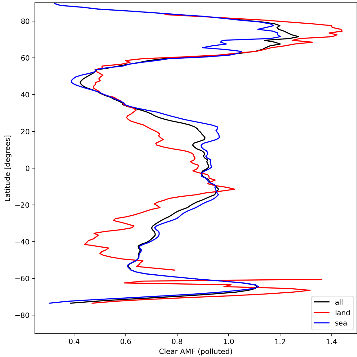
Figure 50: Zonal average of “Clear AMF (polluted)” for 2024-04-19 to 2024-04-21.
