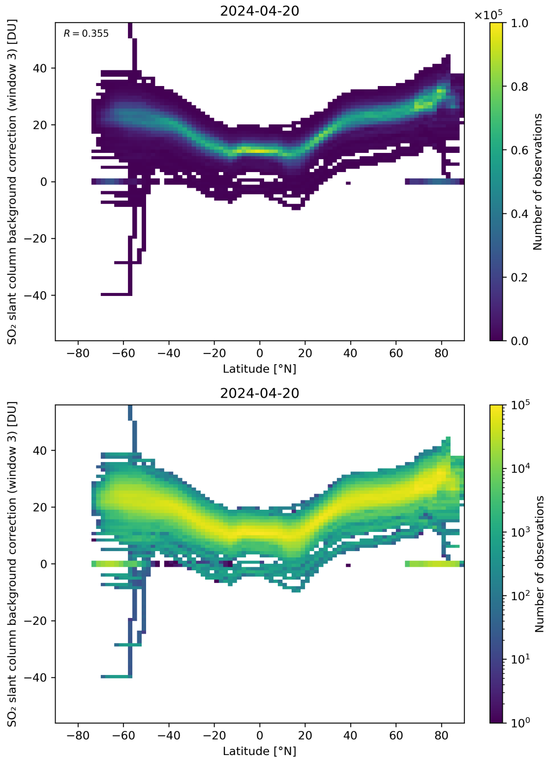
Figure 141: Scatter density plot of “Latitude” against “SO 2 slant column background correction (window 3)” for 2024-04-19 to 2024-04-21.
