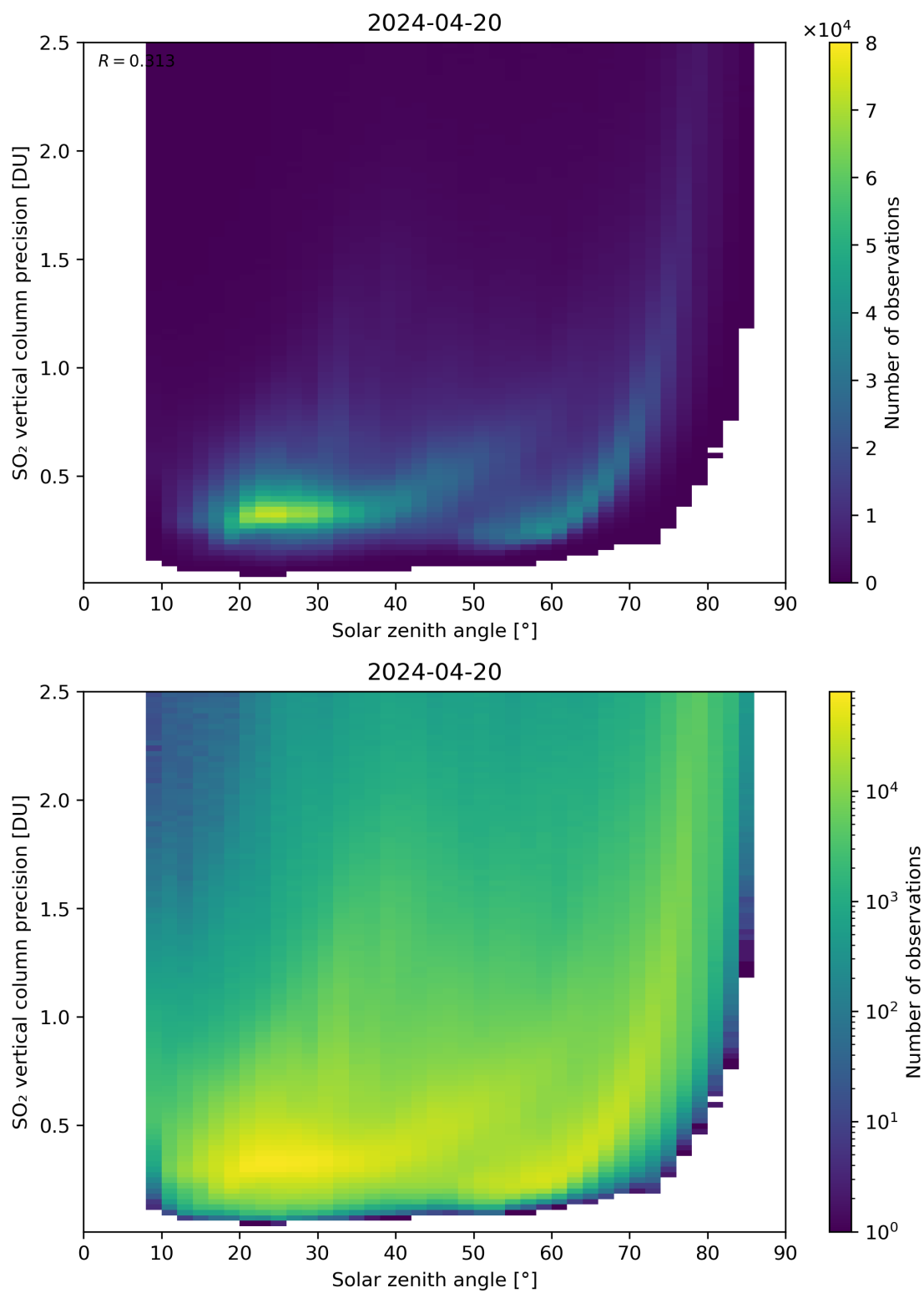
Figure 177: Scatter density plot of “Solar zenith angle” against “SO 2 vertical column precision” for 2024-04-19 to 2024-04-21.
