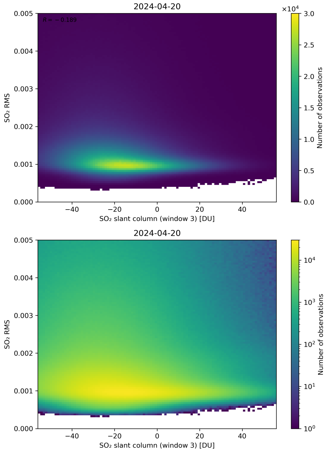
Figure 256: Scatter density plot of “SO 2 slant column (window 3)” against “SO 2 RMS” for 2024-04-19 to 2024-04-21.
