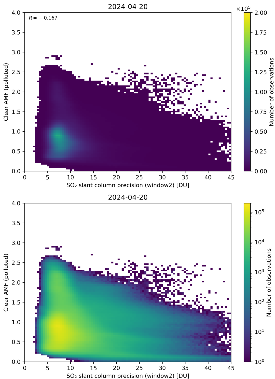
Figure 246: Scatter density plot of “SO 2 slant column precision (window2)” against “Clear AMF (polluted)” for 2024-04-19 to 2024-04-21.
