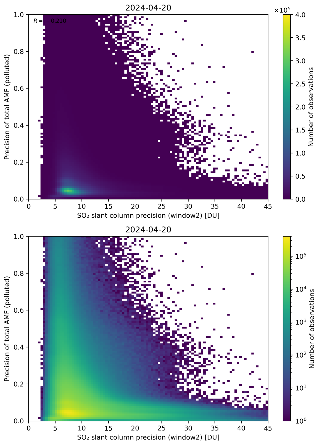
Figure 252: Scatter density plot of “SO 2 slant column precision (window2)” against “Precision of total AMF (polluted)” for 2024-04-19 to 2024-04-21.
