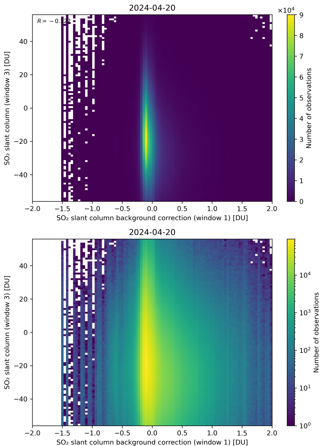
Figure 107: Scatter density plot of “SO 2 slant column background correction (window 1)” against “SO 2 slant column (window 3)” for 2024-04-19 to 2024-04-21.
