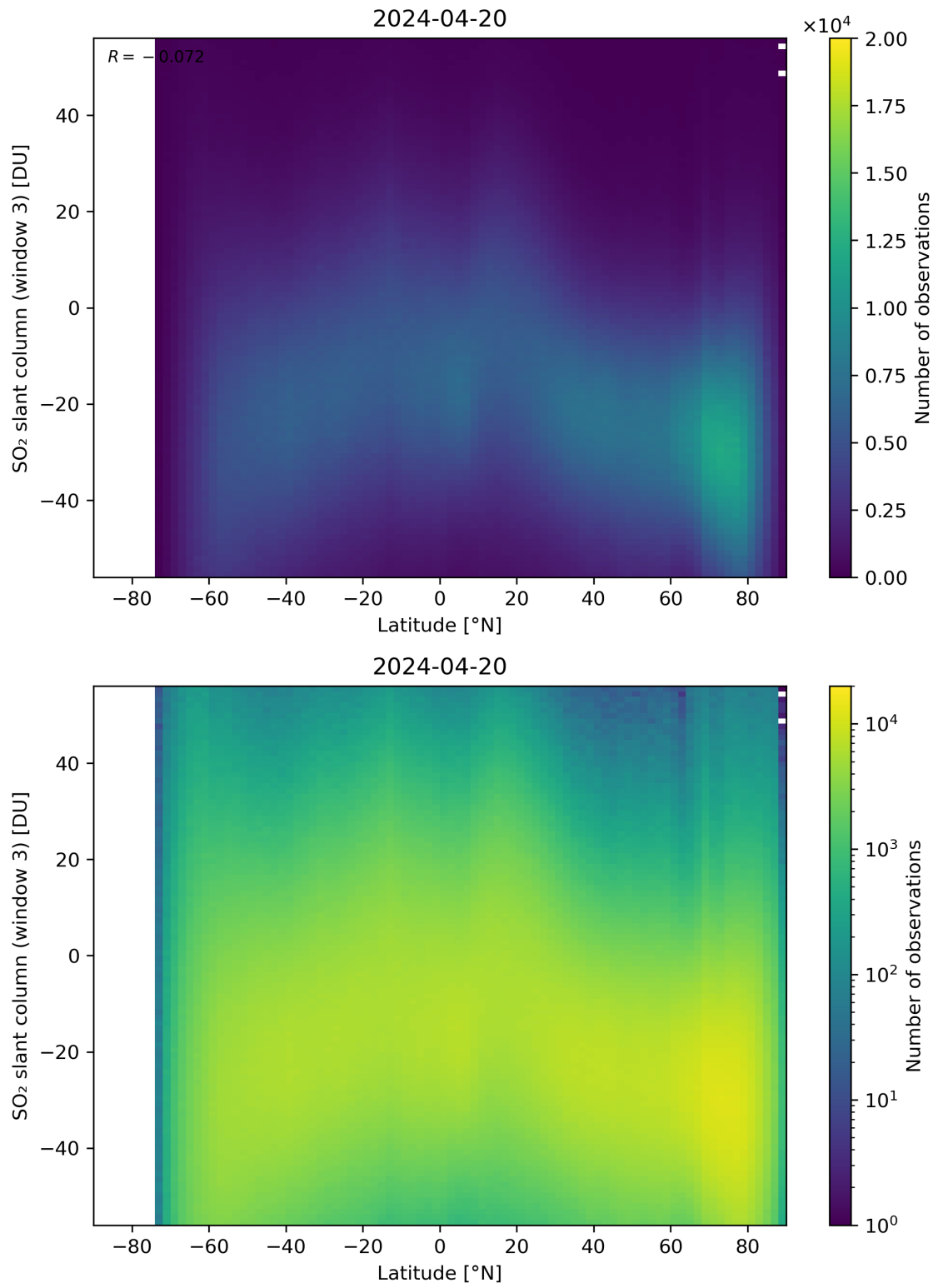
Figure 152: Scatter density plot of “Latitude” against “SO 2 slant column (window 3)” for 2024-04-19 to 2024-04-21.
