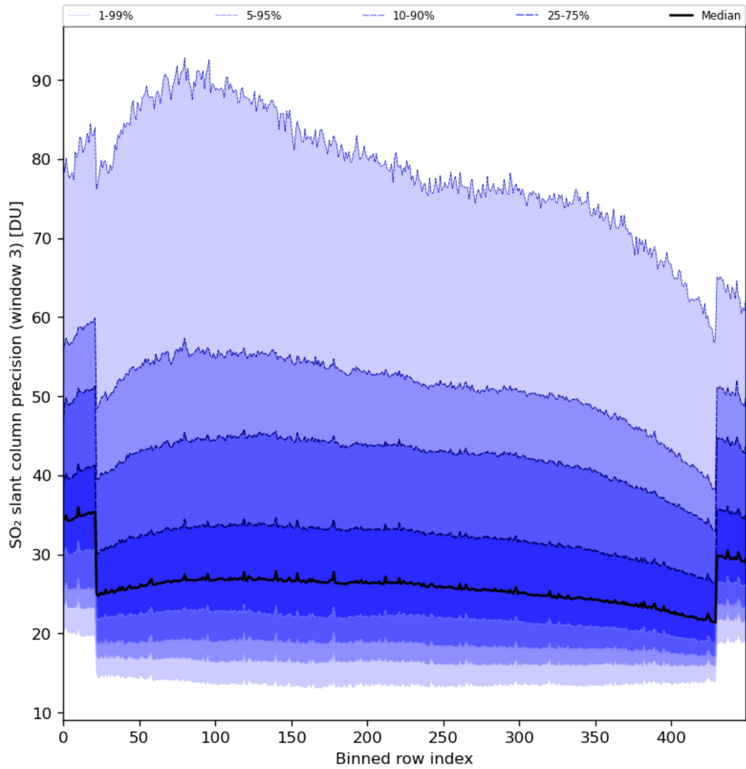
Figure 88: Along track statistics of “SO 2 slant column precision (window 3)” for 2024-04-19 to 2024-04-21
