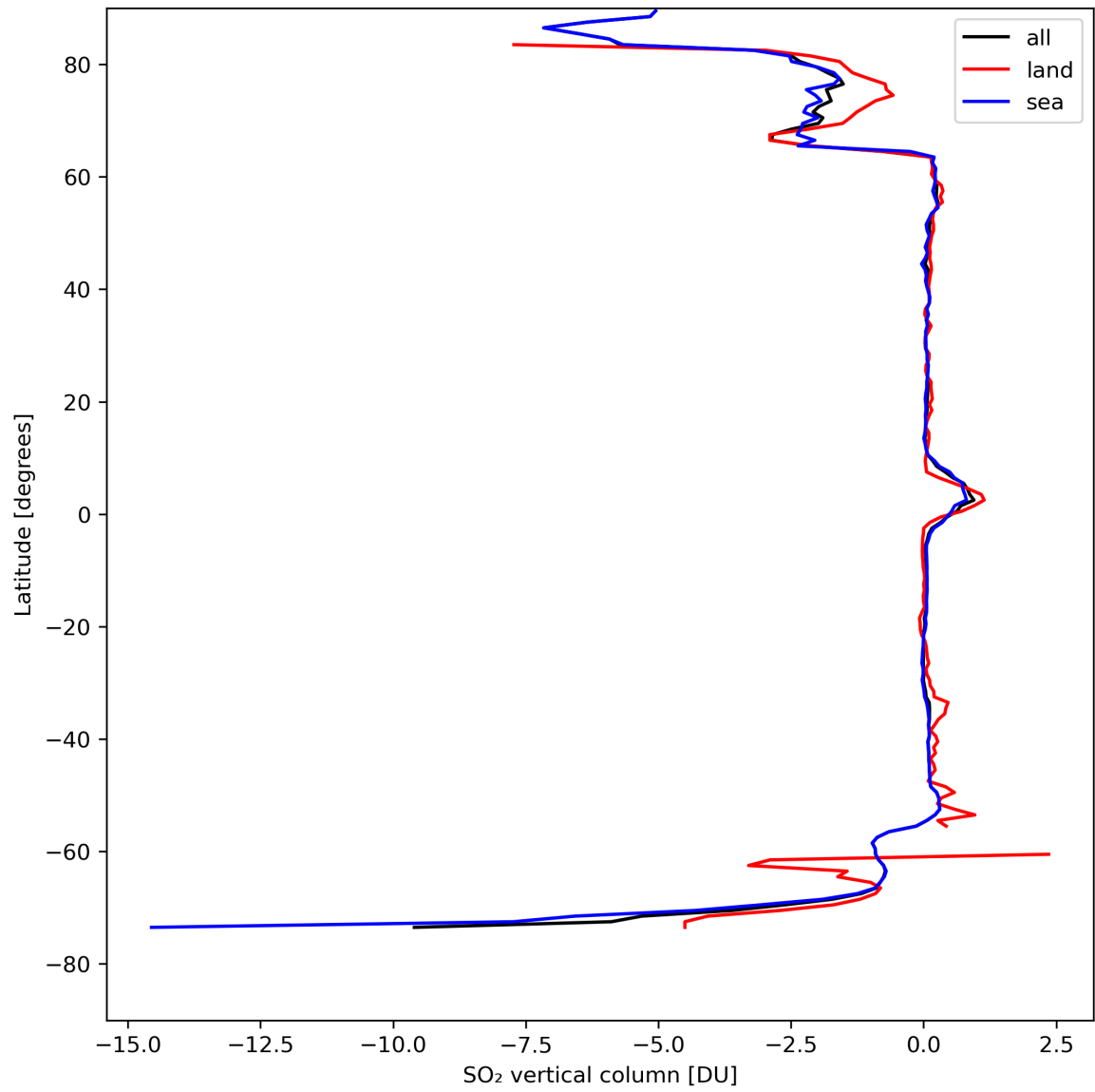
Figure 30: Zonal average of “SO 2 vertical column” for 2024-04-19 to 2024-04-21.
