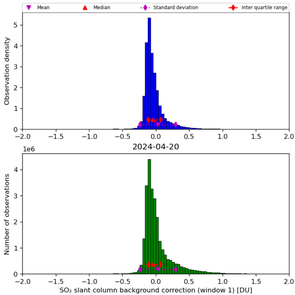
Figure 59: Histogram of “SO 2 slant column background correction (window 1)” for 2024-04-19 to 2024-04-21
