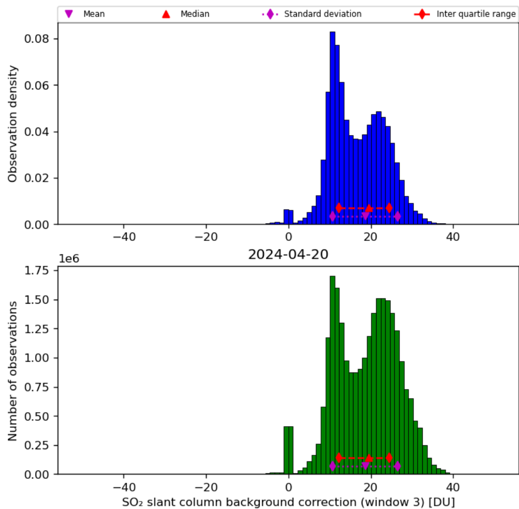
Figure 67: Histogram of “SO 2 slant column background correction (window 3)” for 2024-04-19 to 2024-04-21
