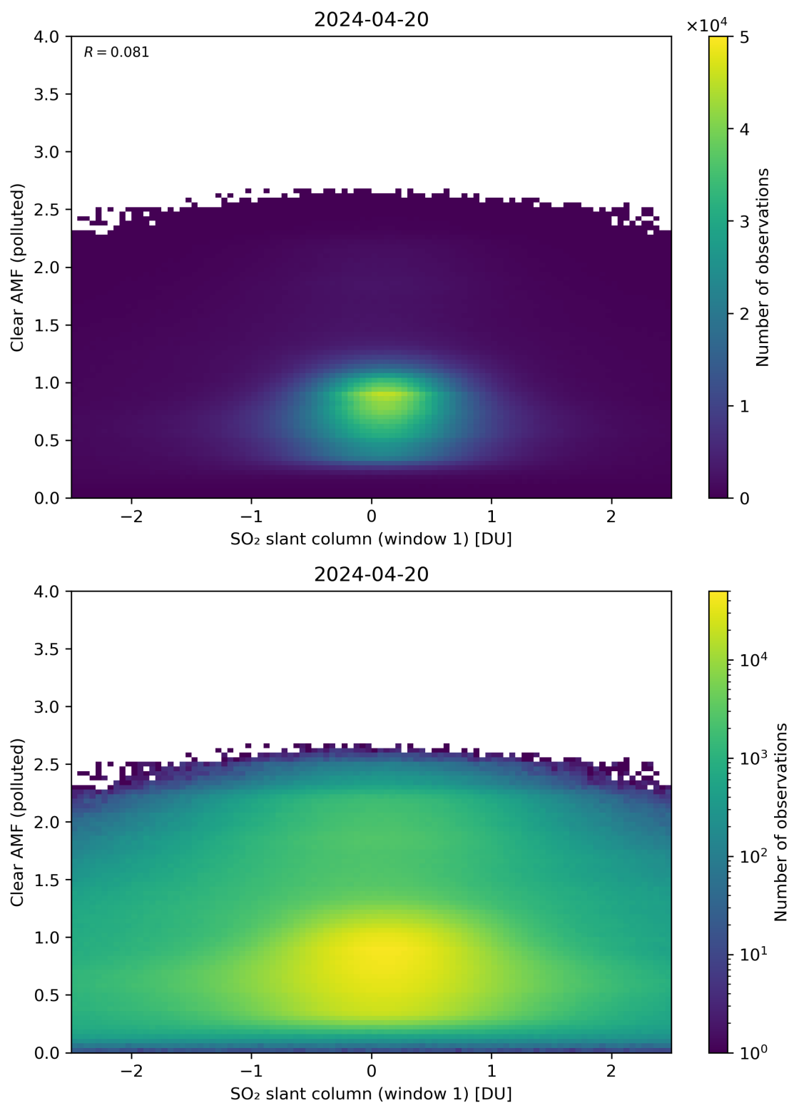
Figure 232: Scatter density plot of “SO 2 slant column (window 1)” against “Clear AMF (polluted)” for 2024-04-19 to 2024-04-21.
