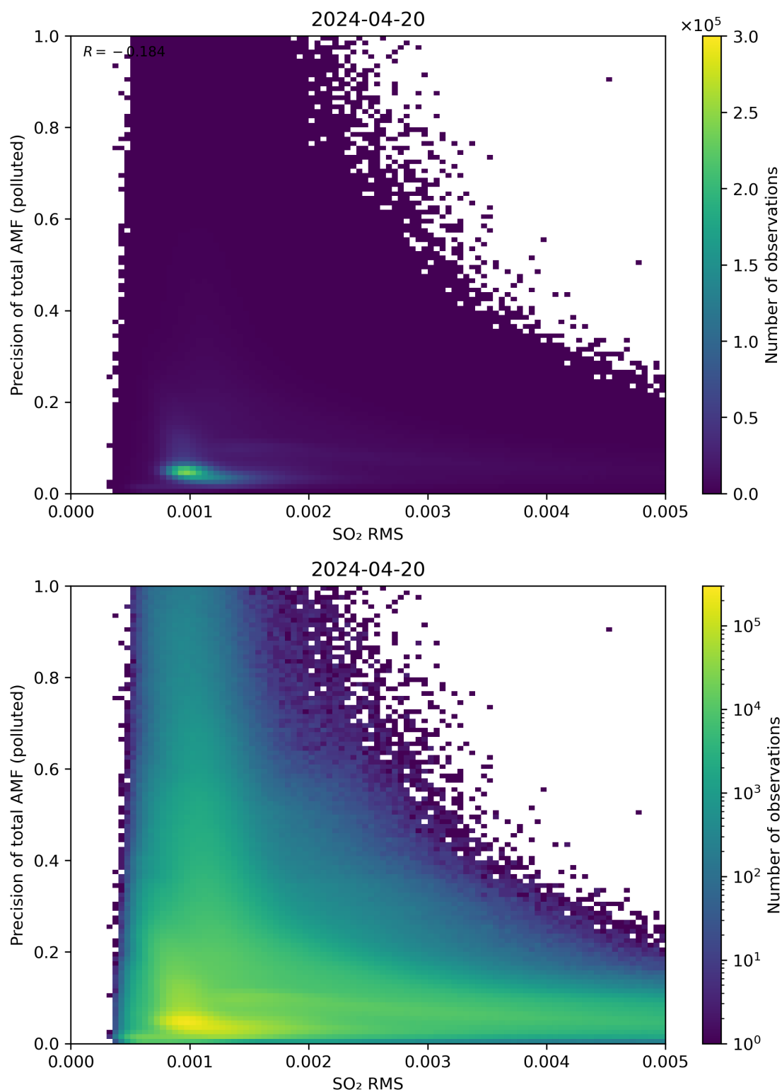
Figure 138: Scatter density plot of “SO 2 RMS” against “Precision of total AMF (polluted)” for 2024-04-19 to 2024-04-21.
