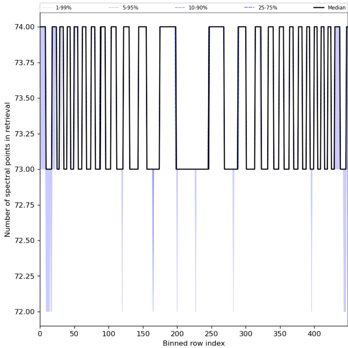
Figure 97: Along track statistics of “Number of spectral points in retrieval” for 2024-04-19 to 2024-04-21
