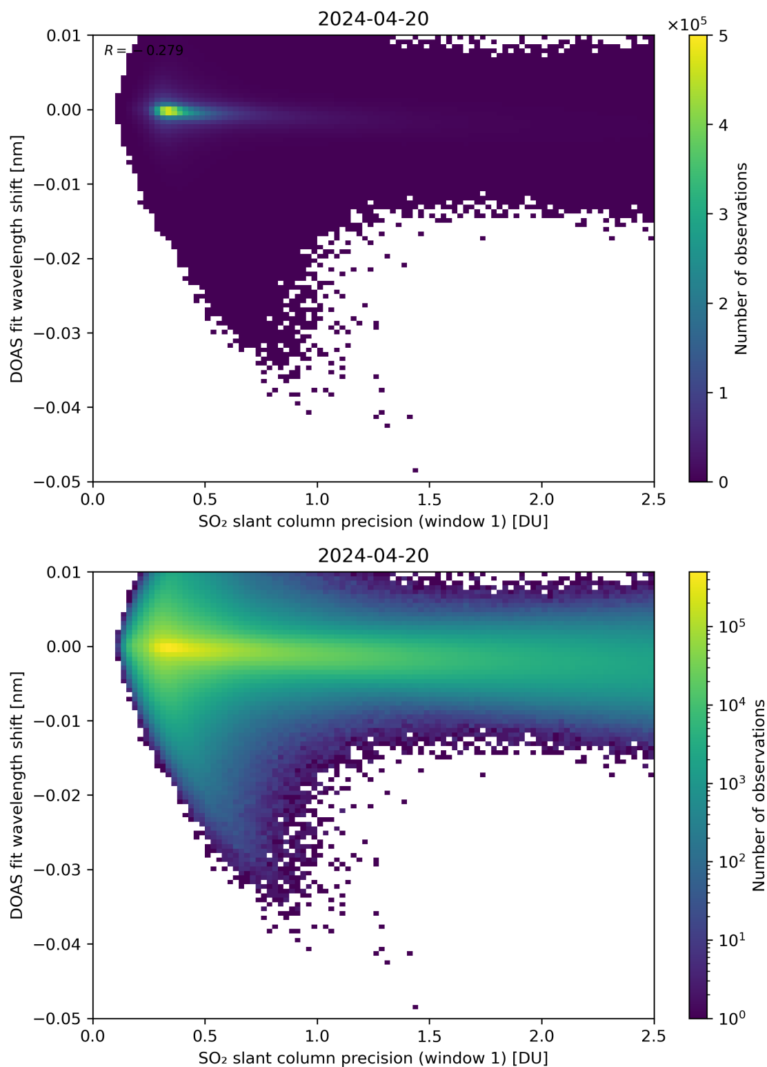
Figure 221: Scatter density plot of “SO 2 slant column precision (window 1)” against “DOAS fit wavelength shift” for 2024-04-19 to 2024-04-21.
