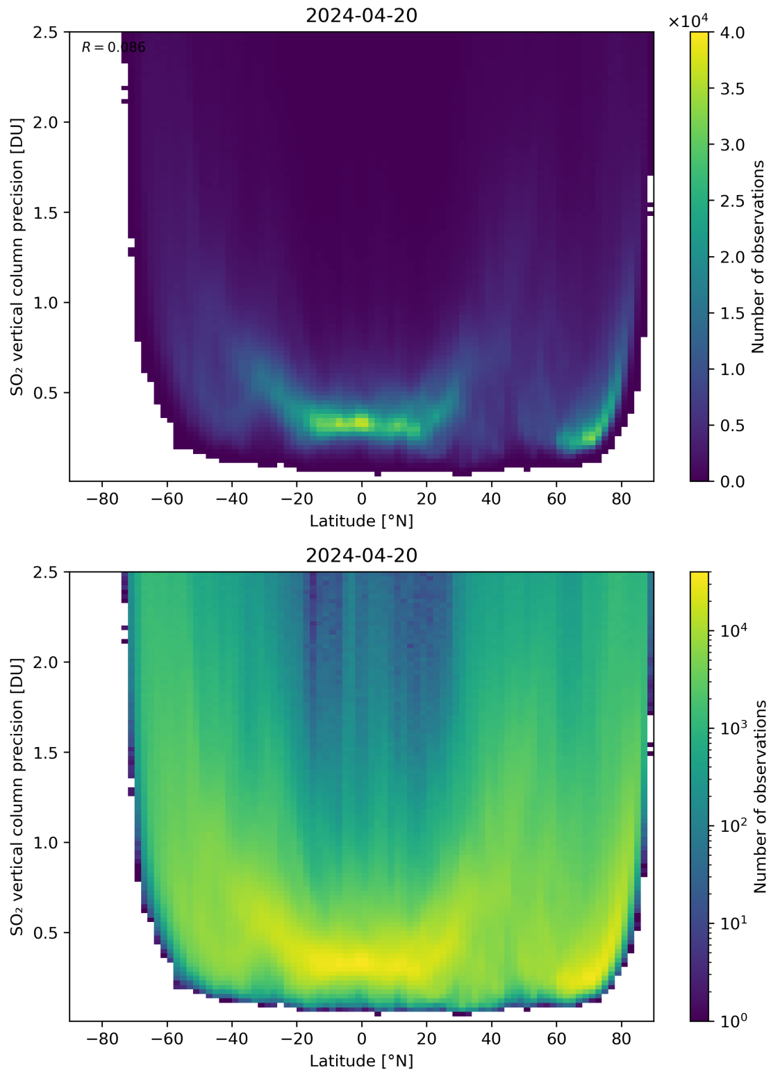
Figure 157: Scatter density plot of “Latitude” against “SO 2 vertical column precision” for 2024-04-19 to 2024-04-21.
