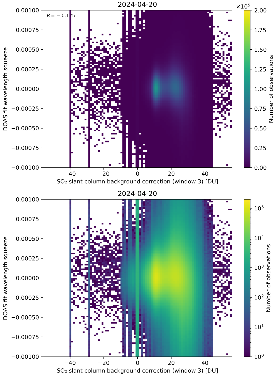
Figure 122: Scatter density plot of “SO 2 slant column background correction (window 3)” against “DOAS fit wavelength squeeze” for 2024-04-19 to 2024-04-21.
