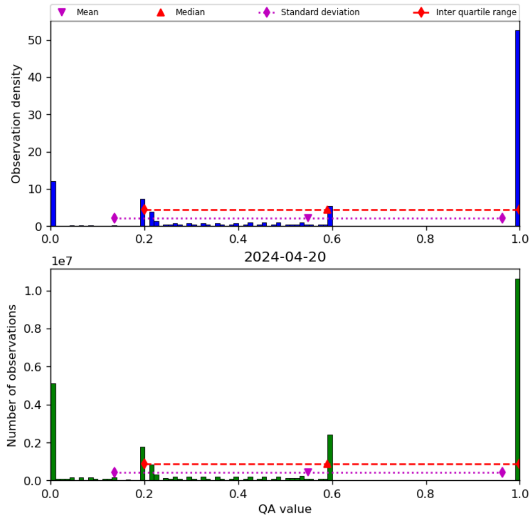
Figure 52: Histogram of “QA value” for 2024-04-19 to 2024-04-21
