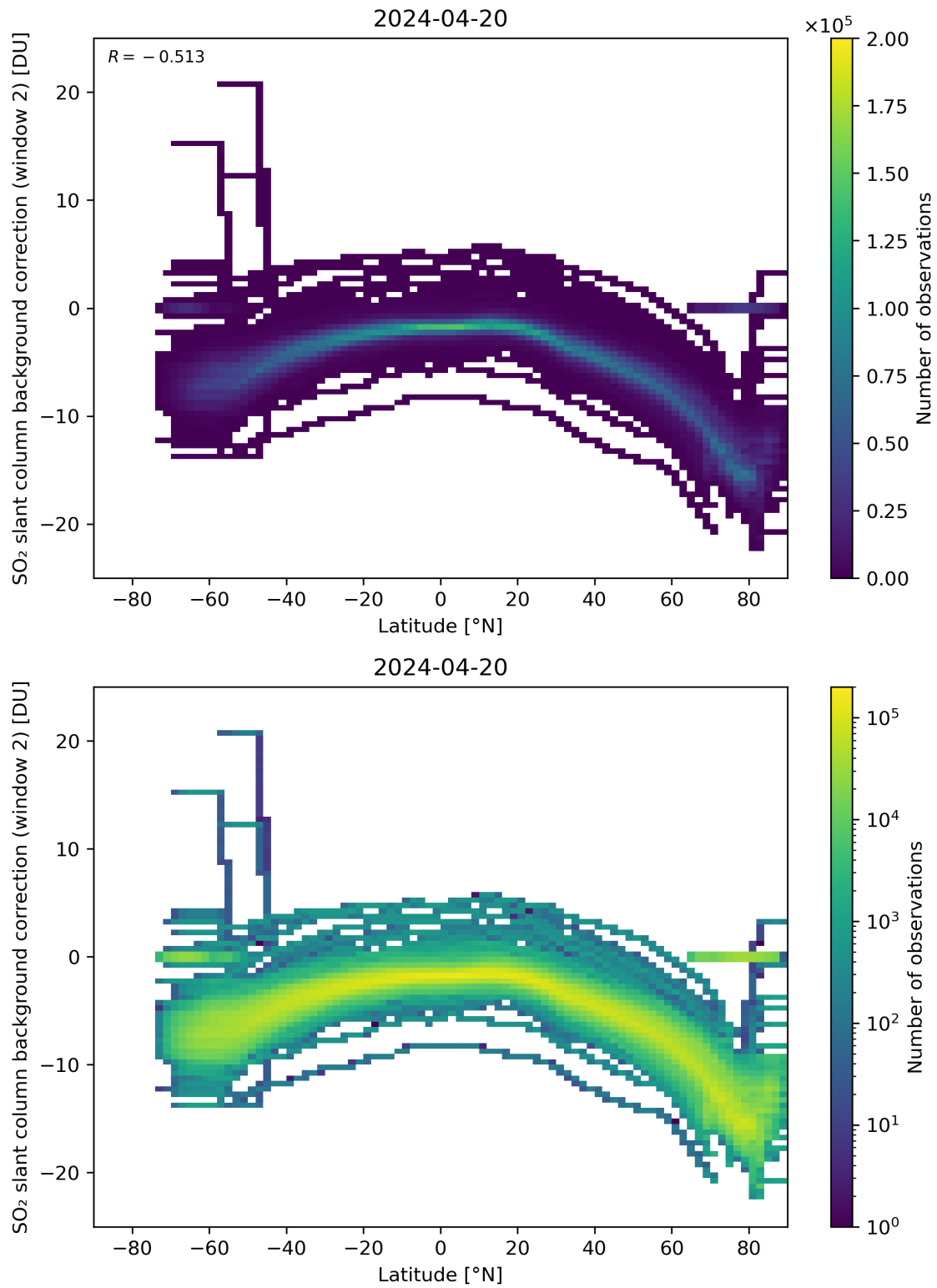
Figure 140: Scatter density plot of “Latitude” against “SO 2 slant column background correction (window 2)” for 2024-04-19 to 2024-04-21.
