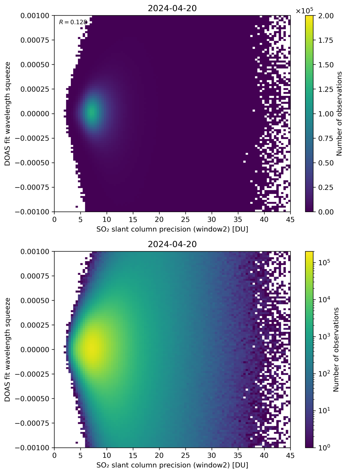
Figure 244: Scatter density plot of “SO 2 slant column precision (window2)” against “DOAS fit wavelength squeeze” for 2024-04-19 to 2024-04-21.
