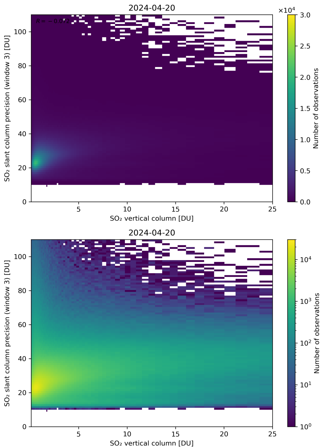
Figure 304: Scatter density plot of “SO 2 vertical column” against “SO 2 slant column precision (window 3)” for 2024-04-19 to 2024-04-21.
