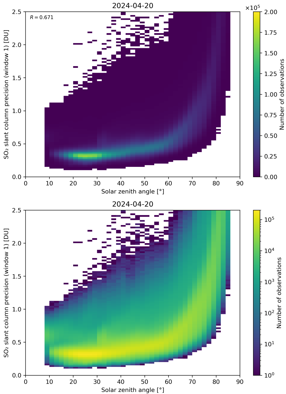
Figure 170: Scatter density plot of “Solar zenith angle” against “SO 2 slant column precision (window 1)” for 2024-04-19 to 2024-04-21.
