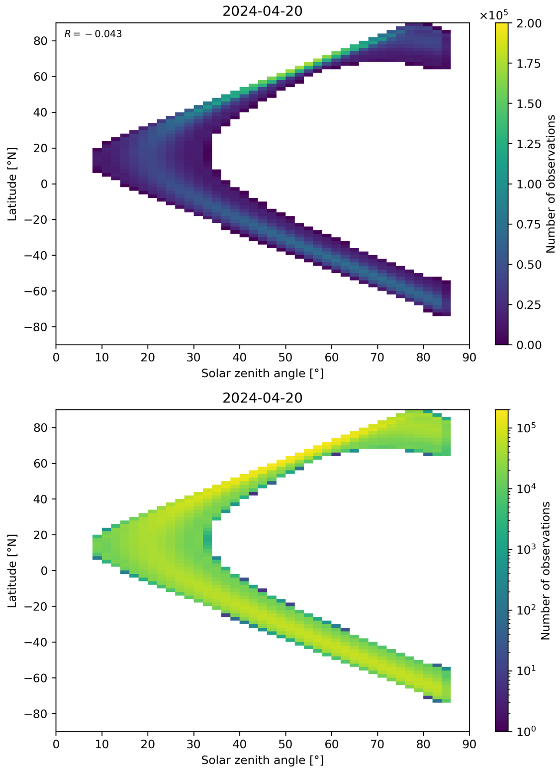
Figure 164: Scatter density plot of “Solar zenith angle” against “Latitude” for 2024-04-19 to 2024-04-21.
