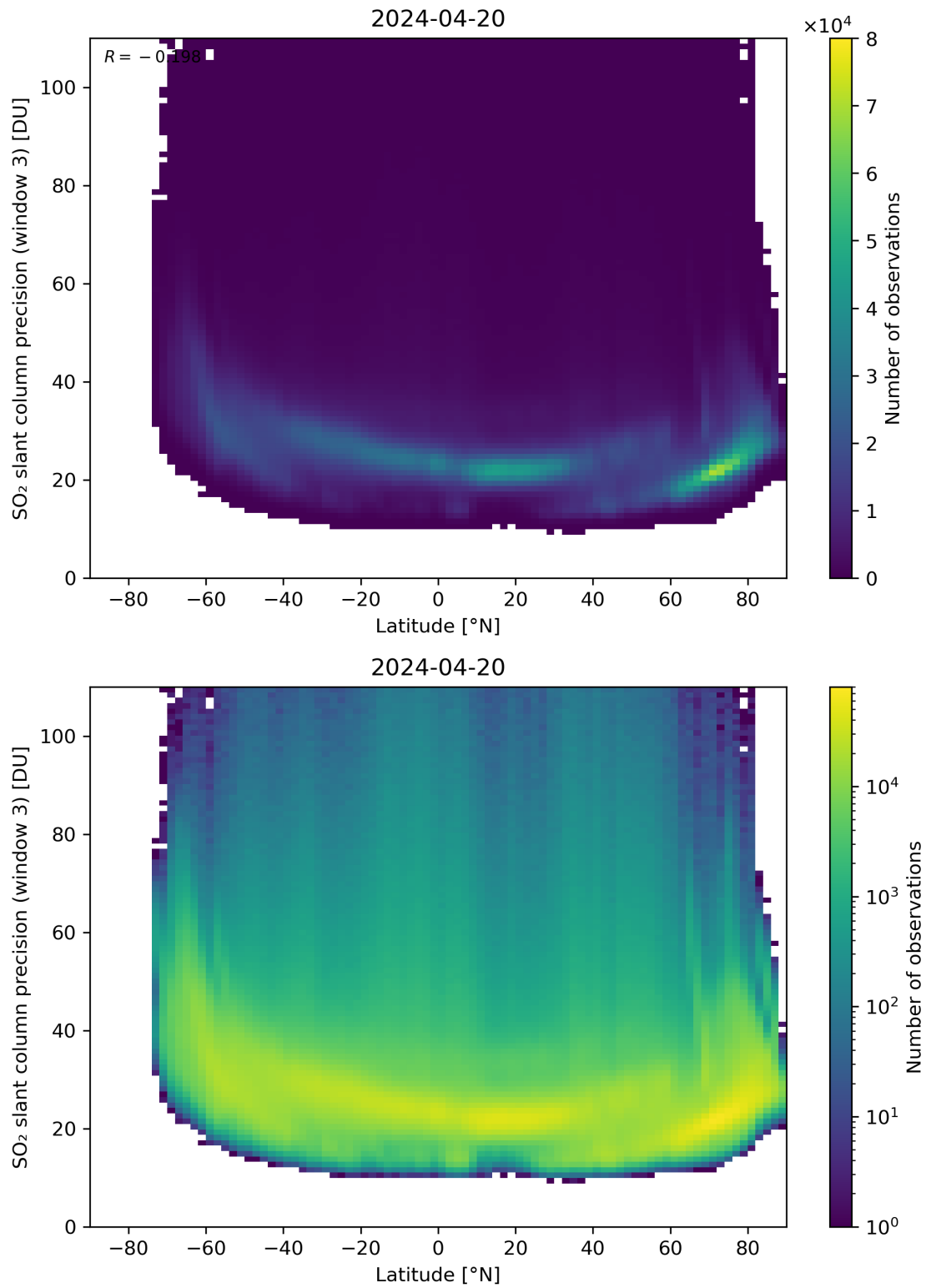
Figure 153: Scatter density plot of “Latitude” against “SO 2 slant column precision (window 3)” for 2024-04-19 to 2024-04-21.
