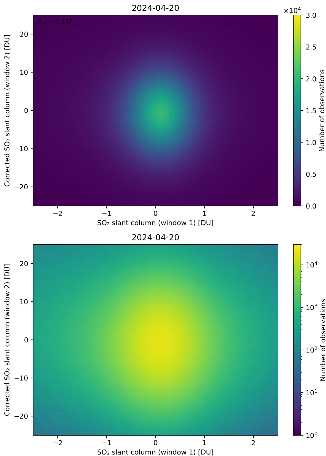
Figure 233: Scatter density plot of “SO 2 slant column (window 1)” against “Corrected SO 2 slant column (window 2)” for 2024-04-19 to 2024-04-21.
