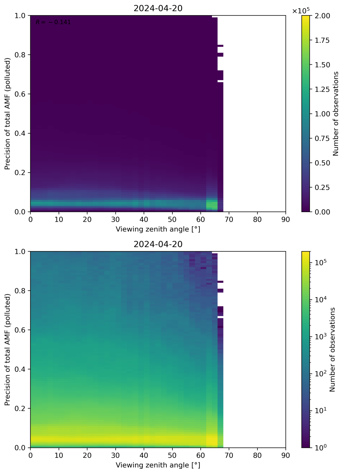
Figure 326: Scatter density plot of “Viewing zenith angle” against “Precision of total AMF (polluted)” for 2024-04-19 to 2024-04-21.
