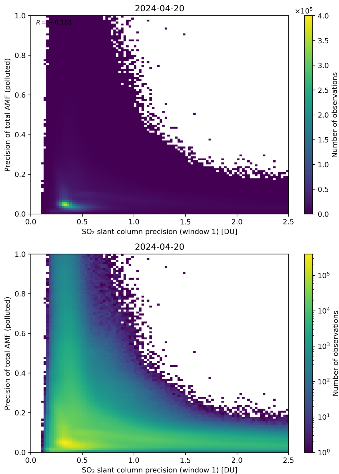
Figure 231: Scatter density plot of “SO 2 slant column precision (window 1)” against “Precision of total AMF (polluted)” for 2024-04-19 to 2024-04-21.
