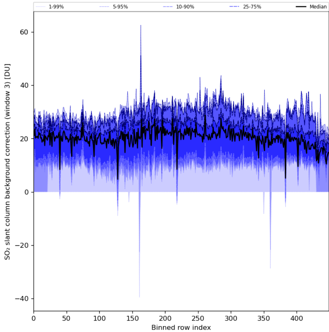
Figure 90: Along track statistics of “SO 2 slant column background correction (window 3)” for 2024-04-19 to 2024-04-21
