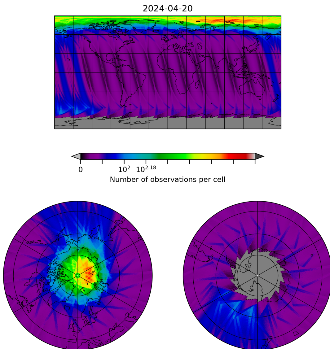
Figure 28: Map of the number of observations for 2024-04-19 to 2024-04-21
