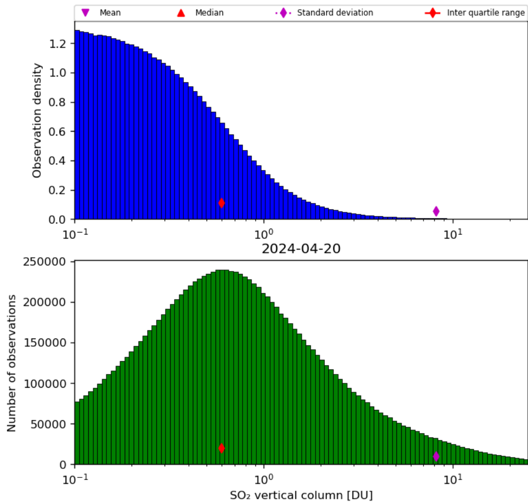
Figure 53: Histogram of “SO 2 vertical column” for 2024-04-19 to 2024-04-21
