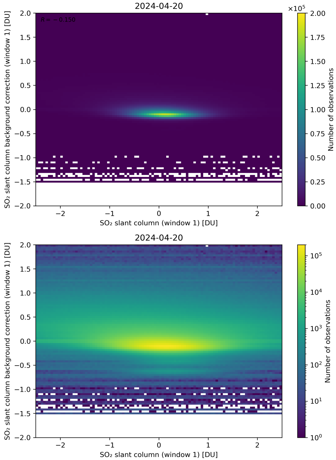
Figure 212: Scatter density plot of “SO 2 slant column (window 1)” against “SO 2 slant column background correction (window 1)” for 2024-04-19 to 2024-04-21.
