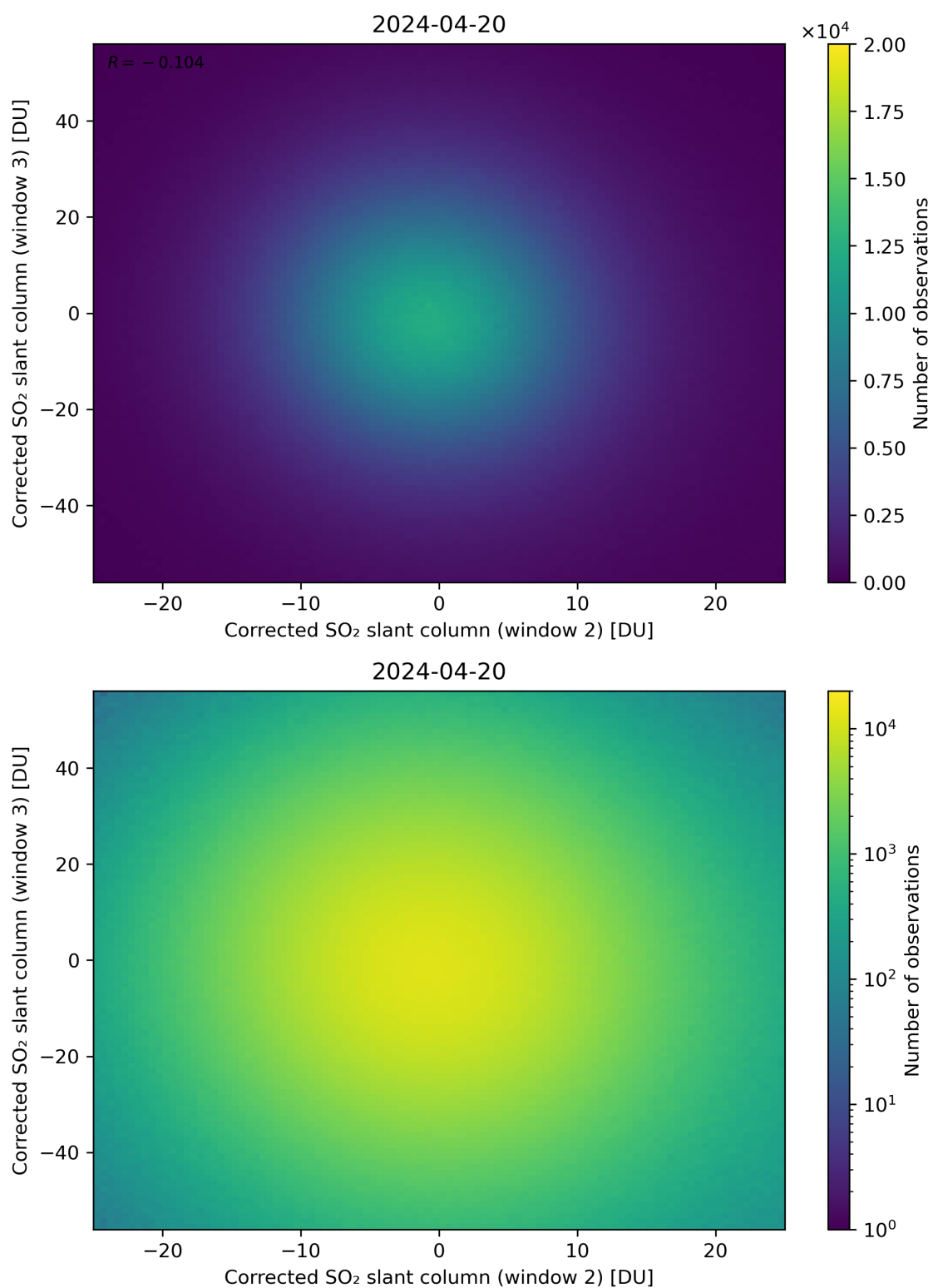
Figure 200: Scatter density plot of “Corrected SO 2 slant column (window 2)” against “Corrected SO 2 slant column (window 3)” for 2024-04-19 to 2024-04-21.
