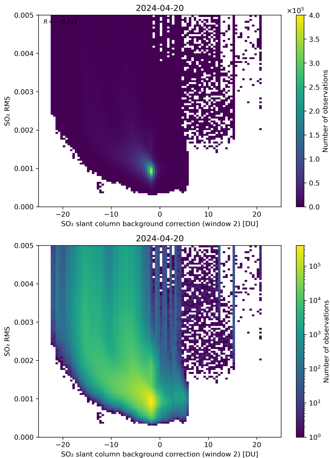
Figure 114: Scatter density plot of “SO 2 slant column background correction (window 2)” against “SO 2 RMS” for 2024-04-19 to 2024-04-21.
