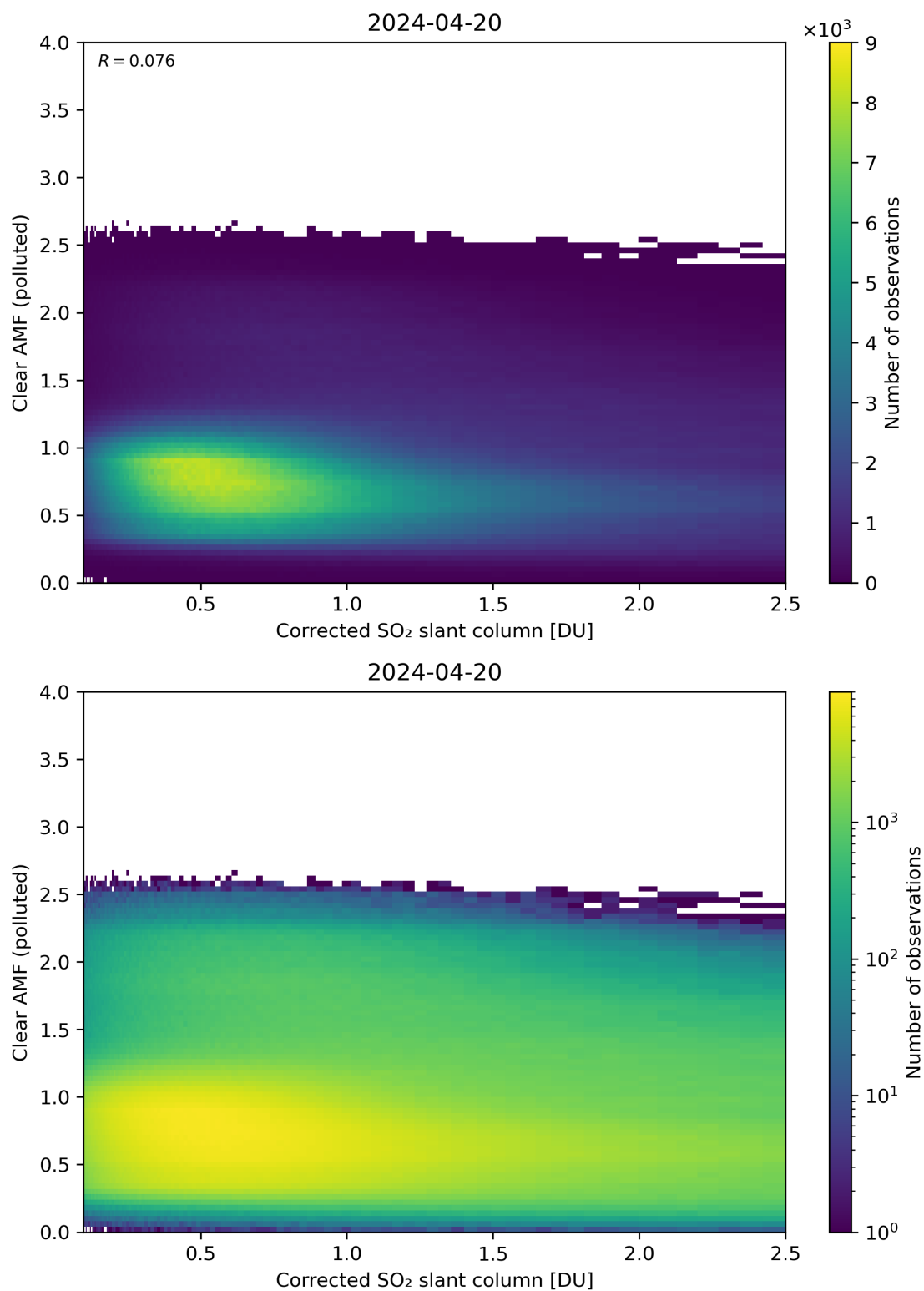
Figure 184: Scatter density plot of “Corrected SO 2 slant column” against “Clear AMF (polluted)” for 2024-04-19 to 2024-04-21.
