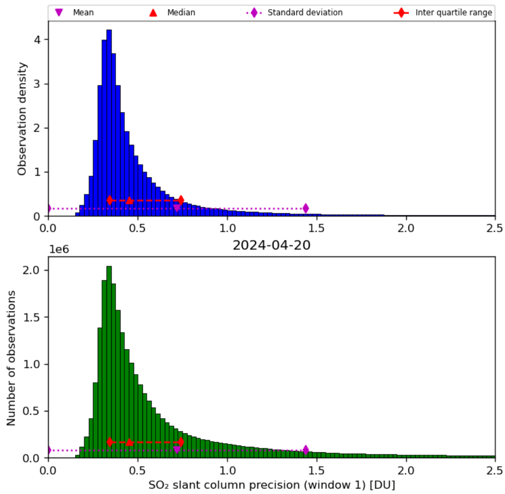
Figure 57: Histogram of “SO 2 slant column precision (window 1)” for 2024-04-19 to 2024-04-21
