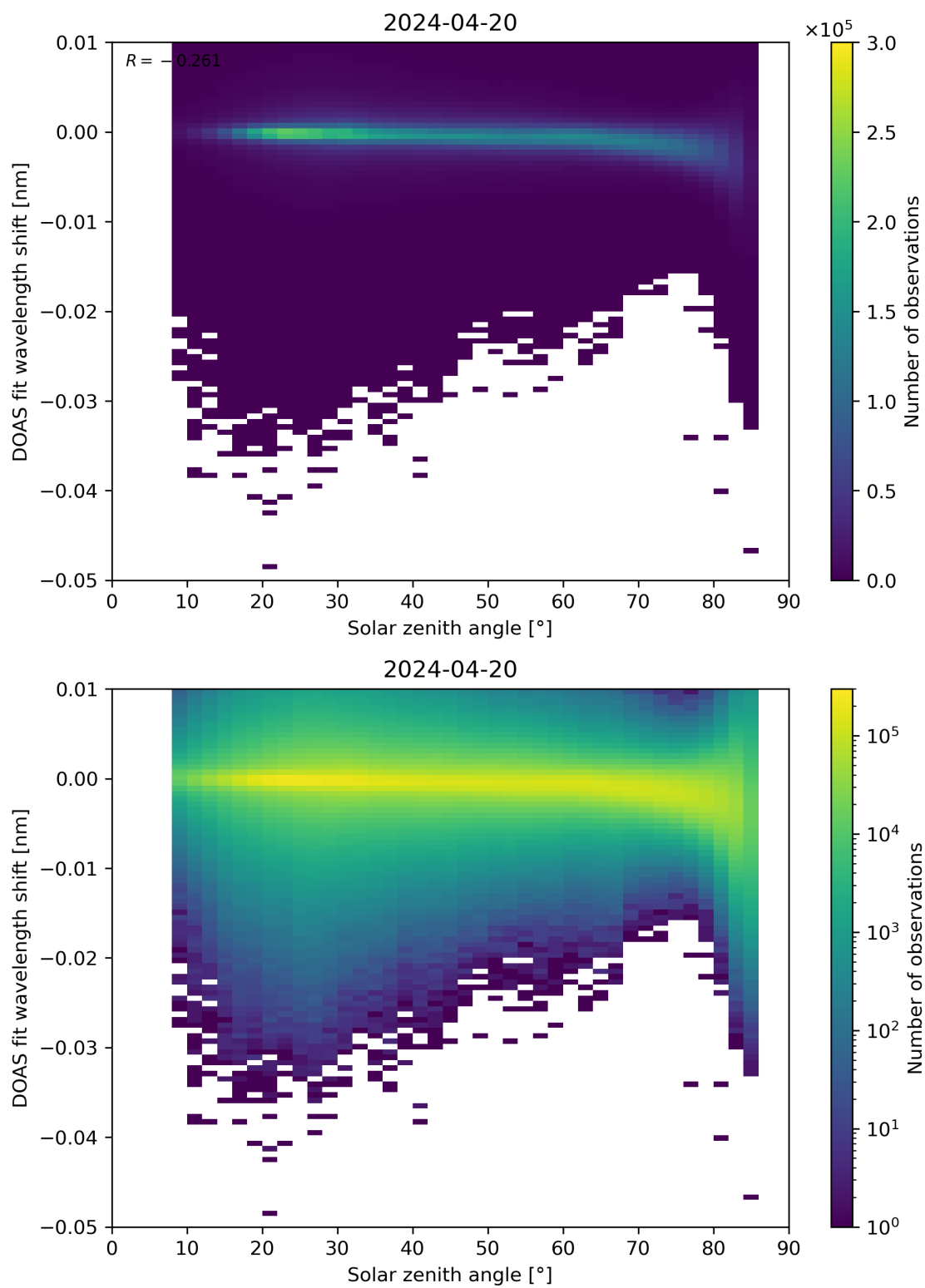
Figure 161: Scatter density plot of “Solar zenith angle” against “DOAS fit wavelength shift” for 2024-04-19 to 2024-04-21.
