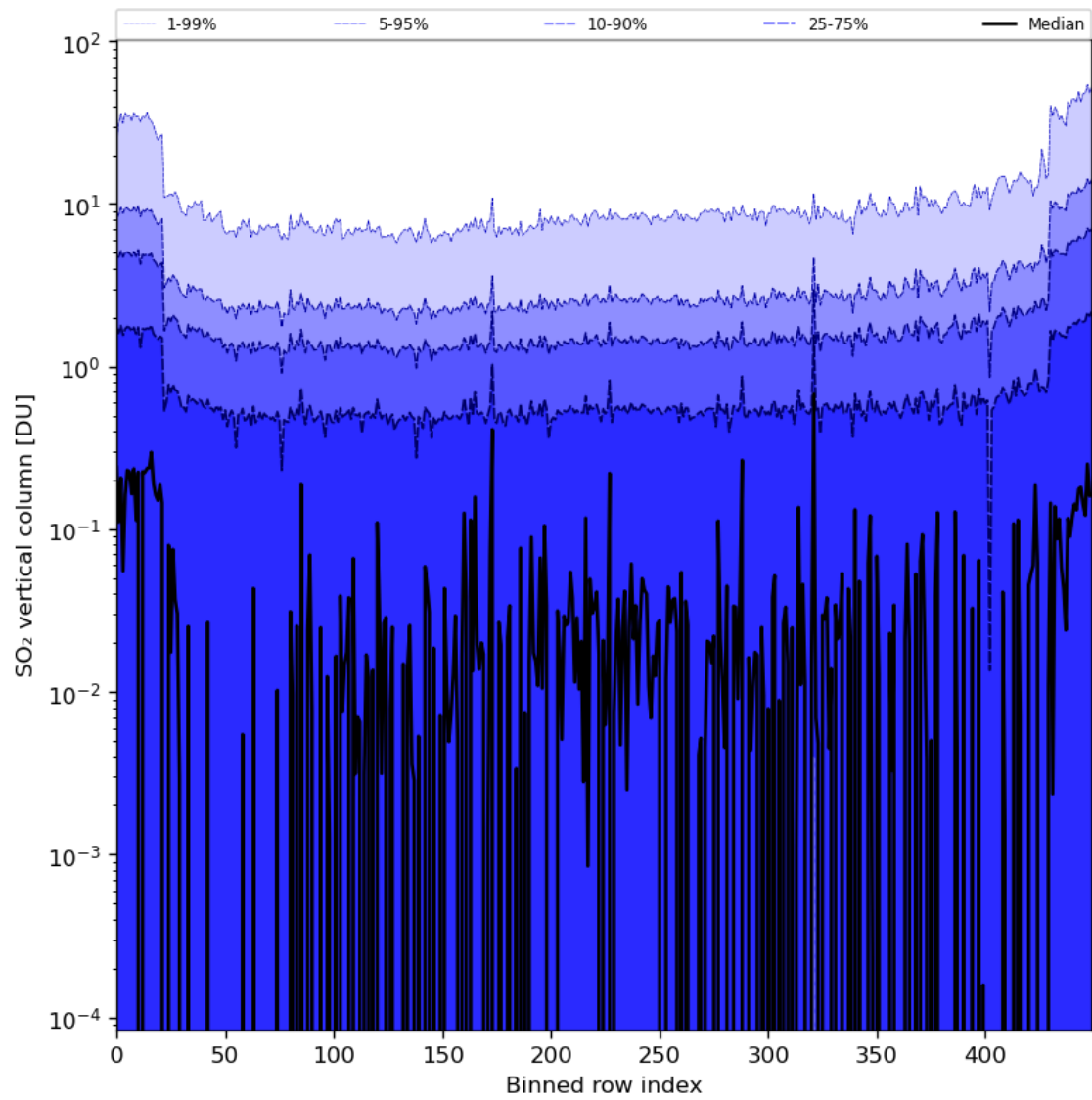
Figure 76: Along track statistics of “SO 2 vertical column” for 2024-04-19 to 2024-04-21
