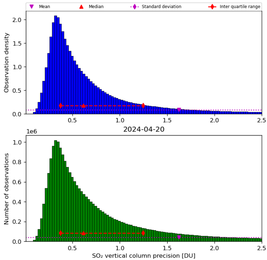
Figure 54: Histogram of “SO 2 vertical column precision” for 2024-04-19 to 2024-04-21
