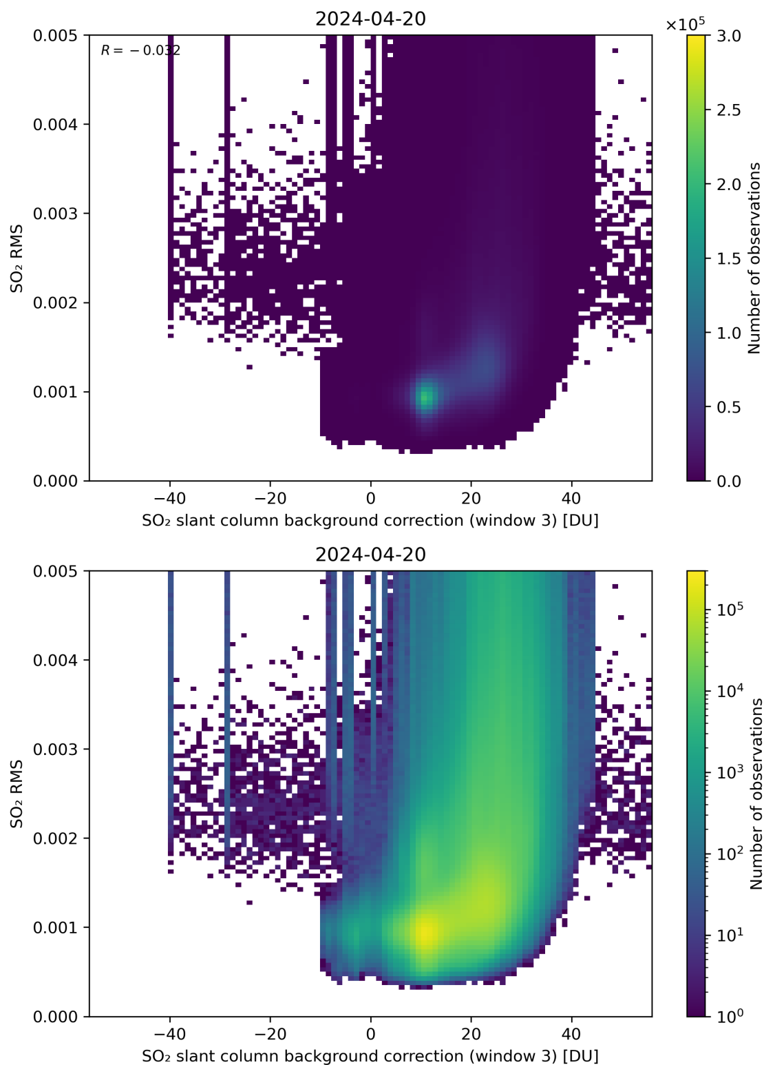
Figure 123: Scatter density plot of “SO 2 slant column background correction (window 3)” against “SO 2 RMS” for 2024-04-19 to 2024-04-21.
