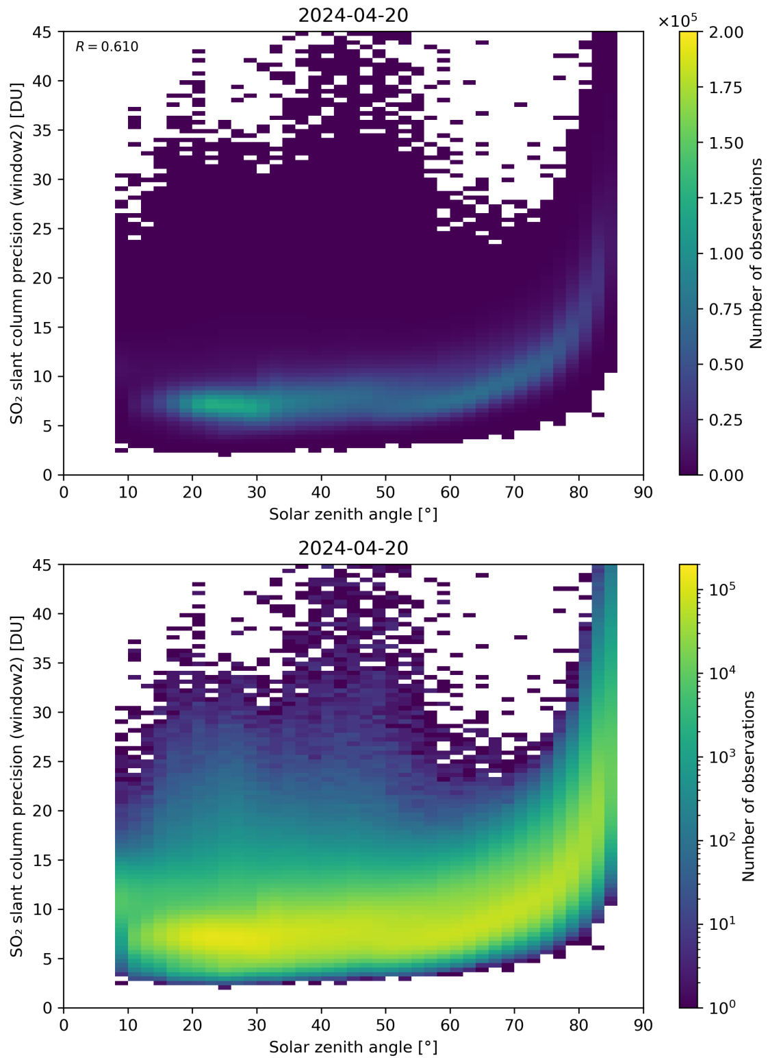
Figure 171: Scatter density plot of “Solar zenith angle” against “SO 2 slant column precision (window2)” for 2024-04-19 to 2024-04-21.
