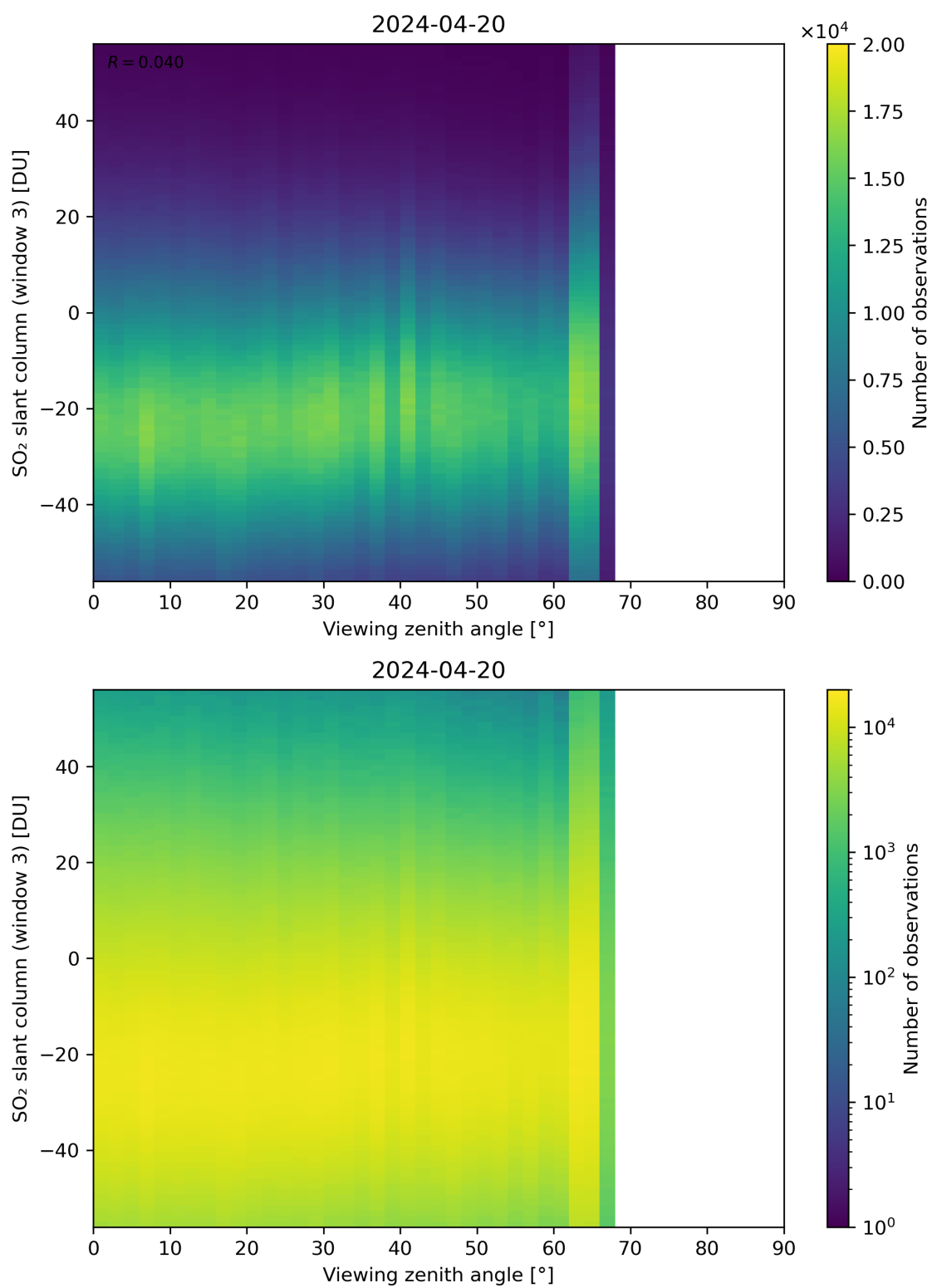
Figure 323: Scatter density plot of “Viewing zenith angle” against “SO 2 slant column (window 3)” for 2024-04-19 to 2024-04-21.
