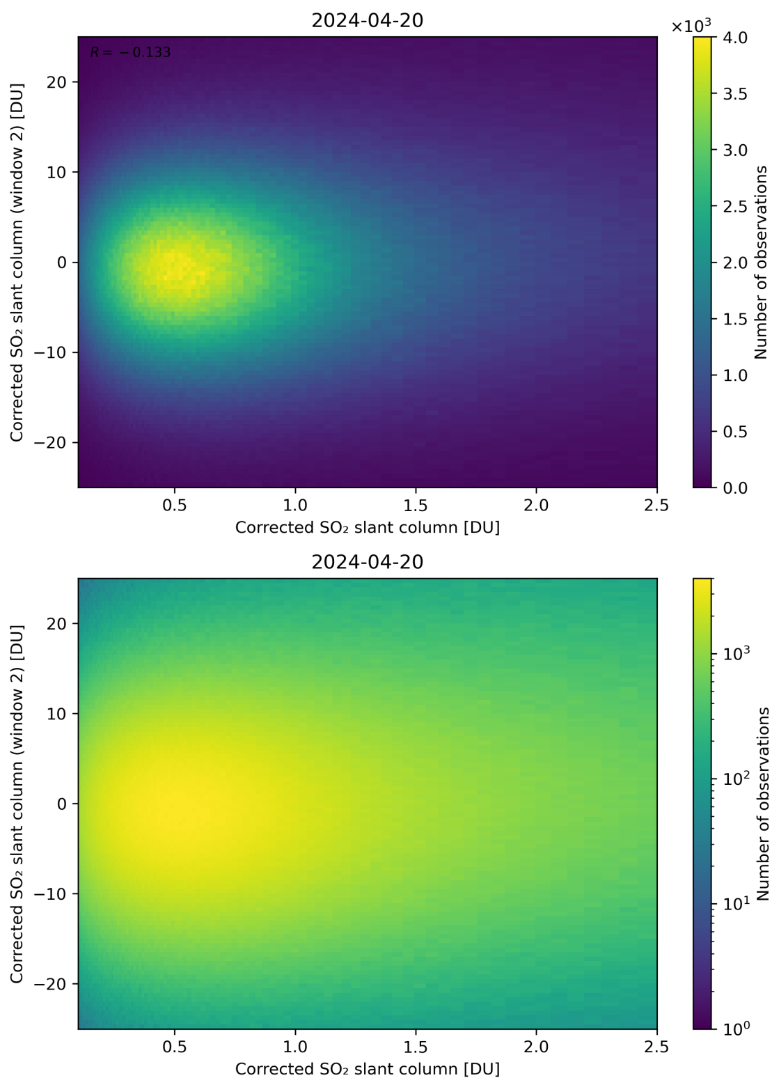
Figure 185: Scatter density plot of “Corrected SO 2 slant column” against “Corrected SO 2 slant column (window 2)” for 2024-04-19 to 2024-04-21.
