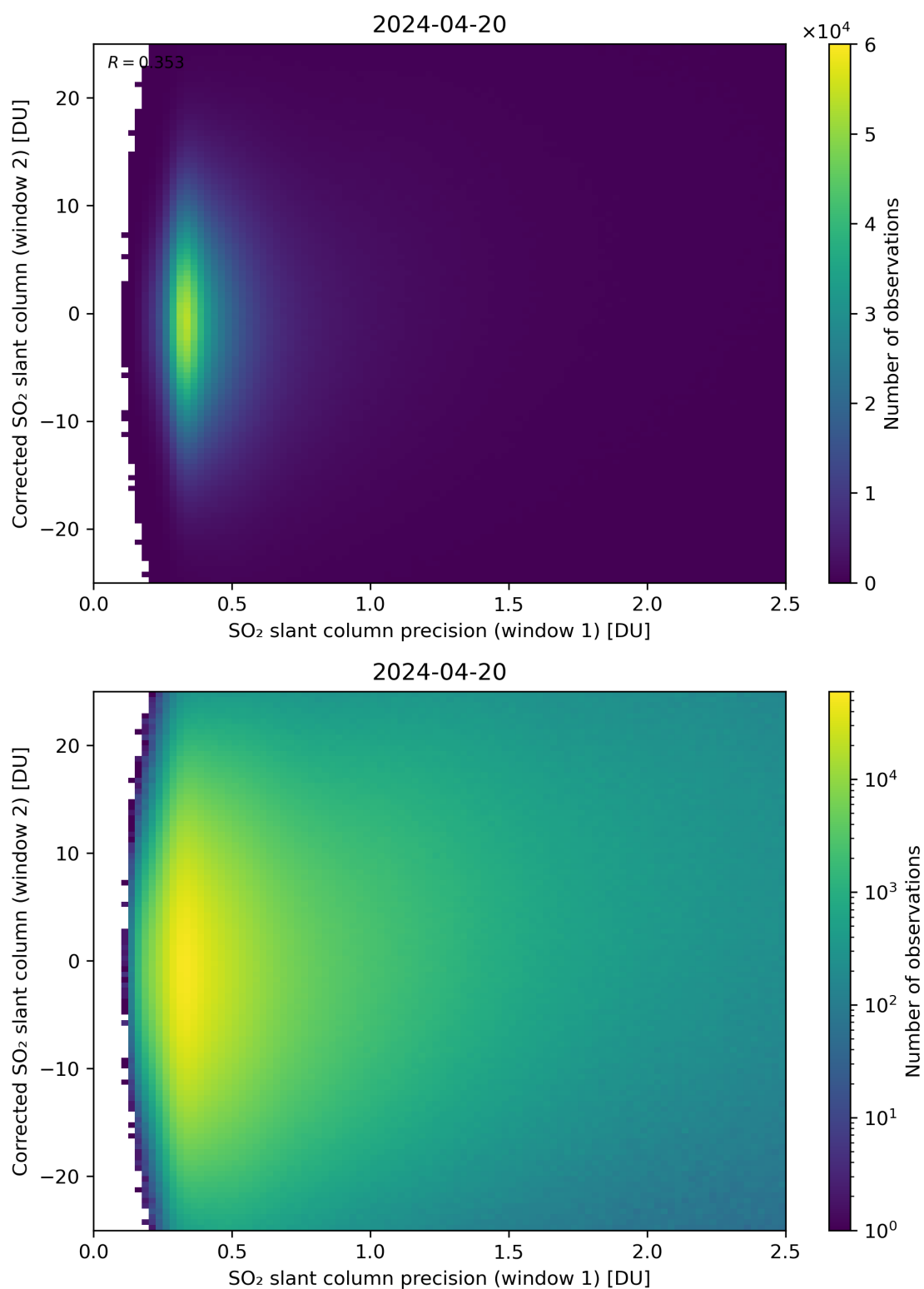
Figure 225: Scatter density plot of “SO 2 slant column precision (window 1)” against “Corrected SO 2 slant column (window 2)” for 2024-04-19 to 2024-04-21.
