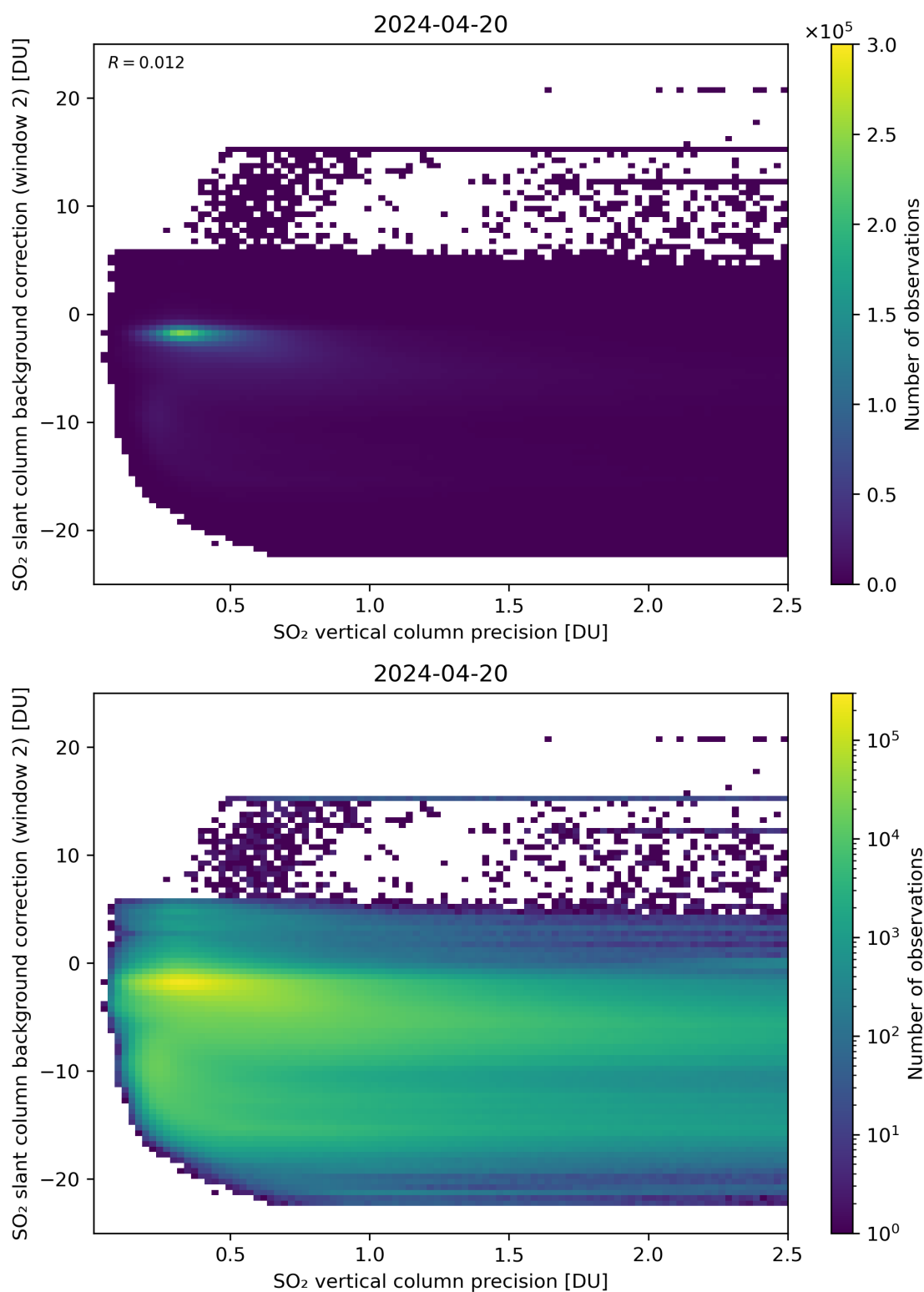
Figure 280: Scatter density plot of “SO 2 vertical column precision” against “SO 2 slant column background correction (window 2)” for 2024-04-19 to 2024-04-21.
