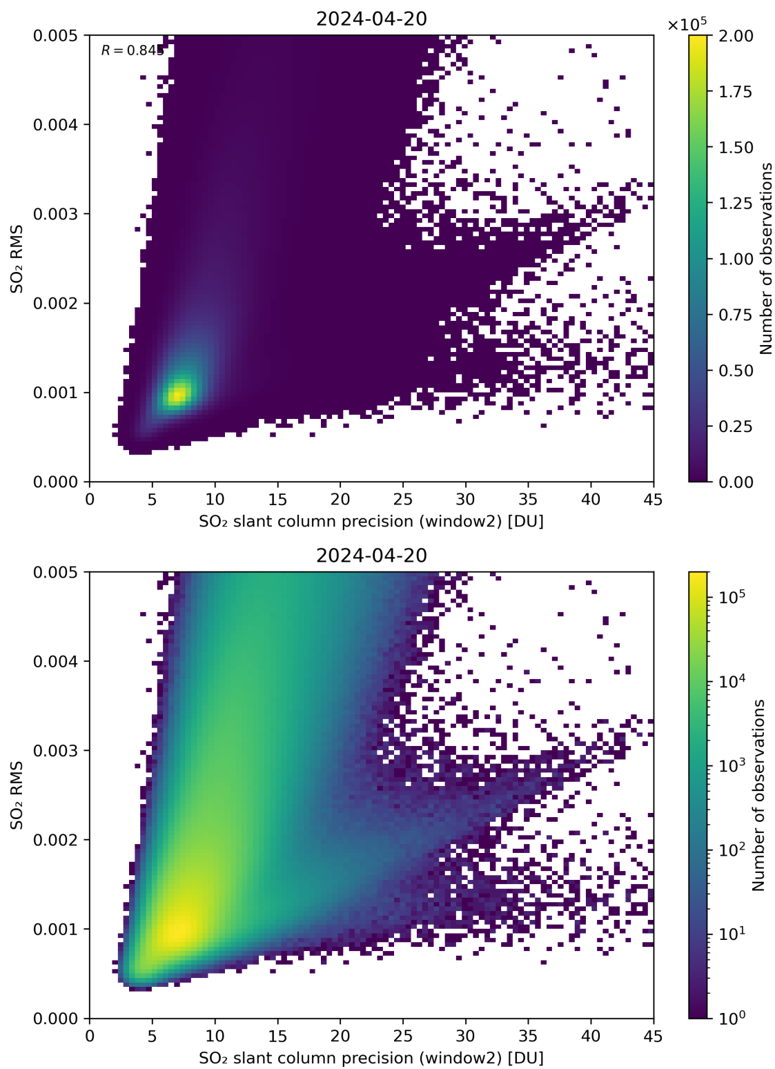
Figure 245: Scatter density plot of “SO 2 slant column precision (window2)” against “SO 2 RMS” for 2024-04-19 to 2024-04-21.
