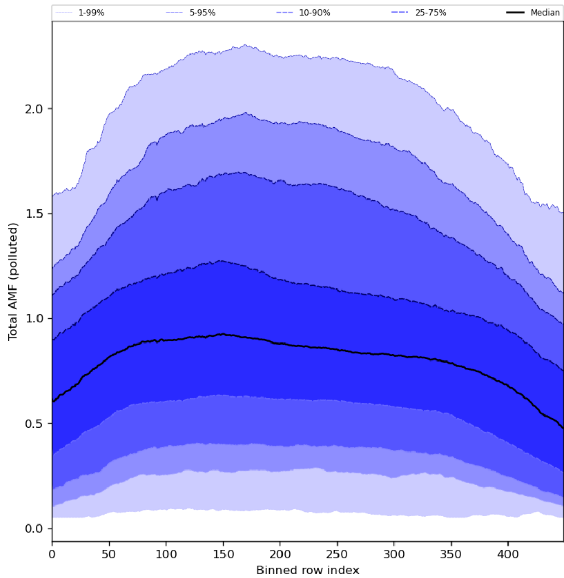
Figure 94: Along track statistics of “Total AMF (polluted)” for 2024-04-19 to 2024-04-21
