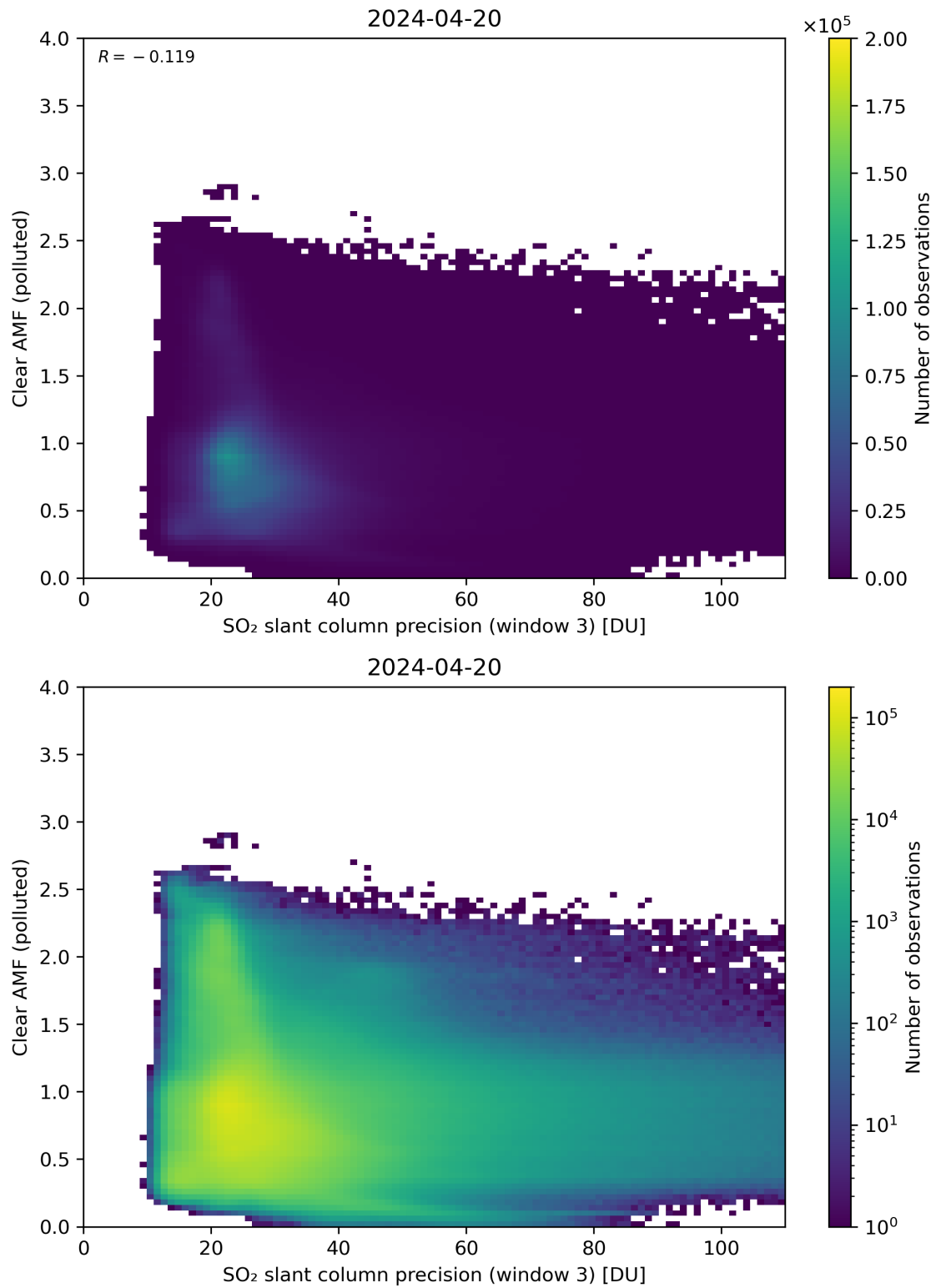
Figure 261: Scatter density plot of “SO 2 slant column precision (window 3)” against “Clear AMF (polluted)” for 2024-04-19 to 2024-04-21.
