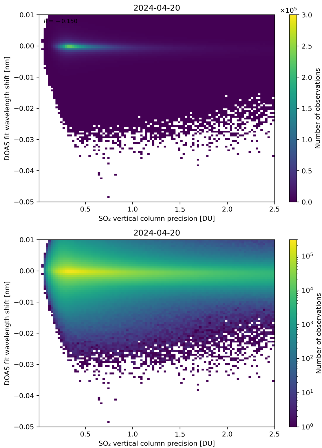
Figure 282: Scatter density plot of “SO 2 vertical column precision” against “DOAS fit wavelength shift” for 2024-04-19 to 2024-04-21.
