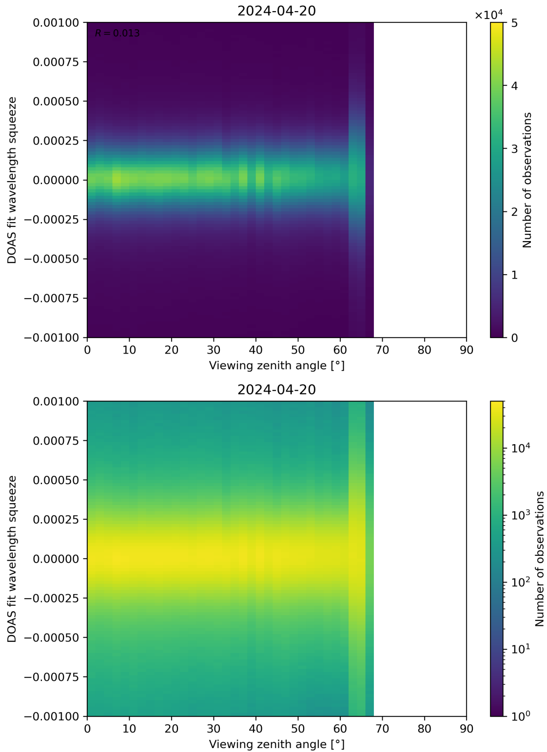
Figure 312: Scatter density plot of “Viewing zenith angle” against “DOAS fit wavelength squeeze” for 2024-04-19 to 2024-04-21.
