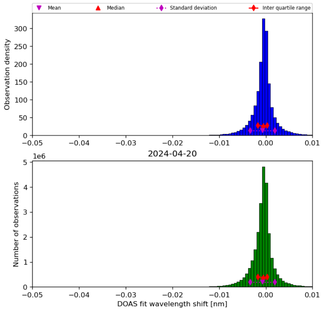
Figure 68: Histogram of “DOAS fit wavelength shift” for 2024-04-19 to 2024-04-21
