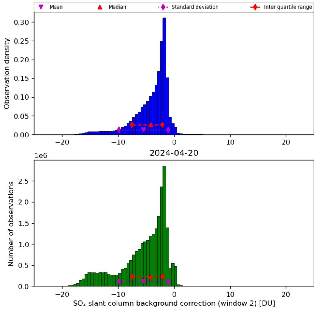
Figure 63: Histogram of “SO 2 slant column background correction (window 2)” for 2024-04-19 to 2024-04-21
