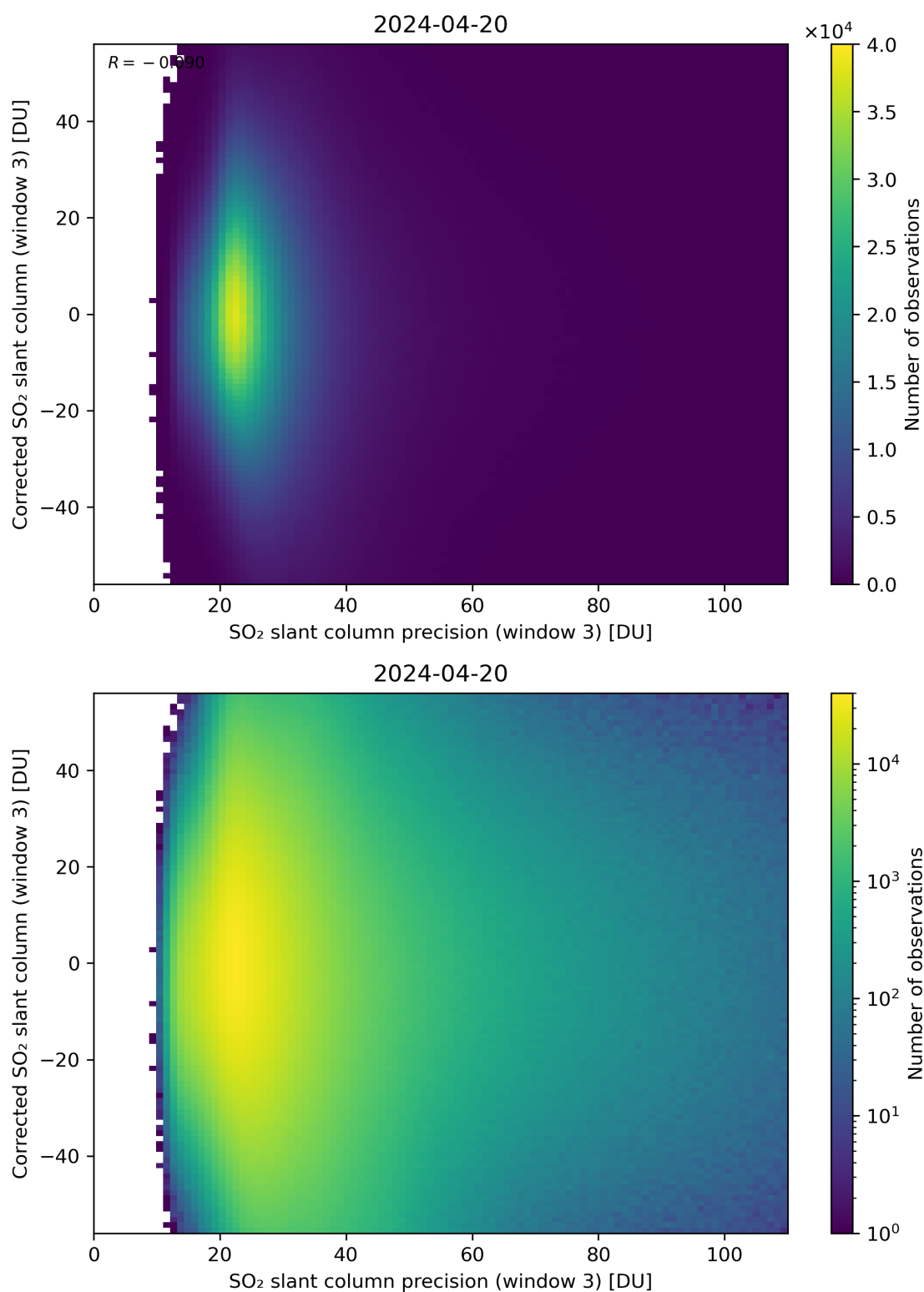
Figure 262: Scatter density plot of “SO 2 slant column precision (window 3)” against “Corrected SO 2 slant column (window 3)” for 2024-04-19 to 2024-04-21.
