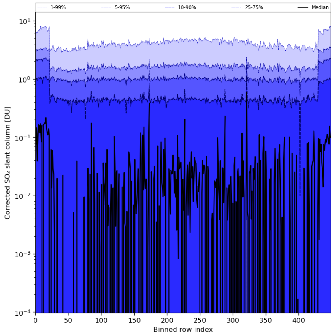
Figure 78: Along track statistics of “Corrected SO 2 slant column” for 2024-04-19 to 2024-04-21
