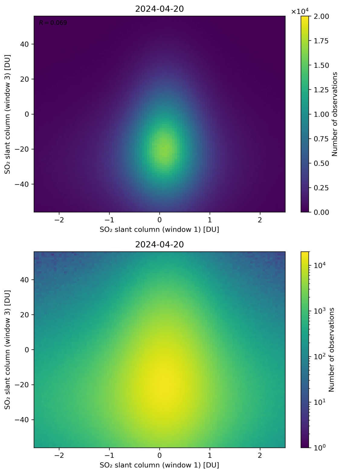
Figure 237: Scatter density plot of “SO 2 slant column (window 1)” against “SO 2 slant column (window 3)” for 2024-04-19 to 2024-04-21.
