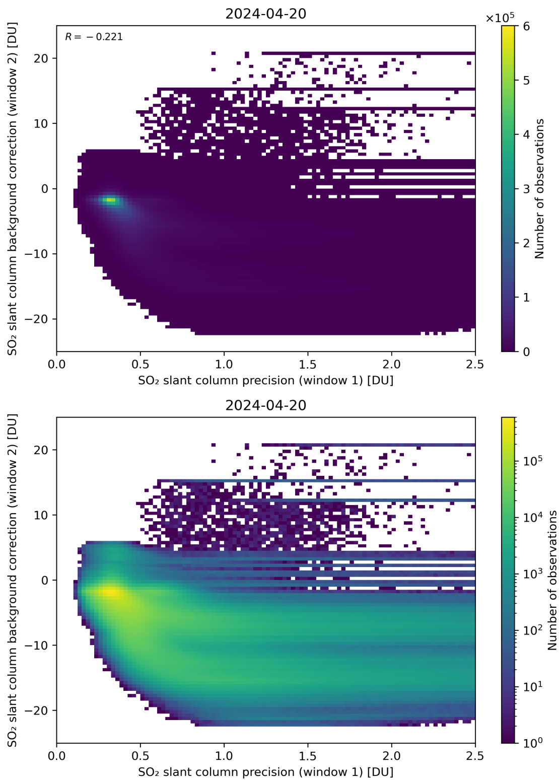
Figure 219: Scatter density plot of “SO 2 slant column precision (window 1)” against “SO 2 slant column background correction (window 2)” for 2024-04-19 to 2024-04-21.
