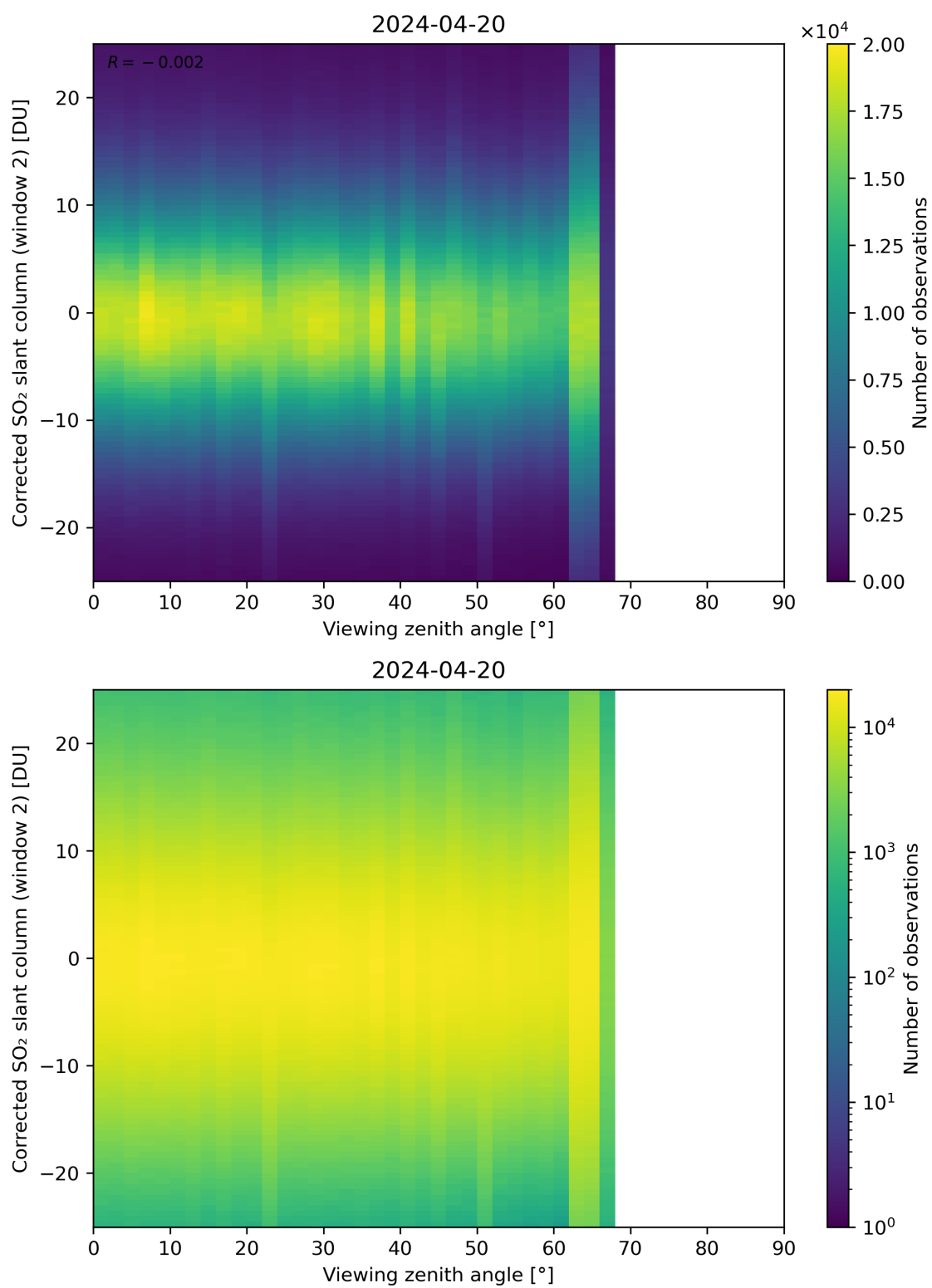
Figure 318: Scatter density plot of “Viewing zenith angle” against “Corrected SO 2 slant column (window 2)” for 2024-04-19 to 2024-04-21.
