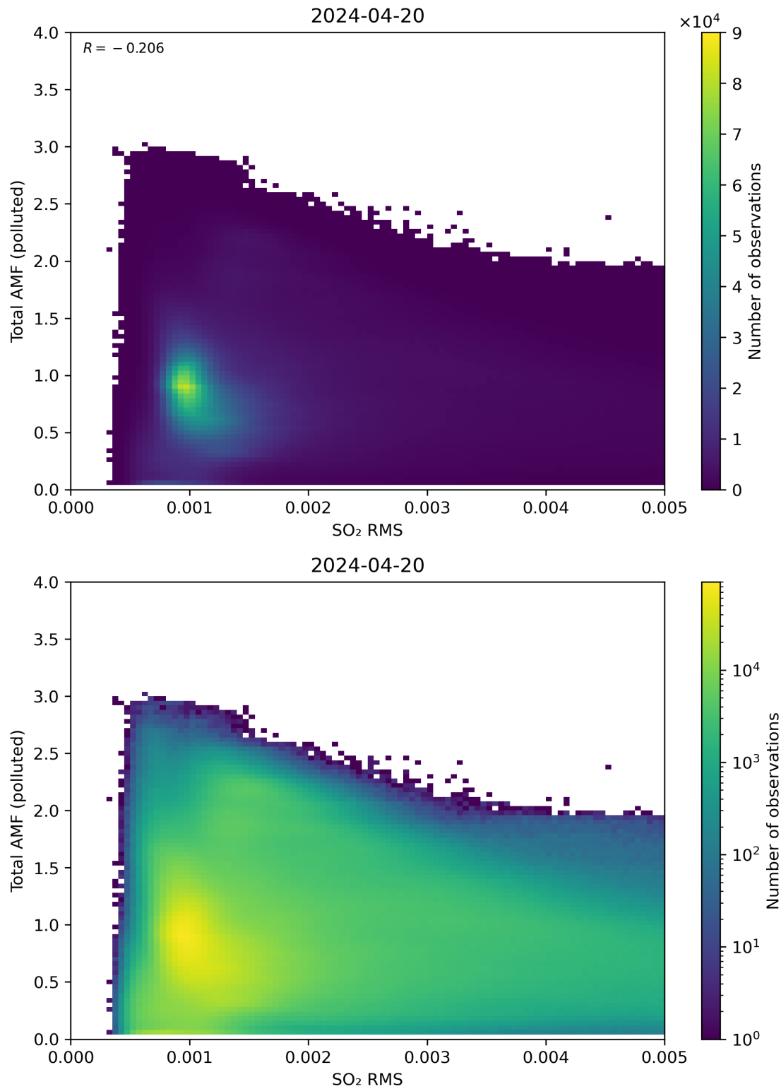
Figure 137: Scatter density plot of “SO 2 RMS” against “Total AMF (polluted)” for 2024-04-19 to 2024-04-21.
