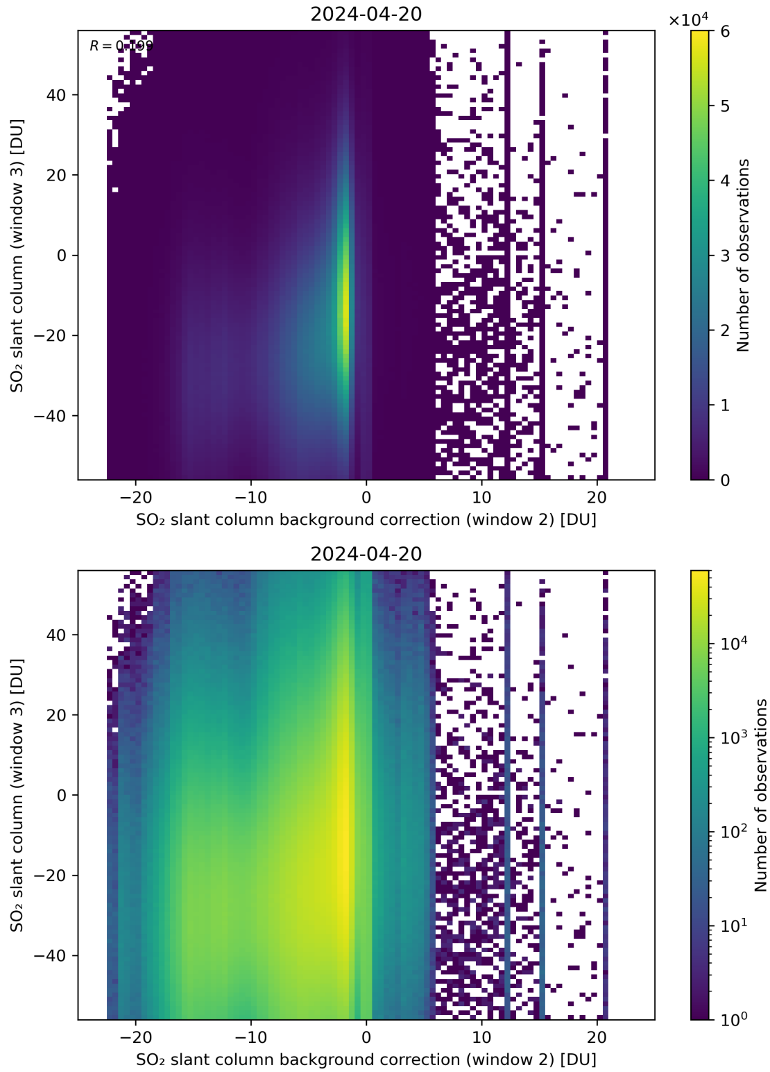
Figure 117: Scatter density plot of “SO 2 slant column background correction (window 2)” against “SO 2 slant column (window 3)” for 2024-04-19 to 2024-04-21.
