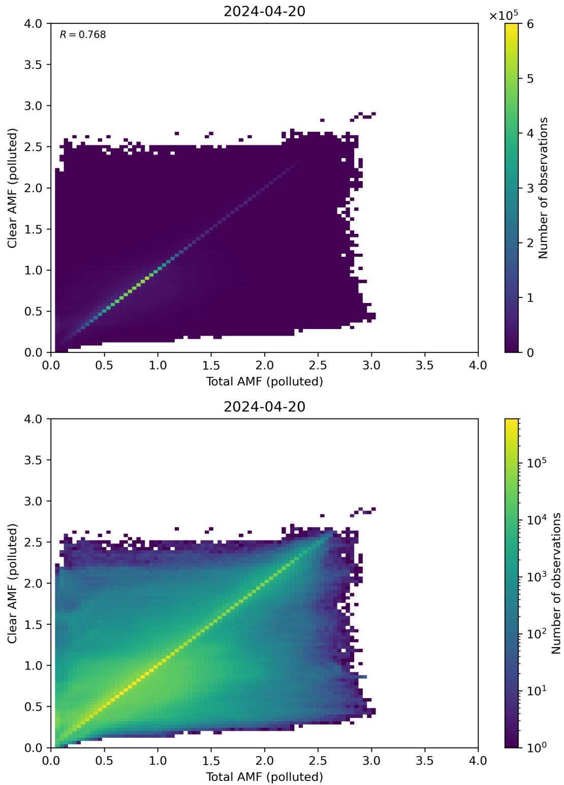
Figure 271: Scatter density plot of “Total AMF (polluted)” against “Clear AMF (polluted)” for 2024-04-19 to 2024-04-21.
