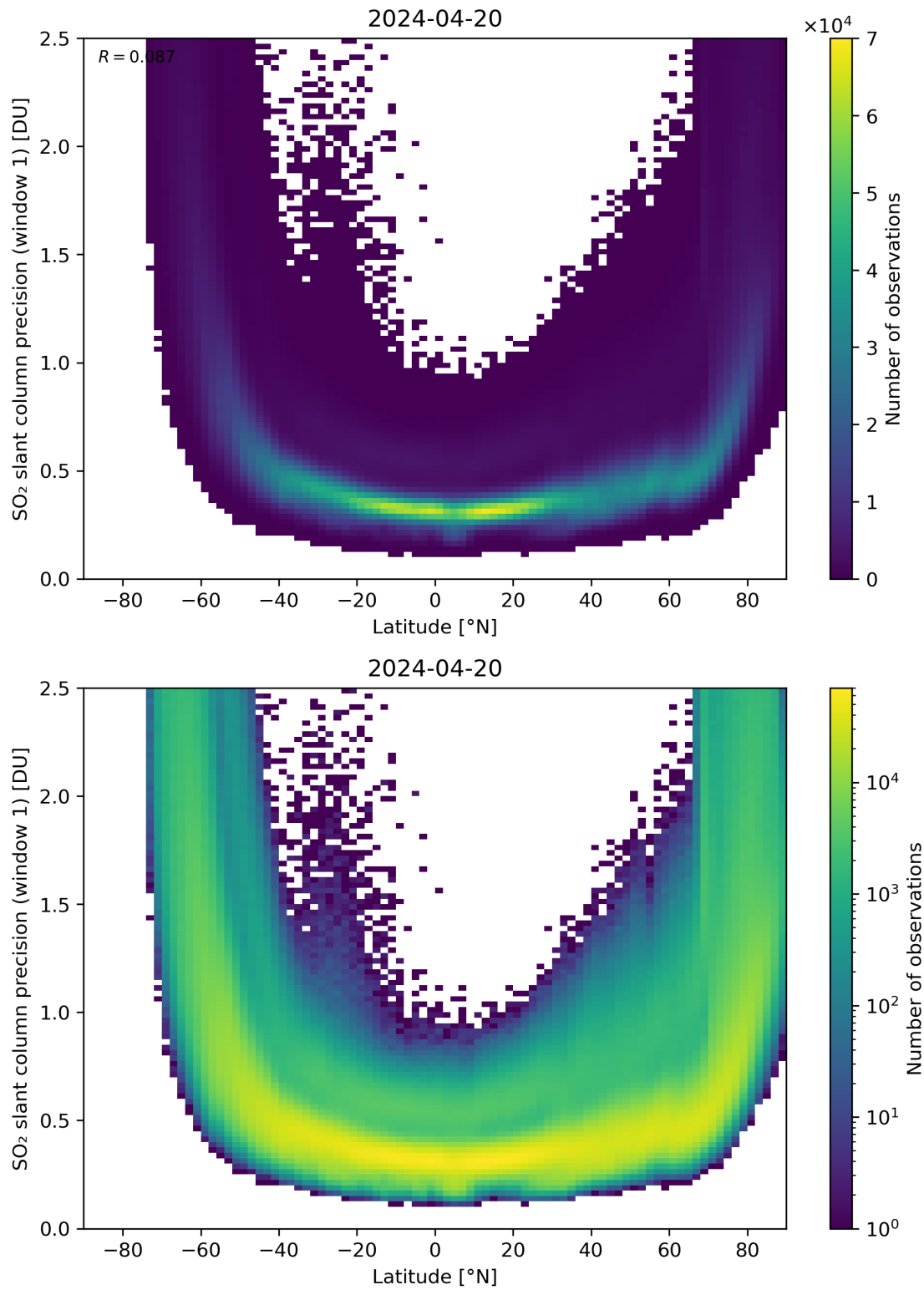
Figure 150: Scatter density plot of “Latitude” against “SO 2 slant column precision (window 1)” for 2024-04-19 to 2024-04-21.
