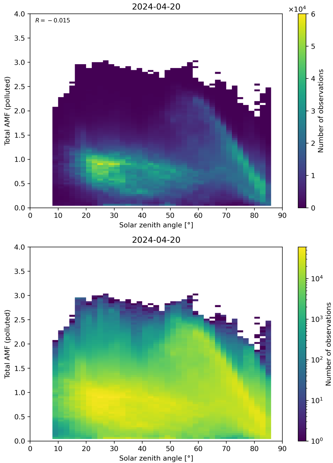
Figure 174: Scatter density plot of “Solar zenith angle” against “Total AMF (polluted)” for 2024-04-19 to 2024-04-21.
