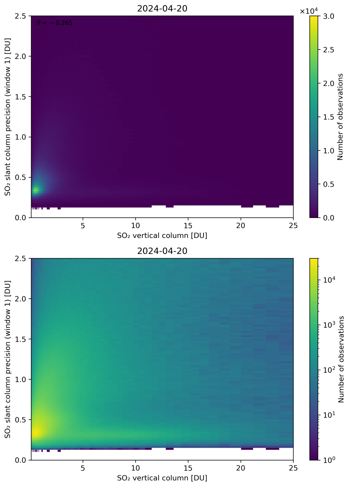
Figure 301: Scatter density plot of “SO 2 vertical column” against “SO 2 slant column precision (window 1)” for 2024-04-19 to 2024-04-21.
