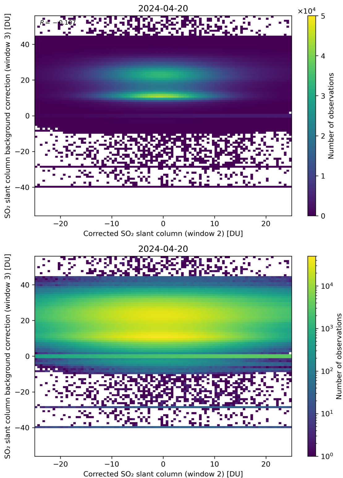
Figure 195: Scatter density plot of “Corrected SO 2 slant column (window 2)” against “SO 2 slant column background correction (window 3)” for 2024-04-19 to 2024-04-21.
