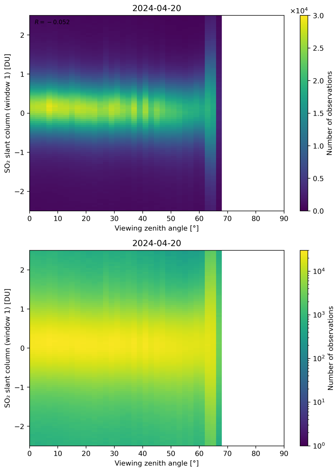
Figure 320: Scatter density plot of “Viewing zenith angle” against “SO 2 slant column (window 1)” for 2024-04-19 to 2024-04-21.
