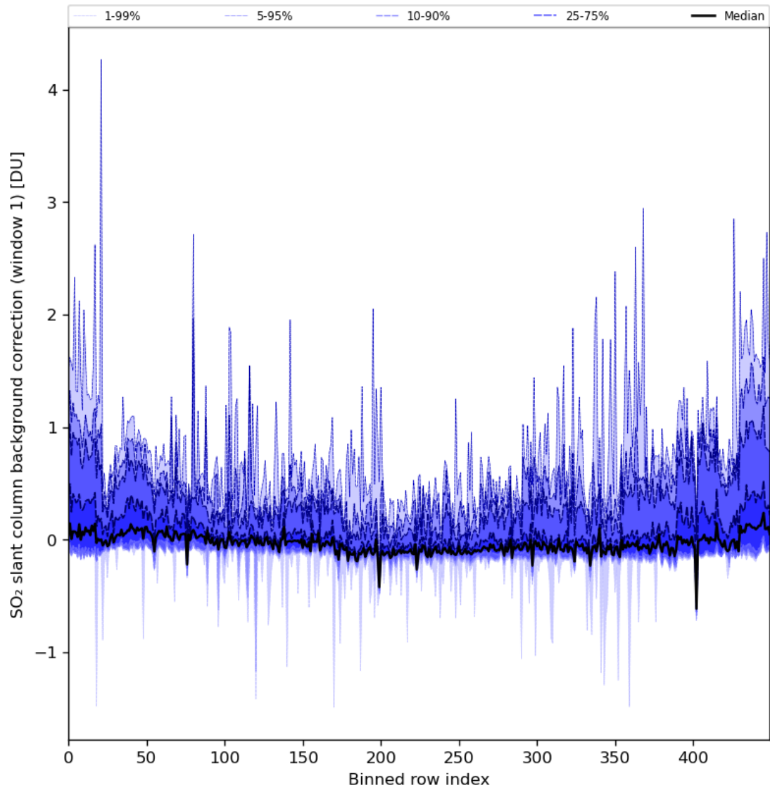
Figure 82: Along track statistics of “SO 2 slant column background correction (window 1)” for 2024-04-19 to 2024-04-21
