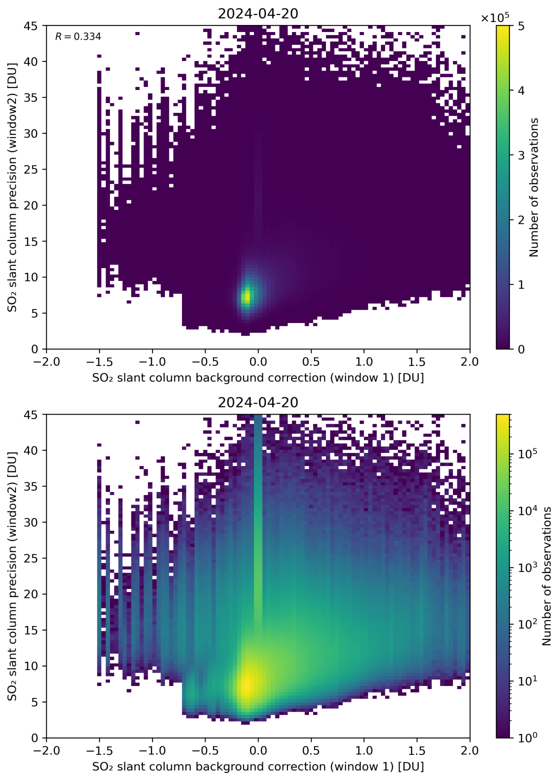
Figure 106: Scatter density plot of “SO 2 slant column background correction (window 1)” against “SO 2 slant column precision (window2)” for 2024-04-19 to 2024-04-21.
