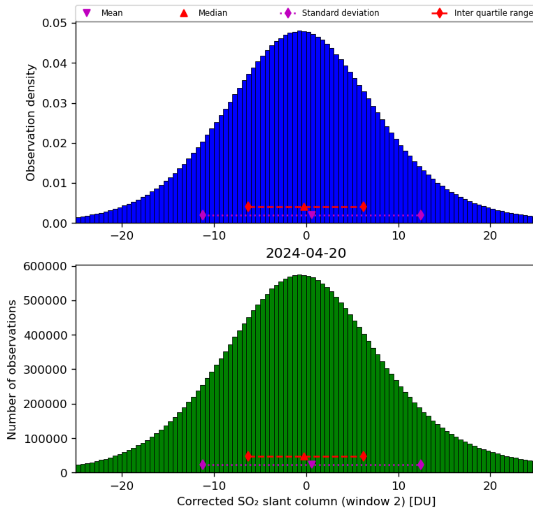
Figure 62: Histogram of “Corrected SO 2 slant column (window 2)” for 2024-04-19 to 2024-04-21
