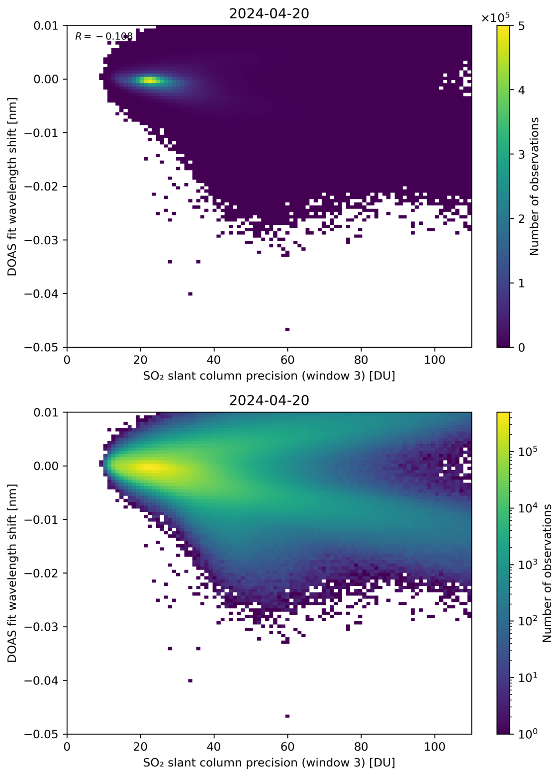
Figure 258: Scatter density plot of “SO 2 slant column precision (window 3)” against “DOAS fit wavelength shift” for 2024-04-19 to 2024-04-21.
