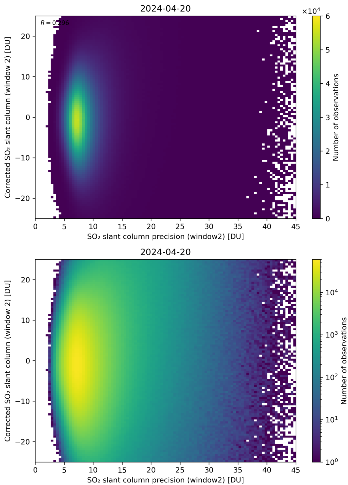
Figure 247: Scatter density plot of “SO 2 slant column precision (window2)” against “Corrected SO 2 slant column (window 2)” for 2024-04-19 to 2024-04-21.
