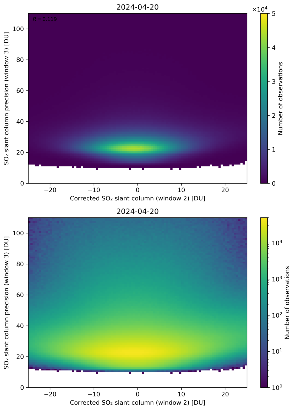
Figure 202: Scatter density plot of “Corrected SO 2 slant column (window 2)” against “SO 2 slant column precision (window 3)” for 2024-04-19 to 2024-04-21.
