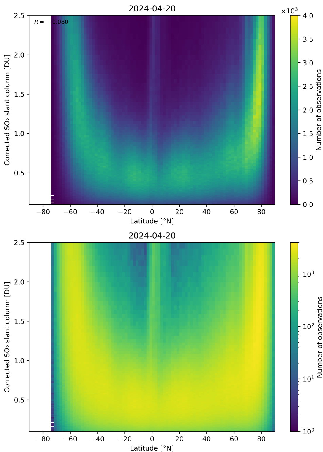
Figure 146: Scatter density plot of “Latitude” against “Corrected SO 2 slant column” for 2024-04-19 to 2024-04-21.
