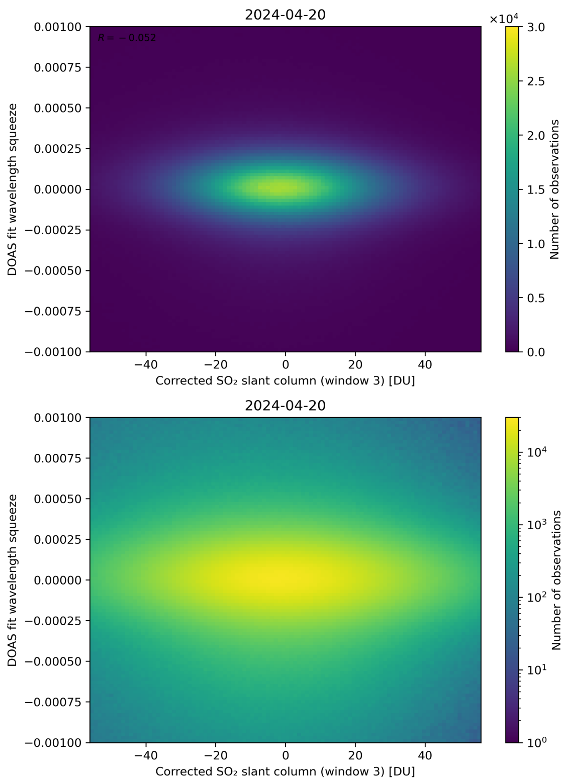
Figure 207: Scatter density plot of “Corrected SO 2 slant column (window 3)” against “DOAS fit wavelength squeeze” for 2024-04-19 to 2024-04-21.
