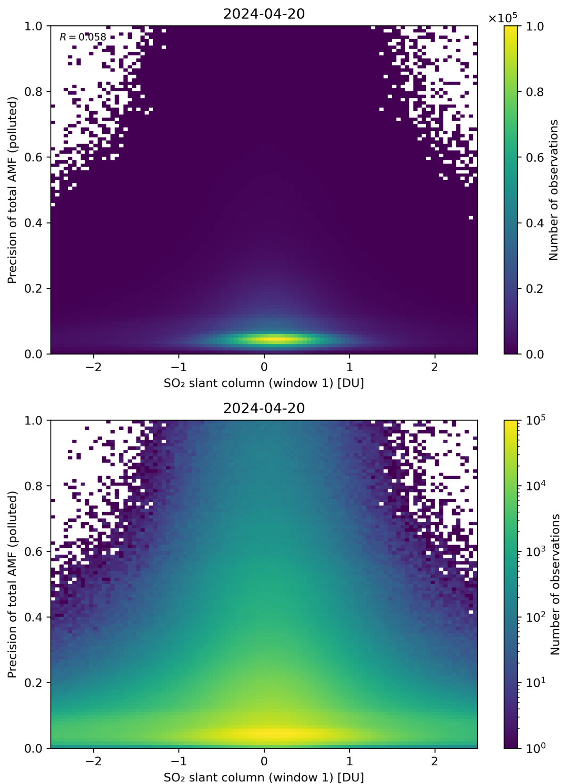
Figure 240: Scatter density plot of “SO 2 slant column (window 1)” against “Precision of total AMF (polluted)” for 2024-04-19 to 2024-04-21.
