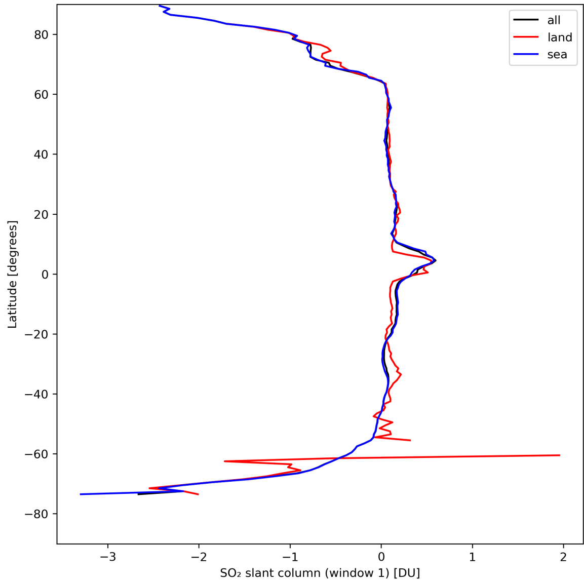
Figure 33: Zonal average of “SO 2 slant column (window 1)” for 2024-04-19 to 2024-04-21.
