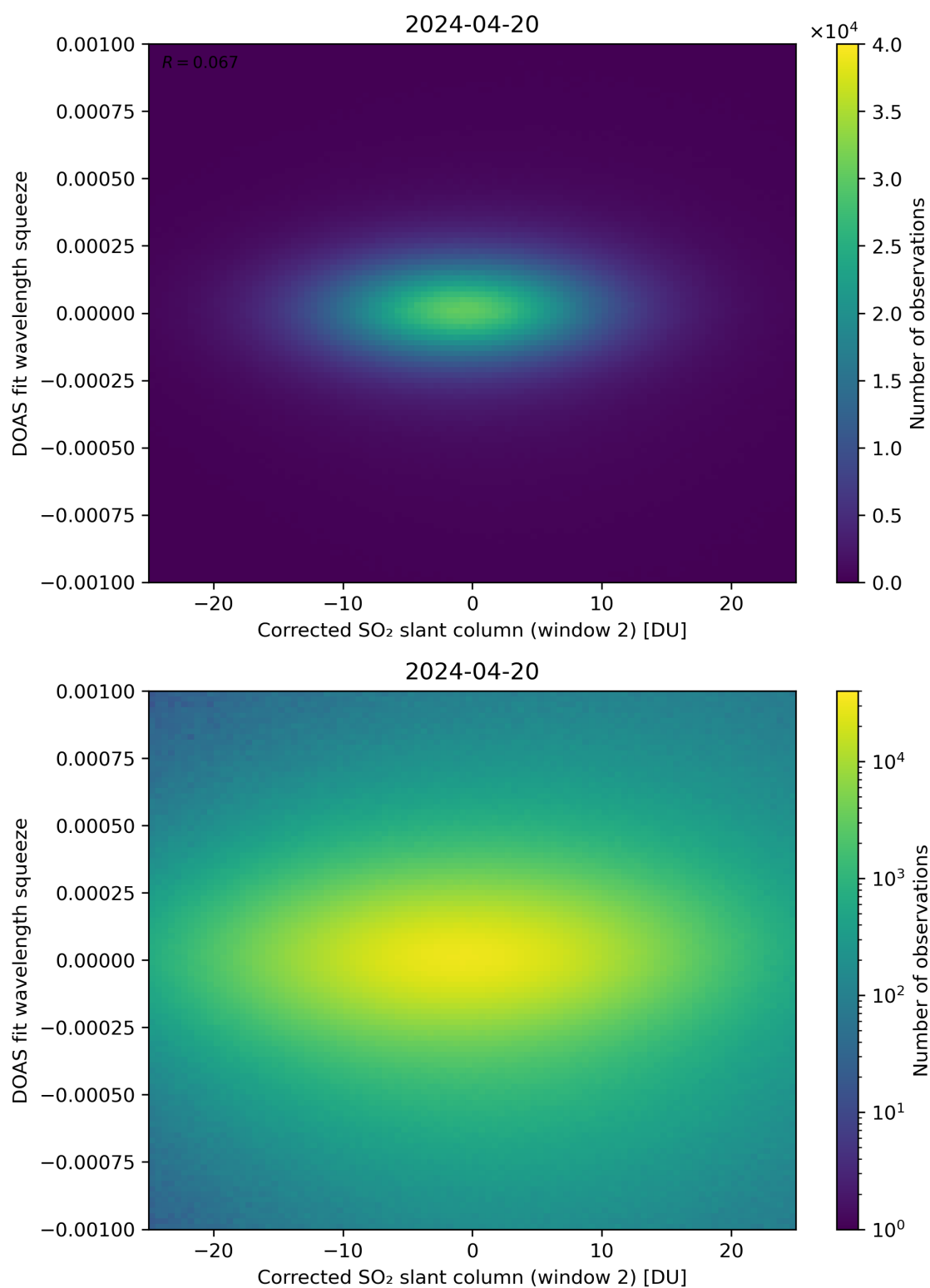
Figure 197: Scatter density plot of “Corrected SO 2 slant column (window 2)” against “DOAS fit wavelength squeeze” for 2024-04-19 to 2024-04-21.
