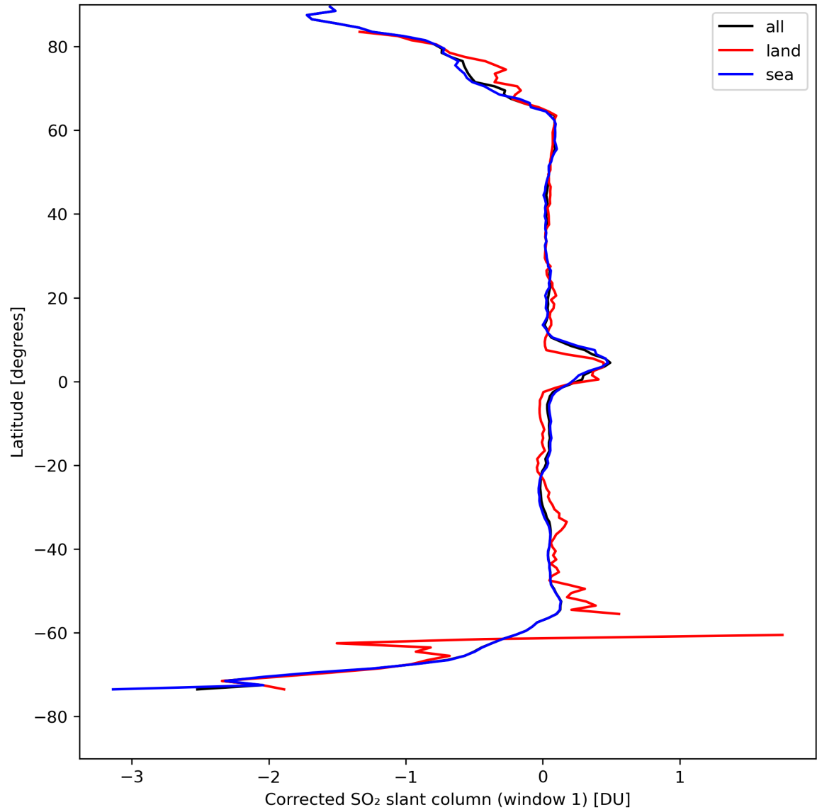
Figure 35: Zonal average of “Corrected SO 2 slant column (window 1)” for 2024-04-19 to 2024-04-21.
