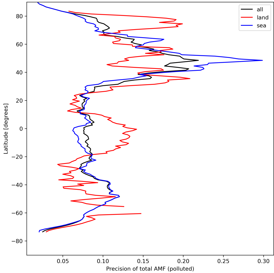
Figure 49: Zonal average of “Precision of total AMF (polluted)” for 2024-04-19 to 2024-04-21.
