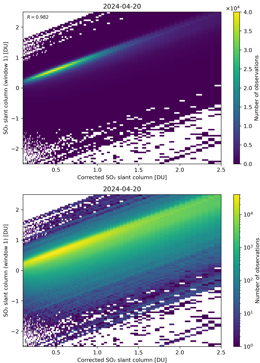
Figure 187: Scatter density plot of “Corrected SO 2 slant column” against “SO 2 slant column (window 1)” for 2024-04-19 to 2024-04-21.
