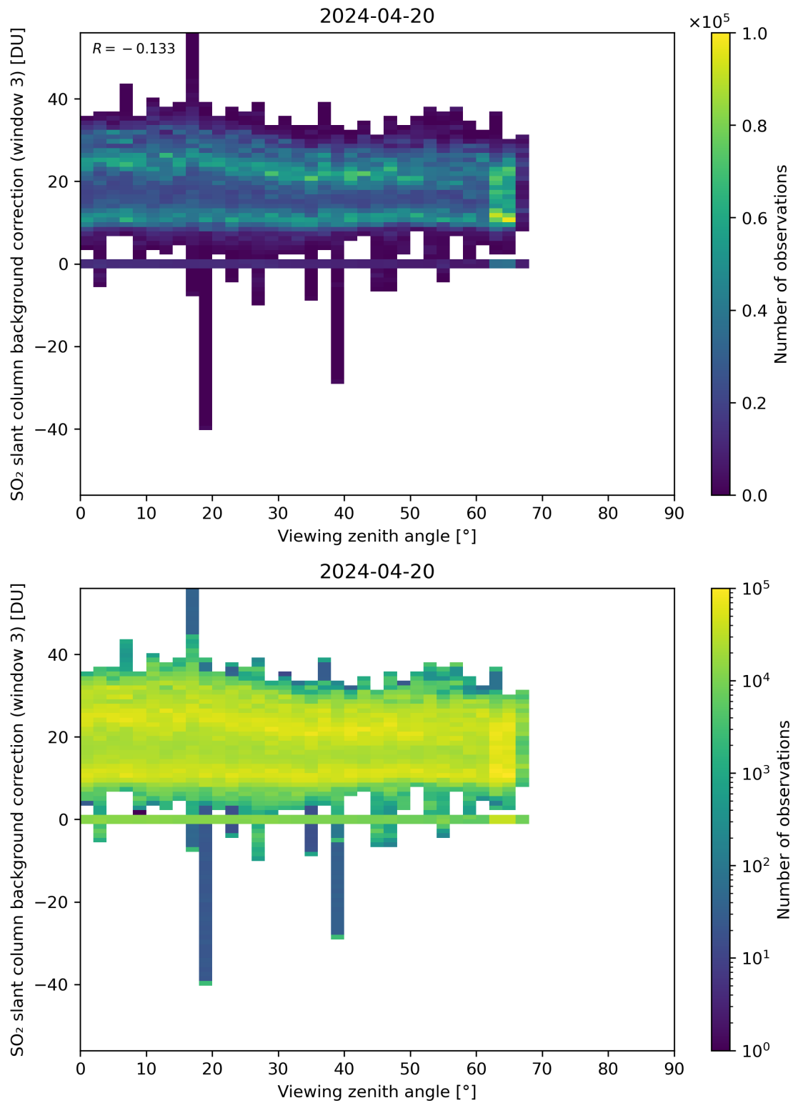
Figure 310: Scatter density plot of “Viewing zenith angle” against “SO 2 slant column background correction (window 3)” for 2024-04-19 to 2024-04-21.
