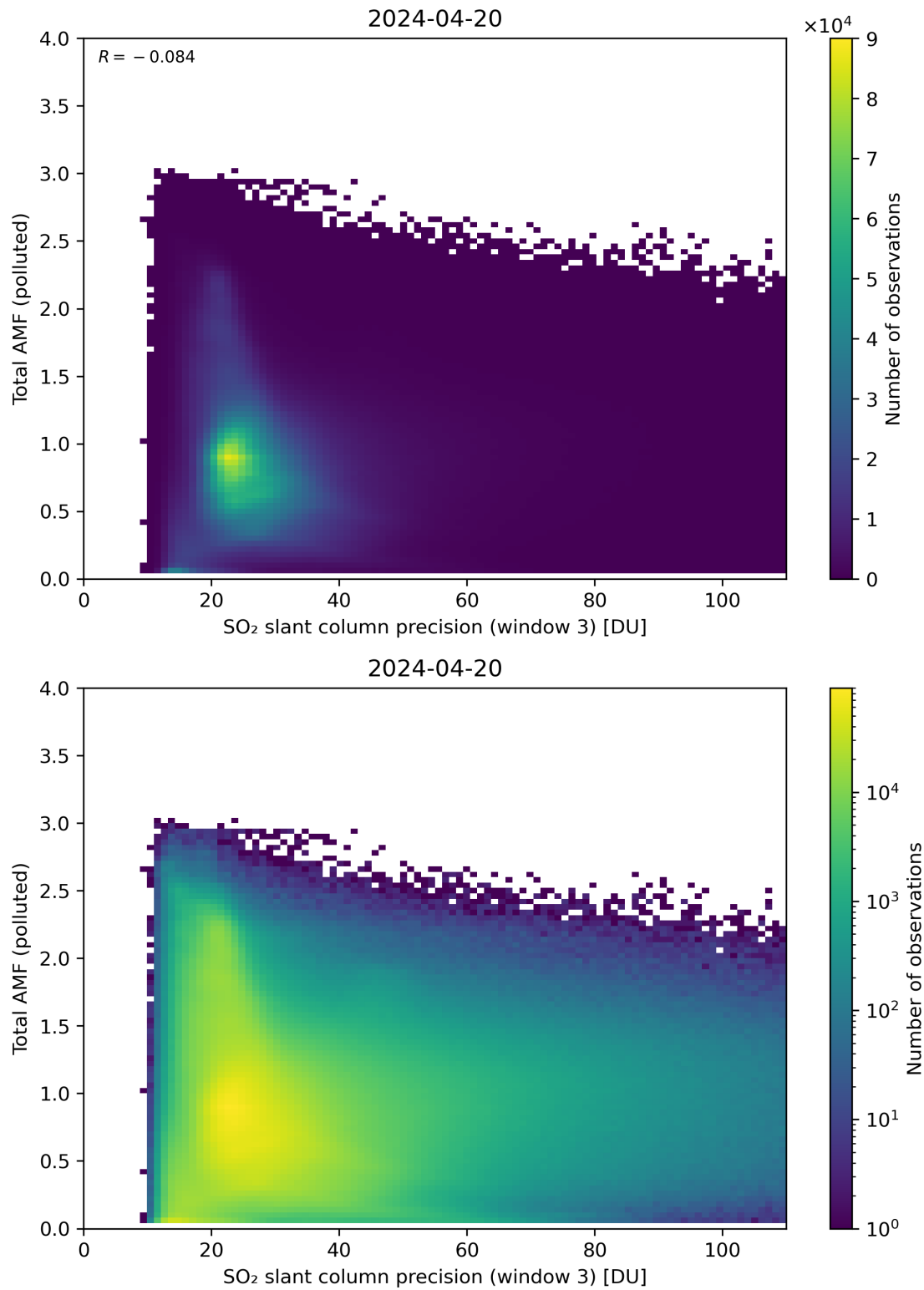
Figure 263: Scatter density plot of “SO 2 slant column precision (window 3)” against “Total AMF (polluted)” for 2024-04-19 to 2024-04-21.
