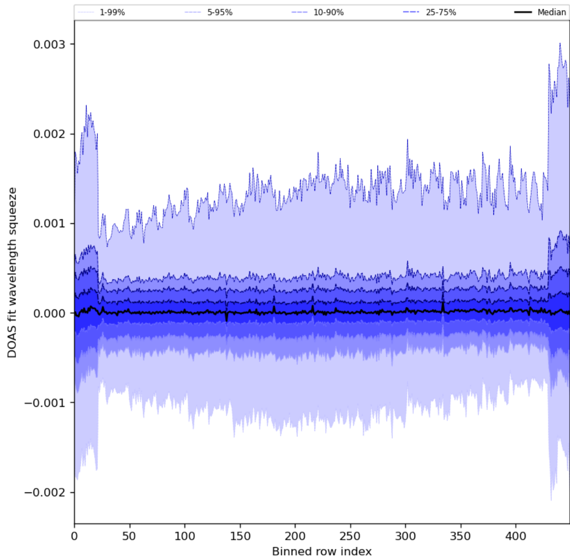
Figure 92: Along track statistics of “DOAS fit wavelength squeeze” for 2024-04-19 to 2024-04-21
