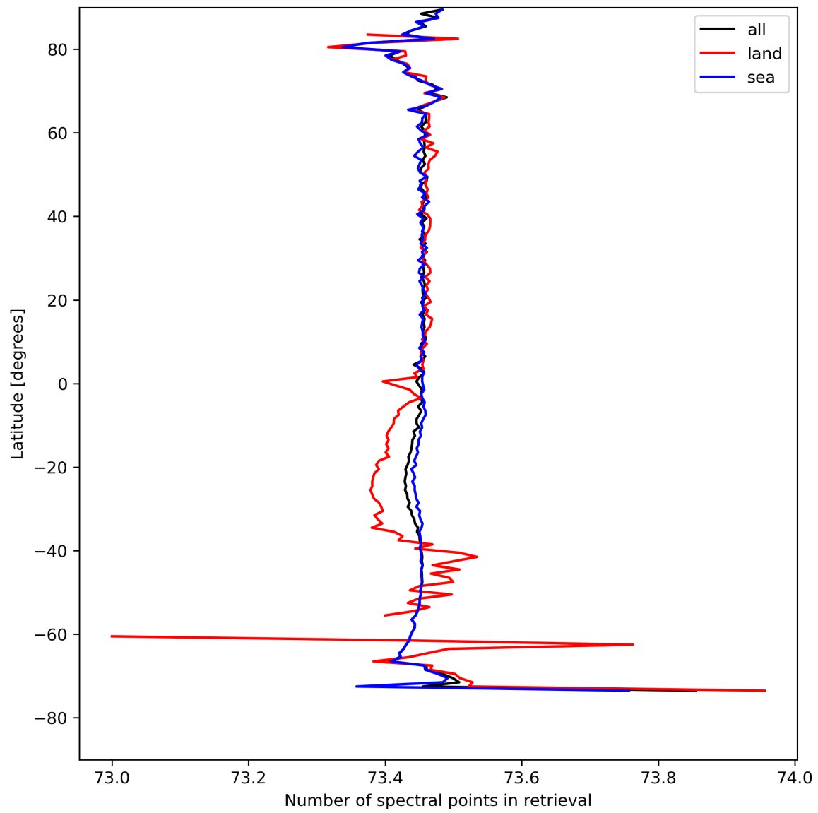
Figure 51: Zonal average of “Number of spectral points in retrieval” for 2024-04-19 to 2024-04-21.
