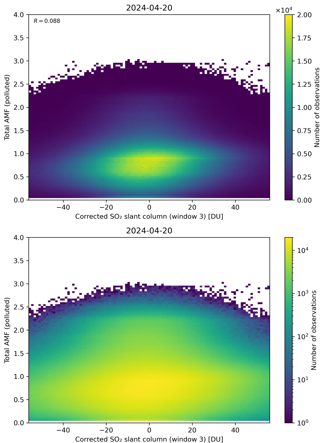
Figure 210: Scatter density plot of “Corrected SO 2 slant column (window 3)” against “Total AMF (polluted)” for 2024-04-19 to 2024-04-21.
