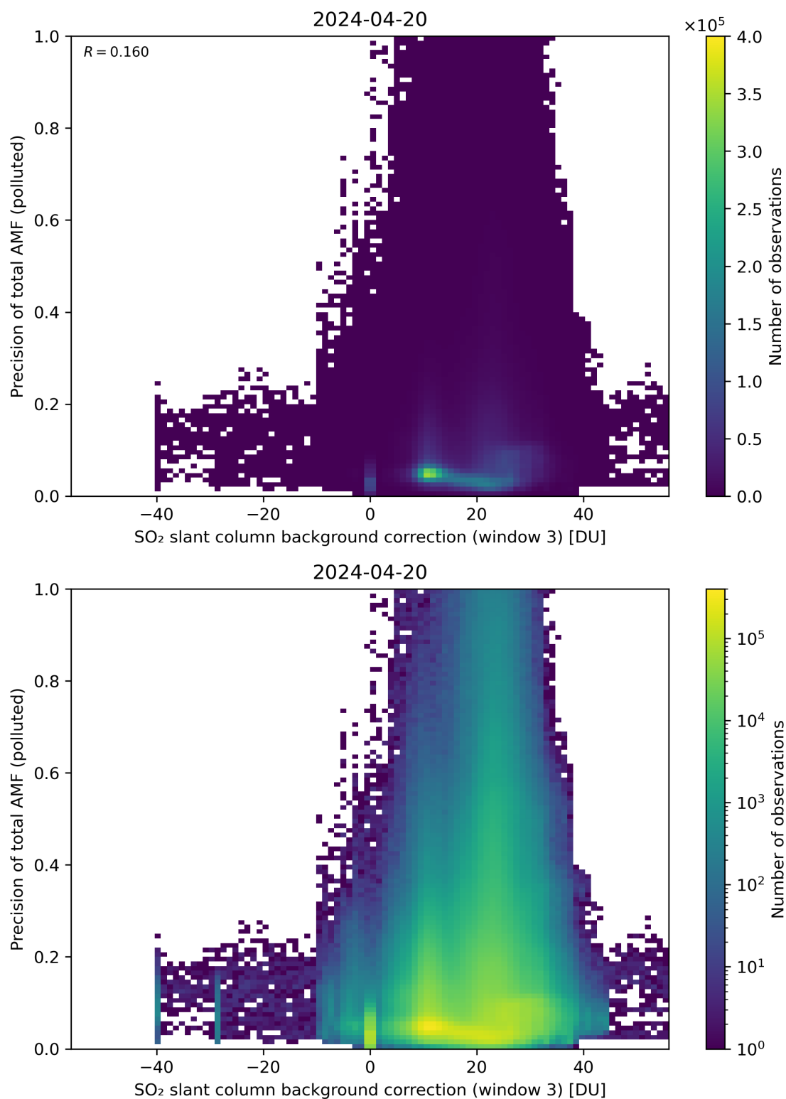
Figure 126: Scatter density plot of “SO 2 slant column background correction (window 3)” against “Precision of total AMF (polluted)” for 2024-04-19 to 2024-04-21.
