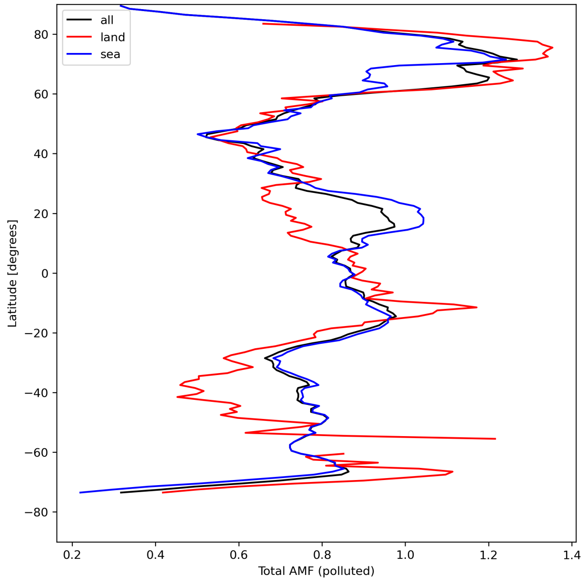
Figure 48: Zonal average of “Total AMF (polluted)” for 2024-04-19 to 2024-04-21.
