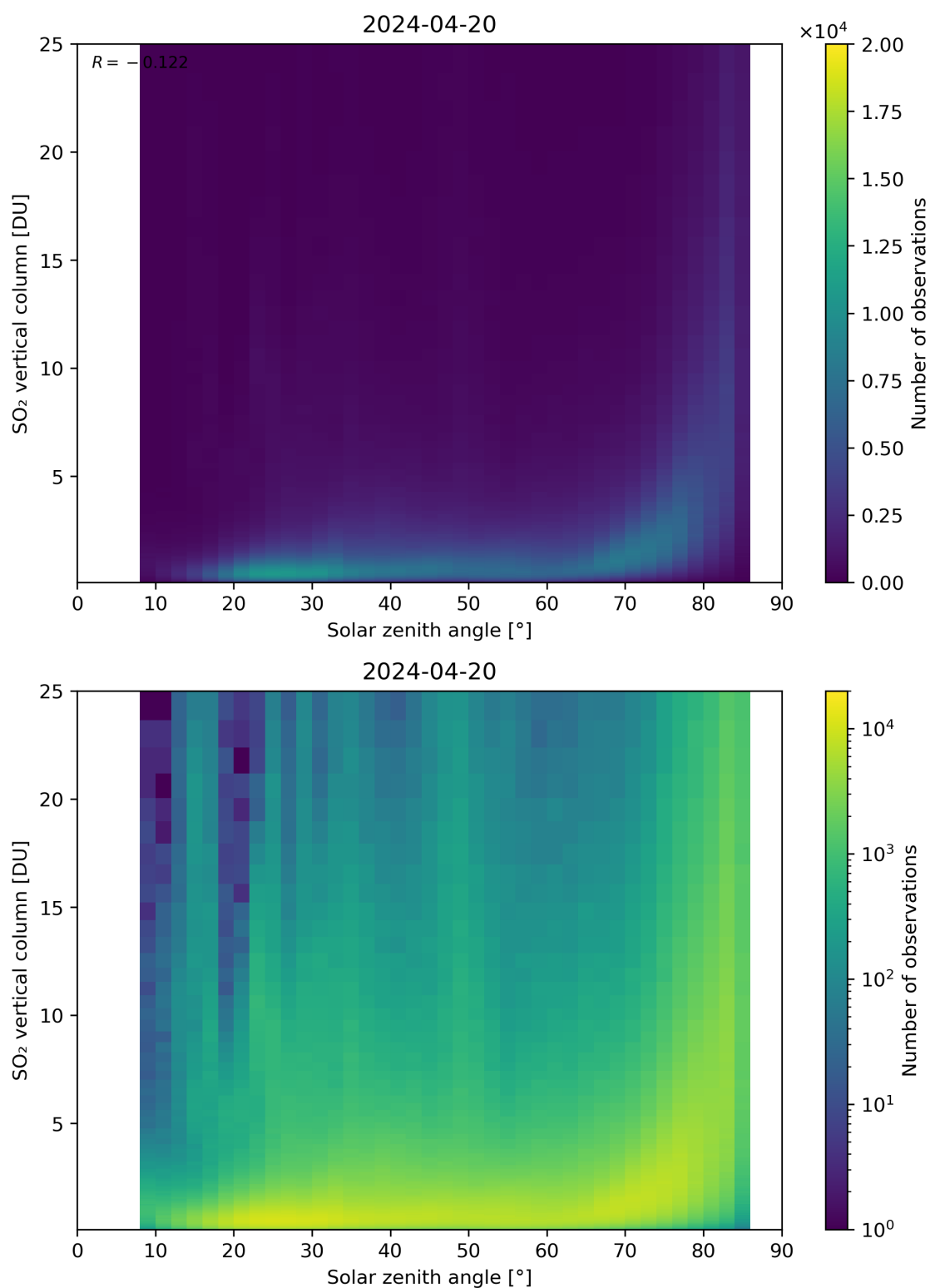
Figure 176: Scatter density plot of “Solar zenith angle” against “SO 2 vertical column” for 2024-04-19 to 2024-04-21.
