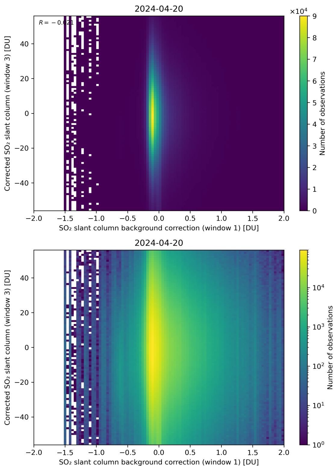
Figure 105: Scatter density plot of “SO 2 slant column background correction (window 1)” against “Corrected SO 2 slant column (window 3)” for 2024-04-19 to 2024-04-21.
