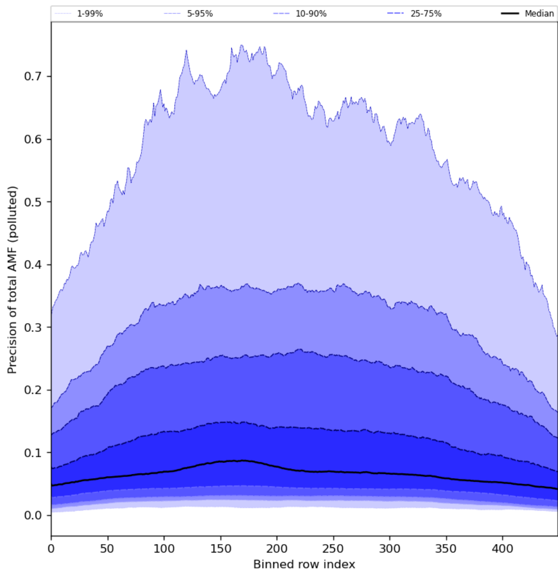
Figure 95: Along track statistics of “Precision of total AMF (polluted)” for 2024-04-19 to 2024-04-21
