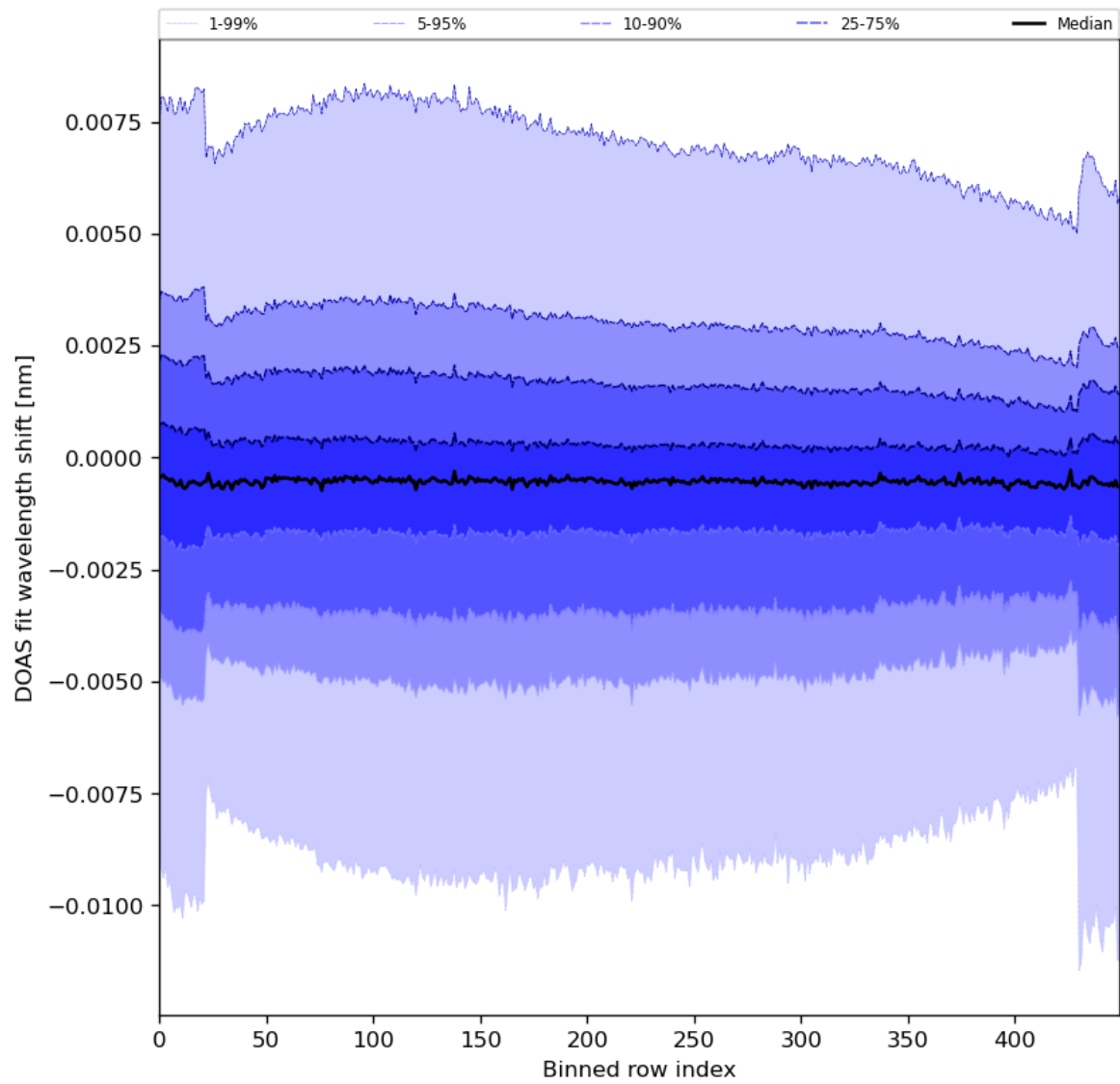
Figure 91: Along track statistics of “DOAS fit wavelength shift” for 2024-04-19 to 2024-04-21
