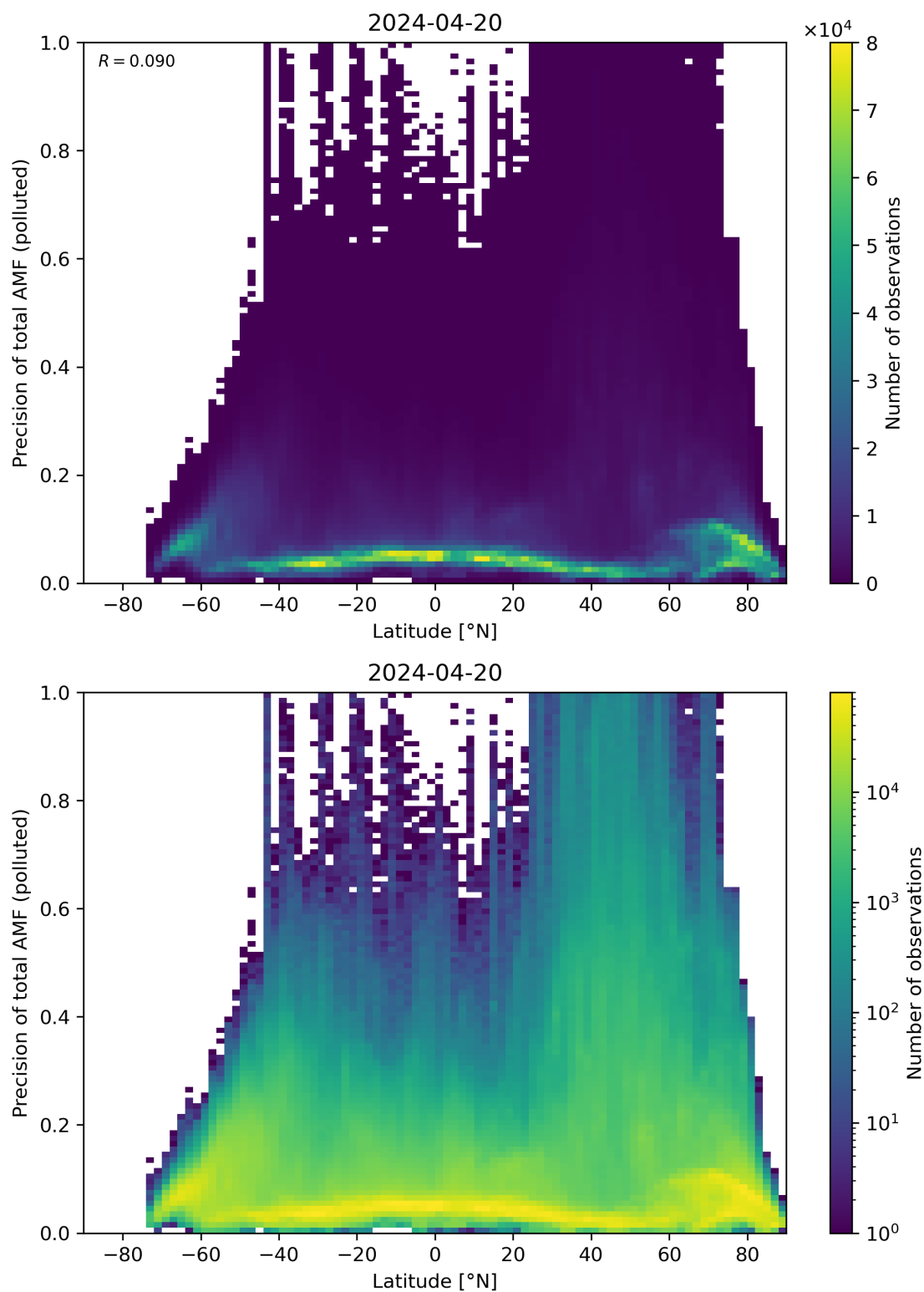
Figure 155: Scatter density plot of “Latitude” against “Precision of total AMF (polluted)” for 2024-04-19 to 2024-04-21.
