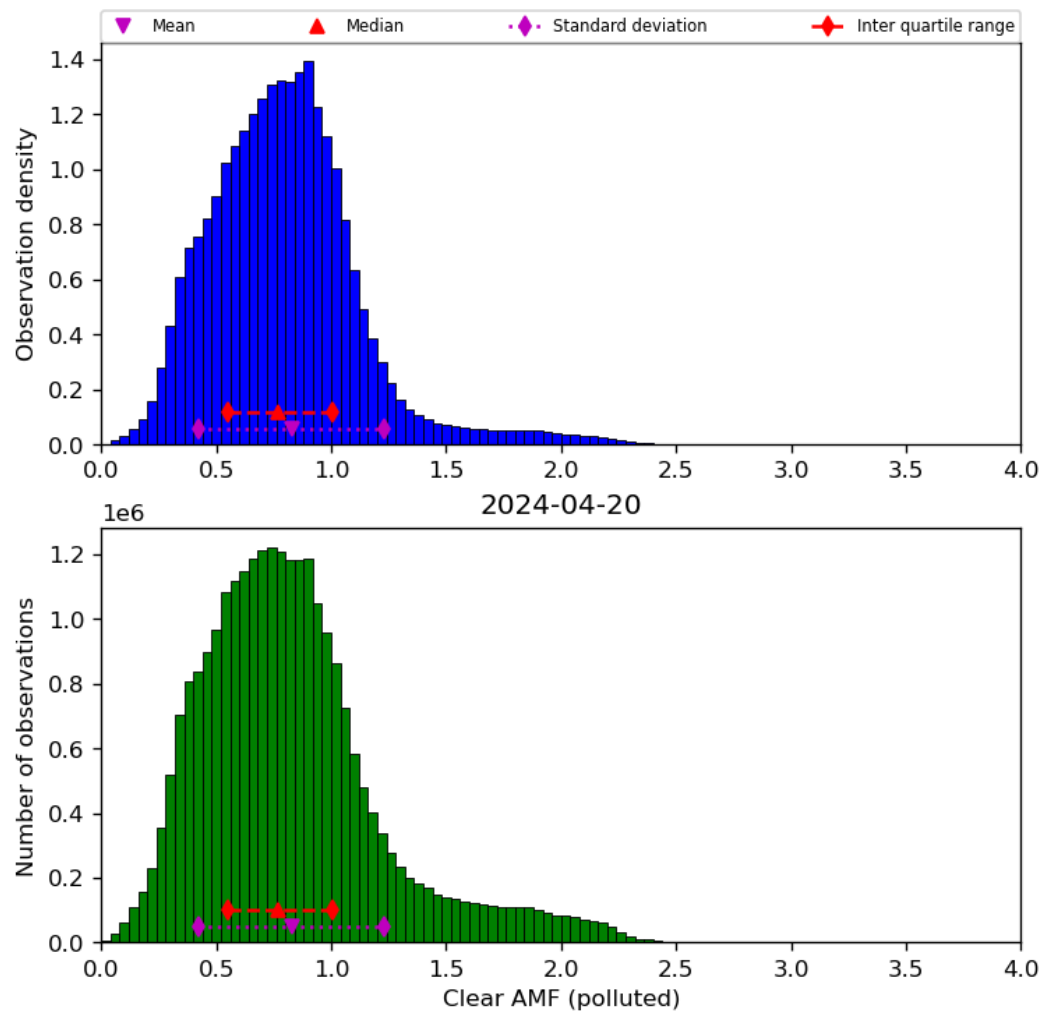
Figure 73: Histogram of “Clear AMF (polluted)” for 2024-04-19 to 2024-04-21
