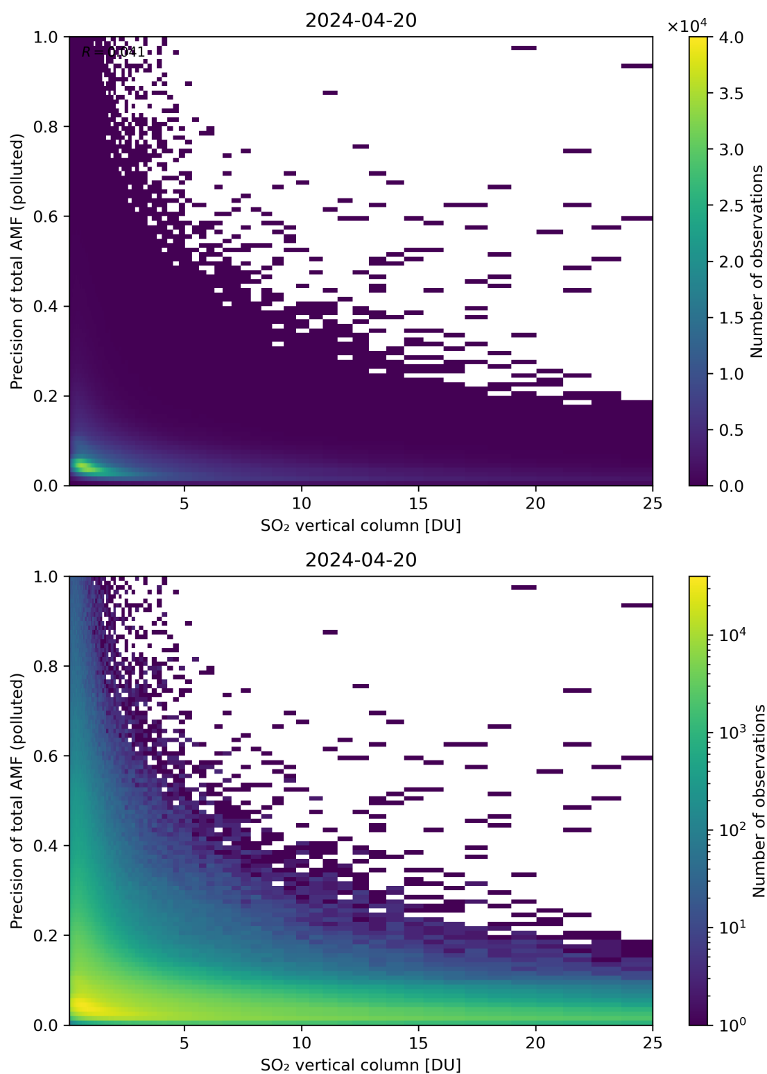
Figure 306: Scatter density plot of “SO 2 vertical column” against “Precision of total AMF (polluted)” for 2024-04-19 to 2024-04-21.
