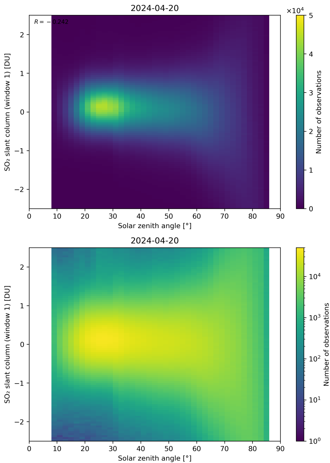
Figure 169: Scatter density plot of “Solar zenith angle” against “SO 2 slant column (window 1)” for 2024-04-19 to 2024-04-21.
