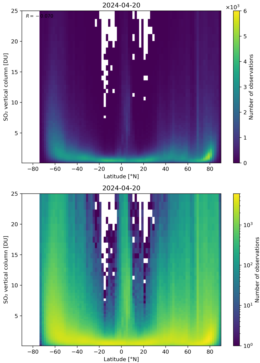
Figure 156: Scatter density plot of “Latitude” against “SO 2 vertical column” for 2024-04-19 to 2024-04-21.
