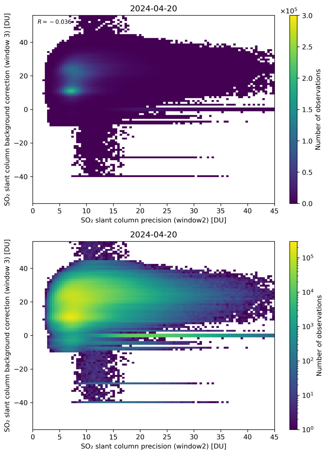
Figure 242: Scatter density plot of “SO 2 slant column precision (window2)” against “SO 2 slant column background correction (window 3)” for 2024-04-19 to 2024-04-21.
