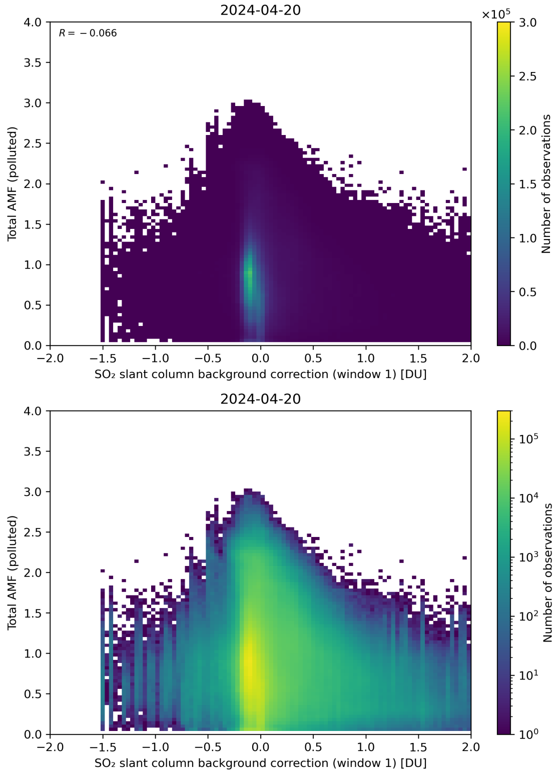
Figure 109: Scatter density plot of “SO 2 slant column background correction (window 1)” against “Total AMF (polluted)” for 2024-04-19 to 2024-04-21.
