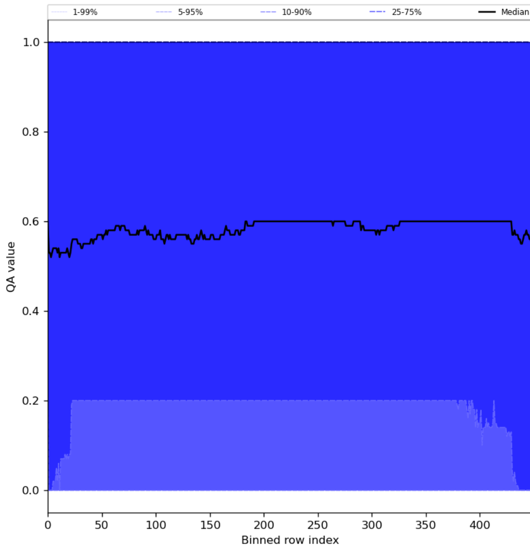
Figure 75: Along track statistics of “QA value” for 2024-04-19 to 2024-04-21
