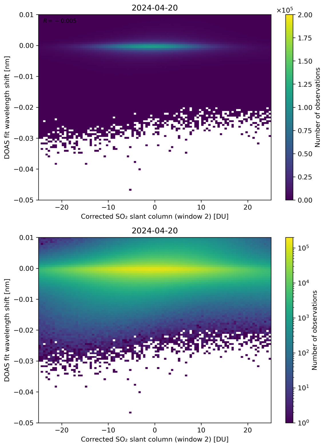
Figure 196: Scatter density plot of “Corrected SO 2 slant column (window 2)” against “DOAS fit wavelength shift” for 2024-04-19 to 2024-04-21.
