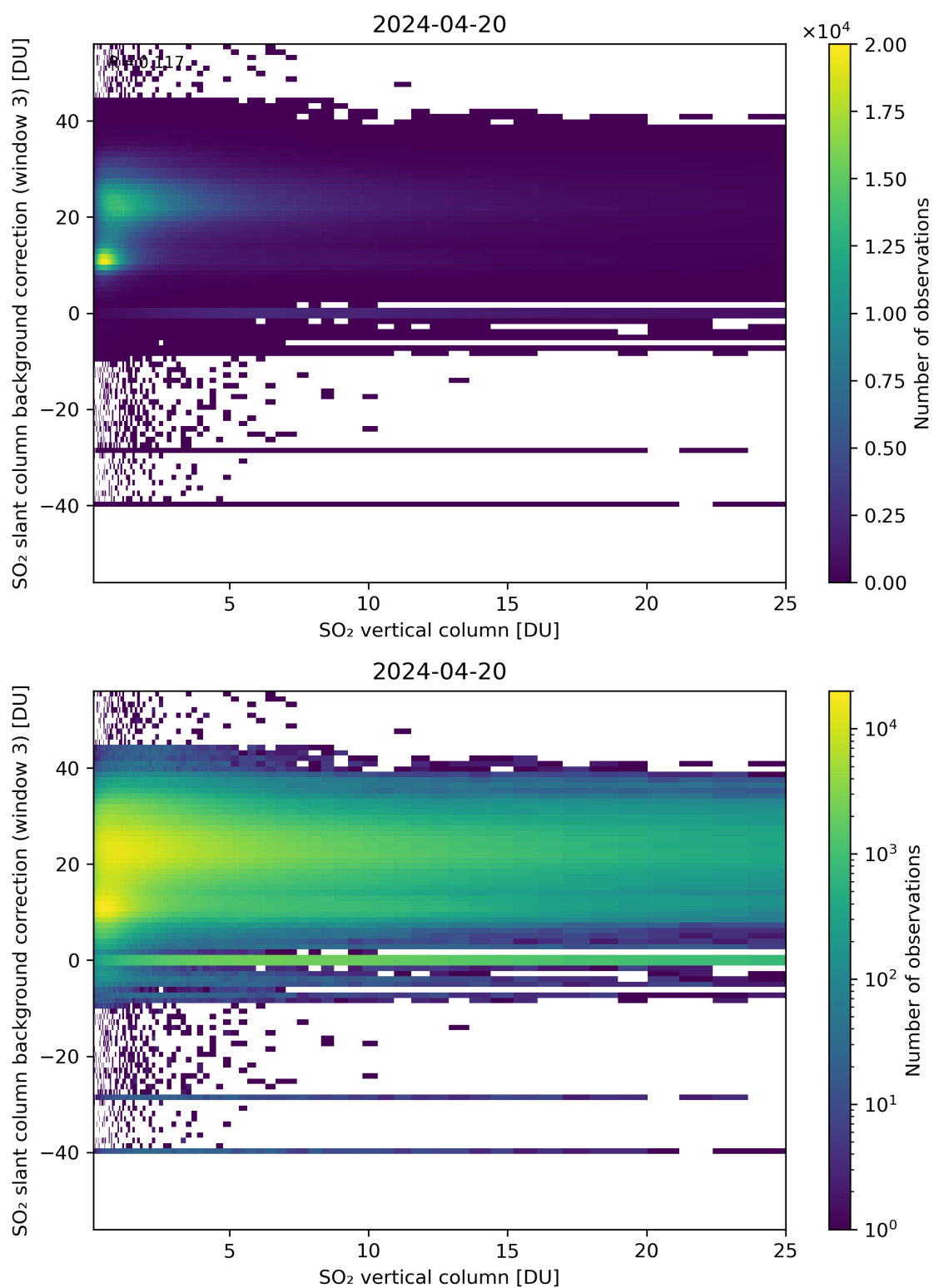
Figure 275: Scatter density plot of “SO 2 vertical column” against “SO 2 slant column background correction (window 3)” for 2024-04-19 to 2024-04-21.
