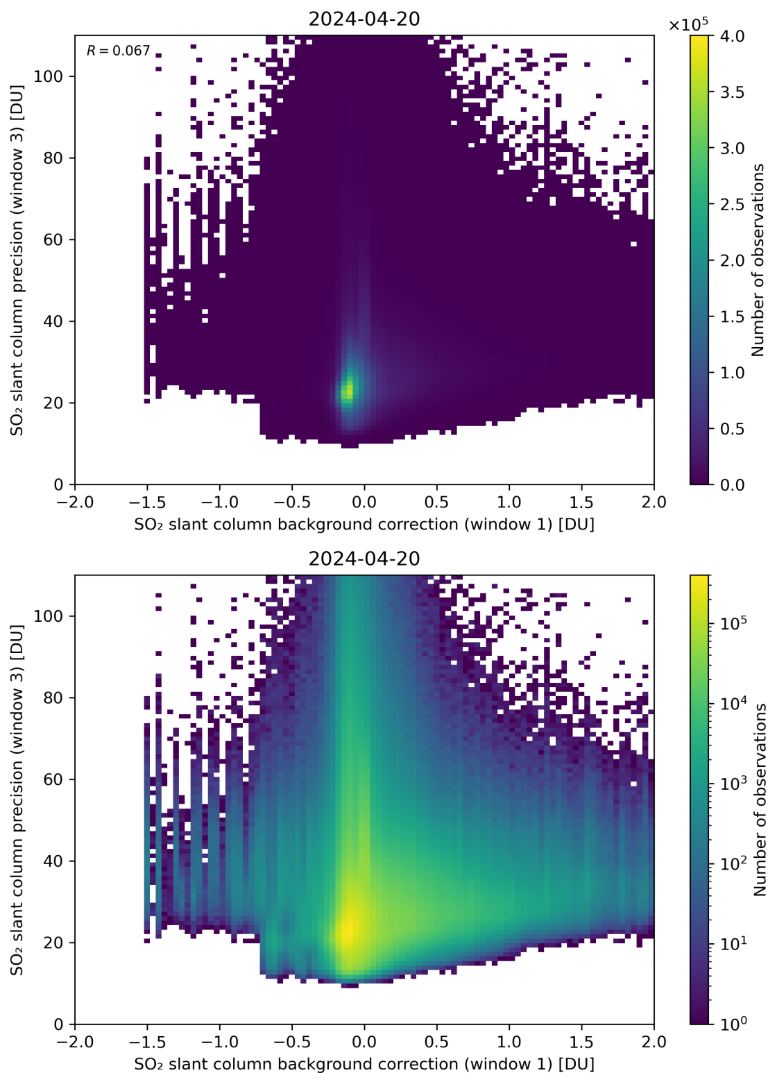
Figure 108: Scatter density plot of “SO 2 slant column background correction (window 1)” against “SO 2 slant column precision (window 3)” for 2024-04-19 to 2024-04-21.
