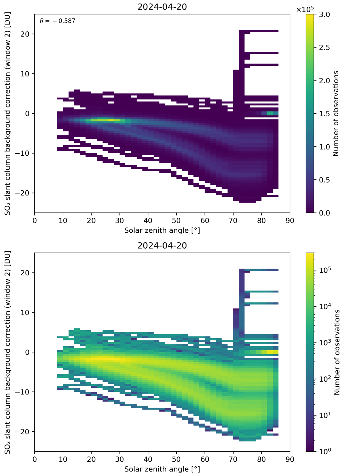
Figure 159: Scatter density plot of “Solar zenith angle” against “SO 2 slant column background correction (window 2)” for 2024-04-19 to 2024-04-21.
