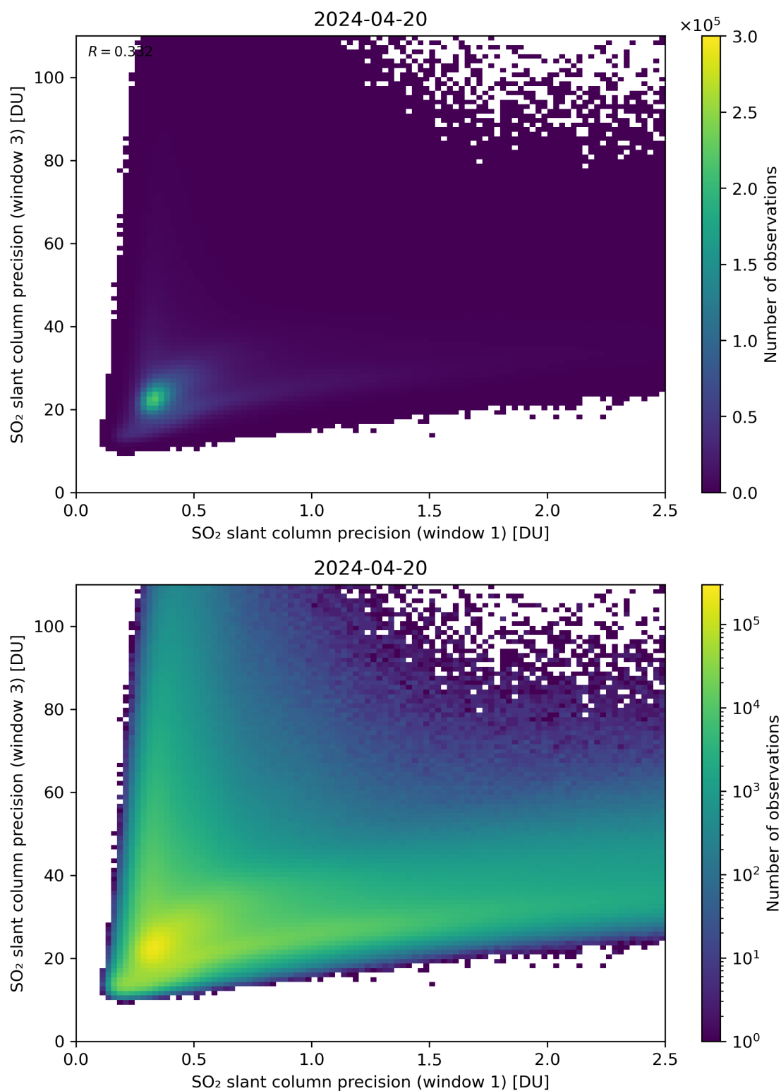
Figure 229: Scatter density plot of “SO 2 slant column precision (window 1)” against “SO 2 slant column precision (window 3)” for 2024-04-19 to 2024-04-21.
