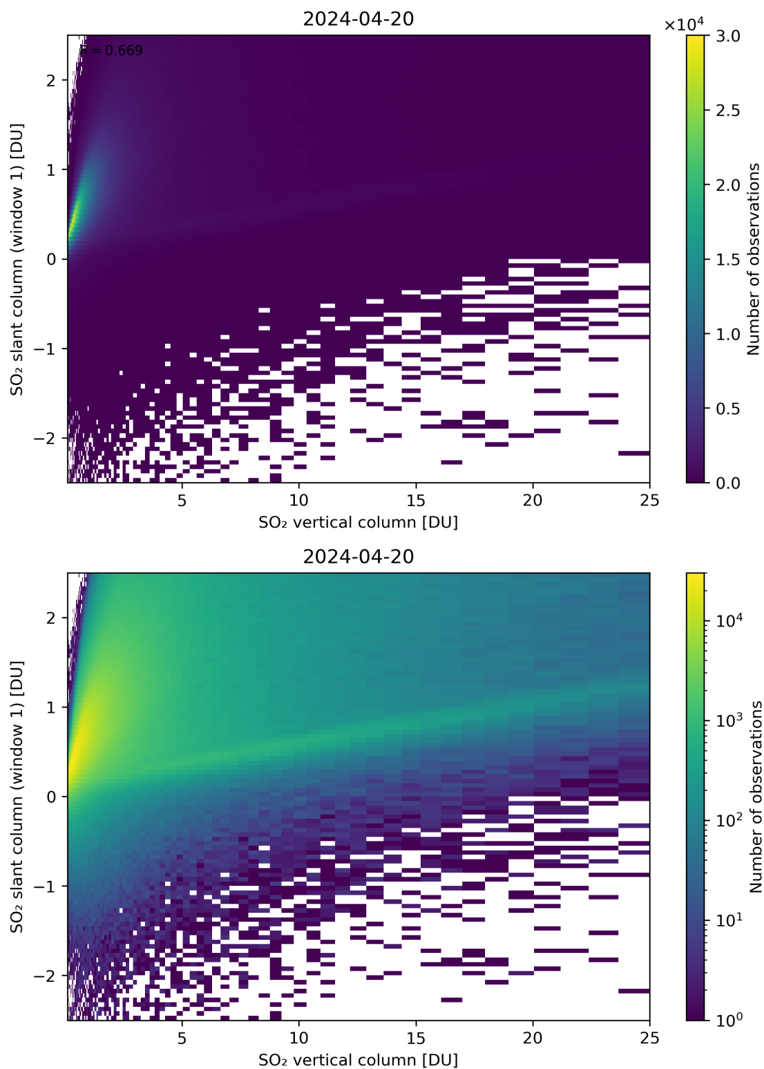
Figure 300: Scatter density plot of “SO 2 vertical column” against “SO 2 slant column (window 1)” for 2024-04-19 to 2024-04-21.
