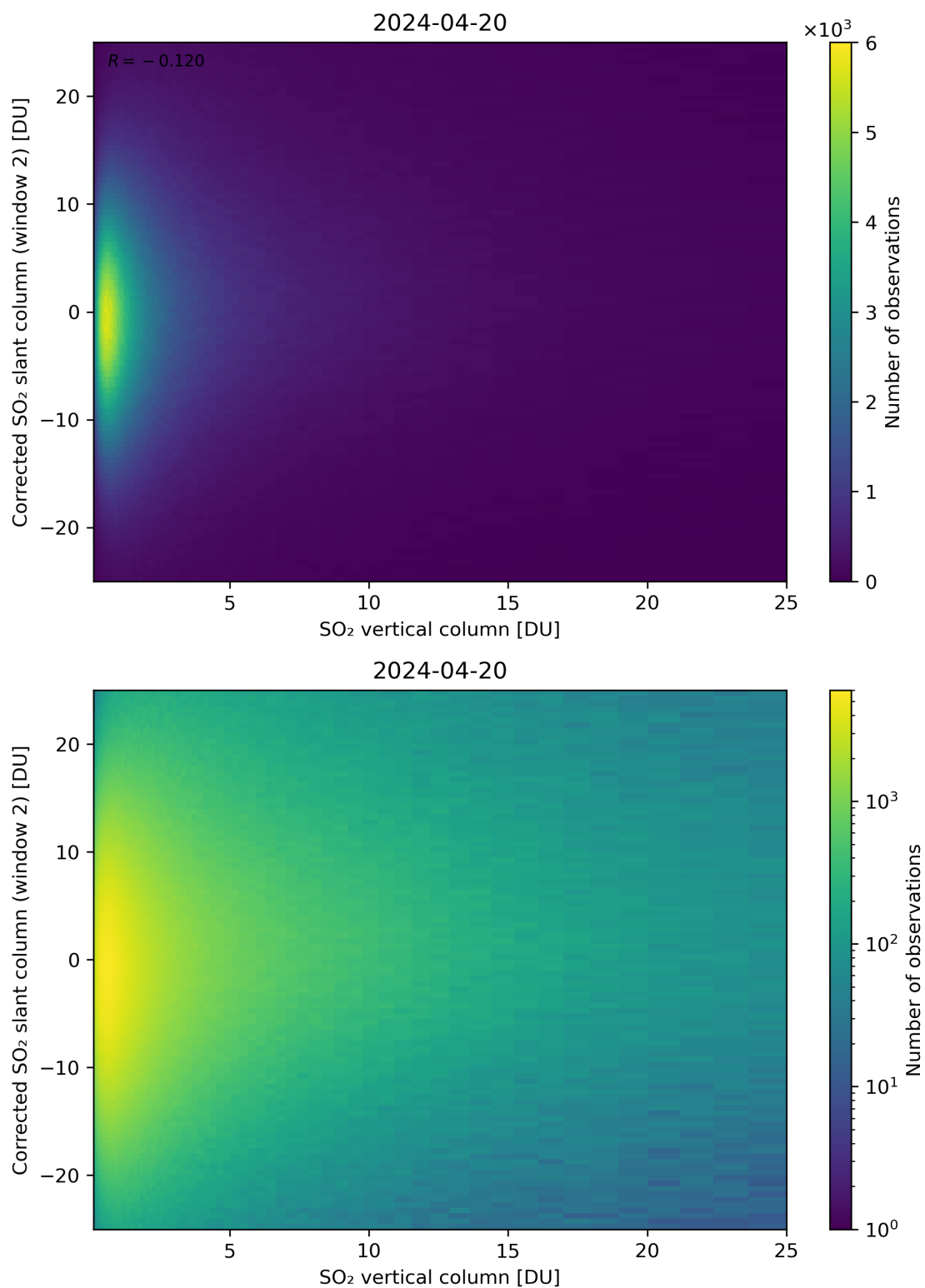
Figure 298: Scatter density plot of “SO 2 vertical column” against “Corrected SO 2 slant column (window 2)” for 2024-04-19 to 2024-04-21.
