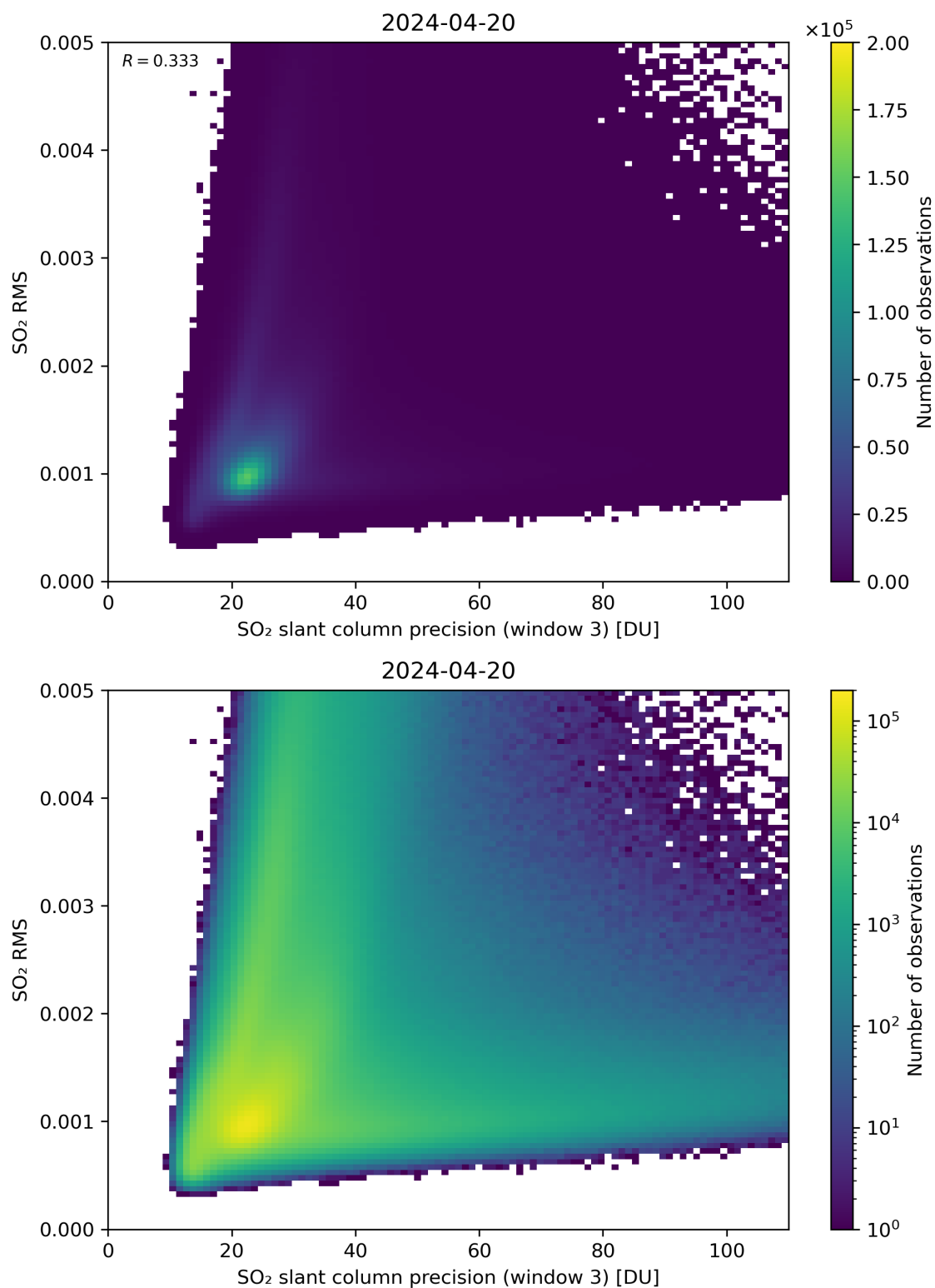
Figure 260: Scatter density plot of “SO 2 slant column precision (window 3)” against “SO 2 RMS” for 2024-04-19 to 2024-04-21.
