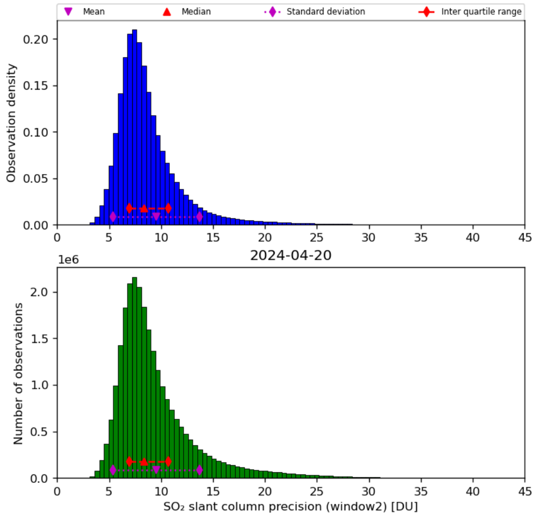
Figure 61: Histogram of “SO 2 slant column precision (window2)” for 2024-04-19 to 2024-04-21
