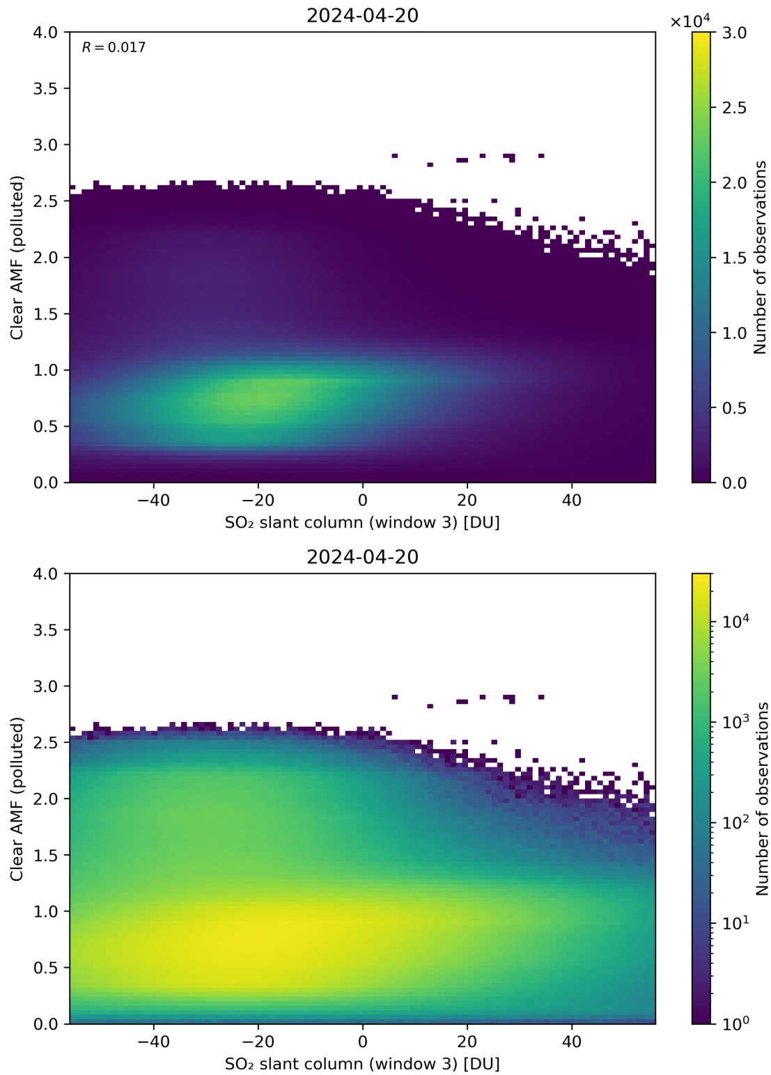
Figure 265: Scatter density plot of “SO 2 slant column (window 3)” against “Clear AMF (polluted)” for 2024-04-19 to 2024-04-21.
