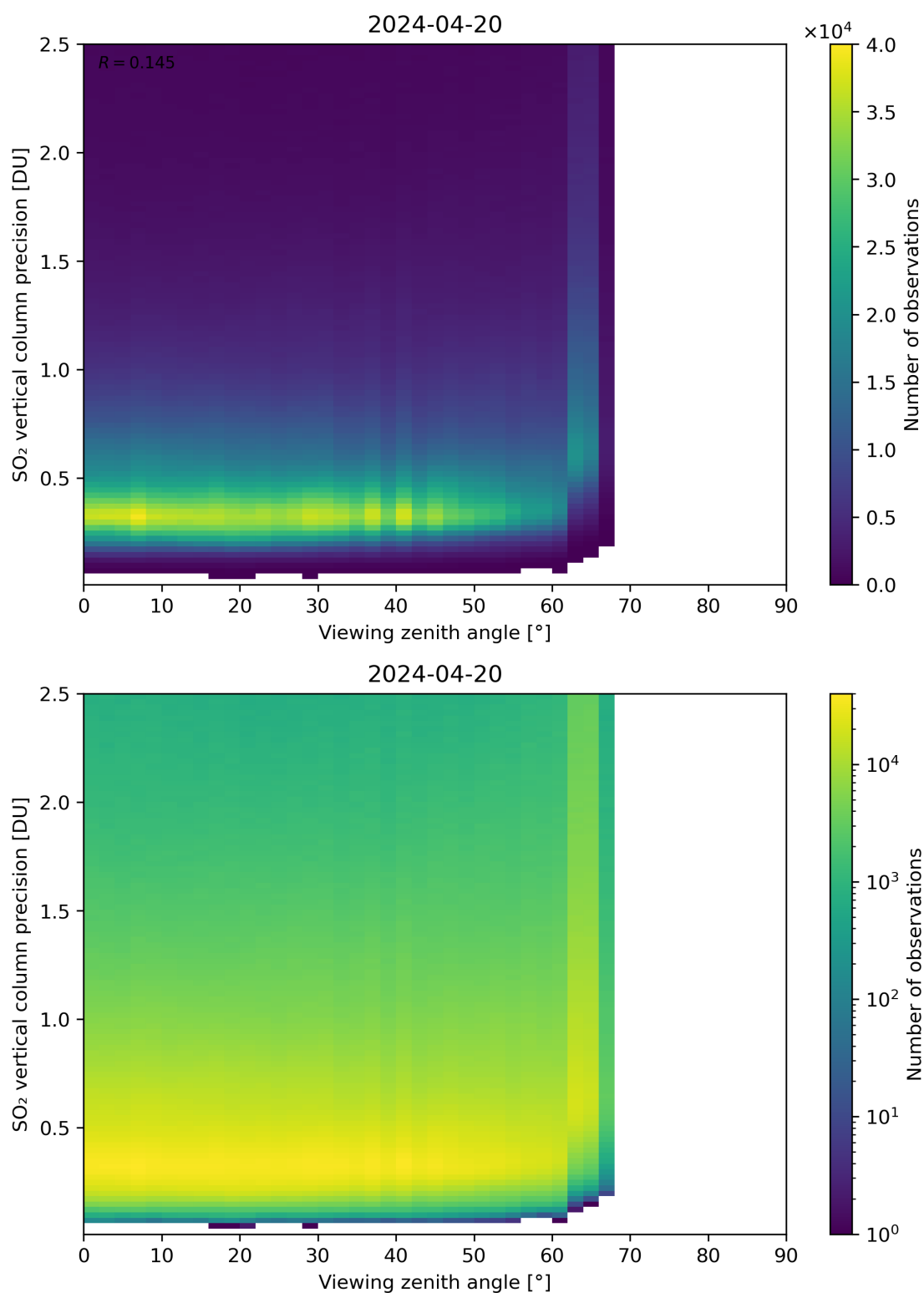
Figure 328: Scatter density plot of “Viewing zenith angle” against “SO 2 vertical column precision” for 2024-04-19 to 2024-04-21.
