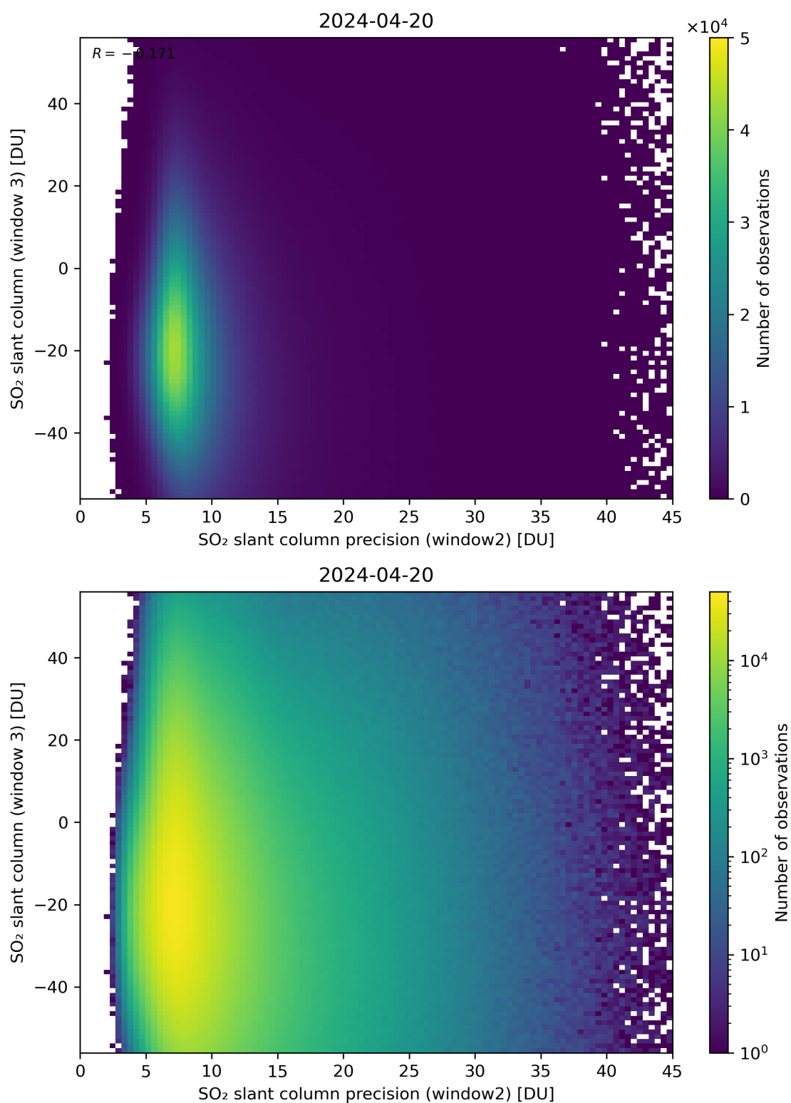
Figure 249: Scatter density plot of “SO 2 slant column precision (window2)” against “SO 2 slant column (window 3)” for 2024-04-19 to 2024-04-21.
