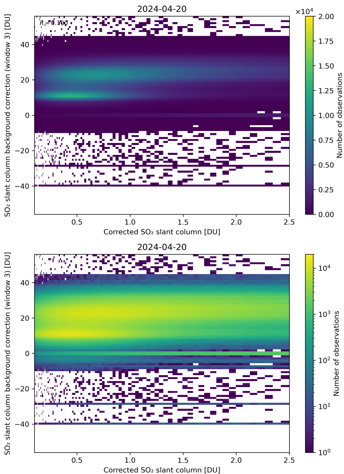
Figure 180: Scatter density plot of “Corrected SO 2 slant column” against “SO 2 slant column background correction (window 3)” for 2024-04-19 to 2024-04-21.
