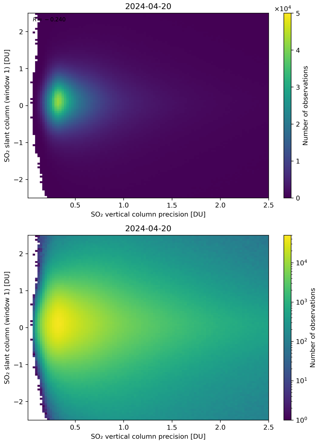
Figure 289: Scatter density plot of “SO 2 vertical column precision” against “SO 2 slant column (window 1)” for 2024-04-19 to 2024-04-21.
