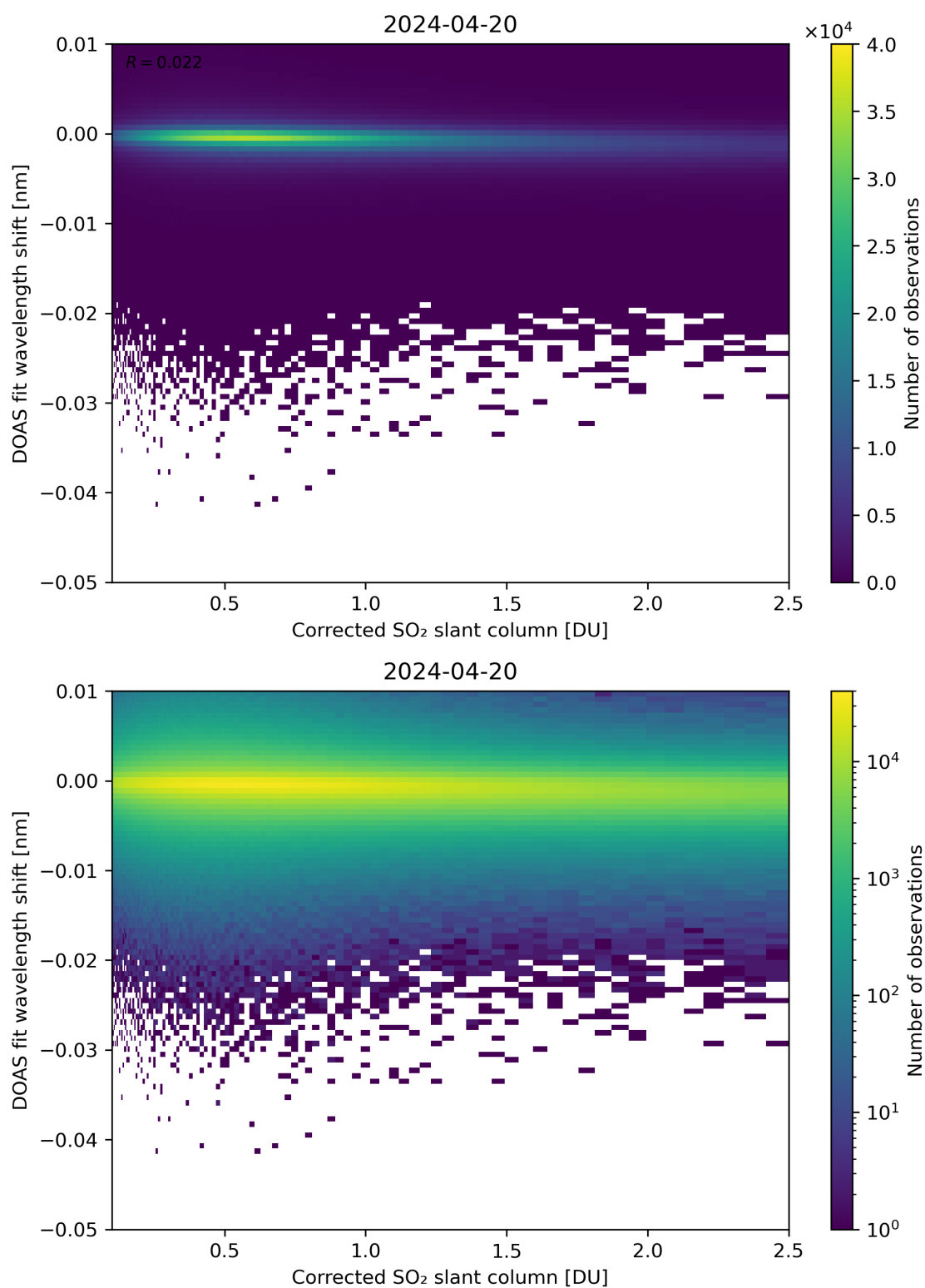
Figure 181: Scatter density plot of “Corrected SO 2 slant column” against “DOAS fit wavelength shift” for 2024-04-19 to 2024-04-21.
