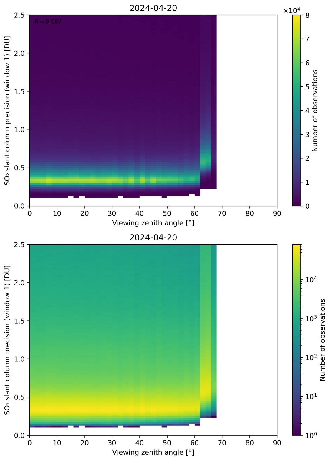
Figure 321: Scatter density plot of “Viewing zenith angle” against “SO 2 slant column precision (window 1)” for 2024-04-19 to 2024-04-21.
