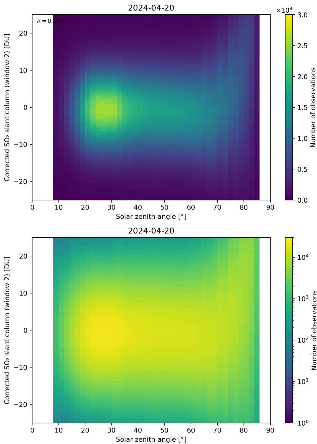
Figure 167: Scatter density plot of “Solar zenith angle” against “Corrected SO 2 slant column (window 2)” for 2024-04-19 to 2024-04-21.
