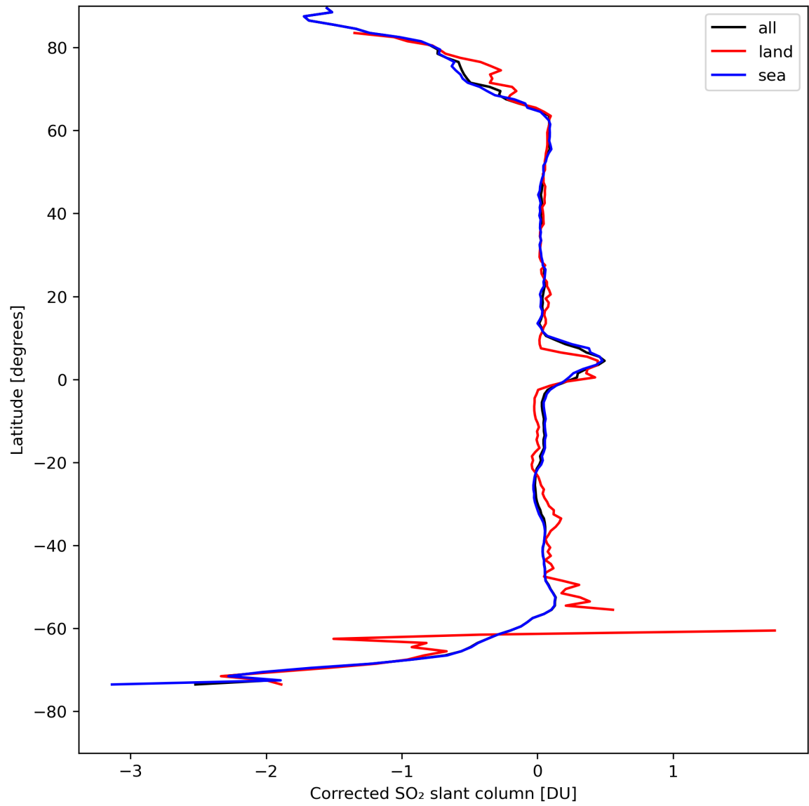
Figure 32: Zonal average of “Corrected SO 2 slant column” for 2024-04-19 to 2024-04-21.
