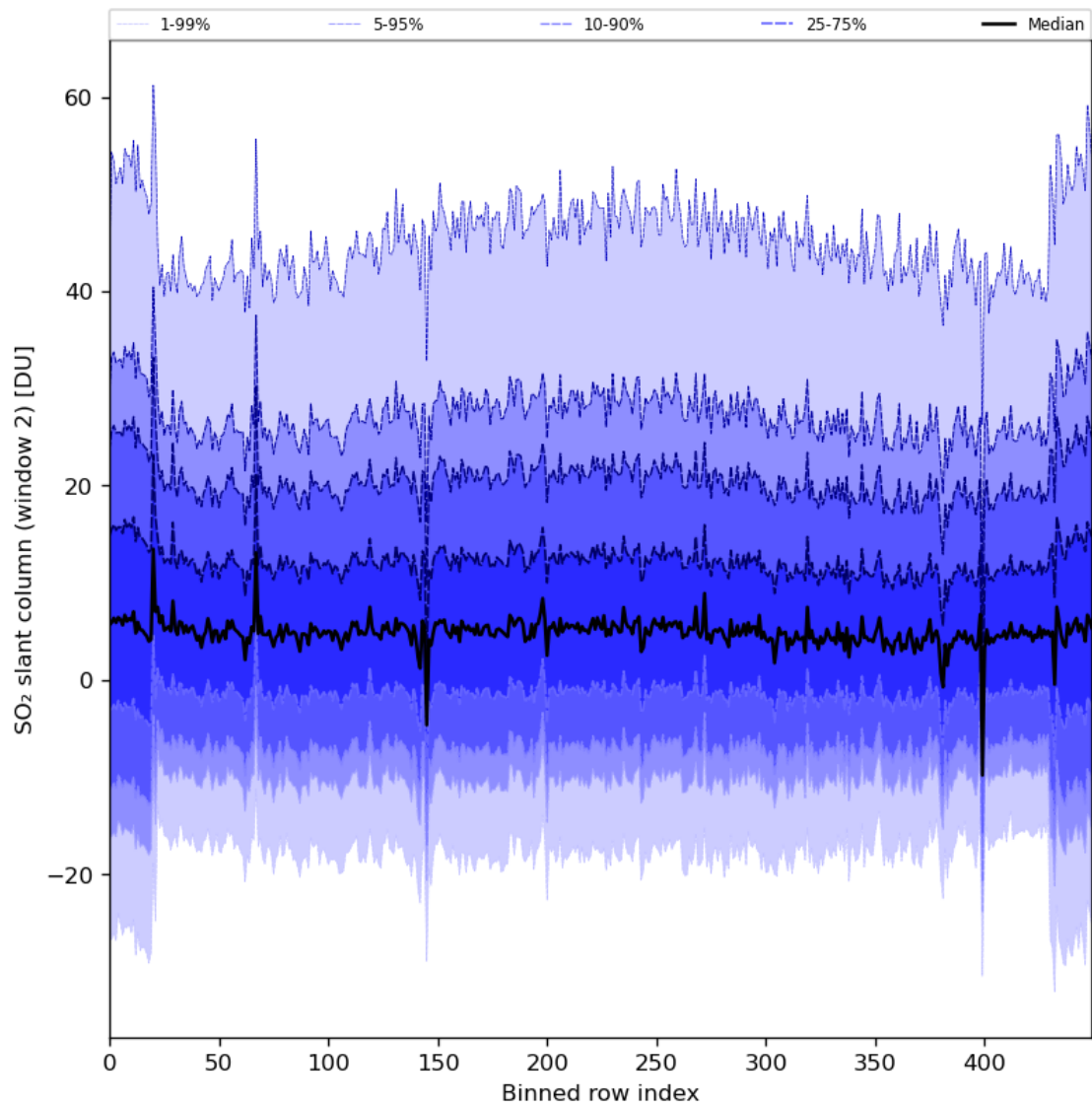
Figure 83: Along track statistics of “SO 2 slant column (window 2)” for 2024-04-19 to 2024-04-21
