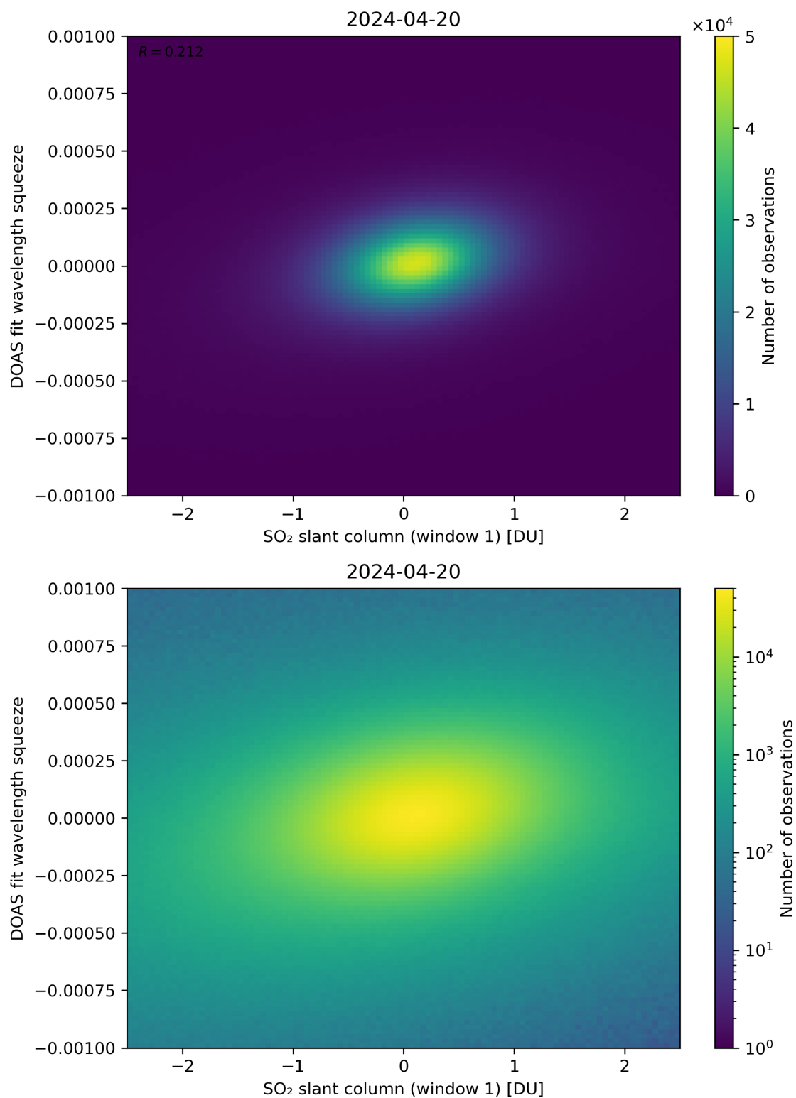
Figure 216: Scatter density plot of “SO 2 slant column (window 1)” against “DOAS fit wavelength squeeze” for 2024-04-19 to 2024-04-21.
