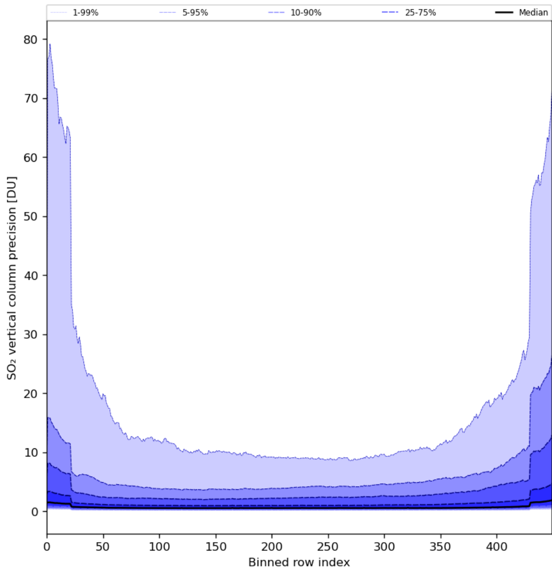
Figure 77: Along track statistics of “SO 2 vertical column precision” for 2024-04-19 to 2024-04-21
