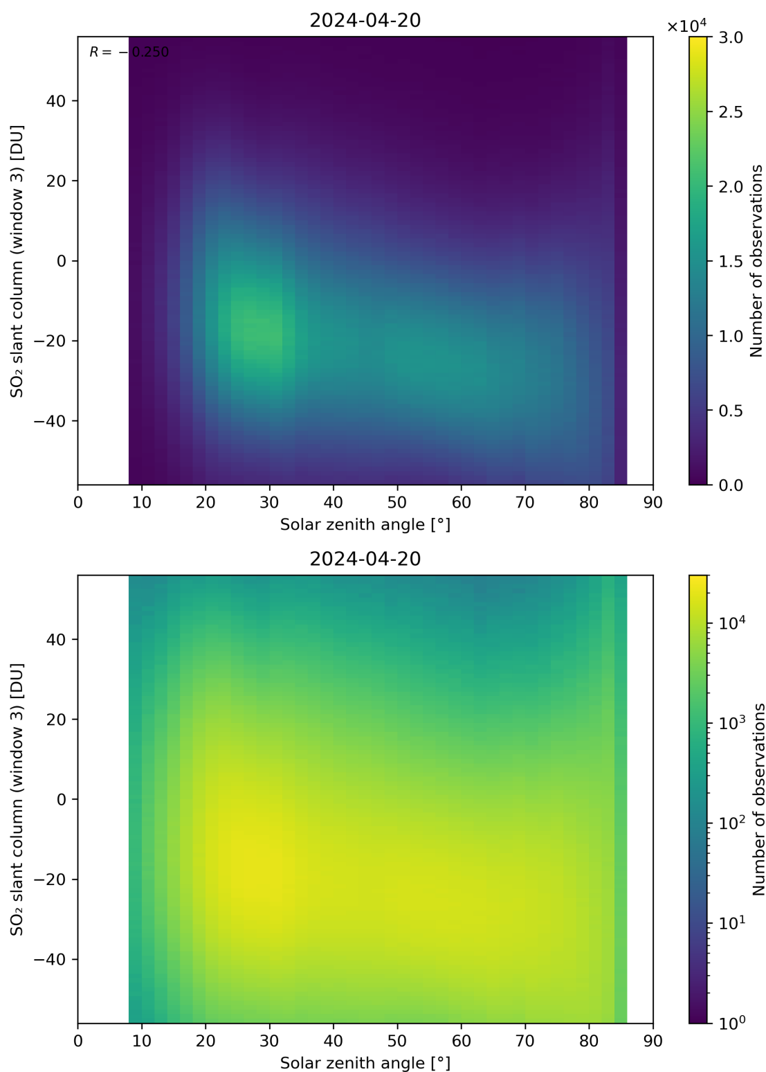
Figure 172: Scatter density plot of “Solar zenith angle” against “SO 2 slant column (window 3)” for 2024-04-19 to 2024-04-21.
