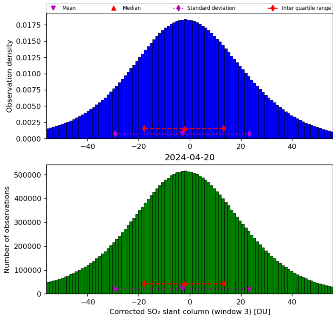
Figure 66: Histogram of “Corrected SO 2 slant column (window 3)” for 2024-04-19 to 2024-04-21
