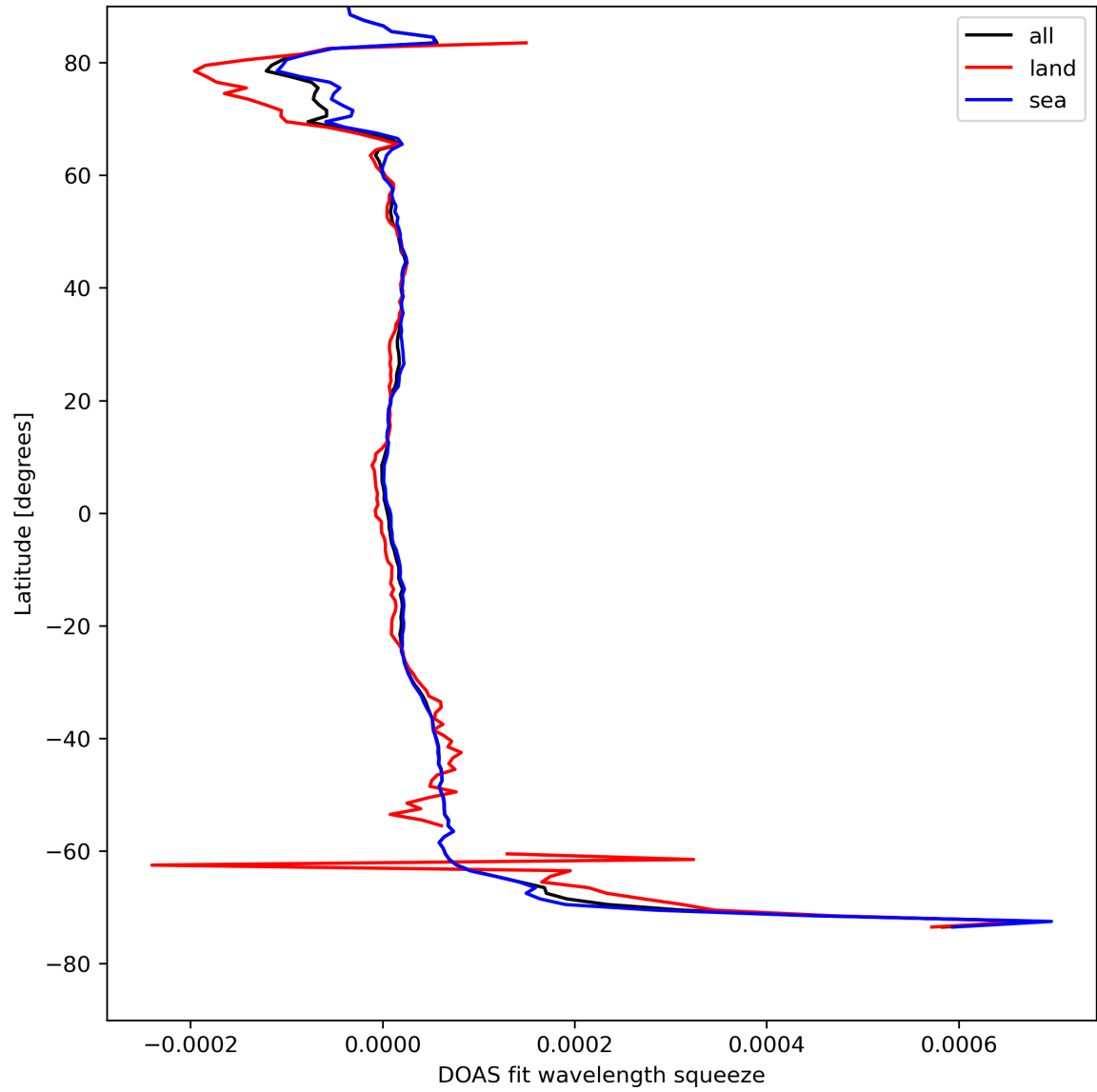
Figure 46: Zonal average of "DOAS fit wavelength squeeze" for 2024-04-19 to 2024-04-21.
