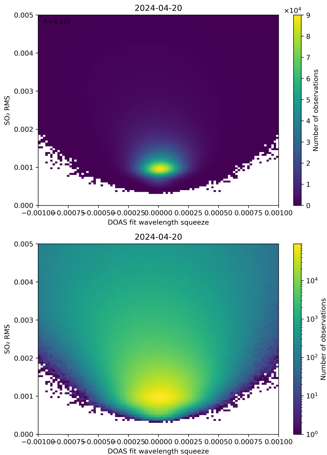
Figure 132: Scatter density plot of “DOAS fit wavelength squeeze” against “SO 2 RMS” for 2024-04-19 to 2024-04-21.
