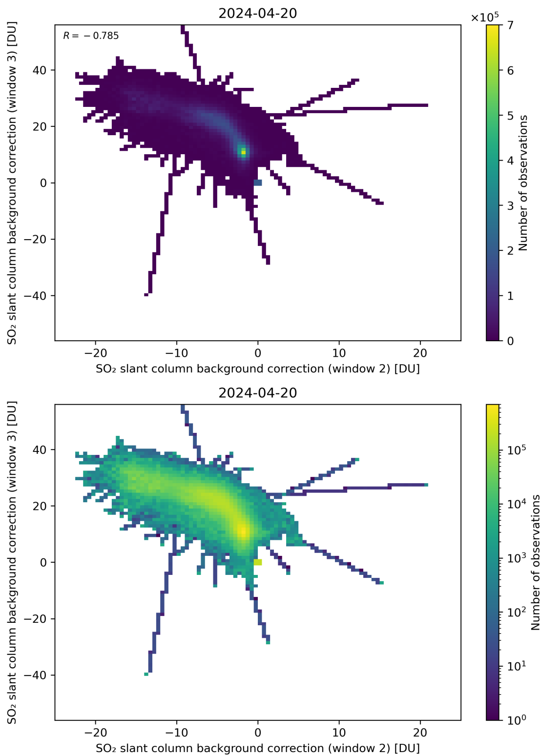
Figure 111: Scatter density plot of “SO 2 slant column background correction (window 2)” against “SO 2 slant column background correction (window 3)” for 2024-04-19 to 2024-04-21.
