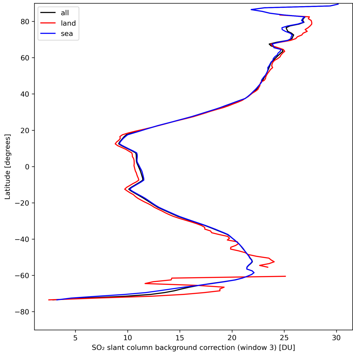
Figure 44: Zonal average of “SO 2 slant column background correction (window 3)” for 2024-04-19 to 2024-04-21.
