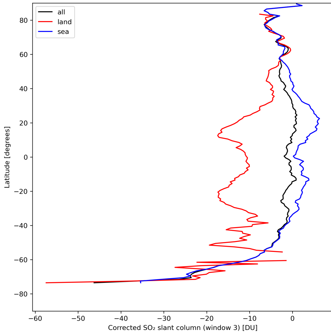
Figure 43: Zonal average of “Corrected SO 2 slant column (window 3)” for 2024-04-19 to 2024-04-21.
