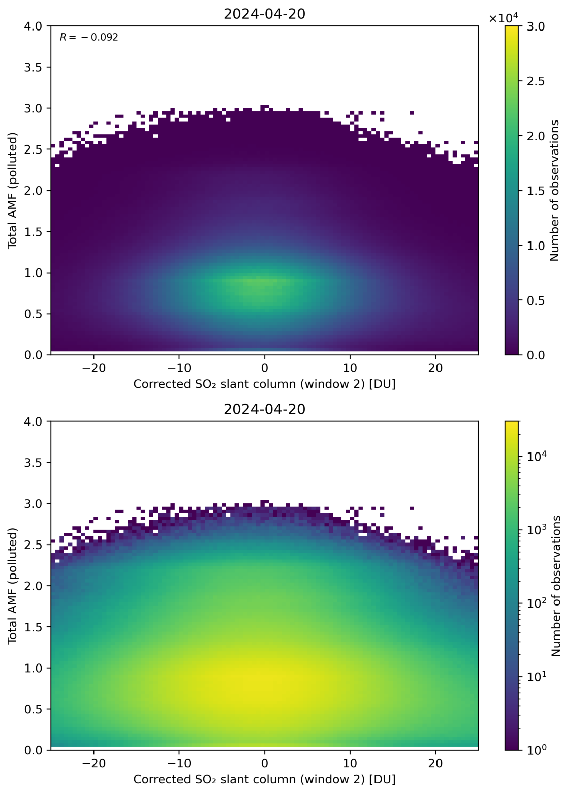
Figure 203: Scatter density plot of “Corrected SO 2 slant column (window 2)” against “Total AMF (polluted)” for 2024-04-19 to 2024-04-21.
