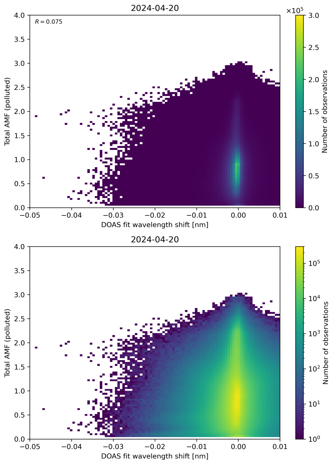
Figure 130: Scatter density plot of “DOAS fit wavelength shift” against “Total AMF (polluted)” for 2024-04-19 to 2024-04-21.
