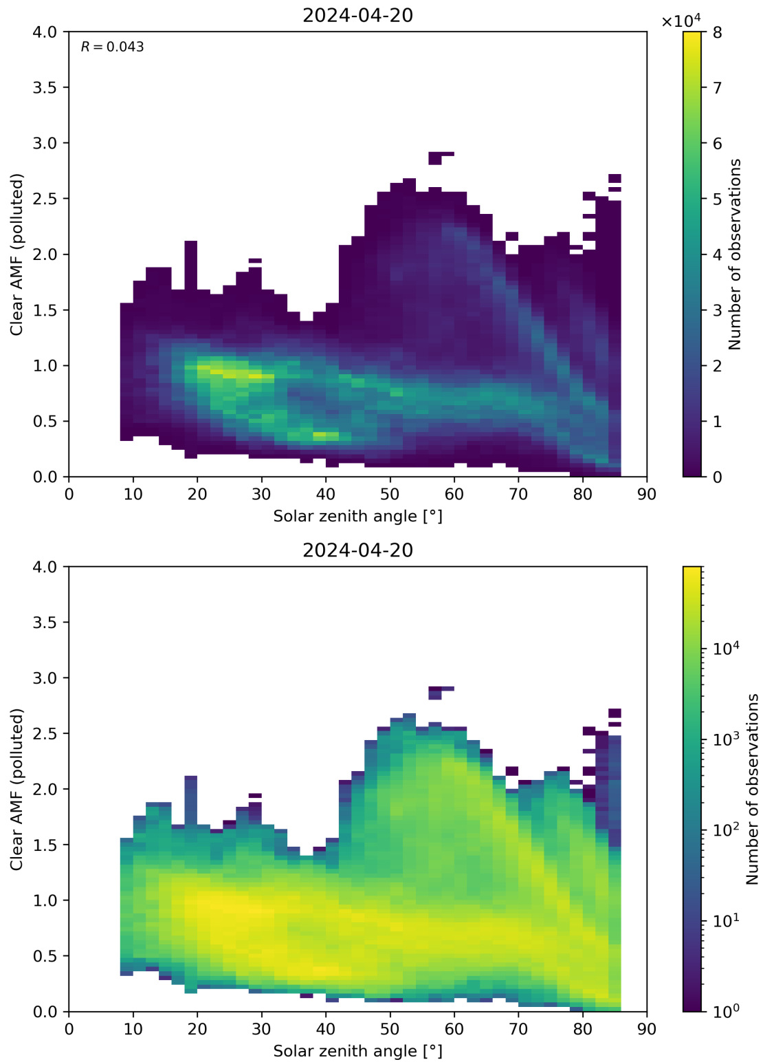
Figure 165: Scatter density plot of “Solar zenith angle” against “Clear AMF (polluted)” for 2024-04-19 to 2024-04-21.
