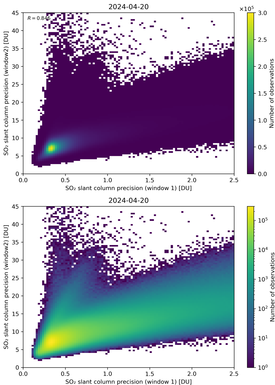
Figure 227: Scatter density plot of “SO 2 slant column precision (window 1)” against “SO 2 slant column precision (window2)” for 2024-04-19 to 2024-04-21.
