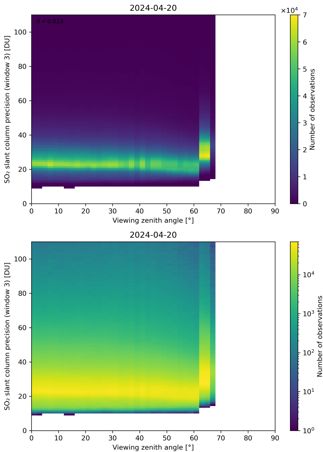
Figure 324: Scatter density plot of “Viewing zenith angle” against “SO 2 slant column precision (window 3)” for 2024-04-19 to 2024-04-21.
