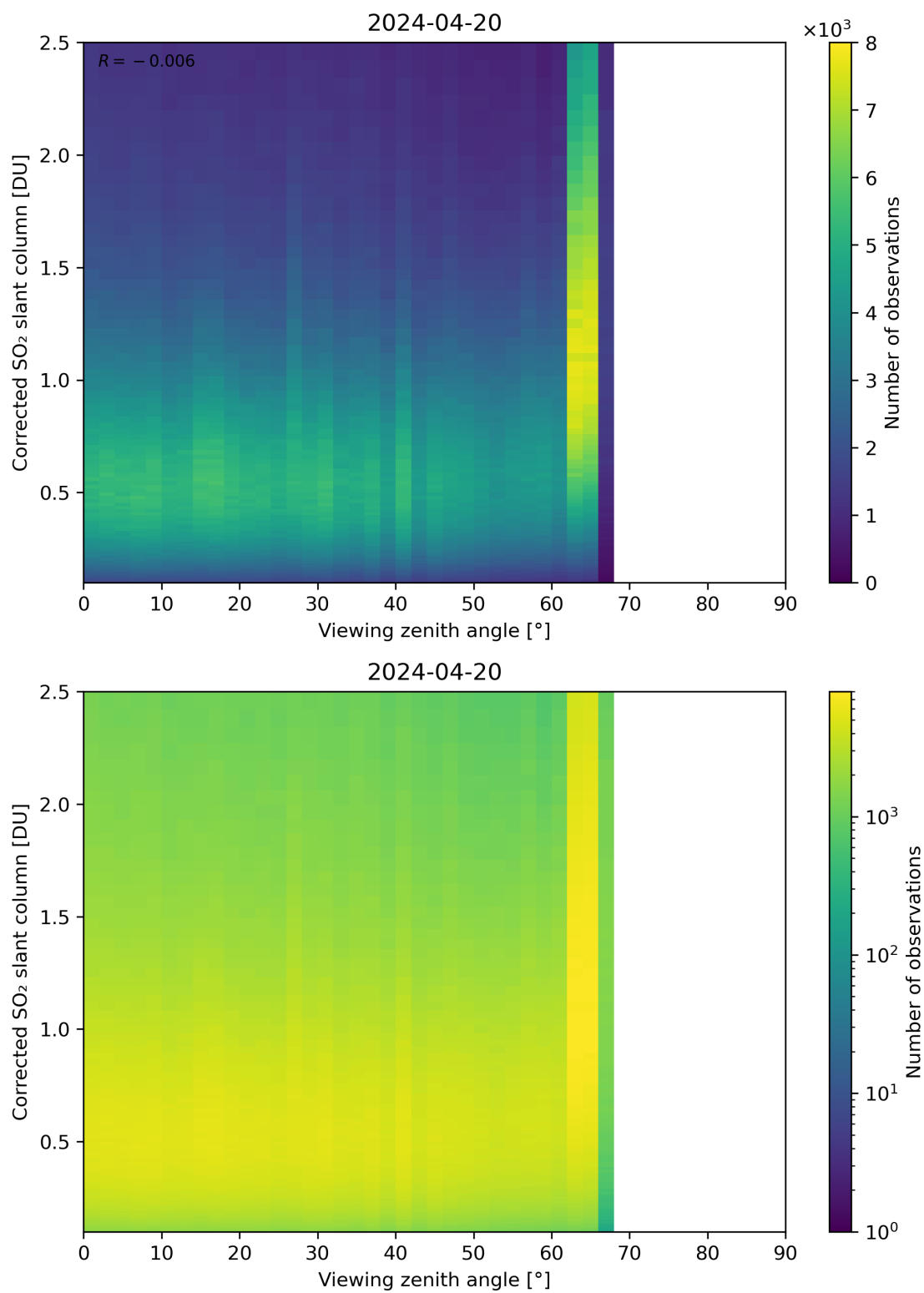
Figure 317: Scatter density plot of “Viewing zenith angle” against “Corrected SO 2 slant column” for 2024-04-19 to 2024-04-21.
