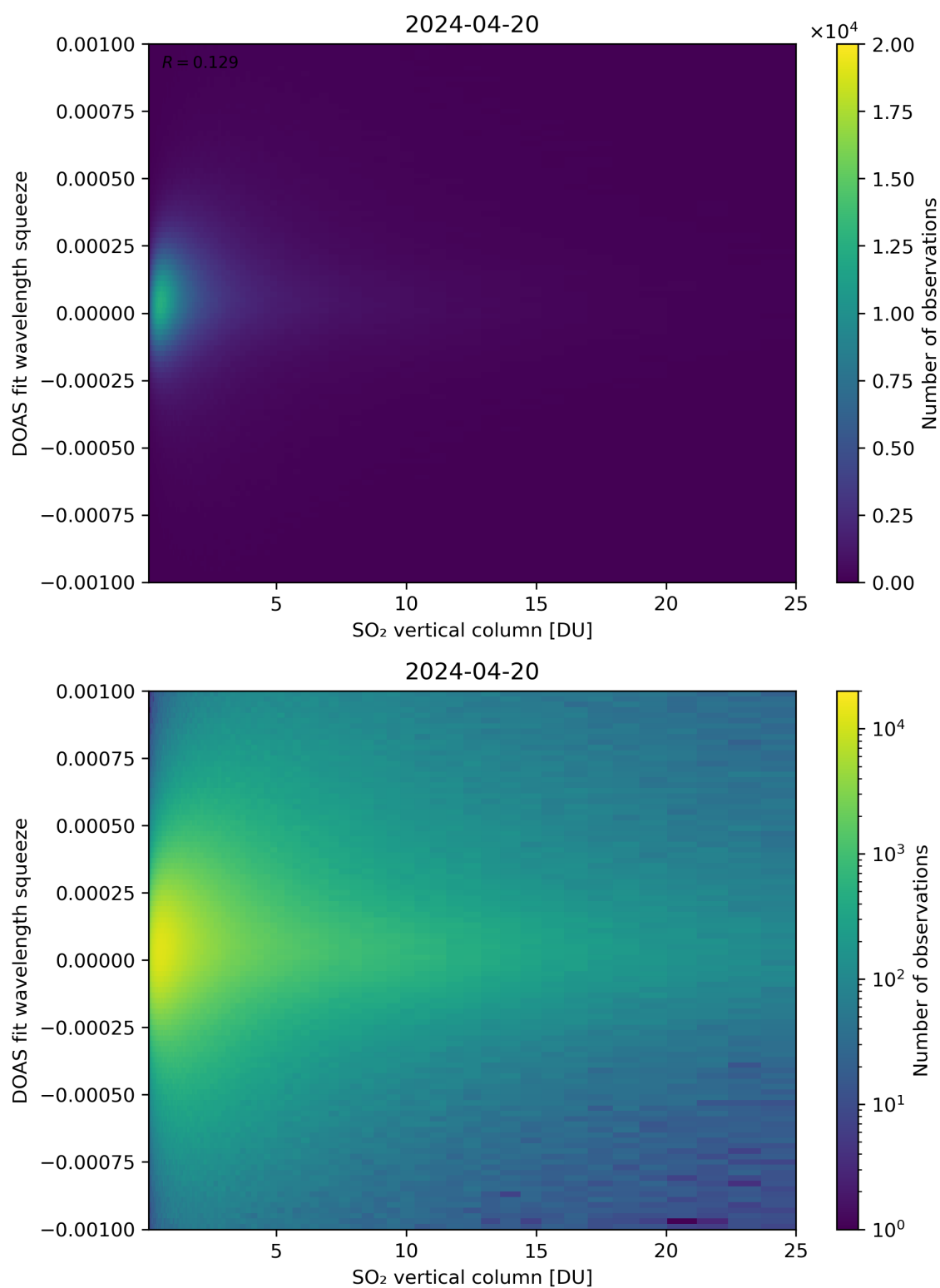
Figure 277: Scatter density plot of “SO 2 vertical column” against “DOAS fit wavelength squeeze” for 2024-04-19 to 2024-04-21.
