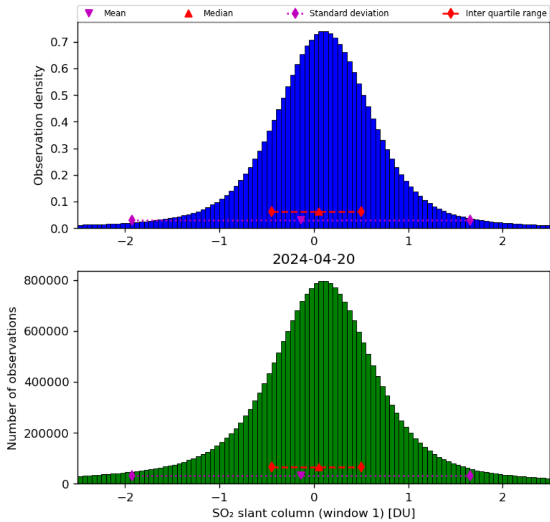
Figure 56: Histogram of “SO 2 slant column (window 1)” for 2024-04-19 to 2024-04-21
