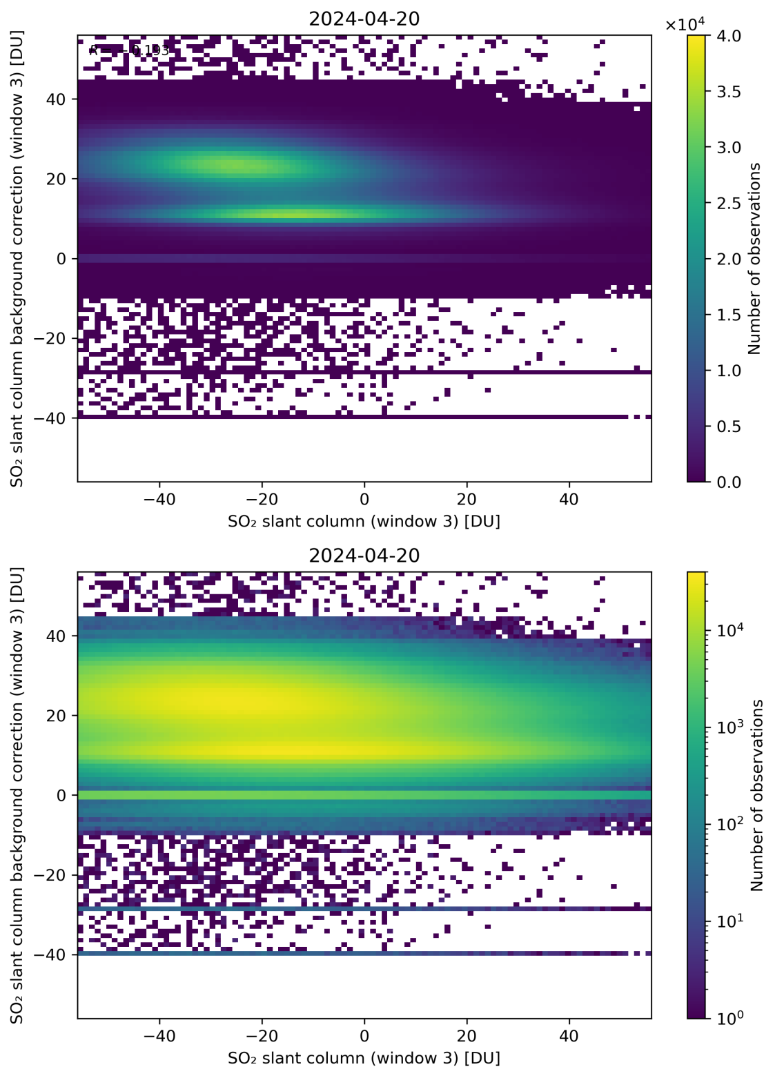
Figure 253: Scatter density plot of “SO 2 slant column (window 3)” against “SO 2 slant column background correction (window 3)” for 2024-04-19 to 2024-04-21.
