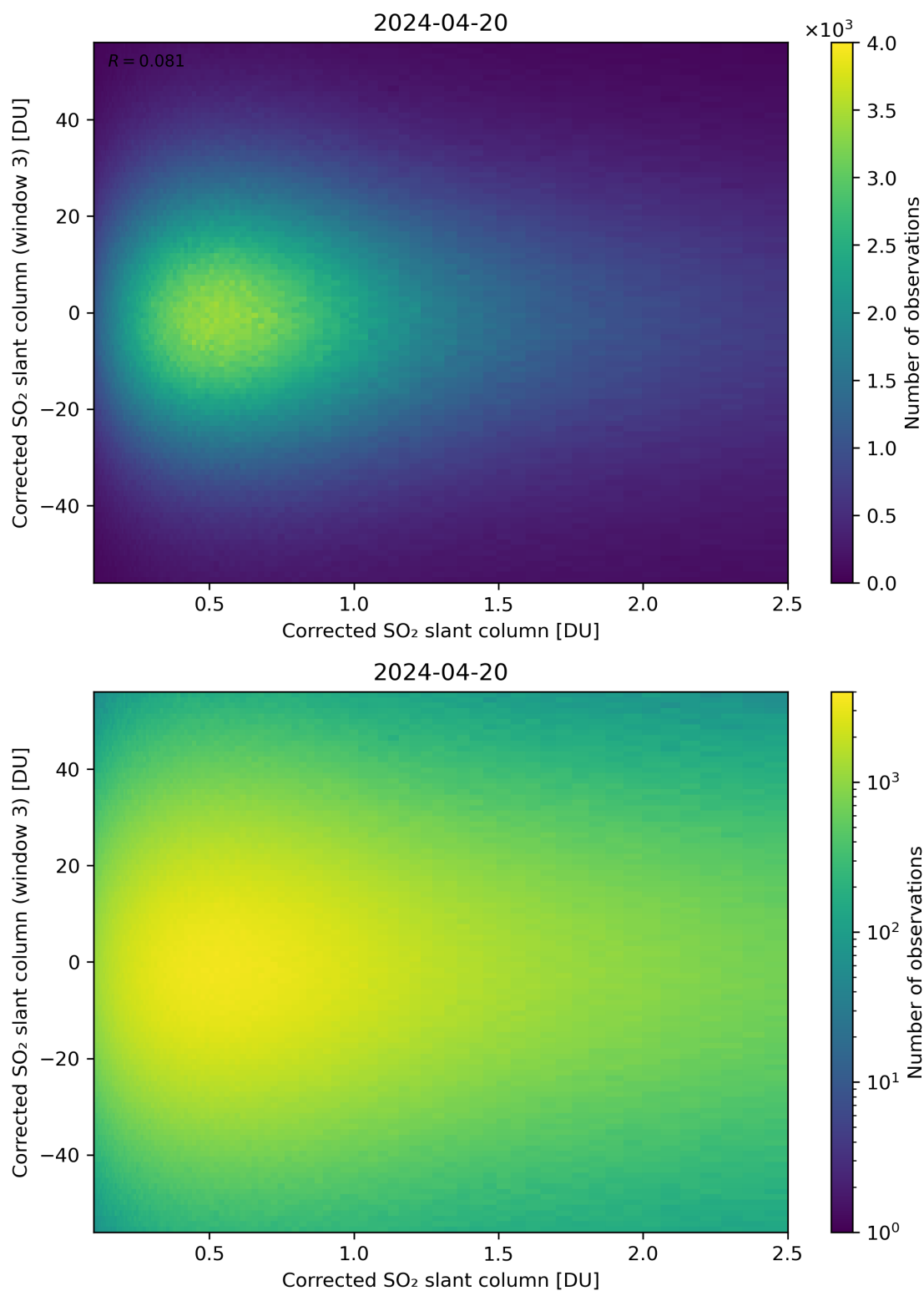
Figure 186: Scatter density plot of “Corrected SO 2 slant column” against “Corrected SO 2 slant column (window 3)” for 2024-04-19 to 2024-04-21.
