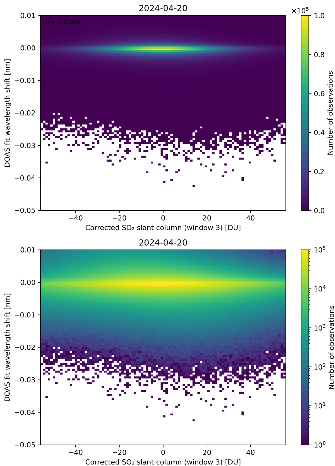
Figure 206: Scatter density plot of “Corrected SO 2 slant column (window 3)” against “DOAS fit wavelength shift” for 2024-04-19 to 2024-04-21.
