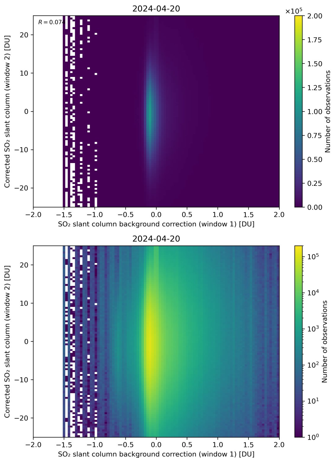
Figure 104: Scatter density plot of “SO 2 slant column background correction (window 1)” against “Corrected SO 2 slant column (window 2)” for 2024-04-19 to 2024-04-21.
