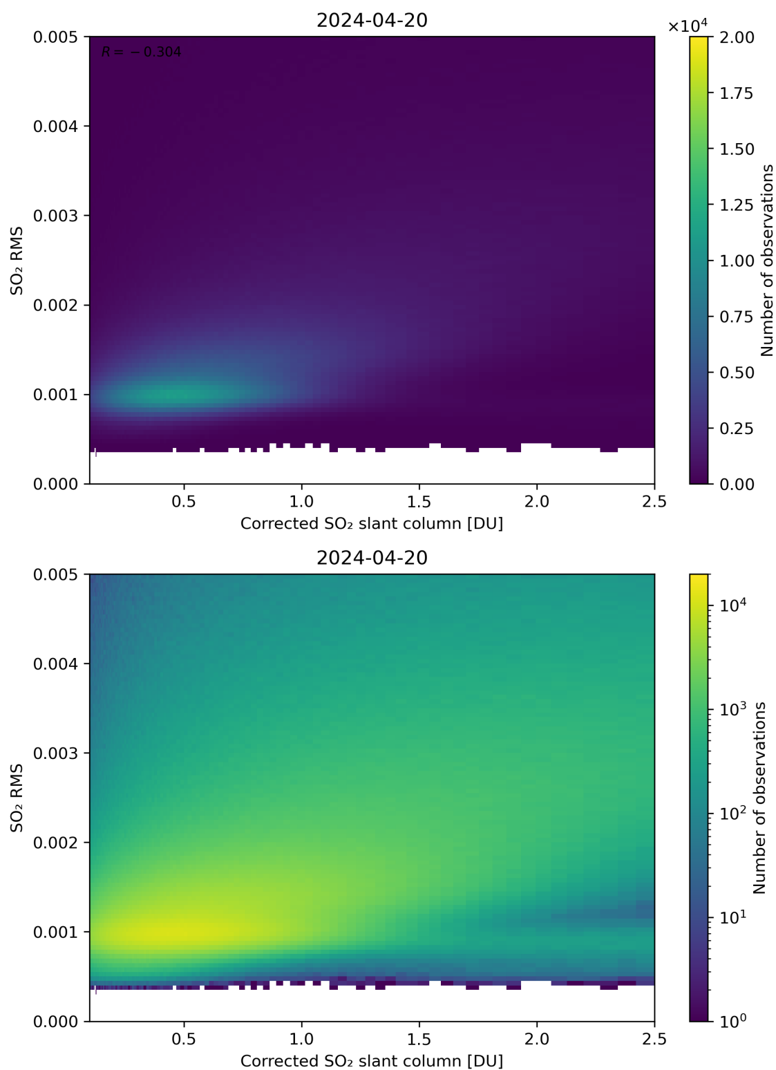
Figure 183: Scatter density plot of “Corrected SO 2 slant column” against “SO 2 RMS” for 2024-04-19 to 2024-04-21.
