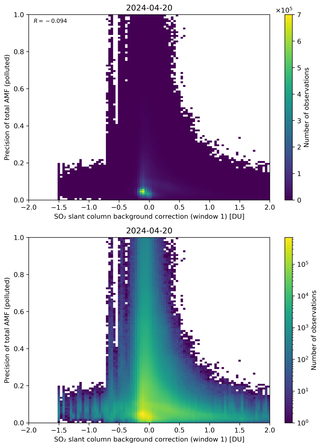
Figure 110: Scatter density plot of “SO 2 slant column background correction (window 1)” against “Precision of total AMF (polluted)” for 2024-04-19 to 2024-04-21.
