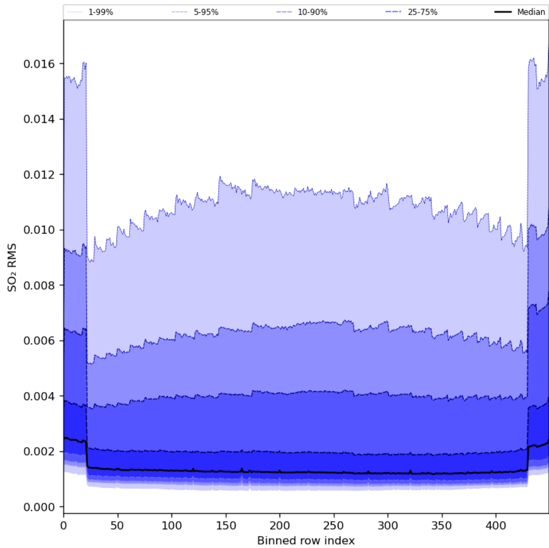
Figure 93: Along track statistics of “SO 2 RMS” for 2024-04-19 to 2024-04-21
