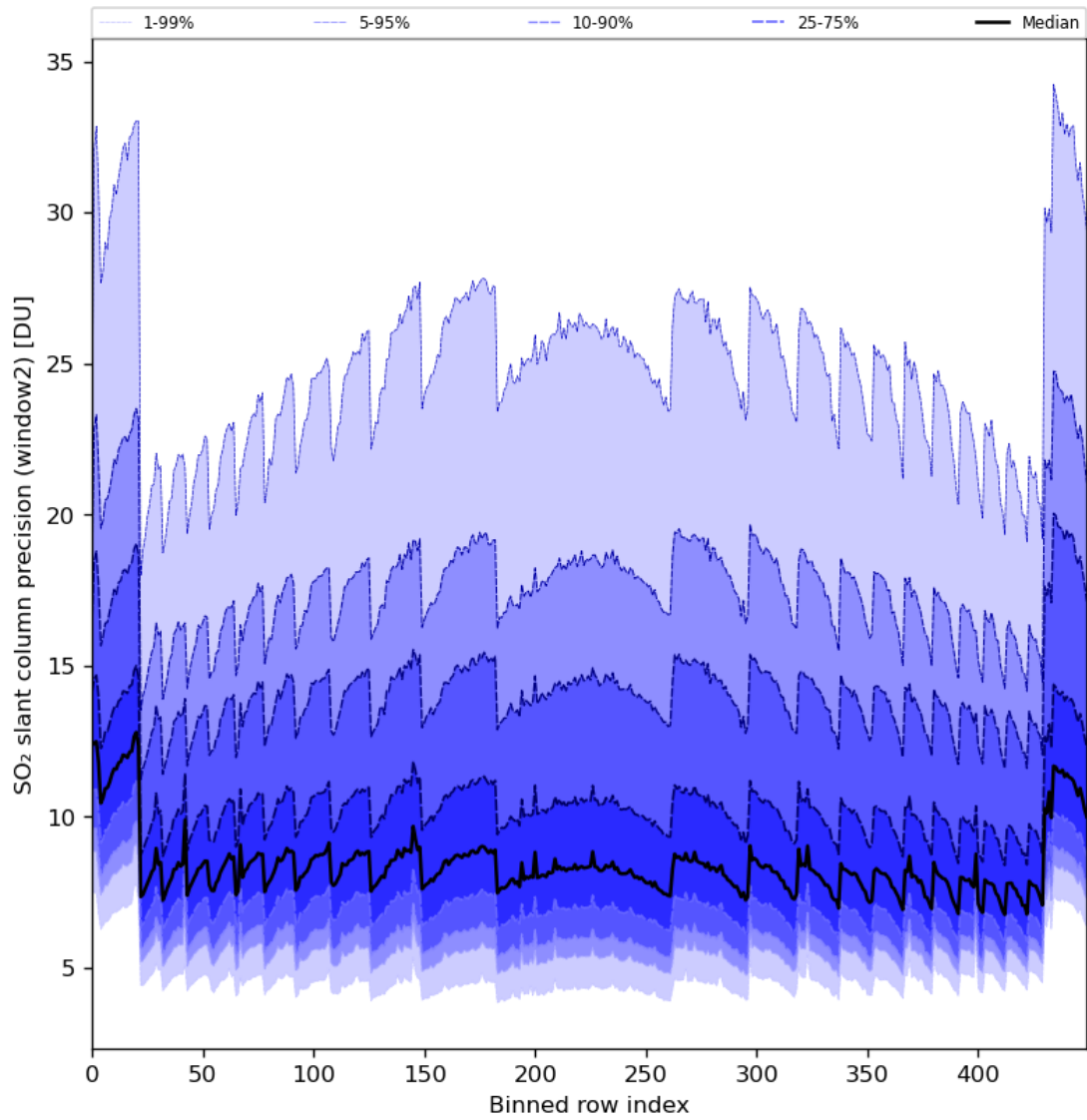
Figure 84: Along track statistics of “SO 2 slant column precision (window2)” for 2024-04-19 to 2024-04-21
