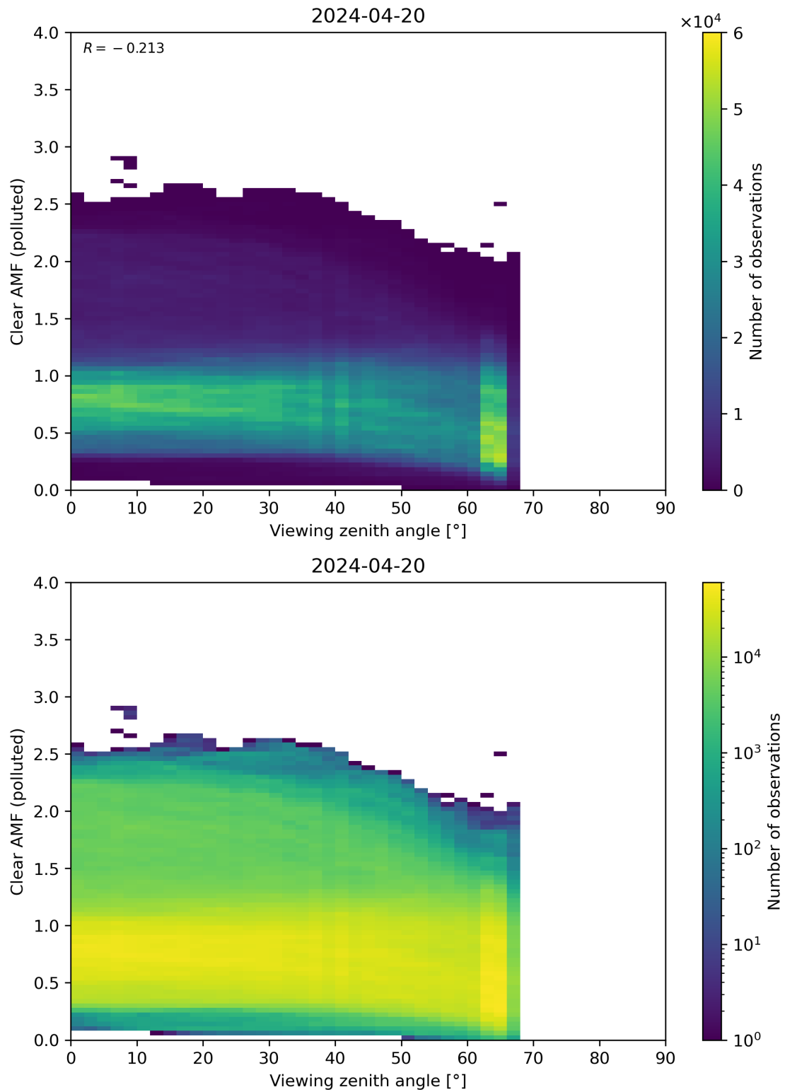
Figure 316: Scatter density plot of “Viewing zenith angle” against “Clear AMF (polluted)” for 2024-04-19 to 2024-04-21.
