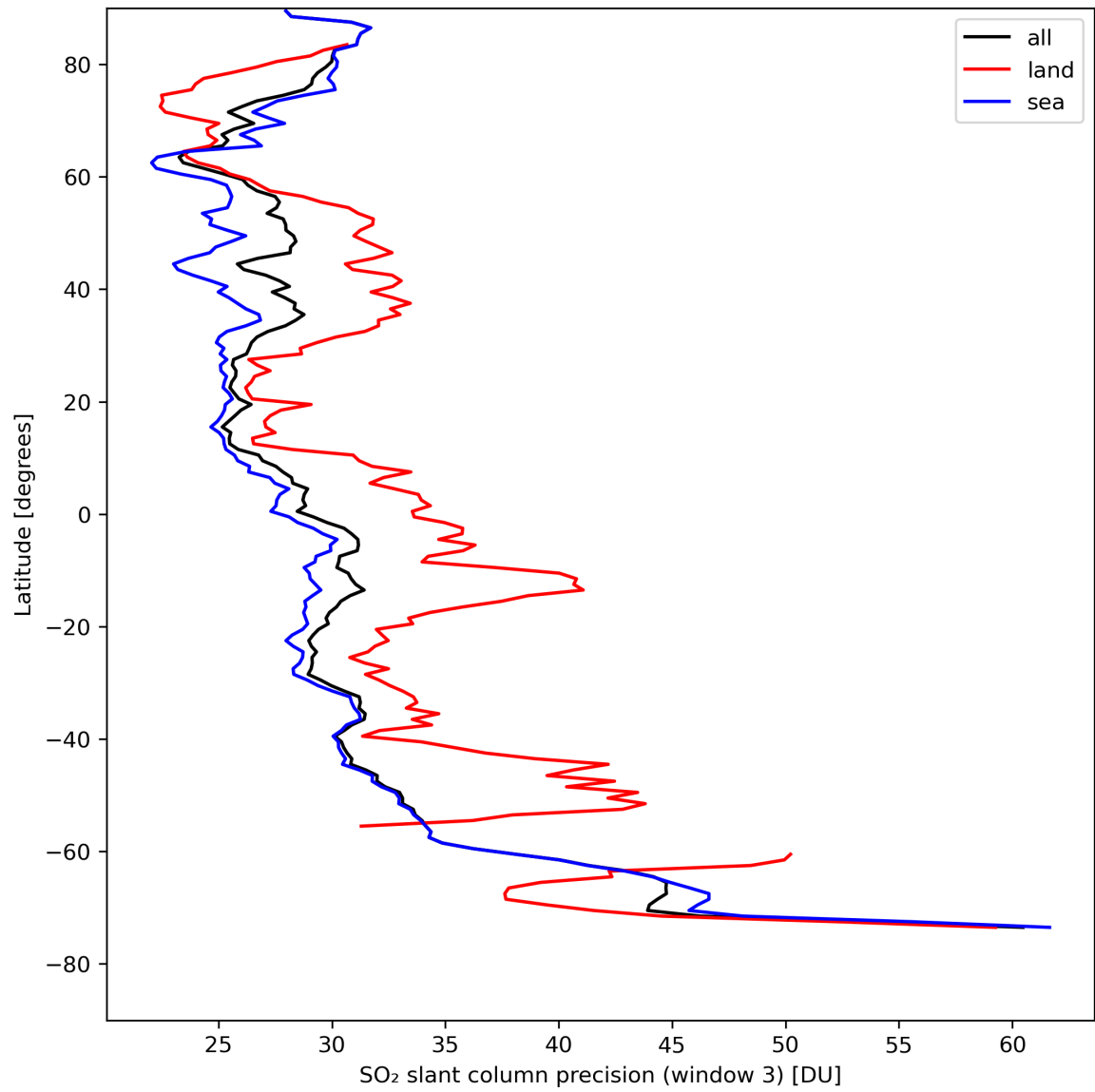
Figure 42: Zonal average of “SO 2 slant column precision (window 3)” for 2024-04-19 to 2024-04-21.
