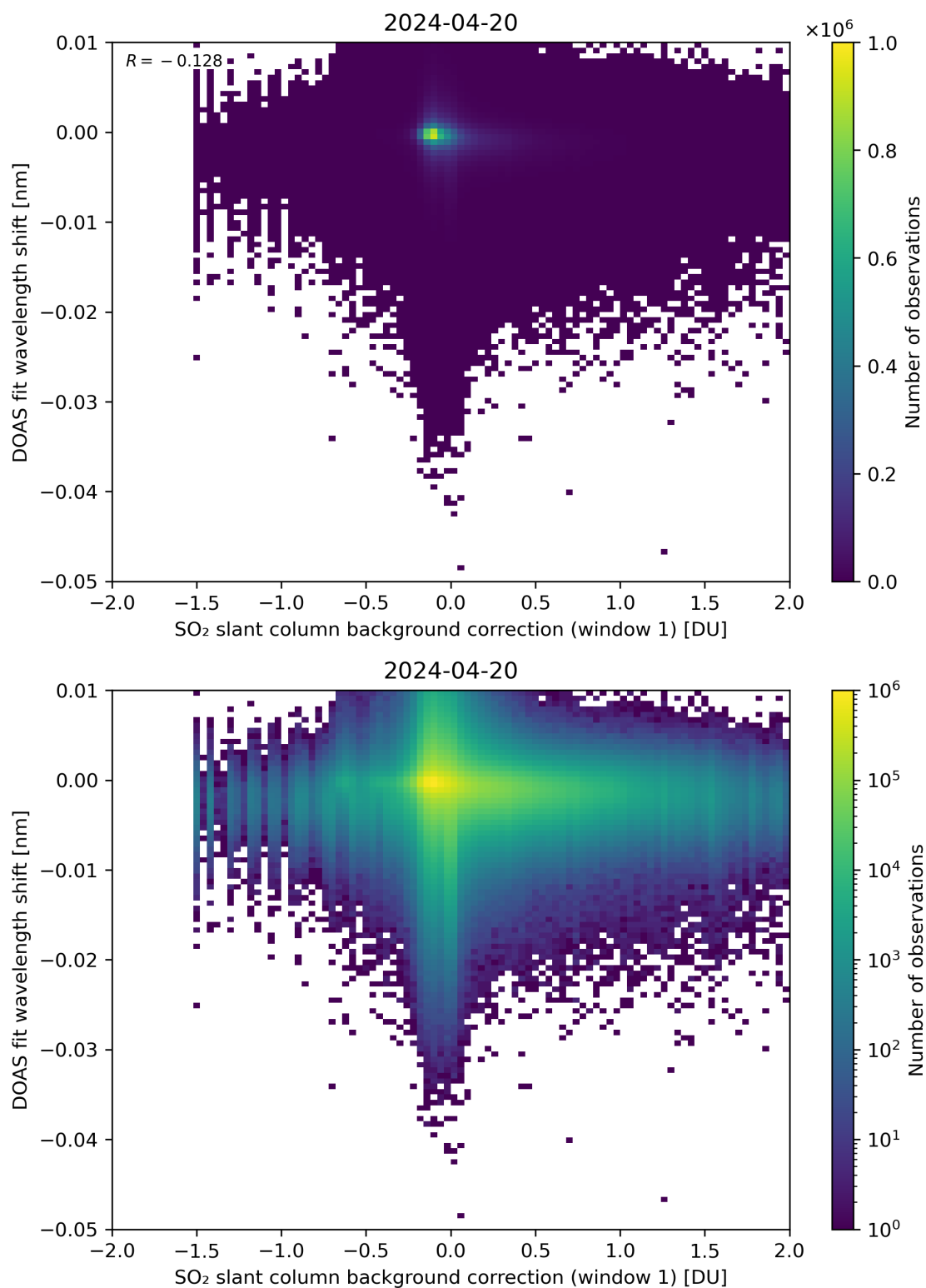
Figure 100: Scatter density plot of “SO 2 slant column background correction (window 1)” against “DOAS fit wavelength shift” for 2024-04-19 to 2024-04-21.
