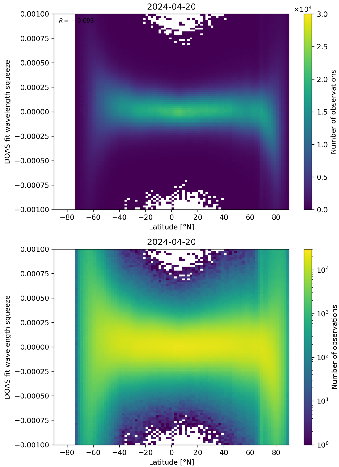
Figure 143: Scatter density plot of “Latitude” against “DOAS fit wavelength squeeze” for 2024-04-19 to 2024-04-21.
