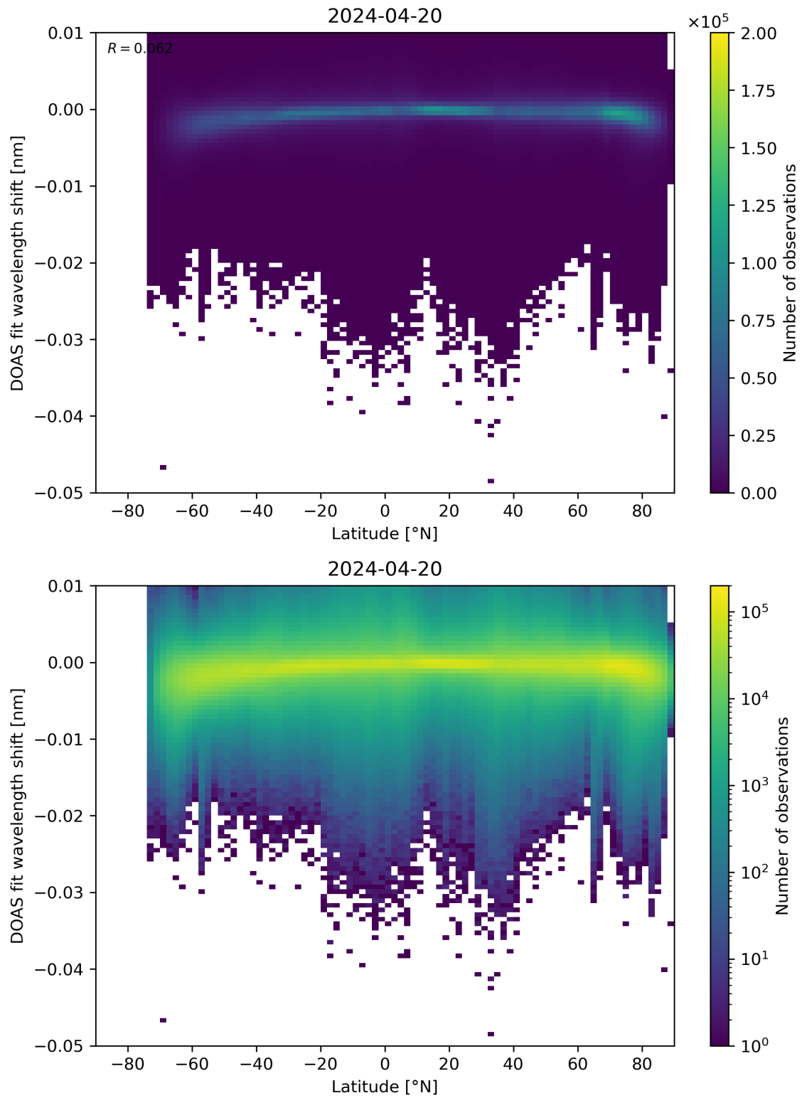
Figure 142: Scatter density plot of “Latitude” against “DOAS fit wavelength shift” for 2024-04-19 to 2024-04-21.
