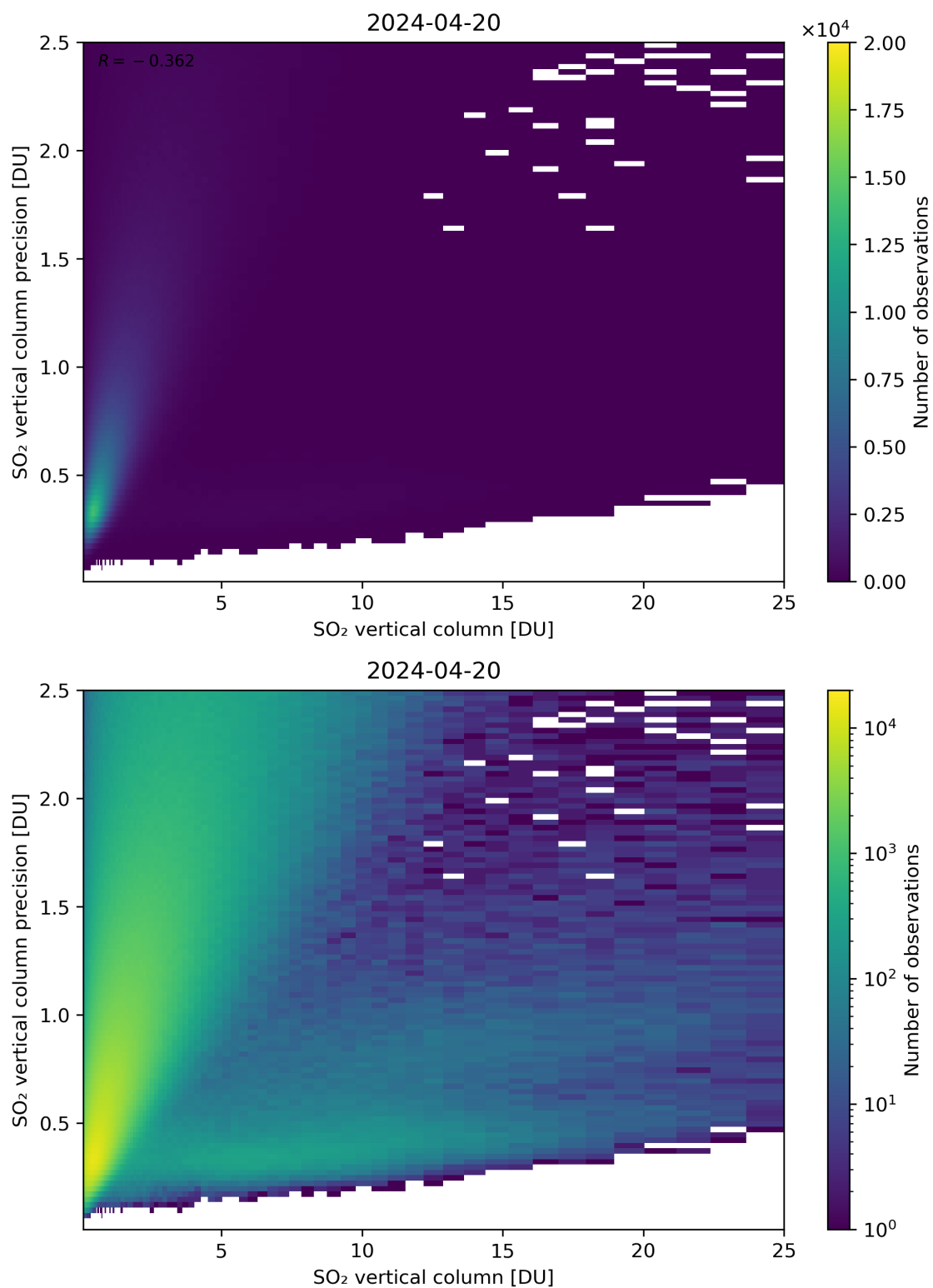
Figure 307: Scatter density plot of “SO 2 vertical column” against “SO 2 vertical column precision” for 2024-04-19 to 2024-04-21.
