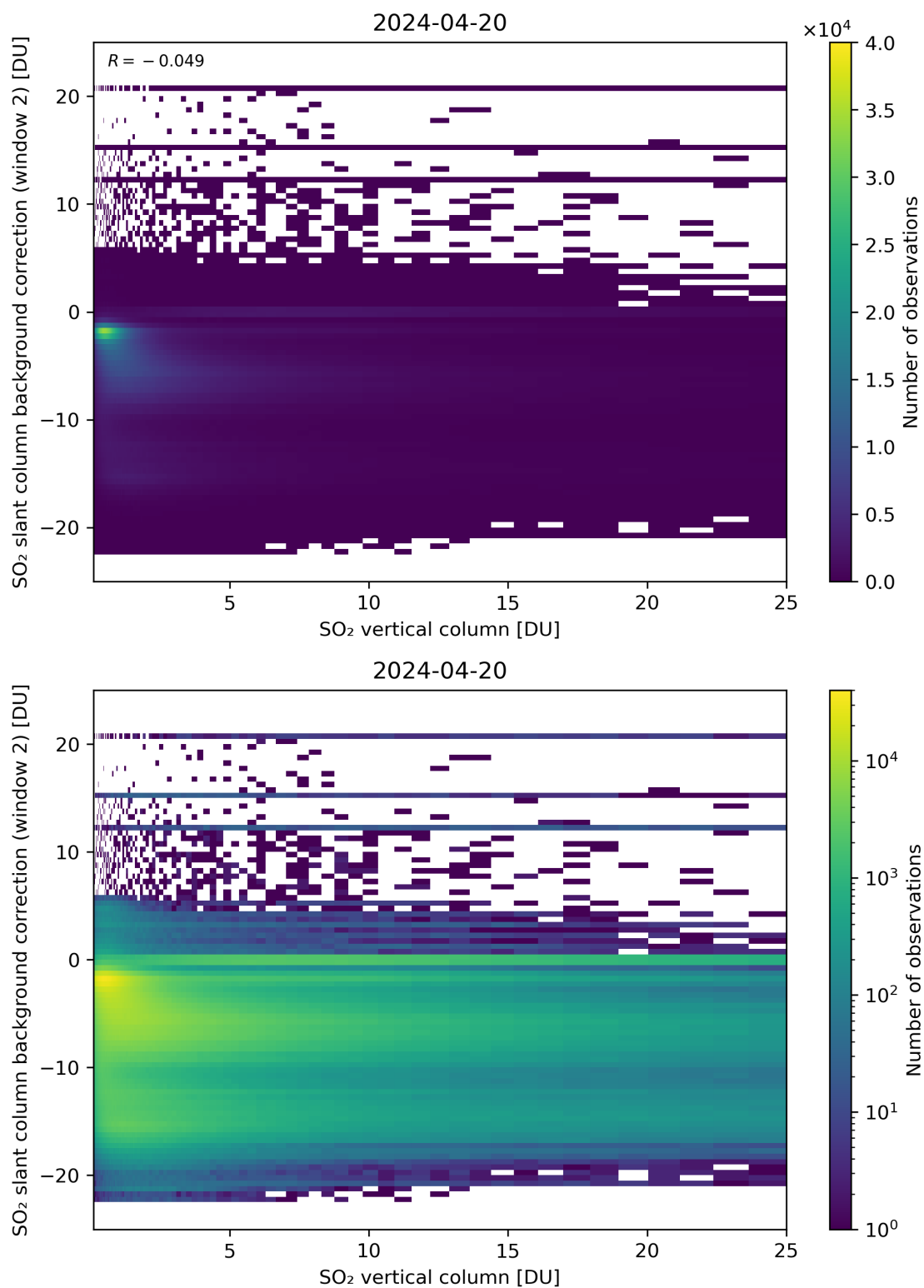
Figure 274: Scatter density plot of “SO 2 vertical column” against “SO 2 slant column background correction (window 2)” for 2024-04-19 to 2024-04-21.
