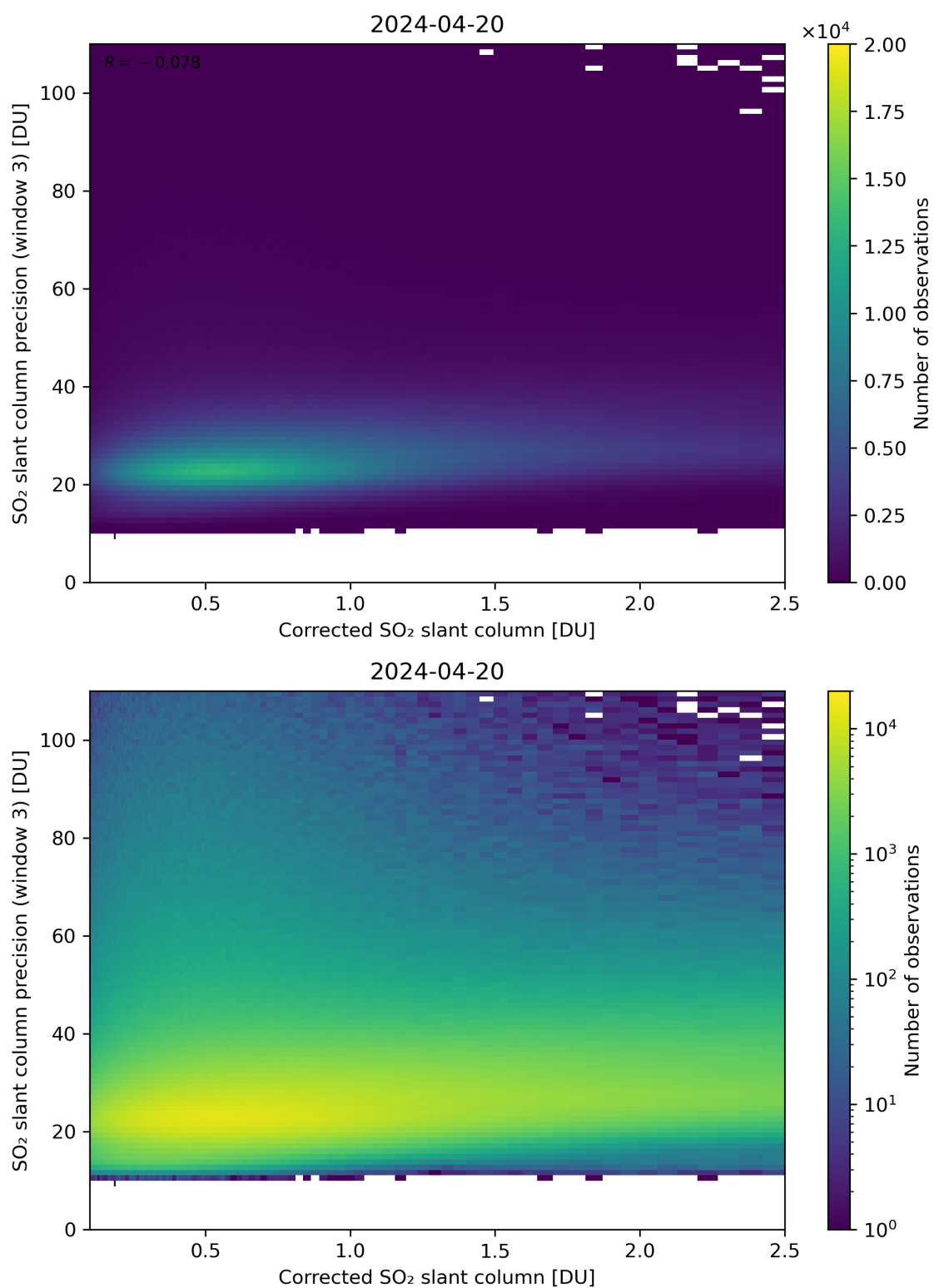
Figure 191: Scatter density plot of “Corrected SO 2 slant column” against “SO 2 slant column precision (window 3)” for 2024-04-19 to 2024-04-21.
