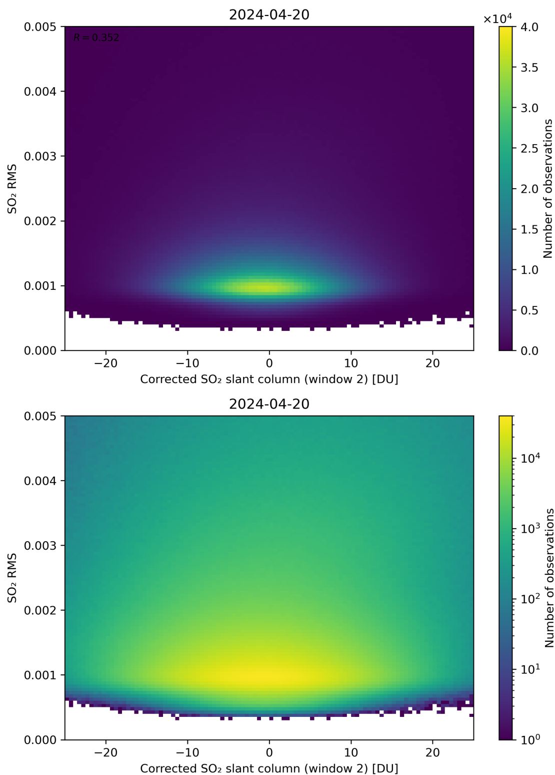
Figure 198: Scatter density plot of “Corrected SO 2 slant column (window 2)” against “SO 2 RMS” for 2024-04-19 to 2024-04-21.
