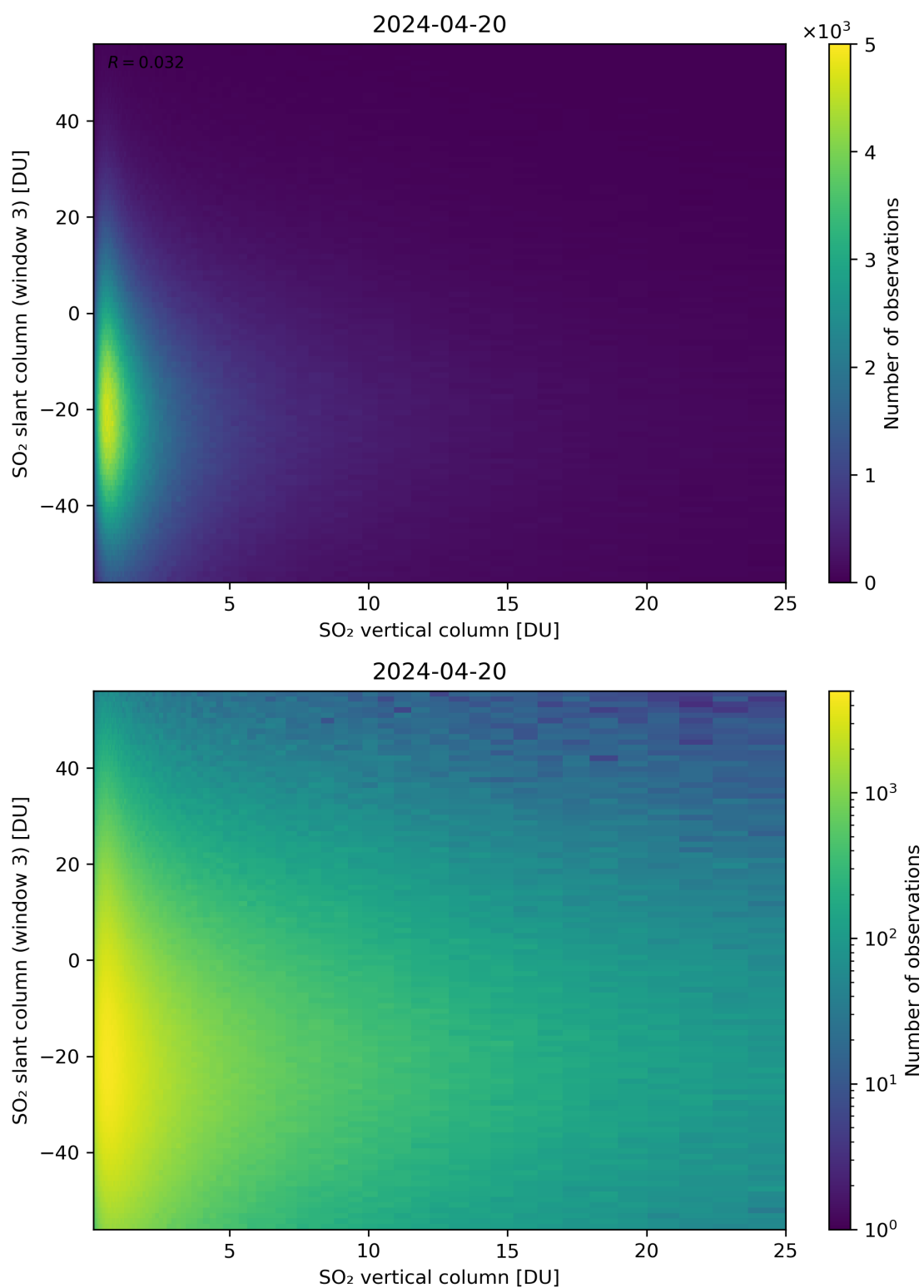
Figure 303: Scatter density plot of “SO 2 vertical column” against “SO 2 slant column (window 3)” for 2024-04-19 to 2024-04-21.
