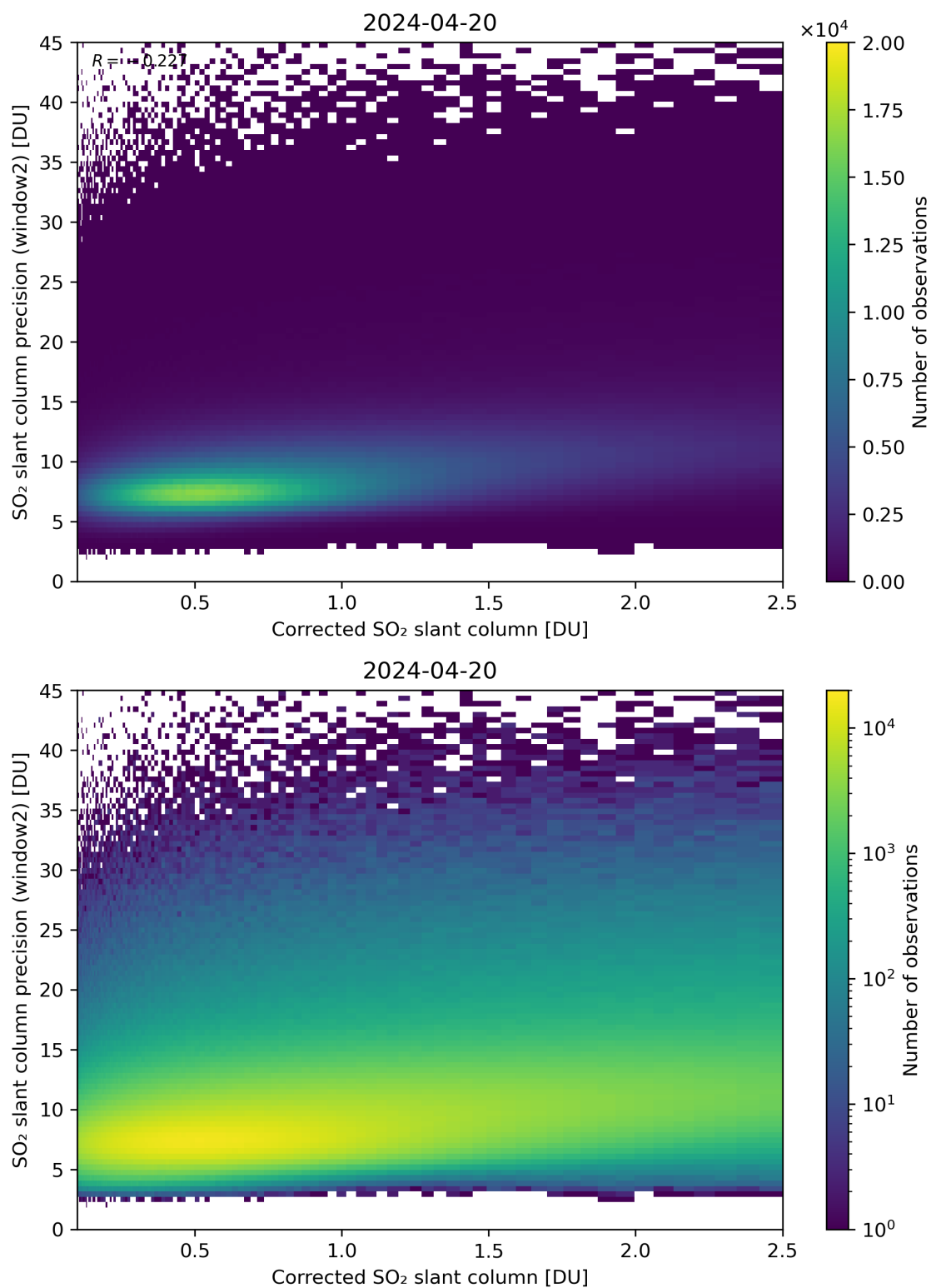
Figure 189: Scatter density plot of “Corrected SO 2 slant column” against “SO 2 slant column precision (window2)” for 2024-04-19 to 2024-04-21.
