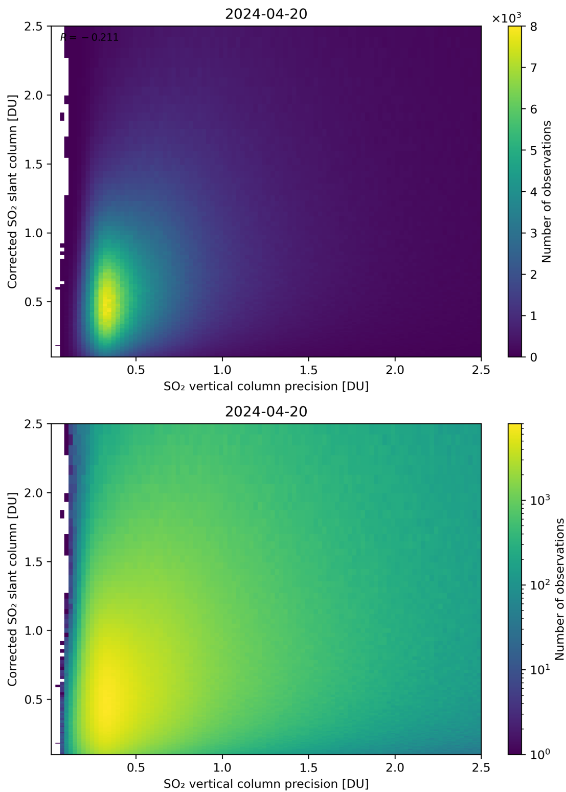
Figure 286: Scatter density plot of “SO 2 vertical column precision” against “Corrected SO 2 slant column” for 2024-04-19 to 2024-04-21.
