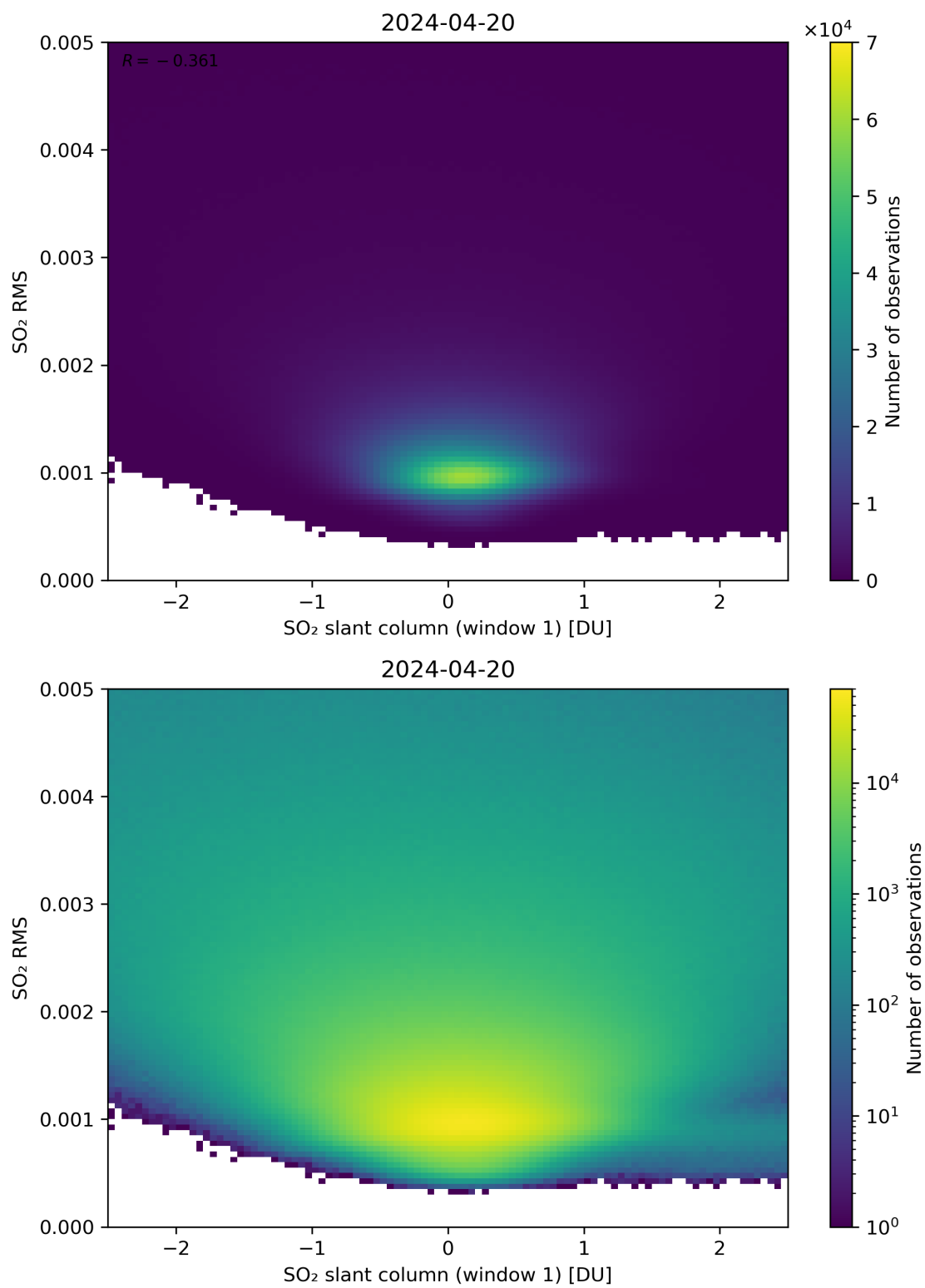
Figure 217: Scatter density plot of “SO 2 slant column (window 1)” against “SO 2 RMS” for 2024-04-19 to 2024-04-21.
