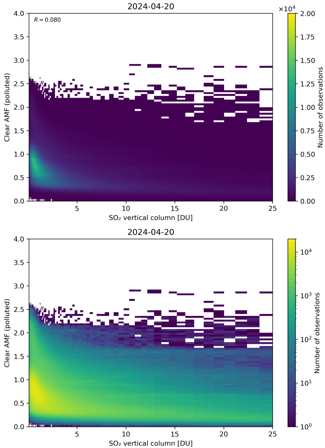
Figure 296: Scatter density plot of “SO 2 vertical column” against “Clear AMF (polluted)” for 2024-04-19 to 2024-04-21.
