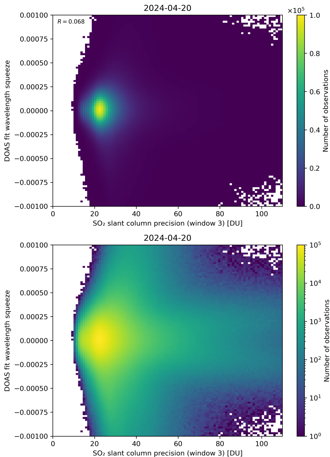
Figure 259: Scatter density plot of “SO 2 slant column precision (window 3)” against “DOAS fit wavelength squeeze” for 2024-04-19 to 2024-04-21.
