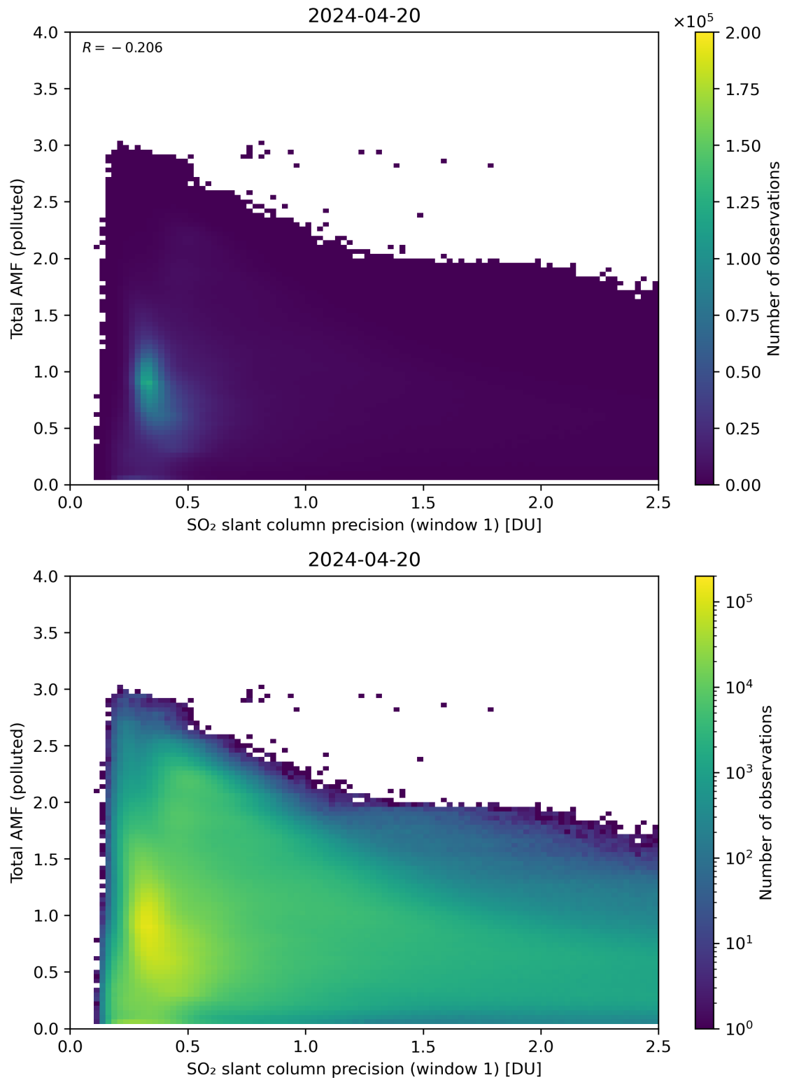
Figure 230: Scatter density plot of “SO 2 slant column precision (window 1)” against “Total AMF (polluted)” for 2024-04-19 to 2024-04-21.
