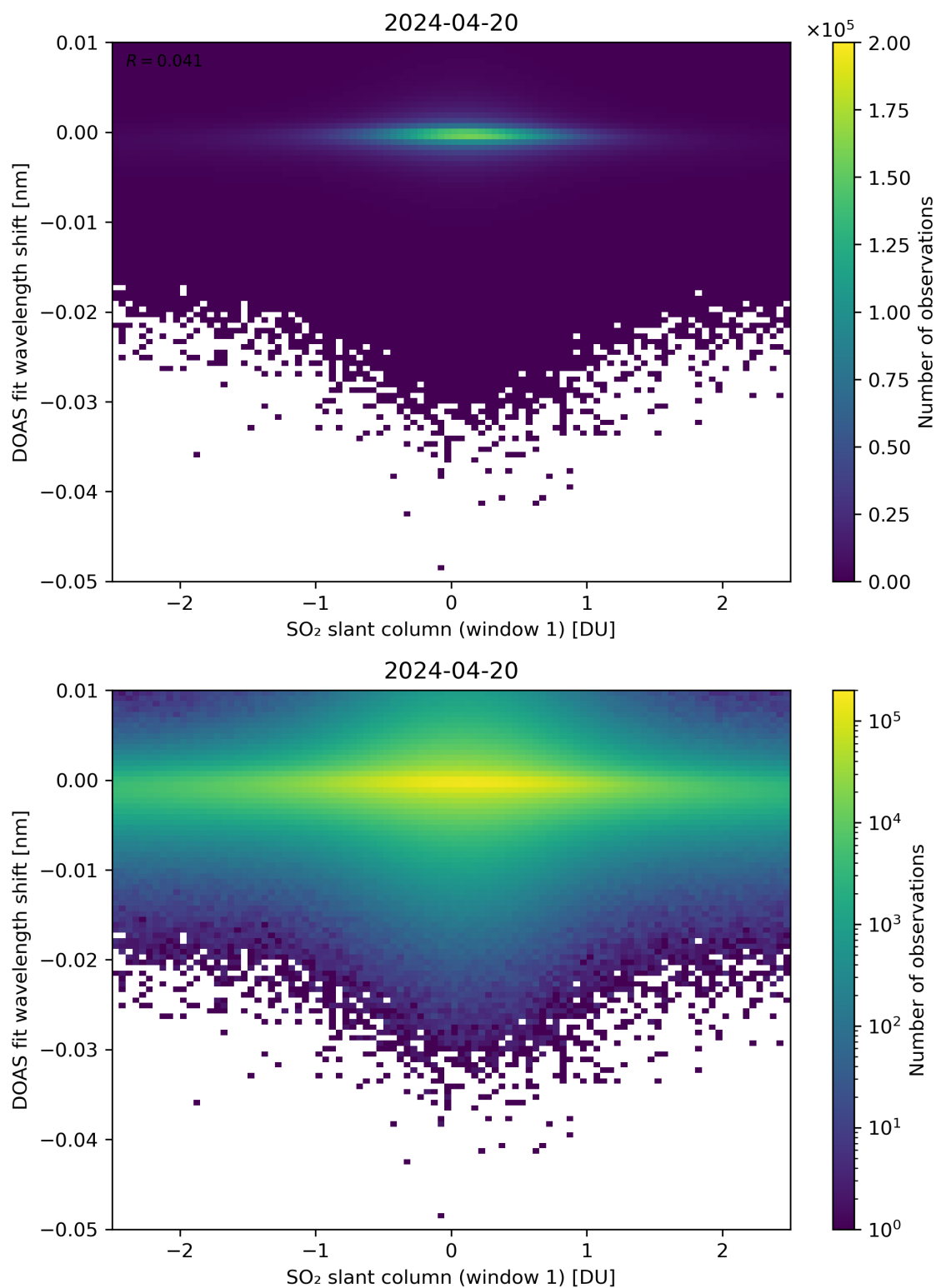
Figure 215: Scatter density plot of “SO 2 slant column (window 1)” against “DOAS fit wavelength shift” for 2024-04-19 to 2024-04-21.
