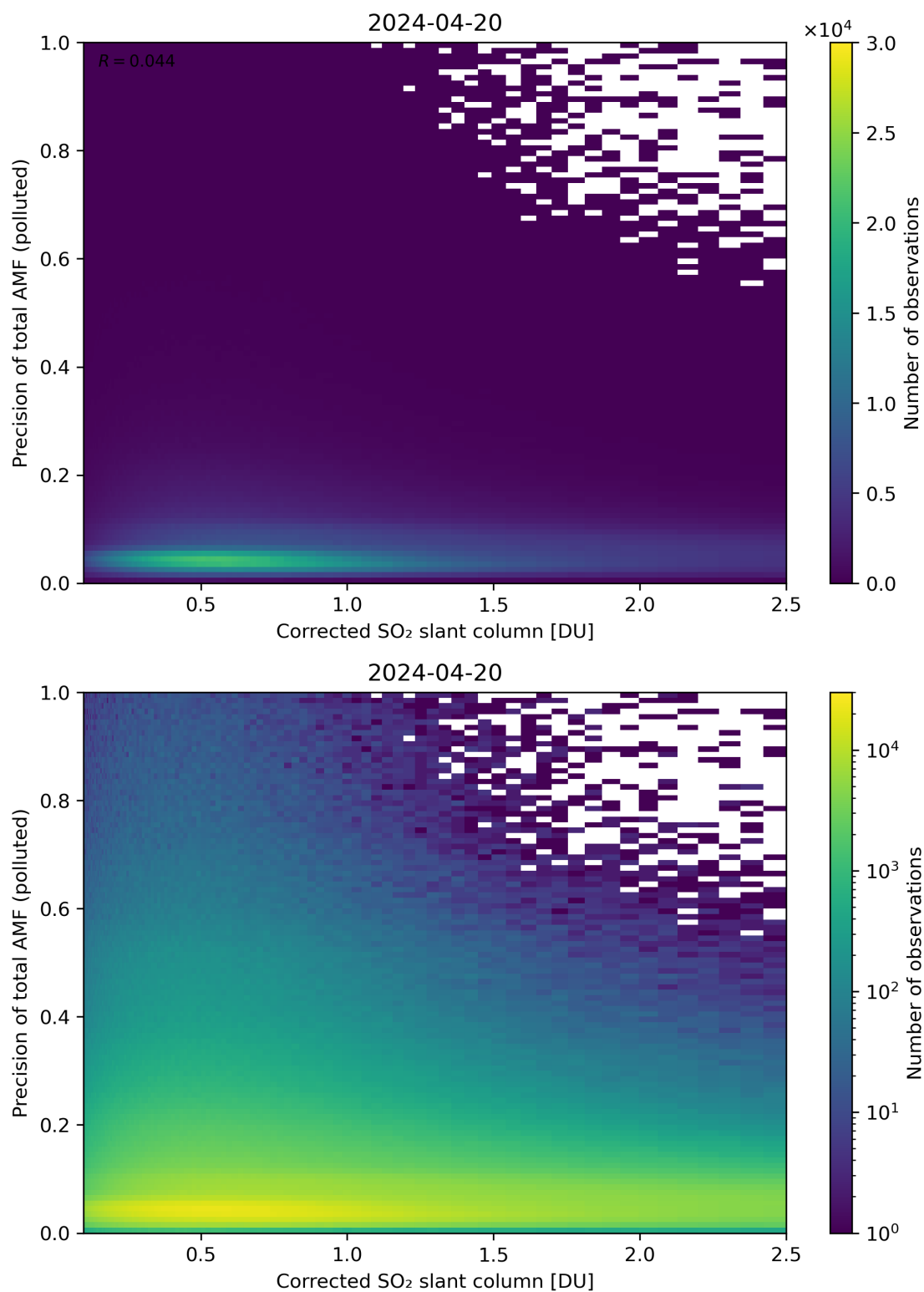
Figure 193: Scatter density plot of “Corrected SO 2 slant column” against “Precision of total AMF (polluted)” for 2024-04-19 to 2024-04-21.
