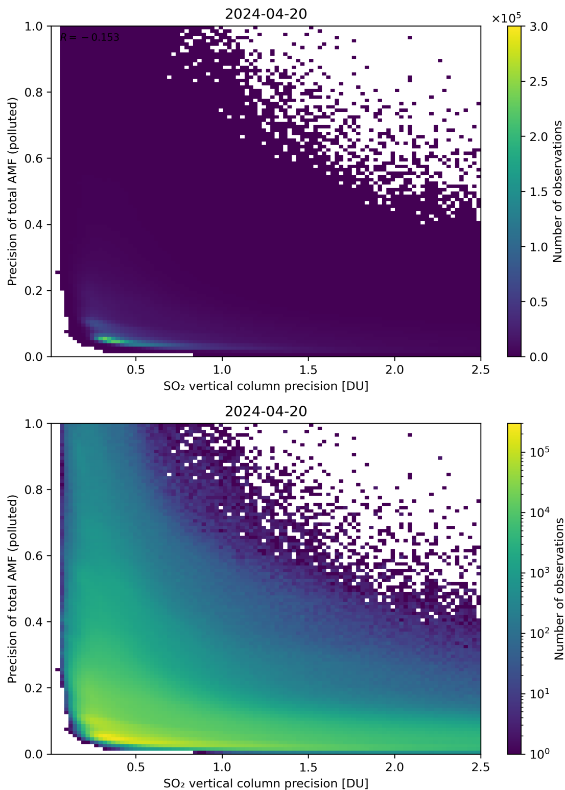
Figure 295: Scatter density plot of “SO 2 vertical column precision” against “Precision of total AMF (polluted)” for 2024-04-19 to 2024-04-21.
