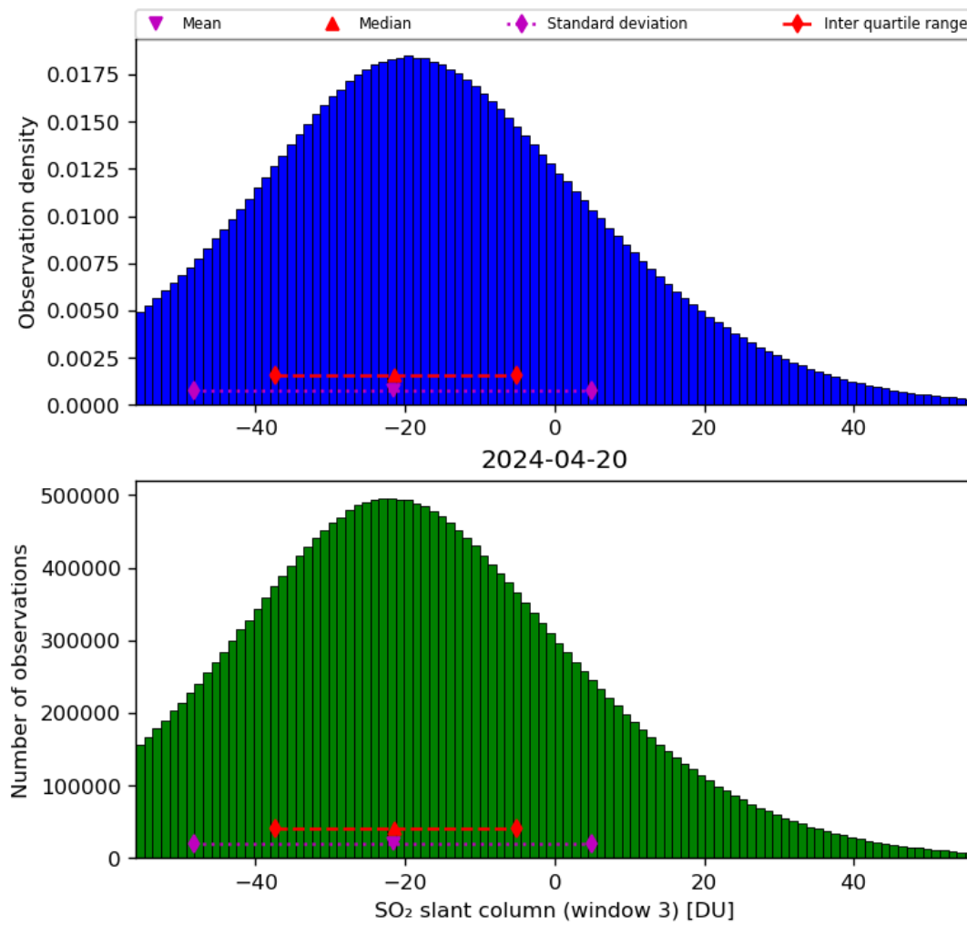
Figure 64: Histogram of “SO 2 slant column (window 3)” for 2024-04-19 to 2024-04-21
