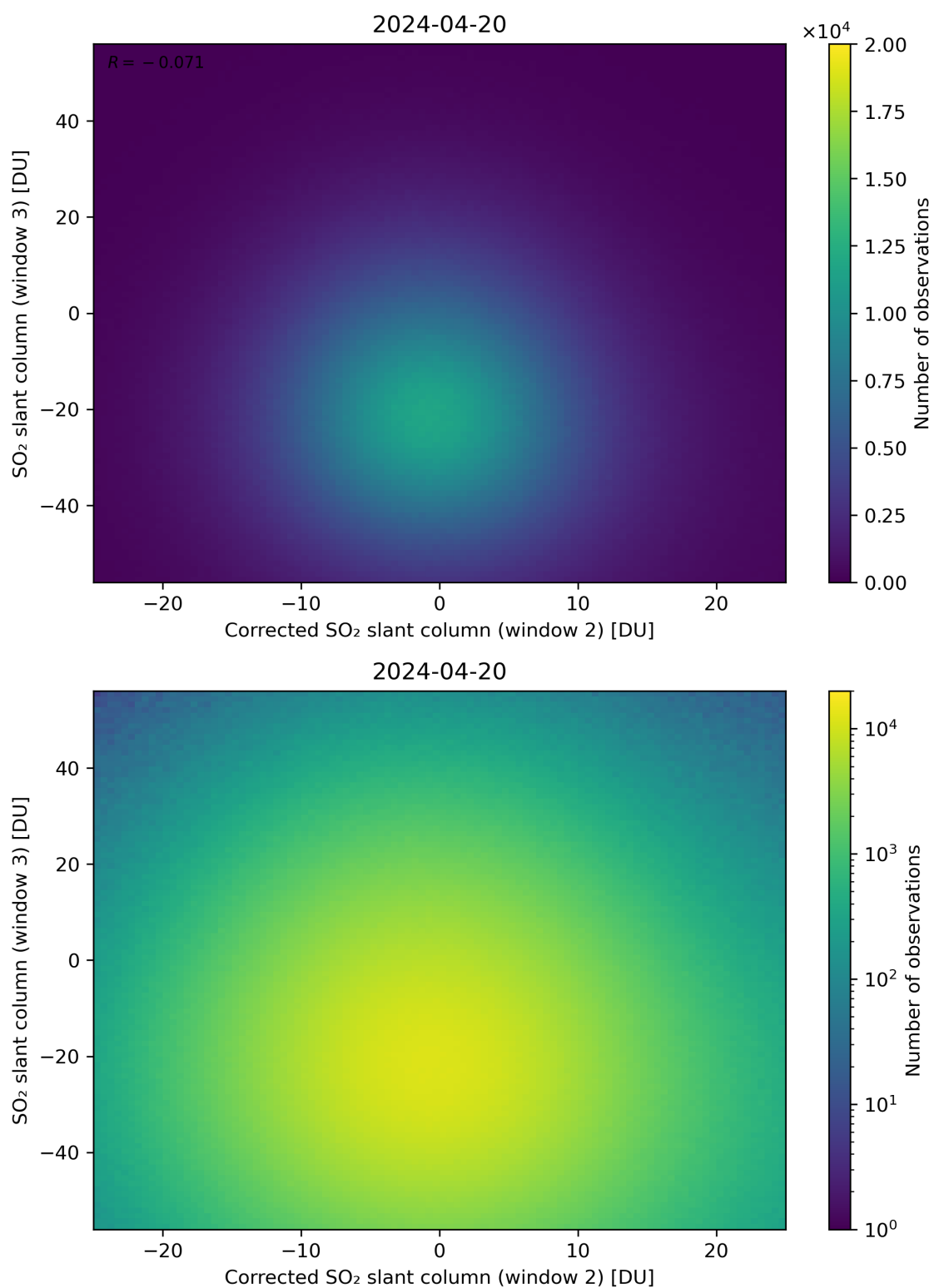
Figure 201: Scatter density plot of “Corrected SO 2 slant column (window 2)” against “SO 2 slant column (window 3)” for 2024-04-19 to 2024-04-21.
