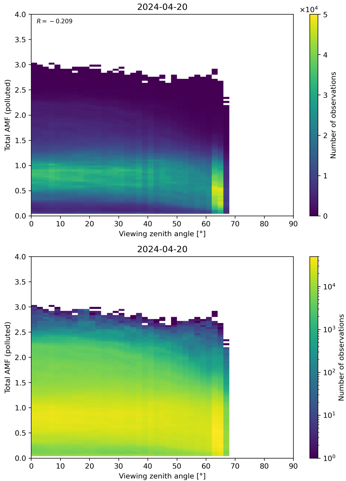
Figure 325: Scatter density plot of “Viewing zenith angle” against “Total AMF (polluted)” for 2024-04-19 to 2024-04-21.
