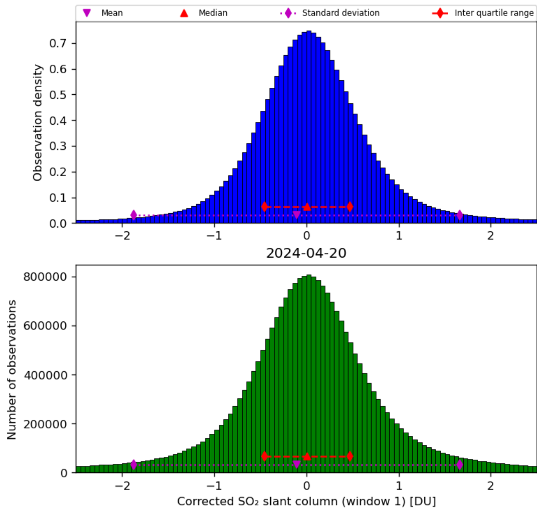
Figure 58: Histogram of “Corrected SO 2 slant column (window 1)” for 2024-04-19 to 2024-04-21
