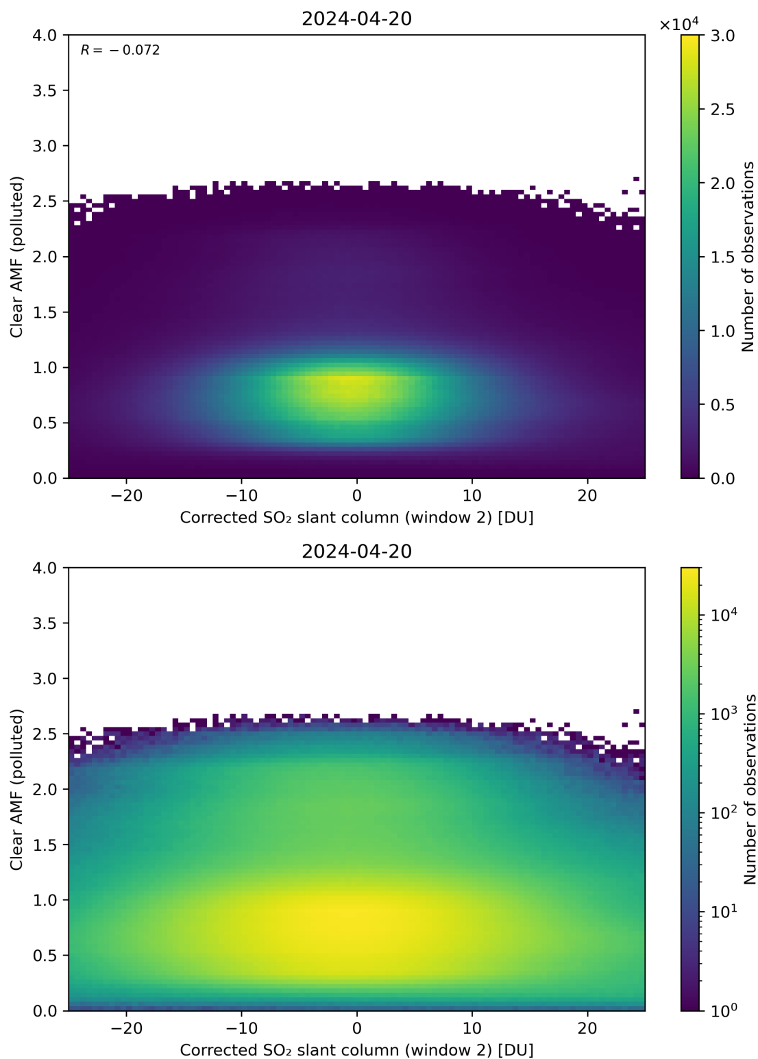
Figure 199: Scatter density plot of “Corrected SO 2 slant column (window 2)” against “Clear AMF (polluted)” for 2024-04-19 to 2024-04-21.
