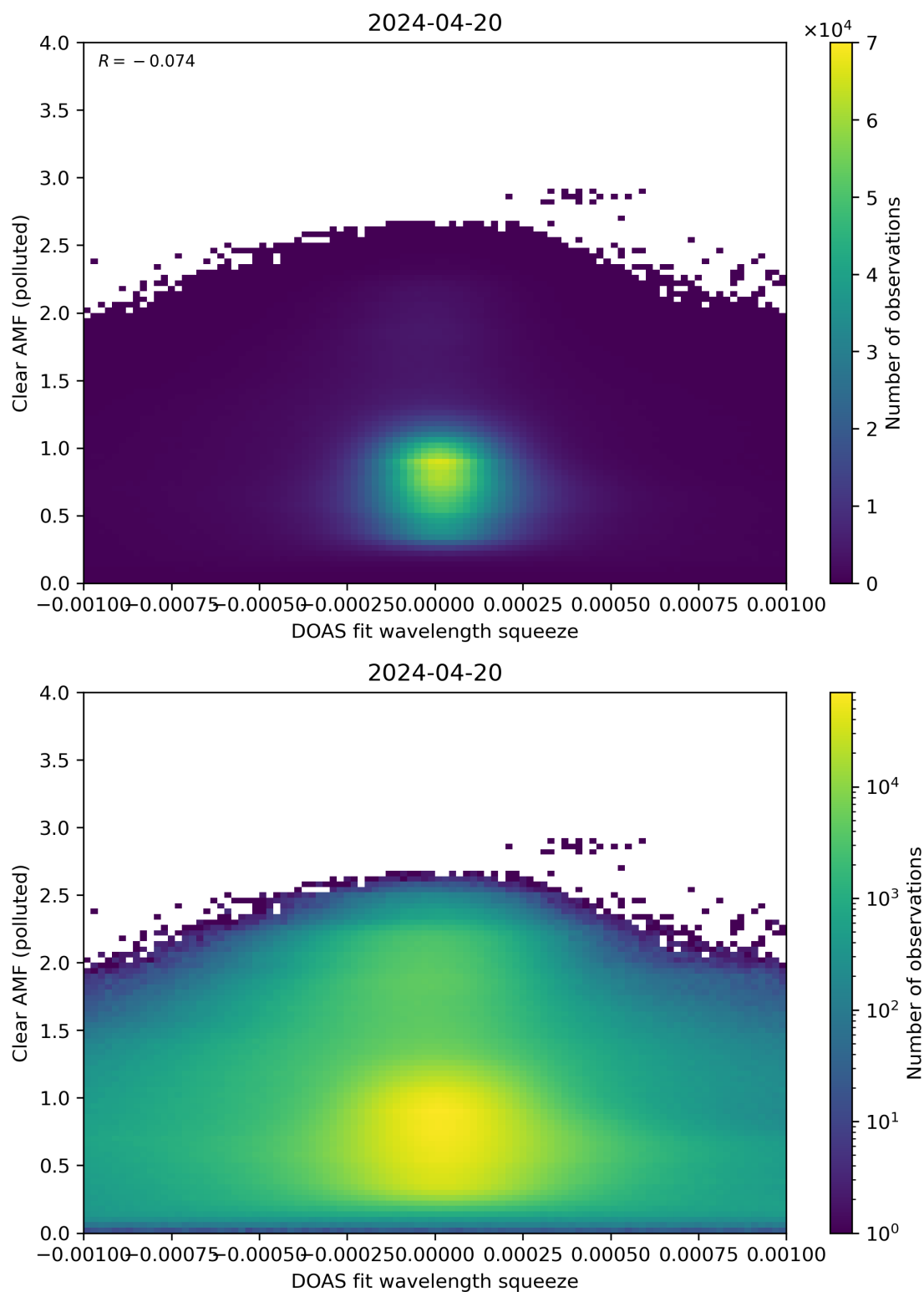
Figure 133: Scatter density plot of “DOAS fit wavelength squeeze” against “Clear AMF (polluted)” for 2024-04-19 to 2024-04-21.
