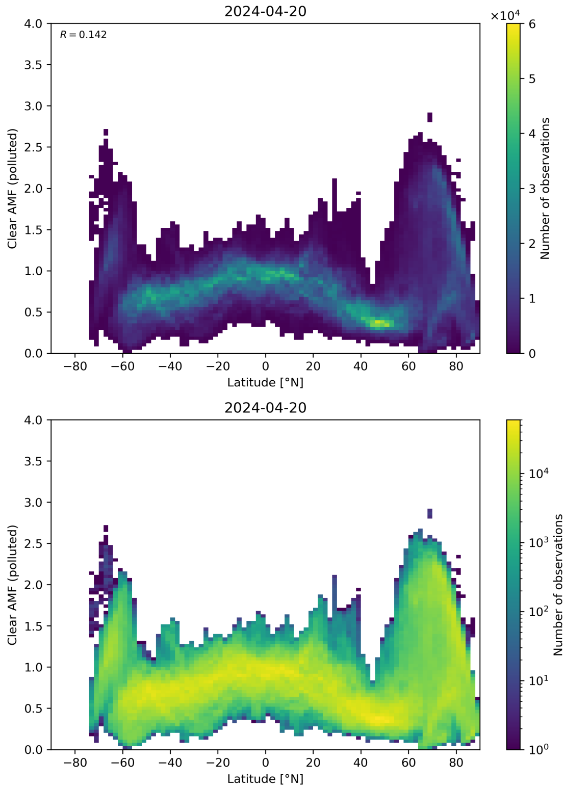
Figure 145: Scatter density plot of “Latitude” against “Clear AMF (polluted)” for 2024-04-19 to 2024-04-21.
