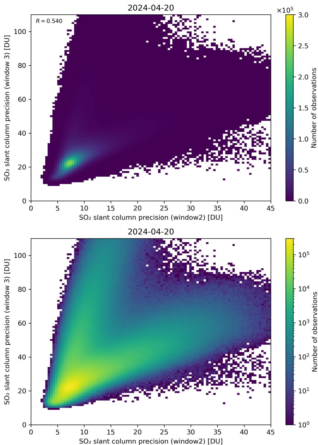
Figure 250: Scatter density plot of “SO 2 slant column precision (window2)” against “SO 2 slant column precision (window 3)” for 2024-04-19 to 2024-04-21.
