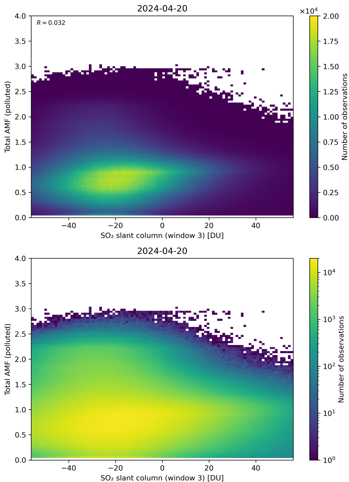
Figure 268: Scatter density plot of “SO 2 slant column (window 3)” against “Total AMF (polluted)” for 2024-04-19 to 2024-04-21.
