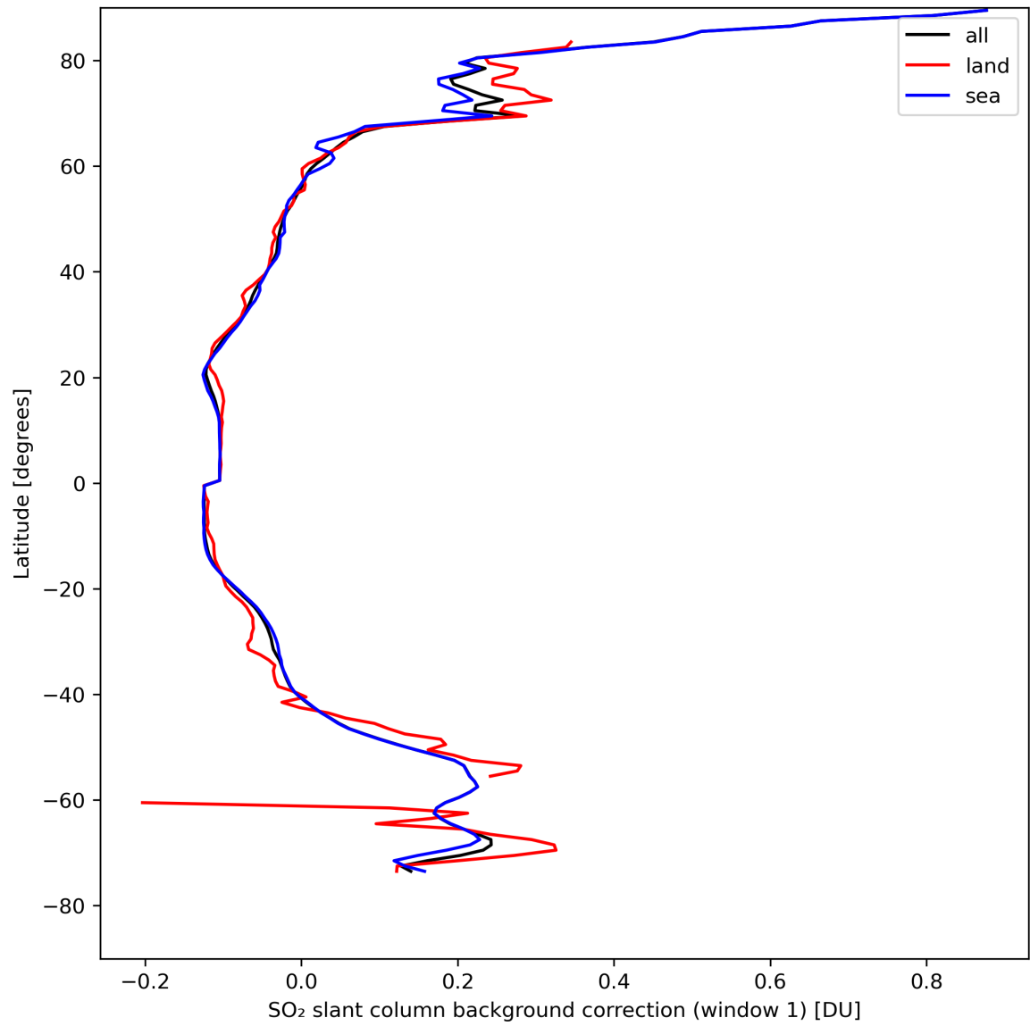
Figure 36: Zonal average of “SO 2 slant column background correction (window 1)” for 2024-04-19 to 2024-04-21.
