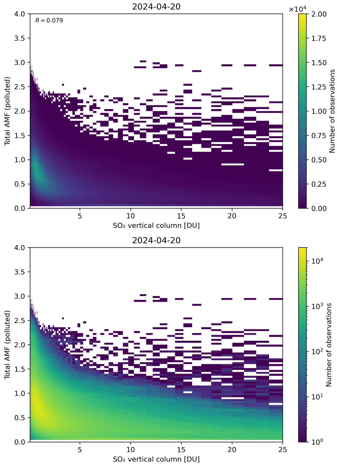
Figure 305: Scatter density plot of “SO 2 vertical column” against “Total AMF (polluted)” for 2024-04-19 to 2024-04-21.
