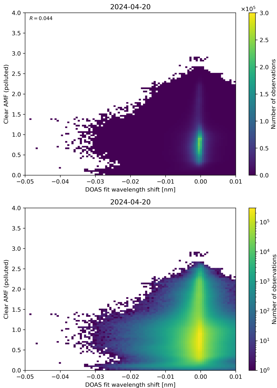
Figure 129: Scatter density plot of “DOAS fit wavelength shift” against “Clear AMF (polluted)” for 2024-04-19 to 2024-04-21.
