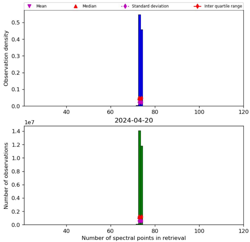
Figure 74: Histogram of “Number of spectral points in retrieval” for 2024-04-19 to 2024-04-21
