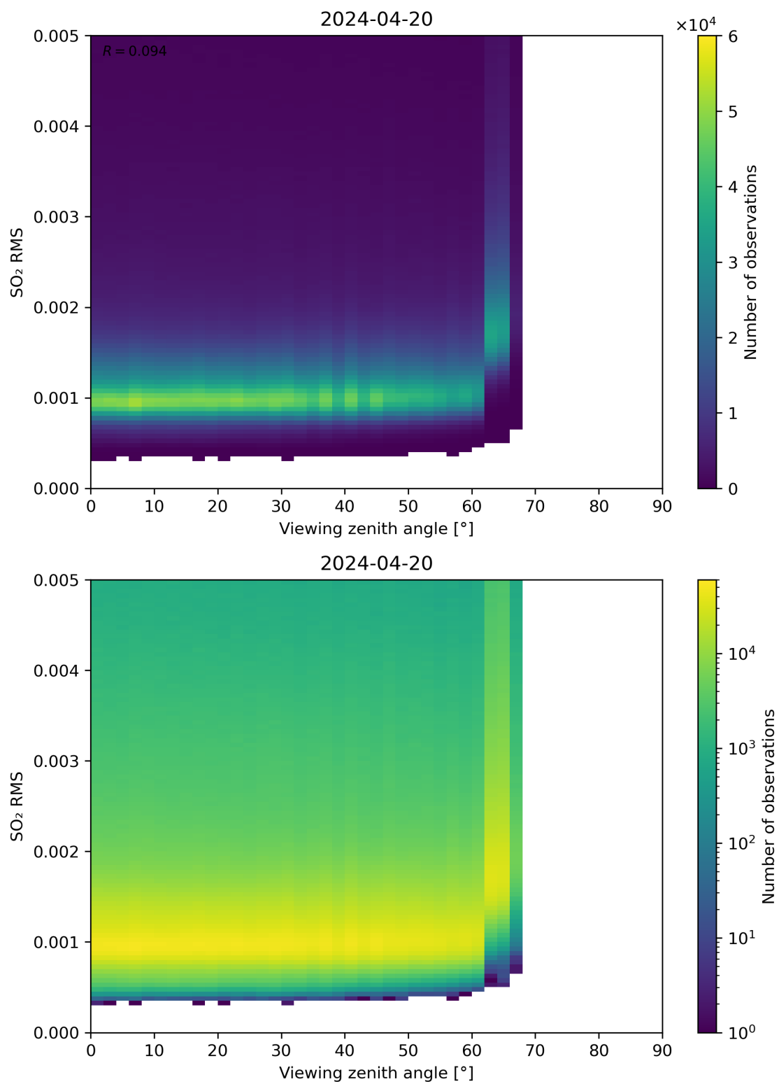
Figure 313: Scatter density plot of “Viewing zenith angle” against “SO 2 RMS” for 2024-04-19 to 2024-04-21.
