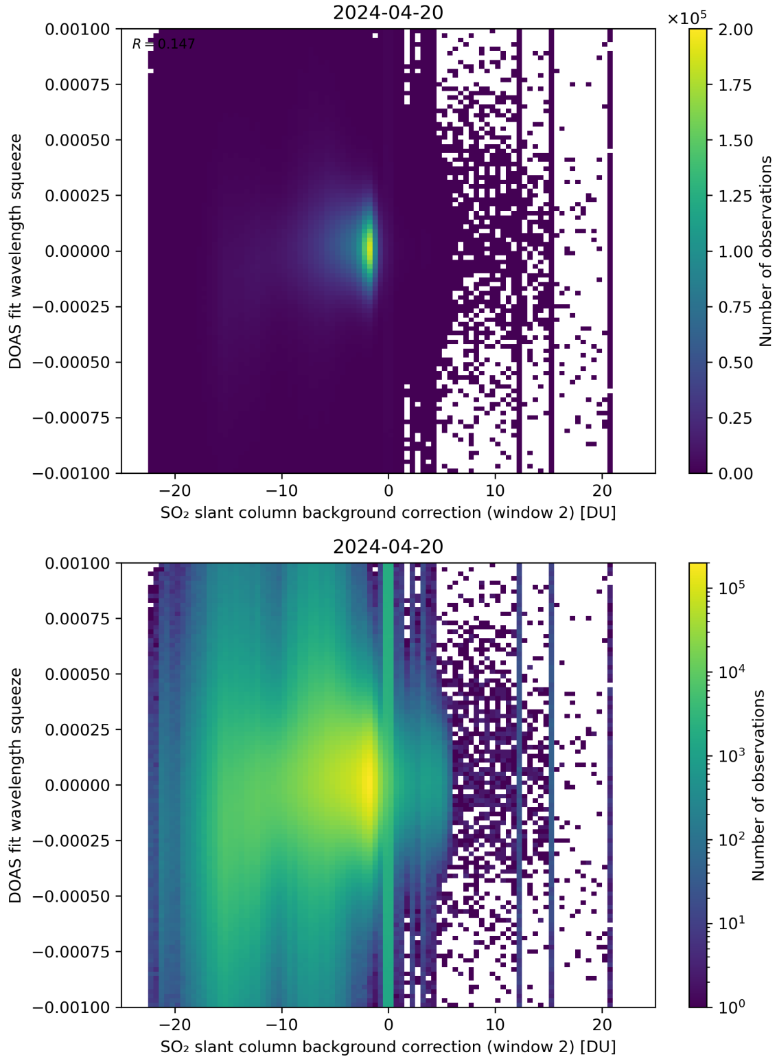
Figure 113: Scatter density plot of “SO 2 slant column background correction (window 2)” against “DOAS fit wavelength squeeze” for 2024-04-19 to 2024-04-21.
