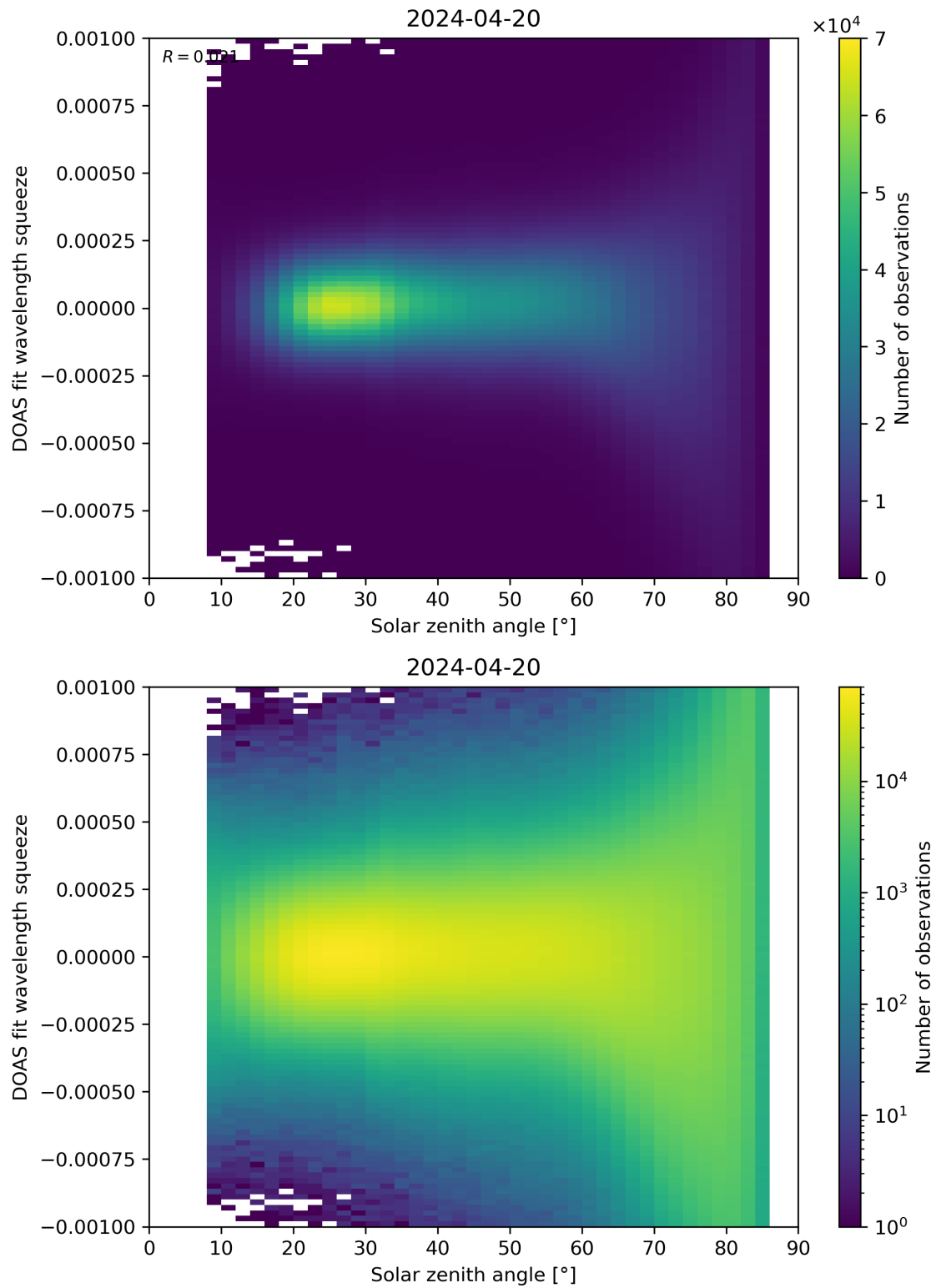
Figure 162: Scatter density plot of “Solar zenith angle” against “DOAS fit wavelength squeeze” for 2024-04-19 to 2024-04-21.
