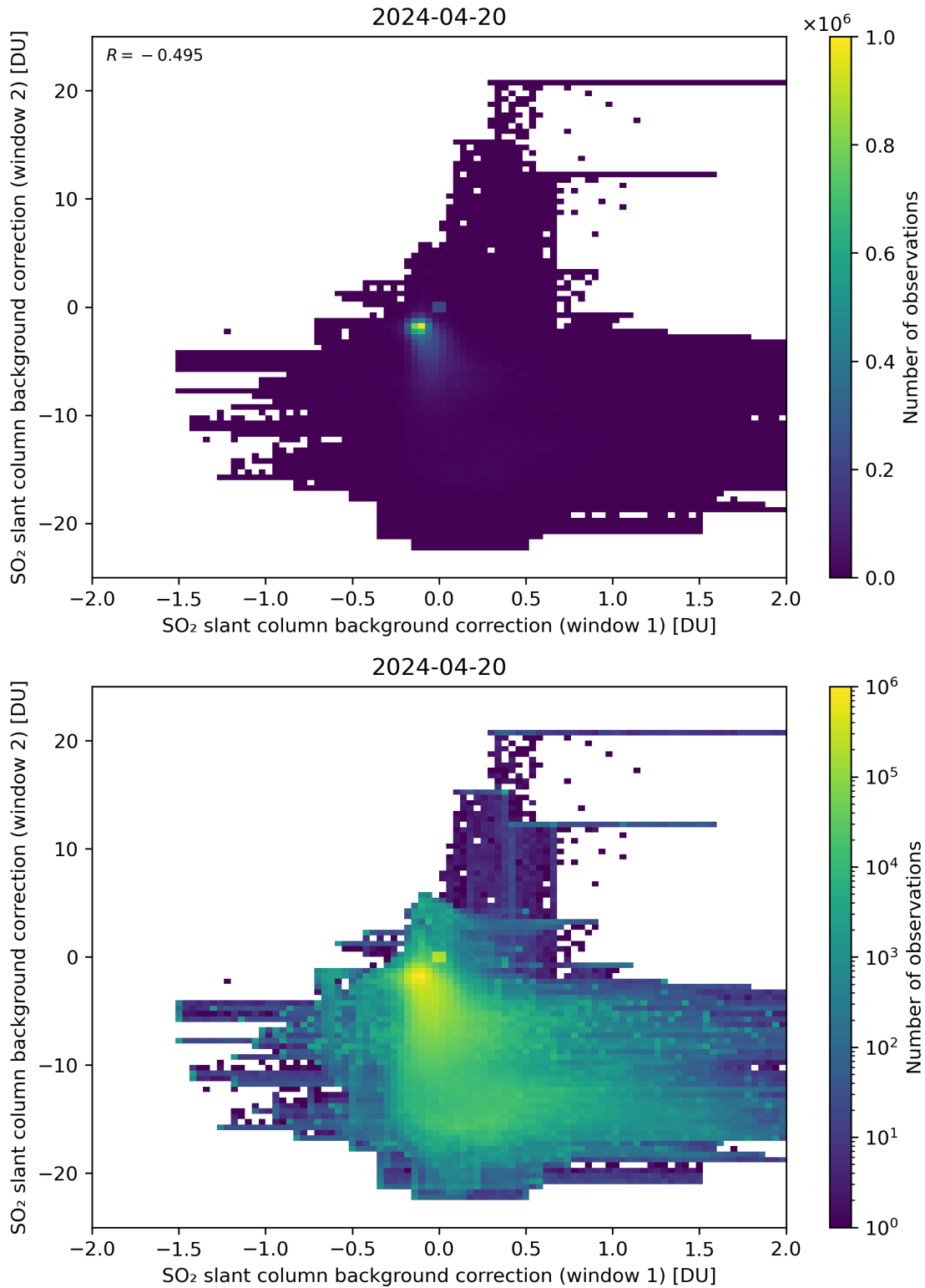
Figure 98: Scatter density plot of “SO 2 slant column background correction (window 1)” against “SO 2 slant column background correction (window 2)” for 2024-04-19 to 2024-04-21.
