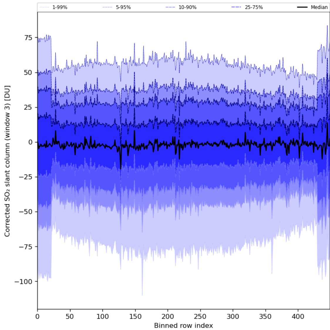
Figure 89: Along track statistics of “Corrected SO 2 slant column (window 3)” for 2024-04-19 to 2024-04-21
