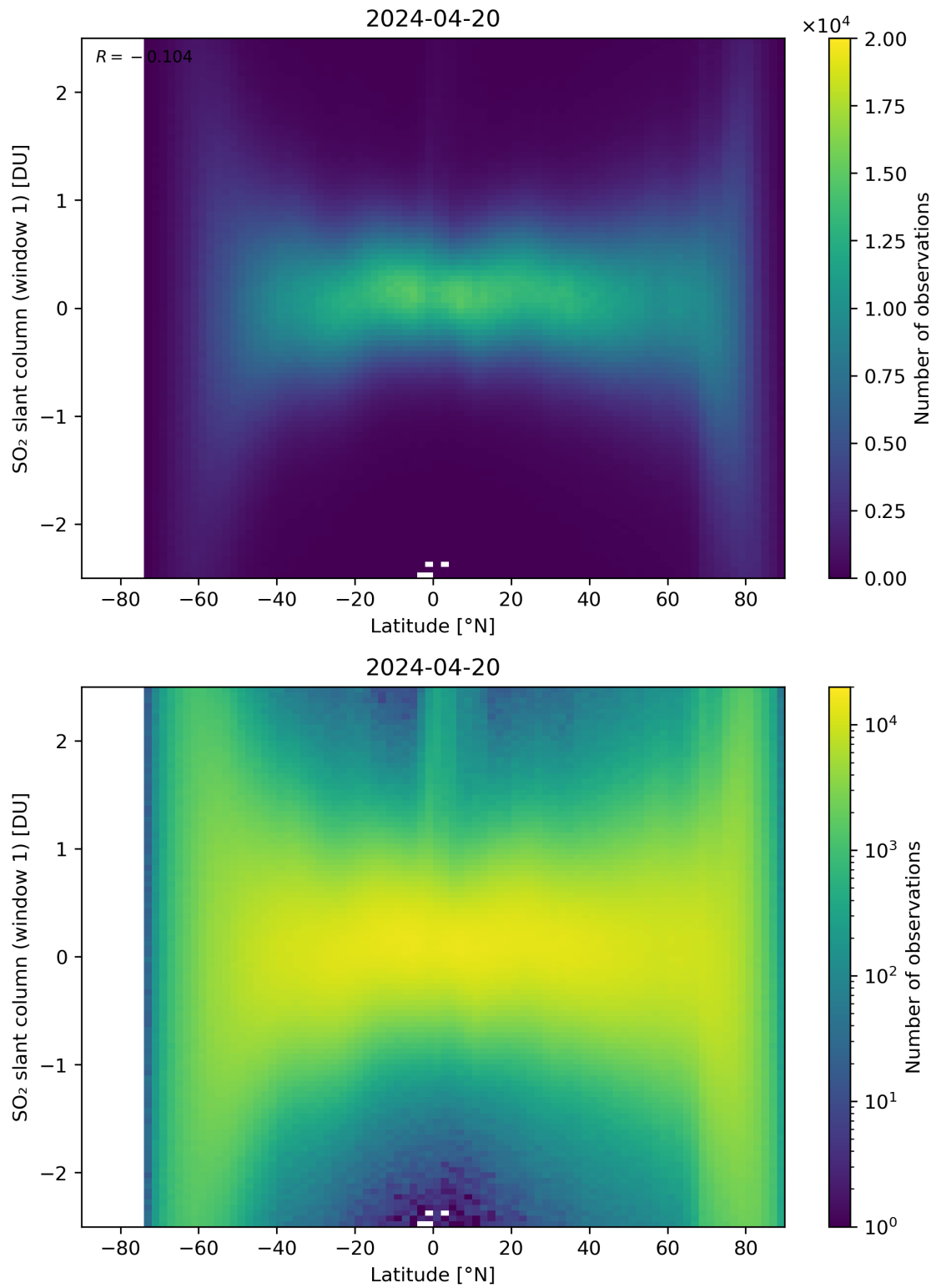
Figure 149: Scatter density plot of “Latitude” against “SO 2 slant column (window 1)” for 2024-04-19 to 2024-04-21.
