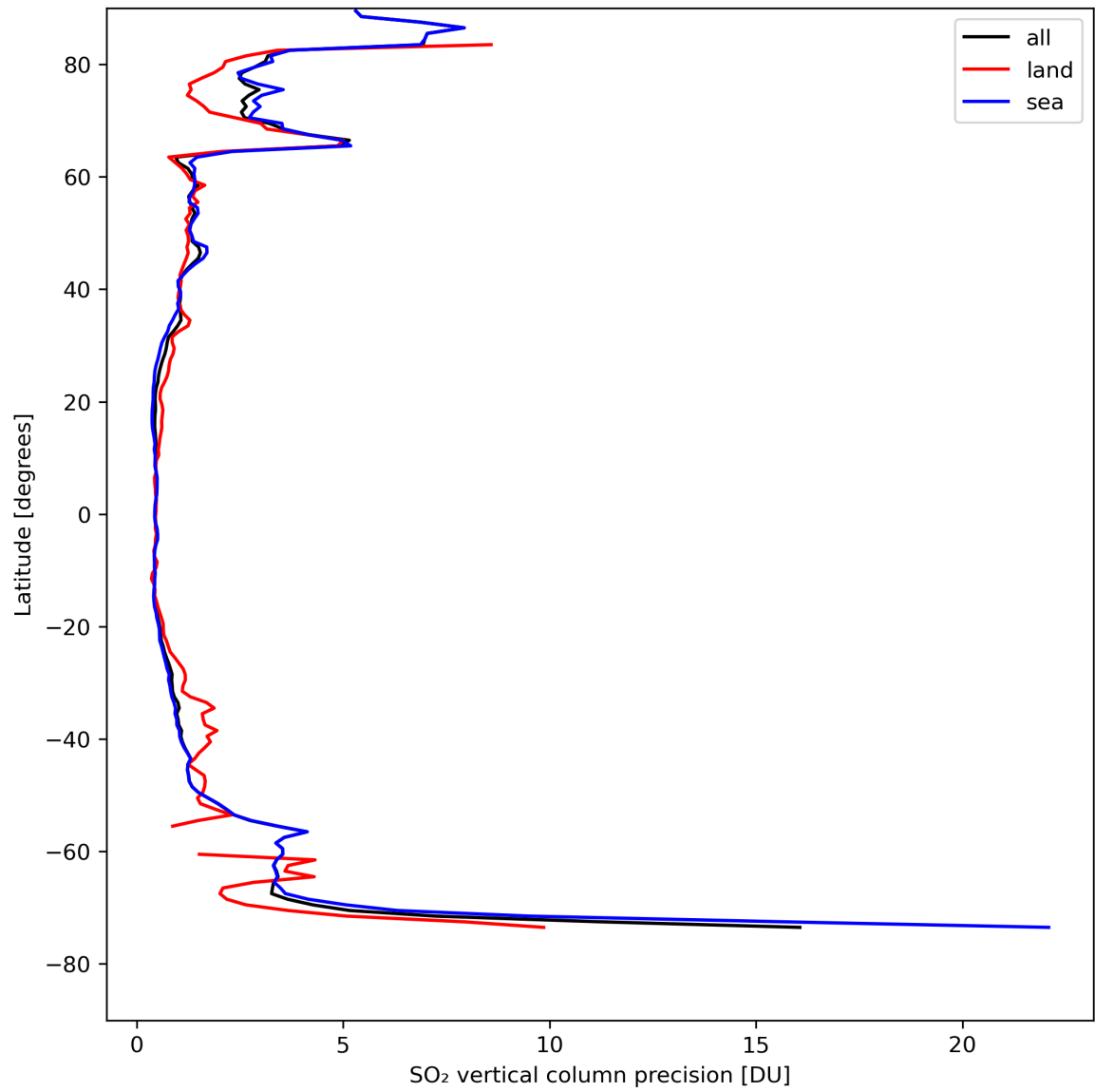
Figure 31: Zonal average of “SO 2 vertical column precision” for 2024-04-19 to 2024-04-21.
