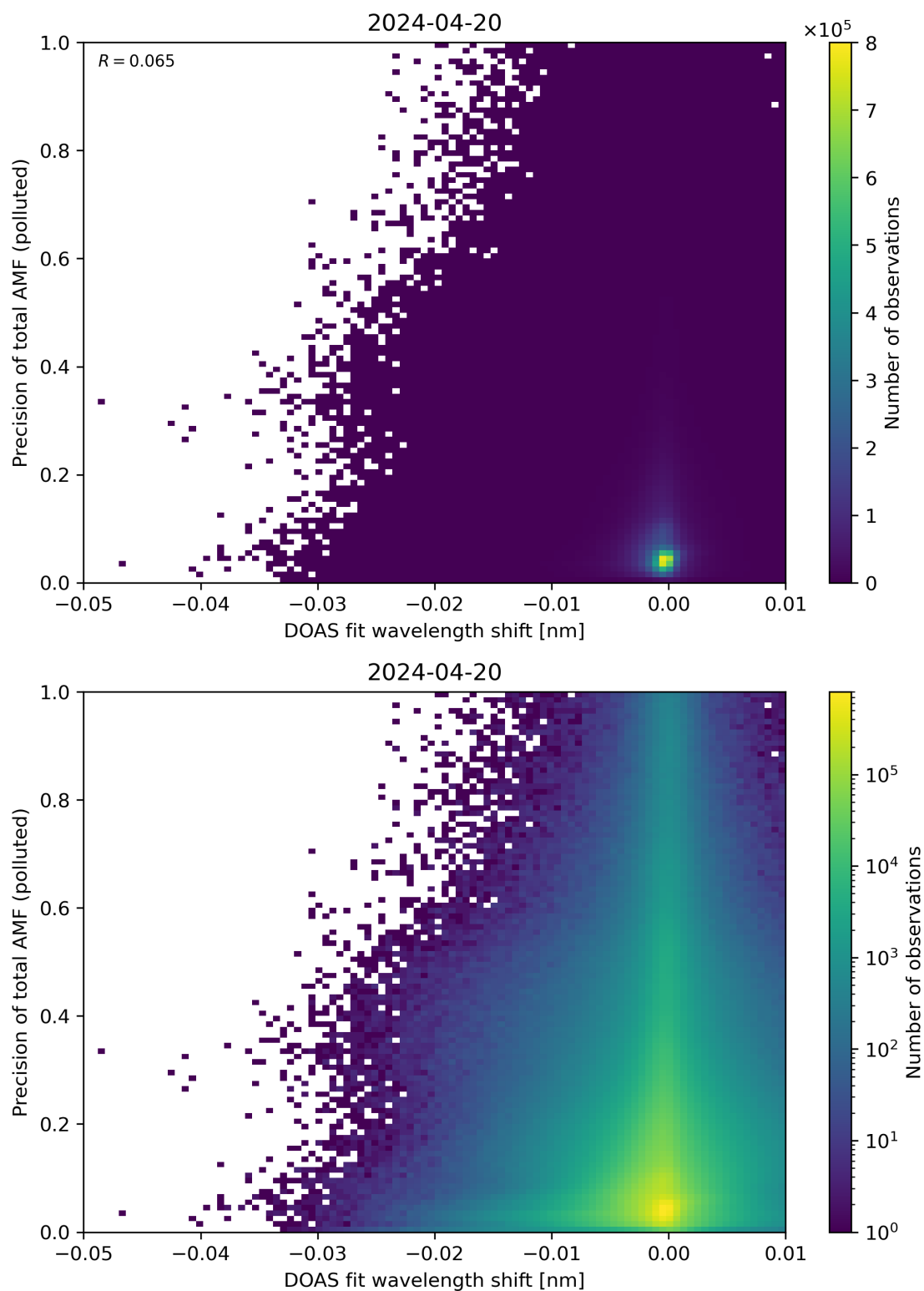
Figure 131: Scatter density plot of “DOAS fit wavelength shift” against “Precision of total AMF (polluted)” for 2024-04-19 to 2024-04-21.
