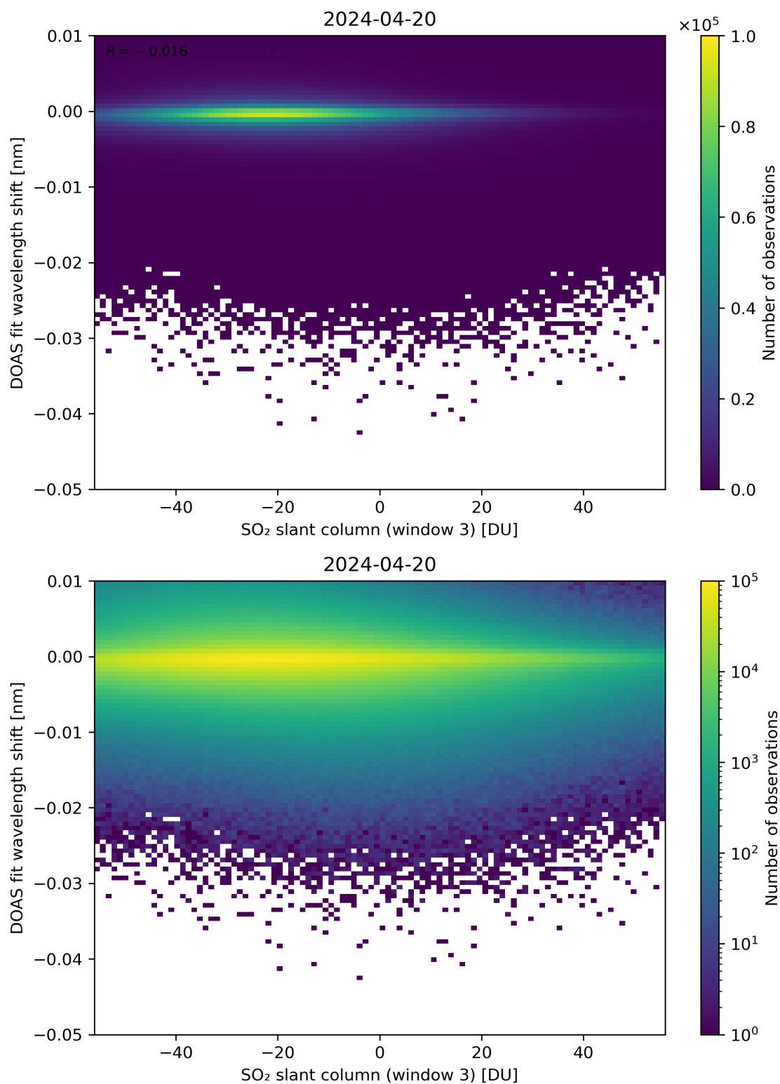
Figure 254: Scatter density plot of “SO 2 slant column (window 3)” against “DOAS fit wavelength shift” for 2024-04-19 to 2024-04-21.
