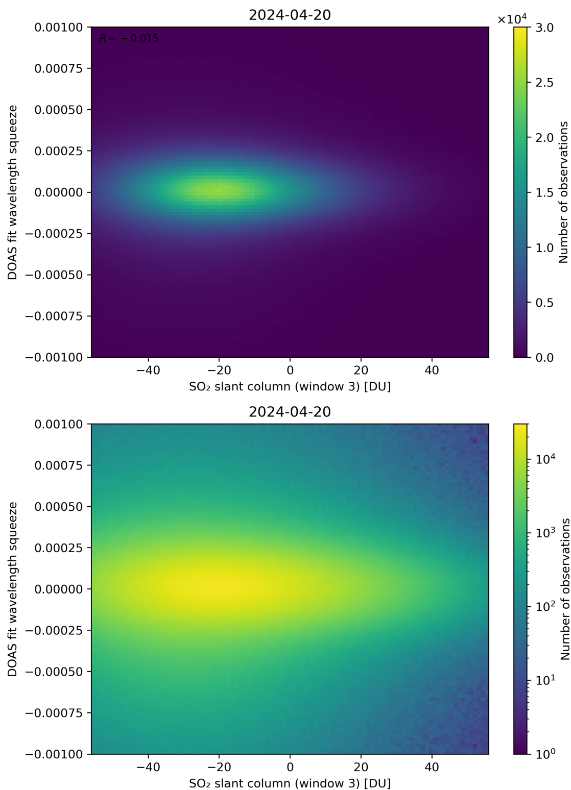
Figure 255: Scatter density plot of “SO 2 slant column (window 3)” against “DOAS fit wavelength squeeze” for 2024-04-19 to 2024-04-21.
