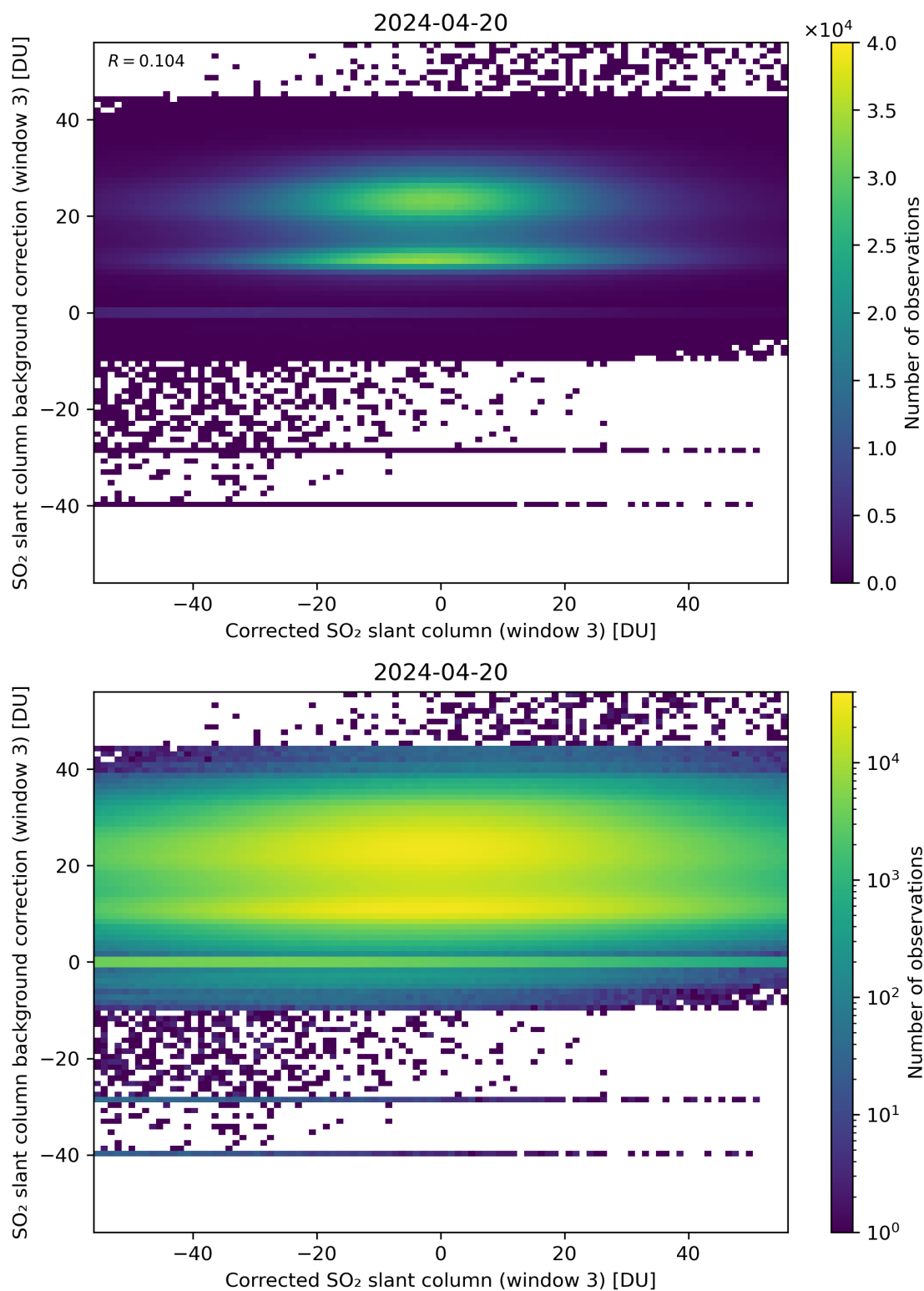
Figure 205: Scatter density plot of “Corrected SO 2 slant column (window 3)” against “SO 2 slant column background correction (window 3)” for 2024-04-19 to 2024-04-21.
