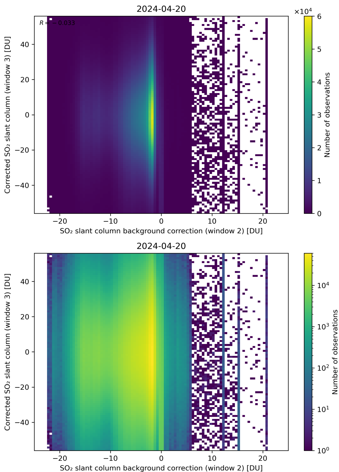
Figure 116: Scatter density plot of “SO 2 slant column background correction (window 2)” against “Corrected SO 2 slant column (window 3)” for 2024-04-19 to 2024-04-21.
