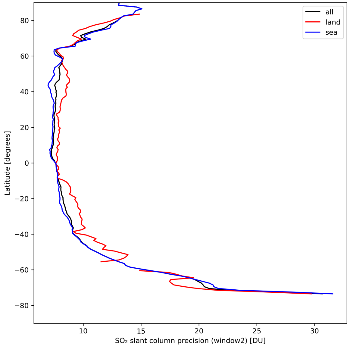
Figure 38: Zonal average of “SO 2 slant column precision (window2)” for 2024-04-19 to 2024-04-21.
