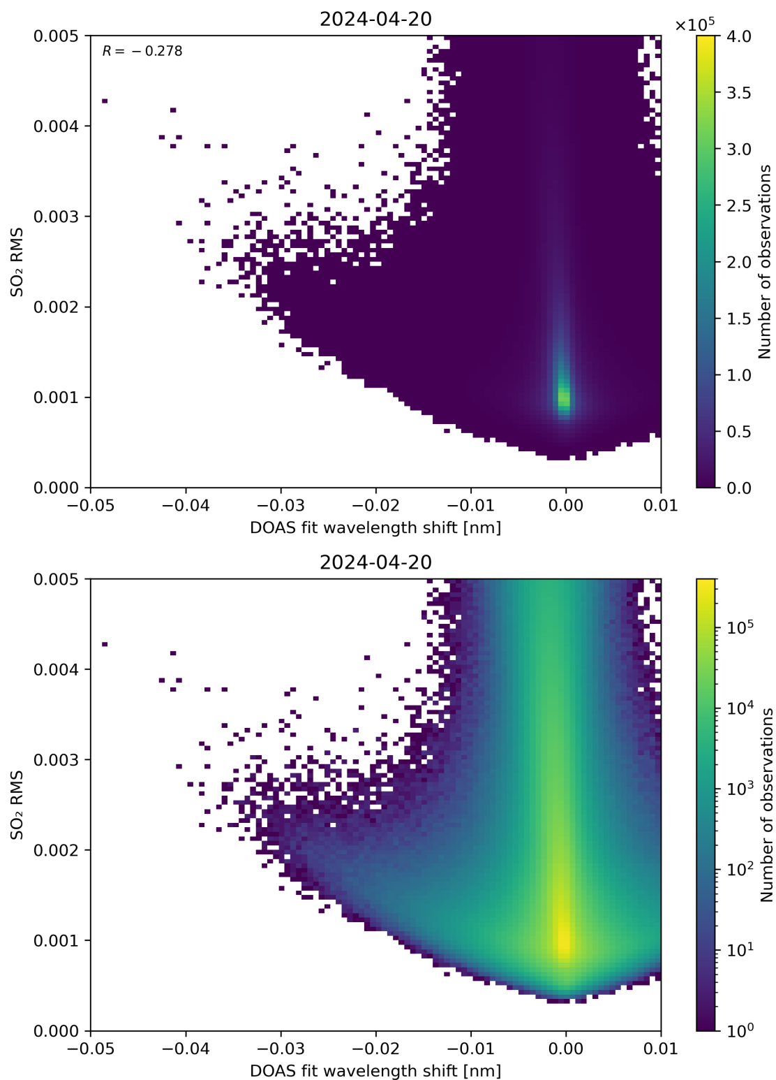
Figure 128: Scatter density plot of “DOAS fit wavelength shift” against “SO 2 RMS” for 2024-04-19 to 2024-04-21.
