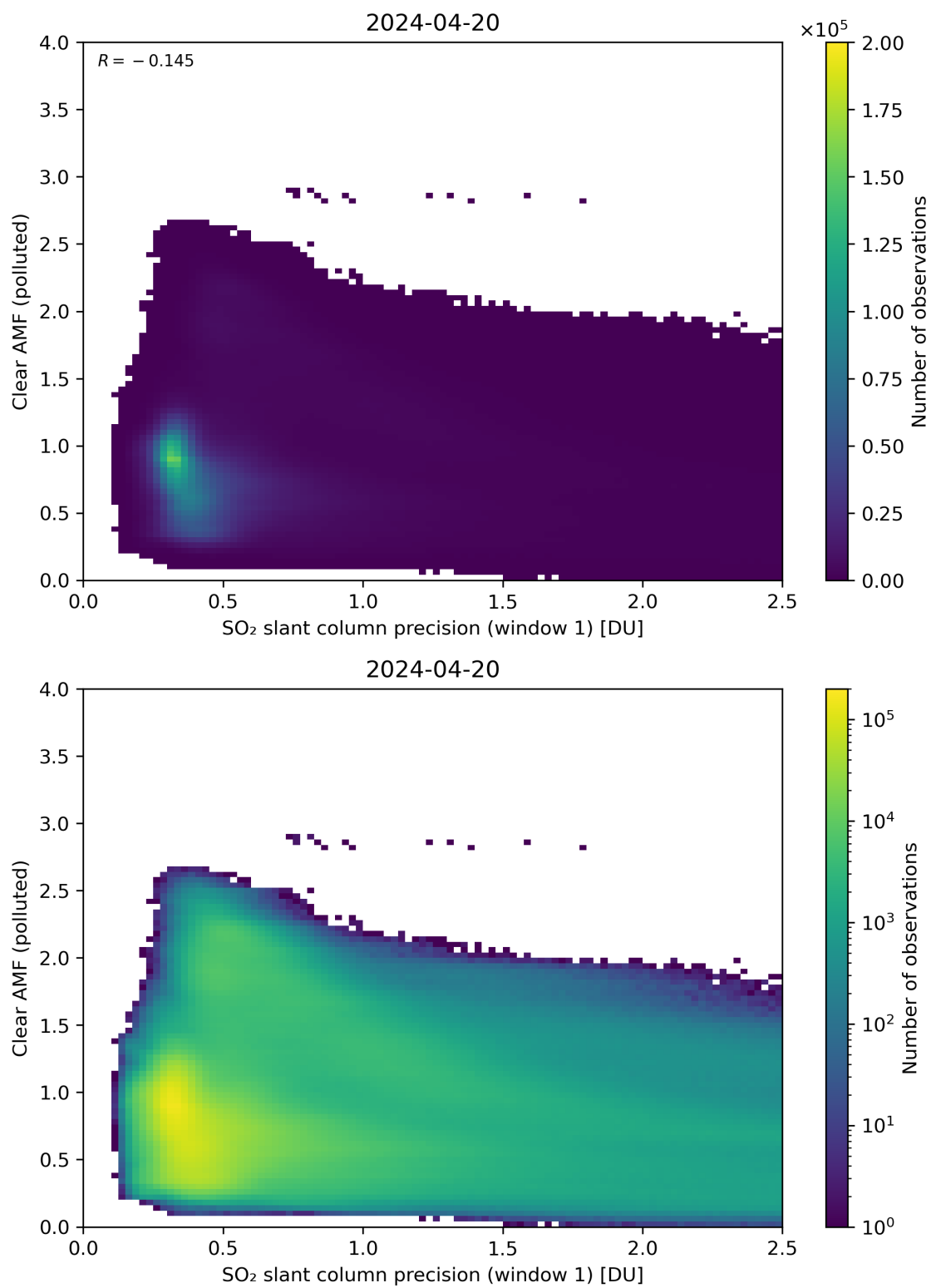
Figure 224: Scatter density plot of “SO 2 slant column precision (window 1)” against “Clear AMF (polluted)” for 2024-04-19 to 2024-04-21.
