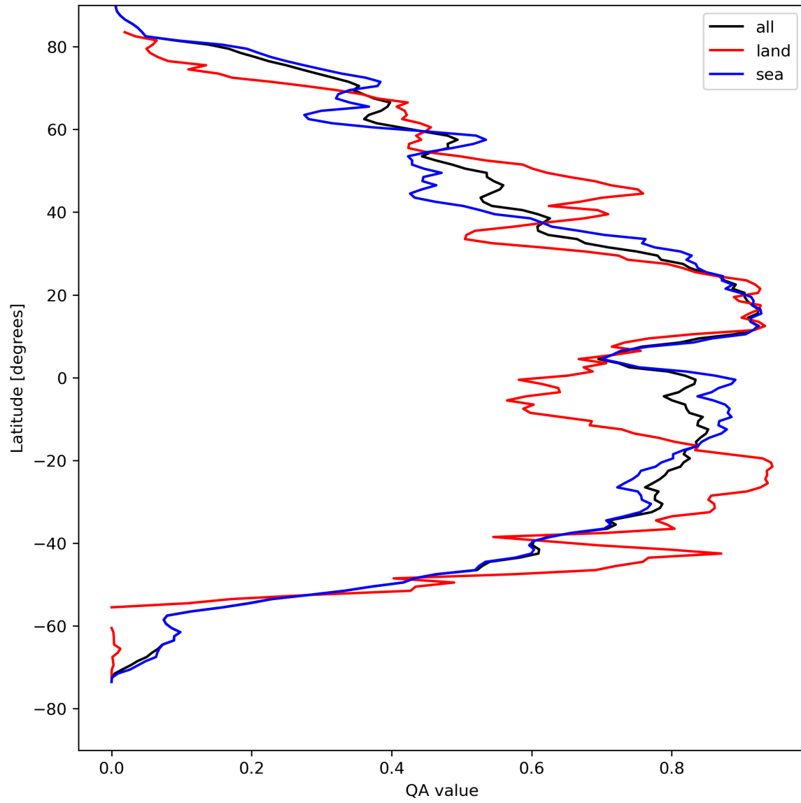
Figure 29: Zonal average of “QA value” for 2024-04-19 to 2024-04-21.
