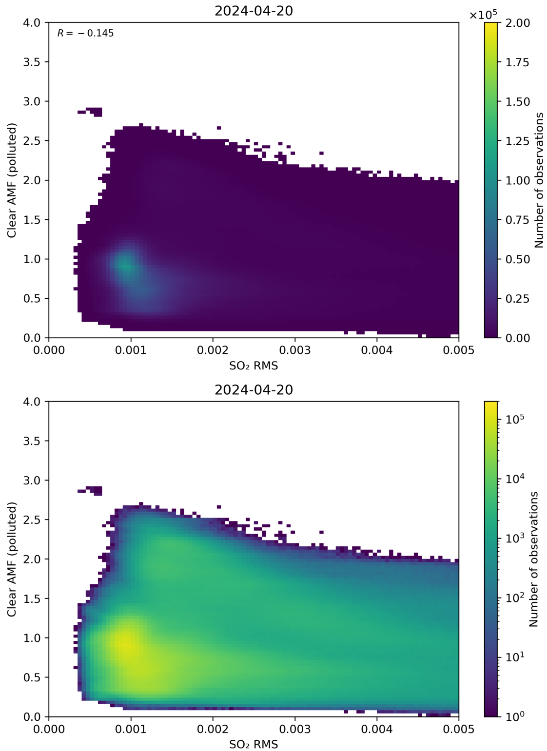
Figure 136: Scatter density plot of “SO 2 RMS” against “Clear AMF (polluted)” for 2024-04-19 to 2024-04-21.
