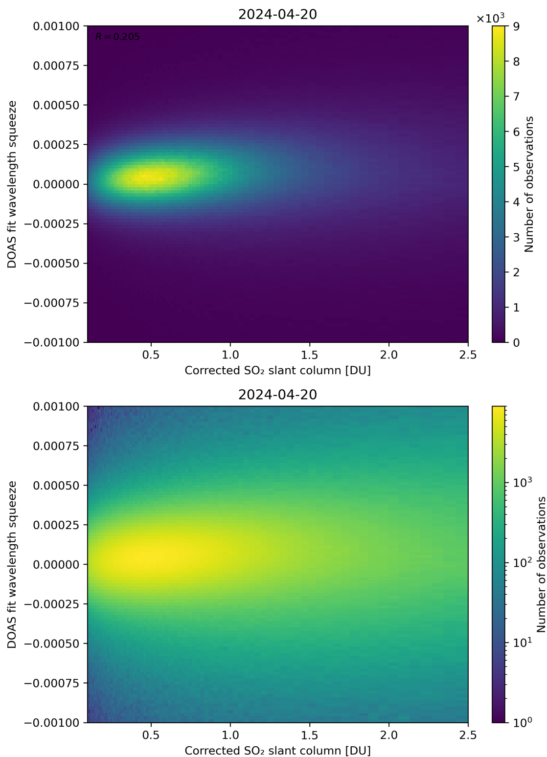
Figure 182: Scatter density plot of “Corrected SO 2 slant column” against “DOAS fit wavelength squeeze” for 2024-04-19 to 2024-04-21.
