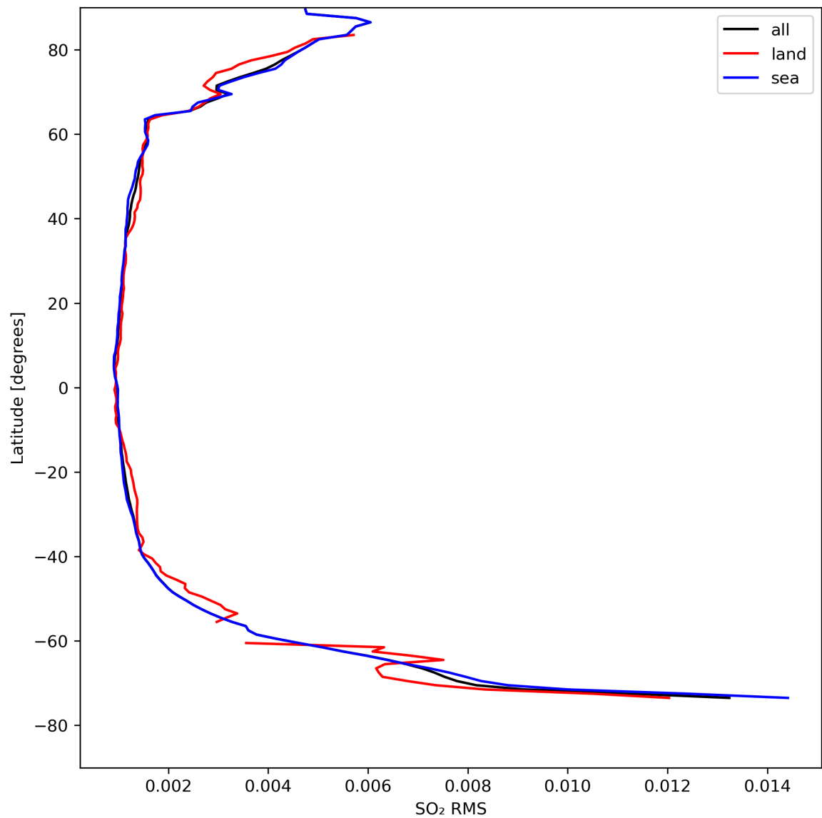
Figure 47: Zonal average of “SO 2 RMS” for 2024-04-19 to 2024-04-21.
