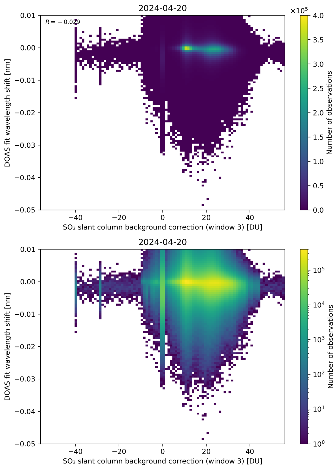
Figure 121: Scatter density plot of “SO 2 slant column background correction (window 3)” against “DOAS fit wavelength shift” for 2024-04-19 to 2024-04-21.
