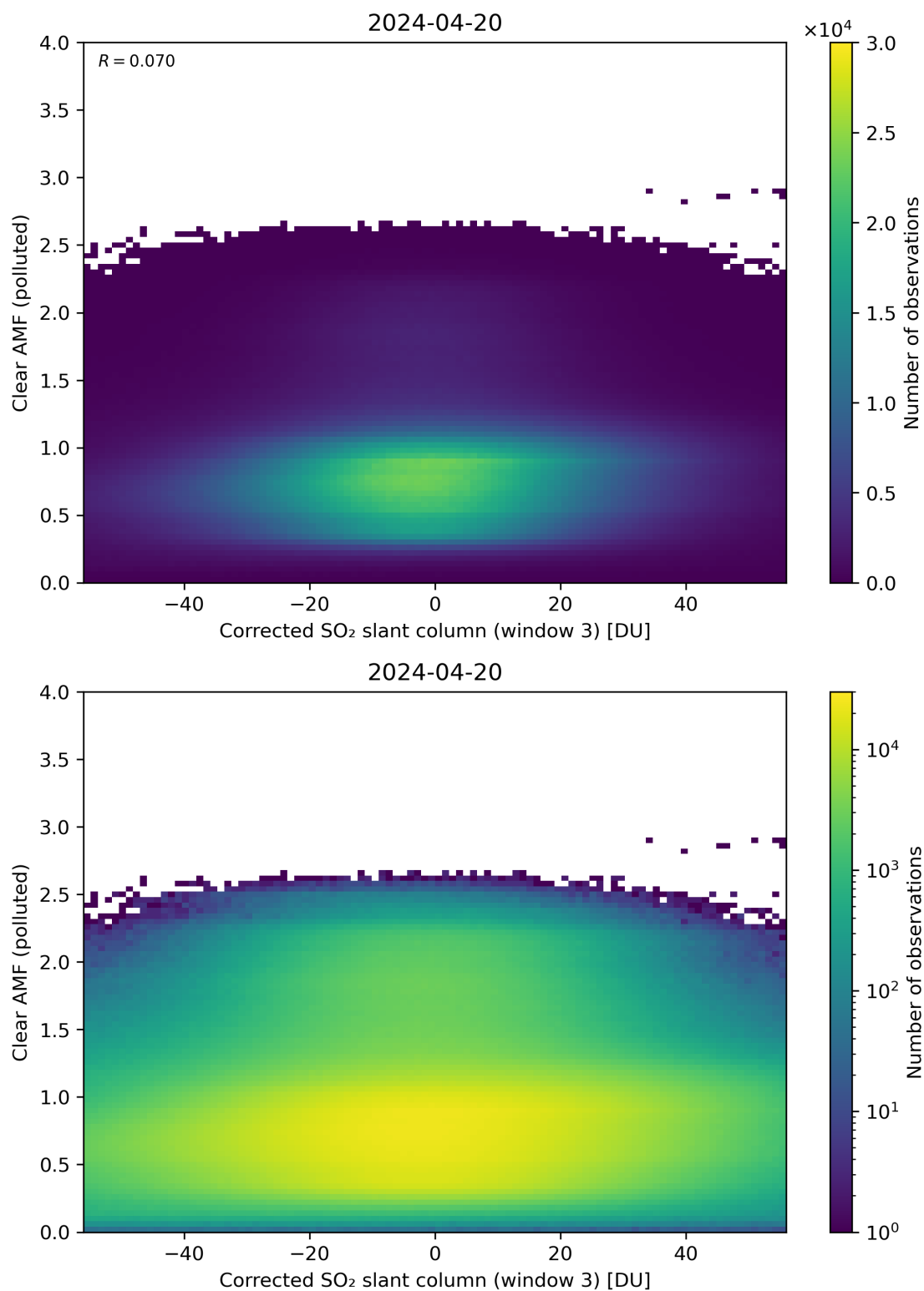
Figure 209: Scatter density plot of “Corrected SO 2 slant column (window 3)” against “Clear AMF (polluted)” for 2024-04-19 to 2024-04-21.
