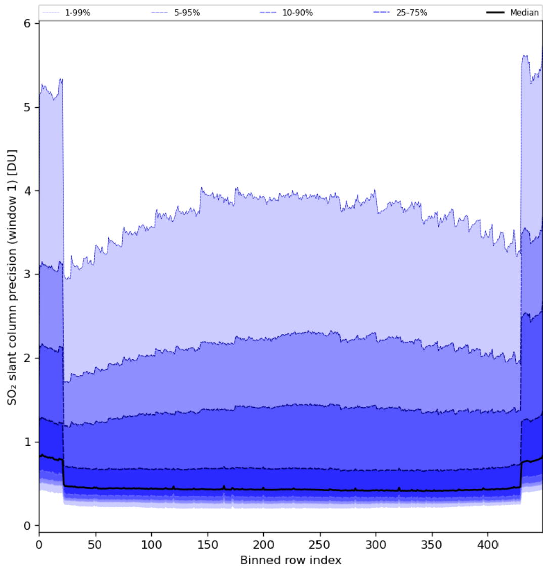
Figure 80: Along track statistics of “SO 2 slant column precision (window 1)” for 2024-04-19 to 2024-04-21
