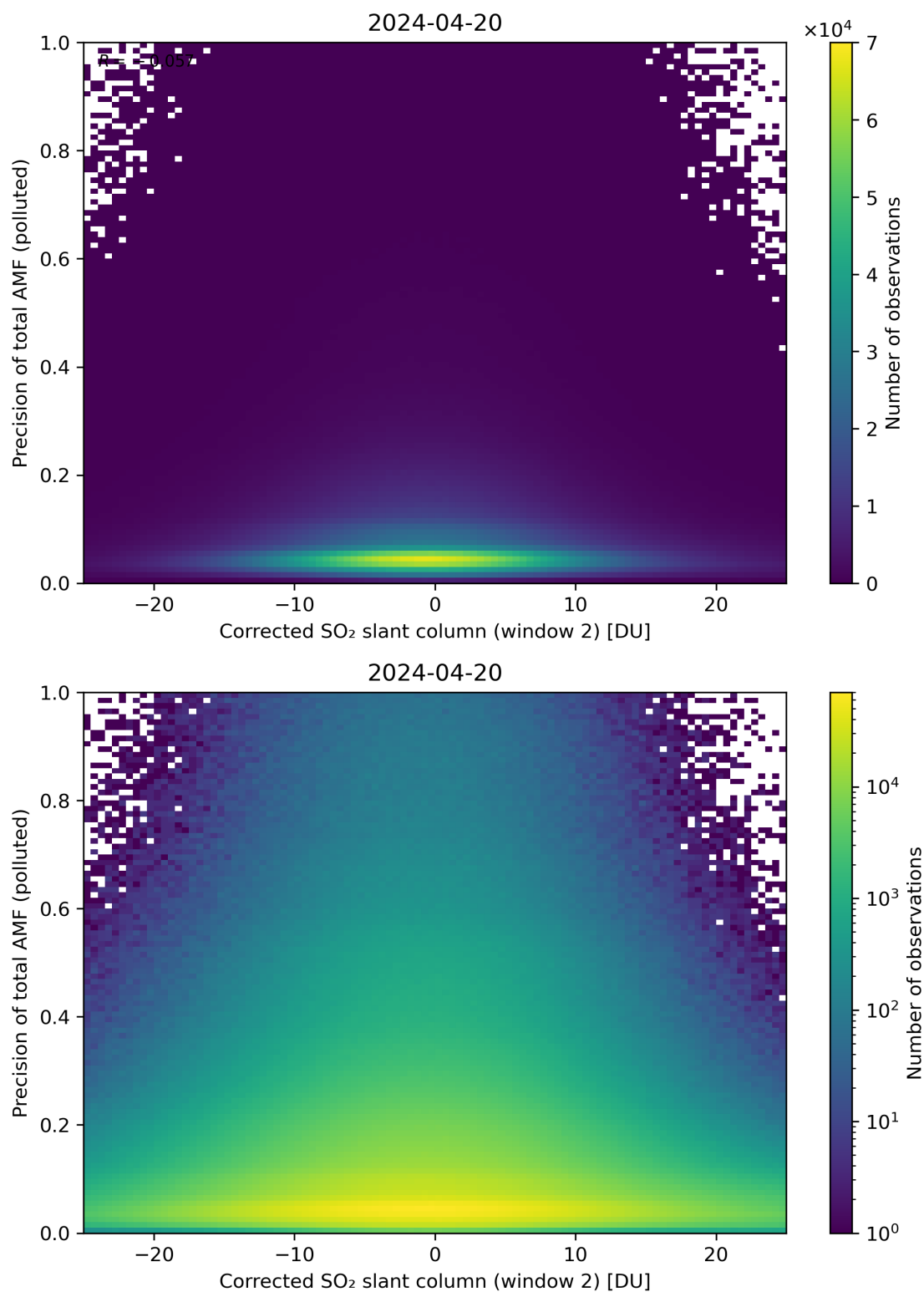
Figure 204: Scatter density plot of “Corrected SO 2 slant column (window 2)” against “Precision of total AMF (polluted)” for 2024-04-19 to 2024-04-21.
