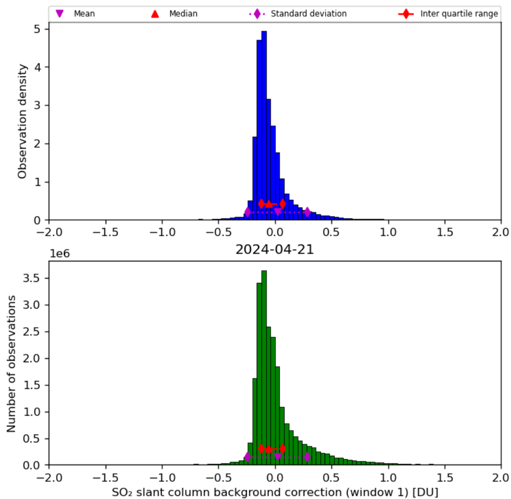
Figure 59: Histogram of “SO 2 slant column background correction (window 1)” for 2024-04-21 to 2024-04-22
