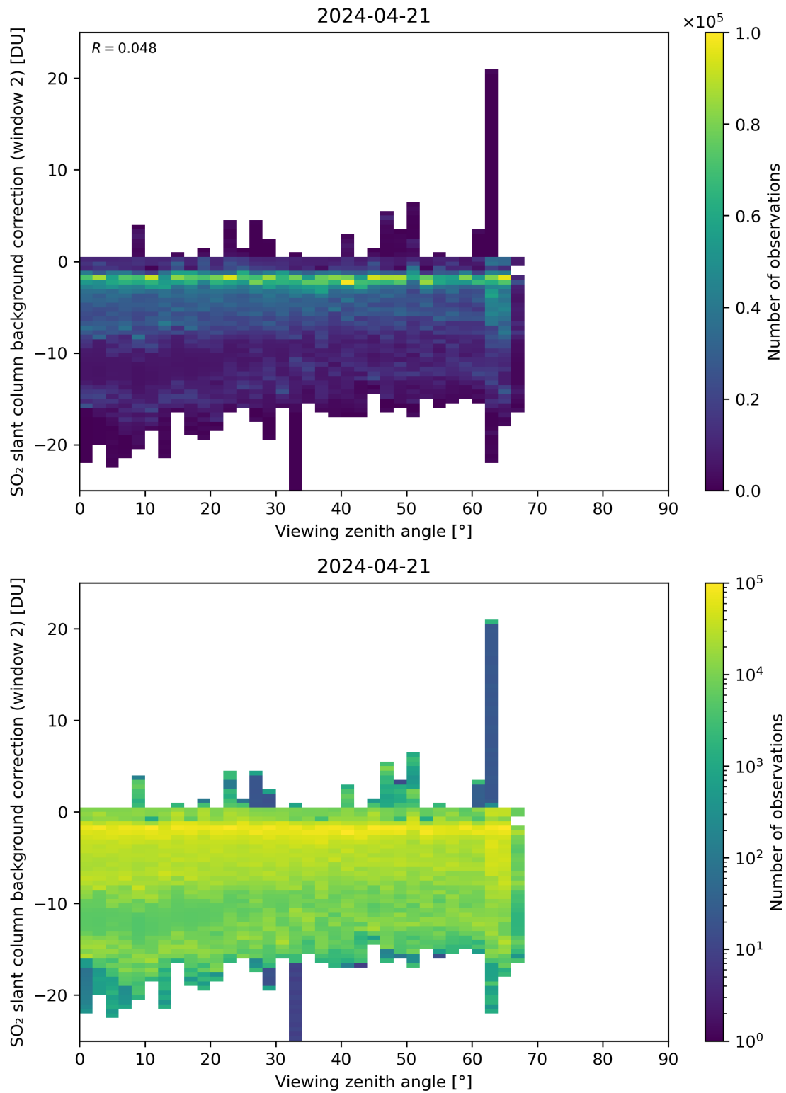
Figure 309: Scatter density plot of “Viewing zenith angle” against “SO 2 slant column background correction (window 2)” for 2024-04-21 to 2024-04-22.
