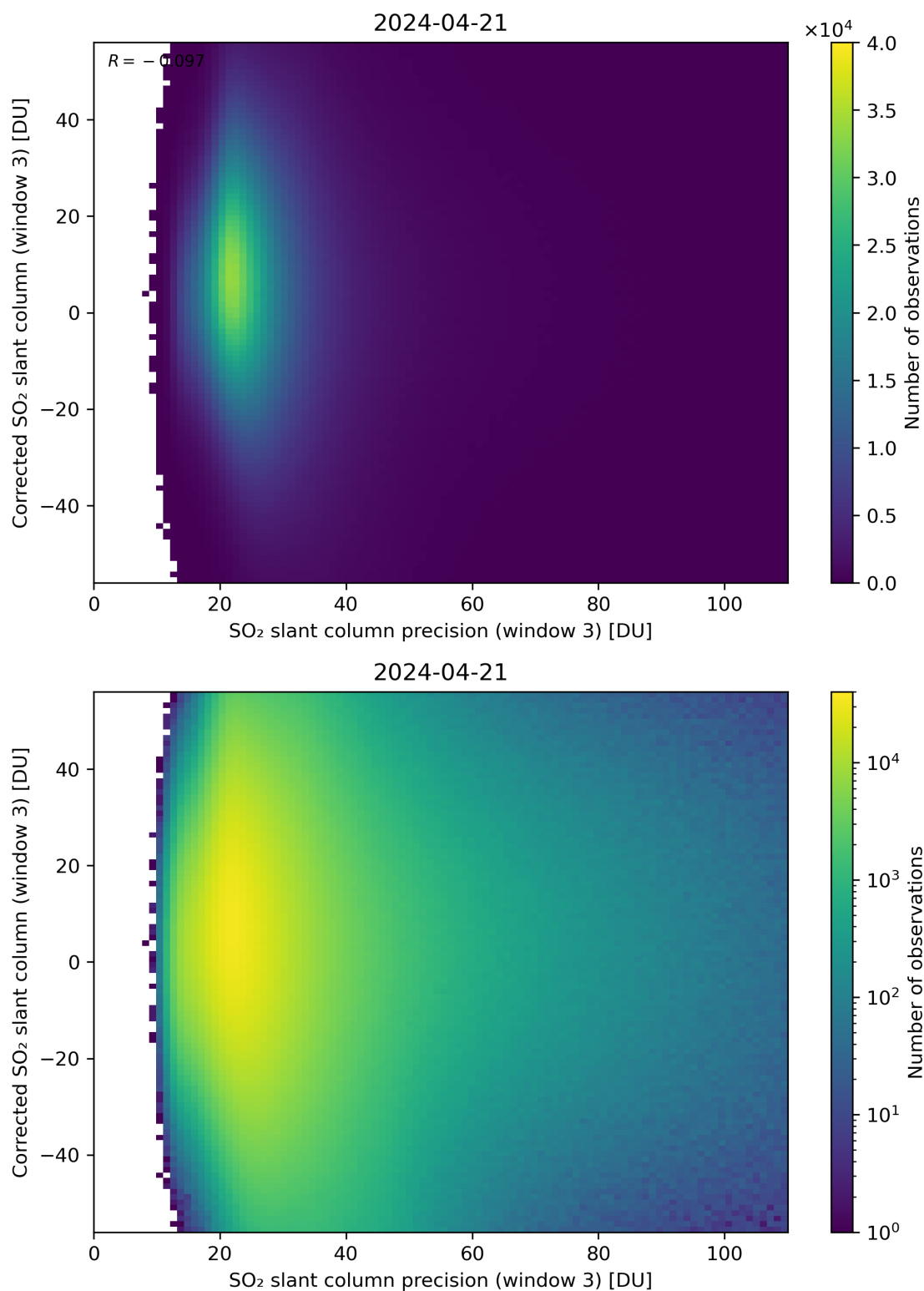
Figure 262: Scatter density plot of “SO 2 slant column precision (window 3)” against “Corrected SO 2 slant column (window 3)” for 2024-04-21 to 2024-04-22.
