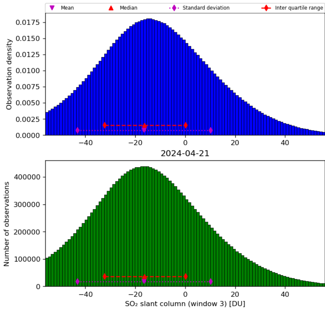
Figure 64: Histogram of “SO 2 slant column (window 3)” for 2024-04-21 to 2024-04-22
