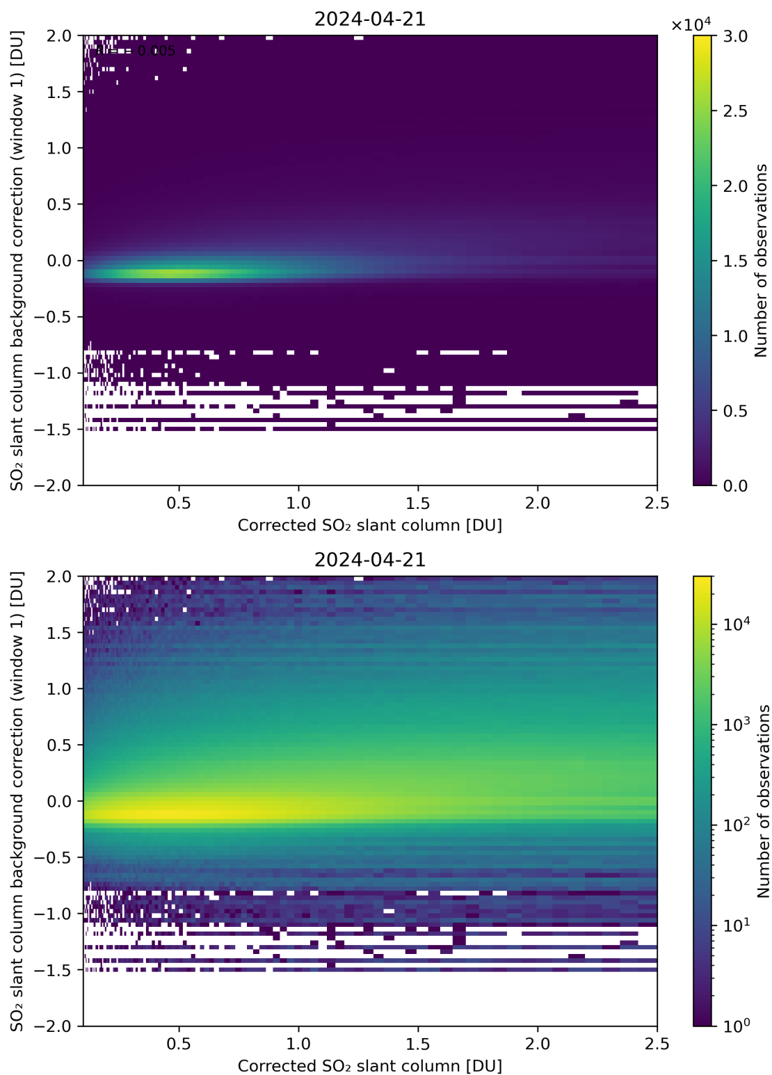
Figure 178: Scatter density plot of “Corrected SO 2 slant column” against “SO 2 slant column background correction (window 1)” for 2024-04-21 to 2024-04-22.
