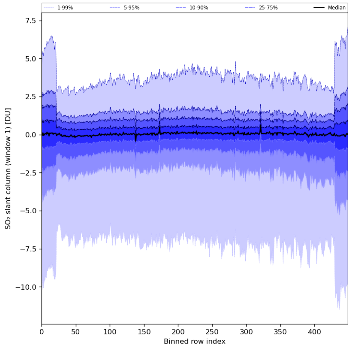
Figure 79: Along track statistics of “SO 2 slant column (window 1)” for 2024-04-21 to 2024-04-22
