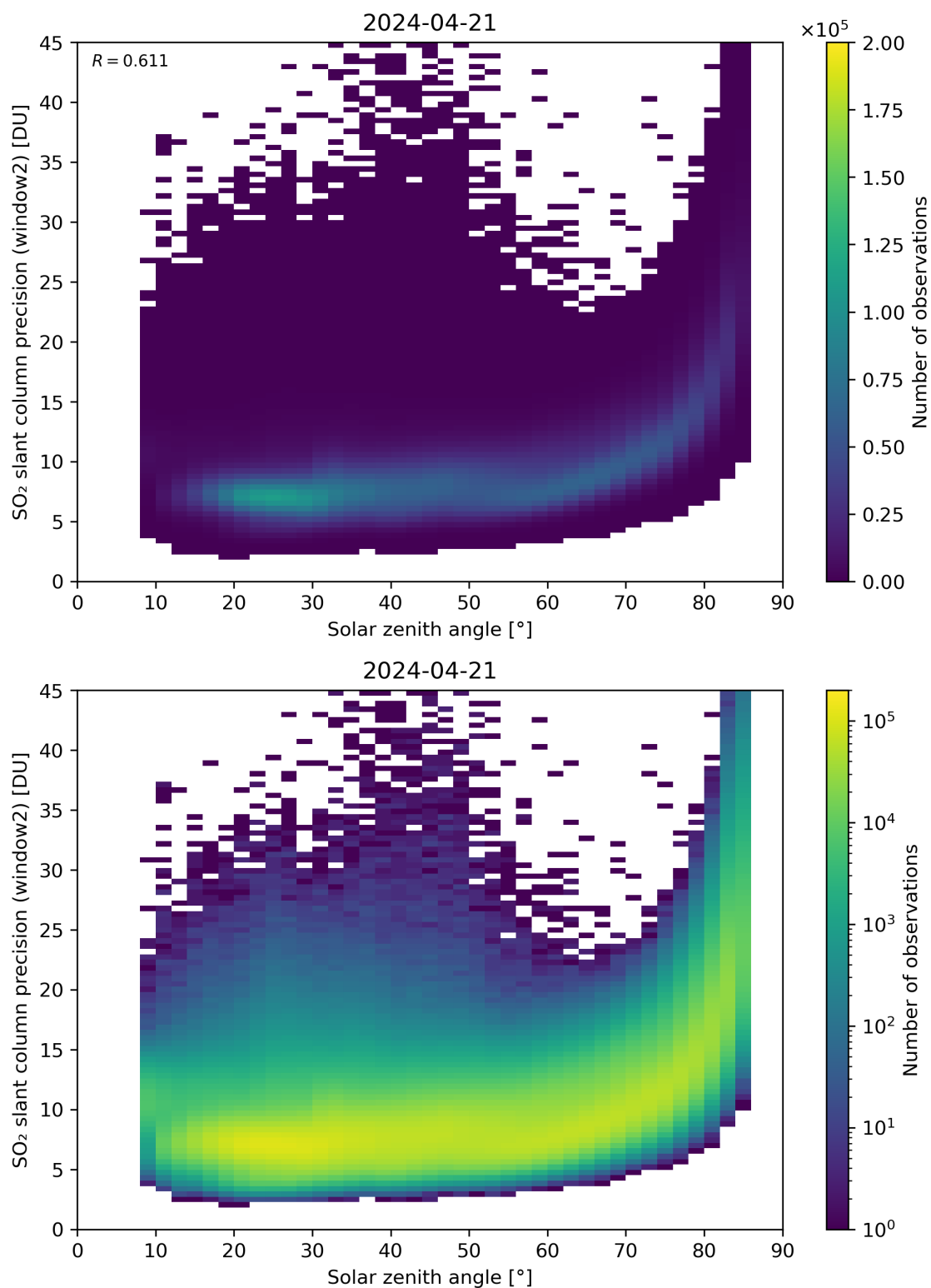
Figure 171: Scatter density plot of “Solar zenith angle” against “SO 2 slant column precision (window2)” for 2024-04-21 to 2024-04-22.
