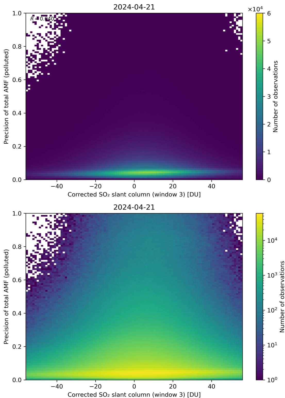
Figure 211: Scatter density plot of “Corrected SO 2 slant column (window 3)” against “Precision of total AMF (polluted)” for 2024-04-21 to 2024-04-22.
