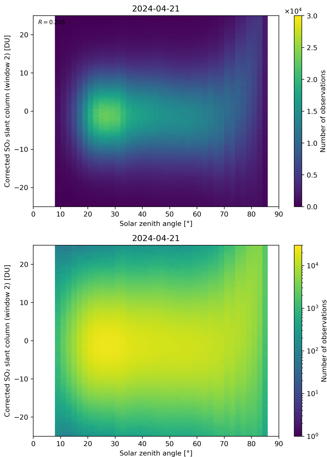
Figure 167: Scatter density plot of “Solar zenith angle” against “Corrected SO 2 slant column (window 2)” for 2024-04-21 to 2024-04-22.
