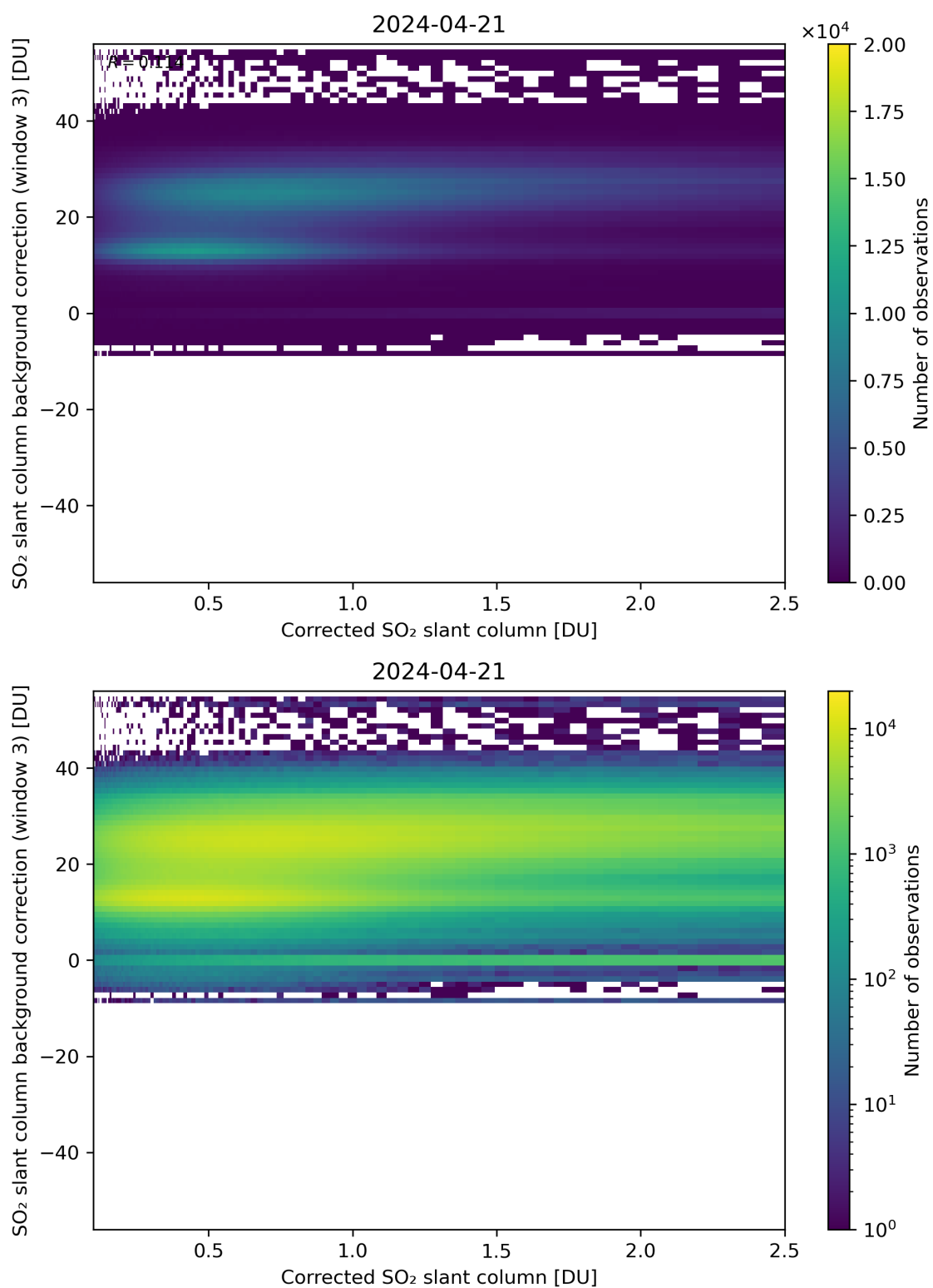
Figure 180: Scatter density plot of “Corrected SO 2 slant column” against “SO 2 slant column background correction (window 3)” for 2024-04-21 to 2024-04-22.
