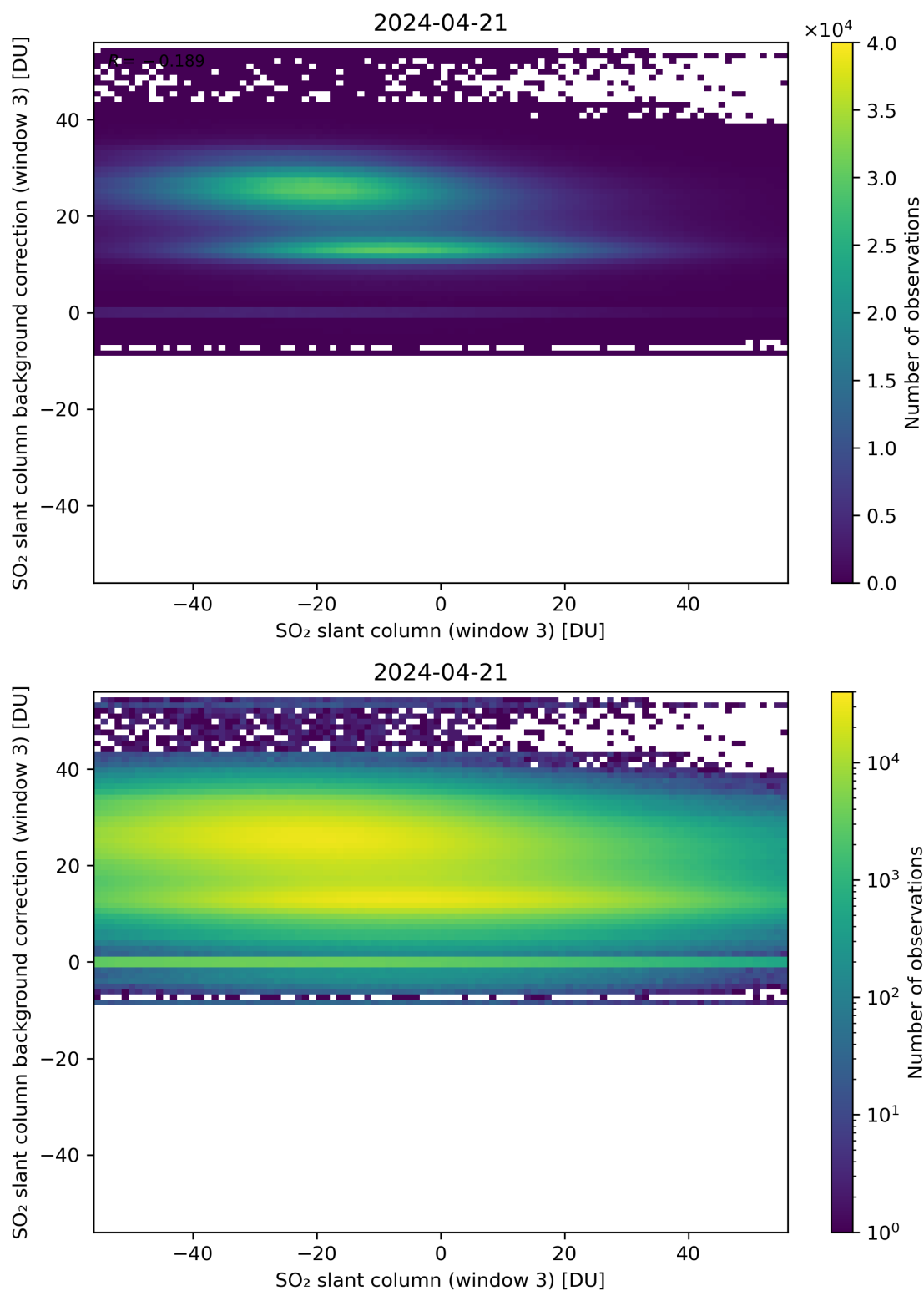
Figure 253: Scatter density plot of “SO 2 slant column (window 3)” against “SO 2 slant column background correction (window 3)” for 2024-04-21 to 2024-04-22.
