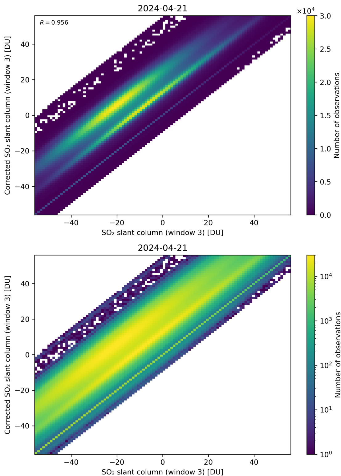
Figure 266: Scatter density plot of “SO 2 slant column (window 3)” against “Corrected SO 2 slant column (window 3)” for 2024-04-21 to 2024-04-22.
