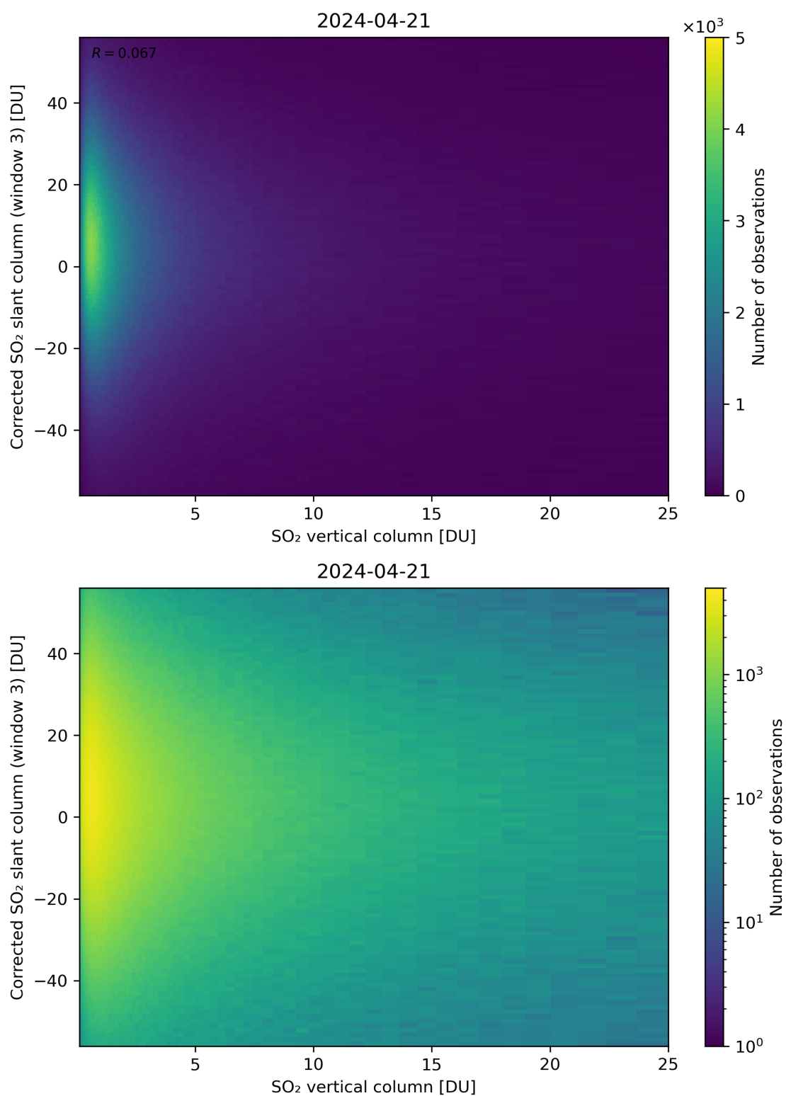
Figure 299: Scatter density plot of “SO 2 vertical column” against “Corrected SO 2 slant column (window 3)” for 2024-04-21 to 2024-04-22.
