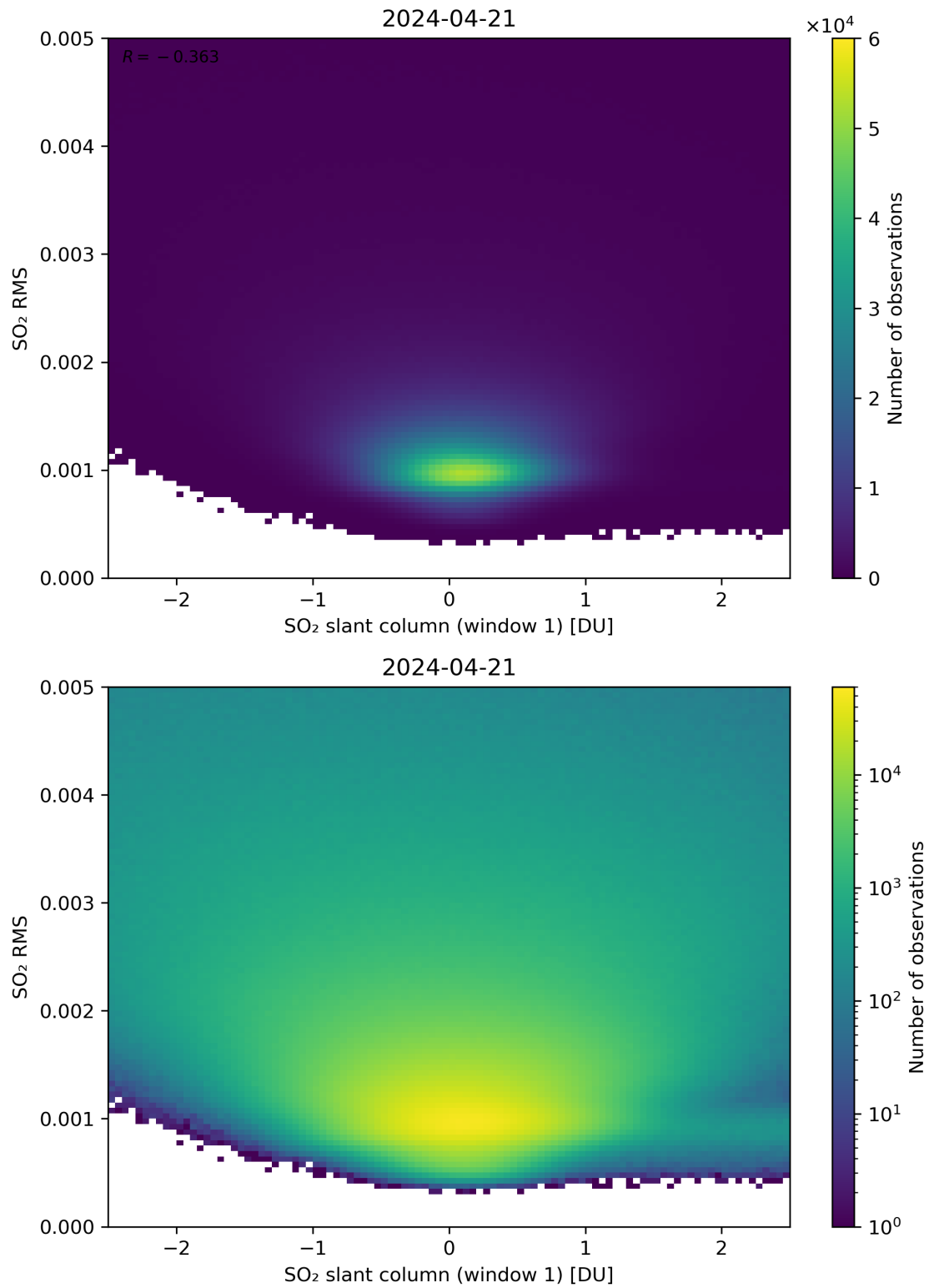
Figure 217: Scatter density plot of “SO 2 slant column (window 1)” against “SO 2 RMS” for 2024-04-21 to 2024-04-22.
