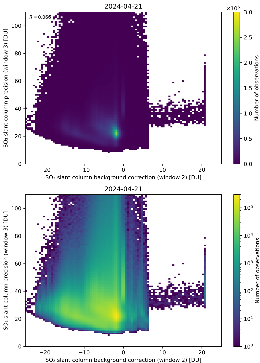
Figure 118: Scatter density plot of “SO 2 slant column background correction (window 2)” against “SO 2 slant column precision (window 3)” for 2024-04-21 to 2024-04-22.
