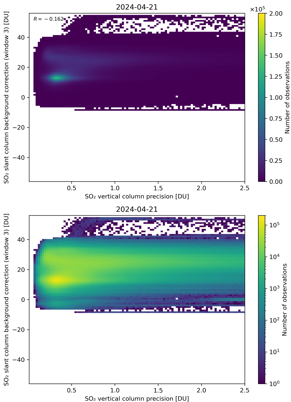
Figure 281: Scatter density plot of “SO 2 vertical column precision” against “SO 2 slant column background correction (window 3)” for 2024-04-21 to 2024-04-22.
