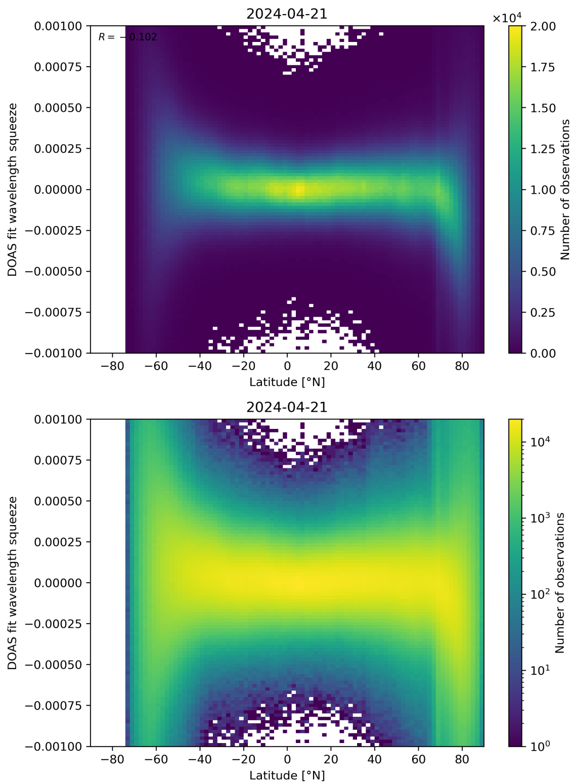
Figure 143: Scatter density plot of “Latitude” against “DOAS fit wavelength squeeze” for 2024-04-21 to 2024-04-22.
