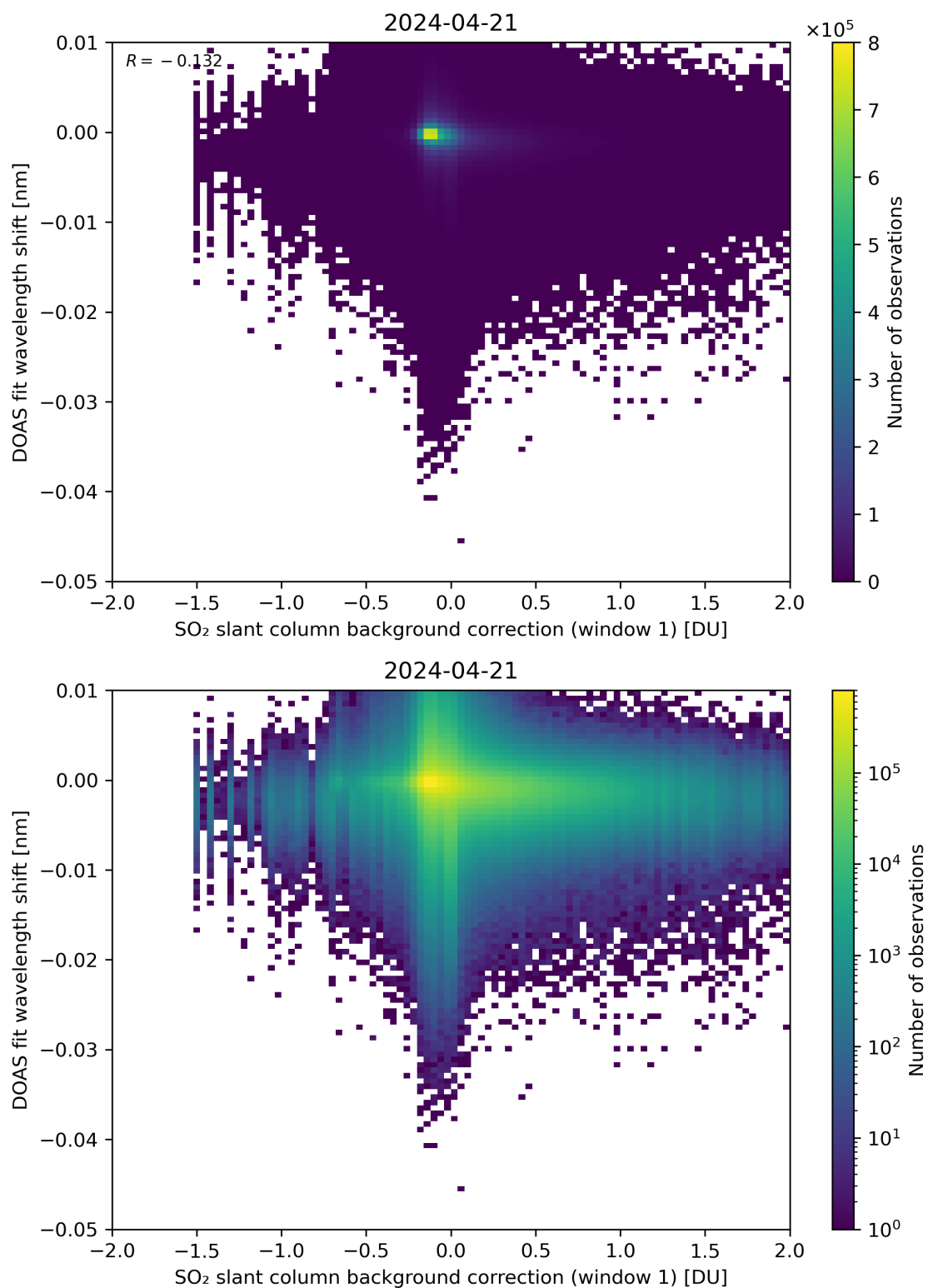
Figure 100: Scatter density plot of “SO 2 slant column background correction (window 1)” against “DOAS fit wavelength shift” for 2024-04-21 to 2024-04-22.
