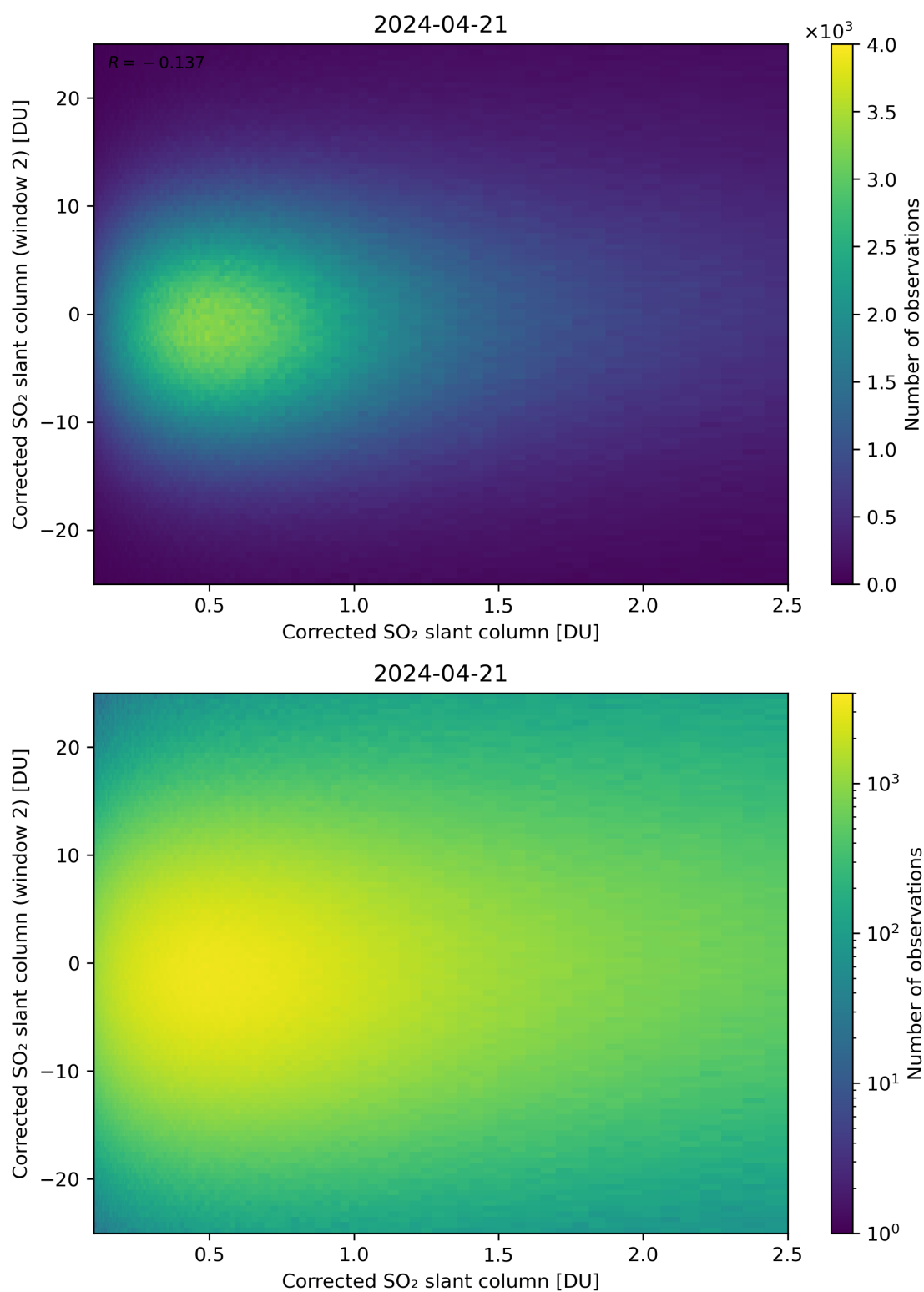
Figure 185: Scatter density plot of “Corrected SO 2 slant column” against “Corrected SO 2 slant column (window 2)” for 2024-04-21 to 2024-04-22.
