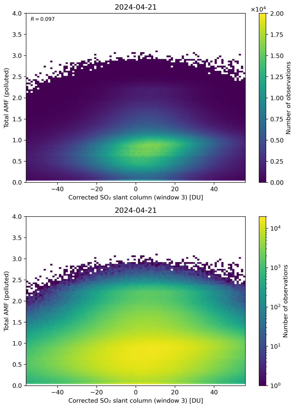
Figure 210: Scatter density plot of “Corrected SO 2 slant column (window 3)” against “Total AMF (polluted)” for 2024-04-21 to 2024-04-22.
