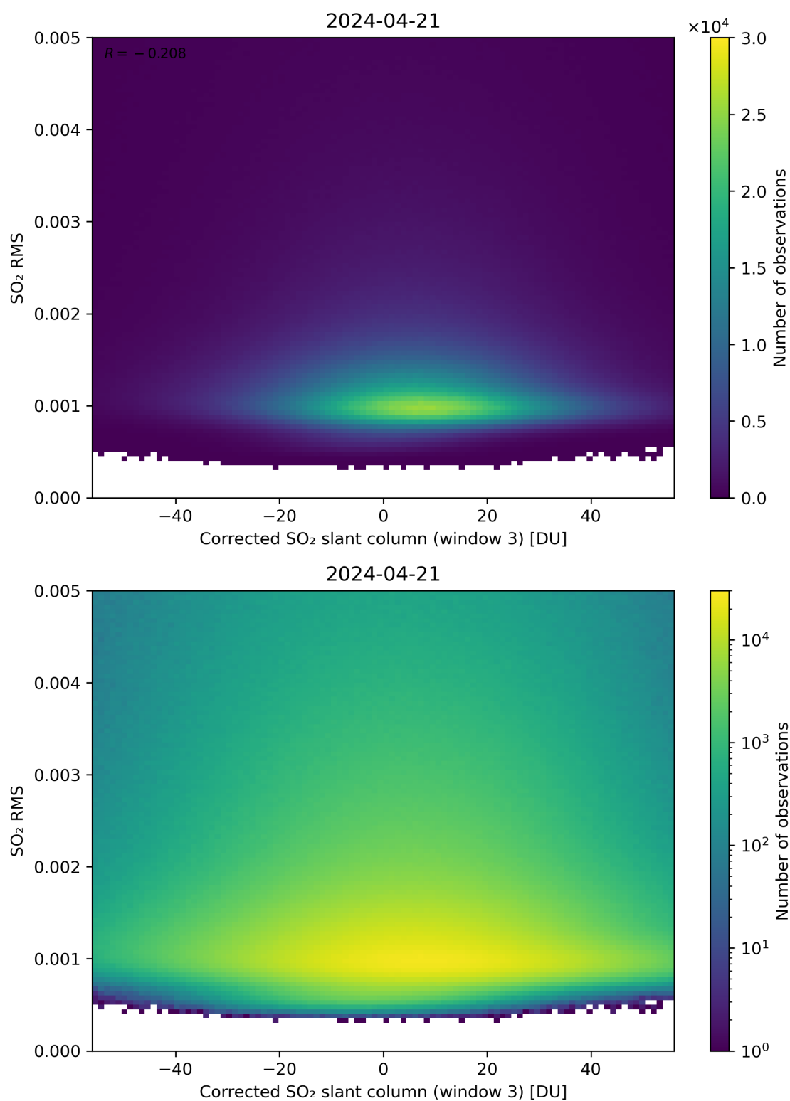
Figure 208: Scatter density plot of “Corrected SO 2 slant column (window 3)” against “SO 2 RMS” for 2024-04-21 to 2024-04-22.
