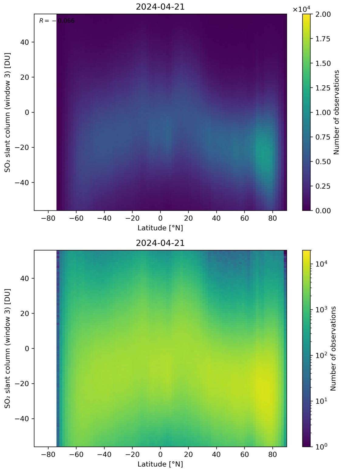
Figure 152: Scatter density plot of “Latitude” against “SO 2 slant column (window 3)” for 2024-04-21 to 2024-04-22.
