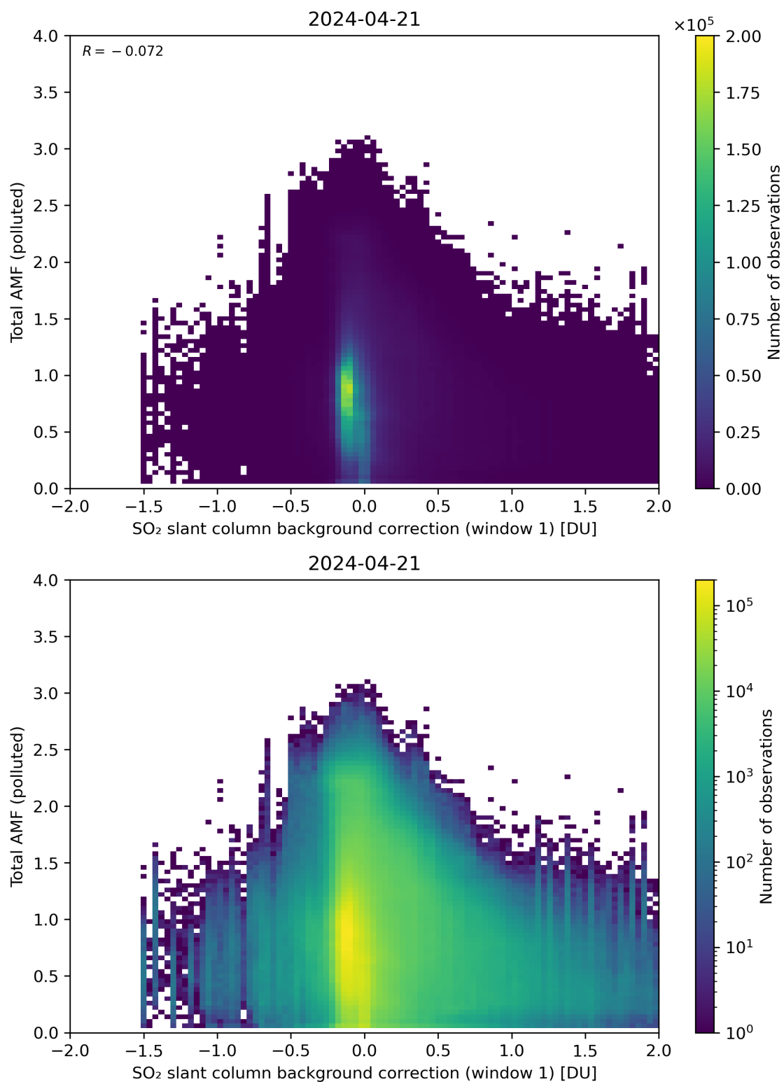
Figure 109: Scatter density plot of “SO 2 slant column background correction (window 1)” against “Total AMF (polluted)” for 2024-04-21 to 2024-04-22.
