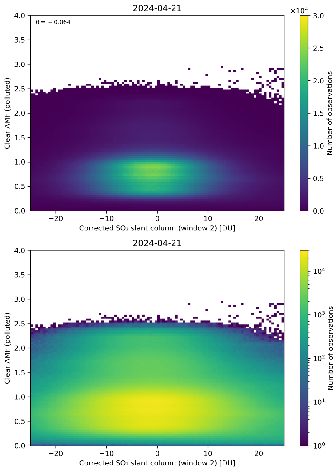
Figure 199: Scatter density plot of “Corrected SO 2 slant column (window 2)” against “Clear AMF (polluted)” for 2024-04-21 to 2024-04-22.
