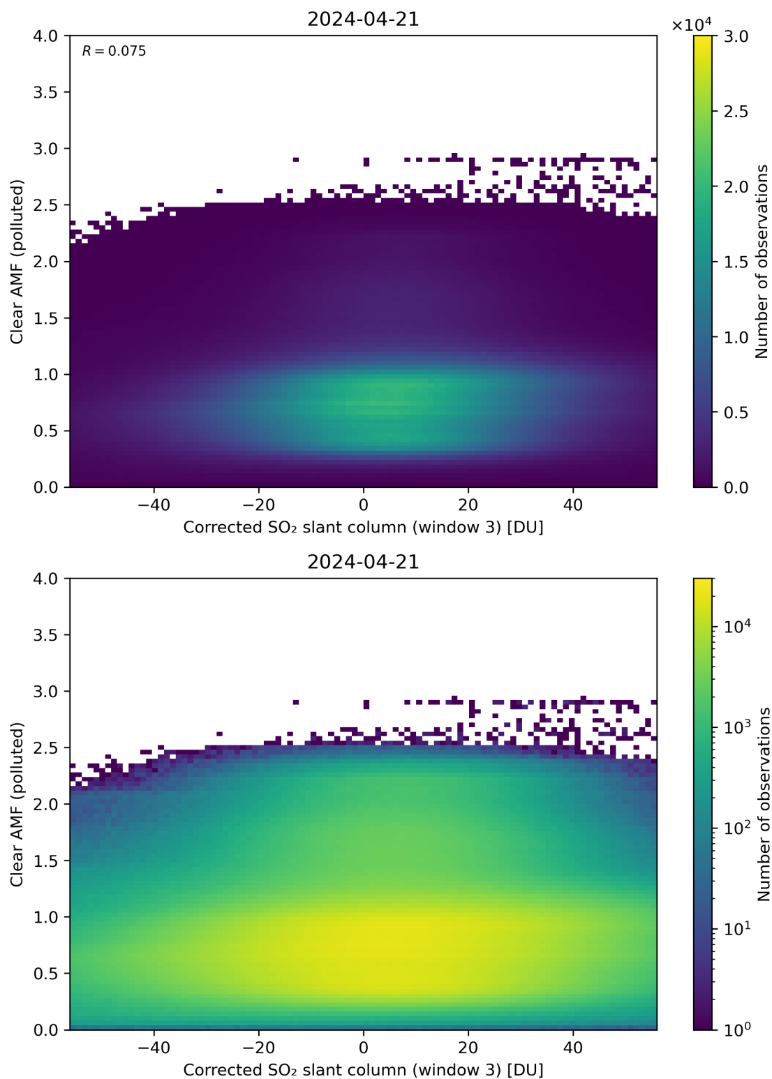
Figure 209: Scatter density plot of “Corrected SO 2 slant column (window 3)” against “Clear AMF (polluted)” for 2024-04-21 to 2024-04-22.
