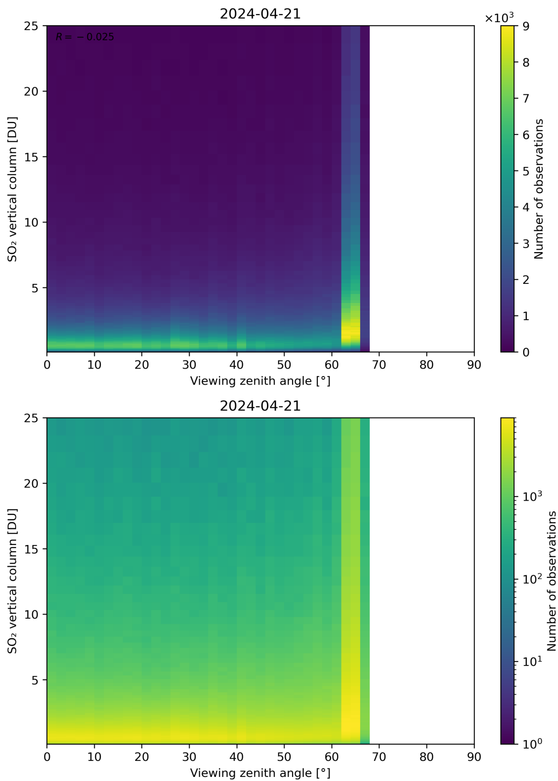
Figure 327: Scatter density plot of “Viewing zenith angle” against “SO 2 vertical column” for 2024-04-21 to 2024-04-22.
