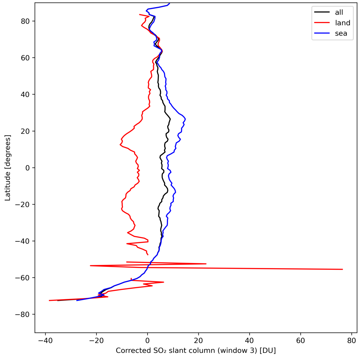
Figure 43: Zonal average of “Corrected SO 2 slant column (window 3)” for 2024-04-21 to 2024-04-22.
