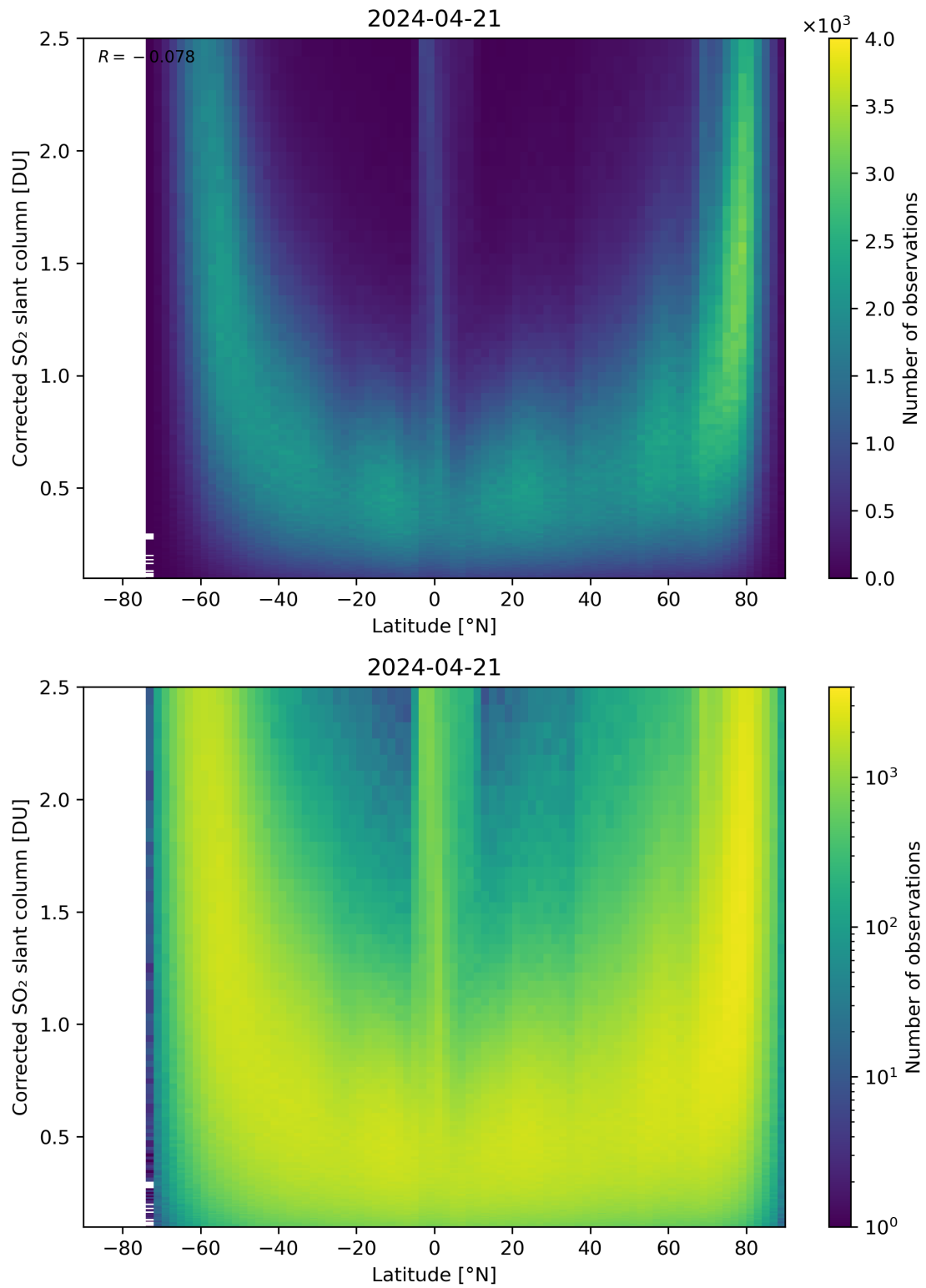
Figure 146: Scatter density plot of “Latitude” against “Corrected SO 2 slant column” for 2024-04-21 to 2024-04-22.
