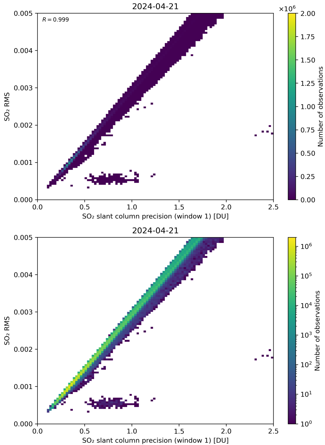
Figure 223: Scatter density plot of “SO 2 slant column precision (window 1)” against “SO 2 RMS” for 2024-04-21 to 2024-04-22.
