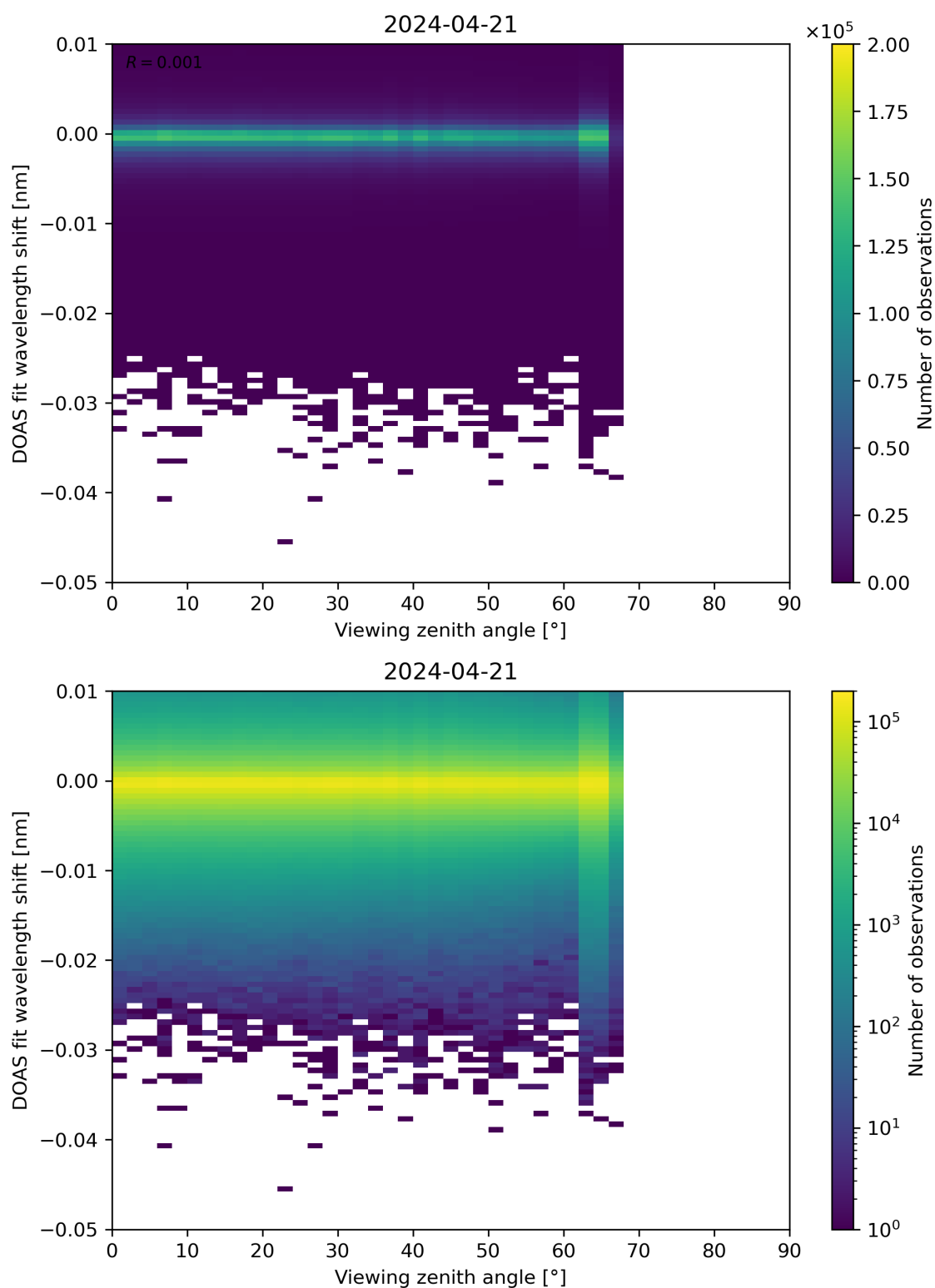
Figure 311: Scatter density plot of “Viewing zenith angle” against “DOAS fit wavelength shift” for 2024-04-21 to 2024-04-22.
