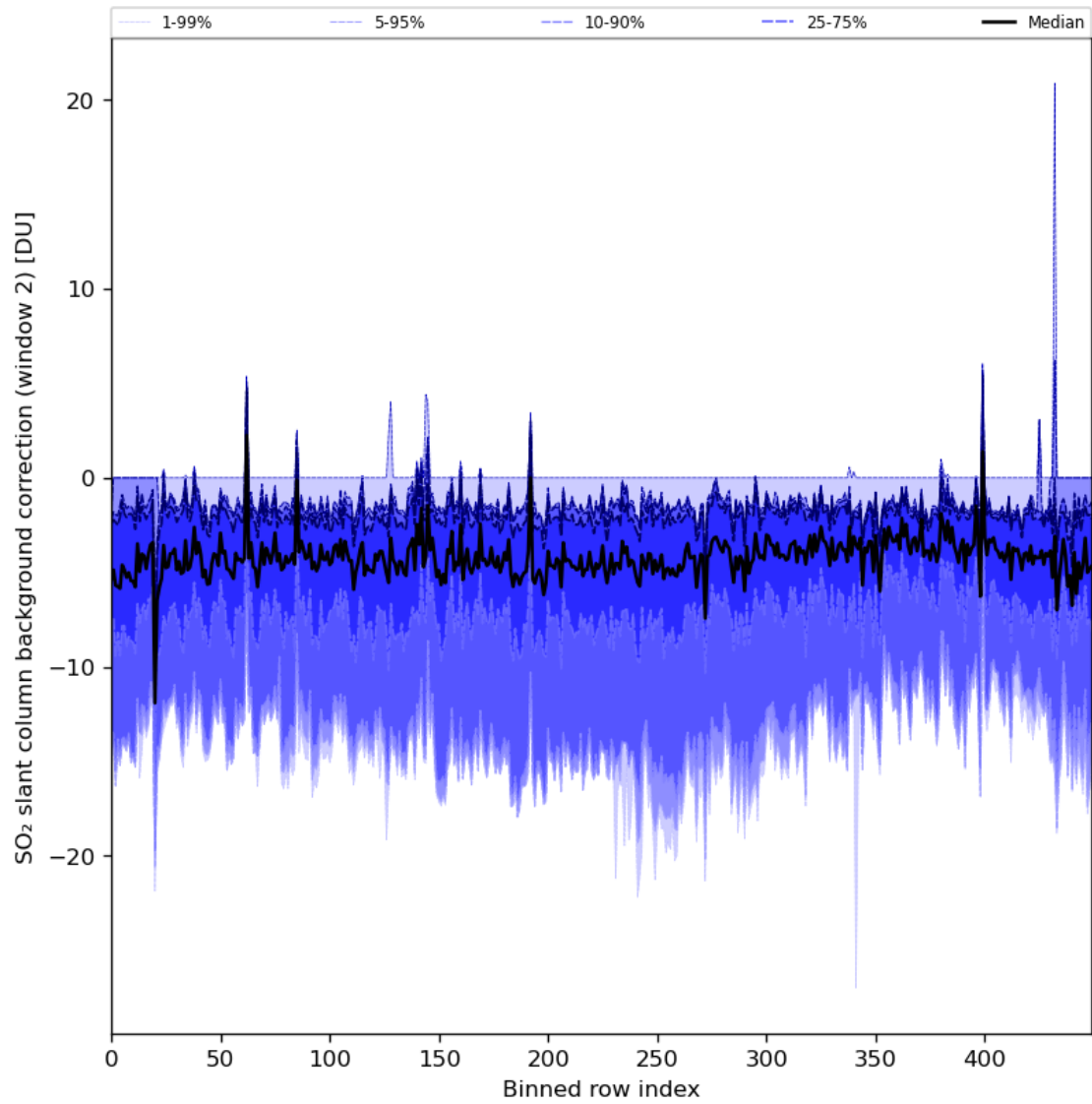
Figure 86: Along track statistics of “SO 2 slant column background correction (window 2)” for 2024-04-21 to 2024-04-22
