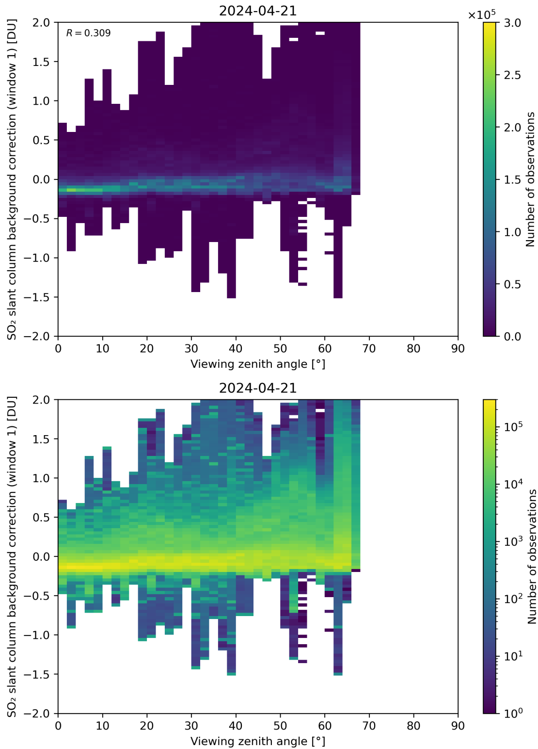
Figure 308: Scatter density plot of “Viewing zenith angle” against “SO 2 slant column background correction (window 1)” for 2024-04-21 to 2024-04-22.
