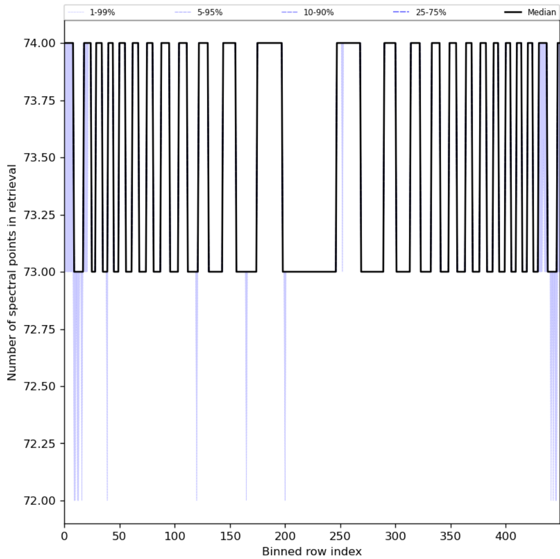
Figure 97: Along track statistics of “Number of spectral points in retrieval” for 2024-04-21 to 2024-04-22
