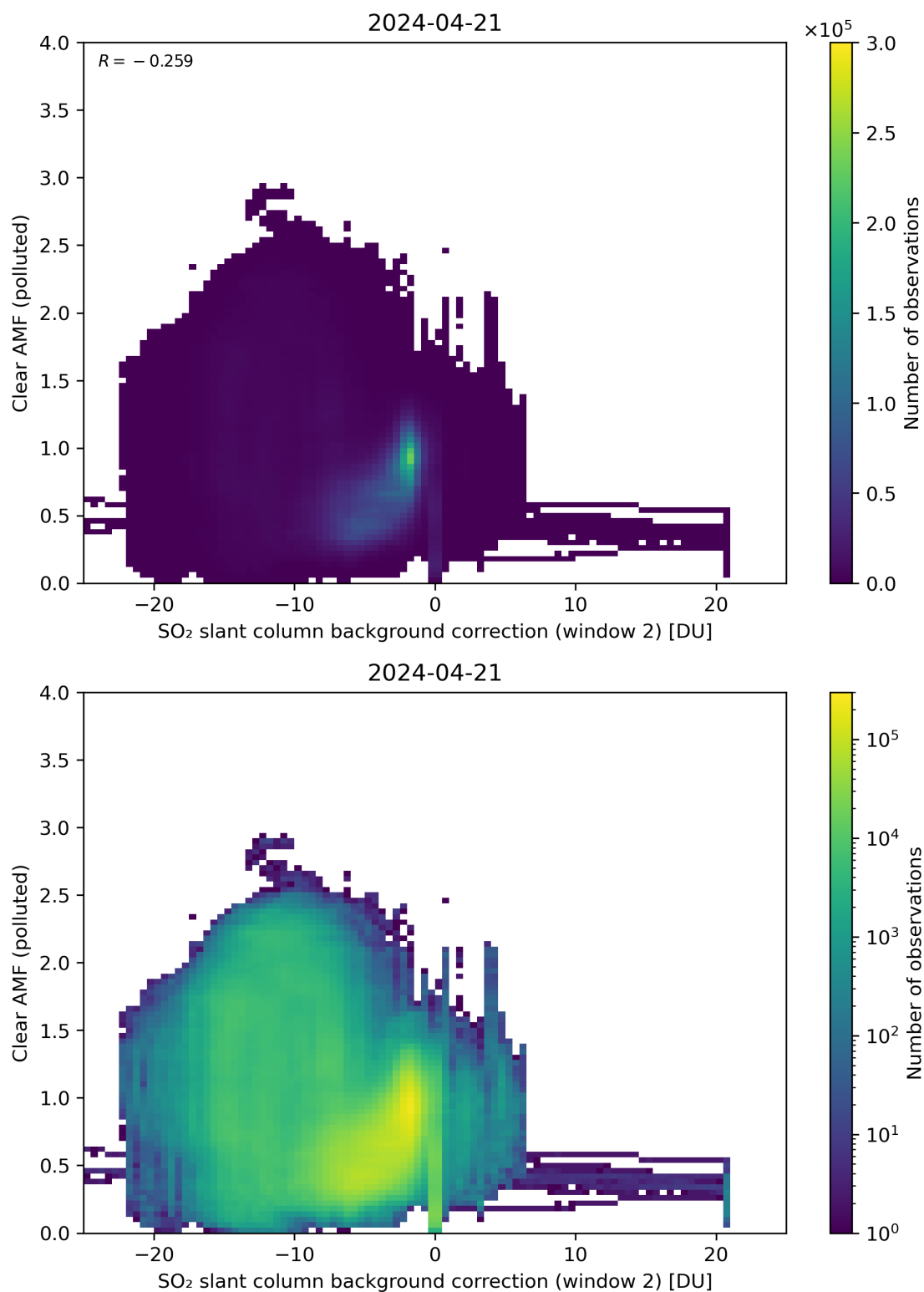
Figure 115: Scatter density plot of “SO 2 slant column background correction (window 2)” against “Clear AMF (polluted)” for 2024-04-21 to 2024-04-22.
