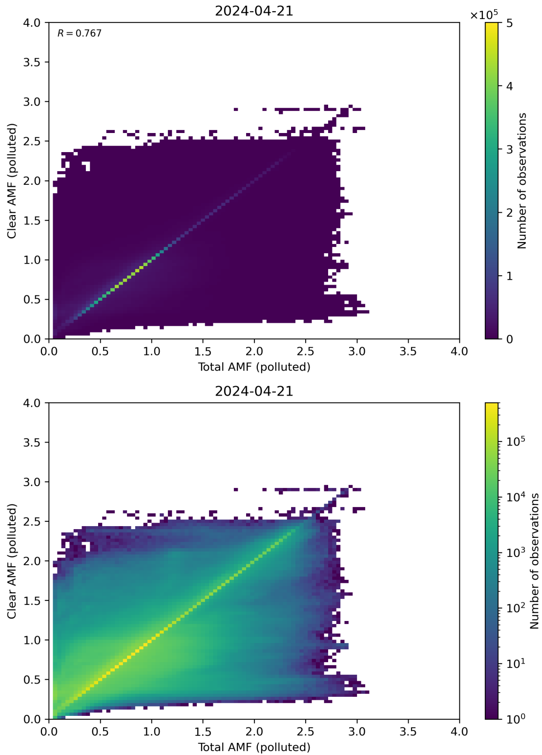
Figure 271: Scatter density plot of “Total AMF (polluted)” against “Clear AMF (polluted)” for 2024-04-21 to 2024-04-22.
