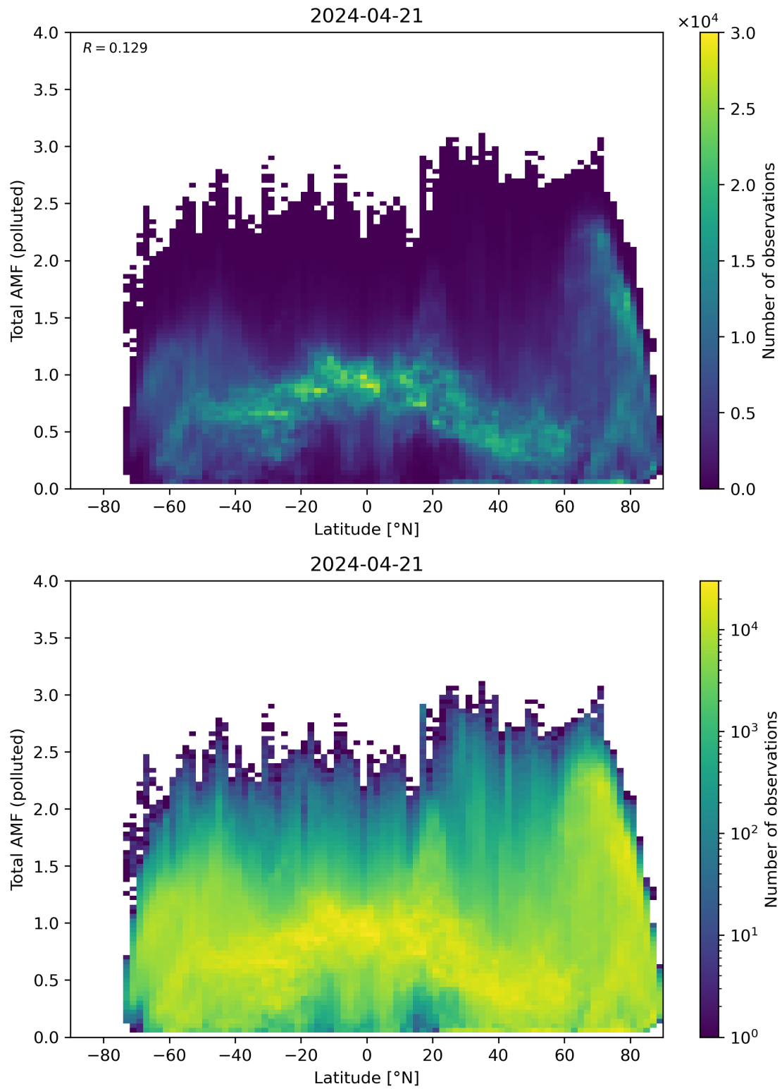
Figure 154: Scatter density plot of “Latitude” against “Total AMF (polluted)” for 2024-04-21 to 2024-04-22.
