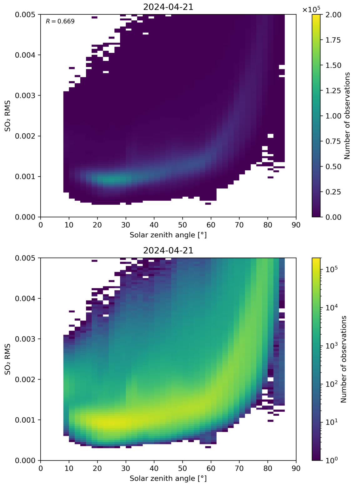
Figure 163: Scatter density plot of “Solar zenith angle” against “SO 2 RMS” for 2024-04-21 to 2024-04-22.
