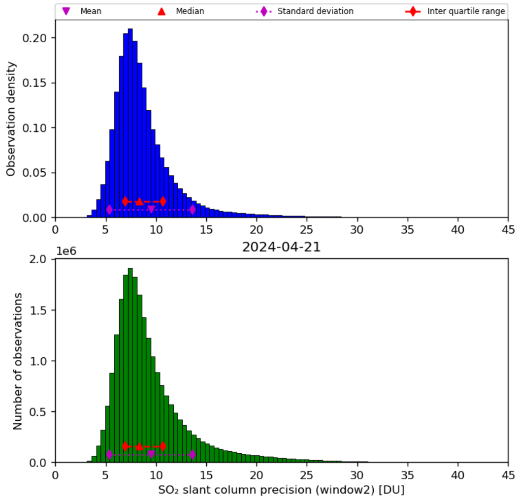
Figure 61: Histogram of “SO 2 slant column precision (window2)” for 2024-04-21 to 2024-04-22
