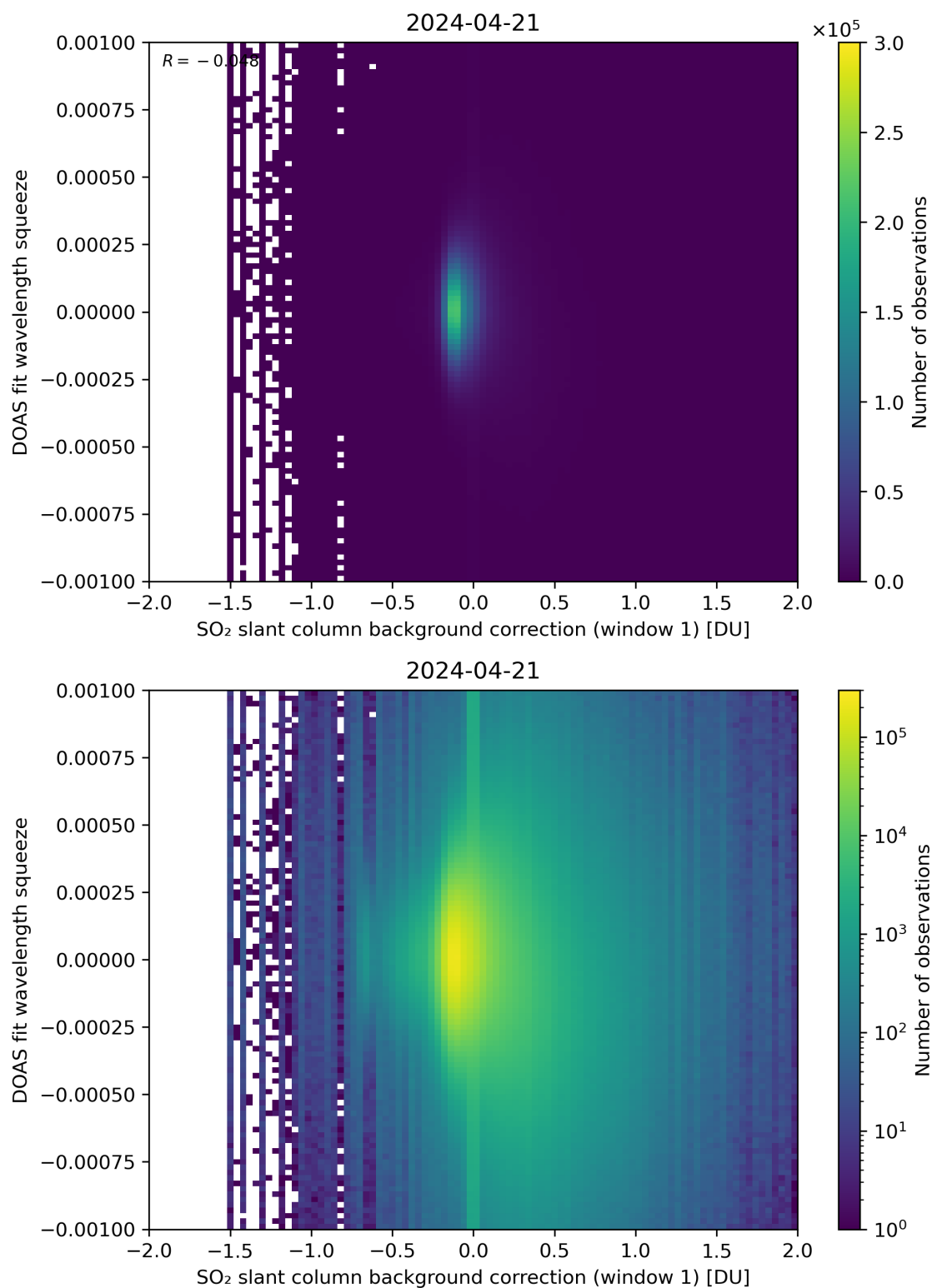
Figure 101: Scatter density plot of “SO 2 slant column background correction (window 1)” against “DOAS fit wavelength squeeze” for 2024-04-21 to 2024-04-22.
