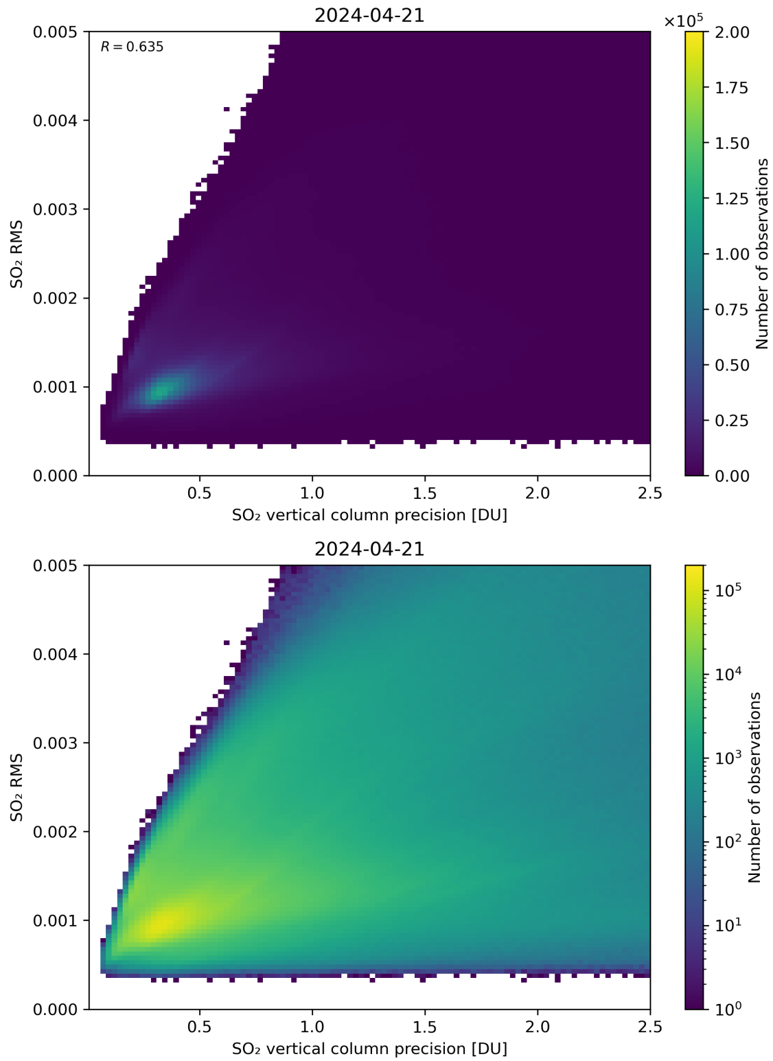
Figure 284: Scatter density plot of “SO 2 vertical column precision” against “SO 2 RMS” for 2024-04-21 to 2024-04-22.
