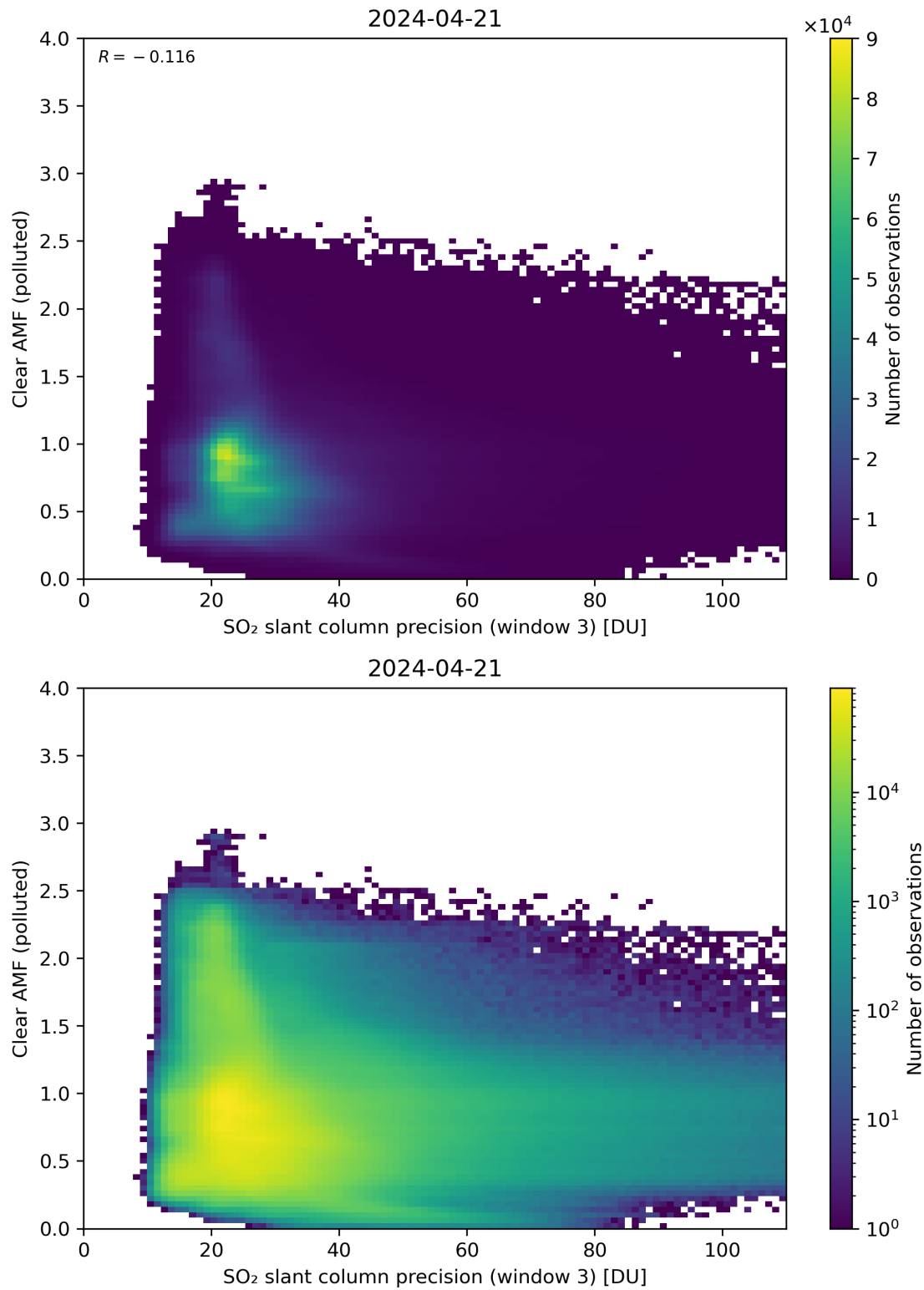
Figure 261: Scatter density plot of “SO 2 slant column precision (window 3)” against “Clear AMF (polluted)” for 2024-04-21 to 2024-04-22.
