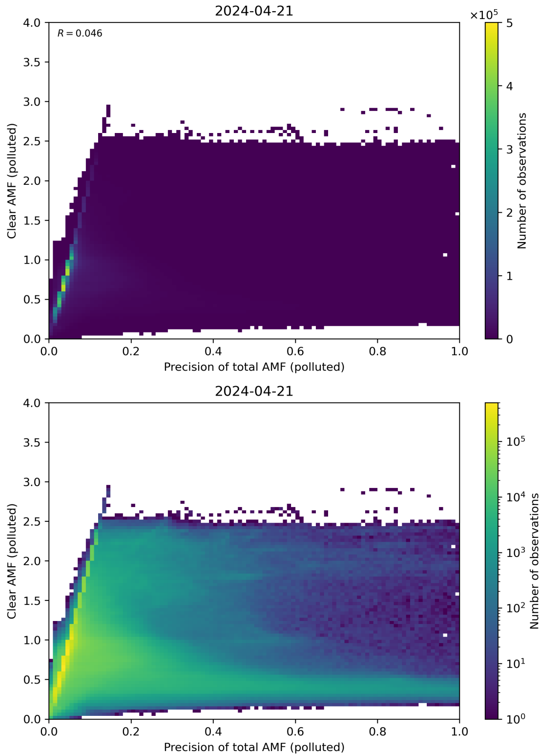
Figure 270: Scatter density plot of “Precision of total AMF (polluted)” against “Clear AMF (polluted)” for 2024-04-21 to 2024-04-22.
