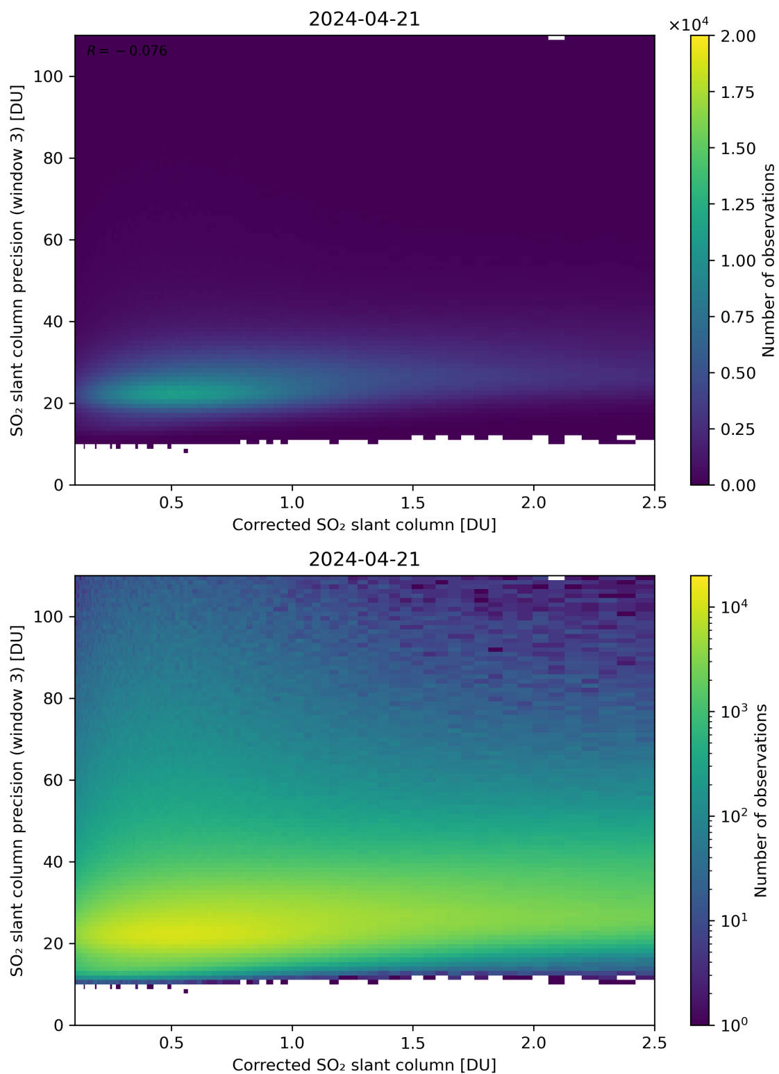
Figure 191: Scatter density plot of “Corrected SO 2 slant column” against “SO 2 slant column precision (window 3)” for 2024-04-21 to 2024-04-22.
