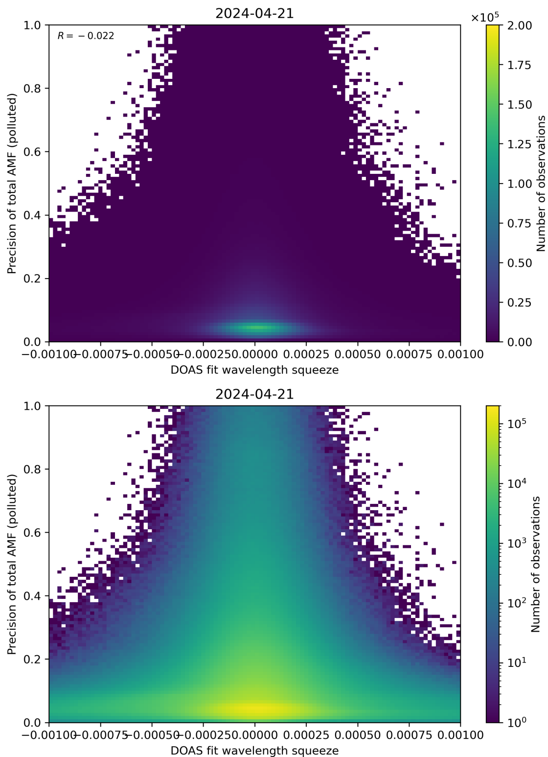
Figure 135: Scatter density plot of “DOAS fit wavelength squeeze” against “Precision of total AMF (polluted)” for 2024-04-21 to 2024-04-22.
