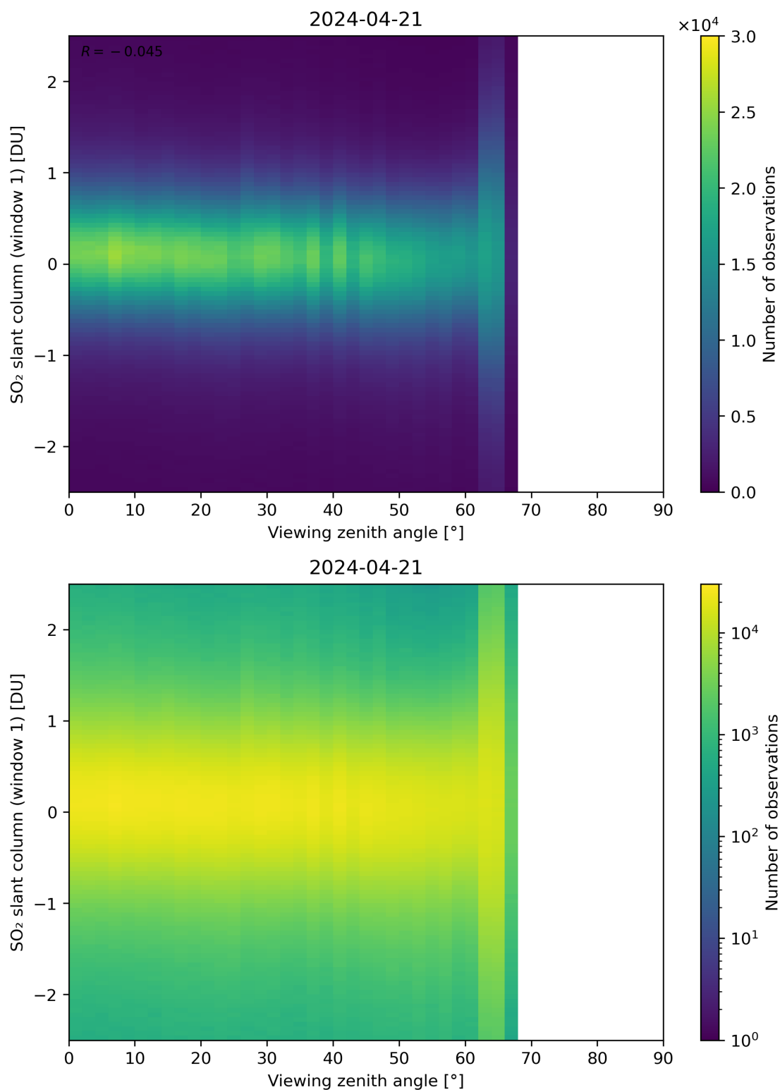
Figure 320: Scatter density plot of “Viewing zenith angle” against “SO 2 slant column (window 1)” for 2024-04-21 to 2024-04-22.
