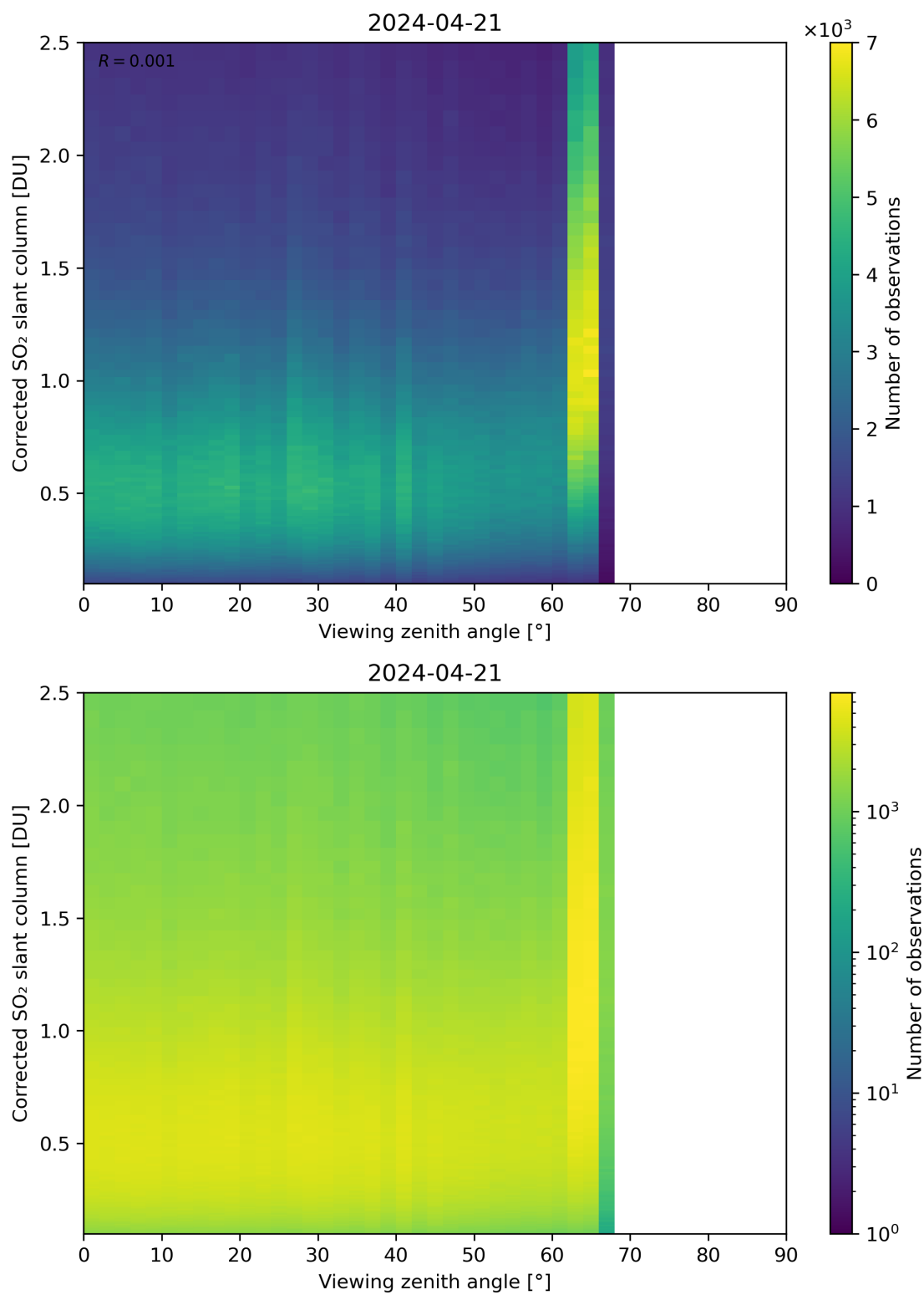
Figure 317: Scatter density plot of “Viewing zenith angle” against “Corrected SO 2 slant column” for 2024-04-21 to 2024-04-22.
