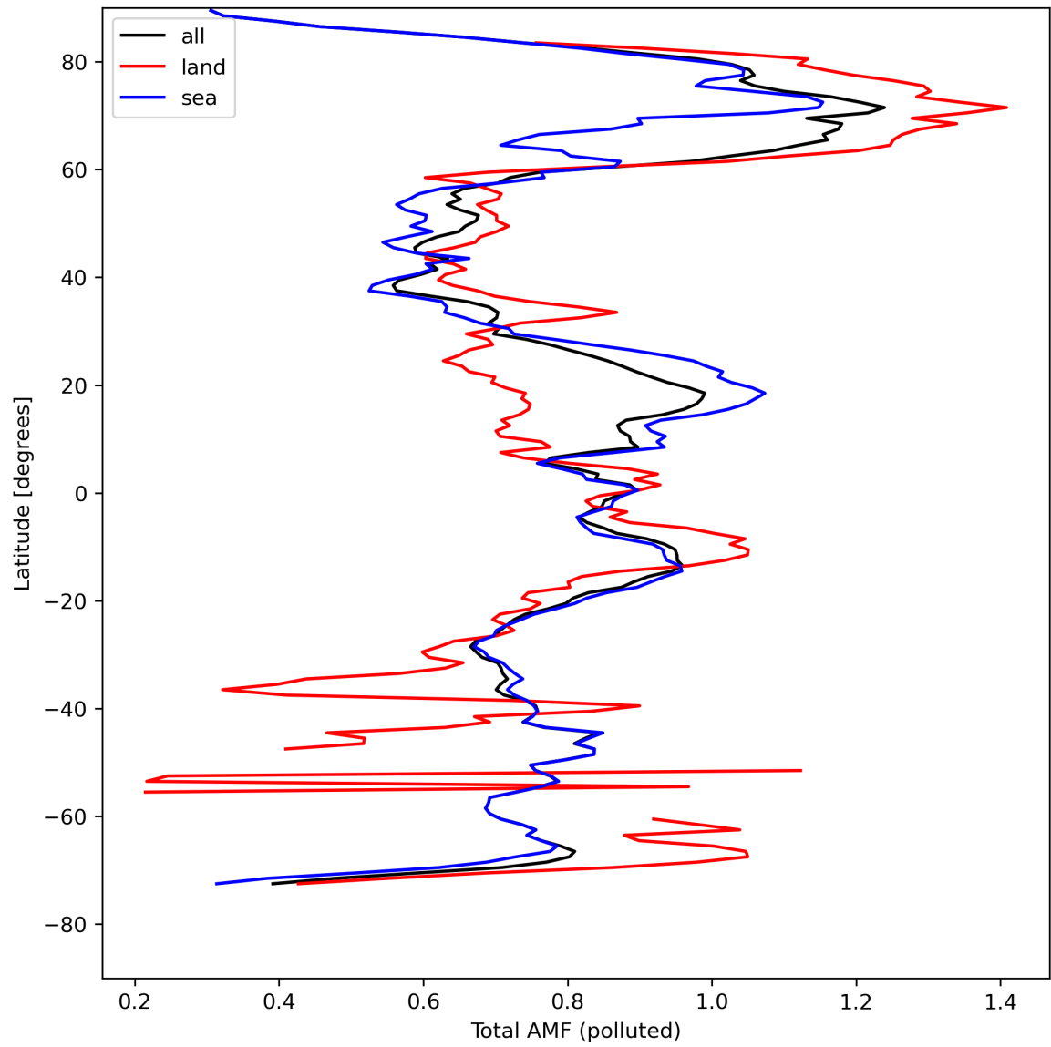
Figure 48: Zonal average of “Total AMF (polluted)” for 2024-04-21 to 2024-04-22.
