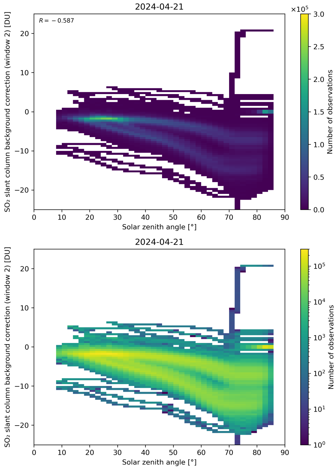
Figure 159: Scatter density plot of “Solar zenith angle” against “SO 2 slant column background correction (window 2)” for 2024-04-21 to 2024-04-22.
