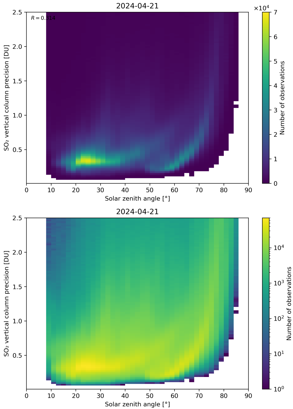
Figure 177: Scatter density plot of “Solar zenith angle” against “SO 2 vertical column precision” for 2024-04-21 to 2024-04-22.
