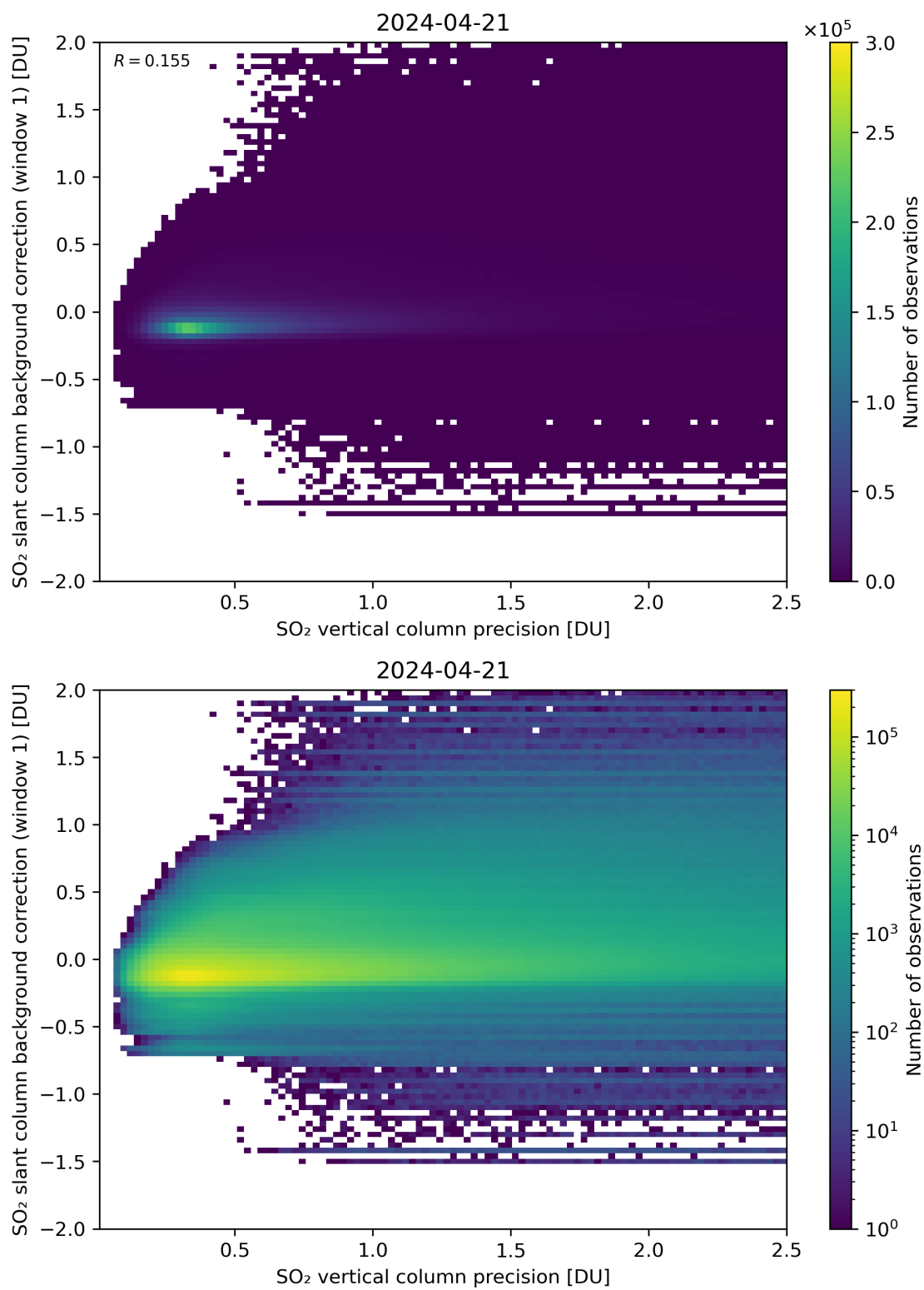
Figure 279: Scatter density plot of “SO 2 vertical column precision” against “SO 2 slant column background correction (window 1)” for 2024-04-21 to 2024-04-22.
