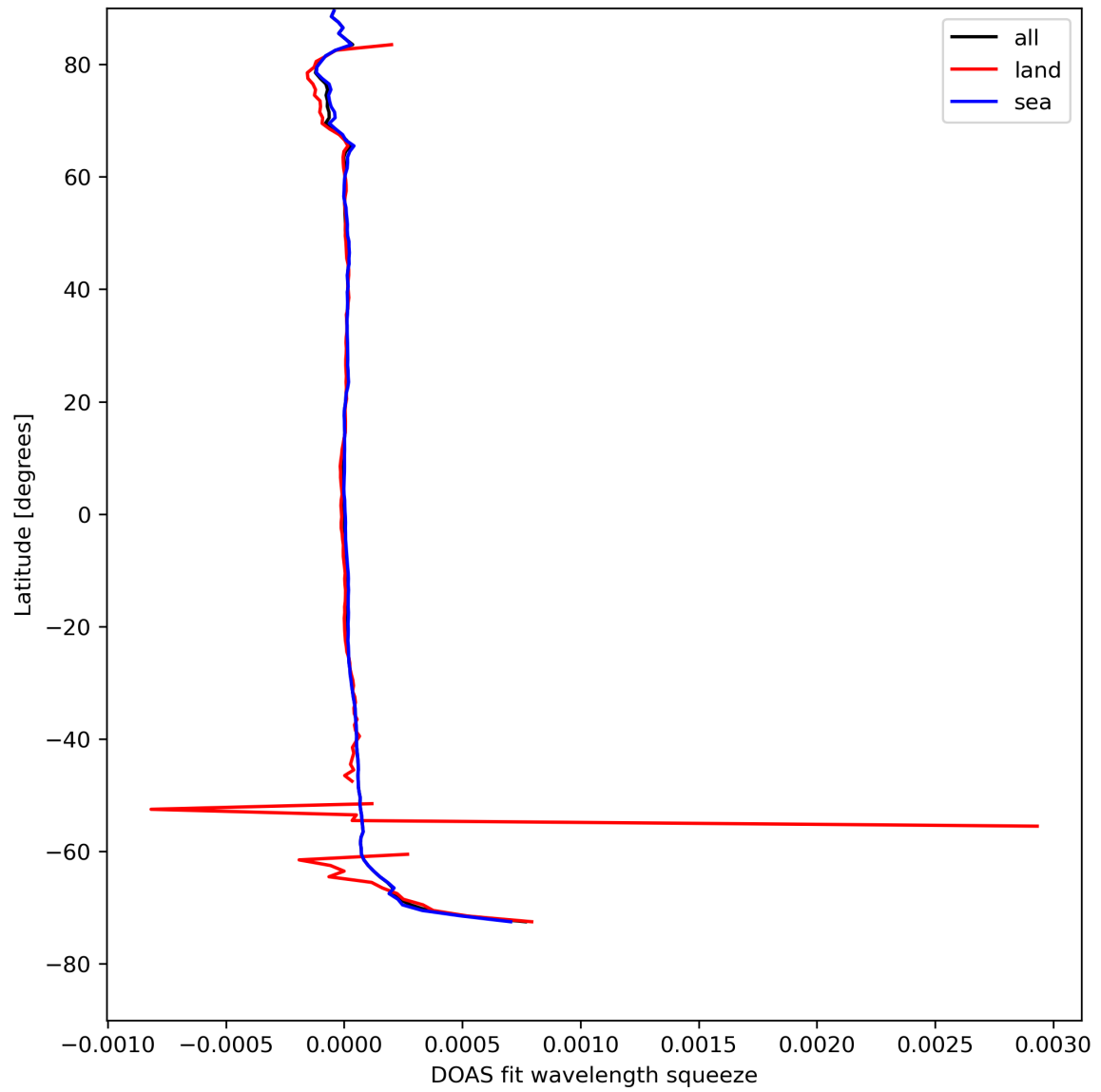
Figure 46: Zonal average of “DOAS fit wavelength squeeze” for 2024-04-21 to 2024-04-22.
