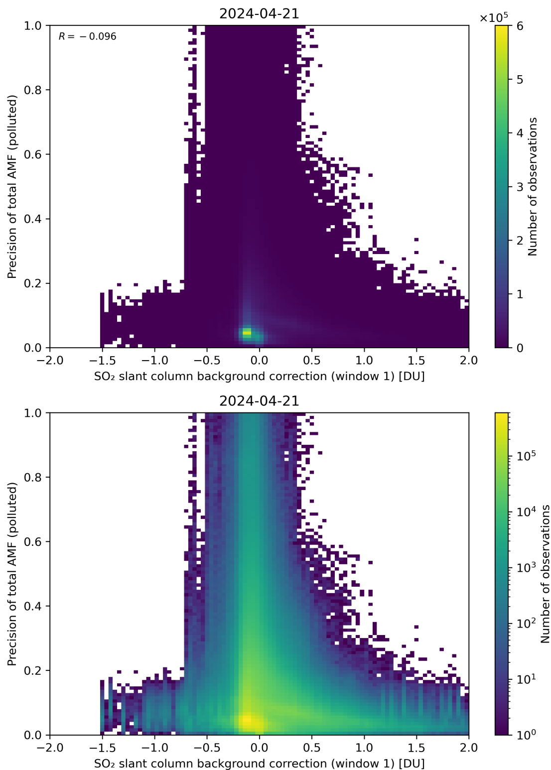
Figure 110: Scatter density plot of “SO 2 slant column background correction (window 1)” against “Precision of total AMF (polluted)” for 2024-04-21 to 2024-04-22.
