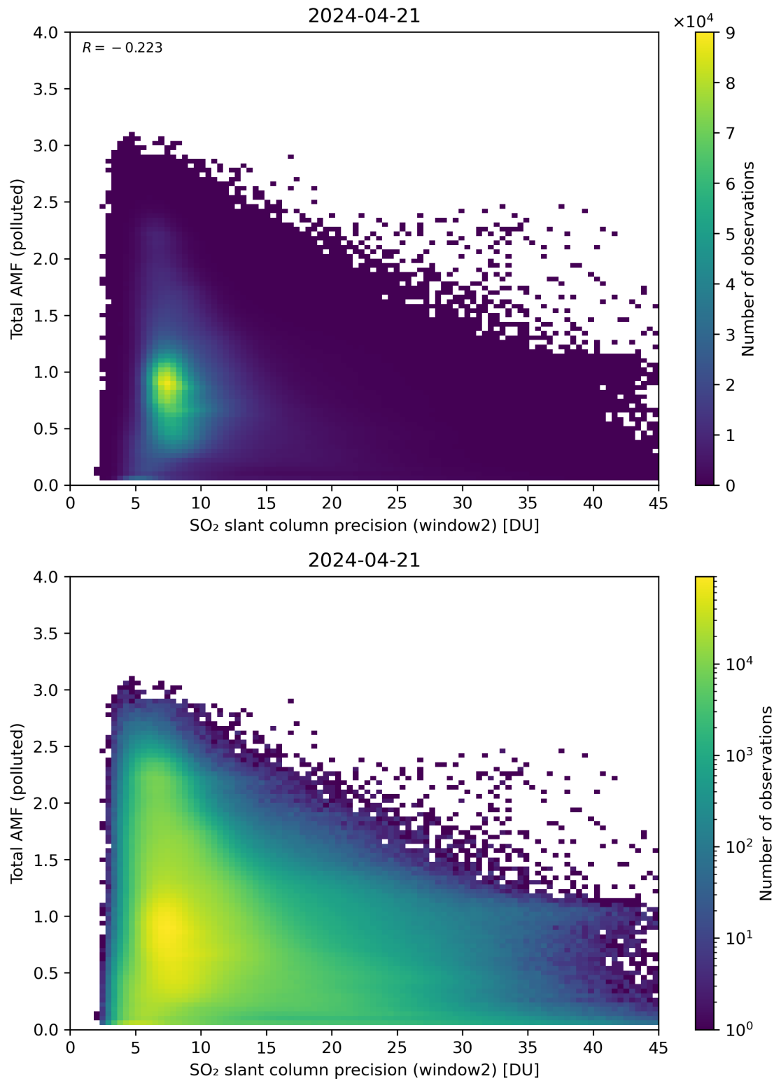
Figure 251: Scatter density plot of “SO 2 slant column precision (window2)” against “Total AMF (polluted)” for 2024-04-21 to 2024-04-22.
