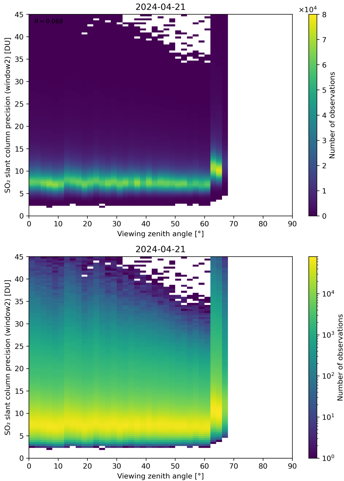
Figure 322: Scatter density plot of “Viewing zenith angle” against “SO 2 slant column precision (window2)” for 2024-04-21 to 2024-04-22.
