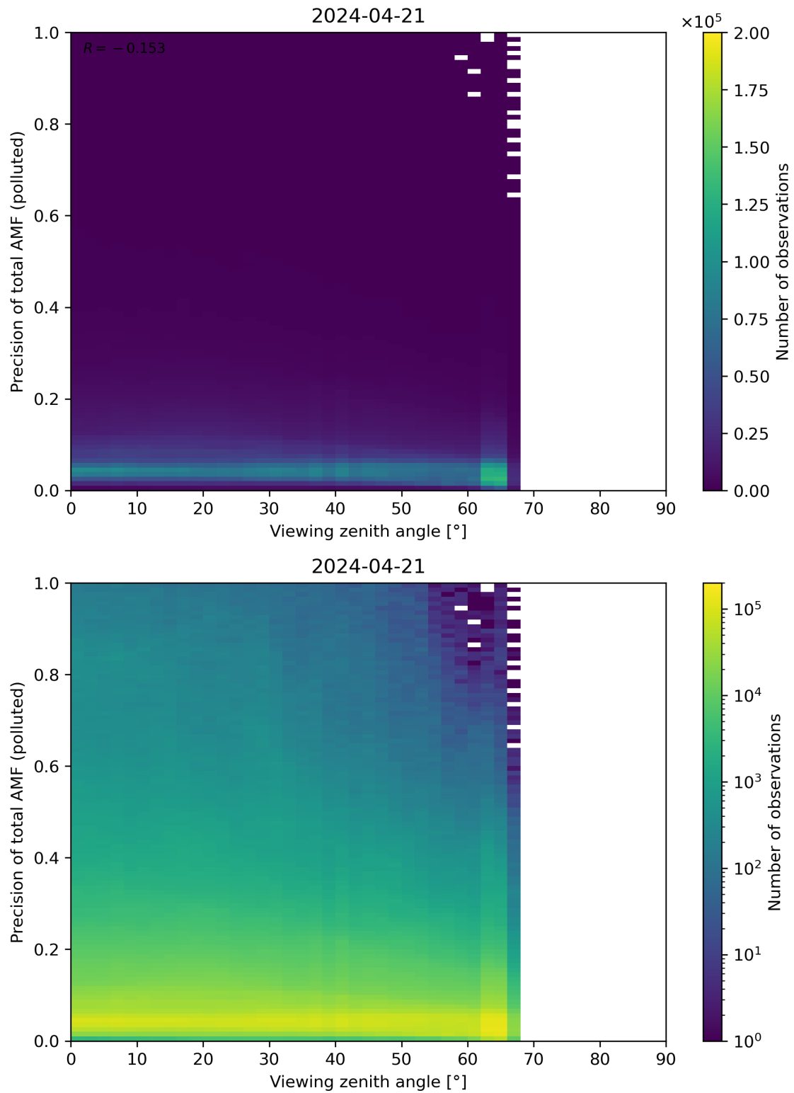
Figure 326: Scatter density plot of “Viewing zenith angle” against “Precision of total AMF (polluted)” for 2024-04-21 to 2024-04-22.
