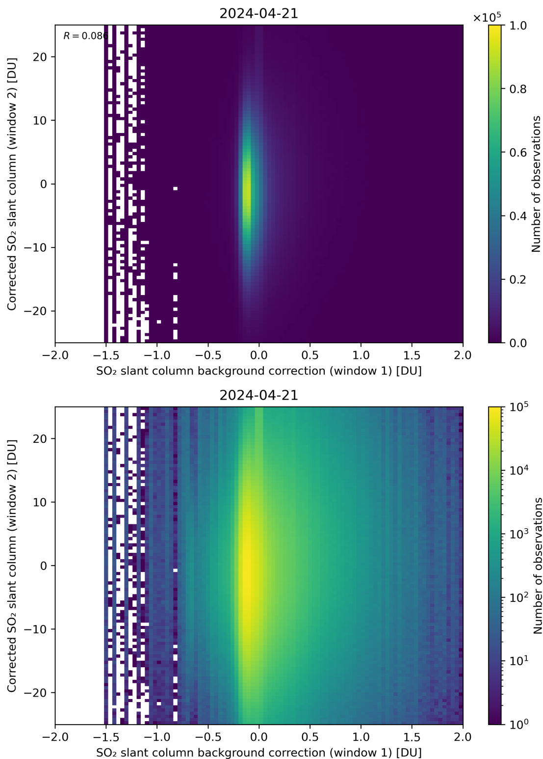
Figure 104: Scatter density plot of “SO 2 slant column background correction (window 1)” against “Corrected SO 2 slant column (window 2)” for 2024-04-21 to 2024-04-22.
