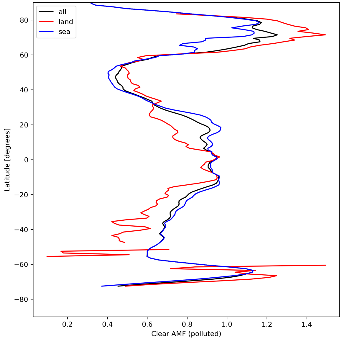
Figure 50: Zonal average of “Clear AMF (polluted)” for 2024-04-21 to 2024-04-22.
