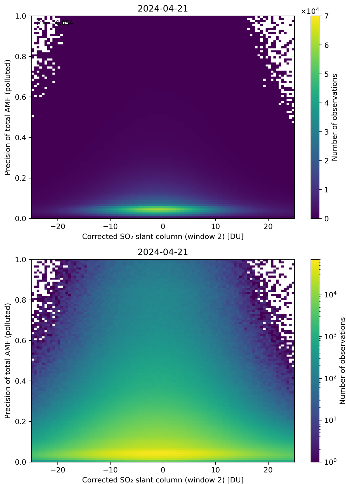
Figure 204: Scatter density plot of “Corrected SO 2 slant column (window 2)” against “Precision of total AMF (polluted)” for 2024-04-21 to 2024-04-22.
