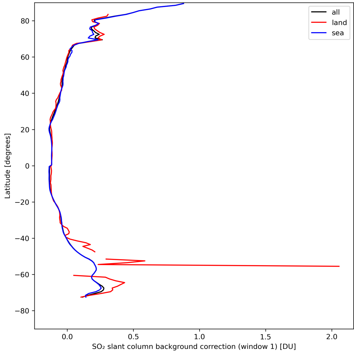
Figure 36: Zonal average of "SO 2 slant column background correction (window 1)" for 2024-04-21 to 2024-04-22.
