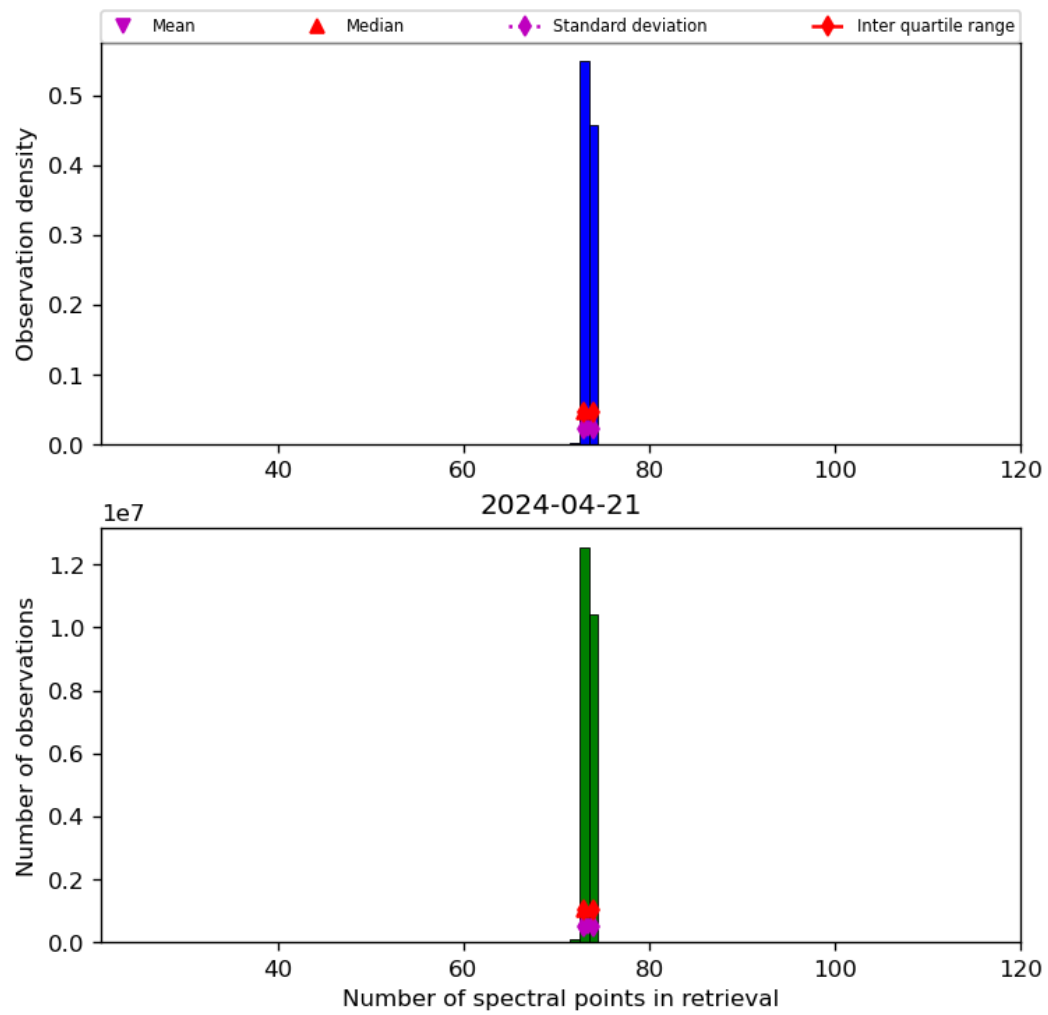
Figure 74: Histogram of “Number of spectral points in retrieval” for 2024-04-21 to 2024-04-22
