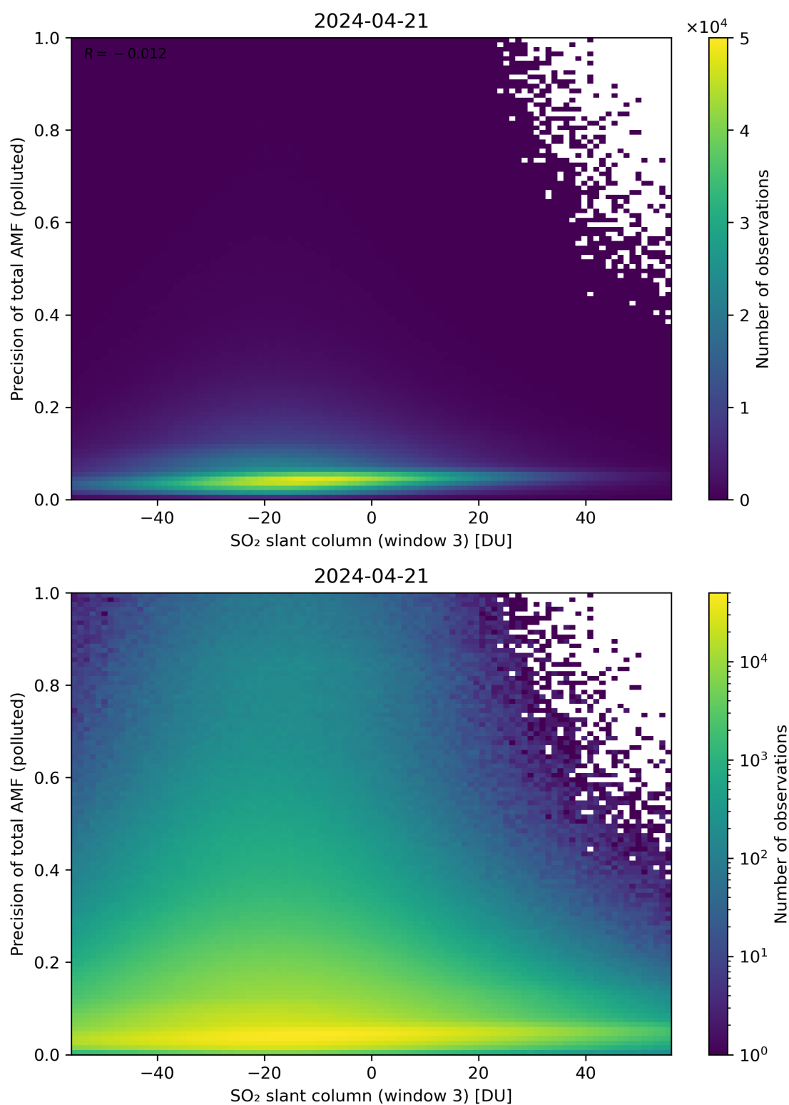
Figure 269: Scatter density plot of “SO 2 slant column (window 3)” against “Precision of total AMF (polluted)” for 2024-04-21 to 2024-04-22.
