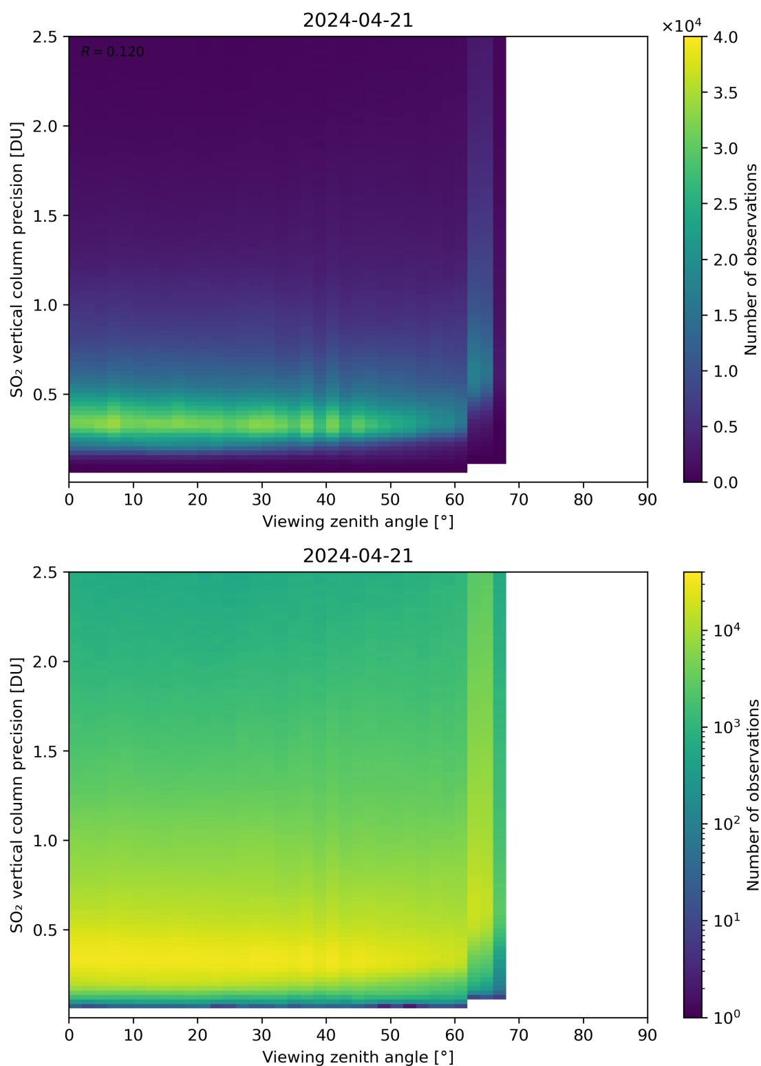
Figure 328: Scatter density plot of “Viewing zenith angle” against “SO 2 vertical column precision” for 2024-04-21 to 2024-04-22.
