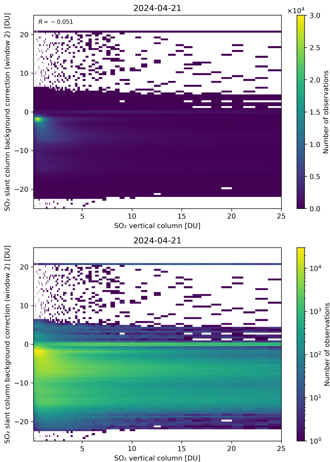
Figure 274: Scatter density plot of “SO 2 vertical column” against “SO 2 slant column background correction (window 2)” for 2024-04-21 to 2024-04-22.
