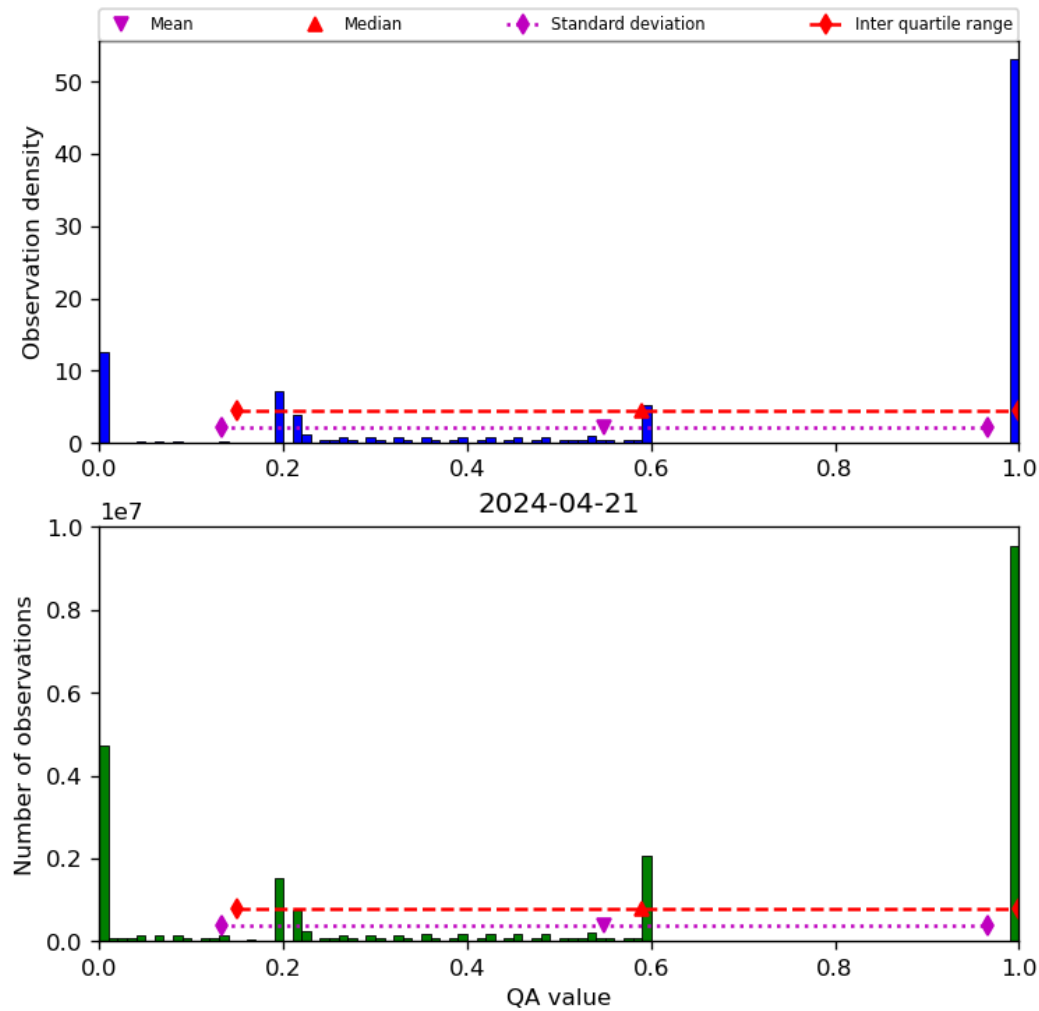
Figure 52: Histogram of “QA value” for 2024-04-21 to 2024-04-22
