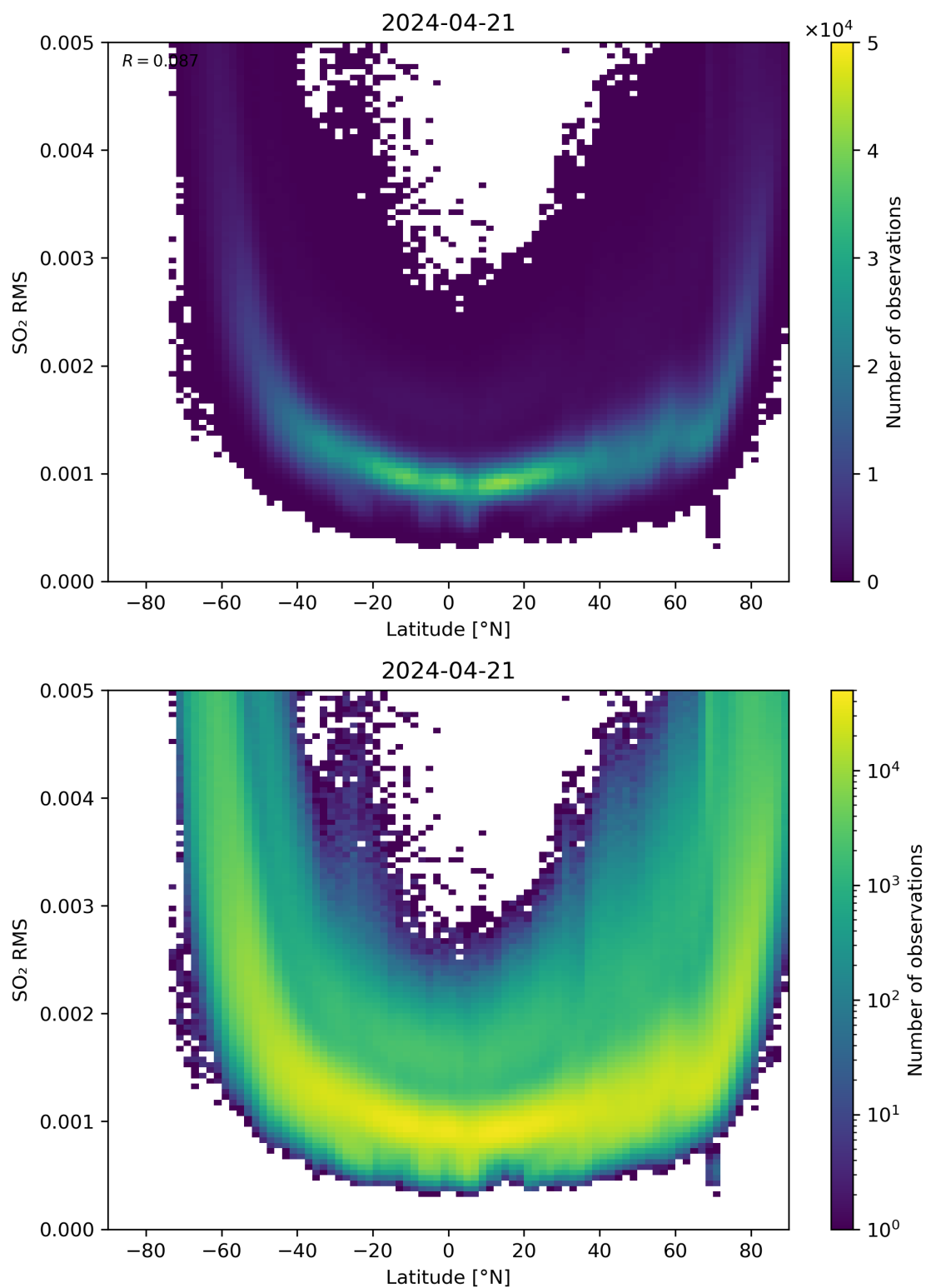
Figure 144: Scatter density plot of “Latitude” against “SO 2 RMS” for 2024-04-21 to 2024-04-22.
