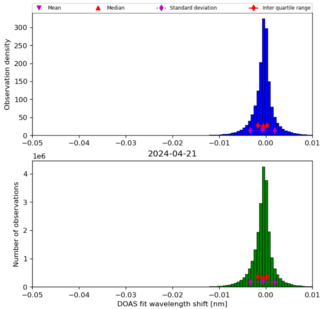
Figure 68: Histogram of “DOAS fit wavelength shift” for 2024-04-21 to 2024-04-22
