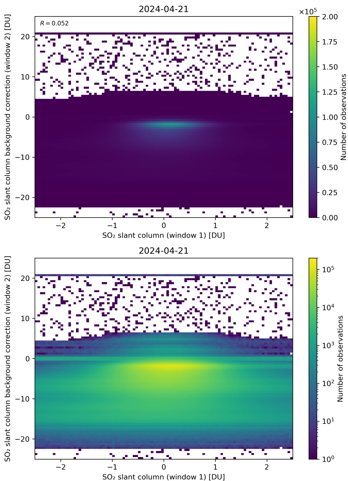
Figure 213: Scatter density plot of “SO 2 slant column (window 1)” against “SO 2 slant column background correction (window 2)” for 2024-04-21 to 2024-04-22.
