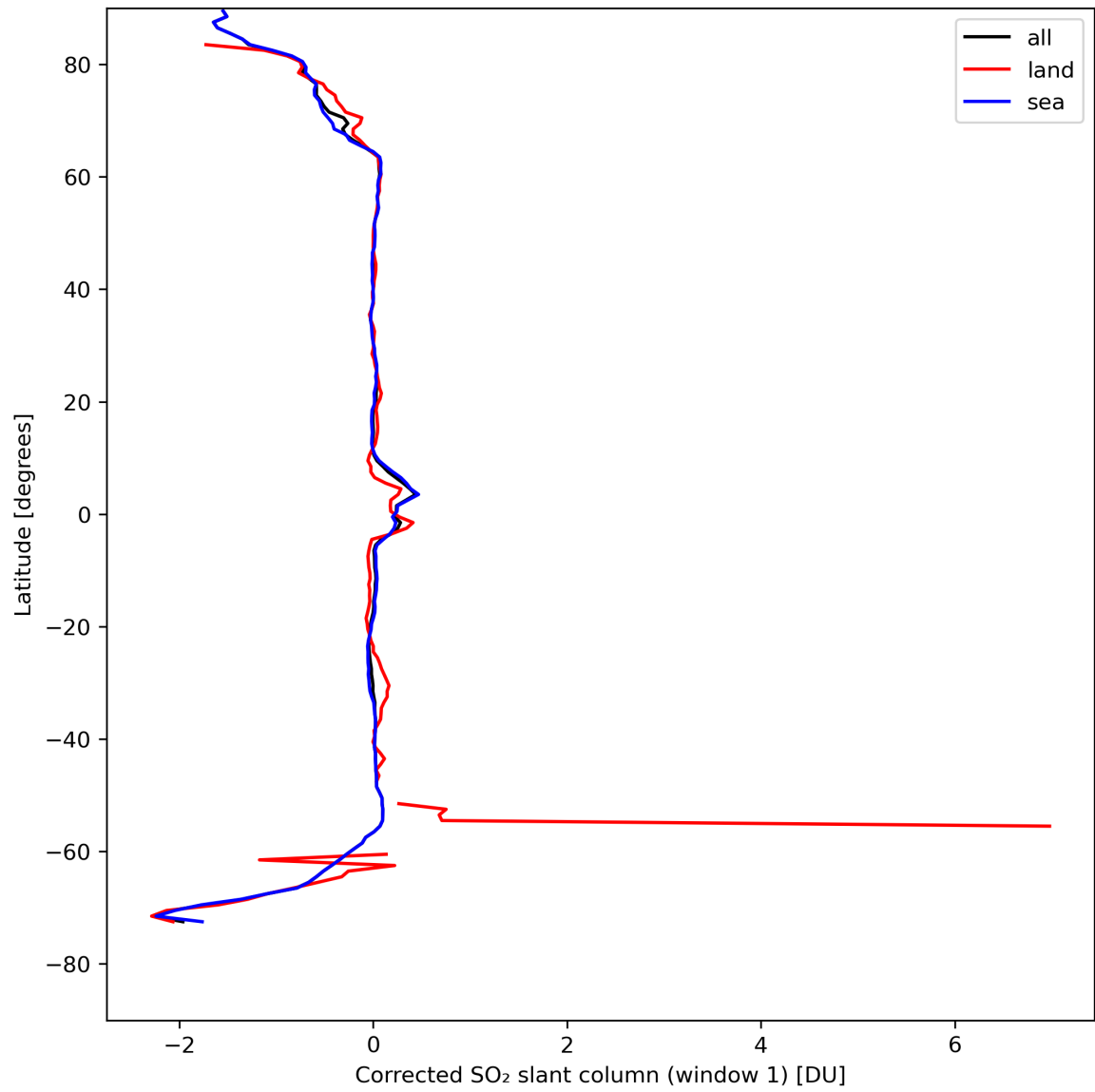
Figure 35: Zonal average of “Corrected SO 2 slant column (window 1)” for 2024-04-21 to 2024-04-22.
