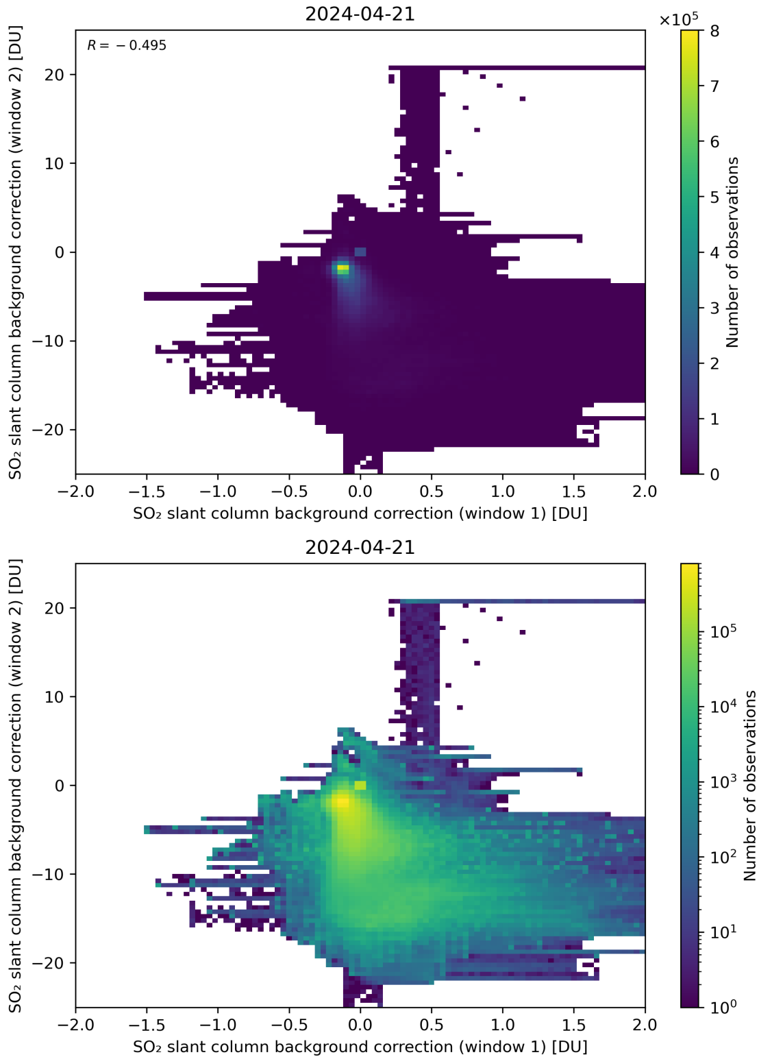
Figure 98: Scatter density plot of “SO 2 slant column background correction (window 1)” against “SO 2 slant column background correction (window 2)” for 2024-04-21 to 2024-04-22.
