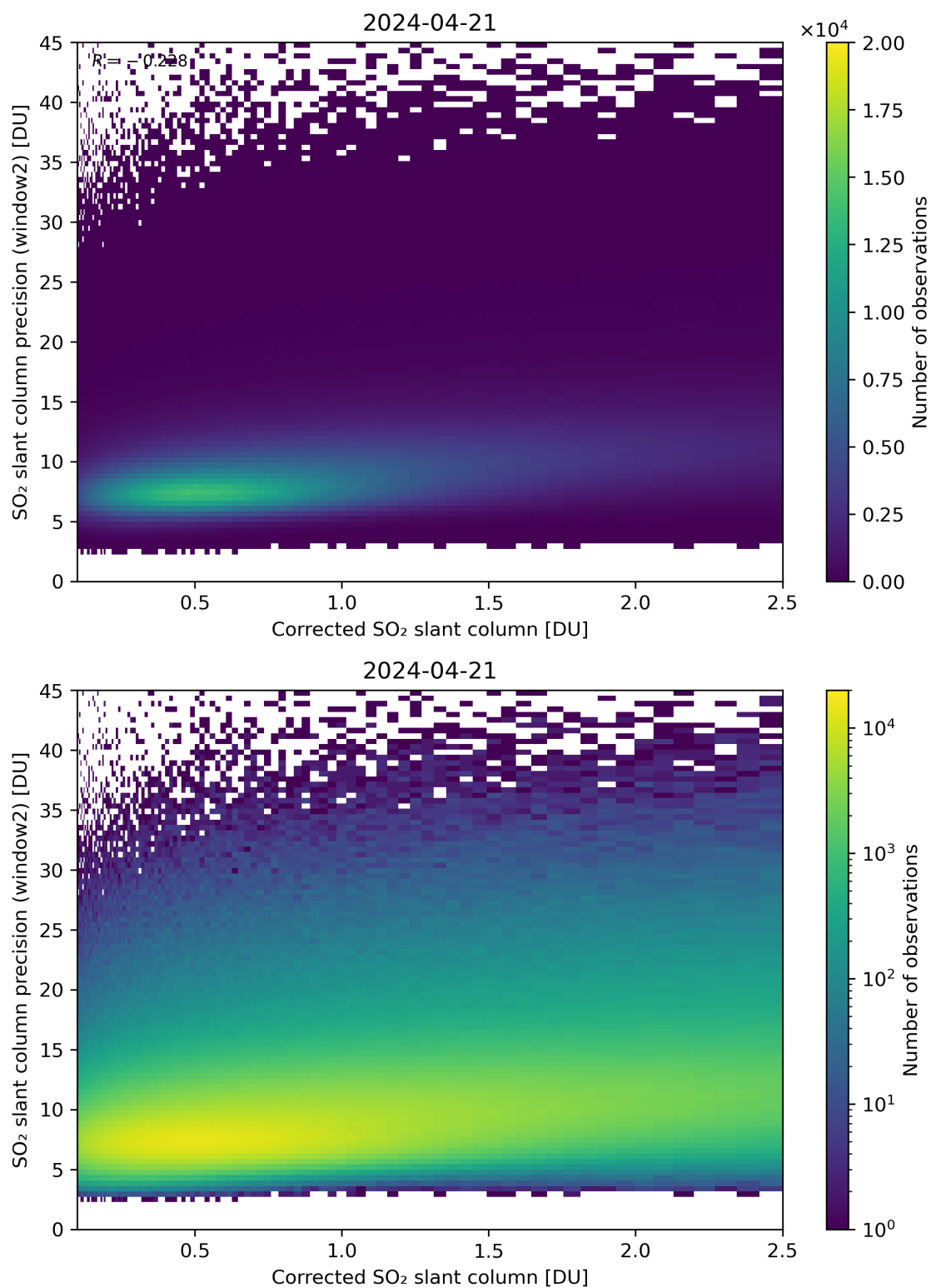
Figure 189: Scatter density plot of “Corrected SO 2 slant column” against “SO 2 slant column precision (window2)” for 2024-04-21 to 2024-04-22.
