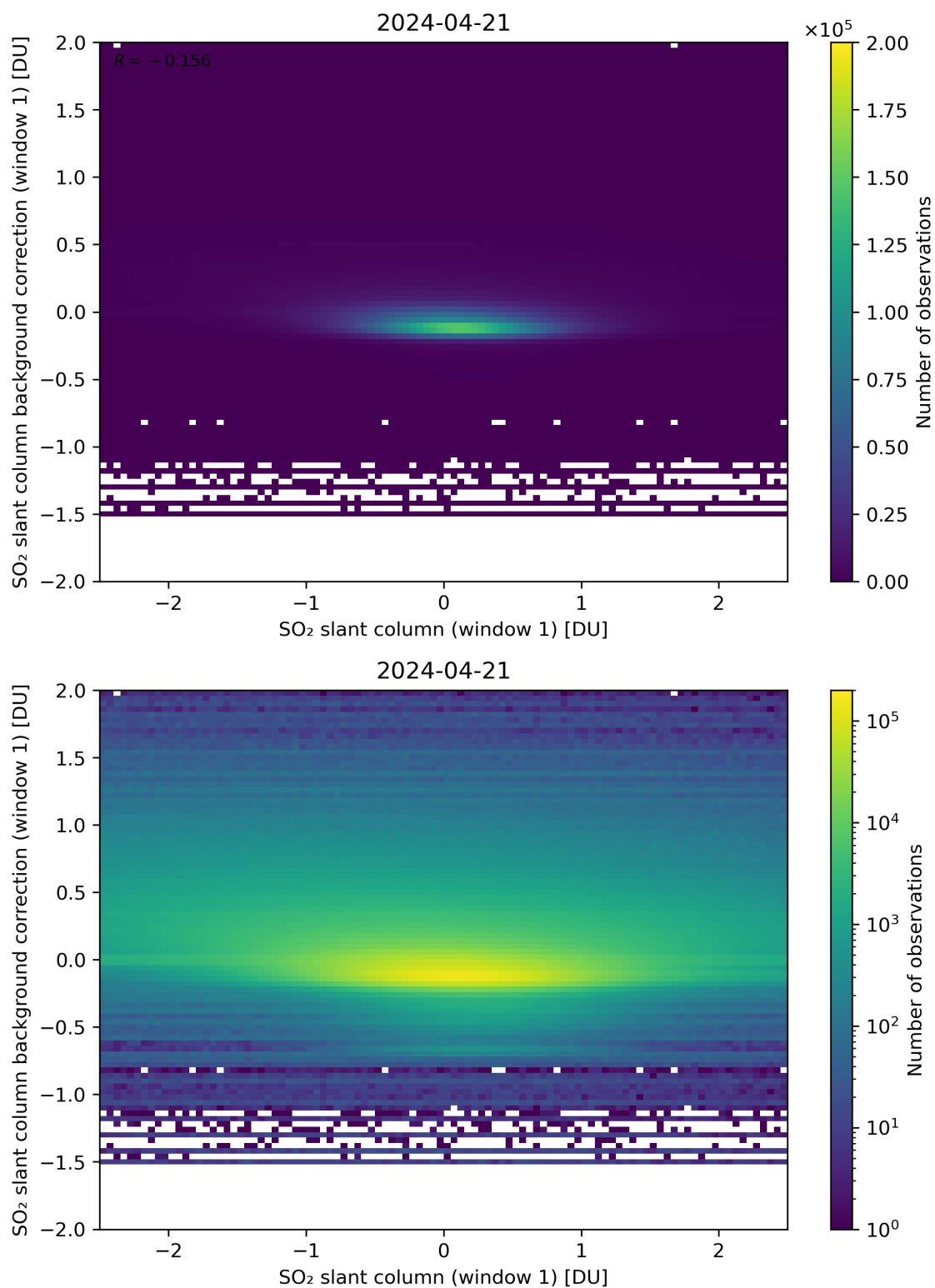
Figure 212: Scatter density plot of “SO 2 slant column (window 1)” against “SO 2 slant column background correction (window 1)” for 2024-04-21 to 2024-04-22.
