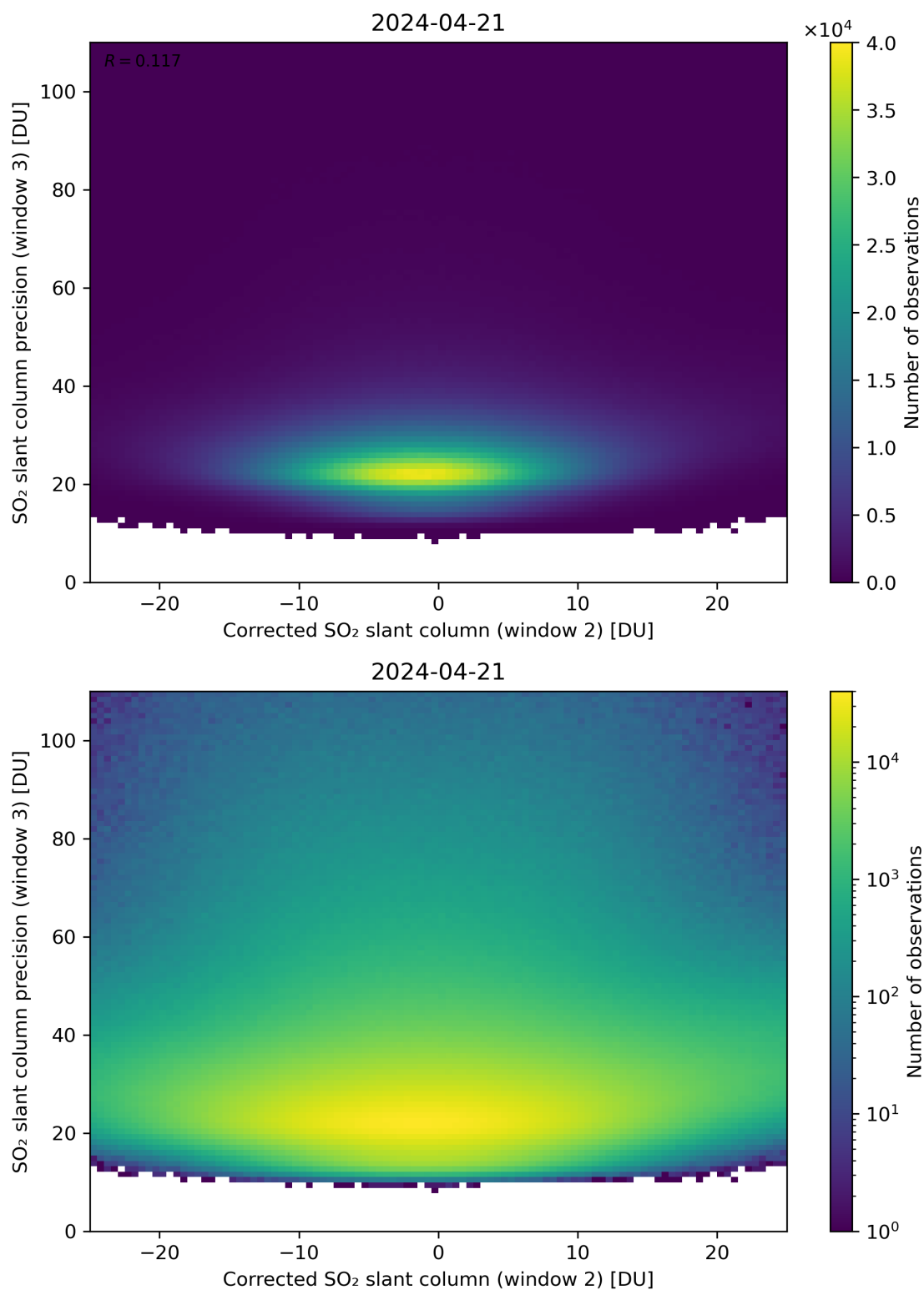
Figure 202: Scatter density plot of “Corrected SO 2 slant column (window 2)” against “SO 2 slant column precision (window 3)” for 2024-04-21 to 2024-04-22.
