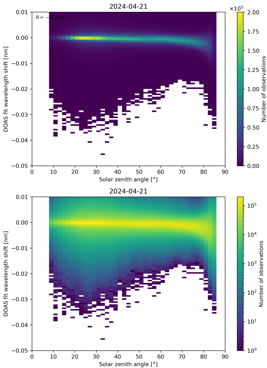
Figure 161: Scatter density plot of “Solar zenith angle” against “DOAS fit wavelength shift” for 2024-04-21 to 2024-04-22.
