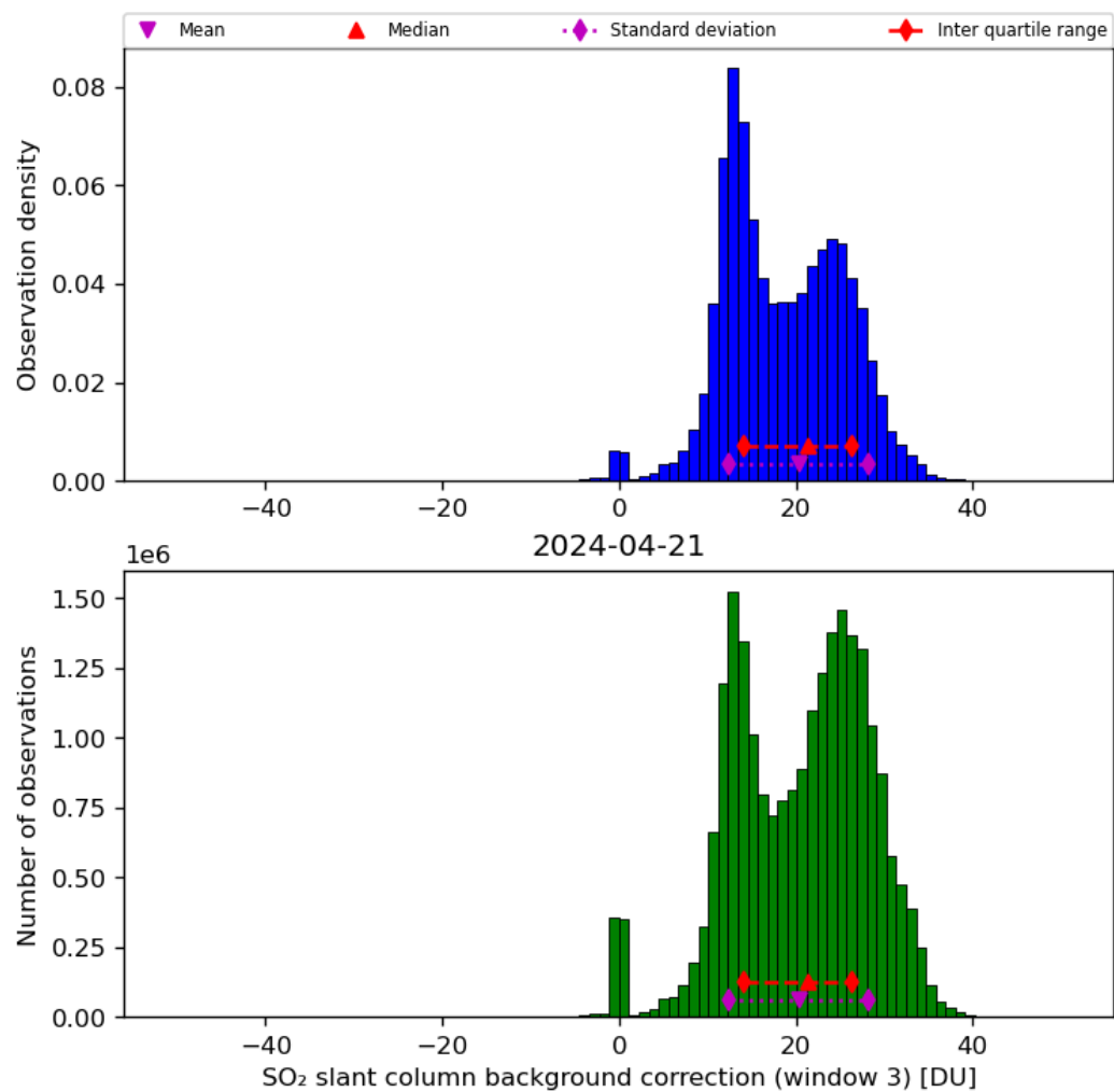
Figure 67: Histogram of “SO 2 slant column background correction (window 3)” for 2024-04-21 to 2024-04-22
