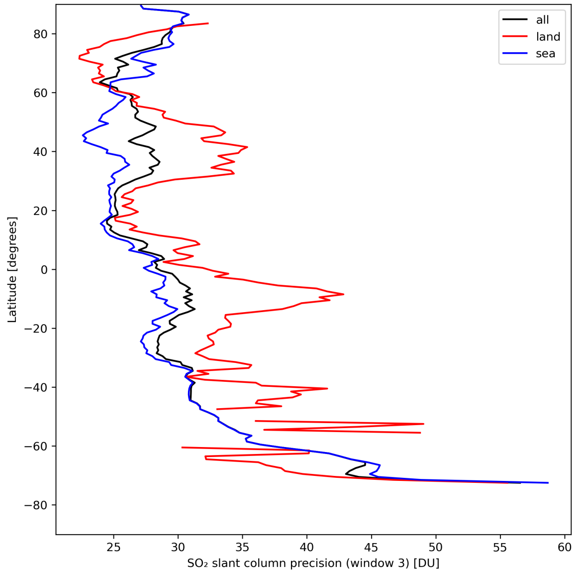
Figure 42: Zonal average of “SO 2 slant column precision (window 3)” for 2024-04-21 to 2024-04-22.
