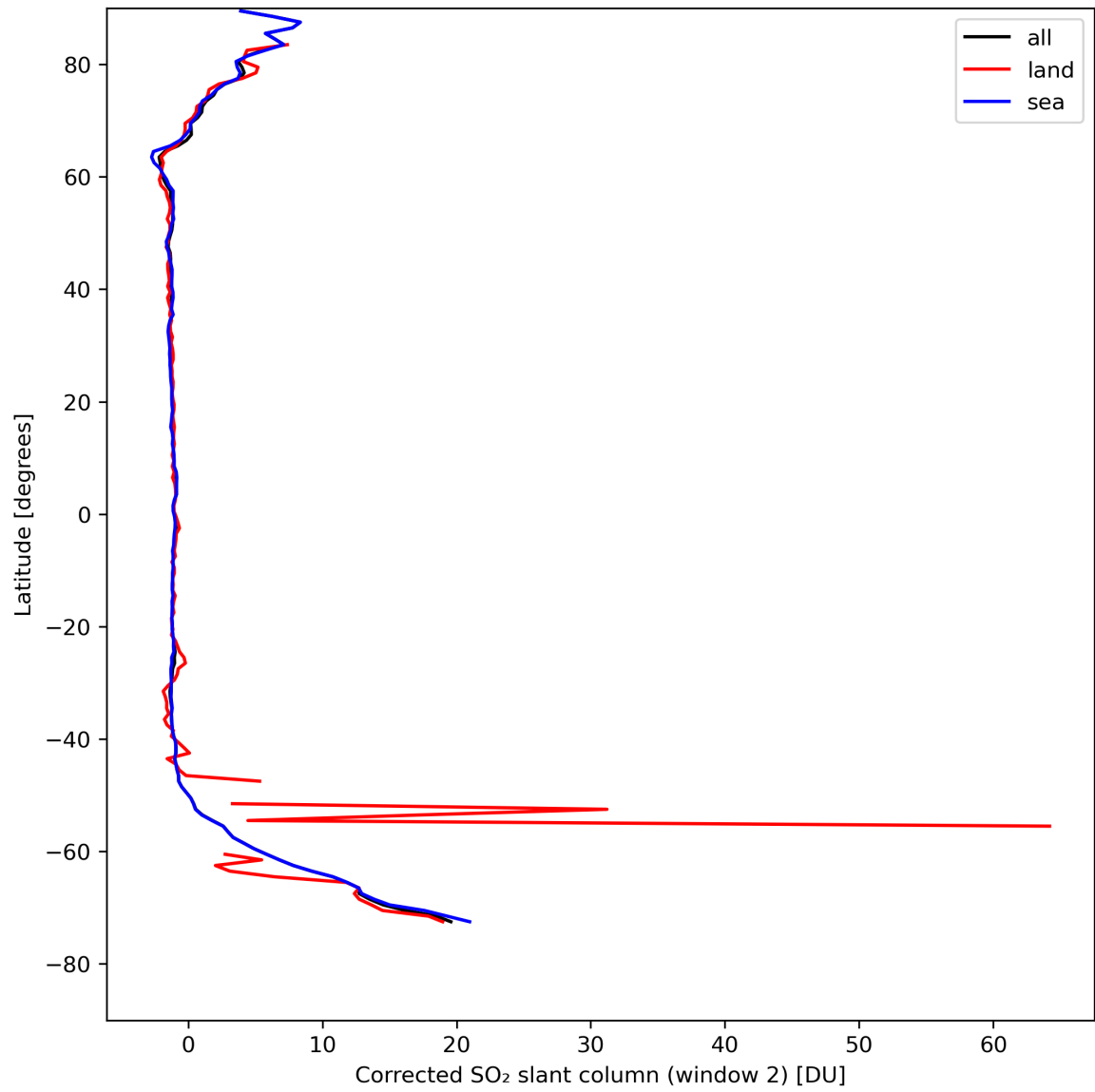
Figure 39: Zonal average of “Corrected SO 2 slant column (window 2)” for 2024-04-21 to 2024-04-22.
