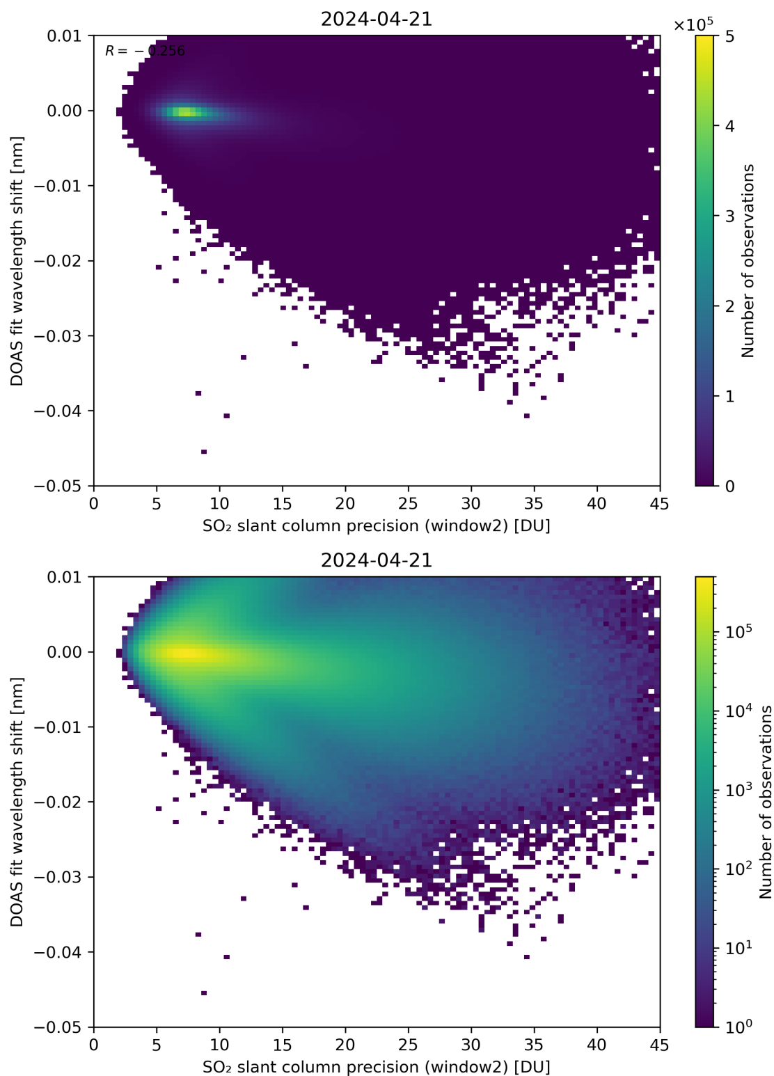
Figure 243: Scatter density plot of “SO 2 slant column precision (window2)” against “DOAS fit wavelength shift” for 2024-04-21 to 2024-04-22.
