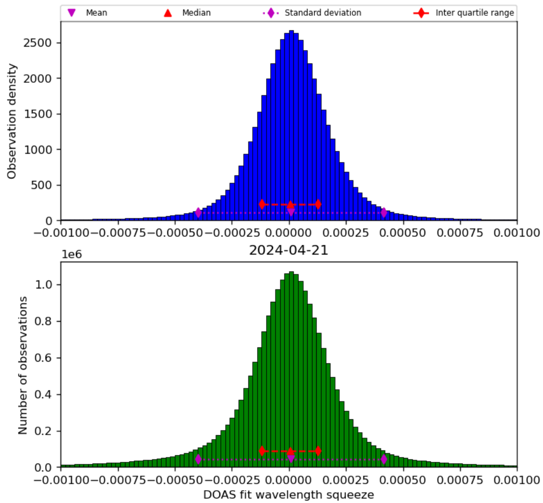
Figure 69: Histogram of “DOAS fit wavelength squeeze” for 2024-04-21 to 2024-04-22
