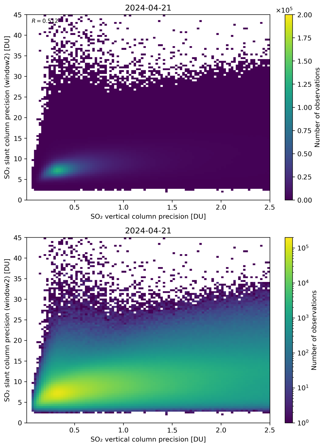
Figure 291: Scatter density plot of “SO 2 vertical column precision” against “SO 2 slant column precision (window2)” for 2024-04-21 to 2024-04-22.
