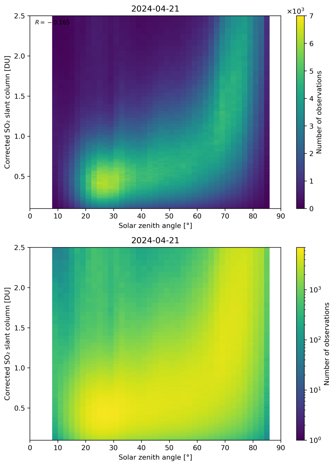
Figure 166: Scatter density plot of “Solar zenith angle” against “Corrected SO 2 slant column” for 2024-04-21 to 2024-04-22.
