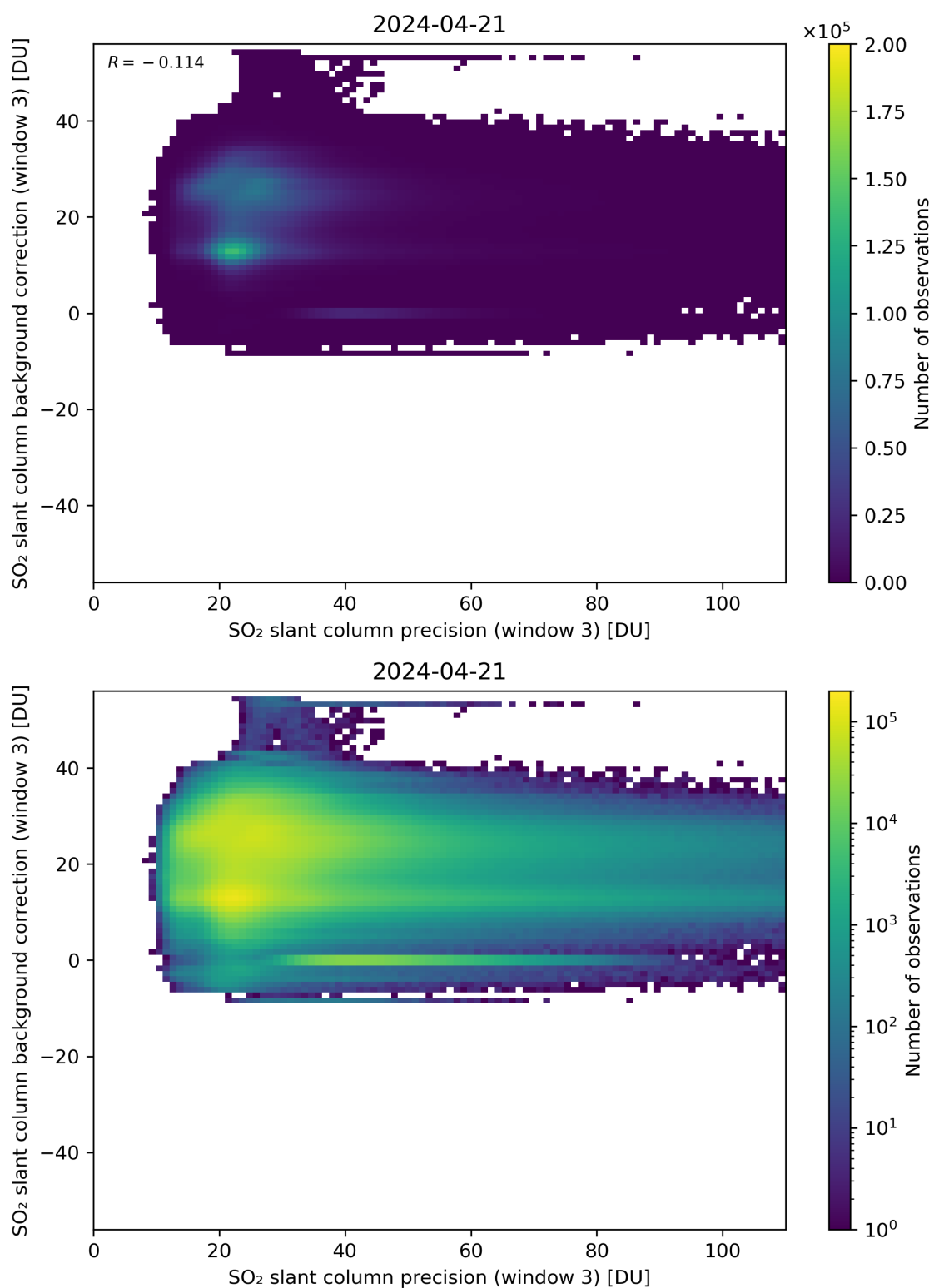
Figure 257: Scatter density plot of “SO 2 slant column precision (window 3)” against “SO 2 slant column background correction (window 3)” for 2024-04-21 to 2024-04-22.
