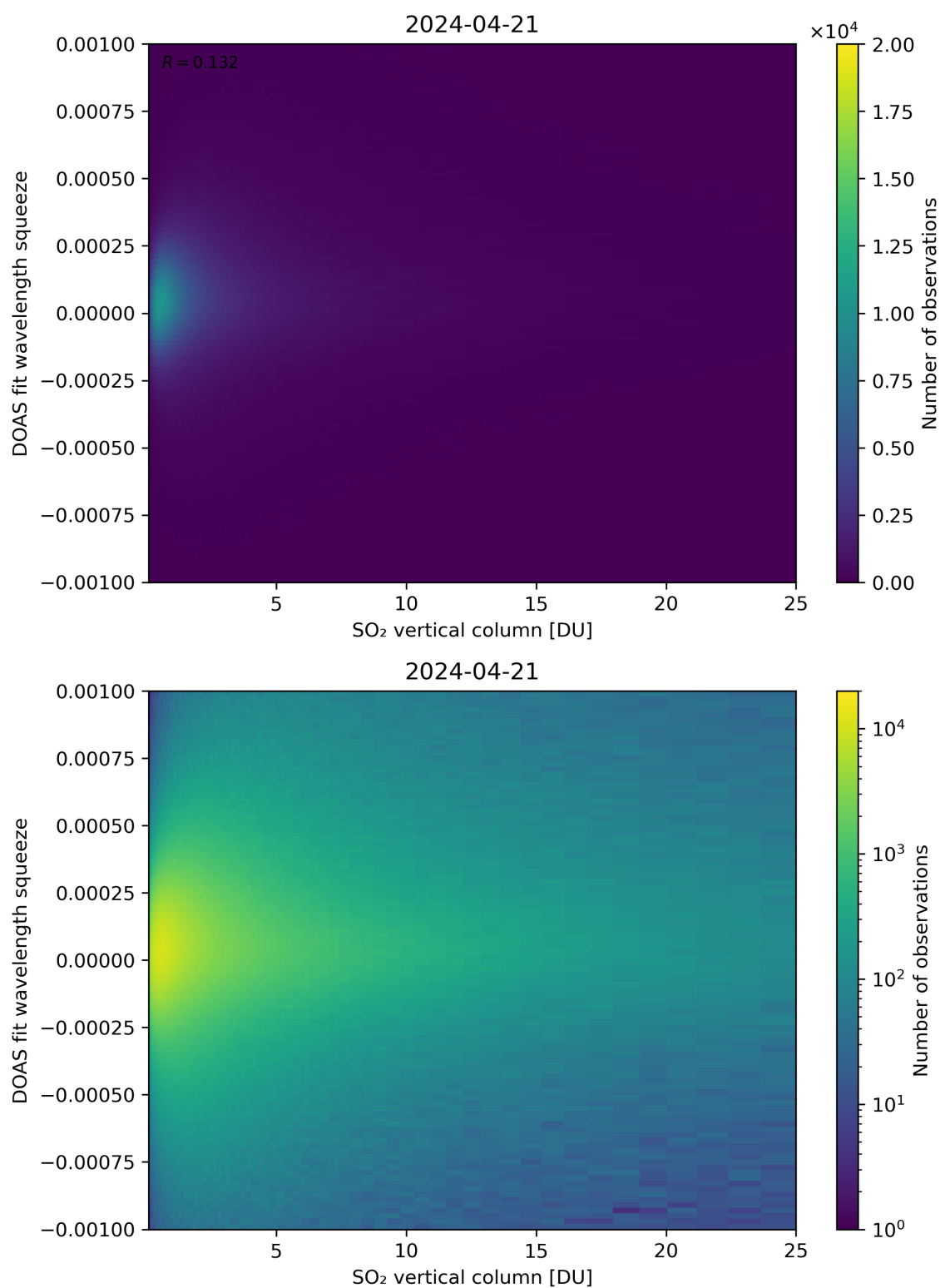
Figure 277: Scatter density plot of “SO 2 vertical column” against “DOAS fit wavelength squeeze” for 2024-04-21 to 2024-04-22.
