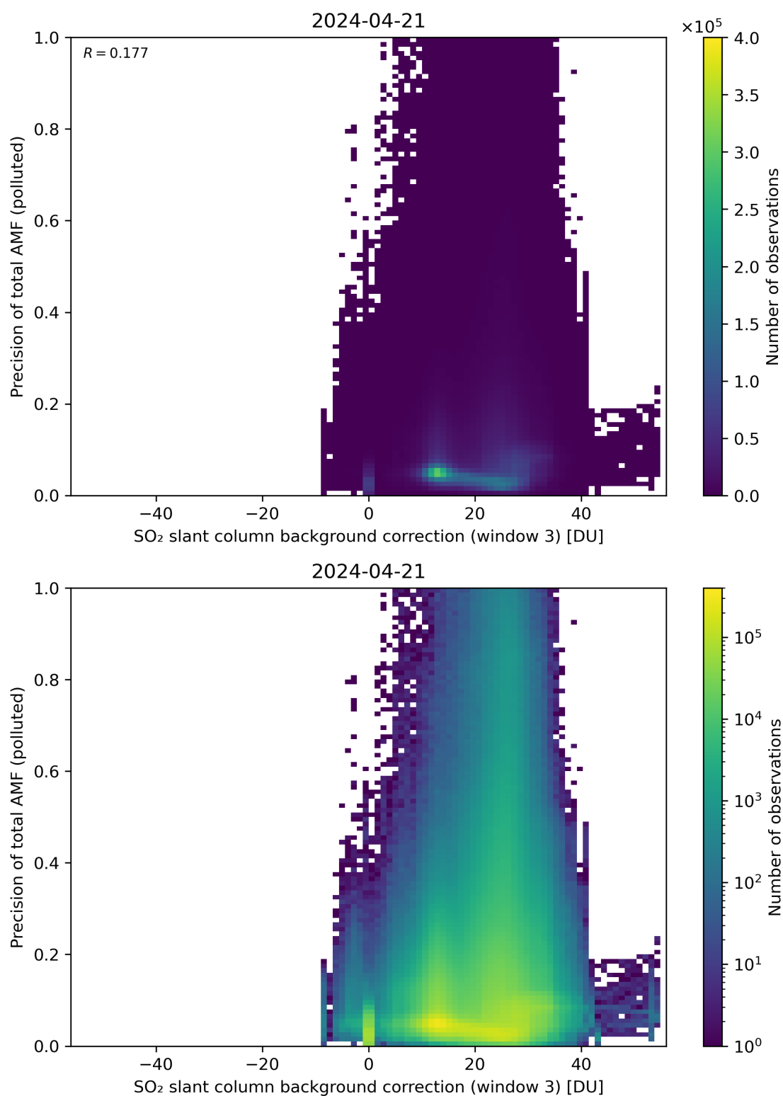
Figure 126: Scatter density plot of “SO 2 slant column background correction (window 3)” against “Precision of total AMF (polluted)” for 2024-04-21 to 2024-04-22.
