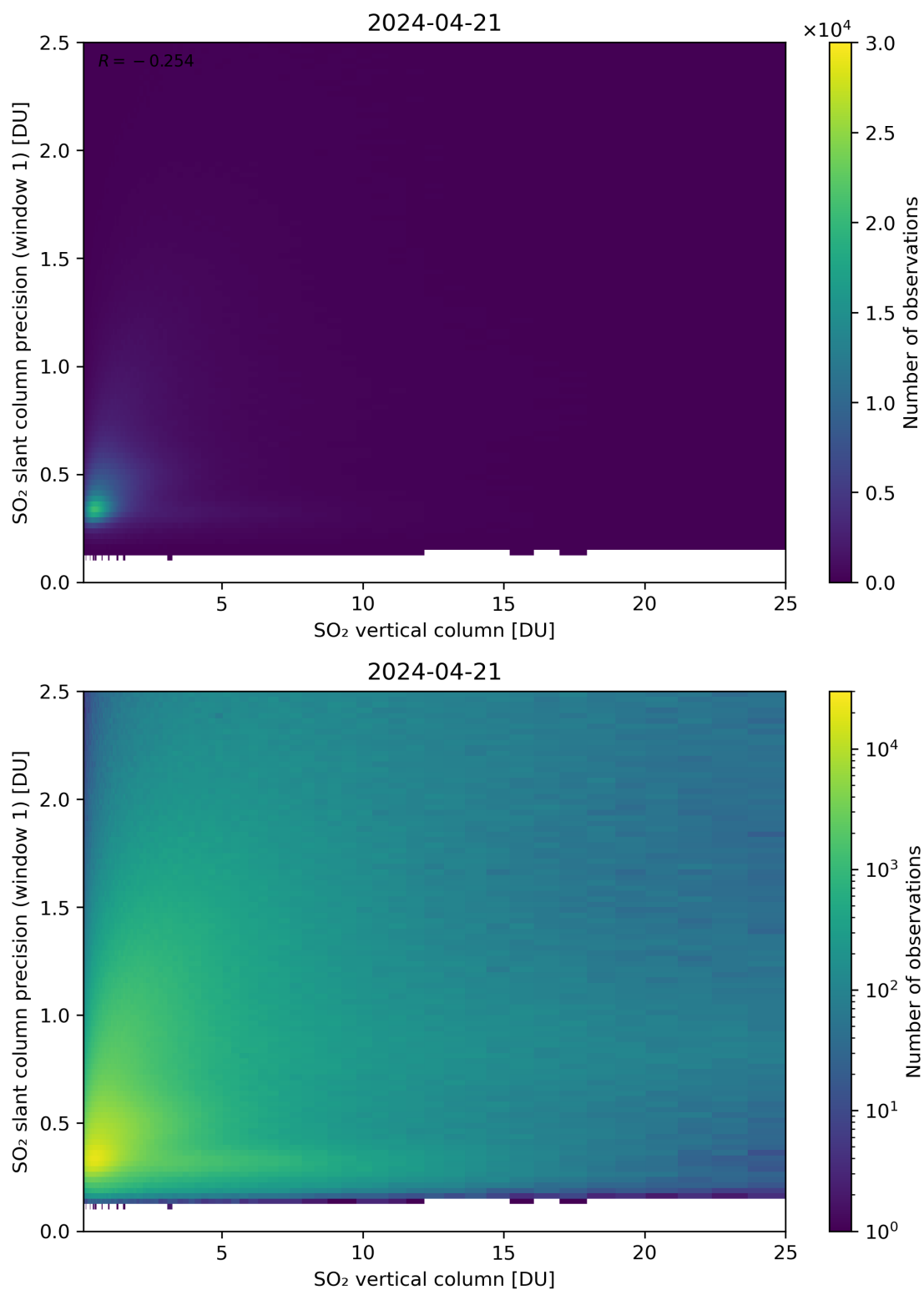
Figure 301: Scatter density plot of “SO 2 vertical column” against “SO 2 slant column precision (window 1)” for 2024-04-21 to 2024-04-22.
