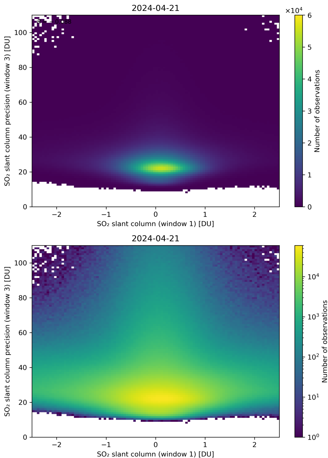
Figure 238: Scatter density plot of “SO 2 slant column (window 1)” against “SO 2 slant column precision (window 3)” for 2024-04-21 to 2024-04-22.
