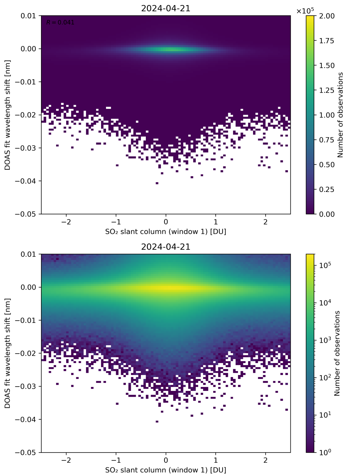
Figure 215: Scatter density plot of “SO 2 slant column (window 1)” against “DOAS fit wavelength shift” for 2024-04-21 to 2024-04-22.
