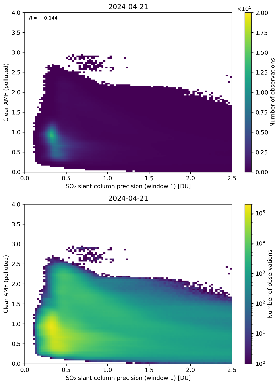
Figure 224: Scatter density plot of “SO 2 slant column precision (window 1)” against “Clear AMF (polluted)” for 2024-04-21 to 2024-04-22.
