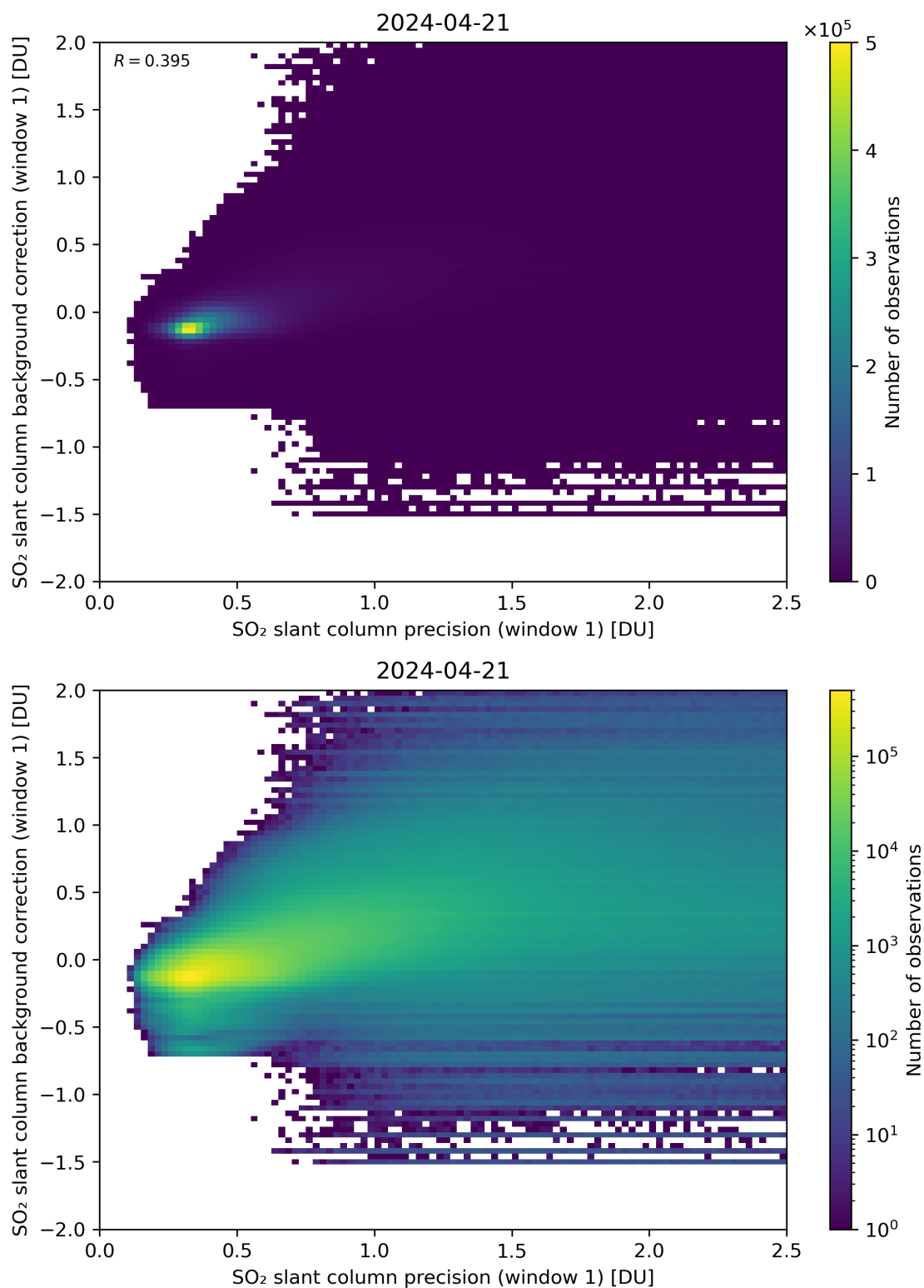
Figure 218: Scatter density plot of “SO 2 slant column precision (window 1)” against “SO 2 slant column background correction (window 1)” for 2024-04-21 to 2024-04-22.
