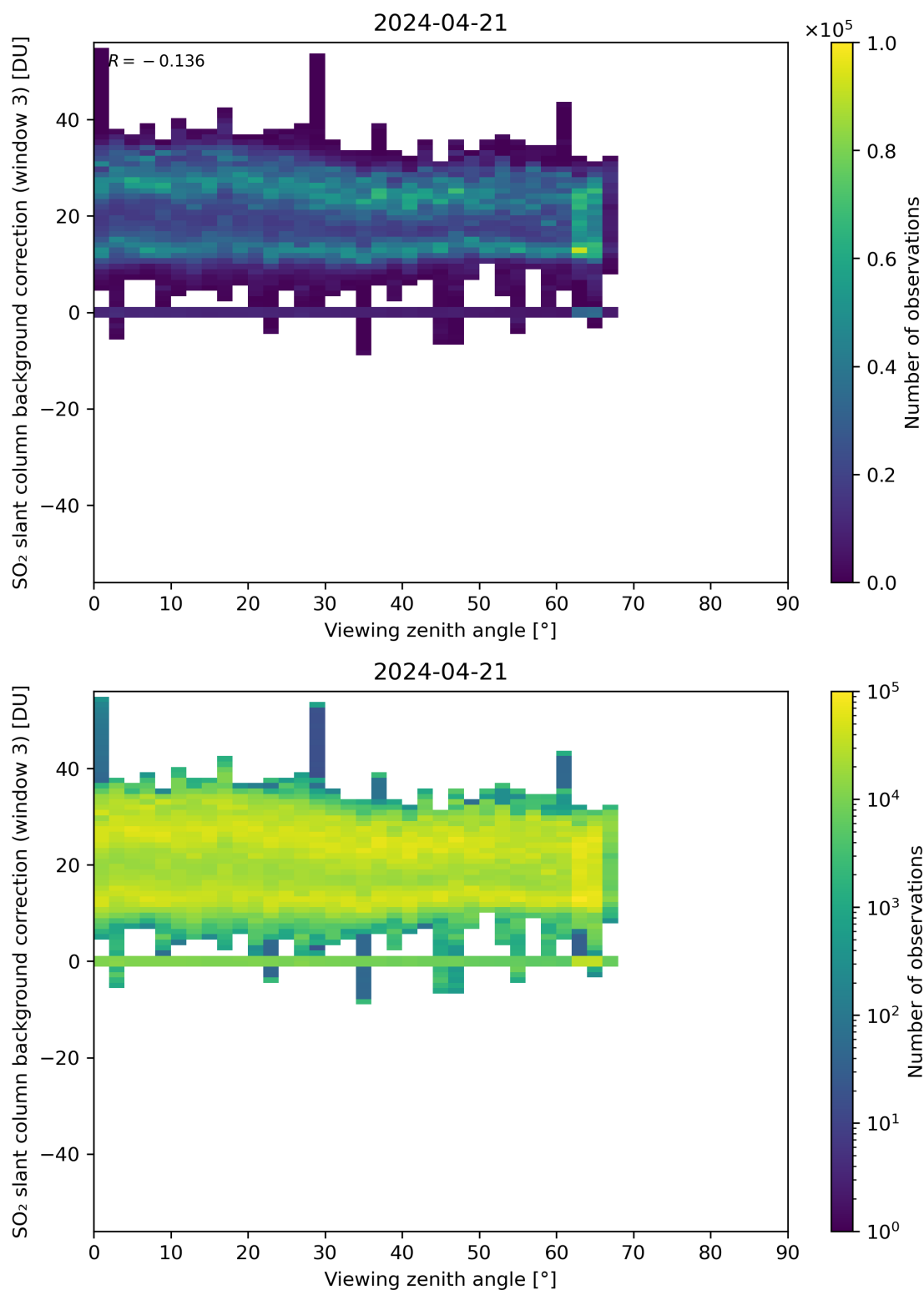
Figure 310: Scatter density plot of “Viewing zenith angle” against “SO 2 slant column background correction (window 3)” for 2024-04-21 to 2024-04-22.
