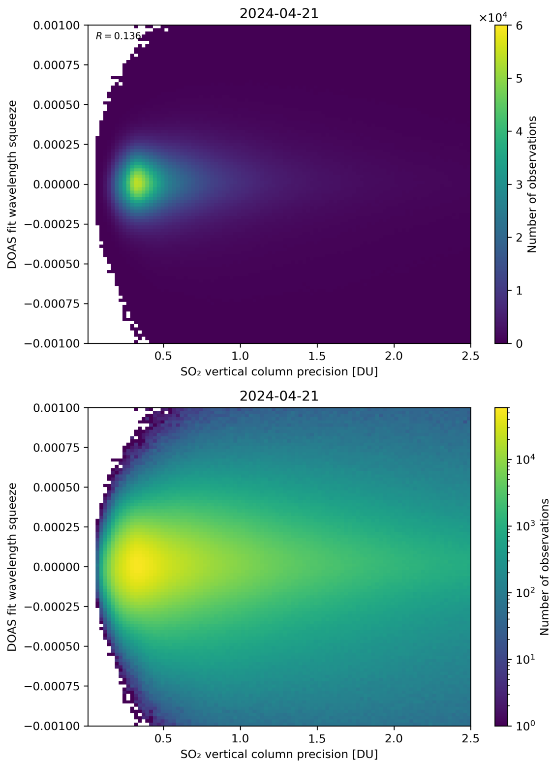
Figure 283: Scatter density plot of “SO 2 vertical column precision” against “DOAS fit wavelength squeeze” for 2024-04-21 to 2024-04-22.
