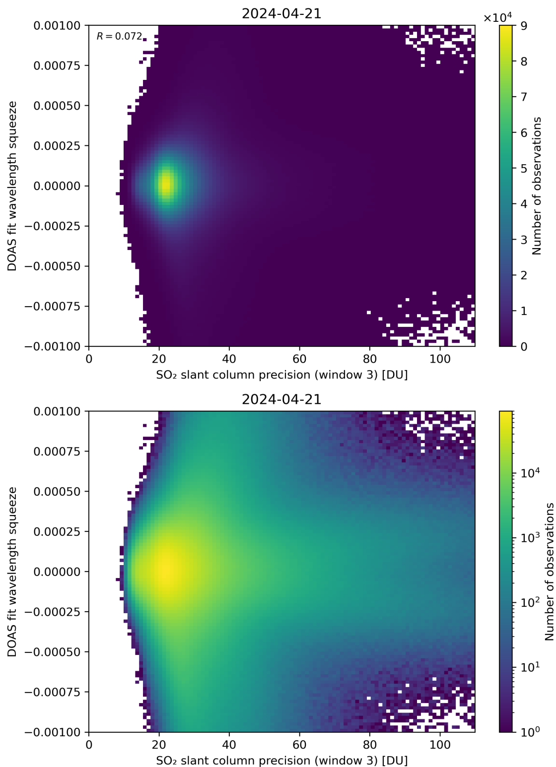
Figure 259: Scatter density plot of “SO 2 slant column precision (window 3)” against “DOAS fit wavelength squeeze” for 2024-04-21 to 2024-04-22.
