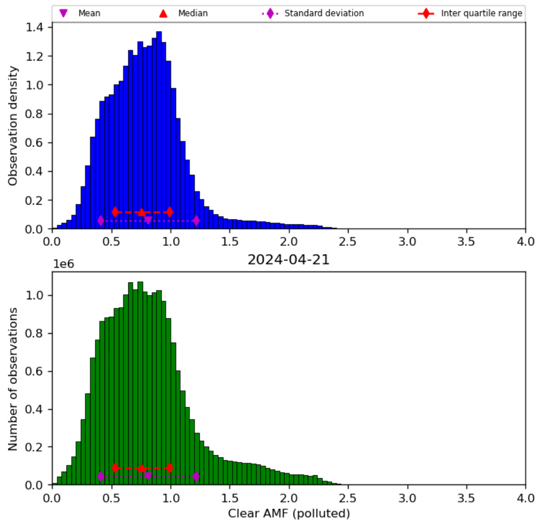
Figure 73: Histogram of “Clear AMF (polluted)” for 2024-04-21 to 2024-04-22
