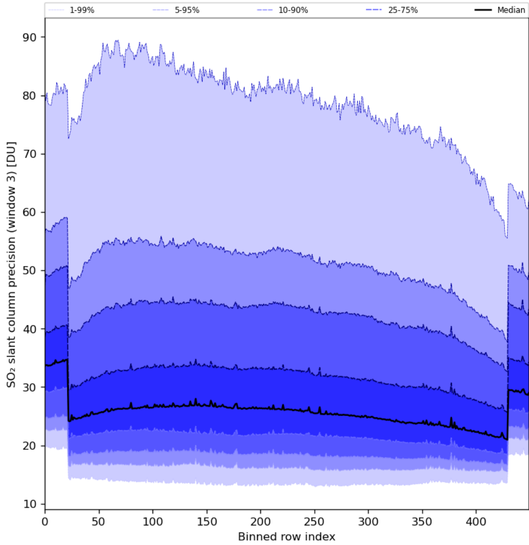
Figure 88: Along track statistics of “SO 2 slant column precision (window 3)” for 2024-04-21 to 2024-04-22
