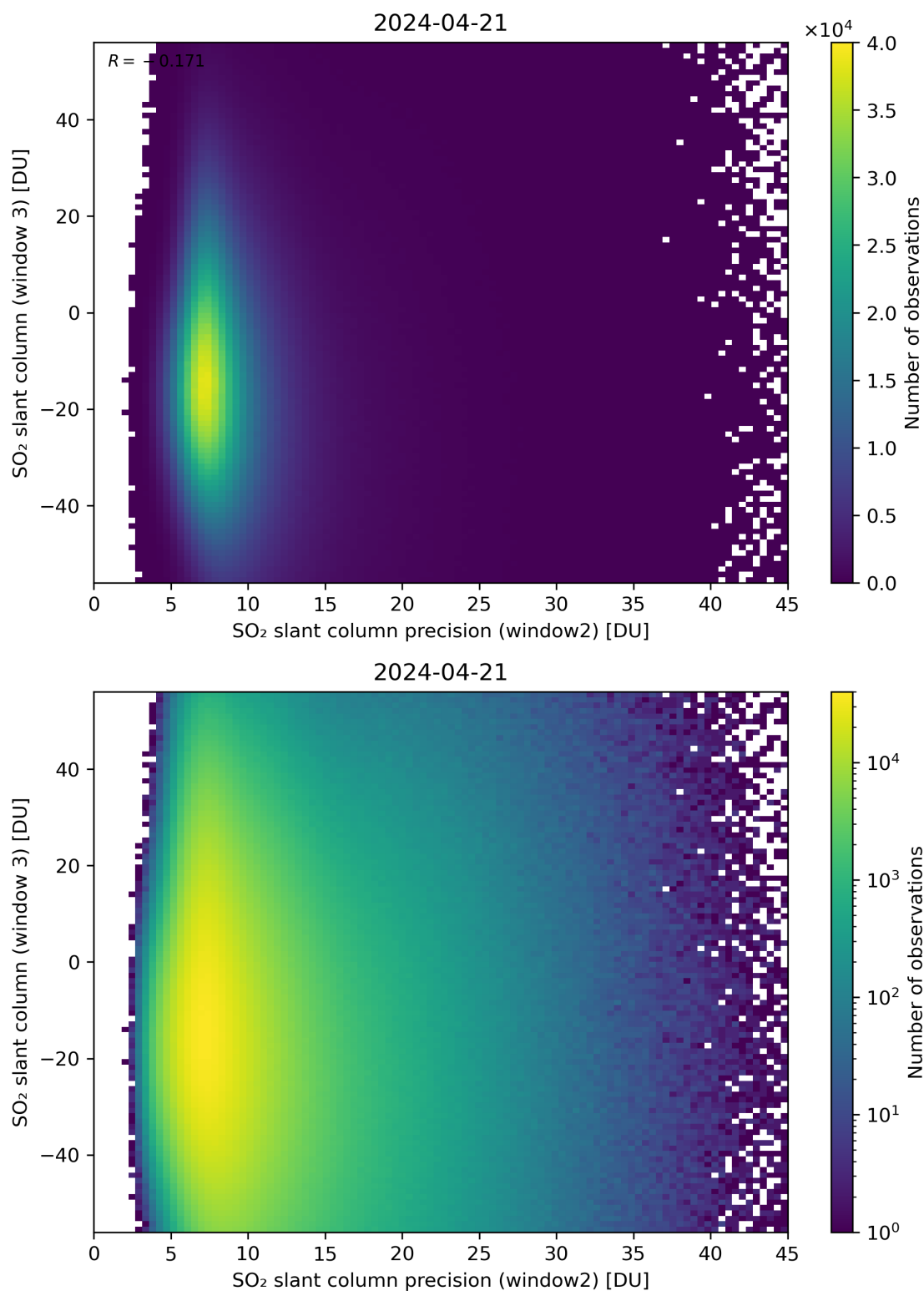
Figure 249: Scatter density plot of “SO 2 slant column precision (window2)” against “SO 2 slant column (window 3)” for 2024-04-21 to 2024-04-22.
