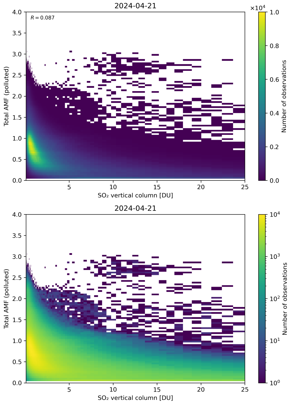
Figure 305: Scatter density plot of “SO 2 vertical column” against “Total AMF (polluted)” for 2024-04-21 to 2024-04-22.
