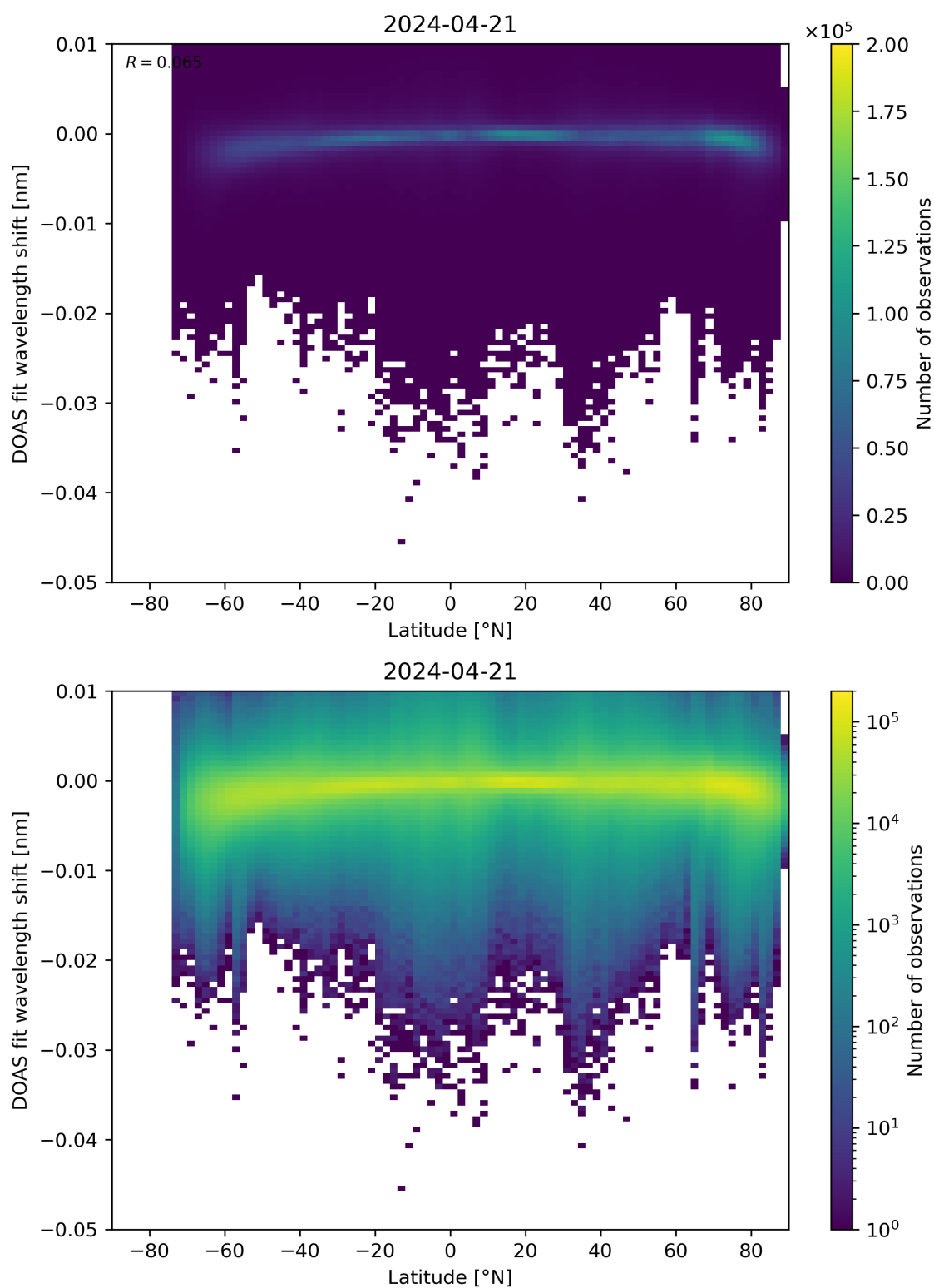
Figure 142: Scatter density plot of “Latitude” against “DOAS fit wavelength shift” for 2024-04-21 to 2024-04-22.
