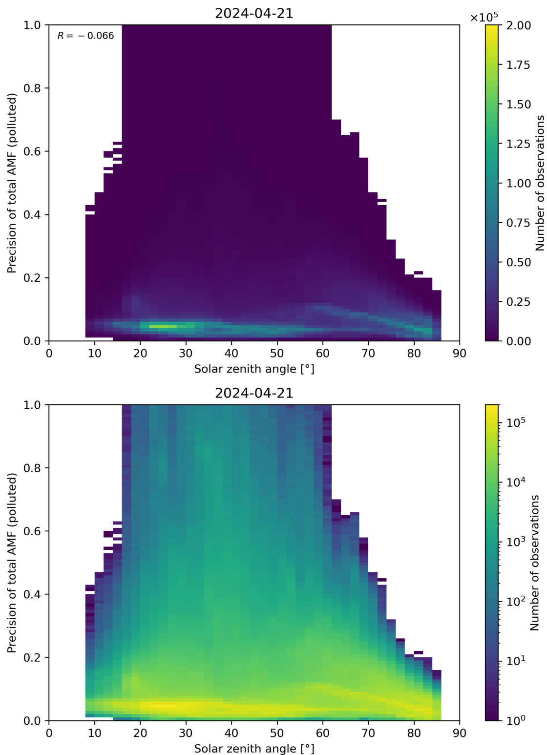
Figure 175: Scatter density plot of “Solar zenith angle” against “Precision of total AMF (polluted)” for 2024-04-21 to 2024-04-22.
