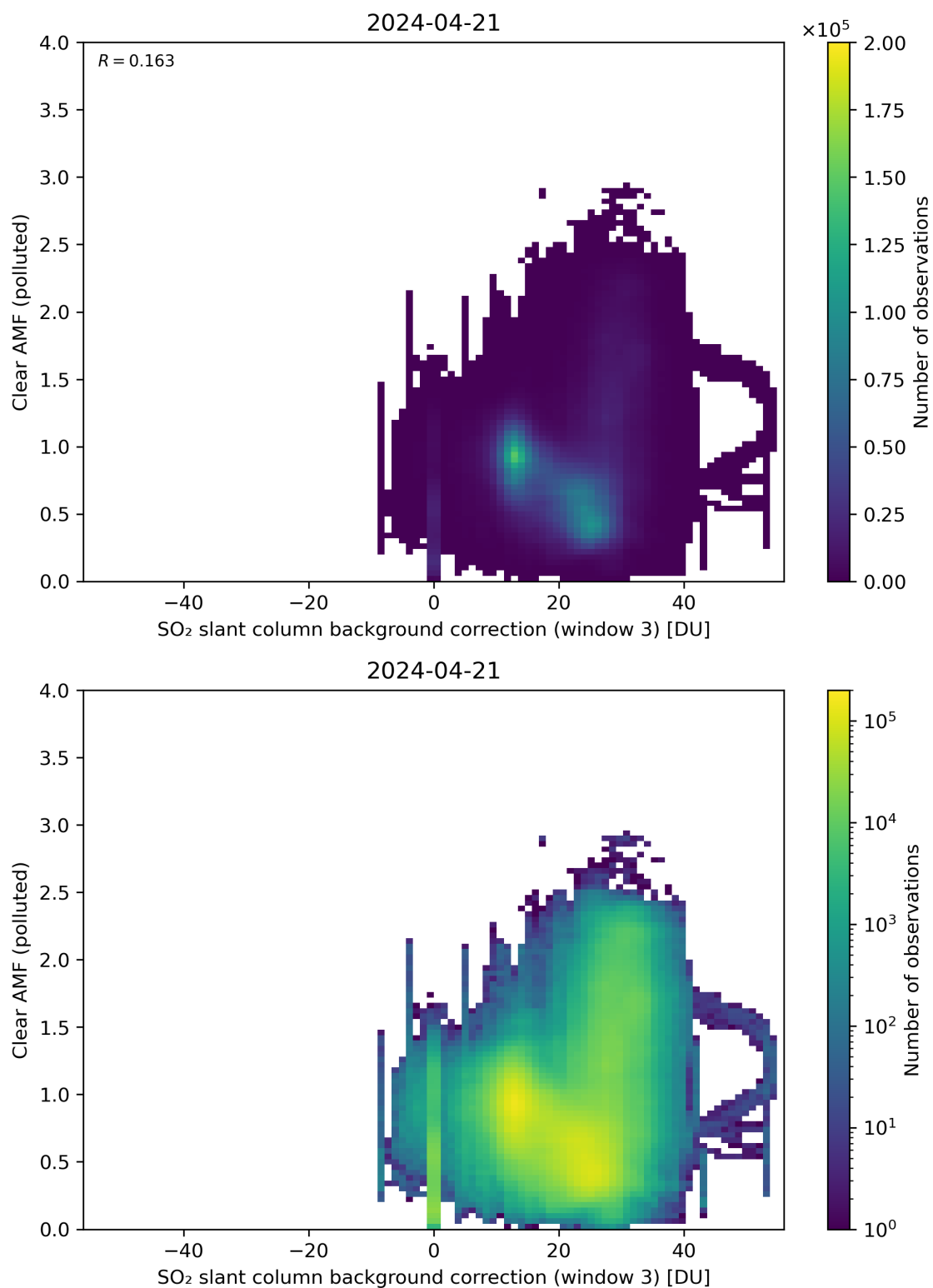
Figure 124: Scatter density plot of “SO 2 slant column background correction (window 3)” against “Clear AMF (polluted)” for 2024-04-21 to 2024-04-22.
