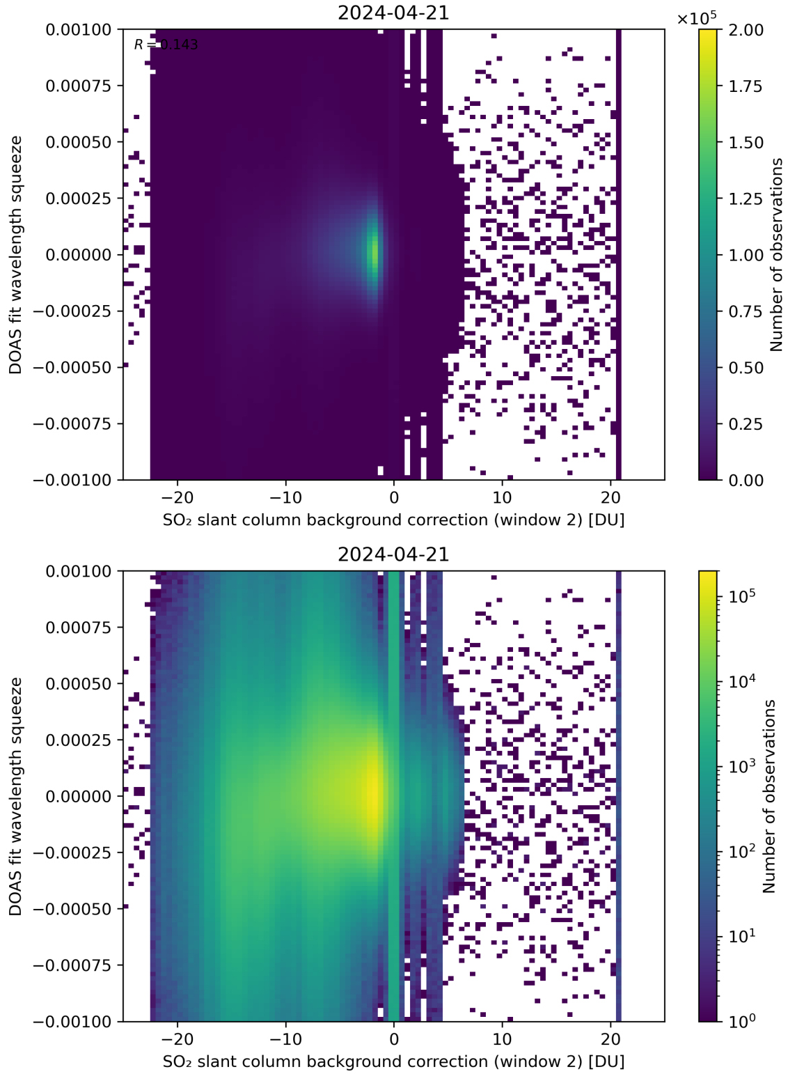
Figure 113: Scatter density plot of “SO 2 slant column background correction (window 2)” against “DOAS fit wavelength squeeze” for 2024-04-21 to 2024-04-22.
