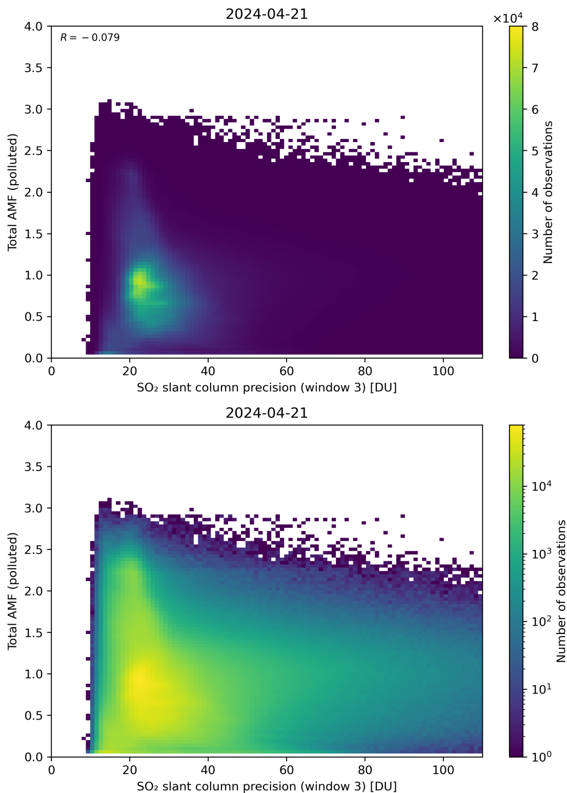
Figure 263: Scatter density plot of “SO 2 slant column precision (window 3)” against “Total AMF (polluted)” for 2024-04-21 to 2024-04-22.
