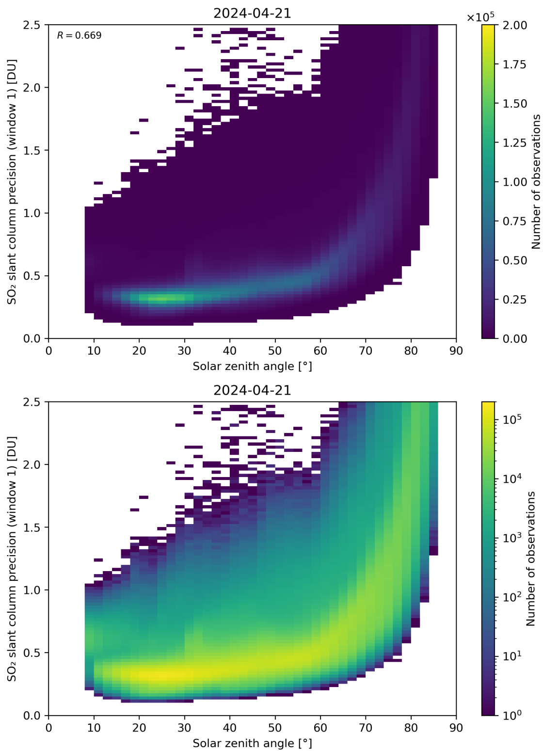
Figure 170: Scatter density plot of “Solar zenith angle” against “SO 2 slant column precision (window 1)” for 2024-04-21 to 2024-04-22.
