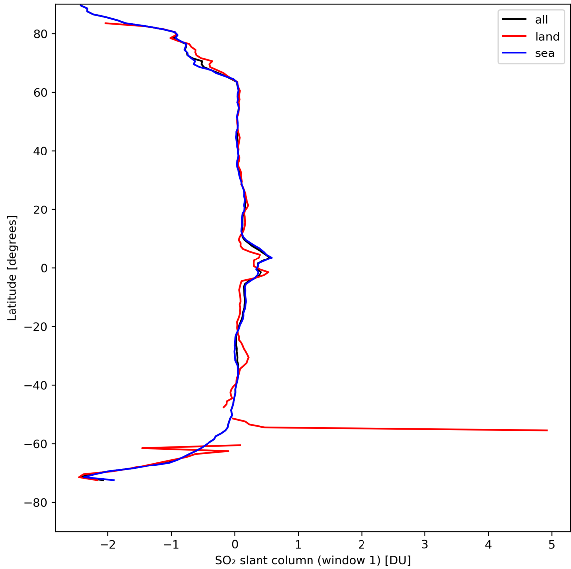
Figure 33: Zonal average of “SO 2 slant column (window 1)” for 2024-04-21 to 2024-04-22.
