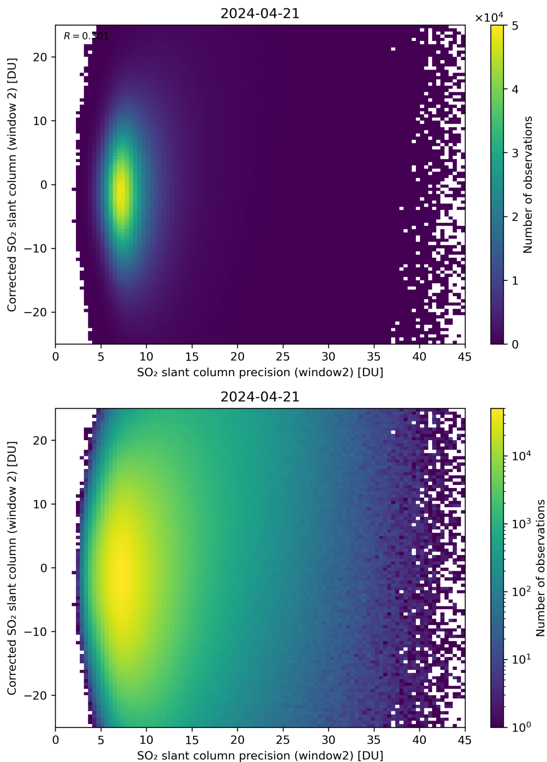
Figure 247: Scatter density plot of “SO 2 slant column precision (window2)” against “Corrected SO 2 slant column (window 2)” for 2024-04-21 to 2024-04-22.
