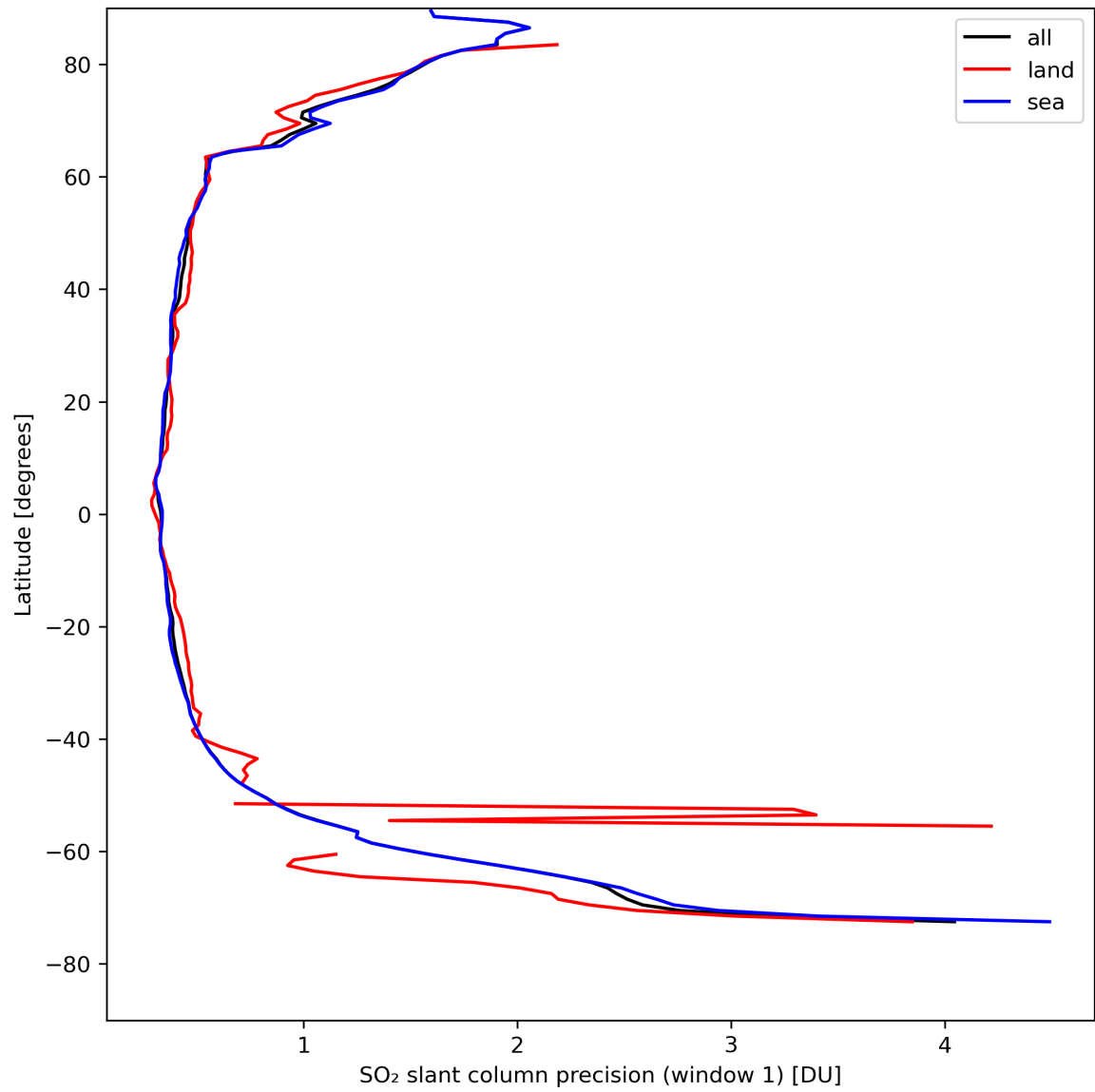
Figure 34: Zonal average of “SO 2 slant column precision (window 1)” for 2024-04-21 to 2024-04-22.
