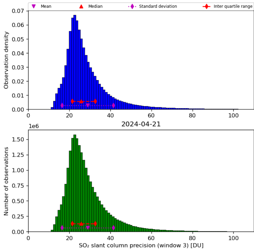
Figure 65: Histogram of “SO 2 slant column precision (window 3)” for 2024-04-21 to 2024-04-22
