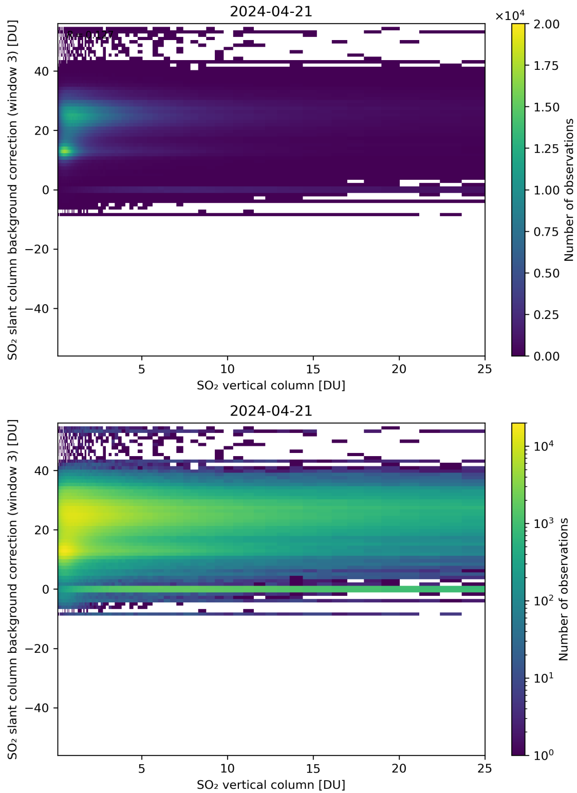
Figure 275: Scatter density plot of “SO 2 vertical column” against “SO 2 slant column background correction (window 3)” for 2024-04-21 to 2024-04-22.
