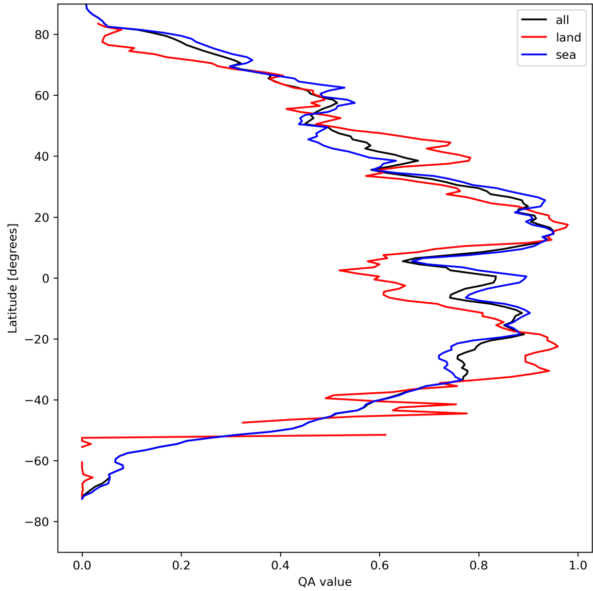
Figure 29: Zonal average of “QA value” for 2024-04-21 to 2024-04-22.
