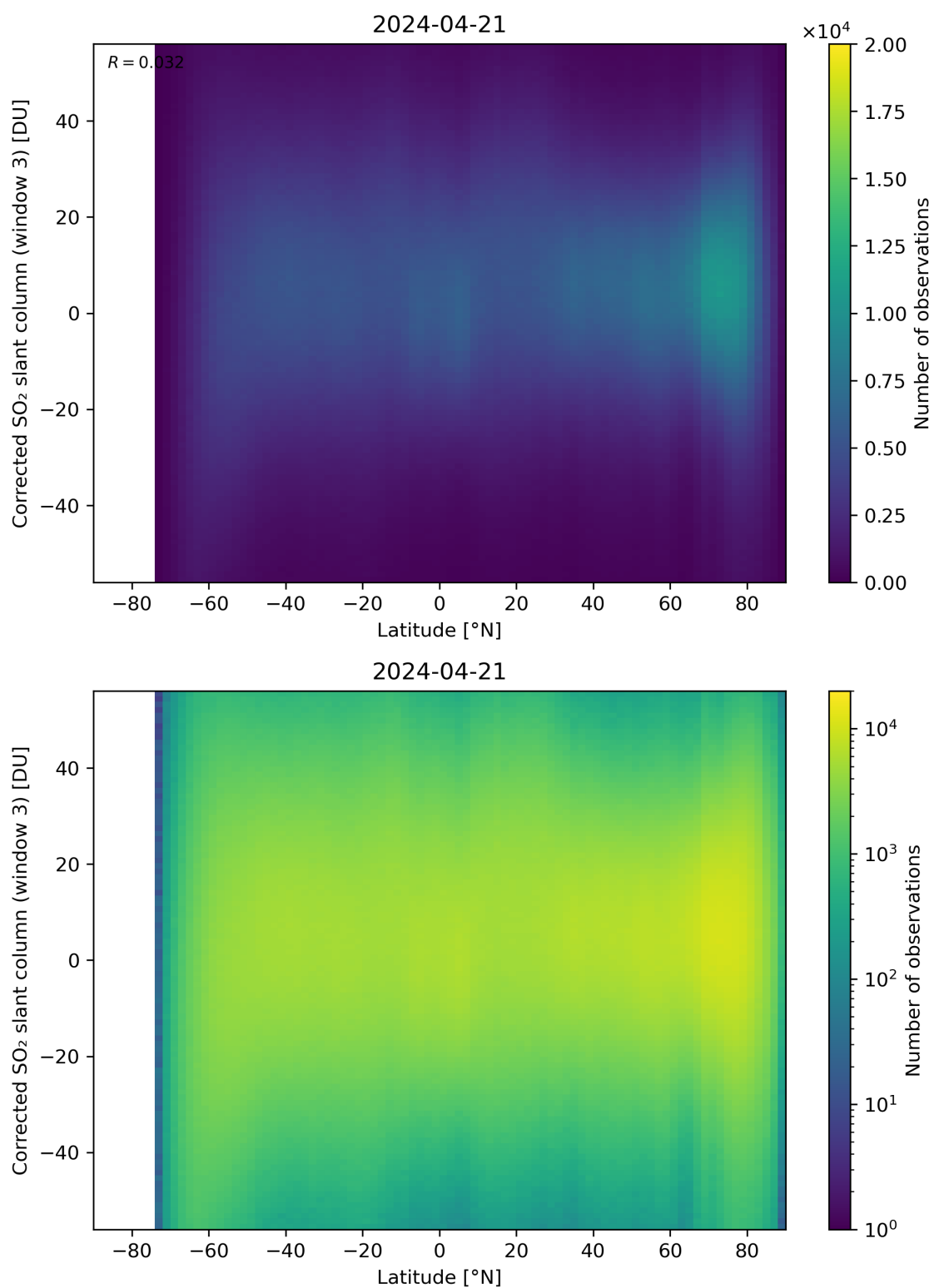
Figure 148: Scatter density plot of “Latitude” against “Corrected SO 2 slant column (window 3)” for 2024-04-21 to 2024-04-22.
