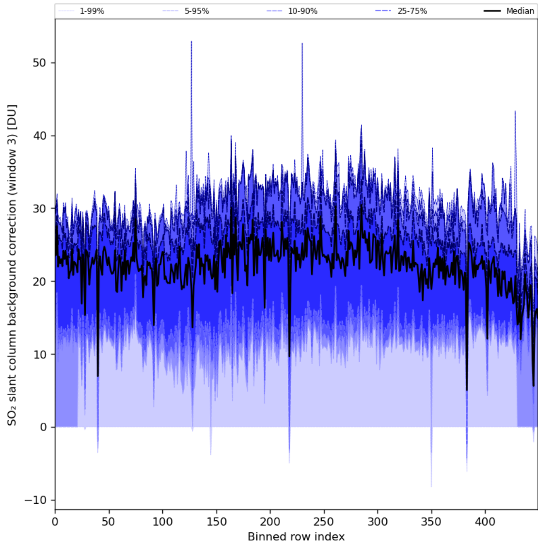
Figure 90: Along track statistics of “SO 2 slant column background correction (window 3)” for 2024-04-21 to 2024-04-22
