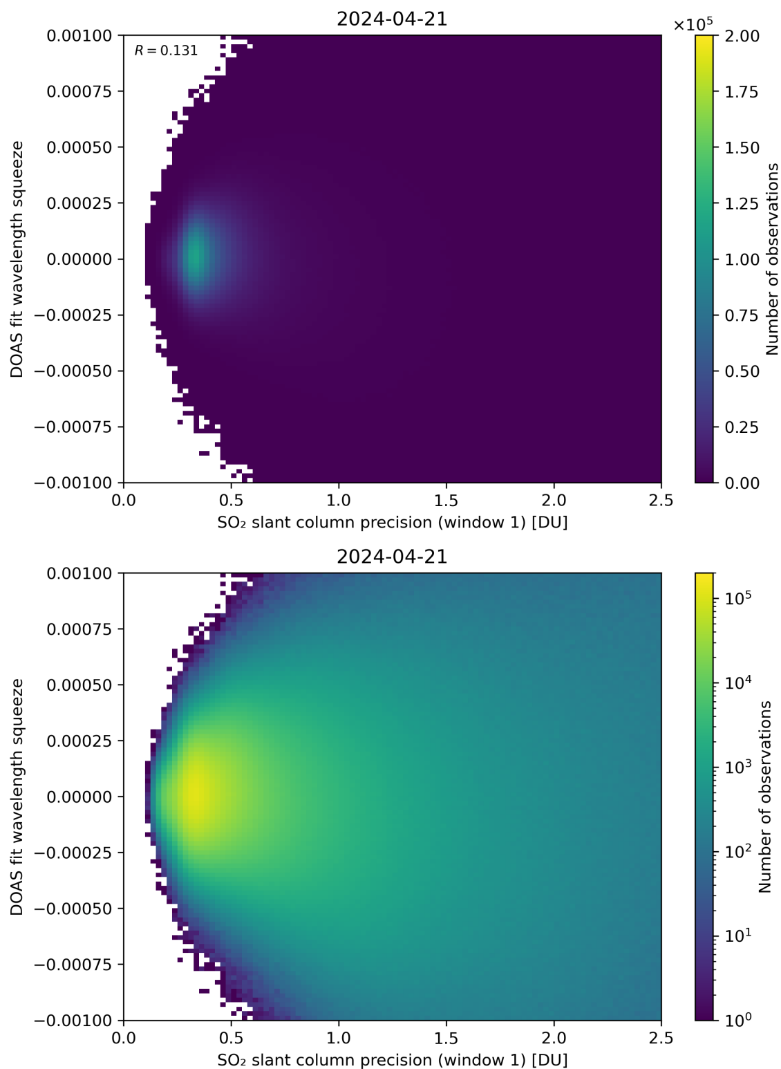
Figure 222: Scatter density plot of “SO 2 slant column precision (window 1)” against “DOAS fit wavelength squeeze” for 2024-04-21 to 2024-04-22.
