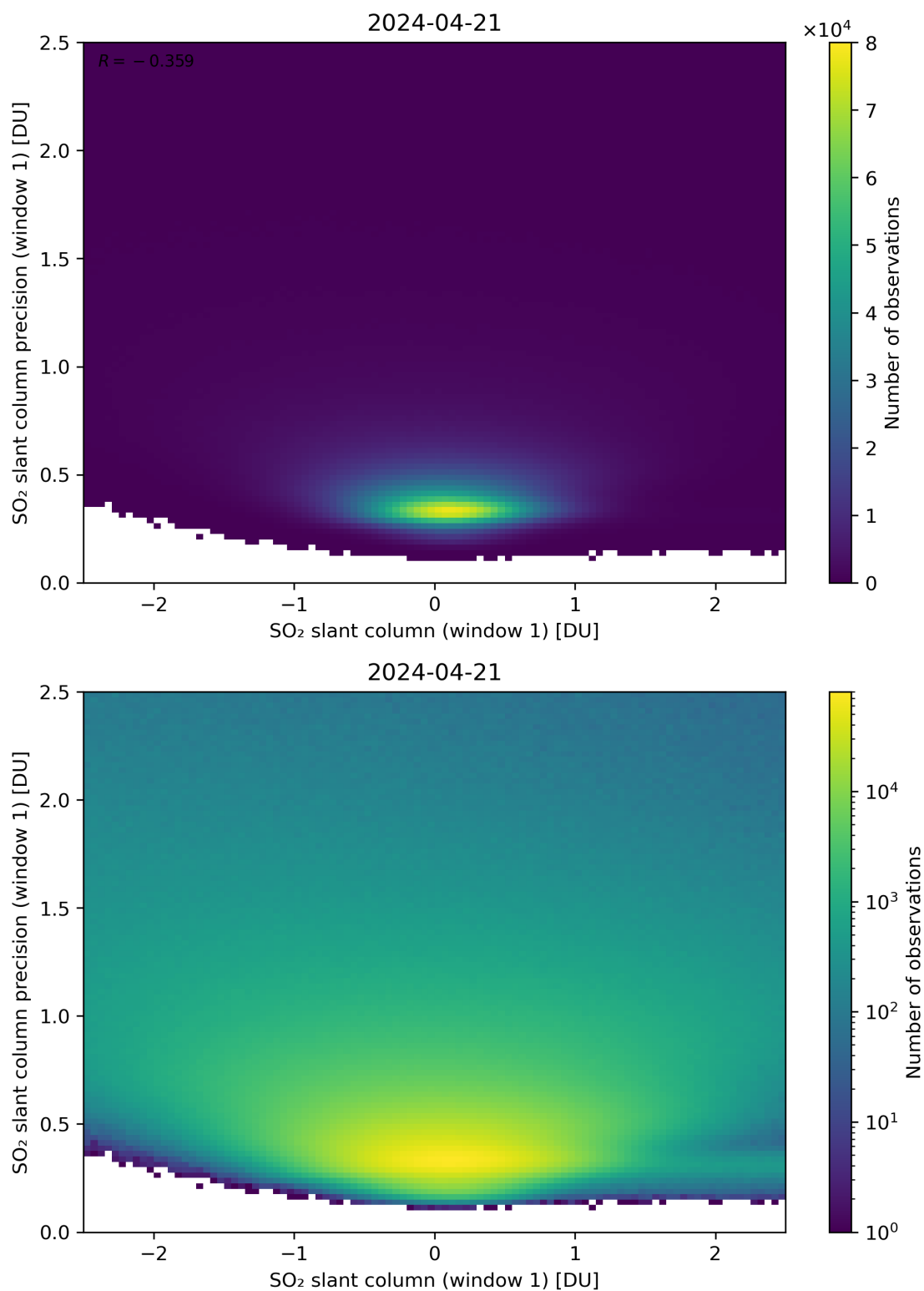
Figure 235: Scatter density plot of “SO 2 slant column (window 1)” against “SO 2 slant column precision (window 1)” for 2024-04-21 to 2024-04-22.
