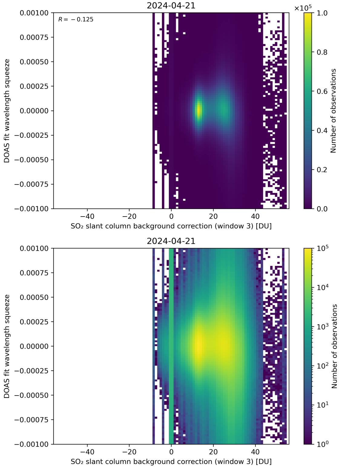
Figure 122: Scatter density plot of “SO 2 slant column background correction (window 3)” against “DOAS fit wavelength squeeze” for 2024-04-21 to 2024-04-22.
