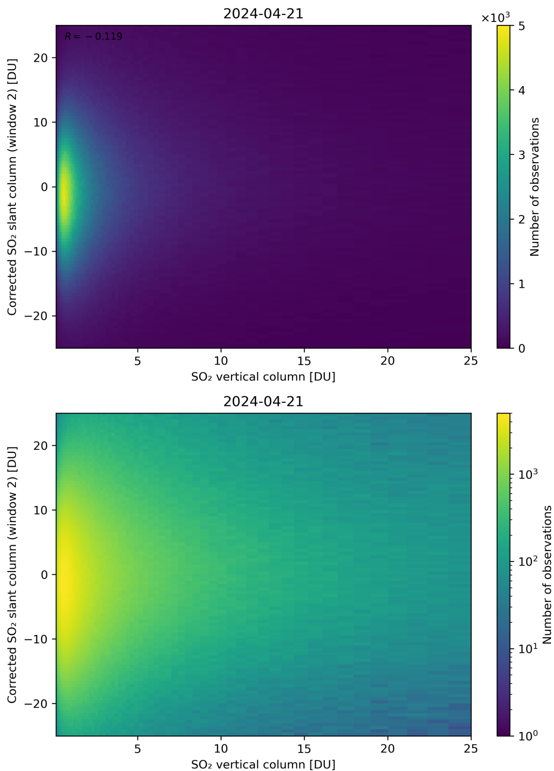
Figure 298: Scatter density plot of “SO 2 vertical column” against “Corrected SO 2 slant column (window 2)” for 2024-04-21 to 2024-04-22.
