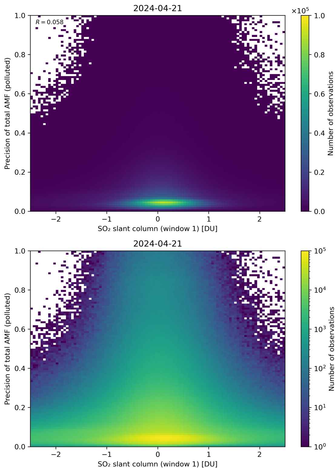
Figure 240: Scatter density plot of “SO 2 slant column (window 1)” against “Precision of total AMF (polluted)” for 2024-04-21 to 2024-04-22.
