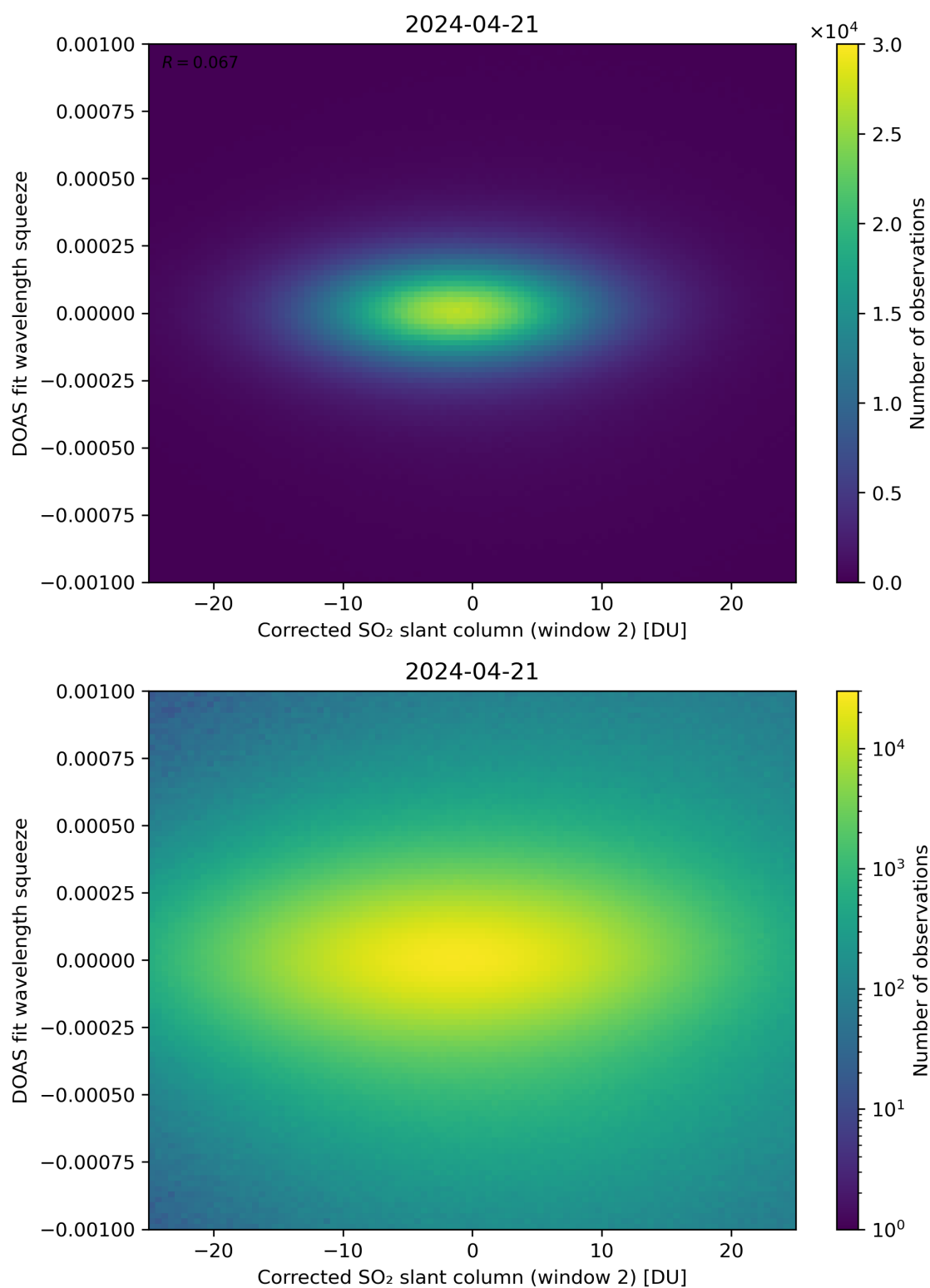
Figure 197: Scatter density plot of “Corrected SO 2 slant column (window 2)” against “DOAS fit wavelength squeeze” for 2024-04-21 to 2024-04-22.
