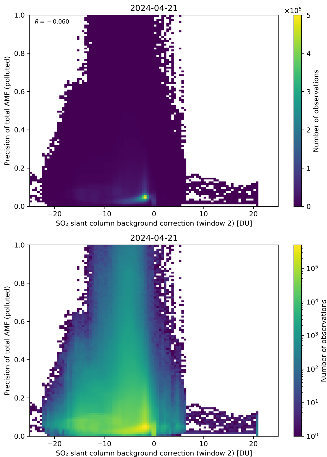
Figure 120: Scatter density plot of “SO 2 slant column background correction (window 2)” against “Precision of total AMF (polluted)” for 2024-04-21 to 2024-04-22.
