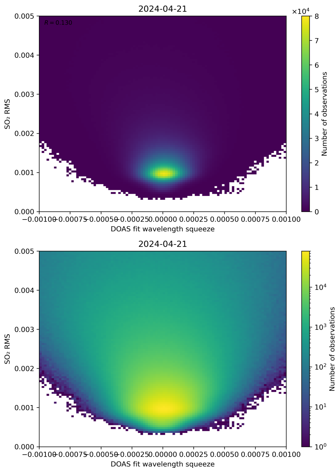
Figure 132: Scatter density plot of “DOAS fit wavelength squeeze” against “SO 2 RMS” for 2024-04-21 to 2024-04-22.
