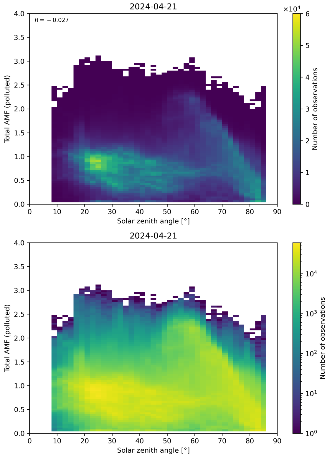
Figure 174: Scatter density plot of “Solar zenith angle” against “Total AMF (polluted)” for 2024-04-21 to 2024-04-22.
