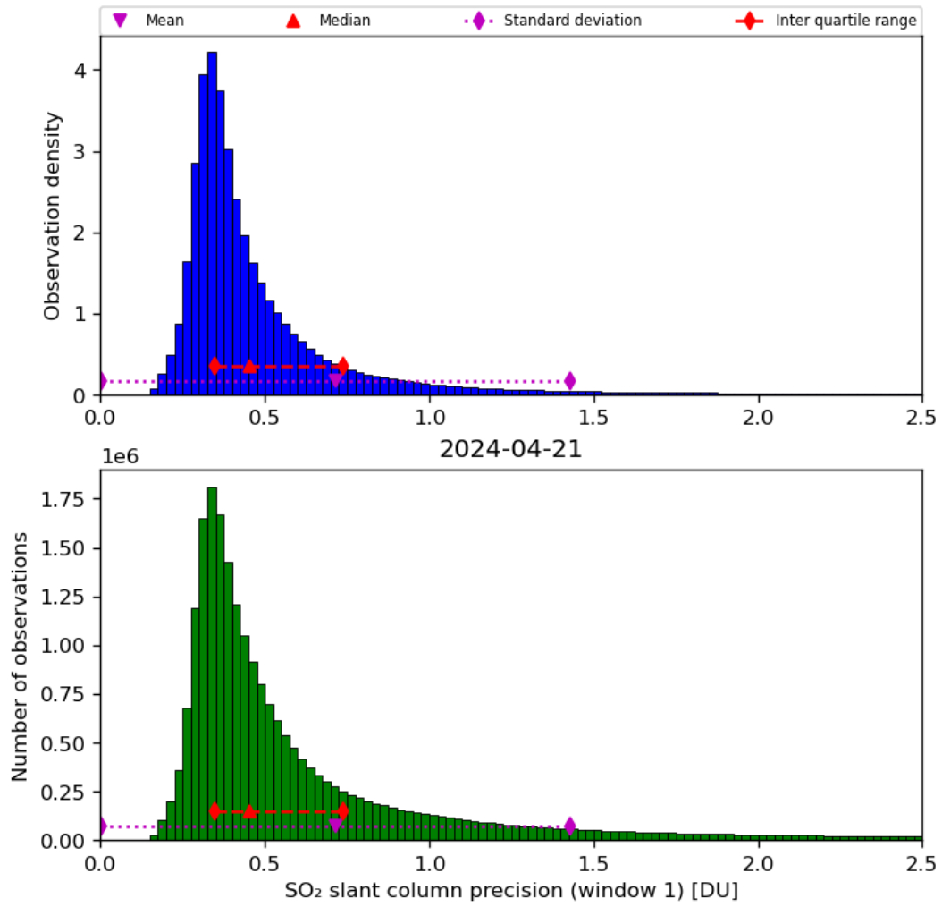
Figure 57: Histogram of “SO 2 slant column precision (window 1)” for 2024-04-21 to 2024-04-22
