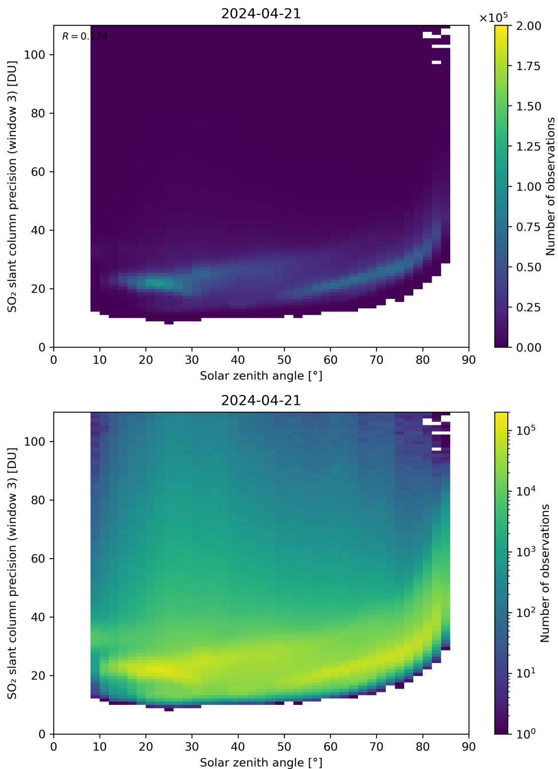
Figure 173: Scatter density plot of “Solar zenith angle” against “SO 2 slant column precision (window 3)” for 2024-04-21 to 2024-04-22.
