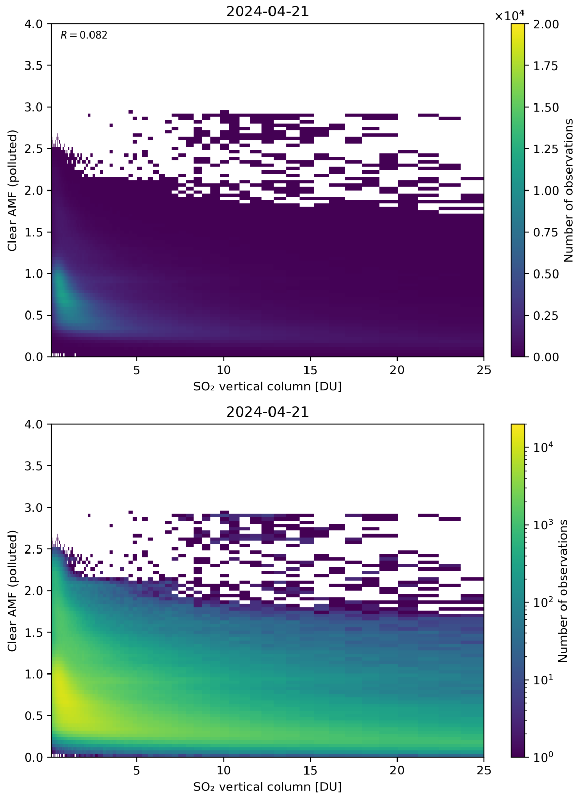
Figure 296: Scatter density plot of “SO 2 vertical column” against “Clear AMF (polluted)” for 2024-04-21 to 2024-04-22.
