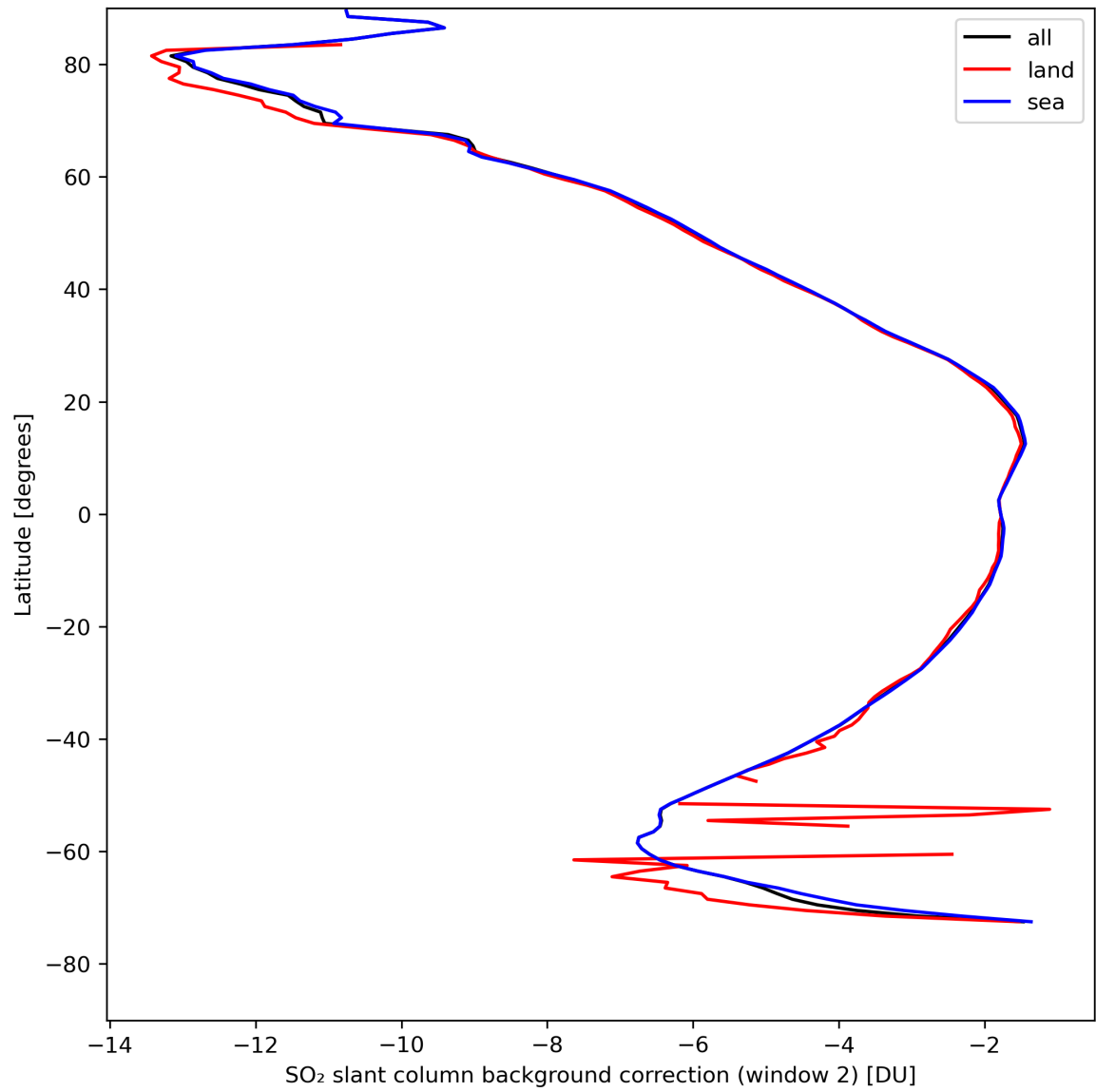
Figure 40: Zonal average of “SO 2 slant column background correction (window 2)” for 2024-04-21 to 2024-04-22.
