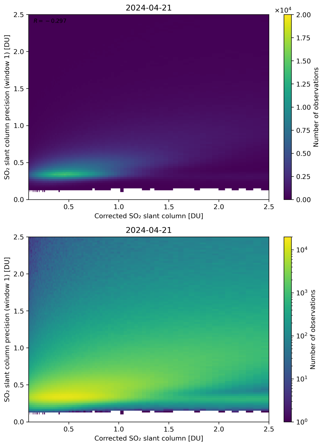
Figure 188: Scatter density plot of “Corrected SO 2 slant column” against “SO 2 slant column precision (window 1)” for 2024-04-21 to 2024-04-22.
