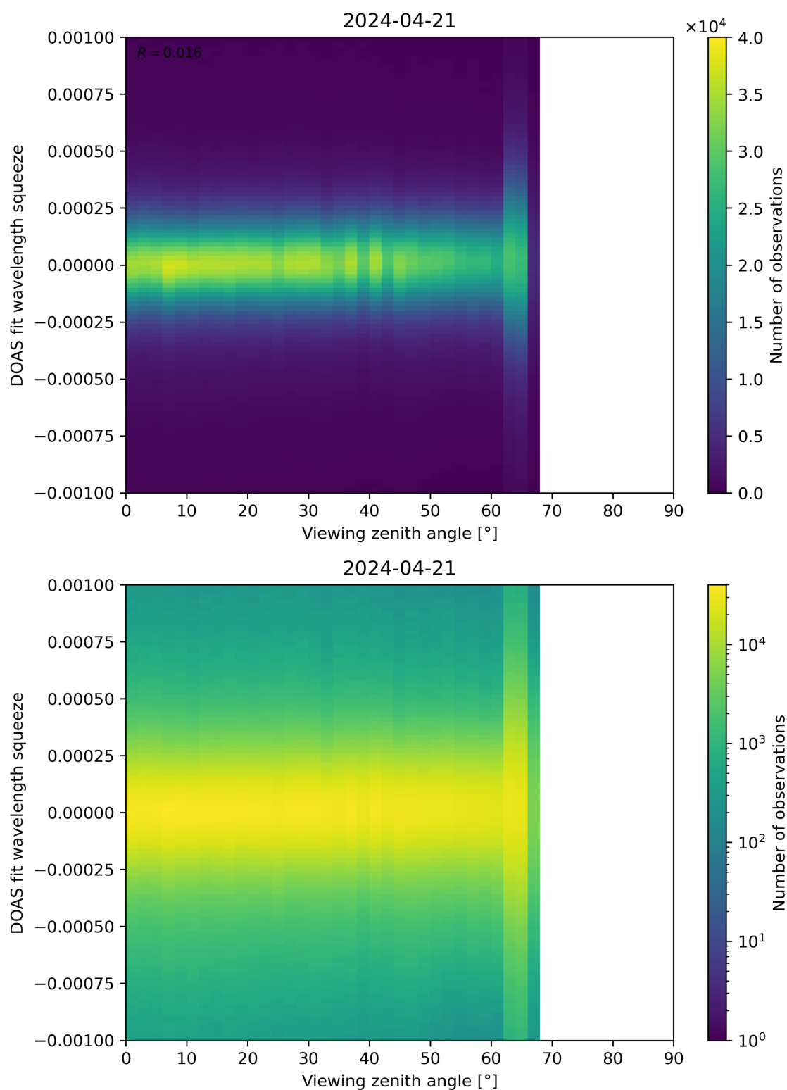
Figure 312: Scatter density plot of “Viewing zenith angle” against “DOAS fit wavelength squeeze” for 2024-04-21 to 2024-04-22.
