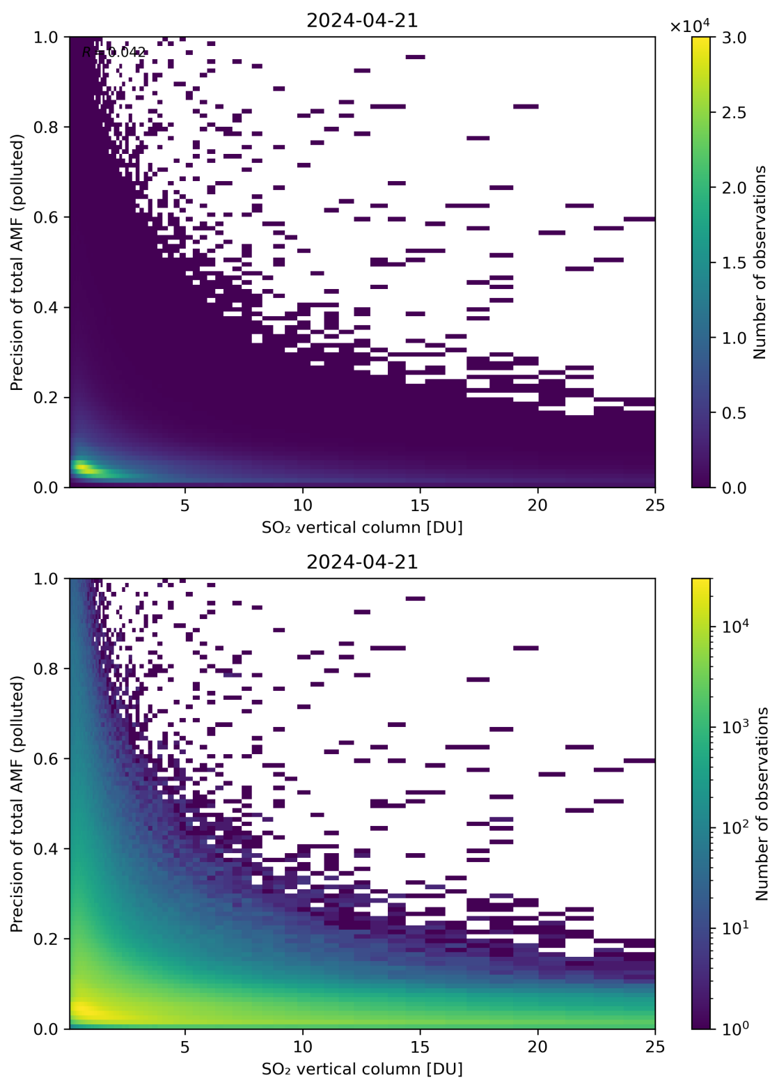
Figure 306: Scatter density plot of “SO 2 vertical column” against “Precision of total AMF (polluted)” for 2024-04-21 to 2024-04-22.
