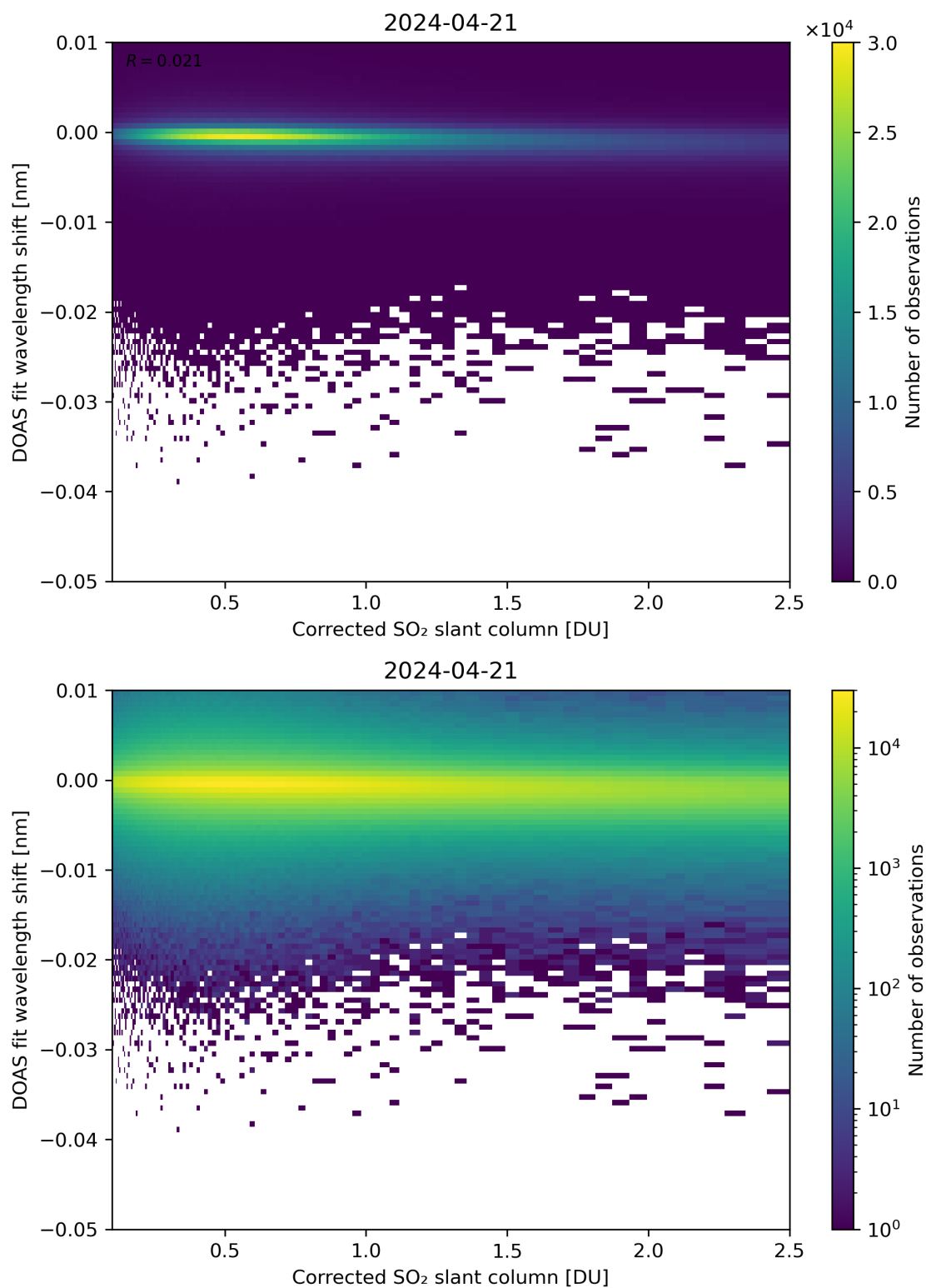
Figure 181: Scatter density plot of “Corrected SO 2 slant column” against “DOAS fit wavelength shift” for 2024-04-21 to 2024-04-22.
