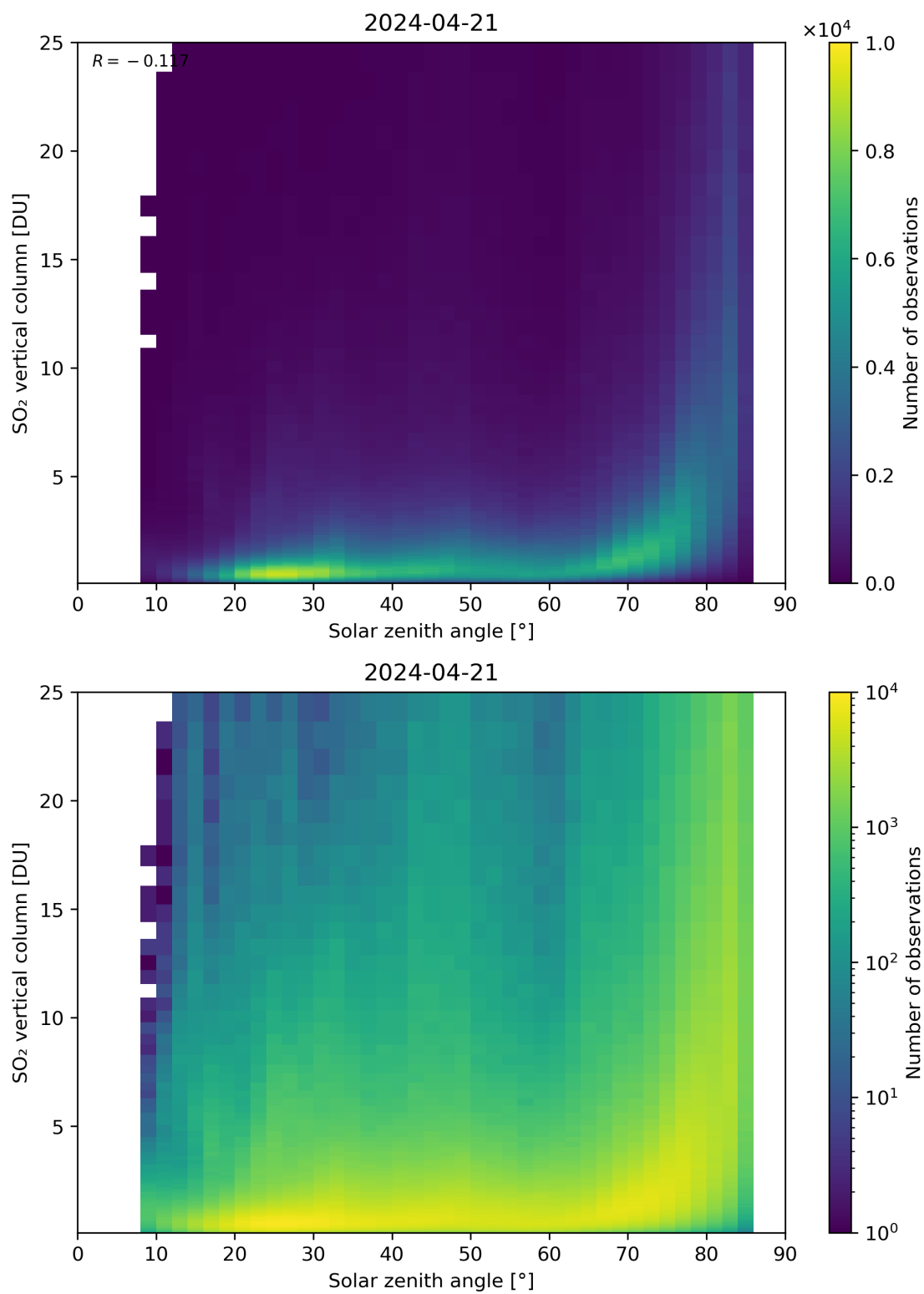
Figure 176: Scatter density plot of “Solar zenith angle” against “SO 2 vertical column” for 2024-04-21 to 2024-04-22.
