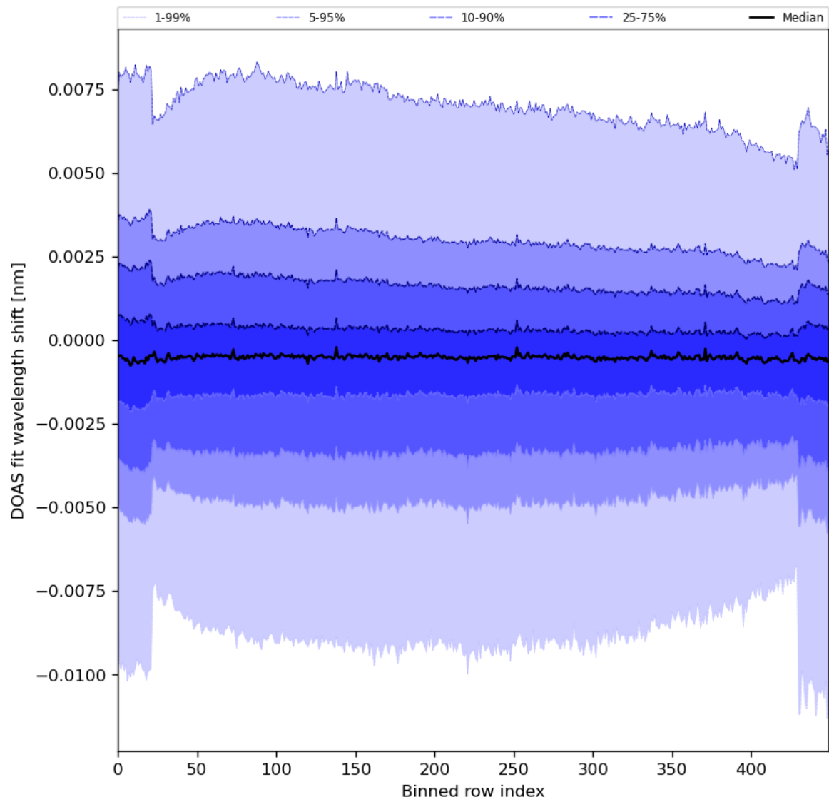
Figure 91: Along track statistics of “DOAS fit wavelength shift” for 2024-04-21 to 2024-04-22
