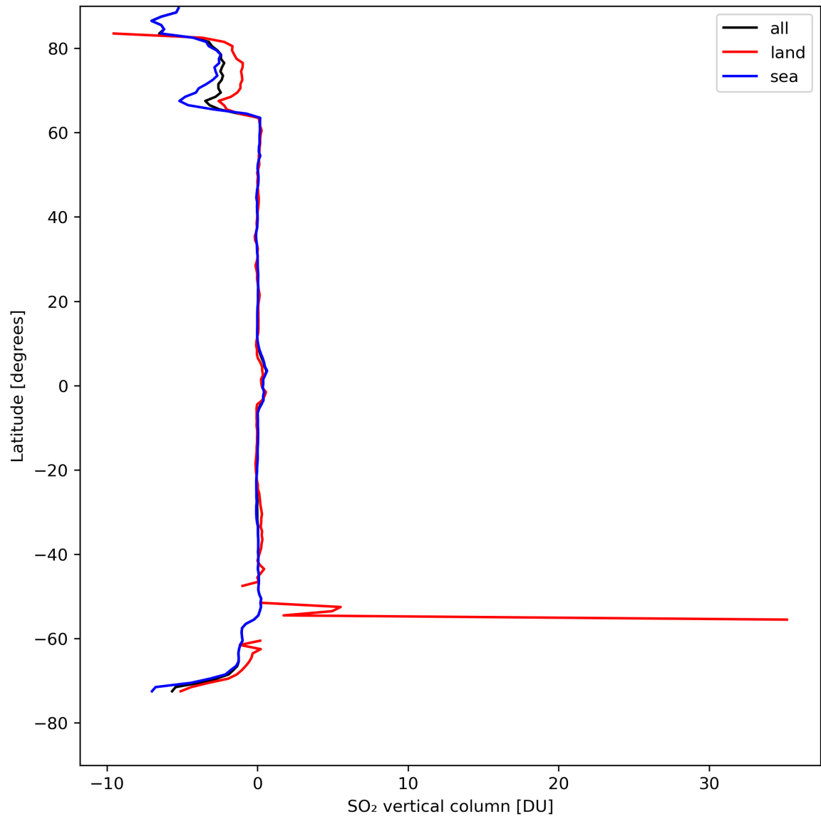
Figure 30: Zonal average of “SO 2 vertical column” for 2024-04-21 to 2024-04-22.
