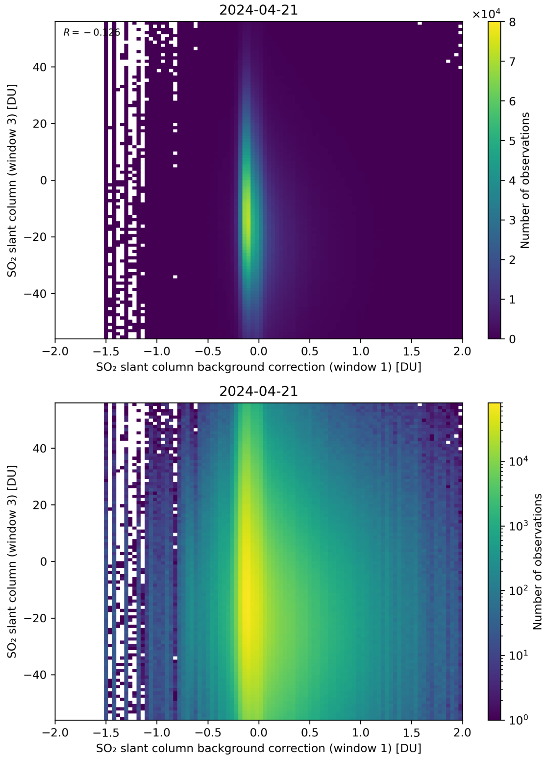
Figure 107: Scatter density plot of “SO 2 slant column background correction (window 1)” against “SO 2 slant column (window 3)” for 2024-04-21 to 2024-04-22.
