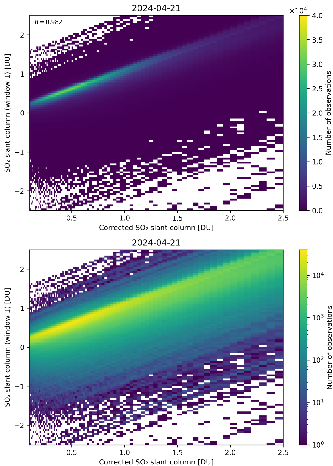
Figure 187: Scatter density plot of “Corrected SO 2 slant column” against “SO 2 slant column (window 1)” for 2024-04-21 to 2024-04-22.
