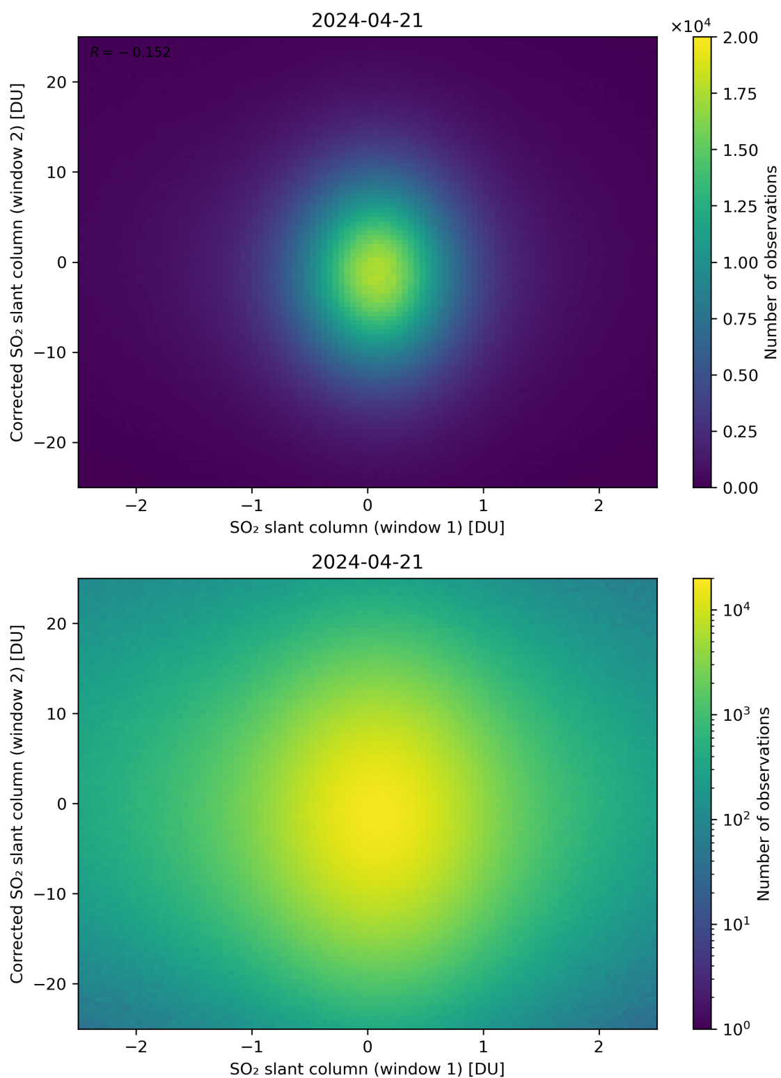
Figure 233: Scatter density plot of “SO 2 slant column (window 1)” against “Corrected SO 2 slant column (window 2)” for 2024-04-21 to 2024-04-22.
