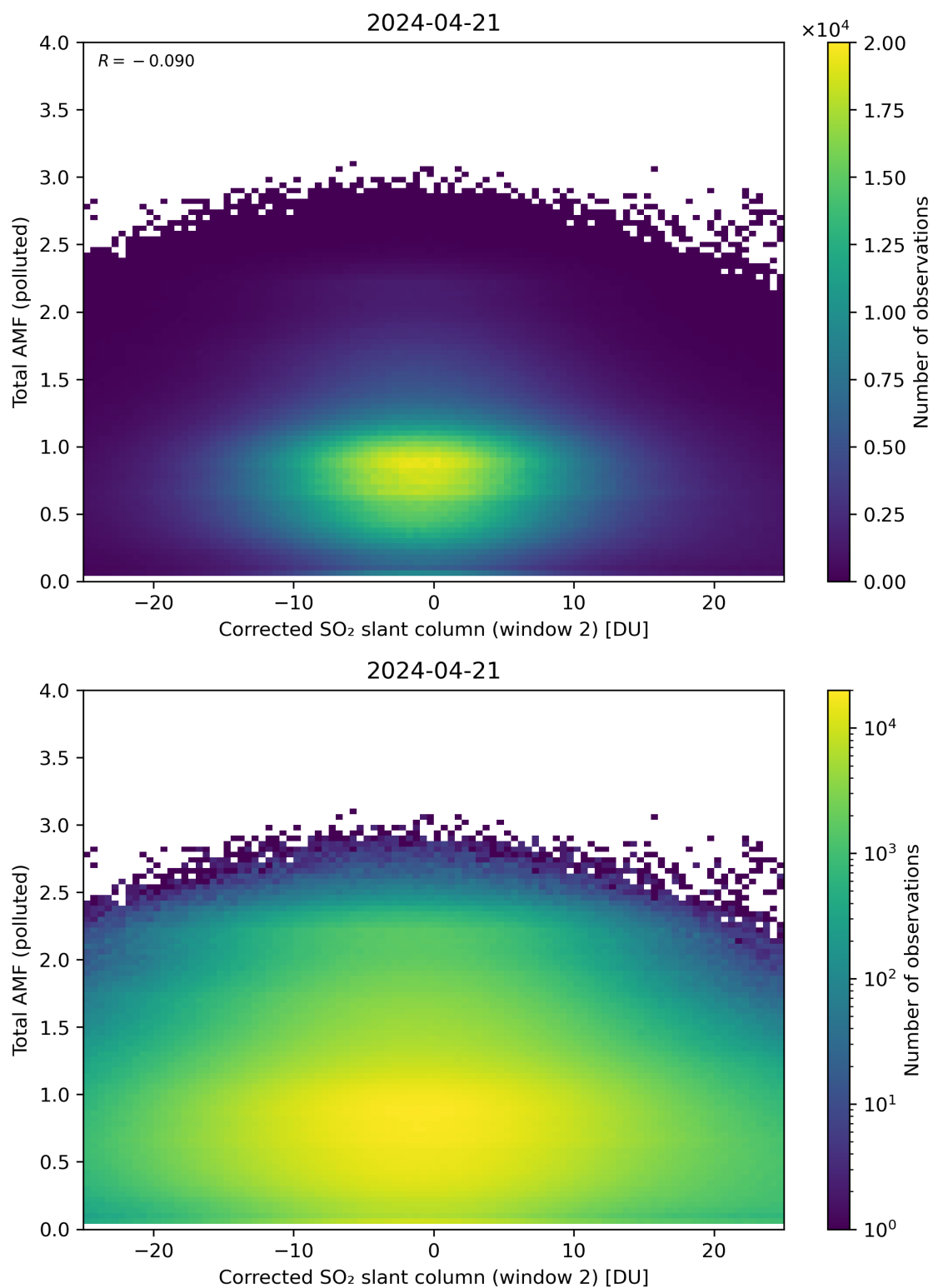
Figure 203: Scatter density plot of “Corrected SO 2 slant column (window 2)” against “Total AMF (polluted)” for 2024-04-21 to 2024-04-22.
