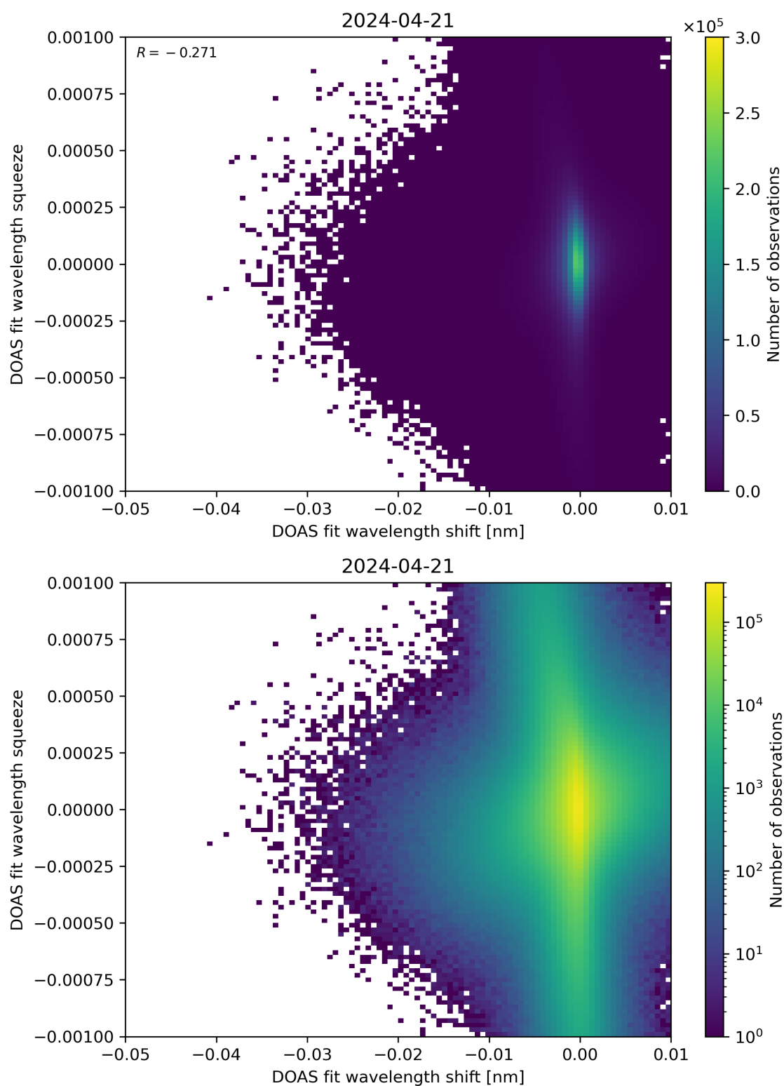
Figure 127: Scatter density plot of “DOAS fit wavelength shift” against “DOAS fit wavelength squeeze” for 2024-04-21 to 2024-04-22.
