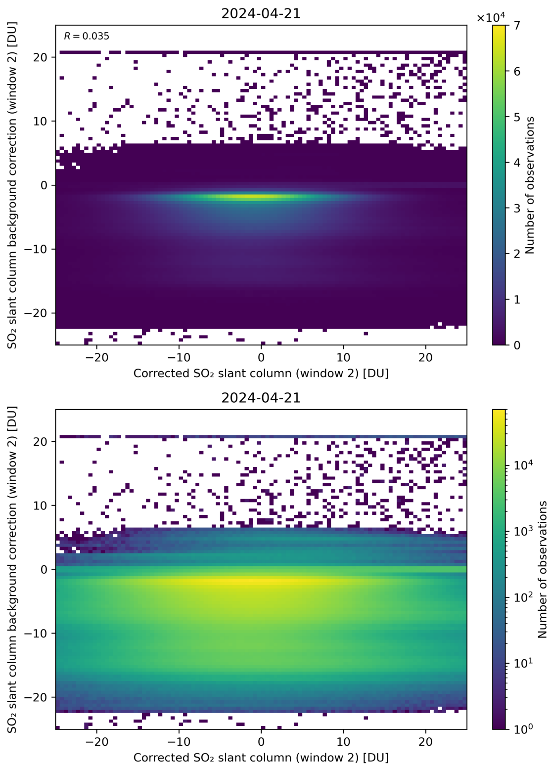
Figure 194: Scatter density plot of “Corrected SO 2 slant column (window 2)” against “SO 2 slant column background correction (window 2)” for 2024-04-21 to 2024-04-22.
