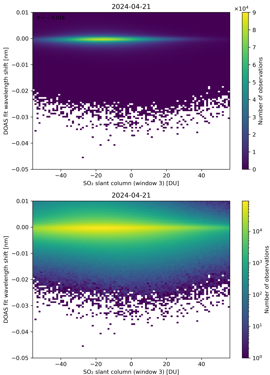
Figure 254: Scatter density plot of “SO 2 slant column (window 3)” against “DOAS fit wavelength shift” for 2024-04-21 to 2024-04-22.
