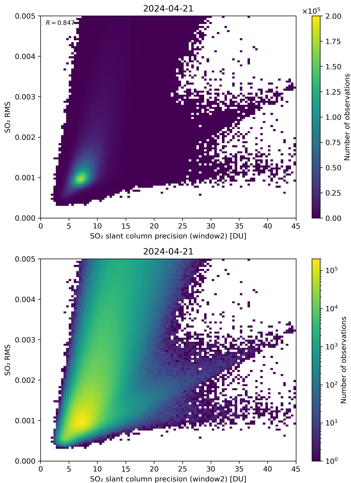
Figure 245: Scatter density plot of “SO 2 slant column precision (window2)” against “SO 2 RMS” for 2024-04-21 to 2024-04-22.
