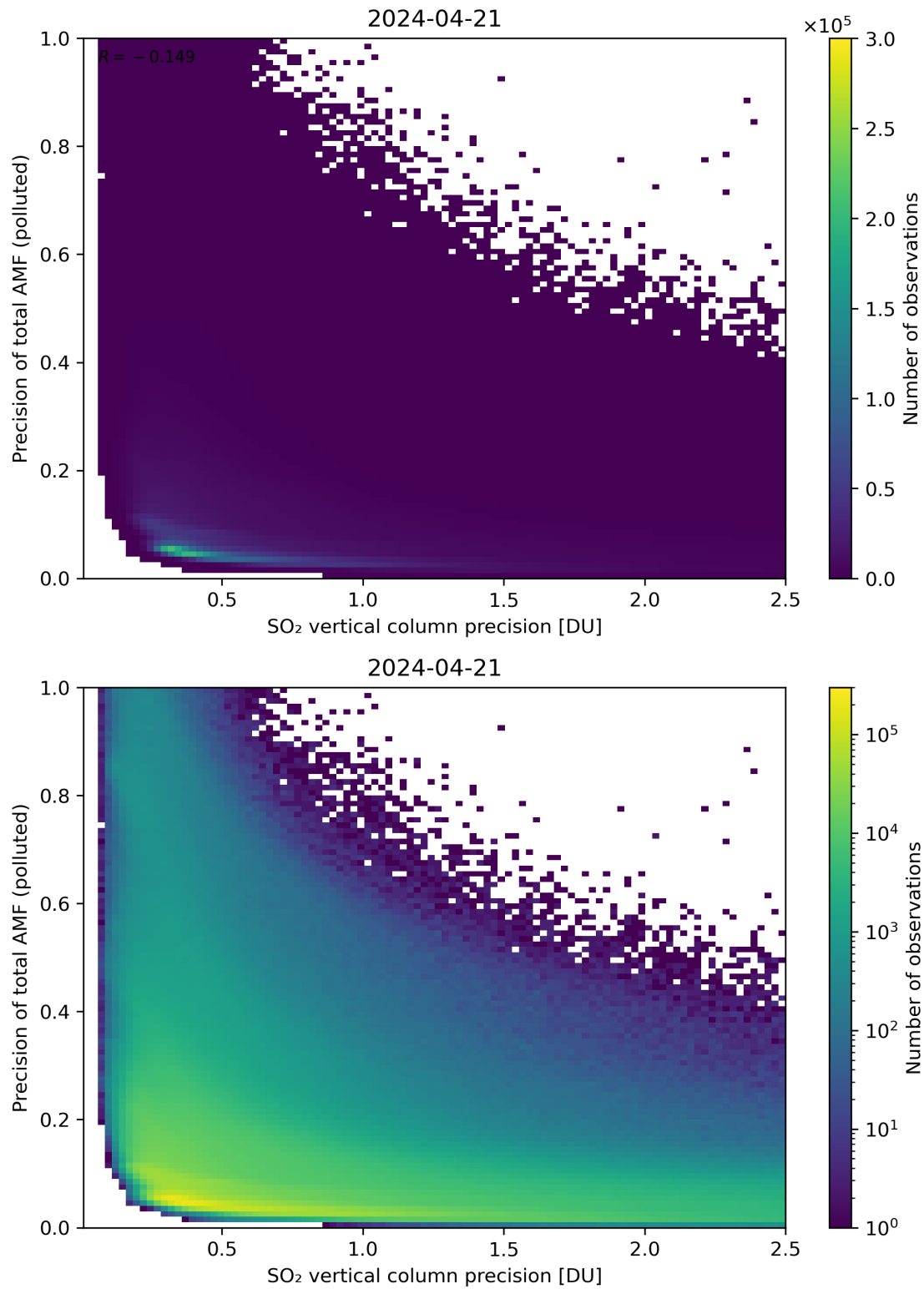
Figure 295: Scatter density plot of “SO 2 vertical column precision” against “Precision of total AMF (polluted)” for 2024-04-21 to 2024-04-22.
