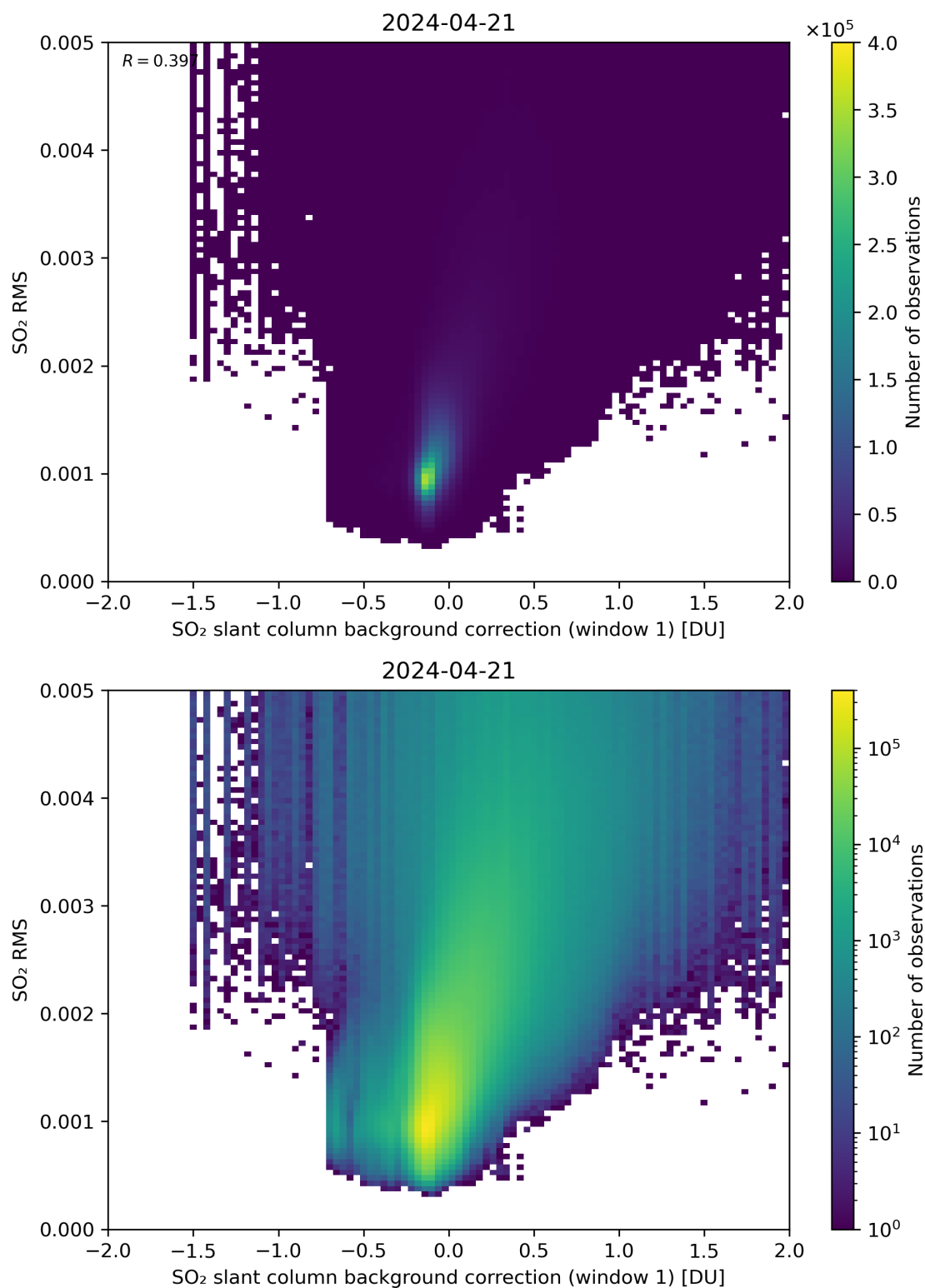
Figure 102: Scatter density plot of “SO 2 slant column background correction (window 1)” against “SO 2 RMS” for 2024-04-21 to 2024-04-22.
