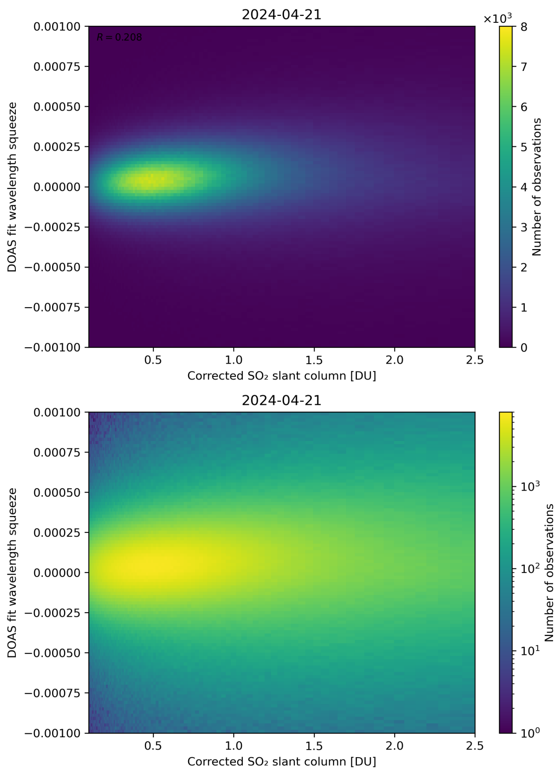
Figure 182: Scatter density plot of “Corrected SO 2 slant column” against “DOAS fit wavelength squeeze” for 2024-04-21 to 2024-04-22.
