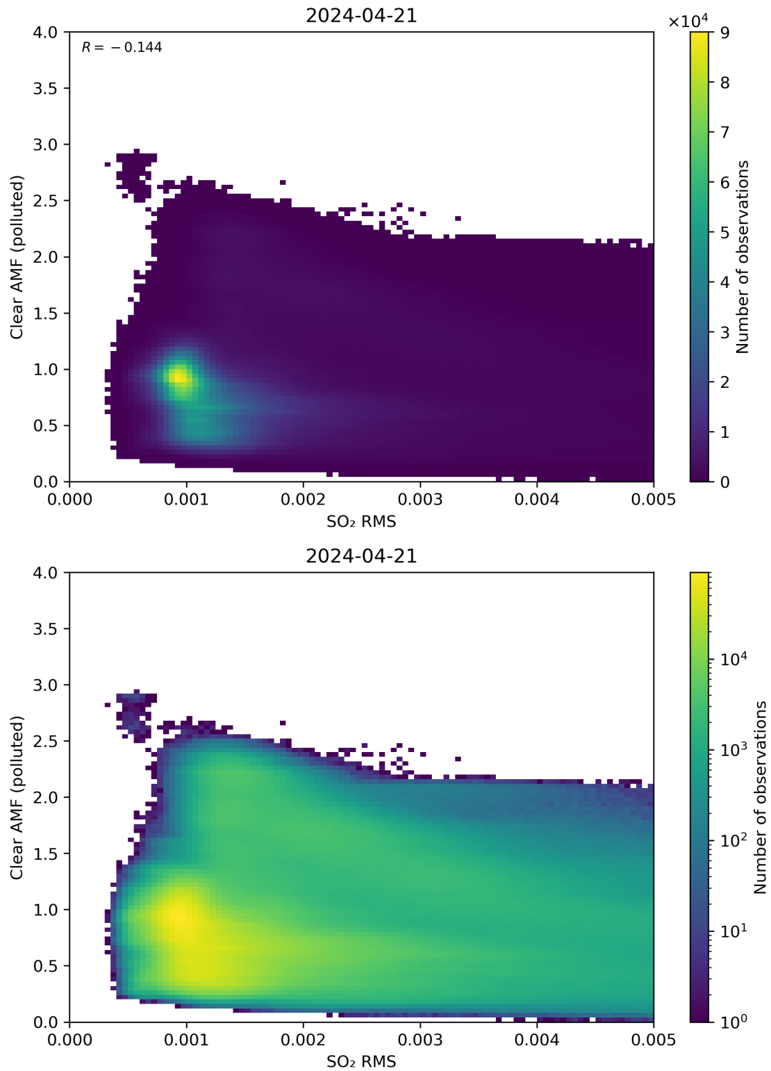
Figure 136: Scatter density plot of “SO 2 RMS” against “Clear AMF (polluted)” for 2024-04-21 to 2024-04-22.
