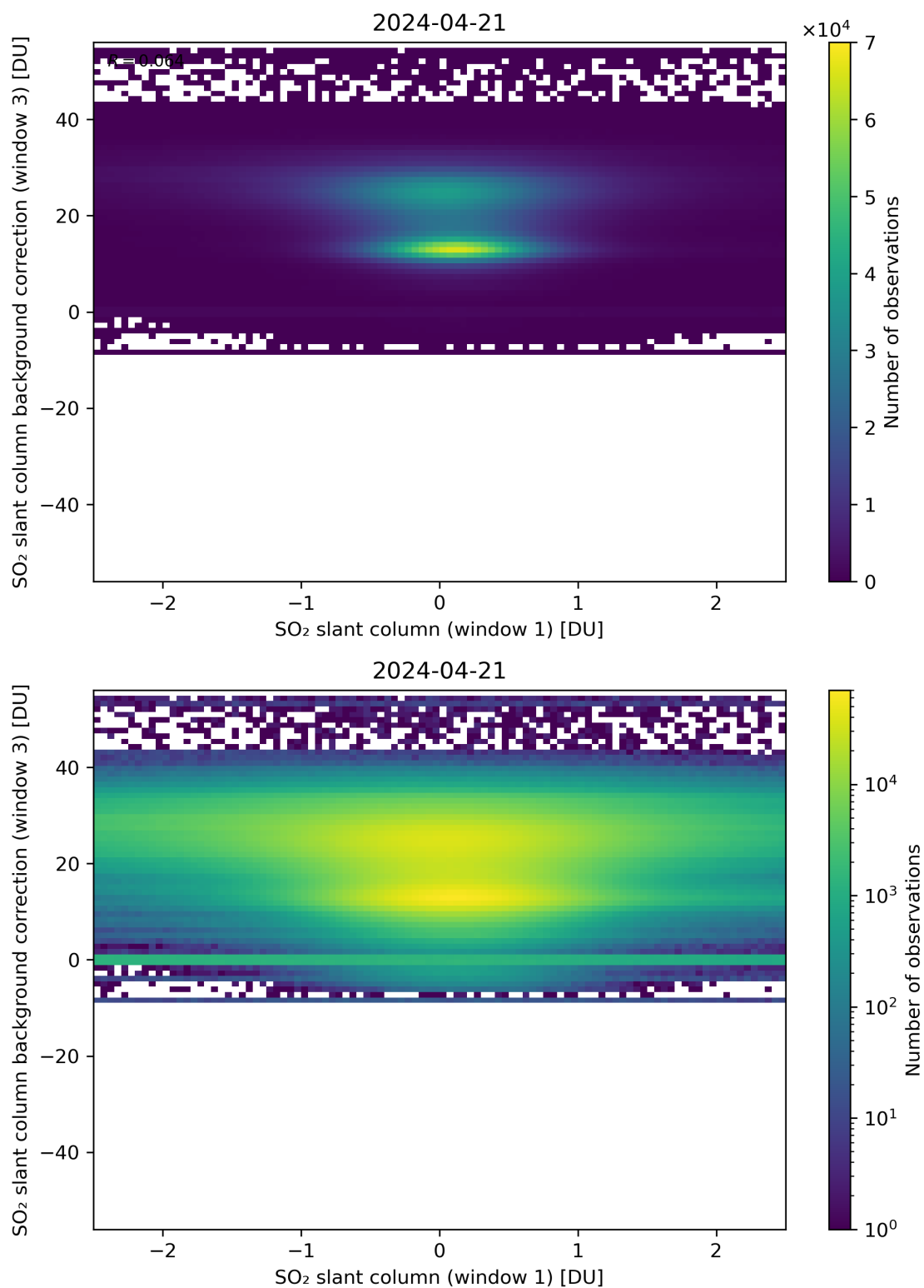
Figure 214: Scatter density plot of “SO 2 slant column (window 1)” against “SO 2 slant column background correction (window 3)” for 2024-04-21 to 2024-04-22.
