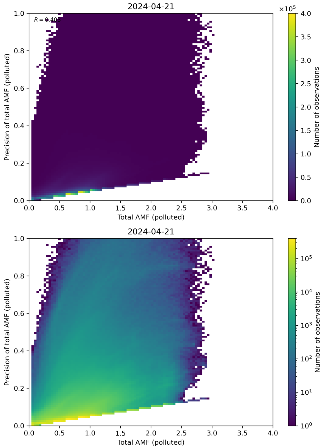
Figure 272: Scatter density plot of “Total AMF (polluted)” against “Precision of total AMF (polluted)” for 2024-04-21 to 2024-04-22.
