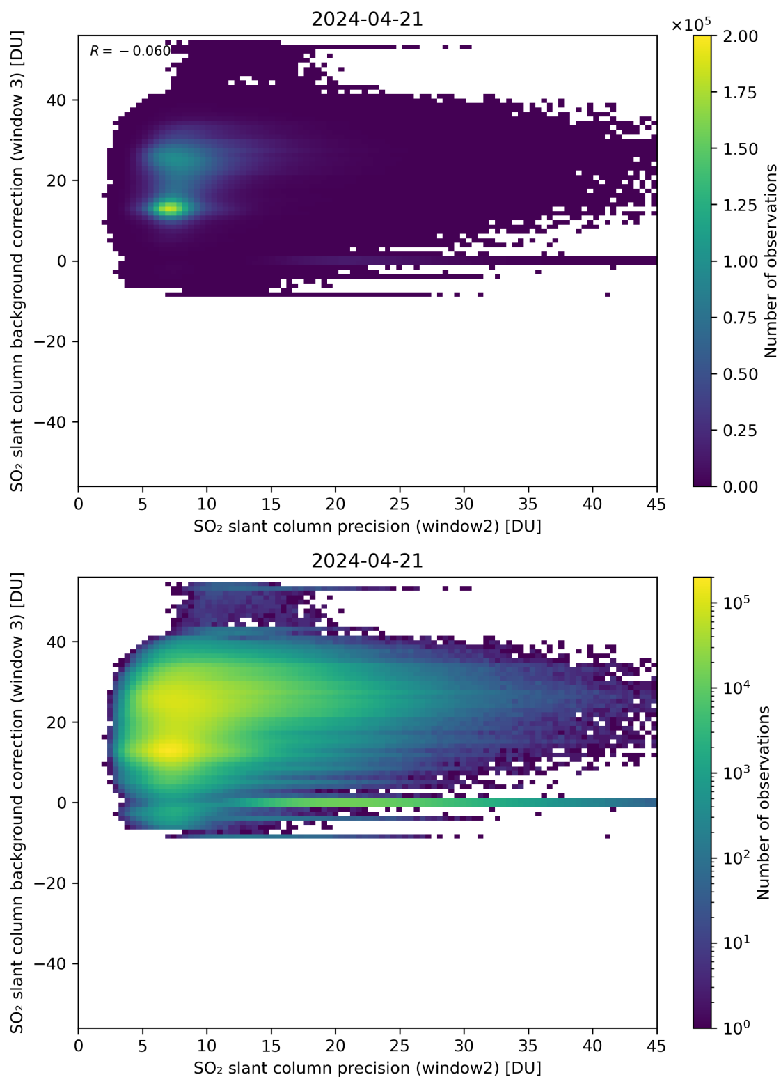
Figure 242: Scatter density plot of “SO 2 slant column precision (window2)” against “SO 2 slant column background correction (window 3)” for 2024-04-21 to 2024-04-22.
