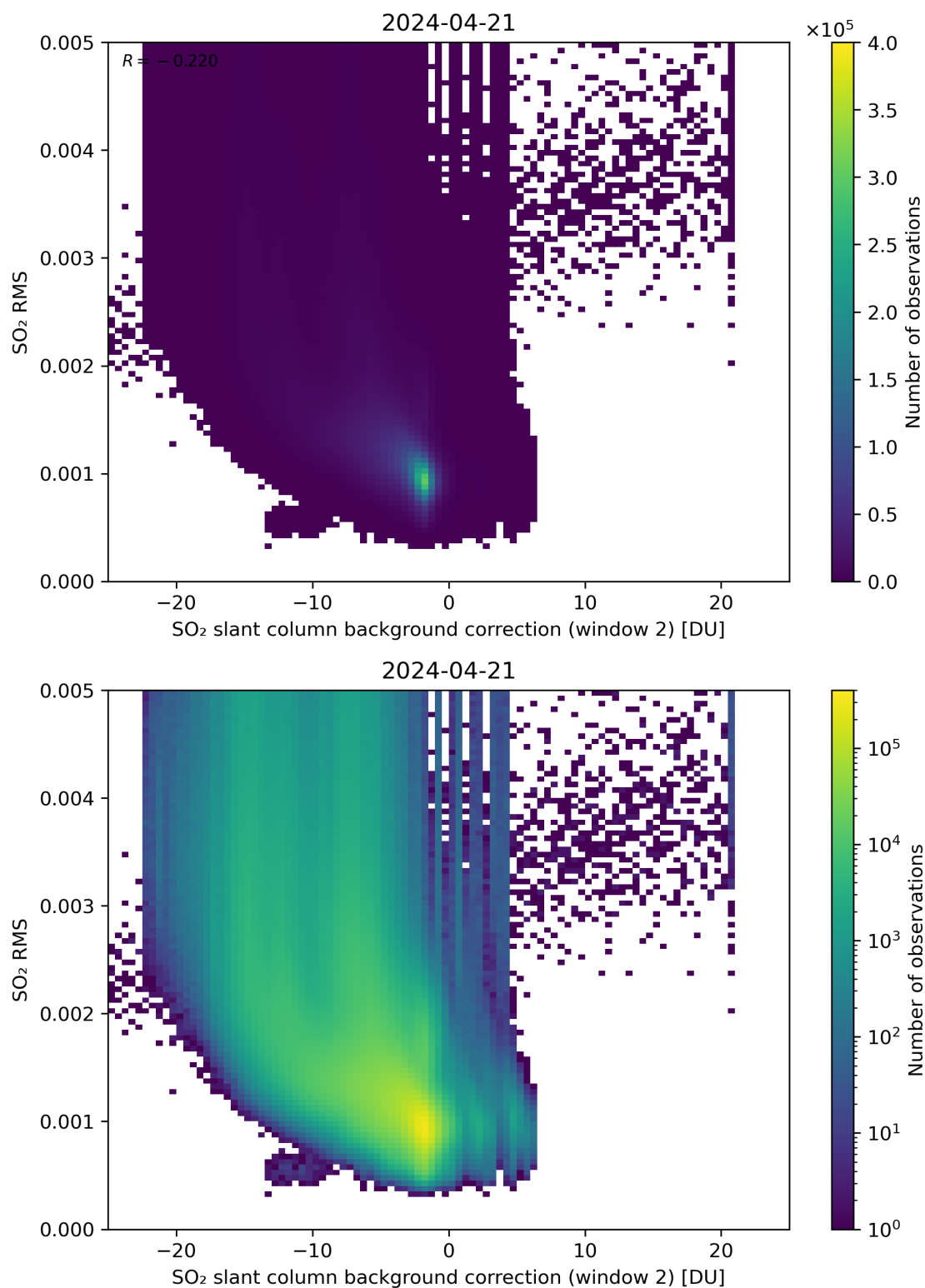
Figure 114: Scatter density plot of “SO 2 slant column background correction (window 2)” against “SO 2 RMS” for 2024-04-21 to 2024-04-22.
