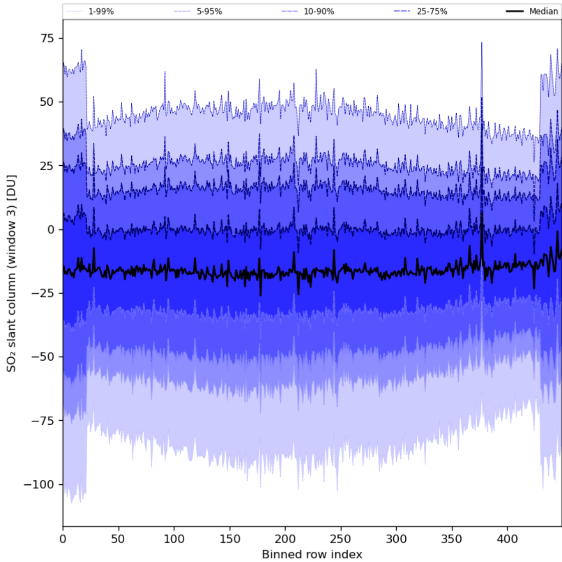
Figure 87: Along track statistics of “SO 2 slant column (window 3)” for 2024-04-21 to 2024-04-22
