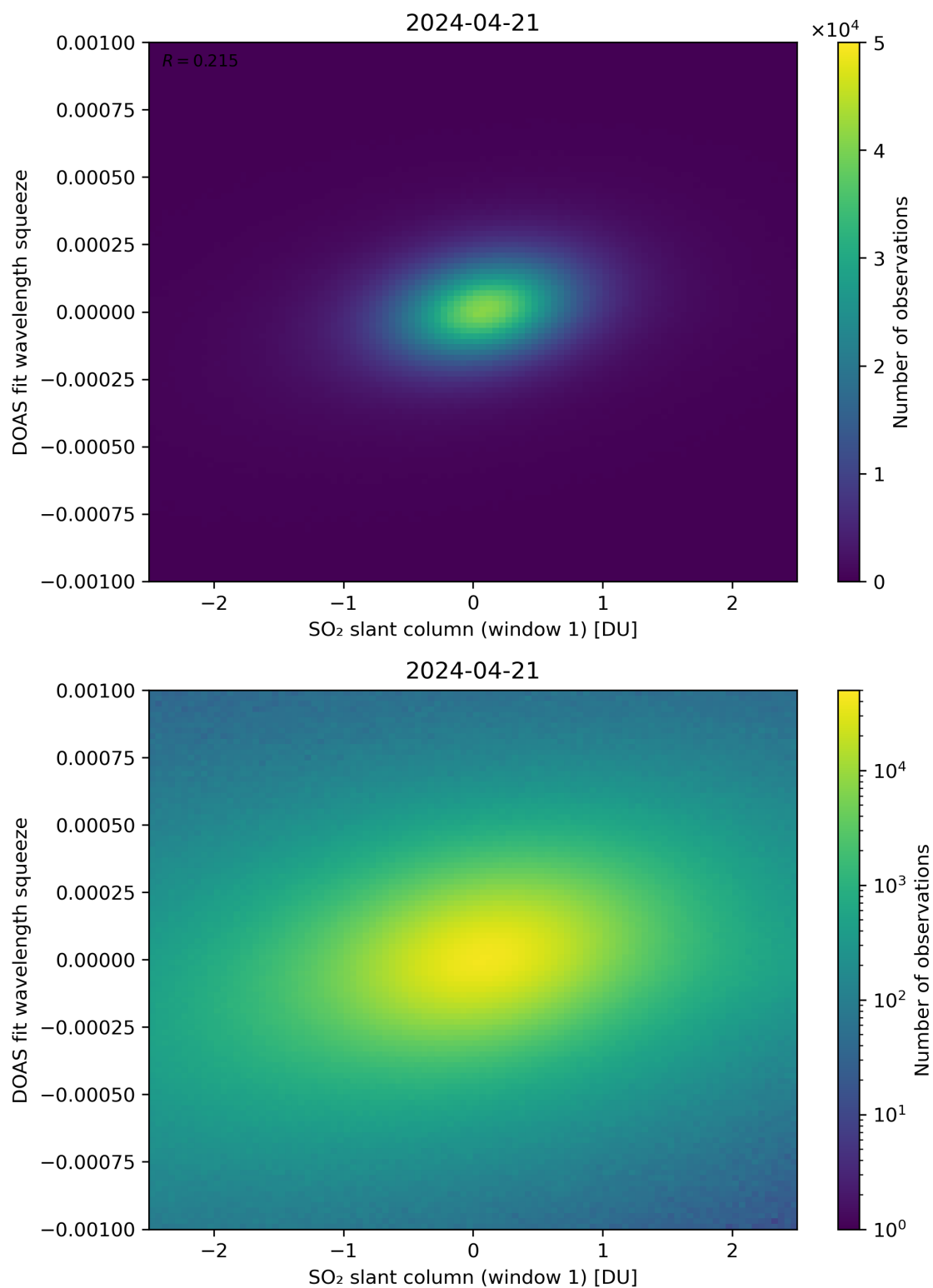
Figure 216: Scatter density plot of “SO 2 slant column (window 1)” against “DOAS fit wavelength squeeze” for 2024-04-21 to 2024-04-22.
