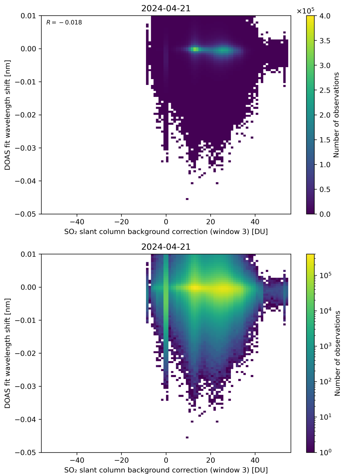
Figure 121: Scatter density plot of “SO 2 slant column background correction (window 3)” against “DOAS fit wavelength shift” for 2024-04-21 to 2024-04-22.
