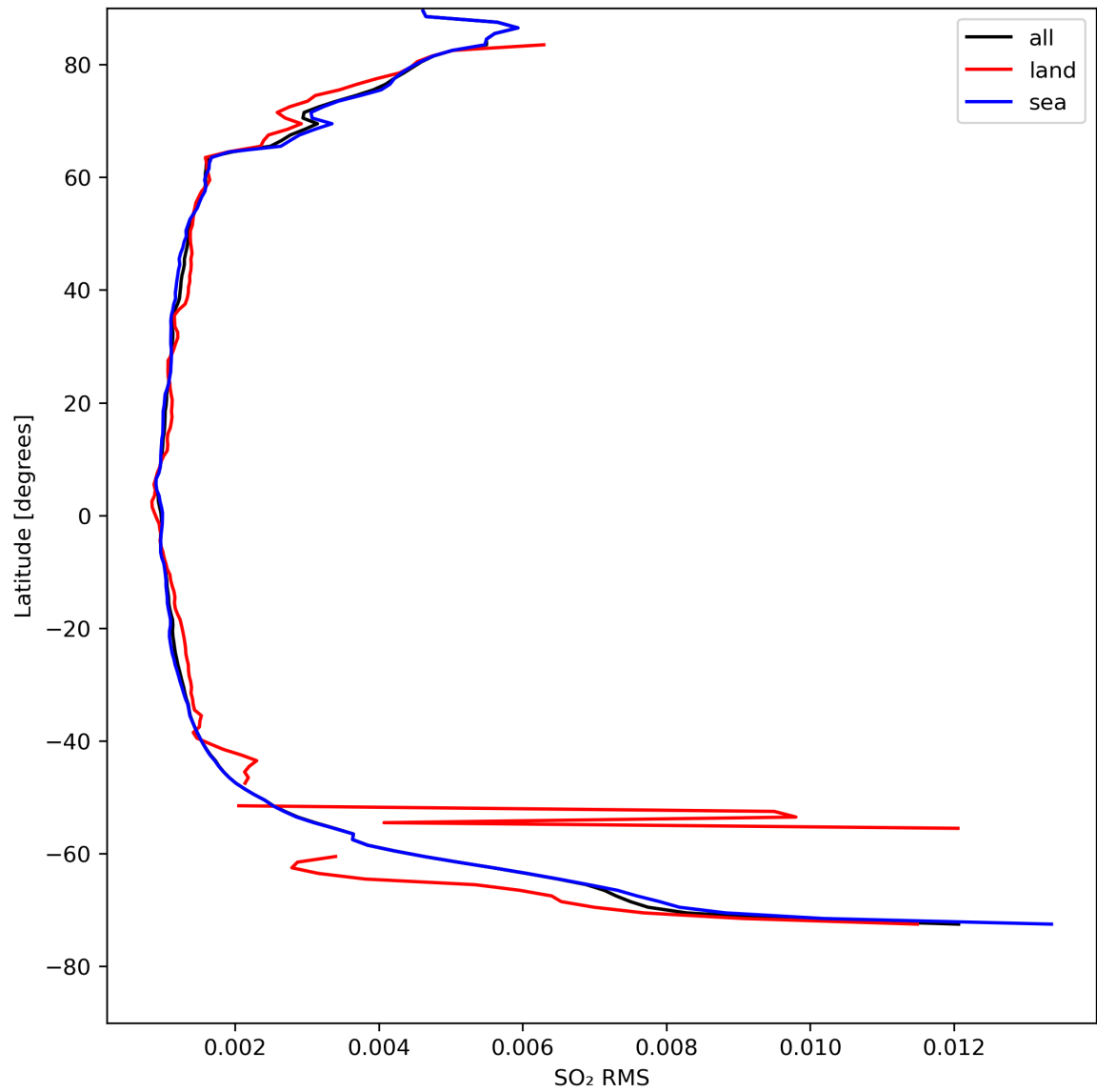
Figure 47: Zonal average of “SO 2 RMS” for 2024-04-21 to 2024-04-22.
