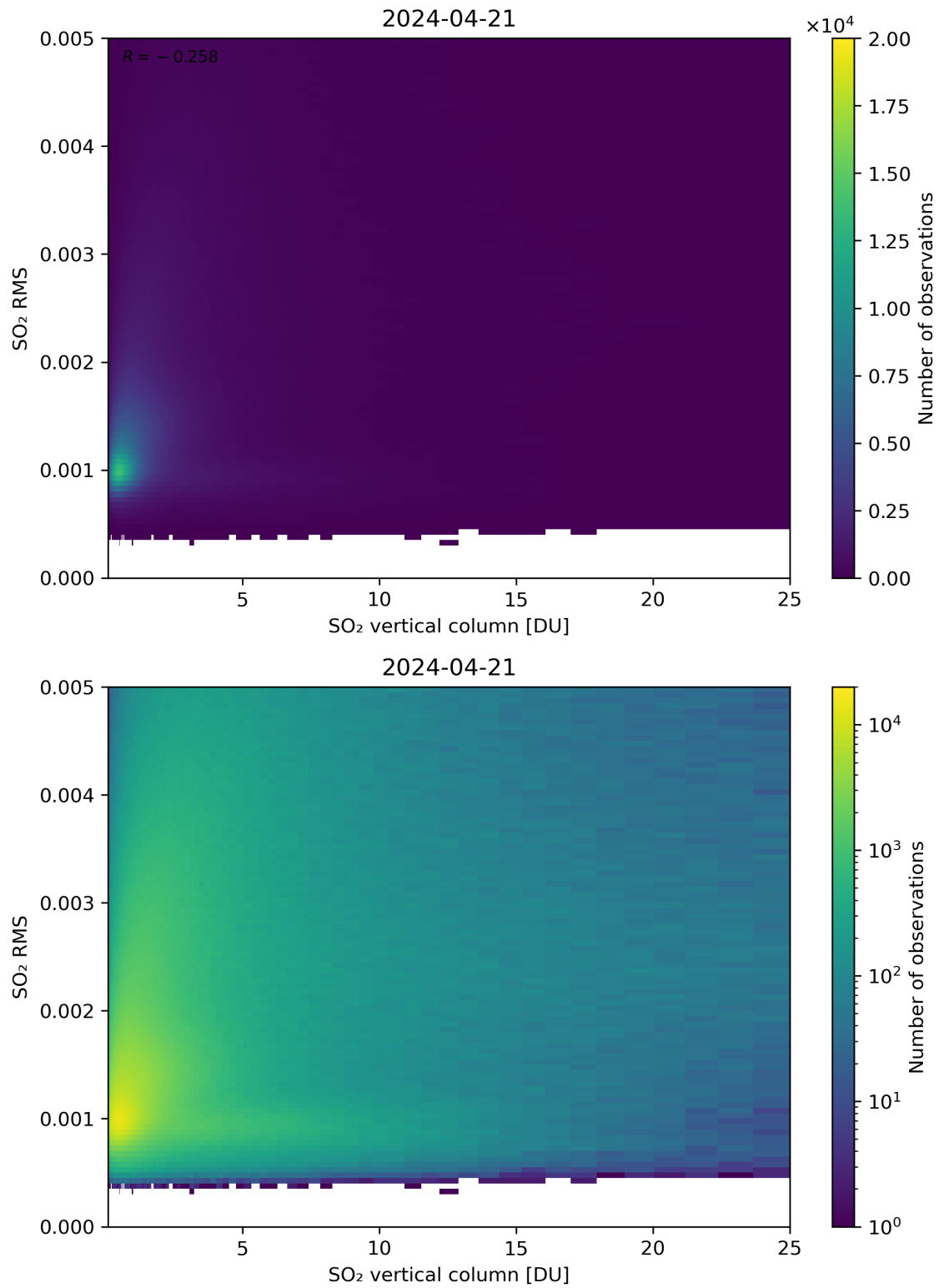
Figure 278: Scatter density plot of “SO 2 vertical column” against “SO 2 RMS” for 2024-04-21 to 2024-04-22.
