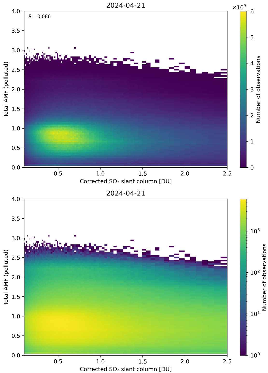
Figure 192: Scatter density plot of “Corrected SO 2 slant column” against “Total AMF (polluted)” for 2024-04-21 to 2024-04-22.
