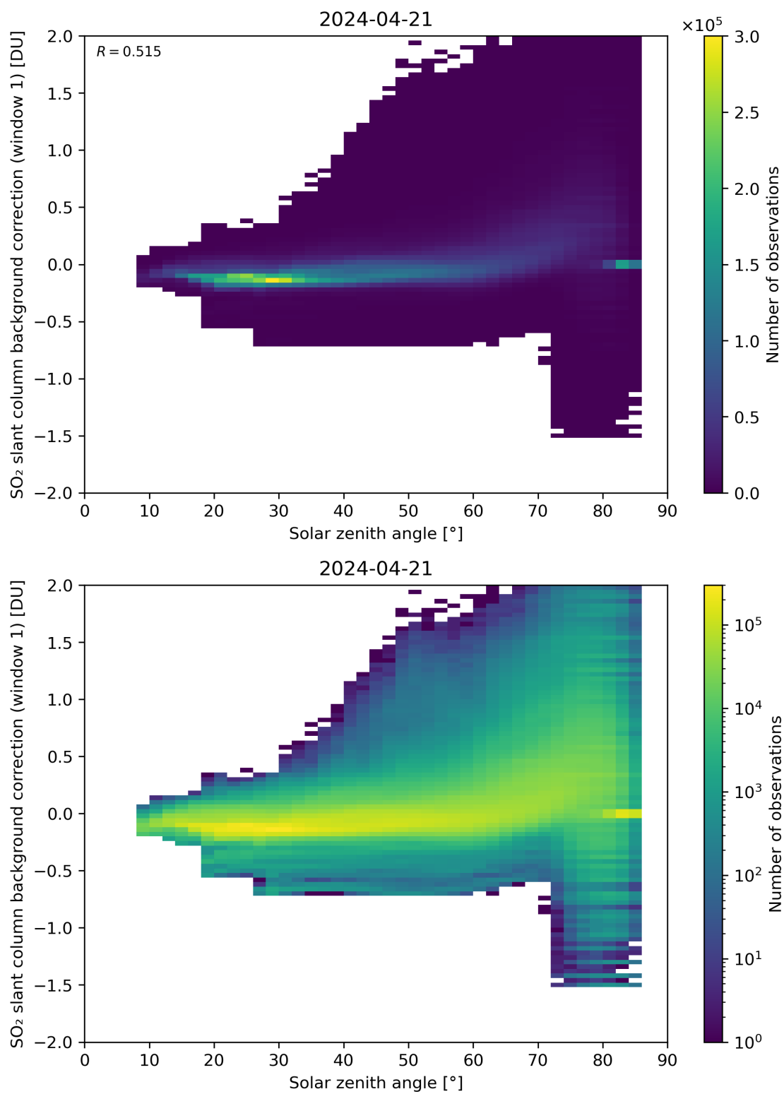
Figure 158: Scatter density plot of “Solar zenith angle” against “SO 2 slant column background correction (window 1)” for 2024-04-21 to 2024-04-22.
