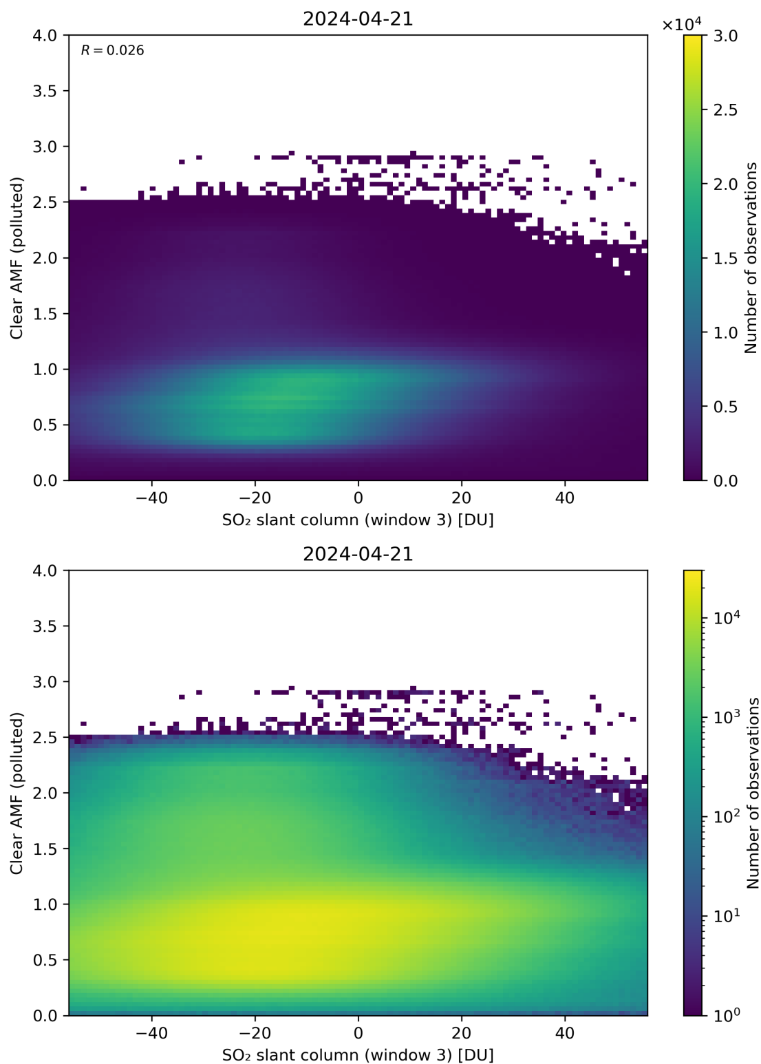
Figure 265: Scatter density plot of “SO 2 slant column (window 3)” against “Clear AMF (polluted)” for 2024-04-21 to 2024-04-22.
