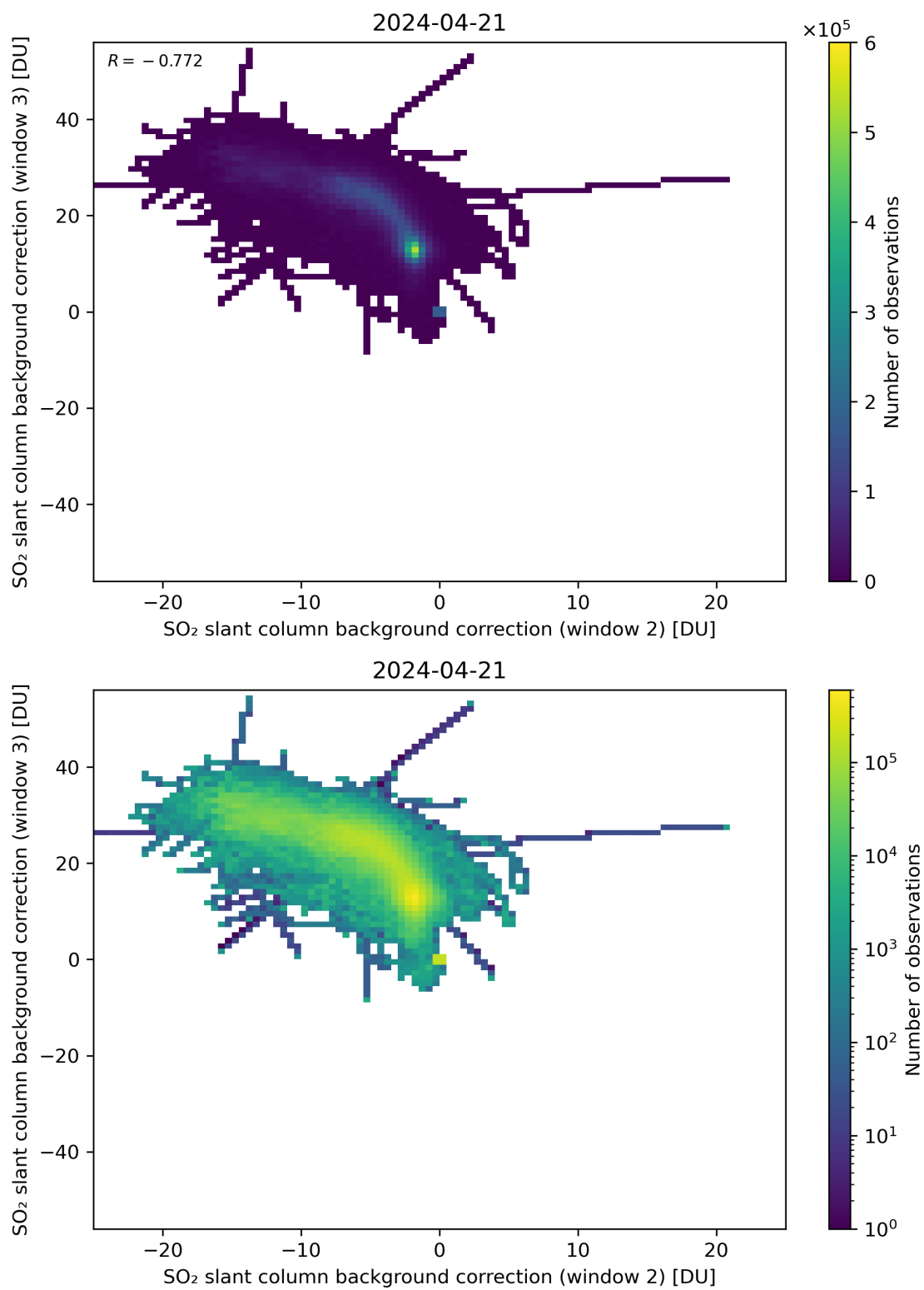
Figure 111: Scatter density plot of “SO 2 slant column background correction (window 2)” against “SO 2 slant column background correction (window 3)” for 2024-04-21 to 2024-04-22.
