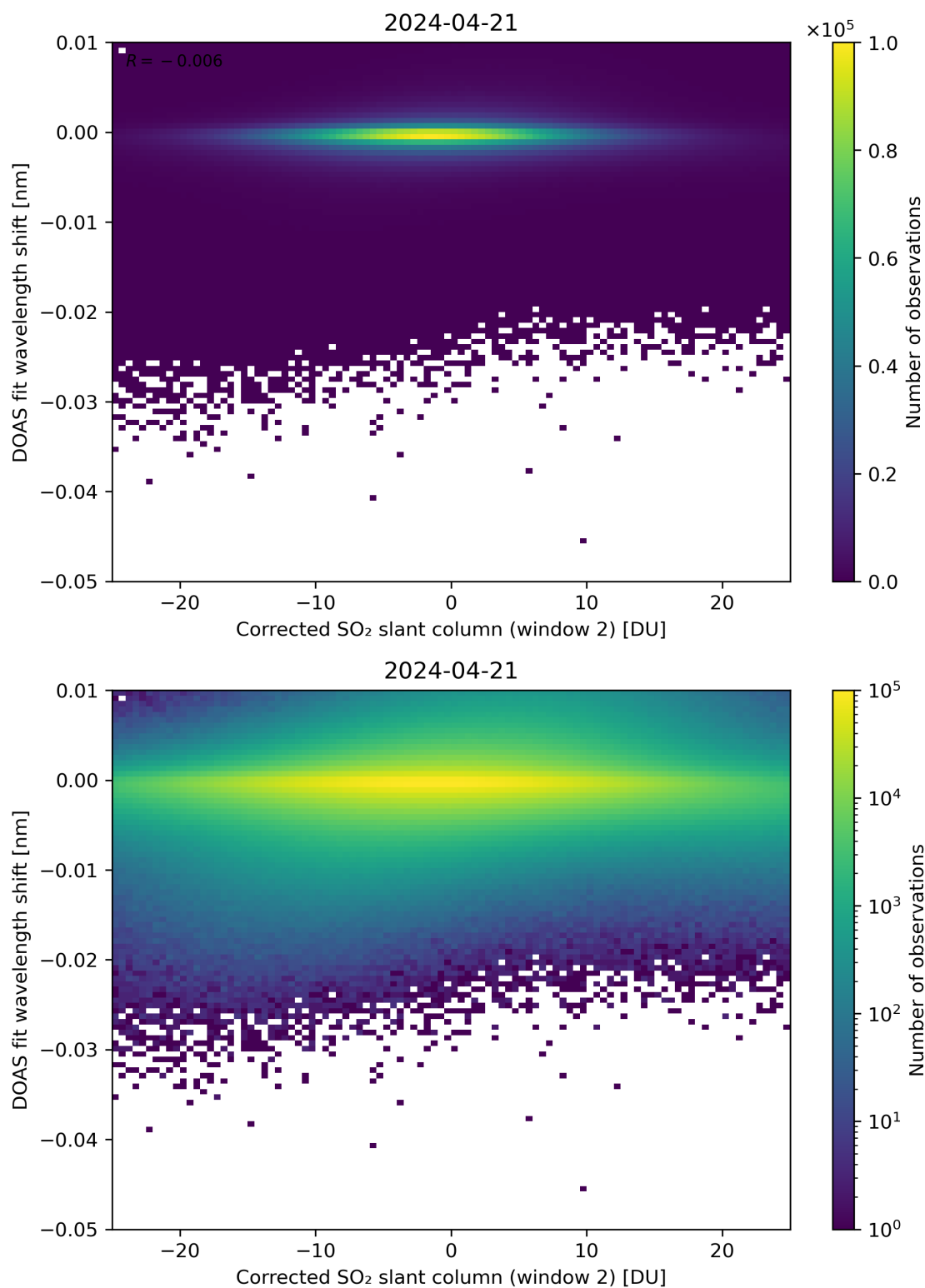
Figure 196: Scatter density plot of “Corrected SO 2 slant column (window 2)” against “DOAS fit wavelength shift” for 2024-04-21 to 2024-04-22.
