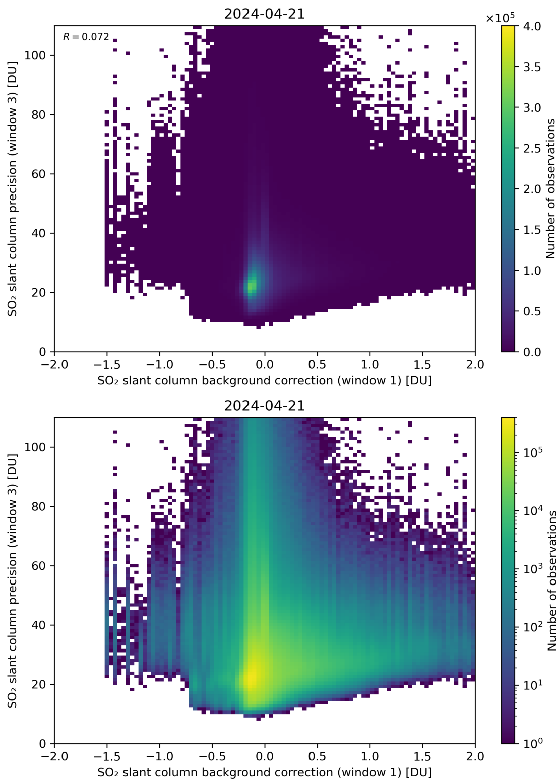
Figure 108: Scatter density plot of “SO 2 slant column background correction (window 1)” against “SO 2 slant column precision (window 3)” for 2024-04-21 to 2024-04-22.
