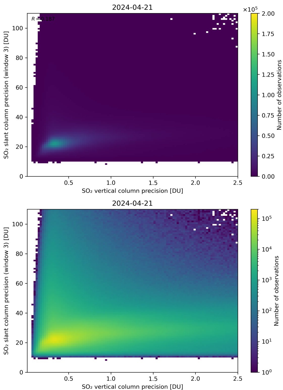
Figure 293: Scatter density plot of “SO 2 vertical column precision” against “SO 2 slant column precision (window 3)” for 2024-04-21 to 2024-04-22.
