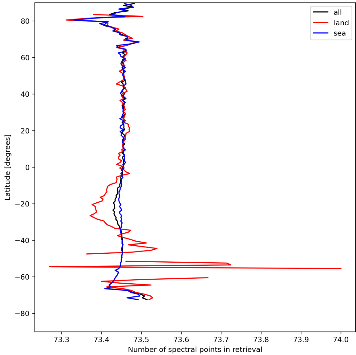
Figure 51: Zonal average of “Number of spectral points in retrieval” for 2024-04-21 to 2024-04-22.
