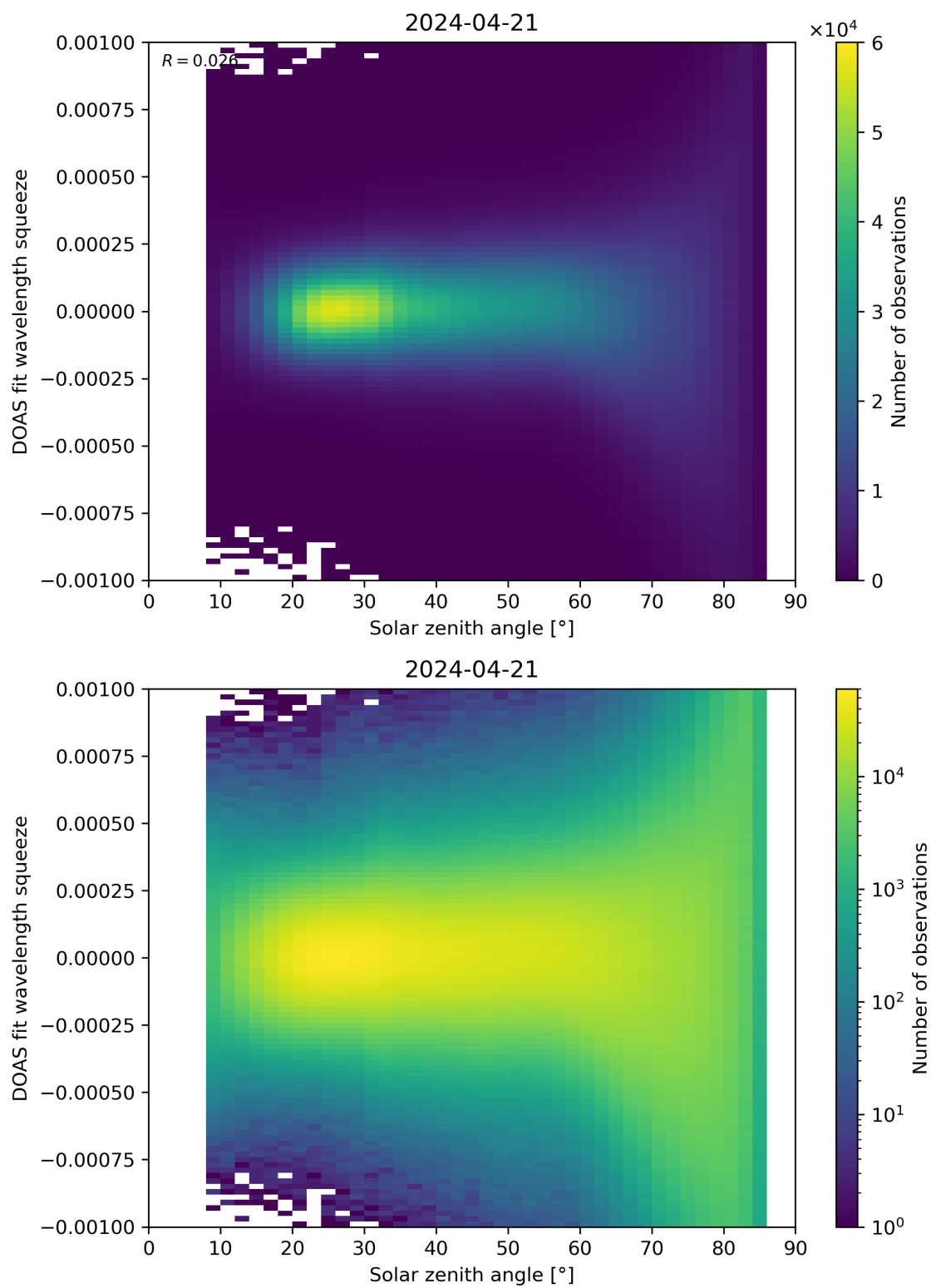
Figure 162: Scatter density plot of “Solar zenith angle” against “DOAS fit wavelength squeeze” for 2024-04-21 to 2024-04-22.
