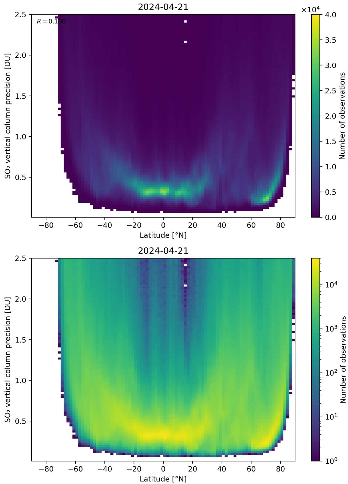
Figure 157: Scatter density plot of “Latitude” against “SO 2 vertical column precision” for 2024-04-21 to 2024-04-22.
