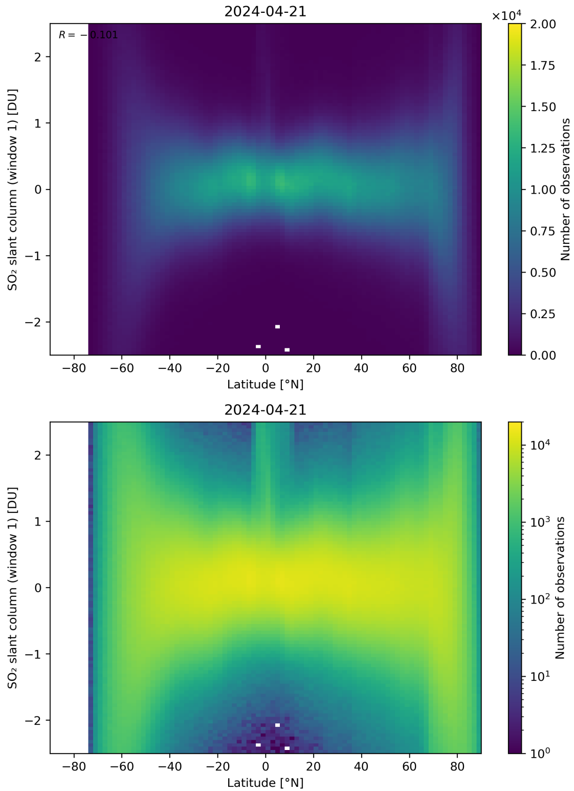
Figure 149: Scatter density plot of “Latitude” against “SO 2 slant column (window 1)” for 2024-04-21 to 2024-04-22.
