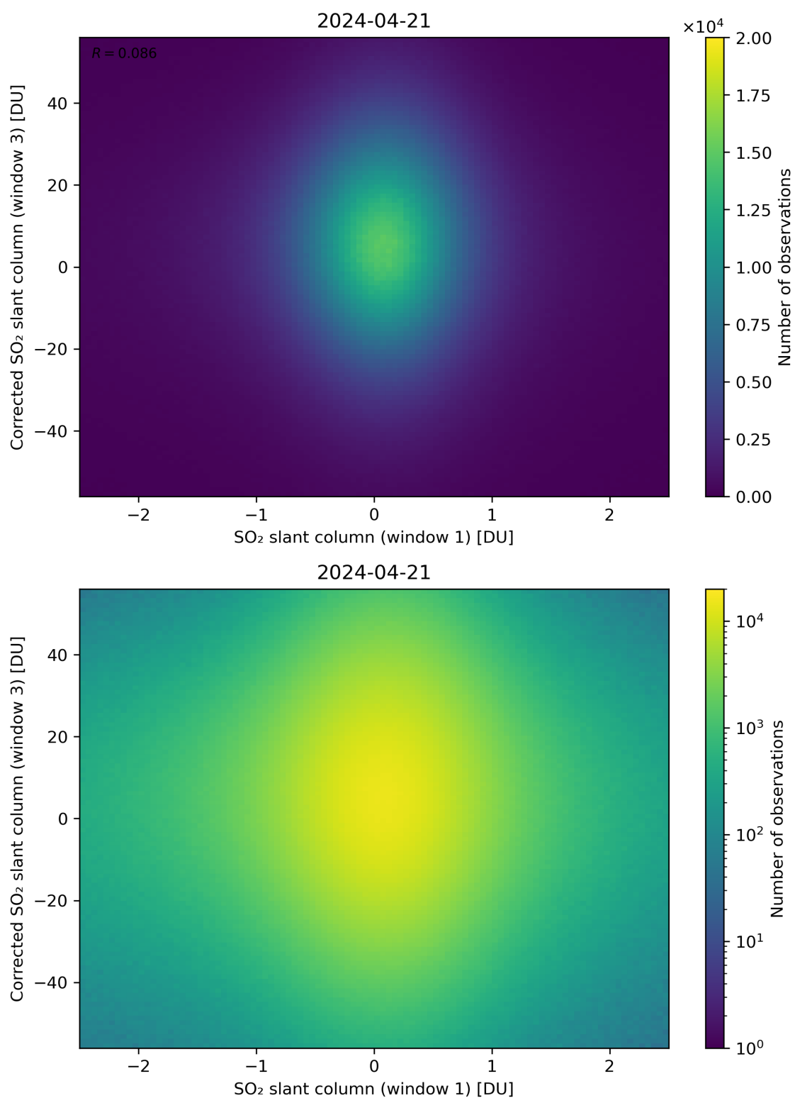
Figure 234: Scatter density plot of “SO 2 slant column (window 1)” against “Corrected SO 2 slant column (window 3)” for 2024-04-21 to 2024-04-22.
