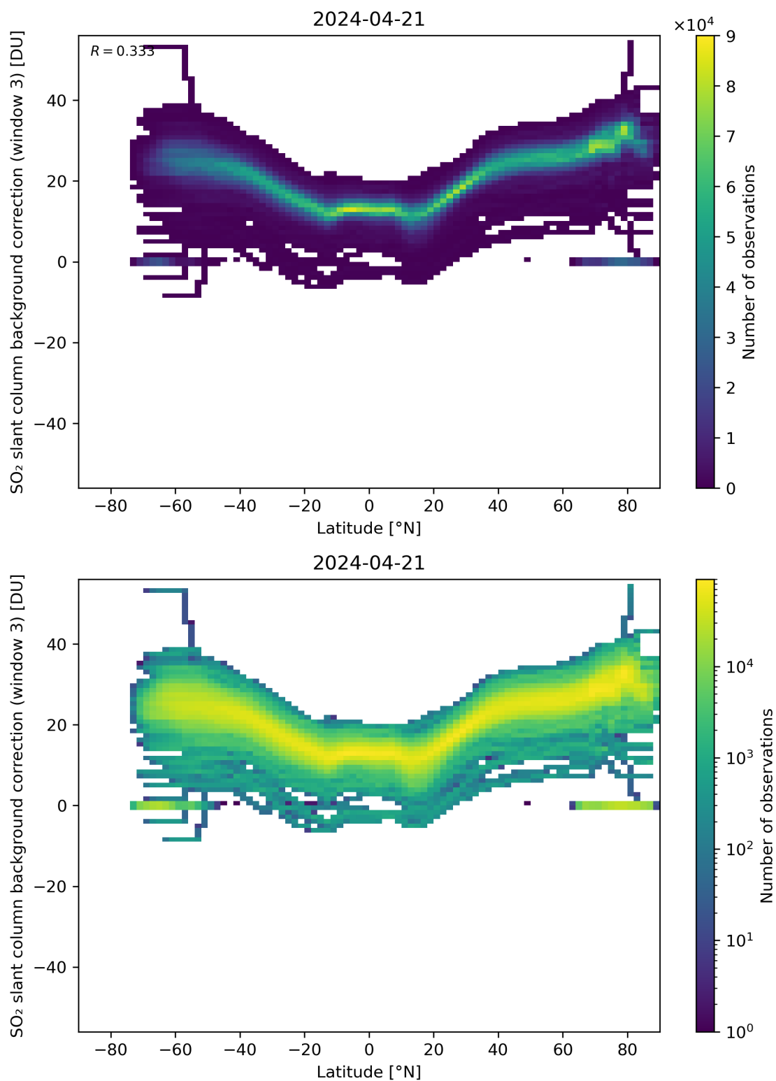
Figure 141: Scatter density plot of “Latitude” against “SO 2 slant column background correction (window 3)” for 2024-04-21 to 2024-04-22.
