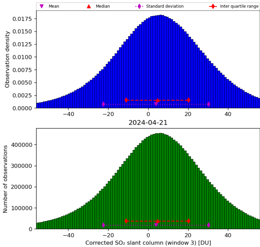
Figure 66: Histogram of “Corrected SO 2 slant column (window 3)” for 2024-04-21 to 2024-04-22
