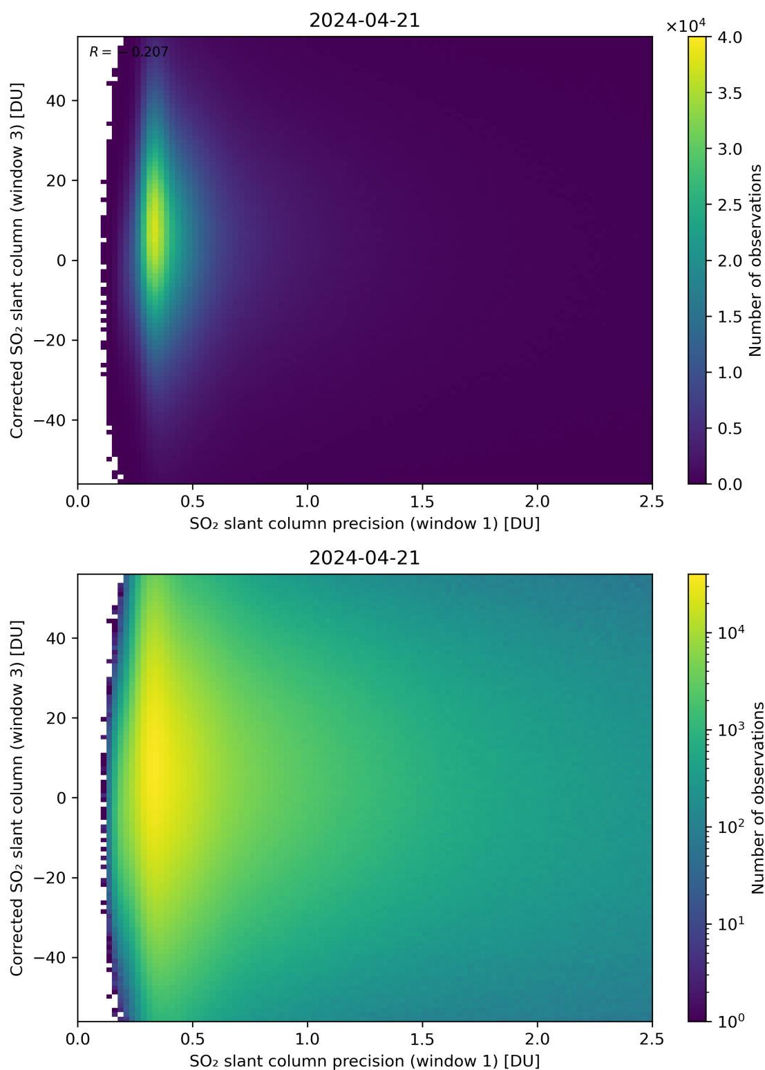
Figure 226: Scatter density plot of “SO 2 slant column precision (window 1)” against “Corrected SO 2 slant column (window 3)” for 2024-04-21 to 2024-04-22.
