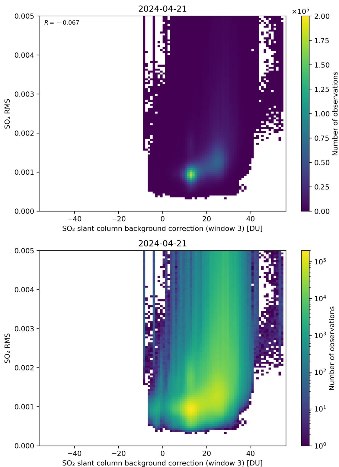
Figure 123: Scatter density plot of “SO 2 slant column background correction (window 3)” against “SO 2 RMS” for 2024-04-21 to 2024-04-22.
