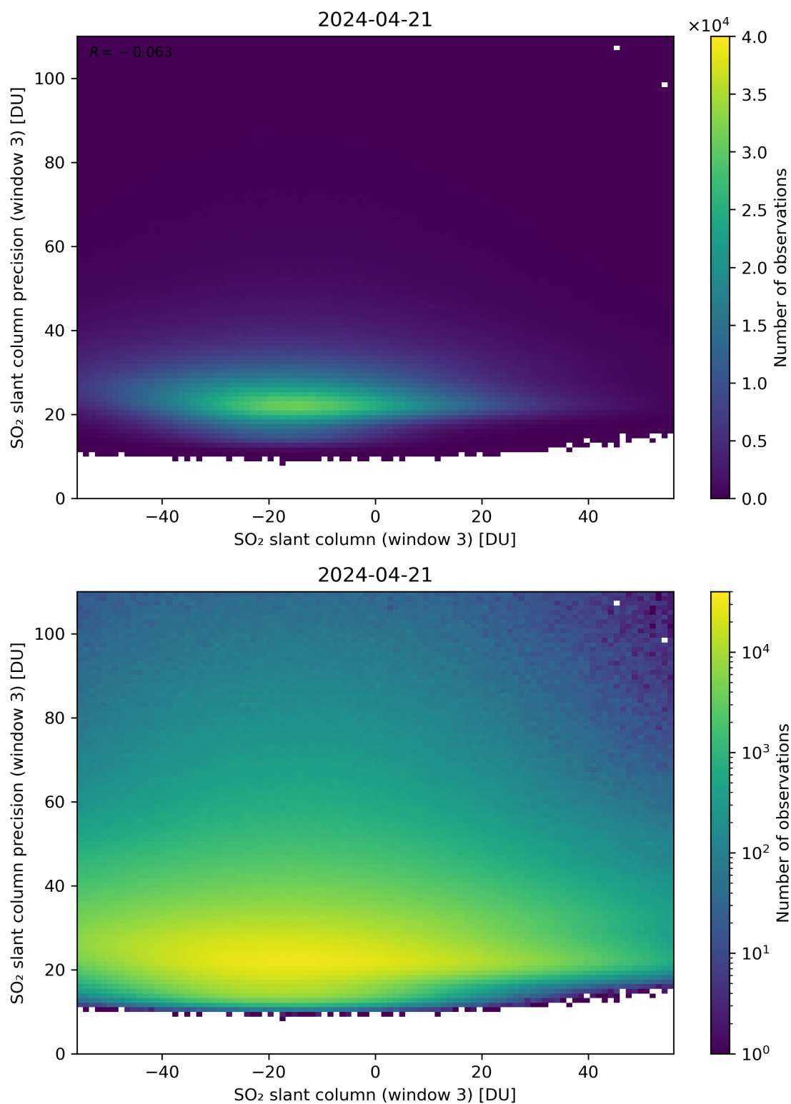
Figure 267: Scatter density plot of “SO 2 slant column (window 3)” against “SO 2 slant column precision (window 3)” for 2024-04-21 to 2024-04-22.
