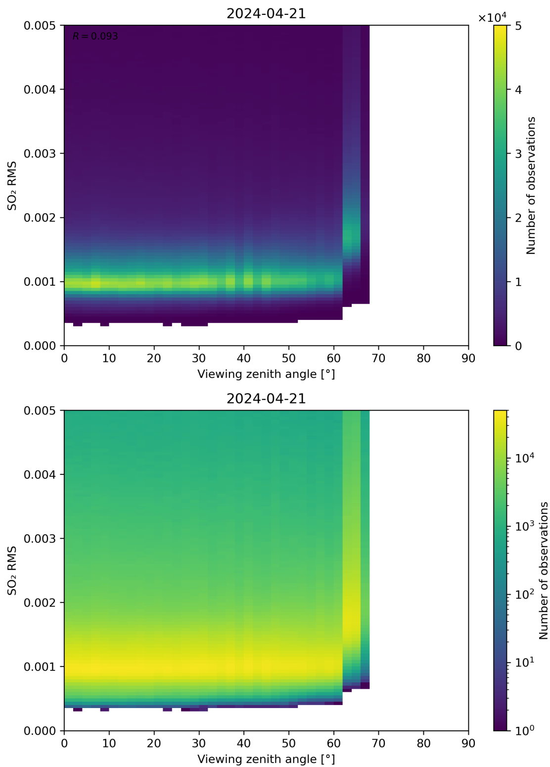
Figure 313: Scatter density plot of “Viewing zenith angle” against “SO 2 RMS” for 2024-04-21 to 2024-04-22.
