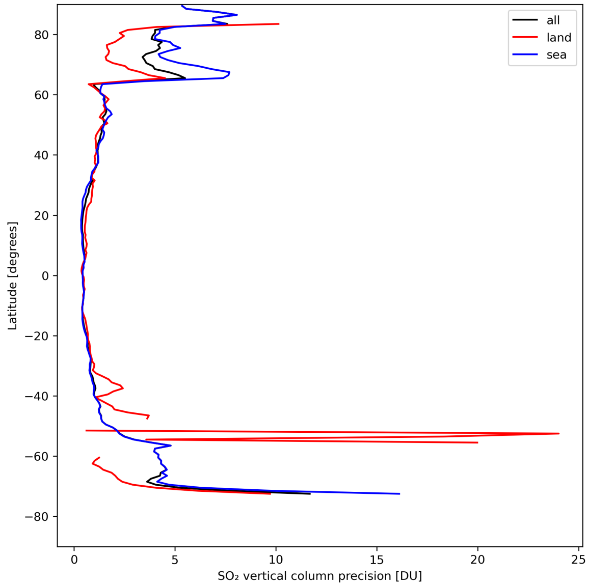
Figure 31: Zonal average of “SO 2 vertical column precision” for 2024-04-21 to 2024-04-22.
