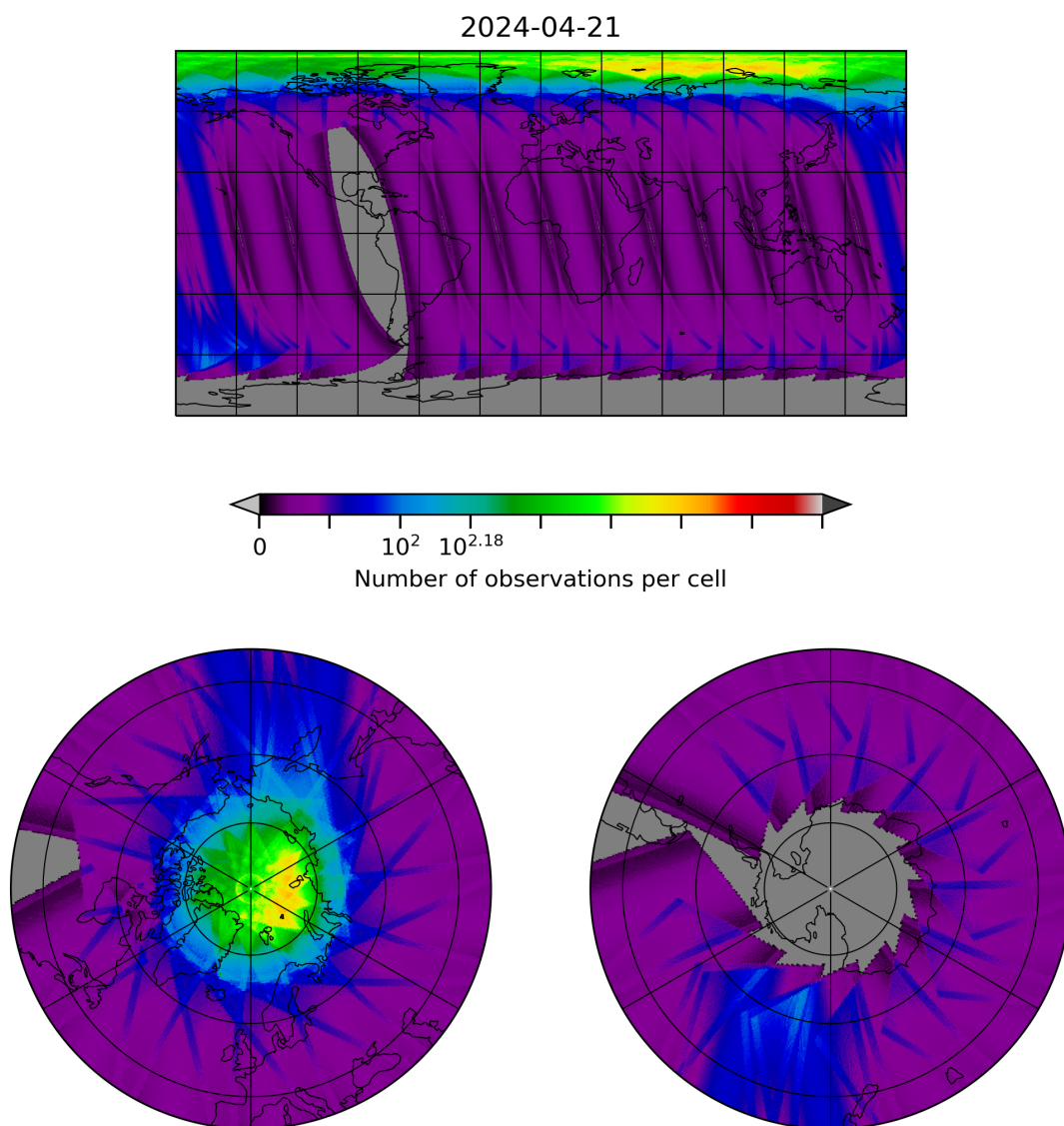
Figure 28: Map of the number of observations for 2024-04-21 to 2024-04-22
