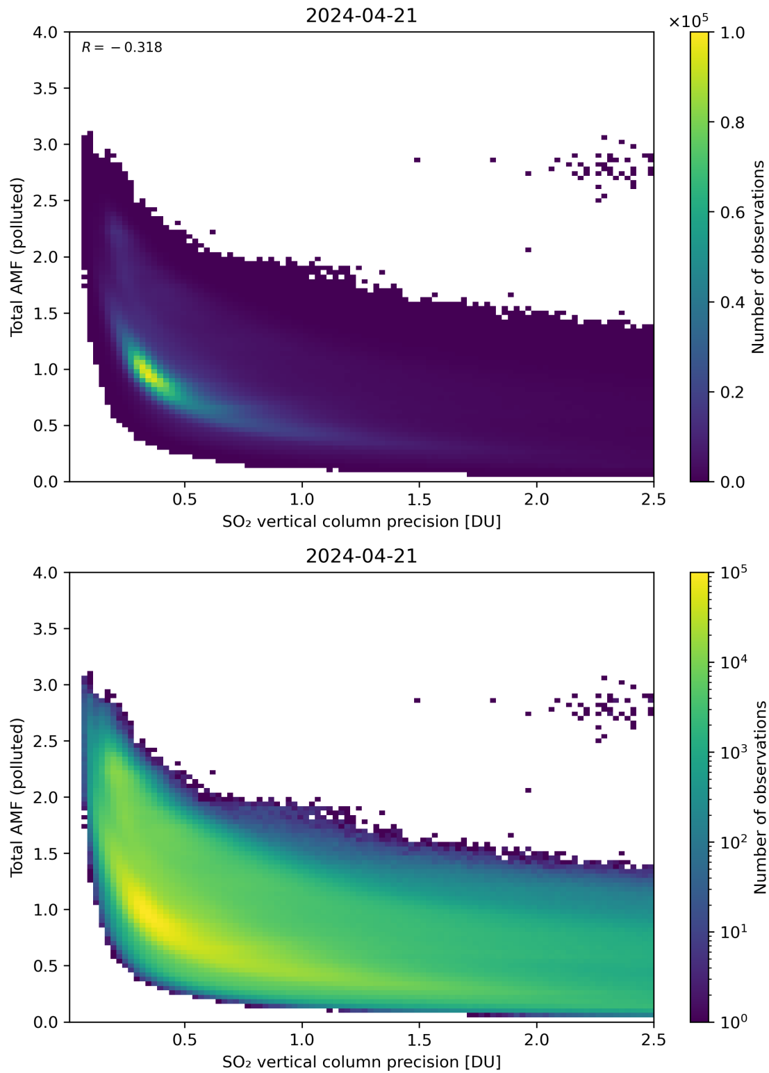
Figure 294: Scatter density plot of “SO 2 vertical column precision” against “Total AMF (polluted)” for 2024-04-21 to 2024-04-22.
