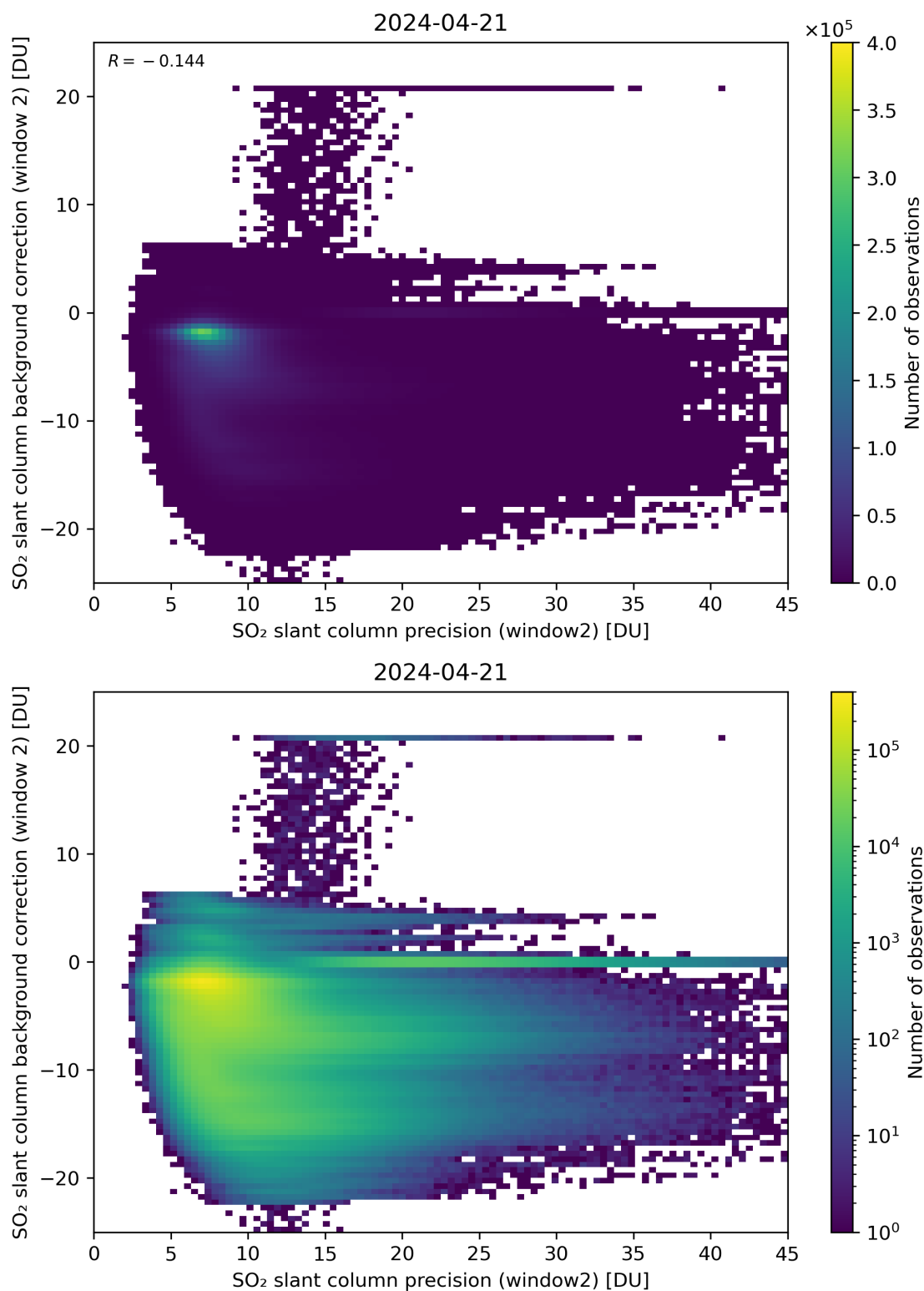
Figure 241: Scatter density plot of “SO 2 slant column precision (window2)” against “SO 2 slant column background correction (window 2)” for 2024-04-21 to 2024-04-22.
