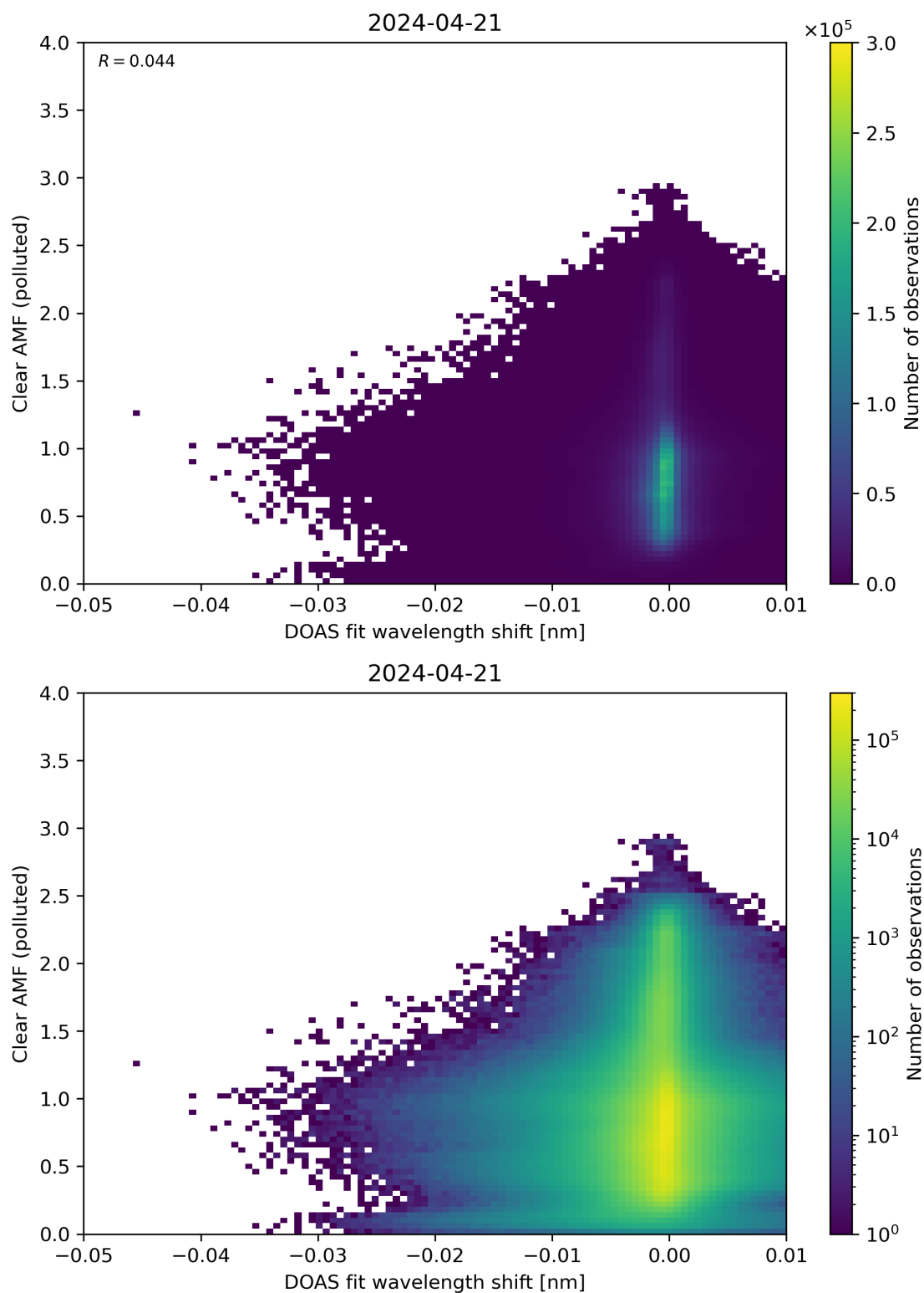
Figure 129: Scatter density plot of “DOAS fit wavelength shift” against “Clear AMF (polluted)” for 2024-04-21 to 2024-04-22.
