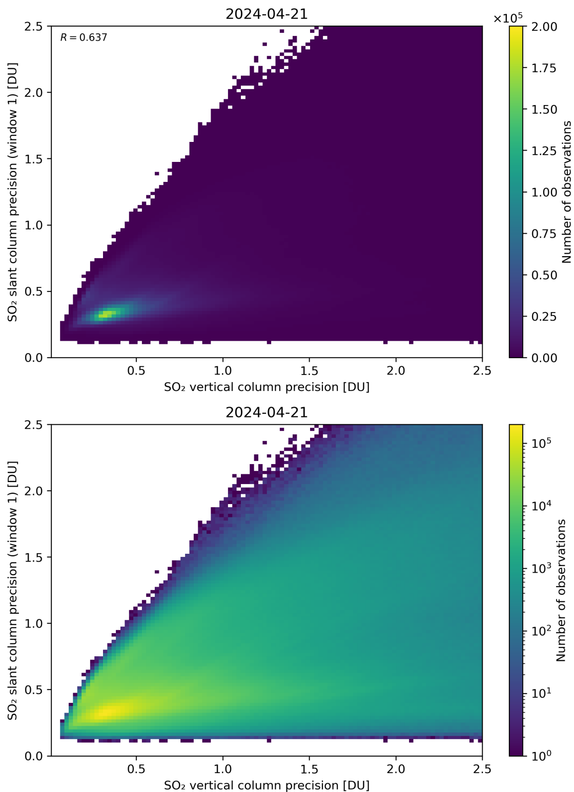
Figure 290: Scatter density plot of “SO 2 vertical column precision” against “SO 2 slant column precision (window 1)” for 2024-04-21 to 2024-04-22.
