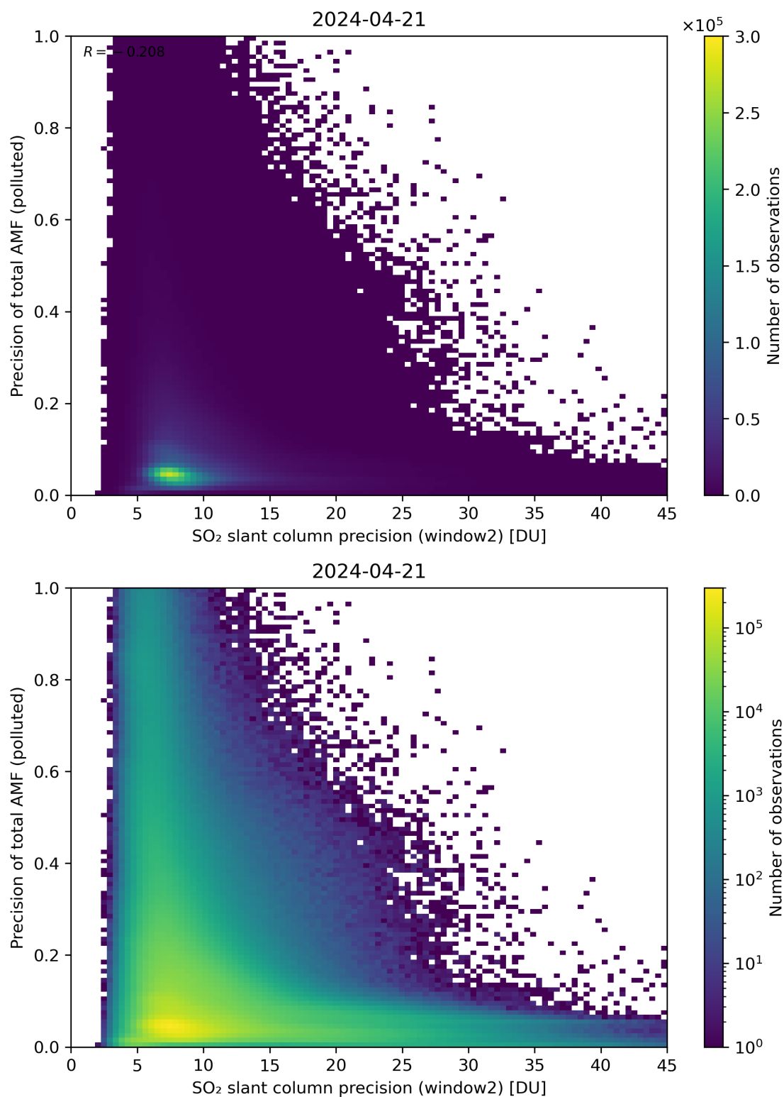
Figure 252: Scatter density plot of “SO 2 slant column precision (window2)” against “Precision of total AMF (polluted)” for 2024-04-21 to 2024-04-22.
