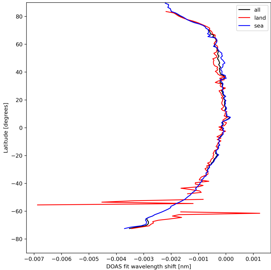
Figure 45: Zonal average of “DOAS fit wavelength shift” for 2024-04-21 to 2024-04-22.
