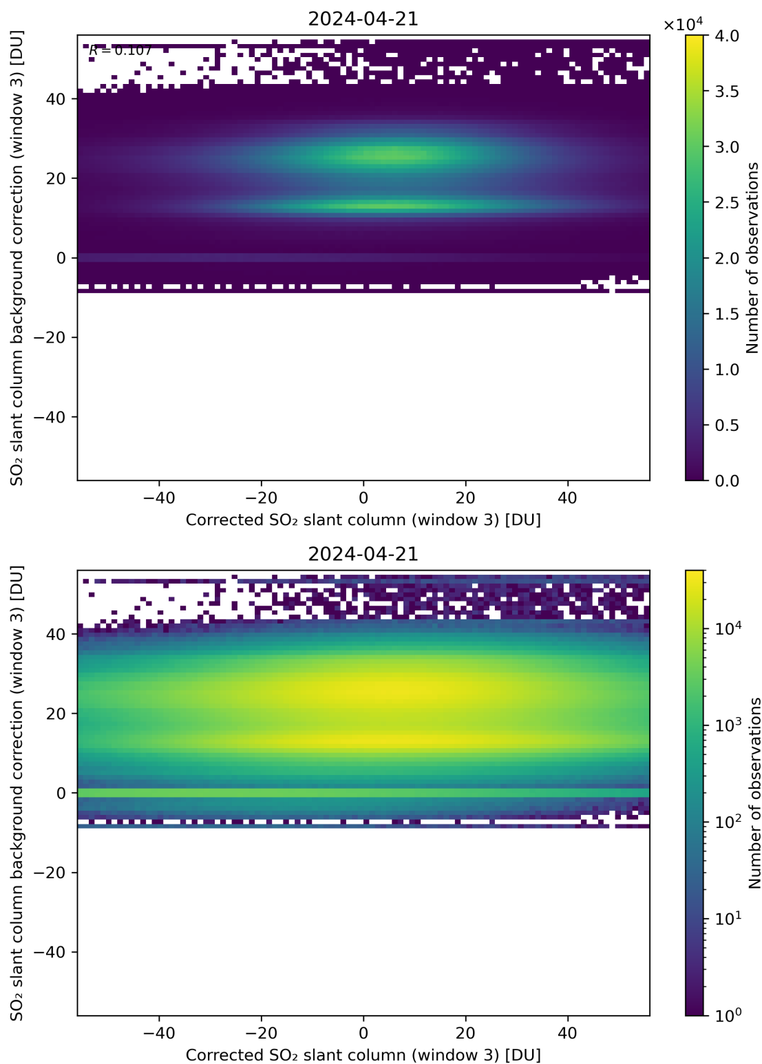
Figure 205: Scatter density plot of “Corrected SO 2 slant column (window 3)” against “SO 2 slant column background correction (window 3)” for 2024-04-21 to 2024-04-22.
