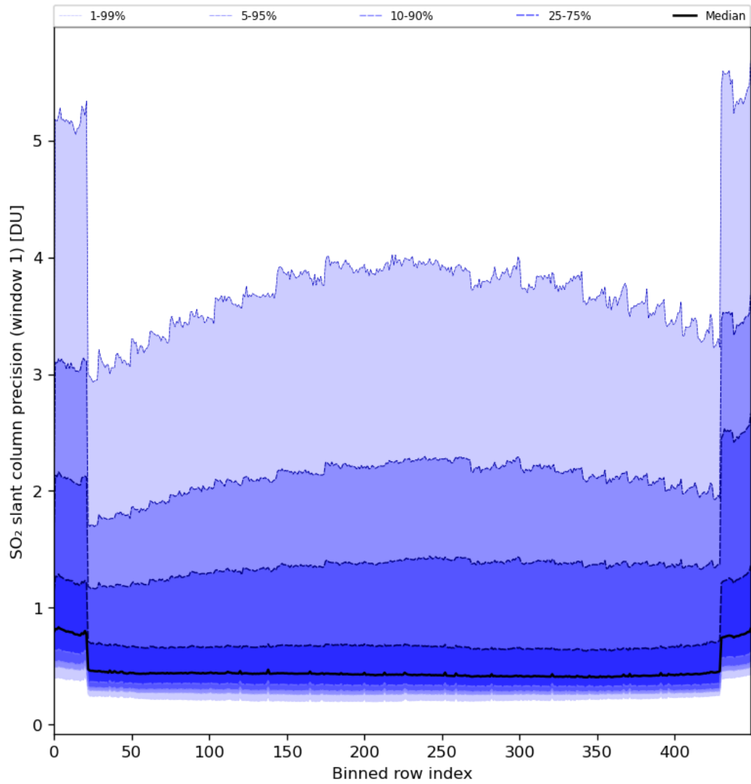
Figure 80: Along track statistics of “SO 2 slant column precision (window 1)” for 2024-04-21 to 2024-04-22
