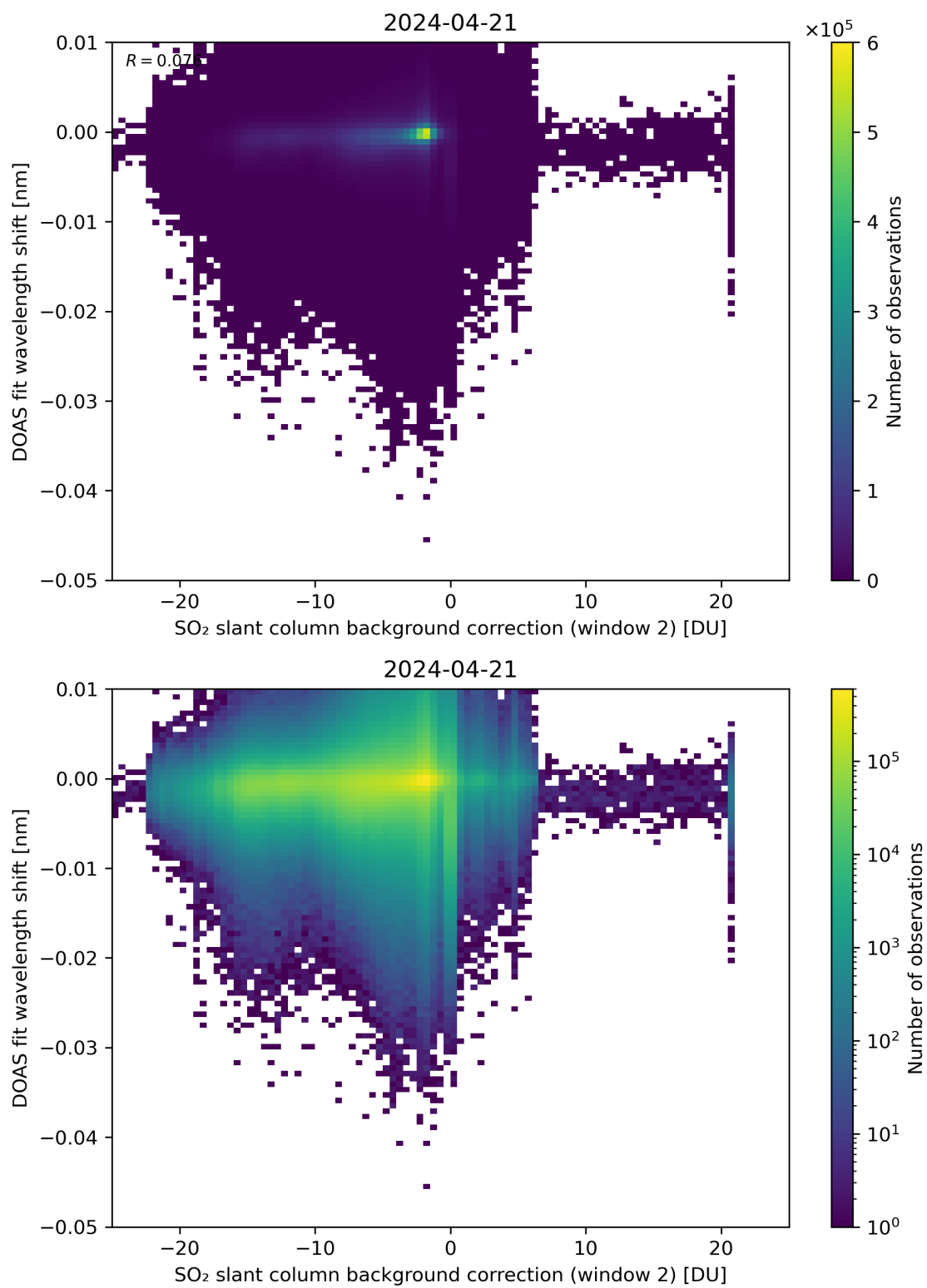
Figure 112: Scatter density plot of “SO 2 slant column background correction (window 2)” against “DOAS fit wavelength shift” for 2024-04-21 to 2024-04-22.
