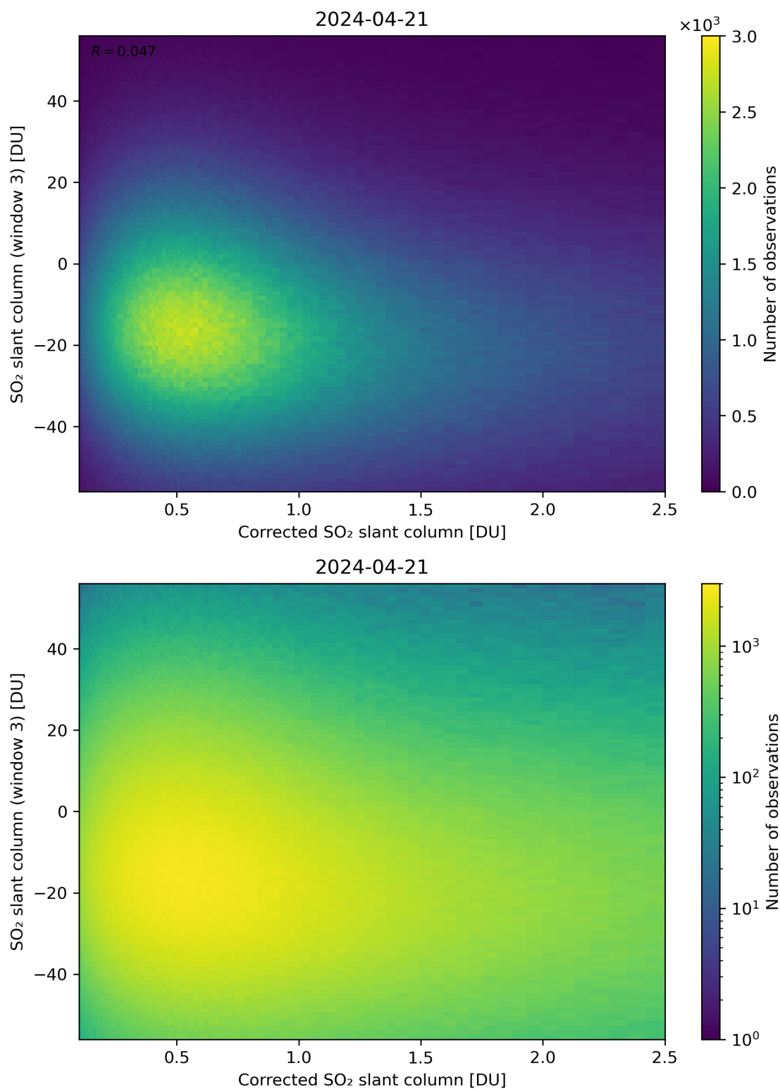
Figure 190: Scatter density plot of “Corrected SO 2 slant column” against “SO 2 slant column (window 3)” for 2024-04-21 to 2024-04-22.
