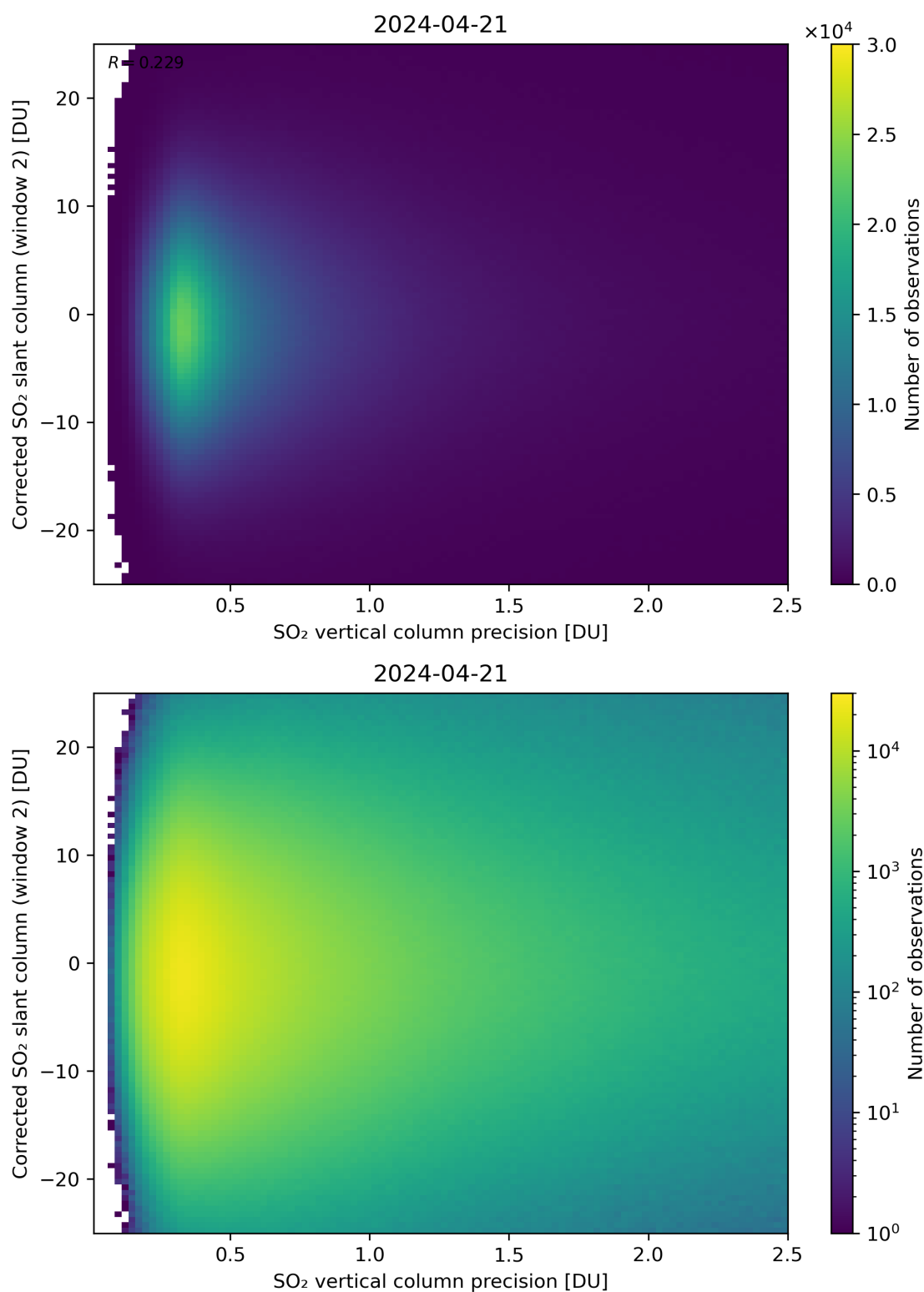
Figure 287: Scatter density plot of “SO 2 vertical column precision” against “Corrected SO 2 slant column (window 2)” for 2024-04-21 to 2024-04-22.
