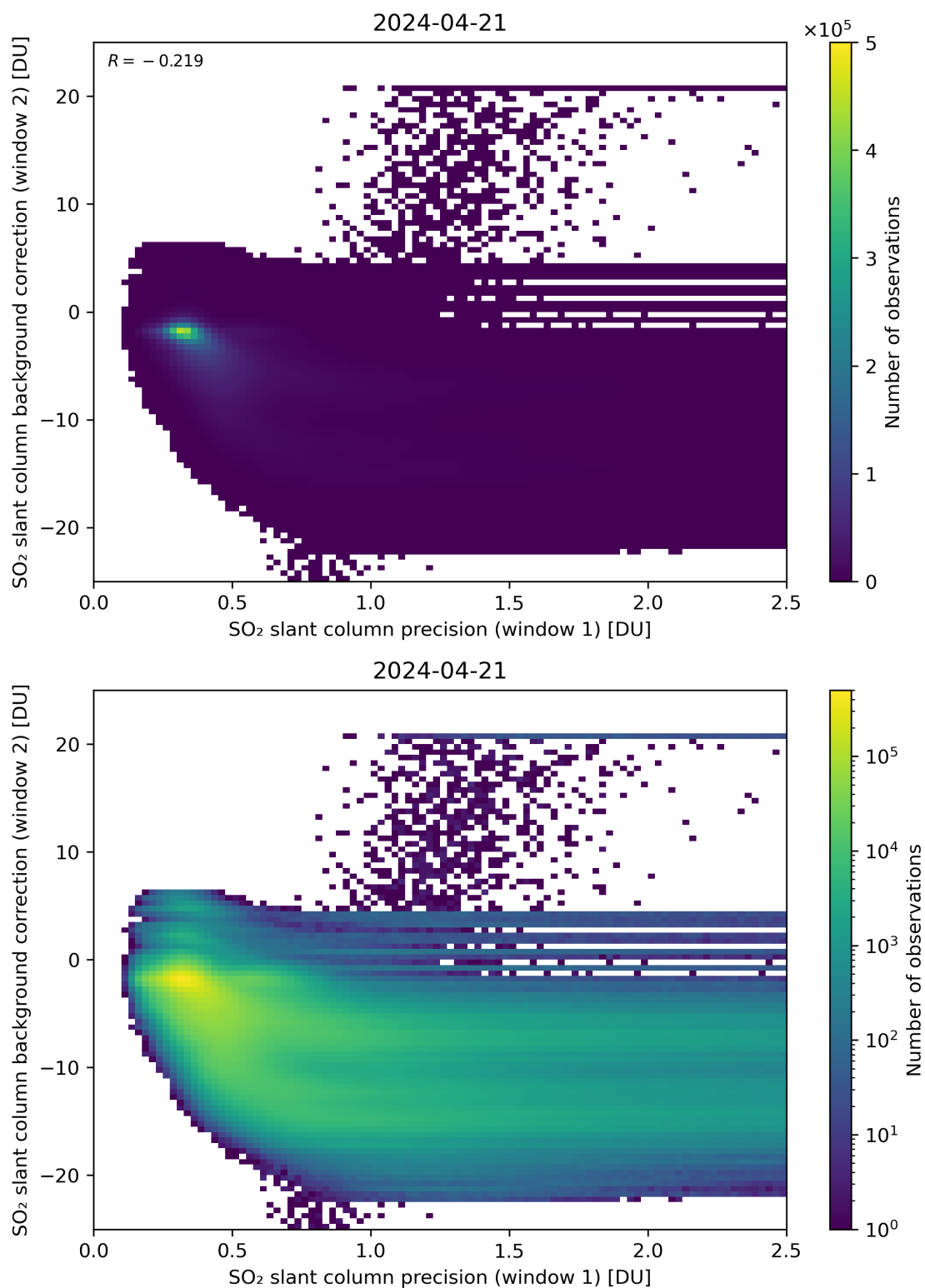
Figure 219: Scatter density plot of “SO 2 slant column precision (window 1)” against “SO 2 slant column background correction (window 2)” for 2024-04-21 to 2024-04-22.
