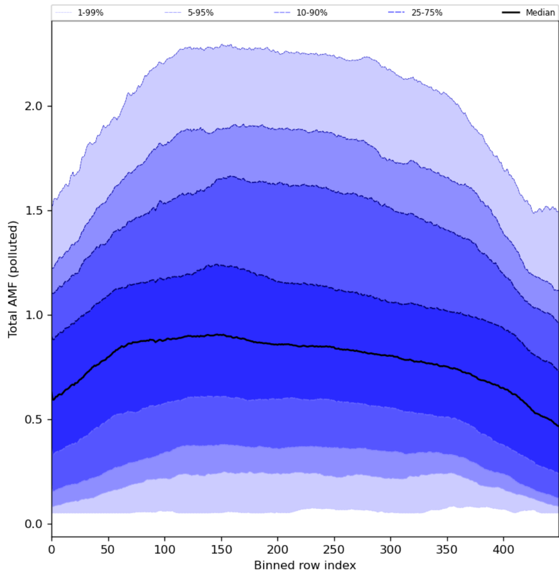
Figure 94: Along track statistics of “Total AMF (polluted)” for 2024-04-21 to 2024-04-22
