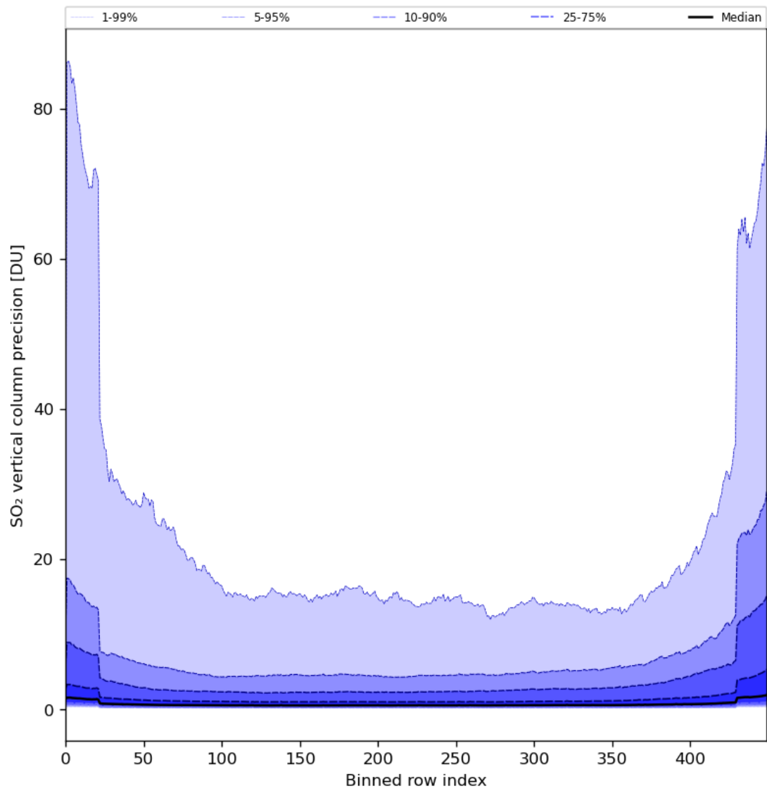
Figure 77: Along track statistics of “SO 2 vertical column precision” for 2024-04-21 to 2024-04-22
