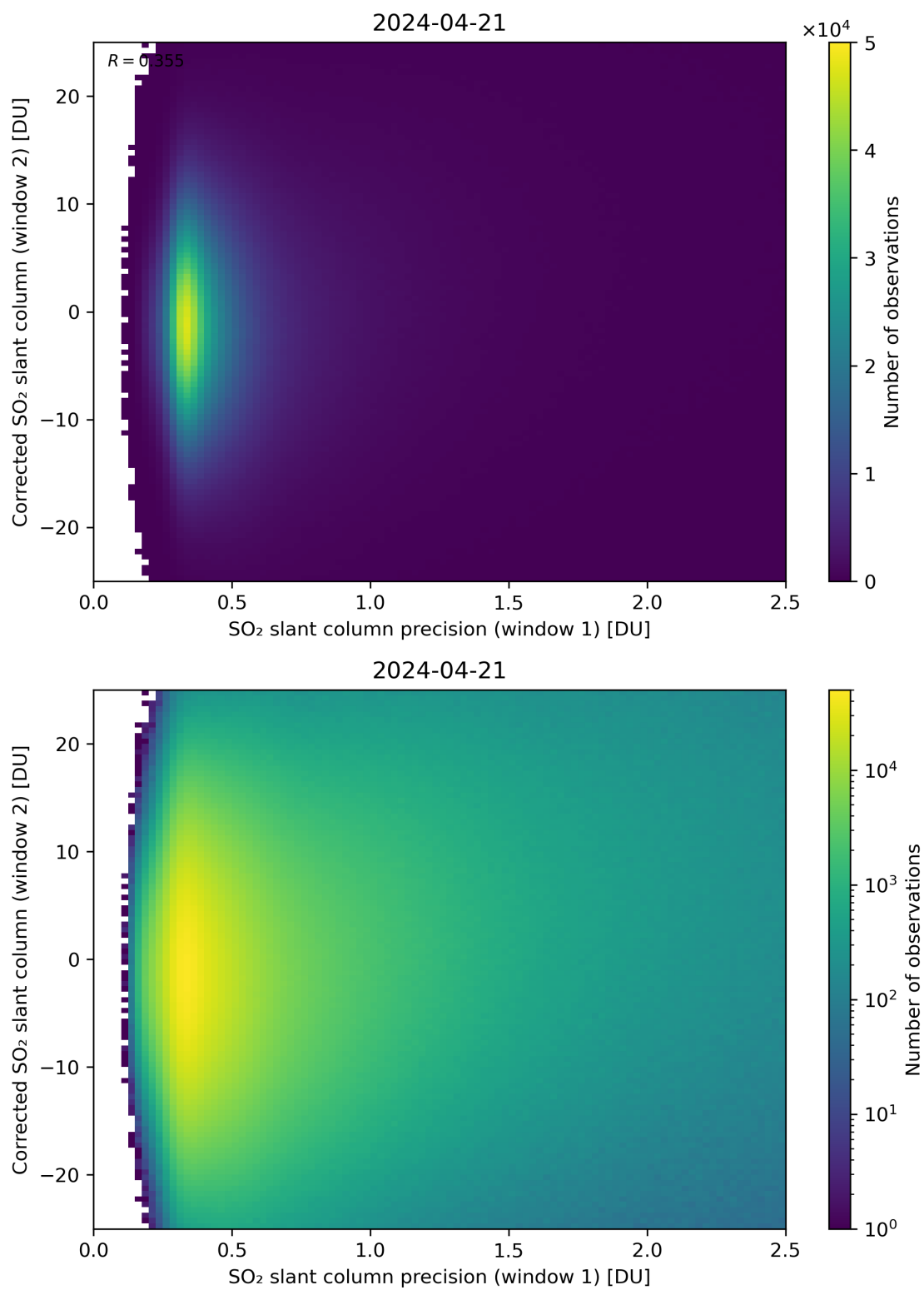
Figure 225: Scatter density plot of “SO 2 slant column precision (window 1)” against “Corrected SO 2 slant column (window 2)” for 2024-04-21 to 2024-04-22.
