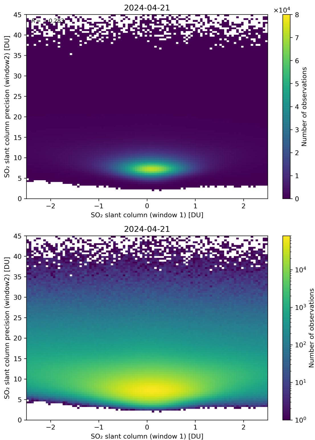
Figure 236: Scatter density plot of “SO 2 slant column (window 1)” against “SO 2 slant column precision (window2)” for 2024-04-21 to 2024-04-22.
