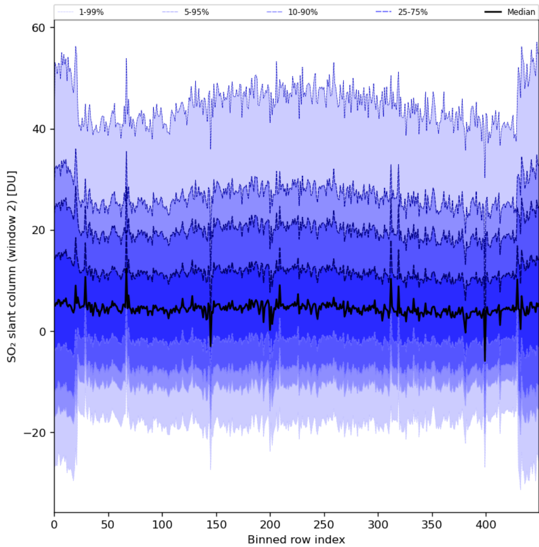
Figure 83: Along track statistics of “SO 2 slant column (window 2)” for 2024-04-21 to 2024-04-22
