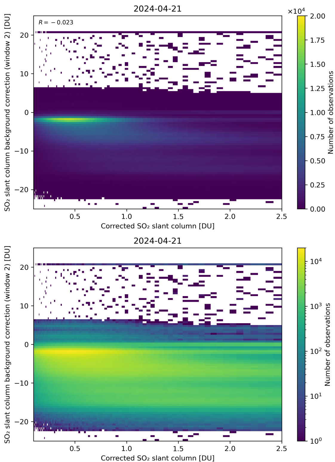
Figure 179: Scatter density plot of “Corrected SO 2 slant column” against “SO 2 slant column background correction (window 2)” for 2024-04-21 to 2024-04-22.
