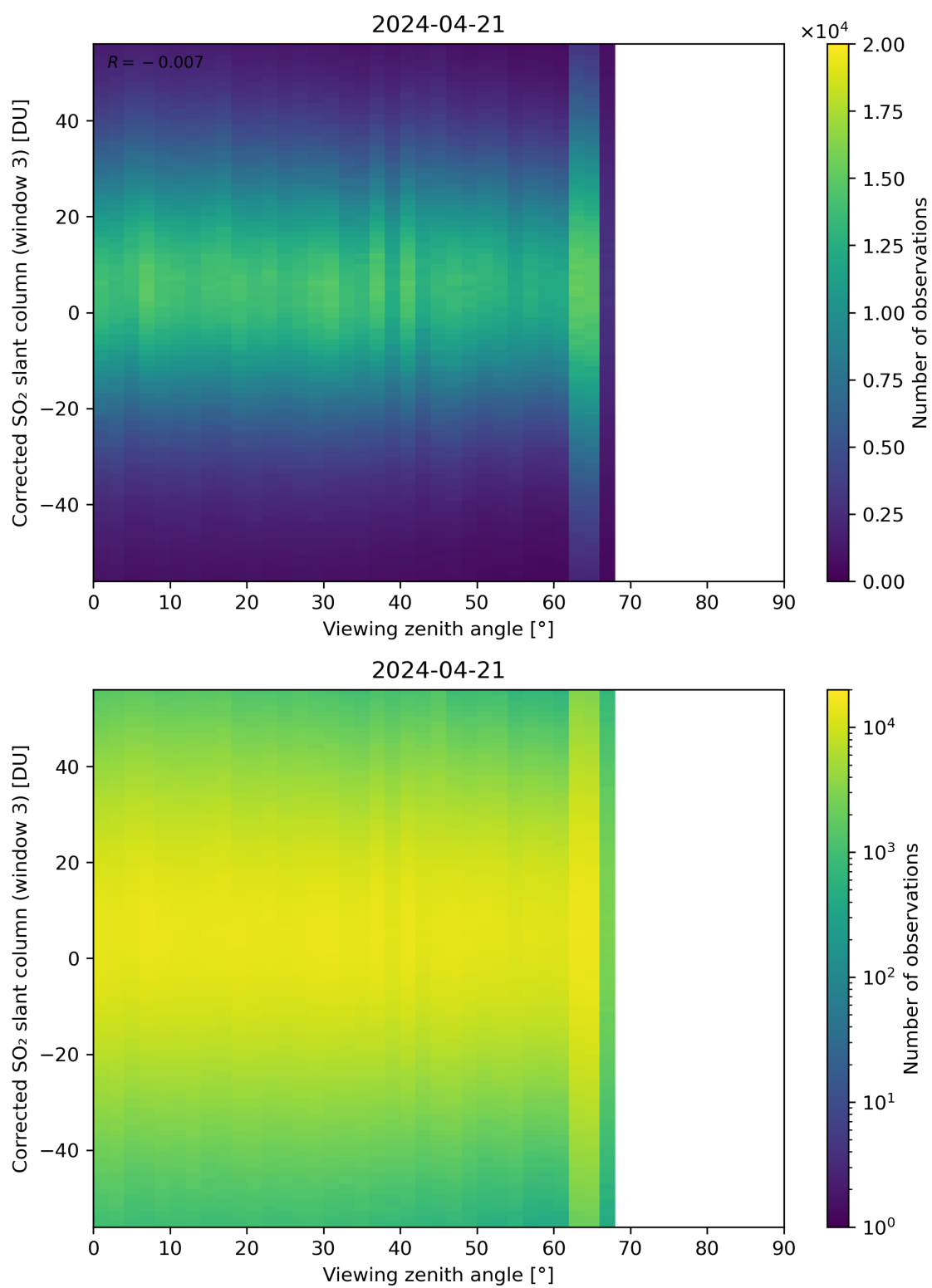
Figure 319: Scatter density plot of “Viewing zenith angle” against “Corrected SO 2 slant column (window 3)” for 2024-04-21 to 2024-04-22.
