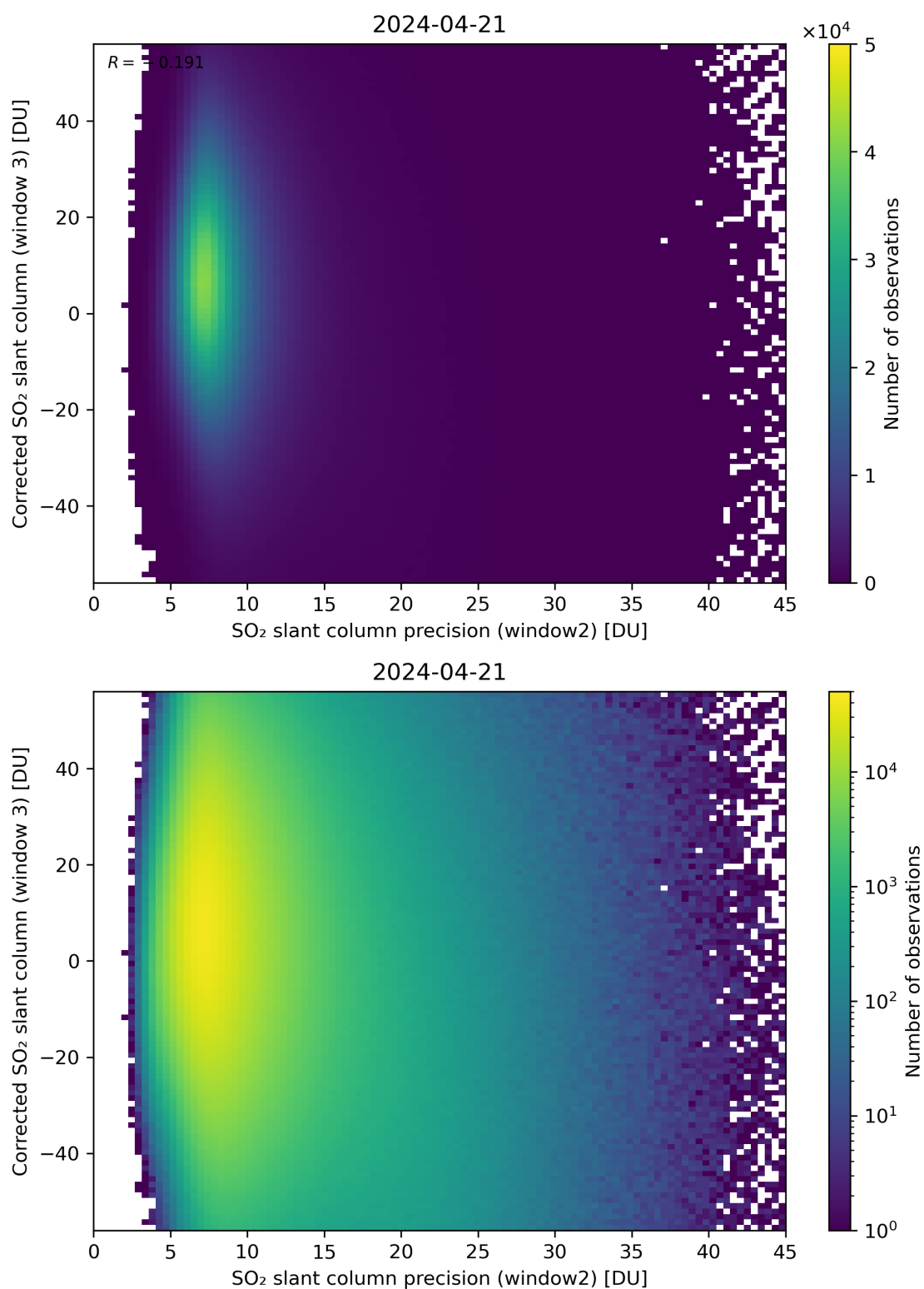
Figure 248: Scatter density plot of “SO 2 slant column precision (window2)” against “Corrected SO 2 slant column (window 3)” for 2024-04-21 to 2024-04-22.
