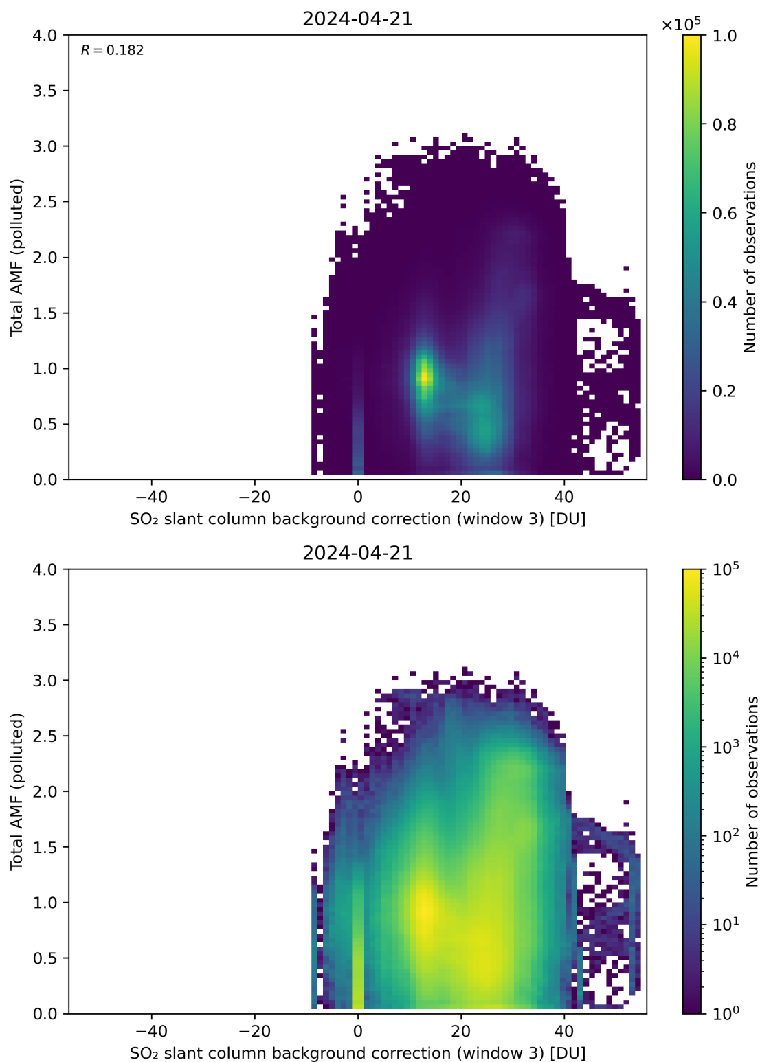
Figure 125: Scatter density plot of “SO 2 slant column background correction (window 3)” against “Total AMF (polluted)” for 2024-04-21 to 2024-04-22.
