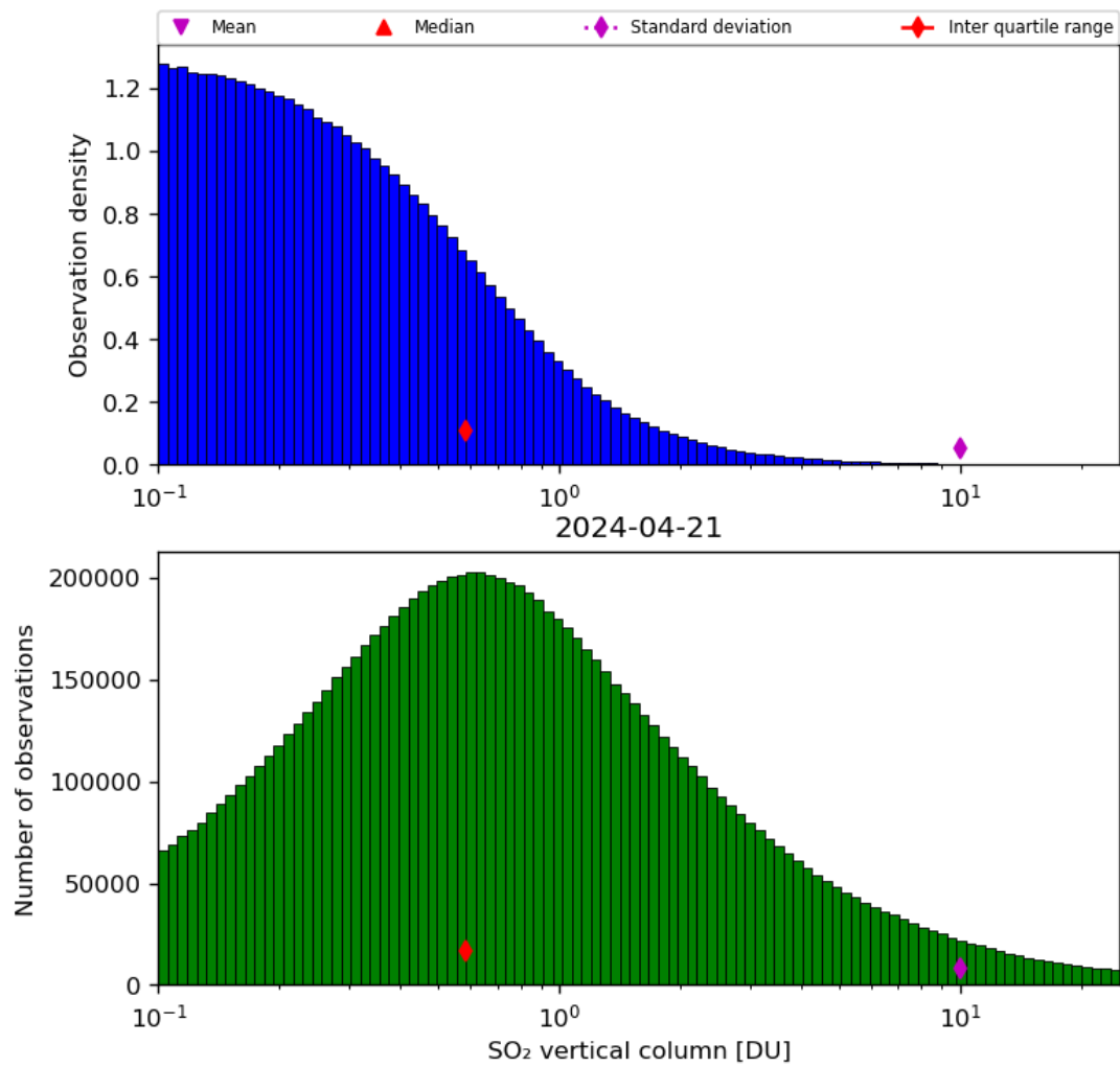
Figure 53: Histogram of “SO 2 vertical column” for 2024-04-21 to 2024-04-22
