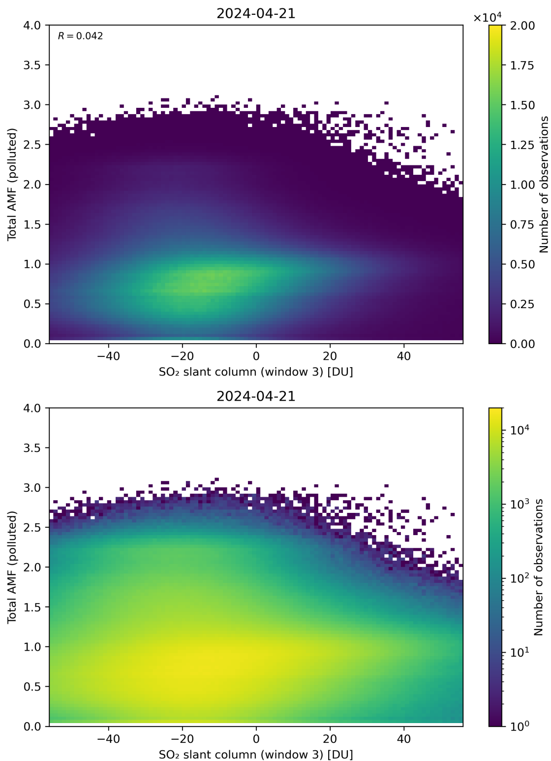
Figure 268: Scatter density plot of “SO 2 slant column (window 3)” against “Total AMF (polluted)” for 2024-04-21 to 2024-04-22.
