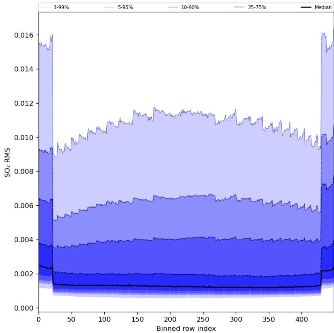
Figure 93: Along track statistics of “SO 2 RMS” for 2024-04-21 to 2024-04-22
