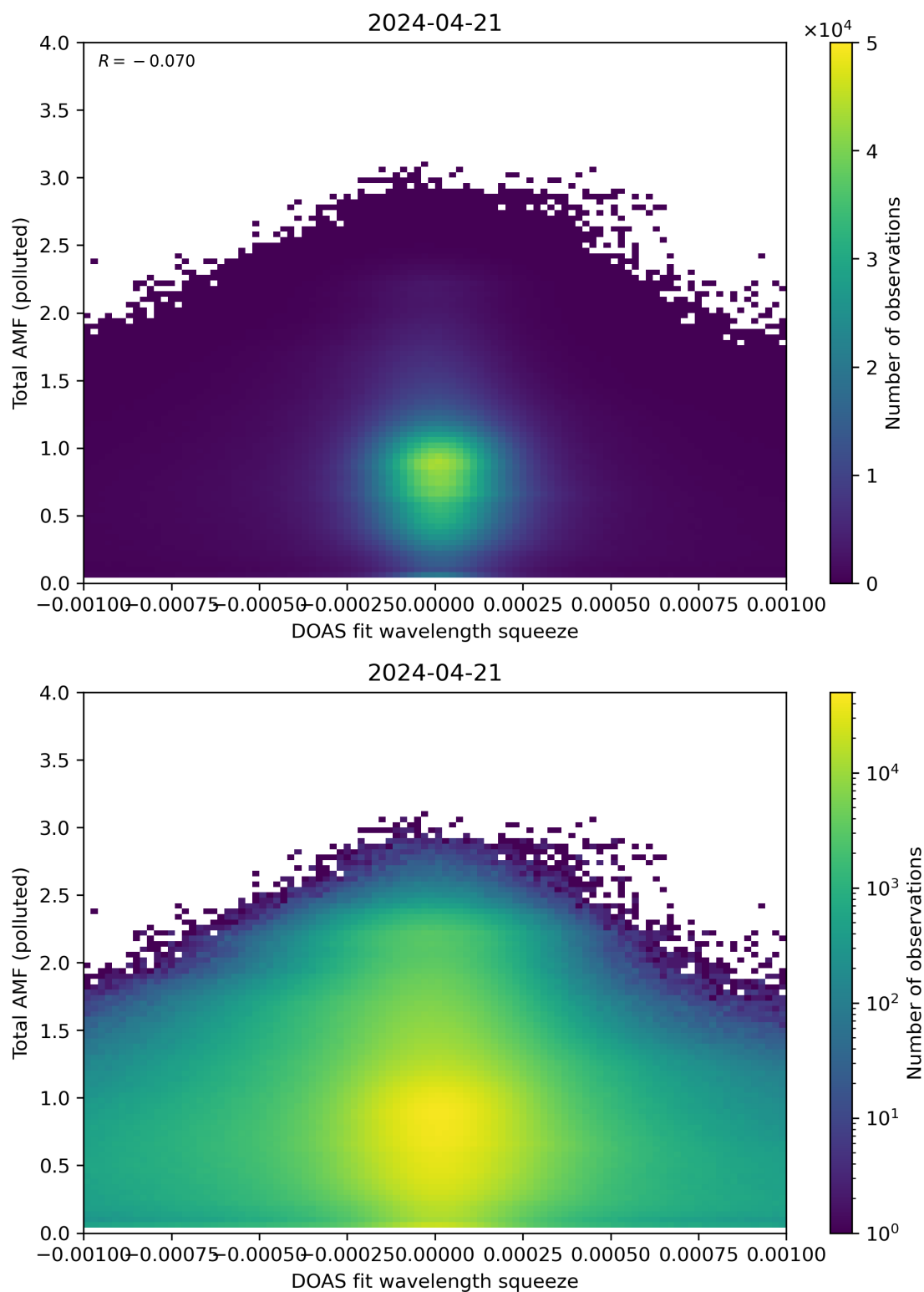
Figure 134: Scatter density plot of “DOAS fit wavelength squeeze” against “Total AMF (polluted)” for 2024-04-21 to 2024-04-22.
