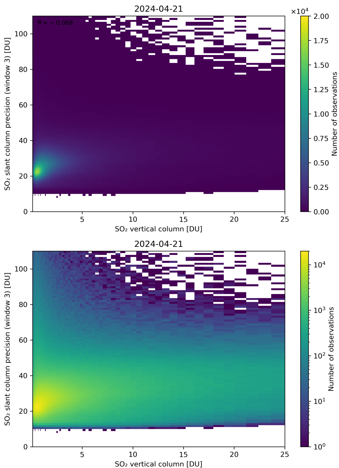
Figure 304: Scatter density plot of “SO 2 vertical column” against “SO 2 slant column precision (window 3)” for 2024-04-21 to 2024-04-22.
