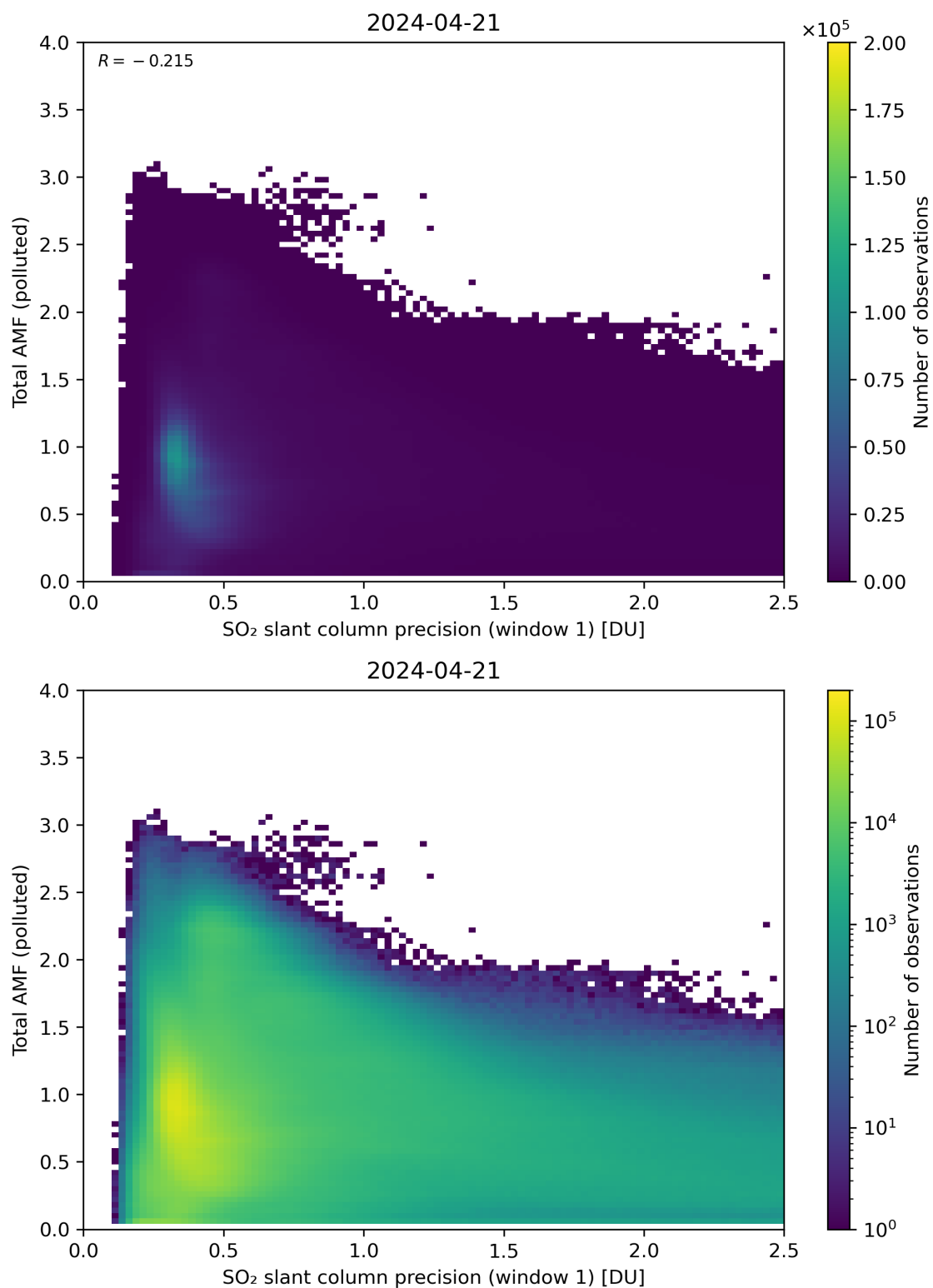
Figure 230: Scatter density plot of “SO 2 slant column precision (window 1)” against “Total AMF (polluted)” for 2024-04-21 to 2024-04-22.
