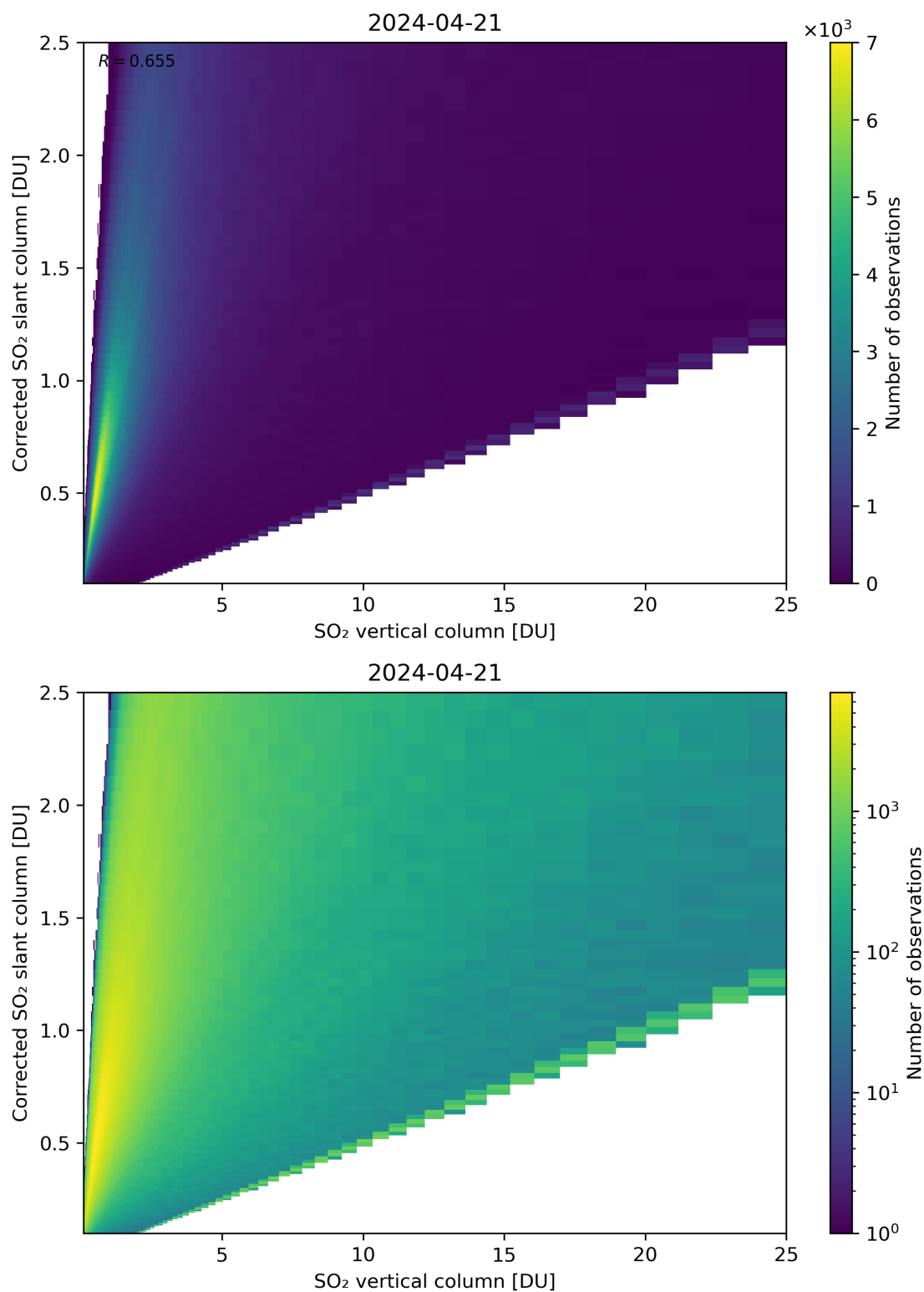
Figure 297: Scatter density plot of “SO 2 vertical column” against “Corrected SO 2 slant column” for 2024-04-21 to 2024-04-22.
