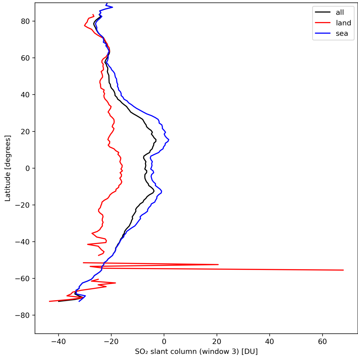
Figure 41: Zonal average of “SO 2 slant column (window 3)” for 2024-04-21 to 2024-04-22.
