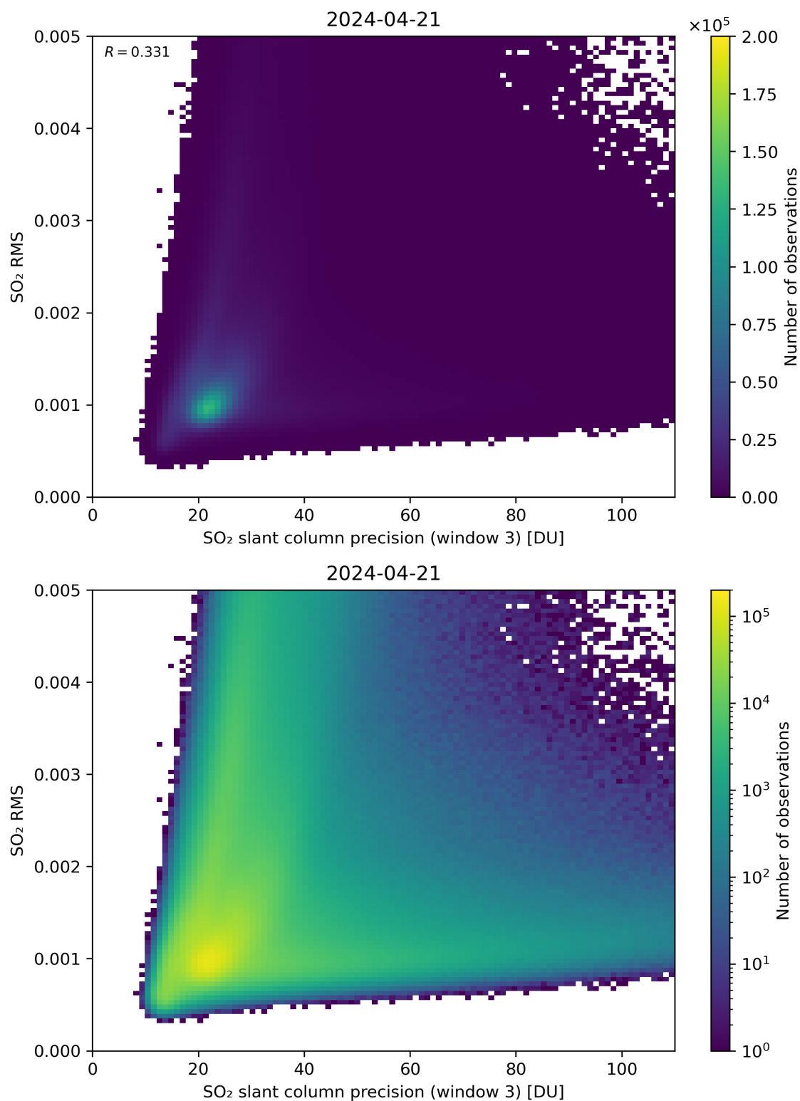
Figure 260: Scatter density plot of “SO 2 slant column precision (window 3)” against “SO 2 RMS” for 2024-04-21 to 2024-04-22.
