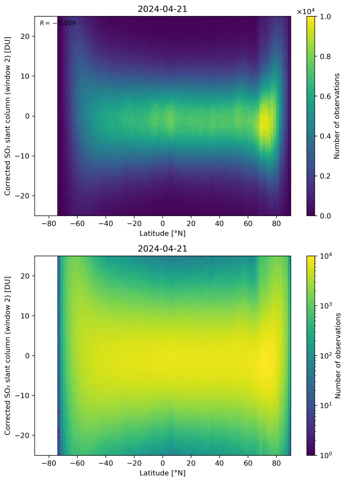
Figure 147: Scatter density plot of “Latitude” against “Corrected SO 2 slant column (window 2)” for 2024-04-21 to 2024-04-22.
