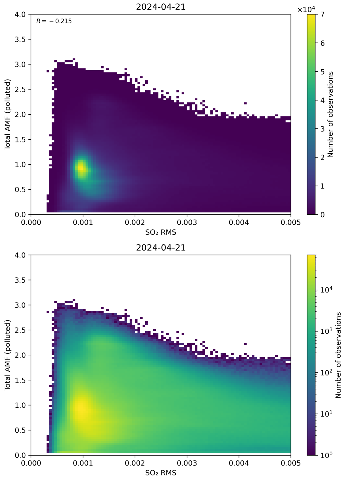
Figure 137: Scatter density plot of “SO 2 RMS” against “Total AMF (polluted)” for 2024-04-21 to 2024-04-22.
