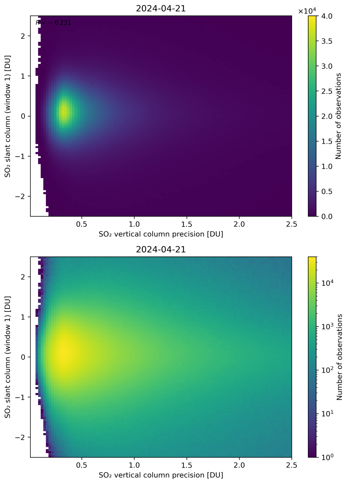
Figure 289: Scatter density plot of “SO 2 vertical column precision” against “SO 2 slant column (window 1)” for 2024-04-21 to 2024-04-22.
