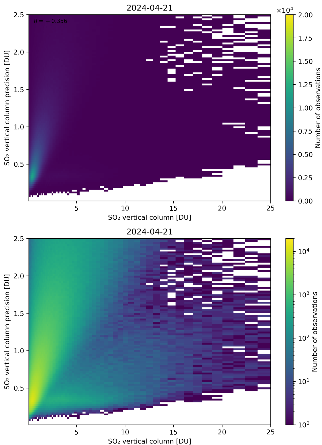
Figure 307: Scatter density plot of “SO 2 vertical column” against “SO 2 vertical column precision” for 2024-04-21 to 2024-04-22.
