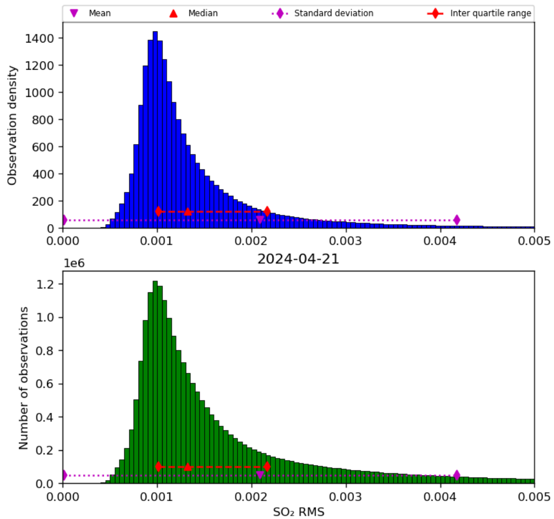
Figure 70: Histogram of “SO 2 RMS” for 2024-04-21 to 2024-04-22
