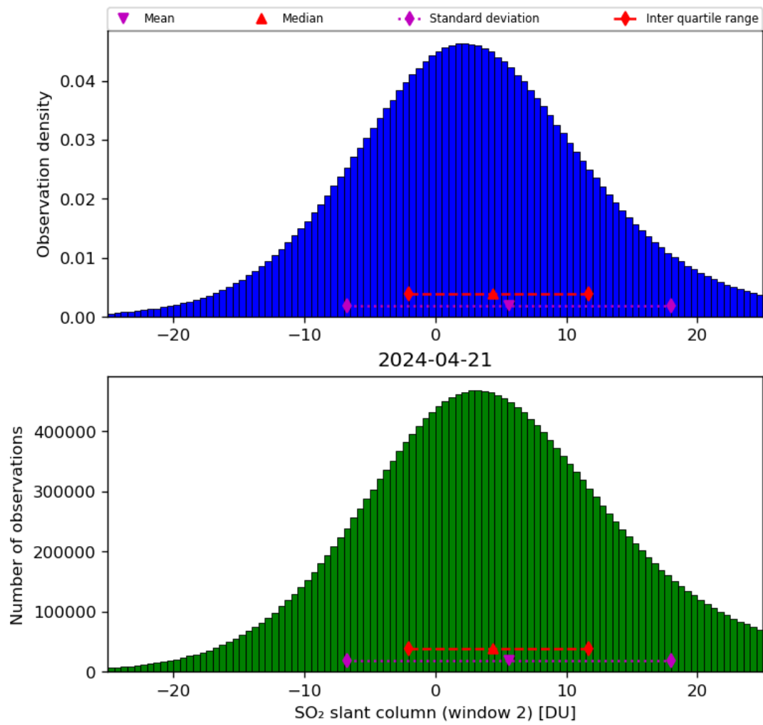
Figure 60: Histogram of “SO 2 slant column (window 2)” for 2024-04-21 to 2024-04-22
