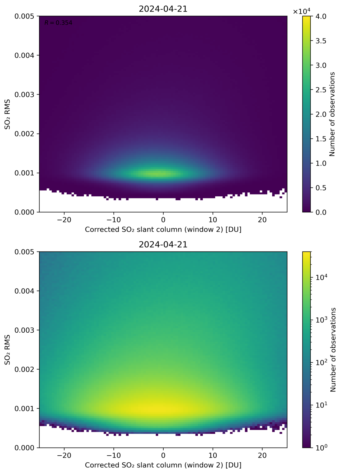
Figure 198: Scatter density plot of “Corrected SO 2 slant column (window 2)” against “SO 2 RMS” for 2024-04-21 to 2024-04-22.
