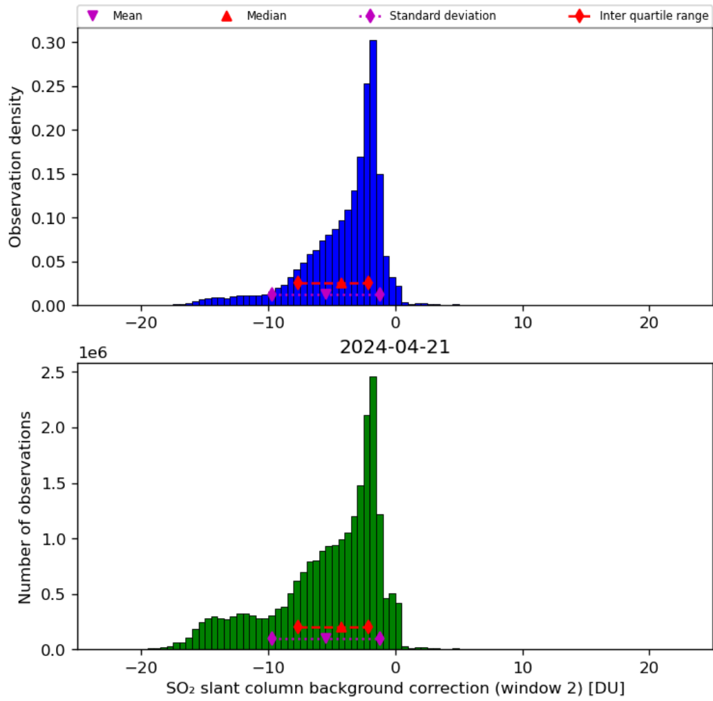
Figure 63: Histogram of “SO 2 slant column background correction (window 2)” for 2024-04-21 to 2024-04-22
