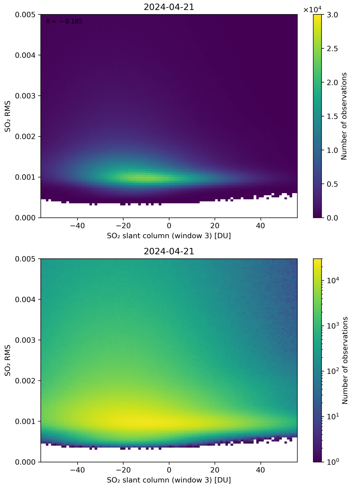
Figure 256: Scatter density plot of “SO 2 slant column (window 3)” against “SO 2 RMS” for 2024-04-21 to 2024-04-22.
