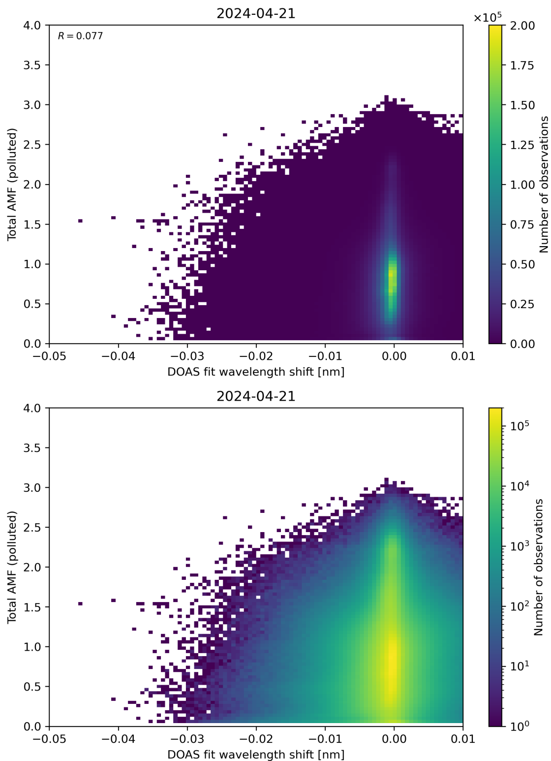
Figure 130: Scatter density plot of “DOAS fit wavelength shift” against “Total AMF (polluted)” for 2024-04-21 to 2024-04-22.
