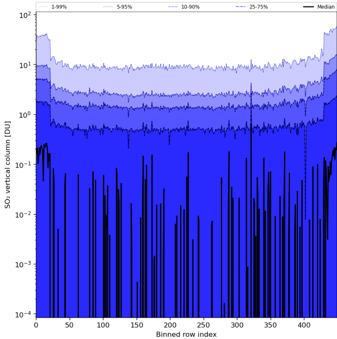
Figure 76: Along track statistics of “SO 2 vertical column” for 2024-04-21 to 2024-04-22
