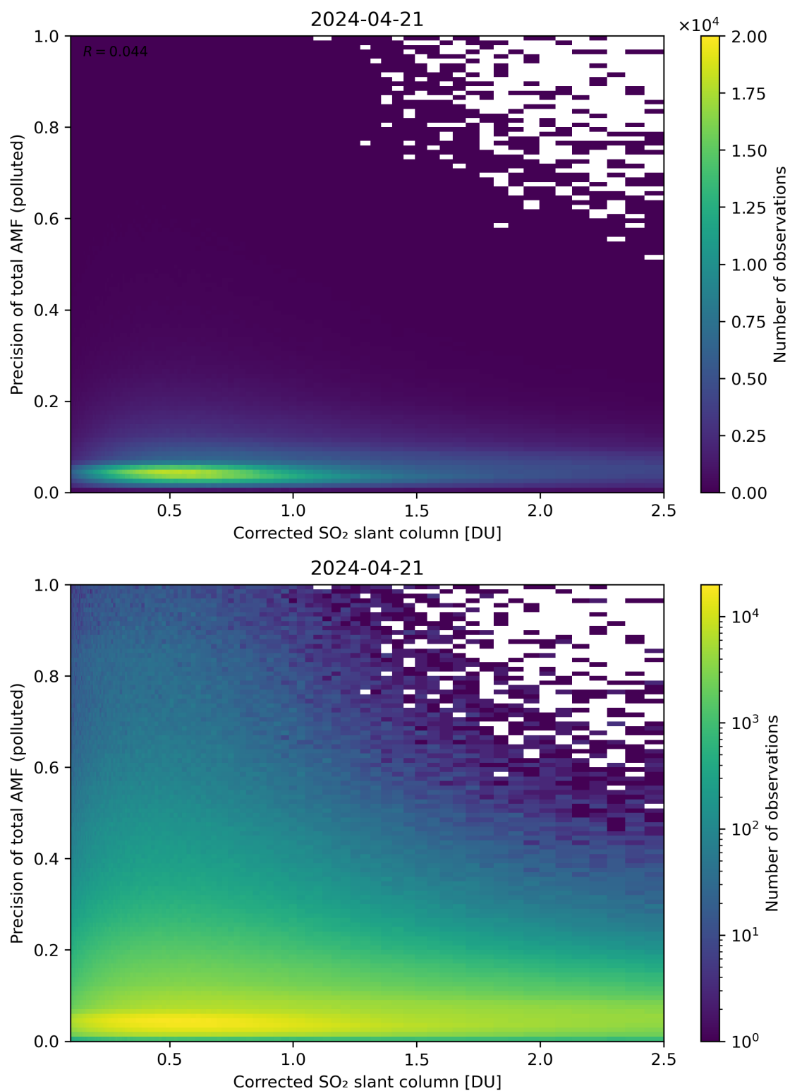
Figure 193: Scatter density plot of “Corrected SO 2 slant column” against “Precision of total AMF (polluted)” for 2024-04-21 to 2024-04-22.
