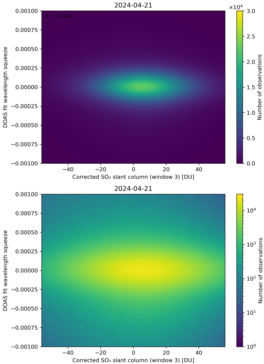
Figure 207: Scatter density plot of “Corrected SO 2 slant column (window 3)” against “DOAS fit wavelength squeeze” for 2024-04-21 to 2024-04-22.
