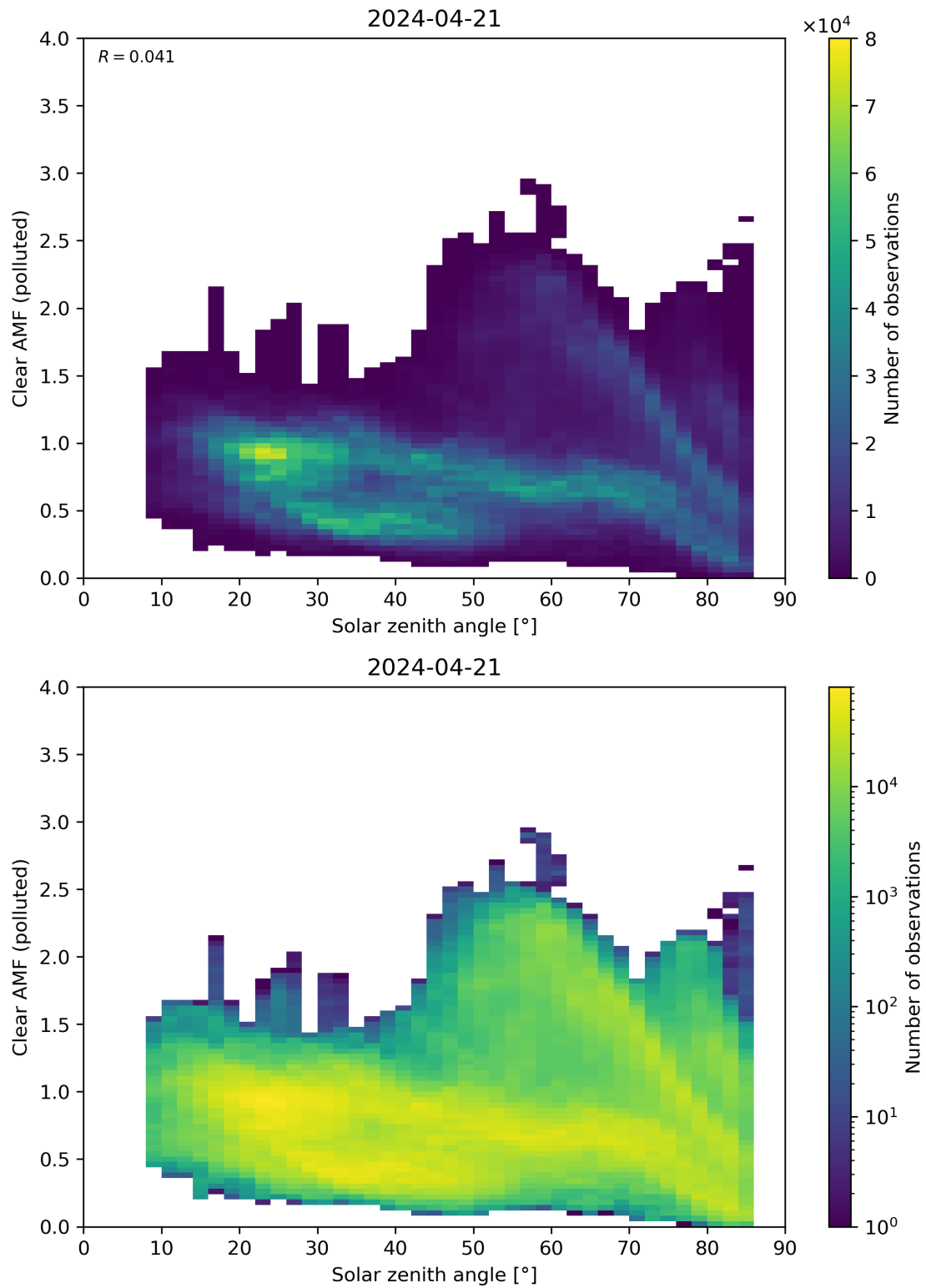
Figure 165: Scatter density plot of “Solar zenith angle” against “Clear AMF (polluted)” for 2024-04-21 to 2024-04-22.
