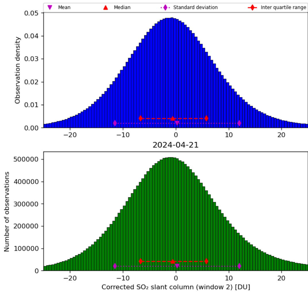
Figure 62: Histogram of “Corrected SO 2 slant column (window 2)” for 2024-04-21 to 2024-04-22
