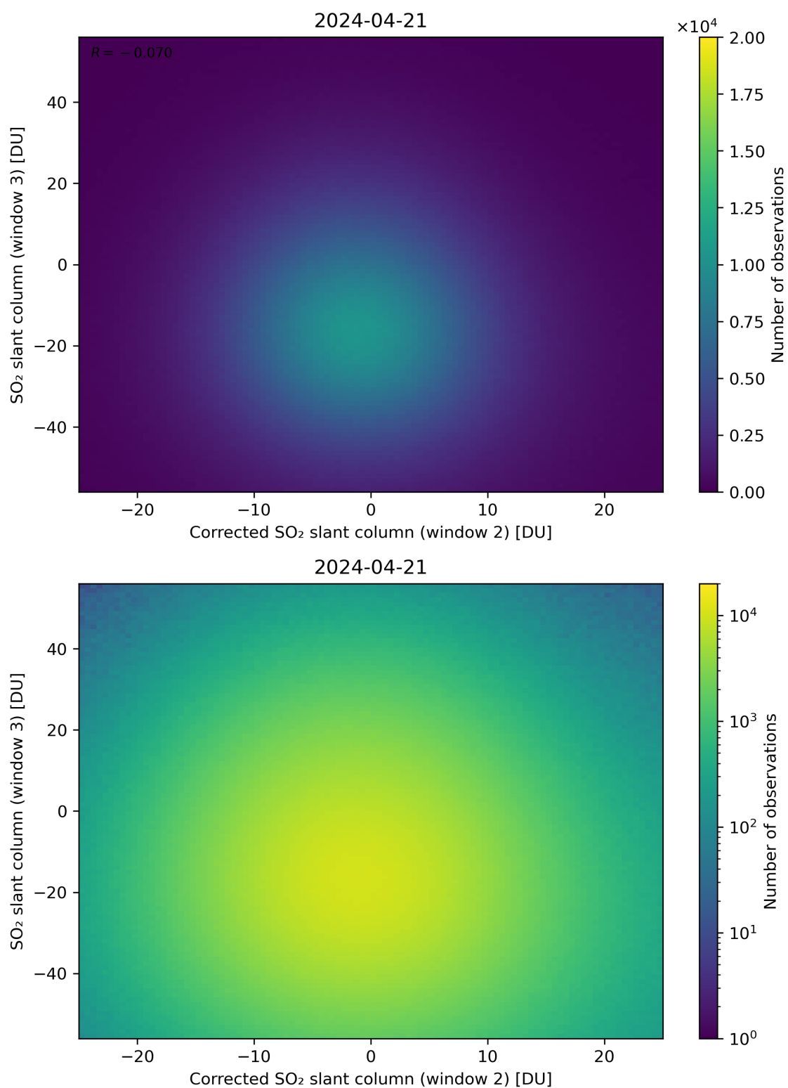
Figure 201: Scatter density plot of “Corrected SO 2 slant column (window 2)” against “SO 2 slant column (window 3)” for 2024-04-21 to 2024-04-22.
