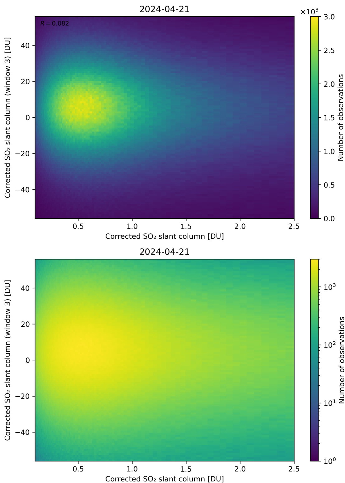
Figure 186: Scatter density plot of “Corrected SO 2 slant column” against “Corrected SO 2 slant column (window 3)” for 2024-04-21 to 2024-04-22.
