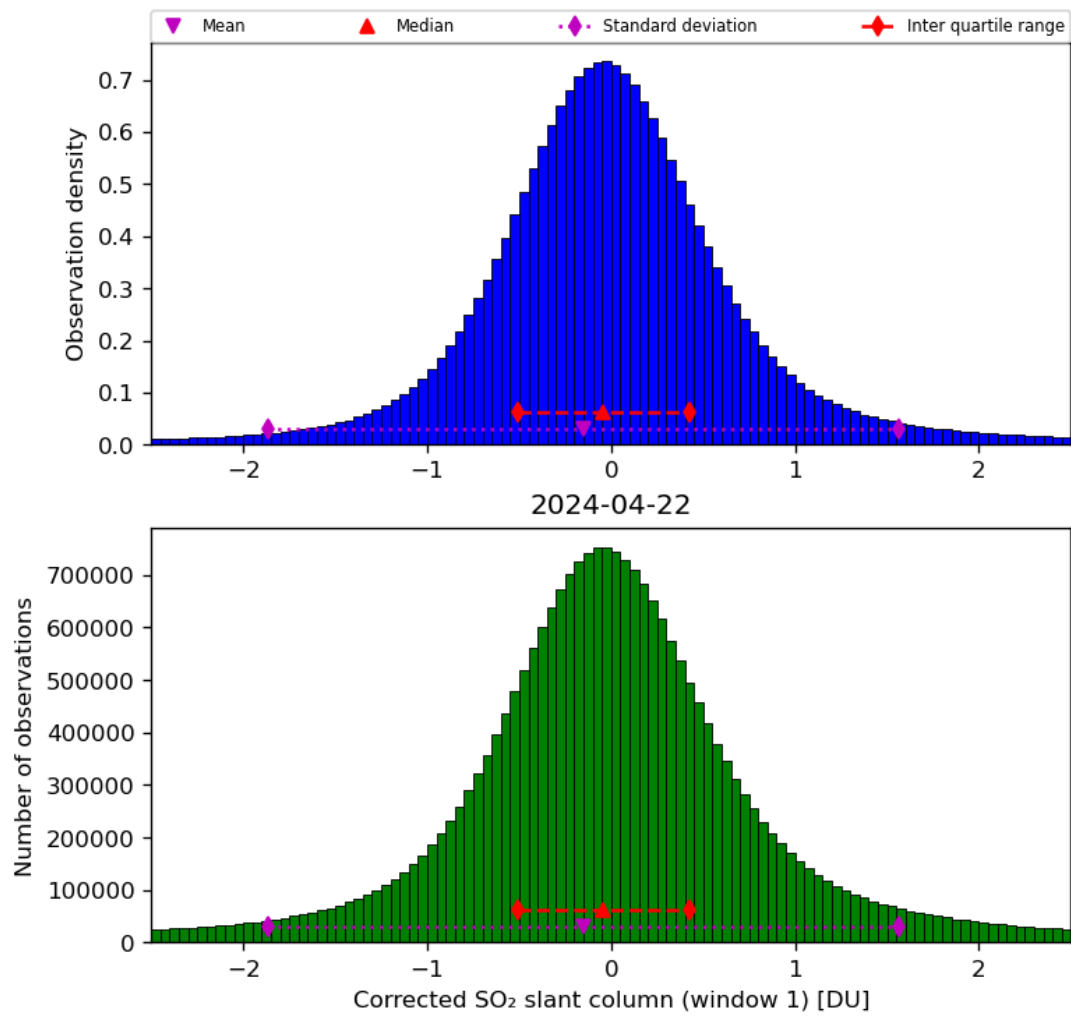
Figure 58: Histogram of “Corrected SO 2 slant column (window 1)” for 2024-04-21 to 2024-04-23
