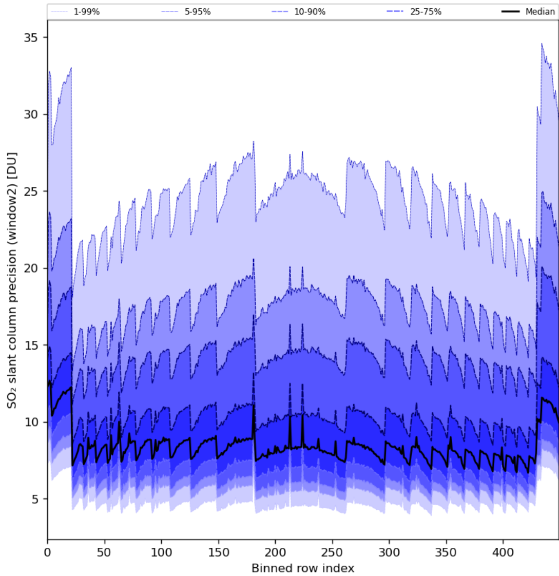
Figure 84: Along track statistics of “SO 2 slant column precision (window2)” for 2024-04-21 to 2024-04-23
