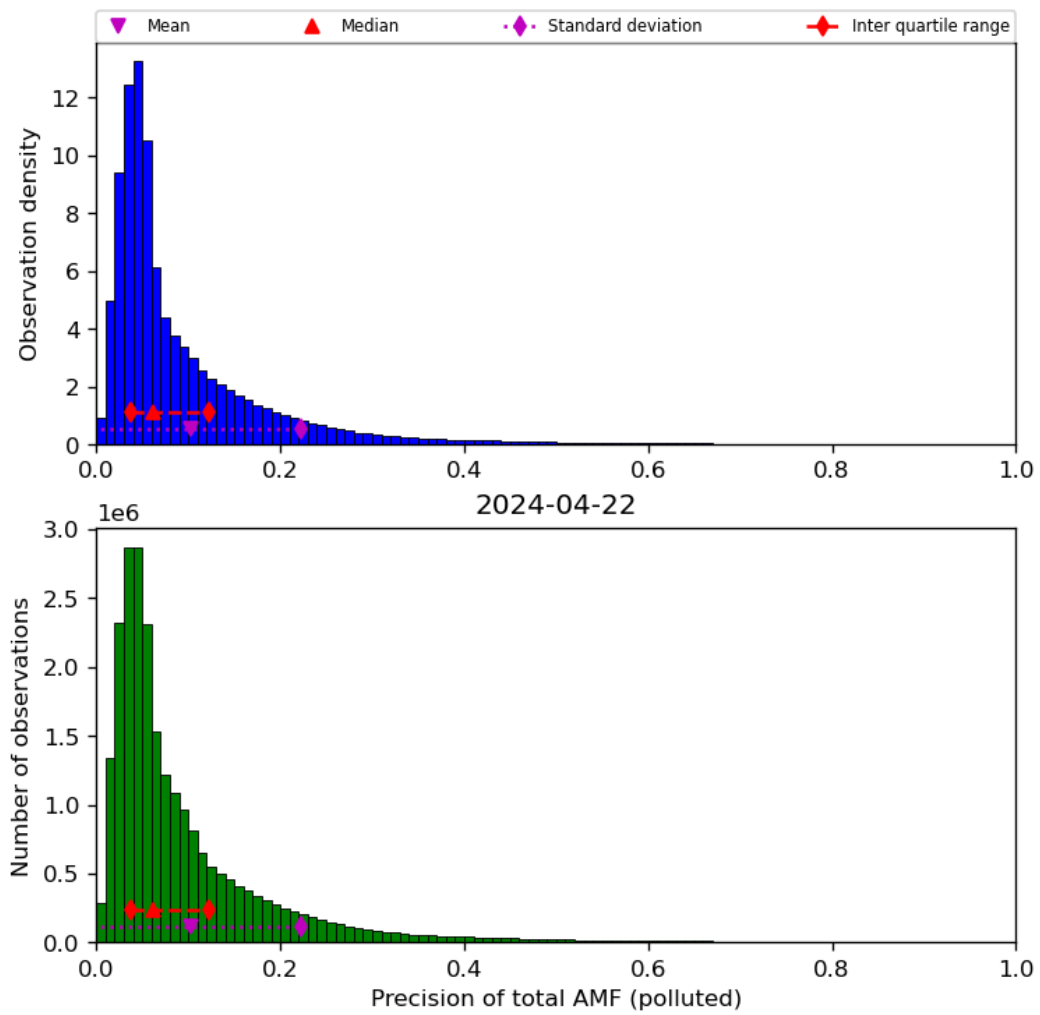
Figure 72: Histogram of “Precision of total AMF (polluted)” for 2024-04-21 to 2024-04-23
