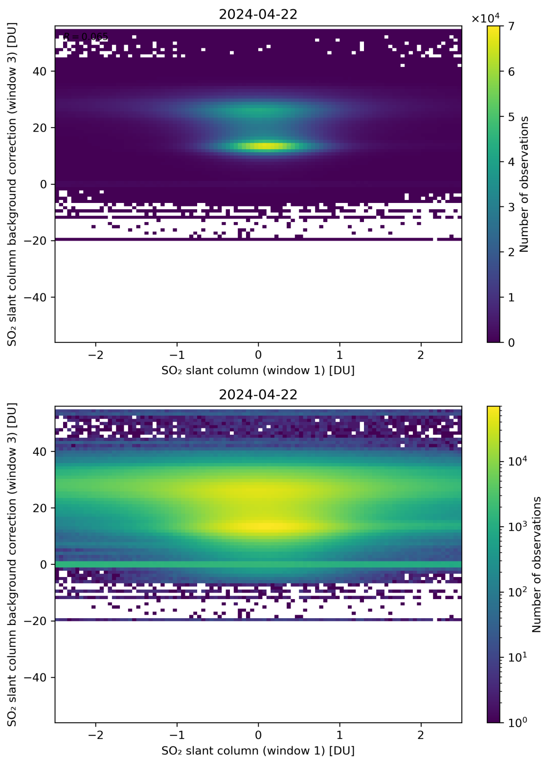
Figure 214: Scatter density plot of “SO 2 slant column (window 1)” against “SO 2 slant column background correction (window 3)” for 2024-04-21 to 2024-04-23.
