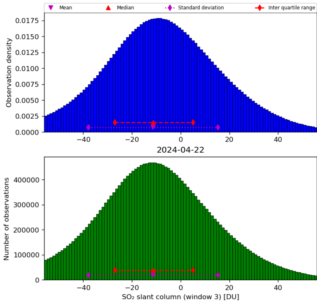
Figure 64: Histogram of “SO 2 slant column (window 3)” for 2024-04-21 to 2024-04-23
