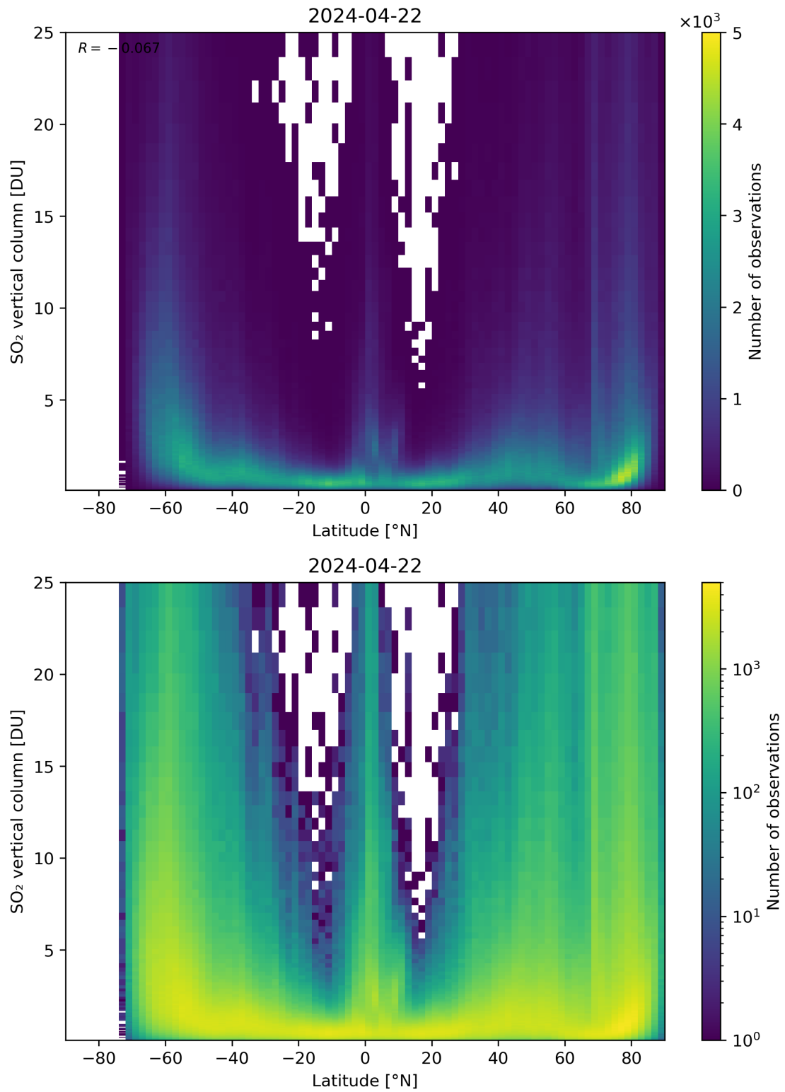
Figure 156: Scatter density plot of “Latitude” against “SO 2 vertical column” for 2024-04-21 to 2024-04-23.
