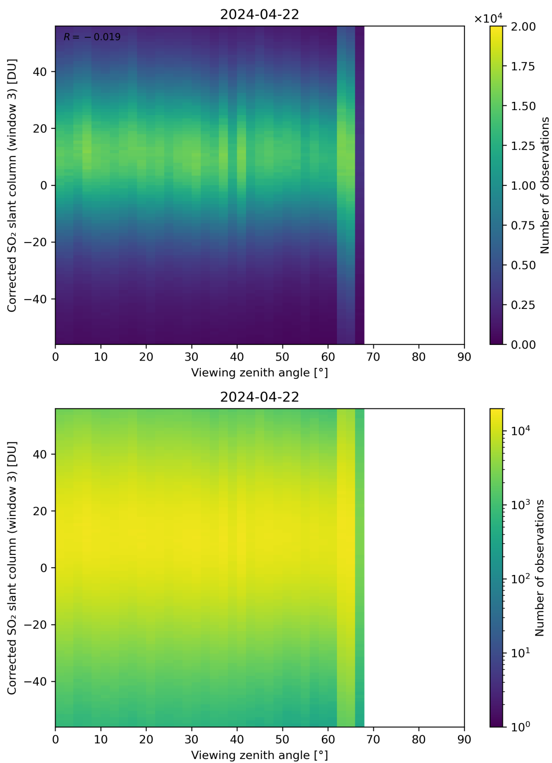
Figure 319: Scatter density plot of “Viewing zenith angle” against “Corrected SO 2 slant column (window 3)” for 2024-04-21 to 2024-04-23.
