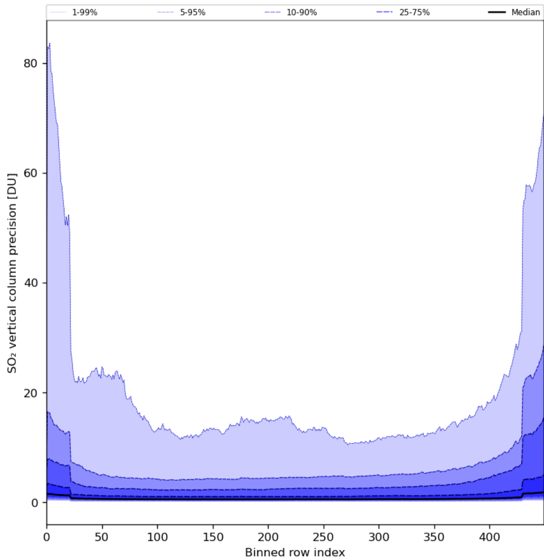
Figure 77: Along track statistics of “SO 2 vertical column precision” for 2024-04-21 to 2024-04-23
