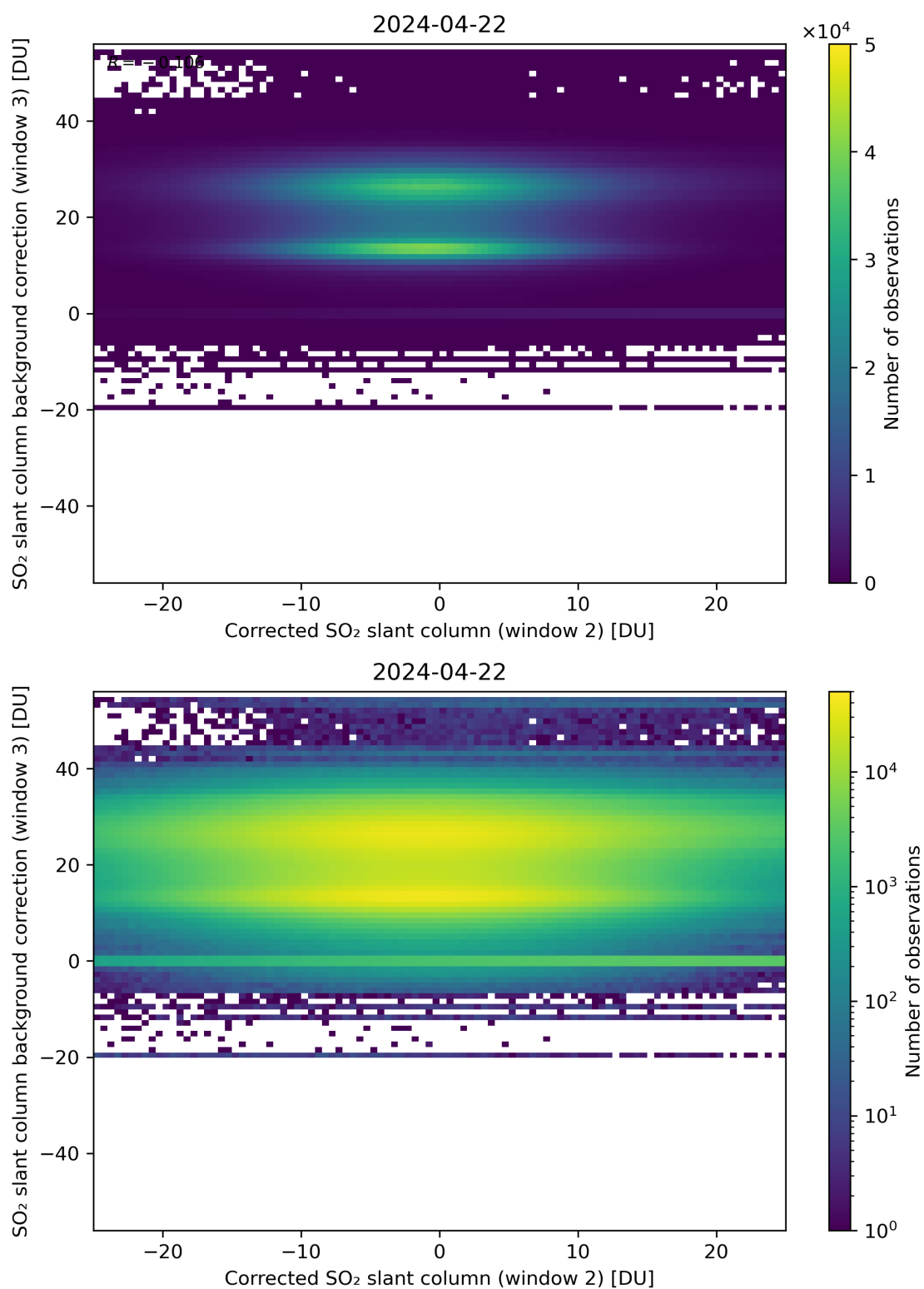
Figure 195: Scatter density plot of “Corrected SO 2 slant column (window 2)” against “SO 2 slant column background correction (window 3)” for 2024-04-21 to 2024-04-23.
