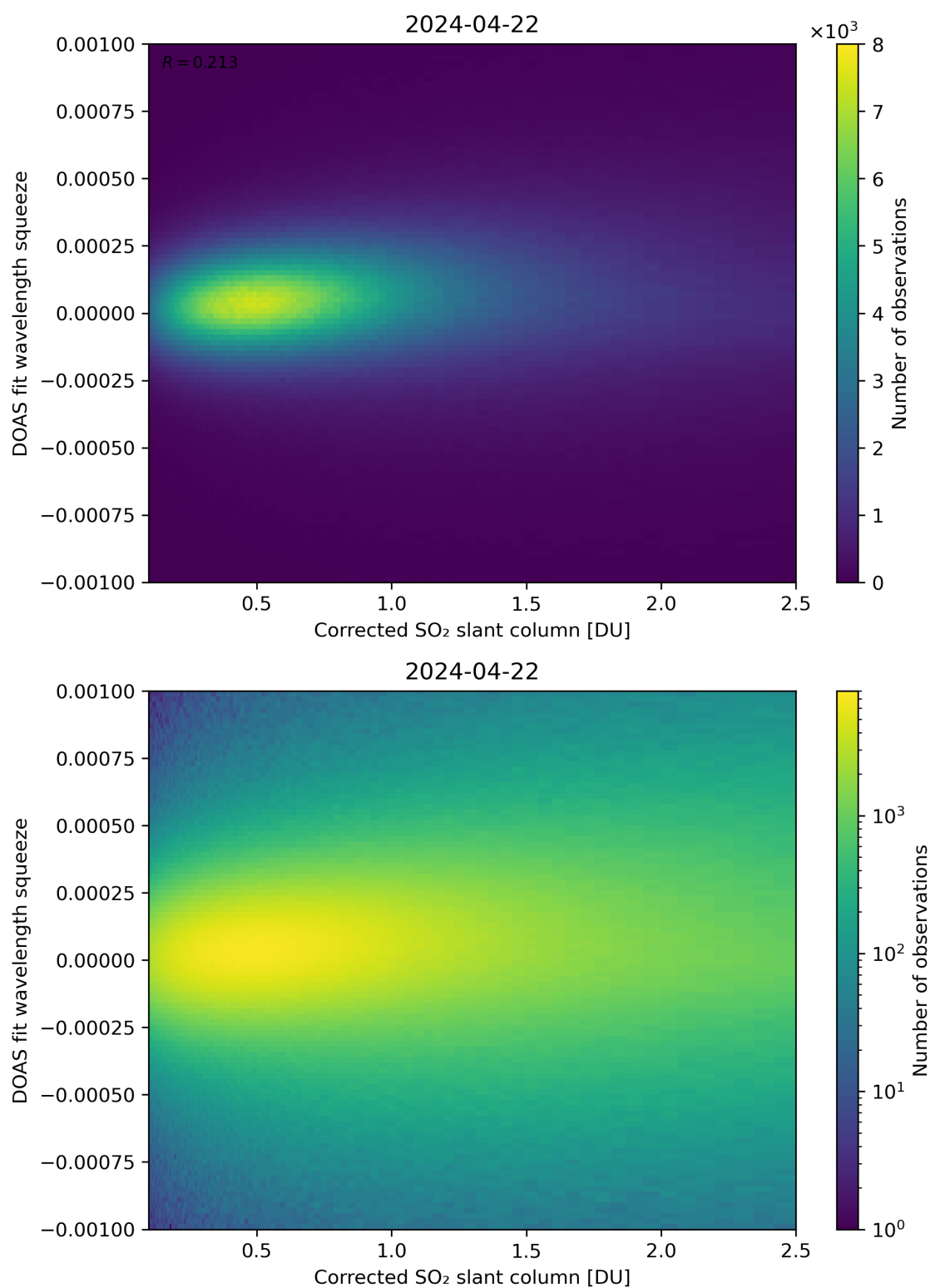
Figure 182: Scatter density plot of “Corrected SO 2 slant column” against “DOAS fit wavelength squeeze” for 2024-04-21 to 2024-04-23.
