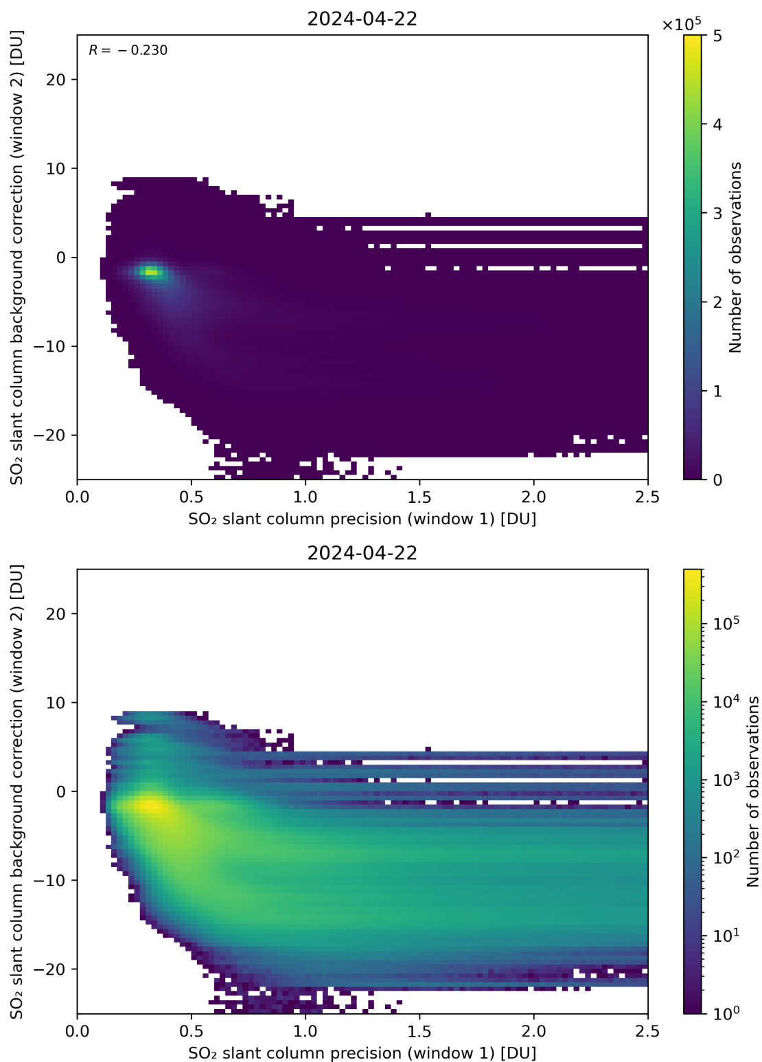
Figure 219: Scatter density plot of “SO 2 slant column precision (window 1)” against “SO 2 slant column background correction (window 2)” for 2024-04-21 to 2024-04-23.
