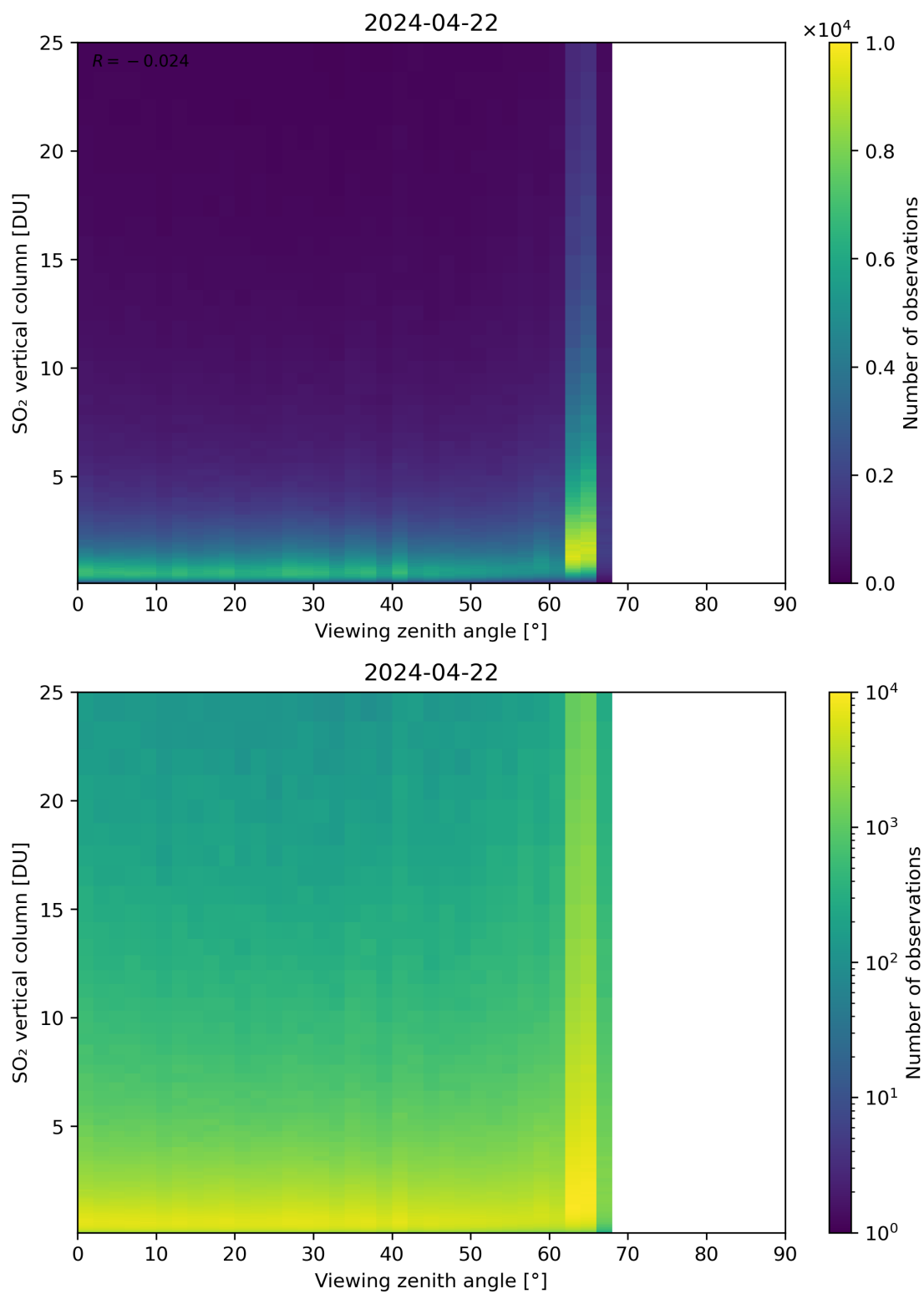
Figure 327: Scatter density plot of “Viewing zenith angle” against “SO 2 vertical column” for 2024-04-21 to 2024-04-23.
