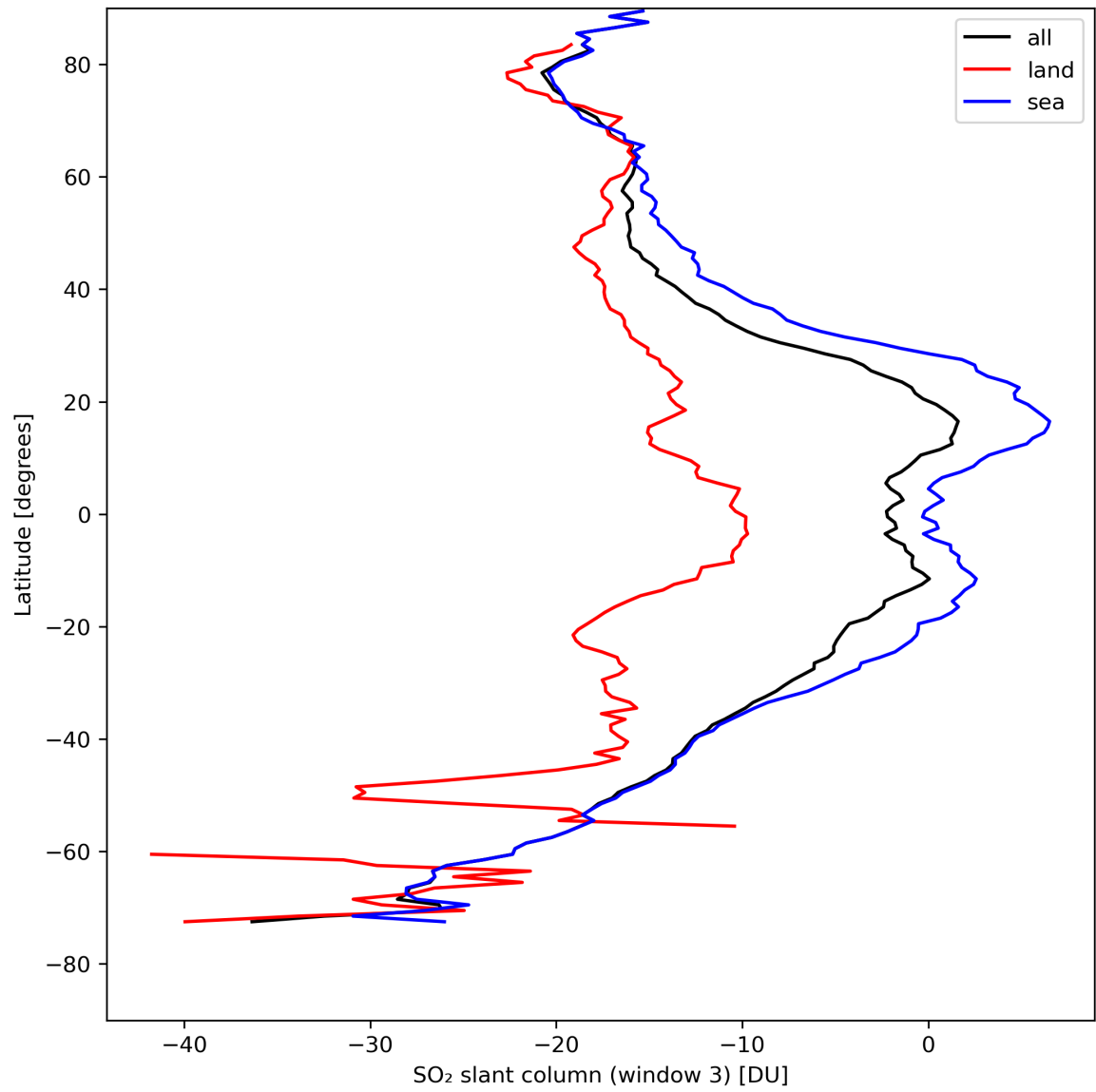
Figure 41: Zonal average of “SO 2 slant column (window 3)” for 2024-04-21 to 2024-04-23.
