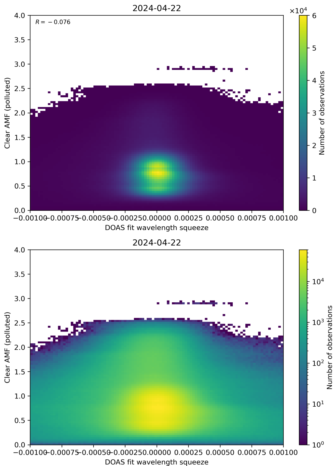
Figure 133: Scatter density plot of “DOAS fit wavelength squeeze” against “Clear AMF (polluted)” for 2024-04-21 to 2024-04-23.
