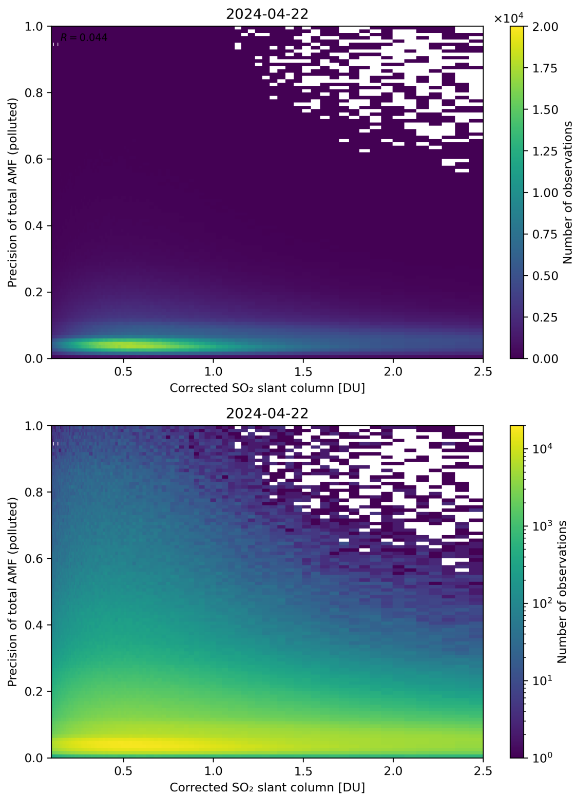
Figure 193: Scatter density plot of “Corrected SO 2 slant column” against “Precision of total AMF (polluted)” for 2024-04-21 to 2024-04-23.
