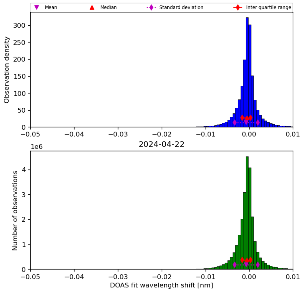
Figure 68: Histogram of “DOAS fit wavelength shift” for 2024-04-21 to 2024-04-23
