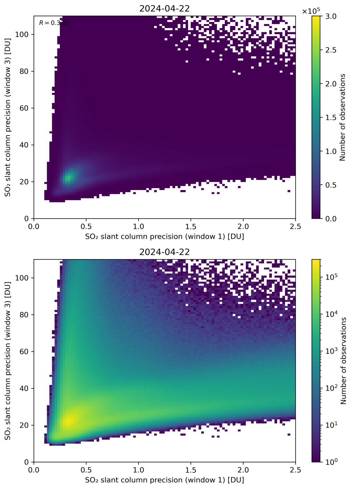
Figure 229: Scatter density plot of “SO 2 slant column precision (window 1)” against “SO 2 slant column precision (window 3)” for 2024-04-21 to 2024-04-23.
