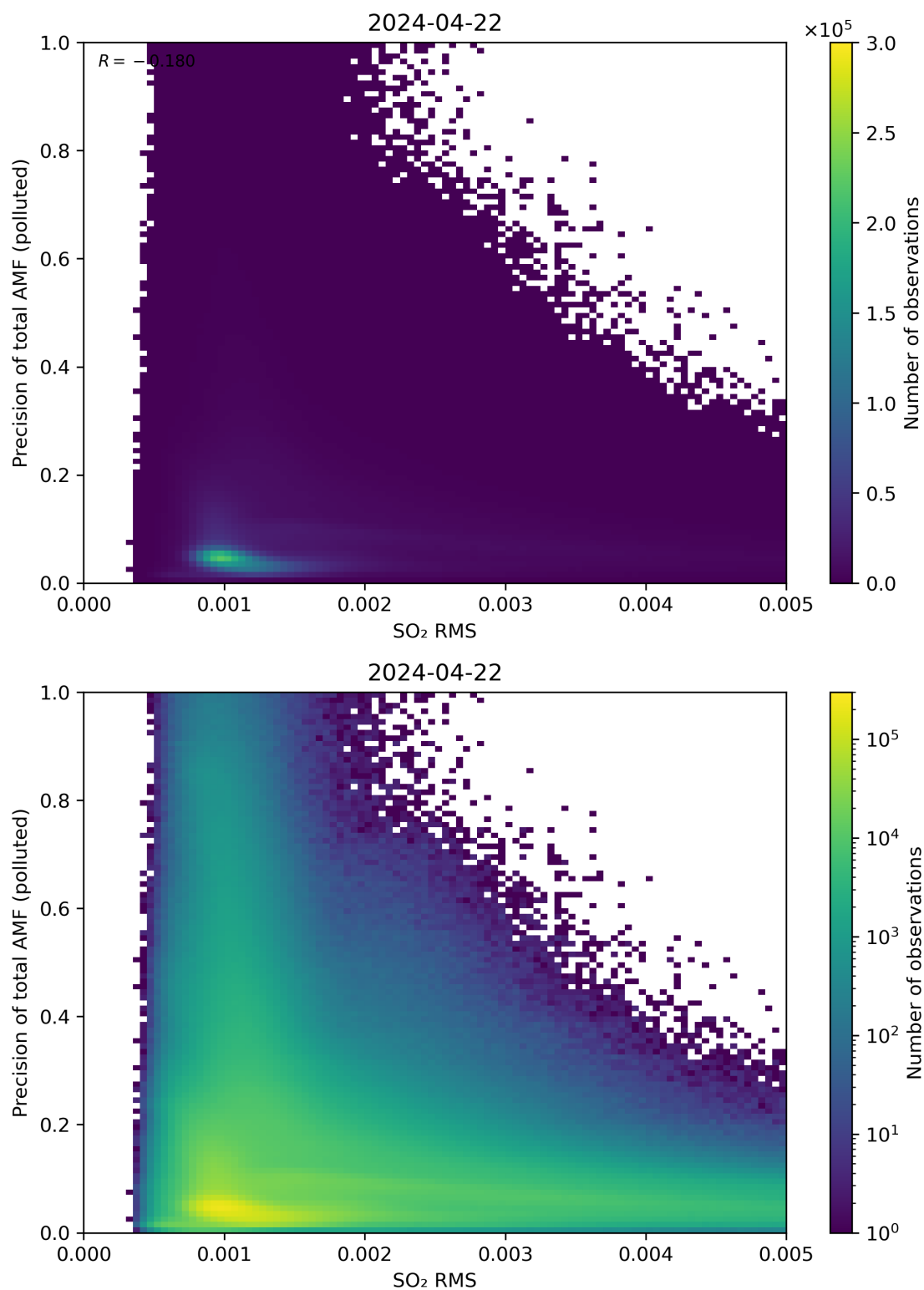
Figure 138: Scatter density plot of “SO 2 RMS” against “Precision of total AMF (polluted)” for 2024-04-21 to 2024-04-23.
