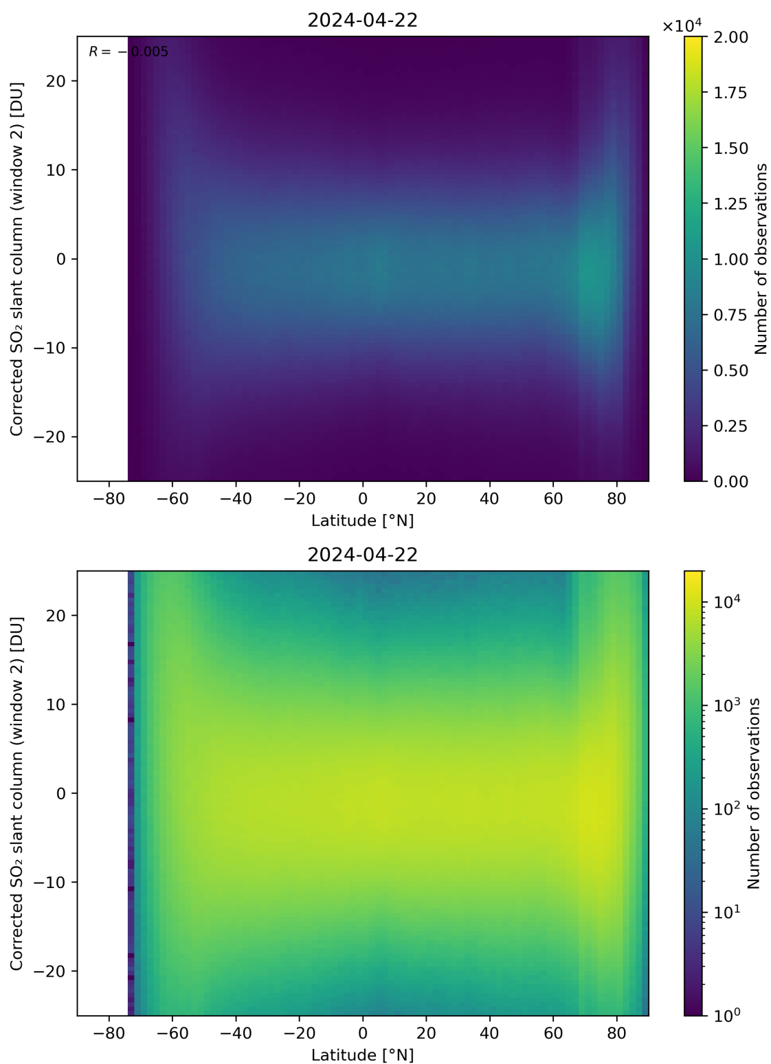
Figure 147: Scatter density plot of “Latitude” against “Corrected SO 2 slant column (window 2)” for 2024-04-21 to 2024-04-23.
