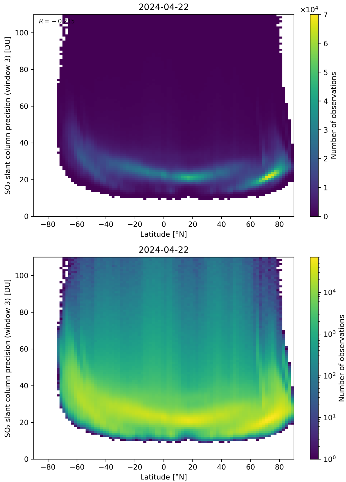
Figure 153: Scatter density plot of “Latitude” against “SO 2 slant column precision (window 3)” for 2024-04-21 to 2024-04-23.
