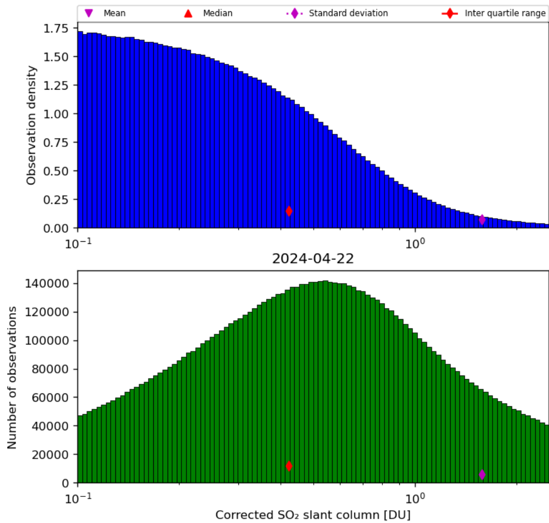
Figure 55: Histogram of “Corrected SO 2 slant column” for 2024-04-21 to 2024-04-23
