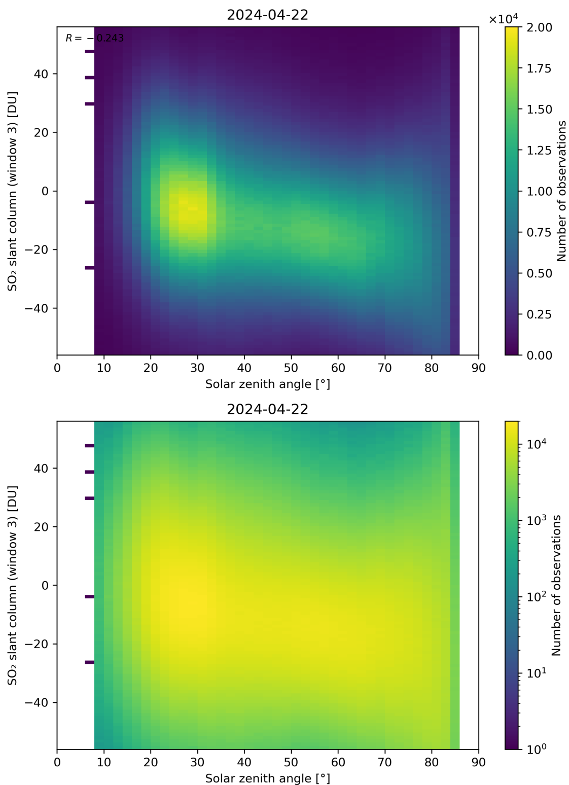
Figure 172: Scatter density plot of “Solar zenith angle” against “SO 2 slant column (window 3)” for 2024-04-21 to 2024-04-23.
