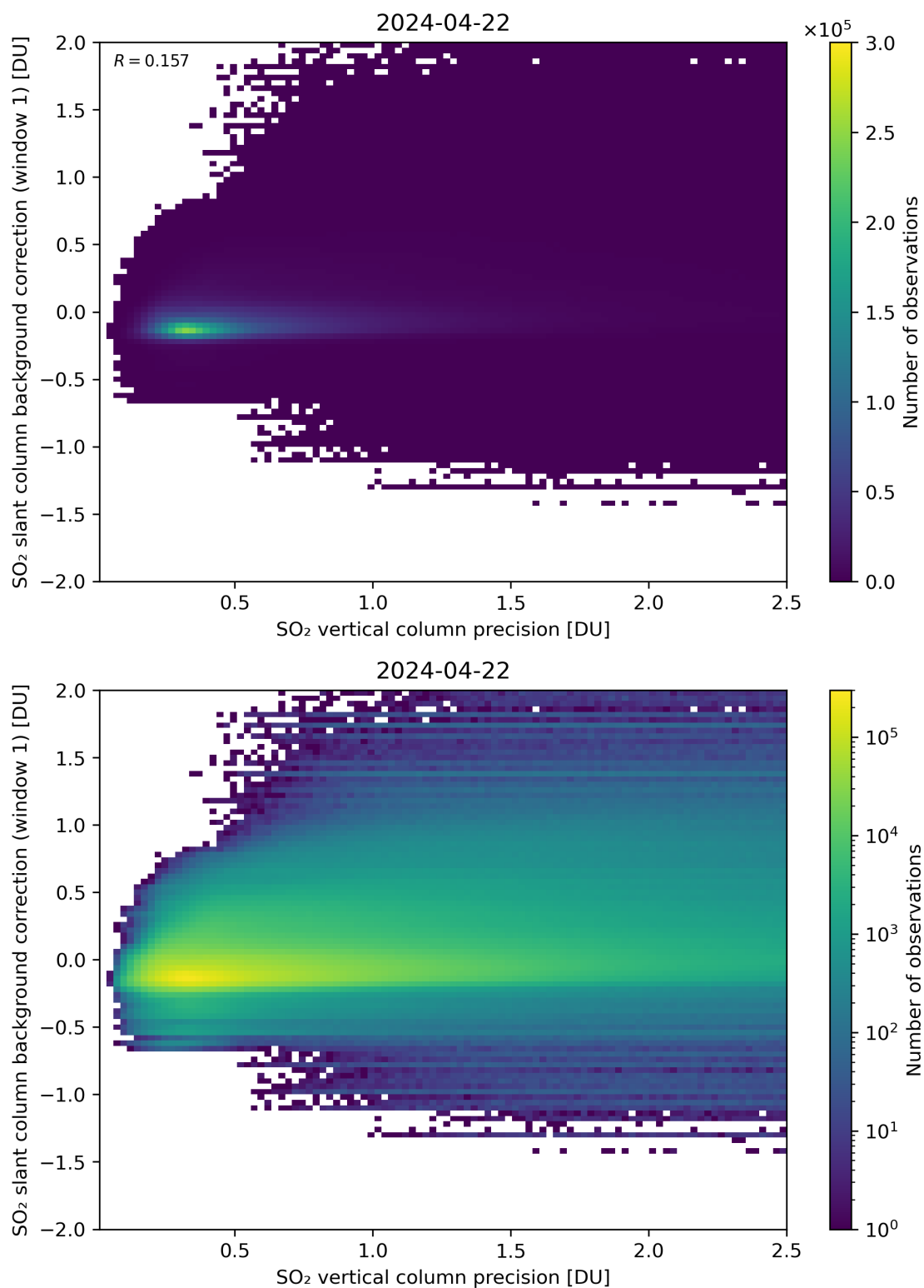
Figure 279: Scatter density plot of “SO 2 vertical column precision” against “SO 2 slant column background correction (window 1)” for 2024-04-21 to 2024-04-23.
