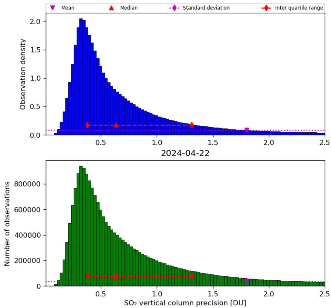
Figure 54: Histogram of “SO 2 vertical column precision” for 2024-04-21 to 2024-04-23
