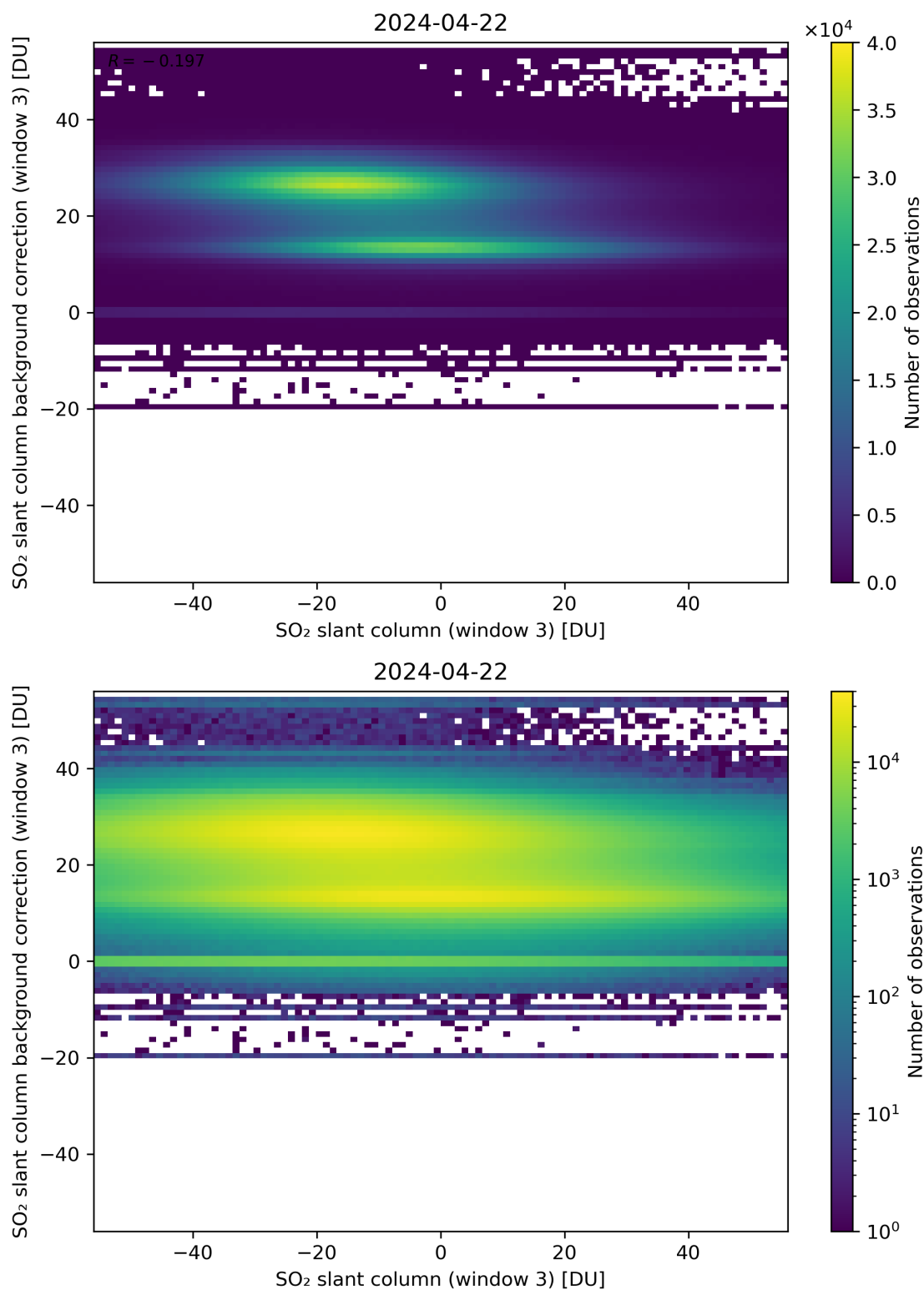
Figure 253: Scatter density plot of “SO 2 slant column (window 3)” against “SO 2 slant column background correction (window 3)” for 2024-04-21 to 2024-04-23.
