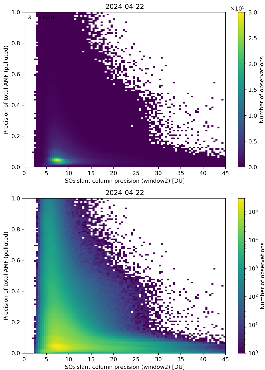
Figure 252: Scatter density plot of “SO 2 slant column precision (window2)” against “Precision of total AMF (polluted)” for 2024-04-21 to 2024-04-23.
