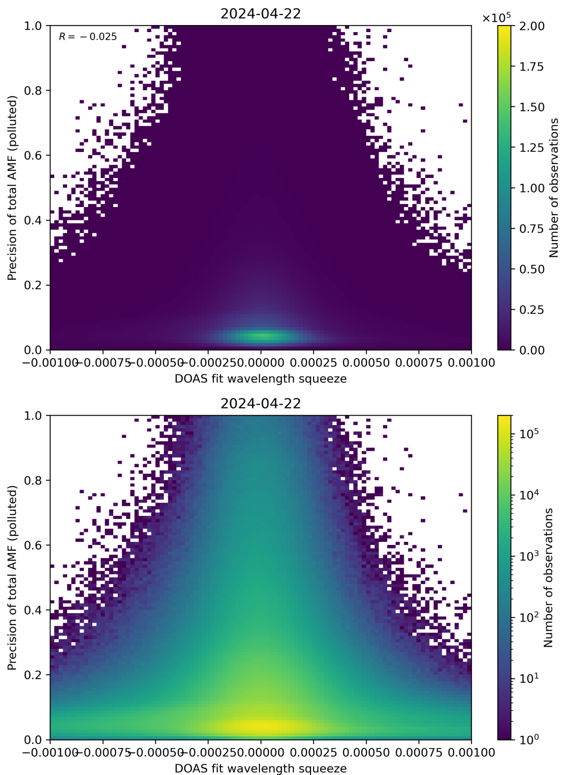
Figure 135: Scatter density plot of “DOAS fit wavelength squeeze” against “Precision of total AMF (polluted)” for 2024-04-21 to 2024-04-23.
