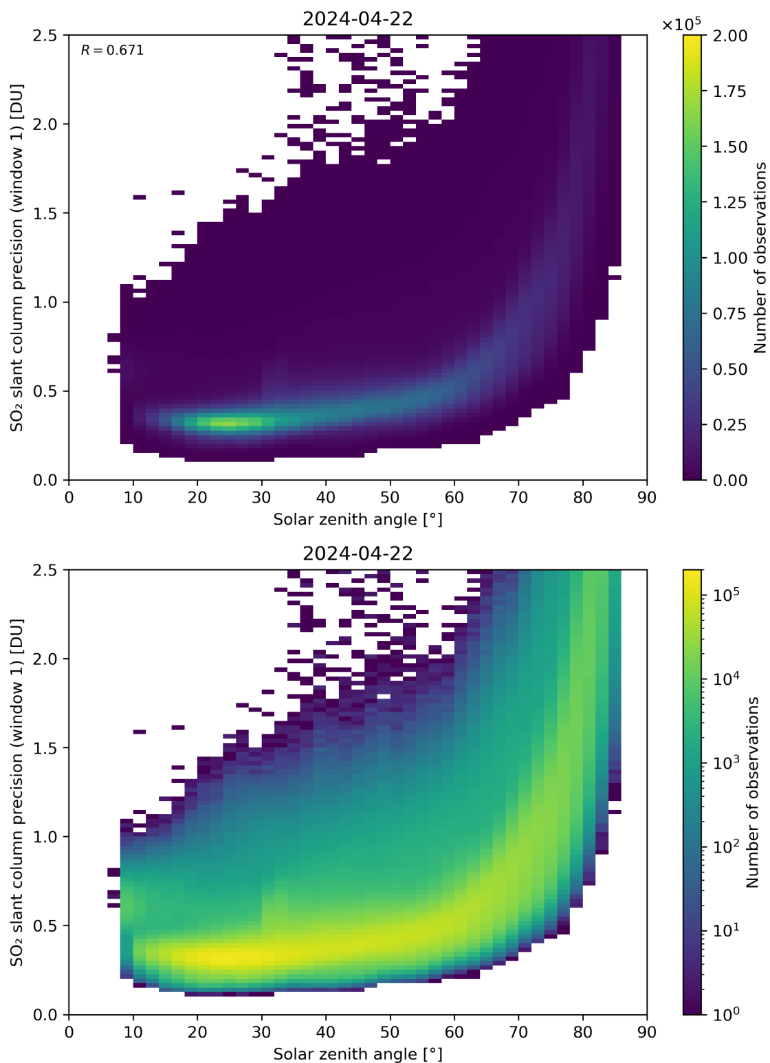
Figure 170: Scatter density plot of “Solar zenith angle” against “SO 2 slant column precision (window 1)” for 2024-04-21 to 2024-04-23.
