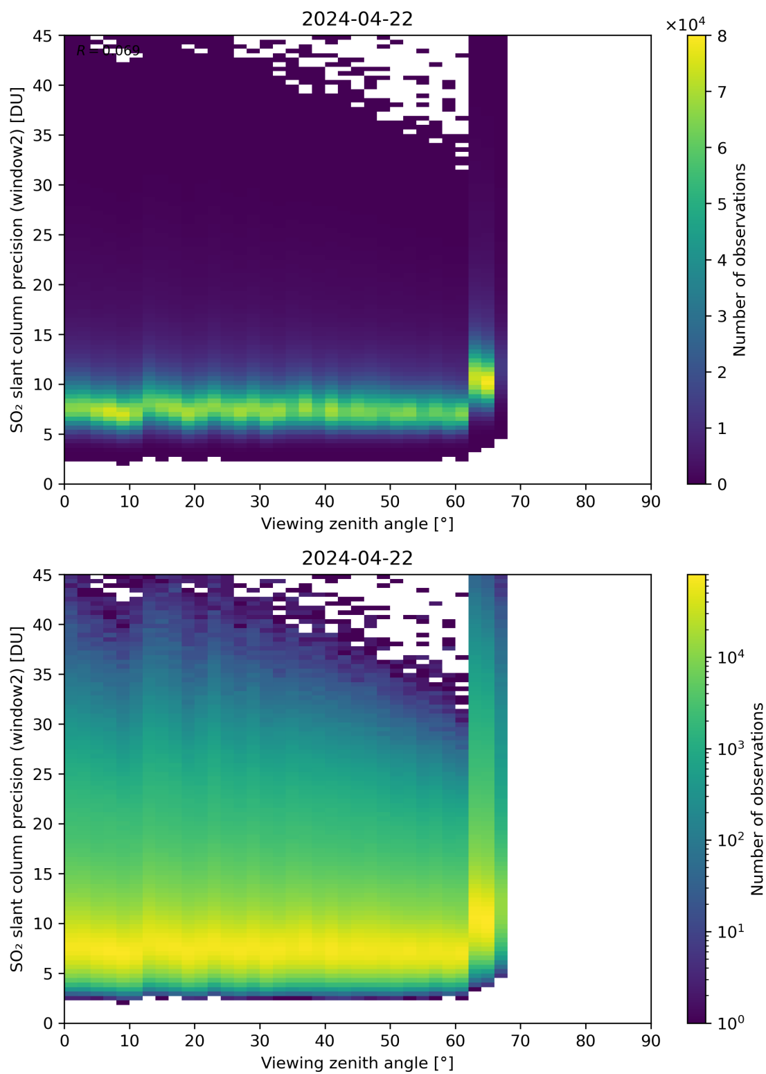
Figure 322: Scatter density plot of “Viewing zenith angle” against “SO 2 slant column precision (window2)” for 2024-04-21 to 2024-04-23.
