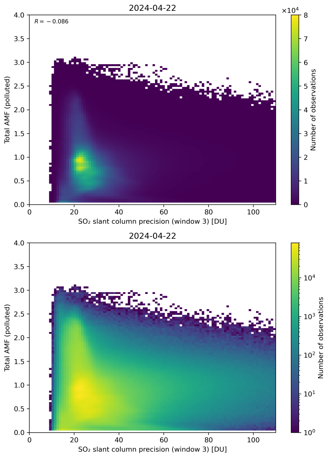
Figure 263: Scatter density plot of “SO 2 slant column precision (window 3)” against “Total AMF (polluted)” for 2024-04-21 to 2024-04-23.
