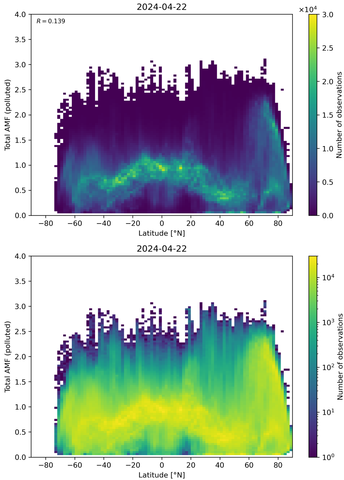
Figure 154: Scatter density plot of “Latitude” against “Total AMF (polluted)” for 2024-04-21 to 2024-04-23.
