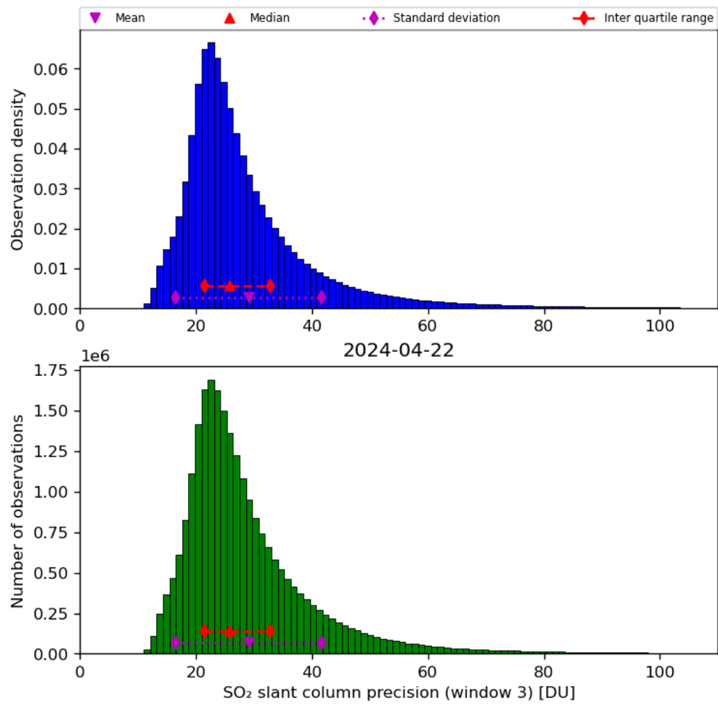
Figure 65: Histogram of “SO 2 slant column precision (window 3)” for 2024-04-21 to 2024-04-23
