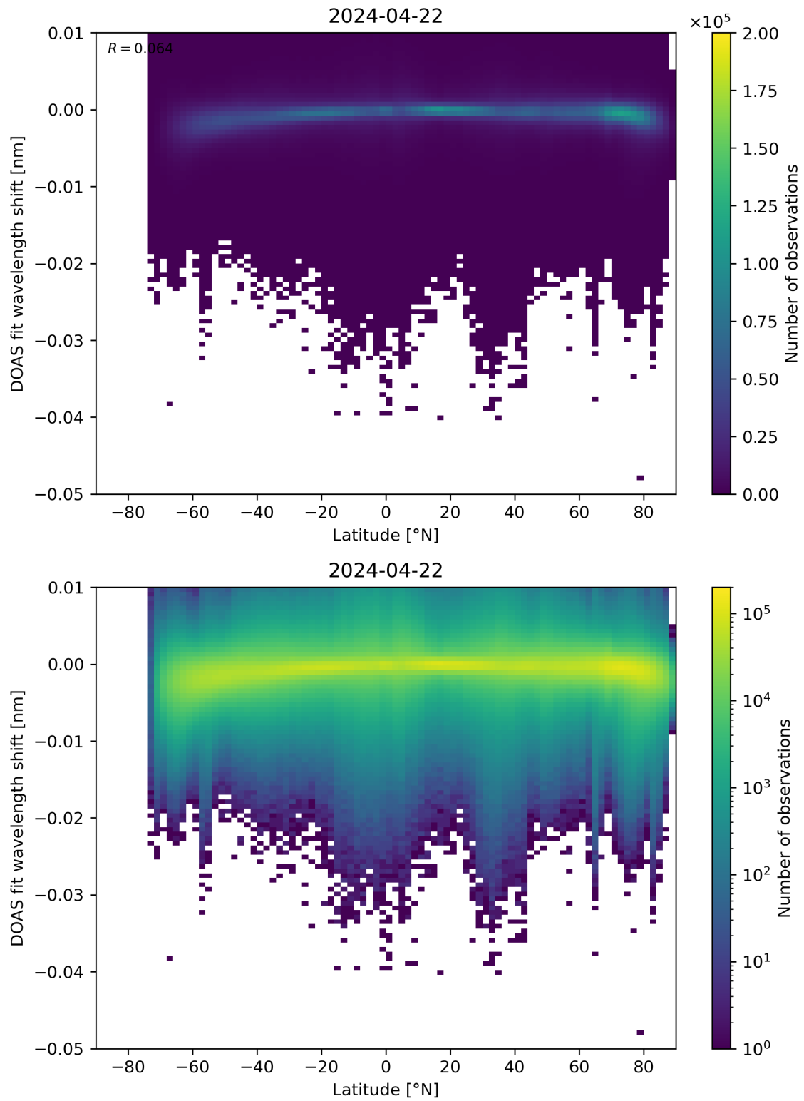
Figure 142: Scatter density plot of “Latitude” against “DOAS fit wavelength shift” for 2024-04-21 to 2024-04-23.
