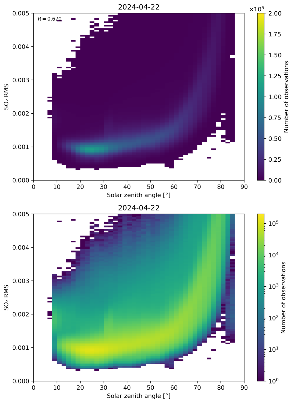
Figure 163: Scatter density plot of “Solar zenith angle” against “SO 2 RMS” for 2024-04-21 to 2024-04-23.
