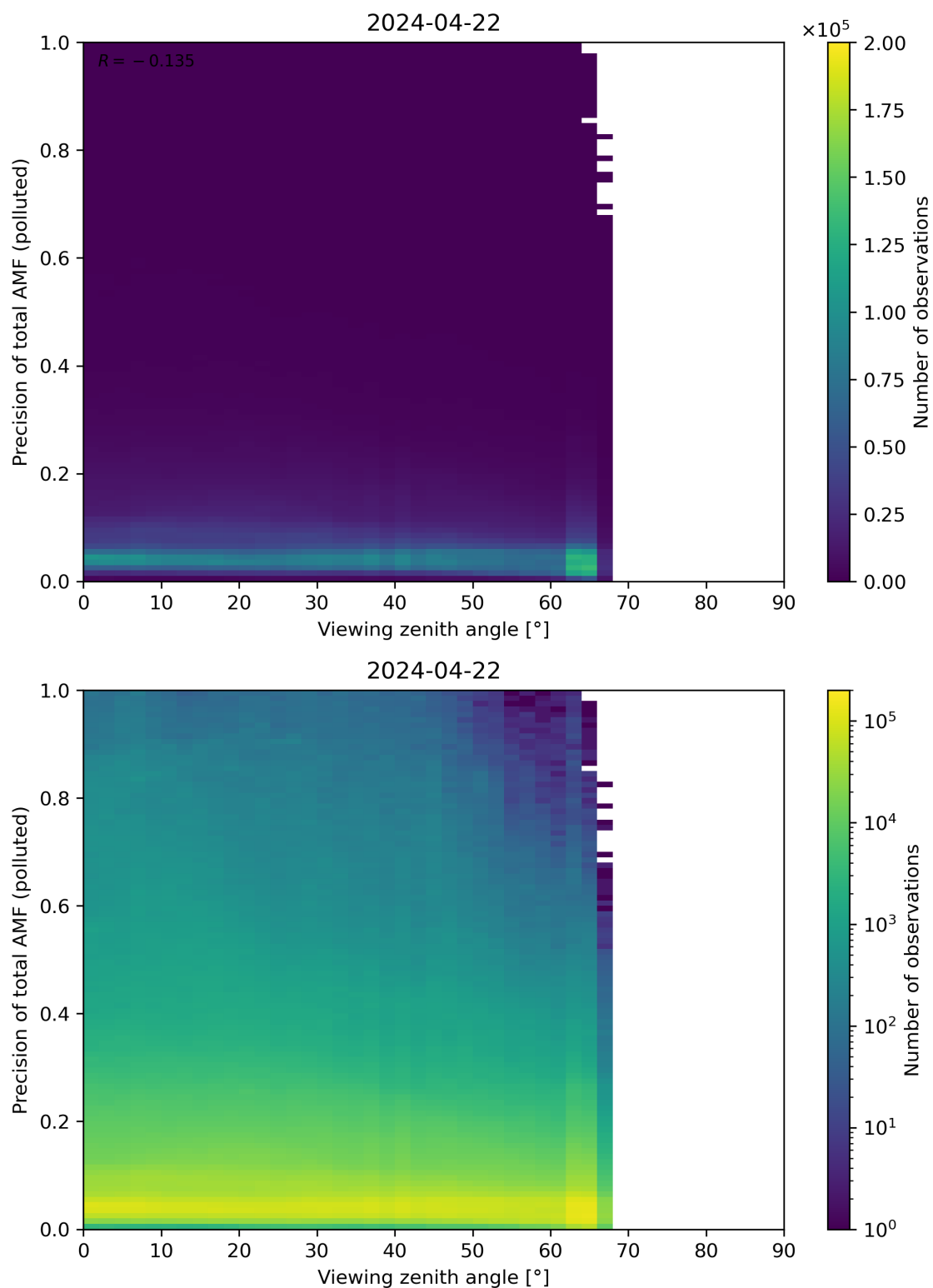
Figure 326: Scatter density plot of “Viewing zenith angle” against “Precision of total AMF (polluted)” for 2024-04-21 to 2024-04-23.
