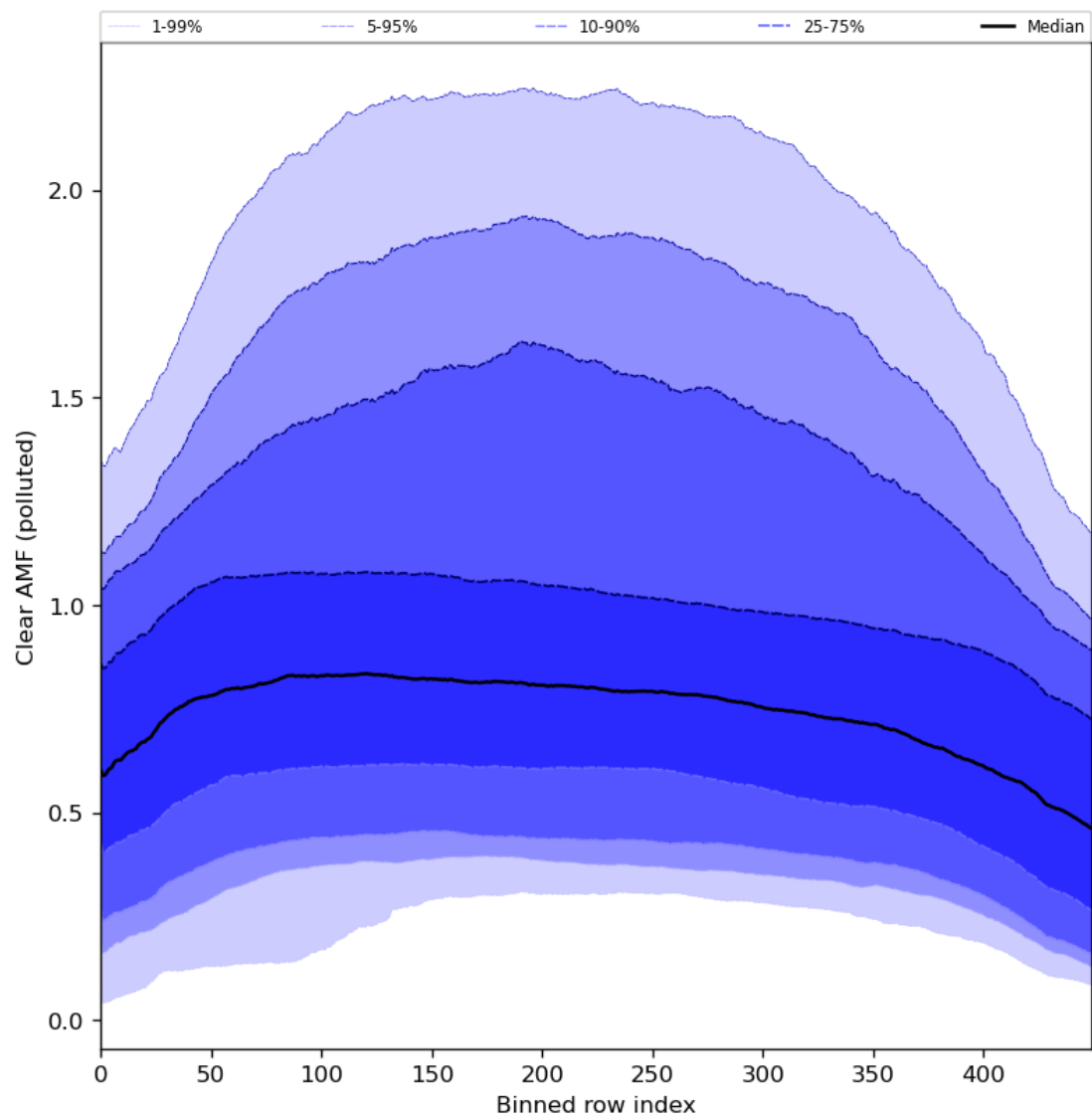
Figure 96: Along track statistics of “Clear AMF (polluted)” for 2024-04-21 to 2024-04-23
