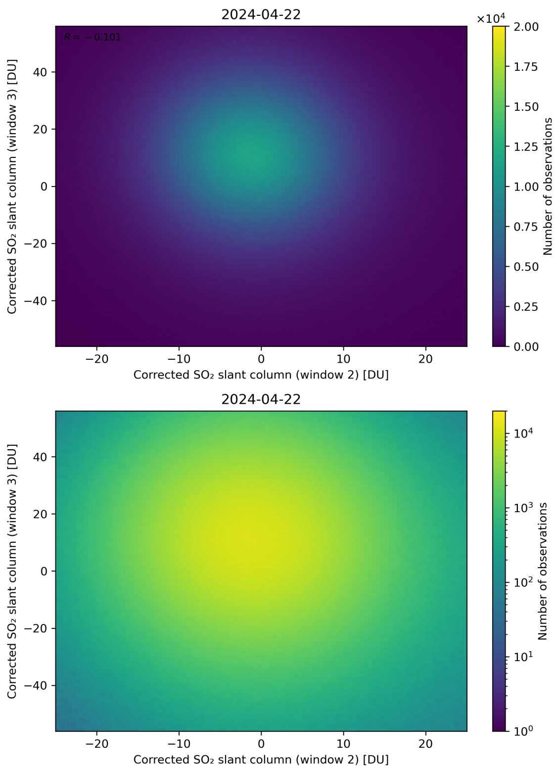
Figure 200: Scatter density plot of “Corrected SO 2 slant column (window 2)” against “Corrected SO 2 slant column (window 3)” for 2024-04-21 to 2024-04-23.
