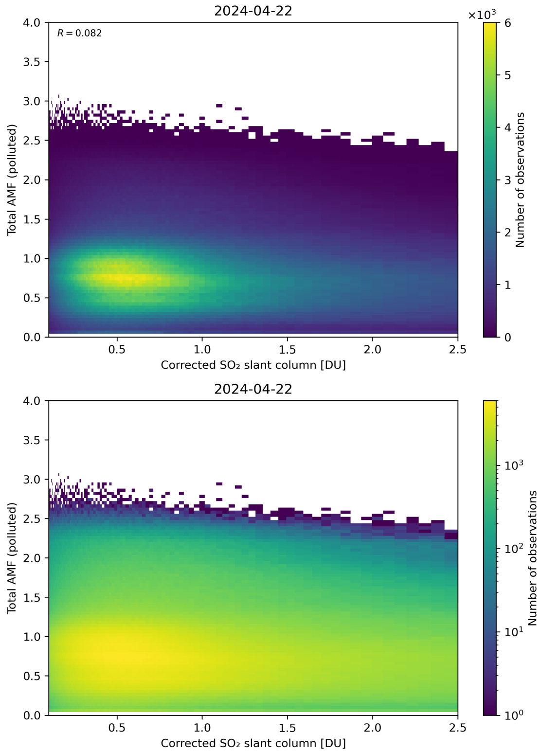
Figure 192: Scatter density plot of “Corrected SO 2 slant column” against “Total AMF (polluted)” for 2024-04-21 to 2024-04-23.
