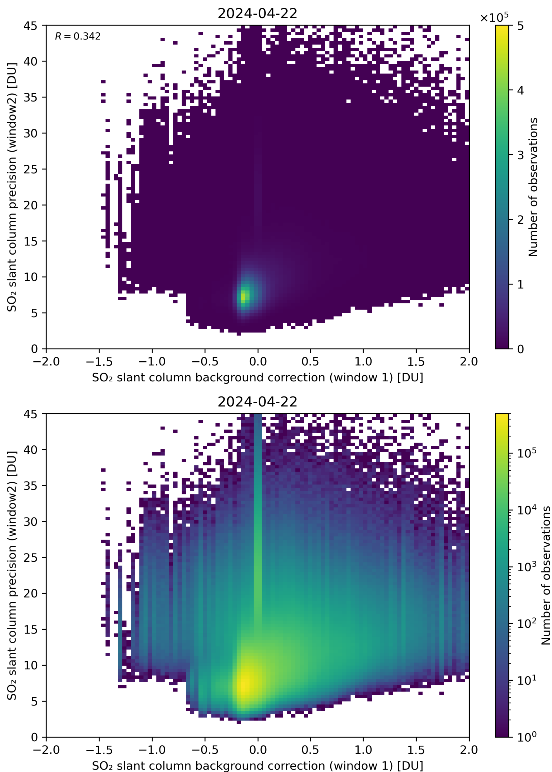
Figure 106: Scatter density plot of “SO 2 slant column background correction (window 1)” against “SO 2 slant column precision (window2)” for 2024-04-21 to 2024-04-23.
