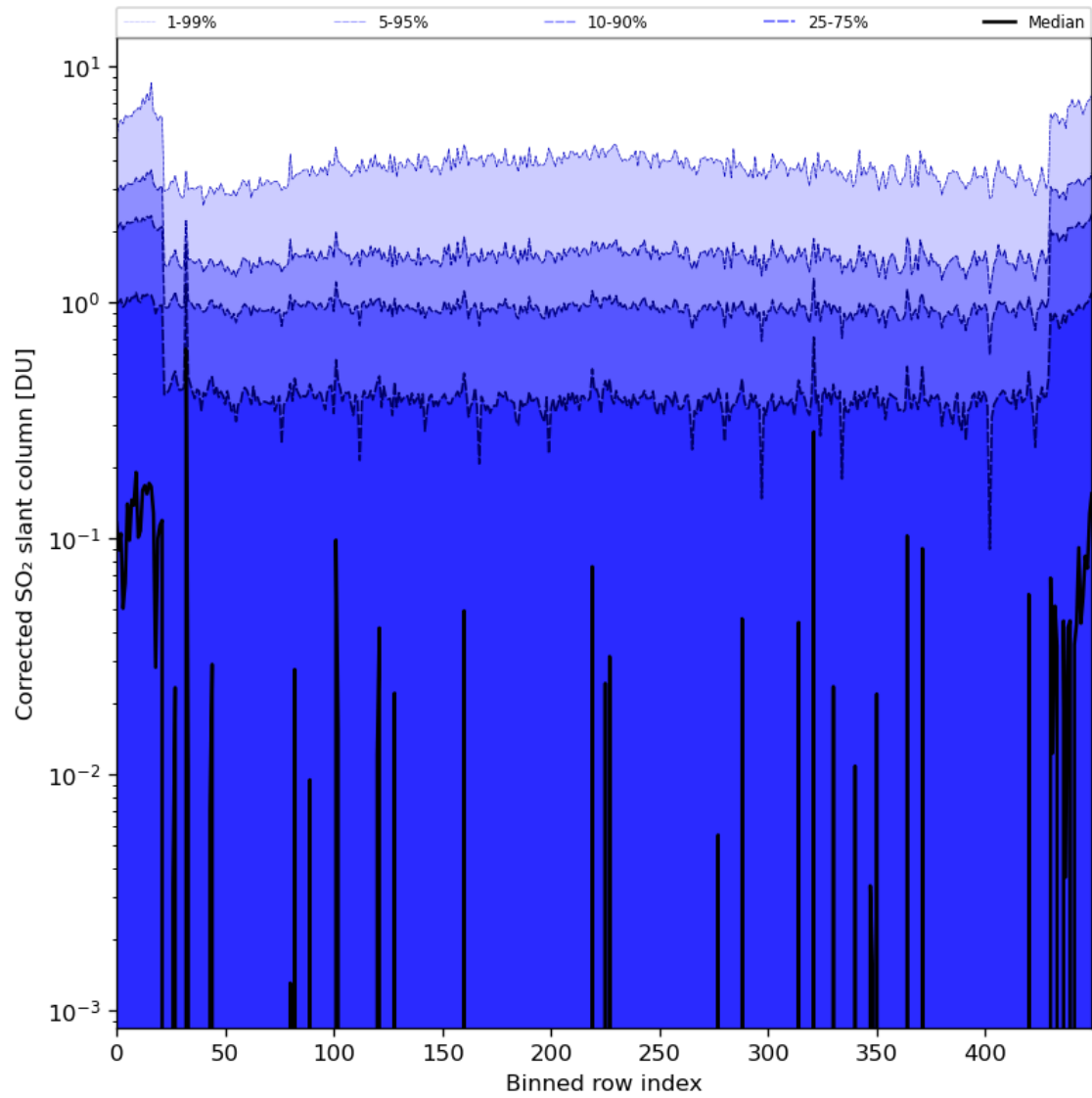
Figure 78: Along track statistics of “Corrected SO 2 slant column” for 2024-04-21 to 2024-04-23
