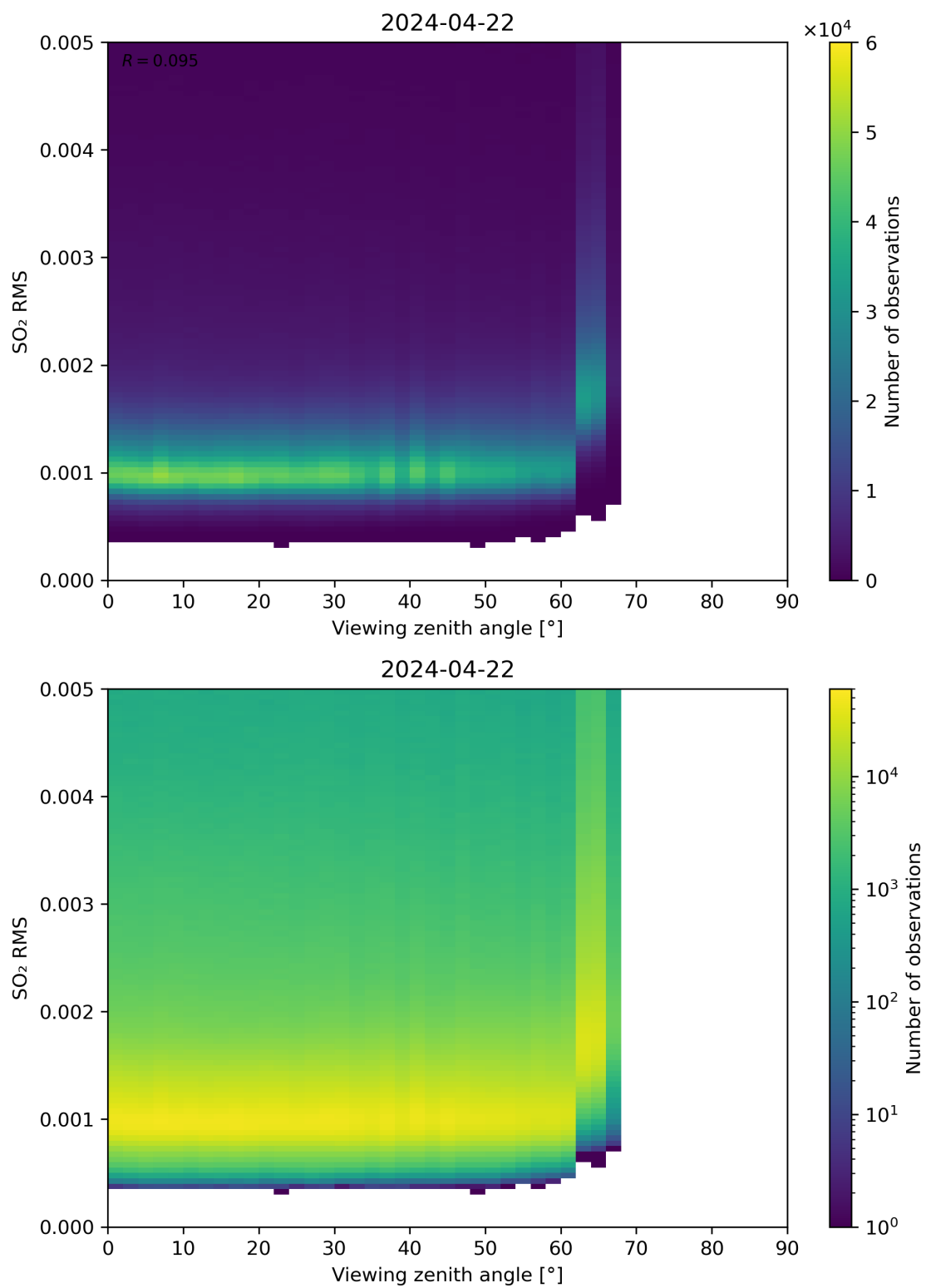
Figure 313: Scatter density plot of “Viewing zenith angle” against “SO 2 RMS” for 2024-04-21 to 2024-04-23.
