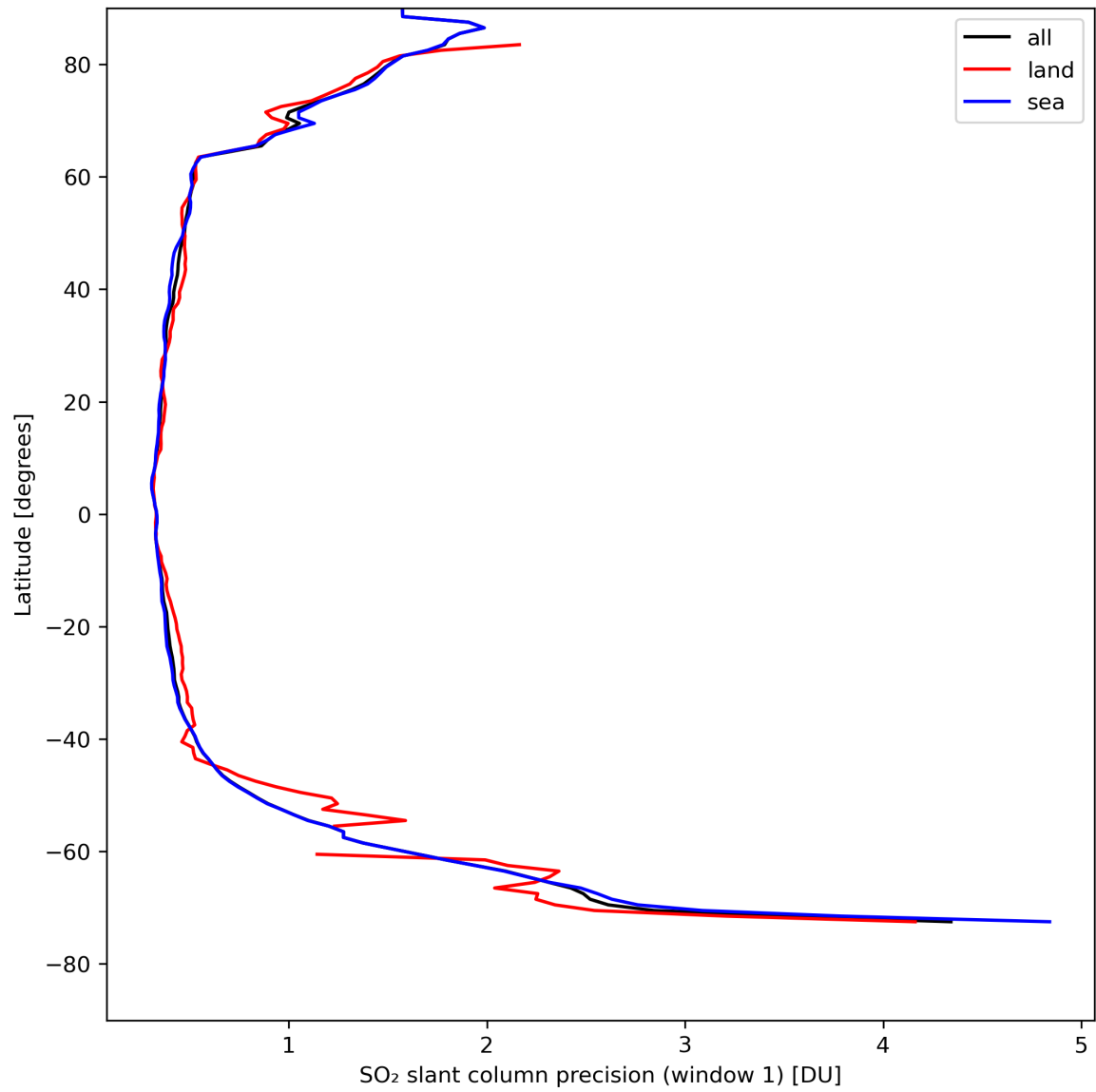
Figure 34: Zonal average of “SO 2 slant column precision (window 1)” for 2024-04-21 to 2024-04-23.
