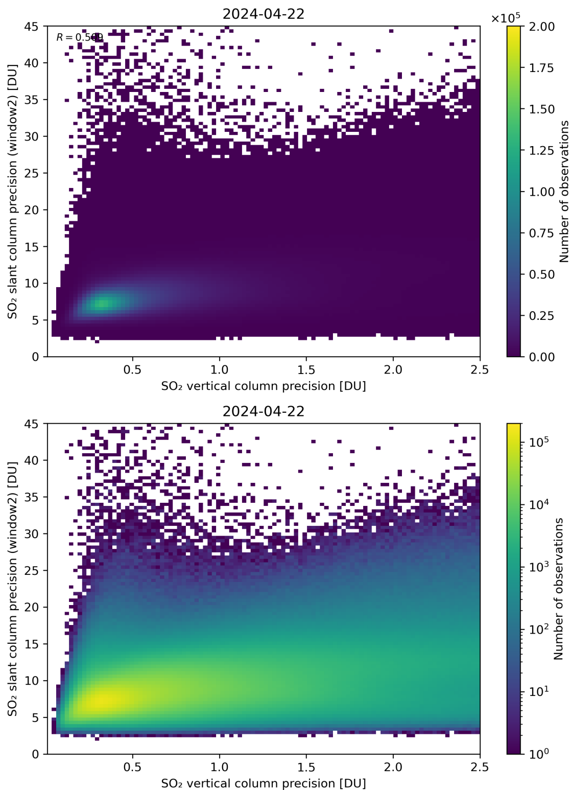
Figure 291: Scatter density plot of “SO 2 vertical column precision” against “SO 2 slant column precision (window2)” for 2024-04-21 to 2024-04-23.
