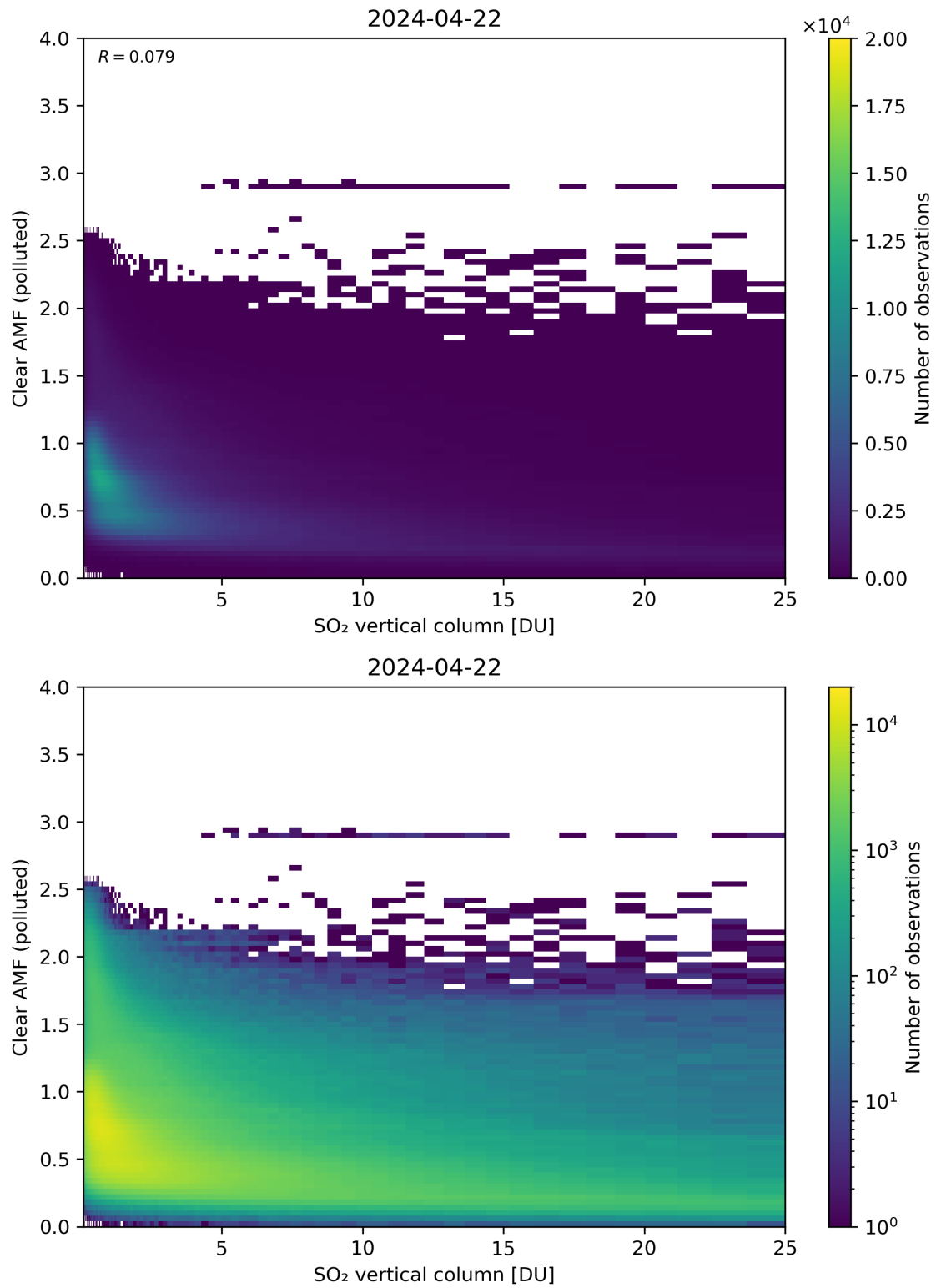
Figure 296: Scatter density plot of “SO 2 vertical column” against “Clear AMF (polluted)” for 2024-04-21 to 2024-04-23.
