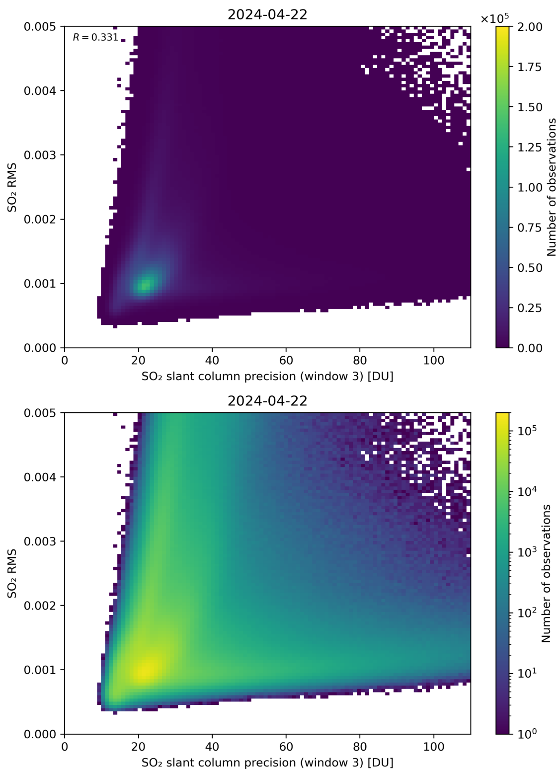
Figure 260: Scatter density plot of “SO 2 slant column precision (window 3)” against “SO 2 RMS” for 2024-04-21 to 2024-04-23.
