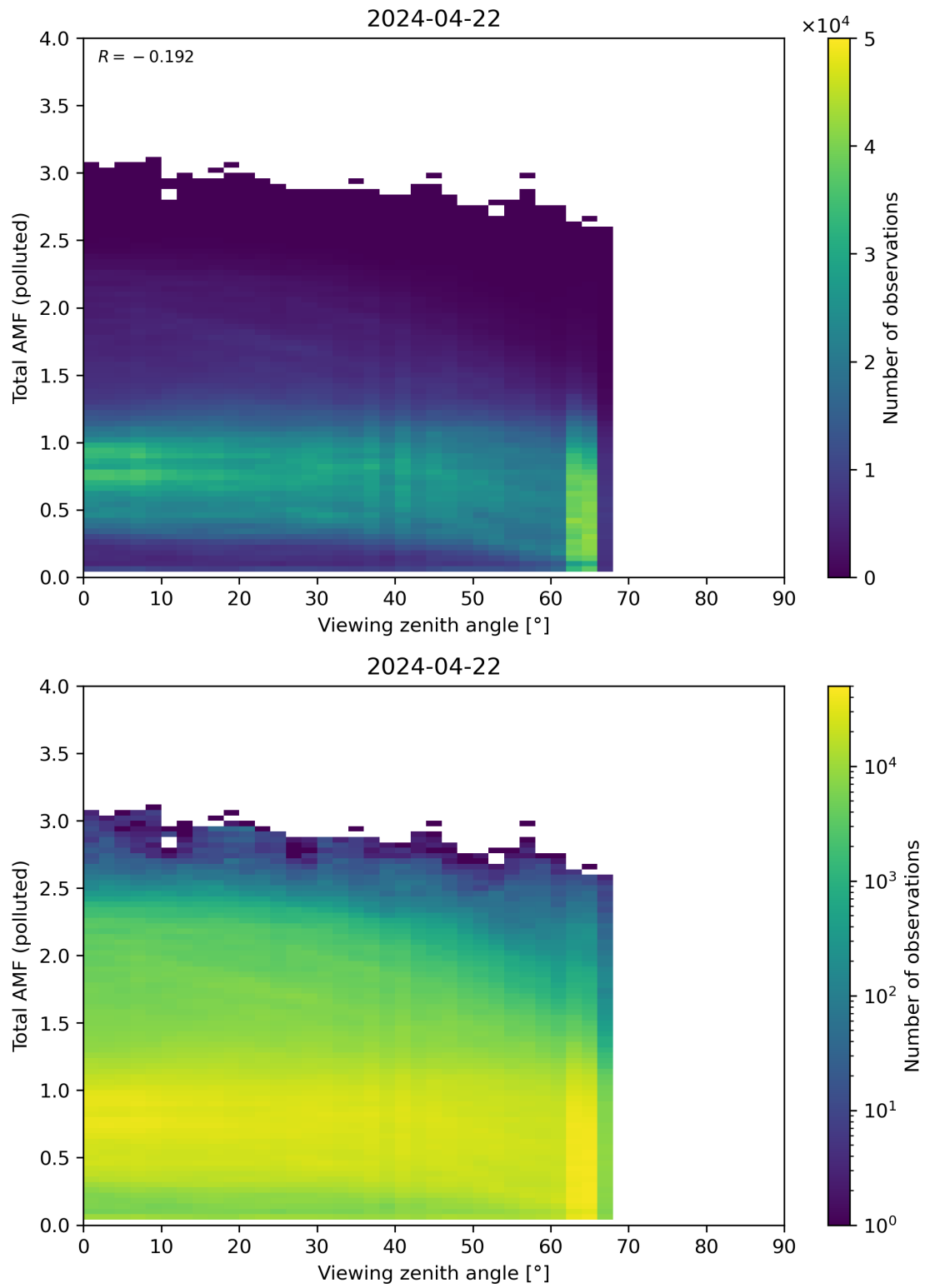
Figure 325: Scatter density plot of “Viewing zenith angle” against “Total AMF (polluted)” for 2024-04-21 to 2024-04-23.
