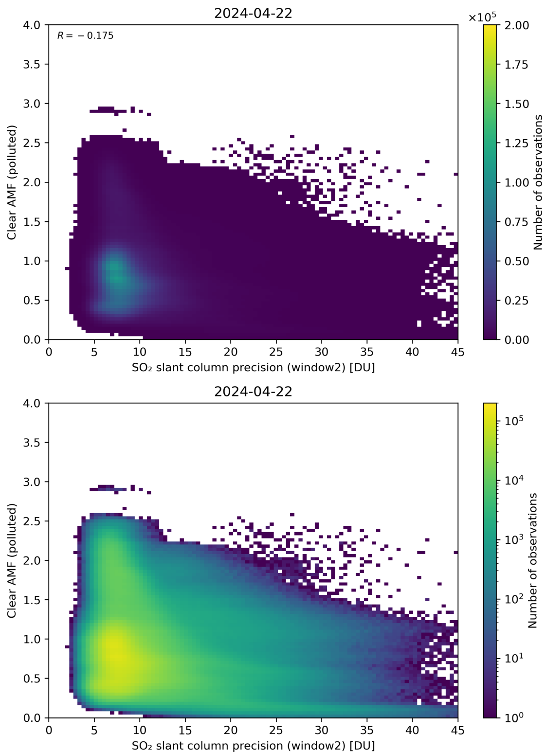
Figure 246: Scatter density plot of “SO 2 slant column precision (window2)” against “Clear AMF (polluted)” for 2024-04-21 to 2024-04-23.
