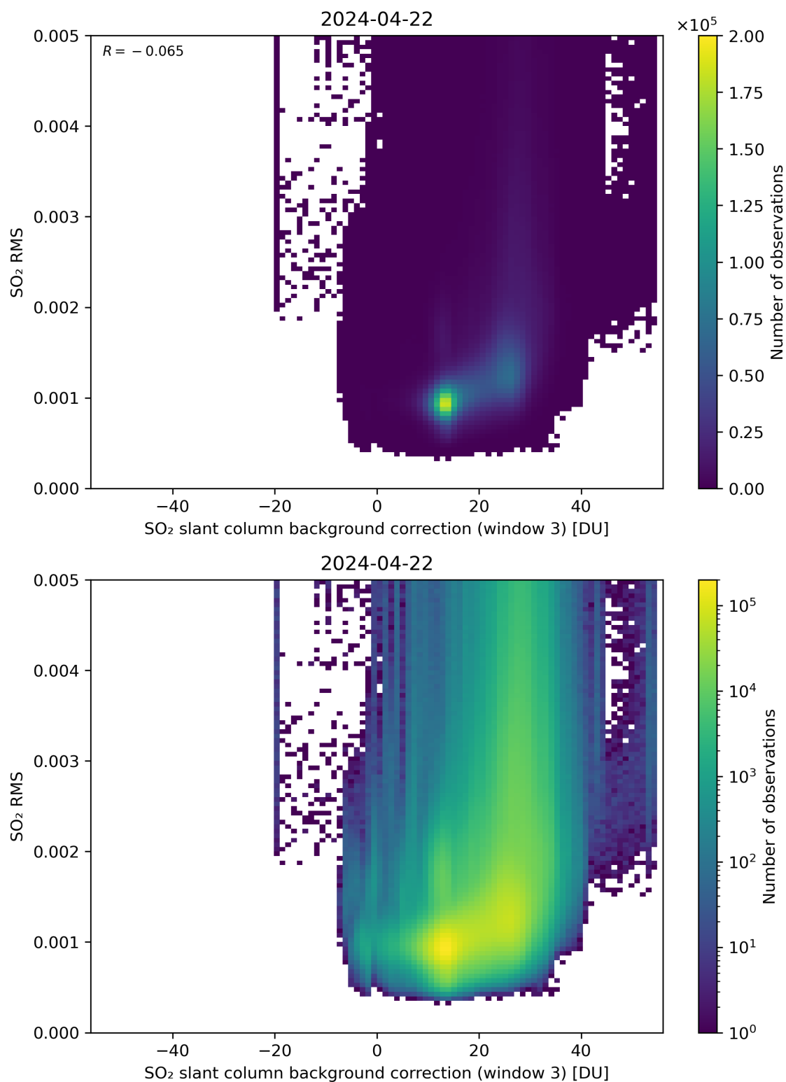
Figure 123: Scatter density plot of “SO 2 slant column background correction (window 3)” against “SO 2 RMS” for 2024-04-21 to 2024-04-23.
