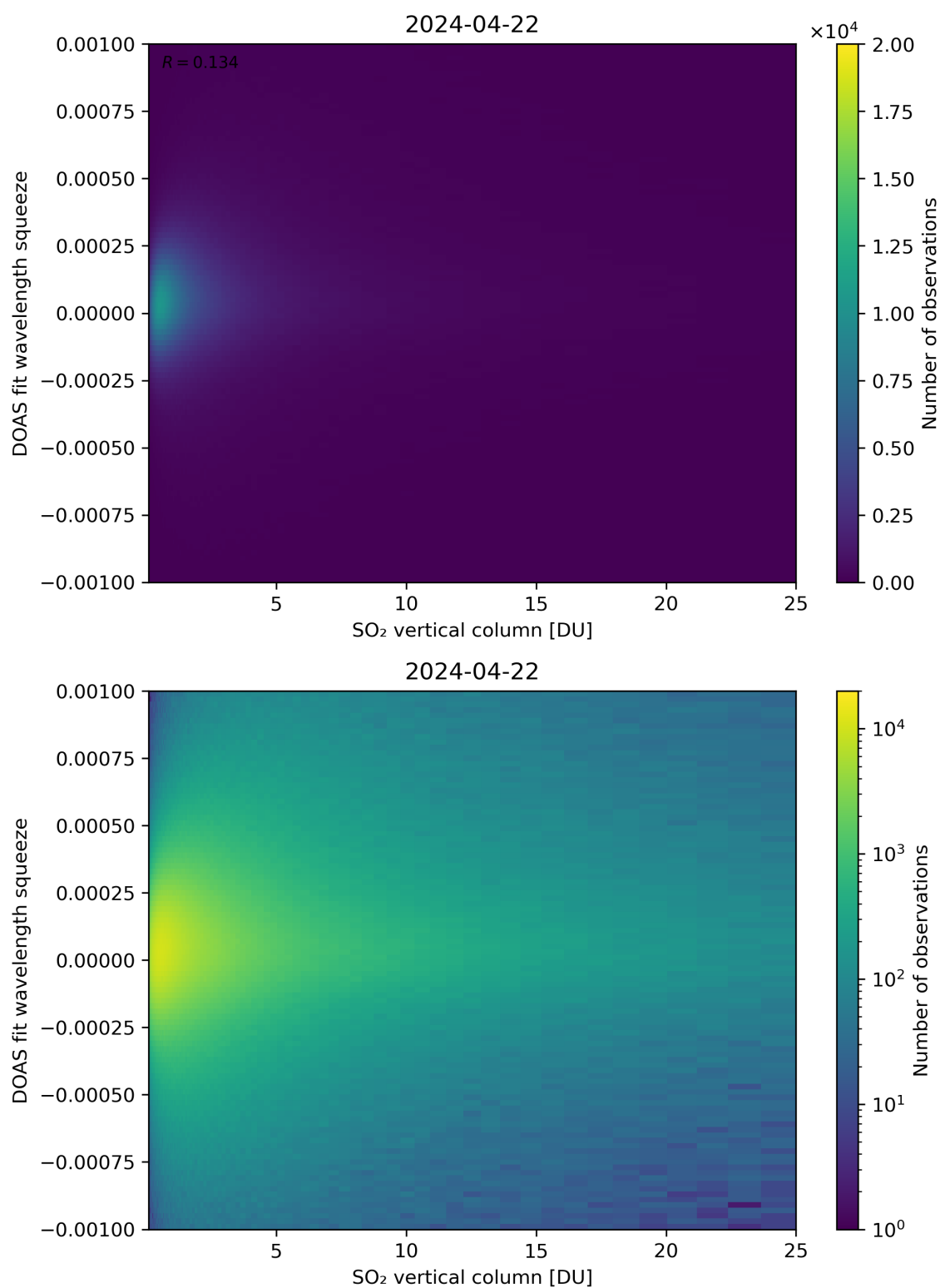
Figure 277: Scatter density plot of “SO 2 vertical column” against “DOAS fit wavelength squeeze” for 2024-04-21 to 2024-04-23.
