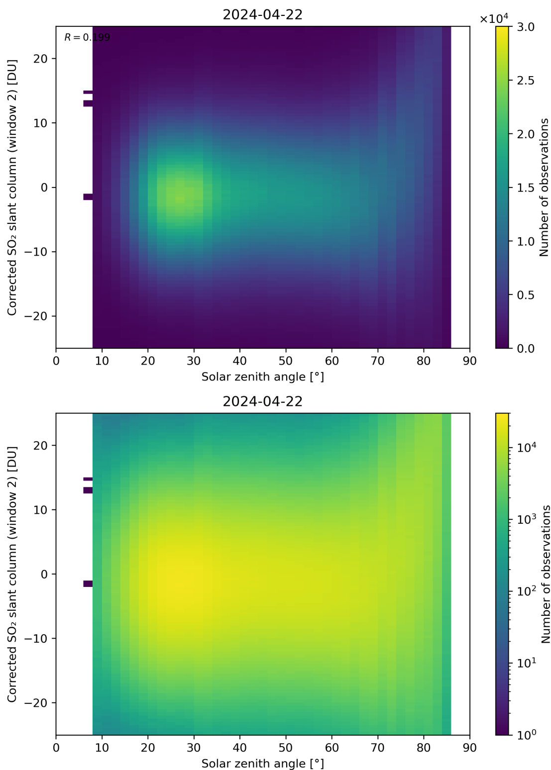
Figure 167: Scatter density plot of “Solar zenith angle” against “Corrected SO 2 slant column (window 2)” for 2024-04-21 to 2024-04-23.
