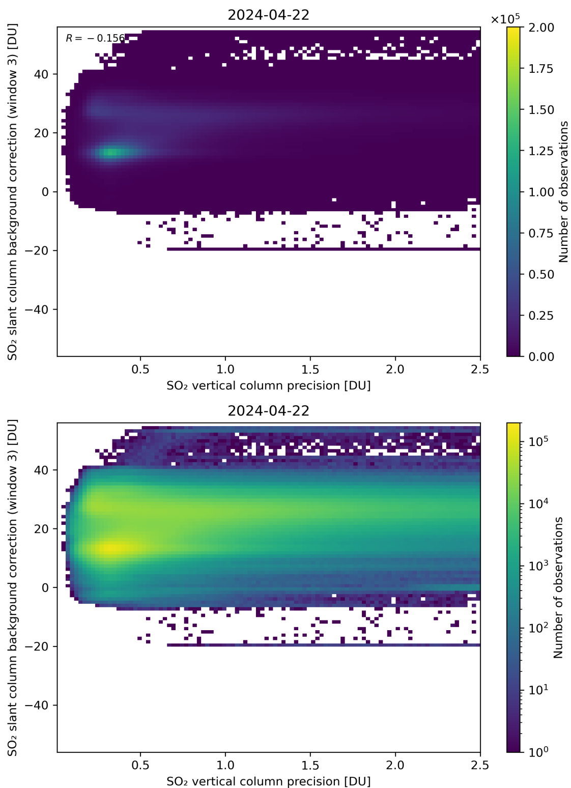
Figure 281: Scatter density plot of “SO 2 vertical column precision” against “SO 2 slant column background correction (window 3)” for 2024-04-21 to 2024-04-23.
