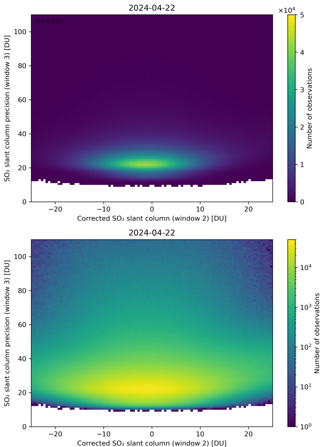
Figure 202: Scatter density plot of “Corrected SO 2 slant column (window 2)” against “SO 2 slant column precision (window 3)” for 2024-04-21 to 2024-04-23.
