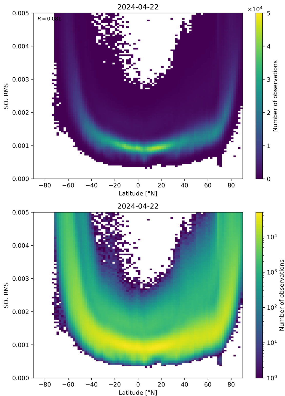
Figure 144: Scatter density plot of “Latitude” against “SO 2 RMS” for 2024-04-21 to 2024-04-23.
