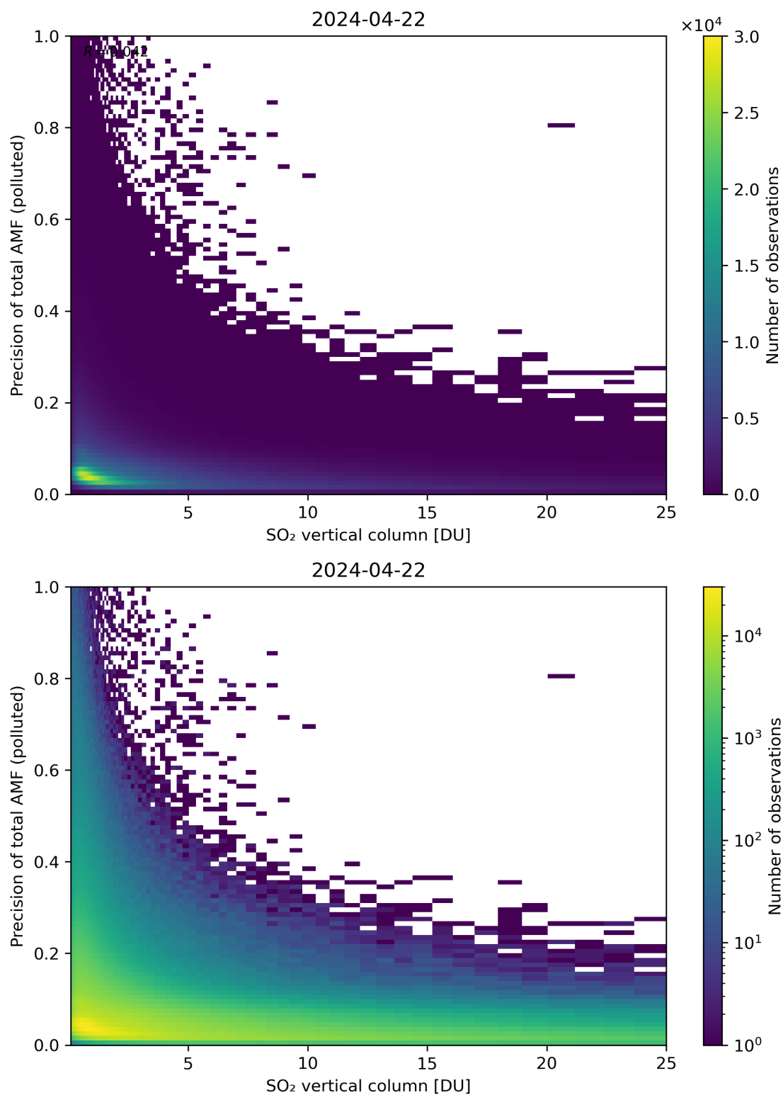
Figure 306: Scatter density plot of “SO 2 vertical column” against “Precision of total AMF (polluted)” for 2024-04-21 to 2024-04-23.
