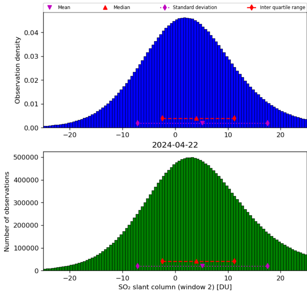
Figure 60: Histogram of “SO 2 slant column (window 2)” for 2024-04-21 to 2024-04-23
