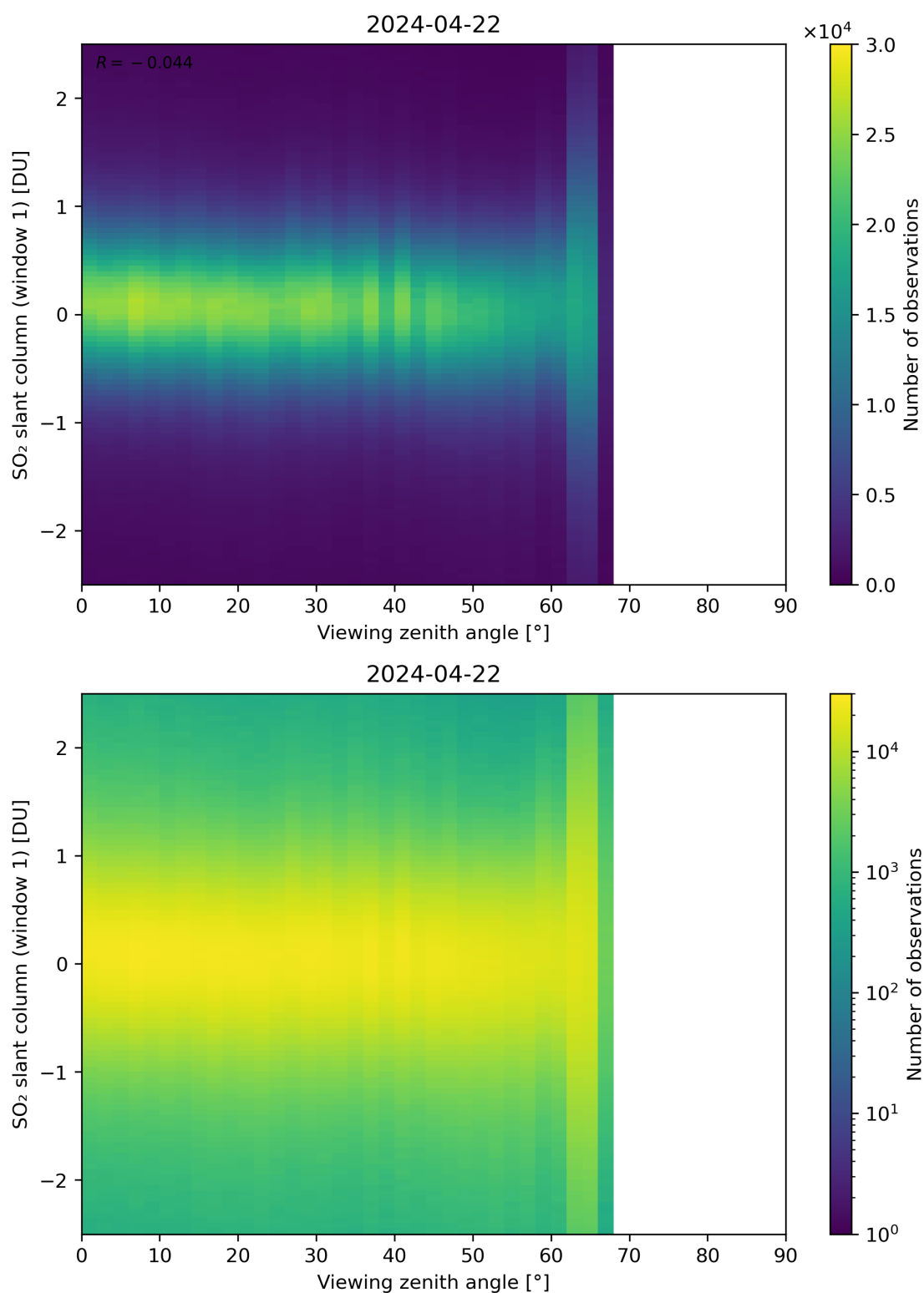
Figure 320: Scatter density plot of “Viewing zenith angle” against “SO 2 slant column (window 1)” for 2024-04-21 to 2024-04-23.
