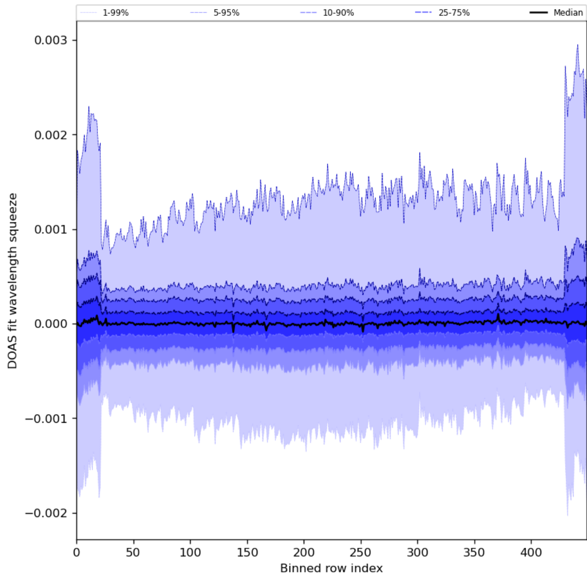
Figure 92: Along track statistics of “DOAS fit wavelength squeeze” for 2024-04-21 to 2024-04-23
