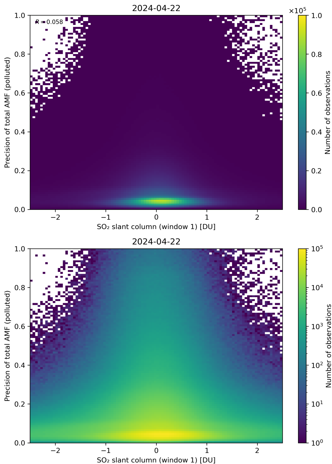
Figure 240: Scatter density plot of “SO 2 slant column (window 1)” against “Precision of total AMF (polluted)” for 2024-04-21 to 2024-04-23.
