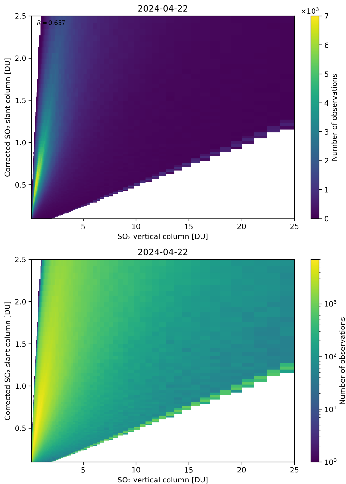
Figure 297: Scatter density plot of “SO 2 vertical column” against “Corrected SO 2 slant column” for 2024-04-21 to 2024-04-23.
