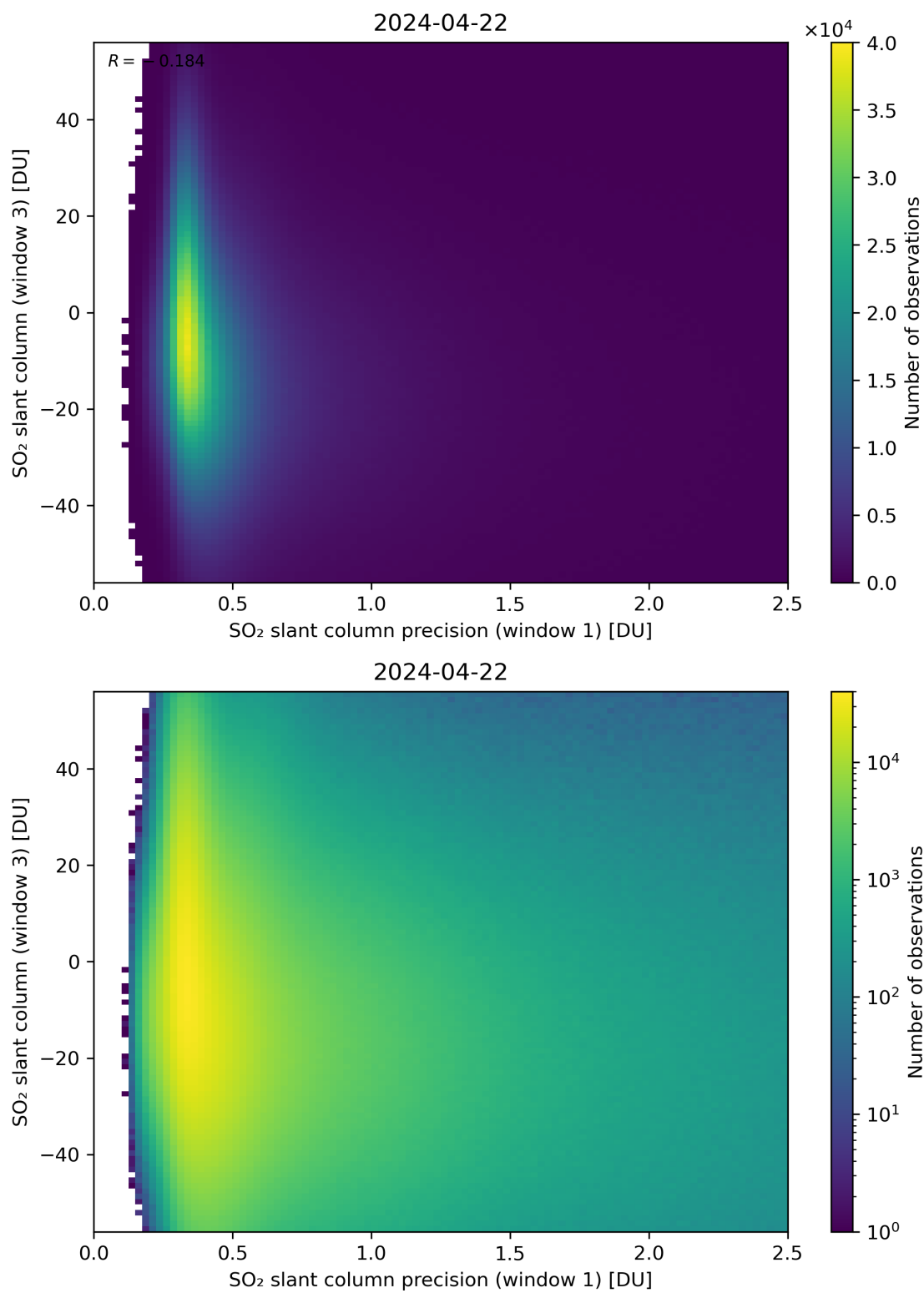
Figure 228: Scatter density plot of “SO 2 slant column precision (window 1)” against “SO 2 slant column (window 3)” for 2024-04-21 to 2024-04-23.
