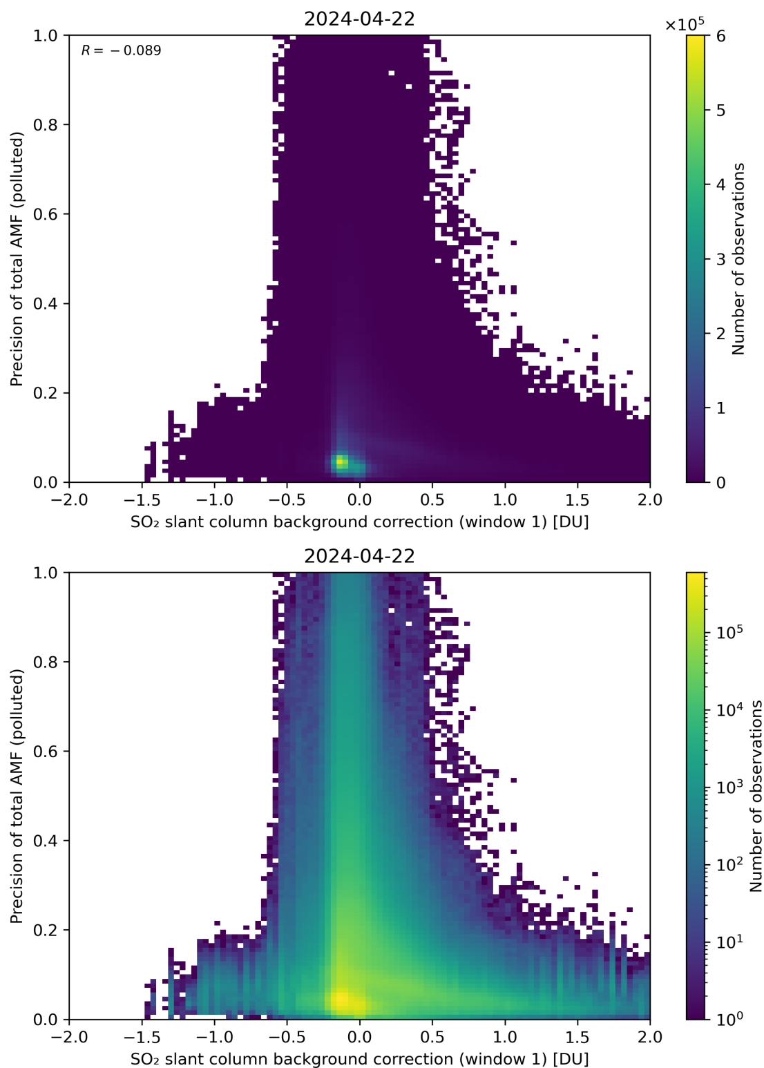
Figure 110: Scatter density plot of “SO 2 slant column background correction (window 1)” against “Precision of total AMF (polluted)” for 2024-04-21 to 2024-04-23.
