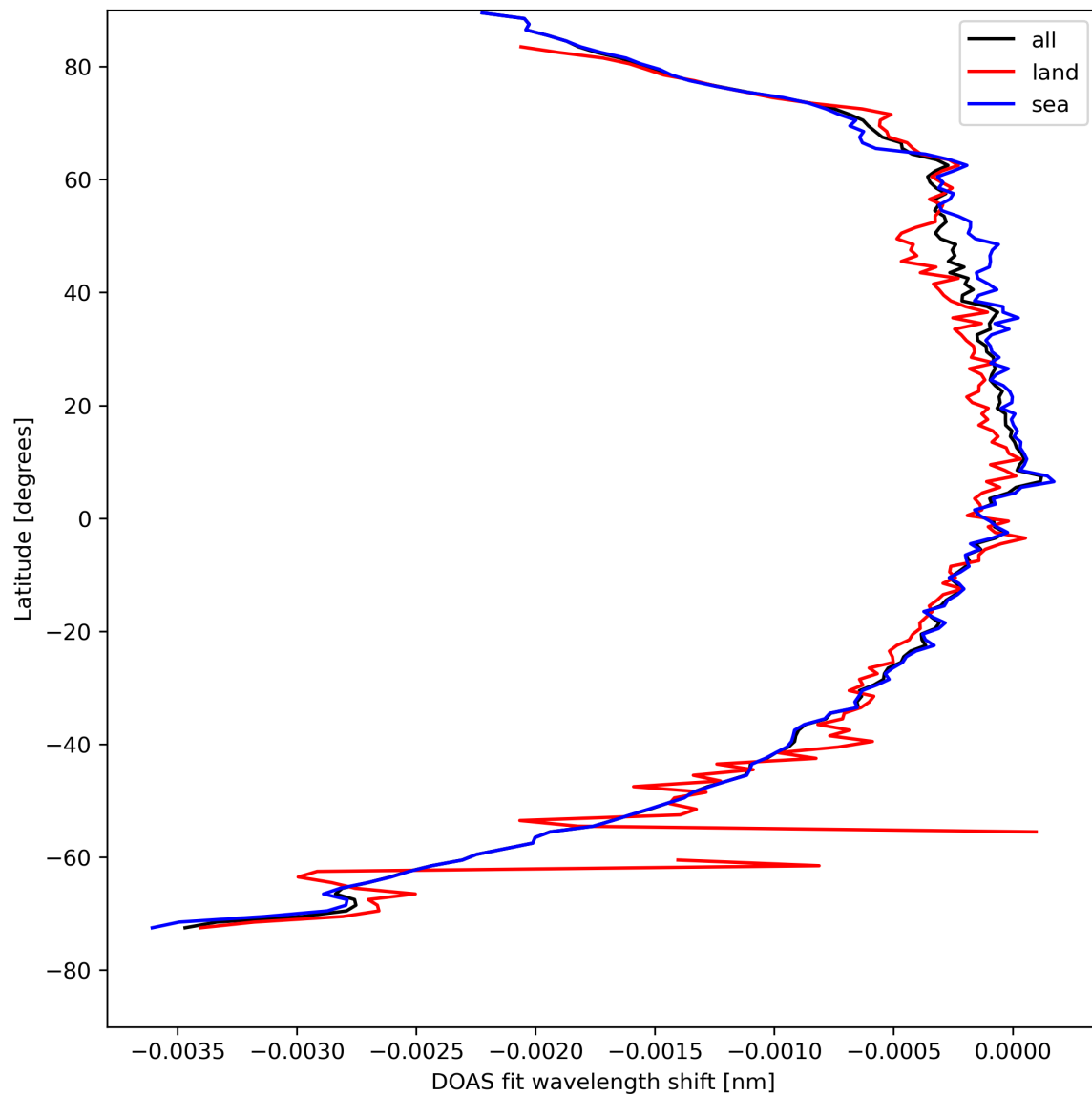
Figure 45: Zonal average of “DOAS fit wavelength shift” for 2024-04-21 to 2024-04-23.
