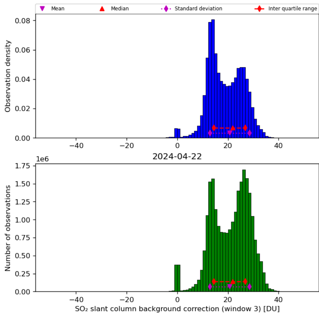
Figure 67: Histogram of “SO 2 slant column background correction (window 3)” for 2024-04-21 to 2024-04-23
