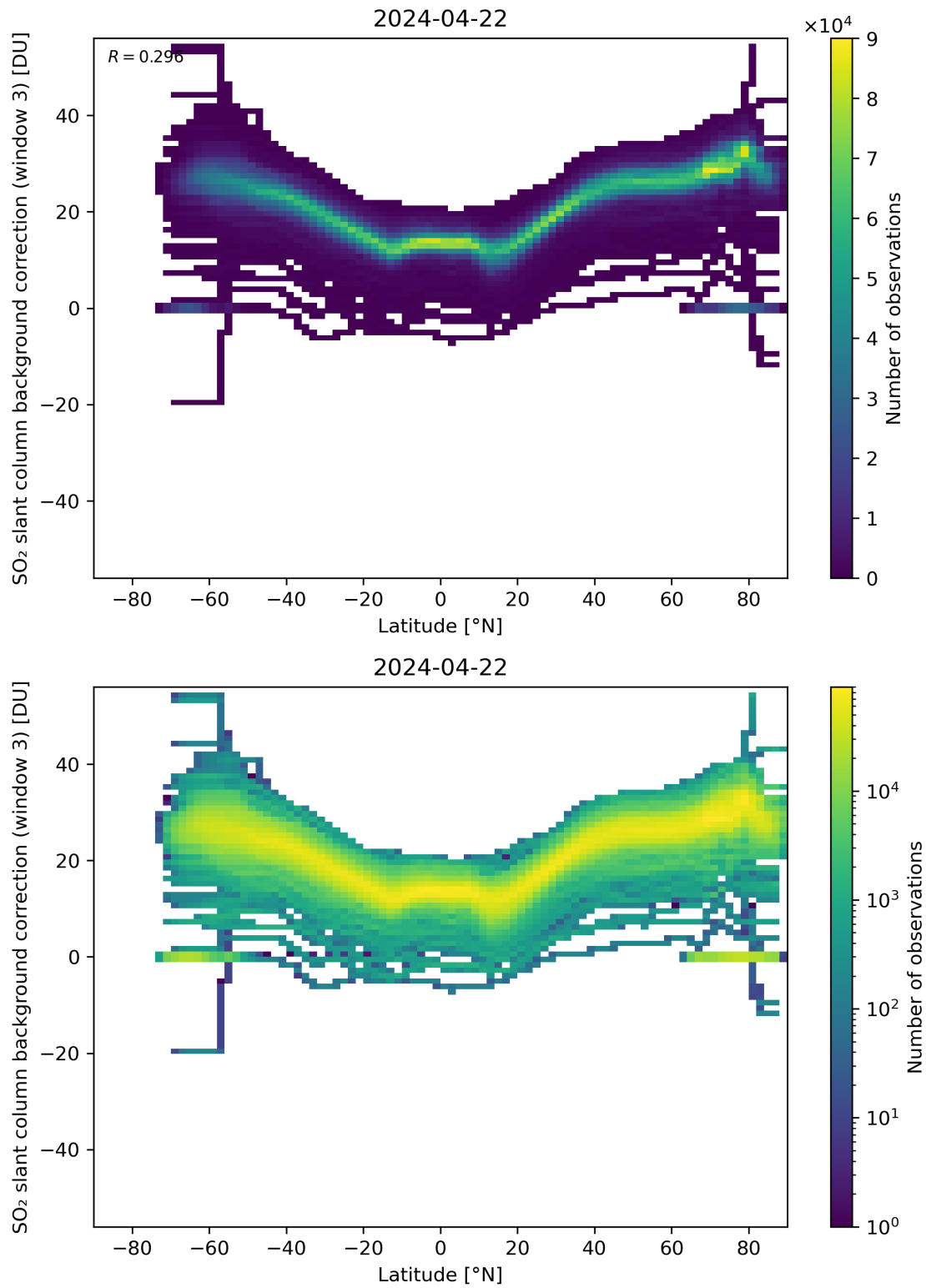
Figure 141: Scatter density plot of “Latitude” against “SO 2 slant column background correction (window 3)” for 2024-04-21 to 2024-04-23.
