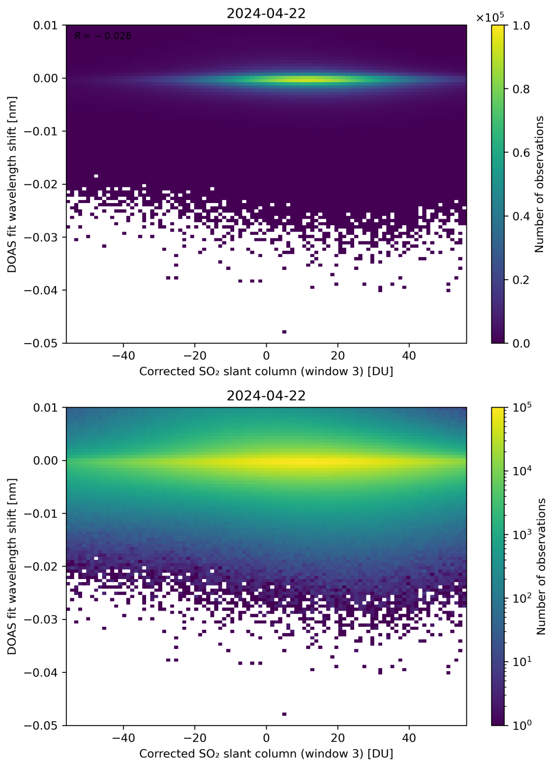
Figure 206: Scatter density plot of “Corrected SO 2 slant column (window 3)” against “DOAS fit wavelength shift” for 2024-04-21 to 2024-04-23.
