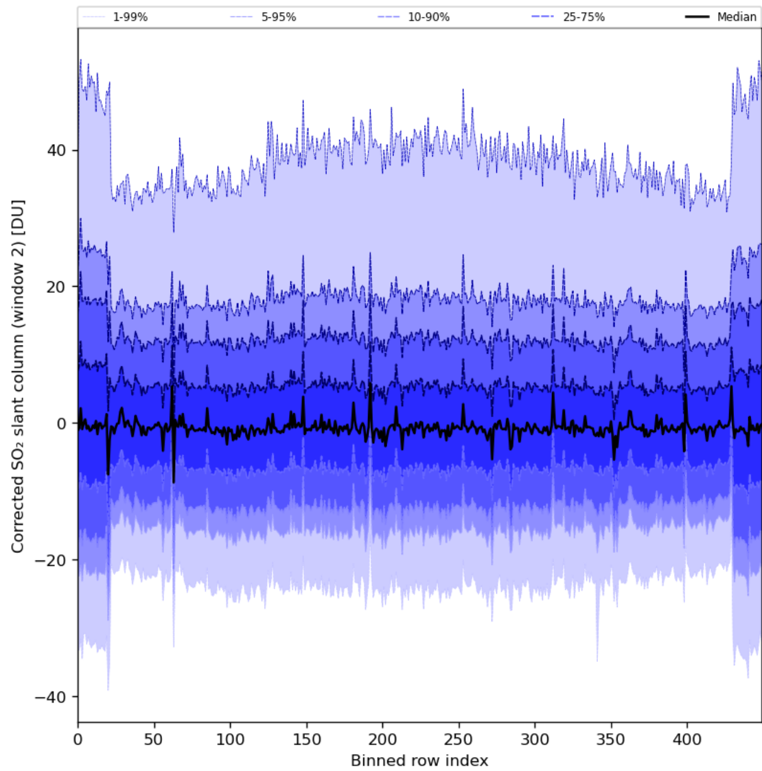
Figure 85: Along track statistics of “Corrected SO 2 slant column (window 2)” for 2024-04-21 to 2024-04-23
