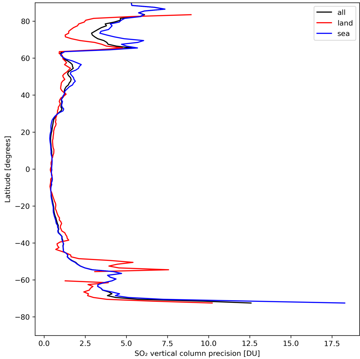
Figure 31: Zonal average of “SO 2 vertical column precision” for 2024-04-21 to 2024-04-23.
