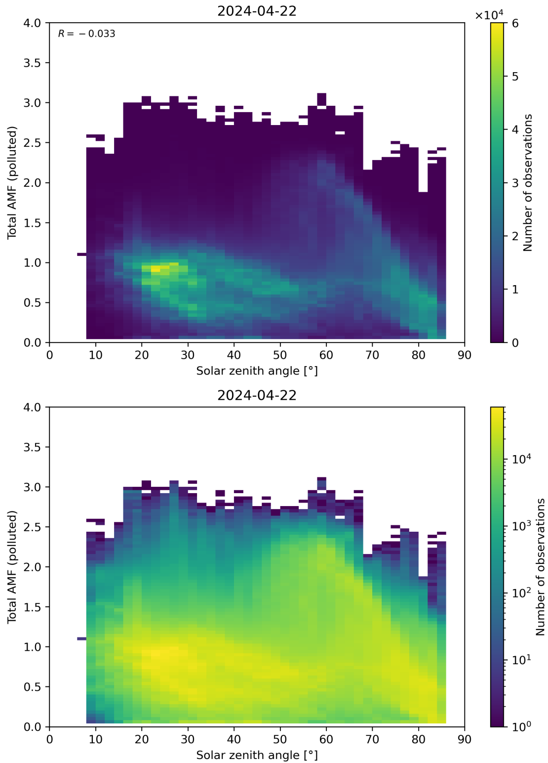
Figure 174: Scatter density plot of “Solar zenith angle” against “Total AMF (polluted)” for 2024-04-21 to 2024-04-23.
