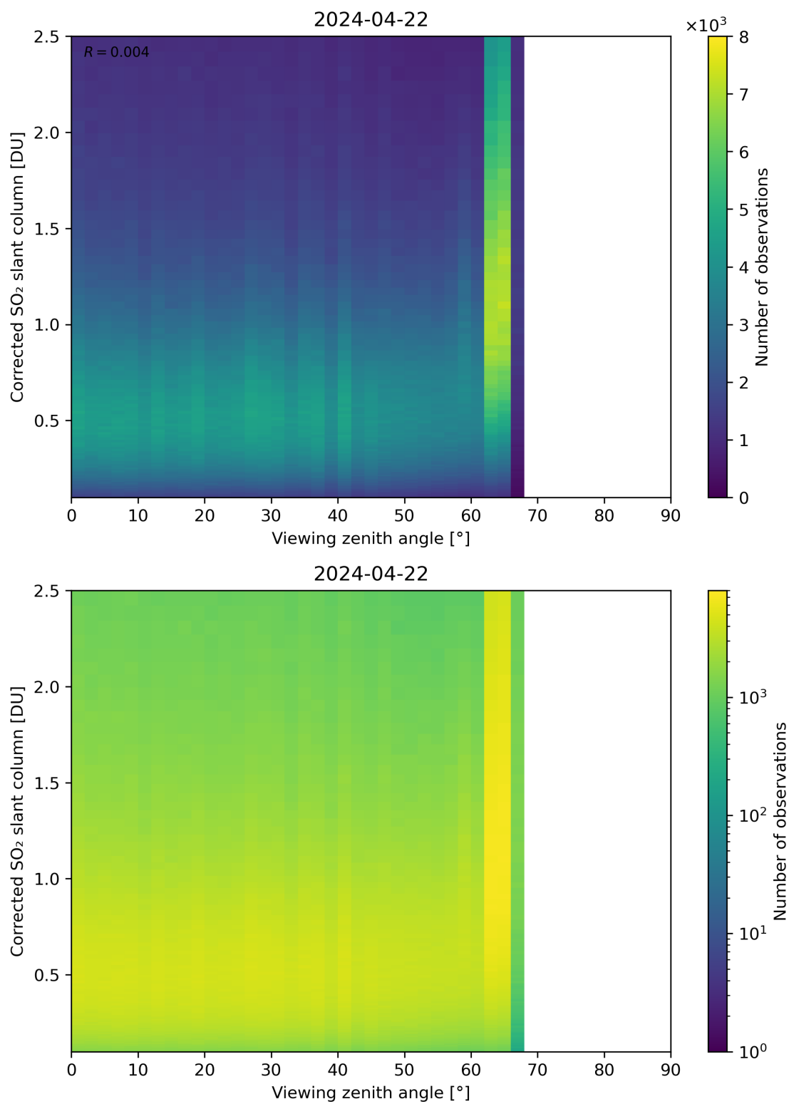
Figure 317: Scatter density plot of “Viewing zenith angle” against “Corrected SO 2 slant column” for 2024-04-21 to 2024-04-23.
