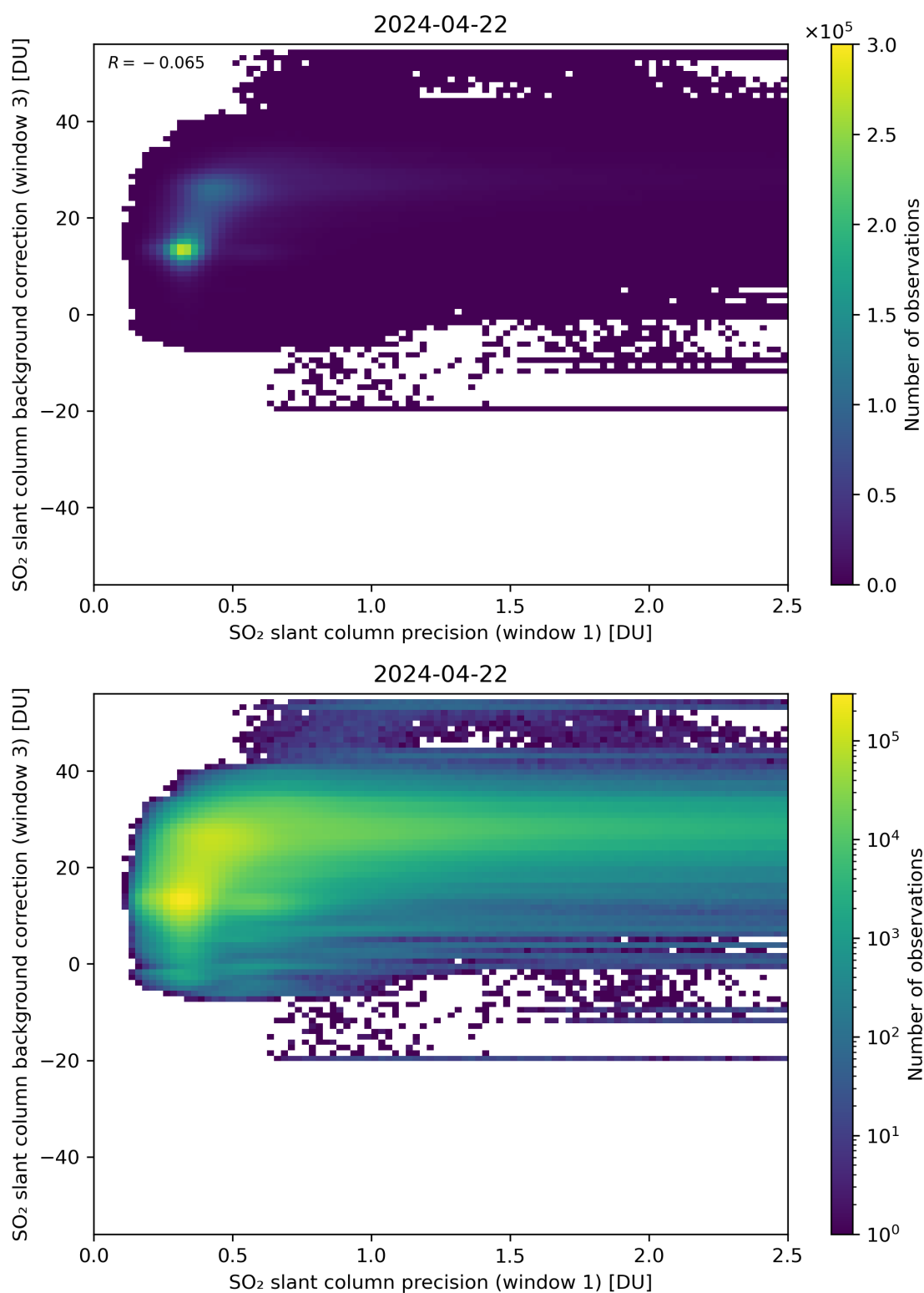
Figure 220: Scatter density plot of “SO 2 slant column precision (window 1)” against “SO 2 slant column background correction (window 3)” for 2024-04-21 to 2024-04-23.
