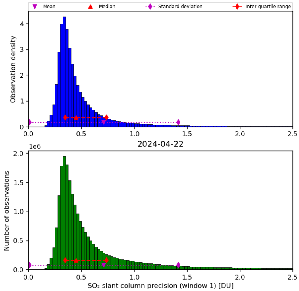
Figure 57: Histogram of “SO 2 slant column precision (window 1)” for 2024-04-21 to 2024-04-23
