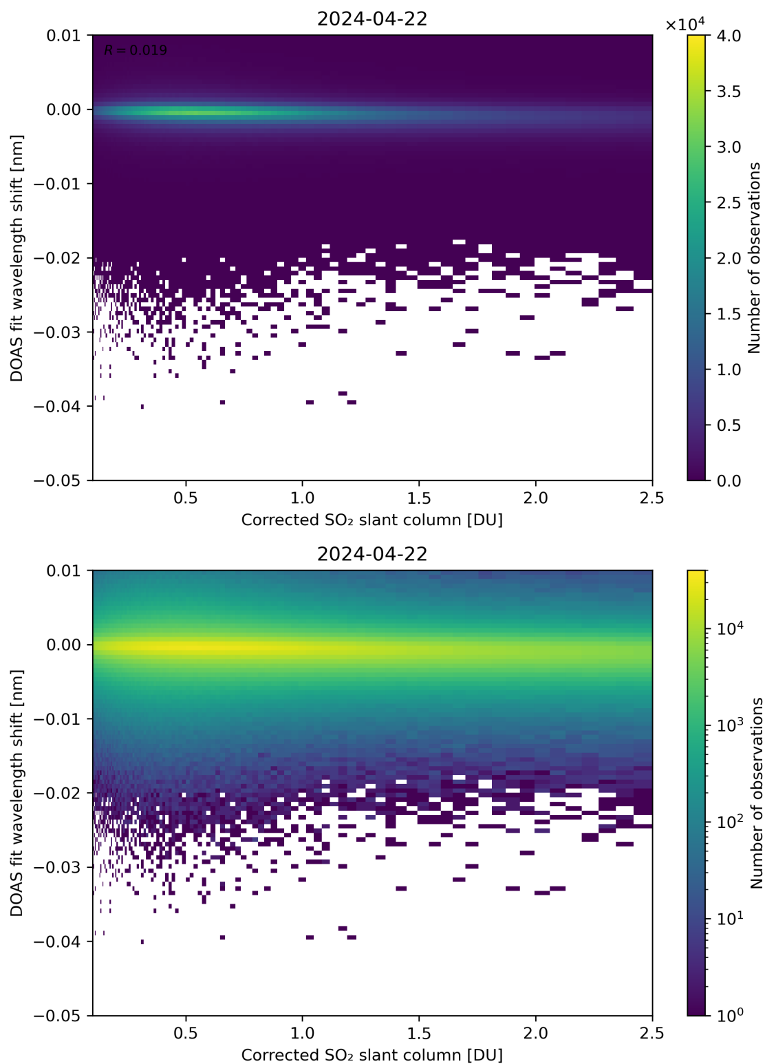
Figure 181: Scatter density plot of “Corrected SO 2 slant column” against “DOAS fit wavelength shift” for 2024-04-21 to 2024-04-23.
