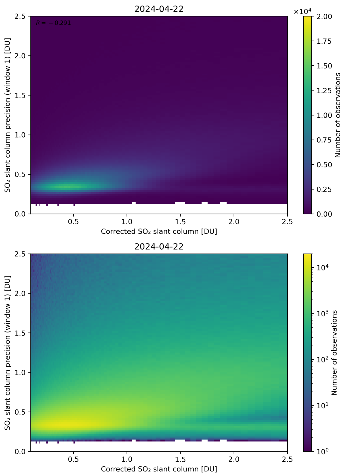
Figure 188: Scatter density plot of “Corrected SO 2 slant column” against “SO 2 slant column precision (window 1)” for 2024-04-21 to 2024-04-23.
