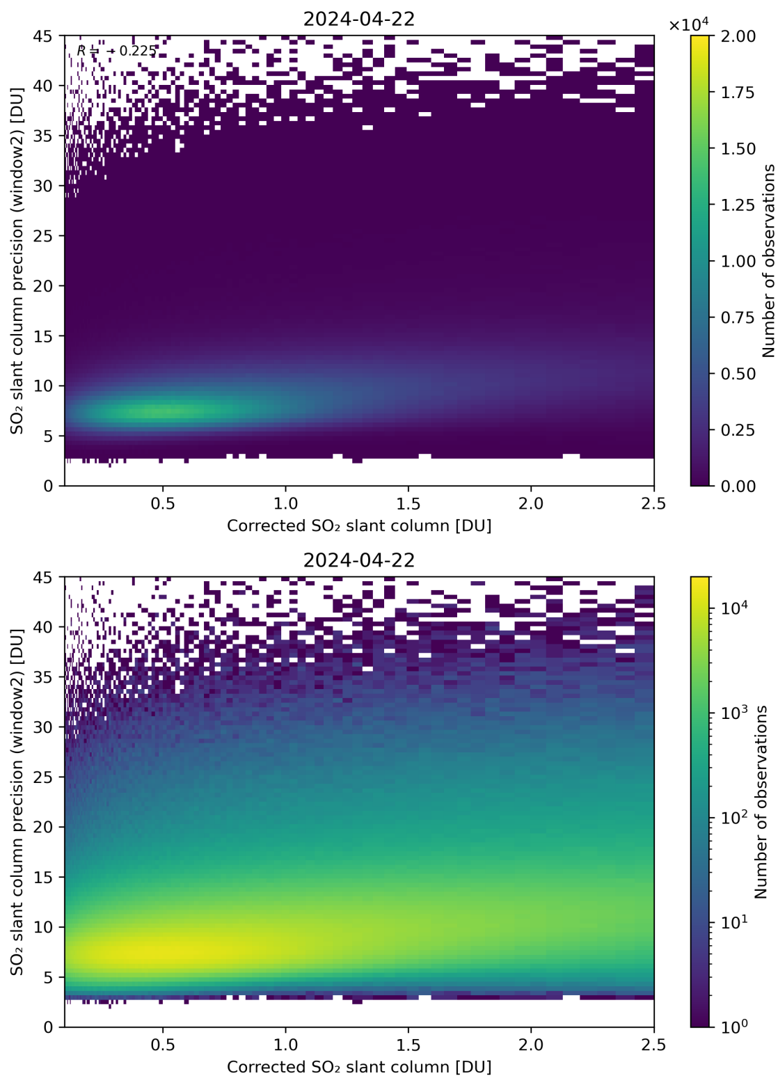
Figure 189: Scatter density plot of “Corrected SO 2 slant column” against “SO 2 slant column precision (window2)” for 2024-04-21 to 2024-04-23.
