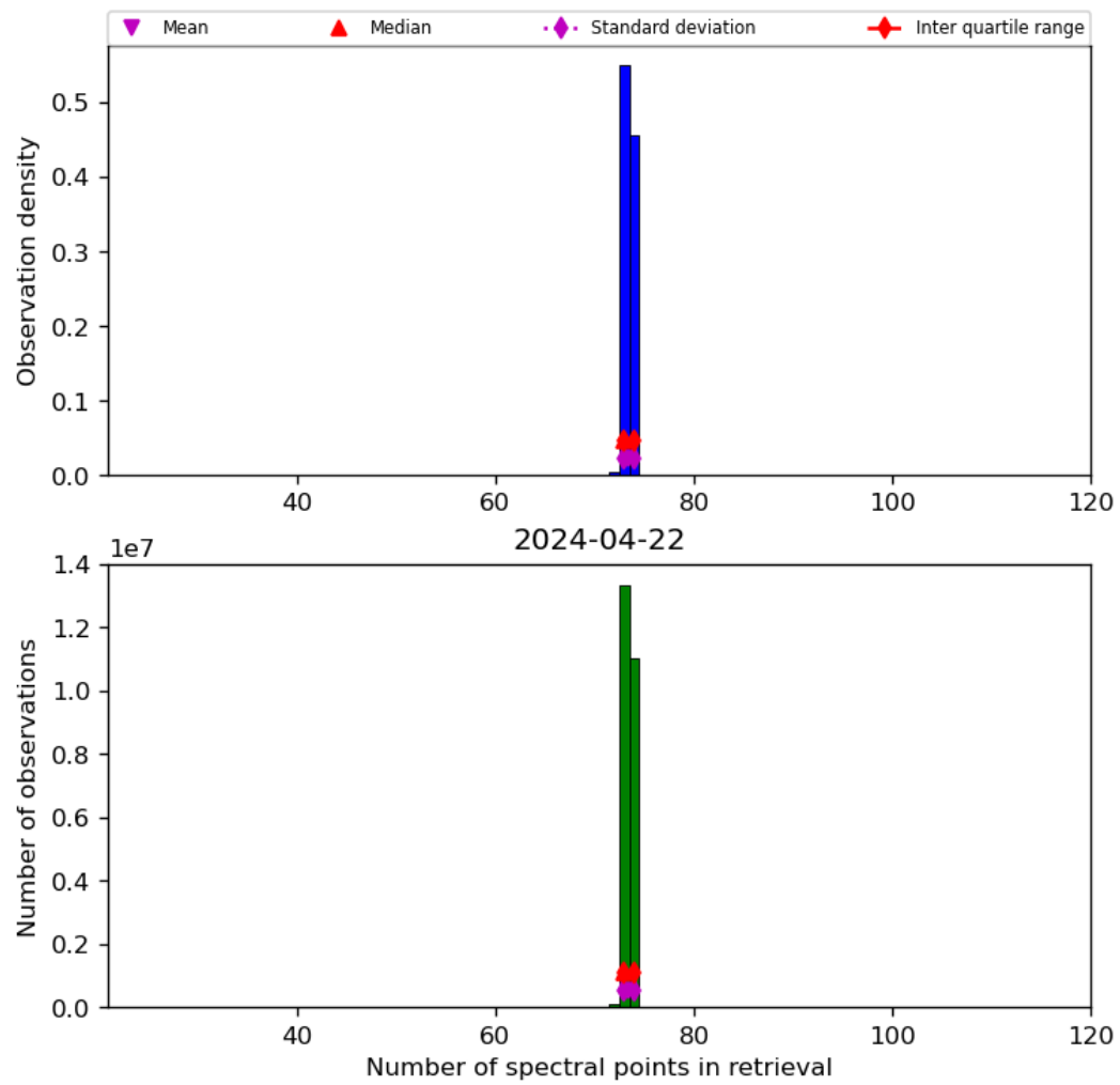
Figure 74: Histogram of “Number of spectral points in retrieval” for 2024-04-21 to 2024-04-23
