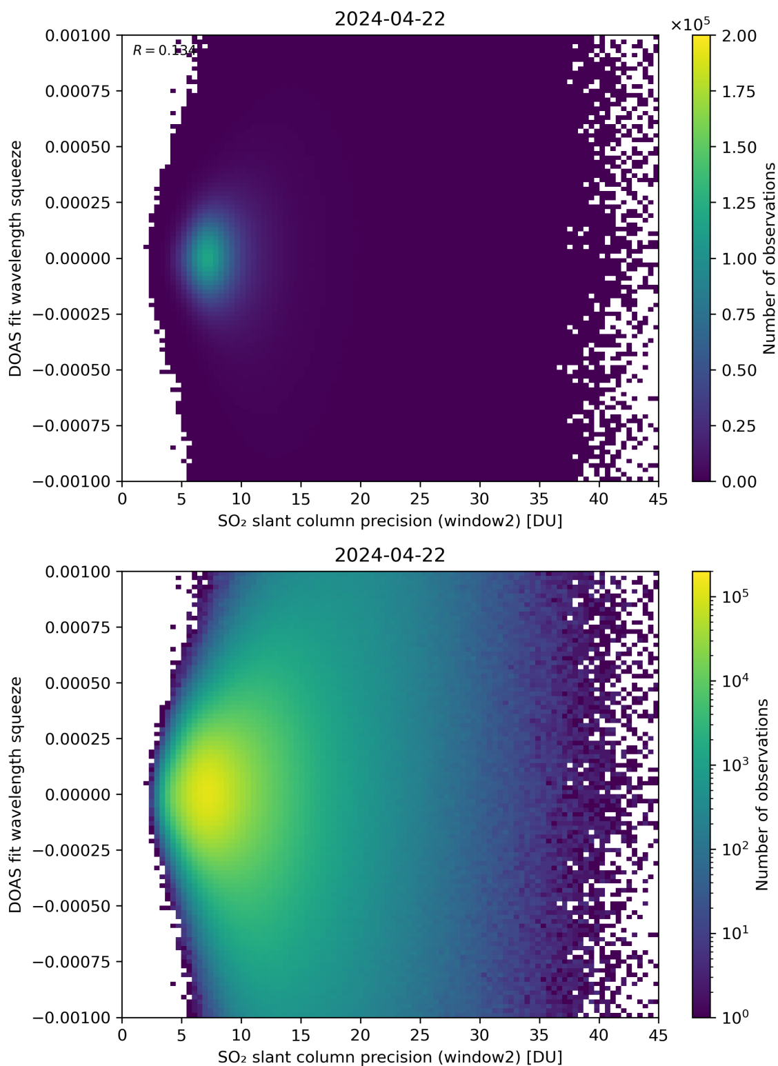
Figure 244: Scatter density plot of “SO 2 slant column precision (window2)” against “DOAS fit wavelength squeeze” for 2024-04-21 to 2024-04-23.
