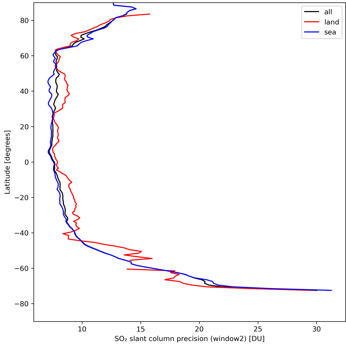
Figure 38: Zonal average of “SO 2 slant column precision (window2)” for 2024-04-21 to 2024-04-23.
