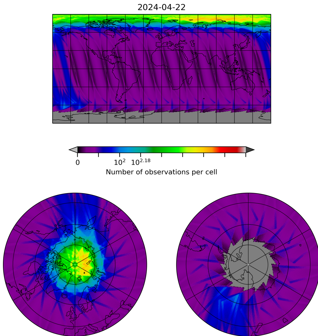
Figure 28: Map of the number of observations for 2024-04-21 to 2024-04-23
