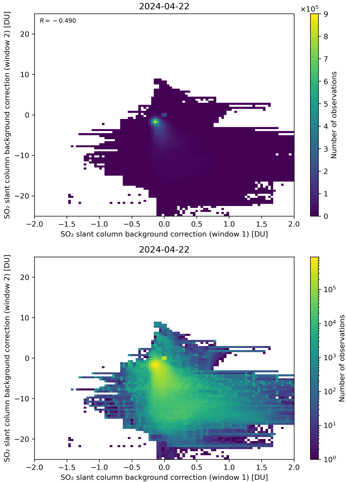
Figure 98: Scatter density plot of “SO 2 slant column background correction (window 1)” against “SO 2 slant column background correction (window 2)” for 2024-04-21 to 2024-04-23.
