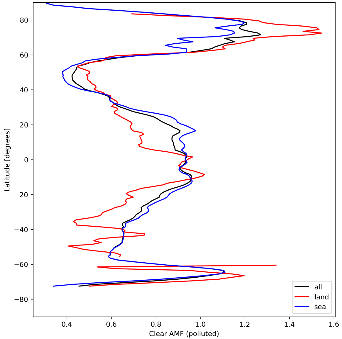
Figure 50: Zonal average of “Clear AMF (polluted)” for 2024-04-21 to 2024-04-23.
