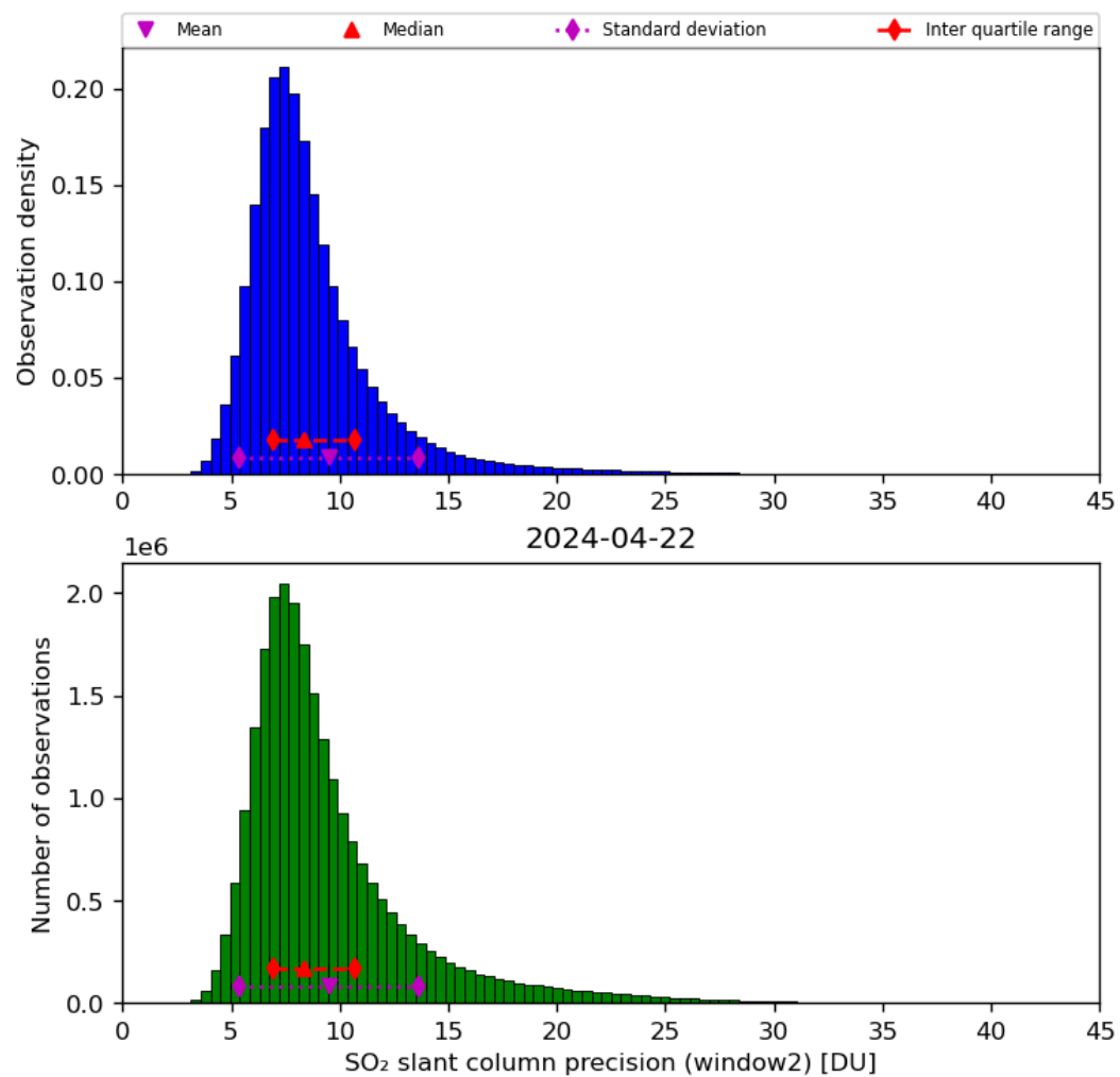
Figure 61: Histogram of “SO 2 slant column precision (window2)” for 2024-04-21 to 2024-04-23
