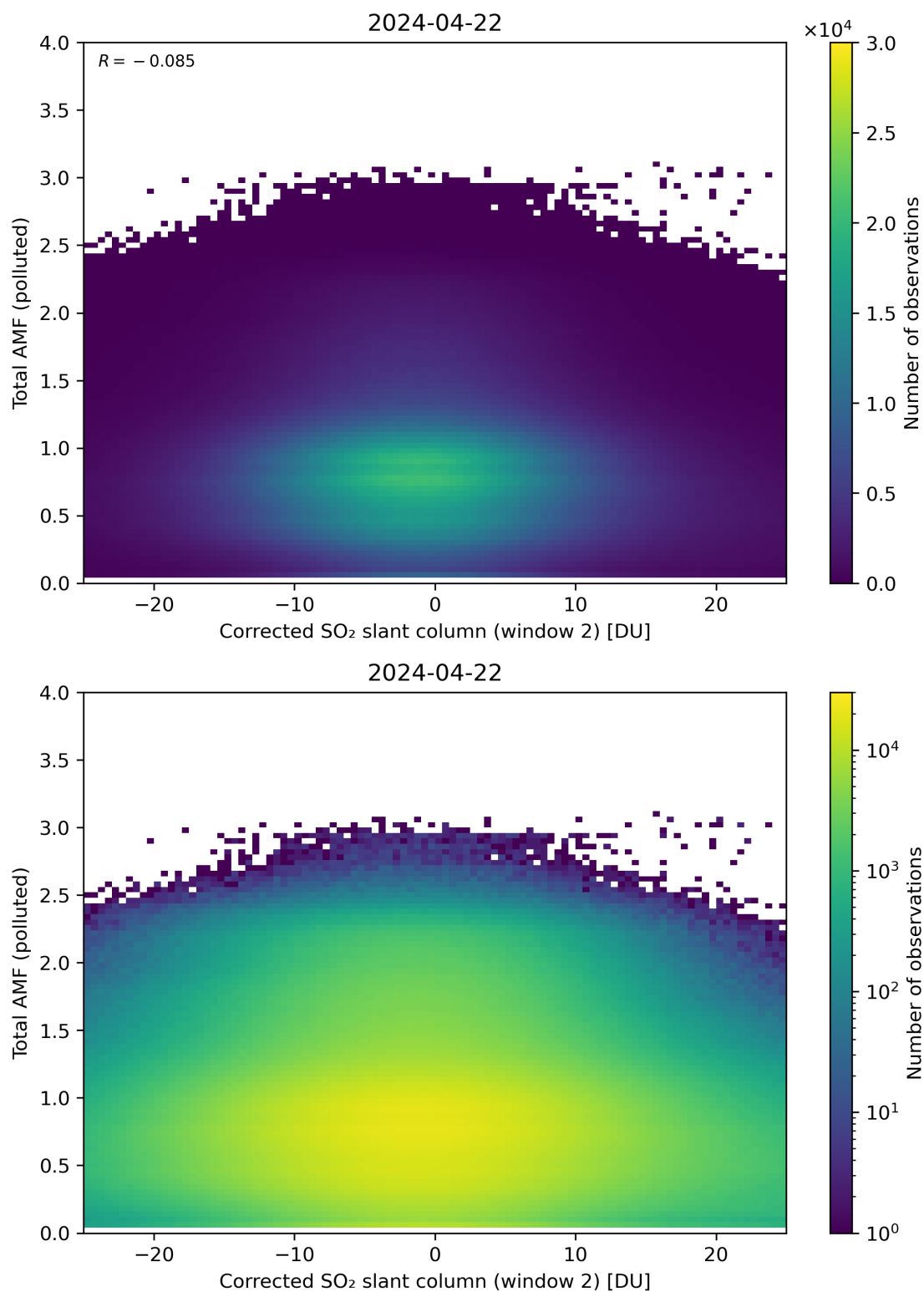
Figure 203: Scatter density plot of “Corrected SO 2 slant column (window 2)” against “Total AMF (polluted)” for 2024-04-21 to 2024-04-23.
