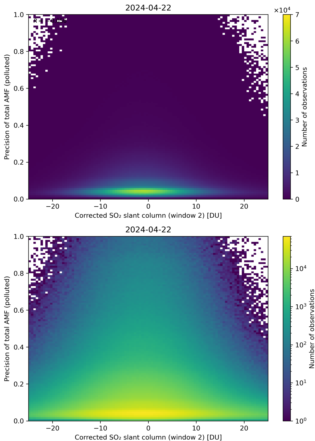
Figure 204: Scatter density plot of “Corrected SO 2 slant column (window 2)” against “Precision of total AMF (polluted)” for 2024-04-21 to 2024-04-23.
