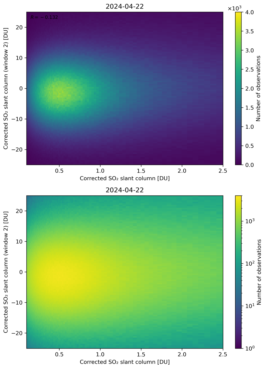
Figure 185: Scatter density plot of “Corrected SO 2 slant column” against “Corrected SO 2 slant column (window 2)” for 2024-04-21 to 2024-04-23.
