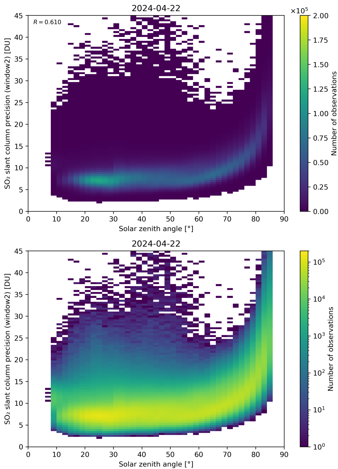
Figure 171: Scatter density plot of “Solar zenith angle” against “SO 2 slant column precision (window2)” for 2024-04-21 to 2024-04-23.
