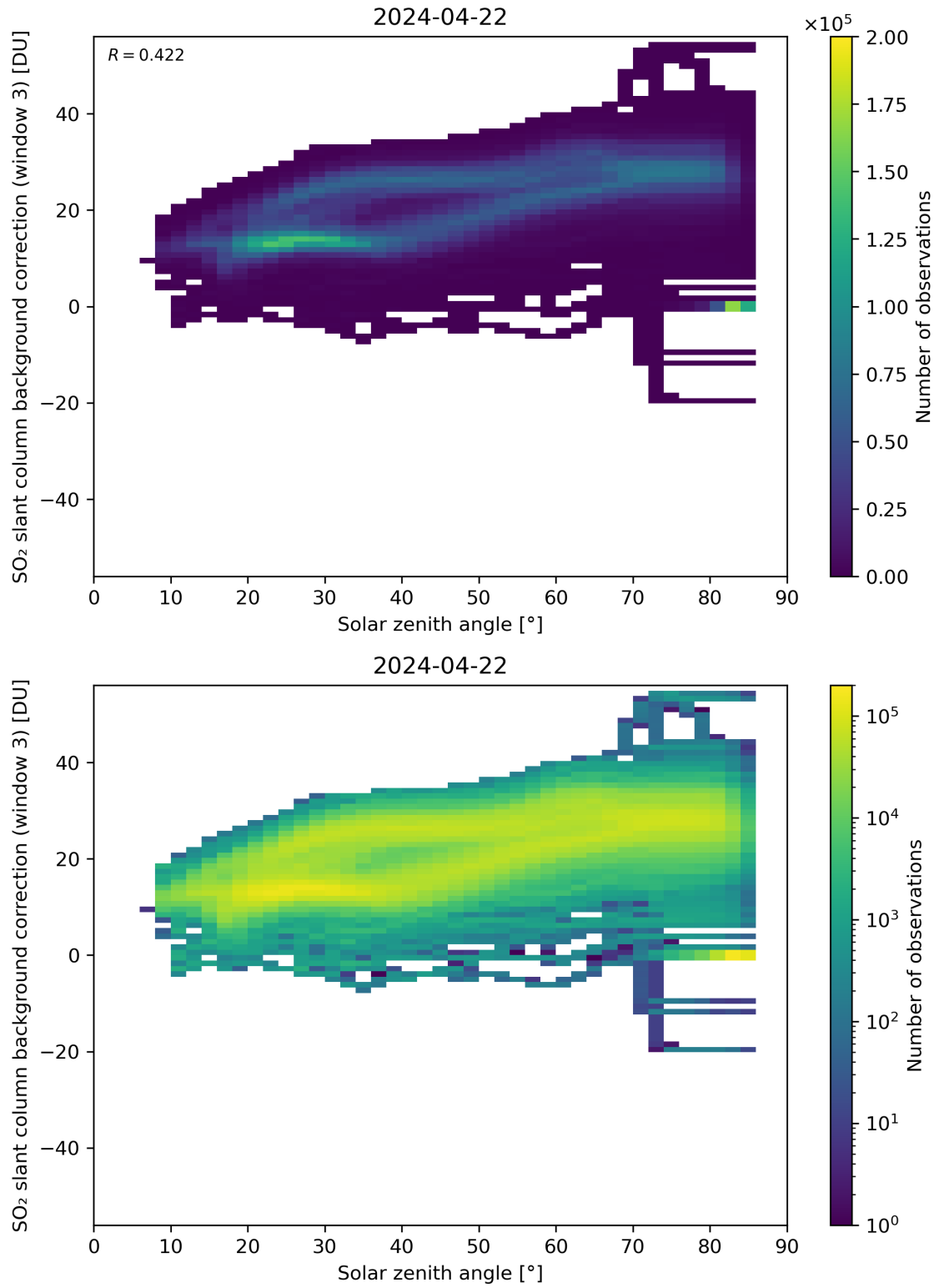
Figure 160: Scatter density plot of “Solar zenith angle” against “SO 2 slant column background correction (window 3)” for 2024-04-21 to 2024-04-23.
