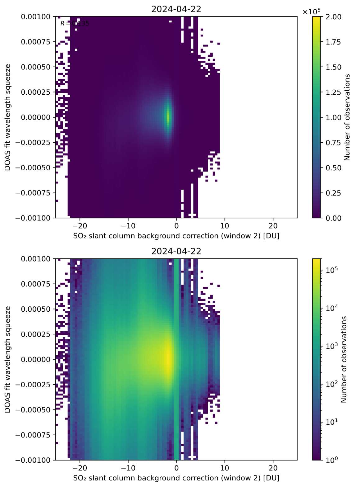
Figure 113: Scatter density plot of “SO 2 slant column background correction (window 2)” against “DOAS fit wavelength squeeze” for 2024-04-21 to 2024-04-23.
