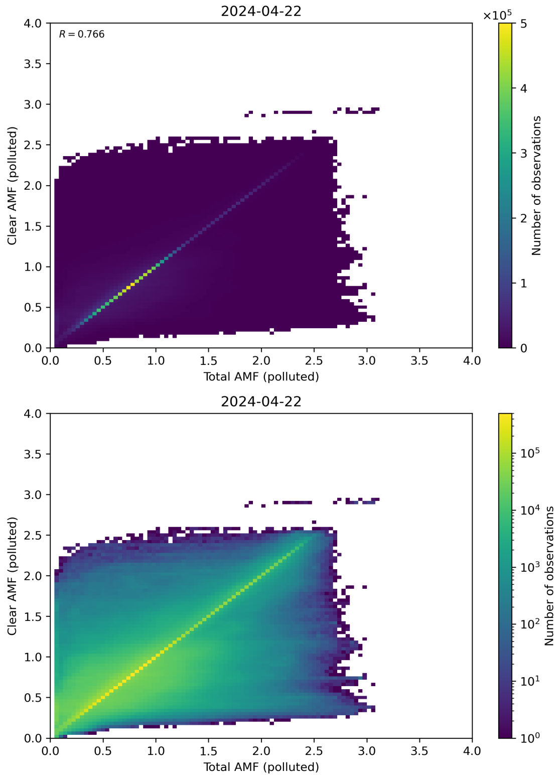
Figure 271: Scatter density plot of “Total AMF (polluted)” against “Clear AMF (polluted)” for 2024-04-21 to 2024-04-23.
