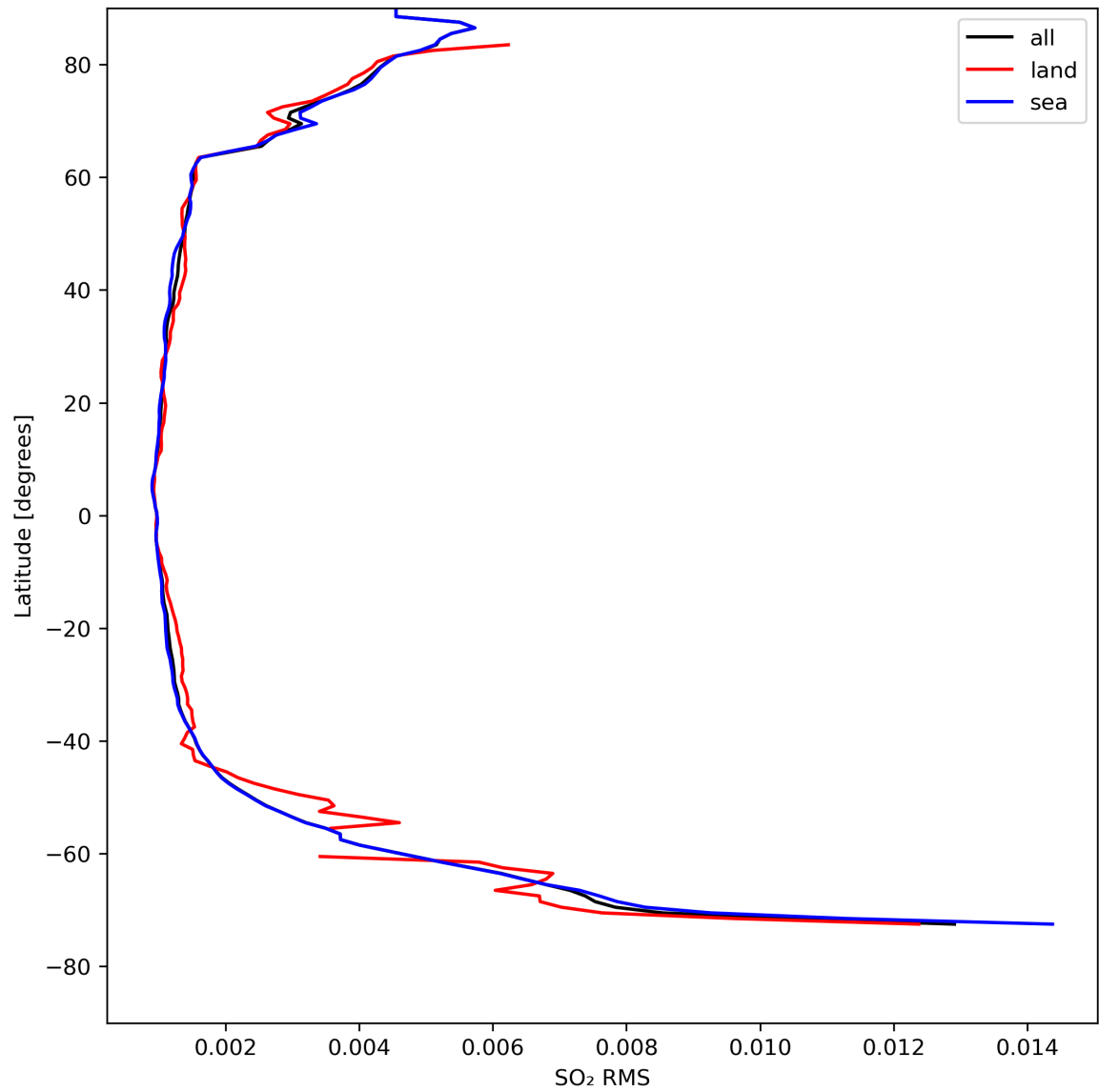
Figure 47: Zonal average of “SO 2 RMS” for 2024-04-21 to 2024-04-23.
