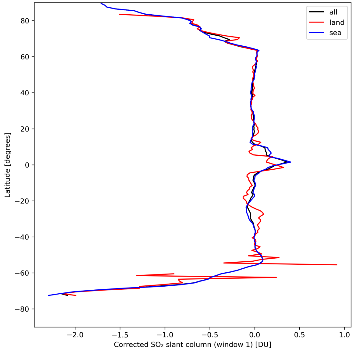
Figure 35: Zonal average of “Corrected SO 2 slant column (window 1)” for 2024-04-21 to 2024-04-23.
