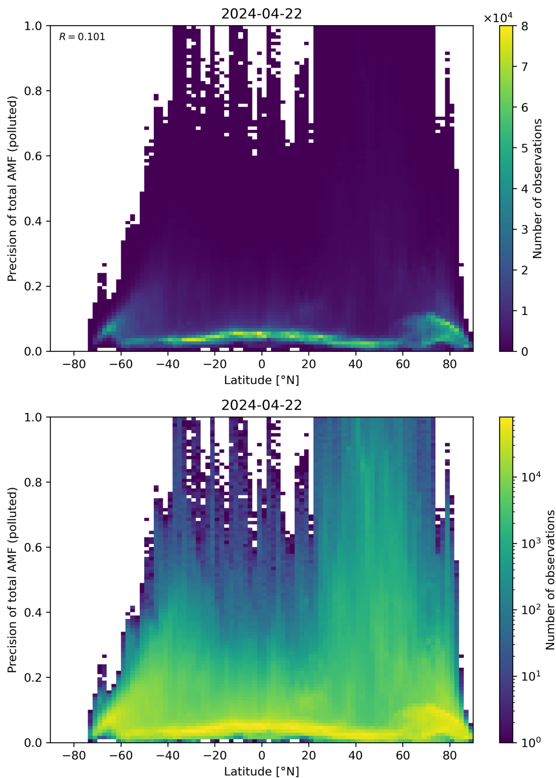
Figure 155: Scatter density plot of “Latitude” against “Precision of total AMF (polluted)” for 2024-04-21 to 2024-04-23.
