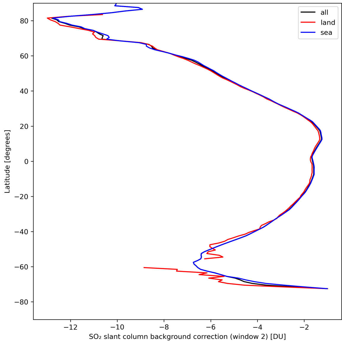
Figure 40: Zonal average of “SO 2 slant column background correction (window 2)” for 2024-04-21 to 2024-04-23.
