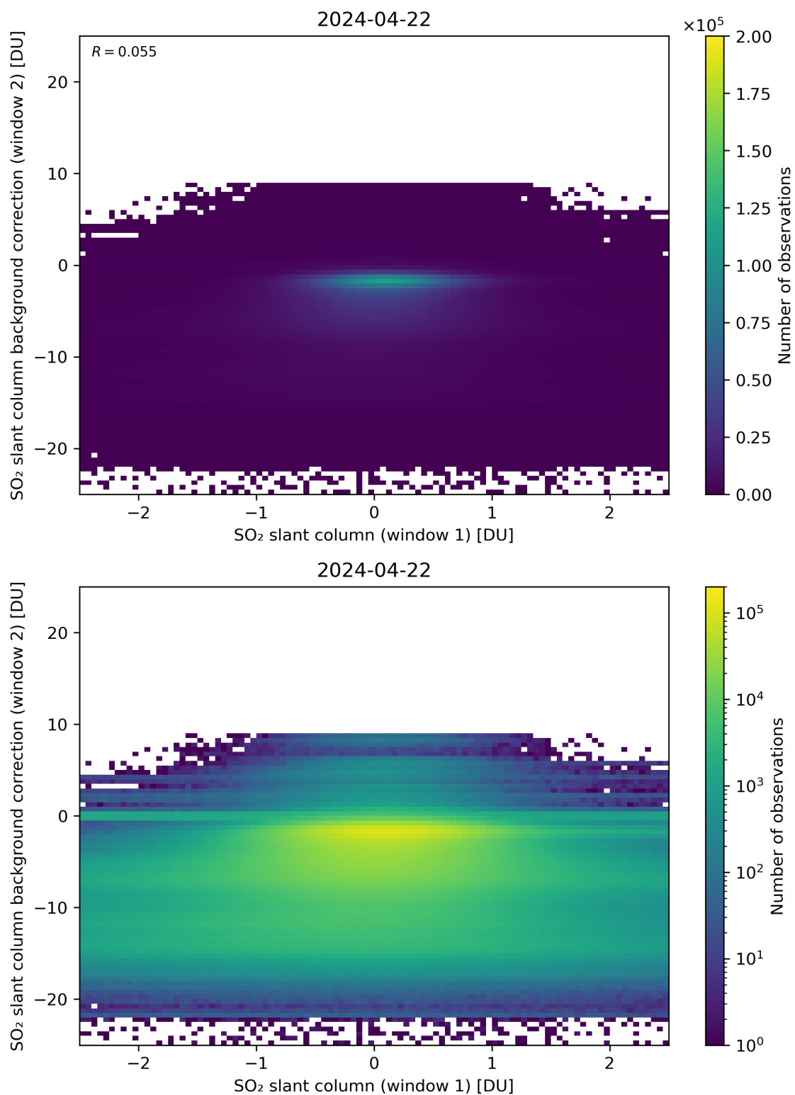
Figure 213: Scatter density plot of “SO 2 slant column (window 1)” against “SO 2 slant column background correction (window 2)” for 2024-04-21 to 2024-04-23.
