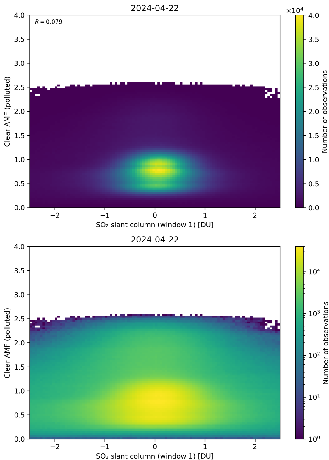
Figure 232: Scatter density plot of “SO 2 slant column (window 1)” against “Clear AMF (polluted)” for 2024-04-21 to 2024-04-23.
