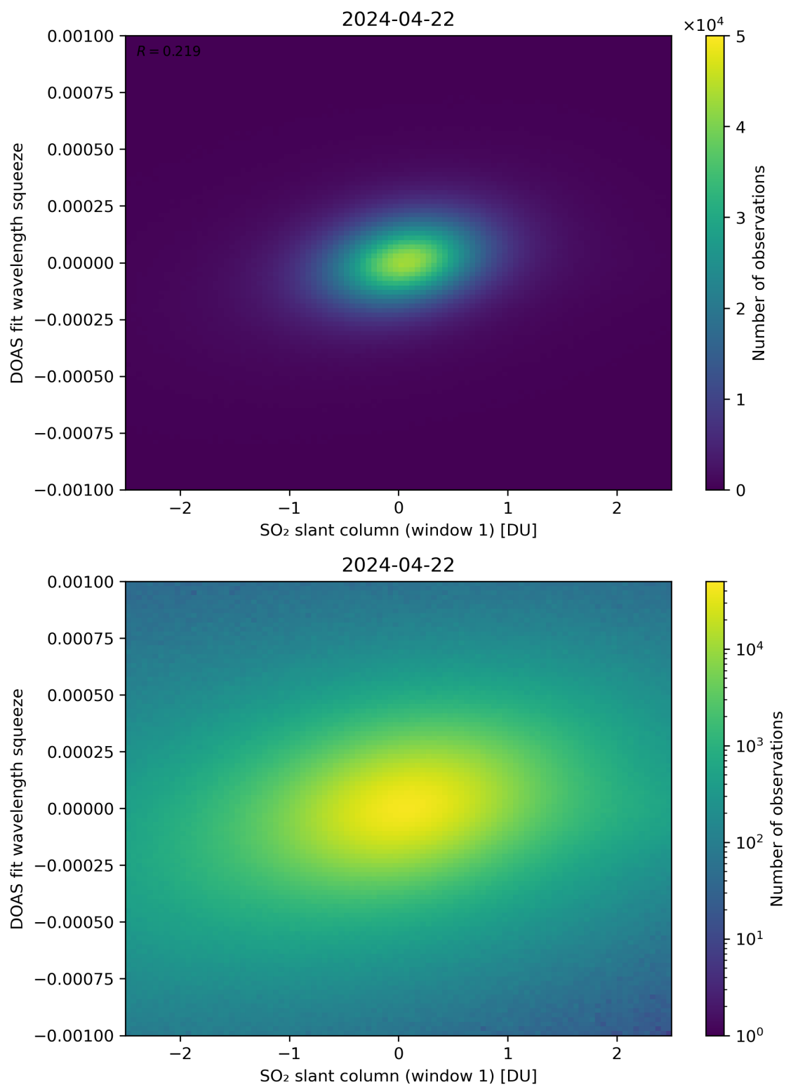
Figure 216: Scatter density plot of “SO 2 slant column (window 1)” against “DOAS fit wavelength squeeze” for 2024-04-21 to 2024-04-23.
