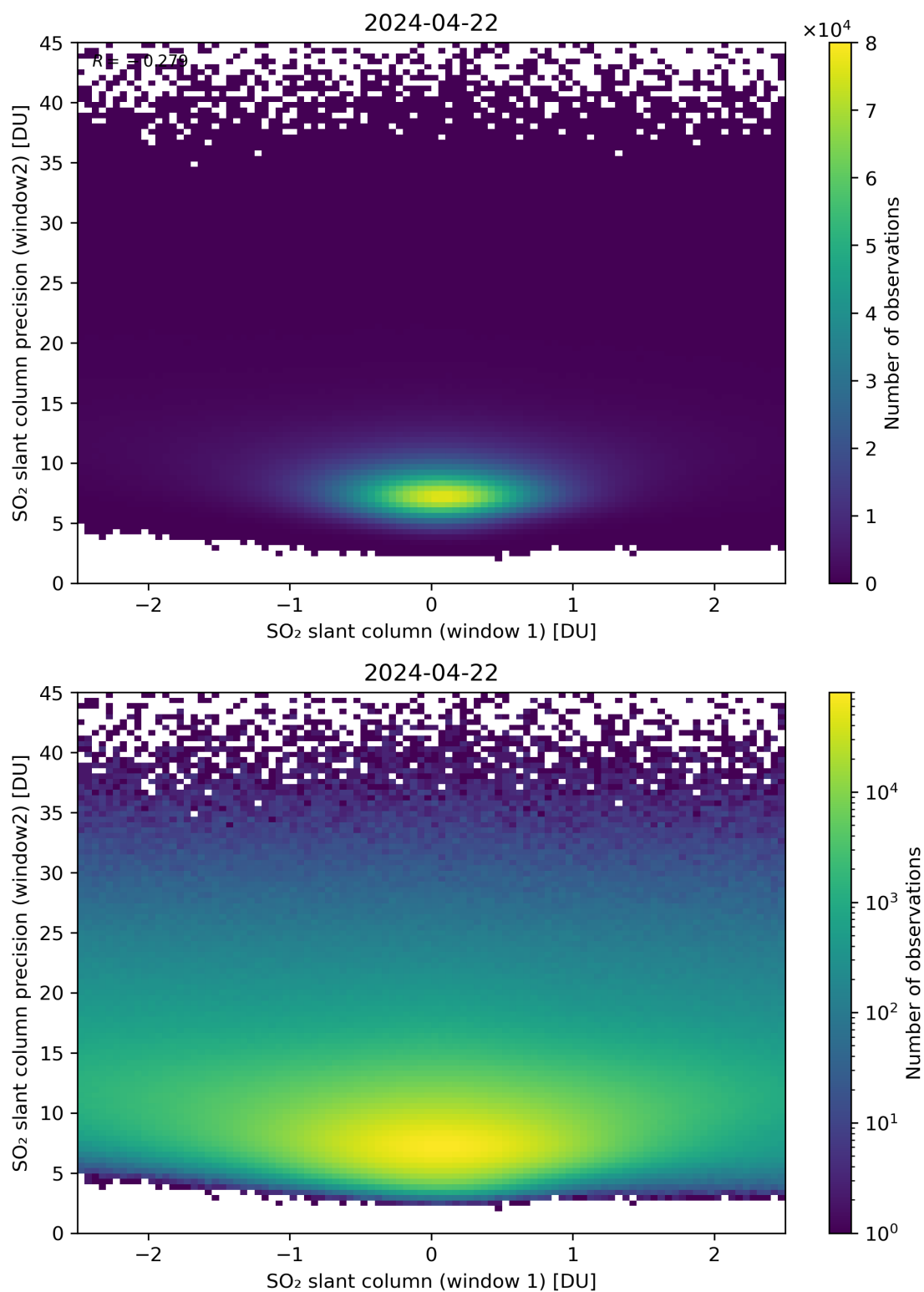
Figure 236: Scatter density plot of “SO 2 slant column (window 1)” against “SO 2 slant column precision (window2)” for 2024-04-21 to 2024-04-23.
