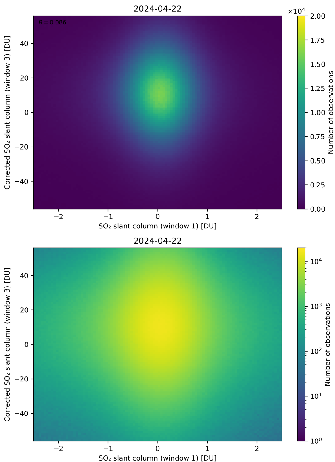
Figure 234: Scatter density plot of “SO 2 slant column (window 1)” against “Corrected SO 2 slant column (window 3)” for 2024-04-21 to 2024-04-23.
