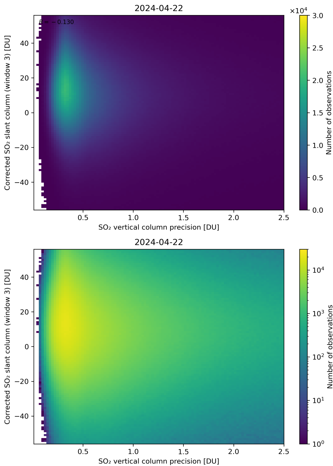
Figure 288: Scatter density plot of “SO 2 vertical column precision” against “Corrected SO 2 slant column (window 3)” for 2024-04-21 to 2024-04-23.
