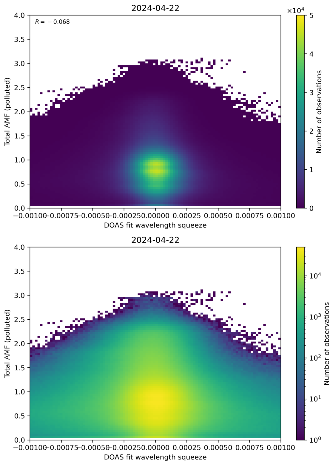
Figure 134: Scatter density plot of “DOAS fit wavelength squeeze” against “Total AMF (polluted)” for 2024-04-21 to 2024-04-23.
