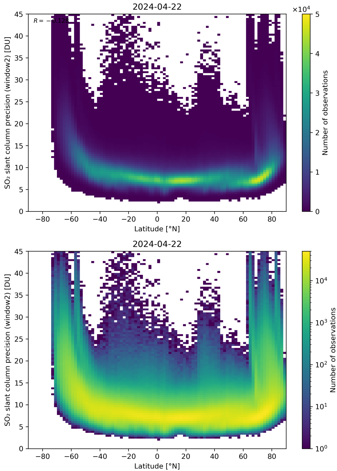
Figure 151: Scatter density plot of “Latitude” against “SO 2 slant column precision (window2)” for 2024-04-21 to 2024-04-23.
