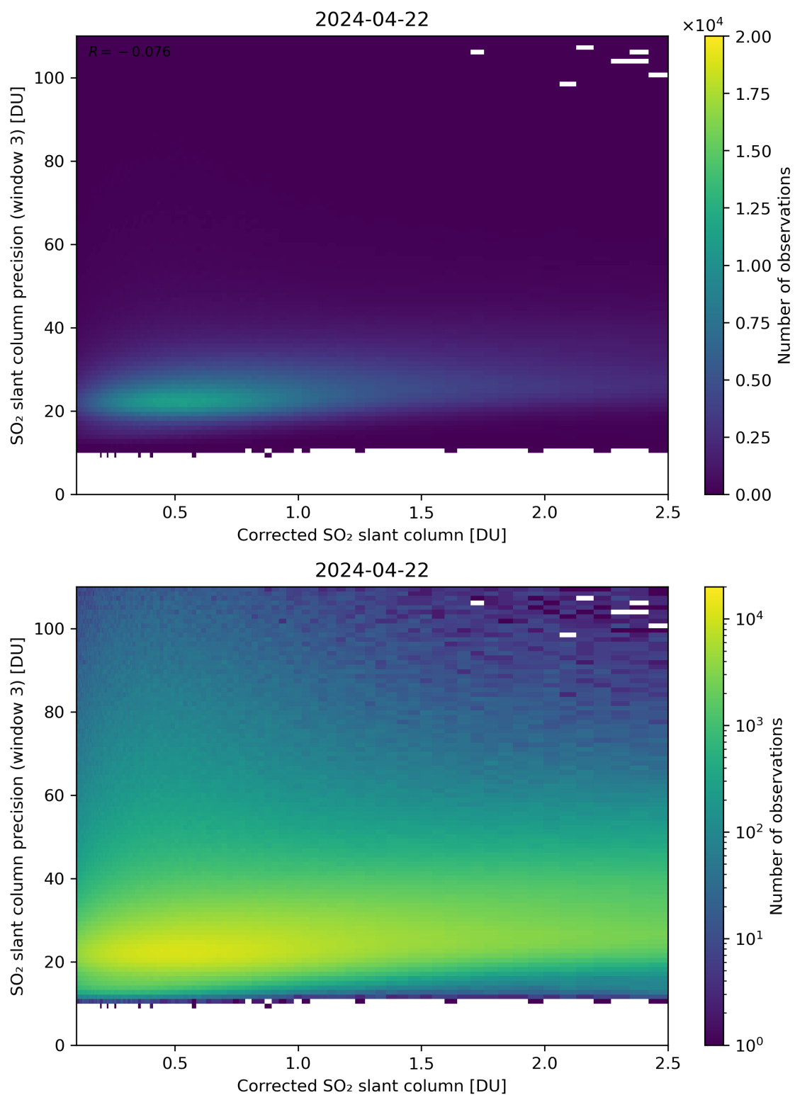
Figure 191: Scatter density plot of “Corrected SO 2 slant column” against “SO 2 slant column precision (window 3)” for 2024-04-21 to 2024-04-23.
