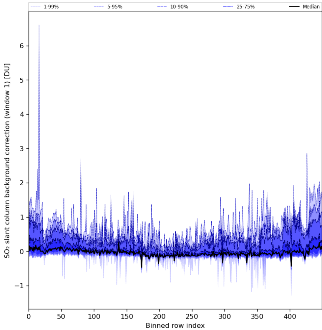
Figure 82: Along track statistics of “SO 2 slant column background correction (window 1)” for 2024-04-21 to 2024-04-23
