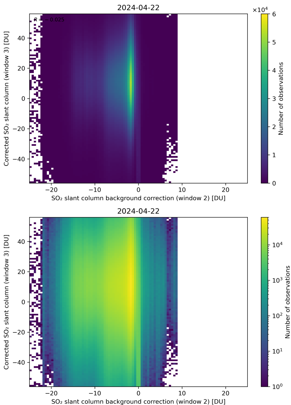
Figure 116: Scatter density plot of “SO 2 slant column background correction (window 2)” against “Corrected SO 2 slant column (window 3)” for 2024-04-21 to 2024-04-23.
