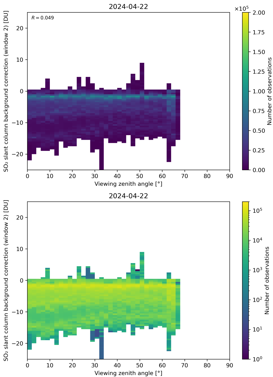
Figure 309: Scatter density plot of “Viewing zenith angle” against “SO 2 slant column background correction (window 2)” for 2024-04-21 to 2024-04-23.
