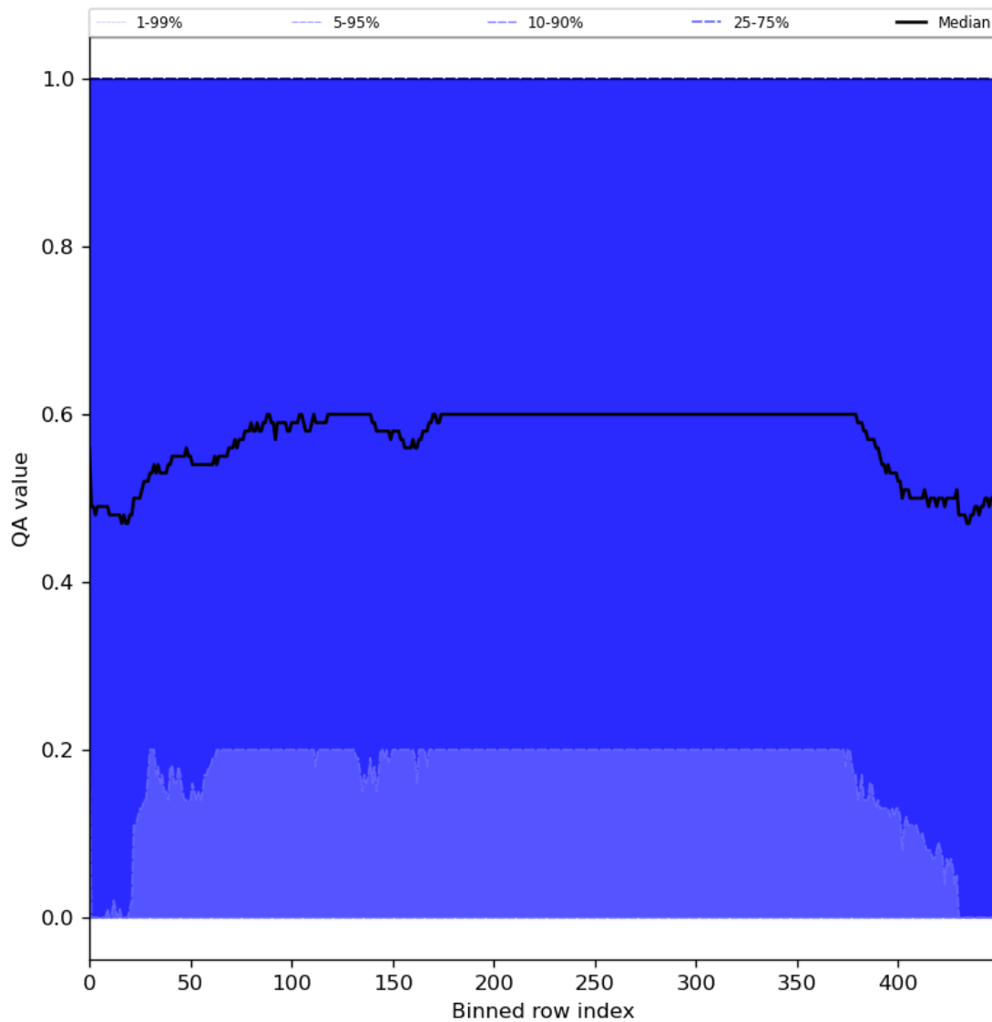
Figure 75: Along track statistics of “QA value” for 2024-04-21 to 2024-04-23
