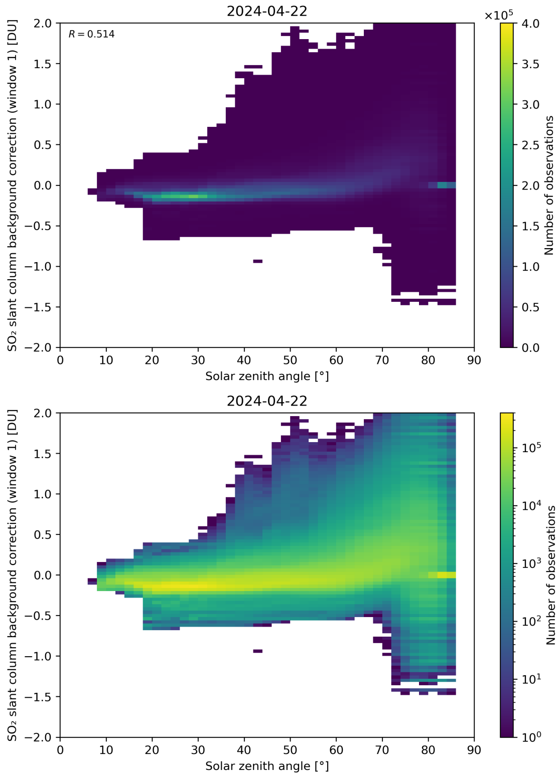
Figure 158: Scatter density plot of “Solar zenith angle” against “SO 2 slant column background correction (window 1)” for 2024-04-21 to 2024-04-23.
