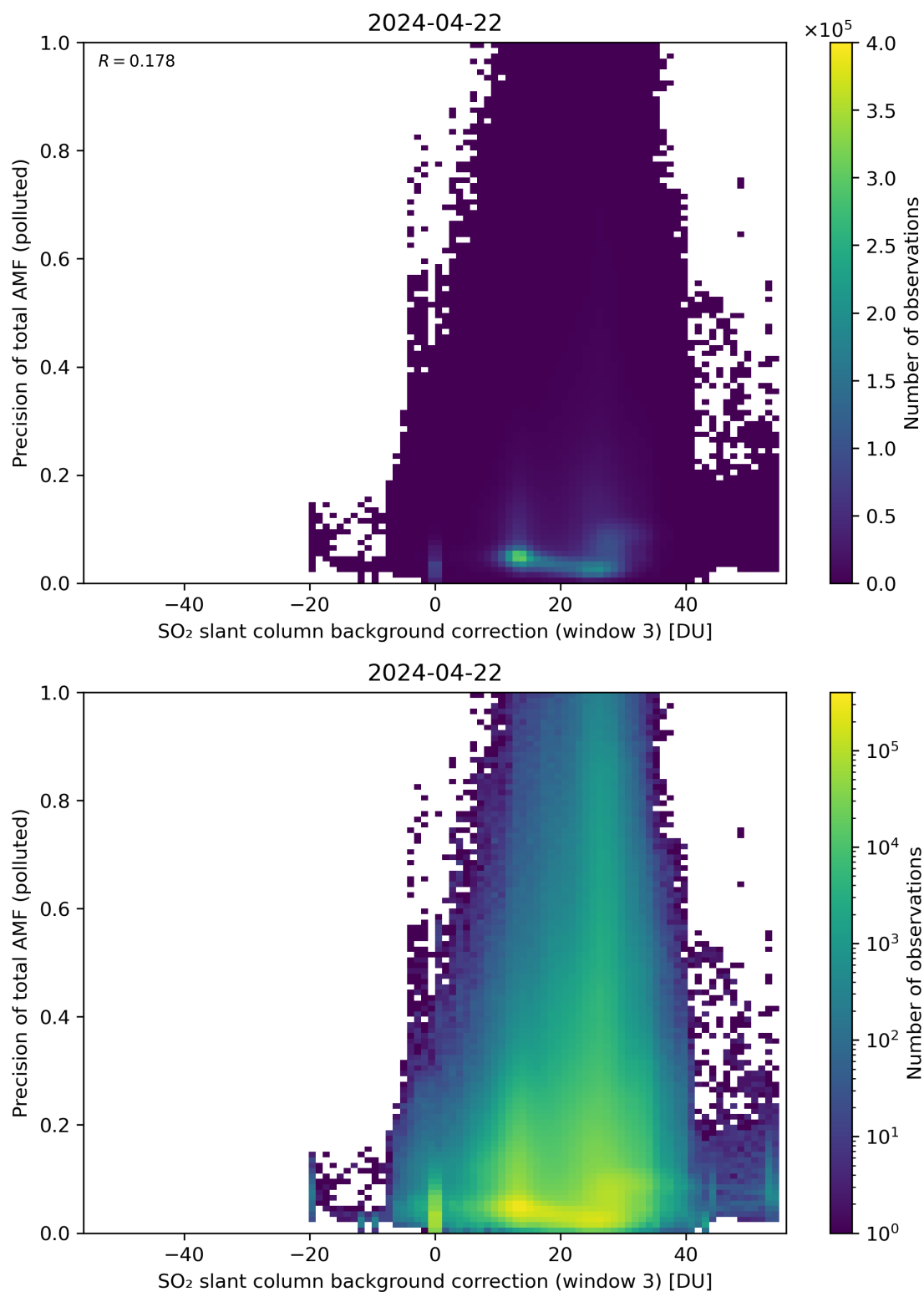
Figure 126: Scatter density plot of “SO 2 slant column background correction (window 3)” against “Precision of total AMF (polluted)” for 2024-04-21 to 2024-04-23.
