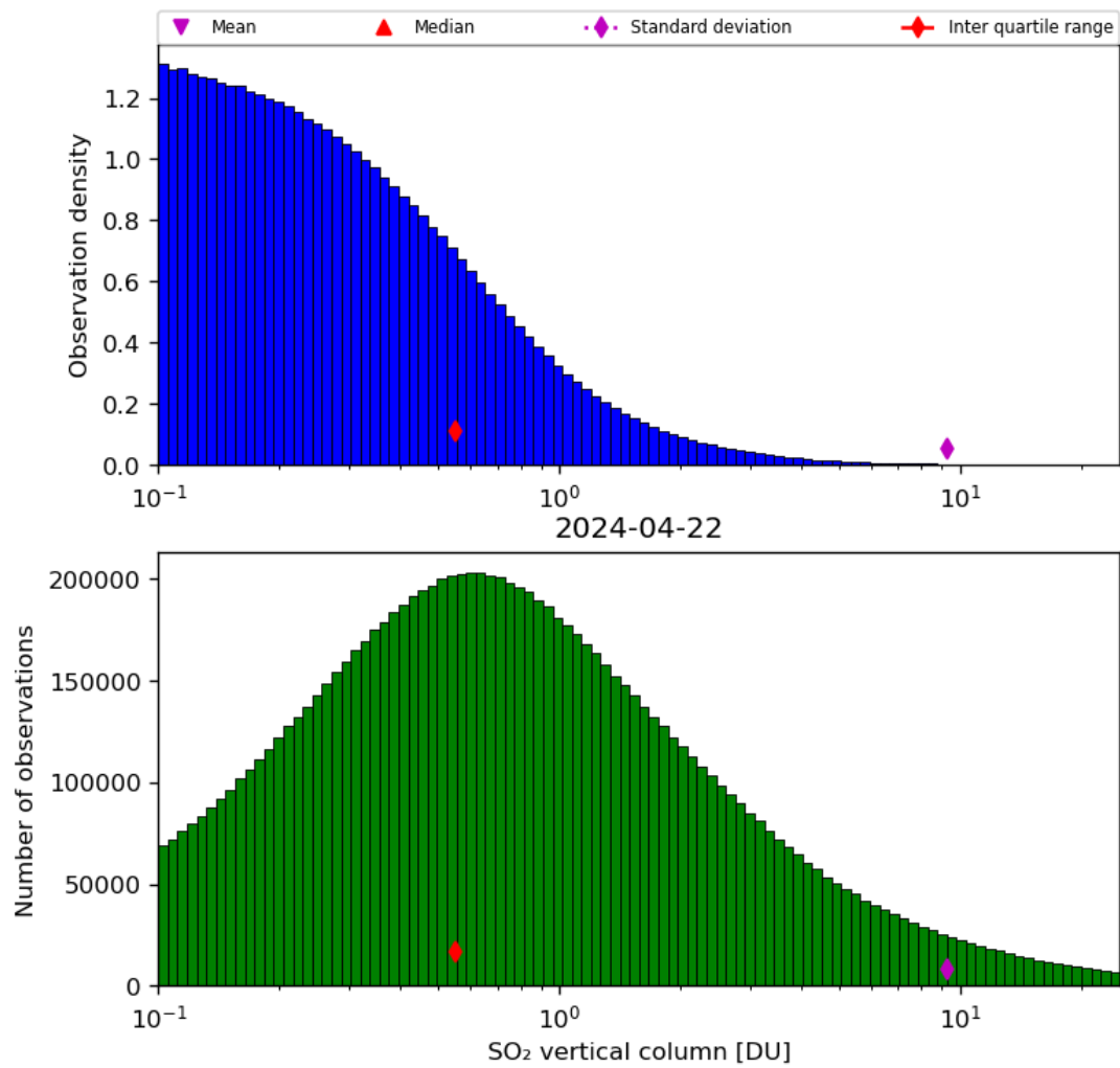
Figure 53: Histogram of “SO 2 vertical column” for 2024-04-21 to 2024-04-23
