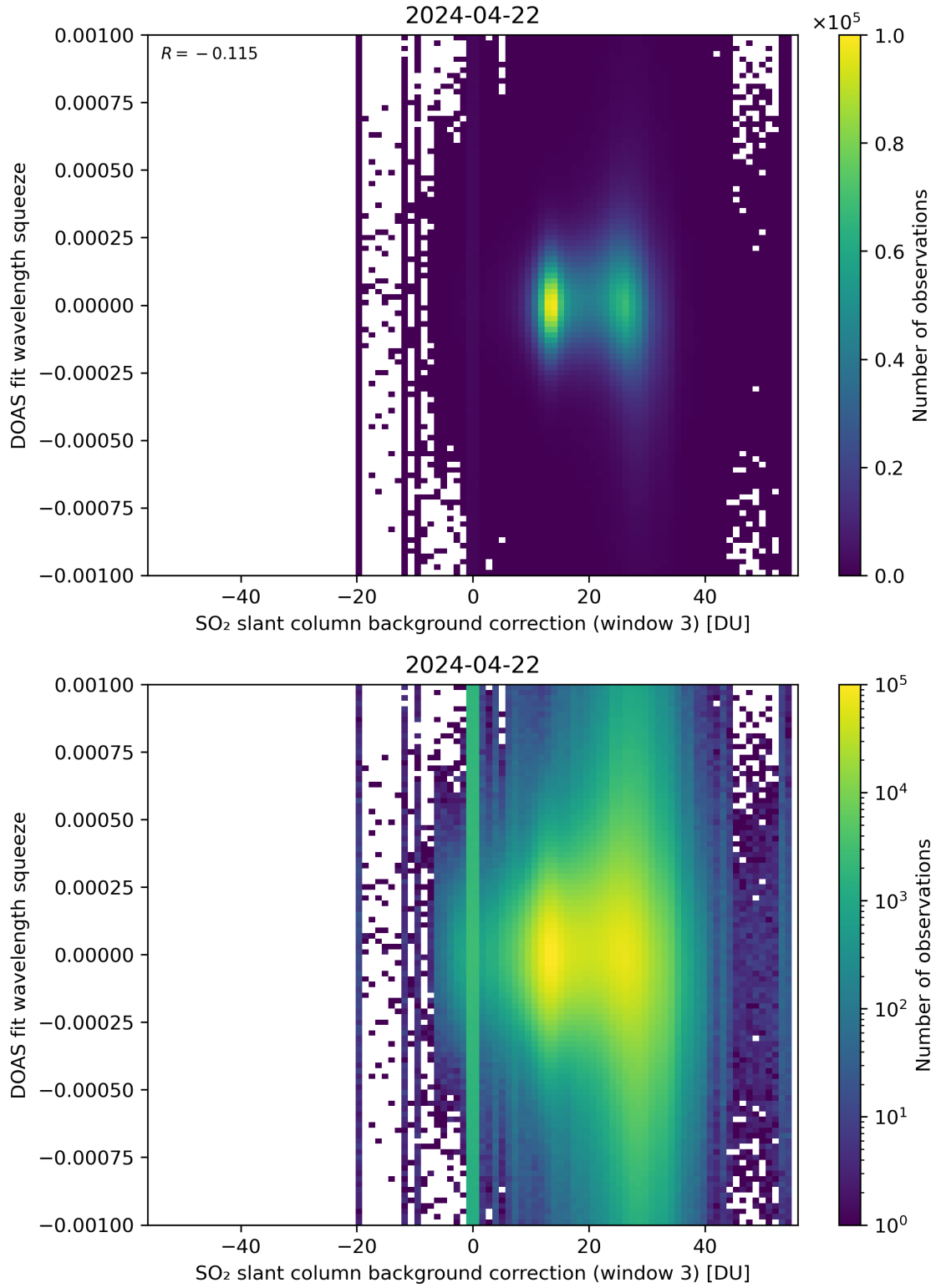
Figure 122: Scatter density plot of “SO 2 slant column background correction (window 3)” against “DOAS fit wavelength squeeze” for 2024-04-21 to 2024-04-23.
