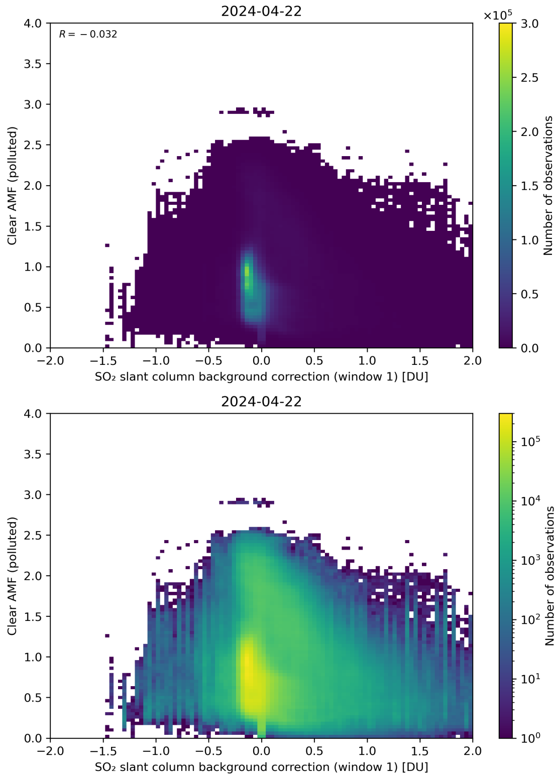
Figure 103: Scatter density plot of “SO 2 slant column background correction (window 1)” against “Clear AMF (polluted)” for 2024-04-21 to 2024-04-23.
