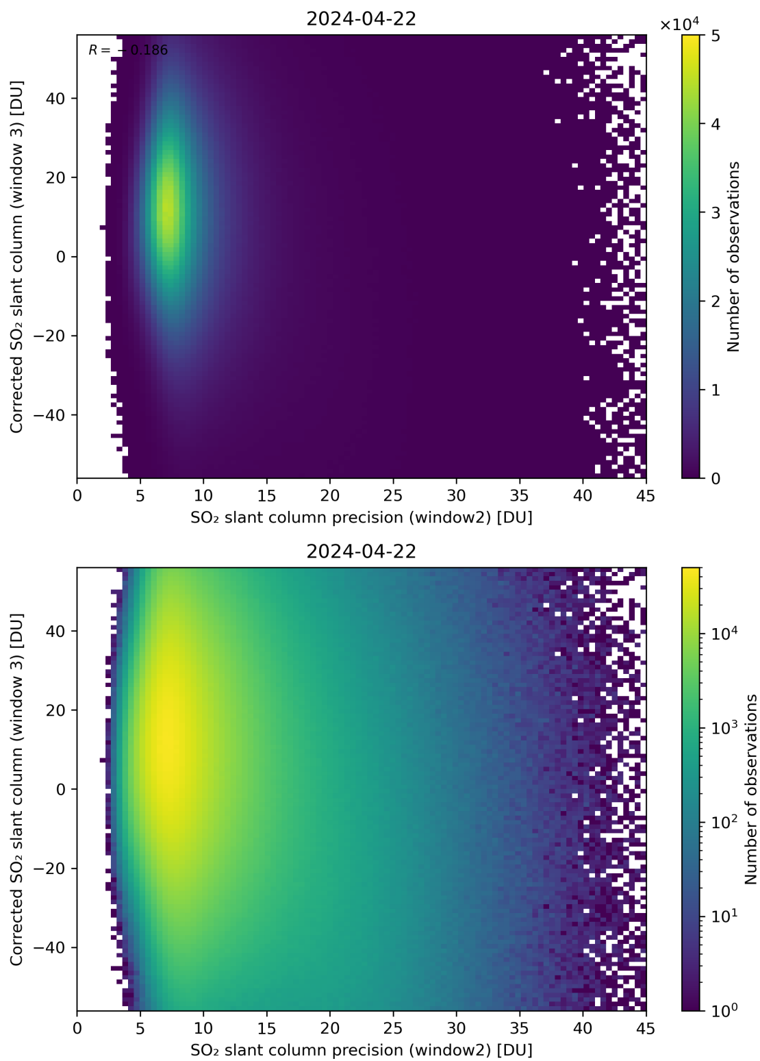
Figure 248: Scatter density plot of “SO 2 slant column precision (window2)” against “Corrected SO 2 slant column (window 3)” for 2024-04-21 to 2024-04-23.
