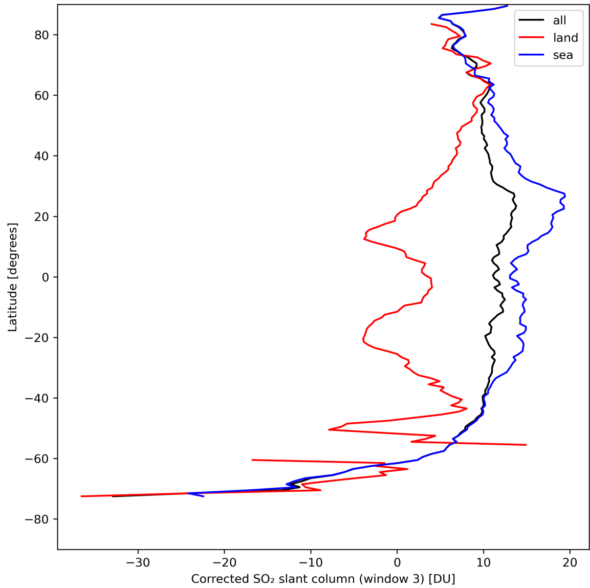
Figure 43: Zonal average of “Corrected SO 2 slant column (window 3)” for 2024-04-21 to 2024-04-23.
