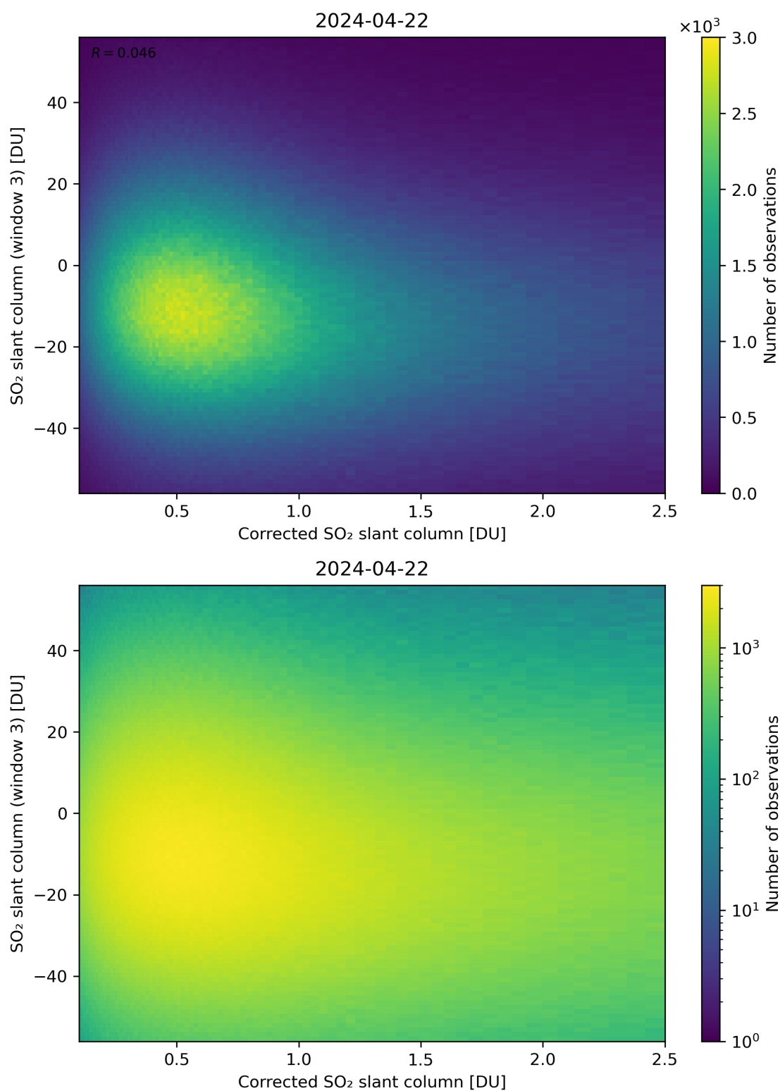
Figure 190: Scatter density plot of “Corrected SO 2 slant column” against “SO 2 slant column (window 3)” for 2024-04-21 to 2024-04-23.
