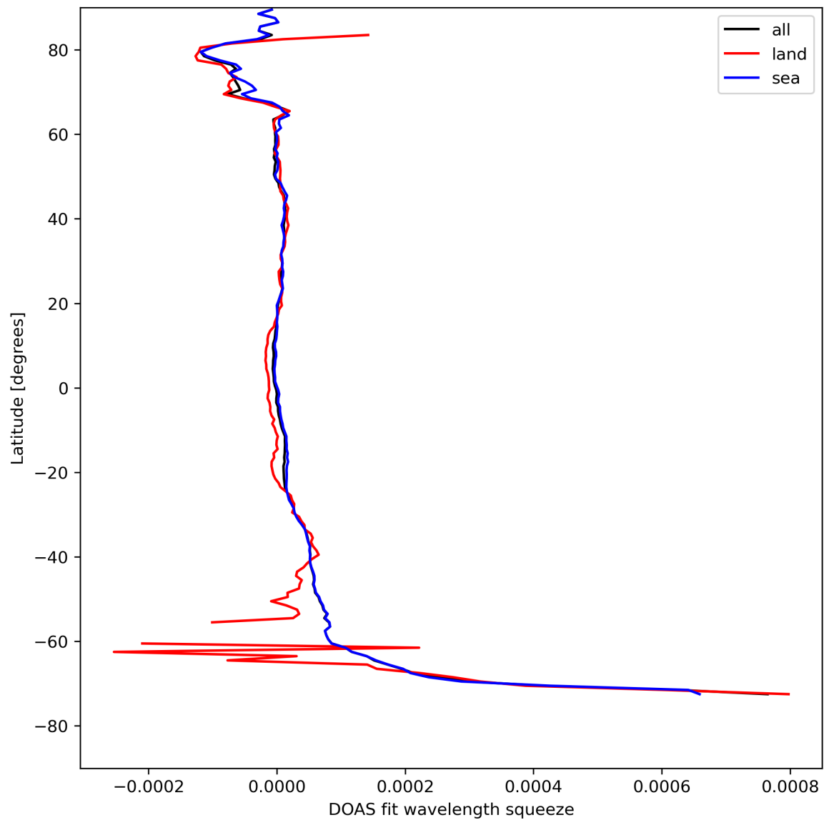
Figure 46: Zonal average of “DOAS fit wavelength squeeze” for 2024-04-21 to 2024-04-23.
