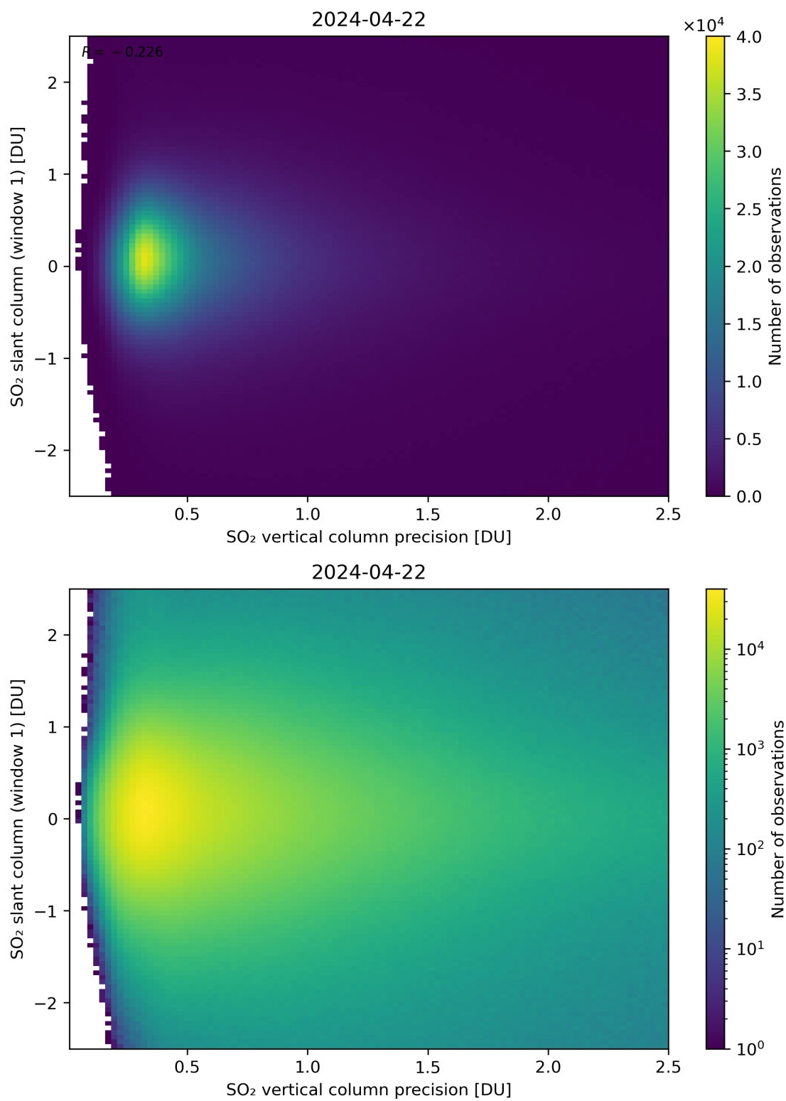
Figure 289: Scatter density plot of “SO 2 vertical column precision” against “SO 2 slant column (window 1)” for 2024-04-21 to 2024-04-23.
