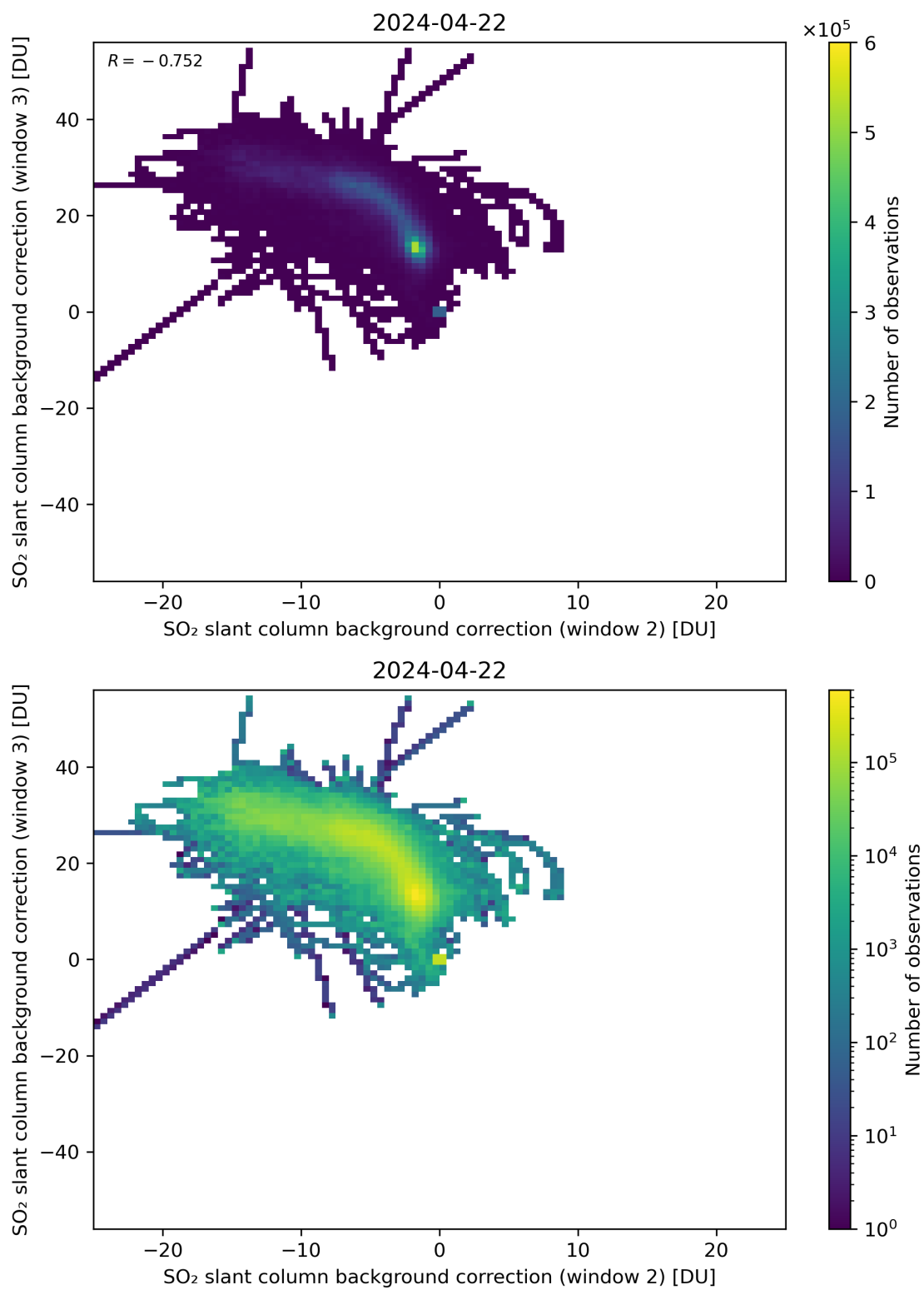
Figure 111: Scatter density plot of “SO 2 slant column background correction (window 2)” against “SO 2 slant column background correction (window 3)” for 2024-04-21 to 2024-04-23.
