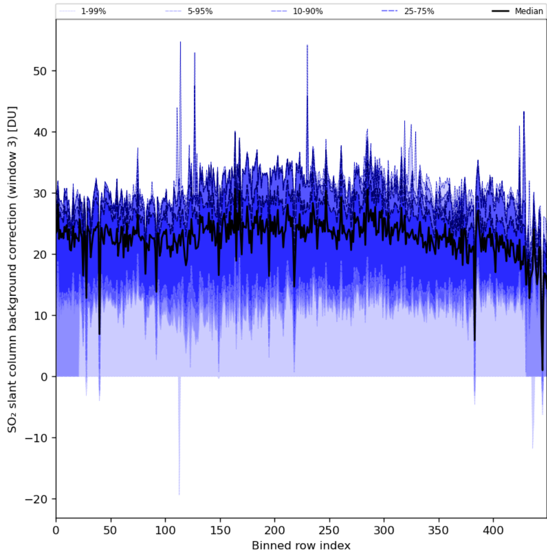
Figure 90: Along track statistics of “SO 2 slant column background correction (window 3)” for 2024-04-21 to 2024-04-23
