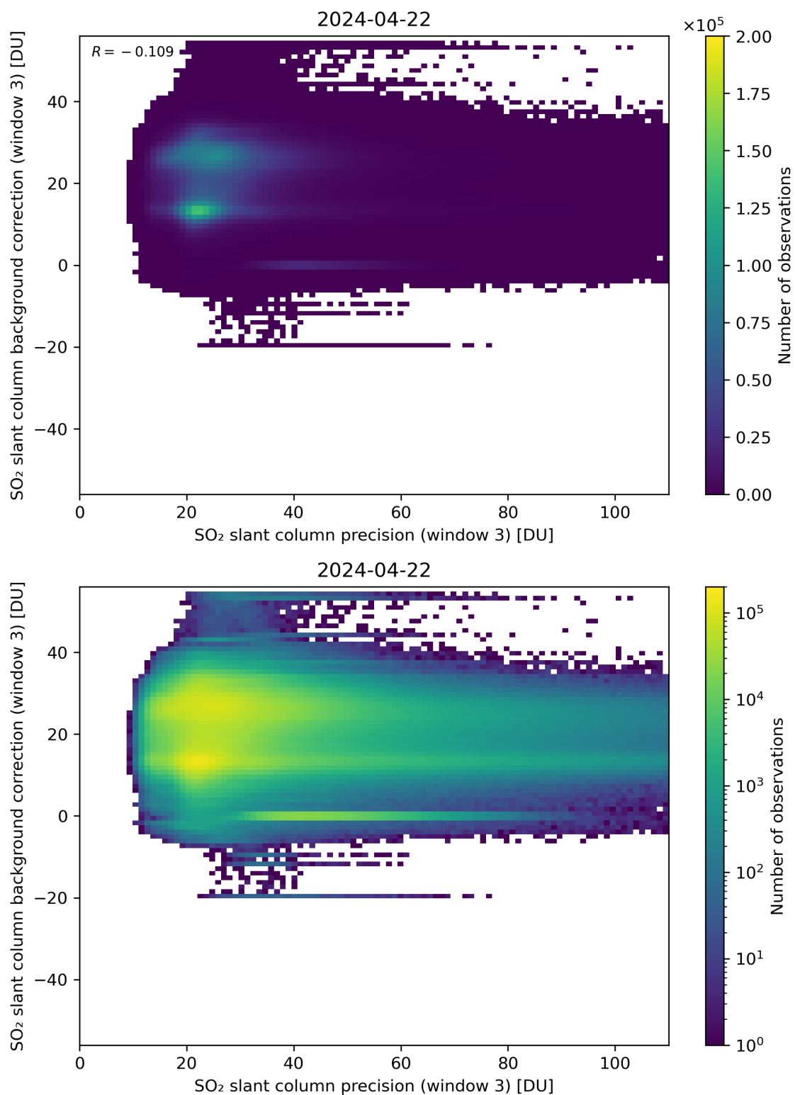
Figure 257: Scatter density plot of “SO 2 slant column precision (window 3)” against “SO 2 slant column background correction (window 3)” for 2024-04-21 to 2024-04-23.
