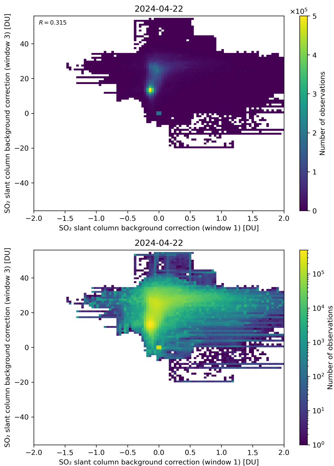
Figure 99: Scatter density plot of “SO 2 slant column background correction (window 1)” against “SO 2 slant column background correction (window 3)” for 2024-04-21 to 2024-04-23.
