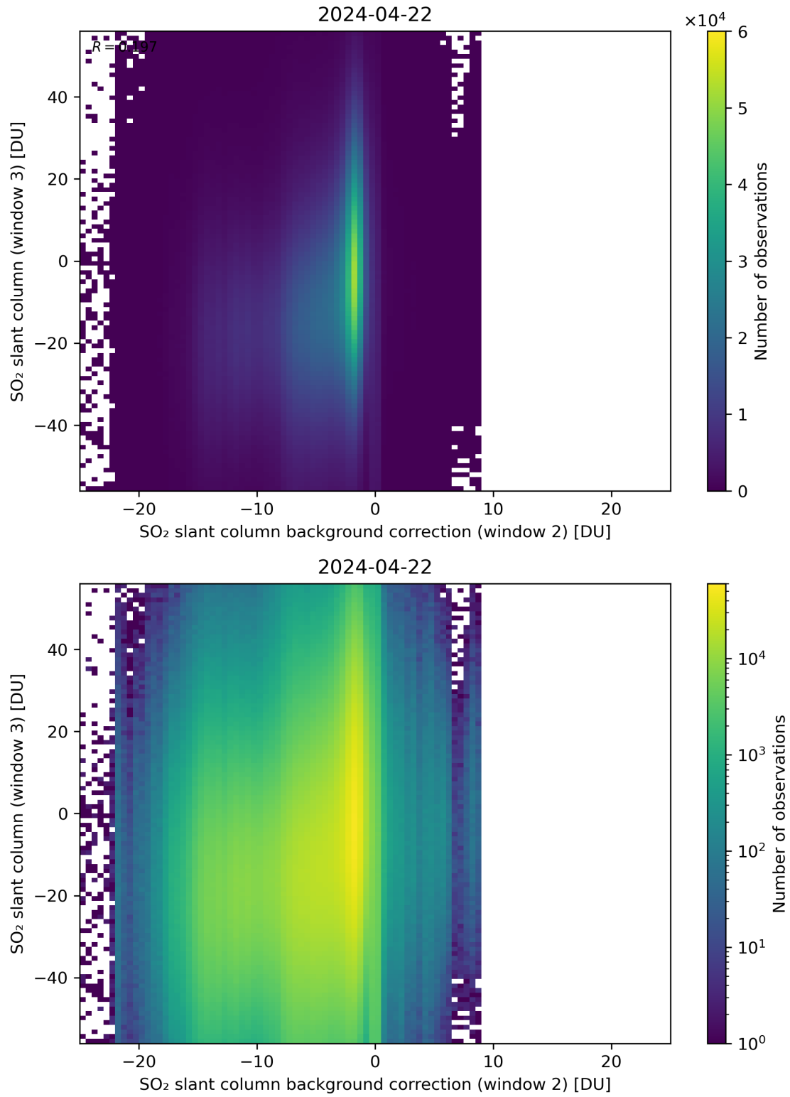
Figure 117: Scatter density plot of “SO 2 slant column background correction (window 2)” against “SO 2 slant column (window 3)” for 2024-04-21 to 2024-04-23.
