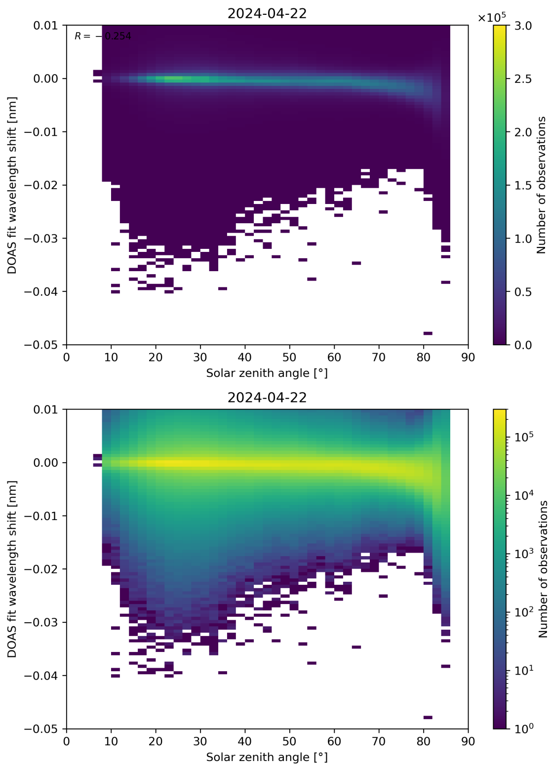
Figure 161: Scatter density plot of “Solar zenith angle” against “DOAS fit wavelength shift” for 2024-04-21 to 2024-04-23.
