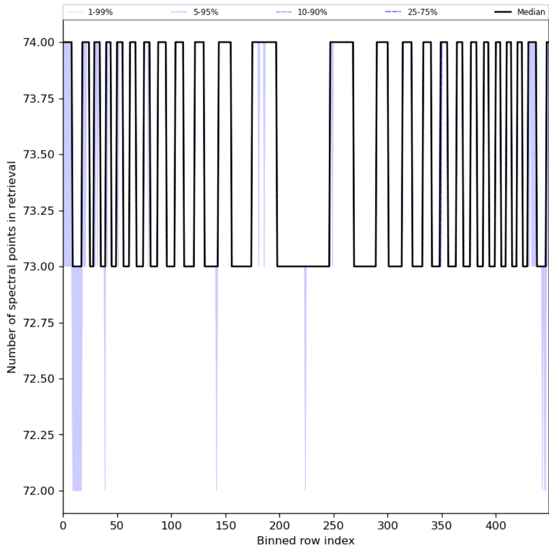
Figure 97: Along track statistics of “Number of spectral points in retrieval” for 2024-04-21 to 2024-04-23
