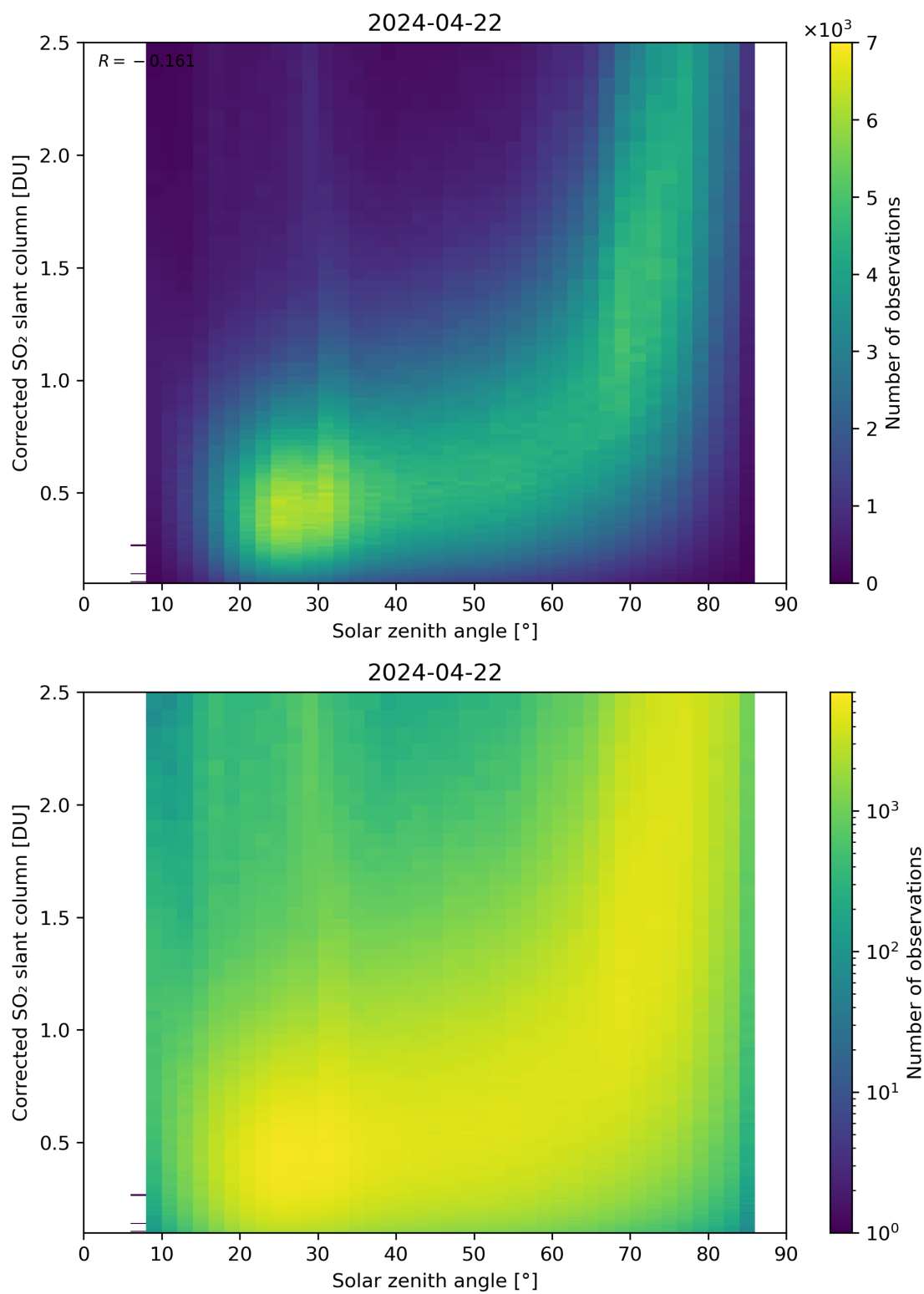
Figure 166: Scatter density plot of “Solar zenith angle” against “Corrected SO 2 slant column” for 2024-04-21 to 2024-04-23.
