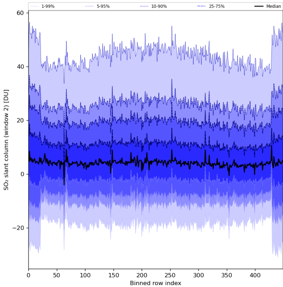
Figure 83: Along track statistics of “SO 2 slant column (window 2)” for 2024-04-21 to 2024-04-23
