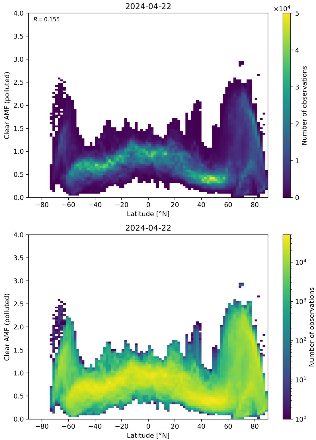
Figure 145: Scatter density plot of “Latitude” against “Clear AMF (polluted)” for 2024-04-21 to 2024-04-23.
