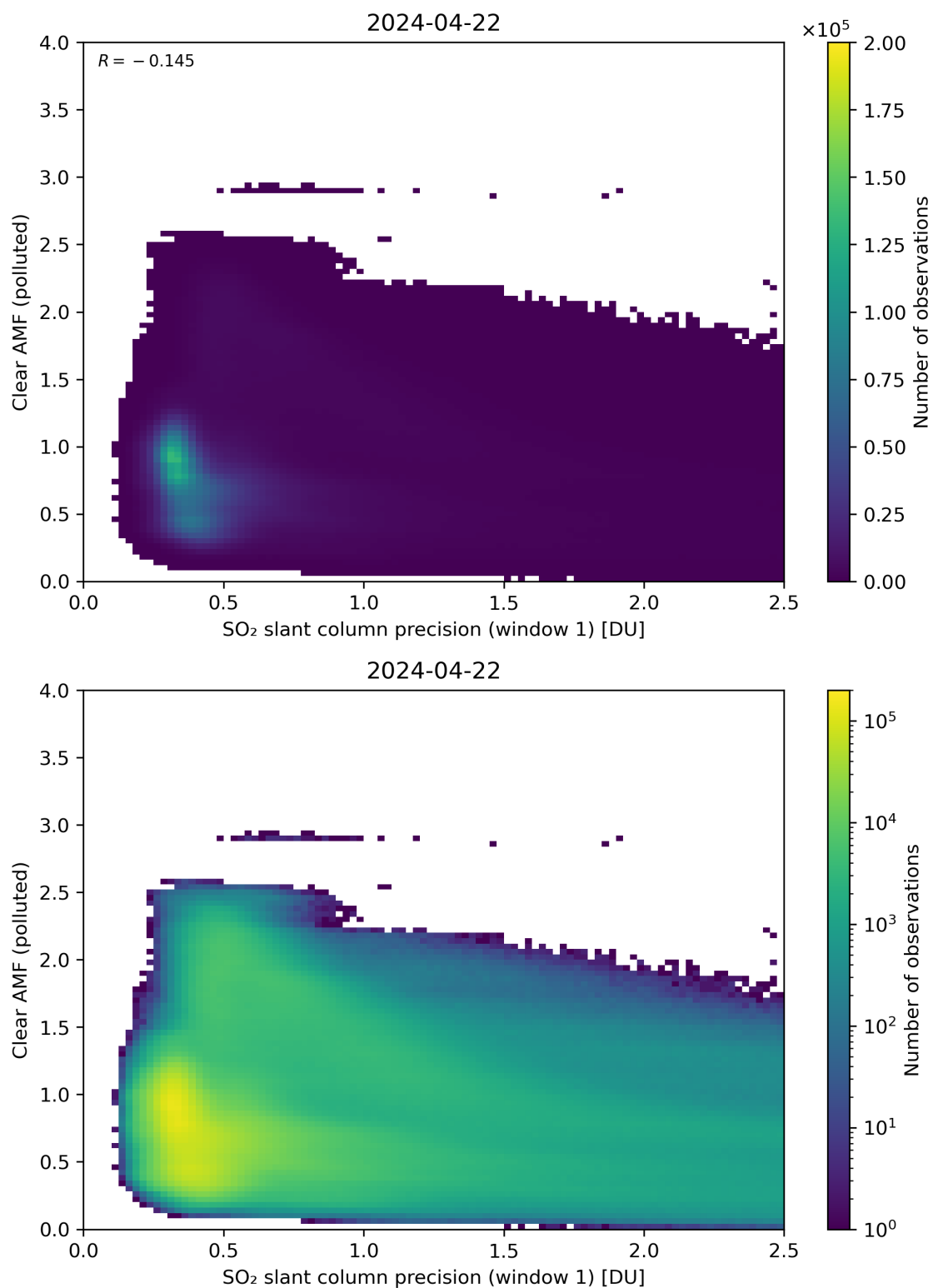
Figure 224: Scatter density plot of “SO 2 slant column precision (window 1)” against “Clear AMF (polluted)” for 2024-04-21 to 2024-04-23.
