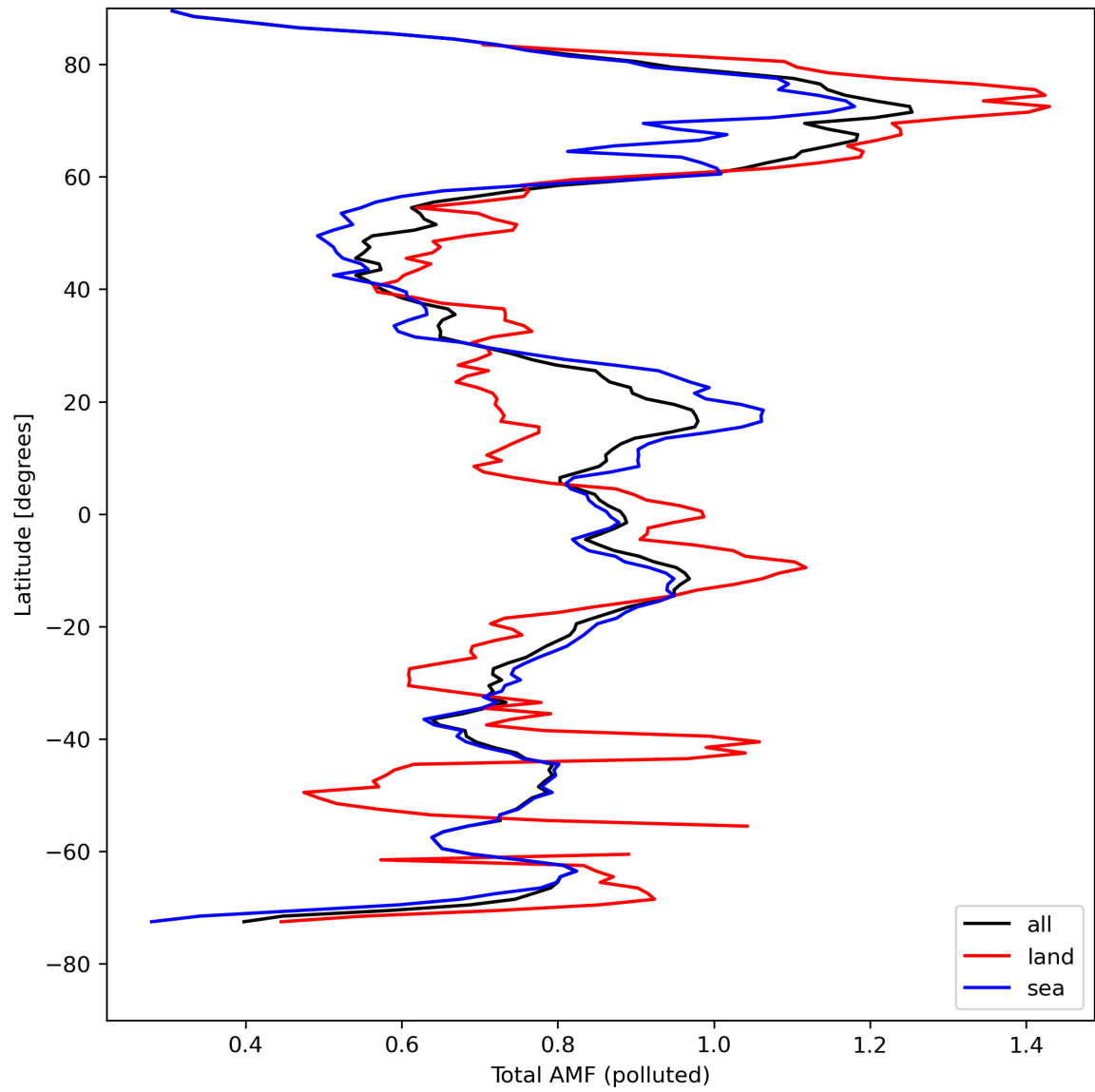
Figure 48: Zonal average of “Total AMF (polluted)” for 2024-04-21 to 2024-04-23.
