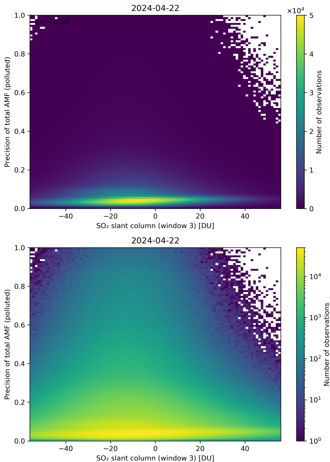
Figure 269: Scatter density plot of “SO 2 slant column (window 3)” against “Precision of total AMF (polluted)” for 2024-04-21 to 2024-04-23.
