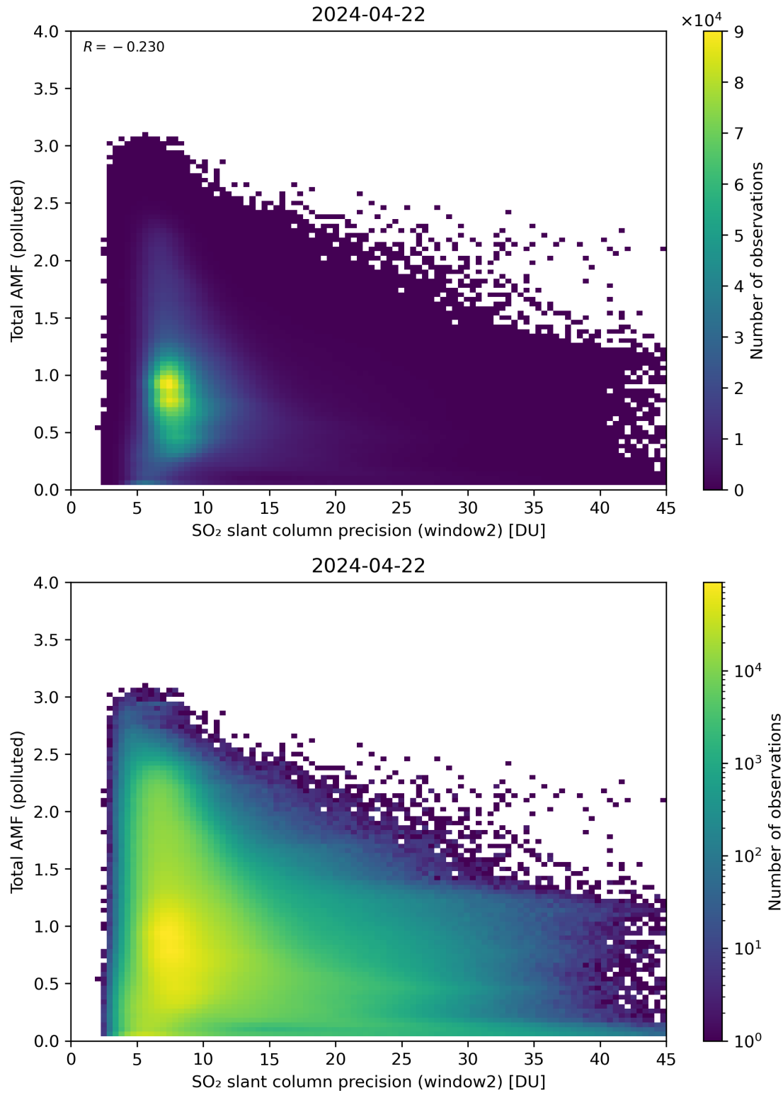
Figure 251: Scatter density plot of “SO 2 slant column precision (window2)” against “Total AMF (polluted)” for 2024-04-21 to 2024-04-23.
