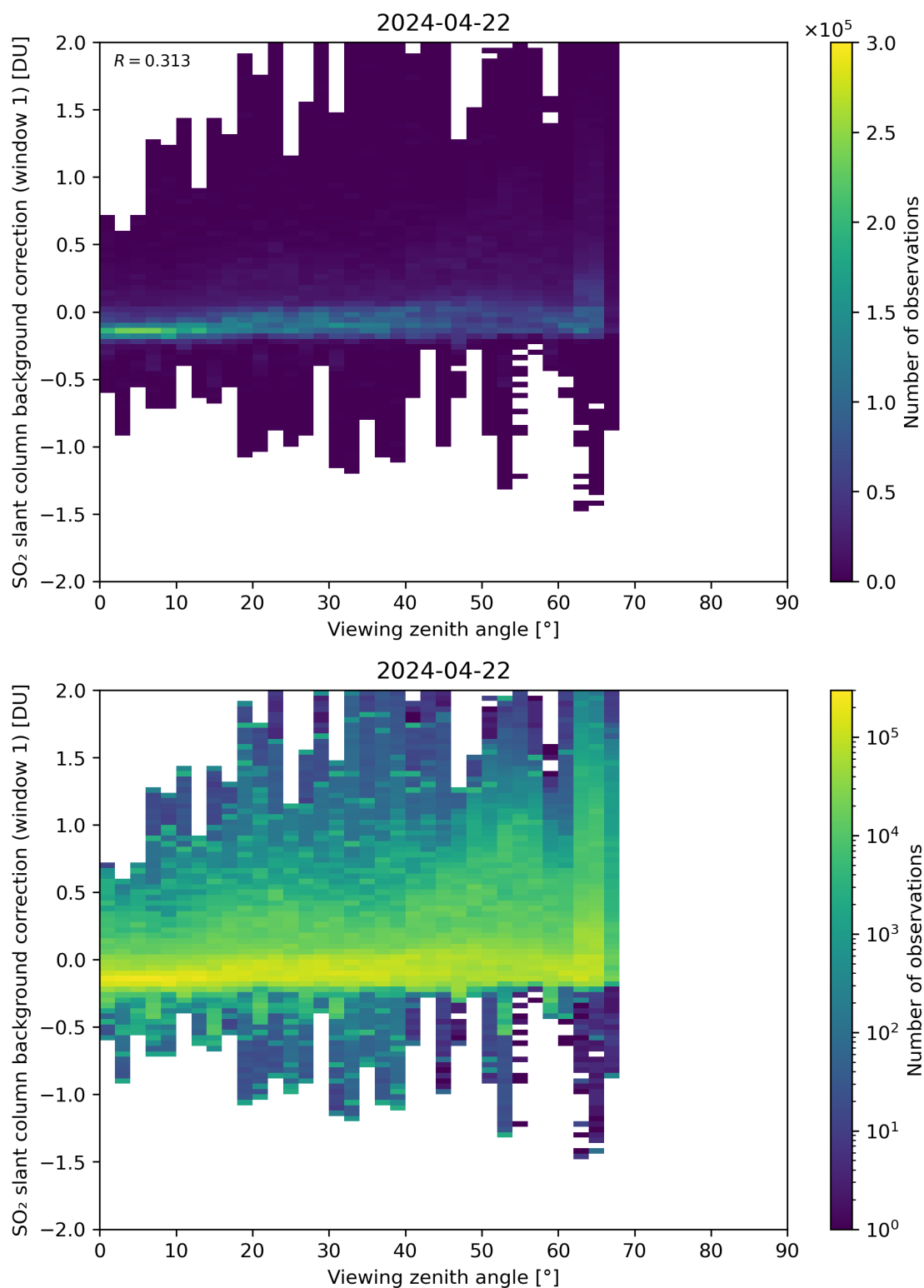
Figure 308: Scatter density plot of “Viewing zenith angle” against “SO 2 slant column background correction (window 1)” for 2024-04-21 to 2024-04-23.
