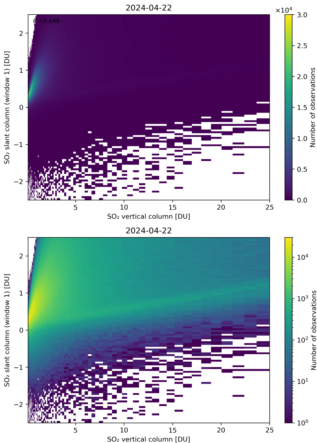
Figure 300: Scatter density plot of “SO 2 vertical column” against “SO 2 slant column (window 1)” for 2024-04-21 to 2024-04-23.
