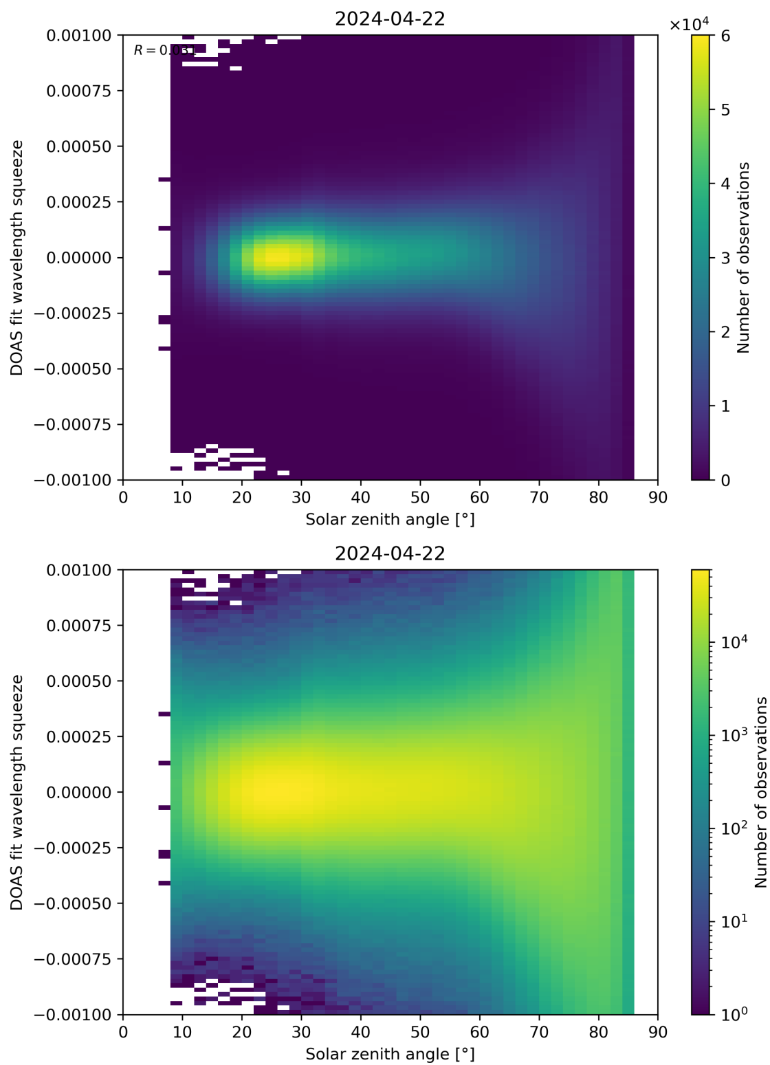
Figure 162: Scatter density plot of “Solar zenith angle” against “DOAS fit wavelength squeeze” for 2024-04-21 to 2024-04-23.
