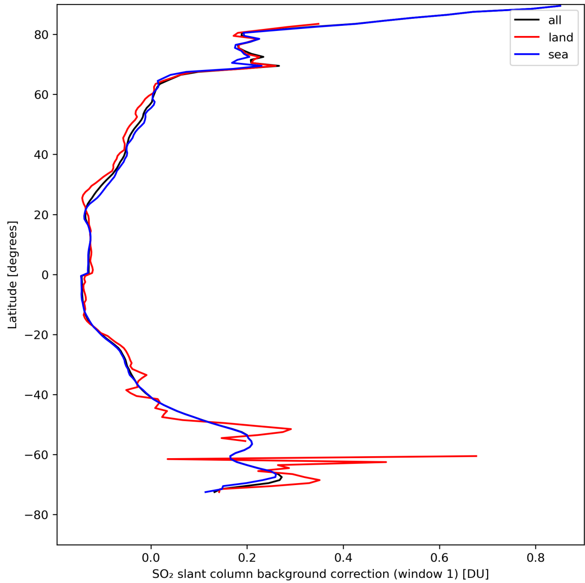
Figure 36: Zonal average of “SO 2 slant column background correction (window 1)” for 2024-04-21 to 2024-04-23.
