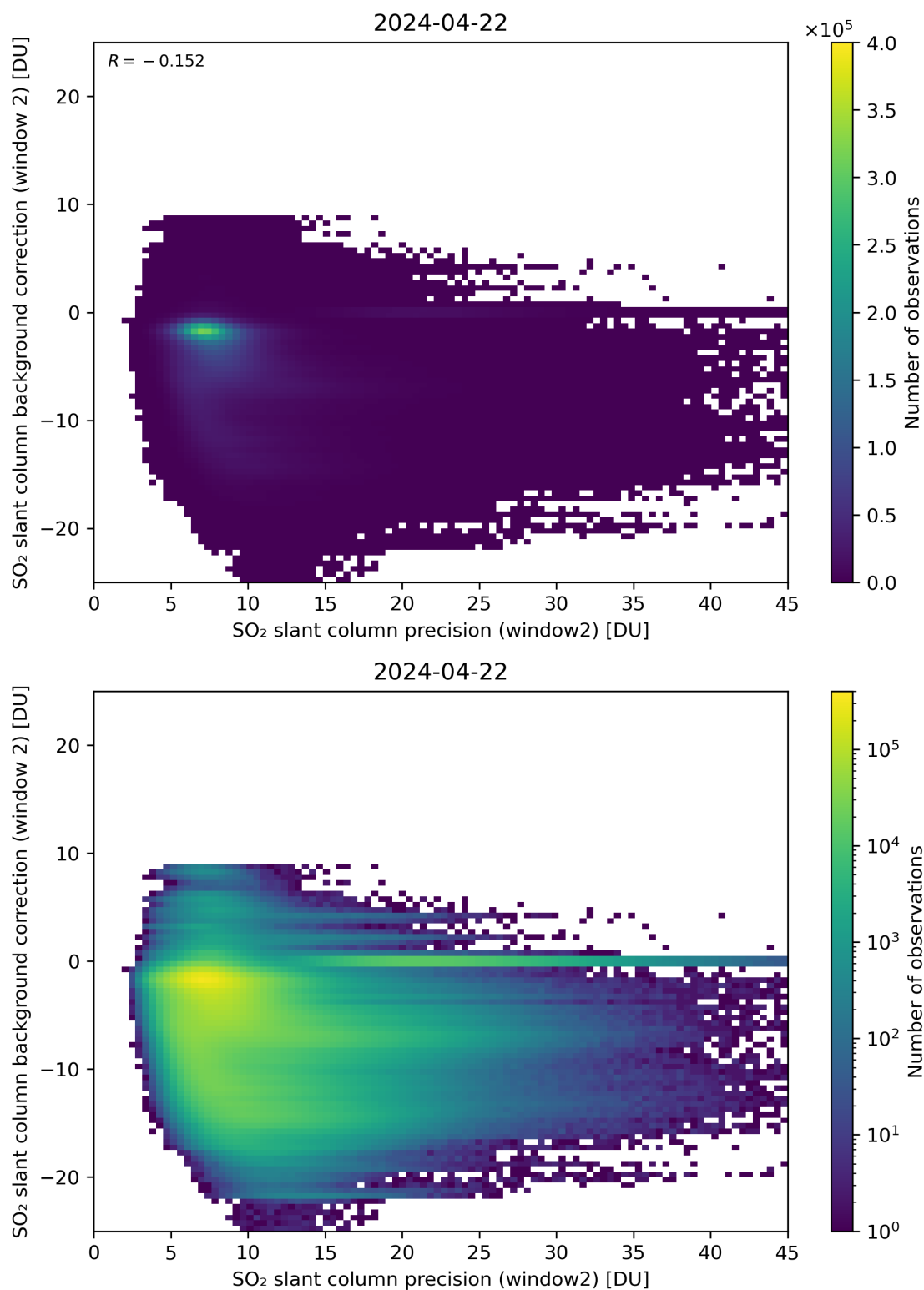
Figure 241: Scatter density plot of “SO 2 slant column precision (window2)” against “SO 2 slant column background correction (window 2)” for 2024-04-21 to 2024-04-23.
