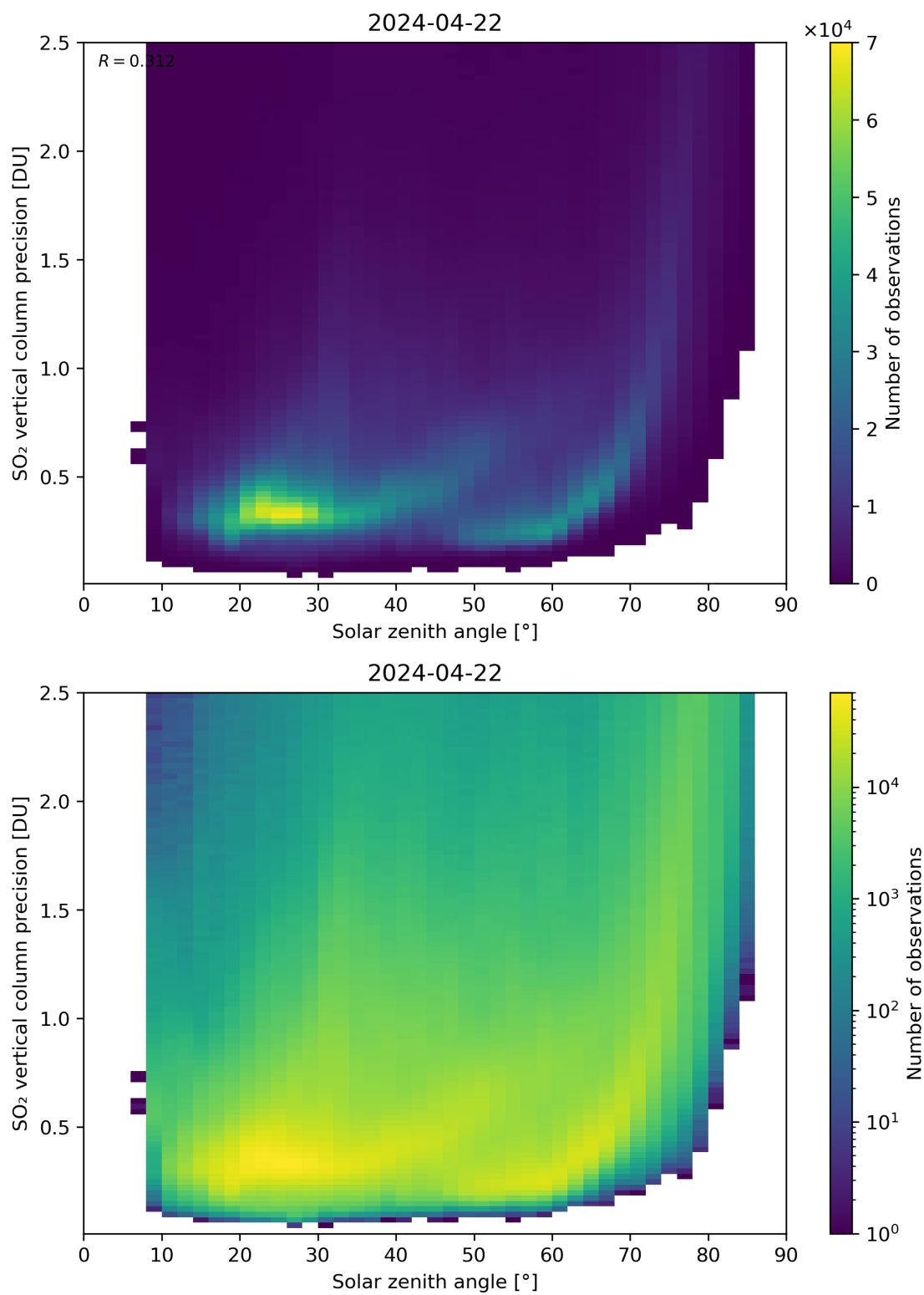
Figure 177: Scatter density plot of “Solar zenith angle” against “SO 2 vertical column precision” for 2024-04-21 to 2024-04-23.
