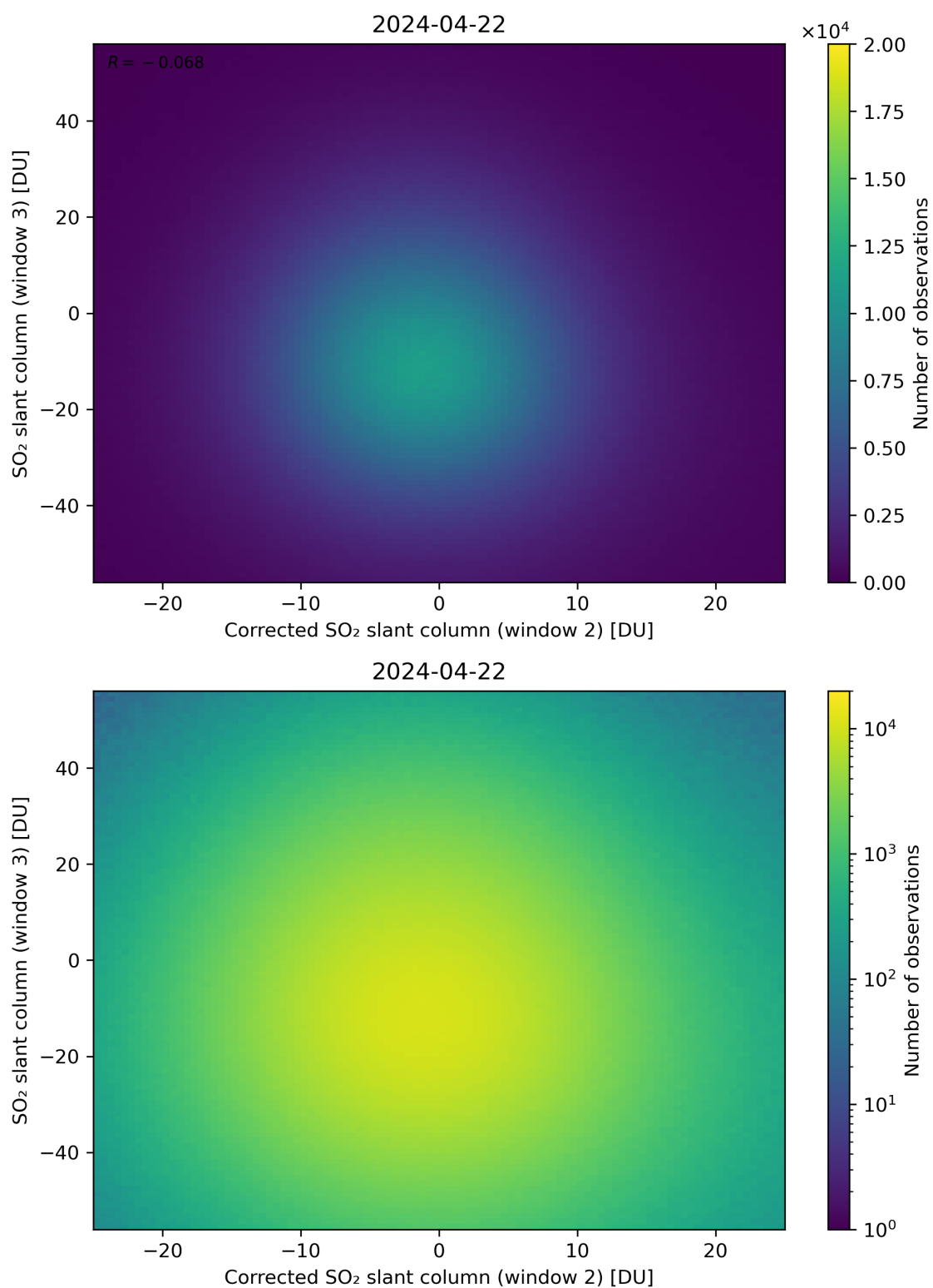
Figure 201: Scatter density plot of “Corrected SO 2 slant column (window 2)” against “SO 2 slant column (window 3)” for 2024-04-21 to 2024-04-23.
