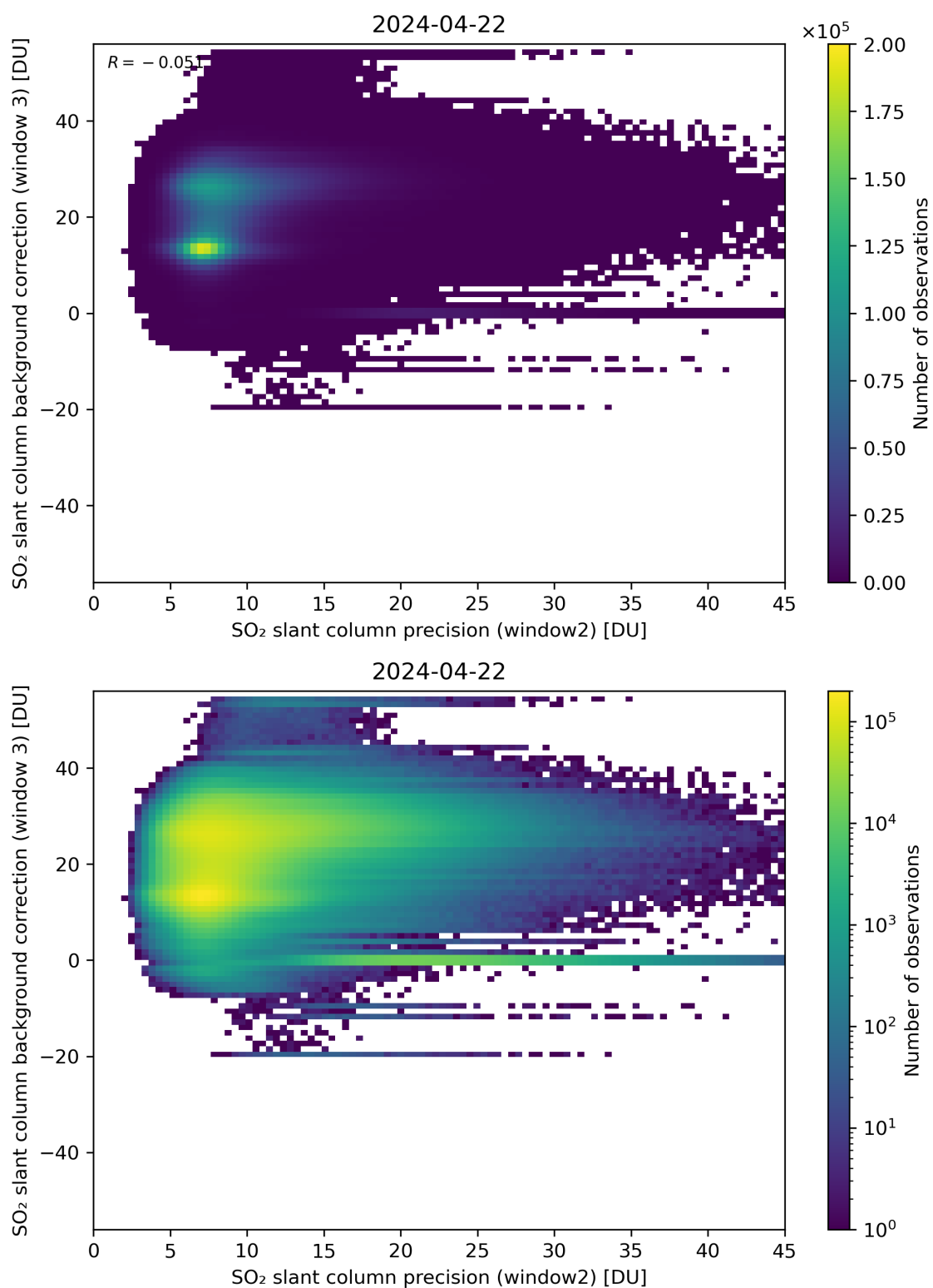
Figure 242: Scatter density plot of “SO 2 slant column precision (window2)” against “SO 2 slant column background correction (window 3)” for 2024-04-21 to 2024-04-23.
