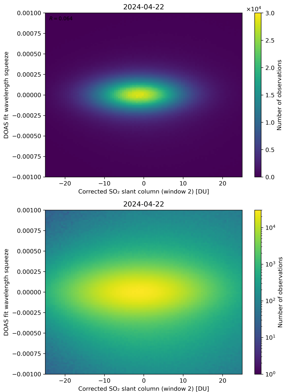
Figure 197: Scatter density plot of “Corrected SO 2 slant column (window 2)” against “DOAS fit wavelength squeeze” for 2024-04-21 to 2024-04-23.
