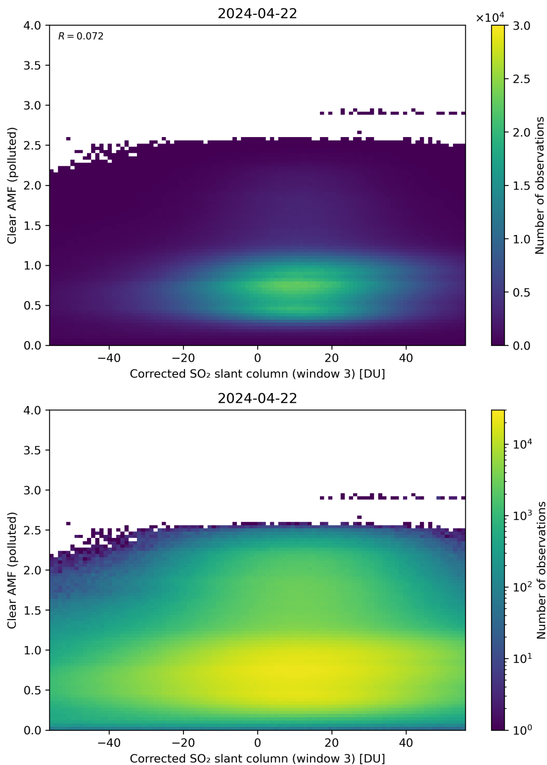
Figure 209: Scatter density plot of “Corrected SO 2 slant column (window 3)” against “Clear AMF (polluted)” for 2024-04-21 to 2024-04-23.
