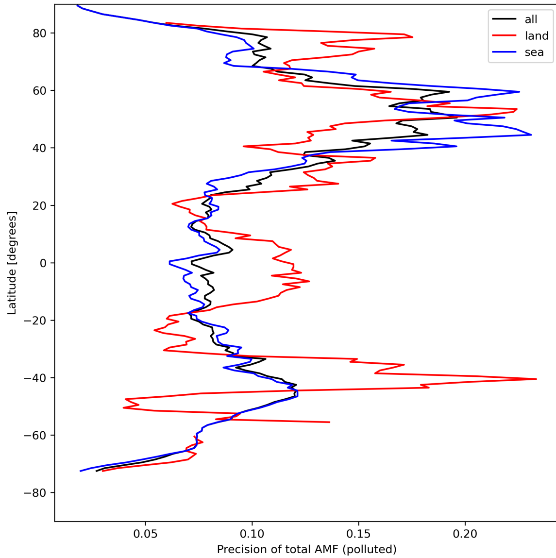
Figure 49: Zonal average of “Precision of total AMF (polluted)” for 2024-04-21 to 2024-04-23.
