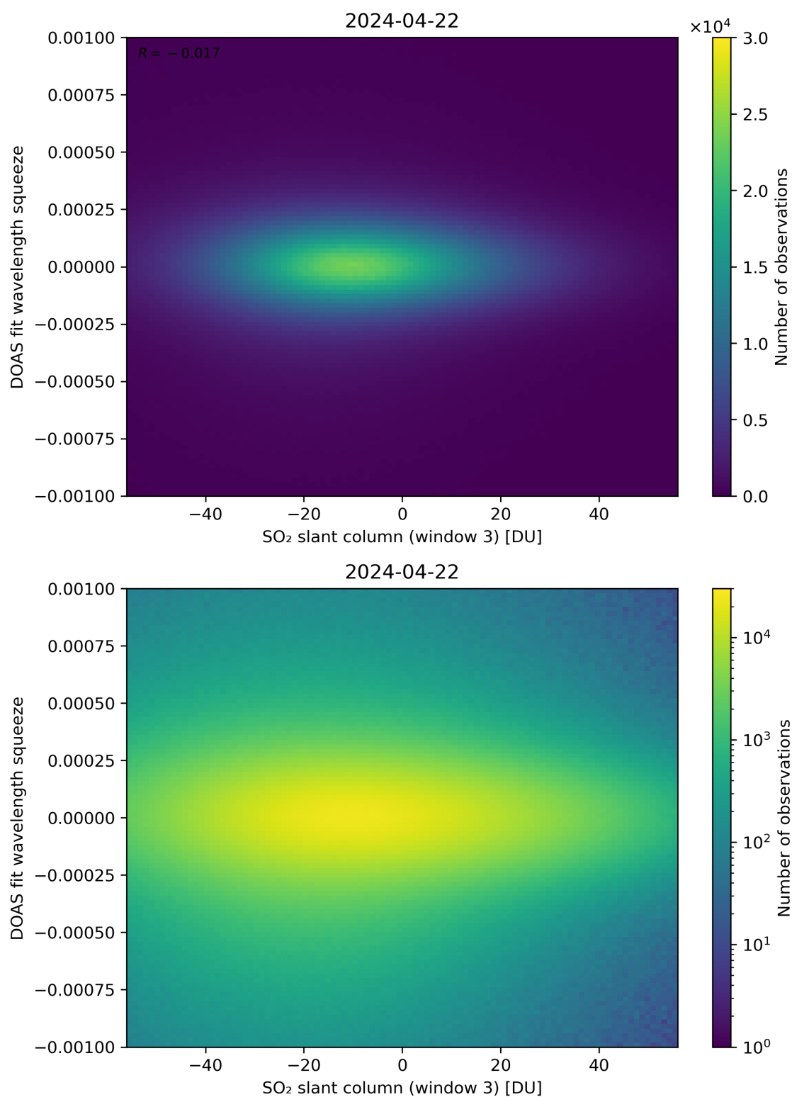
Figure 255: Scatter density plot of “SO 2 slant column (window 3)” against “DOAS fit wavelength squeeze” for 2024-04-21 to 2024-04-23.
