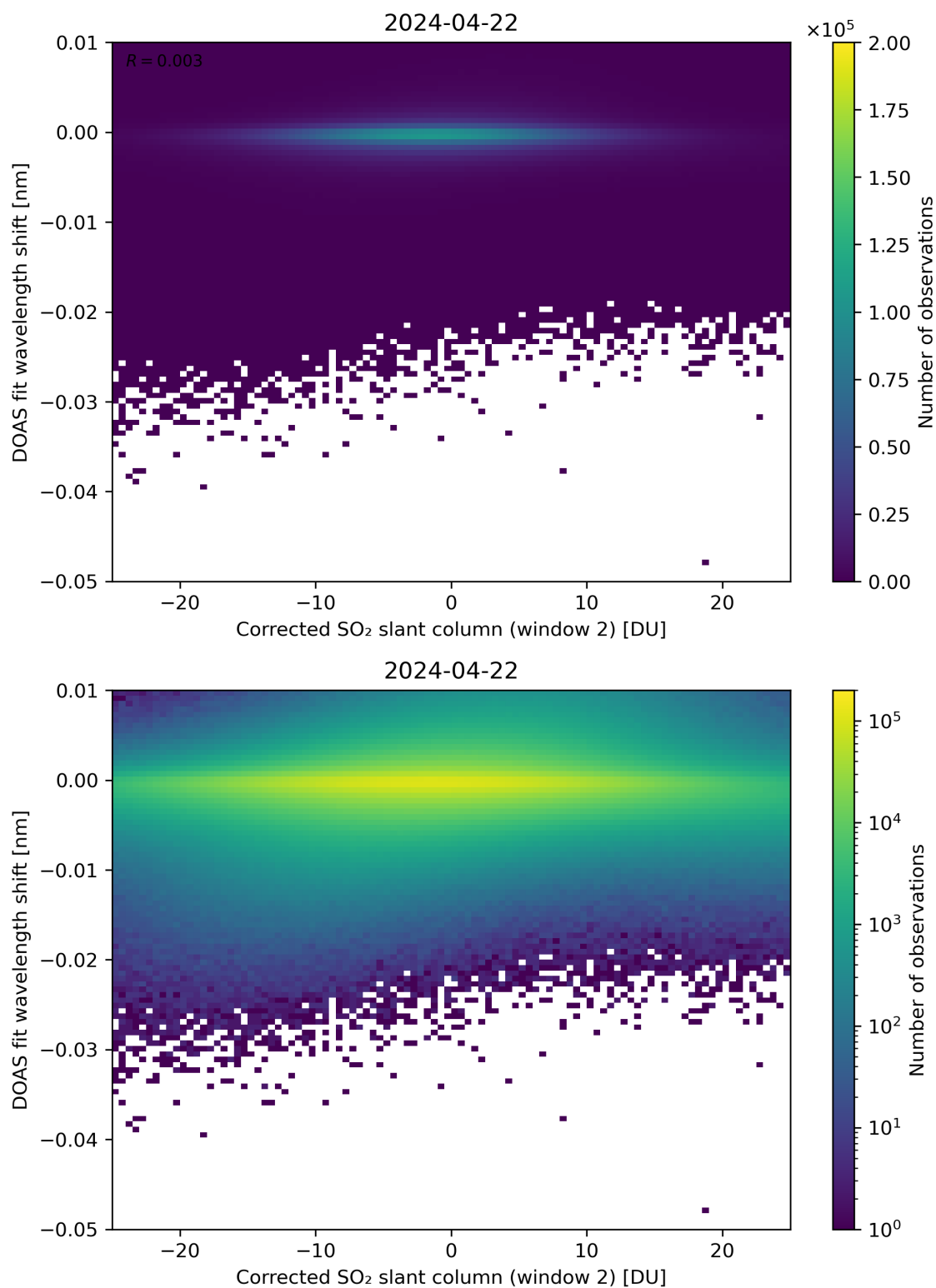
Figure 196: Scatter density plot of “Corrected SO 2 slant column (window 2)” against “DOAS fit wavelength shift” for 2024-04-21 to 2024-04-23.
