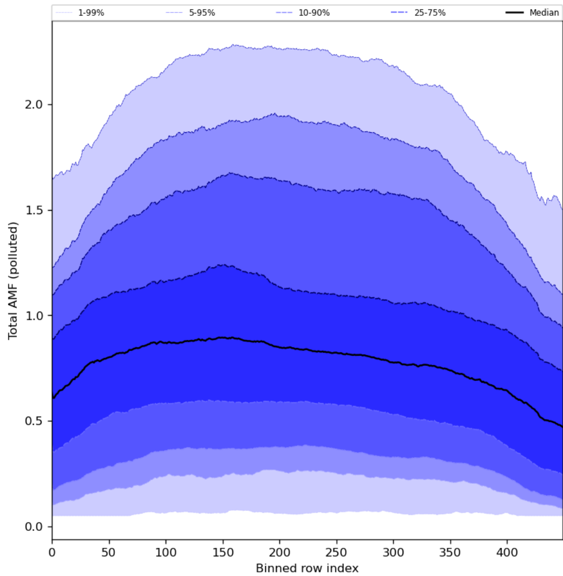
Figure 94: Along track statistics of “Total AMF (polluted)” for 2024-04-21 to 2024-04-23
