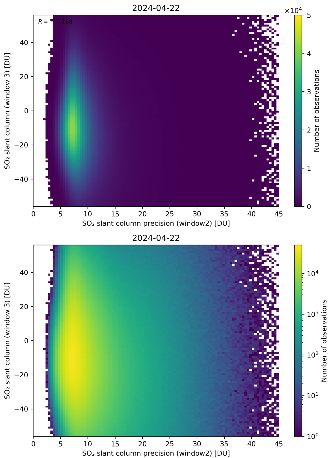
Figure 249: Scatter density plot of “SO 2 slant column precision (window2)” against “SO 2 slant column (window 3)” for 2024-04-21 to 2024-04-23.
