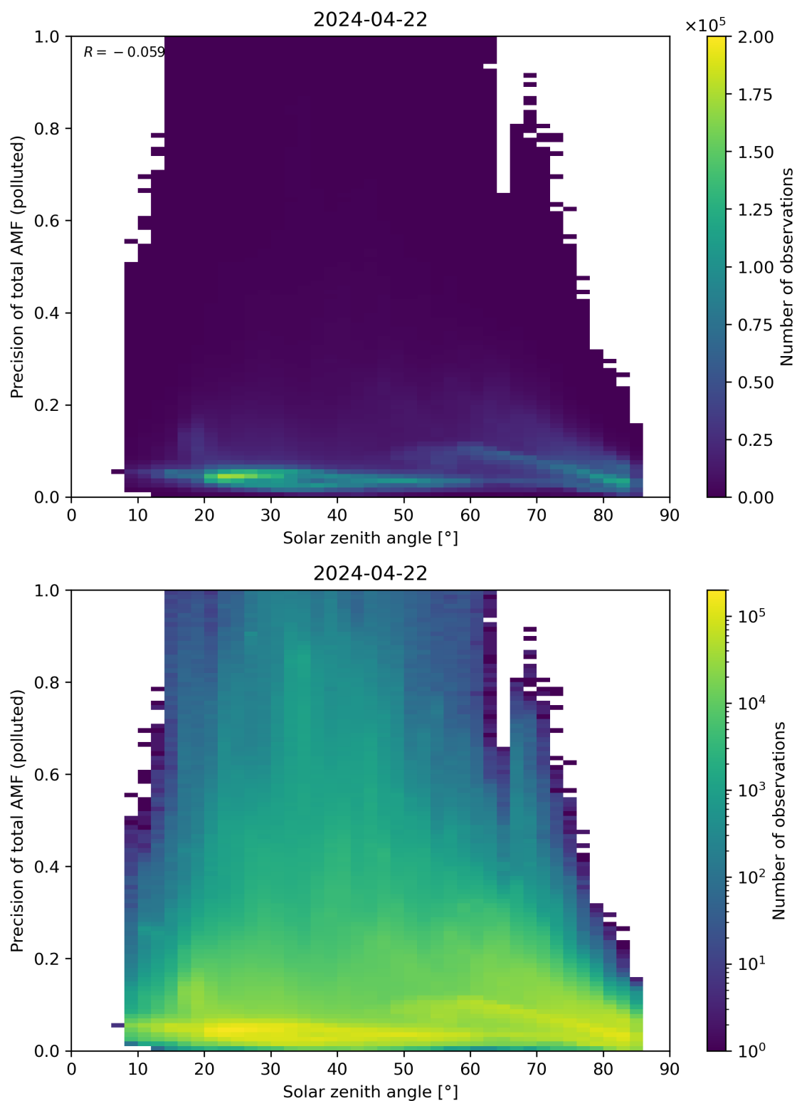
Figure 175: Scatter density plot of “Solar zenith angle” against “Precision of total AMF (polluted)” for 2024-04-21 to 2024-04-23.
