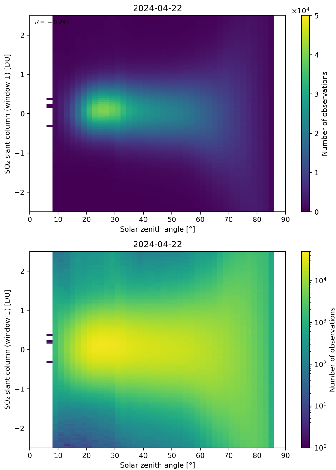
Figure 169: Scatter density plot of “Solar zenith angle” against “SO 2 slant column (window 1)” for 2024-04-21 to 2024-04-23.
