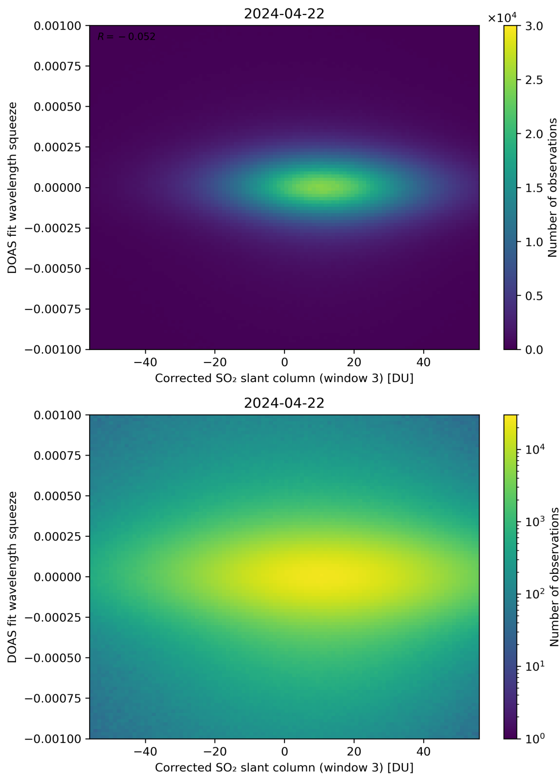
Figure 207: Scatter density plot of “Corrected SO 2 slant column (window 3)” against “DOAS fit wavelength squeeze” for 2024-04-21 to 2024-04-23.
