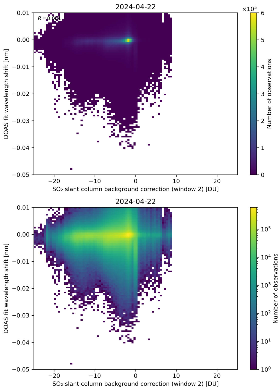
Figure 112: Scatter density plot of “SO 2 slant column background correction (window 2)” against “DOAS fit wavelength shift” for 2024-04-21 to 2024-04-23.
