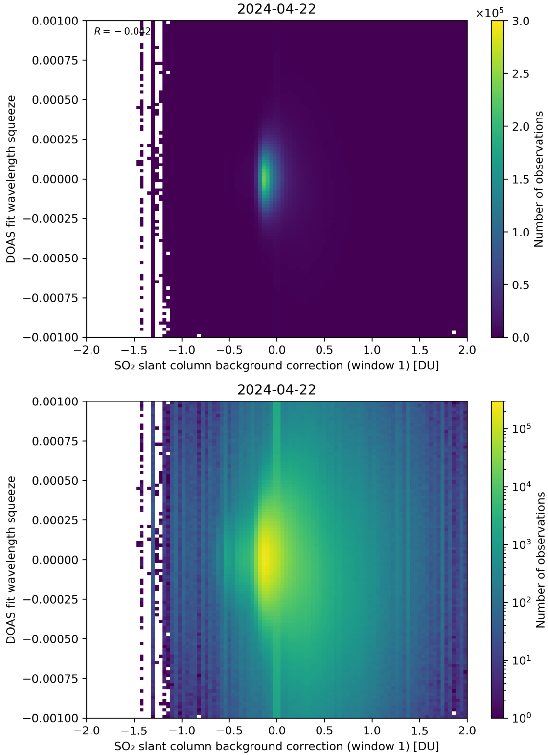
Figure 101: Scatter density plot of “SO 2 slant column background correction (window 1)” against “DOAS fit wavelength squeeze” for 2024-04-21 to 2024-04-23.
