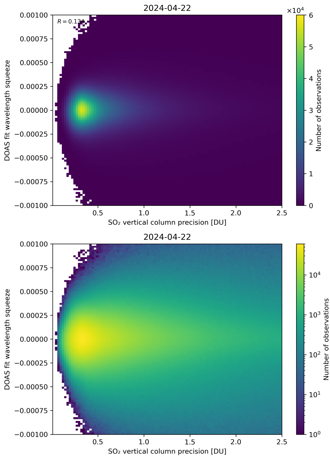
Figure 283: Scatter density plot of “SO 2 vertical column precision” against “DOAS fit wavelength squeeze” for 2024-04-21 to 2024-04-23.
