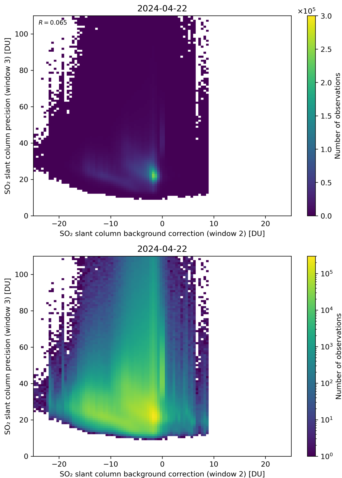
Figure 118: Scatter density plot of “SO 2 slant column background correction (window 2)” against “SO 2 slant column precision (window 3)” for 2024-04-21 to 2024-04-23.
