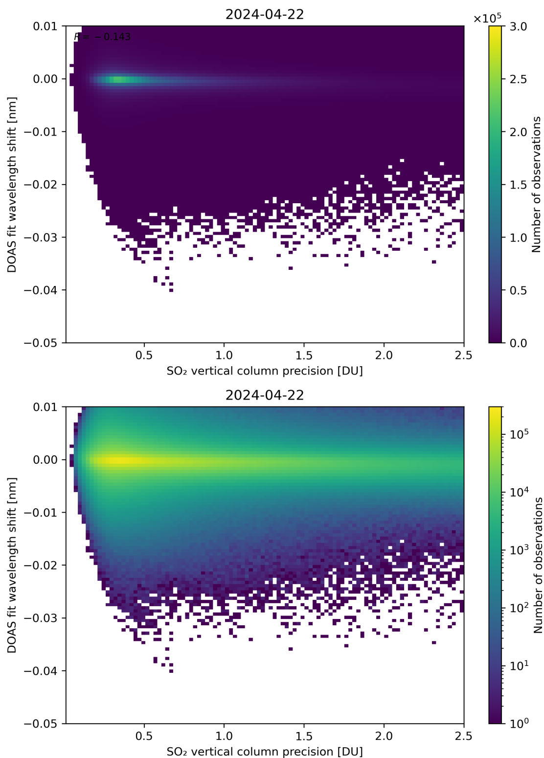
Figure 282: Scatter density plot of “SO 2 vertical column precision” against “DOAS fit wavelength shift” for 2024-04-21 to 2024-04-23.
