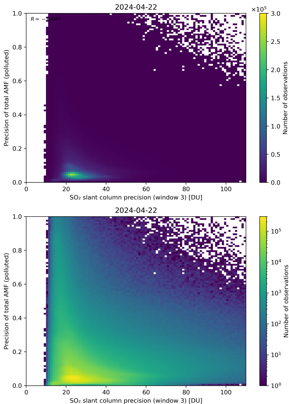
Figure 264: Scatter density plot of “SO 2 slant column precision (window 3)” against “Precision of total AMF (polluted)” for 2024-04-21 to 2024-04-23.
