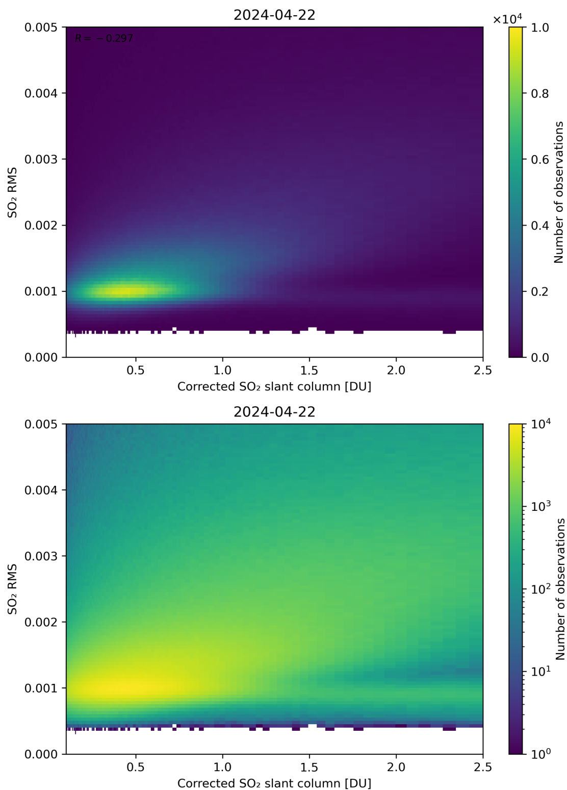
Figure 183: Scatter density plot of “Corrected SO 2 slant column” against “SO 2 RMS” for 2024-04-21 to 2024-04-23.
