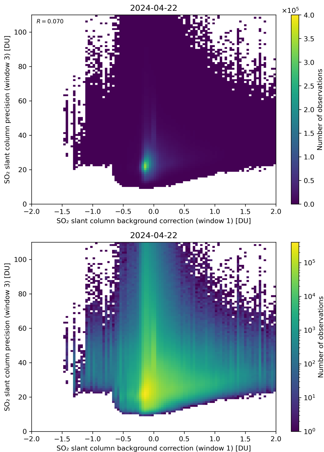
Figure 108: Scatter density plot of “SO 2 slant column background correction (window 1)” against “SO 2 slant column precision (window 3)” for 2024-04-21 to 2024-04-23.
