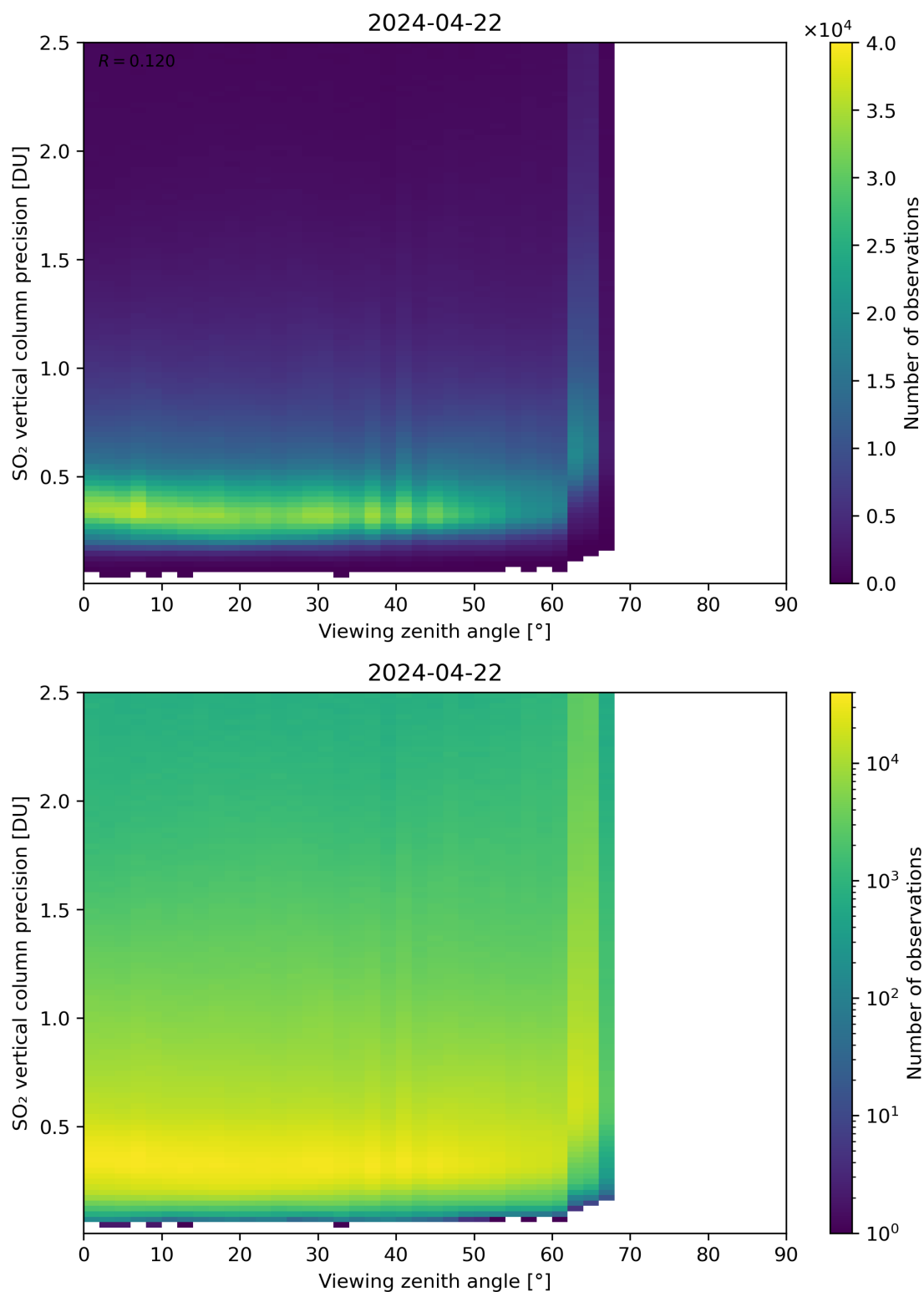
Figure 328: Scatter density plot of “Viewing zenith angle” against “SO 2 vertical column precision” for 2024-04-21 to 2024-04-23.
