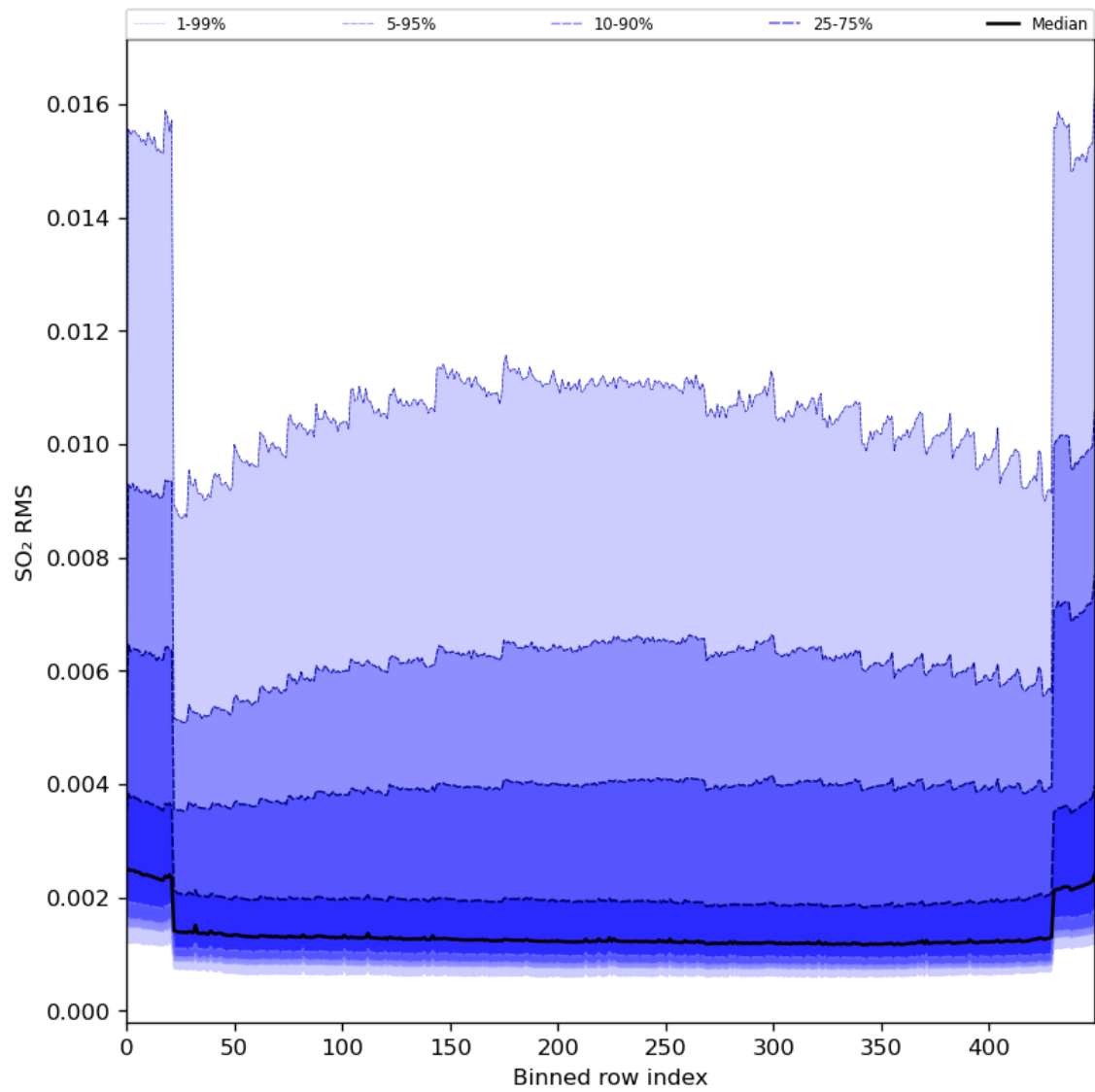
Figure 93: Along track statistics of “SO 2 RMS” for 2024-04-21 to 2024-04-23
