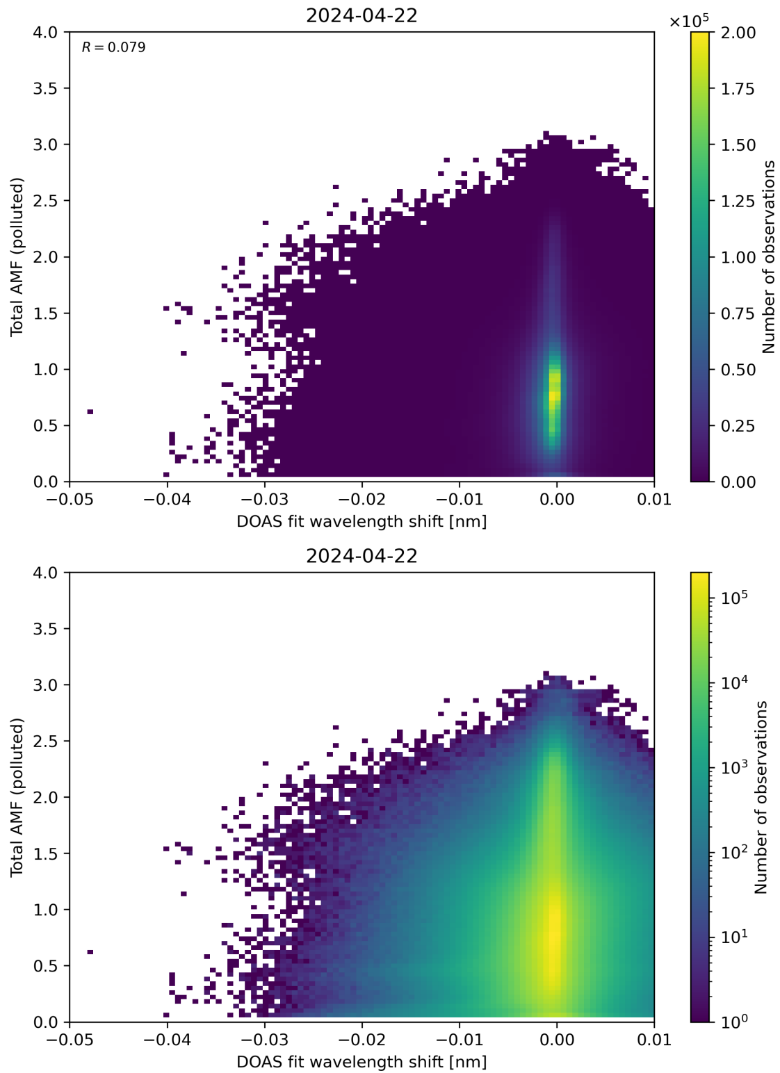
Figure 130: Scatter density plot of “DOAS fit wavelength shift” against “Total AMF (polluted)” for 2024-04-21 to 2024-04-23.
