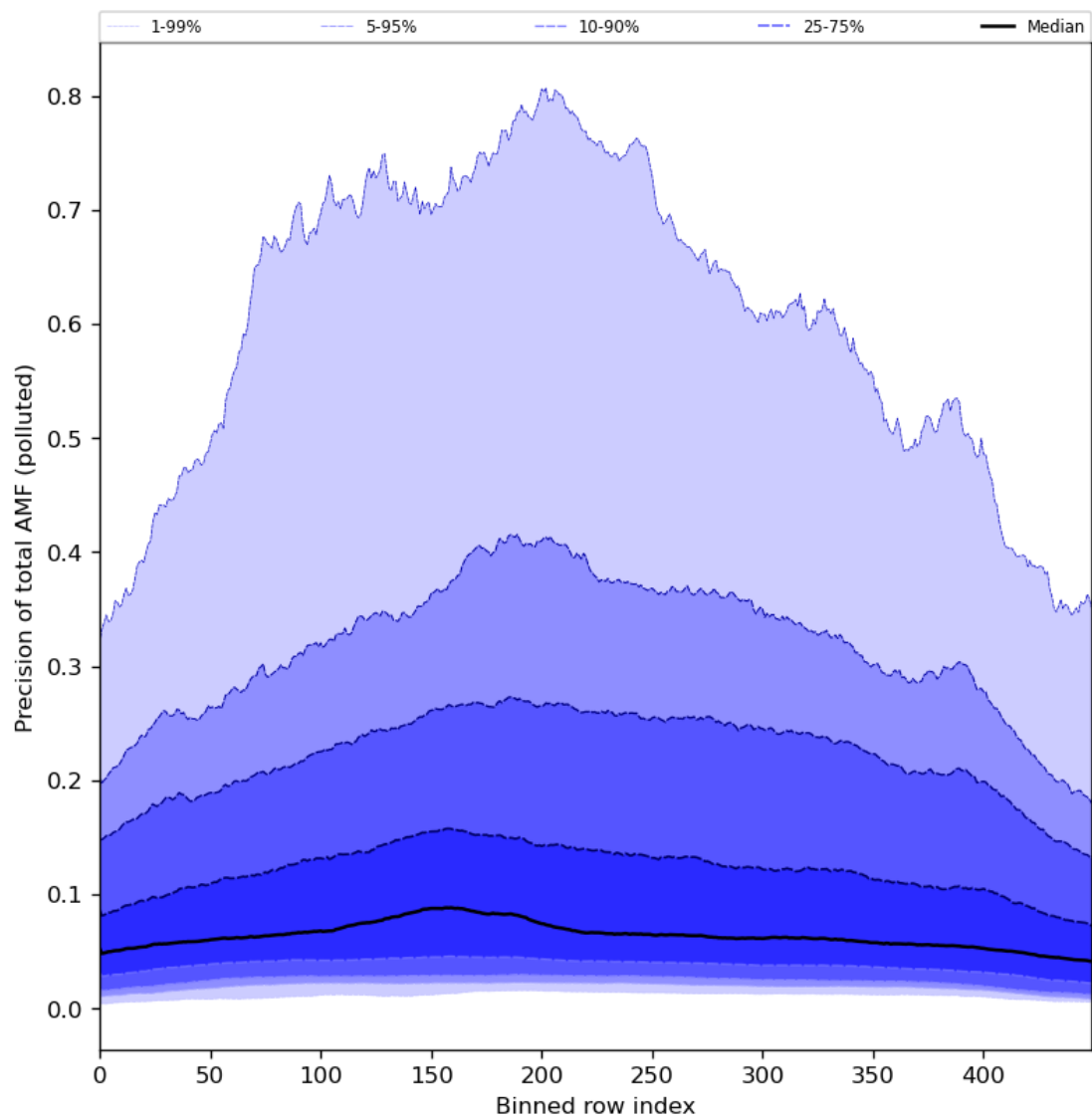
Figure 95: Along track statistics of “Precision of total AMF (polluted)” for 2024-04-21 to 2024-04-23
