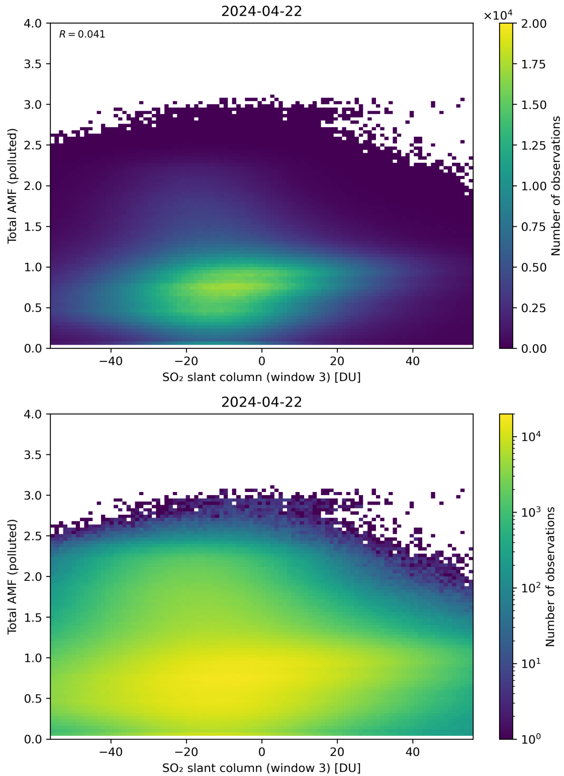
Figure 268: Scatter density plot of “SO 2 slant column (window 3)” against “Total AMF (polluted)” for 2024-04-21 to 2024-04-23.
