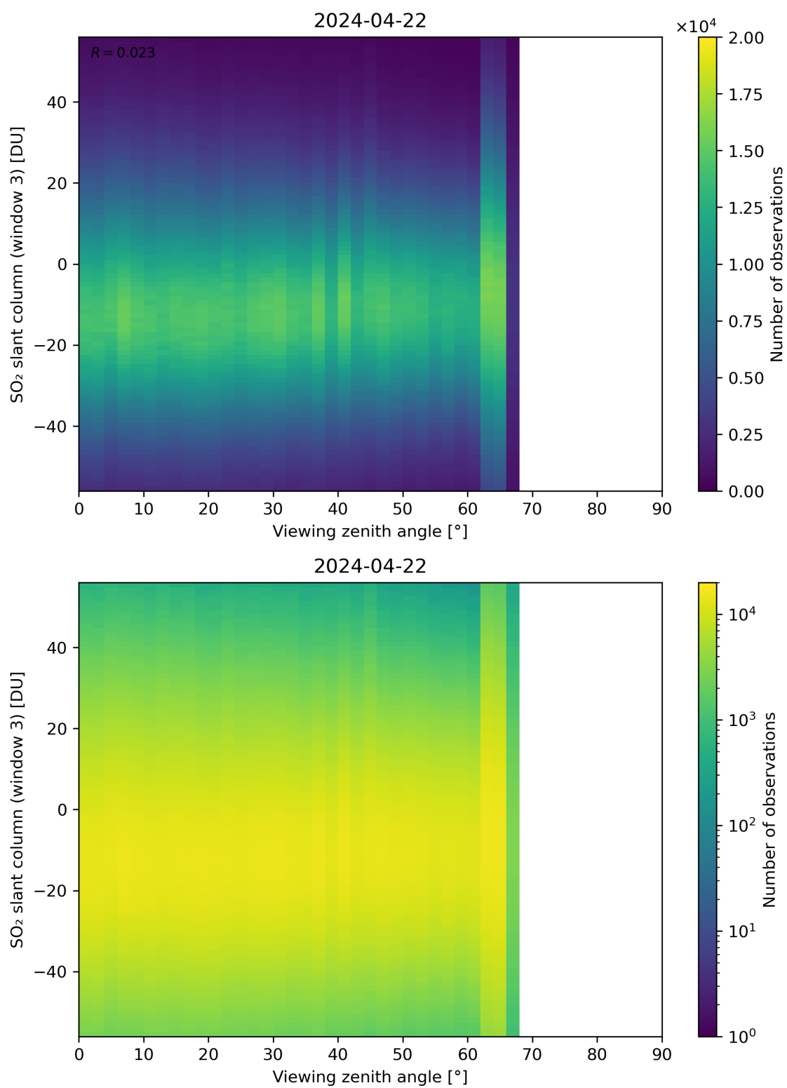
Figure 323: Scatter density plot of “Viewing zenith angle” against “SO 2 slant column (window 3)” for 2024-04-21 to 2024-04-23.
