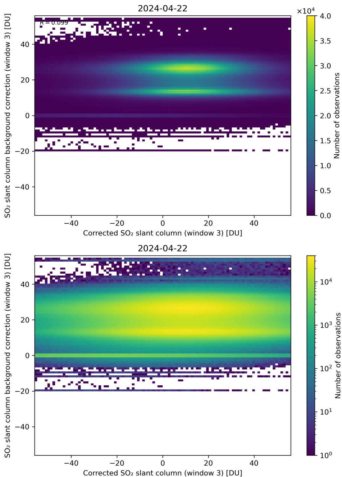
Figure 205: Scatter density plot of “Corrected SO 2 slant column (window 3)” against “SO 2 slant column background correction (window 3)” for 2024-04-21 to 2024-04-23.
