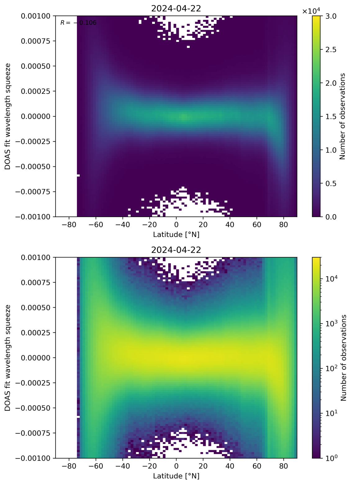
Figure 143: Scatter density plot of “Latitude” against “DOAS fit wavelength squeeze” for 2024-04-21 to 2024-04-23.
