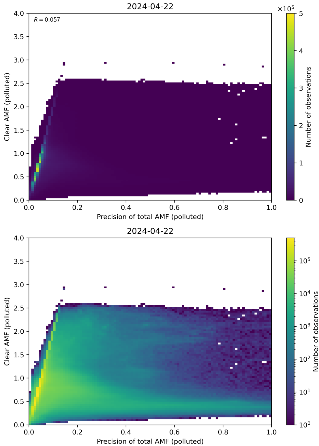
Figure 270: Scatter density plot of “Precision of total AMF (polluted)” against “Clear AMF (polluted)” for 2024-04-21 to 2024-04-23.
