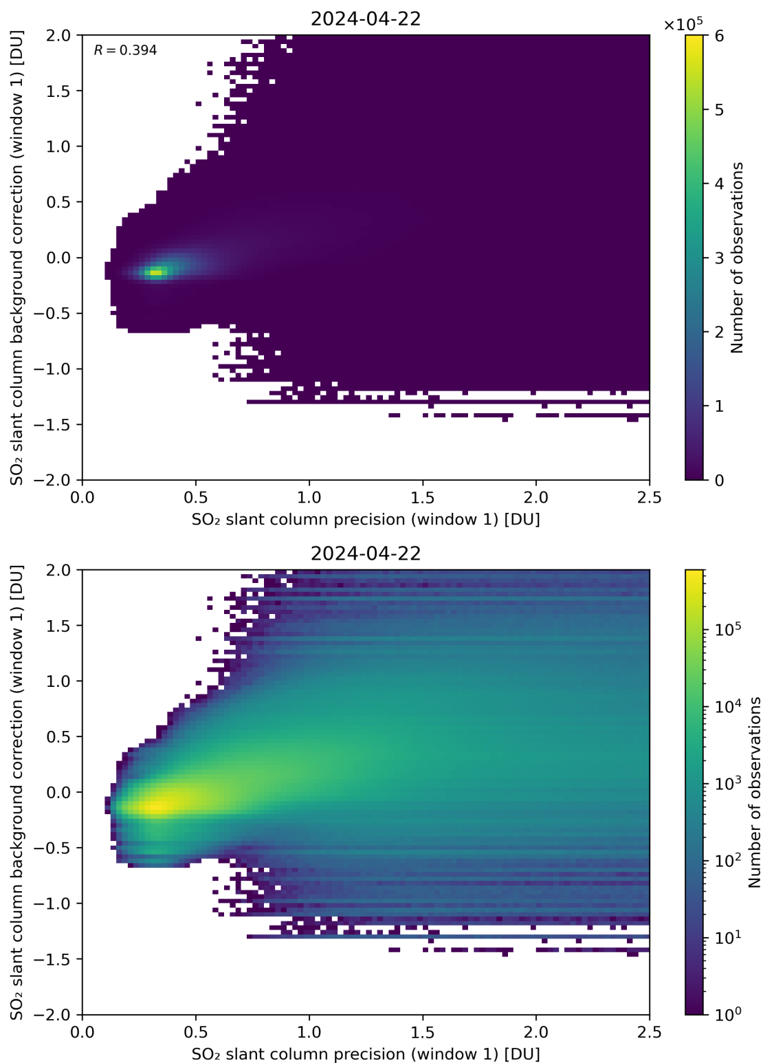
Figure 218: Scatter density plot of “SO 2 slant column precision (window 1)” against “SO 2 slant column background correction (window 1)” for 2024-04-21 to 2024-04-23.
