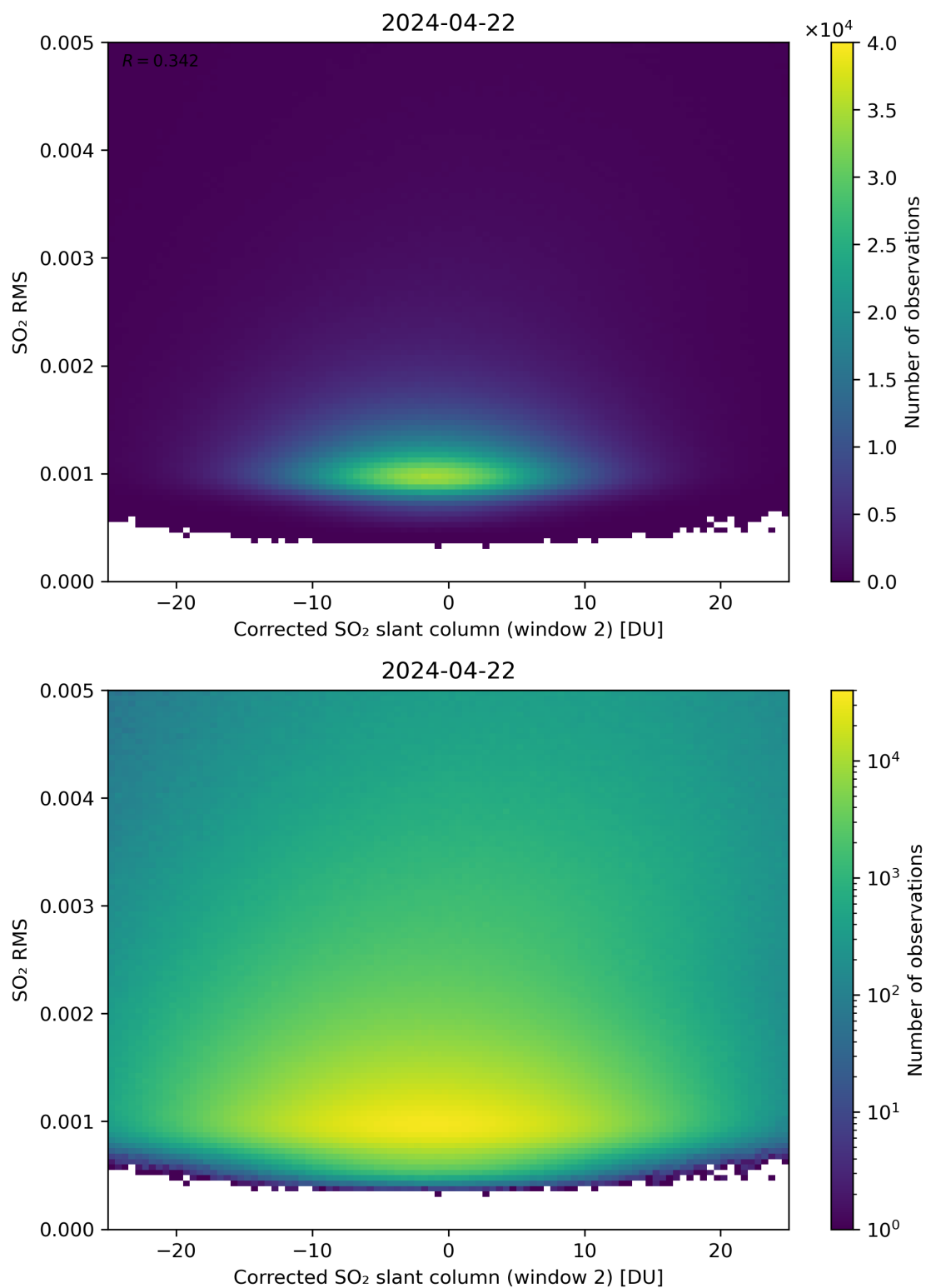
Figure 198: Scatter density plot of “Corrected SO 2 slant column (window 2)” against “SO 2 RMS” for 2024-04-21 to 2024-04-23.
