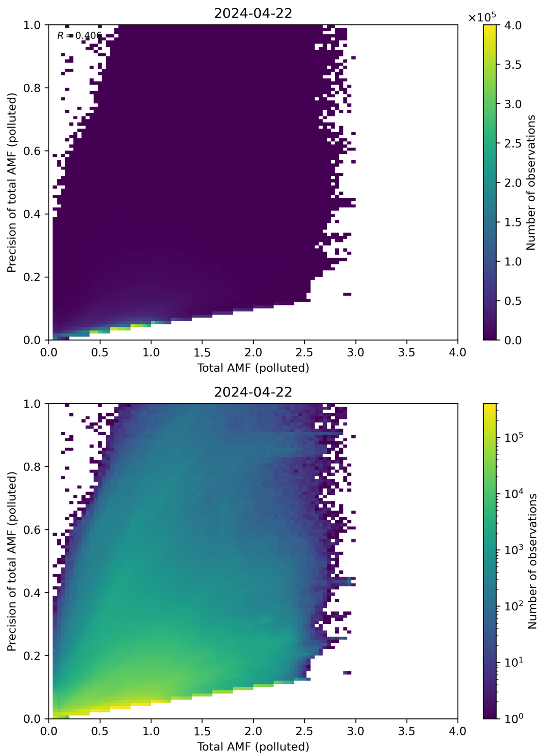
Figure 272: Scatter density plot of “Total AMF (polluted)” against “Precision of total AMF (polluted)” for 2024-04-21 to 2024-04-23.
