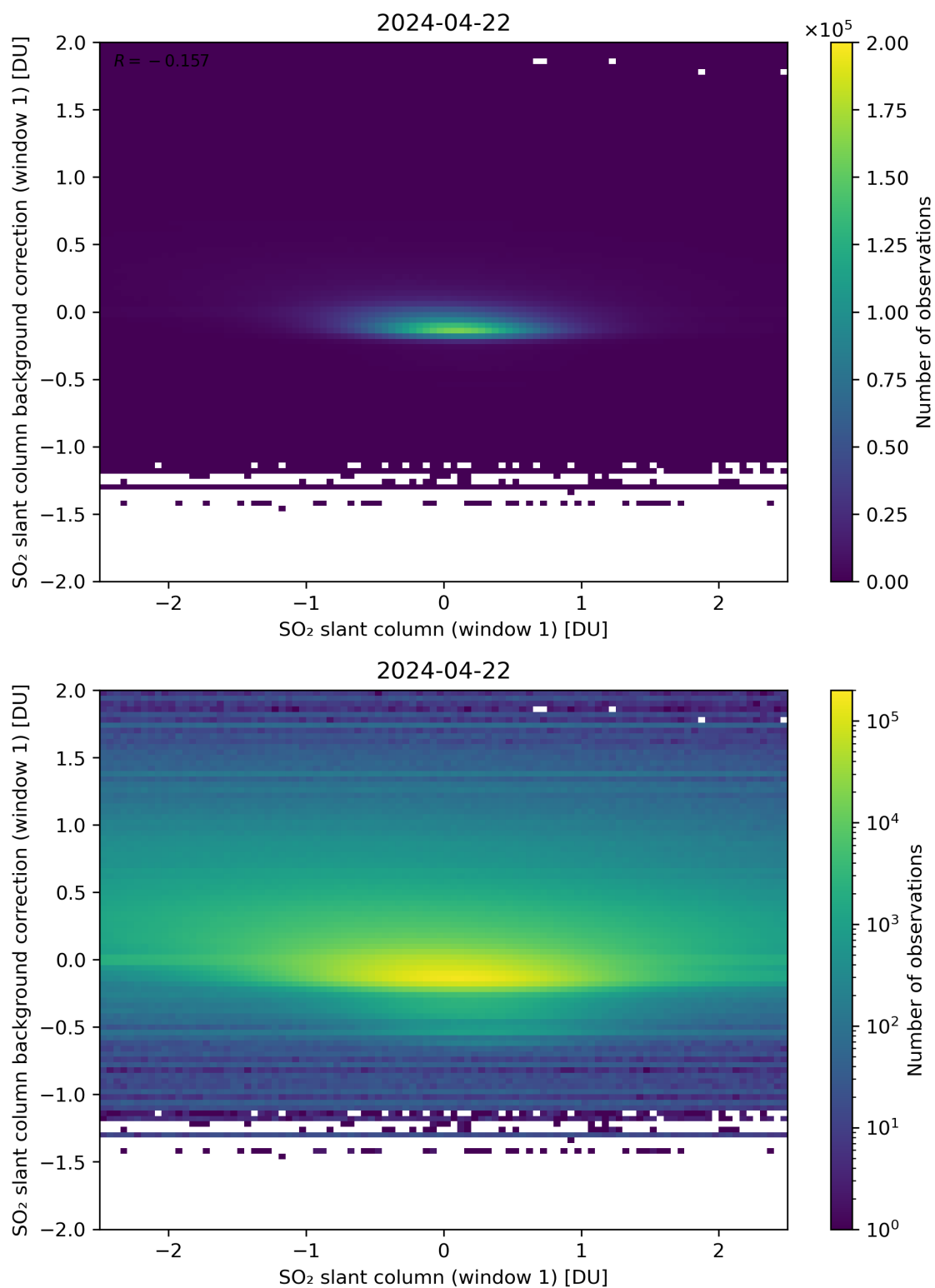
Figure 212: Scatter density plot of “SO 2 slant column (window 1)” against “SO 2 slant column background correction (window 1)” for 2024-04-21 to 2024-04-23.
