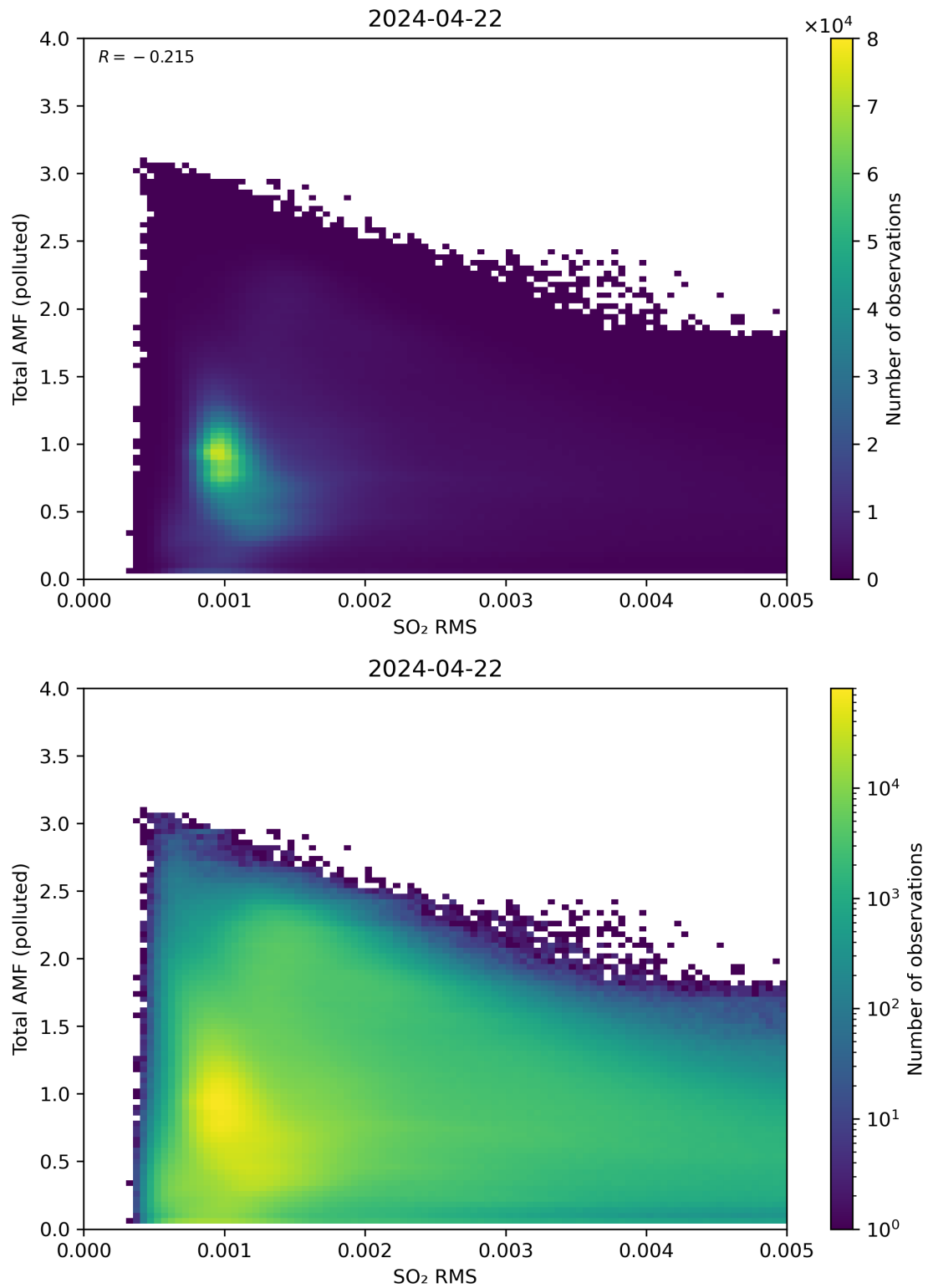
Figure 137: Scatter density plot of “SO 2 RMS” against “Total AMF (polluted)” for 2024-04-21 to 2024-04-23.
