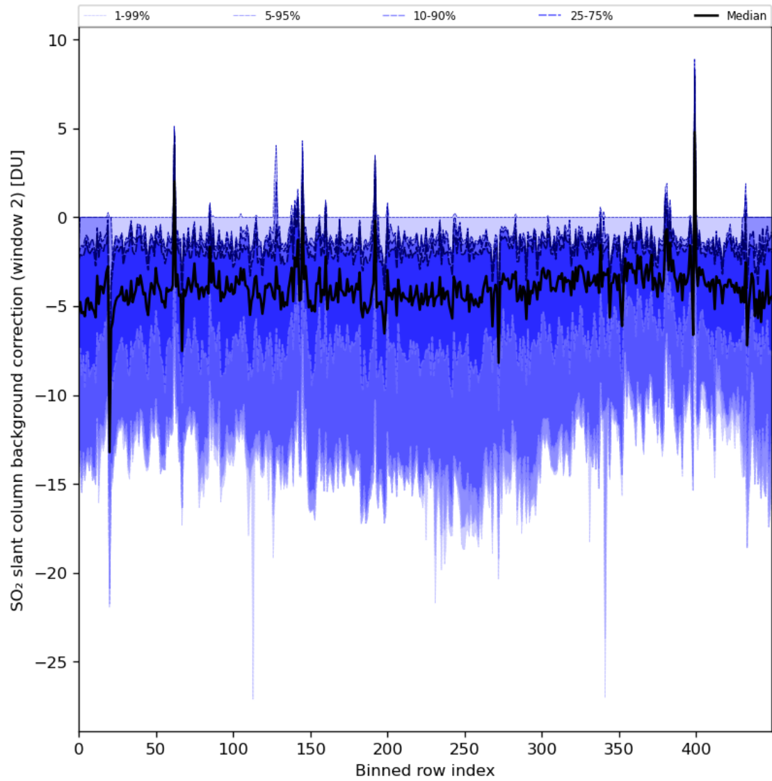
Figure 86: Along track statistics of “SO 2 slant column background correction (window 2)” for 2024-04-21 to 2024-04-23
