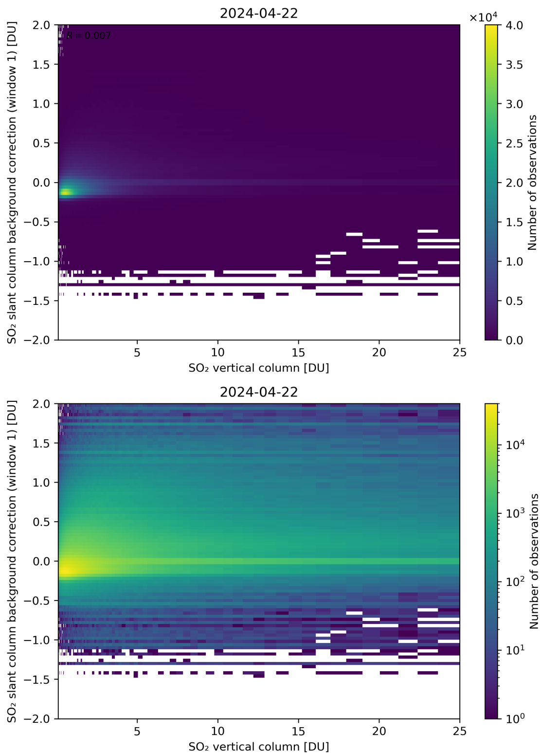
Figure 273: Scatter density plot of “SO 2 vertical column” against “SO 2 slant column background correction (window 1)” for 2024-04-21 to 2024-04-23.
