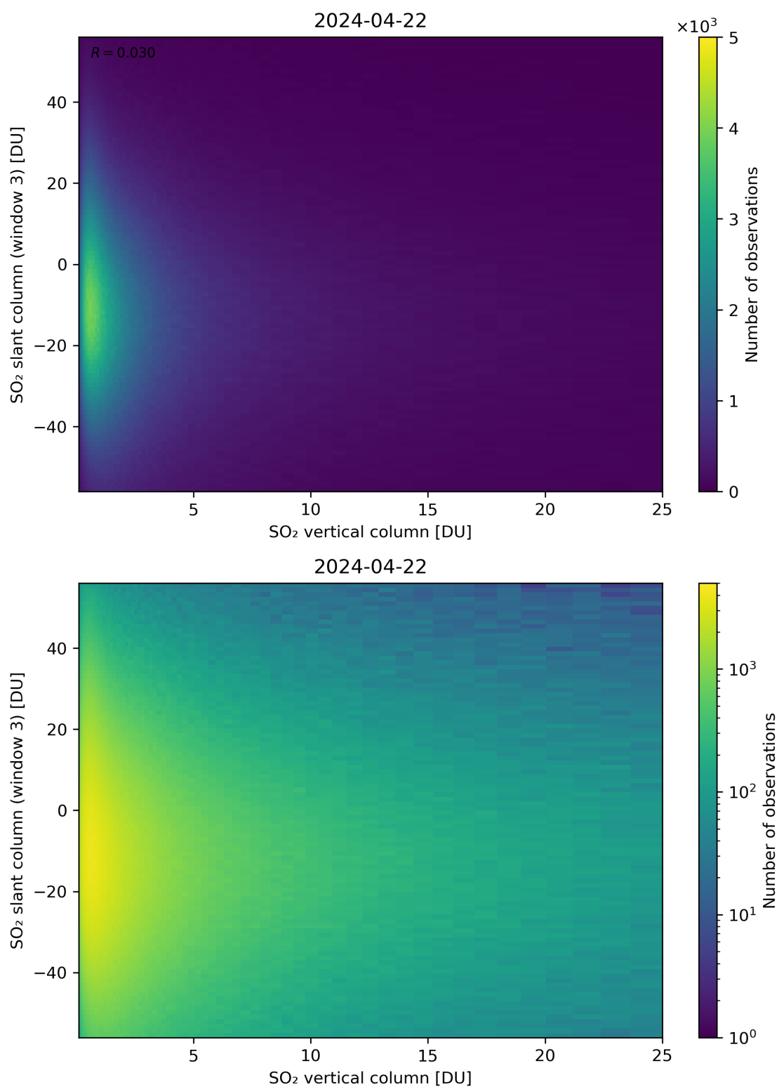
Figure 303: Scatter density plot of “SO 2 vertical column” against “SO 2 slant column (window 3)” for 2024-04-21 to 2024-04-23.
