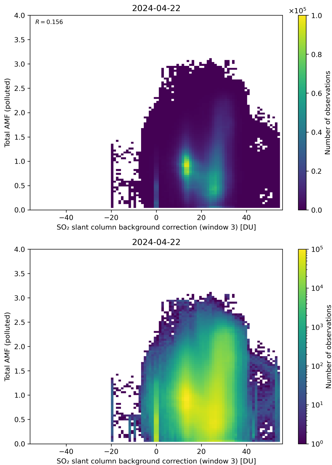
Figure 125: Scatter density plot of “SO 2 slant column background correction (window 3)” against “Total AMF (polluted)” for 2024-04-21 to 2024-04-23.
