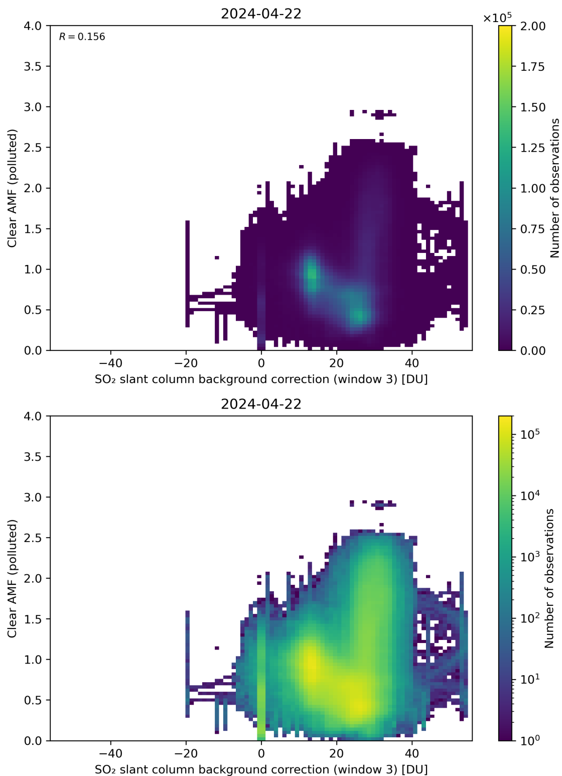
Figure 124: Scatter density plot of “SO 2 slant column background correction (window 3)” against “Clear AMF (polluted)” for 2024-04-21 to 2024-04-23.
