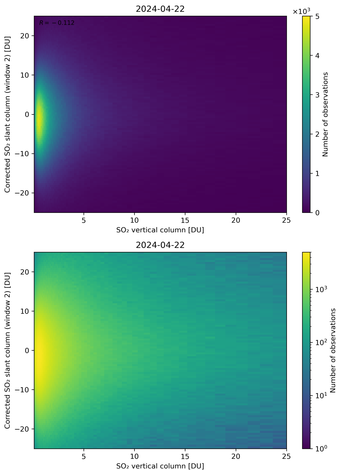
Figure 298: Scatter density plot of “SO 2 vertical column” against “Corrected SO 2 slant column (window 2)” for 2024-04-21 to 2024-04-23.
