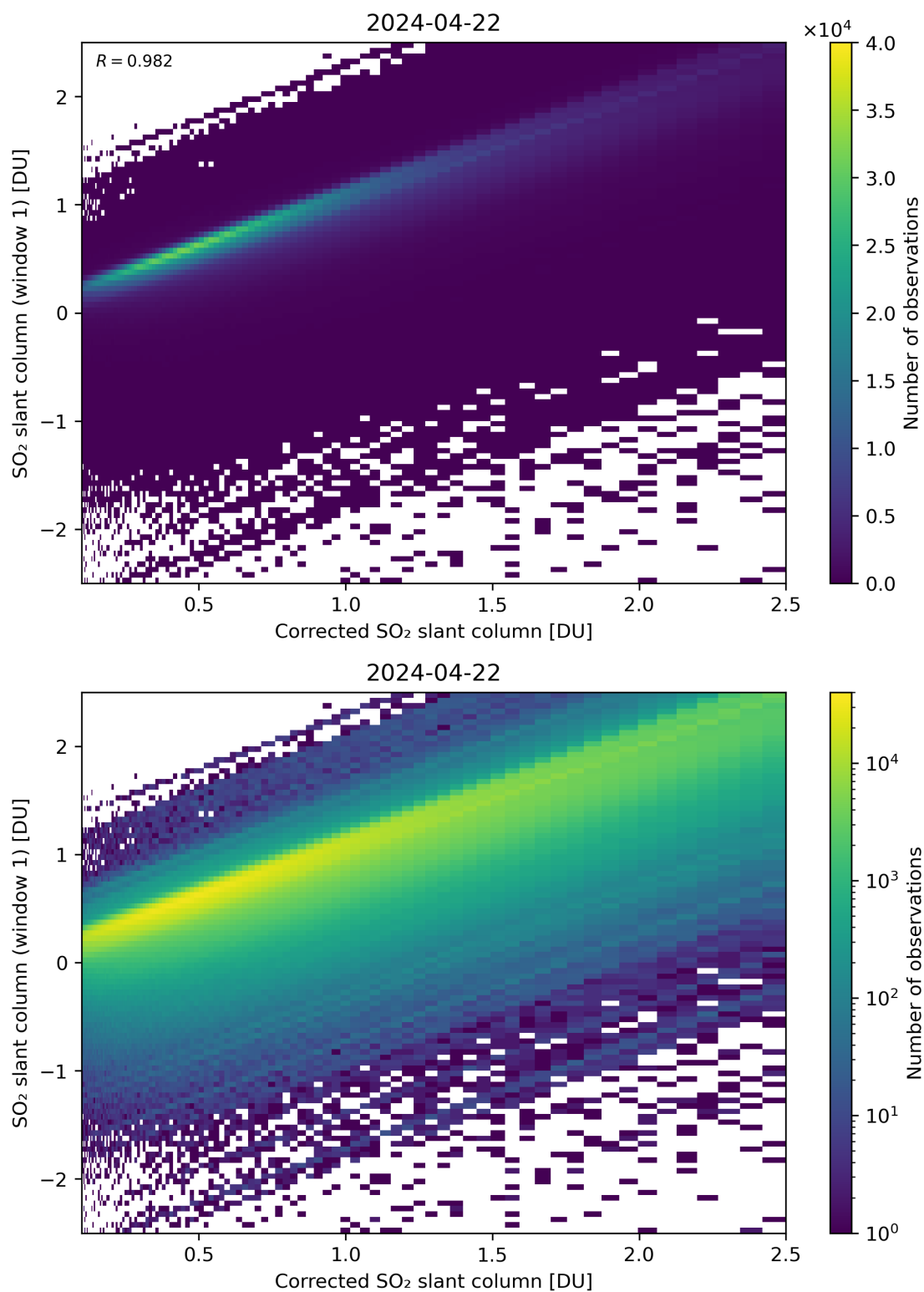
Figure 187: Scatter density plot of “Corrected SO 2 slant column” against “SO 2 slant column (window 1)” for 2024-04-21 to 2024-04-23.
