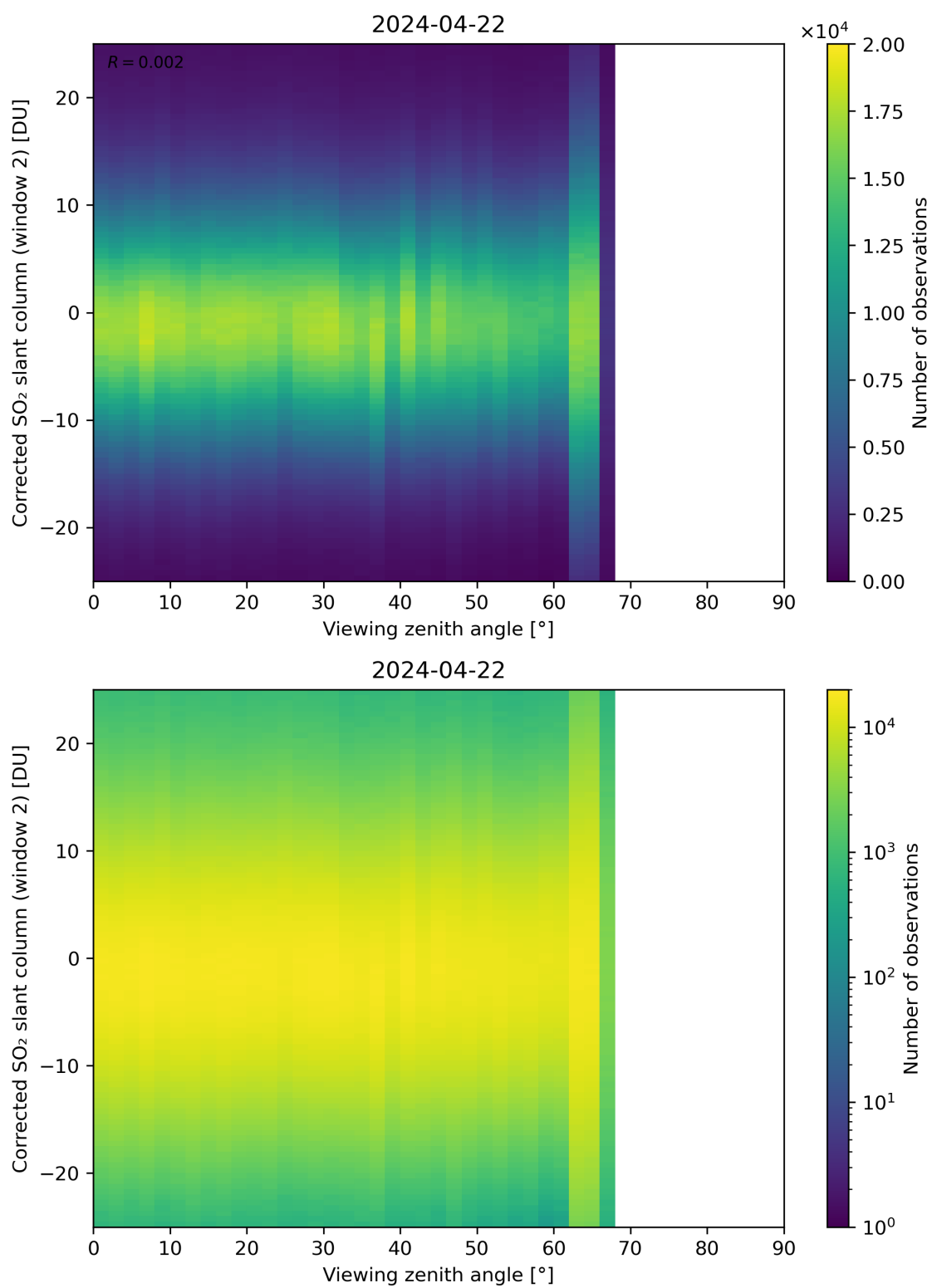
Figure 318: Scatter density plot of “Viewing zenith angle” against “Corrected SO 2 slant column (window 2)” for 2024-04-21 to 2024-04-23.
