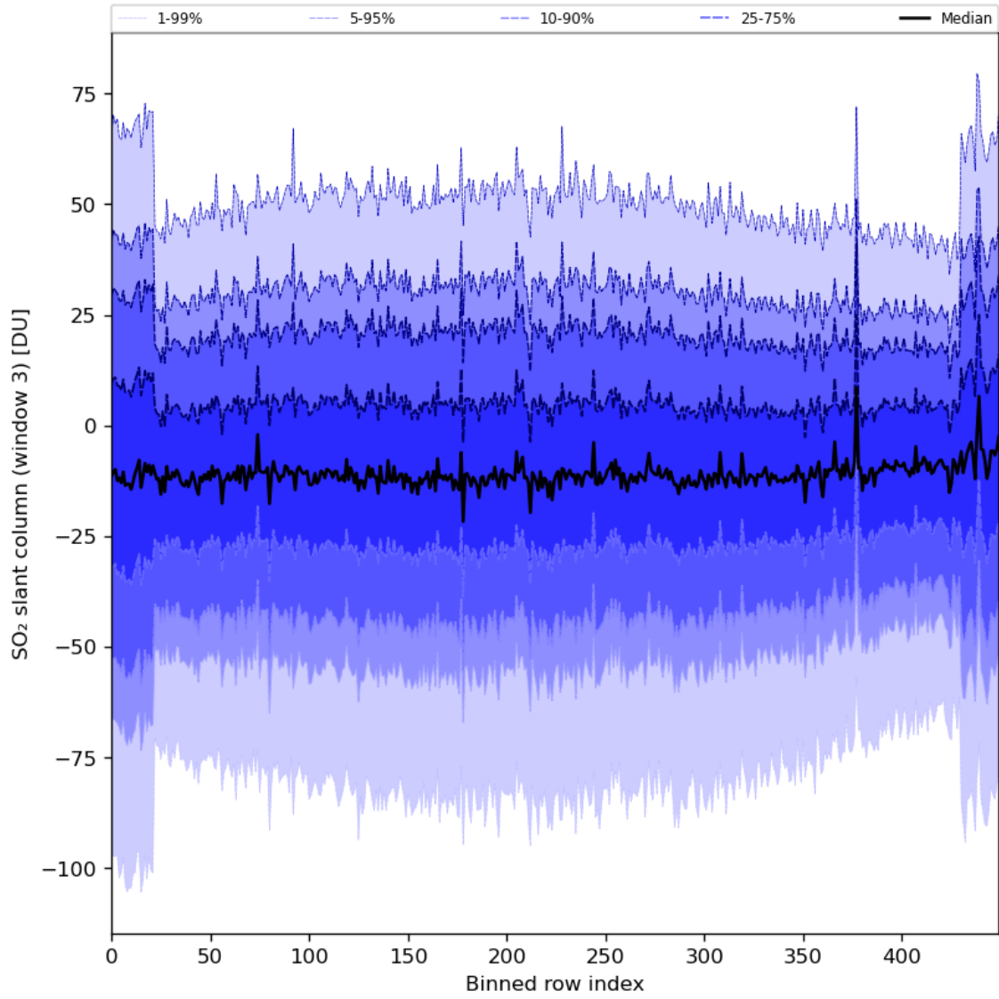
Figure 87: Along track statistics of “SO 2 slant column (window 3)” for 2024-04-21 to 2024-04-23
