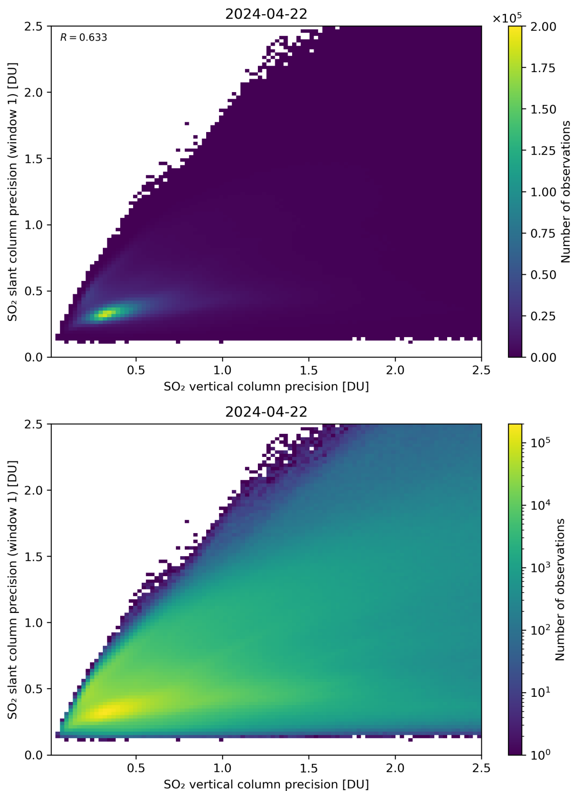
Figure 290: Scatter density plot of “SO 2 vertical column precision” against “SO 2 slant column precision (window 1)” for 2024-04-21 to 2024-04-23.
