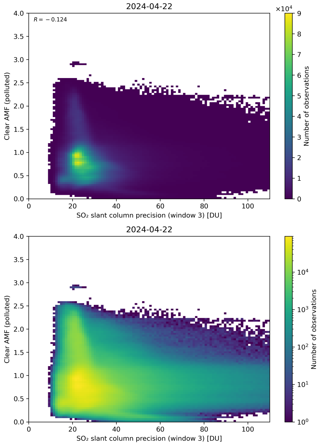
Figure 261: Scatter density plot of “SO 2 slant column precision (window 3)” against “Clear AMF (polluted)” for 2024-04-21 to 2024-04-23.
