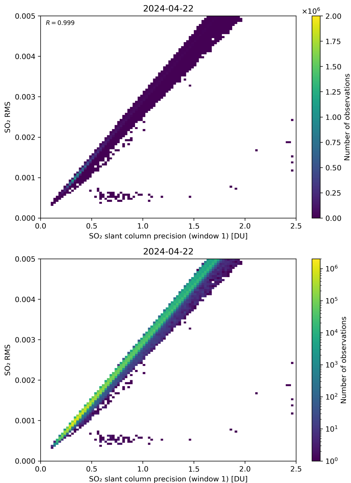
Figure 223: Scatter density plot of “SO 2 slant column precision (window 1)” against “SO 2 RMS” for 2024-04-21 to 2024-04-23.
