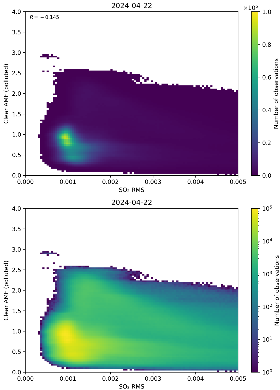
Figure 136: Scatter density plot of “SO 2 RMS” against “Clear AMF (polluted)” for 2024-04-21 to 2024-04-23.
