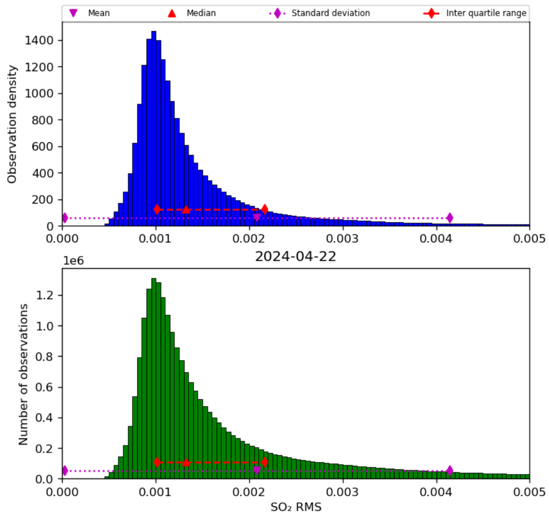
Figure 70: Histogram of “SO 2 RMS” for 2024-04-21 to 2024-04-23
