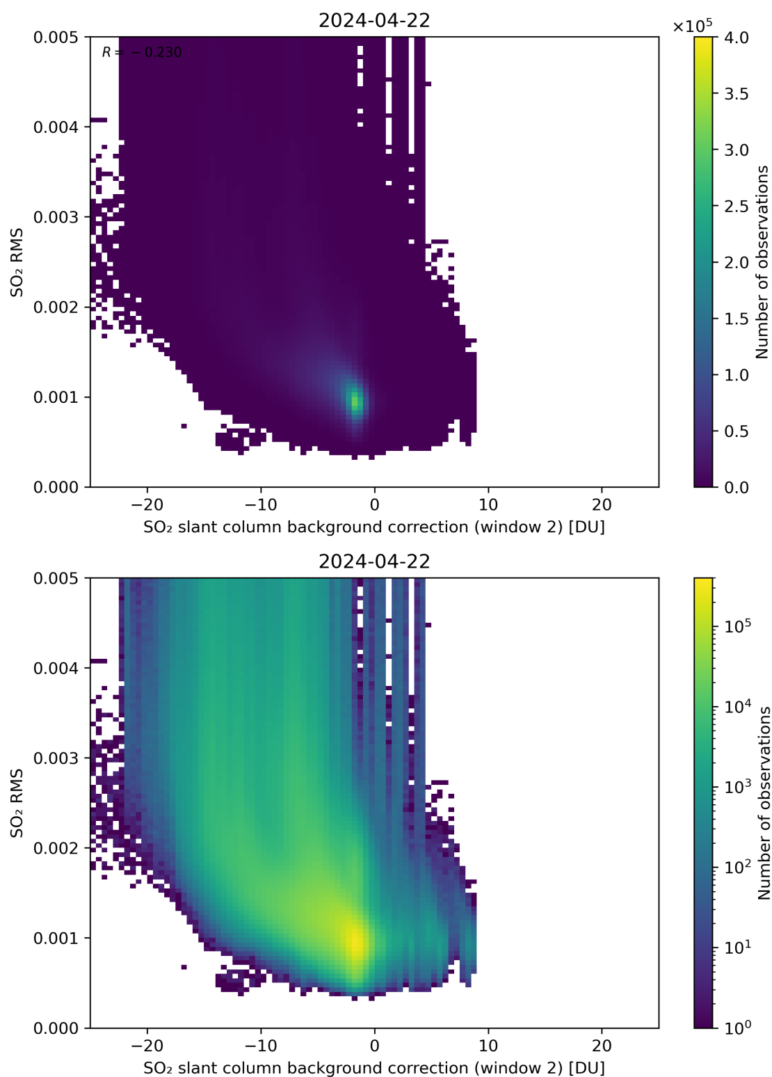
Figure 114: Scatter density plot of “SO 2 slant column background correction (window 2)” against “SO 2 RMS” for 2024-04-21 to 2024-04-23.
