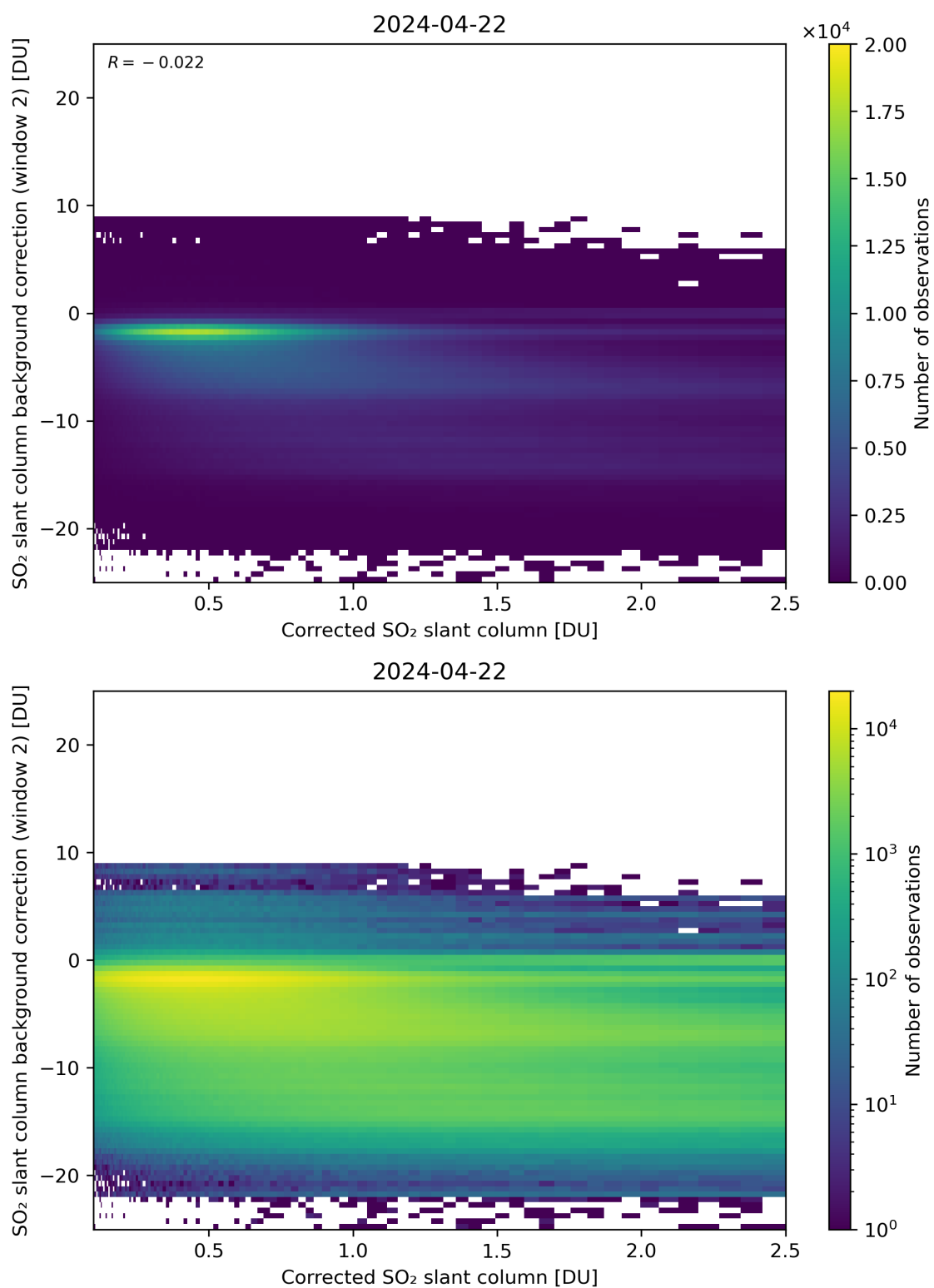
Figure 179: Scatter density plot of “Corrected SO 2 slant column” against “SO 2 slant column background correction (window 2)” for 2024-04-21 to 2024-04-23.
