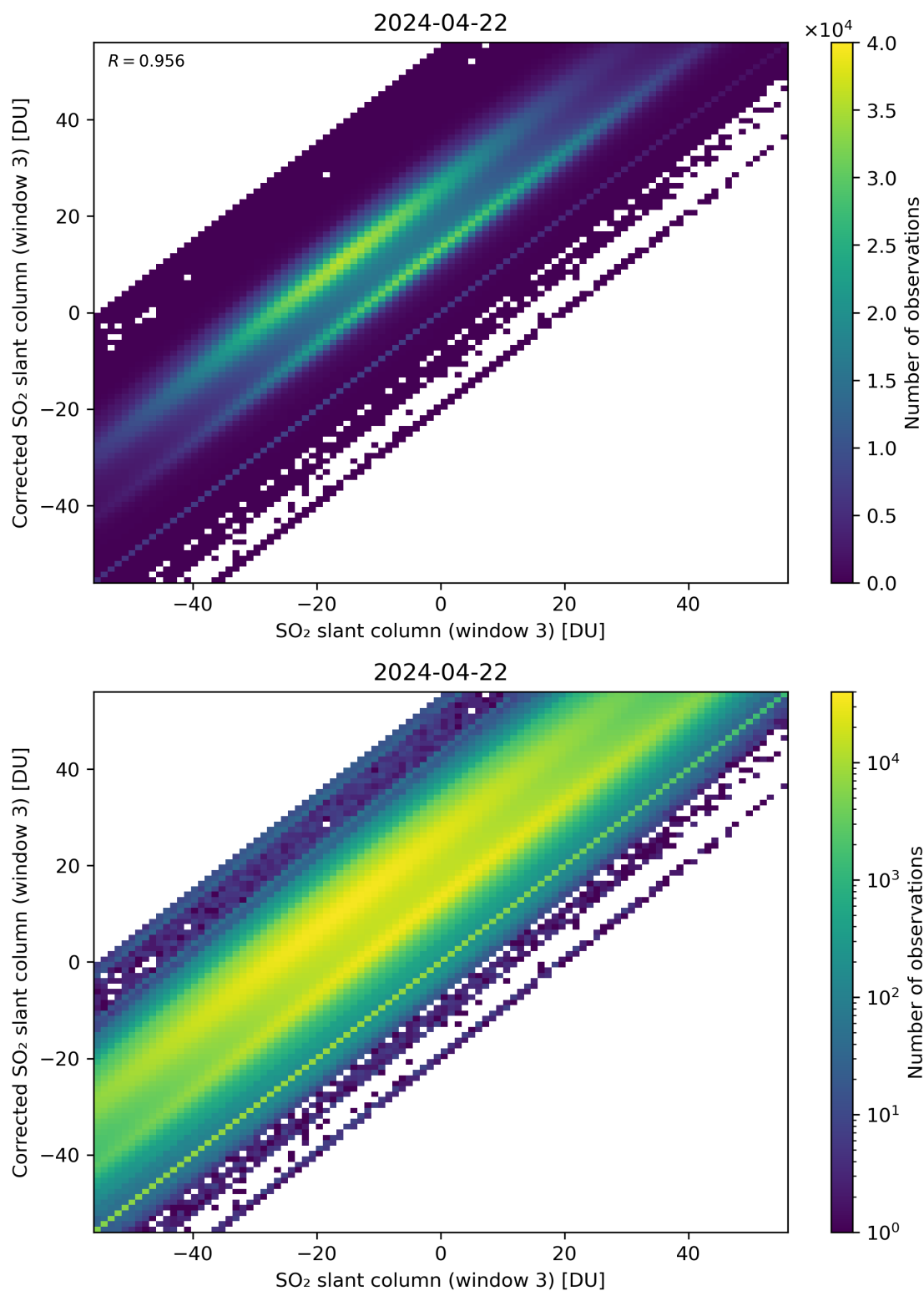
Figure 266: Scatter density plot of “SO 2 slant column (window 3)” against “Corrected SO 2 slant column (window 3)” for 2024-04-21 to 2024-04-23.
