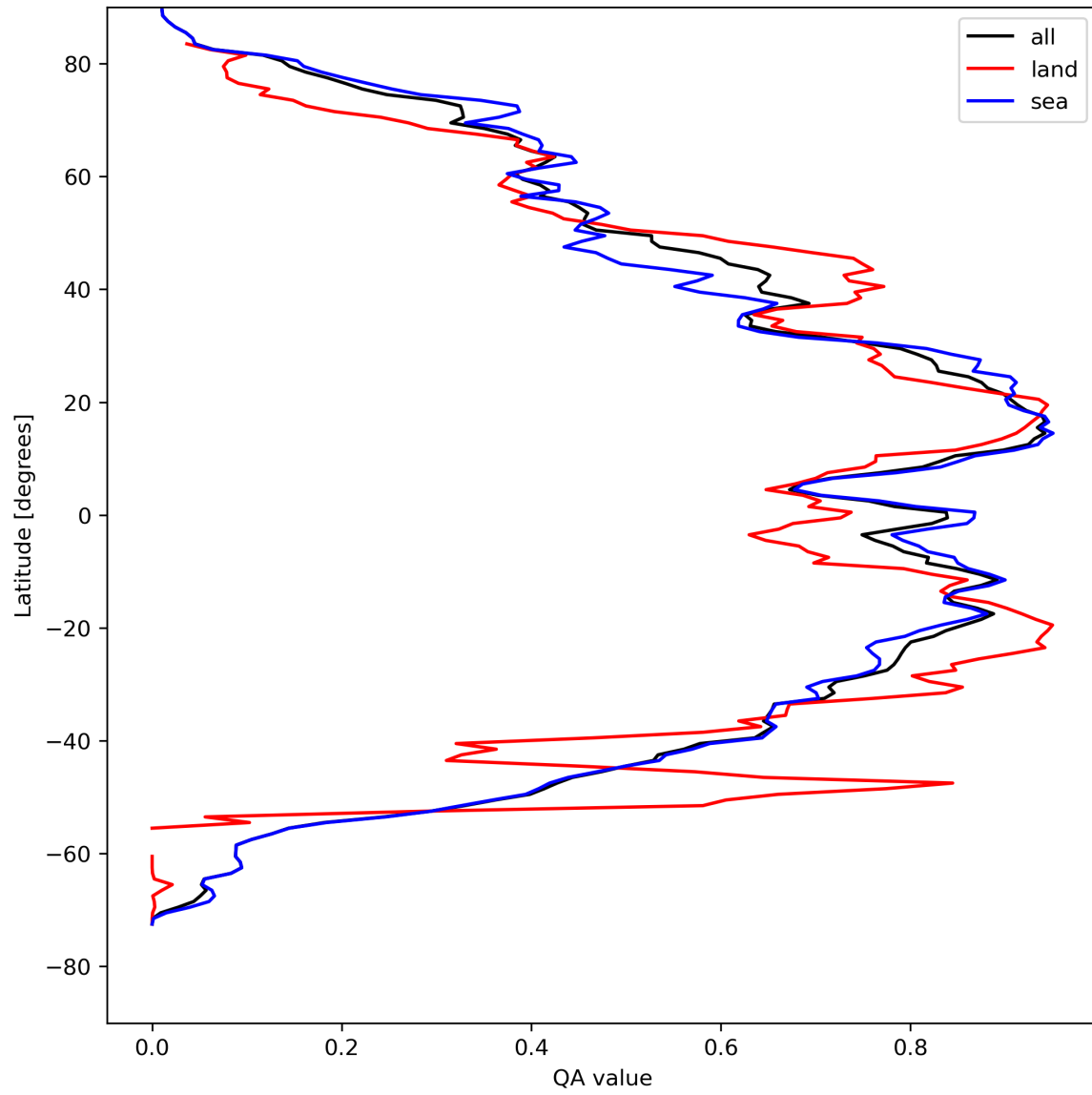
Figure 29: Zonal average of “QA value” for 2024-04-21 to 2024-04-23.
