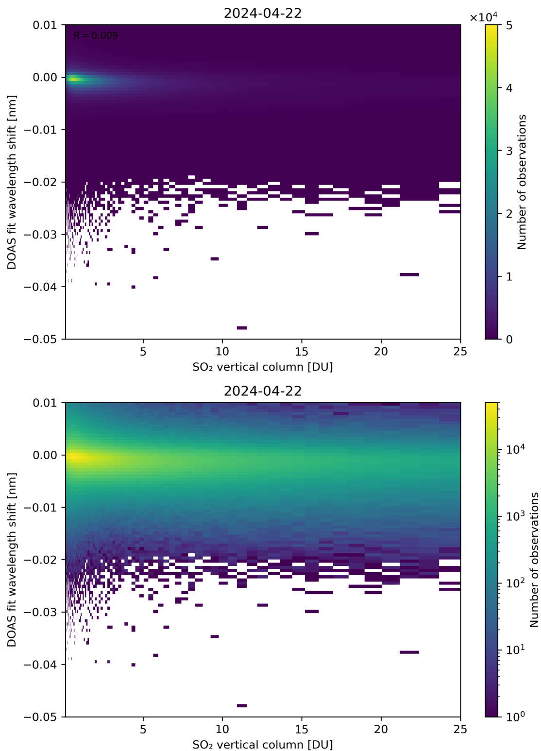
Figure 276: Scatter density plot of “SO 2 vertical column” against “DOAS fit wavelength shift” for 2024-04-21 to 2024-04-23.
