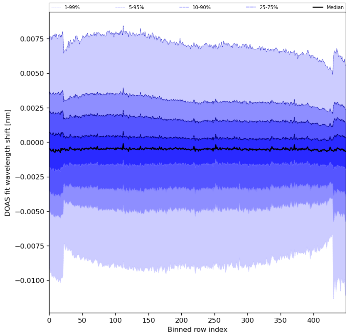
Figure 91: Along track statistics of “DOAS fit wavelength shift” for 2024-04-21 to 2024-04-23
