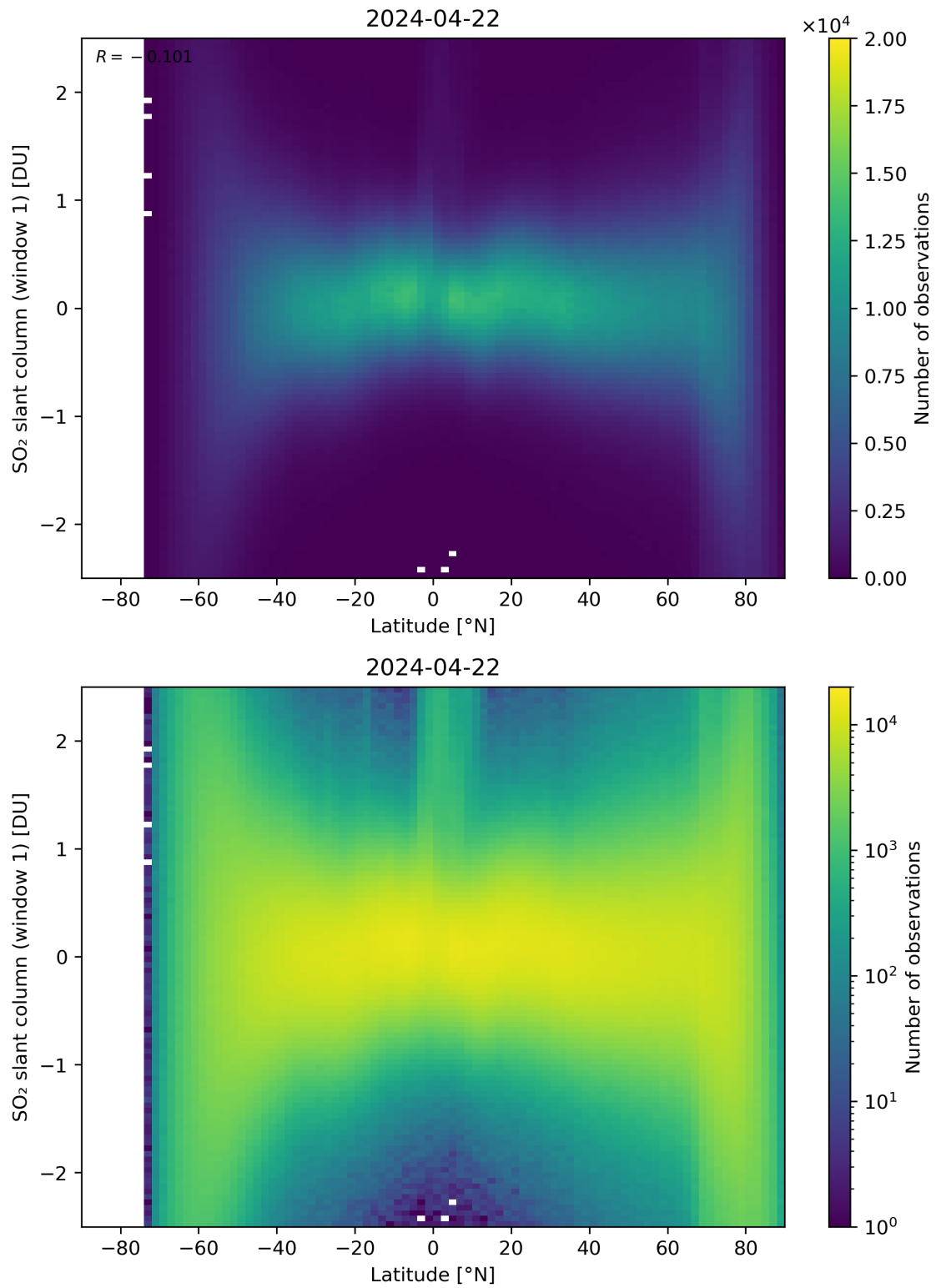
Figure 149: Scatter density plot of “Latitude” against “SO 2 slant column (window 1)” for 2024-04-21 to 2024-04-23.
