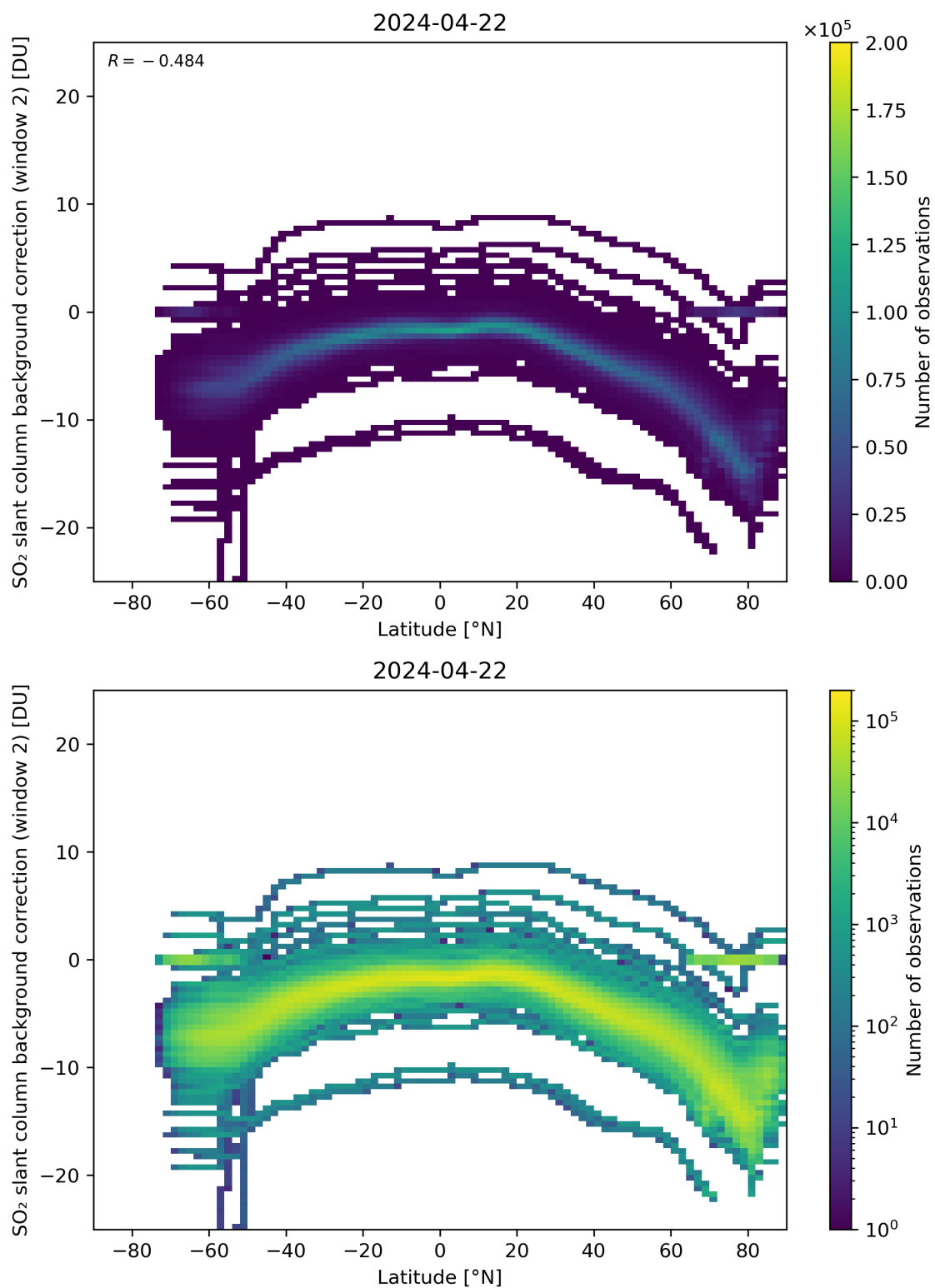
Figure 140: Scatter density plot of “Latitude” against “SO 2 slant column background correction (window 2)” for 2024-04-21 to 2024-04-23.
