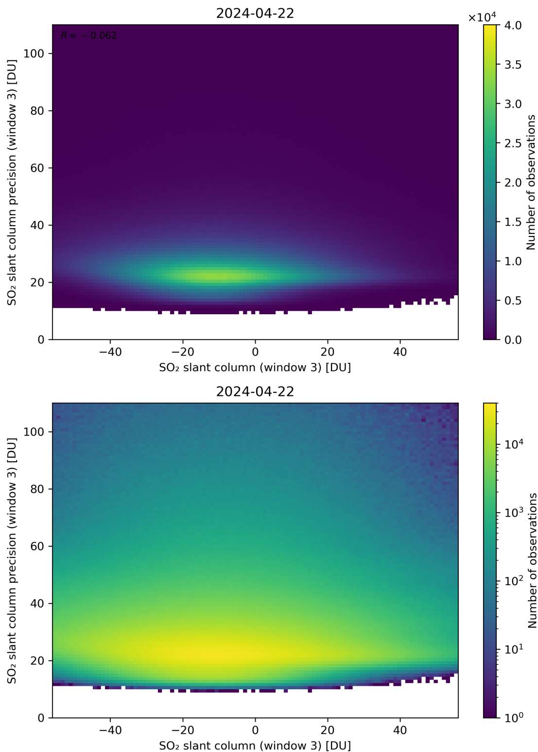
Figure 267: Scatter density plot of “SO 2 slant column (window 3)” against “SO 2 slant column precision (window 3)” for 2024-04-21 to 2024-04-23.
