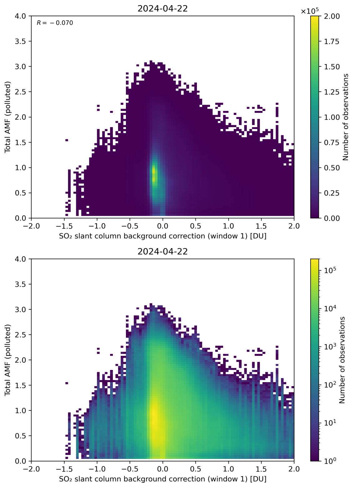
Figure 109: Scatter density plot of “SO 2 slant column background correction (window 1)” against “Total AMF (polluted)” for 2024-04-21 to 2024-04-23.
