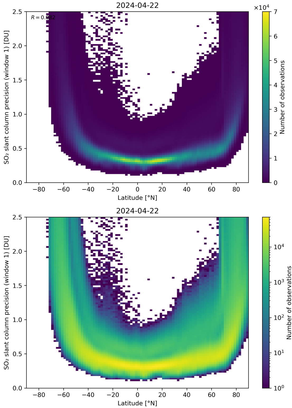
Figure 150: Scatter density plot of “Latitude” against “SO 2 slant column precision (window 1)” for 2024-04-21 to 2024-04-23.
