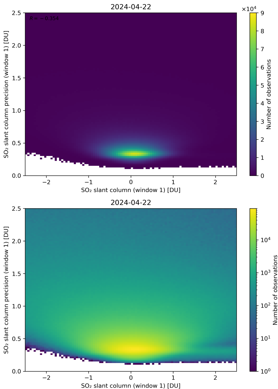
Figure 235: Scatter density plot of “SO 2 slant column (window 1)” against “SO 2 slant column precision (window 1)” for 2024-04-21 to 2024-04-23.
