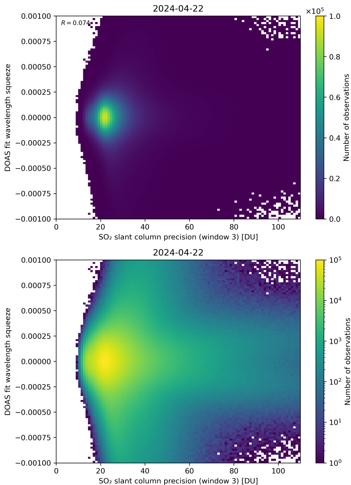
Figure 259: Scatter density plot of “SO 2 slant column precision (window 3)” against “DOAS fit wavelength squeeze” for 2024-04-21 to 2024-04-23.
