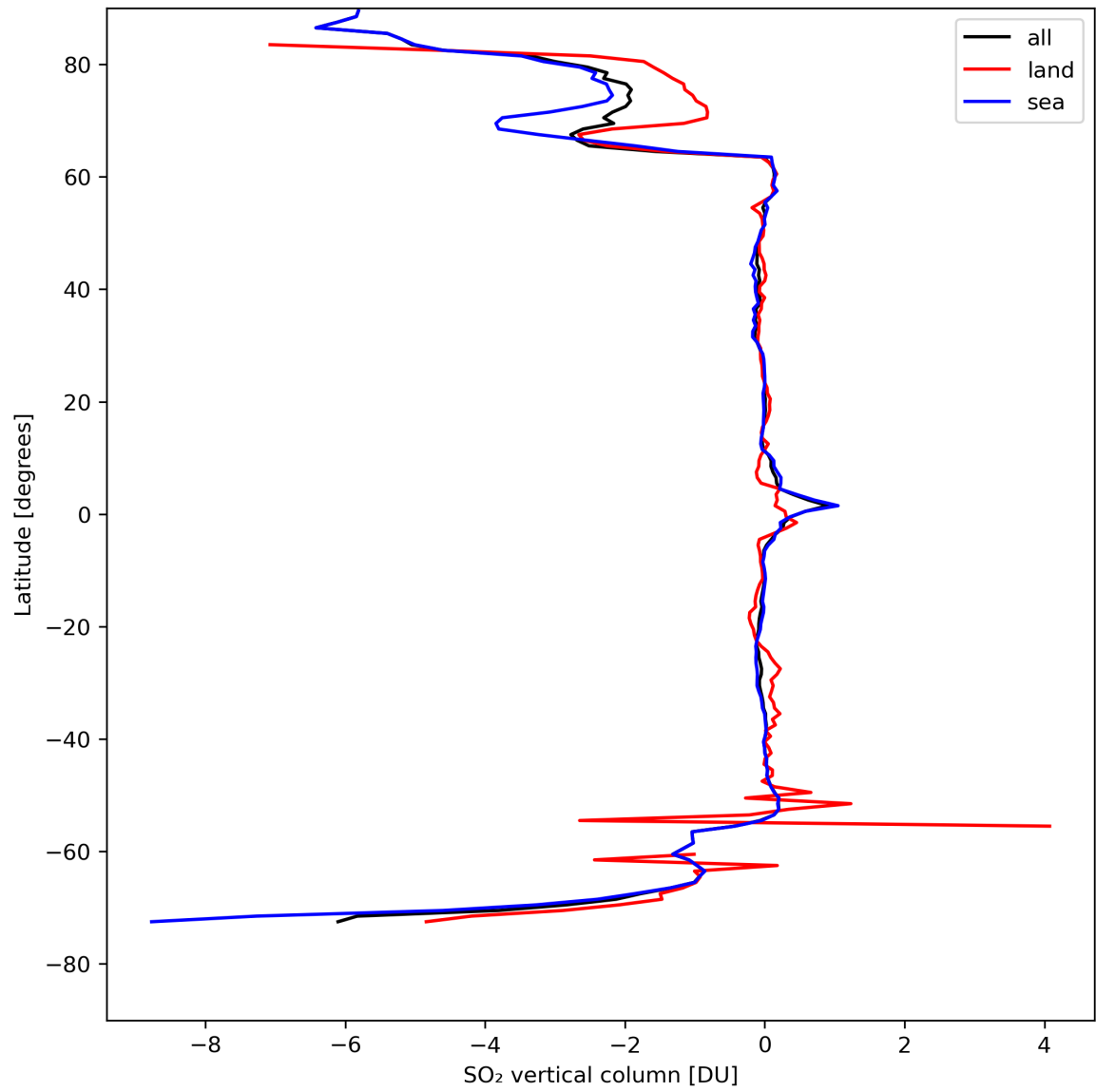
Figure 30: Zonal average of “SO 2 vertical column” for 2024-04-21 to 2024-04-23.
