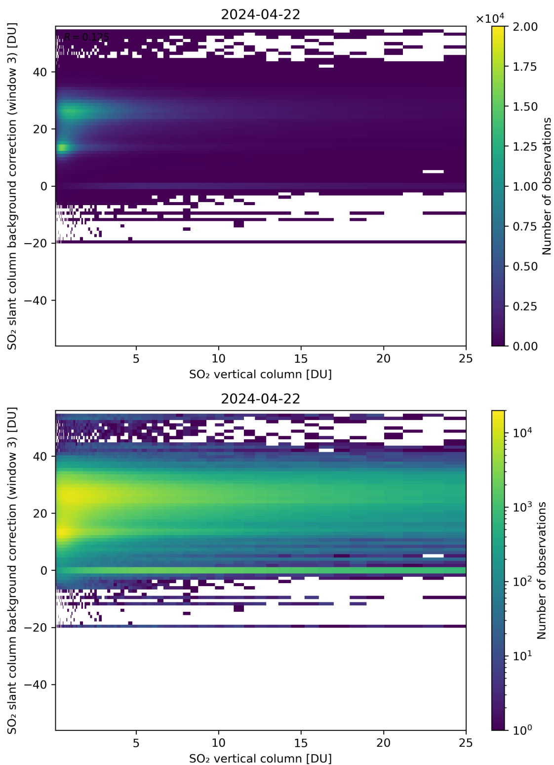
Figure 275: Scatter density plot of “SO 2 vertical column” against “SO 2 slant column background correction (window 3)” for 2024-04-21 to 2024-04-23.
