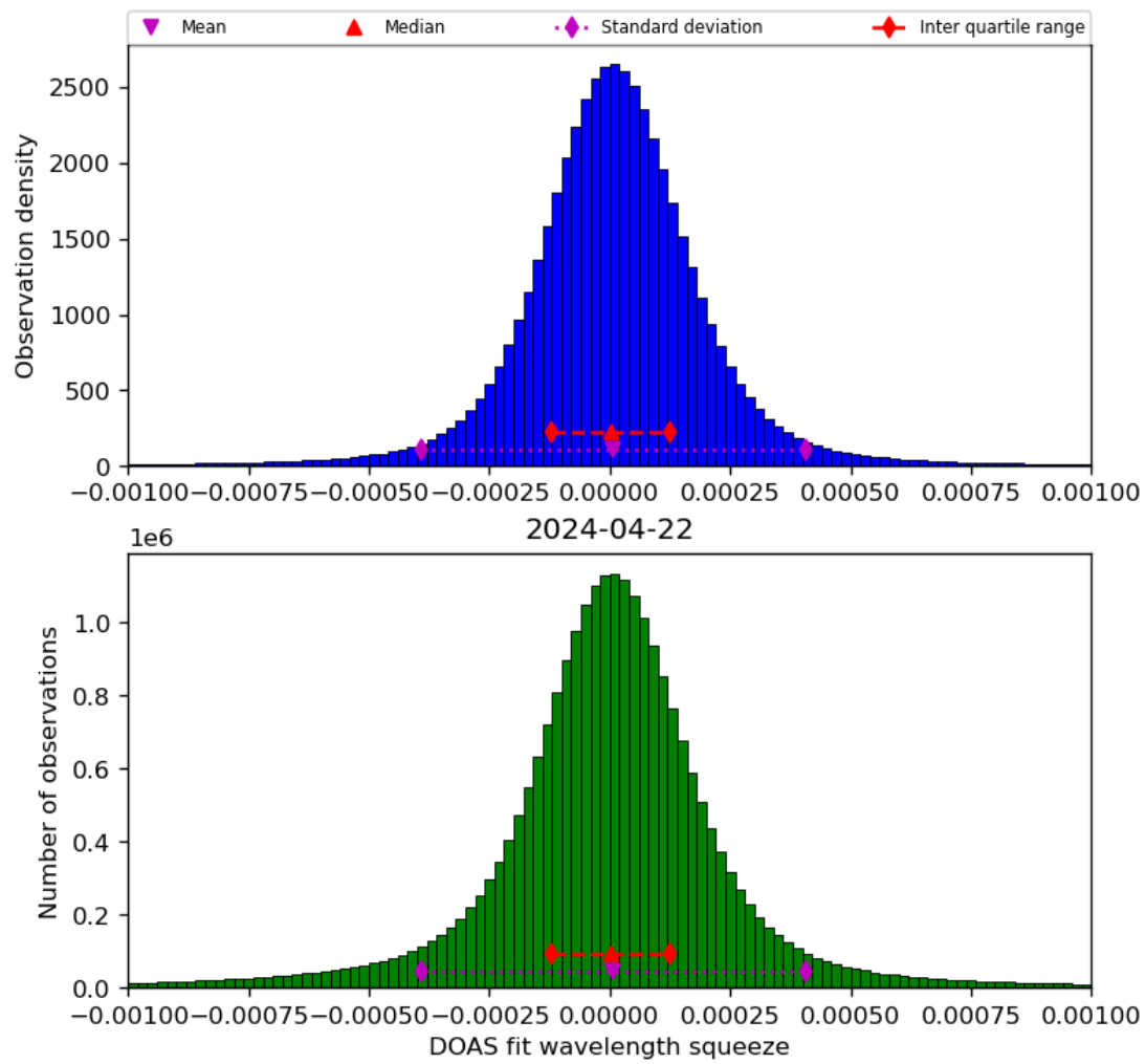
Figure 69: Histogram of “DOAS fit wavelength squeeze” for 2024-04-21 to 2024-04-23
