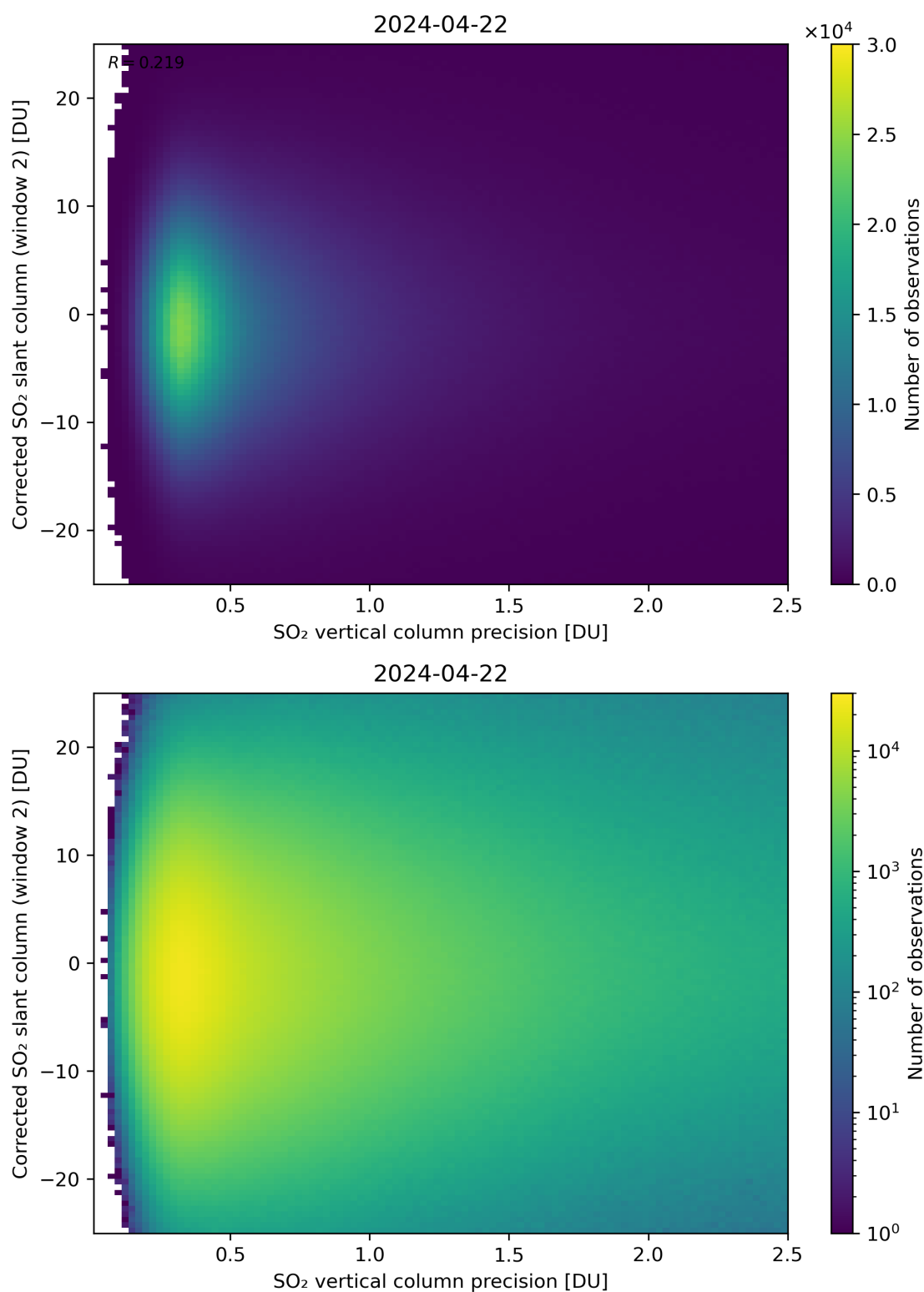
Figure 287: Scatter density plot of “SO 2 vertical column precision” against “Corrected SO 2 slant column (window 2)” for 2024-04-21 to 2024-04-23.
