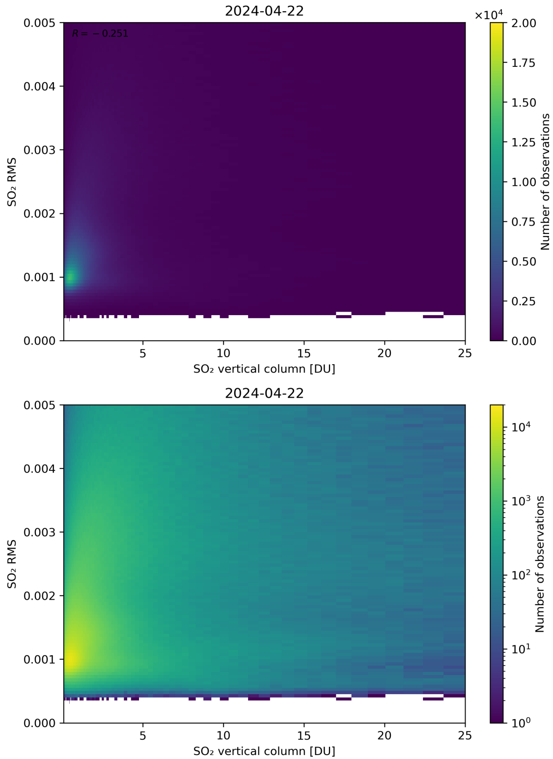
Figure 278: Scatter density plot of “SO 2 vertical column” against “SO 2 RMS” for 2024-04-21 to 2024-04-23.
