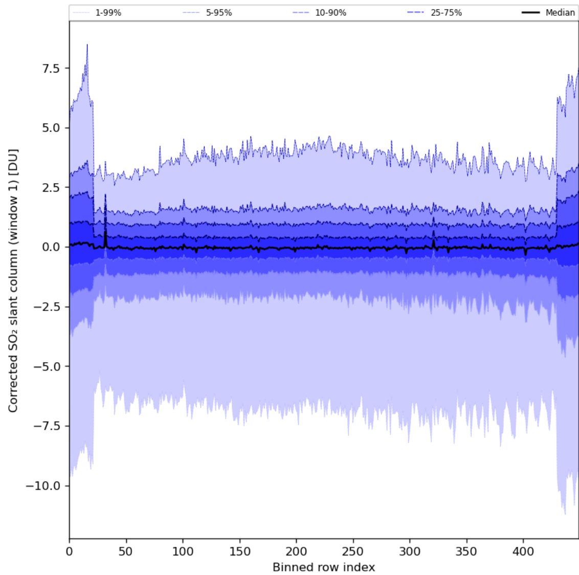
Figure 81: Along track statistics of “Corrected SO 2 slant column (window 1)” for 2024-04-21 to 2024-04-23
