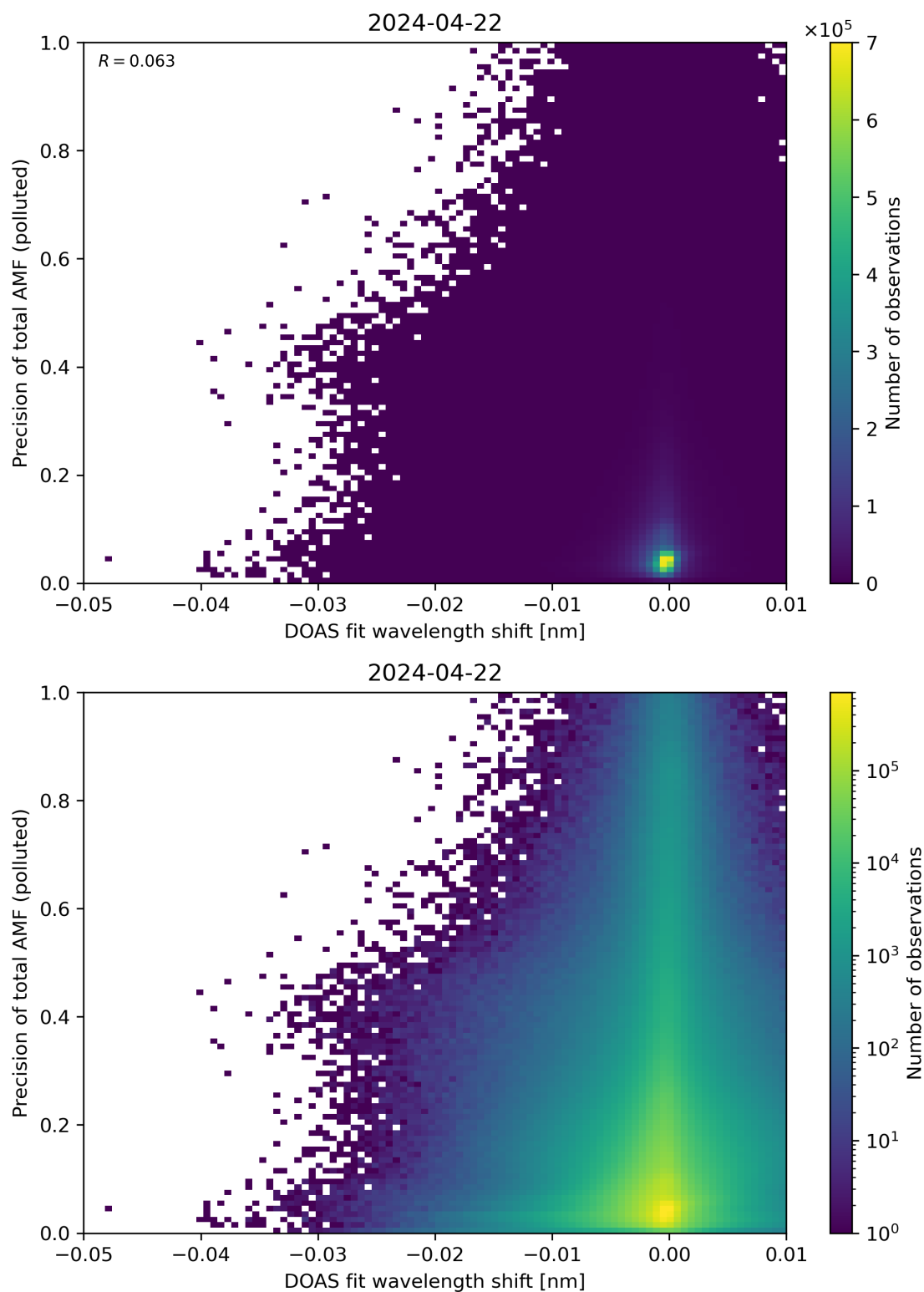
Figure 131: Scatter density plot of “DOAS fit wavelength shift” against “Precision of total AMF (polluted)” for 2024-04-21 to 2024-04-23.
