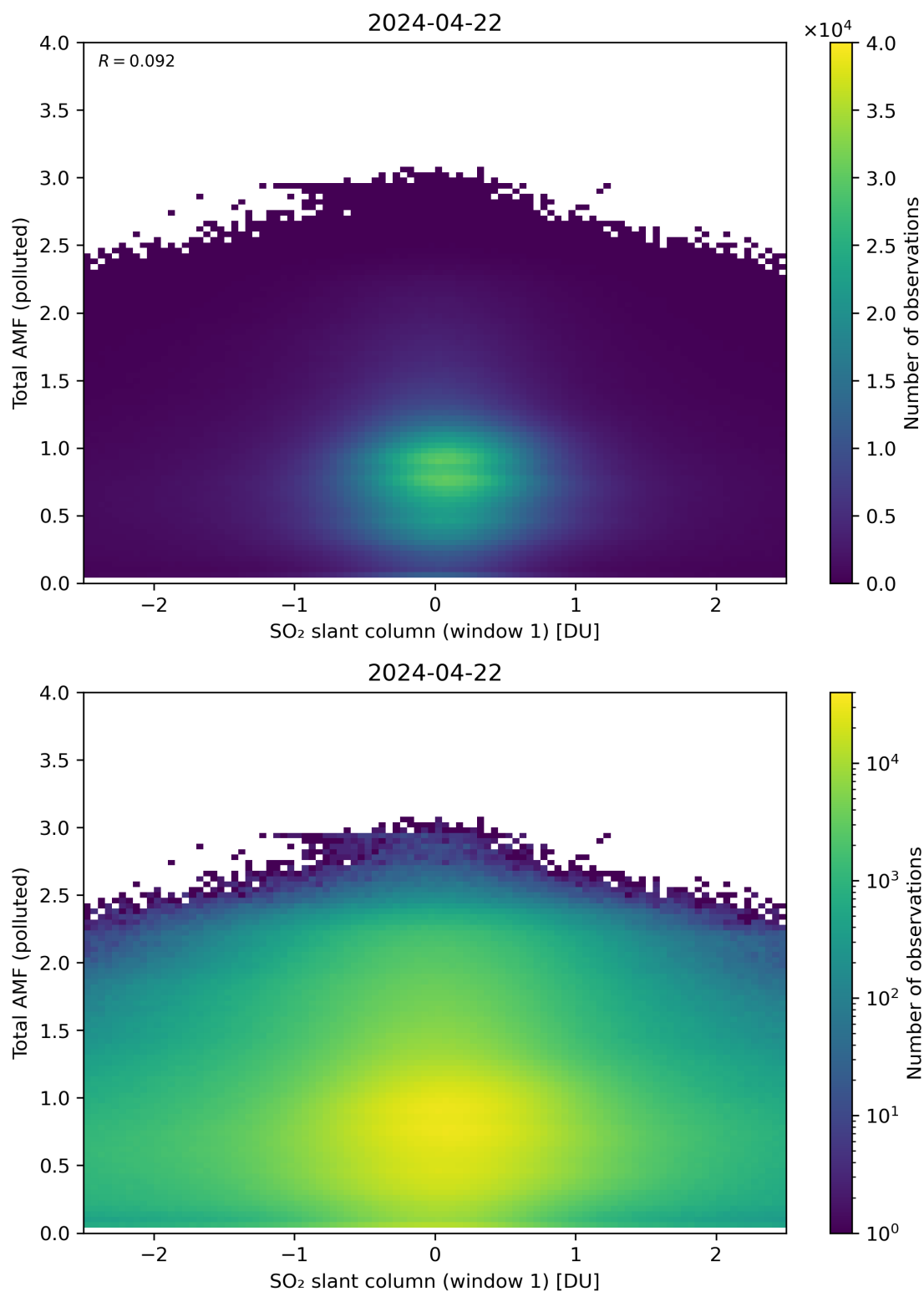
Figure 239: Scatter density plot of “SO 2 slant column (window 1)” against “Total AMF (polluted)” for 2024-04-21 to 2024-04-23.
