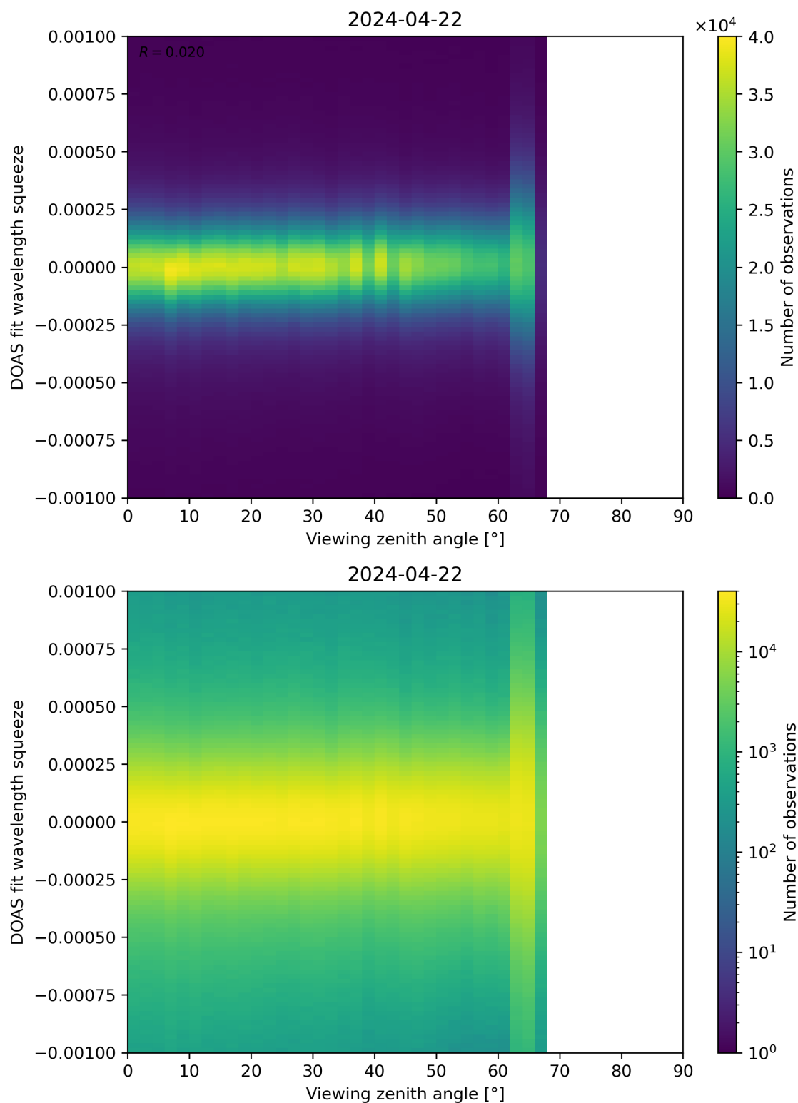
Figure 312: Scatter density plot of “Viewing zenith angle” against “DOAS fit wavelength squeeze” for 2024-04-21 to 2024-04-23.
