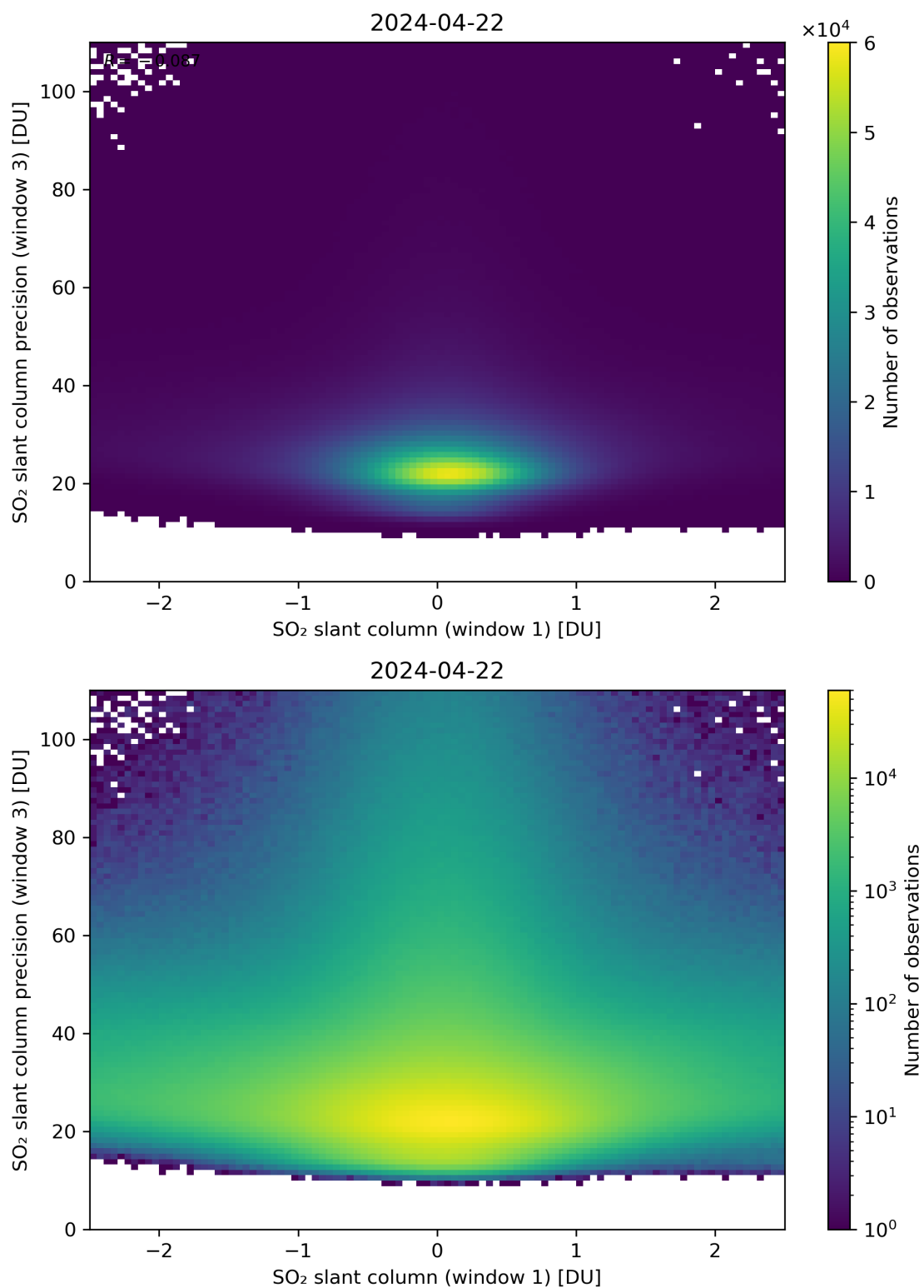
Figure 238: Scatter density plot of “SO 2 slant column (window 1)” against “SO 2 slant column precision (window 3)” for 2024-04-21 to 2024-04-23.
