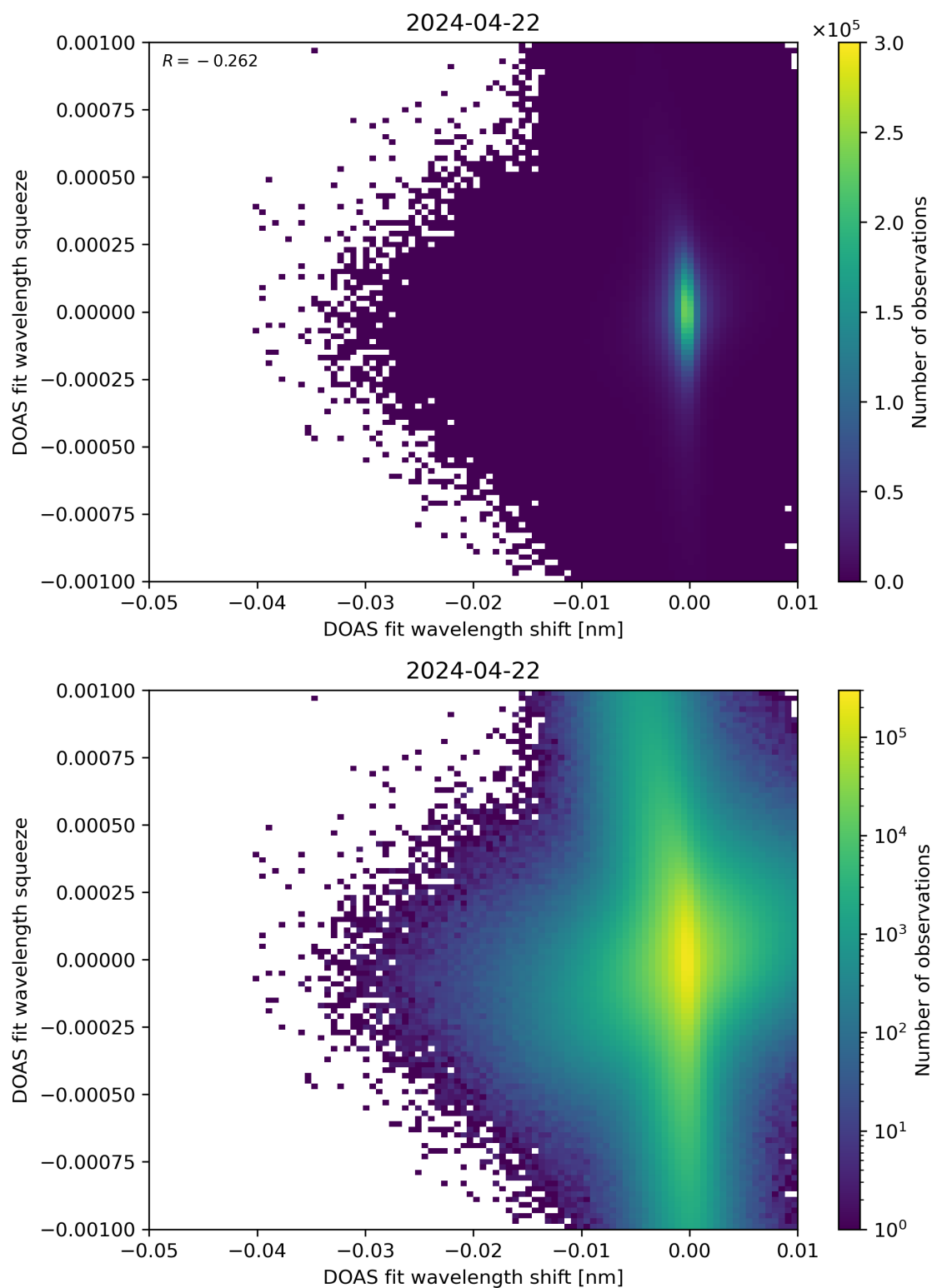
Figure 127: Scatter density plot of “DOAS fit wavelength shift” against “DOAS fit wavelength squeeze” for 2024-04-21 to 2024-04-23.
