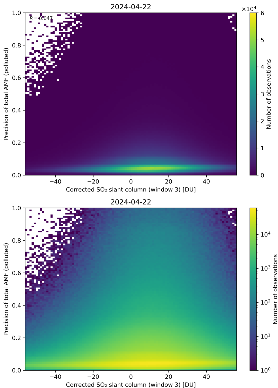
Figure 211: Scatter density plot of “Corrected SO 2 slant column (window 3)” against “Precision of total AMF (polluted)” for 2024-04-21 to 2024-04-23.
