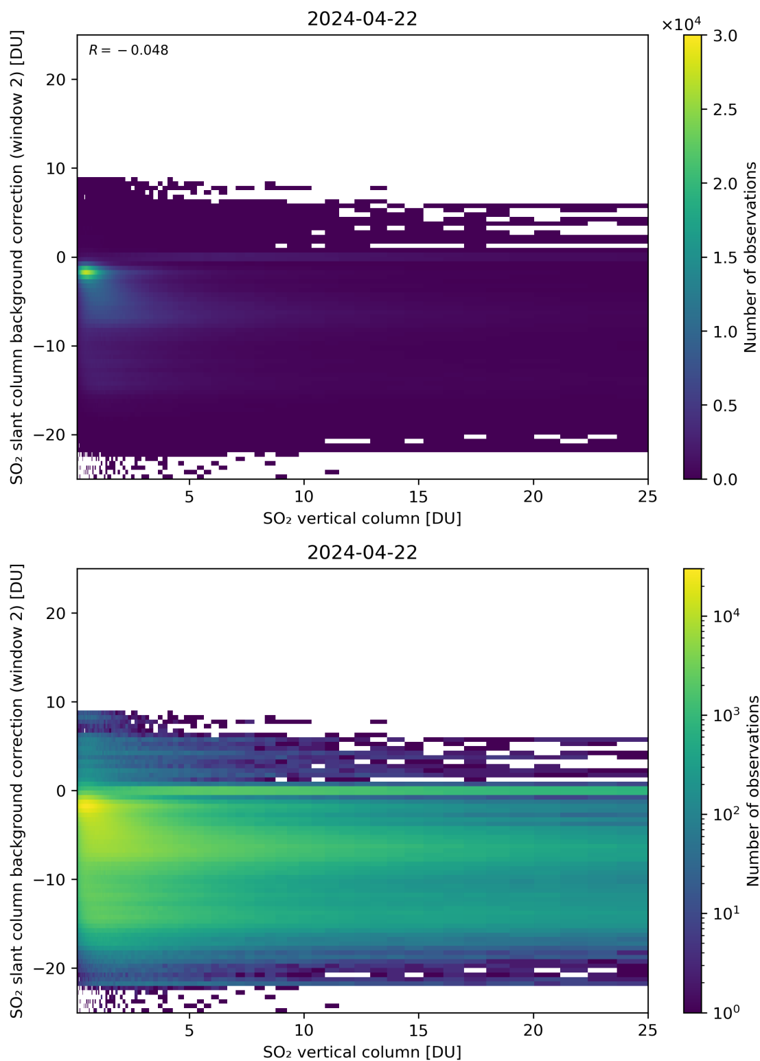
Figure 274: Scatter density plot of “SO 2 vertical column” against “SO 2 slant column background correction (window 2)” for 2024-04-21 to 2024-04-23.
