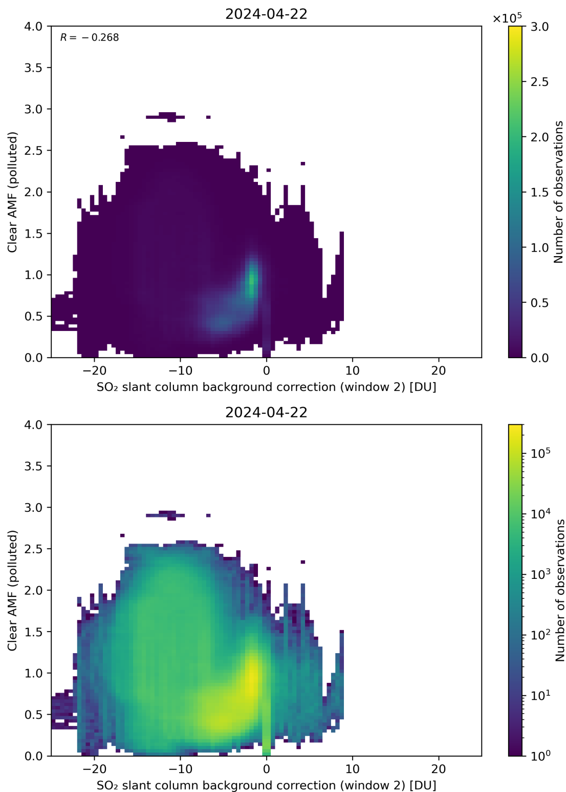
Figure 115: Scatter density plot of “SO 2 slant column background correction (window 2)” against “Clear AMF (polluted)” for 2024-04-21 to 2024-04-23.
