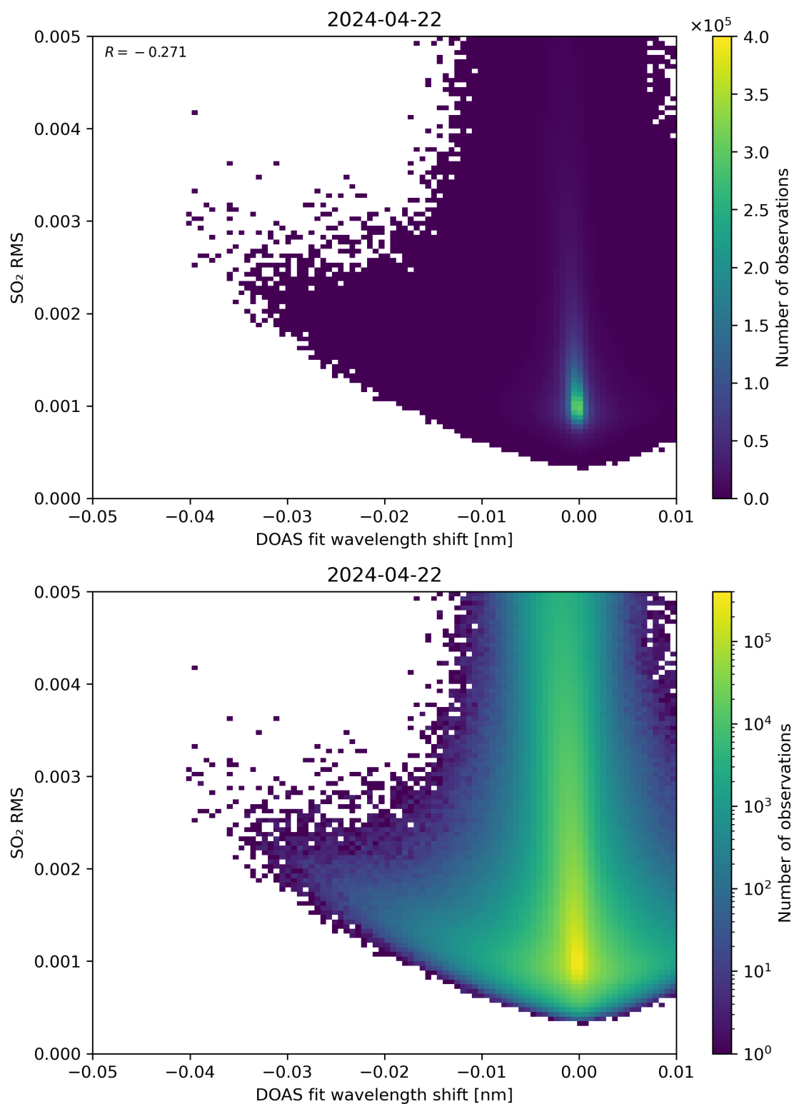
Figure 128: Scatter density plot of “DOAS fit wavelength shift” against “SO 2 RMS” for 2024-04-21 to 2024-04-23.
