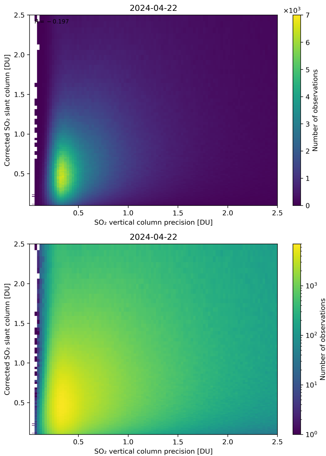
Figure 286: Scatter density plot of “SO 2 vertical column precision” against “Corrected SO 2 slant column” for 2024-04-21 to 2024-04-23.
