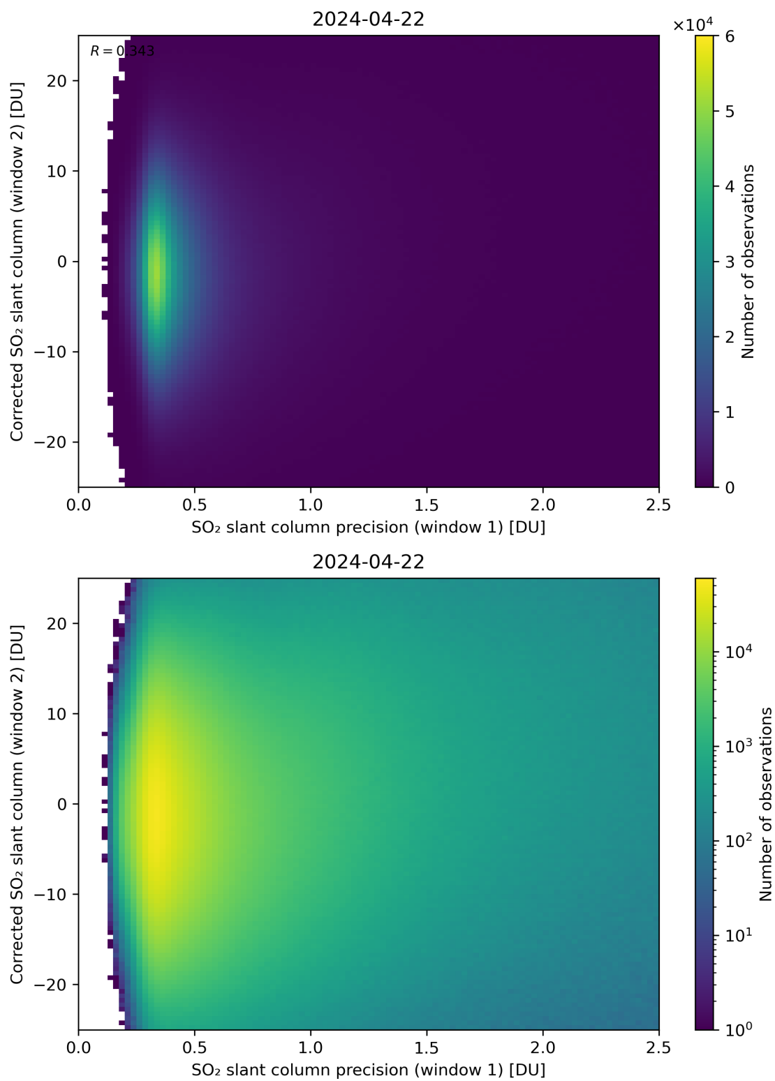
Figure 225: Scatter density plot of “SO 2 slant column precision (window 1)” against “Corrected SO 2 slant column (window 2)” for 2024-04-21 to 2024-04-23.
