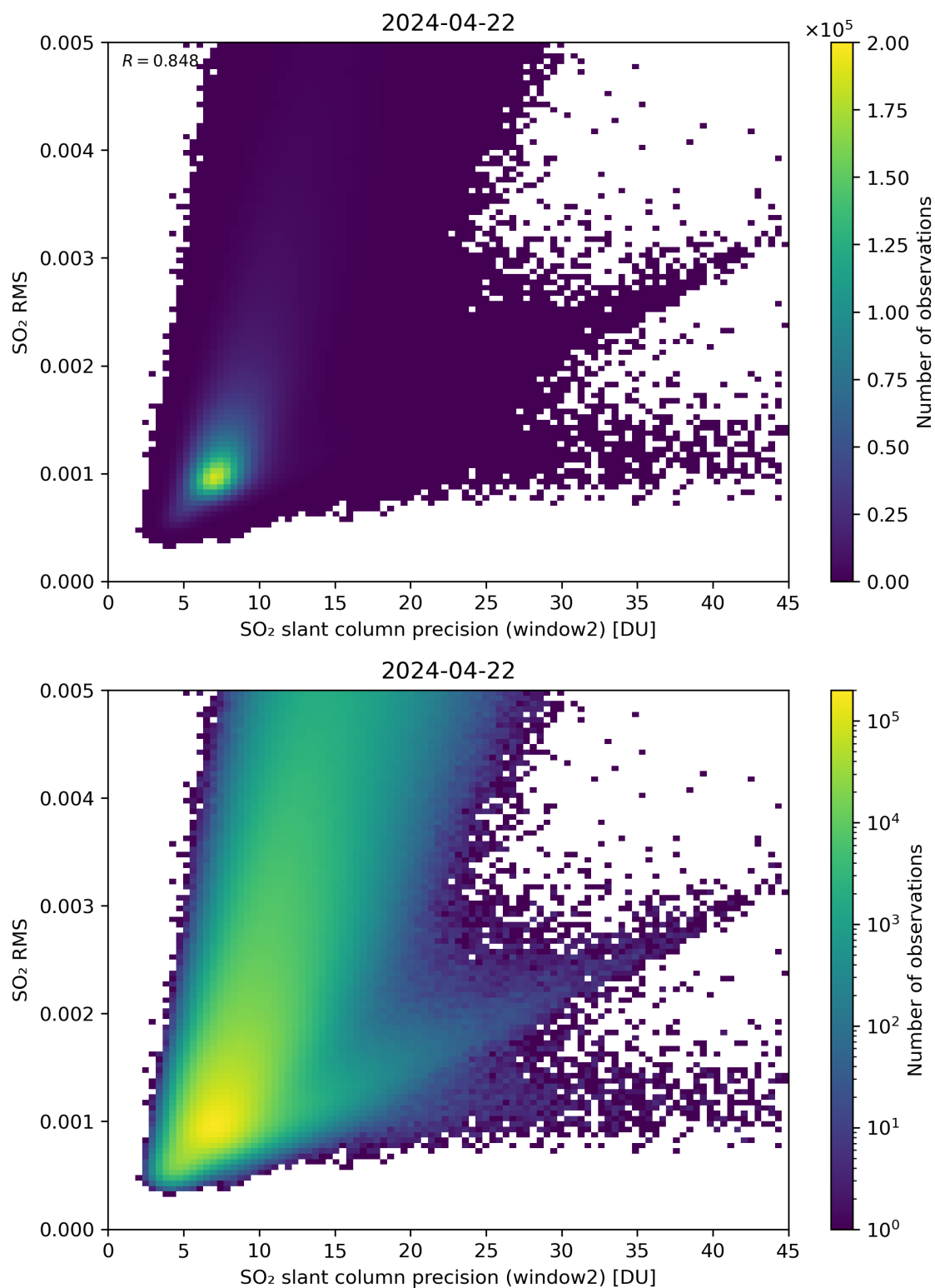
Figure 245: Scatter density plot of “SO 2 slant column precision (window2)” against “SO 2 RMS” for 2024-04-21 to 2024-04-23.
