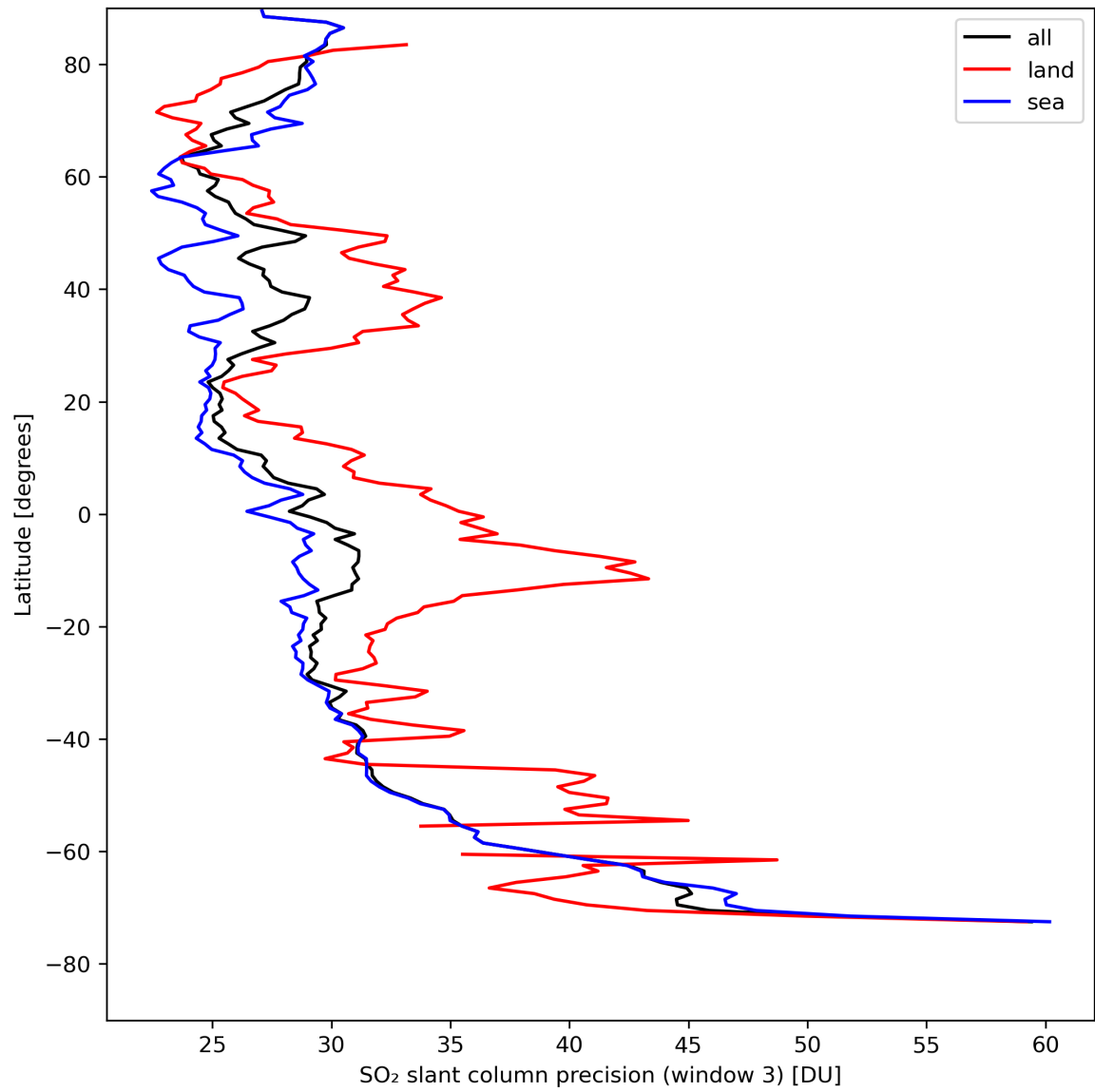
Figure 42: Zonal average of “SO 2 slant column precision (window 3)” for 2024-04-21 to 2024-04-23.
