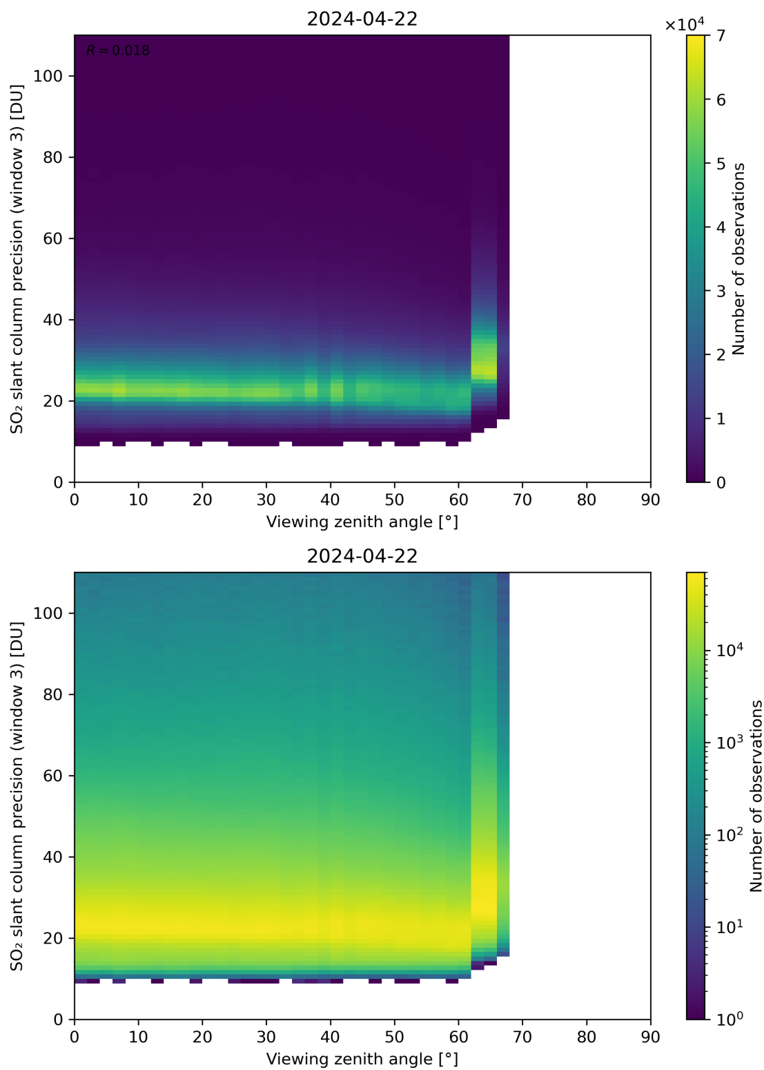
Figure 324: Scatter density plot of “Viewing zenith angle” against “SO 2 slant column precision (window 3)” for 2024-04-21 to 2024-04-23.
