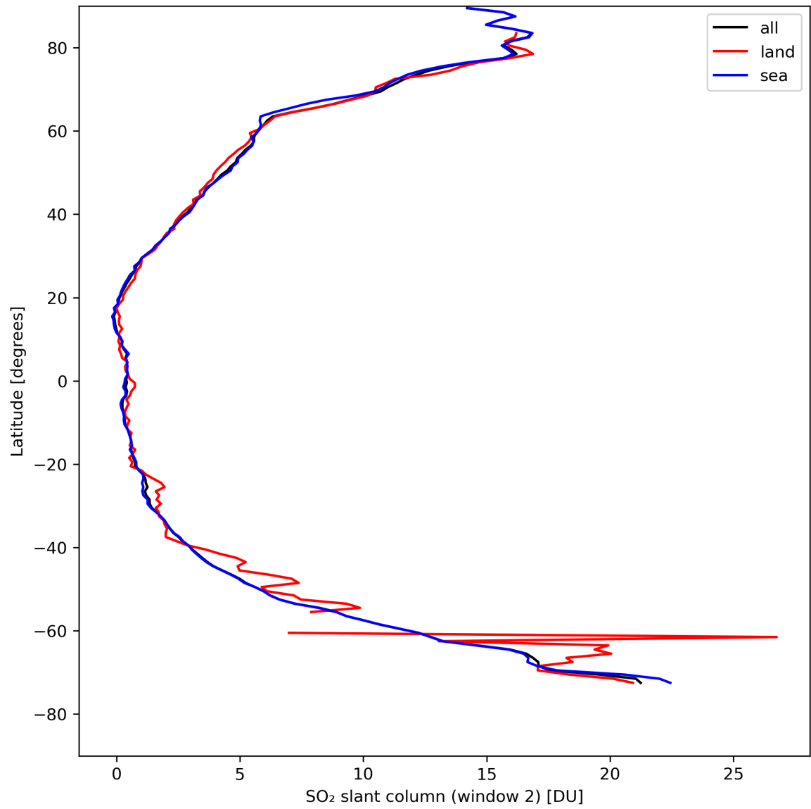
Figure 37: Zonal average of “SO 2 slant column (window 2)” for 2024-04-21 to 2024-04-23.
