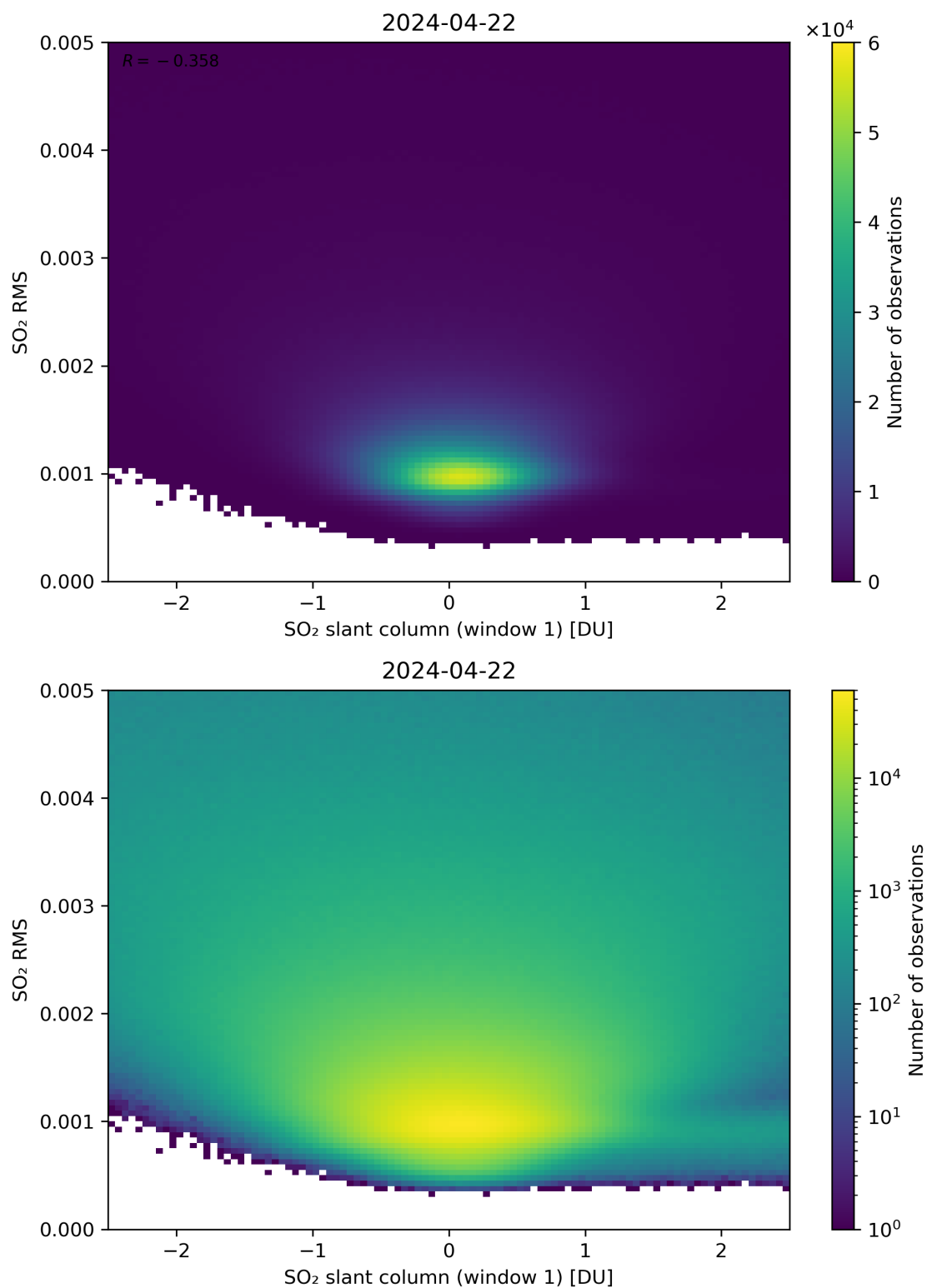
Figure 217: Scatter density plot of “SO 2 slant column (window 1)” against “SO 2 RMS” for 2024-04-21 to 2024-04-23.
