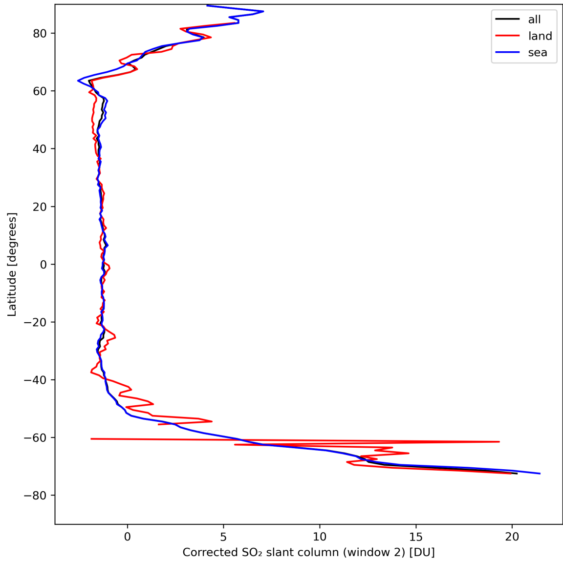
Figure 39: Zonal average of “Corrected SO 2 slant column (window 2)” for 2024-04-21 to 2024-04-23.
