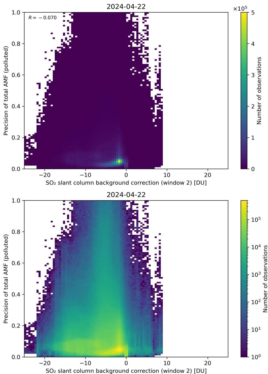
Figure 120: Scatter density plot of “SO 2 slant column background correction (window 2)” against “Precision of total AMF (polluted)” for 2024-04-21 to 2024-04-23.
