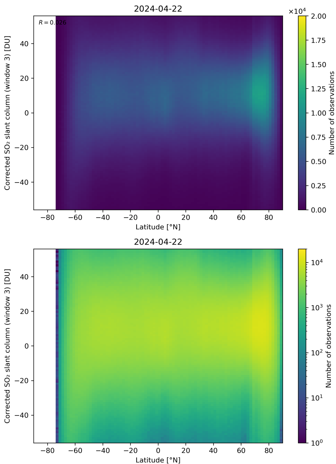
Figure 148: Scatter density plot of “Latitude” against “Corrected SO 2 slant column (window 3)” for 2024-04-21 to 2024-04-23.
