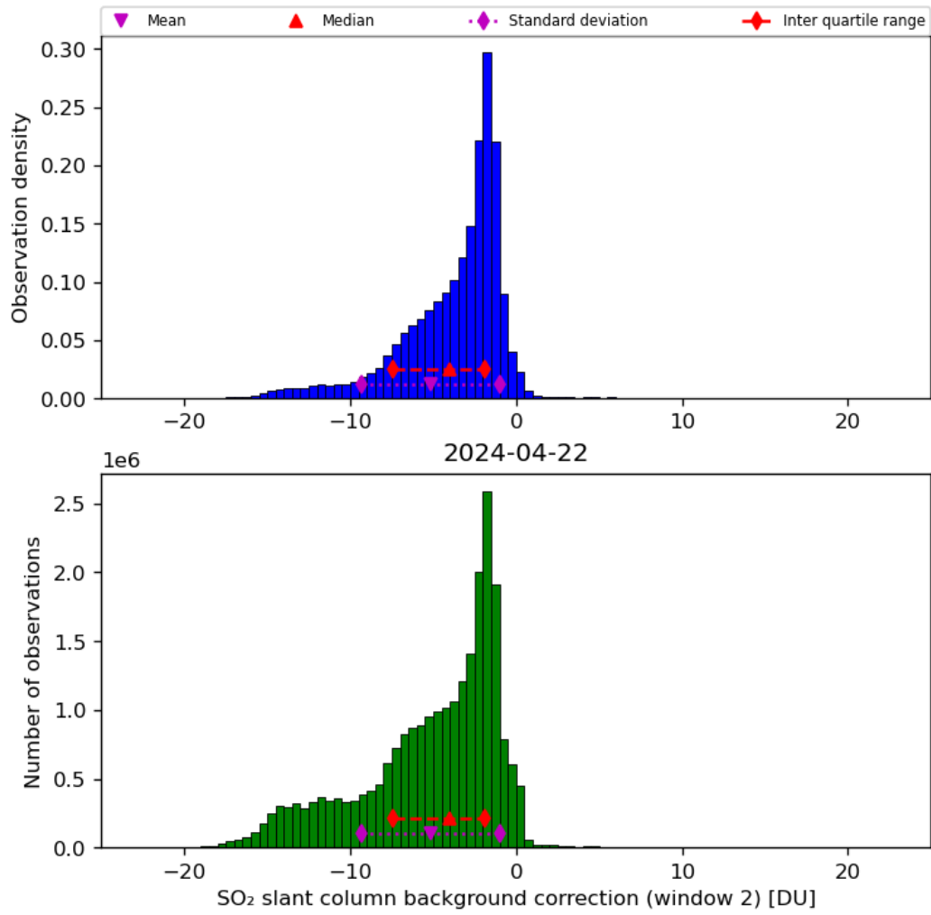
Figure 63: Histogram of “SO 2 slant column background correction (window 2)” for 2024-04-21 to 2024-04-23
