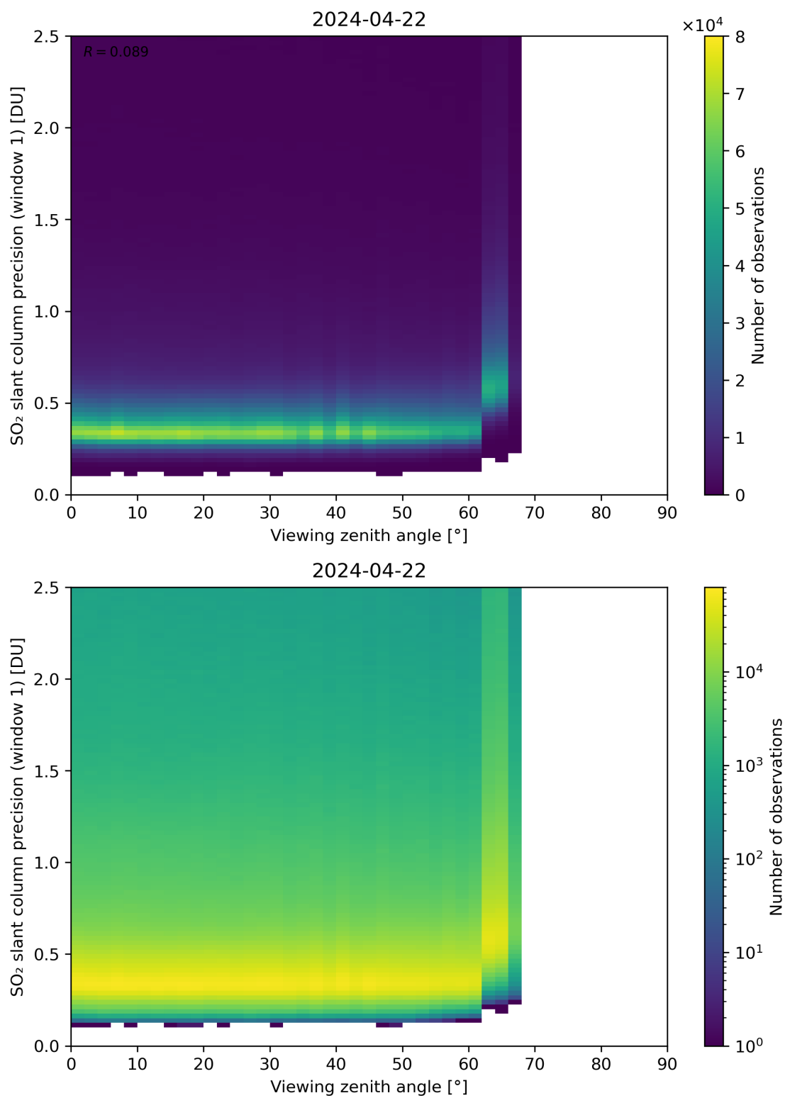
Figure 321: Scatter density plot of “Viewing zenith angle” against “SO 2 slant column precision (window 1)” for 2024-04-21 to 2024-04-23.
