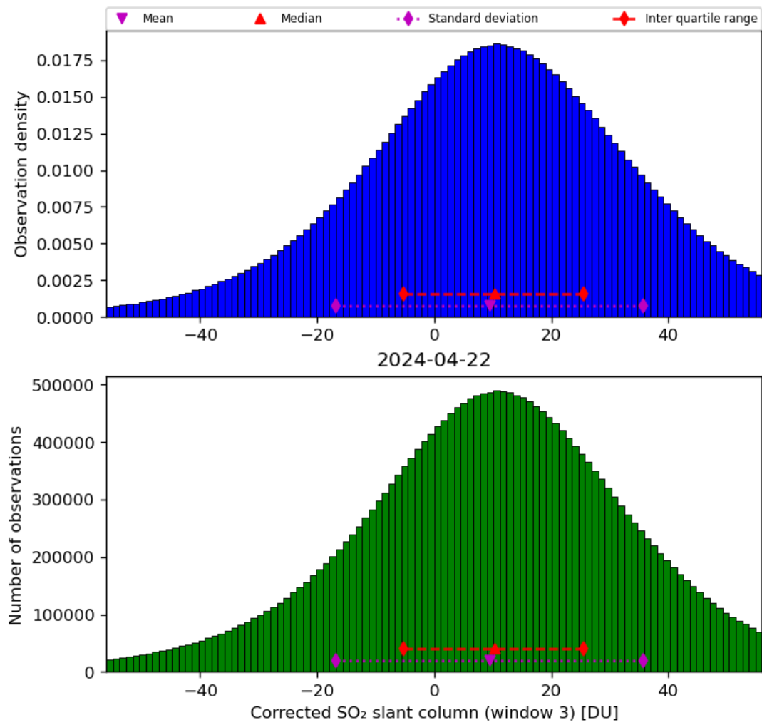
Figure 66: Histogram of “Corrected SO 2 slant column (window 3)” for 2024-04-21 to 2024-04-23
