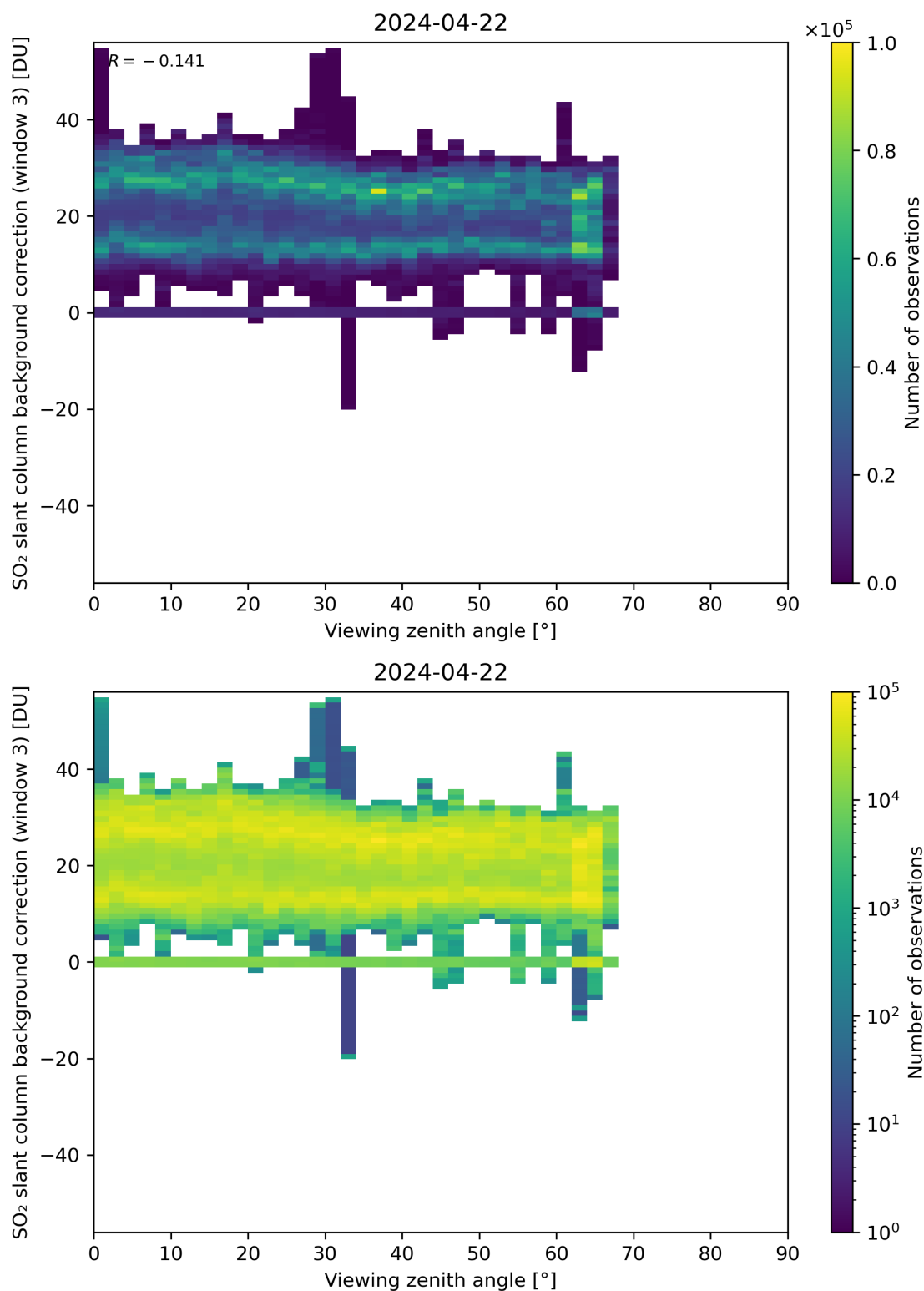
Figure 310: Scatter density plot of “Viewing zenith angle” against “SO 2 slant column background correction (window 3)” for 2024-04-21 to 2024-04-23.
