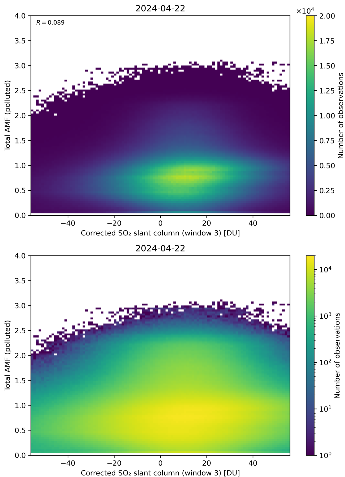
Figure 210: Scatter density plot of “Corrected SO 2 slant column (window 3)” against “Total AMF (polluted)” for 2024-04-21 to 2024-04-23.
