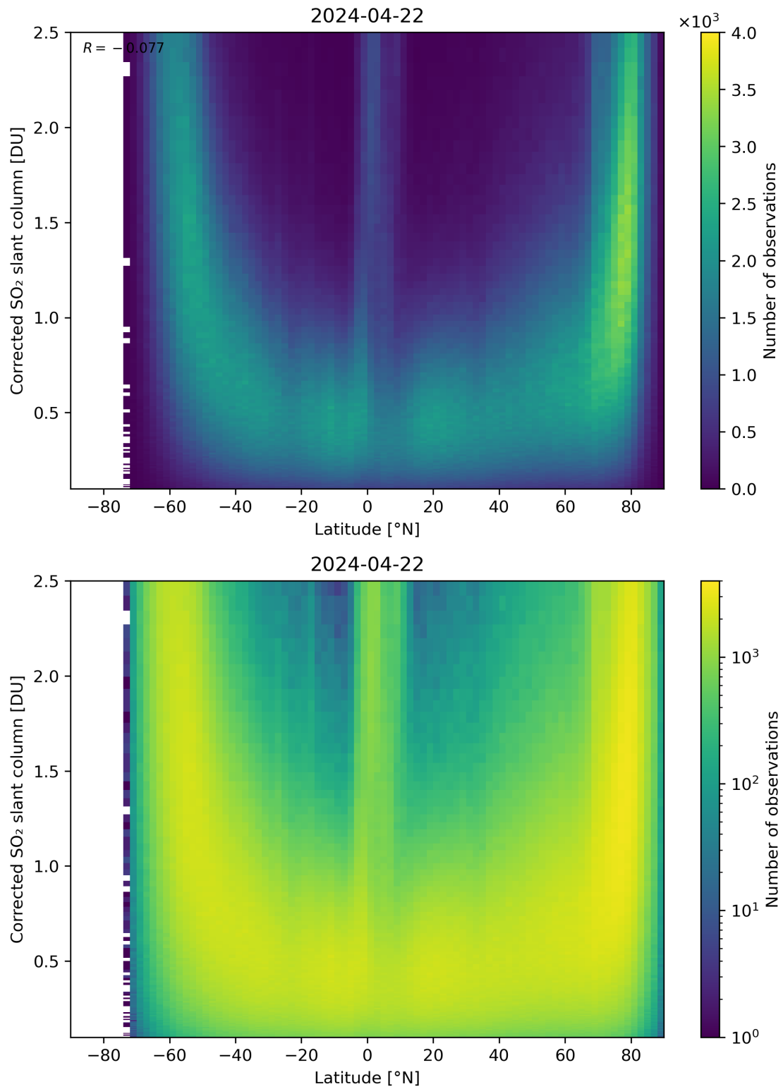
Figure 146: Scatter density plot of “Latitude” against “Corrected SO 2 slant column” for 2024-04-21 to 2024-04-23.
