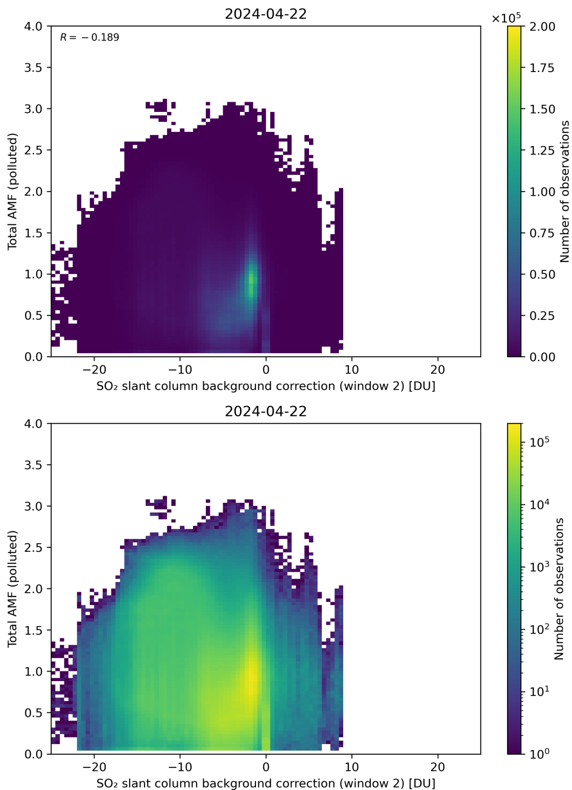
Figure 119: Scatter density plot of “SO 2 slant column background correction (window 2)” against “Total AMF (polluted)” for 2024-04-21 to 2024-04-23.
