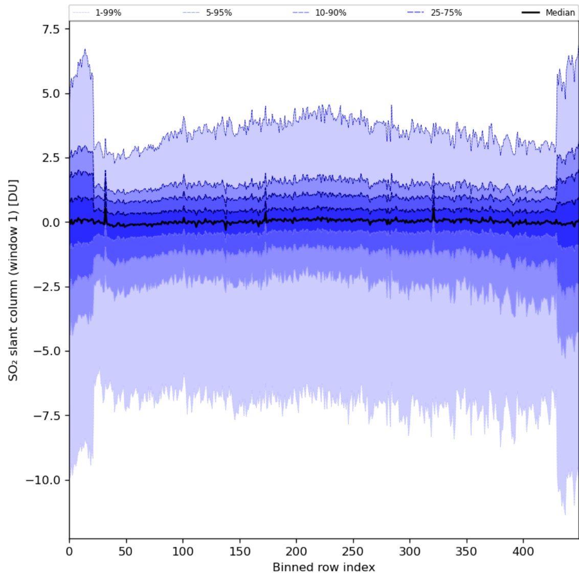
Figure 79: Along track statistics of “SO 2 slant column (window 1)” for 2024-04-21 to 2024-04-23
