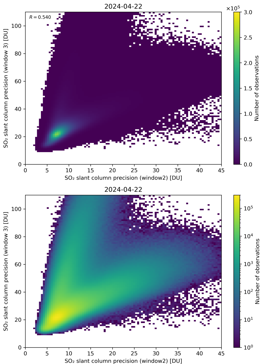
Figure 250: Scatter density plot of “SO 2 slant column precision (window2)” against “SO 2 slant column precision (window 3)” for 2024-04-21 to 2024-04-23.
