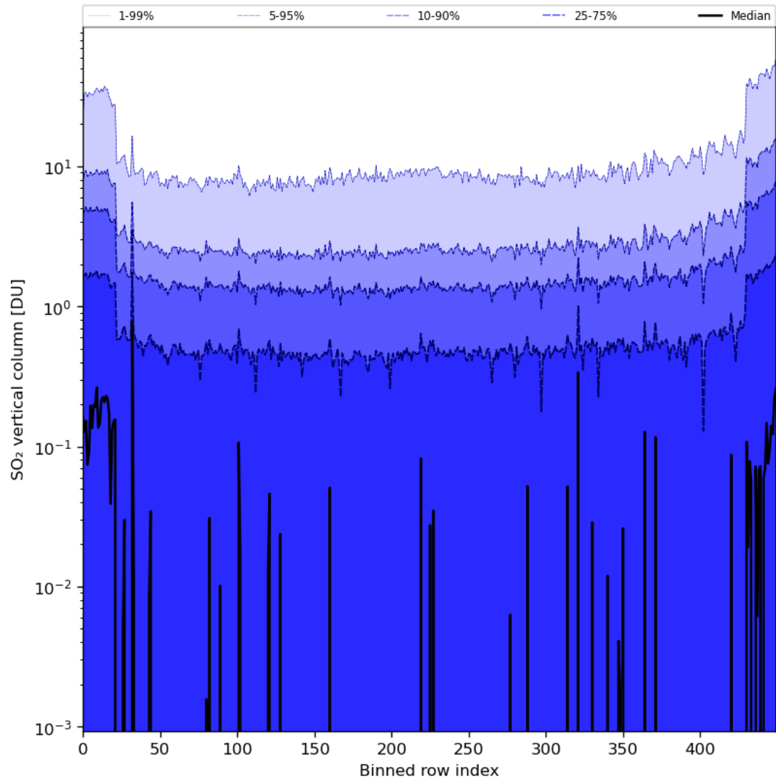
Figure 76: Along track statistics of “SO 2 vertical column” for 2024-04-21 to 2024-04-23
