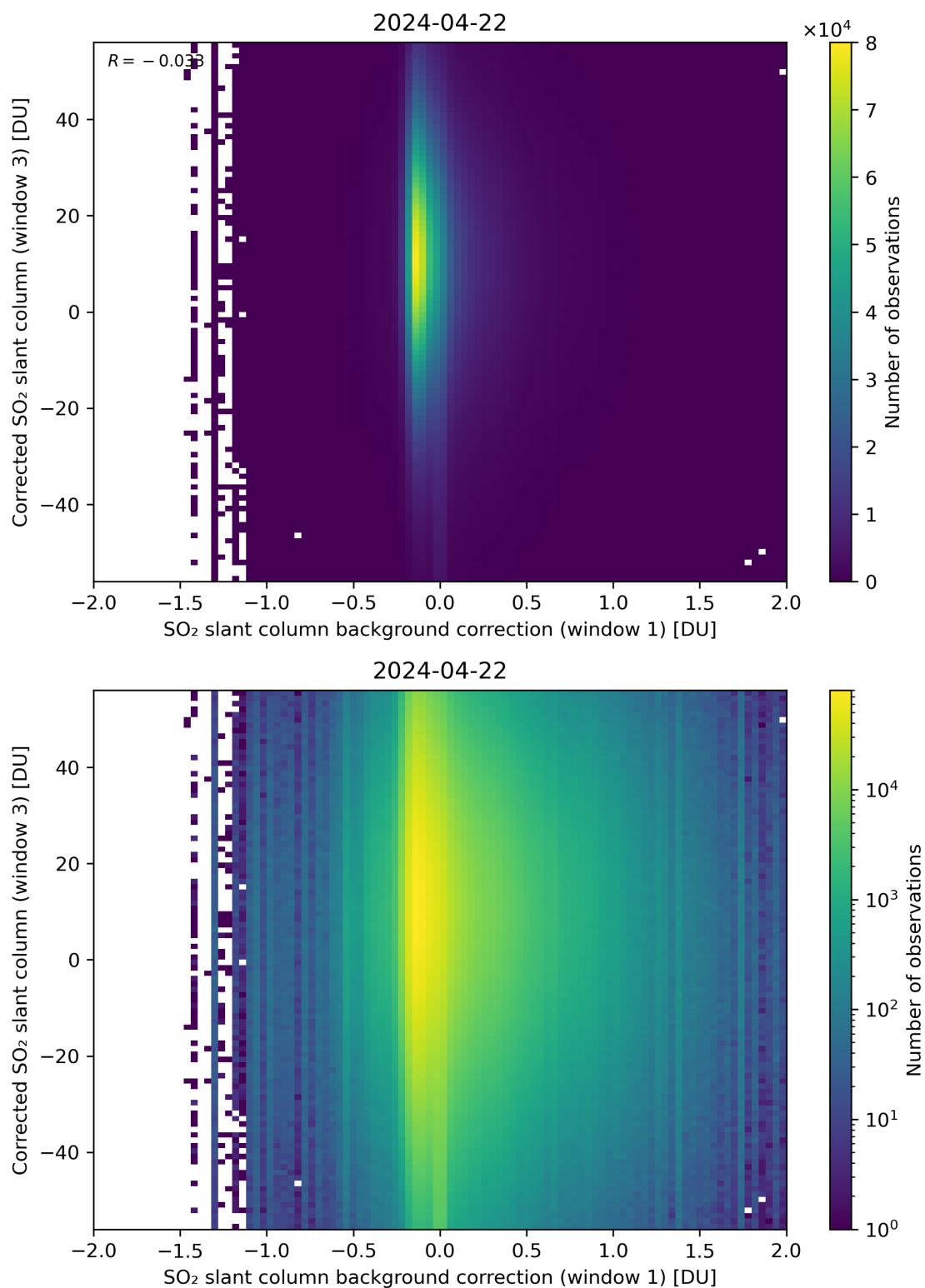
Figure 105: Scatter density plot of “SO 2 slant column background correction (window 1)” against “Corrected SO 2 slant column (window 3)” for 2024-04-21 to 2024-04-23.
