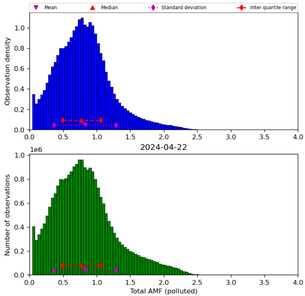
Figure 71: Histogram of “Total AMF (polluted)” for 2024-04-21 to 2024-04-23
