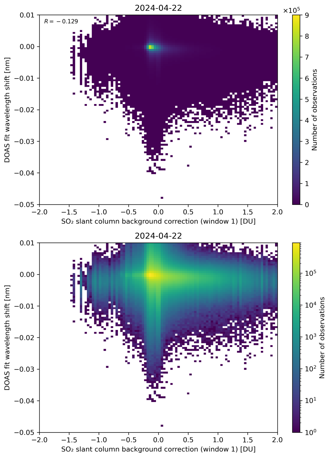
Figure 100: Scatter density plot of “SO 2 slant column background correction (window 1)” against “DOAS fit wavelength shift” for 2024-04-21 to 2024-04-23.
