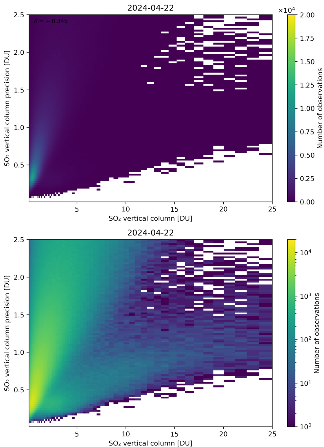
Figure 307: Scatter density plot of “SO 2 vertical column” against “SO 2 vertical column precision” for 2024-04-21 to 2024-04-23.
