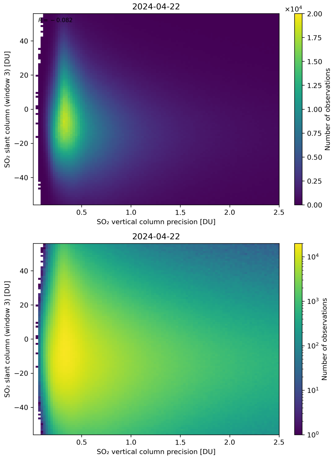
Figure 292: Scatter density plot of “SO 2 vertical column precision” against “SO 2 slant column (window 3)” for 2024-04-21 to 2024-04-23.
