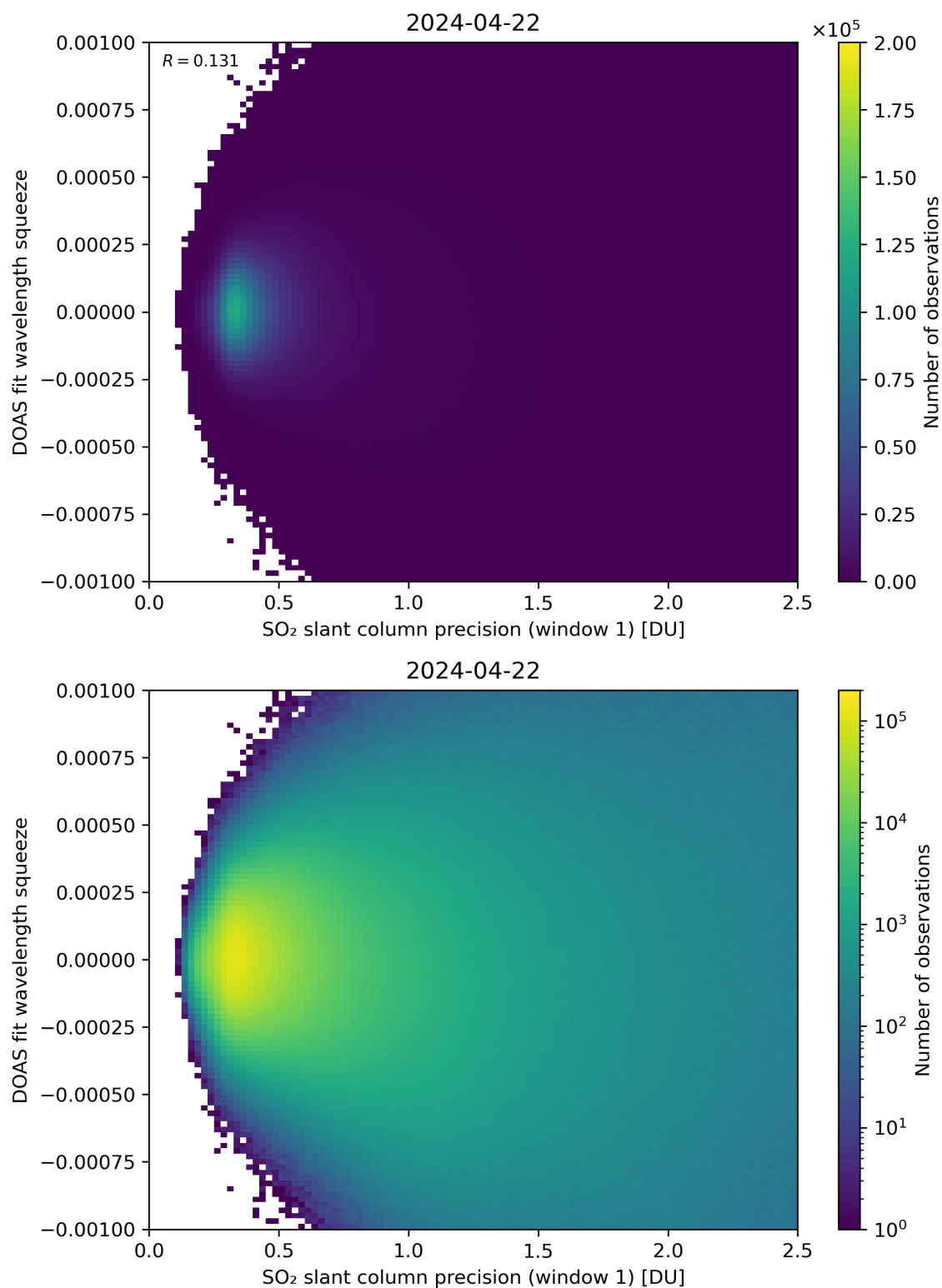
Figure 222: Scatter density plot of “SO 2 slant column precision (window 1)” against “DOAS fit wavelength squeeze” for 2024-04-21 to 2024-04-23.
