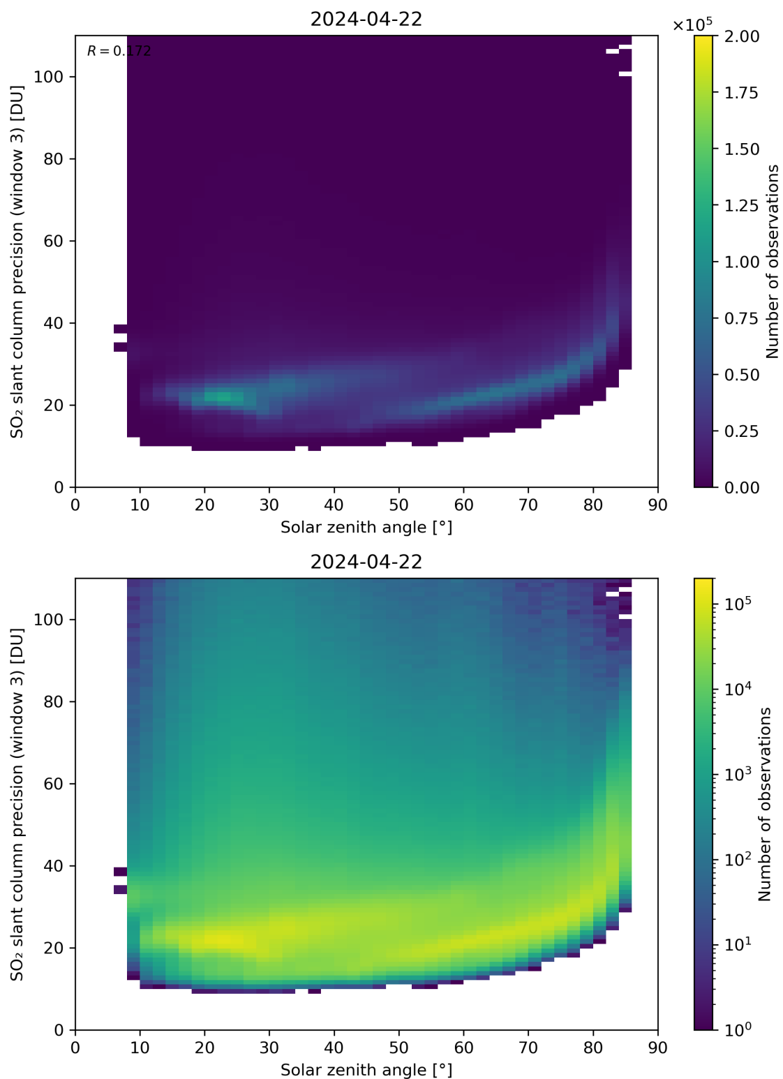
Figure 173: Scatter density plot of “Solar zenith angle” against “SO 2 slant column precision (window 3)” for 2024-04-21 to 2024-04-23.
