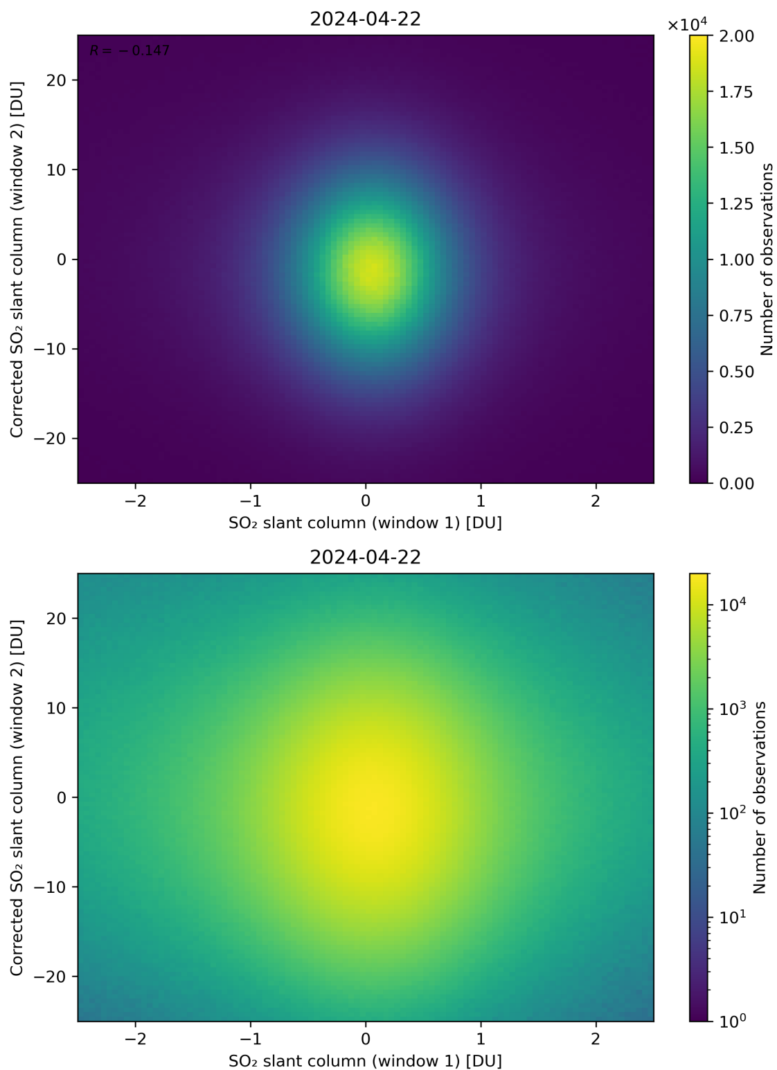
Figure 233: Scatter density plot of “SO 2 slant column (window 1)” against “Corrected SO 2 slant column (window 2)” for 2024-04-21 to 2024-04-23.
