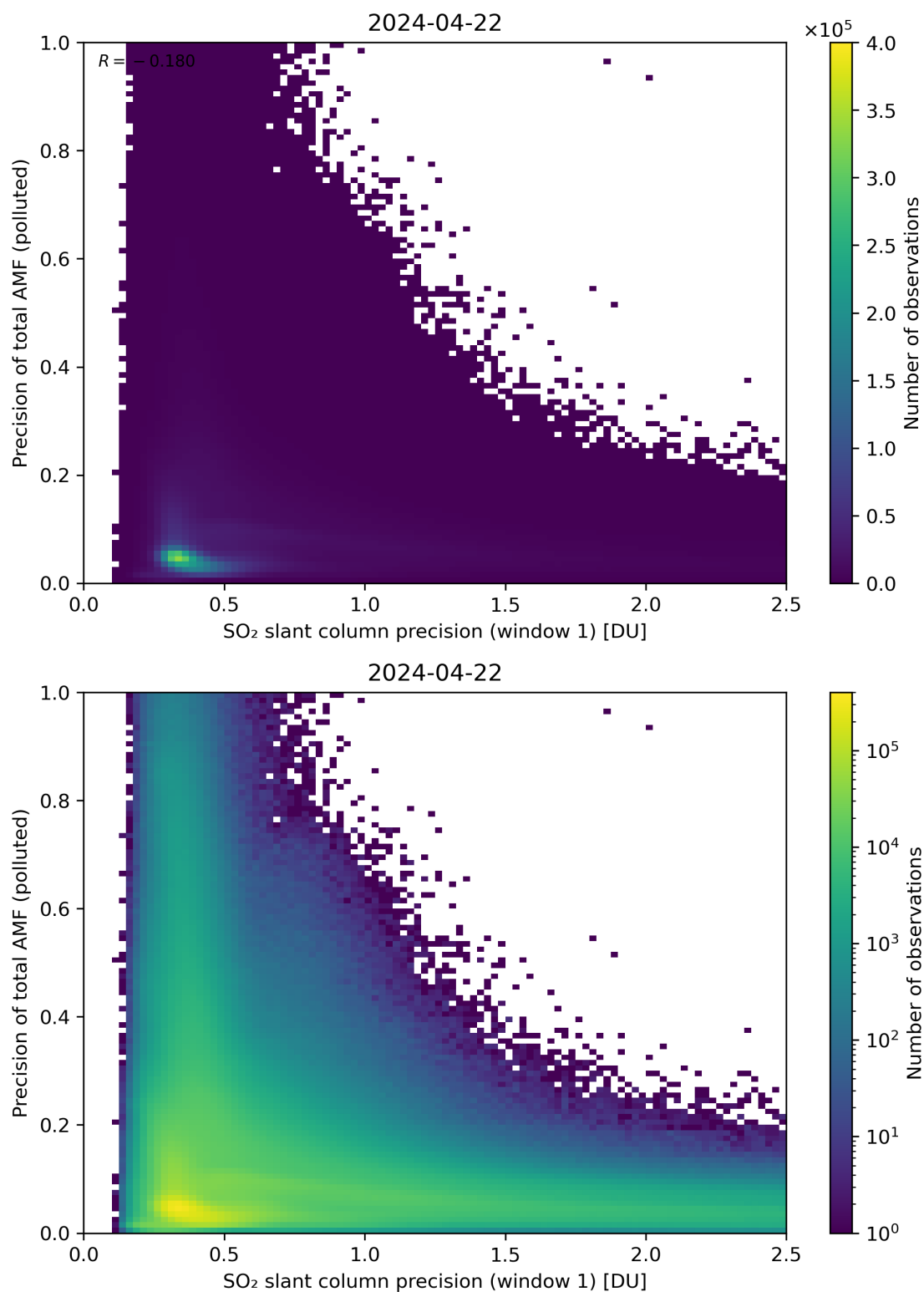
Figure 231: Scatter density plot of “SO 2 slant column precision (window 1)” against “Precision of total AMF (polluted)” for 2024-04-21 to 2024-04-23.
