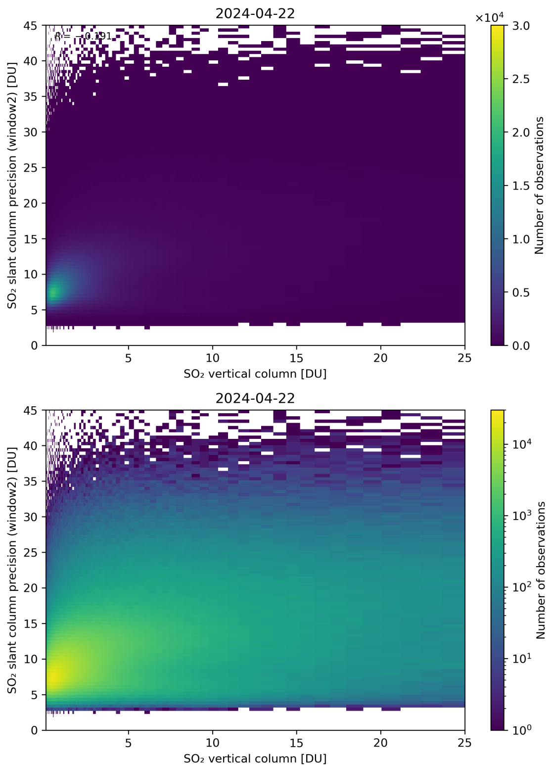
Figure 302: Scatter density plot of “SO 2 vertical column” against “SO 2 slant column precision (window2)” for 2024-04-21 to 2024-04-23.
