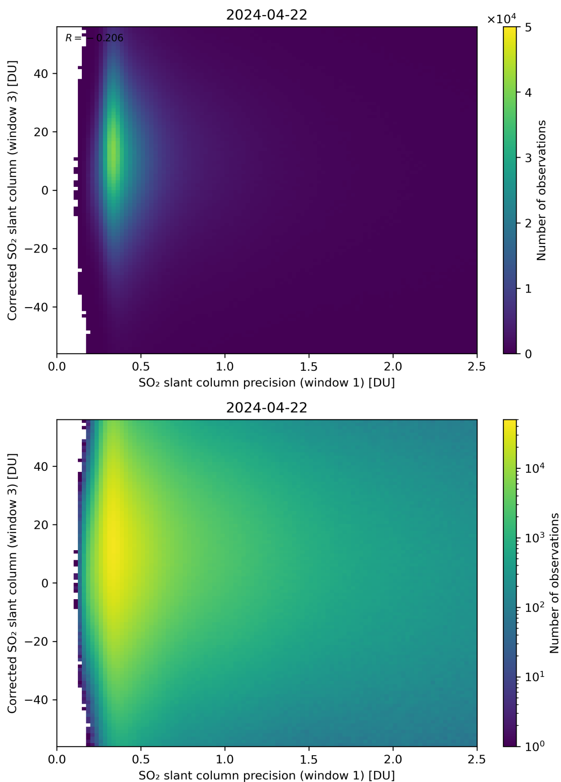
Figure 226: Scatter density plot of “SO 2 slant column precision (window 1)” against “Corrected SO 2 slant column (window 3)” for 2024-04-21 to 2024-04-23.
