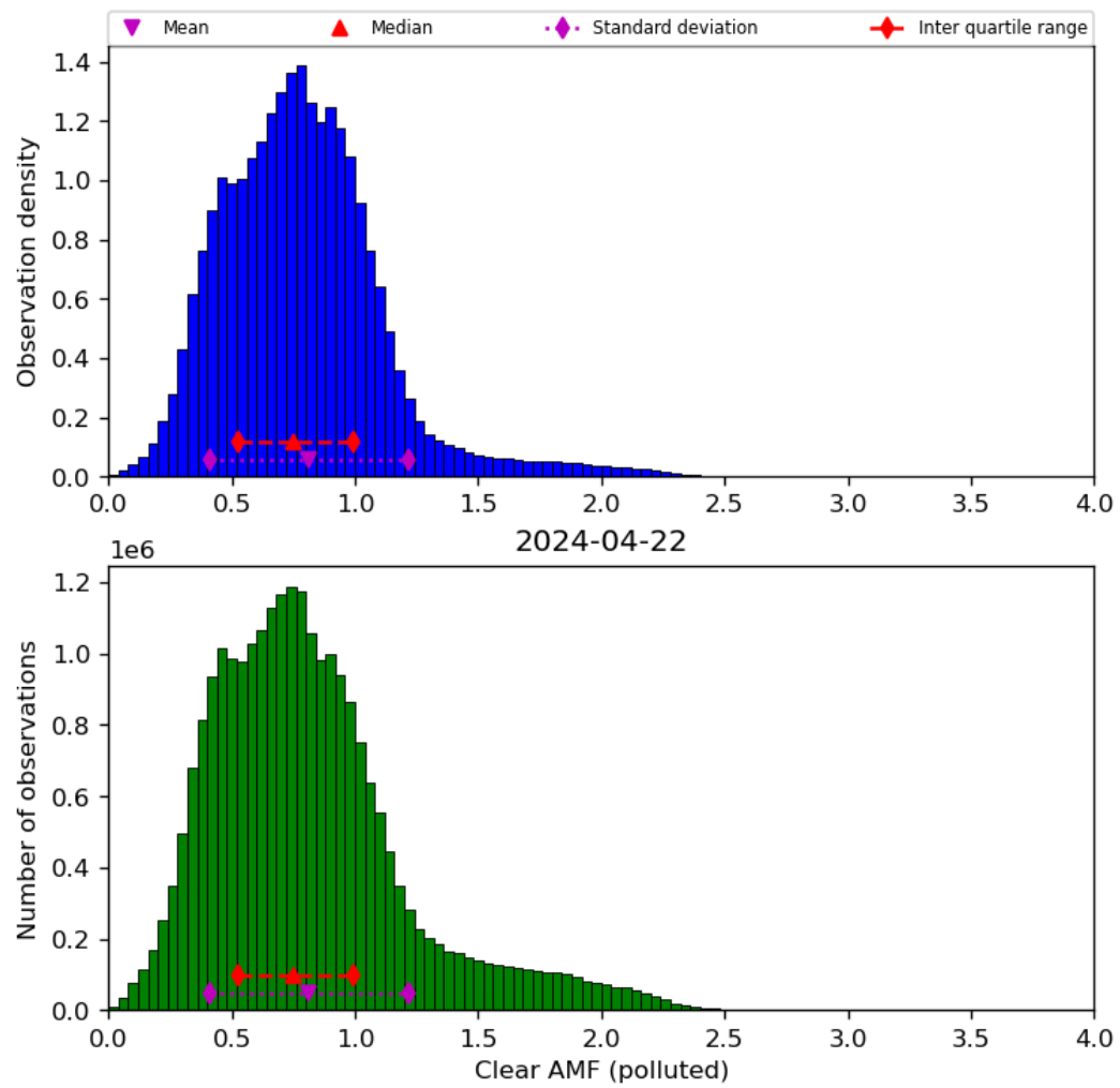
Figure 73: Histogram of “Clear AMF (polluted)” for 2024-04-21 to 2024-04-23
