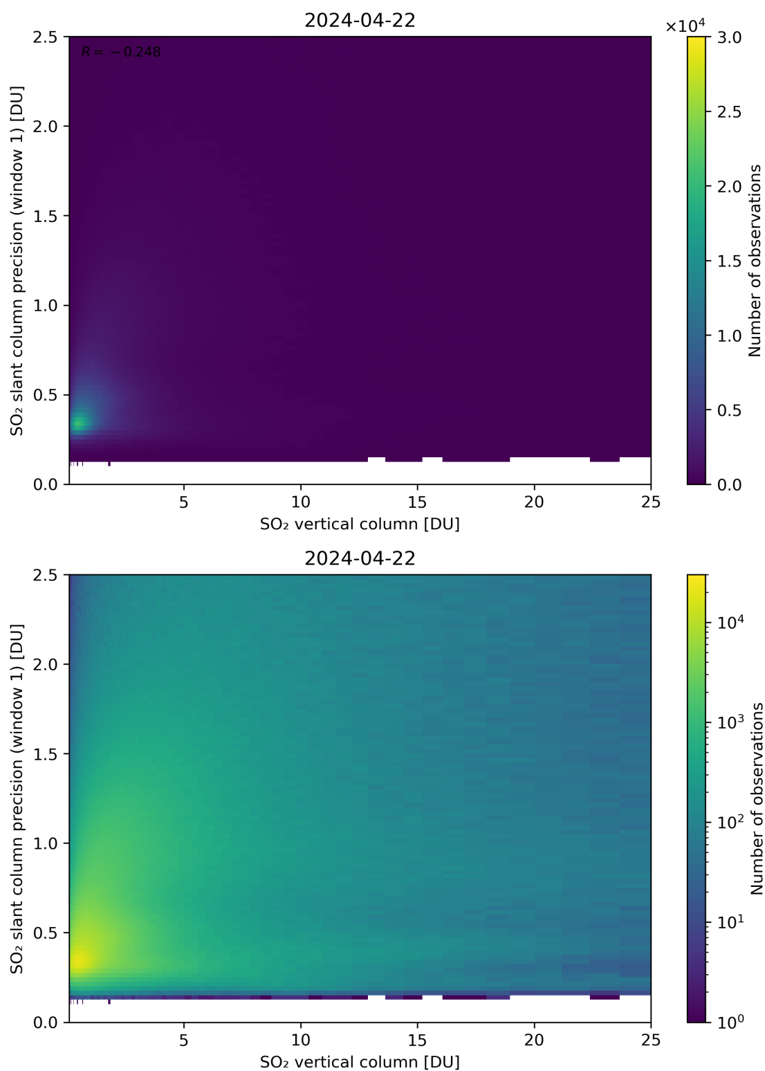
Figure 301: Scatter density plot of “SO 2 vertical column” against “SO 2 slant column precision (window 1)” for 2024-04-21 to 2024-04-23.
