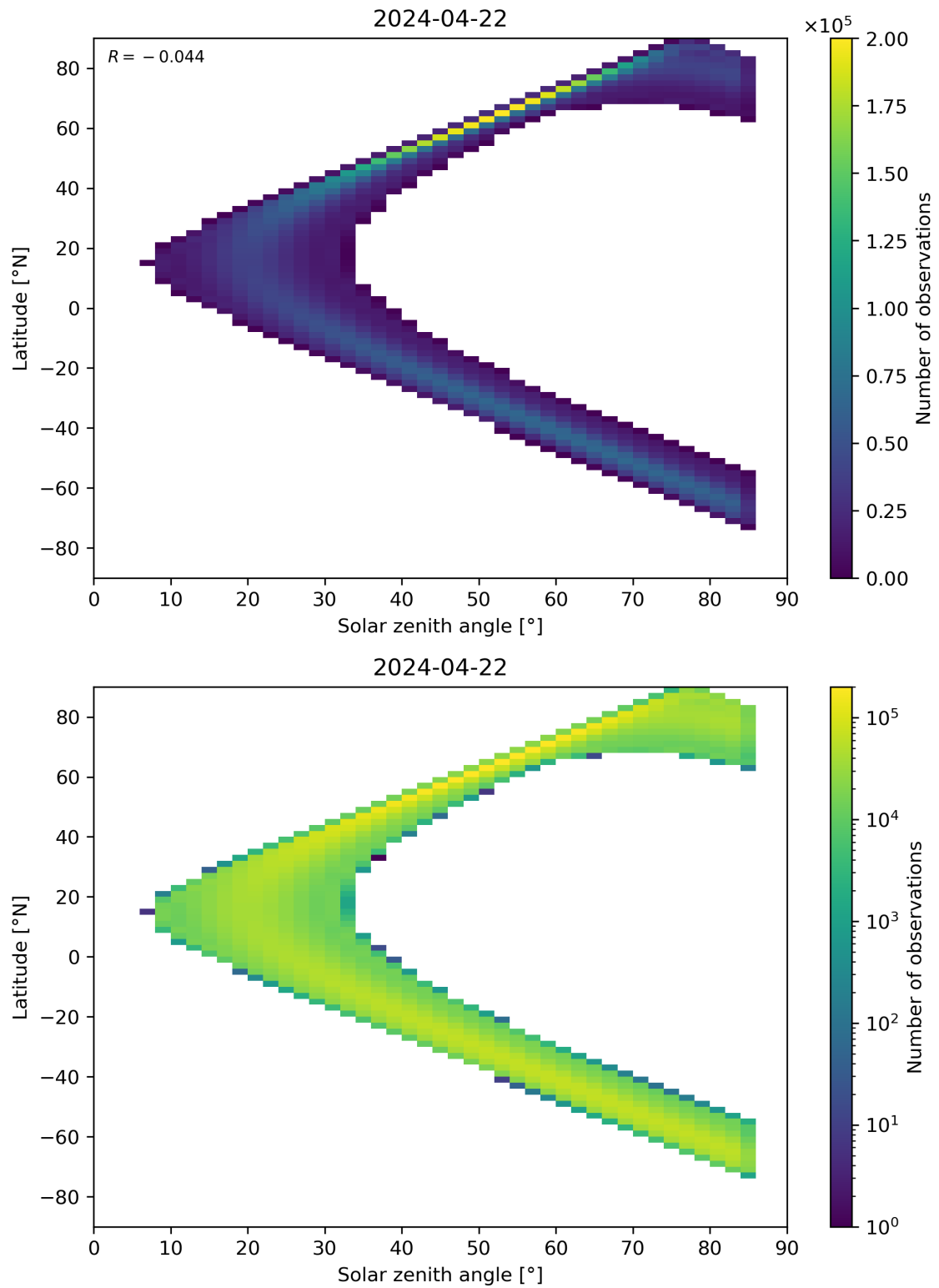
Figure 164: Scatter density plot of “Solar zenith angle” against “Latitude” for 2024-04-21 to 2024-04-23.
