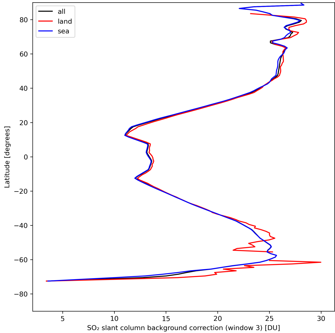
Figure 44: Zonal average of “SO 2 slant column background correction (window 3)” for 2024-04-21 to 2024-04-23.
