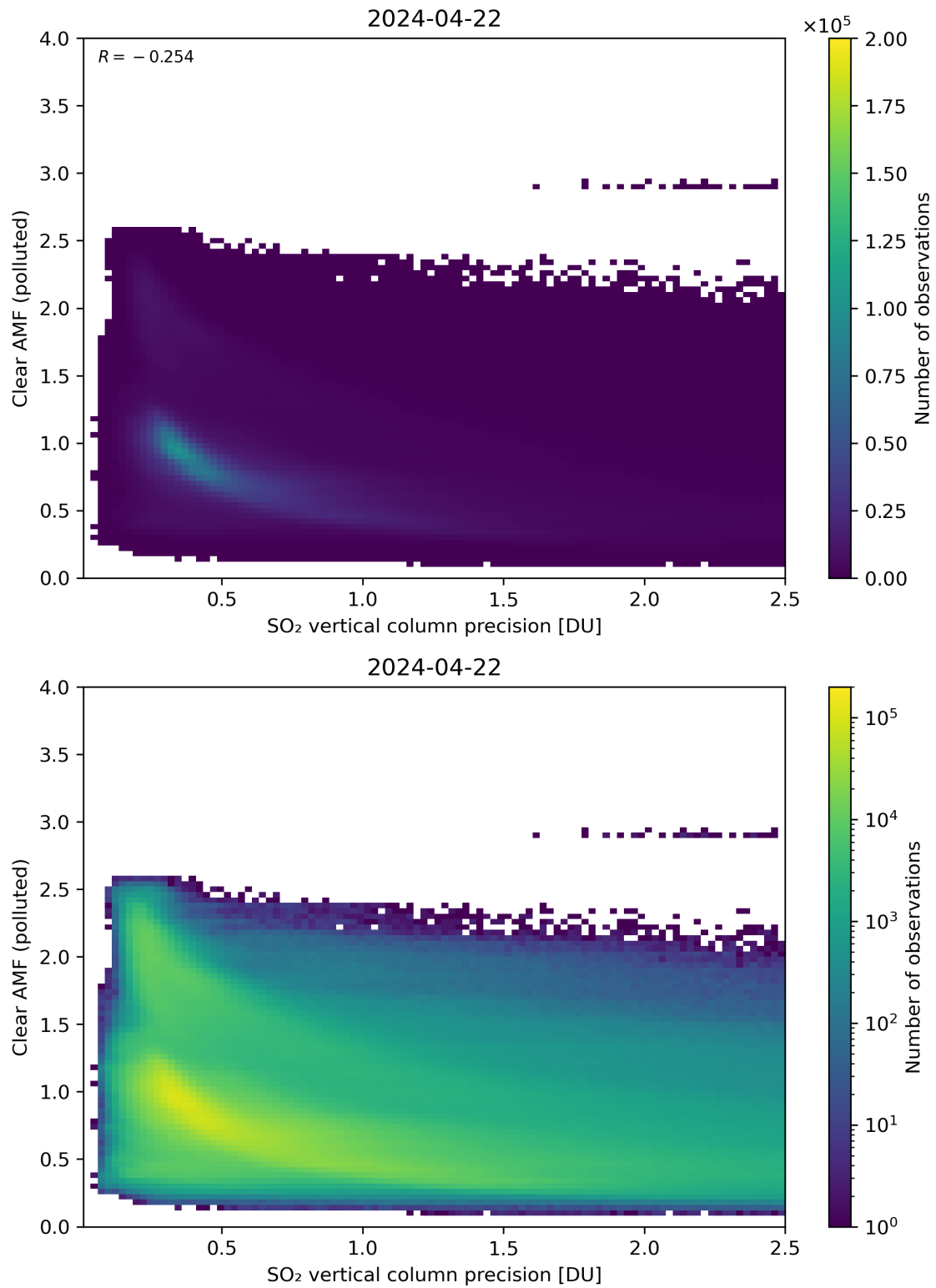
Figure 285: Scatter density plot of “SO 2 vertical column precision” against “Clear AMF (polluted)” for 2024-04-21 to 2024-04-23.
