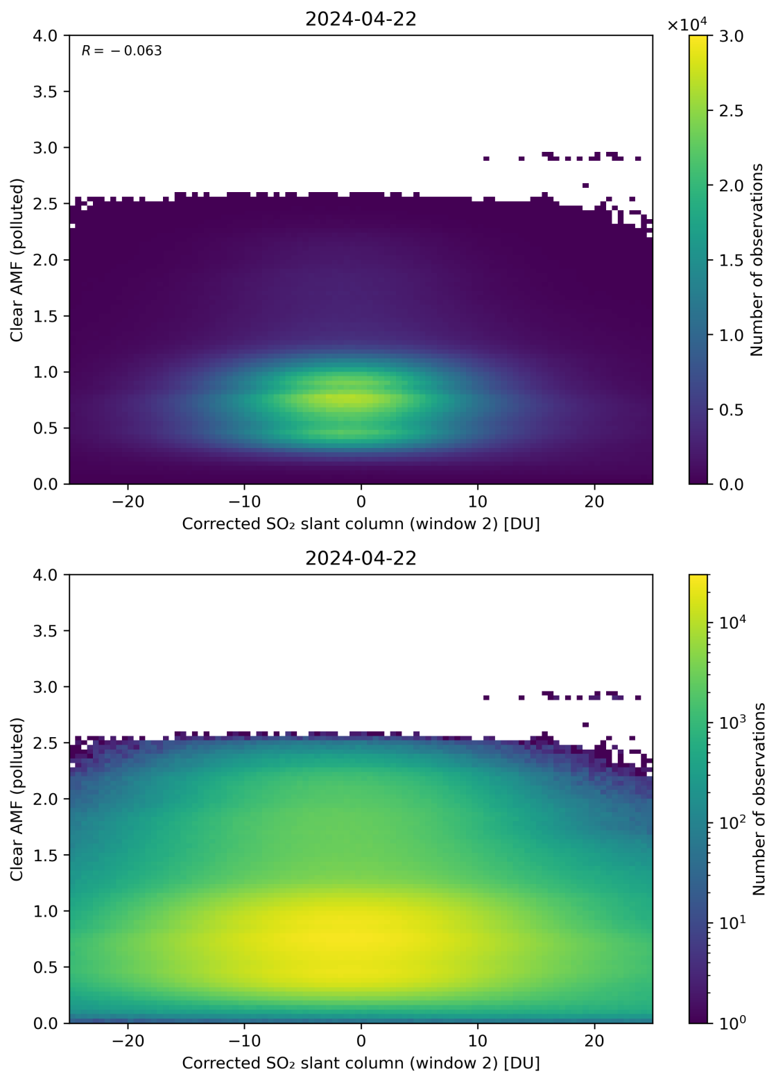
Figure 199: Scatter density plot of “Corrected SO 2 slant column (window 2)” against “Clear AMF (polluted)” for 2024-04-21 to 2024-04-23.
