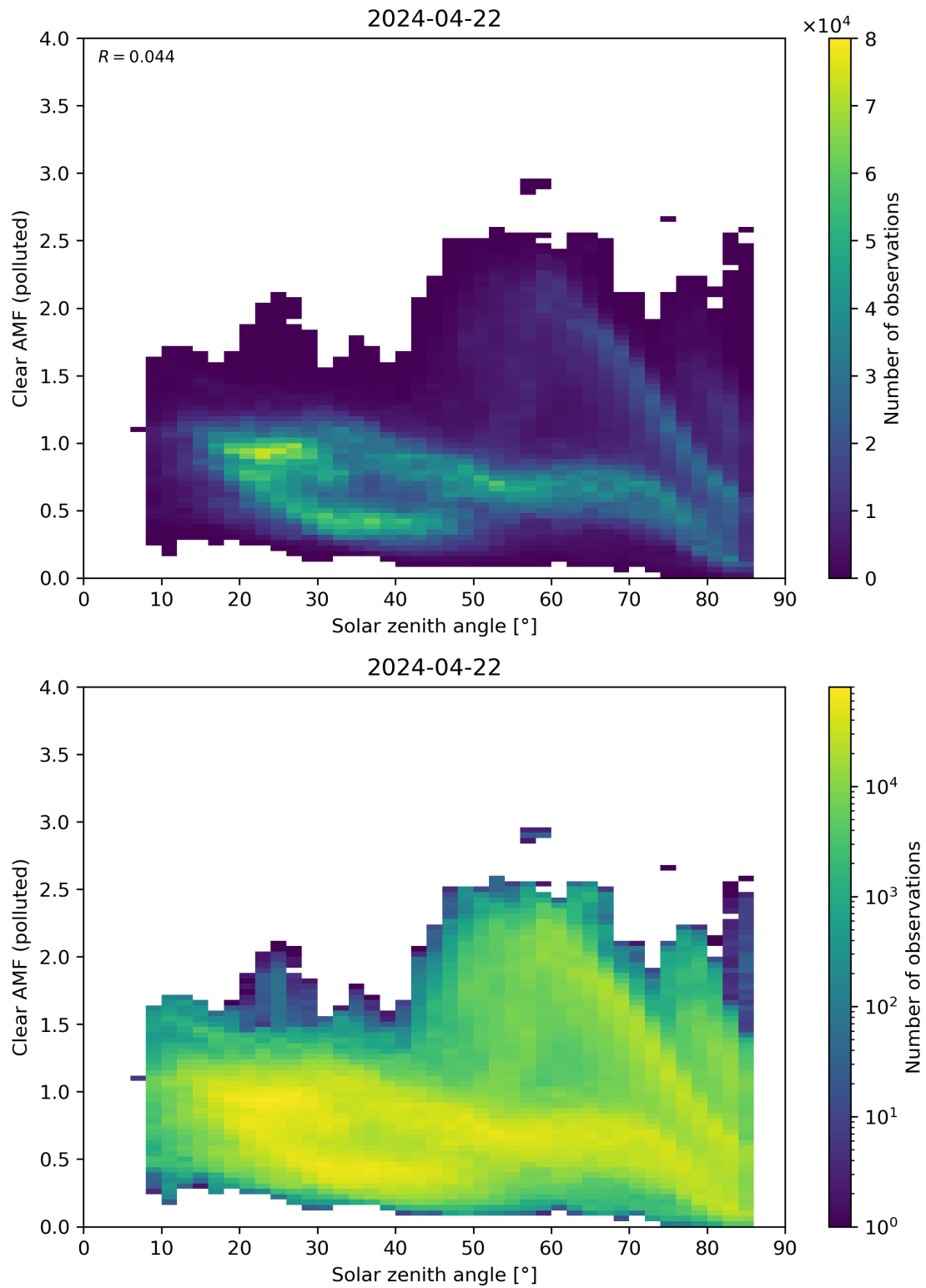
Figure 165: Scatter density plot of “Solar zenith angle” against “Clear AMF (polluted)” for 2024-04-21 to 2024-04-23.
