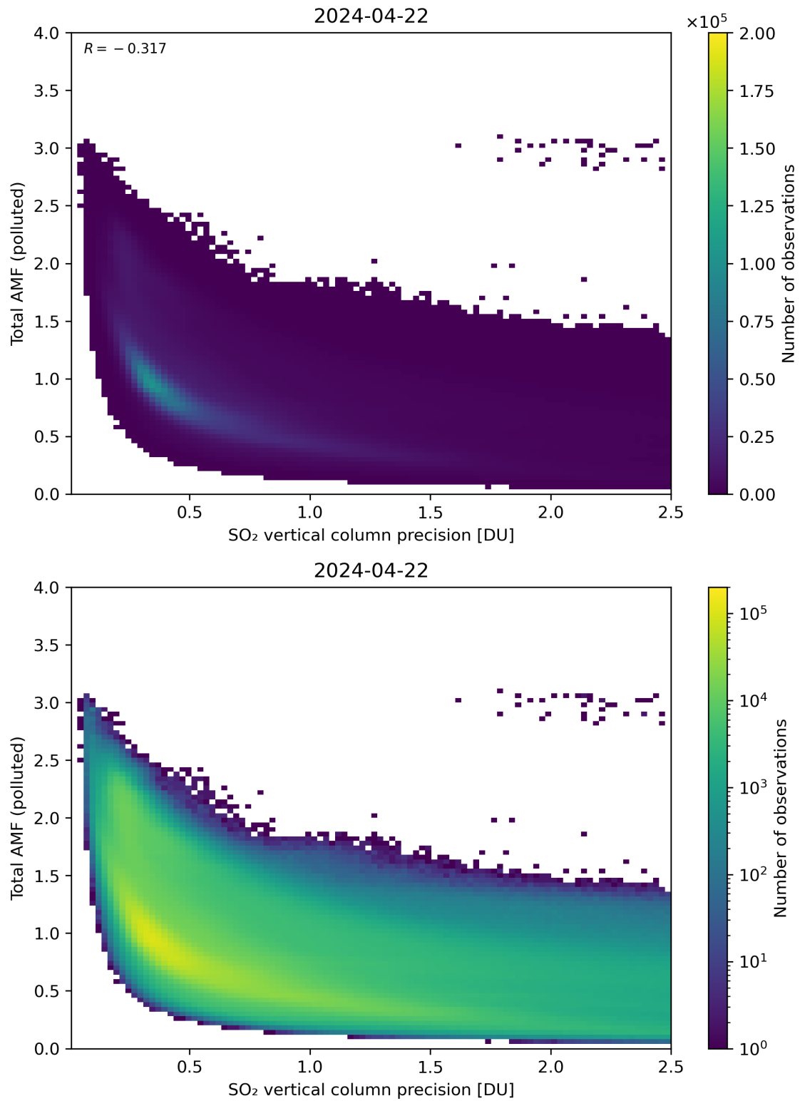
Figure 294: Scatter density plot of “SO 2 vertical column precision” against “Total AMF (polluted)” for 2024-04-21 to 2024-04-23.
