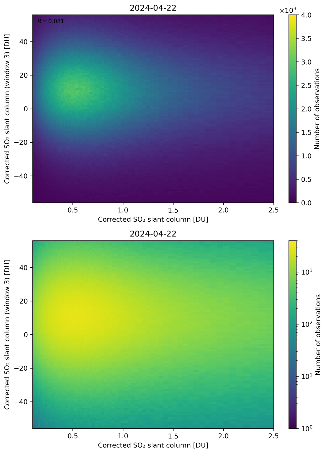
Figure 186: Scatter density plot of “Corrected SO 2 slant column” against “Corrected SO 2 slant column (window 3)” for 2024-04-21 to 2024-04-23.
