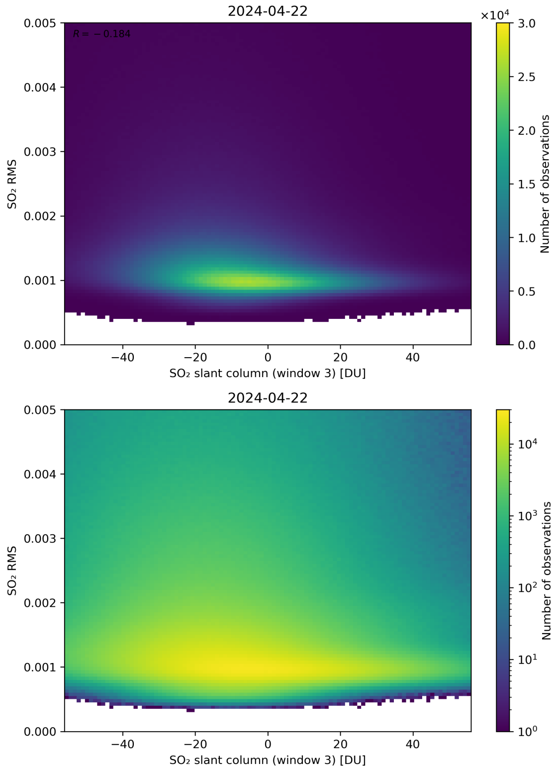
Figure 256: Scatter density plot of “SO 2 slant column (window 3)” against “SO 2 RMS” for 2024-04-21 to 2024-04-23.
