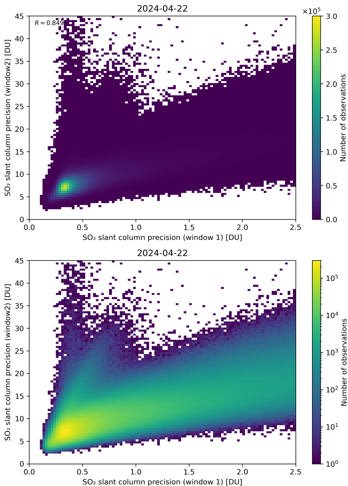
Figure 227: Scatter density plot of “SO 2 slant column precision (window 1)” against “SO 2 slant column precision (window2)” for 2024-04-21 to 2024-04-23.
