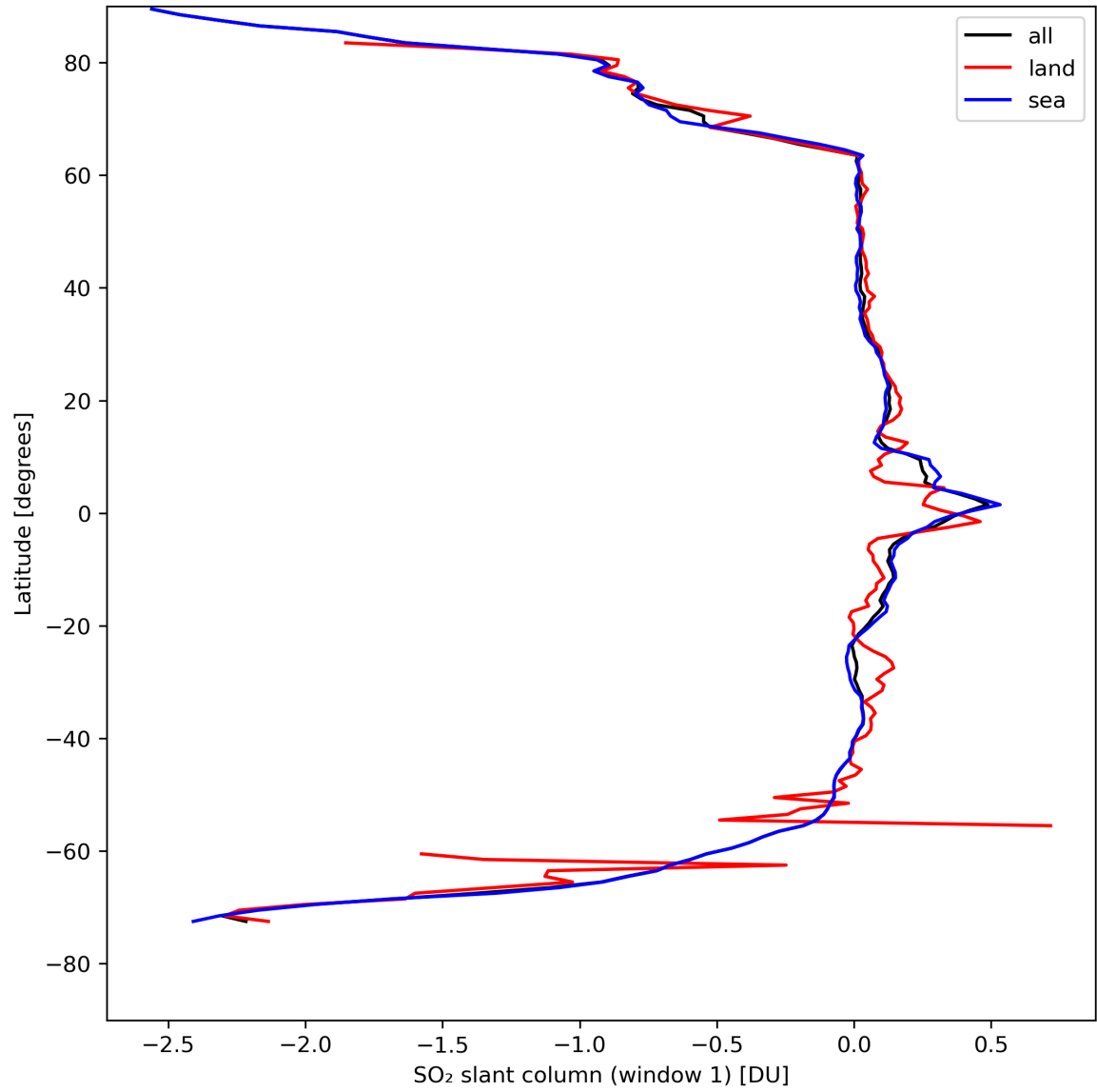
Figure 33: Zonal average of “SO 2 slant column (window 1)” for 2024-04-21 to 2024-04-23.
