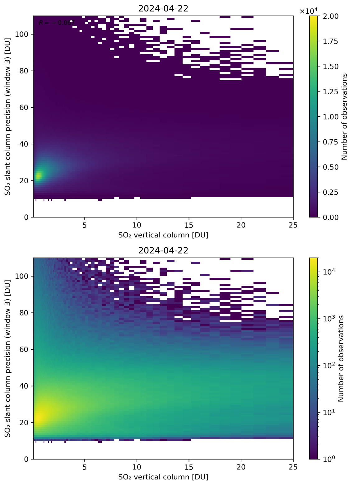
Figure 304: Scatter density plot of “SO 2 vertical column” against “SO 2 slant column precision (window 3)” for 2024-04-21 to 2024-04-23.
