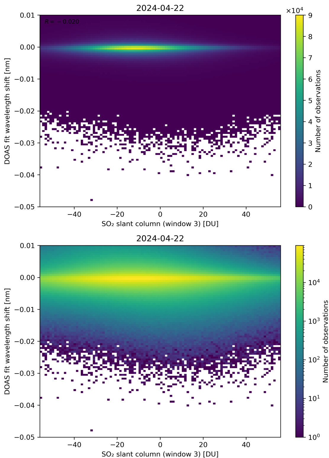
Figure 254: Scatter density plot of “SO 2 slant column (window 3)” against “DOAS fit wavelength shift” for 2024-04-21 to 2024-04-23.
