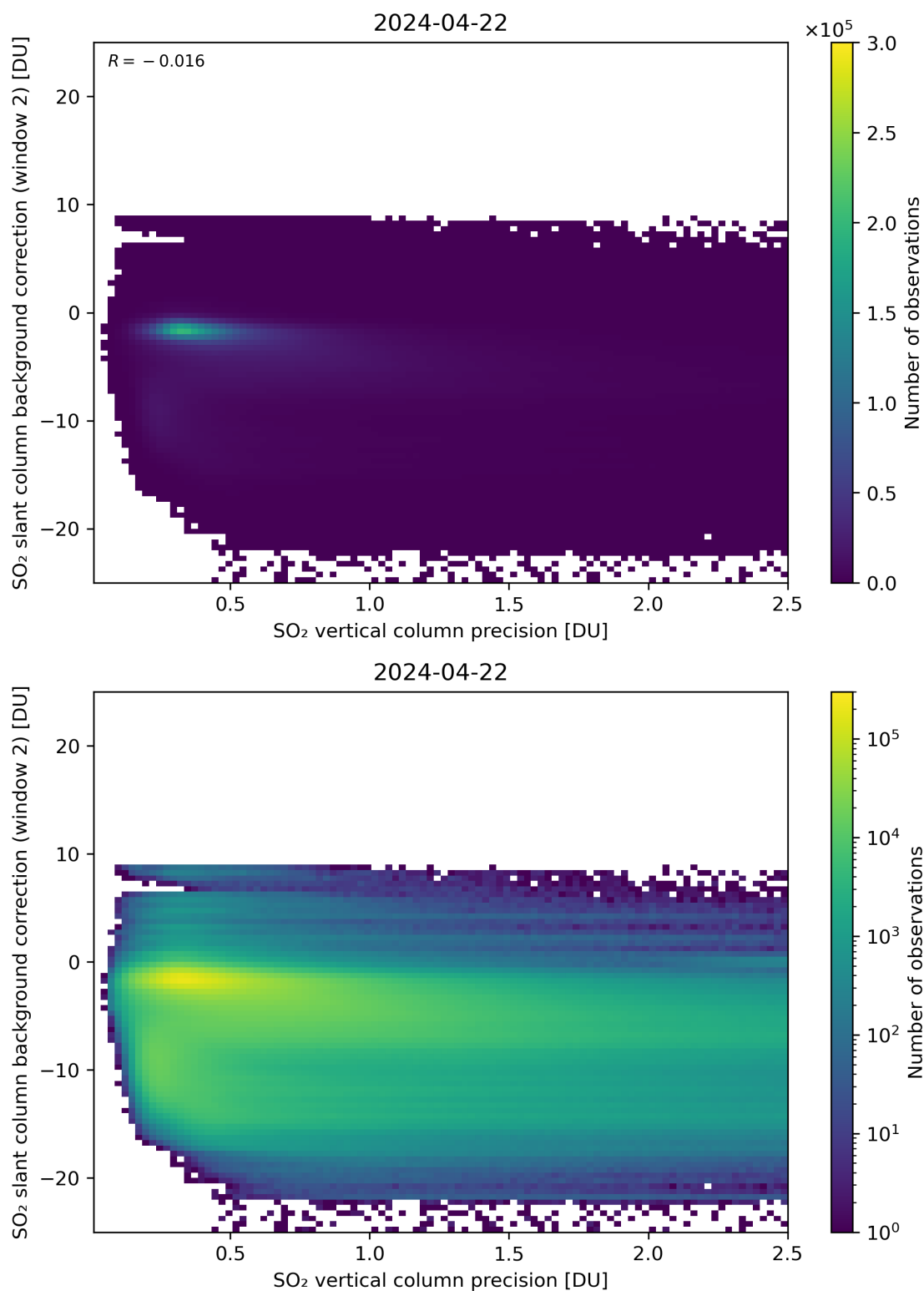
Figure 280: Scatter density plot of “SO 2 vertical column precision” against “SO 2 slant column background correction (window 2)” for 2024-04-21 to 2024-04-23.
