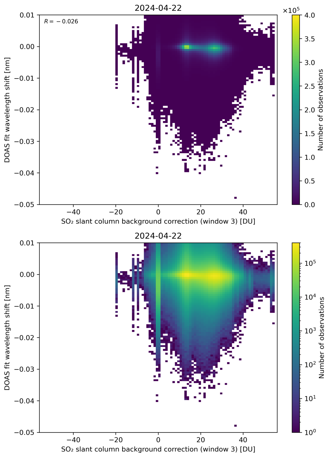
Figure 121: Scatter density plot of “SO 2 slant column background correction (window 3)” against “DOAS fit wavelength shift” for 2024-04-21 to 2024-04-23.
