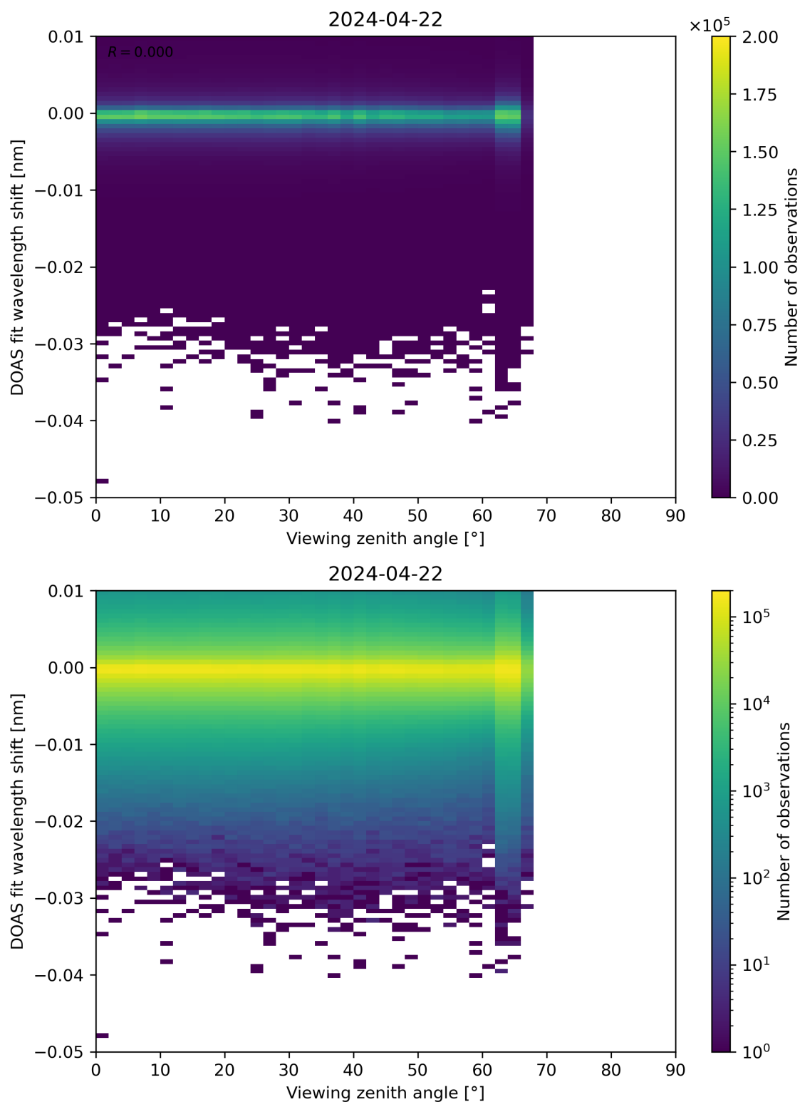
Figure 311: Scatter density plot of “Viewing zenith angle” against “DOAS fit wavelength shift” for 2024-04-21 to 2024-04-23.
