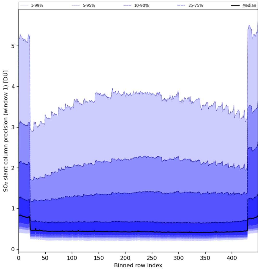
Figure 80: Along track statistics of “SO 2 slant column precision (window 1)” for 2024-04-21 to 2024-04-23
