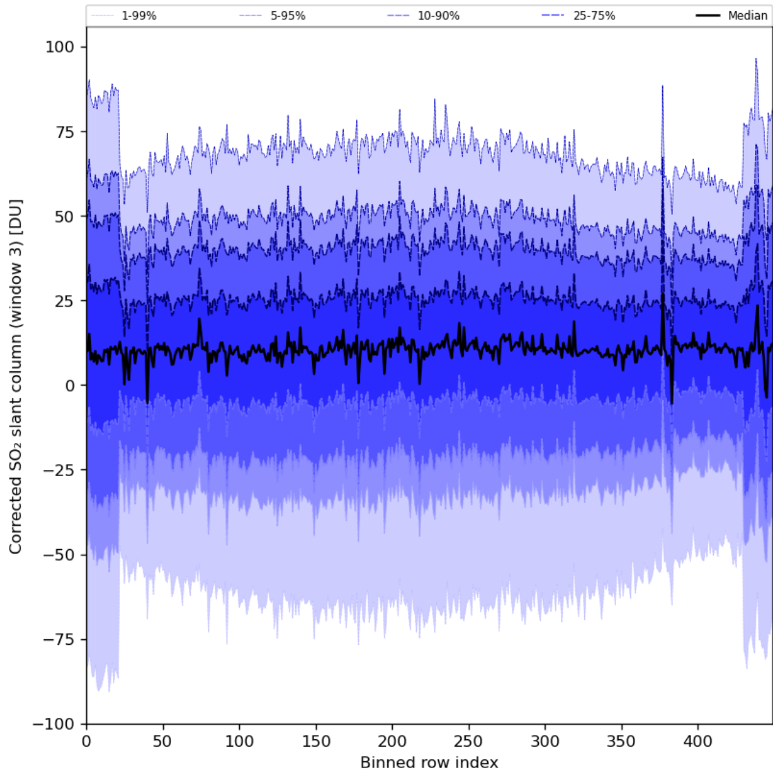
Figure 89: Along track statistics of “Corrected SO 2 slant column (window 3)” for 2024-04-21 to 2024-04-23
