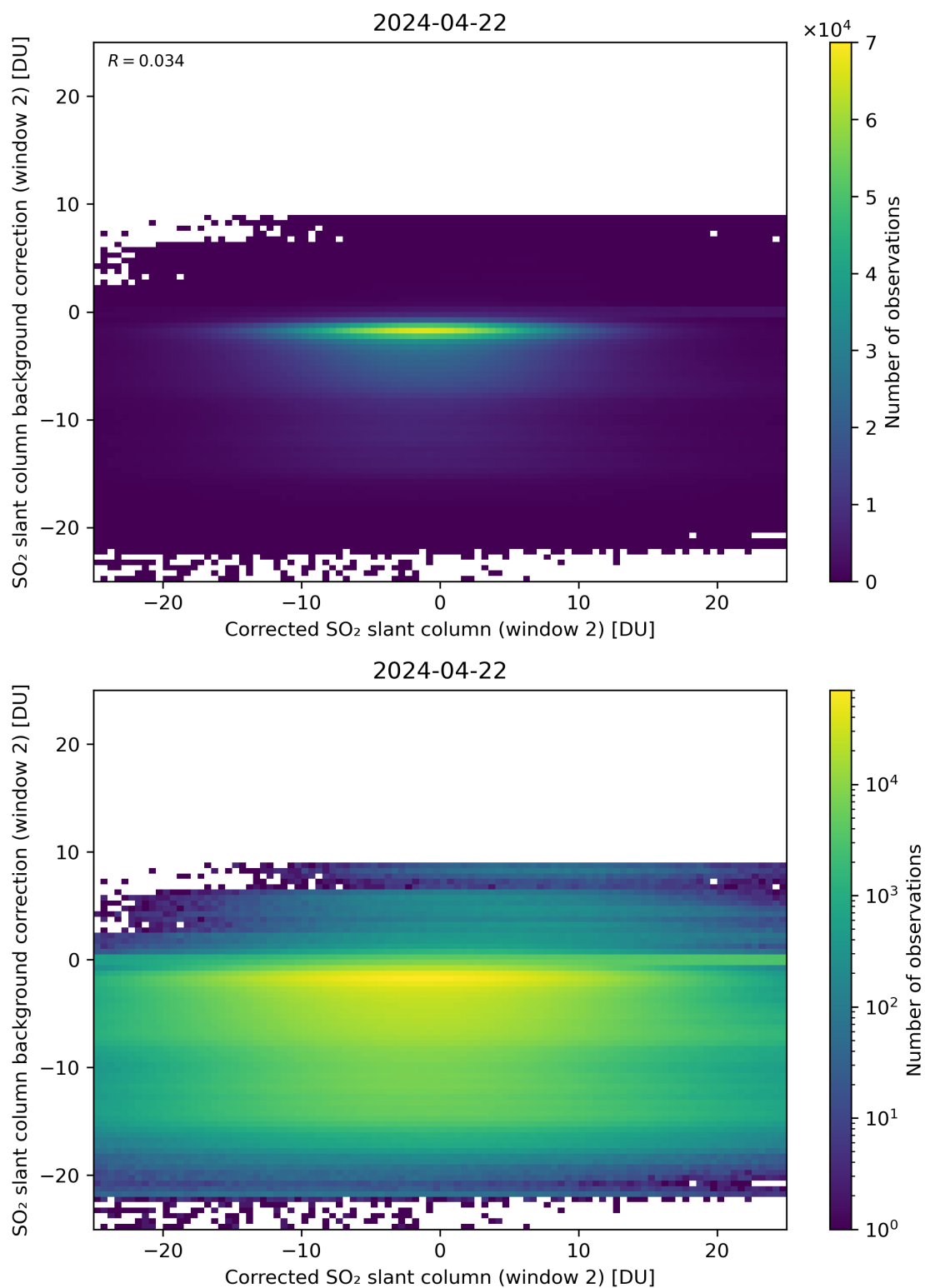
Figure 194: Scatter density plot of “Corrected SO 2 slant column (window 2)” against “SO 2 slant column background correction (window 2)” for 2024-04-21 to 2024-04-23.
