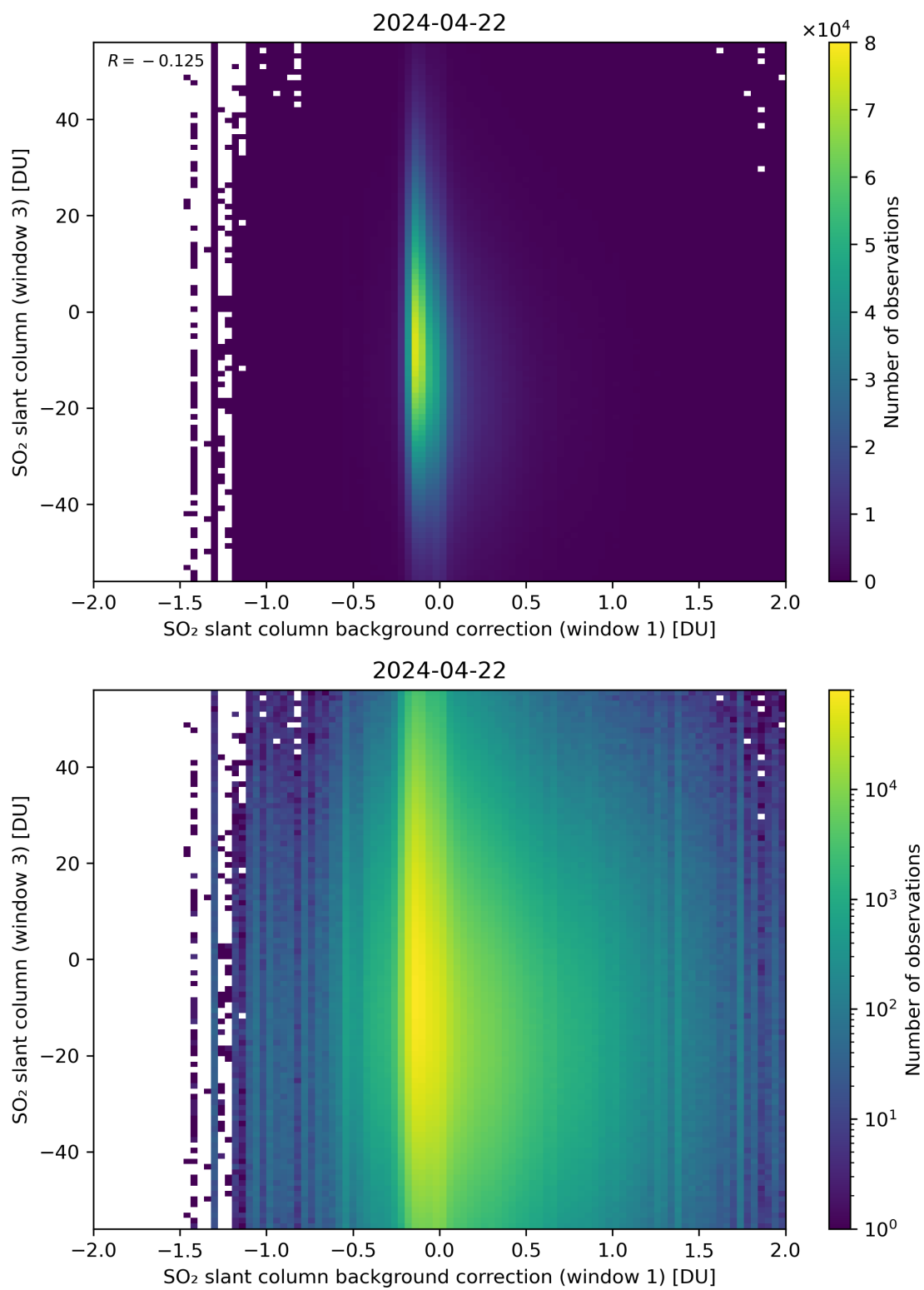
Figure 107: Scatter density plot of “SO 2 slant column background correction (window 1)” against “SO 2 slant column (window 3)” for 2024-04-21 to 2024-04-23.
