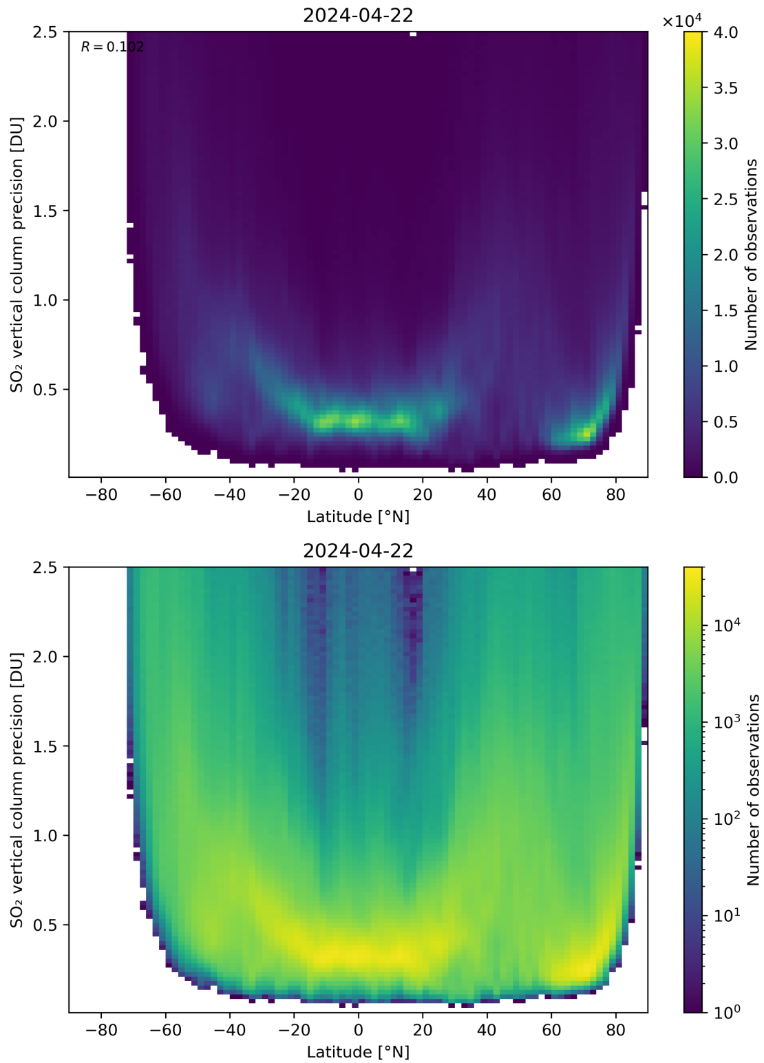
Figure 157: Scatter density plot of “Latitude” against “SO 2 vertical column precision” for 2024-04-21 to 2024-04-23.
