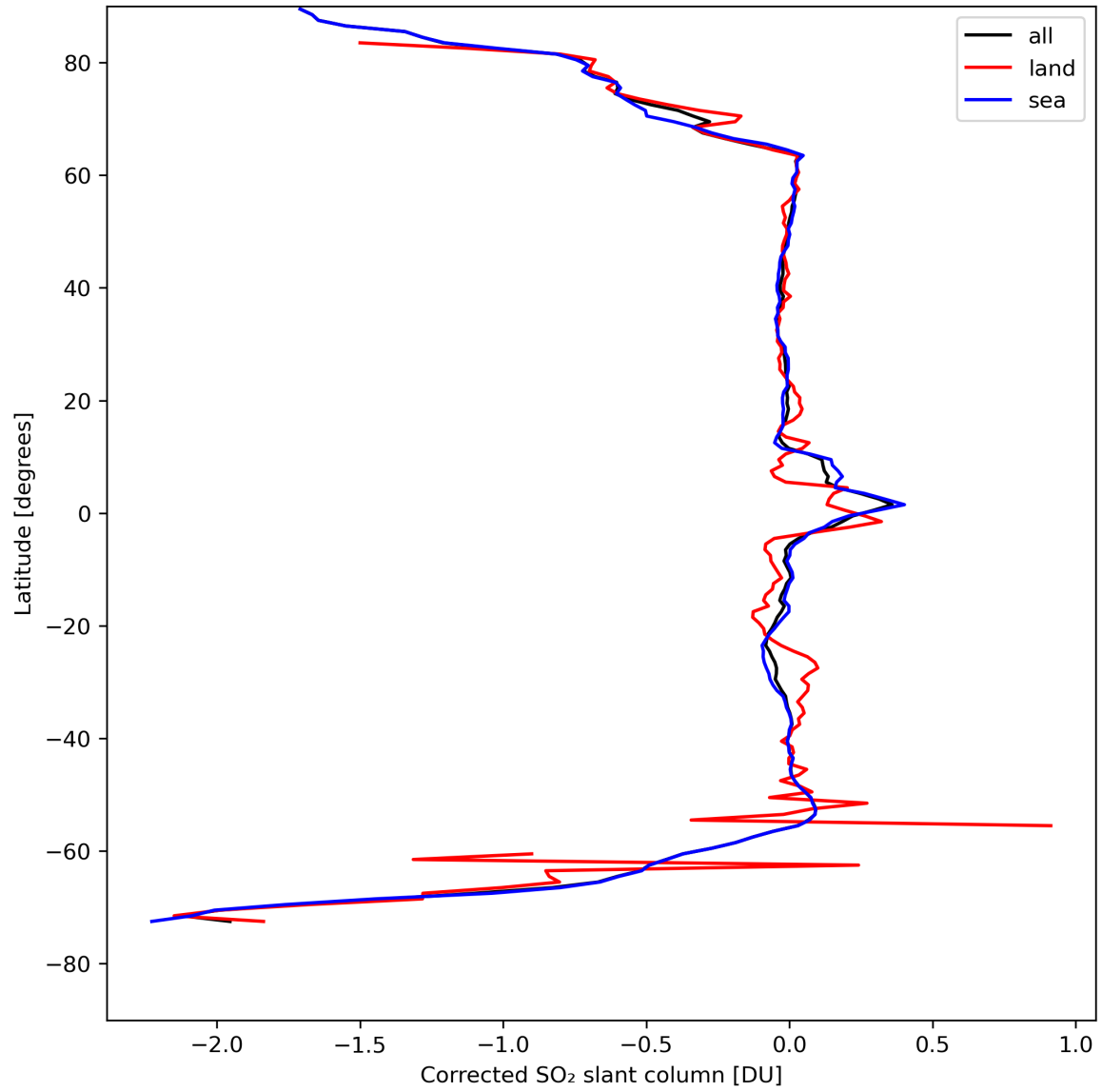
Figure 32: Zonal average of “Corrected SO 2 slant column” for 2024-04-21 to 2024-04-23.
