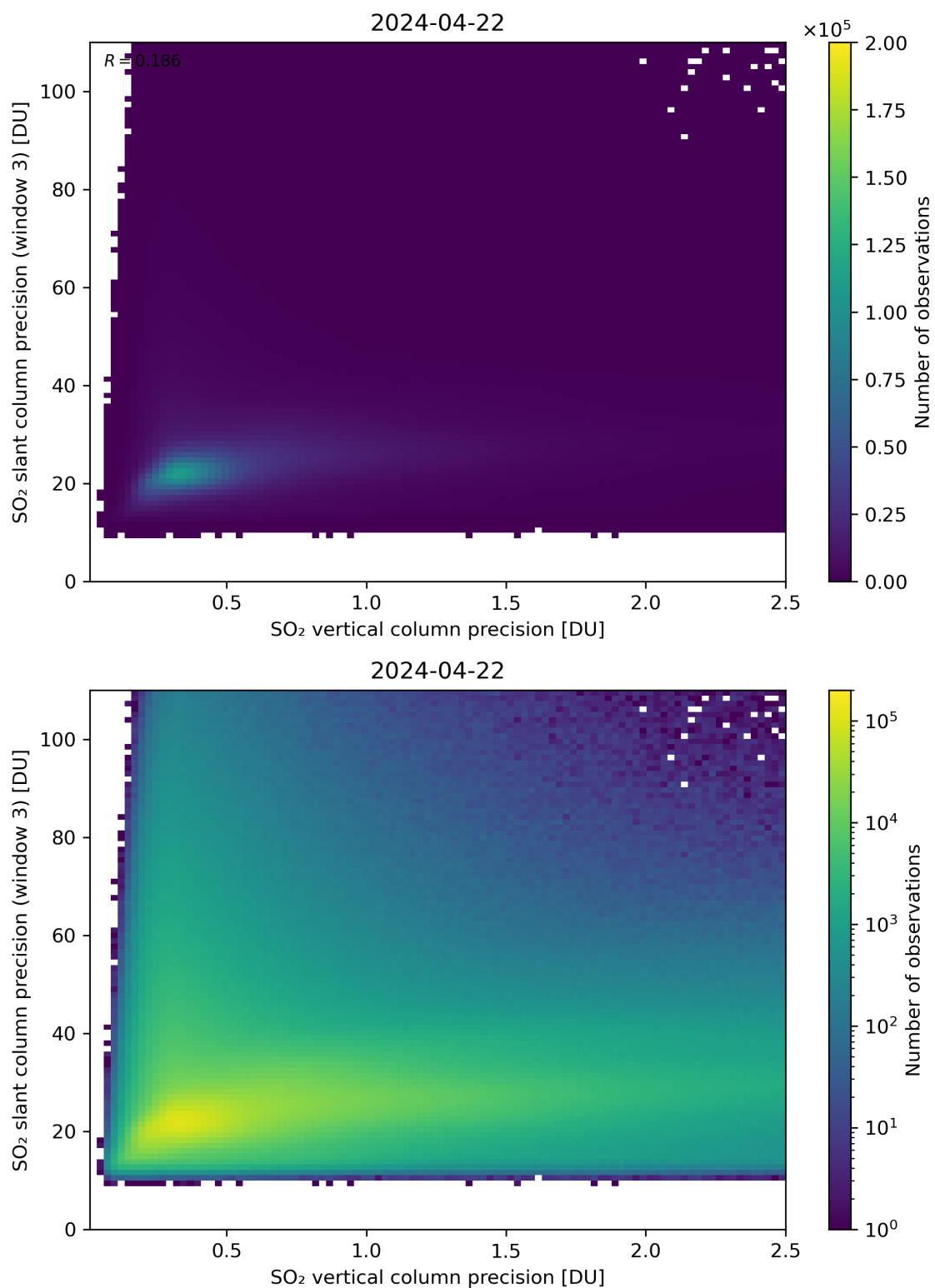
Figure 293: Scatter density plot of “SO 2 vertical column precision” against “SO 2 slant column precision (window 3)” for 2024-04-21 to 2024-04-23.
