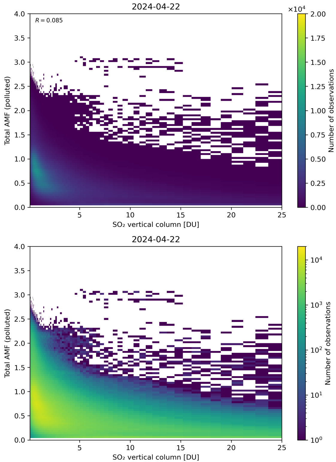
Figure 305: Scatter density plot of “SO 2 vertical column” against “Total AMF (polluted)” for 2024-04-21 to 2024-04-23.
