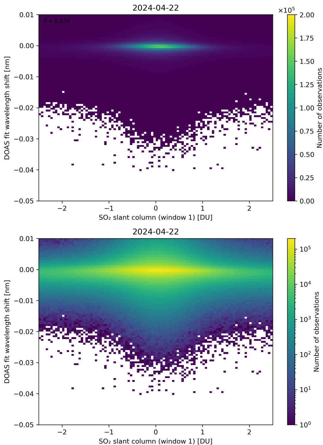
Figure 215: Scatter density plot of “SO 2 slant column (window 1)” against “DOAS fit wavelength shift” for 2024-04-21 to 2024-04-23.
