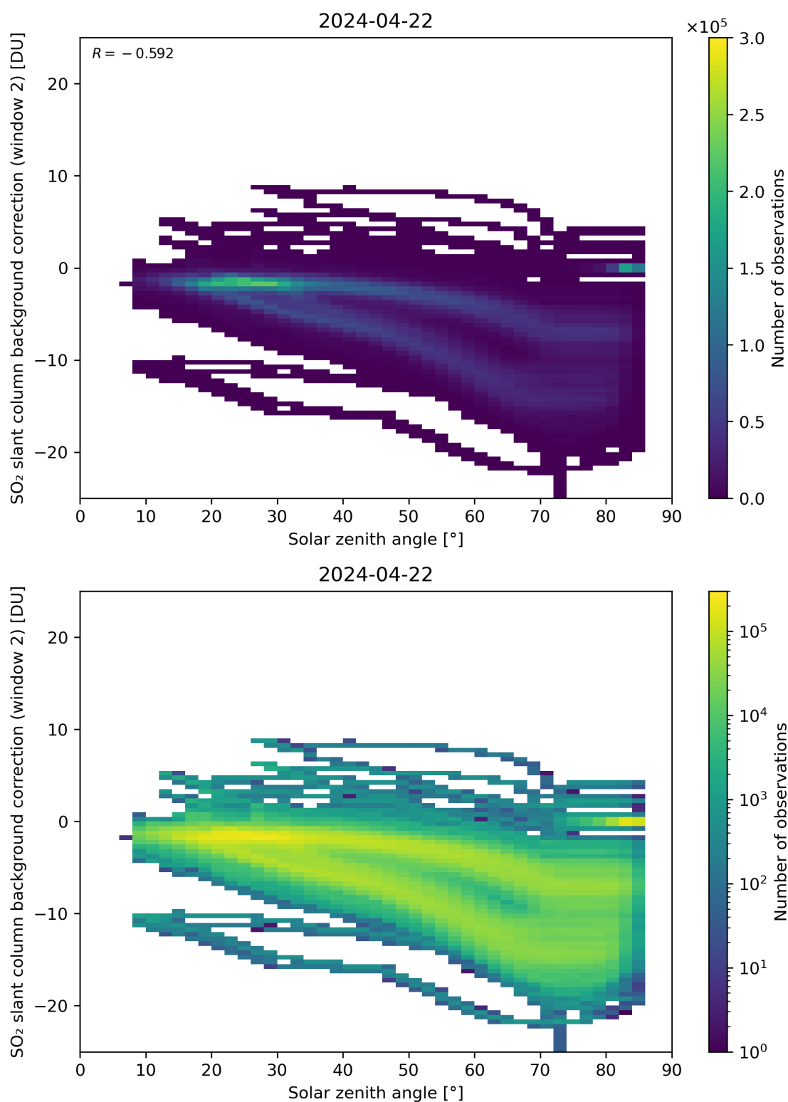
Figure 159: Scatter density plot of “Solar zenith angle” against “SO 2 slant column background correction (window 2)” for 2024-04-21 to 2024-04-23.
