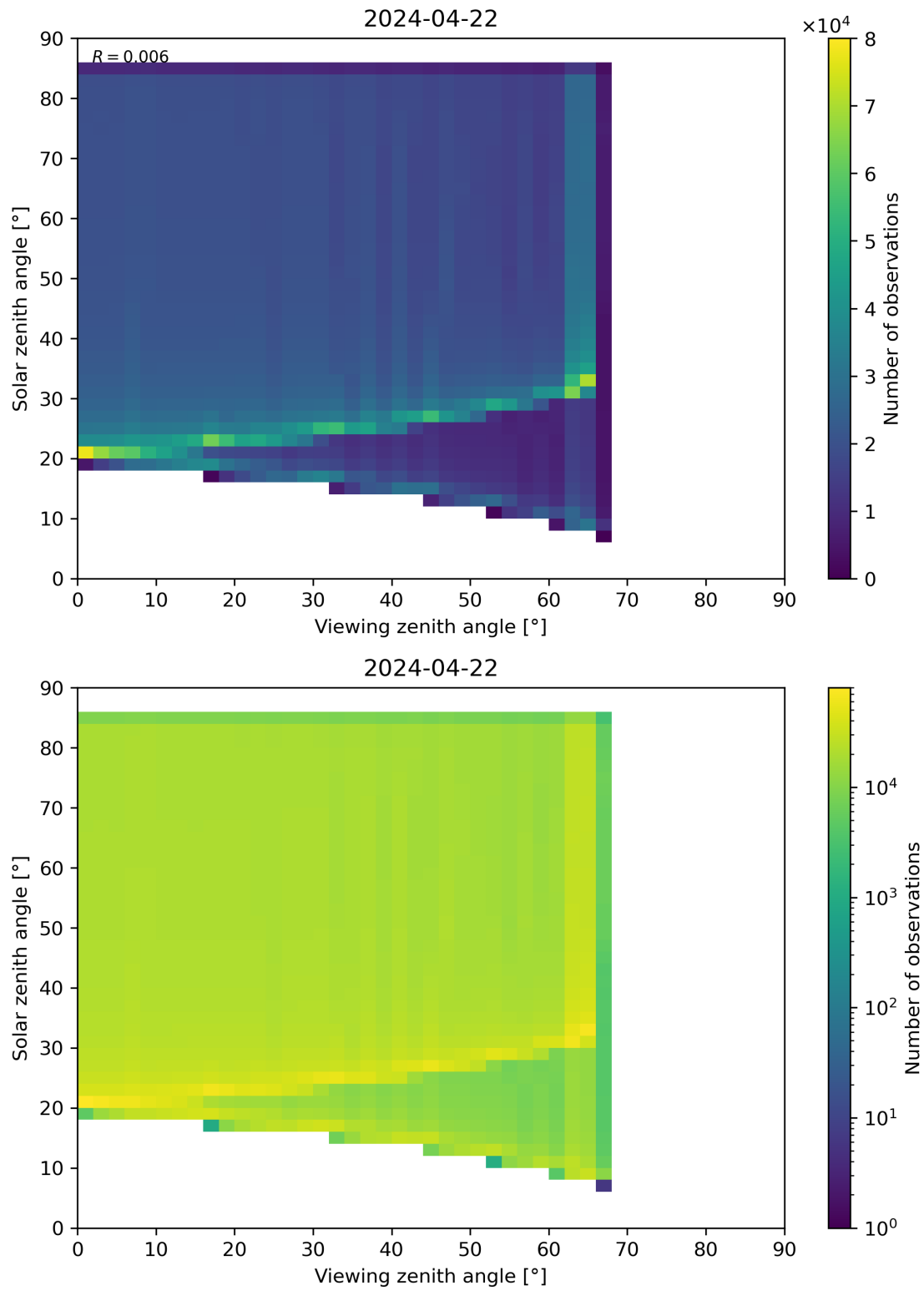
Figure 315: Scatter density plot of “Viewing zenith angle” against “Solar zenith angle” for 2024-04-21 to 2024-04-23.
