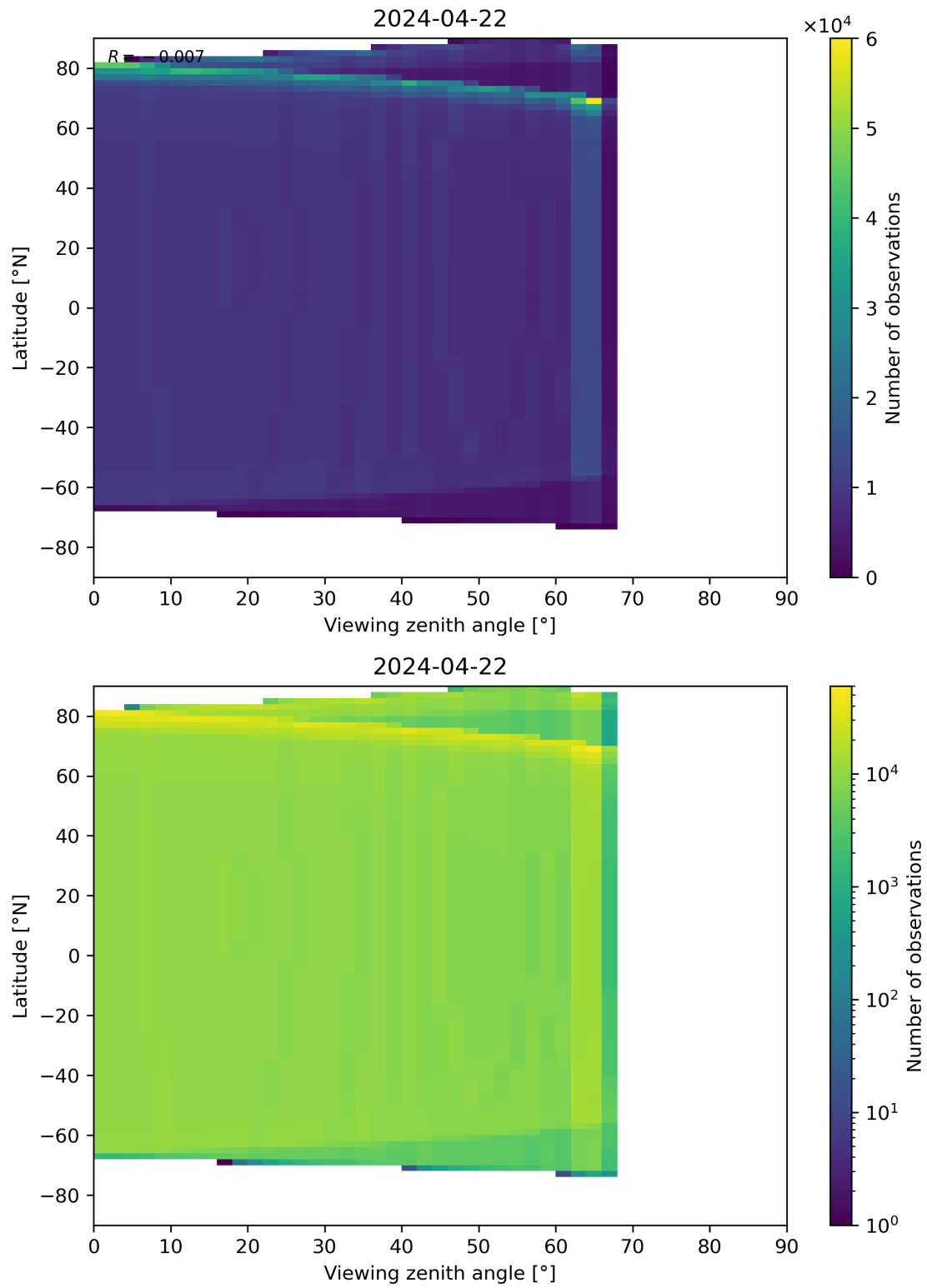
Figure 314: Scatter density plot of “Viewing zenith angle” against “Latitude” for 2024-04-21 to 2024-04-23.
