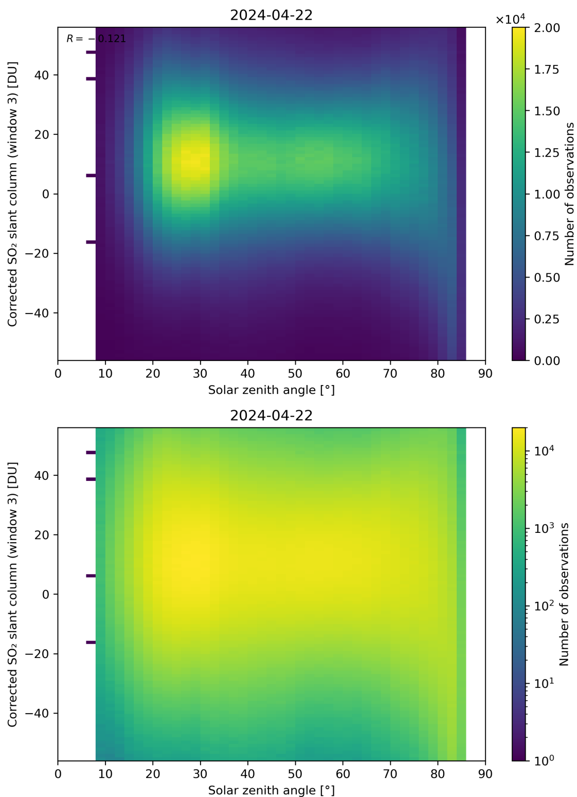
Figure 168: Scatter density plot of “Solar zenith angle” against “Corrected SO 2 slant column (window 3)” for 2024-04-21 to 2024-04-23.
