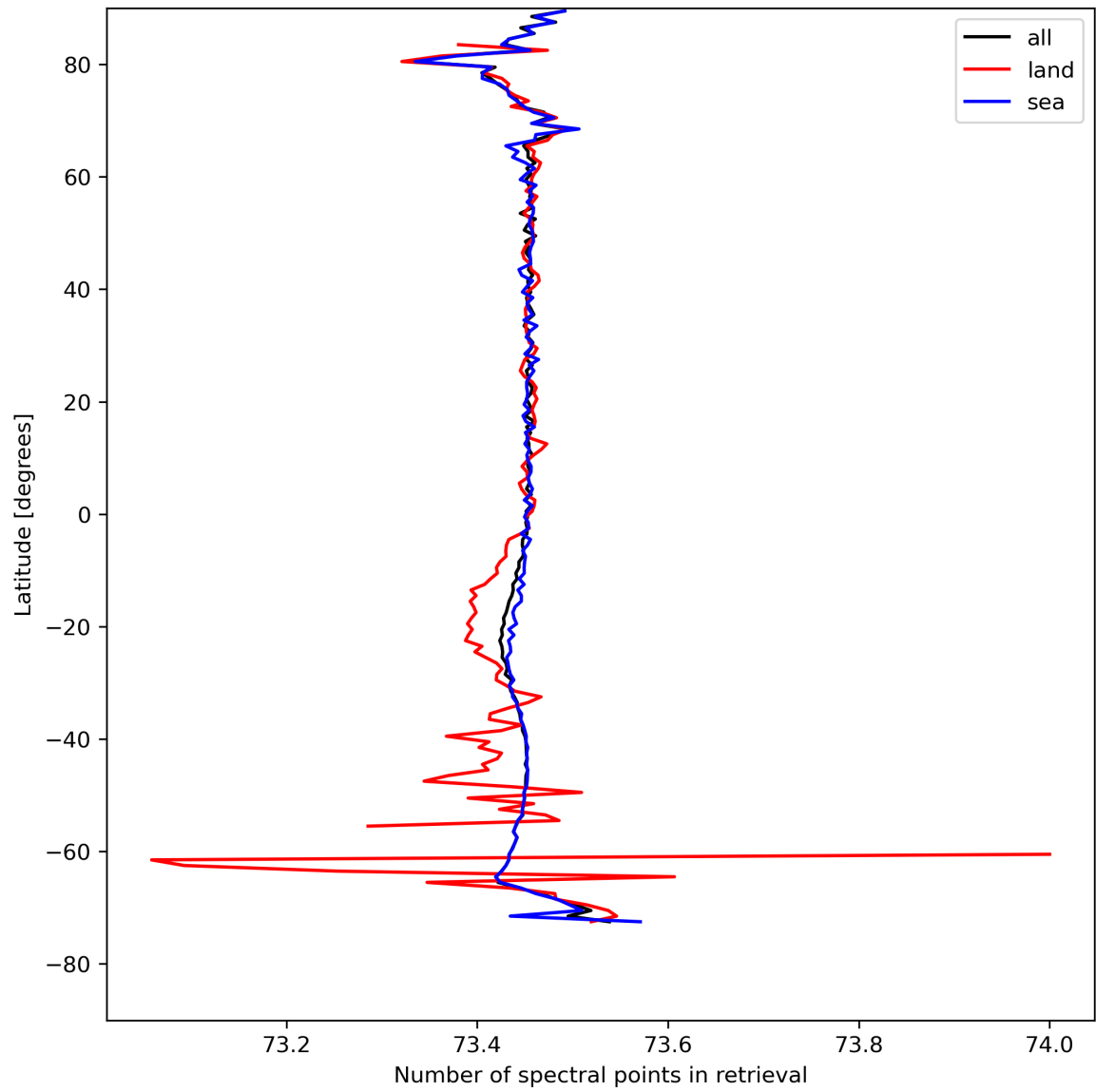
Figure 51: Zonal average of “Number of spectral points in retrieval” for 2024-04-21 to 2024-04-23.
