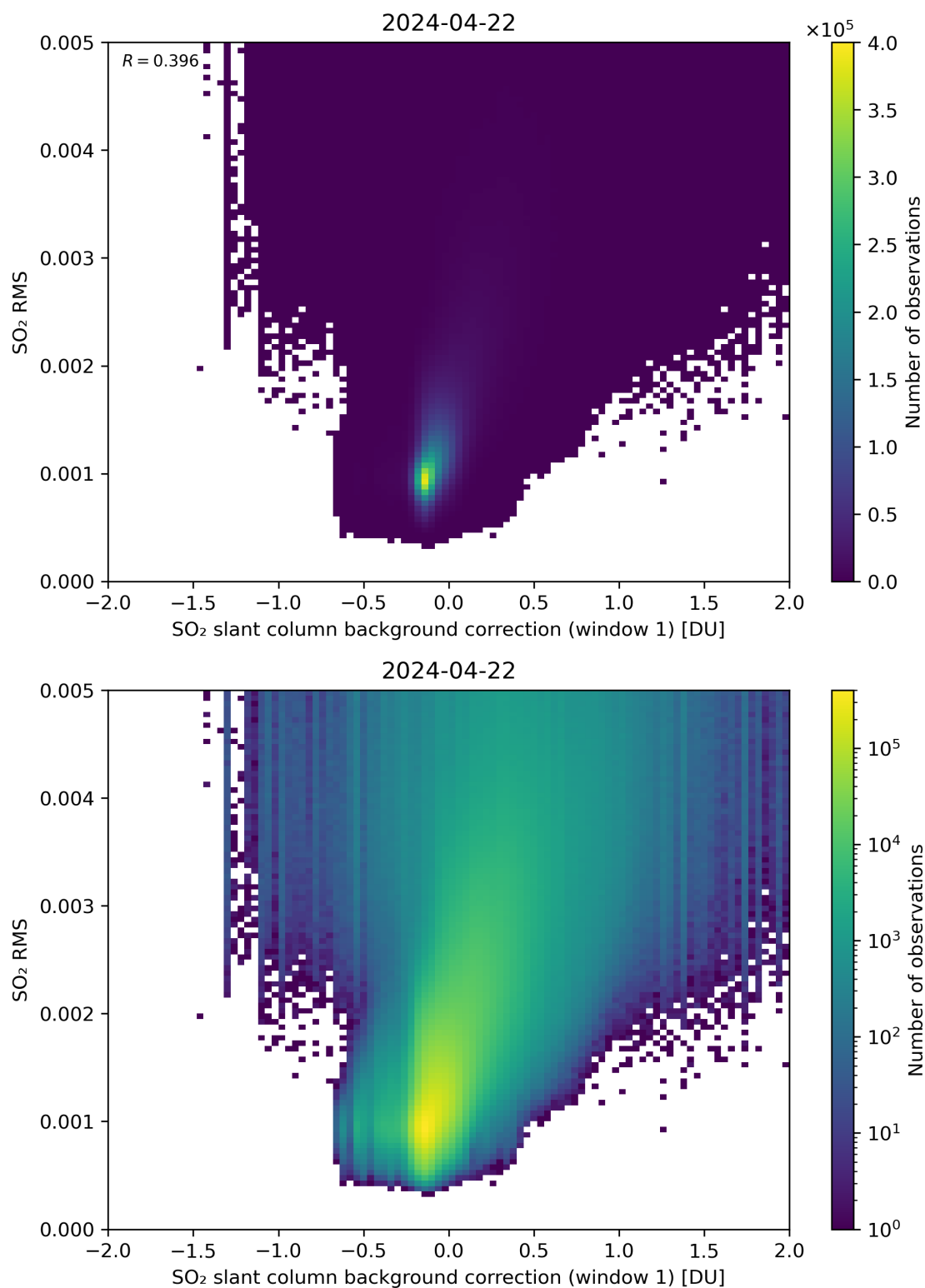
Figure 102: Scatter density plot of “SO 2 slant column background correction (window 1)” against “SO 2 RMS” for 2024-04-21 to 2024-04-23.
