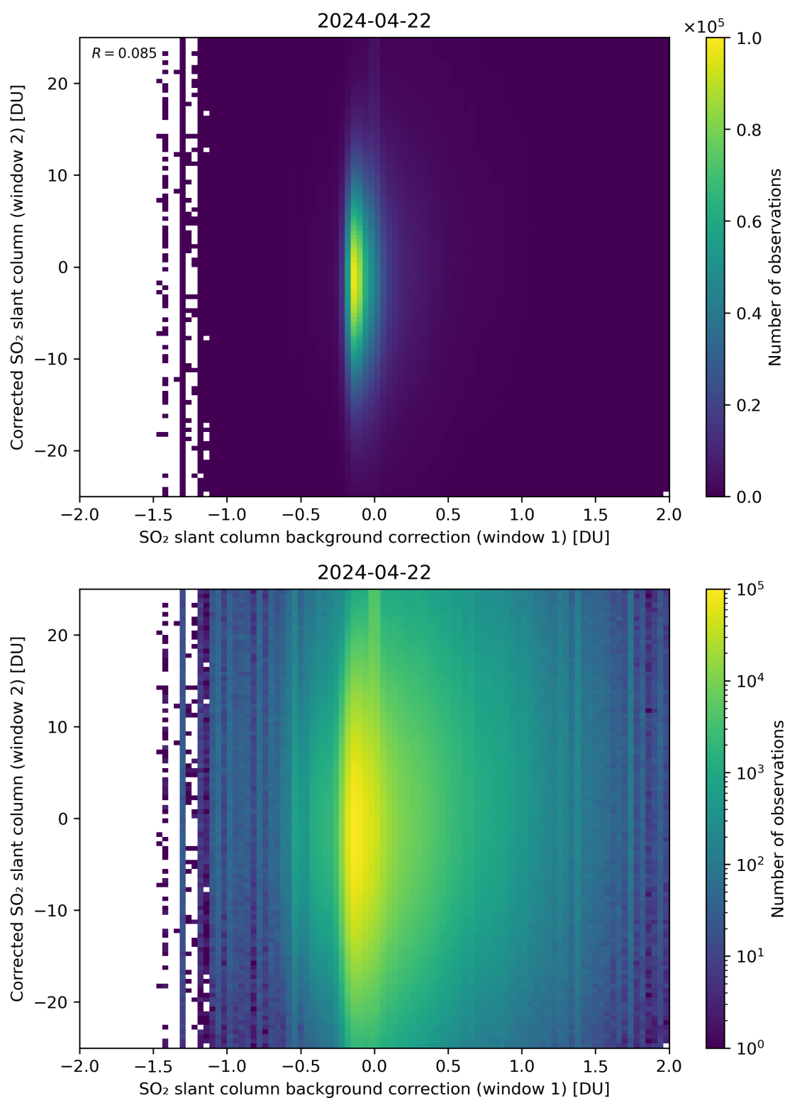
Figure 104: Scatter density plot of “SO 2 slant column background correction (window 1)” against “Corrected SO 2 slant column (window 2)” for 2024-04-21 to 2024-04-23.
