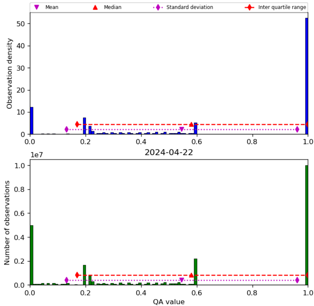
Figure 52: Histogram of “QA value” for 2024-04-21 to 2024-04-23
