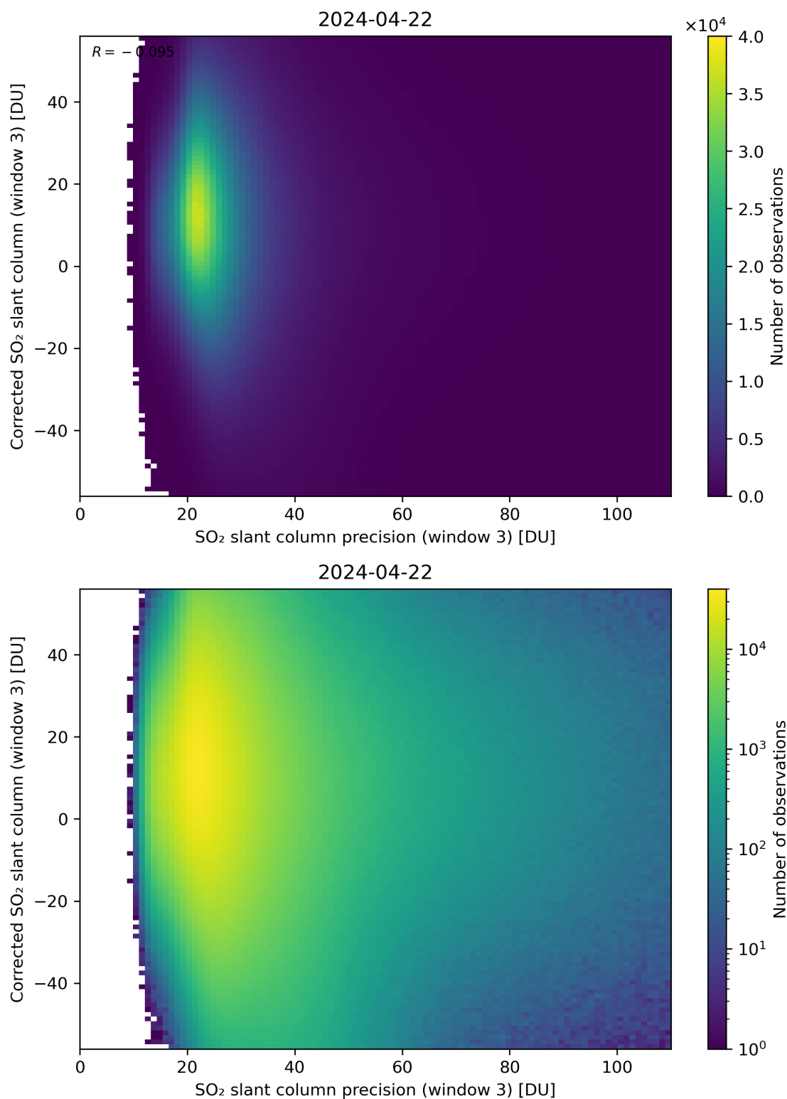
Figure 262: Scatter density plot of “SO 2 slant column precision (window 3)” against “Corrected SO 2 slant column (window 3)” for 2024-04-21 to 2024-04-23.
