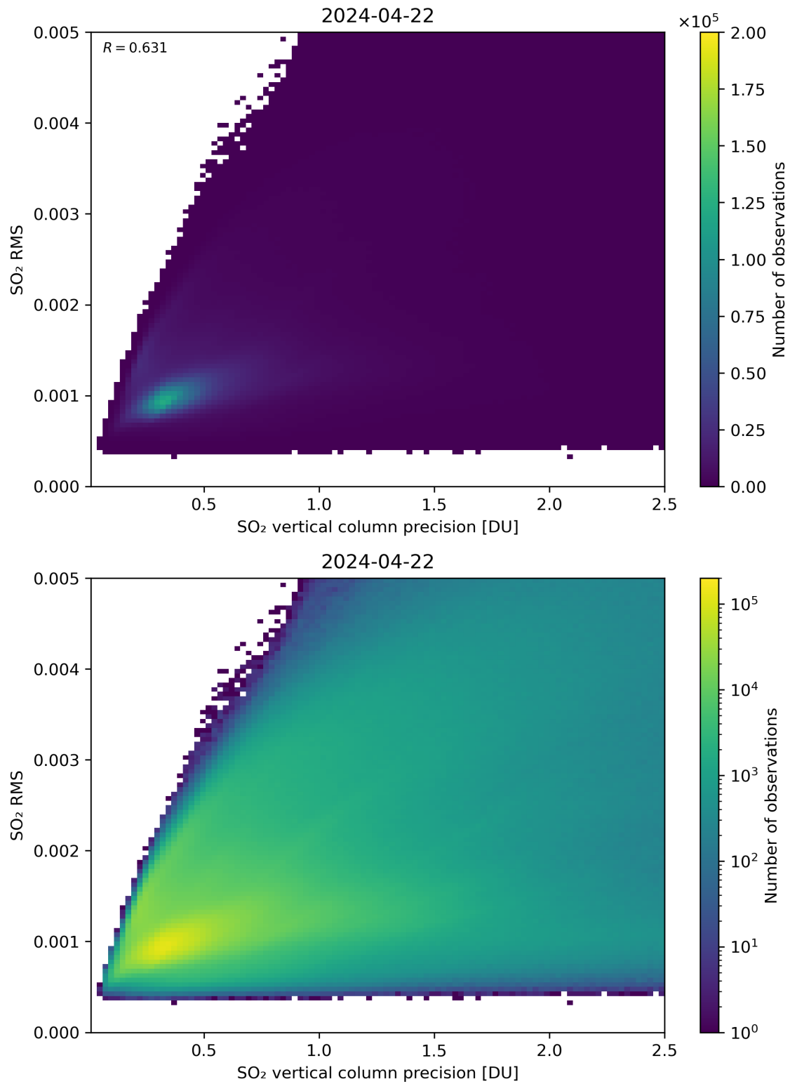
Figure 284: Scatter density plot of “SO 2 vertical column precision” against “SO 2 RMS” for 2024-04-21 to 2024-04-23.
