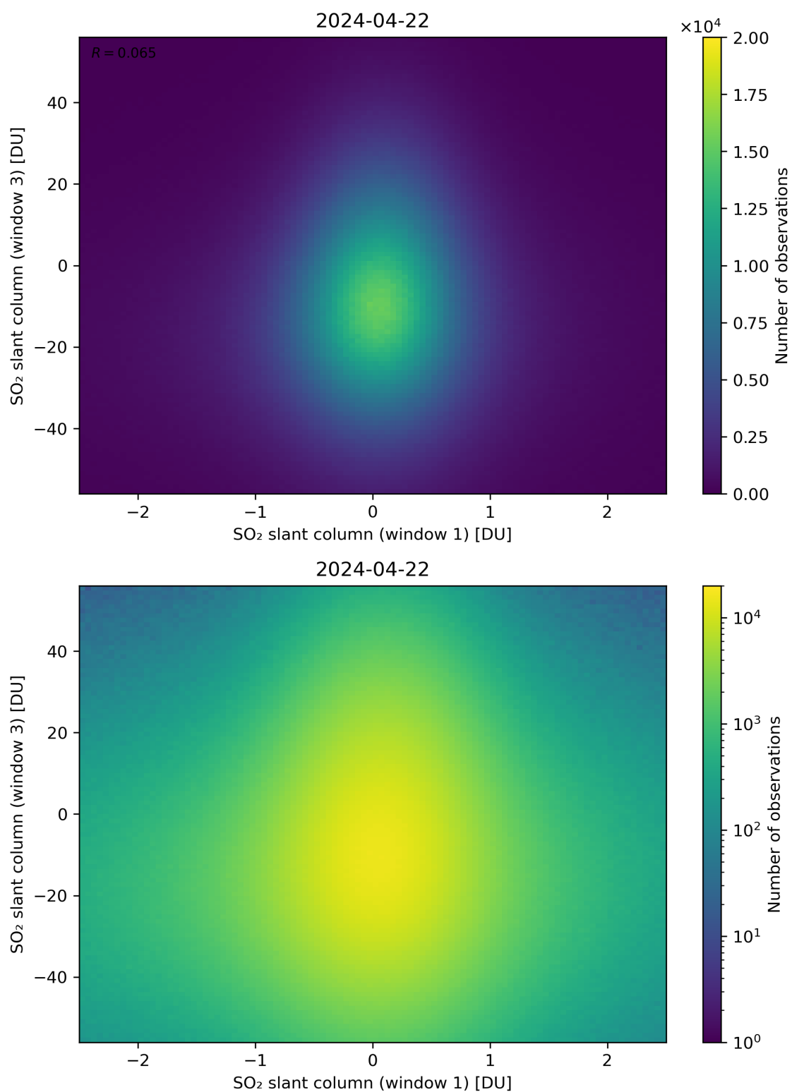
Figure 237: Scatter density plot of “SO 2 slant column (window 1)” against “SO 2 slant column (window 3)” for 2024-04-21 to 2024-04-23.
