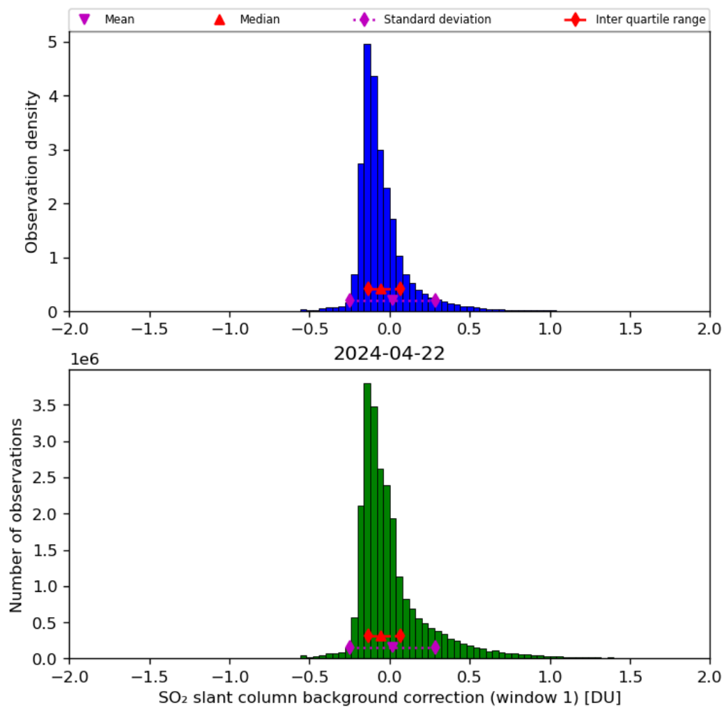
Figure 59: Histogram of “SO 2 slant column background correction (window 1)” for 2024-04-21 to 2024-04-23
