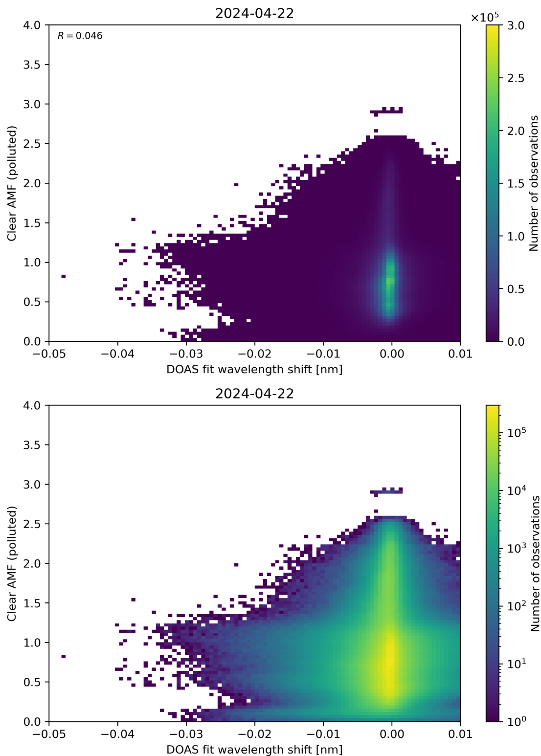
Figure 129: Scatter density plot of “DOAS fit wavelength shift” against “Clear AMF (polluted)” for 2024-04-21 to 2024-04-23.
