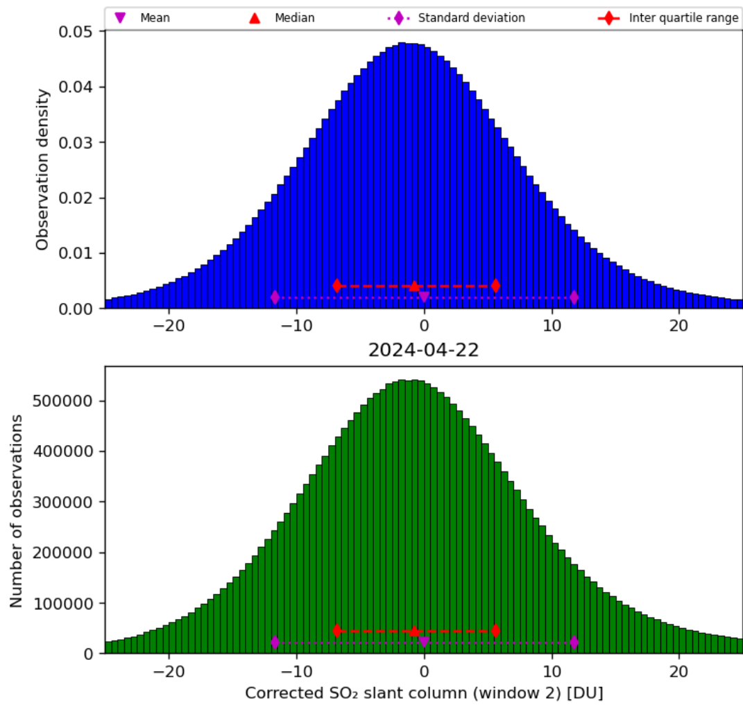
Figure 62: Histogram of “Corrected SO 2 slant column (window 2)” for 2024-04-21 to 2024-04-23
