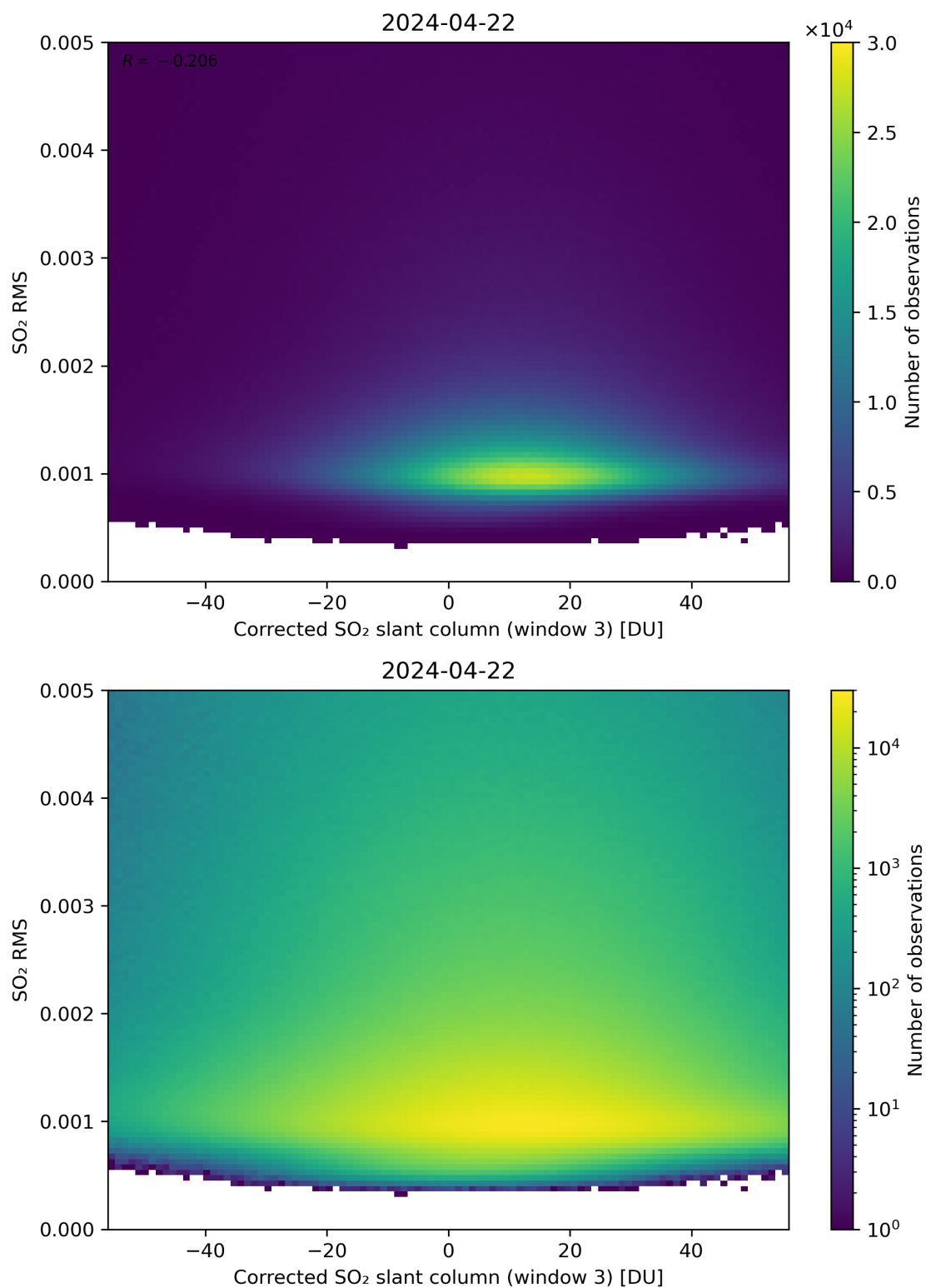
Figure 208: Scatter density plot of “Corrected SO 2 slant column (window 3)” against “SO 2 RMS” for 2024-04-21 to 2024-04-23.
