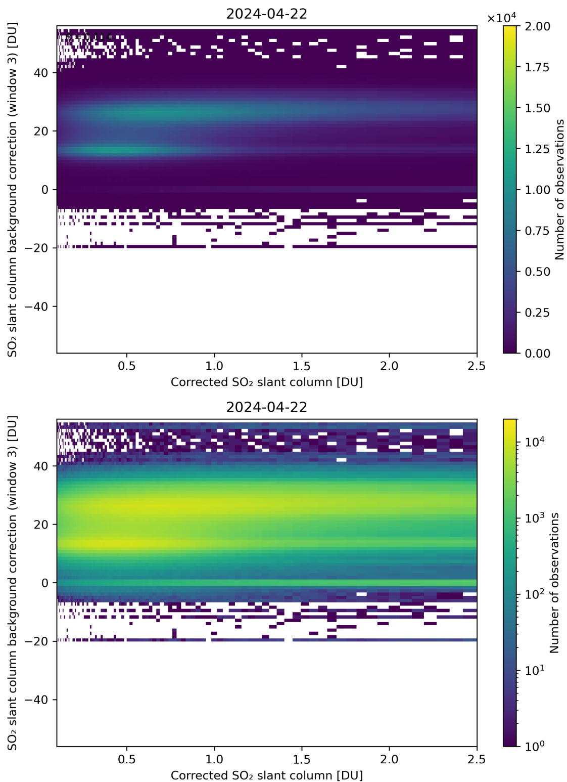
Figure 180: Scatter density plot of “Corrected SO 2 slant column” against “SO 2 slant column background correction (window 3)” for 2024-04-21 to 2024-04-23.
