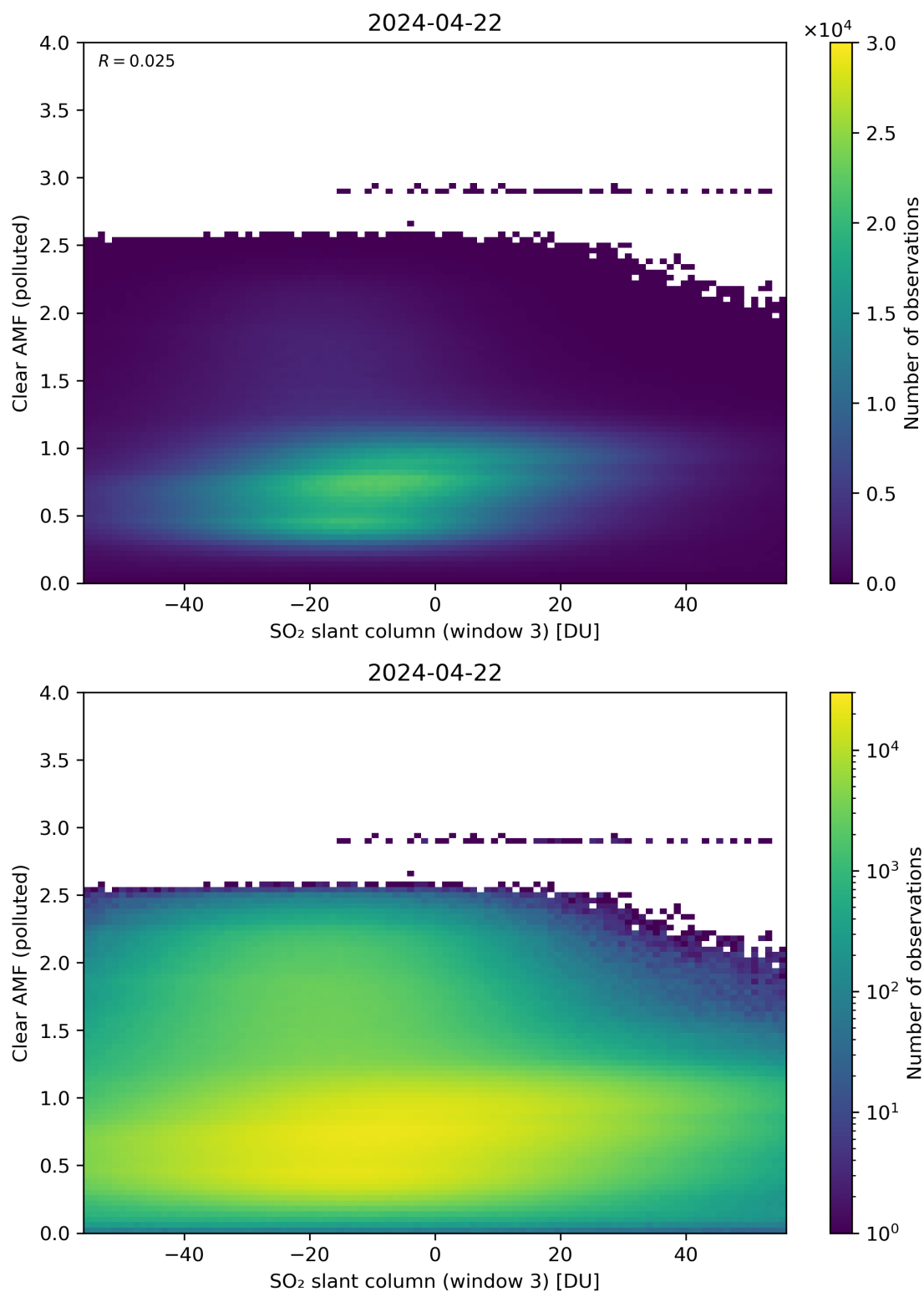
Figure 265: Scatter density plot of “SO 2 slant column (window 3)” against “Clear AMF (polluted)” for 2024-04-21 to 2024-04-23.
