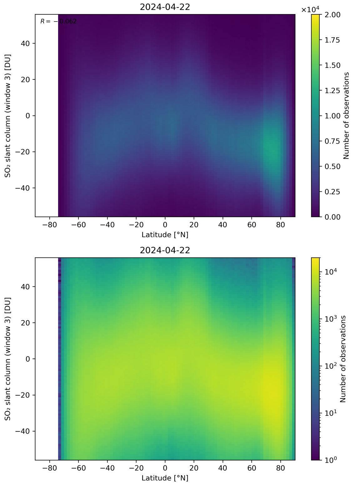
Figure 152: Scatter density plot of “Latitude” against “SO 2 slant column (window 3)” for 2024-04-21 to 2024-04-23.
