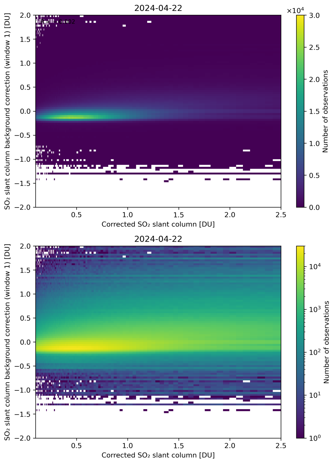
Figure 178: Scatter density plot of “Corrected SO 2 slant column” against “SO 2 slant column background correction (window 1)” for 2024-04-21 to 2024-04-23.
