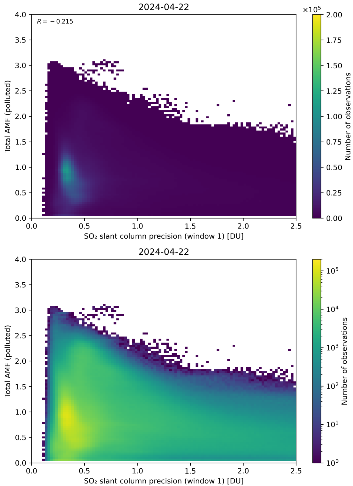
Figure 230: Scatter density plot of “SO 2 slant column precision (window 1)” against “Total AMF (polluted)” for 2024-04-21 to 2024-04-23.
