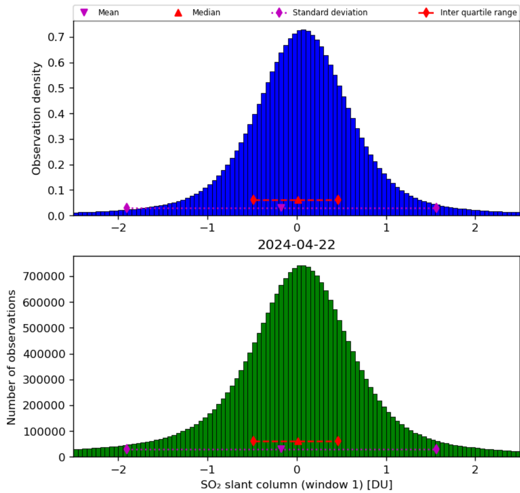
Figure 56: Histogram of “SO 2 slant column (window 1)” for 2024-04-21 to 2024-04-23
