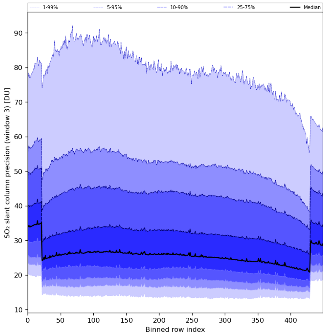
Figure 88: Along track statistics of “SO 2 slant column precision (window 3)” for 2024-04-21 to 2024-04-23
