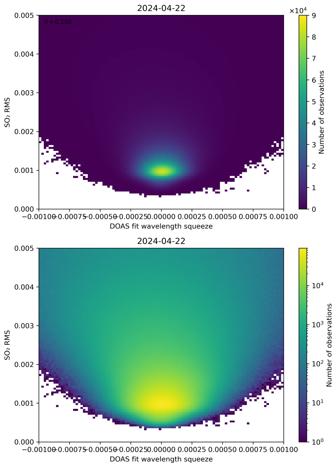
Figure 132: Scatter density plot of “DOAS fit wavelength squeeze” against “SO 2 RMS” for 2024-04-21 to 2024-04-23.
