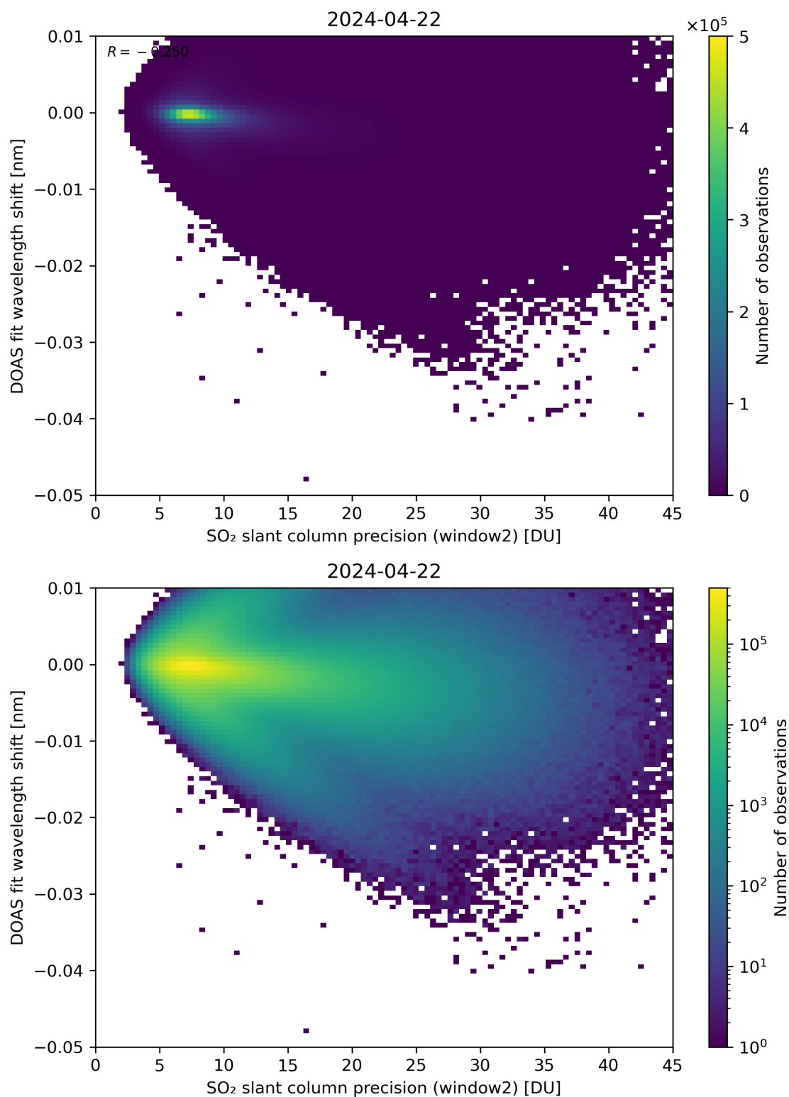
Figure 243: Scatter density plot of “SO 2 slant column precision (window2)” against “DOAS fit wavelength shift” for 2024-04-21 to 2024-04-23.
