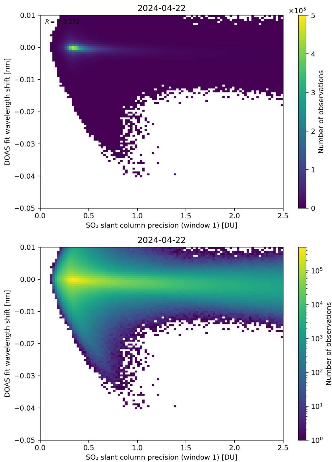
Figure 221: Scatter density plot of “SO 2 slant column precision (window 1)” against “DOAS fit wavelength shift” for 2024-04-21 to 2024-04-23.
