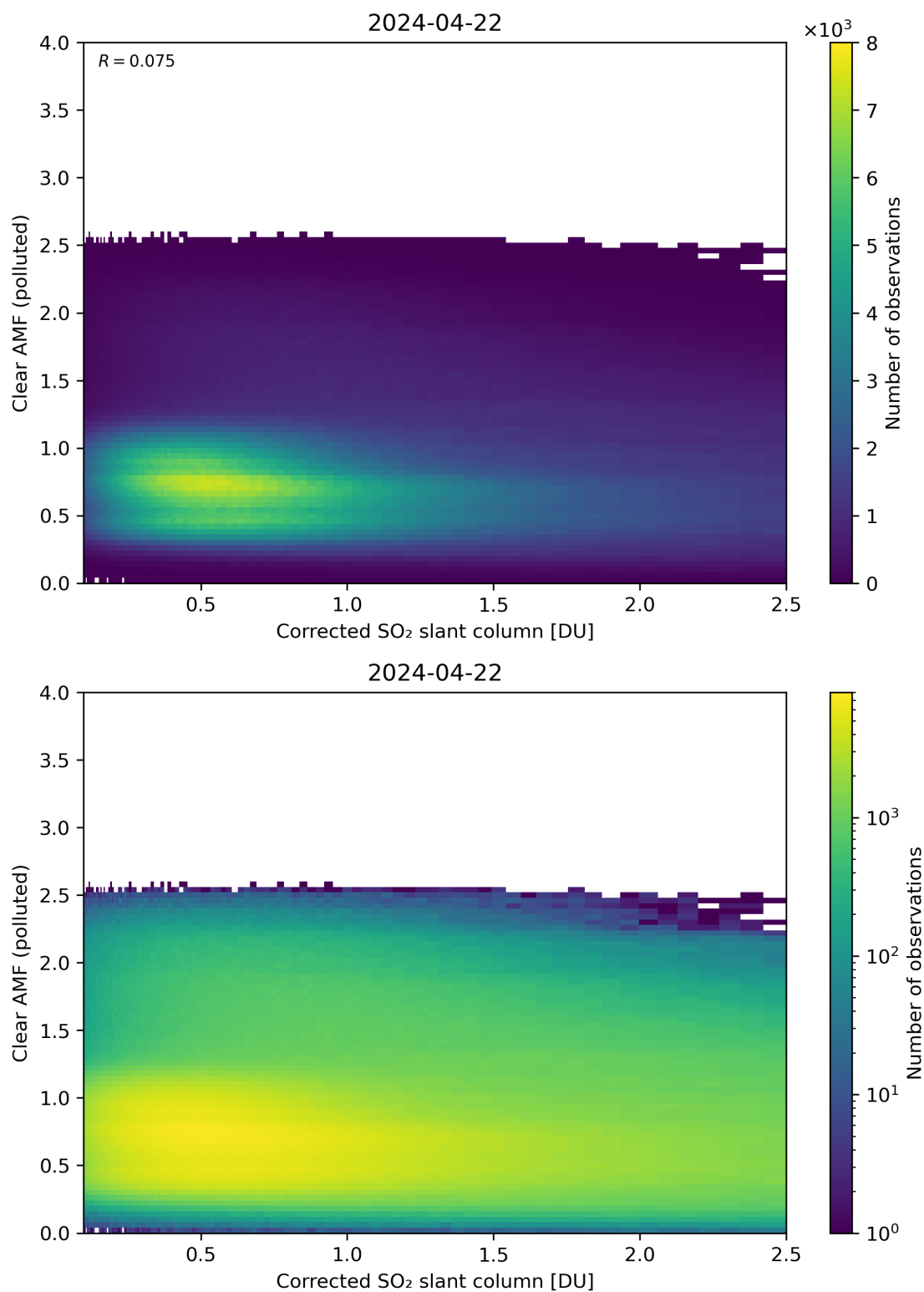
Figure 184: Scatter density plot of “Corrected SO 2 slant column” against “Clear AMF (polluted)” for 2024-04-21 to 2024-04-23.
