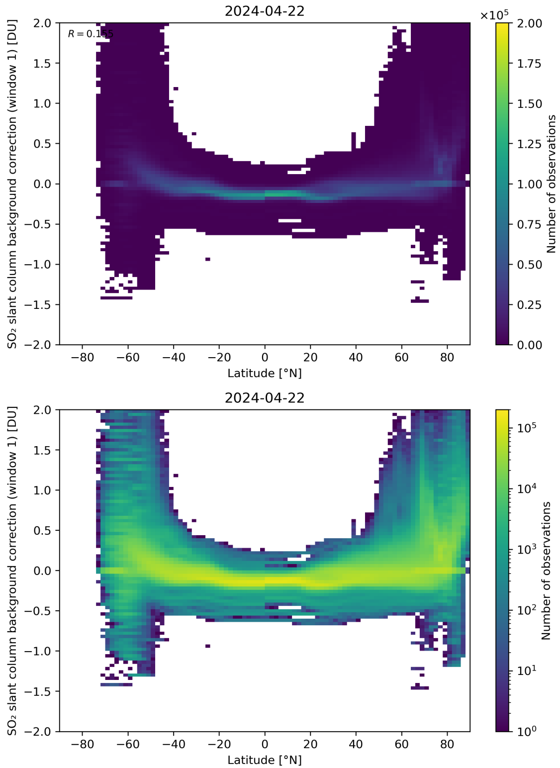
Figure 139: Scatter density plot of “Latitude” against “SO 2 slant column background correction (window 1)” for 2024-04-21 to 2024-04-23.
