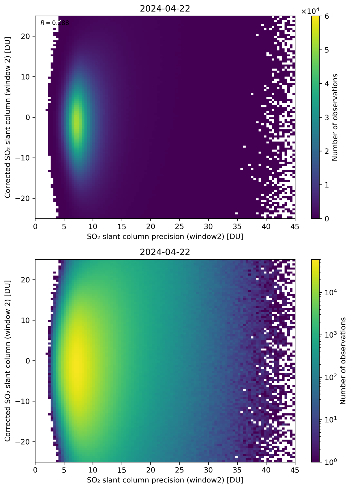
Figure 247: Scatter density plot of “SO 2 slant column precision (window2)” against “Corrected SO 2 slant column (window 2)” for 2024-04-21 to 2024-04-23.
