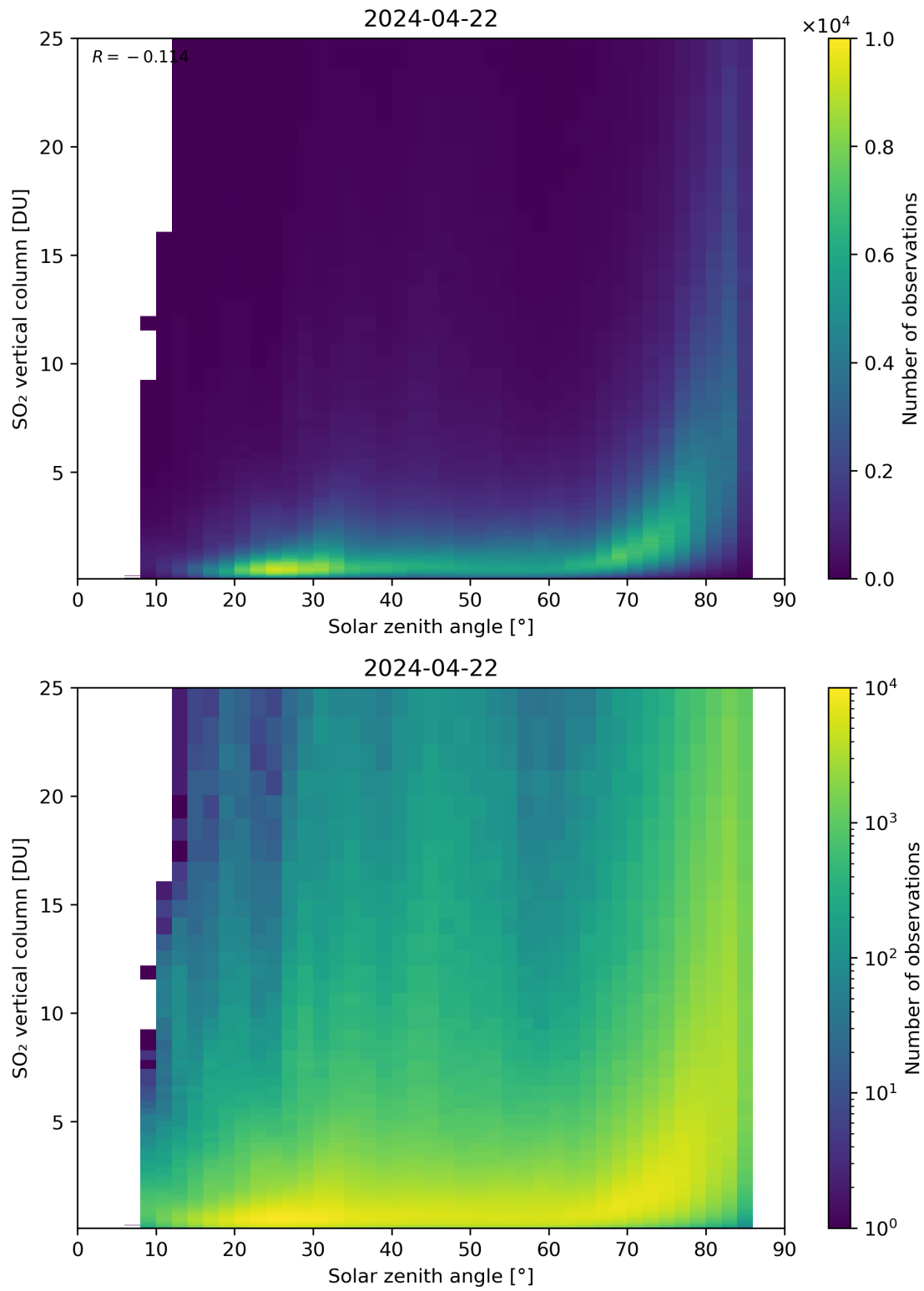
Figure 176: Scatter density plot of “Solar zenith angle” against “SO 2 vertical column” for 2024-04-21 to 2024-04-23.
