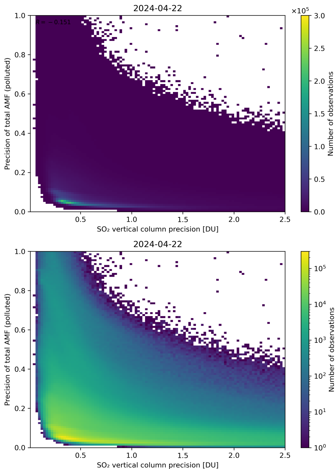
Figure 295: Scatter density plot of “SO 2 vertical column precision” against “Precision of total AMF (polluted)” for 2024-04-21 to 2024-04-23.
