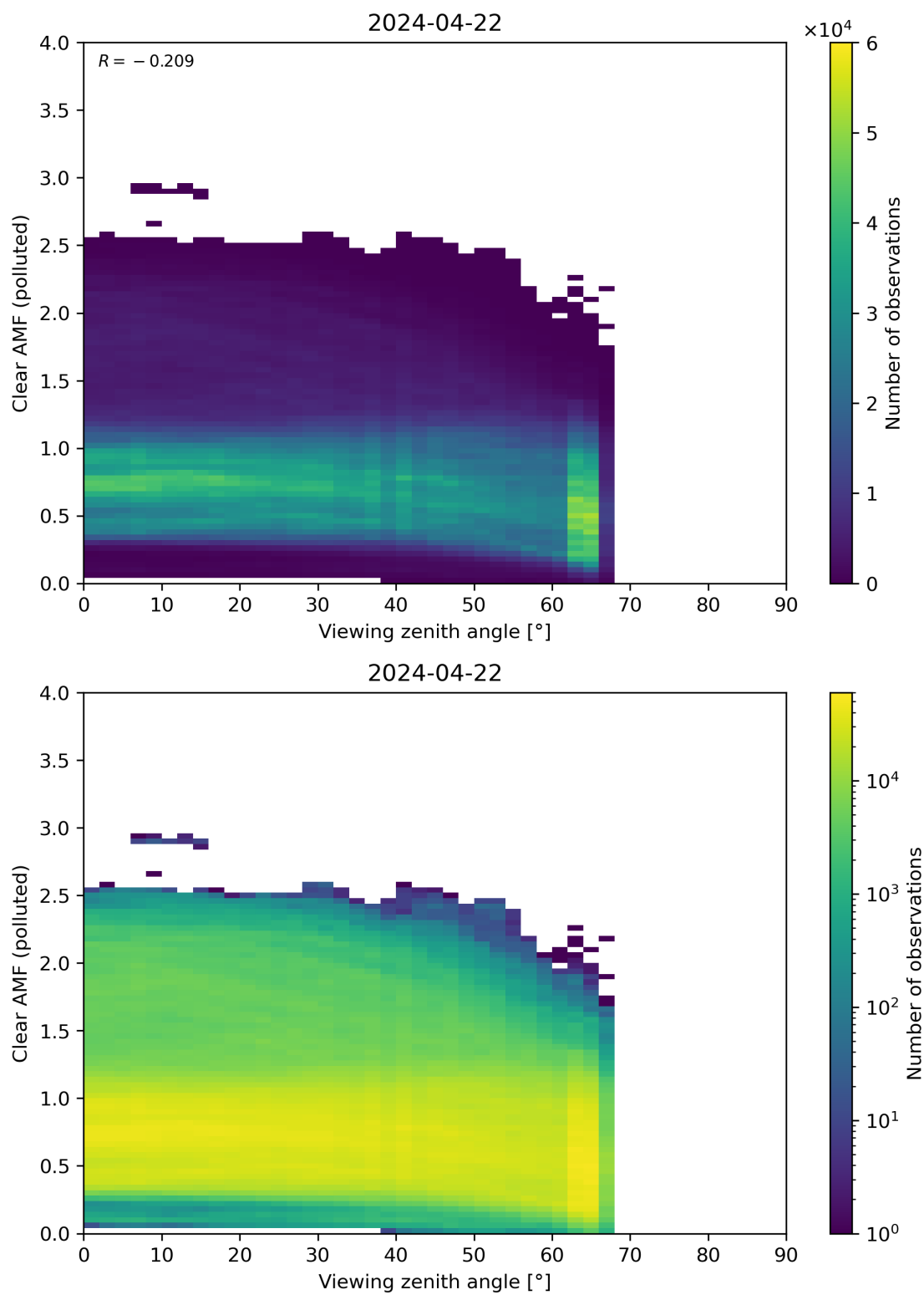
Figure 316: Scatter density plot of “Viewing zenith angle” against “Clear AMF (polluted)” for 2024-04-21 to 2024-04-23.
