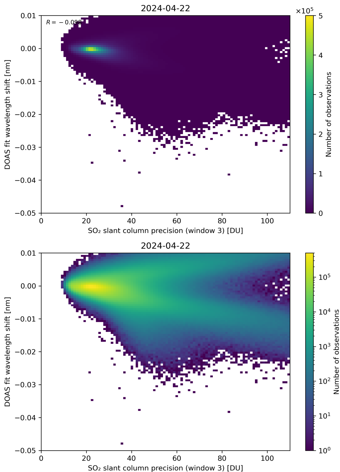
Figure 258: Scatter density plot of “SO 2 slant column precision (window 3)” against “DOAS fit wavelength shift” for 2024-04-21 to 2024-04-23.
