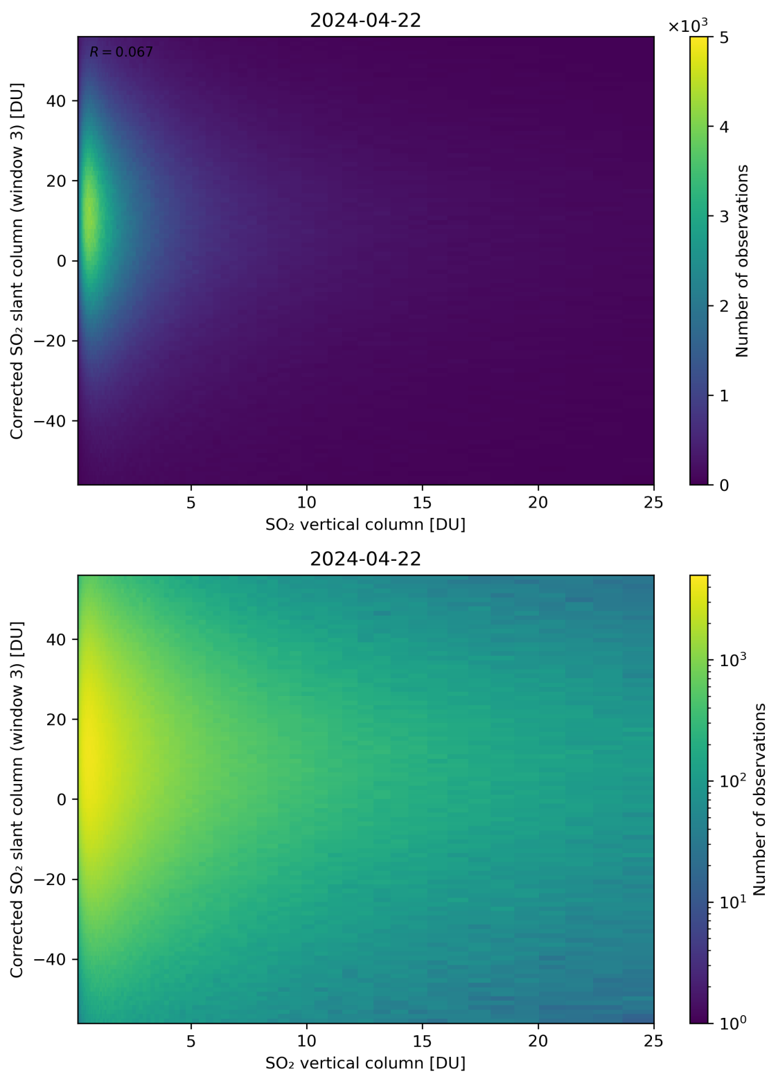
Figure 299: Scatter density plot of “SO 2 vertical column” against “Corrected SO 2 slant column (window 3)” for 2024-04-21 to 2024-04-23.
