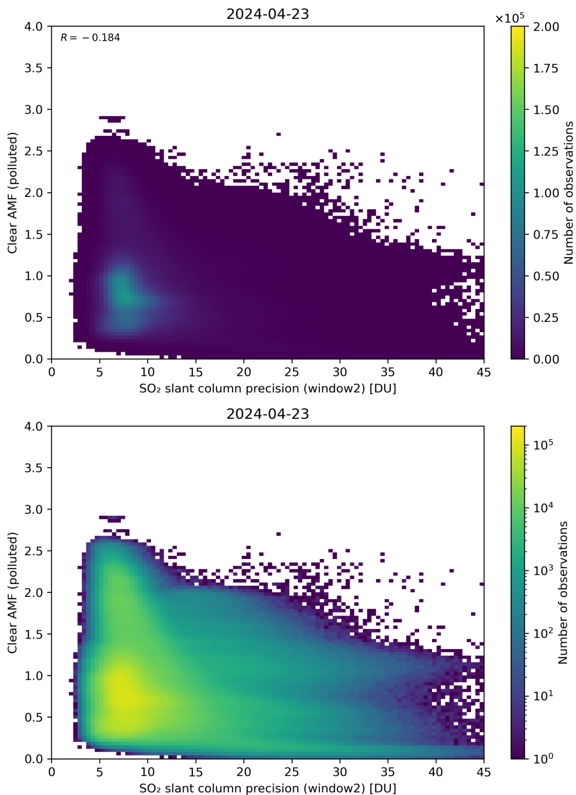
Figure 246: Scatter density plot of “SO 2 slant column precision (window2)” against “Clear AMF (polluted)” for 2024-04-22 to 2024-04-24.
