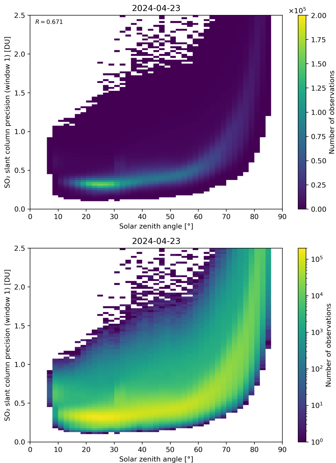
Figure 170: Scatter density plot of “Solar zenith angle” against “SO 2 slant column precision (window 1)” for 2024-04-22 to 2024-04-24.
