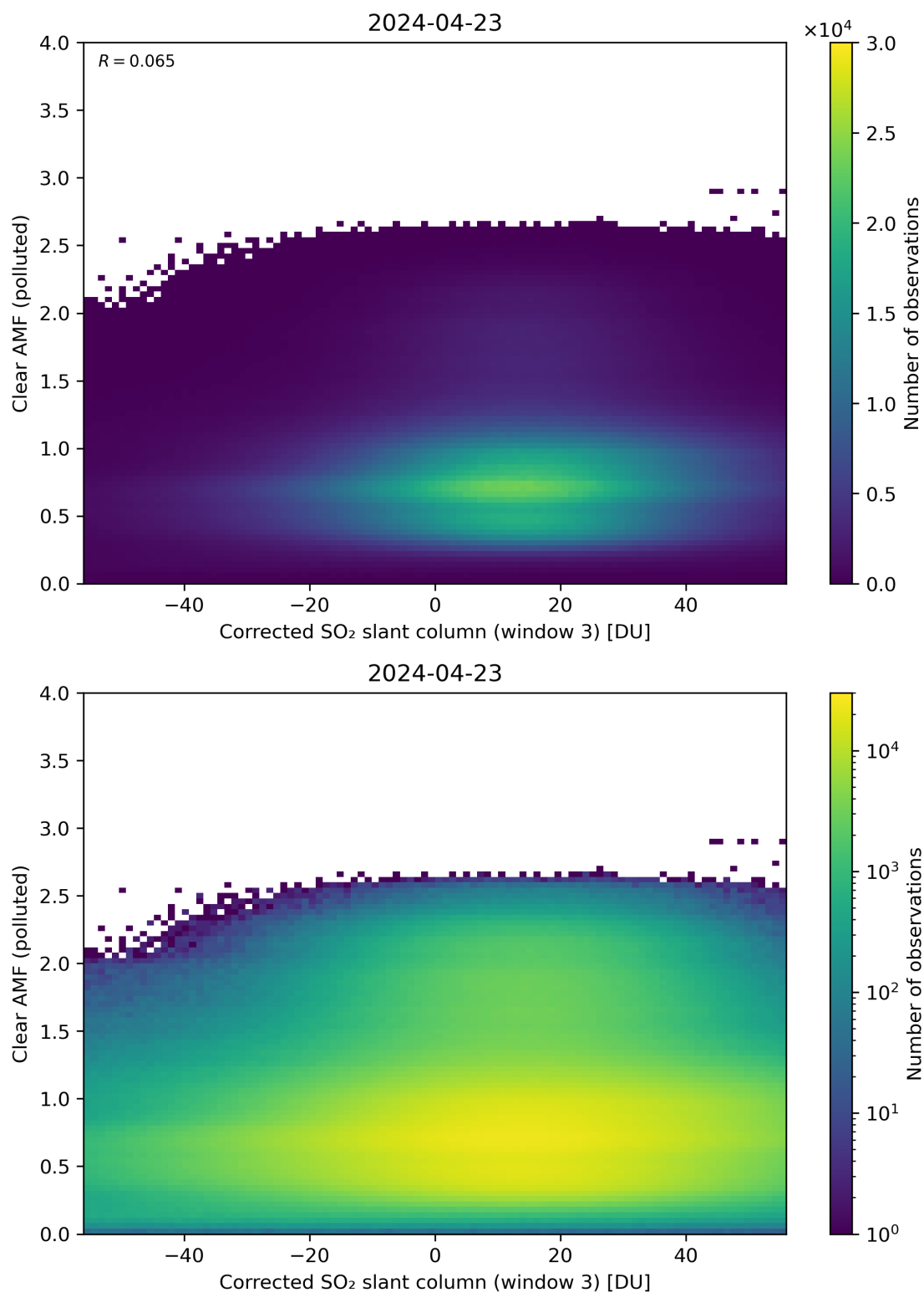
Figure 209: Scatter density plot of “Corrected SO 2 slant column (window 3)” against “Clear AMF (polluted)” for 2024-04-22 to 2024-04-24.
