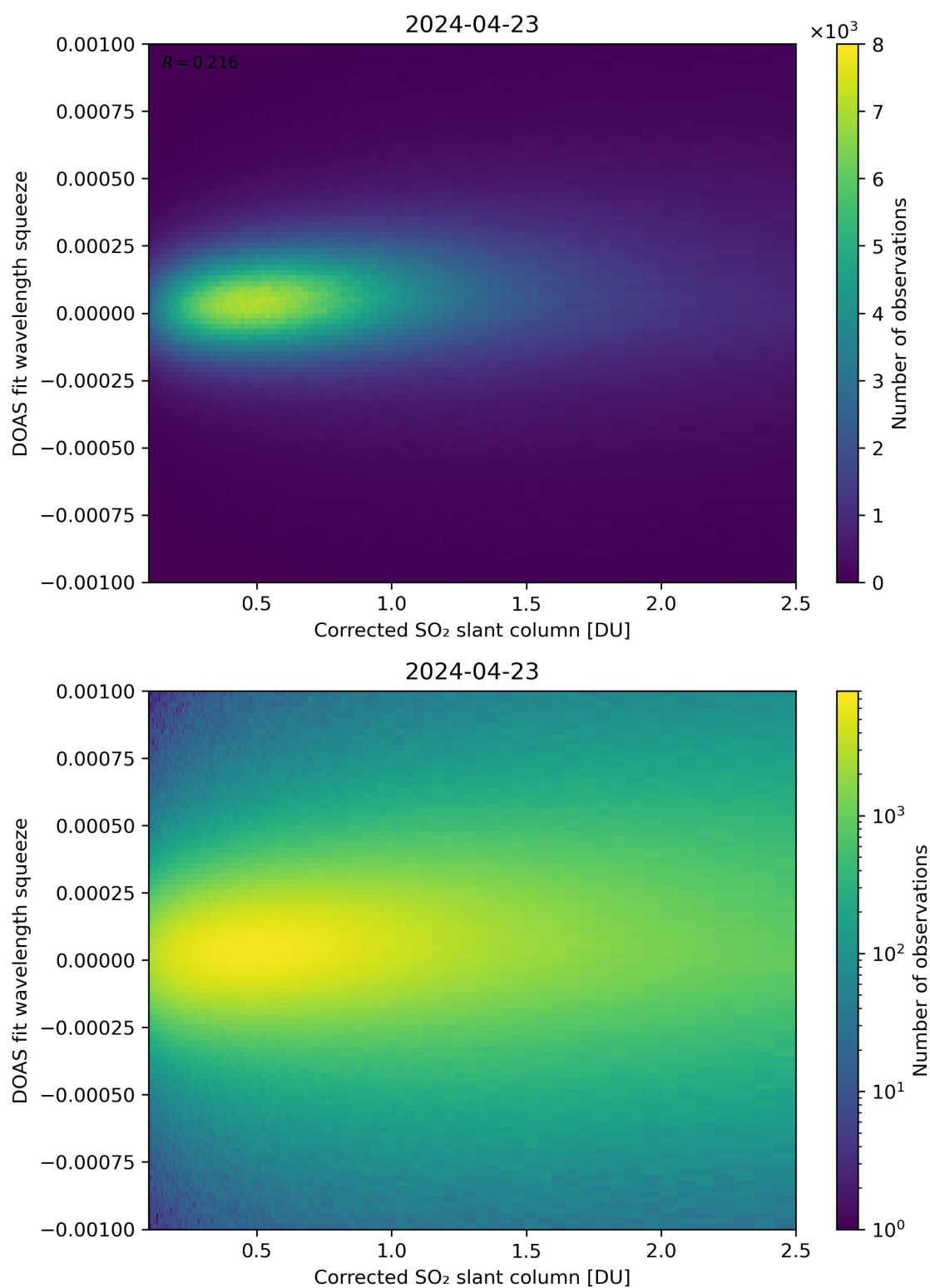
Figure 182: Scatter density plot of “Corrected SO 2 slant column” against “DOAS fit wavelength squeeze” for 2024-04-22 to 2024-04-24.
