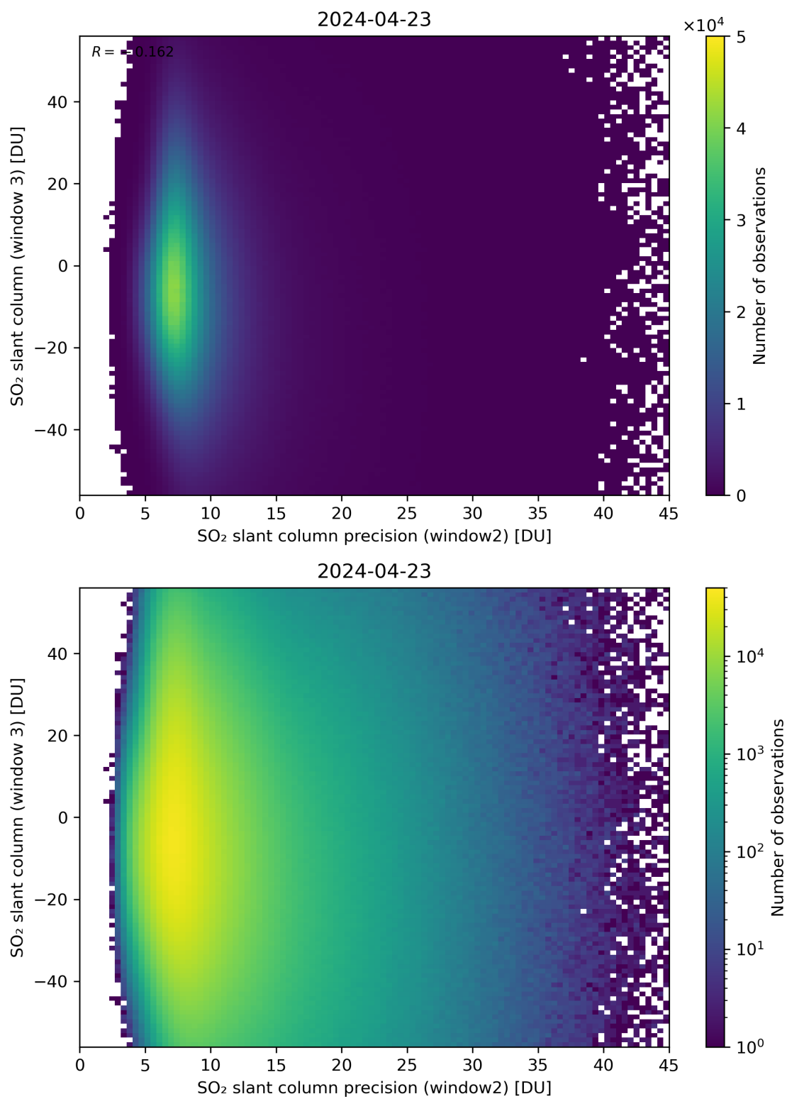
Figure 249: Scatter density plot of “SO 2 slant column precision (window2)” against “SO 2 slant column (window 3)” for 2024-04-22 to 2024-04-24.
