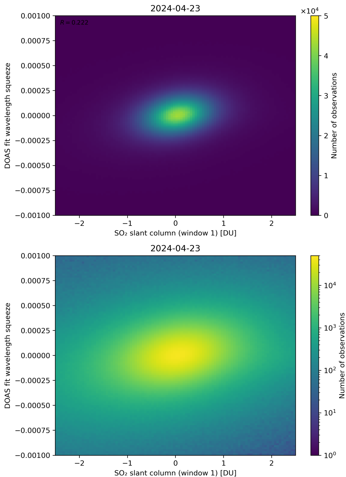
Figure 216: Scatter density plot of “SO 2 slant column (window 1)” against “DOAS fit wavelength squeeze” for 2024-04-22 to 2024-04-24.
