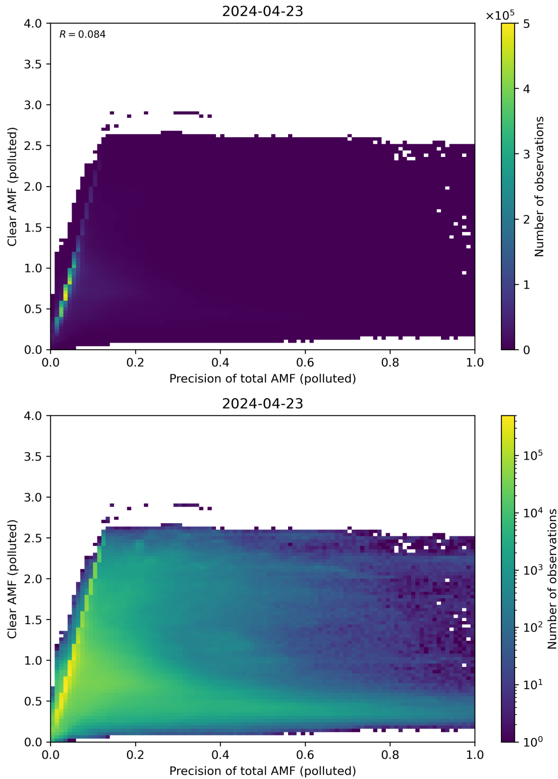
Figure 270: Scatter density plot of “Precision of total AMF (polluted)” against “Clear AMF (polluted)” for 2024-04-22 to 2024-04-24.
