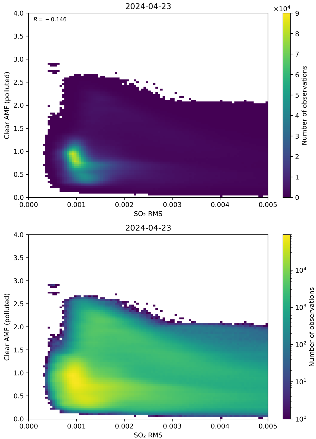
Figure 136: Scatter density plot of “SO 2 RMS” against “Clear AMF (polluted)” for 2024-04-22 to 2024-04-24.
