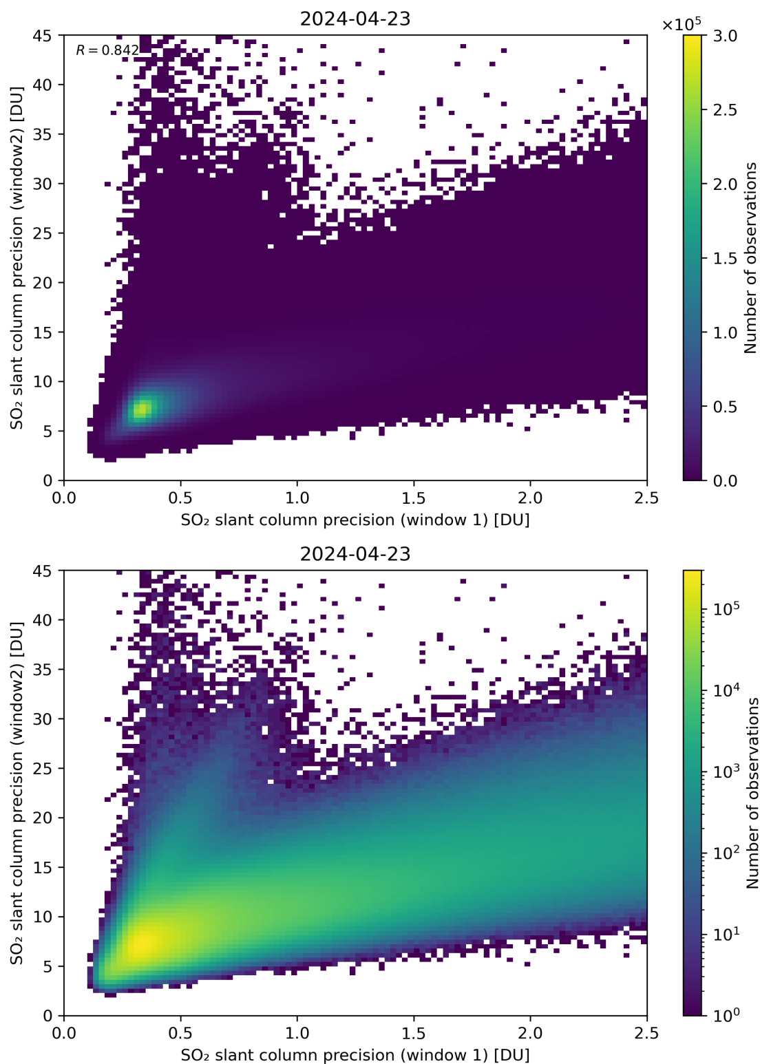
Figure 227: Scatter density plot of “SO 2 slant column precision (window 1)” against “SO 2 slant column precision (window2)” for 2024-04-22 to 2024-04-24.
