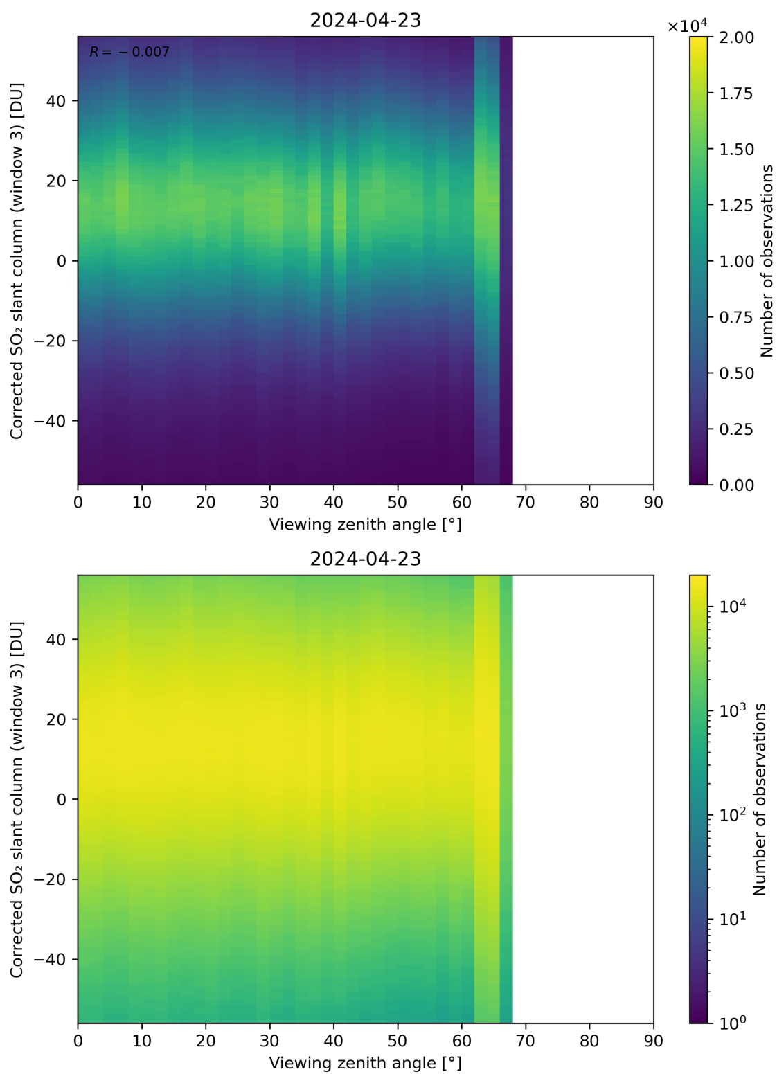
Figure 319: Scatter density plot of “Viewing zenith angle” against “Corrected SO 2 slant column (window 3)” for 2024-04-22 to 2024-04-24.
