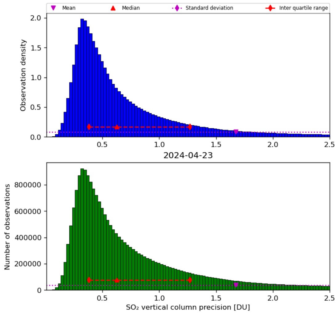
Figure 54: Histogram of “SO 2 vertical column precision” for 2024-04-22 to 2024-04-24
