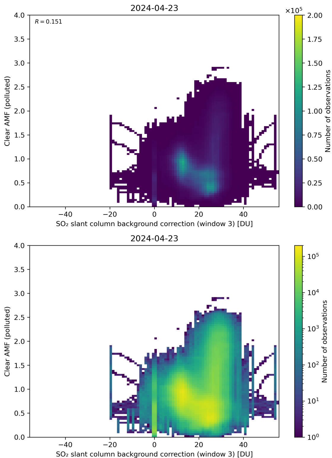
Figure 124: Scatter density plot of “SO 2 slant column background correction (window 3)” against “Clear AMF (polluted)” for 2024-04-22 to 2024-04-24.
