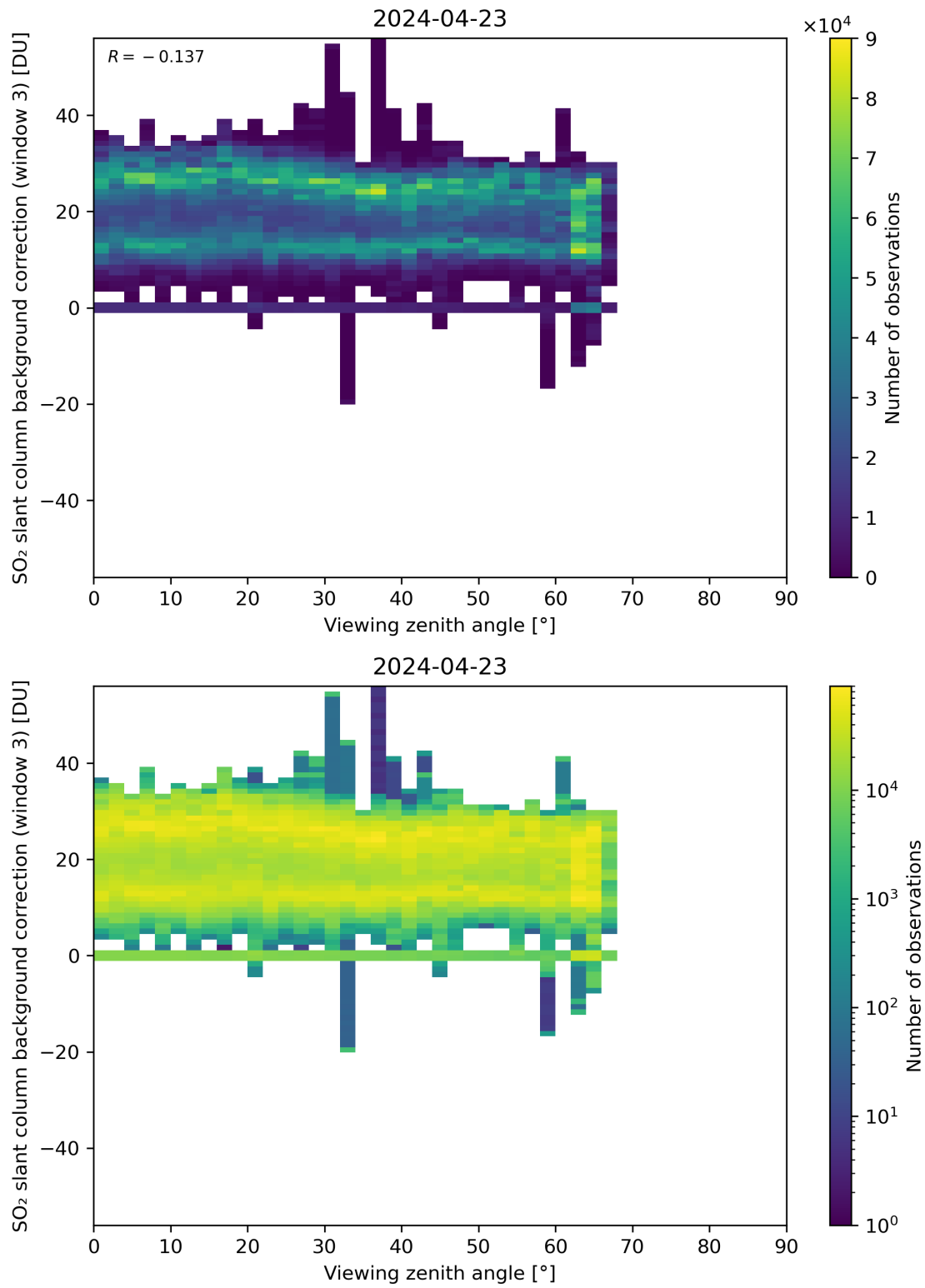
Figure 310: Scatter density plot of “Viewing zenith angle” against “SO 2 slant column background correction (window 3)” for 2024-04-22 to 2024-04-24.
