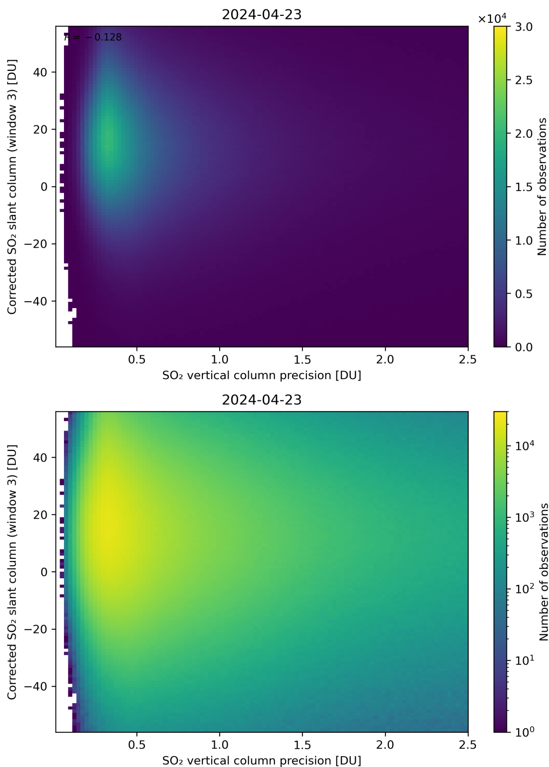
Figure 288: Scatter density plot of “SO 2 vertical column precision” against “Corrected SO 2 slant column (window 3)” for 2024-04-22 to 2024-04-24.
