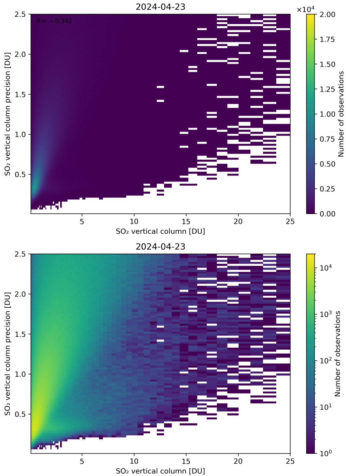
Figure 307: Scatter density plot of “SO 2 vertical column” against “SO 2 vertical column precision” for 2024-04-22 to 2024-04-24.
