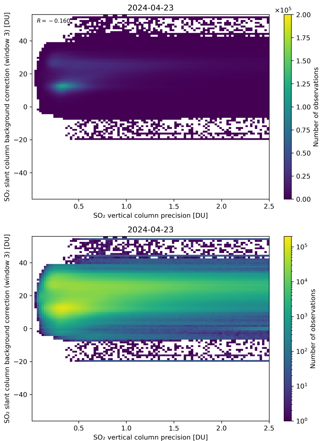
Figure 281: Scatter density plot of “SO 2 vertical column precision” against “SO 2 slant column background correction (window 3)” for 2024-04-22 to 2024-04-24.
