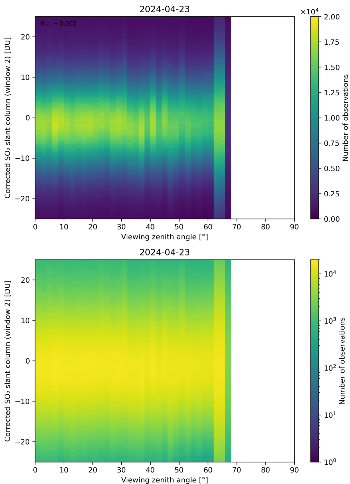
Figure 318: Scatter density plot of “Viewing zenith angle” against “Corrected SO 2 slant column (window 2)” for 2024-04-22 to 2024-04-24.
