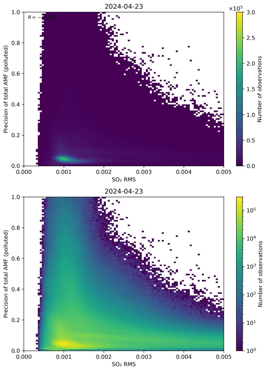
Figure 138: Scatter density plot of “SO 2 RMS” against “Precision of total AMF (polluted)” for 2024-04-22 to 2024-04-24.
