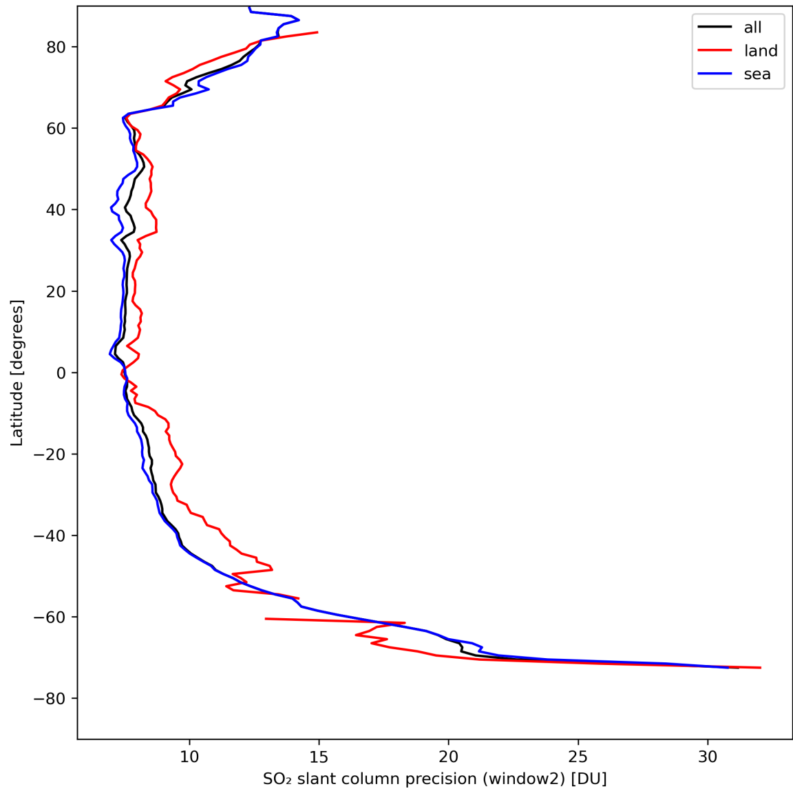
Figure 38: Zonal average of "SO 2 slant column precision (window2)" for 2024-04-22 to 2024-04-24.
