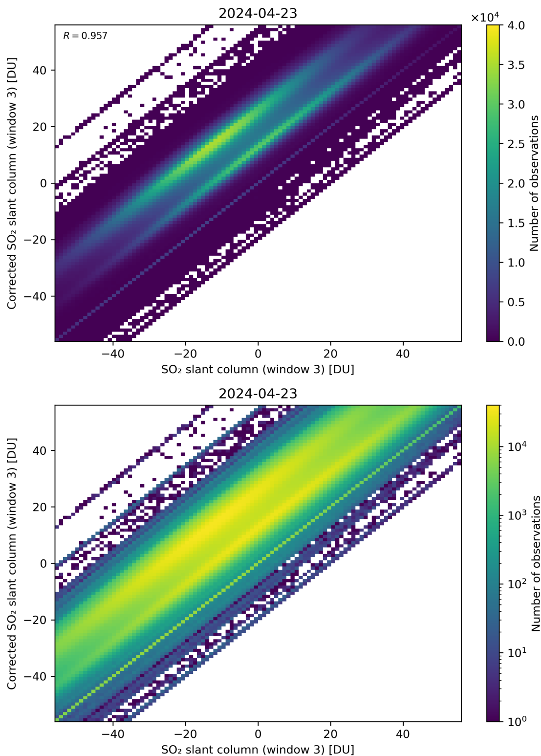
Figure 266: Scatter density plot of “SO 2 slant column (window 3)” against “Corrected SO 2 slant column (window 3)” for 2024-04-22 to 2024-04-24.
