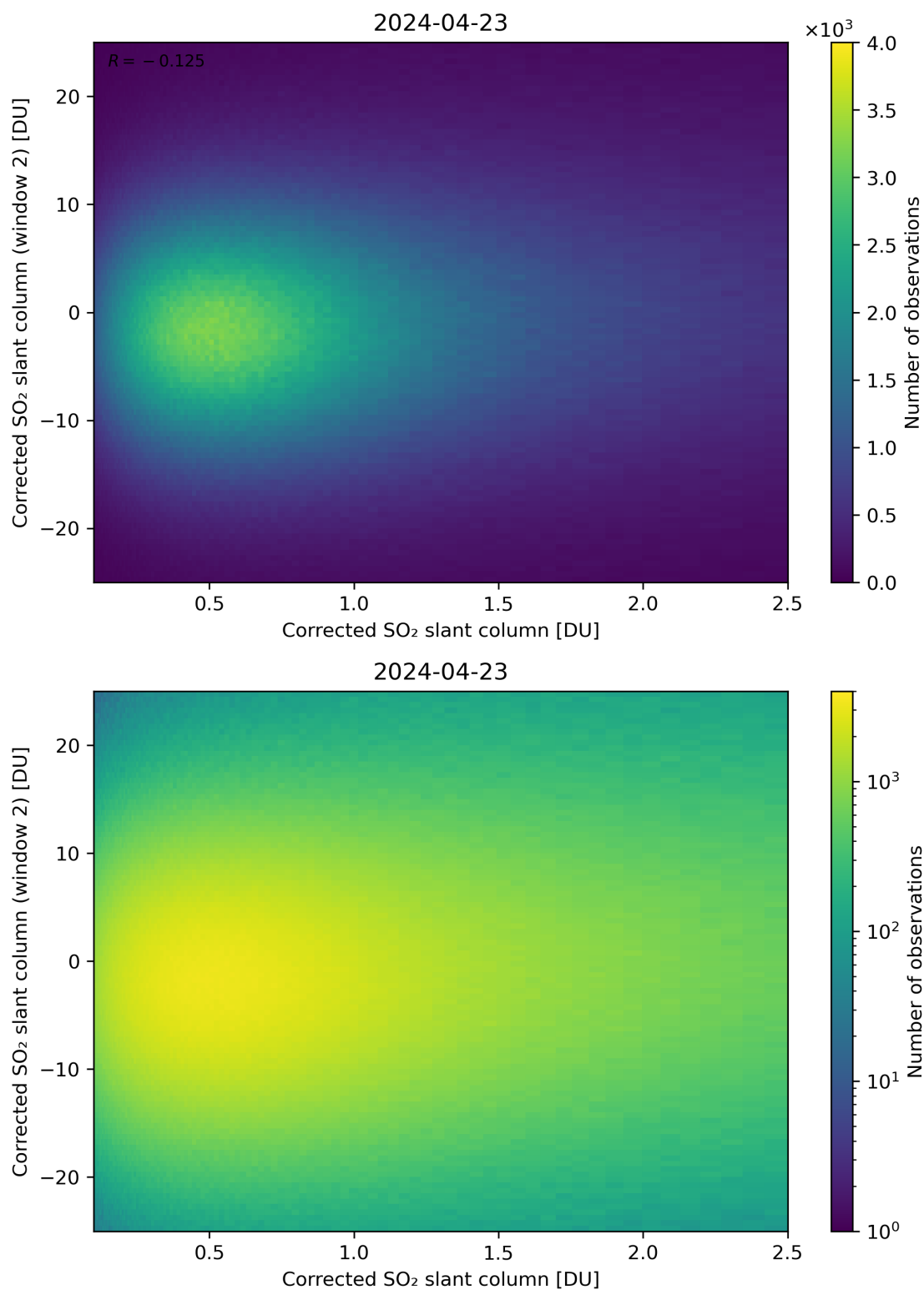
Figure 185: Scatter density plot of “Corrected SO 2 slant column” against “Corrected SO 2 slant column (window 2)” for 2024-04-22 to 2024-04-24.
