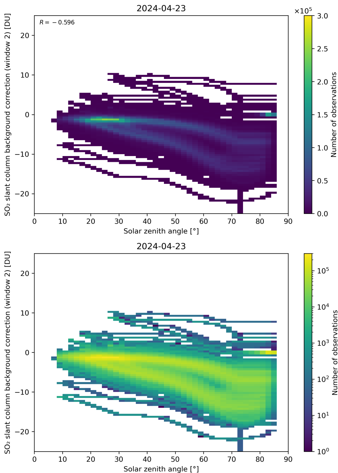
Figure 159: Scatter density plot of “Solar zenith angle” against “SO 2 slant column background correction (window 2)” for 2024-04-22 to 2024-04-24.
