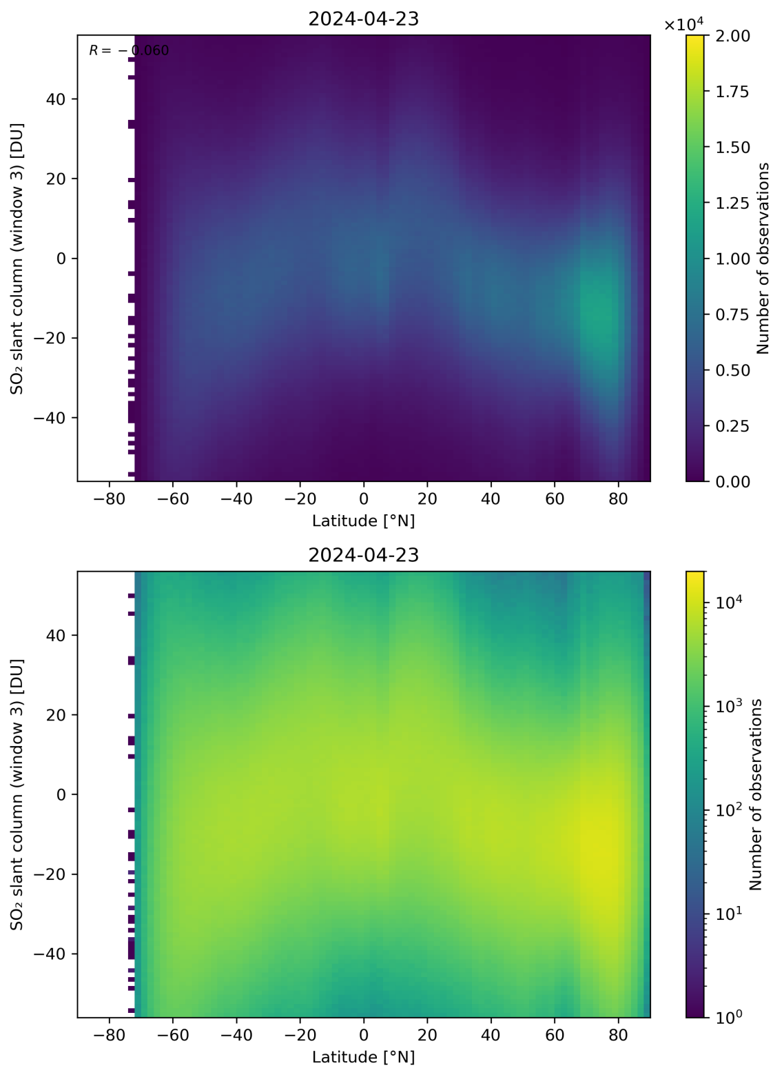
Figure 152: Scatter density plot of “Latitude” against “SO 2 slant column (window 3)” for 2024-04-22 to 2024-04-24.
