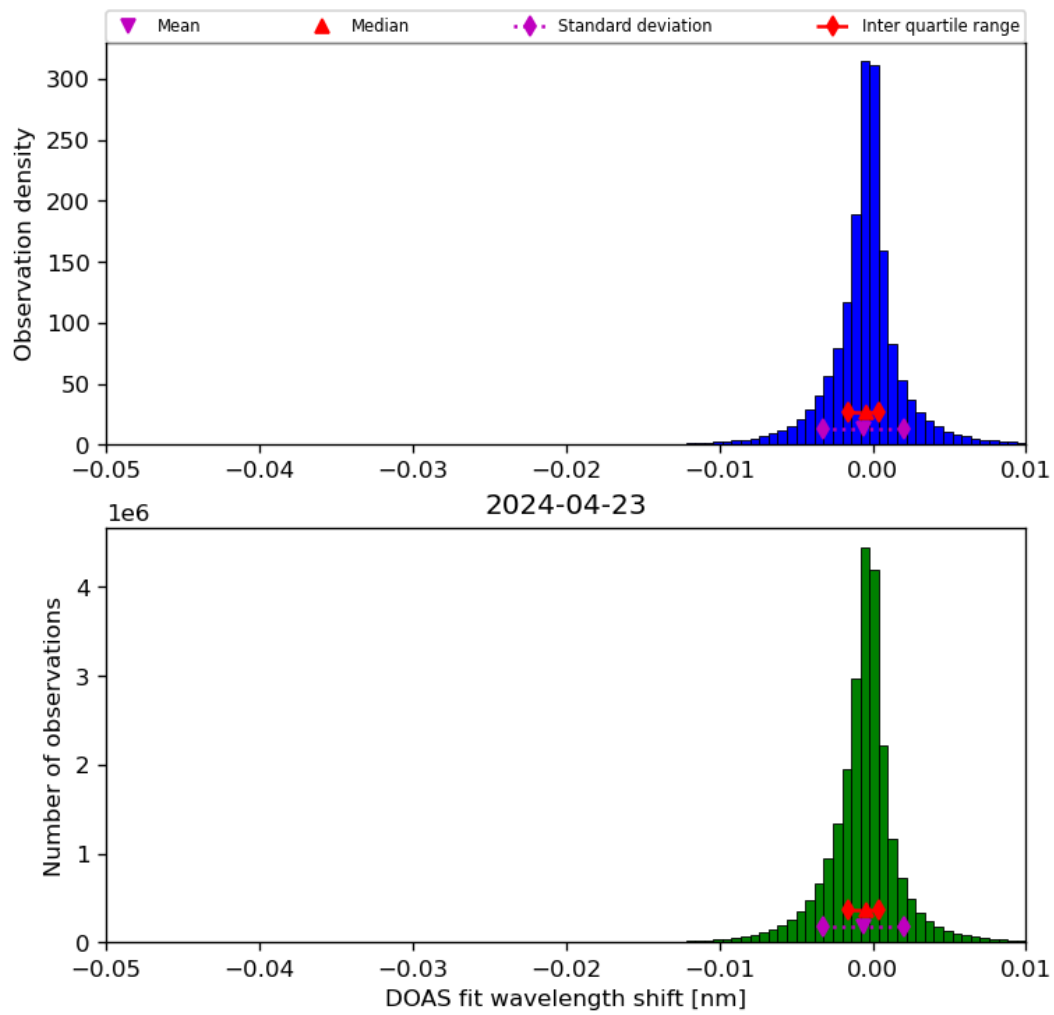
Figure 68: Histogram of “DOAS fit wavelength shift” for 2024-04-22 to 2024-04-24
