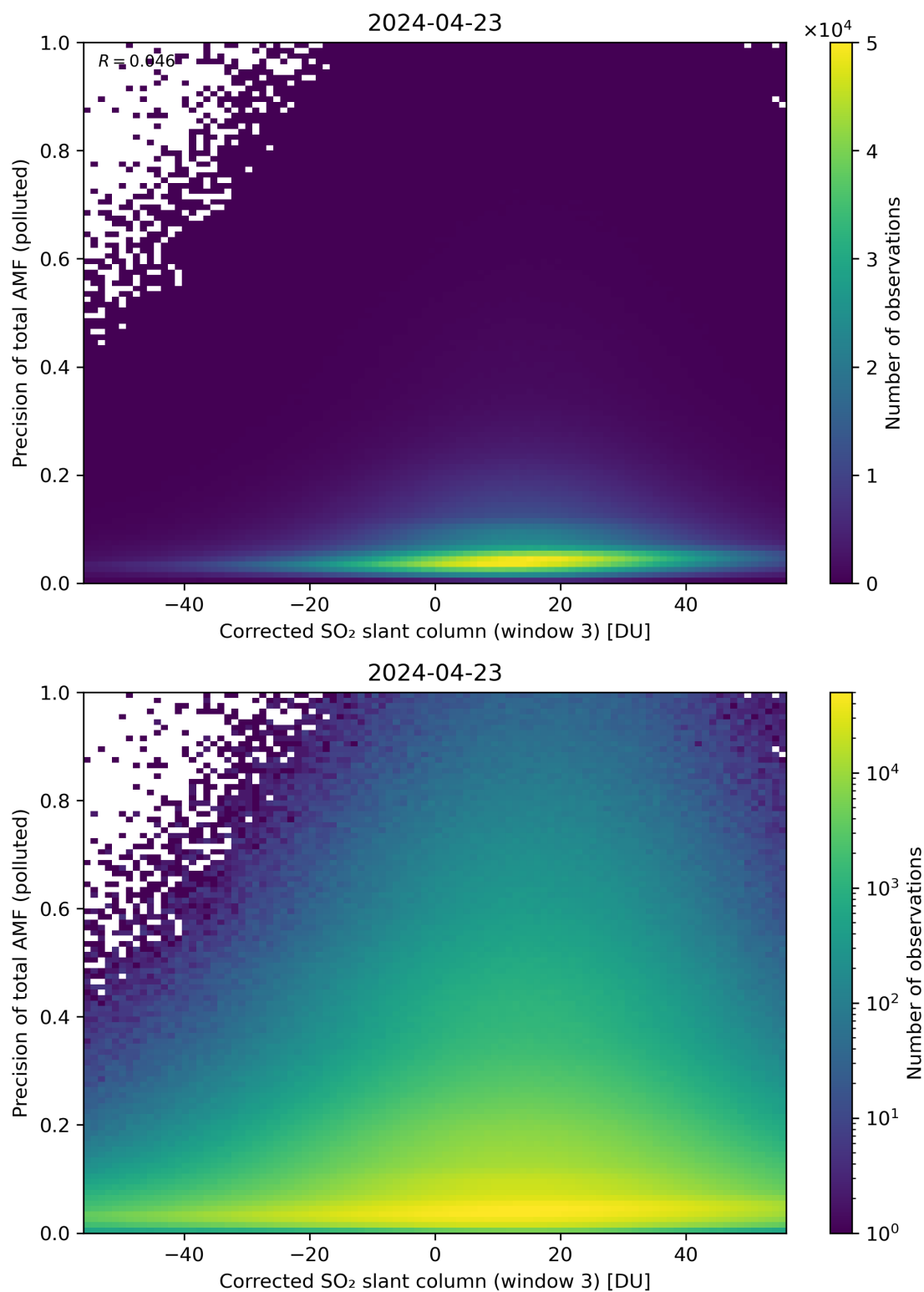
Figure 211: Scatter density plot of “Corrected SO 2 slant column (window 3)” against “Precision of total AMF (polluted)” for 2024-04-22 to 2024-04-24.
