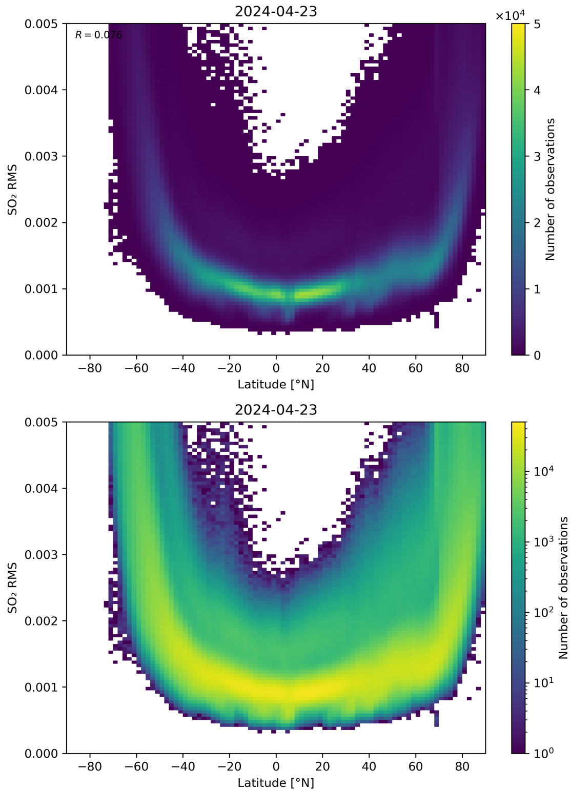
Figure 144: Scatter density plot of “Latitude” against “SO 2 RMS” for 2024-04-22 to 2024-04-24.
