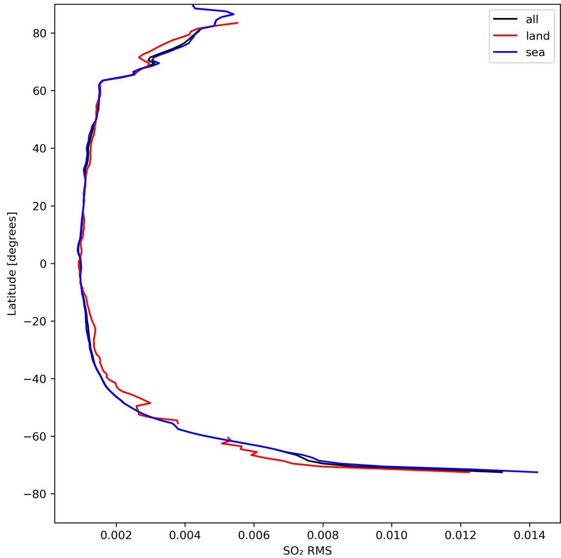
Figure 47: Zonal average of “SO 2 RMS” for 2024-04-22 to 2024-04-24.
