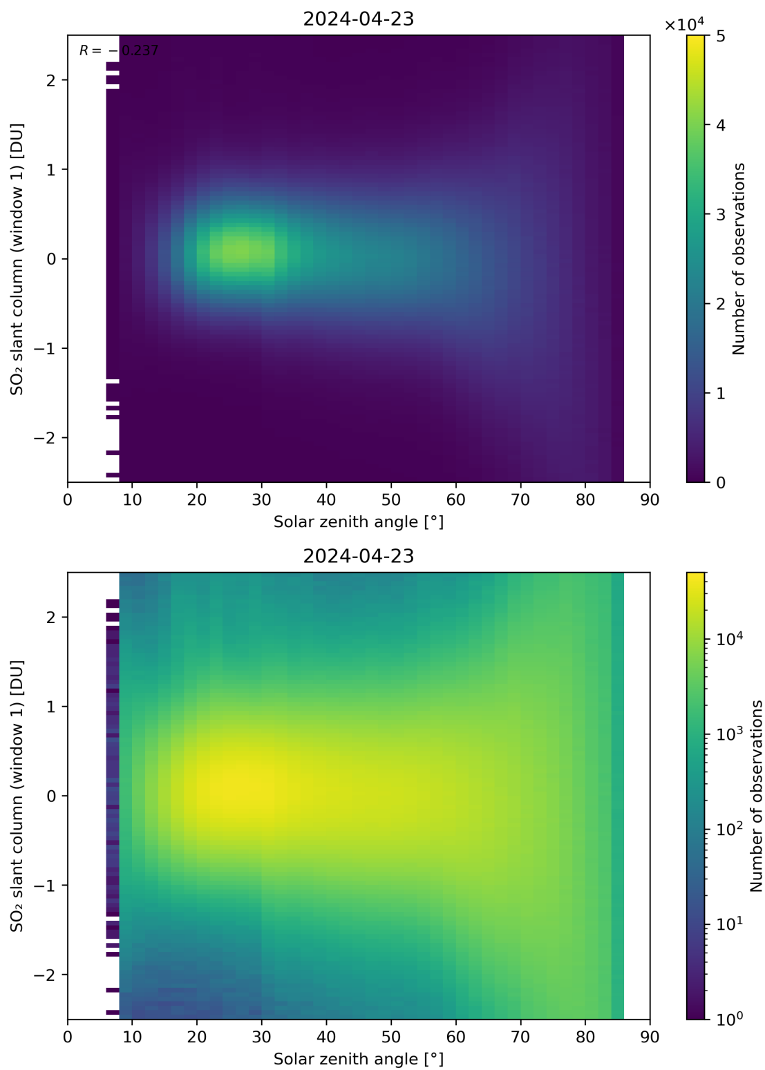
Figure 169: Scatter density plot of “Solar zenith angle” against “SO 2 slant column (window 1)” for 2024-04-22 to 2024-04-24.
