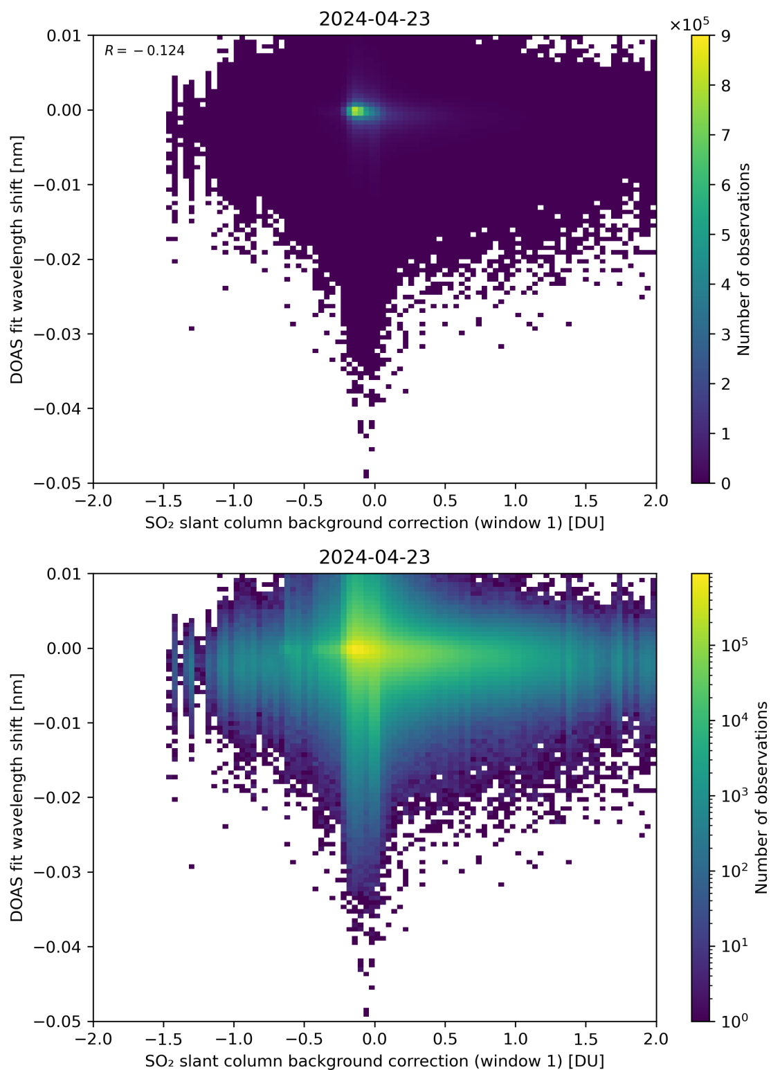
Figure 100: Scatter density plot of “SO 2 slant column background correction (window 1)” against “DOAS fit wavelength shift” for 2024-04-22 to 2024-04-24.
