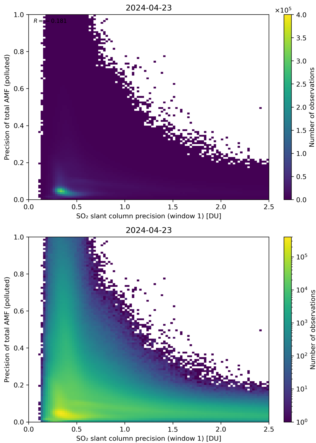
Figure 231: Scatter density plot of “SO 2 slant column precision (window 1)” against “Precision of total AMF (polluted)” for 2024-04-22 to 2024-04-24.
