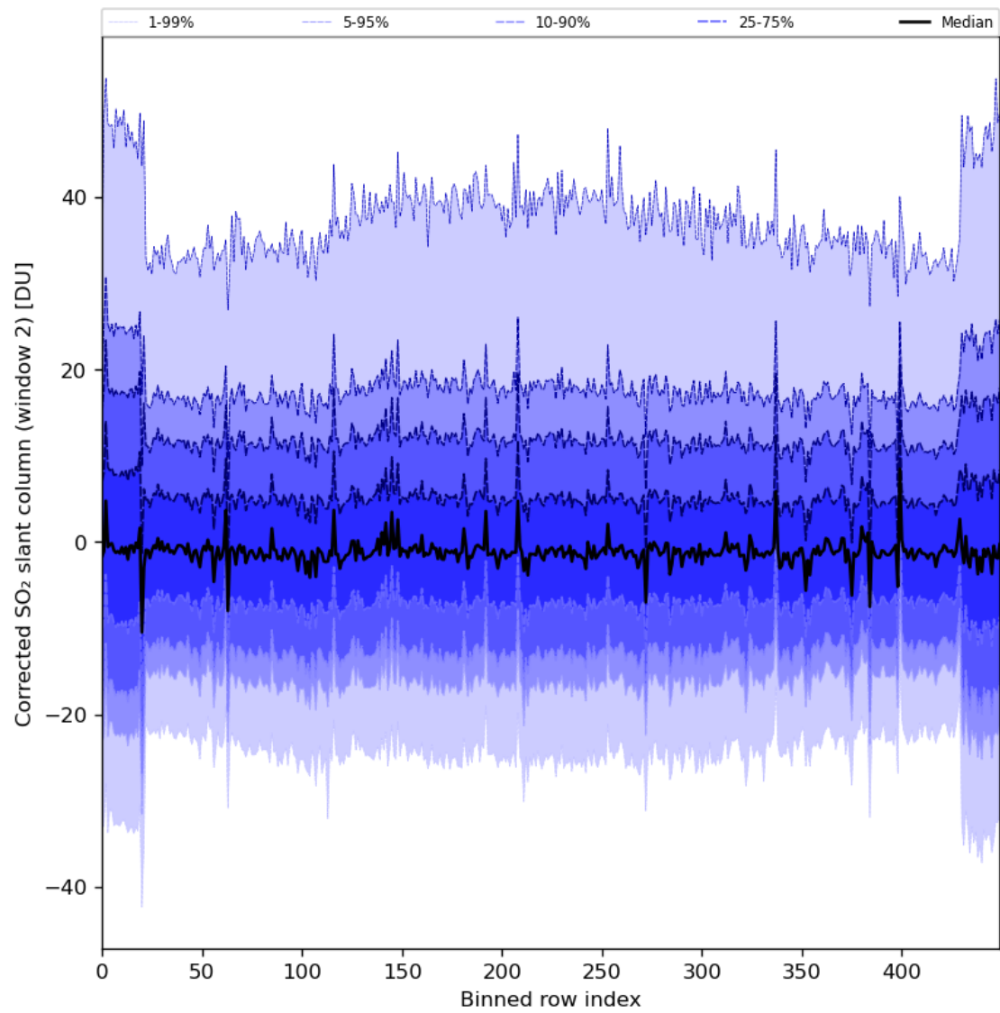
Figure 85: Along track statistics of “Corrected SO 2 slant column (window 2)” for 2024-04-22 to 2024-04-24
