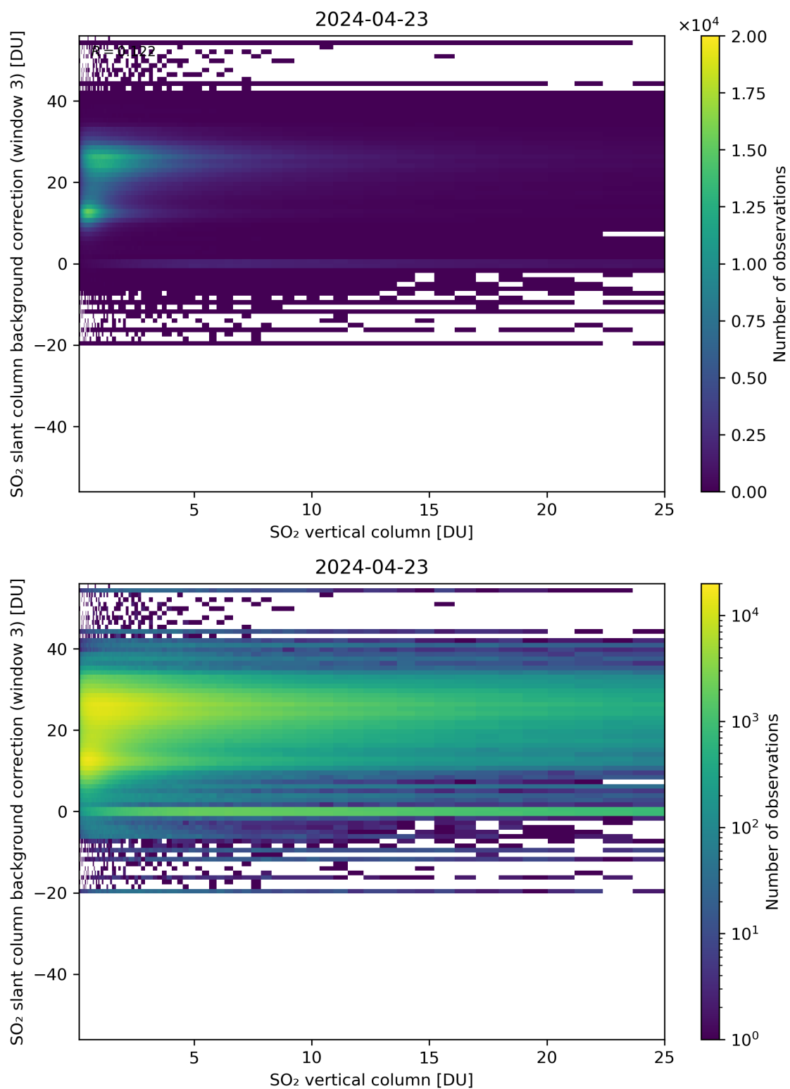
Figure 275: Scatter density plot of “SO 2 vertical column” against “SO 2 slant column background correction (window 3)” for 2024-04-22 to 2024-04-24.
