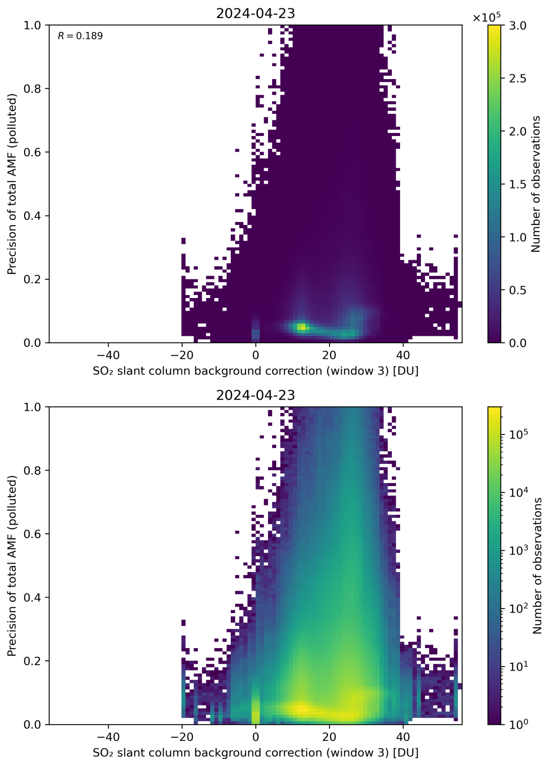
Figure 126: Scatter density plot of “SO 2 slant column background correction (window 3)” against “Precision of total AMF (polluted)” for 2024-04-22 to 2024-04-24.
