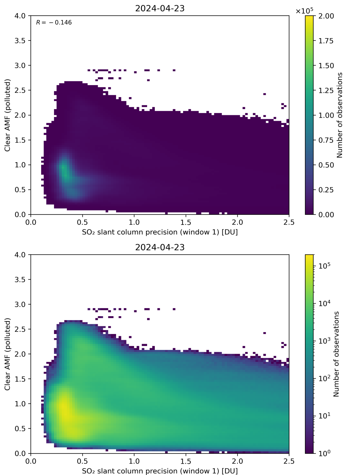
Figure 224: Scatter density plot of “SO 2 slant column precision (window 1)” against “Clear AMF (polluted)” for 2024-04-22 to 2024-04-24.
