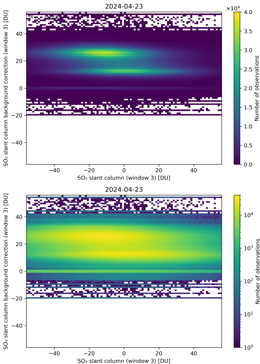
Figure 253: Scatter density plot of “SO 2 slant column (window 3)” against “SO 2 slant column background correction (window 3)” for 2024-04-22 to 2024-04-24.
