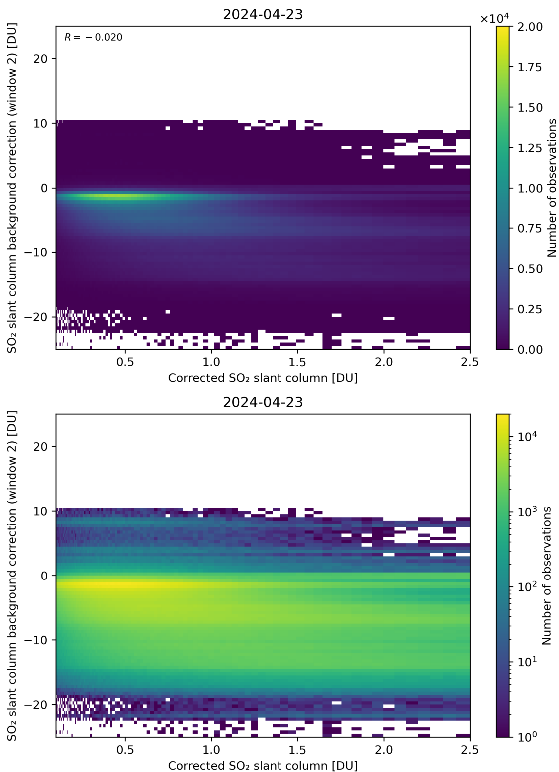
Figure 179: Scatter density plot of “Corrected SO 2 slant column” against “SO 2 slant column background correction (window 2)” for 2024-04-22 to 2024-04-24.
