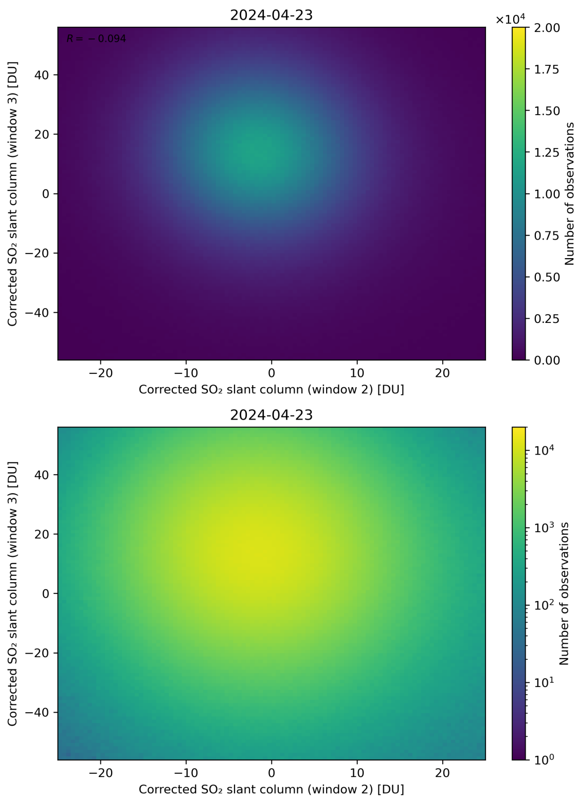
Figure 200: Scatter density plot of “Corrected SO 2 slant column (window 2)” against “Corrected SO 2 slant column (window 3)” for 2024-04-22 to 2024-04-24.
