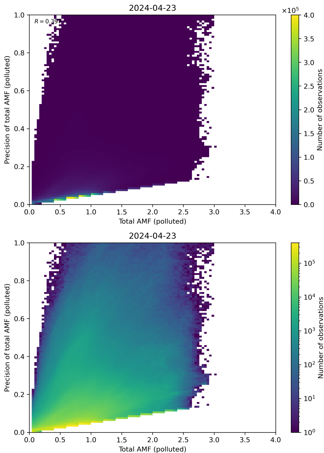
Figure 272: Scatter density plot of “Total AMF (polluted)” against “Precision of total AMF (polluted)” for 2024-04-22 to 2024-04-24.
