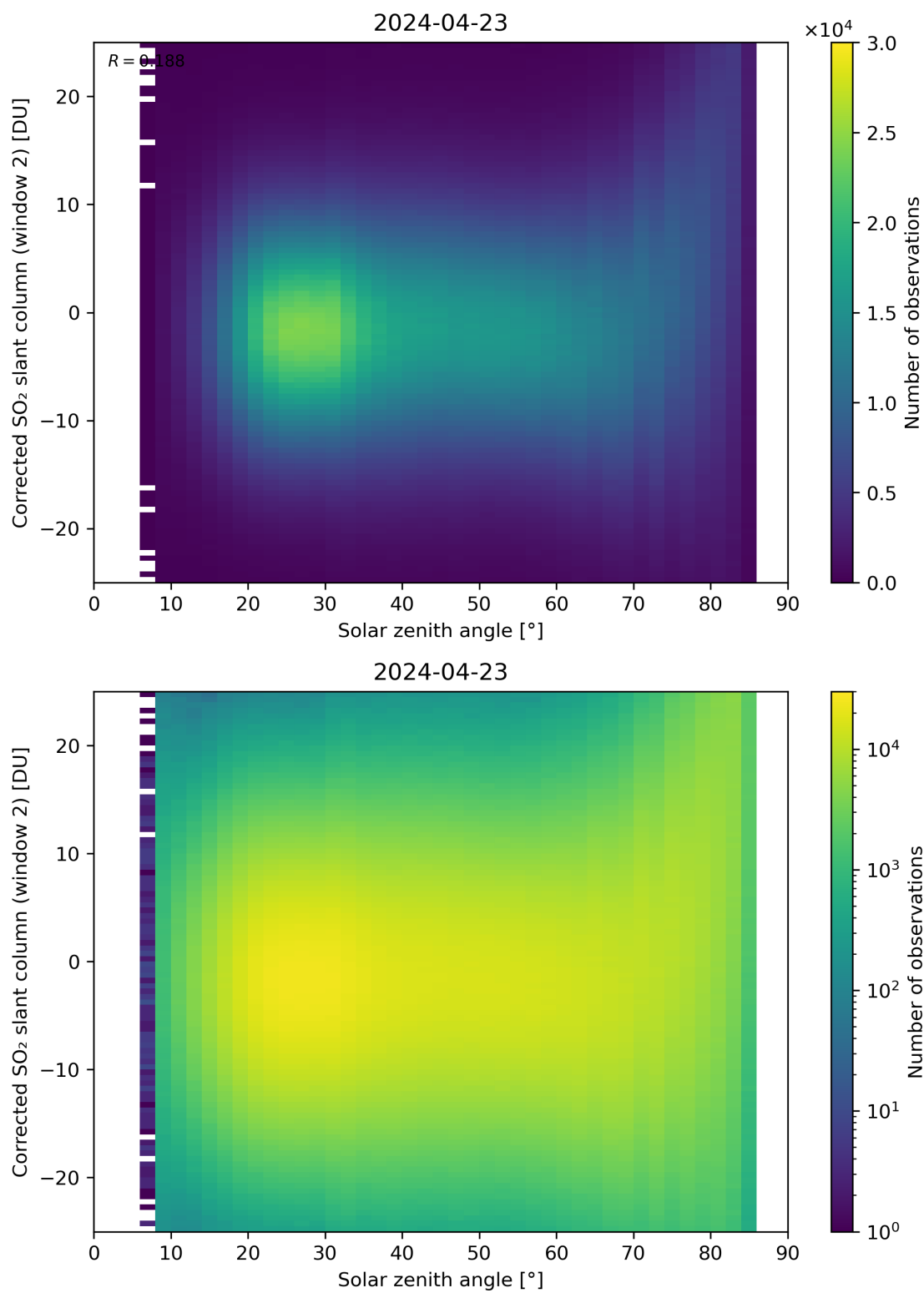
Figure 167: Scatter density plot of “Solar zenith angle” against “Corrected SO 2 slant column (window 2)” for 2024-04-22 to 2024-04-24.
