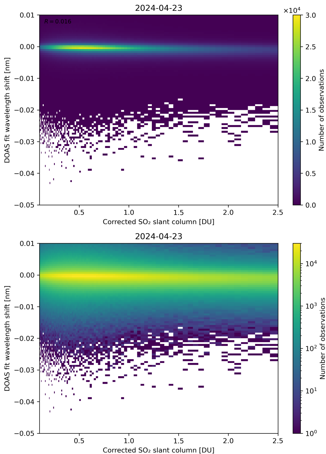
Figure 181: Scatter density plot of “Corrected SO 2 slant column” against “DOAS fit wavelength shift” for 2024-04-22 to 2024-04-24.
