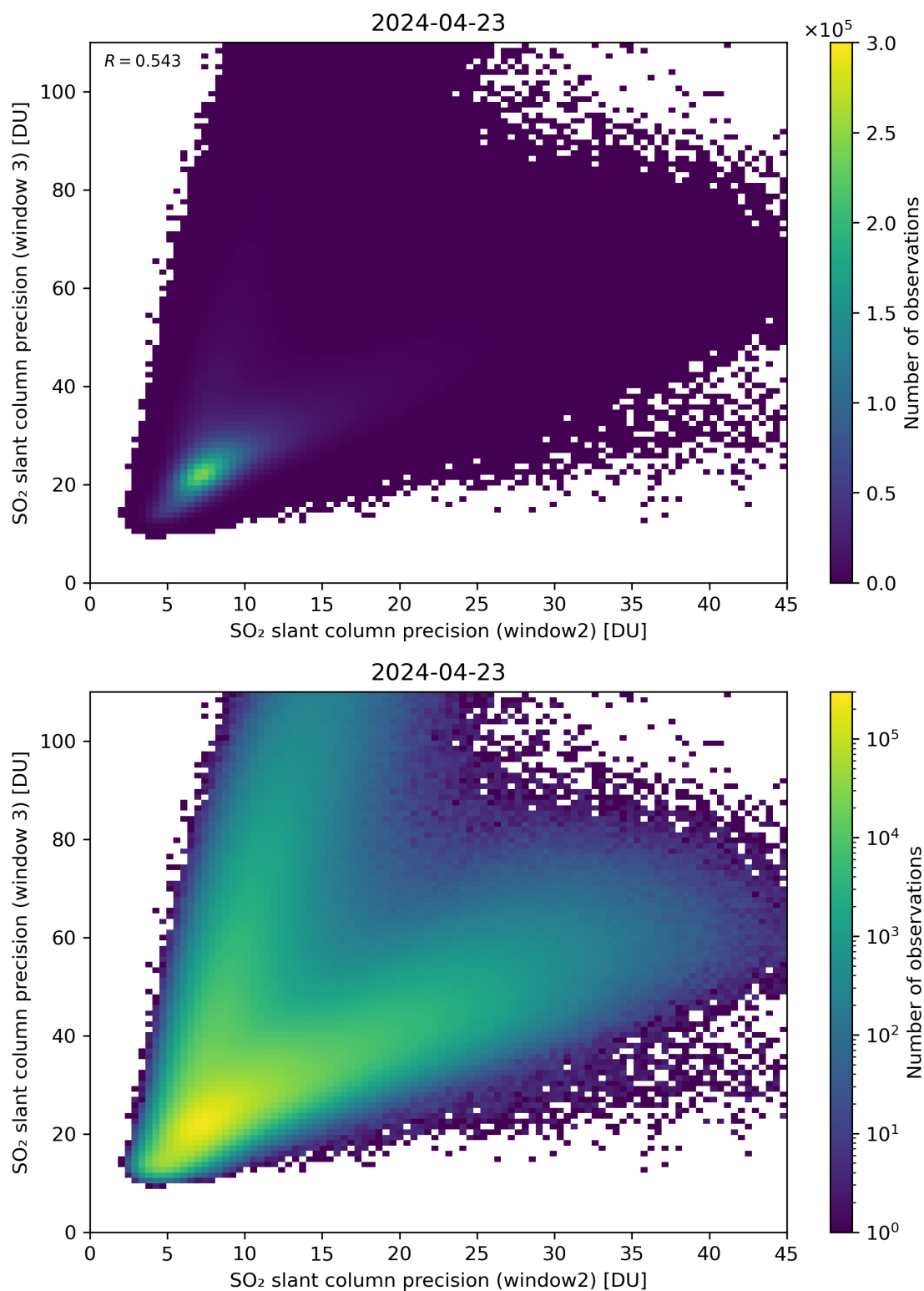
Figure 250: Scatter density plot of “SO 2 slant column precision (window2)” against “SO 2 slant column precision (window 3)” for 2024-04-22 to 2024-04-24.
