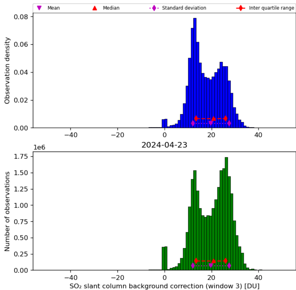
Figure 67: Histogram of “SO 2 slant column background correction (window 3)” for 2024-04-22 to 2024-04-24
