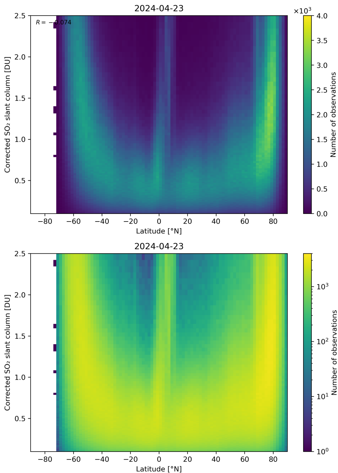
Figure 146: Scatter density plot of “Latitude” against “Corrected SO 2 slant column” for 2024-04-22 to 2024-04-24.
