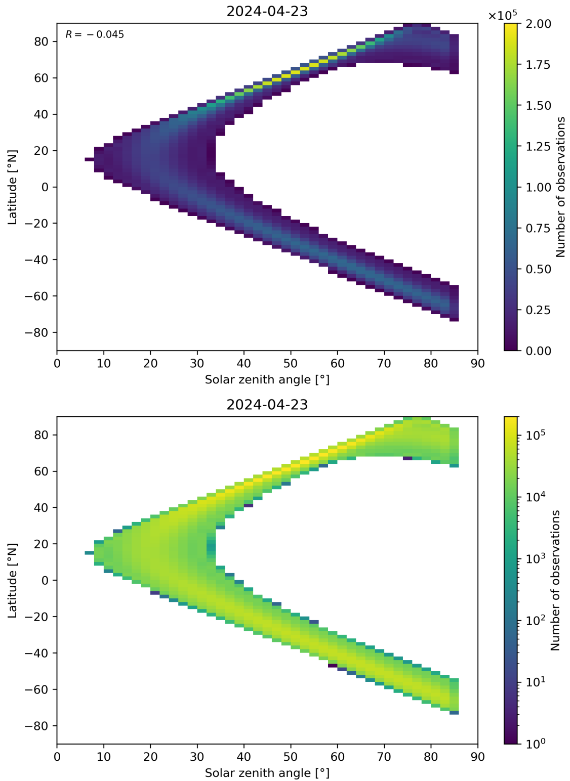
Figure 164: Scatter density plot of “Solar zenith angle” against “Latitude” for 2024-04-22 to 2024-04-24.
