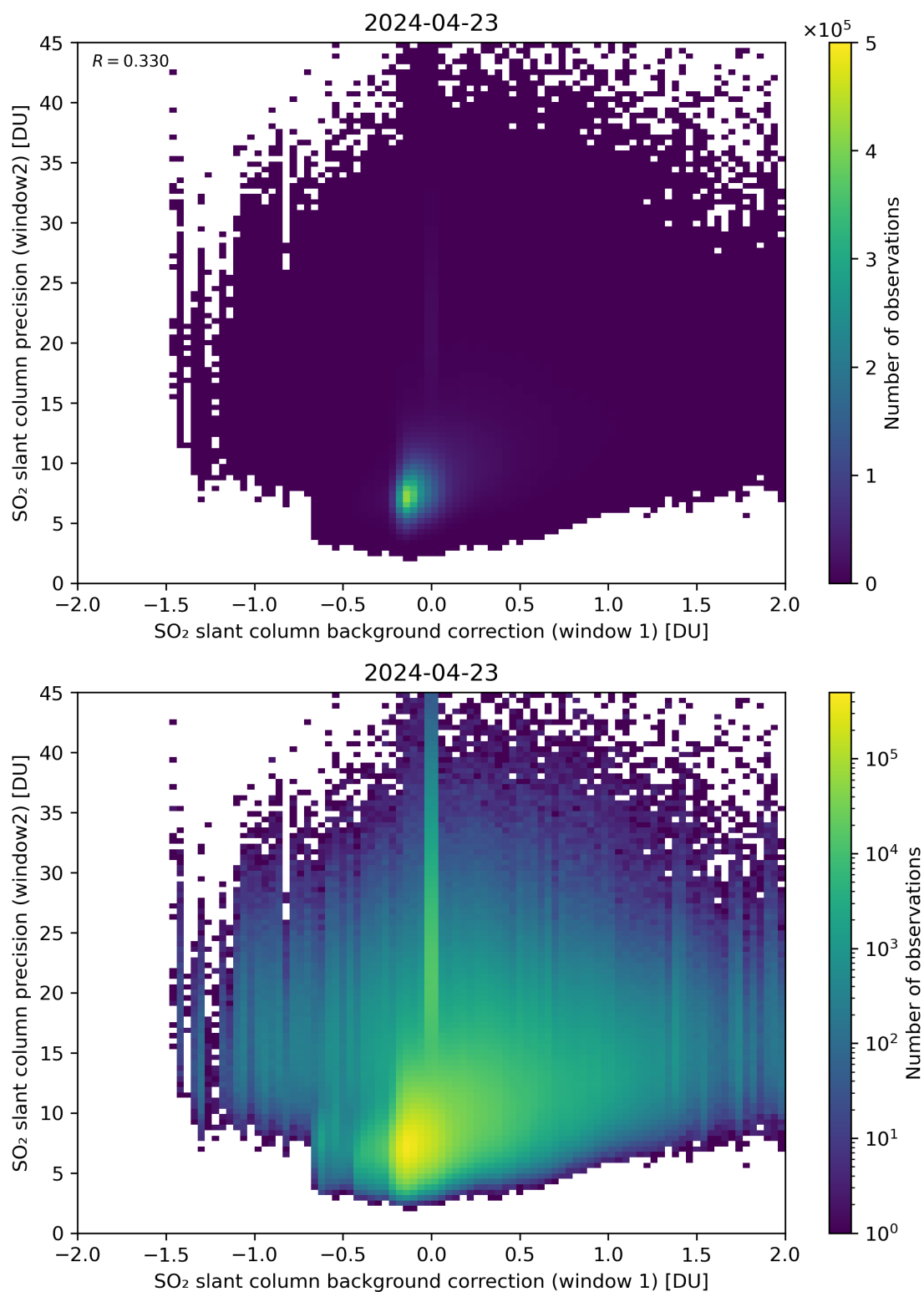
Figure 106: Scatter density plot of “SO 2 slant column background correction (window 1)” against “SO 2 slant column precision (window2)” for 2024-04-22 to 2024-04-24.
