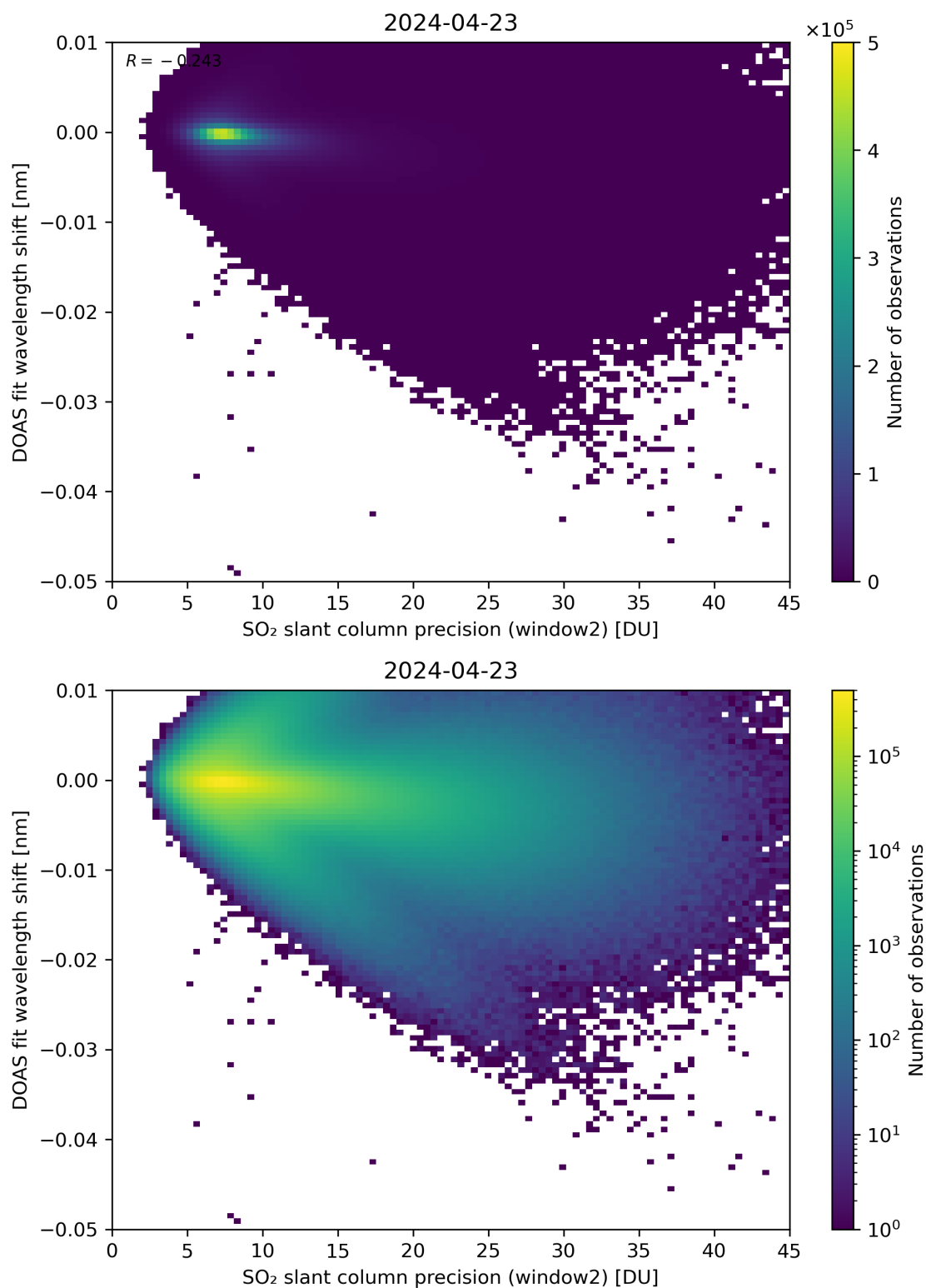
Figure 243: Scatter density plot of “SO 2 slant column precision (window2)” against “DOAS fit wavelength shift” for 2024-04-22 to 2024-04-24.
