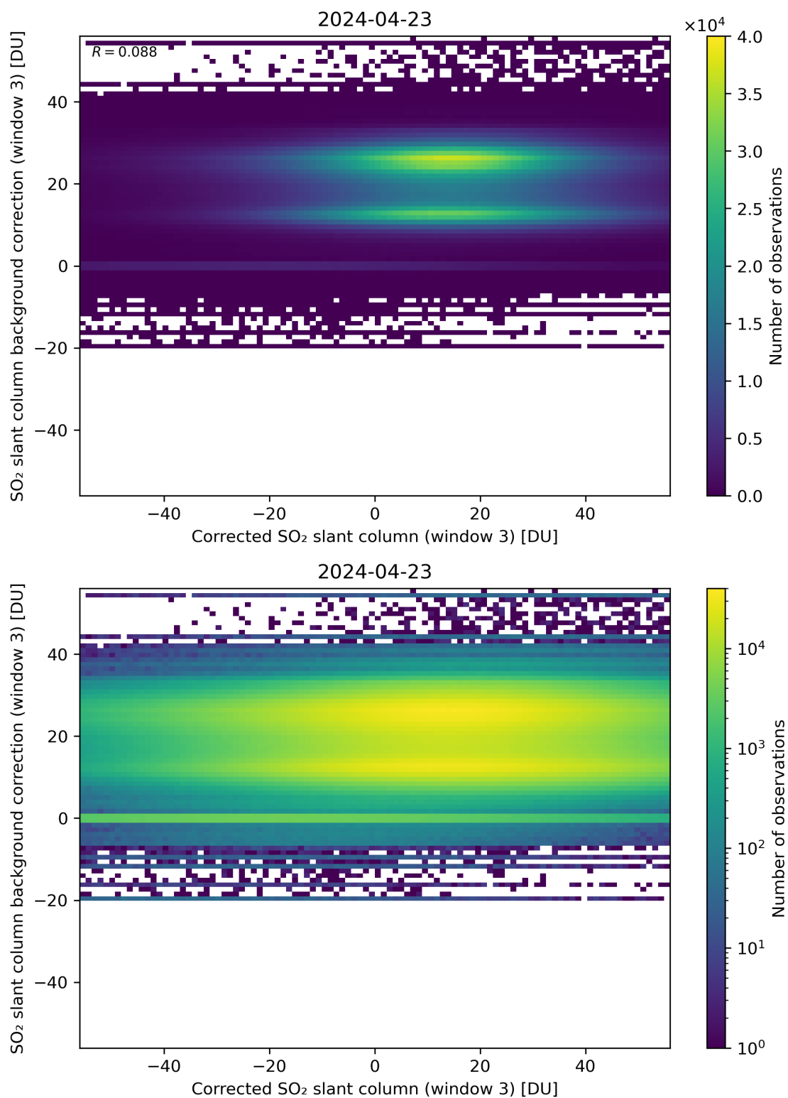
Figure 205: Scatter density plot of “Corrected SO 2 slant column (window 3)” against “SO 2 slant column background correction (window 3)” for 2024-04-22 to 2024-04-24.
