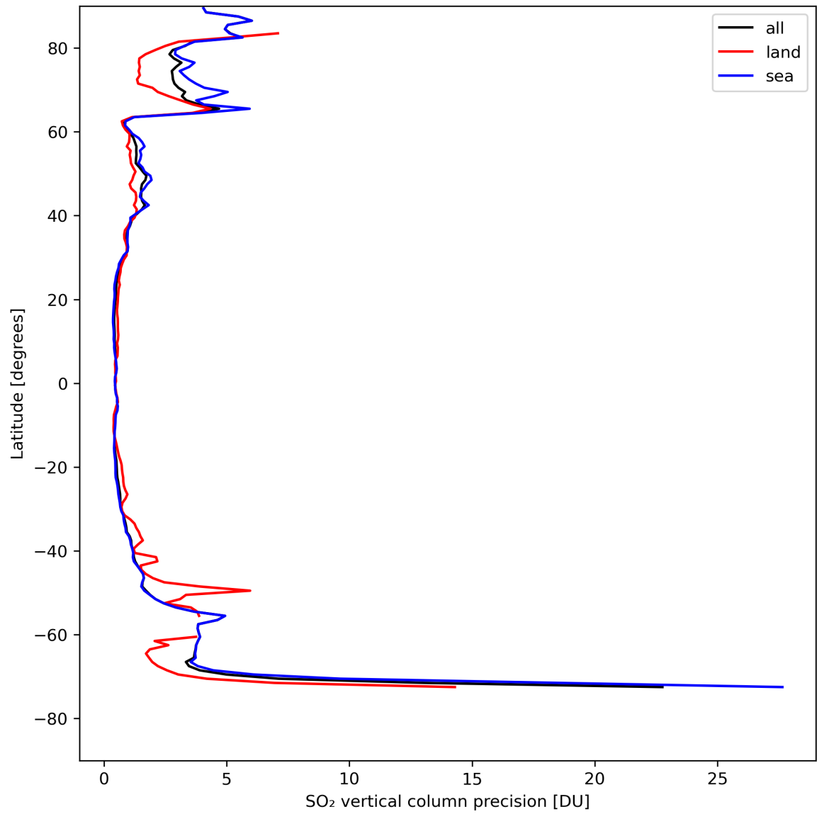
Figure 31: Zonal average of “SO 2 vertical column precision” for 2024-04-22 to 2024-04-24.
