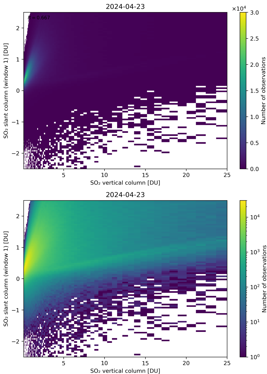
Figure 300: Scatter density plot of “SO 2 vertical column” against “SO 2 slant column (window 1)” for 2024-04-22 to 2024-04-24.
