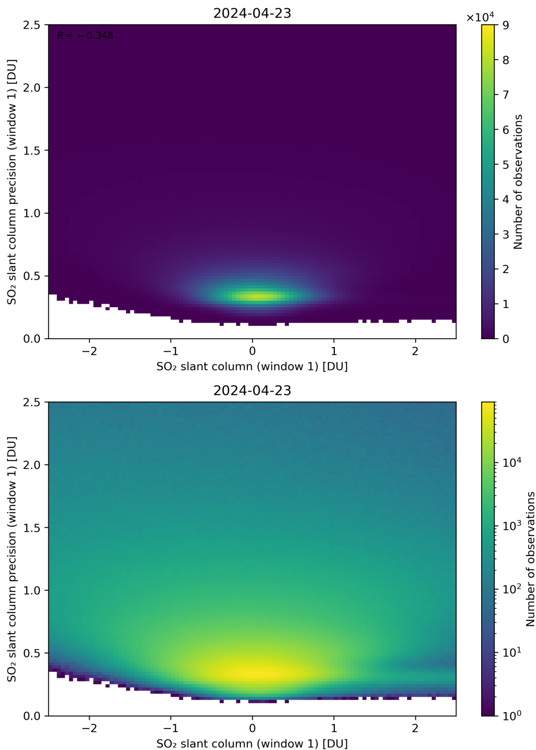
Figure 235: Scatter density plot of “SO 2 slant column (window 1)” against “SO 2 slant column precision (window 1)” for 2024-04-22 to 2024-04-24.
