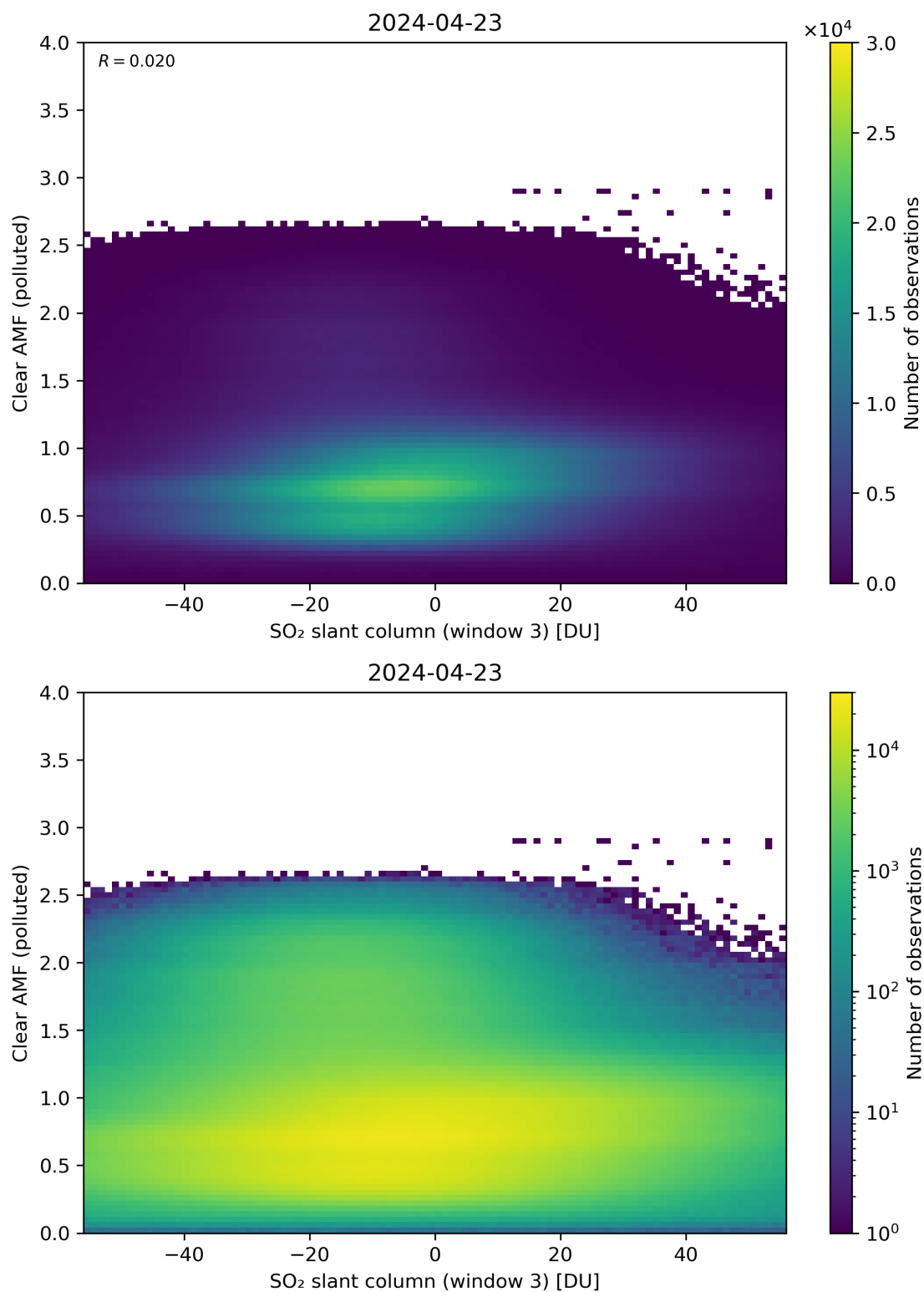
Figure 265: Scatter density plot of “SO 2 slant column (window 3)” against “Clear AMF (polluted)” for 2024-04-22 to 2024-04-24.
