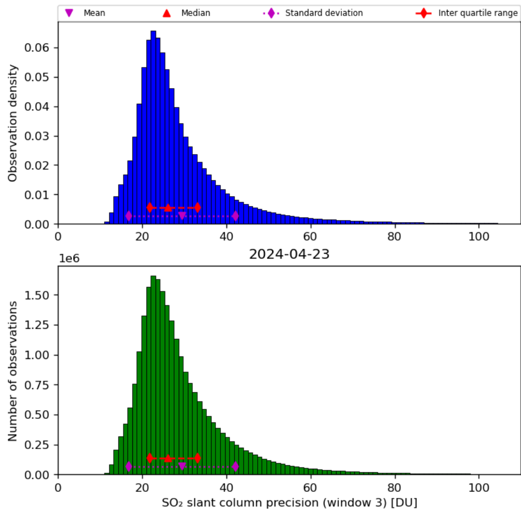
Figure 65: Histogram of “SO 2 slant column precision (window 3)” for 2024-04-22 to 2024-04-24
