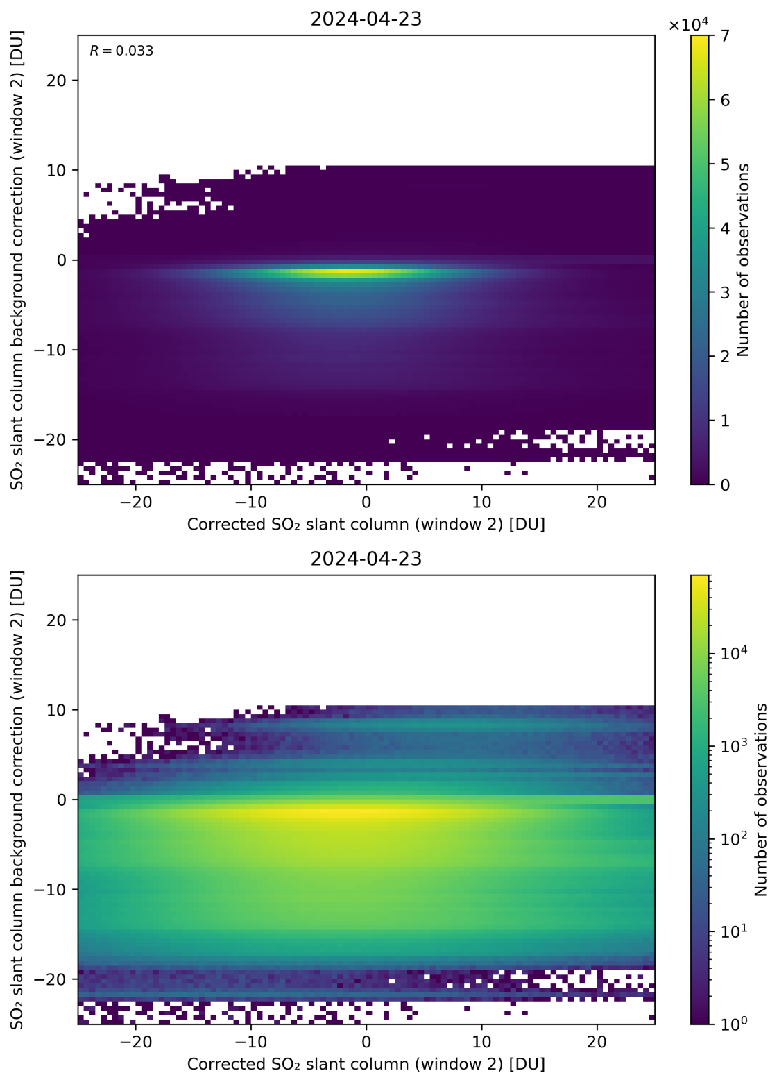
Figure 194: Scatter density plot of “Corrected SO 2 slant column (window 2)” against “SO 2 slant column background correction (window 2)” for 2024-04-22 to 2024-04-24.
