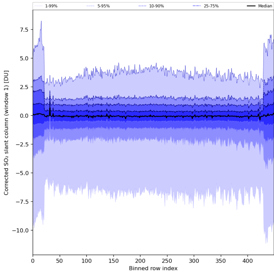
Figure 81: Along track statistics of “Corrected SO 2 slant column (window 1)” for 2024-04-22 to 2024-04-24
