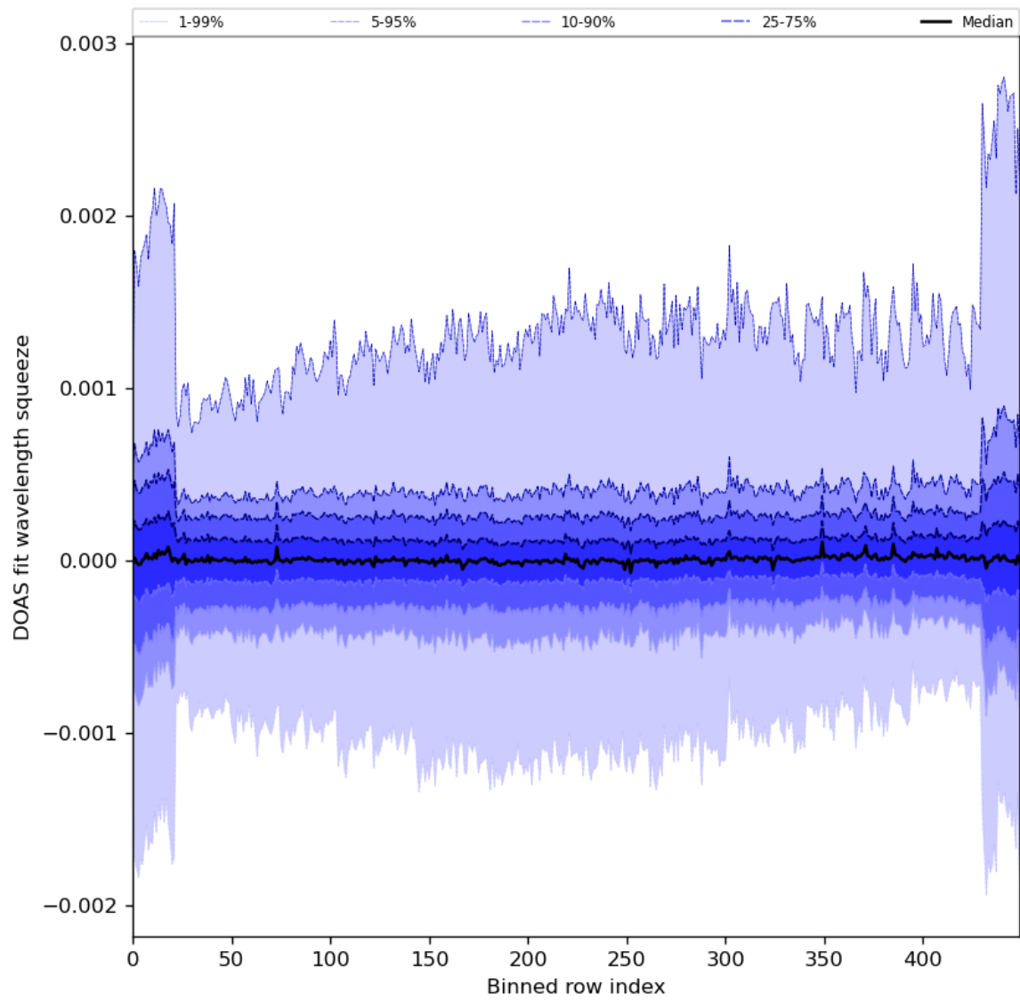
Figure 92: Along track statistics of “DOAS fit wavelength squeeze” for 2024-04-22 to 2024-04-24
