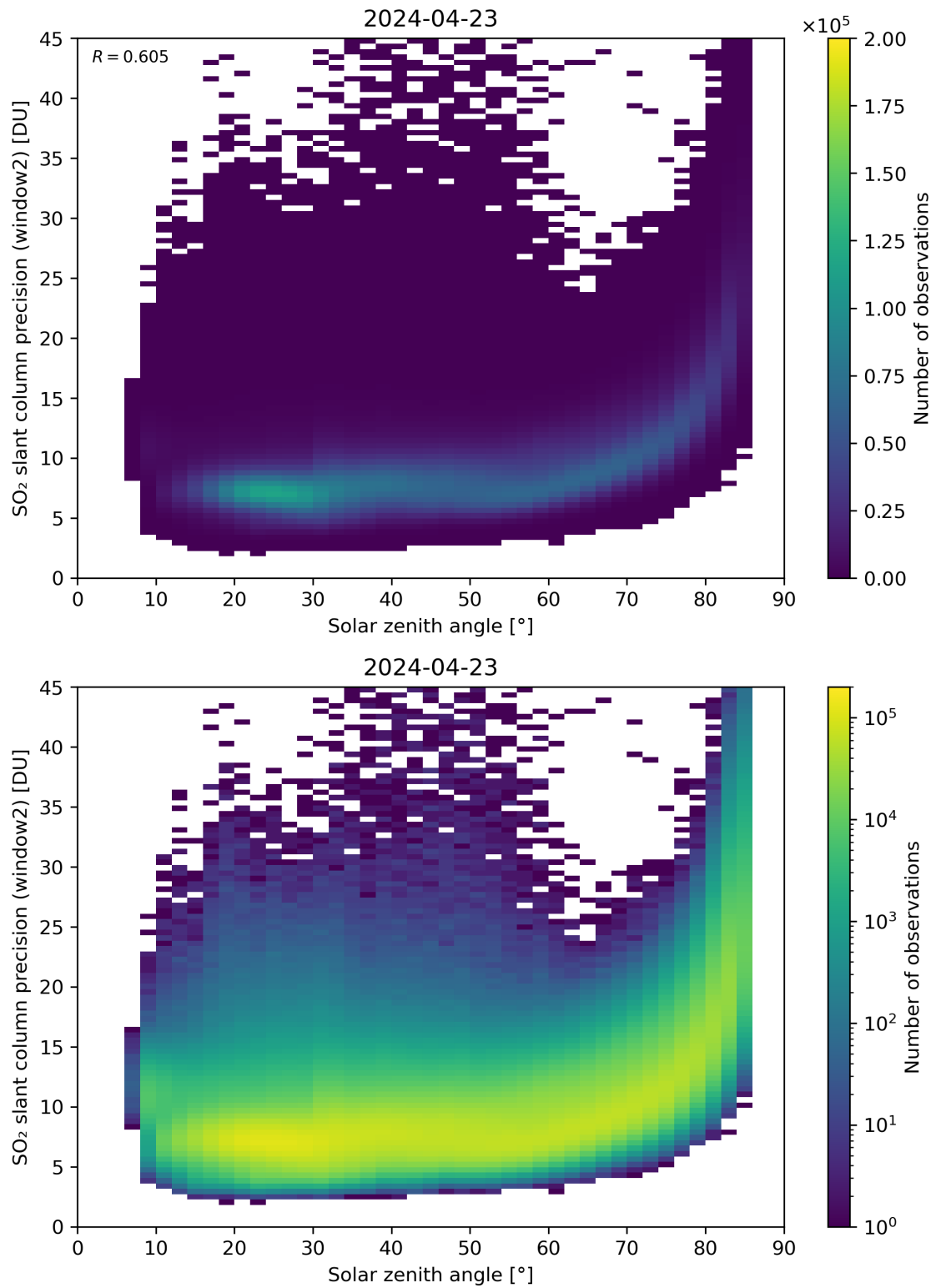
Figure 171: Scatter density plot of “Solar zenith angle” against “SO 2 slant column precision (window2)” for 2024-04-22 to 2024-04-24.
