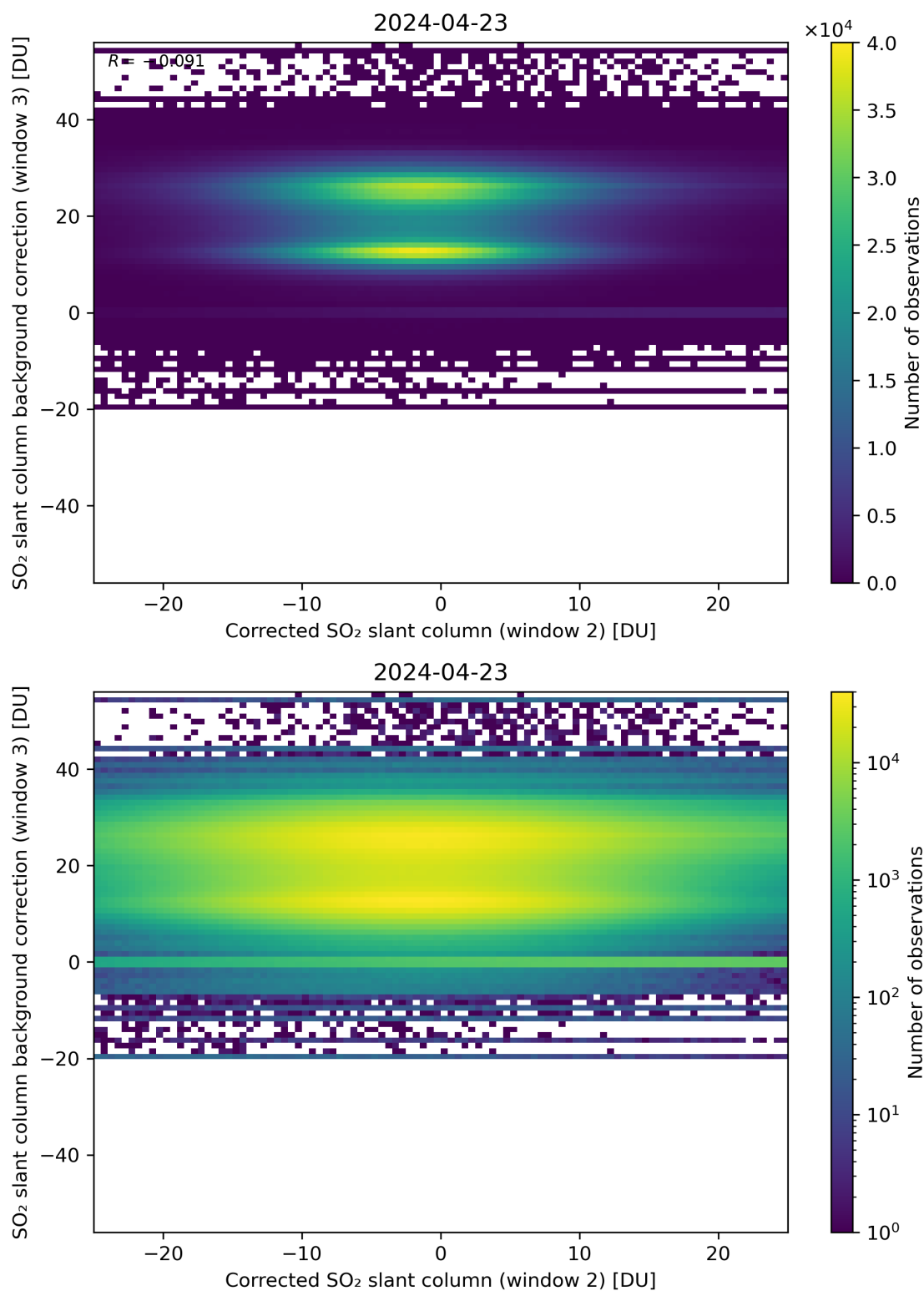
Figure 195: Scatter density plot of “Corrected SO 2 slant column (window 2)” against “SO 2 slant column background correction (window 3)” for 2024-04-22 to 2024-04-24.
