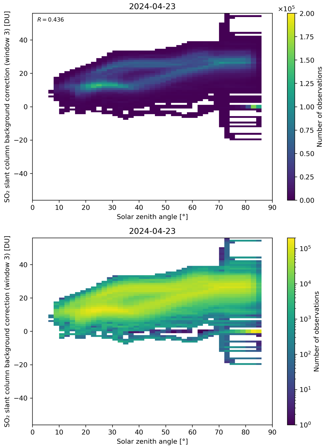
Figure 160: Scatter density plot of “Solar zenith angle” against “SO 2 slant column background correction (window 3)” for 2024-04-22 to 2024-04-24.
