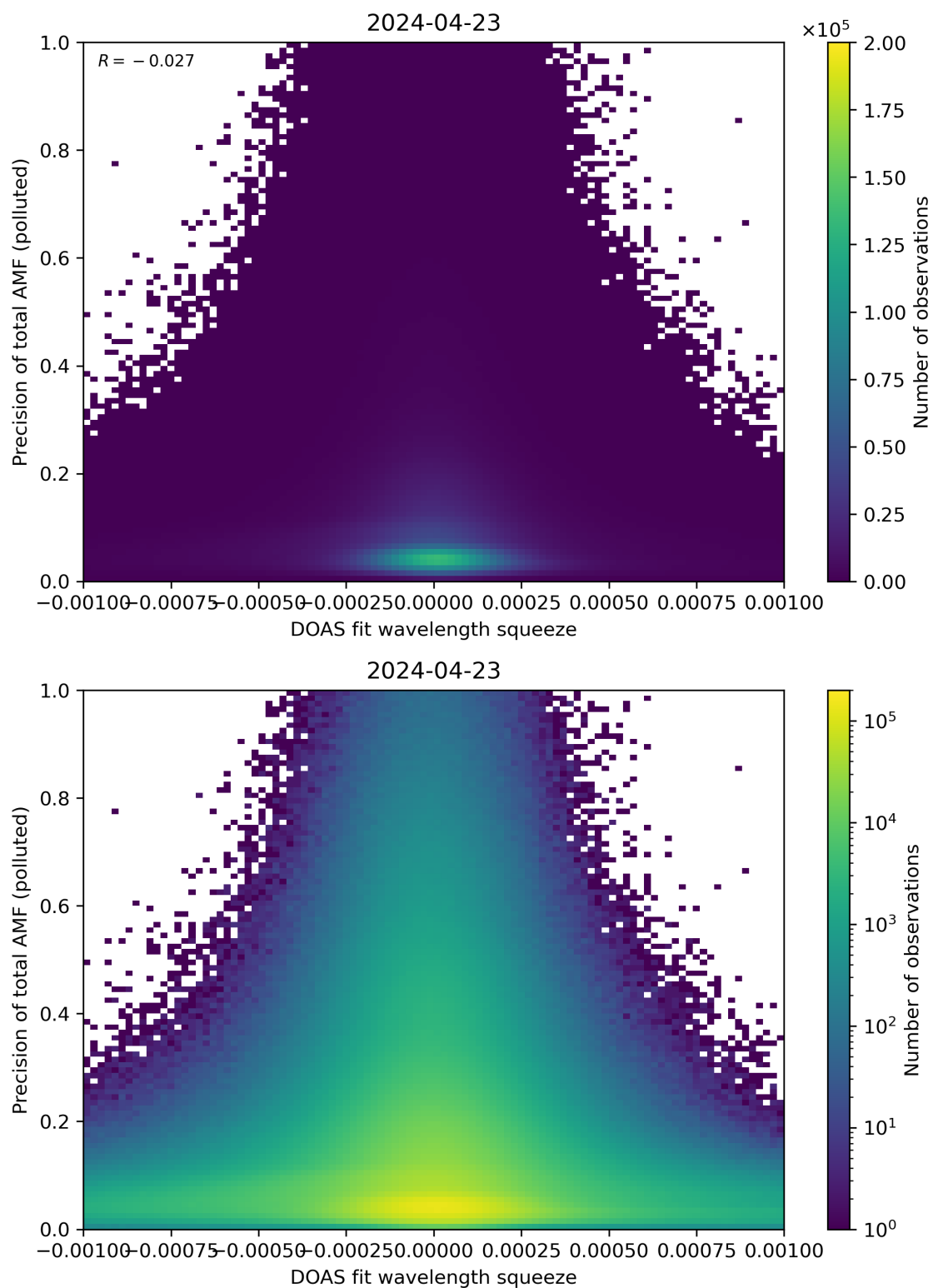
Figure 135: Scatter density plot of “DOAS fit wavelength squeeze” against “Precision of total AMF (polluted)” for 2024-04-22 to 2024-04-24.
