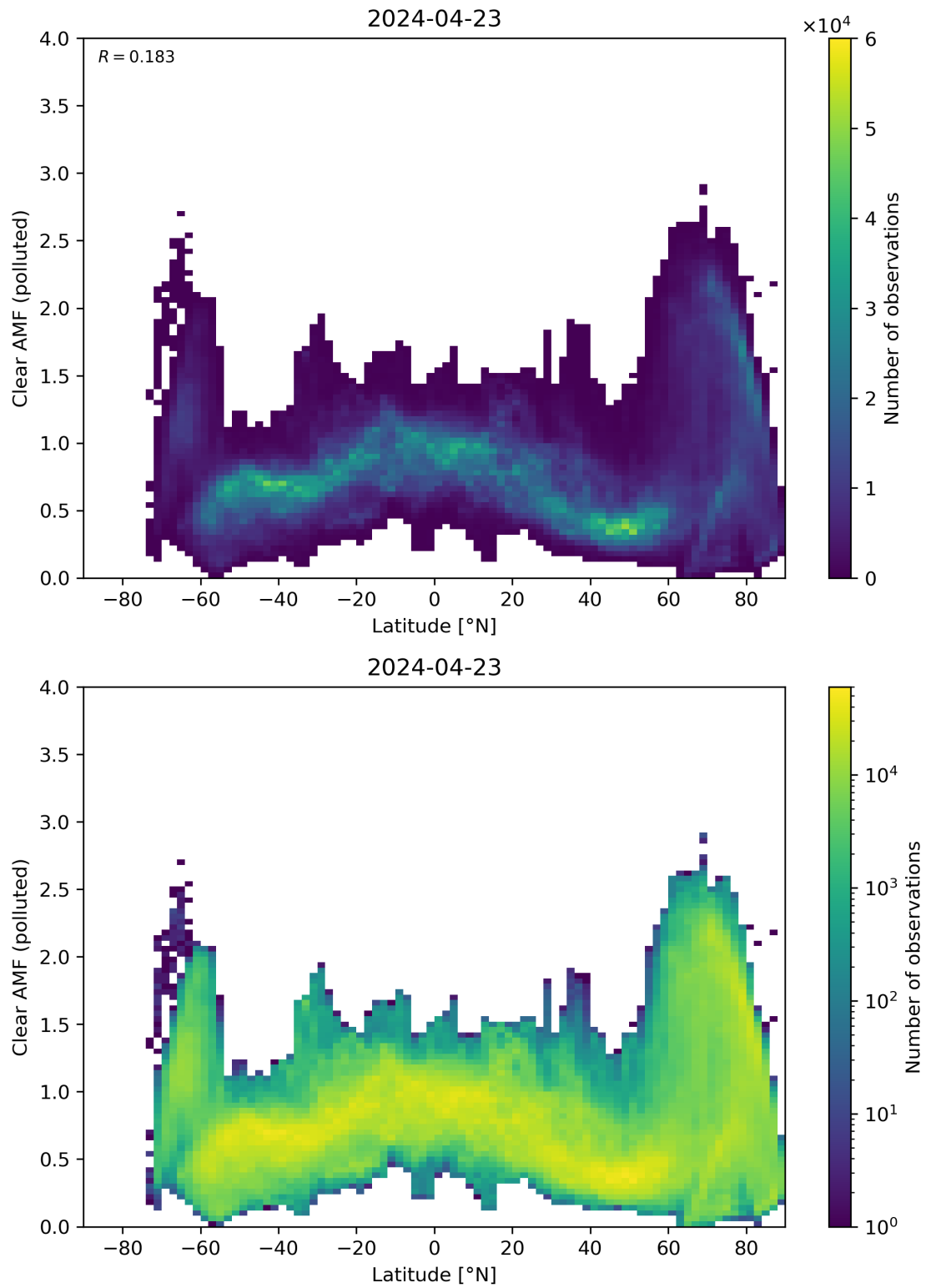
Figure 145: Scatter density plot of “Latitude” against “Clear AMF (polluted)” for 2024-04-22 to 2024-04-24.
