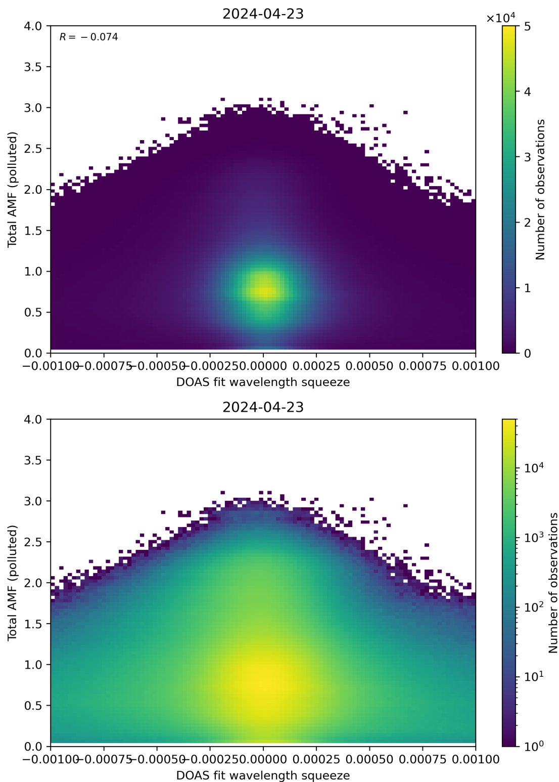
Figure 134: Scatter density plot of “DOAS fit wavelength squeeze” against “Total AMF (polluted)” for 2024-04-22 to 2024-04-24.
