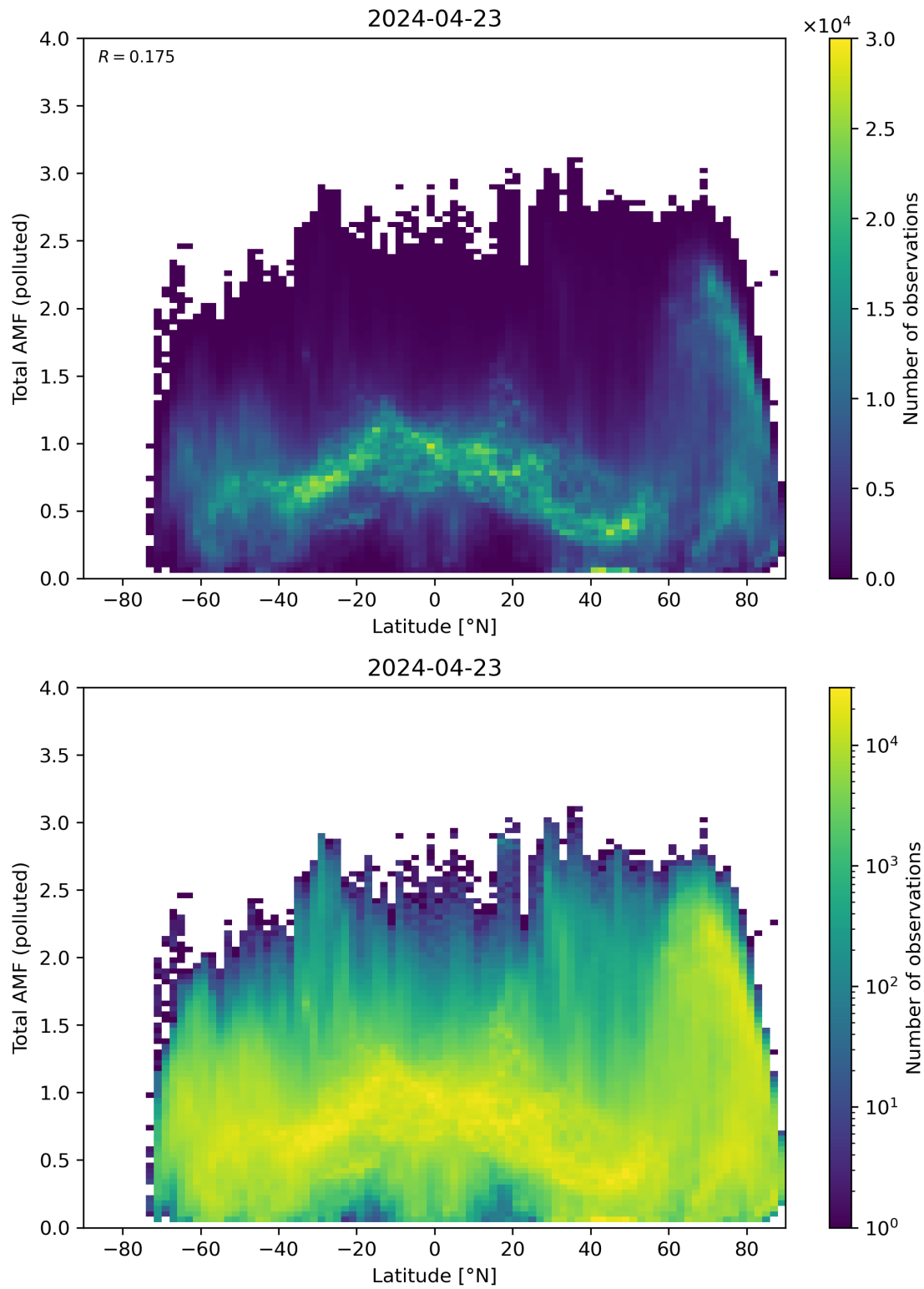
Figure 154: Scatter density plot of “Latitude” against “Total AMF (polluted)” for 2024-04-22 to 2024-04-24.
