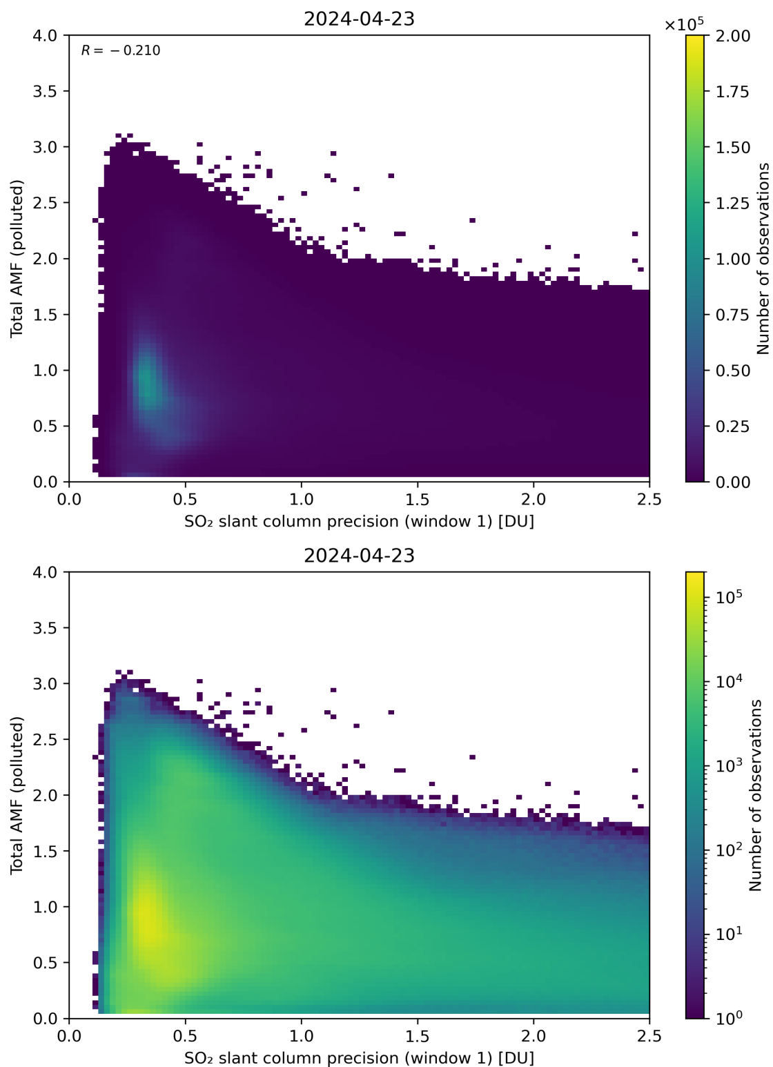
Figure 230: Scatter density plot of “SO 2 slant column precision (window 1)” against “Total AMF (polluted)” for 2024-04-22 to 2024-04-24.
