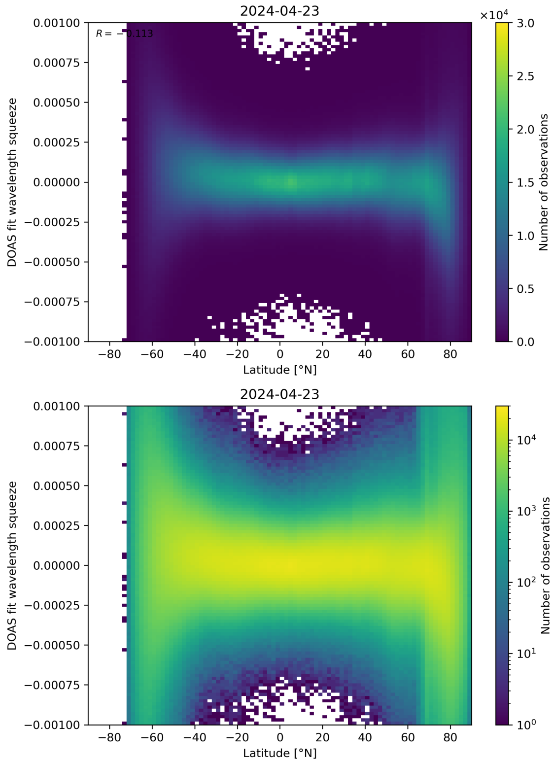
Figure 143: Scatter density plot of “Latitude” against “DOAS fit wavelength squeeze” for 2024-04-22 to 2024-04-24.
