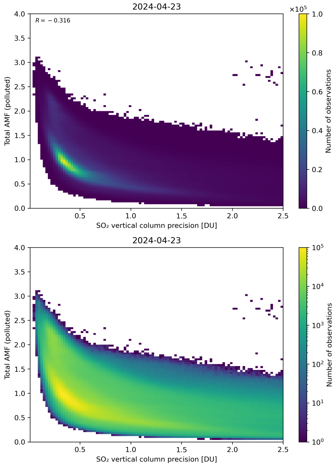
Figure 294: Scatter density plot of “SO 2 vertical column precision” against “Total AMF (polluted)” for 2024-04-22 to 2024-04-24.
