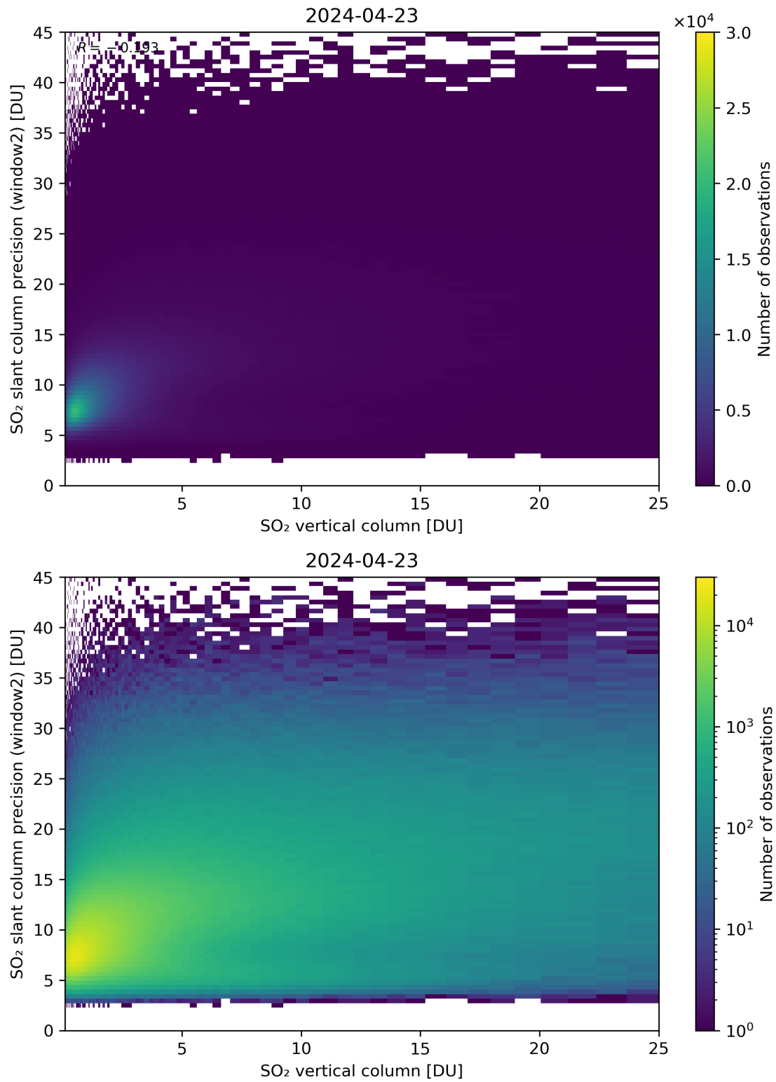
Figure 302: Scatter density plot of “SO 2 vertical column” against “SO 2 slant column precision (window2)” for 2024-04-22 to 2024-04-24.
