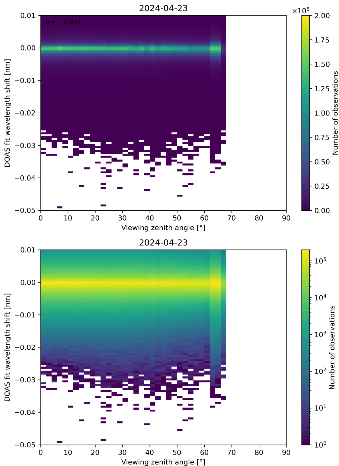
Figure 311: Scatter density plot of “Viewing zenith angle” against “DOAS fit wavelength shift” for 2024-04-22 to 2024-04-24.
