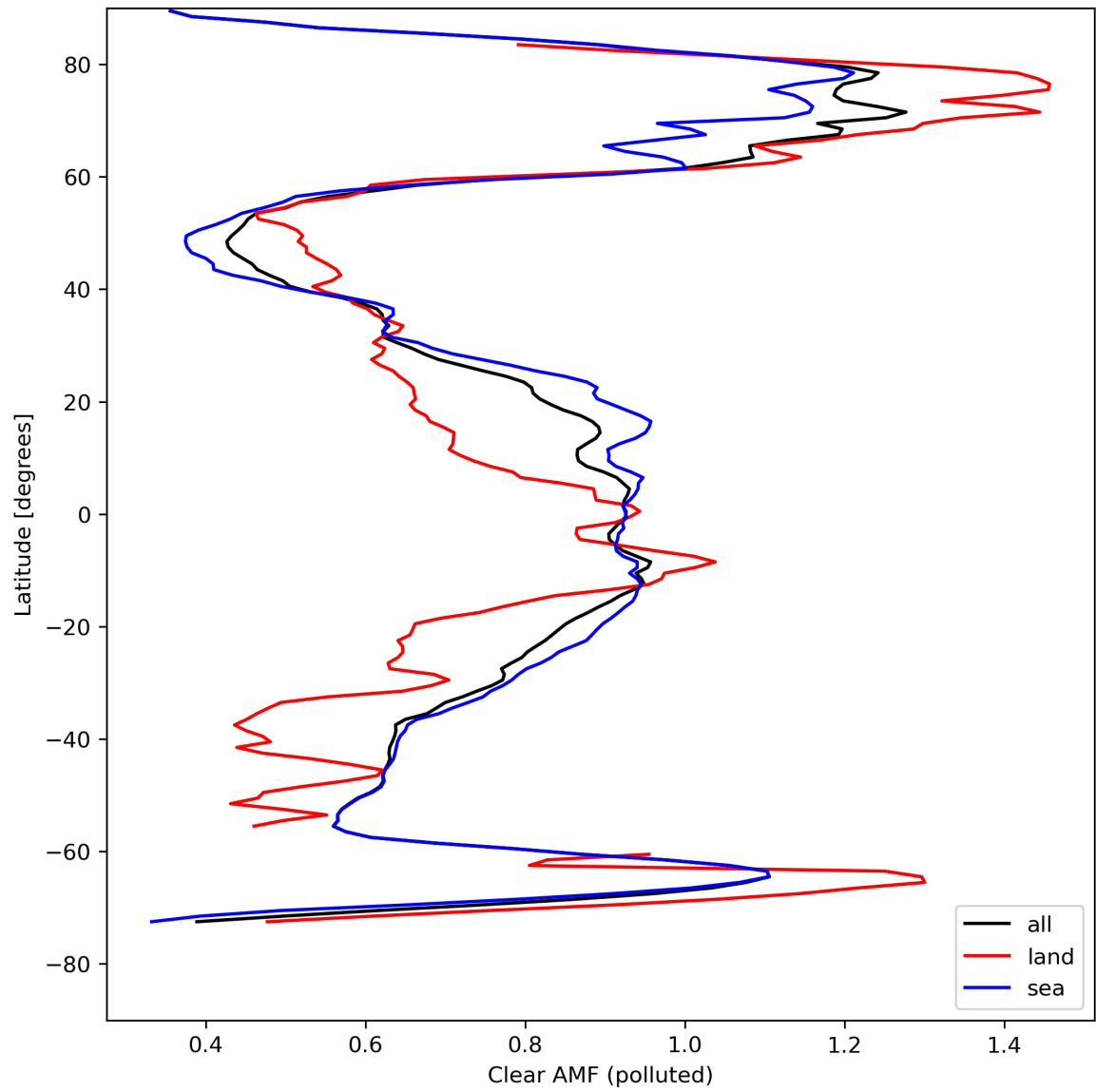
Figure 50: Zonal average of "Clear AMF (polluted)" for 2024-04-22 to 2024-04-24.
