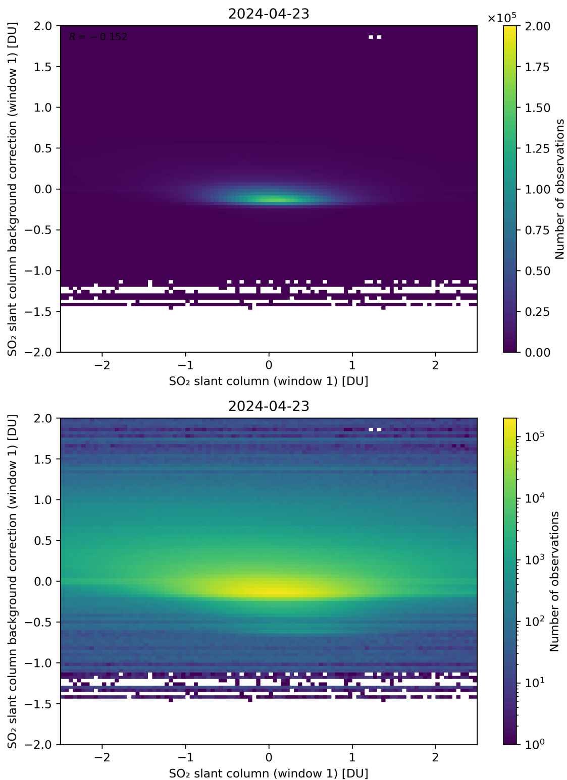
Figure 212: Scatter density plot of “SO 2 slant column (window 1)” against “SO 2 slant column background correction (window 1)” for 2024-04-22 to 2024-04-24.
