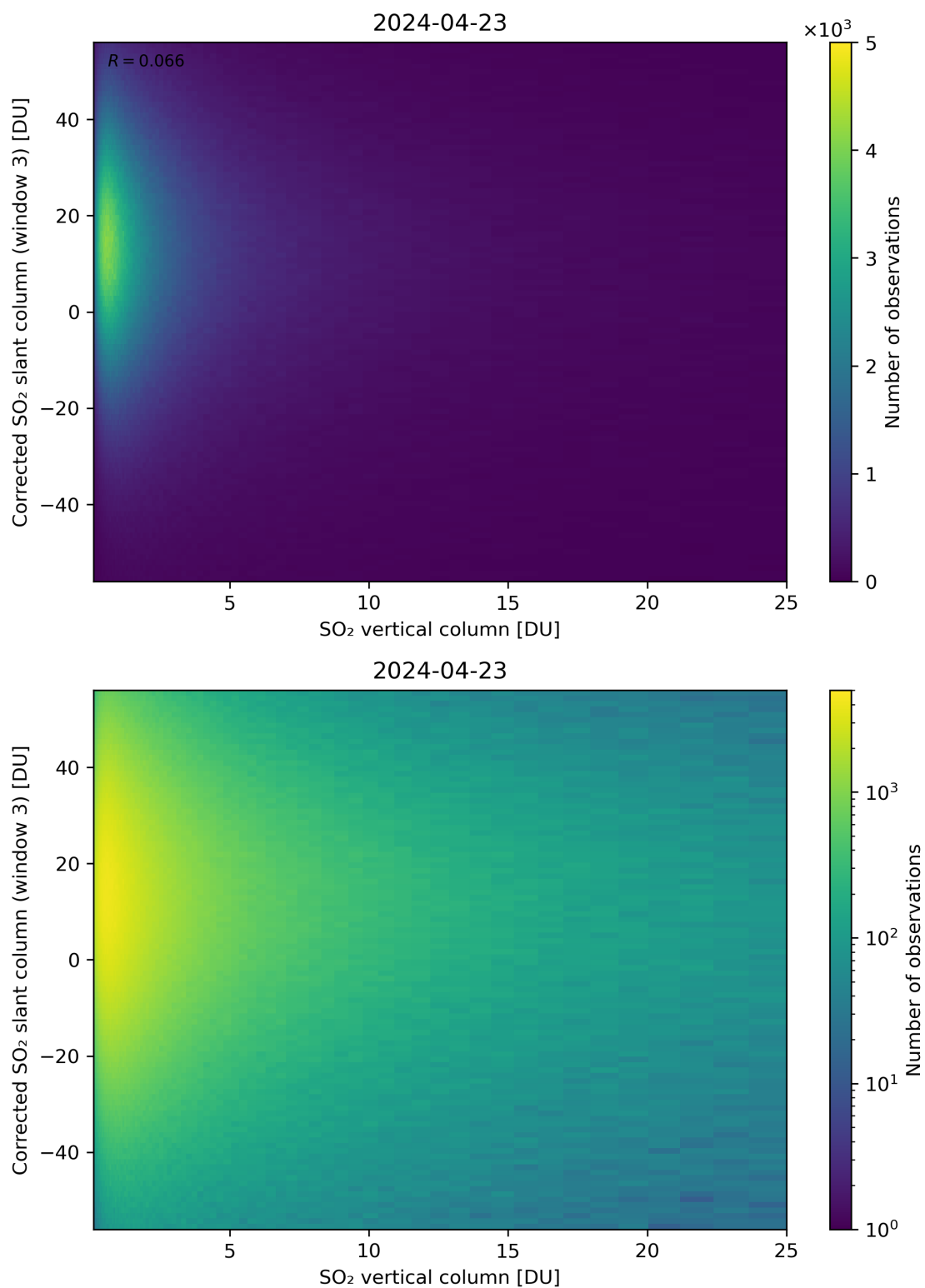
Figure 299: Scatter density plot of “SO 2 vertical column” against “Corrected SO 2 slant column (window 3)” for 2024-04-22 to 2024-04-24.
