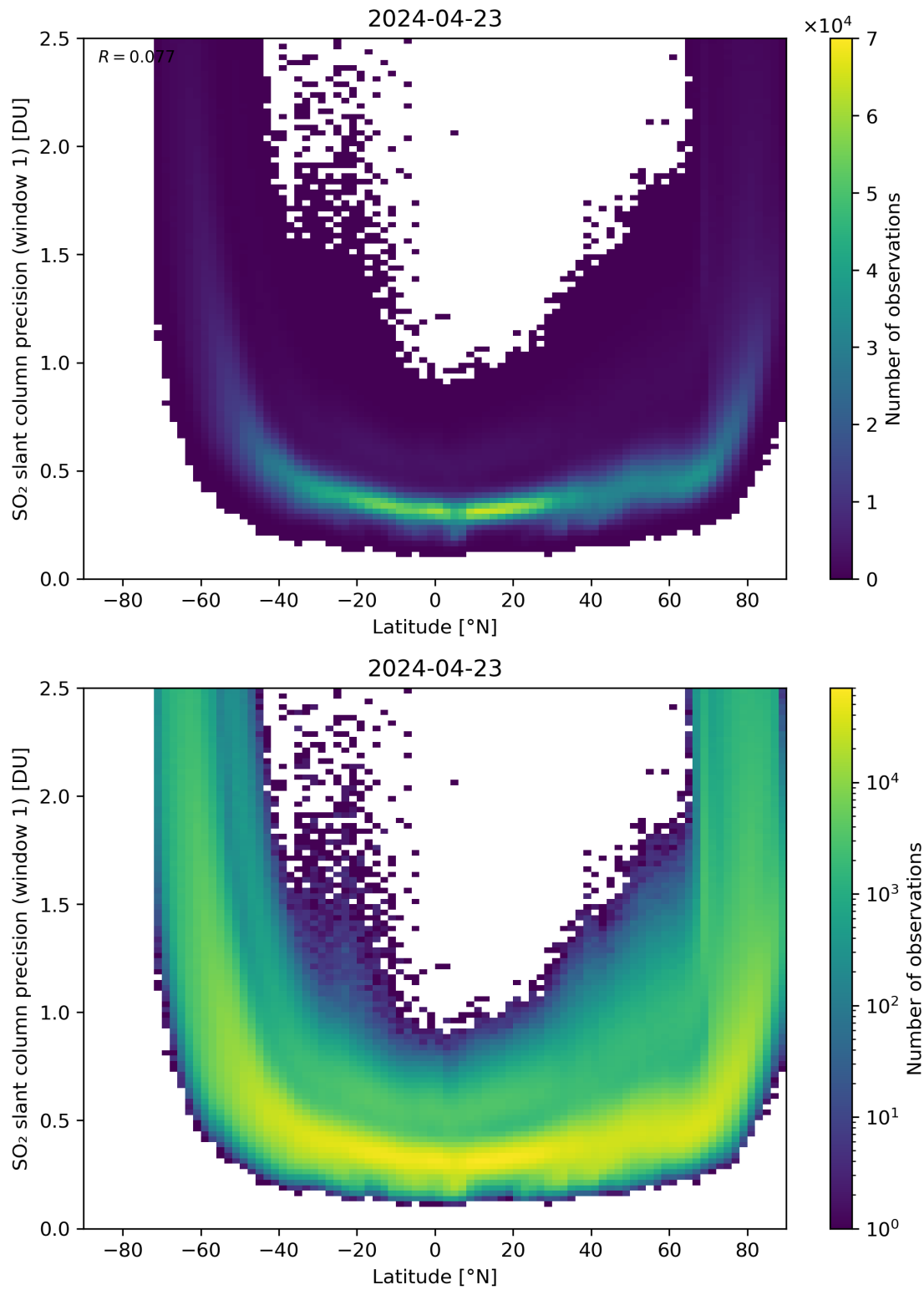
Figure 150: Scatter density plot of “Latitude” against “SO 2 slant column precision (window 1)” for 2024-04-22 to 2024-04-24.
