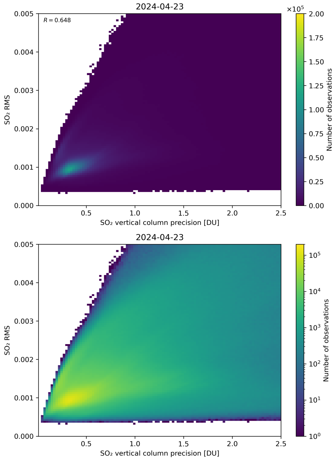
Figure 284: Scatter density plot of “SO 2 vertical column precision” against “SO 2 RMS” for 2024-04-22 to 2024-04-24.
