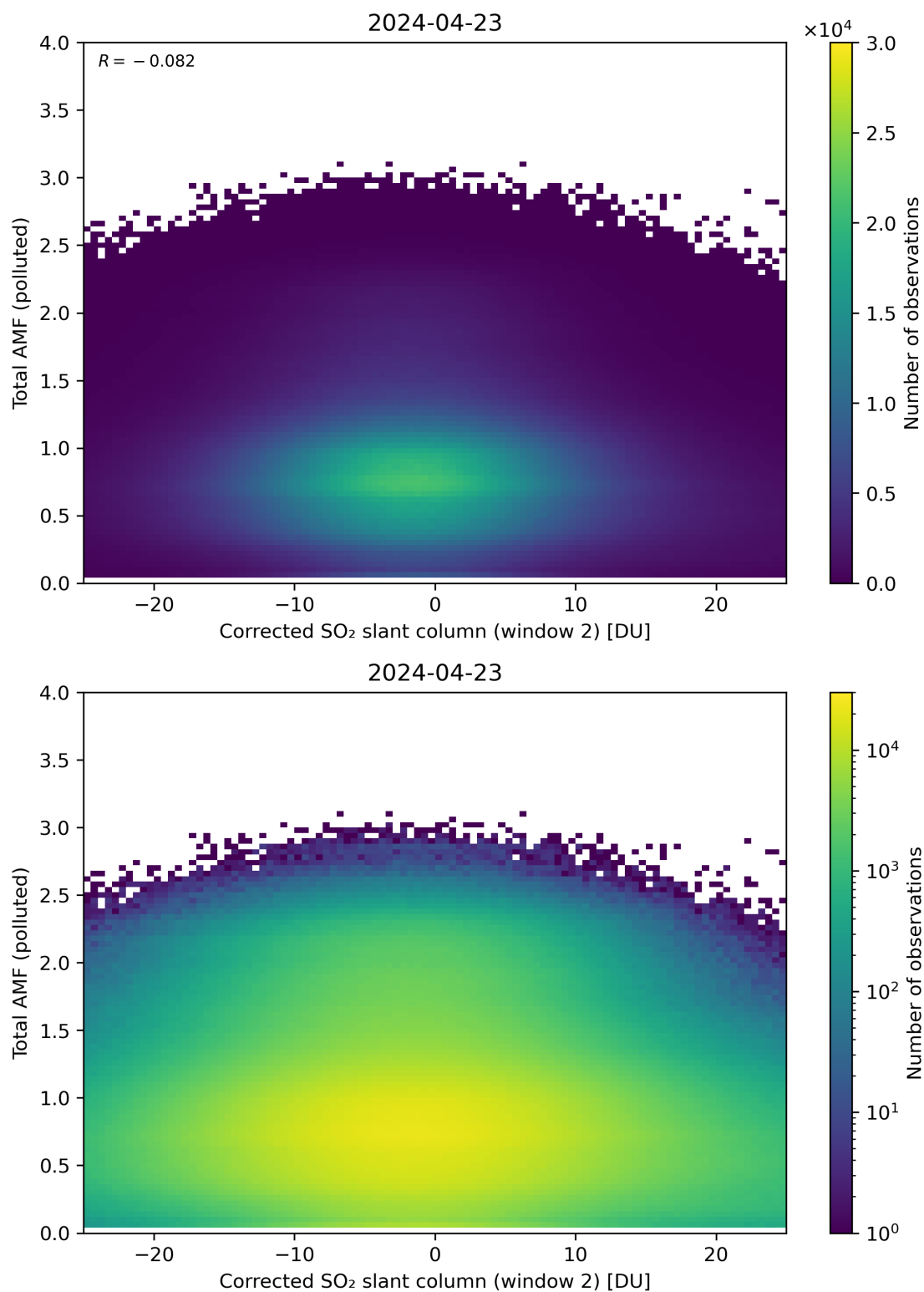
Figure 203: Scatter density plot of “Corrected SO 2 slant column (window 2)” against “Total AMF (polluted)” for 2024-04-22 to 2024-04-24.
