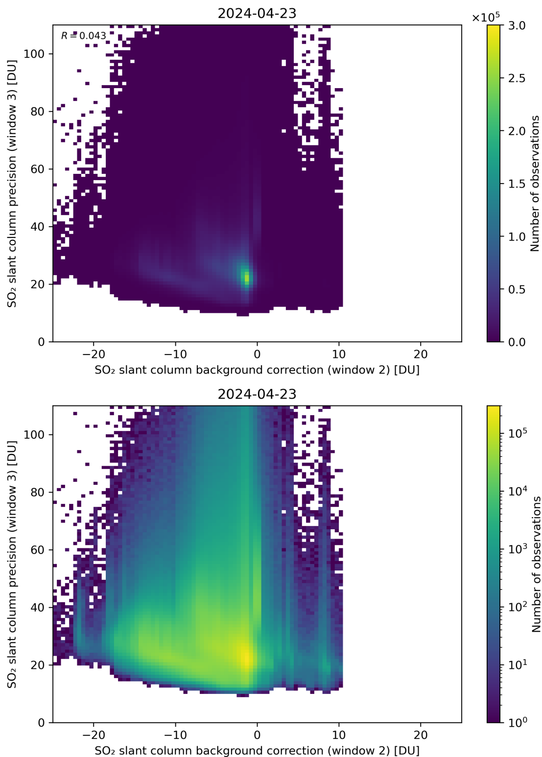
Figure 118: Scatter density plot of “SO 2 slant column background correction (window 2)” against “SO 2 slant column precision (window 3)” for 2024-04-22 to 2024-04-24.
