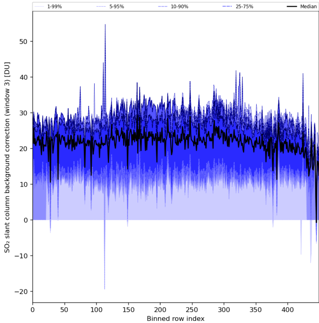
Figure 90: Along track statistics of “SO 2 slant column background correction (window 3)” for 2024-04-22 to 2024-04-24
