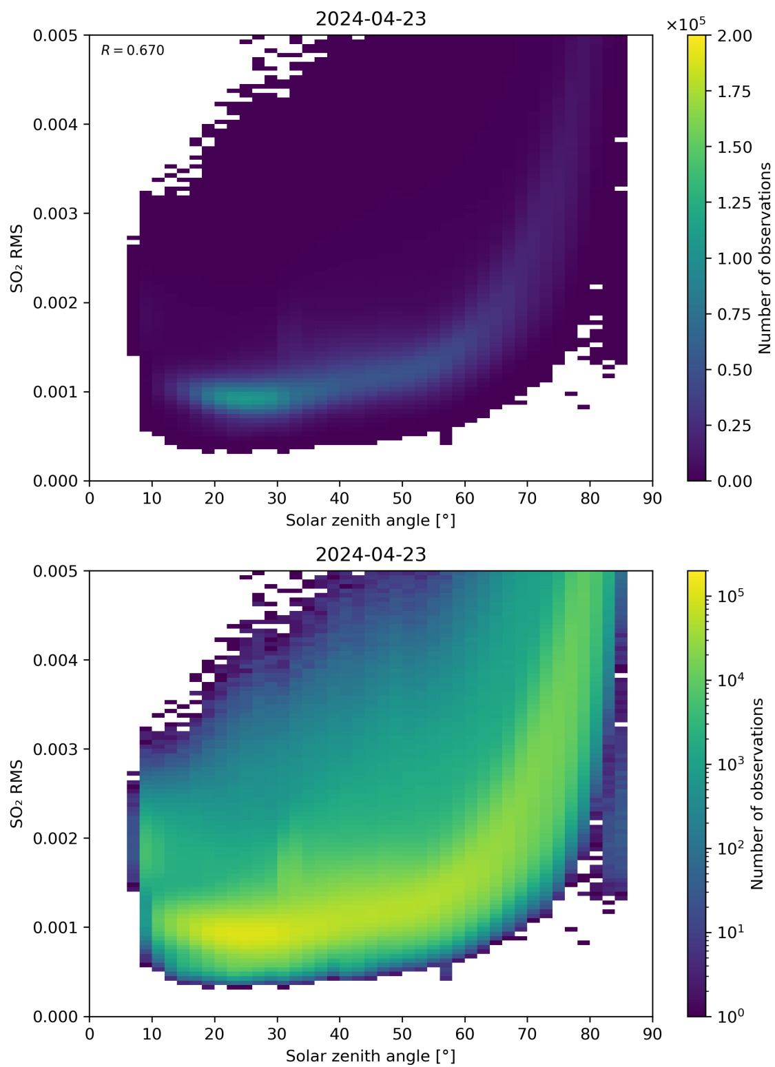
Figure 163: Scatter density plot of “Solar zenith angle” against “SO 2 RMS” for 2024-04-22 to 2024-04-24.
