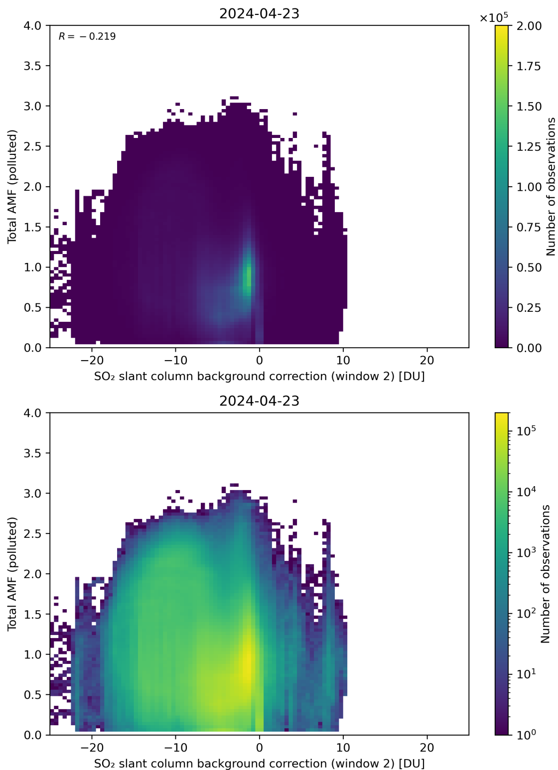
Figure 119: Scatter density plot of “SO 2 slant column background correction (window 2)” against “Total AMF (polluted)” for 2024-04-22 to 2024-04-24.
