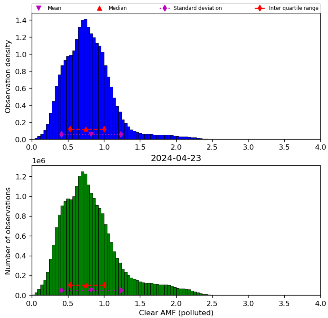
Figure 73: Histogram of “Clear AMF (polluted)” for 2024-04-22 to 2024-04-24
