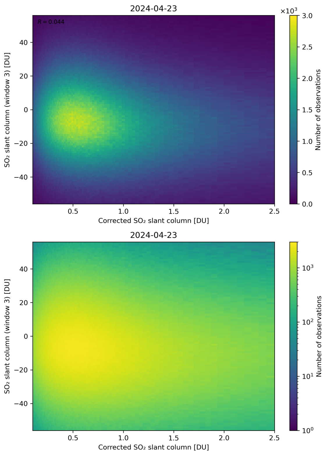
Figure 190: Scatter density plot of “Corrected SO 2 slant column” against “SO 2 slant column (window 3)” for 2024-04-22 to 2024-04-24.
