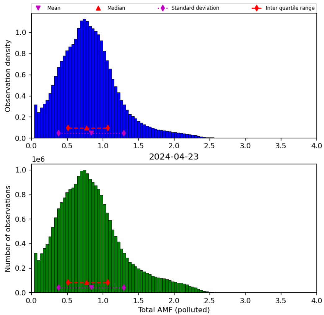
Figure 71: Histogram of “Total AMF (polluted)” for 2024-04-22 to 2024-04-24
