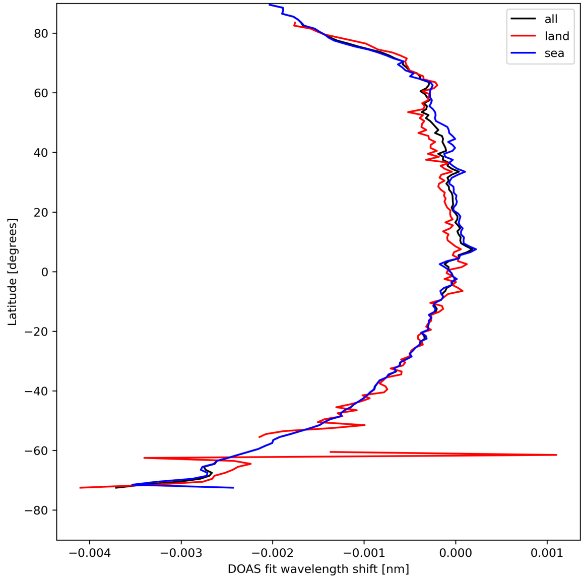
Figure 45: Zonal average of “DOAS fit wavelength shift” for 2024-04-22 to 2024-04-24.
