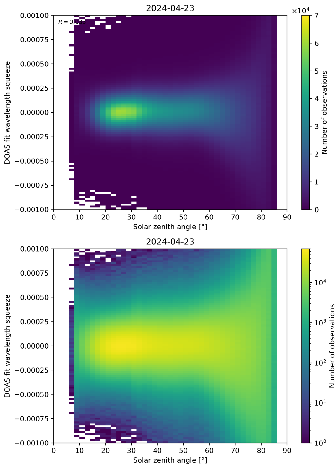
Figure 162: Scatter density plot of “Solar zenith angle” against “DOAS fit wavelength squeeze” for 2024-04-22 to 2024-04-24.
