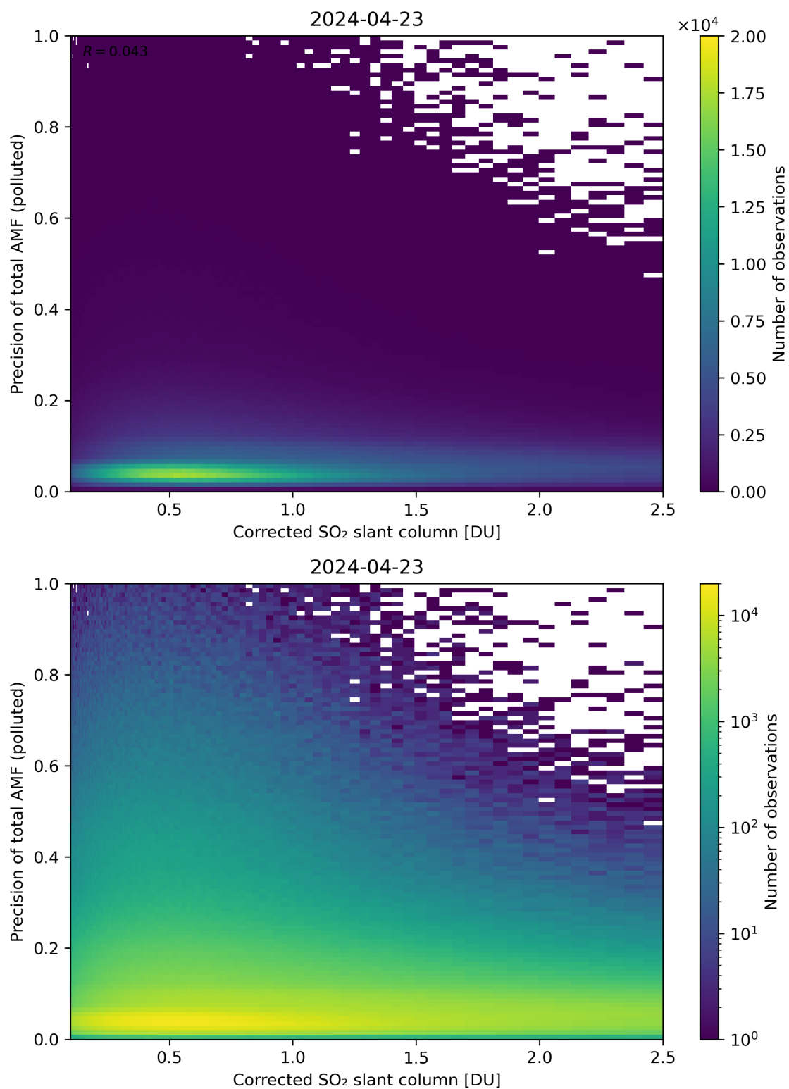
Figure 193: Scatter density plot of “Corrected SO 2 slant column” against “Precision of total AMF (polluted)” for 2024-04-22 to 2024-04-24.
