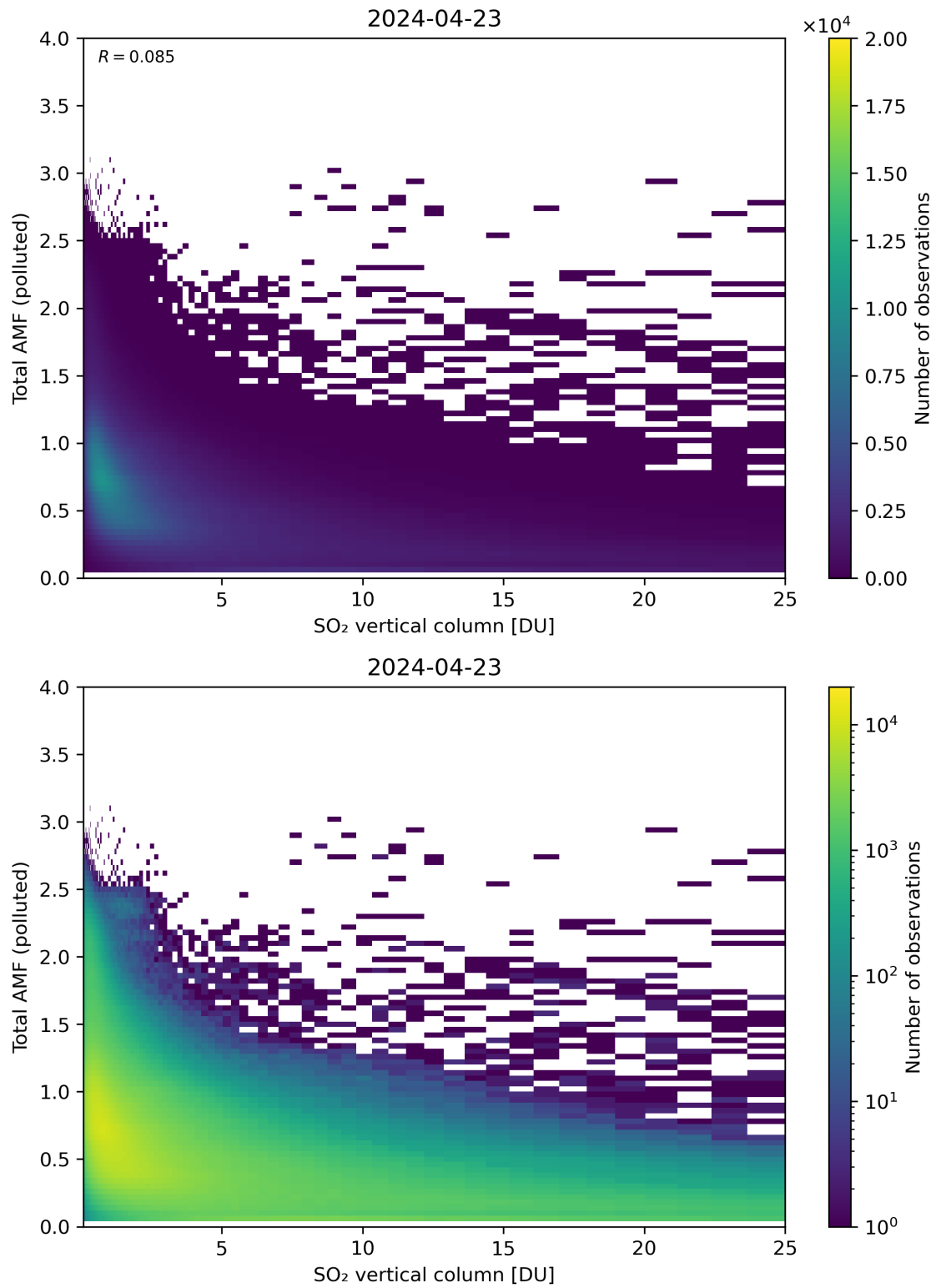
Figure 305: Scatter density plot of “SO 2 vertical column” against “Total AMF (polluted)” for 2024-04-22 to 2024-04-24.
