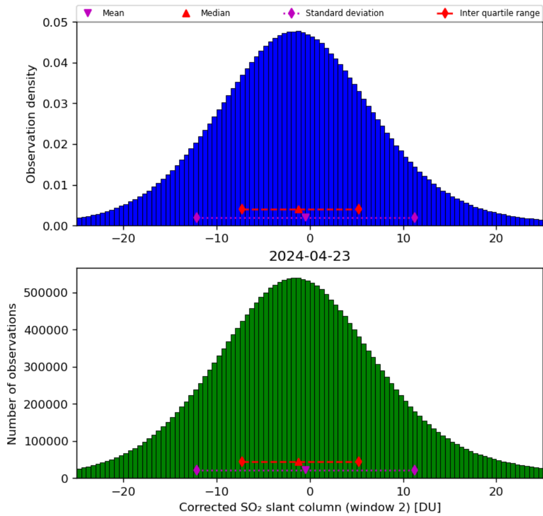
Figure 62: Histogram of “Corrected SO 2 slant column (window 2)” for 2024-04-22 to 2024-04-24
