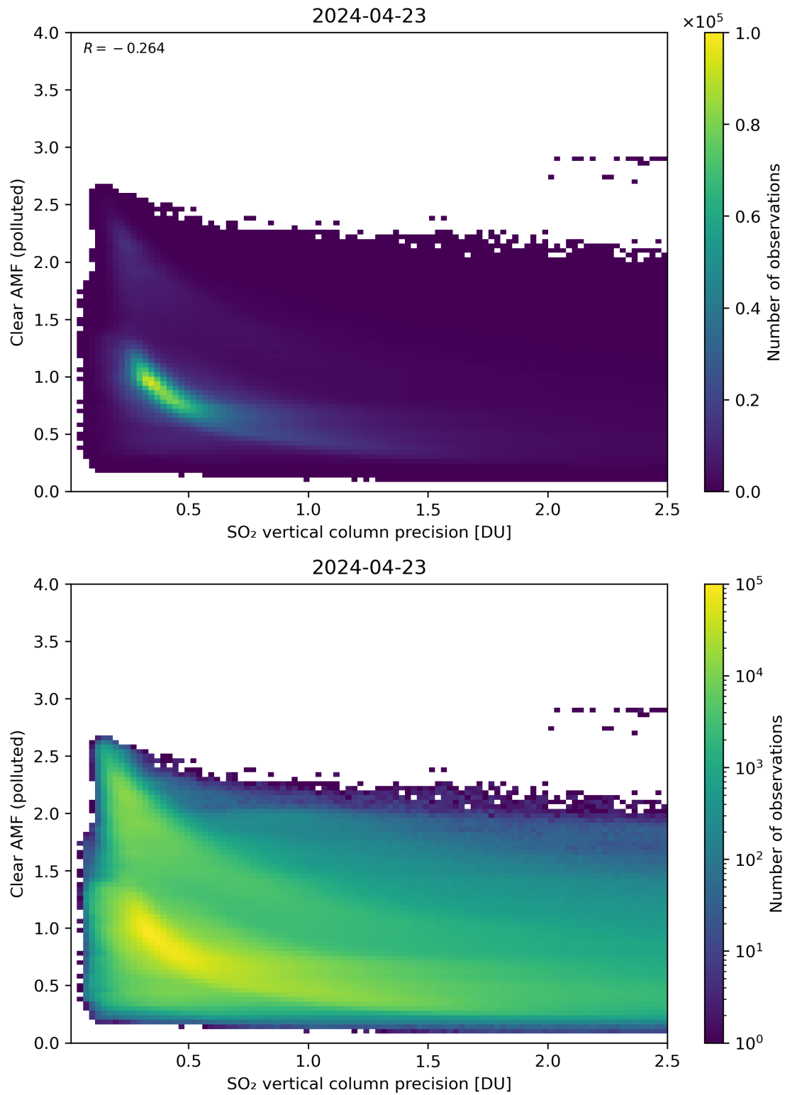
Figure 285: Scatter density plot of “SO 2 vertical column precision” against “Clear AMF (polluted)” for 2024-04-22 to 2024-04-24.
