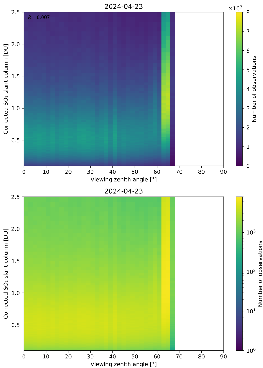
Figure 317: Scatter density plot of “Viewing zenith angle” against “Corrected SO 2 slant column” for 2024-04-22 to 2024-04-24.
