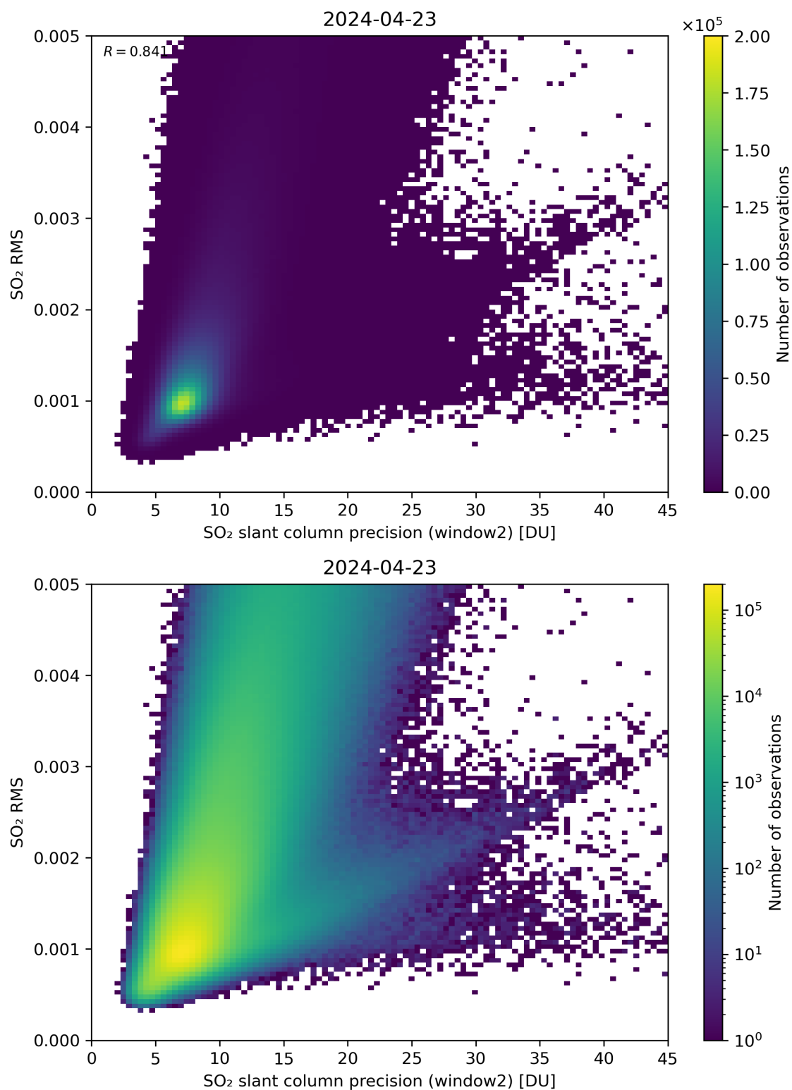
Figure 245: Scatter density plot of “SO 2 slant column precision (window2)” against “SO 2 RMS” for 2024-04-22 to 2024-04-24.
