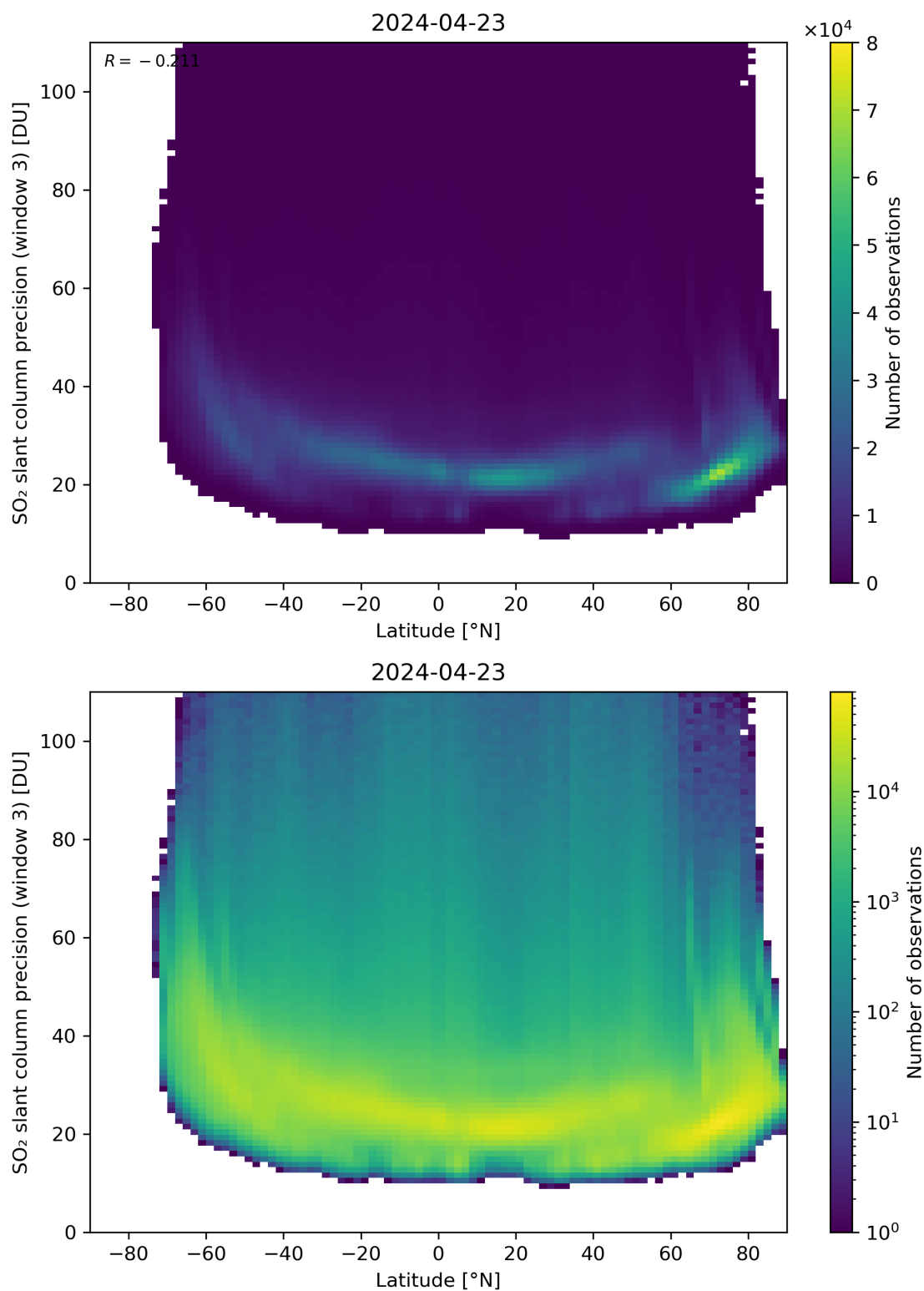
Figure 153: Scatter density plot of “Latitude” against “SO 2 slant column precision (window 3)” for 2024-04-22 to 2024-04-24.
