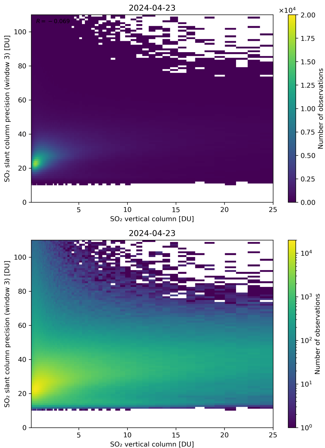
Figure 304: Scatter density plot of “SO 2 vertical column” against “SO 2 slant column precision (window 3)” for 2024-04-22 to 2024-04-24.
