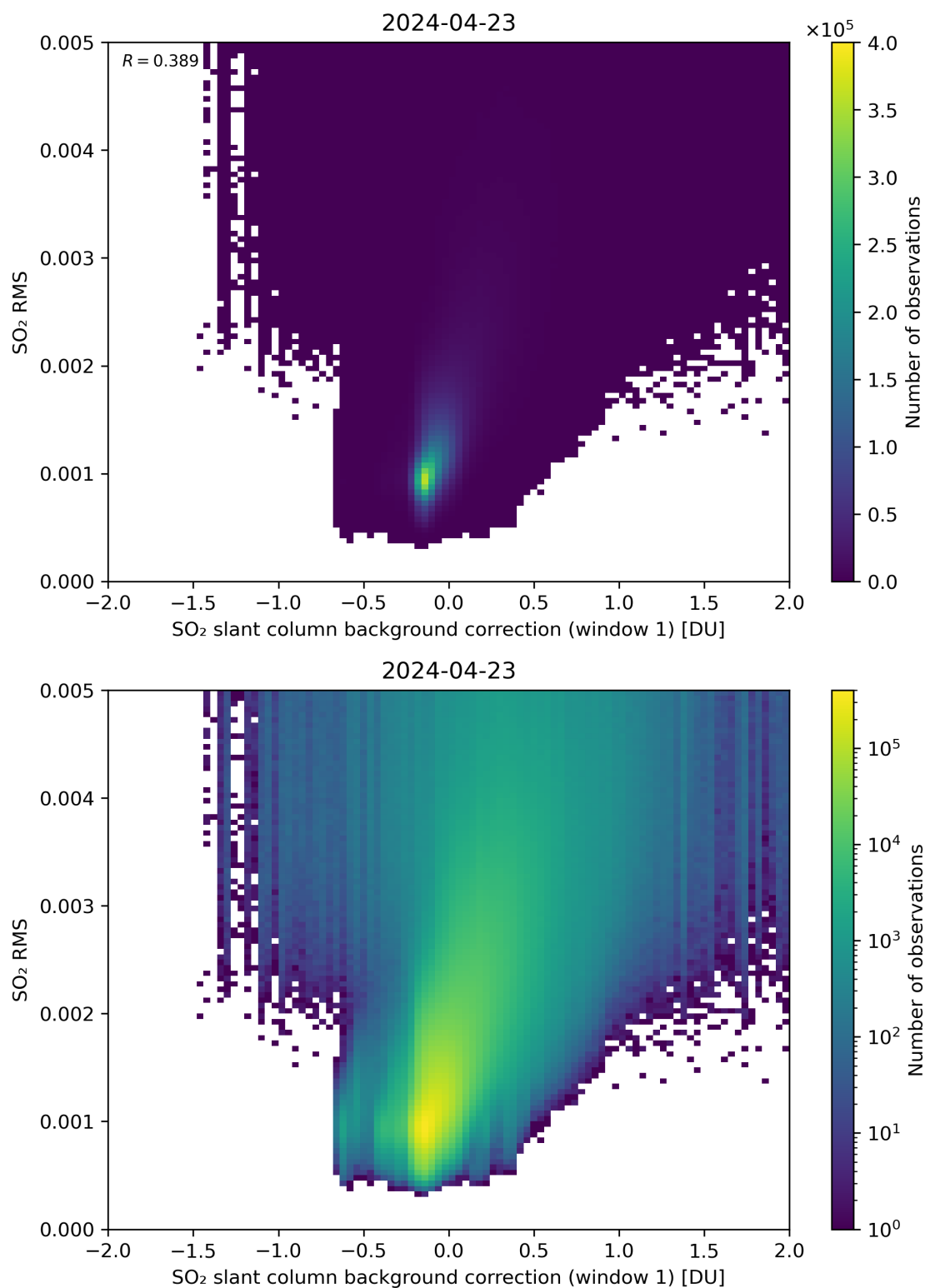
Figure 102: Scatter density plot of “SO 2 slant column background correction (window 1)” against “SO 2 RMS” for 2024-04-22 to 2024-04-24.
