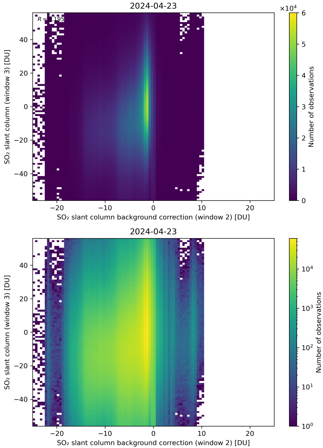
Figure 117: Scatter density plot of “SO 2 slant column background correction (window 2)” against “SO 2 slant column (window 3)” for 2024-04-22 to 2024-04-24.
