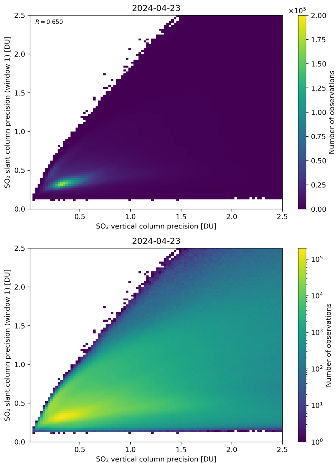
Figure 290: Scatter density plot of “SO 2 vertical column precision” against “SO 2 slant column precision (window 1)” for 2024-04-22 to 2024-04-24.
