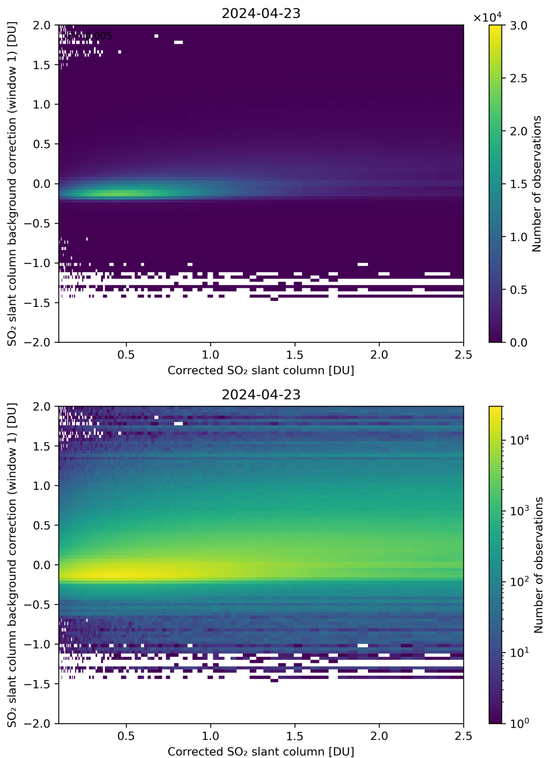
Figure 178: Scatter density plot of “Corrected SO 2 slant column” against “SO 2 slant column background correction (window 1)” for 2024-04-22 to 2024-04-24.
