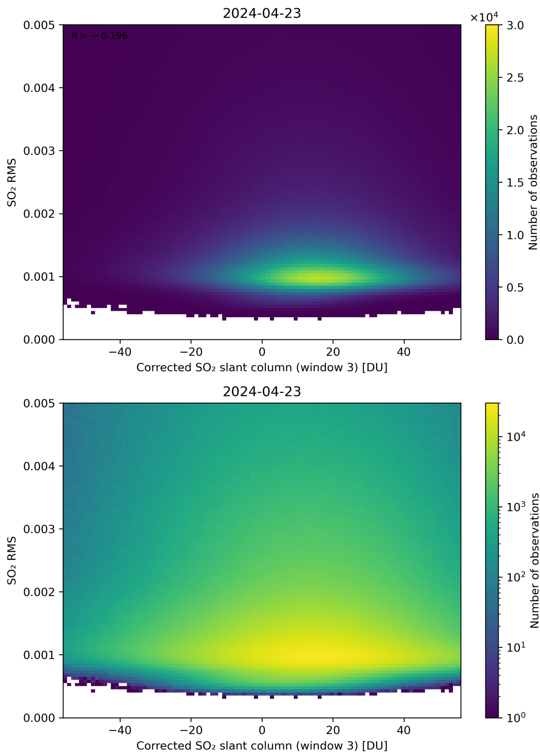
Figure 208: Scatter density plot of “Corrected SO 2 slant column (window 3)” against “SO 2 RMS” for 2024-04-22 to 2024-04-24.
