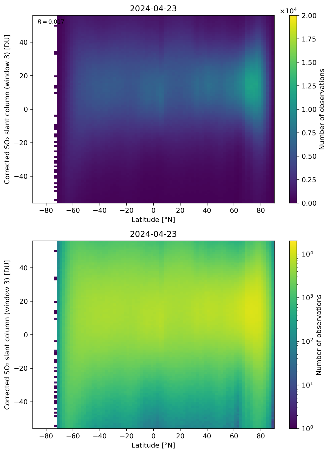
Figure 148: Scatter density plot of “Latitude” against “Corrected SO 2 slant column (window 3)” for 2024-04-22 to 2024-04-24.
