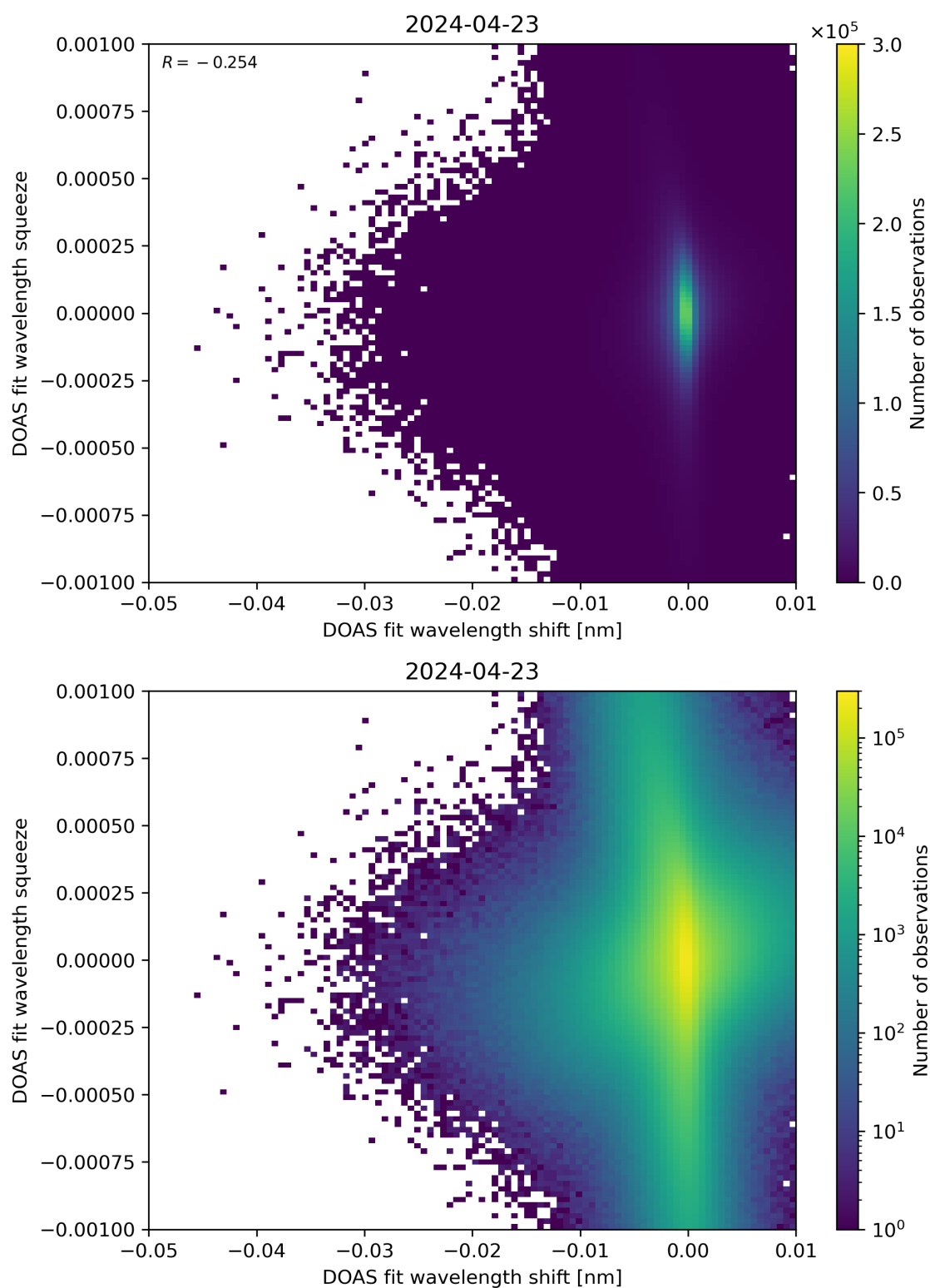
Figure 127: Scatter density plot of “DOAS fit wavelength shift” against “DOAS fit wavelength squeeze” for 2024-04-22 to 2024-04-24.
