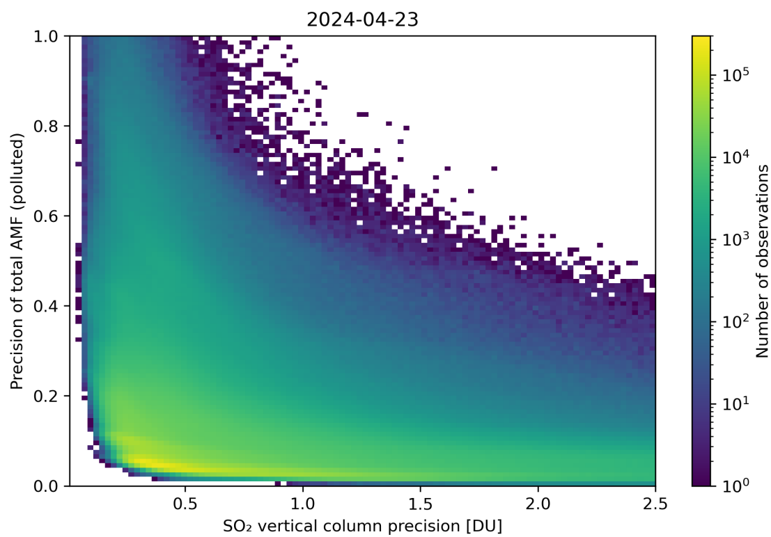
Figure 295: Scatter density plot of “SO 2 vertical column precision” against “Precision of total AMF (polluted)” for 2024-04-22 to 2024-04-24.
