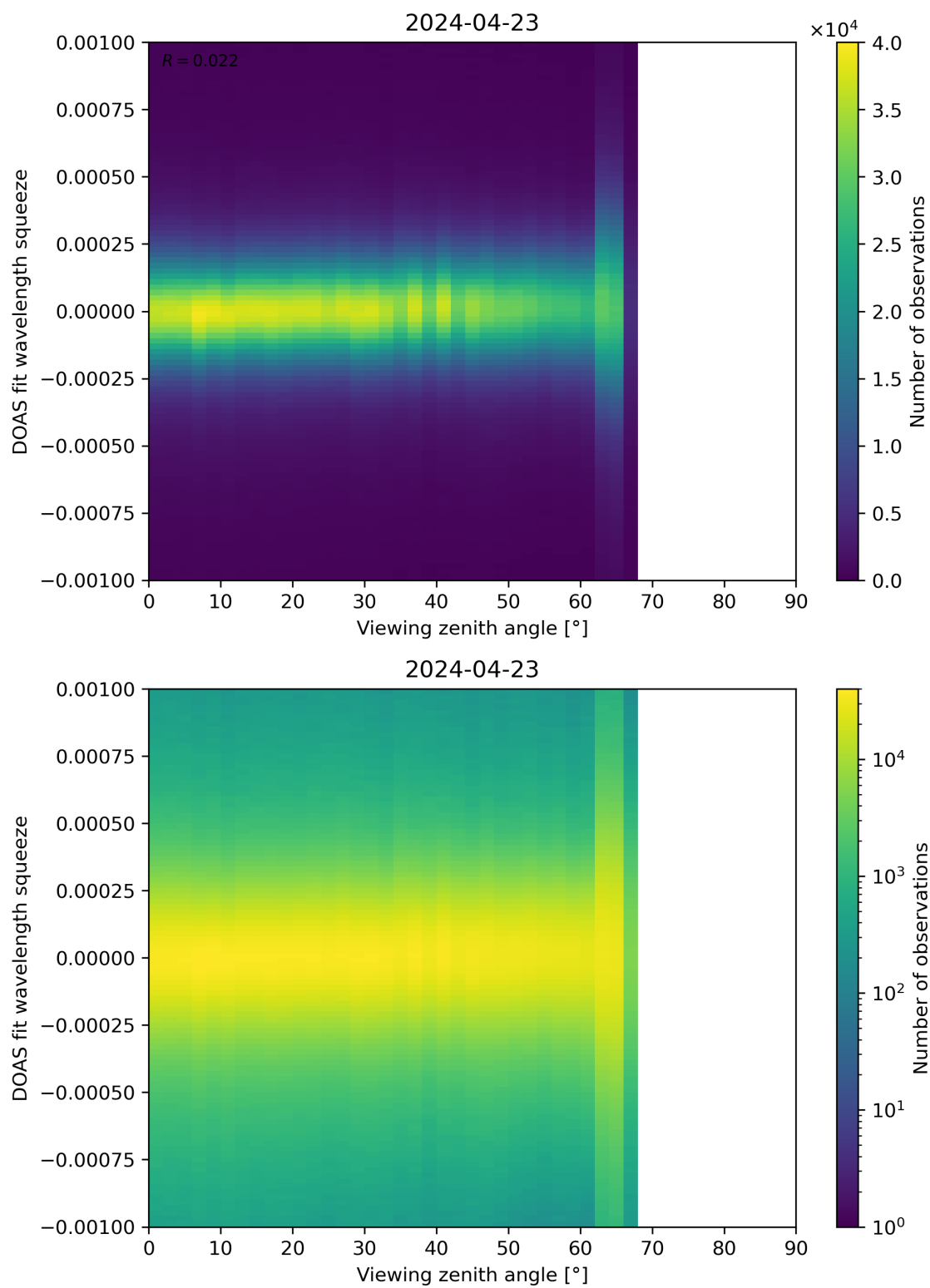
Figure 312: Scatter density plot of “Viewing zenith angle” against “DOAS fit wavelength squeeze” for 2024-04-22 to 2024-04-24.
