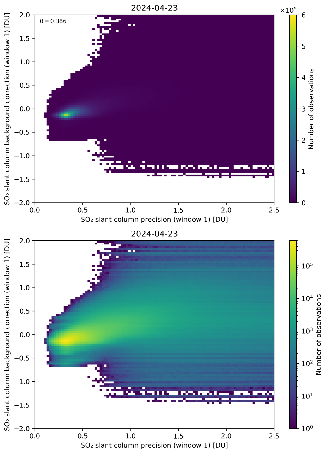
Figure 218: Scatter density plot of “SO 2 slant column precision (window 1)” against “SO 2 slant column background correction (window 1)” for 2024-04-22 to 2024-04-24.
