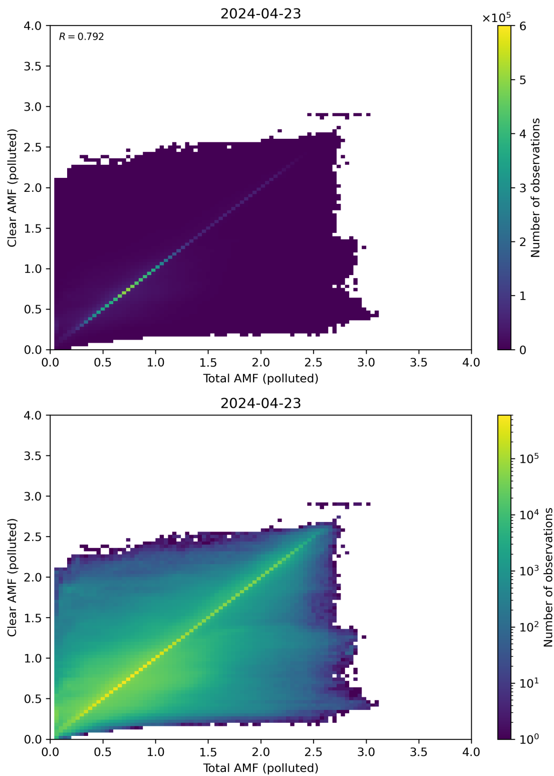
Figure 271: Scatter density plot of “Total AMF (polluted)” against “Clear AMF (polluted)” for 2024-04-22 to 2024-04-24.
