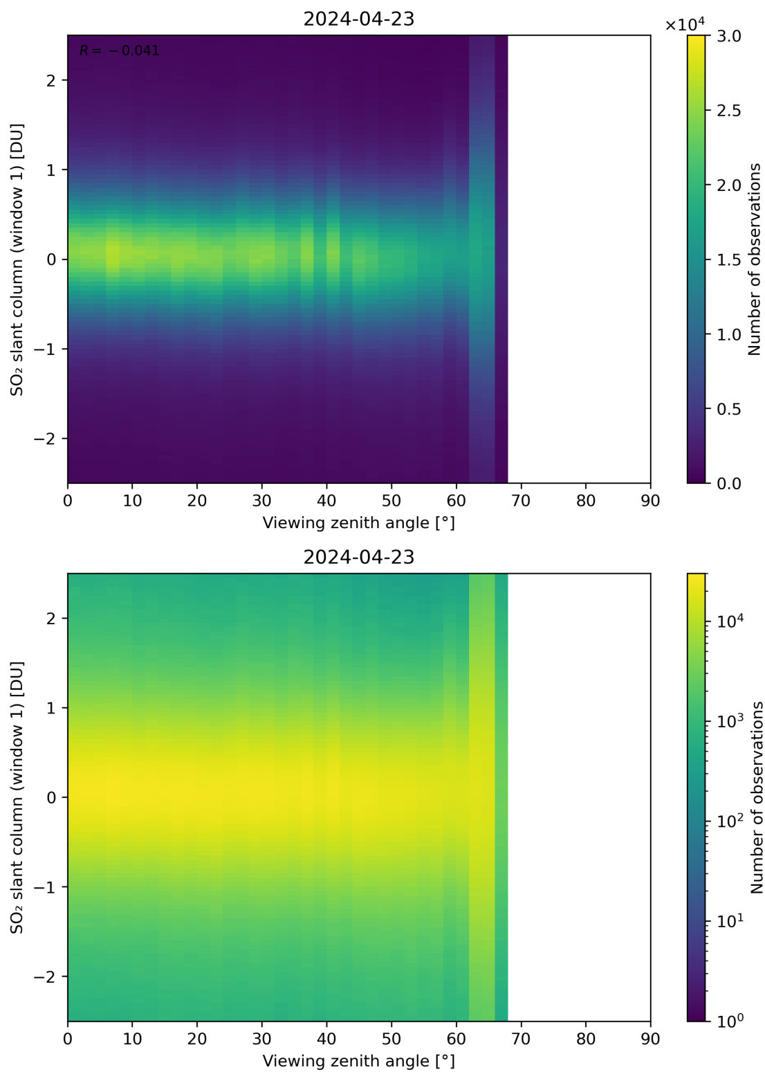
Figure 320: Scatter density plot of “Viewing zenith angle” against “SO 2 slant column (window 1)” for 2024-04-22 to 2024-04-24.
