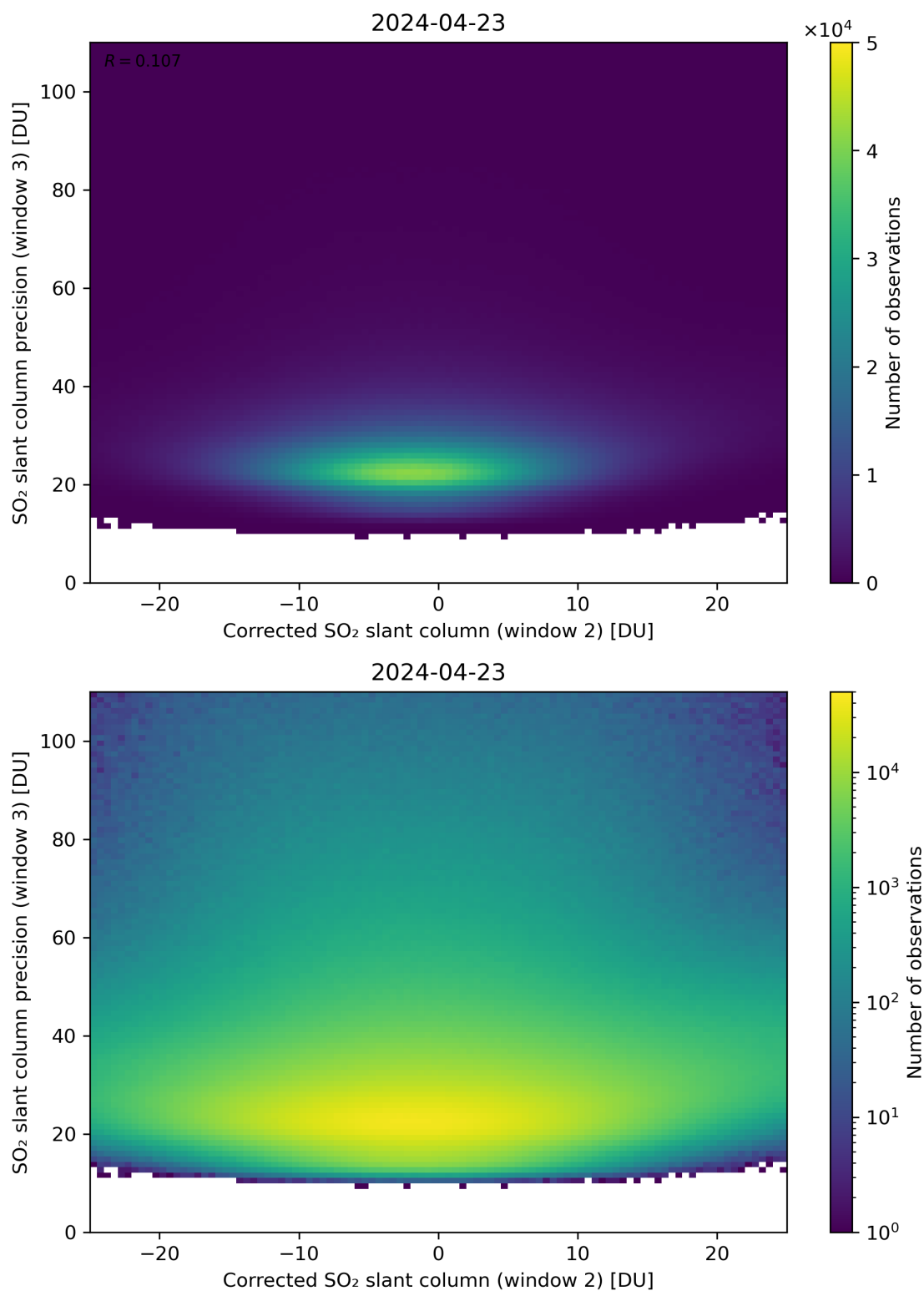
Figure 202: Scatter density plot of “Corrected SO 2 slant column (window 2)” against “SO 2 slant column precision (window 3)” for 2024-04-22 to 2024-04-24.
