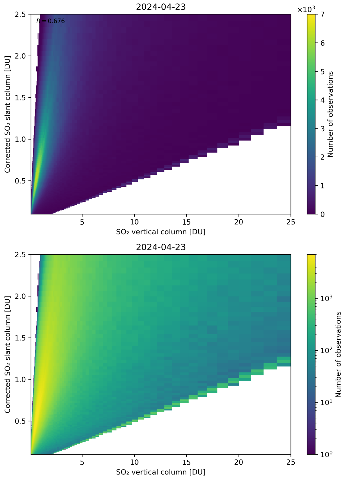
Figure 297: Scatter density plot of “SO 2 vertical column” against “Corrected SO 2 slant column” for 2024-04-22 to 2024-04-24.
