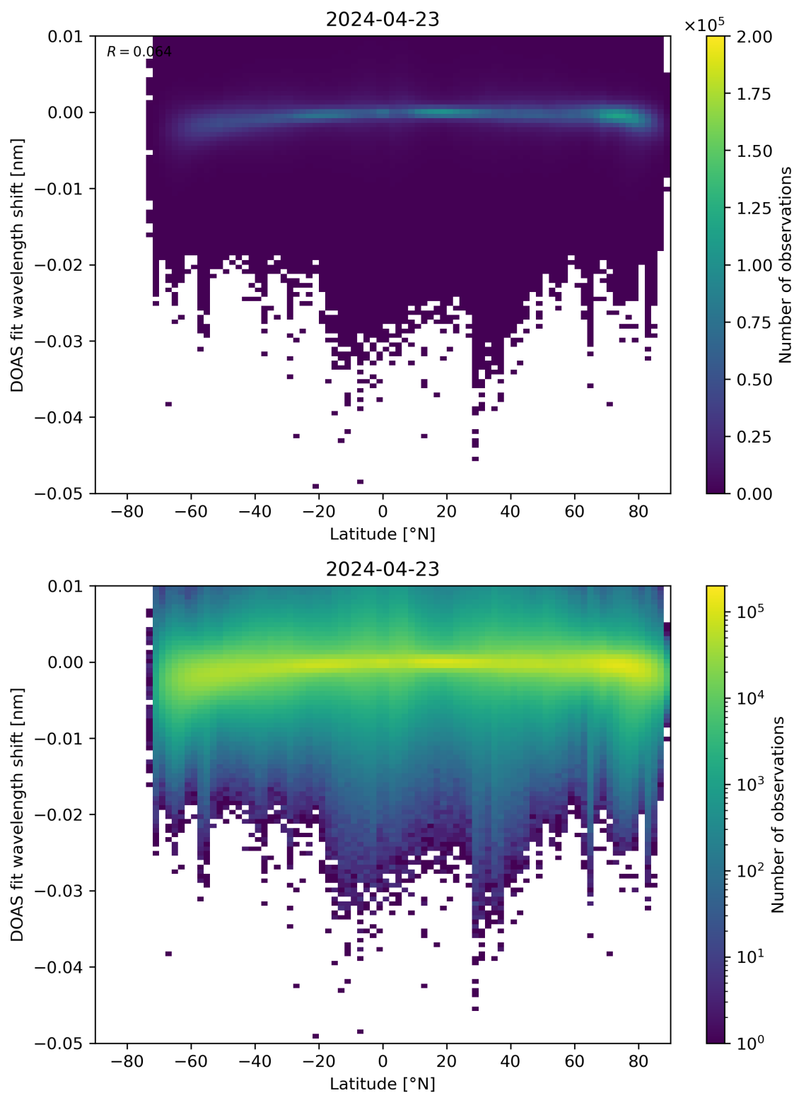
Figure 142: Scatter density plot of “Latitude” against “DOAS fit wavelength shift” for 2024-04-22 to 2024-04-24.
