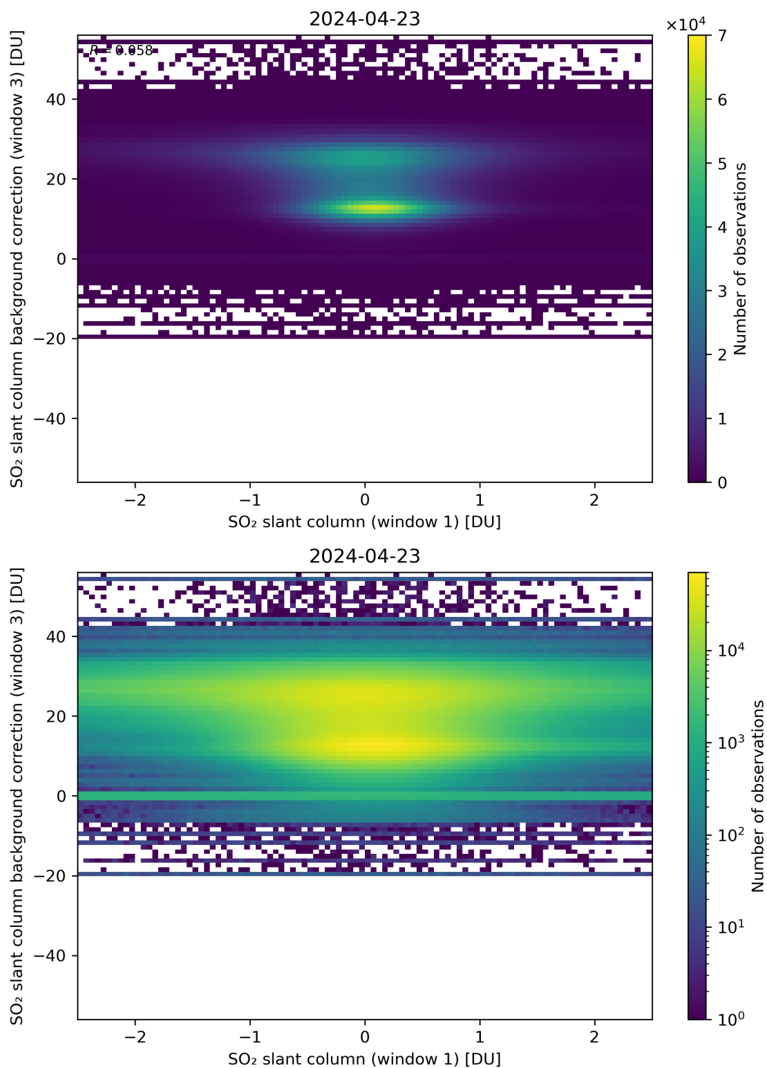
Figure 214: Scatter density plot of “SO 2 slant column (window 1)” against “SO 2 slant column background correction (window 3)” for 2024-04-22 to 2024-04-24.
