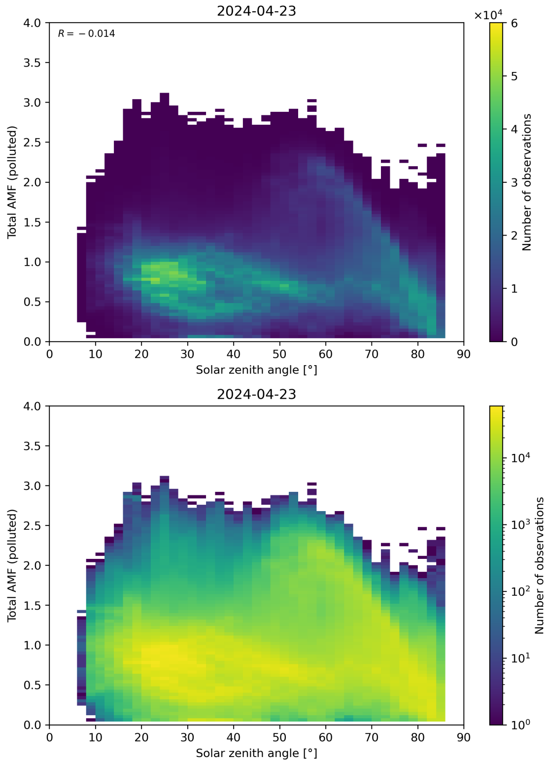
Figure 174: Scatter density plot of “Solar zenith angle” against “Total AMF (polluted)” for 2024-04-22 to 2024-04-24.
