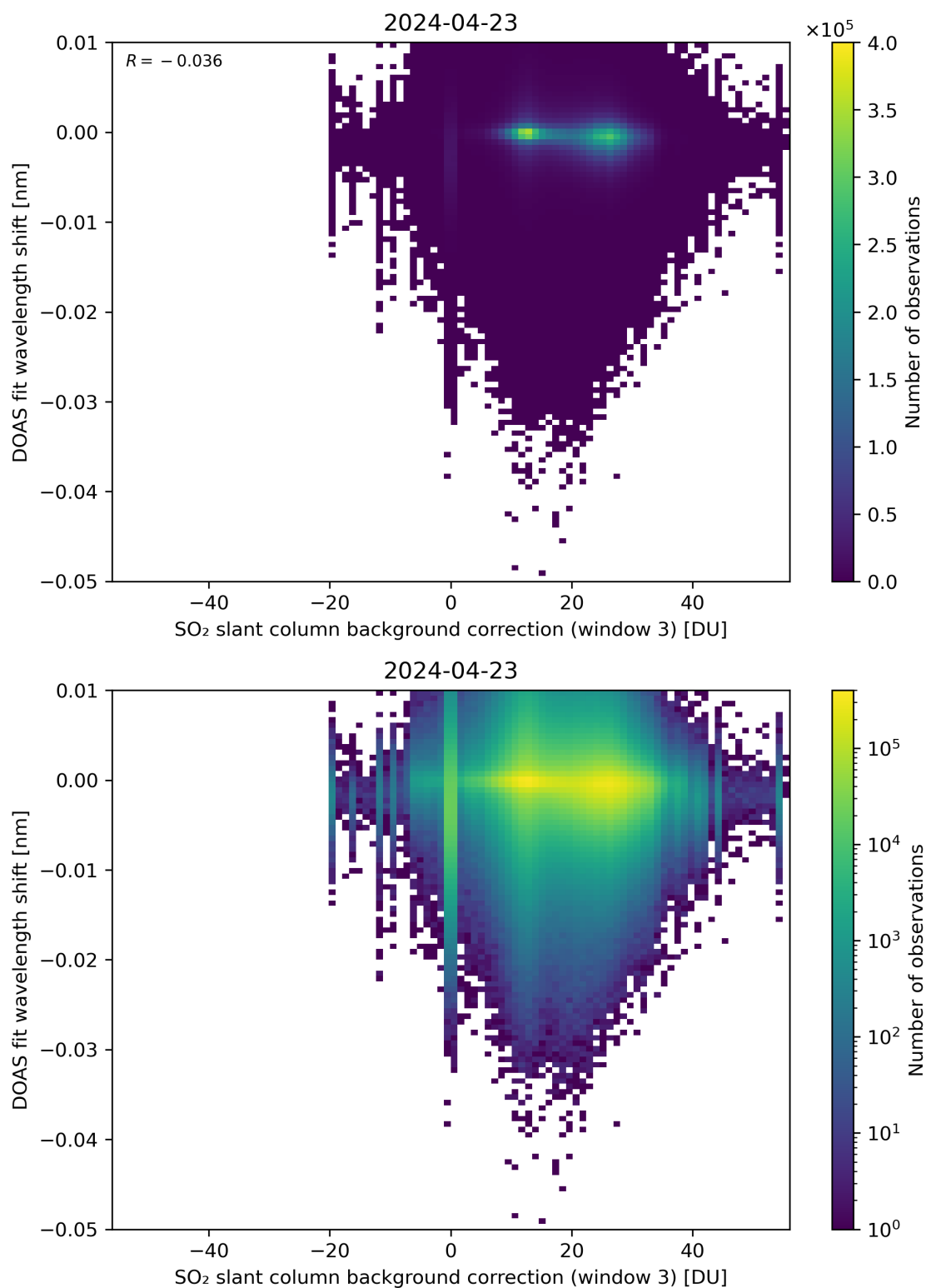
Figure 121: Scatter density plot of “SO 2 slant column background correction (window 3)” against “DOAS fit wavelength shift” for 2024-04-22 to 2024-04-24.
