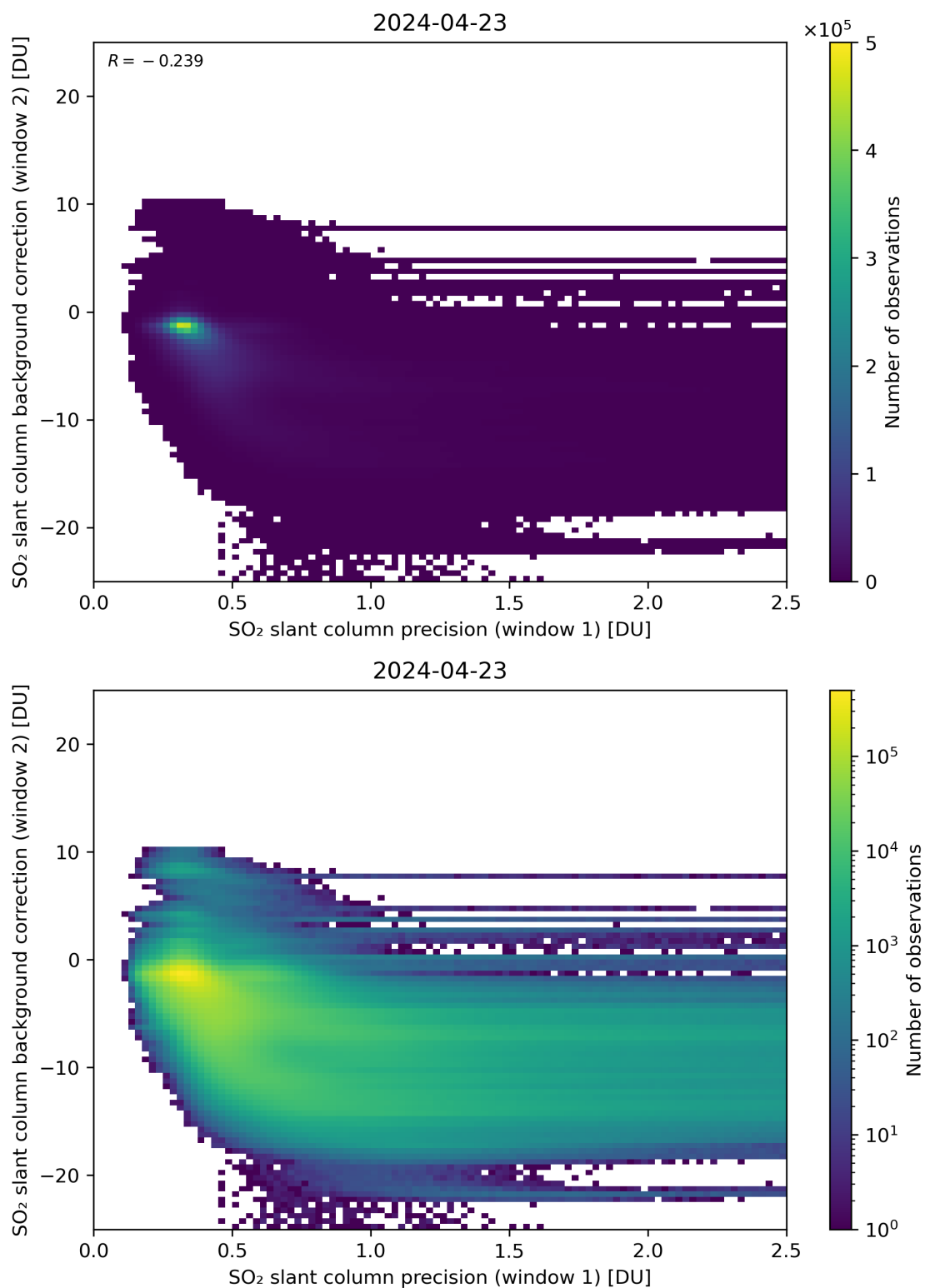
Figure 219: Scatter density plot of “SO 2 slant column precision (window 1)” against “SO 2 slant column background correction (window 2)” for 2024-04-22 to 2024-04-24.
