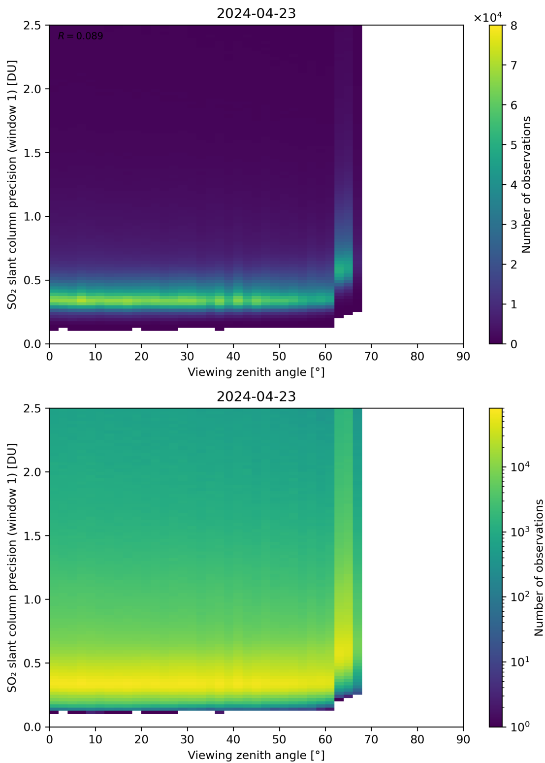
Figure 321: Scatter density plot of “Viewing zenith angle” against “SO 2 slant column precision (window 1)” for 2024-04-22 to 2024-04-24.
