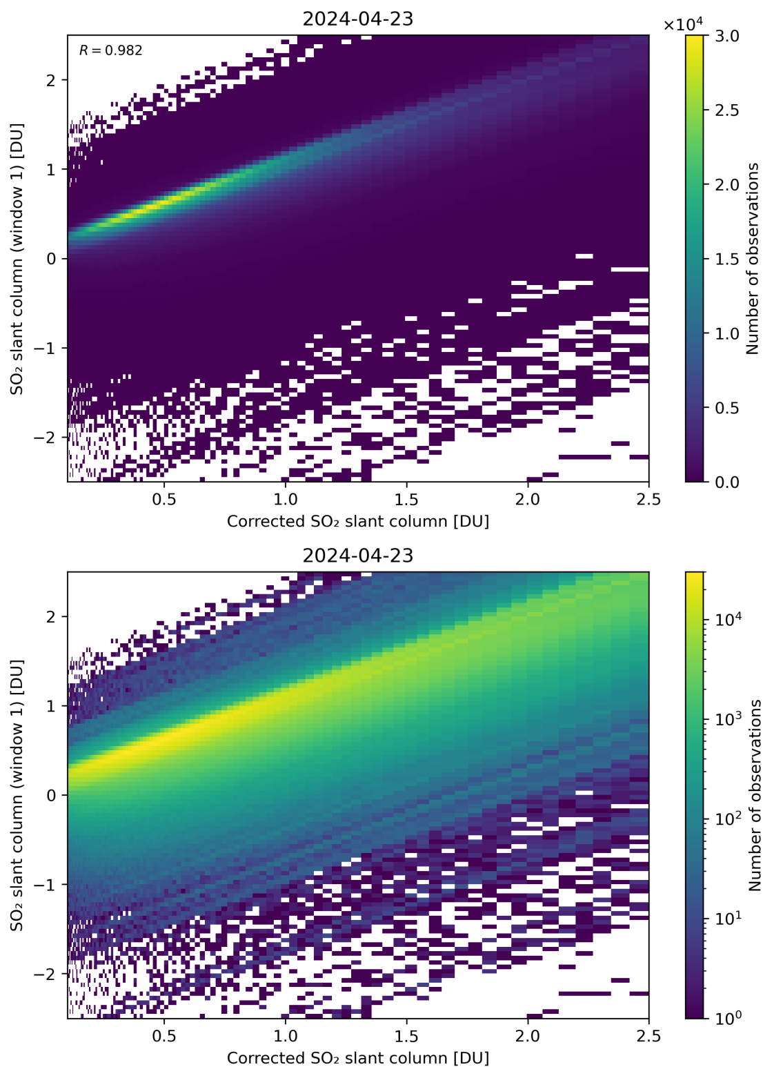
Figure 187: Scatter density plot of “Corrected SO 2 slant column” against “SO 2 slant column (window 1)” for 2024-04-22 to 2024-04-24.
