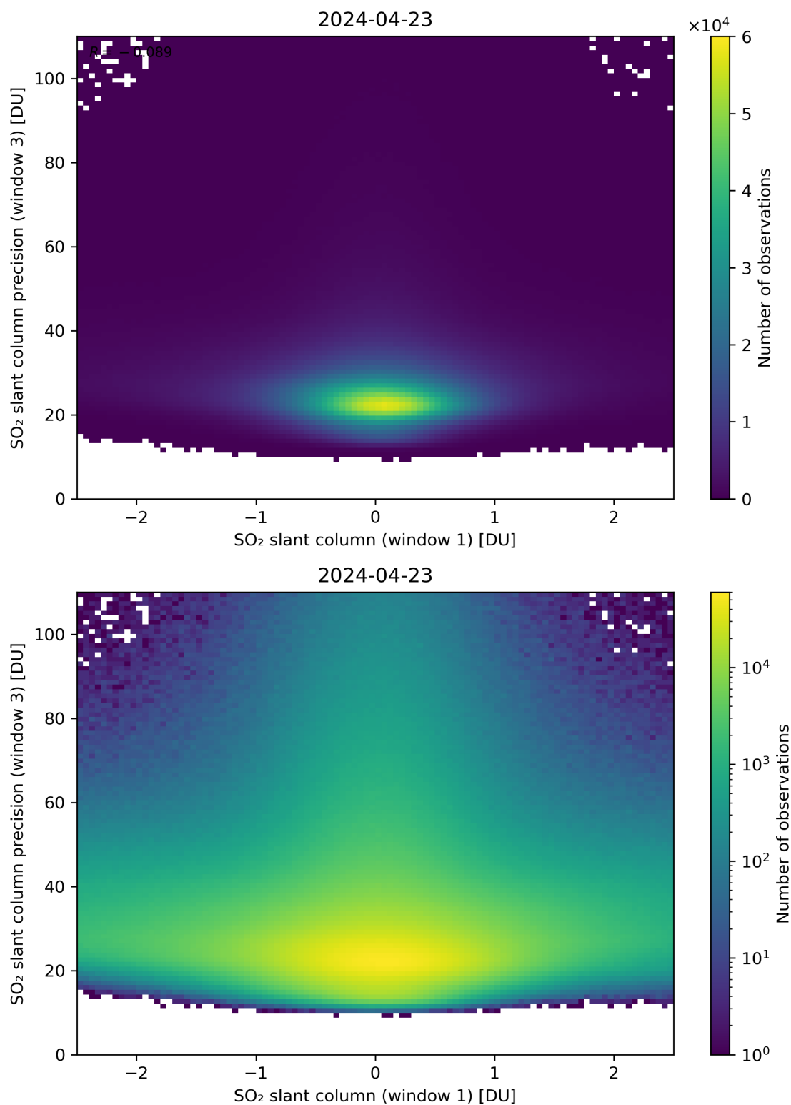
Figure 238: Scatter density plot of “SO 2 slant column (window 1)” against “SO 2 slant column precision (window 3)” for 2024-04-22 to 2024-04-24.
