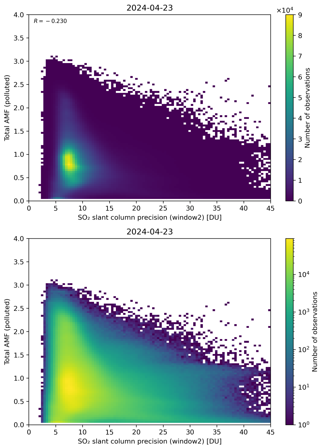
Figure 251: Scatter density plot of “SO 2 slant column precision (window2)” against “Total AMF (polluted)” for 2024-04-22 to 2024-04-24.
