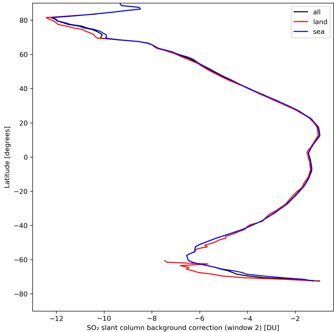
Figure 40: Zonal average of “SO 2 slant column background correction (window 2)” for 2024-04-22 to 2024-04-24.
