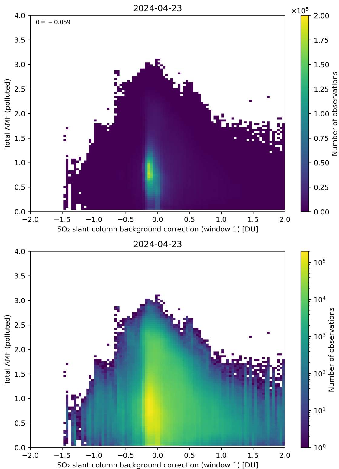
Figure 109: Scatter density plot of “SO 2 slant column background correction (window 1)” against “Total AMF (polluted)” for 2024-04-22 to 2024-04-24.
