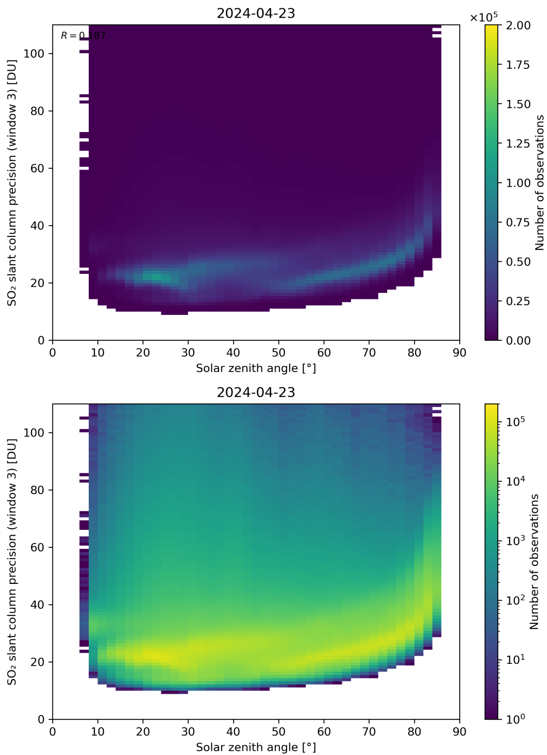
Figure 173: Scatter density plot of “Solar zenith angle” against “SO 2 slant column precision (window 3)” for 2024-04-22 to 2024-04-24.
