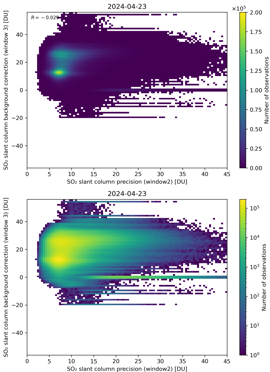
Figure 242: Scatter density plot of “SO 2 slant column precision (window2)” against “SO 2 slant column background correction (window 3)” for 2024-04-22 to 2024-04-24.
