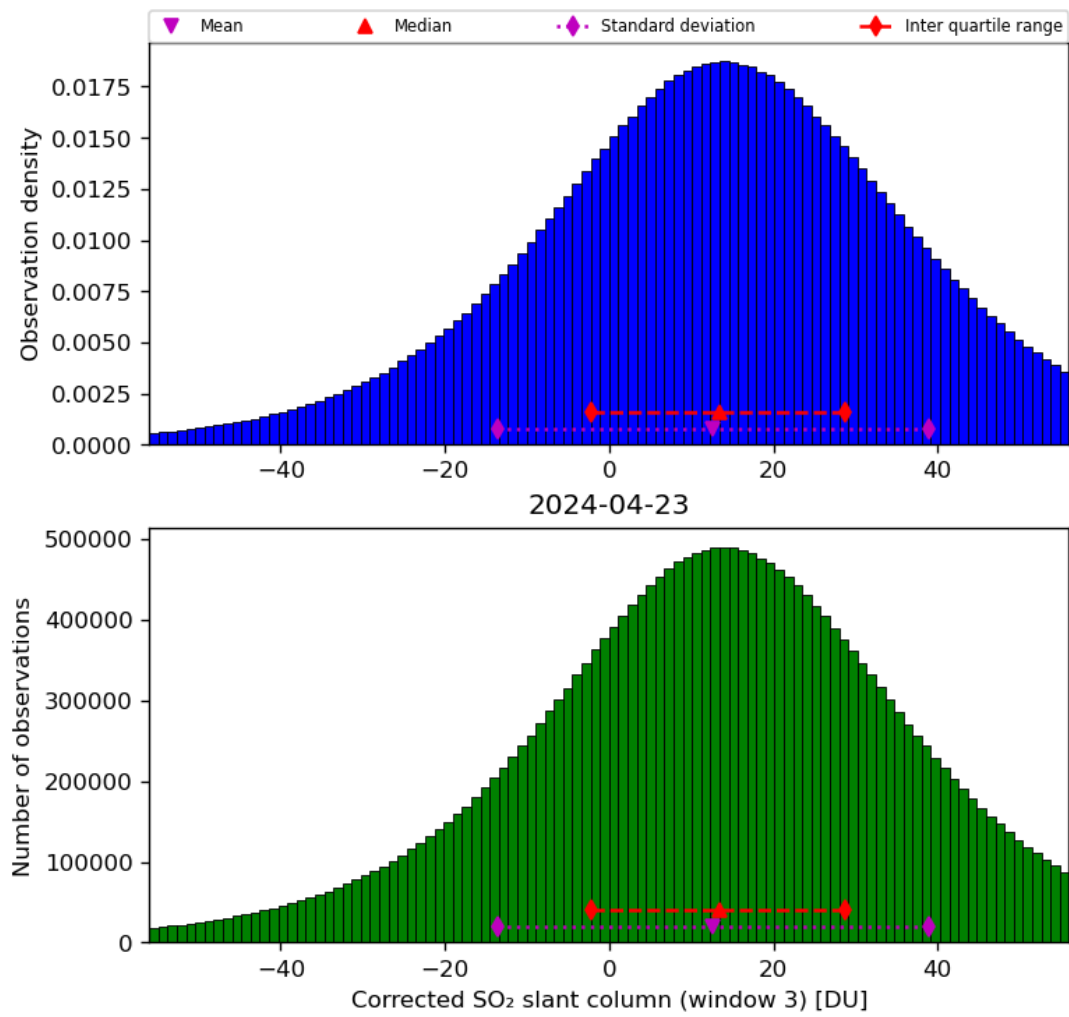
Figure 66: Histogram of “Corrected SO 2 slant column (window 3)” for 2024-04-22 to 2024-04-24
