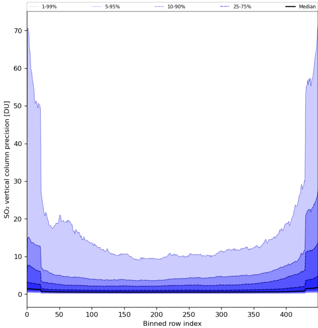
Figure 77: Along track statistics of “SO 2 vertical column precision” for 2024-04-22 to 2024-04-24
