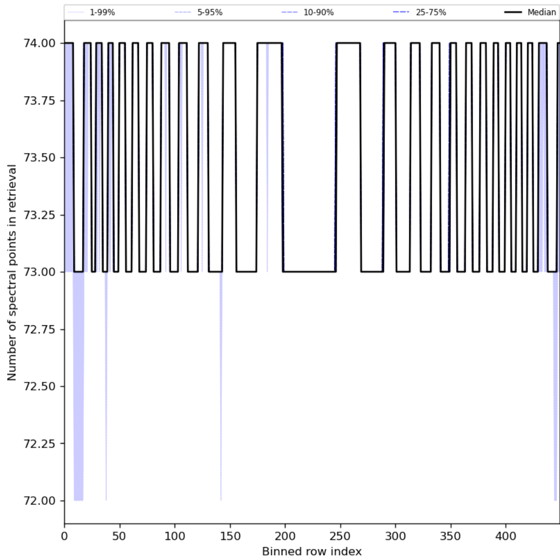
Figure 97: Along track statistics of “Number of spectral points in retrieval” for 2024-04-22 to 2024-04-24
