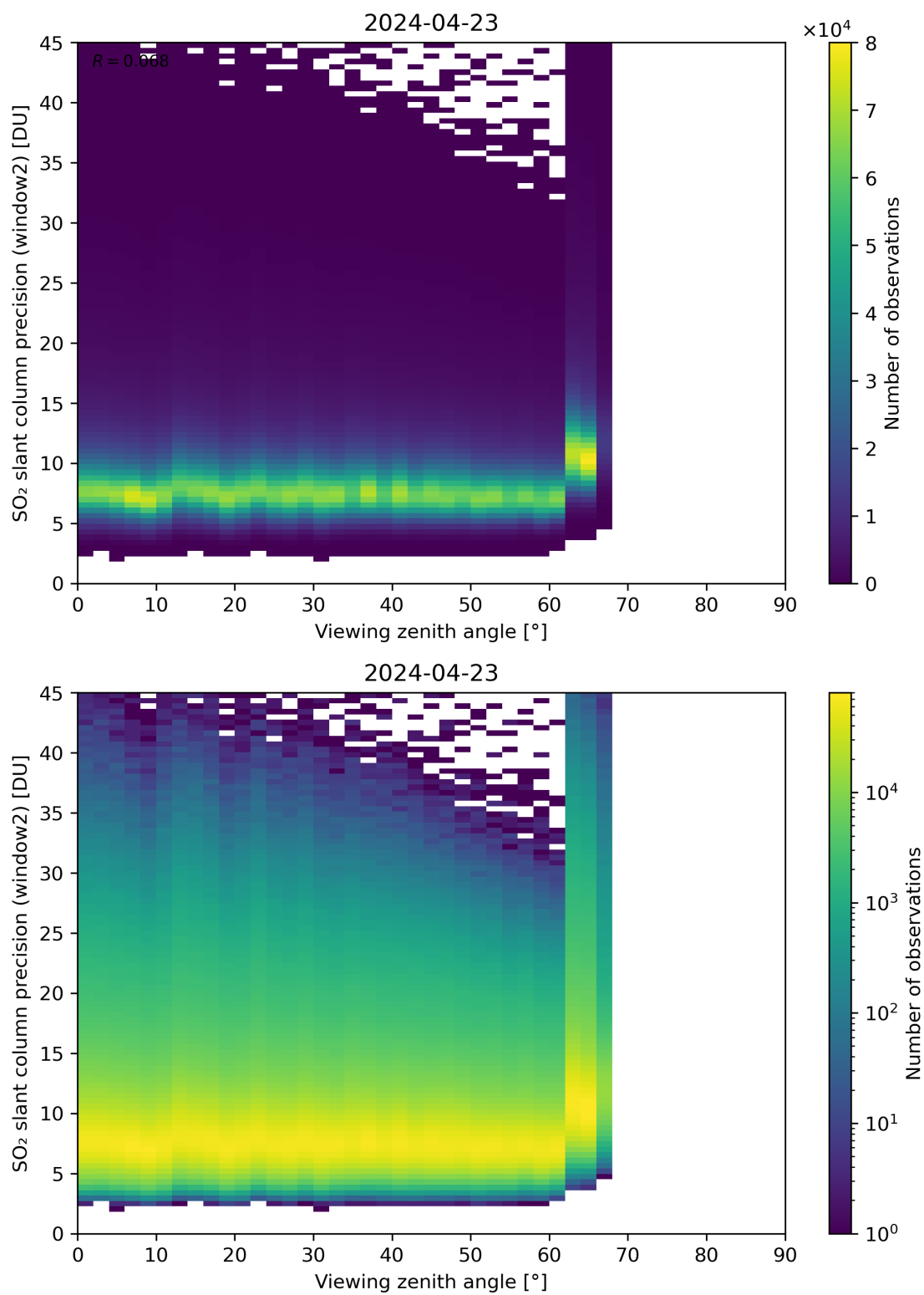
Figure 322: Scatter density plot of “Viewing zenith angle” against “SO 2 slant column precision (window2)” for 2024-04-22 to 2024-04-24.
