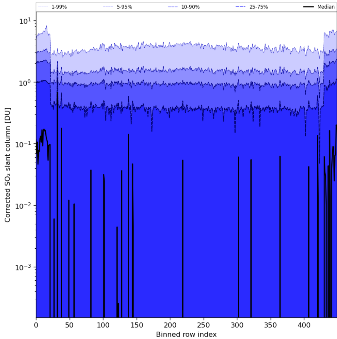
Figure 78: Along track statistics of “Corrected SO 2 slant column” for 2024-04-22 to 2024-04-24
