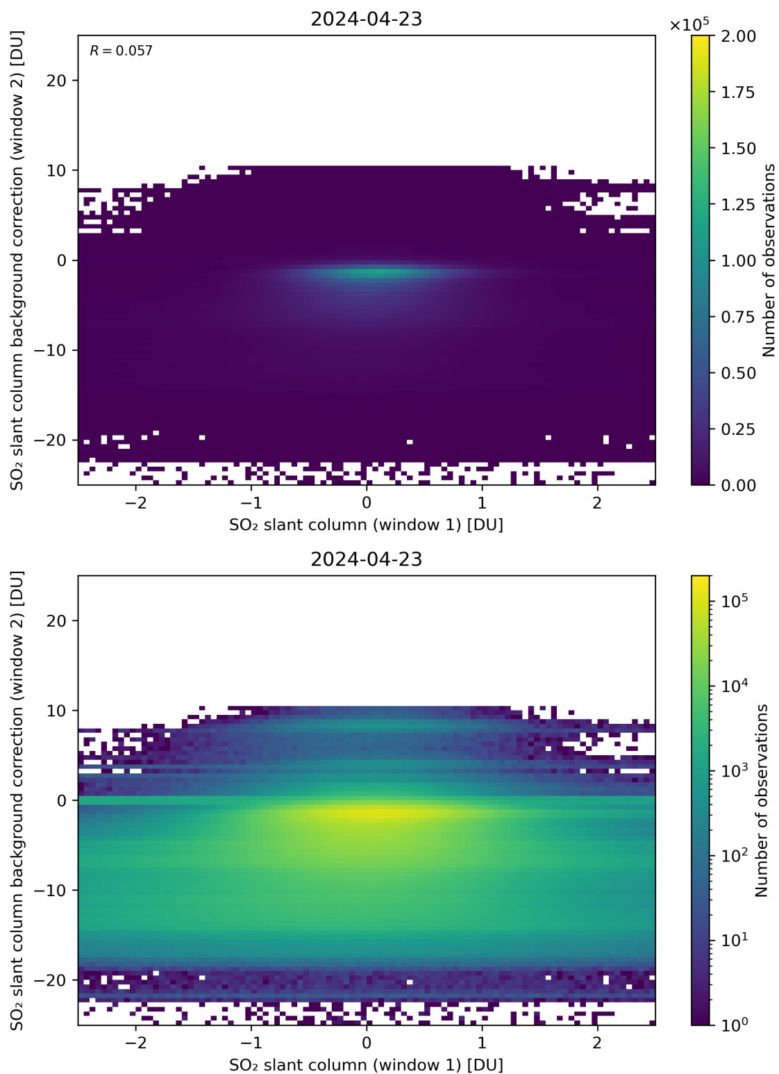
Figure 213: Scatter density plot of “SO 2 slant column (window 1)” against “SO 2 slant column background correction (window 2)” for 2024-04-22 to 2024-04-24.
