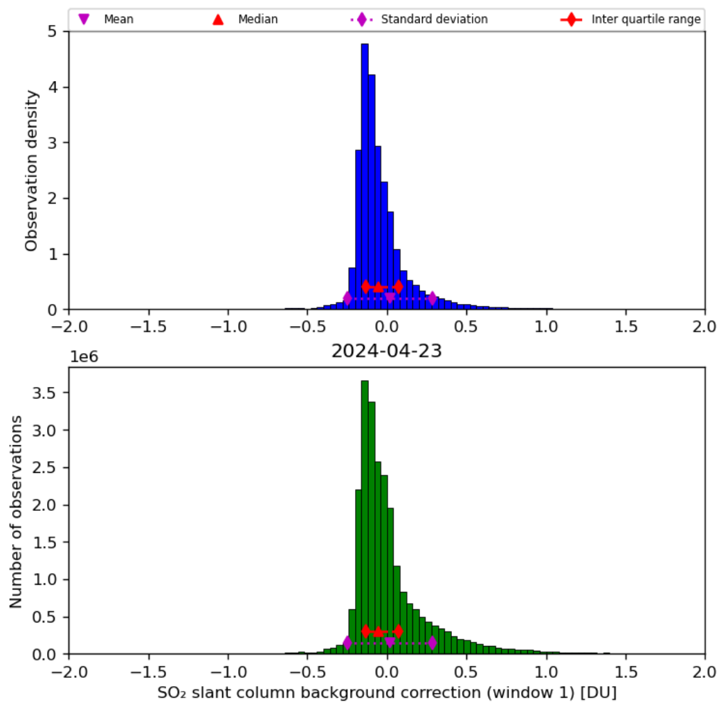
Figure 59: Histogram of “SO 2 slant column background correction (window 1)” for 2024-04-22 to 2024-04-24
