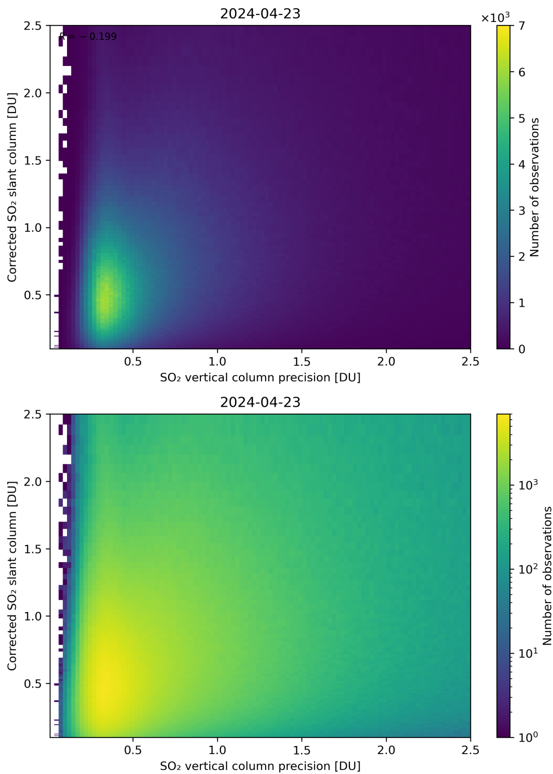
Figure 286: Scatter density plot of “SO 2 vertical column precision” against “Corrected SO 2 slant column” for 2024-04-22 to 2024-04-24.
