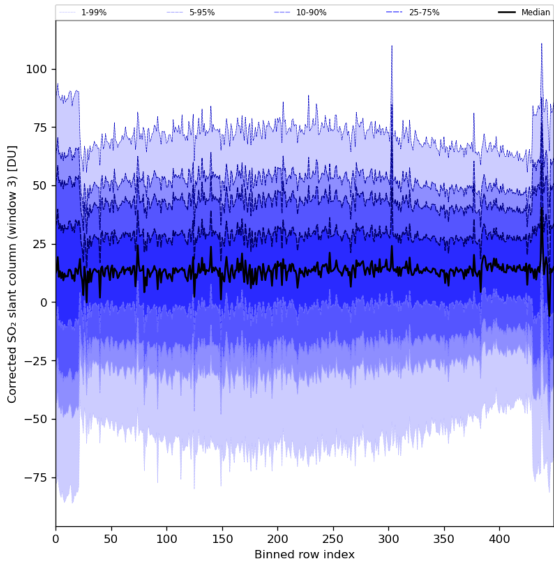
Figure 89: Along track statistics of “Corrected SO 2 slant column (window 3)” for 2024-04-22 to 2024-04-24
