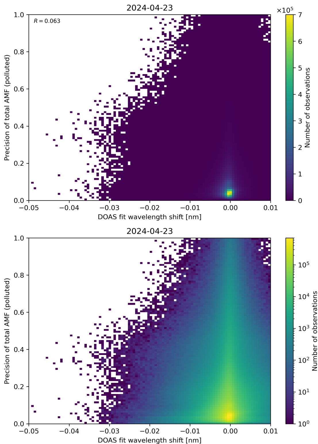
Figure 131: Scatter density plot of “DOAS fit wavelength shift” against “Precision of total AMF (polluted)” for 2024-04-22 to 2024-04-24.
