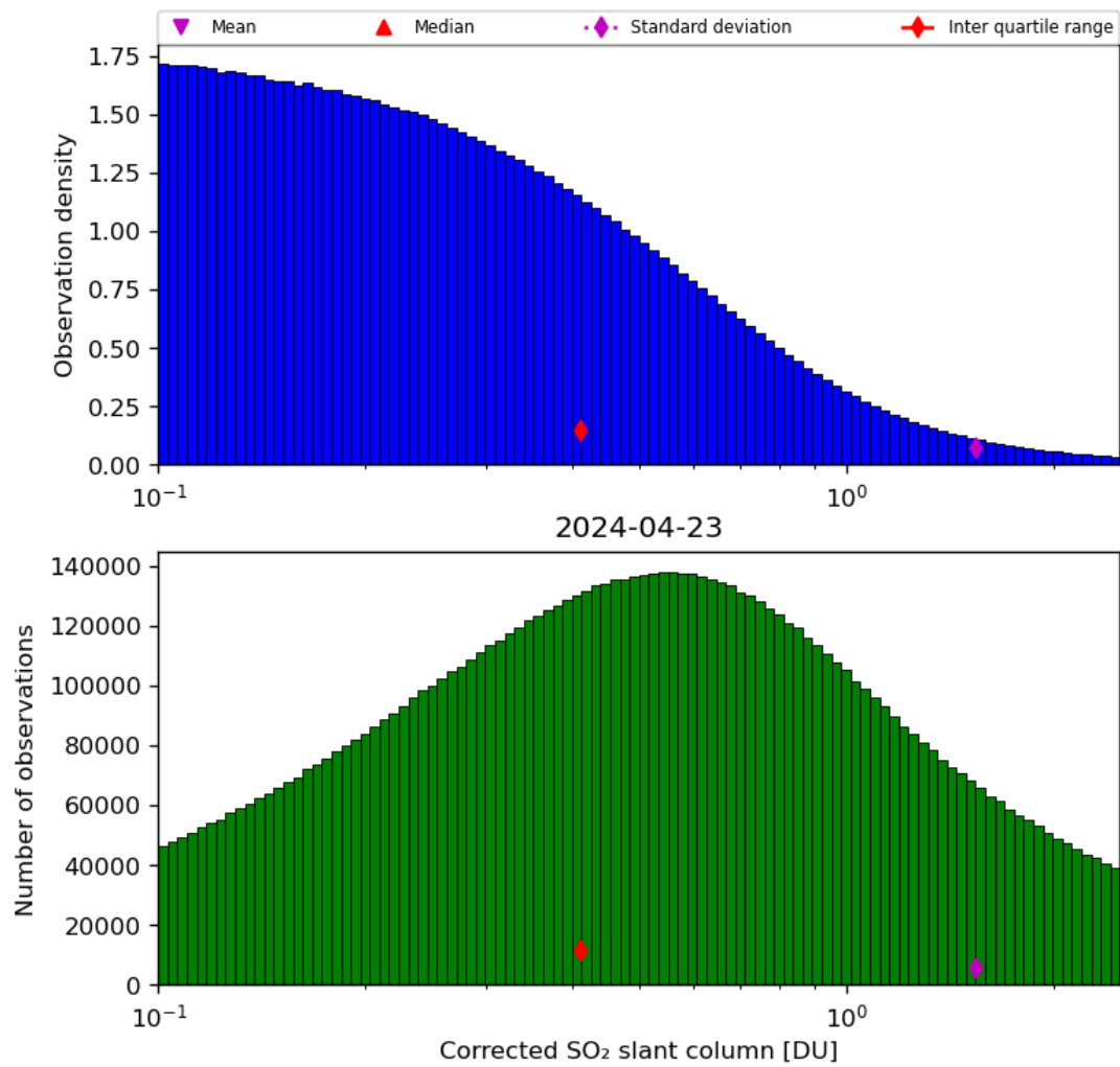
Figure 55: Histogram of “Corrected SO 2 slant column” for 2024-04-22 to 2024-04-24
