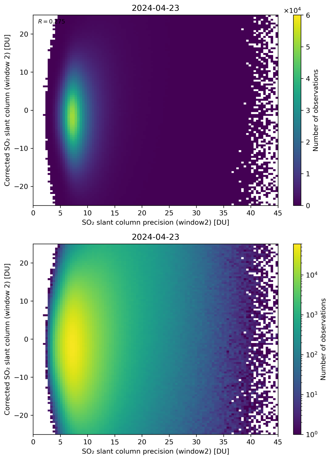
Figure 247: Scatter density plot of “SO 2 slant column precision (window2)” against “Corrected SO 2 slant column (window 2)” for 2024-04-22 to 2024-04-24.
