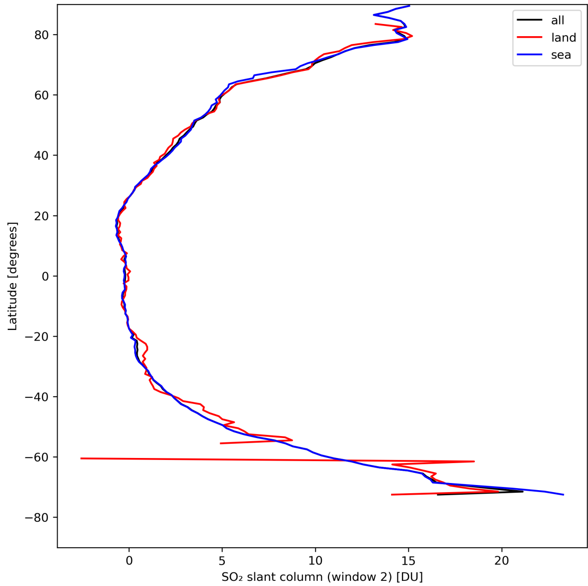
Figure 37: Zonal average of “SO 2 slant column (window 2)” for 2024-04-22 to 2024-04-24.
