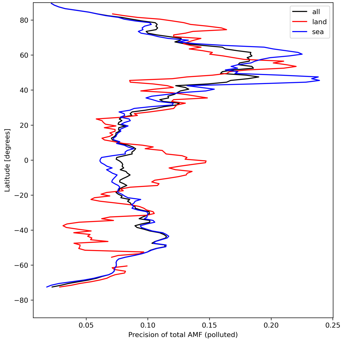
Figure 49: Zonal average of “Precision of total AMF (polluted)” for 2024-04-22 to 2024-04-24.
