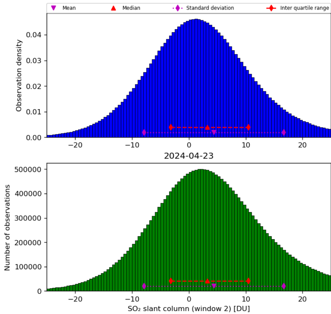
Figure 60: Histogram of “SO 2 slant column (window 2)” for 2024-04-22 to 2024-04-24
