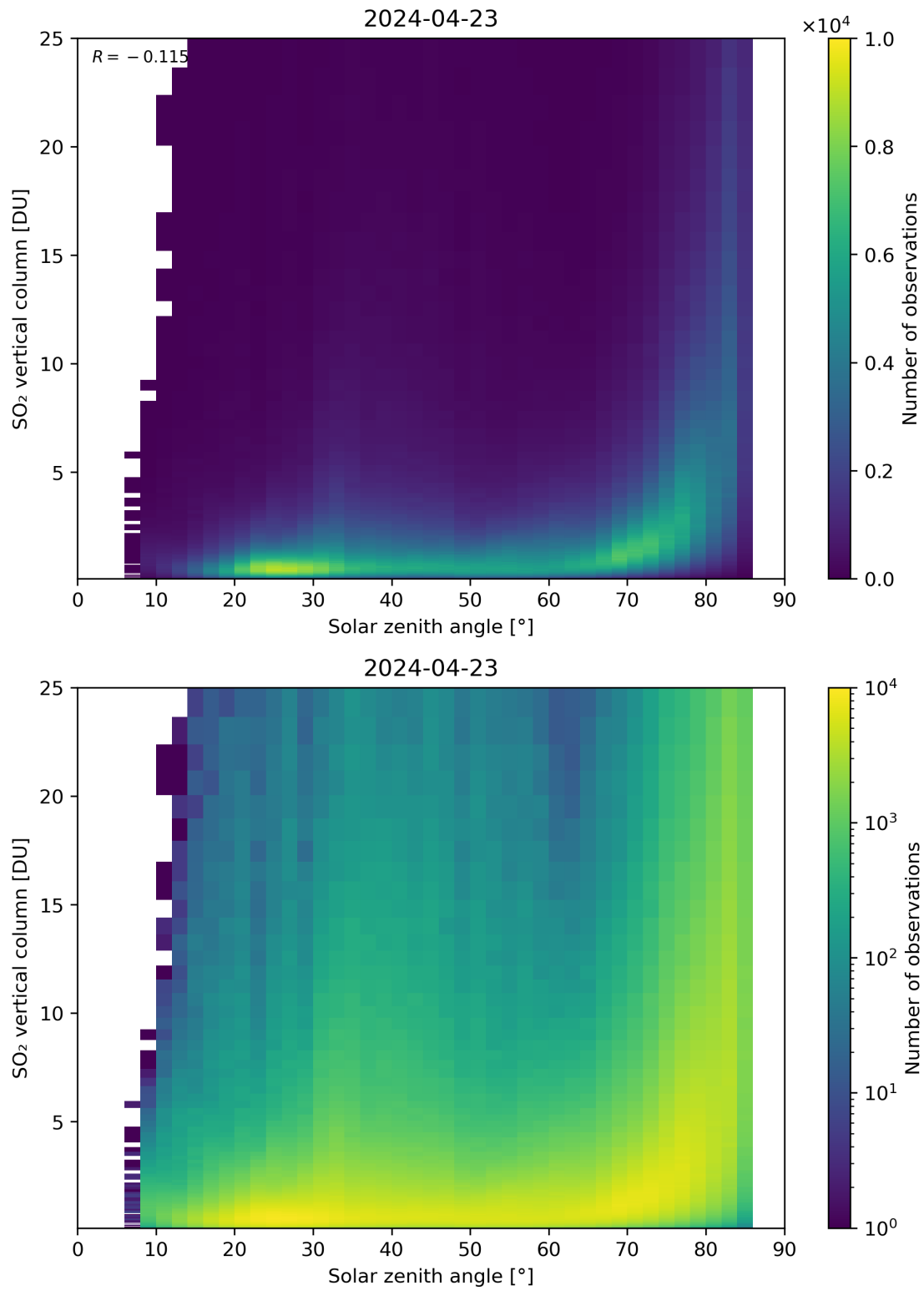
Figure 176: Scatter density plot of “Solar zenith angle” against “SO 2 vertical column” for 2024-04-22 to 2024-04-24.
