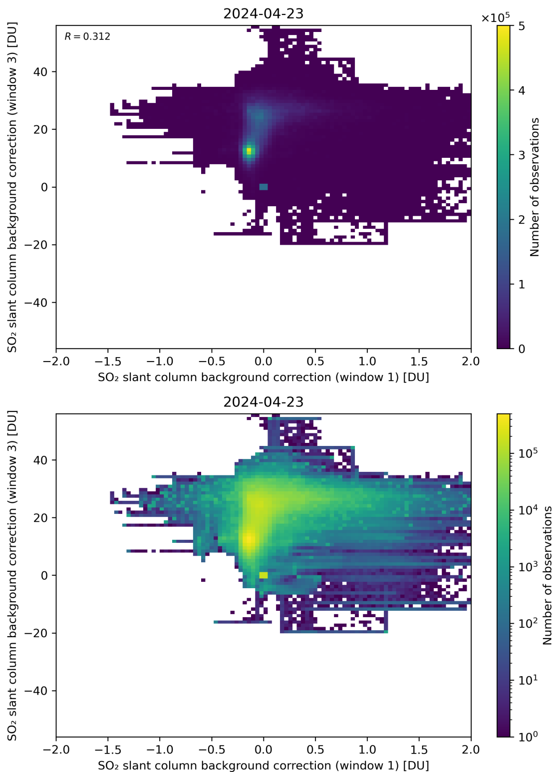
Figure 99: Scatter density plot of “SO 2 slant column background correction (window 1)” against “SO 2 slant column background correction (window 3)” for 2024-04-22 to 2024-04-24.
