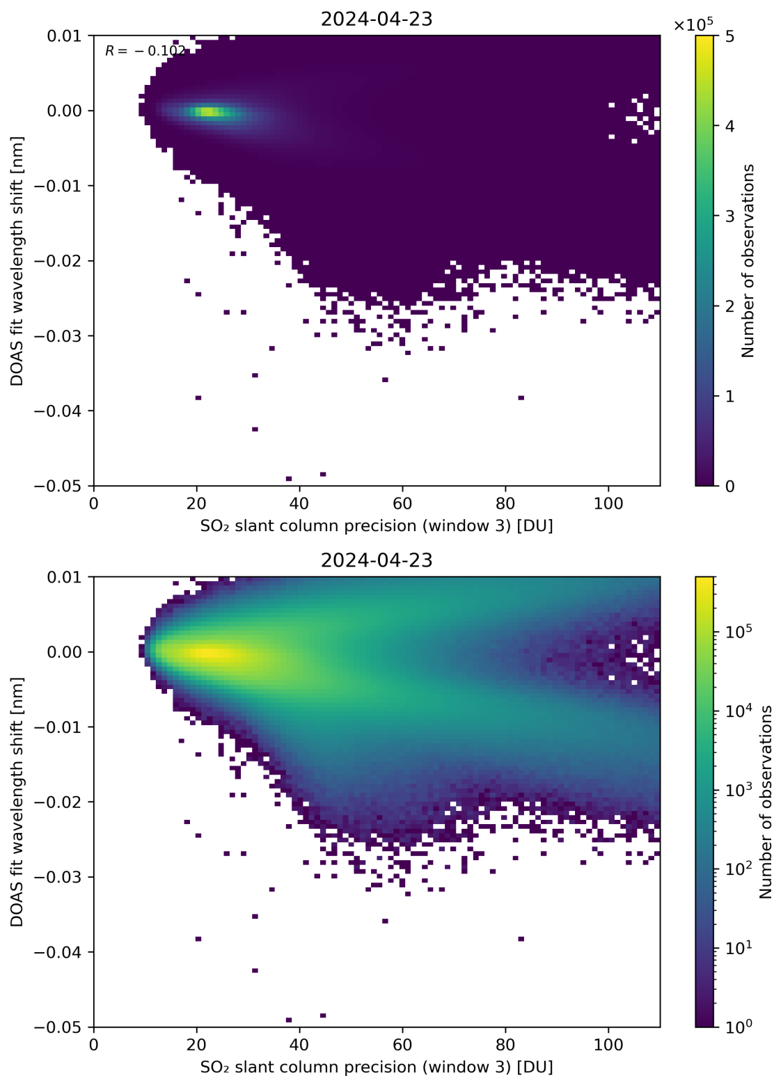
Figure 258: Scatter density plot of “SO 2 slant column precision (window 3)” against “DOAS fit wavelength shift” for 2024-04-22 to 2024-04-24.
