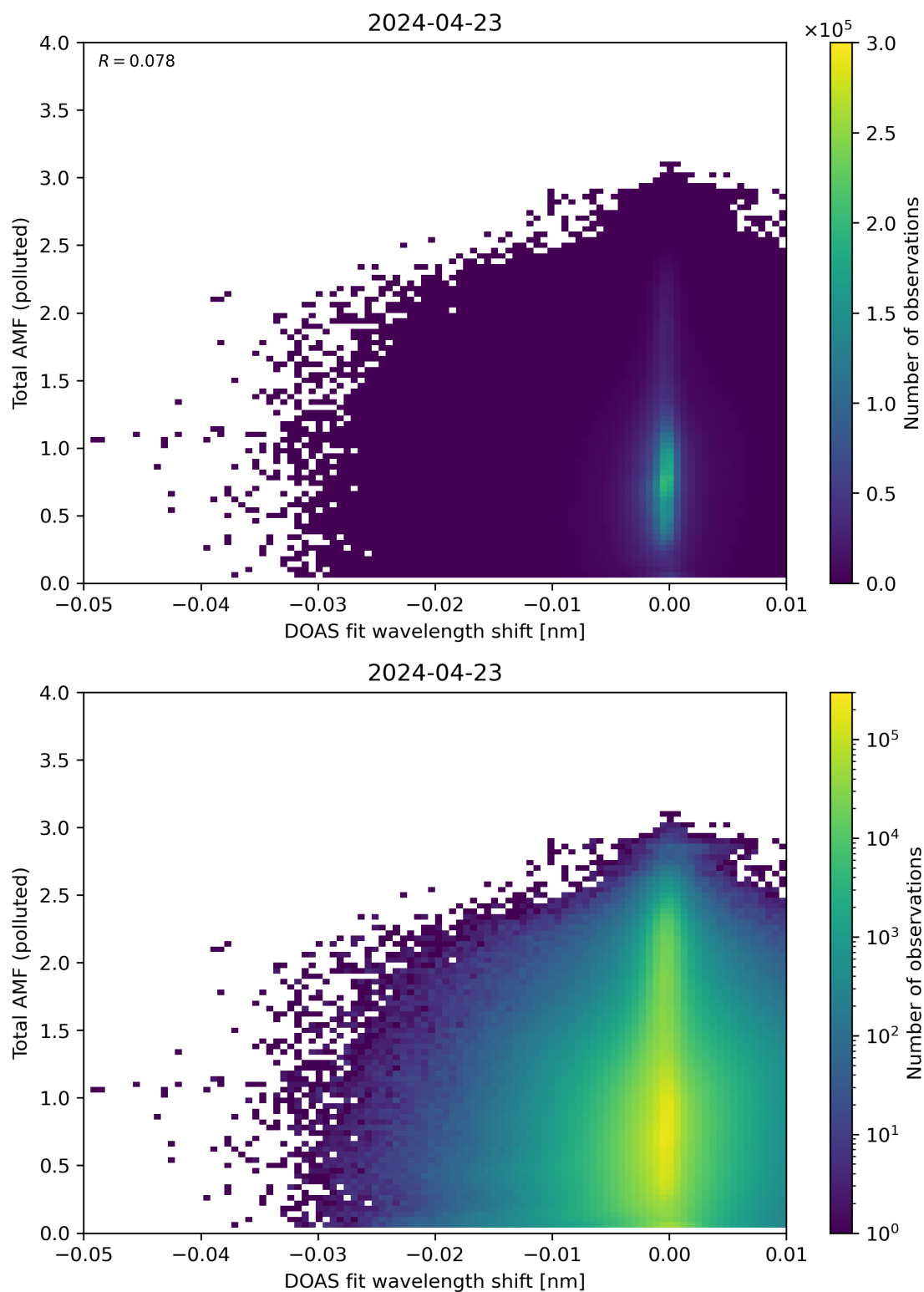
Figure 130: Scatter density plot of “DOAS fit wavelength shift” against “Total AMF (polluted)” for 2024-04-22 to 2024-04-24.
