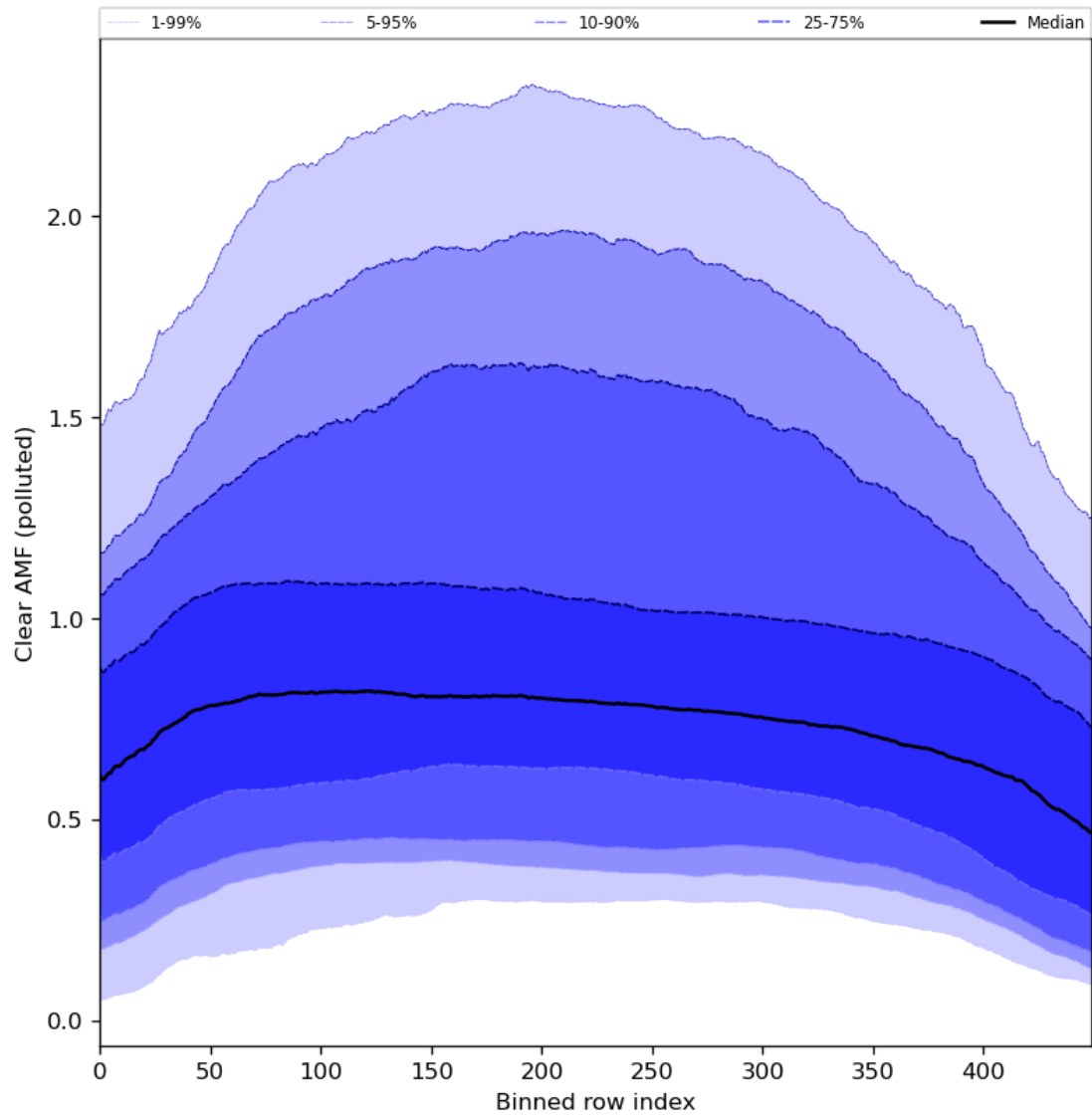
Figure 96: Along track statistics of “Clear AMF (polluted)” for 2024-04-22 to 2024-04-24
