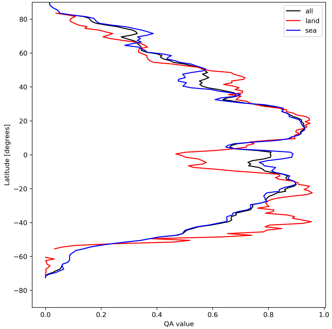
Figure 29: Zonal average of “QA value” for 2024-04-22 to 2024-04-24.
