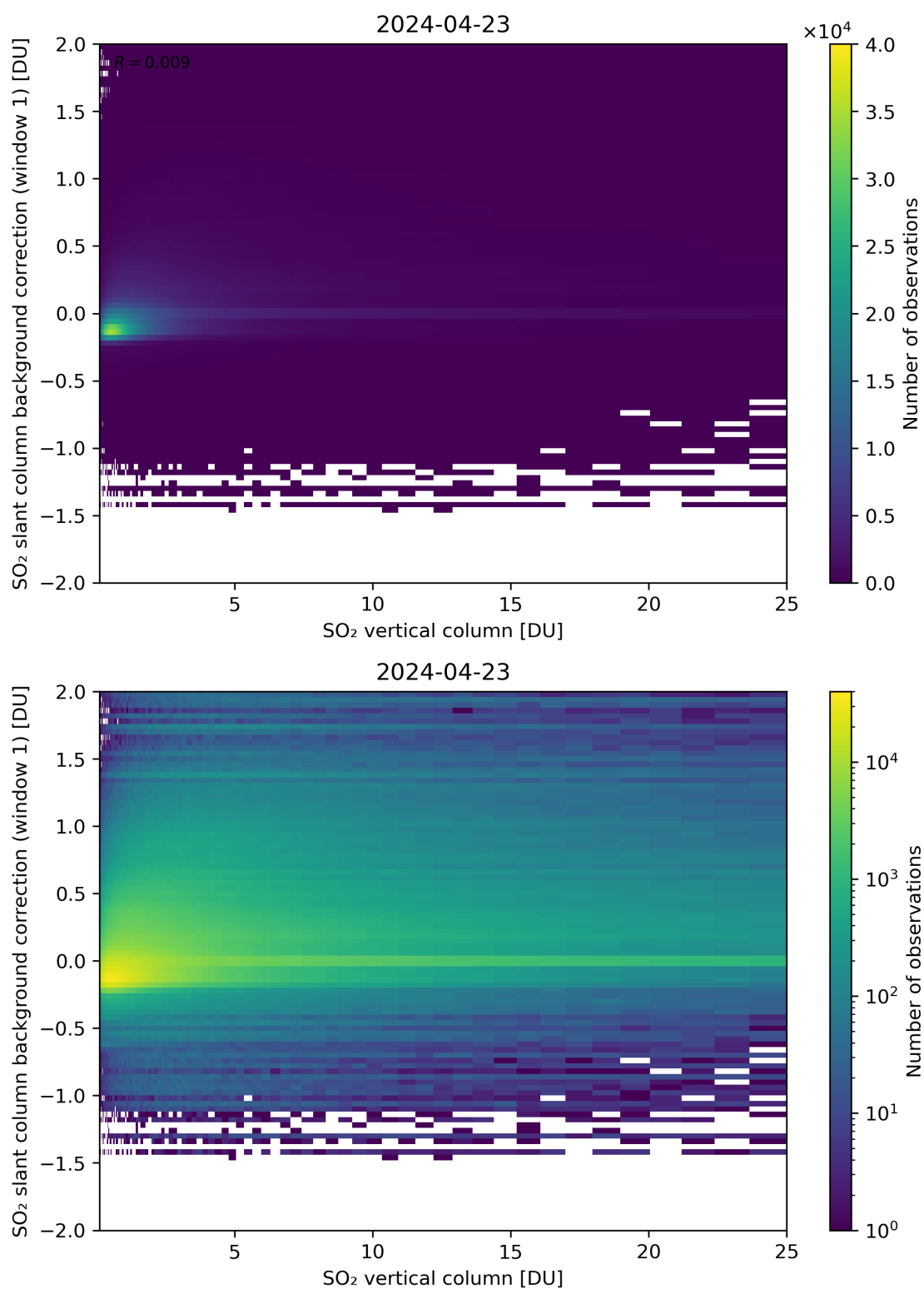
Figure 273: Scatter density plot of “SO 2 vertical column” against “SO 2 slant column background correction (window 1)” for 2024-04-22 to 2024-04-24.
