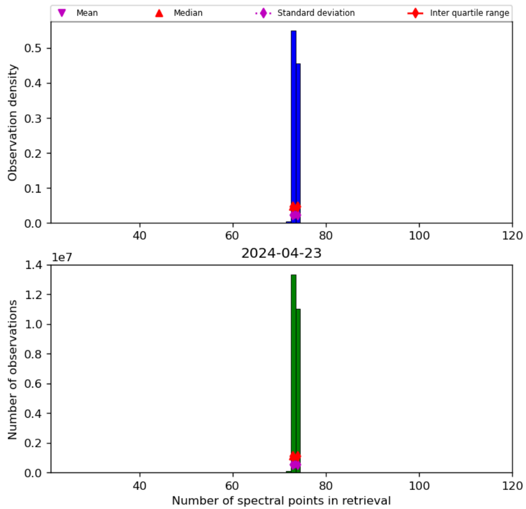
Figure 74: Histogram of “Number of spectral points in retrieval” for 2024-04-22 to 2024-04-24
