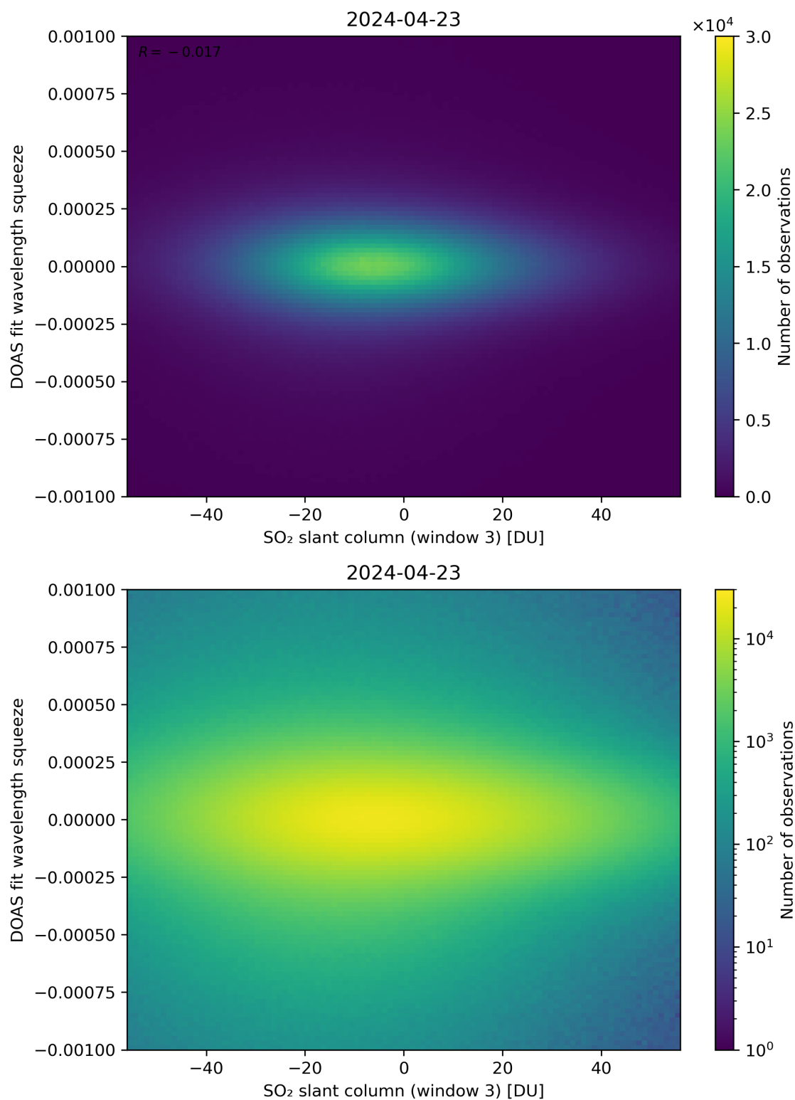
Figure 255: Scatter density plot of “SO 2 slant column (window 3)” against “DOAS fit wavelength squeeze” for 2024-04-22 to 2024-04-24.
