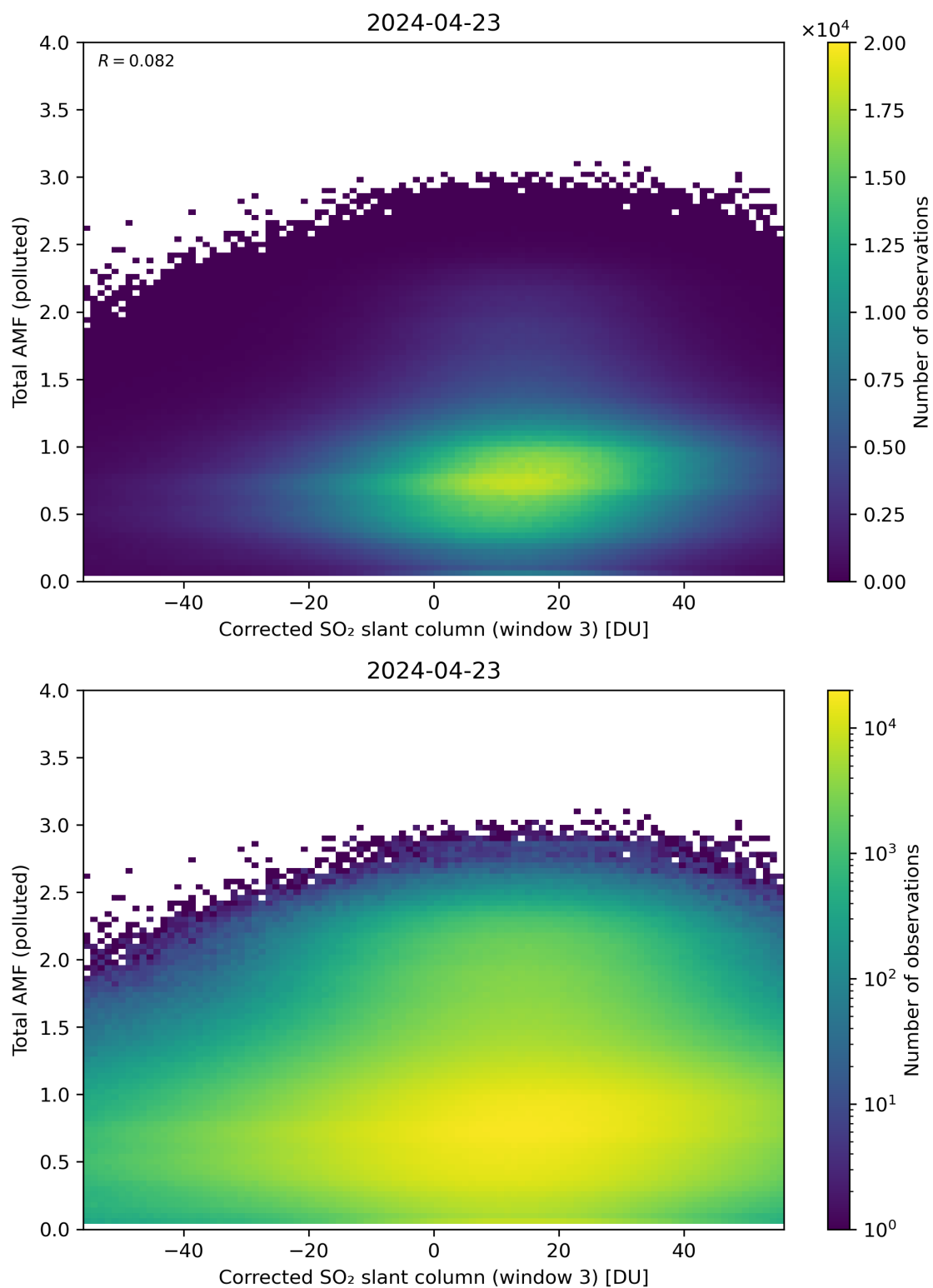
Figure 210: Scatter density plot of “Corrected SO 2 slant column (window 3)” against “Total AMF (polluted)” for 2024-04-22 to 2024-04-24.
