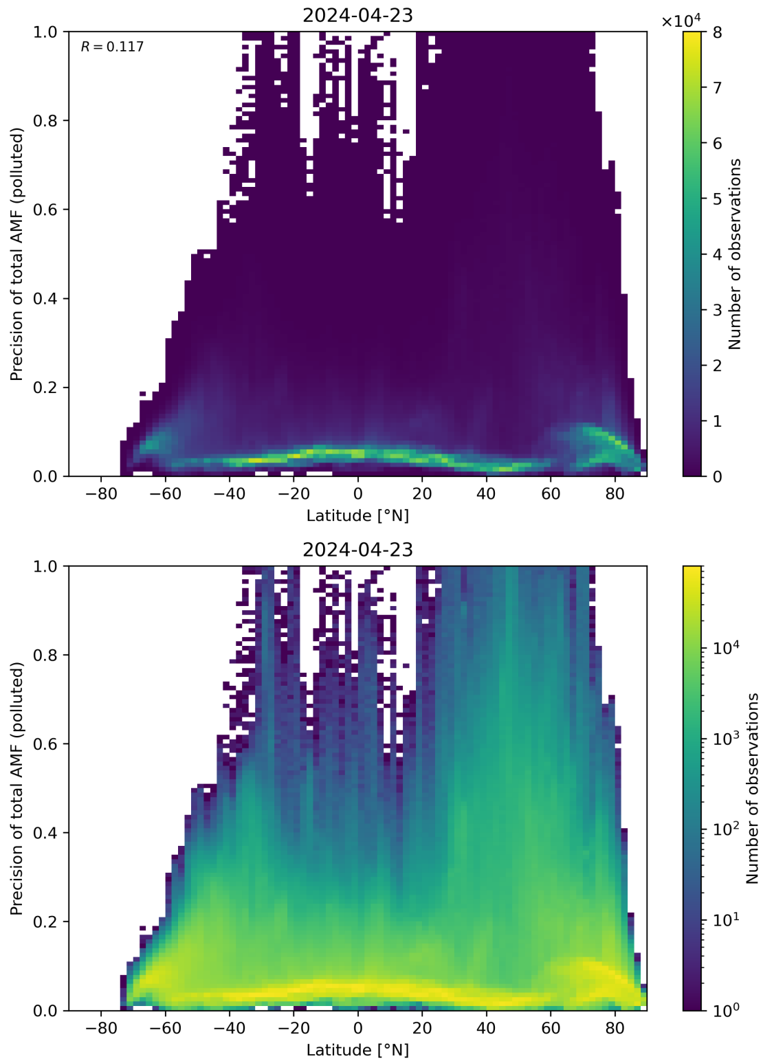
Figure 155: Scatter density plot of “Latitude” against “Precision of total AMF (polluted)” for 2024-04-22 to 2024-04-24.
