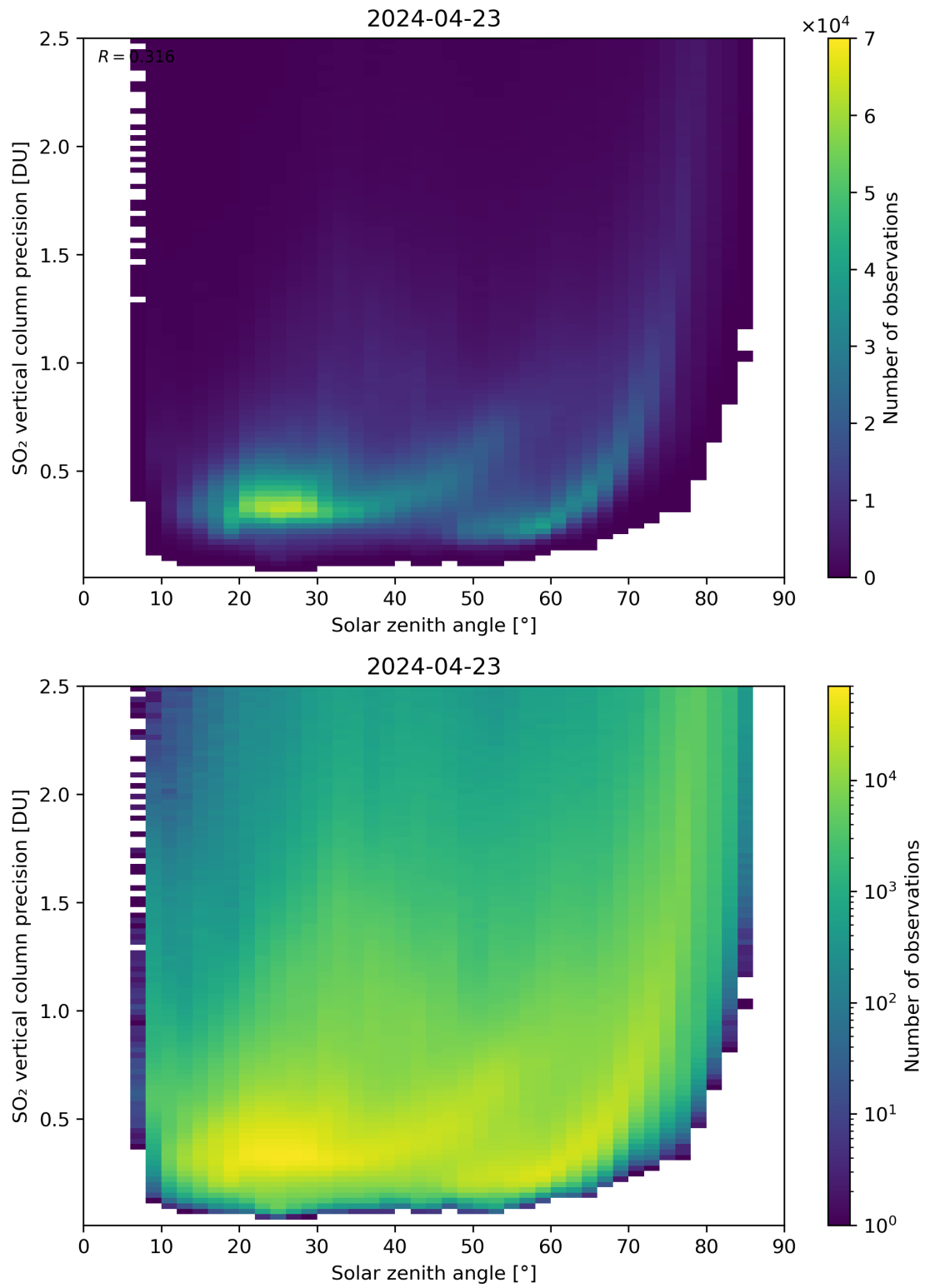
Figure 177: Scatter density plot of “Solar zenith angle” against “SO 2 vertical column precision” for 2024-04-22 to 2024-04-24.
