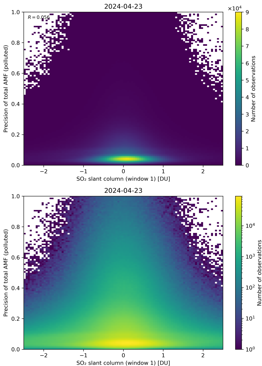
Figure 240: Scatter density plot of “SO 2 slant column (window 1)” against “Precision of total AMF (polluted)” for 2024-04-22 to 2024-04-24.
