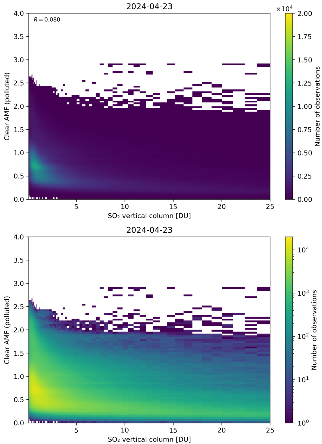
Figure 296: Scatter density plot of “SO 2 vertical column” against “Clear AMF (polluted)” for 2024-04-22 to 2024-04-24.
