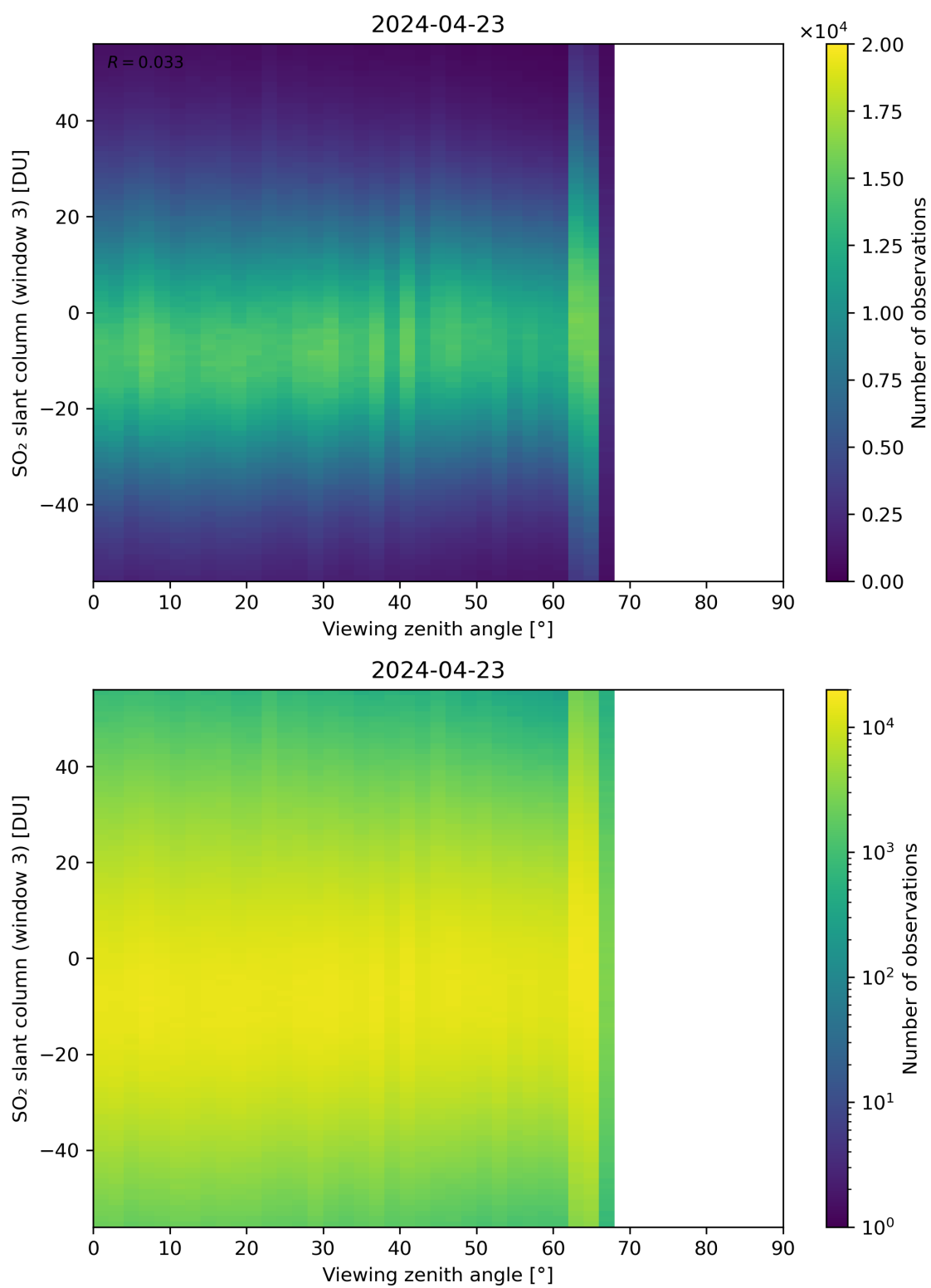
Figure 323: Scatter density plot of “Viewing zenith angle” against “SO 2 slant column (window 3)” for 2024-04-22 to 2024-04-24.
