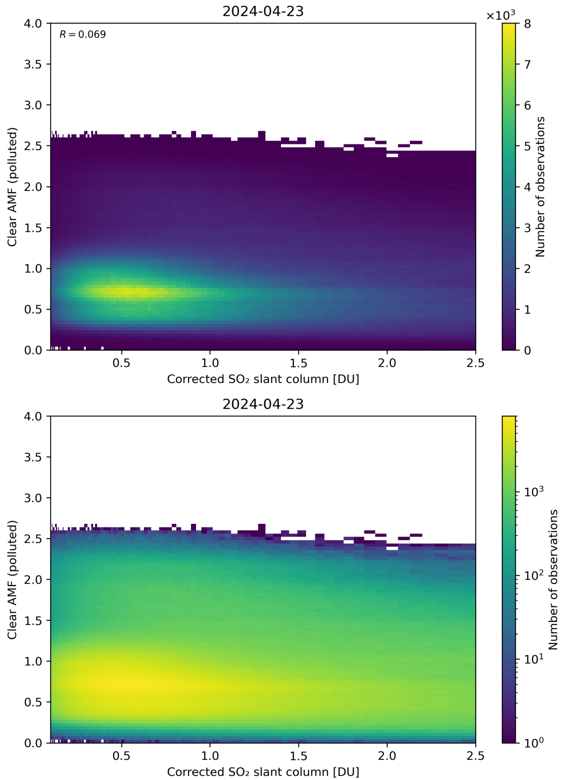
Figure 184: Scatter density plot of “Corrected SO 2 slant column” against “Clear AMF (polluted)” for 2024-04-22 to 2024-04-24.
