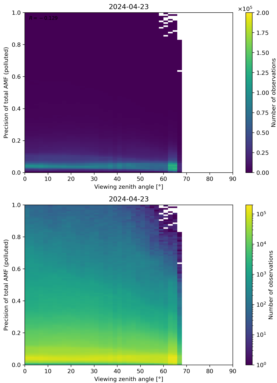
Figure 326: Scatter density plot of “Viewing zenith angle” against “Precision of total AMF (polluted)” for 2024-04-22 to 2024-04-24.
