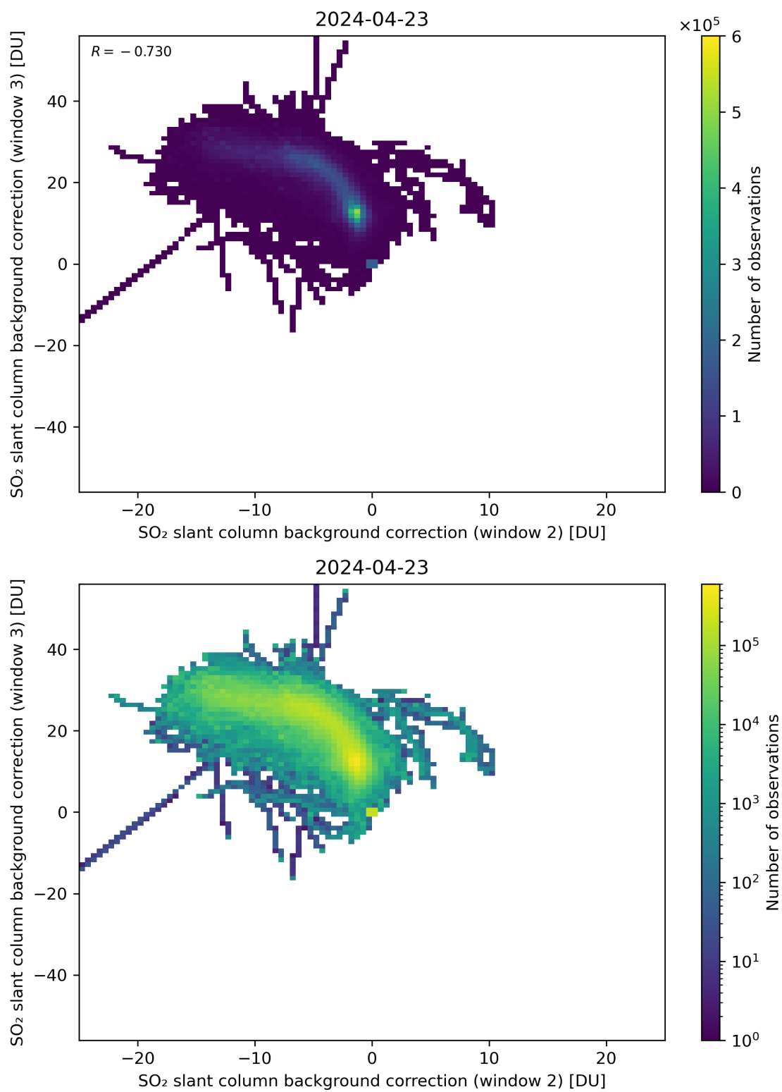
Figure 111: Scatter density plot of “SO 2 slant column background correction (window 2)” against “SO 2 slant column background correction (window 3)” for 2024-04-22 to 2024-04-24.
