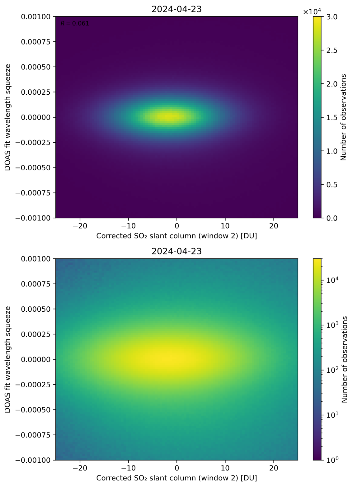
Figure 197: Scatter density plot of “Corrected SO 2 slant column (window 2)” against “DOAS fit wavelength squeeze” for 2024-04-22 to 2024-04-24.
