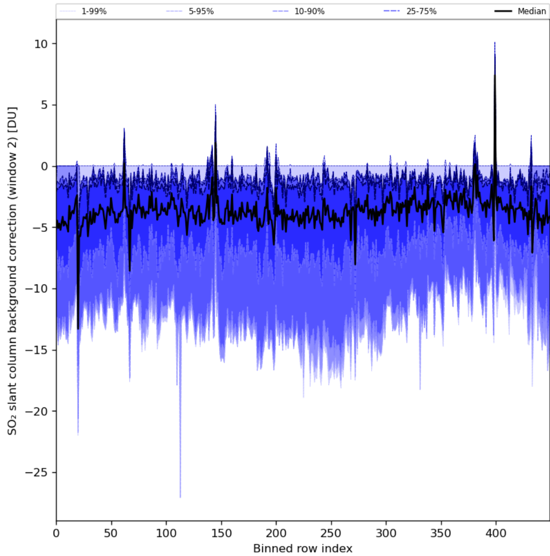
Figure 86: Along track statistics of “SO 2 slant column background correction (window 2)” for 2024-04-22 to 2024-04-24
