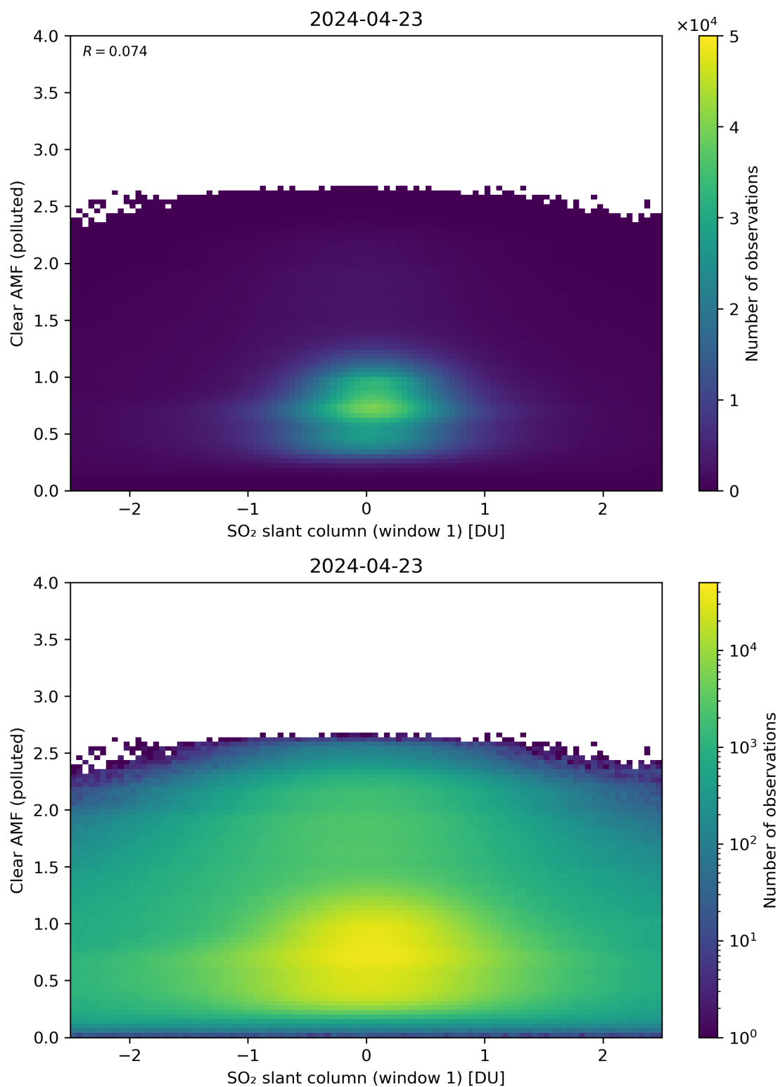
Figure 232: Scatter density plot of “SO 2 slant column (window 1)” against “Clear AMF (polluted)” for 2024-04-22 to 2024-04-24.
