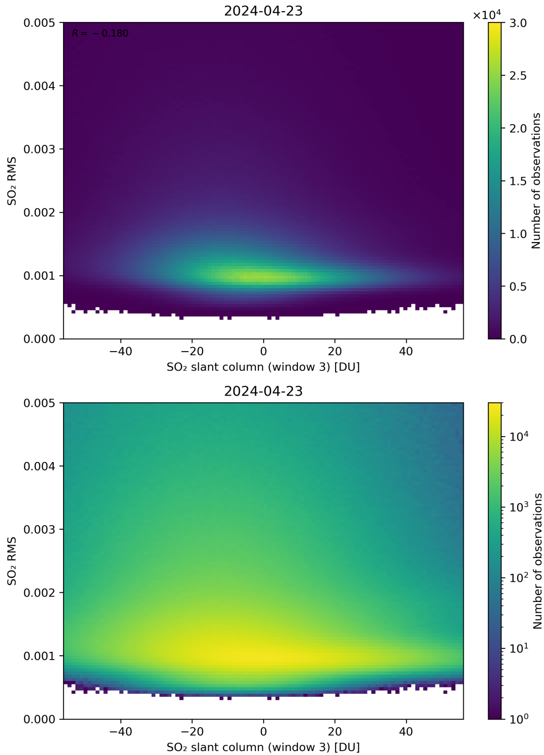
Figure 256: Scatter density plot of “SO 2 slant column (window 3)” against “SO 2 RMS” for 2024-04-22 to 2024-04-24.
