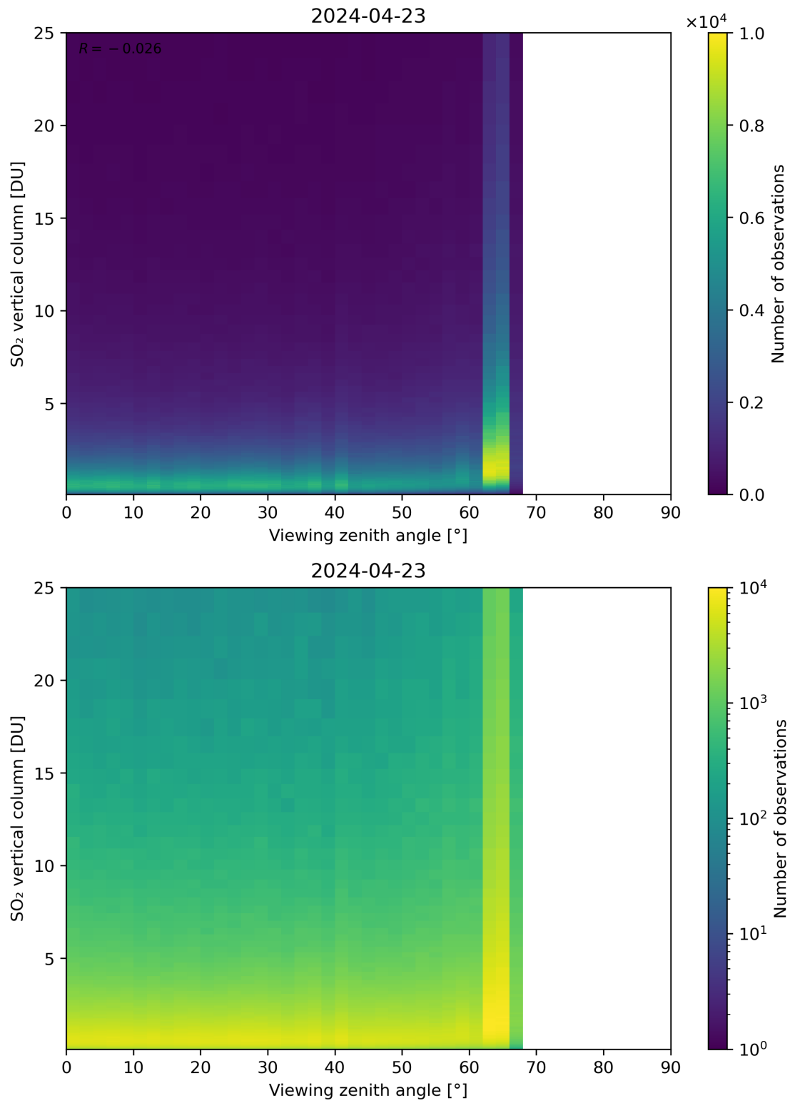
Figure 327: Scatter density plot of “Viewing zenith angle” against “SO 2 vertical column” for 2024-04-22 to 2024-04-24.
