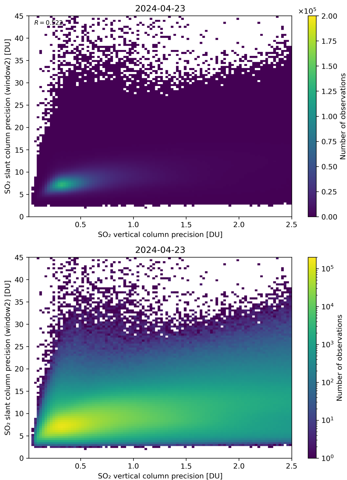
Figure 291: Scatter density plot of “SO 2 vertical column precision” against “SO 2 slant column precision (window2)” for 2024-04-22 to 2024-04-24.
