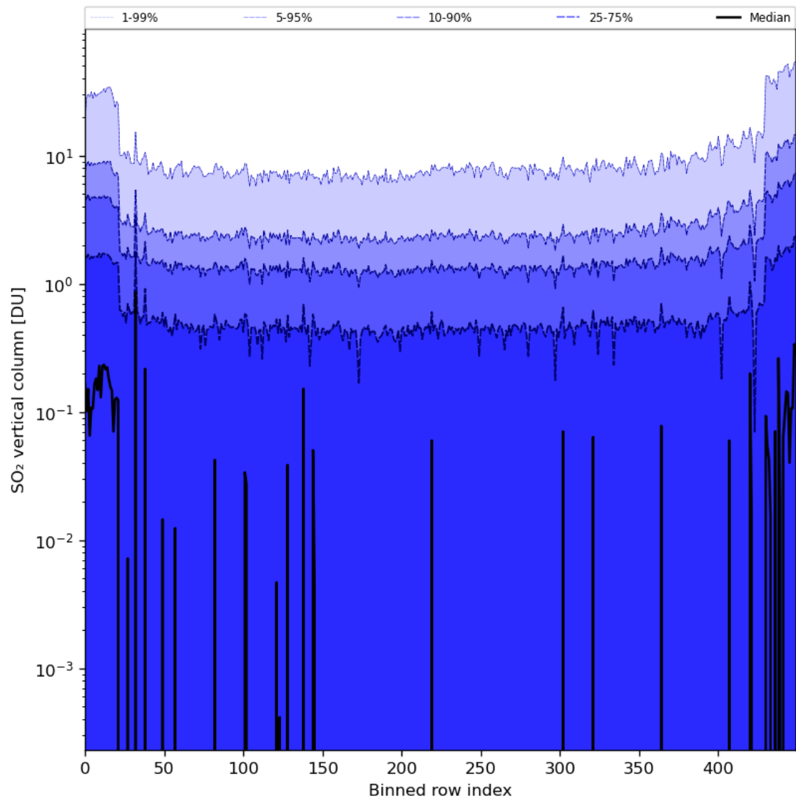
Figure 76: Along track statistics of “SO 2 vertical column” for 2024-04-22 to 2024-04-24
