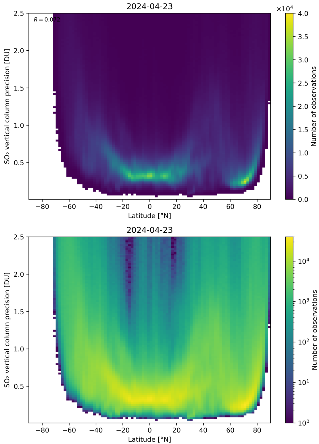
Figure 157: Scatter density plot of “Latitude” against “SO 2 vertical column precision” for 2024-04-22 to 2024-04-24.
