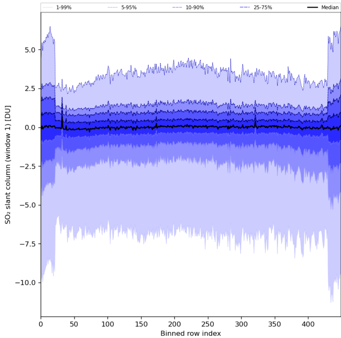
Figure 79: Along track statistics of “SO 2 slant column (window 1)” for 2024-04-22 to 2024-04-24
