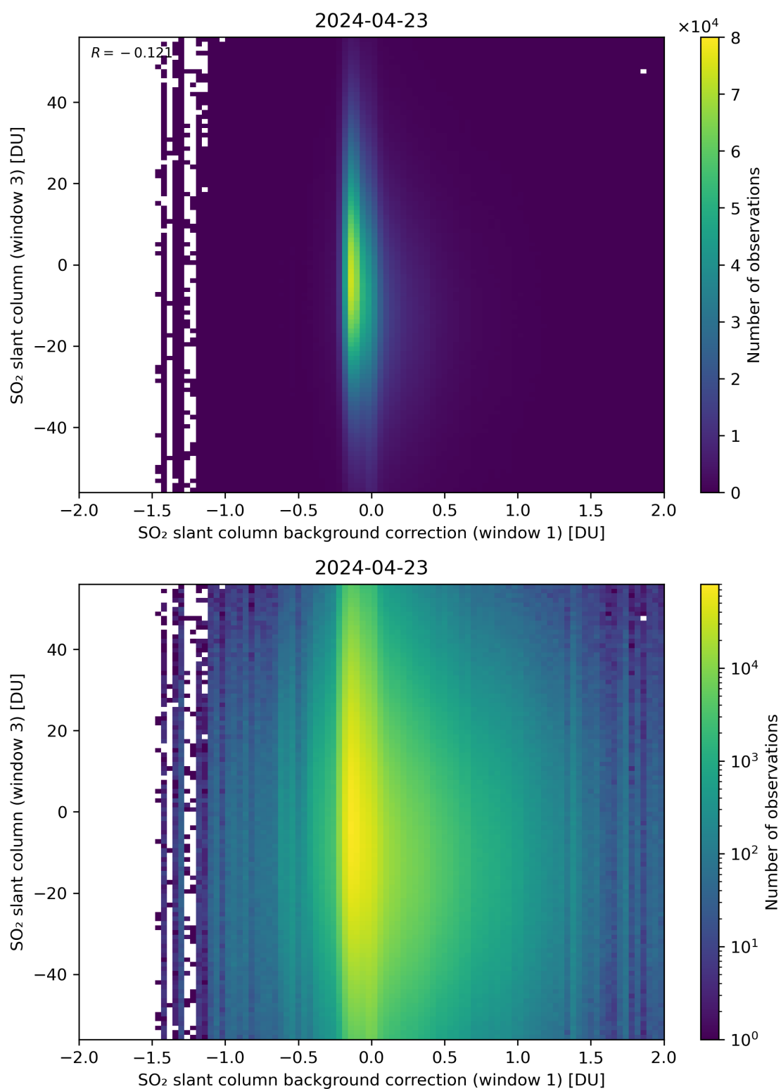
Figure 107: Scatter density plot of “SO 2 slant column background correction (window 1)” against “SO 2 slant column (window 3)” for 2024-04-22 to 2024-04-24.
