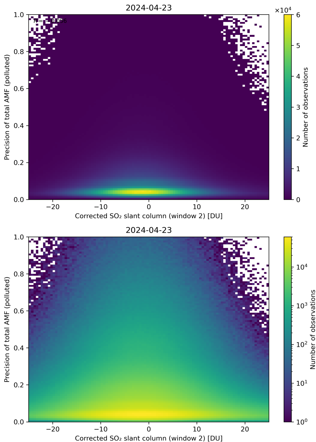
Figure 204: Scatter density plot of “Corrected SO 2 slant column (window 2)” against “Precision of total AMF (polluted)” for 2024-04-22 to 2024-04-24.
