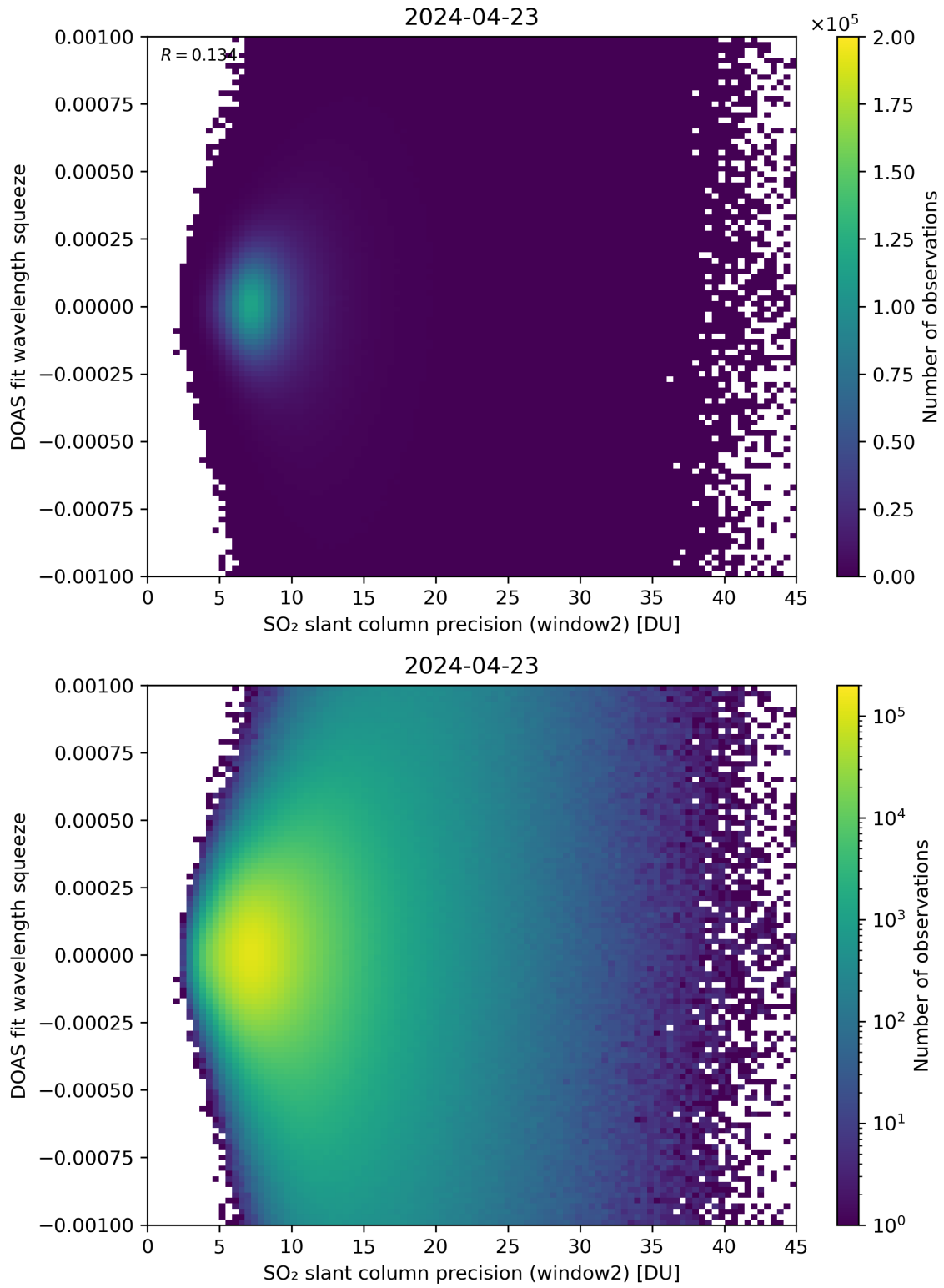
Figure 244: Scatter density plot of “SO 2 slant column precision (window2)” against “DOAS fit wavelength squeeze” for 2024-04-22 to 2024-04-24.
