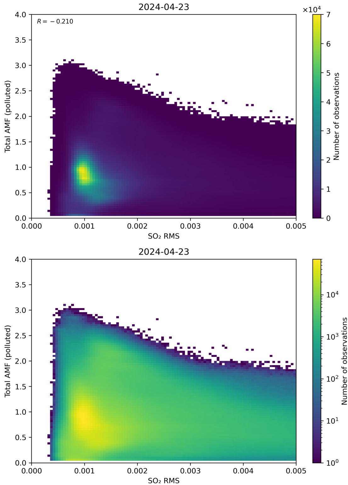
Figure 137: Scatter density plot of “SO 2 RMS” against “Total AMF (polluted)” for 2024-04-22 to 2024-04-24.
