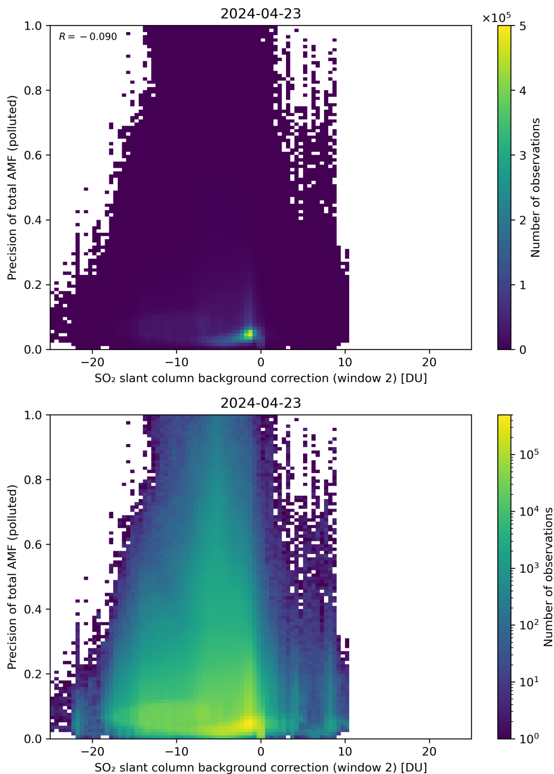
Figure 120: Scatter density plot of “SO 2 slant column background correction (window 2)” against “Precision of total AMF (polluted)” for 2024-04-22 to 2024-04-24.
