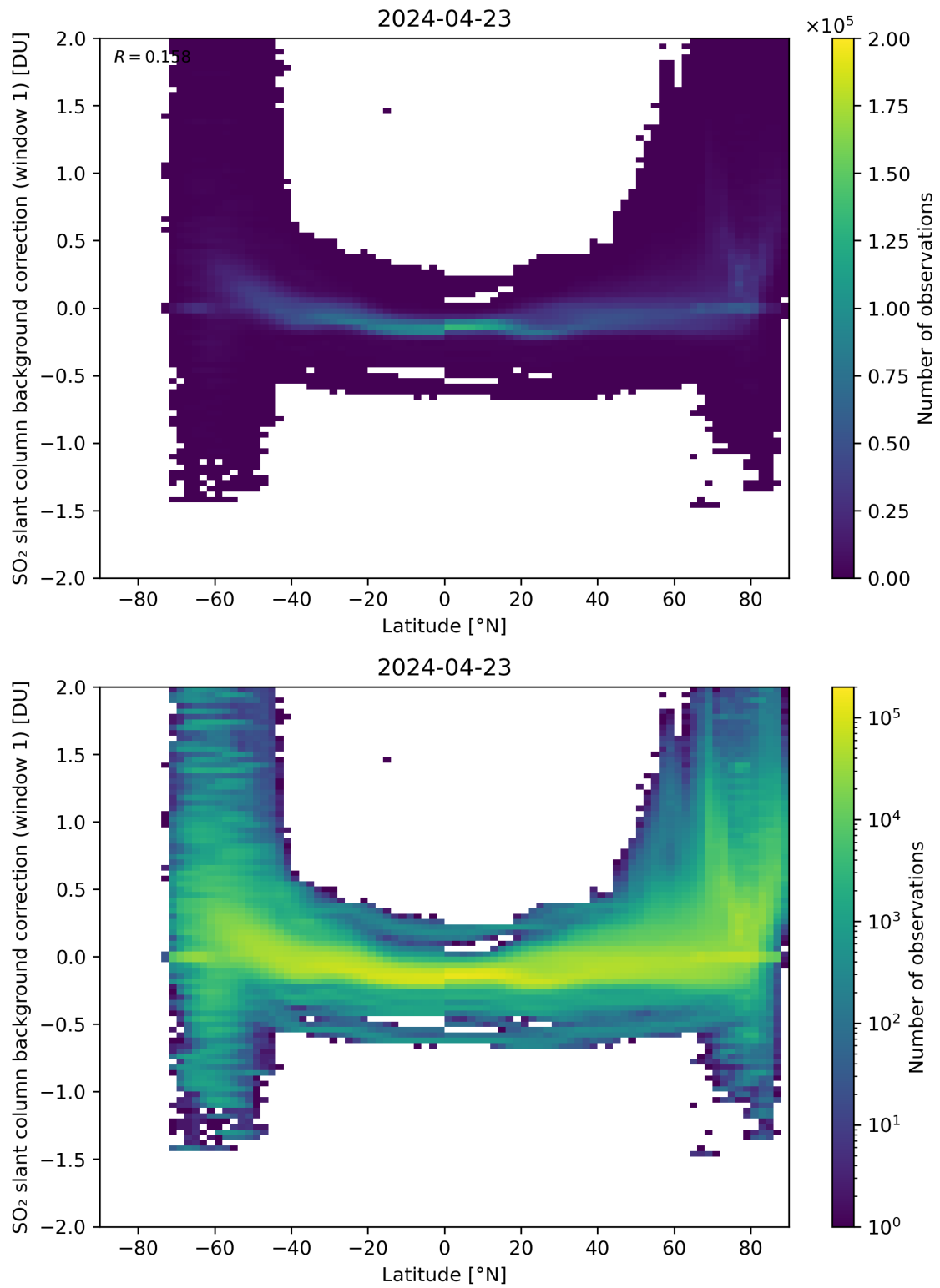
Figure 139: Scatter density plot of “Latitude” against “SO 2 slant column background correction (window 1)” for 2024-04-22 to 2024-04-24.
