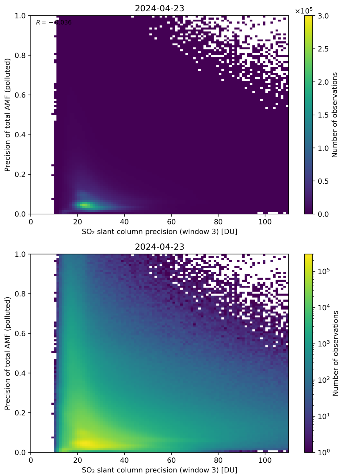
Figure 264: Scatter density plot of “SO 2 slant column precision (window 3)” against “Precision of total AMF (polluted)” for 2024-04-22 to 2024-04-24.
