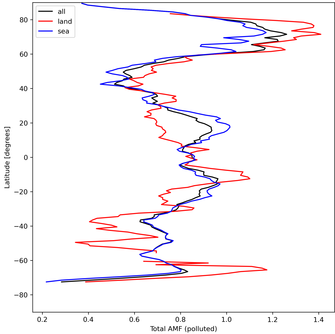
Figure 48: Zonal average of “Total AMF (polluted)” for 2024-04-22 to 2024-04-24.
