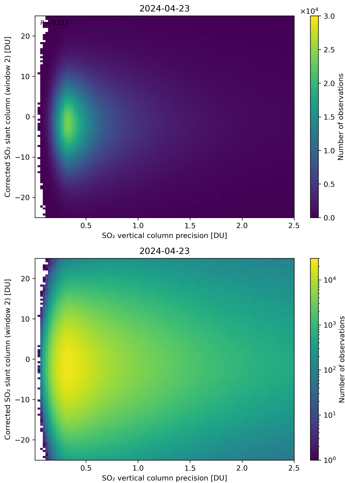
Figure 287: Scatter density plot of “SO 2 vertical column precision” against “Corrected SO 2 slant column (window 2)” for 2024-04-22 to 2024-04-24.
