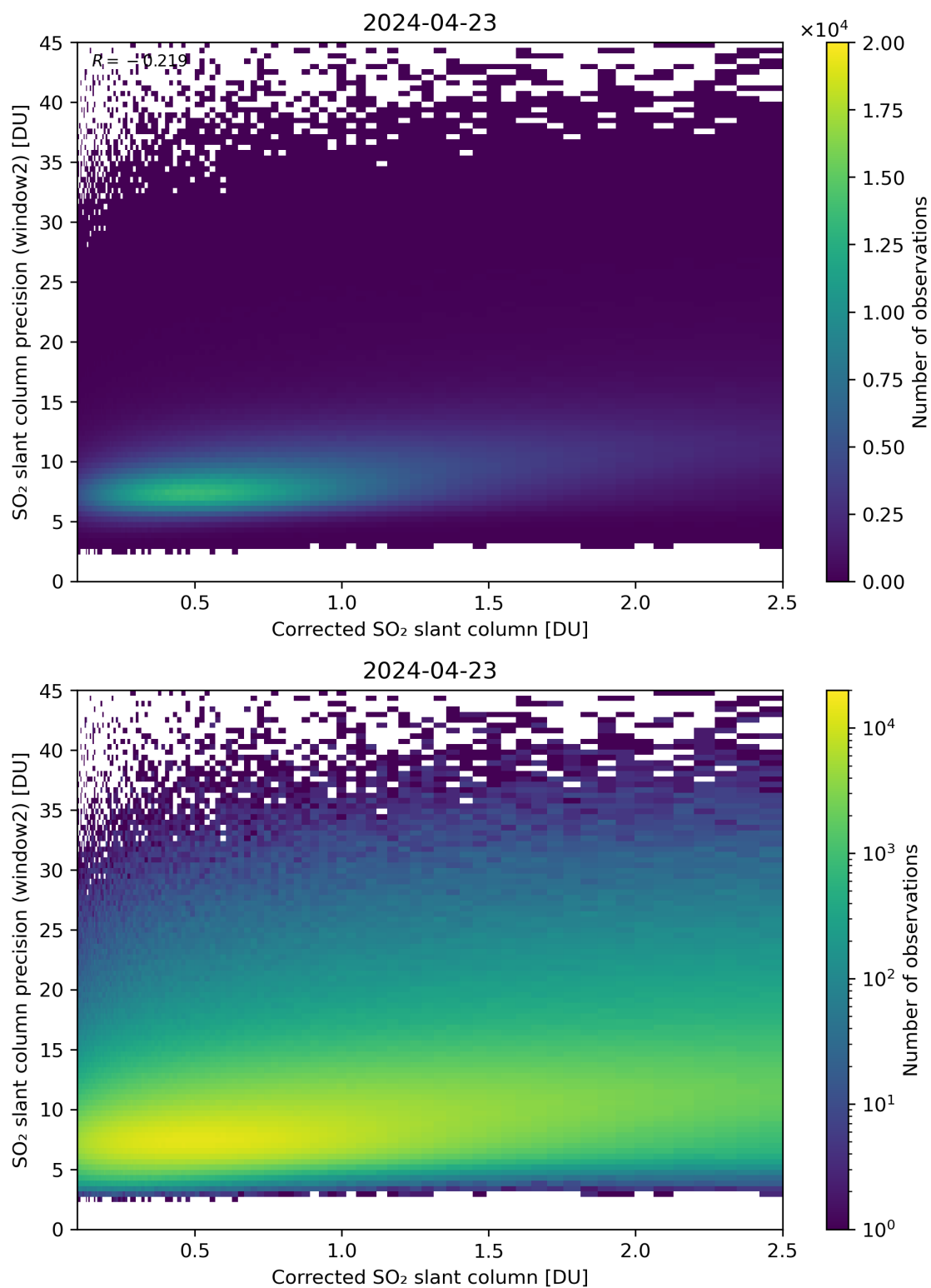
Figure 189: Scatter density plot of “Corrected SO 2 slant column” against “SO 2 slant column precision (window2)” for 2024-04-22 to 2024-04-24.
