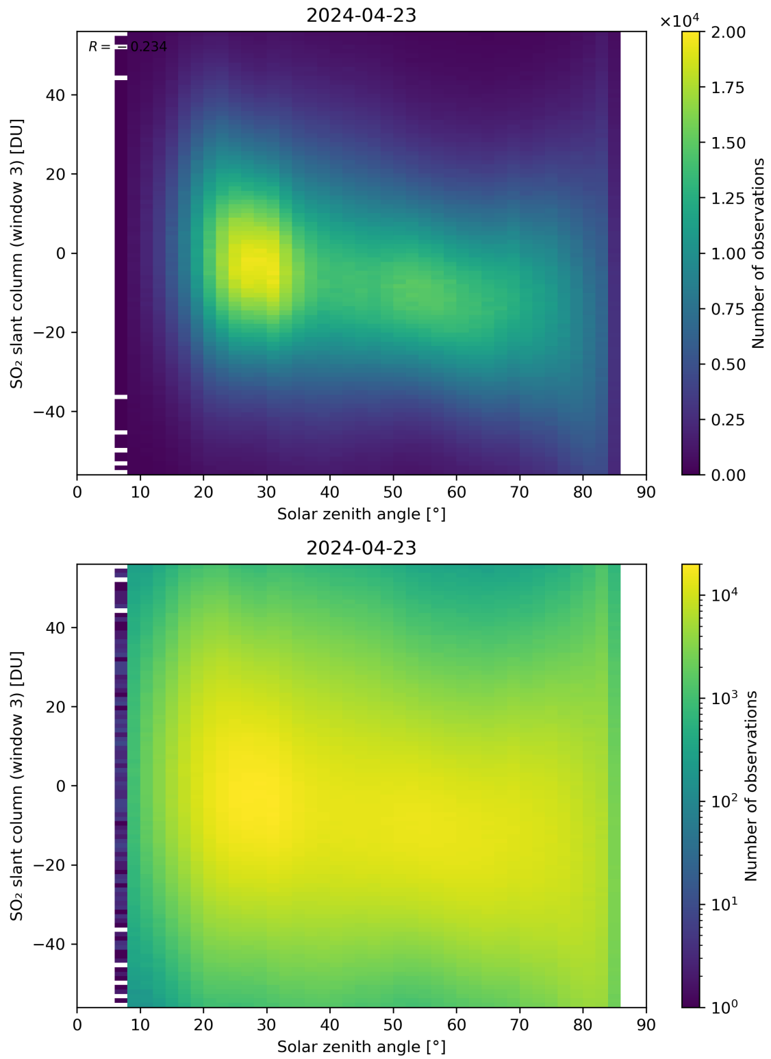
Figure 172: Scatter density plot of “Solar zenith angle” against “SO 2 slant column (window 3)” for 2024-04-22 to 2024-04-24.
