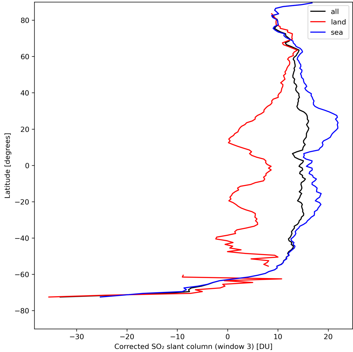
Figure 43: Zonal average of “Corrected SO 2 slant column (window 3)” for 2024-04-22 to 2024-04-24.
