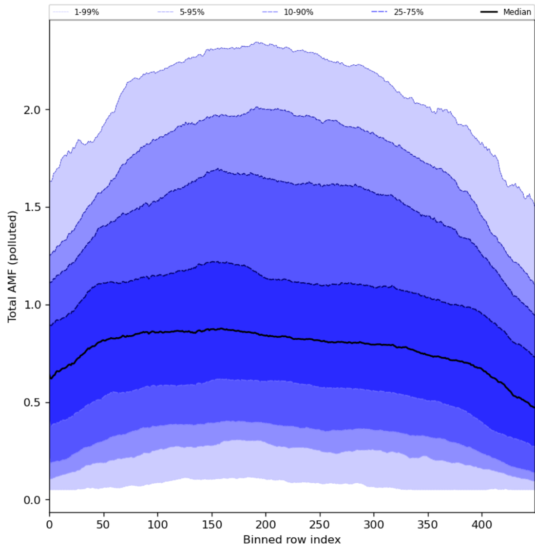
Figure 94: Along track statistics of “Total AMF (polluted)” for 2024-04-22 to 2024-04-24
