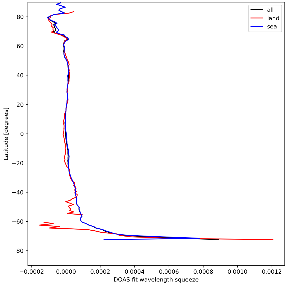
Figure 46: Zonal average of “DOAS fit wavelength squeeze” for 2024-04-22 to 2024-04-24.
