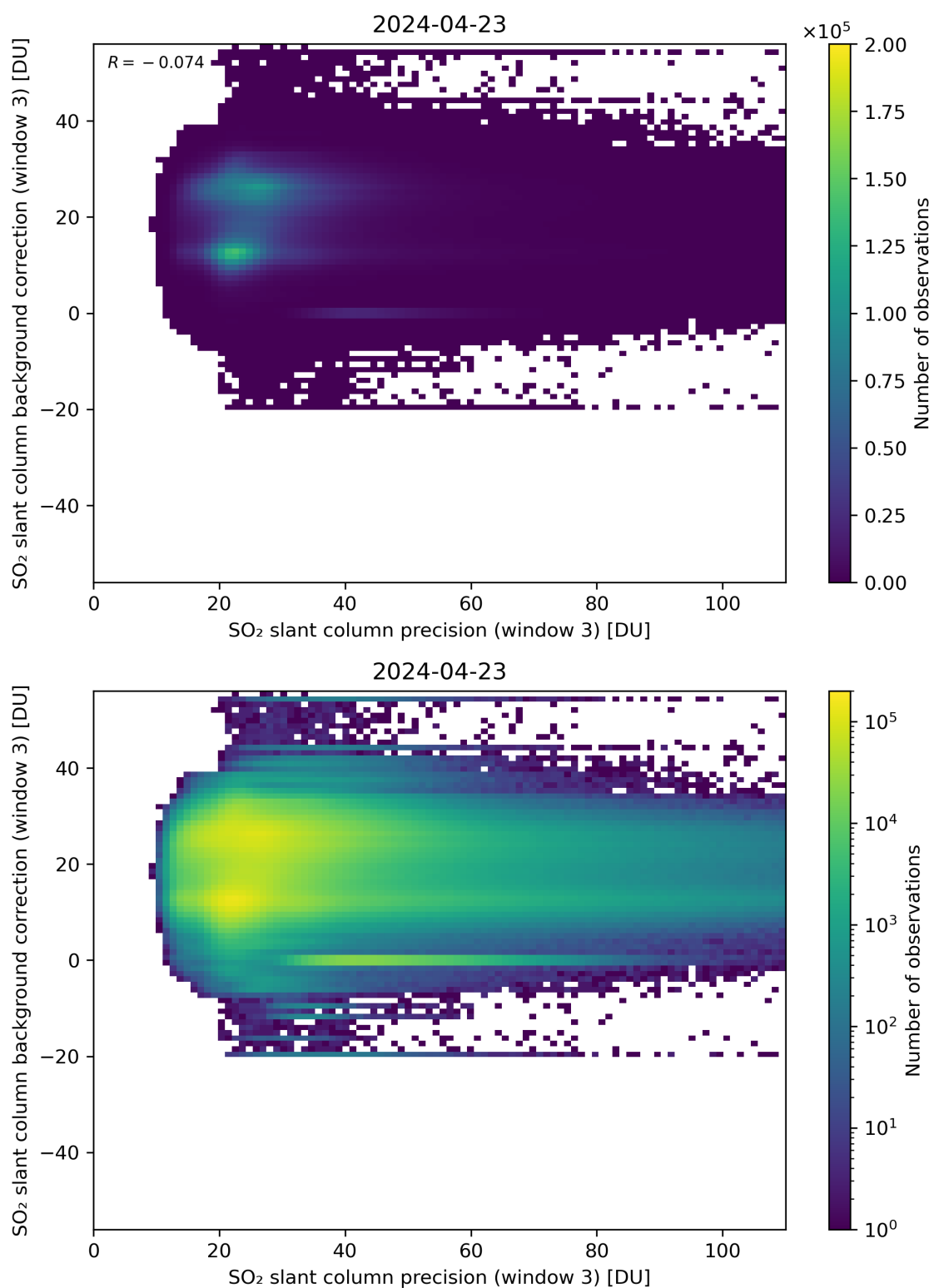
Figure 257: Scatter density plot of “SO 2 slant column precision (window 3)” against “SO 2 slant column background correction (window 3)” for 2024-04-22 to 2024-04-24.
