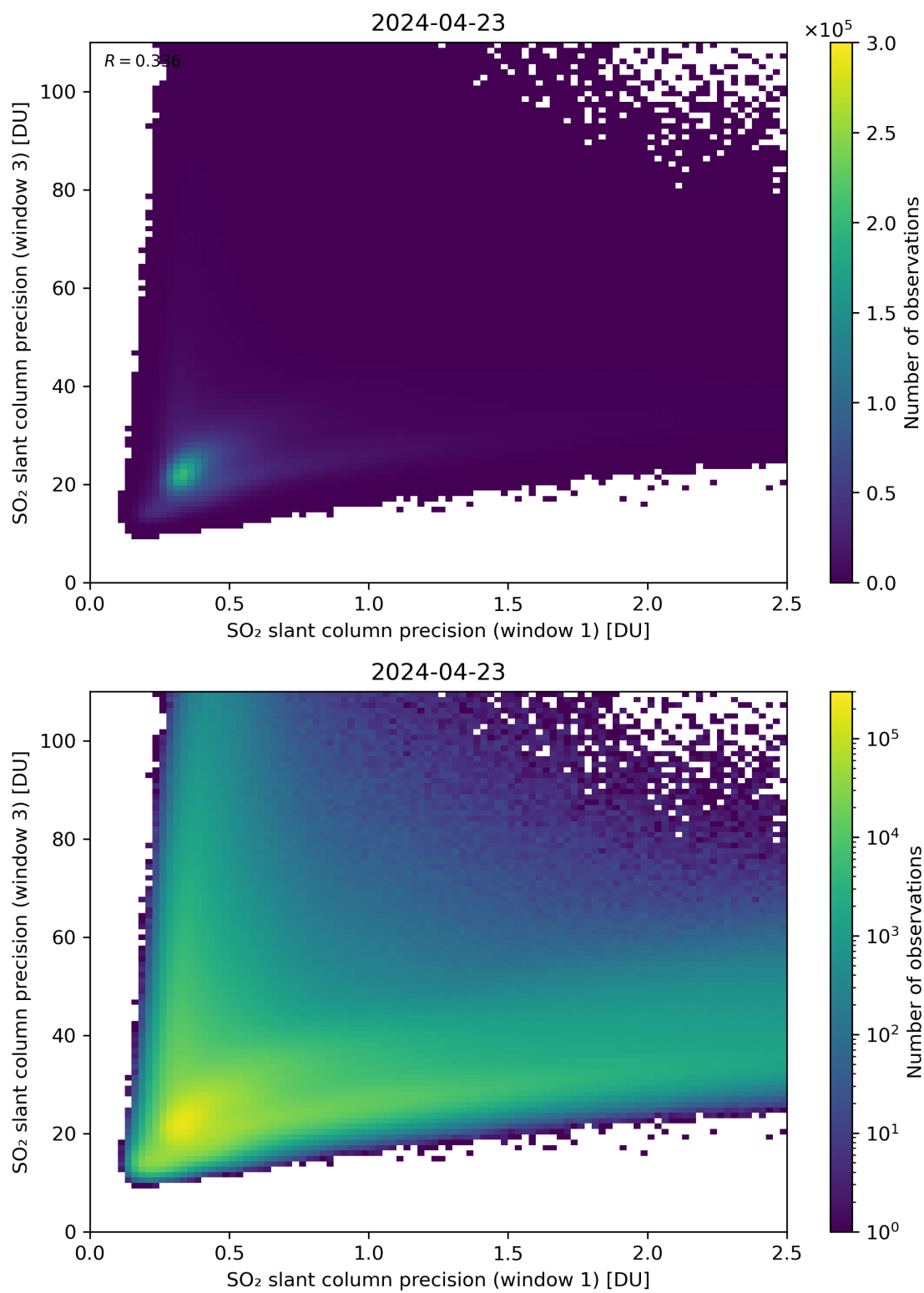
Figure 229: Scatter density plot of “SO 2 slant column precision (window 1)” against “SO 2 slant column precision (window 3)” for 2024-04-22 to 2024-04-24.
