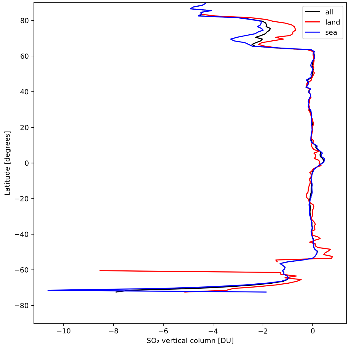
Figure 30: Zonal average of “SO 2 vertical column” for 2024-04-22 to 2024-04-24.
