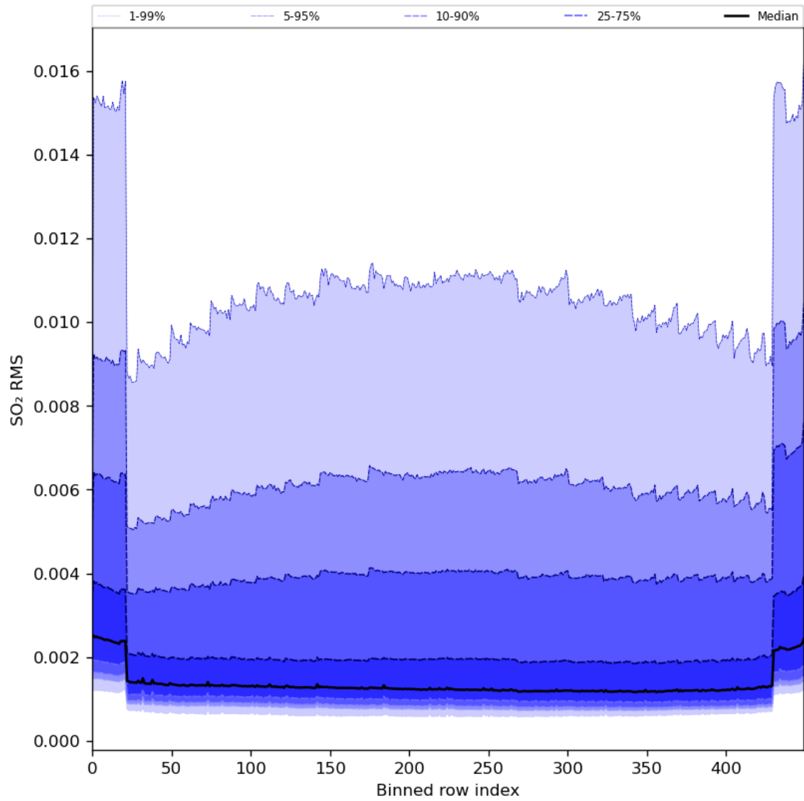
Figure 93: Along track statistics of “SO 2 RMS” for 2024-04-22 to 2024-04-24
