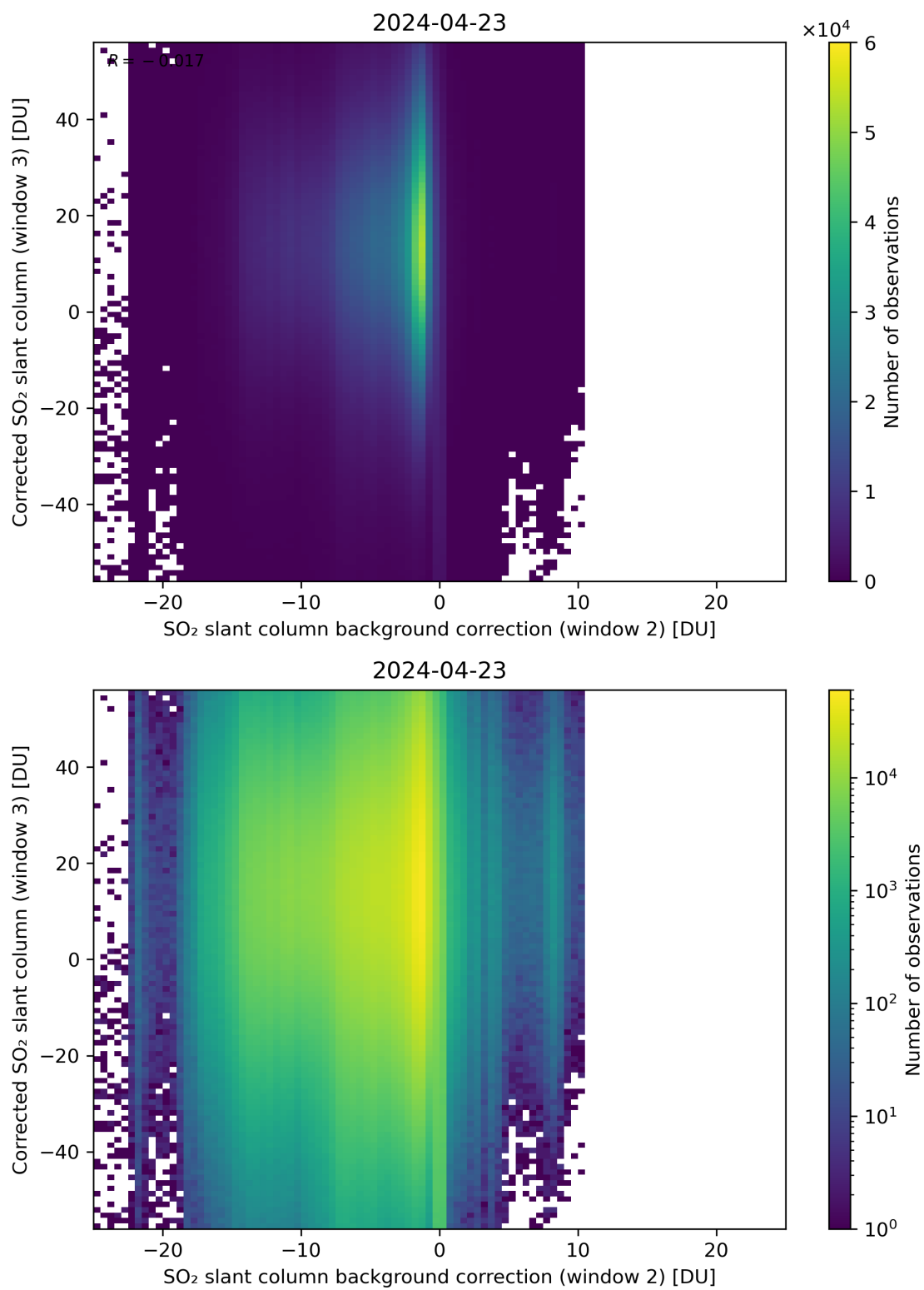
Figure 116: Scatter density plot of “SO 2 slant column background correction (window 2)” against “Corrected SO 2 slant column (window 3)” for 2024-04-22 to 2024-04-24.
