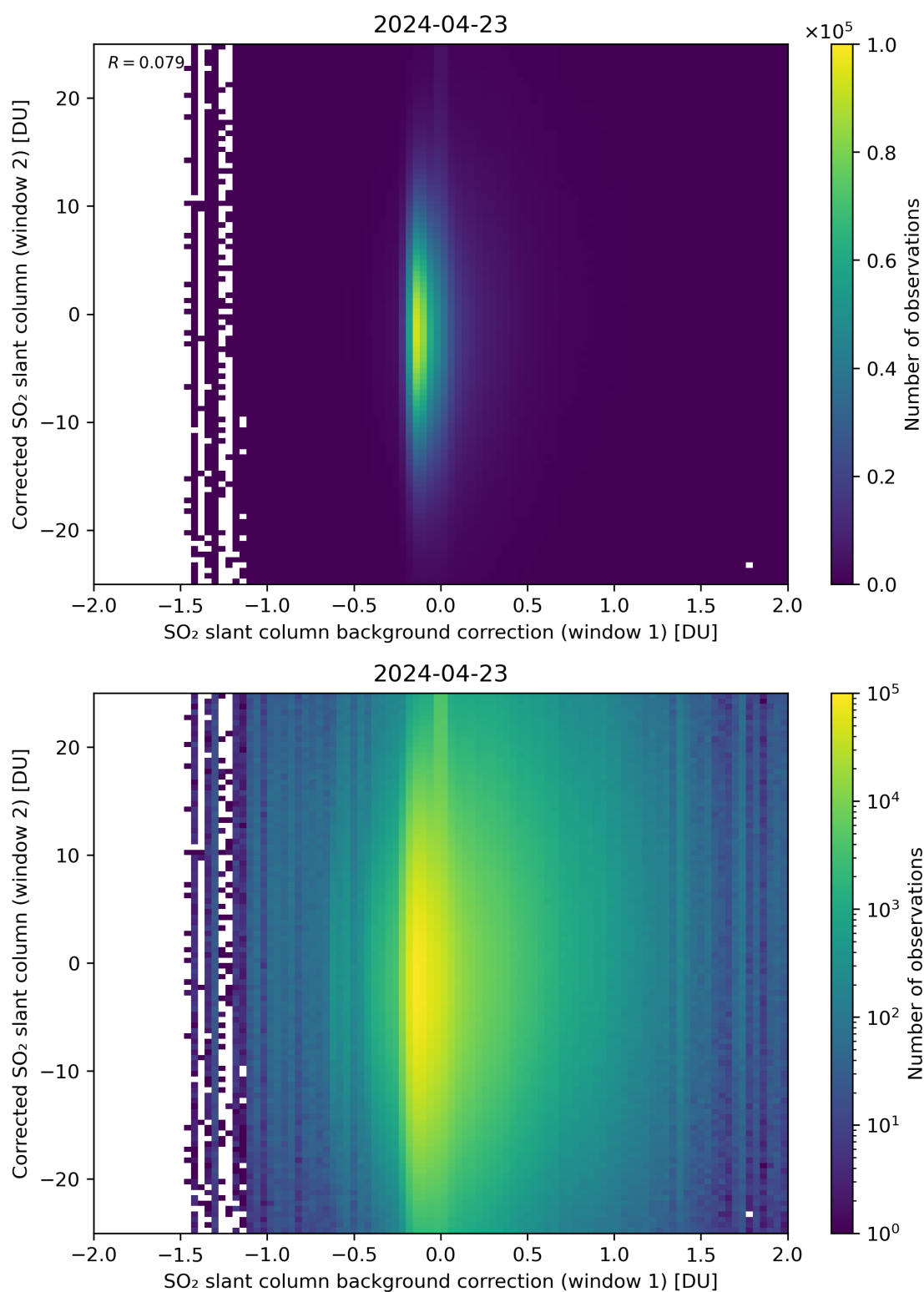
Figure 104: Scatter density plot of “SO 2 slant column background correction (window 1)” against “Corrected SO 2 slant column (window 2)” for 2024-04-22 to 2024-04-24.
