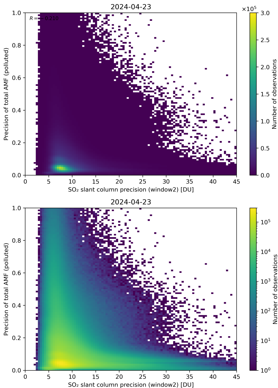
Figure 252: Scatter density plot of “SO 2 slant column precision (window2)” against “Precision of total AMF (polluted)” for 2024-04-22 to 2024-04-24.
