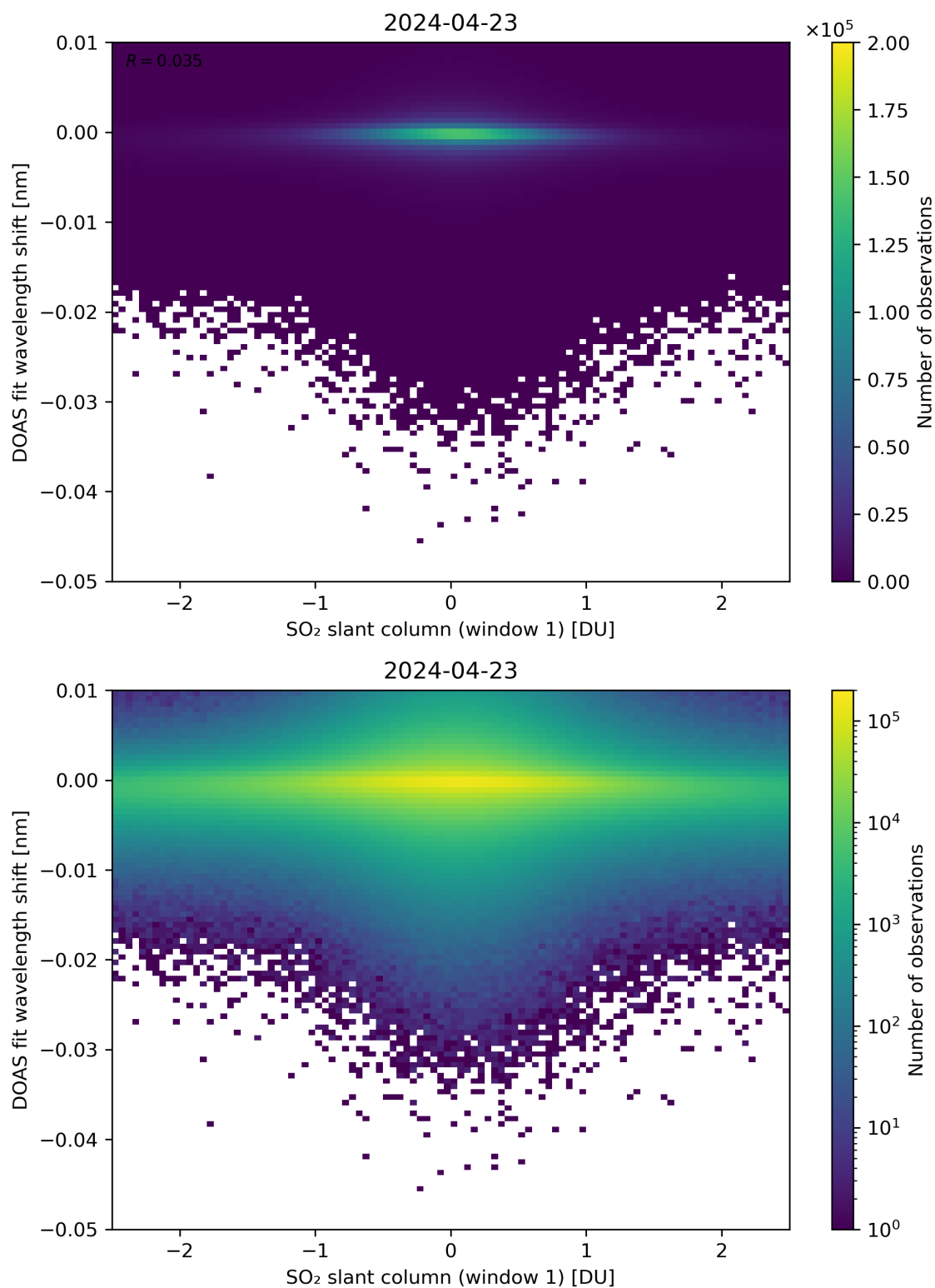
Figure 215: Scatter density plot of “SO 2 slant column (window 1)” against “DOAS fit wavelength shift” for 2024-04-22 to 2024-04-24.
