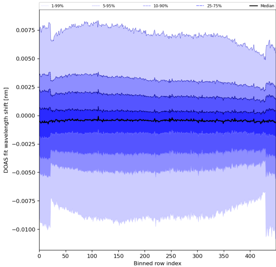
Figure 91: Along track statistics of “DOAS fit wavelength shift” for 2024-04-22 to 2024-04-24
