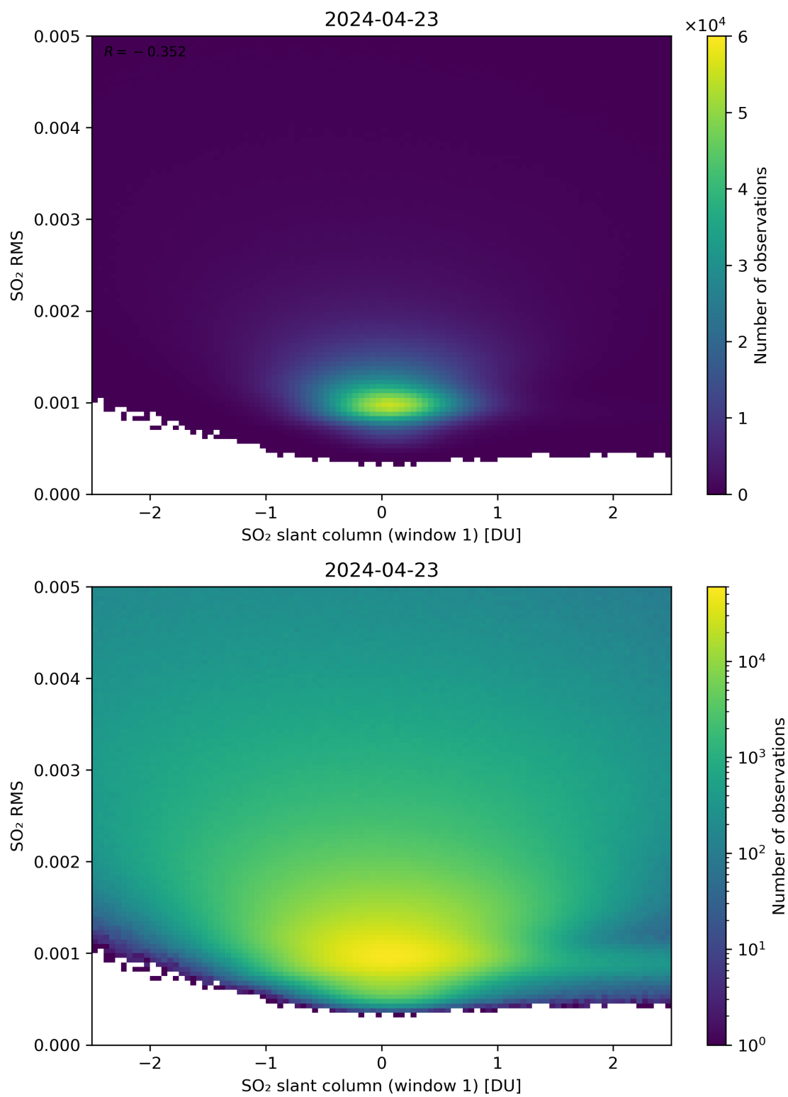
Figure 217: Scatter density plot of “SO 2 slant column (window 1)” against “SO 2 RMS” for 2024-04-22 to 2024-04-24.
