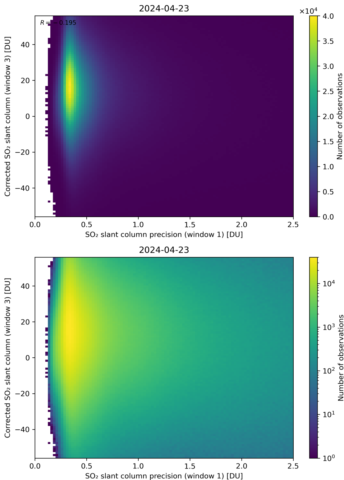
Figure 226: Scatter density plot of “SO 2 slant column precision (window 1)” against “Corrected SO 2 slant column (window 3)” for 2024-04-22 to 2024-04-24.
