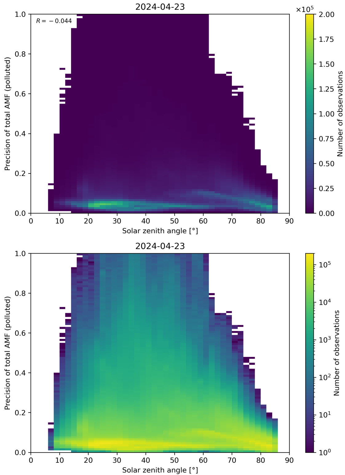
Figure 175: Scatter density plot of “Solar zenith angle” against “Precision of total AMF (polluted)” for 2024-04-22 to 2024-04-24.
