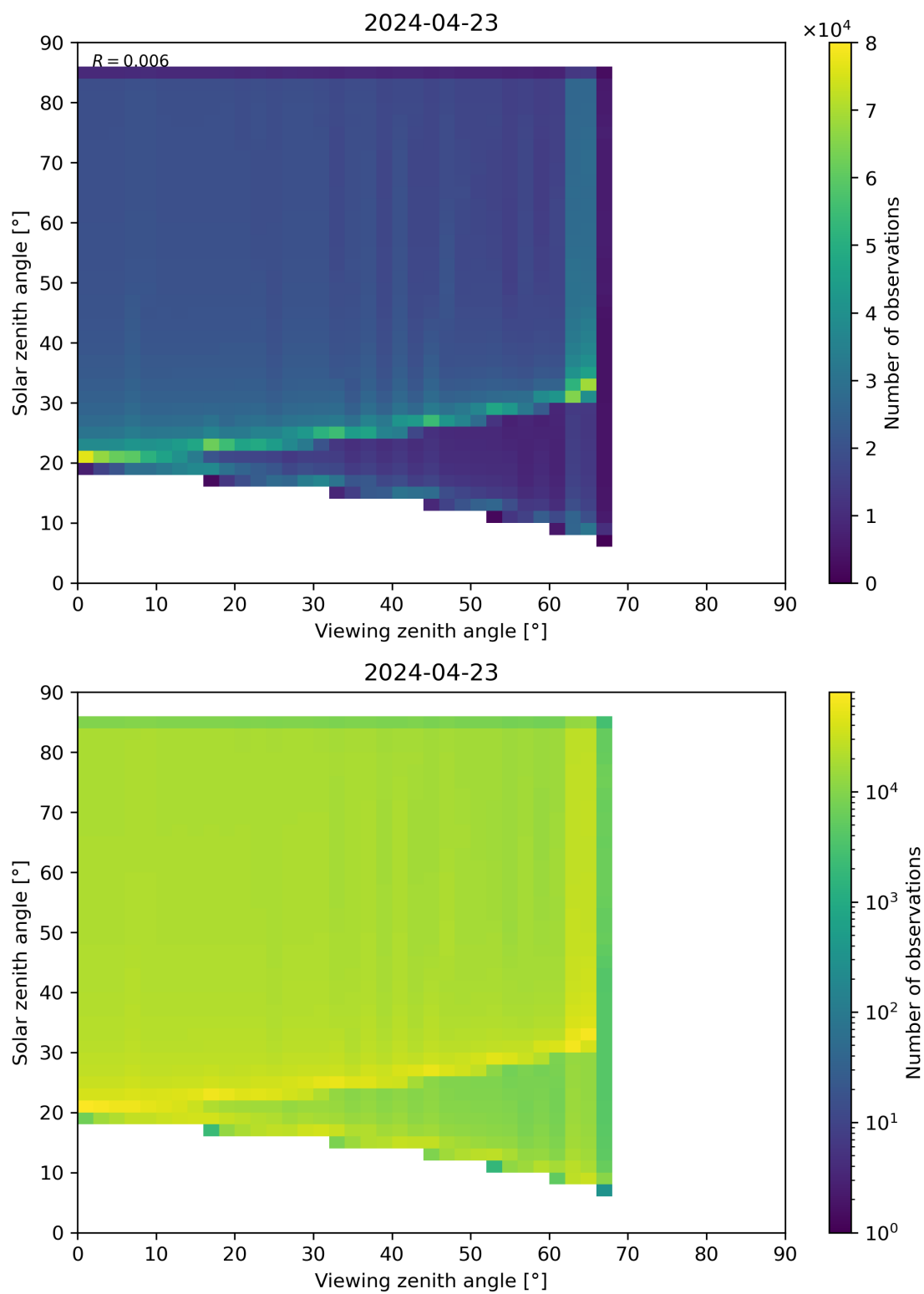
Figure 315: Scatter density plot of “Viewing zenith angle” against “Solar zenith angle” for 2024-04-22 to 2024-04-24.
