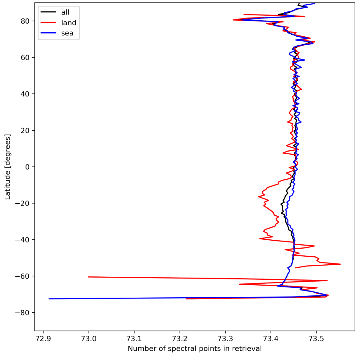
Figure 51: Zonal average of “Number of spectral points in retrieval” for 2024-04-22 to 2024-04-24.
