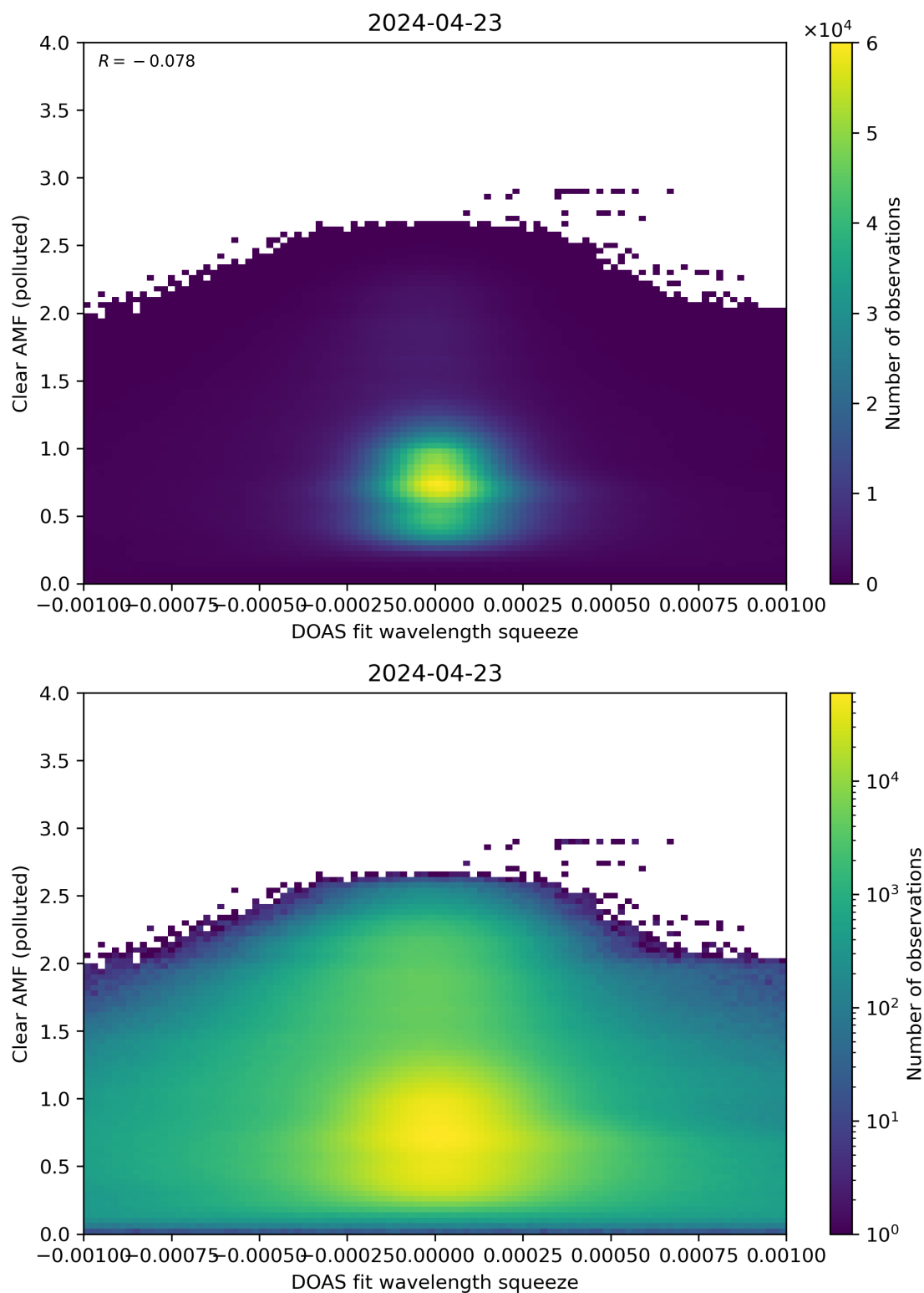
Figure 133: Scatter density plot of “DOAS fit wavelength squeeze” against “Clear AMF (polluted)” for 2024-04-22 to 2024-04-24.
