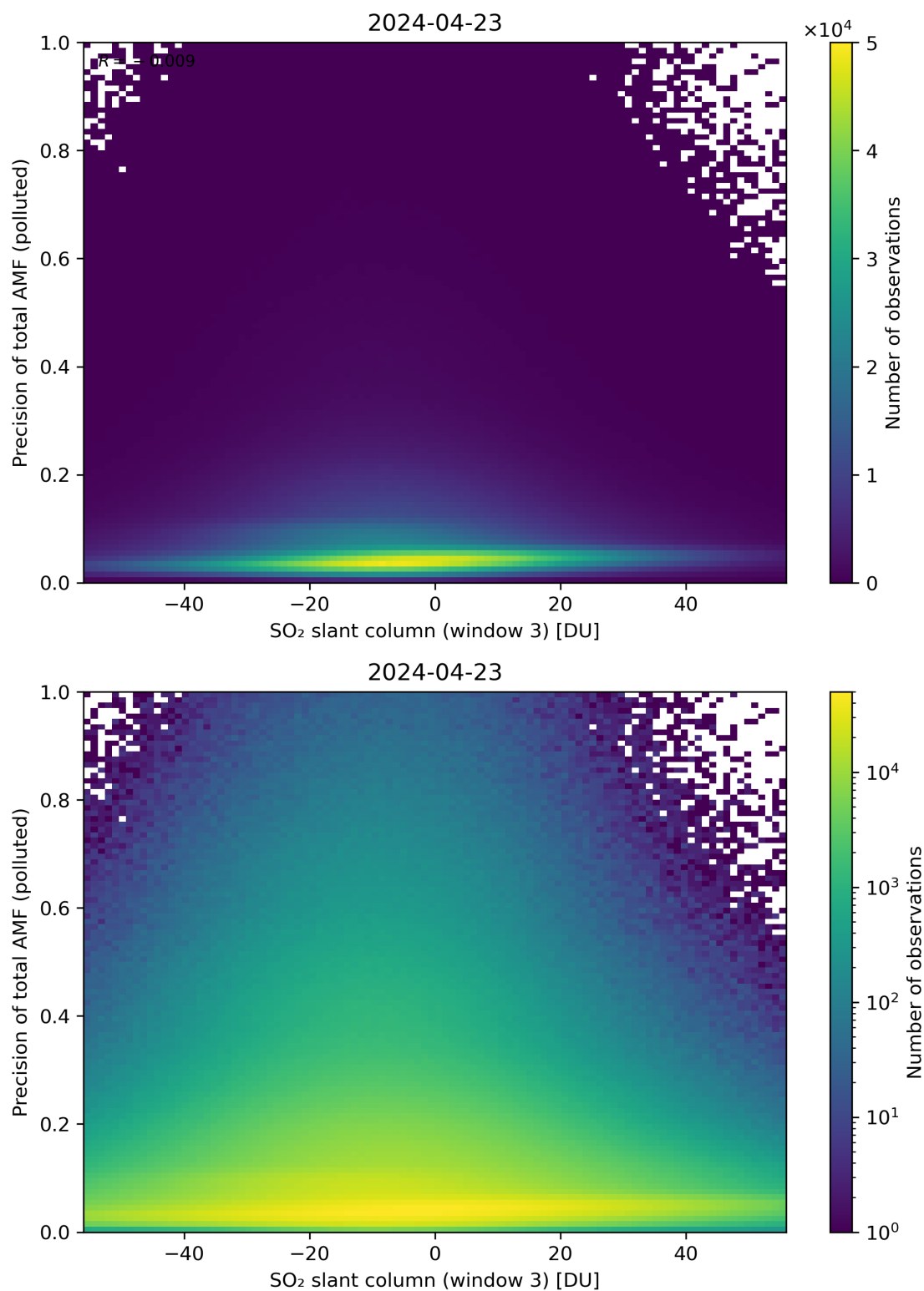
Figure 269: Scatter density plot of “SO 2 slant column (window 3)” against “Precision of total AMF (polluted)” for 2024-04-22 to 2024-04-24.
