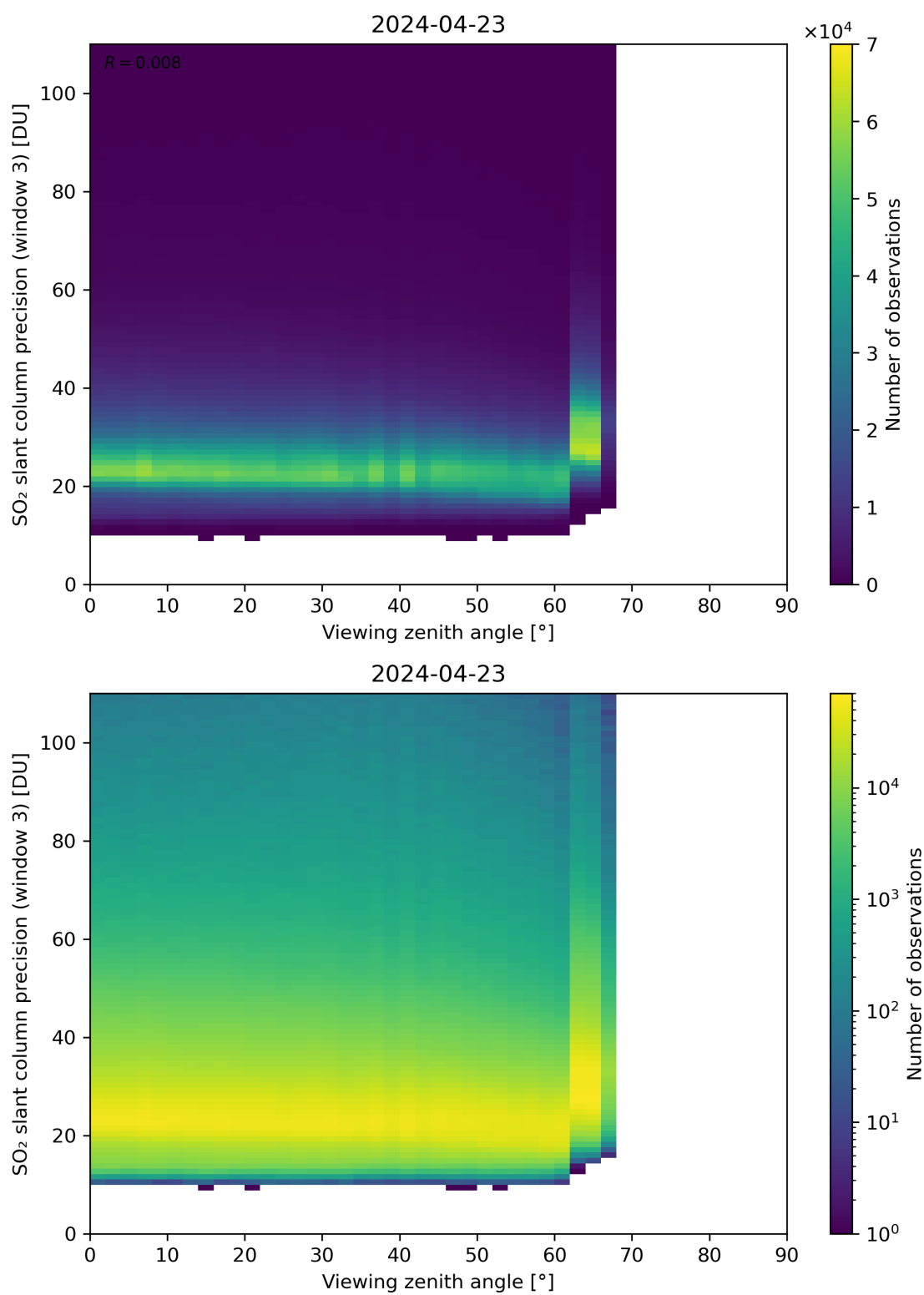
Figure 324: Scatter density plot of “Viewing zenith angle” against “SO 2 slant column precision (window 3)” for 2024-04-22 to 2024-04-24.
