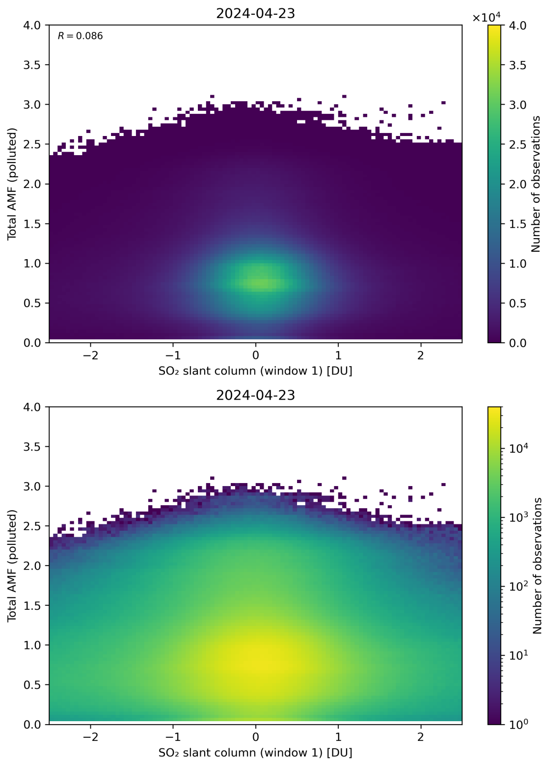
Figure 239: Scatter density plot of “SO 2 slant column (window 1)” against “Total AMF (polluted)” for 2024-04-22 to 2024-04-24.
