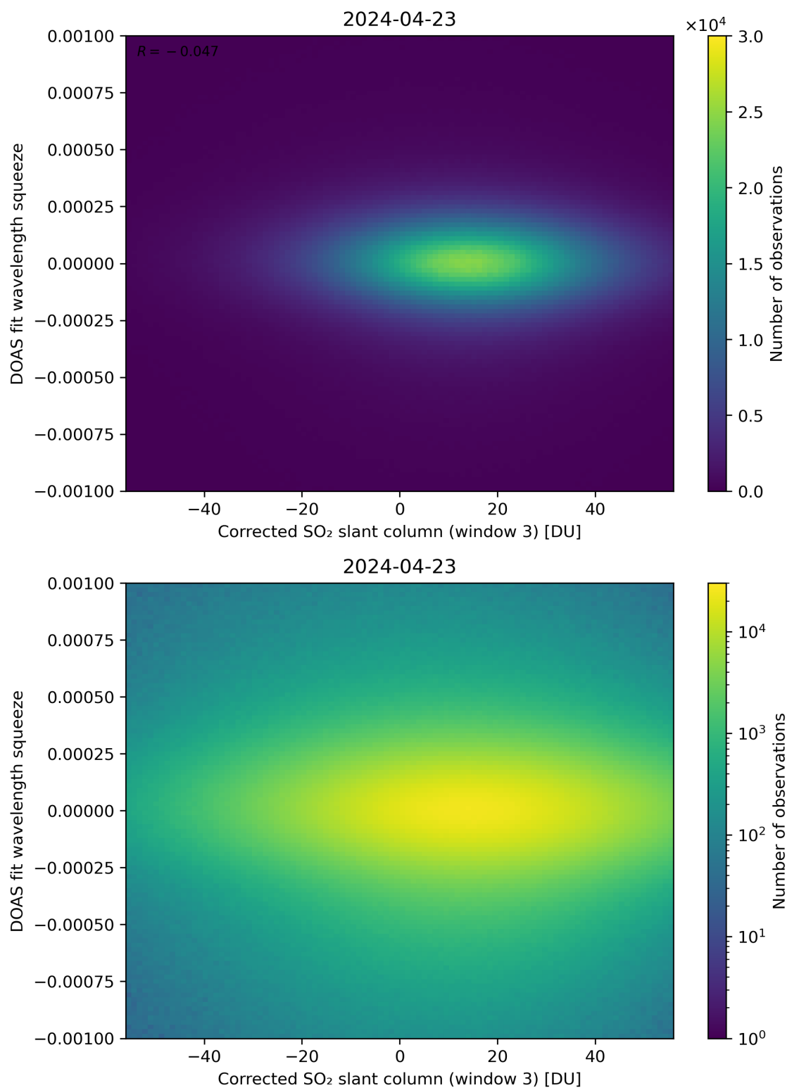
Figure 207: Scatter density plot of “Corrected SO 2 slant column (window 3)” against “DOAS fit wavelength squeeze” for 2024-04-22 to 2024-04-24.
