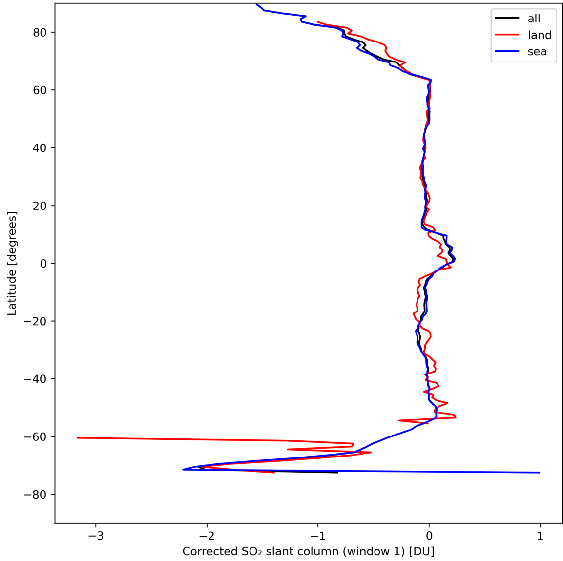
Figure 35: Zonal average of “Corrected SO 2 slant column (window 1)” for 2024-04-22 to 2024-04-24.
