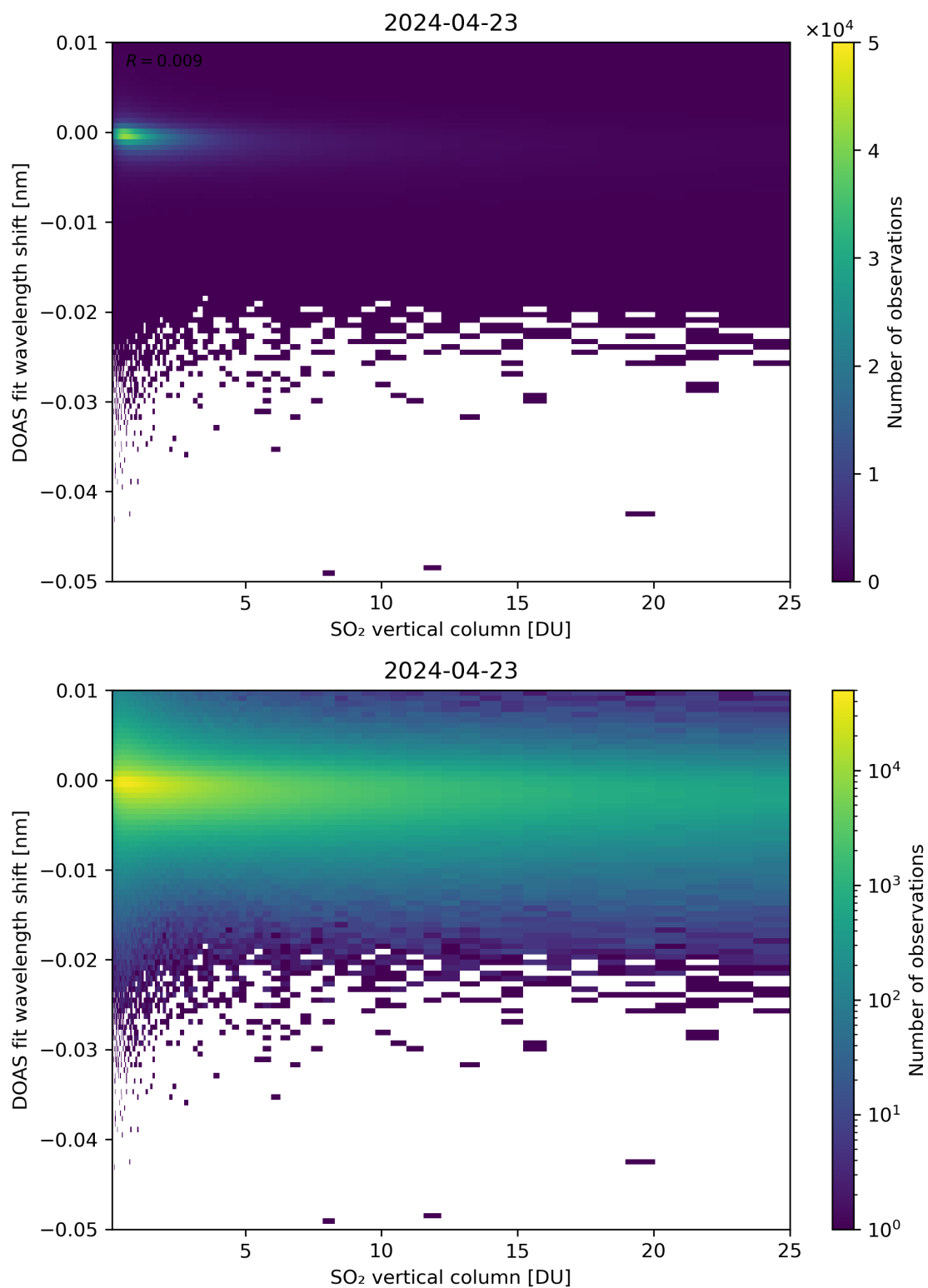
Figure 276: Scatter density plot of “SO 2 vertical column” against “DOAS fit wavelength shift” for 2024-04-22 to 2024-04-24.
