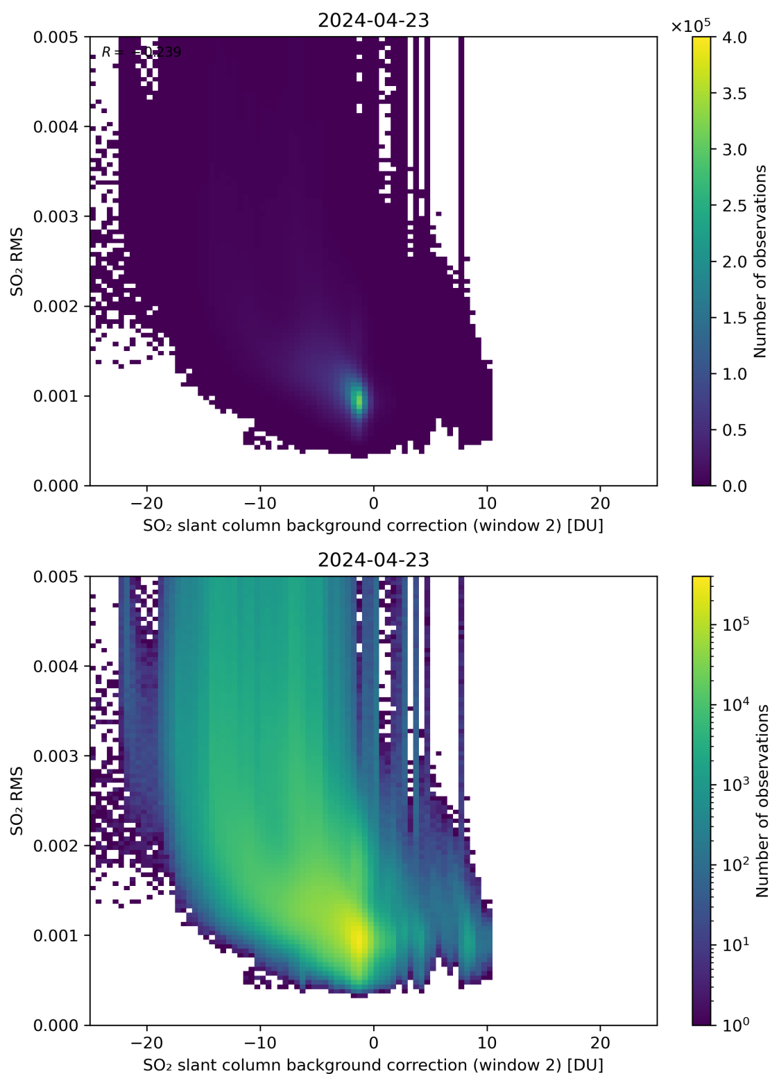
Figure 114: Scatter density plot of “SO 2 slant column background correction (window 2)” against “SO 2 RMS” for 2024-04-22 to 2024-04-24.
