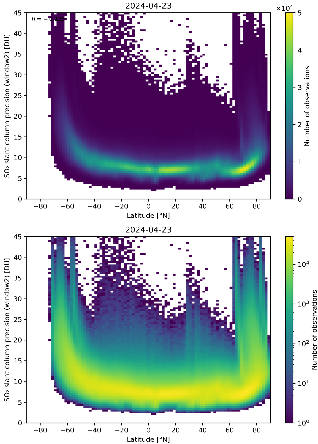
Figure 151: Scatter density plot of “Latitude” against “SO 2 slant column precision (window2)” for 2024-04-22 to 2024-04-24.
