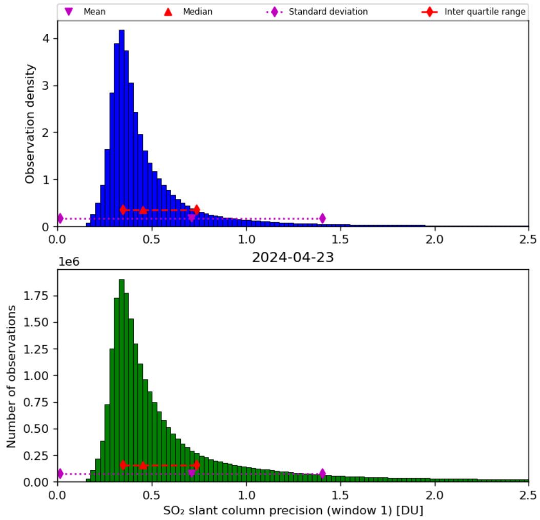
Figure 57: Histogram of “SO 2 slant column precision (window 1)” for 2024-04-22 to 2024-04-24
