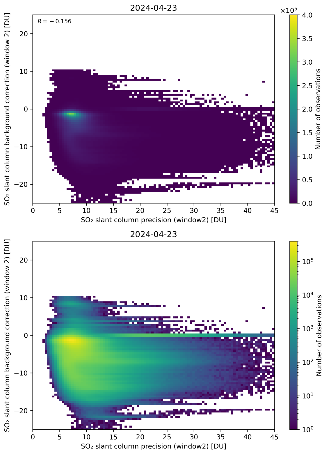
Figure 241: Scatter density plot of “SO 2 slant column precision (window2)” against “SO 2 slant column background correction (window 2)” for 2024-04-22 to 2024-04-24.
