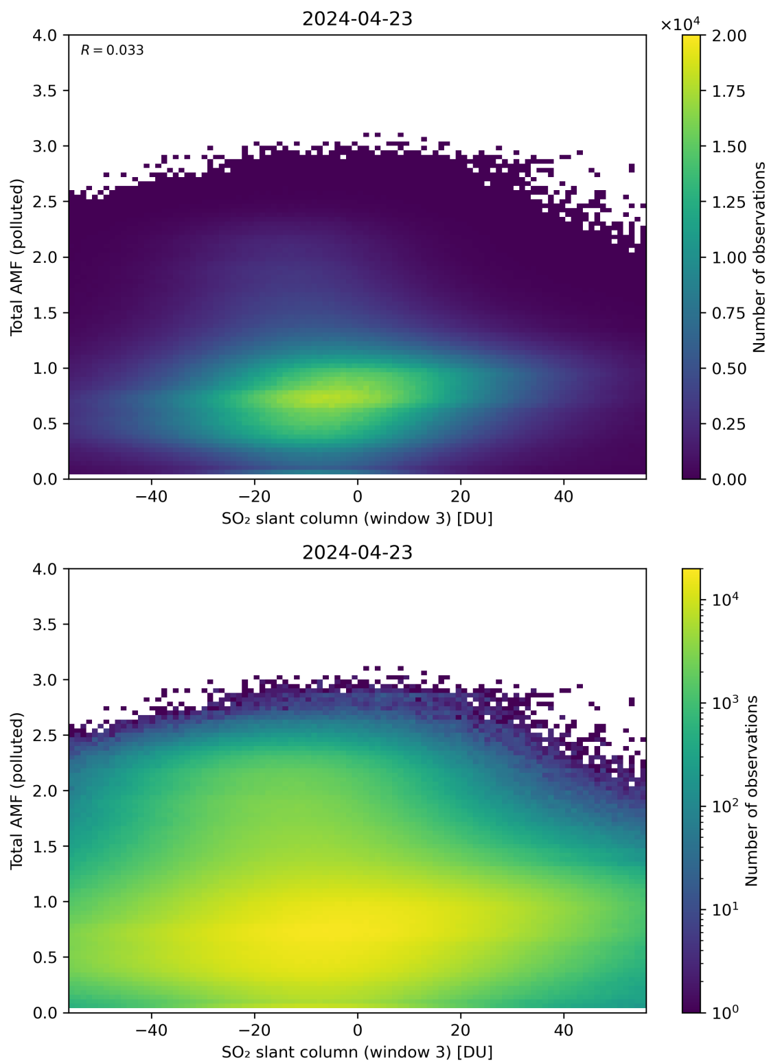
Figure 268: Scatter density plot of “SO 2 slant column (window 3)” against “Total AMF (polluted)” for 2024-04-22 to 2024-04-24.
