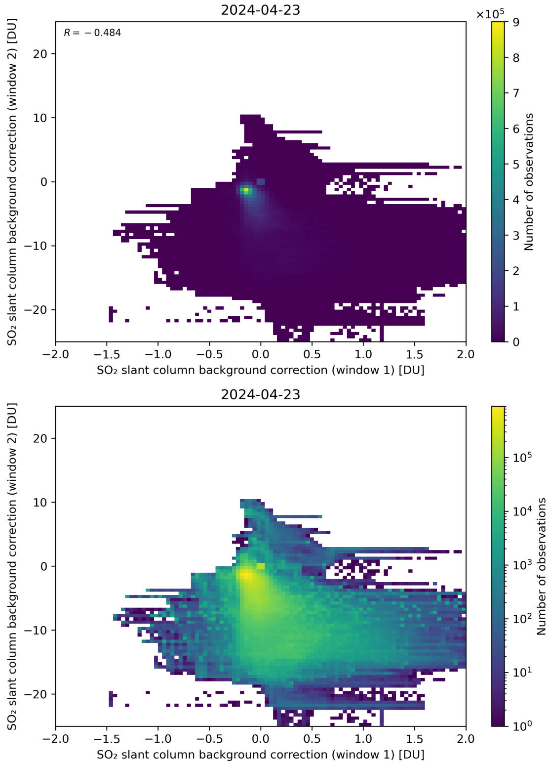
Figure 98: Scatter density plot of “SO 2 slant column background correction (window 1)” against “SO 2 slant column background correction (window 2)” for 2024-04-22 to 2024-04-24.
