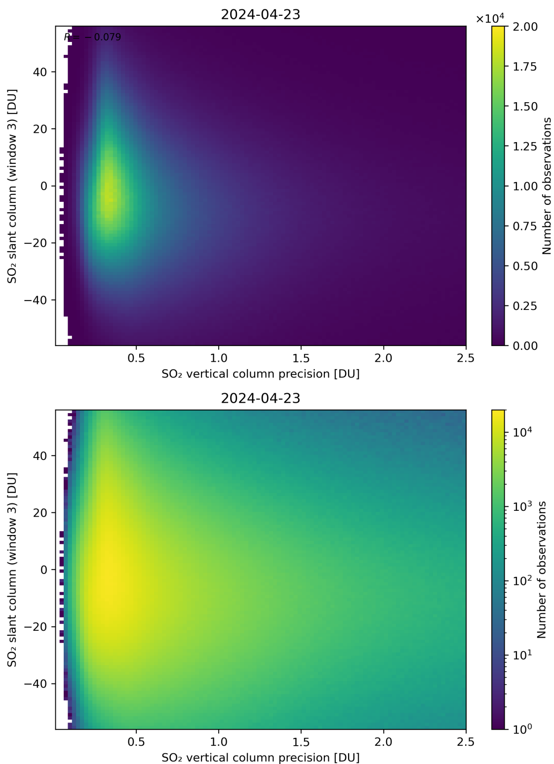
Figure 292: Scatter density plot of “SO 2 vertical column precision” against “SO 2 slant column (window 3)” for 2024-04-22 to 2024-04-24.
