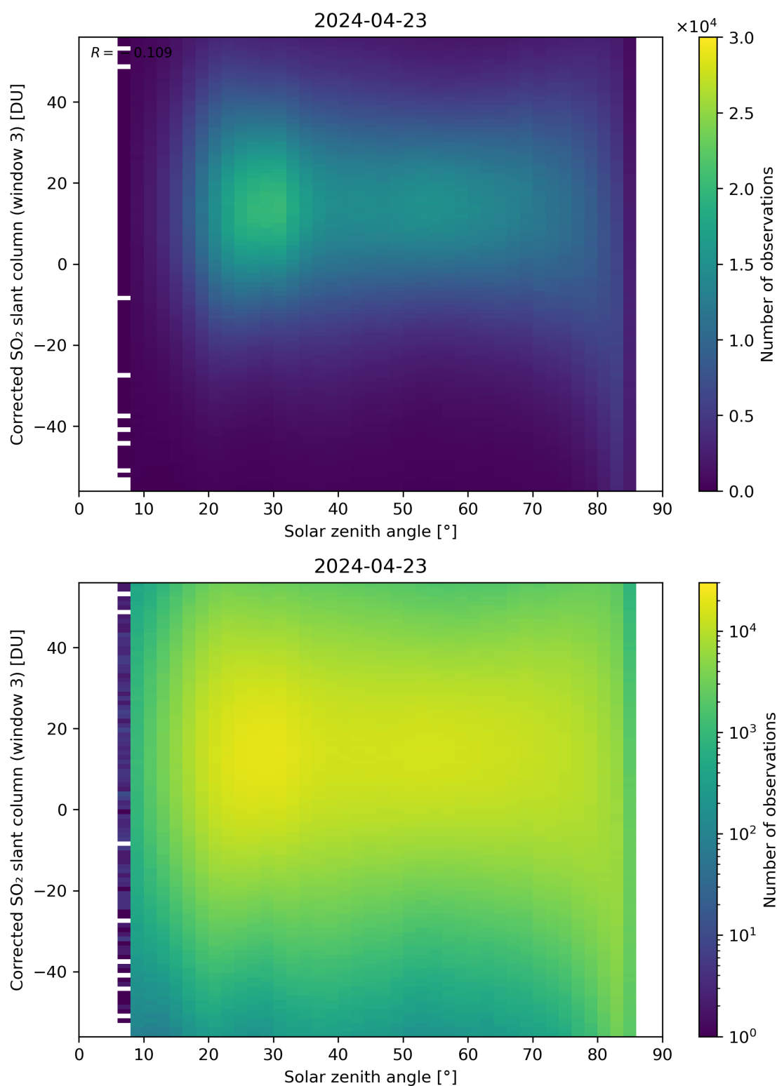
Figure 168: Scatter density plot of “Solar zenith angle” against “Corrected SO 2 slant column (window 3)” for 2024-04-22 to 2024-04-24.
