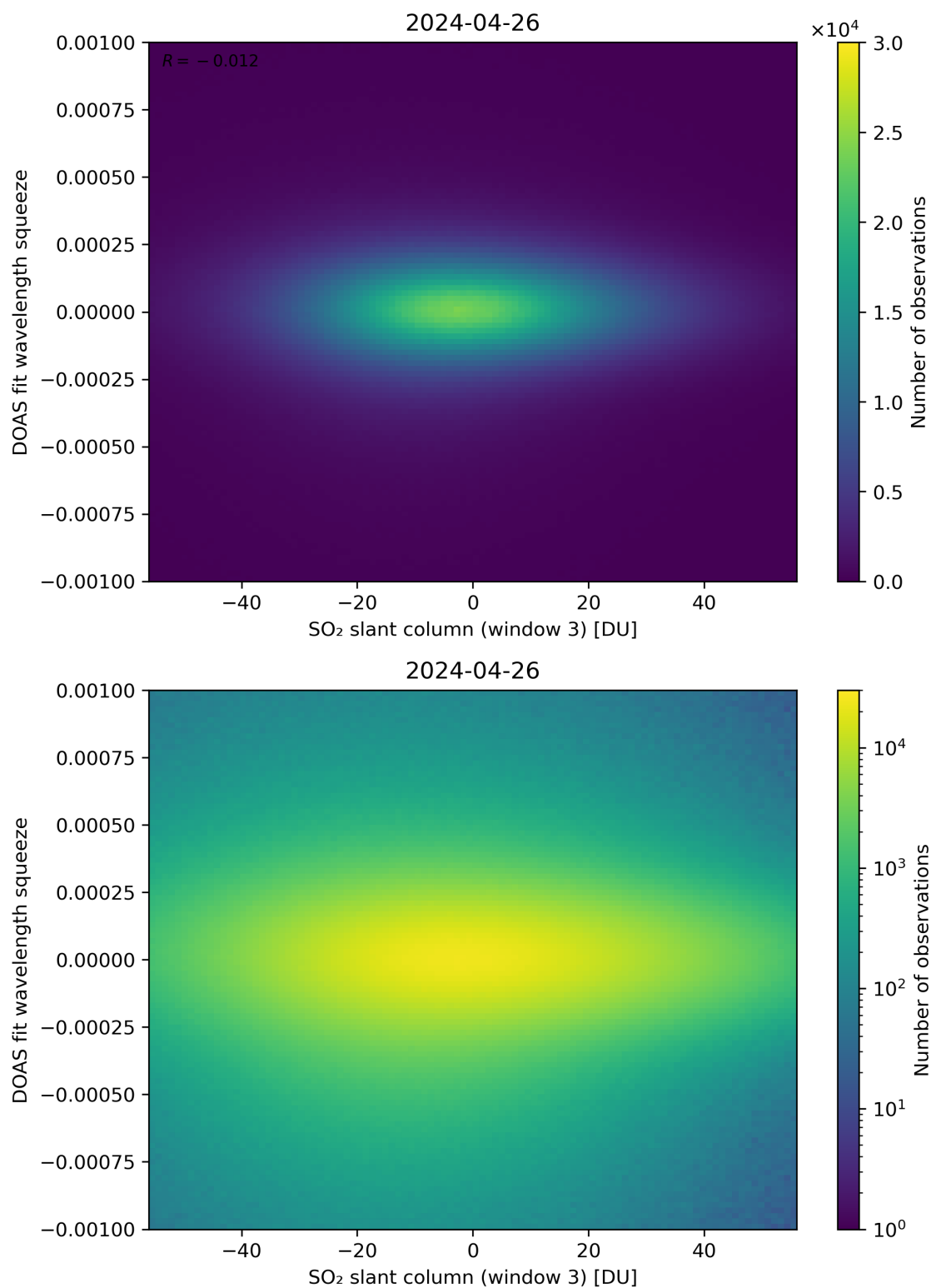
Figure 255: Scatter density plot of “SO 2 slant column (window 3)” against “DOAS fit wavelength squeeze” for 2024-04-26 to 2024-04-27.
