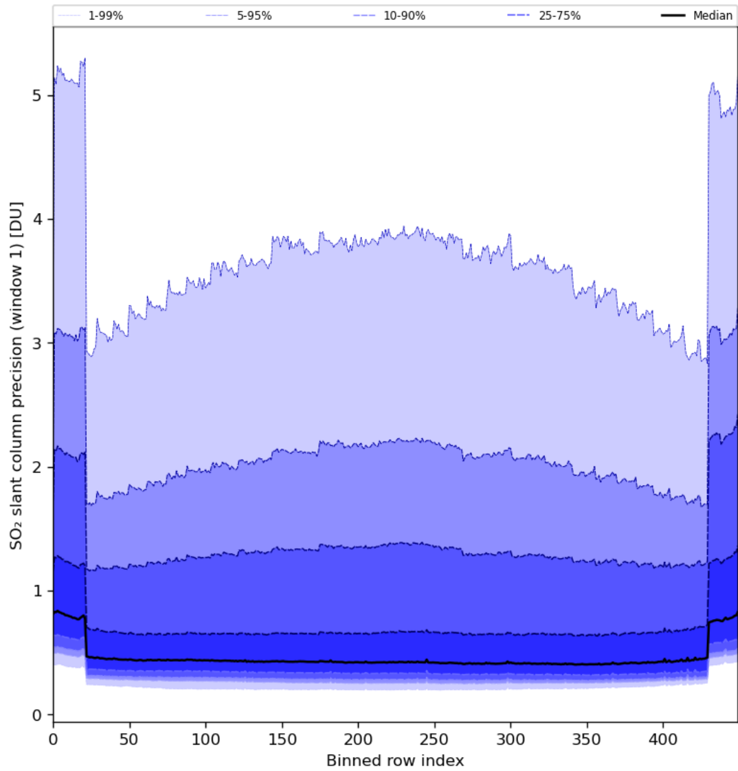
Figure 80: Along track statistics of “SO 2 slant column precision (window 1)” for 2024-04-26 to 2024-04-27
