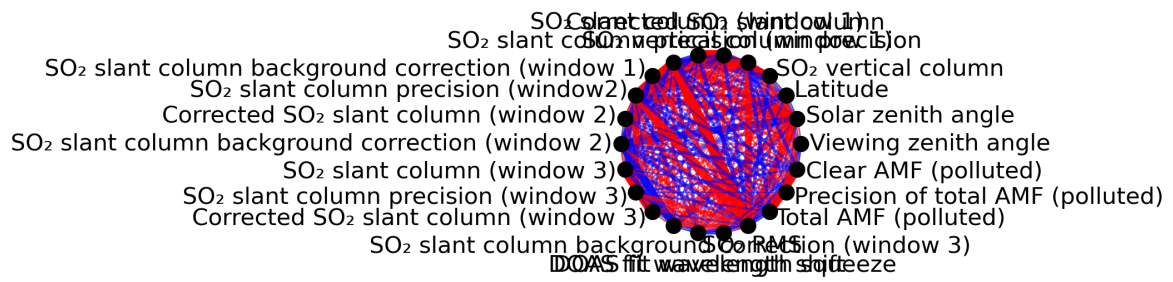
Figure 1: Map of correlation graph for 2024-04-26 to 2024-04-27.
