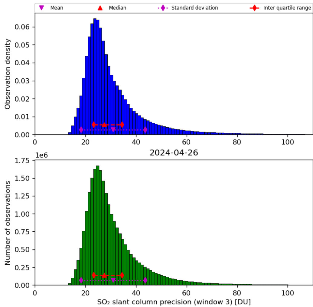
Figure 65: Histogram of “SO 2 slant column precision (window 3)” for 2024-04-26 to 2024-04-27
