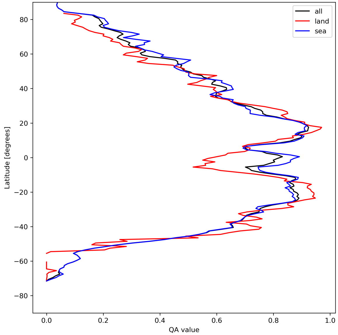
Figure 29: Zonal average of “QA value” for 2024-04-26 to 2024-04-27.
