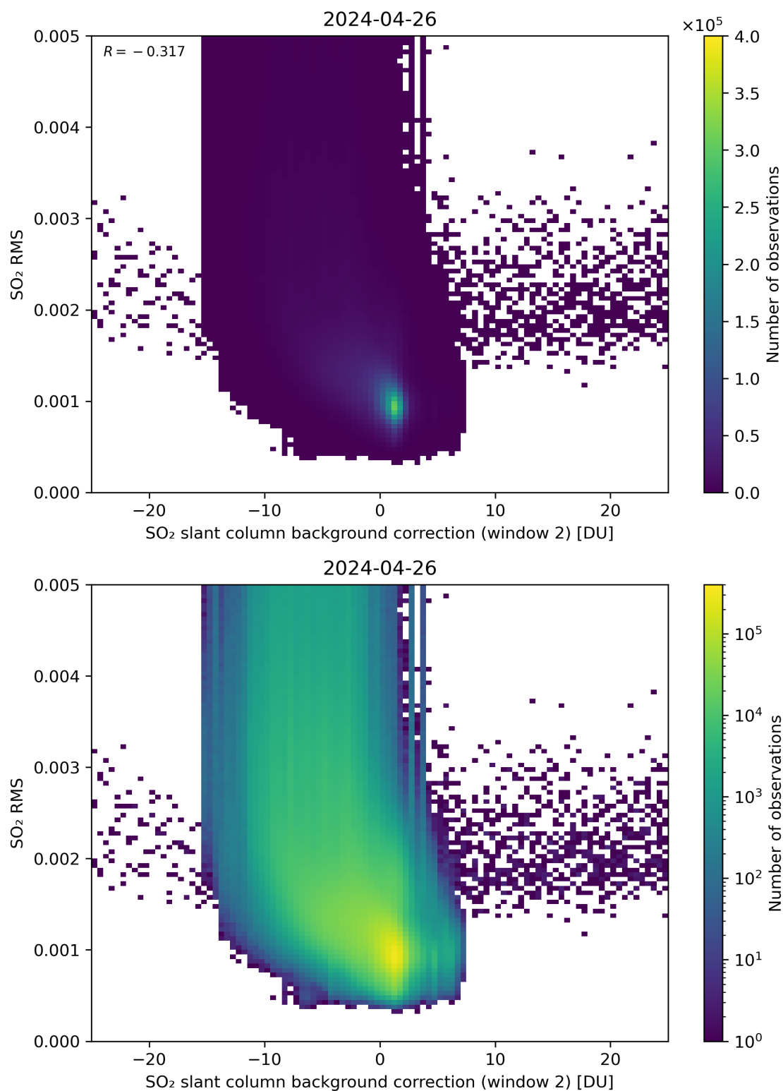
Figure 114: Scatter density plot of “SO 2 slant column background correction (window 2)” against “SO 2 RMS” for 2024-04-26 to 2024-04-27.
