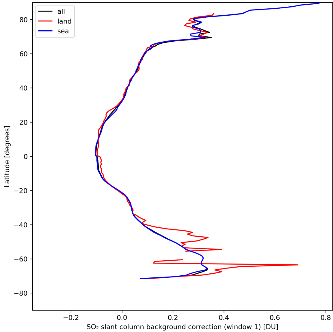
Figure 36: Zonal average of “SO 2 slant column background correction (window 1)” for 2024-04-26 to 2024-04-27.
