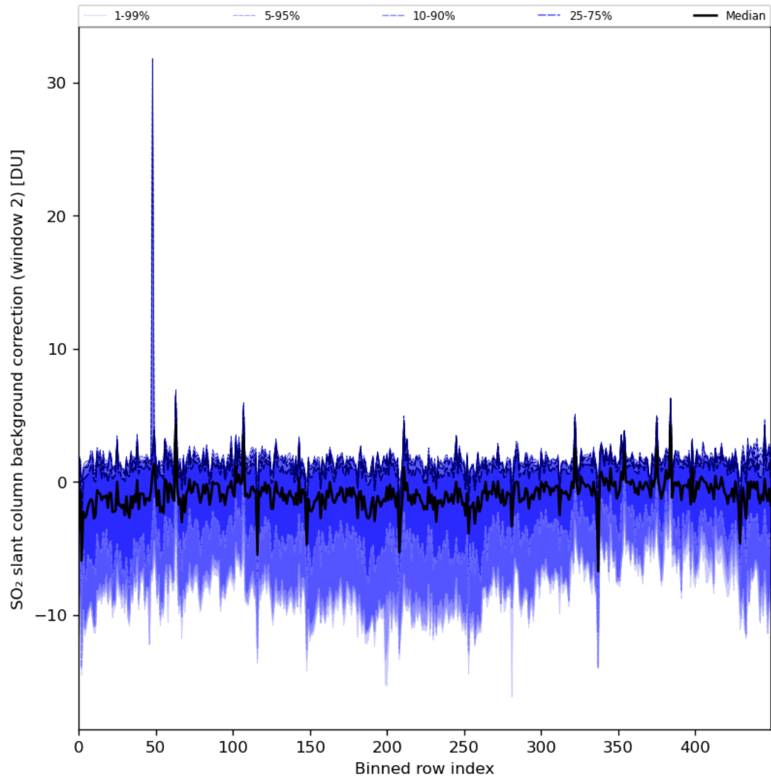
Figure 86: Along track statistics of “SO 2 slant column background correction (window 2)” for 2024-04-26 to 2024-04-27
