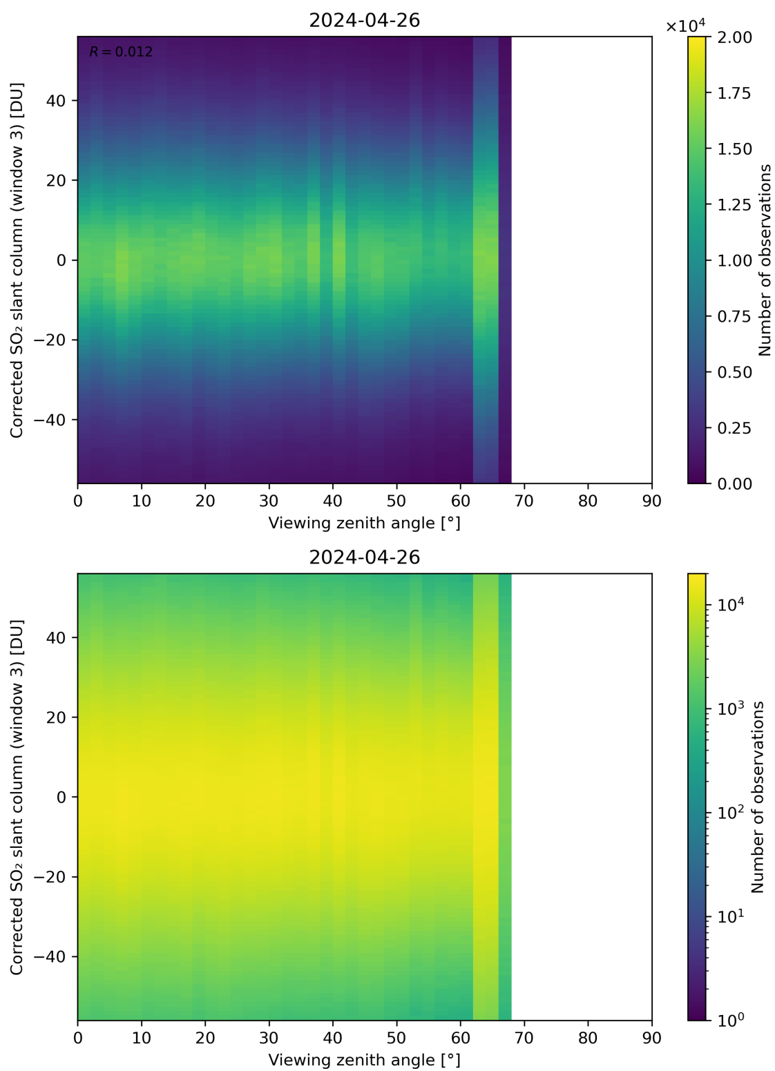
Figure 319: Scatter density plot of “Viewing zenith angle” against “Corrected SO 2 slant column (window 3)” for 2024-04-26 to 2024-04-27.
