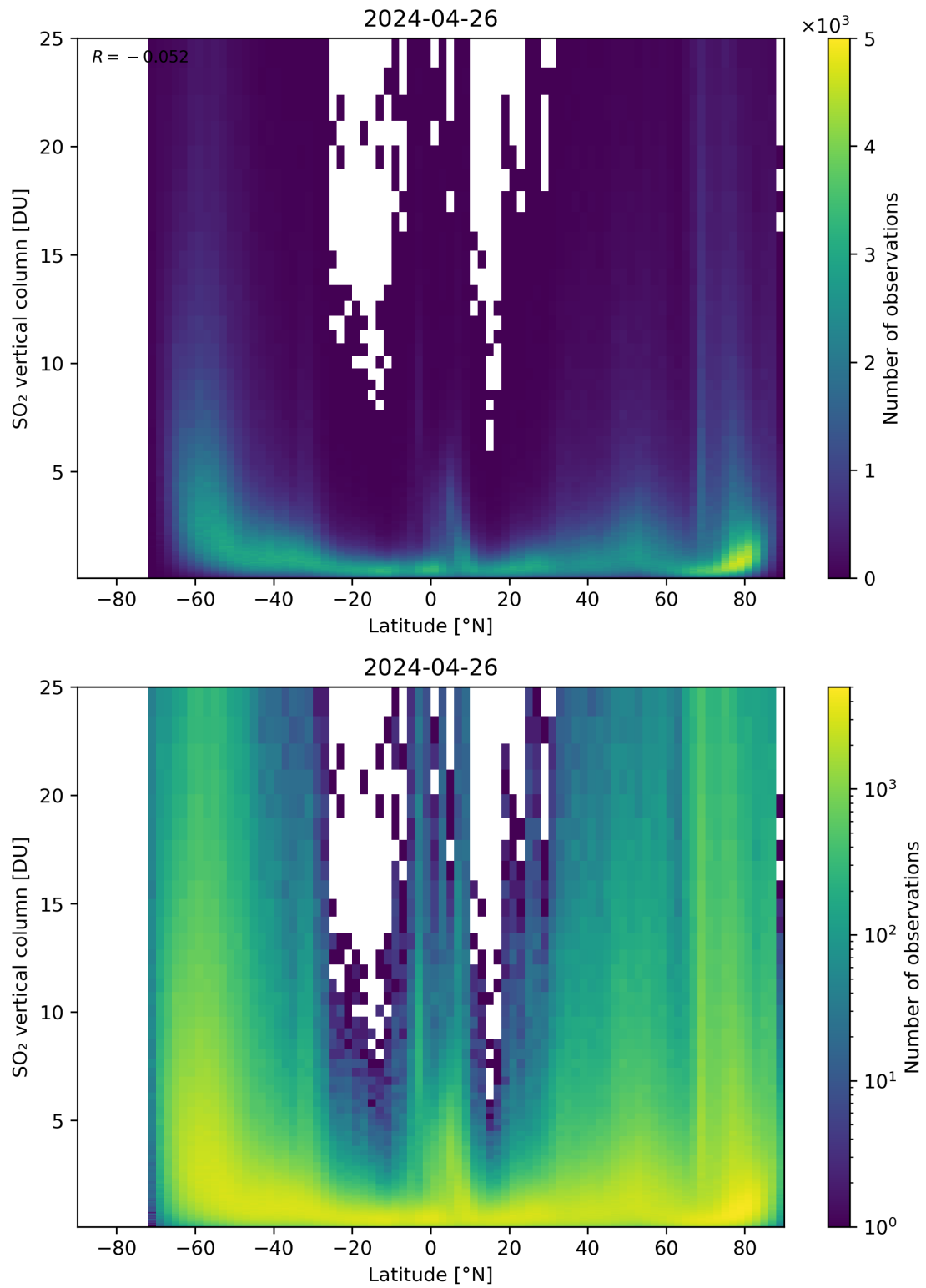
Figure 156: Scatter density plot of “Latitude” against “SO 2 vertical column” for 2024-04-26 to 2024-04-27.
