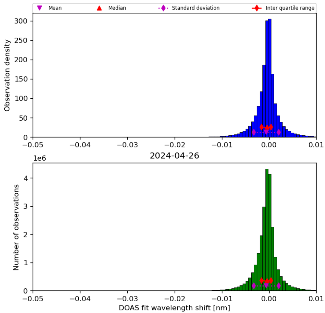
Figure 68: Histogram of “DOAS fit wavelength shift” for 2024-04-26 to 2024-04-27
