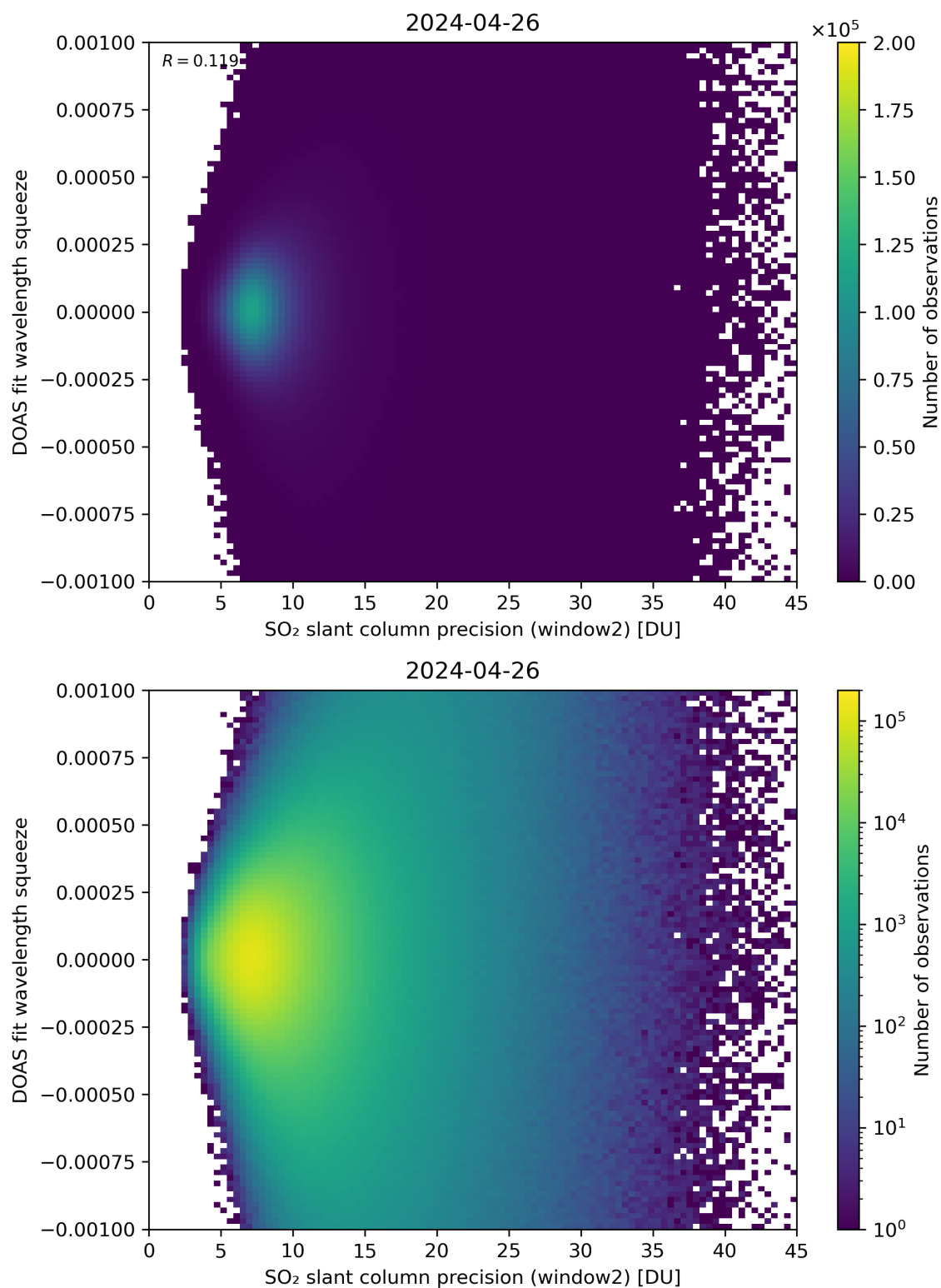
Figure 244: Scatter density plot of “SO 2 slant column precision (window2)” against “DOAS fit wavelength squeeze” for 2024-04-26 to 2024-04-27.
