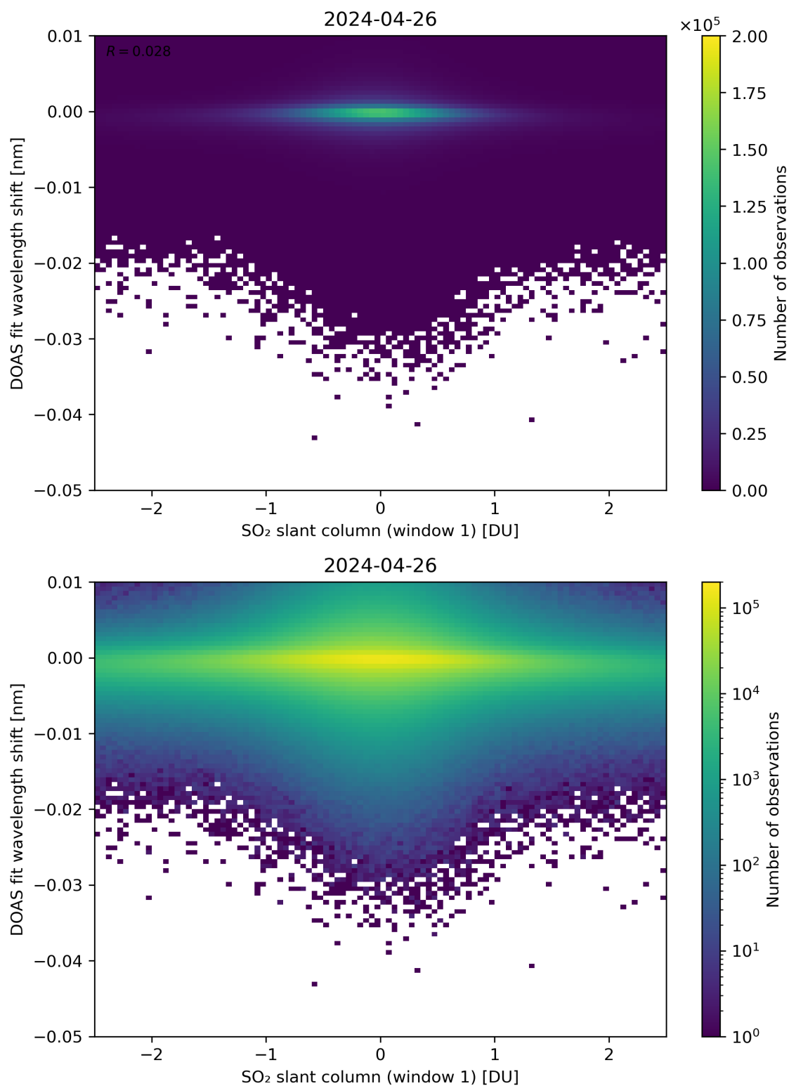
Figure 215: Scatter density plot of “SO 2 slant column (window 1)” against “DOAS fit wavelength shift” for 2024-04-26 to 2024-04-27.
