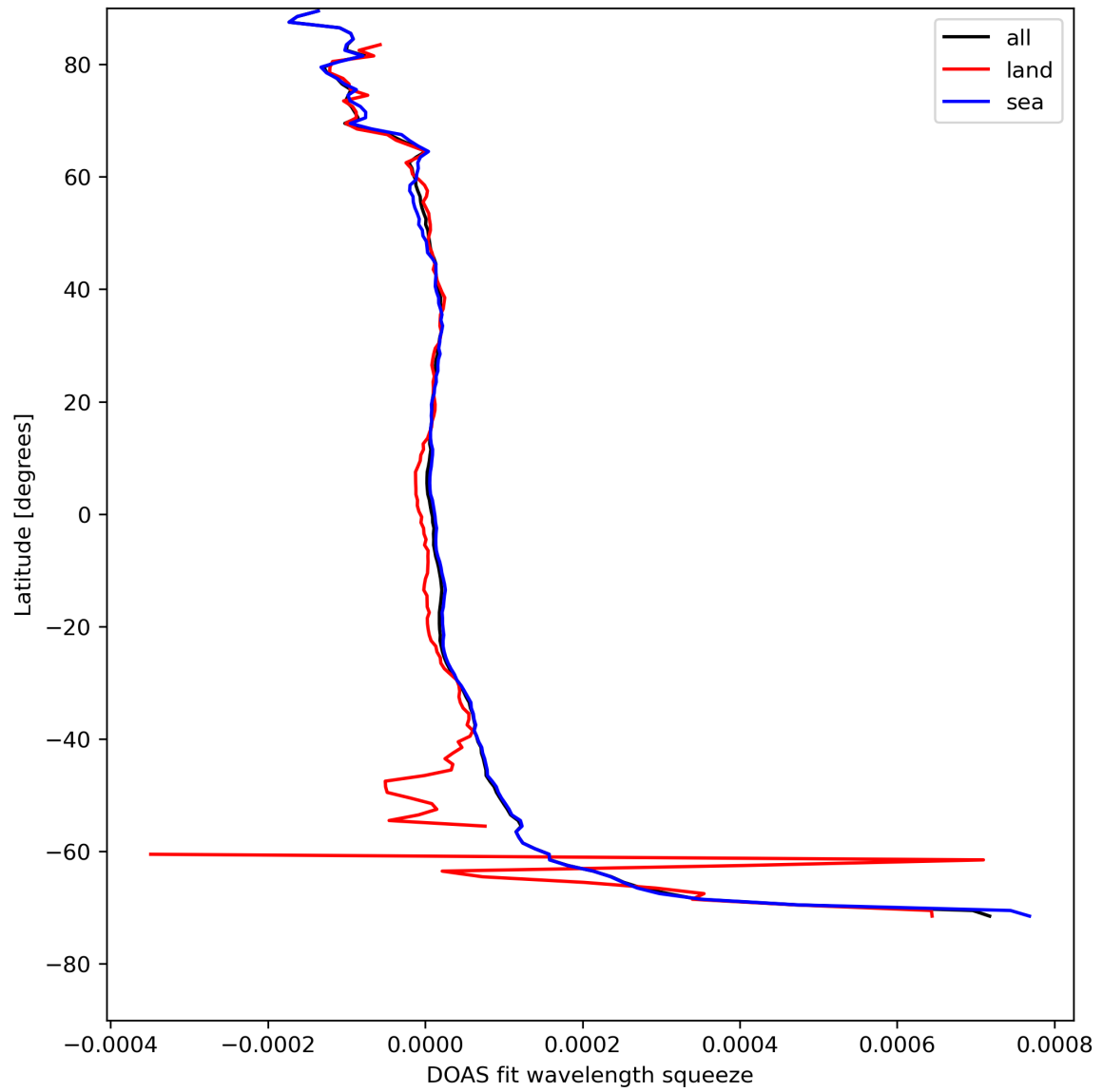
Figure 46: Zonal average of “DOAS fit wavelength squeeze” for 2024-04-26 to 2024-04-27.
