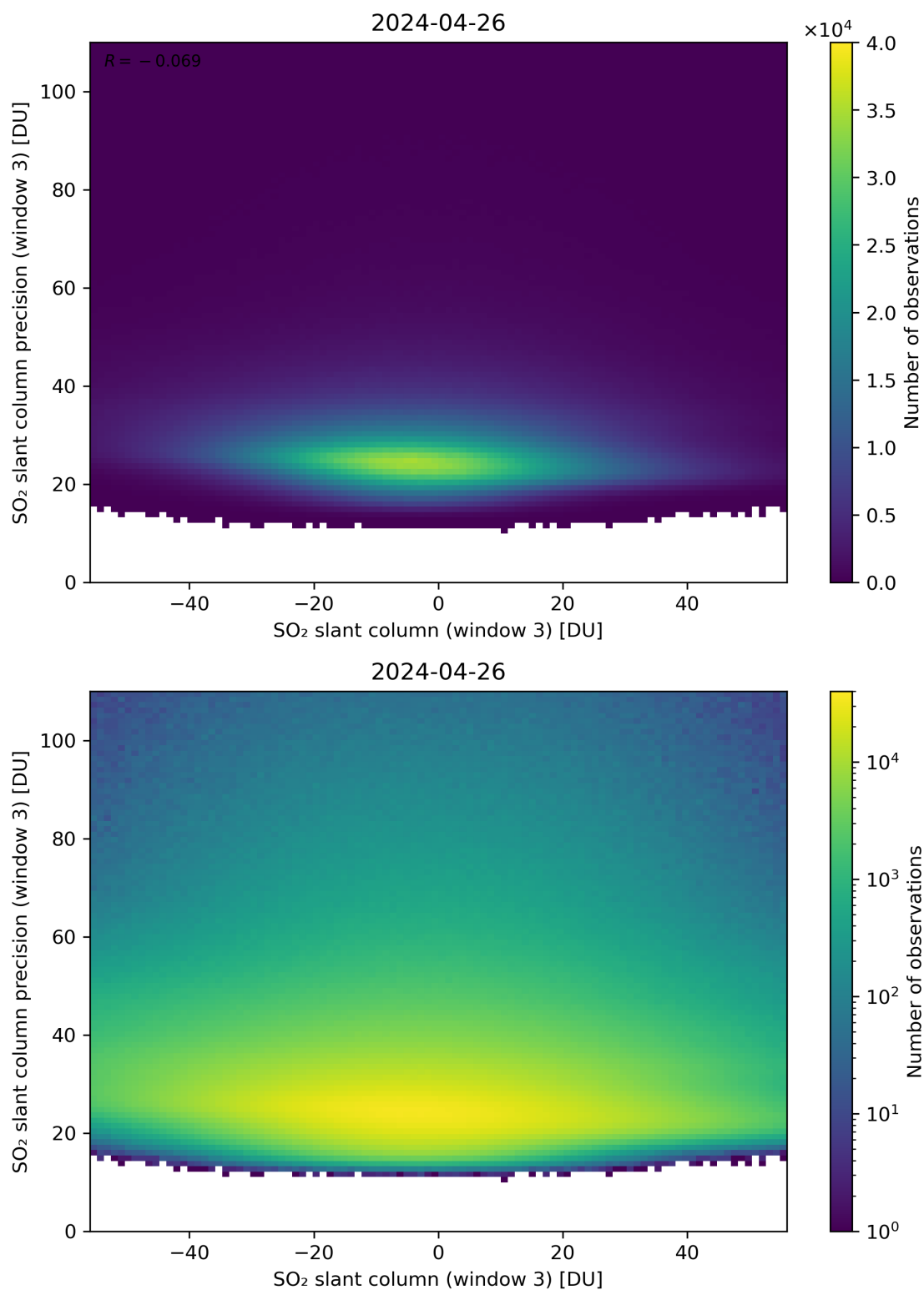
Figure 267: Scatter density plot of “SO 2 slant column (window 3)” against “SO 2 slant column precision (window 3)” for 2024-04-26 to 2024-04-27.
