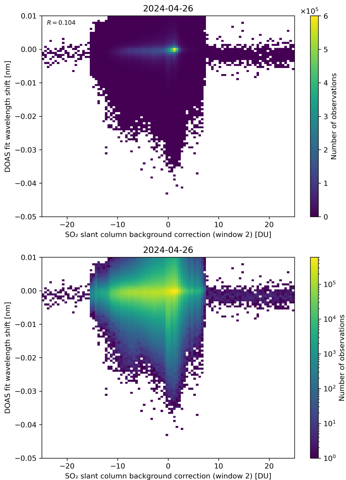
Figure 112: Scatter density plot of “SO 2 slant column background correction (window 2)” against “DOAS fit wavelength shift” for 2024-04-26 to 2024-04-27.
