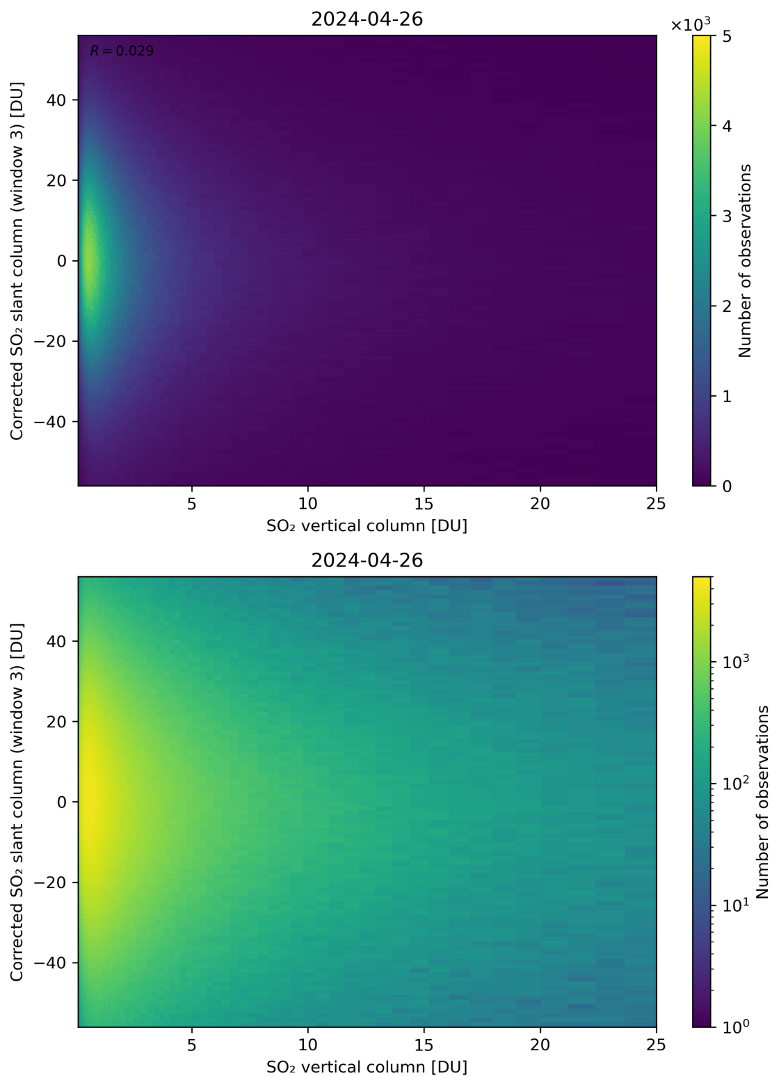
Figure 299: Scatter density plot of “SO 2 vertical column” against “Corrected SO 2 slant column (window 3)” for 2024-04-26 to 2024-04-27.
