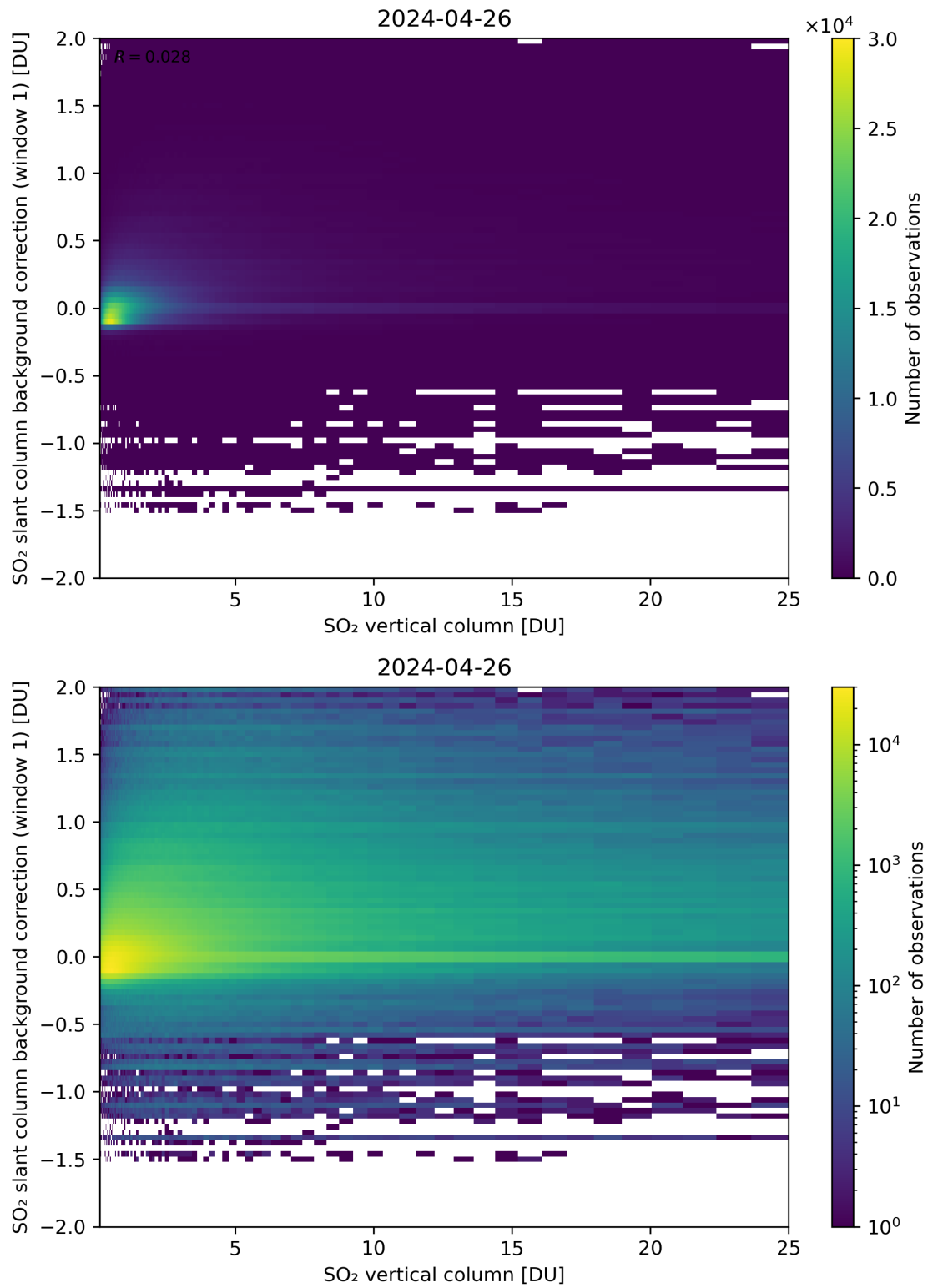
Figure 273: Scatter density plot of “SO 2 vertical column” against “SO 2 slant column background correction (window 1)” for 2024-04-26 to 2024-04-27.
