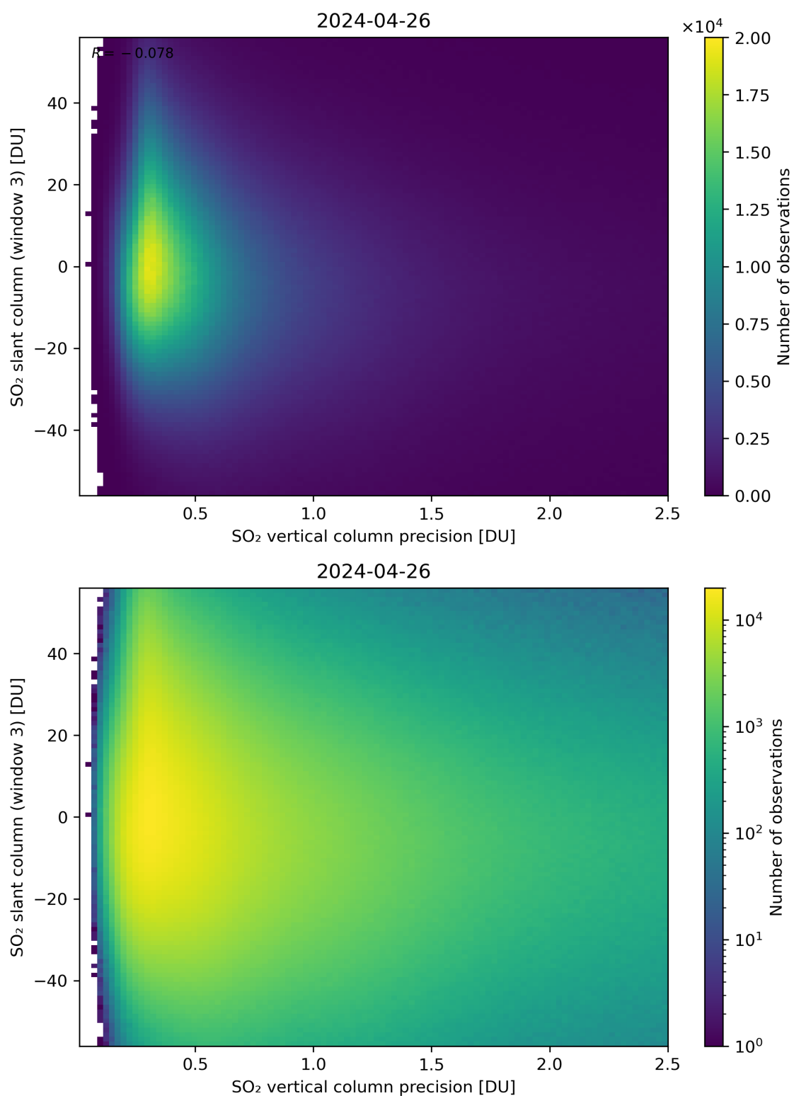
Figure 292: Scatter density plot of “SO 2 vertical column precision” against “SO 2 slant column (window 3)” for 2024-04-26 to 2024-04-27.
