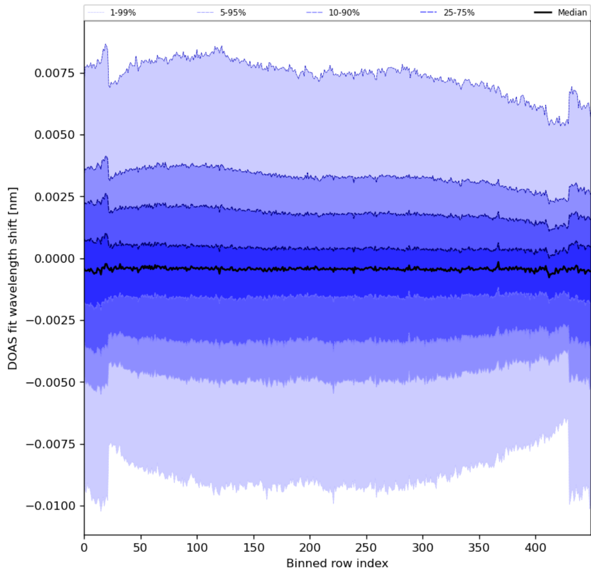
Figure 91: Along track statistics of “DOAS fit wavelength shift” for 2024-04-26 to 2024-04-27
