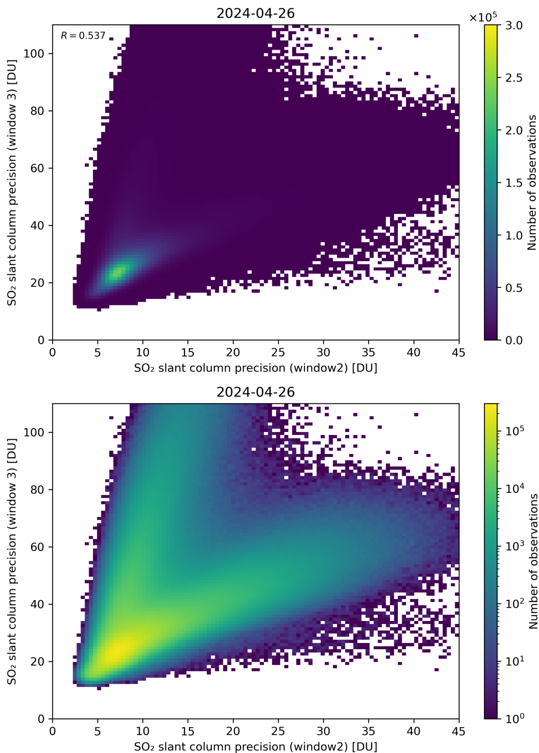
Figure 250: Scatter density plot of “SO 2 slant column precision (window2)” against “SO 2 slant column precision (window 3)” for 2024-04-26 to 2024-04-27.
