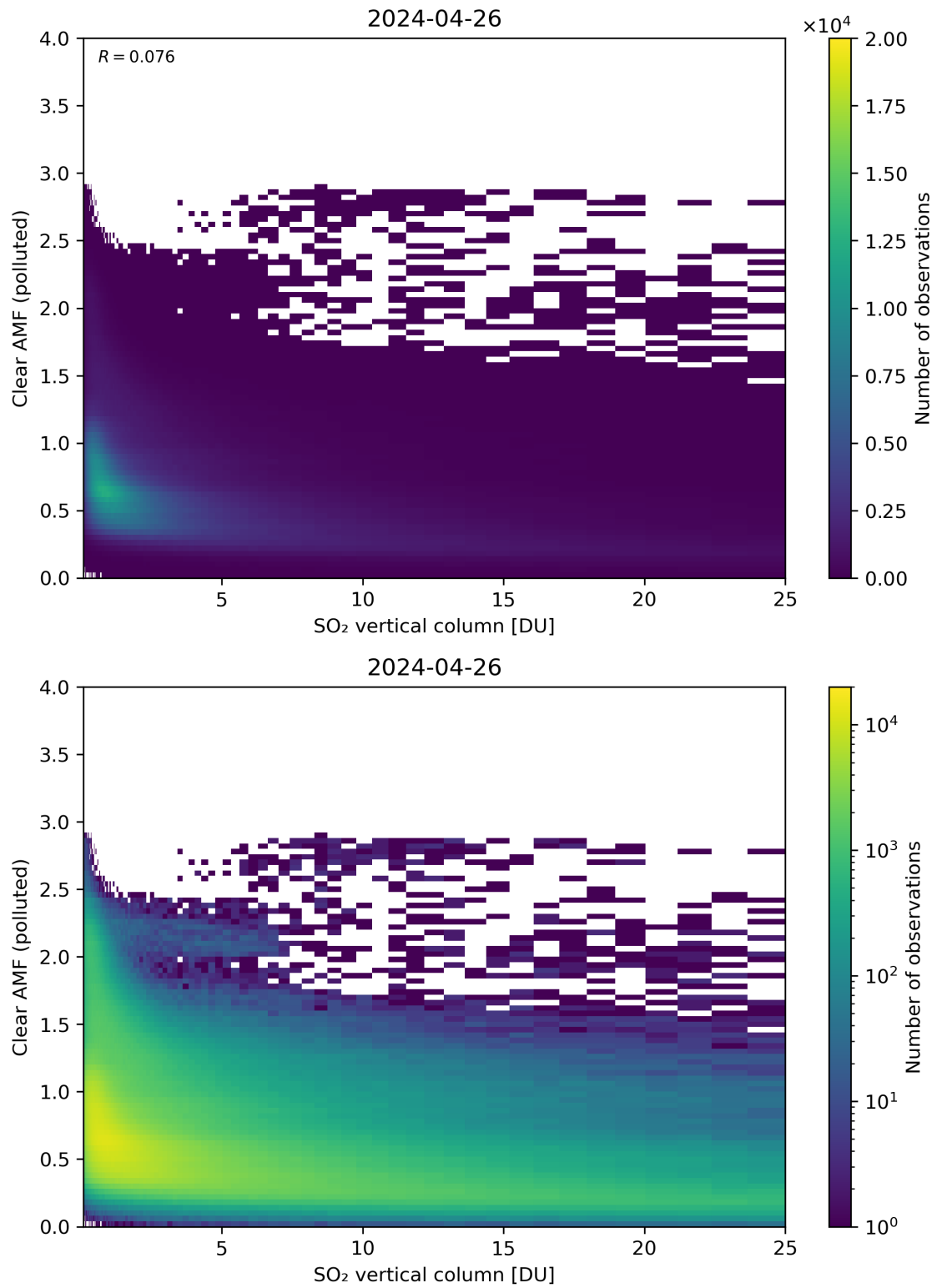
Figure 296: Scatter density plot of “SO 2 vertical column” against “Clear AMF (polluted)” for 2024-04-26 to 2024-04-27.
