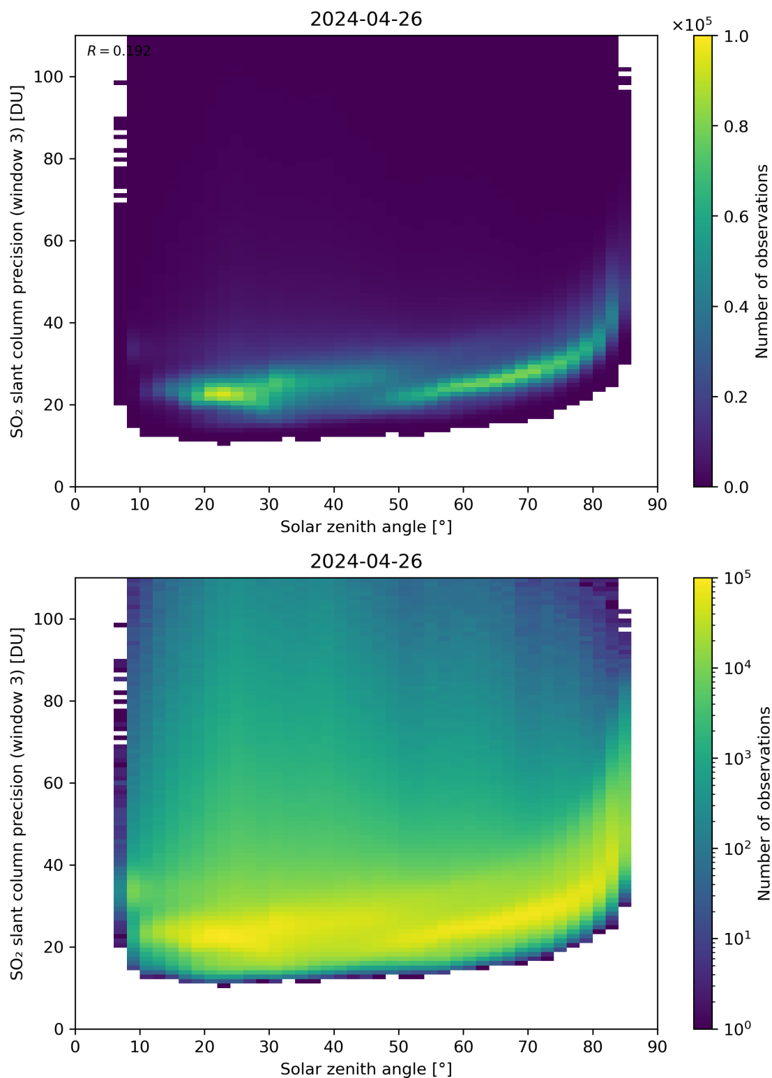
Figure 173: Scatter density plot of “Solar zenith angle” against “SO 2 slant column precision (window 3)” for 2024-04-26 to 2024-04-27.
