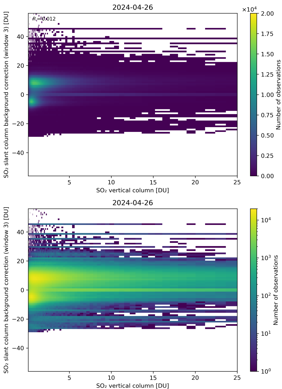
Figure 275: Scatter density plot of “SO 2 vertical column” against “SO 2 slant column background correction (window 3)” for 2024-04-26 to 2024-04-27.
