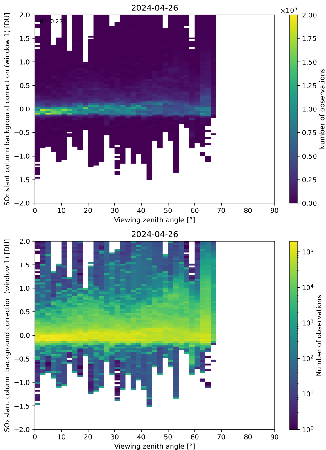
Figure 308: Scatter density plot of “Viewing zenith angle” against “SO 2 slant column background correction (window 1)” for 2024-04-26 to 2024-04-27.
