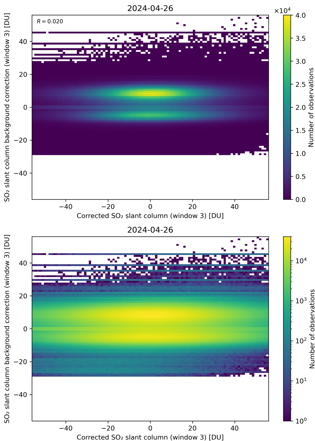
Figure 205: Scatter density plot of “Corrected SO 2 slant column (window 3)” against “SO 2 slant column background correction (window 3)” for 2024-04-26 to 2024-04-27.
