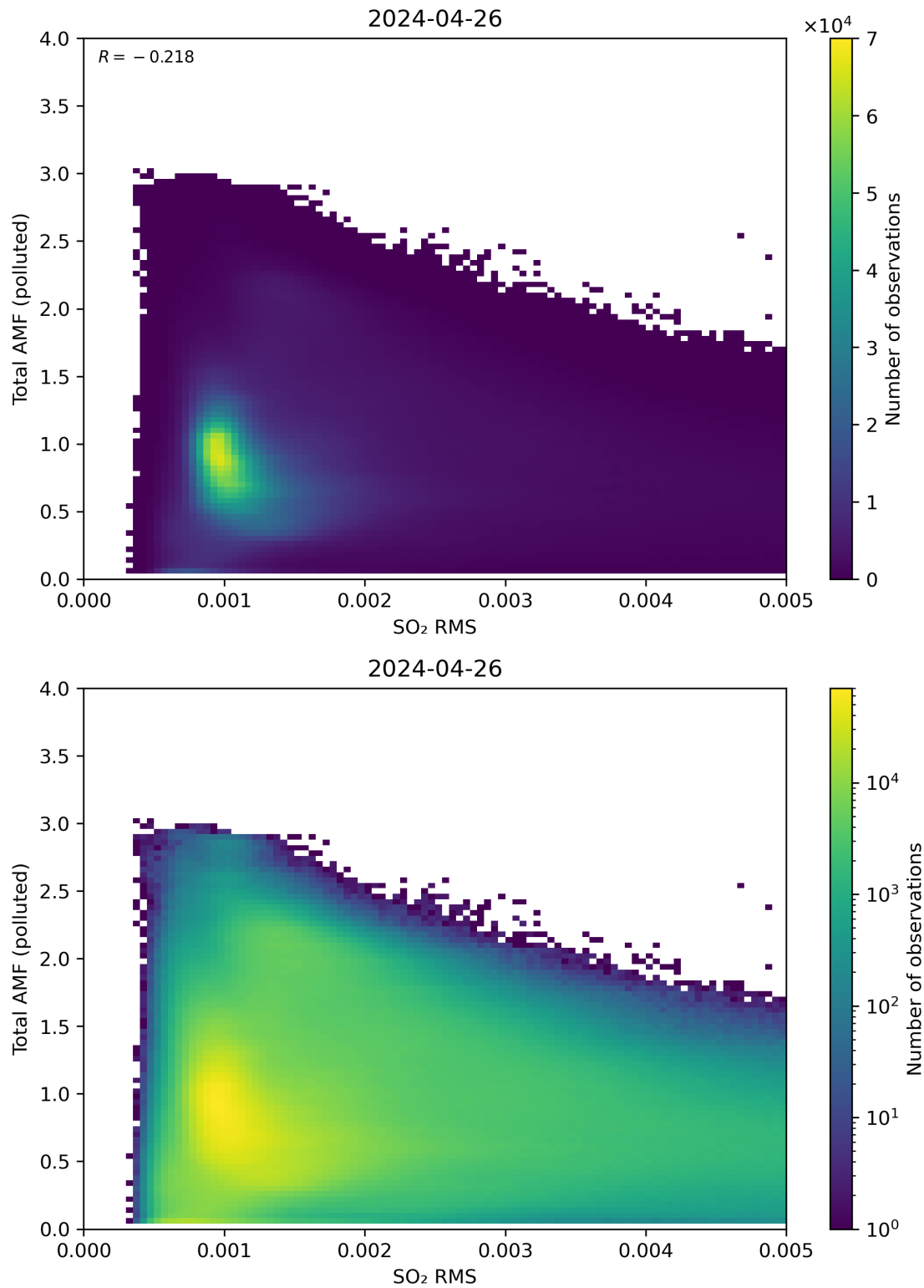
Figure 137: Scatter density plot of “SO 2 RMS” against “Total AMF (polluted)” for 2024-04-26 to 2024-04-27.
