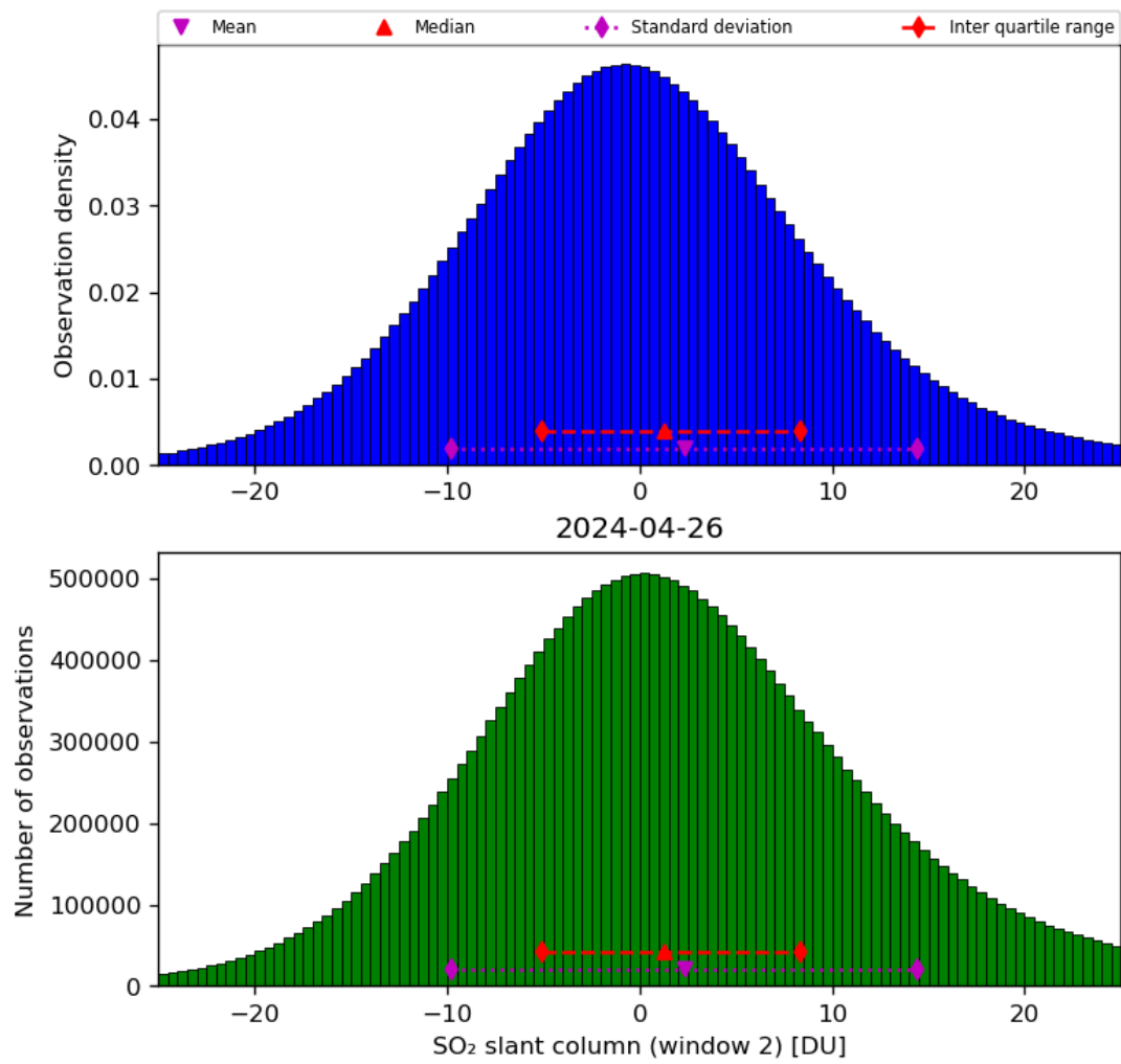
Figure 60: Histogram of “SO 2 slant column (window 2)” for 2024-04-26 to 2024-04-27
