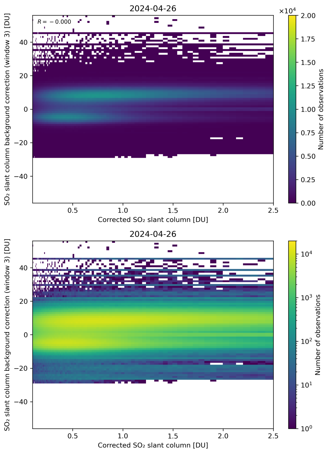
Figure 180: Scatter density plot of “Corrected SO 2 slant column” against “SO 2 slant column background correction (window 3)” for 2024-04-26 to 2024-04-27.
