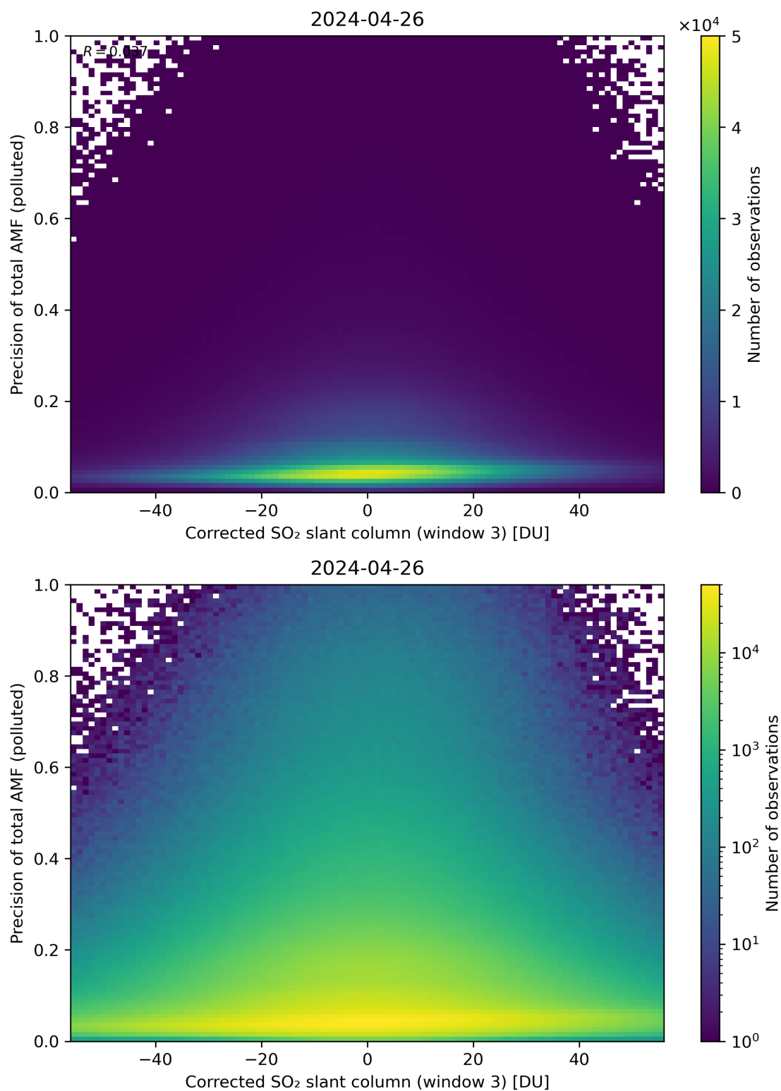
Figure 211: Scatter density plot of “Corrected SO 2 slant column (window 3)” against “Precision of total AMF (polluted)” for 2024-04-26 to 2024-04-27.
