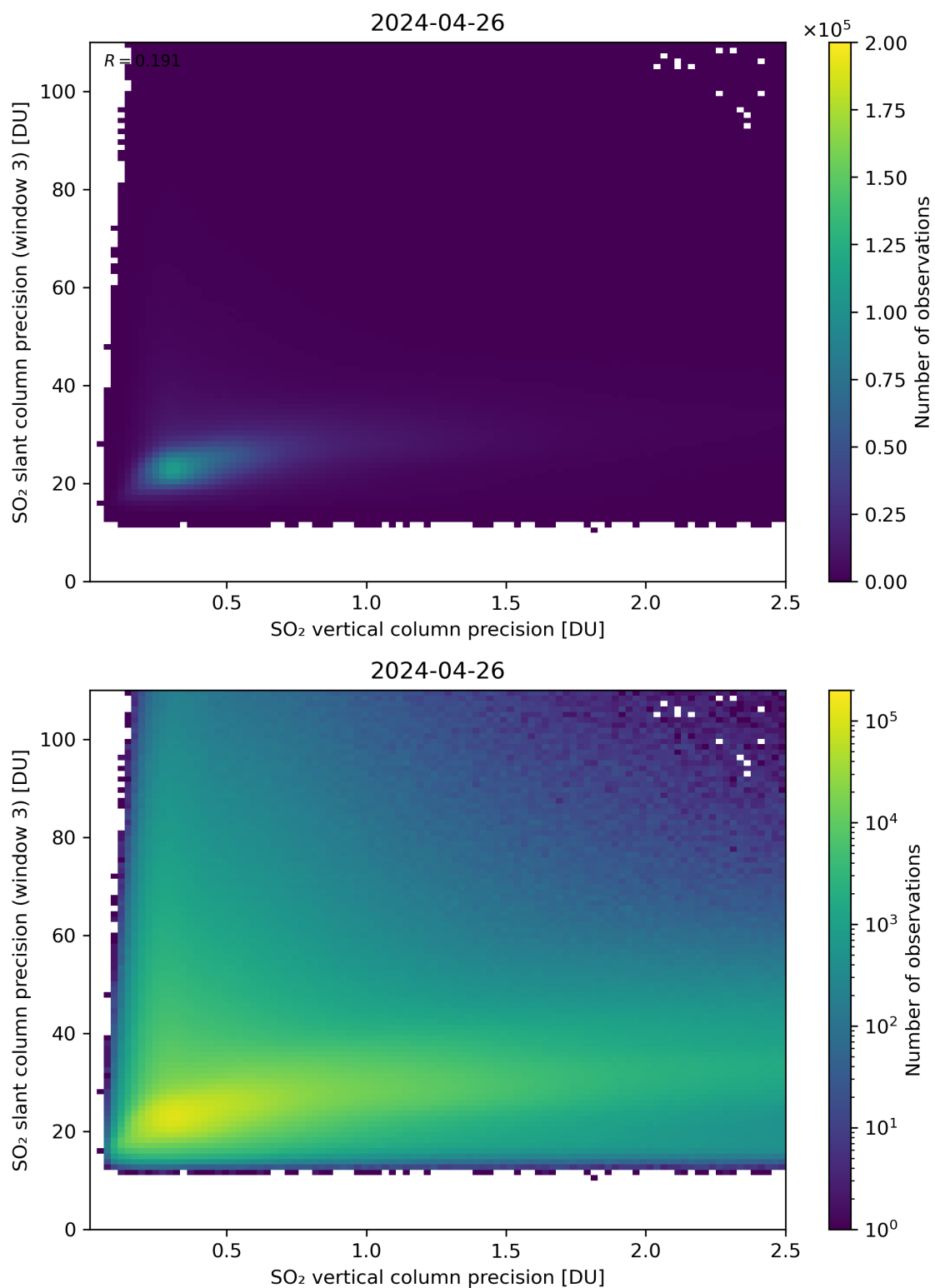
Figure 293: Scatter density plot of “SO 2 vertical column precision” against “SO 2 slant column precision (window 3)” for 2024-04-26 to 2024-04-27.
