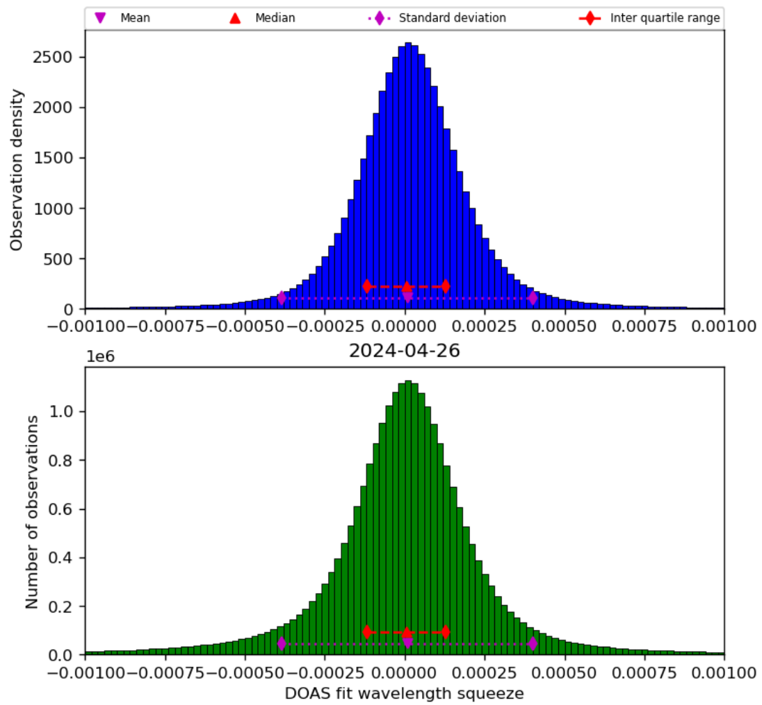
Figure 69: Histogram of “DOAS fit wavelength squeeze” for 2024-04-26 to 2024-04-27
