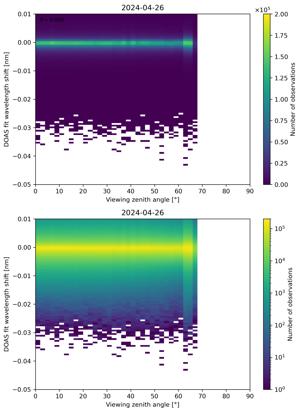
Figure 311: Scatter density plot of “Viewing zenith angle” against “DOAS fit wavelength shift” for 2024-04-26 to 2024-04-27.
