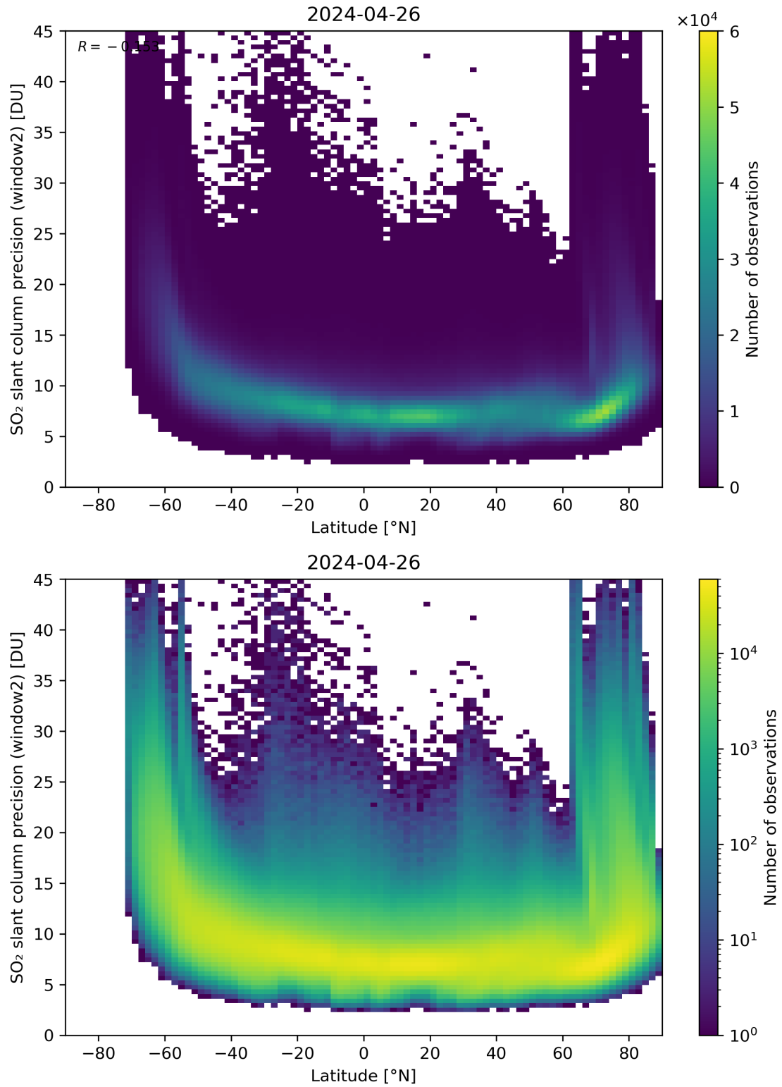
Figure 151: Scatter density plot of “Latitude” against “SO 2 slant column precision (window2)” for 2024-04-26 to 2024-04-27.
