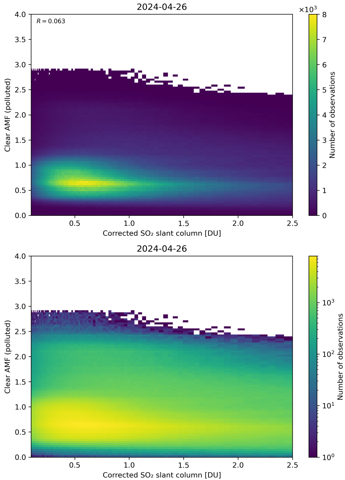
Figure 184: Scatter density plot of “Corrected SO 2 slant column” against “Clear AMF (polluted)” for 2024-04-26 to 2024-04-27.
