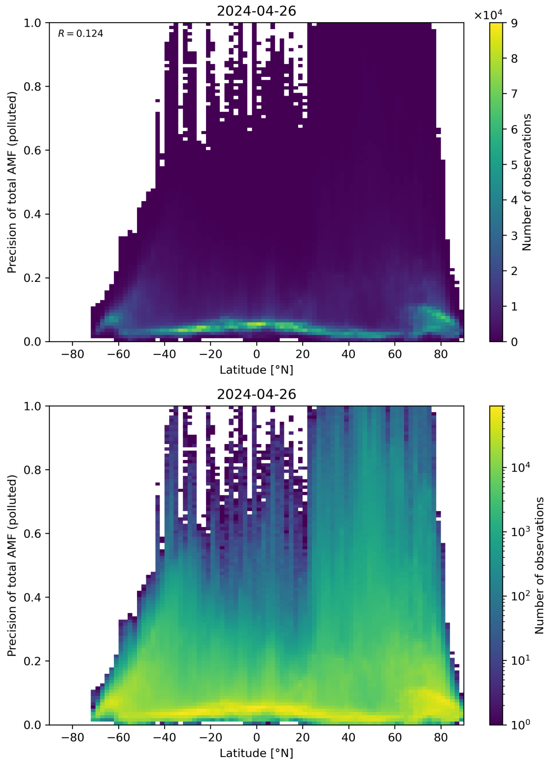
Figure 155: Scatter density plot of “Latitude” against “Precision of total AMF (polluted)” for 2024-04-26 to 2024-04-27.
