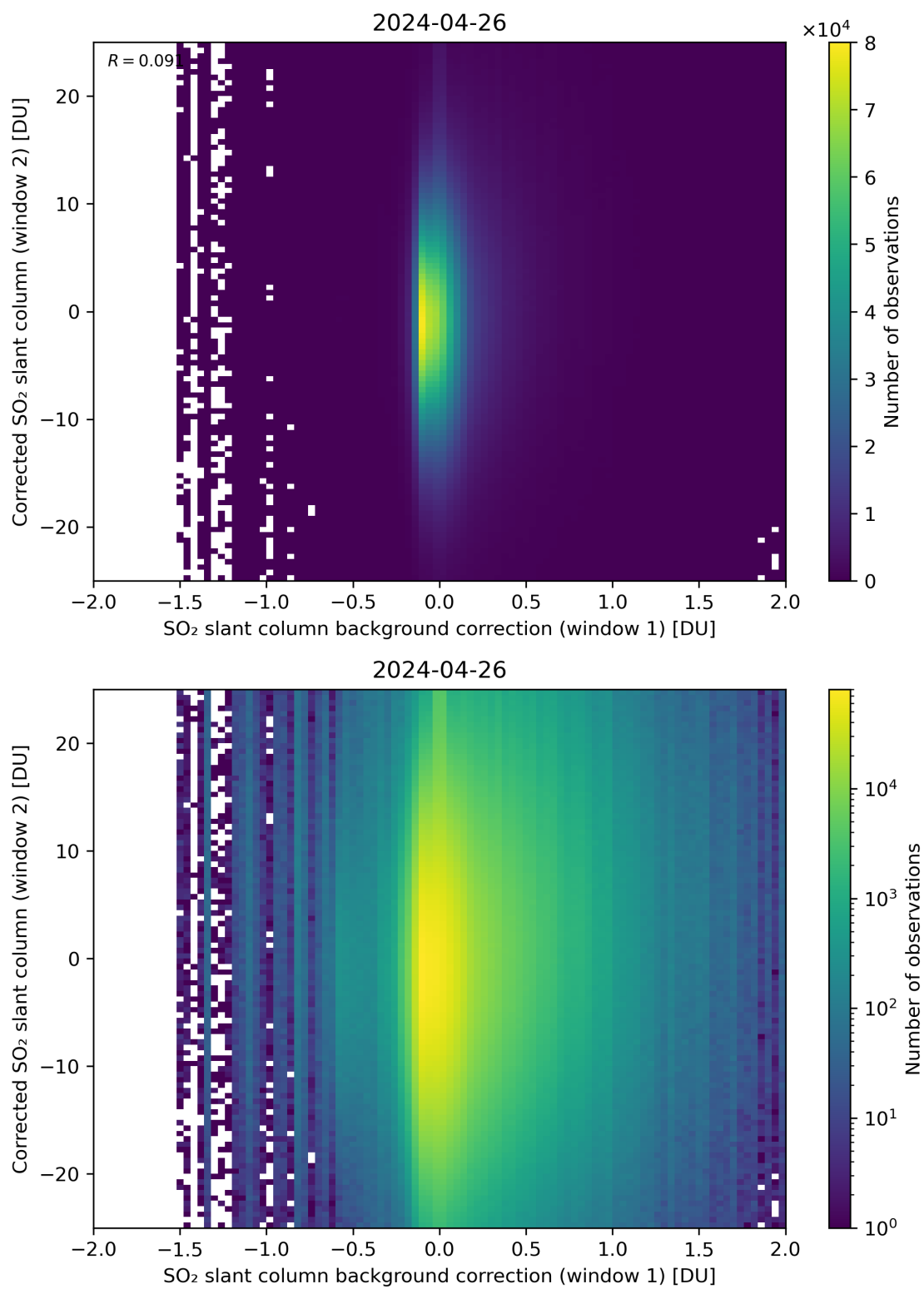
Figure 104: Scatter density plot of “SO 2 slant column background correction (window 1)” against “Corrected SO 2 slant column (window 2)” for 2024-04-26 to 2024-04-27.
