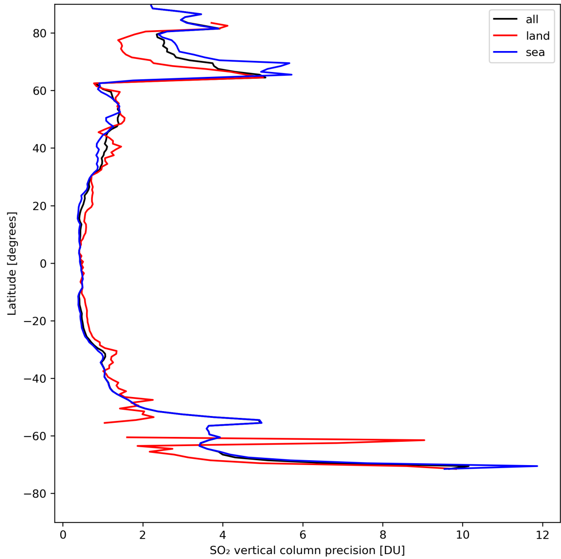
Figure 31: Zonal average of “SO 2 vertical column precision” for 2024-04-26 to 2024-04-27.
