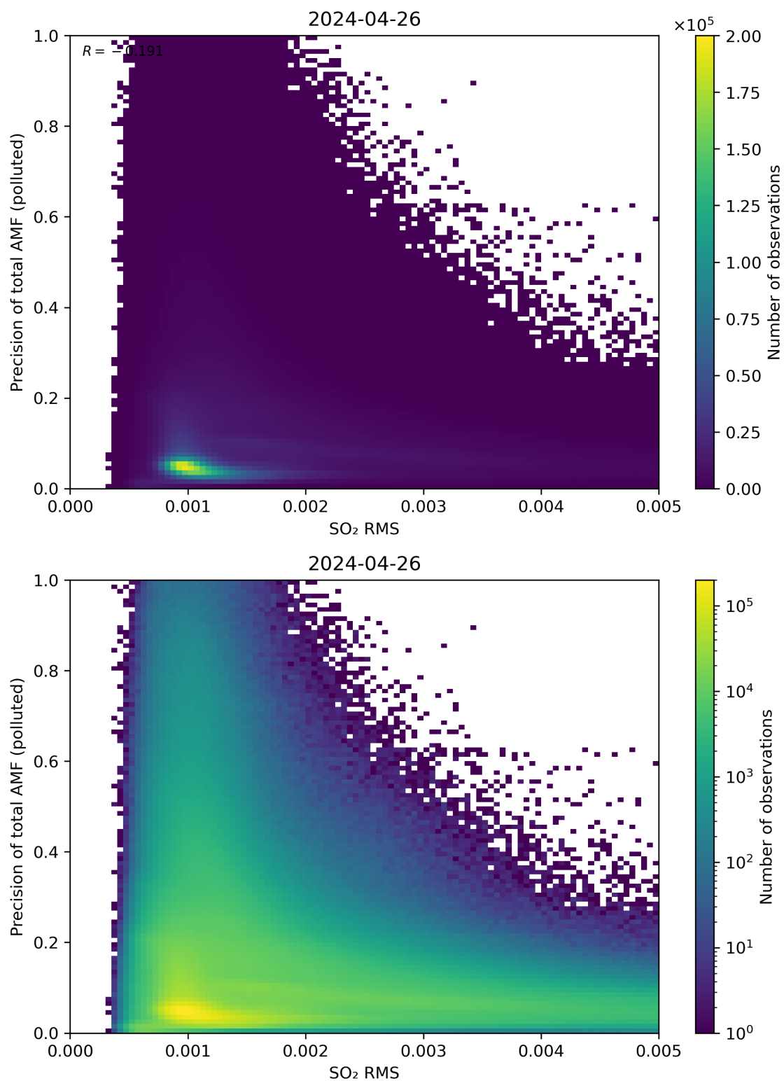
Figure 138: Scatter density plot of “SO 2 RMS” against “Precision of total AMF (polluted)” for 2024-04-26 to 2024-04-27.
