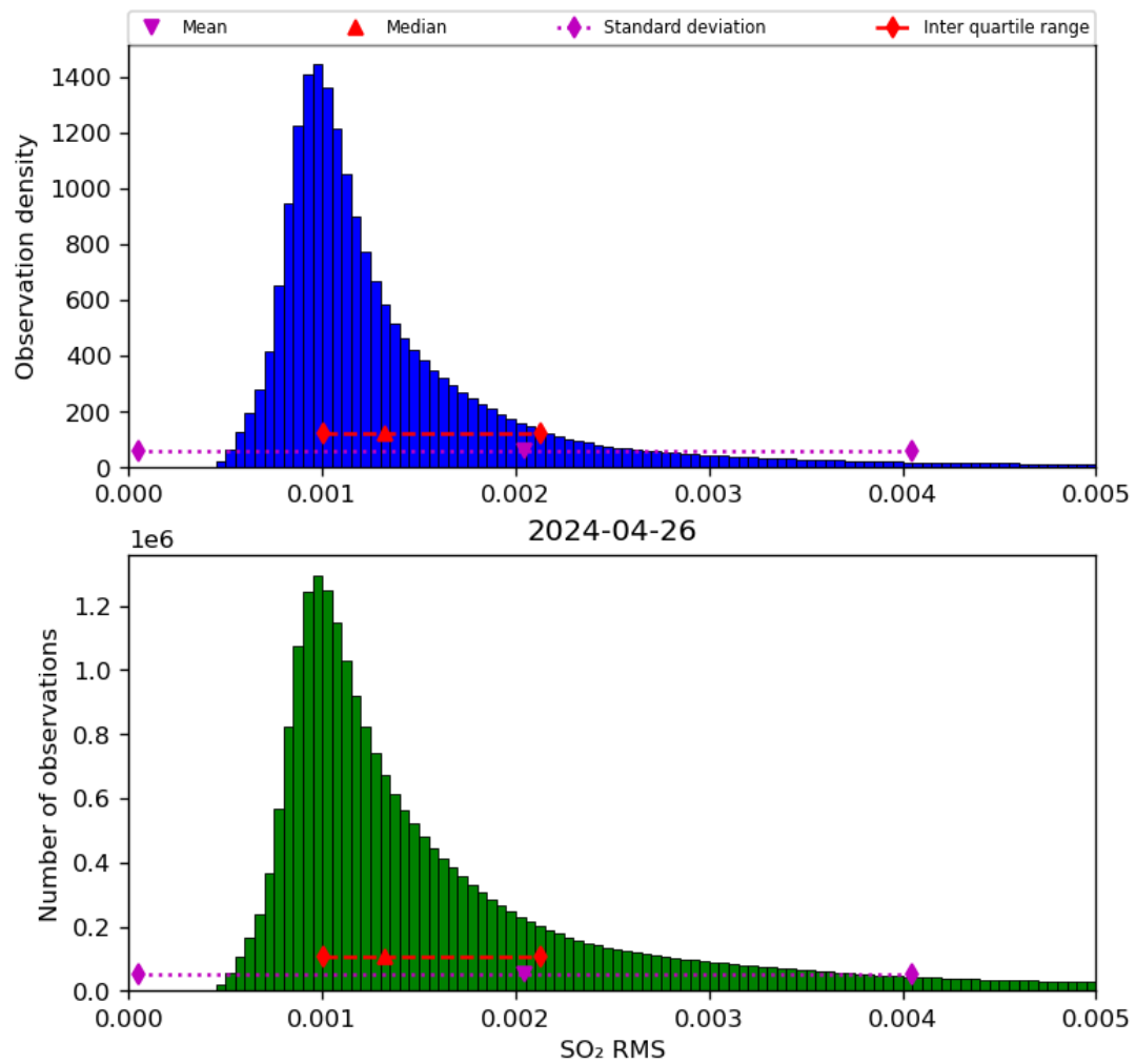
Figure 70: Histogram of “SO 2 RMS” for 2024-04-26 to 2024-04-27
