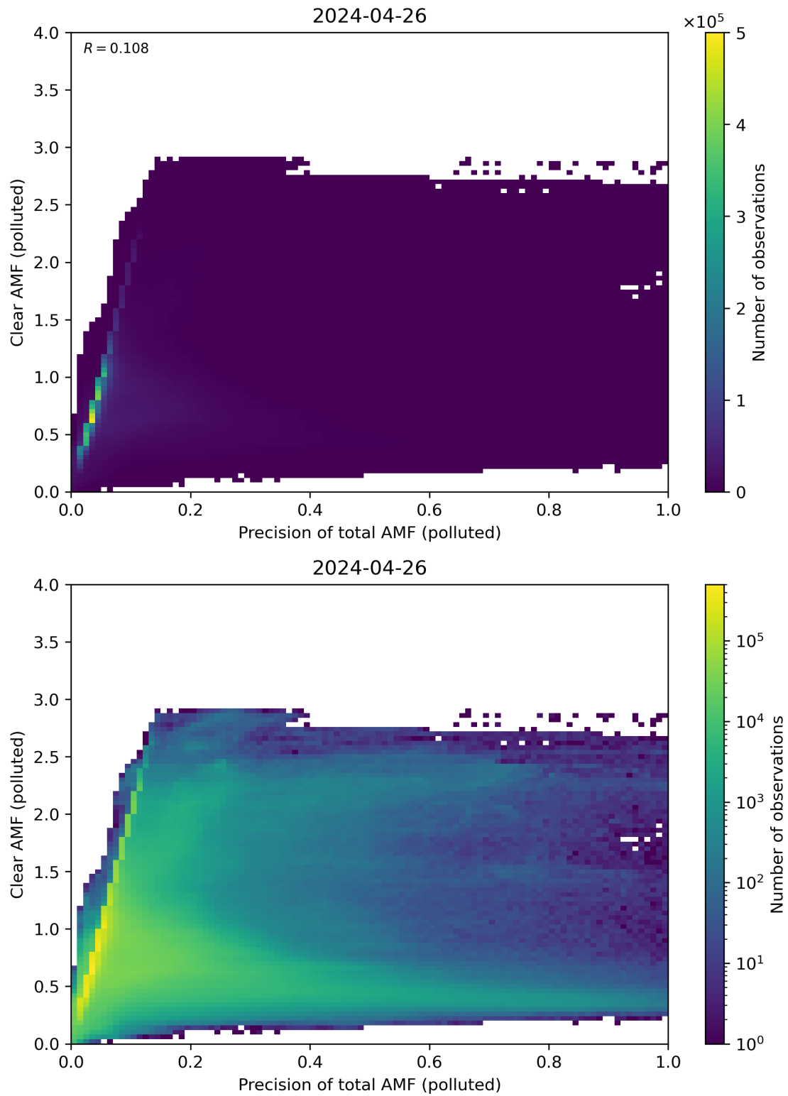
Figure 270: Scatter density plot of “Precision of total AMF (polluted)” against “Clear AMF (polluted)” for 2024-04-26 to 2024-04-27.
