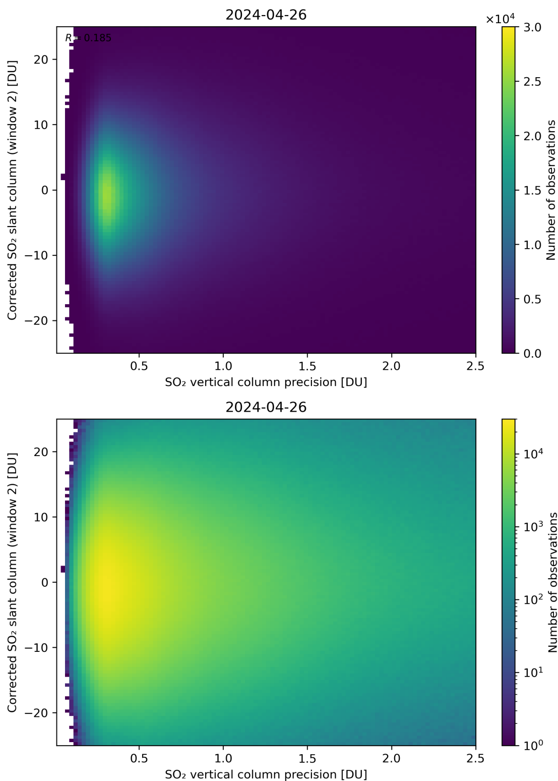
Figure 287: Scatter density plot of “SO 2 vertical column precision” against “Corrected SO 2 slant column (window 2)” for 2024-04-26 to 2024-04-27.
