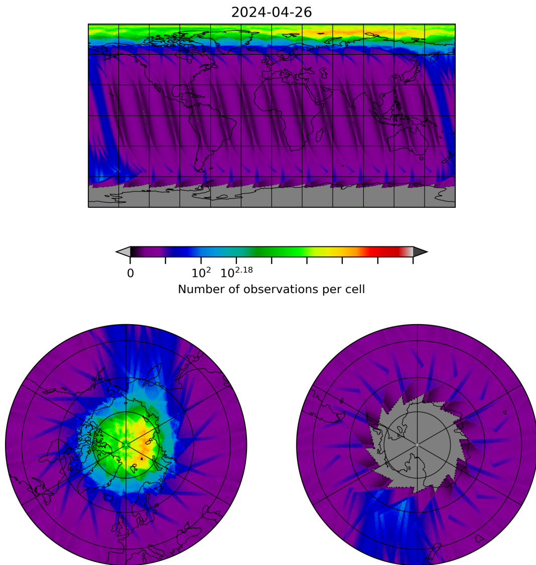
Figure 28: Map of the number of observations for 2024-04-26 to 2024-04-27
