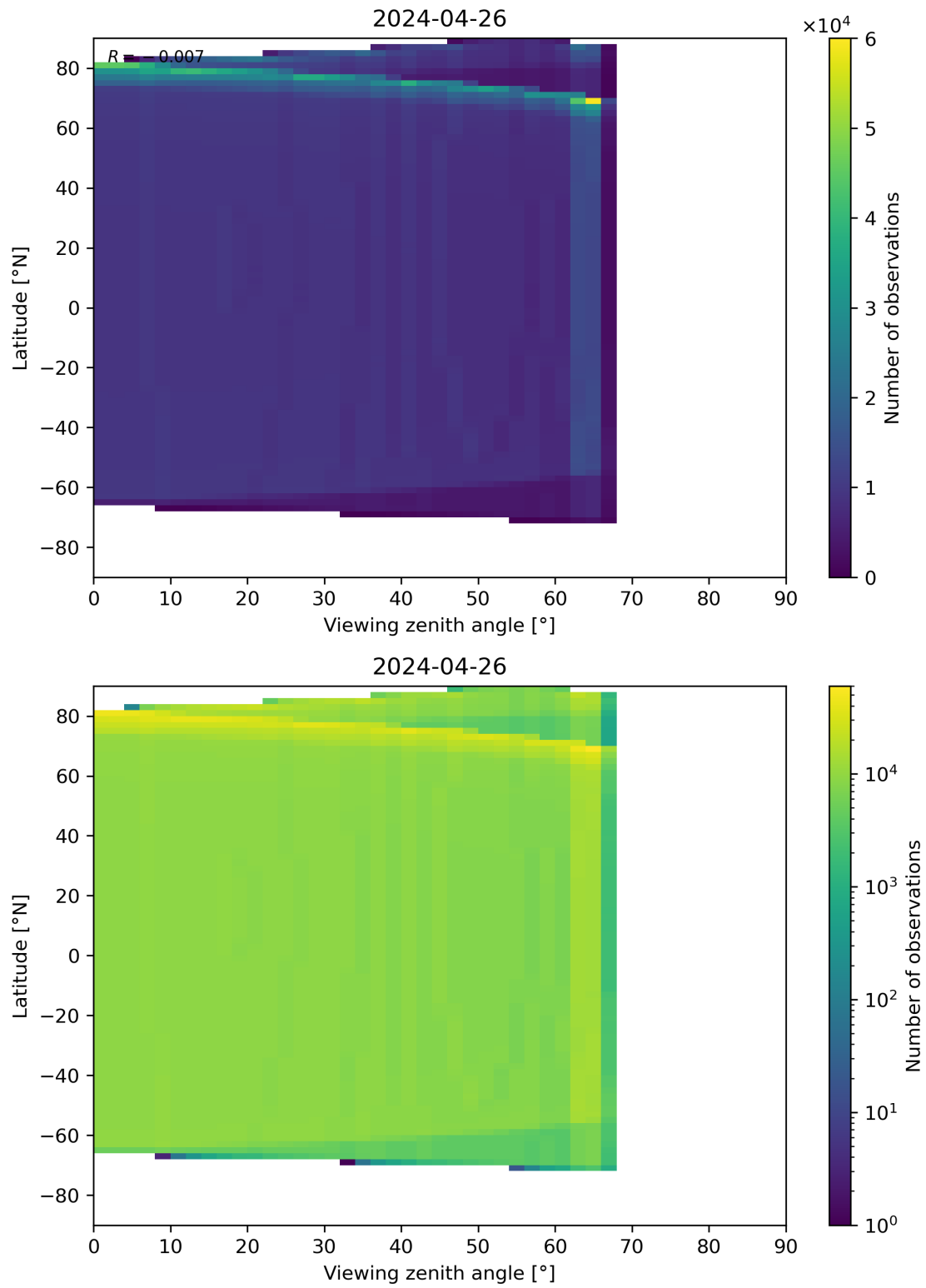
Figure 314: Scatter density plot of “Viewing zenith angle” against “Latitude” for 2024-04-26 to 2024-04-27.
