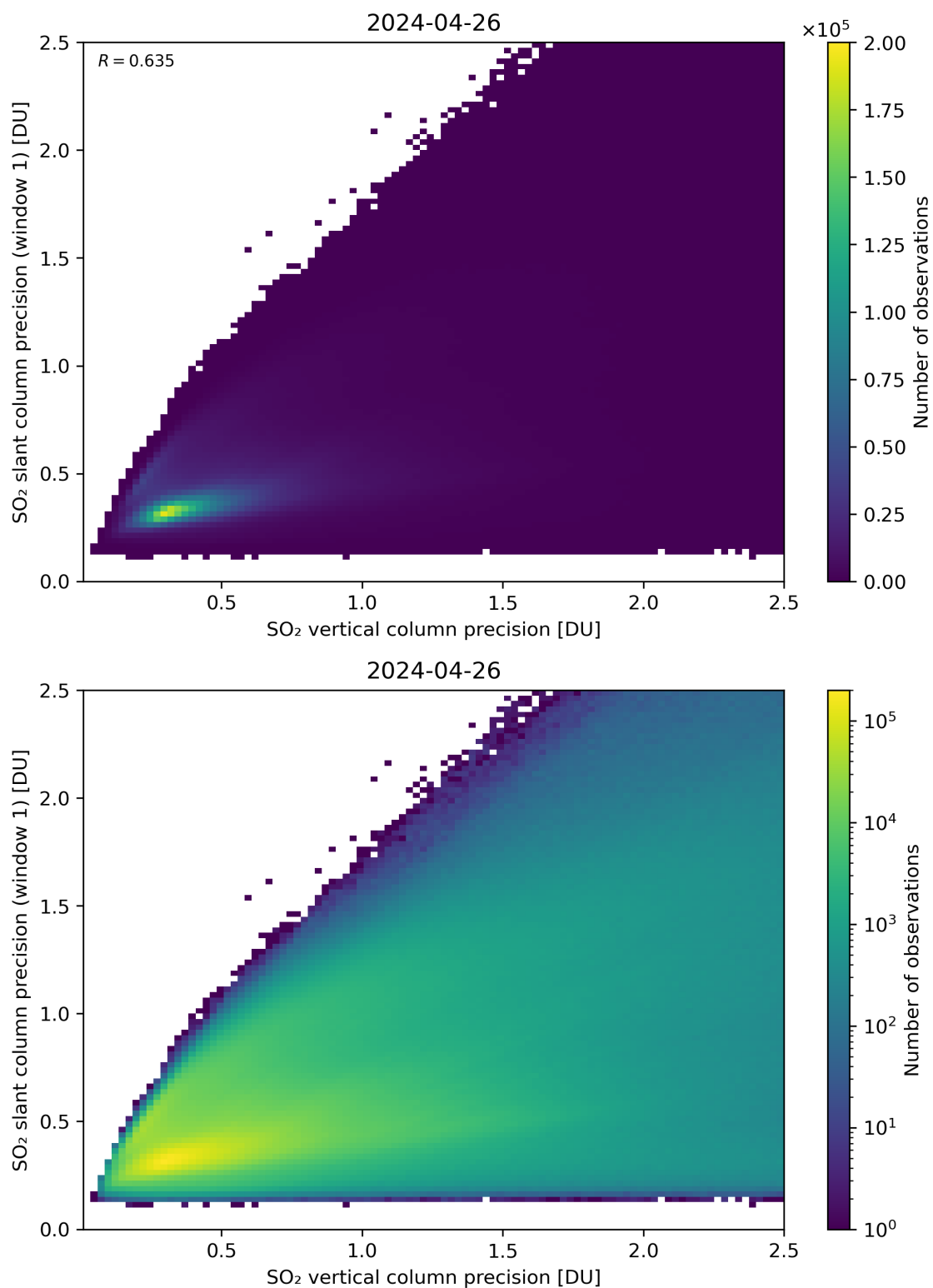
Figure 290: Scatter density plot of “SO 2 vertical column precision” against “SO 2 slant column precision (window 1)” for 2024-04-26 to 2024-04-27.
