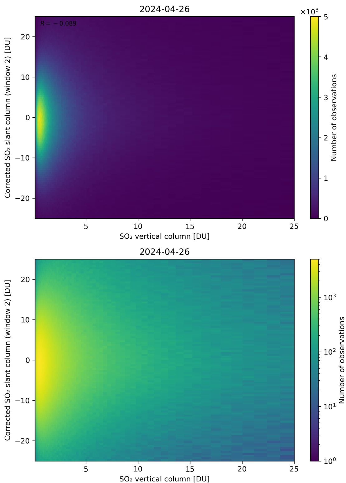
Figure 298: Scatter density plot of “SO 2 vertical column” against “Corrected SO 2 slant column (window 2)” for 2024-04-26 to 2024-04-27.
