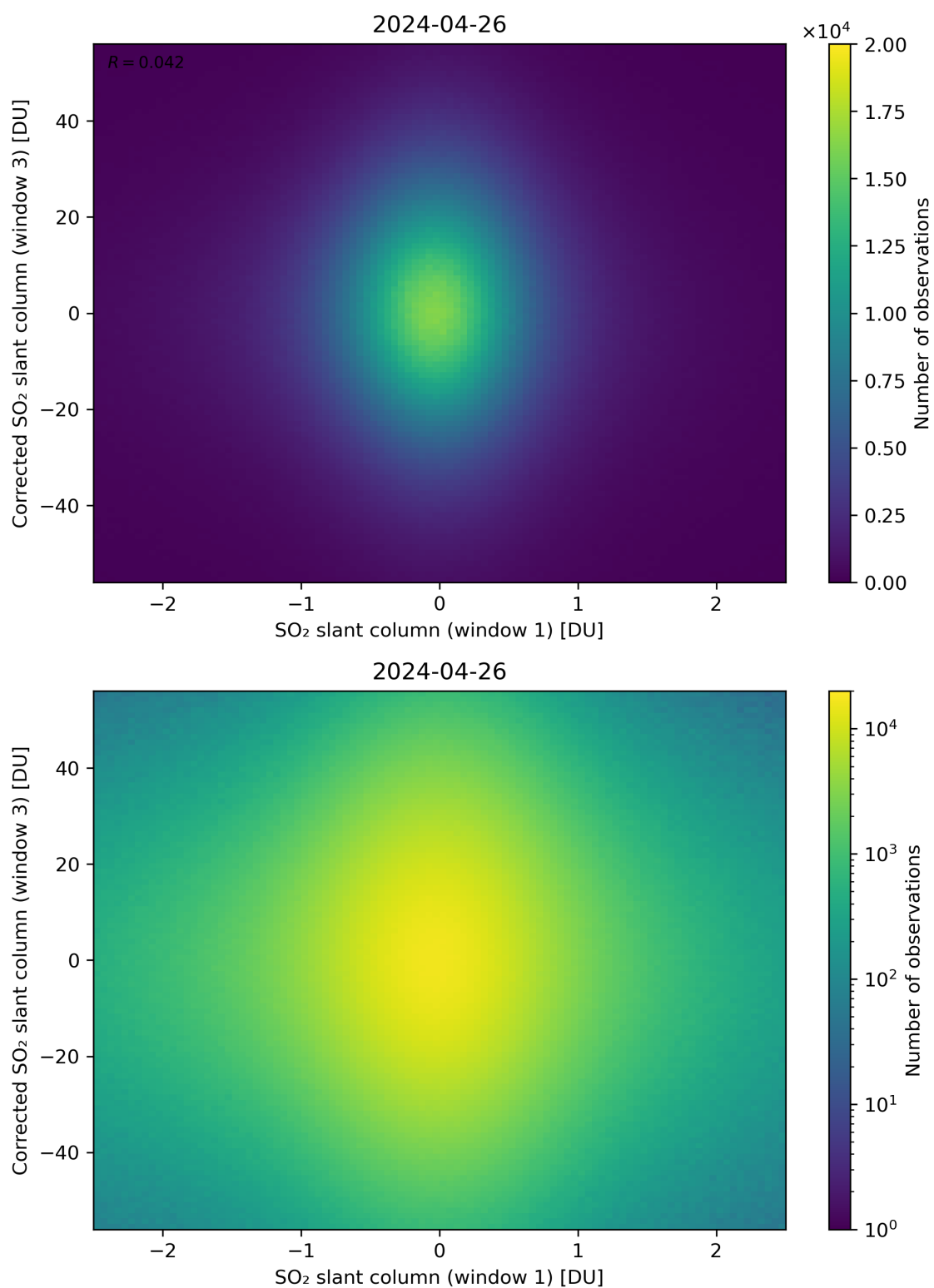
Figure 234: Scatter density plot of “SO 2 slant column (window 1)” against “Corrected SO 2 slant column (window 3)” for 2024-04-26 to 2024-04-27.
