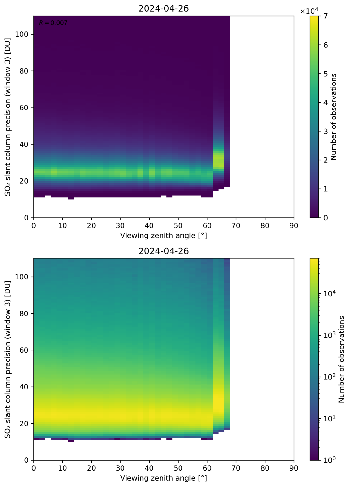
Figure 324: Scatter density plot of “Viewing zenith angle” against “SO 2 slant column precision (window 3)” for 2024-04-26 to 2024-04-27.
