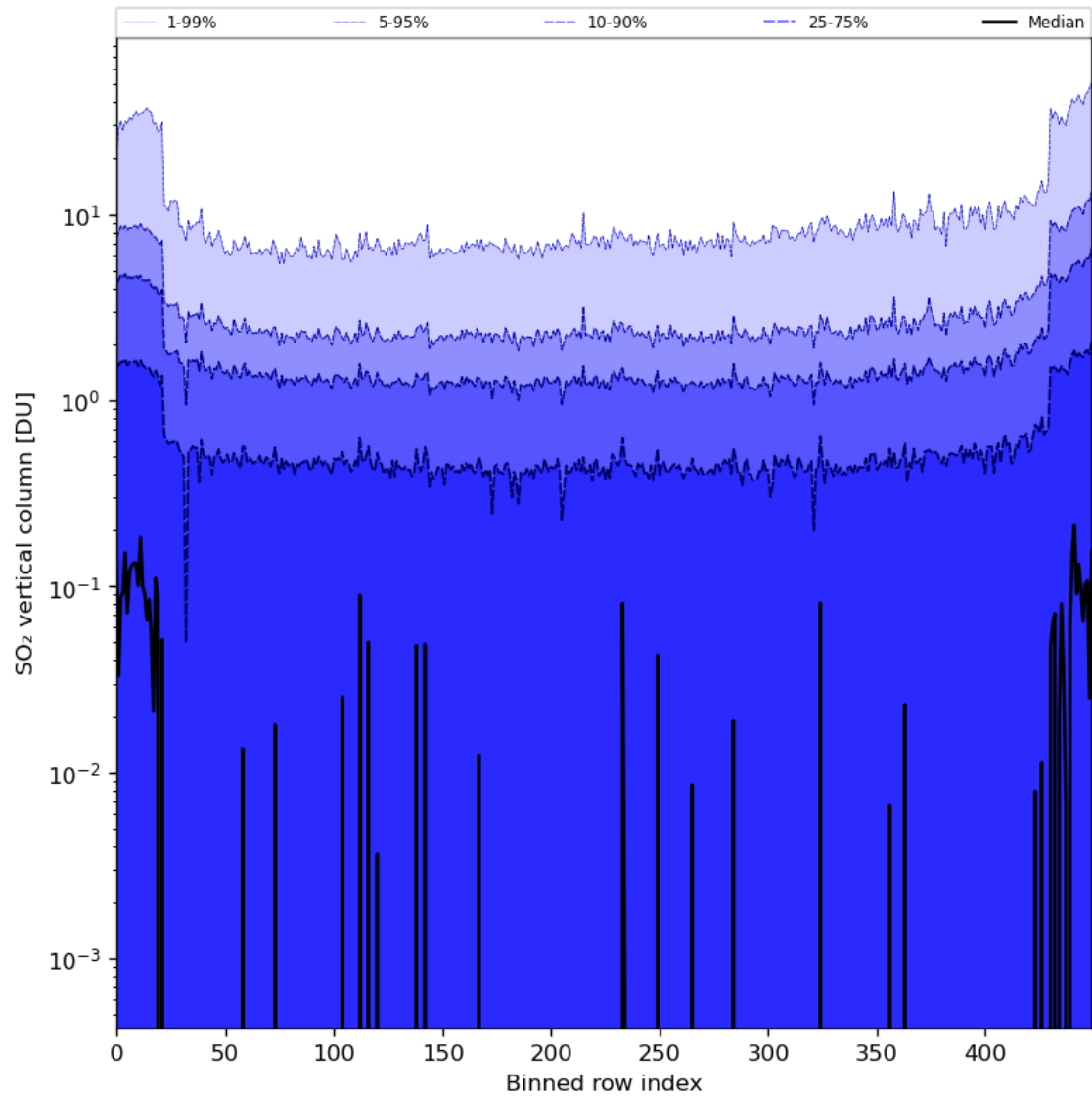
Figure 76: Along track statistics of “SO 2 vertical column” for 2024-04-26 to 2024-04-27
