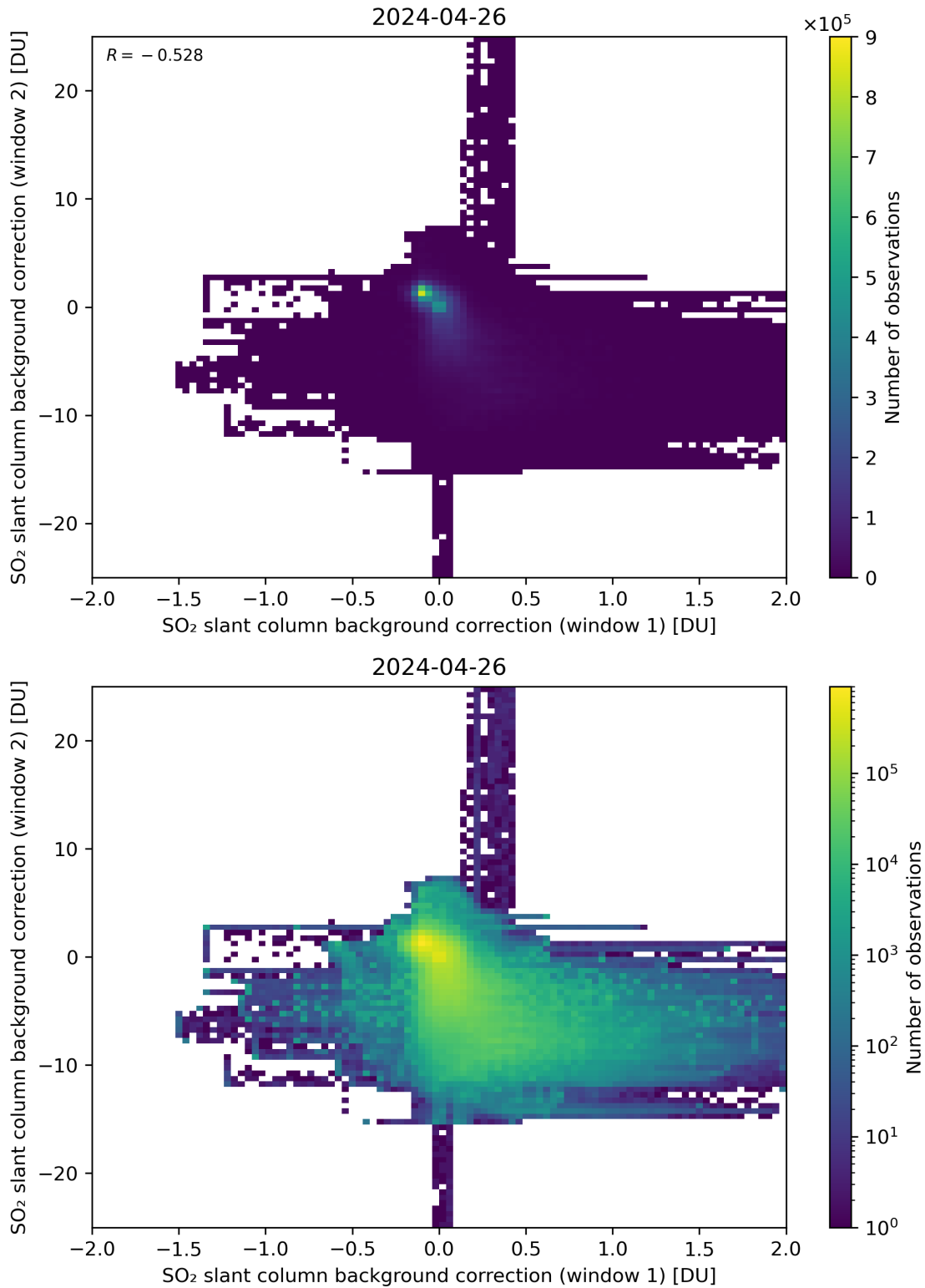
Figure 98: Scatter density plot of “SO 2 slant column background correction (window 1)” against “SO 2 slant column background correction (window 2)” for 2024-04-26 to 2024-04-27.
