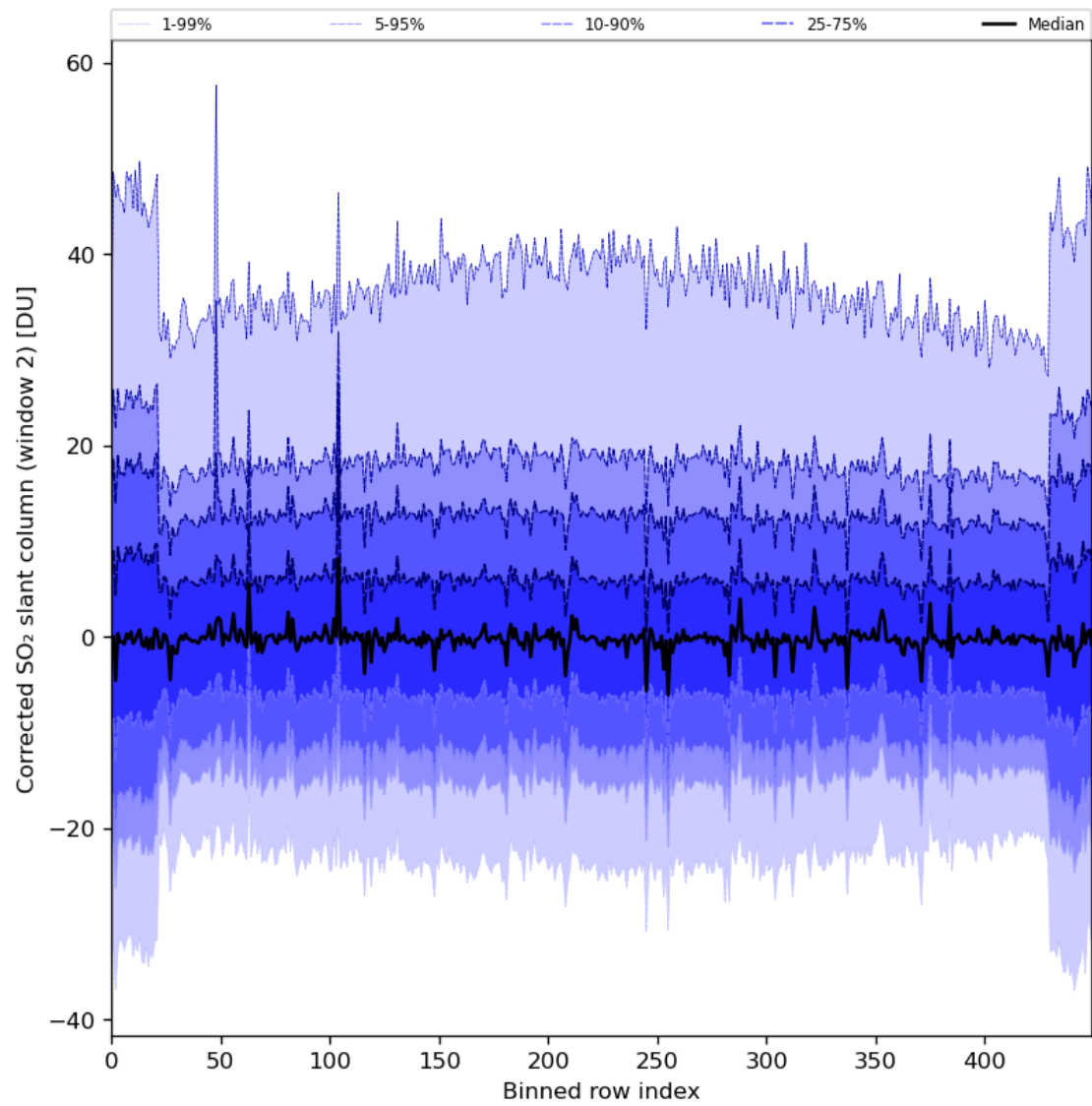
Figure 85: Along track statistics of “Corrected SO 2 slant column (window 2)” for 2024-04-26 to 2024-04-27
