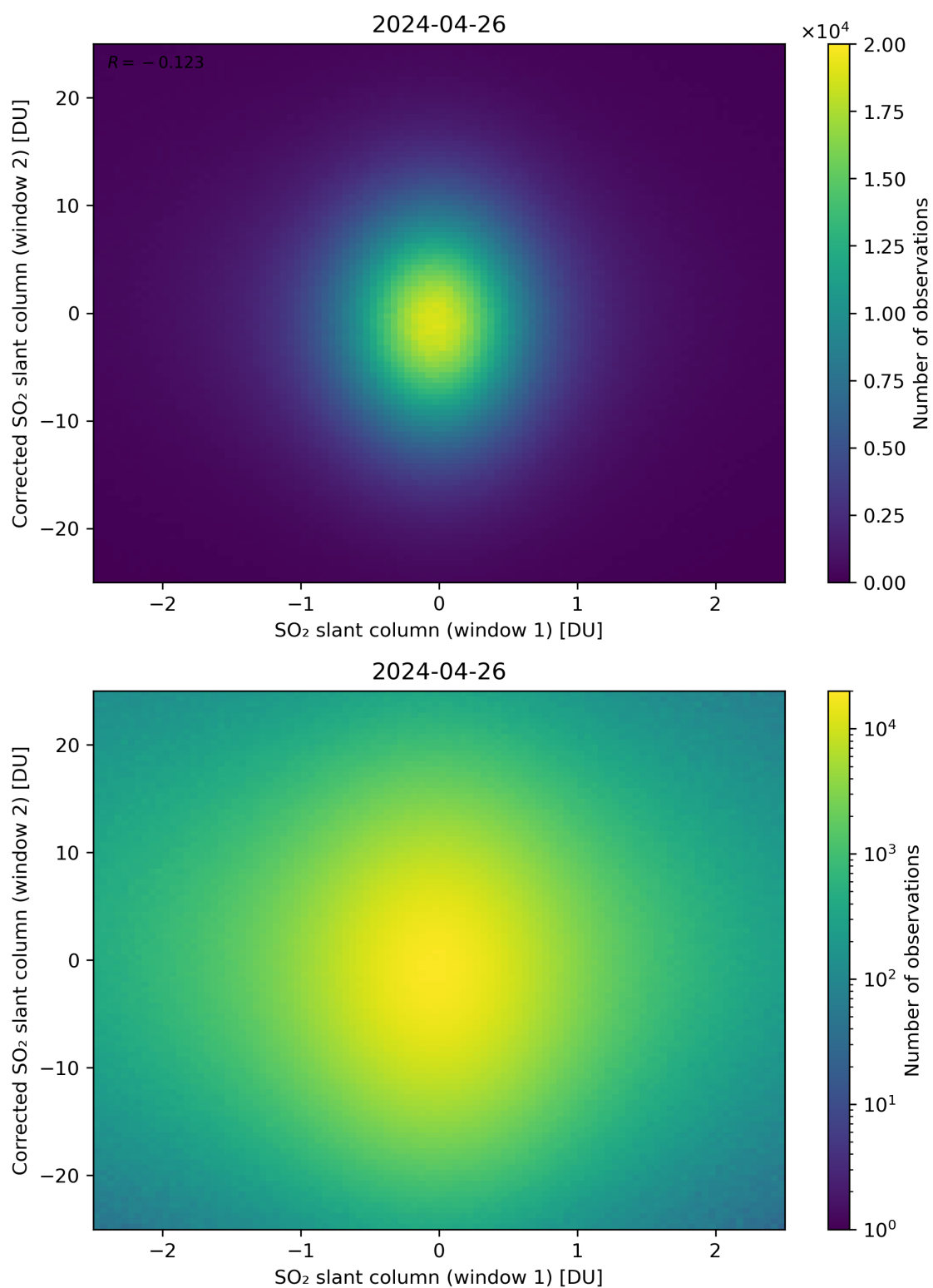
Figure 233: Scatter density plot of “SO 2 slant column (window 1)” against “Corrected SO 2 slant column (window 2)” for 2024-04-26 to 2024-04-27.
