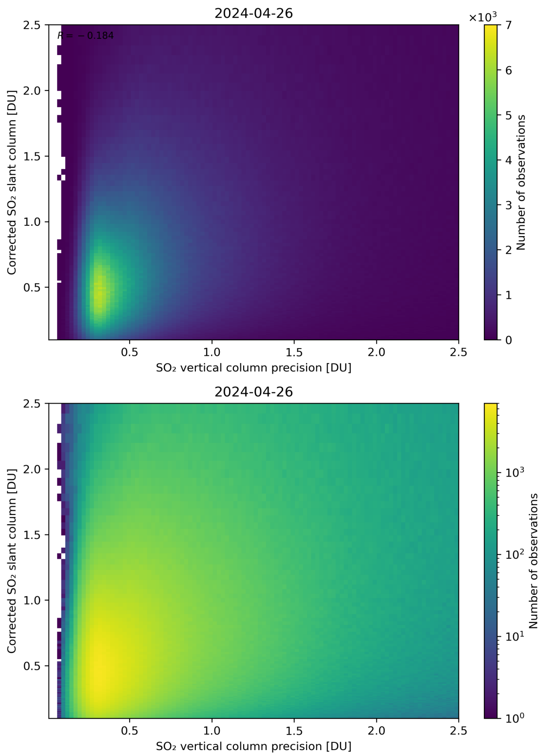
Figure 286: Scatter density plot of “SO 2 vertical column precision” against “Corrected SO 2 slant column” for 2024-04-26 to 2024-04-27.
