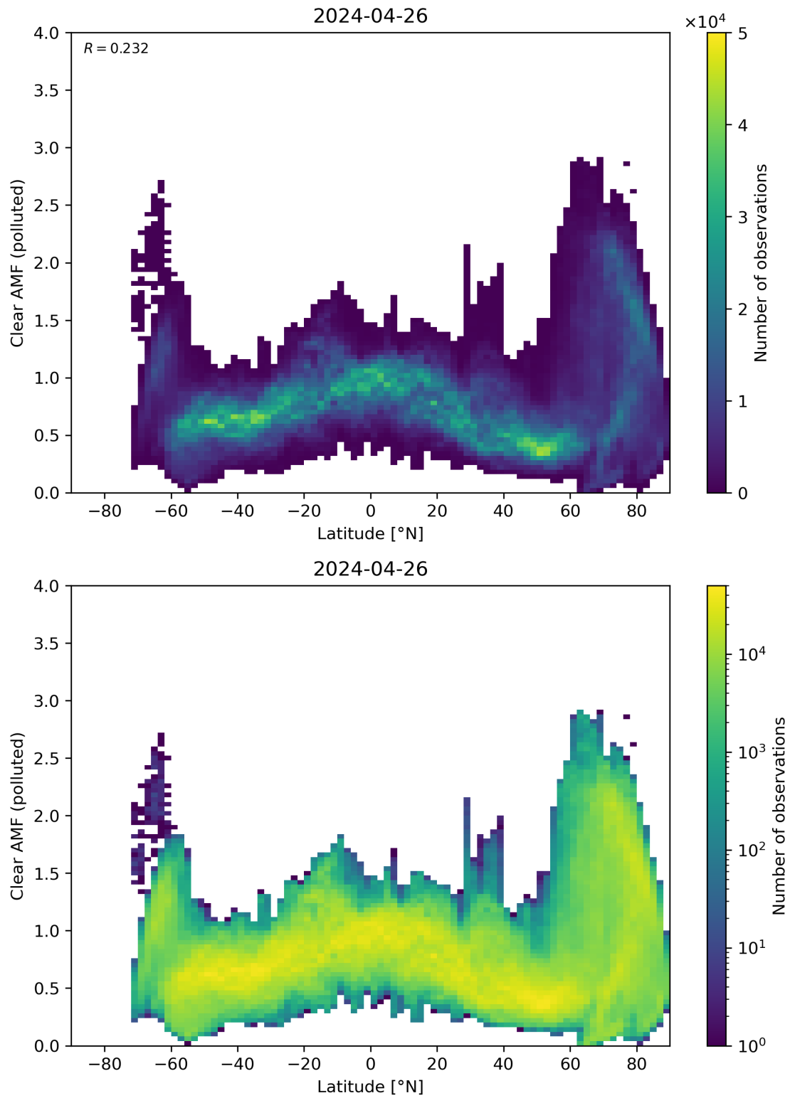
Figure 145: Scatter density plot of “Latitude” against “Clear AMF (polluted)” for 2024-04-26 to 2024-04-27.
