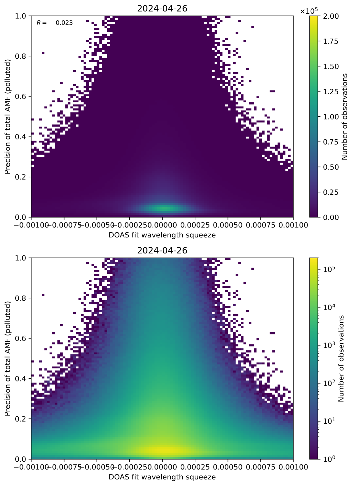
Figure 135: Scatter density plot of “DOAS fit wavelength squeeze” against “Precision of total AMF (polluted)” for 2024-04-26 to 2024-04-27.
