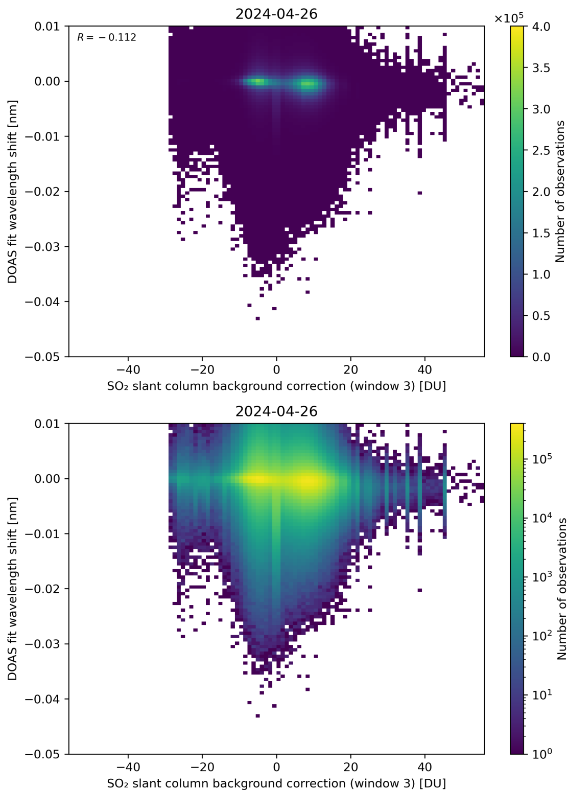
Figure 121: Scatter density plot of “SO 2 slant column background correction (window 3)” against “DOAS fit wavelength shift” for 2024-04-26 to 2024-04-27.
