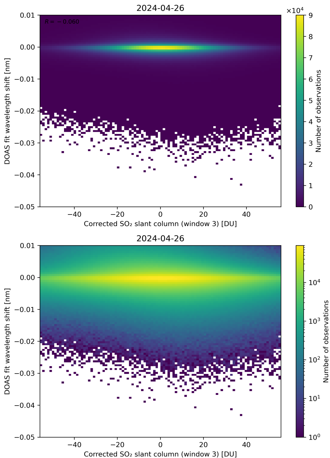
Figure 206: Scatter density plot of “Corrected SO 2 slant column (window 3)” against “DOAS fit wavelength shift” for 2024-04-26 to 2024-04-27.
