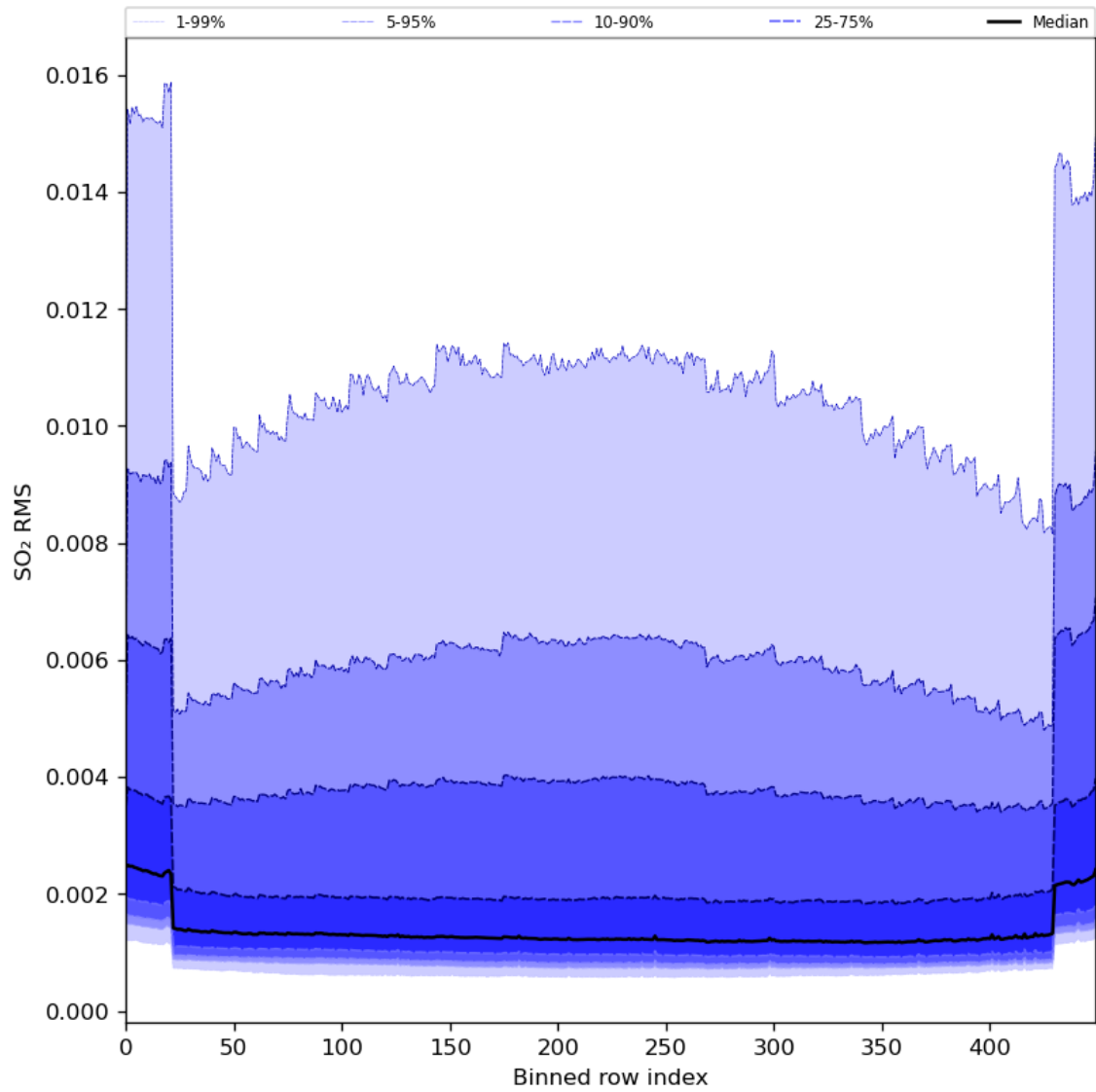
Figure 93: Along track statistics of “SO 2 RMS” for 2024-04-26 to 2024-04-27
