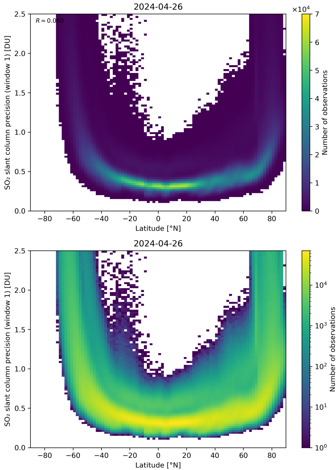
Figure 150: Scatter density plot of “Latitude” against “SO 2 slant column precision (window 1)” for 2024-04-26 to 2024-04-27.
