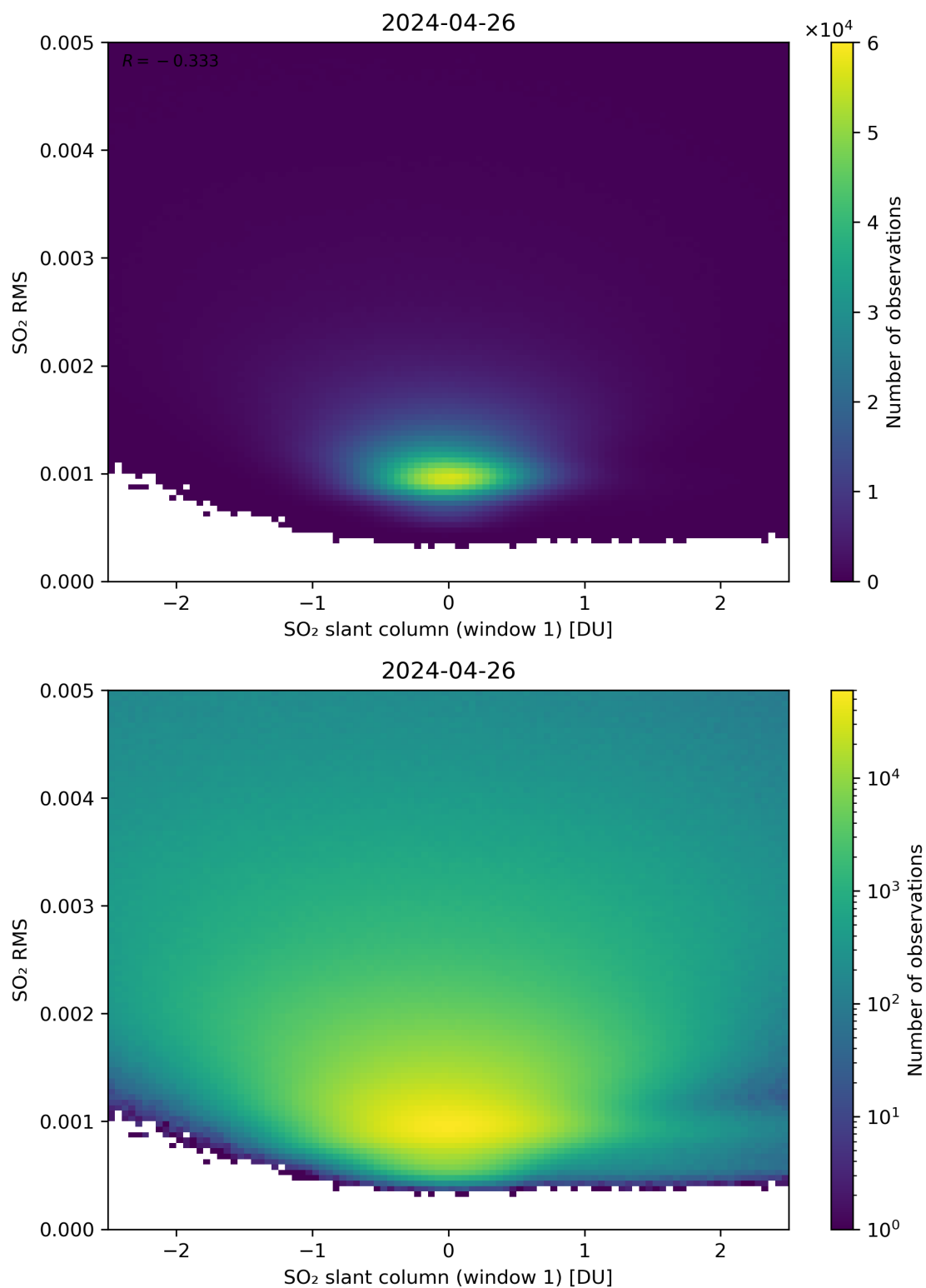
Figure 217: Scatter density plot of “SO 2 slant column (window 1)” against “SO 2 RMS” for 2024-04-26 to 2024-04-27.
