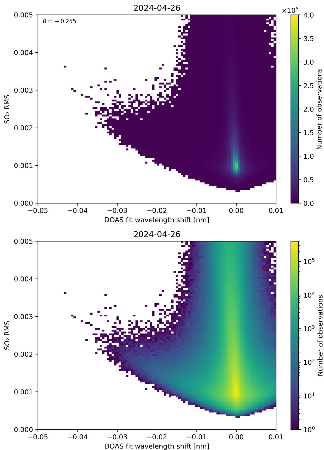
Figure 128: Scatter density plot of “DOAS fit wavelength shift” against “SO 2 RMS” for 2024-04-26 to 2024-04-27.
