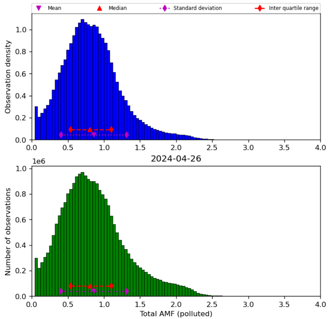
Figure 71: Histogram of “Total AMF (polluted)” for 2024-04-26 to 2024-04-27
