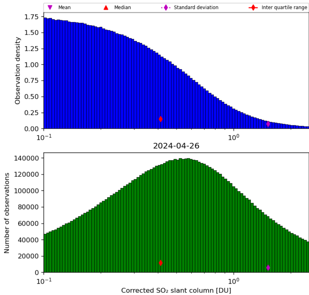
Figure 55: Histogram of “Corrected SO 2 slant column” for 2024-04-26 to 2024-04-27
