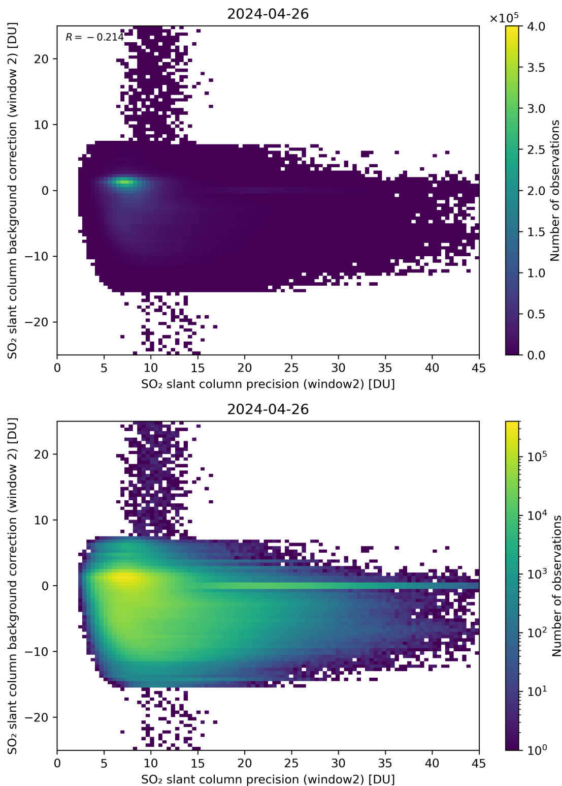
Figure 241: Scatter density plot of “SO 2 slant column precision (window2)” against “SO 2 slant column background correction (window 2)” for 2024-04-26 to 2024-04-27.
