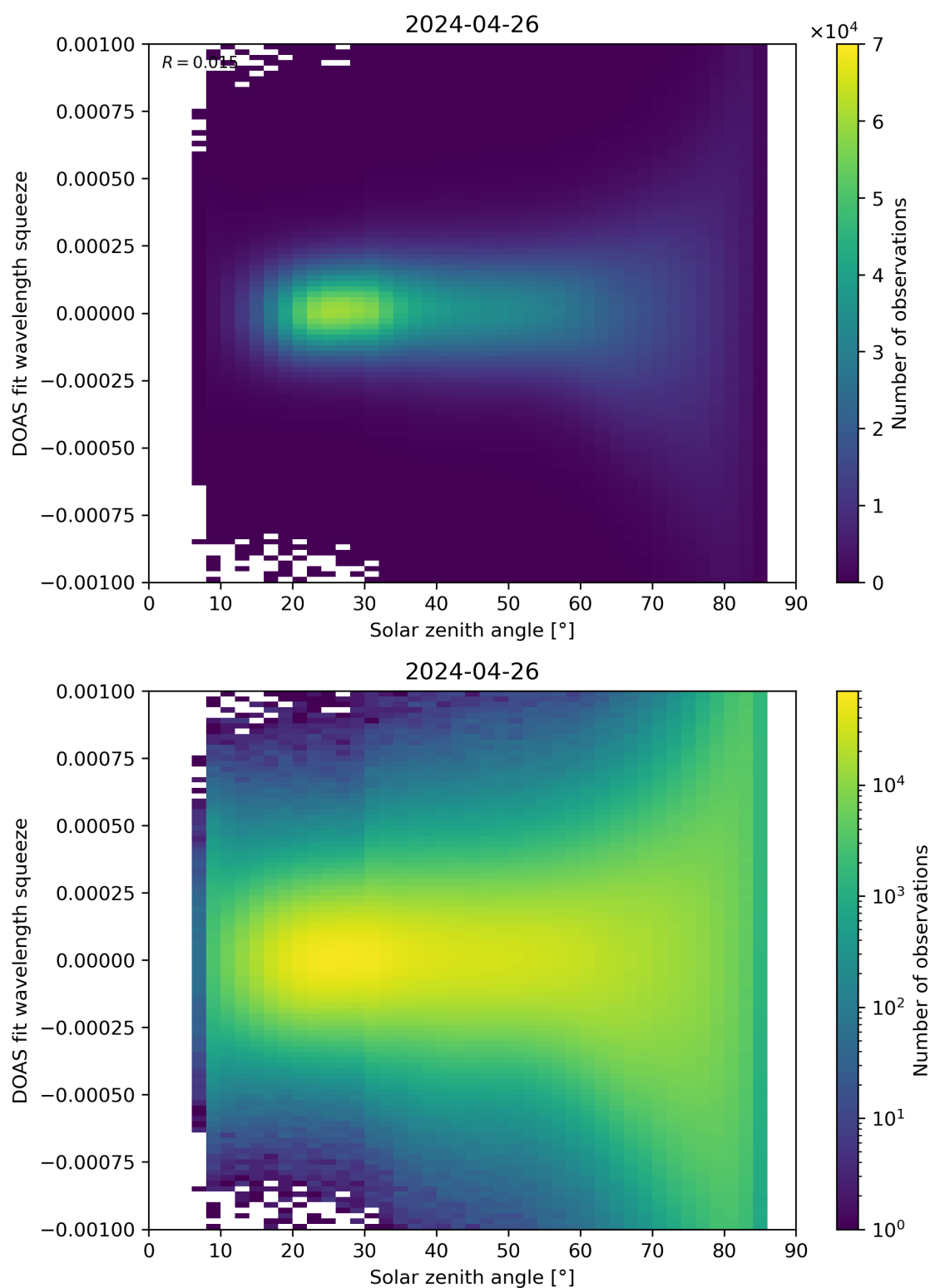
Figure 162: Scatter density plot of “Solar zenith angle” against “DOAS fit wavelength squeeze” for 2024-04-26 to 2024-04-27.
