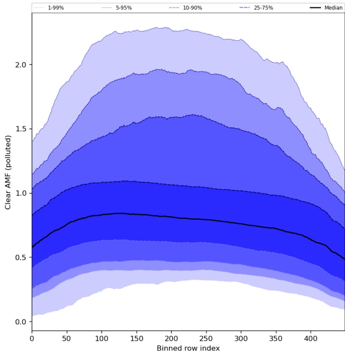
Figure 96: Along track statistics of “Clear AMF (polluted)” for 2024-04-26 to 2024-04-27
