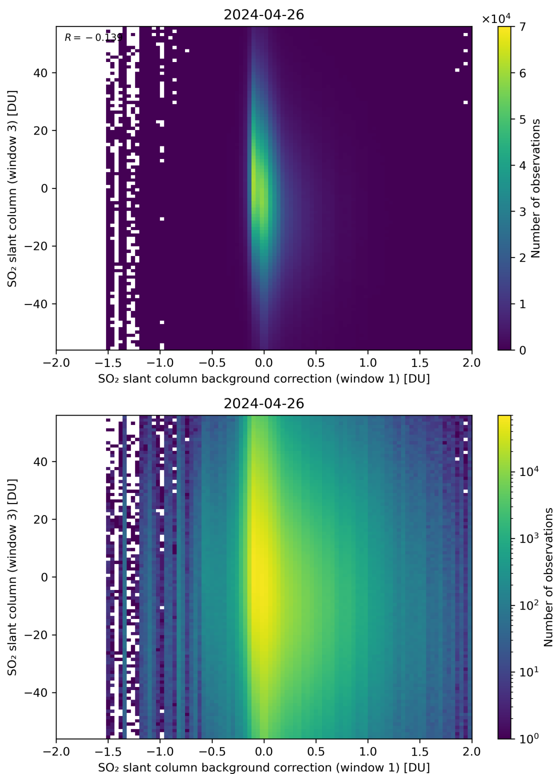
Figure 107: Scatter density plot of “SO 2 slant column background correction (window 1)” against “SO 2 slant column (window 3)” for 2024-04-26 to 2024-04-27.
