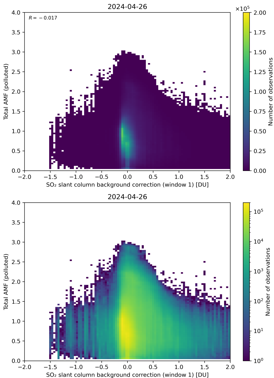
Figure 109: Scatter density plot of “SO 2 slant column background correction (window 1)” against “Total AMF (polluted)” for 2024-04-26 to 2024-04-27.
