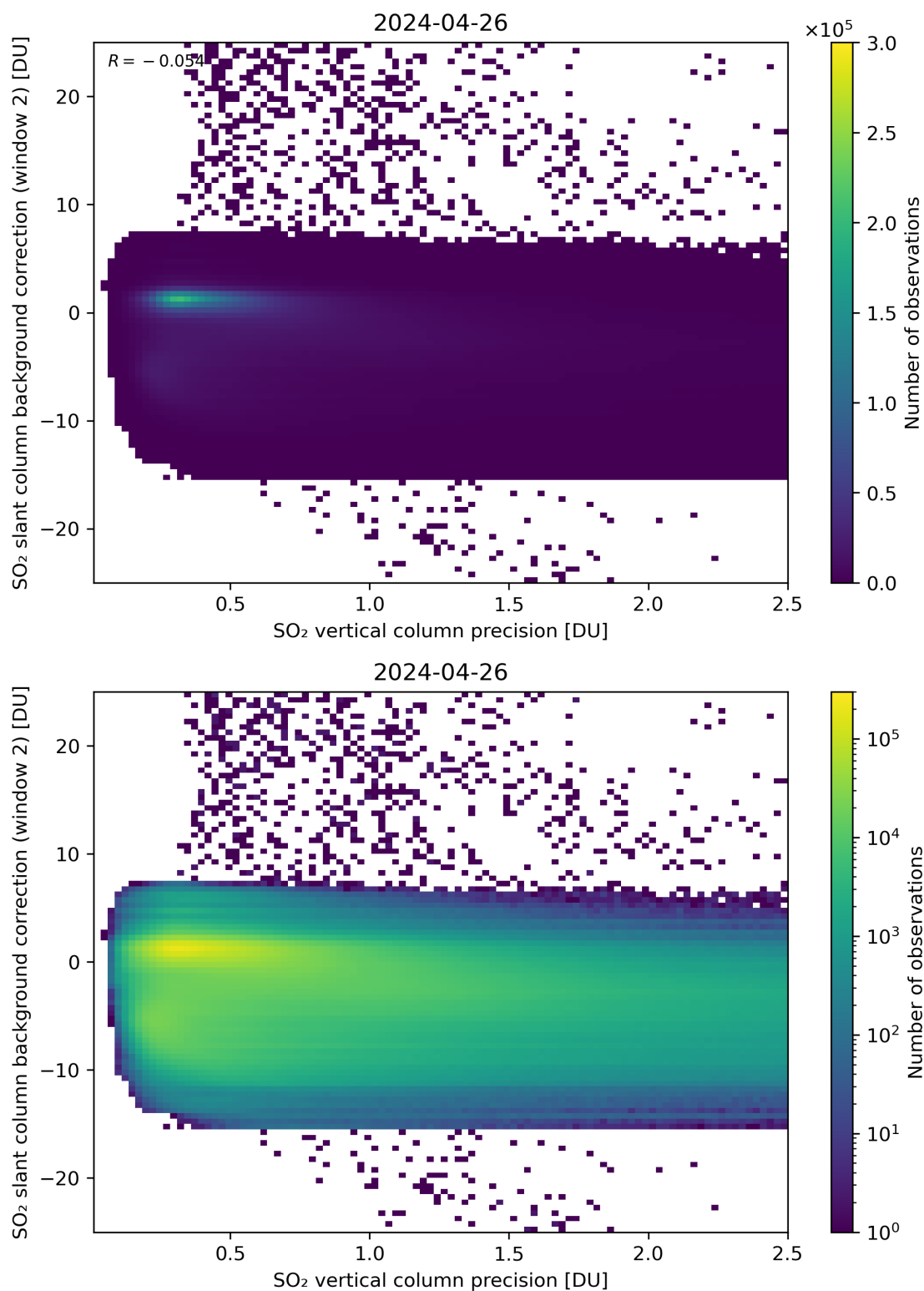
Figure 280: Scatter density plot of “SO 2 vertical column precision” against “SO 2 slant column background correction (window 2)” for 2024-04-26 to 2024-04-27.
