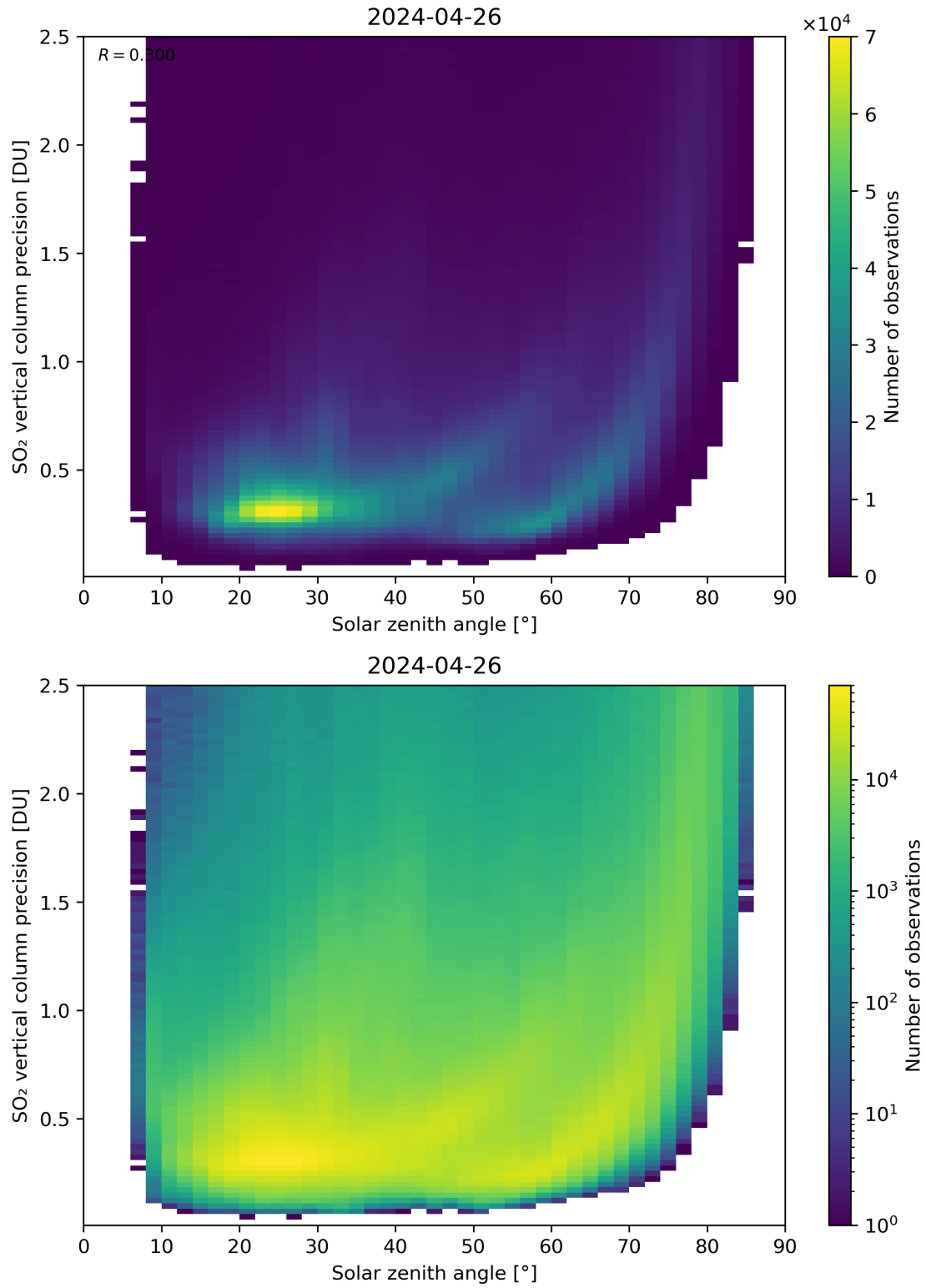
Figure 177: Scatter density plot of “Solar zenith angle” against “SO 2 vertical column precision” for 2024-04-26 to 2024-04-27.
