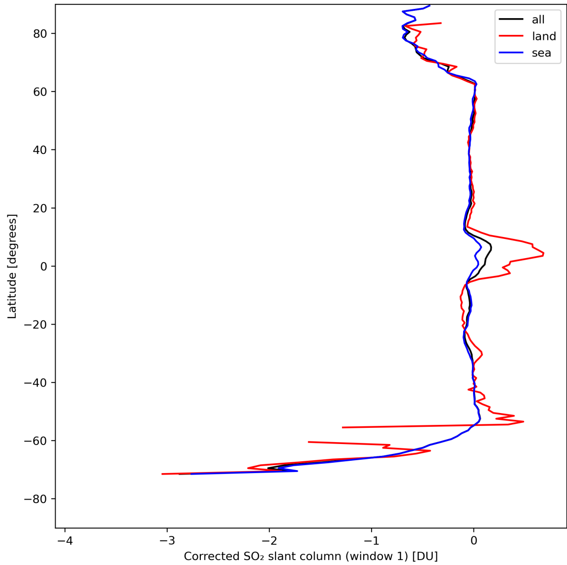
Figure 35: Zonal average of “Corrected SO 2 slant column (window 1)” for 2024-04-26 to 2024-04-27.
