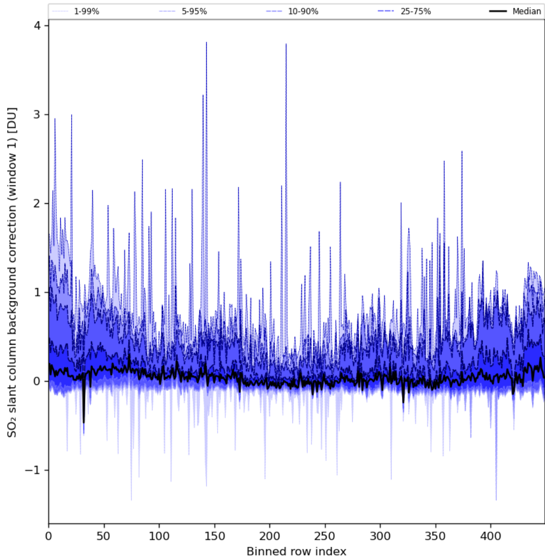
Figure 82: Along track statistics of “SO 2 slant column background correction (window 1)” for 2024-04-26 to 2024-04-27
