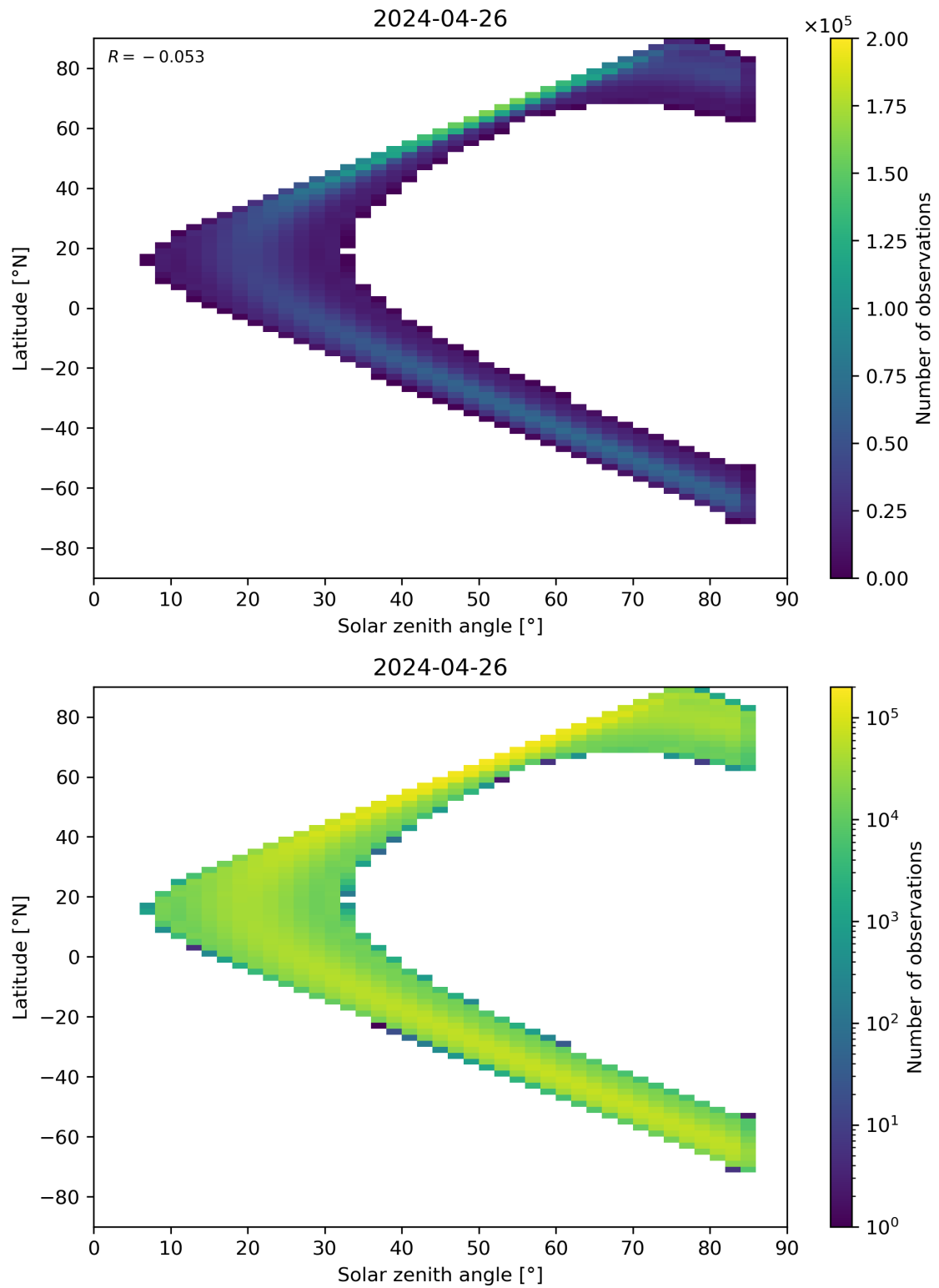
Figure 164: Scatter density plot of “Solar zenith angle” against “Latitude” for 2024-04-26 to 2024-04-27.
