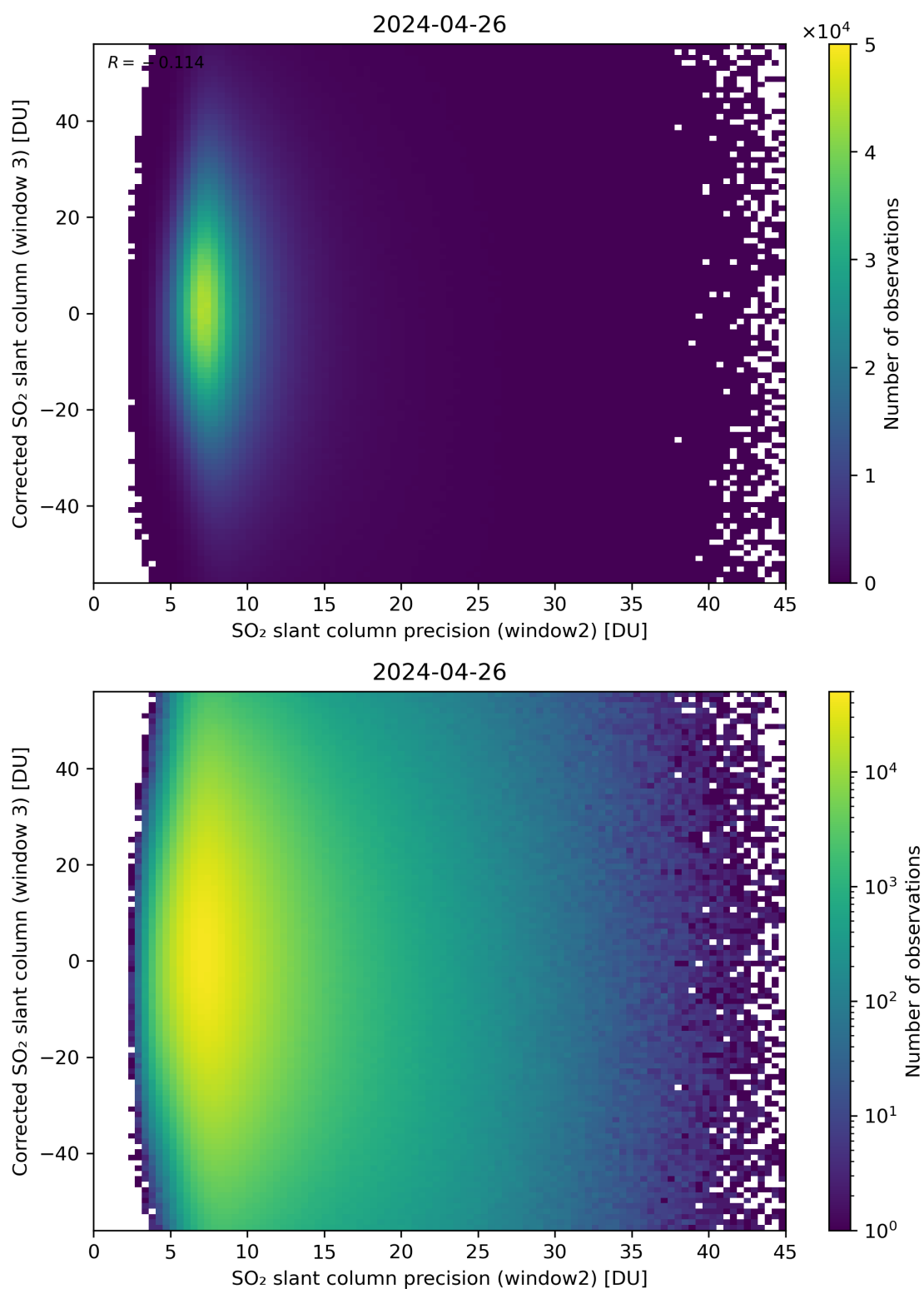
Figure 248: Scatter density plot of “SO 2 slant column precision (window2)” against “Corrected SO 2 slant column (window 3)” for 2024-04-26 to 2024-04-27.
