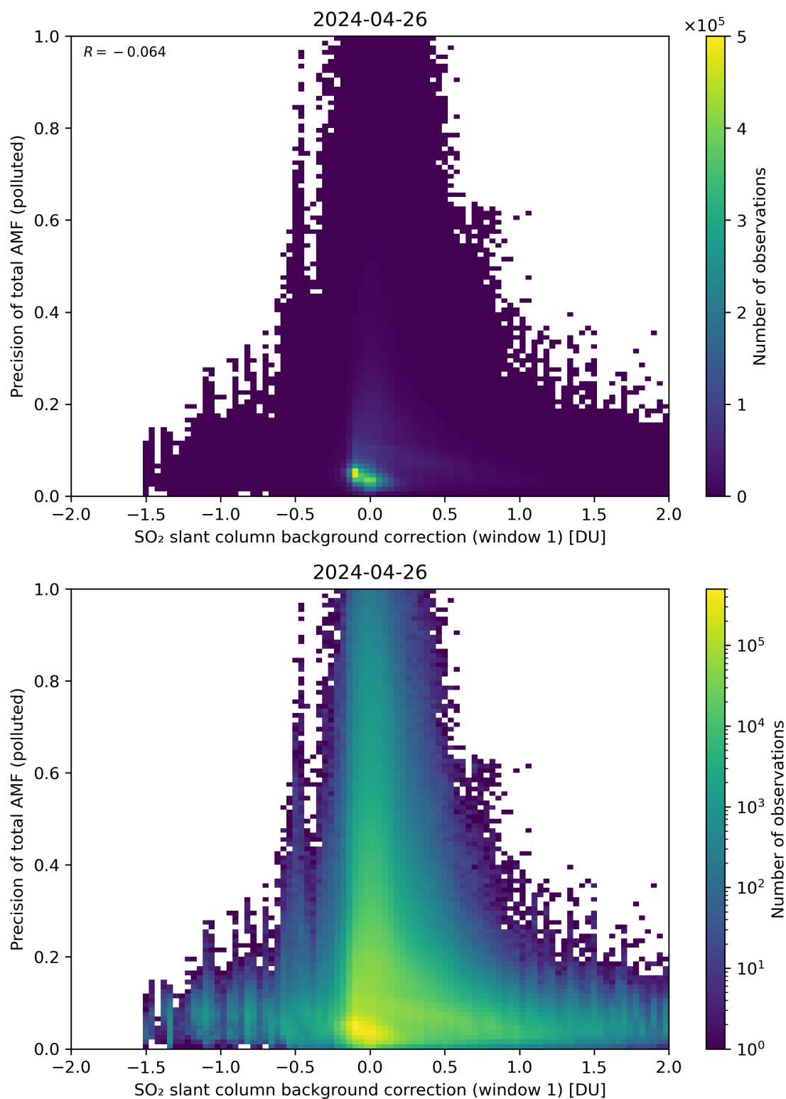
Figure 110: Scatter density plot of “SO 2 slant column background correction (window 1)” against “Precision of total AMF (polluted)” for 2024-04-26 to 2024-04-27.
