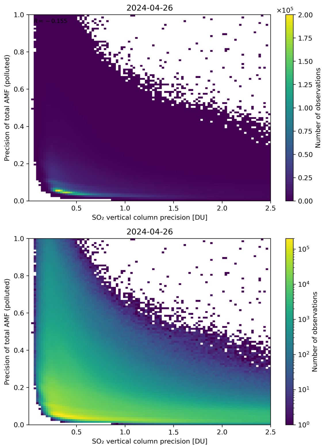
Figure 295: Scatter density plot of “SO 2 vertical column precision” against “Precision of total AMF (polluted)” for 2024-04-26 to 2024-04-27.
