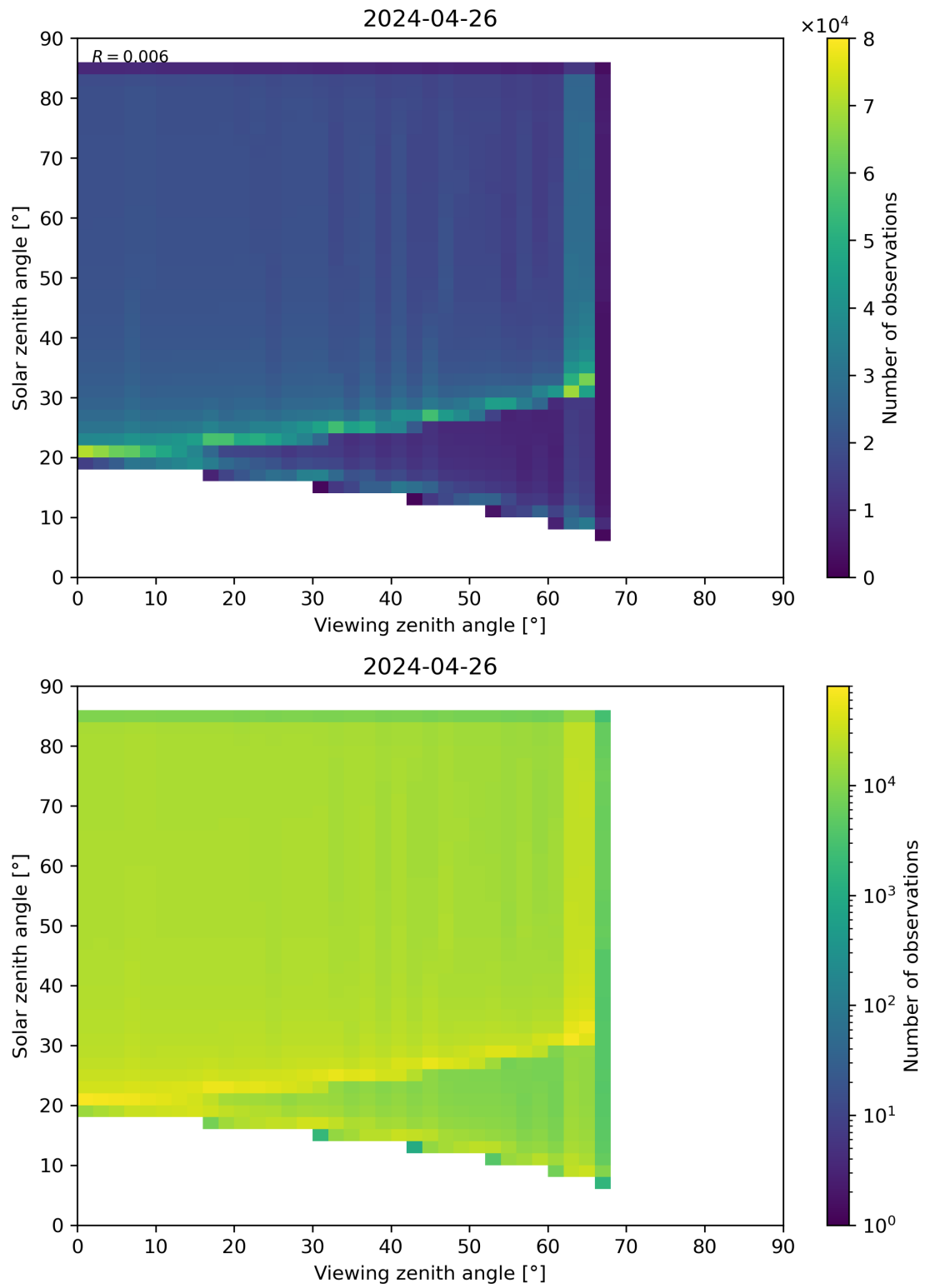
Figure 315: Scatter density plot of “Viewing zenith angle” against “Solar zenith angle” for 2024-04-26 to 2024-04-27.
