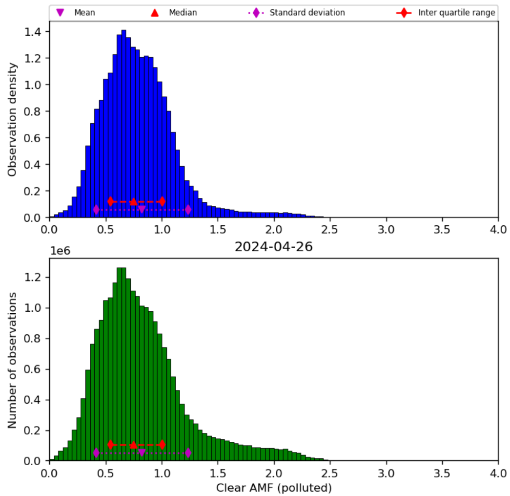
Figure 73: Histogram of “Clear AMF (polluted)” for 2024-04-26 to 2024-04-27
