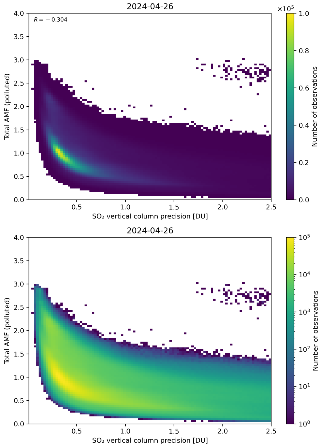
Figure 294: Scatter density plot of “SO 2 vertical column precision” against “Total AMF (polluted)” for 2024-04-26 to 2024-04-27.
