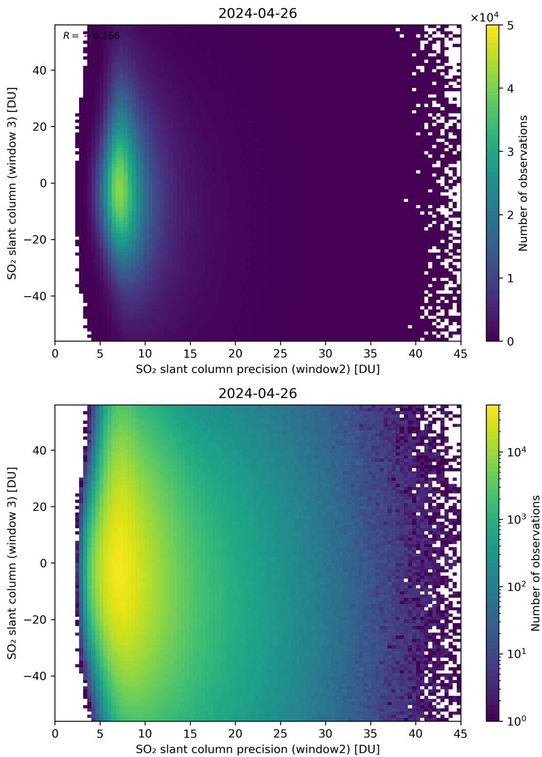
Figure 249: Scatter density plot of “SO 2 slant column precision (window2)” against “SO 2 slant column (window 3)” for 2024-04-26 to 2024-04-27.
