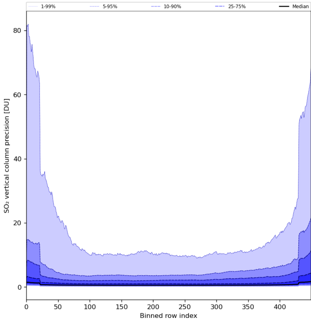
Figure 77: Along track statistics of “SO 2 vertical column precision” for 2024-04-26 to 2024-04-27
