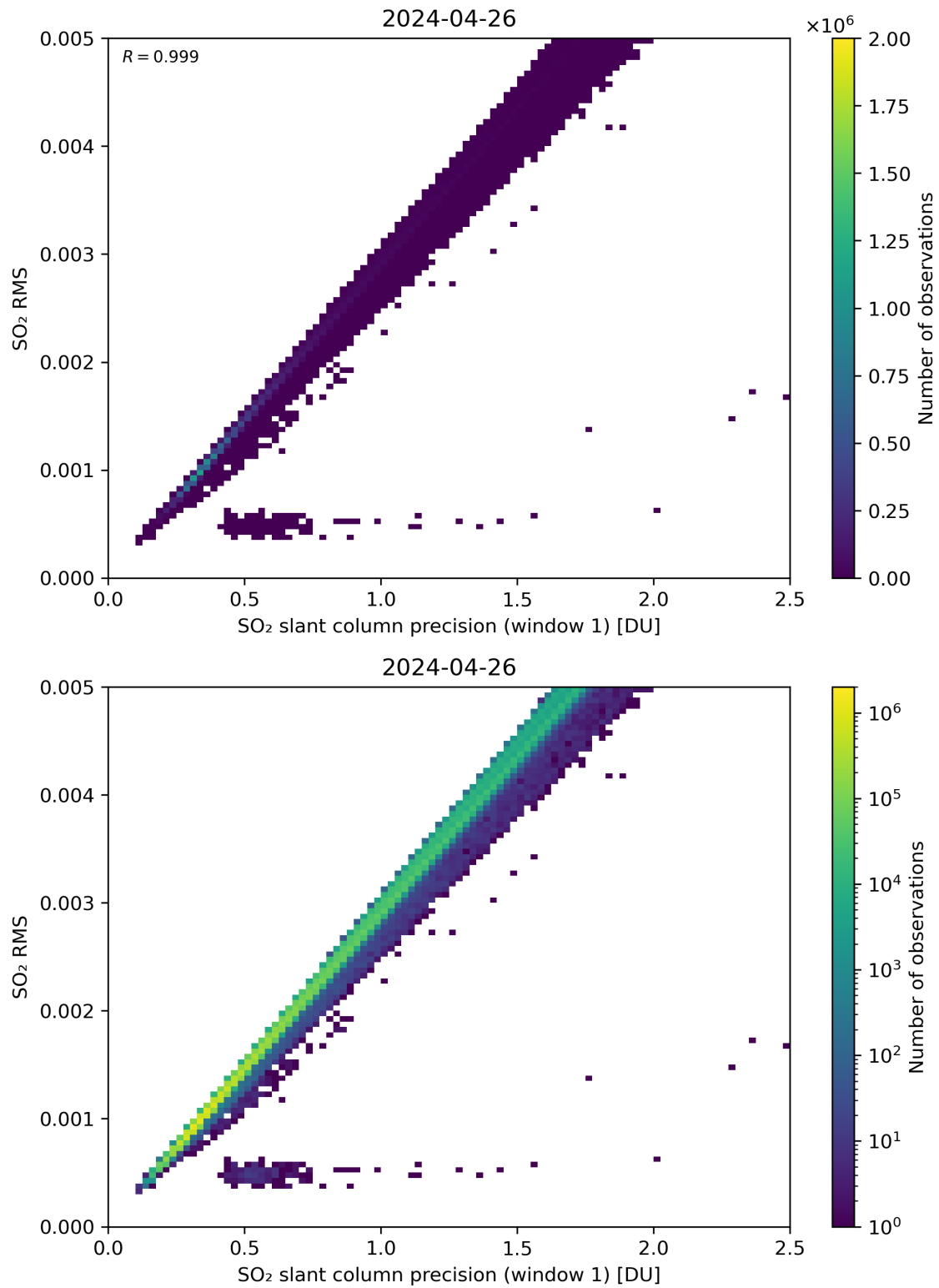
Figure 223: Scatter density plot of “SO 2 slant column precision (window 1)” against “SO 2 RMS” for 2024-04-26 to 2024-04-27.
