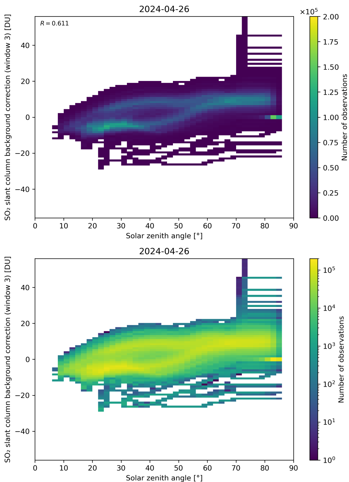
Figure 160: Scatter density plot of “Solar zenith angle” against “SO 2 slant column background correction (window 3)” for 2024-04-26 to 2024-04-27.
