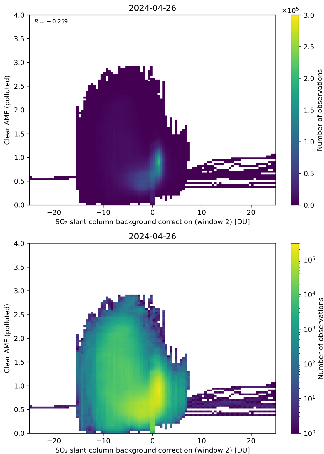
Figure 115: Scatter density plot of “SO 2 slant column background correction (window 2)” against “Clear AMF (polluted)” for 2024-04-26 to 2024-04-27.
