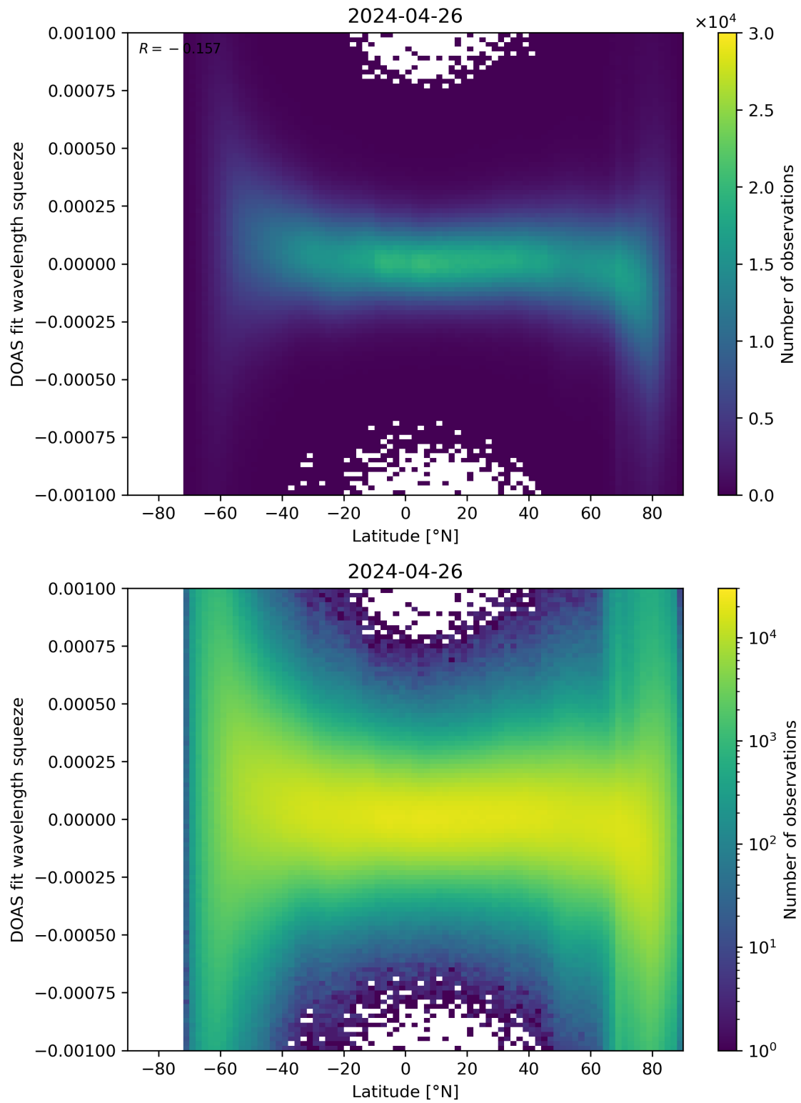
Figure 143: Scatter density plot of “Latitude” against “DOAS fit wavelength squeeze” for 2024-04-26 to 2024-04-27.
