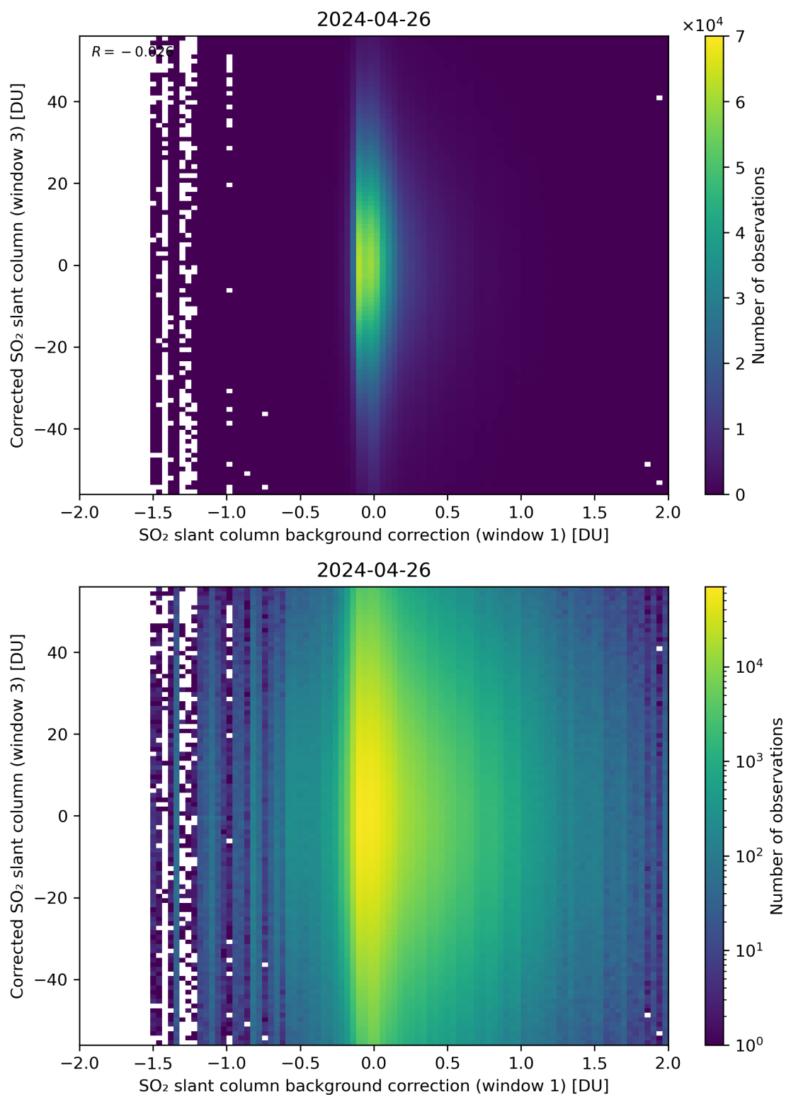
Figure 105: Scatter density plot of “SO 2 slant column background correction (window 1)” against “Corrected SO 2 slant column (window 3)” for 2024-04-26 to 2024-04-27.
