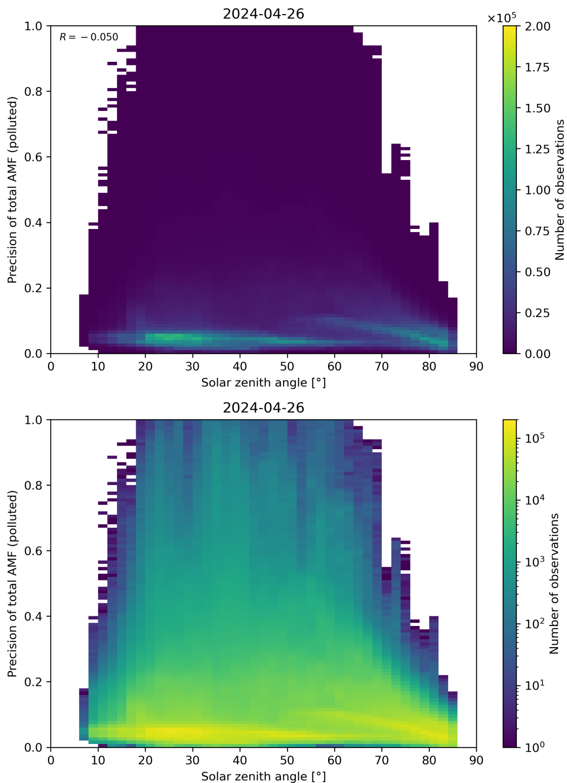
Figure 175: Scatter density plot of “Solar zenith angle” against “Precision of total AMF (polluted)” for 2024-04-26 to 2024-04-27.
