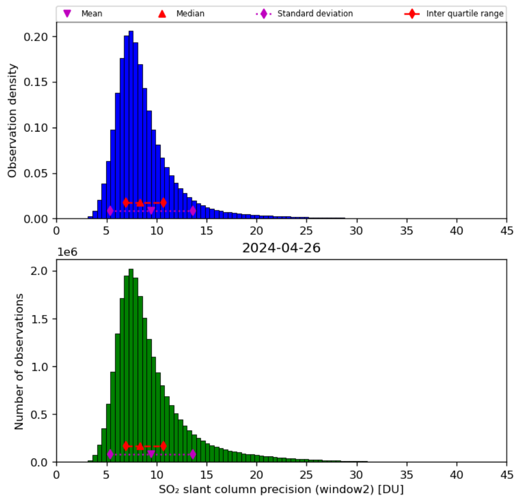
Figure 61: Histogram of “SO 2 slant column precision (window2)” for 2024-04-26 to 2024-04-27
