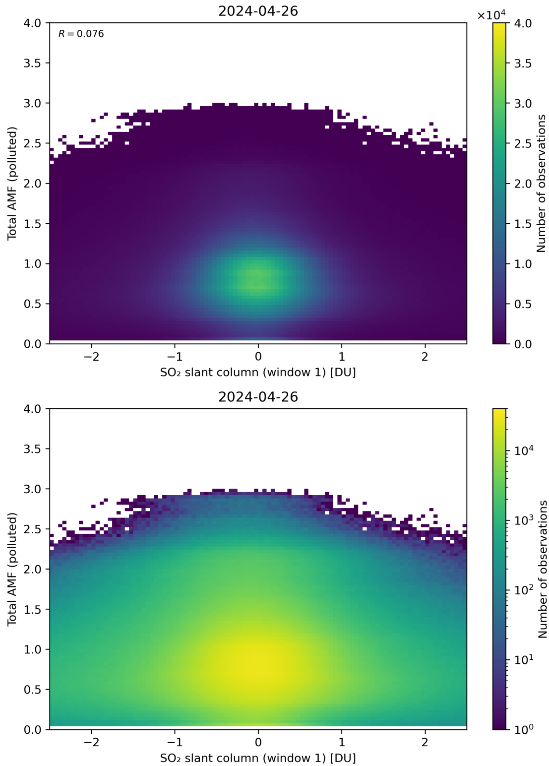
Figure 239: Scatter density plot of “SO 2 slant column (window 1)” against “Total AMF (polluted)” for 2024-04-26 to 2024-04-27.
