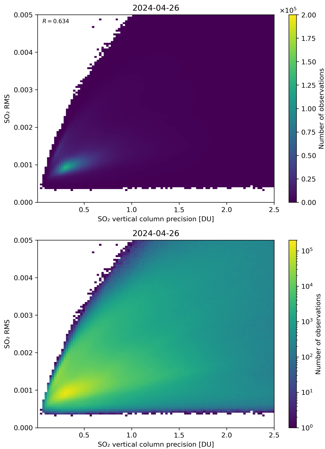
Figure 284: Scatter density plot of “SO 2 vertical column precision” against “SO 2 RMS” for 2024-04-26 to 2024-04-27.
