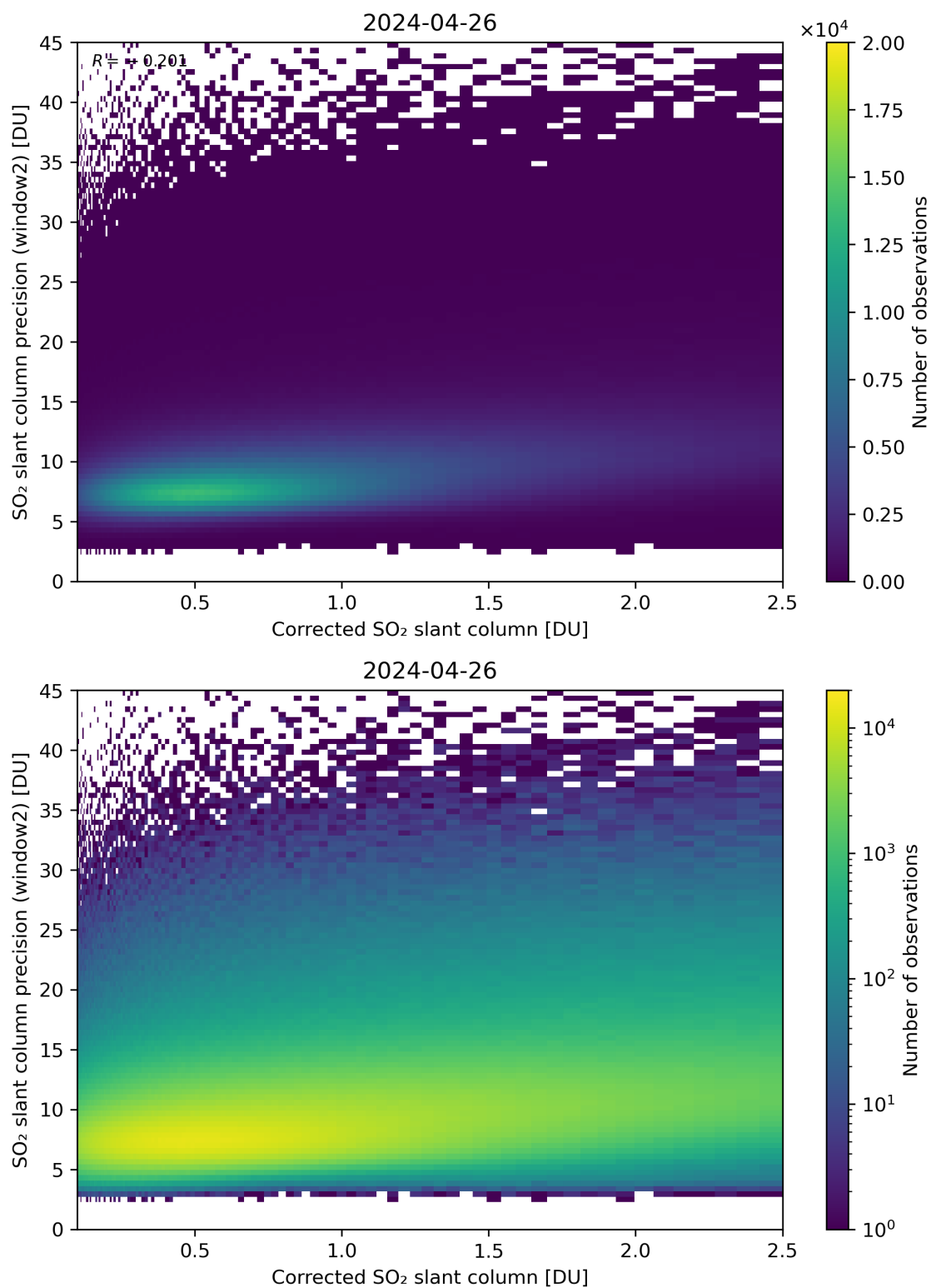
Figure 189: Scatter density plot of “Corrected SO 2 slant column” against “SO 2 slant column precision (window2)” for 2024-04-26 to 2024-04-27.
