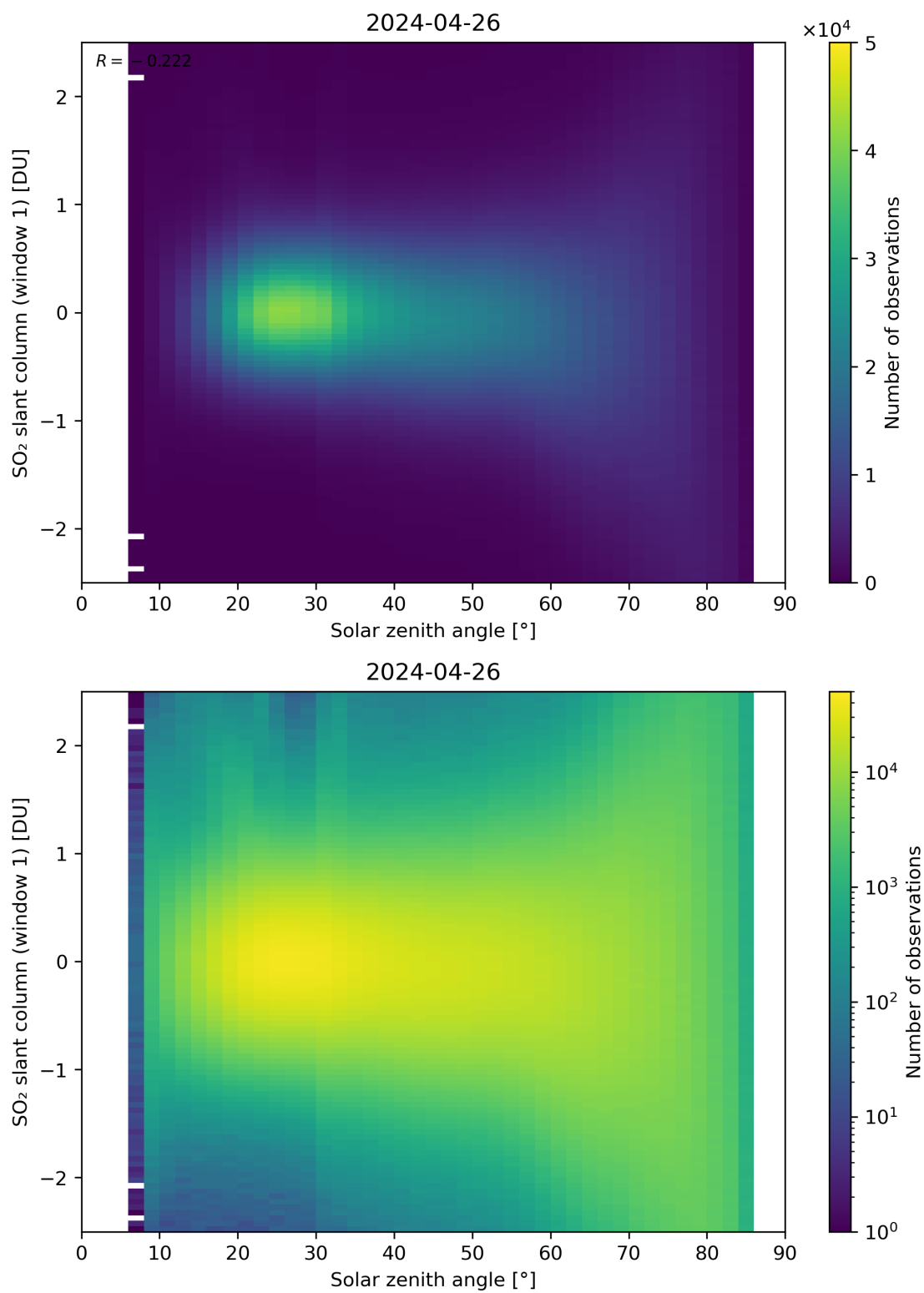
Figure 169: Scatter density plot of “Solar zenith angle” against “SO 2 slant column (window 1)” for 2024-04-26 to 2024-04-27.
