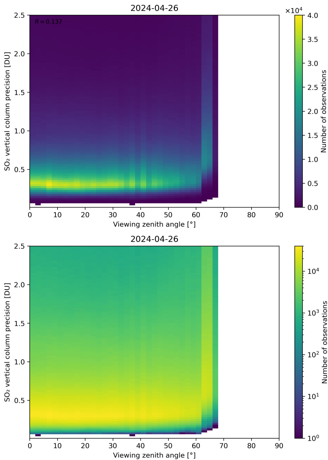
Figure 328: Scatter density plot of “Viewing zenith angle” against “SO 2 vertical column precision” for 2024-04-26 to 2024-04-27.
