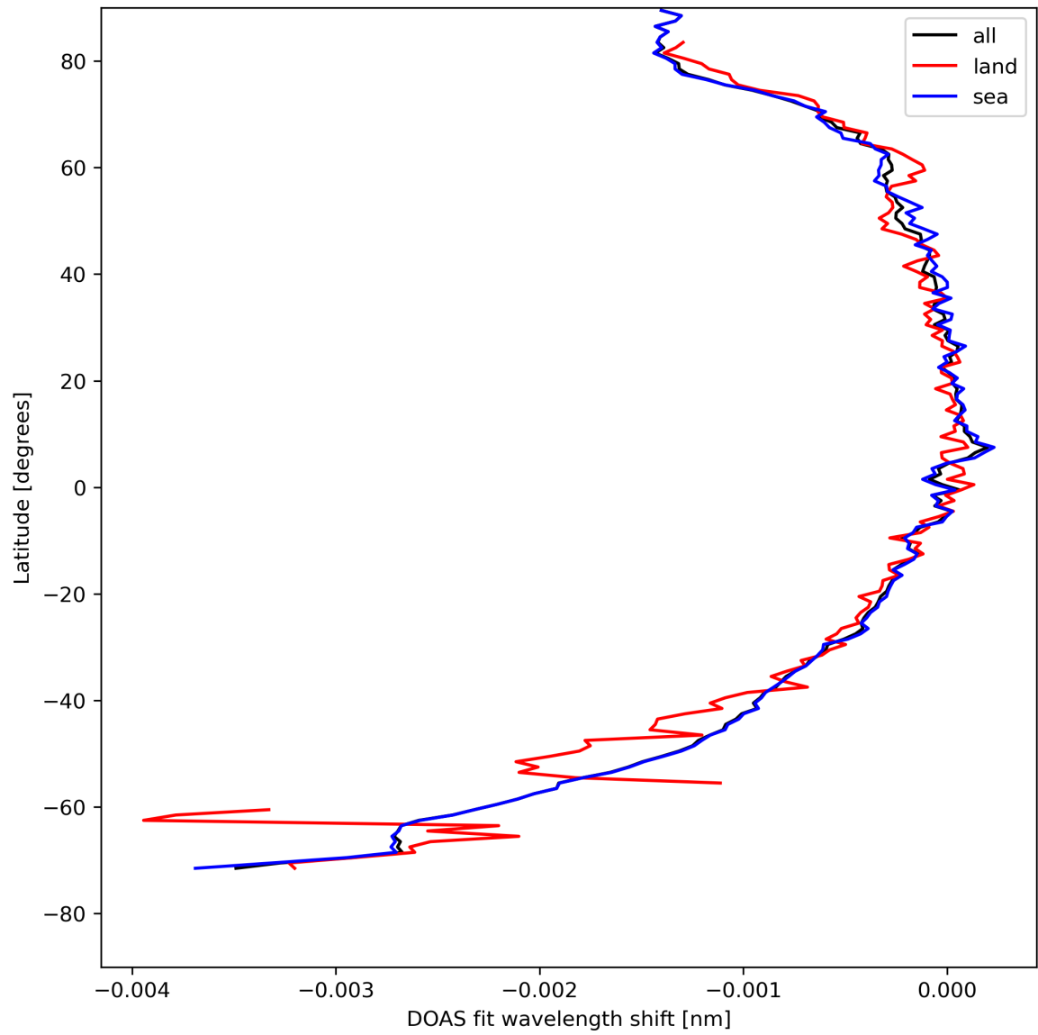
Figure 45: Zonal average of “DOAS fit wavelength shift” for 2024-04-26 to 2024-04-27.
