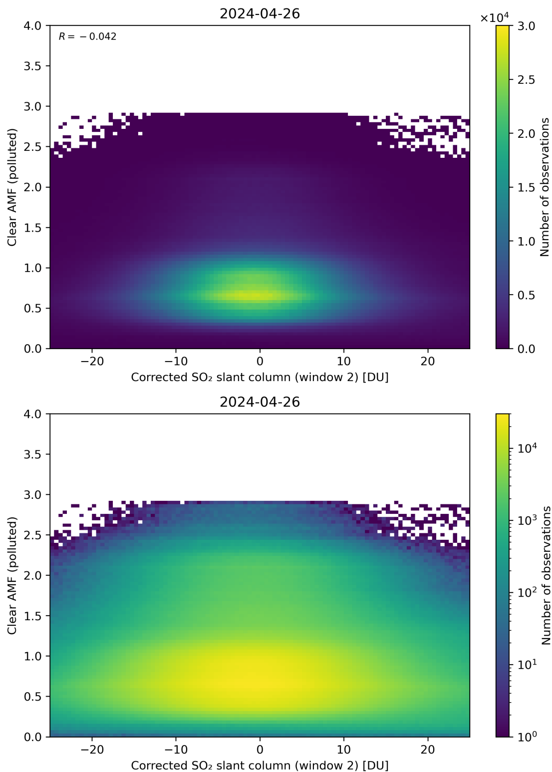
Figure 199: Scatter density plot of “Corrected SO 2 slant column (window 2)” against “Clear AMF (polluted)” for 2024-04-26 to 2024-04-27.
