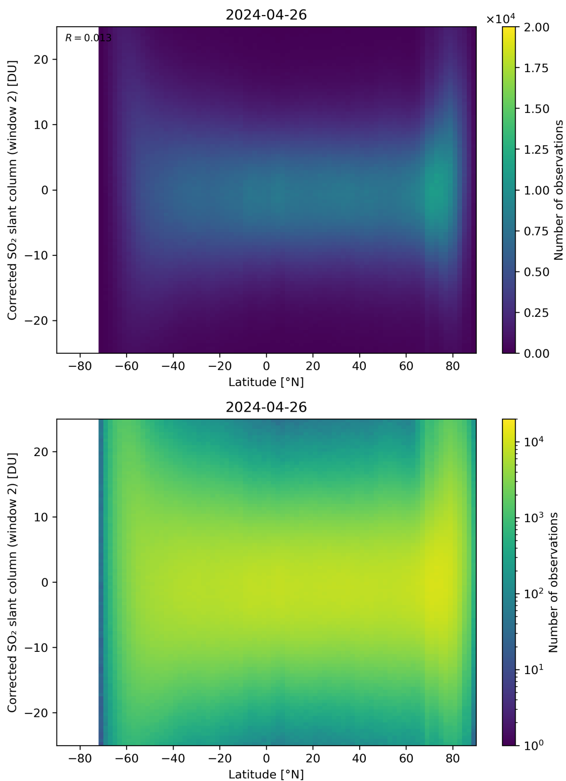
Figure 147: Scatter density plot of “Latitude” against “Corrected SO 2 slant column (window 2)” for 2024-04-26 to 2024-04-27.
