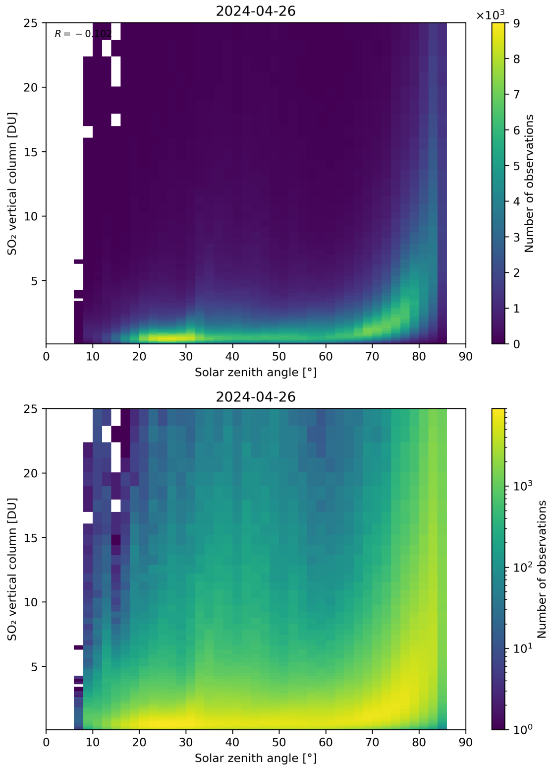
Figure 176: Scatter density plot of “Solar zenith angle” against “SO 2 vertical column” for 2024-04-26 to 2024-04-27.
