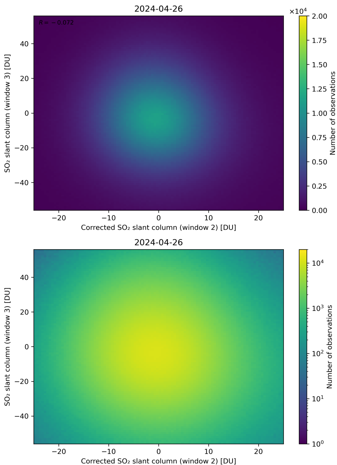
Figure 201: Scatter density plot of “Corrected SO 2 slant column (window 2)” against “SO 2 slant column (window 3)” for 2024-04-26 to 2024-04-27.
