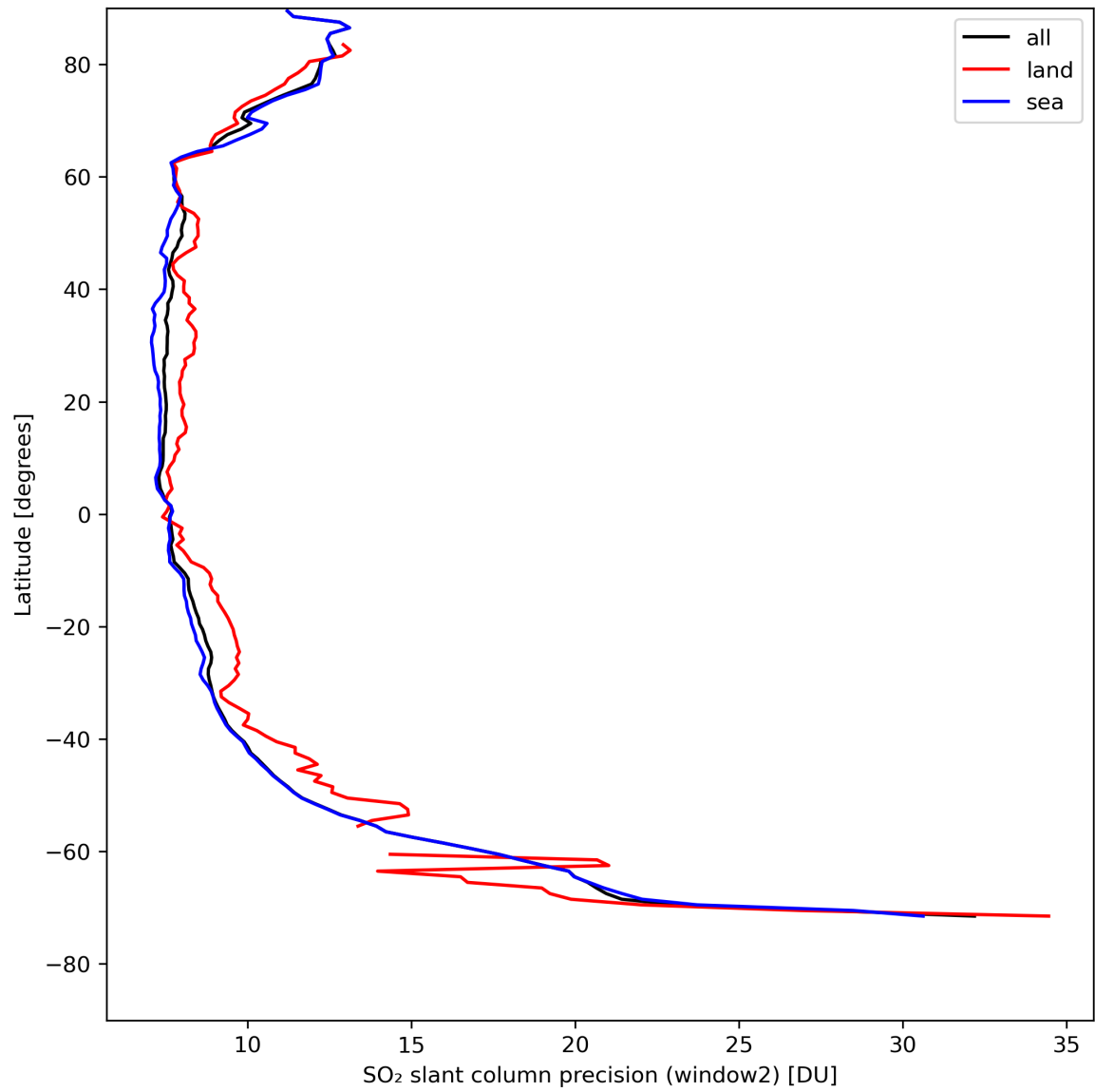
Figure 38: Zonal average of “SO 2 slant column precision (window2)” for 2024-04-26 to 2024-04-27.
