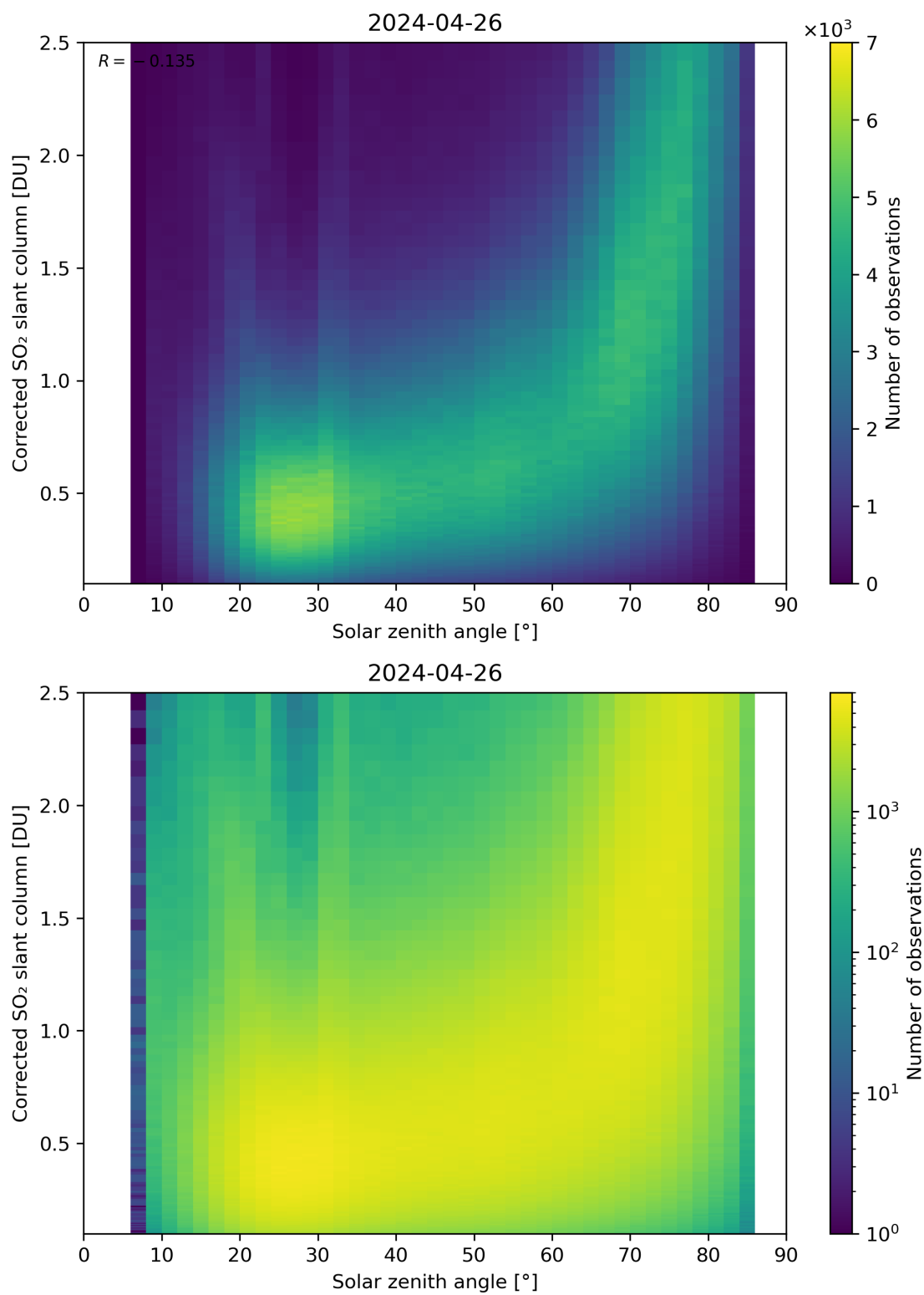
Figure 166: Scatter density plot of “Solar zenith angle” against “Corrected SO 2 slant column” for 2024-04-26 to 2024-04-27.
