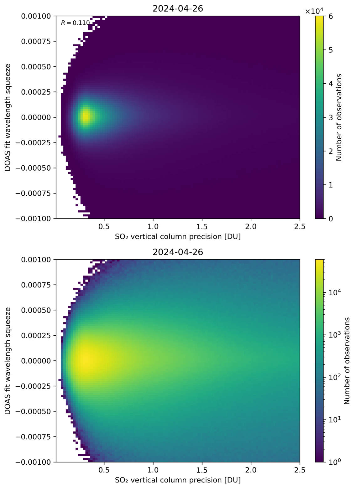
Figure 283: Scatter density plot of “SO 2 vertical column precision” against “DOAS fit wavelength squeeze” for 2024-04-26 to 2024-04-27.
