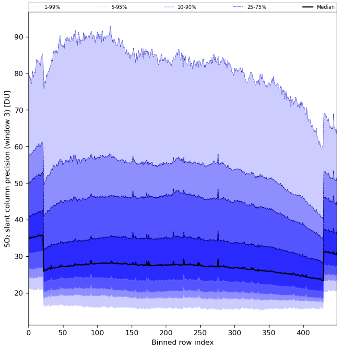
Figure 88: Along track statistics of “SO 2 slant column precision (window 3)” for 2024-04-26 to 2024-04-27
