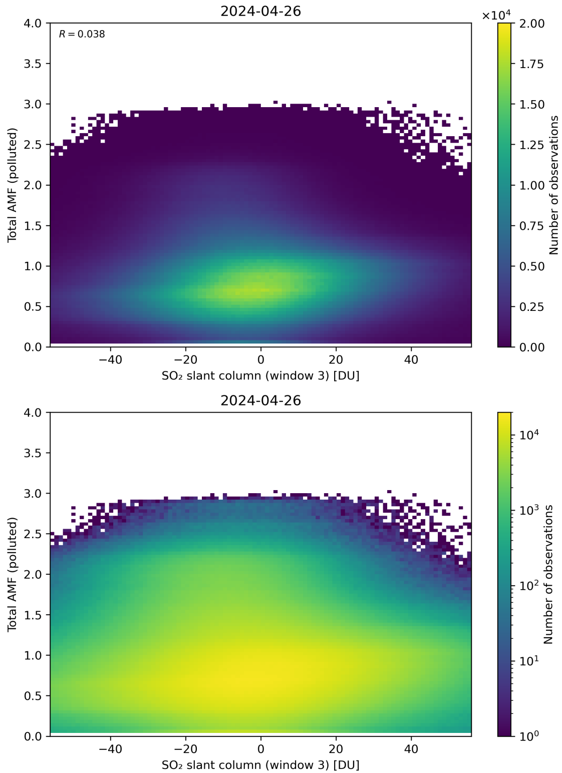
Figure 268: Scatter density plot of “SO 2 slant column (window 3)” against “Total AMF (polluted)” for 2024-04-26 to 2024-04-27.
