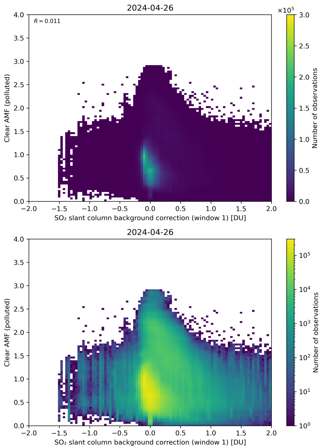
Figure 103: Scatter density plot of “SO 2 slant column background correction (window 1)” against “Clear AMF (polluted)” for 2024-04-26 to 2024-04-27.
