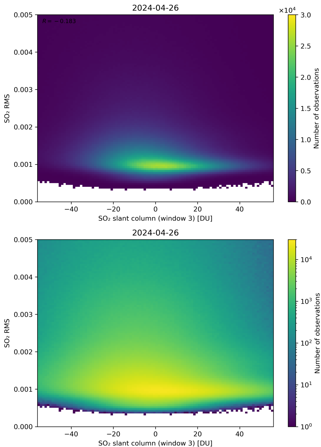
Figure 256: Scatter density plot of “SO 2 slant column (window 3)” against “SO 2 RMS” for 2024-04-26 to 2024-04-27.
