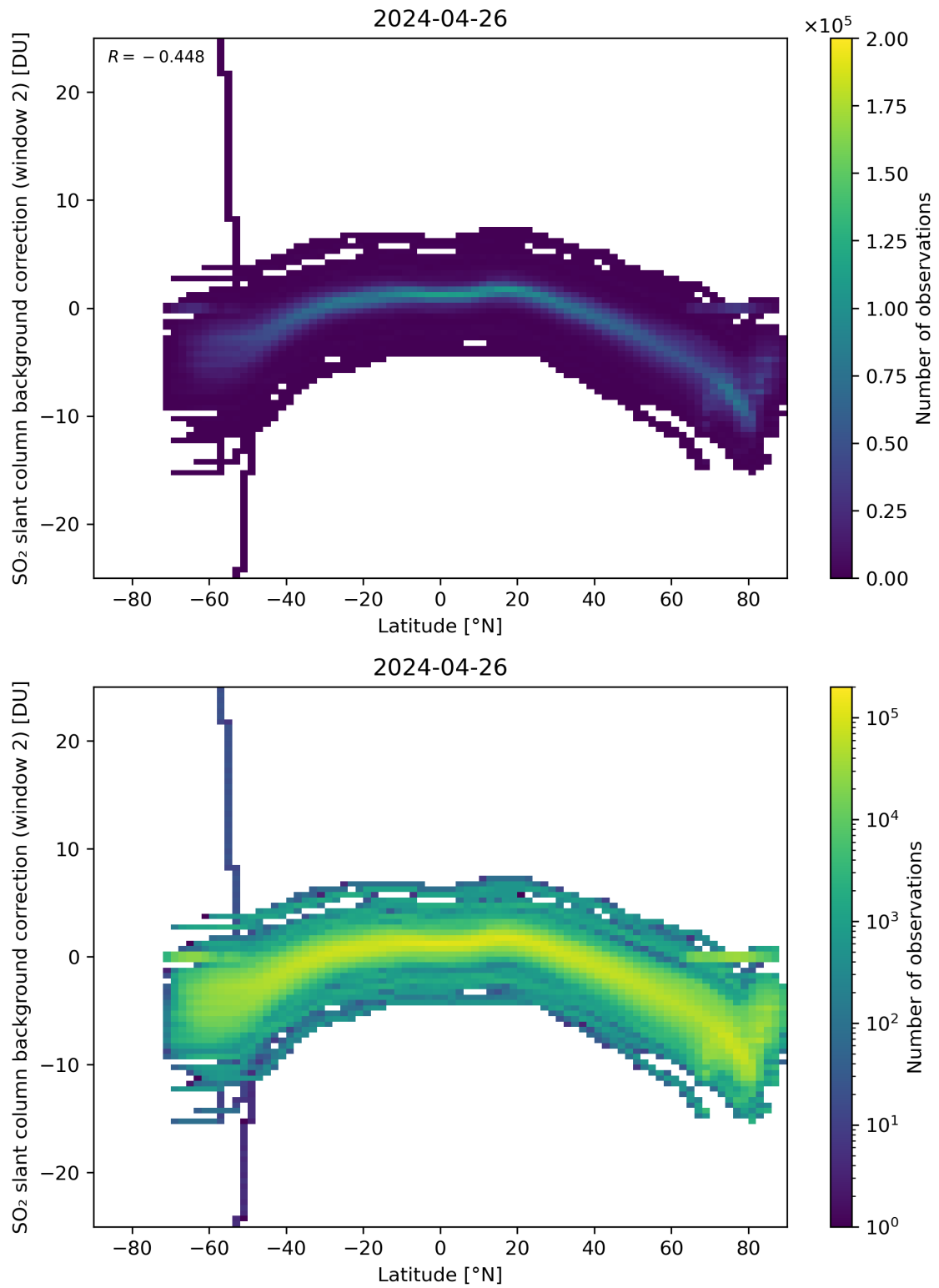
Figure 140: Scatter density plot of “Latitude” against “SO 2 slant column background correction (window 2)” for 2024-04-26 to 2024-04-27.
