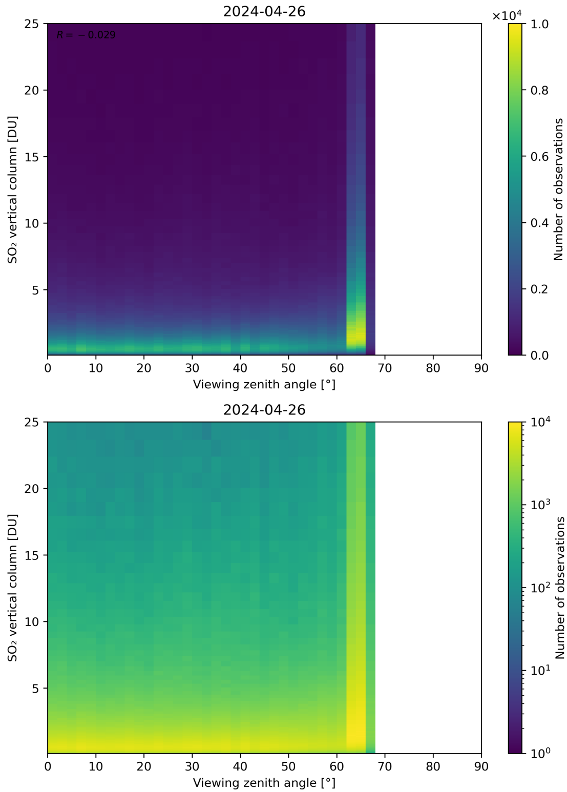
Figure 327: Scatter density plot of “Viewing zenith angle” against “SO 2 vertical column” for 2024-04-26 to 2024-04-27.
