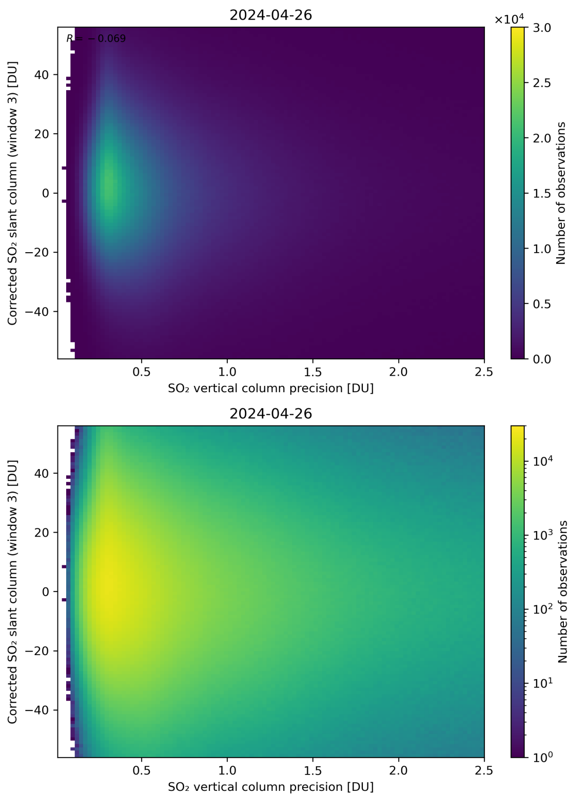
Figure 288: Scatter density plot of “SO 2 vertical column precision” against “Corrected SO 2 slant column (window 3)” for 2024-04-26 to 2024-04-27.
