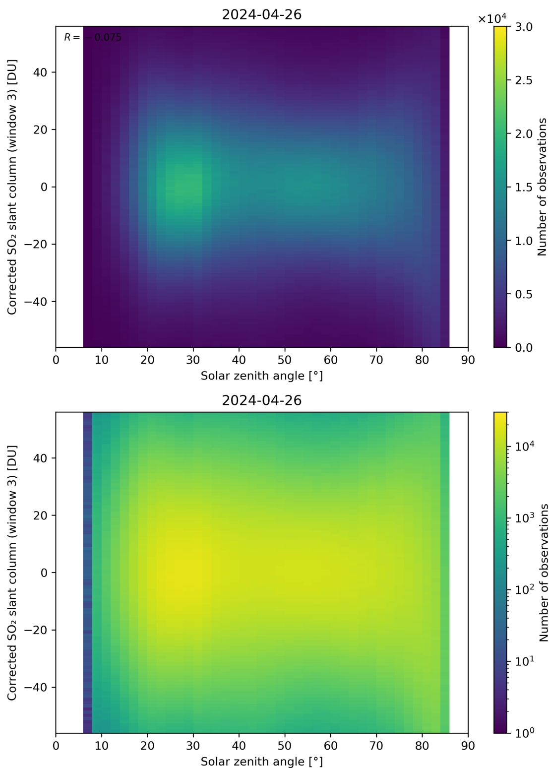
Figure 168: Scatter density plot of “Solar zenith angle” against “Corrected SO 2 slant column (window 3)” for 2024-04-26 to 2024-04-27.
