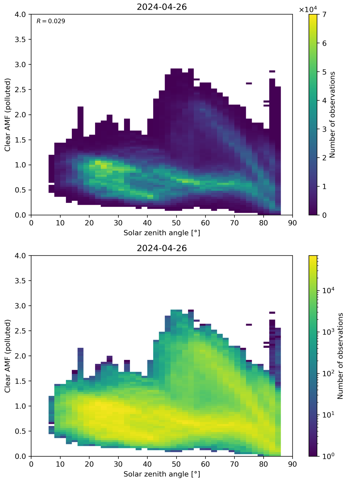
Figure 165: Scatter density plot of “Solar zenith angle” against “Clear AMF (polluted)” for 2024-04-26 to 2024-04-27.
