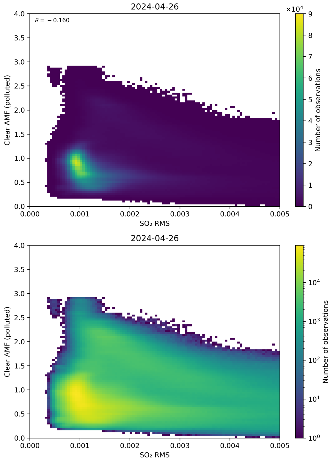
Figure 136: Scatter density plot of “SO 2 RMS” against “Clear AMF (polluted)” for 2024-04-26 to 2024-04-27.
