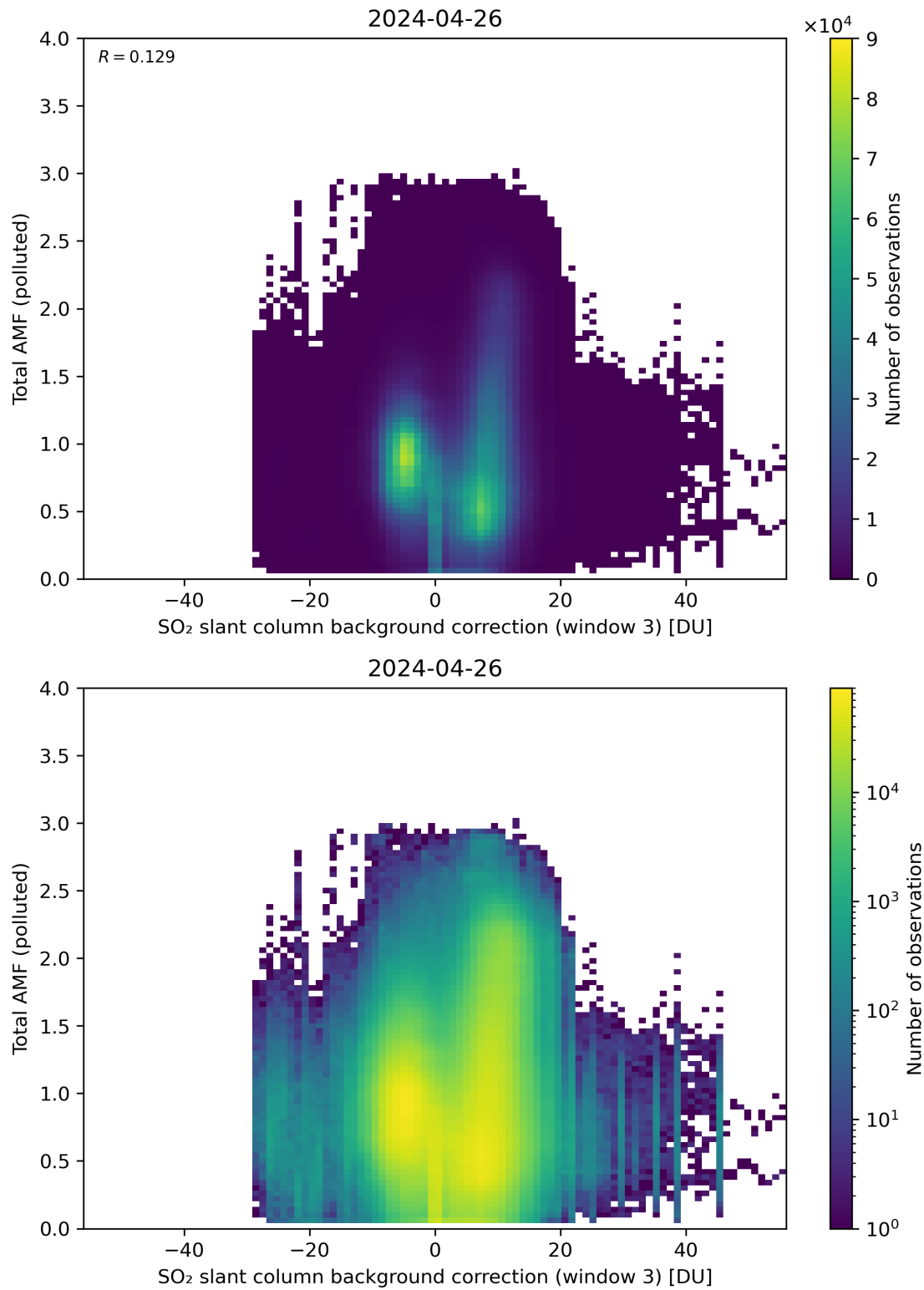
Figure 125: Scatter density plot of “SO 2 slant column background correction (window 3)” against “Total AMF (polluted)” for 2024-04-26 to 2024-04-27.
