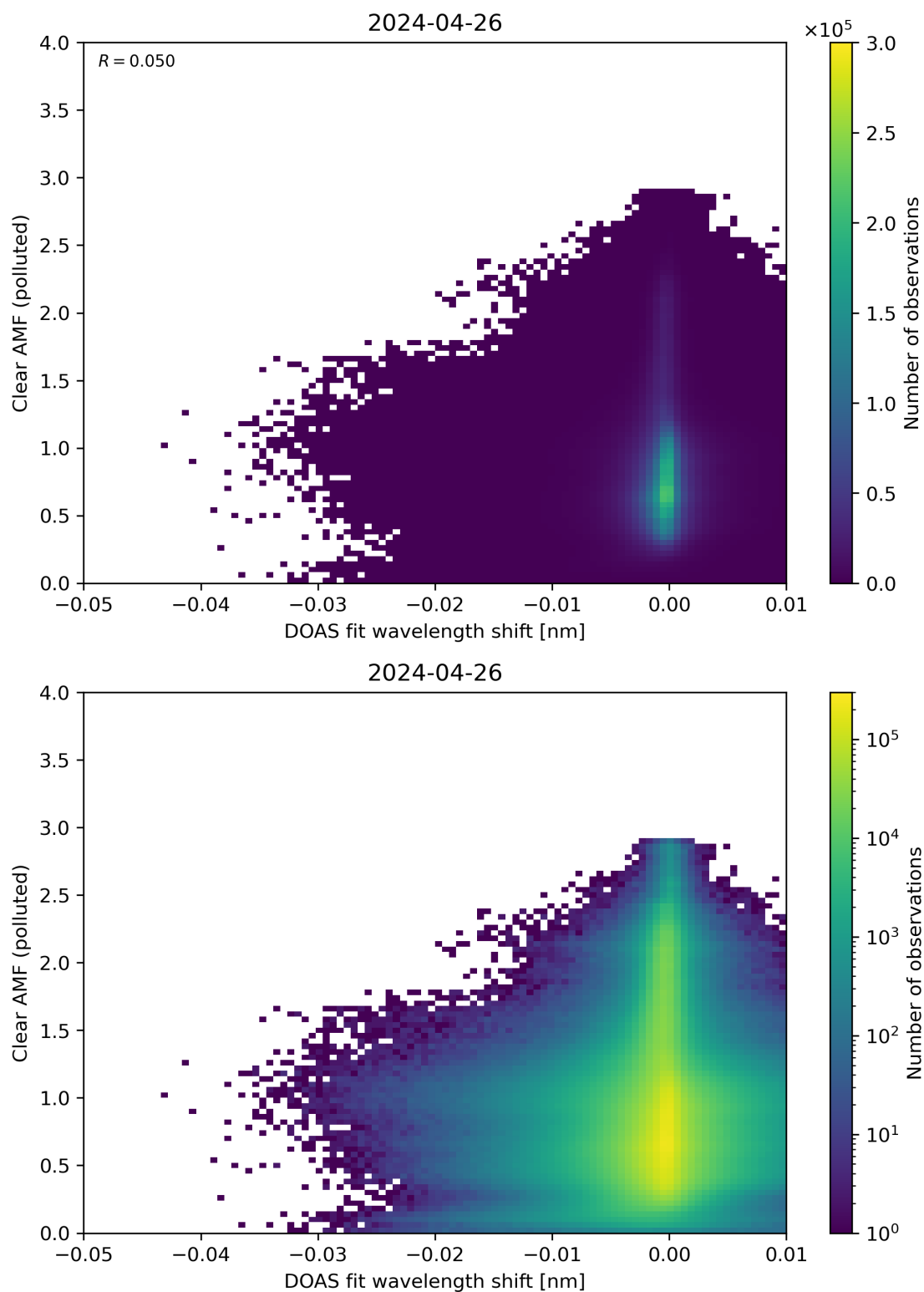
Figure 129: Scatter density plot of “DOAS fit wavelength shift” against “Clear AMF (polluted)” for 2024-04-26 to 2024-04-27.
