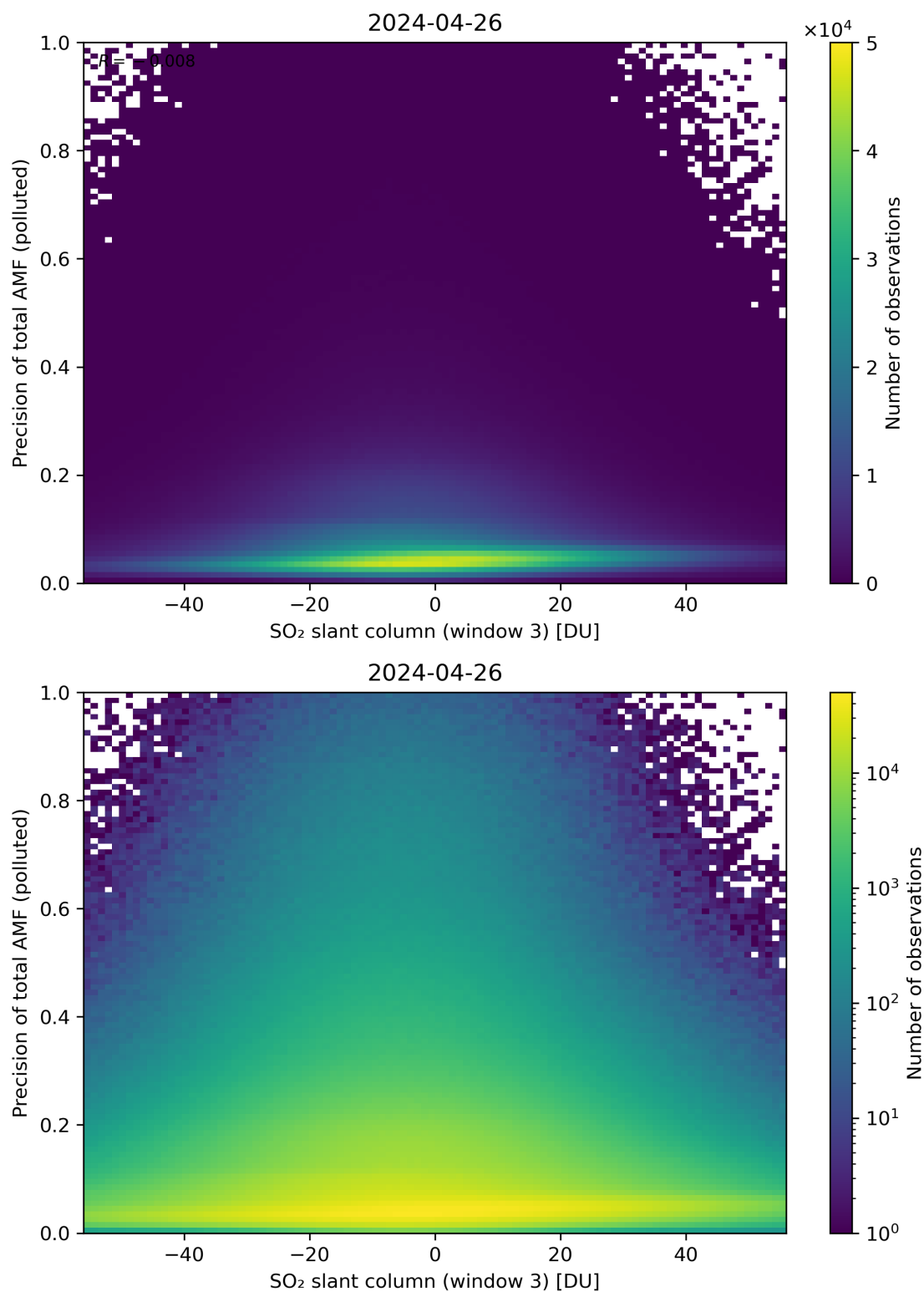
Figure 269: Scatter density plot of “SO 2 slant column (window 3)” against “Precision of total AMF (polluted)” for 2024-04-26 to 2024-04-27.
