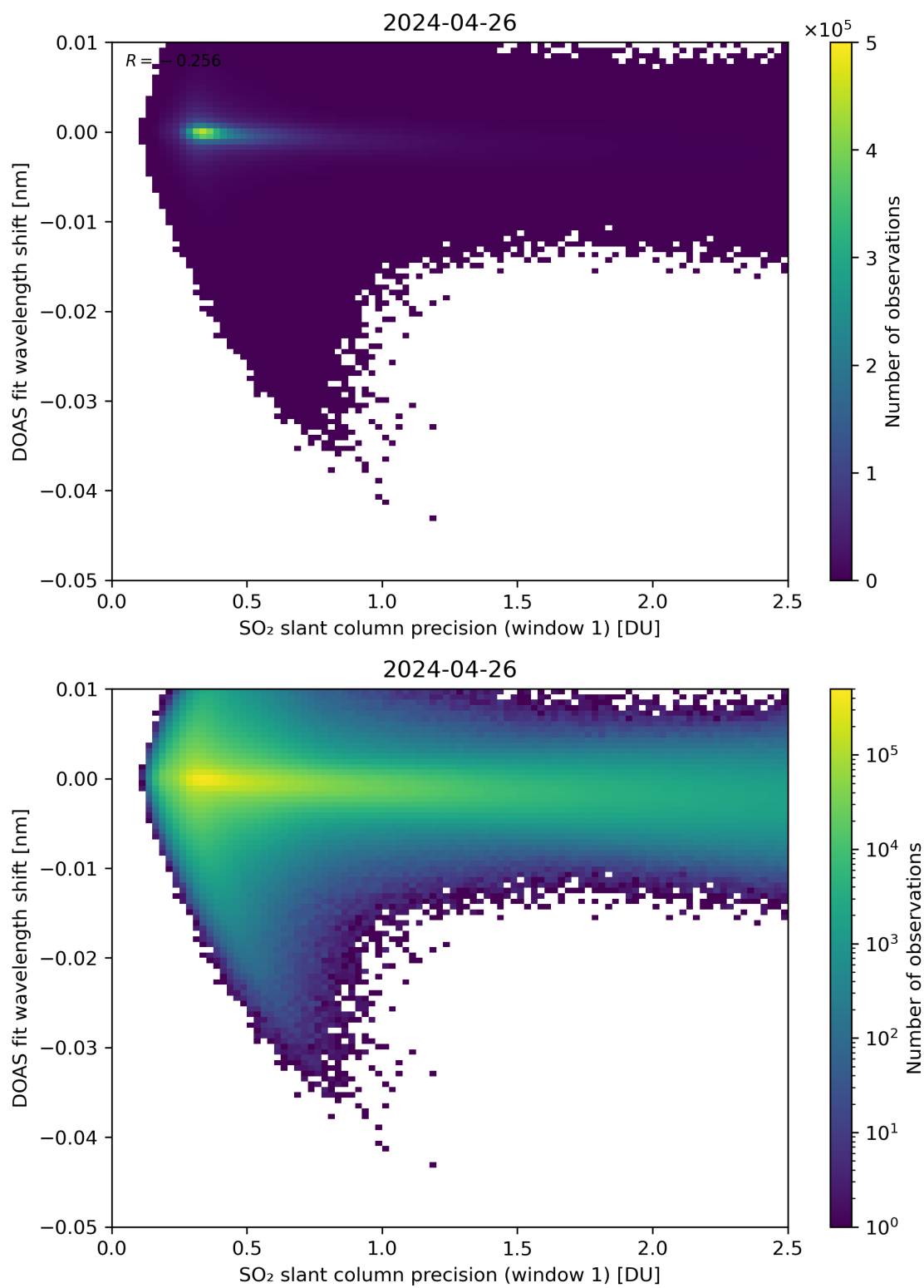
Figure 221: Scatter density plot of “SO 2 slant column precision (window 1)” against “DOAS fit wavelength shift” for 2024-04-26 to 2024-04-27.
