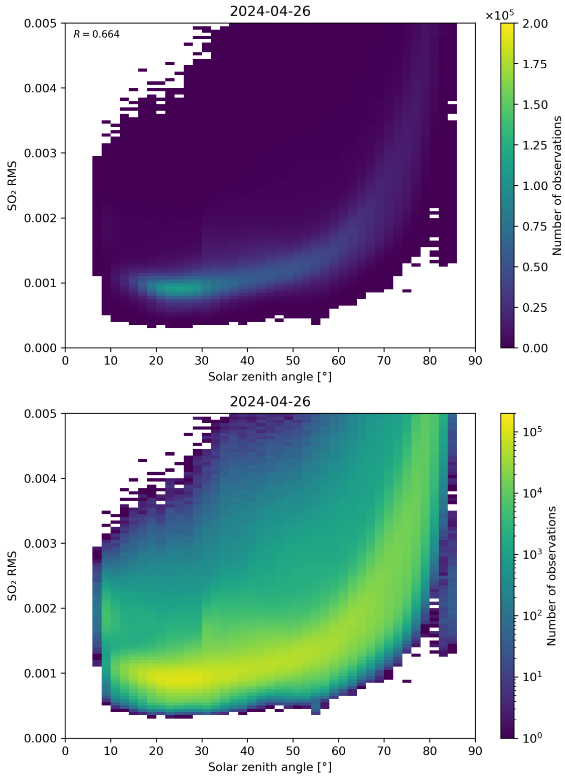
Figure 163: Scatter density plot of “Solar zenith angle” against “SO 2 RMS” for 2024-04-26 to 2024-04-27.
