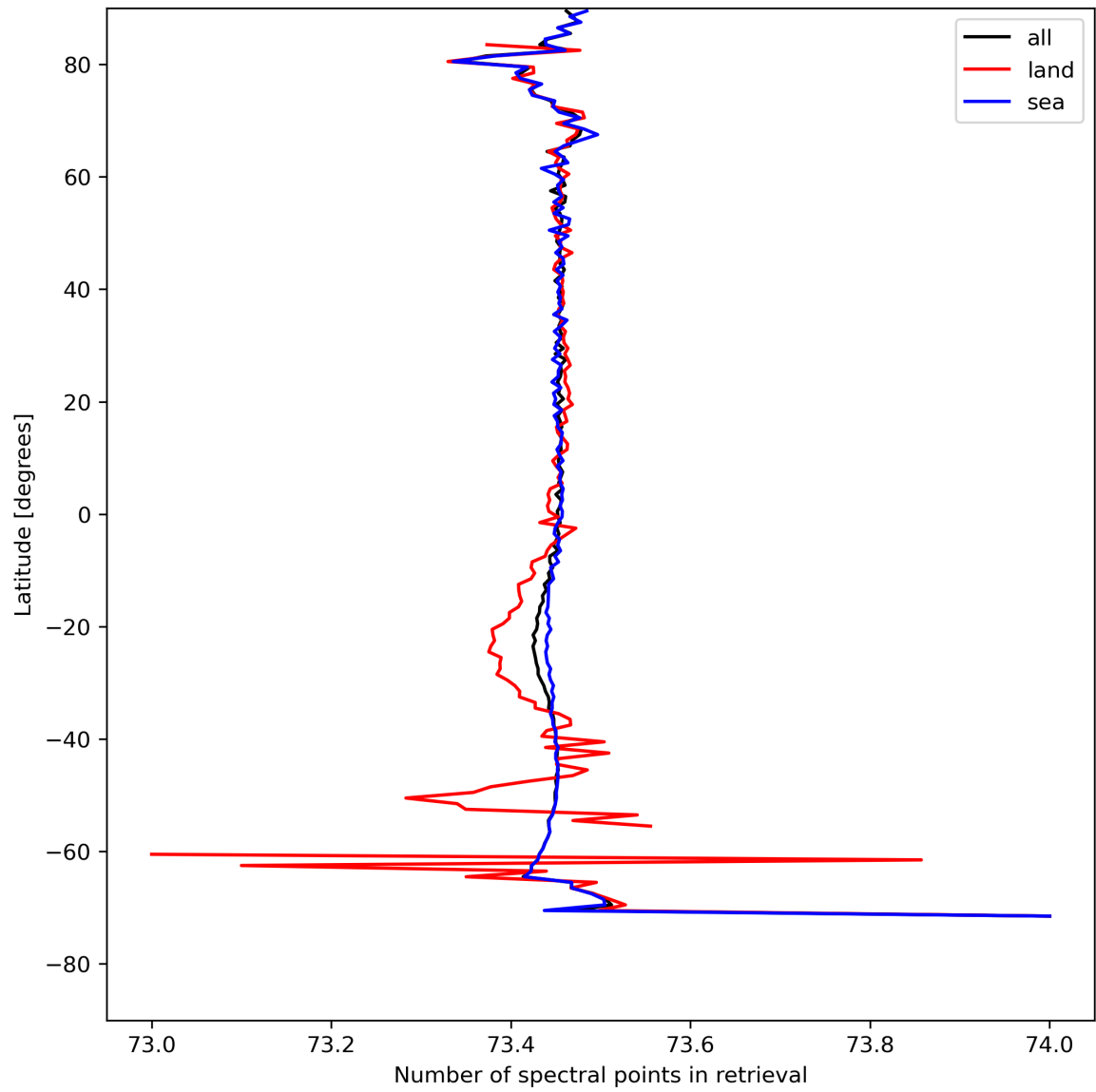
Figure 51: Zonal average of “Number of spectral points in retrieval” for 2024-04-26 to 2024-04-27.
