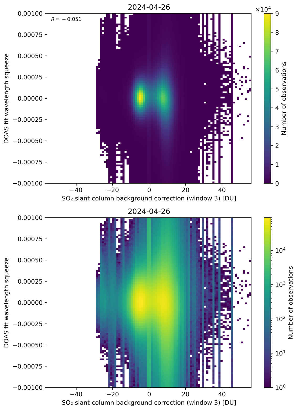
Figure 122: Scatter density plot of “SO 2 slant column background correction (window 3)” against “DOAS fit wavelength squeeze” for 2024-04-26 to 2024-04-27.
