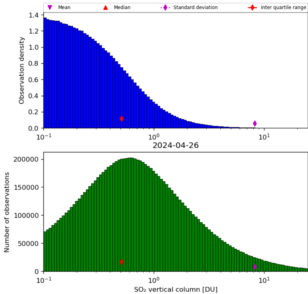
Figure 53: Histogram of “SO 2 vertical column” for 2024-04-26 to 2024-04-27
