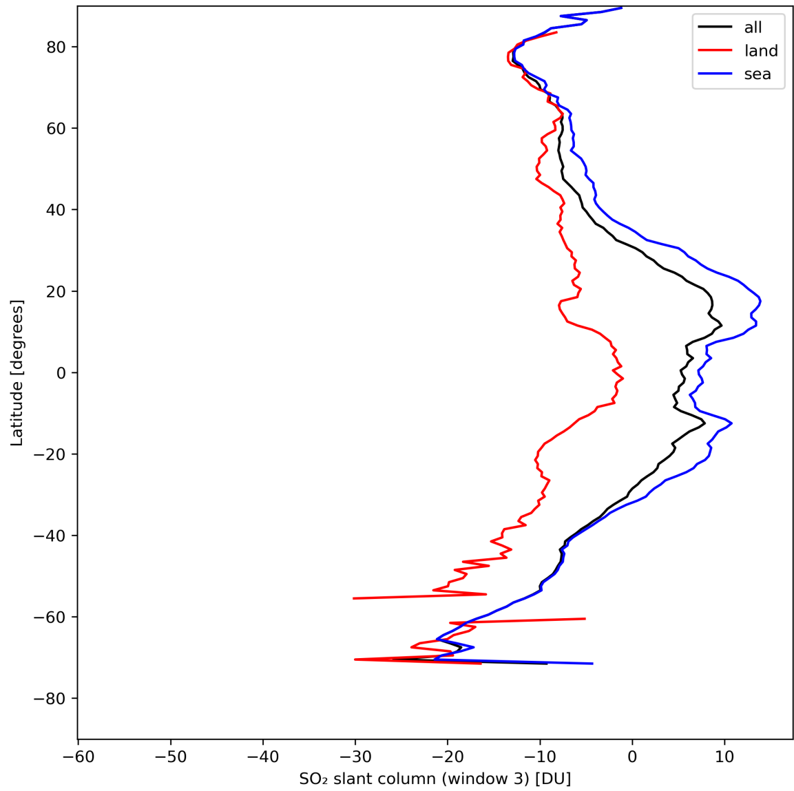
Figure 41: Zonal average of “SO 2 slant column (window 3)” for 2024-04-26 to 2024-04-27.
