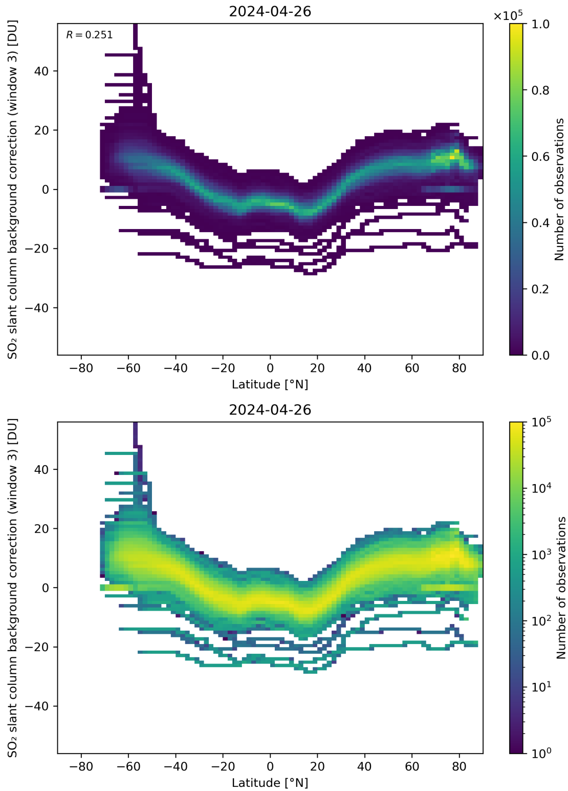
Figure 141: Scatter density plot of “Latitude” against “SO 2 slant column background correction (window 3)” for 2024-04-26 to 2024-04-27.
