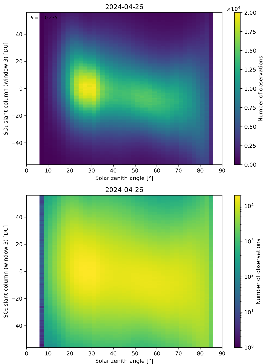
Figure 172: Scatter density plot of “Solar zenith angle” against “SO 2 slant column (window 3)” for 2024-04-26 to 2024-04-27.
