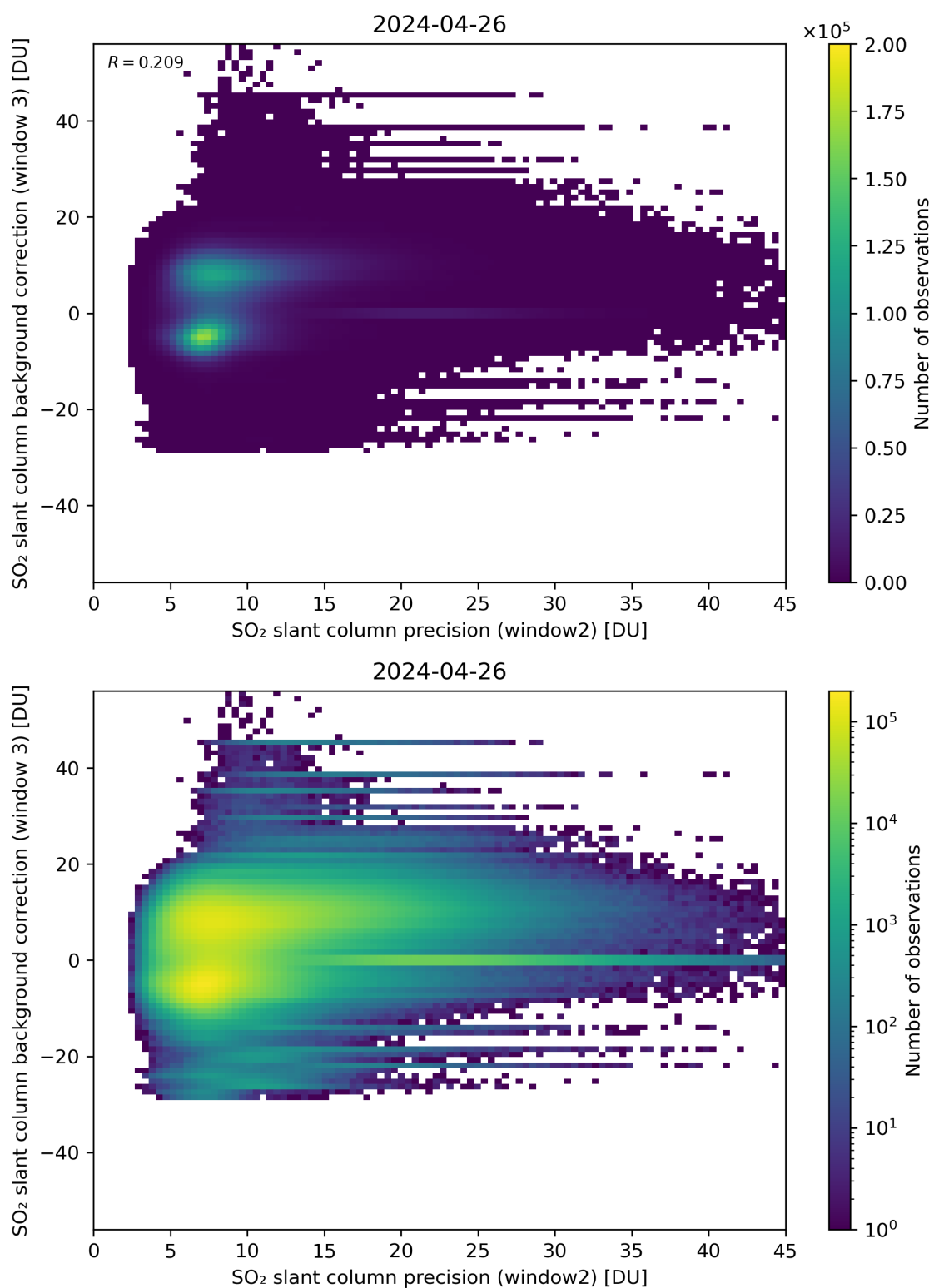
Figure 242: Scatter density plot of “SO 2 slant column precision (window2)” against “SO 2 slant column background correction (window 3)” for 2024-04-26 to 2024-04-27.
