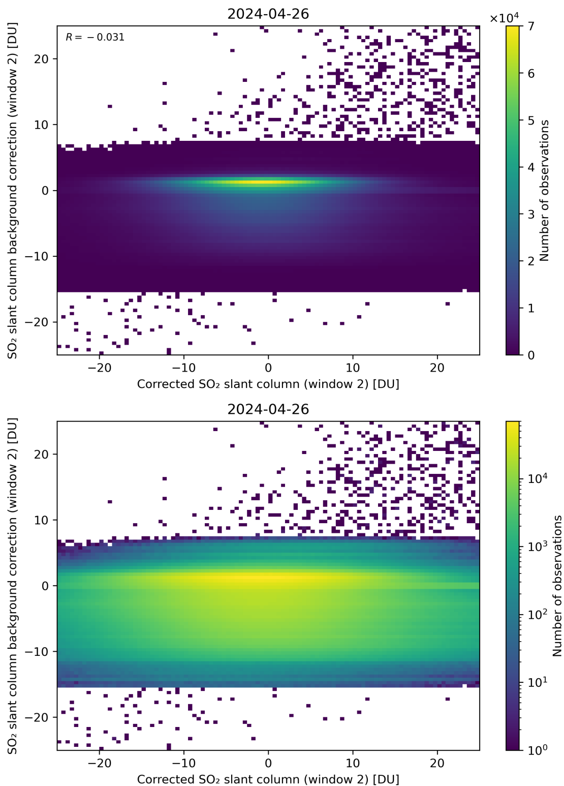
Figure 194: Scatter density plot of “Corrected SO 2 slant column (window 2)” against “SO 2 slant column background correction (window 2)” for 2024-04-26 to 2024-04-27.
