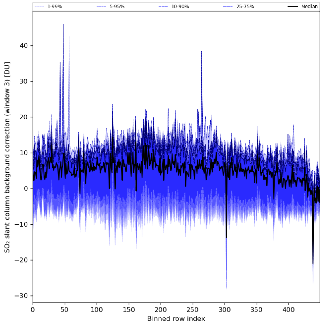
Figure 90: Along track statistics of “SO 2 slant column background correction (window 3)” for 2024-04-26 to 2024-04-27
