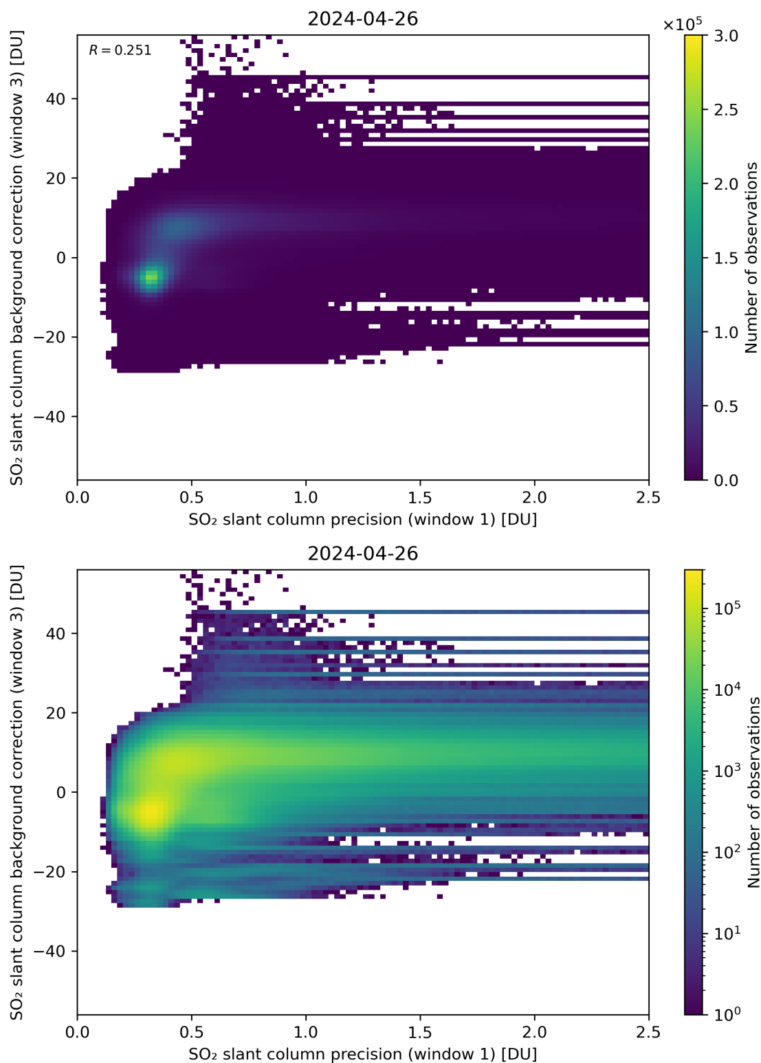
Figure 220: Scatter density plot of “SO 2 slant column precision (window 1)” against “SO 2 slant column background correction (window 3)” for 2024-04-26 to 2024-04-27.
