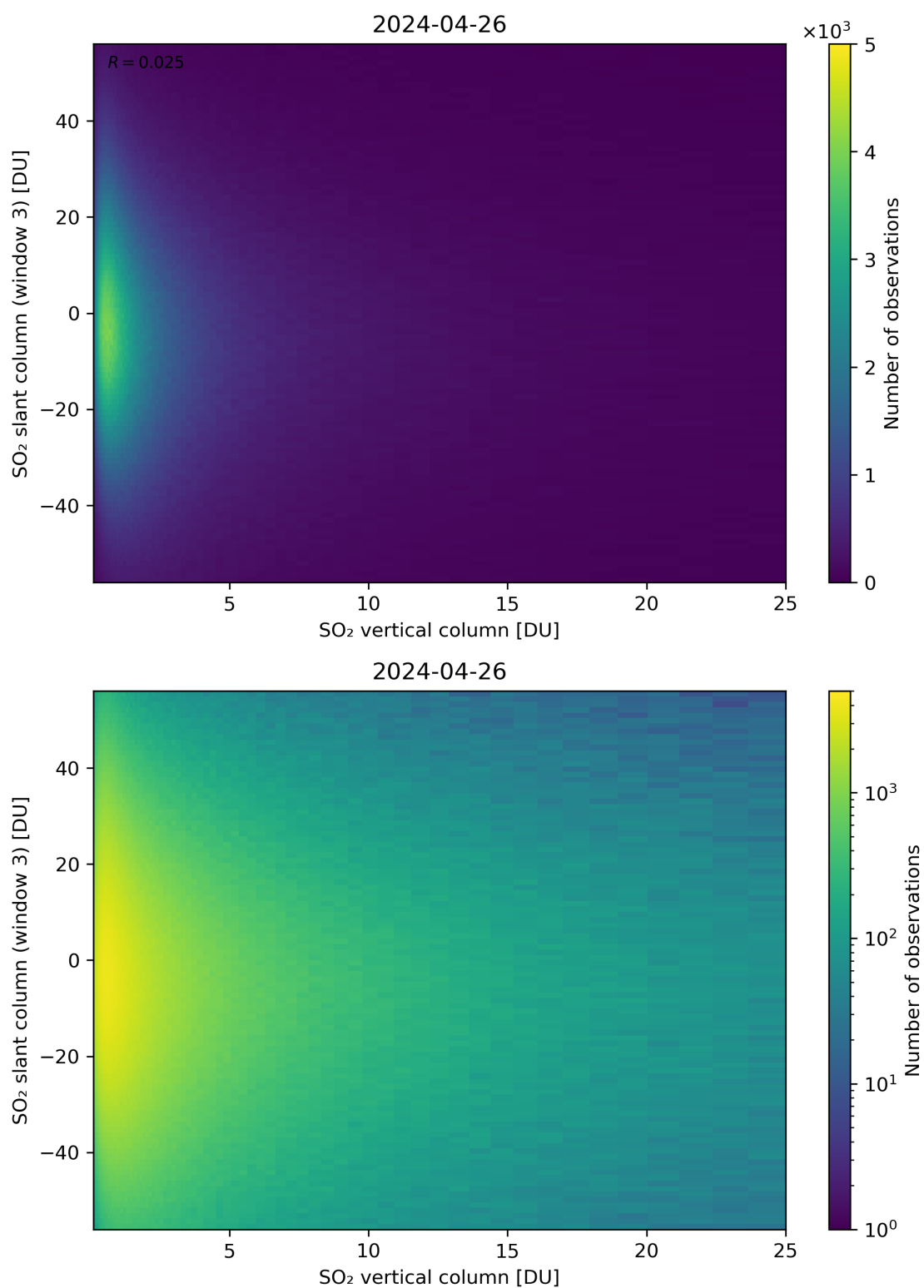
Figure 303: Scatter density plot of “SO 2 vertical column” against “SO 2 slant column (window 3)” for 2024-04-26 to 2024-04-27.
