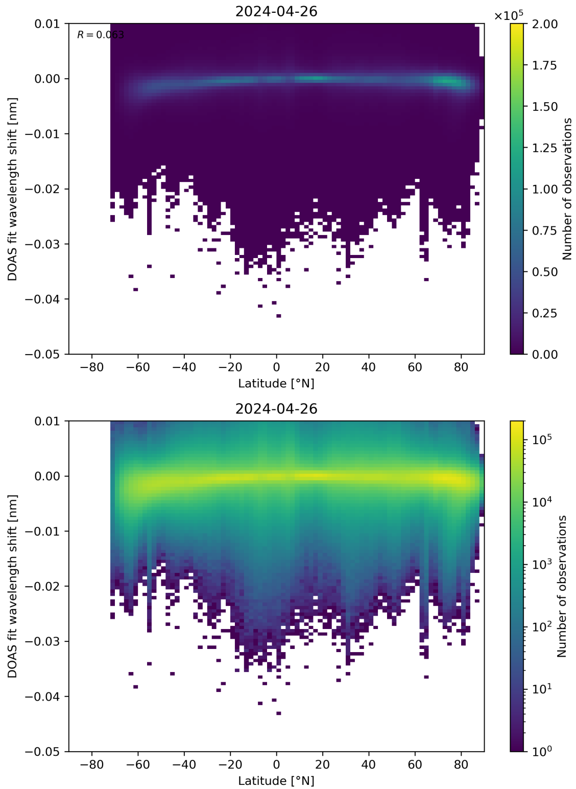
Figure 142: Scatter density plot of “Latitude” against “DOAS fit wavelength shift” for 2024-04-26 to 2024-04-27.
