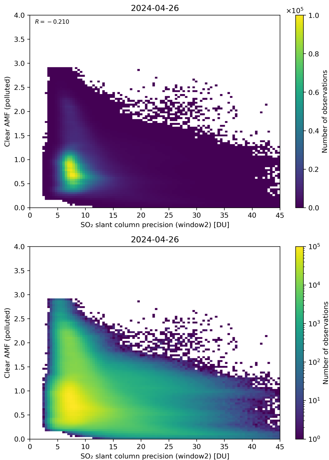
Figure 246: Scatter density plot of “SO 2 slant column precision (window2)” against “Clear AMF (polluted)” for 2024-04-26 to 2024-04-27.
