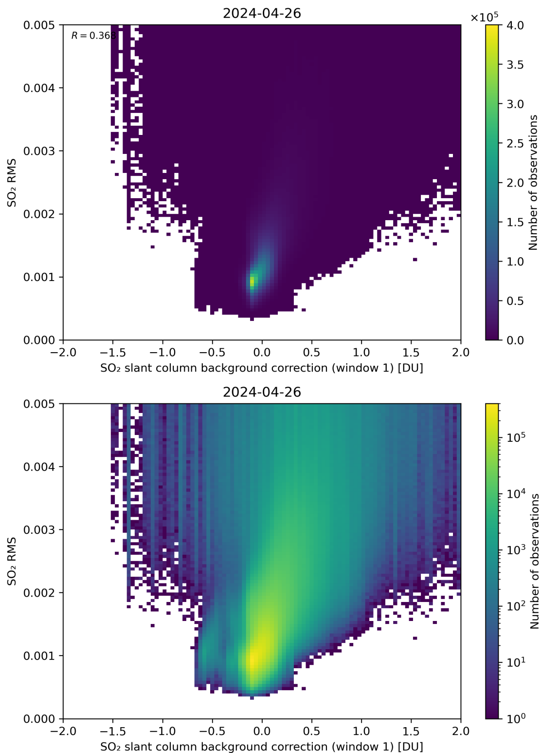
Figure 102: Scatter density plot of “SO 2 slant column background correction (window 1)” against “SO 2 RMS” for 2024-04-26 to 2024-04-27.
