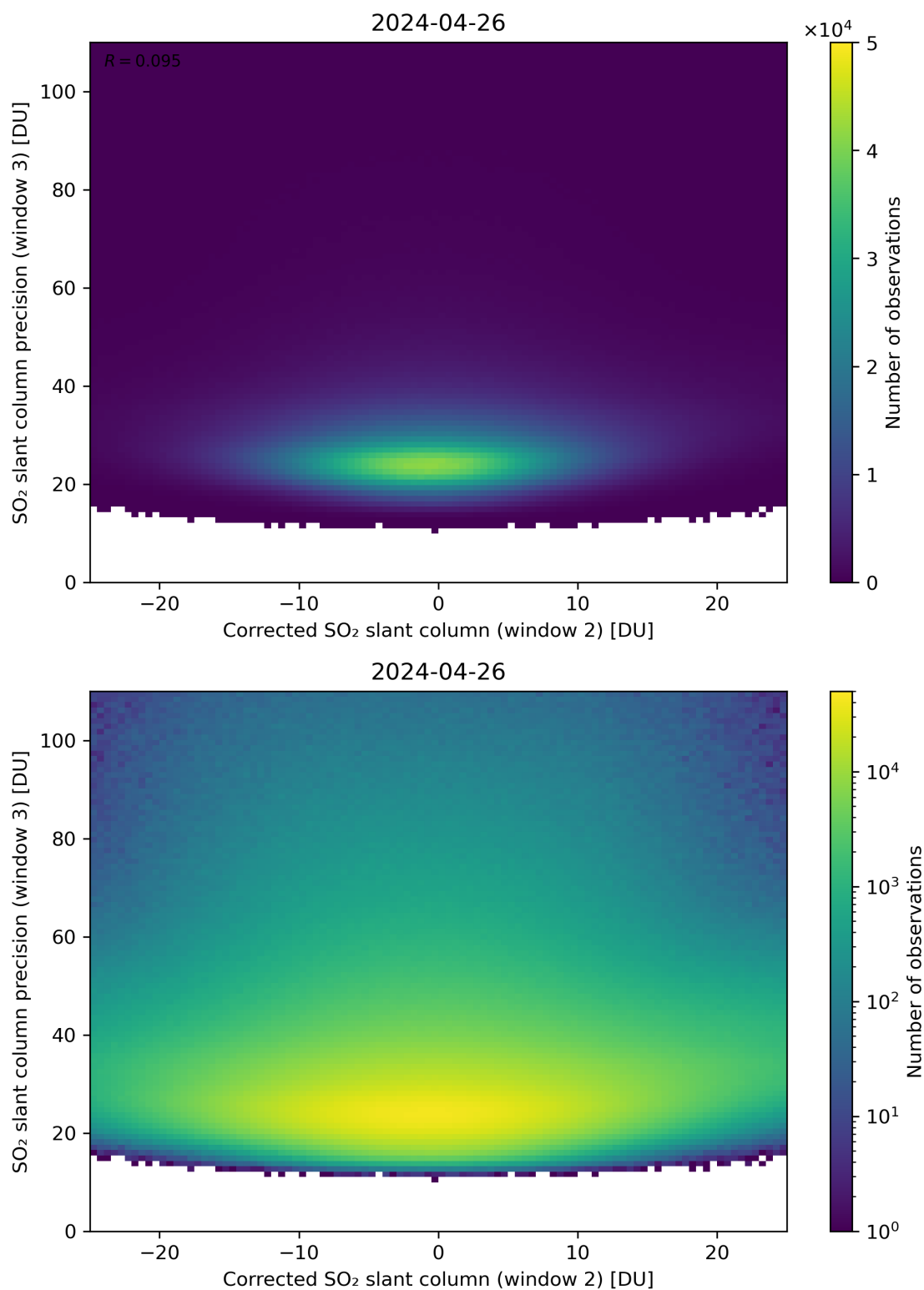
Figure 202: Scatter density plot of “Corrected SO 2 slant column (window 2)” against “SO 2 slant column precision (window 3)” for 2024-04-26 to 2024-04-27.
