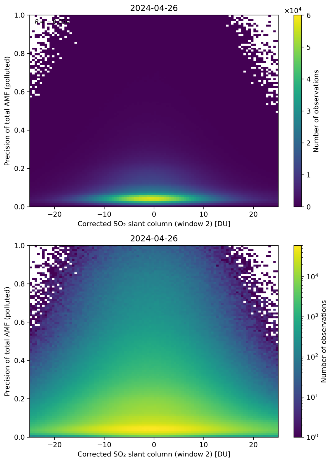
Figure 204: Scatter density plot of “Corrected SO 2 slant column (window 2)” against “Precision of total AMF (polluted)” for 2024-04-26 to 2024-04-27.
