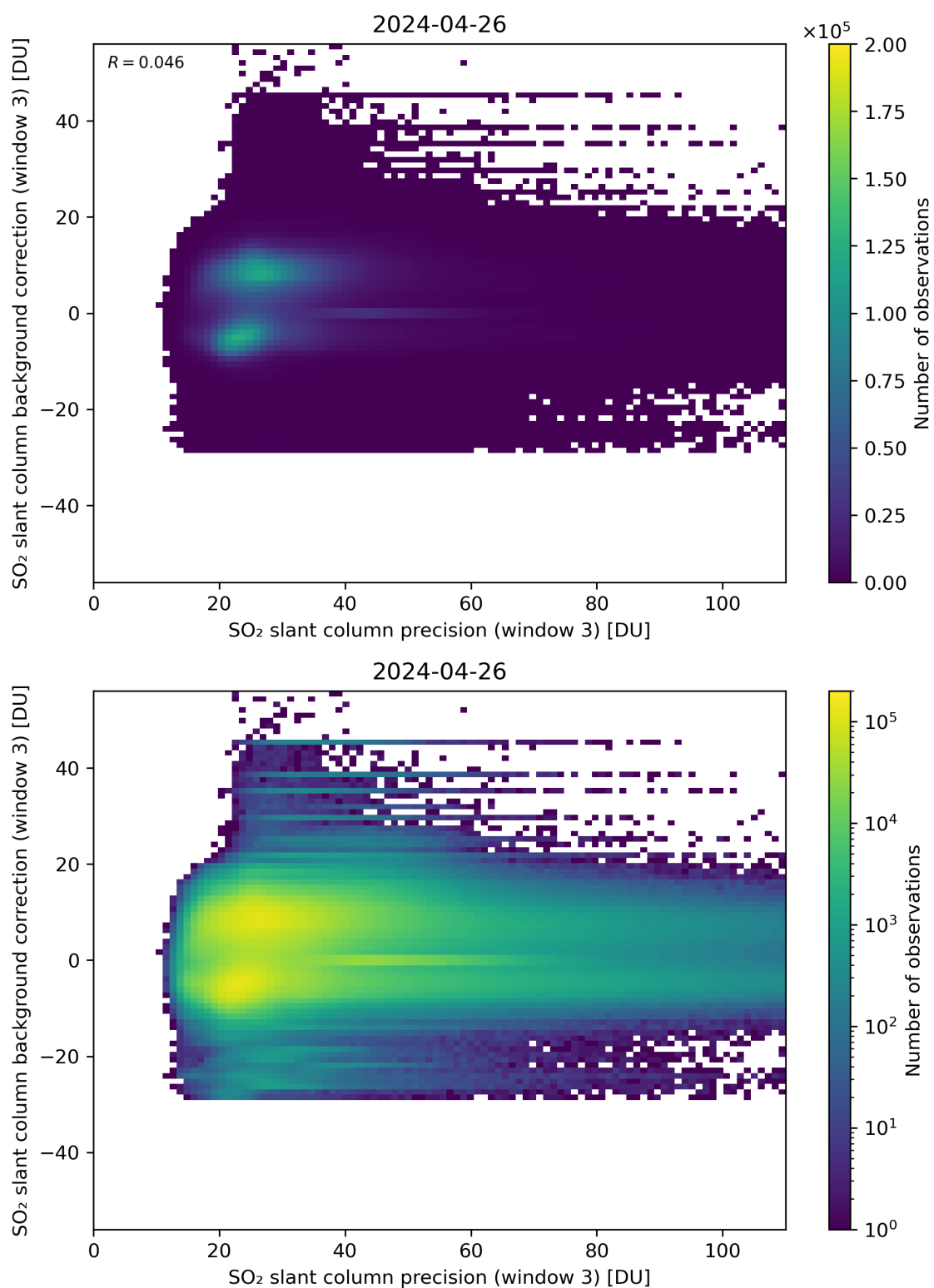
Figure 257: Scatter density plot of “SO 2 slant column precision (window 3)” against “SO 2 slant column background correction (window 3)” for 2024-04-26 to 2024-04-27.
