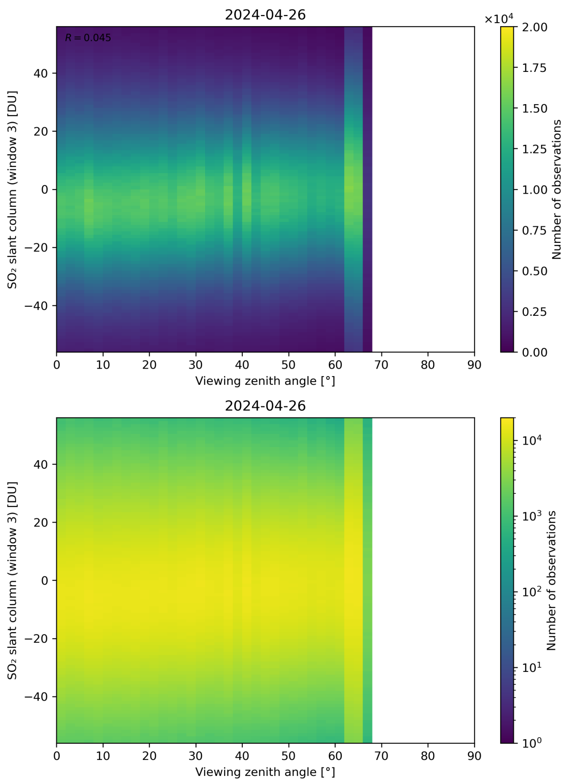
Figure 323: Scatter density plot of “Viewing zenith angle” against “SO 2 slant column (window 3)” for 2024-04-26 to 2024-04-27.
