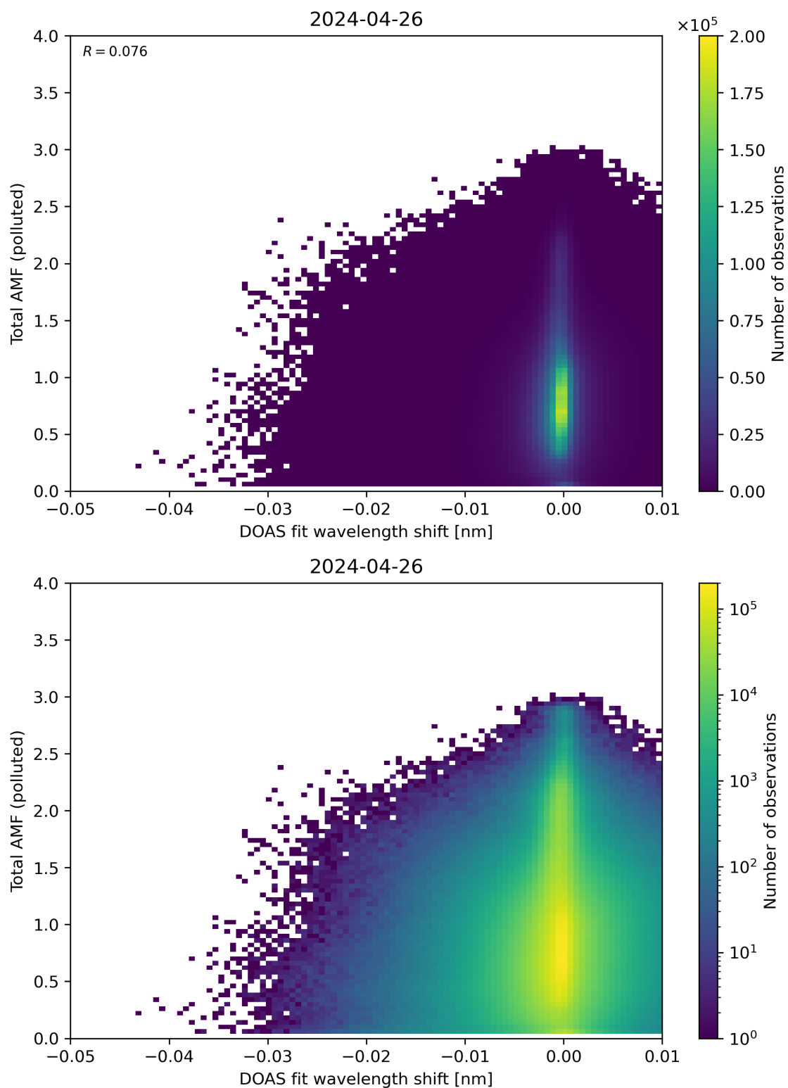
Figure 130: Scatter density plot of “DOAS fit wavelength shift” against “Total AMF (polluted)” for 2024-04-26 to 2024-04-27.
