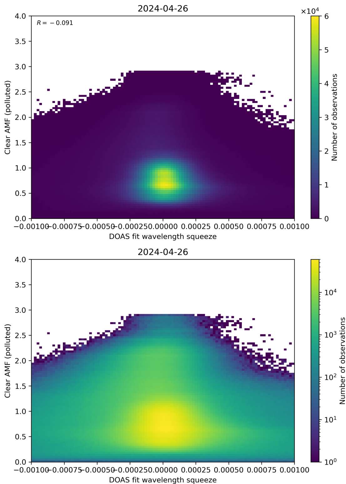
Figure 133: Scatter density plot of “DOAS fit wavelength squeeze” against “Clear AMF (polluted)” for 2024-04-26 to 2024-04-27.
