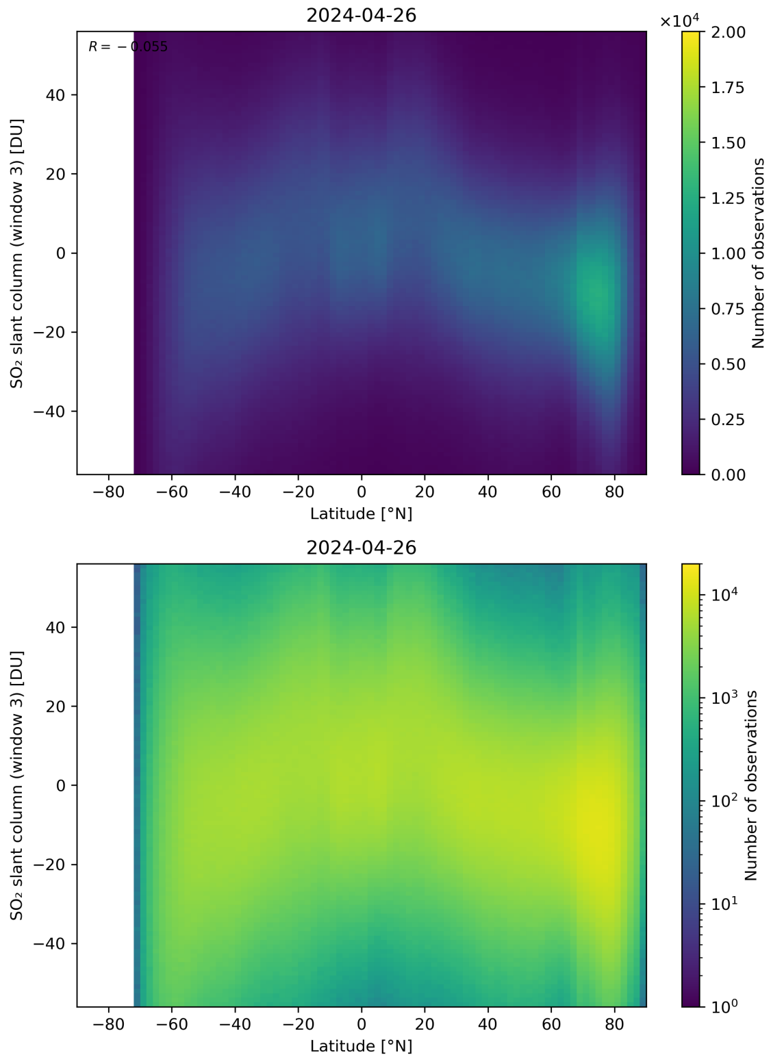
Figure 152: Scatter density plot of “Latitude” against “SO 2 slant column (window 3)” for 2024-04-26 to 2024-04-27.
