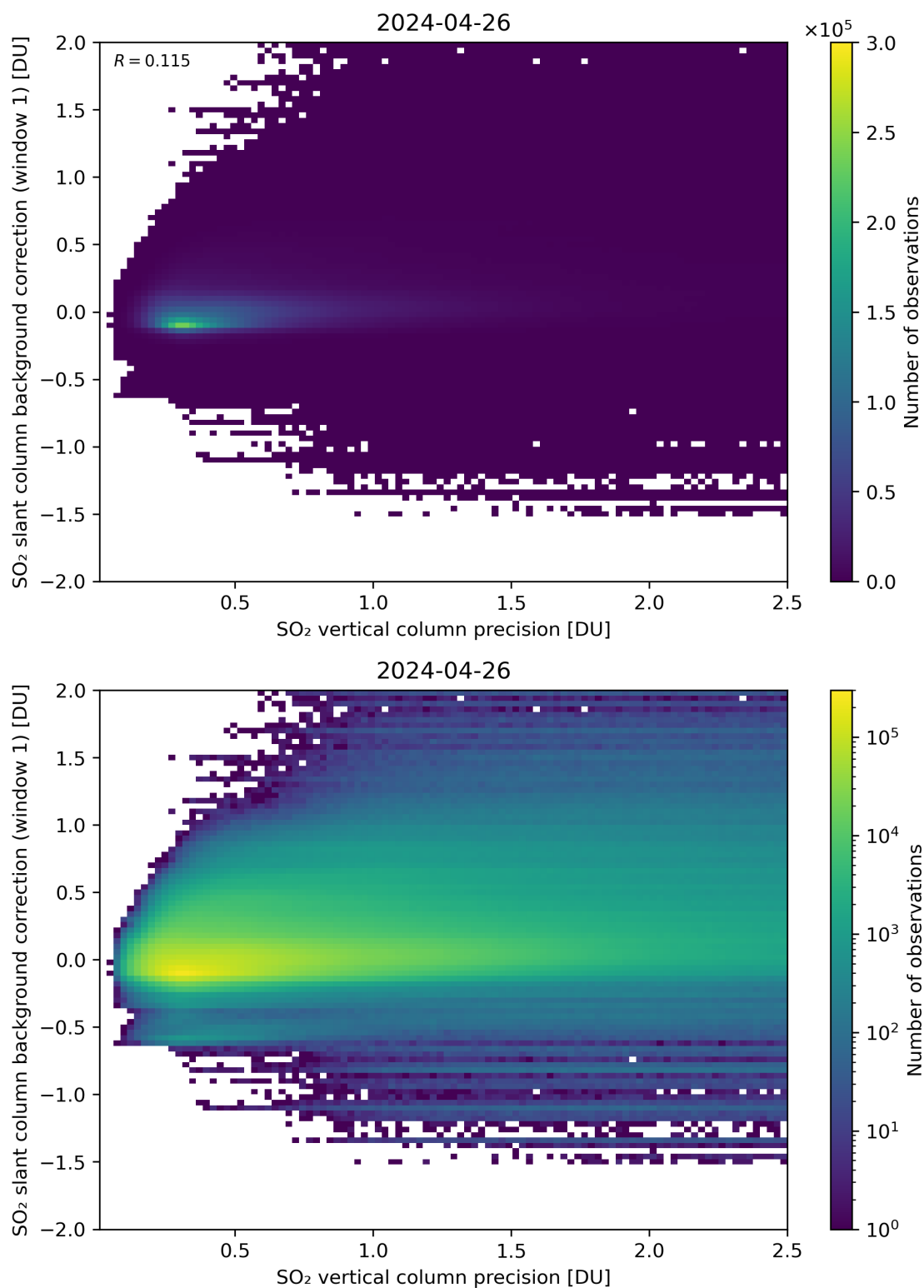
Figure 279: Scatter density plot of “SO 2 vertical column precision” against “SO 2 slant column background correction (window 1)” for 2024-04-26 to 2024-04-27.
