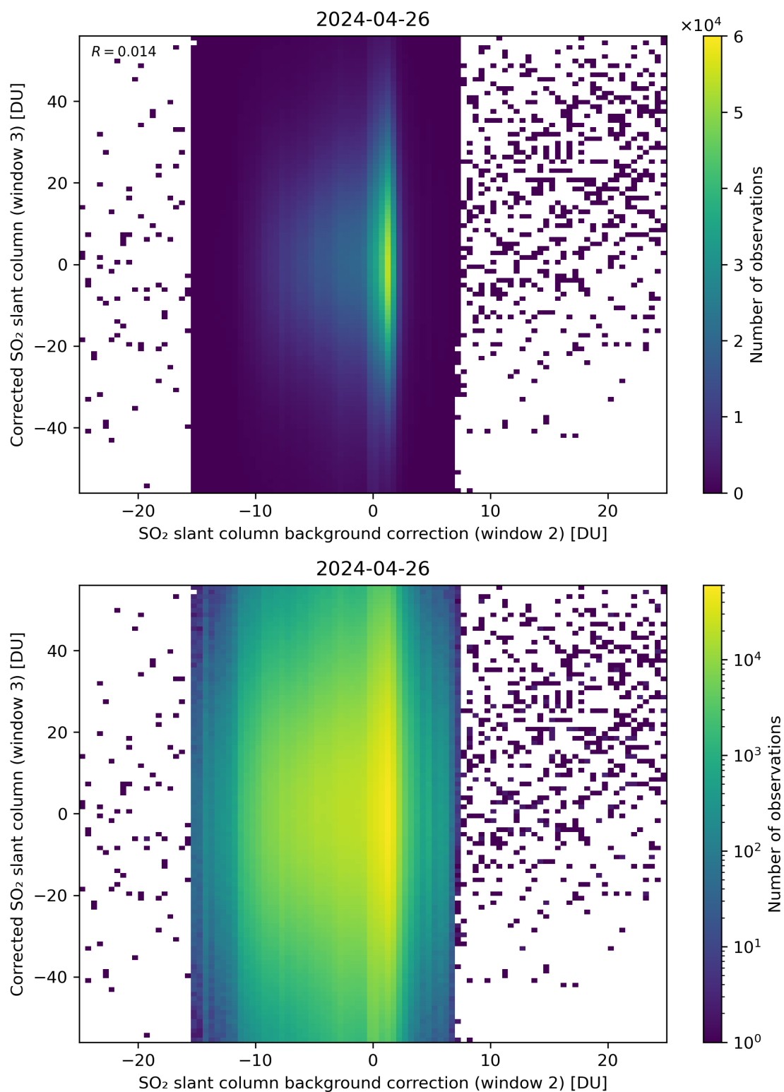
Figure 116: Scatter density plot of “SO 2 slant column background correction (window 2)” against “Corrected SO 2 slant column (window 3)” for 2024-04-26 to 2024-04-27.
