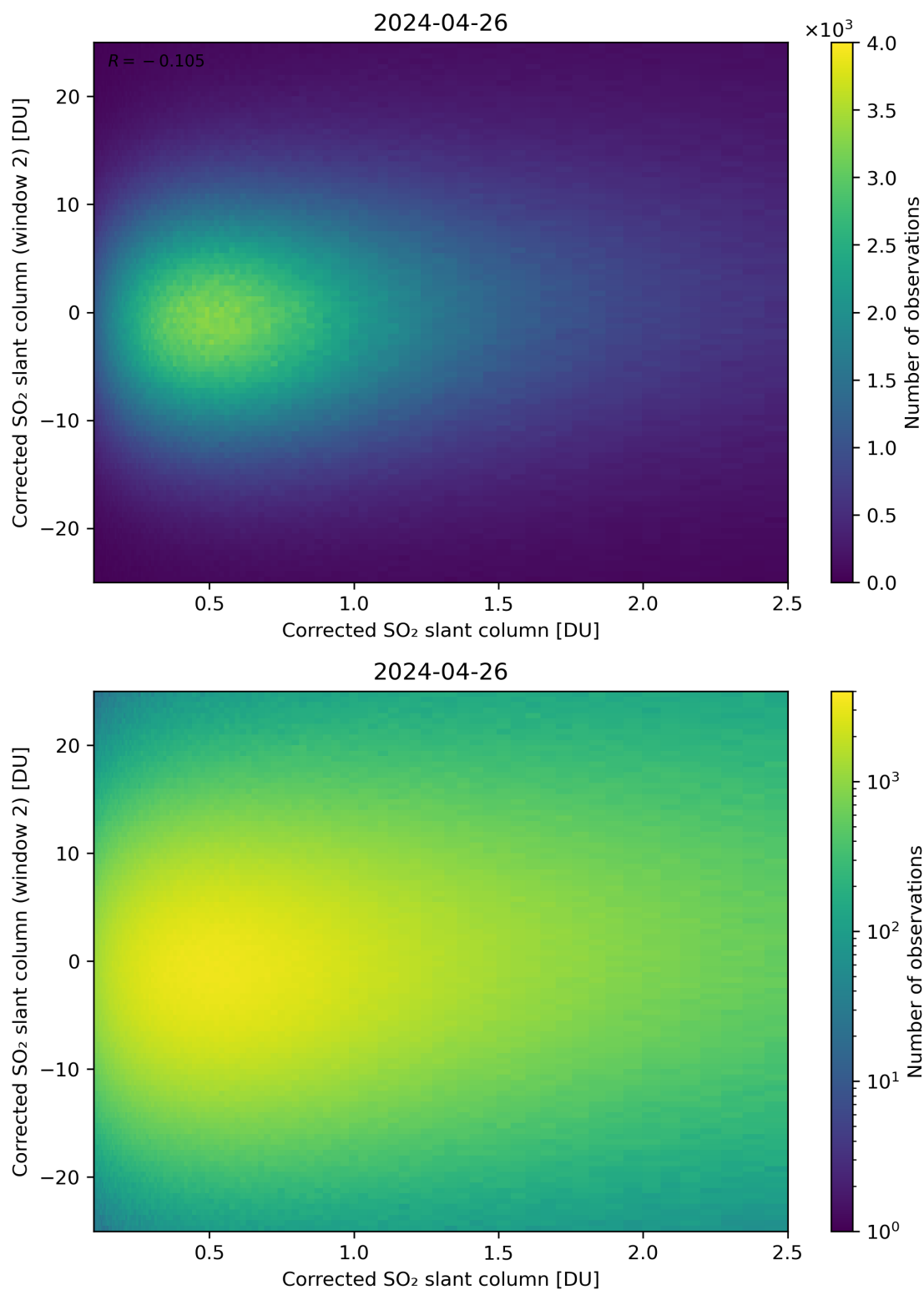
Figure 185: Scatter density plot of “Corrected SO 2 slant column” against “Corrected SO 2 slant column (window 2)” for 2024-04-26 to 2024-04-27.
