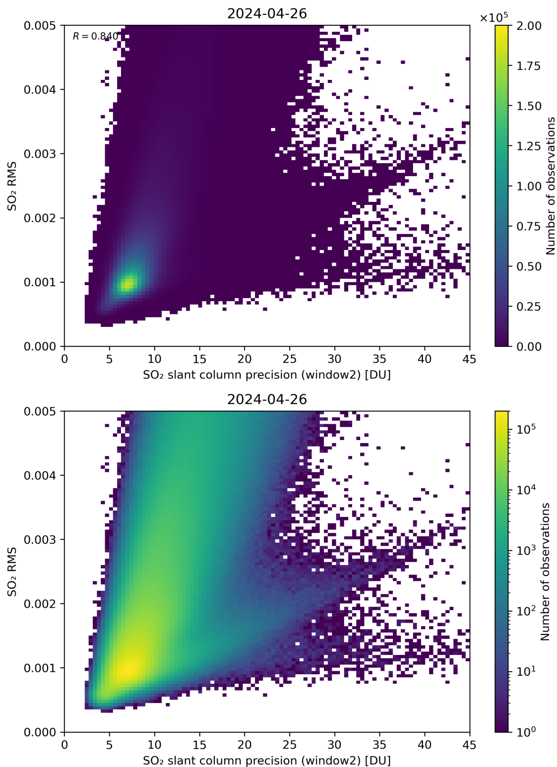
Figure 245: Scatter density plot of “SO 2 slant column precision (window2)” against “SO 2 RMS” for 2024-04-26 to 2024-04-27.
