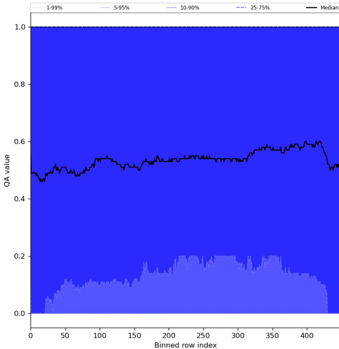
Figure 75: Along track statistics of “QA value” for 2024-04-26 to 2024-04-27
