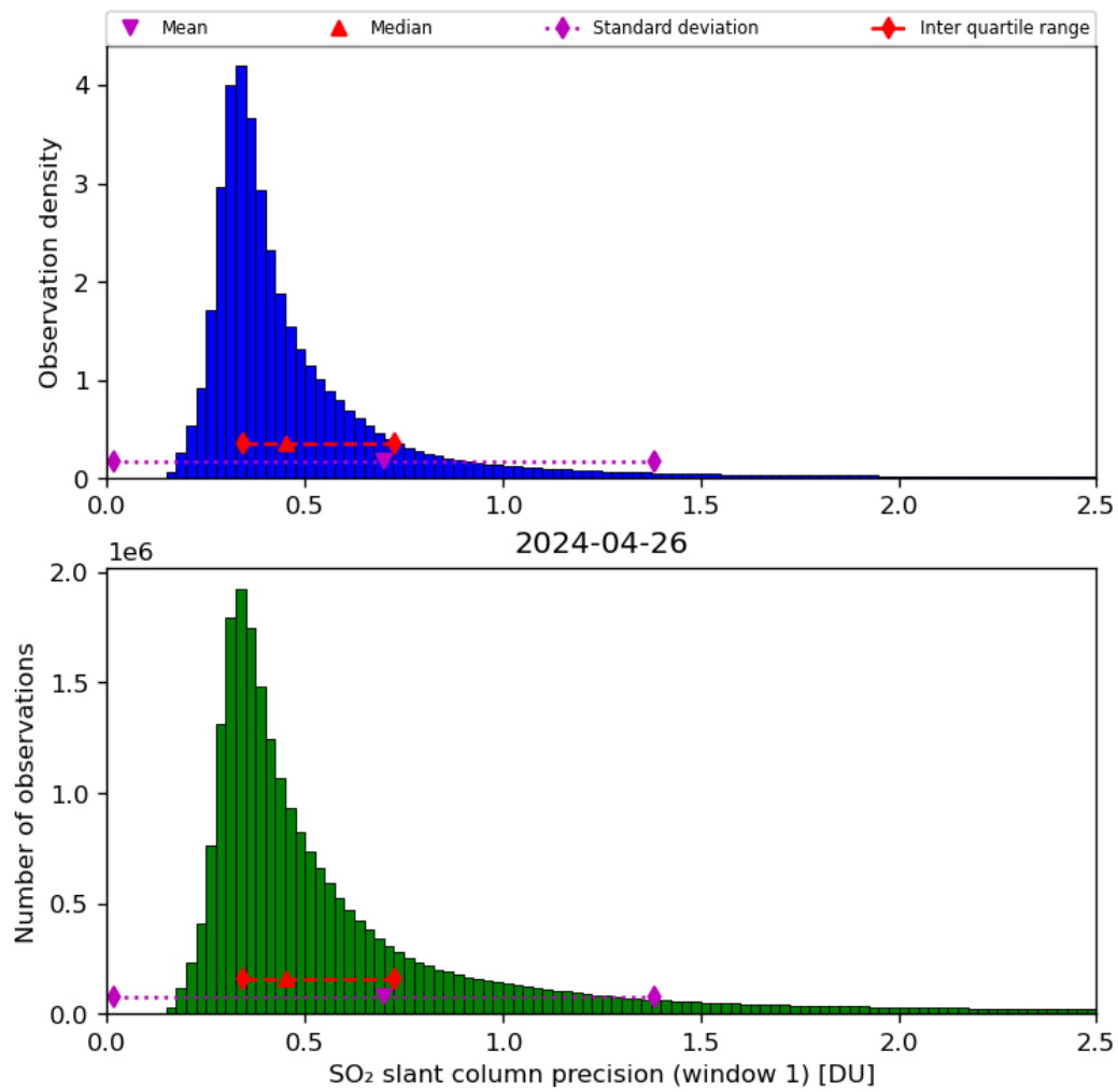
Figure 57: Histogram of “SO 2 slant column precision (window 1)” for 2024-04-26 to 2024-04-27
