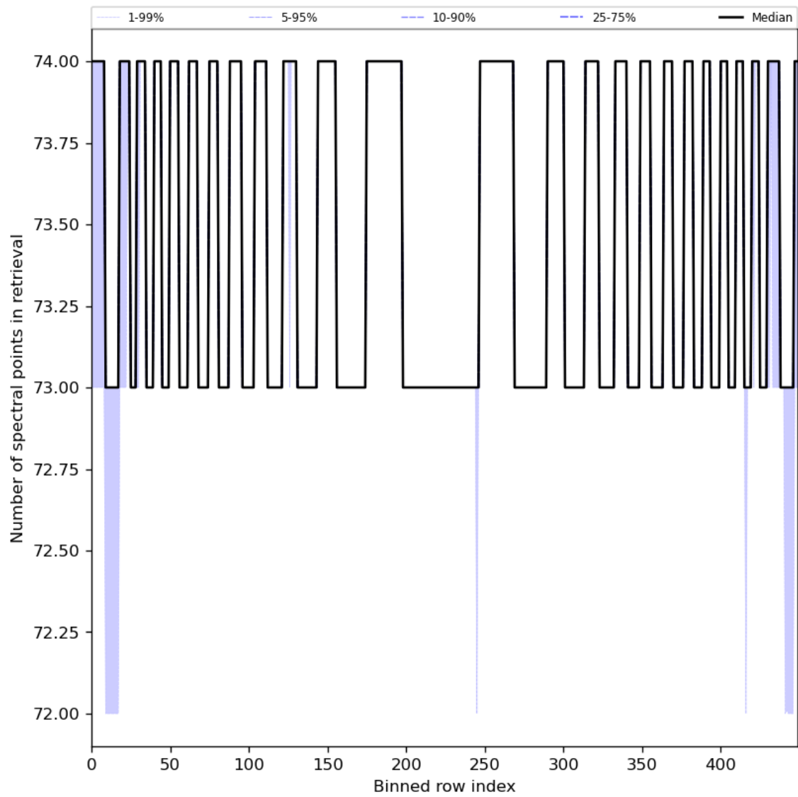
Figure 97: Along track statistics of “Number of spectral points in retrieval” for 2024-04-26 to 2024-04-27
