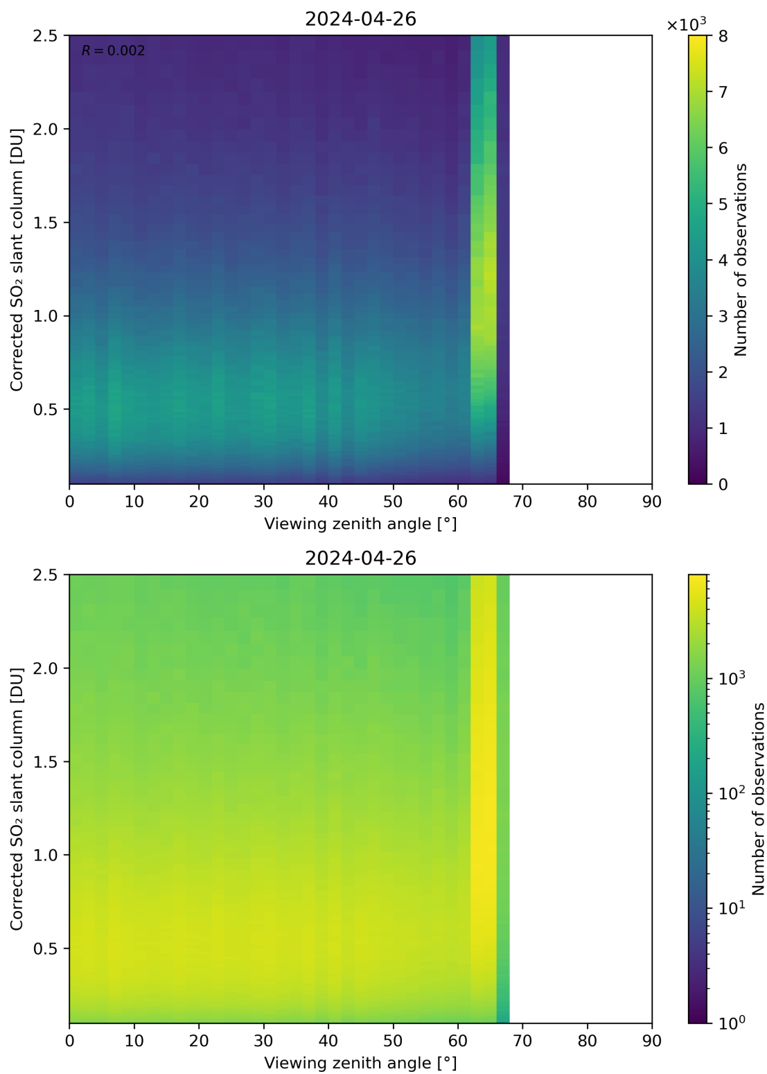
Figure 317: Scatter density plot of “Viewing zenith angle” against “Corrected SO 2 slant column” for 2024-04-26 to 2024-04-27.
