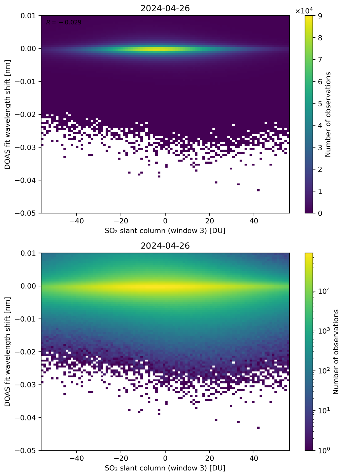
Figure 254: Scatter density plot of “SO 2 slant column (window 3)” against “DOAS fit wavelength shift” for 2024-04-26 to 2024-04-27.
