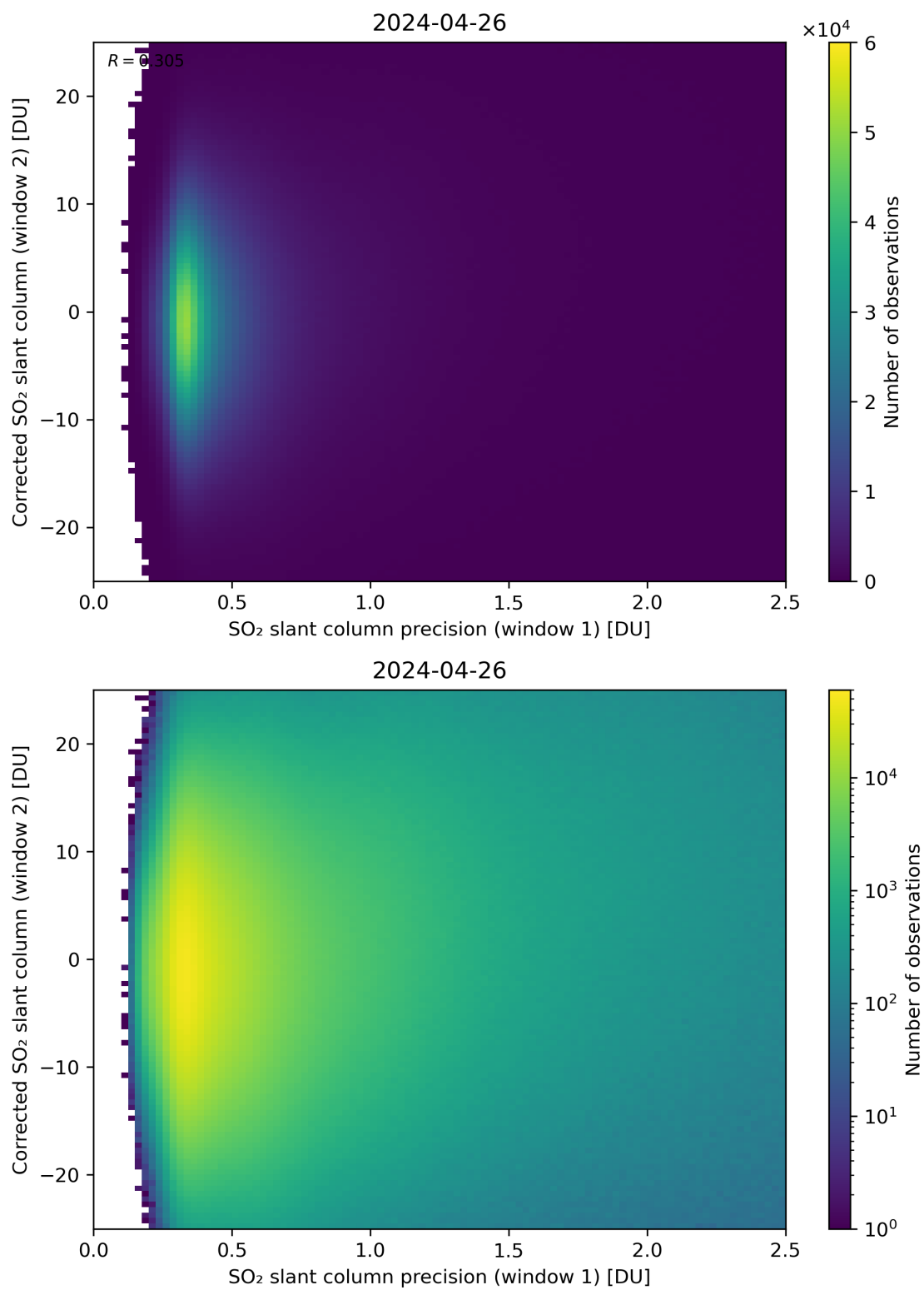
Figure 225: Scatter density plot of “SO 2 slant column precision (window 1)” against “Corrected SO 2 slant column (window 2)” for 2024-04-26 to 2024-04-27.
