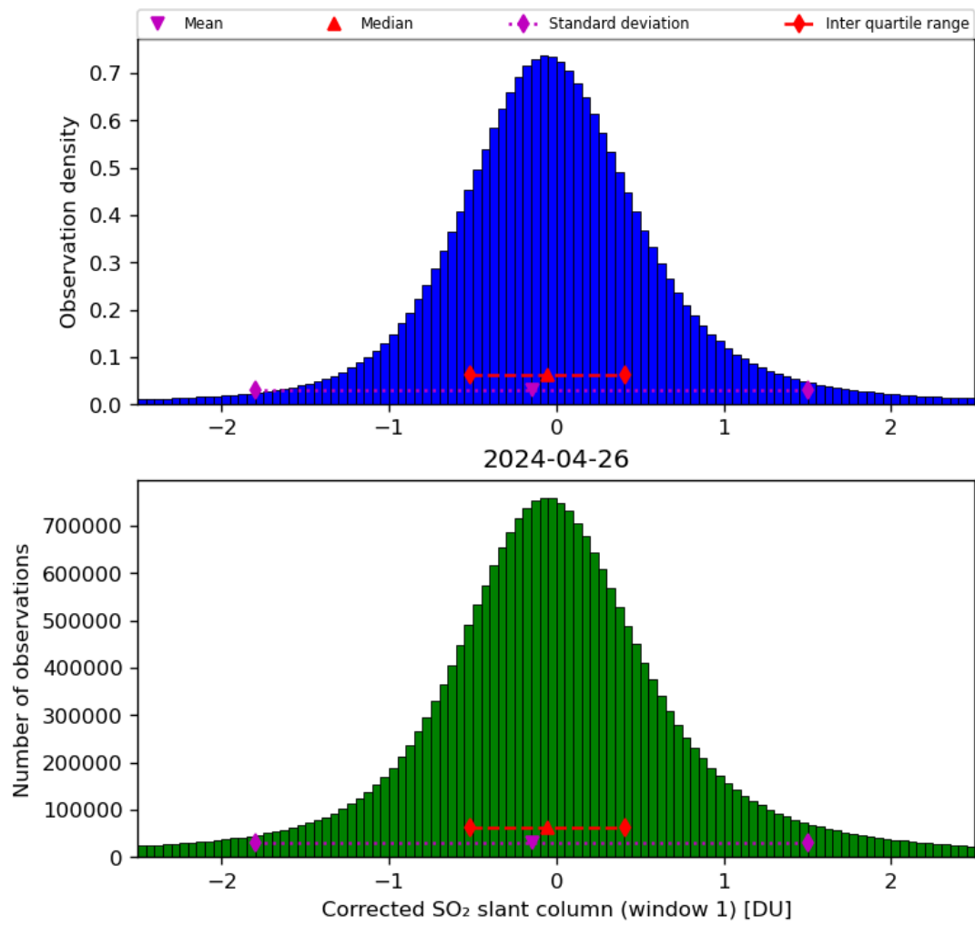
Figure 58: Histogram of “Corrected SO 2 slant column (window 1)” for 2024-04-26 to 2024-04-27
