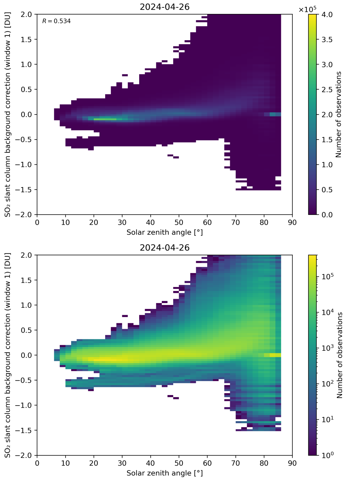
Figure 158: Scatter density plot of “Solar zenith angle” against “SO 2 slant column background correction (window 1)” for 2024-04-26 to 2024-04-27.
