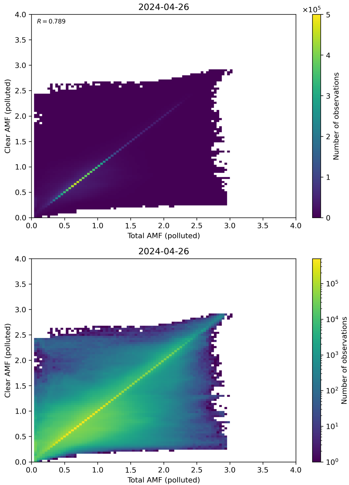
Figure 271: Scatter density plot of “Total AMF (polluted)” against “Clear AMF (polluted)” for 2024-04-26 to 2024-04-27.
