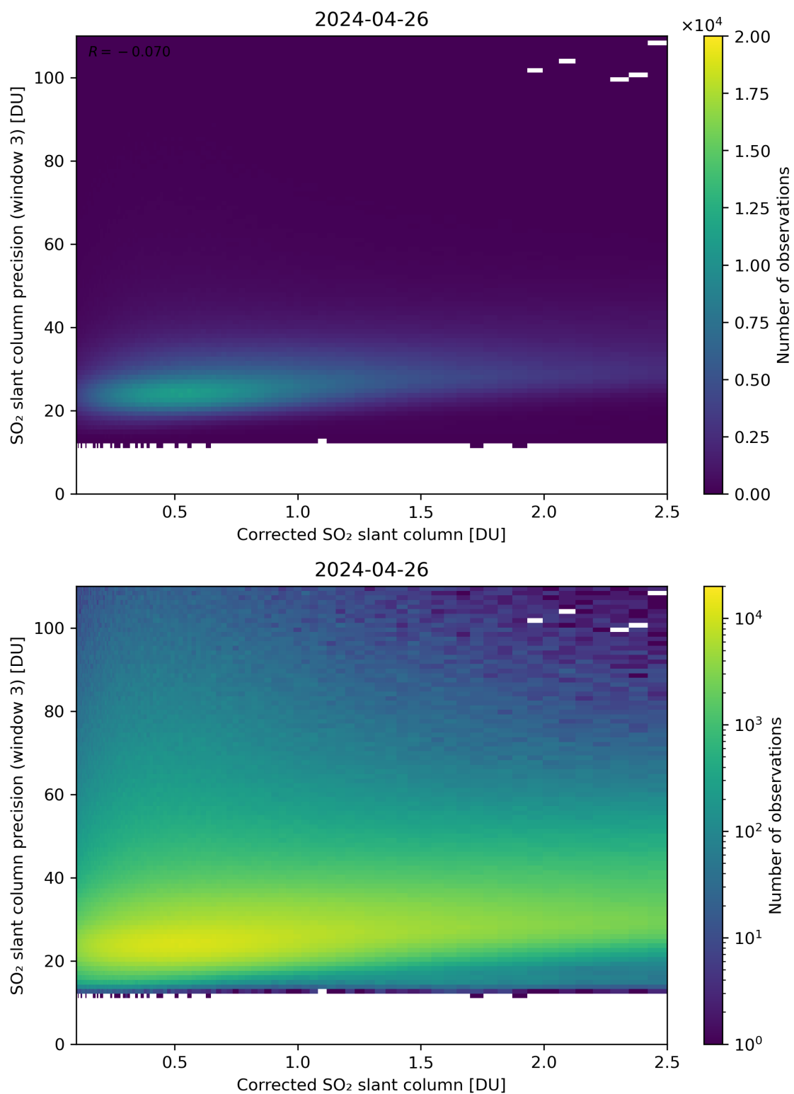
Figure 191: Scatter density plot of “Corrected SO 2 slant column” against “SO 2 slant column precision (window 3)” for 2024-04-26 to 2024-04-27.
