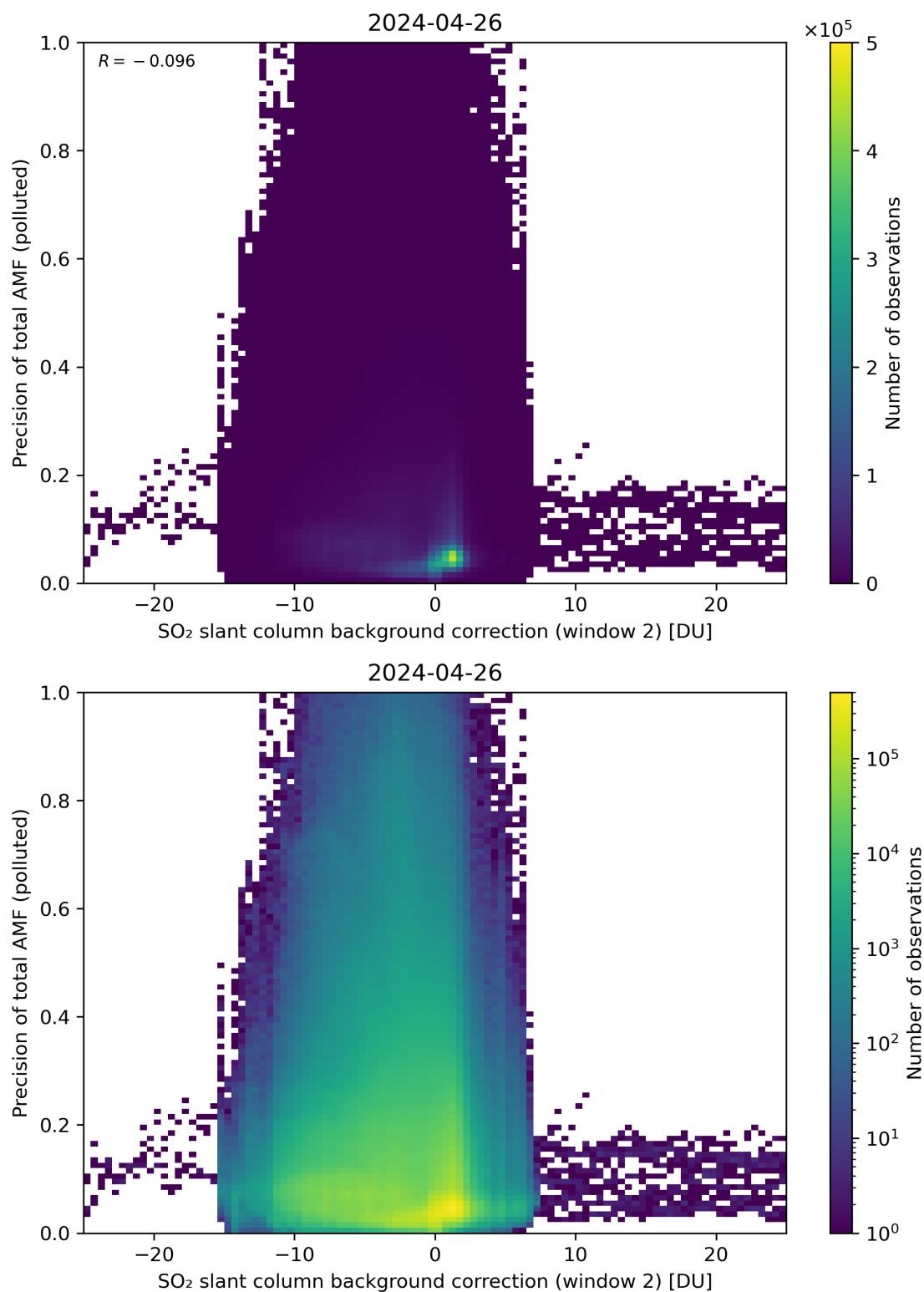
Figure 120: Scatter density plot of “SO 2 slant column background correction (window 2)” against “Precision of total AMF (polluted)” for 2024-04-26 to 2024-04-27.
