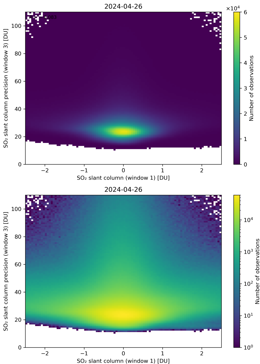
Figure 238: Scatter density plot of “SO 2 slant column (window 1)” against “SO 2 slant column precision (window 3)” for 2024-04-26 to 2024-04-27.
