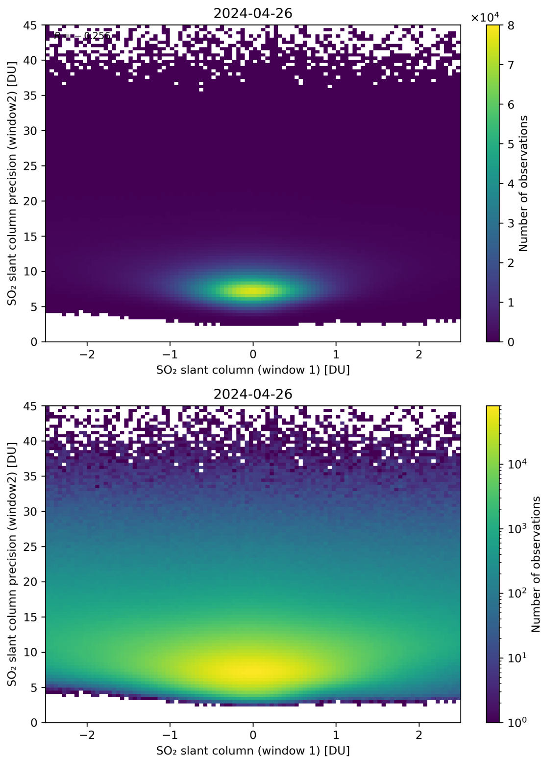
Figure 236: Scatter density plot of “SO 2 slant column (window 1)” against “SO 2 slant column precision (window2)” for 2024-04-26 to 2024-04-27.
