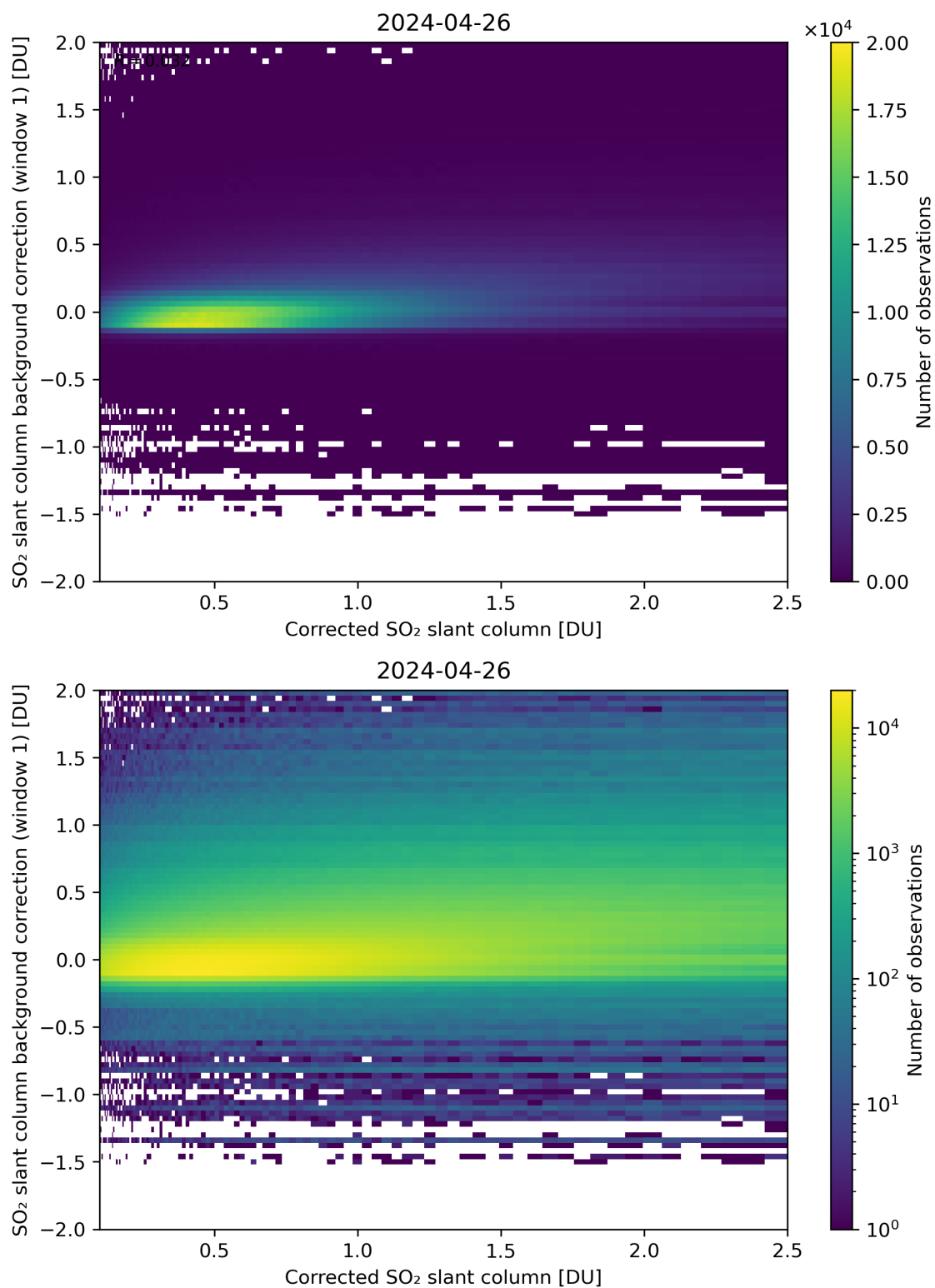
Figure 178: Scatter density plot of “Corrected SO 2 slant column” against “SO 2 slant column background correction (window 1)” for 2024-04-26 to 2024-04-27.
