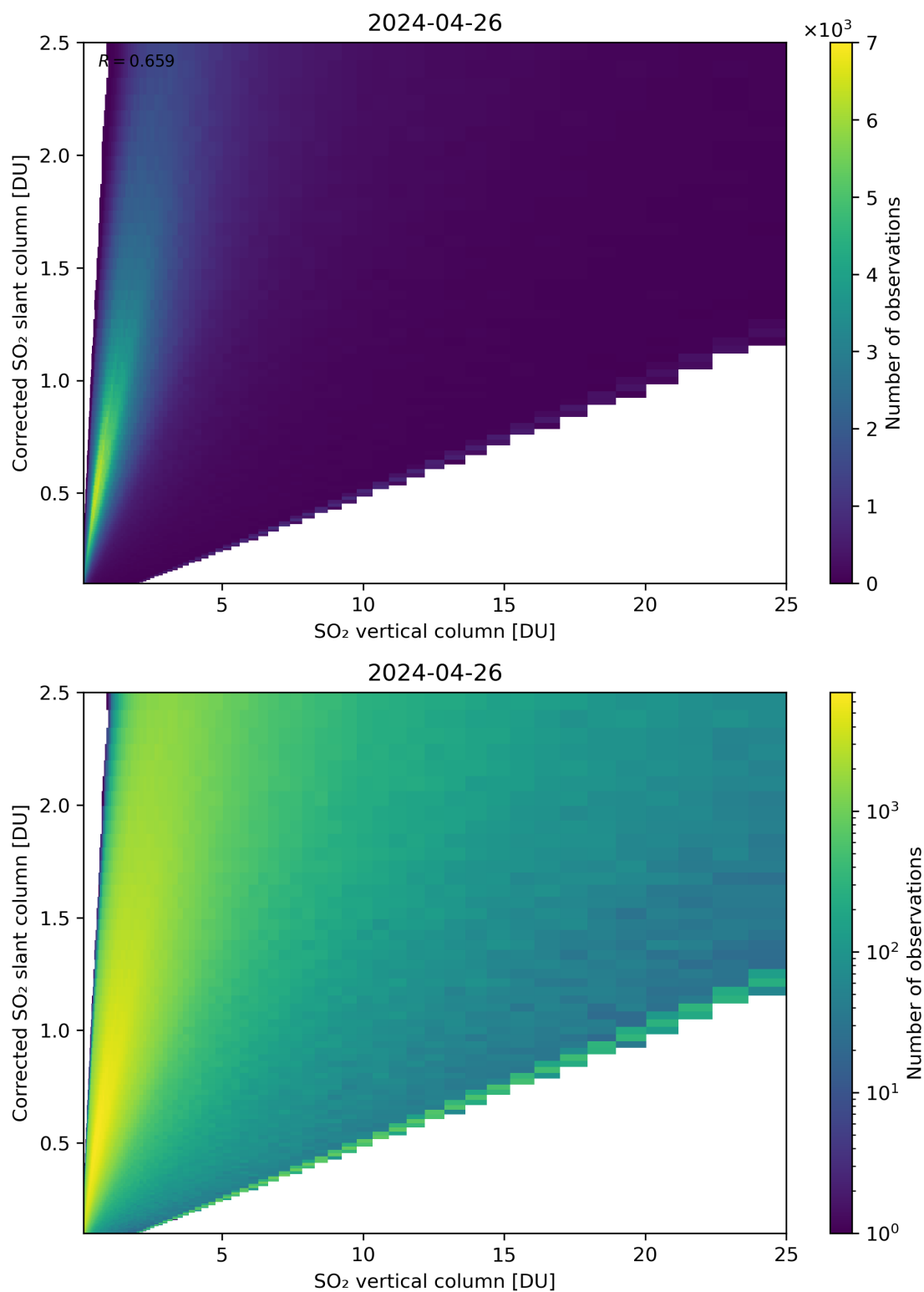
Figure 297: Scatter density plot of “SO 2 vertical column” against “Corrected SO 2 slant column” for 2024-04-26 to 2024-04-27.
