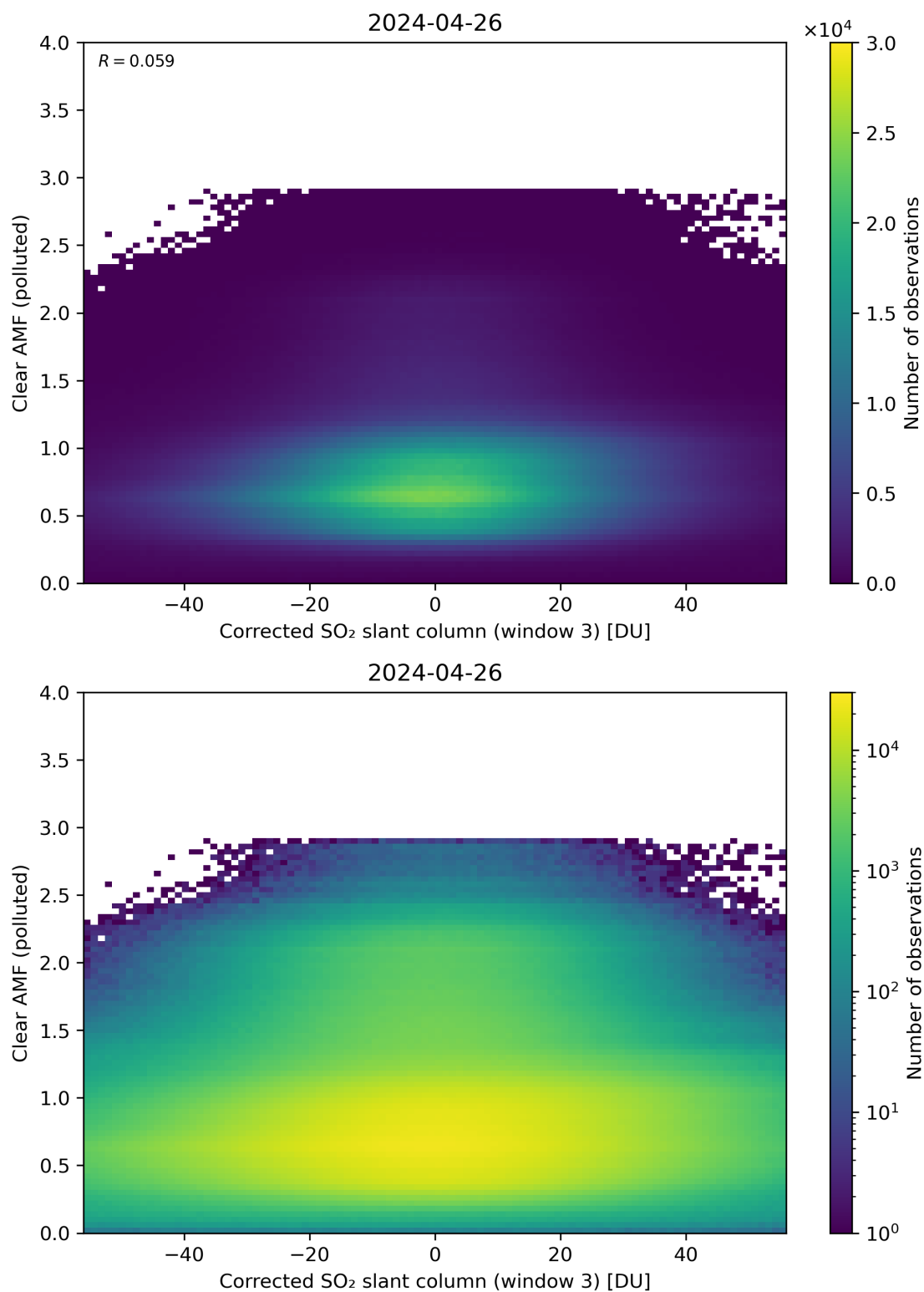
Figure 209: Scatter density plot of “Corrected SO 2 slant column (window 3)” against “Clear AMF (polluted)” for 2024-04-26 to 2024-04-27.
