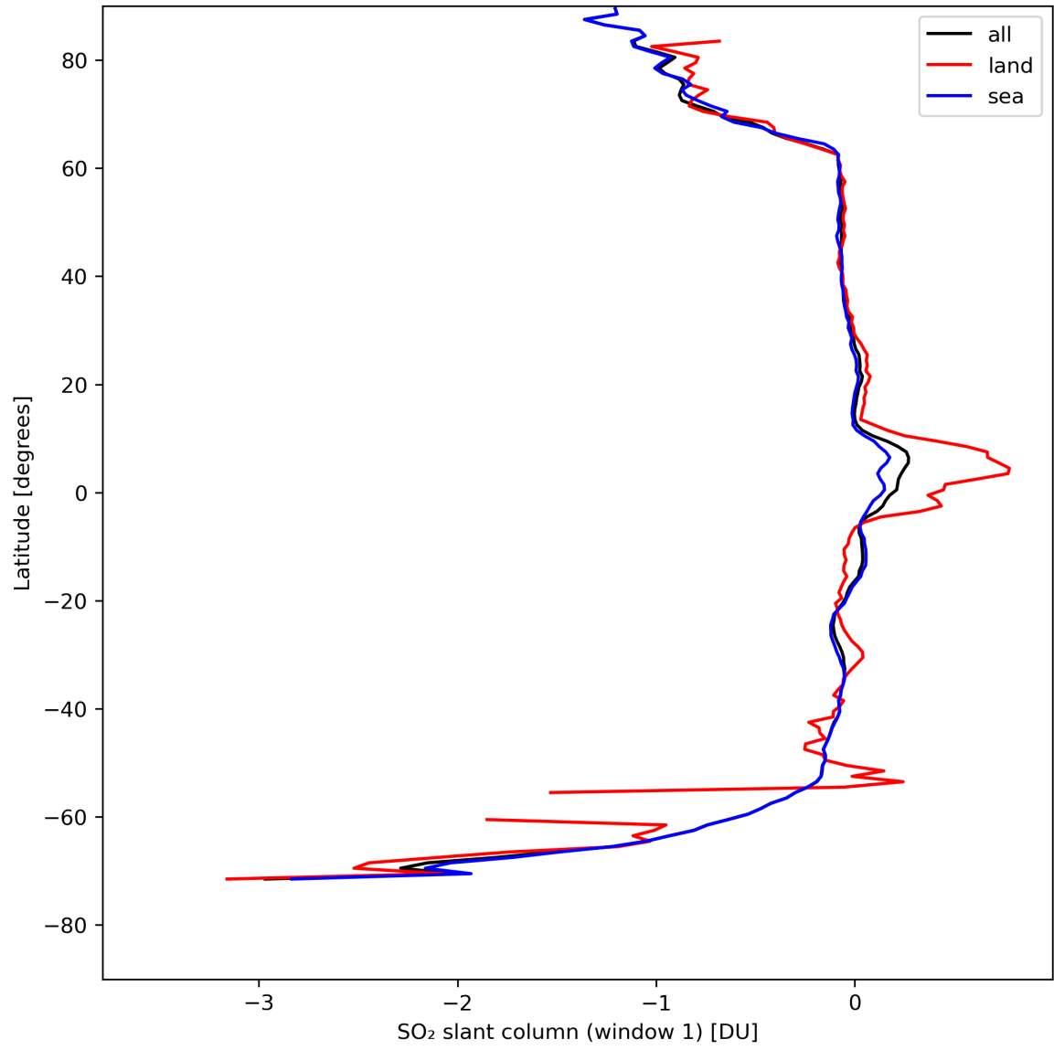
Figure 33: Zonal average of “SO 2 slant column (window 1)” for 2024-04-26 to 2024-04-27.
