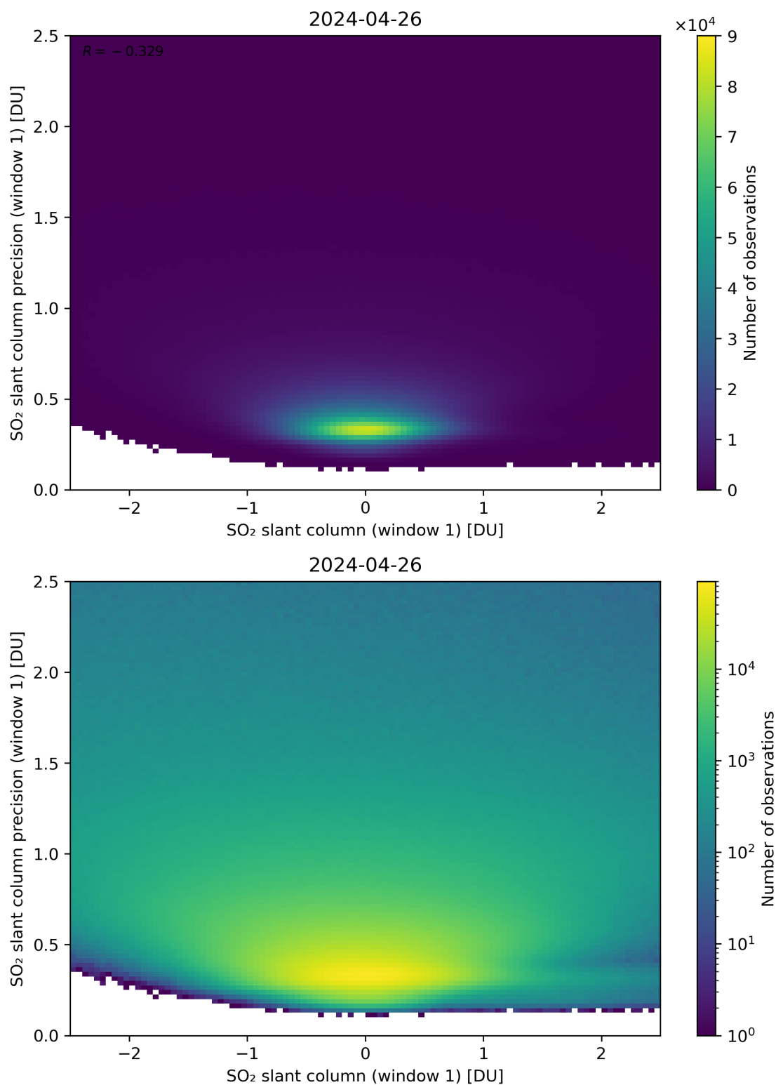
Figure 235: Scatter density plot of “SO 2 slant column (window 1)” against “SO 2 slant column precision (window 1)” for 2024-04-26 to 2024-04-27.
