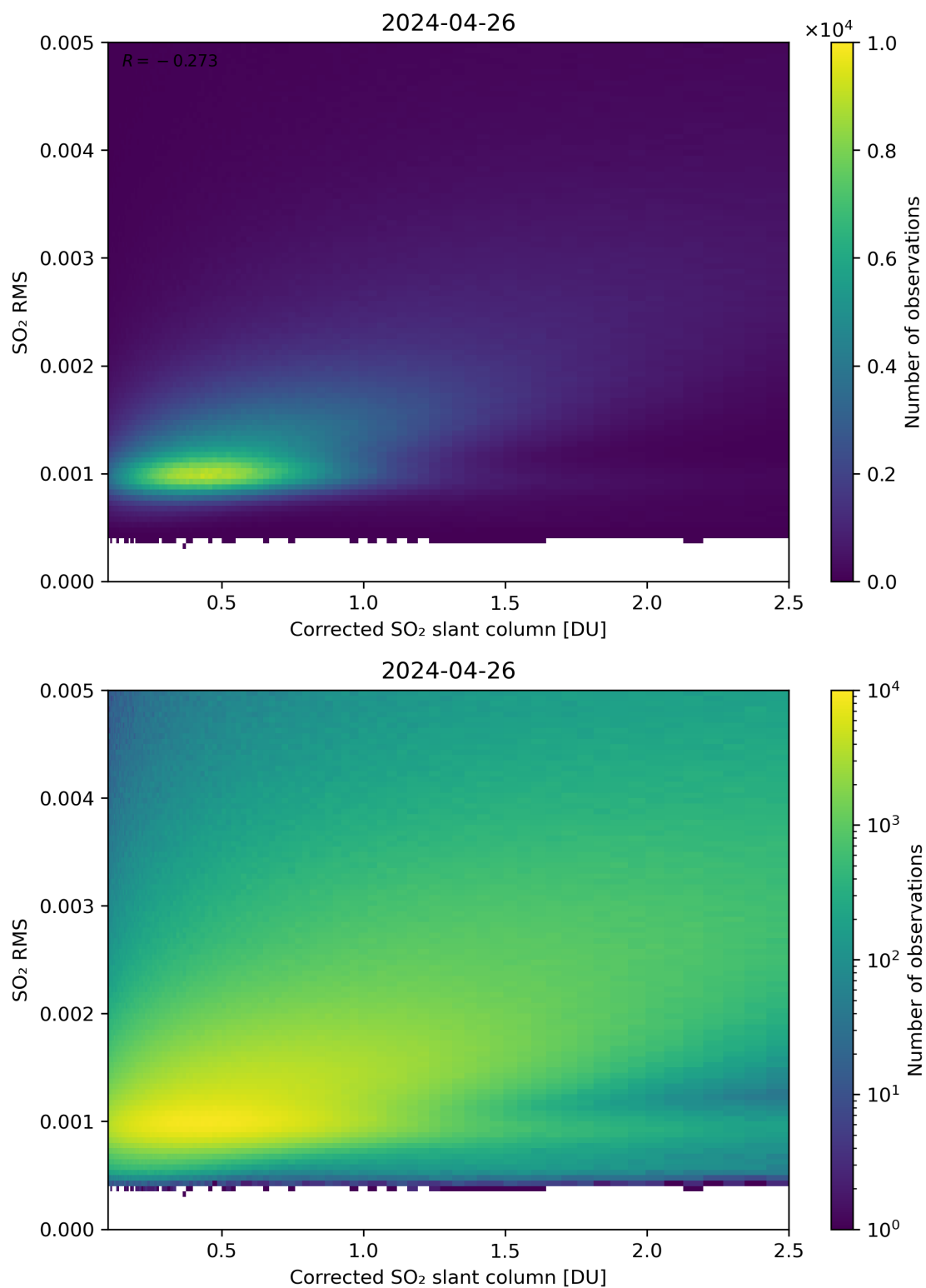
Figure 183: Scatter density plot of “Corrected SO 2 slant column” against “SO 2 RMS” for 2024-04-26 to 2024-04-27.
