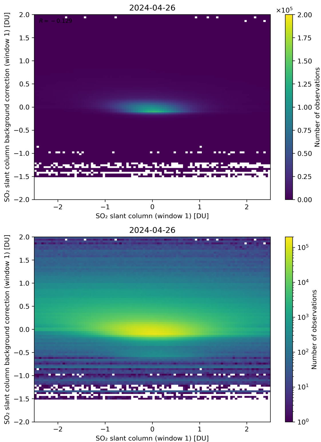
Figure 212: Scatter density plot of “SO 2 slant column (window 1)” against “SO 2 slant column background correction (window 1)” for 2024-04-26 to 2024-04-27.
