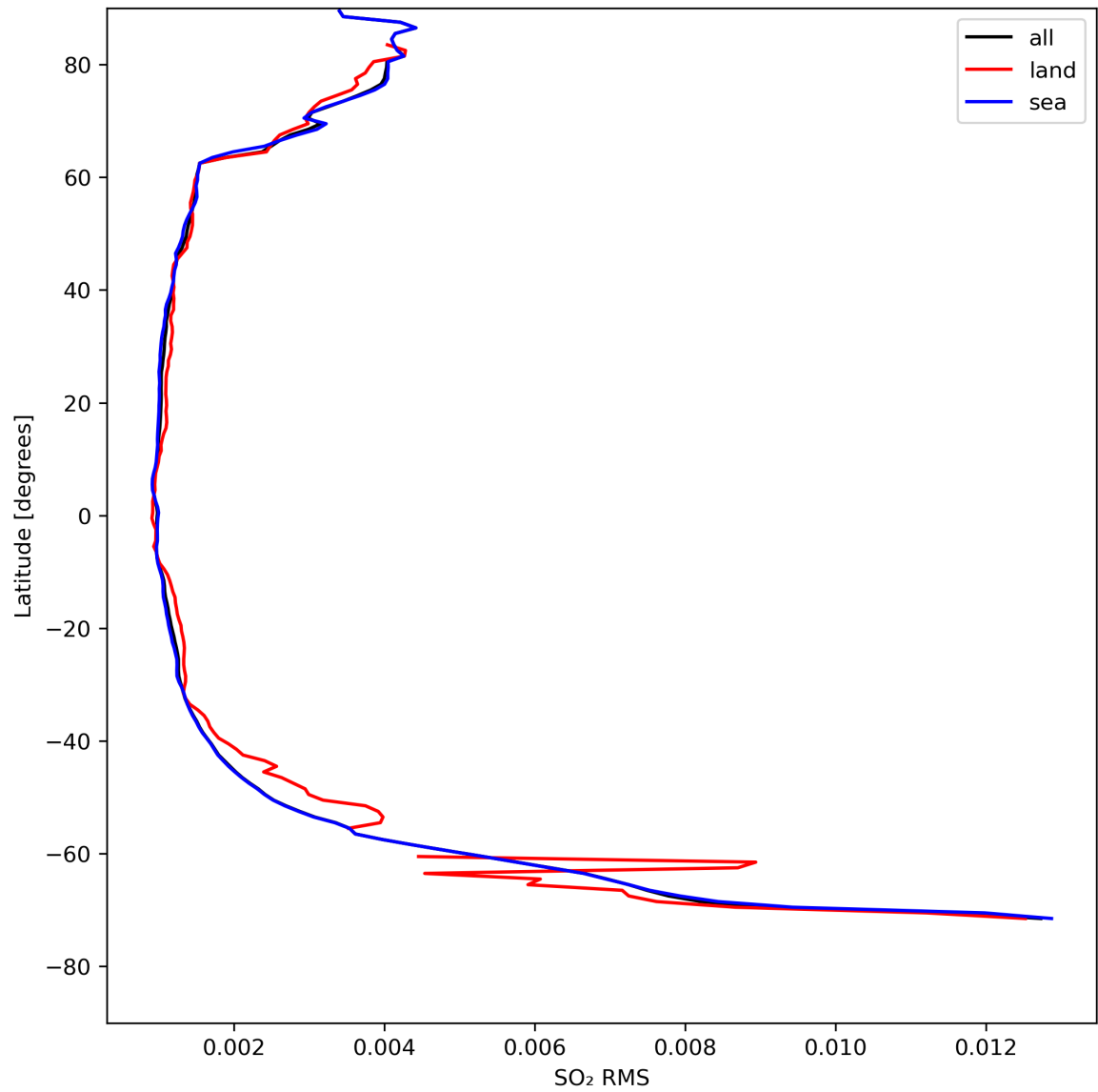
Figure 47: Zonal average of “SO 2 RMS” for 2024-04-26 to 2024-04-27.
