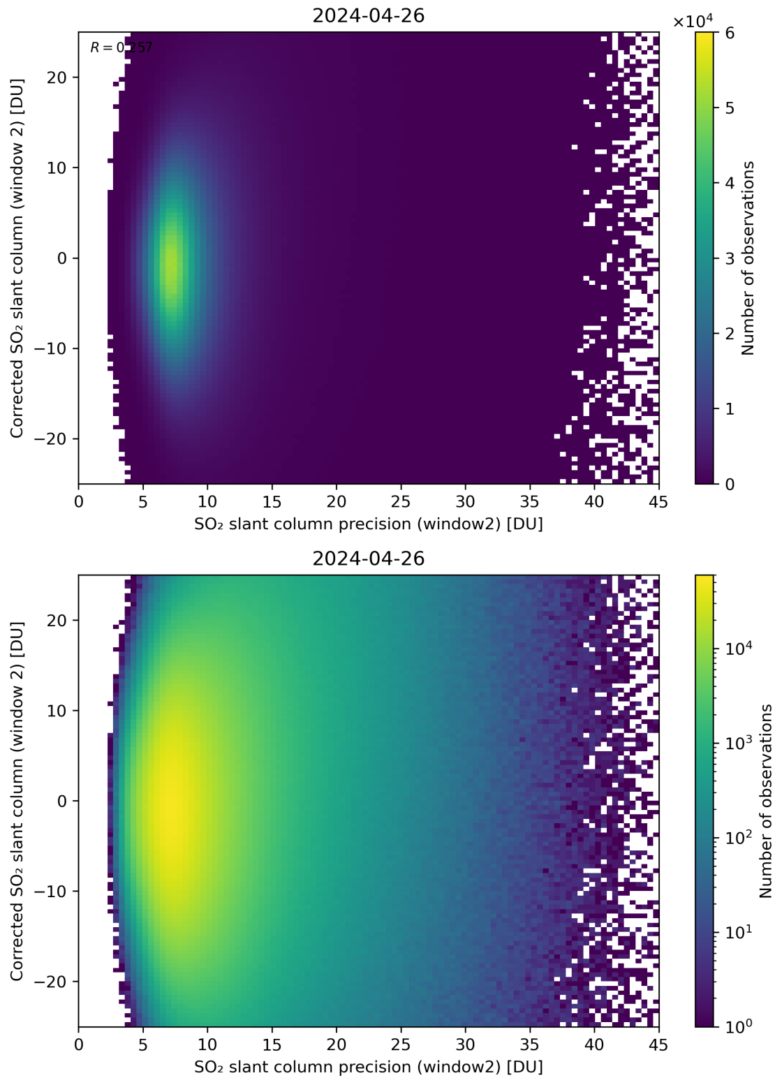
Figure 247: Scatter density plot of “SO 2 slant column precision (window2)” against “Corrected SO 2 slant column (window 2)” for 2024-04-26 to 2024-04-27.
