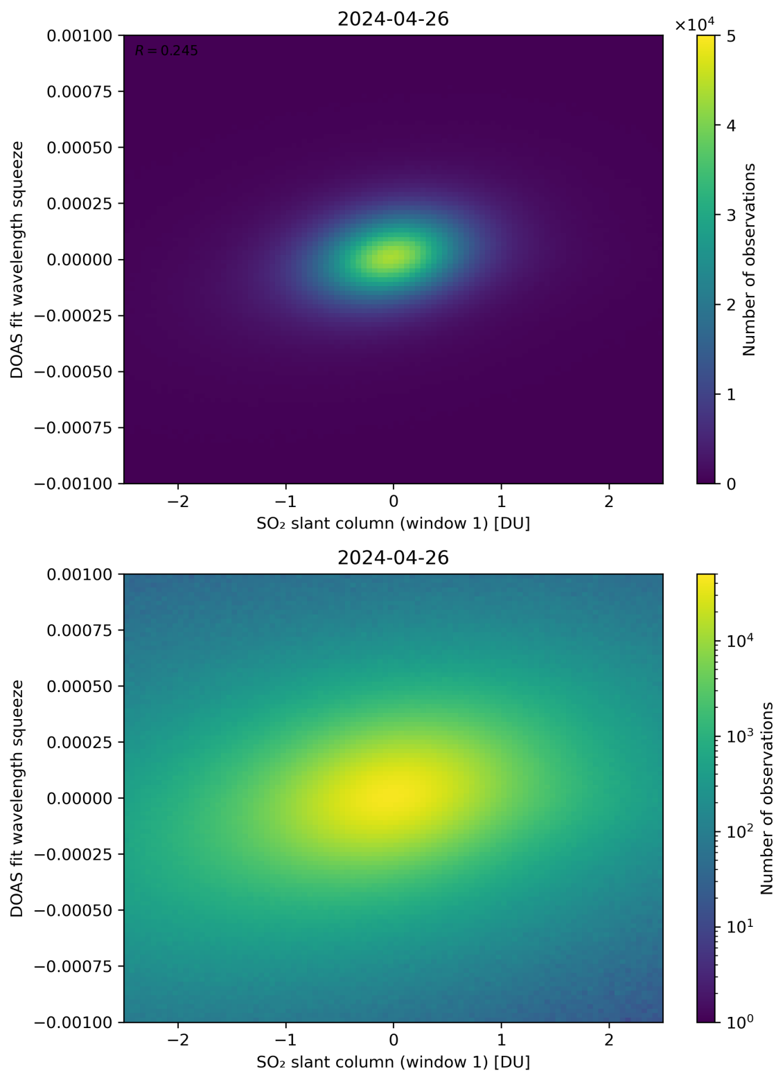
Figure 216: Scatter density plot of “SO 2 slant column (window 1)” against “DOAS fit wavelength squeeze” for 2024-04-26 to 2024-04-27.
