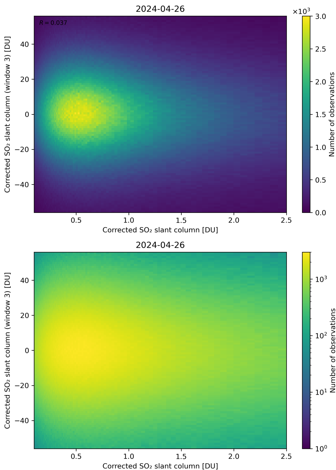
Figure 186: Scatter density plot of “Corrected SO 2 slant column” against “Corrected SO 2 slant column (window 3)” for 2024-04-26 to 2024-04-27.
