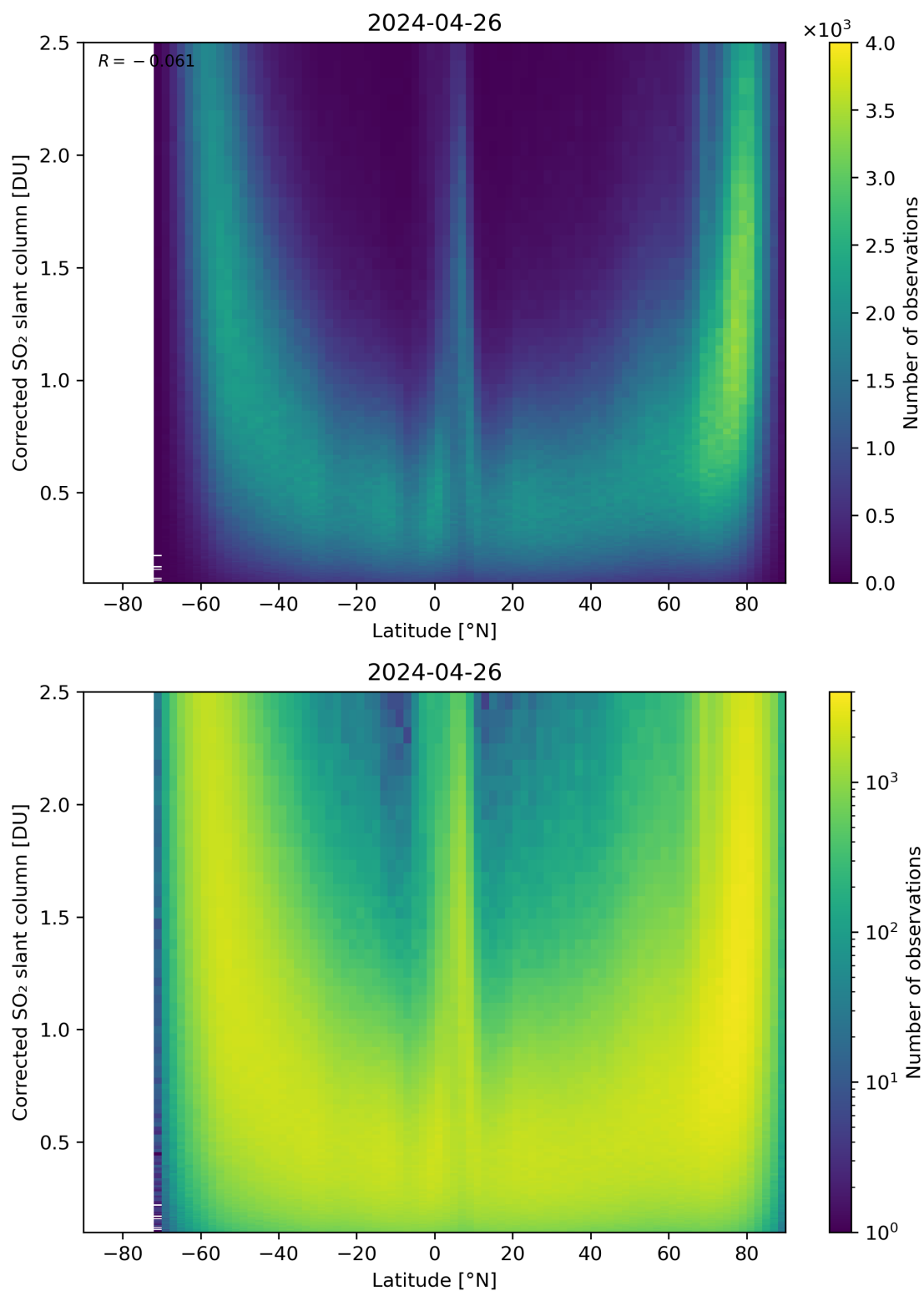
Figure 146: Scatter density plot of “Latitude” against “Corrected SO 2 slant column” for 2024-04-26 to 2024-04-27.
