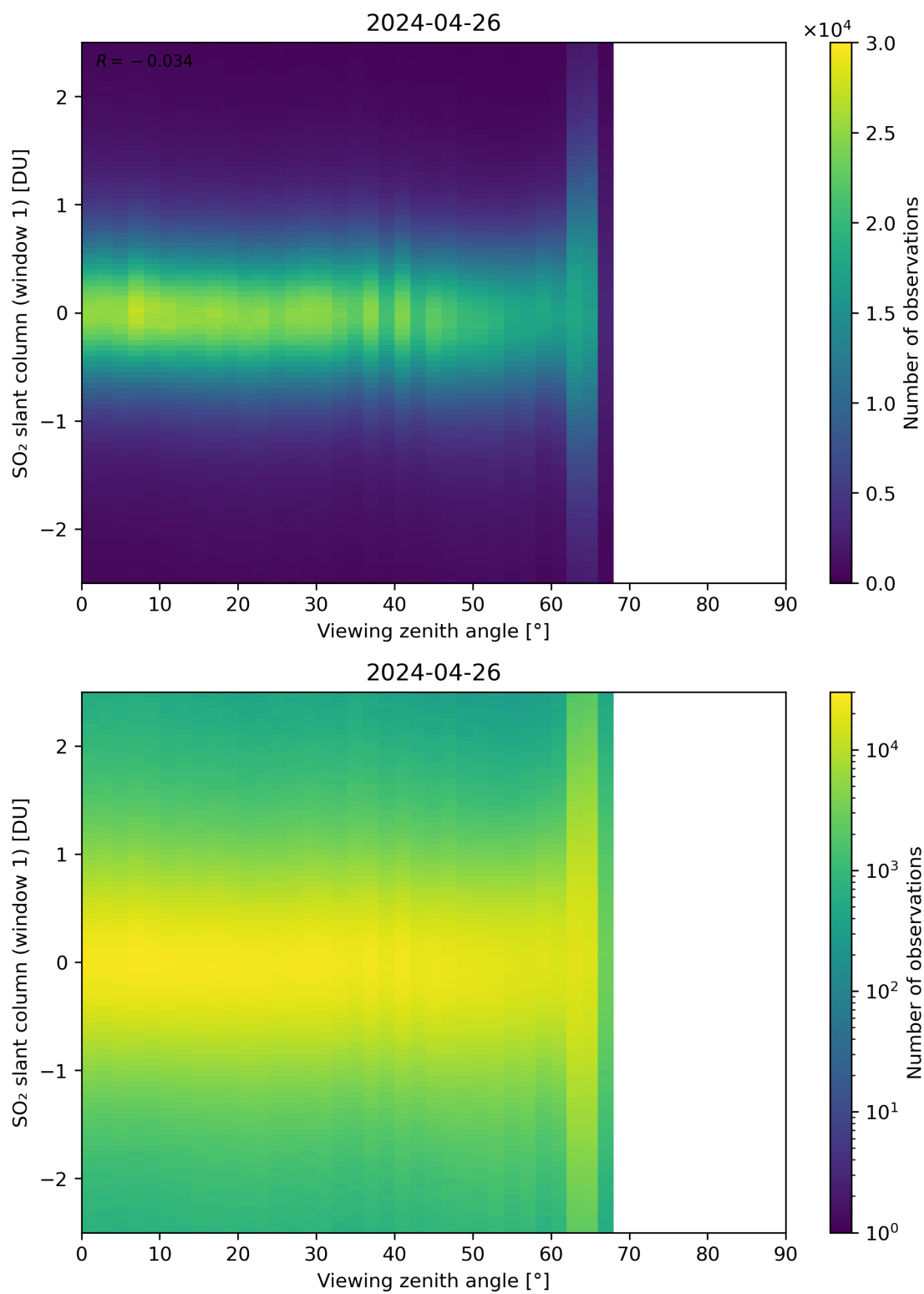
Figure 320: Scatter density plot of “Viewing zenith angle” against “SO 2 slant column (window 1)” for 2024-04-26 to 2024-04-27.
