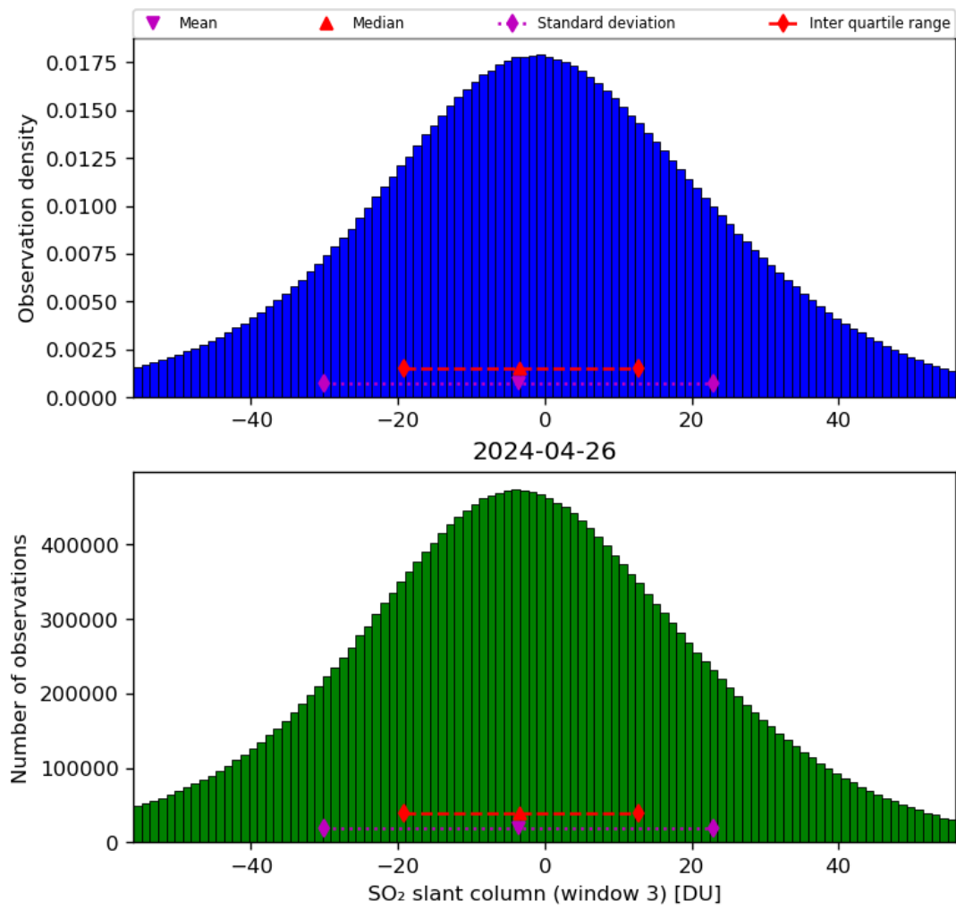
Figure 64: Histogram of “SO 2 slant column (window 3)” for 2024-04-26 to 2024-04-27
