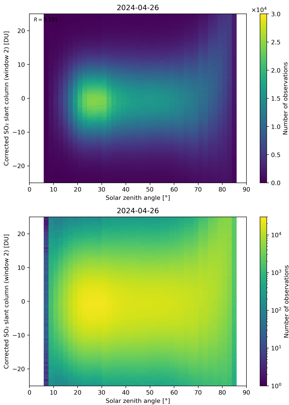
Figure 167: Scatter density plot of “Solar zenith angle” against “Corrected SO 2 slant column (window 2)” for 2024-04-26 to 2024-04-27.
