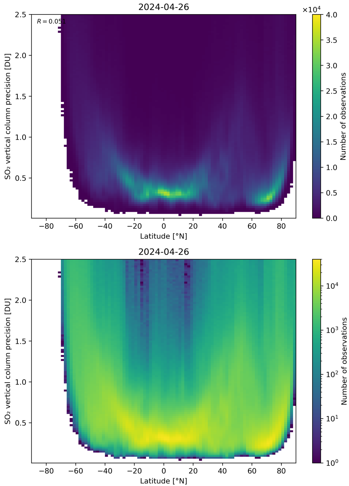
Figure 157: Scatter density plot of “Latitude” against “SO 2 vertical column precision” for 2024-04-26 to 2024-04-27.
