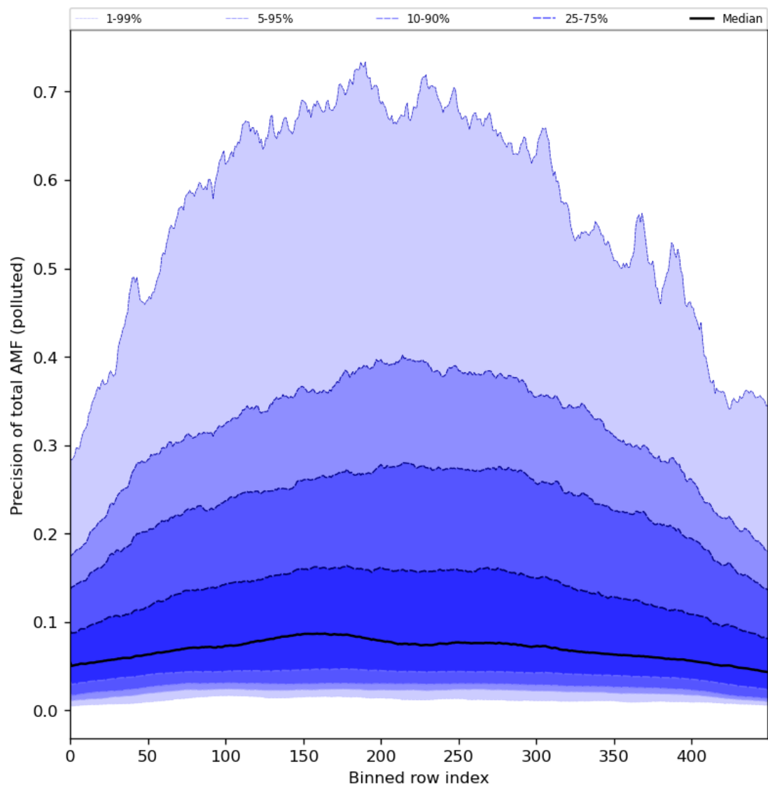
Figure 95: Along track statistics of “Precision of total AMF (polluted)” for 2024-04-26 to 2024-04-27
