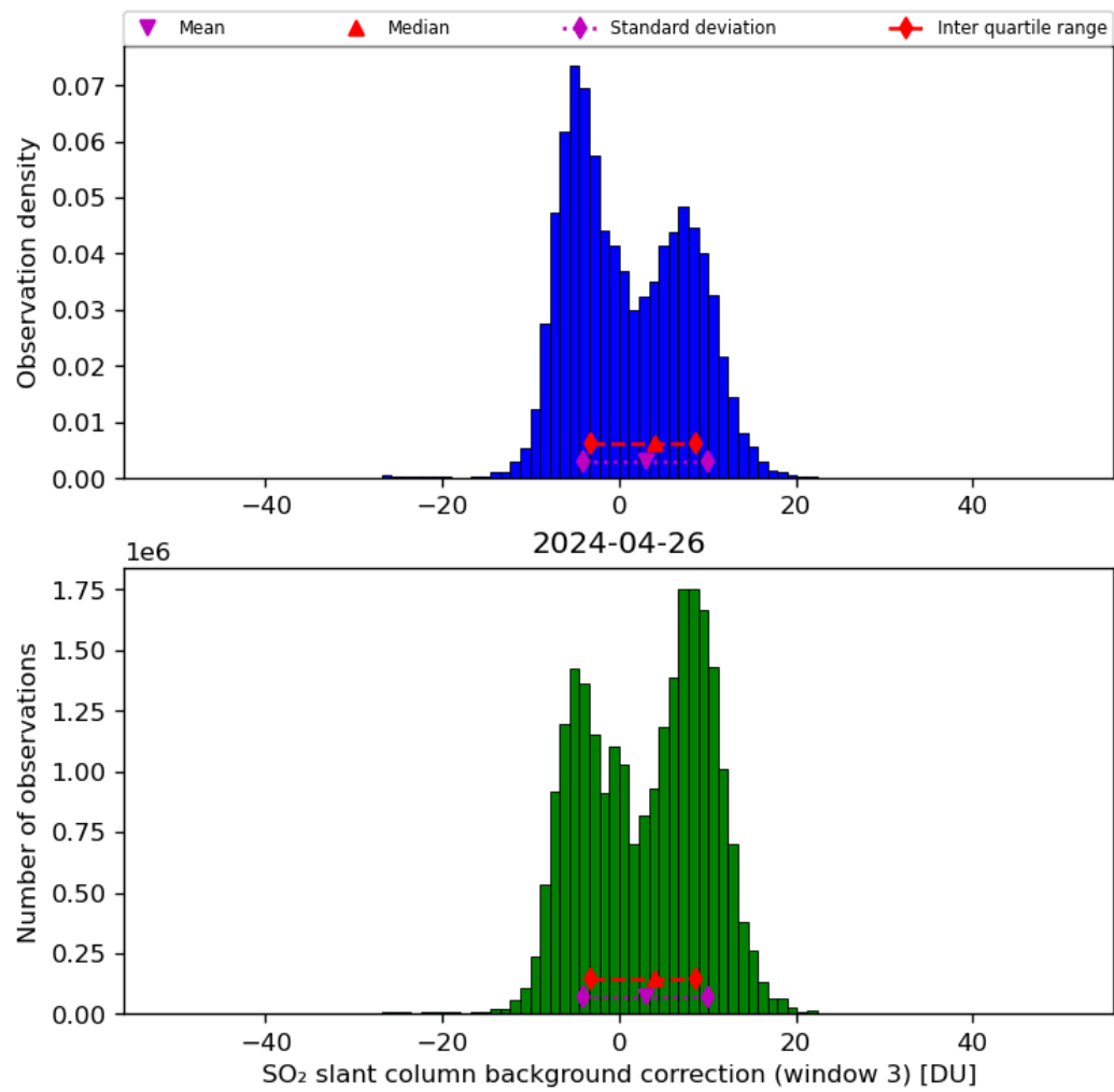
Figure 67: Histogram of “SO 2 slant column background correction (window 3)” for 2024-04-26 to 2024-04-27
