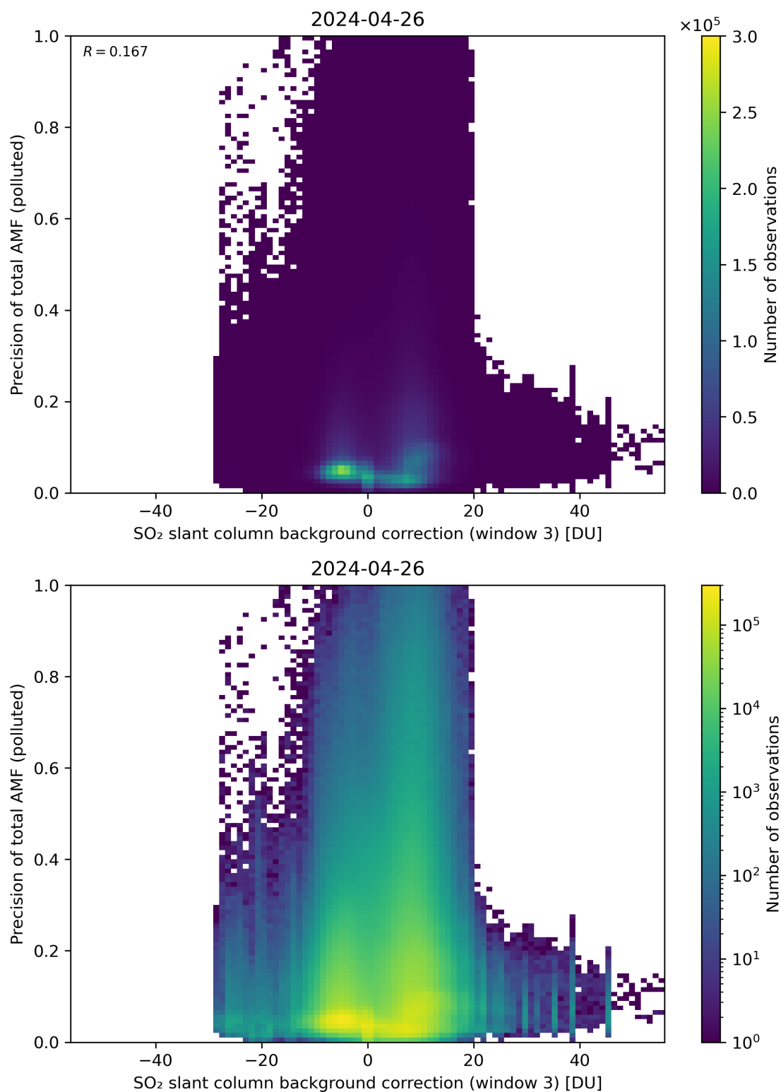
Figure 126: Scatter density plot of “SO 2 slant column background correction (window 3)” against “Precision of total AMF (polluted)” for 2024-04-26 to 2024-04-27.
