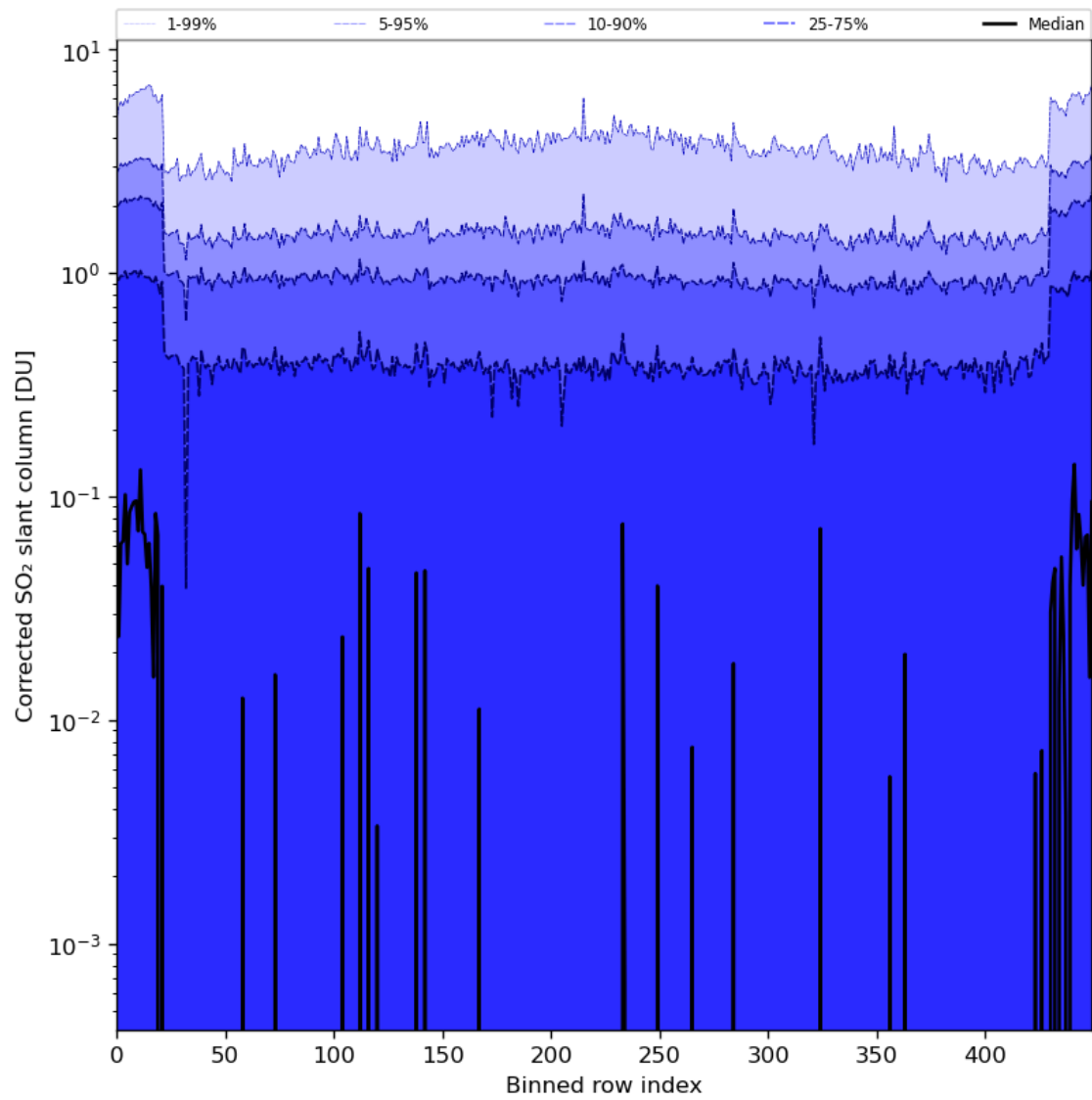
Figure 78: Along track statistics of “Corrected SO 2 slant column” for 2024-04-26 to 2024-04-27
