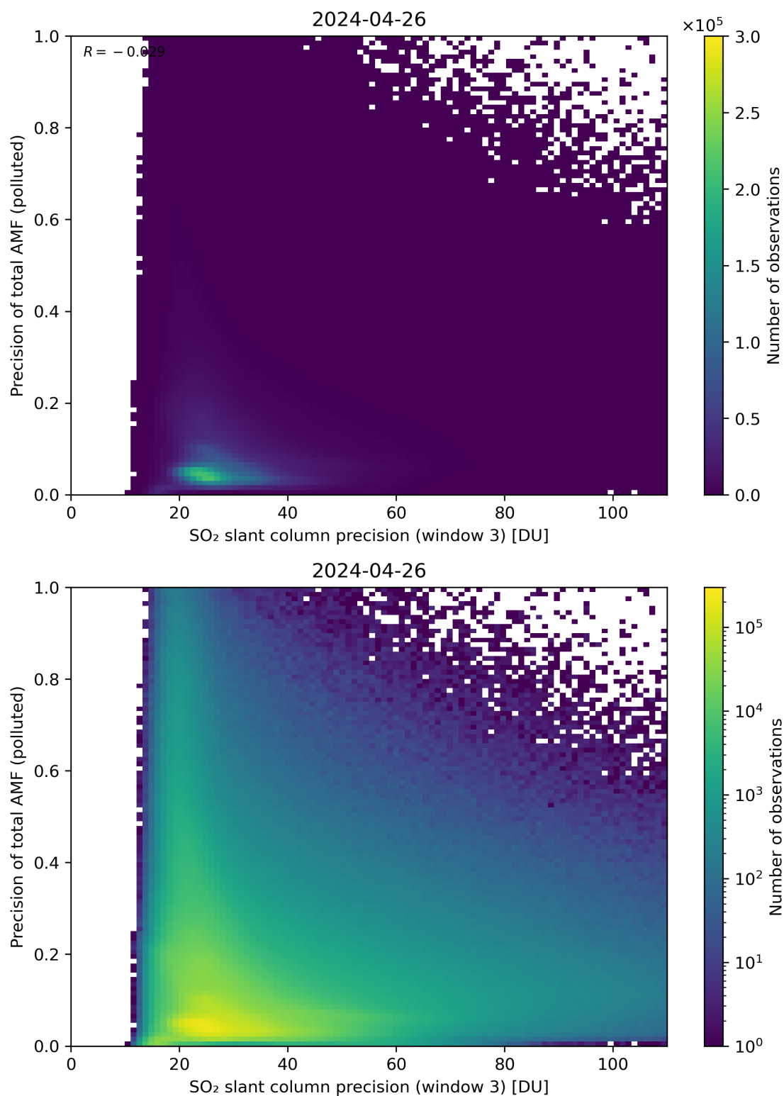
Figure 264: Scatter density plot of “SO 2 slant column precision (window 3)” against “Precision of total AMF (polluted)” for 2024-04-26 to 2024-04-27.
