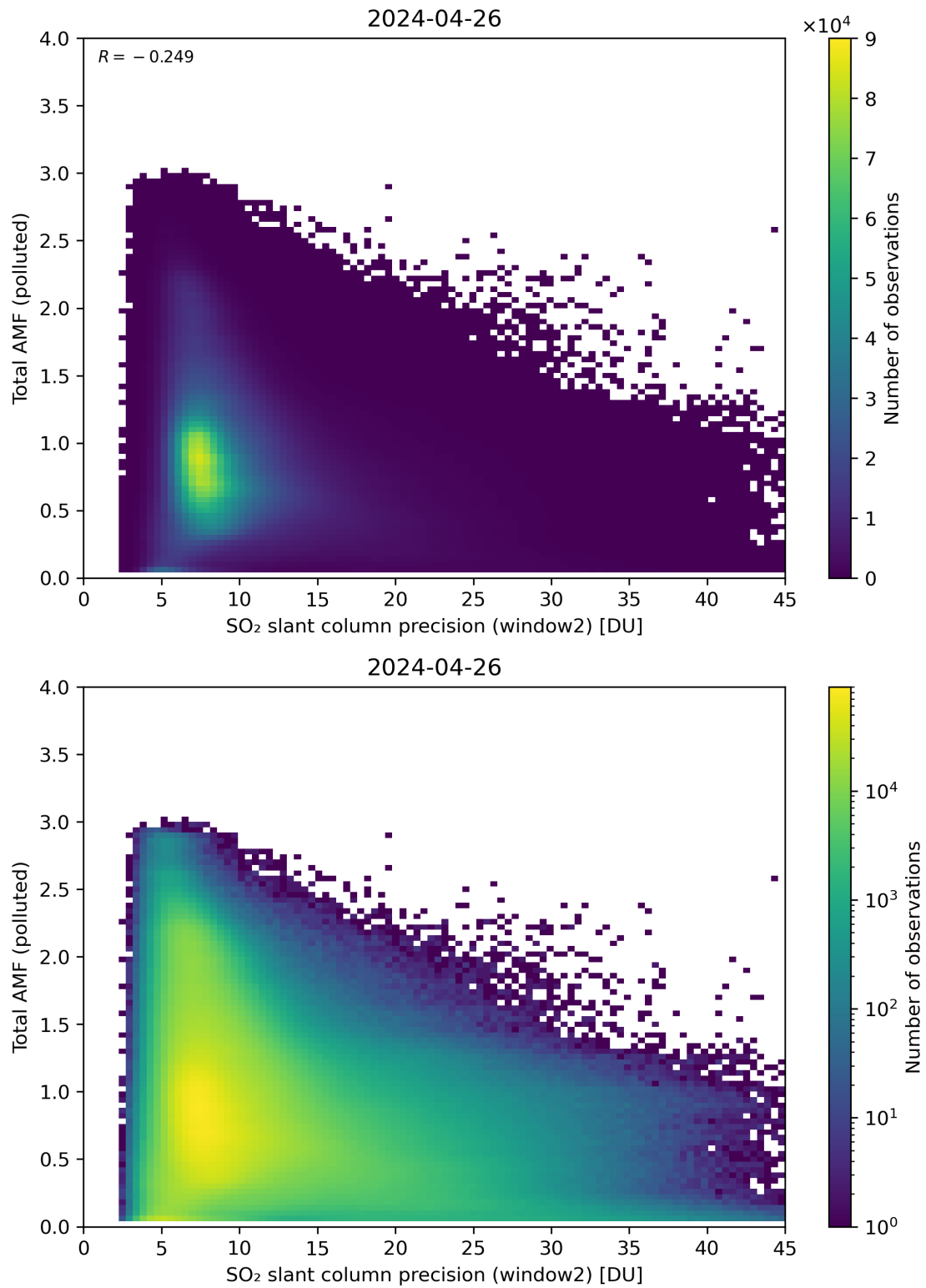
Figure 251: Scatter density plot of “SO 2 slant column precision (window2)” against “Total AMF (polluted)” for 2024-04-26 to 2024-04-27.
