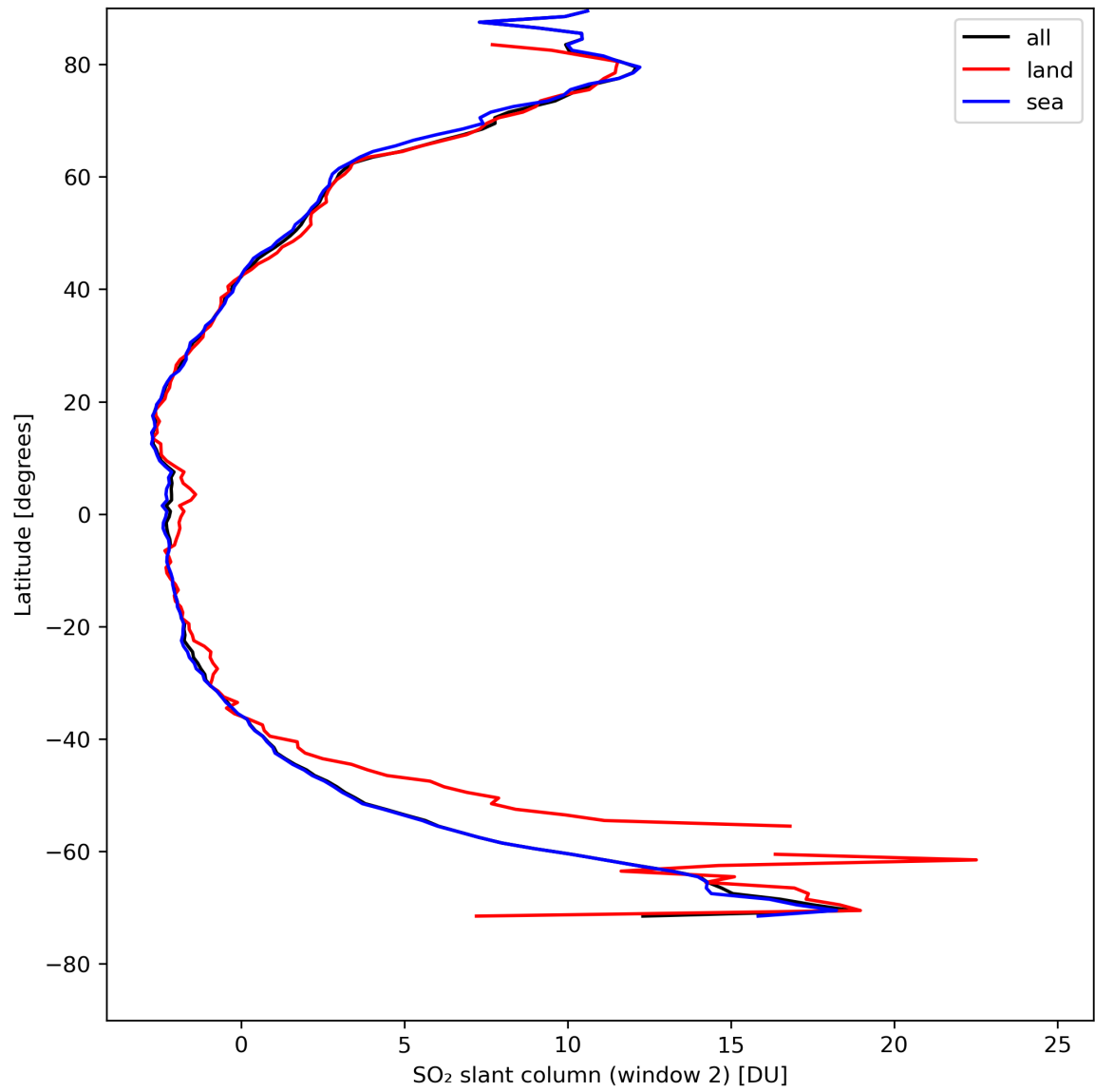
Figure 37: Zonal average of “SO 2 slant column (window 2)” for 2024-04-26 to 2024-04-27.
