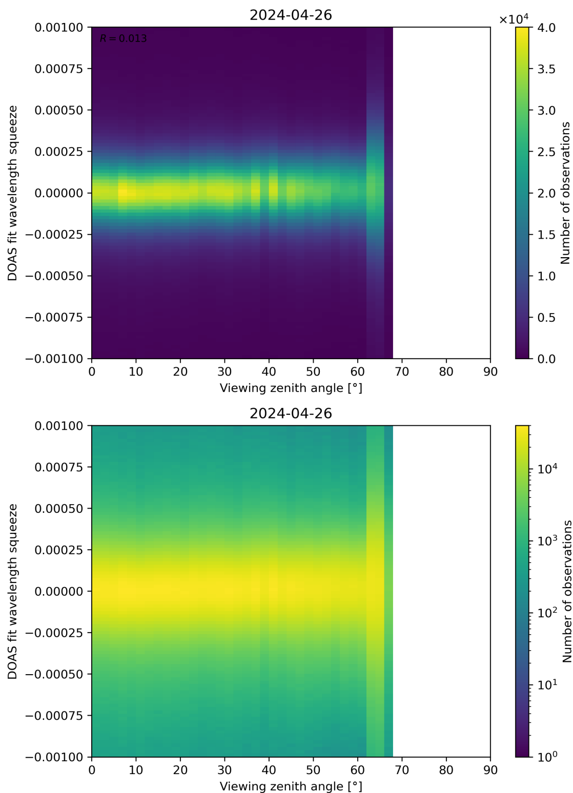
Figure 312: Scatter density plot of “Viewing zenith angle” against “DOAS fit wavelength squeeze” for 2024-04-26 to 2024-04-27.
