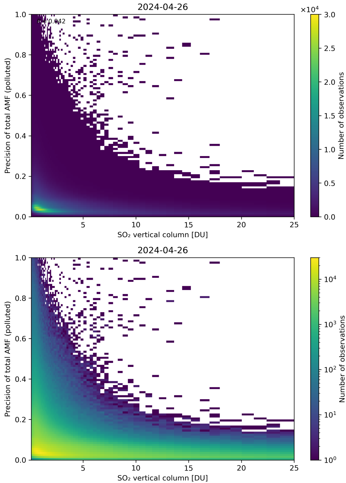
Figure 306: Scatter density plot of “SO 2 vertical column” against “Precision of total AMF (polluted)” for 2024-04-26 to 2024-04-27.
