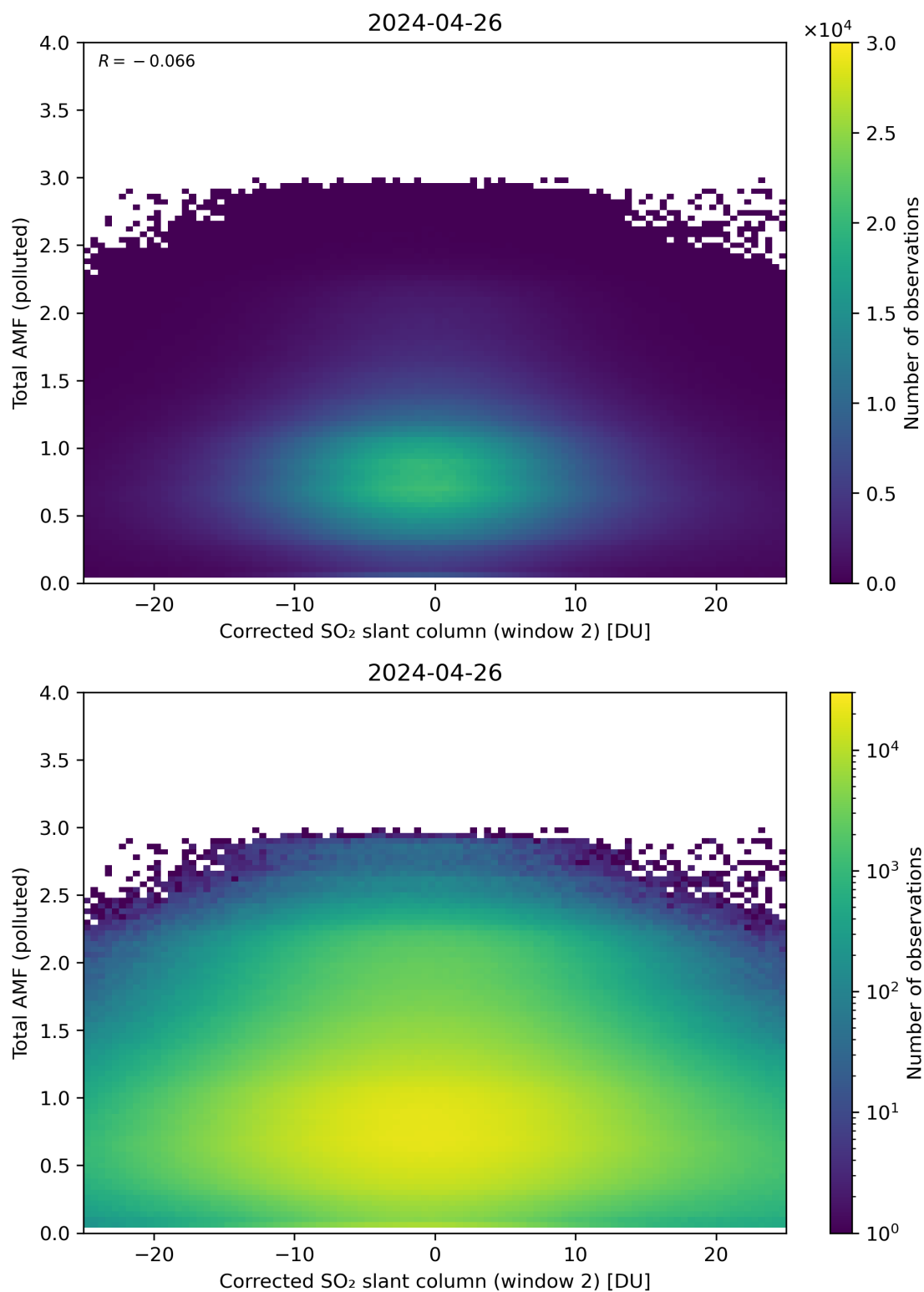
Figure 203: Scatter density plot of “Corrected SO 2 slant column (window 2)” against “Total AMF (polluted)” for 2024-04-26 to 2024-04-27.
