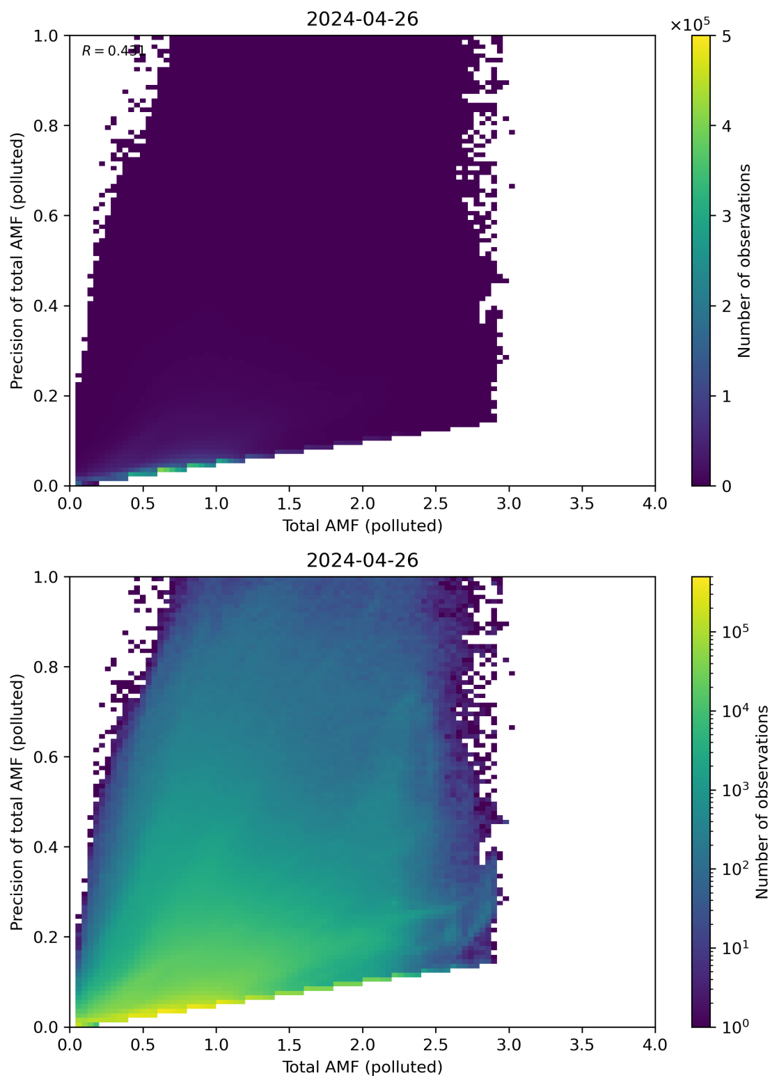
Figure 272: Scatter density plot of “Total AMF (polluted)” against “Precision of total AMF (polluted)” for 2024-04-26 to 2024-04-27.
