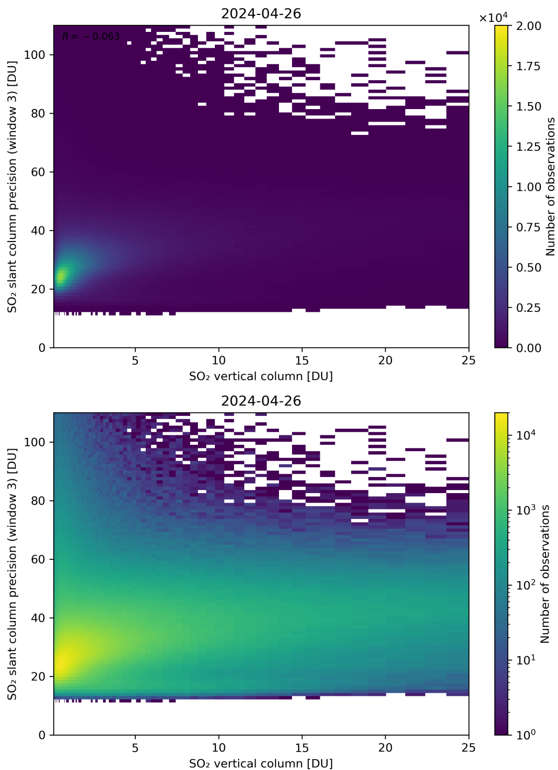
Figure 304: Scatter density plot of “SO 2 vertical column” against “SO 2 slant column precision (window 3)” for 2024-04-26 to 2024-04-27.
