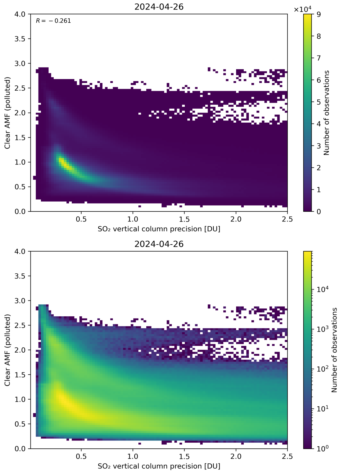
Figure 285: Scatter density plot of “SO 2 vertical column precision” against “Clear AMF (polluted)” for 2024-04-26 to 2024-04-27.
