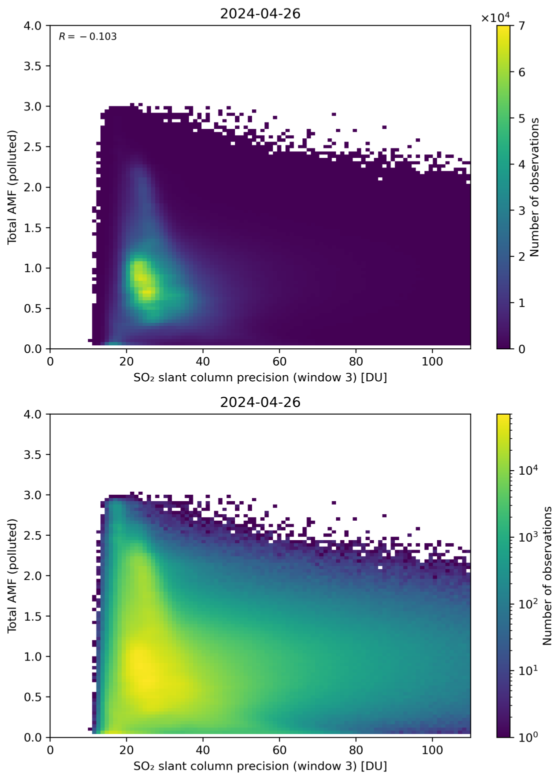
Figure 263: Scatter density plot of “SO 2 slant column precision (window 3)” against “Total AMF (polluted)” for 2024-04-26 to 2024-04-27.
