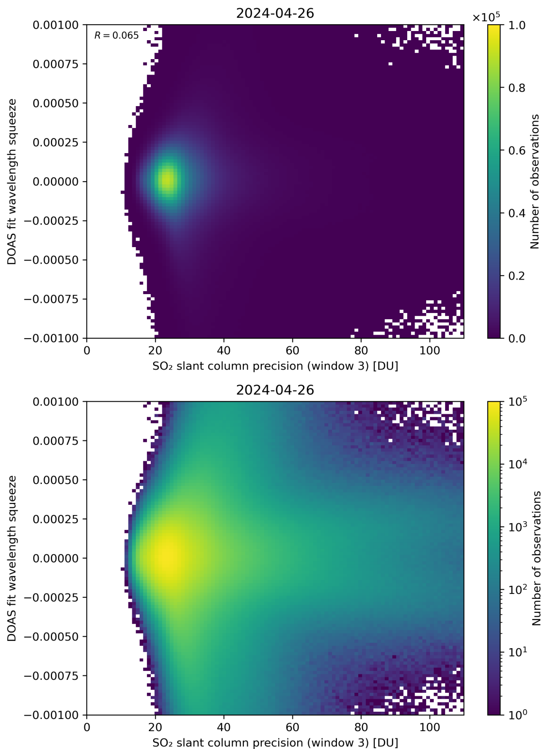
Figure 259: Scatter density plot of “SO 2 slant column precision (window 3)” against “DOAS fit wavelength squeeze” for 2024-04-26 to 2024-04-27.
