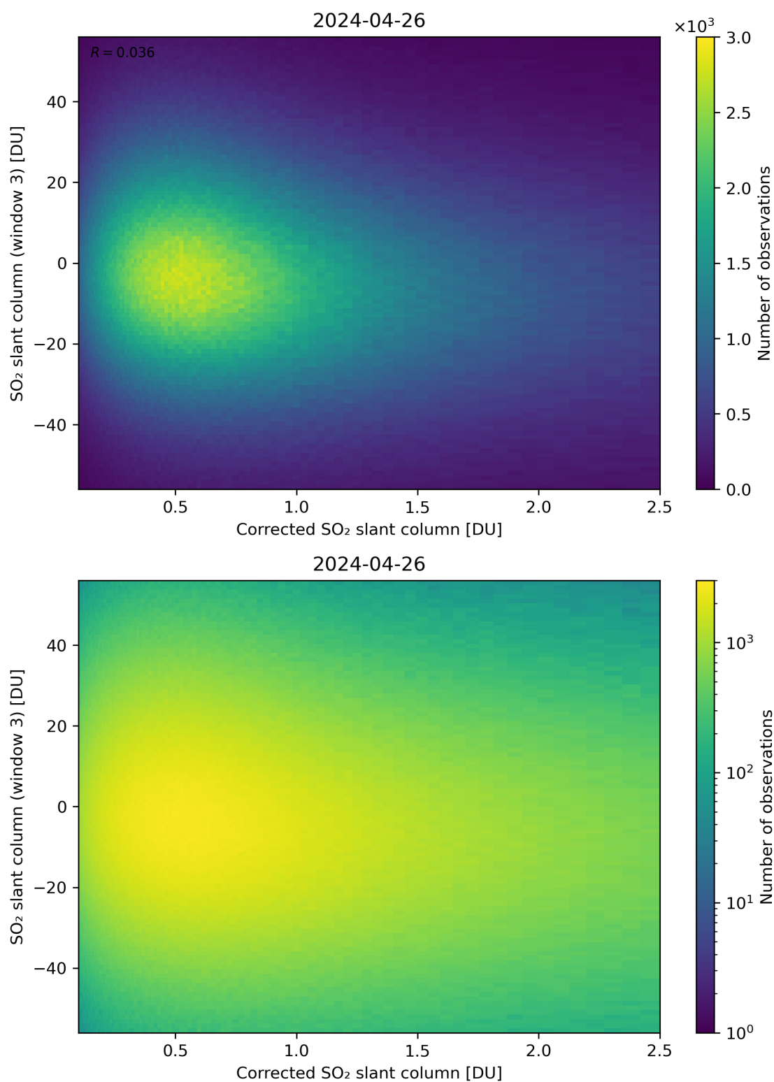
Figure 190: Scatter density plot of “Corrected SO 2 slant column” against “SO 2 slant column (window 3)” for 2024-04-26 to 2024-04-27.
