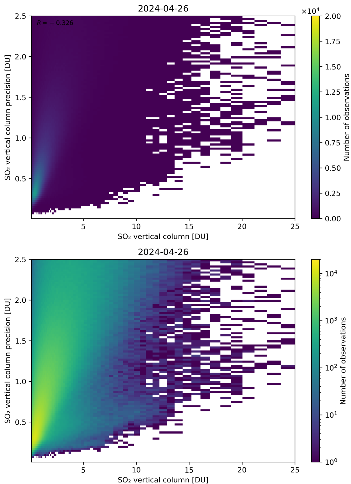
Figure 307: Scatter density plot of “SO 2 vertical column” against “SO 2 vertical column precision” for 2024-04-26 to 2024-04-27.
