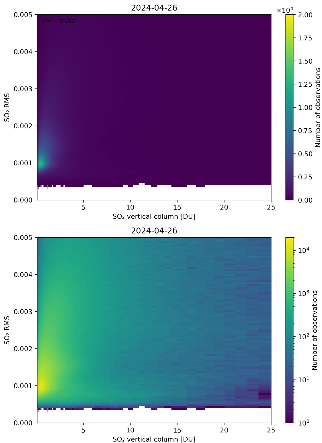
Figure 278: Scatter density plot of “SO 2 vertical column” against “SO 2 RMS” for 2024-04-26 to 2024-04-27.
