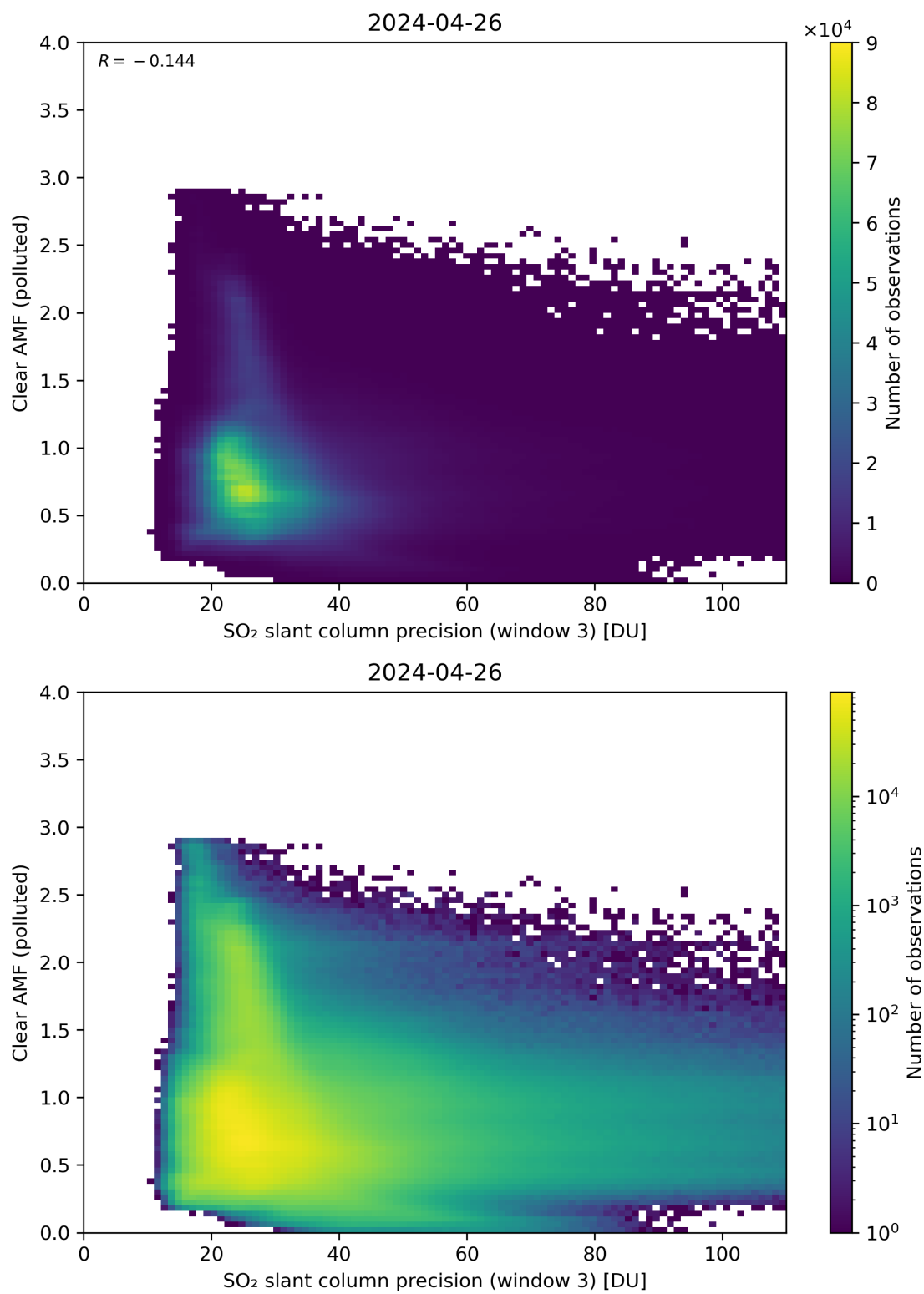
Figure 261: Scatter density plot of “SO 2 slant column precision (window 3)” against “Clear AMF (polluted)” for 2024-04-26 to 2024-04-27.
