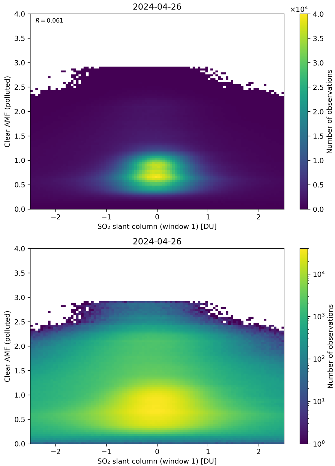
Figure 232: Scatter density plot of “SO 2 slant column (window 1)” against “Clear AMF (polluted)” for 2024-04-26 to 2024-04-27.
