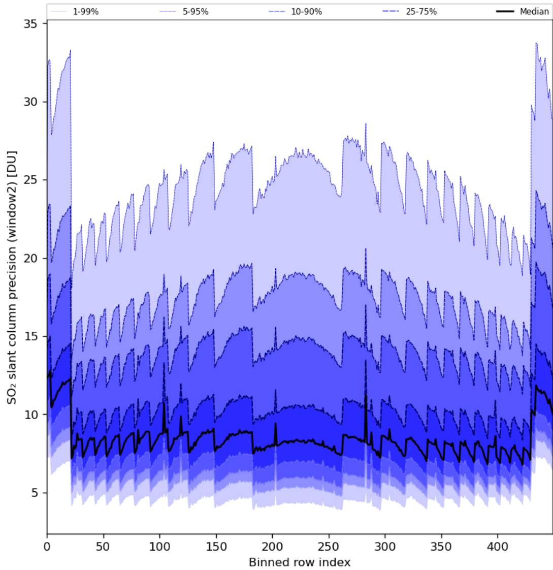
Figure 84: Along track statistics of “SO 2 slant column precision (window2)” for 2024-04-26 to 2024-04-27
