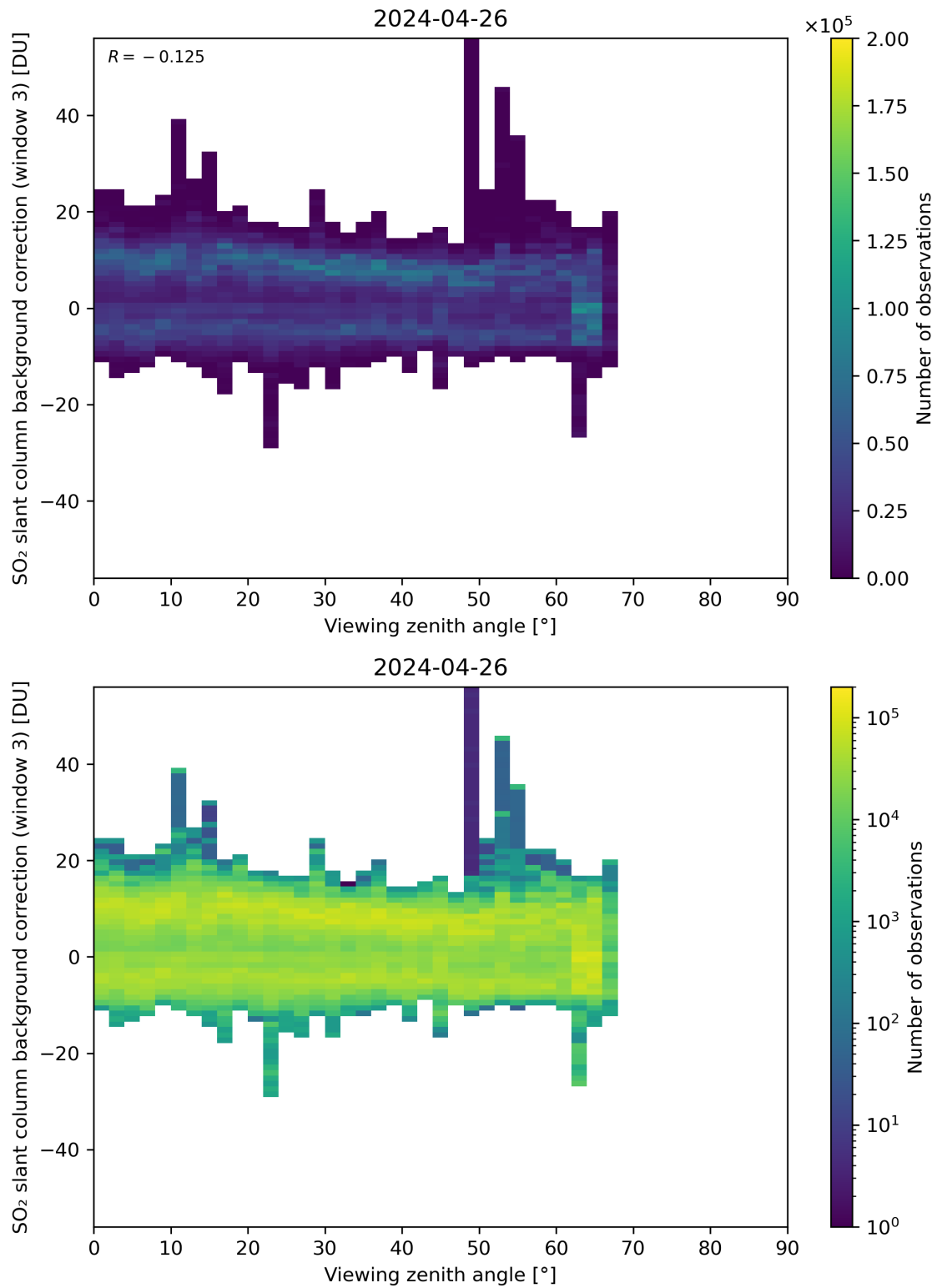
Figure 310: Scatter density plot of “Viewing zenith angle” against “SO 2 slant column background correction (window 3)” for 2024-04-26 to 2024-04-27.
