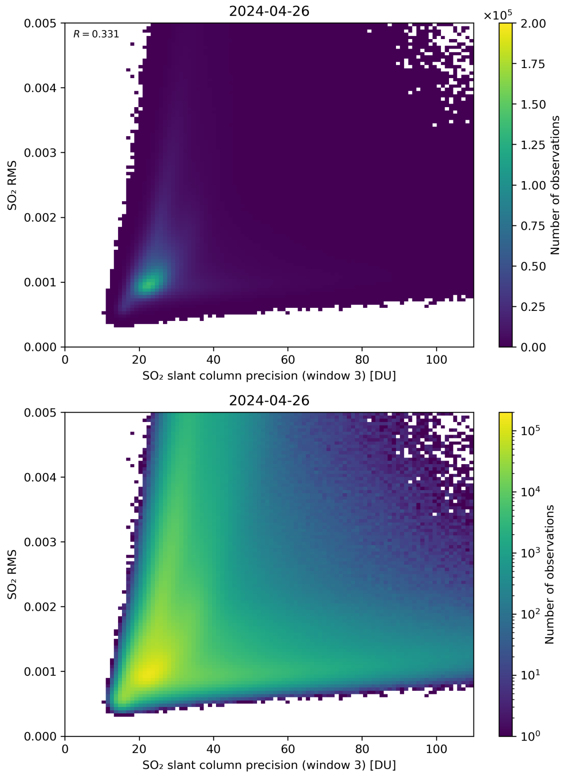
Figure 260: Scatter density plot of “SO 2 slant column precision (window 3)” against “SO 2 RMS” for 2024-04-26 to 2024-04-27.
