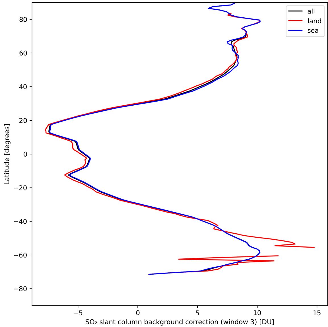
Figure 44: Zonal average of “SO 2 slant column background correction (window 3)” for 2024-04-26 to 2024-04-27.
