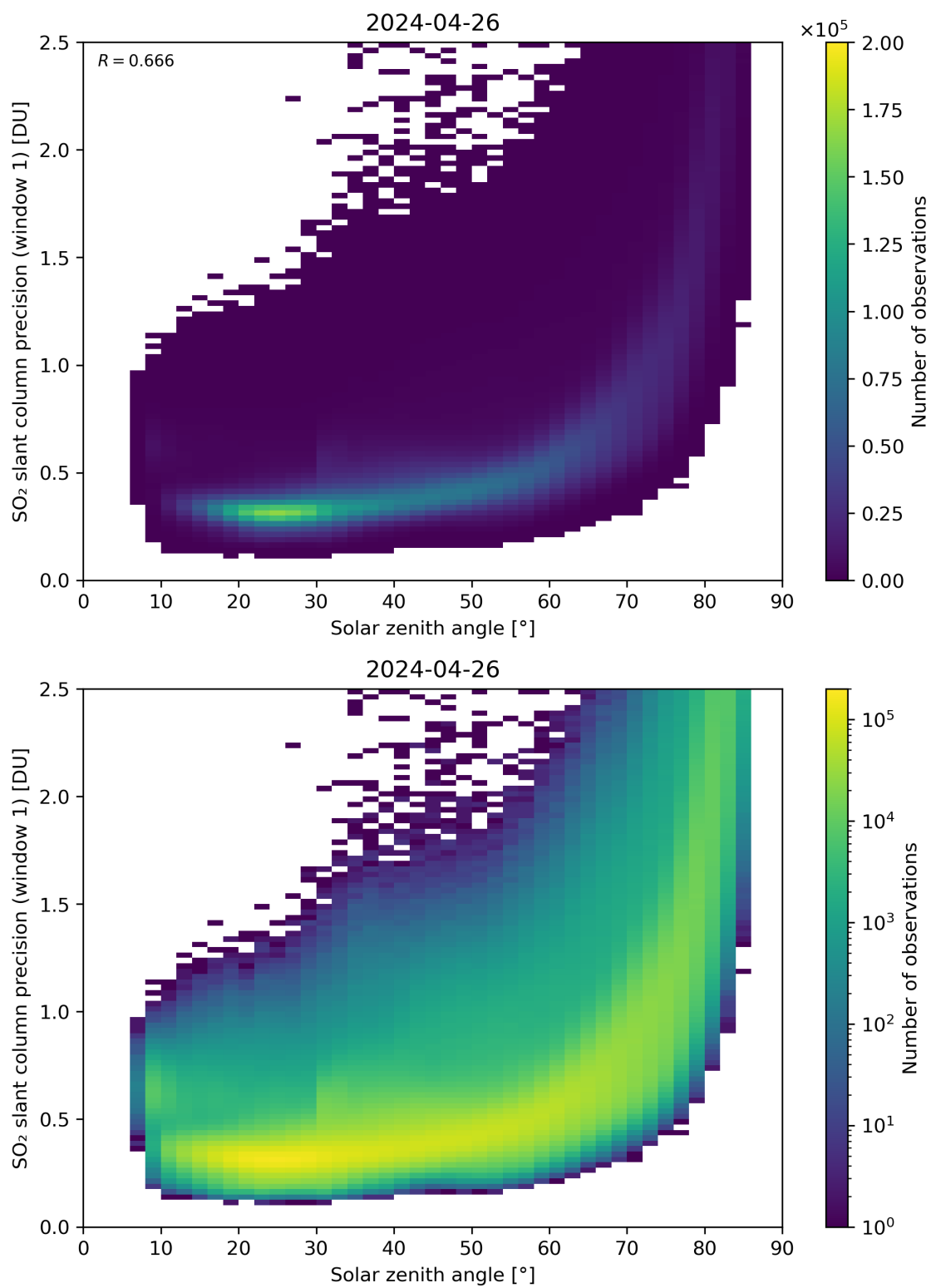
Figure 170: Scatter density plot of “Solar zenith angle” against “SO 2 slant column precision (window 1)” for 2024-04-26 to 2024-04-27.
