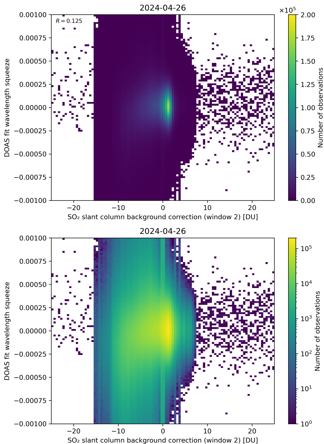
Figure 113: Scatter density plot of “SO 2 slant column background correction (window 2)” against “DOAS fit wavelength squeeze” for 2024-04-26 to 2024-04-27.
