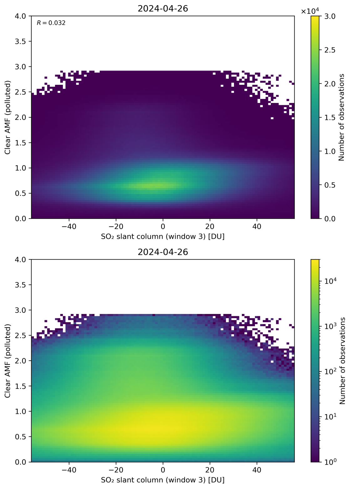
Figure 265: Scatter density plot of “SO 2 slant column (window 3)” against “Clear AMF (polluted)” for 2024-04-26 to 2024-04-27.
