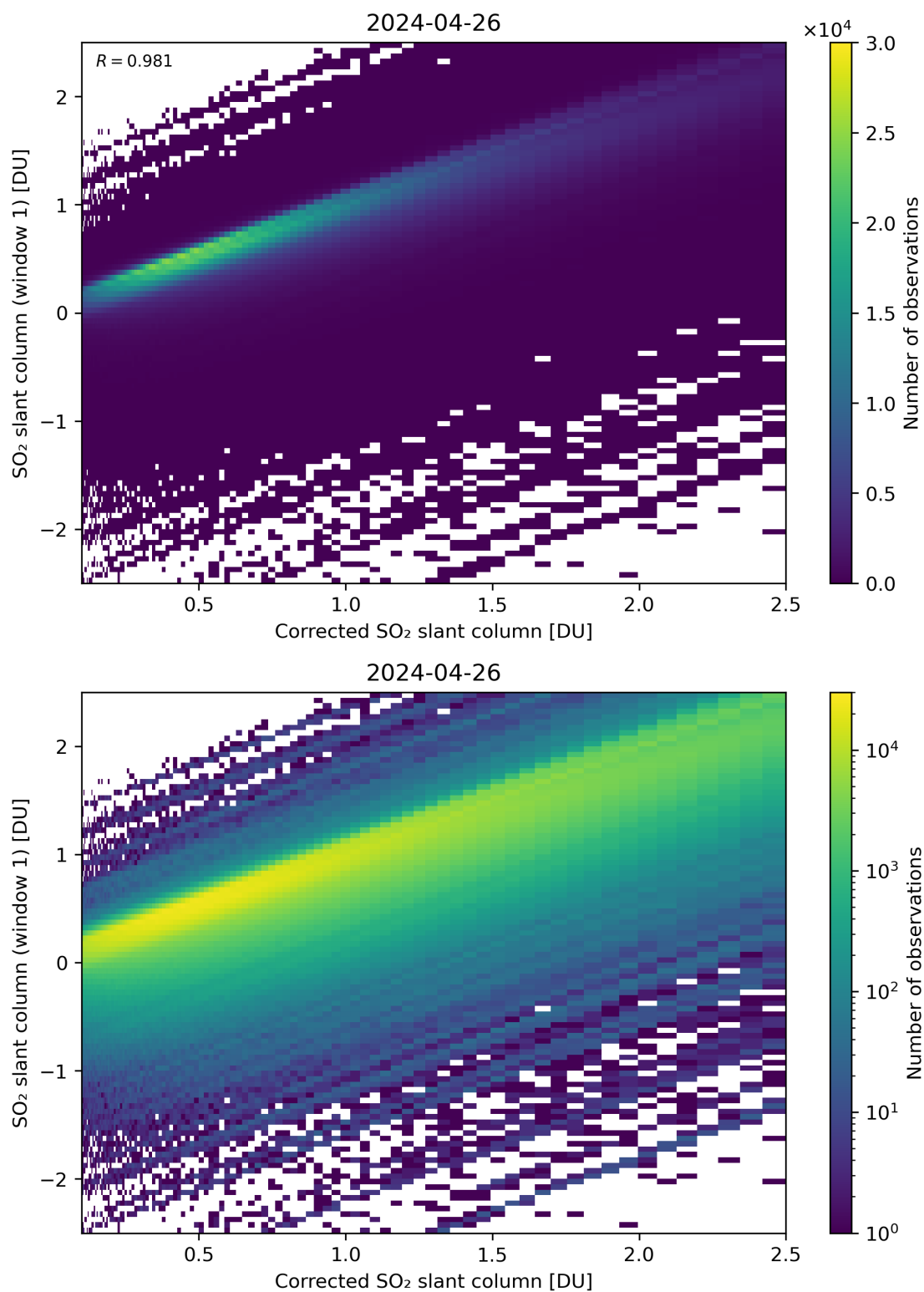
Figure 187: Scatter density plot of “Corrected SO 2 slant column” against “SO 2 slant column (window 1)” for 2024-04-26 to 2024-04-27.
