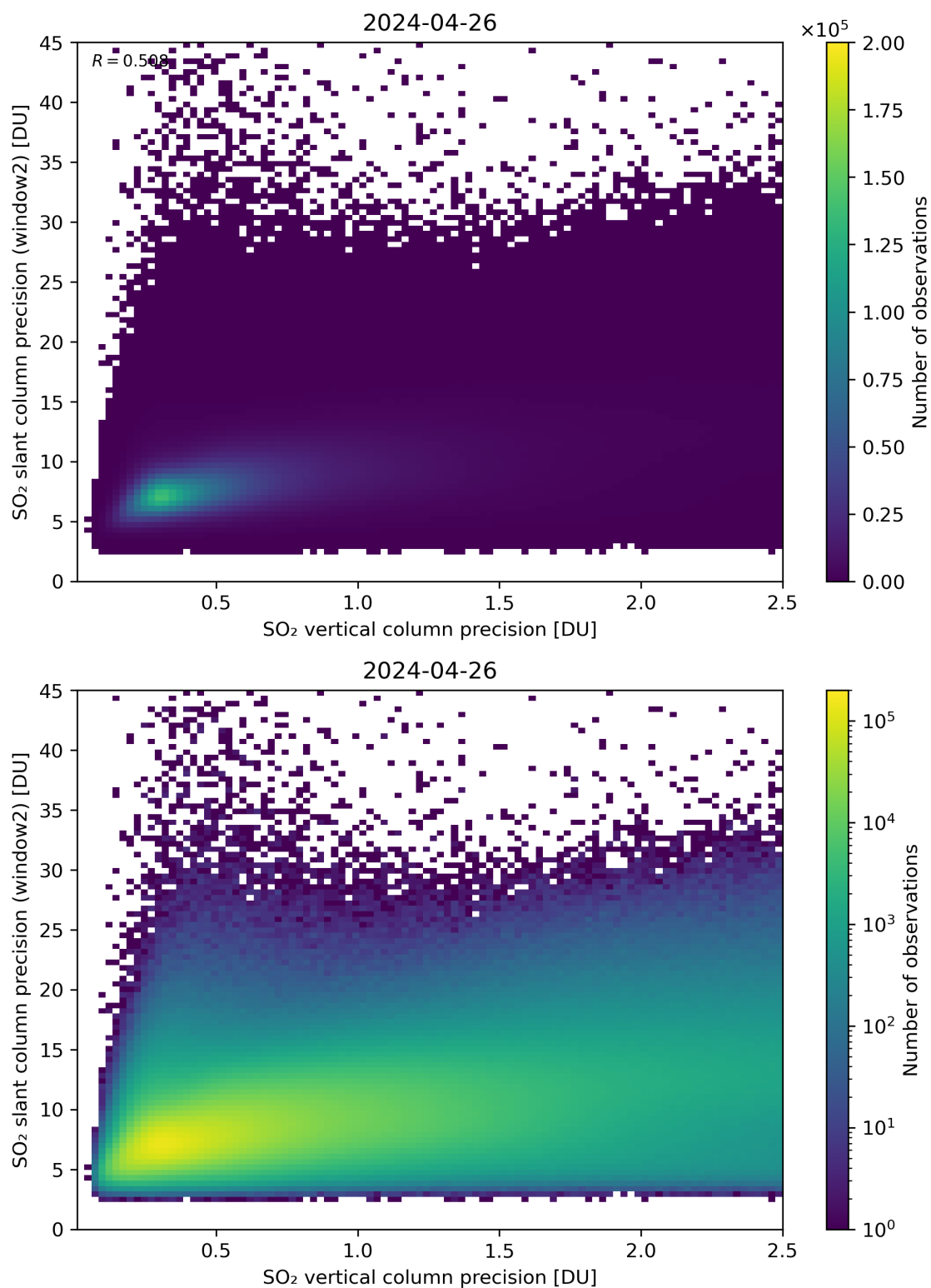
Figure 291: Scatter density plot of “SO 2 vertical column precision” against “SO 2 slant column precision (window2)” for 2024-04-26 to 2024-04-27.
