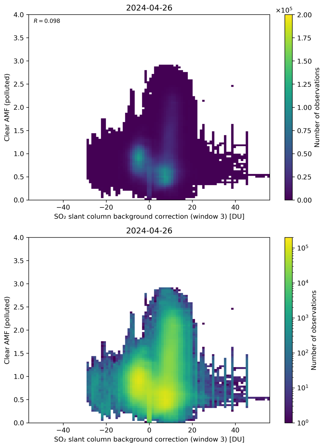
Figure 124: Scatter density plot of “SO 2 slant column background correction (window 3)” against “Clear AMF (polluted)” for 2024-04-26 to 2024-04-27.
