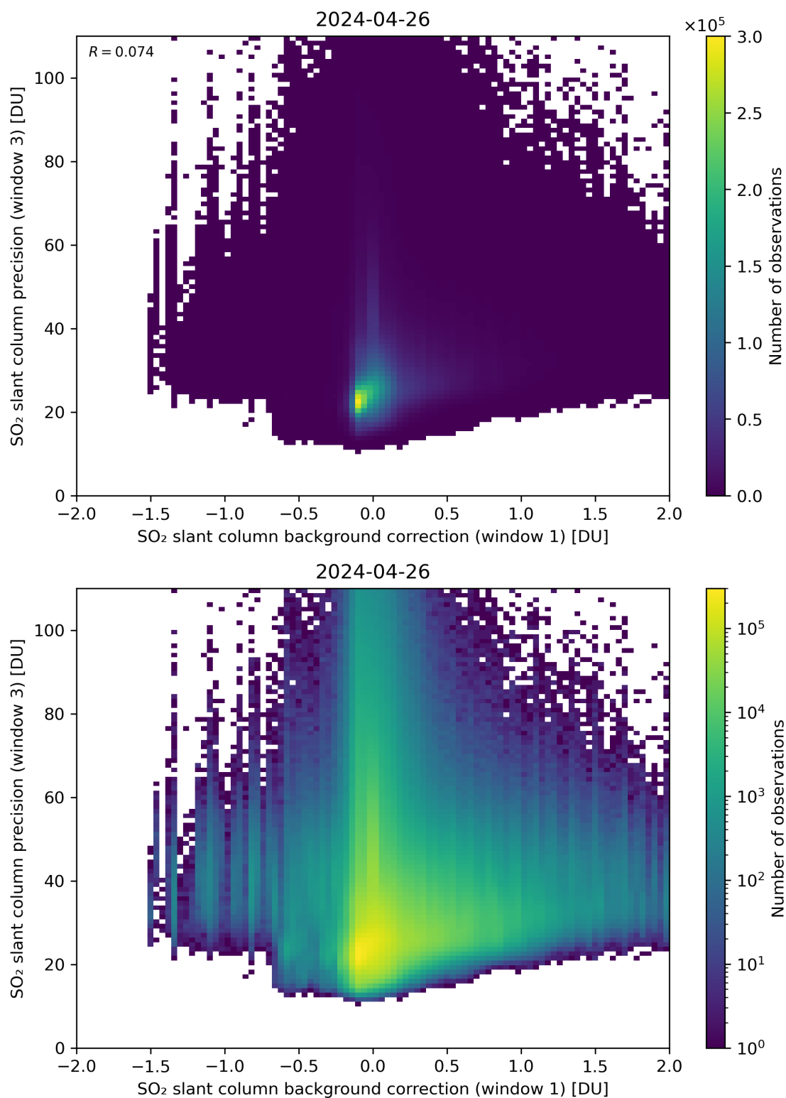
Figure 108: Scatter density plot of “SO 2 slant column background correction (window 1)” against “SO 2 slant column precision (window 3)” for 2024-04-26 to 2024-04-27.
