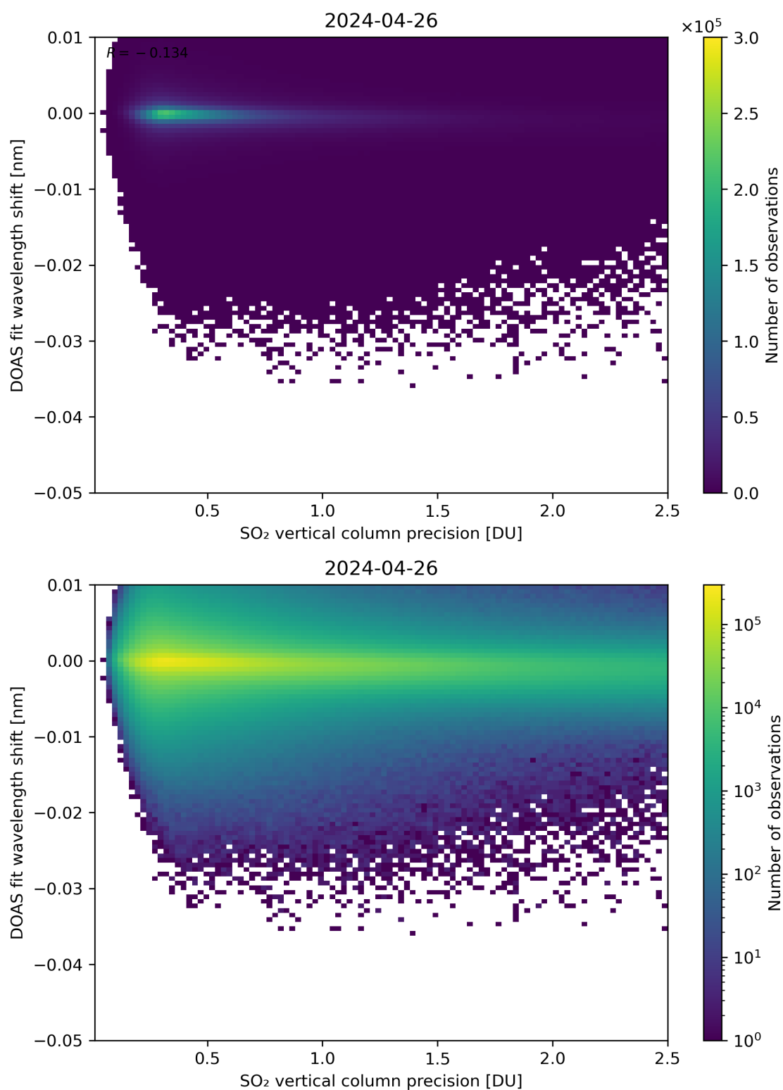
Figure 282: Scatter density plot of “SO 2 vertical column precision” against “DOAS fit wavelength shift” for 2024-04-26 to 2024-04-27.
