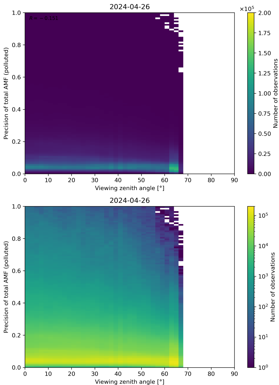
Figure 326: Scatter density plot of “Viewing zenith angle” against “Precision of total AMF (polluted)” for 2024-04-26 to 2024-04-27.
