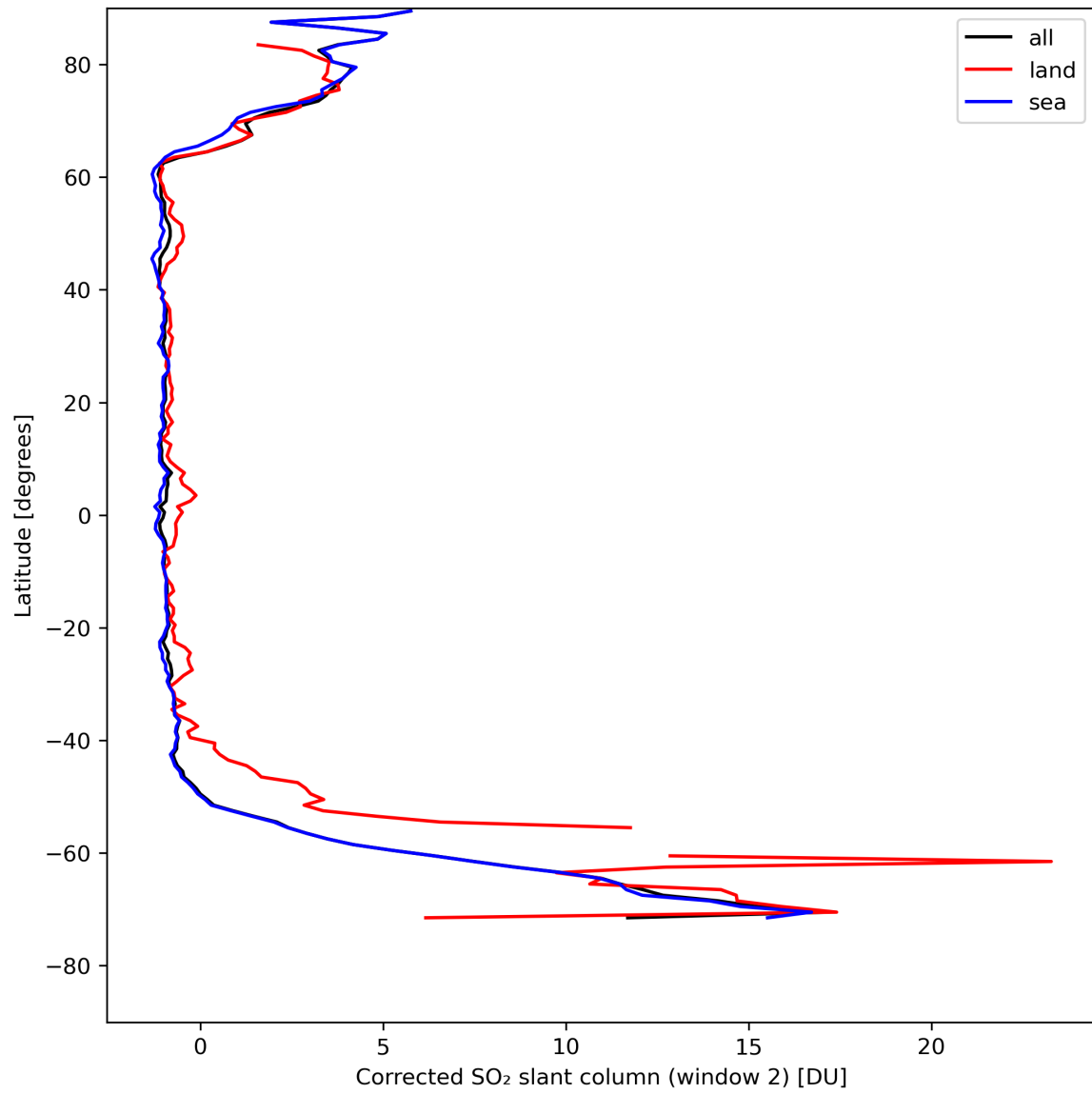
Figure 39: Zonal average of “Corrected SO 2 slant column (window 2)” for 2024-04-26 to 2024-04-27.
