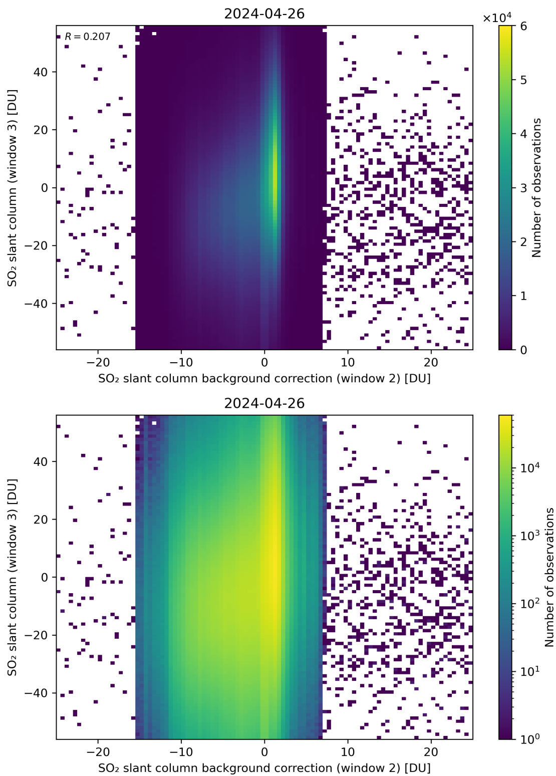
Figure 117: Scatter density plot of “SO 2 slant column background correction (window 2)” against “SO 2 slant column (window 3)” for 2024-04-26 to 2024-04-27.
