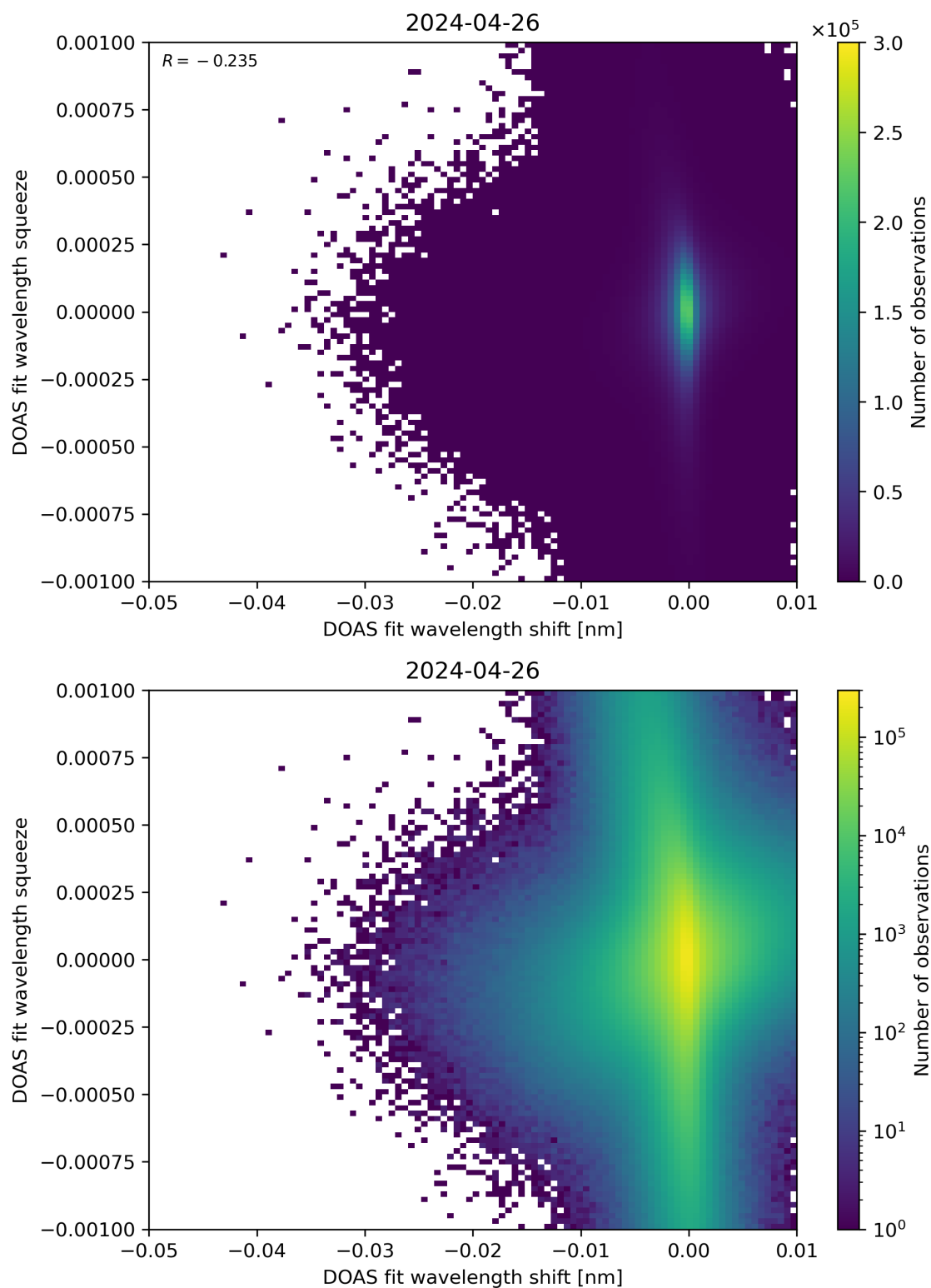
Figure 127: Scatter density plot of “DOAS fit wavelength shift” against “DOAS fit wavelength squeeze” for 2024-04-26 to 2024-04-27.
