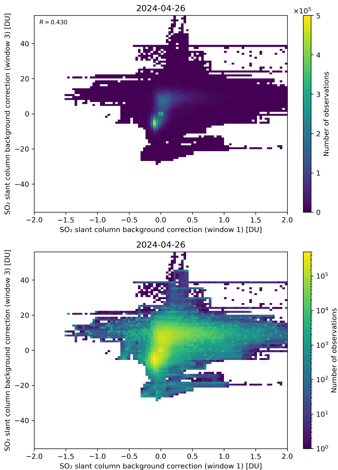
Figure 99: Scatter density plot of “SO 2 slant column background correction (window 1)” against “SO 2 slant column background correction (window 3)” for 2024-04-26 to 2024-04-27.
