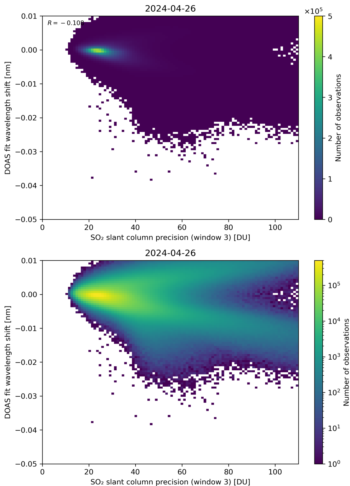
Figure 258: Scatter density plot of “SO 2 slant column precision (window 3)” against “DOAS fit wavelength shift” for 2024-04-26 to 2024-04-27.
