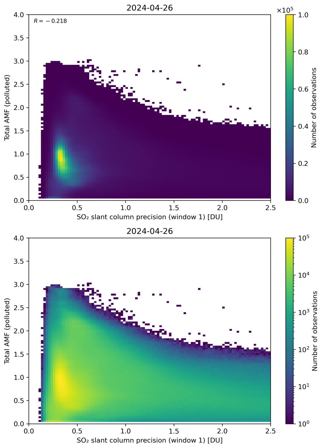
Figure 230: Scatter density plot of “SO 2 slant column precision (window 1)” against “Total AMF (polluted)” for 2024-04-26 to 2024-04-27.
