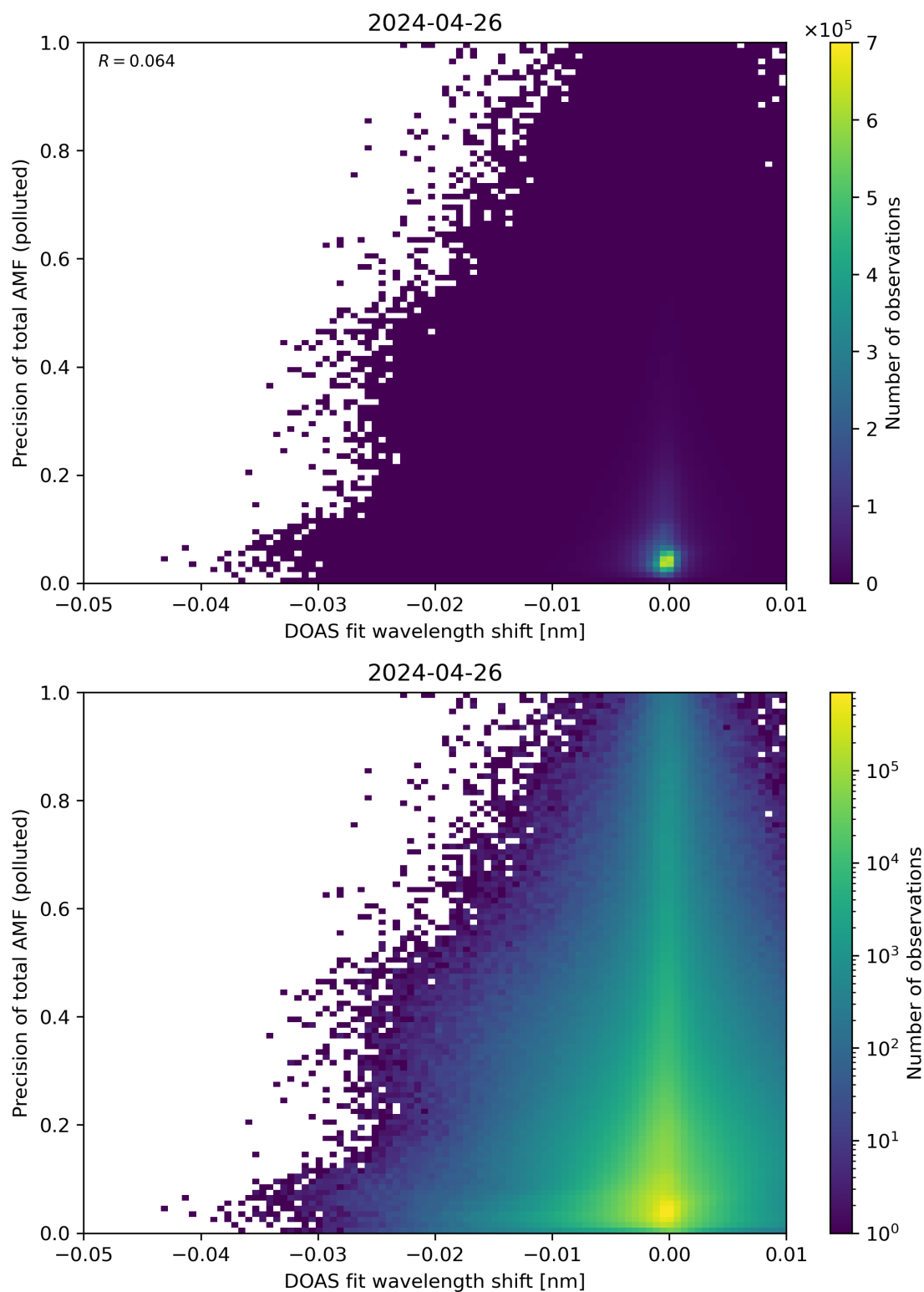
Figure 131: Scatter density plot of “DOAS fit wavelength shift” against “Precision of total AMF (polluted)” for 2024-04-26 to 2024-04-27.
