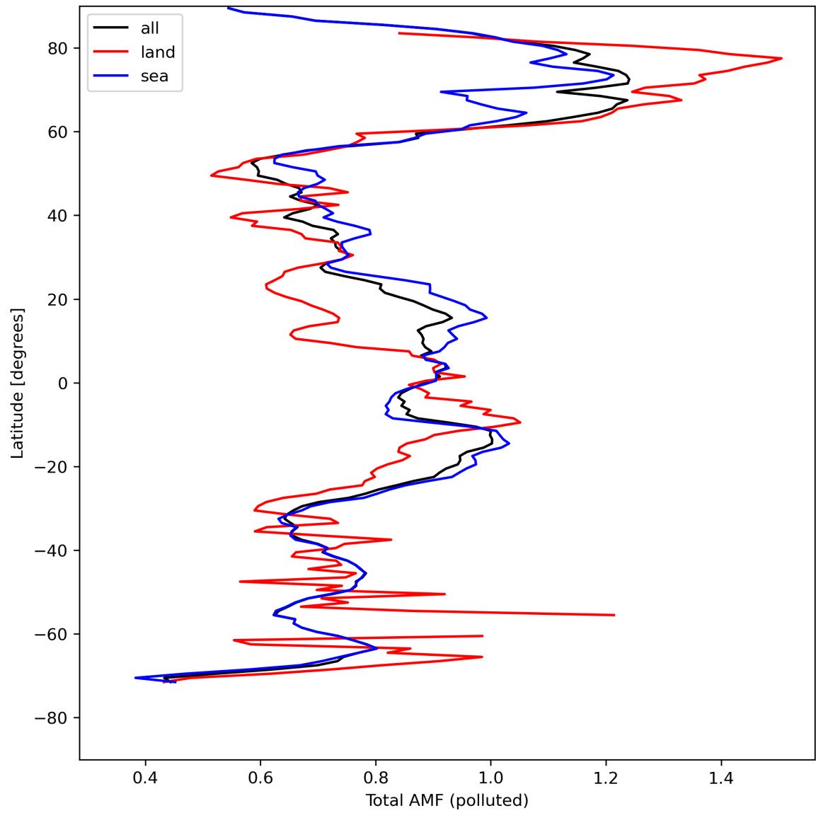
Figure 48: Zonal average of “Total AMF (polluted)” for 2024-04-26 to 2024-04-27.
