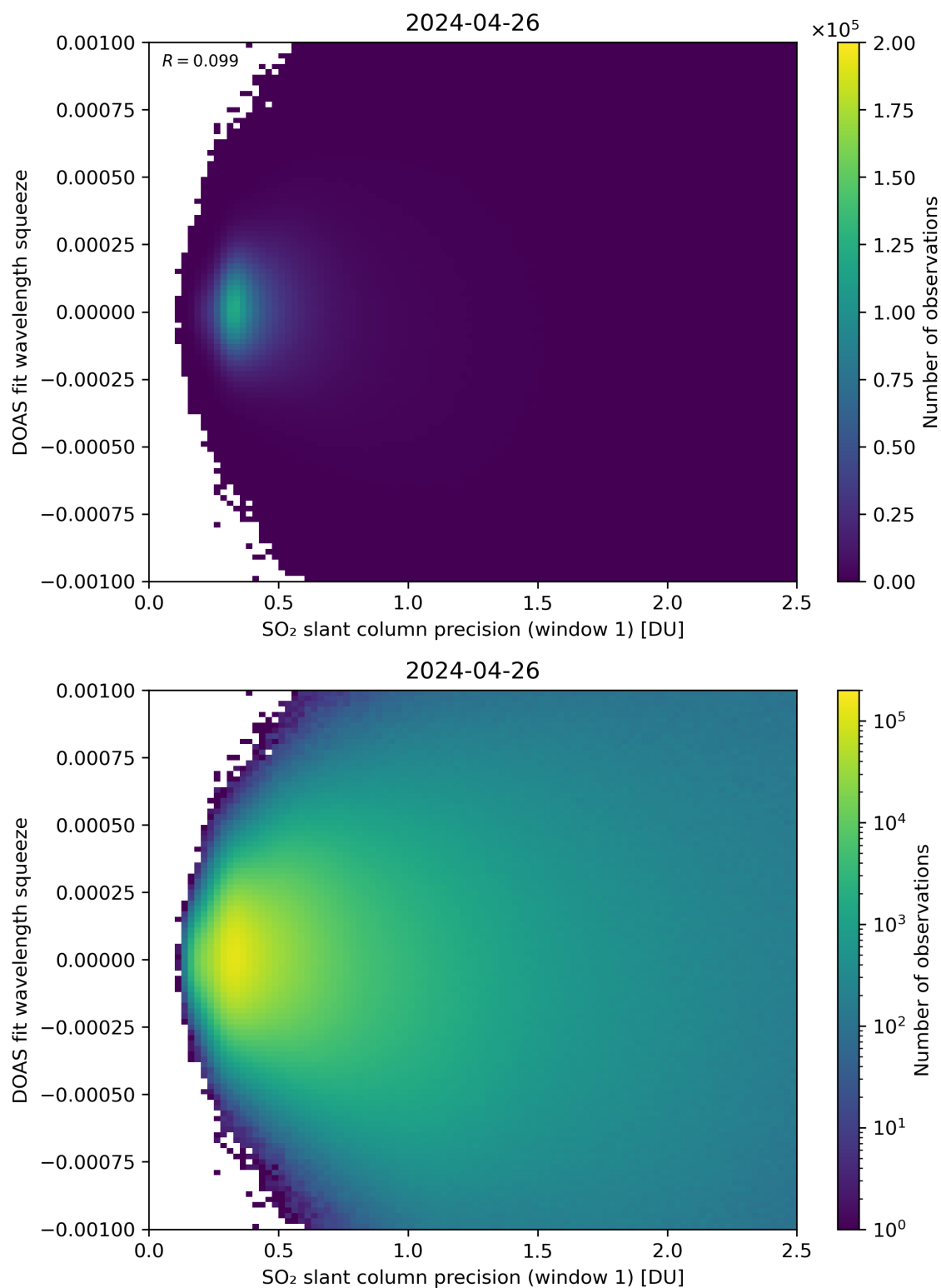
Figure 222: Scatter density plot of “SO 2 slant column precision (window 1)” against “DOAS fit wavelength squeeze” for 2024-04-26 to 2024-04-27.
