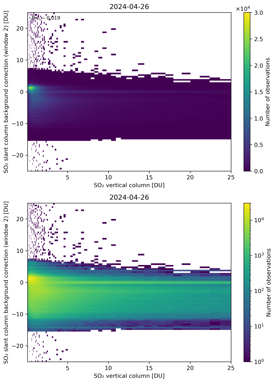
Figure 274: Scatter density plot of “SO 2 vertical column” against “SO 2 slant column background correction (window 2)” for 2024-04-26 to 2024-04-27.
