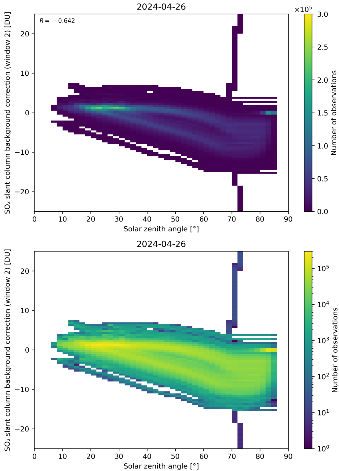
Figure 159: Scatter density plot of “Solar zenith angle” against “SO 2 slant column background correction (window 2)” for 2024-04-26 to 2024-04-27.
