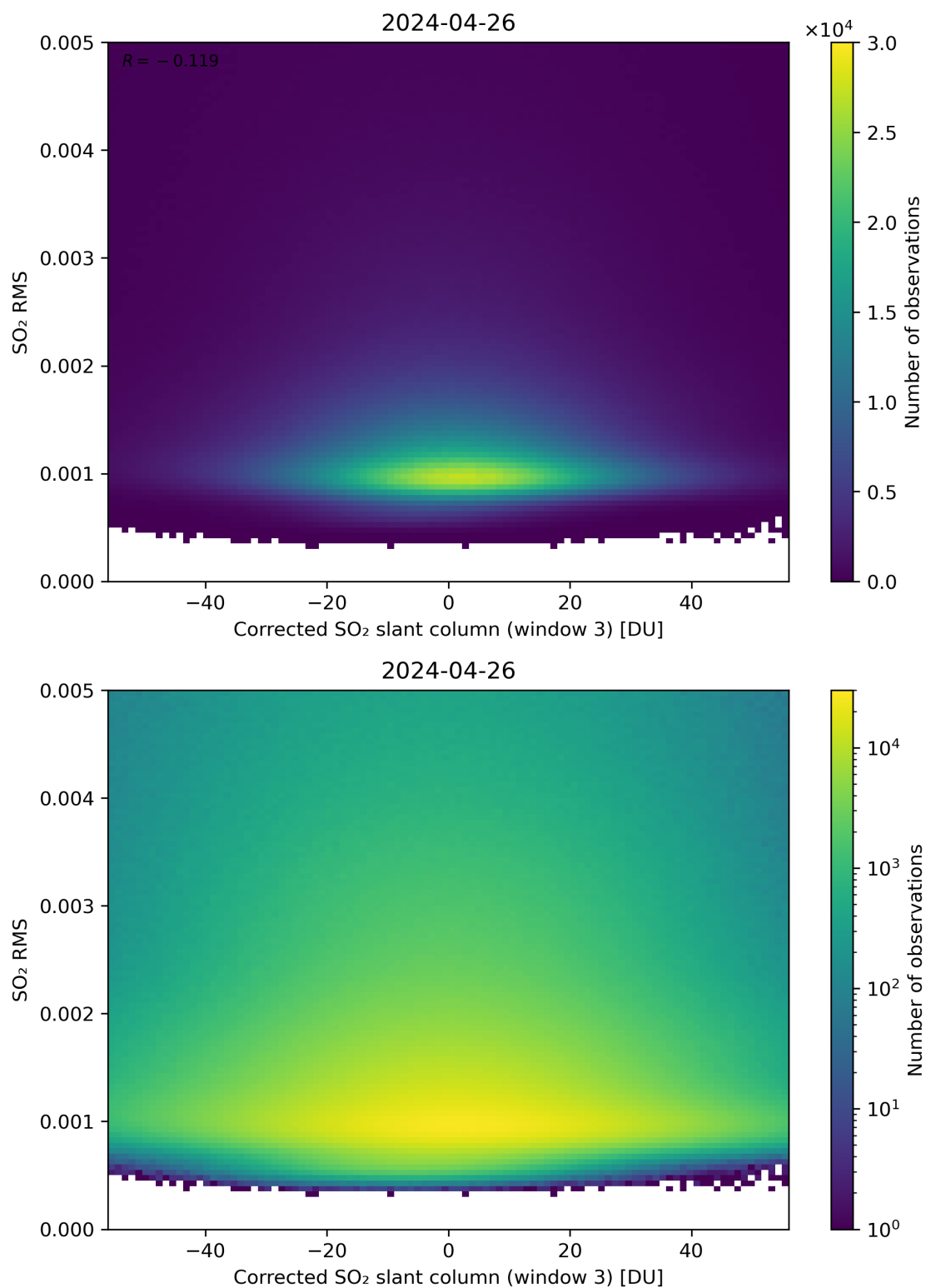
Figure 208: Scatter density plot of “Corrected SO 2 slant column (window 3)” against “SO 2 RMS” for 2024-04-26 to 2024-04-27.
