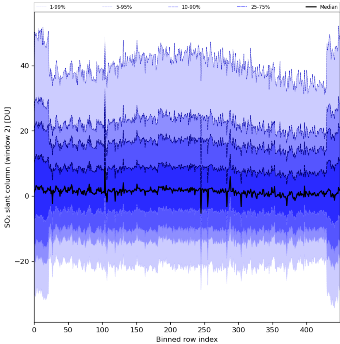
Figure 83: Along track statistics of “SO 2 slant column (window 2)” for 2024-04-26 to 2024-04-27
