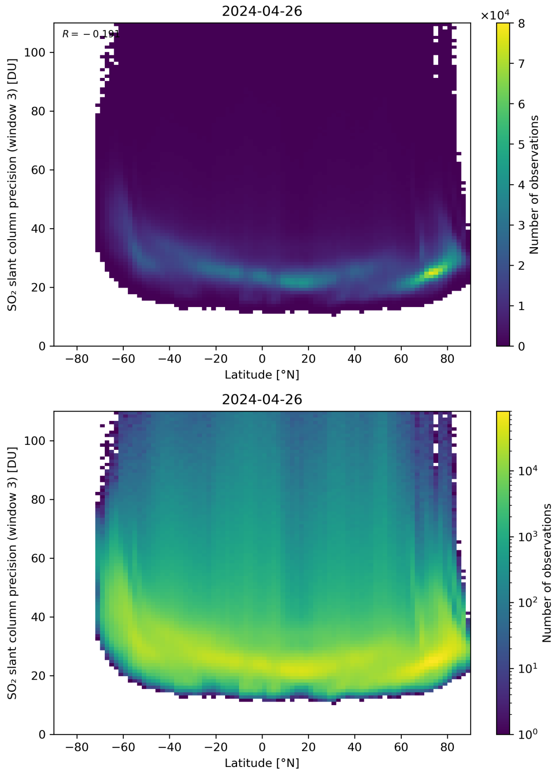
Figure 153: Scatter density plot of “Latitude” against “SO 2 slant column precision (window 3)” for 2024-04-26 to 2024-04-27.
