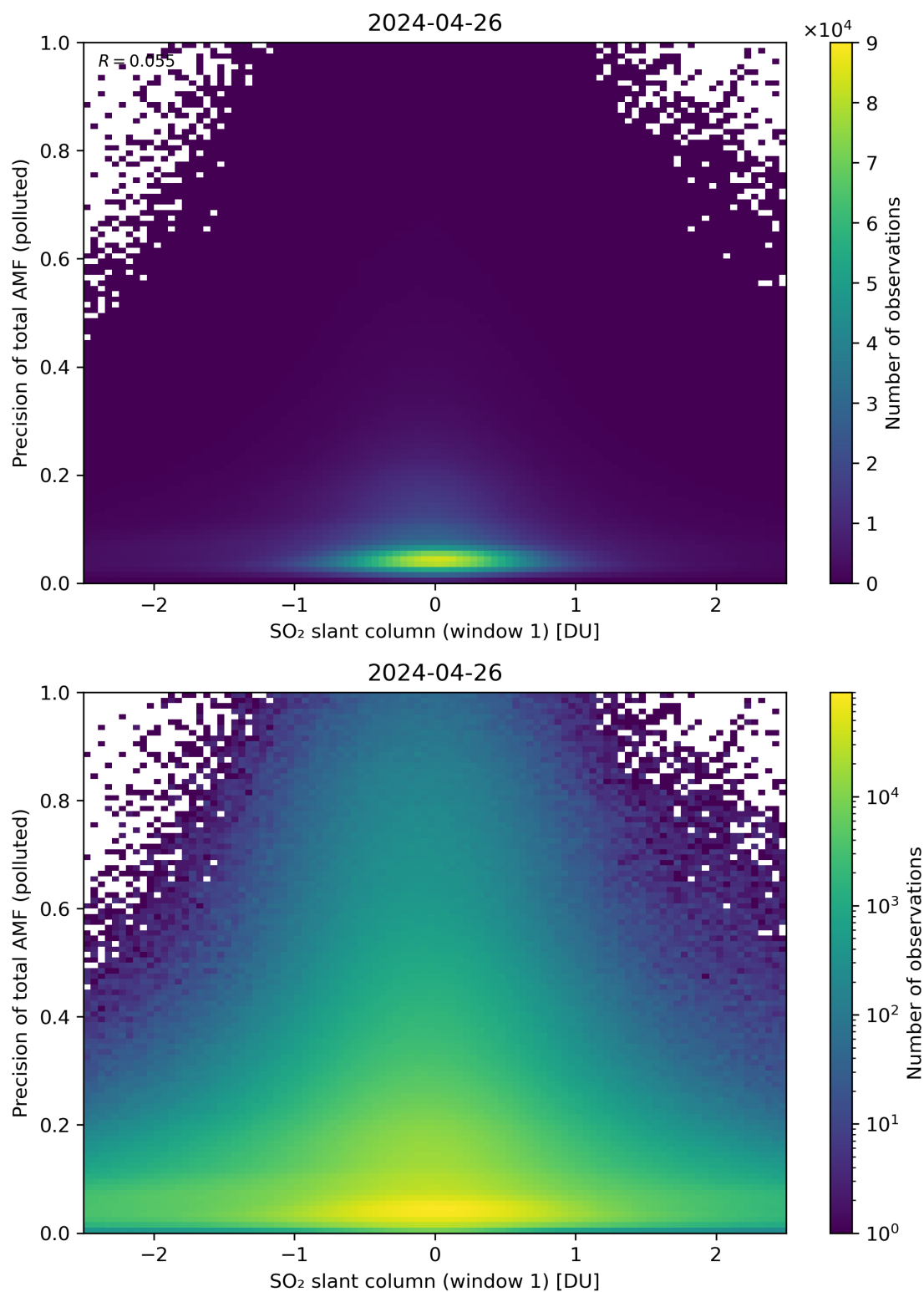
Figure 240: Scatter density plot of “SO 2 slant column (window 1)” against “Precision of total AMF (polluted)” for 2024-04-26 to 2024-04-27.
