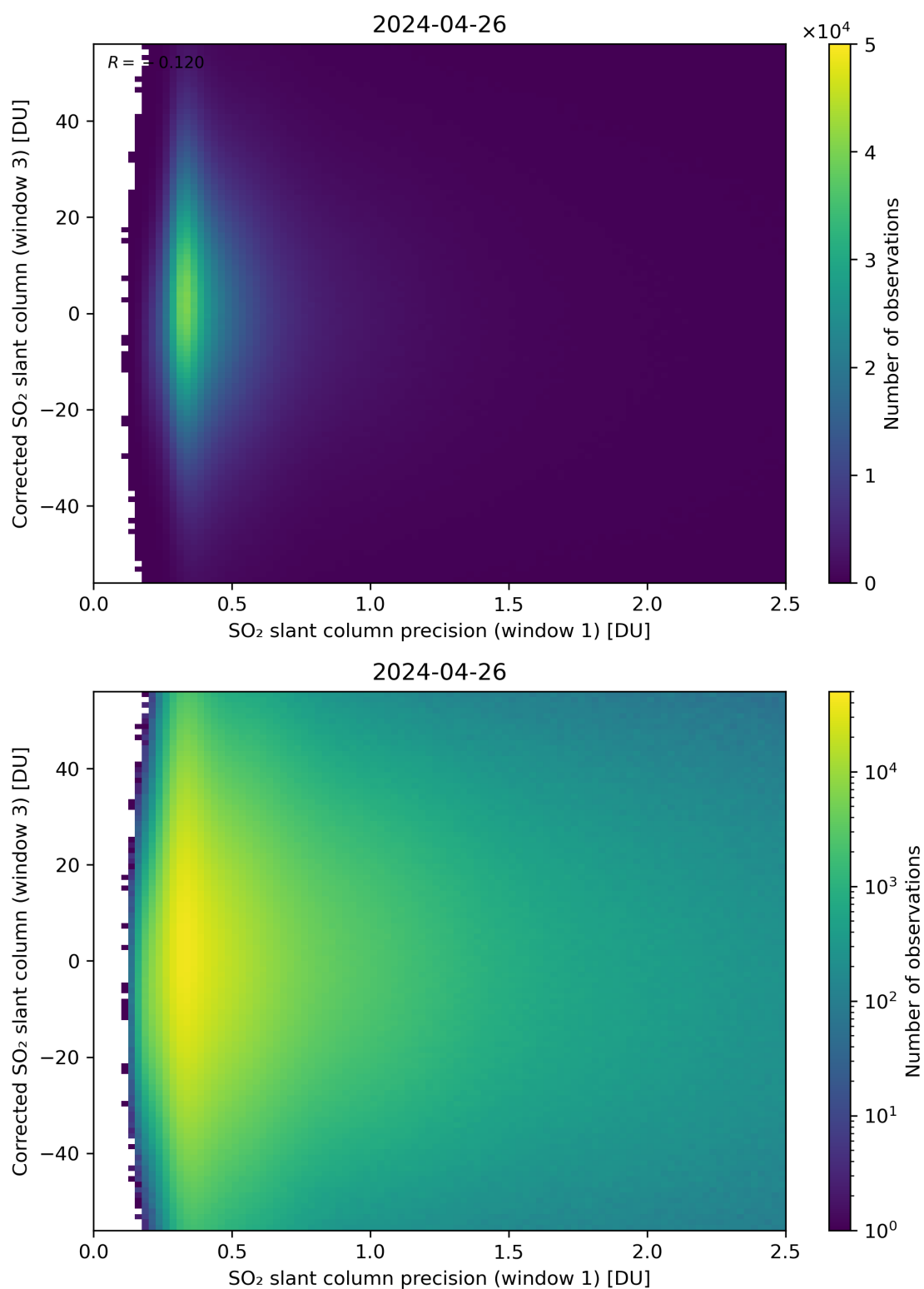
Figure 226: Scatter density plot of “SO 2 slant column precision (window 1)” against “Corrected SO 2 slant column (window 3)” for 2024-04-26 to 2024-04-27.
