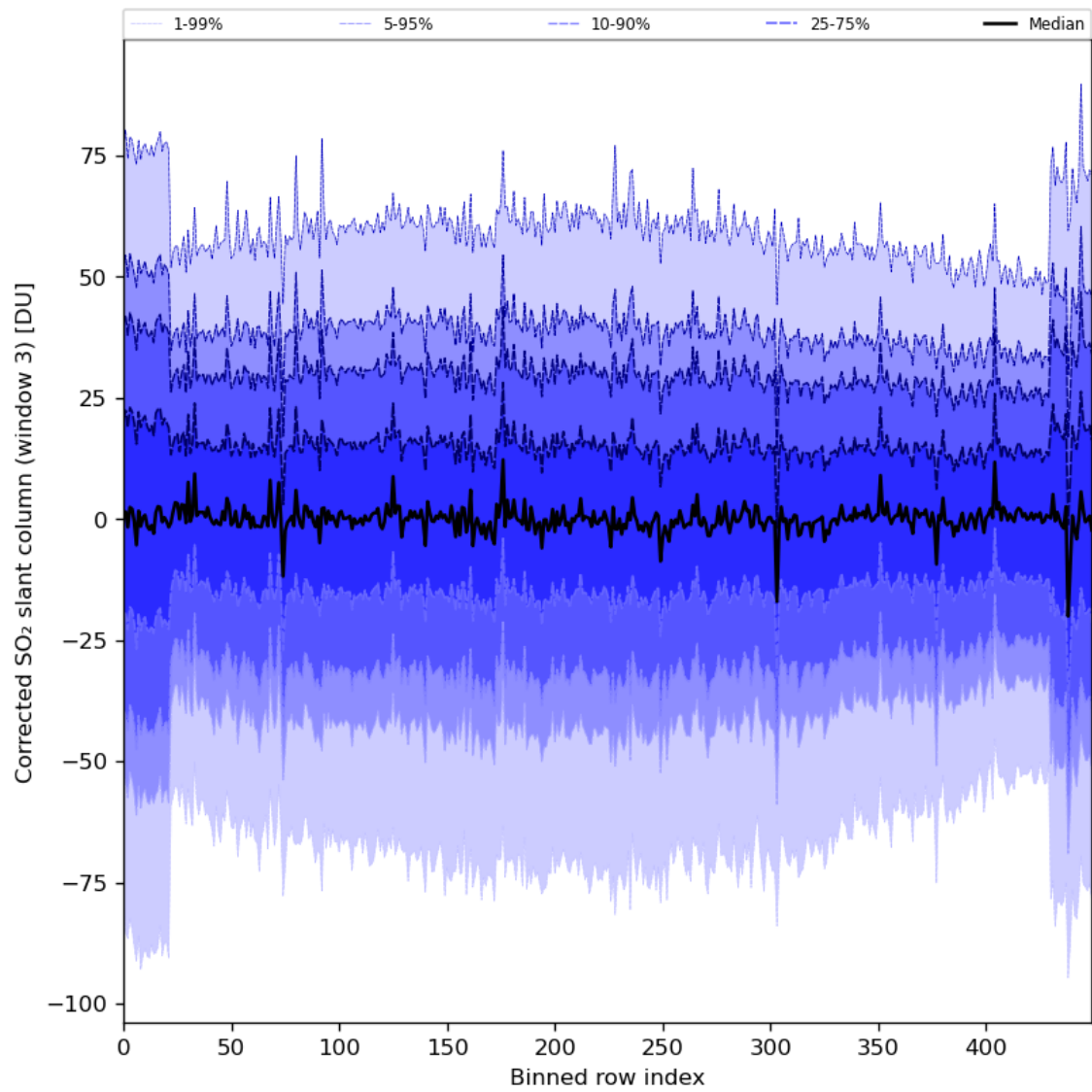
Figure 89: Along track statistics of “Corrected SO 2 slant column (window 3)” for 2024-04-26 to 2024-04-27
