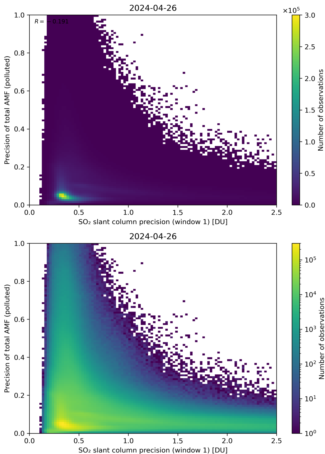
Figure 231: Scatter density plot of “SO 2 slant column precision (window 1)” against “Precision of total AMF (polluted)” for 2024-04-26 to 2024-04-27.
