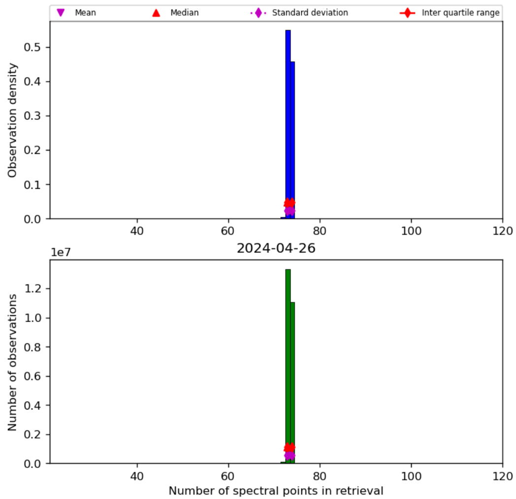
Figure 74: Histogram of “Number of spectral points in retrieval” for 2024-04-26 to 2024-04-27
