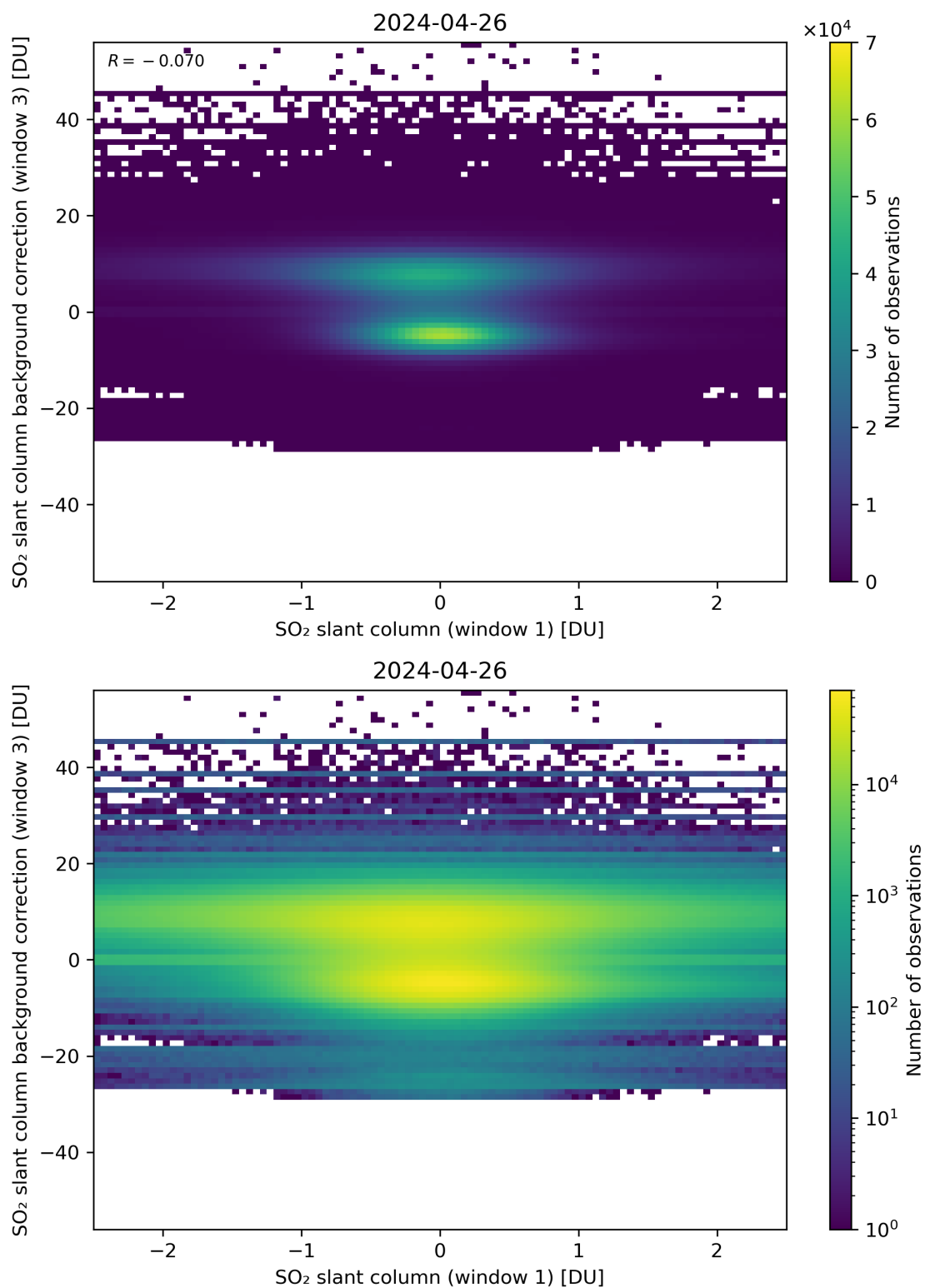
Figure 214: Scatter density plot of “SO 2 slant column (window 1)” against “SO 2 slant column background correction (window 3)” for 2024-04-26 to 2024-04-27.
