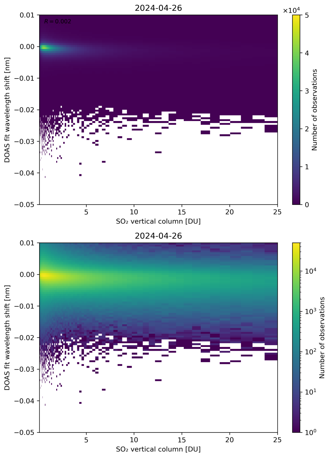
Figure 276: Scatter density plot of “SO 2 vertical column” against “DOAS fit wavelength shift” for 2024-04-26 to 2024-04-27.
