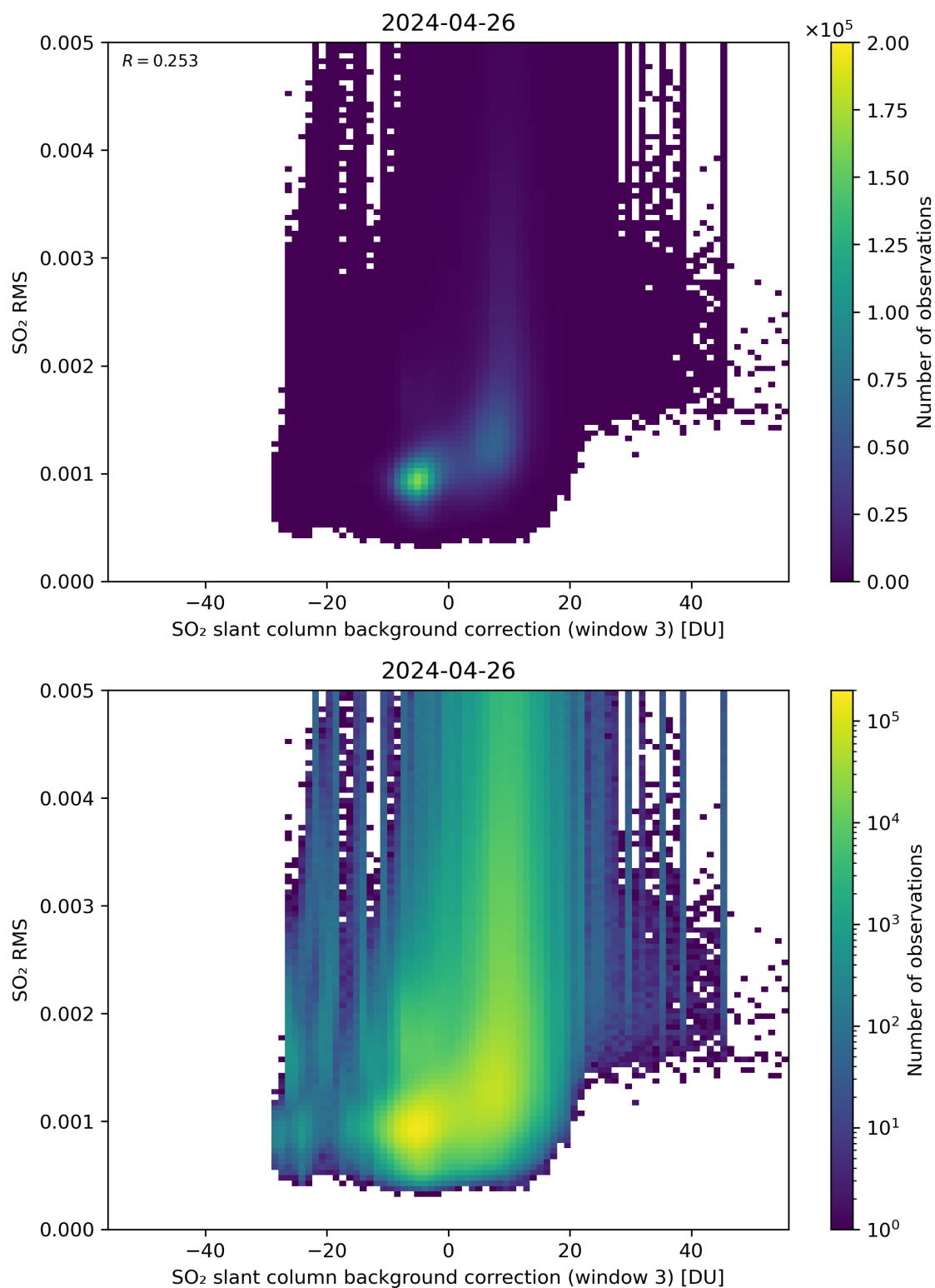
Figure 123: Scatter density plot of “SO 2 slant column background correction (window 3)” against “SO 2 RMS” for 2024-04-26 to 2024-04-27.
