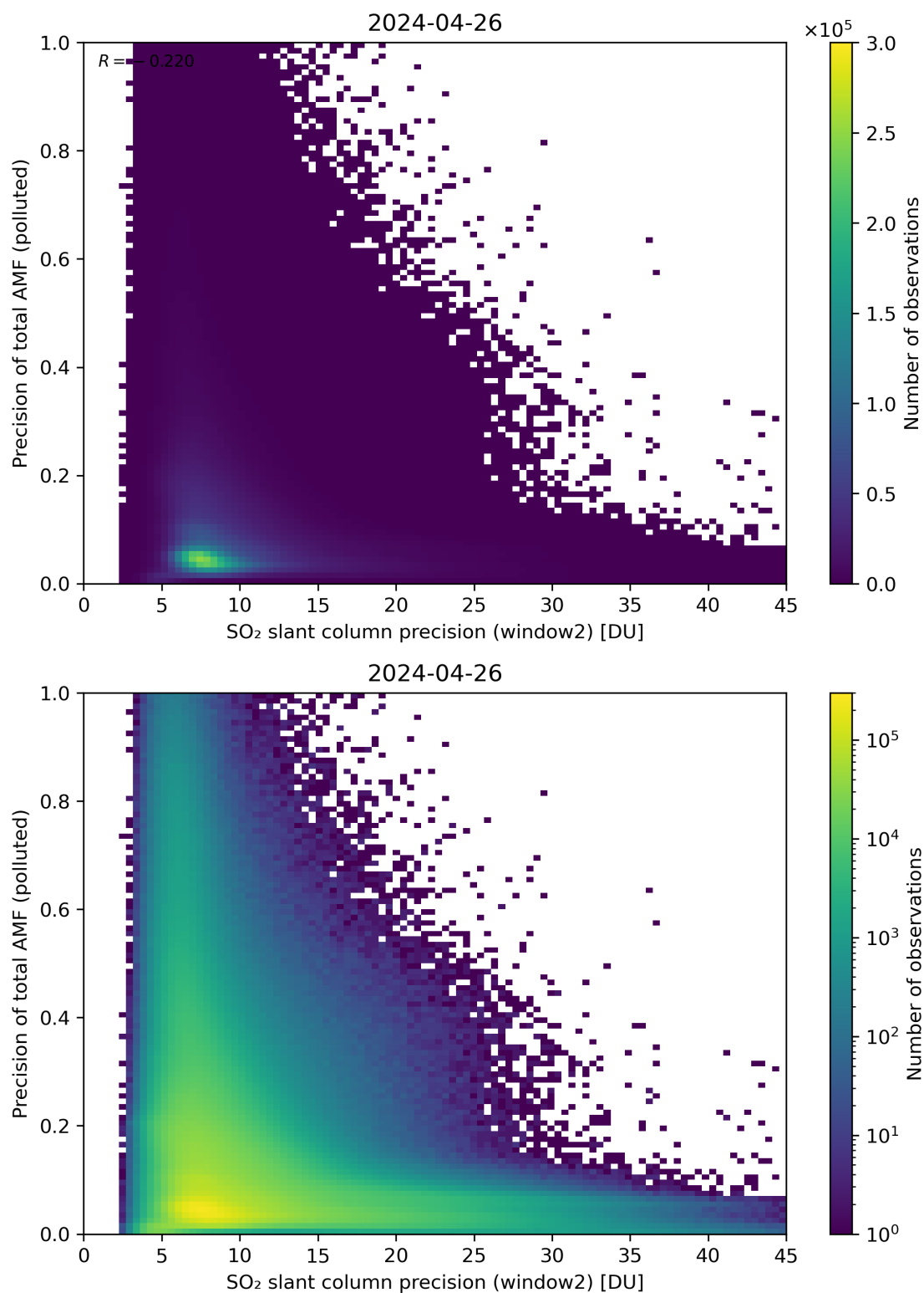
Figure 252: Scatter density plot of “SO 2 slant column precision (window2)” against “Precision of total AMF (polluted)” for 2024-04-26 to 2024-04-27.
