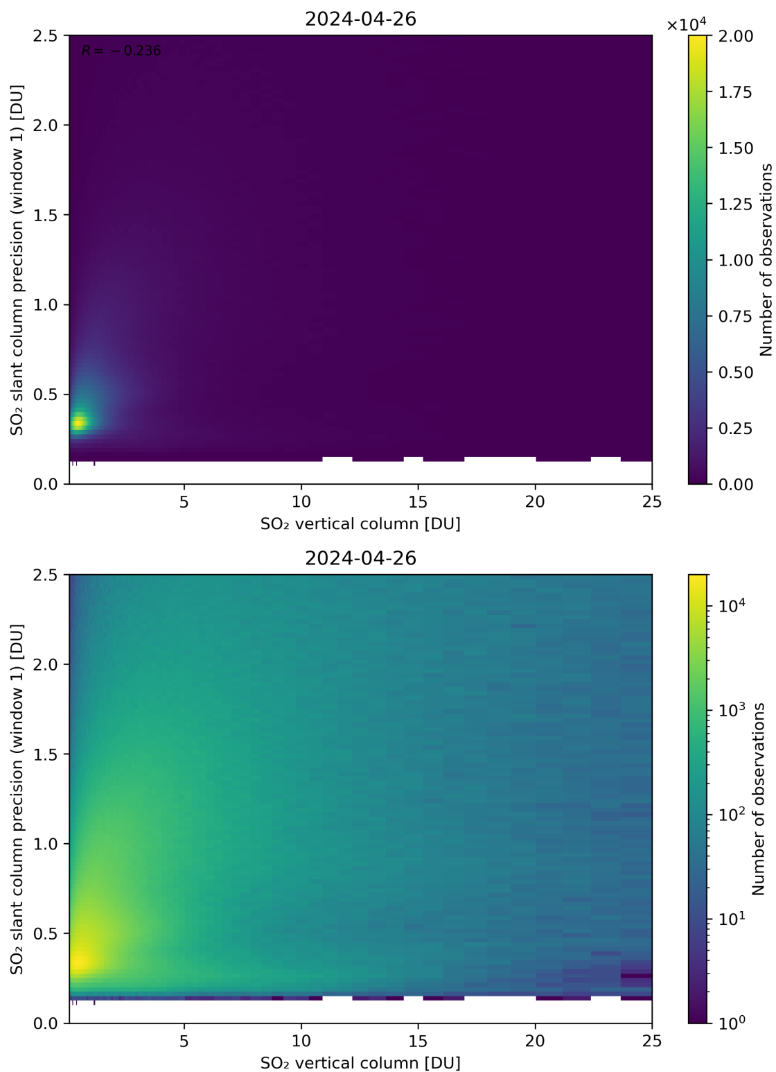
Figure 301: Scatter density plot of “SO 2 vertical column” against “SO 2 slant column precision (window 1)” for 2024-04-26 to 2024-04-27.
