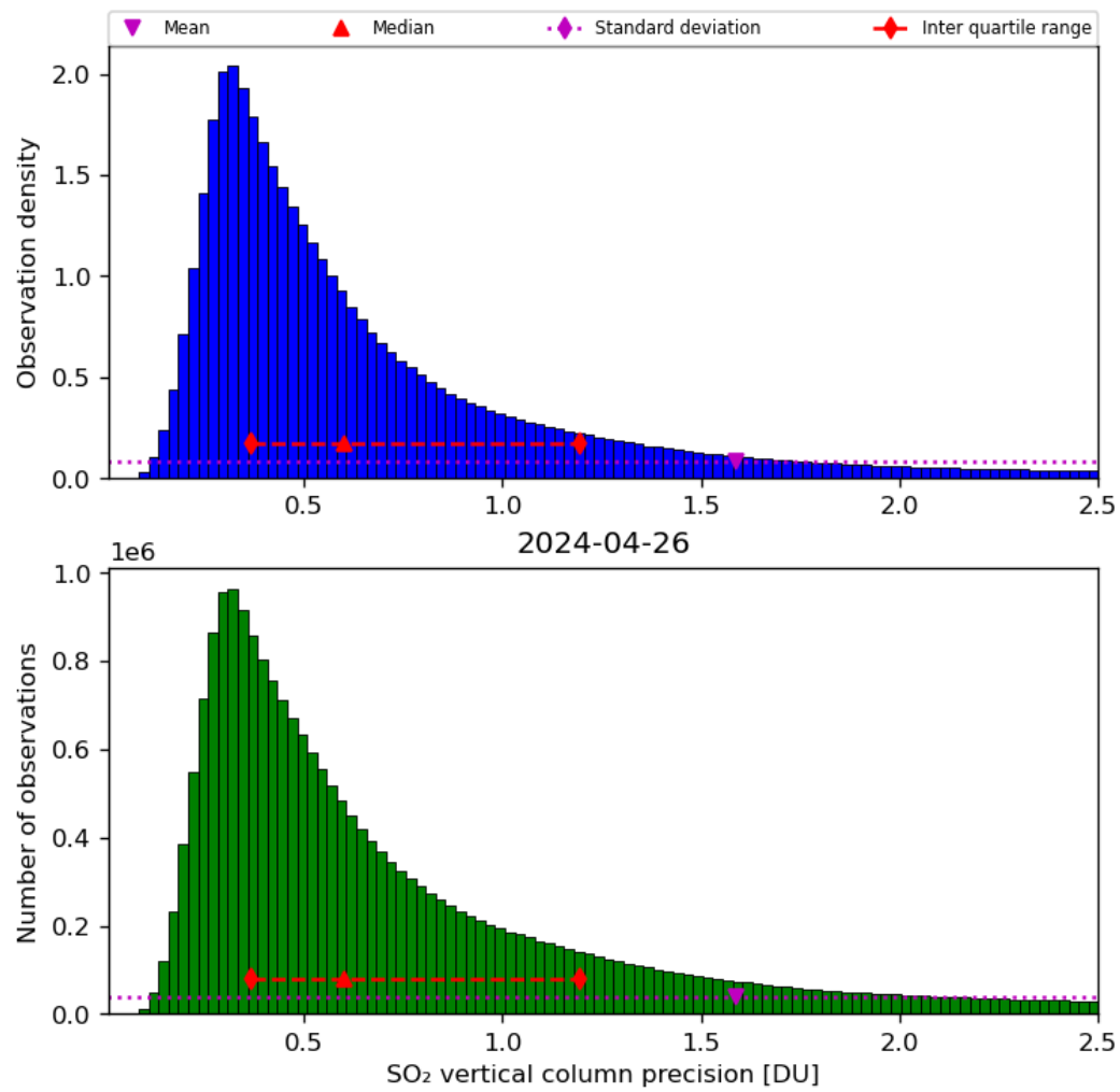
Figure 54: Histogram of “SO 2 vertical column precision” for 2024-04-26 to 2024-04-27
