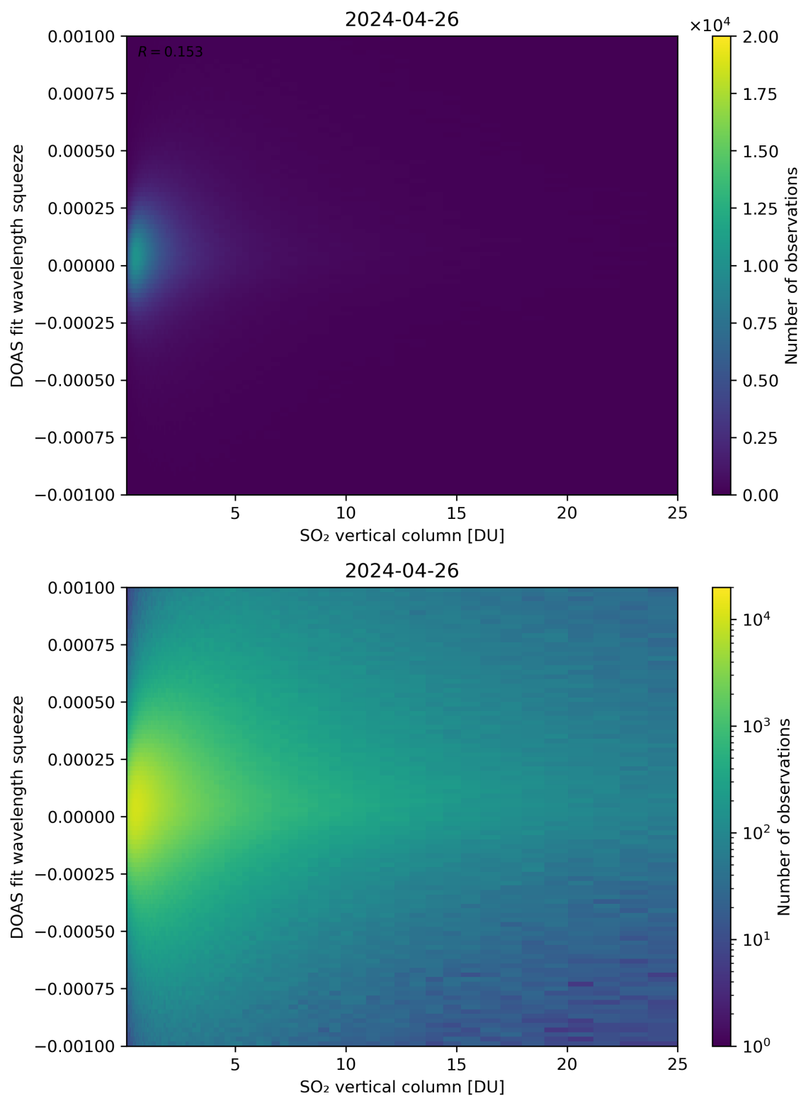
Figure 277: Scatter density plot of “SO 2 vertical column” against “DOAS fit wavelength squeeze” for 2024-04-26 to 2024-04-27.
