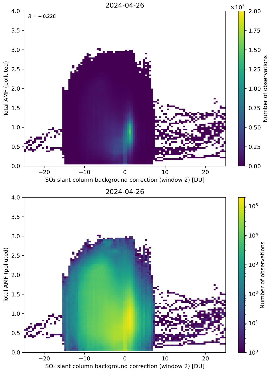
Figure 119: Scatter density plot of “SO 2 slant column background correction (window 2)” against “Total AMF (polluted)” for 2024-04-26 to 2024-04-27.
