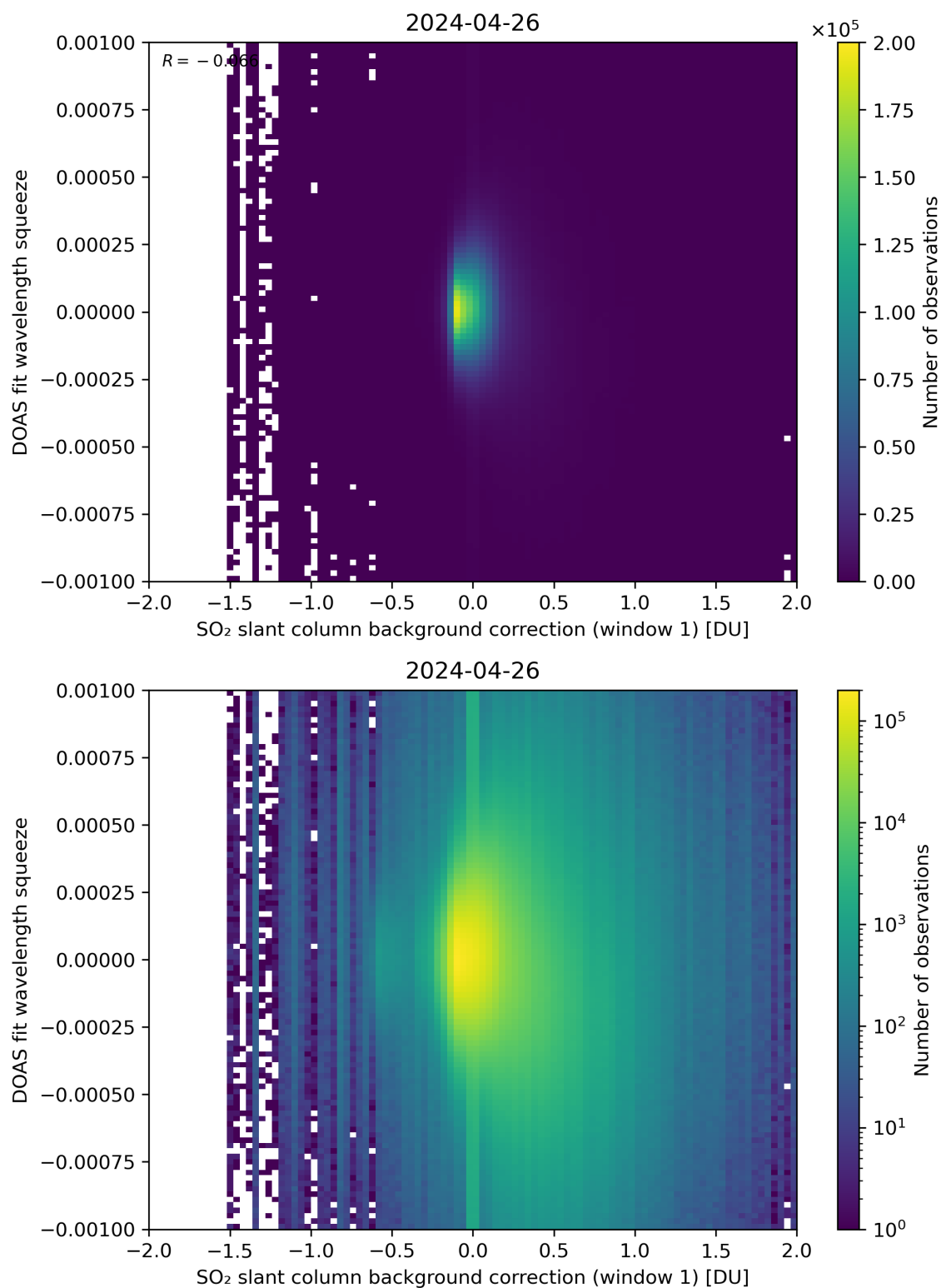
Figure 101: Scatter density plot of “SO 2 slant column background correction (window 1)” against “DOAS fit wavelength squeeze” for 2024-04-26 to 2024-04-27.
