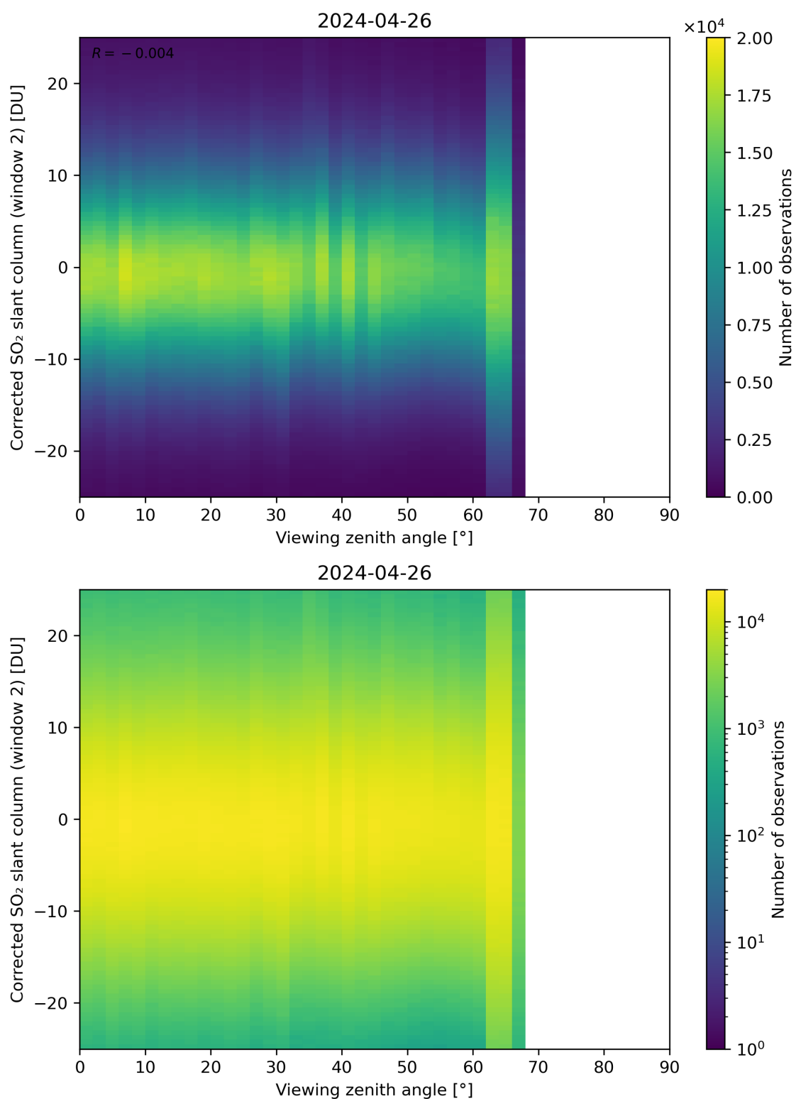
Figure 318: Scatter density plot of “Viewing zenith angle” against “Corrected SO 2 slant column (window 2)” for 2024-04-26 to 2024-04-27.
