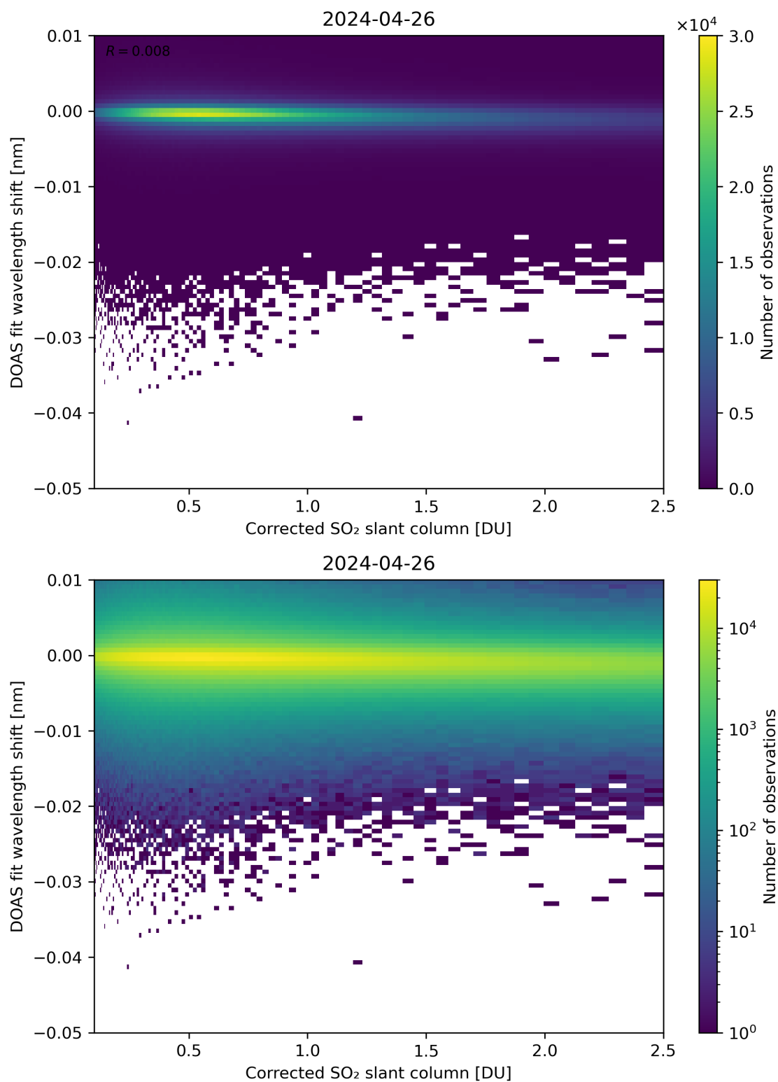
Figure 181: Scatter density plot of “Corrected SO 2 slant column” against “DOAS fit wavelength shift” for 2024-04-26 to 2024-04-27.
