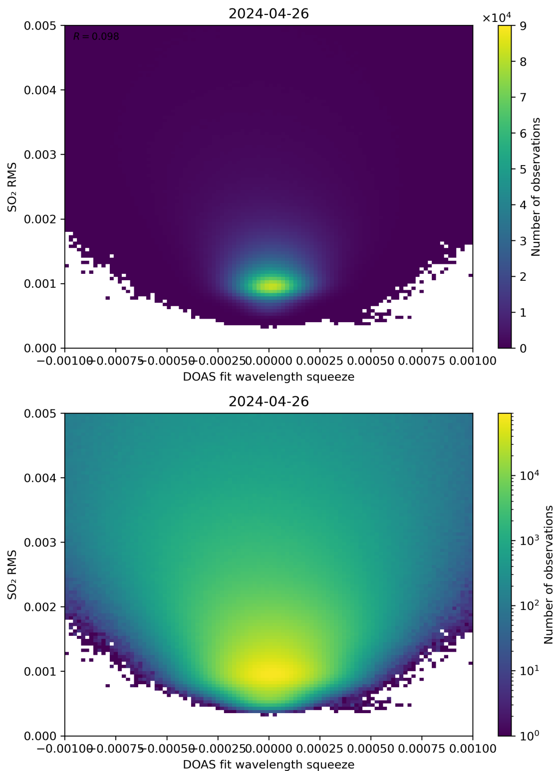
Figure 132: Scatter density plot of “DOAS fit wavelength squeeze” against “SO 2 RMS” for 2024-04-26 to 2024-04-27.
