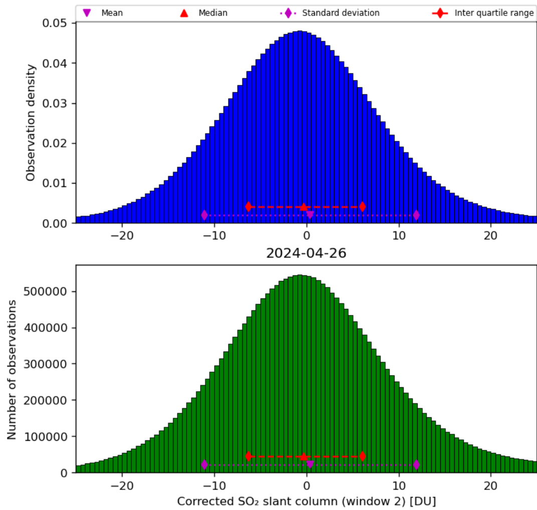
Figure 62: Histogram of “Corrected SO 2 slant column (window 2)” for 2024-04-26 to 2024-04-27
