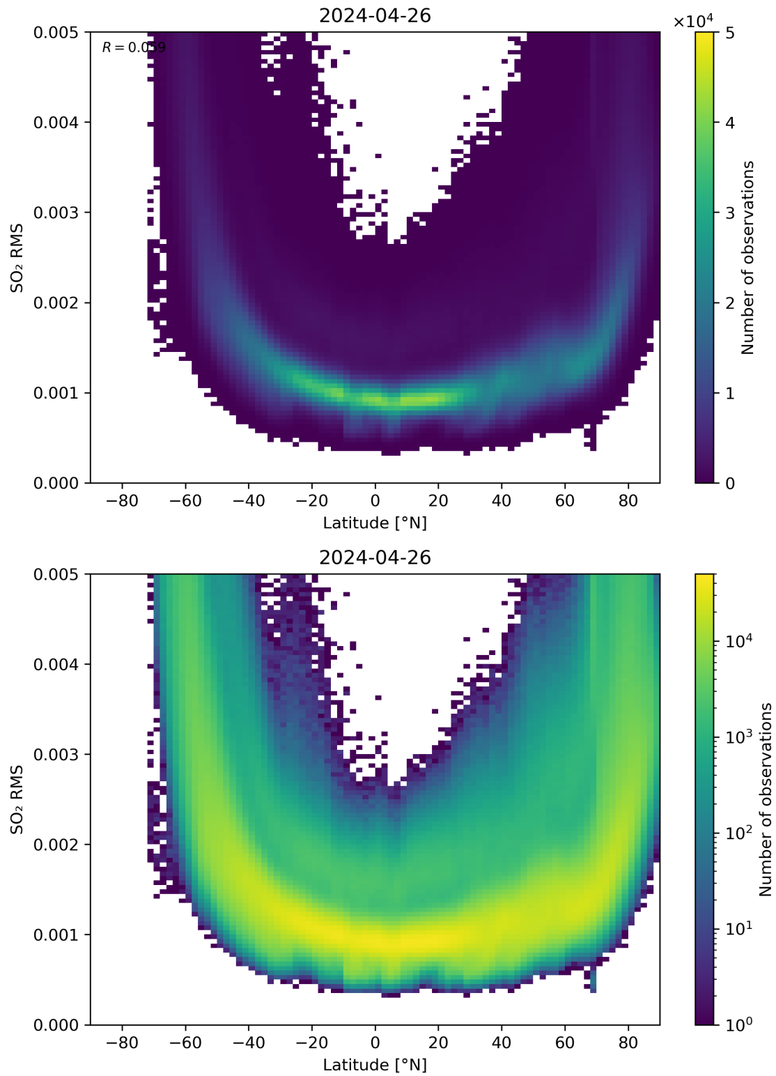
Figure 144: Scatter density plot of “Latitude” against “SO 2 RMS” for 2024-04-26 to 2024-04-27.
