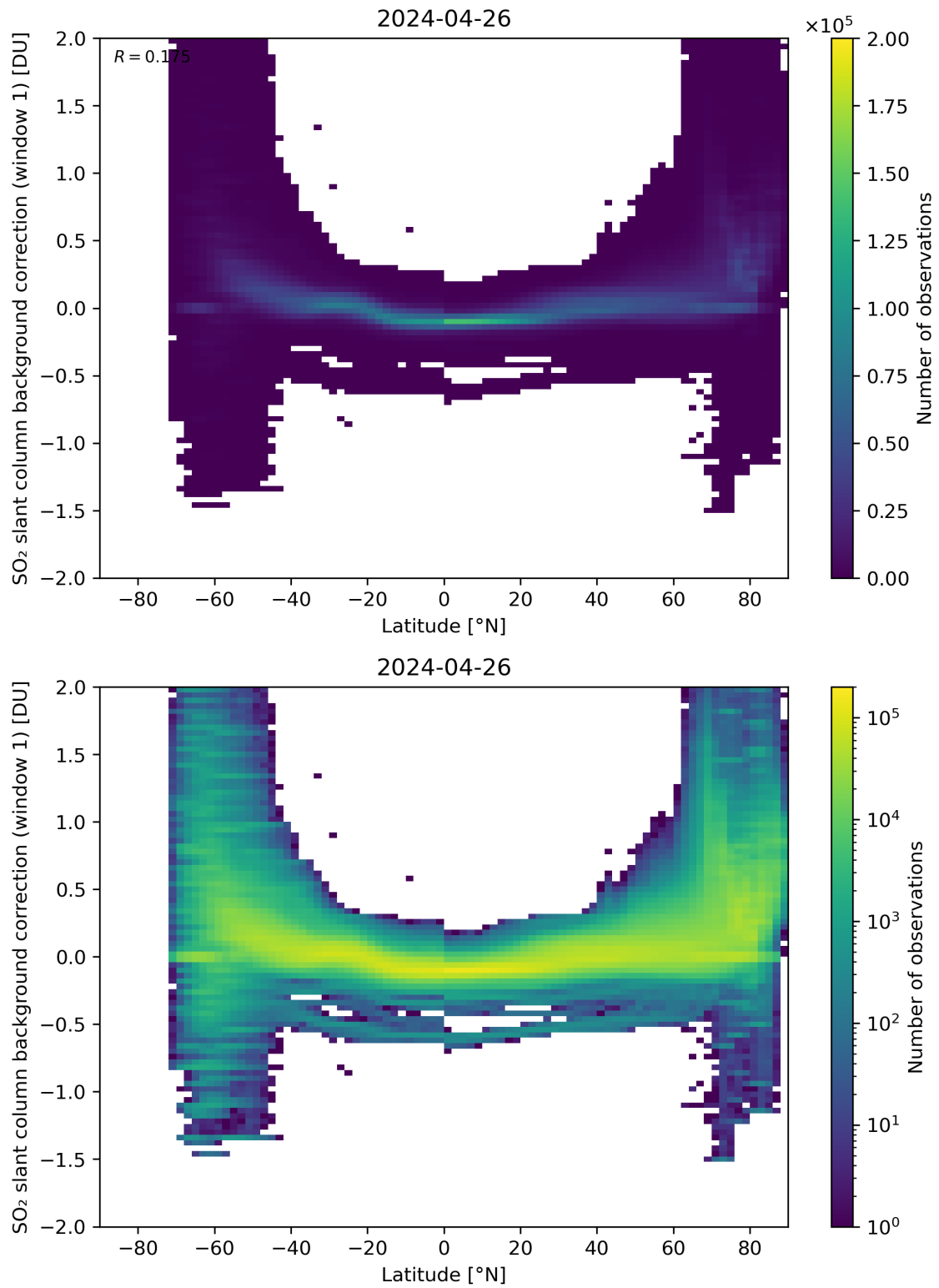
Figure 139: Scatter density plot of “Latitude” against “SO 2 slant column background correction (window 1)” for 2024-04-26 to 2024-04-27.
