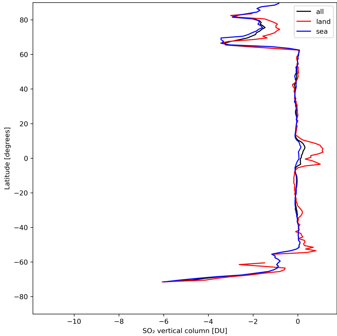
Figure 30: Zonal average of “SO 2 vertical column” for 2024-04-26 to 2024-04-27.
