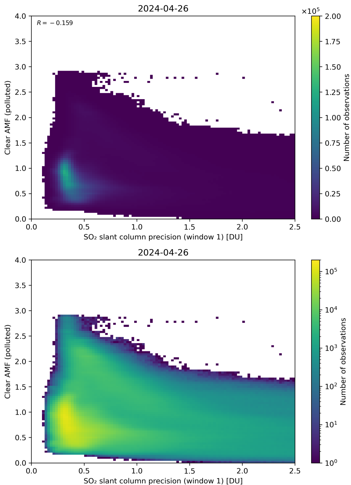
Figure 224: Scatter density plot of “SO 2 slant column precision (window 1)” against “Clear AMF (polluted)” for 2024-04-26 to 2024-04-27.
