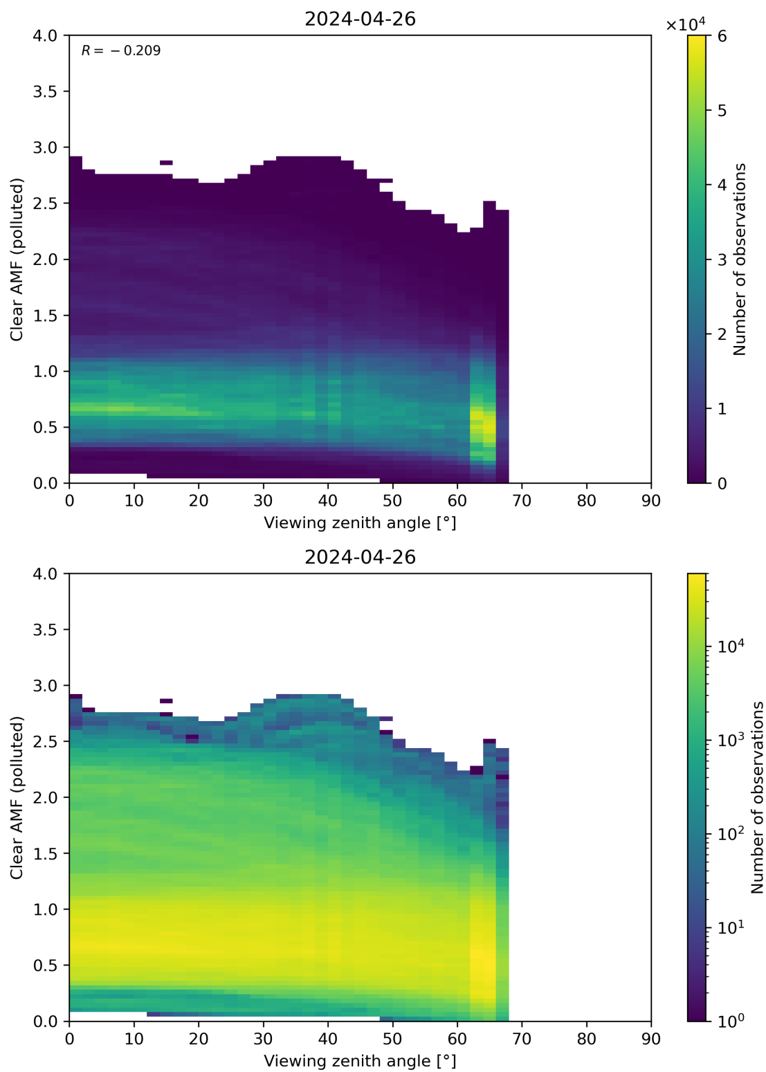
Figure 316: Scatter density plot of “Viewing zenith angle” against “Clear AMF (polluted)” for 2024-04-26 to 2024-04-27.
