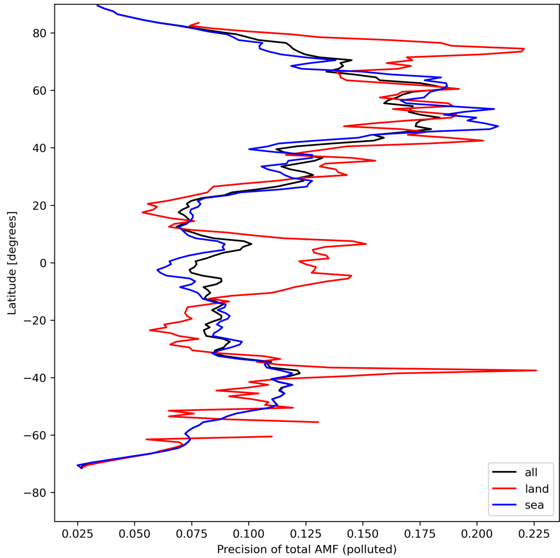
Figure 49: Zonal average of “Precision of total AMF (polluted)” for 2024-04-26 to 2024-04-27.
