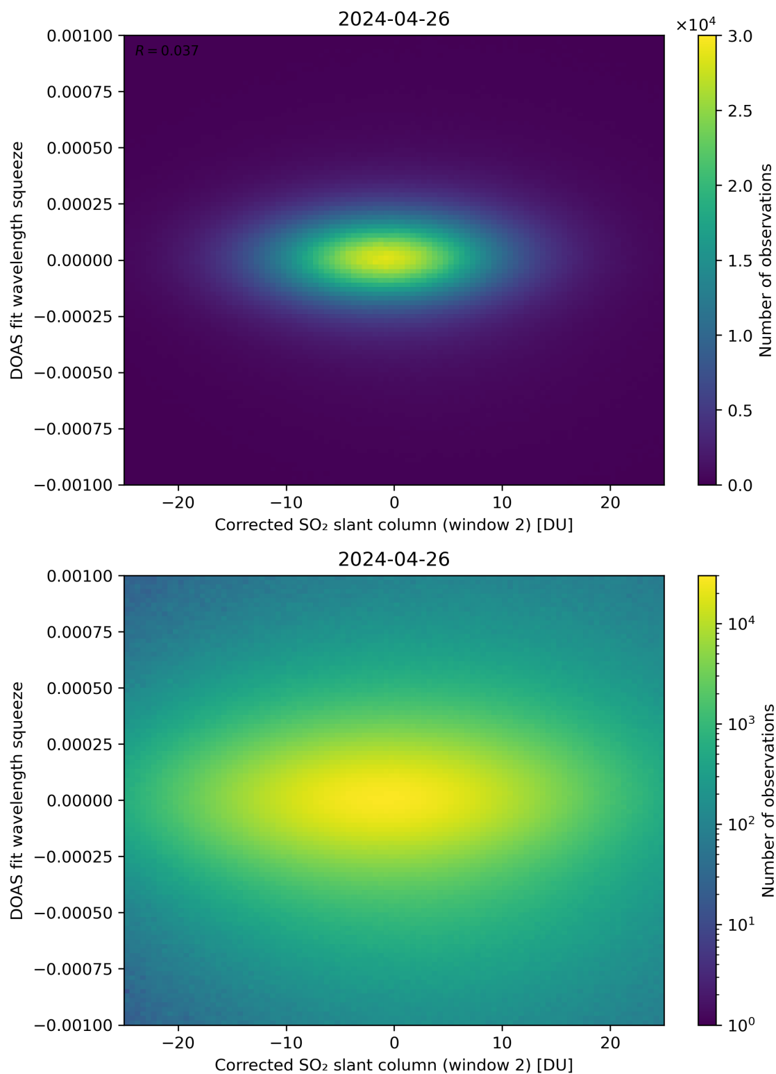
Figure 197: Scatter density plot of “Corrected SO 2 slant column (window 2)” against “DOAS fit wavelength squeeze” for 2024-04-26 to 2024-04-27.
