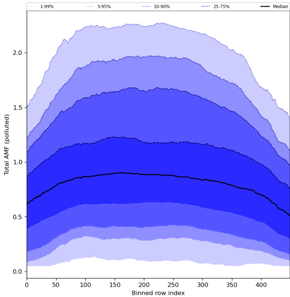
Figure 94: Along track statistics of “Total AMF (polluted)” for 2024-04-26 to 2024-04-27
