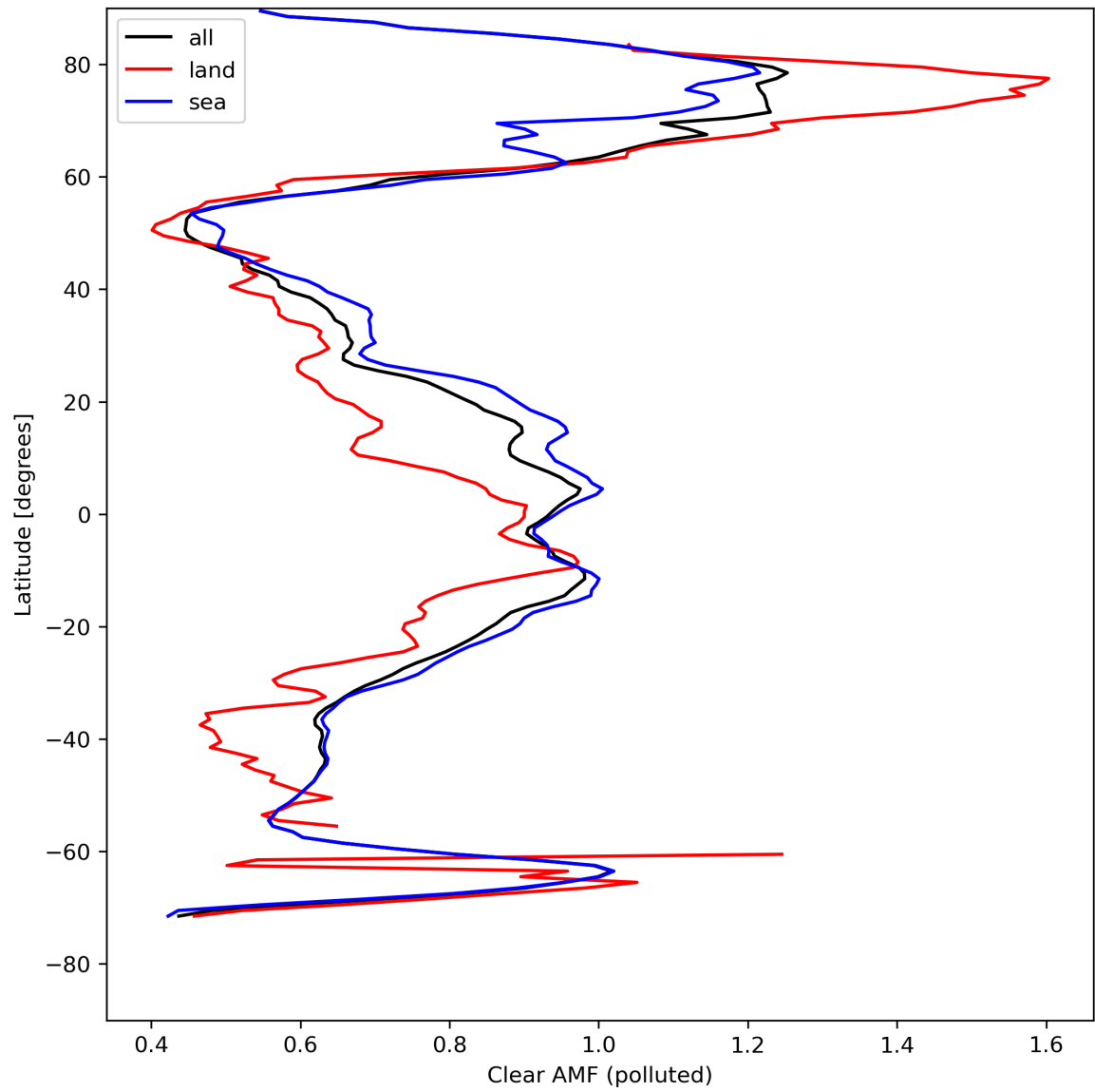
Figure 50: Zonal average of “Clear AMF (polluted)” for 2024-04-26 to 2024-04-27.
