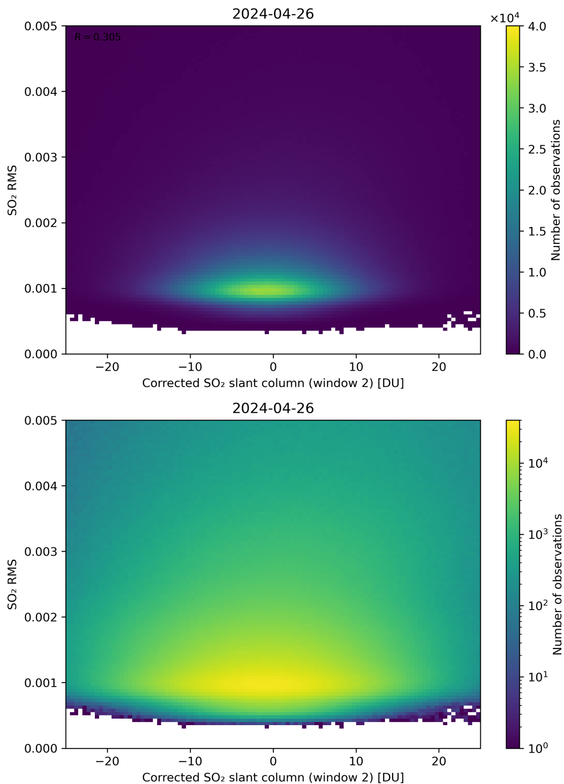
Figure 198: Scatter density plot of “Corrected SO 2 slant column (window 2)” against “SO 2 RMS” for 2024-04-26 to 2024-04-27.
