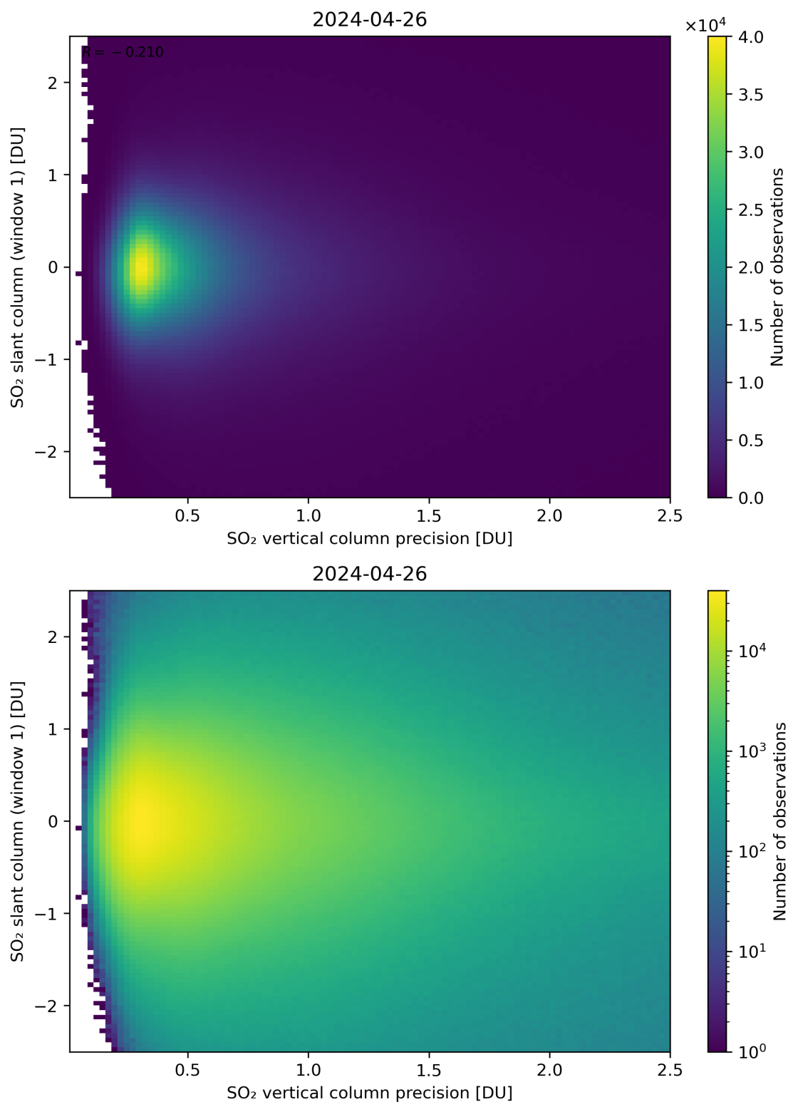
Figure 289: Scatter density plot of “SO 2 vertical column precision” against “SO 2 slant column (window 1)” for 2024-04-26 to 2024-04-27.
