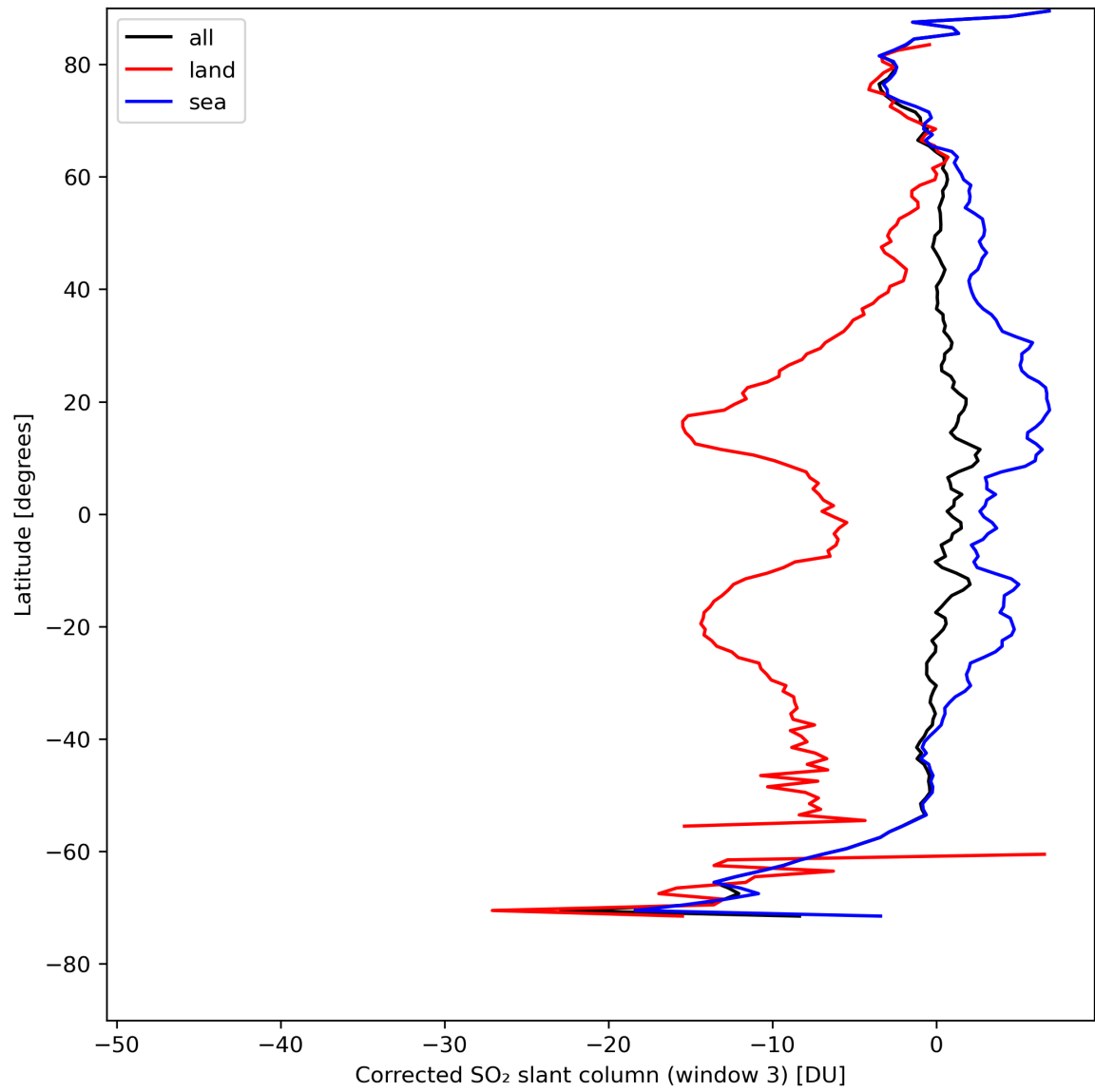
Figure 43: Zonal average of “Corrected SO 2 slant column (window 3)” for 2024-04-26 to 2024-04-27.
