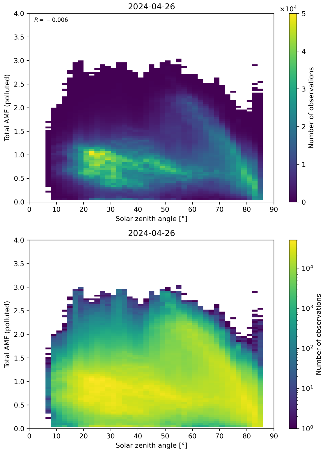
Figure 174: Scatter density plot of “Solar zenith angle” against “Total AMF (polluted)” for 2024-04-26 to 2024-04-27.
