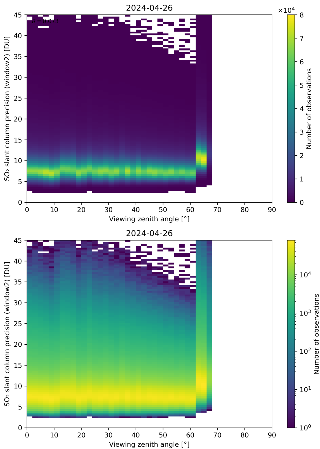
Figure 322: Scatter density plot of “Viewing zenith angle” against “SO 2 slant column precision (window2)” for 2024-04-26 to 2024-04-27.
