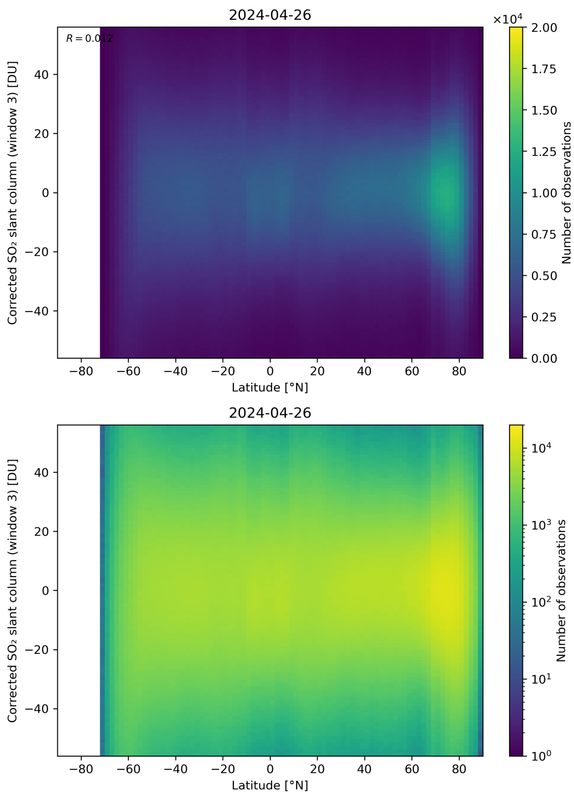
Figure 148: Scatter density plot of “Latitude” against “Corrected SO 2 slant column (window 3)” for 2024-04-26 to 2024-04-27.
