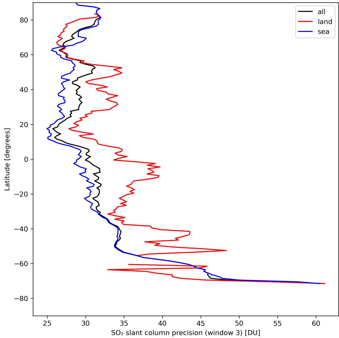
Figure 42: Zonal average of “SO 2 slant column precision (window 3)” for 2024-04-26 to 2024-04-27.
