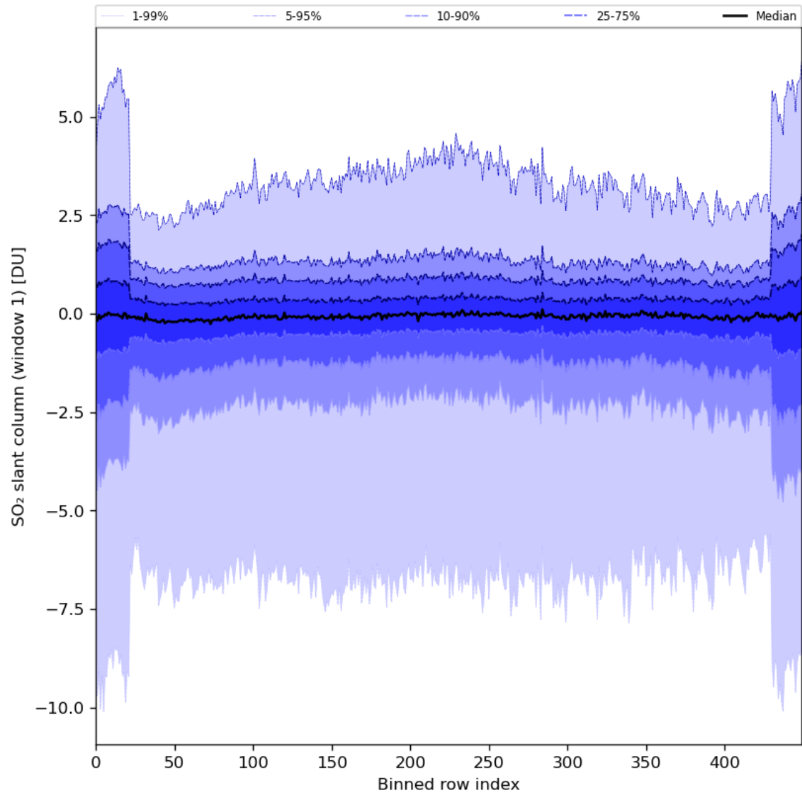
Figure 79: Along track statistics of “SO 2 slant column (window 1)” for 2024-04-26 to 2024-04-27
