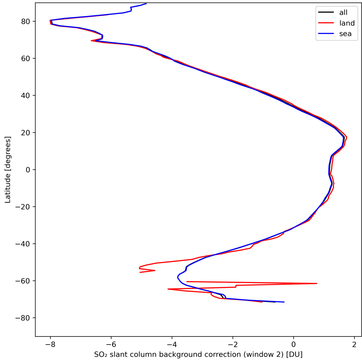
Figure 40: Zonal average of “SO 2 slant column background correction (window 2)” for 2024-04-26 to 2024-04-27.
