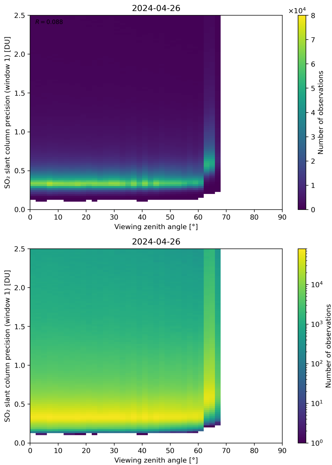
Figure 321: Scatter density plot of “Viewing zenith angle” against “SO 2 slant column precision (window 1)” for 2024-04-26 to 2024-04-27.
