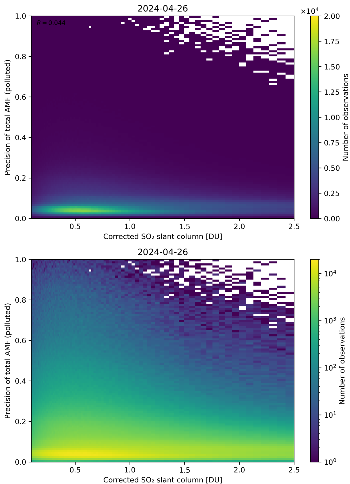
Figure 193: Scatter density plot of “Corrected SO 2 slant column” against “Precision of total AMF (polluted)” for 2024-04-26 to 2024-04-27.
