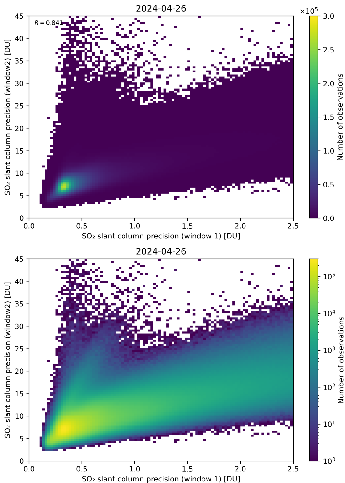
Figure 227: Scatter density plot of “SO 2 slant column precision (window 1)” against “SO 2 slant column precision (window2)” for 2024-04-26 to 2024-04-27.
