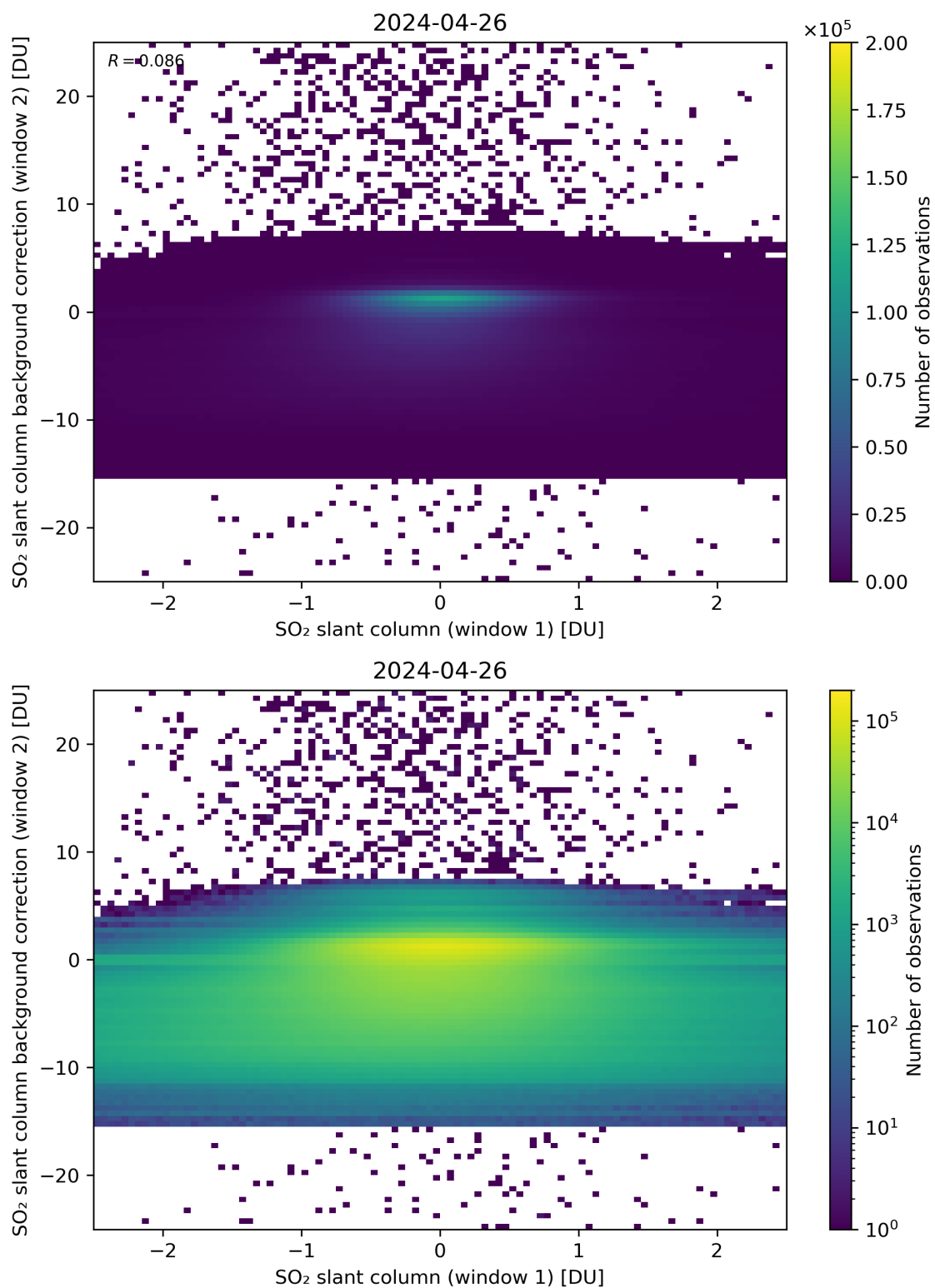
Figure 213: Scatter density plot of “SO 2 slant column (window 1)” against “SO 2 slant column background correction (window 2)” for 2024-04-26 to 2024-04-27.
