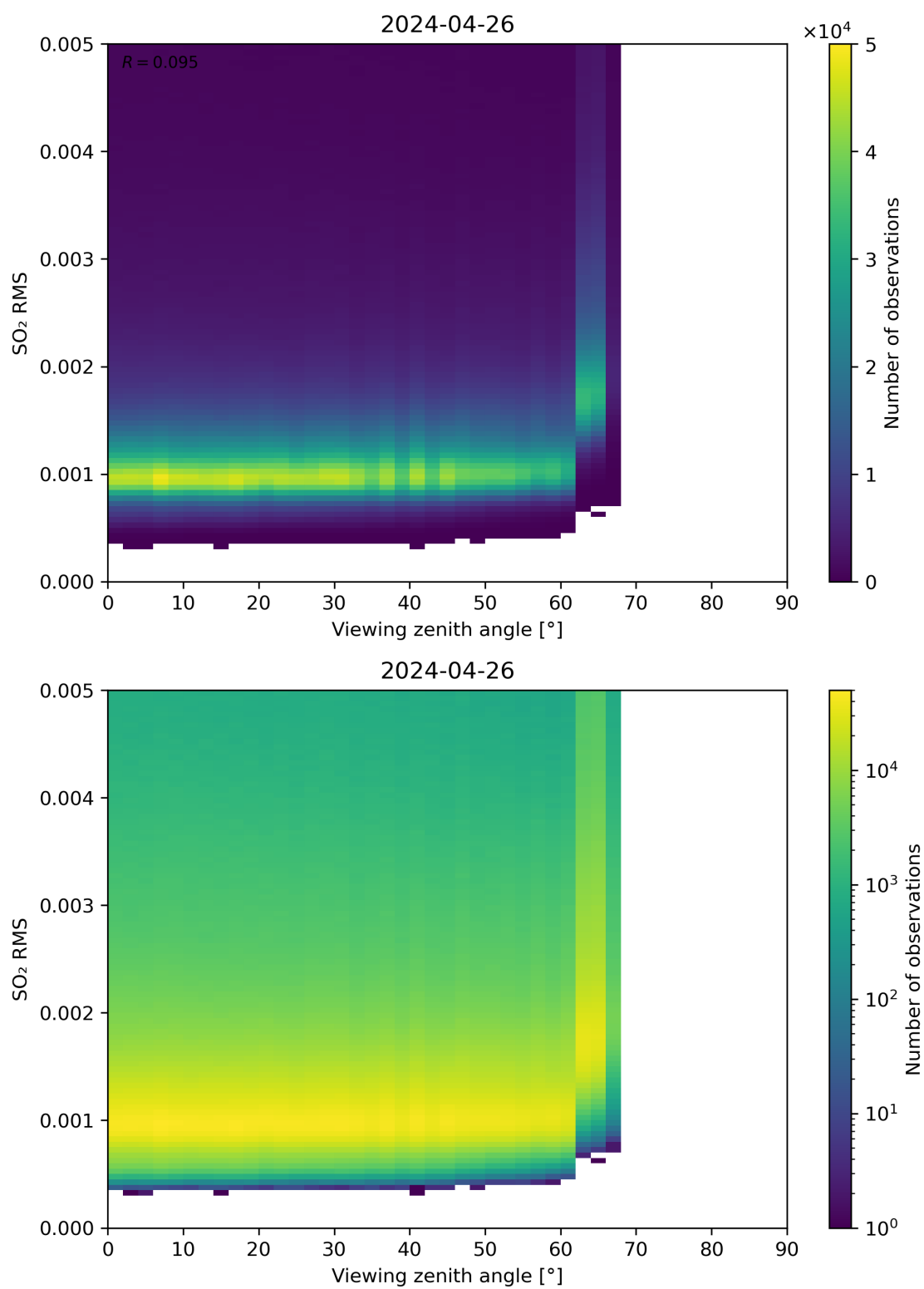
Figure 313: Scatter density plot of “Viewing zenith angle” against “SO 2 RMS” for 2024-04-26 to 2024-04-27.
