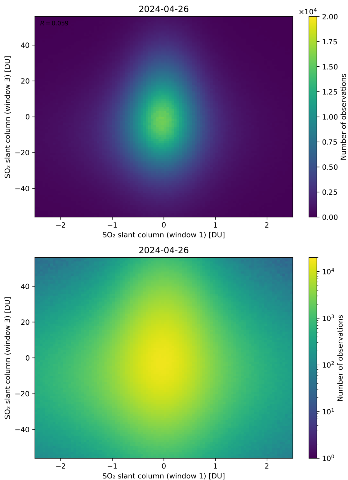
Figure 237: Scatter density plot of “SO 2 slant column (window 1)” against “SO 2 slant column (window 3)” for 2024-04-26 to 2024-04-27.
