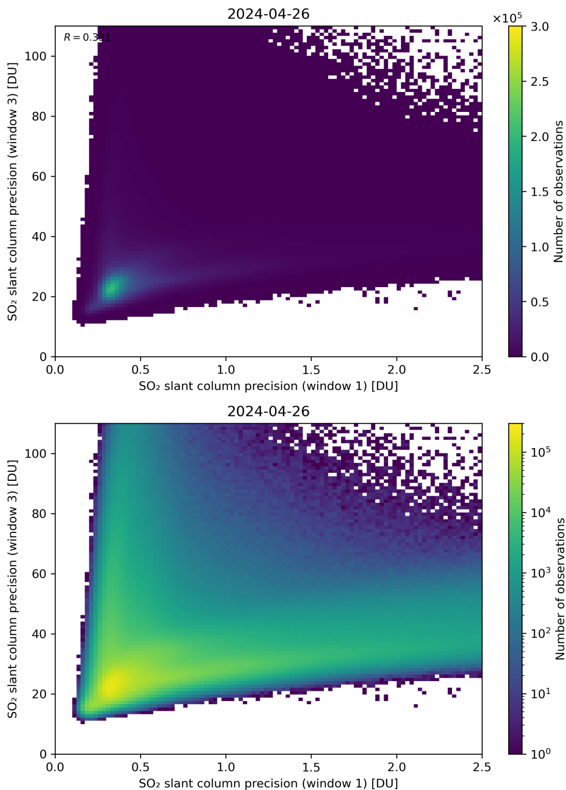
Figure 229: Scatter density plot of “SO 2 slant column precision (window 1)” against “SO 2 slant column precision (window 3)” for 2024-04-26 to 2024-04-27.
