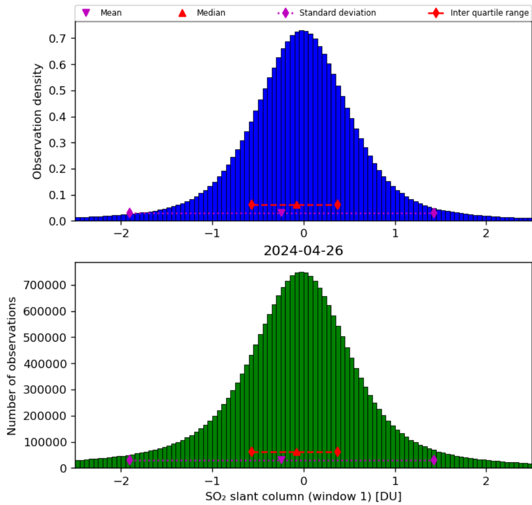
Figure 56: Histogram of “SO 2 slant column (window 1)” for 2024-04-26 to 2024-04-27
