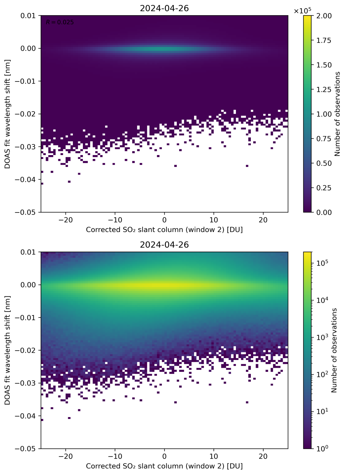
Figure 196: Scatter density plot of “Corrected SO 2 slant column (window 2)” against “DOAS fit wavelength shift” for 2024-04-26 to 2024-04-27.
