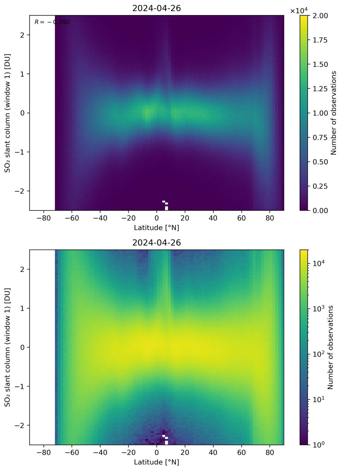
Figure 149: Scatter density plot of “Latitude” against “SO 2 slant column (window 1)” for 2024-04-26 to 2024-04-27.
