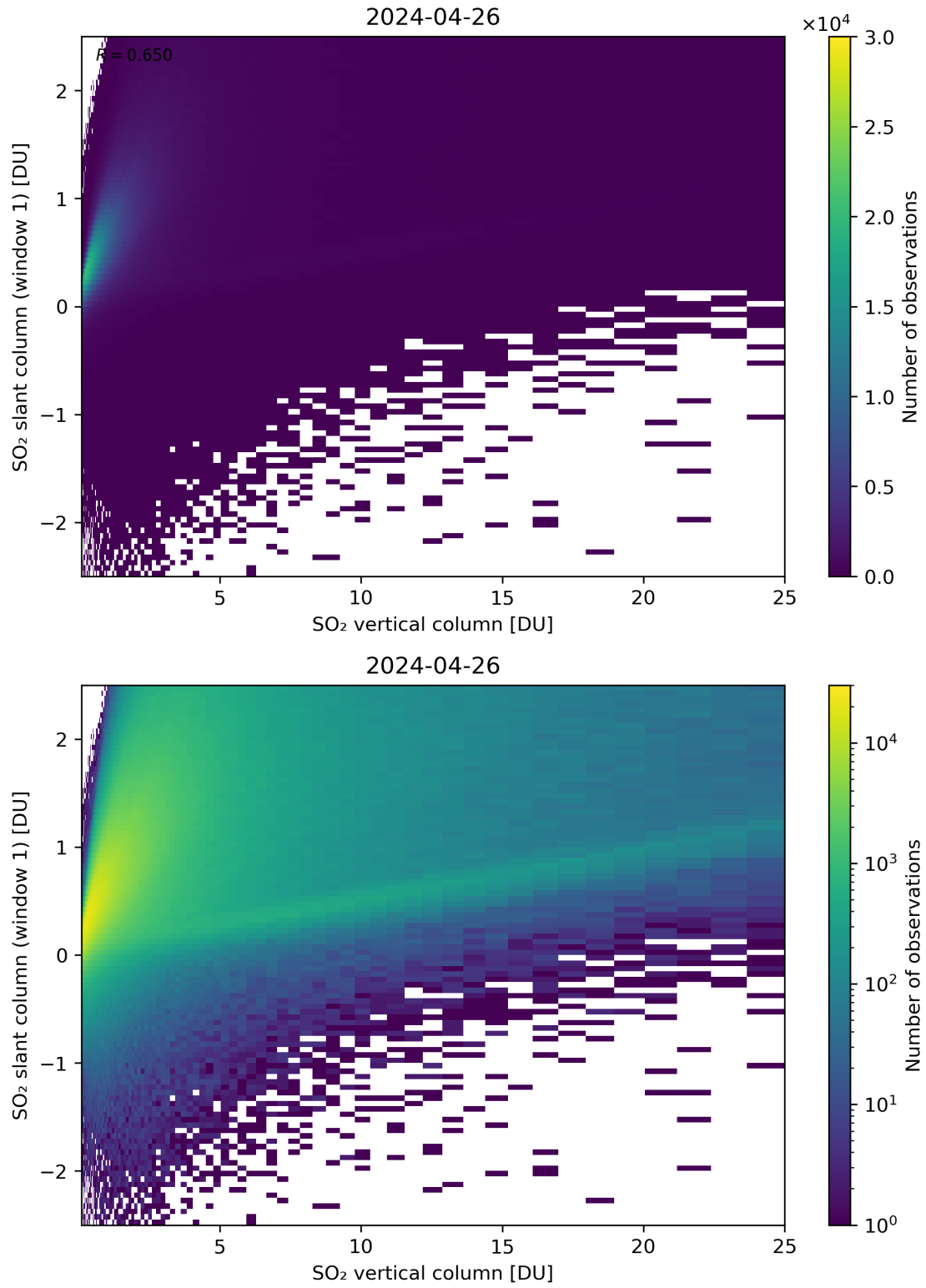
Figure 300: Scatter density plot of “SO 2 vertical column” against “SO 2 slant column (window 1)” for 2024-04-26 to 2024-04-27.
