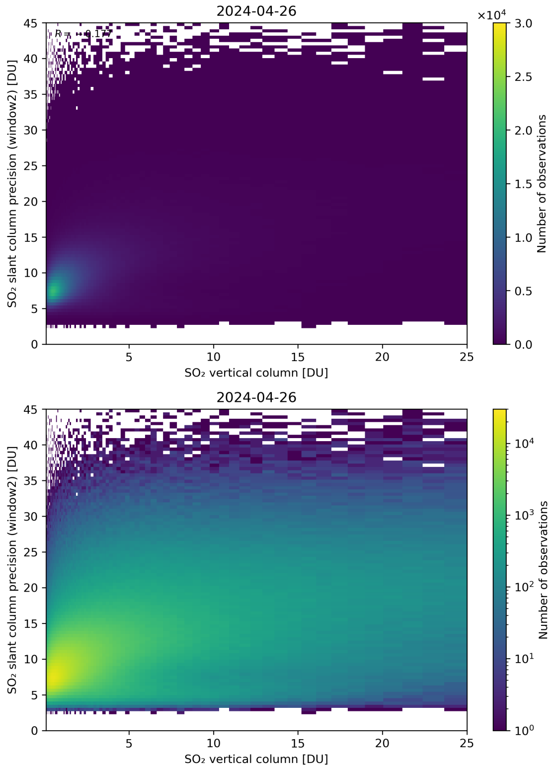
Figure 302: Scatter density plot of “SO 2 vertical column” against “SO 2 slant column precision (window2)” for 2024-04-26 to 2024-04-27.
