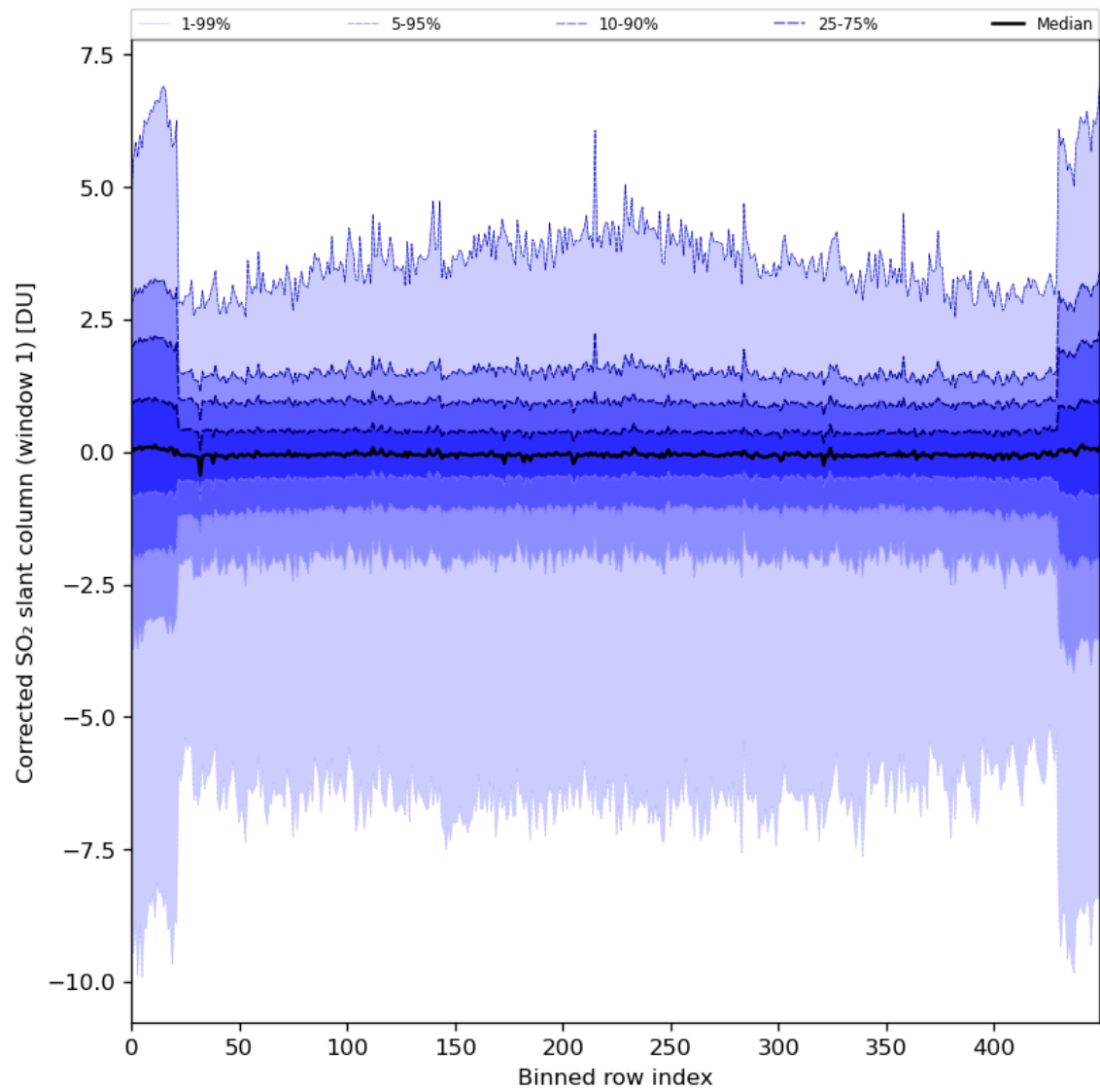
Figure 81: Along track statistics of “Corrected SO 2 slant column (window 1)” for 2024-04-26 to 2024-04-27
