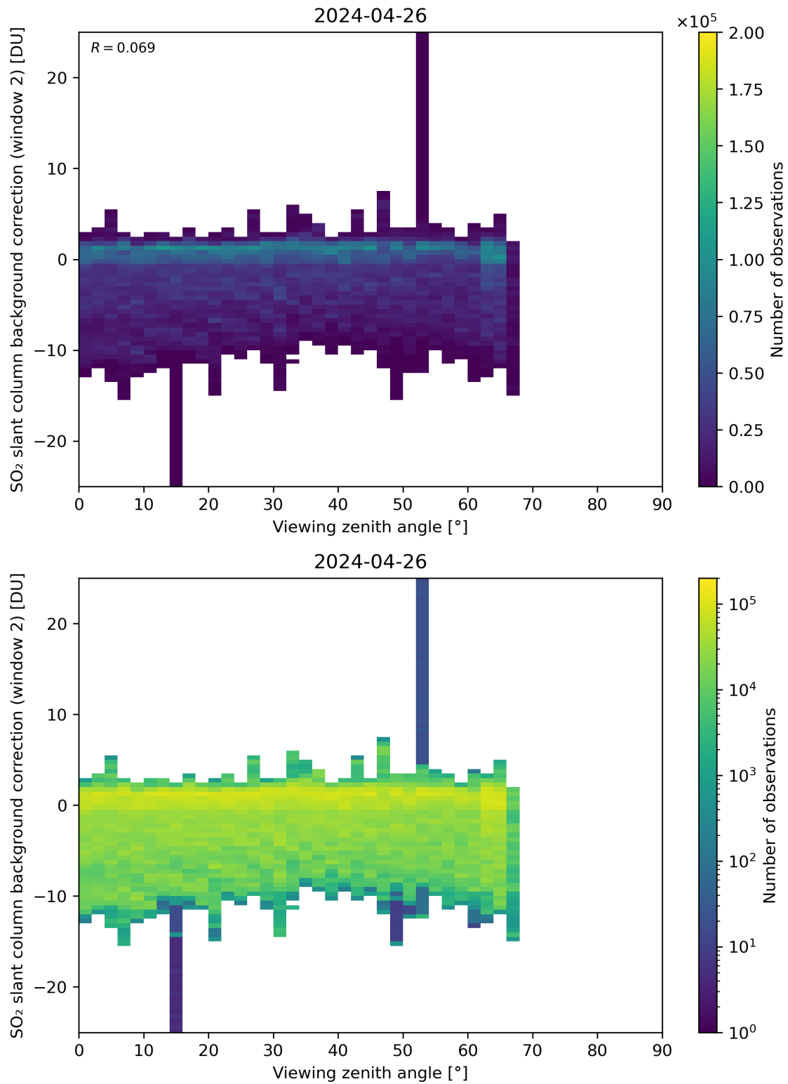
Figure 309: Scatter density plot of “Viewing zenith angle” against “SO 2 slant column background correction (window 2)” for 2024-04-26 to 2024-04-27.
