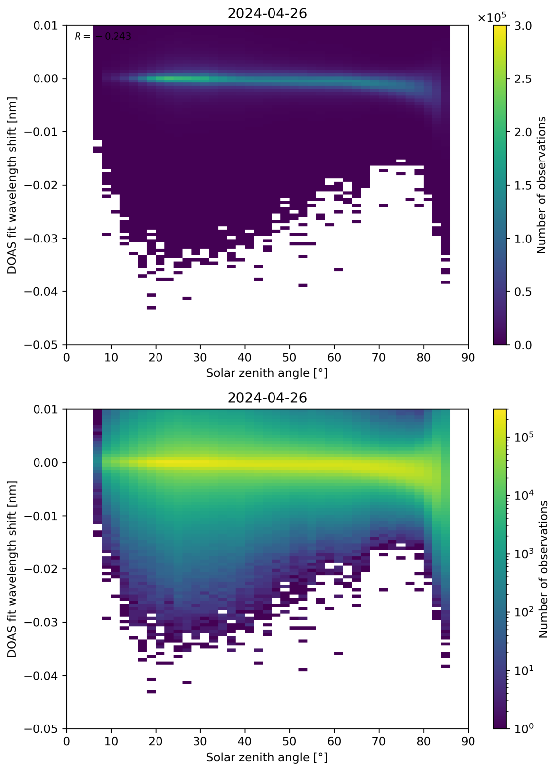
Figure 161: Scatter density plot of “Solar zenith angle” against “DOAS fit wavelength shift” for 2024-04-26 to 2024-04-27.
