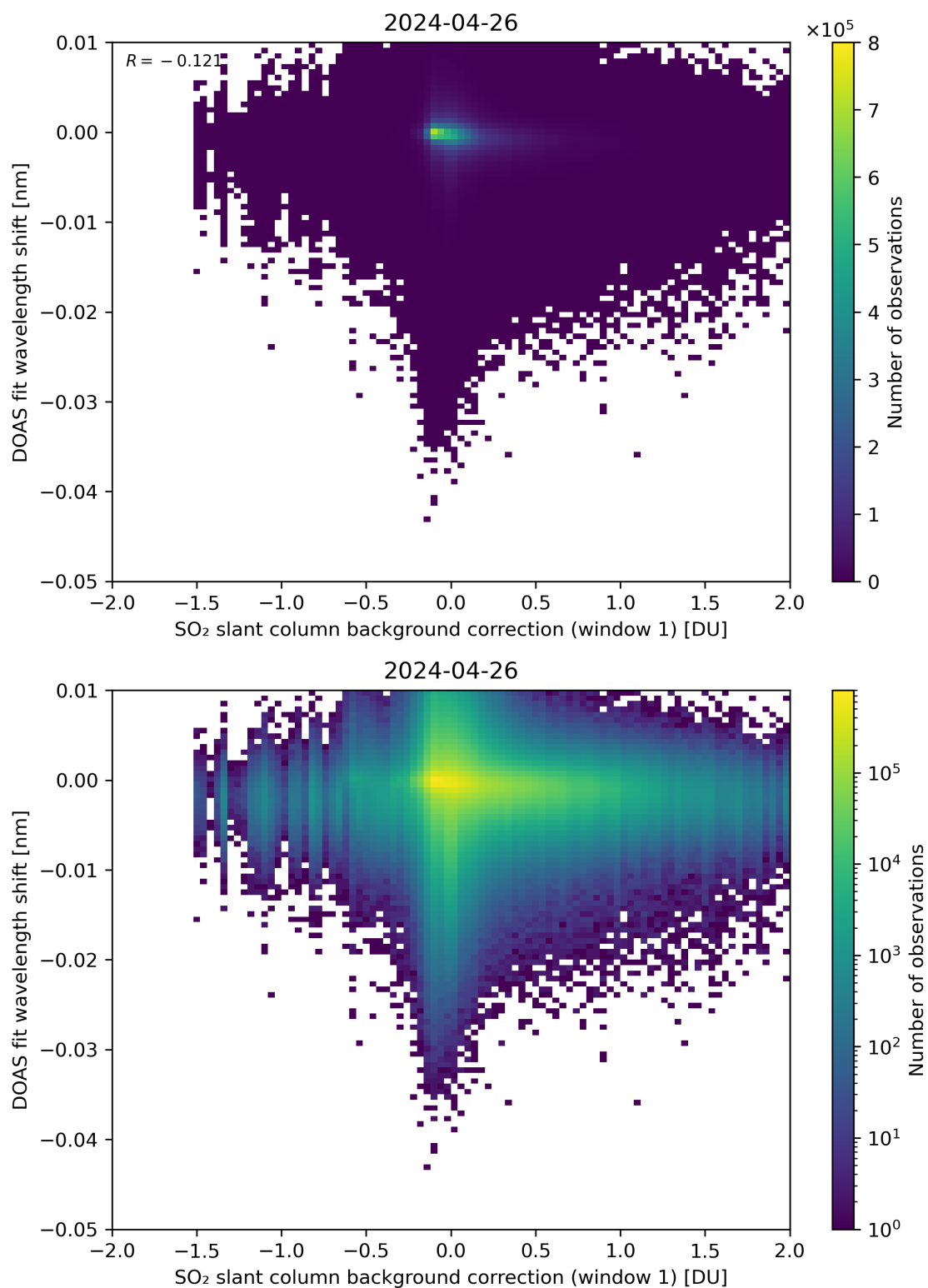
Figure 100: Scatter density plot of “SO 2 slant column background correction (window 1)” against “DOAS fit wavelength shift” for 2024-04-26 to 2024-04-27.
