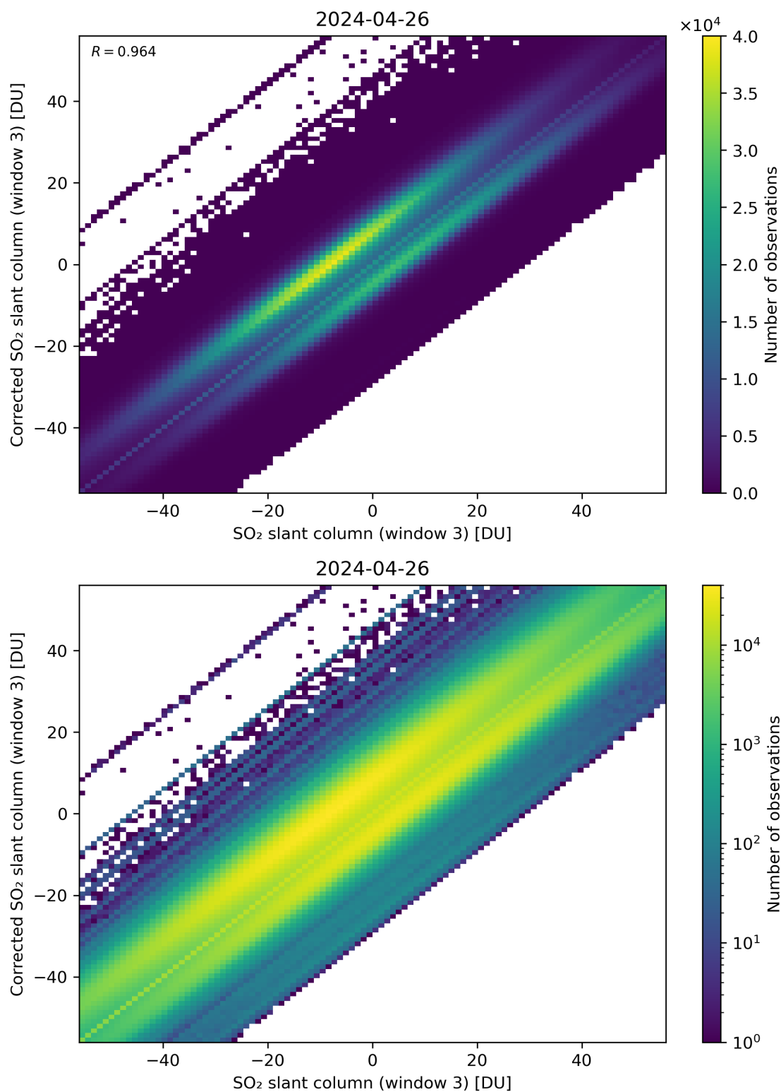
Figure 266: Scatter density plot of “SO 2 slant column (window 3)” against “Corrected SO 2 slant column (window 3)” for 2024-04-26 to 2024-04-27.
