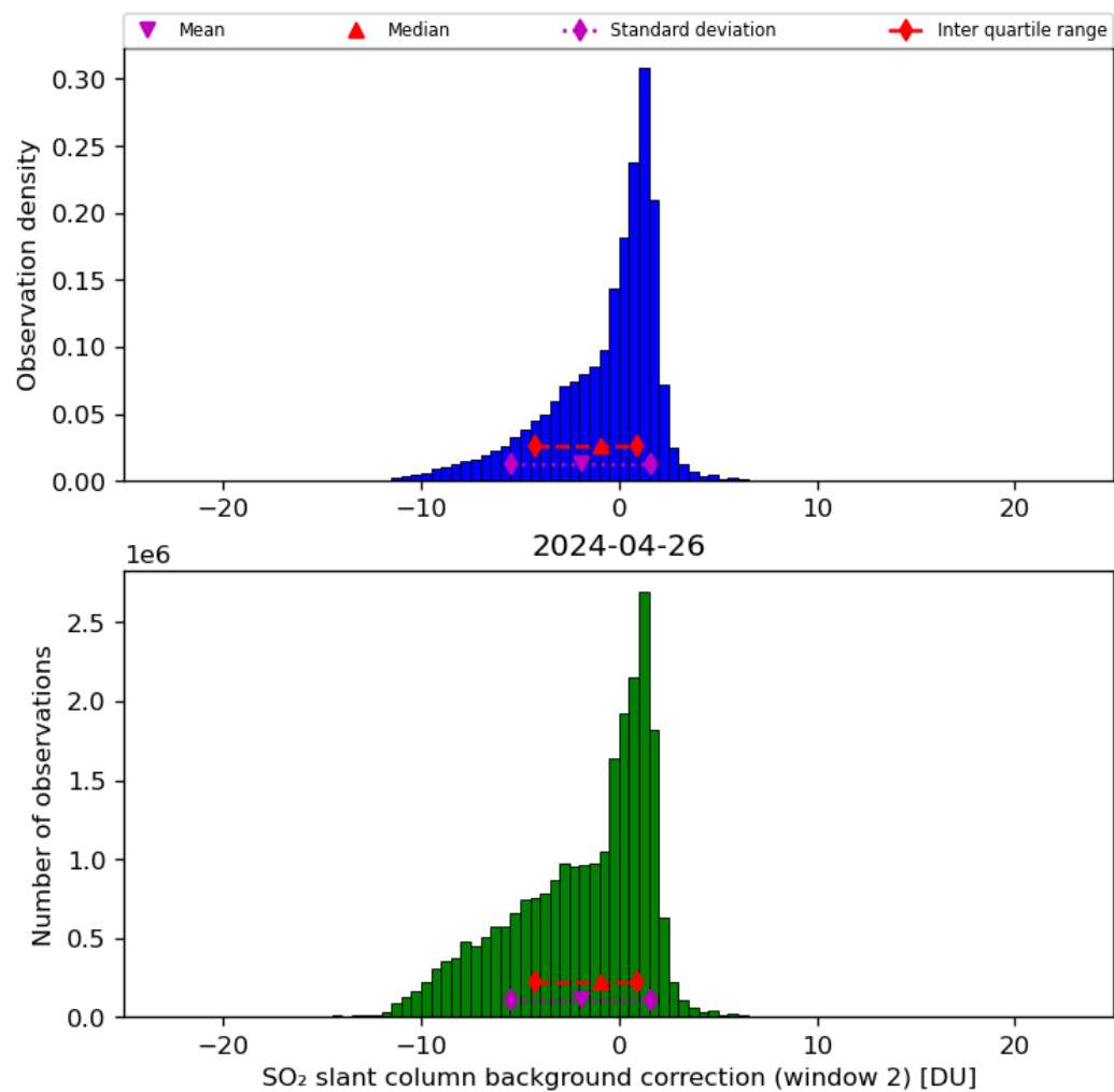
Figure 63: Histogram of “SO 2 slant column background correction (window 2)” for 2024-04-26 to 2024-04-27
