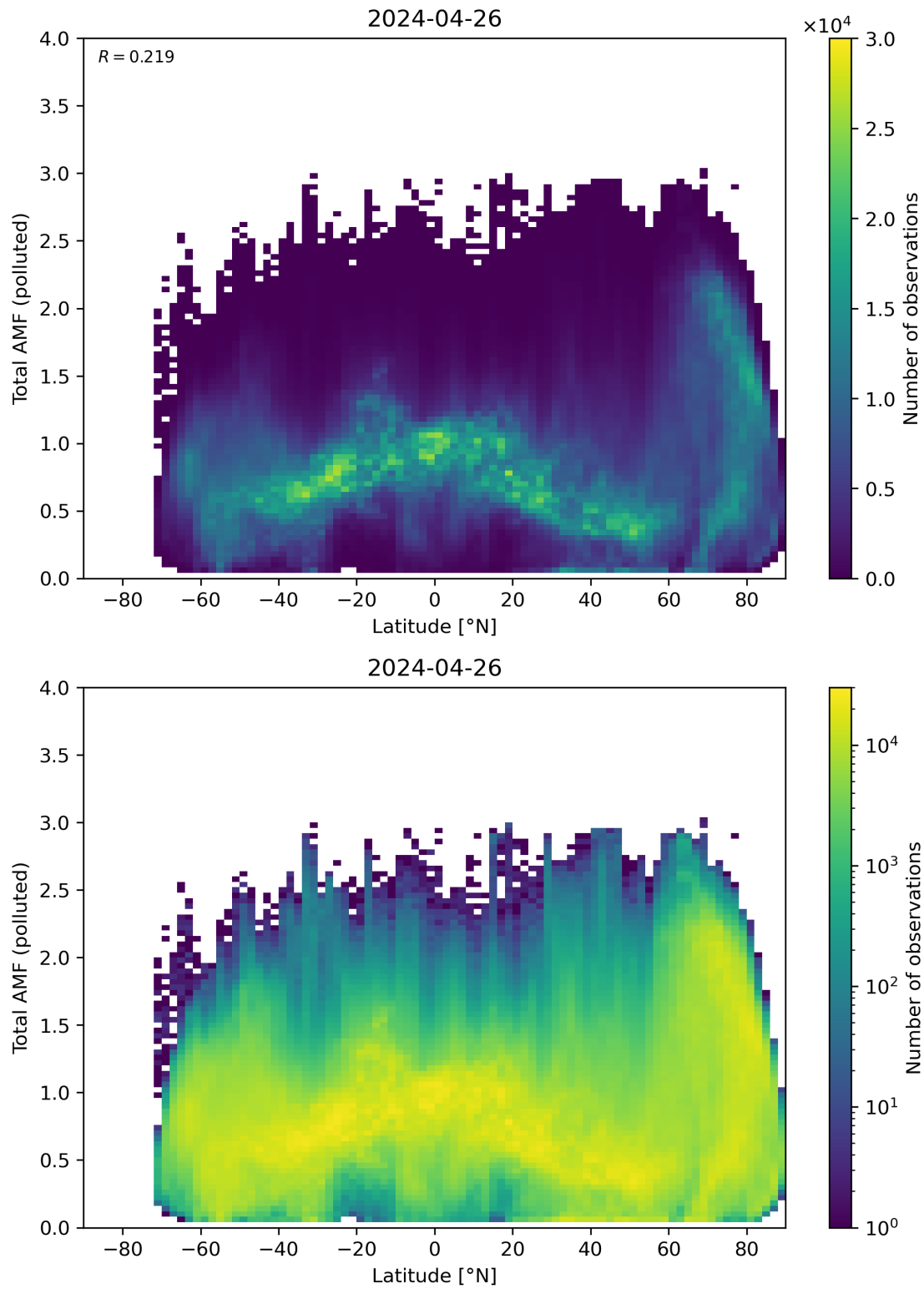
Figure 154: Scatter density plot of “Latitude” against “Total AMF (polluted)” for 2024-04-26 to 2024-04-27.
