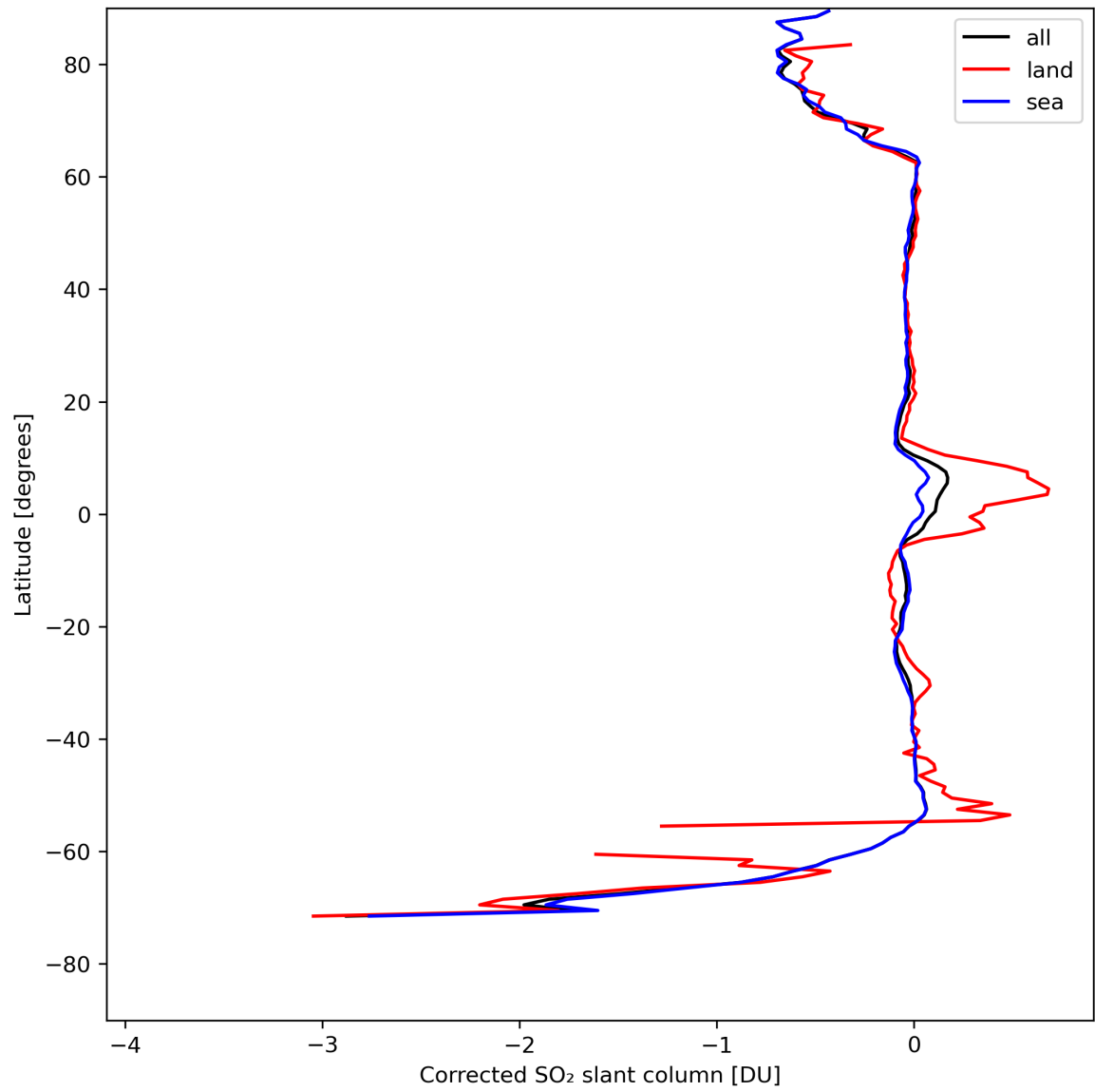
Figure 32: Zonal average of “Corrected SO 2 slant column” for 2024-04-26 to 2024-04-27.
