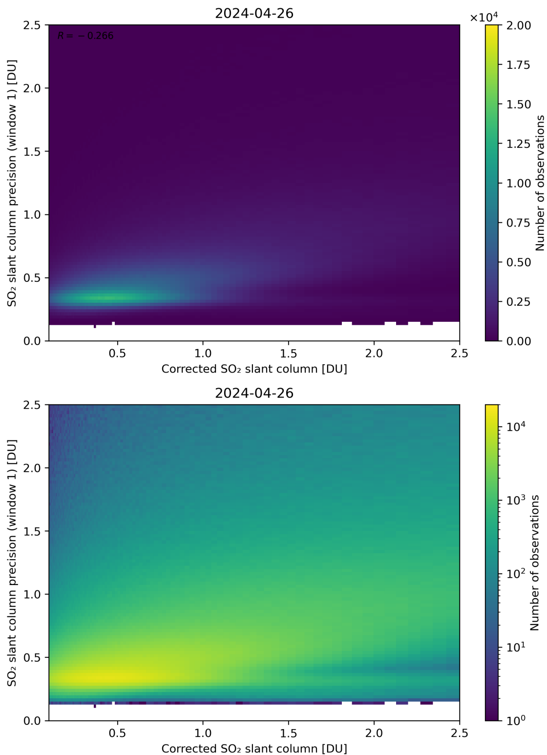
Figure 188: Scatter density plot of “Corrected SO 2 slant column” against “SO 2 slant column precision (window 1)” for 2024-04-26 to 2024-04-27.
