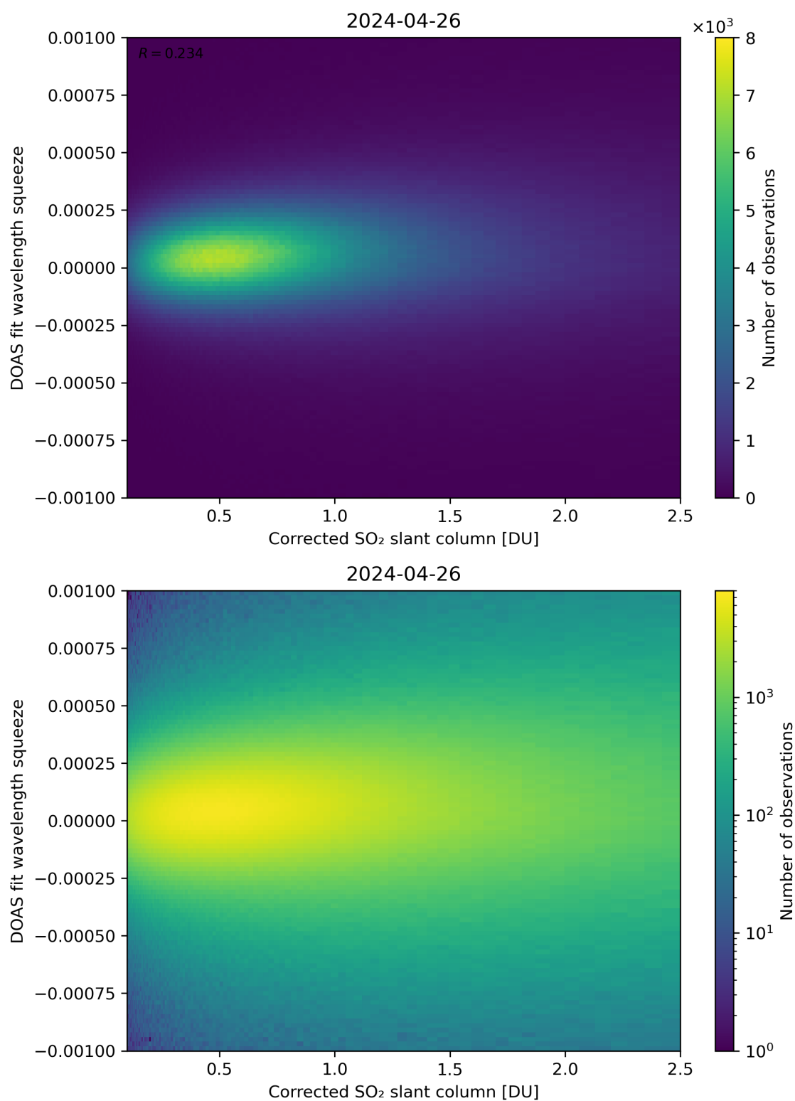
Figure 182: Scatter density plot of “Corrected SO 2 slant column” against “DOAS fit wavelength squeeze” for 2024-04-26 to 2024-04-27.
