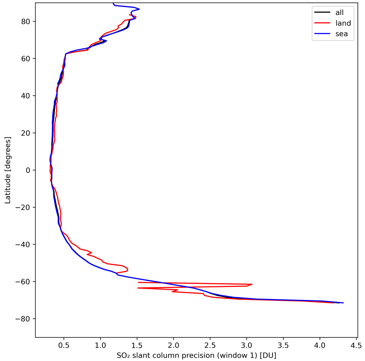
Figure 34: Zonal average of “SO 2 slant column precision (window 1)” for 2024-04-26 to 2024-04-27.
