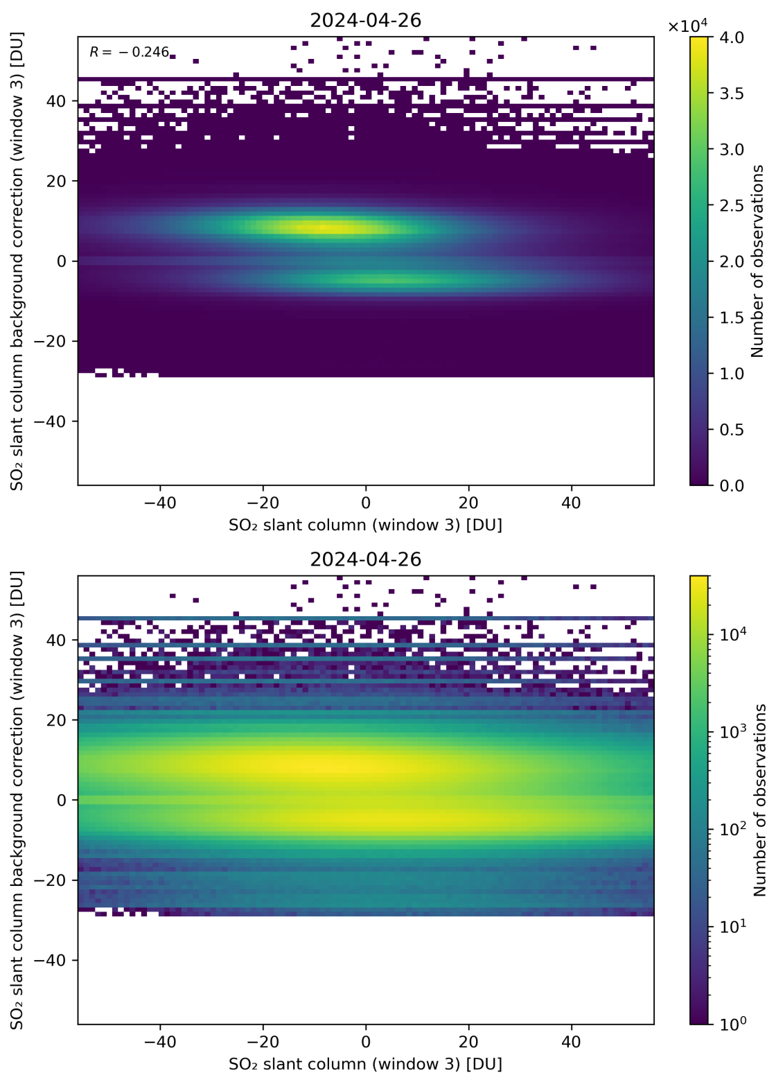
Figure 253: Scatter density plot of “SO 2 slant column (window 3)” against “SO 2 slant column background correction (window 3)” for 2024-04-26 to 2024-04-27.
