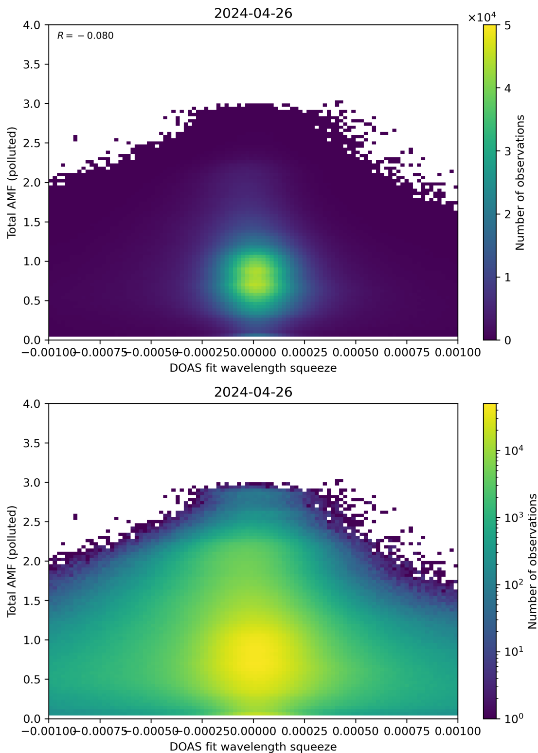
Figure 134: Scatter density plot of “DOAS fit wavelength squeeze” against “Total AMF (polluted)” for 2024-04-26 to 2024-04-27.
