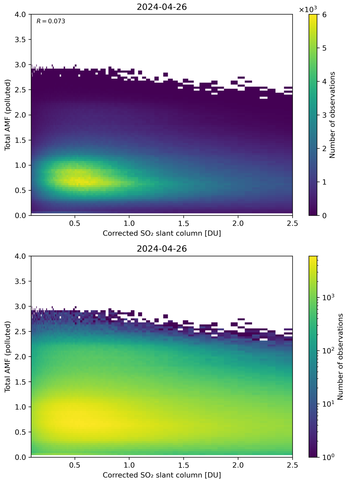
Figure 192: Scatter density plot of “Corrected SO 2 slant column” against “Total AMF (polluted)” for 2024-04-26 to 2024-04-27.
