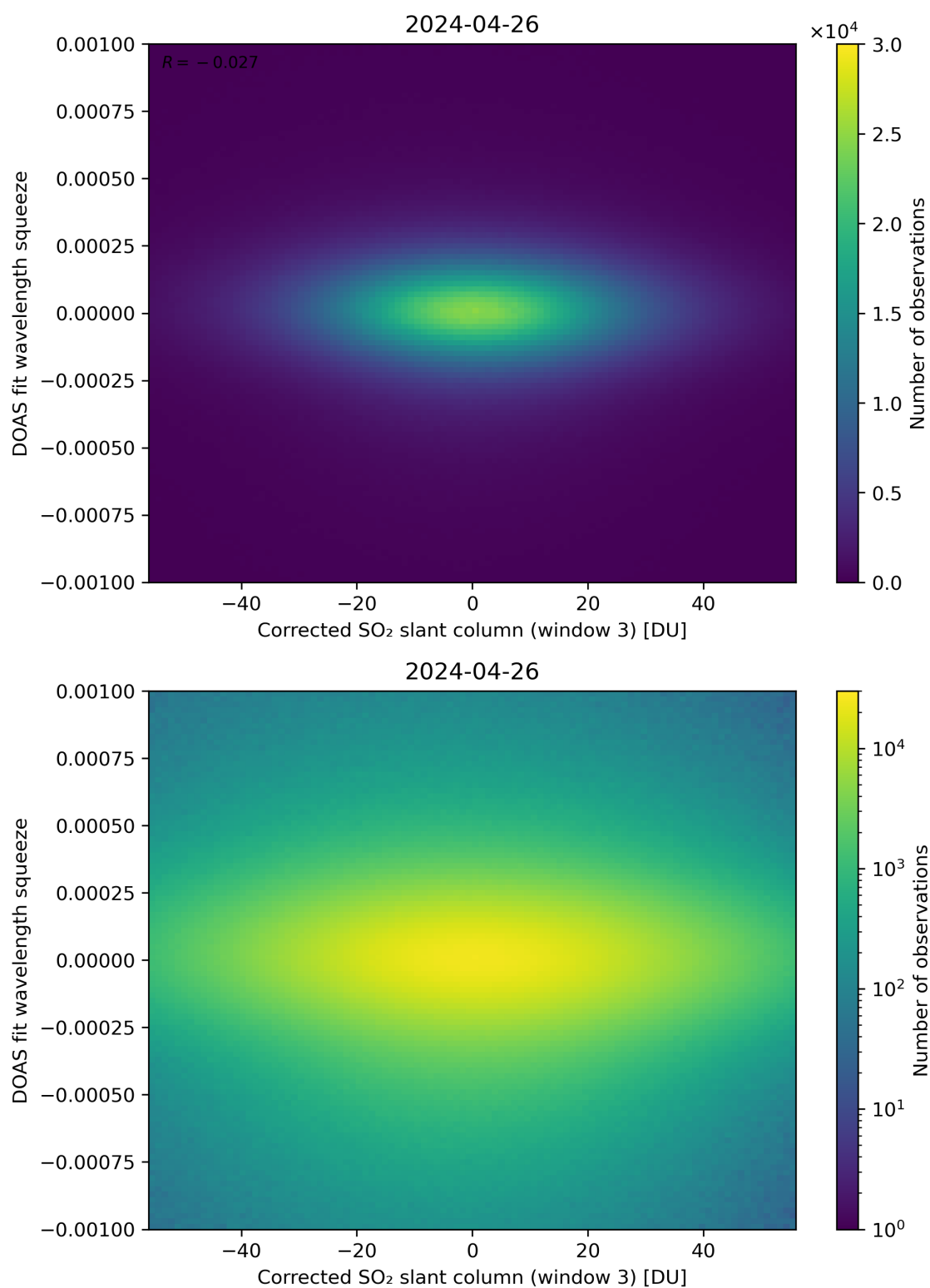
Figure 207: Scatter density plot of “Corrected SO 2 slant column (window 3)” against “DOAS fit wavelength squeeze” for 2024-04-26 to 2024-04-27.
