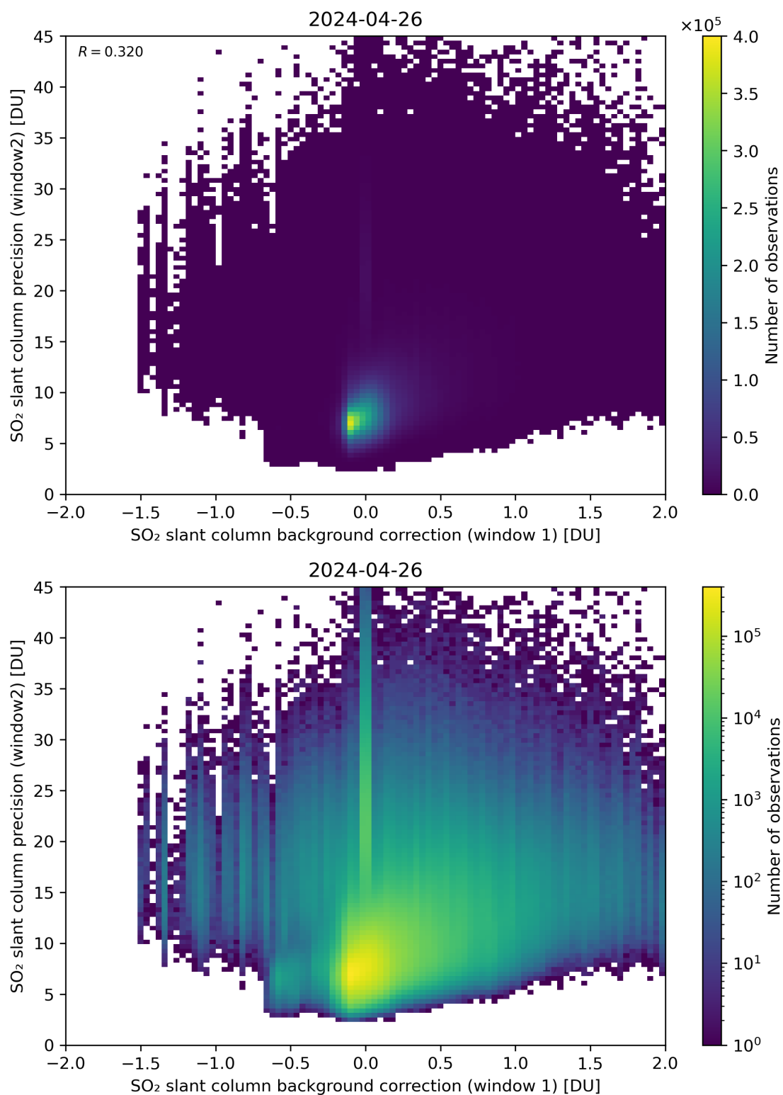
Figure 106: Scatter density plot of “SO 2 slant column background correction (window 1)” against “SO 2 slant column precision (window2)” for 2024-04-26 to 2024-04-27.
