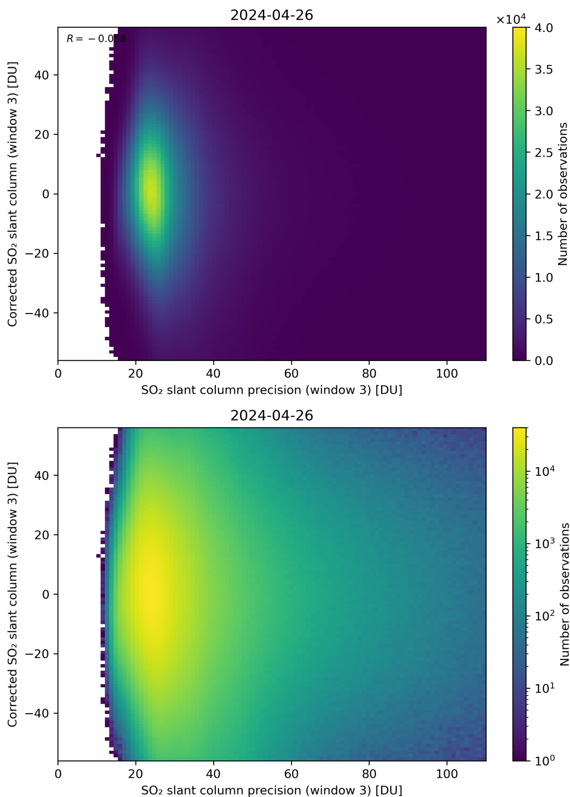
Figure 262: Scatter density plot of “SO 2 slant column precision (window 3)” against “Corrected SO 2 slant column (window 3)” for 2024-04-26 to 2024-04-27.
