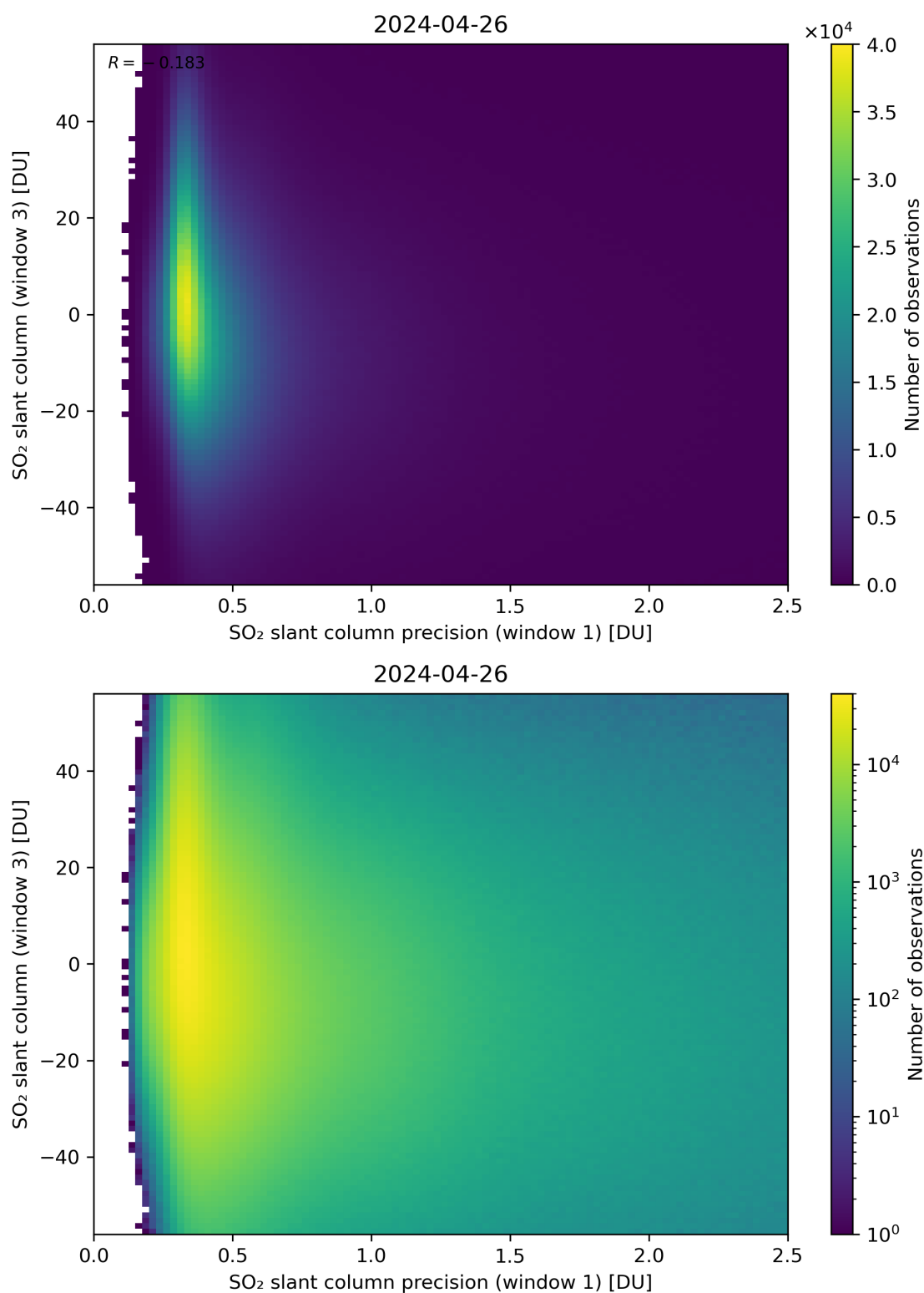
Figure 228: Scatter density plot of “SO 2 slant column precision (window 1)” against “SO 2 slant column (window 3)” for 2024-04-26 to 2024-04-27.
