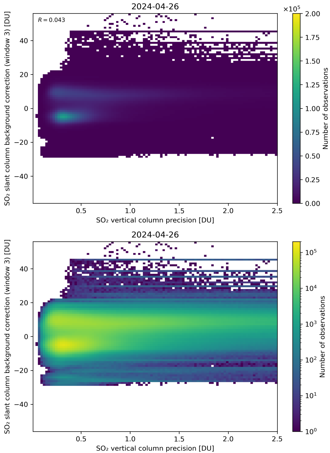
Figure 281: Scatter density plot of “SO 2 vertical column precision” against “SO 2 slant column background correction (window 3)” for 2024-04-26 to 2024-04-27.
