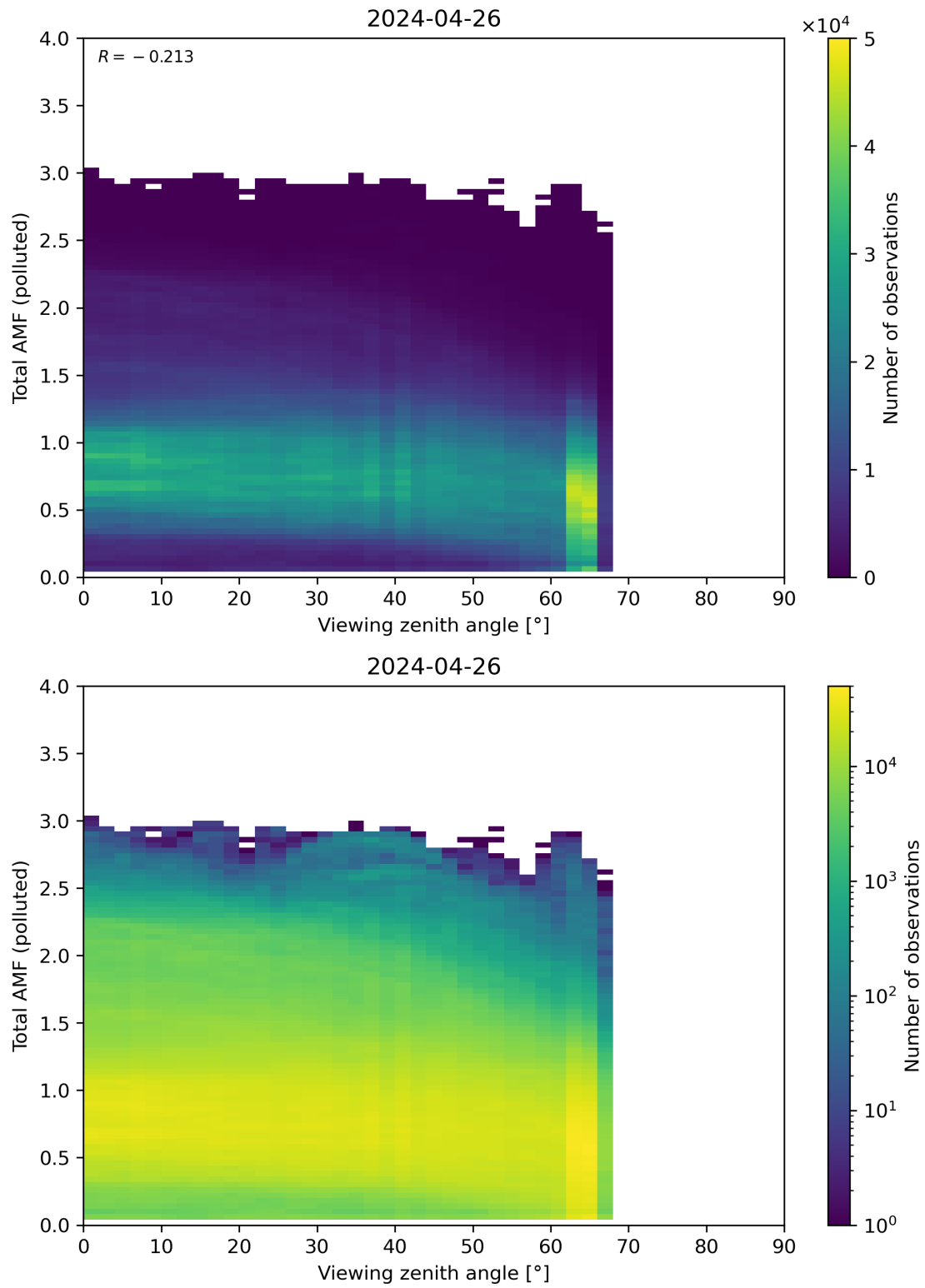
Figure 325: Scatter density plot of “Viewing zenith angle” against “Total AMF (polluted)” for 2024-04-26 to 2024-04-27.
