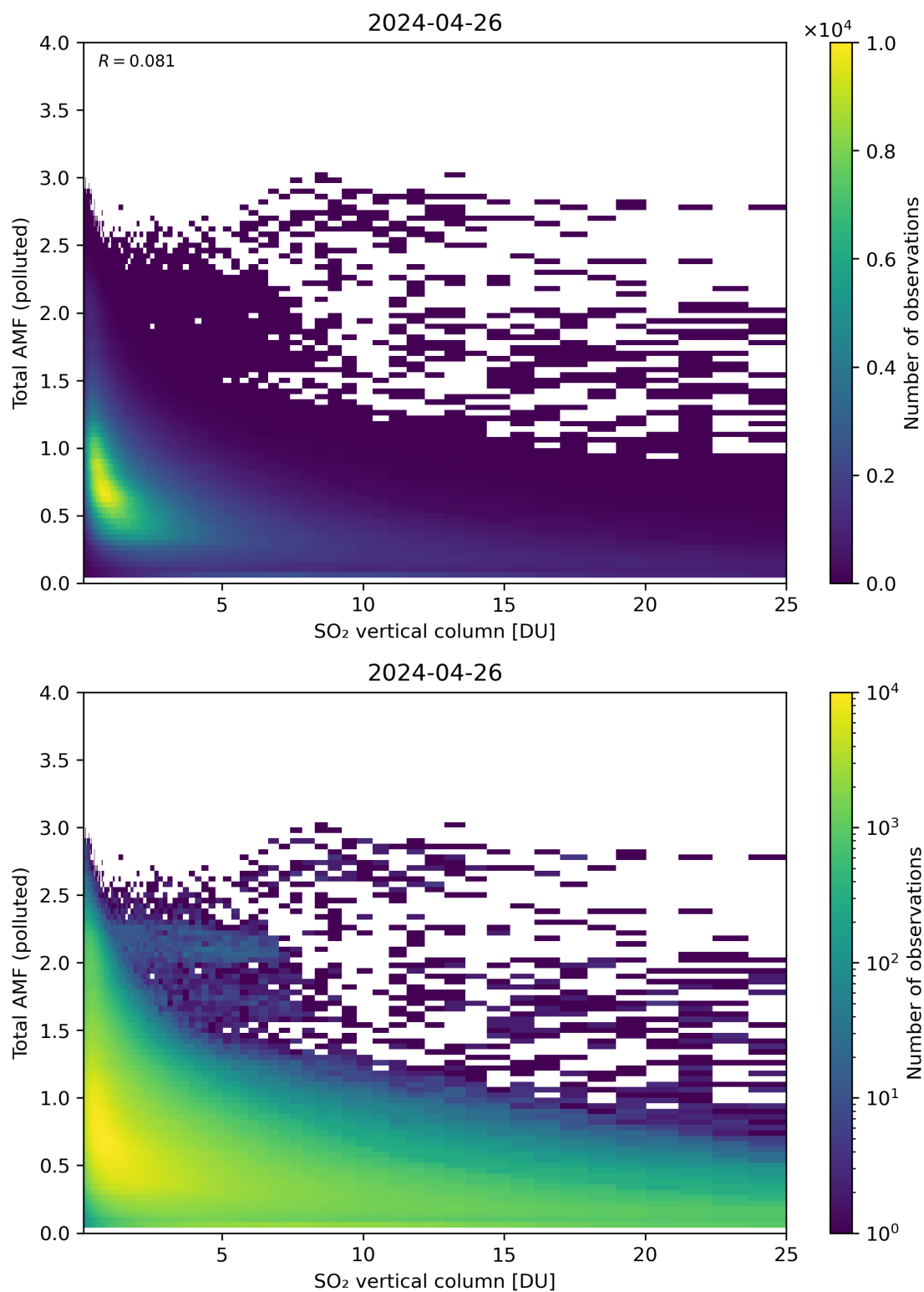
Figure 305: Scatter density plot of “SO 2 vertical column” against “Total AMF (polluted)” for 2024-04-26 to 2024-04-27.
