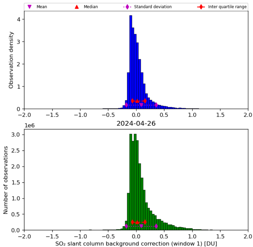
Figure 59: Histogram of “SO 2 slant column background correction (window 1)” for 2024-04-26 to 2024-04-27
