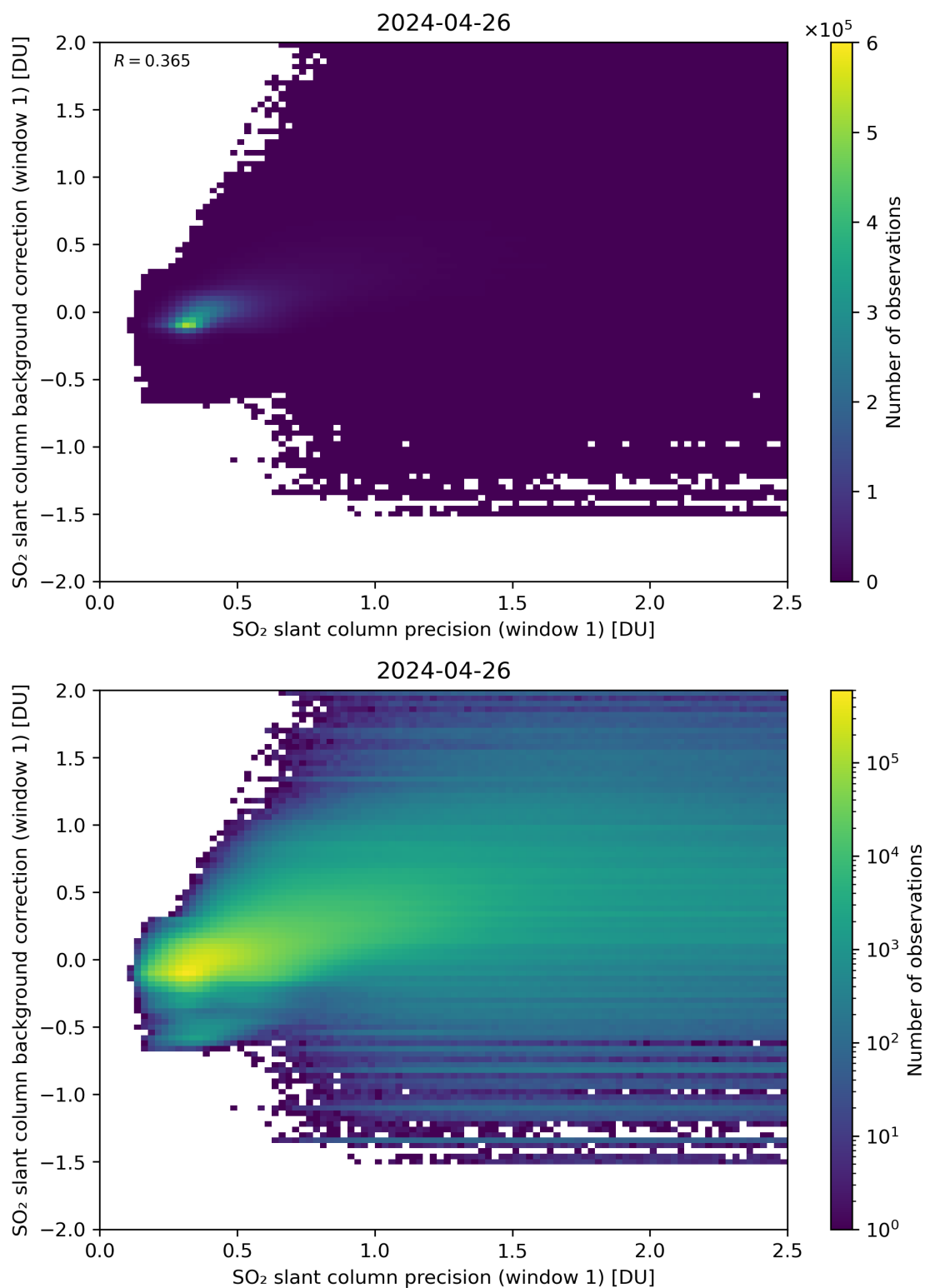
Figure 218: Scatter density plot of “SO 2 slant column precision (window 1)” against “SO 2 slant column background correction (window 1)” for 2024-04-26 to 2024-04-27.
