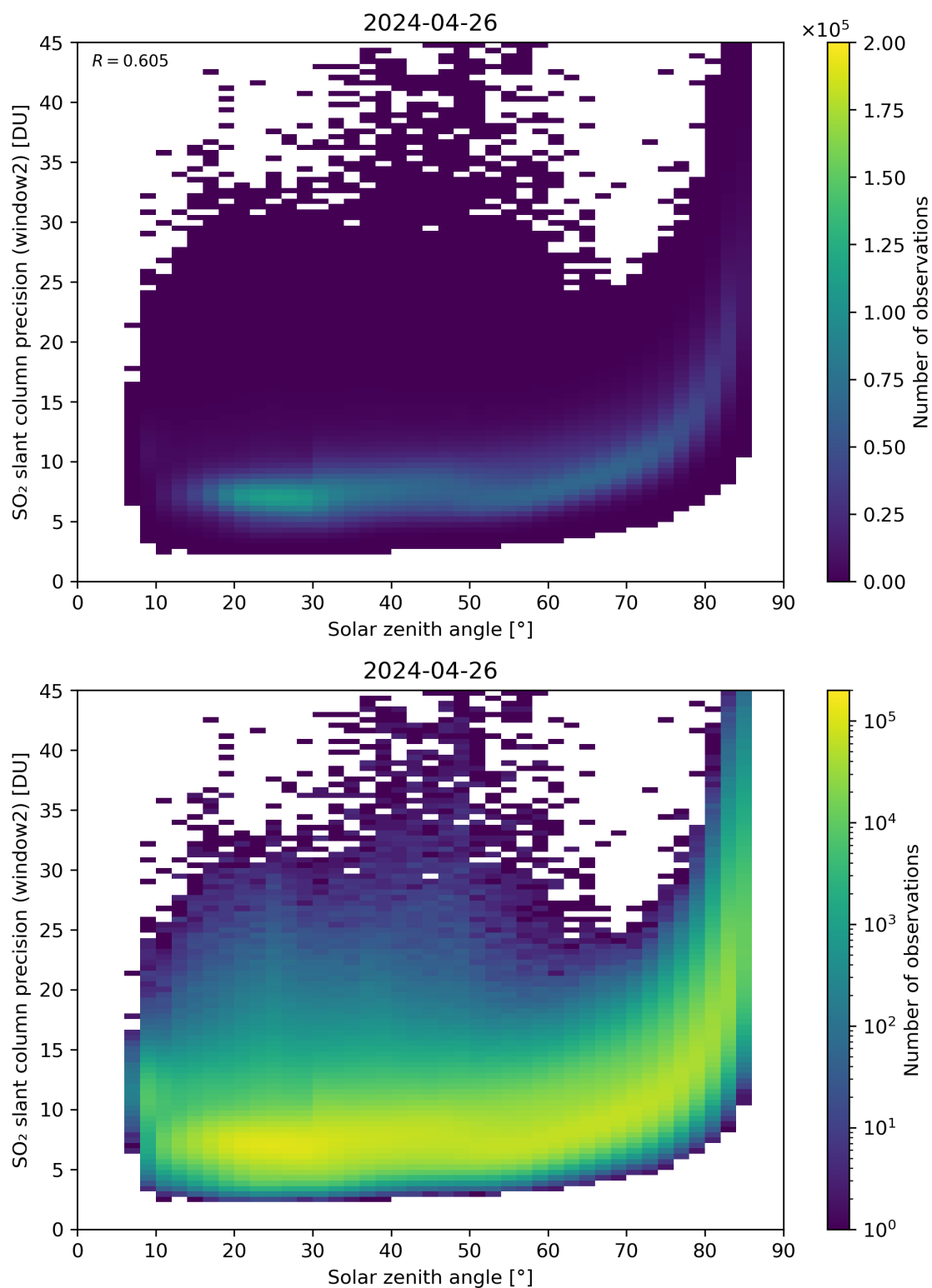
Figure 171: Scatter density plot of “Solar zenith angle” against “SO 2 slant column precision (window2)” for 2024-04-26 to 2024-04-27.
