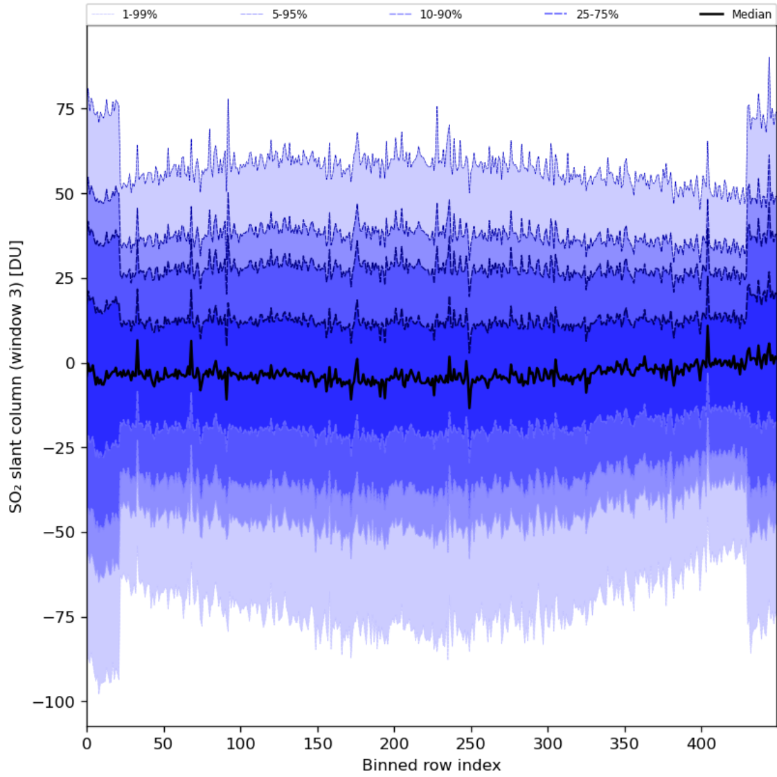
Figure 87: Along track statistics of “SO 2 slant column (window 3)” for 2024-04-26 to 2024-04-27
