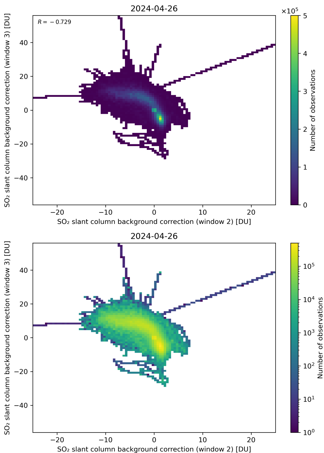
Figure 111: Scatter density plot of “SO 2 slant column background correction (window 2)” against “SO 2 slant column background correction (window 3)” for 2024-04-26 to 2024-04-27.
