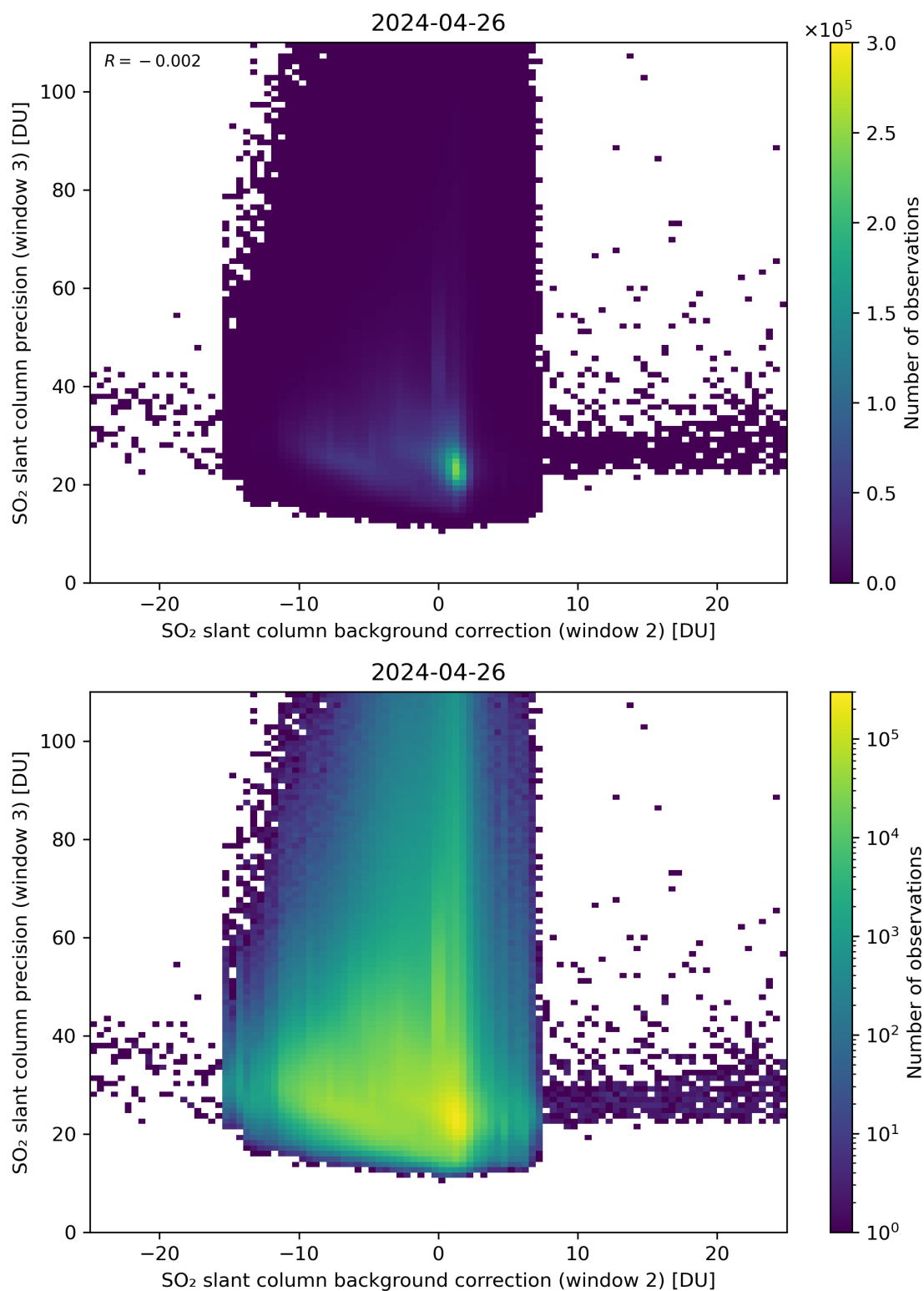
Figure 118: Scatter density plot of “SO 2 slant column background correction (window 2)” against “SO 2 slant column precision (window 3)” for 2024-04-26 to 2024-04-27.
