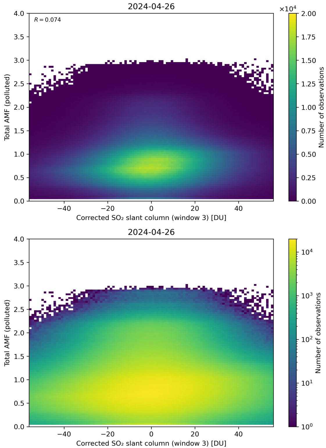
Figure 210: Scatter density plot of “Corrected SO 2 slant column (window 3)” against “Total AMF (polluted)” for 2024-04-26 to 2024-04-27.
