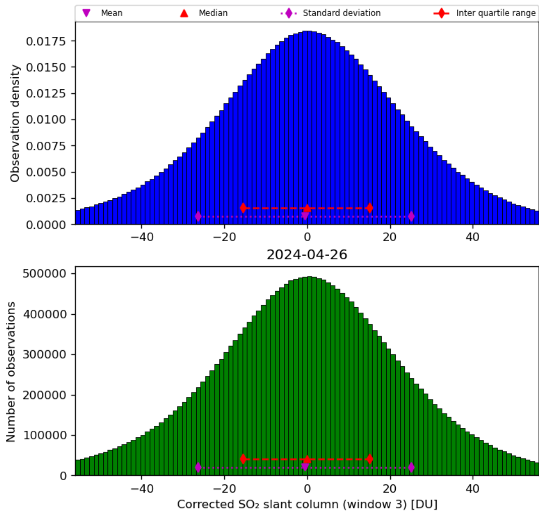
Figure 66: Histogram of “Corrected SO 2 slant column (window 3)” for 2024-04-26 to 2024-04-27
