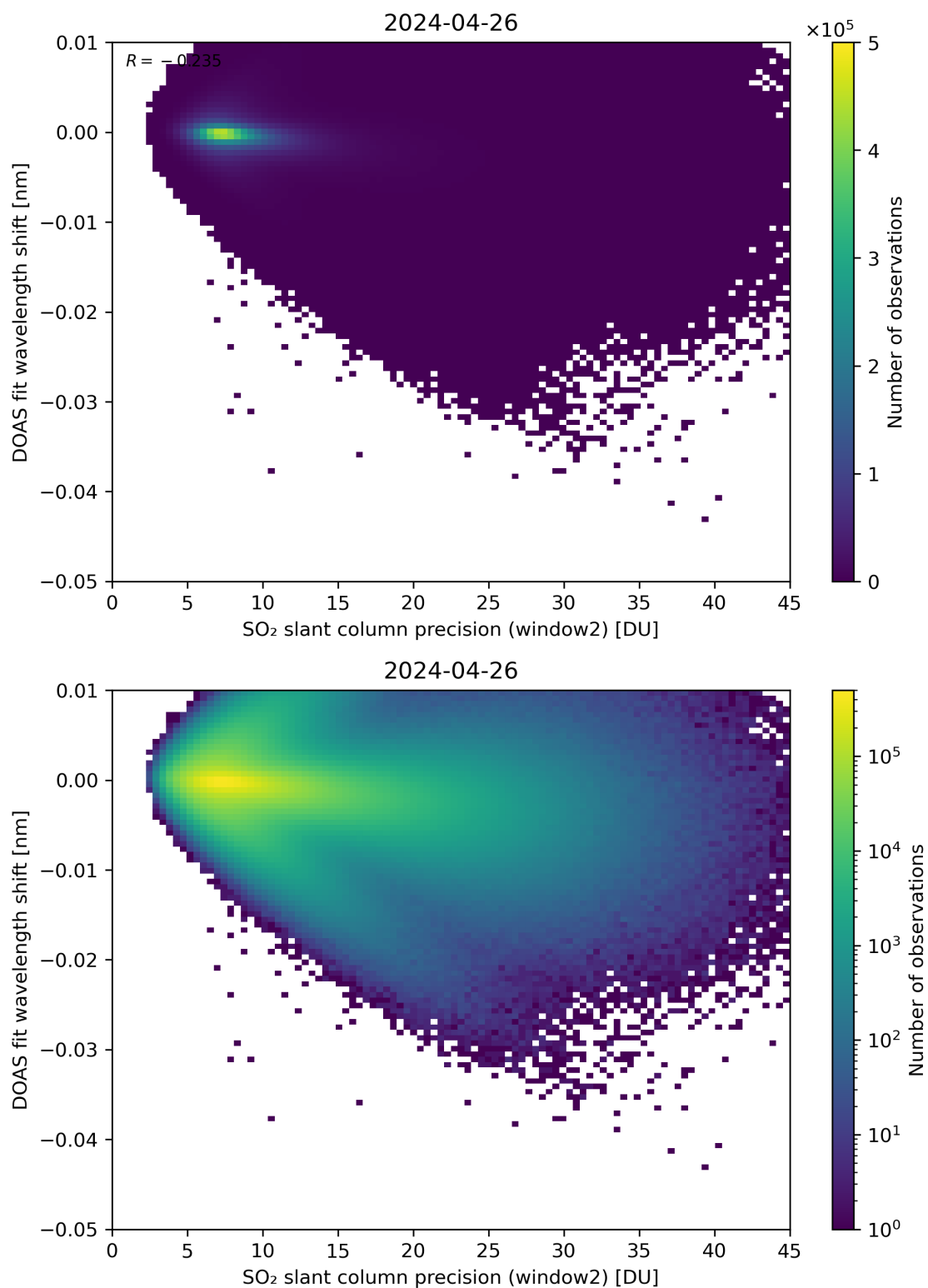
Figure 243: Scatter density plot of “SO 2 slant column precision (window2)” against “DOAS fit wavelength shift” for 2024-04-26 to 2024-04-27.
