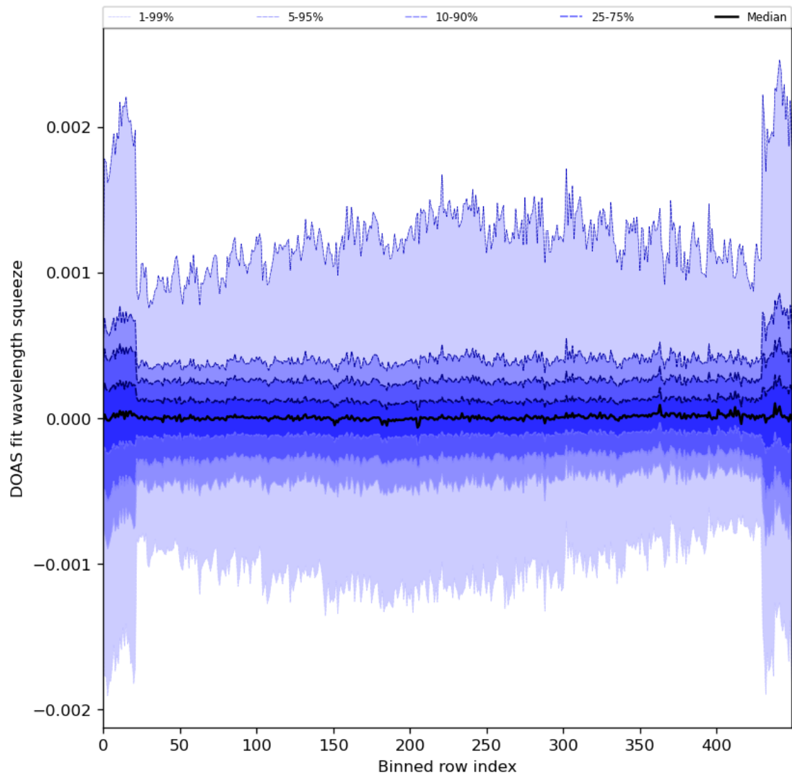
Figure 92: Along track statistics of “DOAS fit wavelength squeeze” for 2024-04-26 to 2024-04-27
