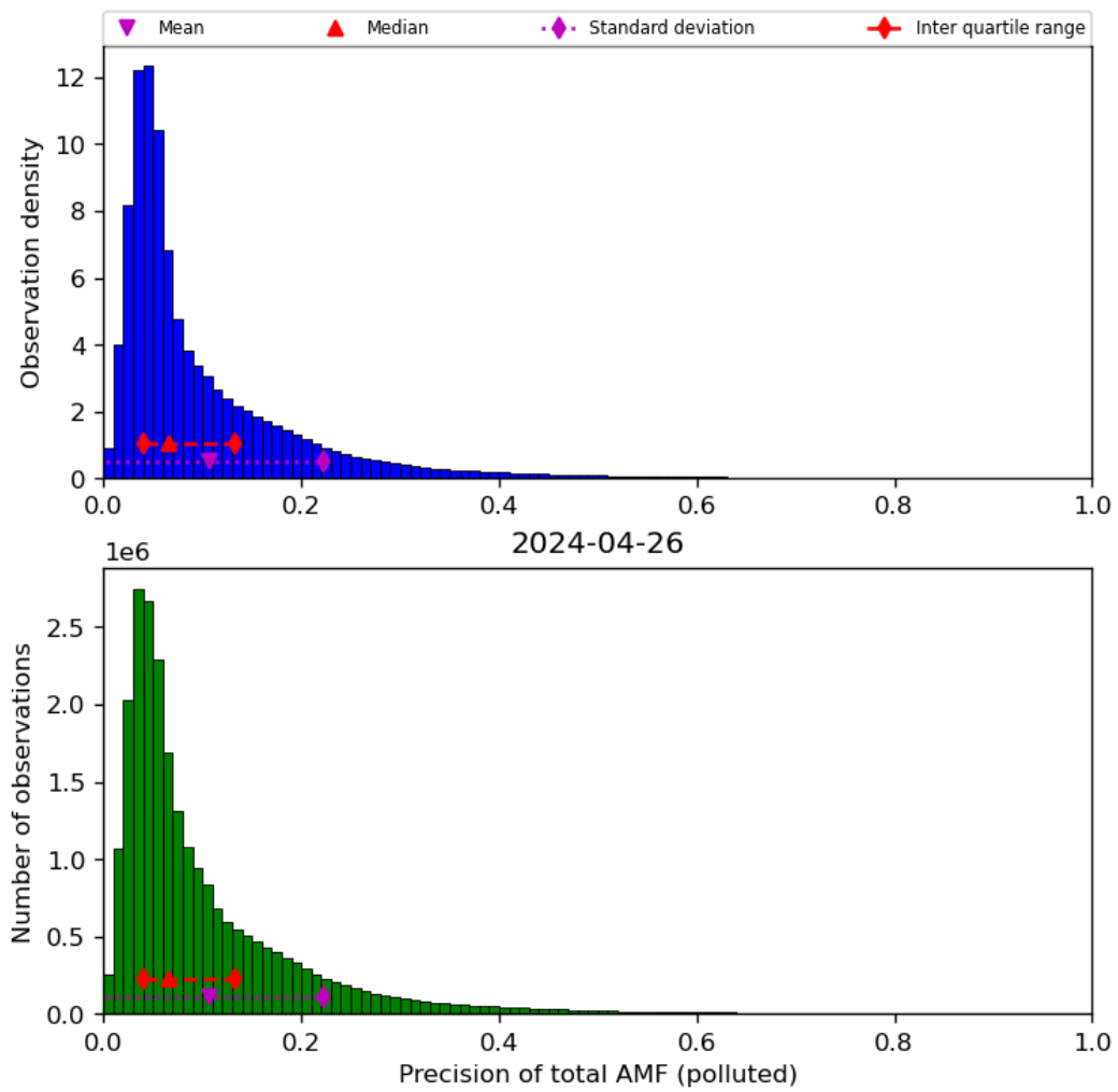
Figure 72: Histogram of “Precision of total AMF (polluted)” for 2024-04-26 to 2024-04-27
