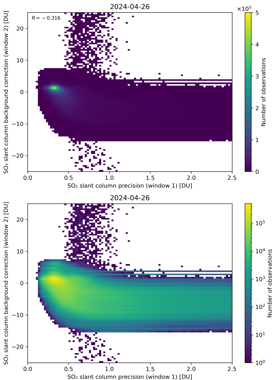
Figure 219: Scatter density plot of “SO 2 slant column precision (window 1)” against “SO 2 slant column background correction (window 2)” for 2024-04-26 to 2024-04-27.
