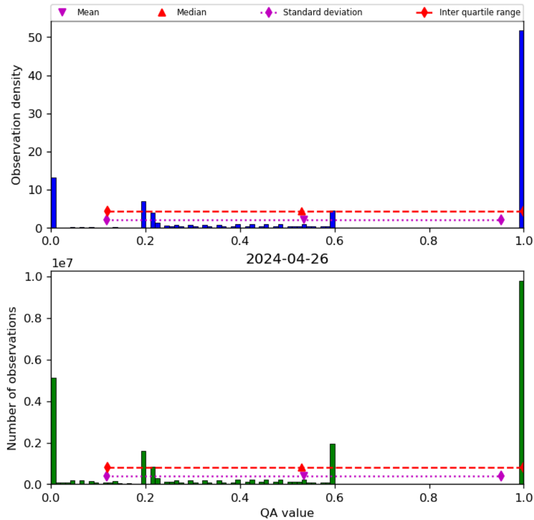
Figure 52: Histogram of “QA value” for 2024-04-26 to 2024-04-27
