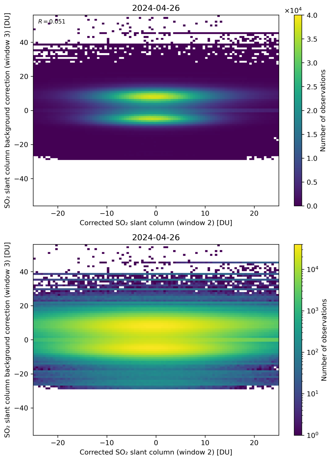
Figure 195: Scatter density plot of “Corrected SO 2 slant column (window 2)” against “SO 2 slant column background correction (window 3)” for 2024-04-26 to 2024-04-27.
