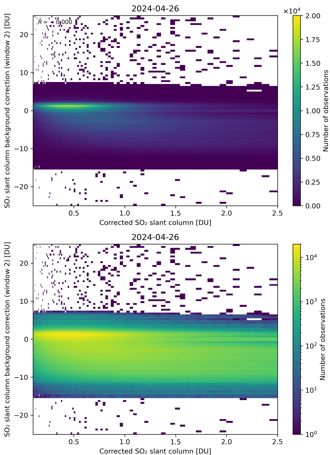
Figure 179: Scatter density plot of “Corrected SO 2 slant column” against “SO 2 slant column background correction (window 2)” for 2024-04-26 to 2024-04-27.
