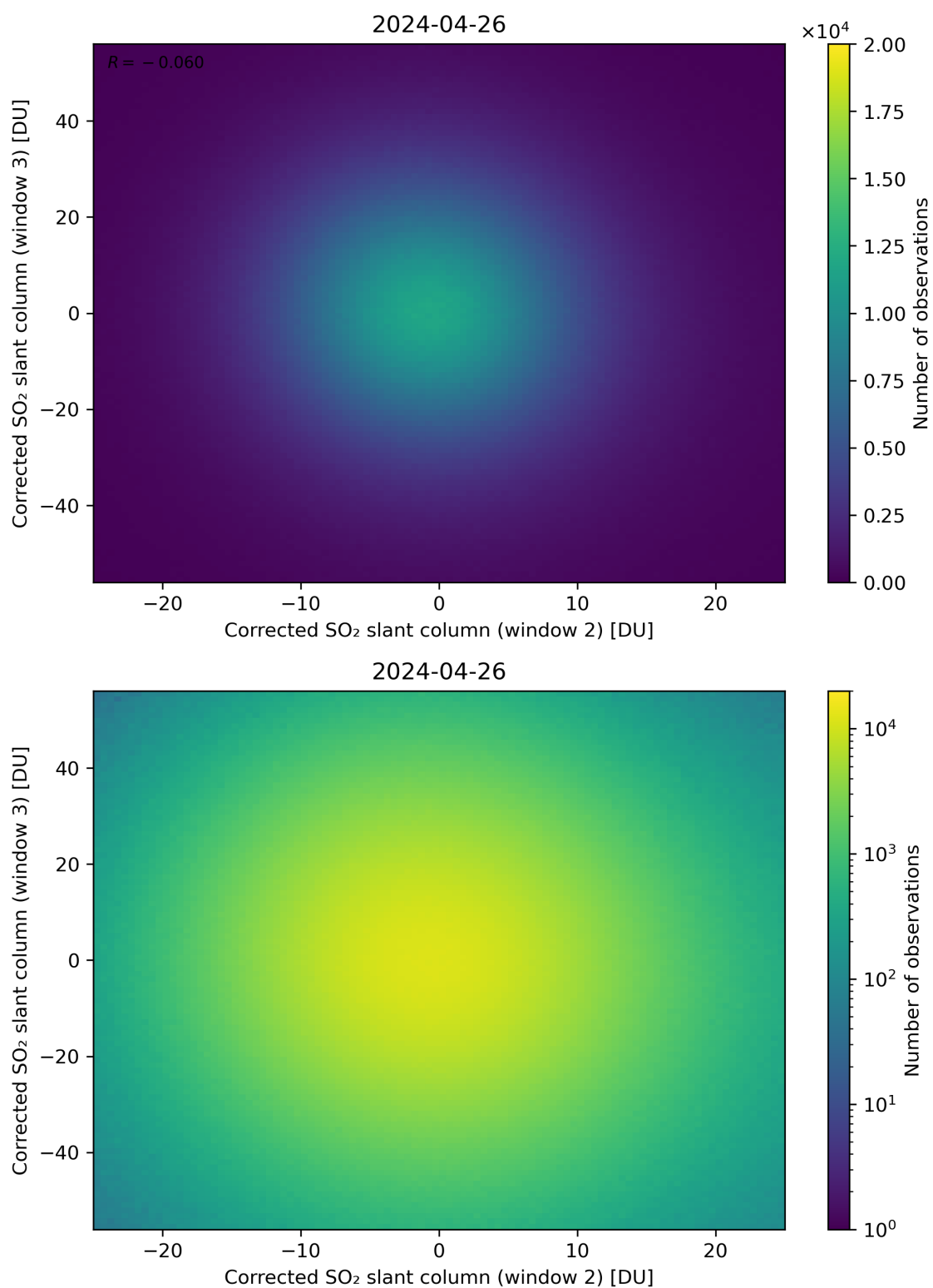
Figure 200: Scatter density plot of “Corrected SO 2 slant column (window 2)” against “Corrected SO 2 slant column (window 3)” for 2024-04-26 to 2024-04-27.
