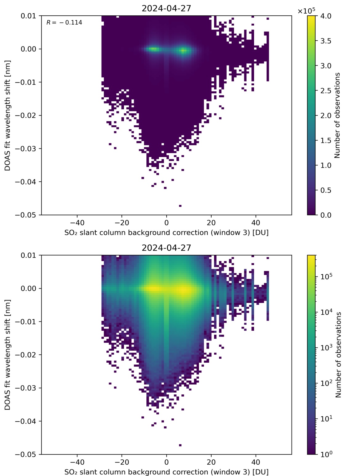
Figure 121: Scatter density plot of “SO 2 slant column background correction (window 3)” against “DOAS fit wavelength shift” for 2024-04-26 to 2024-04-28.
