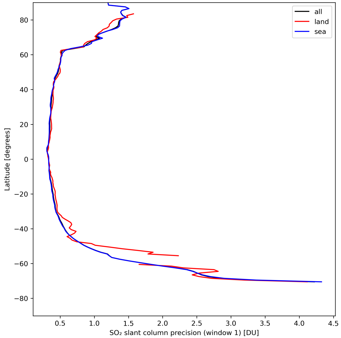
Figure 34: Zonal average of “SO 2 slant column precision (window 1)” for 2024-04-26 to 2024-04-28.
