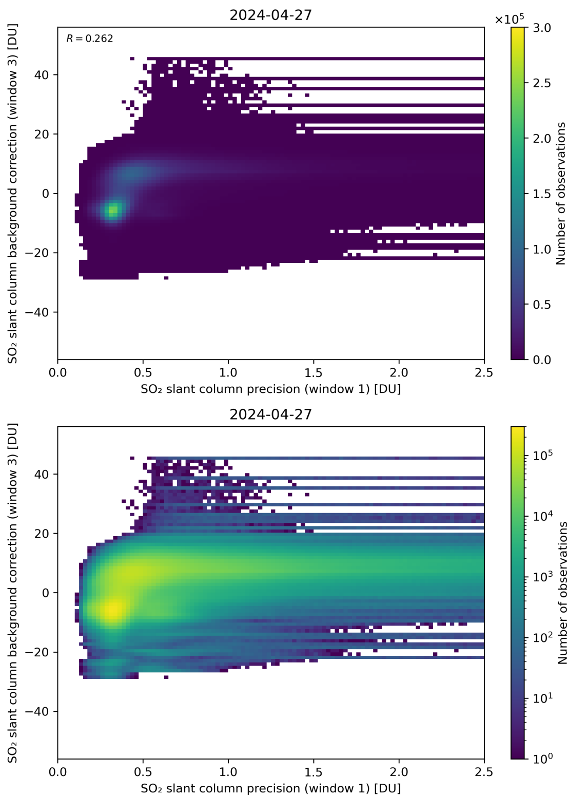
Figure 220: Scatter density plot of “SO 2 slant column precision (window 1)” against “SO 2 slant column background correction (window 3)” for 2024-04-26 to 2024-04-28.
