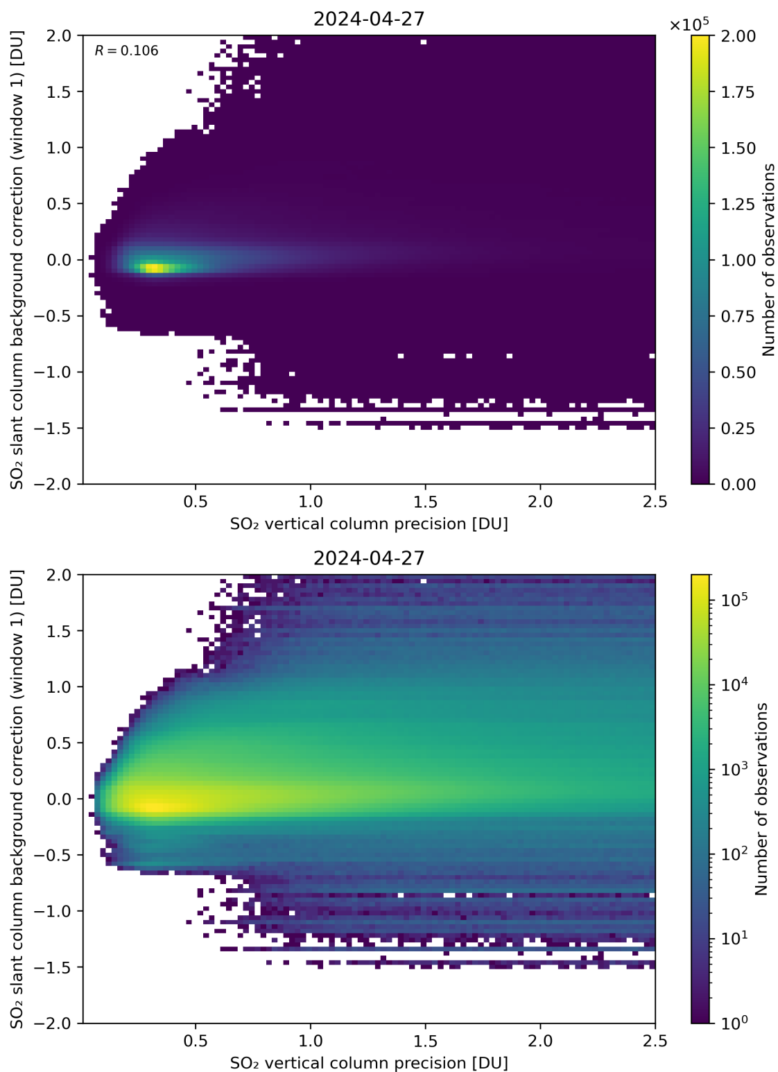
Figure 279: Scatter density plot of “SO 2 vertical column precision” against “SO 2 slant column background correction (window 1)” for 2024-04-26 to 2024-04-28.
