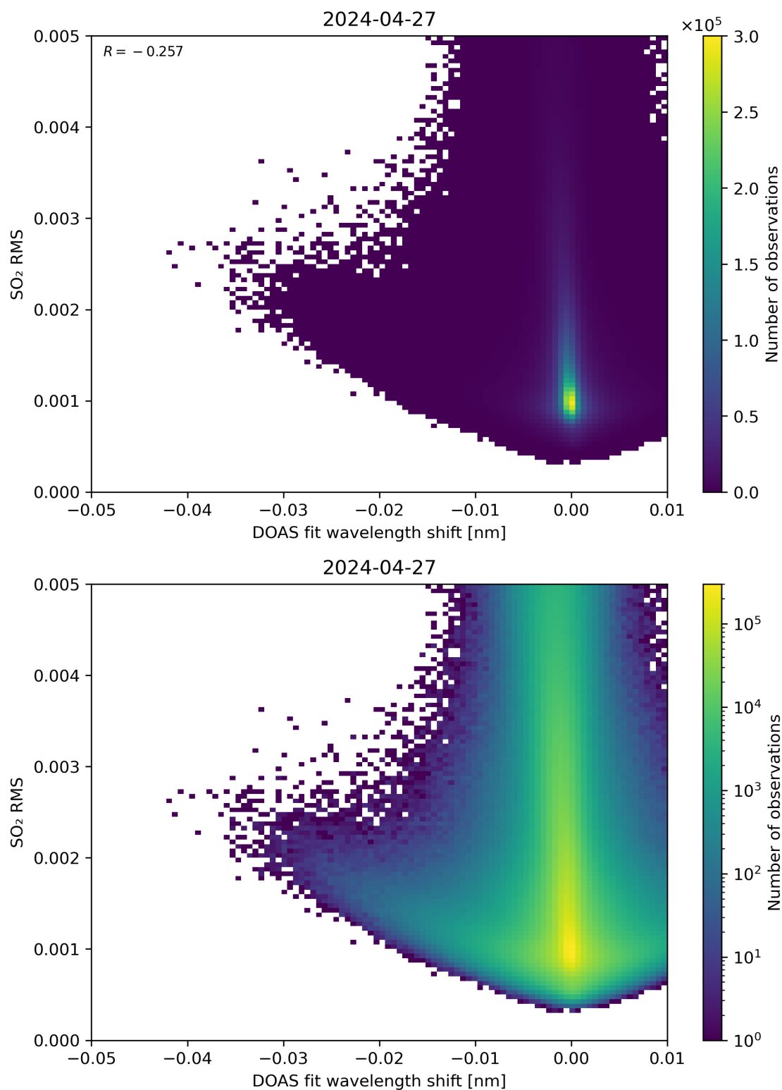
Figure 128: Scatter density plot of “DOAS fit wavelength shift” against “SO 2 RMS” for 2024-04-26 to 2024-04-28.
