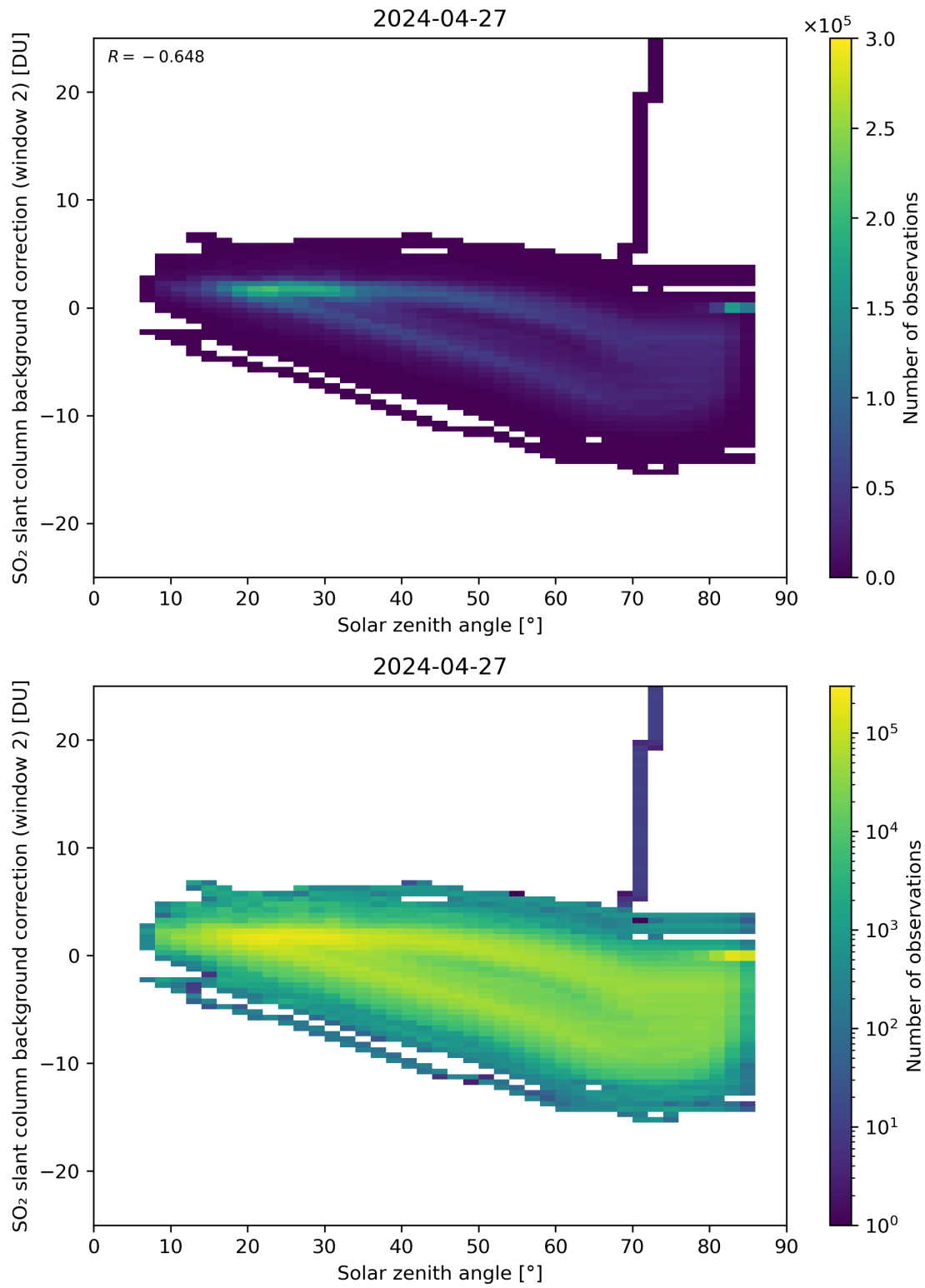
Figure 159: Scatter density plot of “Solar zenith angle” against “SO 2 slant column background correction (window 2)” for 2024-04-26 to 2024-04-28.
