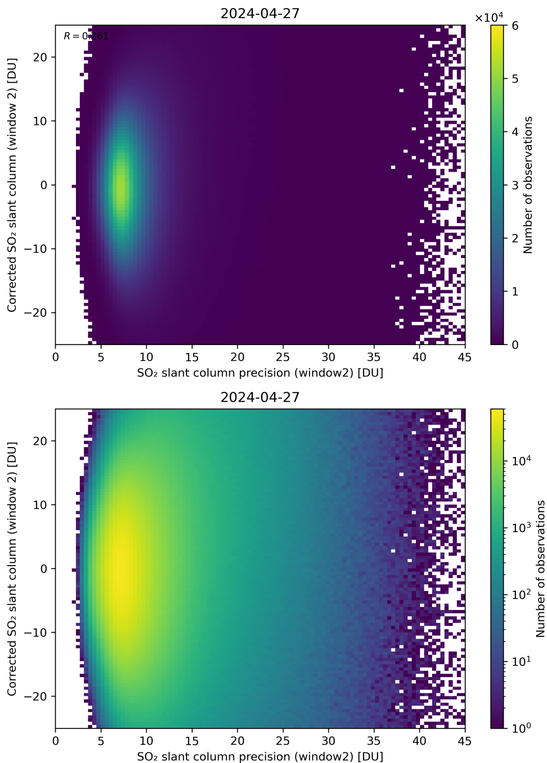
Figure 247: Scatter density plot of “SO 2 slant column precision (window2)” against “Corrected SO 2 slant column (window 2)” for 2024-04-26 to 2024-04-28.
