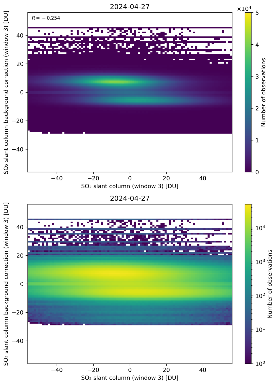
Figure 253: Scatter density plot of “SO 2 slant column (window 3)” against “SO 2 slant column background correction (window 3)” for 2024-04-26 to 2024-04-28.
