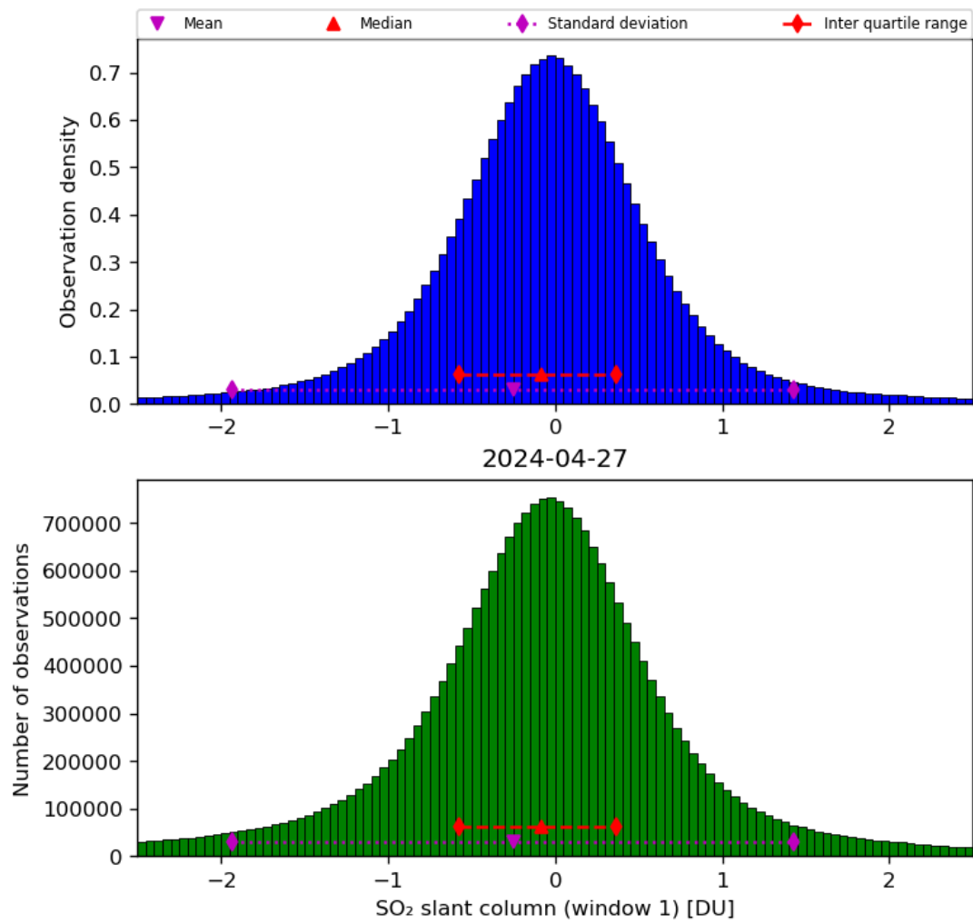
Figure 56: Histogram of “SO 2 slant column (window 1)” for 2024-04-26 to 2024-04-28
