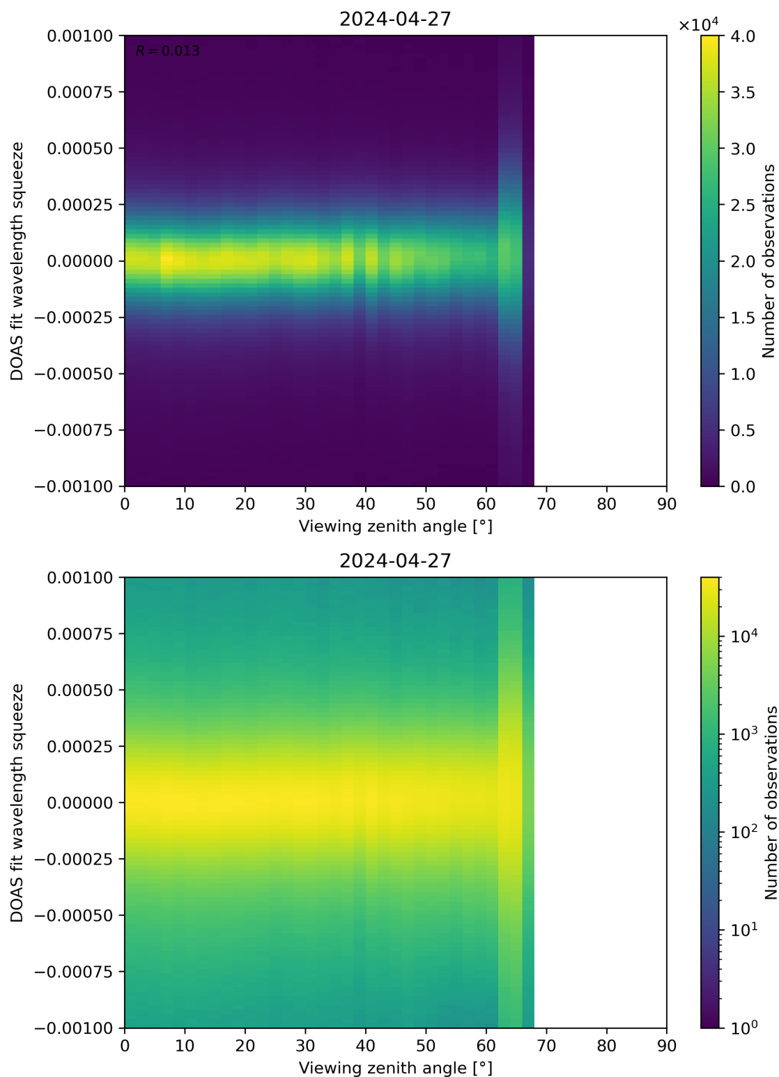
Figure 312: Scatter density plot of “Viewing zenith angle” against “DOAS fit wavelength squeeze” for 2024-04-26 to 2024-04-28.
