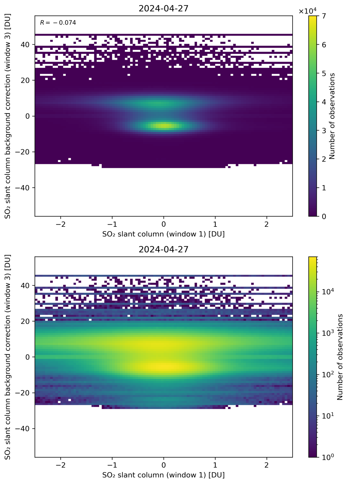
Figure 214: Scatter density plot of “SO 2 slant column (window 1)” against “SO 2 slant column background correction (window 3)” for 2024-04-26 to 2024-04-28.
