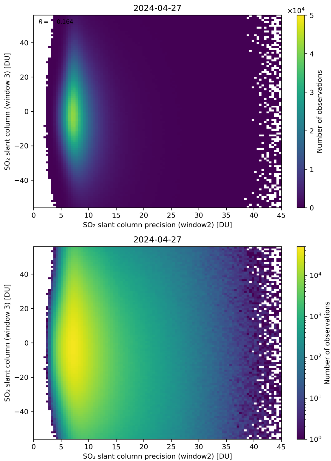
Figure 249: Scatter density plot of “SO 2 slant column precision (window2)” against “SO 2 slant column (window 3)” for 2024-04-26 to 2024-04-28.
