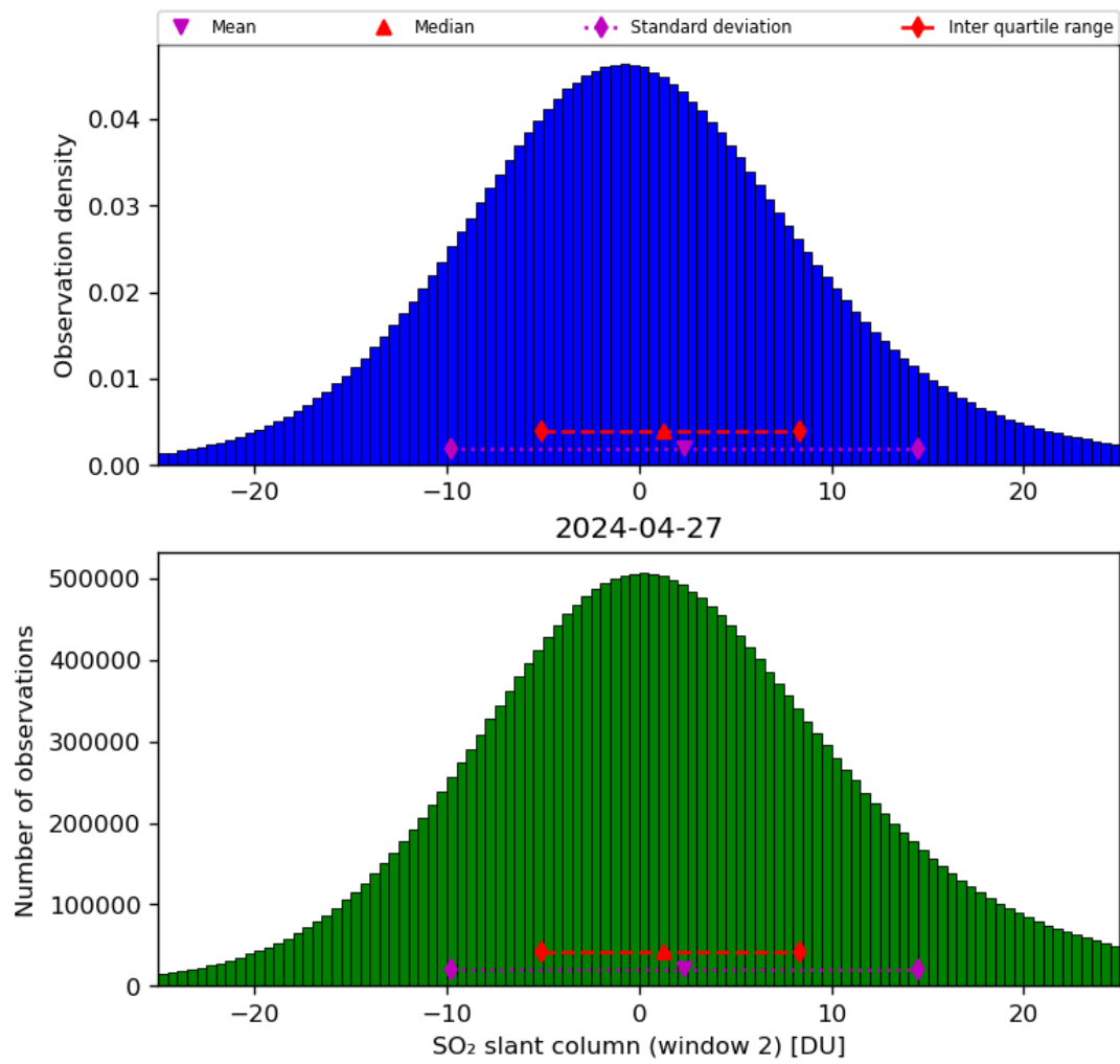
Figure 60: Histogram of “SO 2 slant column (window 2)” for 2024-04-26 to 2024-04-28
