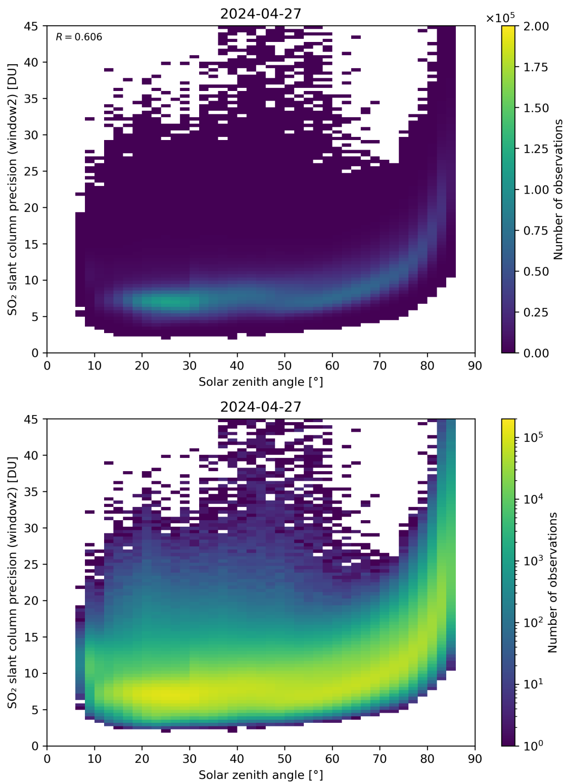
Figure 171: Scatter density plot of “Solar zenith angle” against “SO 2 slant column precision (window2)” for 2024-04-26 to 2024-04-28.
