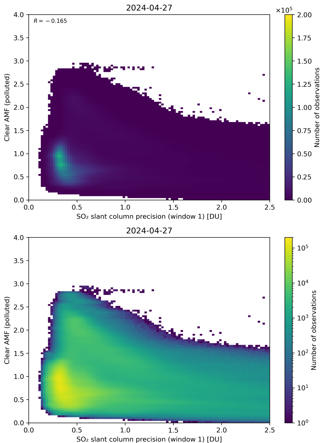
Figure 224: Scatter density plot of “SO 2 slant column precision (window 1)” against “Clear AMF (polluted)” for 2024-04-26 to 2024-04-28.
