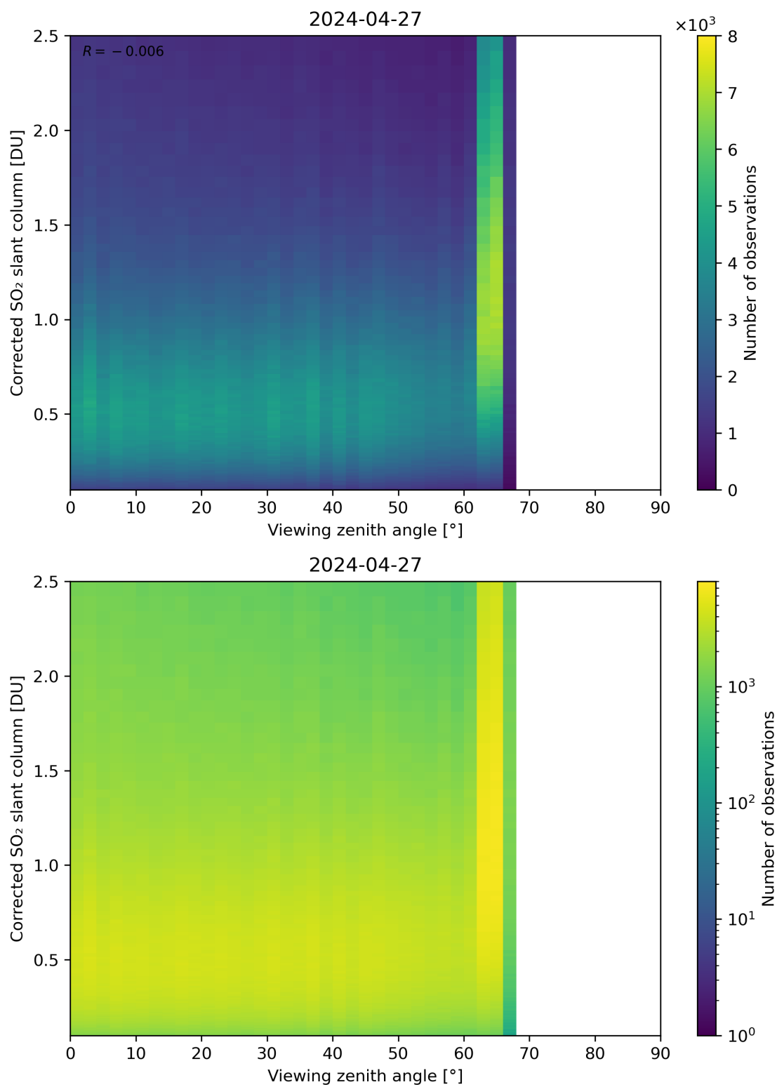
Figure 317: Scatter density plot of “Viewing zenith angle” against “Corrected SO 2 slant column” for 2024-04-26 to 2024-04-28.
