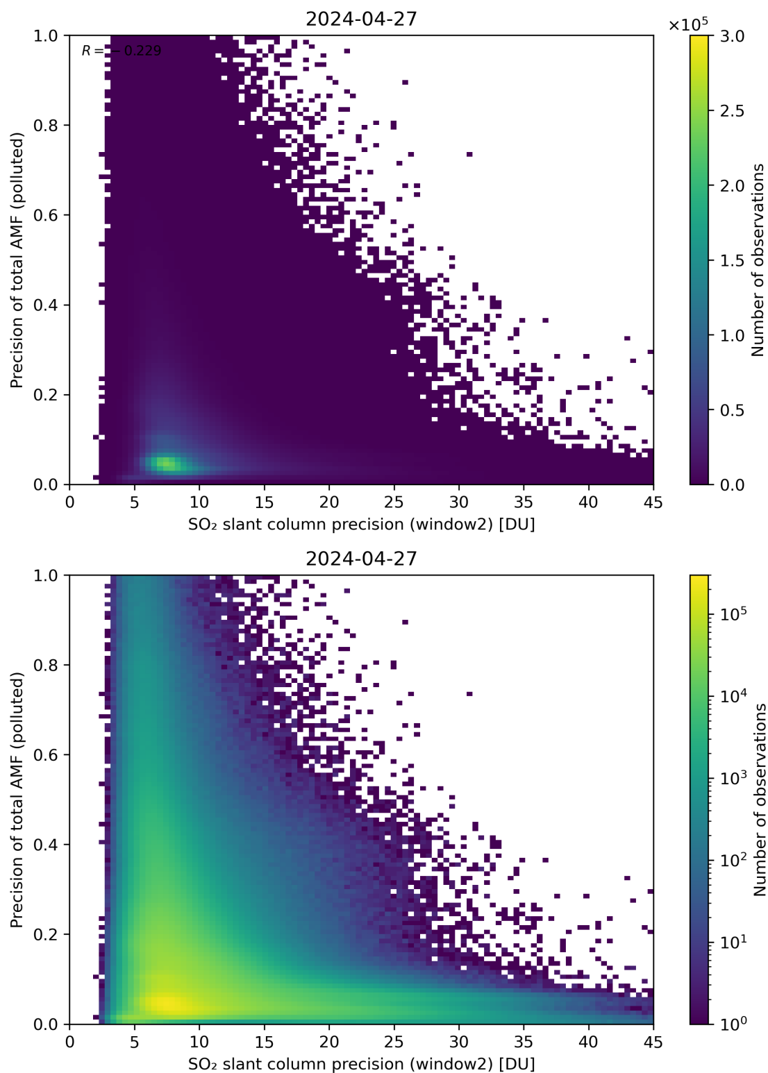
Figure 252: Scatter density plot of “SO 2 slant column precision (window2)” against “Precision of total AMF (polluted)” for 2024-04-26 to 2024-04-28.
