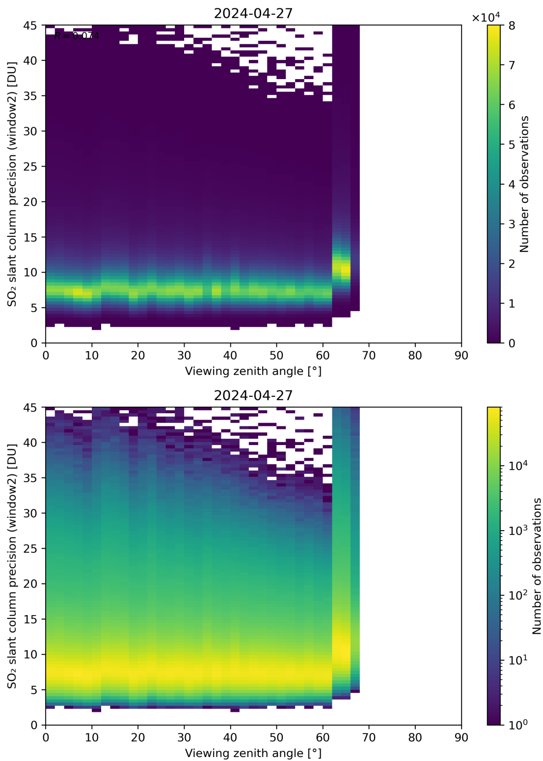
Figure 322: Scatter density plot of “Viewing zenith angle” against “SO 2 slant column precision (window2)” for 2024-04-26 to 2024-04-28.
