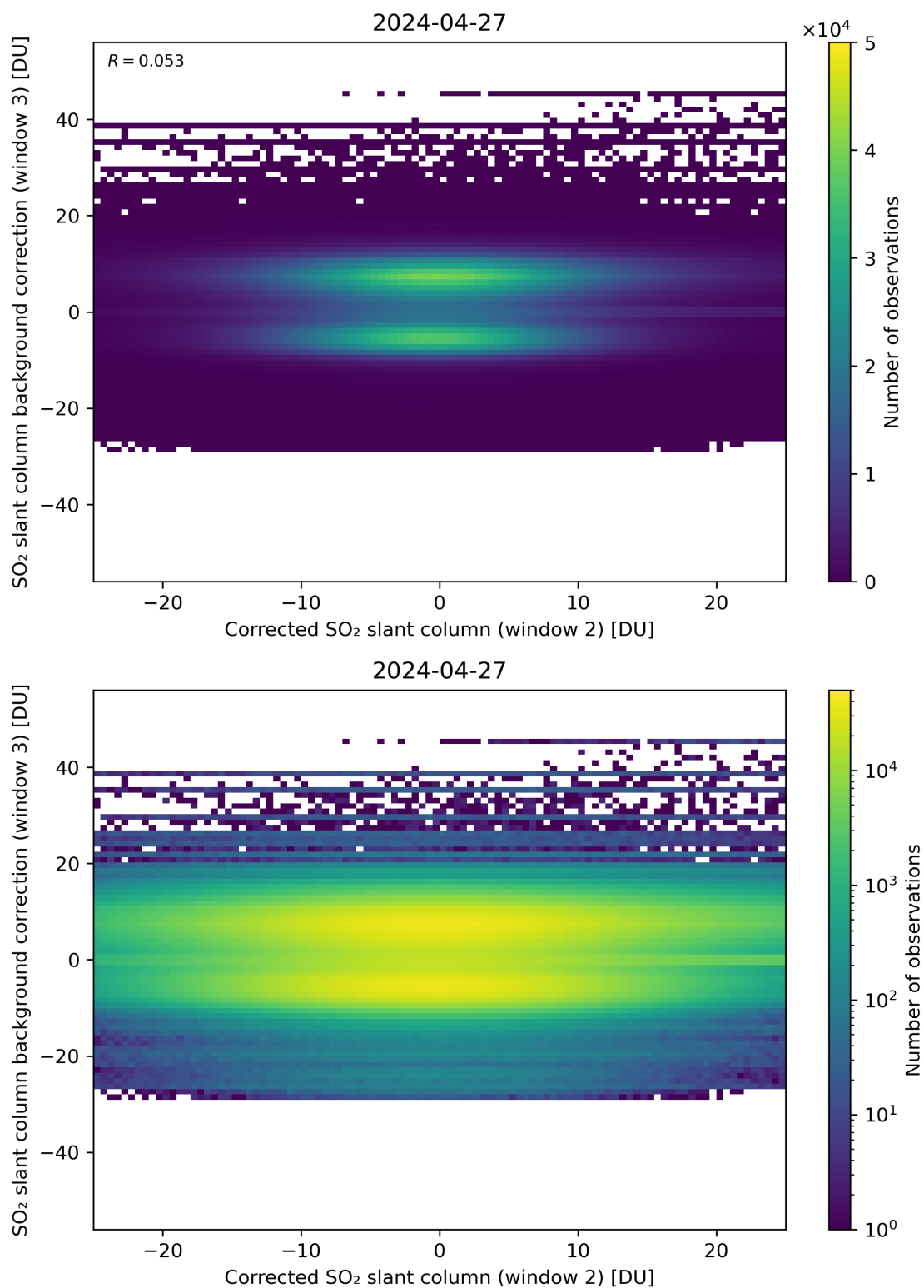
Figure 195: Scatter density plot of “Corrected SO 2 slant column (window 2)” against “SO 2 slant column background correction (window 3)” for 2024-04-26 to 2024-04-28.
