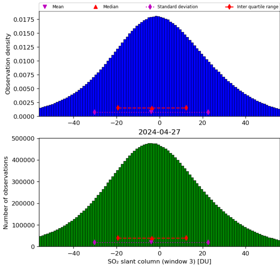
Figure 64: Histogram of “SO 2 slant column (window 3)” for 2024-04-26 to 2024-04-28
