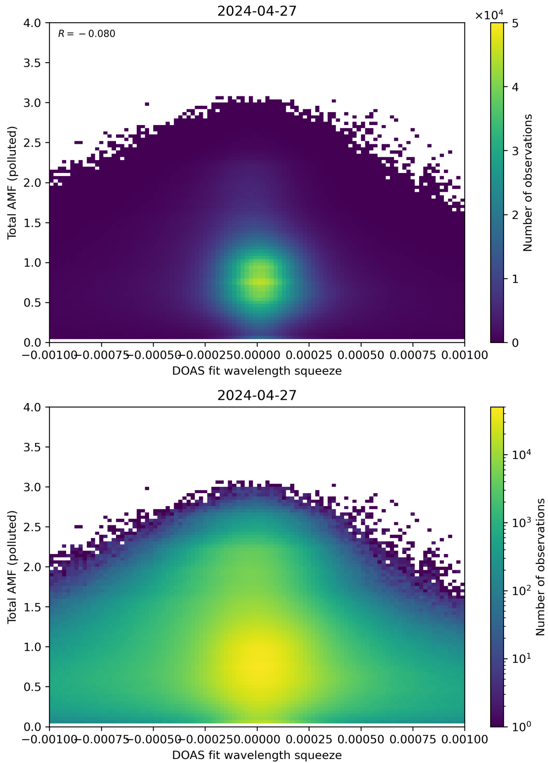
Figure 134: Scatter density plot of “DOAS fit wavelength squeeze” against “Total AMF (polluted)” for 2024-04-26 to 2024-04-28.
