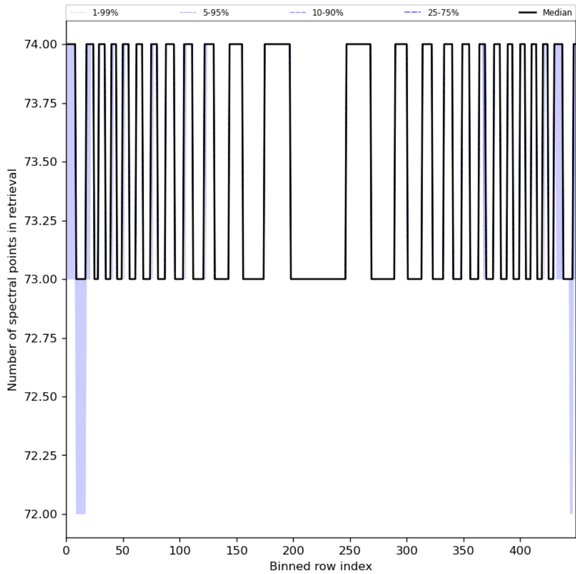
Figure 97: Along track statistics of “Number of spectral points in retrieval” for 2024-04-26 to 2024-04-28
