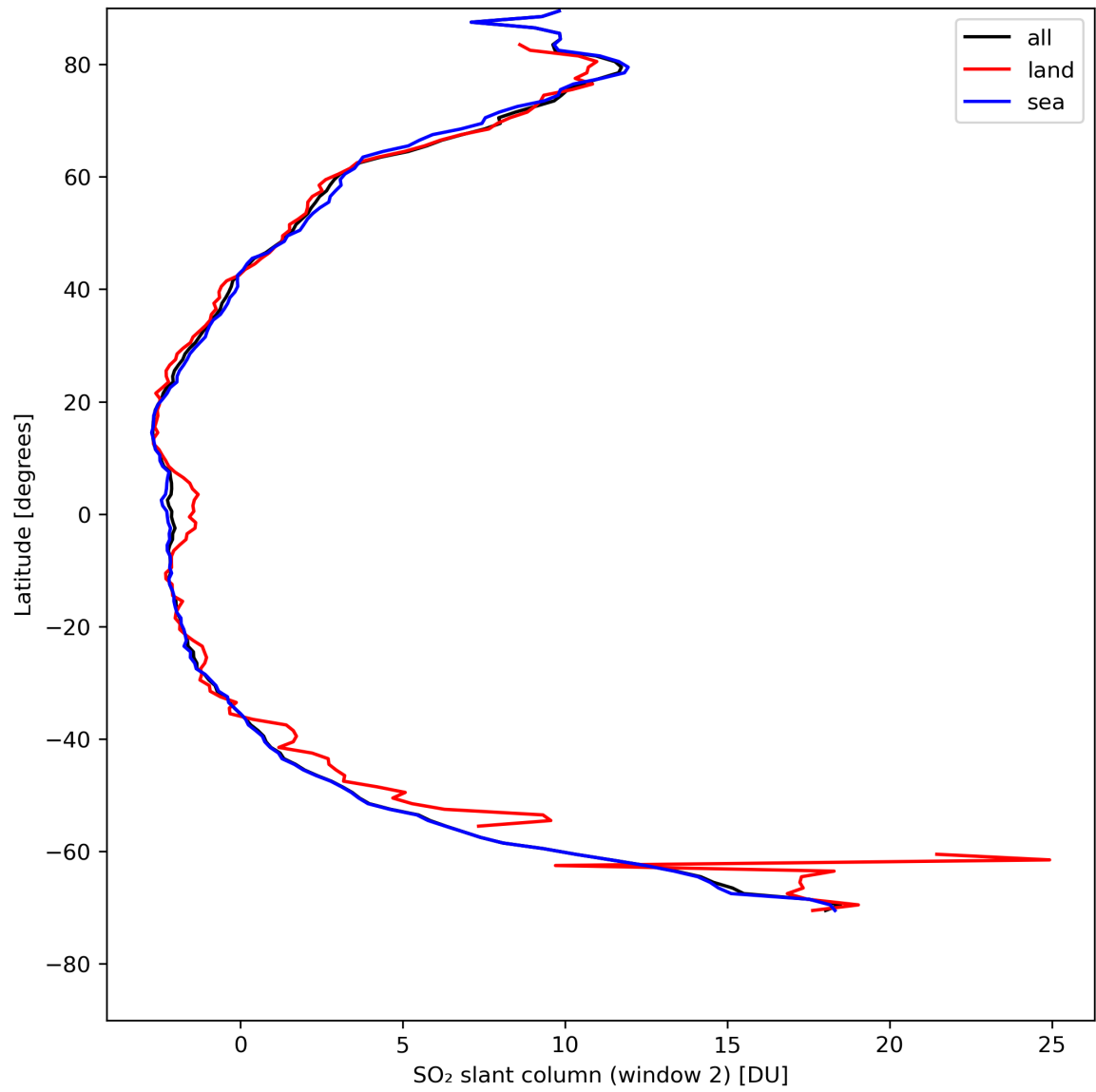
Figure 37: Zonal average of “SO 2 slant column (window 2)” for 2024-04-26 to 2024-04-28.
