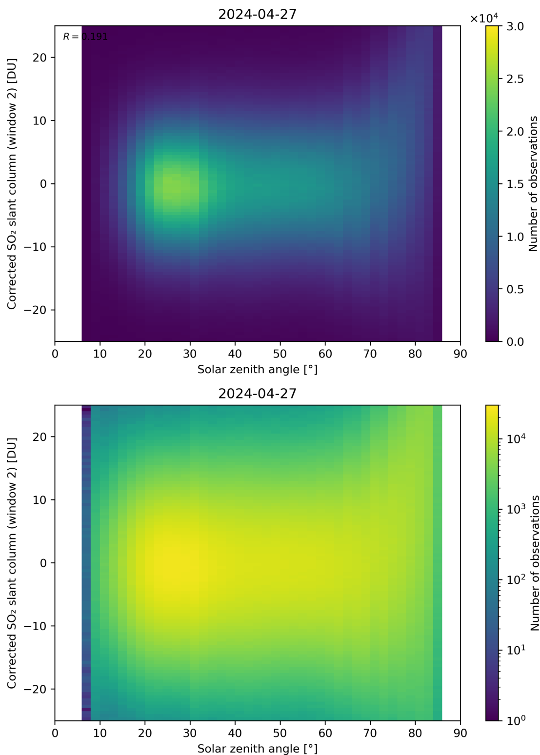
Figure 167: Scatter density plot of “Solar zenith angle” against “Corrected SO 2 slant column (window 2)” for 2024-04-26 to 2024-04-28.
