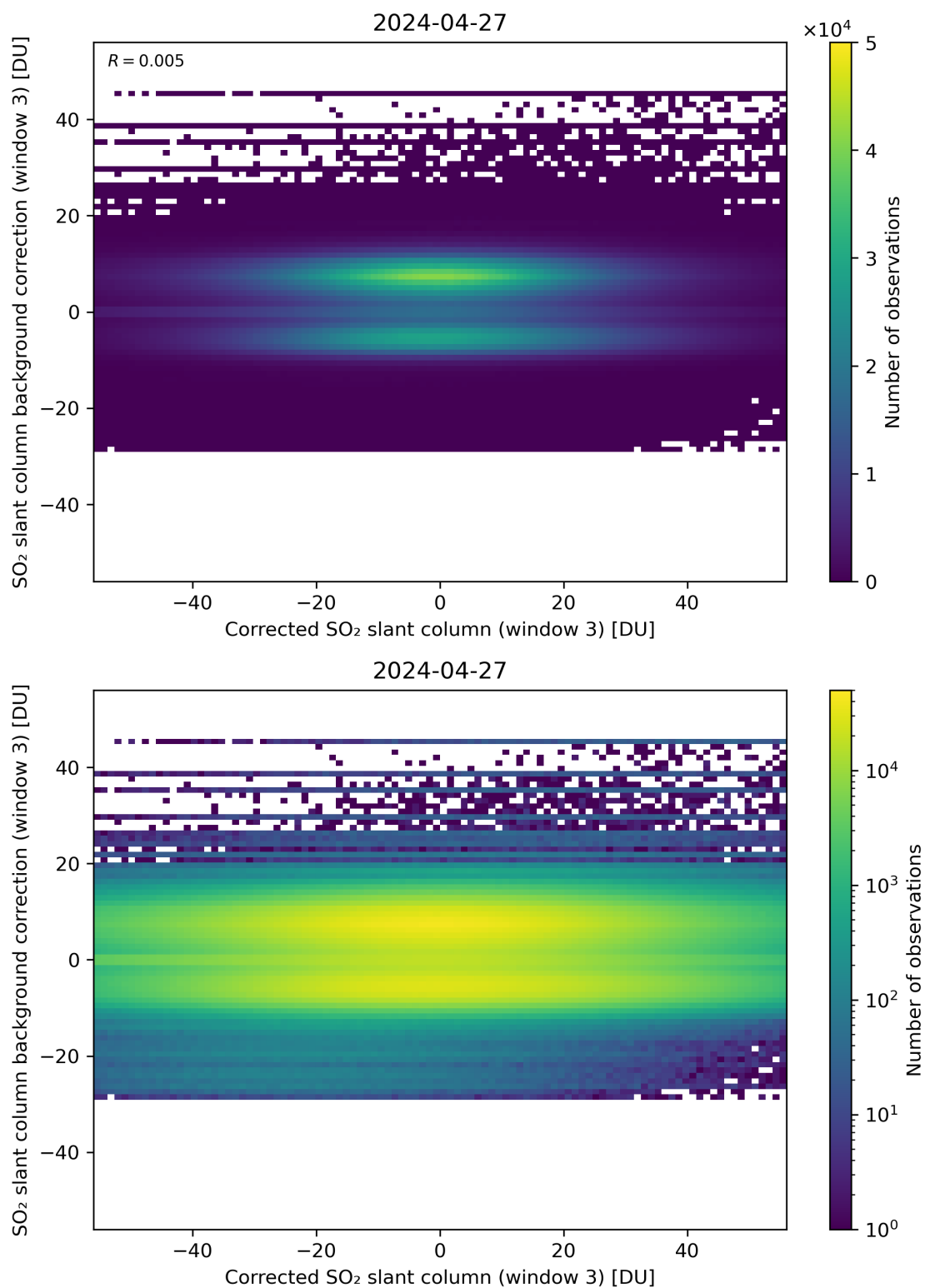
Figure 205: Scatter density plot of “Corrected SO 2 slant column (window 3)” against “SO 2 slant column background correction (window 3)” for 2024-04-26 to 2024-04-28.
