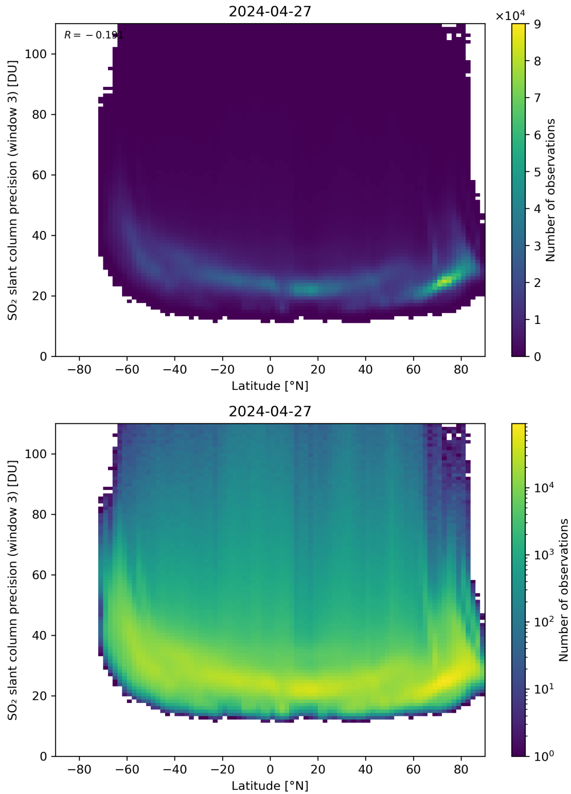
Figure 153: Scatter density plot of “Latitude” against “SO 2 slant column precision (window 3)” for 2024-04-26 to 2024-04-28.
