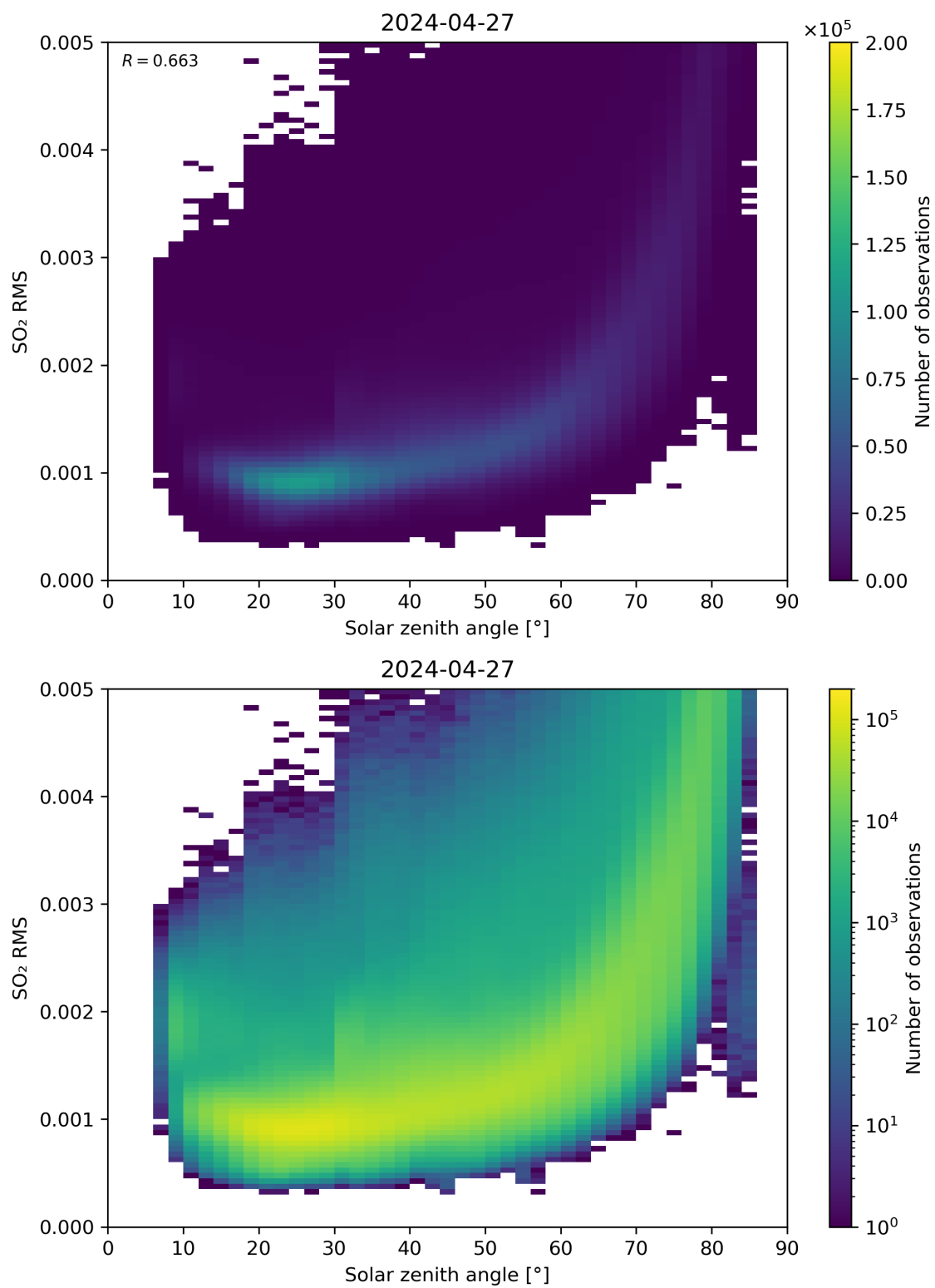
Figure 163: Scatter density plot of “Solar zenith angle” against “SO 2 RMS” for 2024-04-26 to 2024-04-28.
