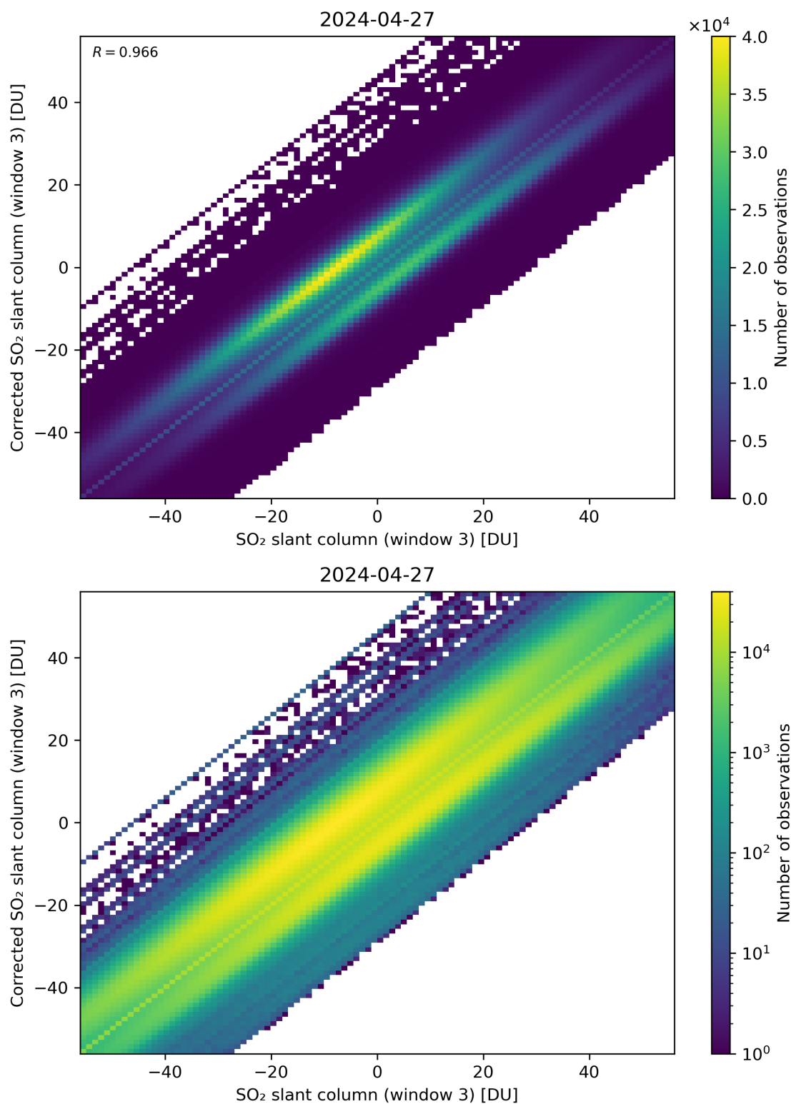
Figure 266: Scatter density plot of “SO 2 slant column (window 3)” against “Corrected SO 2 slant column (window 3)” for 2024-04-26 to 2024-04-28.
