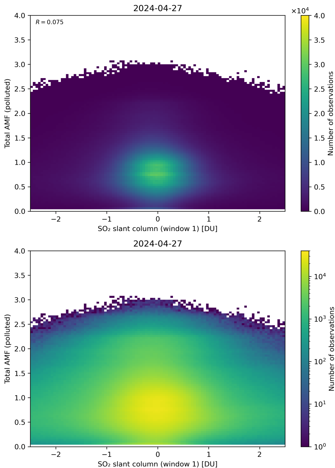
Figure 239: Scatter density plot of “SO 2 slant column (window 1)” against “Total AMF (polluted)” for 2024-04-26 to 2024-04-28.
