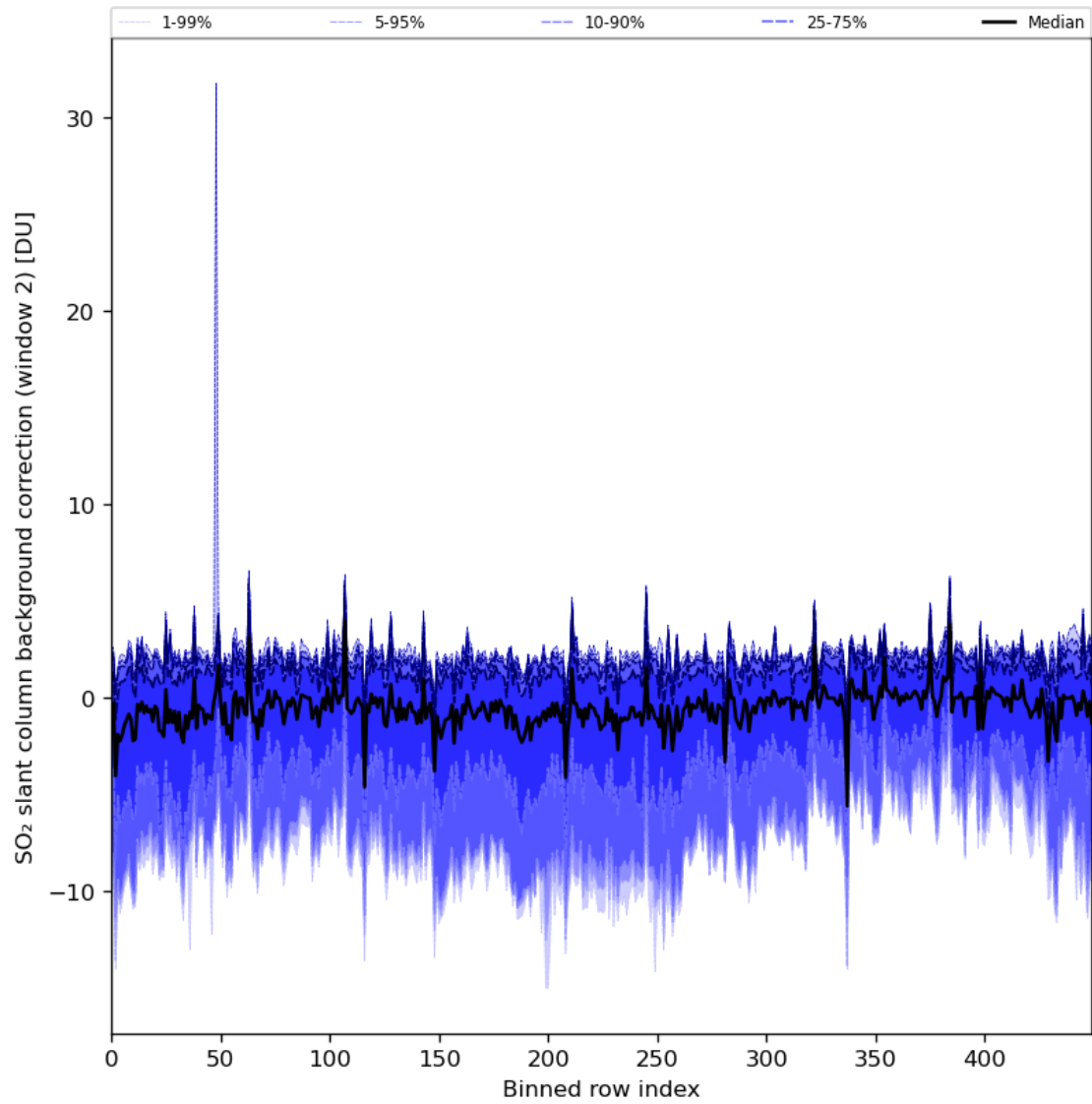
Figure 86: Along track statistics of “SO 2 slant column background correction (window 2)” for 2024-04-26 to 2024-04-28
