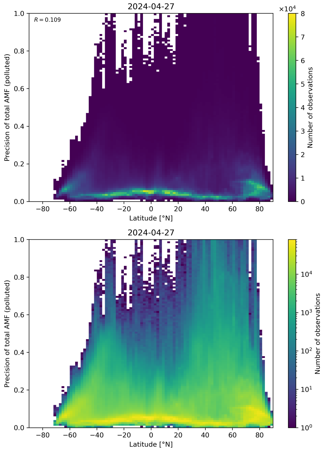
Figure 155: Scatter density plot of “Latitude” against “Precision of total AMF (polluted)” for 2024-04-26 to 2024-04-28.
