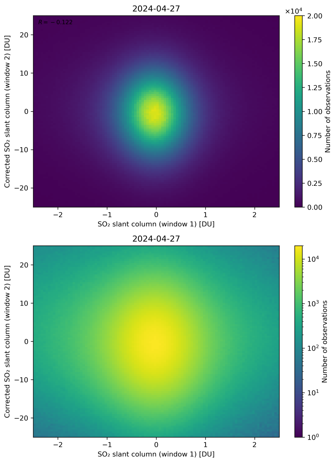
Figure 233: Scatter density plot of “SO 2 slant column (window 1)” against “Corrected SO 2 slant column (window 2)” for 2024-04-26 to 2024-04-28.
