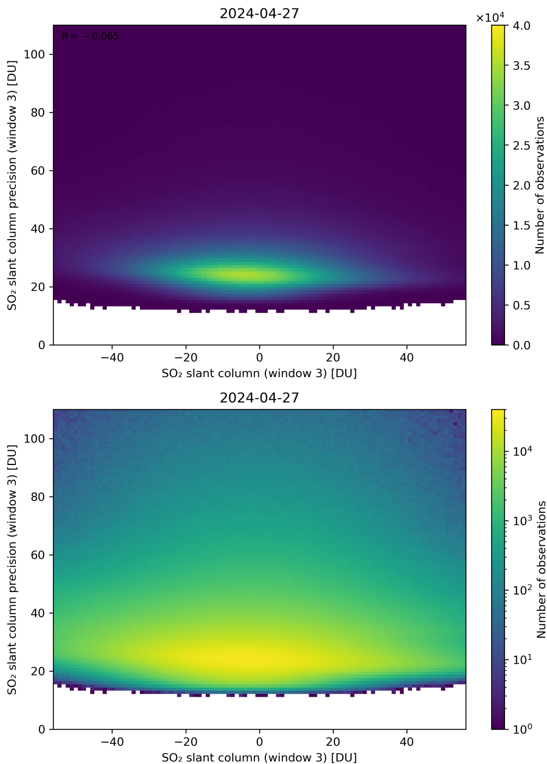
Figure 267: Scatter density plot of “SO 2 slant column (window 3)” against “SO 2 slant column precision (window 3)” for 2024-04-26 to 2024-04-28.
