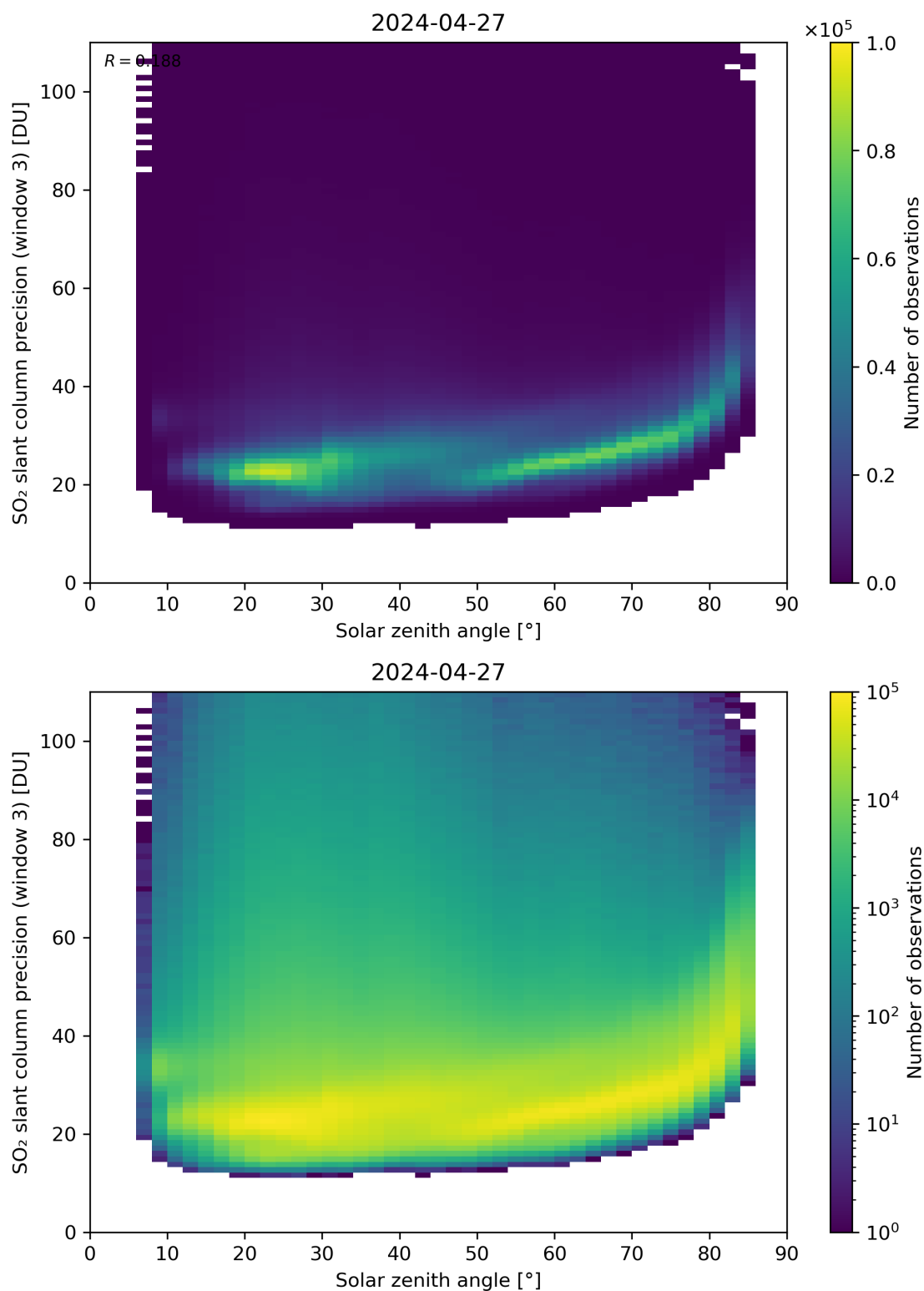
Figure 173: Scatter density plot of “Solar zenith angle” against “SO 2 slant column precision (window 3)” for 2024-04-26 to 2024-04-28.
