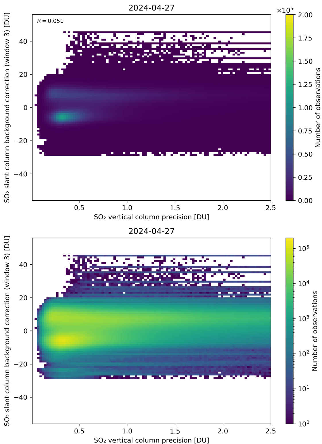
Figure 281: Scatter density plot of “SO 2 vertical column precision” against “SO 2 slant column background correction (window 3)” for 2024-04-26 to 2024-04-28.
