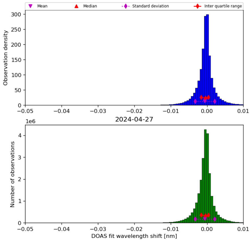
Figure 68: Histogram of “DOAS fit wavelength shift” for 2024-04-26 to 2024-04-28
