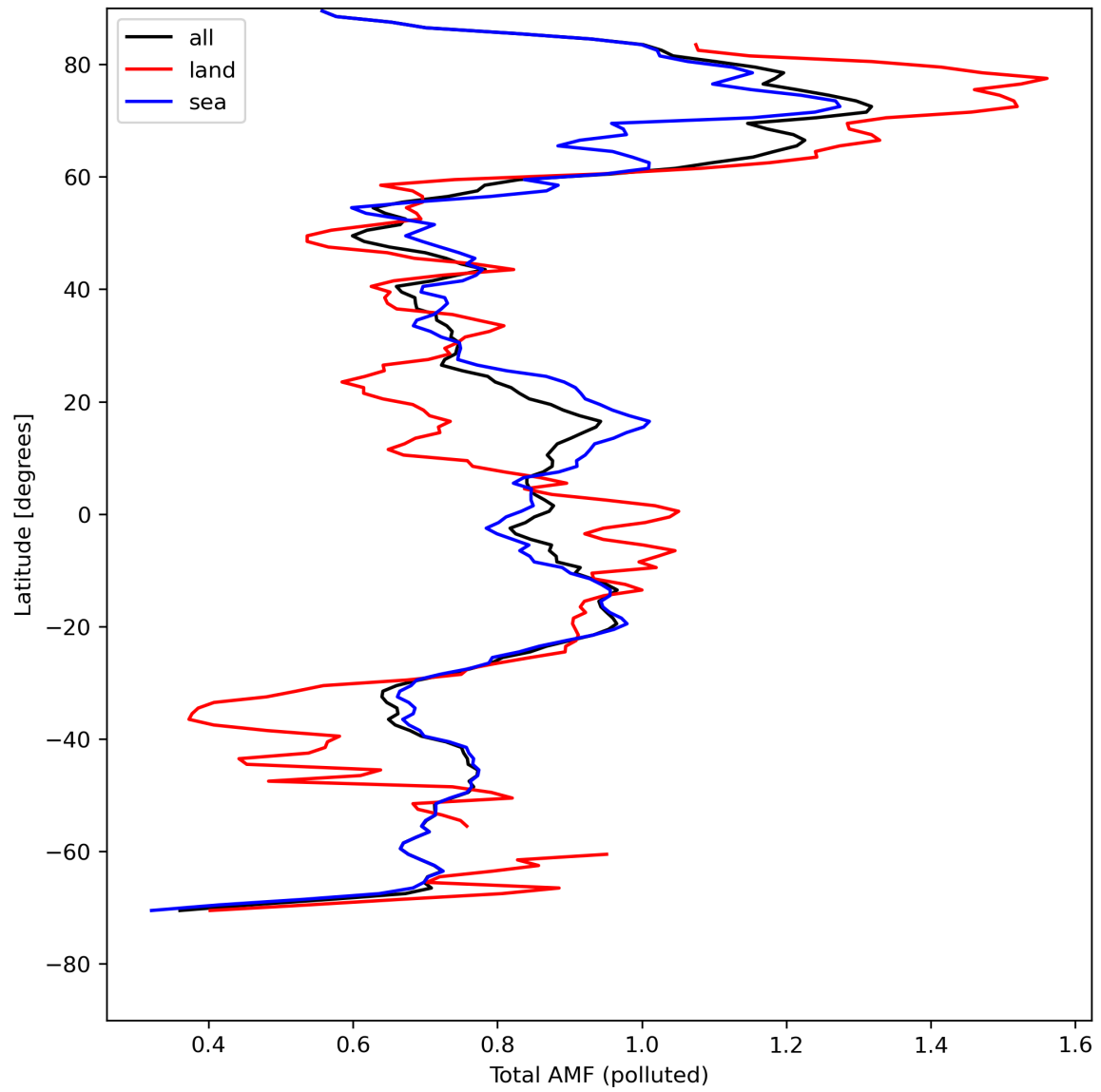
Figure 48: Zonal average of “Total AMF (polluted)” for 2024-04-26 to 2024-04-28.
