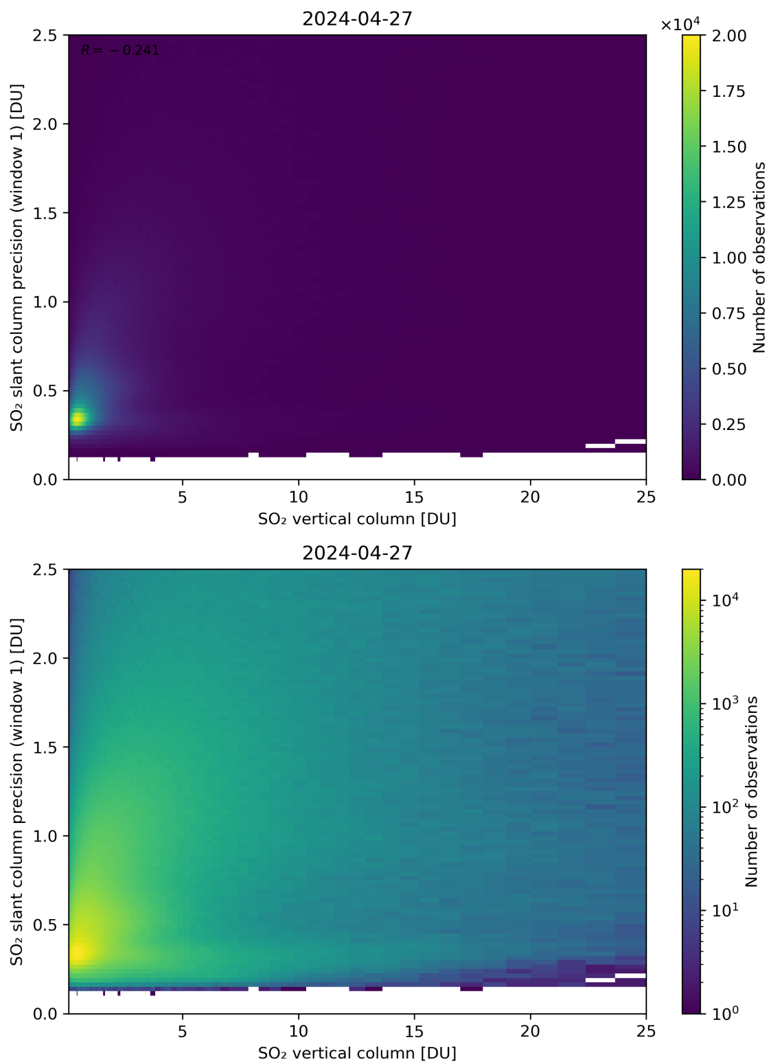
Figure 301: Scatter density plot of “SO 2 vertical column” against “SO 2 slant column precision (window 1)” for 2024-04-26 to 2024-04-28.
