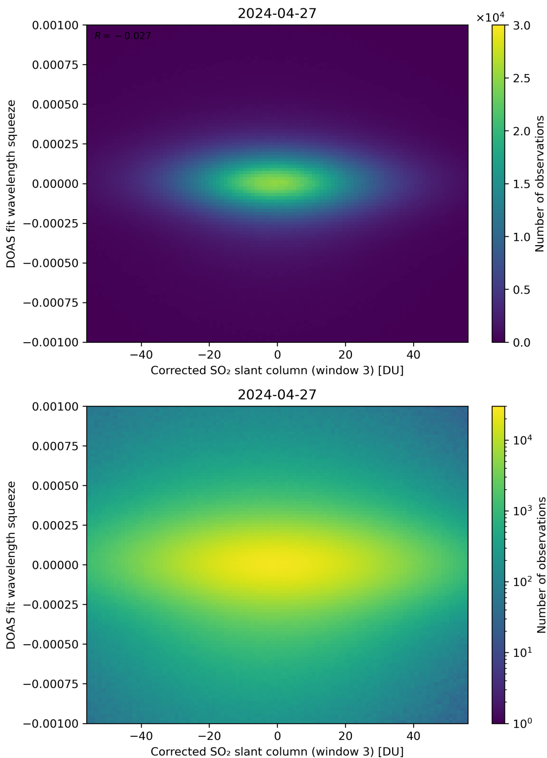
Figure 207: Scatter density plot of “Corrected SO 2 slant column (window 3)” against “DOAS fit wavelength squeeze” for 2024-04-26 to 2024-04-28.
