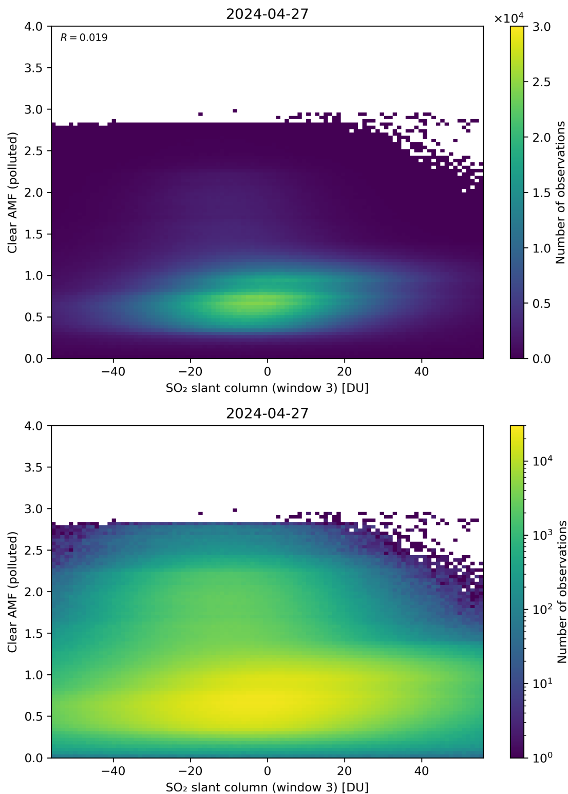
Figure 265: Scatter density plot of “SO 2 slant column (window 3)” against “Clear AMF (polluted)” for 2024-04-26 to 2024-04-28.
