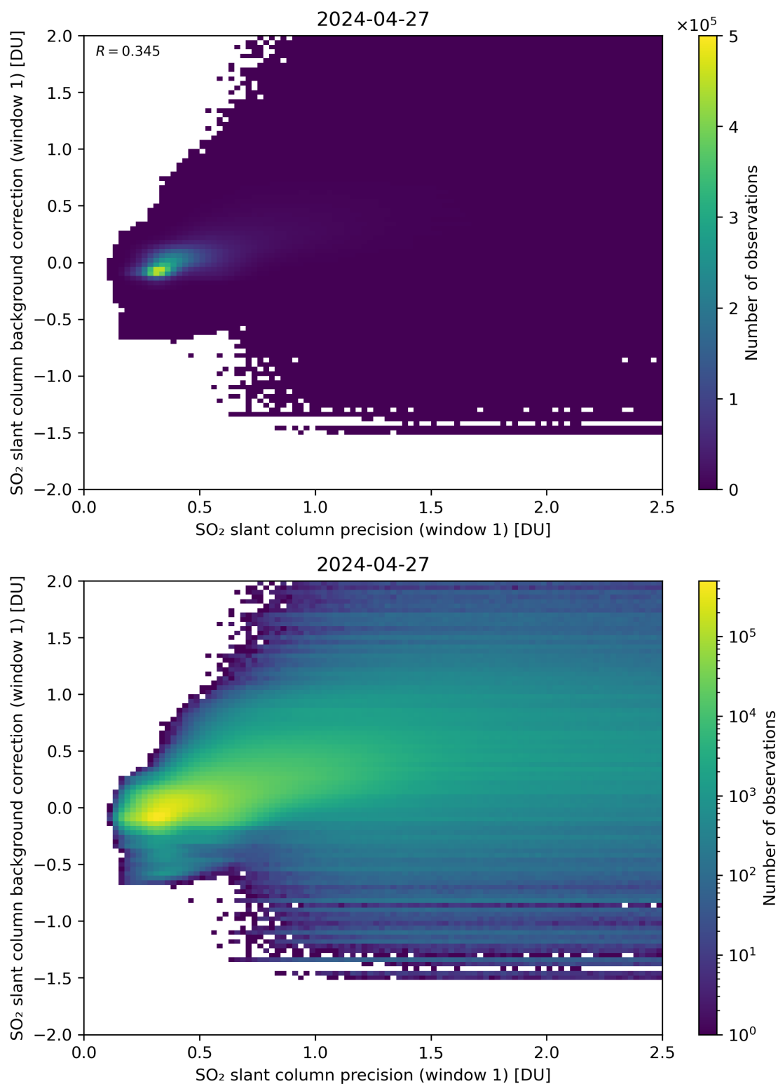
Figure 218: Scatter density plot of “SO 2 slant column precision (window 1)” against “SO 2 slant column background correction (window 1)” for 2024-04-26 to 2024-04-28.
