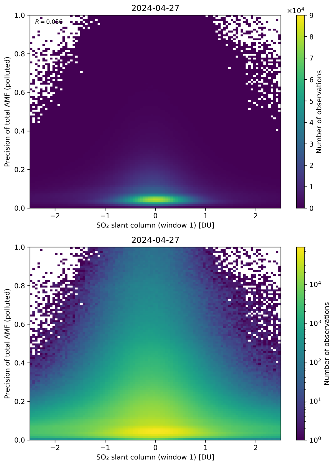
Figure 240: Scatter density plot of “SO 2 slant column (window 1)” against “Precision of total AMF (polluted)” for 2024-04-26 to 2024-04-28.
