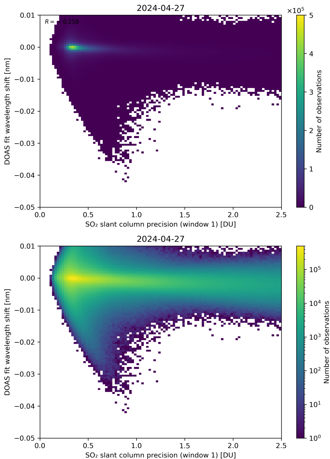
Figure 221: Scatter density plot of “SO 2 slant column precision (window 1)” against “DOAS fit wavelength shift” for 2024-04-26 to 2024-04-28.
