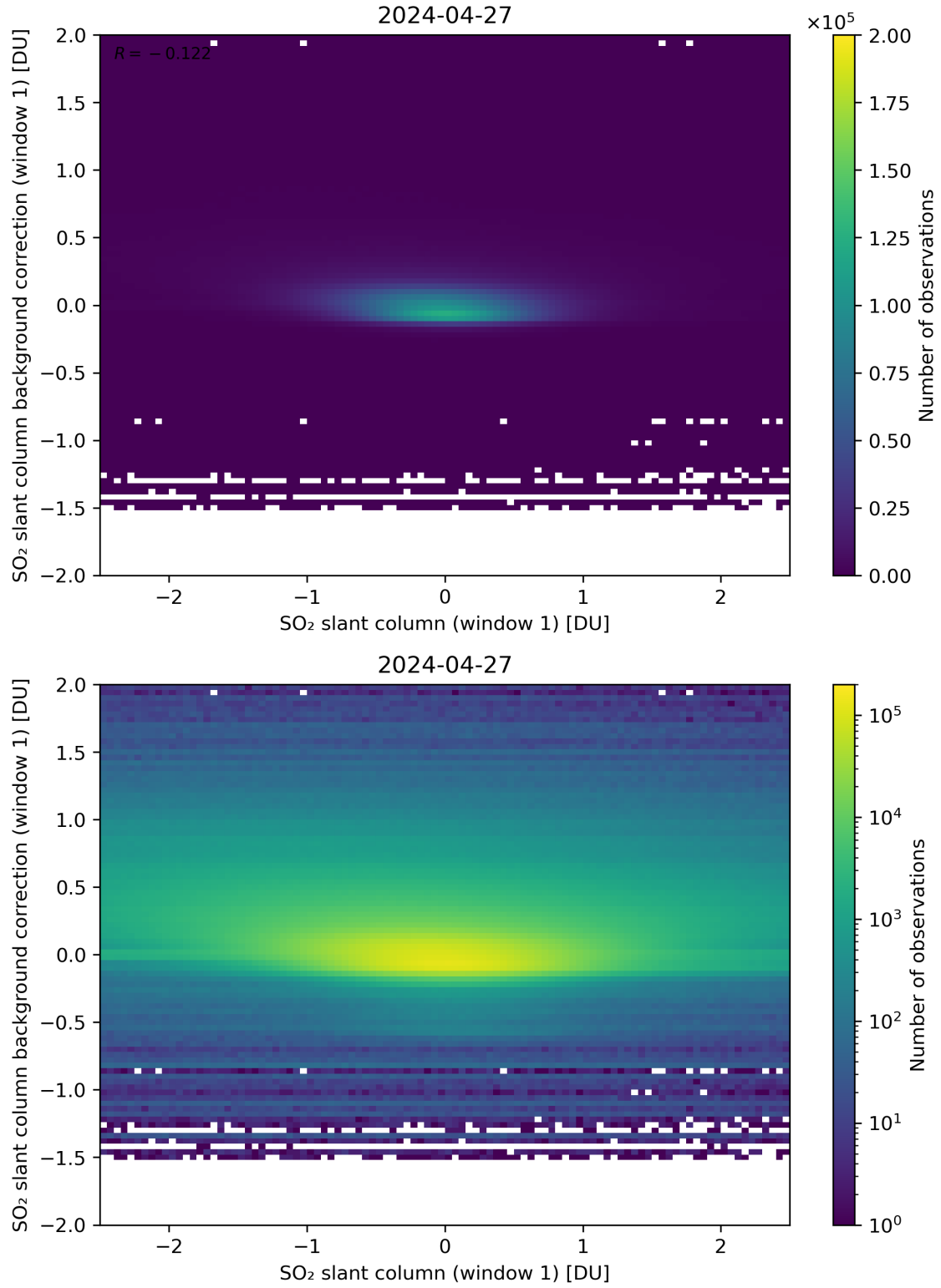
Figure 212: Scatter density plot of “SO 2 slant column (window 1)” against “SO 2 slant column background correction (window 1)” for 2024-04-26 to 2024-04-28.
