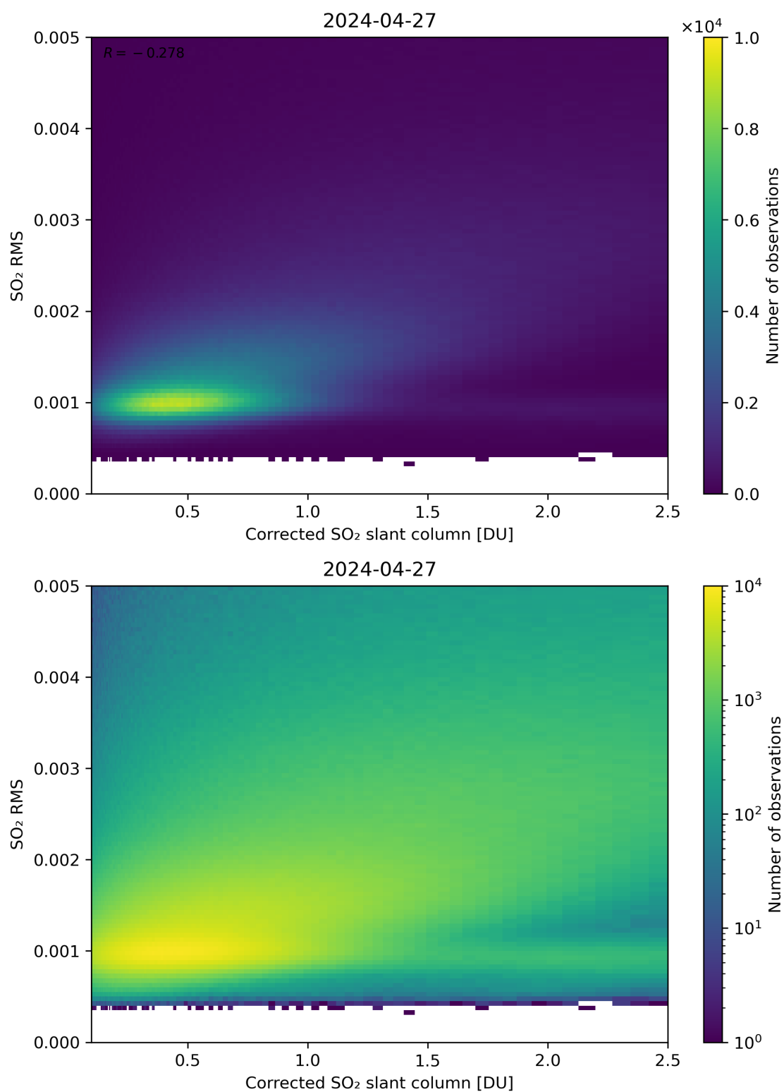
Figure 183: Scatter density plot of “Corrected SO 2 slant column” against “SO 2 RMS” for 2024-04-26 to 2024-04-28.
