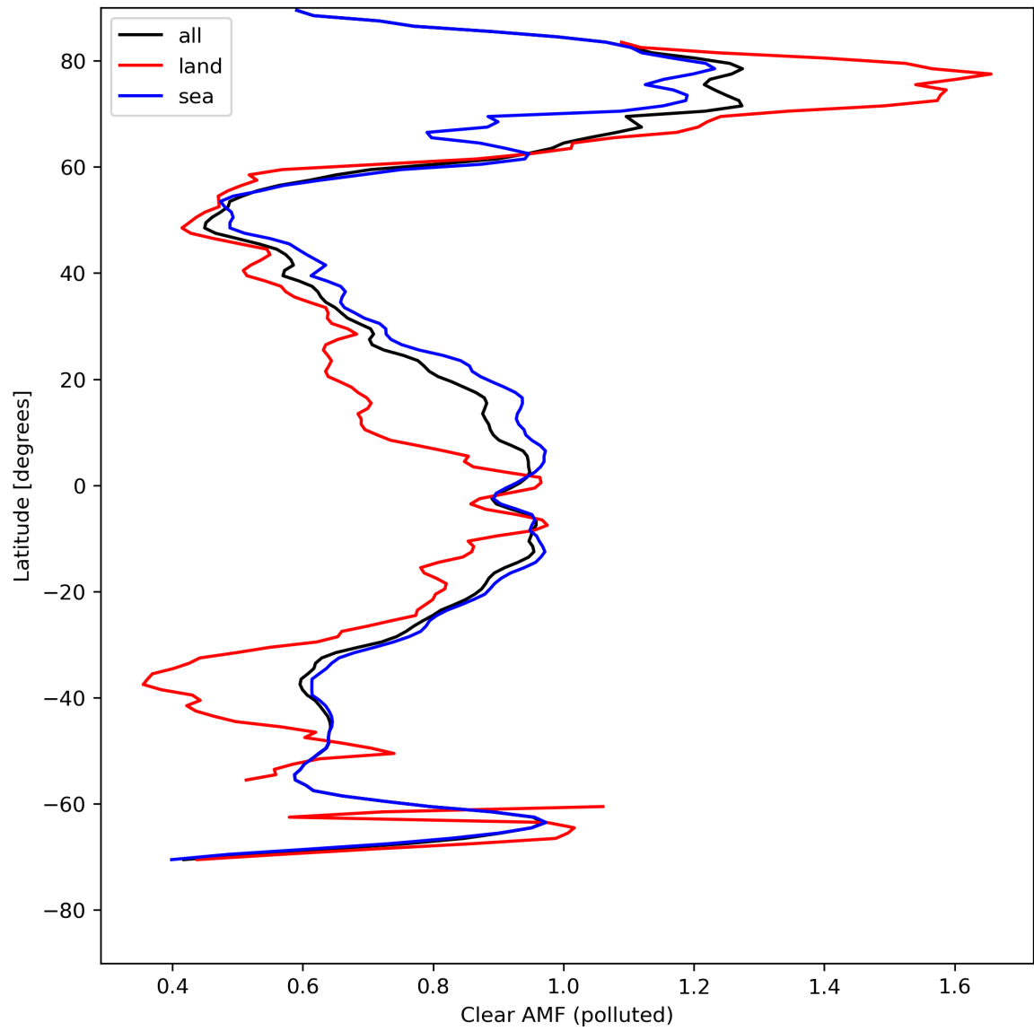
Figure 50: Zonal average of “Clear AMF (polluted)” for 2024-04-26 to 2024-04-28.
