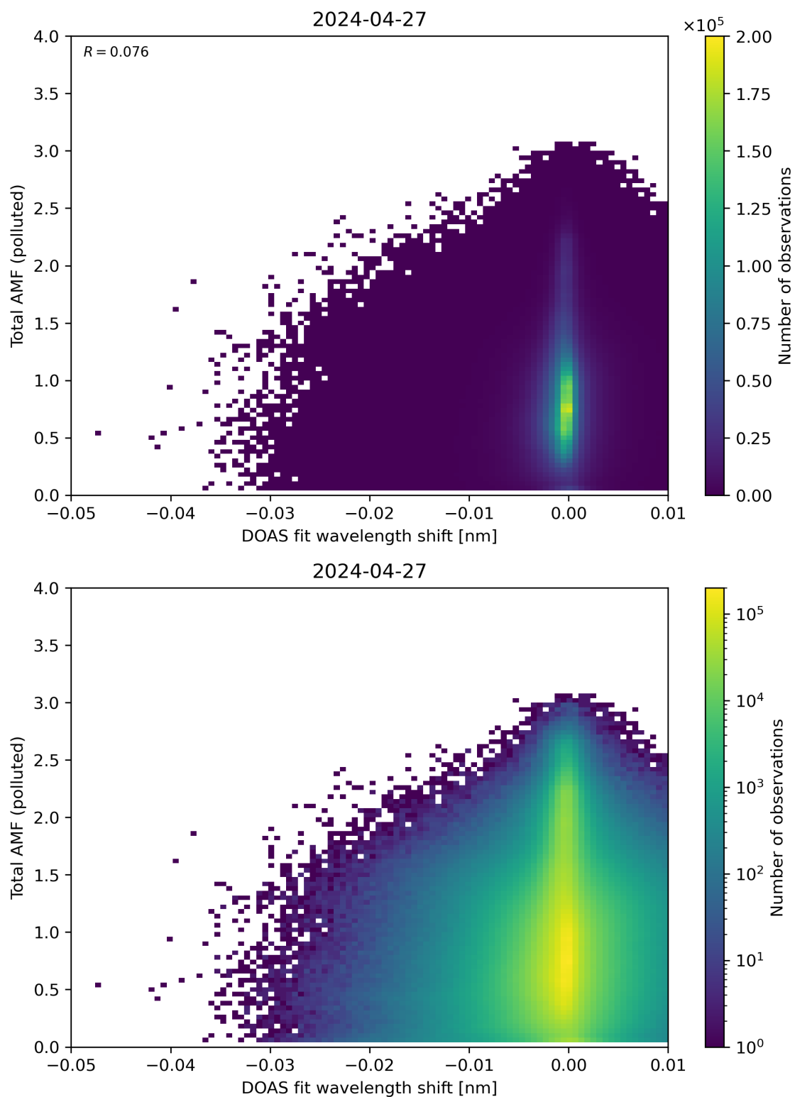
Figure 130: Scatter density plot of “DOAS fit wavelength shift” against “Total AMF (polluted)” for 2024-04-26 to 2024-04-28.
