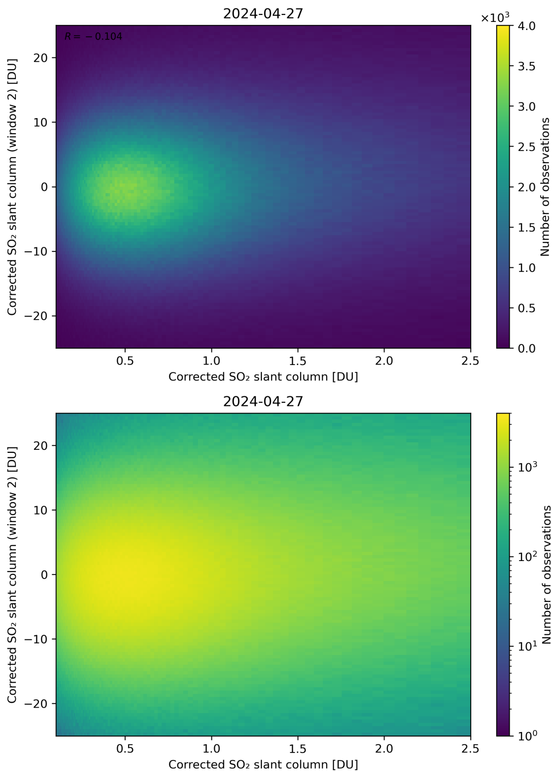
Figure 185: Scatter density plot of “Corrected SO 2 slant column” against “Corrected SO 2 slant column (window 2)” for 2024-04-26 to 2024-04-28.
