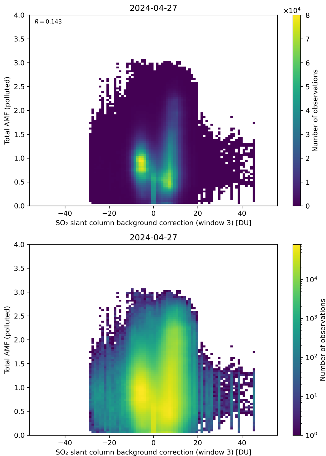
Figure 125: Scatter density plot of “SO 2 slant column background correction (window 3)” against “Total AMF (polluted)” for 2024-04-26 to 2024-04-28.
