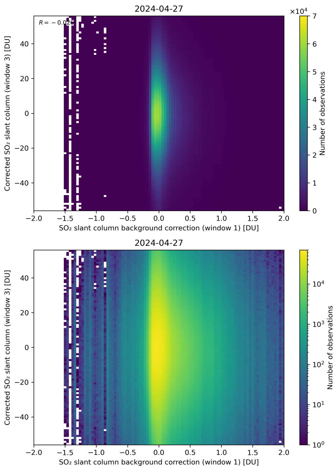
Figure 105: Scatter density plot of “SO 2 slant column background correction (window 1)” against “Corrected SO 2 slant column (window 3)” for 2024-04-26 to 2024-04-28.
