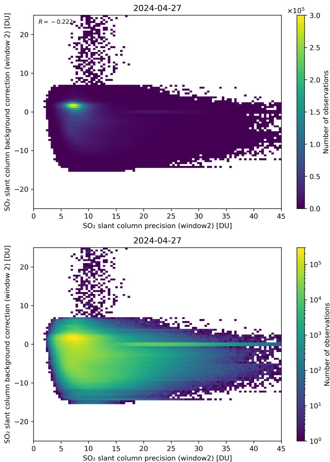
Figure 241: Scatter density plot of “SO 2 slant column precision (window2)” against “SO 2 slant column background correction (window 2)” for 2024-04-26 to 2024-04-28.
