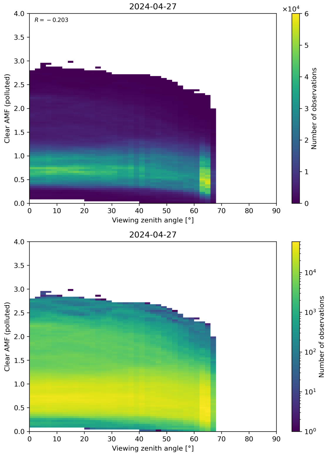
Figure 316: Scatter density plot of “Viewing zenith angle” against “Clear AMF (polluted)” for 2024-04-26 to 2024-04-28.
