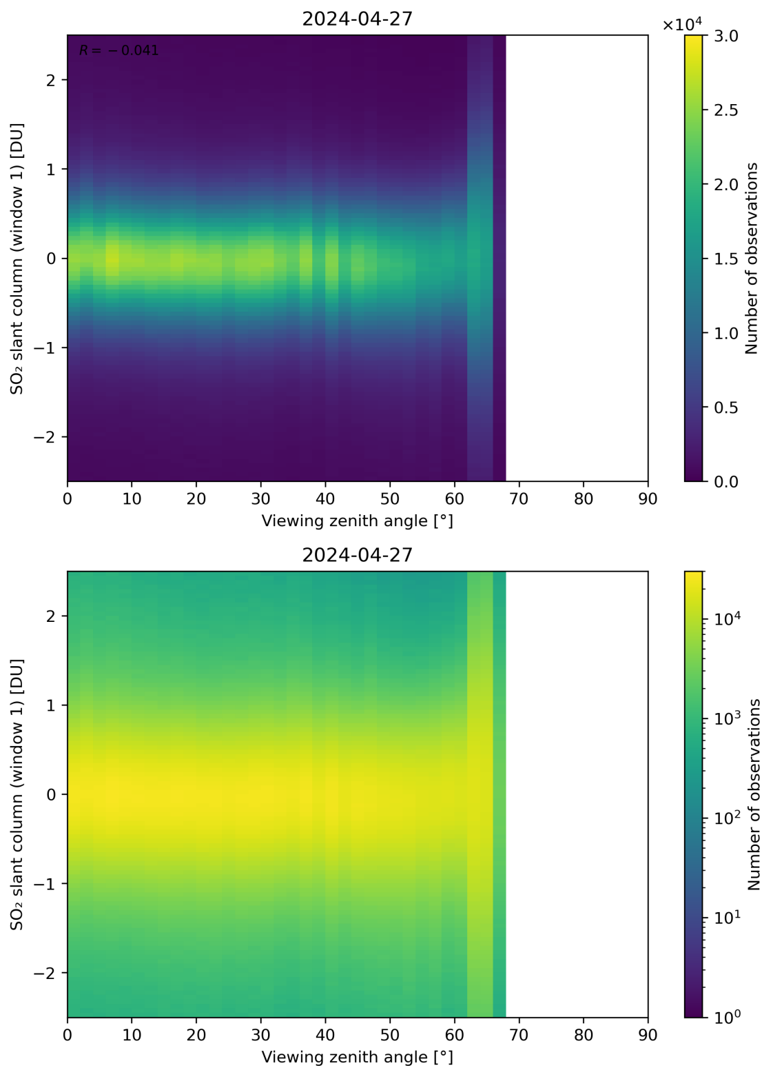
Figure 320: Scatter density plot of “Viewing zenith angle” against “SO 2 slant column (window 1)” for 2024-04-26 to 2024-04-28.
