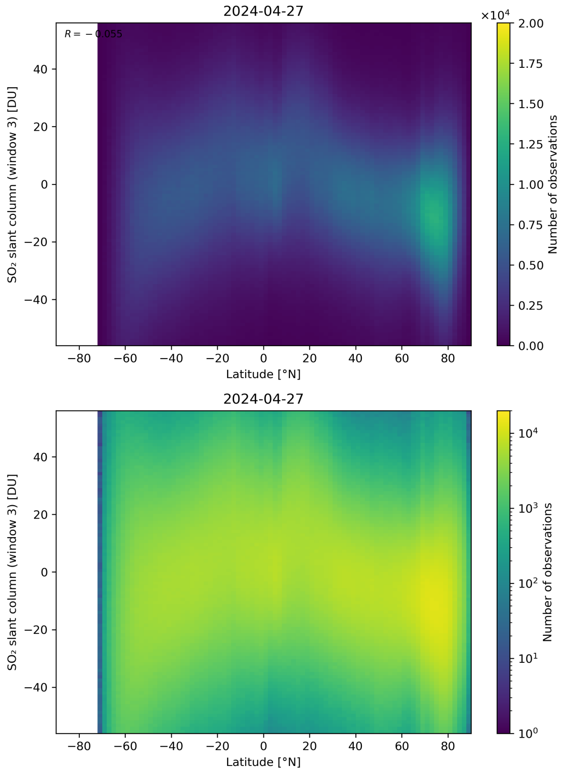
Figure 152: Scatter density plot of “Latitude” against “SO 2 slant column (window 3)” for 2024-04-26 to 2024-04-28.
