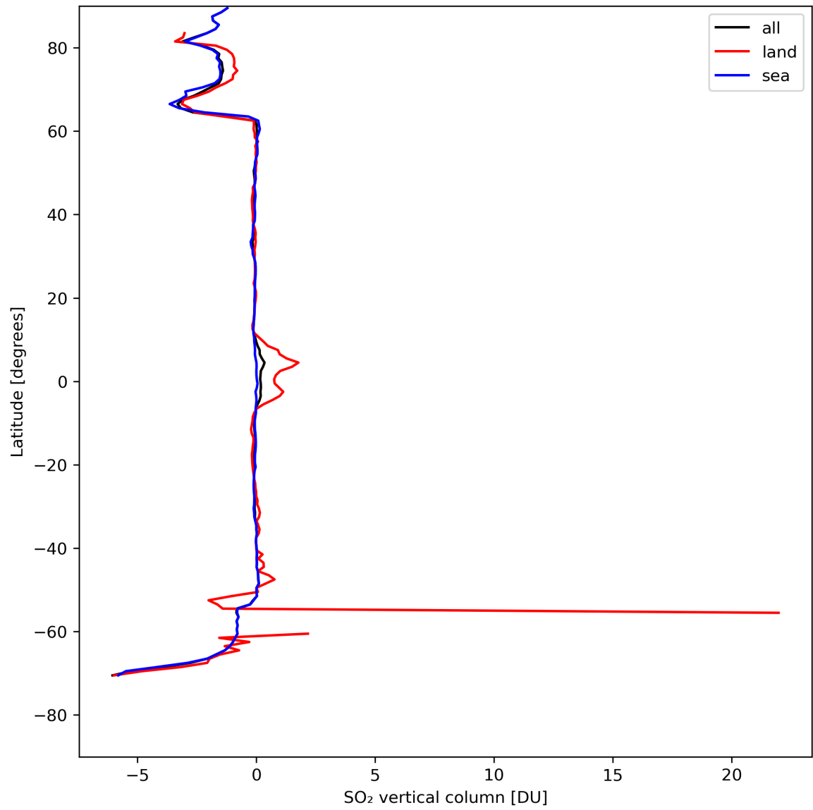
Figure 30: Zonal average of “SO 2 vertical column” for 2024-04-26 to 2024-04-28.
