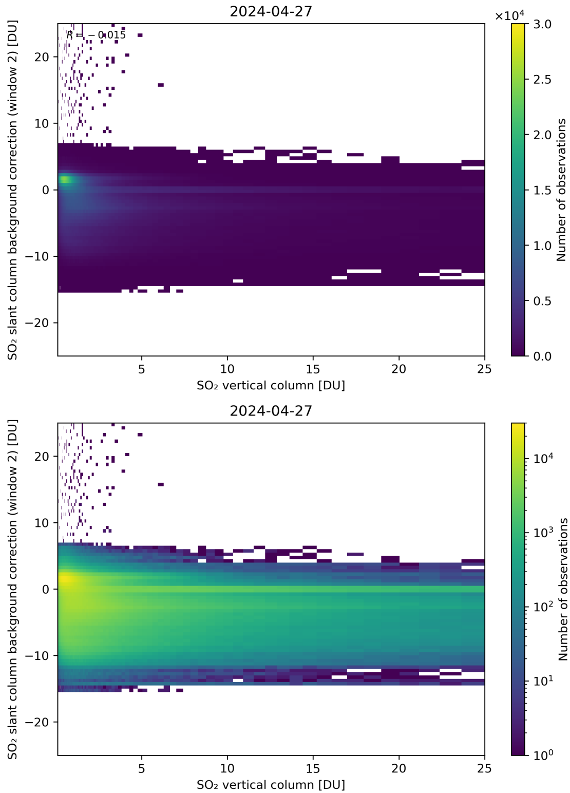
Figure 274: Scatter density plot of “SO 2 vertical column” against “SO 2 slant column background correction (window 2)” for 2024-04-26 to 2024-04-28.
