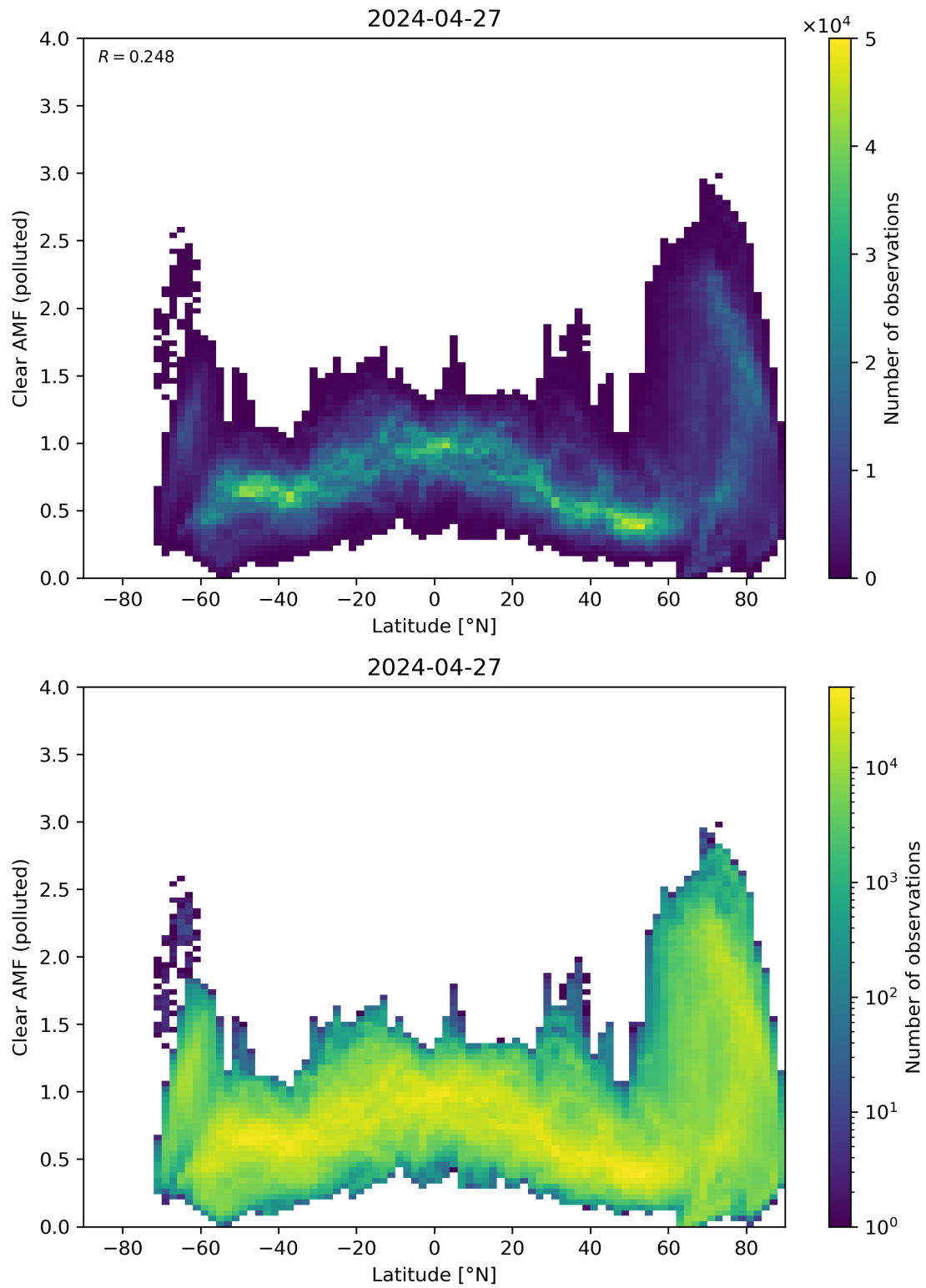
Figure 145: Scatter density plot of “Latitude” against “Clear AMF (polluted)” for 2024-04-26 to 2024-04-28.
