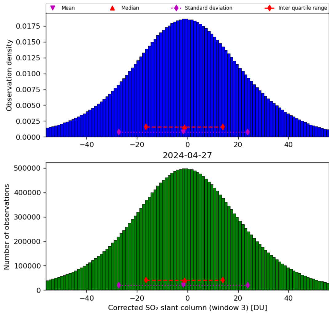
Figure 66: Histogram of “Corrected SO 2 slant column (window 3)” for 2024-04-26 to 2024-04-28
