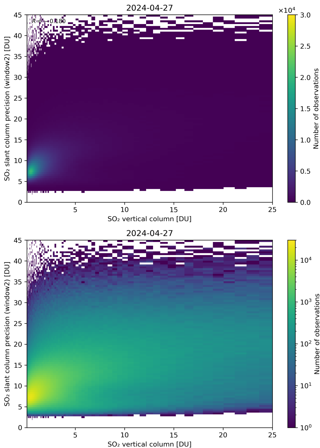
Figure 302: Scatter density plot of “SO 2 vertical column” against “SO 2 slant column precision (window2)” for 2024-04-26 to 2024-04-28.
