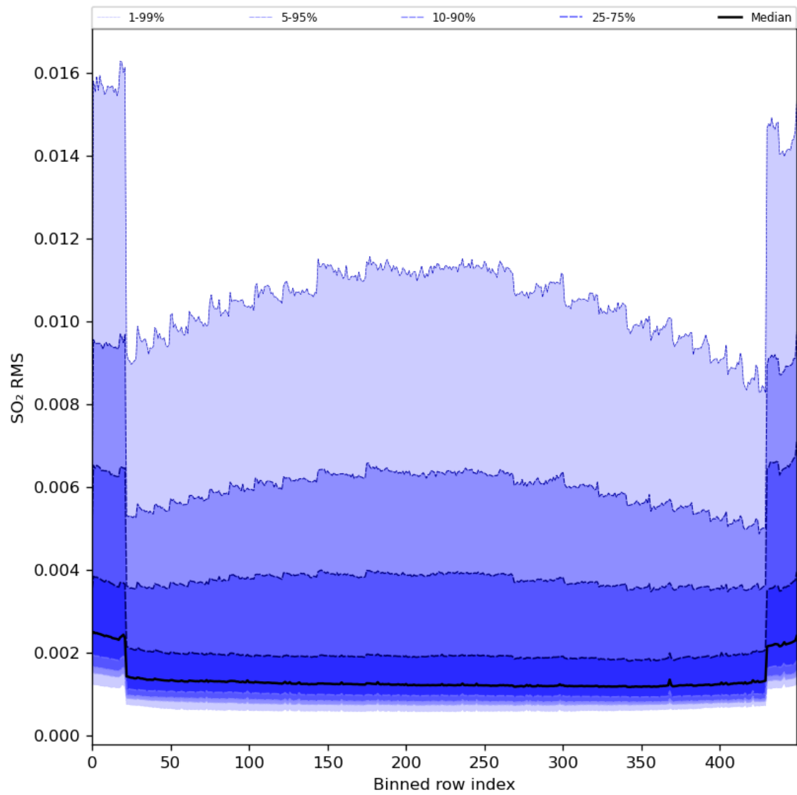
Figure 93: Along track statistics of “SO 2 RMS” for 2024-04-26 to 2024-04-28
