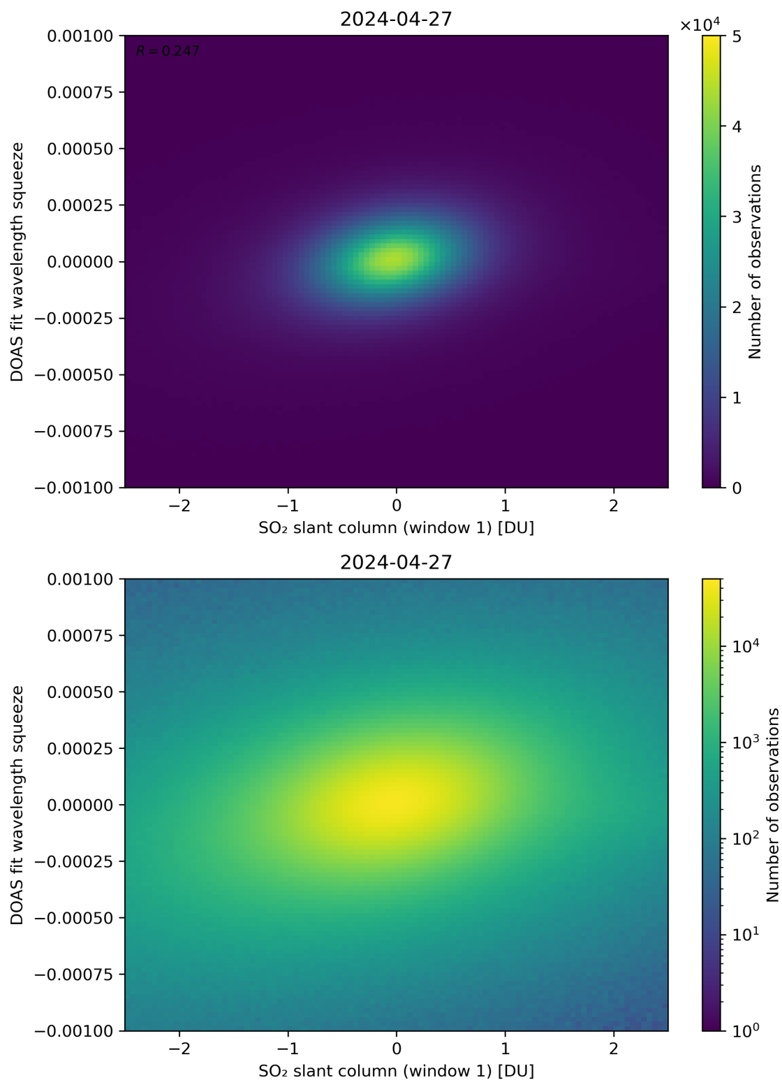
Figure 216: Scatter density plot of “SO 2 slant column (window 1)” against “DOAS fit wavelength squeeze” for 2024-04-26 to 2024-04-28.
