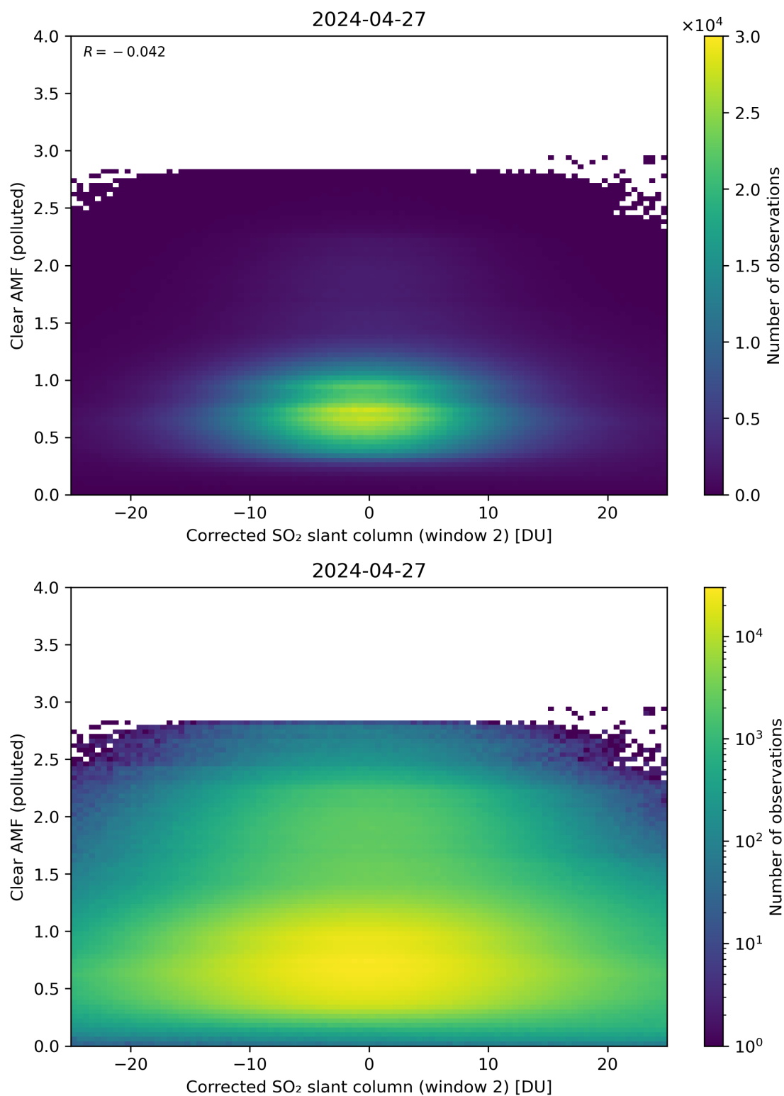
Figure 199: Scatter density plot of “Corrected SO 2 slant column (window 2)” against “Clear AMF (polluted)” for 2024-04-26 to 2024-04-28.
