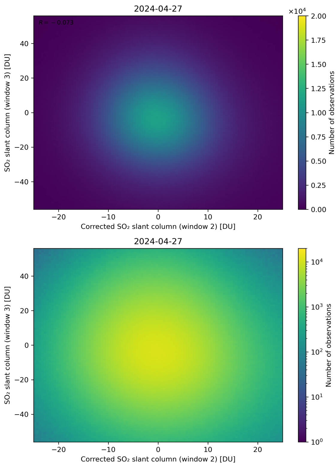
Figure 201: Scatter density plot of “Corrected SO 2 slant column (window 2)” against “SO 2 slant column (window 3)” for 2024-04-26 to 2024-04-28.
