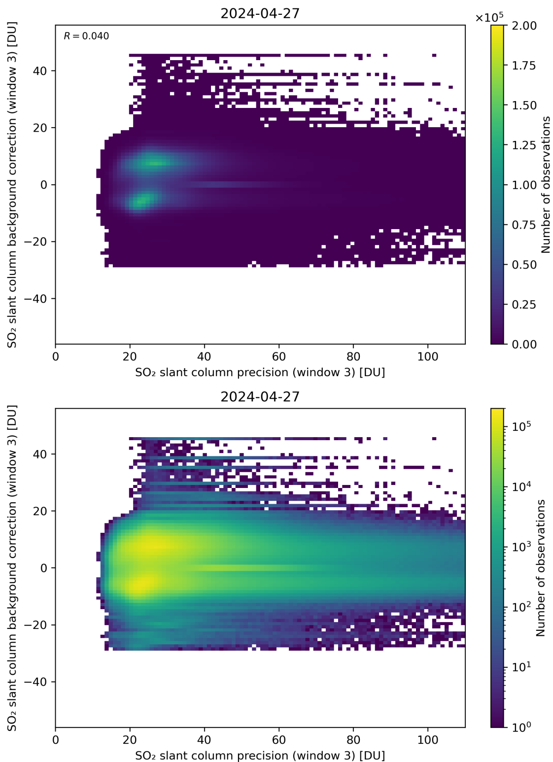
Figure 257: Scatter density plot of “SO 2 slant column precision (window 3)” against “SO 2 slant column background correction (window 3)” for 2024-04-26 to 2024-04-28.
