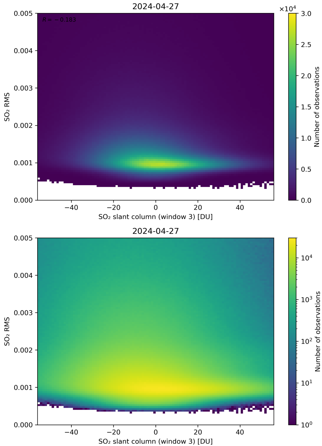
Figure 256: Scatter density plot of “SO 2 slant column (window 3)” against “SO 2 RMS” for 2024-04-26 to 2024-04-28.
