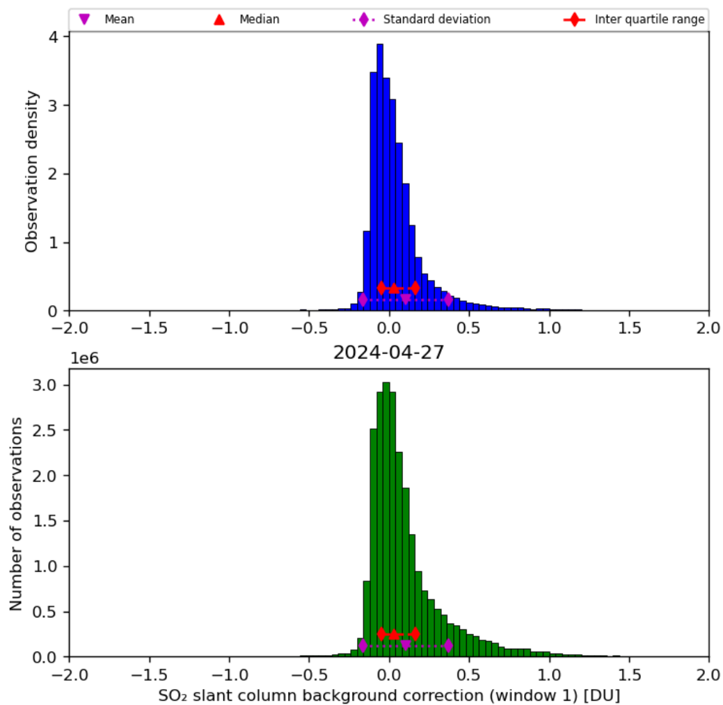
Figure 59: Histogram of “SO 2 slant column background correction (window 1)” for 2024-04-26 to 2024-04-28
