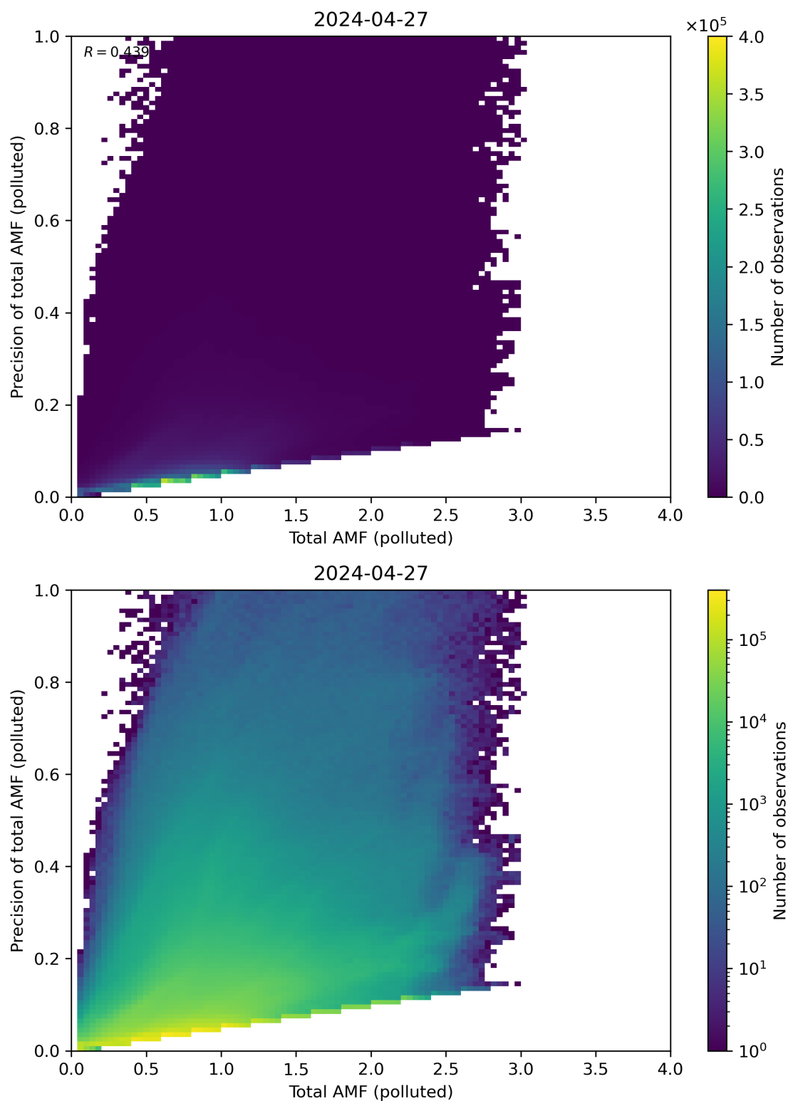
Figure 272: Scatter density plot of “Total AMF (polluted)” against “Precision of total AMF (polluted)” for 2024-04-26 to 2024-04-28.
