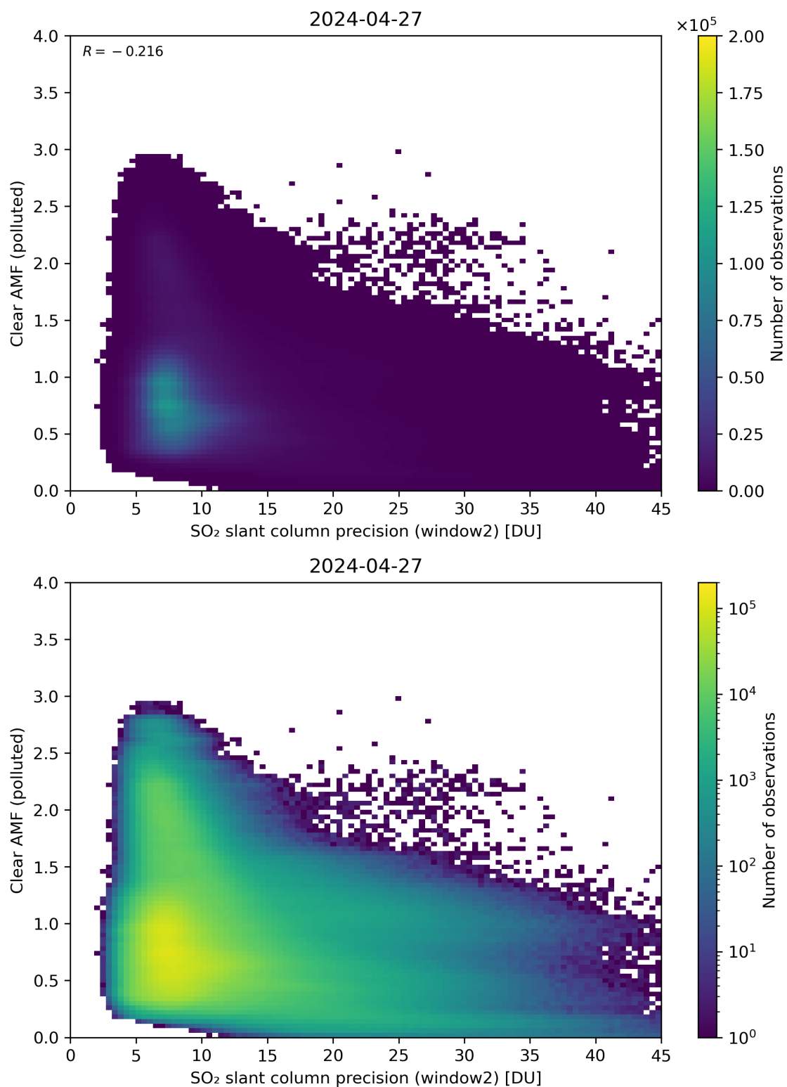
Figure 246: Scatter density plot of “SO 2 slant column precision (window2)” against “Clear AMF (polluted)” for 2024-04-26 to 2024-04-28.
