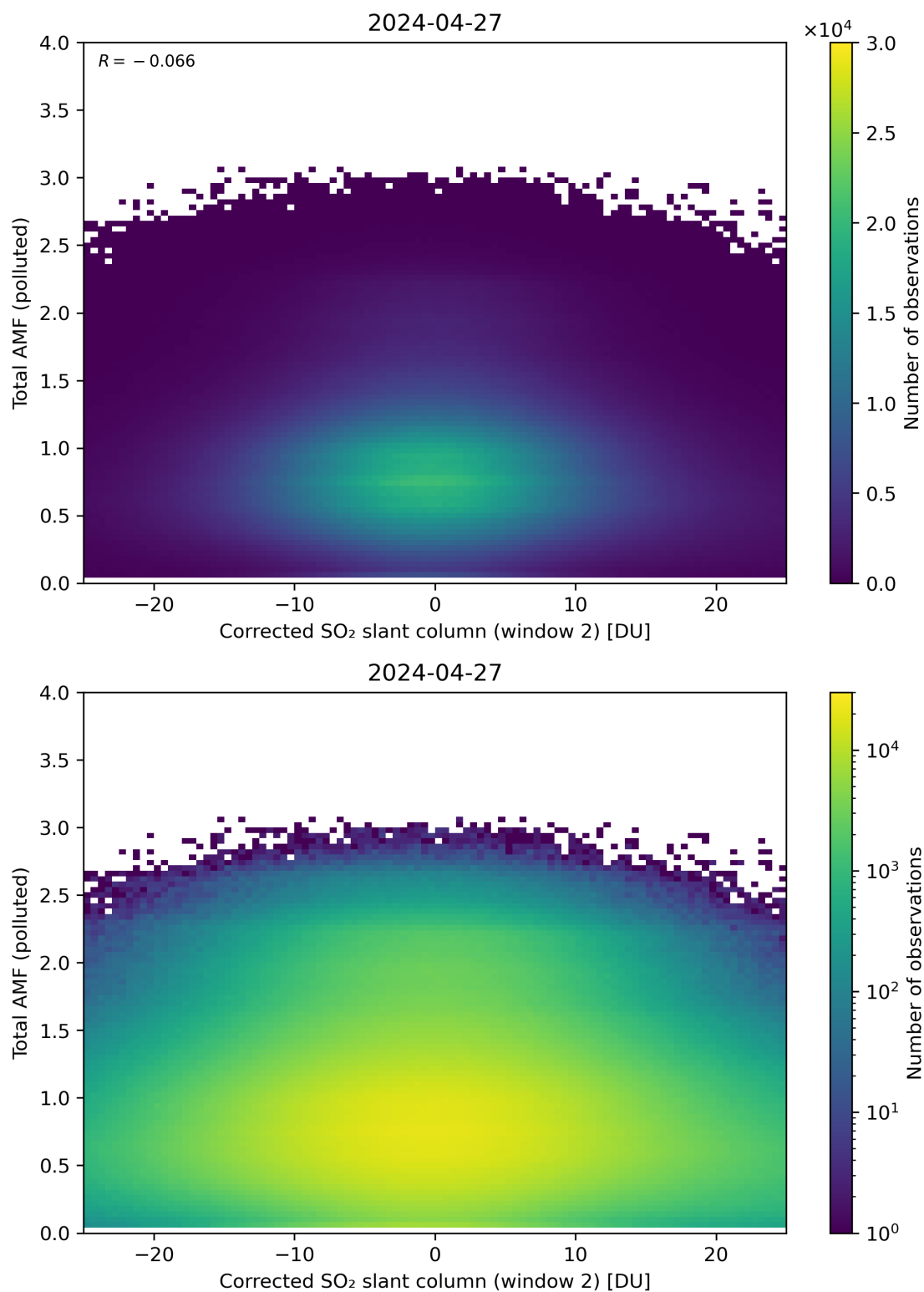
Figure 203: Scatter density plot of “Corrected SO 2 slant column (window 2)” against “Total AMF (polluted)” for 2024-04-26 to 2024-04-28.
