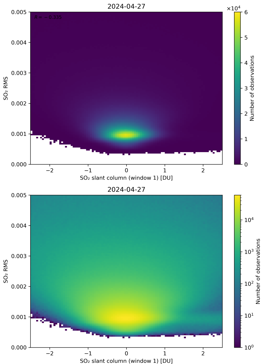
Figure 217: Scatter density plot of “SO 2 slant column (window 1)” against “SO 2 RMS” for 2024-04-26 to 2024-04-28.
