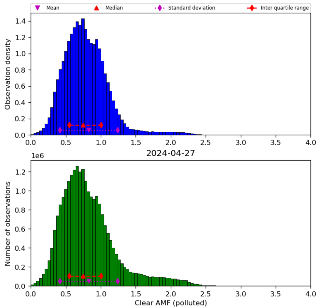
Figure 73: Histogram of “Clear AMF (polluted)” for 2024-04-26 to 2024-04-28
