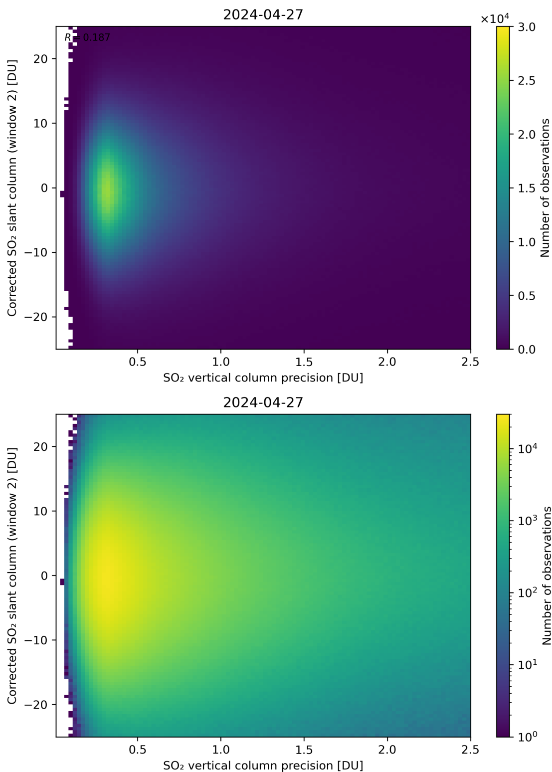
Figure 287: Scatter density plot of “SO 2 vertical column precision” against “Corrected SO 2 slant column (window 2)” for 2024-04-26 to 2024-04-28.
