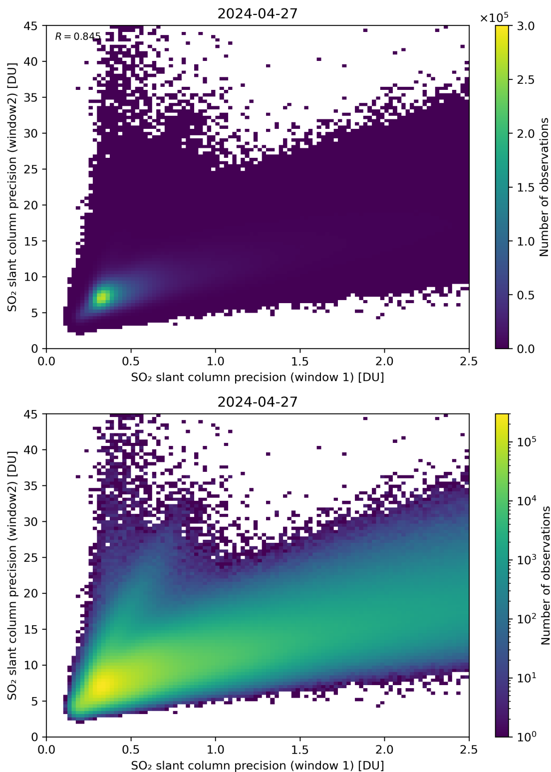
Figure 227: Scatter density plot of “SO 2 slant column precision (window 1)” against “SO 2 slant column precision (window2)” for 2024-04-26 to 2024-04-28.
