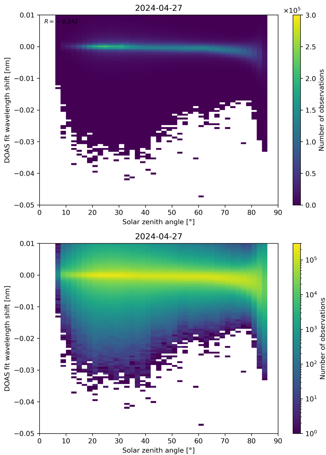
Figure 161: Scatter density plot of “Solar zenith angle” against “DOAS fit wavelength shift” for 2024-04-26 to 2024-04-28.
