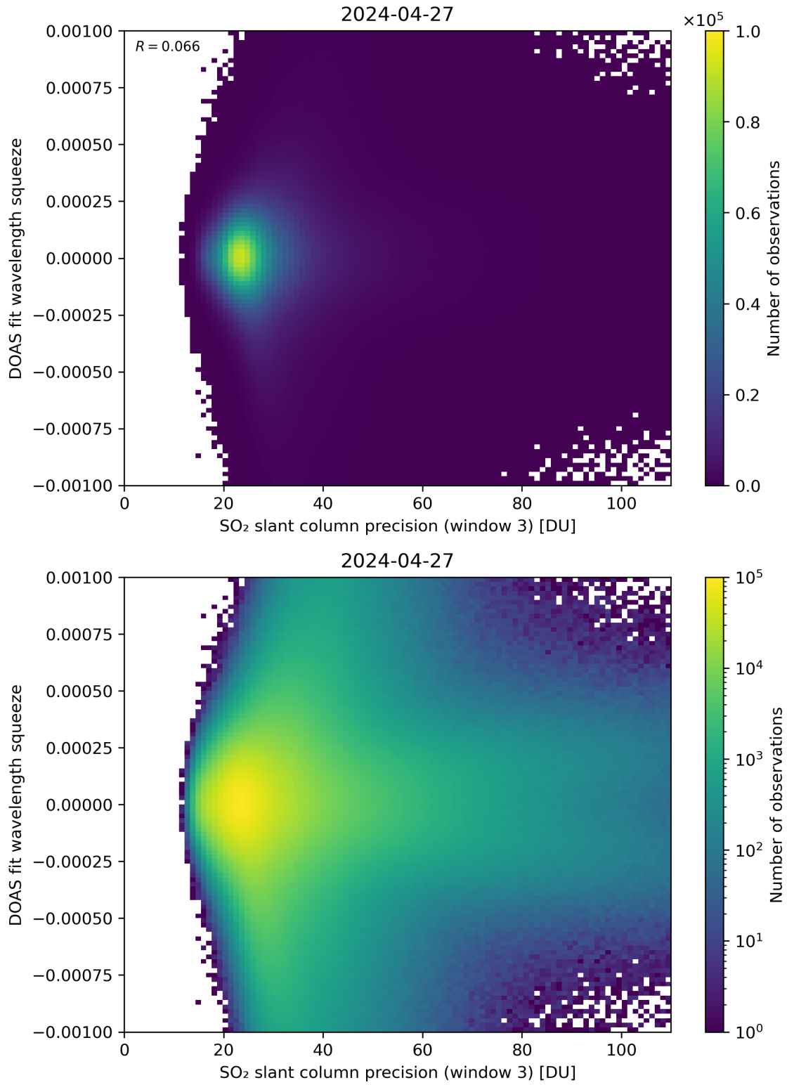
Figure 259: Scatter density plot of “SO 2 slant column precision (window 3)” against “DOAS fit wavelength squeeze” for 2024-04-26 to 2024-04-28.
