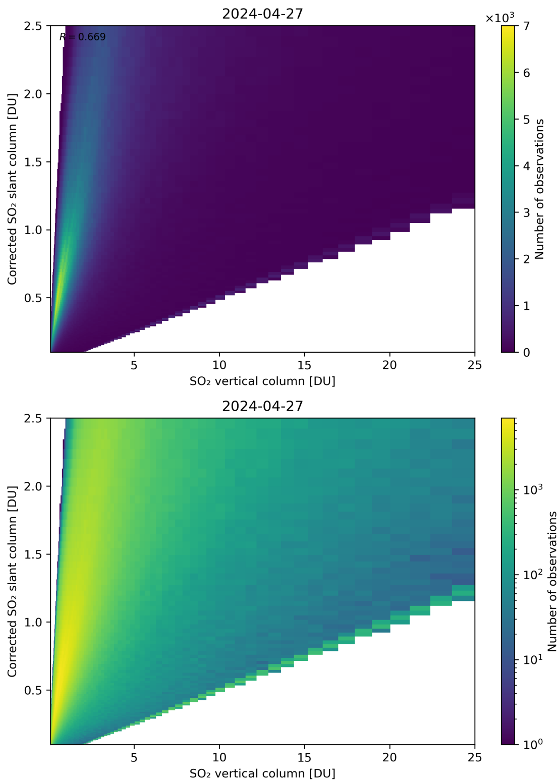
Figure 297: Scatter density plot of “SO 2 vertical column” against “Corrected SO 2 slant column” for 2024-04-26 to 2024-04-28.
