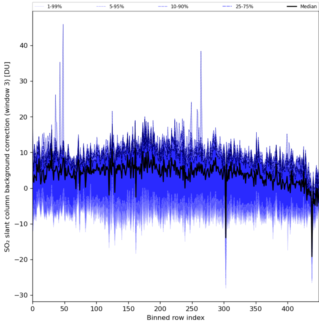
Figure 90: Along track statistics of “SO 2 slant column background correction (window 3)” for 2024-04-26 to 2024-04-28
