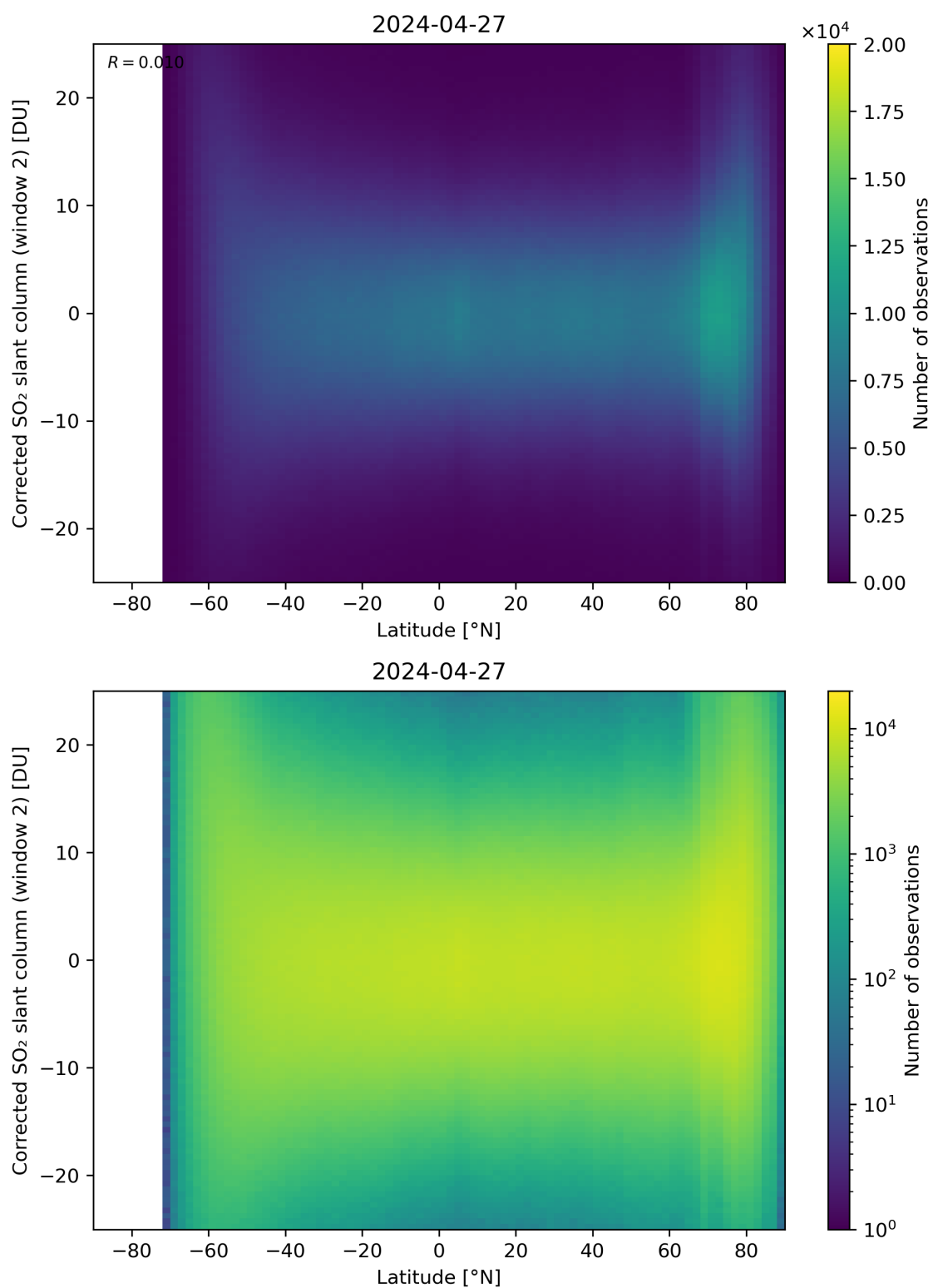
Figure 147: Scatter density plot of “Latitude” against “Corrected SO 2 slant column (window 2)” for 2024-04-26 to 2024-04-28.
