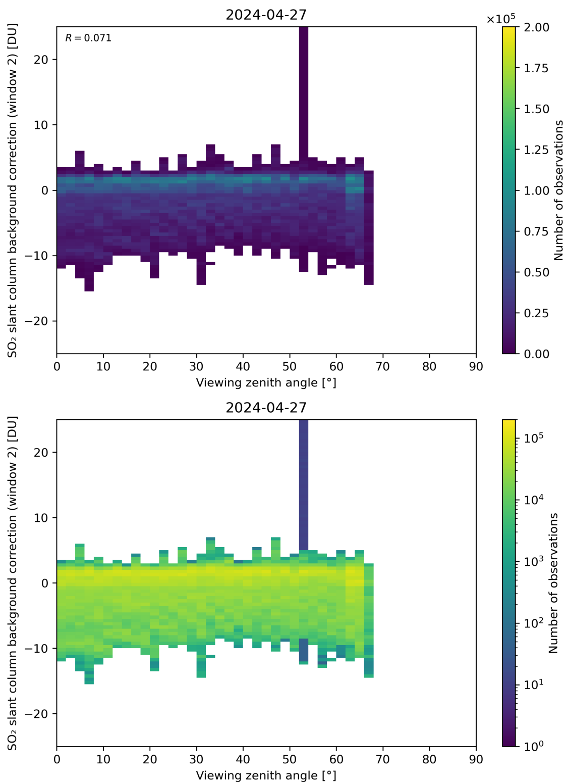
Figure 309: Scatter density plot of “Viewing zenith angle” against “SO 2 slant column background correction (window 2)” for 2024-04-26 to 2024-04-28.
