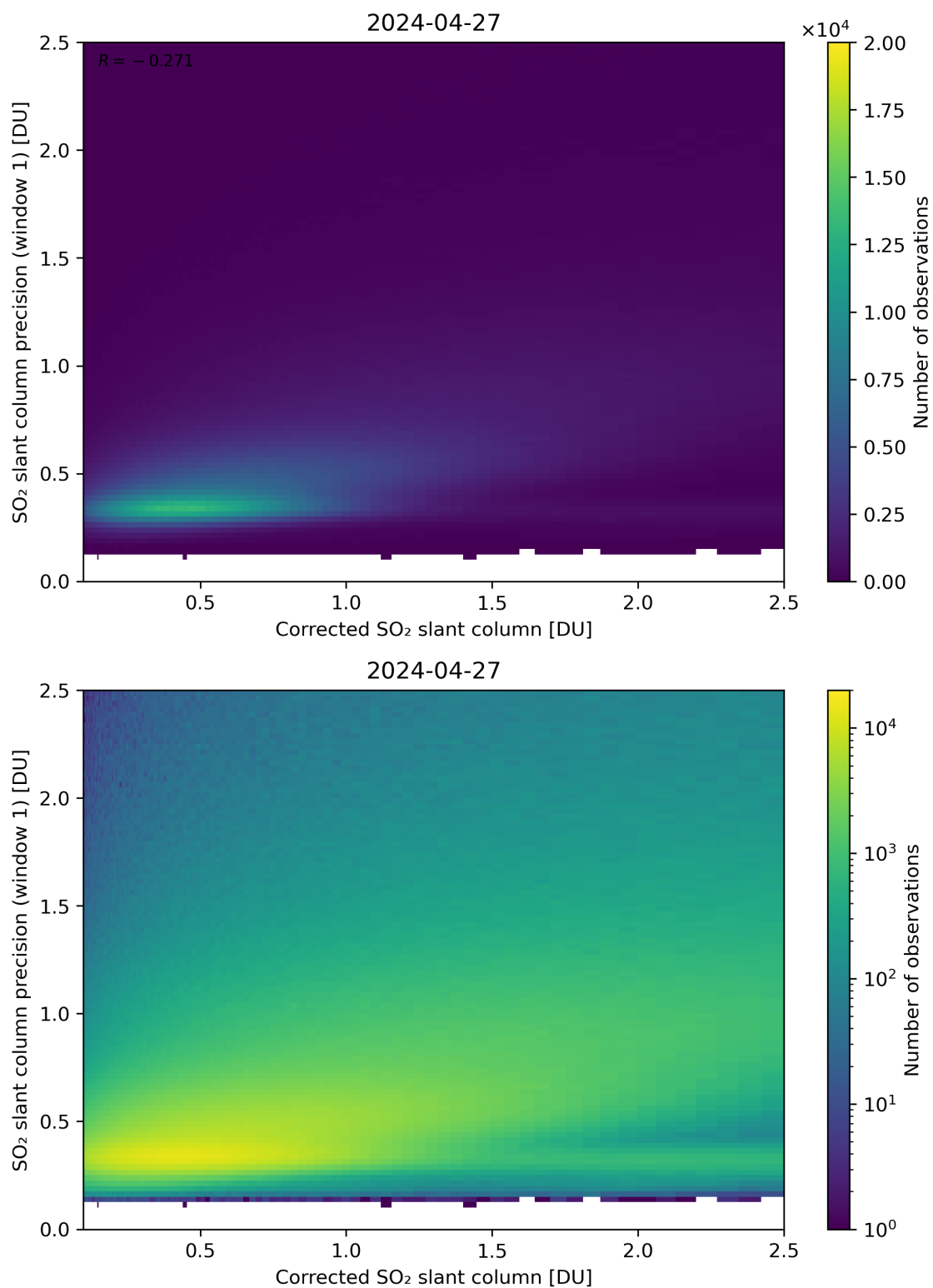
Figure 188: Scatter density plot of “Corrected SO 2 slant column” against “SO 2 slant column precision (window 1)” for 2024-04-26 to 2024-04-28.
