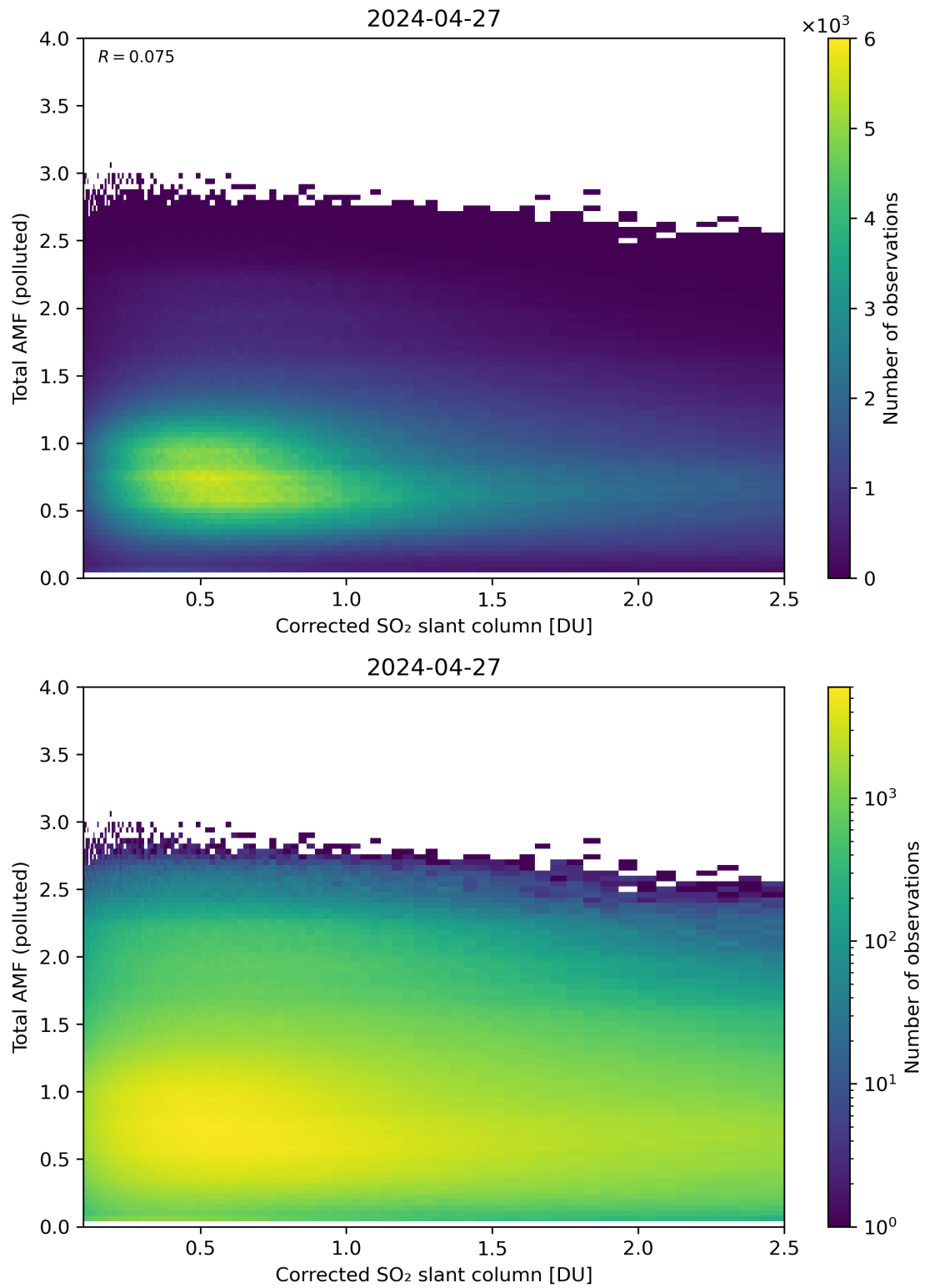
Figure 192: Scatter density plot of “Corrected SO 2 slant column” against “Total AMF (polluted)” for 2024-04-26 to 2024-04-28.
