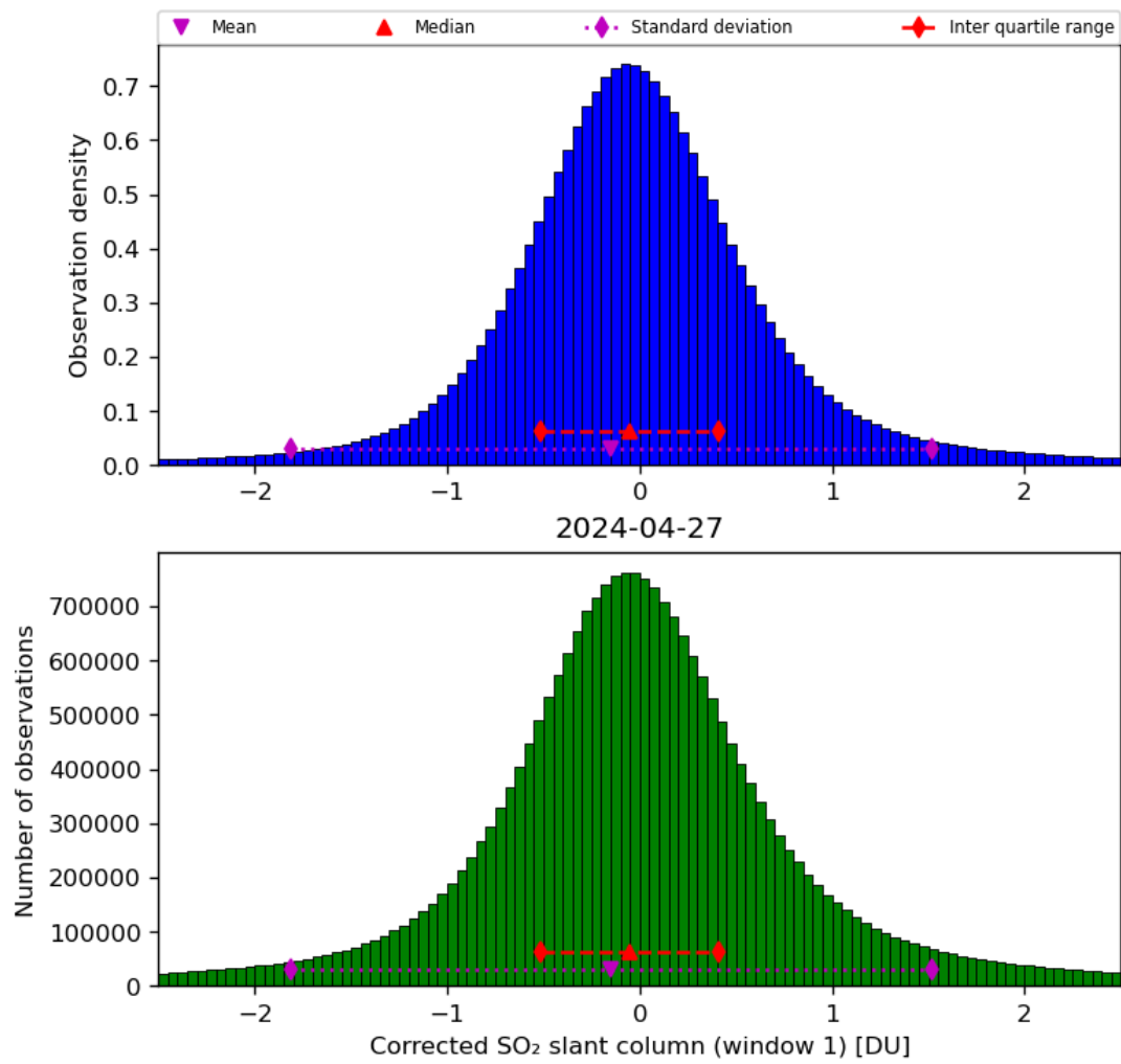
Figure 58: Histogram of “Corrected SO 2 slant column (window 1)” for 2024-04-26 to 2024-04-28
