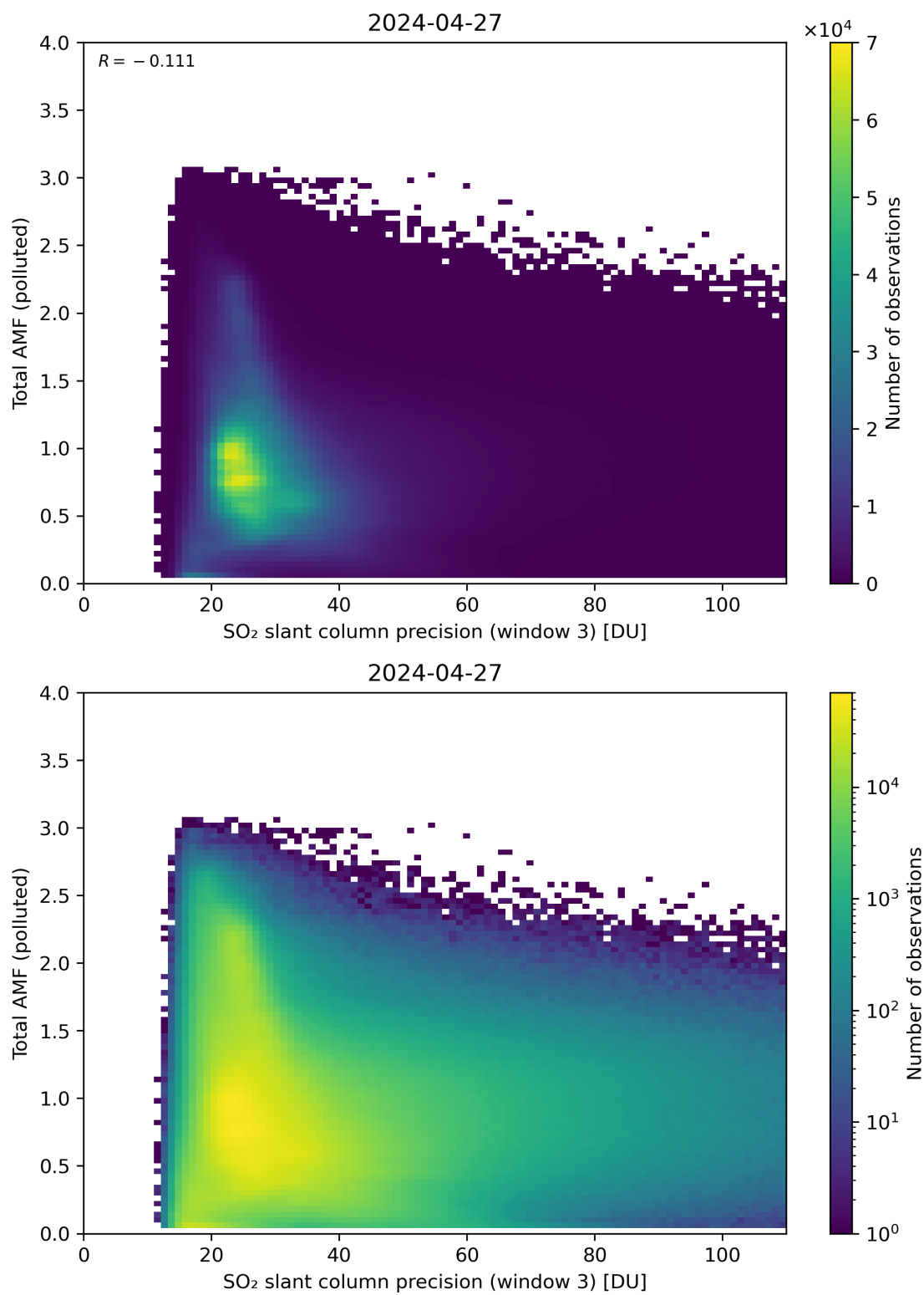
Figure 263: Scatter density plot of “SO 2 slant column precision (window 3)” against “Total AMF (polluted)” for 2024-04-26 to 2024-04-28.
