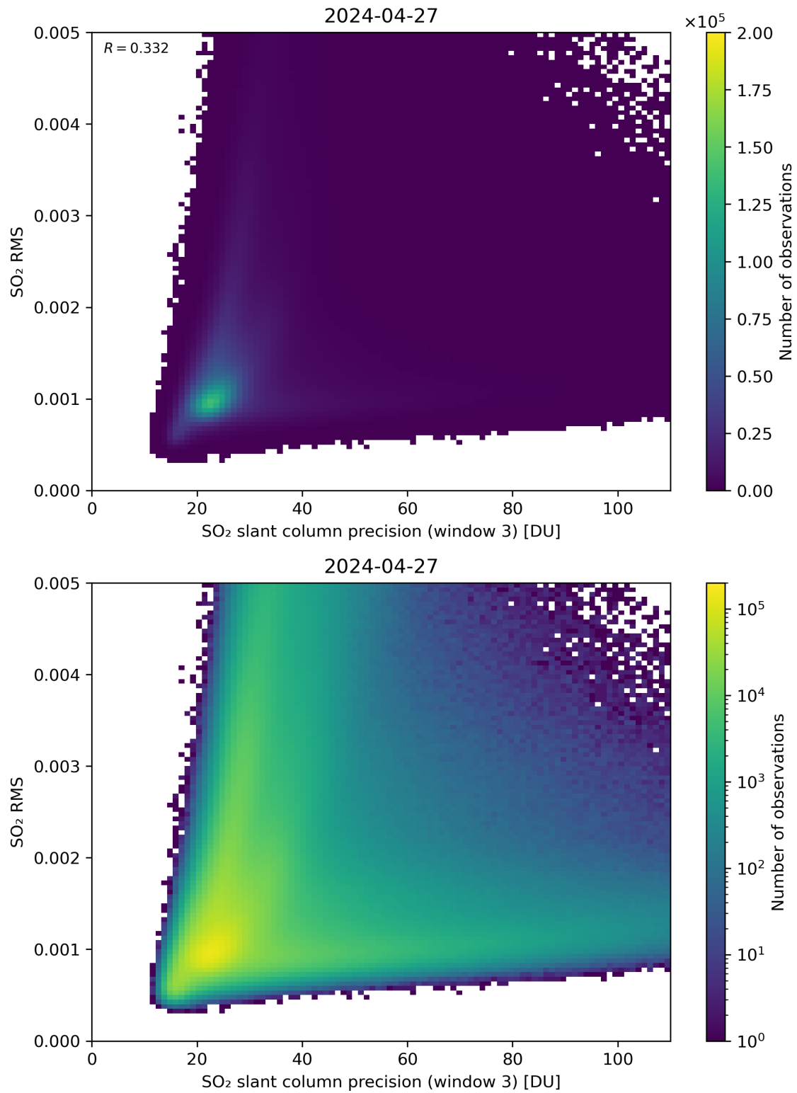
Figure 260: Scatter density plot of “SO 2 slant column precision (window 3)” against “SO 2 RMS” for 2024-04-26 to 2024-04-28.
