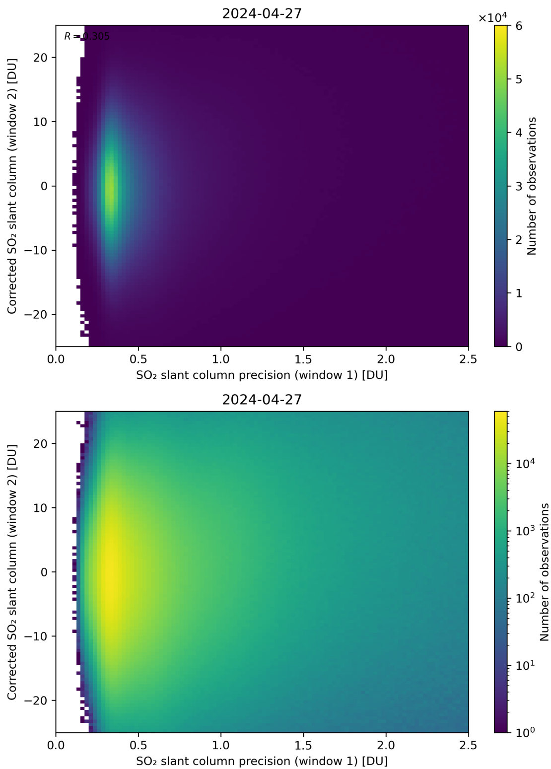
Figure 225: Scatter density plot of “SO 2 slant column precision (window 1)” against “Corrected SO 2 slant column (window 2)” for 2024-04-26 to 2024-04-28.
