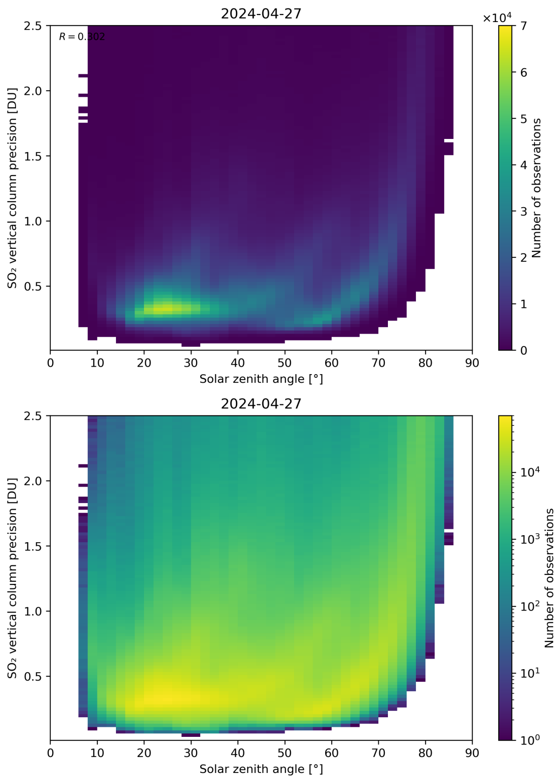
Figure 177: Scatter density plot of “Solar zenith angle” against “SO 2 vertical column precision” for 2024-04-26 to 2024-04-28.
