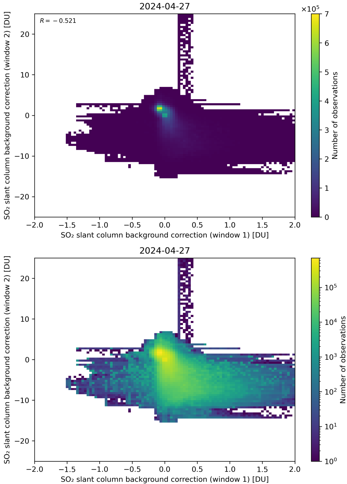
Figure 98: Scatter density plot of “SO 2 slant column background correction (window 1)” against “SO 2 slant column background correction (window 2)” for 2024-04-26 to 2024-04-28.
