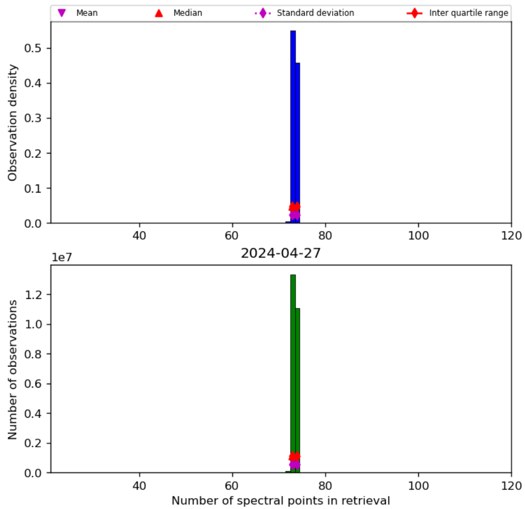
Figure 74: Histogram of “Number of spectral points in retrieval” for 2024-04-26 to 2024-04-28
