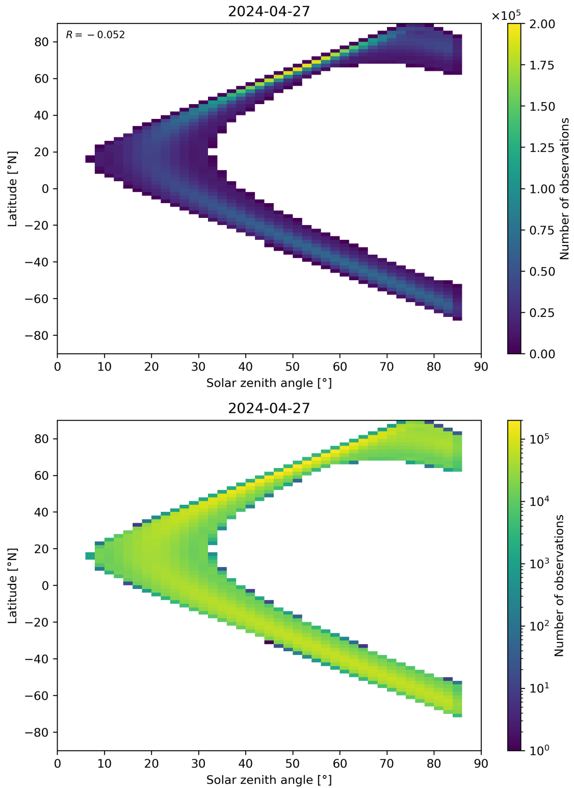
Figure 164: Scatter density plot of “Solar zenith angle” against “Latitude” for 2024-04-26 to 2024-04-28.
