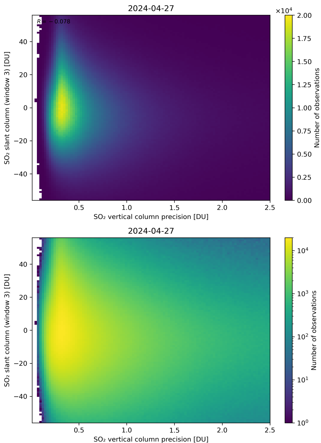
Figure 292: Scatter density plot of “SO 2 vertical column precision” against “SO 2 slant column (window 3)” for 2024-04-26 to 2024-04-28.
