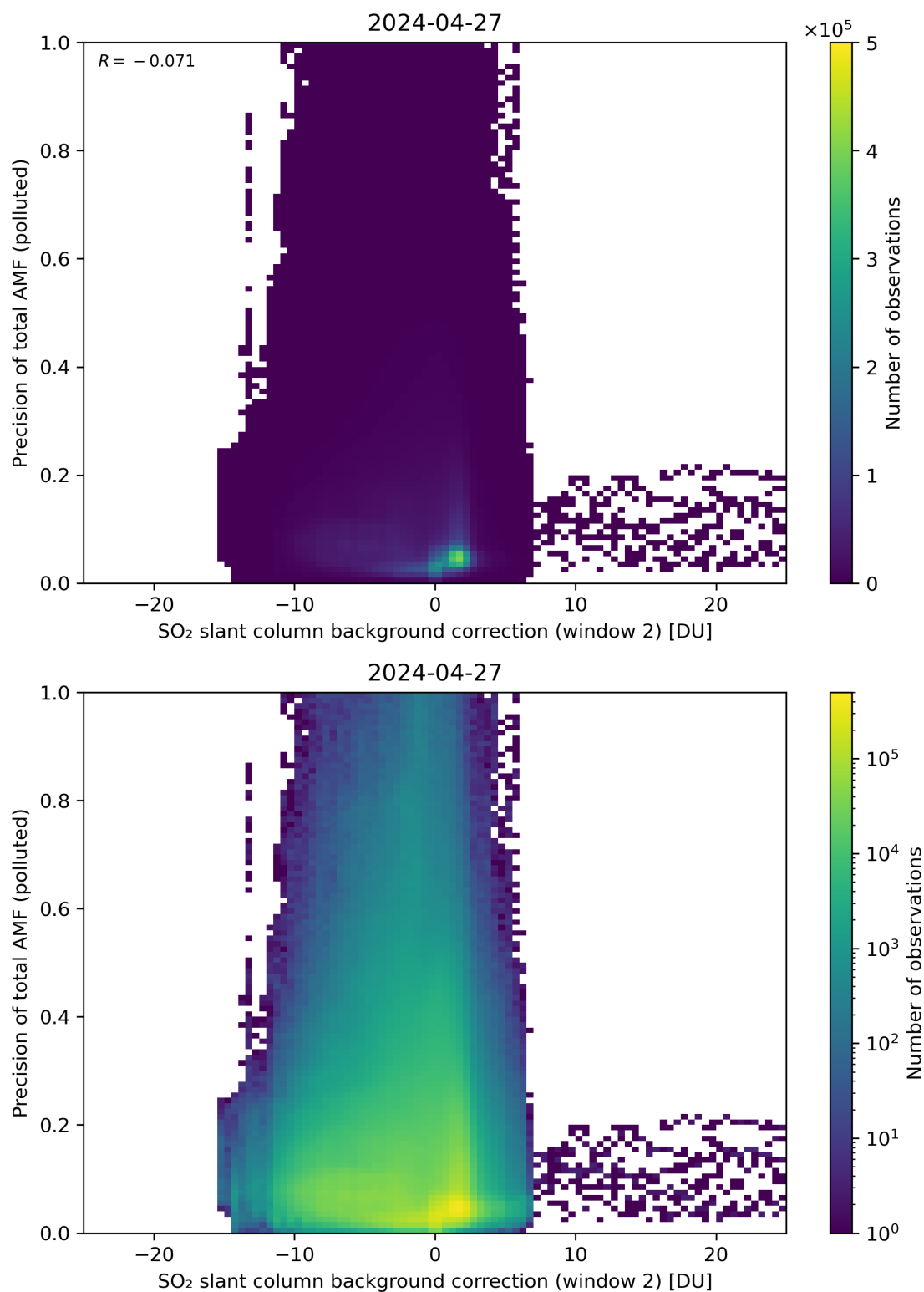
Figure 120: Scatter density plot of “SO 2 slant column background correction (window 2)” against “Precision of total AMF (polluted)” for 2024-04-26 to 2024-04-28.
