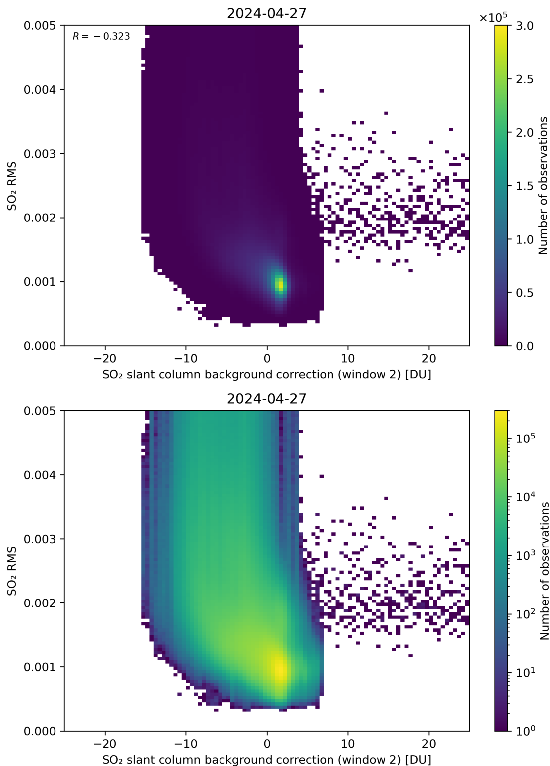
Figure 114: Scatter density plot of “SO 2 slant column background correction (window 2)” against “SO 2 RMS” for 2024-04-26 to 2024-04-28.
