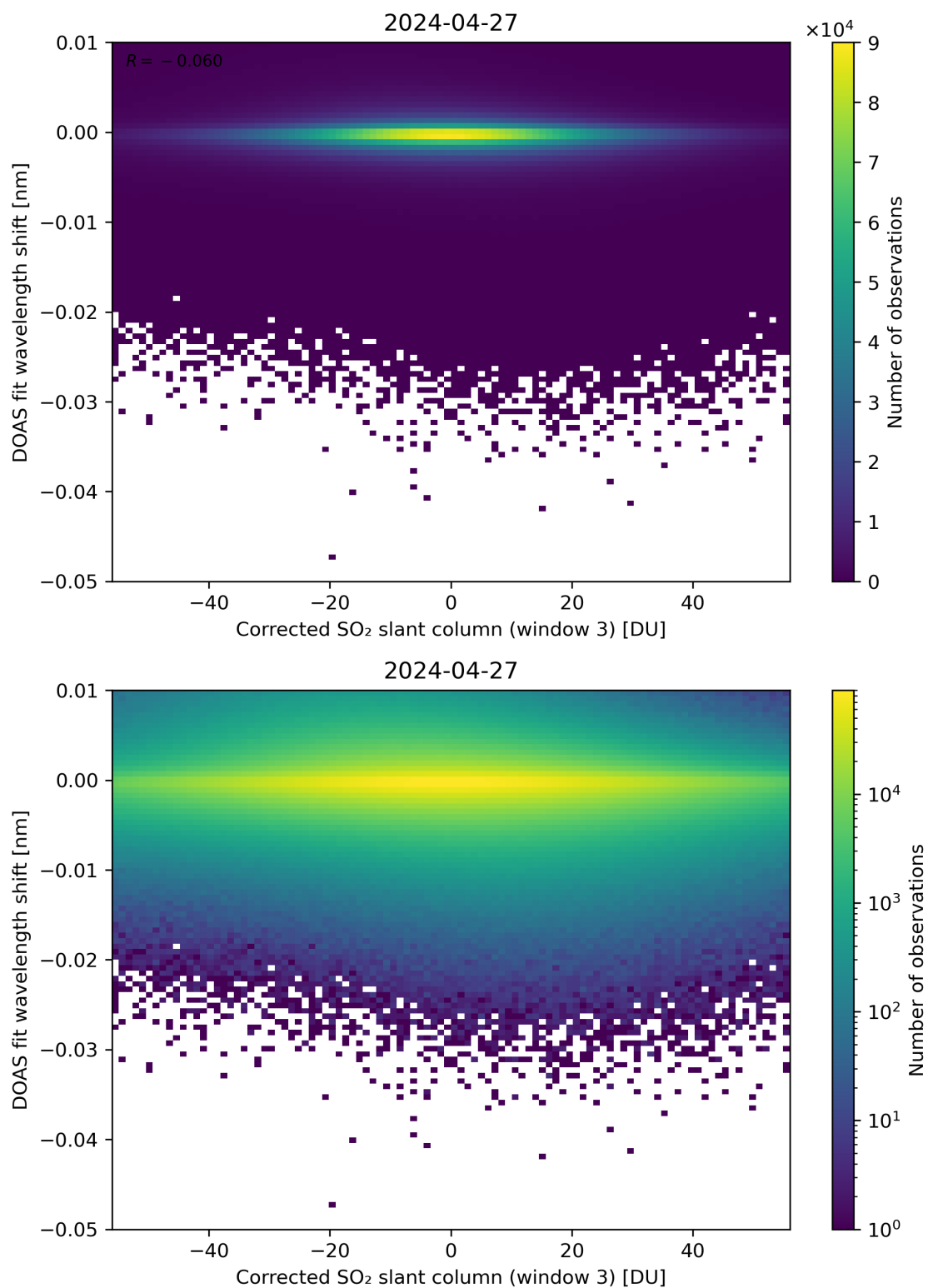
Figure 206: Scatter density plot of “Corrected SO 2 slant column (window 3)” against “DOAS fit wavelength shift” for 2024-04-26 to 2024-04-28.
