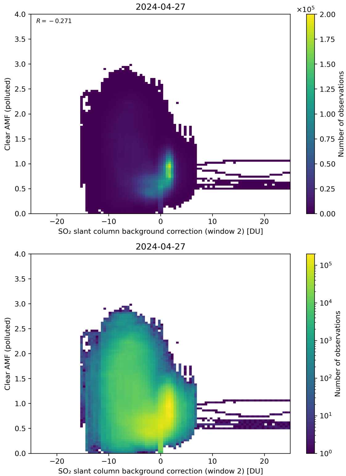
Figure 115: Scatter density plot of “SO 2 slant column background correction (window 2)” against “Clear AMF (polluted)” for 2024-04-26 to 2024-04-28.
