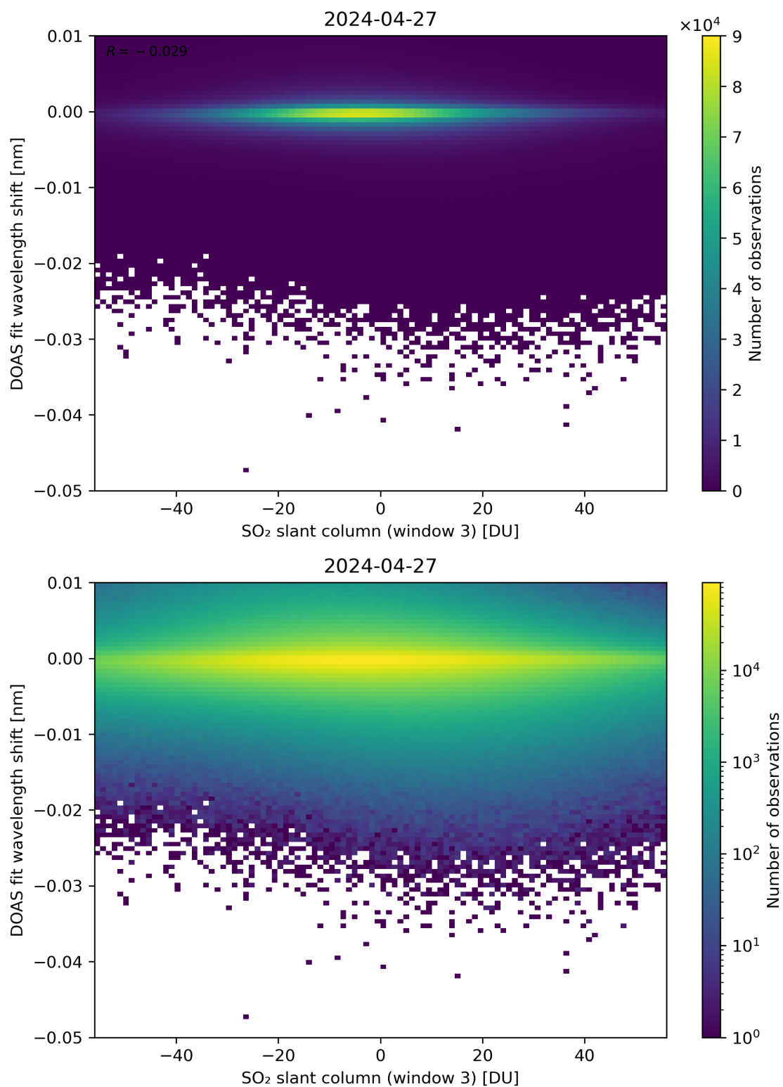
Figure 254: Scatter density plot of “SO 2 slant column (window 3)” against “DOAS fit wavelength shift” for 2024-04-26 to 2024-04-28.
