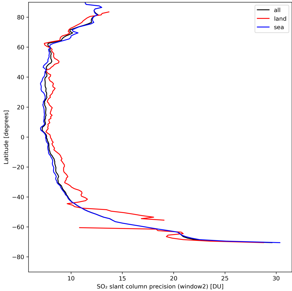
Figure 38: Zonal average of “SO 2 slant column precision (window2)” for 2024-04-26 to 2024-04-28.
