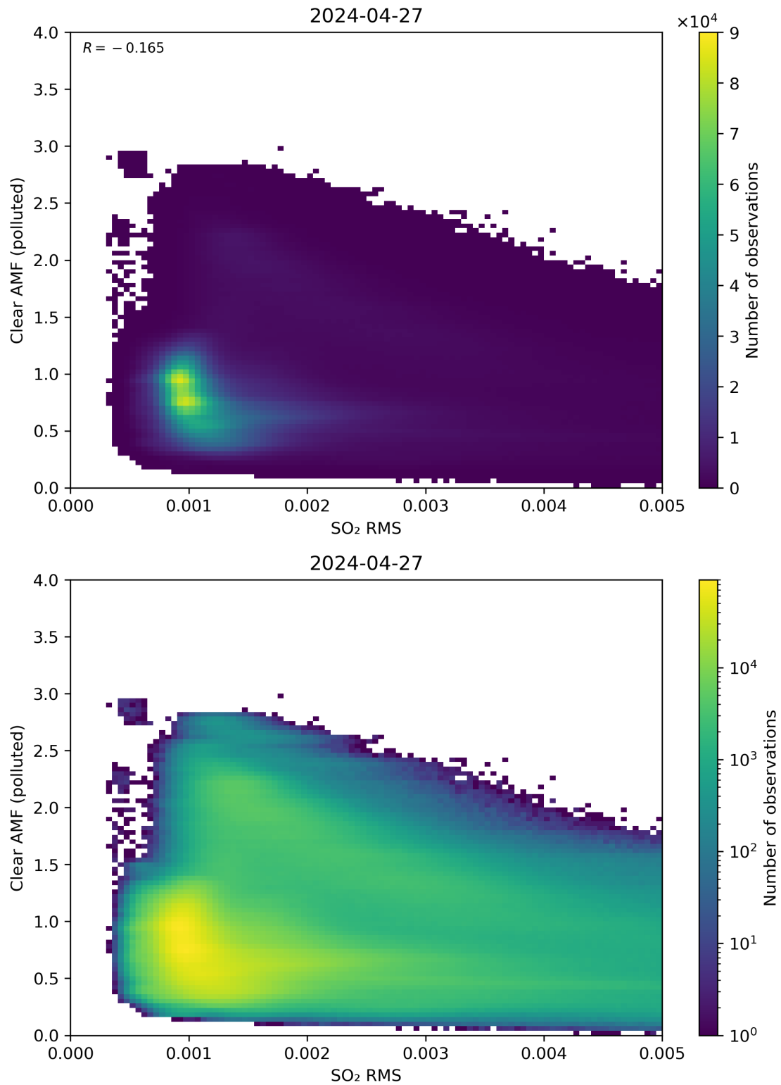
Figure 136: Scatter density plot of “SO 2 RMS” against “Clear AMF (polluted)” for 2024-04-26 to 2024-04-28.
