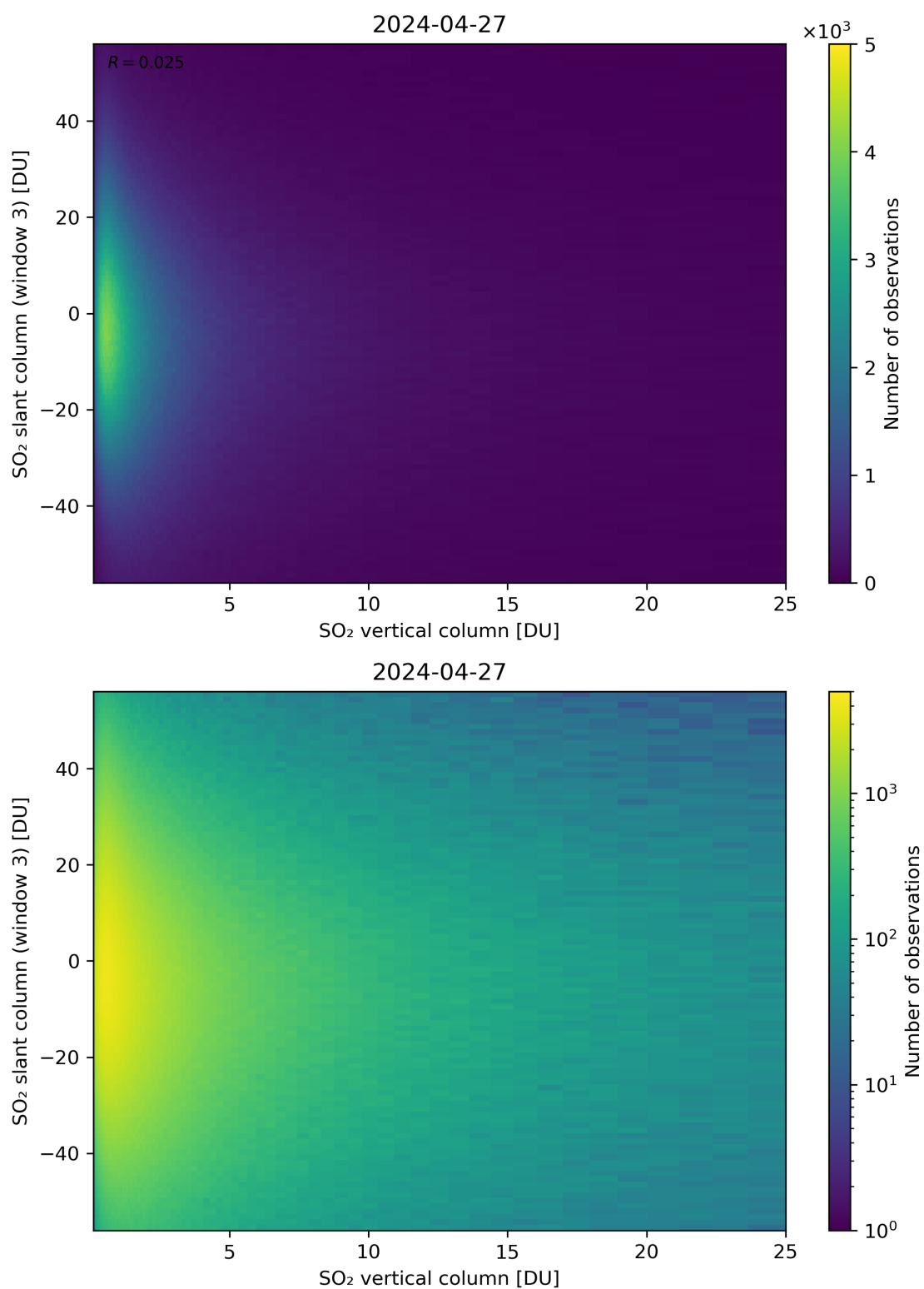
Figure 303: Scatter density plot of “SO 2 vertical column” against “SO 2 slant column (window 3)” for 2024-04-26 to 2024-04-28.
