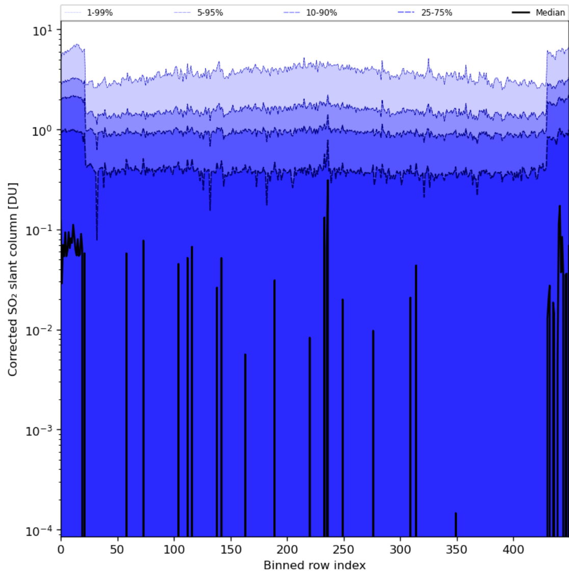
Figure 78: Along track statistics of “Corrected SO 2 slant column” for 2024-04-26 to 2024-04-28
