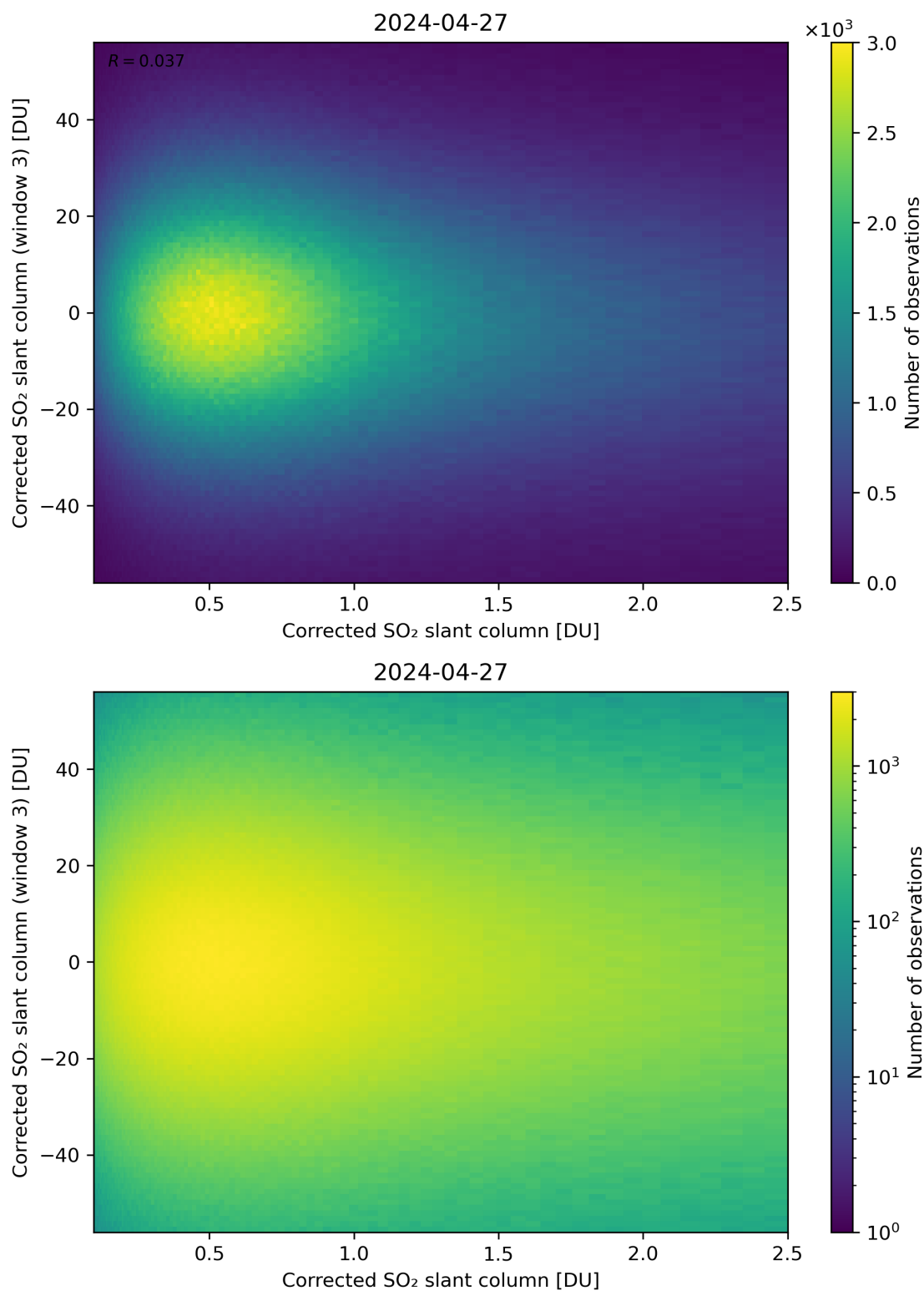
Figure 186: Scatter density plot of “Corrected SO 2 slant column” against “Corrected SO 2 slant column (window 3)” for 2024-04-26 to 2024-04-28.
