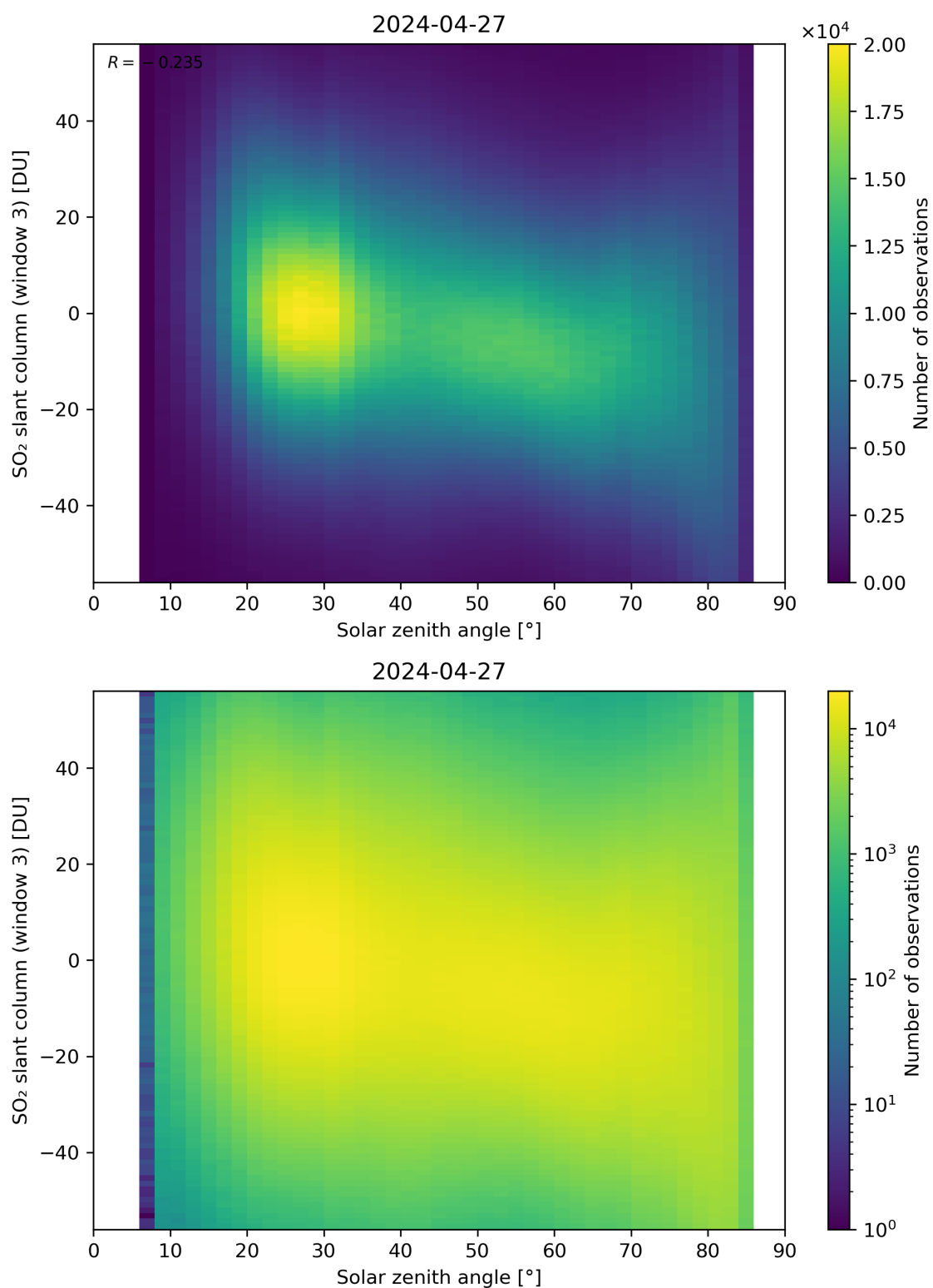
Figure 172: Scatter density plot of “Solar zenith angle” against “SO 2 slant column (window 3)” for 2024-04-26 to 2024-04-28.
