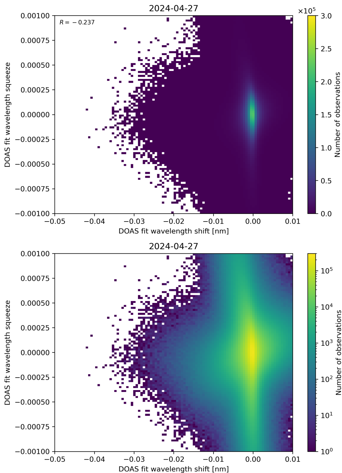
Figure 127: Scatter density plot of “DOAS fit wavelength shift” against “DOAS fit wavelength squeeze” for 2024-04-26 to 2024-04-28.
