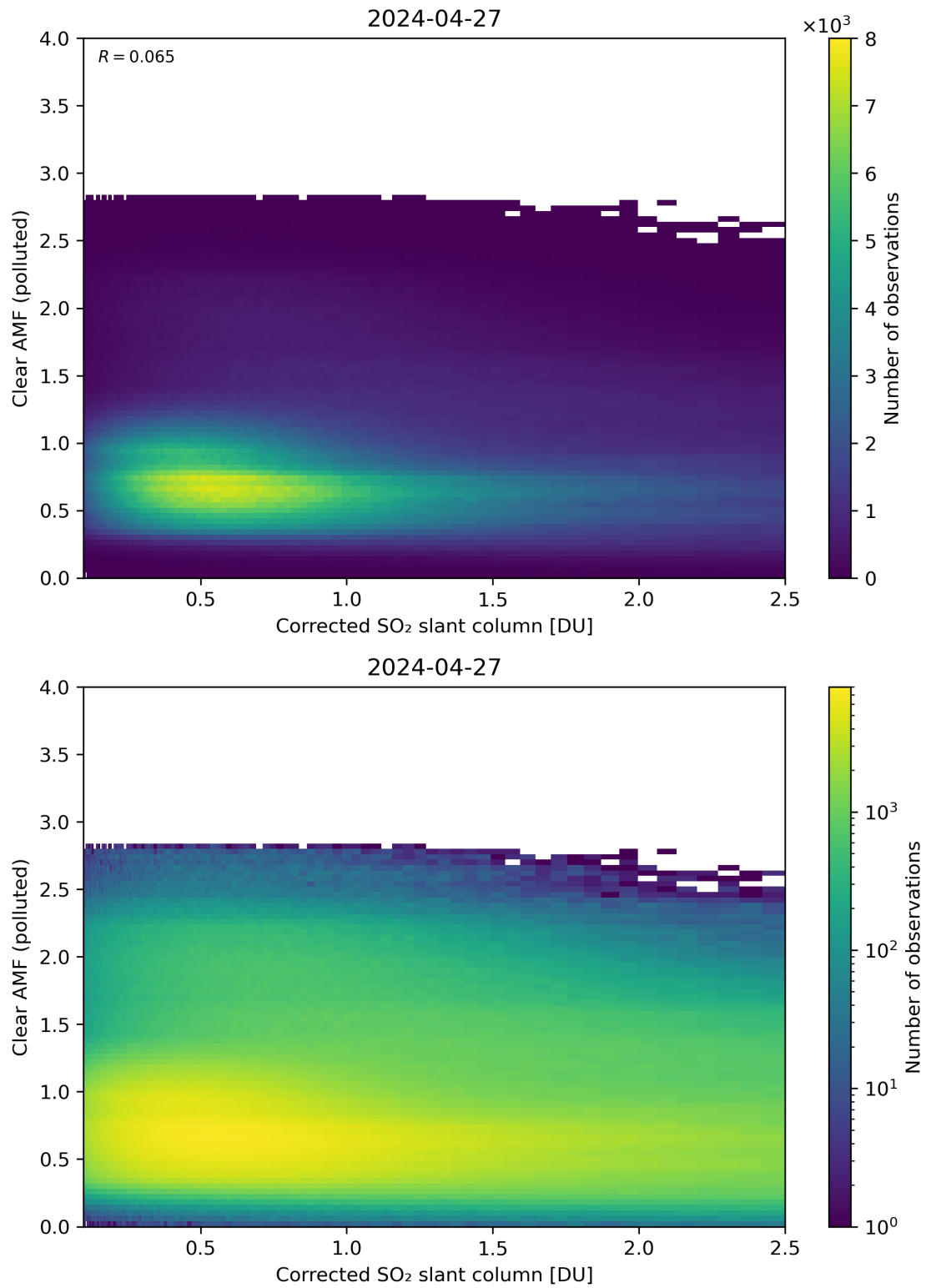
Figure 184: Scatter density plot of “Corrected SO 2 slant column” against “Clear AMF (polluted)” for 2024-04-26 to 2024-04-28.
