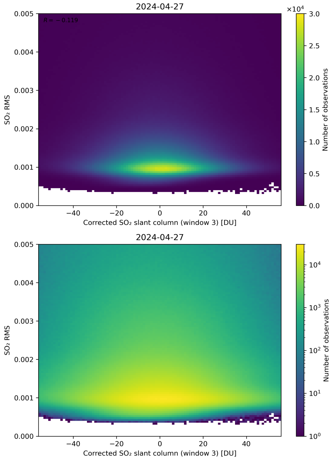
Figure 208: Scatter density plot of “Corrected SO 2 slant column (window 3)” against “SO 2 RMS” for 2024-04-26 to 2024-04-28.
