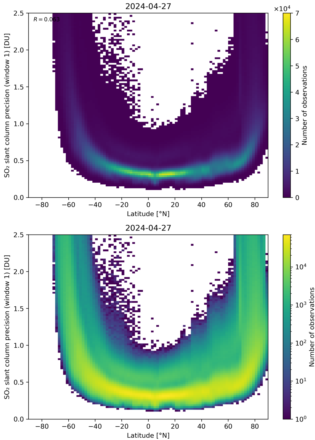
Figure 150: Scatter density plot of “Latitude” against “SO 2 slant column precision (window 1)” for 2024-04-26 to 2024-04-28.
