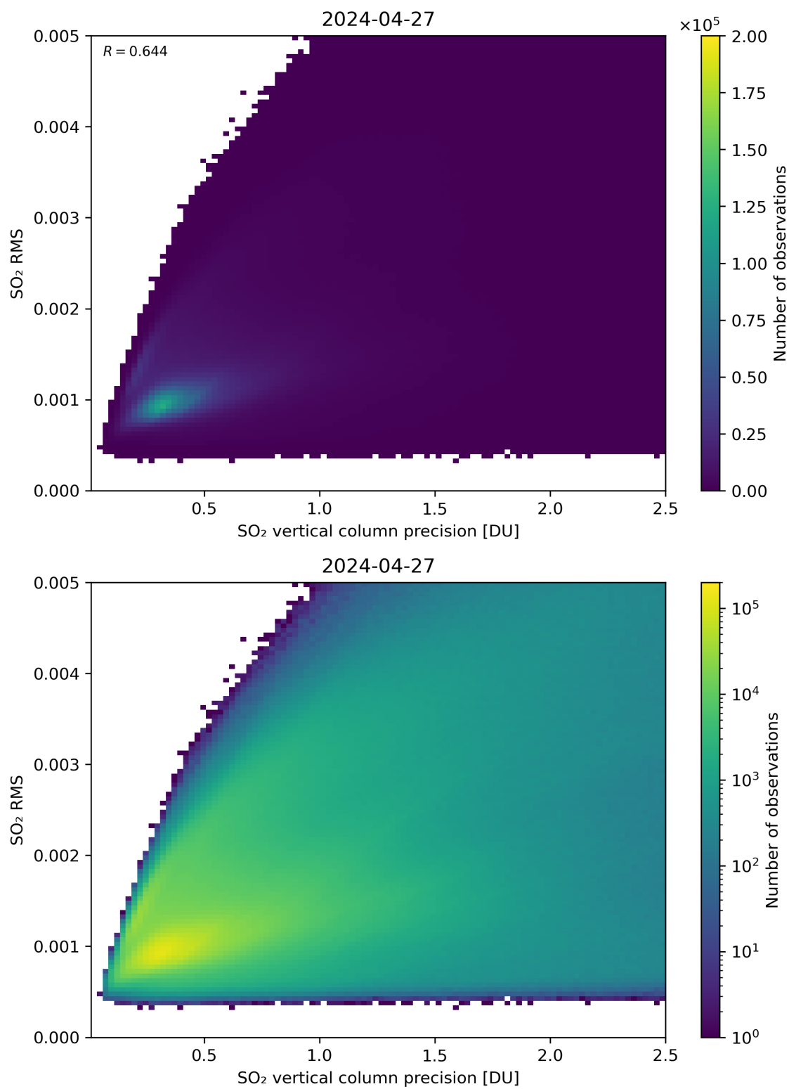
Figure 284: Scatter density plot of “SO 2 vertical column precision” against “SO 2 RMS” for 2024-04-26 to 2024-04-28.
