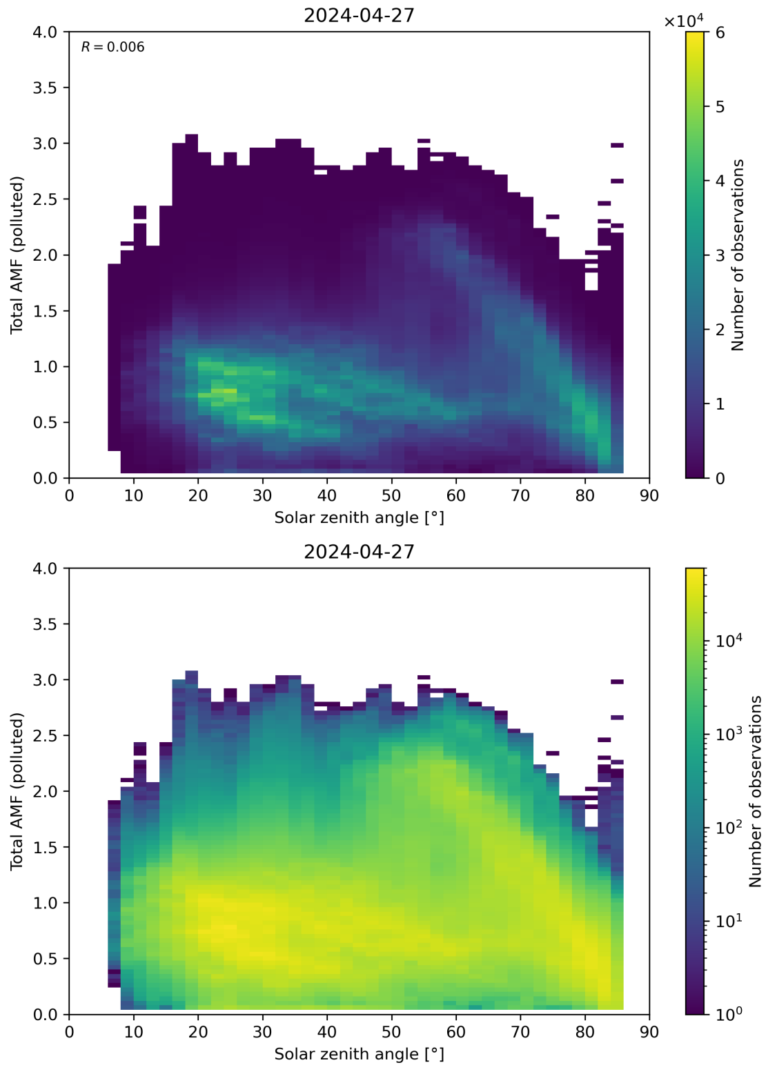
Figure 174: Scatter density plot of “Solar zenith angle” against “Total AMF (polluted)” for 2024-04-26 to 2024-04-28.
