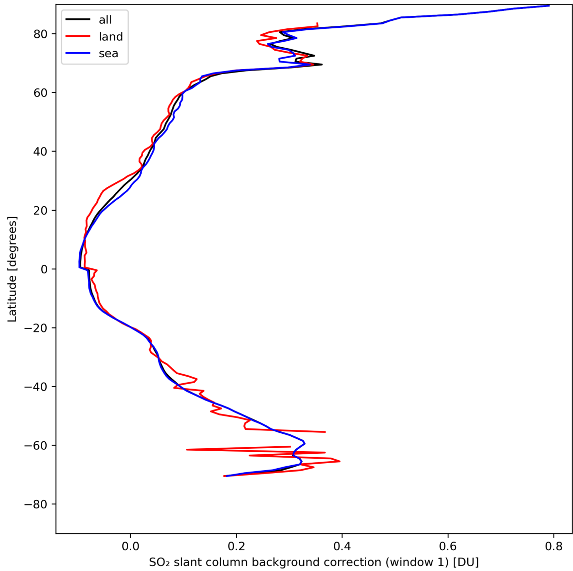
Figure 36: Zonal average of “SO 2 slant column background correction (window 1)” for 2024-04-26 to 2024-04-28.
