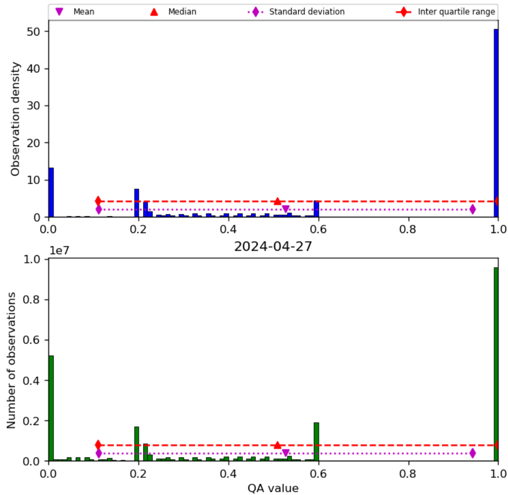
Figure 52: Histogram of “QA value” for 2024-04-26 to 2024-04-28
