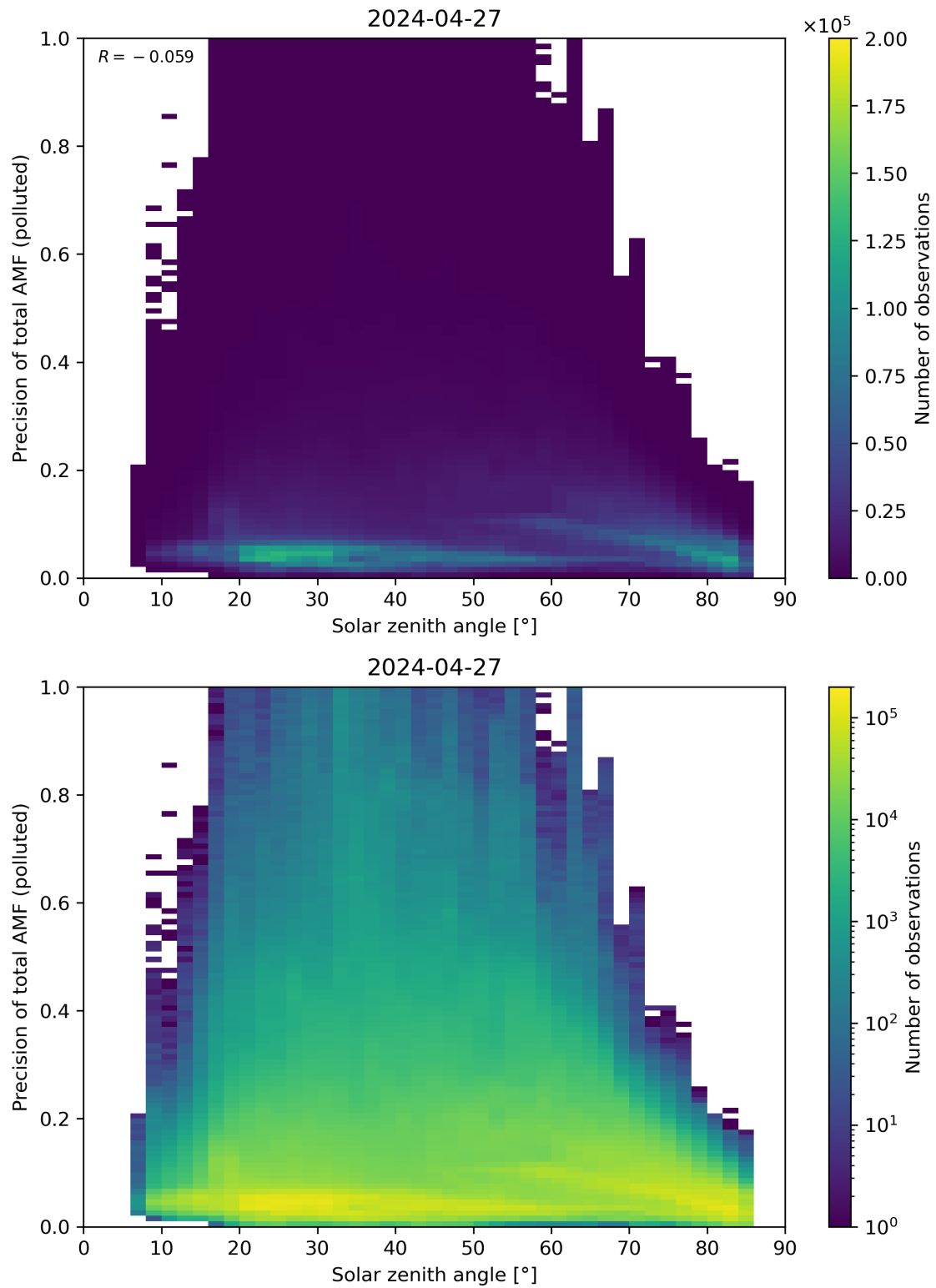
Figure 175: Scatter density plot of “Solar zenith angle” against “Precision of total AMF (polluted)” for 2024-04-26 to 2024-04-28.
