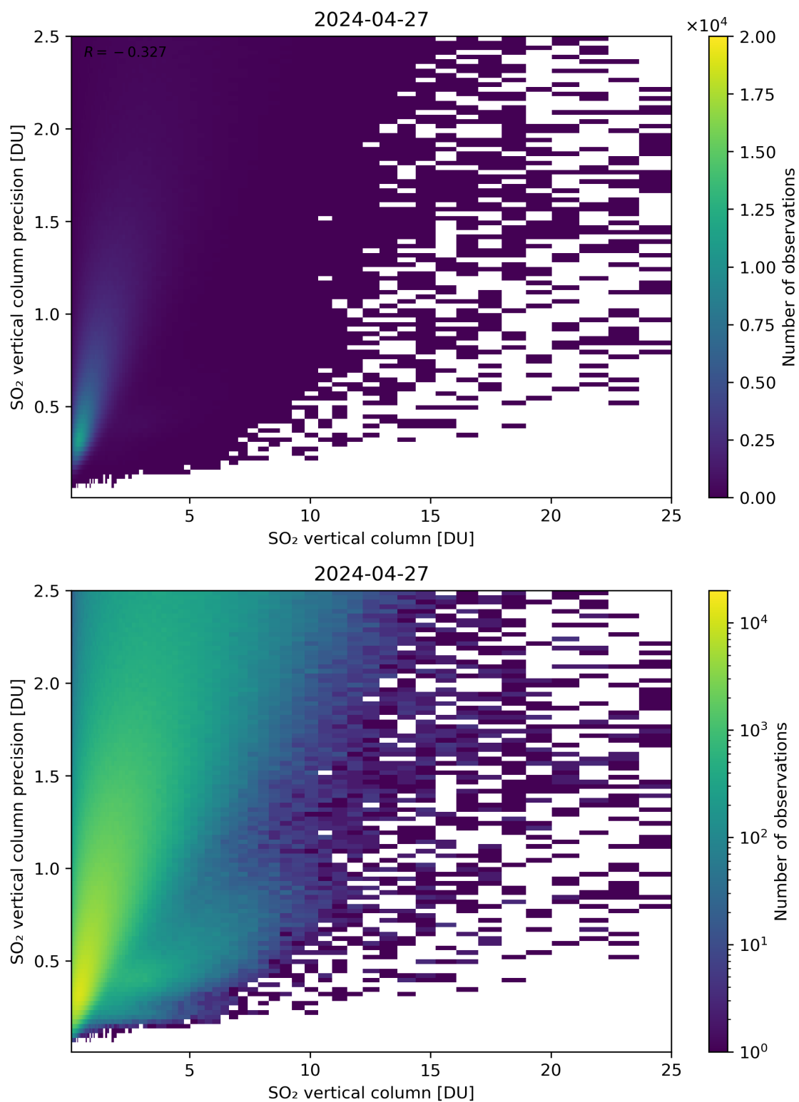
Figure 307: Scatter density plot of “SO 2 vertical column” against “SO 2 vertical column precision” for 2024-04-26 to 2024-04-28.
