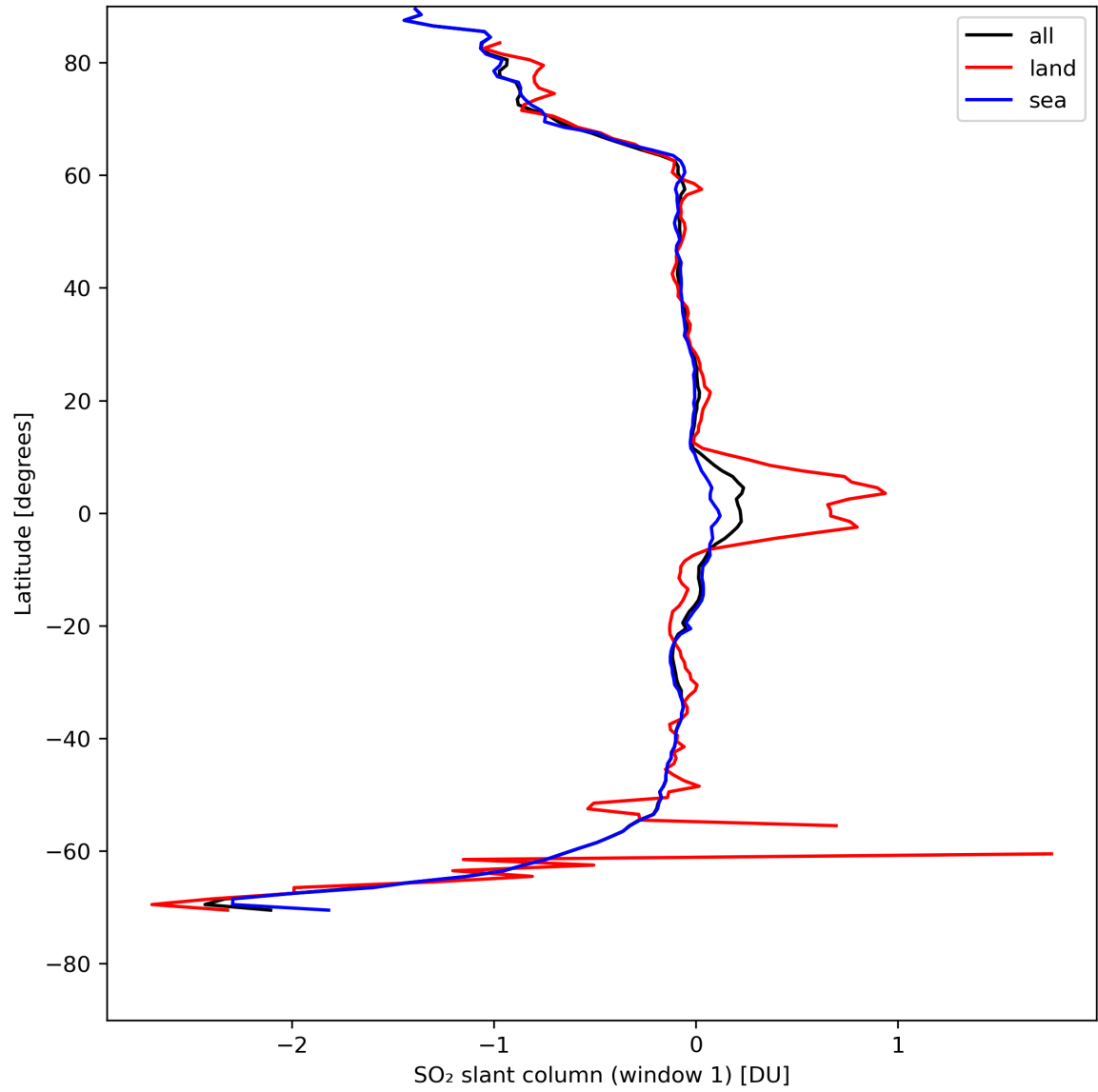
Figure 33: Zonal average of “SO 2 slant column (window 1)” for 2024-04-26 to 2024-04-28.
