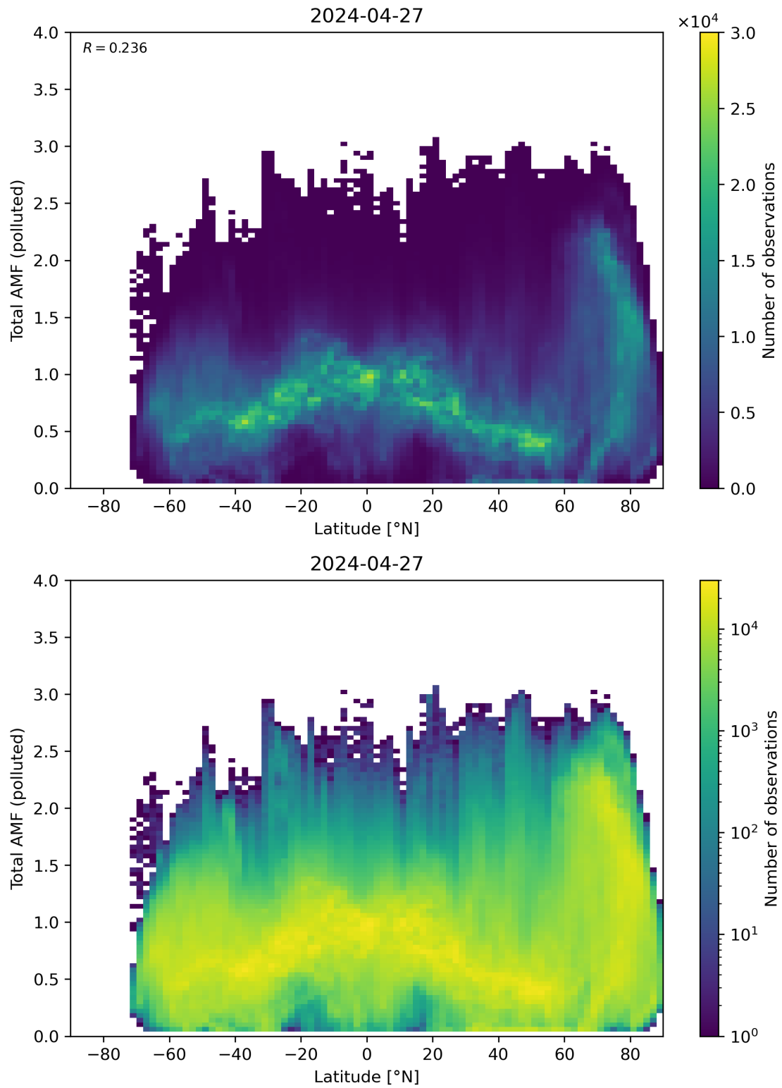
Figure 154: Scatter density plot of “Latitude” against “Total AMF (polluted)” for 2024-04-26 to 2024-04-28.
