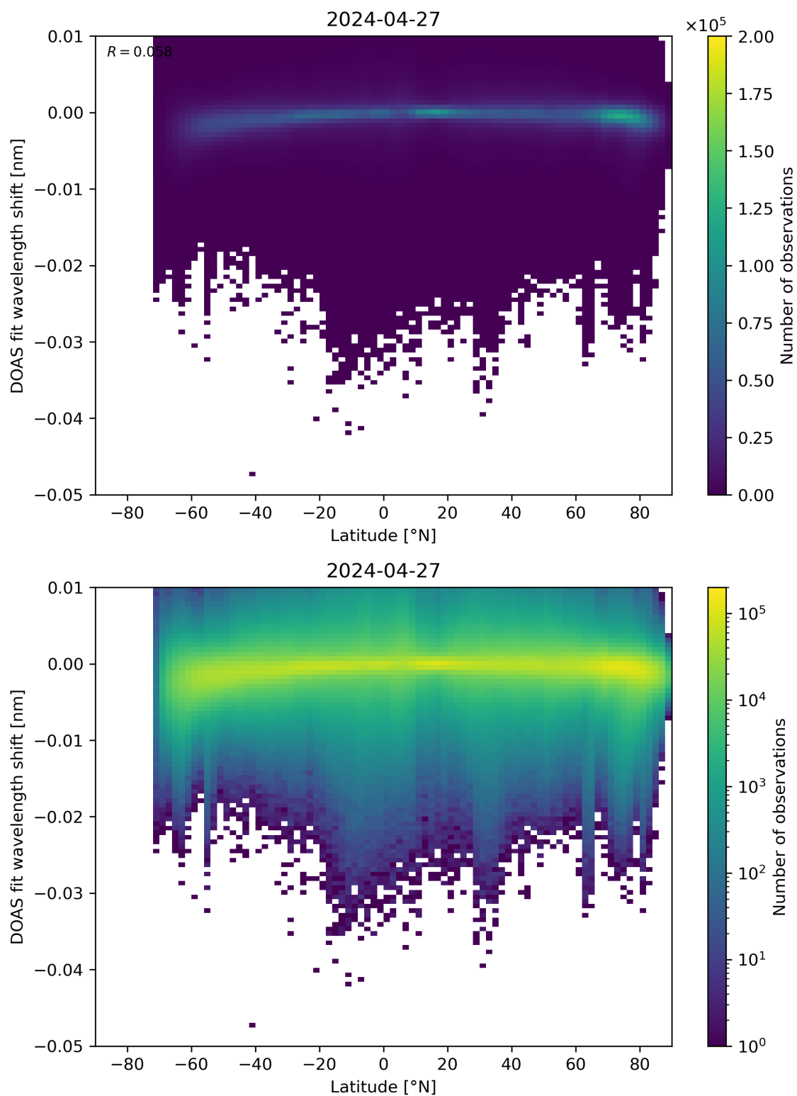
Figure 142: Scatter density plot of “Latitude” against “DOAS fit wavelength shift” for 2024-04-26 to 2024-04-28.
