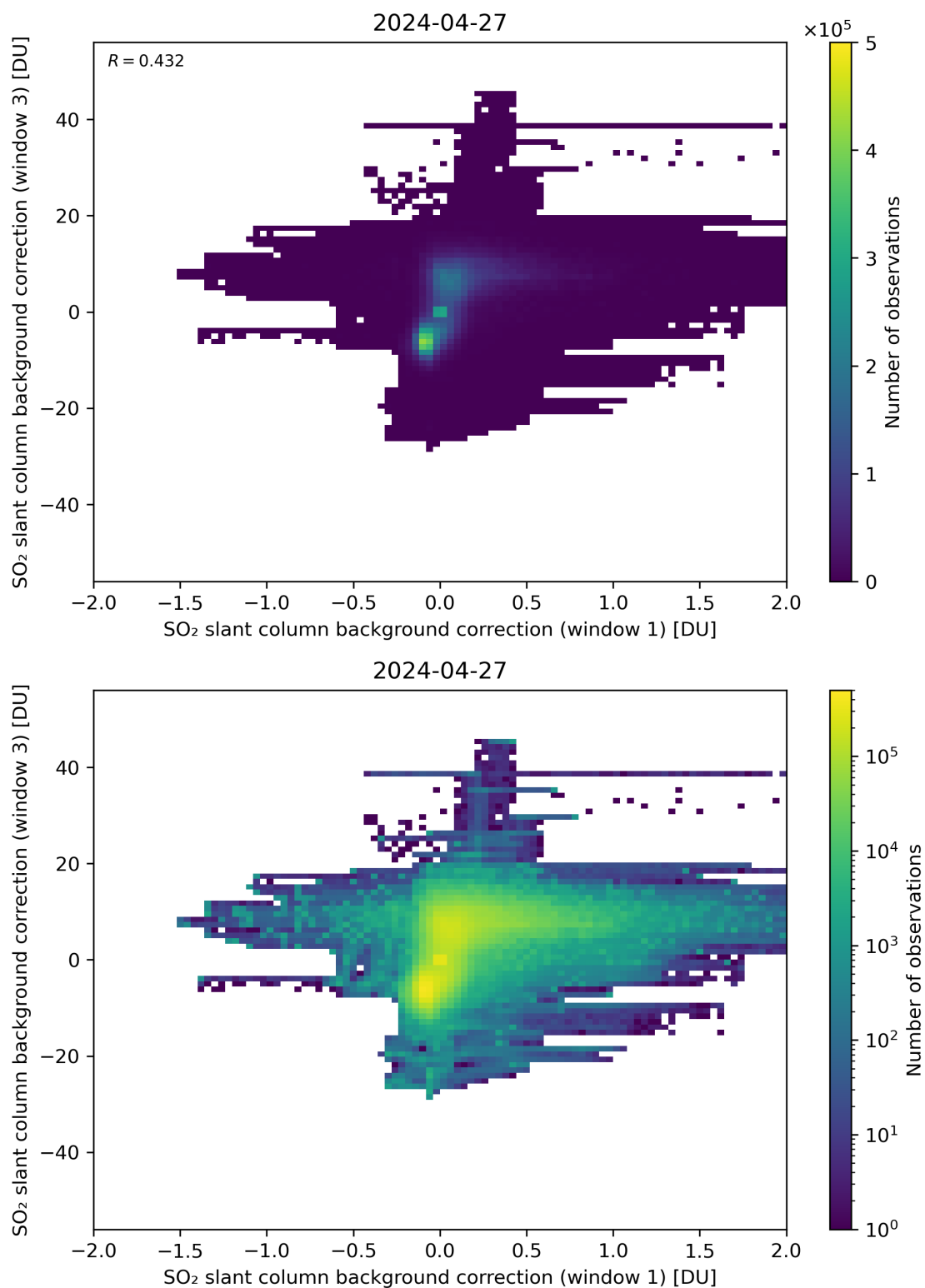
Figure 99: Scatter density plot of “SO 2 slant column background correction (window 1)” against “SO 2 slant column background correction (window 3)” for 2024-04-26 to 2024-04-28.
