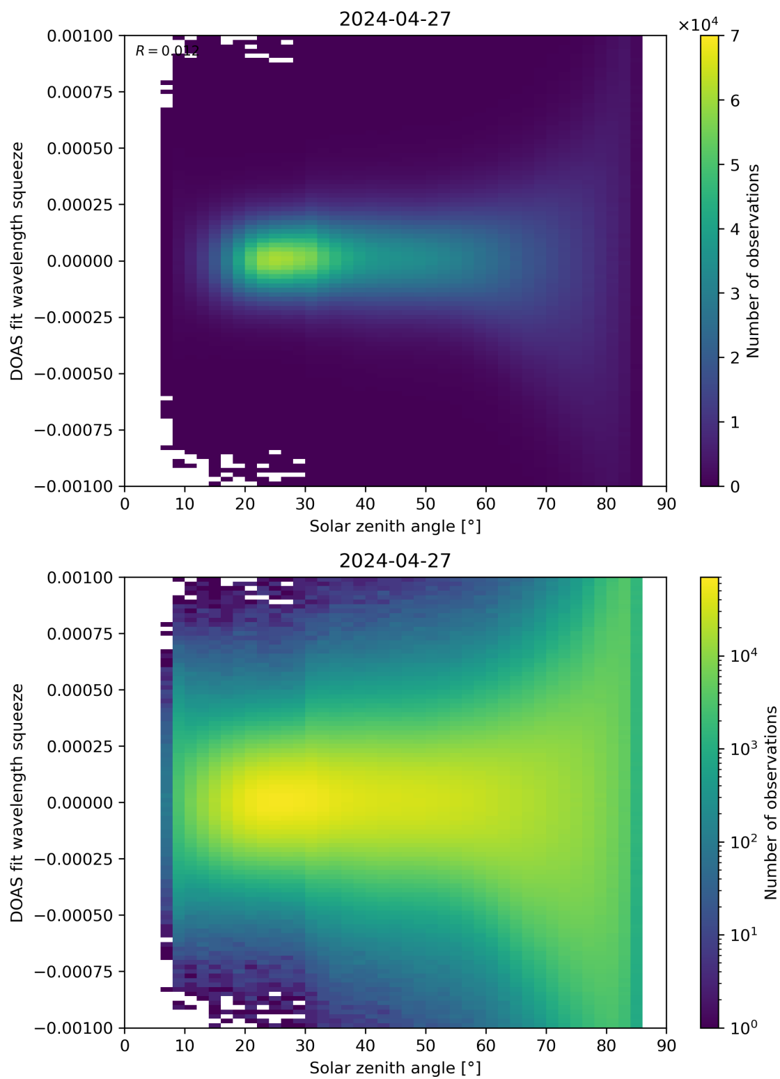
Figure 162: Scatter density plot of “Solar zenith angle” against “DOAS fit wavelength squeeze” for 2024-04-26 to 2024-04-28.
