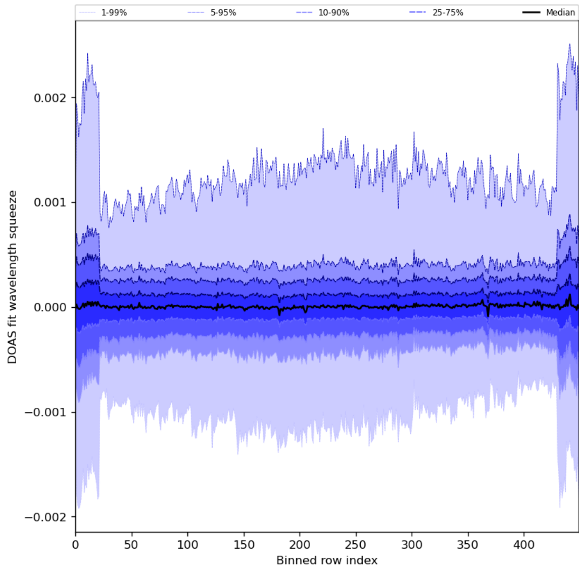
Figure 92: Along track statistics of “DOAS fit wavelength squeeze” for 2024-04-26 to 2024-04-28
