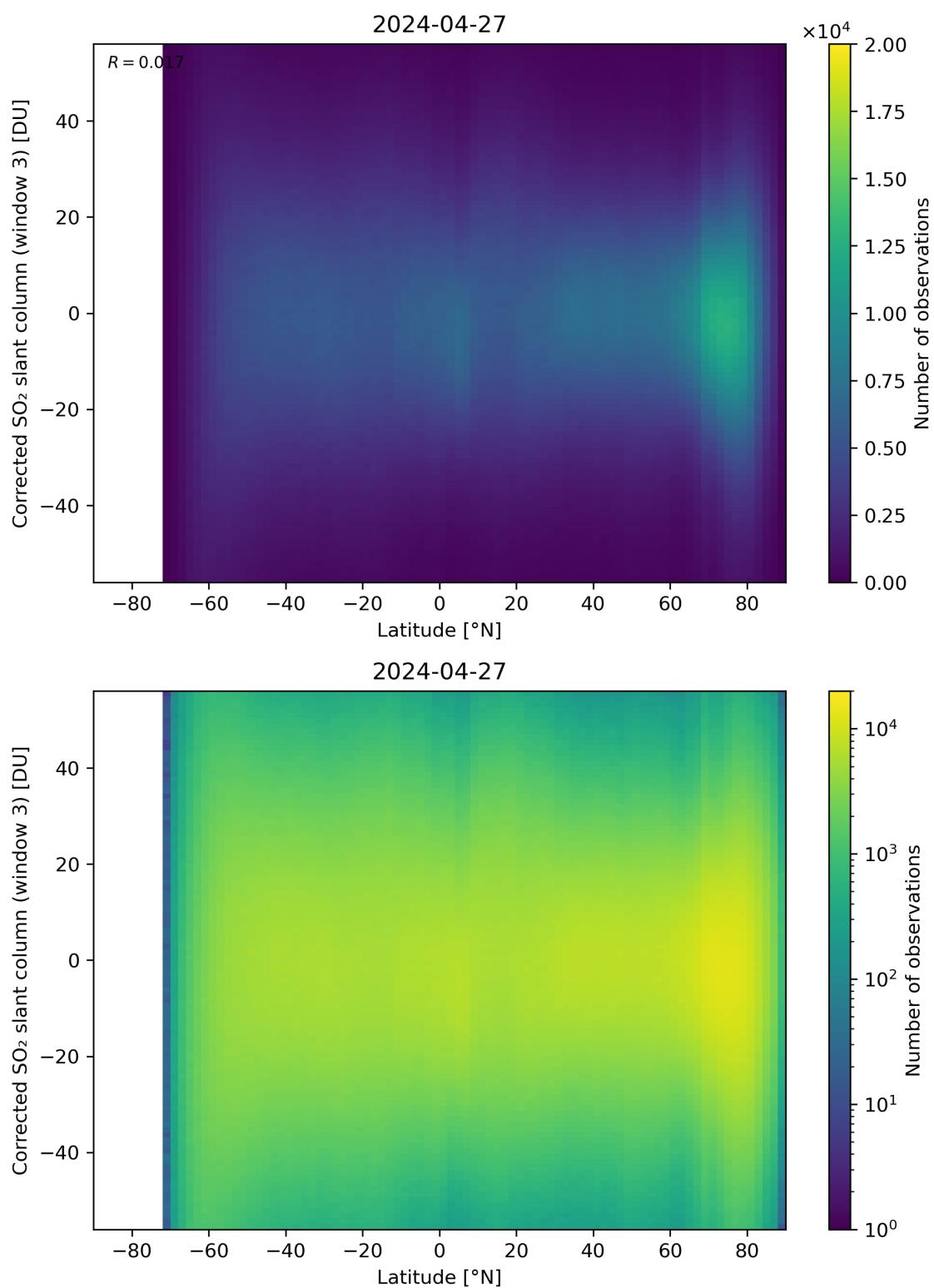
Figure 148: Scatter density plot of “Latitude” against “Corrected SO 2 slant column (window 3)” for 2024-04-26 to 2024-04-28.
