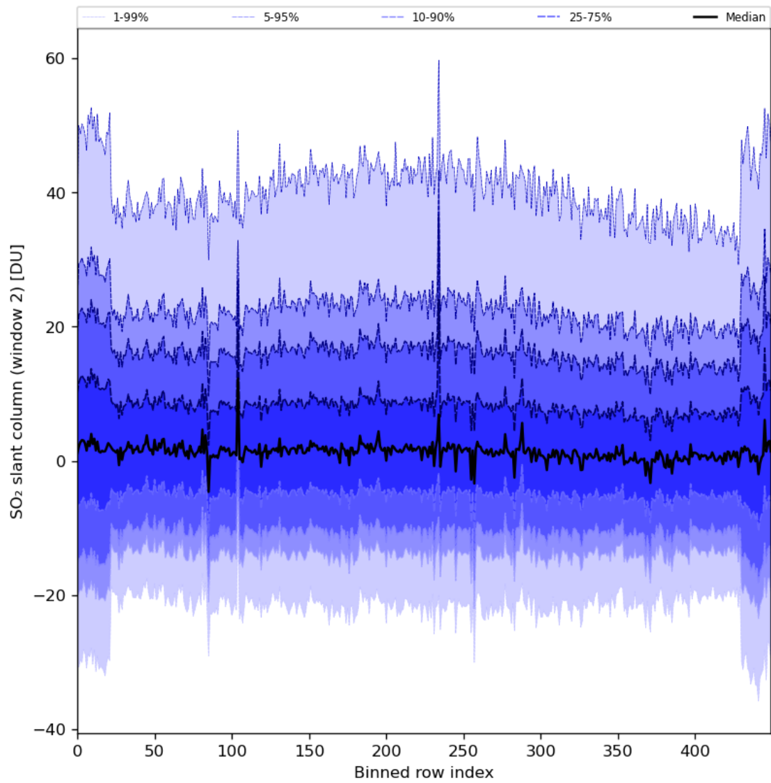
Figure 83: Along track statistics of “SO 2 slant column (window 2)” for 2024-04-26 to 2024-04-28
