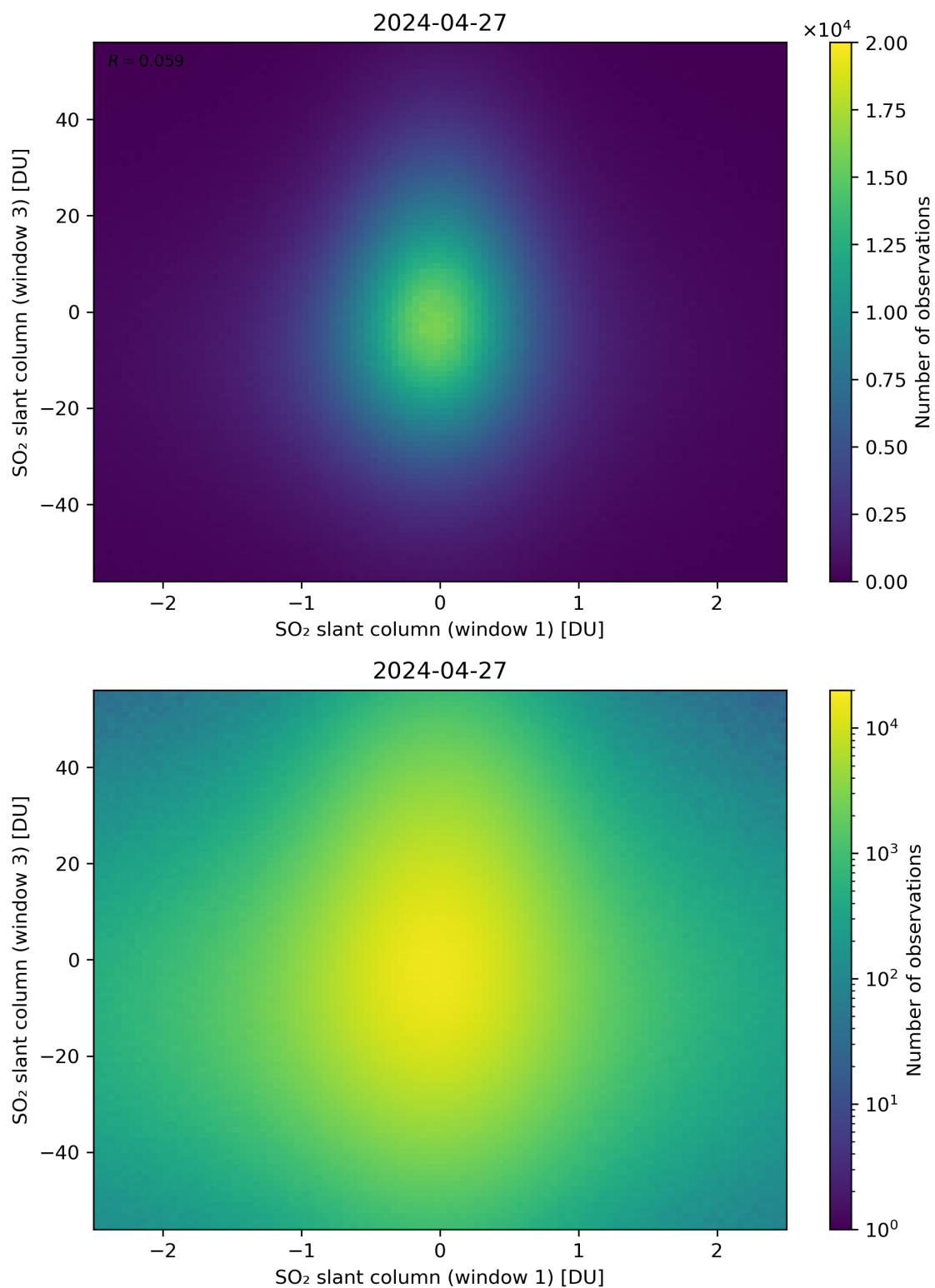
Figure 237: Scatter density plot of “SO 2 slant column (window 1)” against “SO 2 slant column (window 3)” for 2024-04-26 to 2024-04-28.
