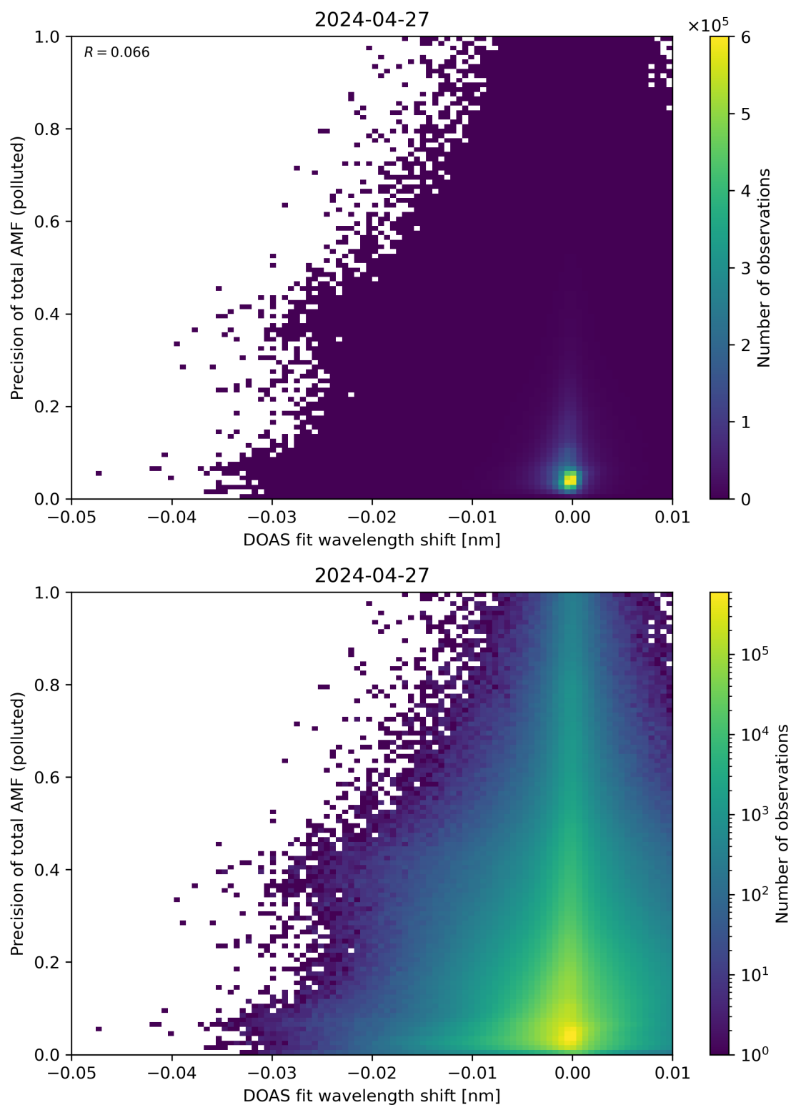
Figure 131: Scatter density plot of “DOAS fit wavelength shift” against “Precision of total AMF (polluted)” for 2024-04-26 to 2024-04-28.
