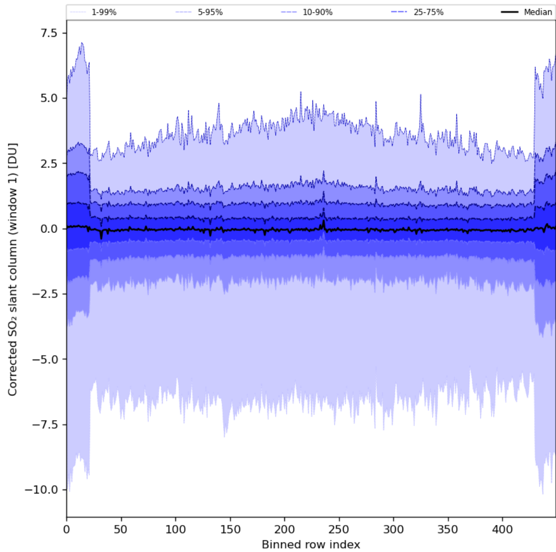
Figure 81: Along track statistics of “Corrected SO 2 slant column (window 1)” for 2024-04-26 to 2024-04-28
