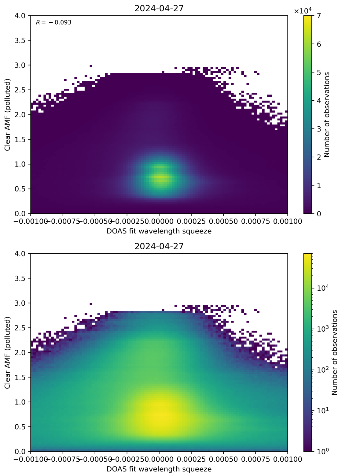
Figure 133: Scatter density plot of “DOAS fit wavelength squeeze” against “Clear AMF (polluted)” for 2024-04-26 to 2024-04-28.
