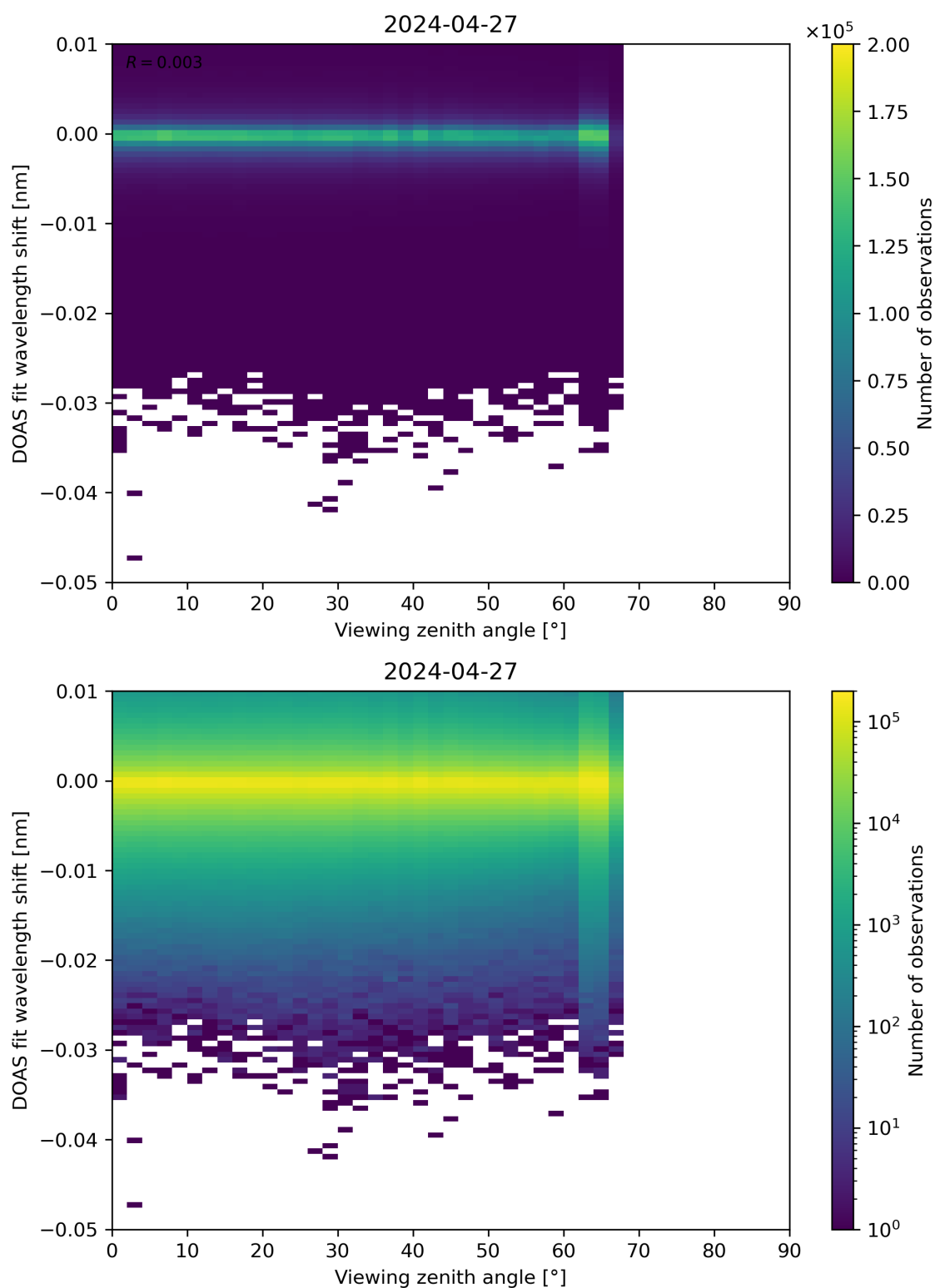
Figure 311: Scatter density plot of “Viewing zenith angle” against “DOAS fit wavelength shift” for 2024-04-26 to 2024-04-28.
