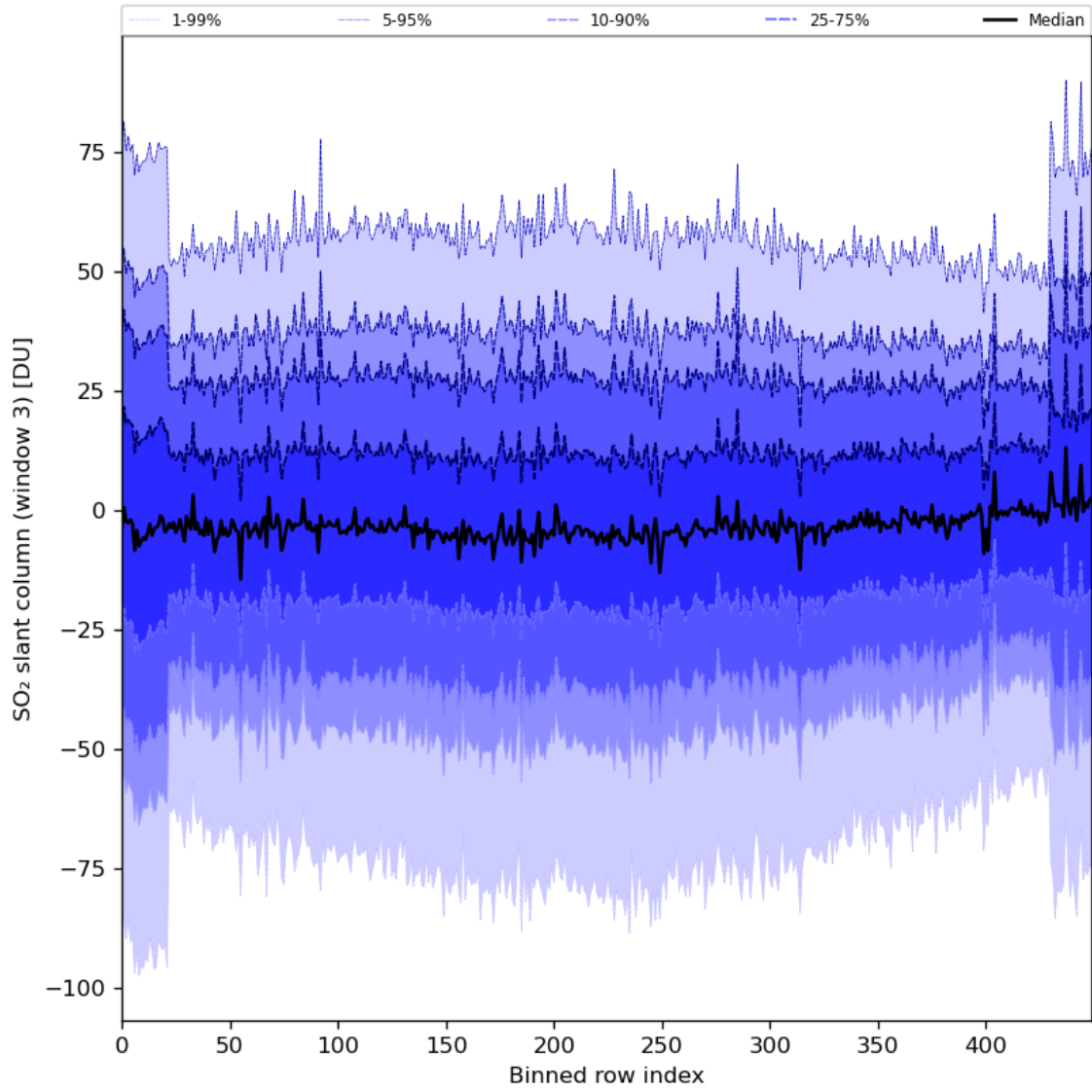
Figure 87: Along track statistics of “SO 2 slant column (window 3)” for 2024-04-26 to 2024-04-28
