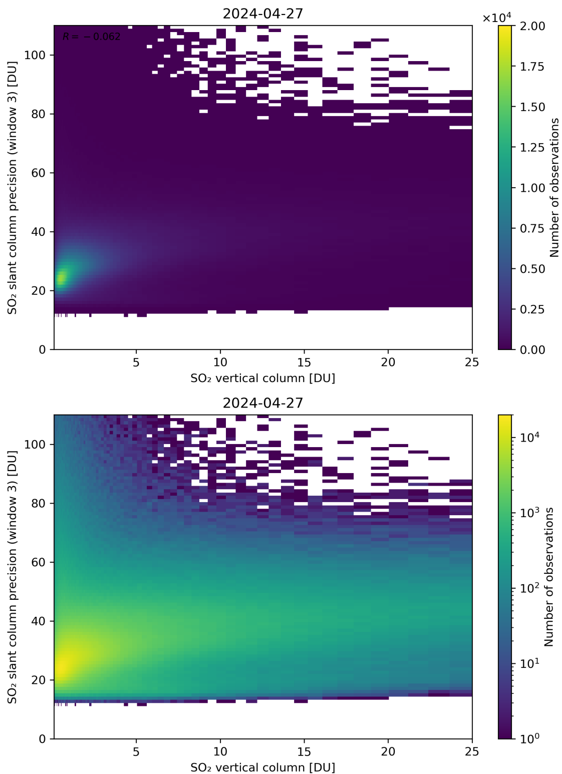
Figure 304: Scatter density plot of “SO 2 vertical column” against “SO 2 slant column precision (window 3)” for 2024-04-26 to 2024-04-28.
