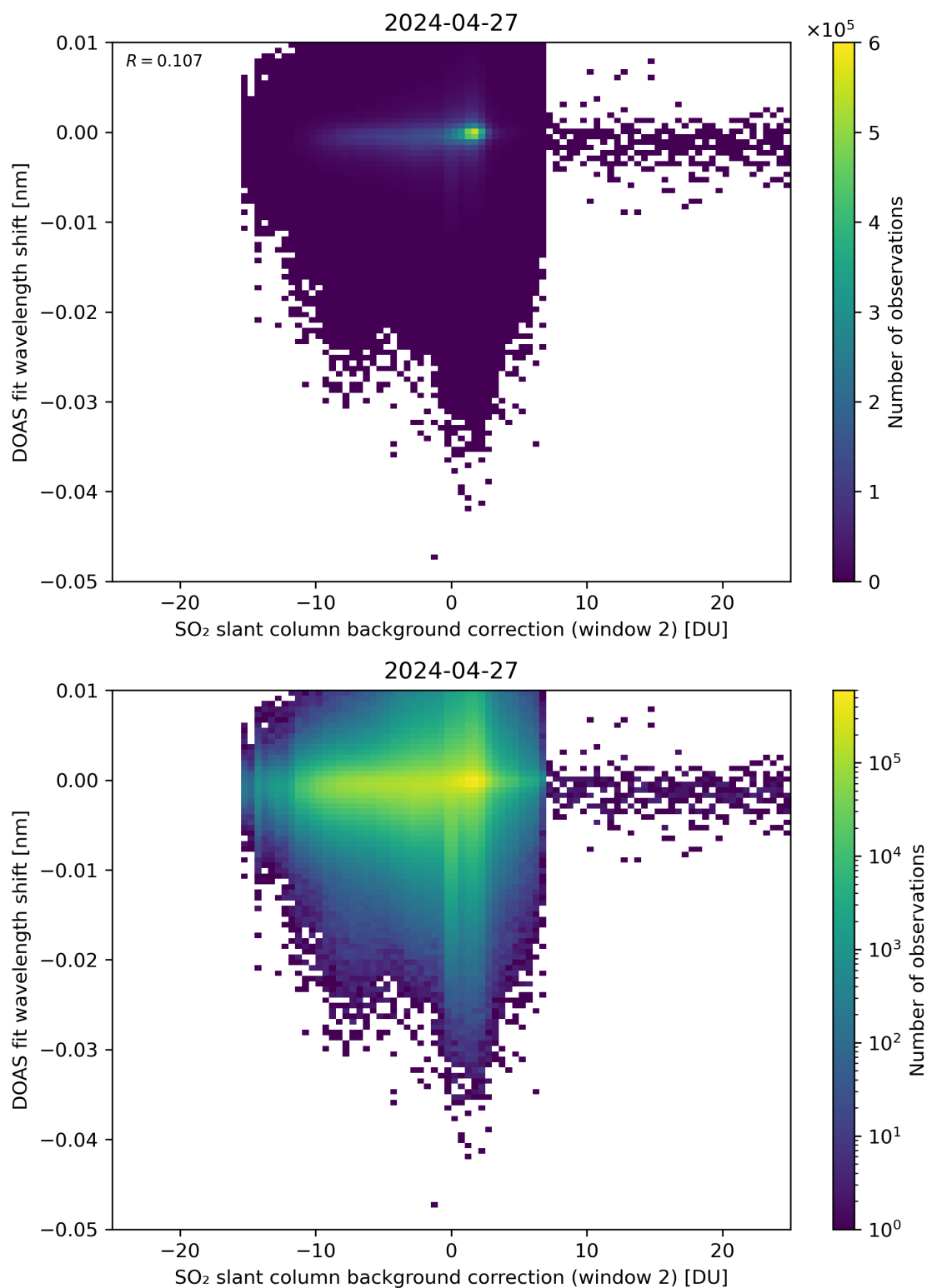
Figure 112: Scatter density plot of “SO 2 slant column background correction (window 2)” against “DOAS fit wavelength shift” for 2024-04-26 to 2024-04-28.
