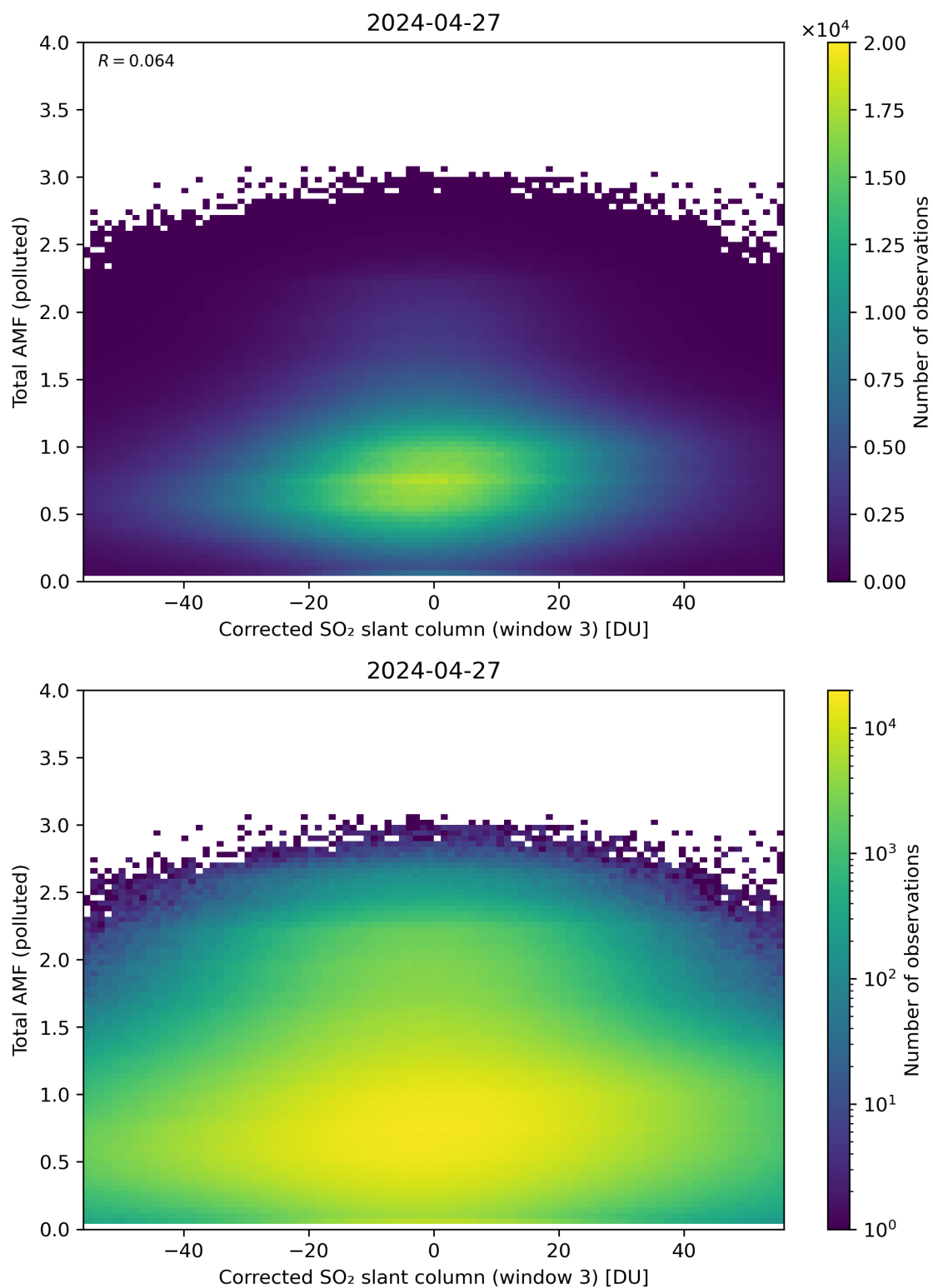
Figure 210: Scatter density plot of “Corrected SO 2 slant column (window 3)” against “Total AMF (polluted)” for 2024-04-26 to 2024-04-28.
