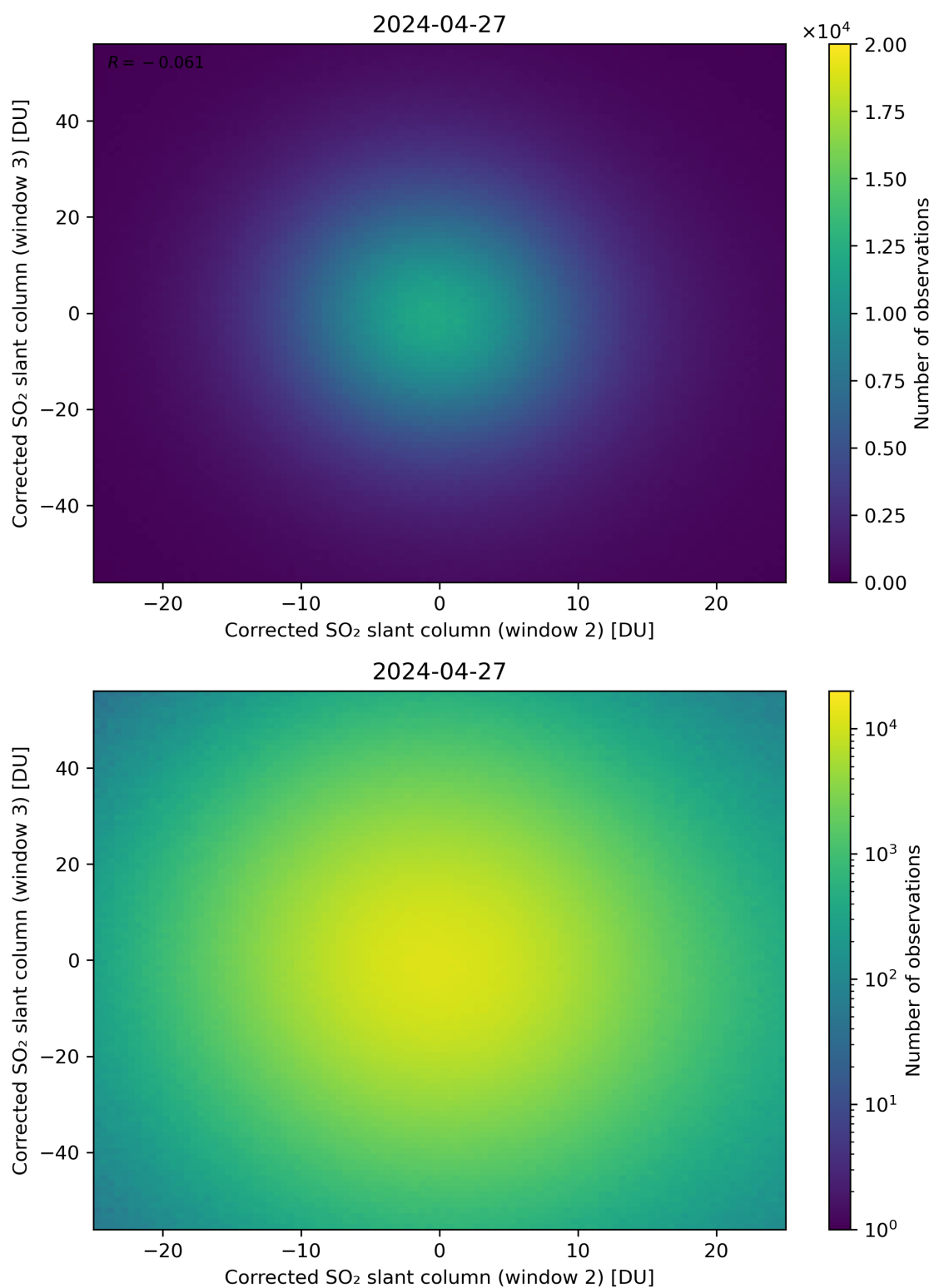
Figure 200: Scatter density plot of “Corrected SO 2 slant column (window 2)” against “Corrected SO 2 slant column (window 3)” for 2024-04-26 to 2024-04-28.
