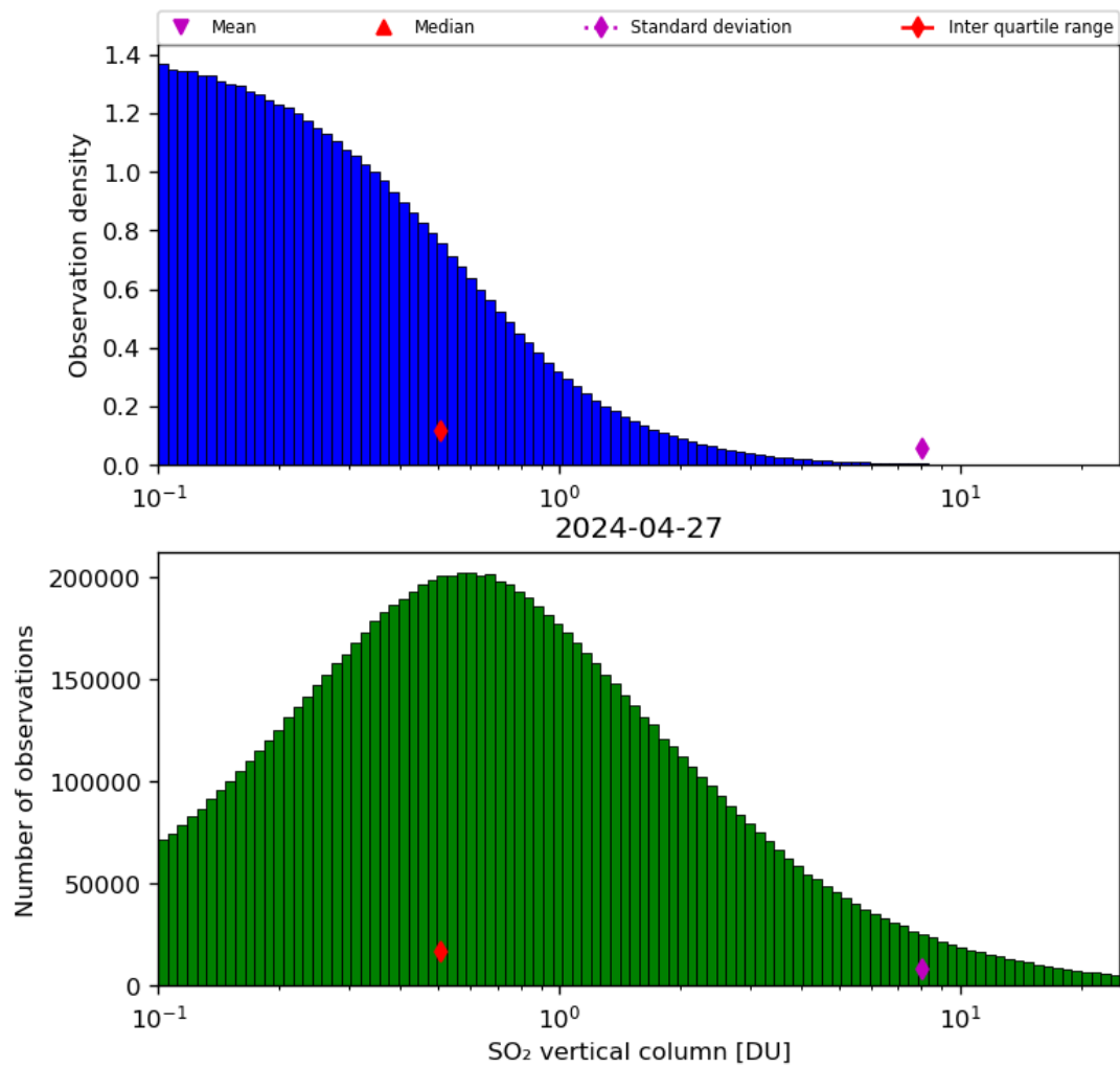
Figure 53: Histogram of “SO 2 vertical column” for 2024-04-26 to 2024-04-28
