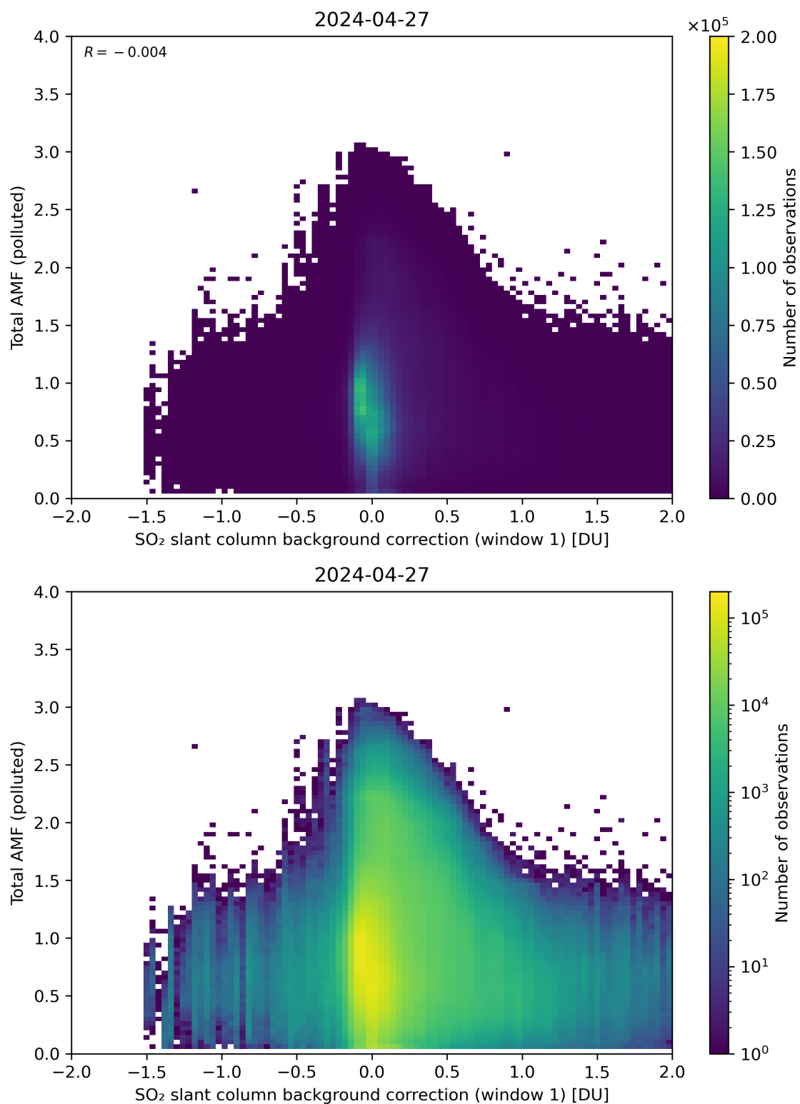
Figure 109: Scatter density plot of “SO 2 slant column background correction (window 1)” against “Total AMF (polluted)” for 2024-04-26 to 2024-04-28.
