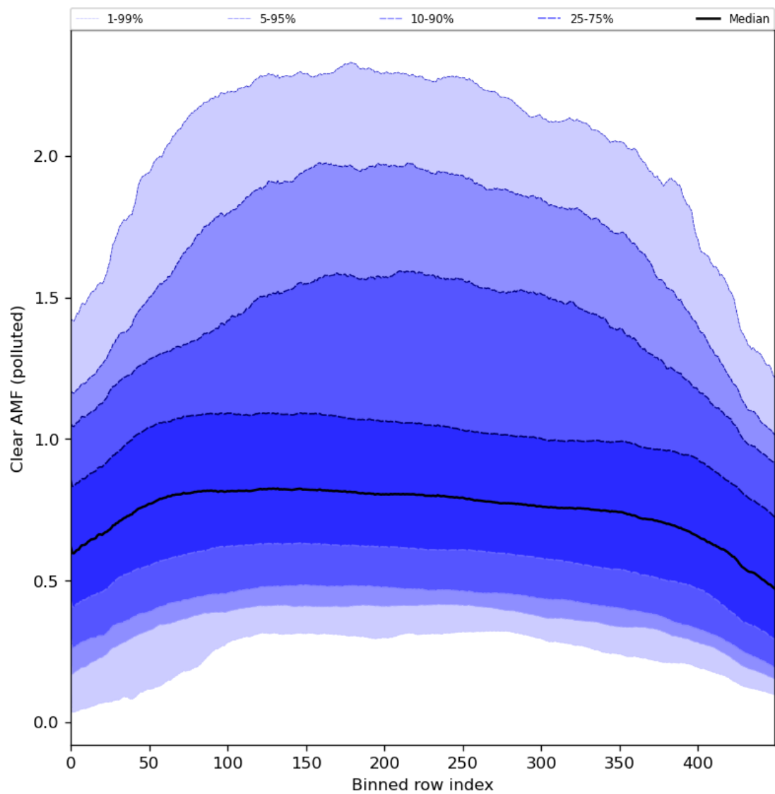
Figure 96: Along track statistics of “Clear AMF (polluted)” for 2024-04-26 to 2024-04-28
