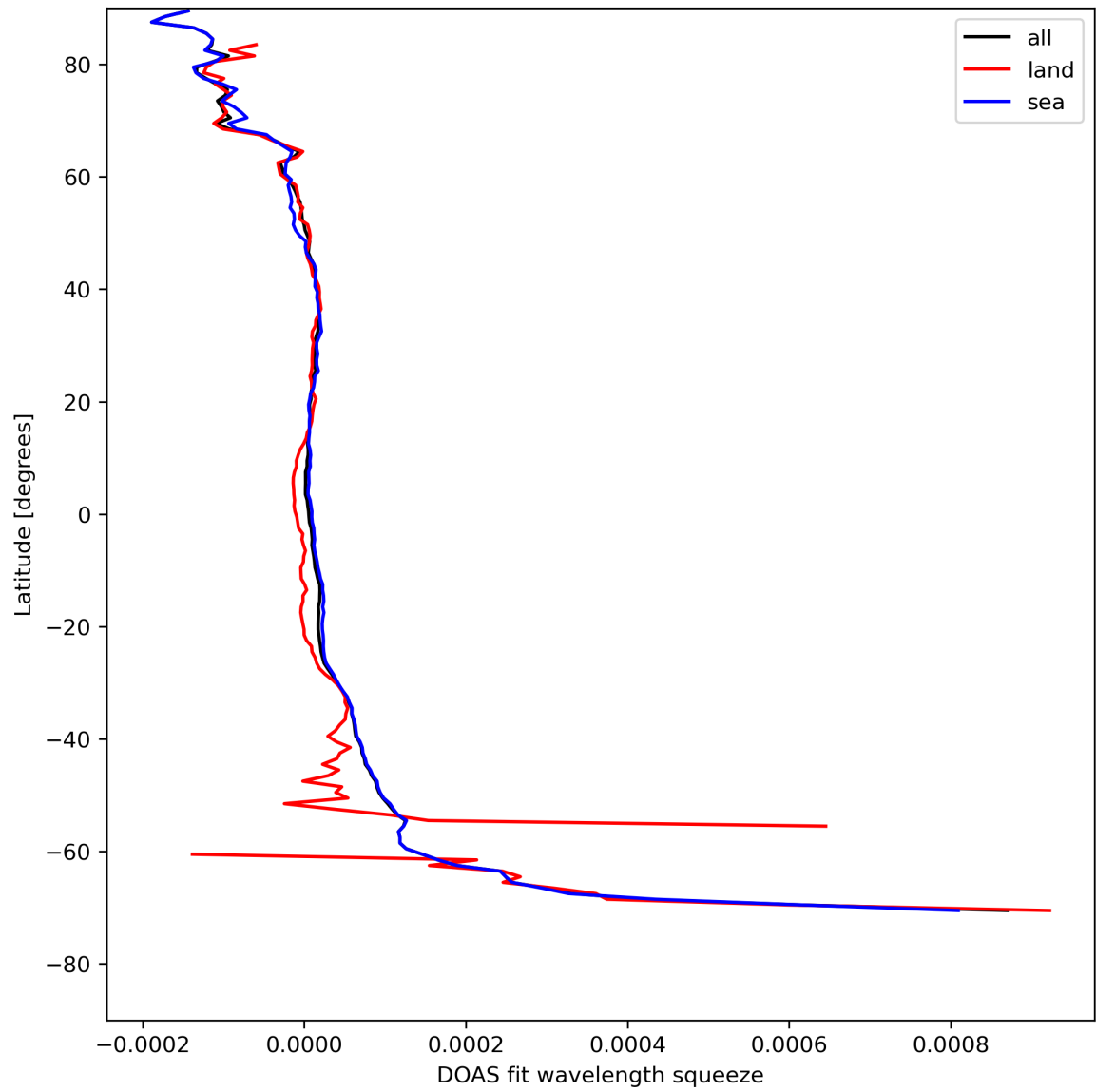
Figure 46: Zonal average of “DOAS fit wavelength squeeze” for 2024-04-26 to 2024-04-28.
