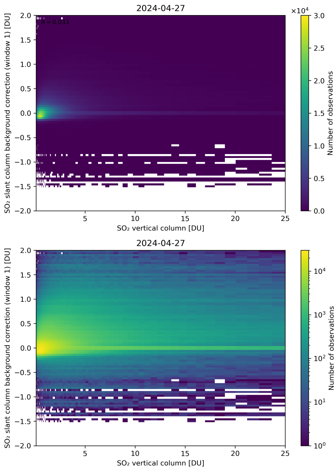
Figure 273: Scatter density plot of “SO 2 vertical column” against “SO 2 slant column background correction (window 1)” for 2024-04-26 to 2024-04-28.
