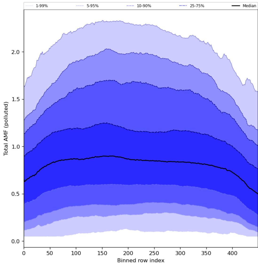
Figure 94: Along track statistics of “Total AMF (polluted)” for 2024-04-26 to 2024-04-28
