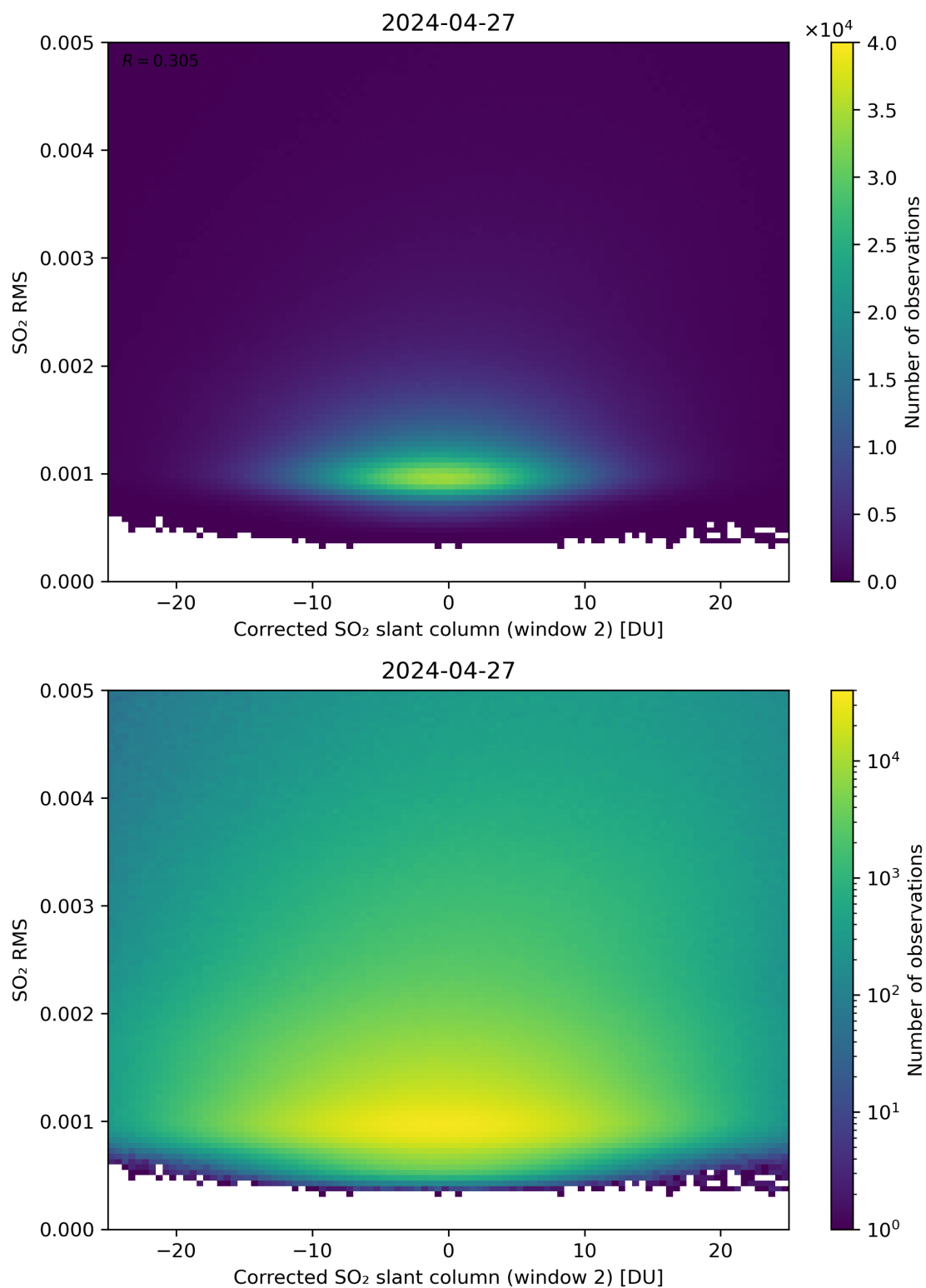
Figure 198: Scatter density plot of “Corrected SO 2 slant column (window 2)” against “SO 2 RMS” for 2024-04-26 to 2024-04-28.
