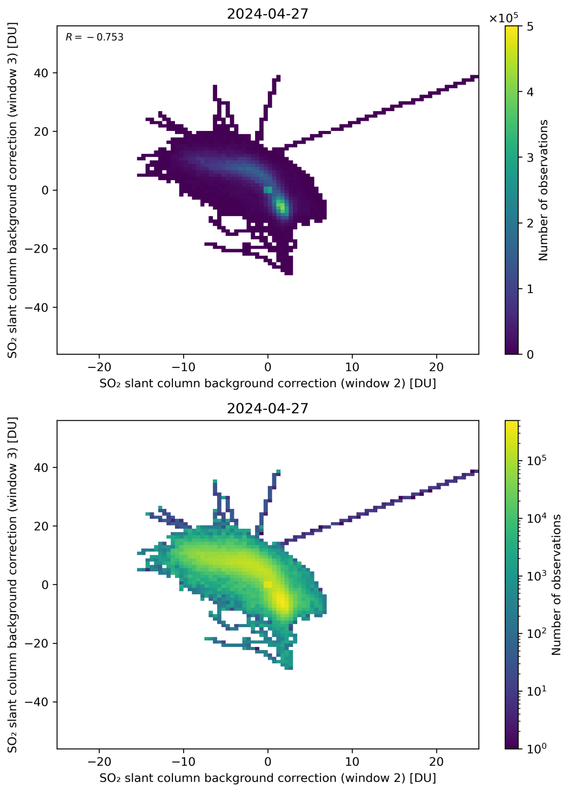
Figure 111: Scatter density plot of “SO 2 slant column background correction (window 2)” against “SO 2 slant column background correction (window 3)” for 2024-04-26 to 2024-04-28.
