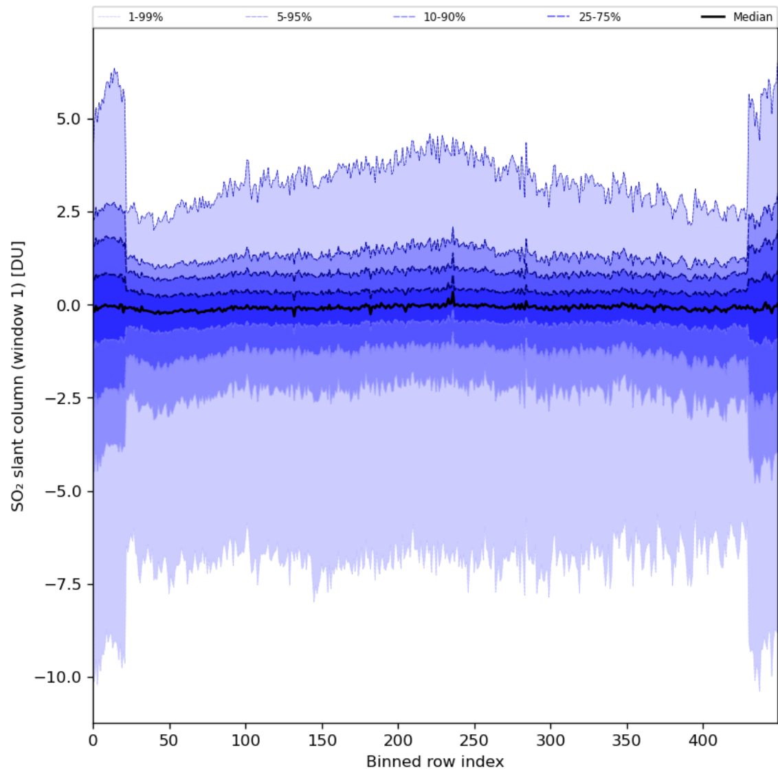
Figure 79: Along track statistics of “SO 2 slant column (window 1)” for 2024-04-26 to 2024-04-28
