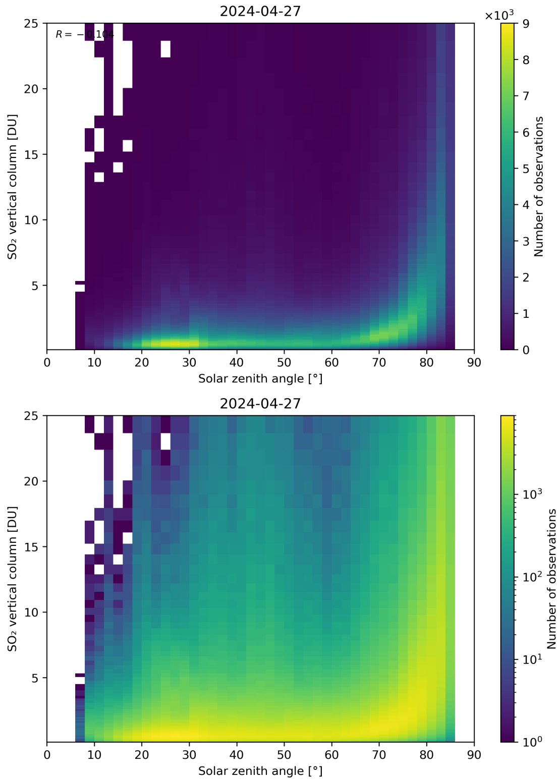
Figure 176: Scatter density plot of “Solar zenith angle” against “SO 2 vertical column” for 2024-04-26 to 2024-04-28.
