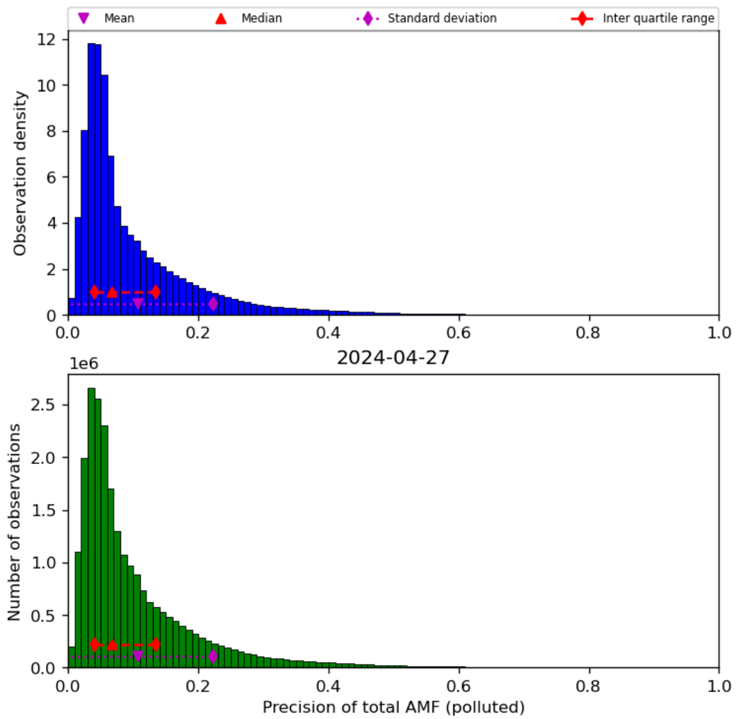
Figure 72: Histogram of “Precision of total AMF (polluted)” for 2024-04-26 to 2024-04-28
