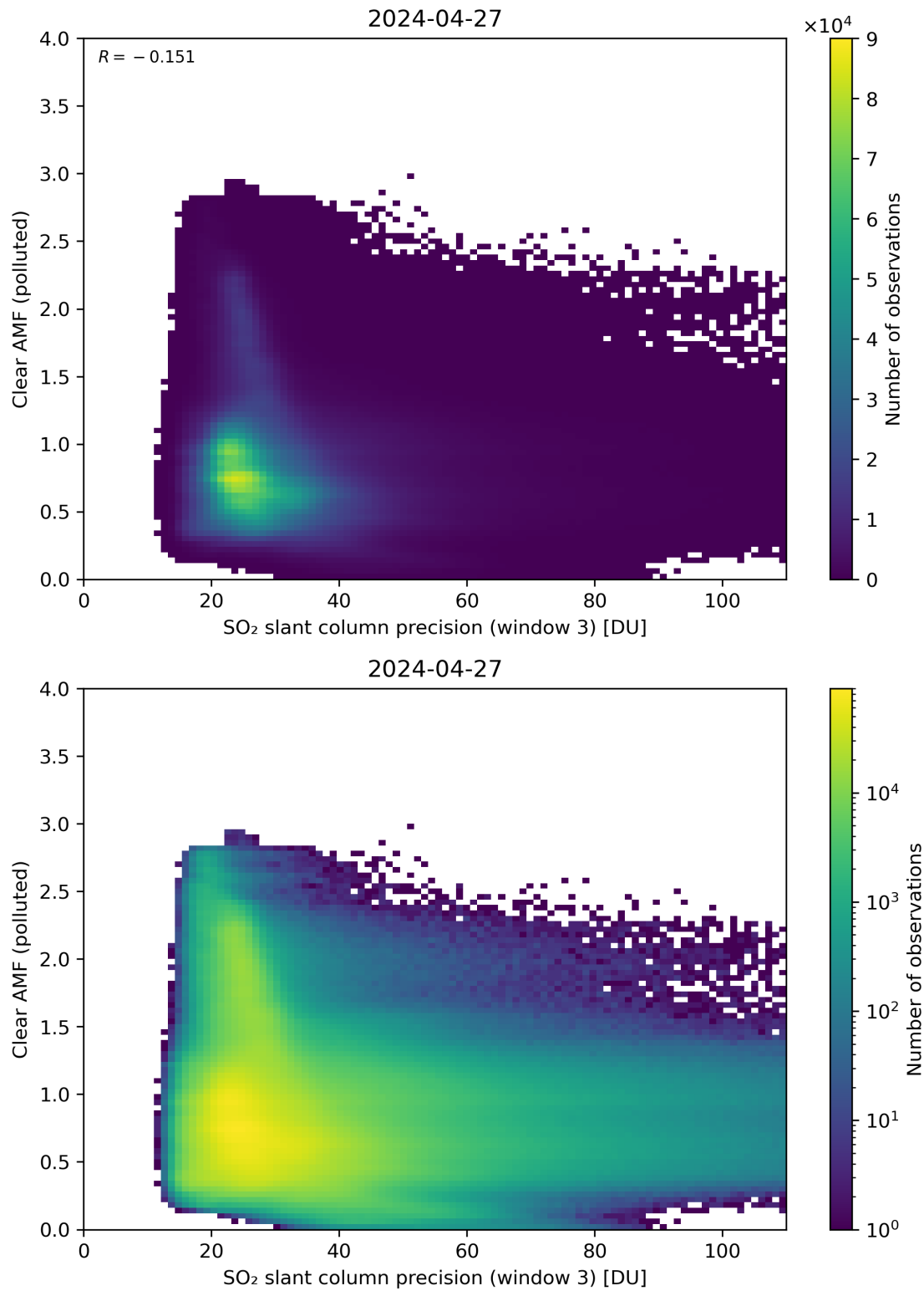
Figure 261: Scatter density plot of “SO 2 slant column precision (window 3)” against “Clear AMF (polluted)” for 2024-04-26 to 2024-04-28.
