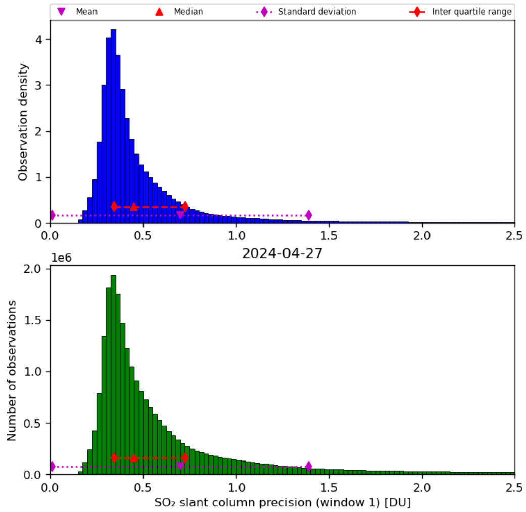
Figure 57: Histogram of “SO 2 slant column precision (window 1)” for 2024-04-26 to 2024-04-28
