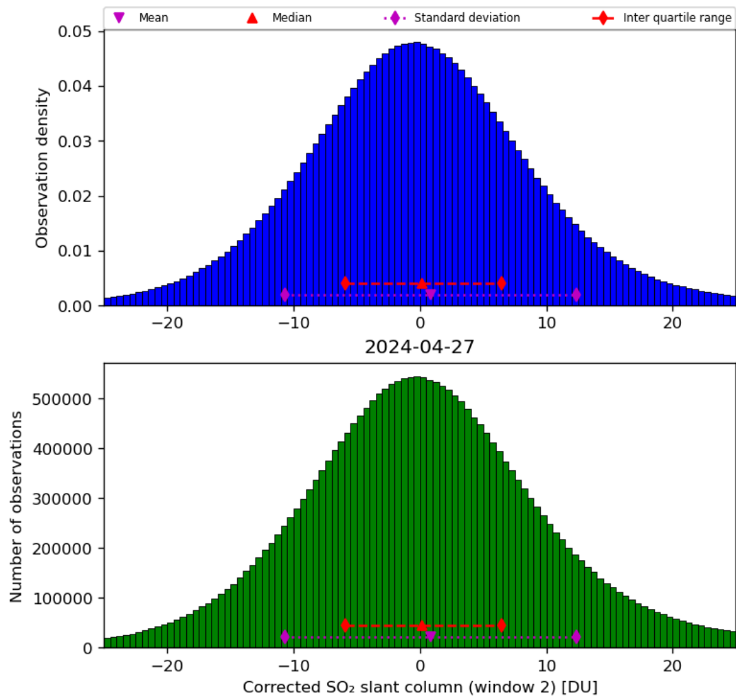
Figure 62: Histogram of “Corrected SO 2 slant column (window 2)” for 2024-04-26 to 2024-04-28
