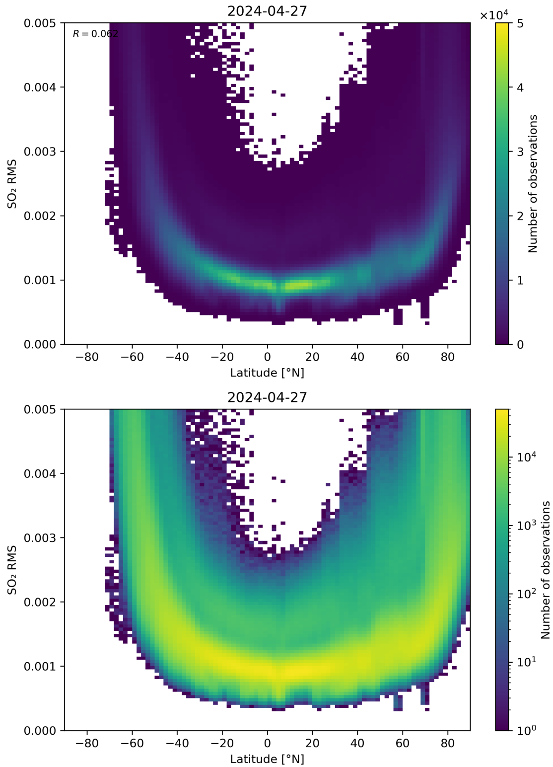
Figure 144: Scatter density plot of “Latitude” against “SO 2 RMS” for 2024-04-26 to 2024-04-28.
