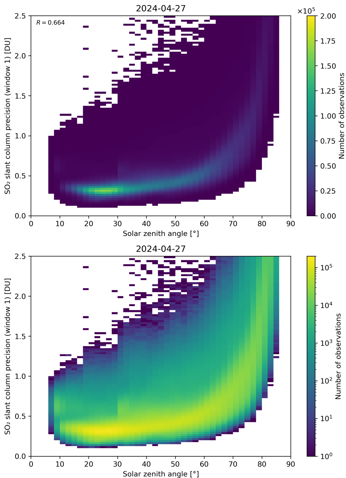
Figure 170: Scatter density plot of “Solar zenith angle” against “SO 2 slant column precision (window 1)” for 2024-04-26 to 2024-04-28.
