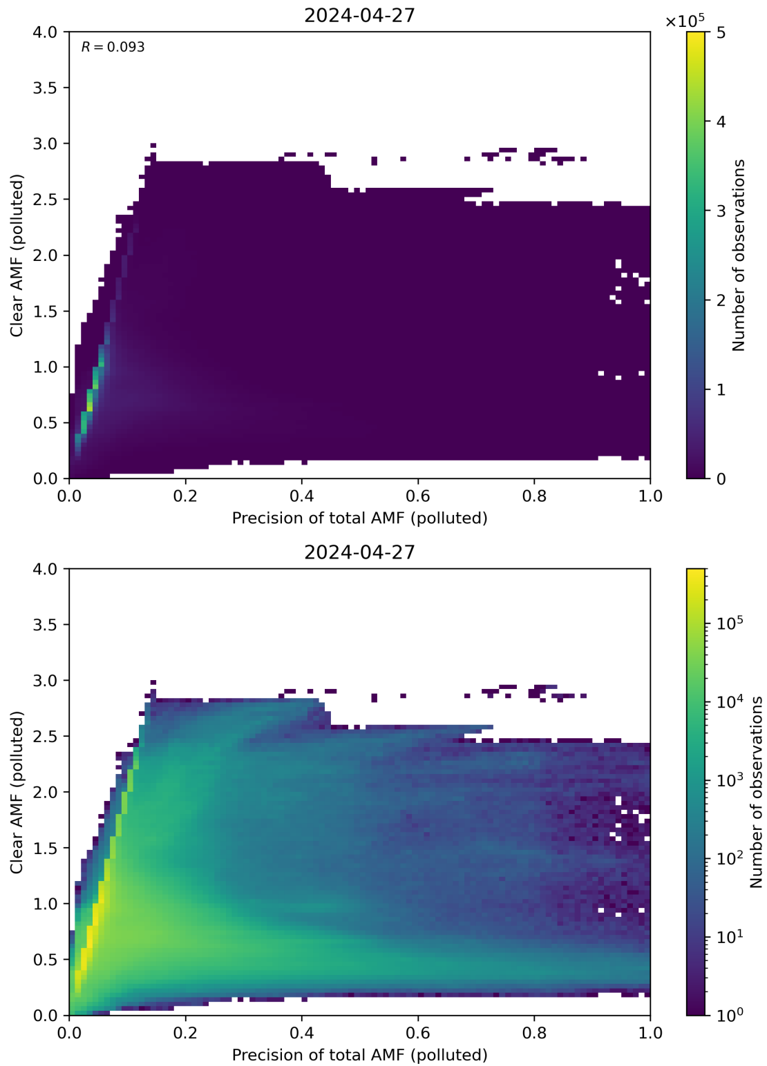
Figure 270: Scatter density plot of “Precision of total AMF (polluted)” against “Clear AMF (polluted)” for 2024-04-26 to 2024-04-28.
