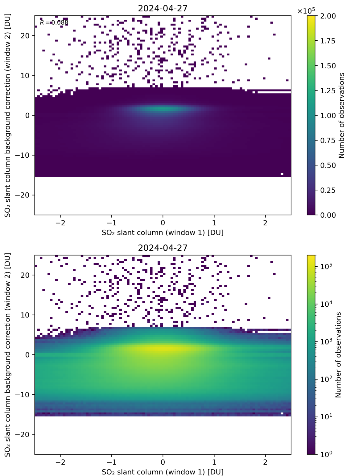
Figure 213: Scatter density plot of “SO 2 slant column (window 1)” against “SO 2 slant column background correction (window 2)” for 2024-04-26 to 2024-04-28.
