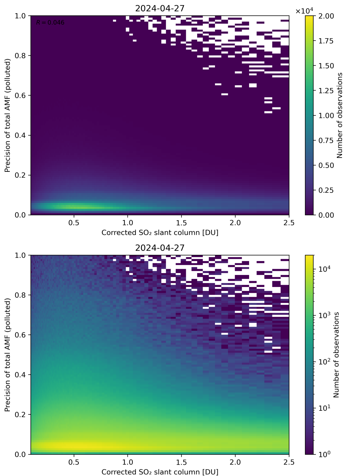
Figure 193: Scatter density plot of “Corrected SO 2 slant column” against “Precision of total AMF (polluted)” for 2024-04-26 to 2024-04-28.
