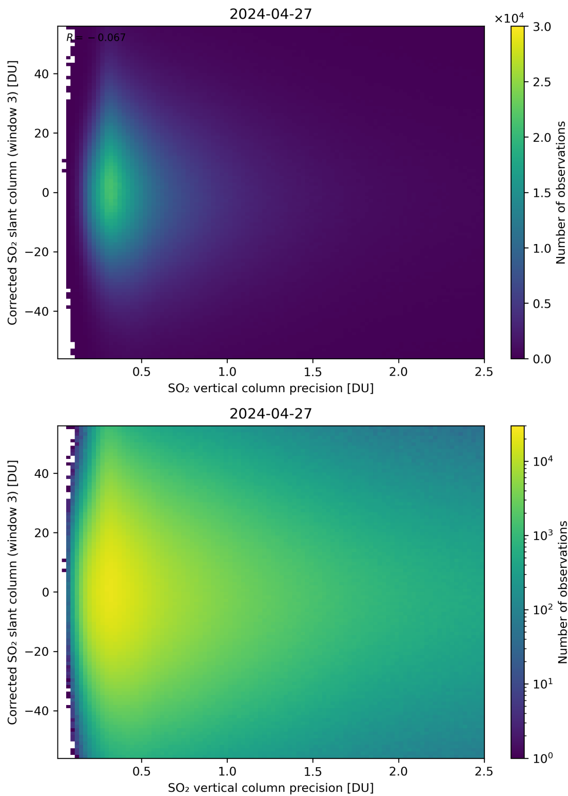
Figure 288: Scatter density plot of “SO 2 vertical column precision” against “Corrected SO 2 slant column (window 3)” for 2024-04-26 to 2024-04-28.
