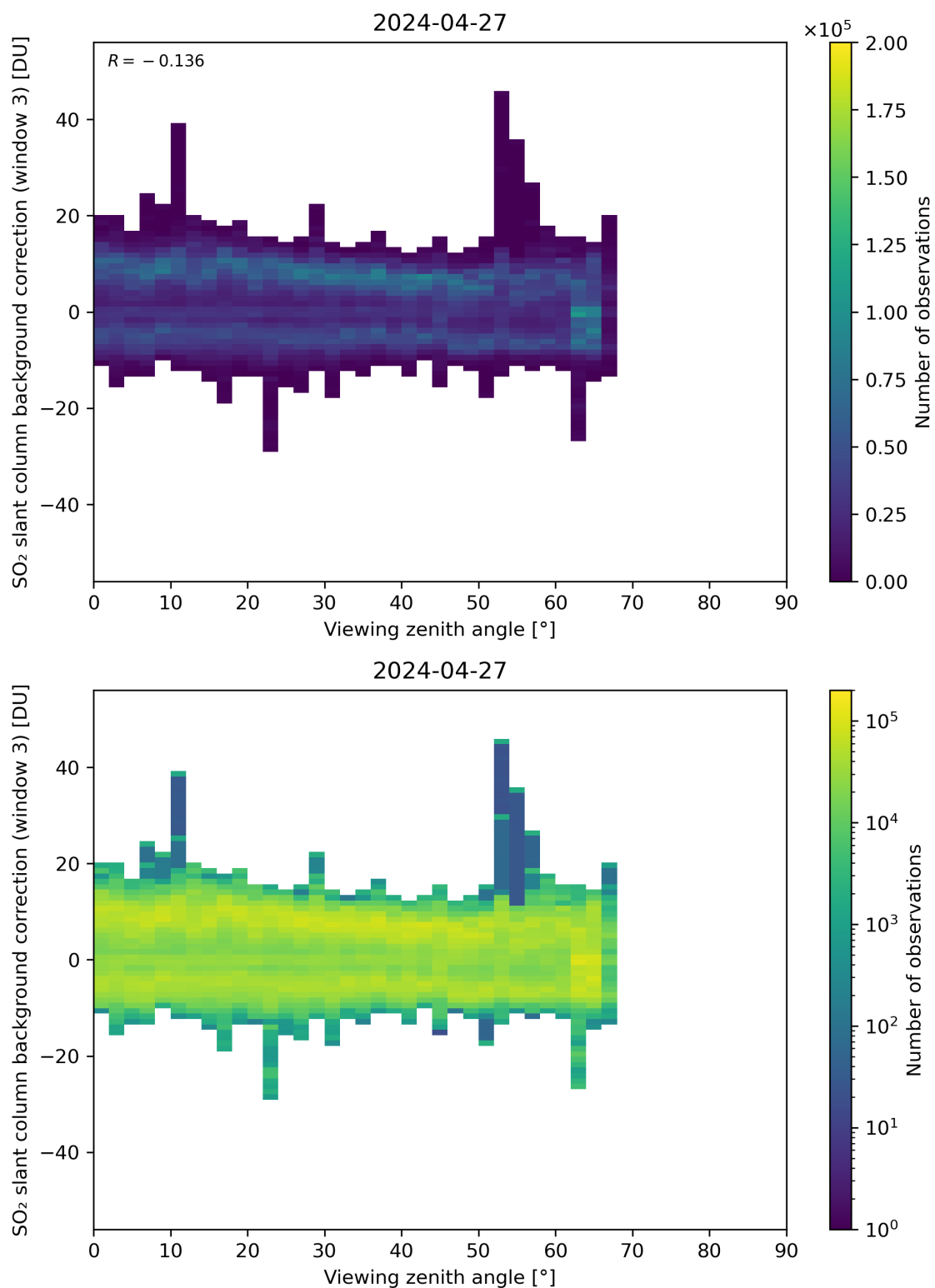
Figure 310: Scatter density plot of “Viewing zenith angle” against “SO 2 slant column background correction (window 3)” for 2024-04-26 to 2024-04-28.
