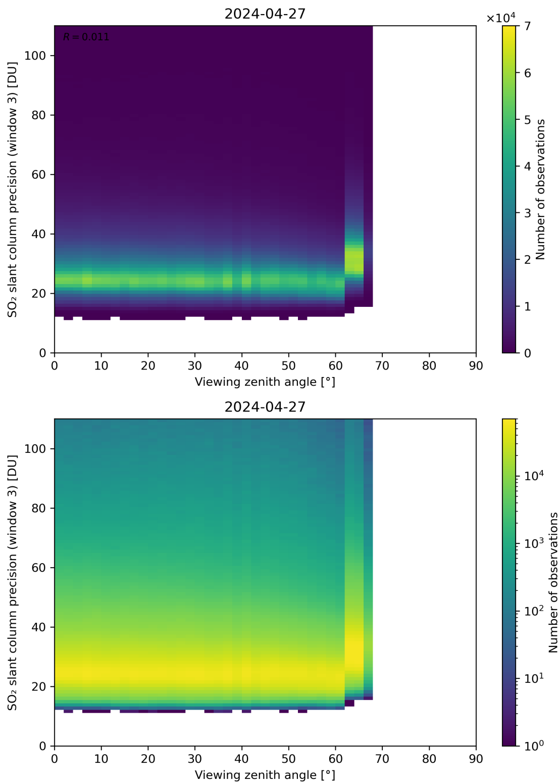
Figure 324: Scatter density plot of “Viewing zenith angle” against “SO 2 slant column precision (window 3)” for 2024-04-26 to 2024-04-28.
