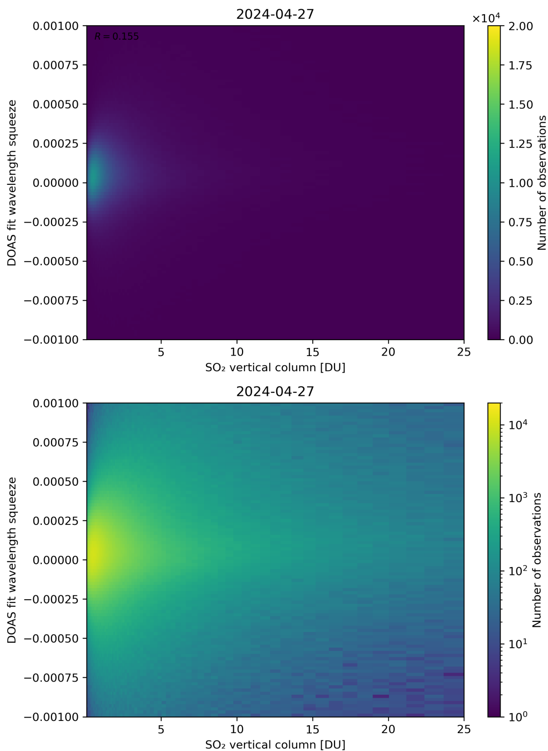
Figure 277: Scatter density plot of “SO 2 vertical column” against “DOAS fit wavelength squeeze” for 2024-04-26 to 2024-04-28.
