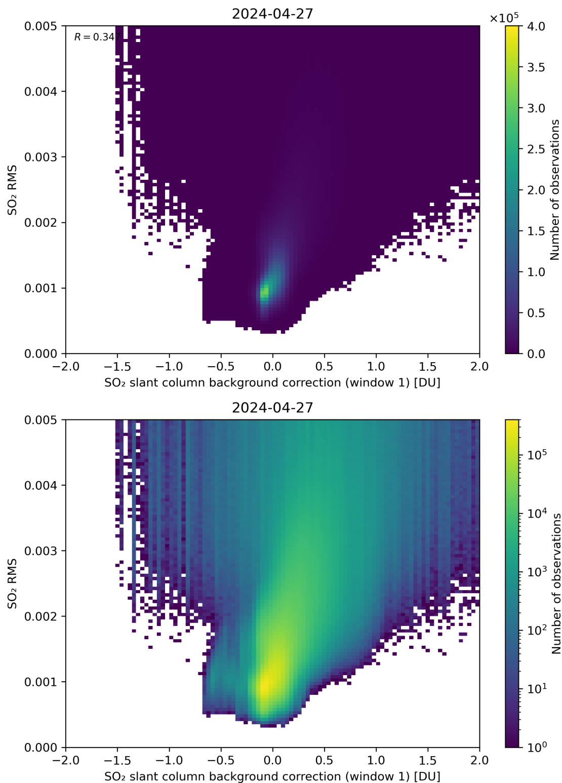
Figure 102: Scatter density plot of “SO 2 slant column background correction (window 1)” against “SO 2 RMS” for 2024-04-26 to 2024-04-28.
