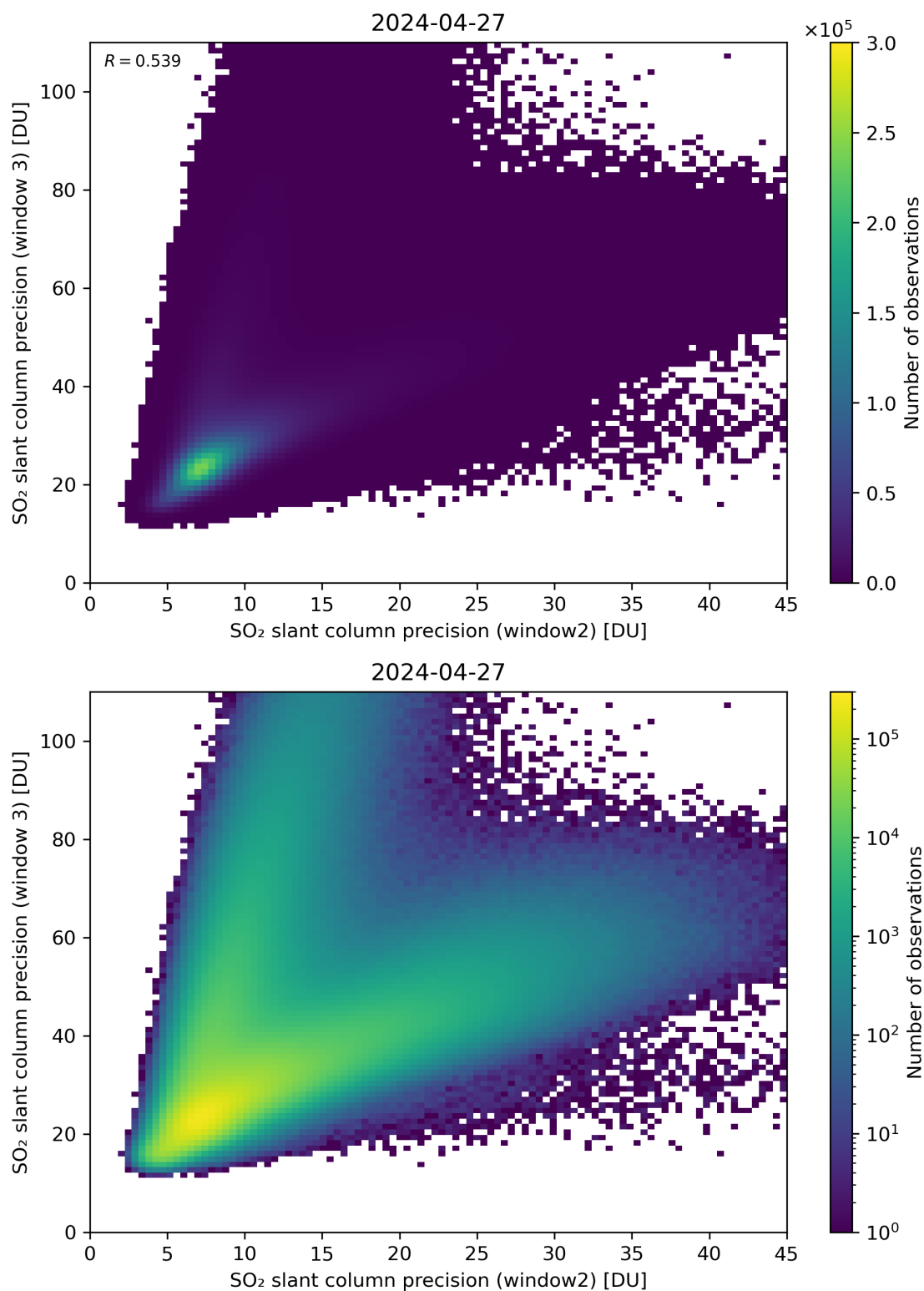
Figure 250: Scatter density plot of “SO 2 slant column precision (window2)” against “SO 2 slant column precision (window 3)” for 2024-04-26 to 2024-04-28.
