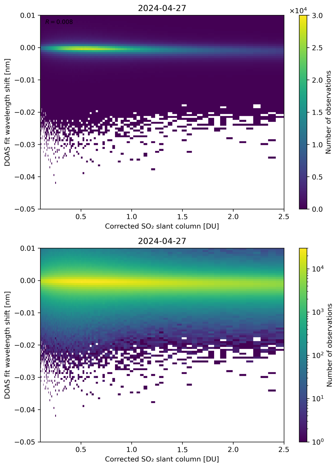
Figure 181: Scatter density plot of “Corrected SO 2 slant column” against “DOAS fit wavelength shift” for 2024-04-26 to 2024-04-28.
