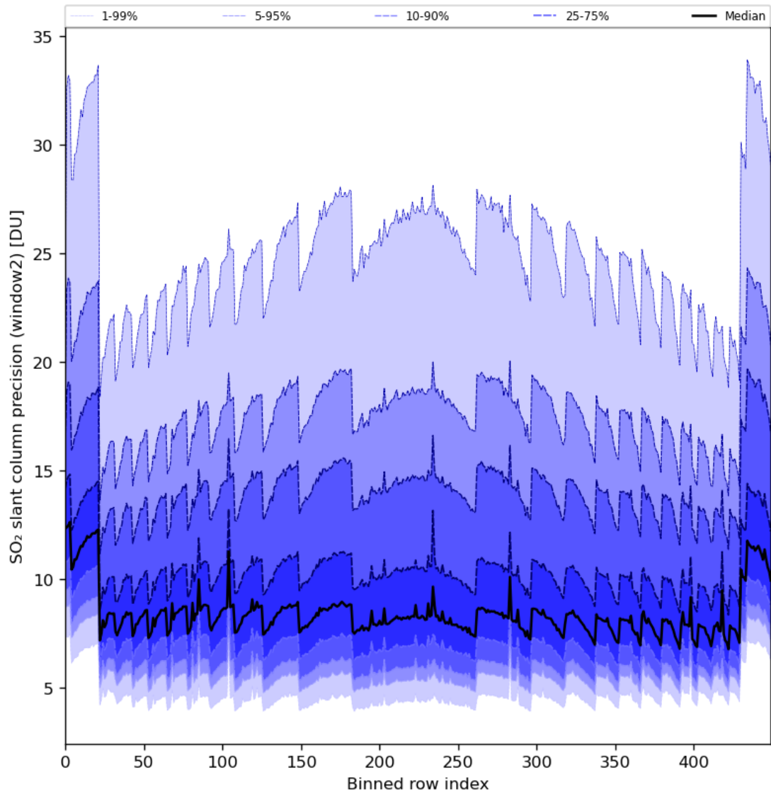
Figure 84: Along track statistics of “SO 2 slant column precision (window2)” for 2024-04-26 to 2024-04-28
