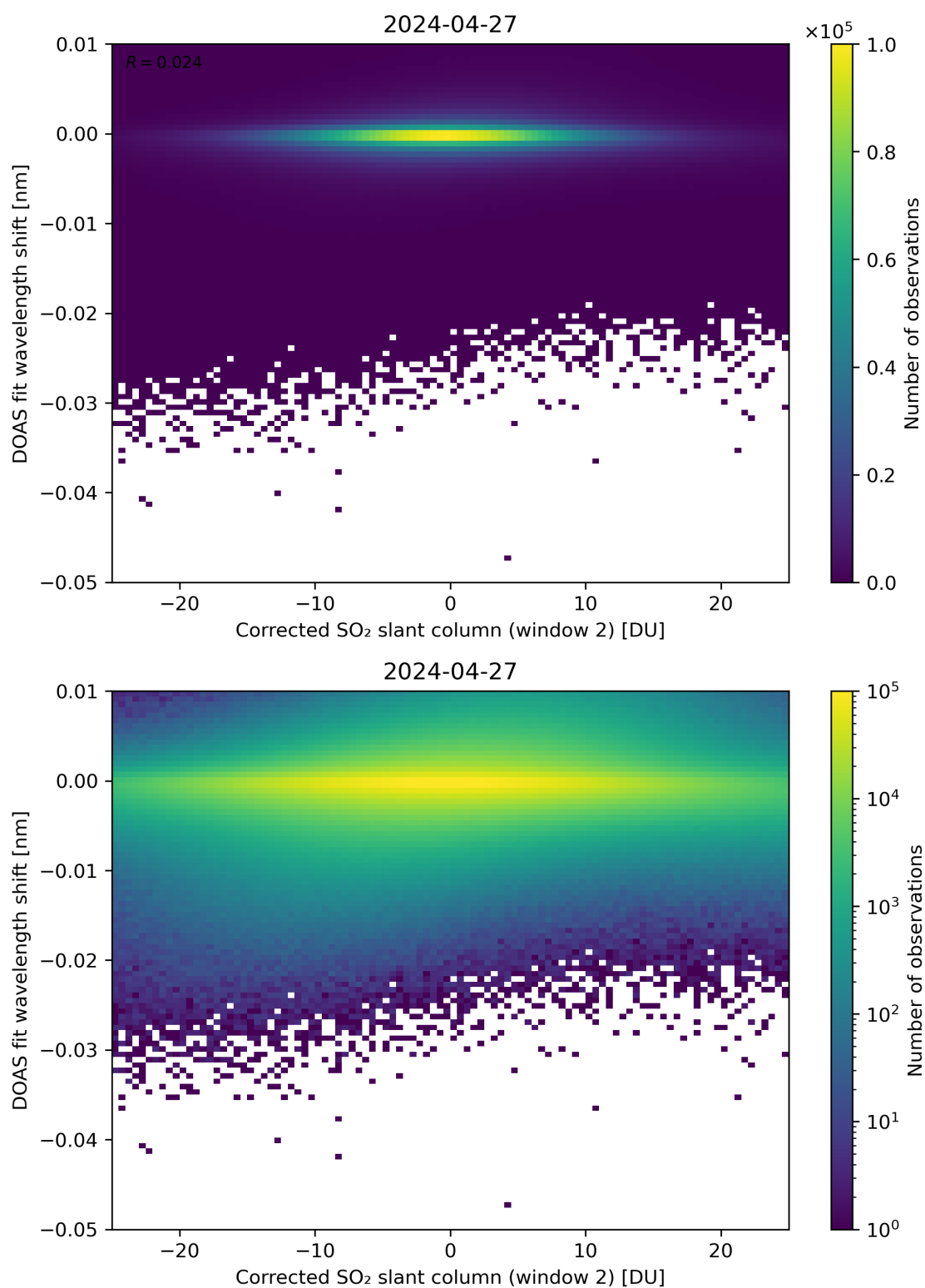
Figure 196: Scatter density plot of “Corrected SO 2 slant column (window 2)” against “DOAS fit wavelength shift” for 2024-04-26 to 2024-04-28.
