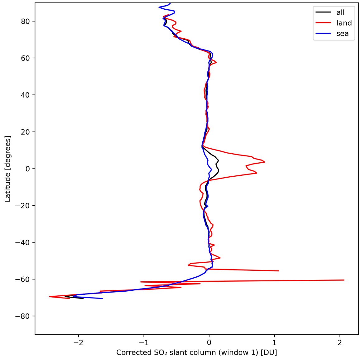
Figure 35: Zonal average of “Corrected SO 2 slant column (window 1)” for 2024-04-26 to 2024-04-28.
