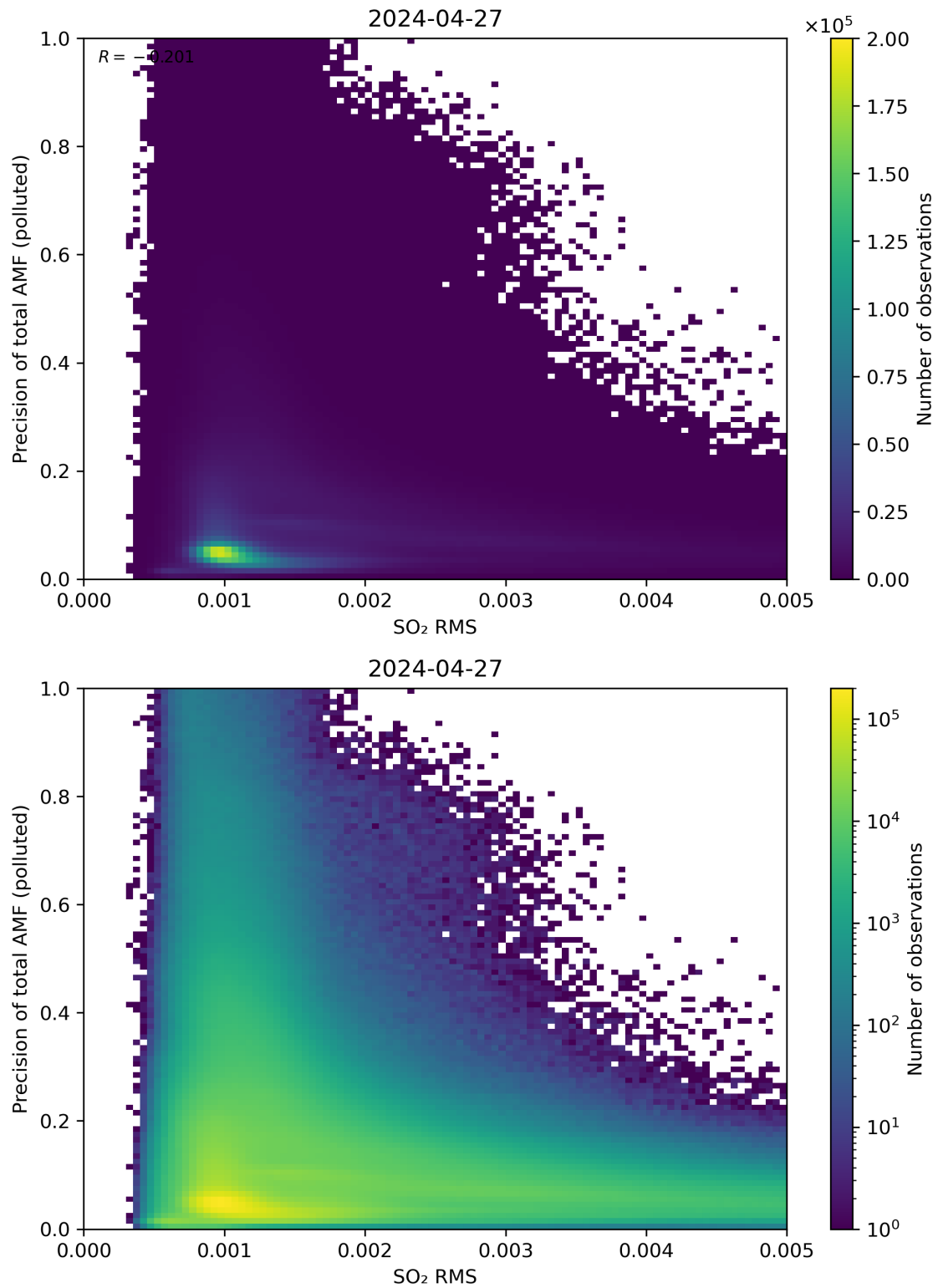
Figure 138: Scatter density plot of “SO 2 RMS” against “Precision of total AMF (polluted)” for 2024-04-26 to 2024-04-28.
