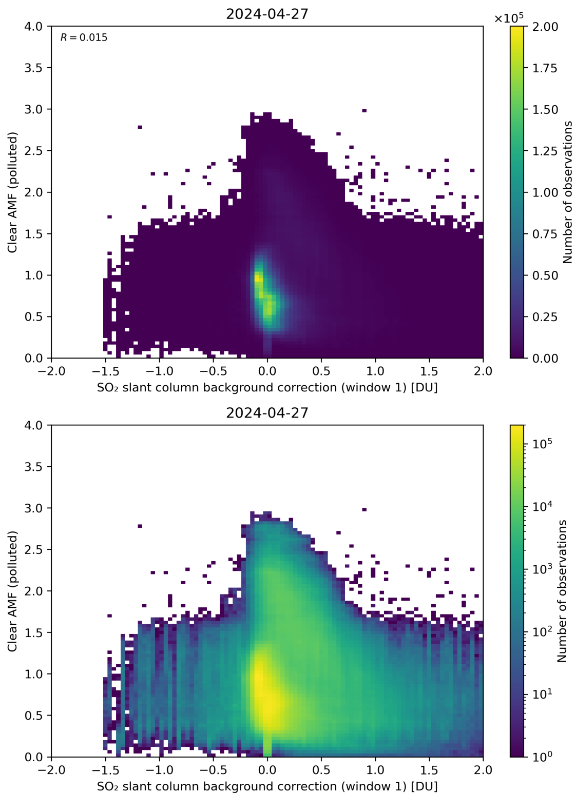
Figure 103: Scatter density plot of “SO 2 slant column background correction (window 1)” against “Clear AMF (polluted)” for 2024-04-26 to 2024-04-28.
