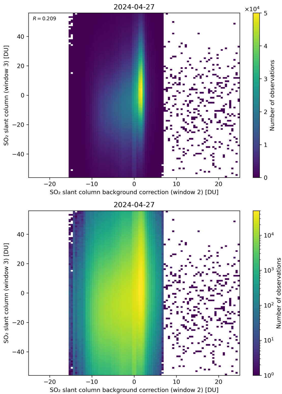
Figure 117: Scatter density plot of “SO 2 slant column background correction (window 2)” against “SO 2 slant column (window 3)” for 2024-04-26 to 2024-04-28.
