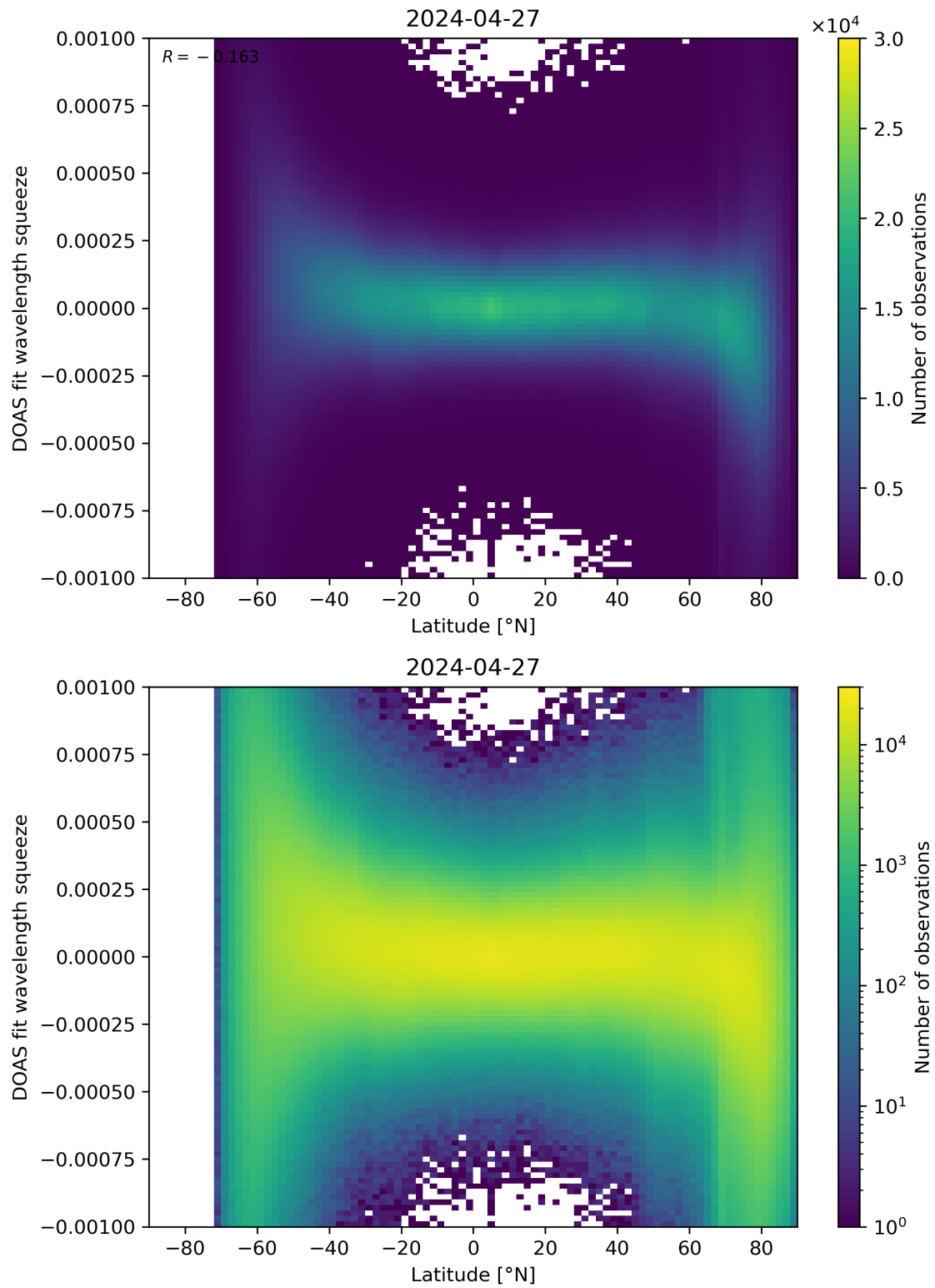
Figure 143: Scatter density plot of “Latitude” against “DOAS fit wavelength squeeze” for 2024-04-26 to 2024-04-28.
