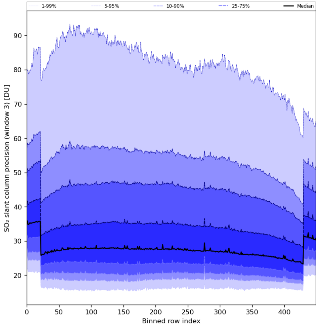
Figure 88: Along track statistics of “SO 2 slant column precision (window 3)” for 2024-04-26 to 2024-04-28
