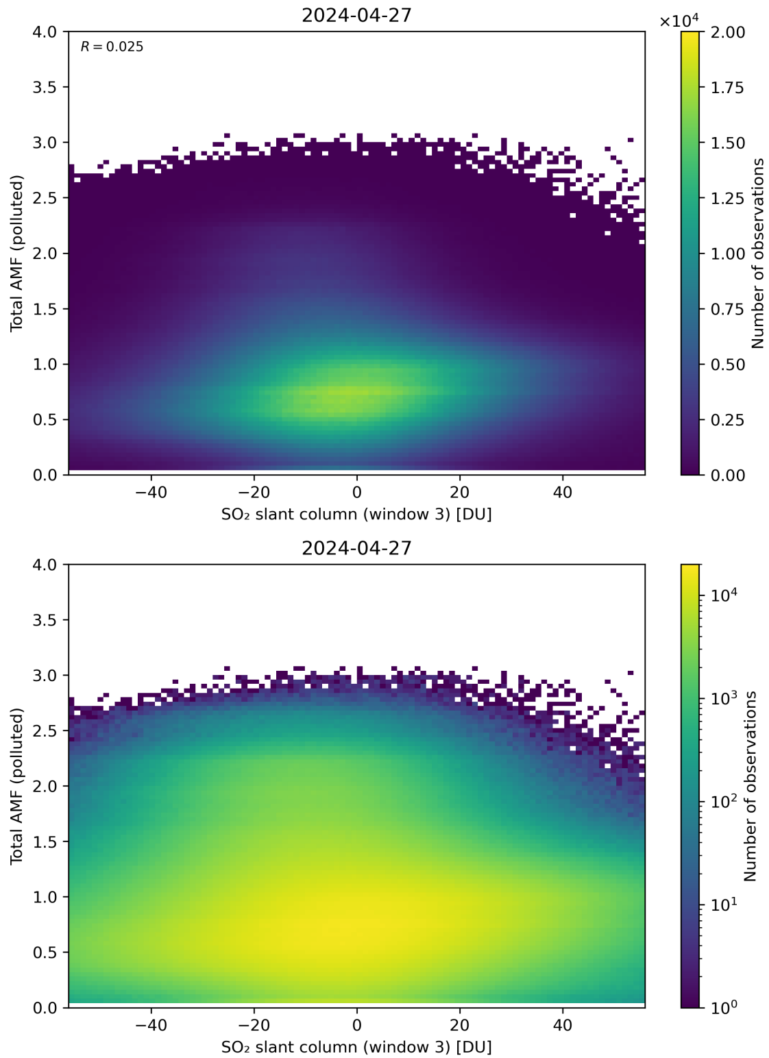
Figure 268: Scatter density plot of “SO 2 slant column (window 3)” against “Total AMF (polluted)” for 2024-04-26 to 2024-04-28.
