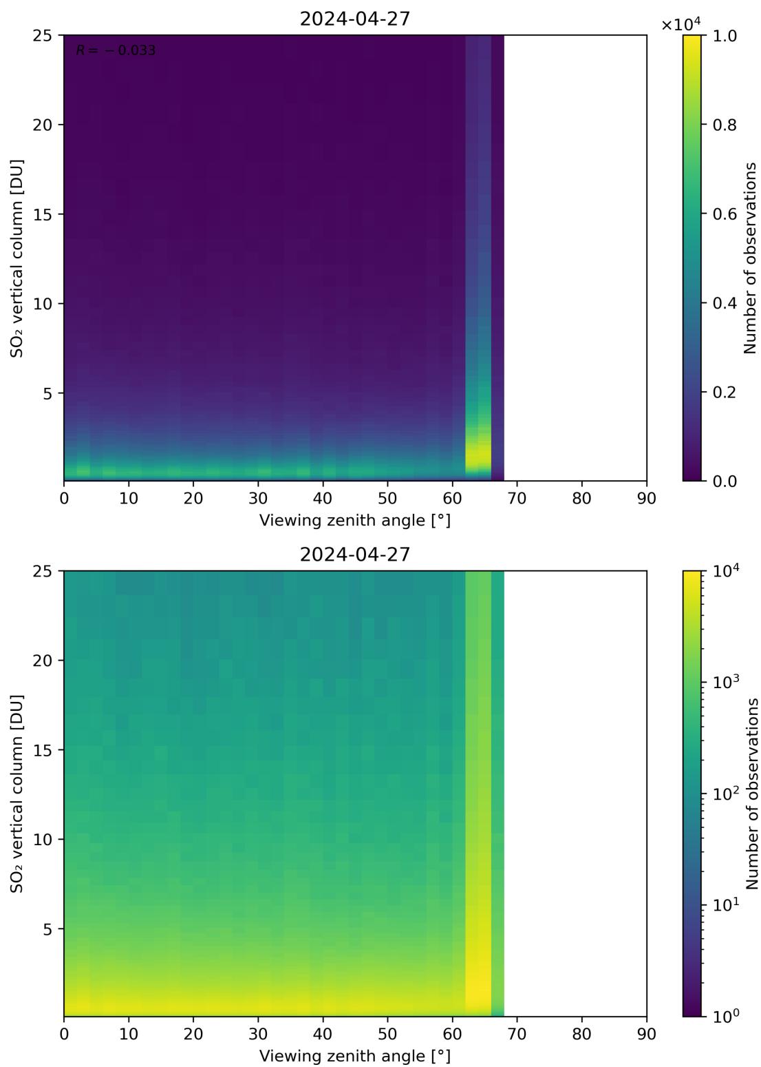
Figure 327: Scatter density plot of “Viewing zenith angle” against “SO 2 vertical column” for 2024-04-26 to 2024-04-28.
