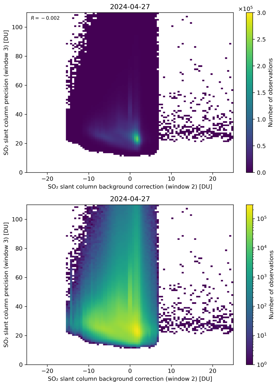
Figure 118: Scatter density plot of “SO 2 slant column background correction (window 2)” against “SO 2 slant column precision (window 3)” for 2024-04-26 to 2024-04-28.
