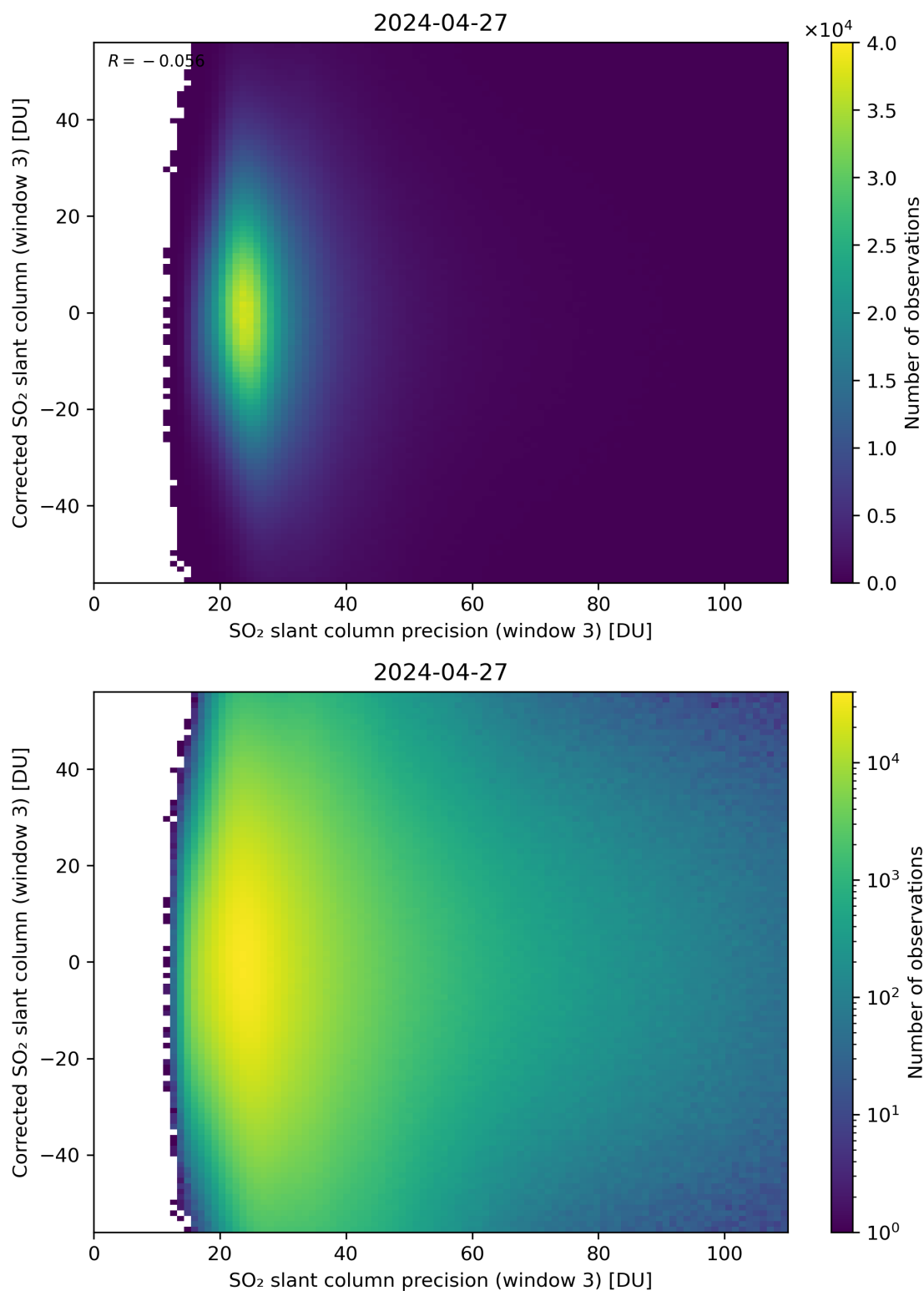
Figure 262: Scatter density plot of “SO 2 slant column precision (window 3)” against “Corrected SO 2 slant column (window 3)” for 2024-04-26 to 2024-04-28.
