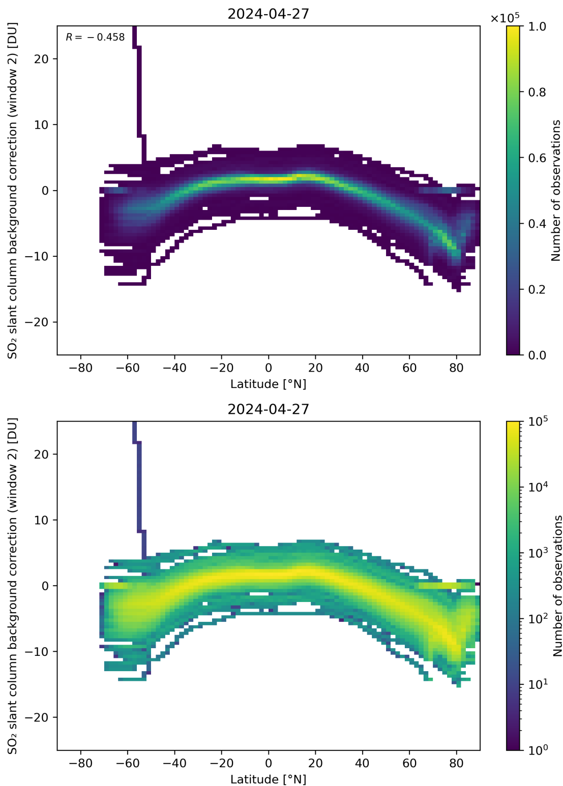
Figure 140: Scatter density plot of “Latitude” against “SO 2 slant column background correction (window 2)” for 2024-04-26 to 2024-04-28.
