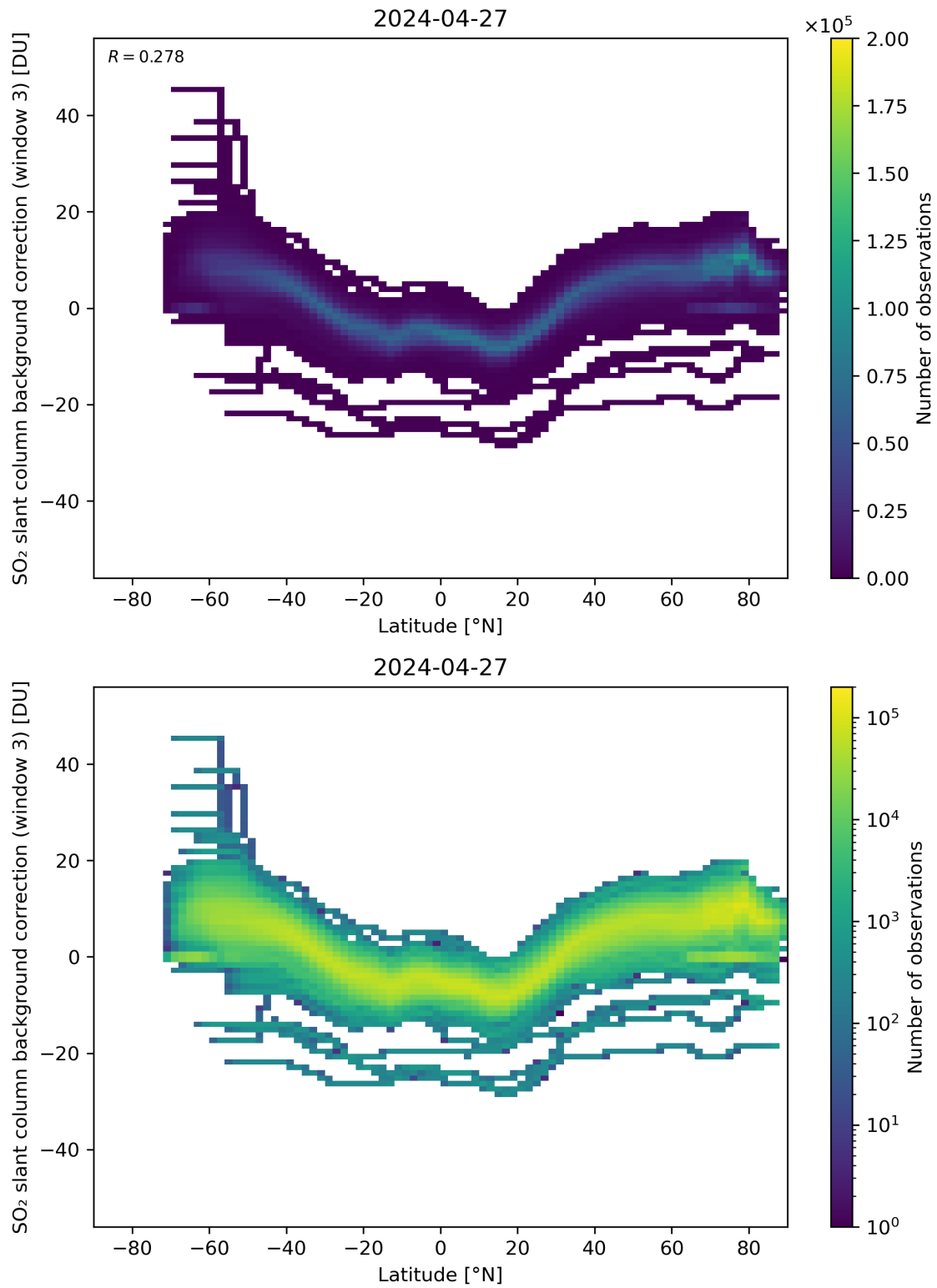
Figure 141: Scatter density plot of “Latitude” against “SO 2 slant column background correction (window 3)” for 2024-04-26 to 2024-04-28.
