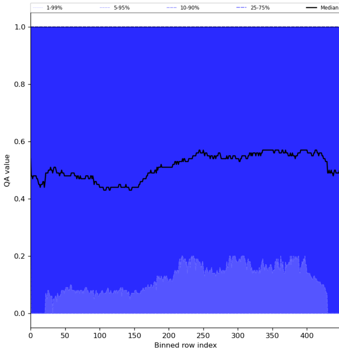
Figure 75: Along track statistics of “QA value” for 2024-04-26 to 2024-04-28
