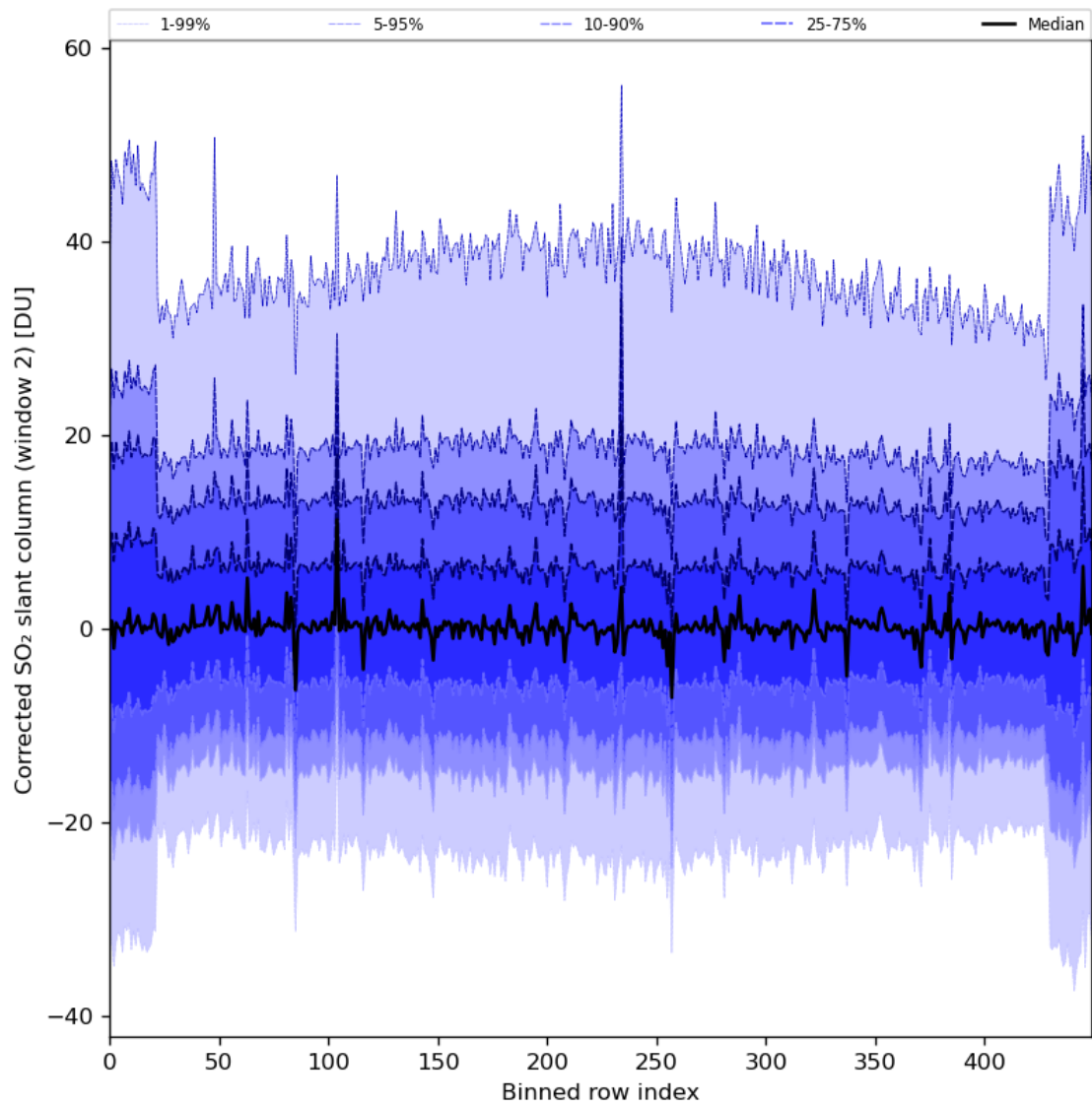
Figure 85: Along track statistics of “Corrected SO 2 slant column (window 2)” for 2024-04-26 to 2024-04-28
