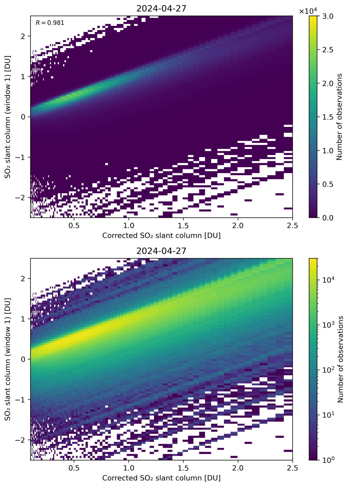
Figure 187: Scatter density plot of “Corrected SO 2 slant column” against “SO 2 slant column (window 1)” for 2024-04-26 to 2024-04-28.
