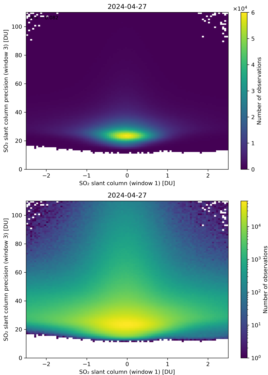
Figure 238: Scatter density plot of “SO 2 slant column (window 1)” against “SO 2 slant column precision (window 3)” for 2024-04-26 to 2024-04-28.
