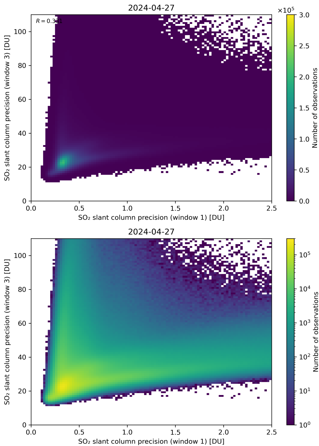
Figure 229: Scatter density plot of “SO 2 slant column precision (window 1)” against “SO 2 slant column precision (window 3)” for 2024-04-26 to 2024-04-28.
