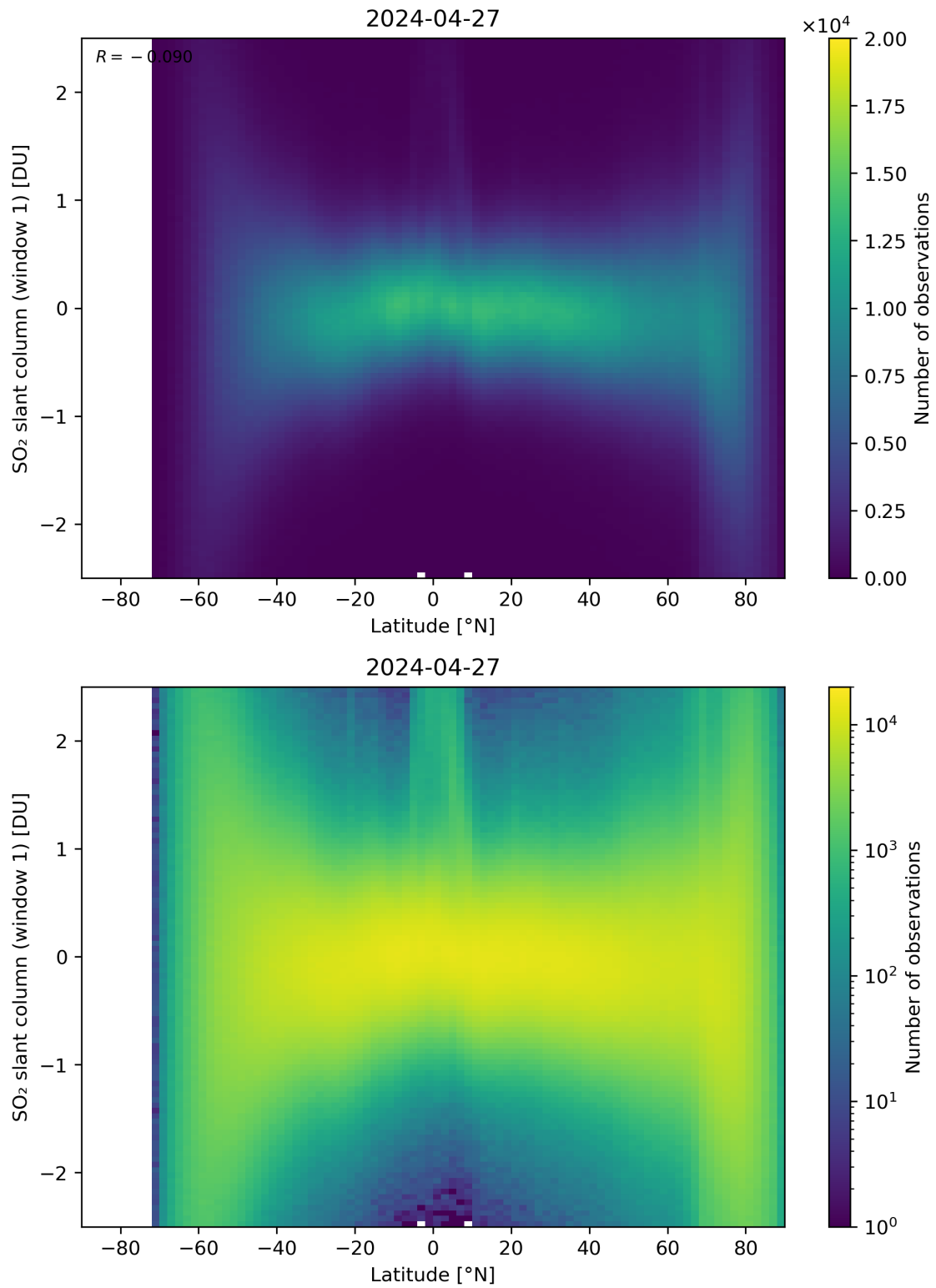
Figure 149: Scatter density plot of “Latitude” against “SO 2 slant column (window 1)” for 2024-04-26 to 2024-04-28.
