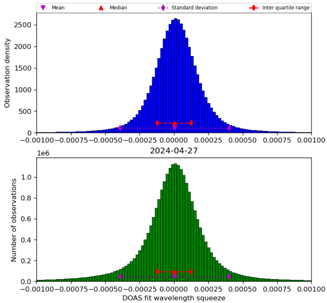
Figure 69: Histogram of “DOAS fit wavelength squeeze” for 2024-04-26 to 2024-04-28
