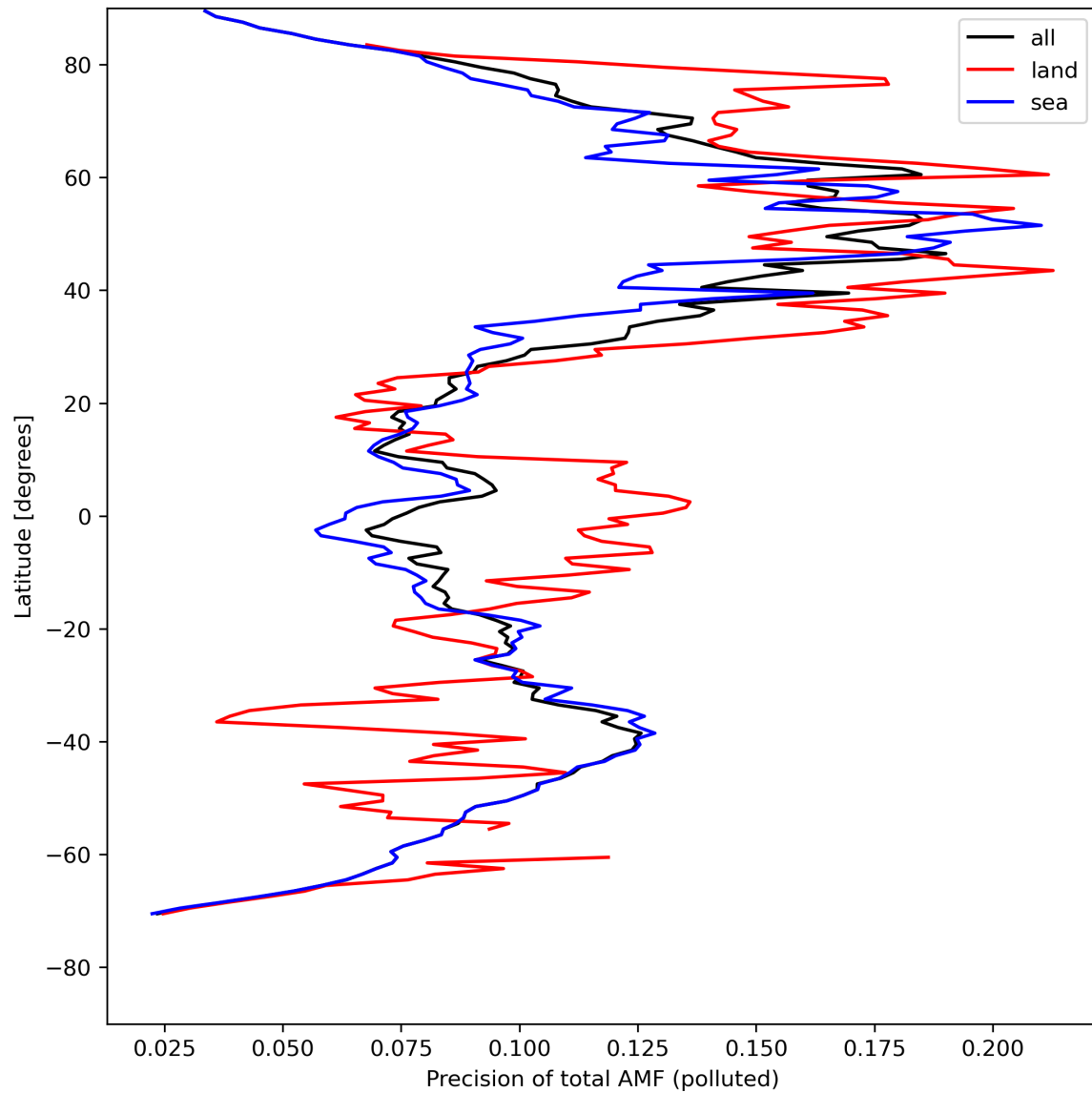
Figure 49: Zonal average of “Precision of total AMF (polluted)” for 2024-04-26 to 2024-04-28.
