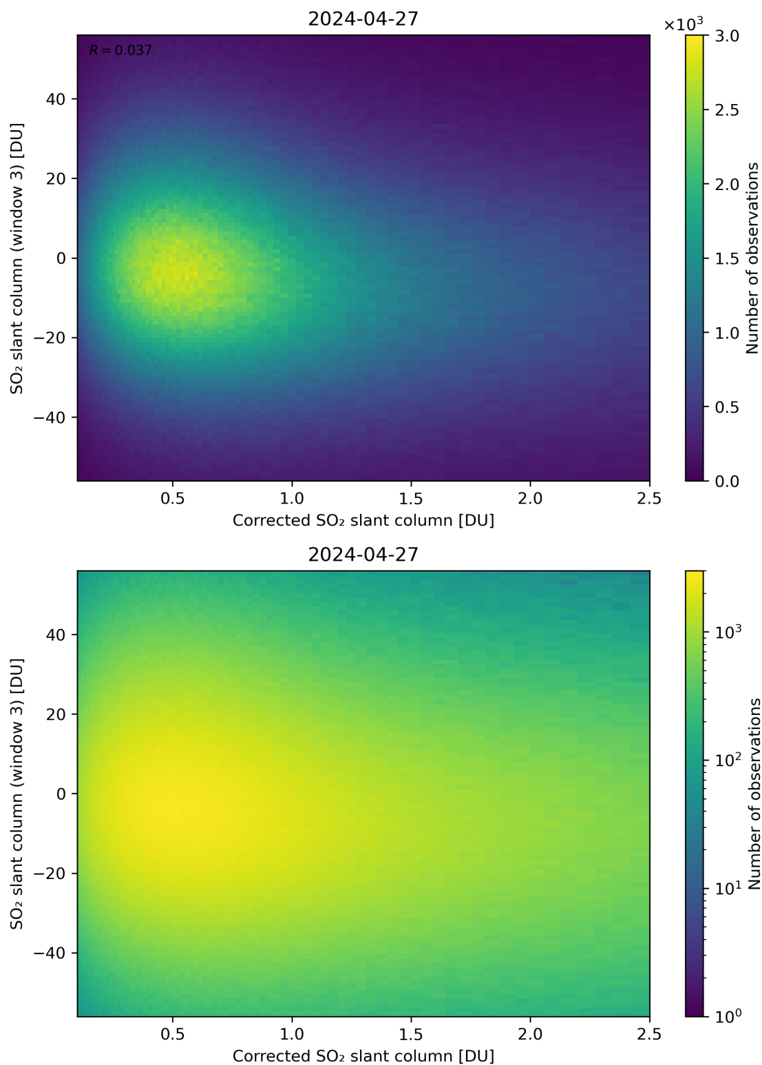
Figure 190: Scatter density plot of “Corrected SO 2 slant column” against “SO 2 slant column (window 3)” for 2024-04-26 to 2024-04-28.
