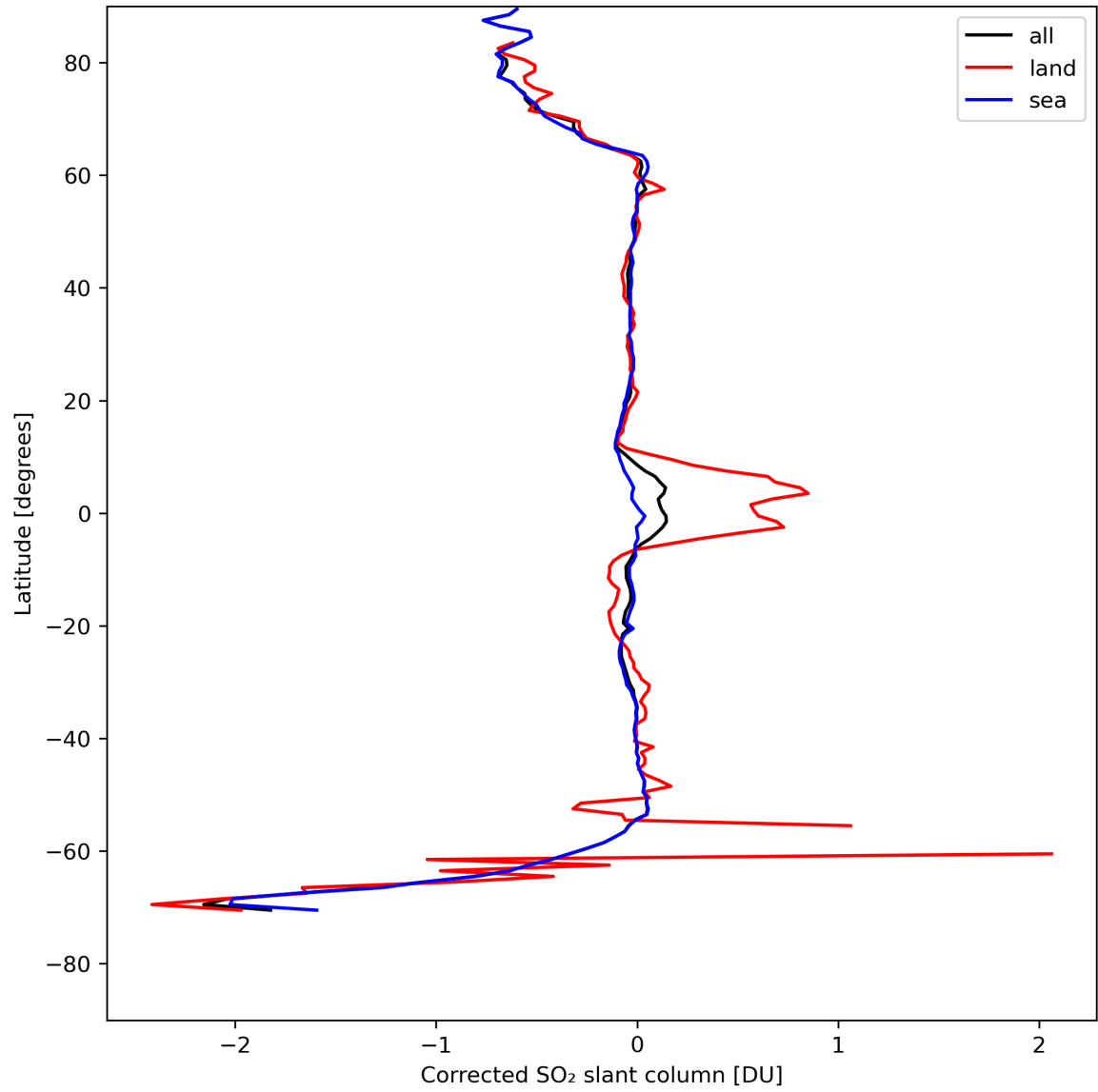
Figure 32: Zonal average of "Corrected SO 2 slant column" for 2024-04-26 to 2024-04-28.
