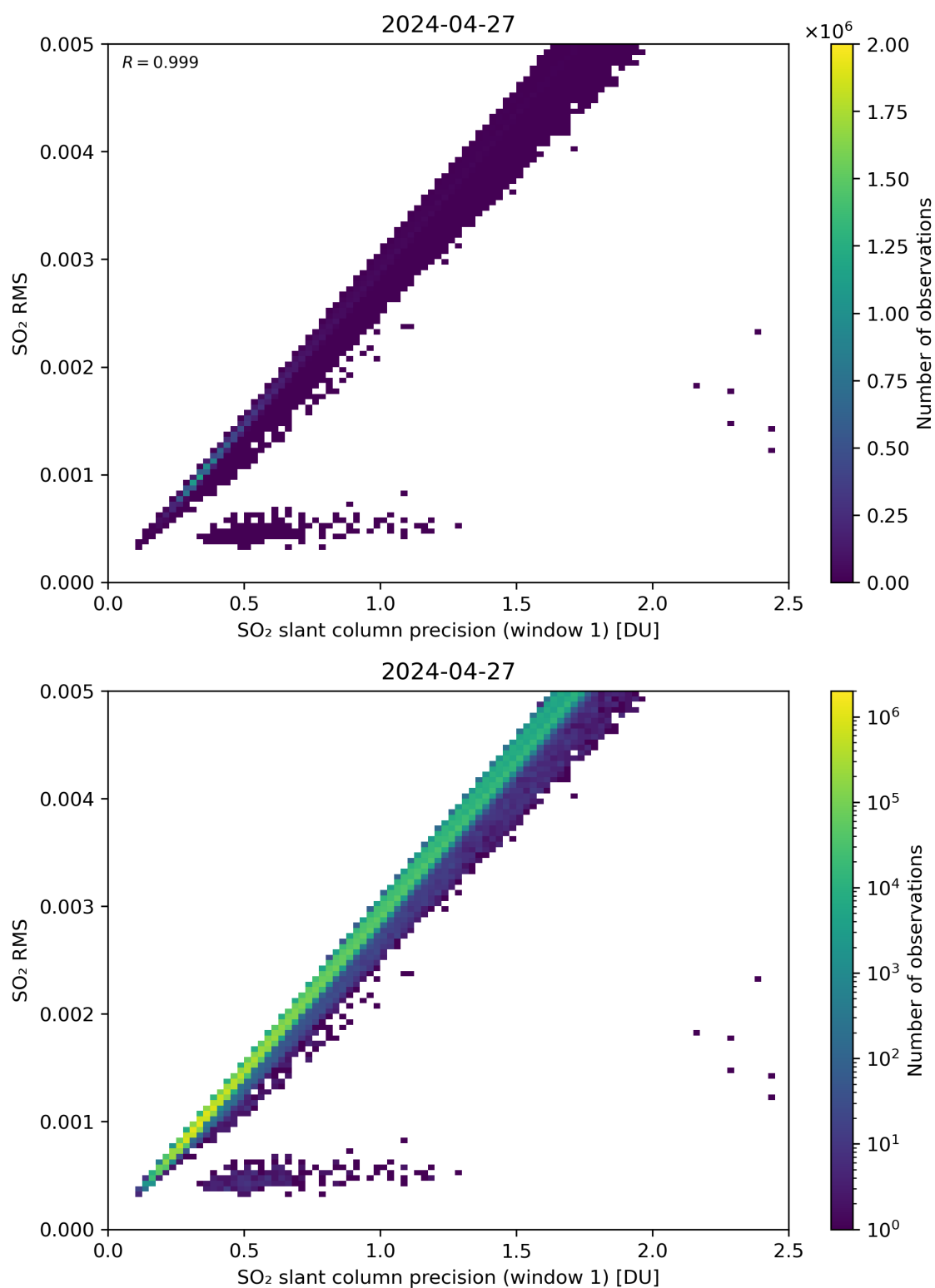
Figure 223: Scatter density plot of “SO 2 slant column precision (window 1)” against “SO 2 RMS” for 2024-04-26 to 2024-04-28.
