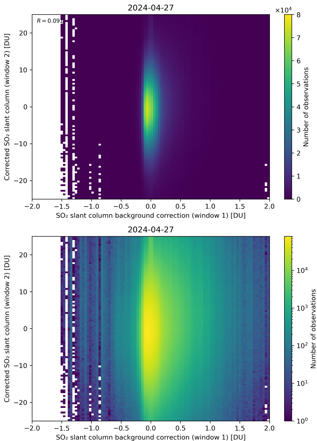
Figure 104: Scatter density plot of “SO 2 slant column background correction (window 1)” against “Corrected SO 2 slant column (window 2)” for 2024-04-26 to 2024-04-28.
