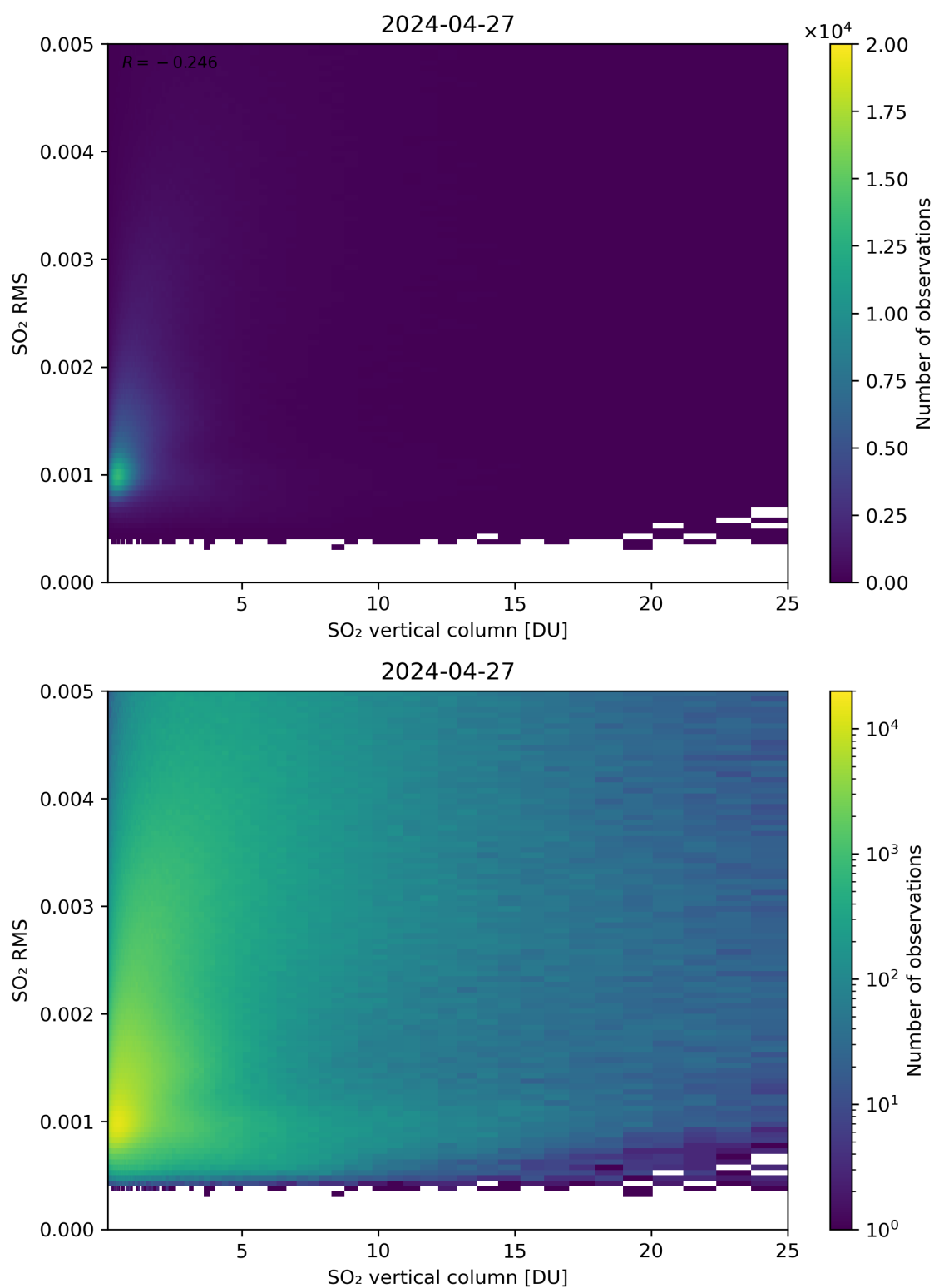
Figure 278: Scatter density plot of “SO 2 vertical column” against “SO 2 RMS” for 2024-04-26 to 2024-04-28.
