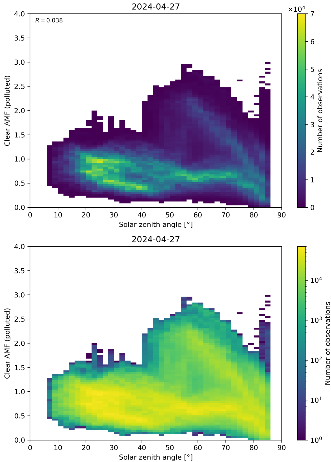
Figure 165: Scatter density plot of “Solar zenith angle” against “Clear AMF (polluted)” for 2024-04-26 to 2024-04-28.
