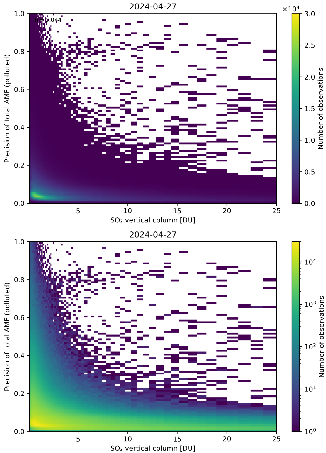
Figure 306: Scatter density plot of “SO 2 vertical column” against “Precision of total AMF (polluted)” for 2024-04-26 to 2024-04-28.
