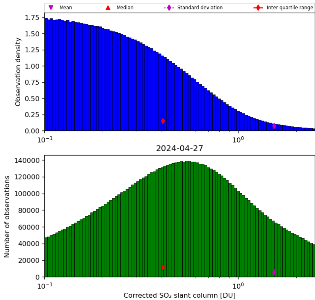
Figure 55: Histogram of “Corrected SO 2 slant column” for 2024-04-26 to 2024-04-28
