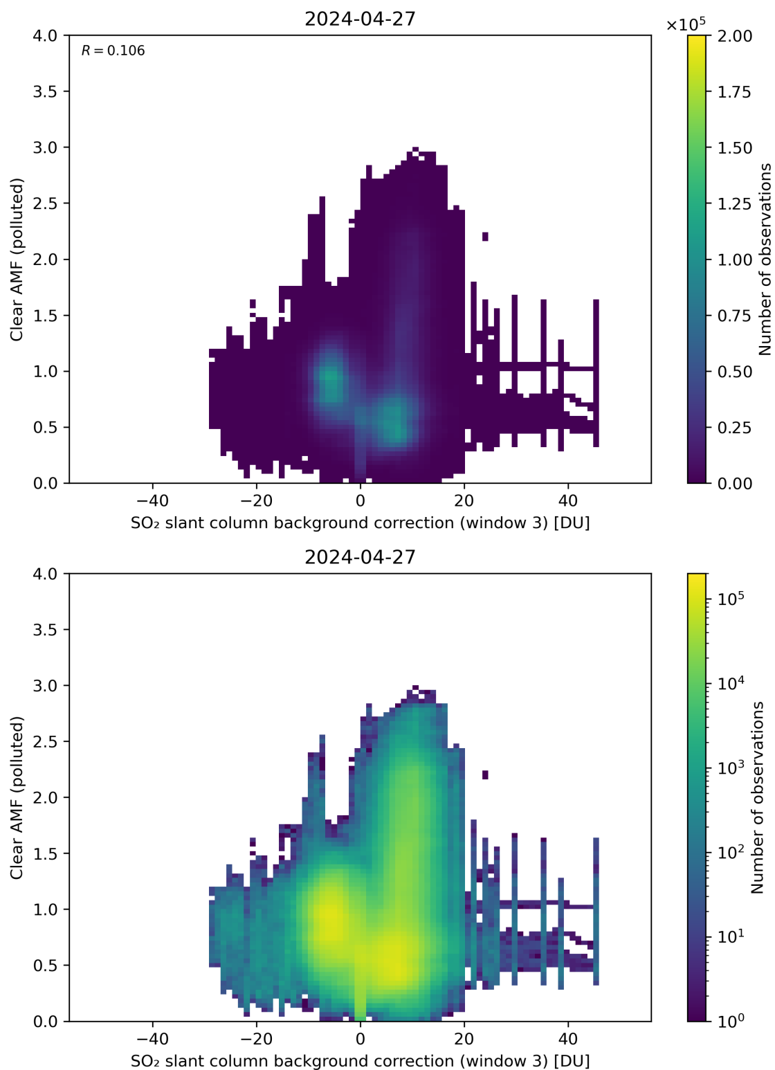
Figure 124: Scatter density plot of “SO 2 slant column background correction (window 3)” against “Clear AMF (polluted)” for 2024-04-26 to 2024-04-28.
