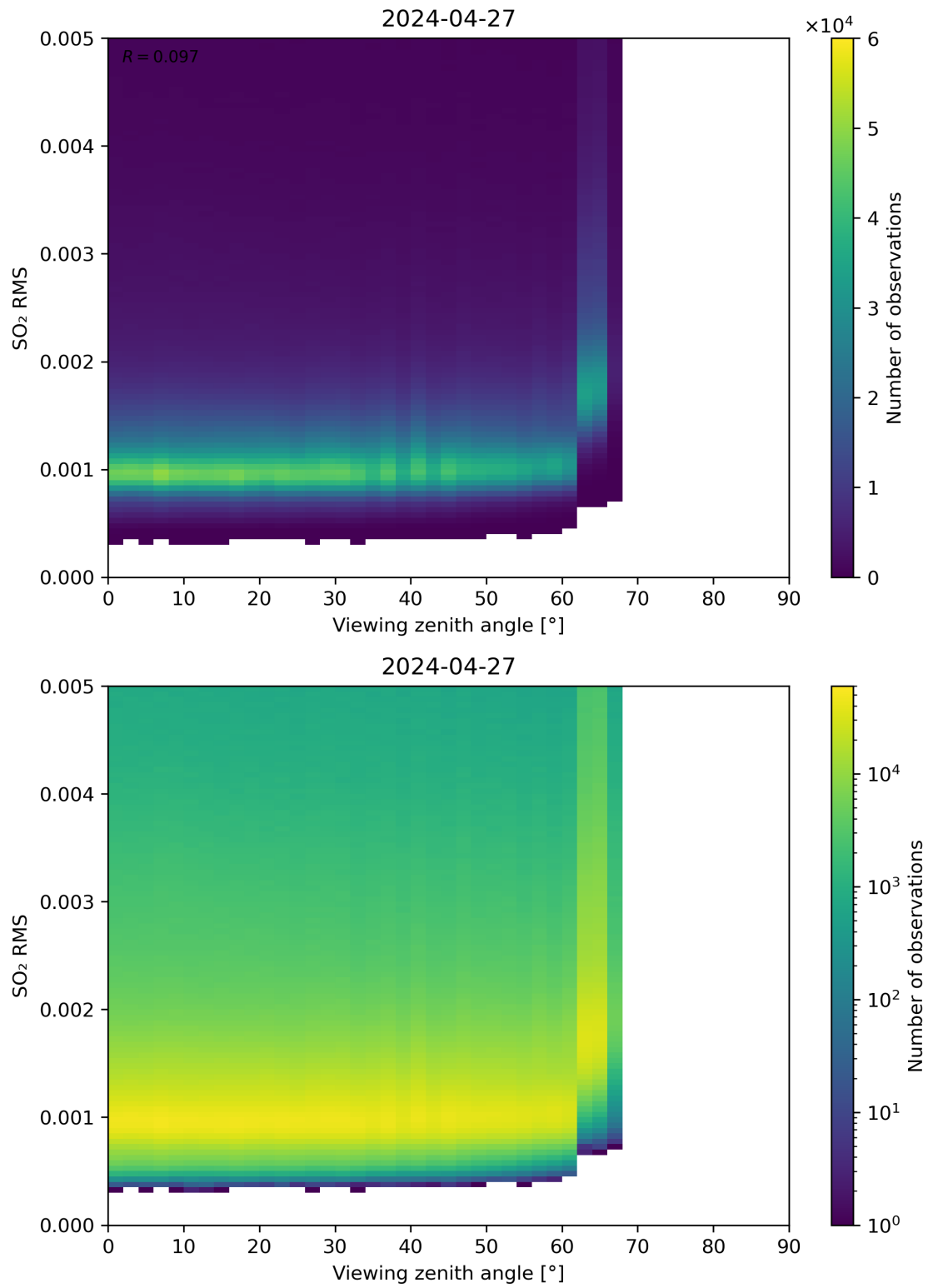
Figure 313: Scatter density plot of “Viewing zenith angle” against “SO 2 RMS” for 2024-04-26 to 2024-04-28.
