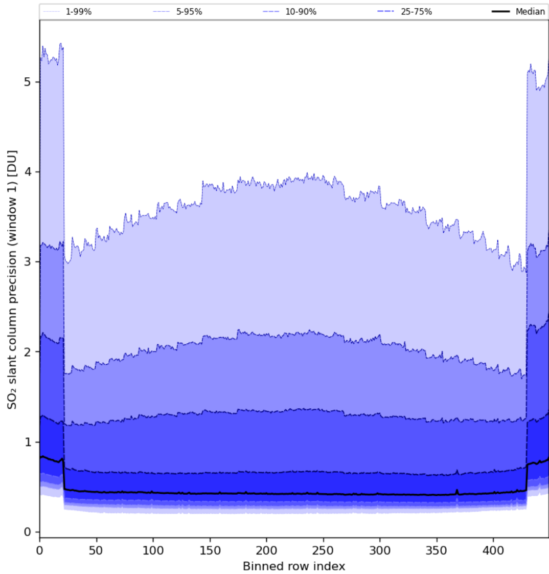
Figure 80: Along track statistics of “SO 2 slant column precision (window 1)” for 2024-04-26 to 2024-04-28
