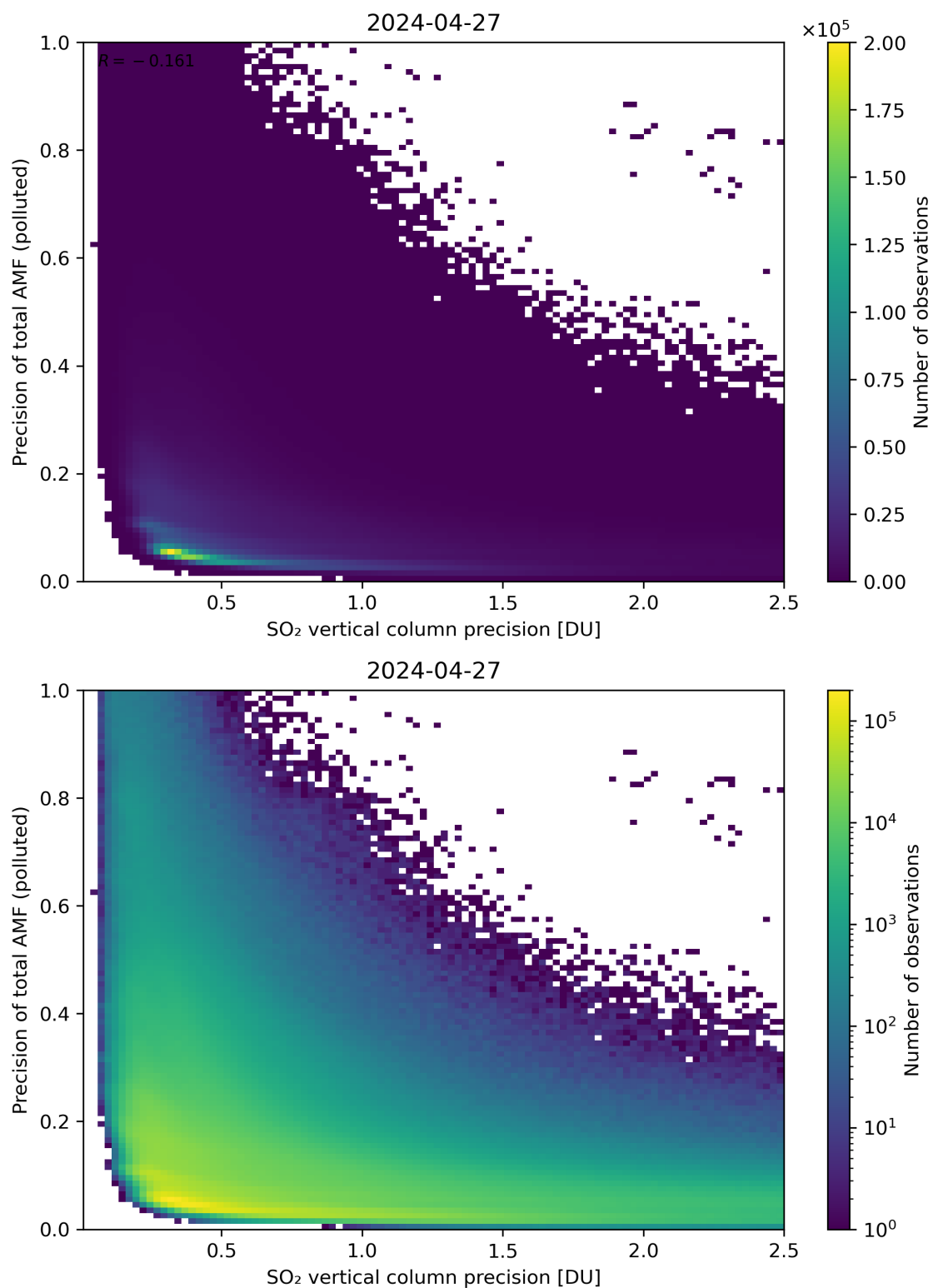
Figure 295: Scatter density plot of “SO 2 vertical column precision” against “Precision of total AMF (polluted)” for 2024-04-26 to 2024-04-28.
