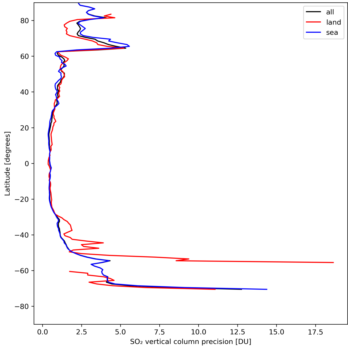
Figure 31: Zonal average of “SO 2 vertical column precision” for 2024-04-26 to 2024-04-28.
