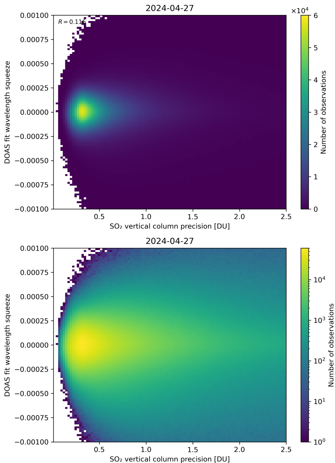
Figure 283: Scatter density plot of “SO 2 vertical column precision” against “DOAS fit wavelength squeeze” for 2024-04-26 to 2024-04-28.
