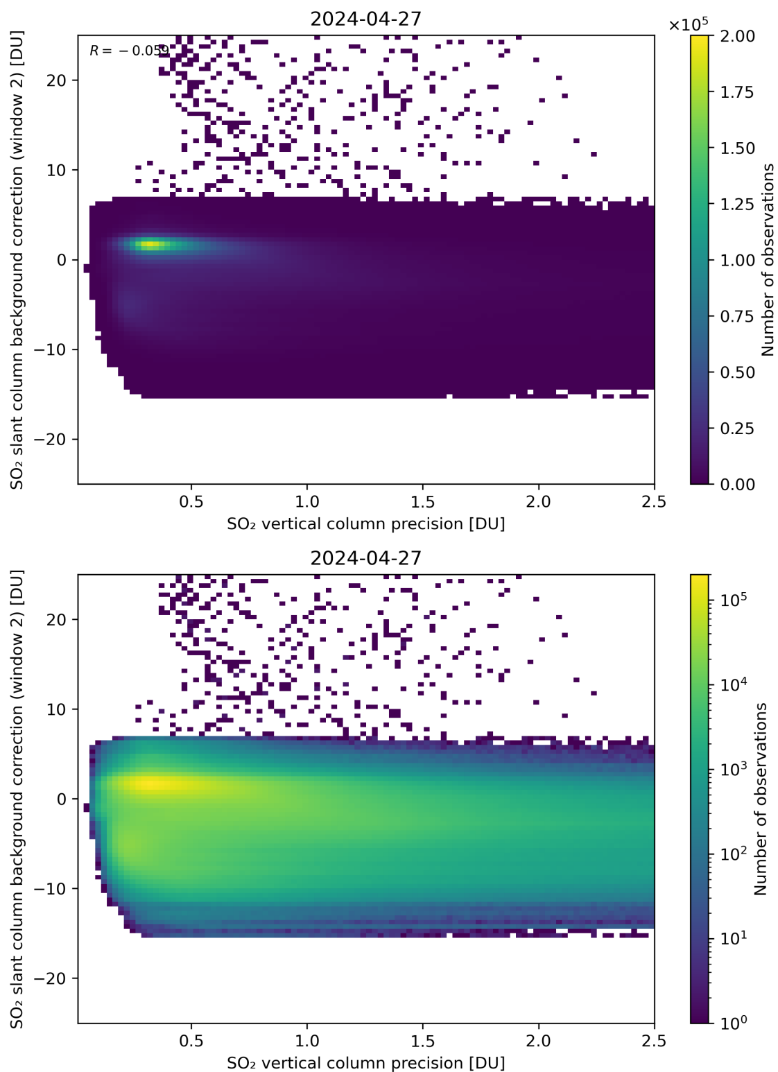
Figure 280: Scatter density plot of “SO 2 vertical column precision” against “SO 2 slant column background correction (window 2)” for 2024-04-26 to 2024-04-28.
