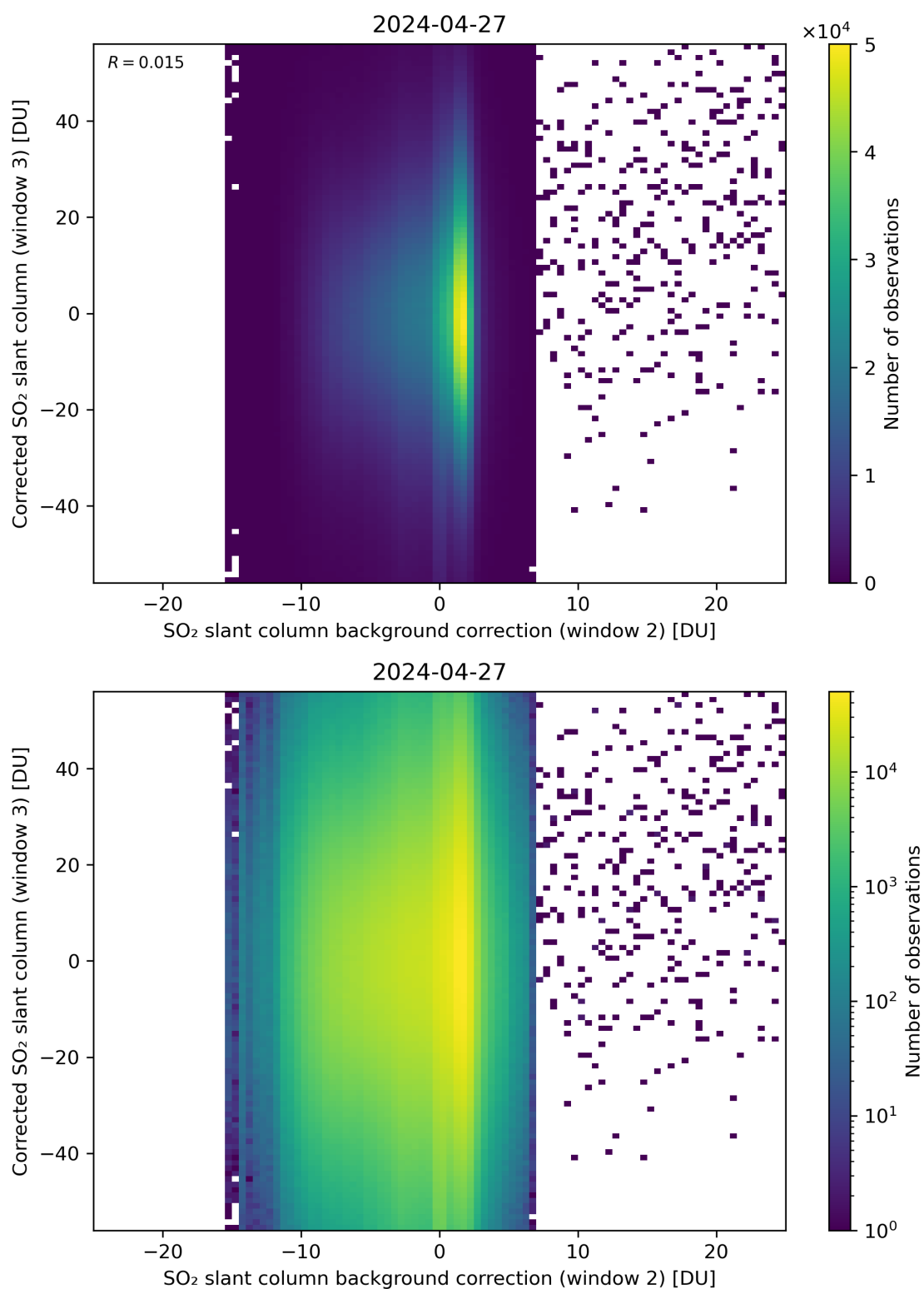
Figure 116: Scatter density plot of “SO 2 slant column background correction (window 2)” against “Corrected SO 2 slant column (window 3)” for 2024-04-26 to 2024-04-28.
