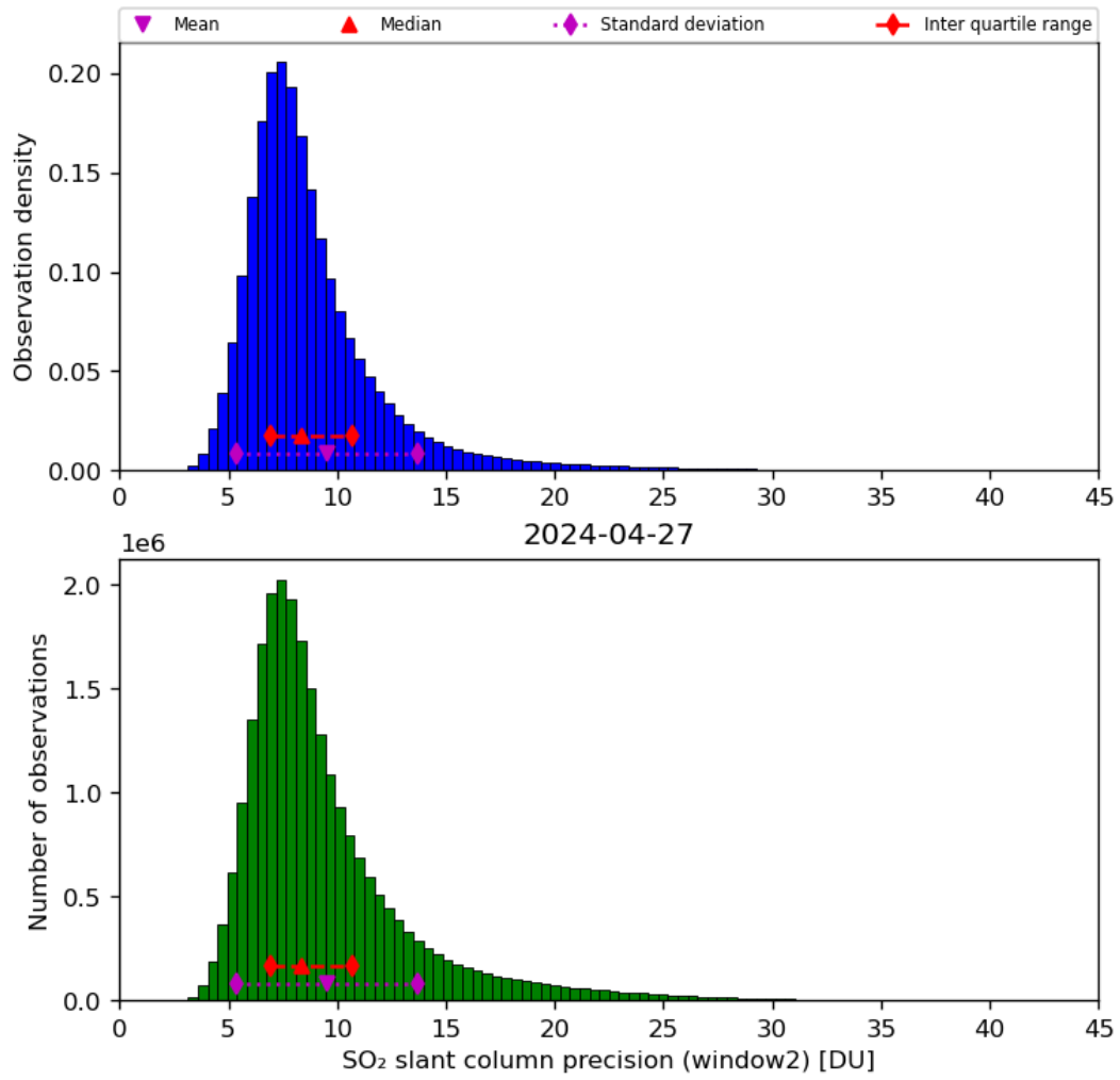
Figure 61: Histogram of “SO 2 slant column precision (window2)” for 2024-04-26 to 2024-04-28
