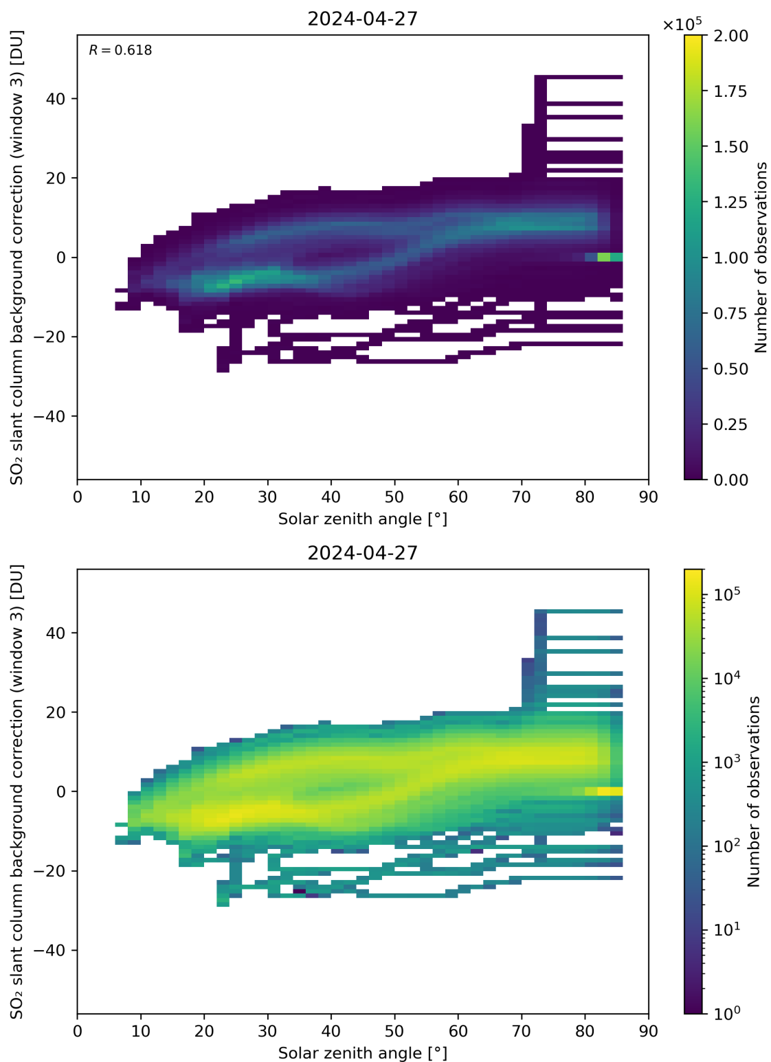
Figure 160: Scatter density plot of “Solar zenith angle” against “SO 2 slant column background correction (window 3)” for 2024-04-26 to 2024-04-28.
