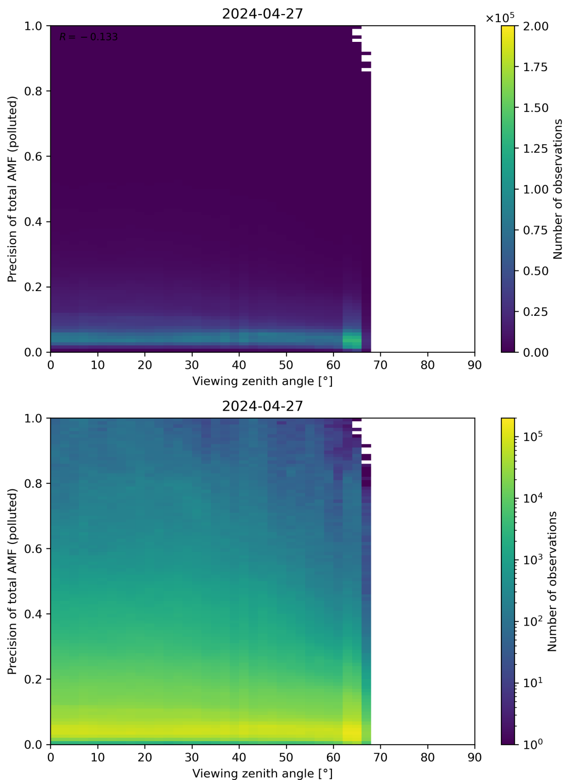
Figure 326: Scatter density plot of “Viewing zenith angle” against “Precision of total AMF (polluted)” for 2024-04-26 to 2024-04-28.
