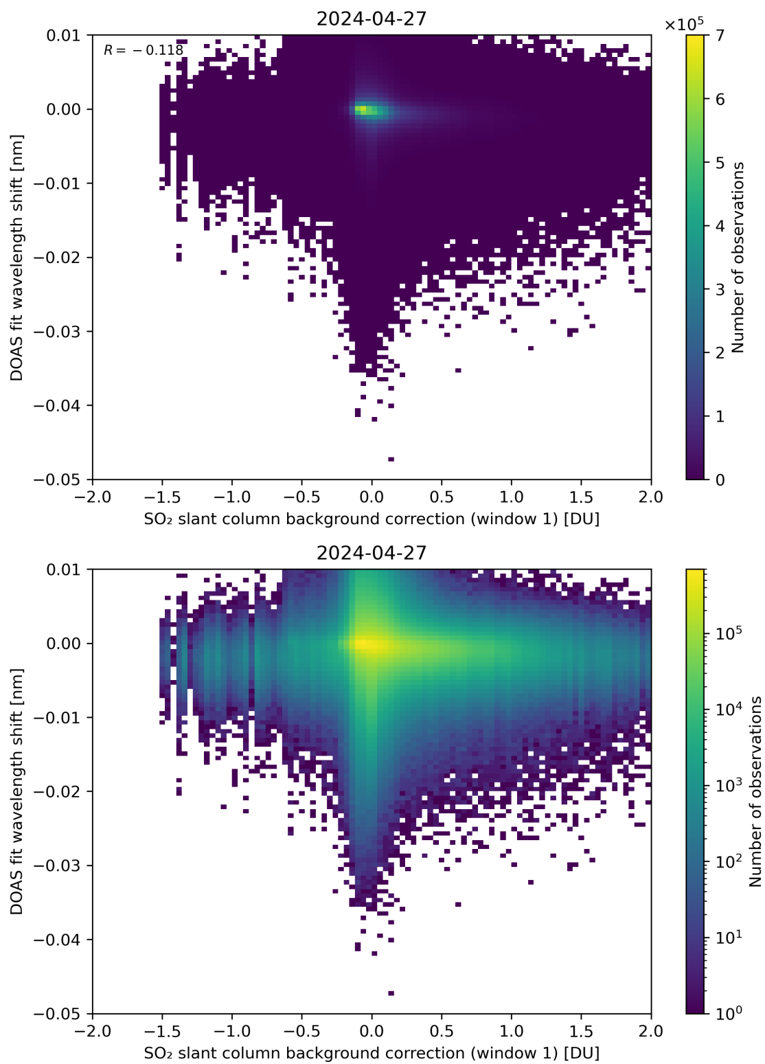
Figure 100: Scatter density plot of “SO 2 slant column background correction (window 1)” against “DOAS fit wavelength shift” for 2024-04-26 to 2024-04-28.
