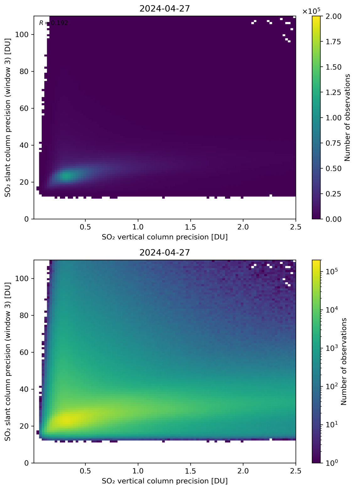
Figure 293: Scatter density plot of “SO 2 vertical column precision” against “SO 2 slant column precision (window 3)” for 2024-04-26 to 2024-04-28.
