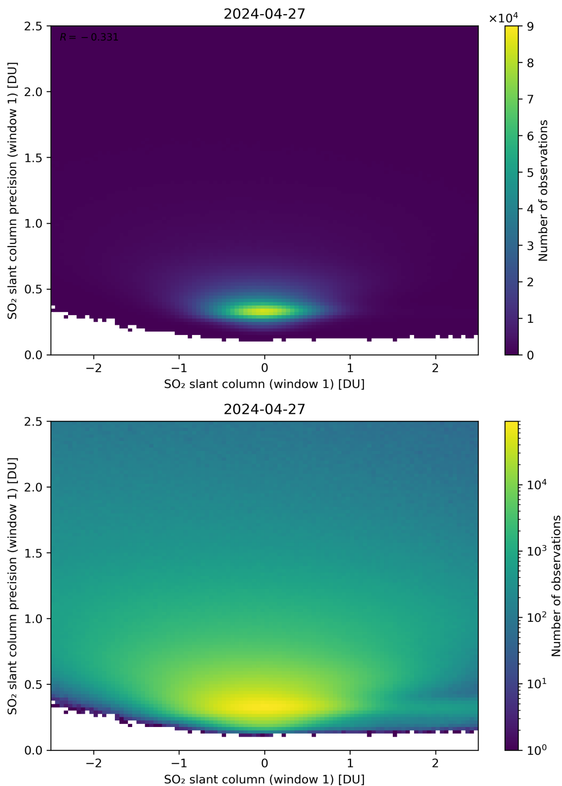
Figure 235: Scatter density plot of “SO 2 slant column (window 1)” against “SO 2 slant column precision (window 1)” for 2024-04-26 to 2024-04-28.
