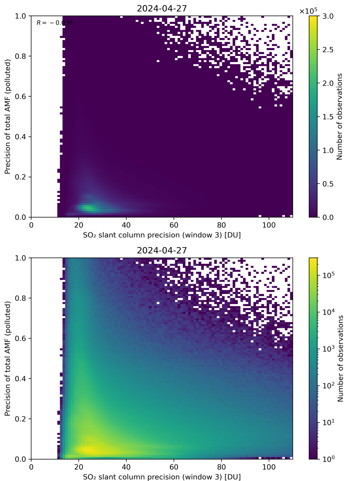
Figure 264: Scatter density plot of “SO 2 slant column precision (window 3)” against “Precision of total AMF (polluted)” for 2024-04-26 to 2024-04-28.
