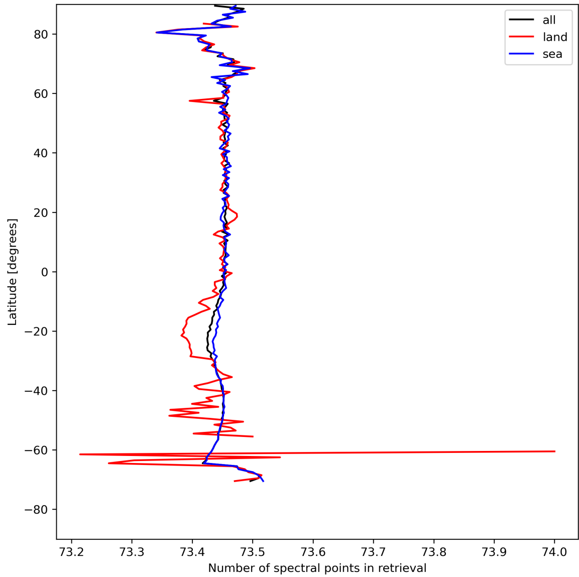
Figure 51: Zonal average of “Number of spectral points in retrieval” for 2024-04-26 to 2024-04-28.
