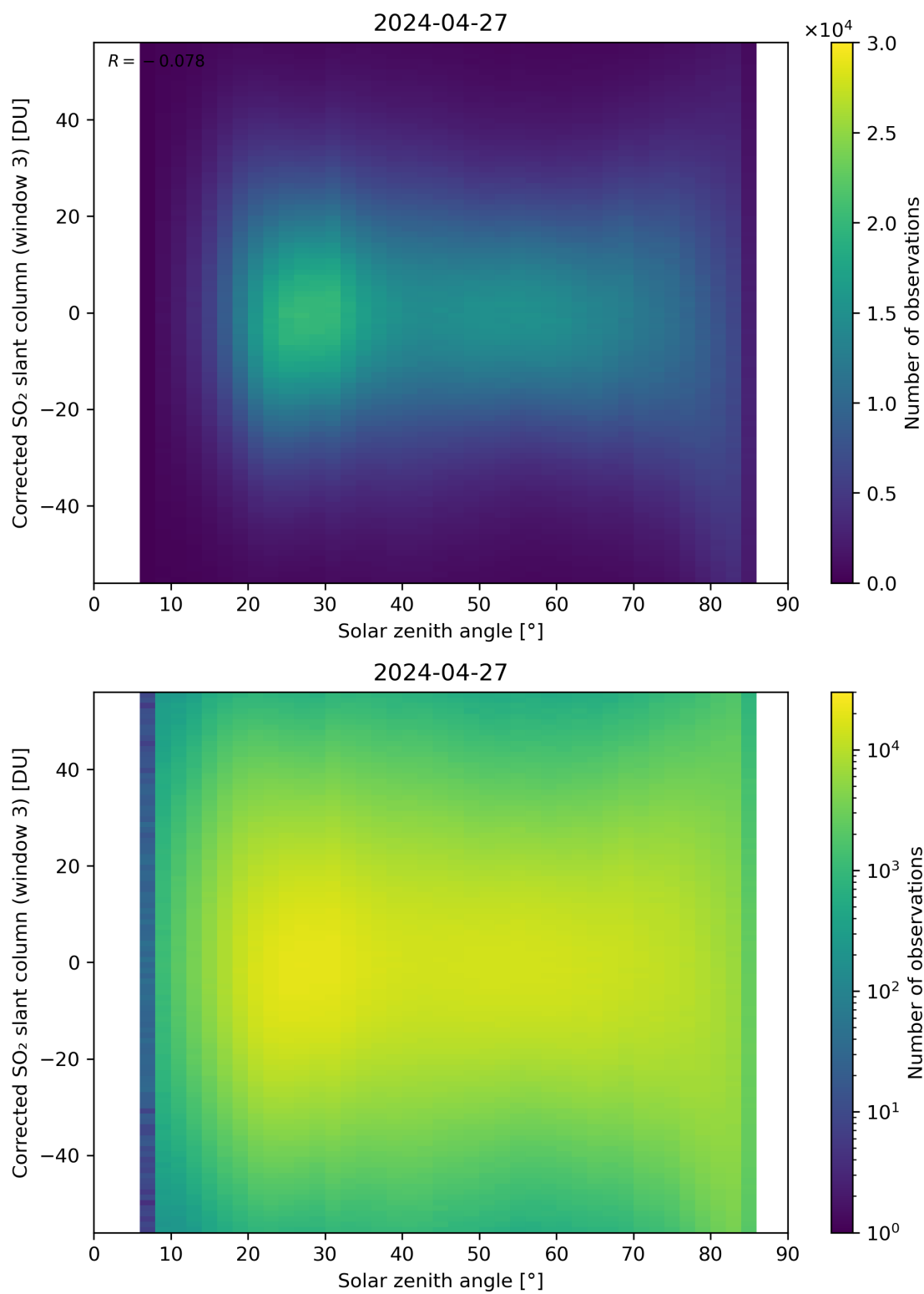
Figure 168: Scatter density plot of “Solar zenith angle” against “Corrected SO 2 slant column (window 3)” for 2024-04-26 to 2024-04-28.
