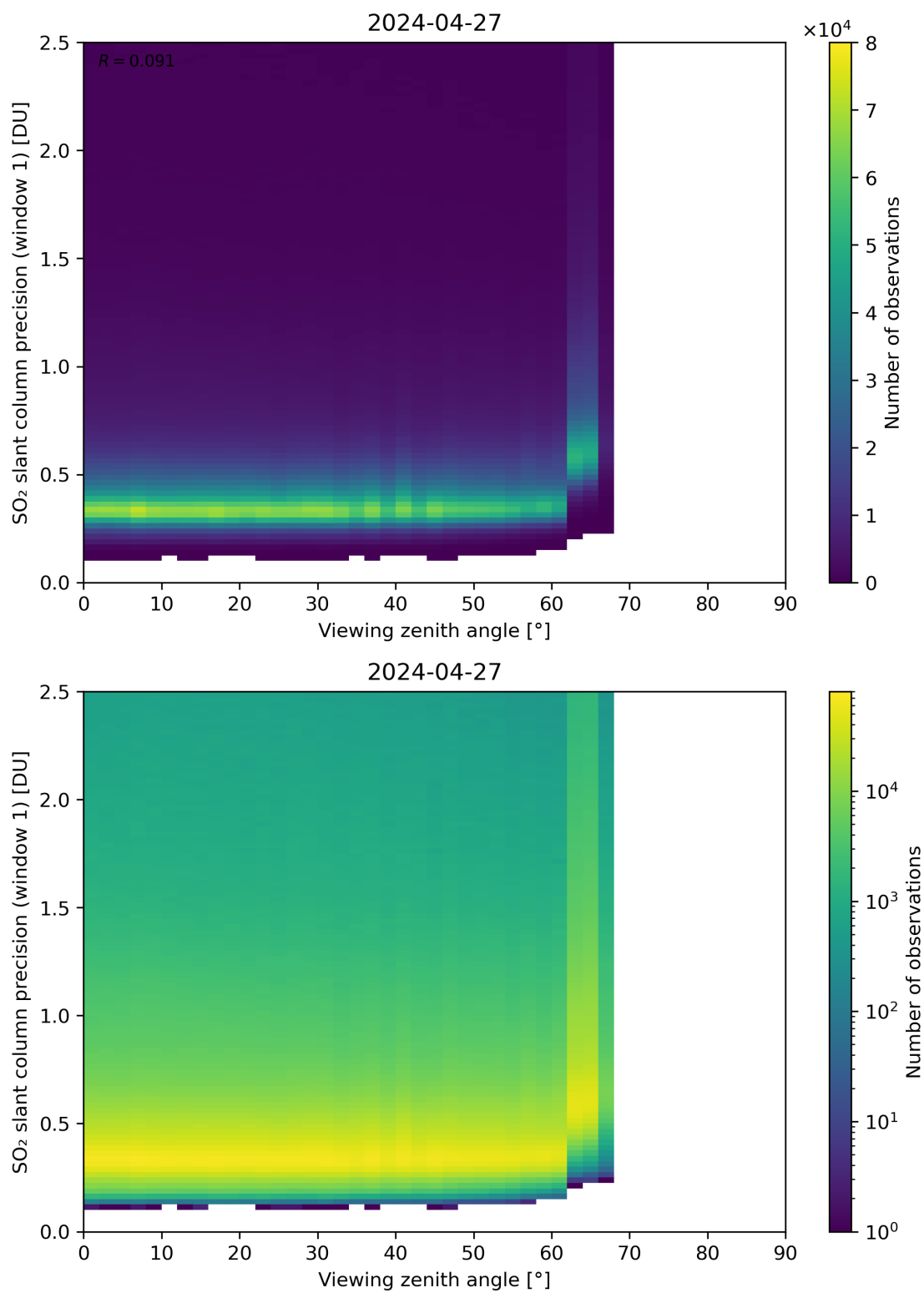
Figure 321: Scatter density plot of “Viewing zenith angle” against “SO 2 slant column precision (window 1)” for 2024-04-26 to 2024-04-28.
