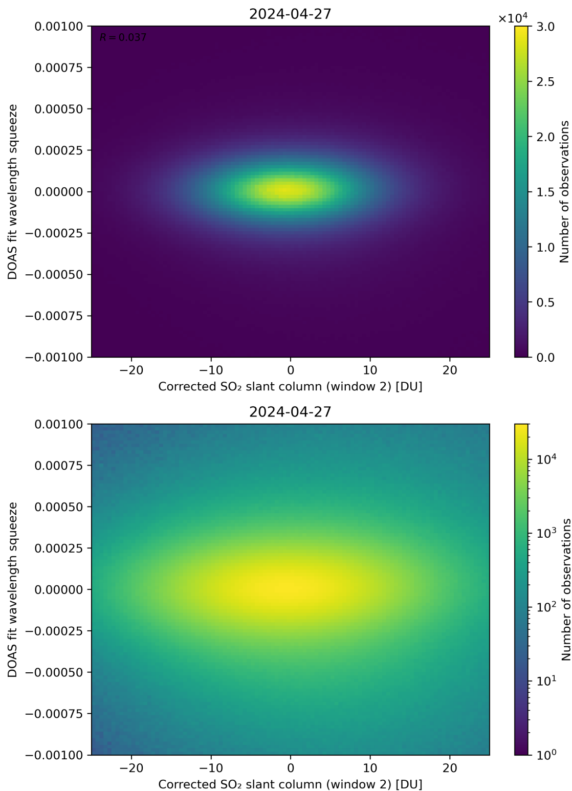
Figure 197: Scatter density plot of “Corrected SO 2 slant column (window 2)” against “DOAS fit wavelength squeeze” for 2024-04-26 to 2024-04-28.
