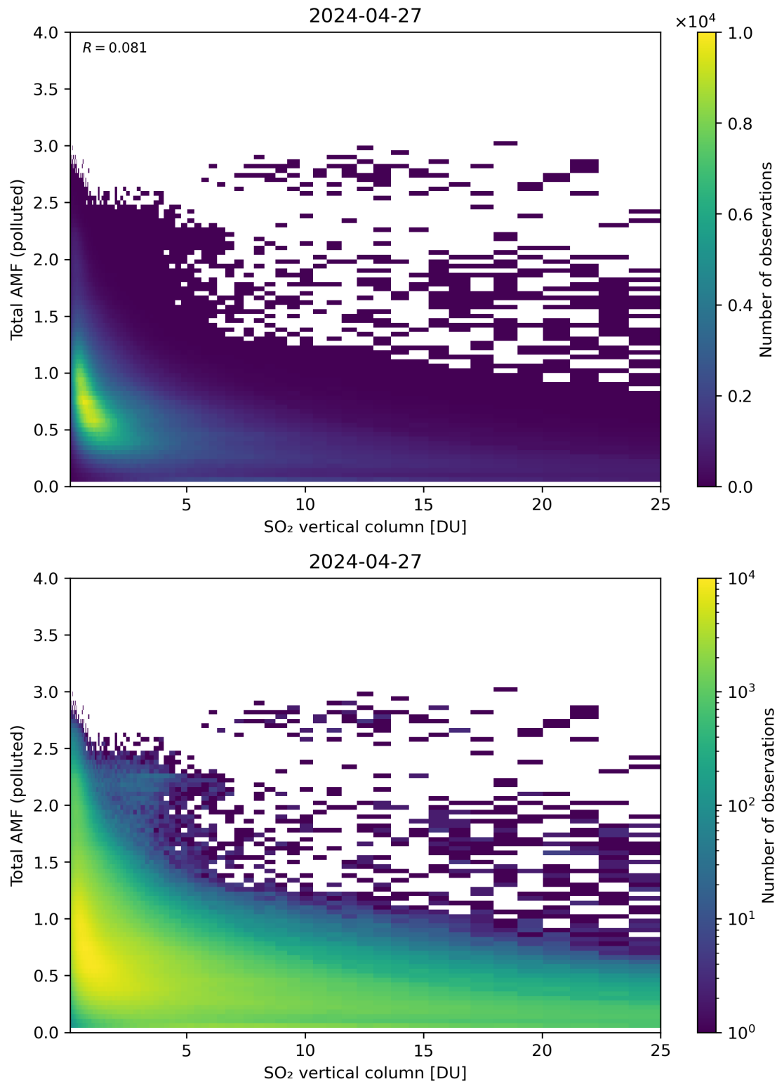
Figure 305: Scatter density plot of “SO 2 vertical column” against “Total AMF (polluted)” for 2024-04-26 to 2024-04-28.
