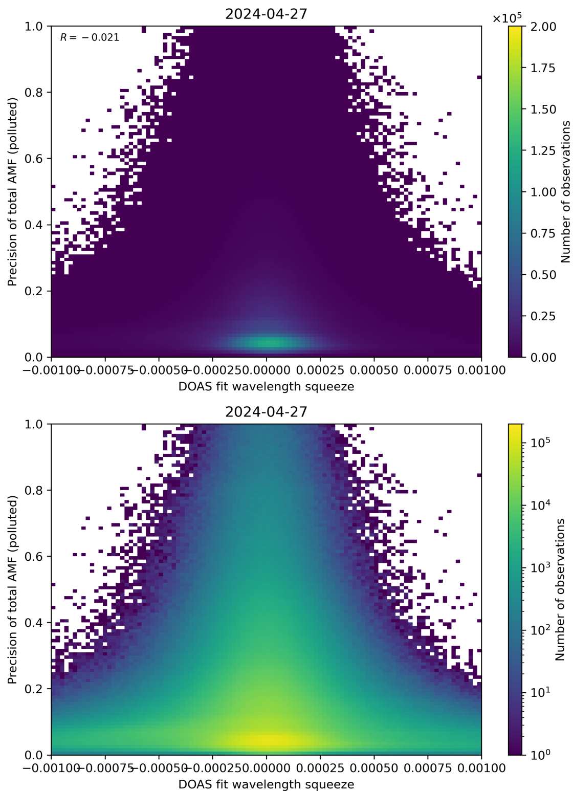
Figure 135: Scatter density plot of “DOAS fit wavelength squeeze” against “Precision of total AMF (polluted)” for 2024-04-26 to 2024-04-28.
