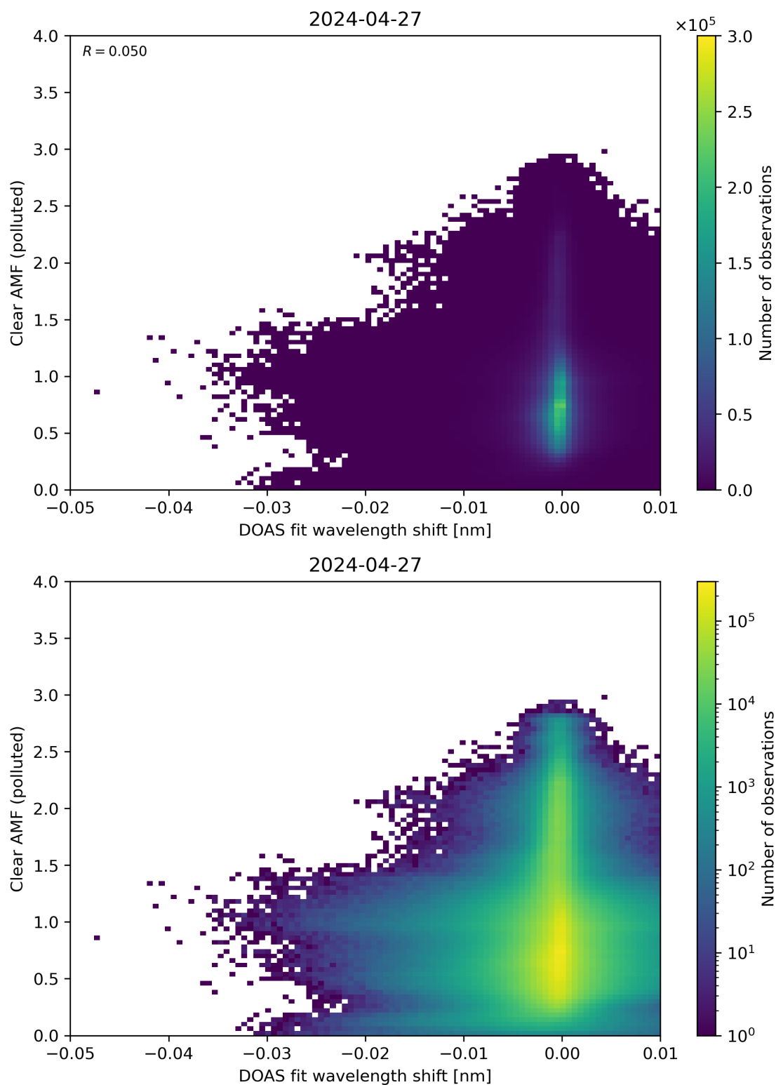
Figure 129: Scatter density plot of “DOAS fit wavelength shift” against “Clear AMF (polluted)” for 2024-04-26 to 2024-04-28.
