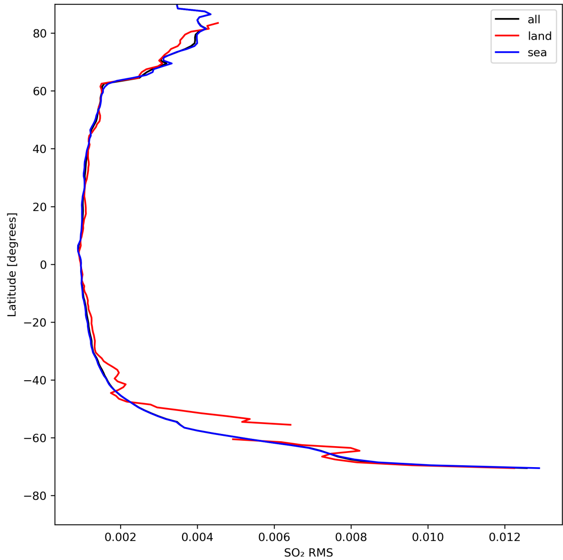
Figure 47: Zonal average of “SO 2 RMS” for 2024-04-26 to 2024-04-28.
