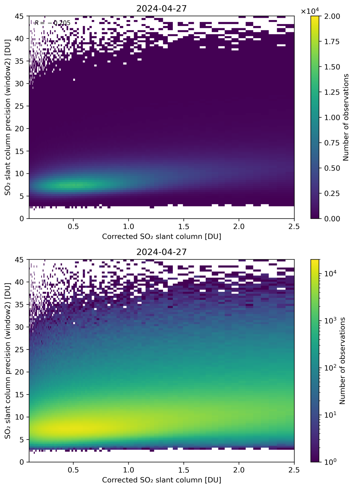
Figure 189: Scatter density plot of “Corrected SO 2 slant column” against “SO 2 slant column precision (window2)” for 2024-04-26 to 2024-04-28.
