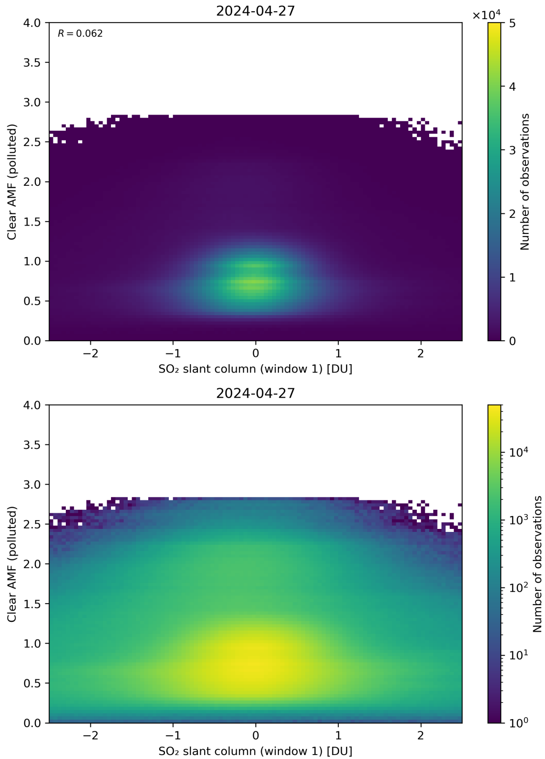
Figure 232: Scatter density plot of “SO 2 slant column (window 1)” against “Clear AMF (polluted)” for 2024-04-26 to 2024-04-28.
