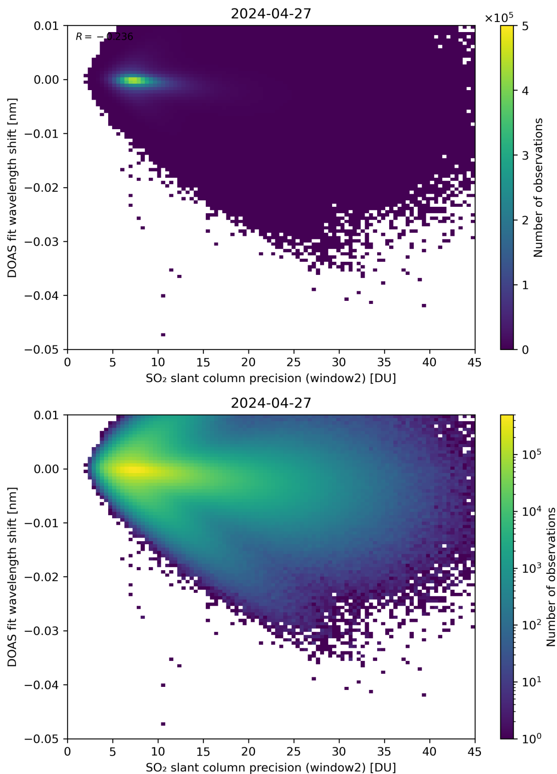
Figure 243: Scatter density plot of “SO 2 slant column precision (window2)” against “DOAS fit wavelength shift” for 2024-04-26 to 2024-04-28.
