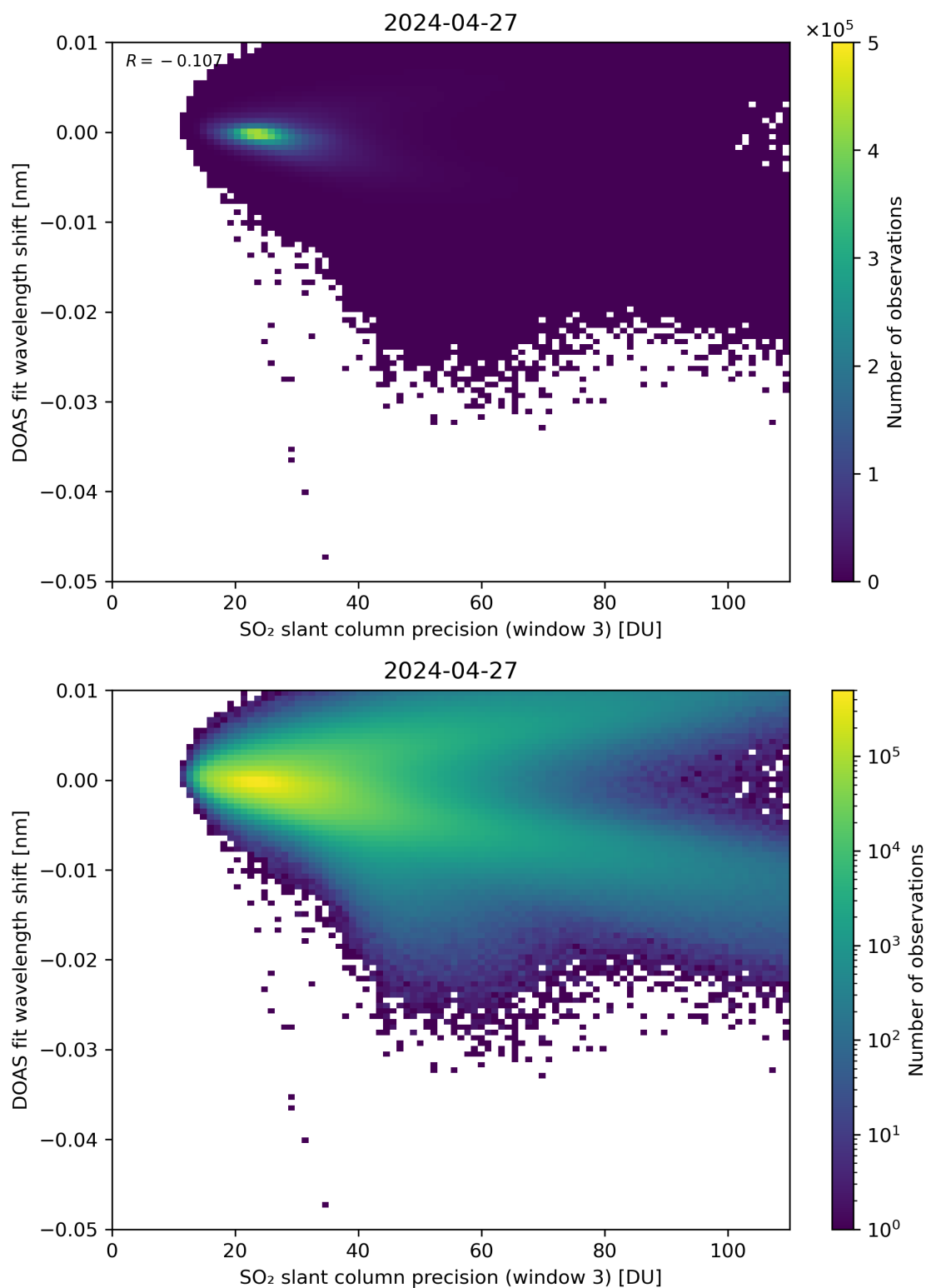
Figure 258: Scatter density plot of “SO 2 slant column precision (window 3)” against “DOAS fit wavelength shift” for 2024-04-26 to 2024-04-28.
