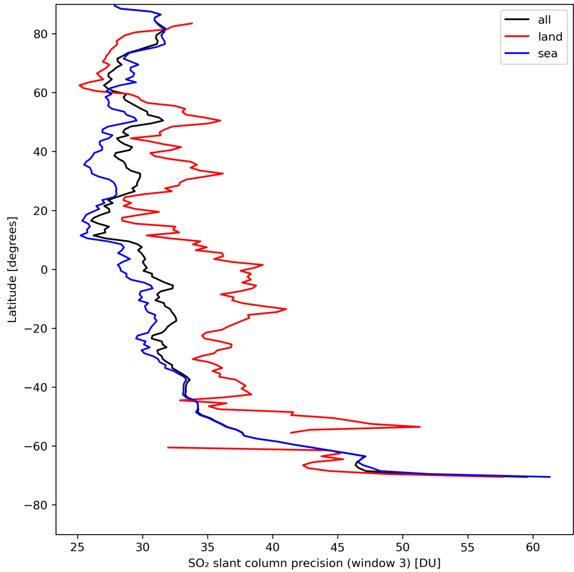
Figure 42: Zonal average of “SO 2 slant column precision (window 3)” for 2024-04-26 to 2024-04-28.
