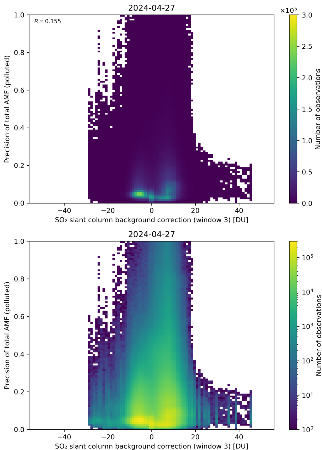
Figure 126: Scatter density plot of “SO 2 slant column background correction (window 3)” against “Precision of total AMF (polluted)” for 2024-04-26 to 2024-04-28.
