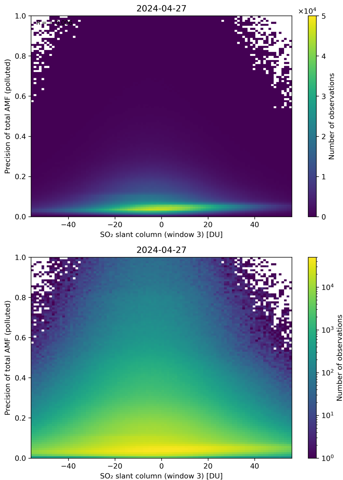
Figure 269: Scatter density plot of “SO 2 slant column (window 3)” against “Precision of total AMF (polluted)” for 2024-04-26 to 2024-04-28.
