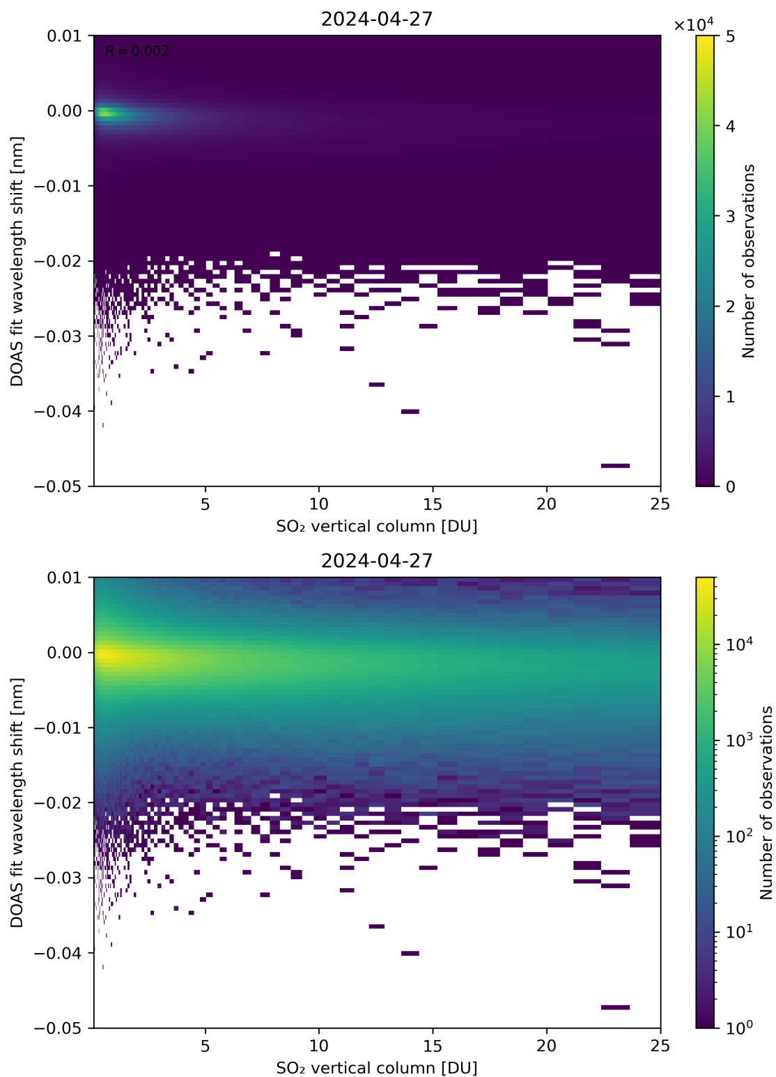
Figure 276: Scatter density plot of “SO 2 vertical column” against “DOAS fit wavelength shift” for 2024-04-26 to 2024-04-28.
