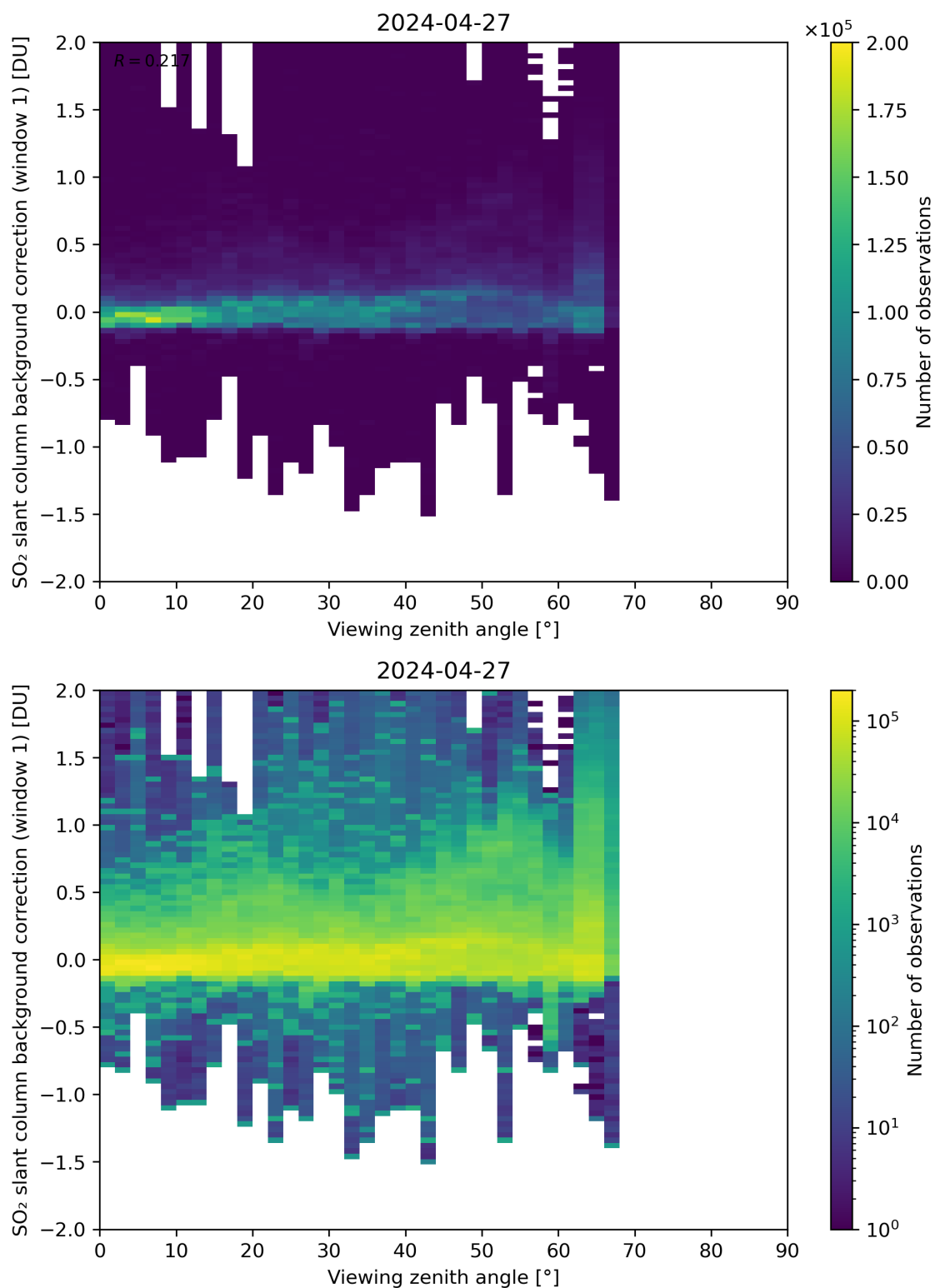
Figure 308: Scatter density plot of “Viewing zenith angle” against “SO 2 slant column background correction (window 1)” for 2024-04-26 to 2024-04-28.
