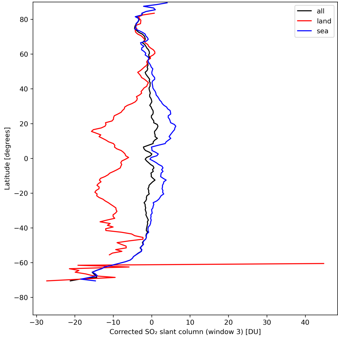
Figure 43: Zonal average of “Corrected SO 2 slant column (window 3)” for 2024-04-26 to 2024-04-28.
