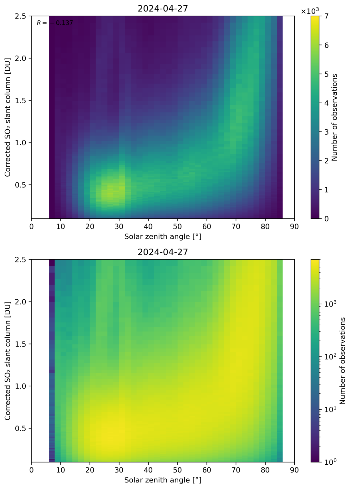
Figure 166: Scatter density plot of “Solar zenith angle” against “Corrected SO 2 slant column” for 2024-04-26 to 2024-04-28.
