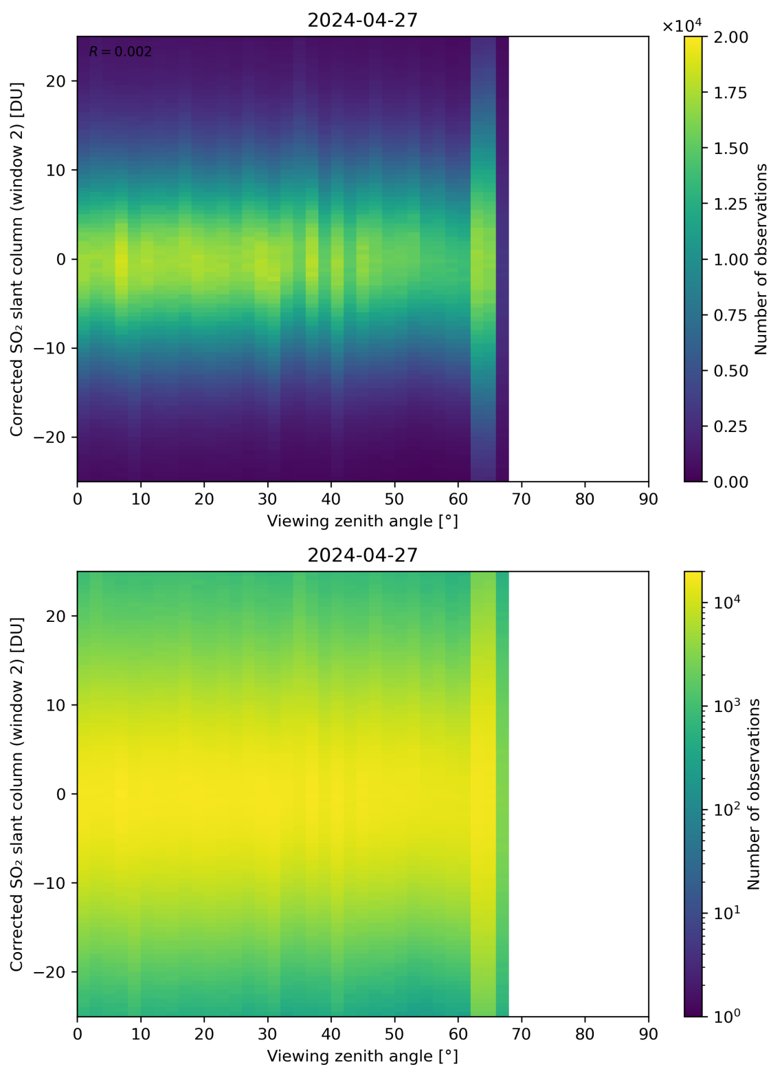
Figure 318: Scatter density plot of “Viewing zenith angle” against “Corrected SO 2 slant column (window 2)” for 2024-04-26 to 2024-04-28.
