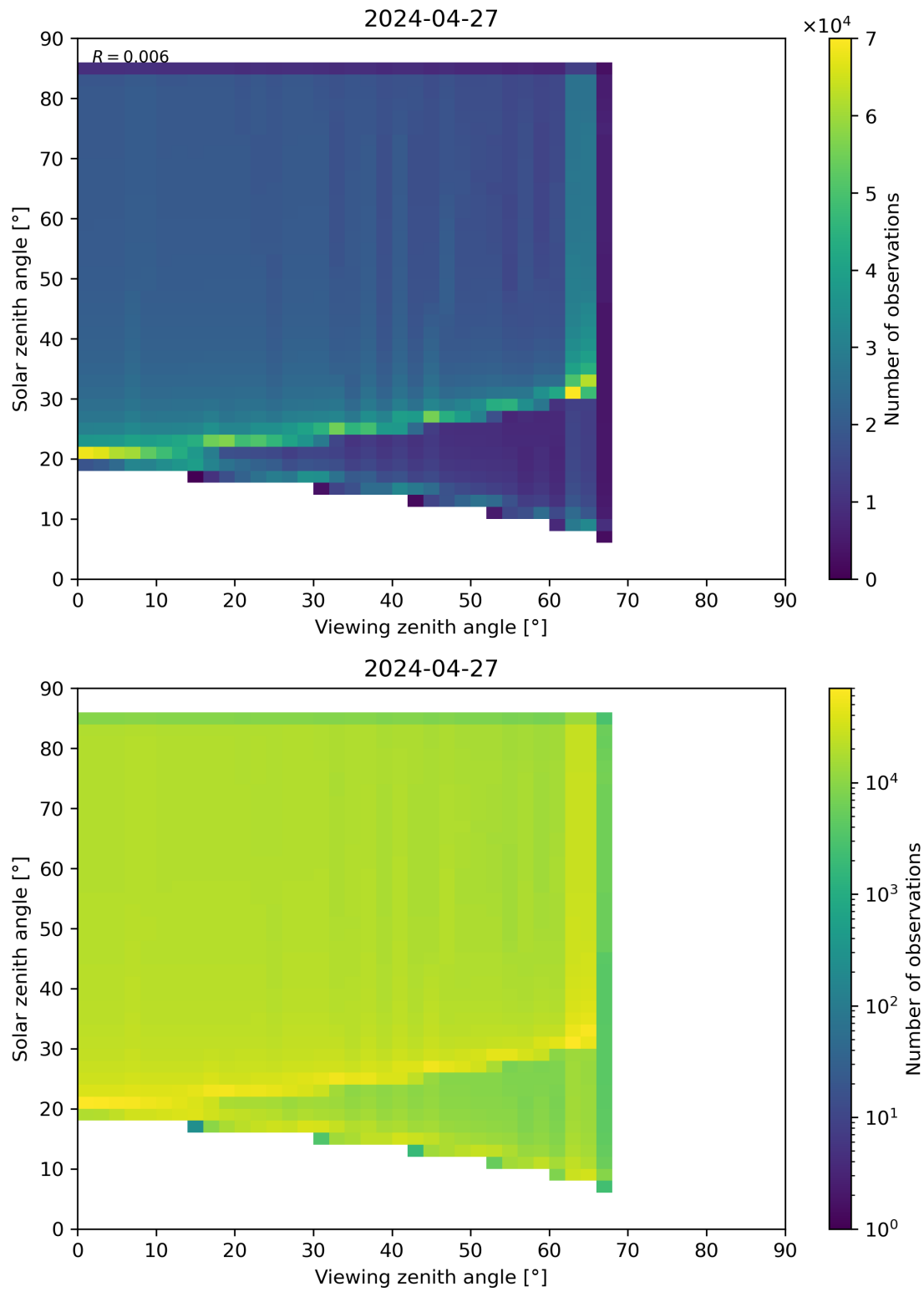
Figure 315: Scatter density plot of “Viewing zenith angle” against “Solar zenith angle” for 2024-04-26 to 2024-04-28.
