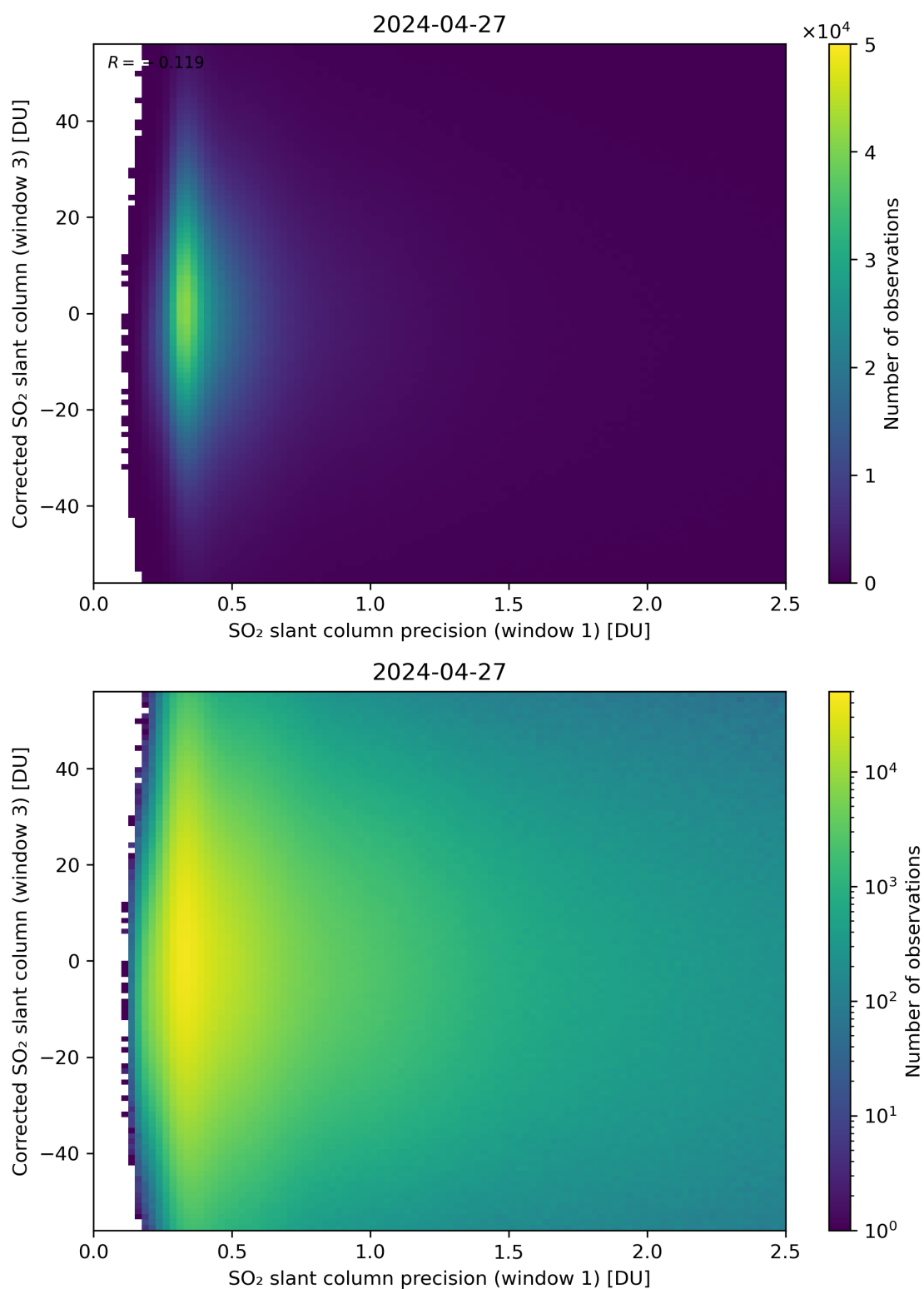
Figure 226: Scatter density plot of “SO 2 slant column precision (window 1)” against “Corrected SO 2 slant column (window 3)” for 2024-04-26 to 2024-04-28.
