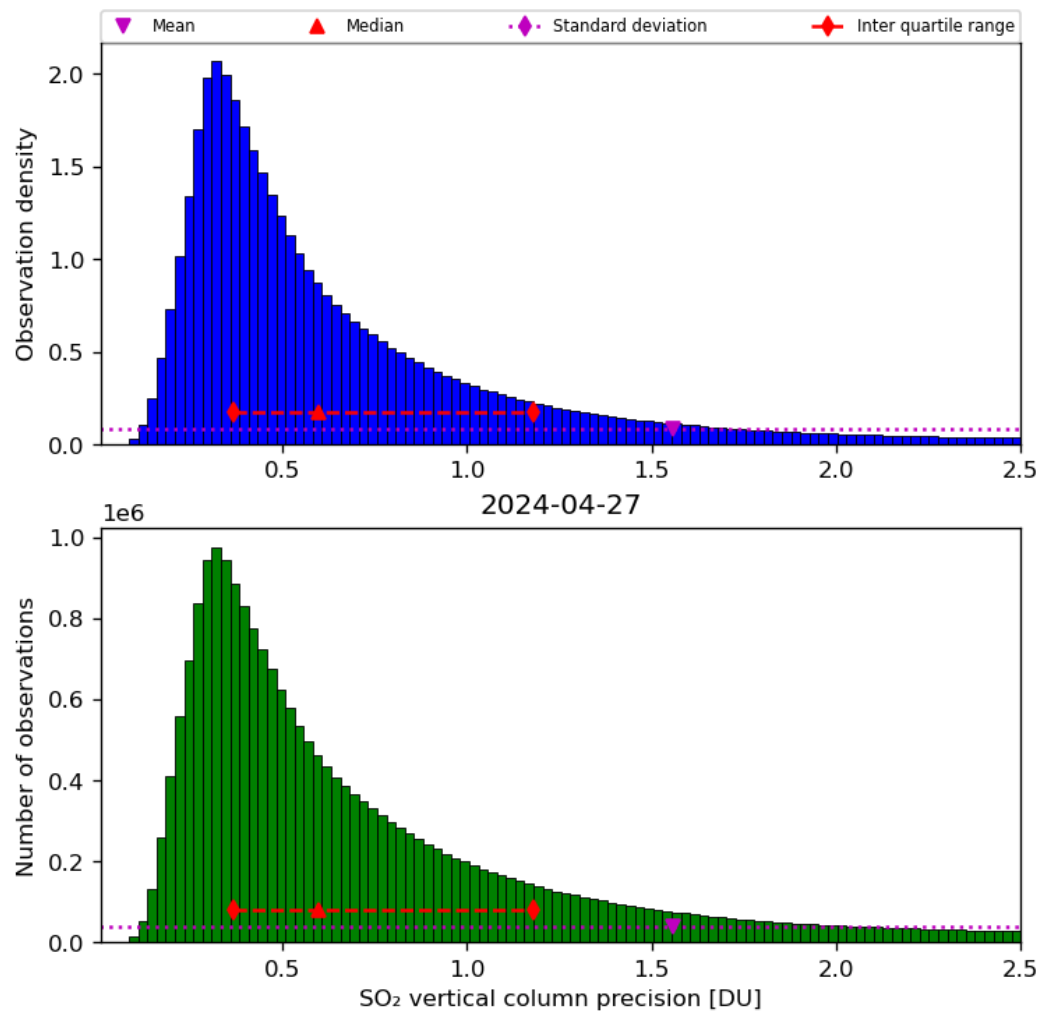
Figure 54: Histogram of “SO 2 vertical column precision” for 2024-04-26 to 2024-04-28
