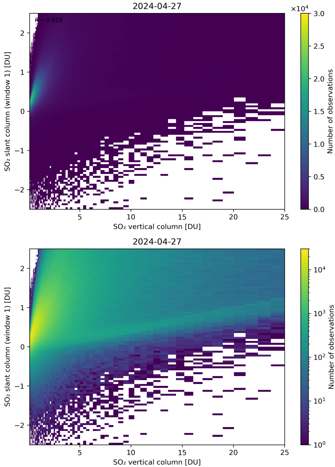
Figure 300: Scatter density plot of “SO 2 vertical column” against “SO 2 slant column (window 1)” for 2024-04-26 to 2024-04-28.
