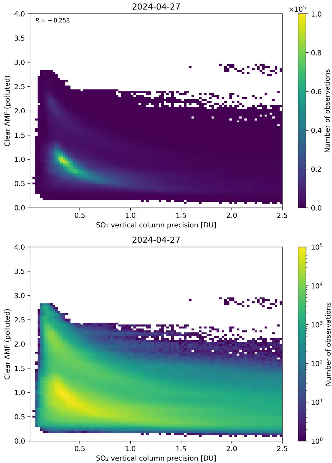
Figure 285: Scatter density plot of “SO 2 vertical column precision” against “Clear AMF (polluted)” for 2024-04-26 to 2024-04-28.
