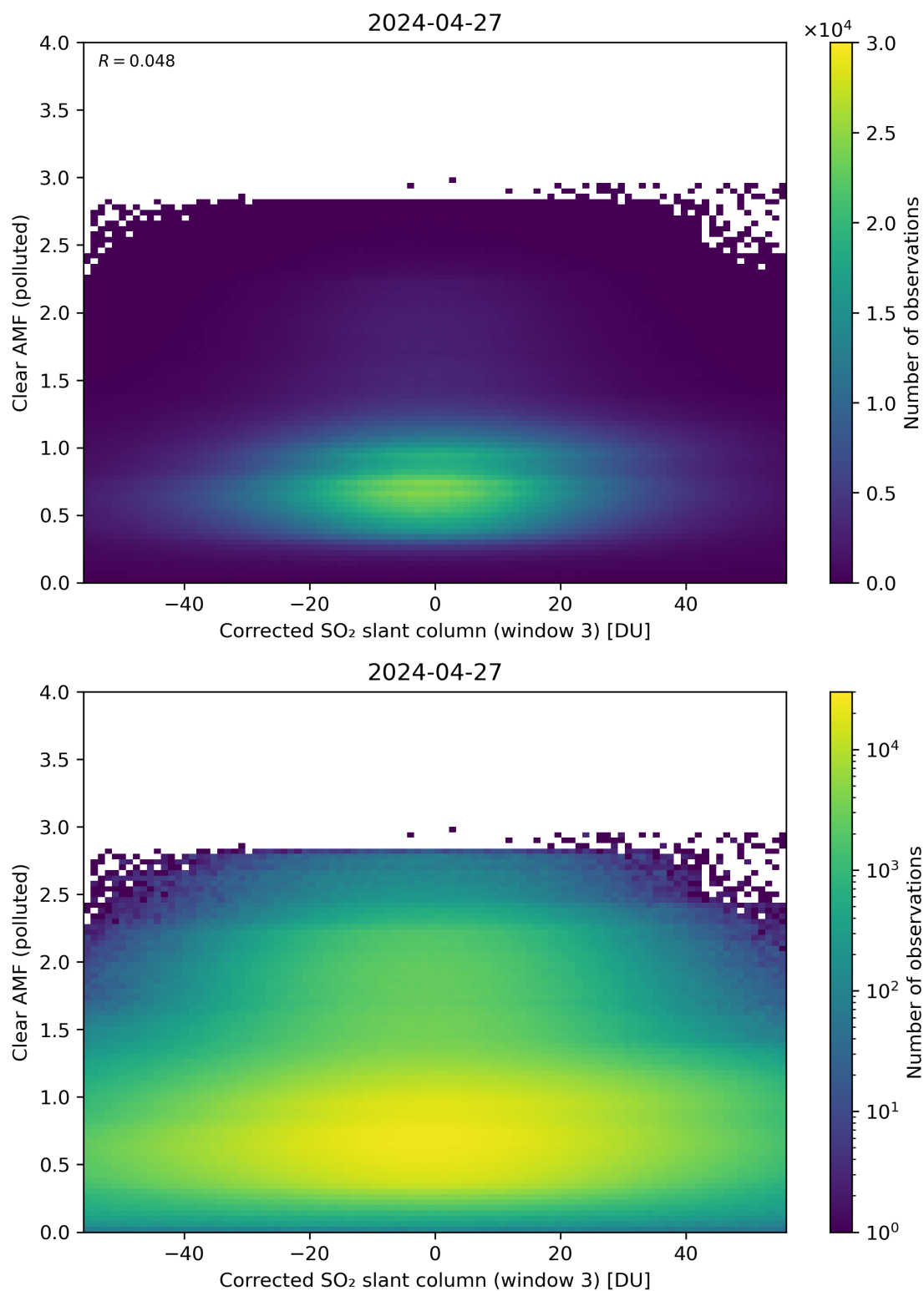
Figure 209: Scatter density plot of “Corrected SO 2 slant column (window 3)” against “Clear AMF (polluted)” for 2024-04-26 to 2024-04-28.
