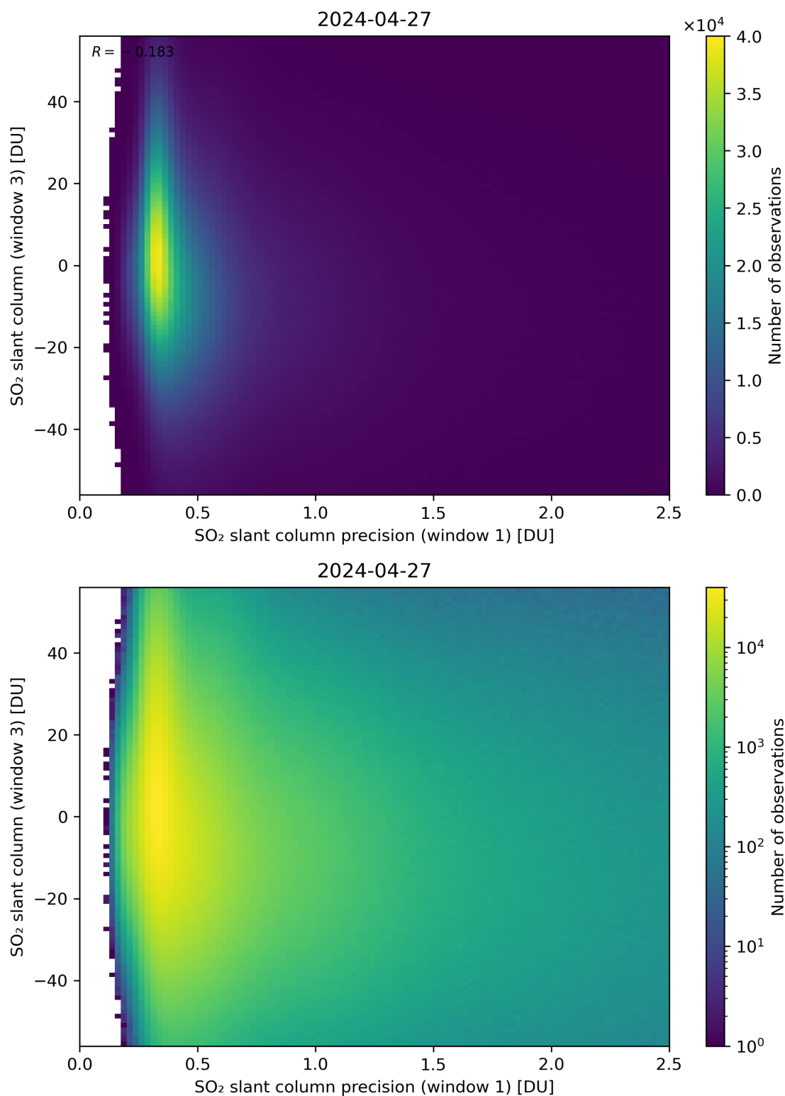
Figure 228: Scatter density plot of “SO 2 slant column precision (window 1)” against “SO 2 slant column (window 3)” for 2024-04-26 to 2024-04-28.
