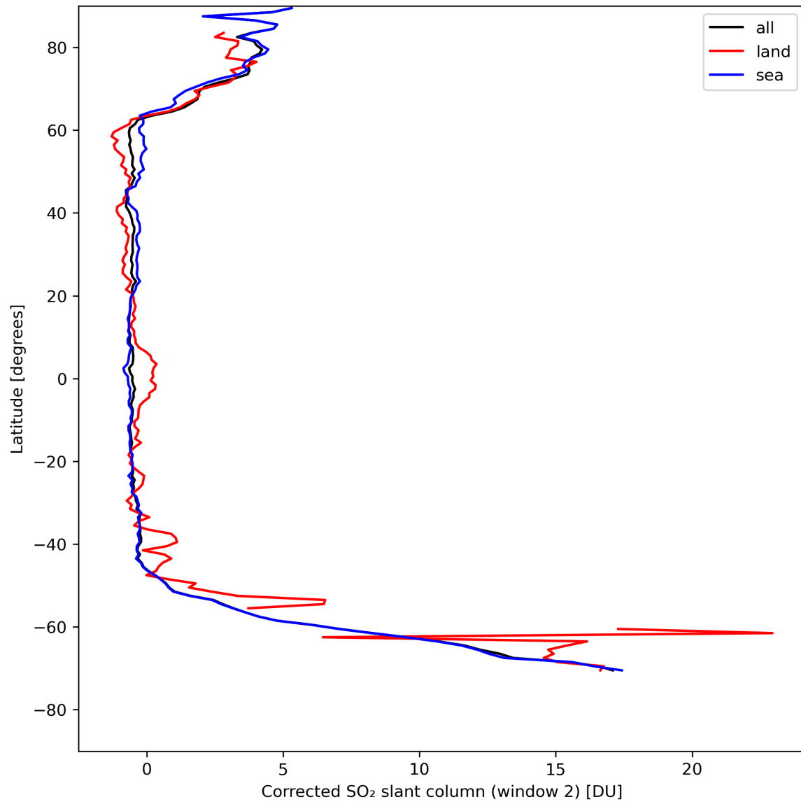
Figure 39: Zonal average of “Corrected SO 2 slant column (window 2)” for 2024-04-26 to 2024-04-28.
