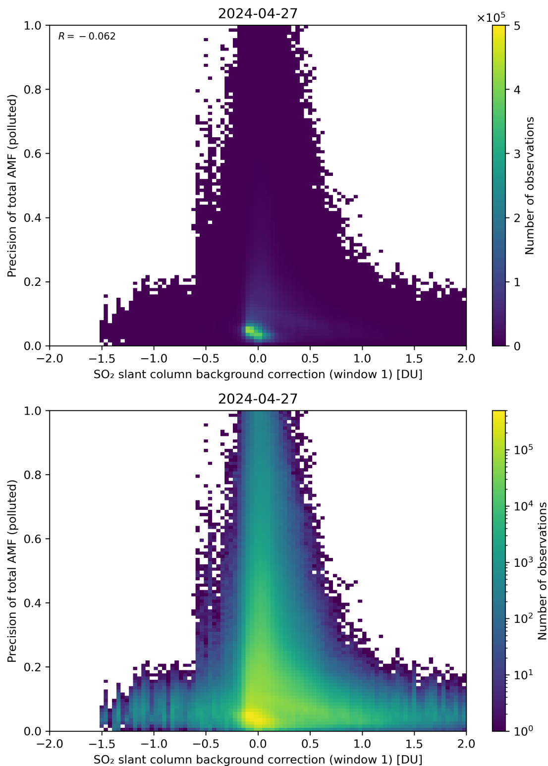
Figure 110: Scatter density plot of “SO 2 slant column background correction (window 1)” against “Precision of total AMF (polluted)” for 2024-04-26 to 2024-04-28.
