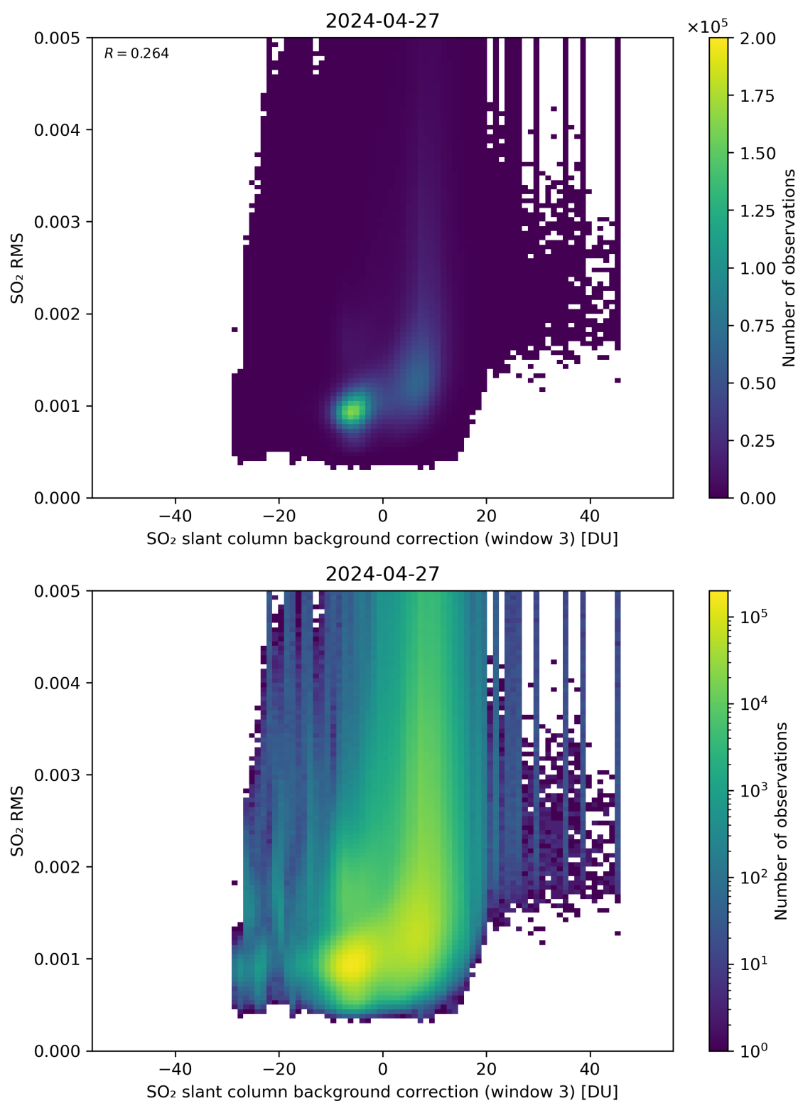
Figure 123: Scatter density plot of “SO 2 slant column background correction (window 3)” against “SO 2 RMS” for 2024-04-26 to 2024-04-28.
