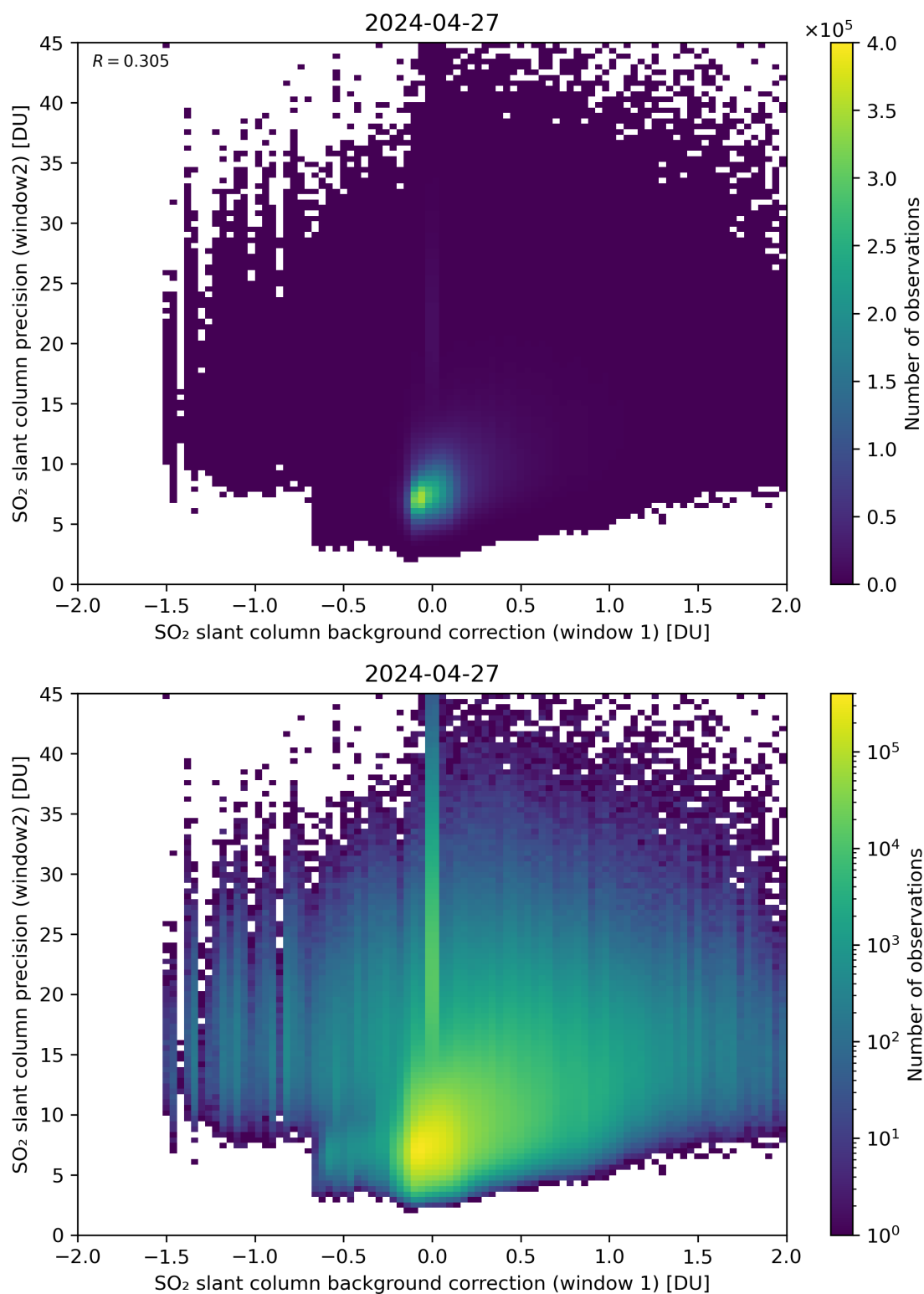
Figure 106: Scatter density plot of “SO 2 slant column background correction (window 1)” against “SO 2 slant column precision (window2)” for 2024-04-26 to 2024-04-28.
