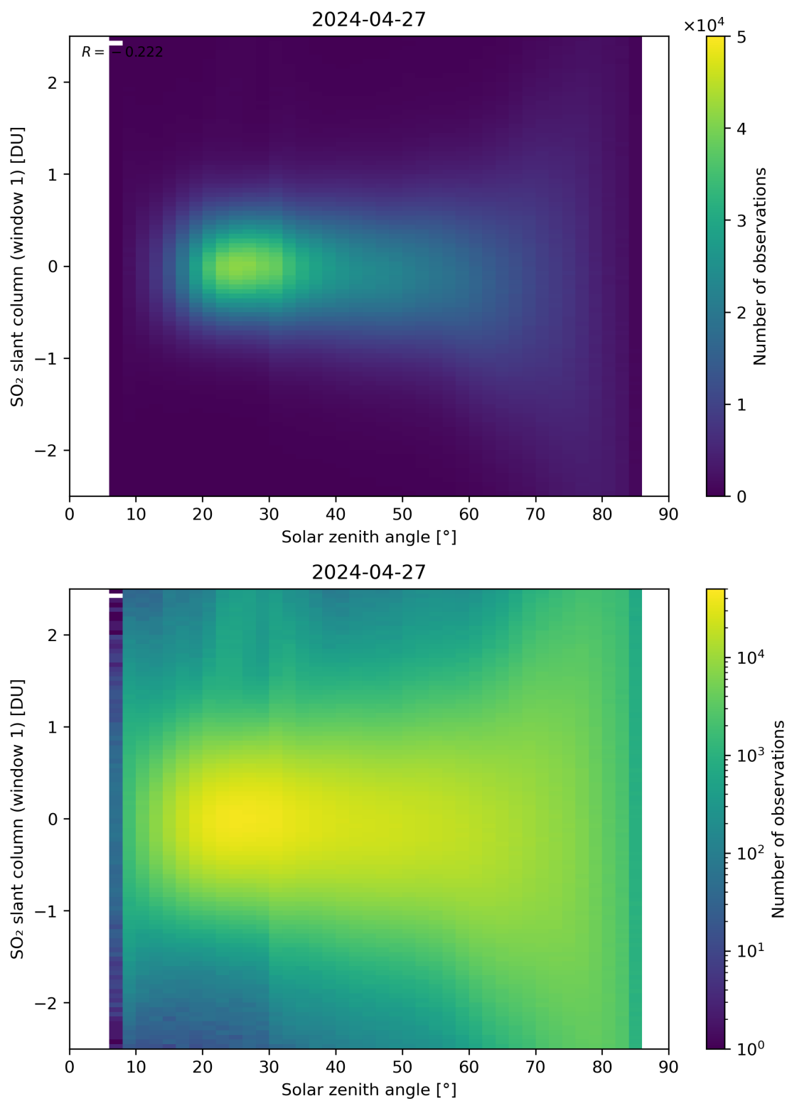
Figure 169: Scatter density plot of “Solar zenith angle” against “SO 2 slant column (window 1)” for 2024-04-26 to 2024-04-28.
