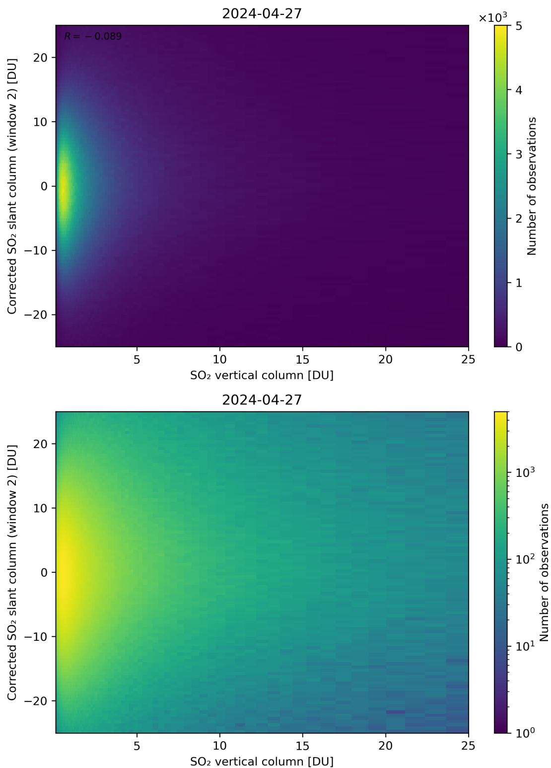
Figure 298: Scatter density plot of “SO 2 vertical column” against “Corrected SO 2 slant column (window 2)” for 2024-04-26 to 2024-04-28.
