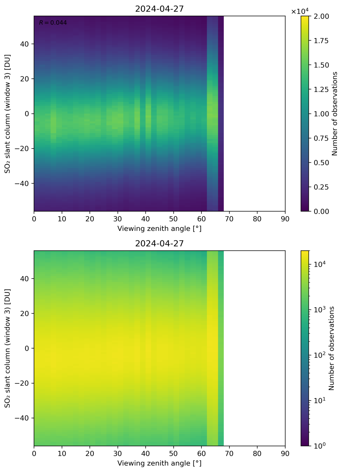
Figure 323: Scatter density plot of “Viewing zenith angle” against “SO 2 slant column (window 3)” for 2024-04-26 to 2024-04-28.
