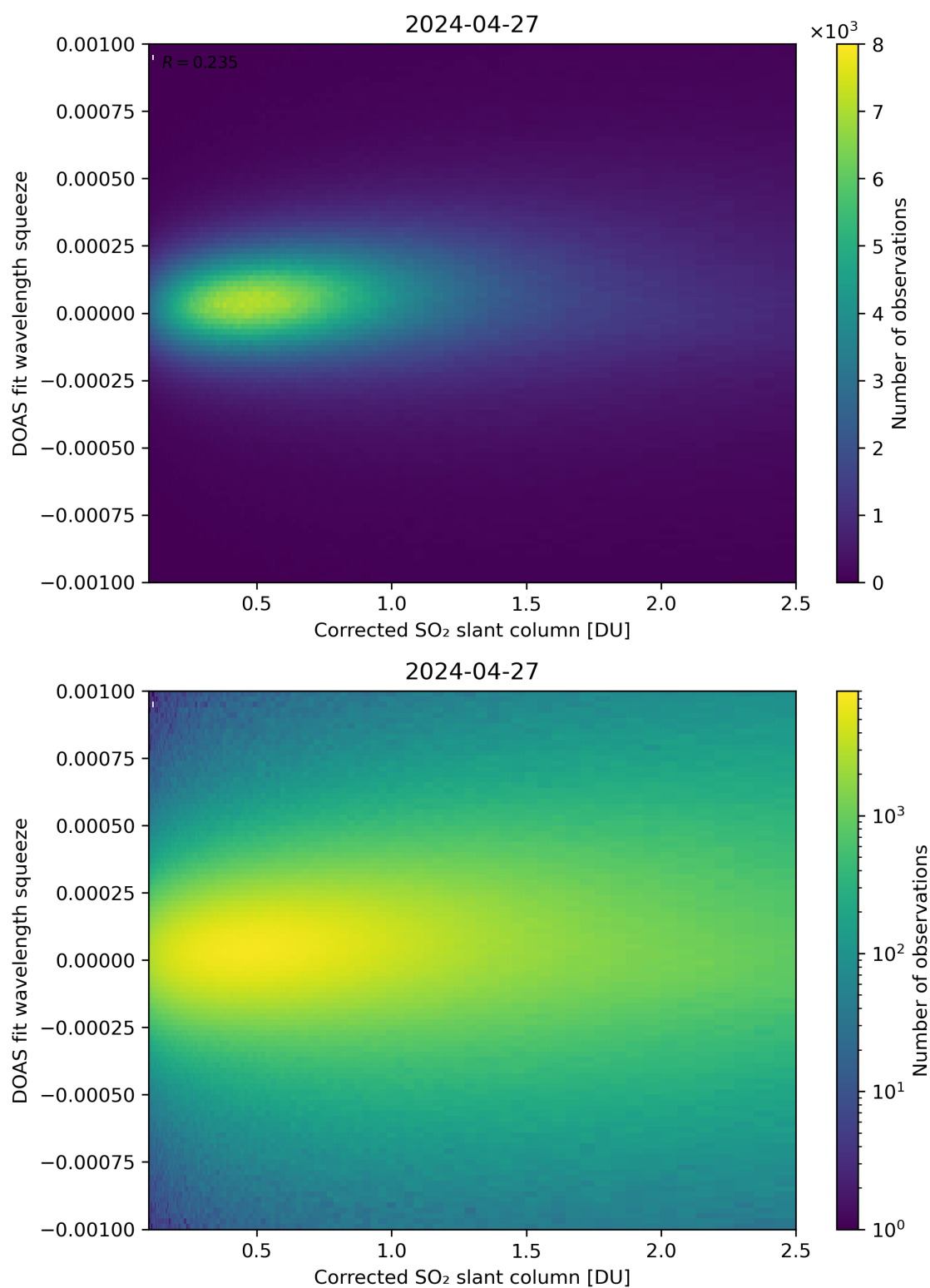
Figure 182: Scatter density plot of “Corrected SO 2 slant column” against “DOAS fit wavelength squeeze” for 2024-04-26 to 2024-04-28.
