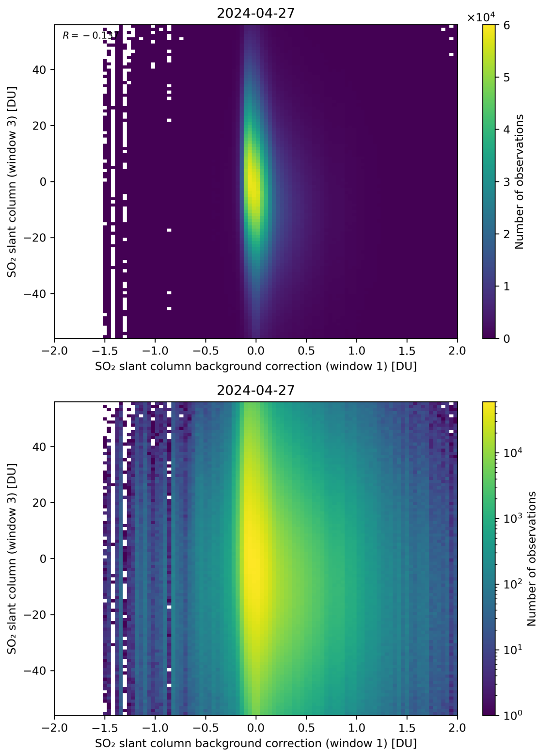
Figure 107: Scatter density plot of “SO 2 slant column background correction (window 1)” against “SO 2 slant column (window 3)” for 2024-04-26 to 2024-04-28.
