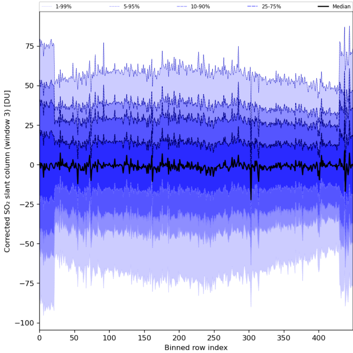
Figure 89: Along track statistics of “Corrected SO 2 slant column (window 3)” for 2024-04-26 to 2024-04-28
