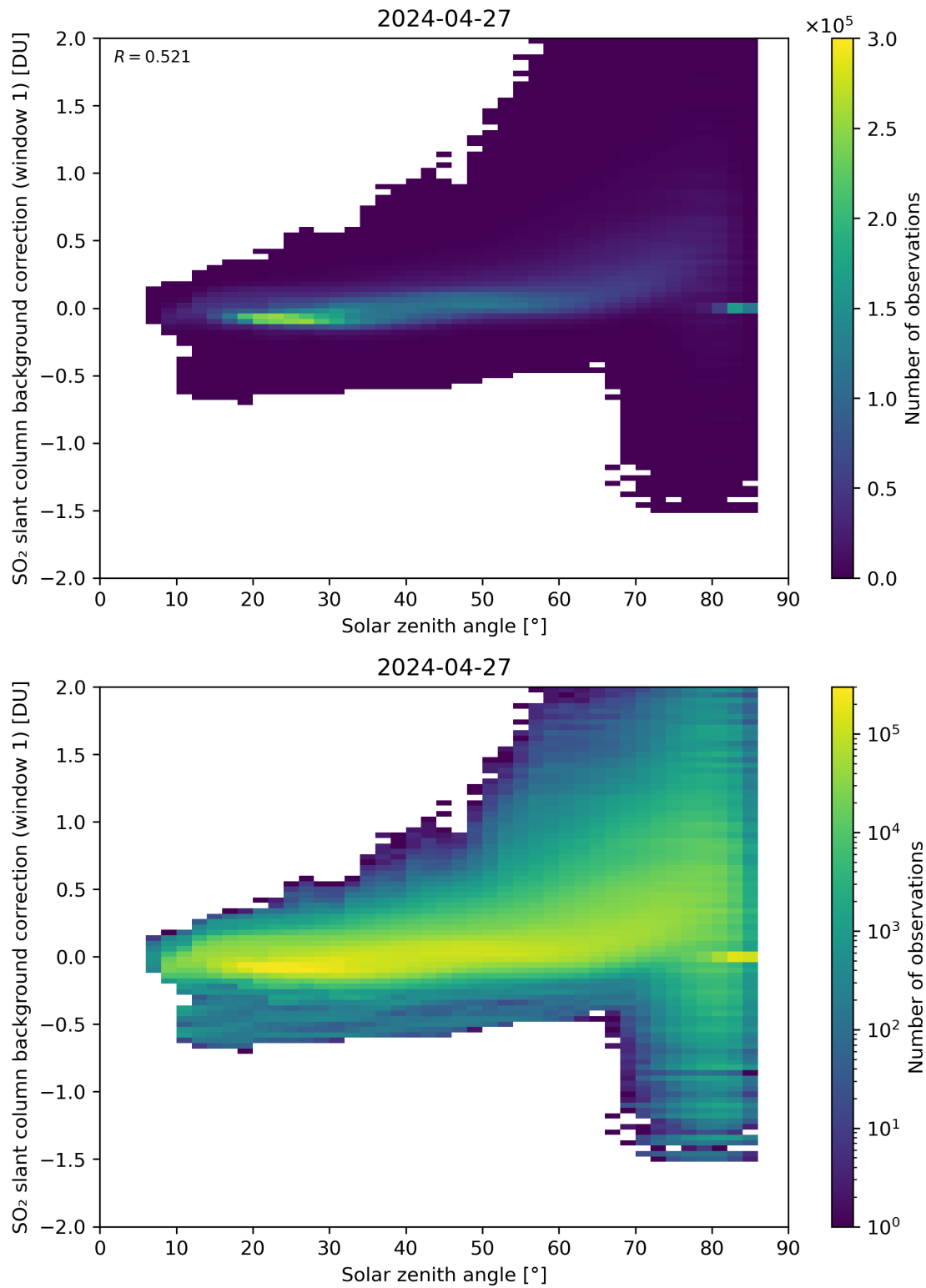
Figure 158: Scatter density plot of “Solar zenith angle” against “SO 2 slant column background correction (window 1)” for 2024-04-26 to 2024-04-28.
