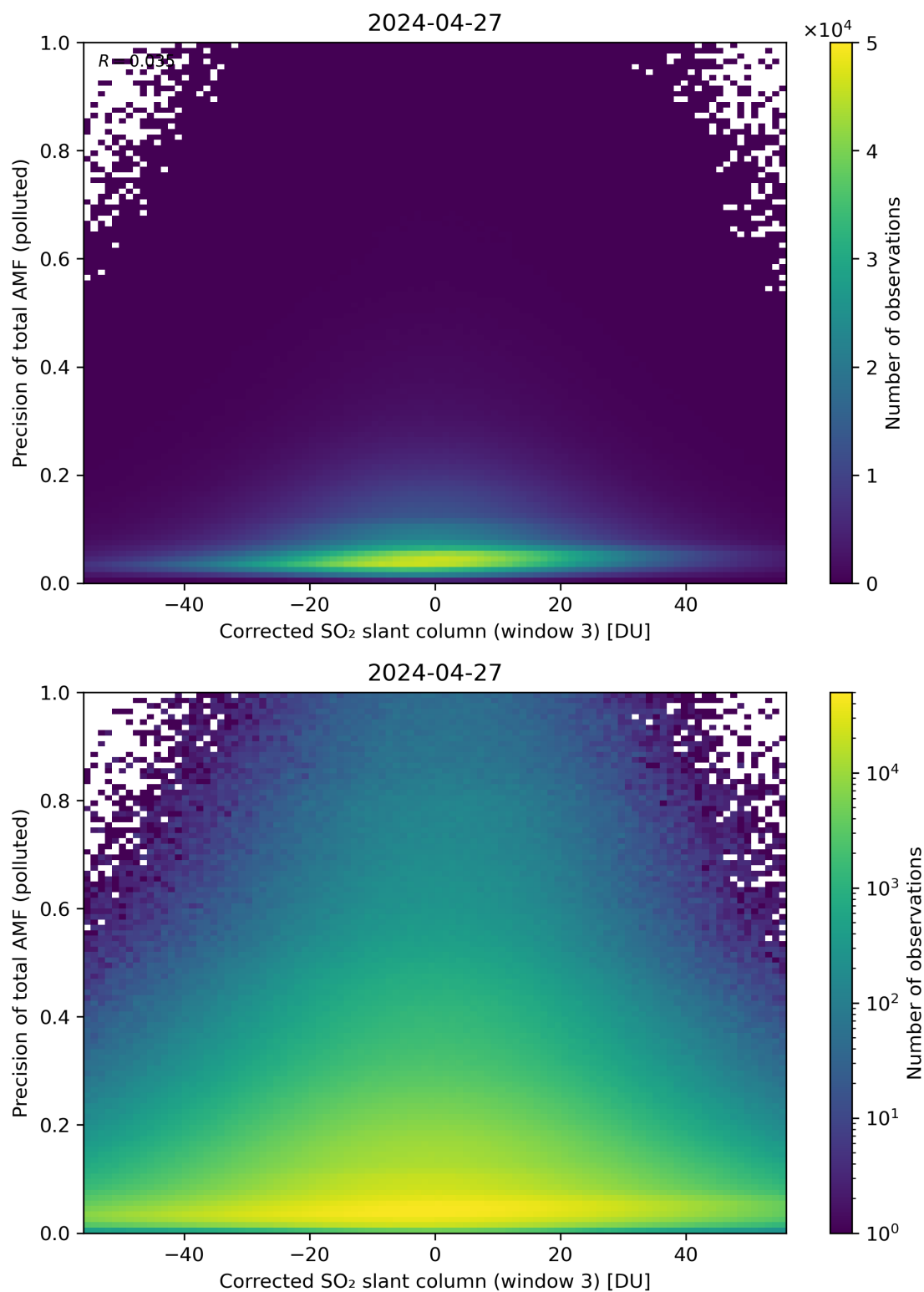
Figure 211: Scatter density plot of “Corrected SO 2 slant column (window 3)” against “Precision of total AMF (polluted)” for 2024-04-26 to 2024-04-28.
