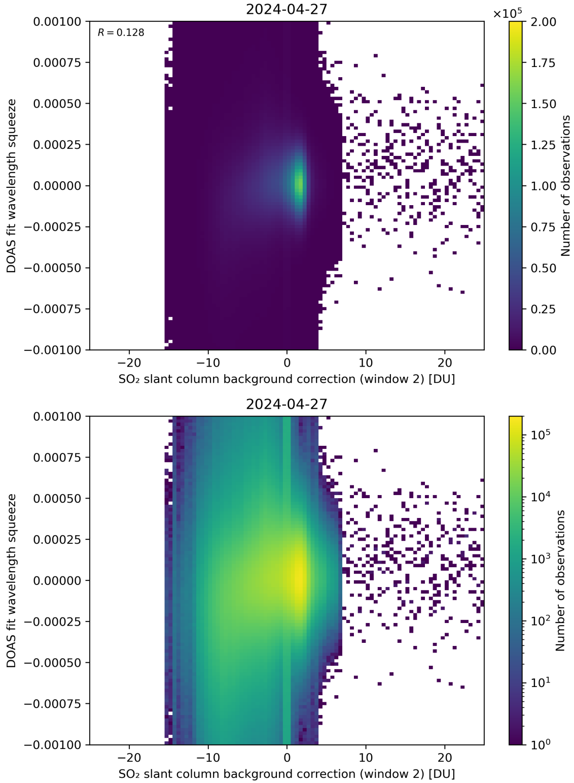
Figure 113: Scatter density plot of “SO 2 slant column background correction (window 2)” against “DOAS fit wavelength squeeze” for 2024-04-26 to 2024-04-28.
