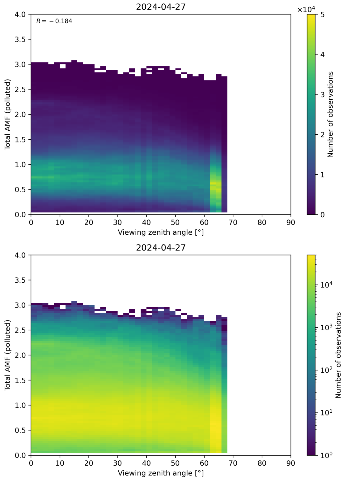
Figure 325: Scatter density plot of “Viewing zenith angle” against “Total AMF (polluted)” for 2024-04-26 to 2024-04-28.
