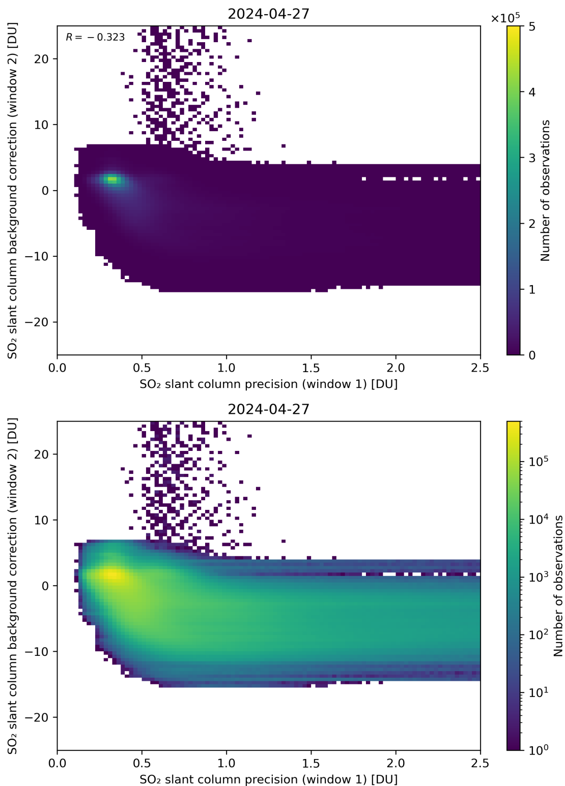
Figure 219: Scatter density plot of “SO 2 slant column precision (window 1)” against “SO 2 slant column background correction (window 2)” for 2024-04-26 to 2024-04-28.
