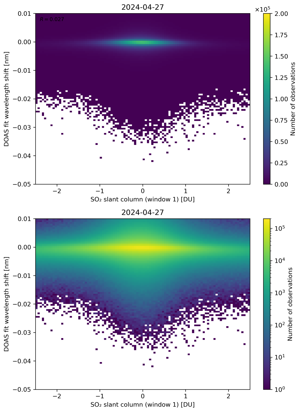
Figure 215: Scatter density plot of “SO 2 slant column (window 1)” against “DOAS fit wavelength shift” for 2024-04-26 to 2024-04-28.
