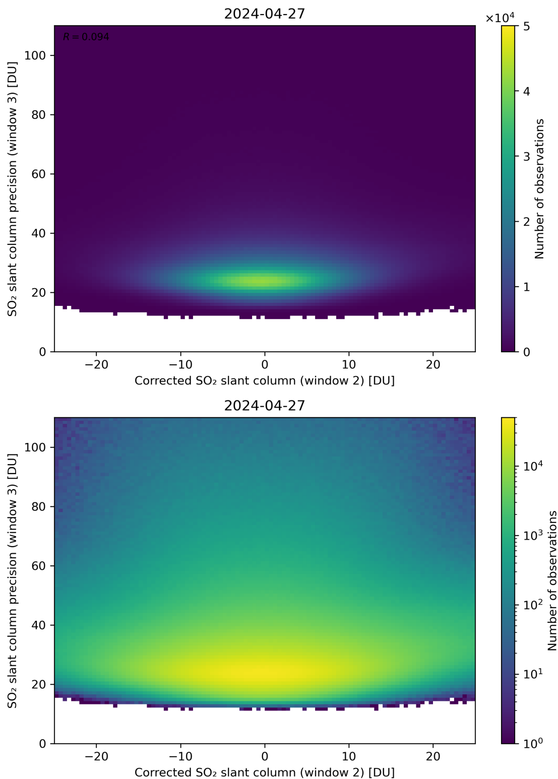
Figure 202: Scatter density plot of “Corrected SO 2 slant column (window 2)” against “SO 2 slant column precision (window 3)” for 2024-04-26 to 2024-04-28.
