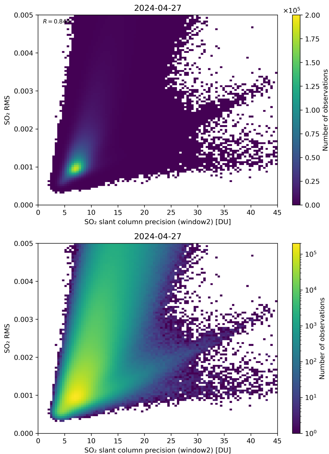
Figure 245: Scatter density plot of “SO 2 slant column precision (window2)” against “SO 2 RMS” for 2024-04-26 to 2024-04-28.
