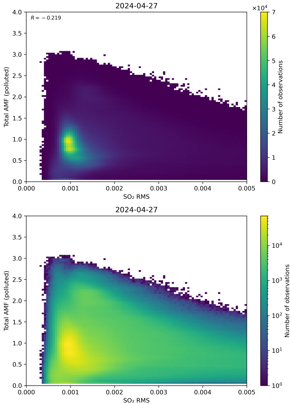
Figure 137: Scatter density plot of “SO 2 RMS” against “Total AMF (polluted)” for 2024-04-26 to 2024-04-28.
