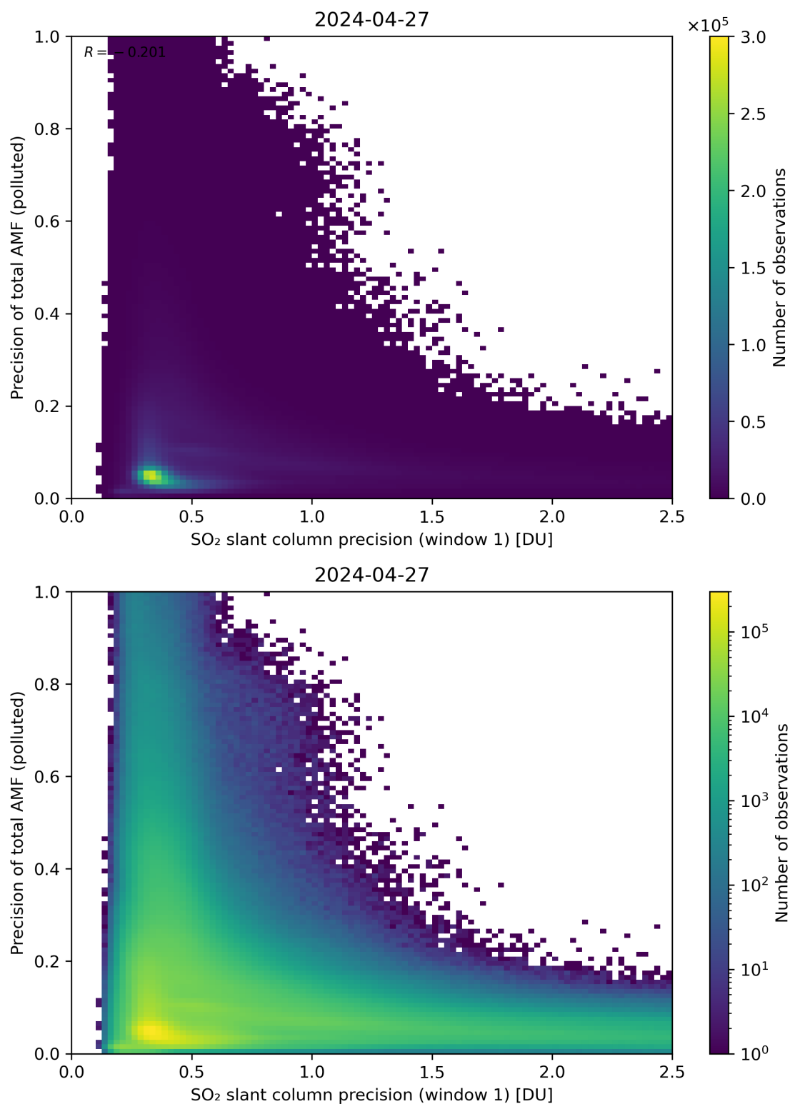
Figure 231: Scatter density plot of “SO 2 slant column precision (window 1)” against “Precision of total AMF (polluted)” for 2024-04-26 to 2024-04-28.
