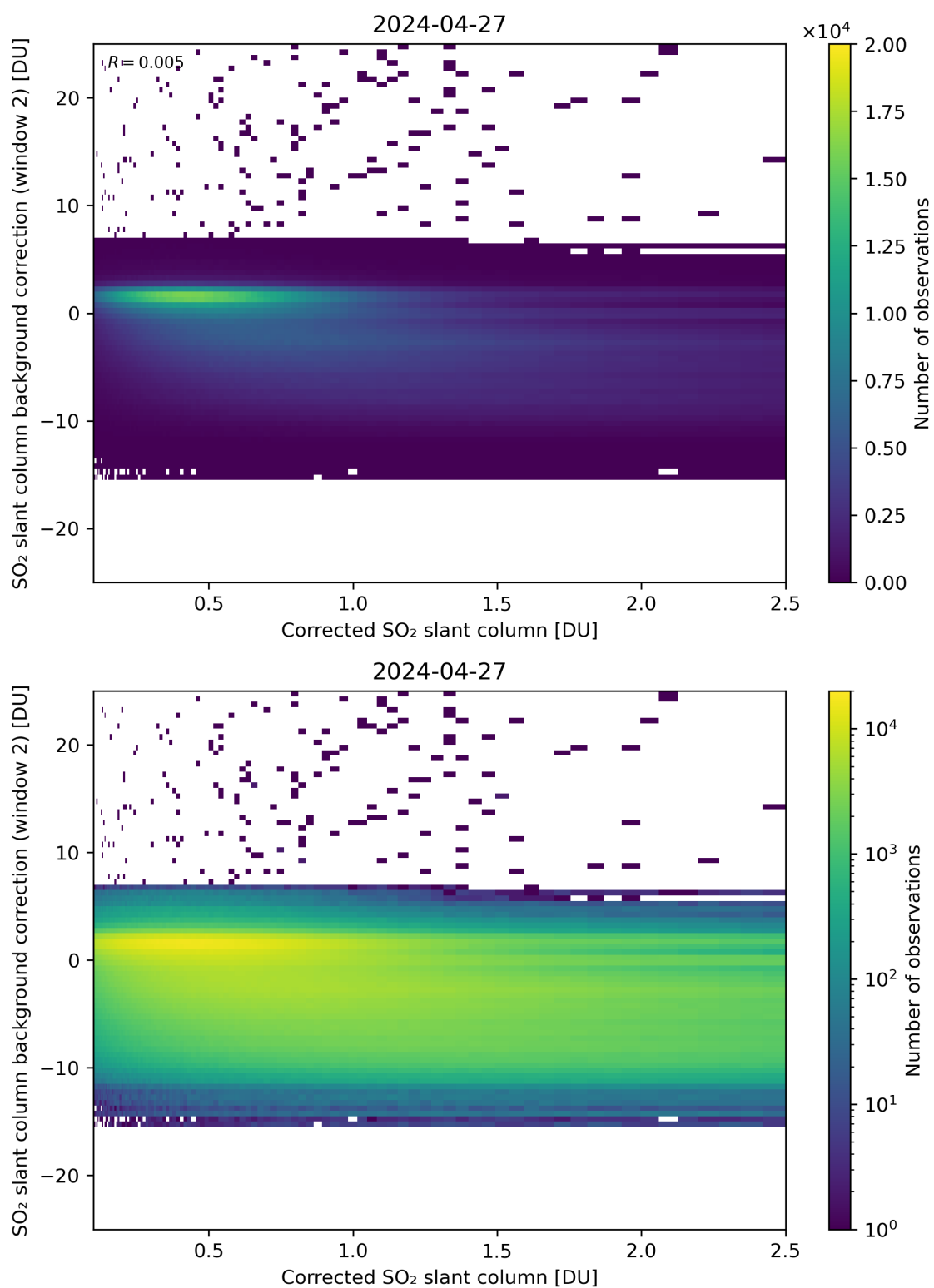
Figure 179: Scatter density plot of “Corrected SO 2 slant column” against “SO 2 slant column background correction (window 2)” for 2024-04-26 to 2024-04-28.
