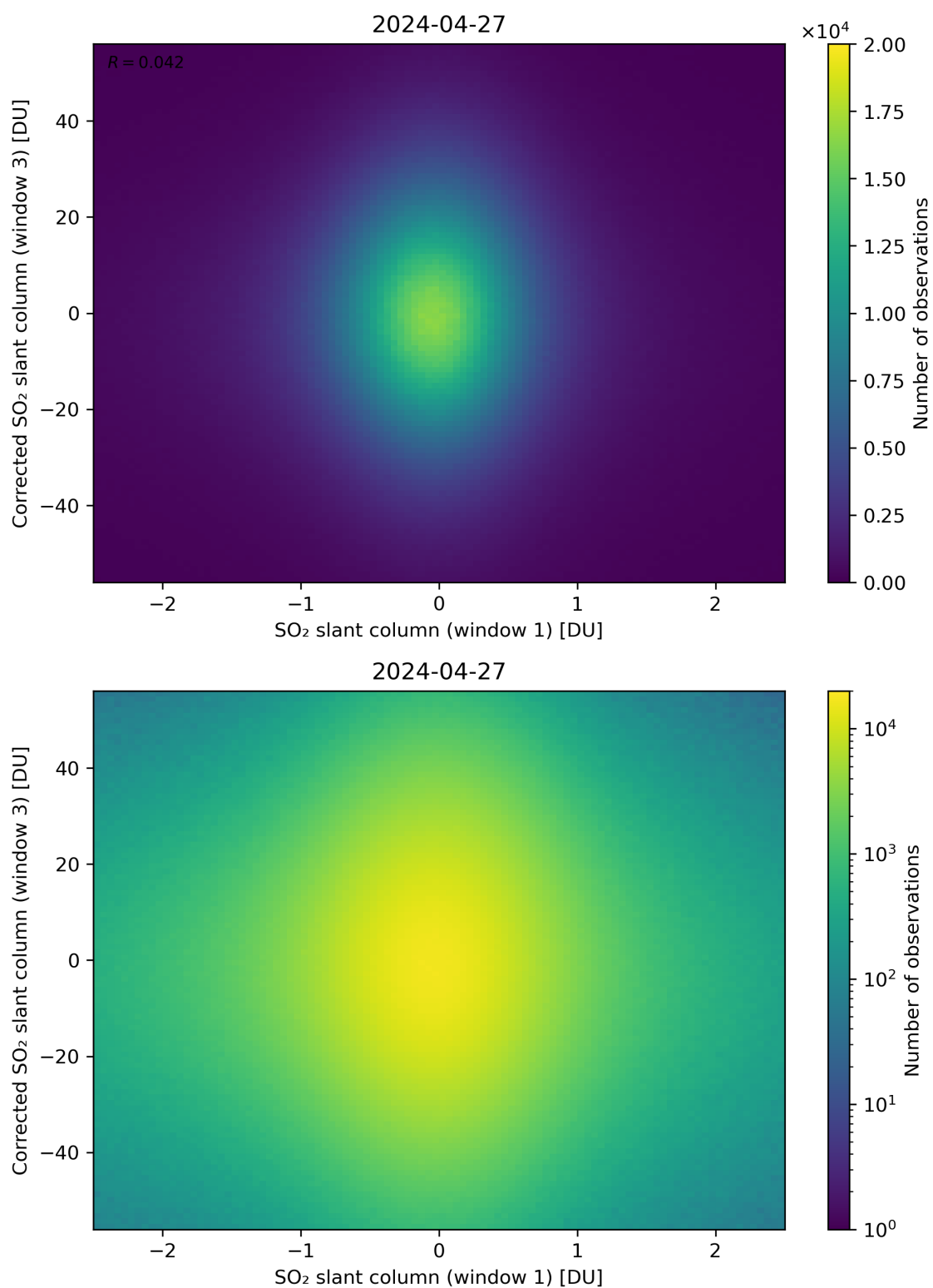
Figure 234: Scatter density plot of “SO 2 slant column (window 1)” against “Corrected SO 2 slant column (window 3)” for 2024-04-26 to 2024-04-28.
