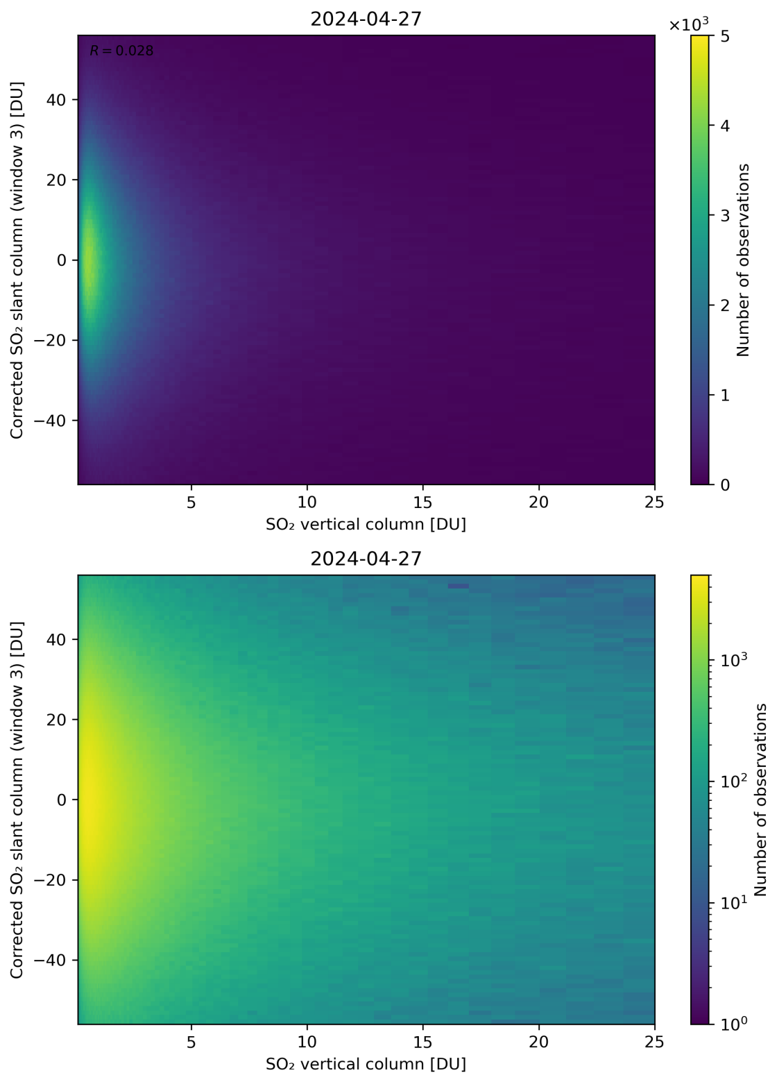
Figure 299: Scatter density plot of “SO 2 vertical column” against “Corrected SO 2 slant column (window 3)” for 2024-04-26 to 2024-04-28.
