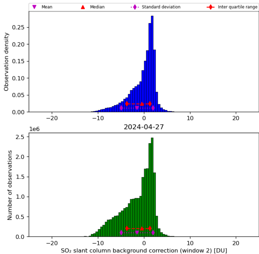
Figure 63: Histogram of “SO 2 slant column background correction (window 2)” for 2024-04-26 to 2024-04-28
