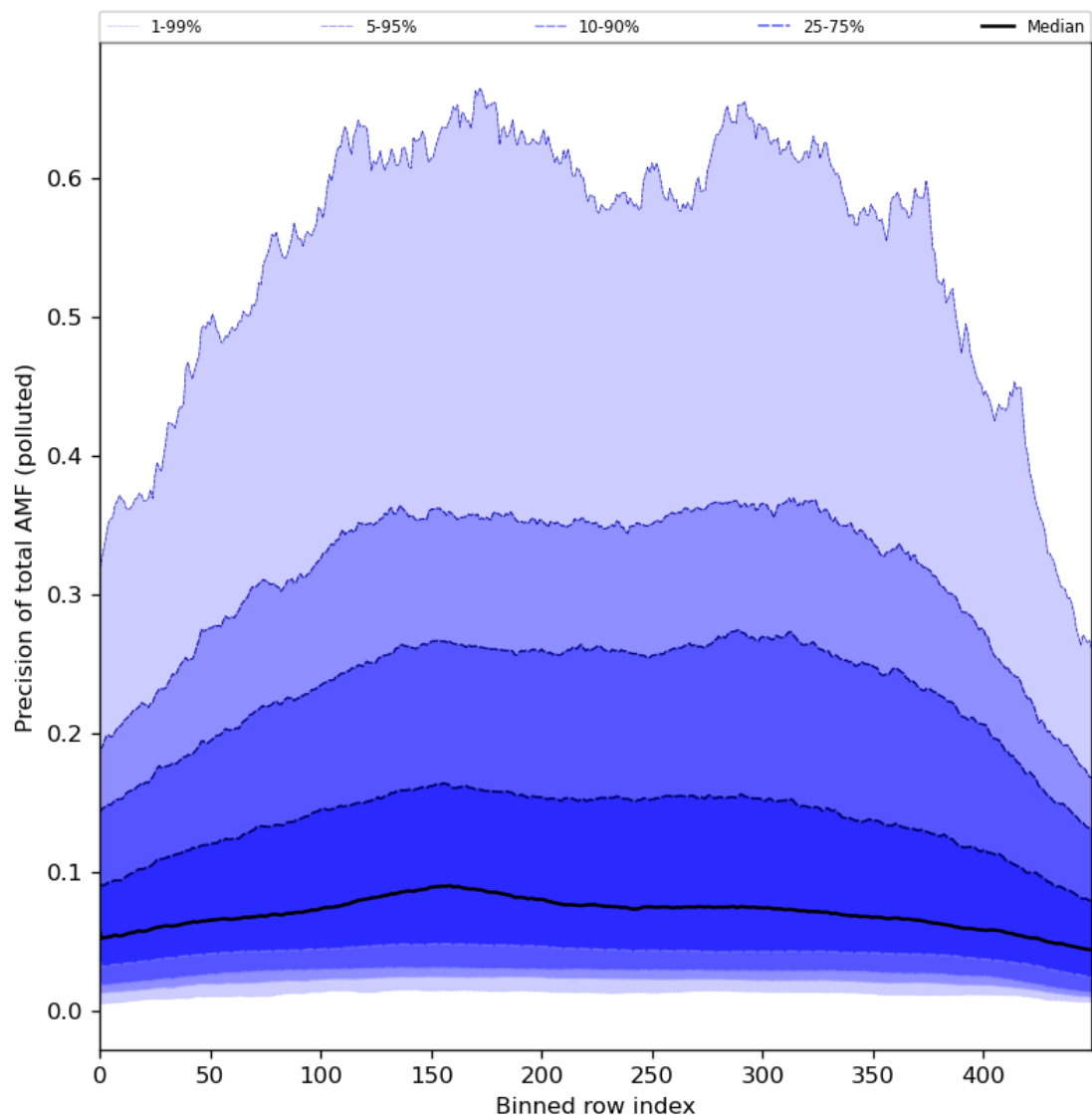
Figure 95: Along track statistics of “Precision of total AMF (polluted)” for 2024-04-26 to 2024-04-28
