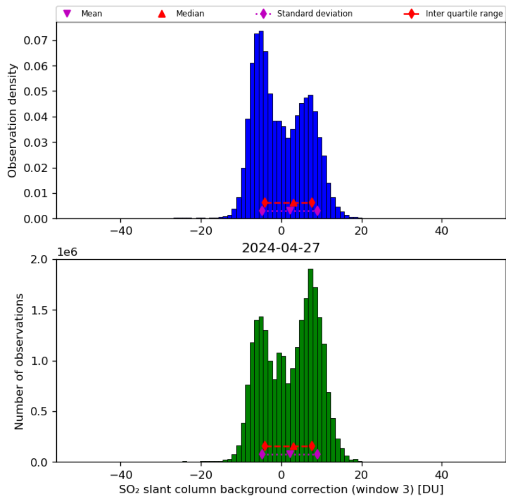
Figure 67: Histogram of “SO 2 slant column background correction (window 3)” for 2024-04-26 to 2024-04-28
