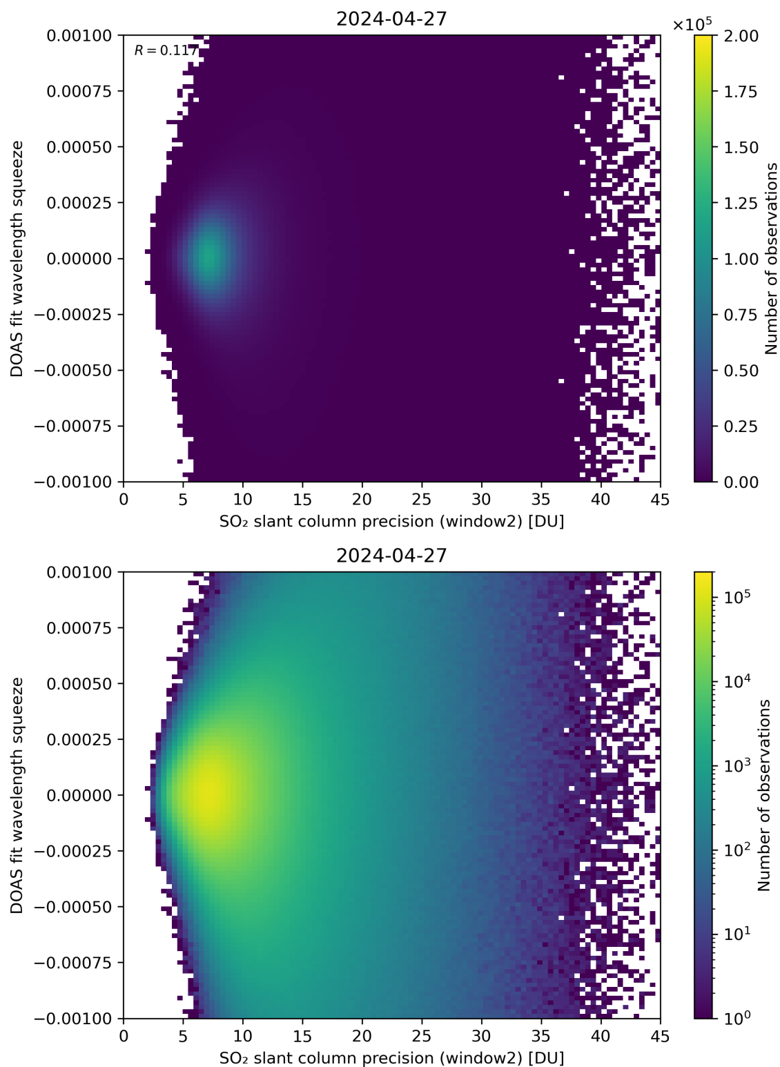
Figure 244: Scatter density plot of “SO 2 slant column precision (window2)” against “DOAS fit wavelength squeeze” for 2024-04-26 to 2024-04-28.
