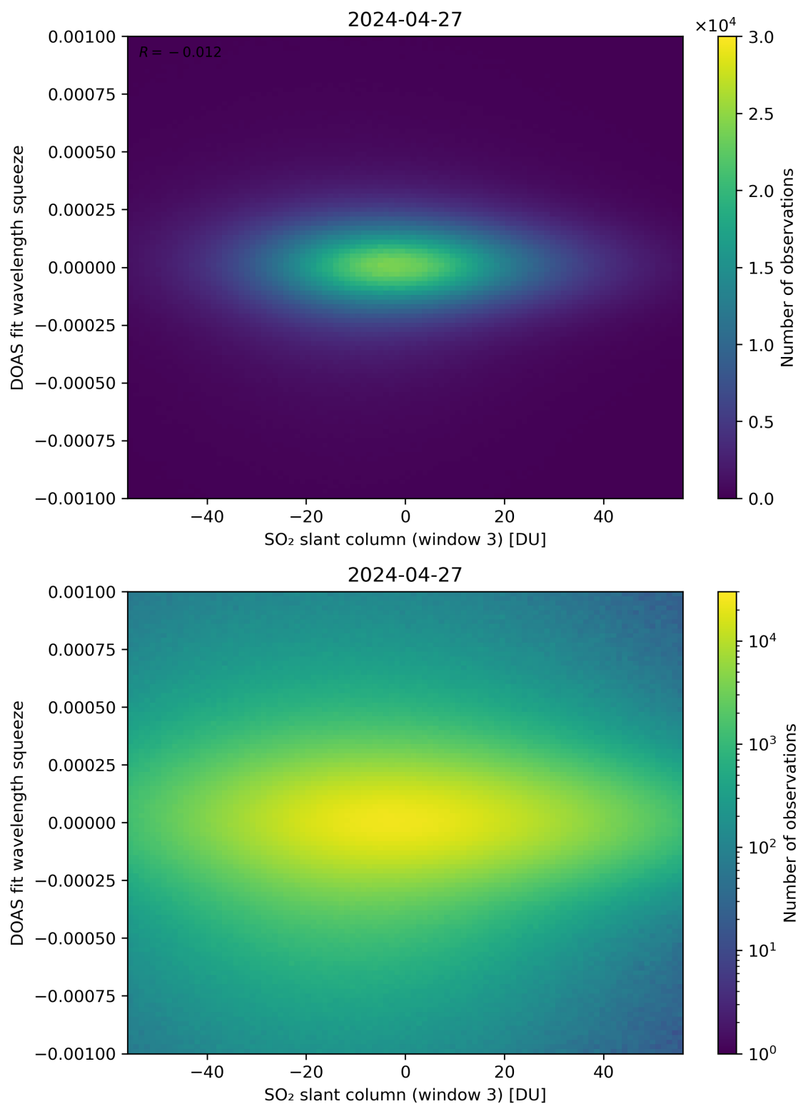
Figure 255: Scatter density plot of “SO 2 slant column (window 3)” against “DOAS fit wavelength squeeze” for 2024-04-26 to 2024-04-28.
