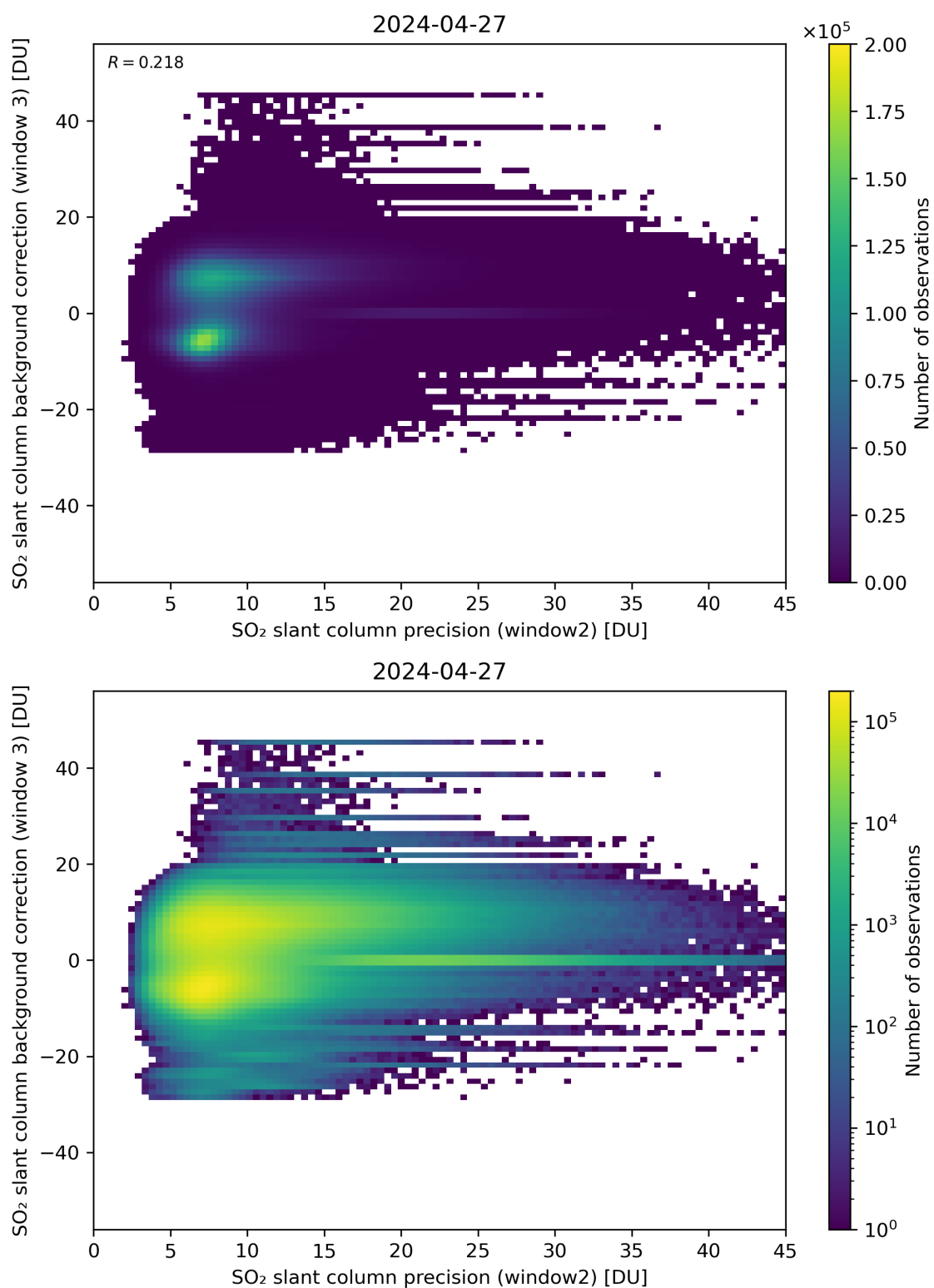
Figure 242: Scatter density plot of “SO 2 slant column precision (window2)” against “SO 2 slant column background correction (window 3)” for 2024-04-26 to 2024-04-28.
