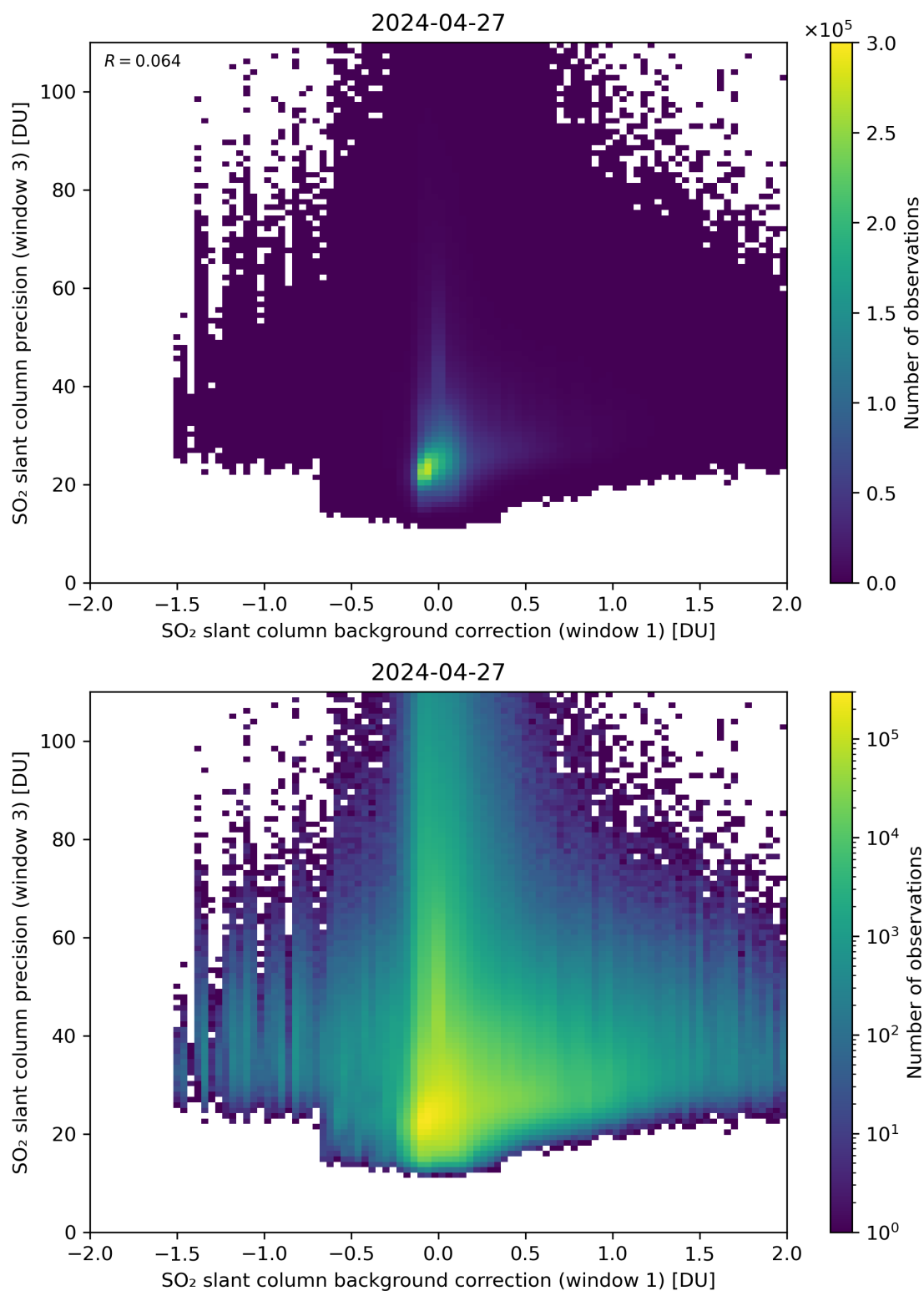
Figure 108: Scatter density plot of “SO 2 slant column background correction (window 1)” against “SO 2 slant column precision (window 3)” for 2024-04-26 to 2024-04-28.
