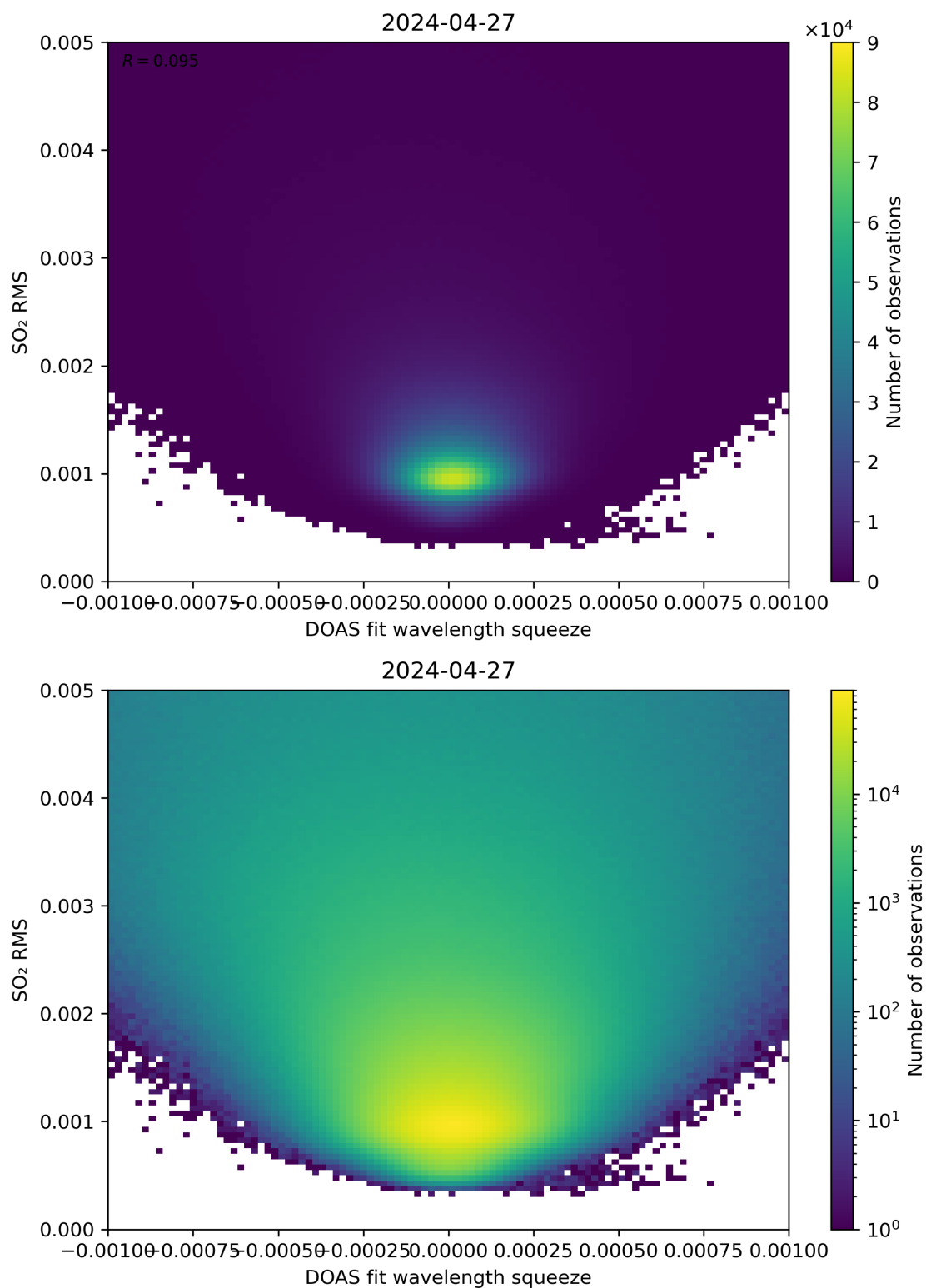
Figure 132: Scatter density plot of “DOAS fit wavelength squeeze” against “SO 2 RMS” for 2024-04-26 to 2024-04-28.
