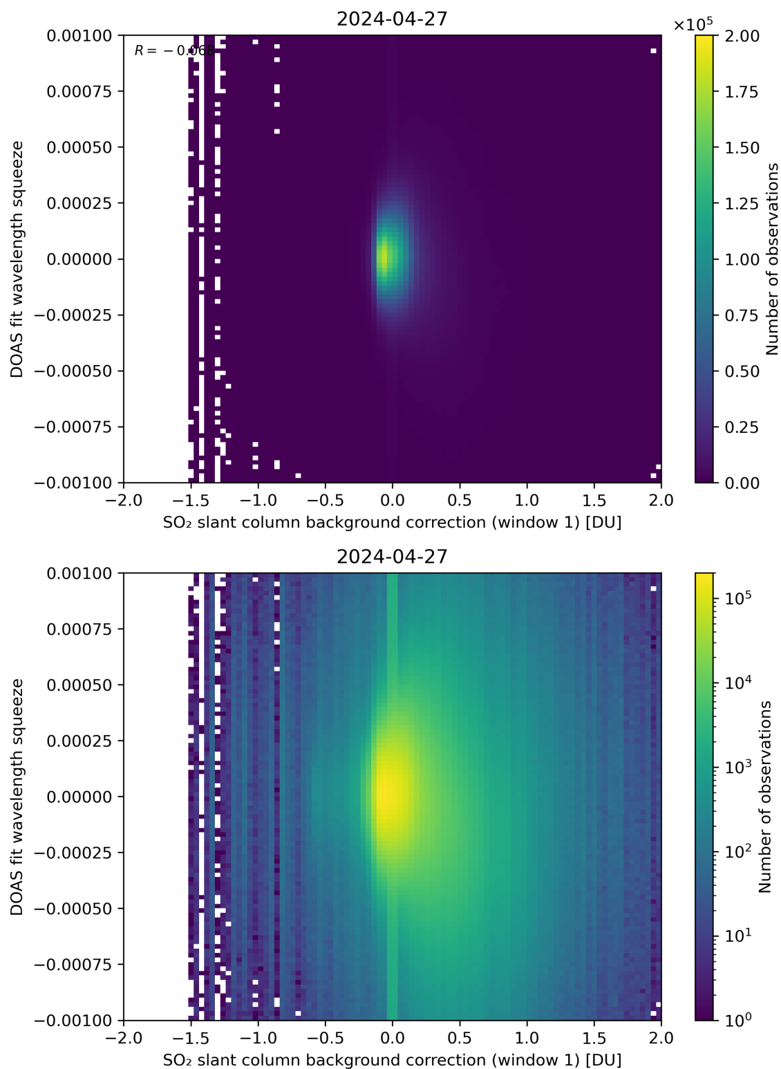
Figure 101: Scatter density plot of “SO 2 slant column background correction (window 1)” against “DOAS fit wavelength squeeze” for 2024-04-26 to 2024-04-28.
