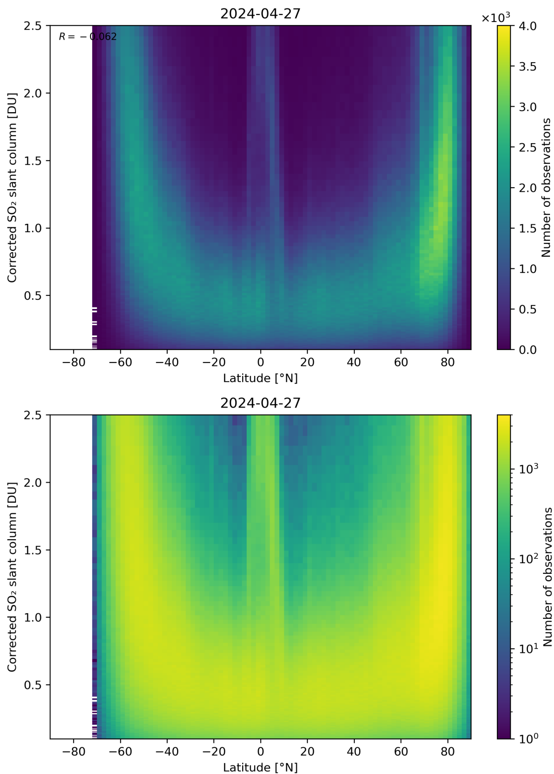
Figure 146: Scatter density plot of “Latitude” against “Corrected SO 2 slant column” for 2024-04-26 to 2024-04-28.
