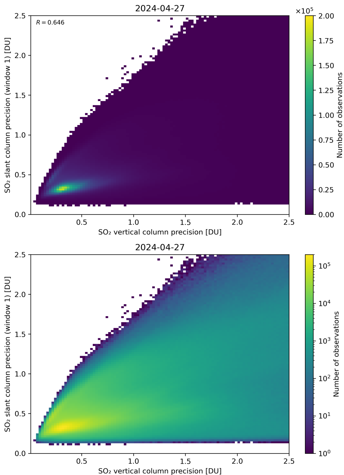
Figure 290: Scatter density plot of “SO 2 vertical column precision” against “SO 2 slant column precision (window 1)” for 2024-04-26 to 2024-04-28.
