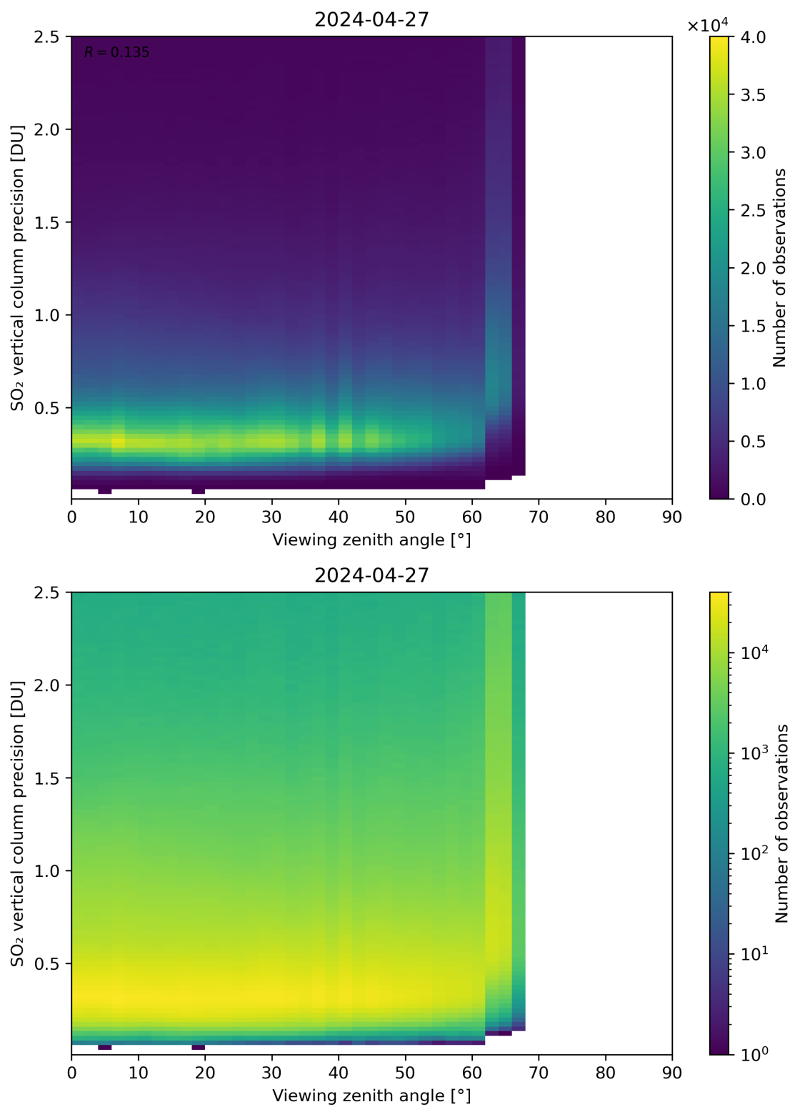
Figure 328: Scatter density plot of “Viewing zenith angle” against “SO 2 vertical column precision” for 2024-04-26 to 2024-04-28.
