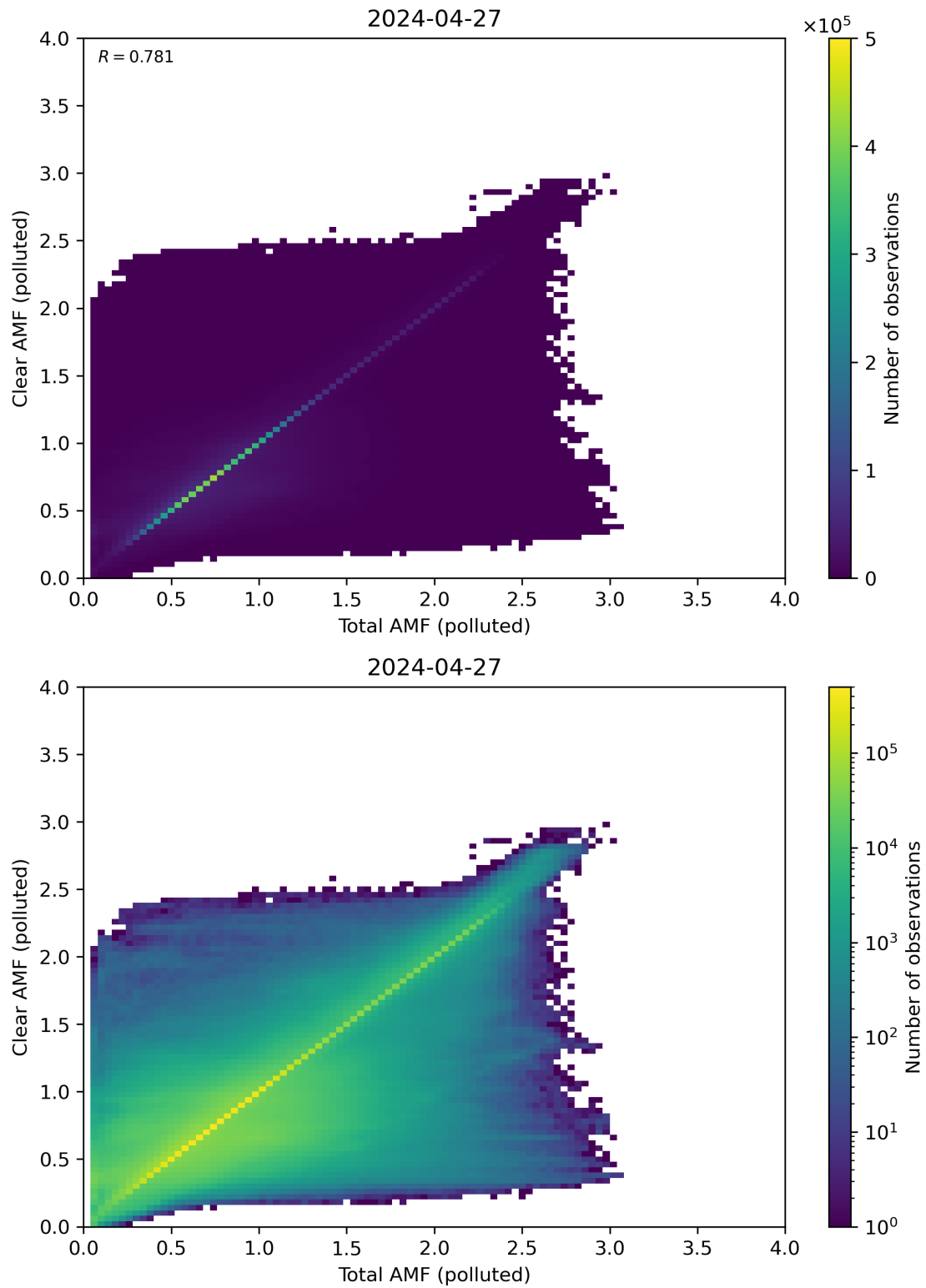
Figure 271: Scatter density plot of “Total AMF (polluted)” against “Clear AMF (polluted)” for 2024-04-26 to 2024-04-28.
