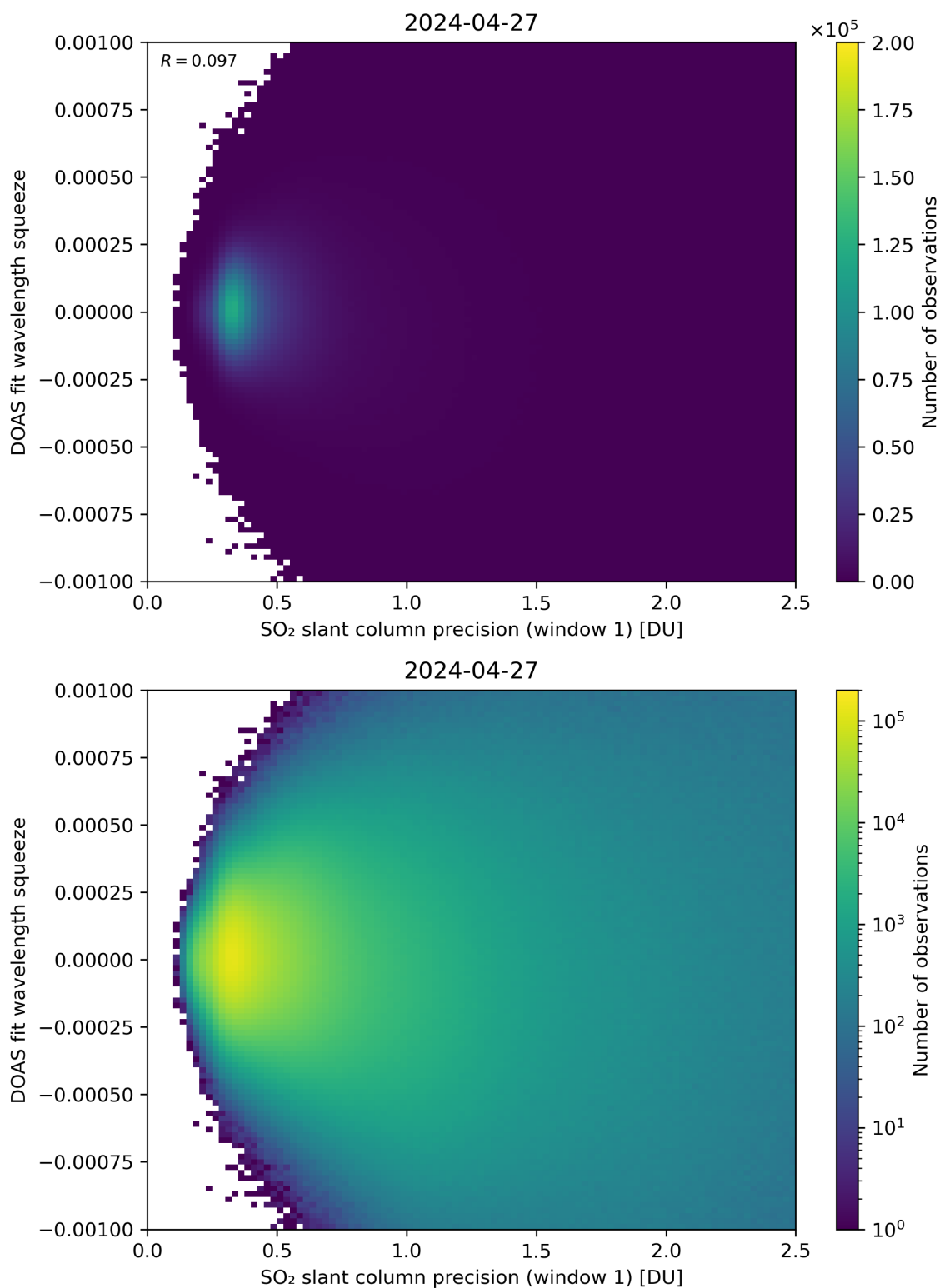
Figure 222: Scatter density plot of “SO 2 slant column precision (window 1)” against “DOAS fit wavelength squeeze” for 2024-04-26 to 2024-04-28.
