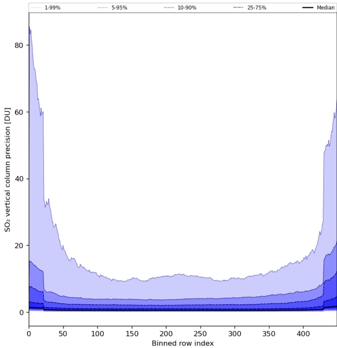
Figure 77: Along track statistics of “SO 2 vertical column precision” for 2024-04-26 to 2024-04-28
