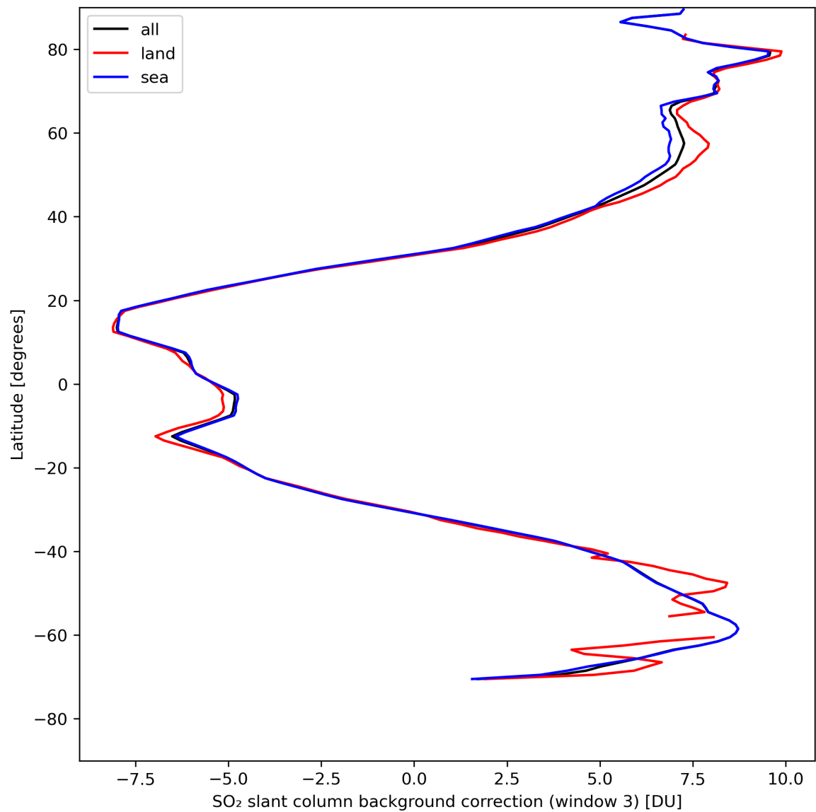
Figure 44: Zonal average of “SO 2 slant column background correction (window 3)” for 2024-04-26 to 2024-04-28.
