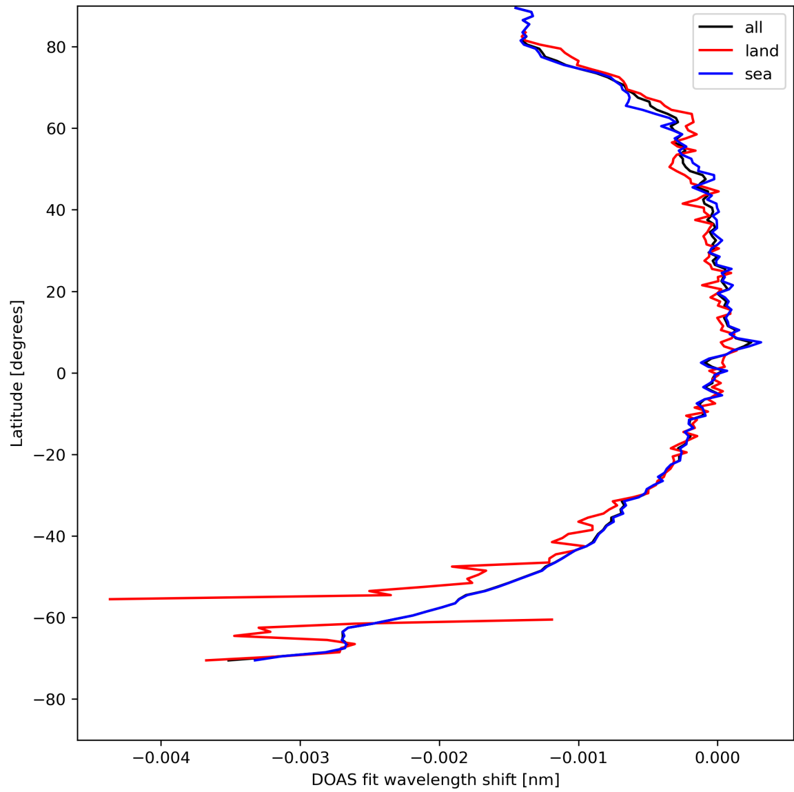
Figure 45: Zonal average of “DOAS fit wavelength shift” for 2024-04-26 to 2024-04-28.
