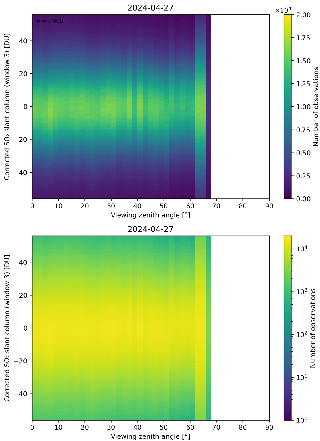
Figure 319: Scatter density plot of “Viewing zenith angle” against “Corrected SO 2 slant column (window 3)” for 2024-04-26 to 2024-04-28.
