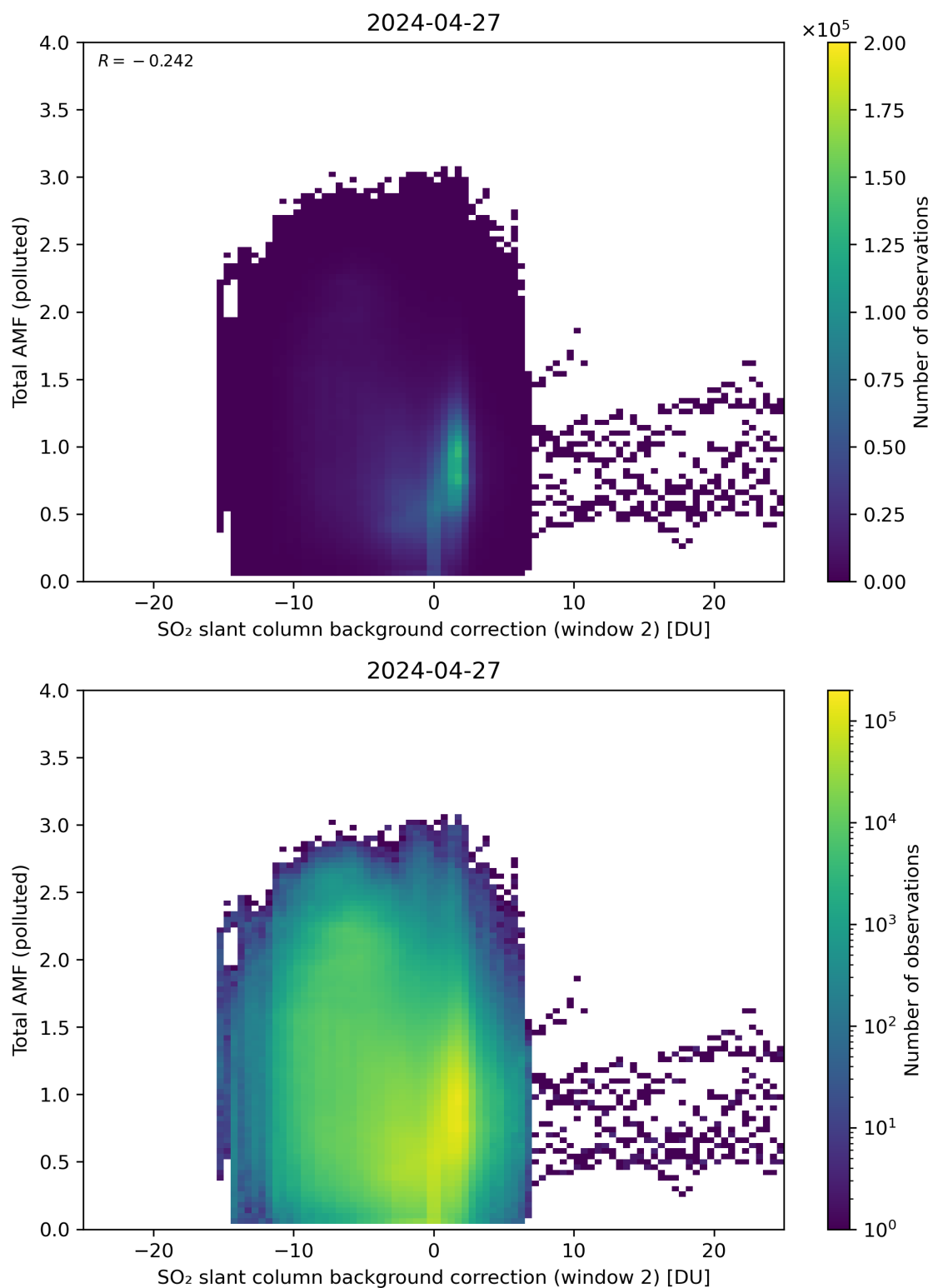
Figure 119: Scatter density plot of “SO 2 slant column background correction (window 2)” against “Total AMF (polluted)” for 2024-04-26 to 2024-04-28.
