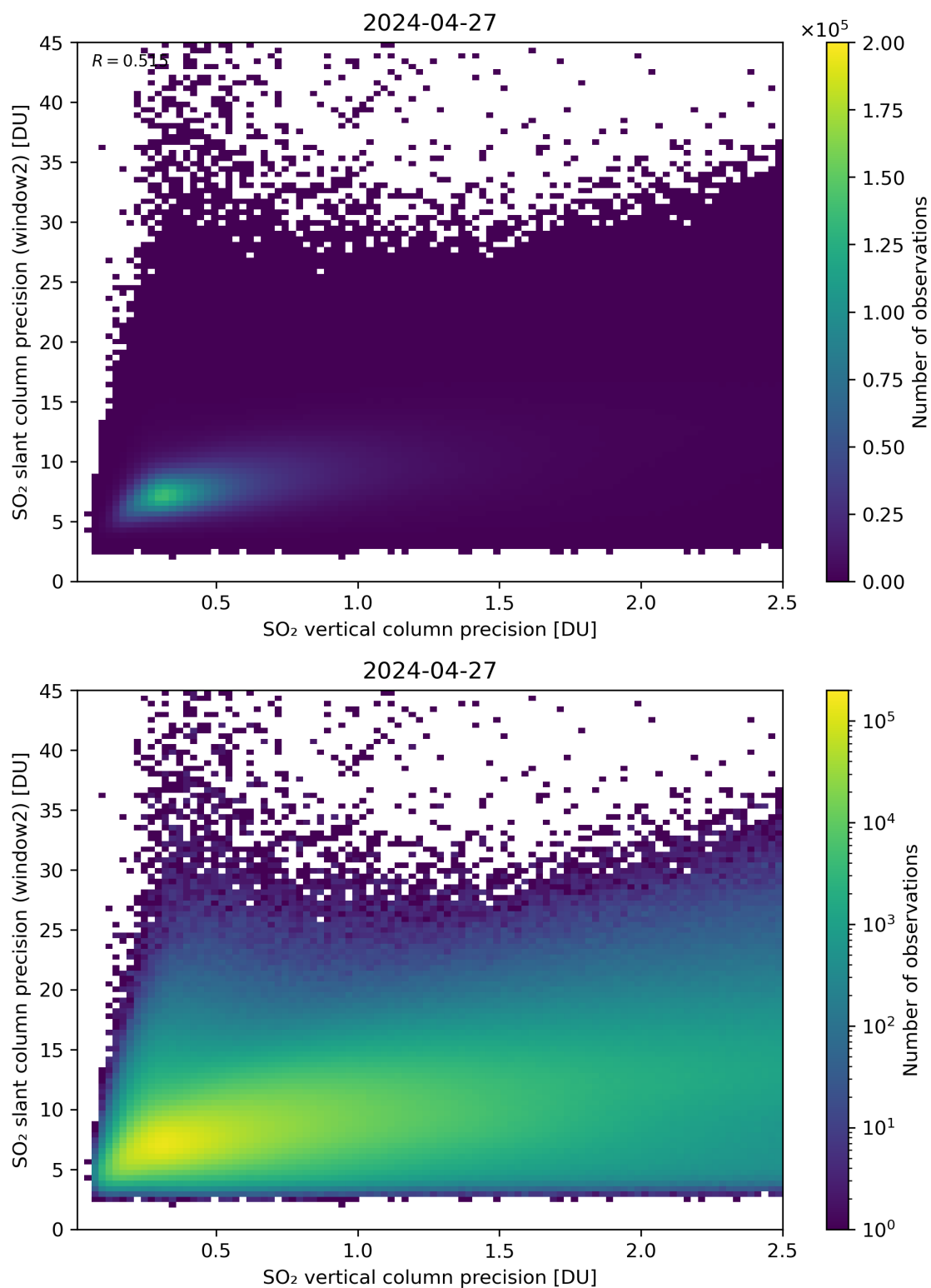
Figure 291: Scatter density plot of “SO 2 vertical column precision” against “SO 2 slant column precision (window2)” for 2024-04-26 to 2024-04-28.
