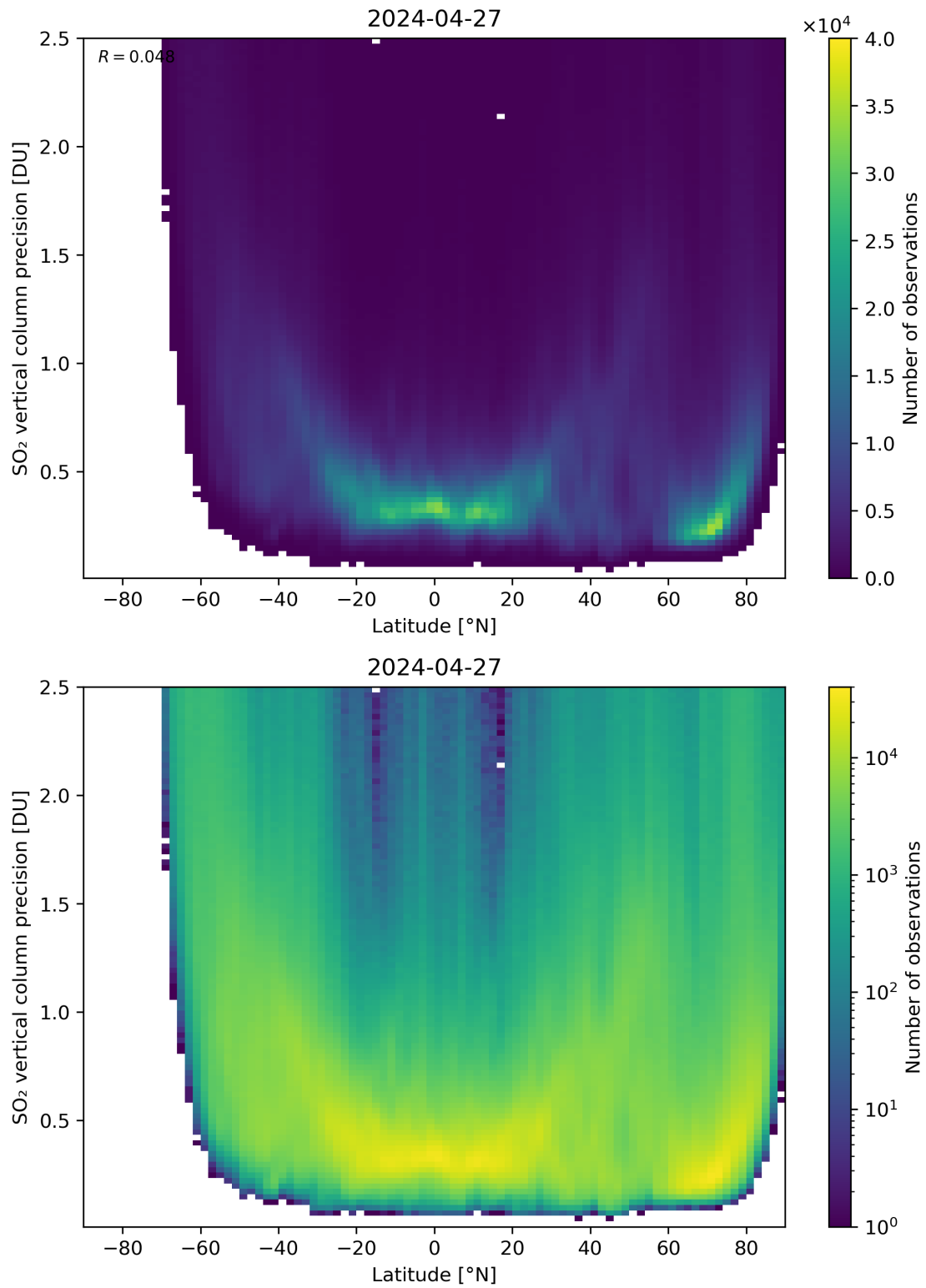
Figure 157: Scatter density plot of “Latitude” against “SO 2 vertical column precision” for 2024-04-26 to 2024-04-28.
