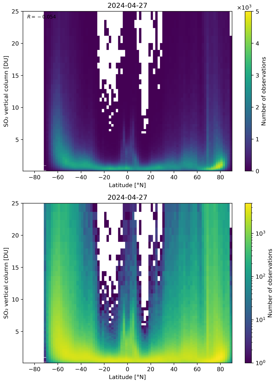
Figure 156: Scatter density plot of “Latitude” against “SO 2 vertical column” for 2024-04-26 to 2024-04-28.
