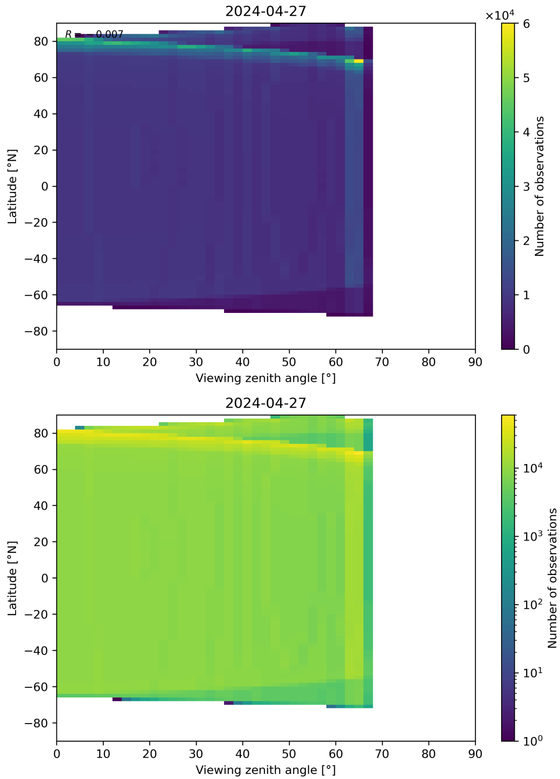
Figure 314: Scatter density plot of “Viewing zenith angle” against “Latitude” for 2024-04-26 to 2024-04-28.
