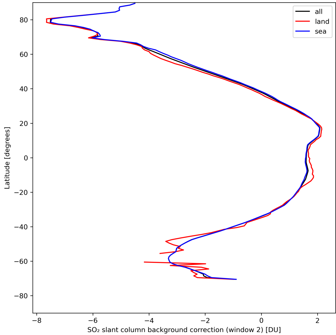
Figure 40: Zonal average of “SO 2 slant column background correction (window 2)” for 2024-04-26 to 2024-04-28.
