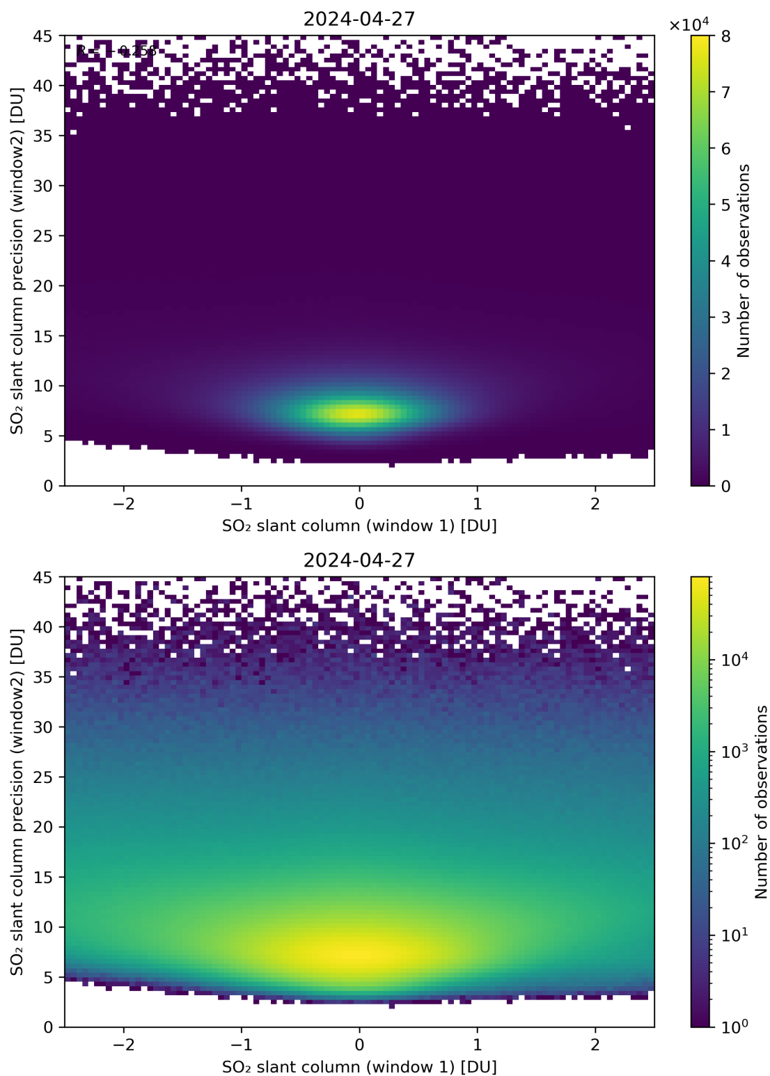
Figure 236: Scatter density plot of “SO 2 slant column (window 1)” against “SO 2 slant column precision (window2)” for 2024-04-26 to 2024-04-28.
