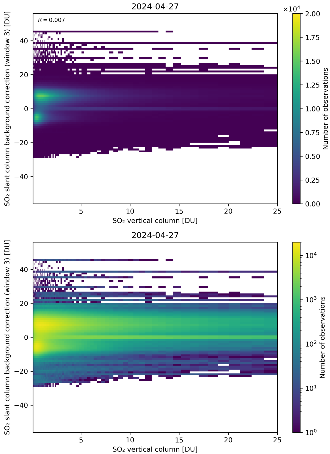
Figure 275: Scatter density plot of “SO 2 vertical column” against “SO 2 slant column background correction (window 3)” for 2024-04-26 to 2024-04-28.
