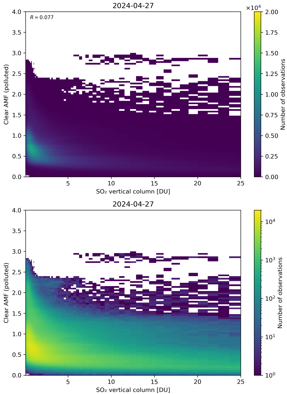
Figure 296: Scatter density plot of “SO 2 vertical column” against “Clear AMF (polluted)” for 2024-04-26 to 2024-04-28.
