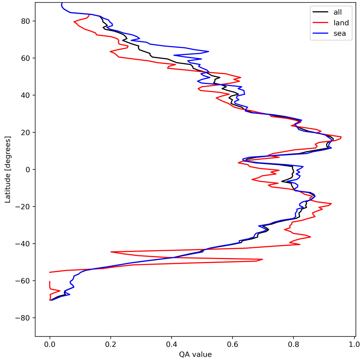
Figure 29: Zonal average of “QA value” for 2024-04-26 to 2024-04-28.
