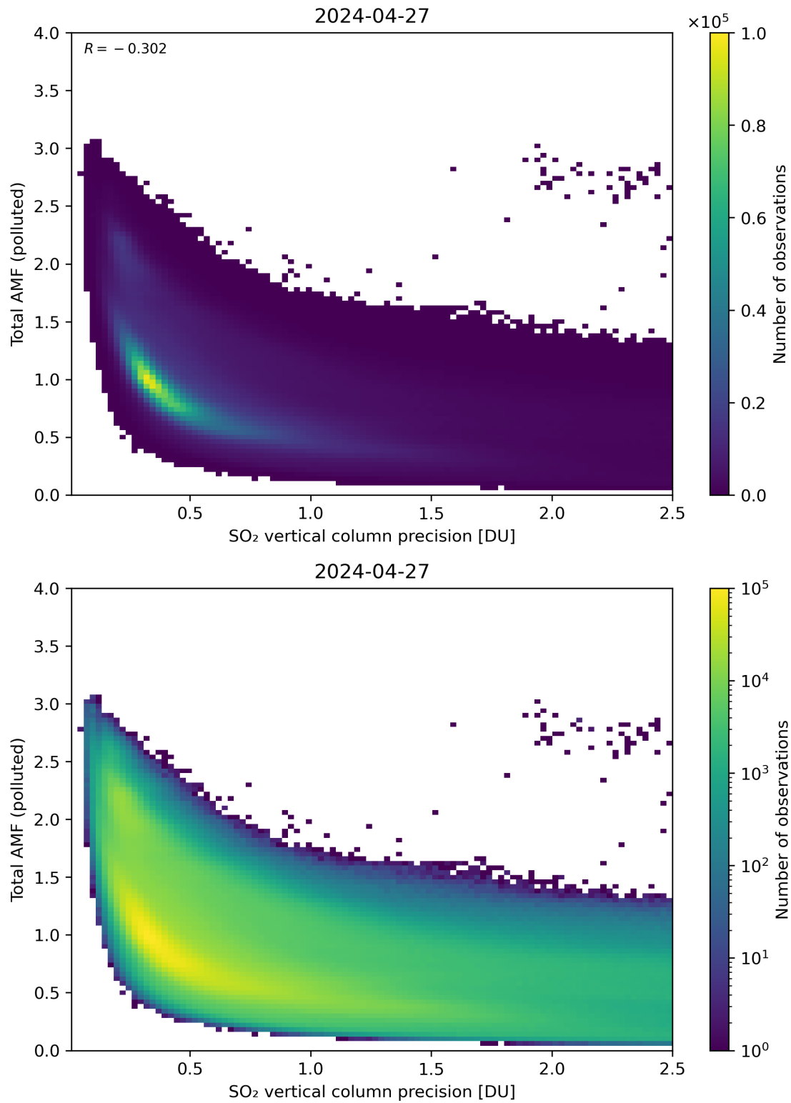
Figure 294: Scatter density plot of “SO 2 vertical column precision” against “Total AMF (polluted)” for 2024-04-26 to 2024-04-28.
