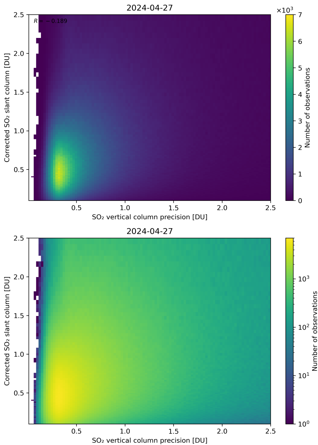
Figure 286: Scatter density plot of “SO 2 vertical column precision” against “Corrected SO 2 slant column” for 2024-04-26 to 2024-04-28.
