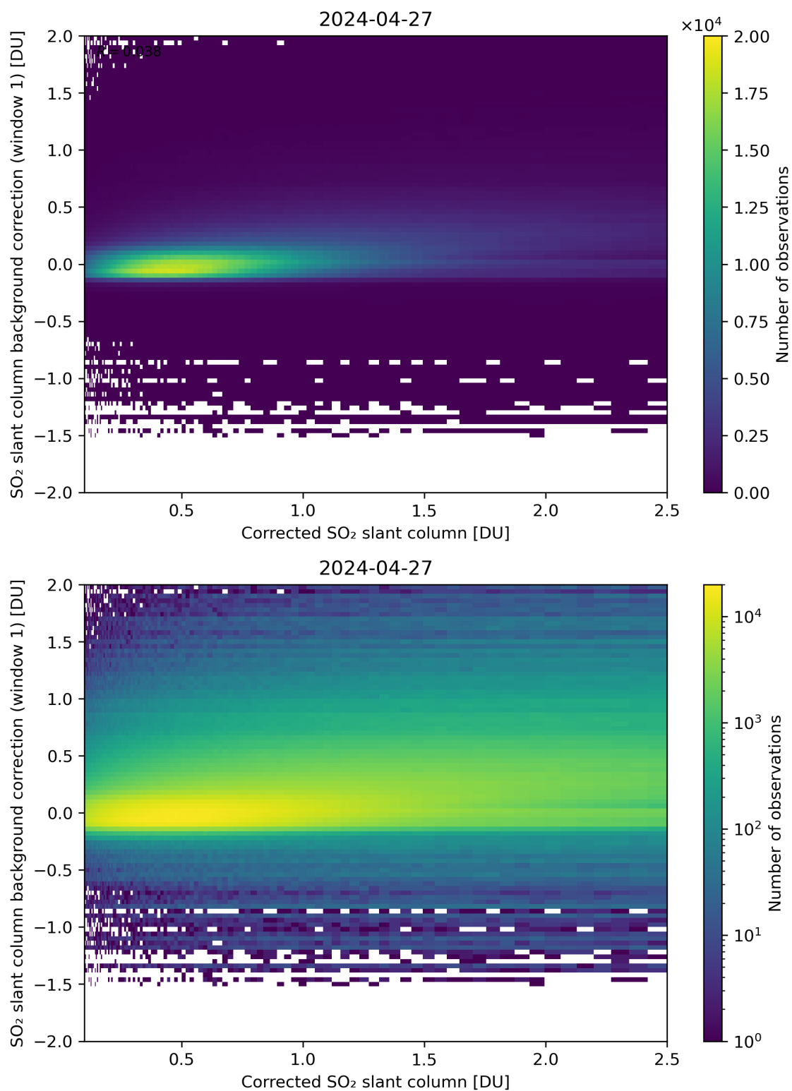
Figure 178: Scatter density plot of “Corrected SO 2 slant column” against “SO 2 slant column background correction (window 1)” for 2024-04-26 to 2024-04-28.
