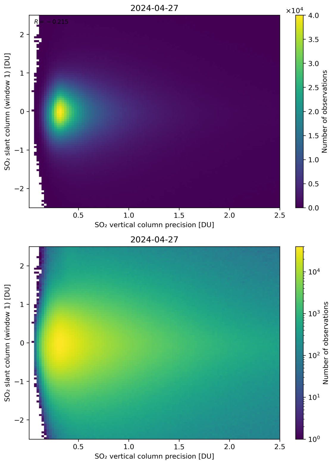
Figure 289: Scatter density plot of “SO 2 vertical column precision” against “SO 2 slant column (window 1)” for 2024-04-26 to 2024-04-28.
