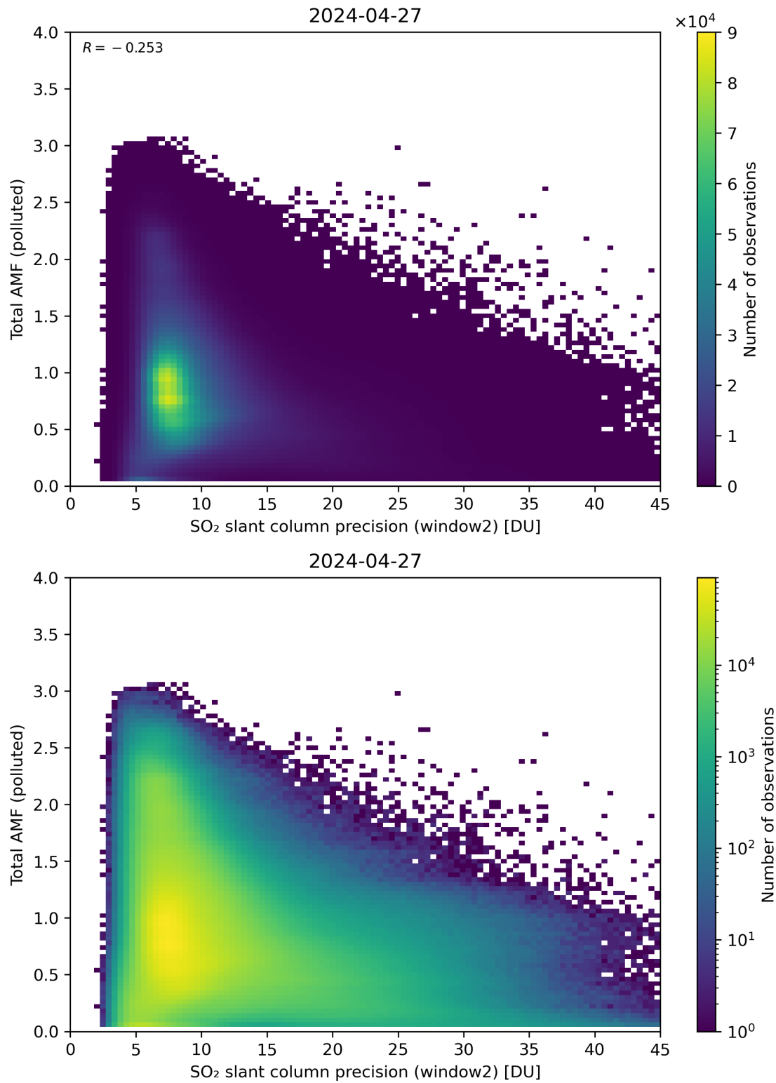
Figure 251: Scatter density plot of “SO 2 slant column precision (window2)” against “Total AMF (polluted)” for 2024-04-26 to 2024-04-28.
