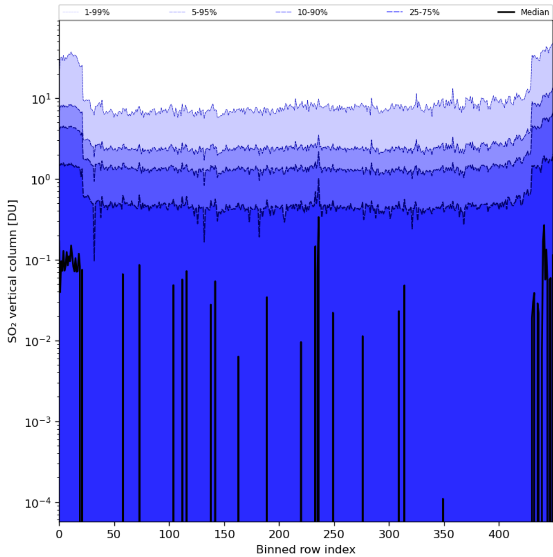
Figure 76: Along track statistics of “SO 2 vertical column” for 2024-04-26 to 2024-04-28
