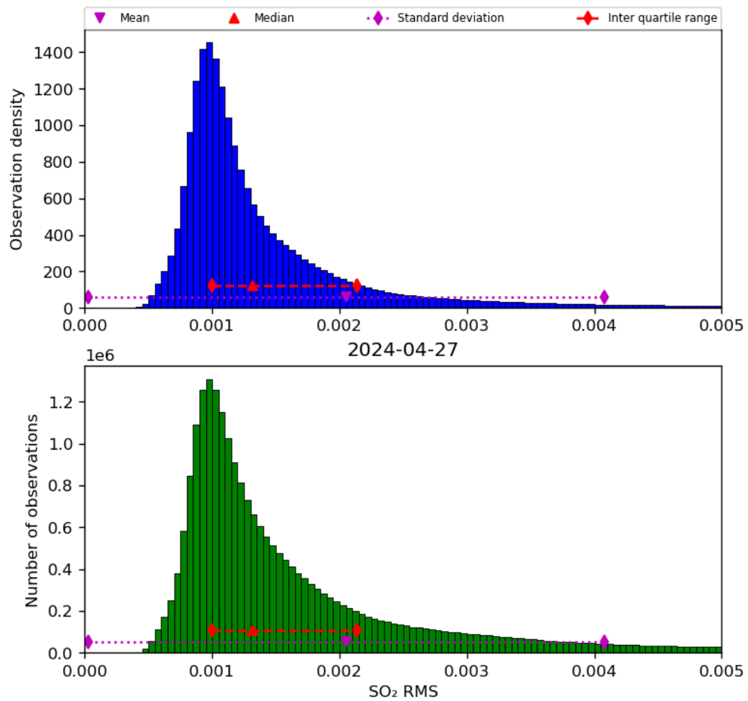
Figure 70: Histogram of “SO 2 RMS” for 2024-04-26 to 2024-04-28
