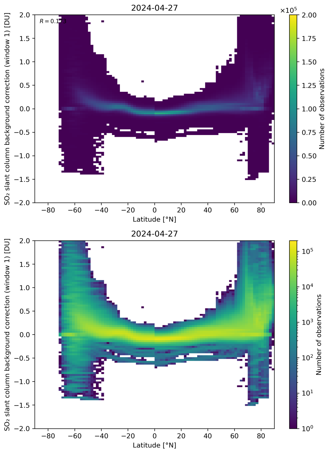
Figure 139: Scatter density plot of “Latitude” against “SO 2 slant column background correction (window 1)” for 2024-04-26 to 2024-04-28.
