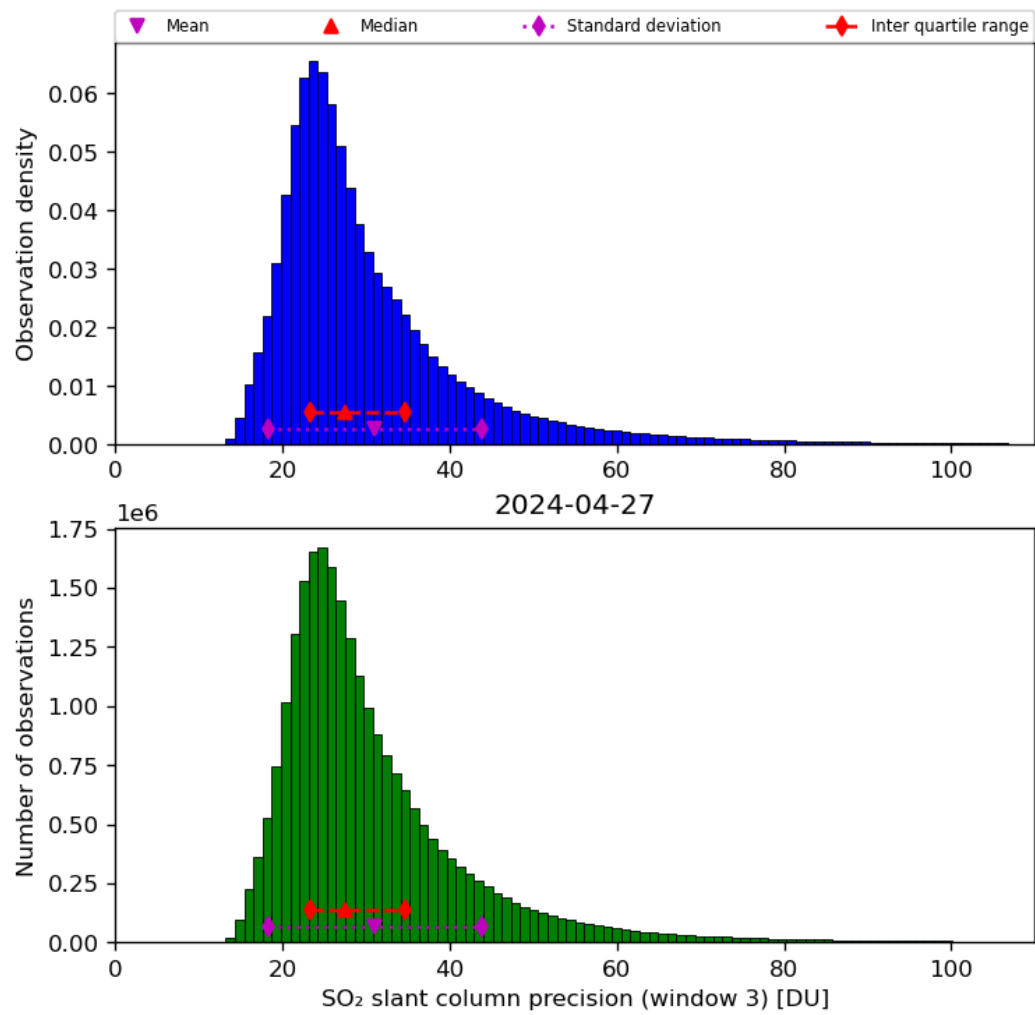
Figure 65: Histogram of “SO 2 slant column precision (window 3)” for 2024-04-26 to 2024-04-28
