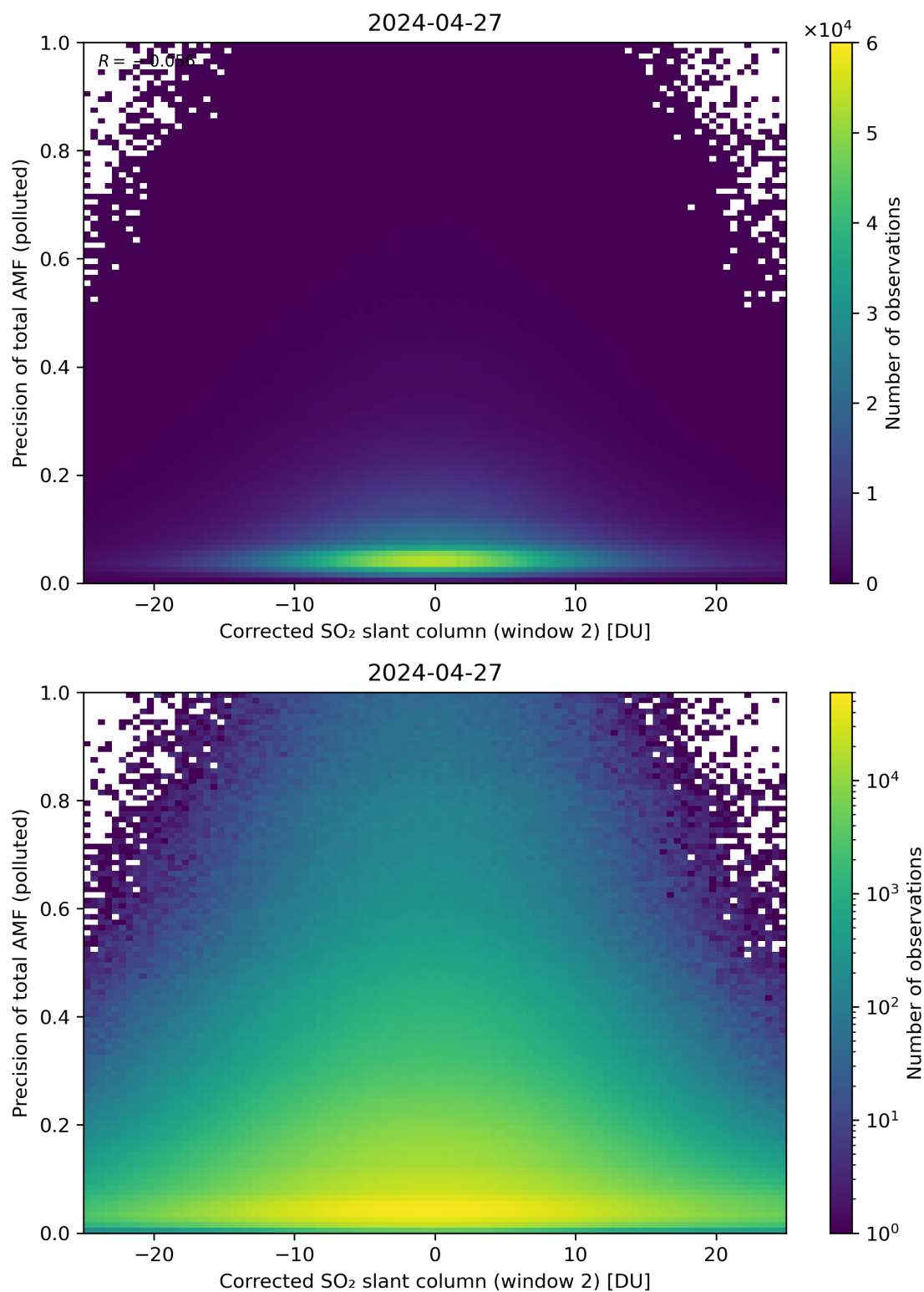
Figure 204: Scatter density plot of “Corrected SO 2 slant column (window 2)” against “Precision of total AMF (polluted)” for 2024-04-26 to 2024-04-28.
