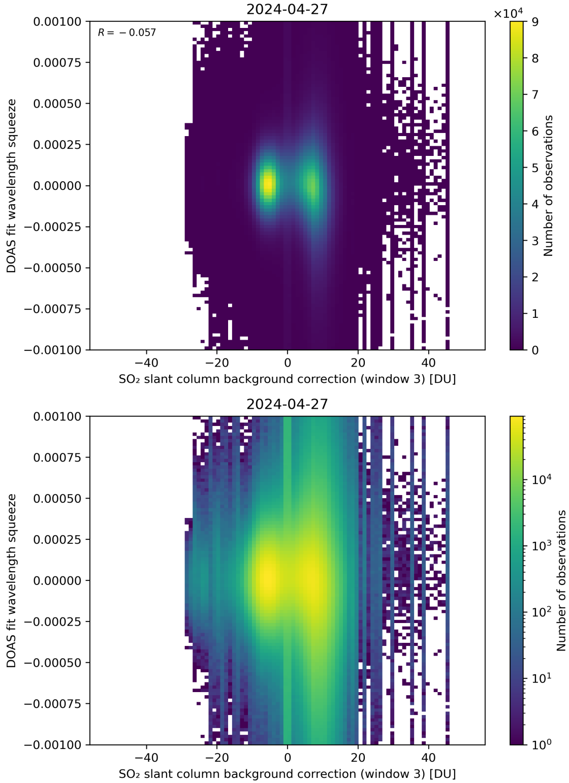
Figure 122: Scatter density plot of “SO 2 slant column background correction (window 3)” against “DOAS fit wavelength squeeze” for 2024-04-26 to 2024-04-28.
