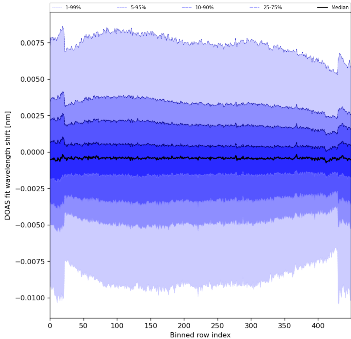
Figure 91: Along track statistics of “DOAS fit wavelength shift” for 2024-04-26 to 2024-04-28
