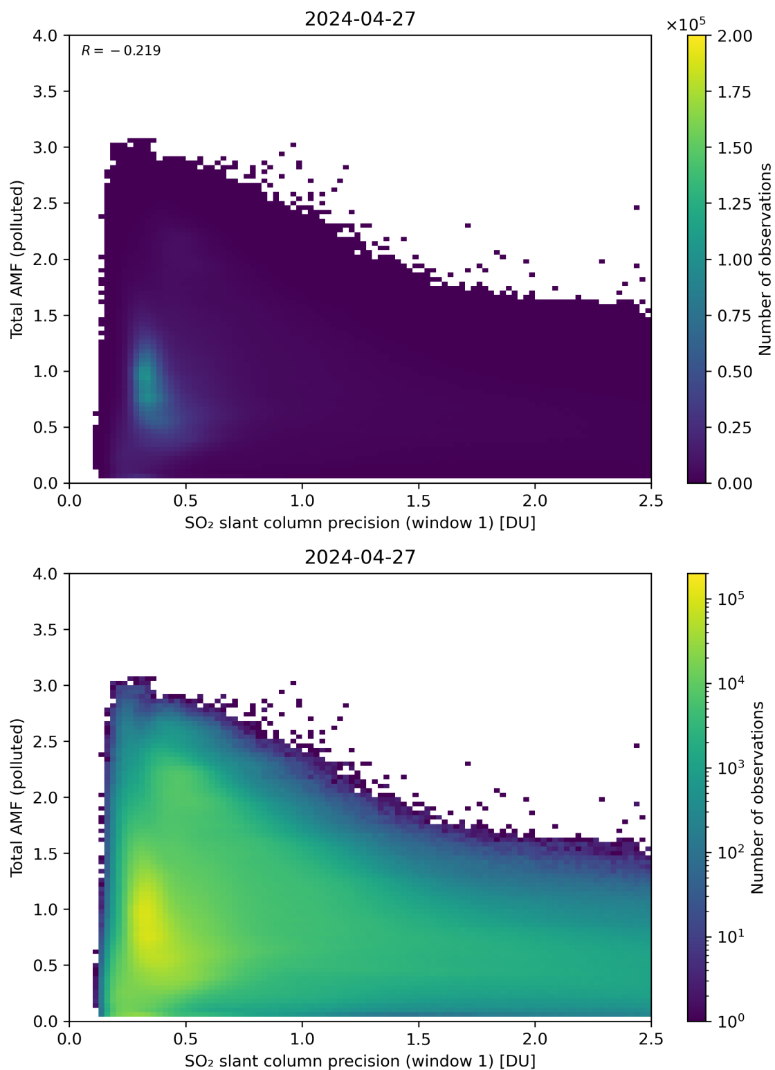
Figure 230: Scatter density plot of “SO 2 slant column precision (window 1)” against “Total AMF (polluted)” for 2024-04-26 to 2024-04-28.
