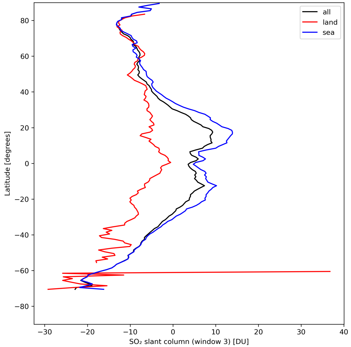
Figure 41: Zonal average of “SO 2 slant column (window 3)” for 2024-04-26 to 2024-04-28.
