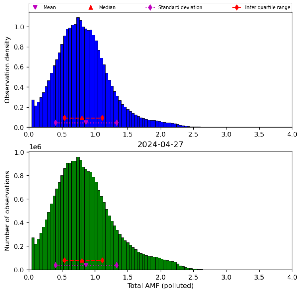
Figure 71: Histogram of “Total AMF (polluted)” for 2024-04-26 to 2024-04-28
