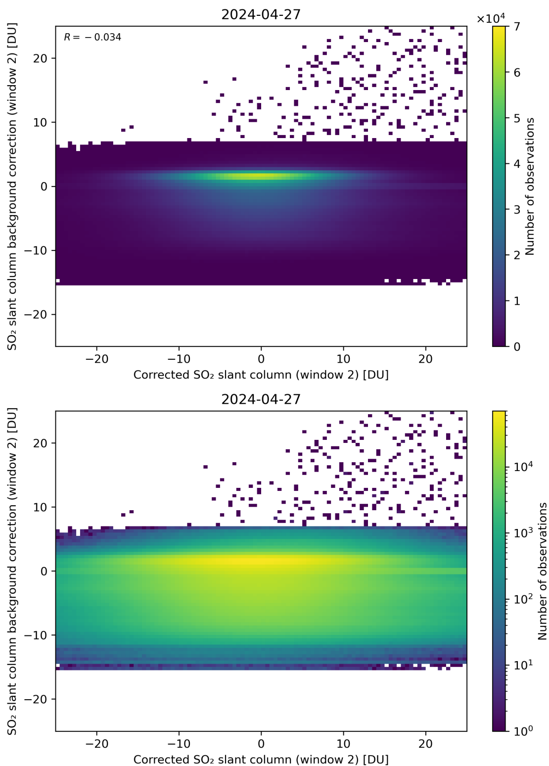
Figure 194: Scatter density plot of “Corrected SO 2 slant column (window 2)” against “SO 2 slant column background correction (window 2)” for 2024-04-26 to 2024-04-28.
