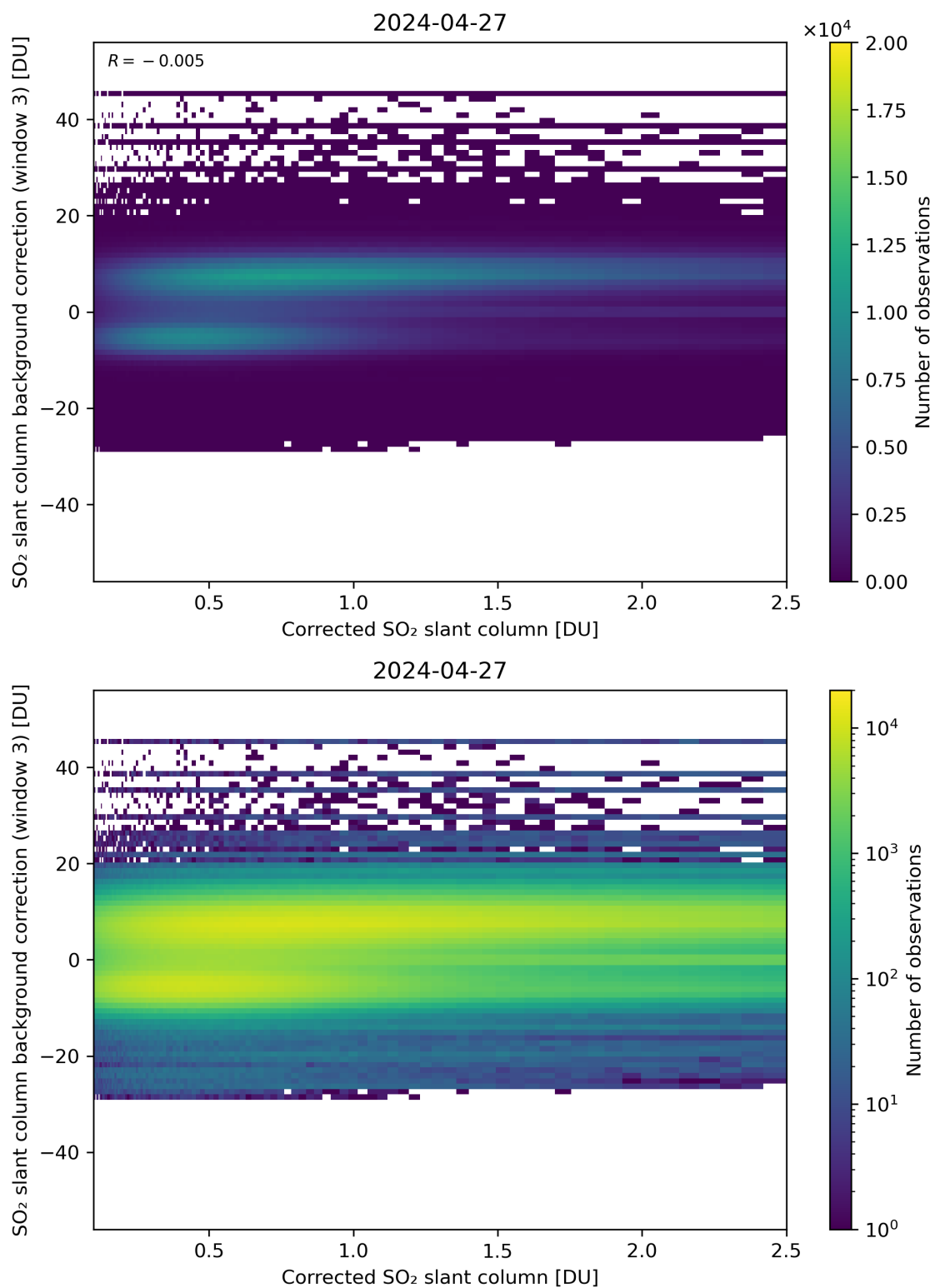
Figure 180: Scatter density plot of “Corrected SO 2 slant column” against “SO 2 slant column background correction (window 3)” for 2024-04-26 to 2024-04-28.
