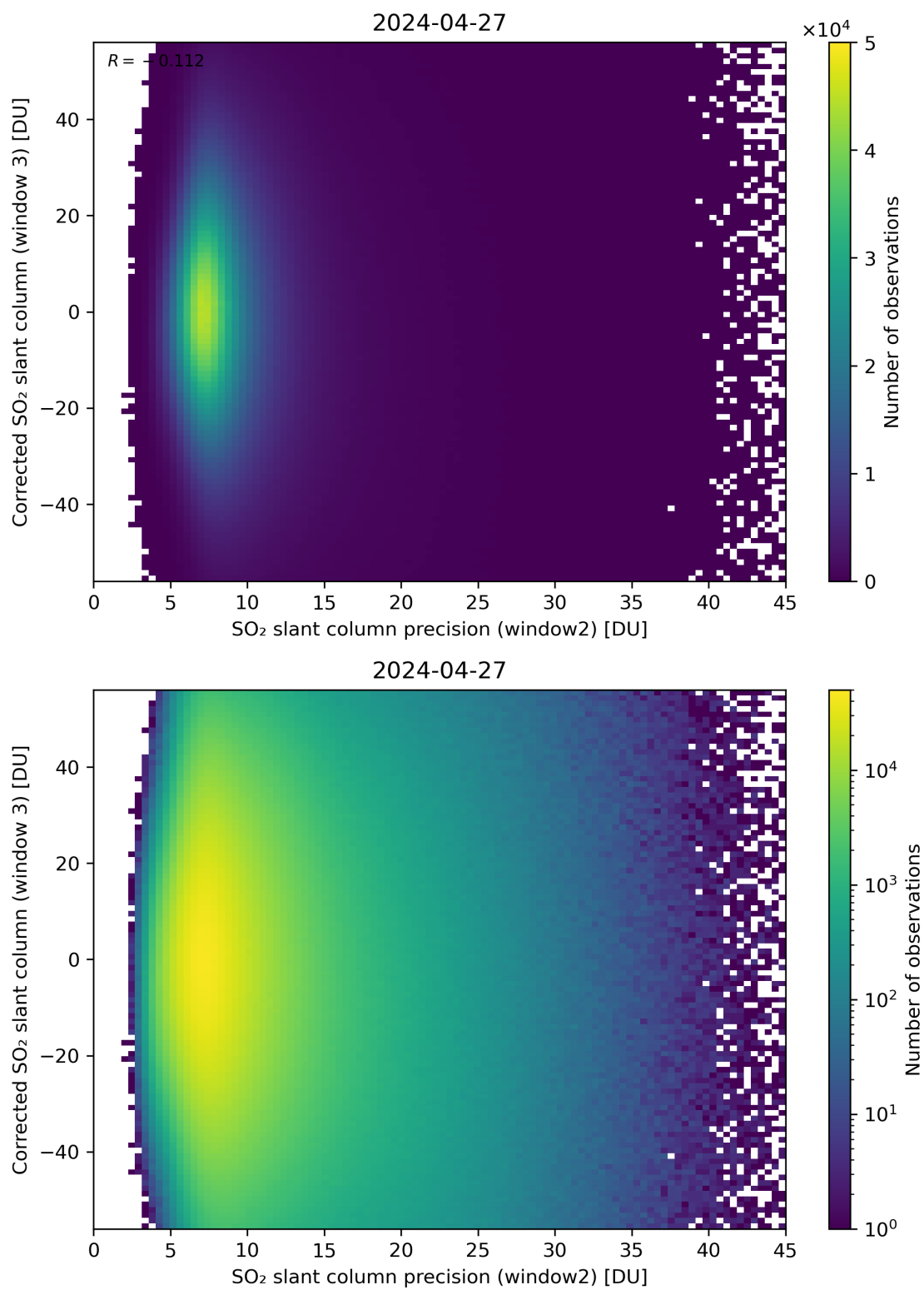
Figure 248: Scatter density plot of “SO 2 slant column precision (window2)” against “Corrected SO 2 slant column (window 3)” for 2024-04-26 to 2024-04-28.
