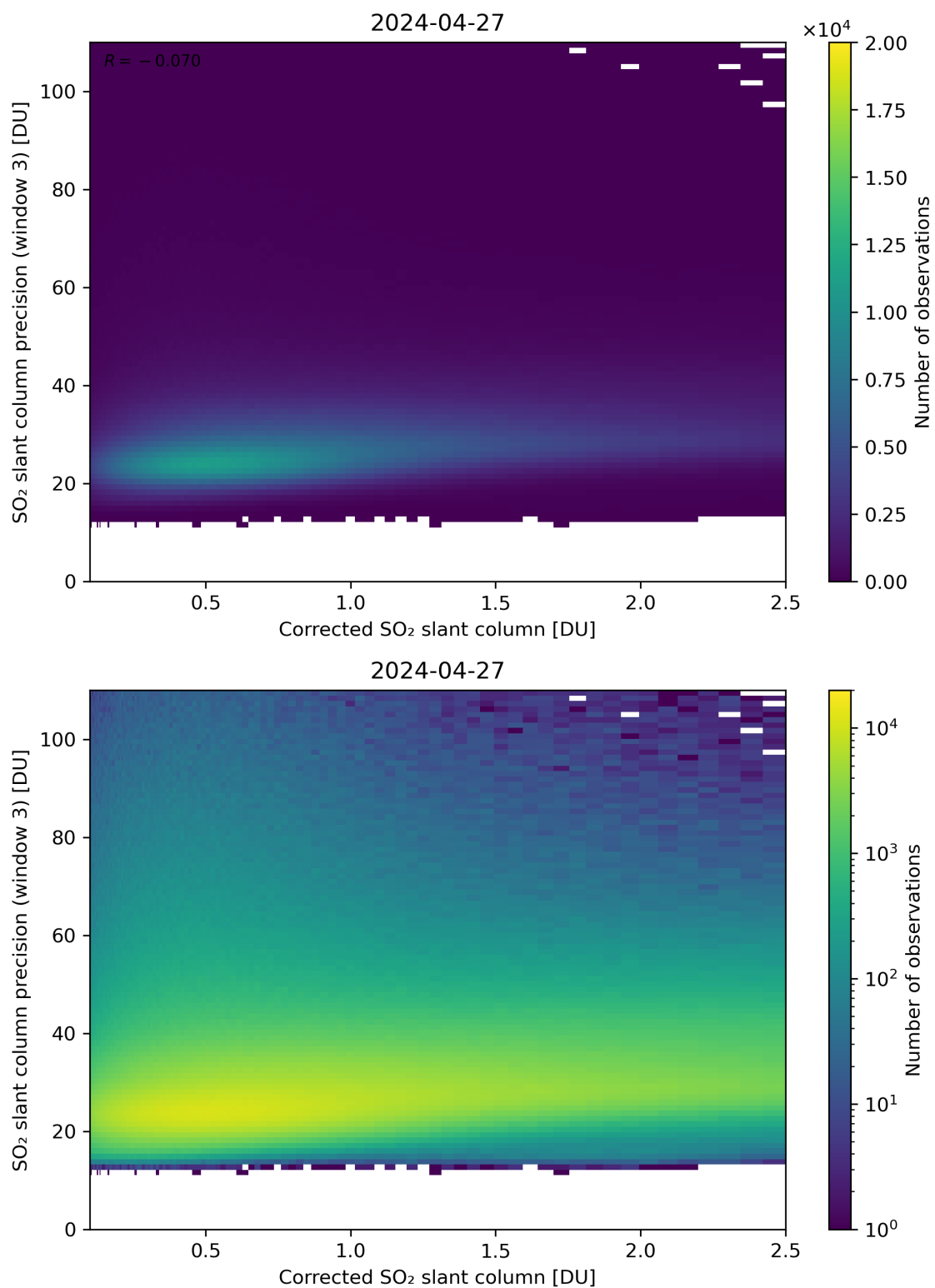
Figure 191: Scatter density plot of “Corrected SO 2 slant column” against “SO 2 slant column precision (window 3)” for 2024-04-26 to 2024-04-28.
