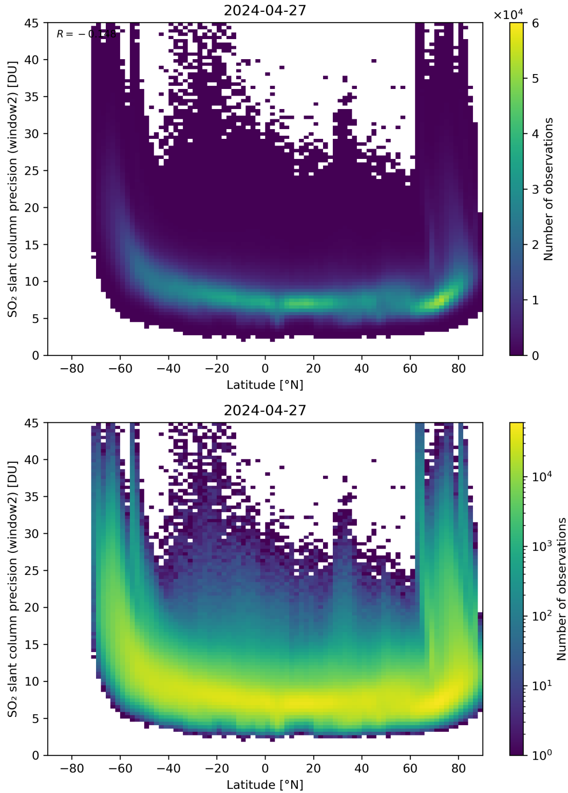
Figure 151: Scatter density plot of “Latitude” against “SO 2 slant column precision (window2)” for 2024-04-26 to 2024-04-28.
