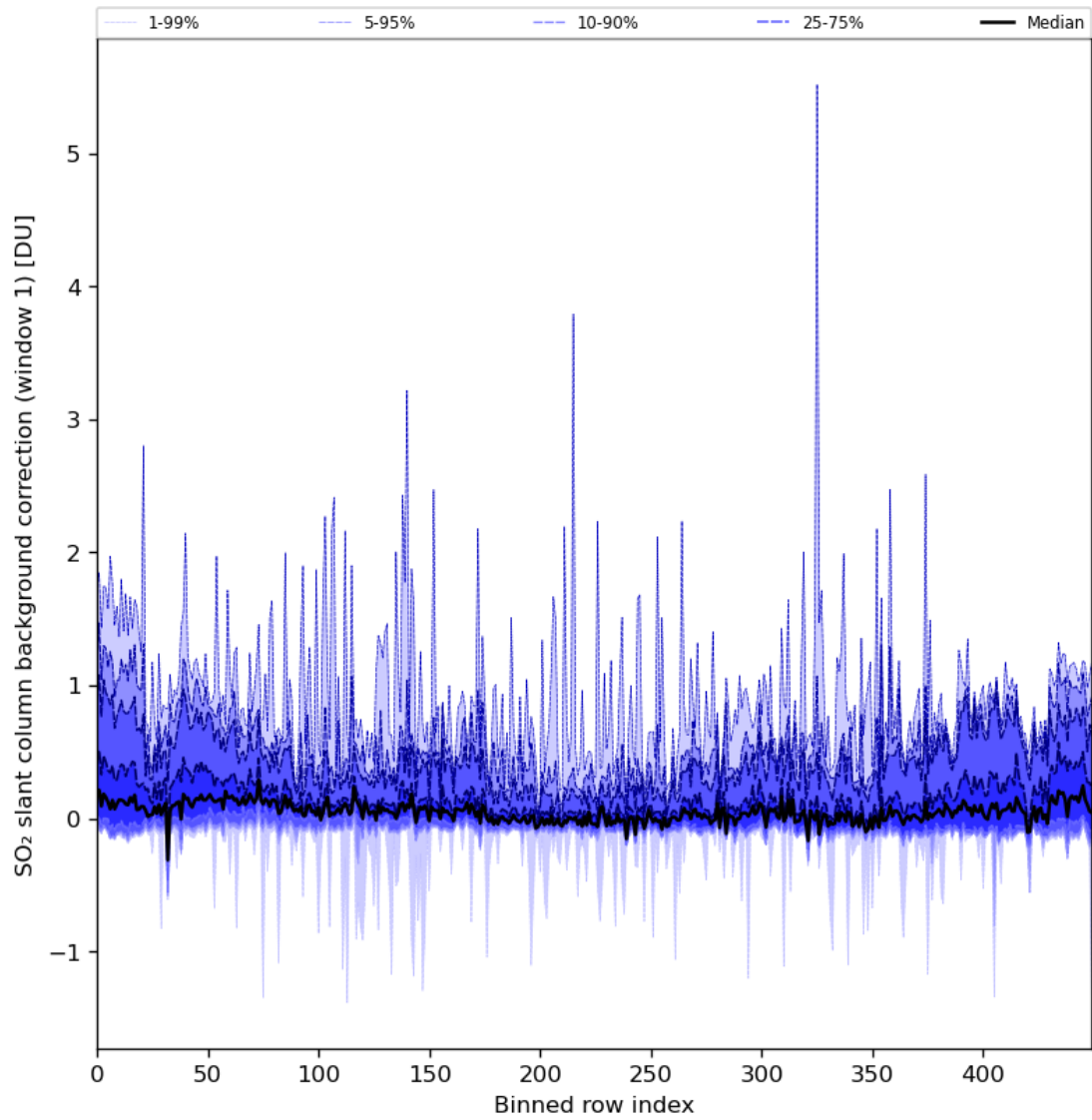
Figure 82: Along track statistics of “SO 2 slant column background correction (window 1)” for 2024-04-26 to 2024-04-28
