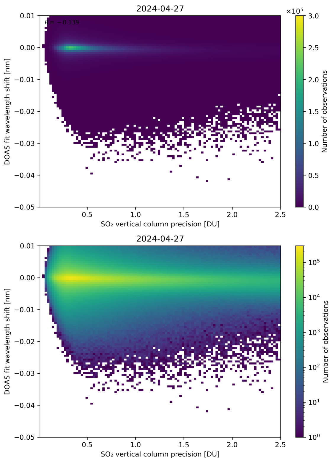
Figure 282: Scatter density plot of “SO 2 vertical column precision” against “DOAS fit wavelength shift” for 2024-04-26 to 2024-04-28.
