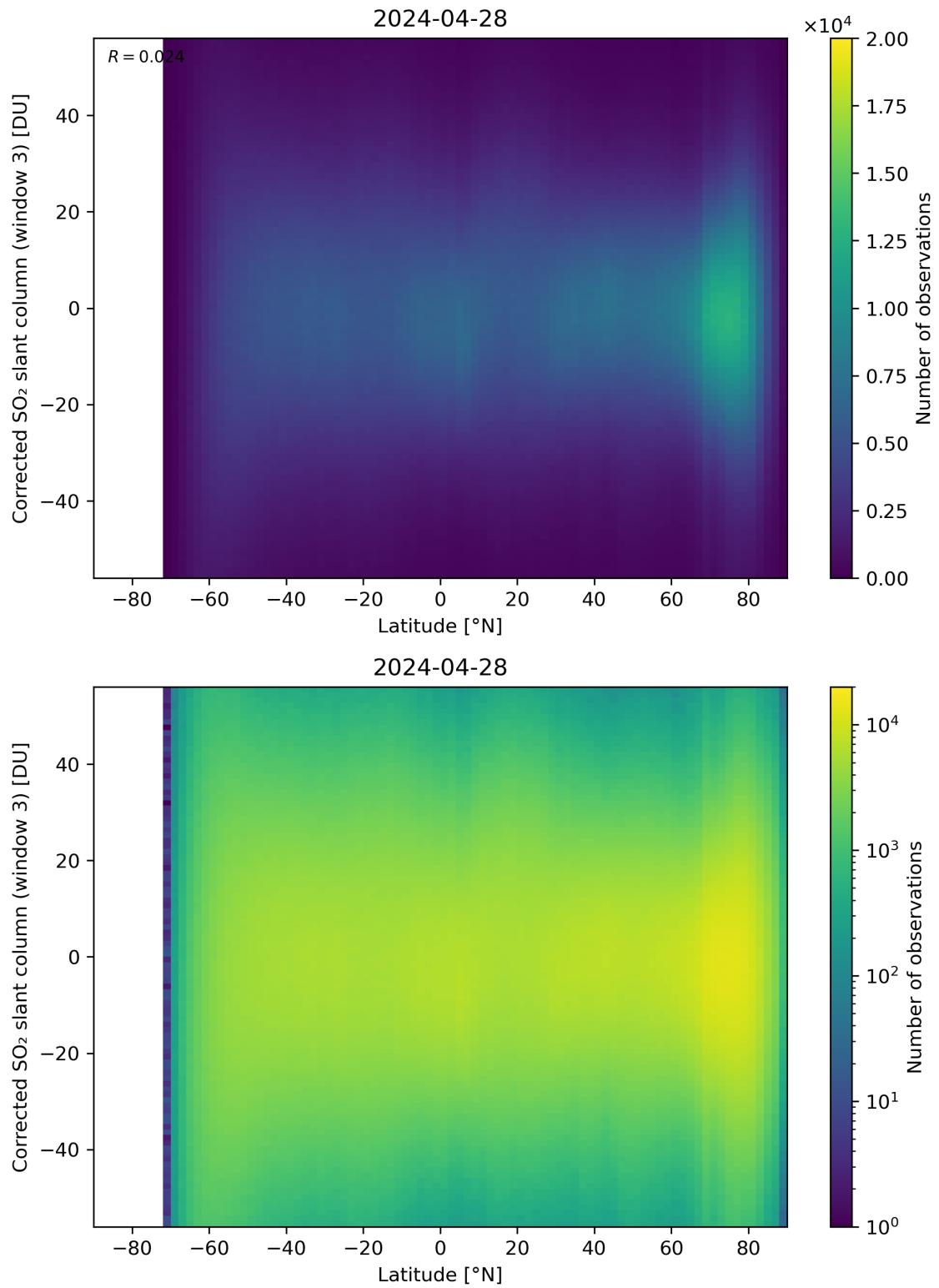
Figure 148: Scatter density plot of “Latitude” against “Corrected SO 2 slant column (window 3)” for 2024-04-27 to 2024-04-29.
