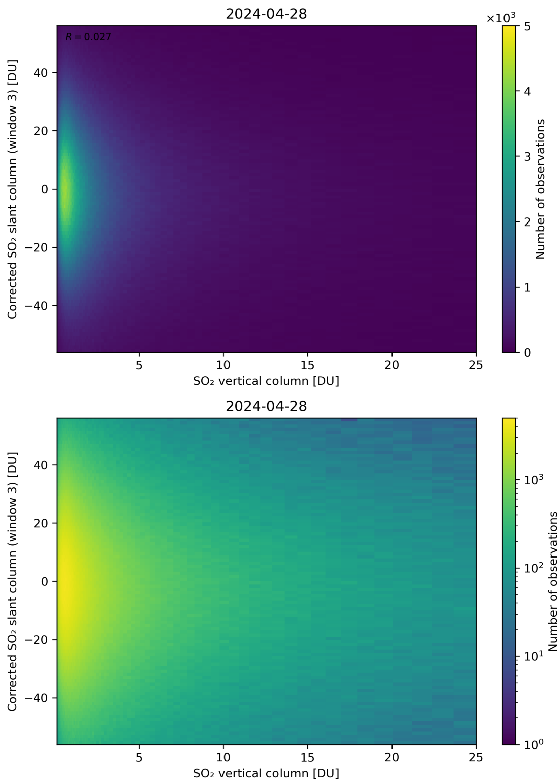
Figure 299: Scatter density plot of “SO 2 vertical column” against “Corrected SO 2 slant column (window 3)” for 2024-04-27 to 2024-04-29.
