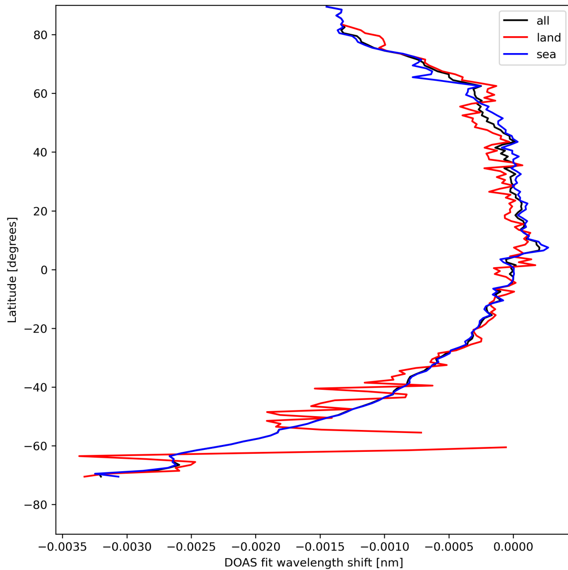
Figure 45: Zonal average of “DOAS fit wavelength shift” for 2024-04-27 to 2024-04-29.
