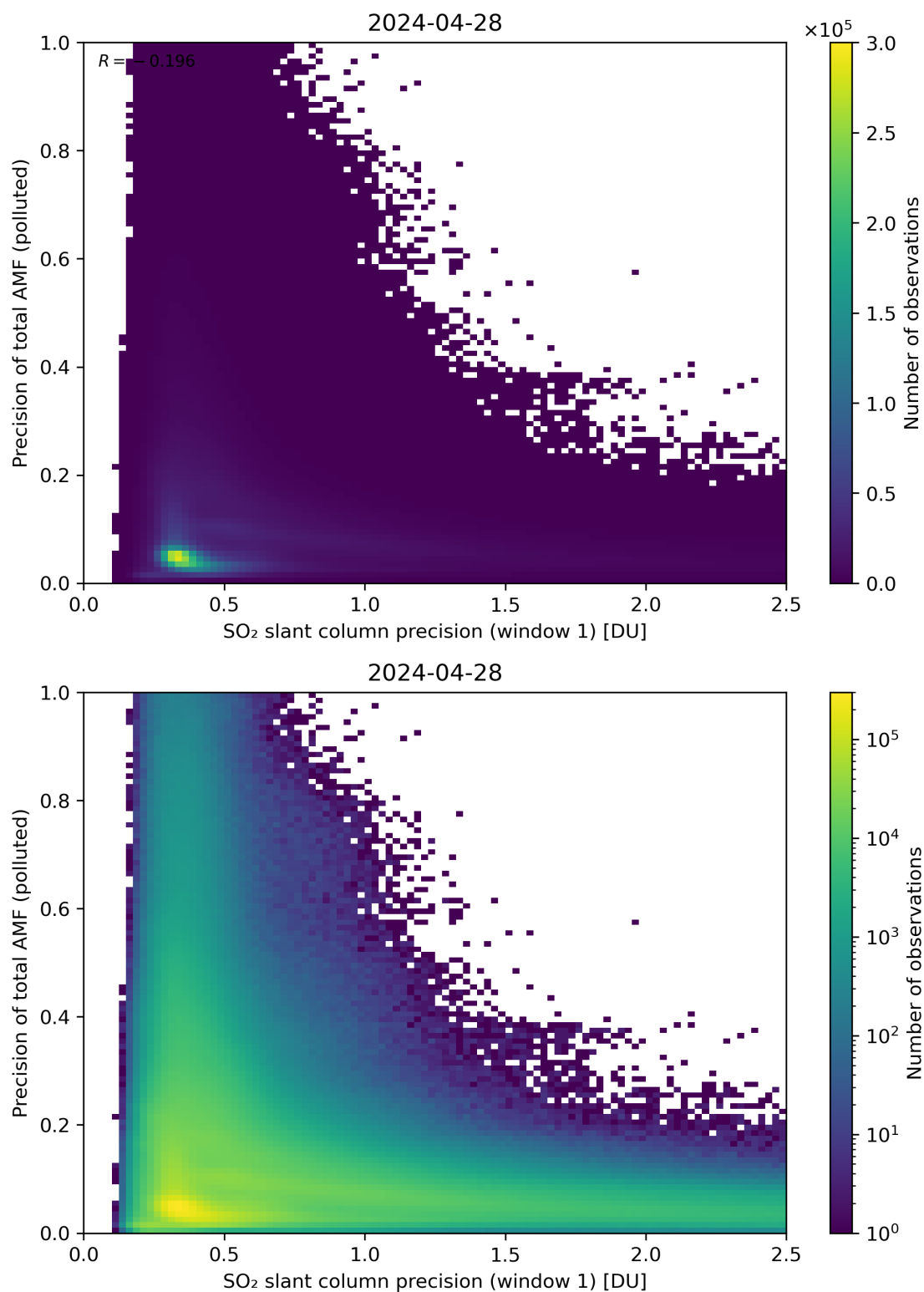
Figure 231: Scatter density plot of “SO 2 slant column precision (window 1)” against “Precision of total AMF (polluted)” for 2024-04-27 to 2024-04-29.
