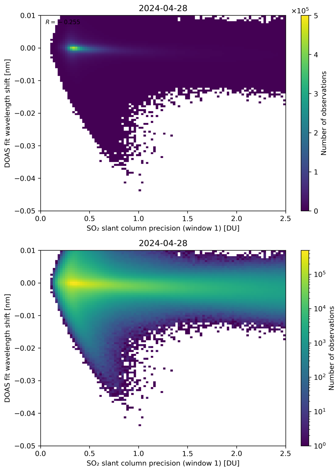
Figure 221: Scatter density plot of “SO 2 slant column precision (window 1)” against “DOAS fit wavelength shift” for 2024-04-27 to 2024-04-29.
