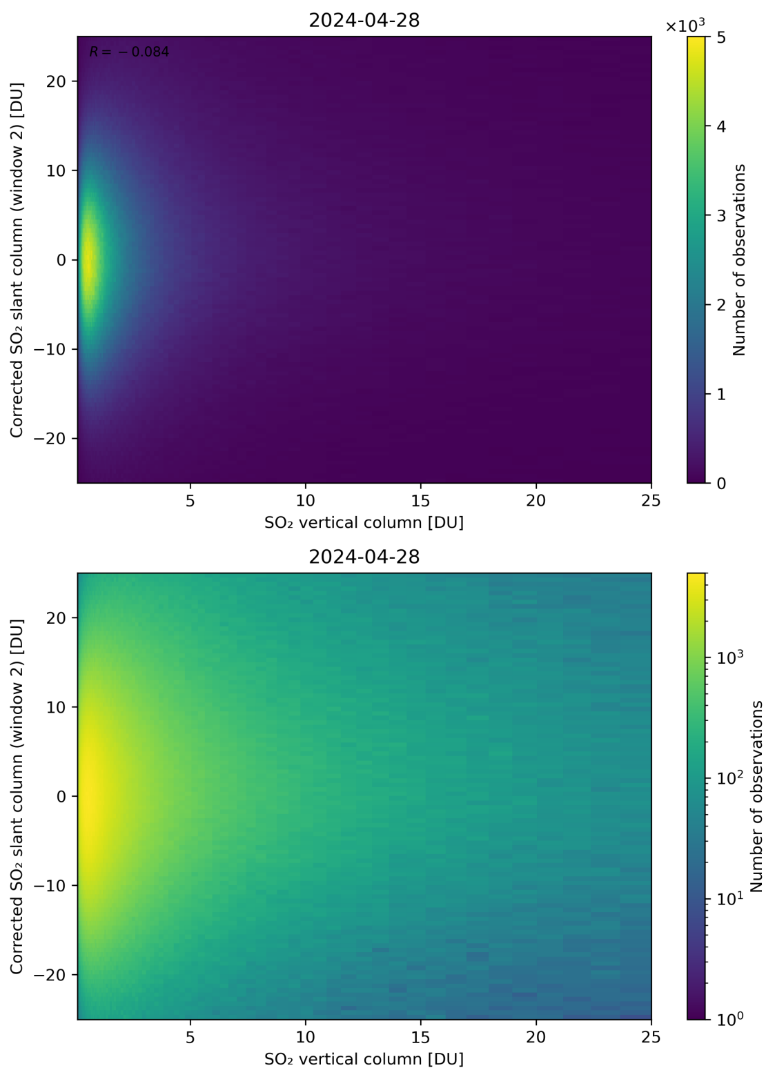
Figure 298: Scatter density plot of “SO 2 vertical column” against “Corrected SO 2 slant column (window 2)” for 2024-04-27 to 2024-04-29.
