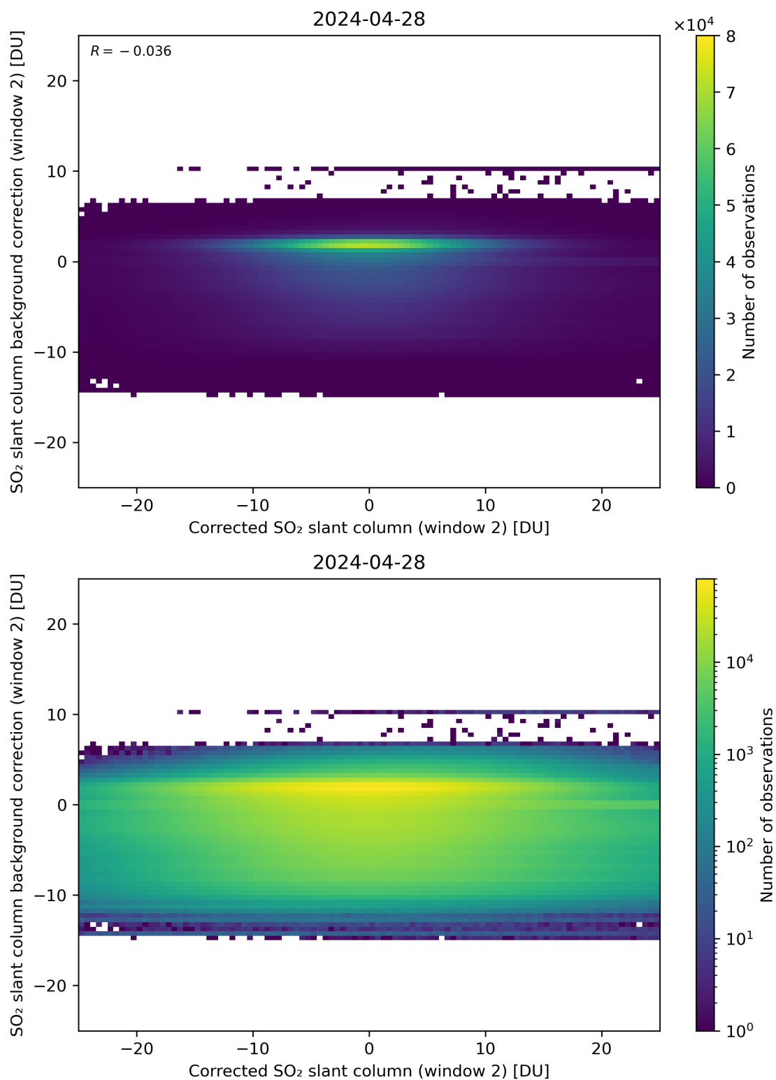
Figure 194: Scatter density plot of “Corrected SO 2 slant column (window 2)” against “SO 2 slant column background correction (window 2)” for 2024-04-27 to 2024-04-29.
