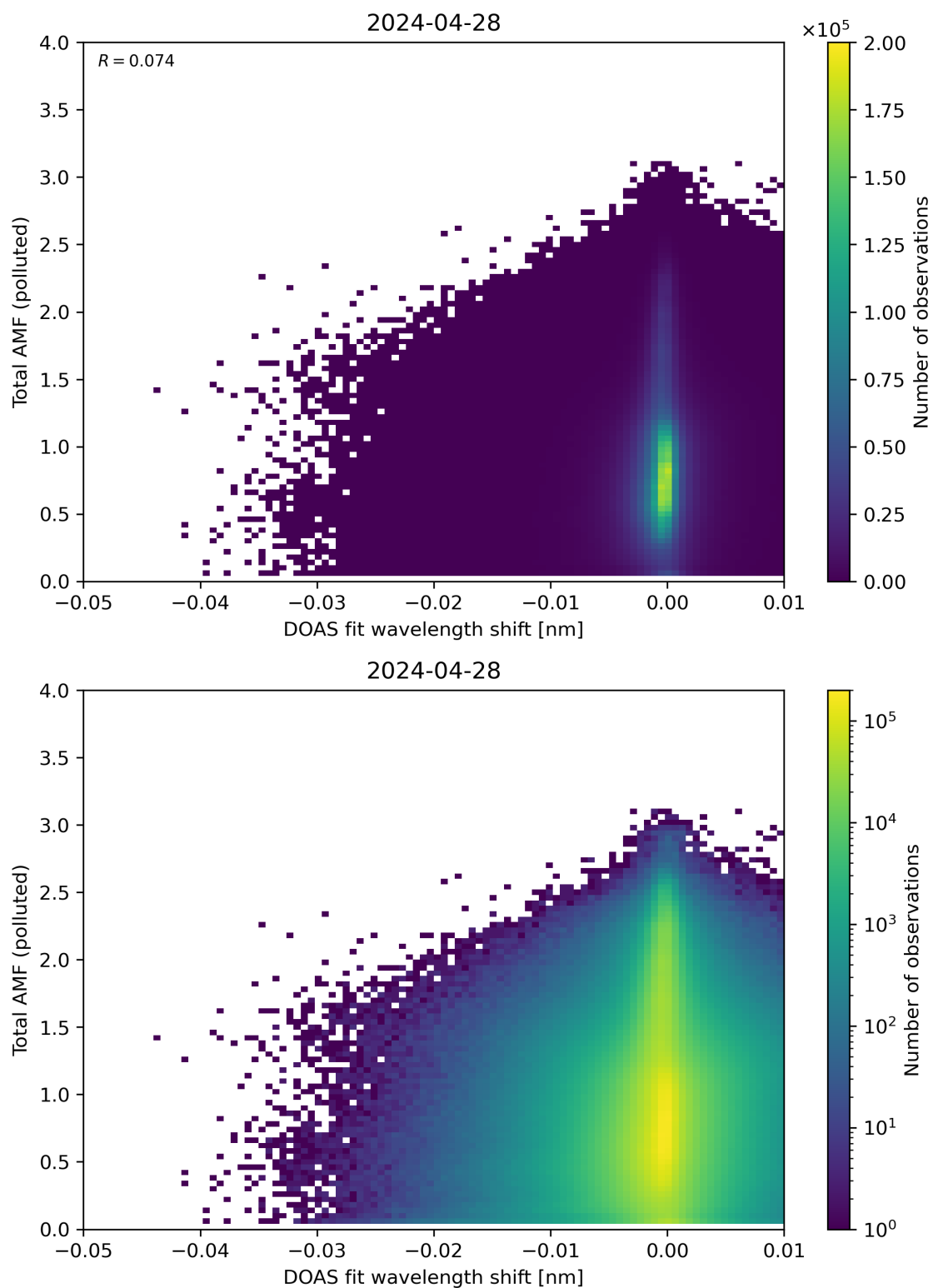
Figure 130: Scatter density plot of “DOAS fit wavelength shift” against “Total AMF (polluted)” for 2024-04-27 to 2024-04-29.
