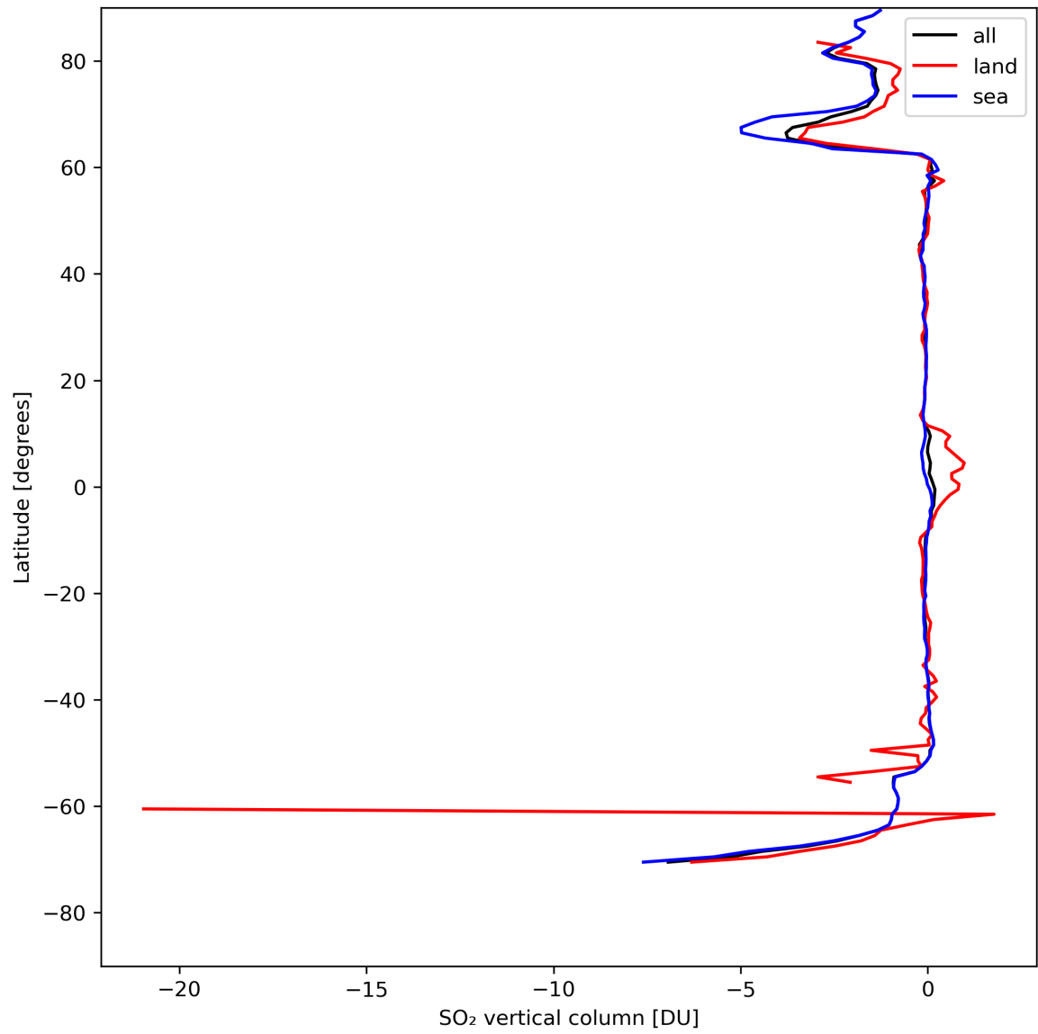
Figure 30: Zonal average of “SO 2 vertical column” for 2024-04-27 to 2024-04-29.
