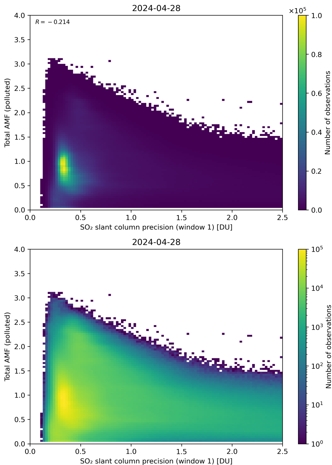
Figure 230: Scatter density plot of “SO 2 slant column precision (window 1)” against “Total AMF (polluted)” for 2024-04-27 to 2024-04-29.
