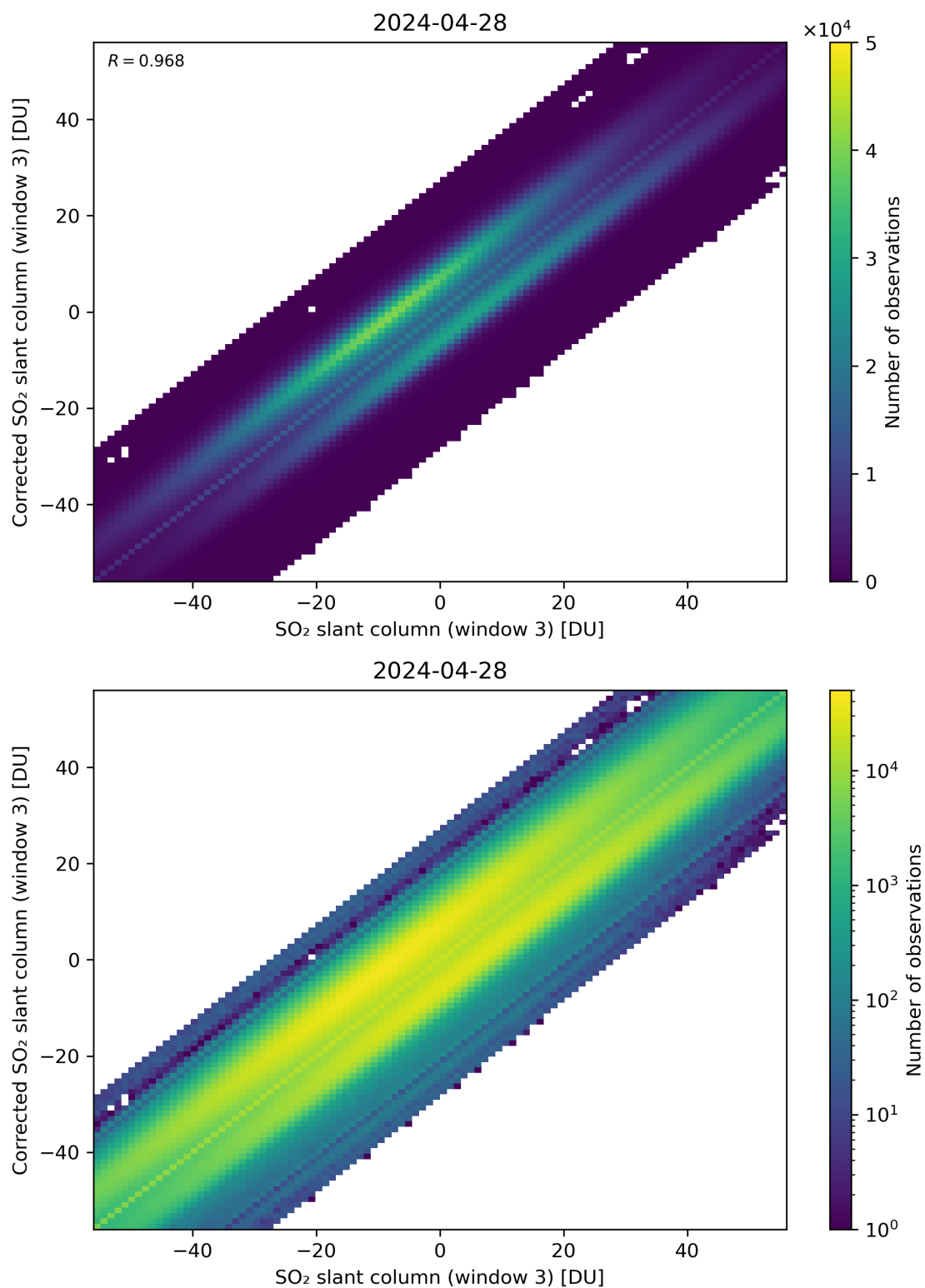
Figure 266: Scatter density plot of “SO 2 slant column (window 3)” against “Corrected SO 2 slant column (window 3)” for 2024-04-27 to 2024-04-29.
