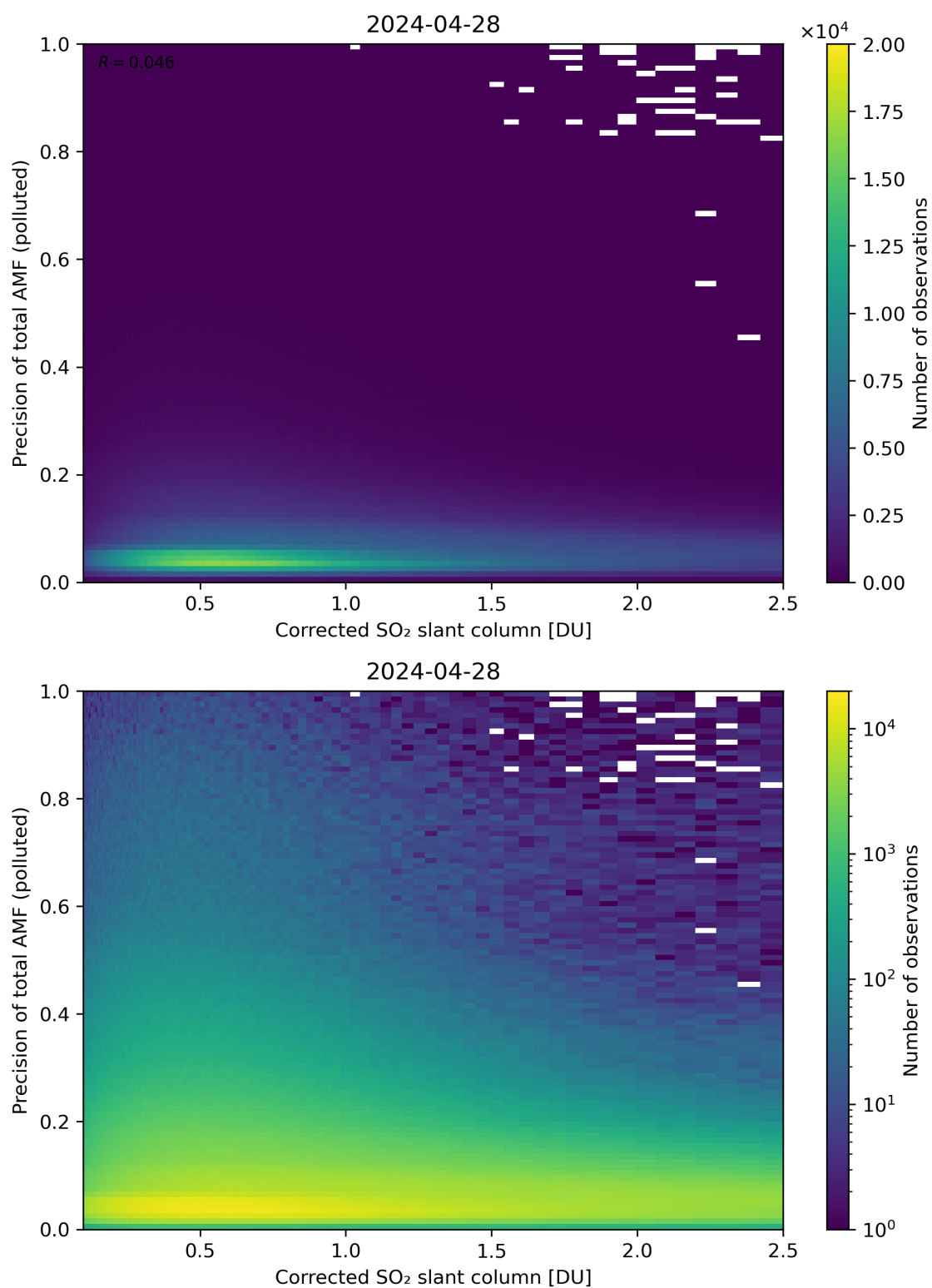
Figure 193: Scatter density plot of “Corrected SO 2 slant column” against “Precision of total AMF (polluted)” for 2024-04-27 to 2024-04-29.
