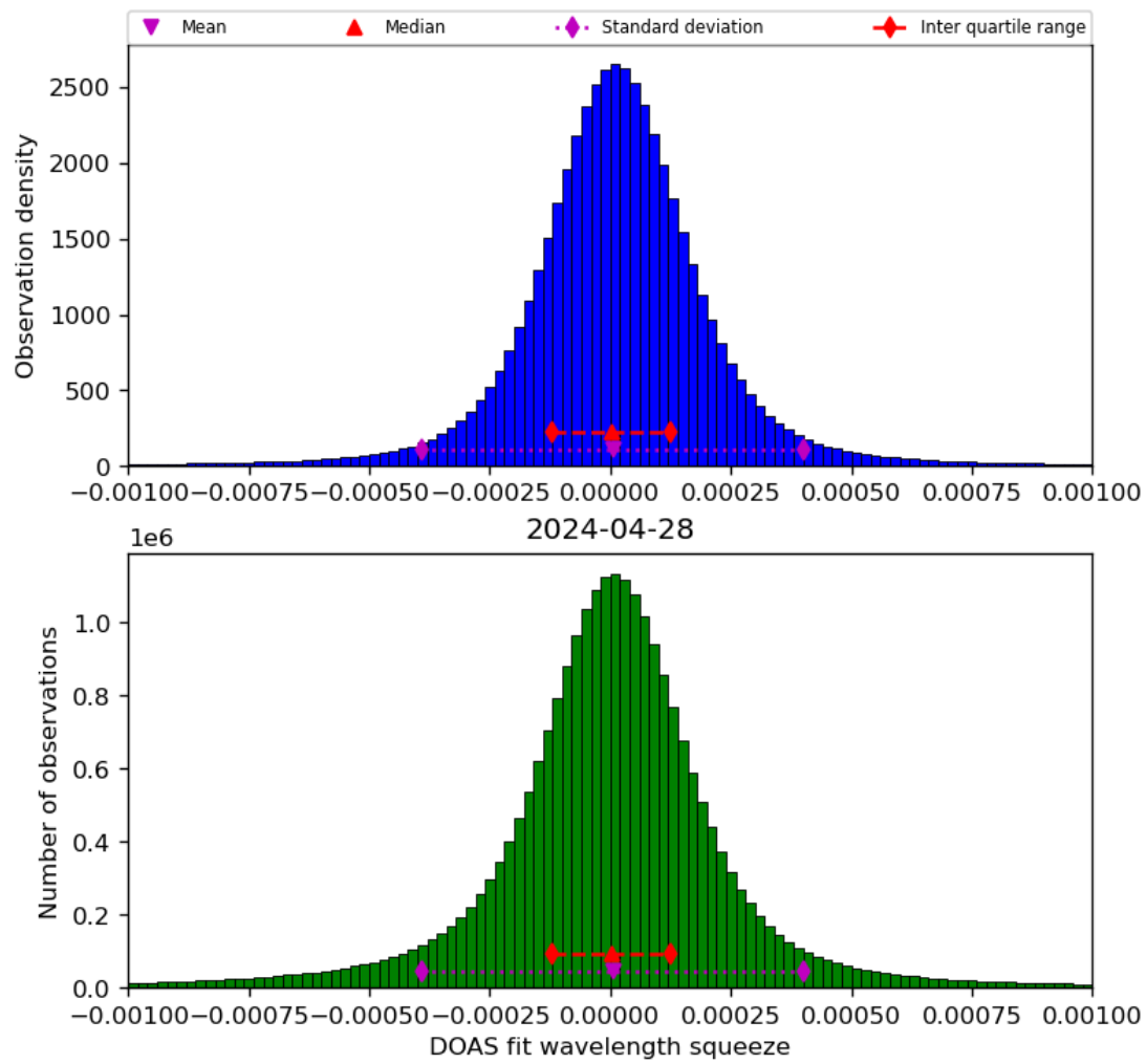
Figure 69: Histogram of “DOAS fit wavelength squeeze” for 2024-04-27 to 2024-04-29
