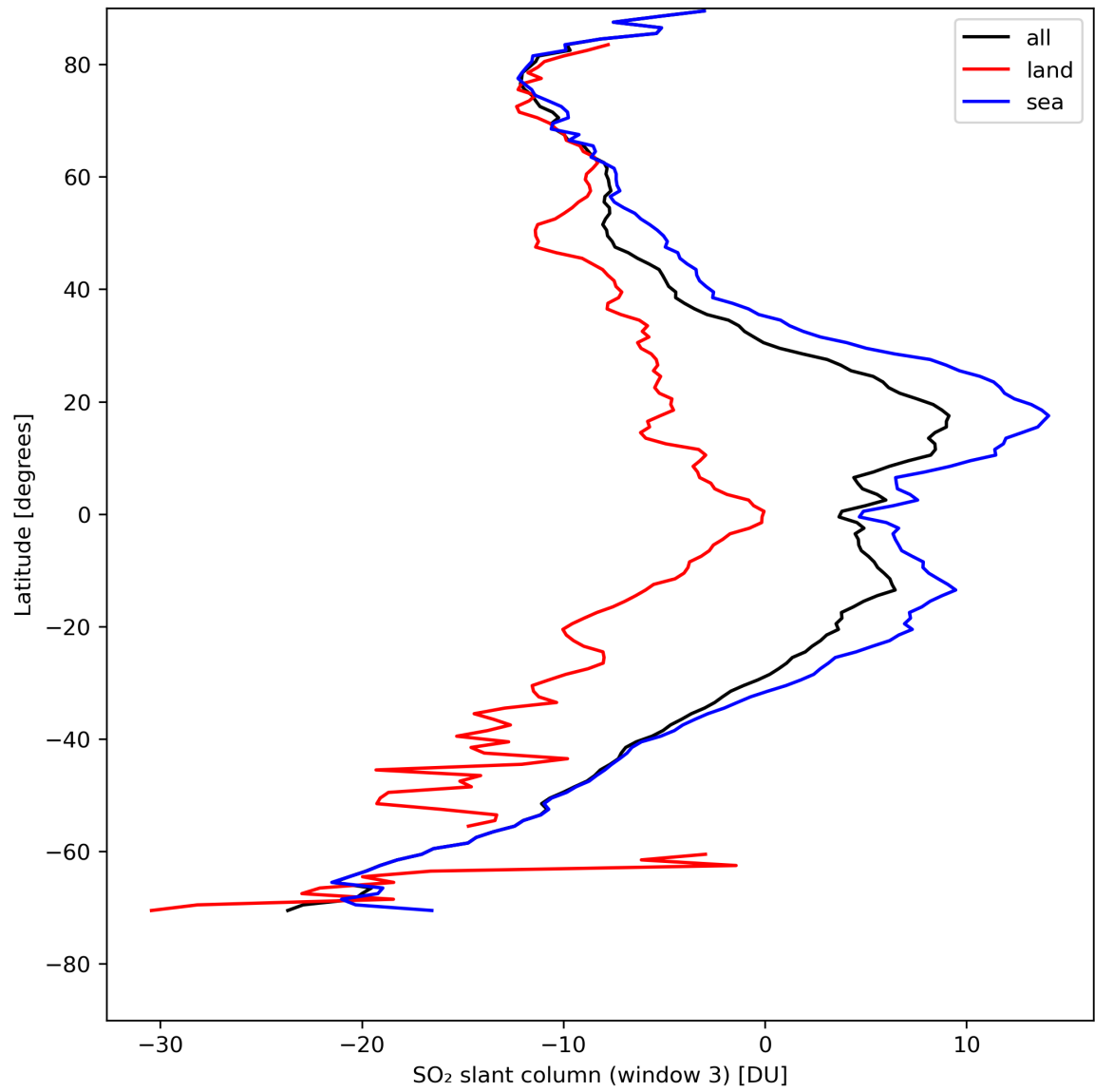
Figure 41: Zonal average of “SO 2 slant column (window 3)” for 2024-04-27 to 2024-04-29.
