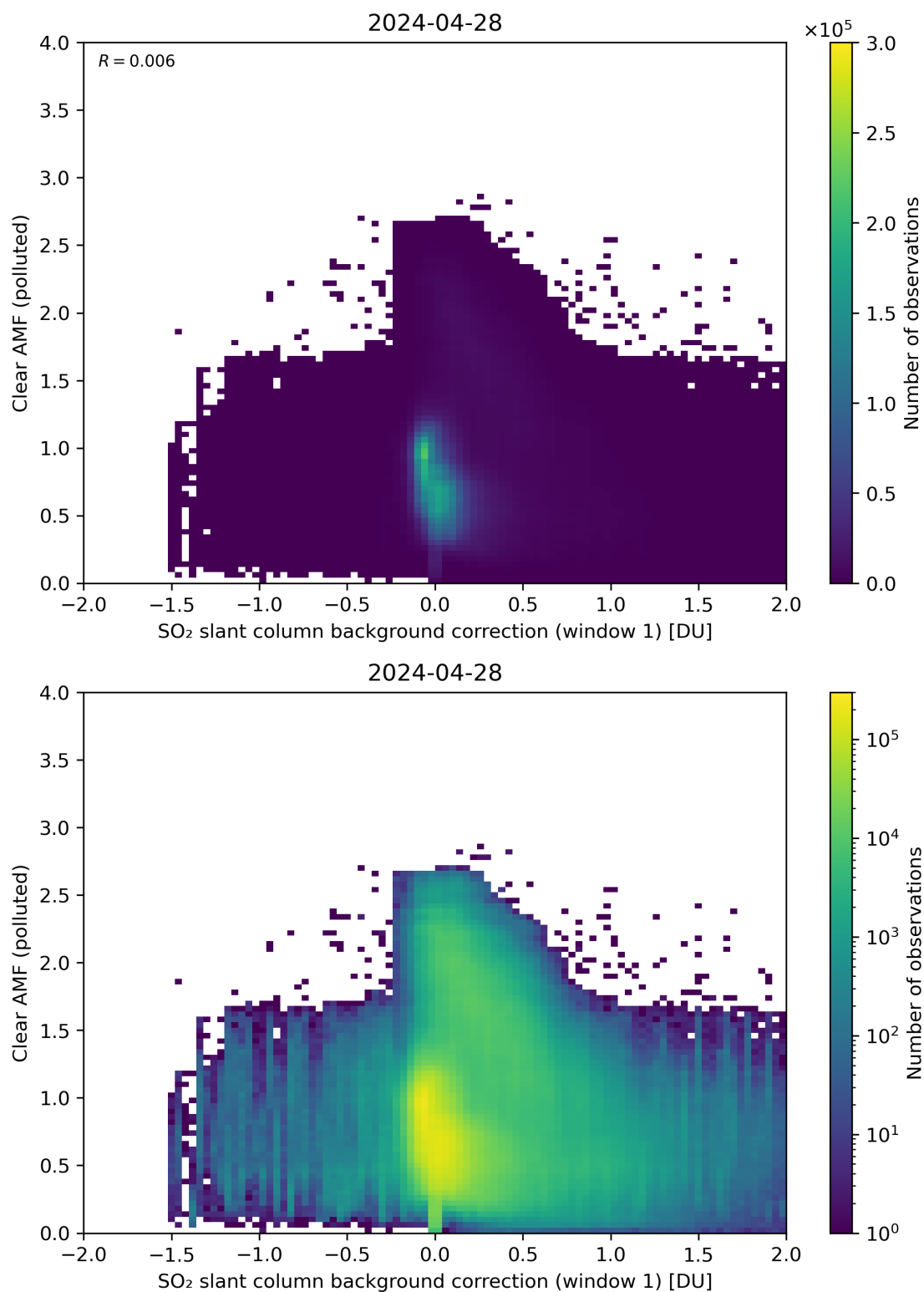
Figure 103: Scatter density plot of “SO 2 slant column background correction (window 1)” against “Clear AMF (polluted)” for 2024-04-27 to 2024-04-29.
