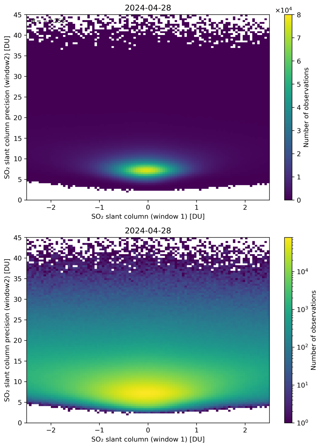
Figure 236: Scatter density plot of “SO 2 slant column (window 1)” against “SO 2 slant column precision (window2)” for 2024-04-27 to 2024-04-29.
