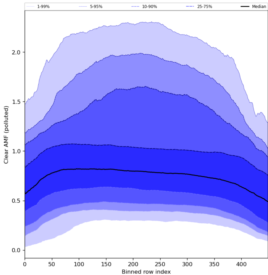
Figure 96: Along track statistics of “Clear AMF (polluted)” for 2024-04-27 to 2024-04-29
