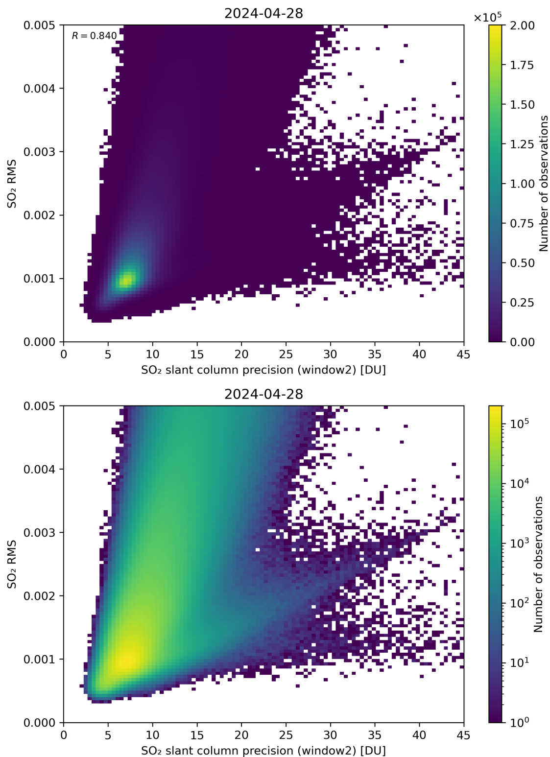
Figure 245: Scatter density plot of “SO 2 slant column precision (window2)” against “SO 2 RMS” for 2024-04-27 to 2024-04-29.
