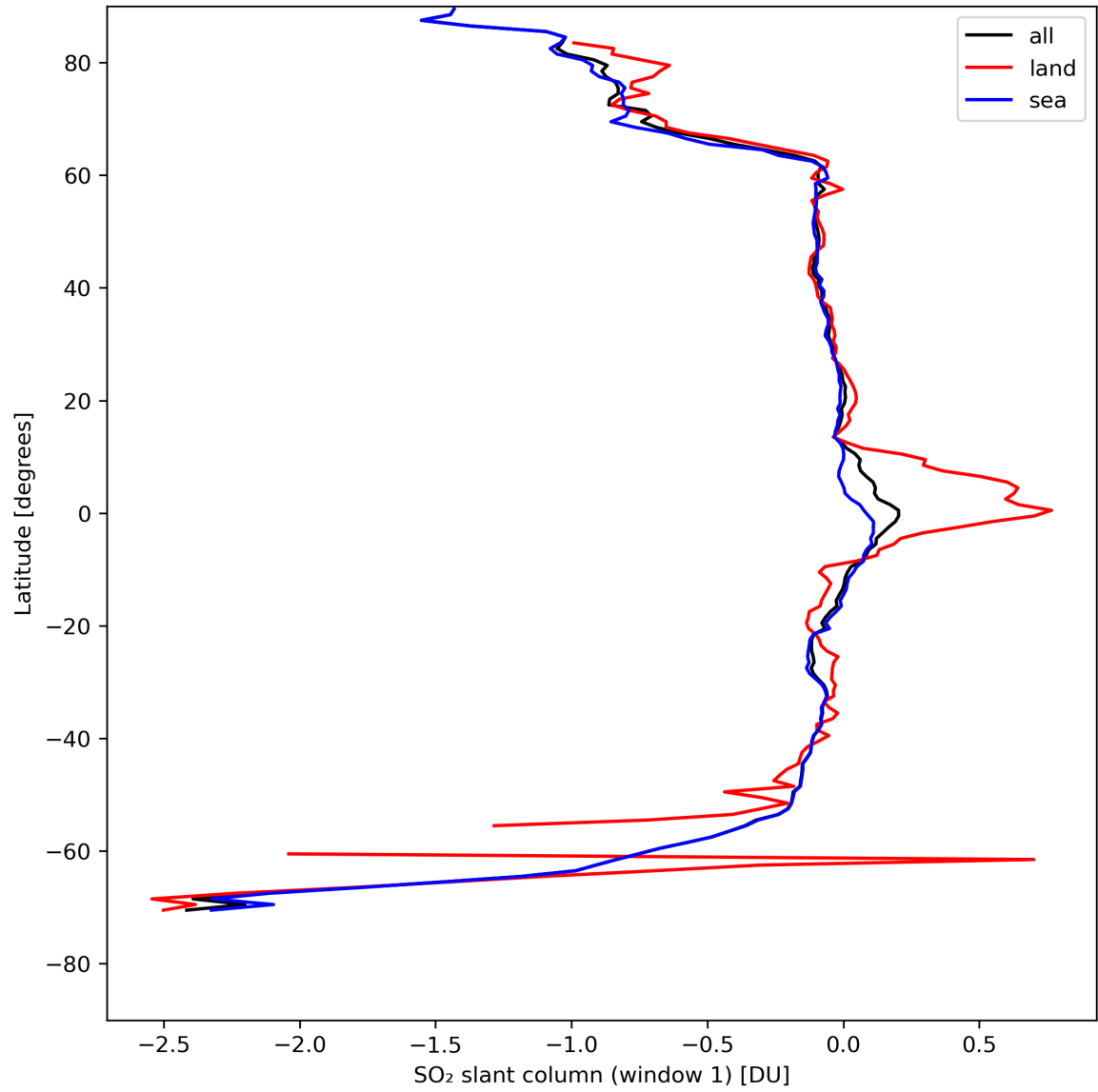
Figure 33: Zonal average of “SO 2 slant column (window 1)” for 2024-04-27 to 2024-04-29.
