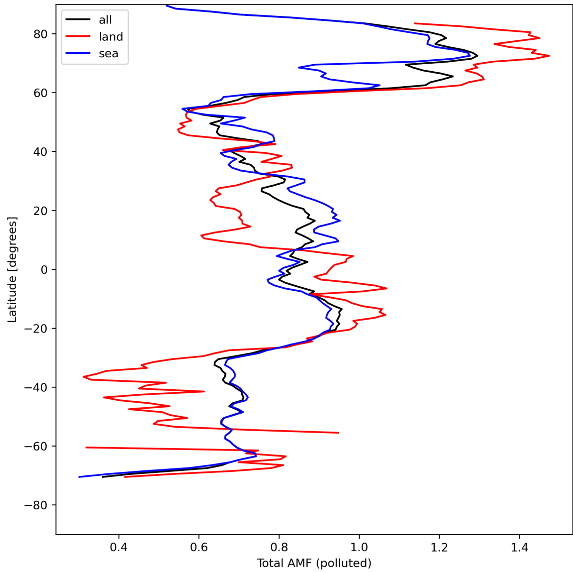
Figure 48: Zonal average of “Total AMF (polluted)” for 2024-04-27 to 2024-04-29.
