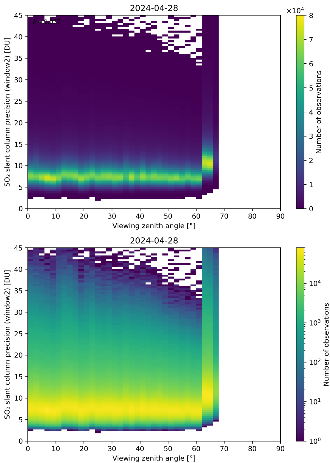
Figure 322: Scatter density plot of “Viewing zenith angle” against “SO 2 slant column precision (window2)” for 2024-04-27 to 2024-04-29.
