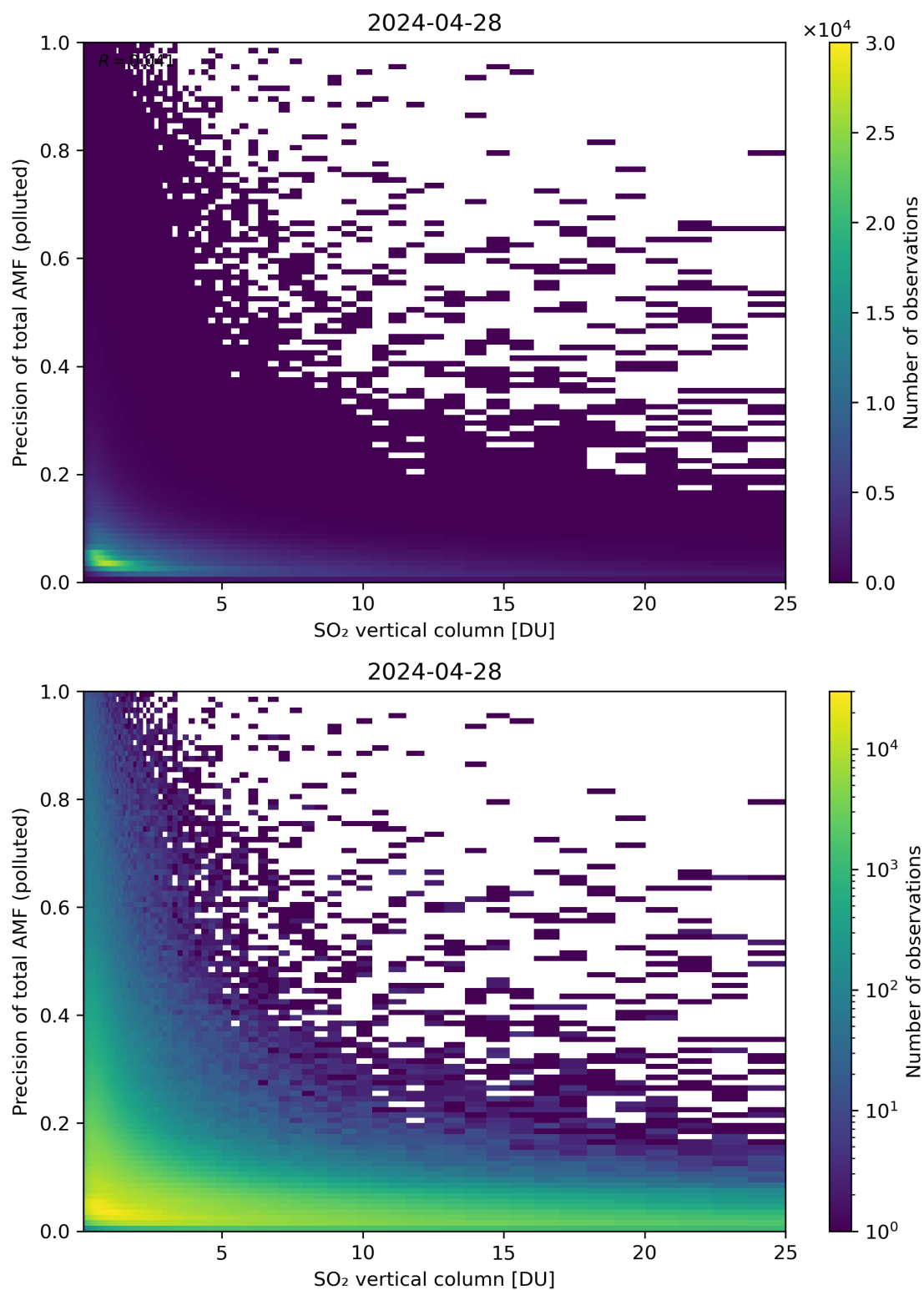
Figure 306: Scatter density plot of “SO 2 vertical column” against “Precision of total AMF (polluted)” for 2024-04-27 to 2024-04-29.
