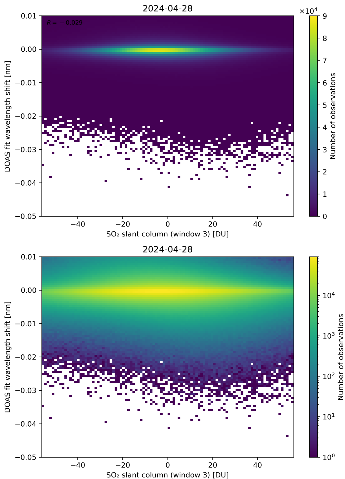
Figure 254: Scatter density plot of “SO 2 slant column (window 3)” against “DOAS fit wavelength shift” for 2024-04-27 to 2024-04-29.
