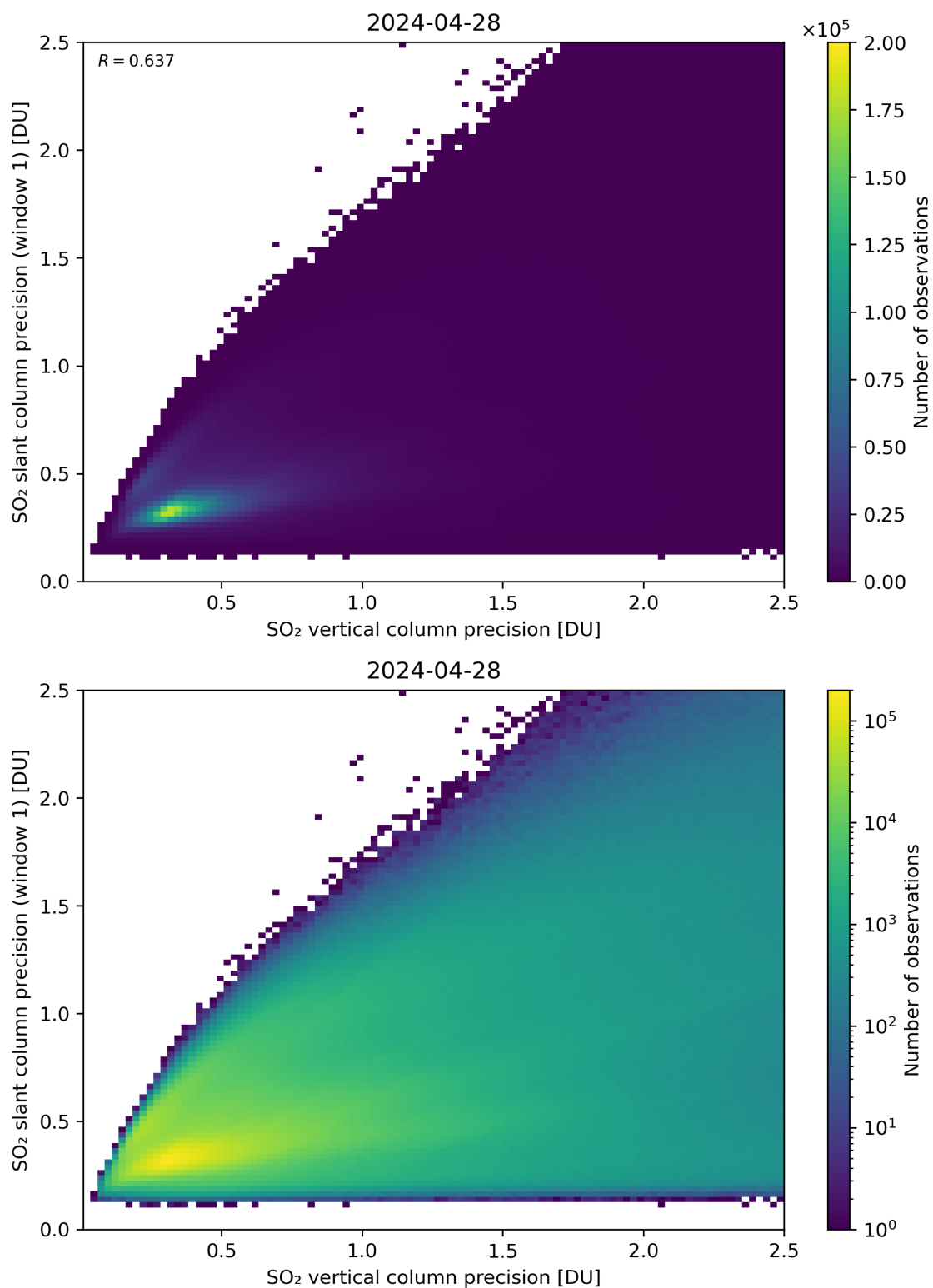
Figure 290: Scatter density plot of “SO 2 vertical column precision” against “SO 2 slant column precision (window 1)” for 2024-04-27 to 2024-04-29.
