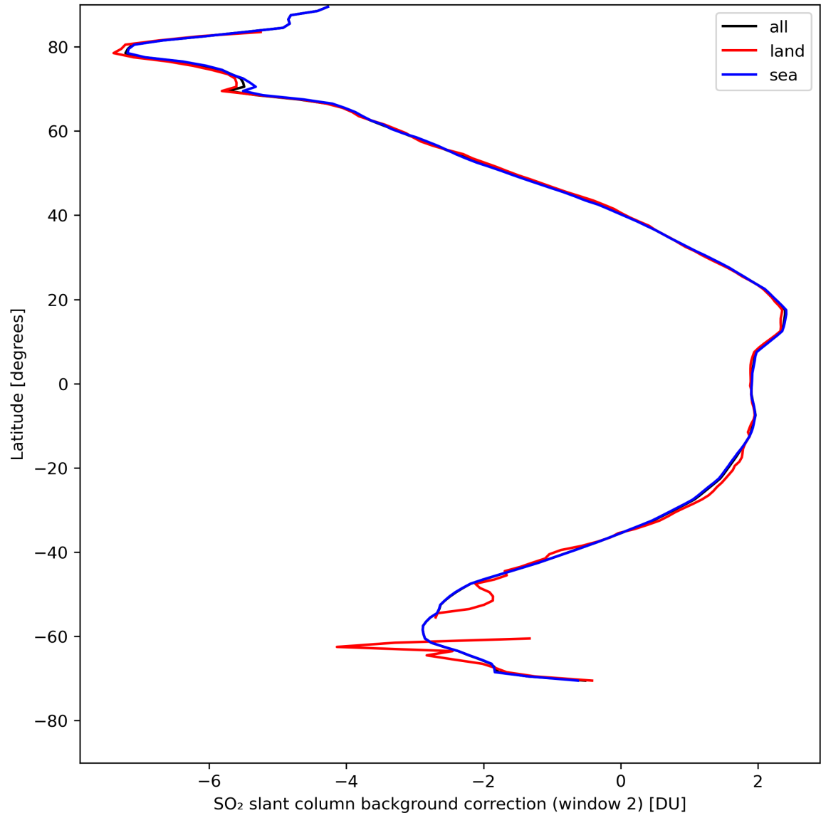
Figure 40: Zonal average of “SO 2 slant column background correction (window 2)” for 2024-04-27 to 2024-04-29.
