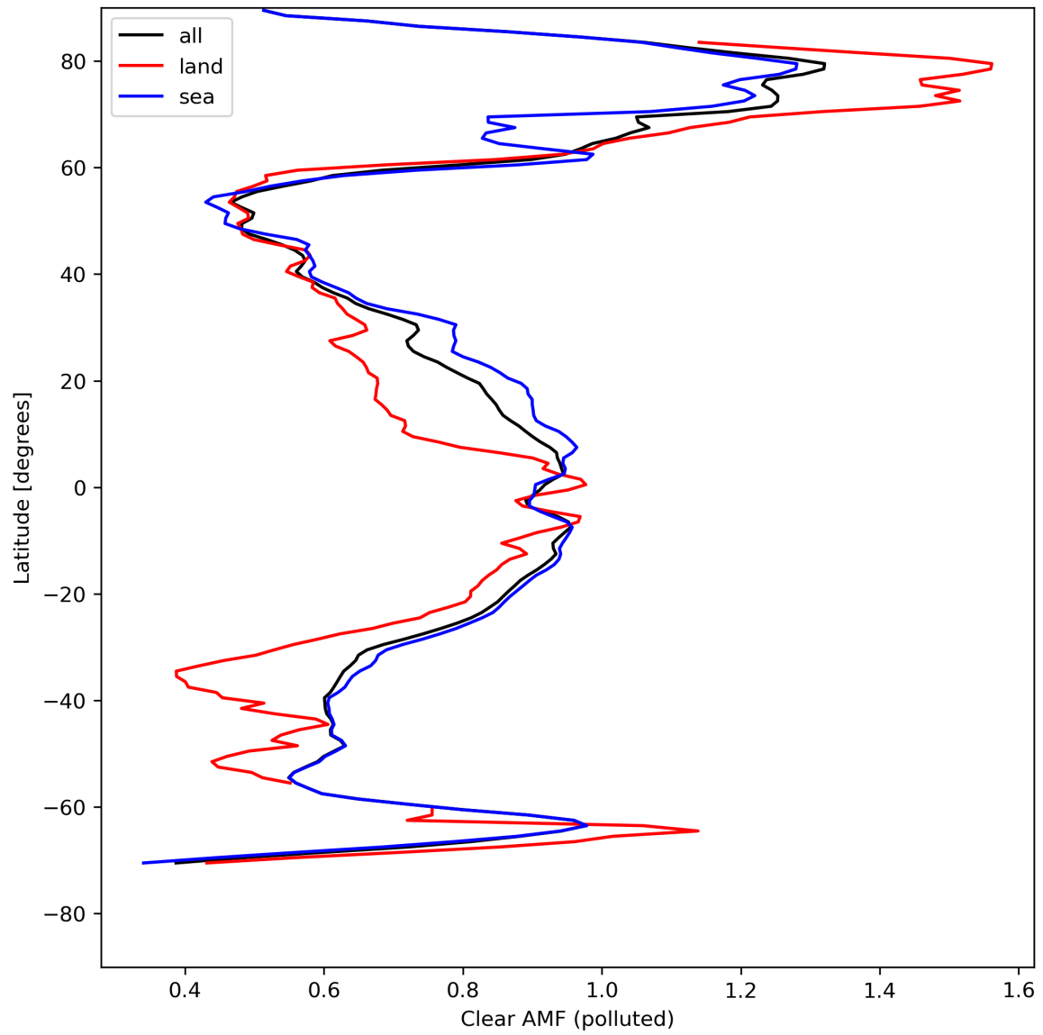
Figure 50: Zonal average of “Clear AMF (polluted)” for 2024-04-27 to 2024-04-29.
