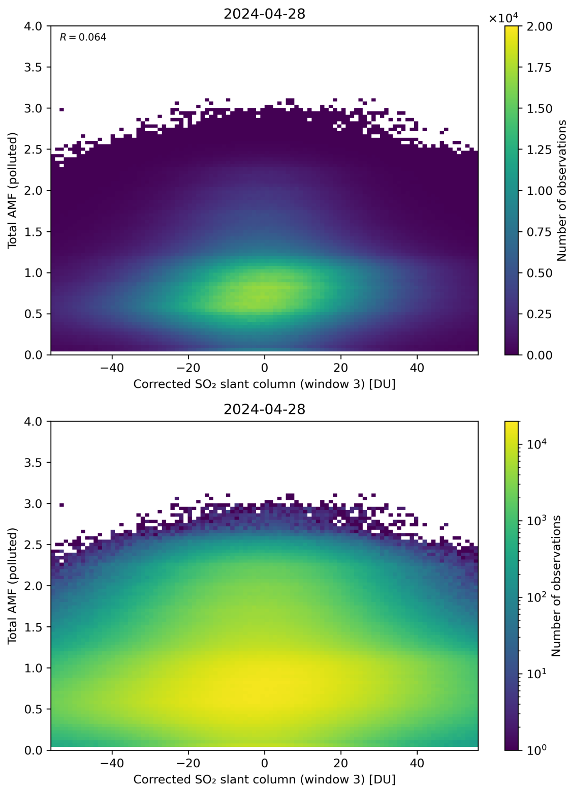
Figure 210: Scatter density plot of “Corrected SO 2 slant column (window 3)” against “Total AMF (polluted)” for 2024-04-27 to 2024-04-29.
