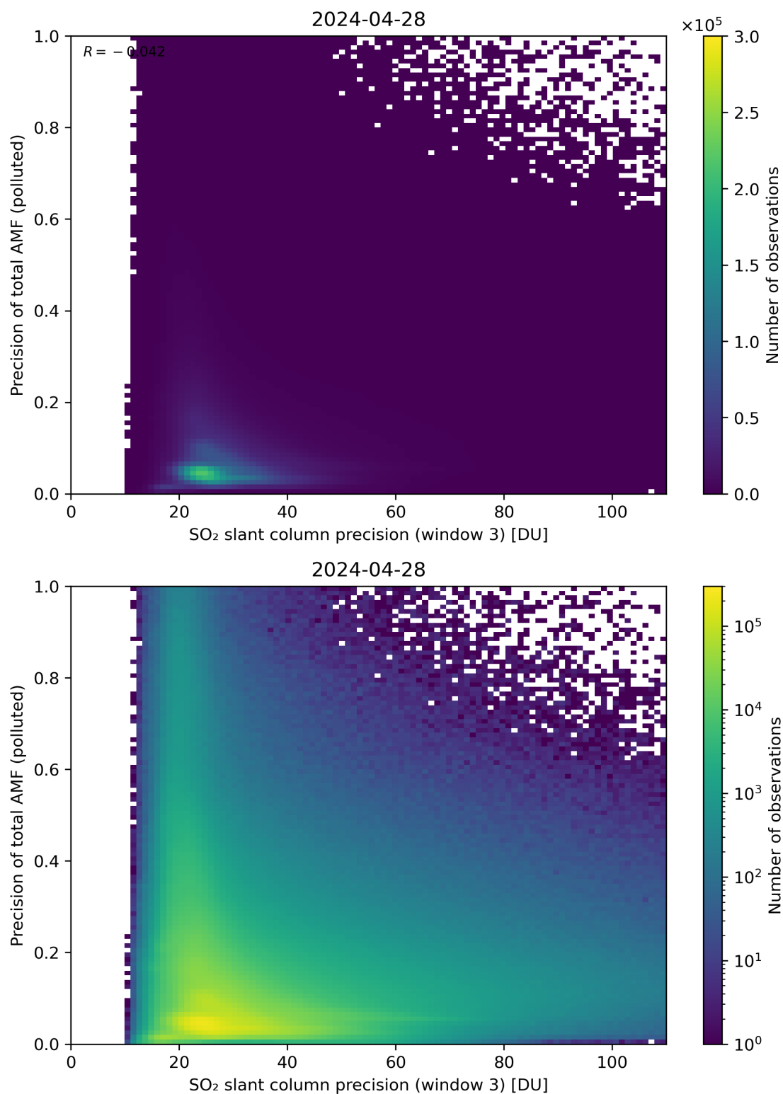
Figure 264: Scatter density plot of “SO 2 slant column precision (window 3)” against “Precision of total AMF (polluted)” for 2024-04-27 to 2024-04-29.
