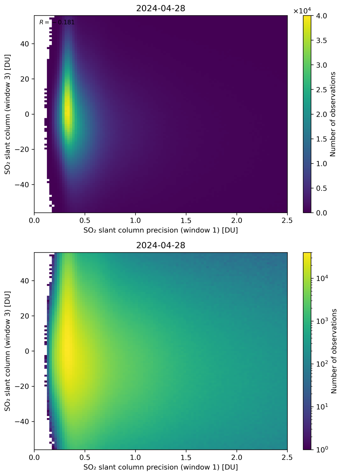
Figure 228: Scatter density plot of “SO 2 slant column precision (window 1)” against “SO 2 slant column (window 3)” for 2024-04-27 to 2024-04-29.
