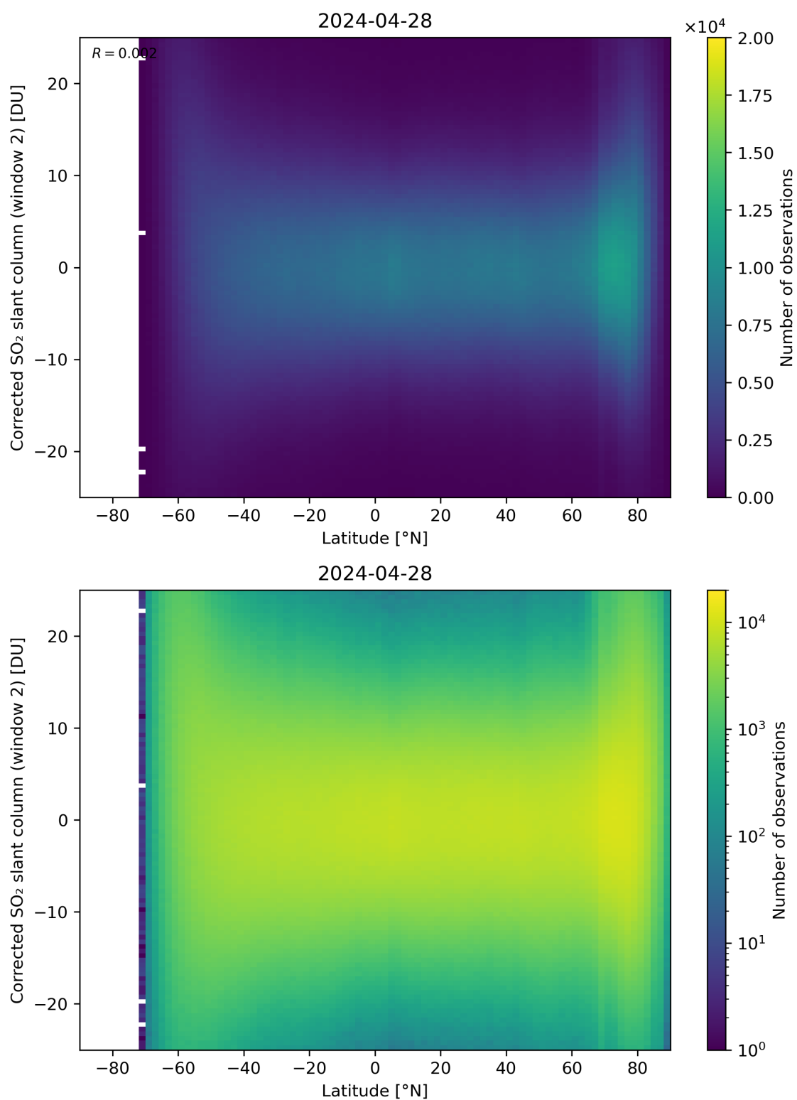
Figure 147: Scatter density plot of “Latitude” against “Corrected SO 2 slant column (window 2)” for 2024-04-27 to 2024-04-29.
