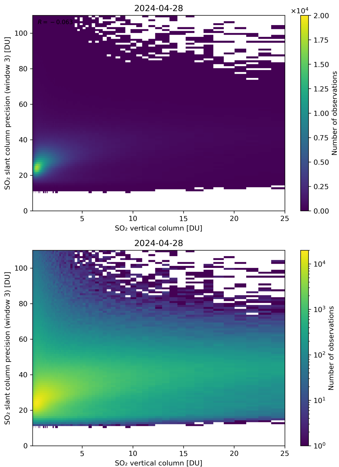
Figure 304: Scatter density plot of “SO 2 vertical column” against “SO 2 slant column precision (window 3)” for 2024-04-27 to 2024-04-29.
