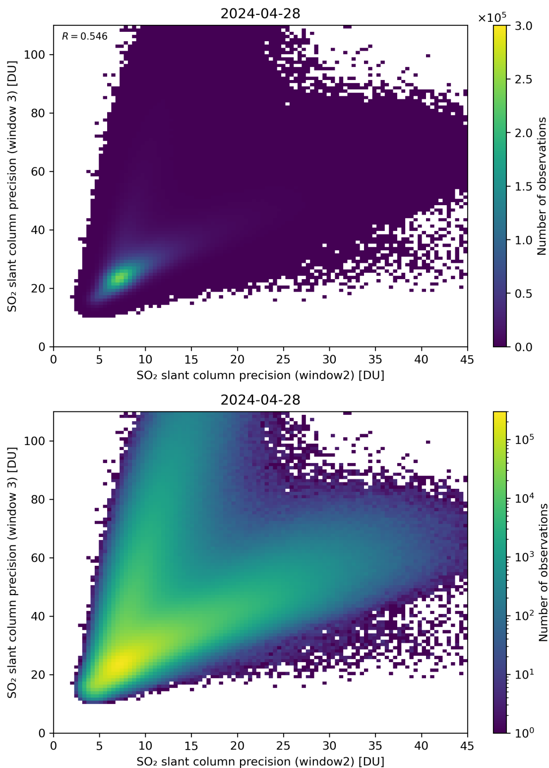
Figure 250: Scatter density plot of “SO 2 slant column precision (window2)” against “SO 2 slant column precision (window 3)” for 2024-04-27 to 2024-04-29.
