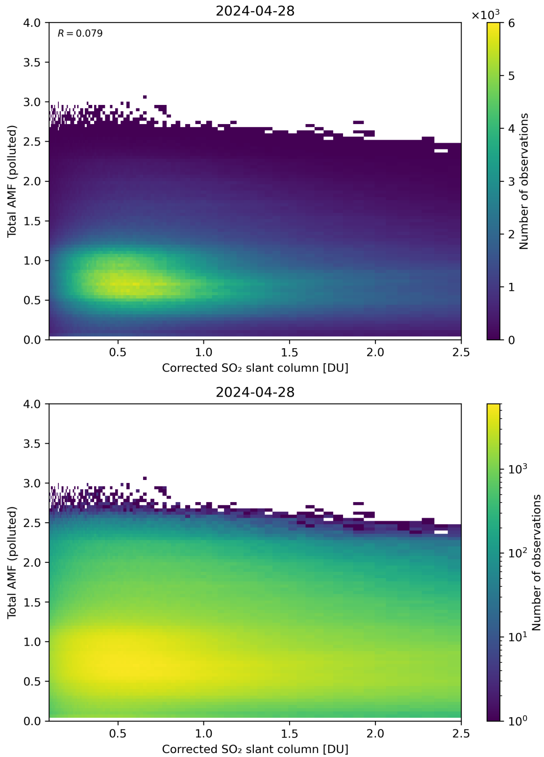
Figure 192: Scatter density plot of “Corrected SO 2 slant column” against “Total AMF (polluted)” for 2024-04-27 to 2024-04-29.
