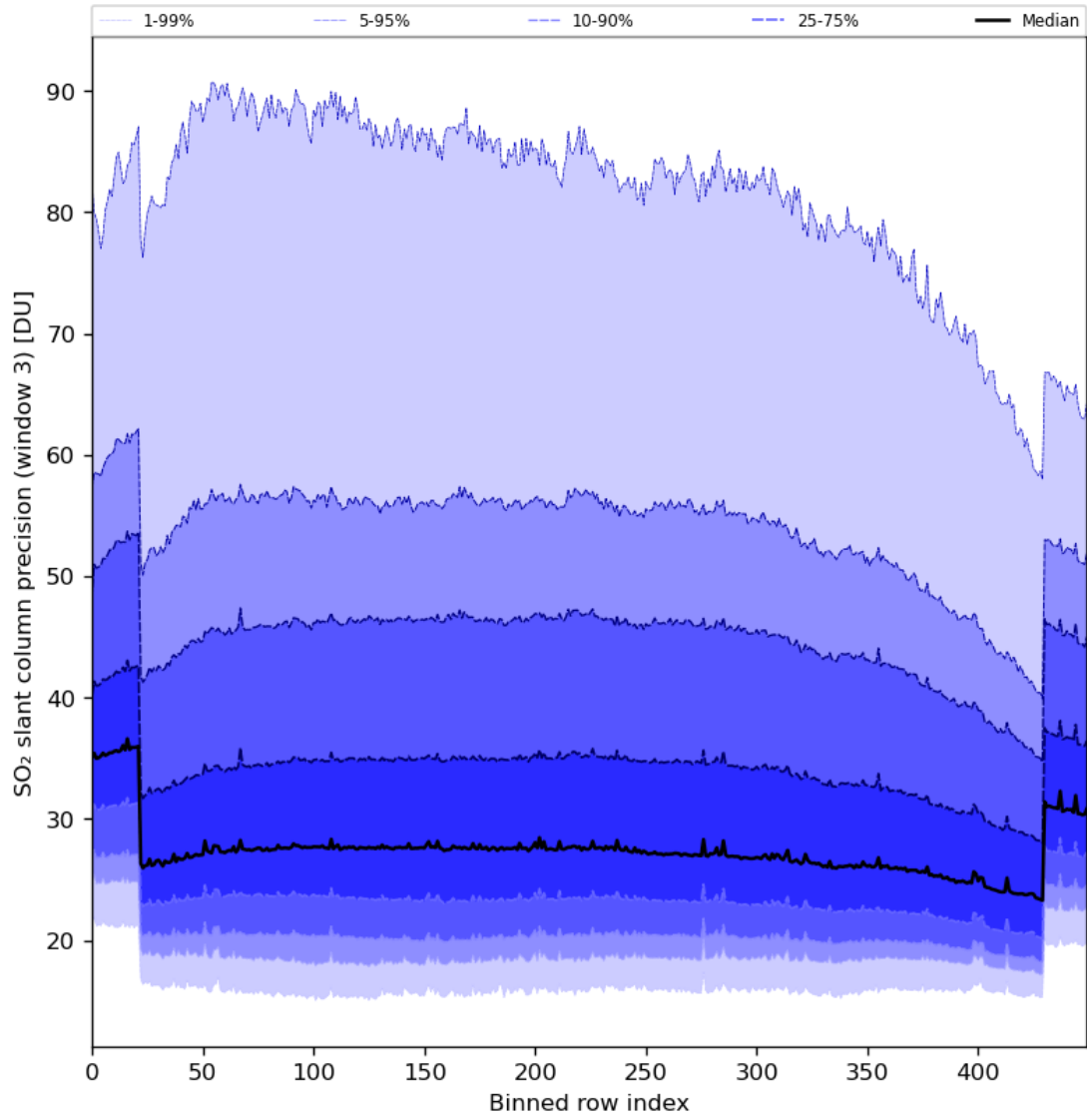
Figure 88: Along track statistics of “SO 2 slant column precision (window 3)” for 2024-04-27 to 2024-04-29
