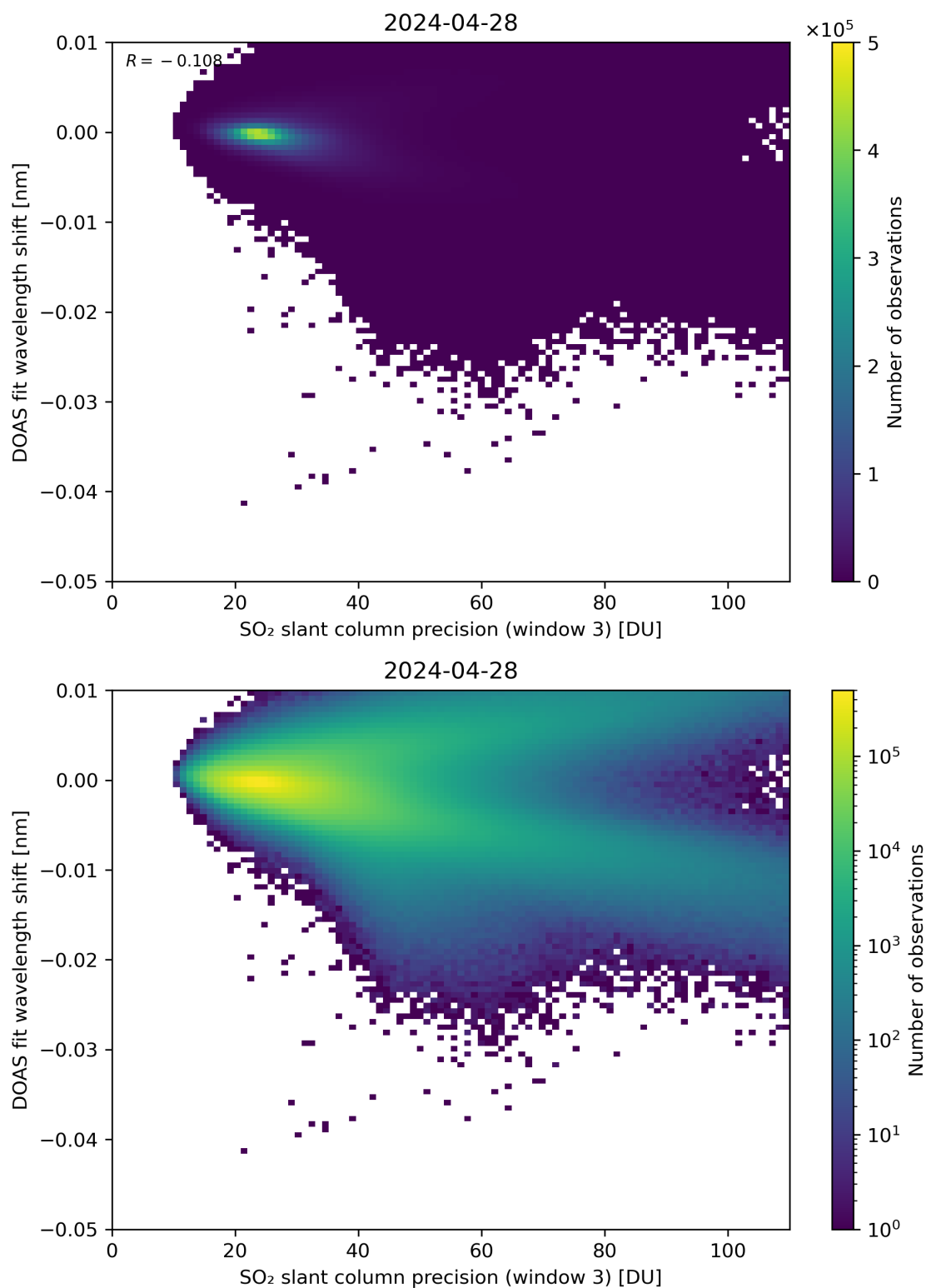
Figure 258: Scatter density plot of “SO 2 slant column precision (window 3)” against “DOAS fit wavelength shift” for 2024-04-27 to 2024-04-29.
