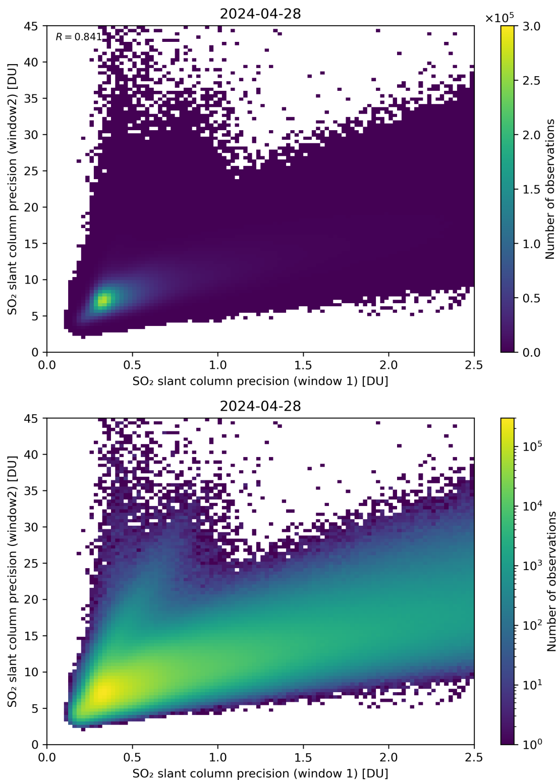
Figure 227: Scatter density plot of “SO 2 slant column precision (window 1)” against “SO 2 slant column precision (window2)” for 2024-04-27 to 2024-04-29.
