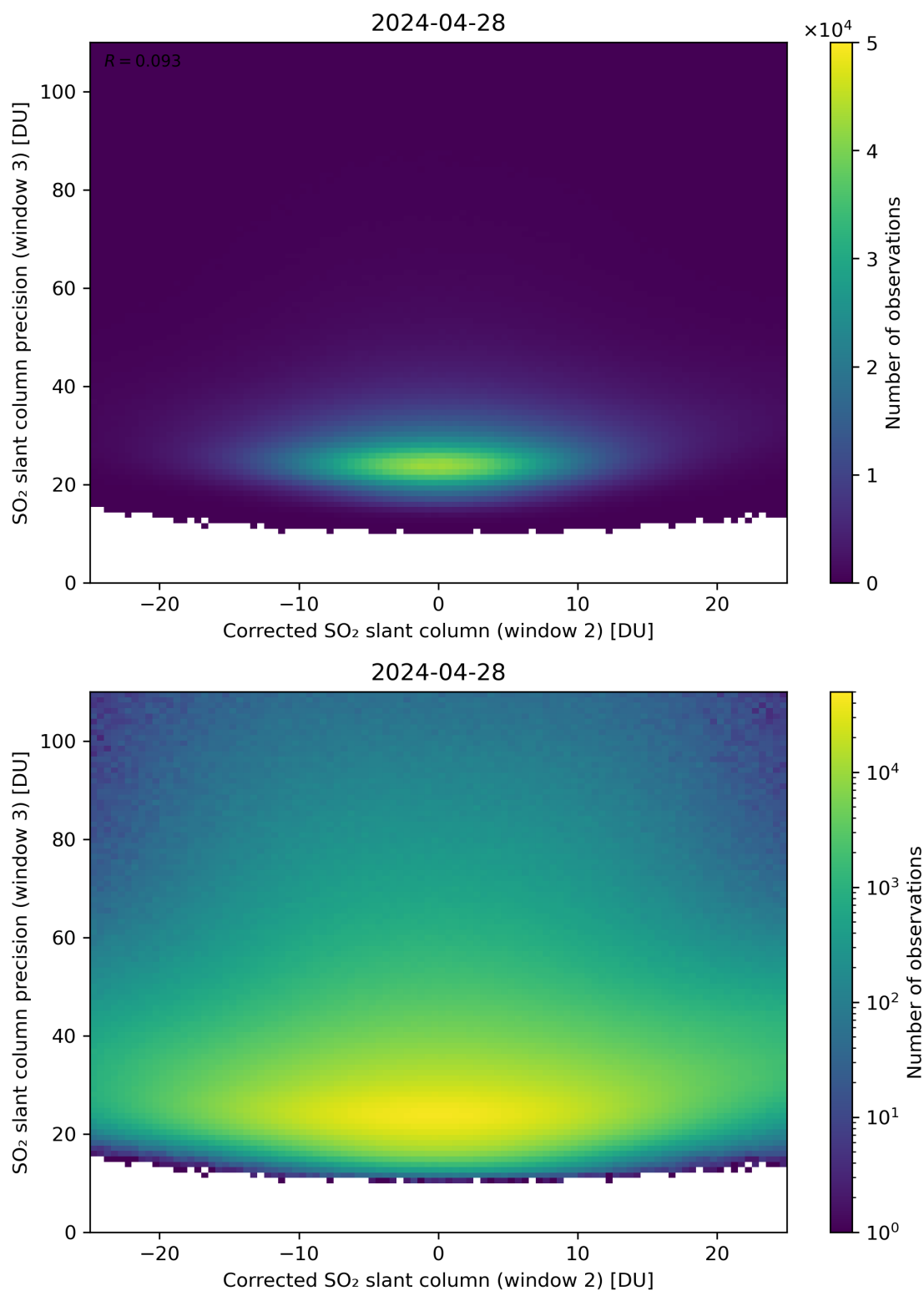
Figure 202: Scatter density plot of “Corrected SO 2 slant column (window 2)” against “SO 2 slant column precision (window 3)” for 2024-04-27 to 2024-04-29.
