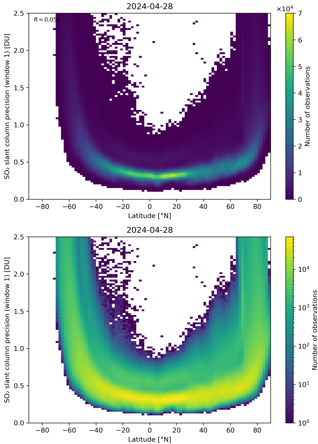
Figure 150: Scatter density plot of “Latitude” against “SO 2 slant column precision (window 1)” for 2024-04-27 to 2024-04-29.
