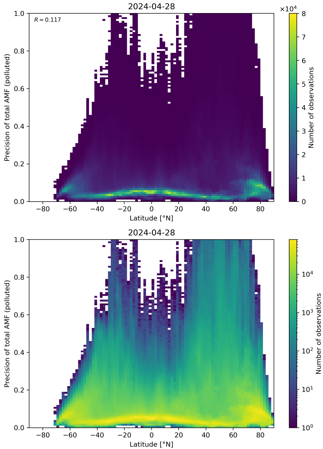
Figure 155: Scatter density plot of “Latitude” against “Precision of total AMF (polluted)” for 2024-04-27 to 2024-04-29.
