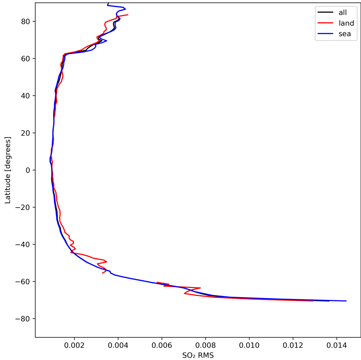
Figure 47: Zonal average of “SO 2 RMS” for 2024-04-27 to 2024-04-29.
