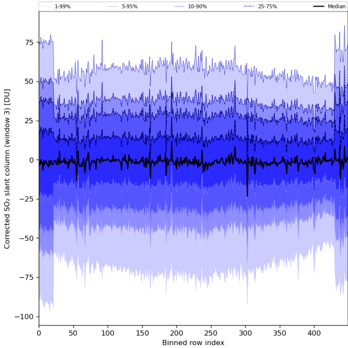
Figure 89: Along track statistics of “Corrected SO 2 slant column (window 3)” for 2024-04-27 to 2024-04-29
