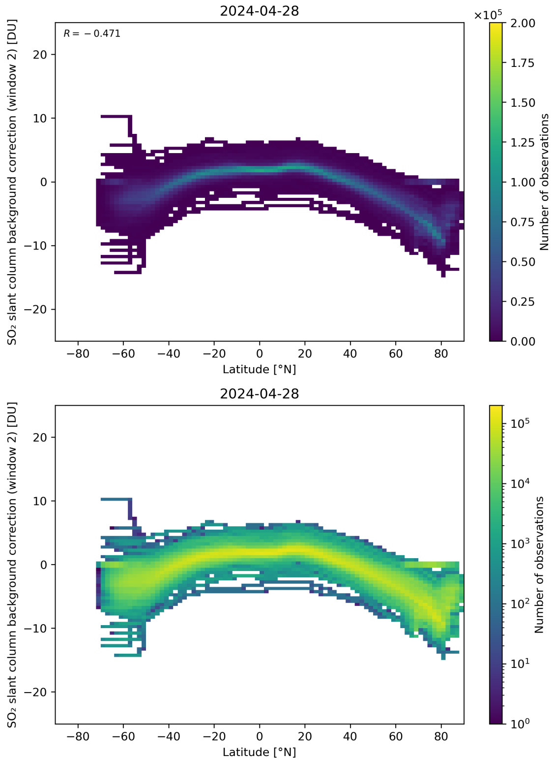
Figure 140: Scatter density plot of “Latitude” against “SO 2 slant column background correction (window 2)” for 2024-04-27 to 2024-04-29.
