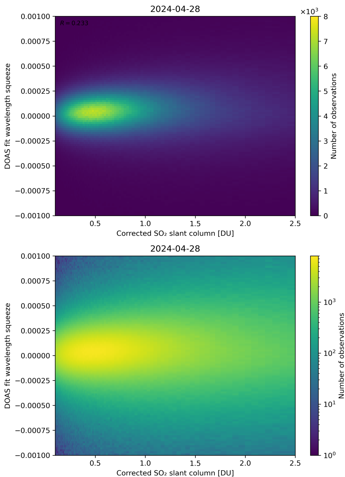
Figure 182: Scatter density plot of “Corrected SO 2 slant column” against “DOAS fit wavelength squeeze” for 2024-04-27 to 2024-04-29.
