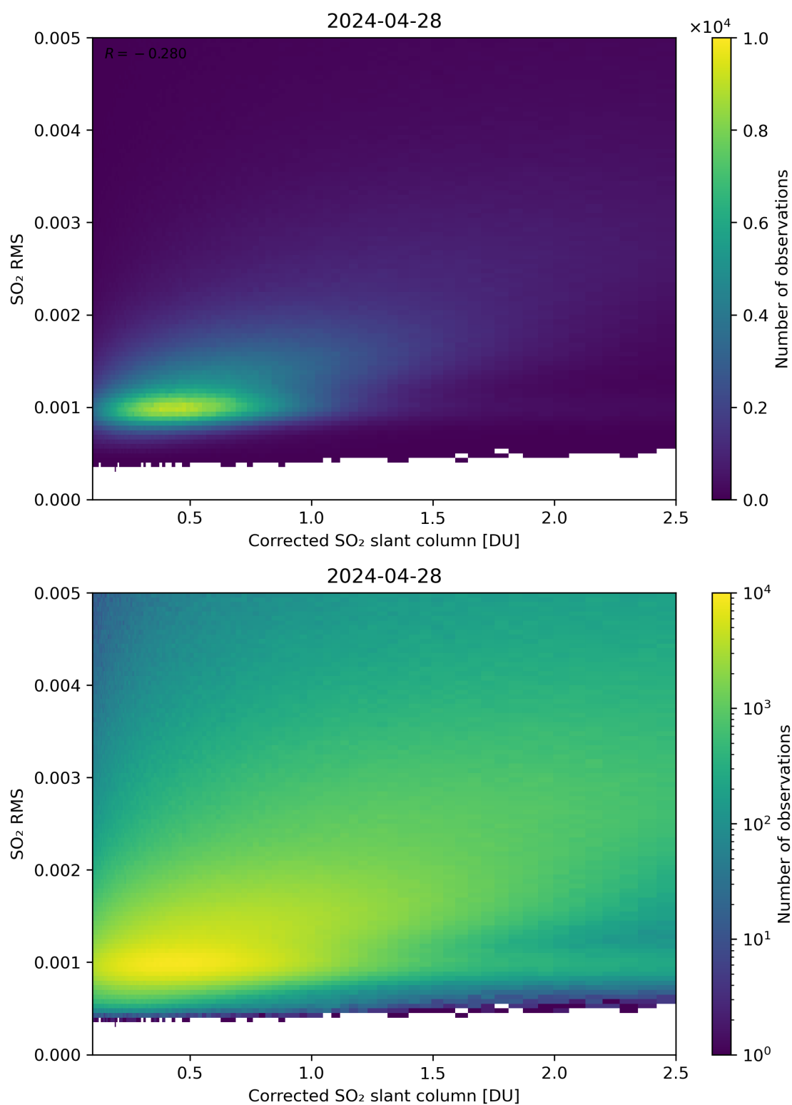
Figure 183: Scatter density plot of “Corrected SO 2 slant column” against “SO 2 RMS” for 2024-04-27 to 2024-04-29.
