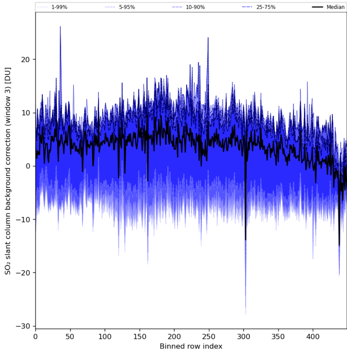
Figure 90: Along track statistics of “SO 2 slant column background correction (window 3)” for 2024-04-27 to 2024-04-29
