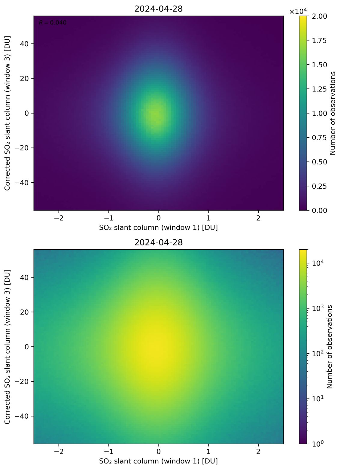
Figure 234: Scatter density plot of “SO 2 slant column (window 1)” against “Corrected SO 2 slant column (window 3)” for 2024-04-27 to 2024-04-29.
