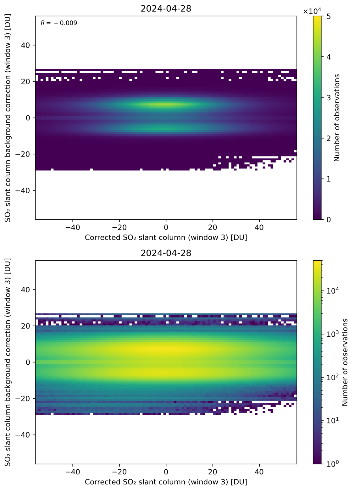
Figure 205: Scatter density plot of “Corrected SO 2 slant column (window 3)” against “SO 2 slant column background correction (window 3)” for 2024-04-27 to 2024-04-29.
