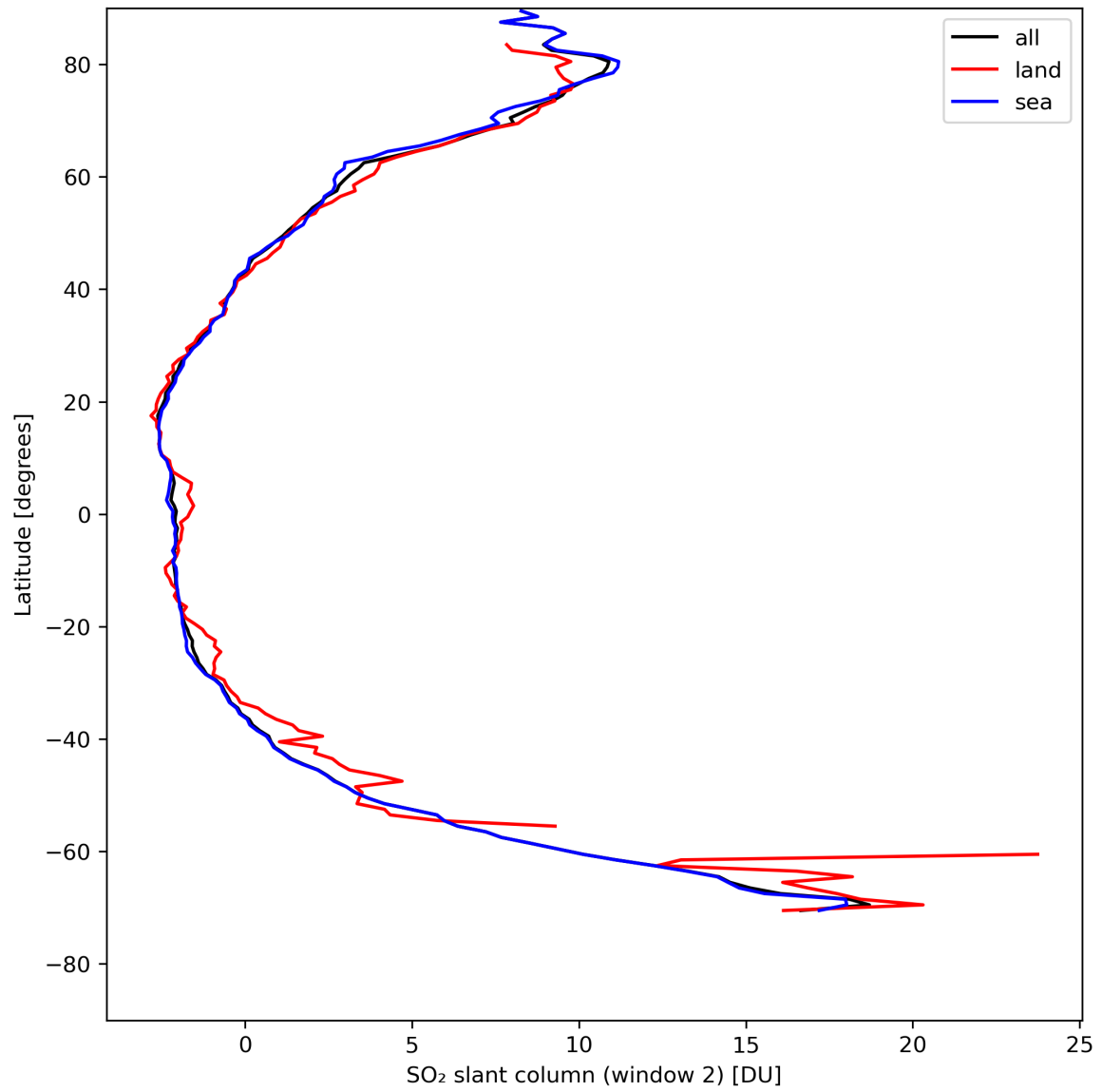
Figure 37: Zonal average of “SO 2 slant column (window 2)” for 2024-04-27 to 2024-04-29.
