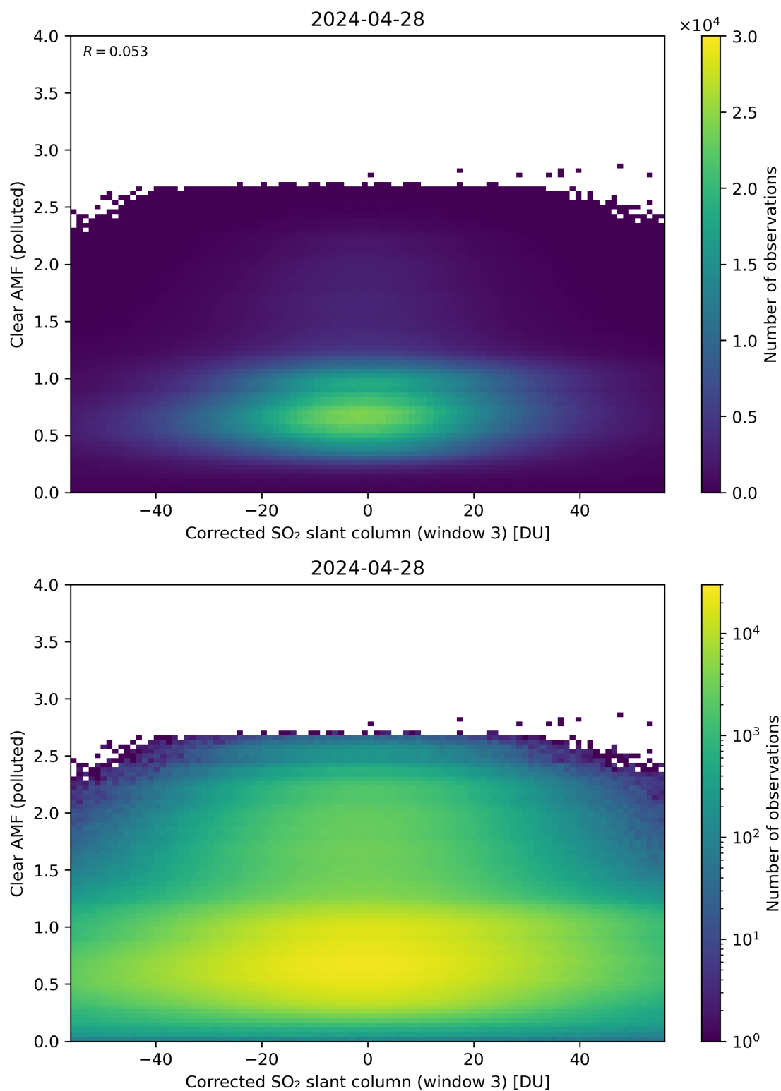
Figure 209: Scatter density plot of “Corrected SO 2 slant column (window 3)” against “Clear AMF (polluted)” for 2024-04-27 to 2024-04-29.
