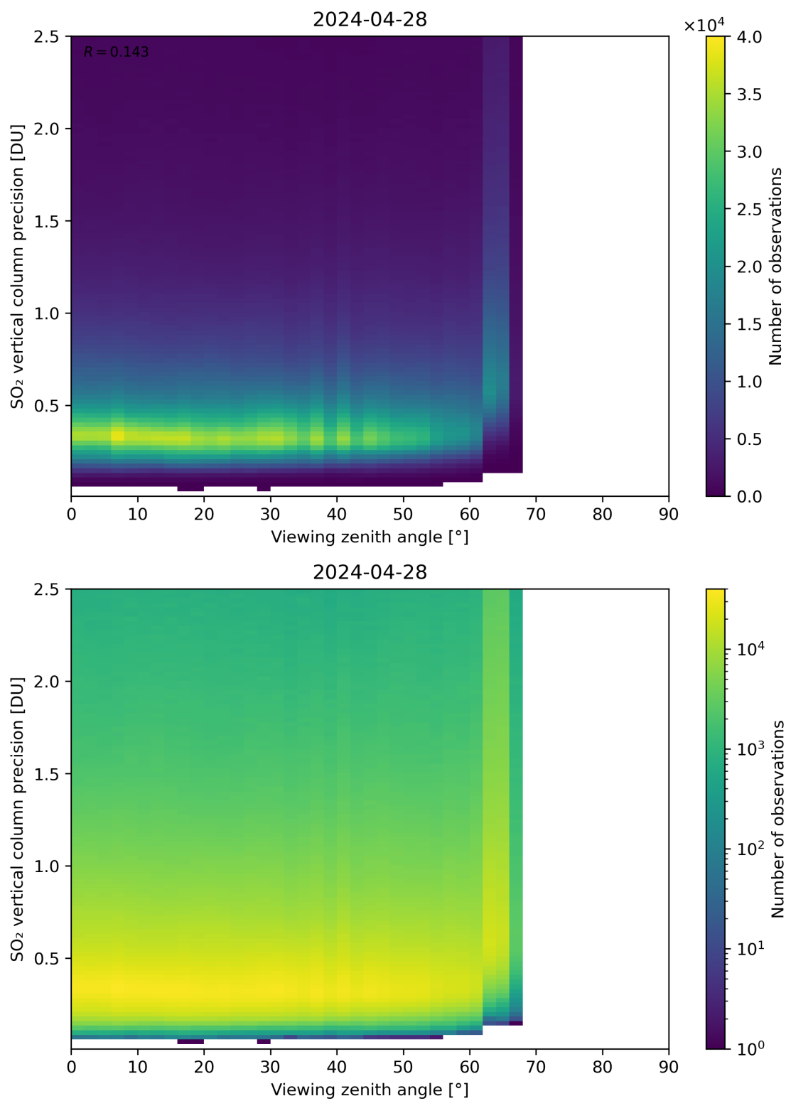
Figure 328: Scatter density plot of “Viewing zenith angle” against “SO 2 vertical column precision” for 2024-04-27 to 2024-04-29.
