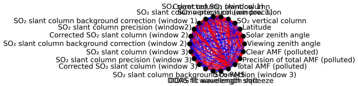
Figure 1: Map of correlation graph for 2024-04-27 to 2024-04-29.
