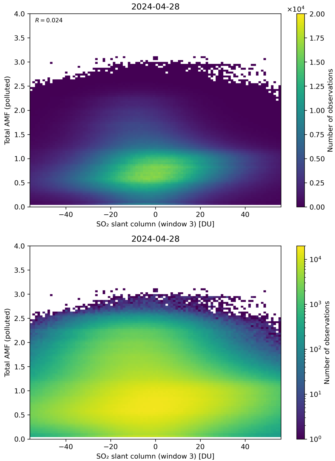
Figure 268: Scatter density plot of “SO 2 slant column (window 3)” against “Total AMF (polluted)” for 2024-04-27 to 2024-04-29.
