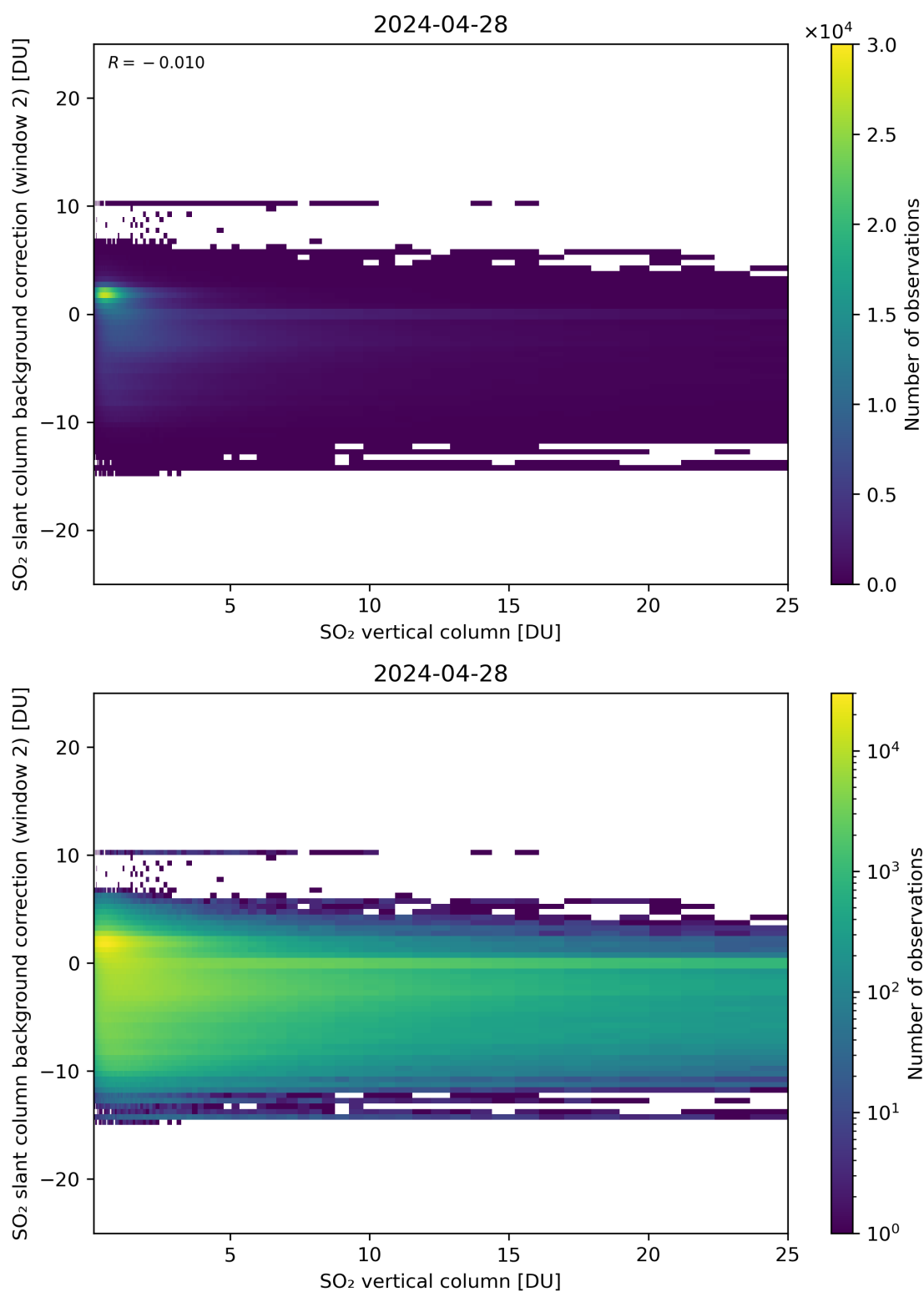
Figure 274: Scatter density plot of “SO 2 vertical column” against “SO 2 slant column background correction (window 2)” for 2024-04-27 to 2024-04-29.
