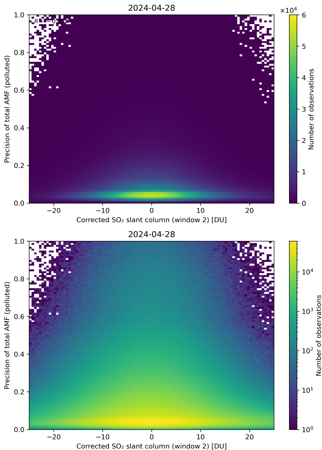
Figure 204: Scatter density plot of “Corrected SO 2 slant column (window 2)” against “Precision of total AMF (polluted)” for 2024-04-27 to 2024-04-29.
