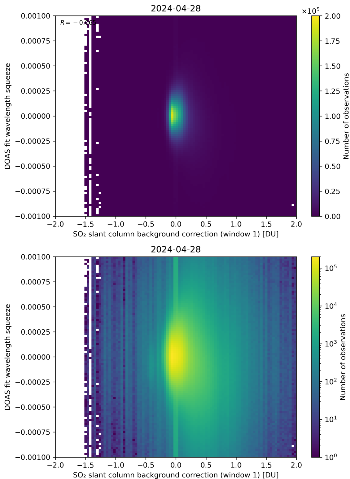
Figure 101: Scatter density plot of “SO 2 slant column background correction (window 1)” against “DOAS fit wavelength squeeze” for 2024-04-27 to 2024-04-29.
