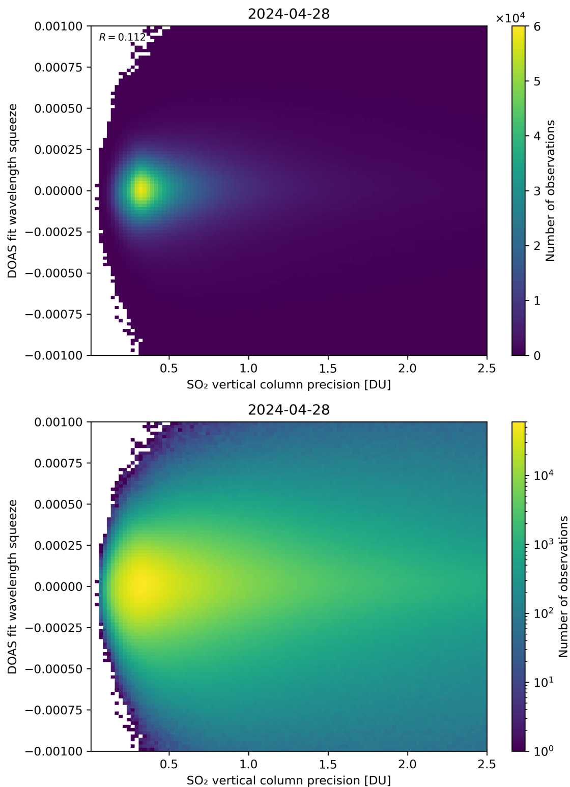
Figure 283: Scatter density plot of “SO 2 vertical column precision” against “DOAS fit wavelength squeeze” for 2024-04-27 to 2024-04-29.
