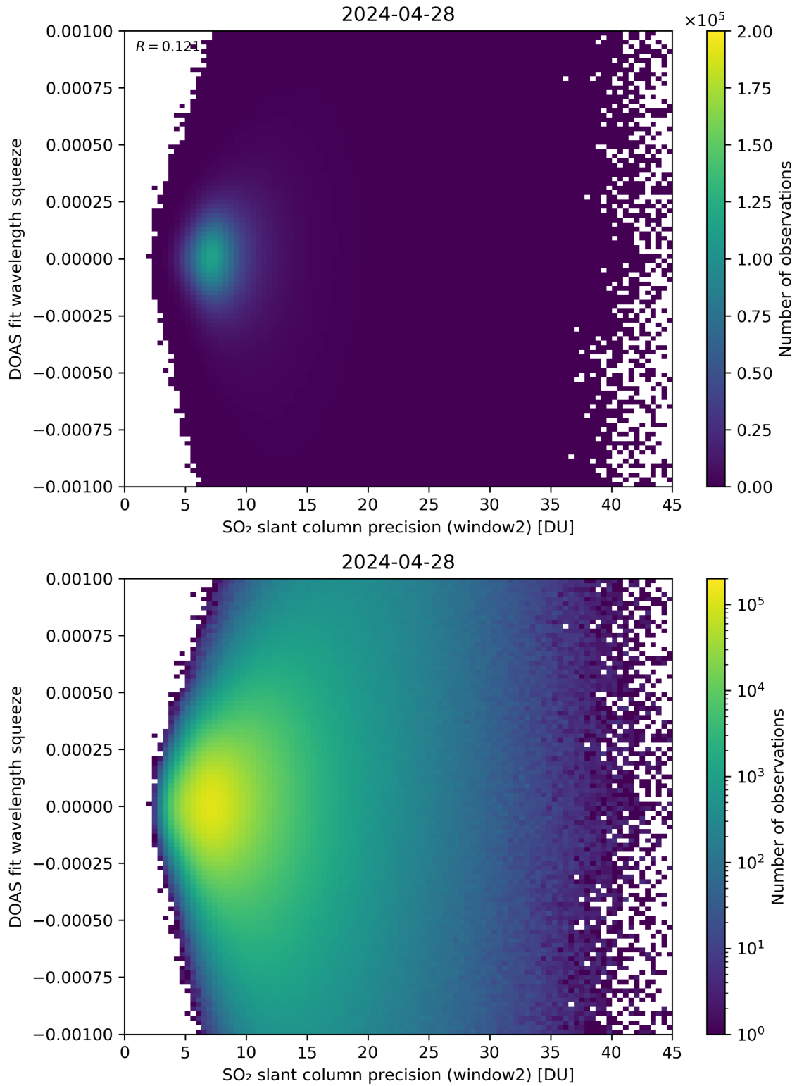
Figure 244: Scatter density plot of “SO 2 slant column precision (window2)” against “DOAS fit wavelength squeeze” for 2024-04-27 to 2024-04-29.
