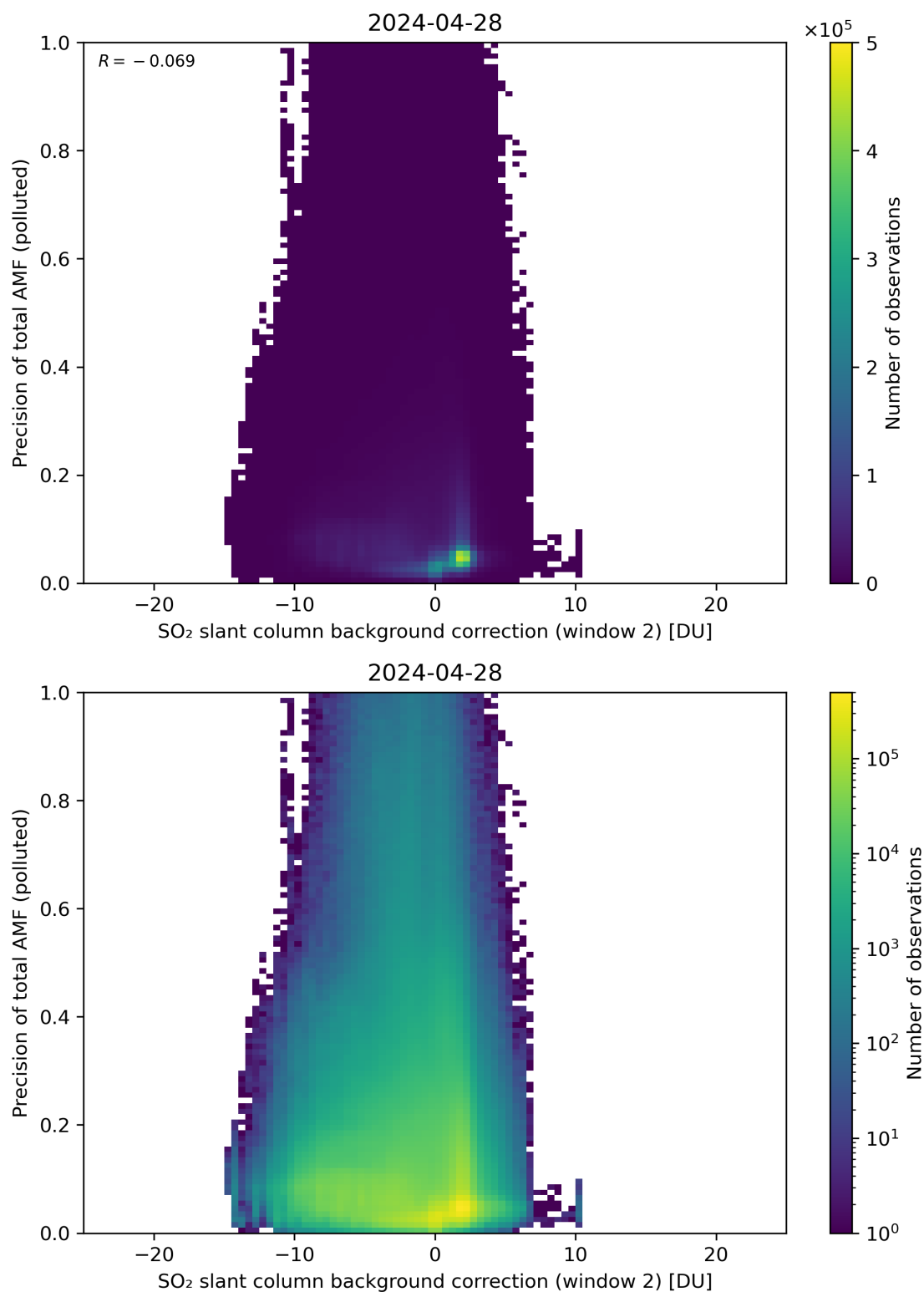
Figure 120: Scatter density plot of “SO 2 slant column background correction (window 2)” against “Precision of total AMF (polluted)” for 2024-04-27 to 2024-04-29.
