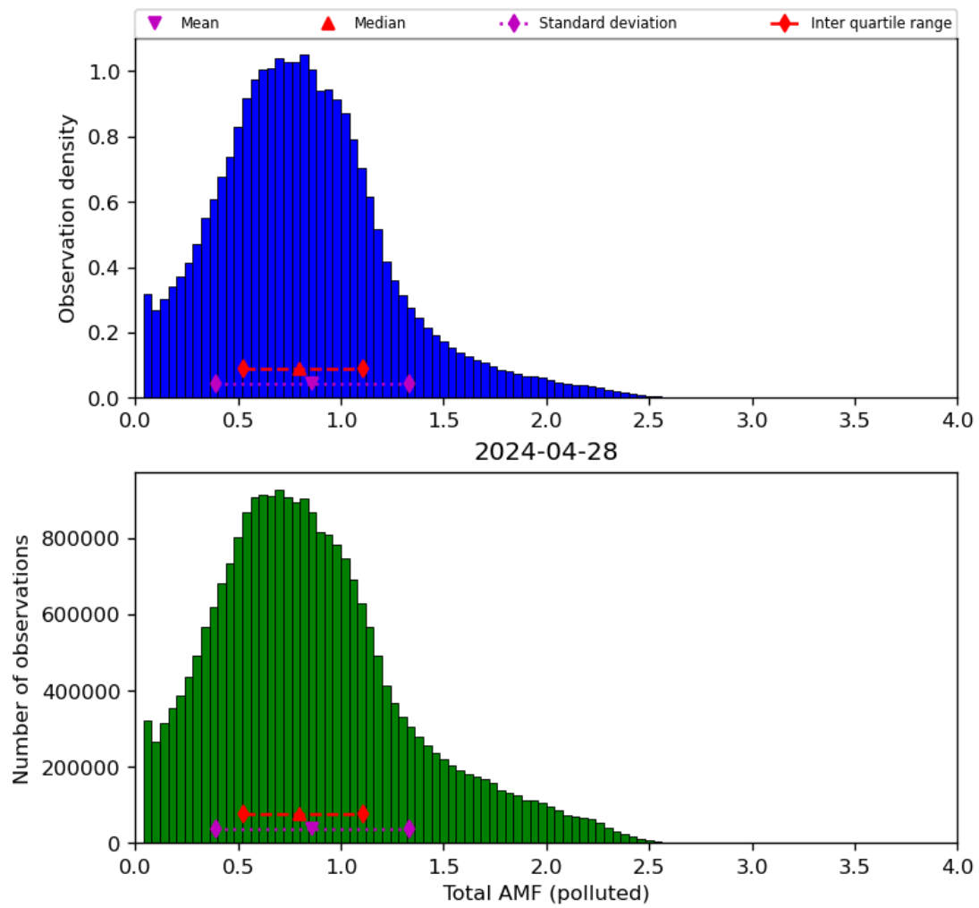
Figure 71: Histogram of “Total AMF (polluted)” for 2024-04-27 to 2024-04-29
