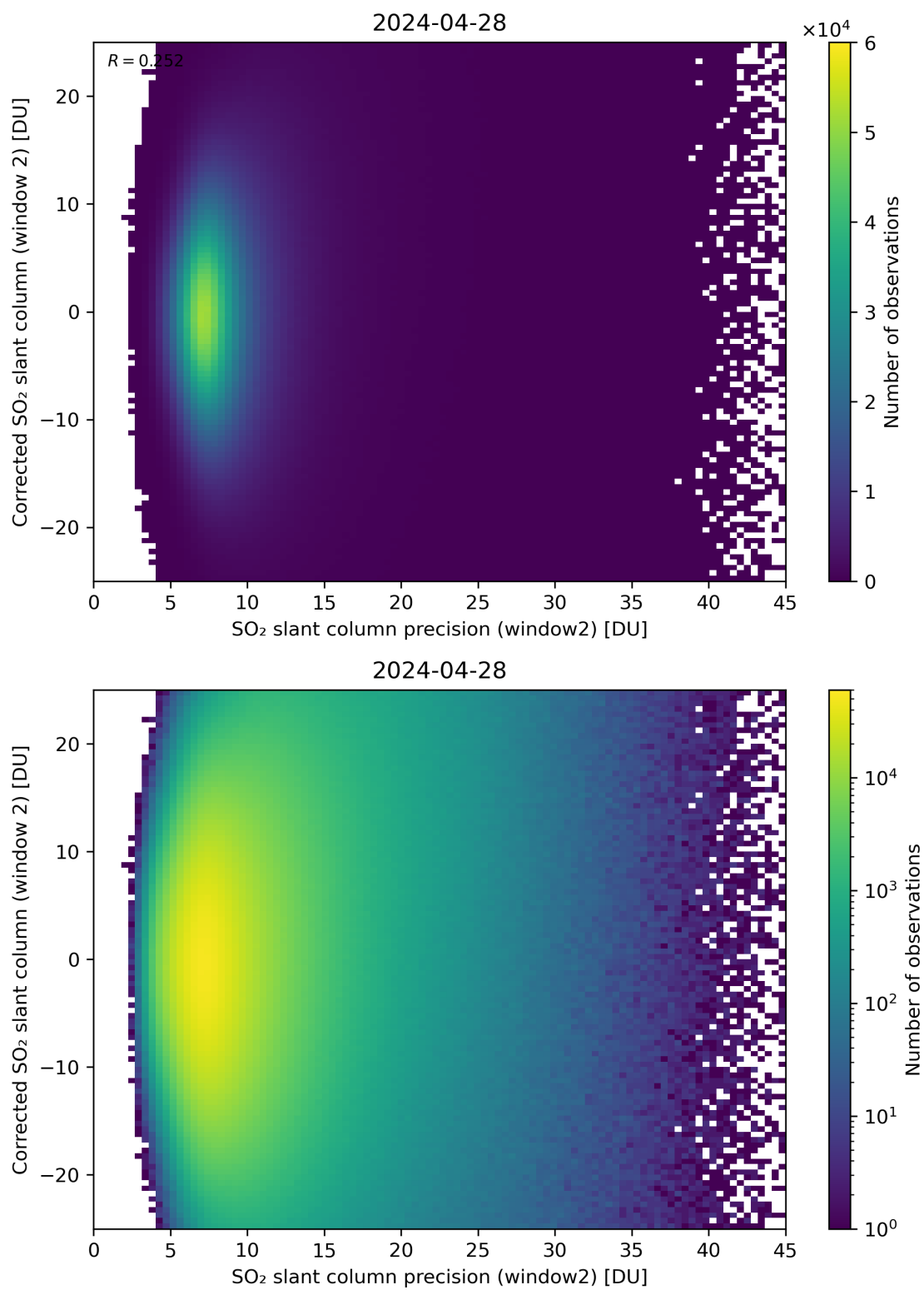
Figure 247: Scatter density plot of “SO 2 slant column precision (window2)” against “Corrected SO 2 slant column (window 2)” for 2024-04-27 to 2024-04-29.
