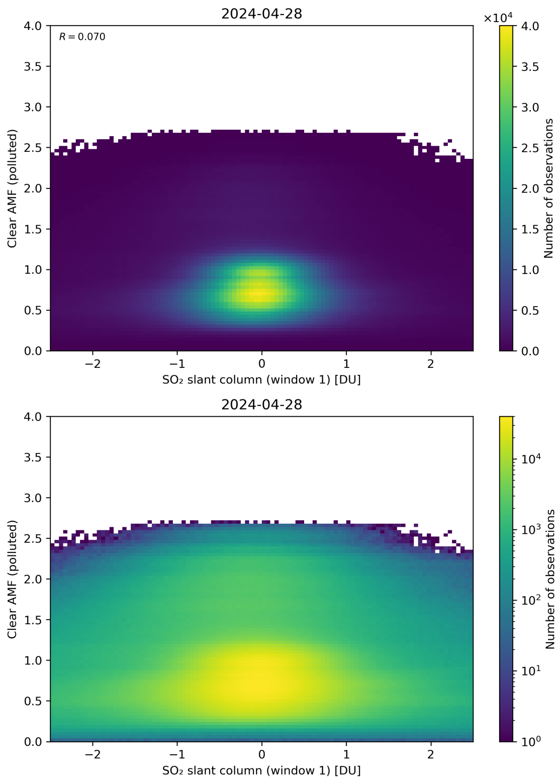
Figure 232: Scatter density plot of “SO 2 slant column (window 1)” against “Clear AMF (polluted)” for 2024-04-27 to 2024-04-29.
