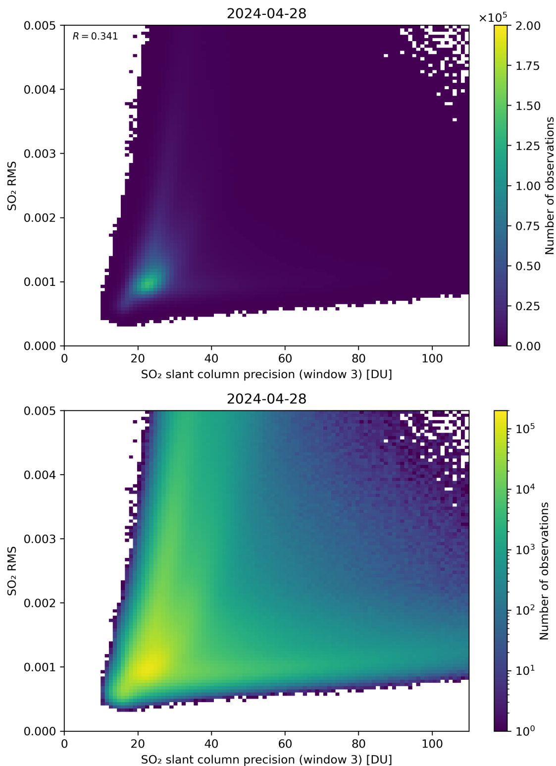
Figure 260: Scatter density plot of “SO 2 slant column precision (window 3)” against “SO 2 RMS” for 2024-04-27 to 2024-04-29.
