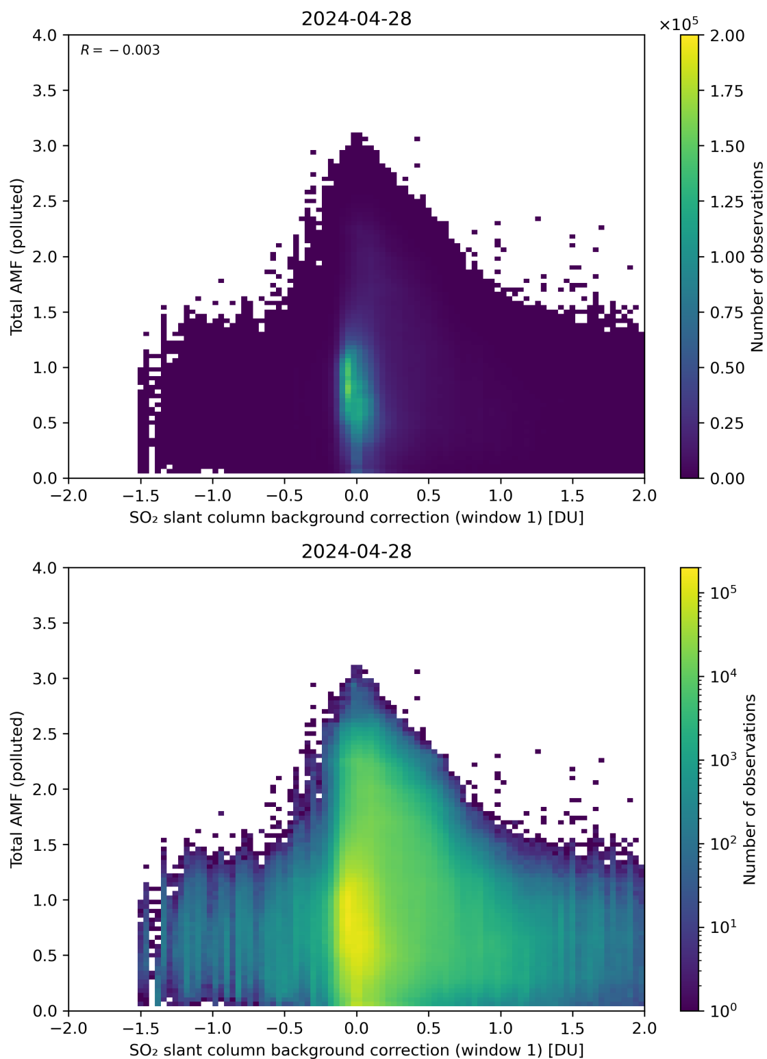
Figure 109: Scatter density plot of “SO 2 slant column background correction (window 1)” against “Total AMF (polluted)” for 2024-04-27 to 2024-04-29.
