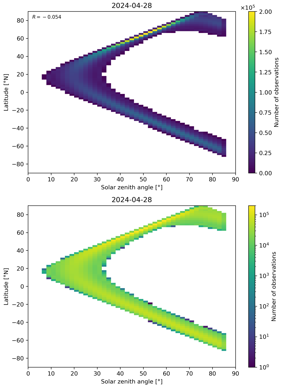
Figure 164: Scatter density plot of “Solar zenith angle” against “Latitude” for 2024-04-27 to 2024-04-29.
