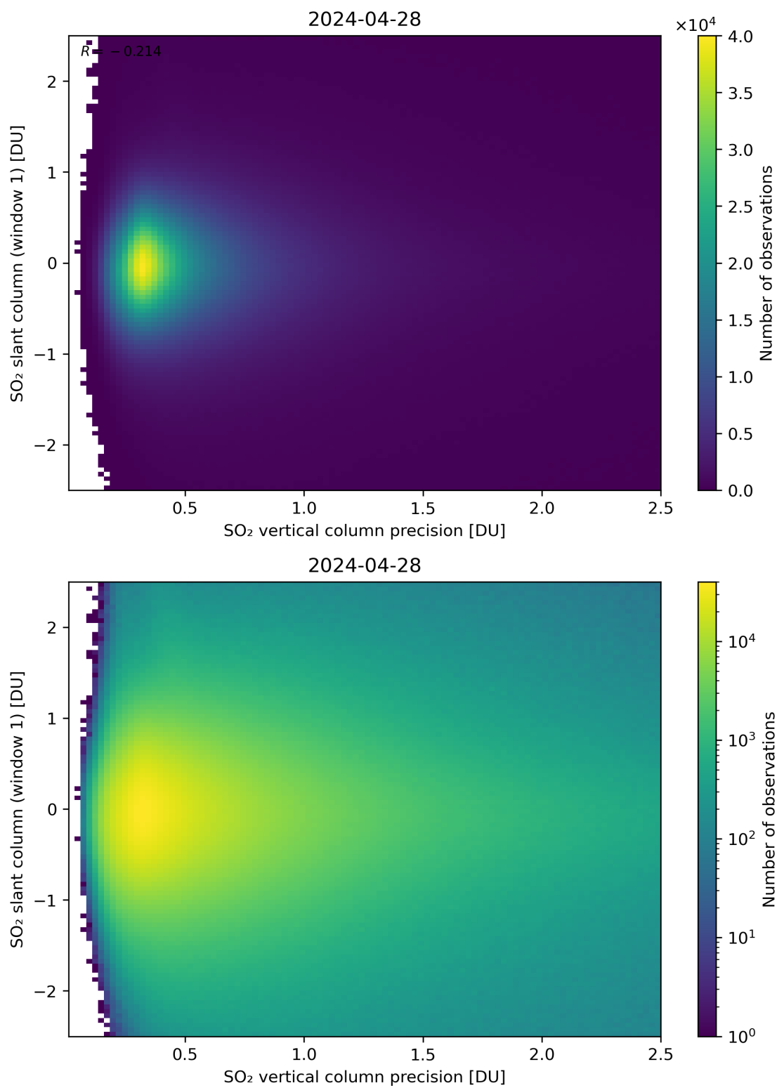
Figure 289: Scatter density plot of “SO 2 vertical column precision” against “SO 2 slant column (window 1)” for 2024-04-27 to 2024-04-29.
