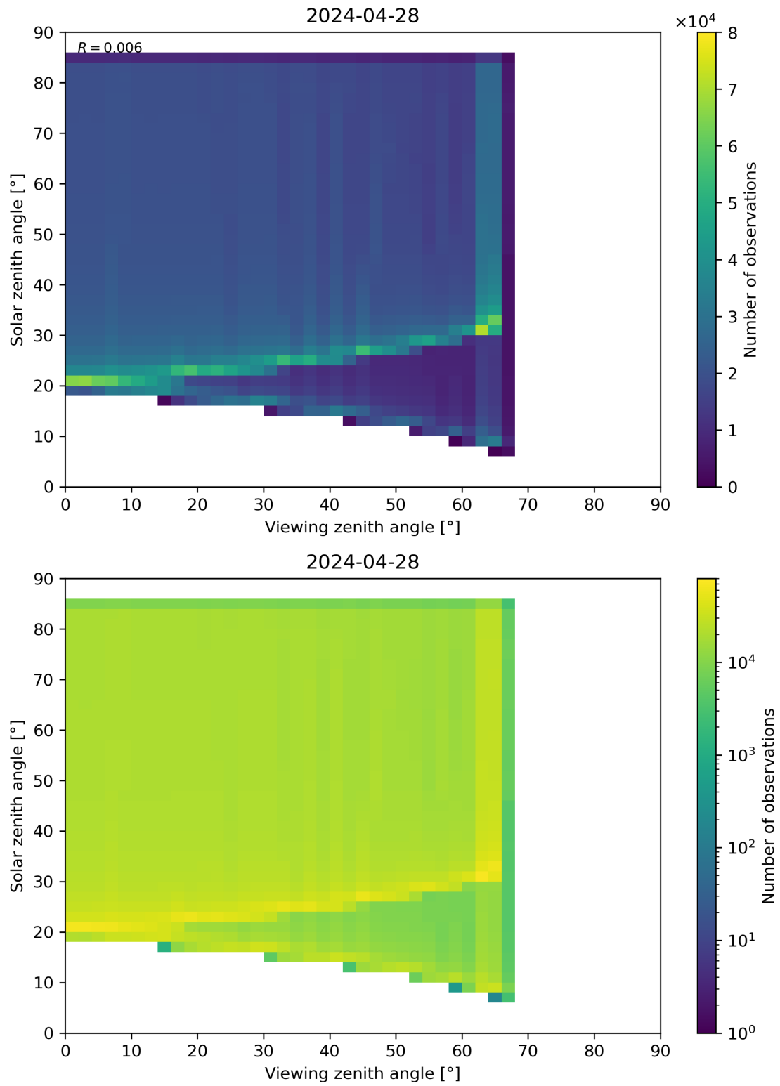
Figure 315: Scatter density plot of “Viewing zenith angle” against “Solar zenith angle” for 2024-04-27 to 2024-04-29.
