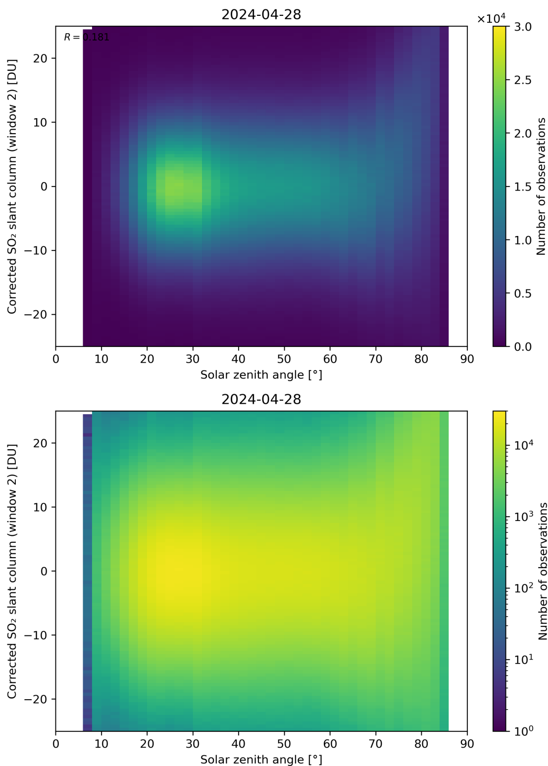
Figure 167: Scatter density plot of “Solar zenith angle” against “Corrected SO 2 slant column (window 2)” for 2024-04-27 to 2024-04-29.
