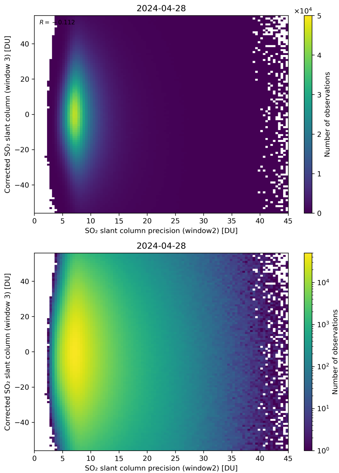
Figure 248: Scatter density plot of “SO 2 slant column precision (window2)” against “Corrected SO 2 slant column (window 3)” for 2024-04-27 to 2024-04-29.
