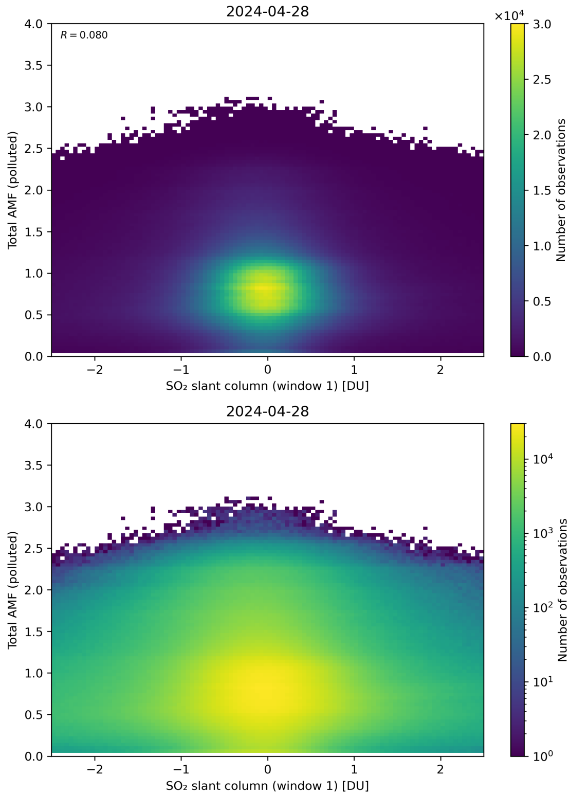
Figure 239: Scatter density plot of “SO 2 slant column (window 1)” against “Total AMF (polluted)” for 2024-04-27 to 2024-04-29.
