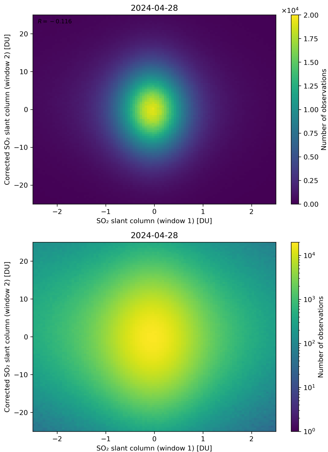
Figure 233: Scatter density plot of “SO 2 slant column (window 1)” against “Corrected SO 2 slant column (window 2)” for 2024-04-27 to 2024-04-29.
