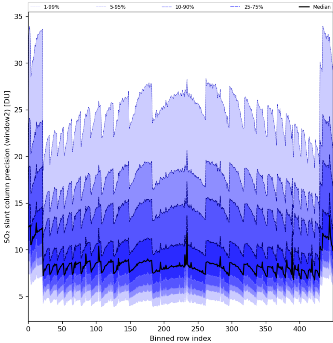
Figure 84: Along track statistics of “SO 2 slant column precision (window2)” for 2024-04-27 to 2024-04-29
