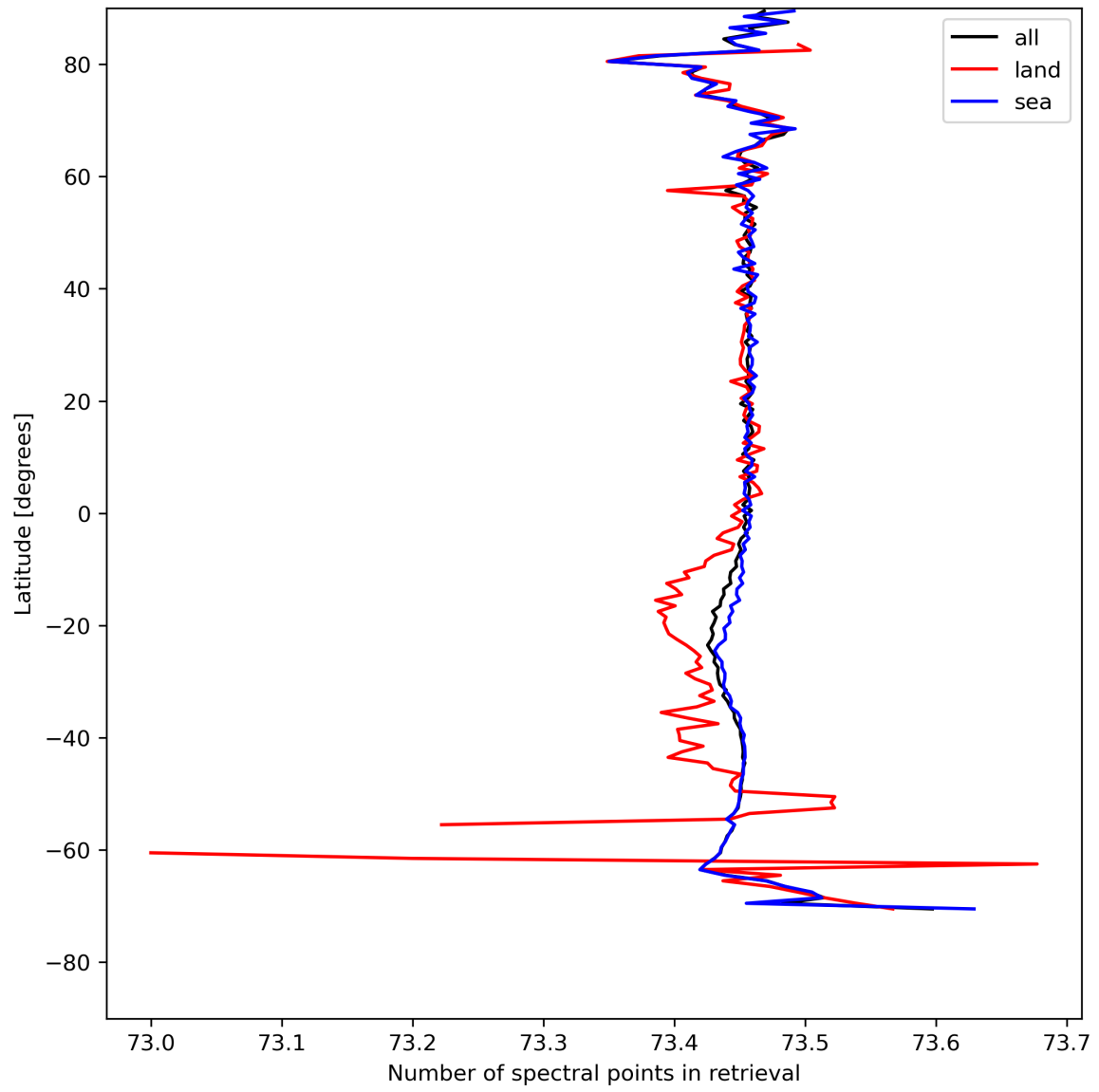
Figure 51: Zonal average of “Number of spectral points in retrieval” for 2024-04-27 to 2024-04-29.
