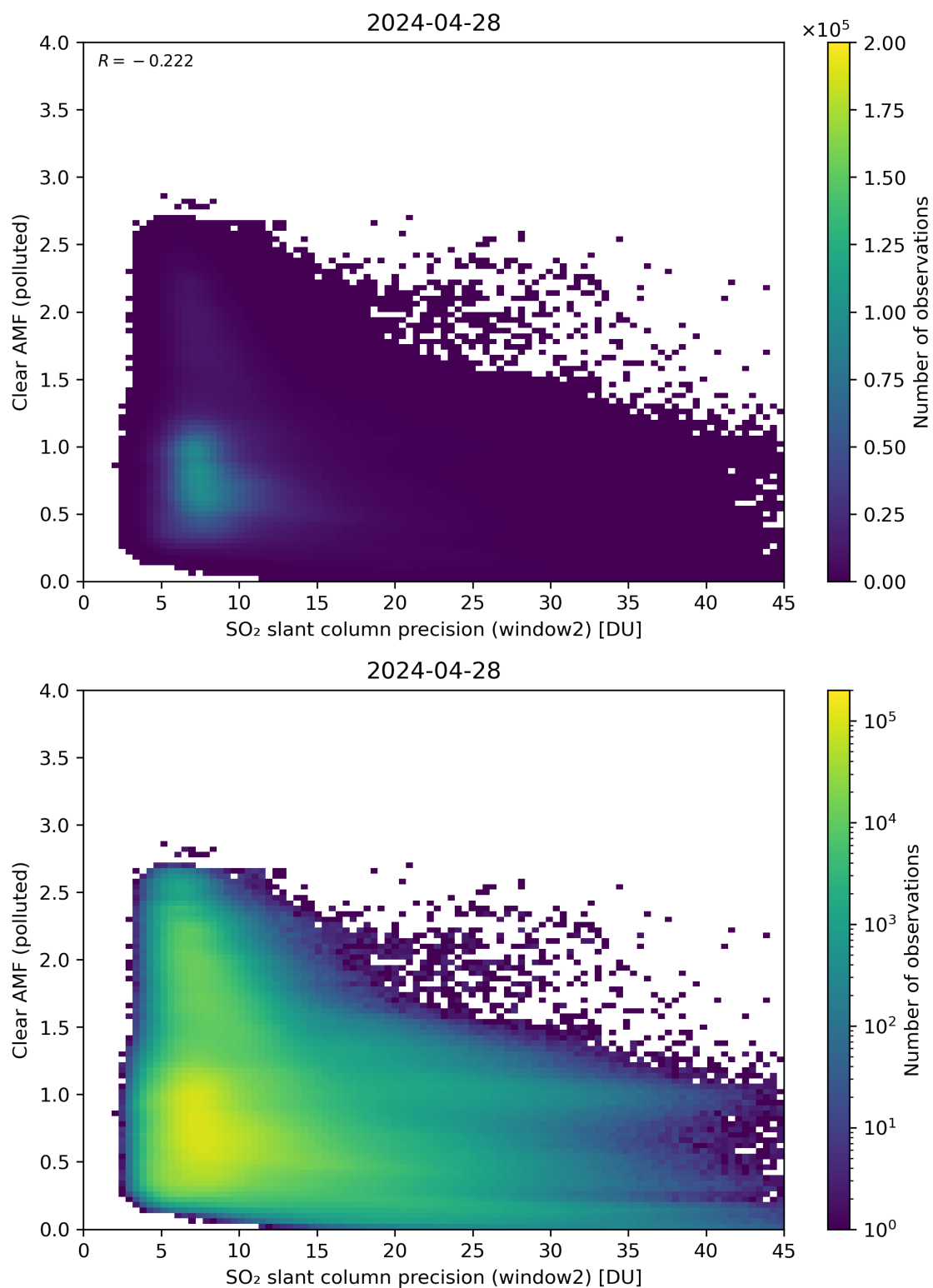
Figure 246: Scatter density plot of “SO 2 slant column precision (window2)” against “Clear AMF (polluted)” for 2024-04-27 to 2024-04-29.
