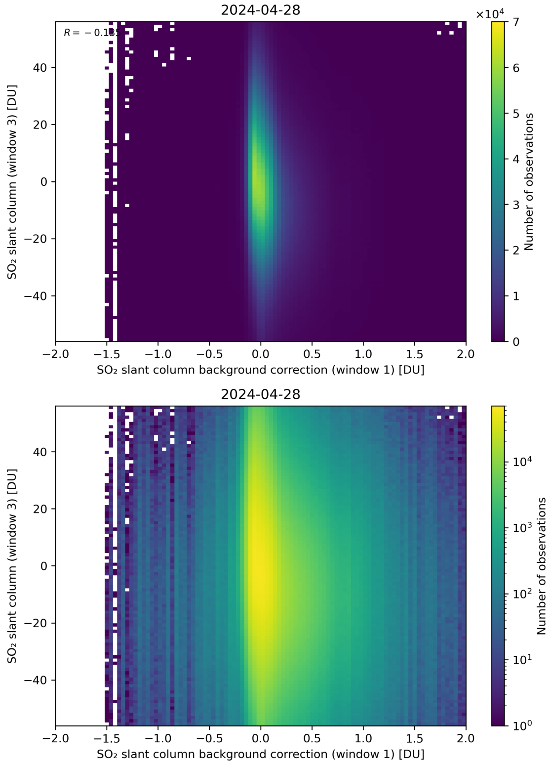
Figure 107: Scatter density plot of “SO 2 slant column background correction (window 1)” against “SO 2 slant column (window 3)” for 2024-04-27 to 2024-04-29.
