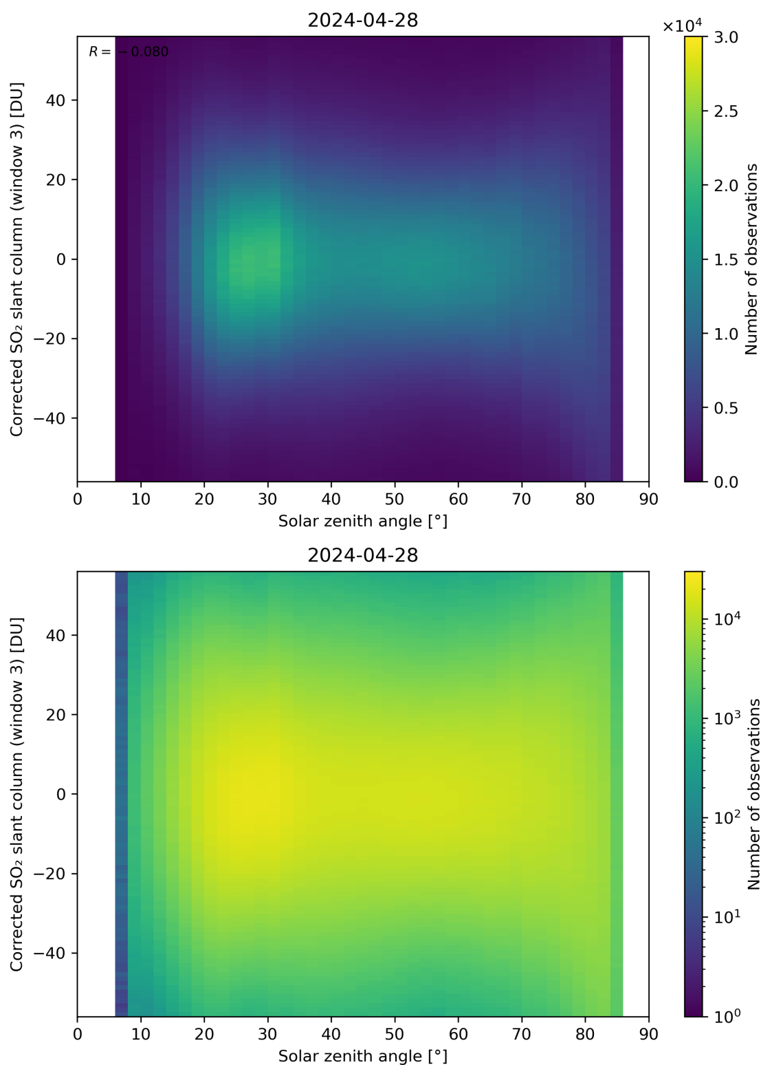
Figure 168: Scatter density plot of “Solar zenith angle” against “Corrected SO 2 slant column (window 3)” for 2024-04-27 to 2024-04-29.
