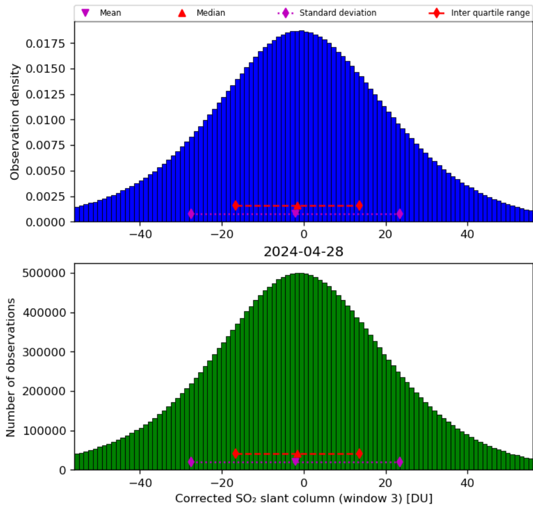
Figure 66: Histogram of “Corrected SO 2 slant column (window 3)” for 2024-04-27 to 2024-04-29
