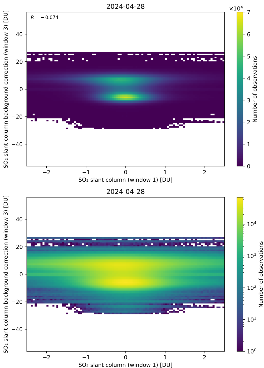
Figure 214: Scatter density plot of “SO 2 slant column (window 1)” against “SO 2 slant column background correction (window 3)” for 2024-04-27 to 2024-04-29.
