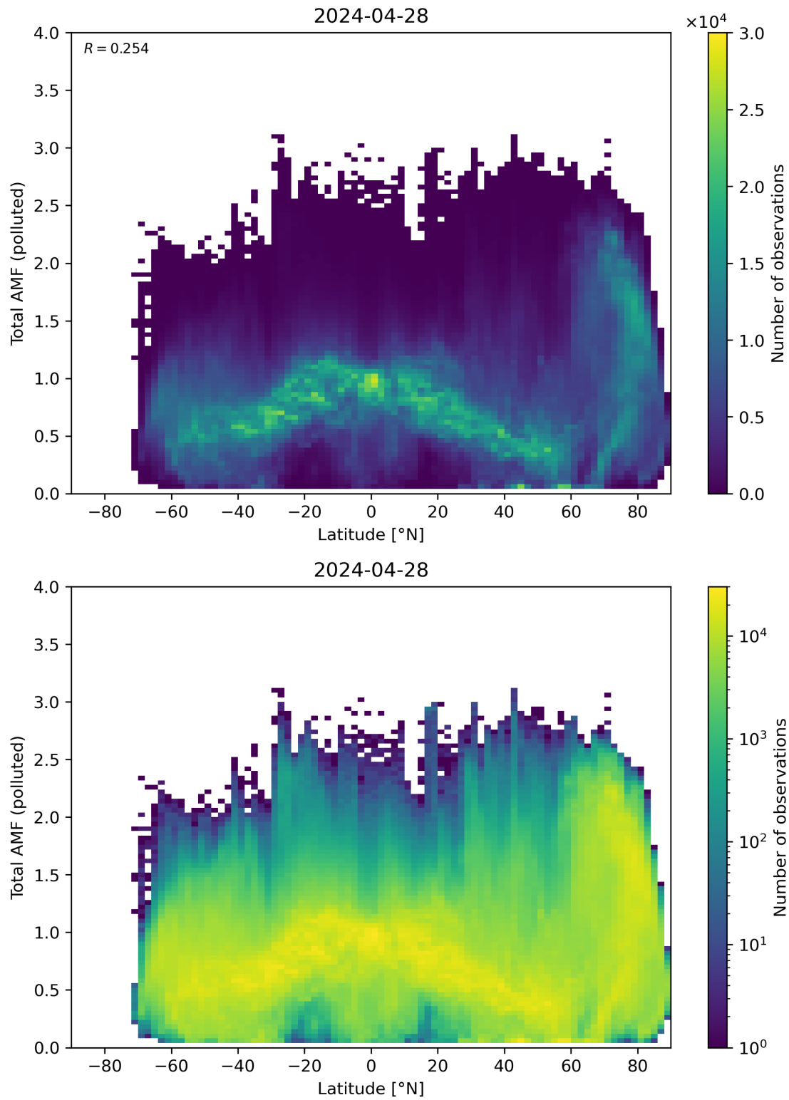
Figure 154: Scatter density plot of “Latitude” against “Total AMF (polluted)” for 2024-04-27 to 2024-04-29.
