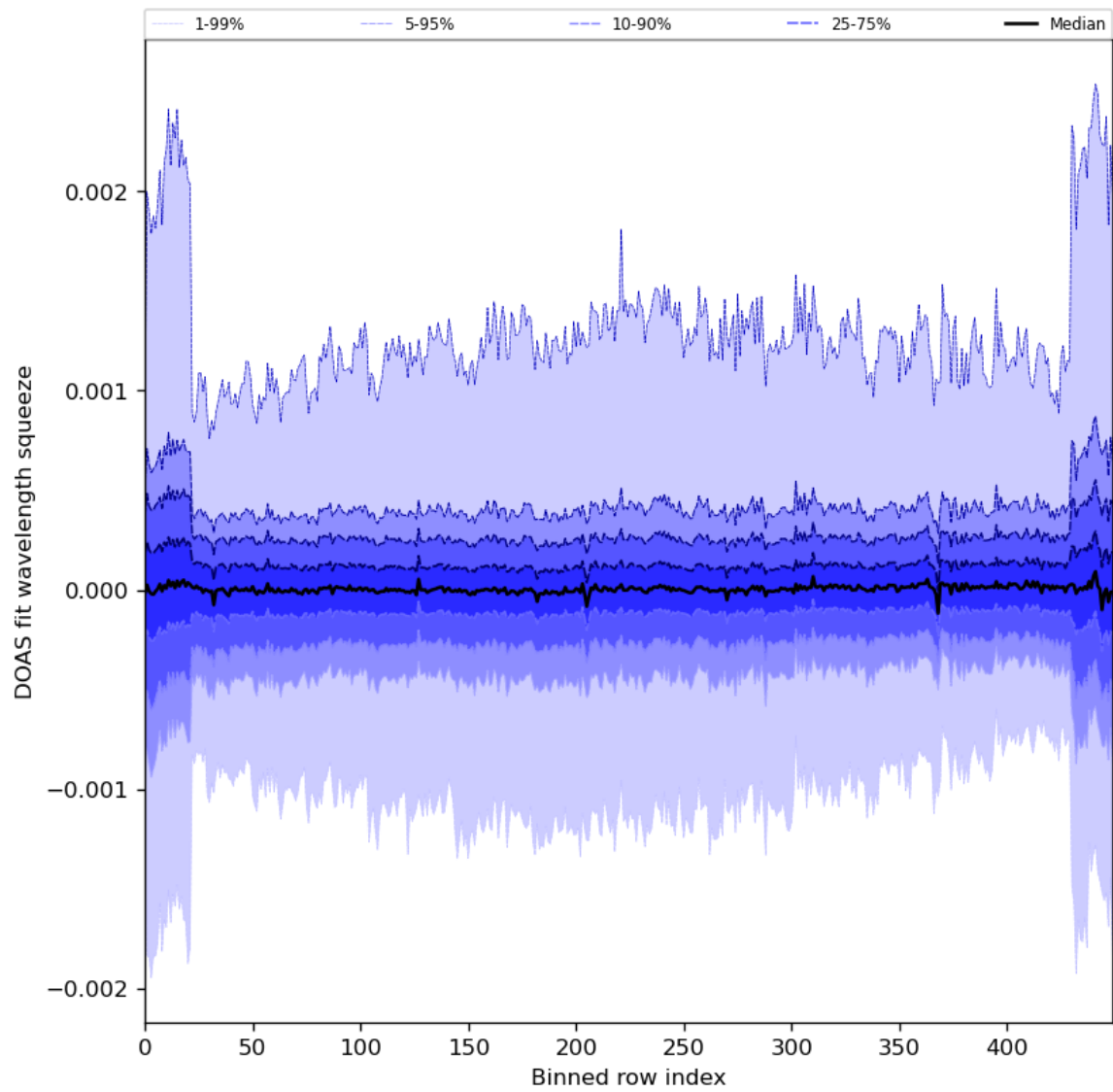
Figure 92: Along track statistics of “DOAS fit wavelength squeeze” for 2024-04-27 to 2024-04-29
