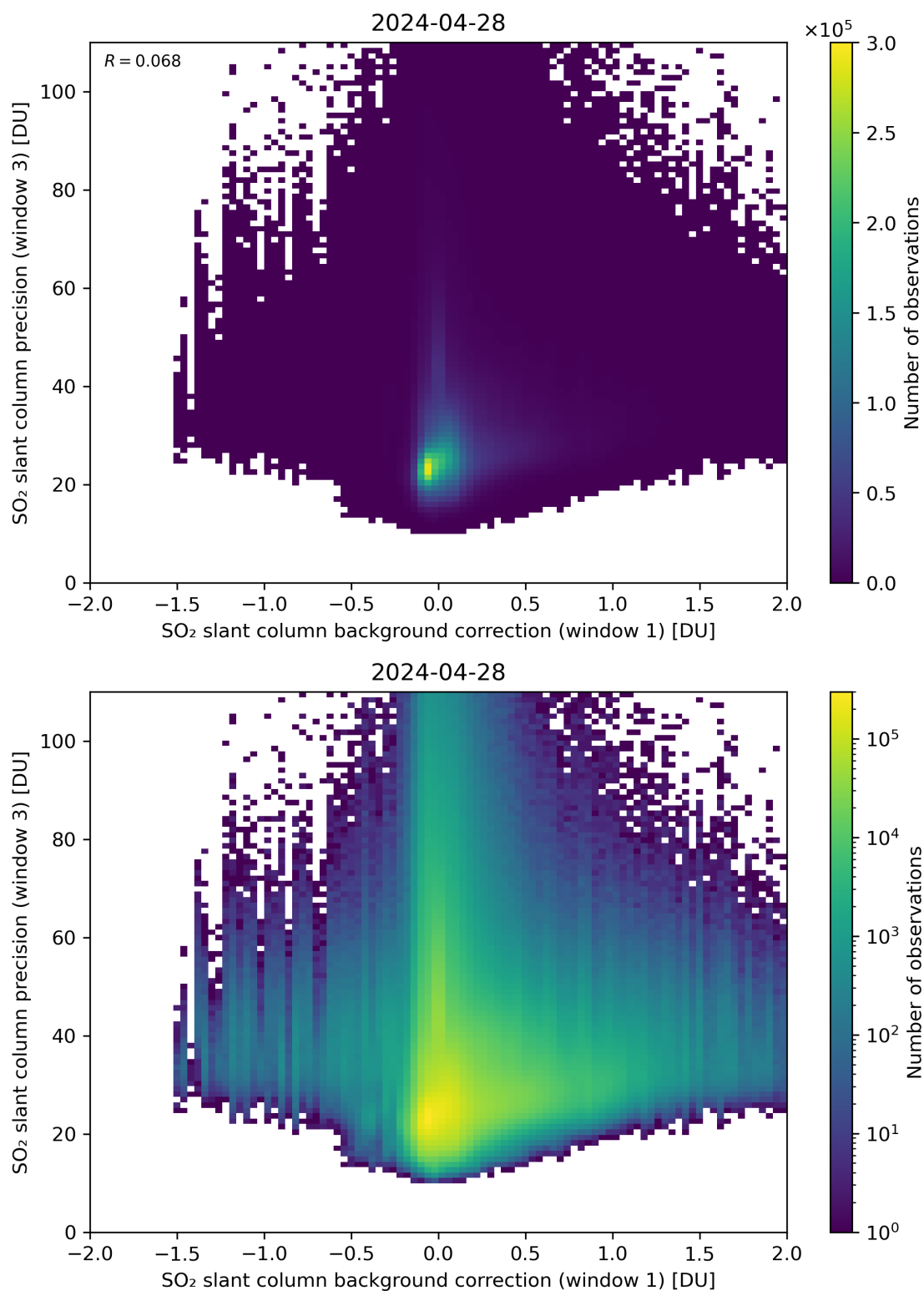
Figure 108: Scatter density plot of “SO 2 slant column background correction (window 1)” against “SO 2 slant column precision (window 3)” for 2024-04-27 to 2024-04-29.
