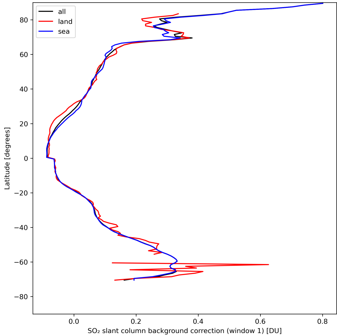
Figure 36: Zonal average of “SO 2 slant column background correction (window 1)” for 2024-04-27 to 2024-04-29.
