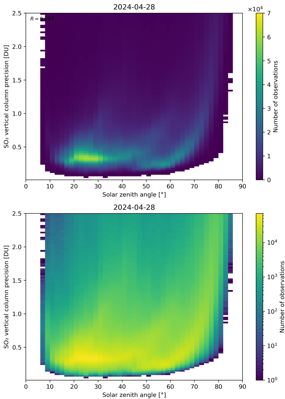
Figure 177: Scatter density plot of “Solar zenith angle” against “SO 2 vertical column precision” for 2024-04-27 to 2024-04-29.
