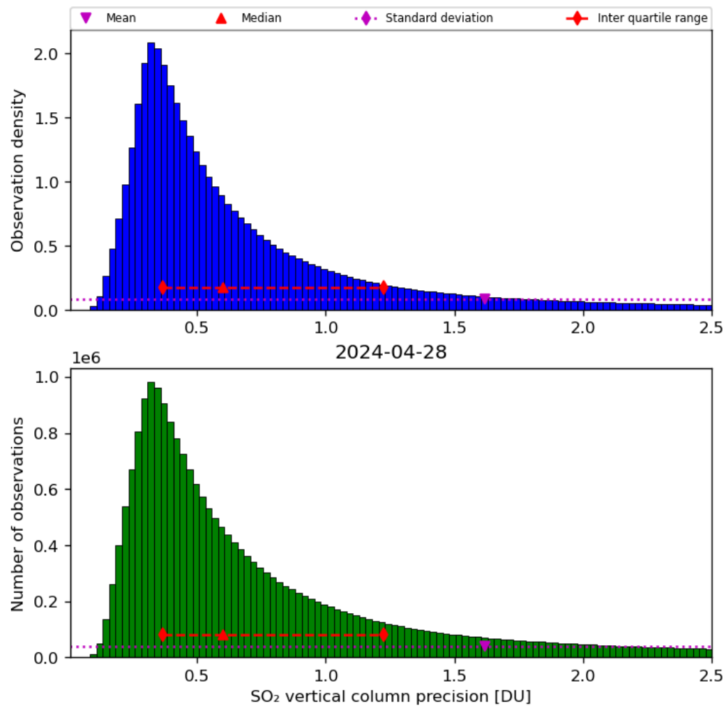
Figure 54: Histogram of “SO 2 vertical column precision” for 2024-04-27 to 2024-04-29
