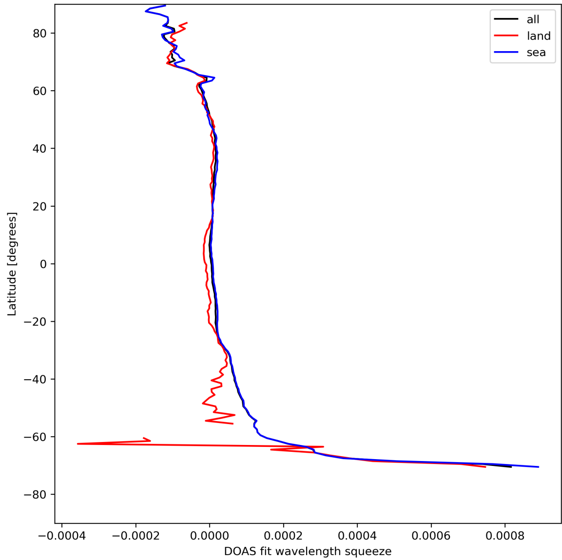
Figure 46: Zonal average of "DOAS fit wavelength squeeze" for 2024-04-27 to 2024-04-29.
