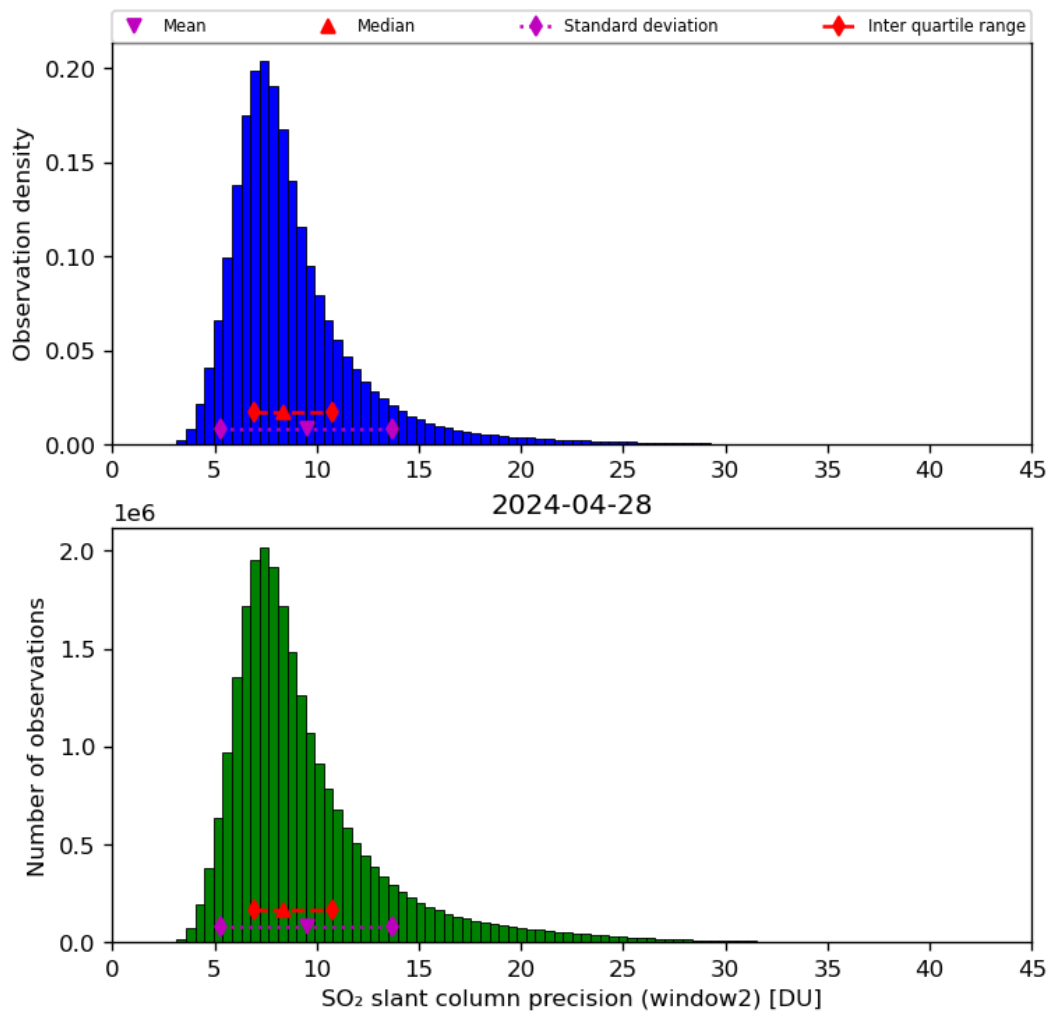
Figure 61: Histogram of “SO 2 slant column precision (window2)” for 2024-04-27 to 2024-04-29
