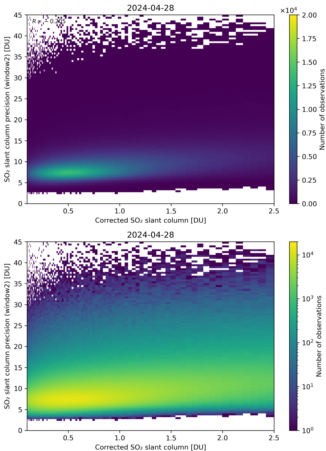
Figure 189: Scatter density plot of “Corrected SO 2 slant column” against “SO 2 slant column precision (window2)” for 2024-04-27 to 2024-04-29.
