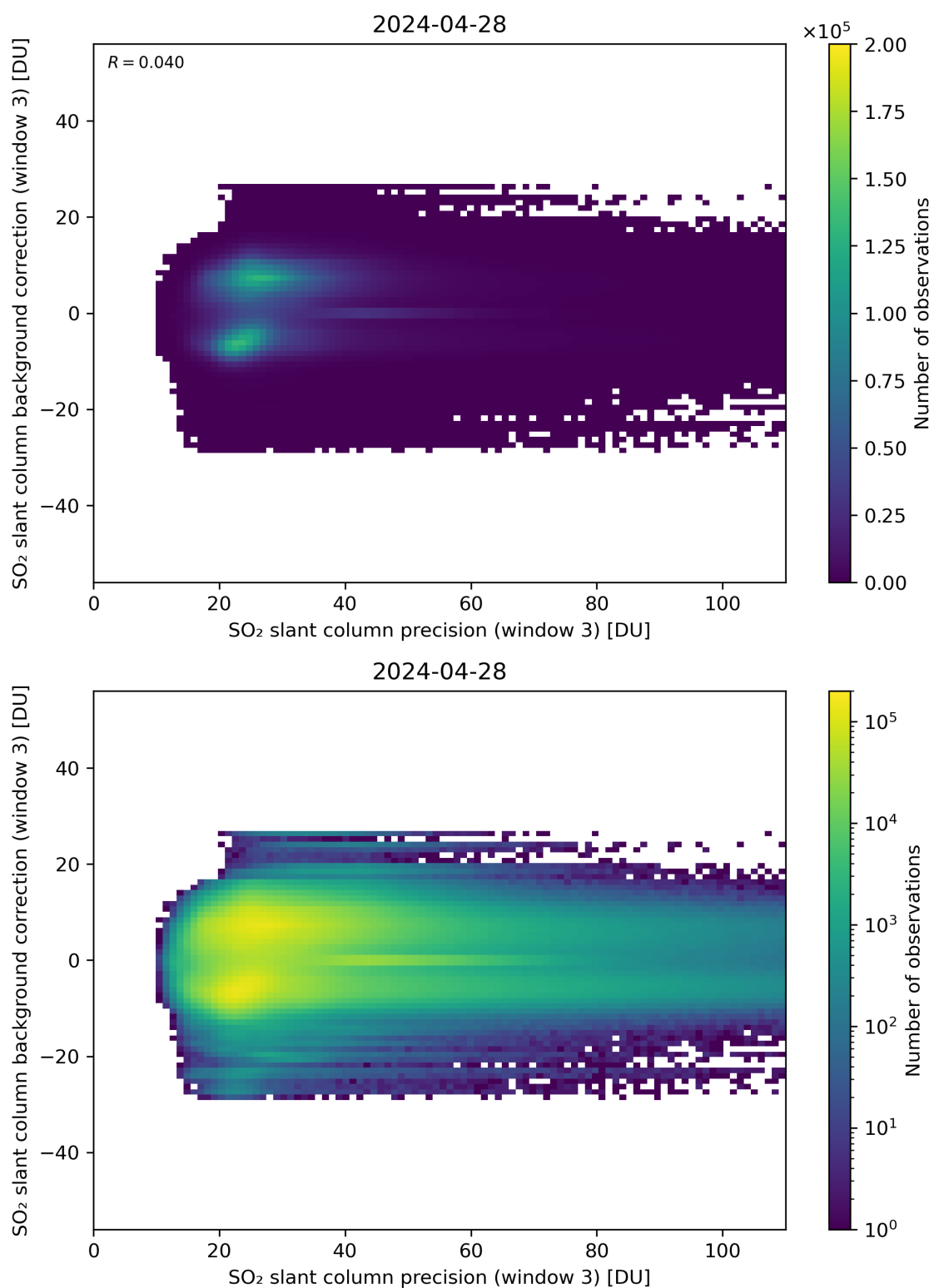
Figure 257: Scatter density plot of “SO 2 slant column precision (window 3)” against “SO 2 slant column background correction (window 3)” for 2024-04-27 to 2024-04-29.
