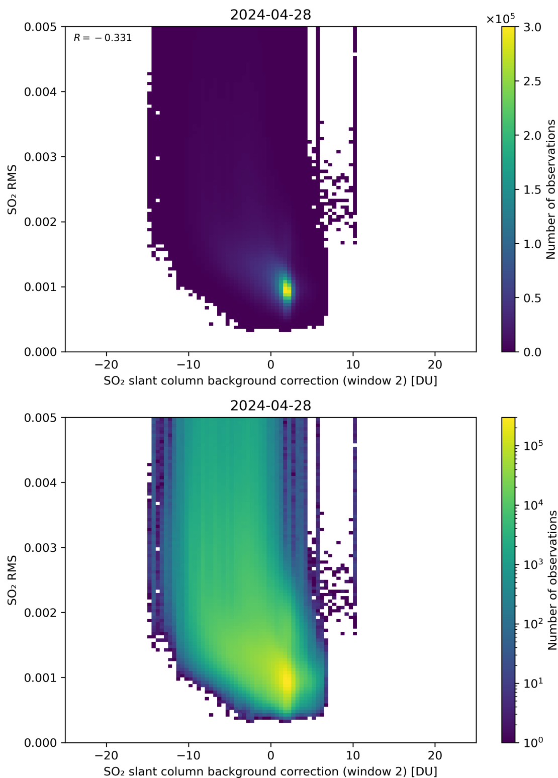
Figure 114: Scatter density plot of “SO 2 slant column background correction (window 2)” against “SO 2 RMS” for 2024-04-27 to 2024-04-29.
