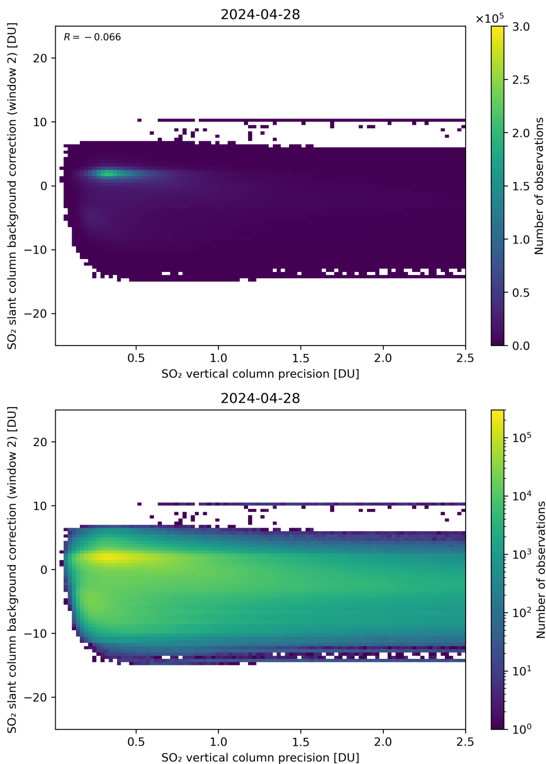
Figure 280: Scatter density plot of “SO 2 vertical column precision” against “SO 2 slant column background correction (window 2)” for 2024-04-27 to 2024-04-29.
