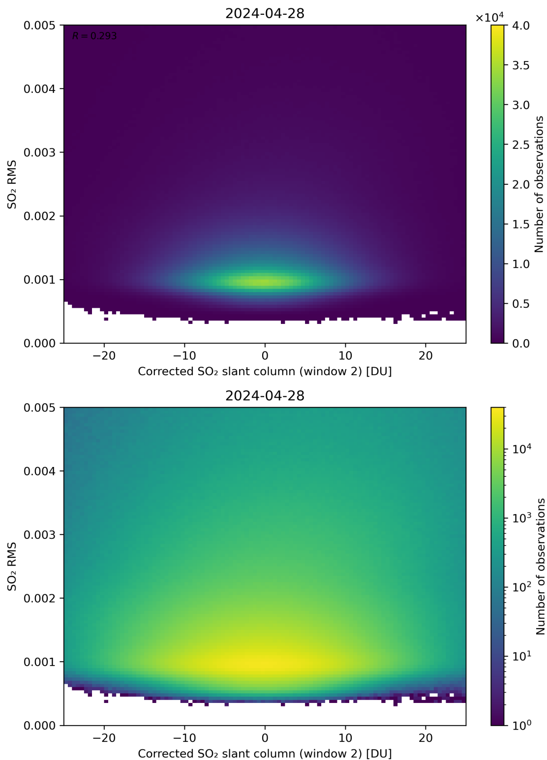
Figure 198: Scatter density plot of “Corrected SO 2 slant column (window 2)” against “SO 2 RMS” for 2024-04-27 to 2024-04-29.
