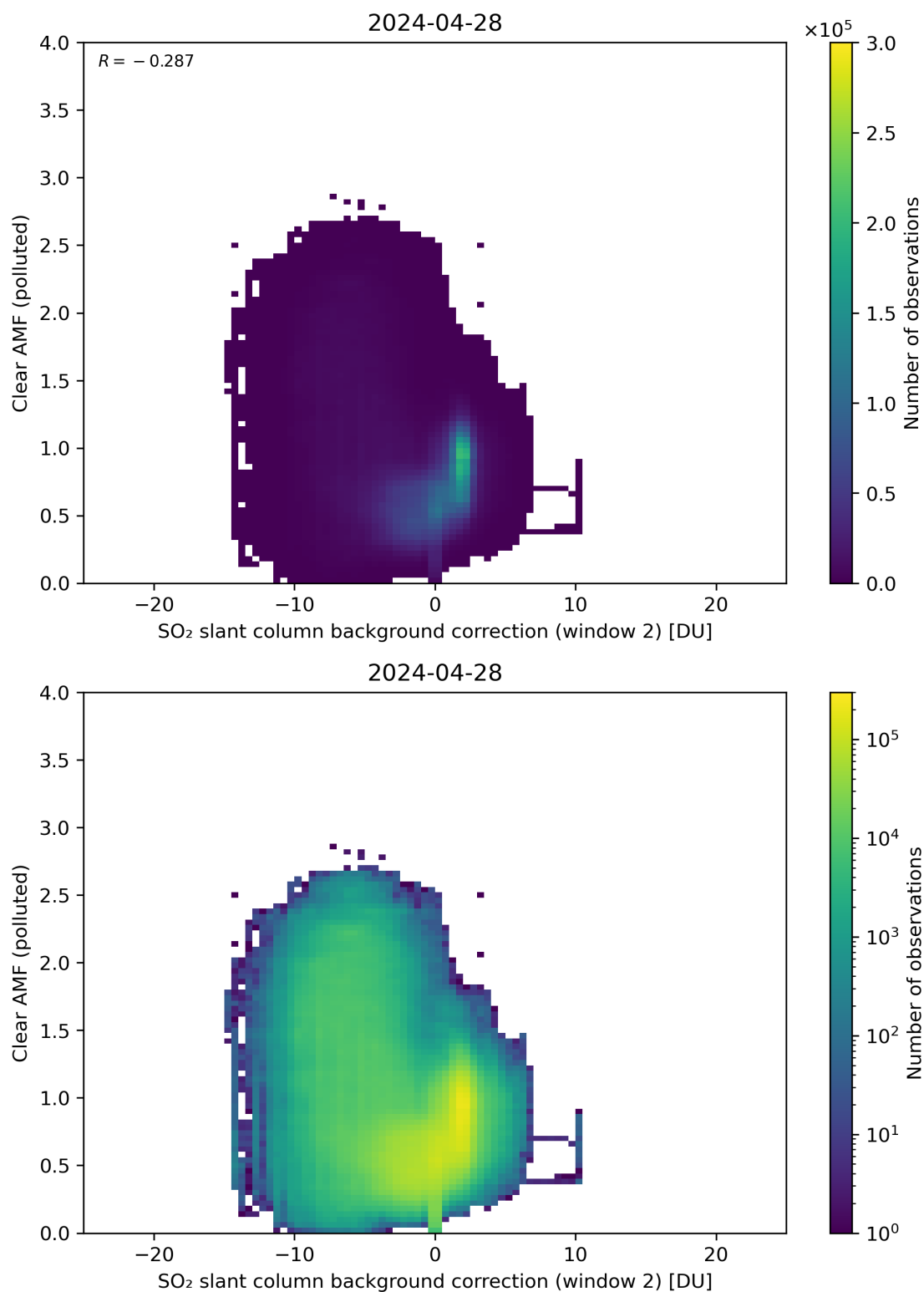
Figure 115: Scatter density plot of “SO 2 slant column background correction (window 2)” against “Clear AMF (polluted)” for 2024-04-27 to 2024-04-29.
