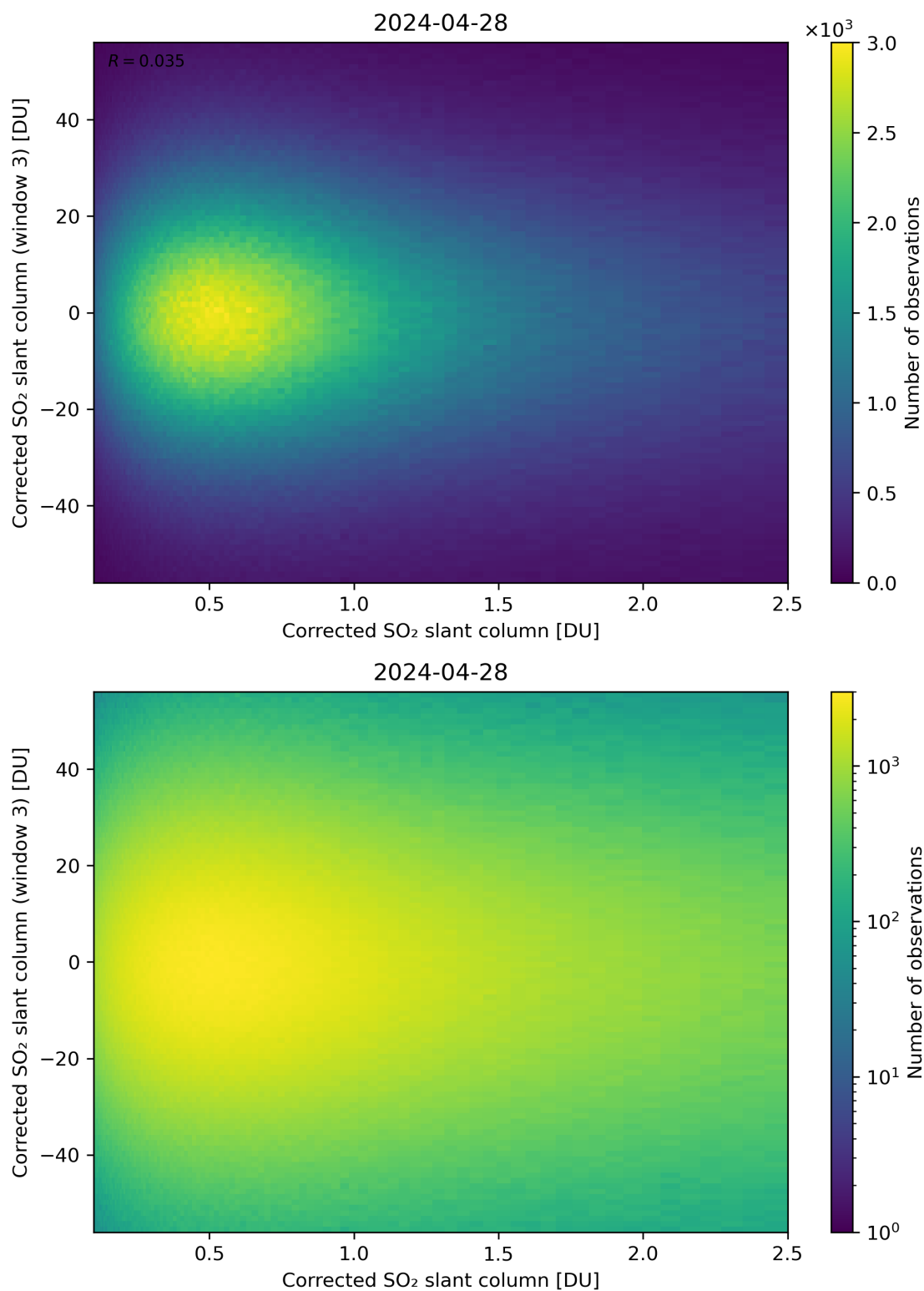
Figure 186: Scatter density plot of “Corrected SO 2 slant column” against “Corrected SO 2 slant column (window 3)” for 2024-04-27 to 2024-04-29.
