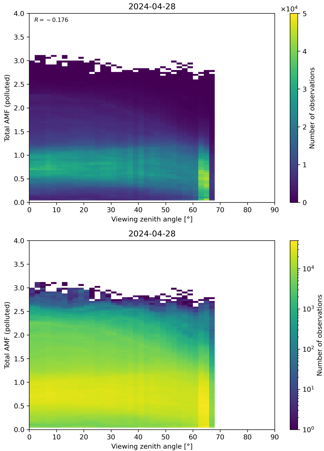
Figure 325: Scatter density plot of “Viewing zenith angle” against “Total AMF (polluted)” for 2024-04-27 to 2024-04-29.
