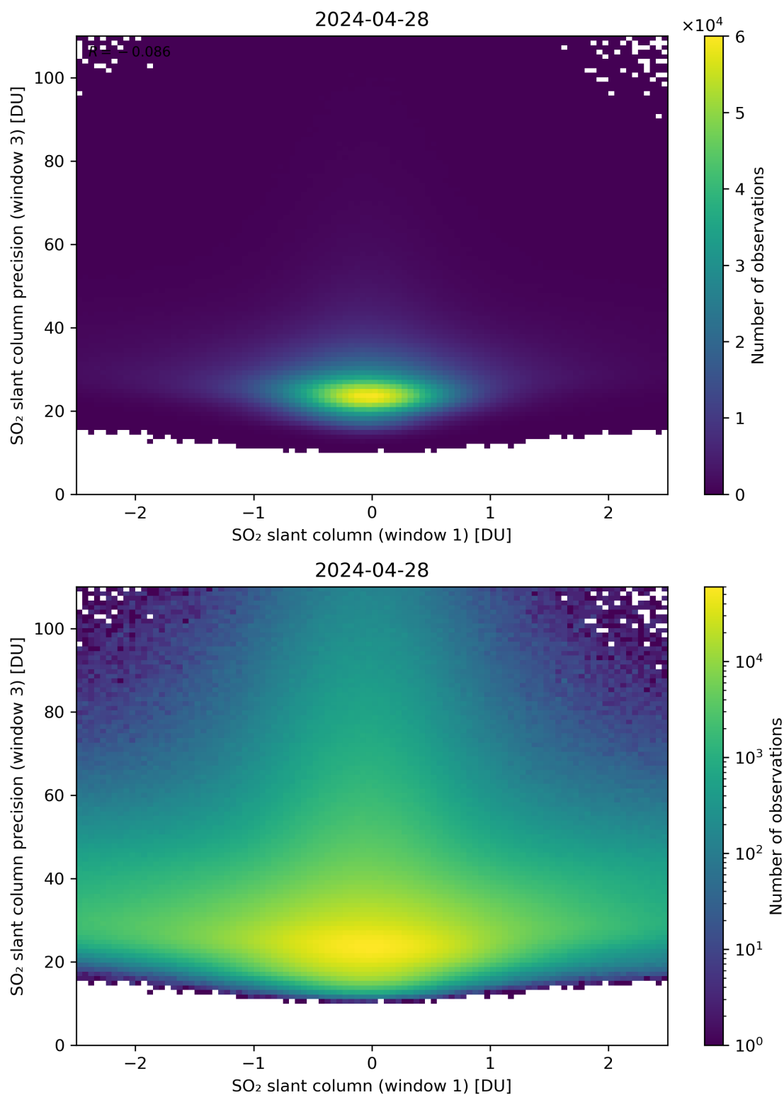
Figure 238: Scatter density plot of “SO 2 slant column (window 1)” against “SO 2 slant column precision (window 3)” for 2024-04-27 to 2024-04-29.
