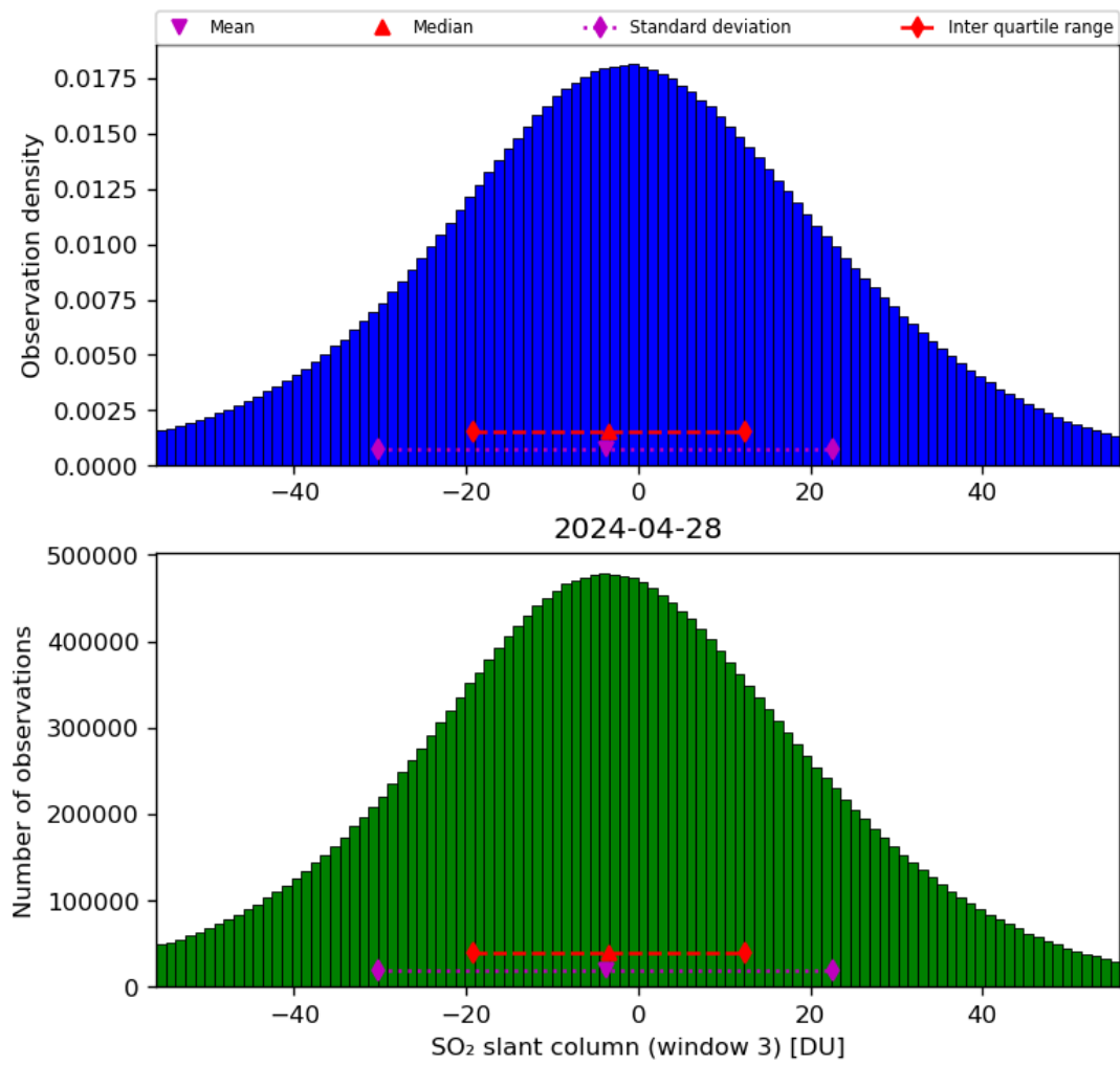
Figure 64: Histogram of “SO 2 slant column (window 3)” for 2024-04-27 to 2024-04-29
