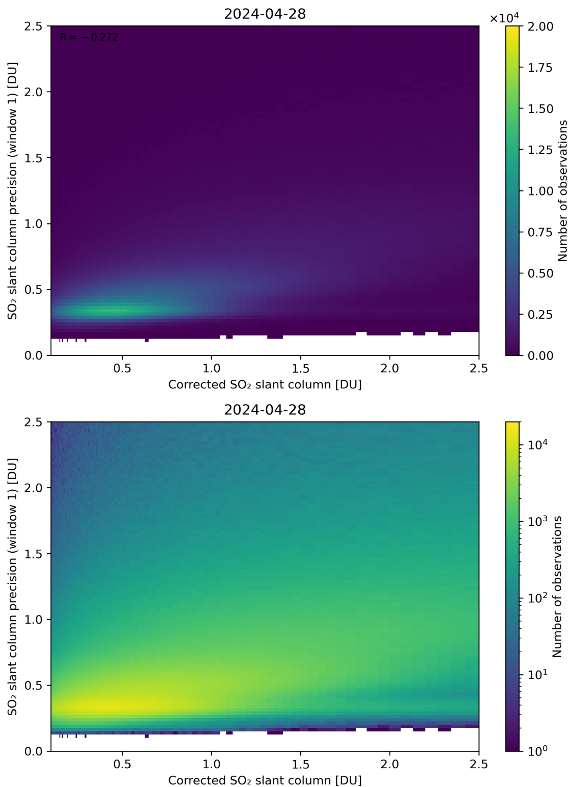
Figure 188: Scatter density plot of “Corrected SO 2 slant column” against “SO 2 slant column precision (window 1)” for 2024-04-27 to 2024-04-29.
