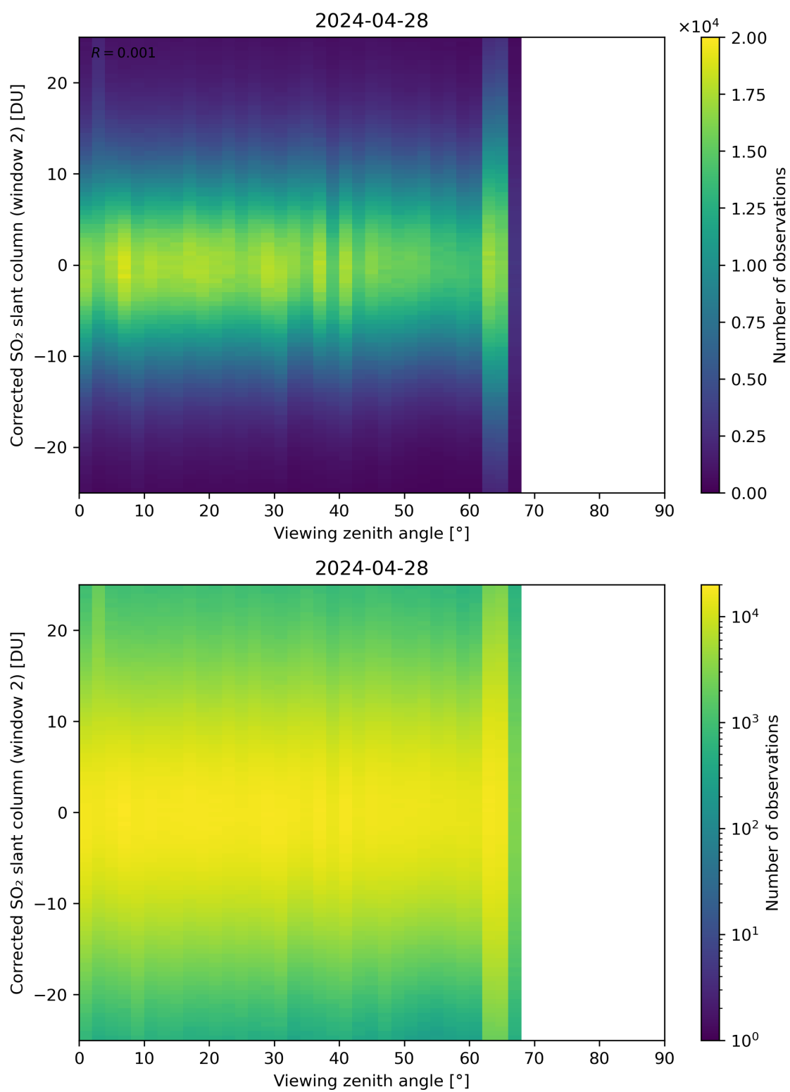
Figure 318: Scatter density plot of “Viewing zenith angle” against “Corrected SO 2 slant column (window 2)” for 2024-04-27 to 2024-04-29.
