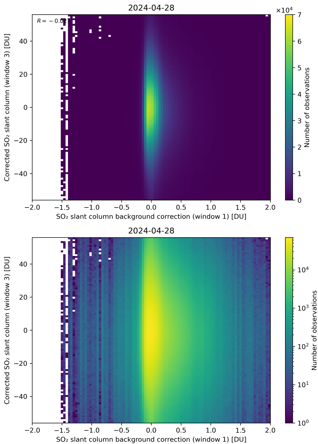
Figure 105: Scatter density plot of “SO 2 slant column background correction (window 1)” against “Corrected SO 2 slant column (window 3)” for 2024-04-27 to 2024-04-29.
