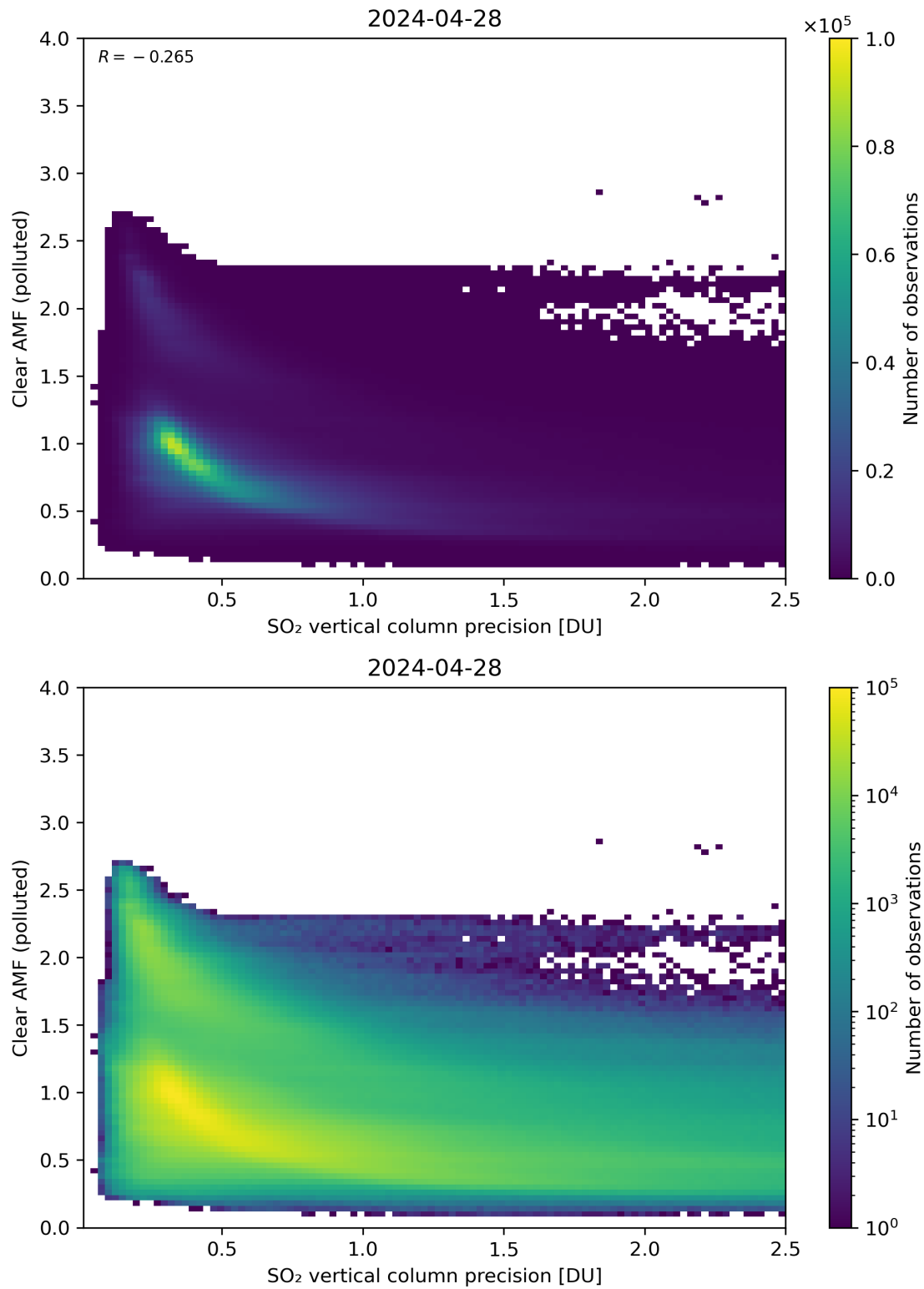
Figure 285: Scatter density plot of “SO 2 vertical column precision” against “Clear AMF (polluted)” for 2024-04-27 to 2024-04-29.
