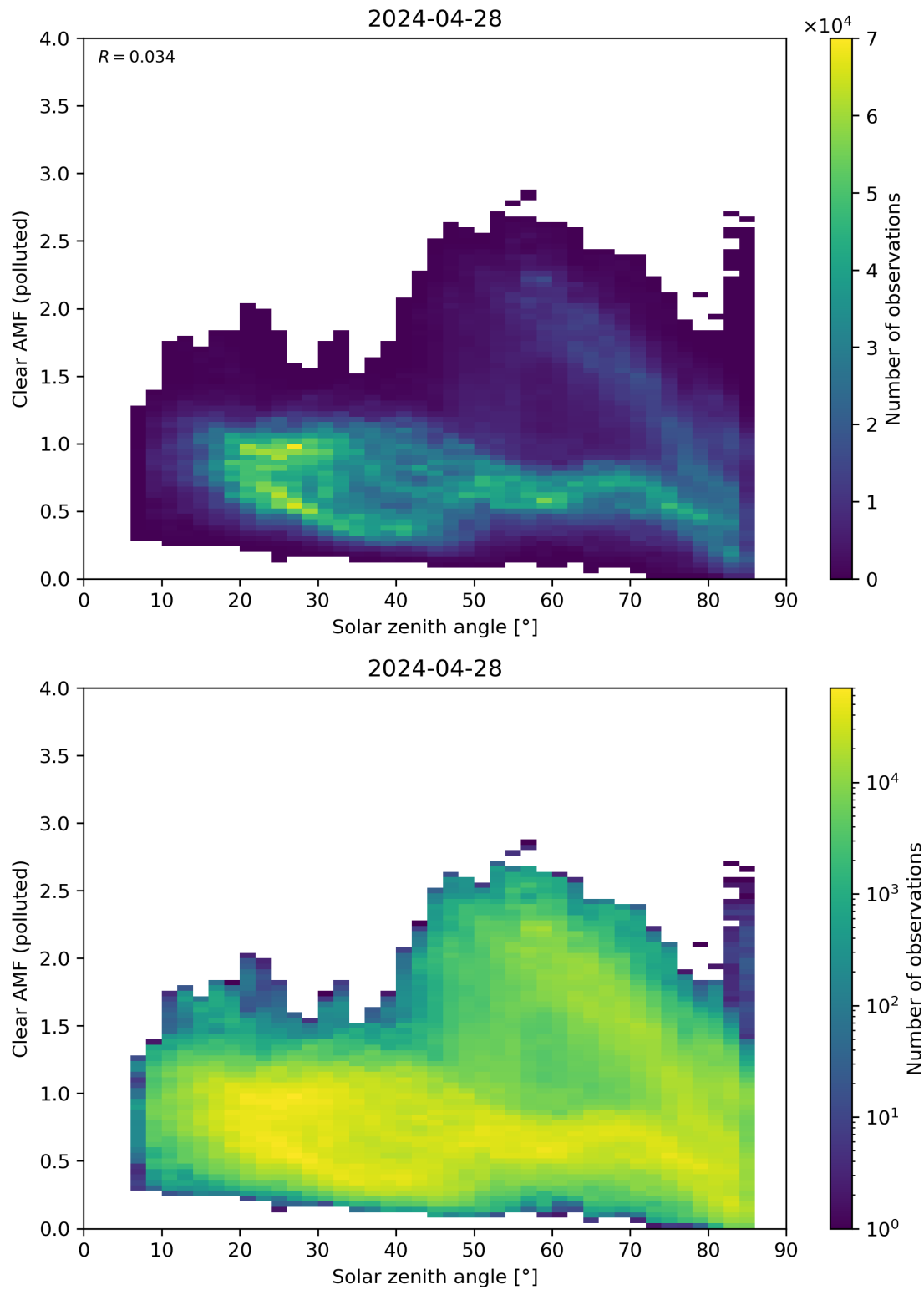
Figure 165: Scatter density plot of “Solar zenith angle” against “Clear AMF (polluted)” for 2024-04-27 to 2024-04-29.
