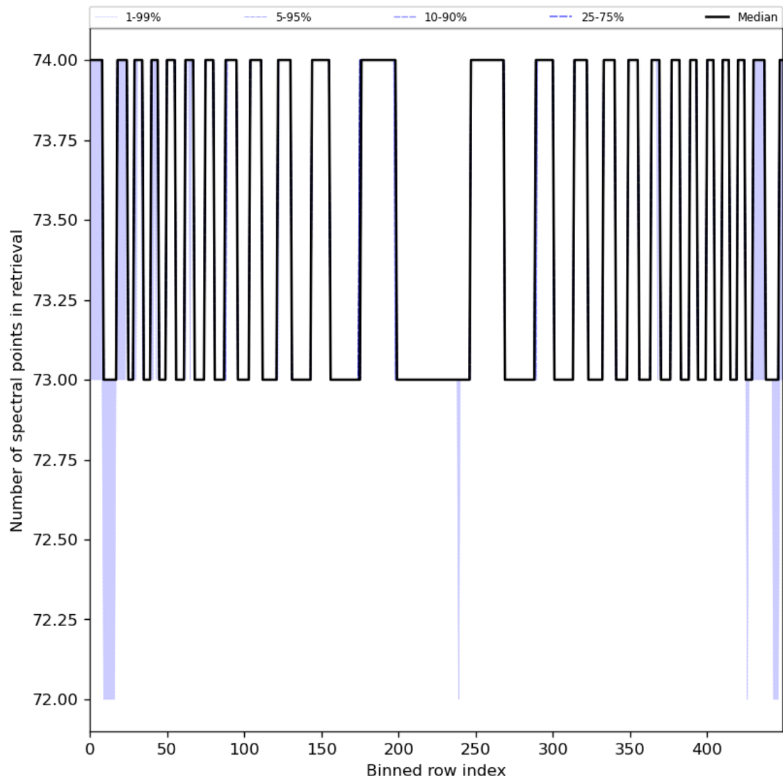
Figure 97: Along track statistics of “Number of spectral points in retrieval” for 2024-04-27 to 2024-04-29
