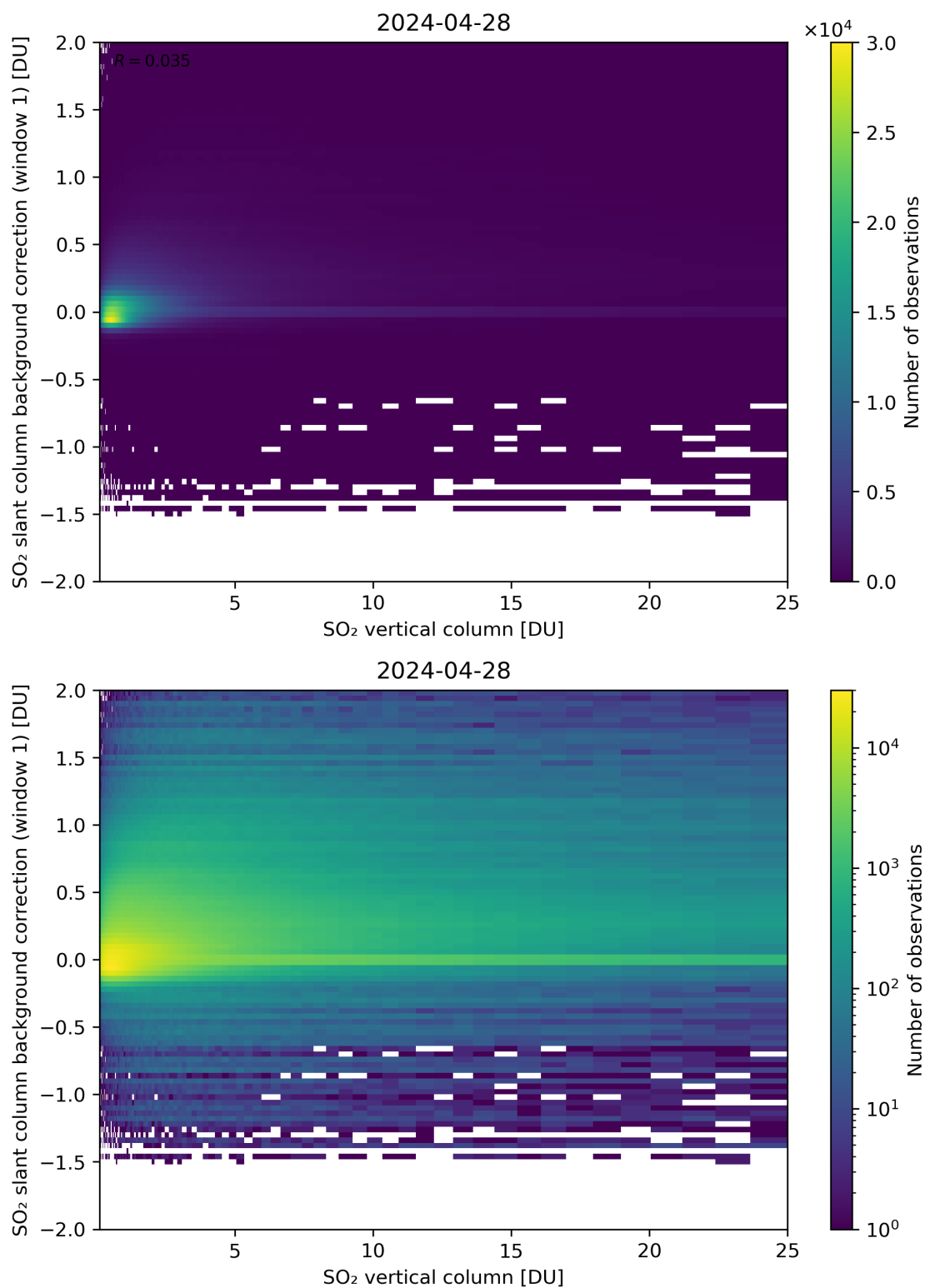
Figure 273: Scatter density plot of “SO 2 vertical column” against “SO 2 slant column background correction (window 1)” for 2024-04-27 to 2024-04-29.
