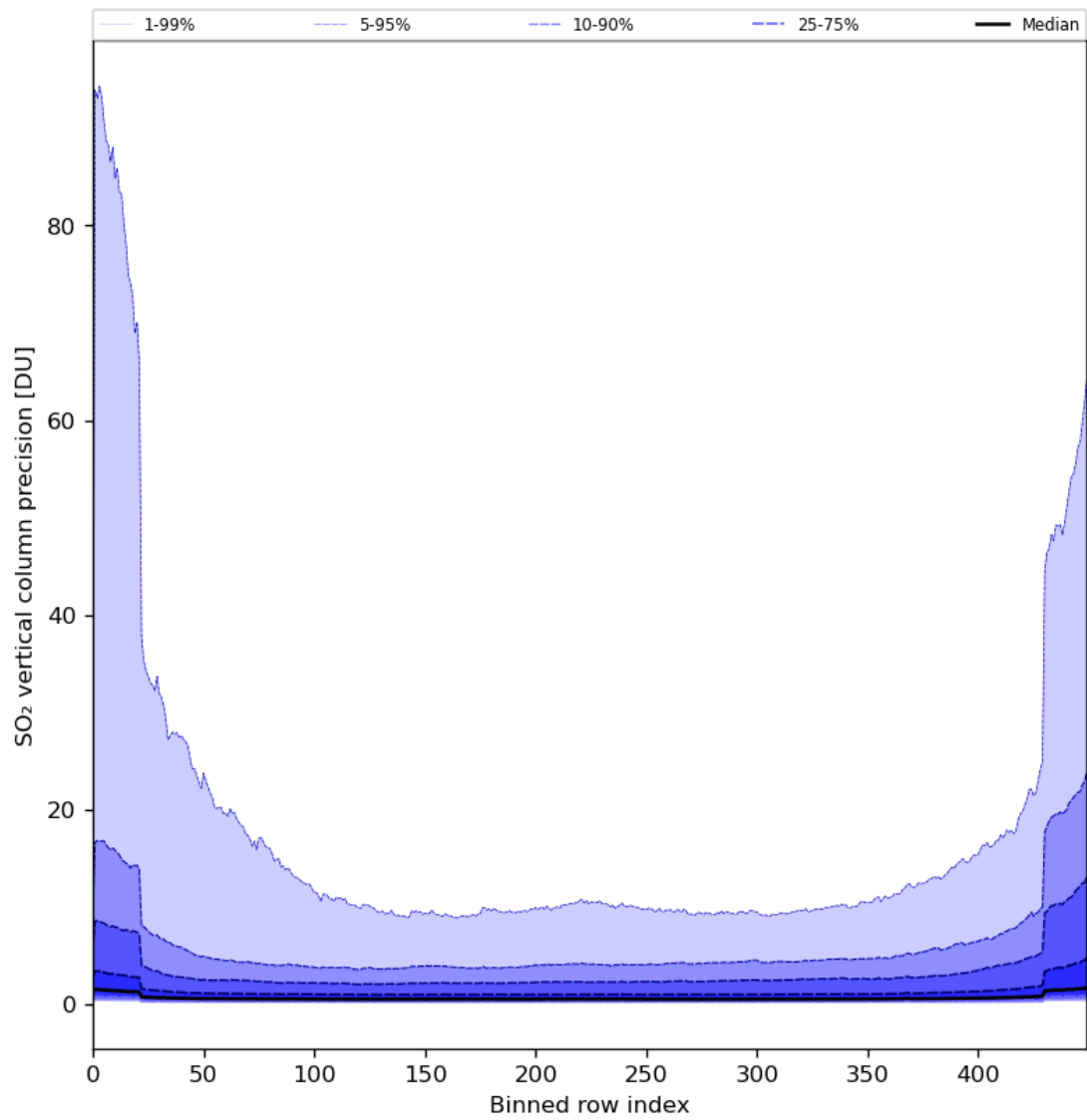
Figure 77: Along track statistics of “SO 2 vertical column precision” for 2024-04-27 to 2024-04-29
