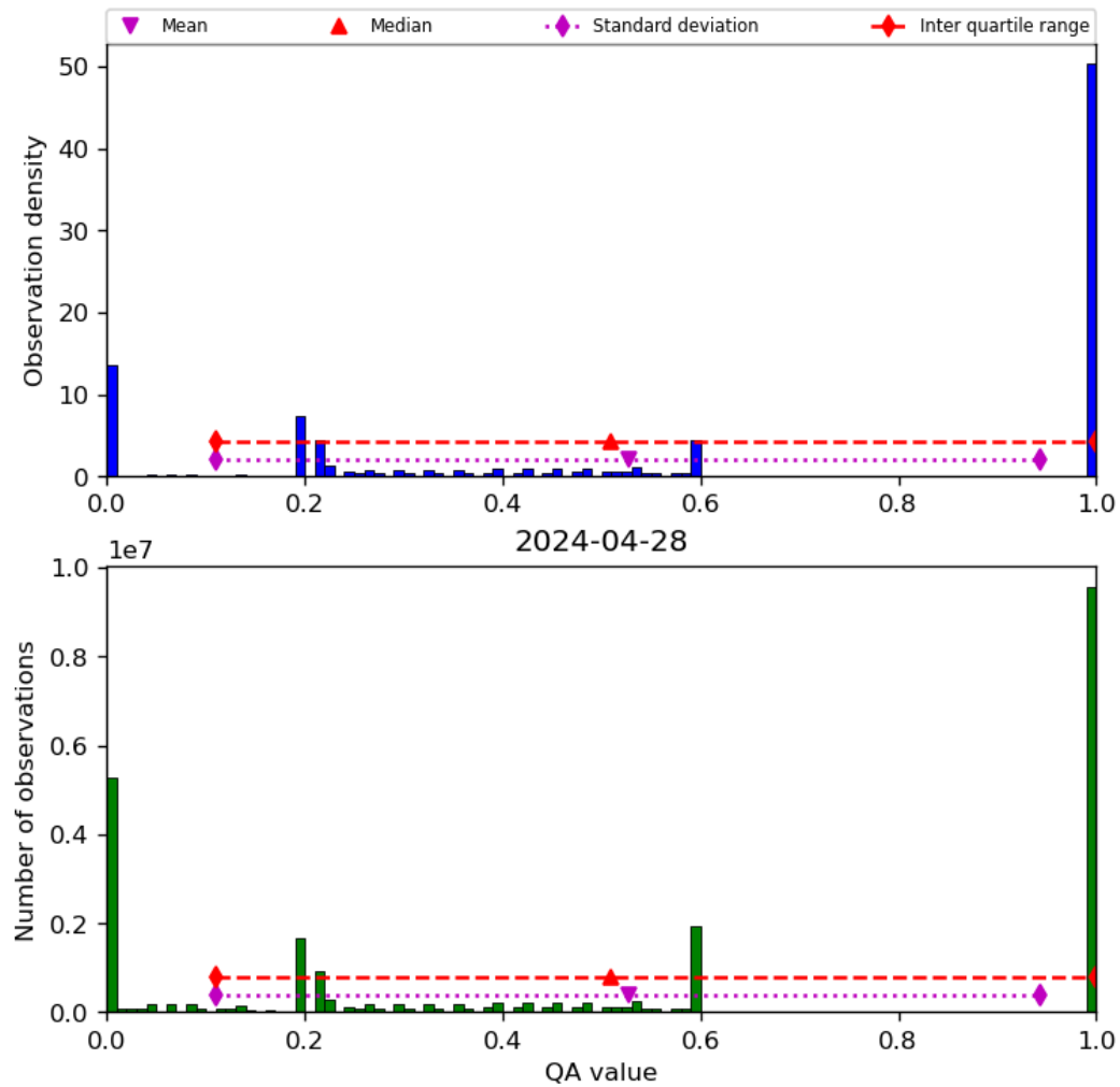
Figure 52: Histogram of “QA value” for 2024-04-27 to 2024-04-29
