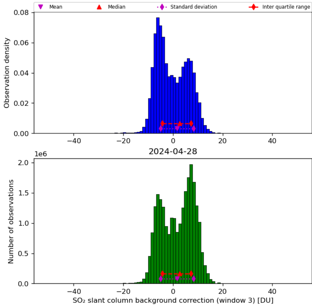
Figure 67: Histogram of “SO 2 slant column background correction (window 3)” for 2024-04-27 to 2024-04-29
