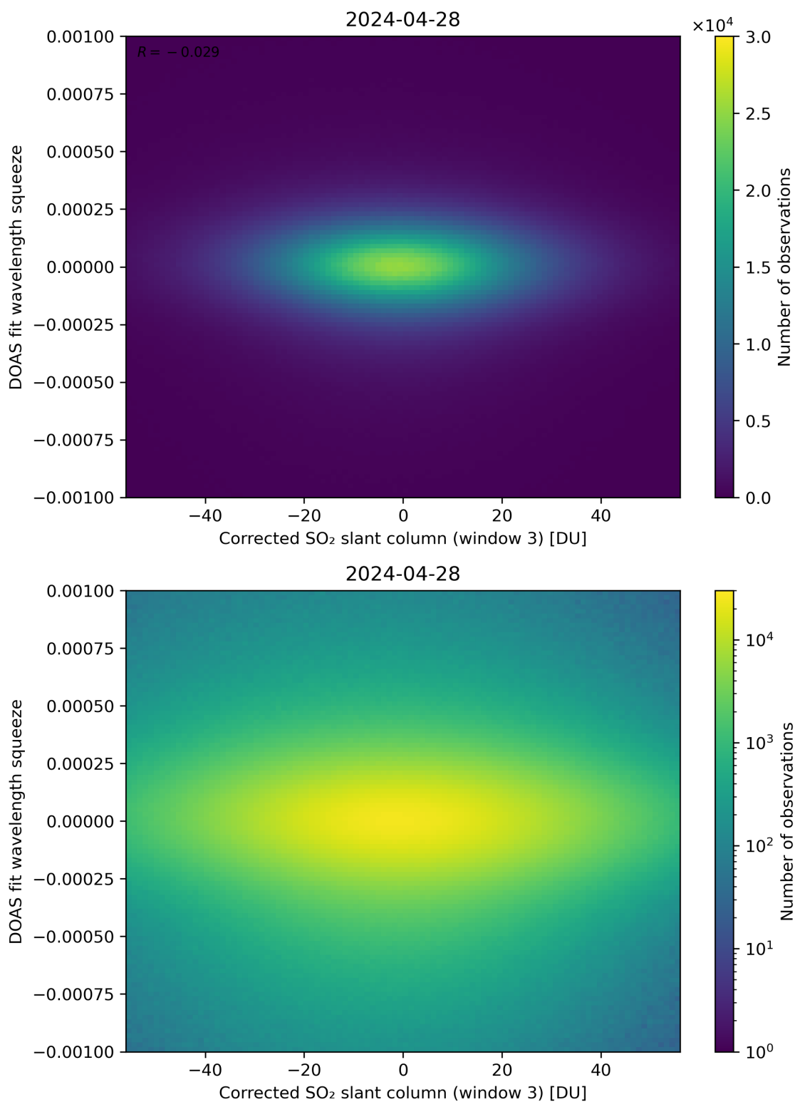
Figure 207: Scatter density plot of “Corrected SO 2 slant column (window 3)” against “DOAS fit wavelength squeeze” for 2024-04-27 to 2024-04-29.
