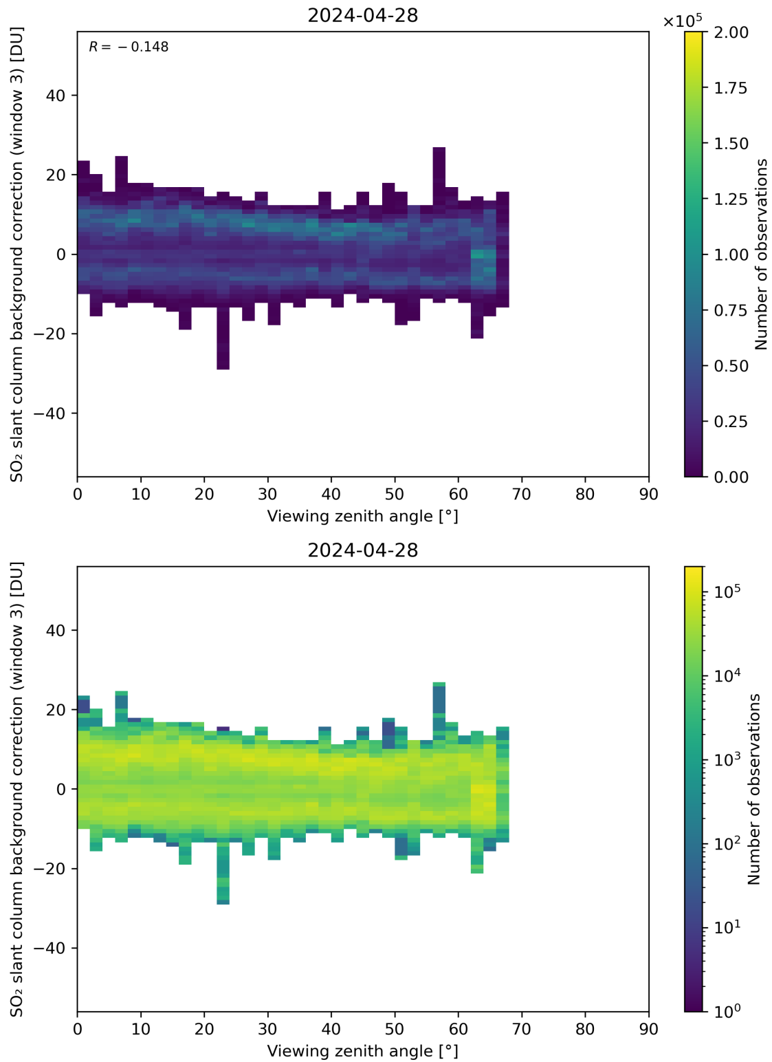
Figure 310: Scatter density plot of “Viewing zenith angle” against “SO 2 slant column background correction (window 3)” for 2024-04-27 to 2024-04-29.
