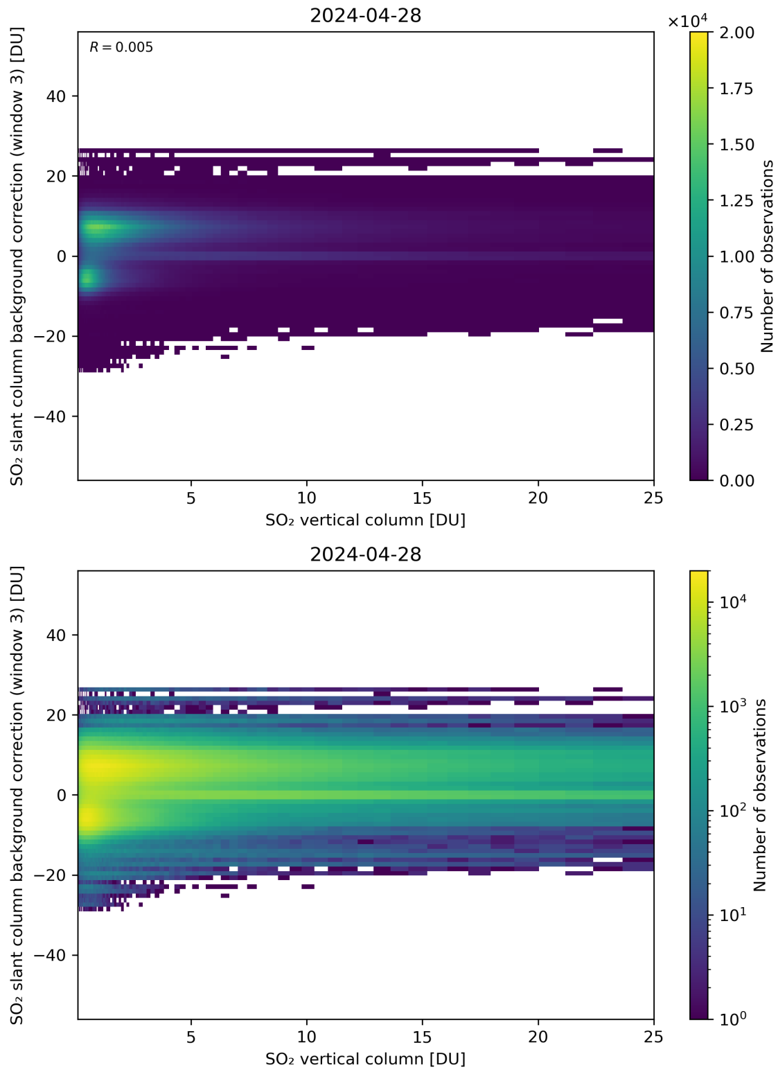
Figure 275: Scatter density plot of “SO 2 vertical column” against “SO 2 slant column background correction (window 3)” for 2024-04-27 to 2024-04-29.
