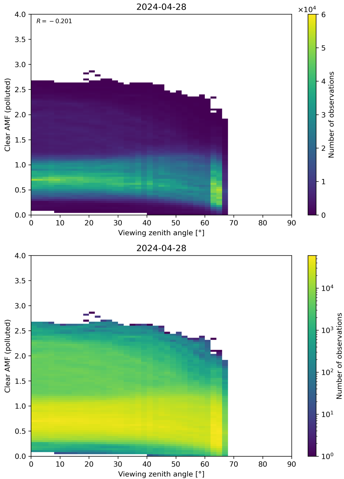
Figure 316: Scatter density plot of “Viewing zenith angle” against “Clear AMF (polluted)” for 2024-04-27 to 2024-04-29.
