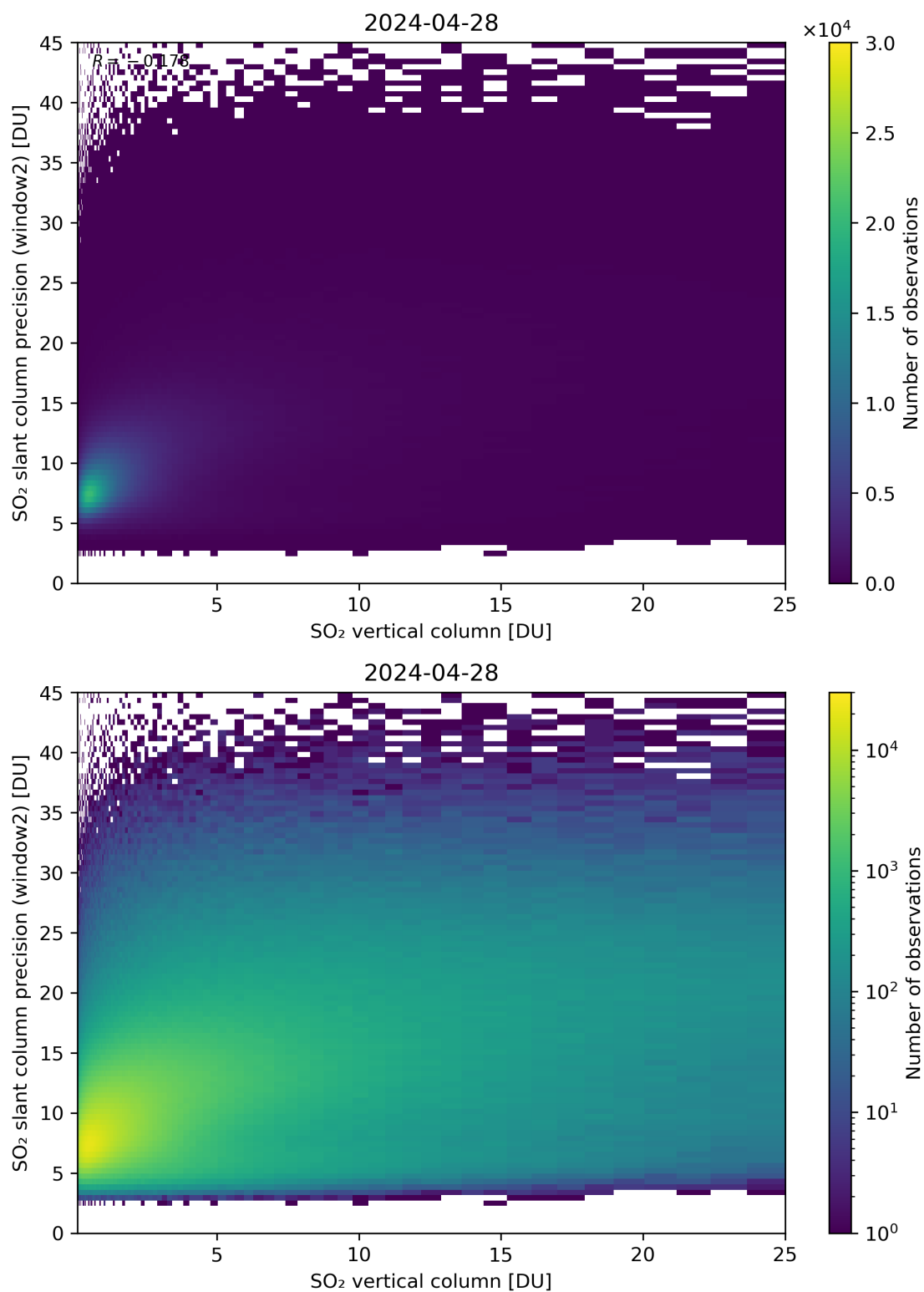
Figure 302: Scatter density plot of “SO 2 vertical column” against “SO 2 slant column precision (window2)” for 2024-04-27 to 2024-04-29.
