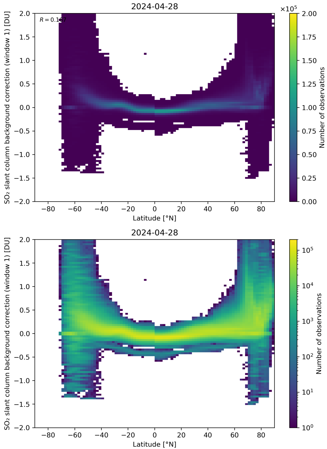
Figure 139: Scatter density plot of “Latitude” against “SO 2 slant column background correction (window 1)” for 2024-04-27 to 2024-04-29.
