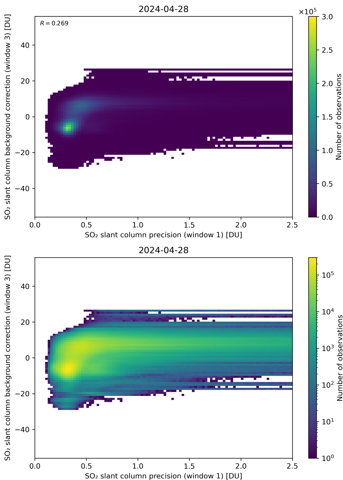
Figure 220: Scatter density plot of “SO 2 slant column precision (window 1)” against “SO 2 slant column background correction (window 3)” for 2024-04-27 to 2024-04-29.
