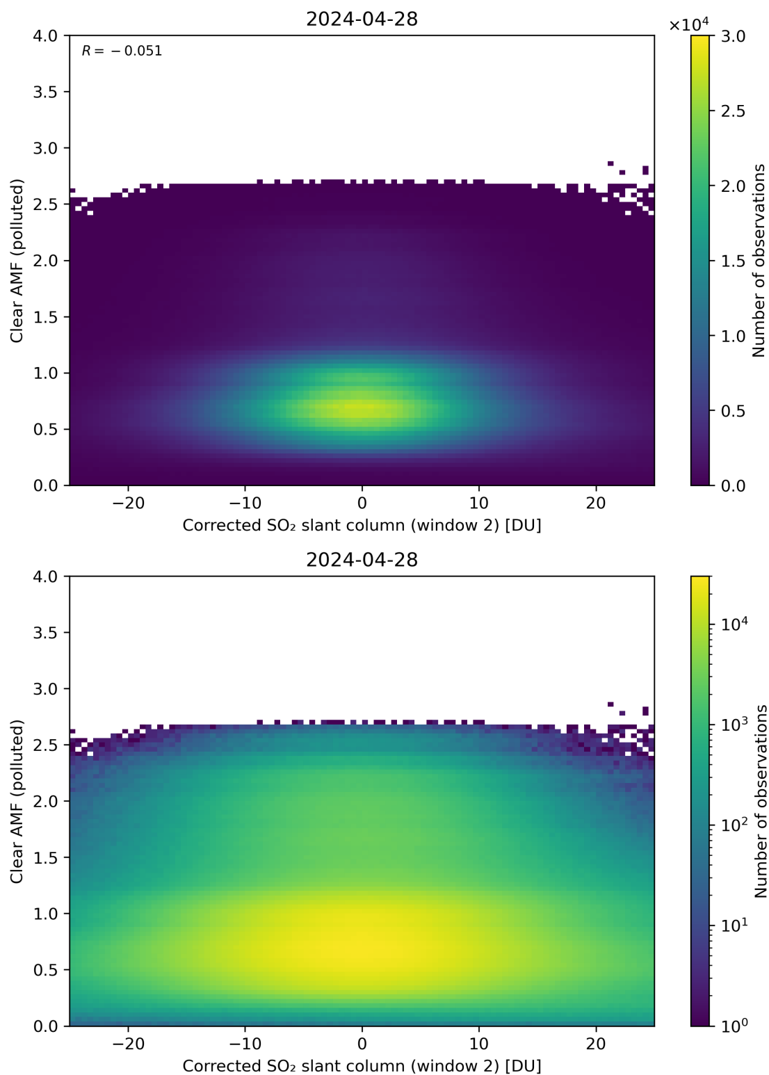
Figure 199: Scatter density plot of “Corrected SO 2 slant column (window 2)” against “Clear AMF (polluted)” for 2024-04-27 to 2024-04-29.
