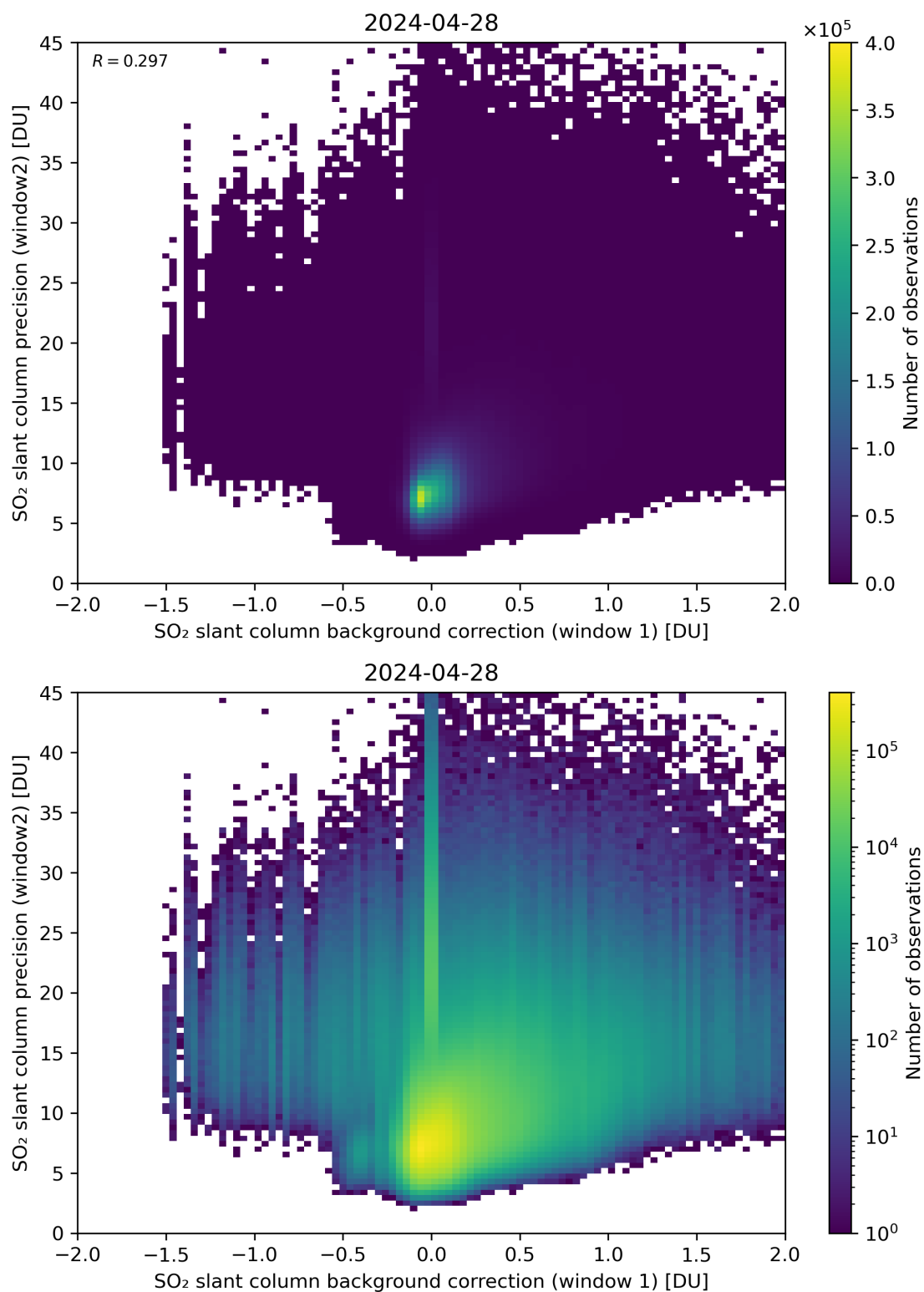
Figure 106: Scatter density plot of “SO 2 slant column background correction (window 1)” against “SO 2 slant column precision (window2)” for 2024-04-27 to 2024-04-29.
