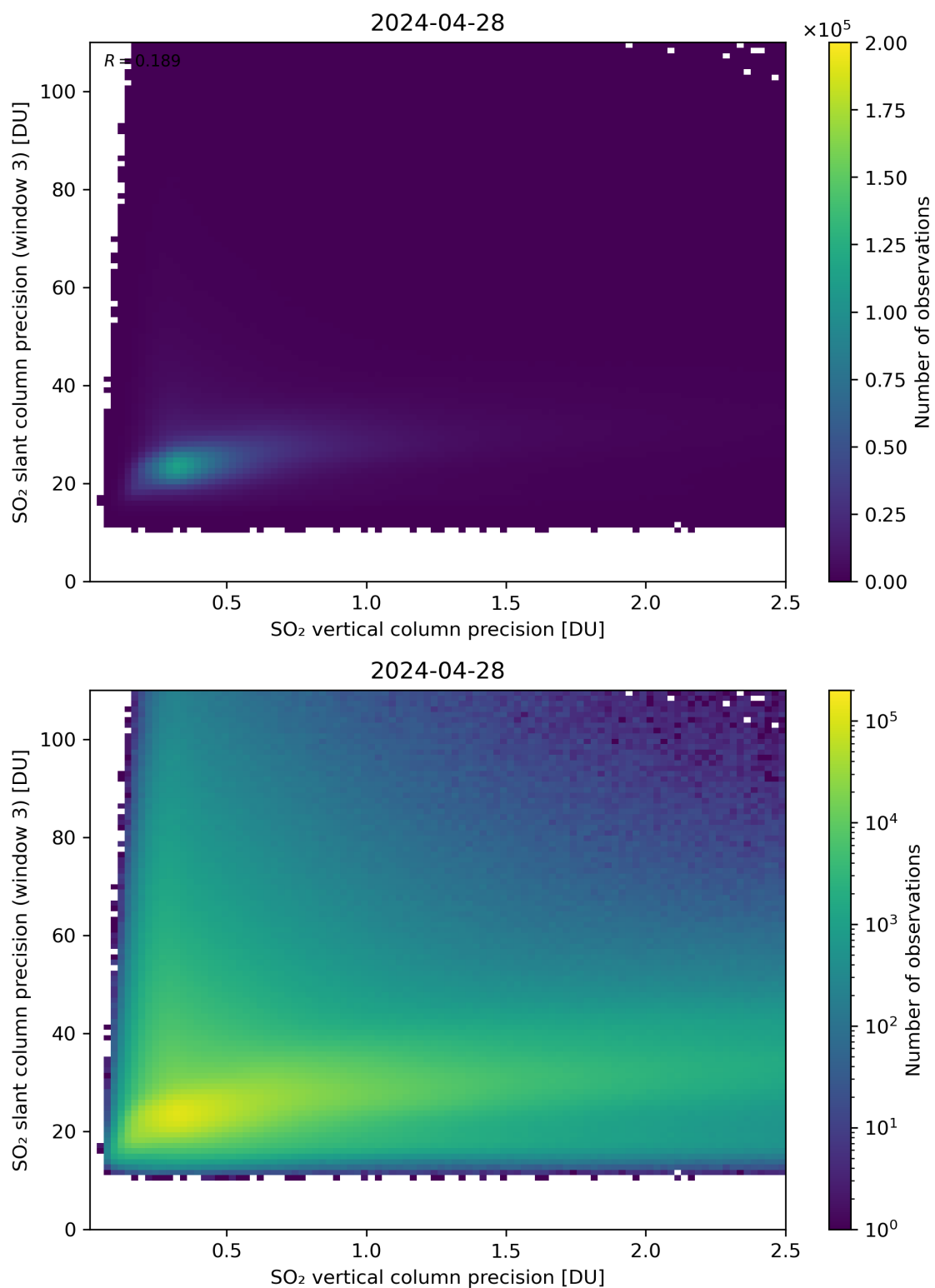
Figure 293: Scatter density plot of “SO 2 vertical column precision” against “SO 2 slant column precision (window 3)” for 2024-04-27 to 2024-04-29.
