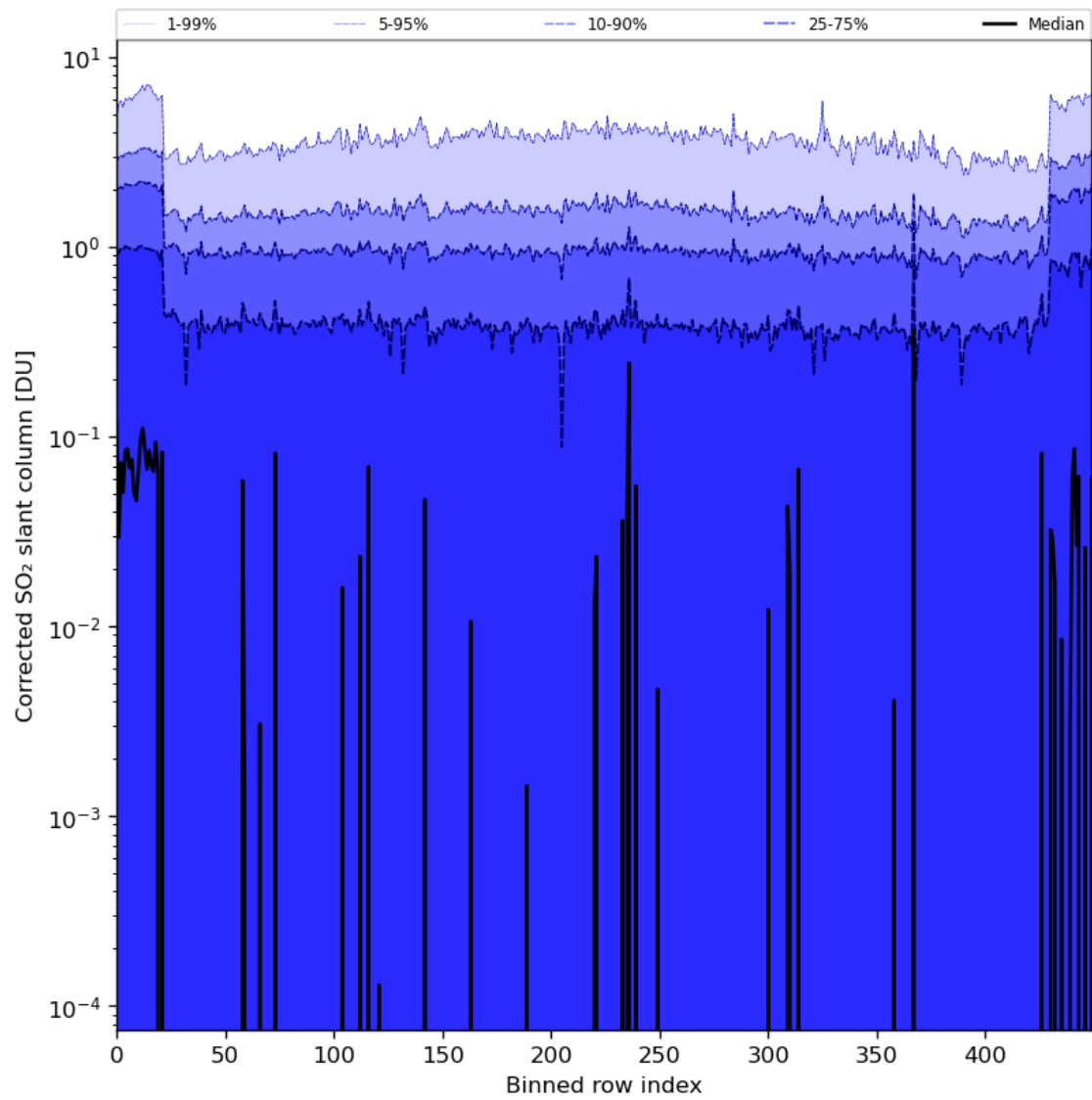
Figure 78: Along track statistics of “Corrected SO 2 slant column” for 2024-04-27 to 2024-04-29
