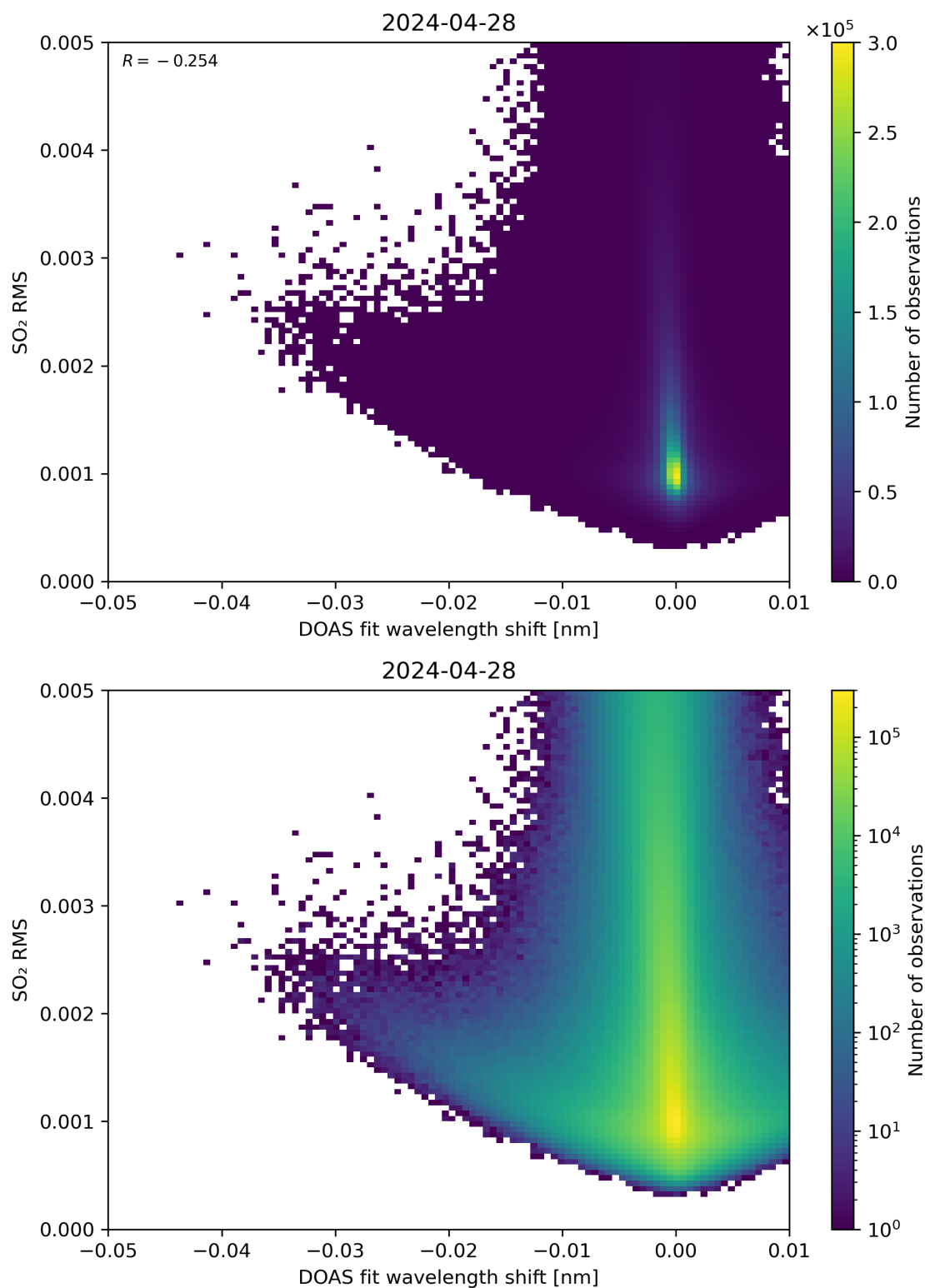
Figure 128: Scatter density plot of “DOAS fit wavelength shift” against “SO 2 RMS” for 2024-04-27 to 2024-04-29.
