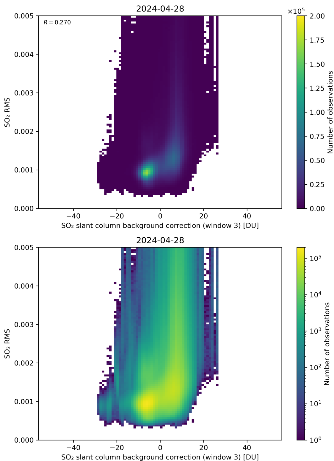
Figure 123: Scatter density plot of “SO 2 slant column background correction (window 3)” against “SO 2 RMS” for 2024-04-27 to 2024-04-29.
