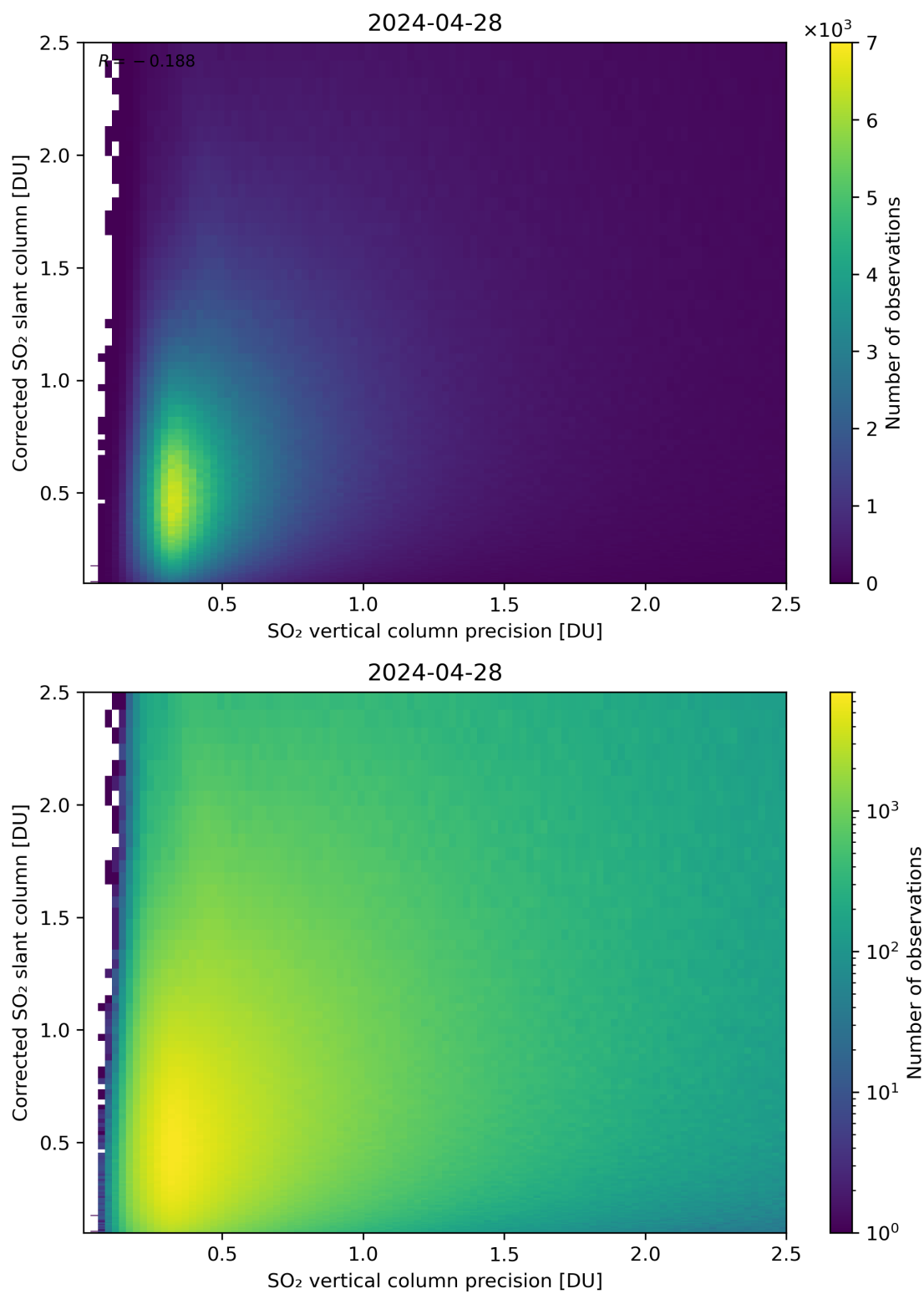
Figure 286: Scatter density plot of “SO 2 vertical column precision” against “Corrected SO 2 slant column” for 2024-04-27 to 2024-04-29.
