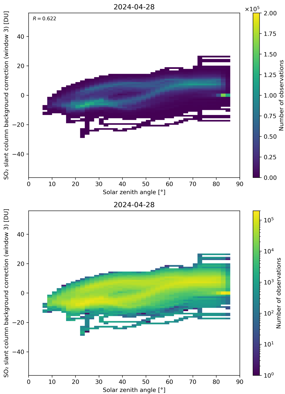
Figure 160: Scatter density plot of “Solar zenith angle” against “SO 2 slant column background correction (window 3)” for 2024-04-27 to 2024-04-29.
