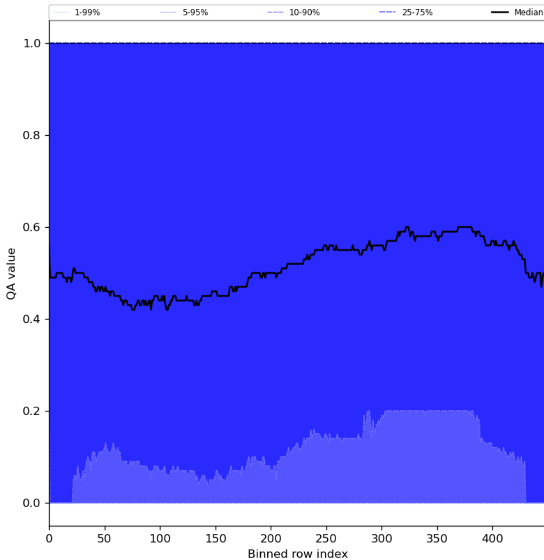
Figure 75: Along track statistics of “QA value” for 2024-04-27 to 2024-04-29
