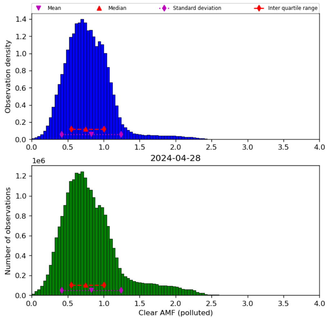
Figure 73: Histogram of “Clear AMF (polluted)” for 2024-04-27 to 2024-04-29
