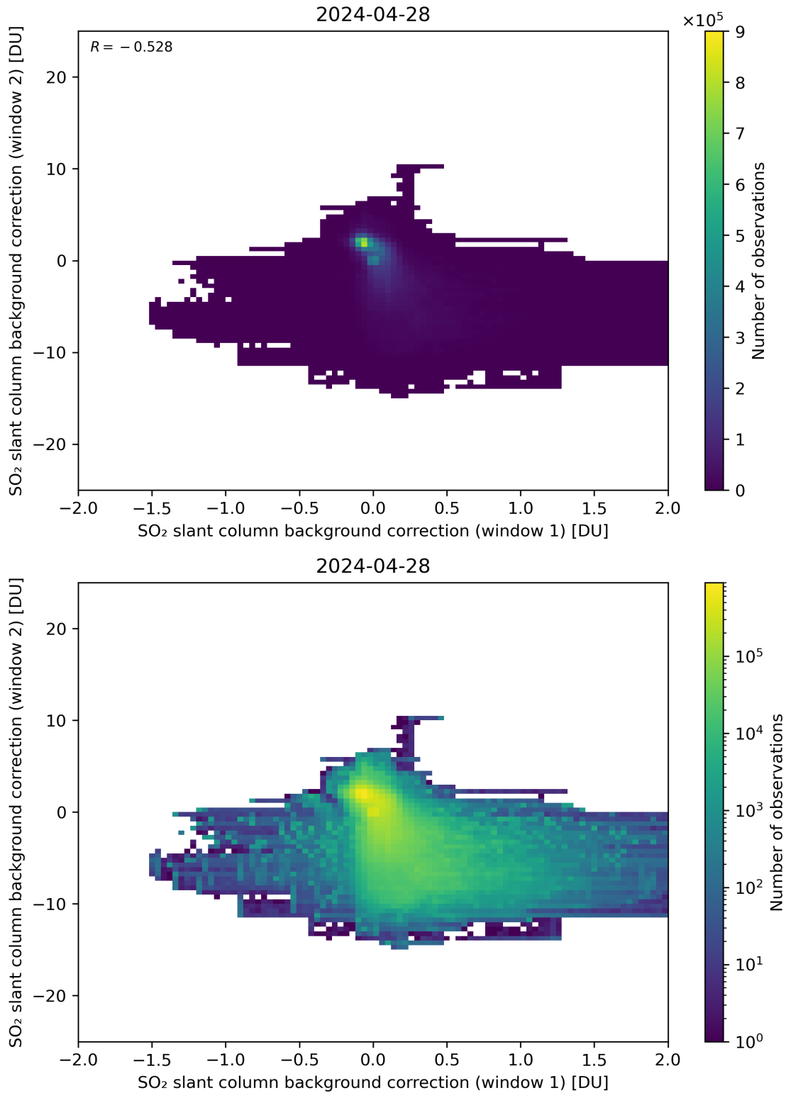
Figure 98: Scatter density plot of “SO 2 slant column background correction (window 1)” against “SO 2 slant column background correction (window 2)” for 2024-04-27 to 2024-04-29.
