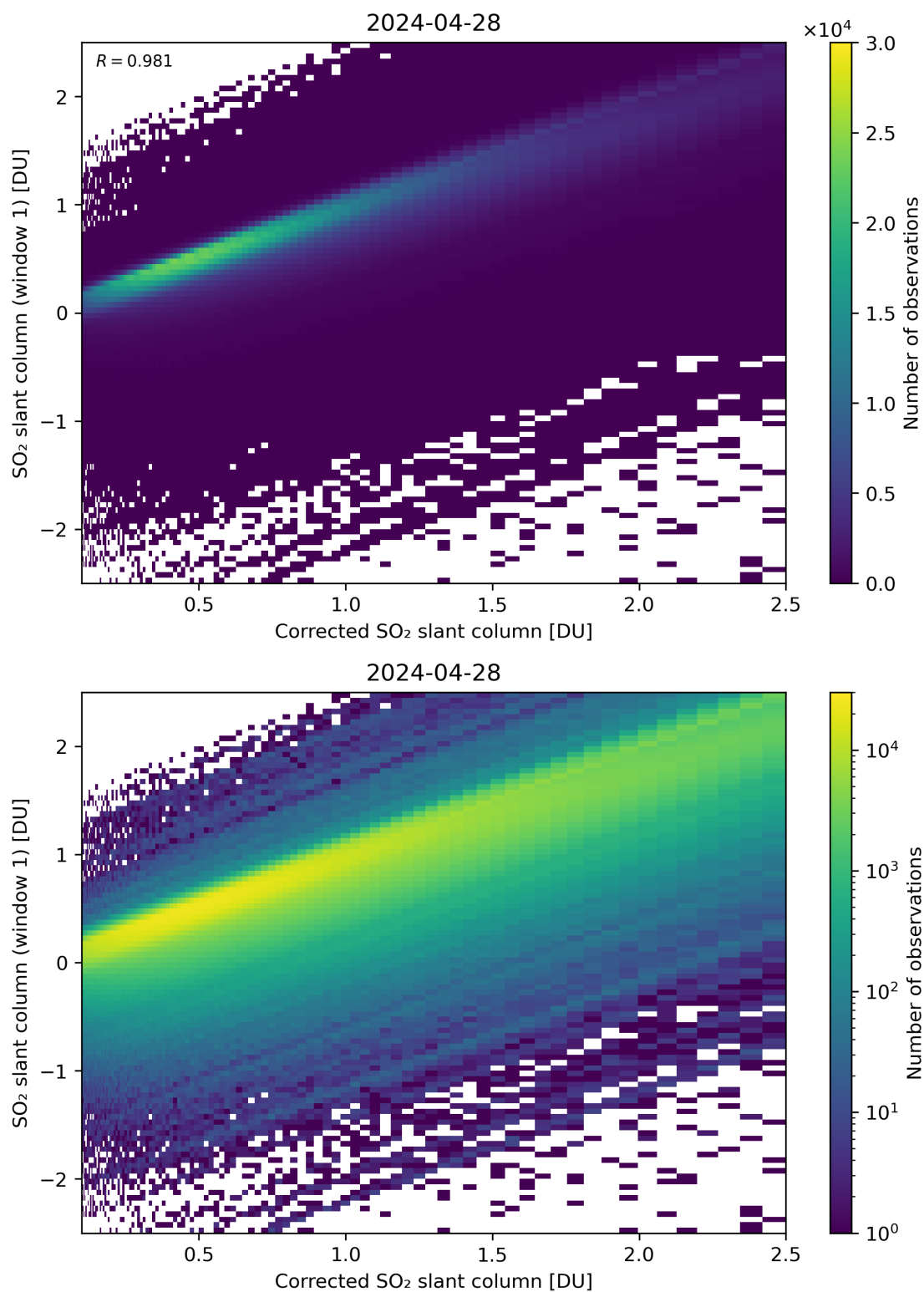
Figure 187: Scatter density plot of “Corrected SO 2 slant column” against “SO 2 slant column (window 1)” for 2024-04-27 to 2024-04-29.
