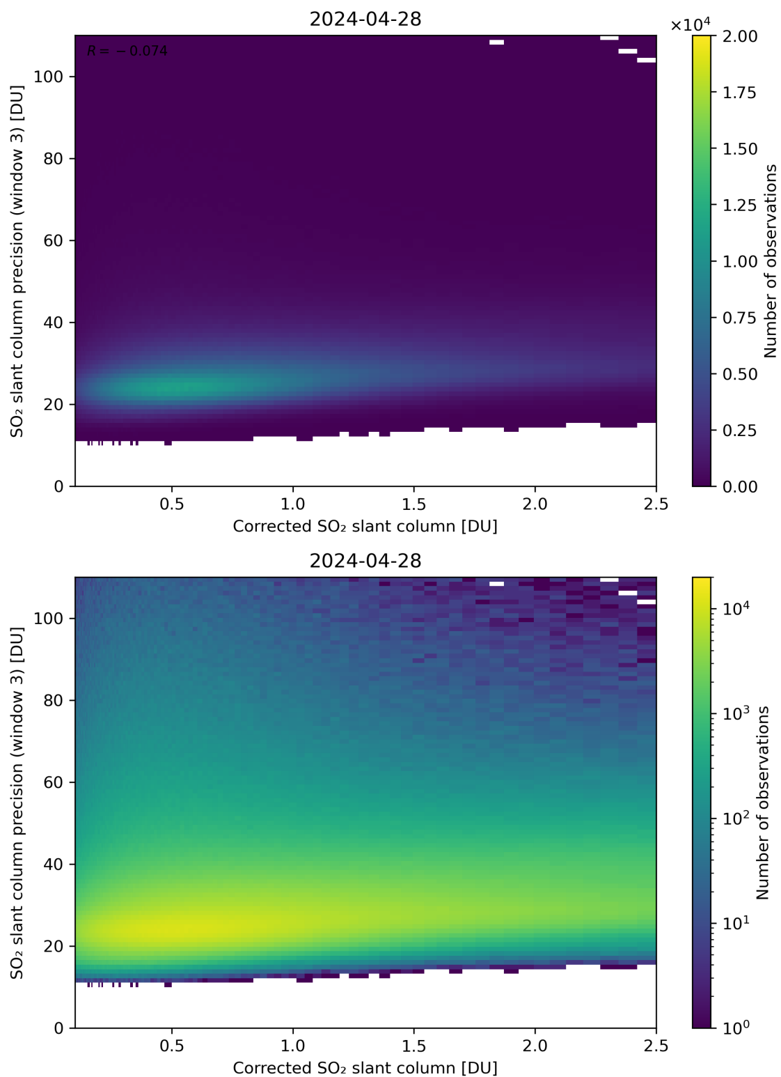
Figure 191: Scatter density plot of “Corrected SO 2 slant column” against “SO 2 slant column precision (window 3)” for 2024-04-27 to 2024-04-29.
