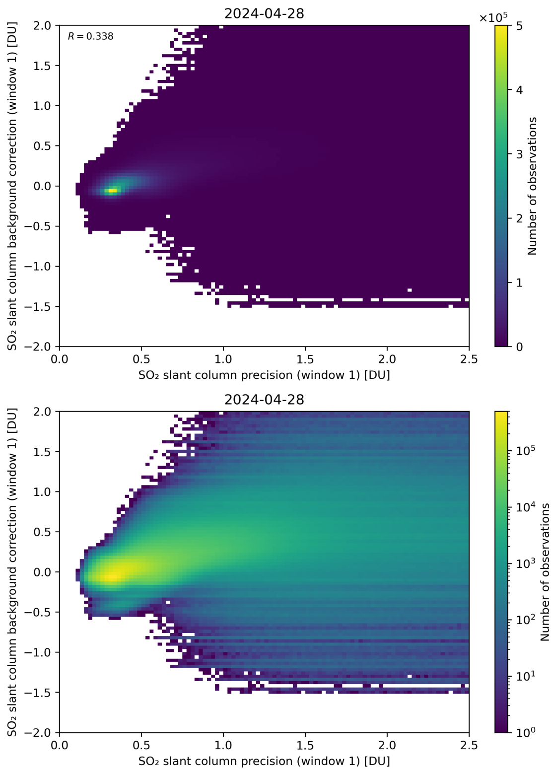
Figure 218: Scatter density plot of “SO 2 slant column precision (window 1)” against “SO 2 slant column background correction (window 1)” for 2024-04-27 to 2024-04-29.
