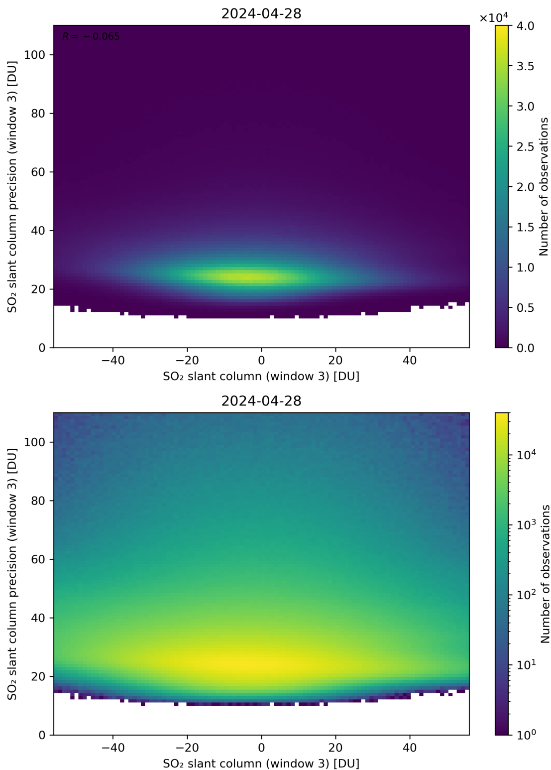
Figure 267: Scatter density plot of “SO 2 slant column (window 3)” against “SO 2 slant column precision (window 3)” for 2024-04-27 to 2024-04-29.
