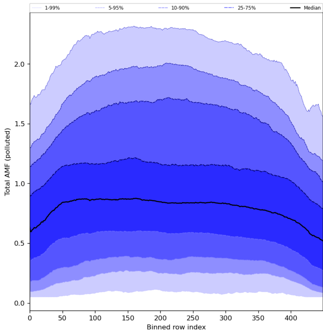
Figure 94: Along track statistics of “Total AMF (polluted)” for 2024-04-27 to 2024-04-29
