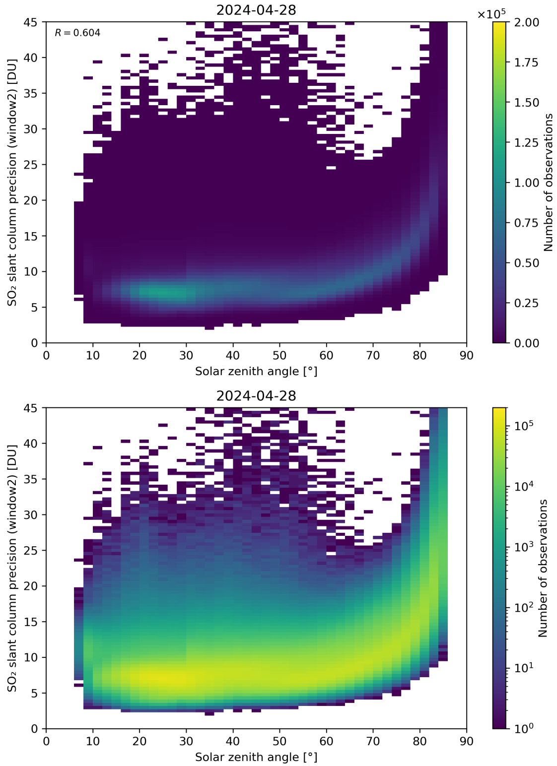
Figure 171: Scatter density plot of “Solar zenith angle” against “SO 2 slant column precision (window2)” for 2024-04-27 to 2024-04-29.
