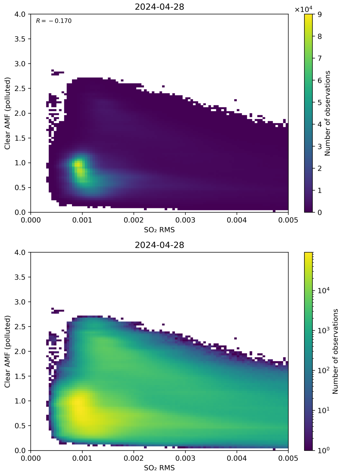
Figure 136: Scatter density plot of “SO 2 RMS” against “Clear AMF (polluted)” for 2024-04-27 to 2024-04-29.
