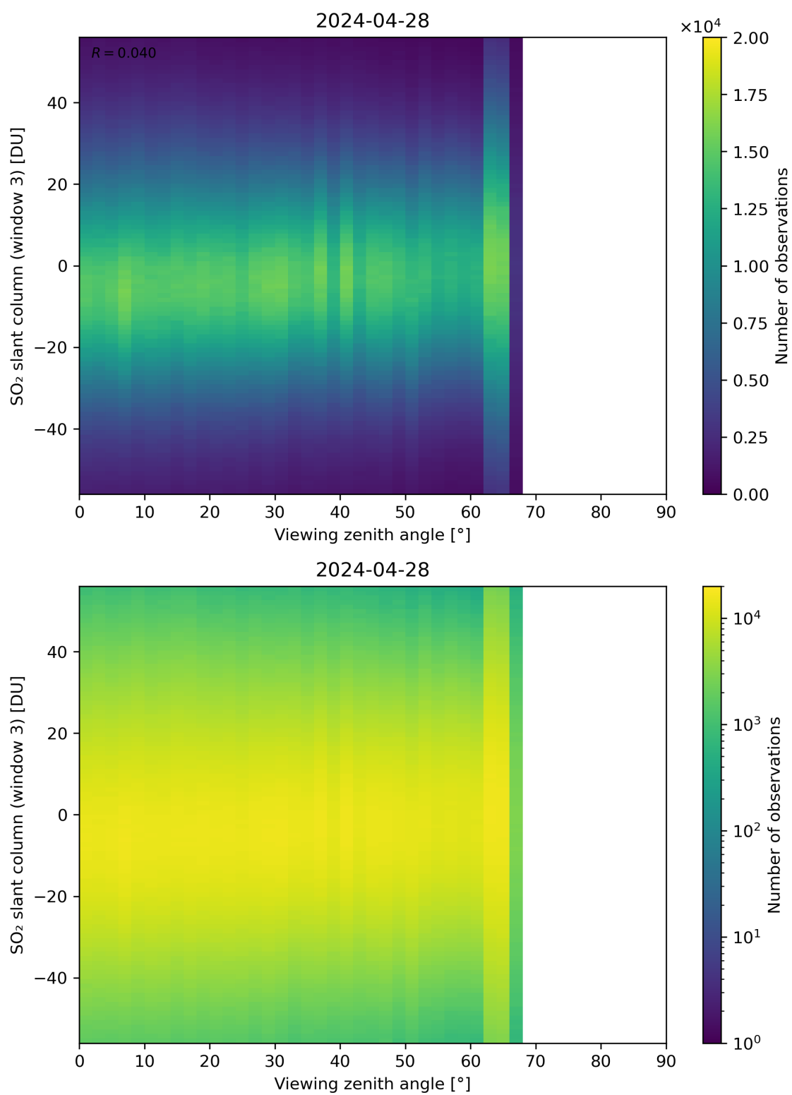
Figure 323: Scatter density plot of “Viewing zenith angle” against “SO 2 slant column (window 3)” for 2024-04-27 to 2024-04-29.
