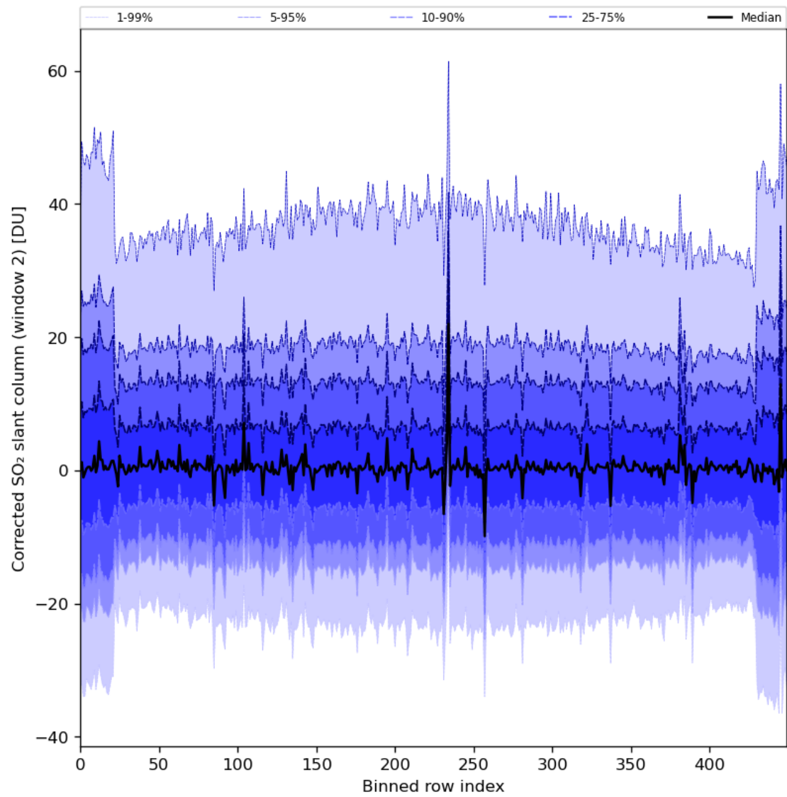
Figure 85: Along track statistics of “Corrected SO 2 slant column (window 2)” for 2024-04-27 to 2024-04-29
