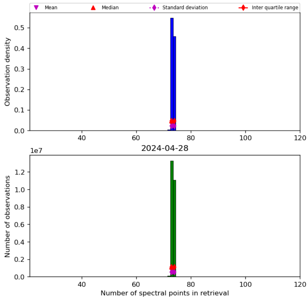
Figure 74: Histogram of “Number of spectral points in retrieval” for 2024-04-27 to 2024-04-29
