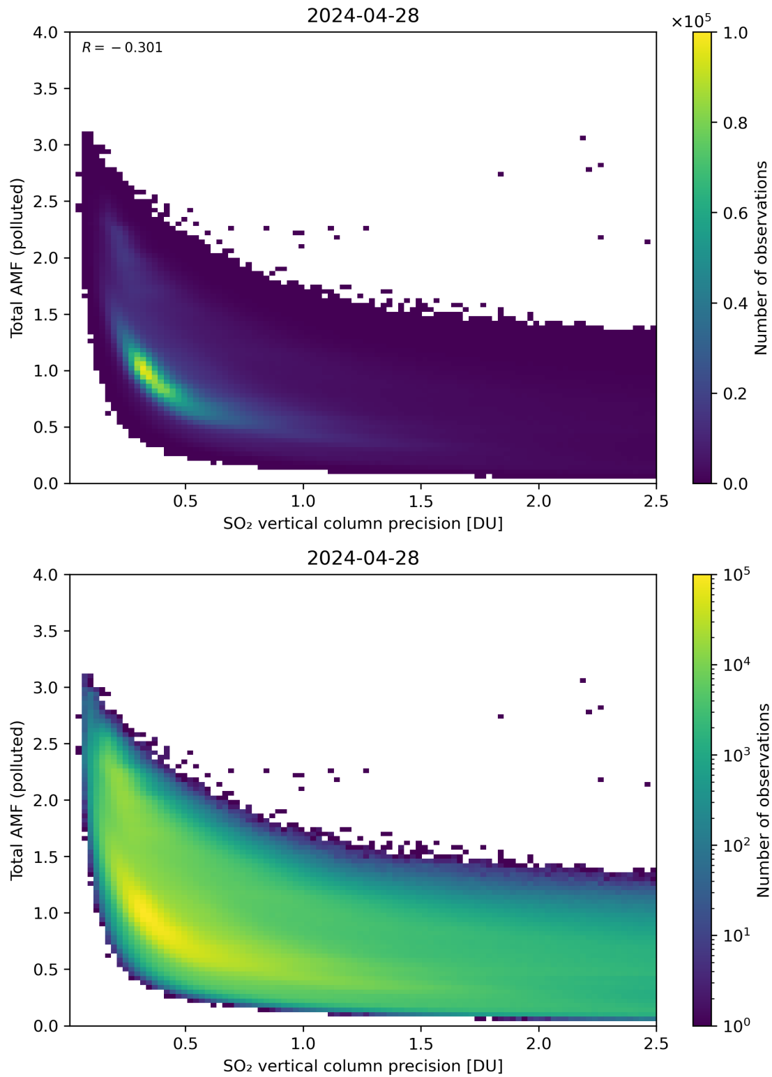
Figure 294: Scatter density plot of “SO 2 vertical column precision” against “Total AMF (polluted)” for 2024-04-27 to 2024-04-29.
