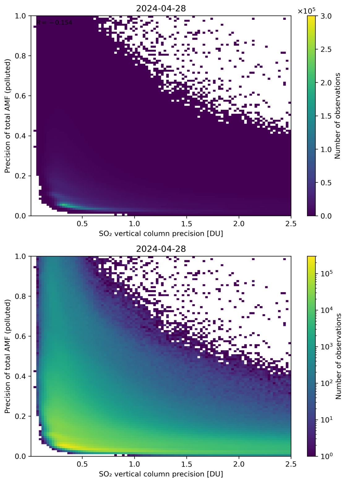
Figure 295: Scatter density plot of “SO 2 vertical column precision” against “Precision of total AMF (polluted)” for 2024-04-27 to 2024-04-29.
