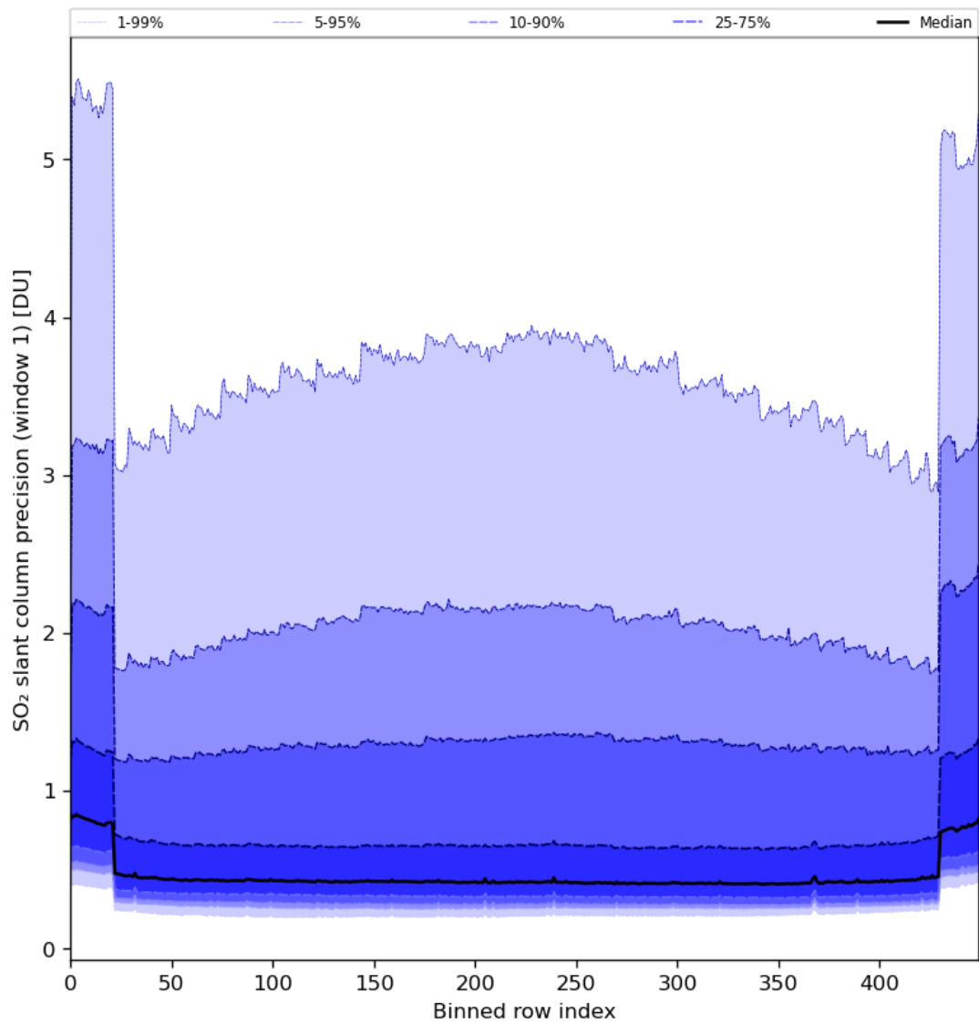
Figure 80: Along track statistics of “SO 2 slant column precision (window 1)” for 2024-04-27 to 2024-04-29
