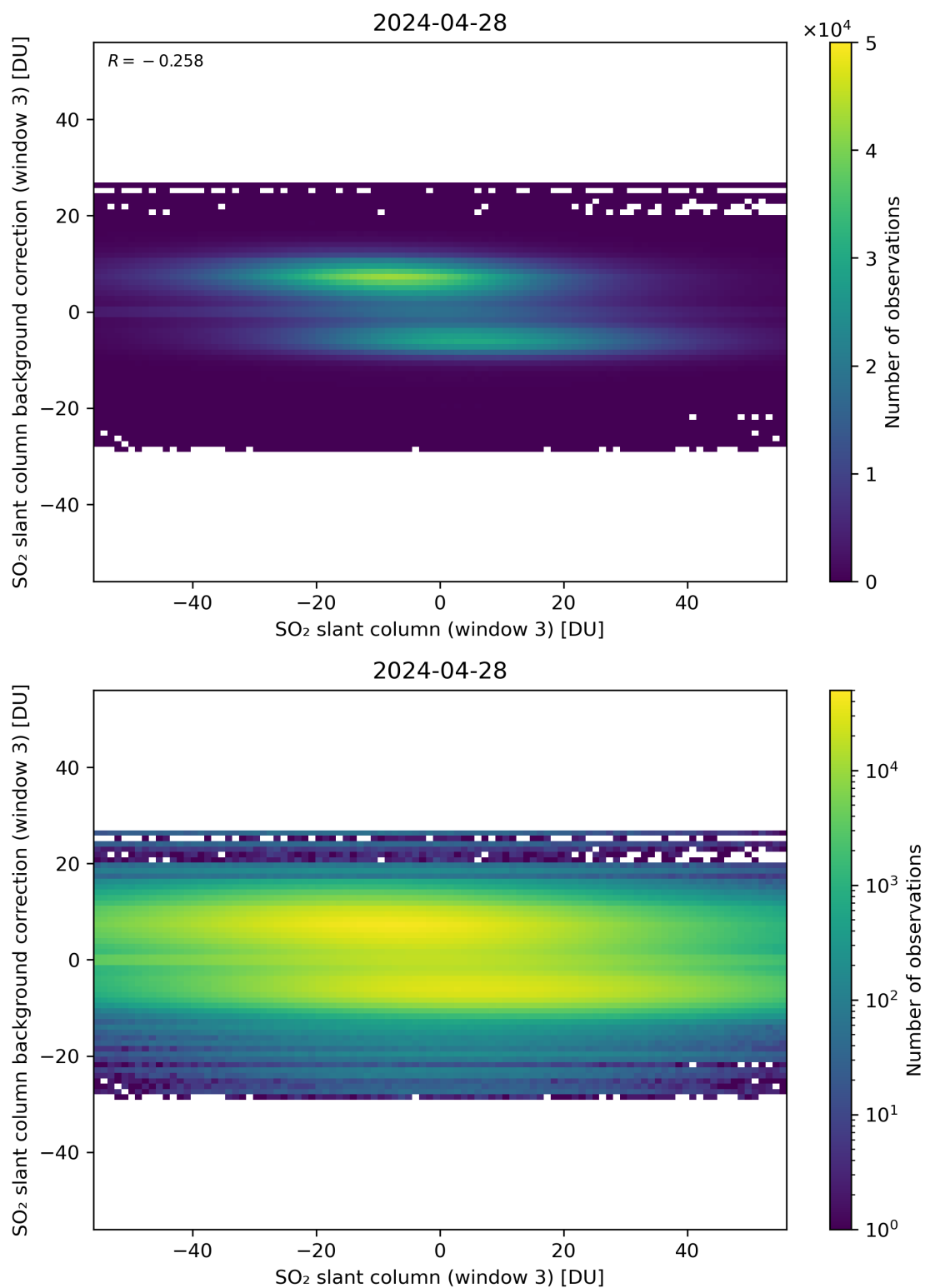
Figure 253: Scatter density plot of “SO 2 slant column (window 3)” against “SO 2 slant column background correction (window 3)” for 2024-04-27 to 2024-04-29.
