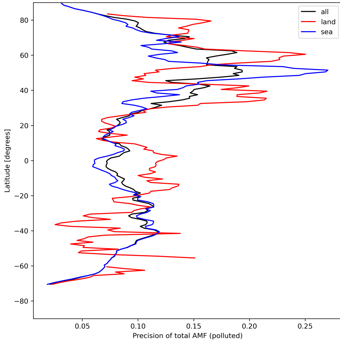
Figure 49: Zonal average of “Precision of total AMF (polluted)” for 2024-04-27 to 2024-04-29.
