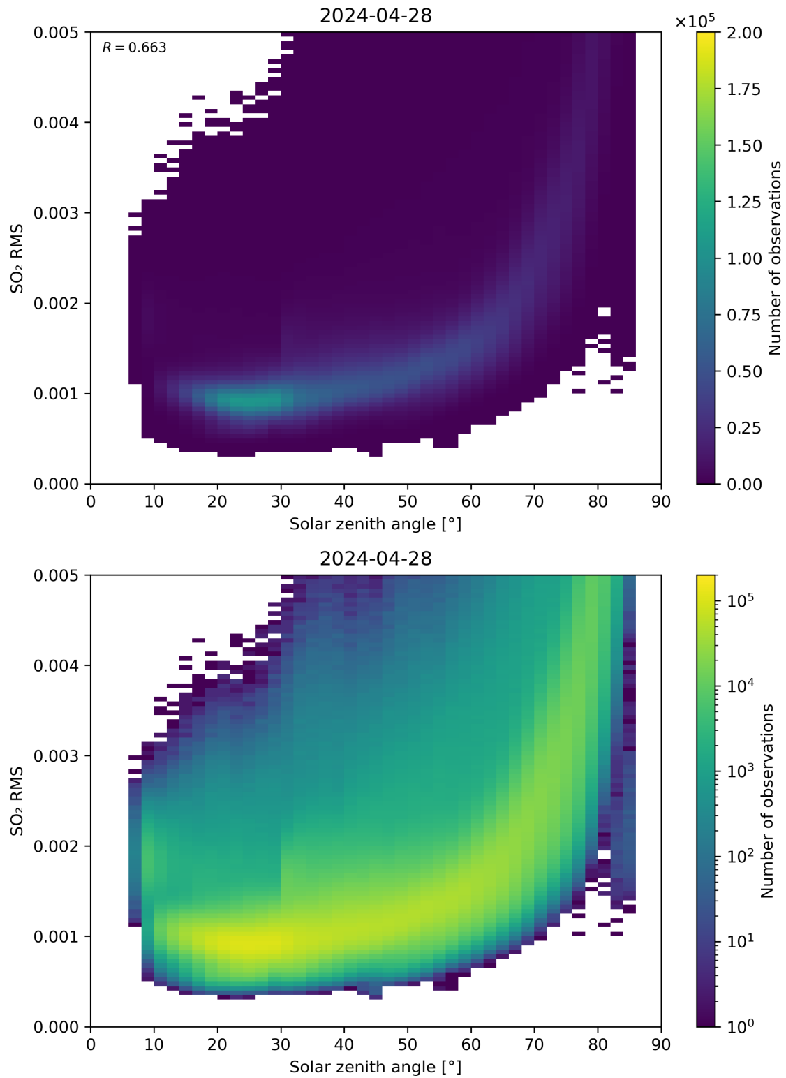
Figure 163: Scatter density plot of “Solar zenith angle” against “SO 2 RMS” for 2024-04-27 to 2024-04-29.
