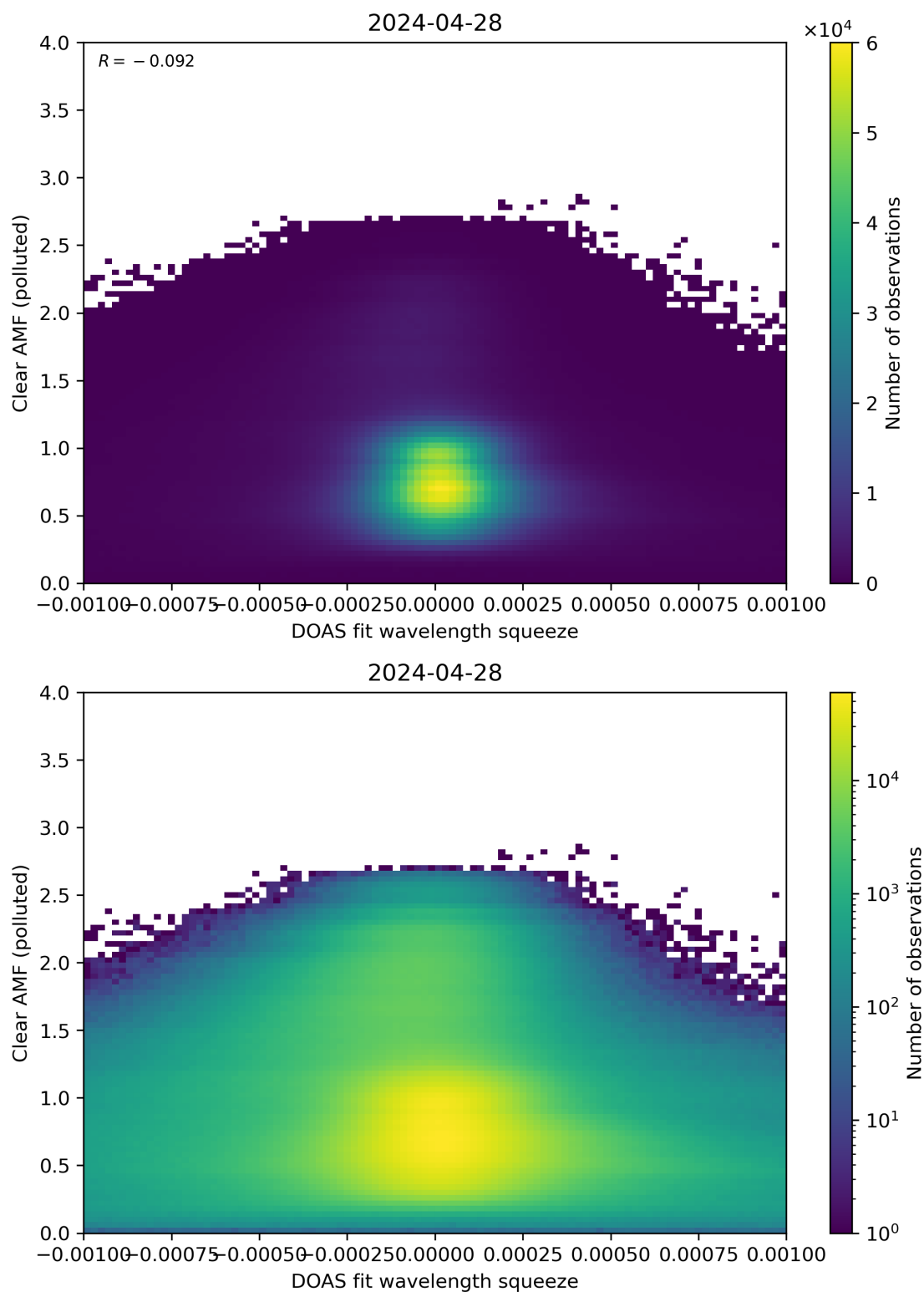
Figure 133: Scatter density plot of “DOAS fit wavelength squeeze” against “Clear AMF (polluted)” for 2024-04-27 to 2024-04-29.
