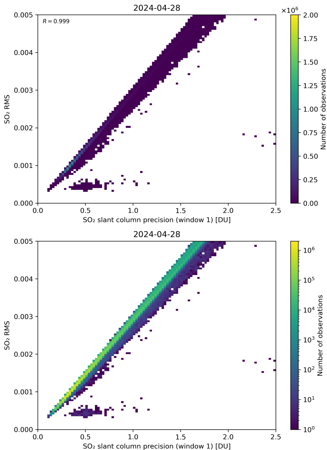
Figure 223: Scatter density plot of “SO 2 slant column precision (window 1)” against “SO 2 RMS” for 2024-04-27 to 2024-04-29.
