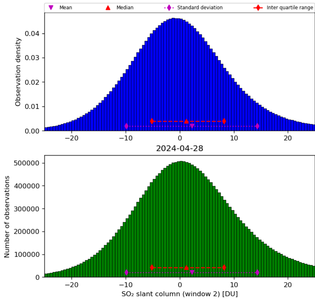
Figure 60: Histogram of “SO 2 slant column (window 2)” for 2024-04-27 to 2024-04-29
