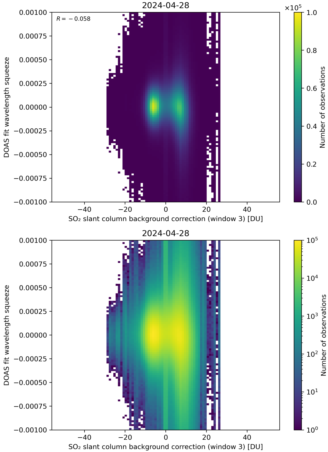
Figure 122: Scatter density plot of “SO 2 slant column background correction (window 3)” against “DOAS fit wavelength squeeze” for 2024-04-27 to 2024-04-29.
