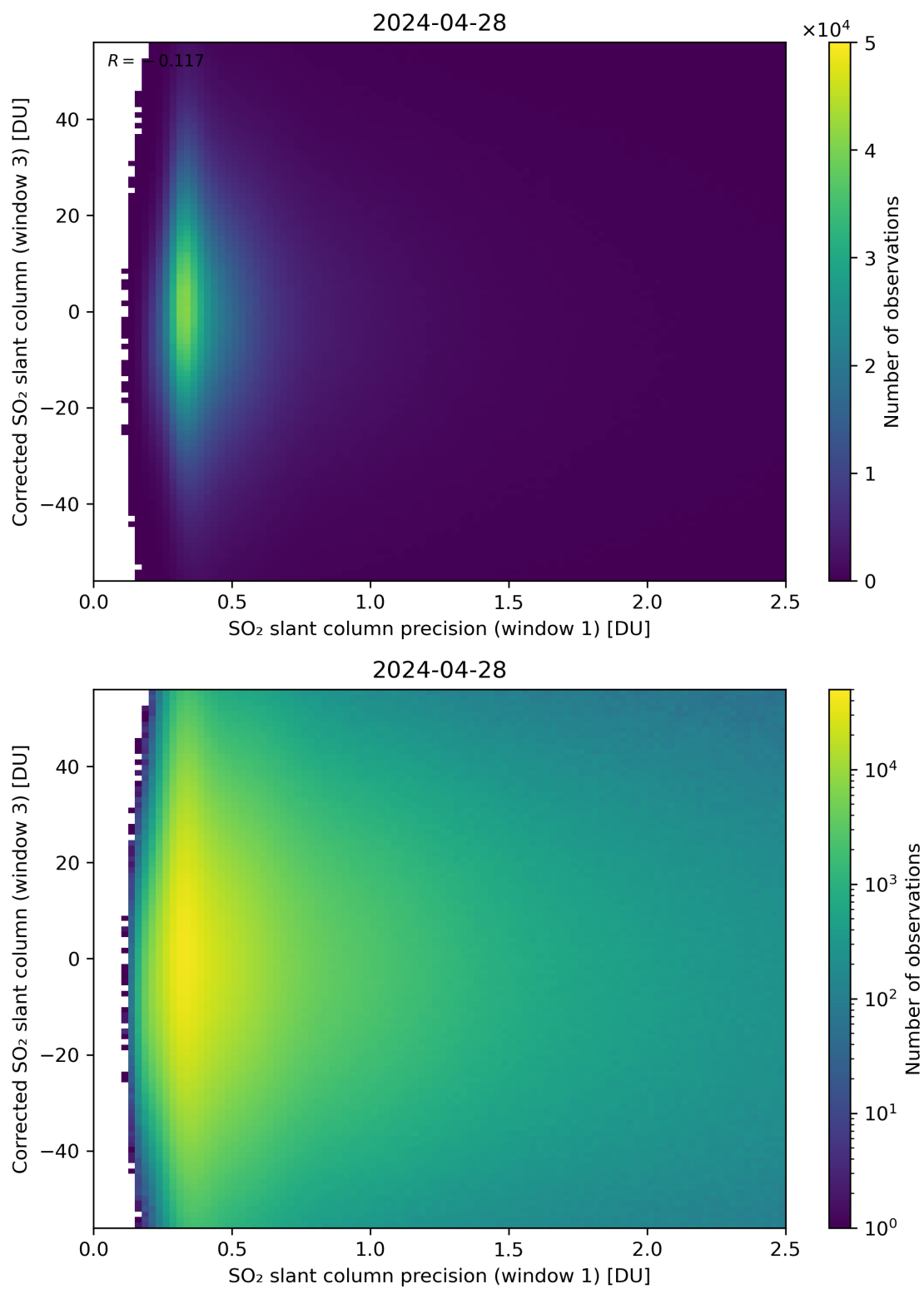
Figure 226: Scatter density plot of “SO 2 slant column precision (window 1)” against “Corrected SO 2 slant column (window 3)” for 2024-04-27 to 2024-04-29.
