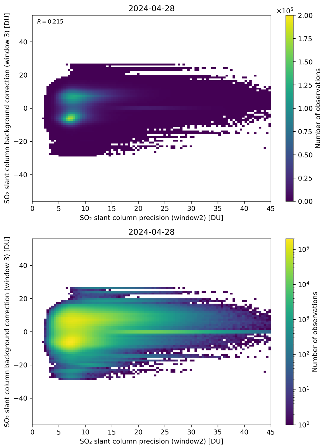
Figure 242: Scatter density plot of “SO 2 slant column precision (window2)” against “SO 2 slant column background correction (window 3)” for 2024-04-27 to 2024-04-29.
