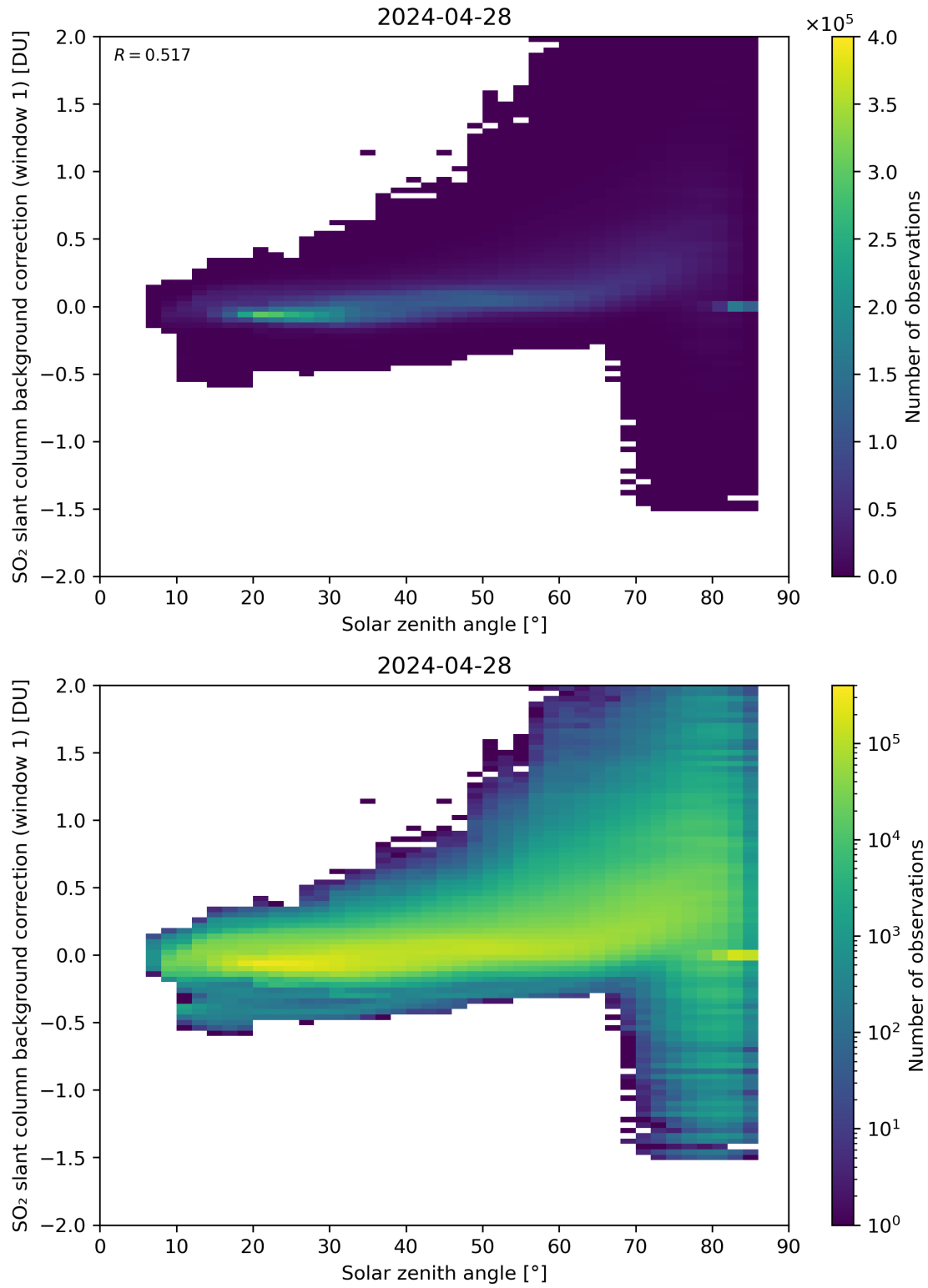
Figure 158: Scatter density plot of “Solar zenith angle” against “SO 2 slant column background correction (window 1)” for 2024-04-27 to 2024-04-29.
