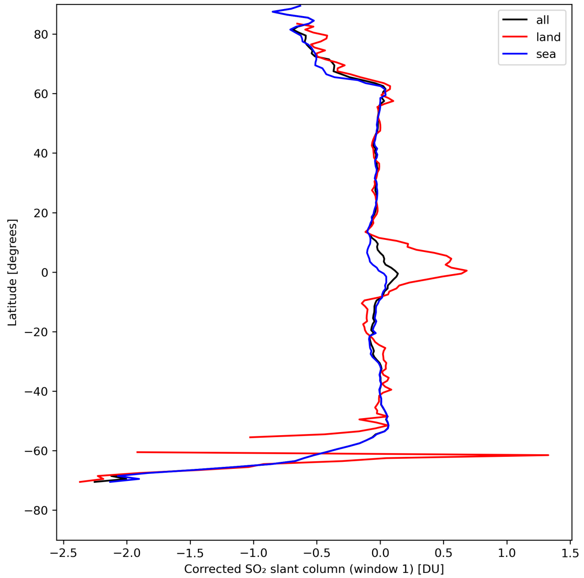
Figure 35: Zonal average of “Corrected SO 2 slant column (window 1)” for 2024-04-27 to 2024-04-29.
