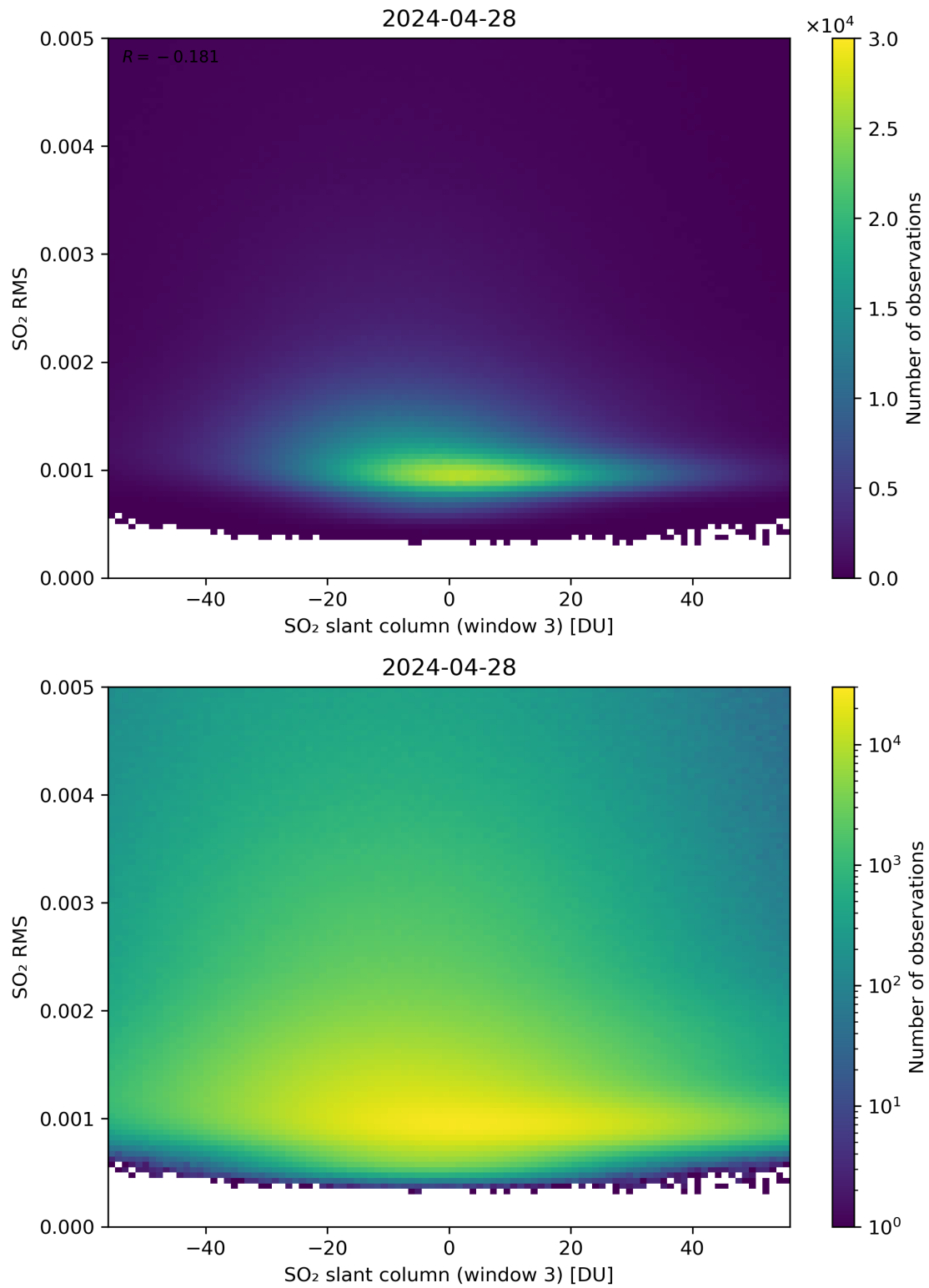
Figure 256: Scatter density plot of “SO 2 slant column (window 3)” against “SO 2 RMS” for 2024-04-27 to 2024-04-29.
