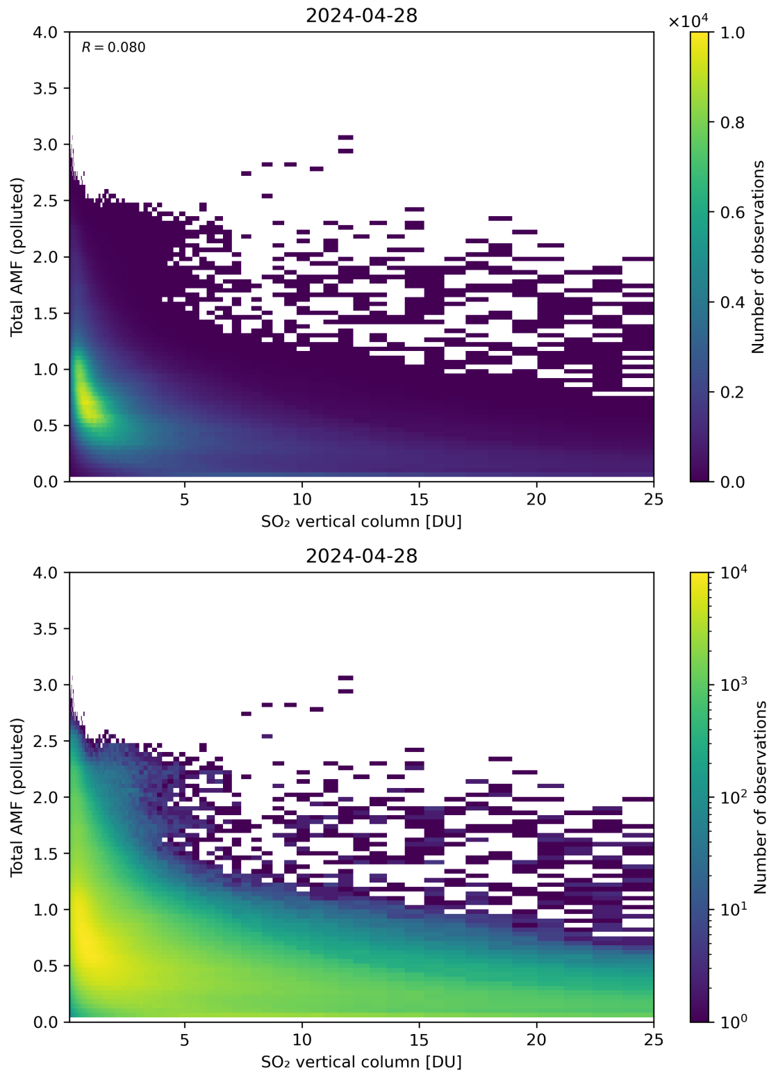
Figure 305: Scatter density plot of “SO 2 vertical column” against “Total AMF (polluted)” for 2024-04-27 to 2024-04-29.
