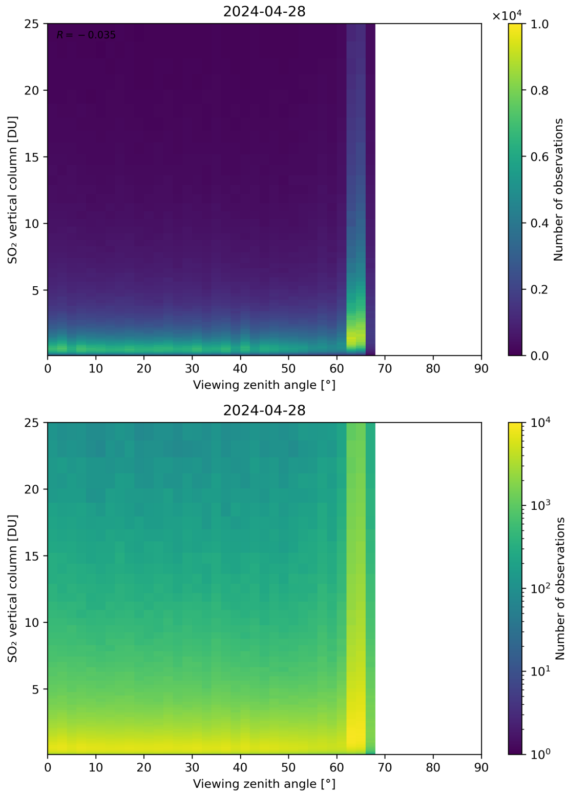
Figure 327: Scatter density plot of “Viewing zenith angle” against “SO 2 vertical column” for 2024-04-27 to 2024-04-29.
