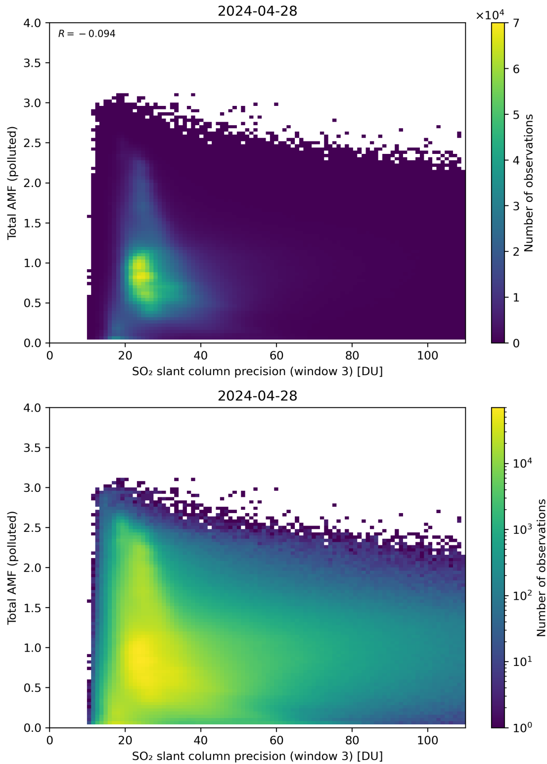
Figure 263: Scatter density plot of “SO 2 slant column precision (window 3)” against “Total AMF (polluted)” for 2024-04-27 to 2024-04-29.
