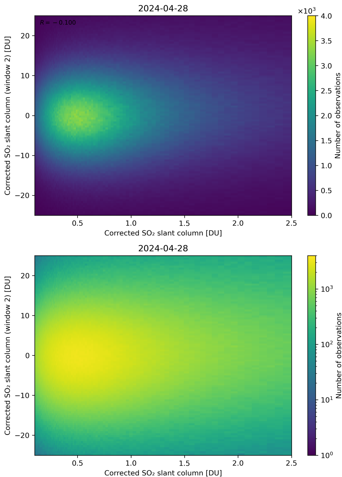
Figure 185: Scatter density plot of “Corrected SO 2 slant column” against “Corrected SO 2 slant column (window 2)” for 2024-04-27 to 2024-04-29.
