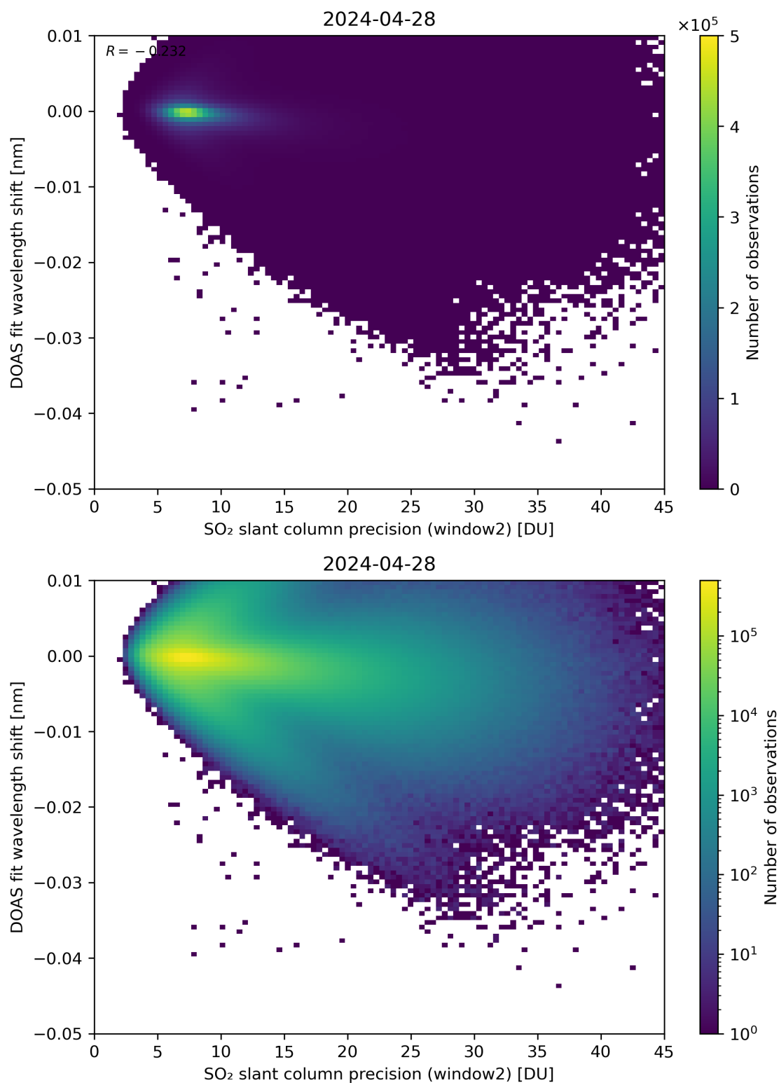
Figure 243: Scatter density plot of “SO 2 slant column precision (window2)” against “DOAS fit wavelength shift” for 2024-04-27 to 2024-04-29.
