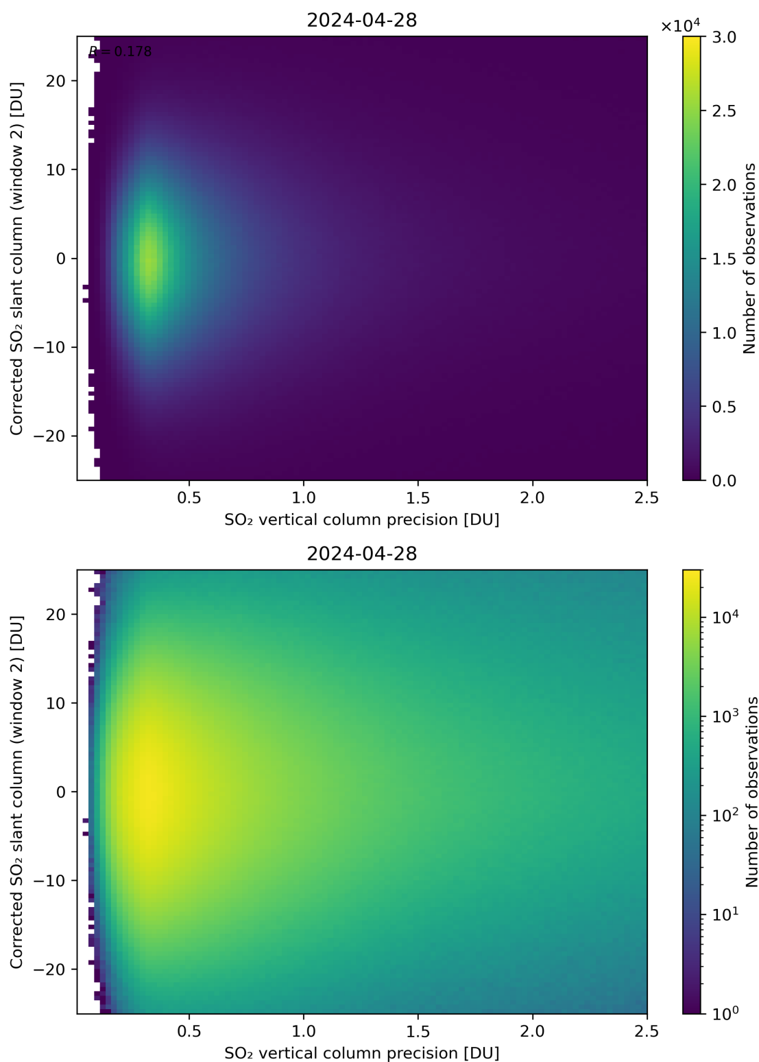
Figure 287: Scatter density plot of “SO 2 vertical column precision” against “Corrected SO 2 slant column (window 2)” for 2024-04-27 to 2024-04-29.
