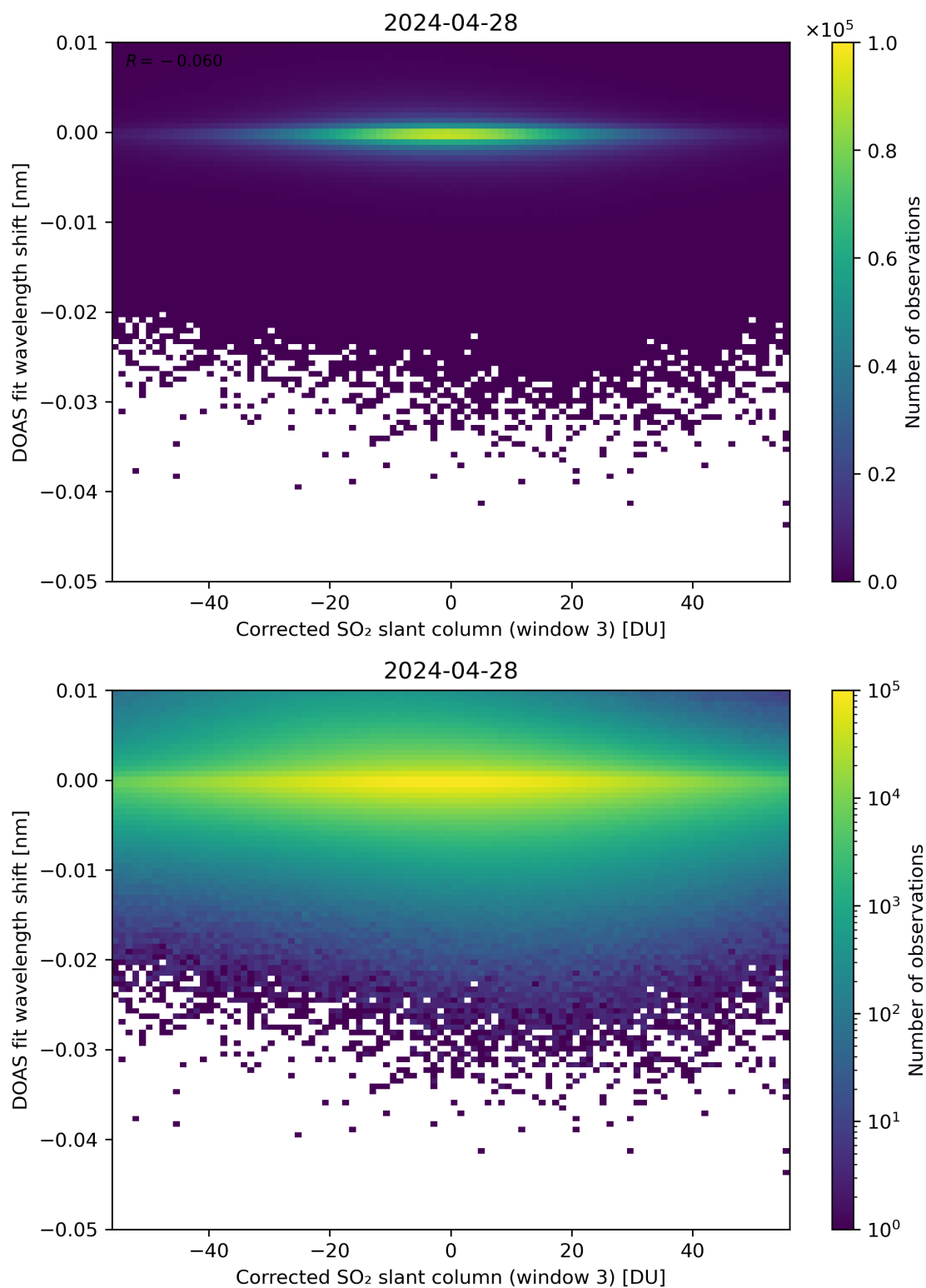
Figure 206: Scatter density plot of “Corrected SO 2 slant column (window 3)” against “DOAS fit wavelength shift” for 2024-04-27 to 2024-04-29.
