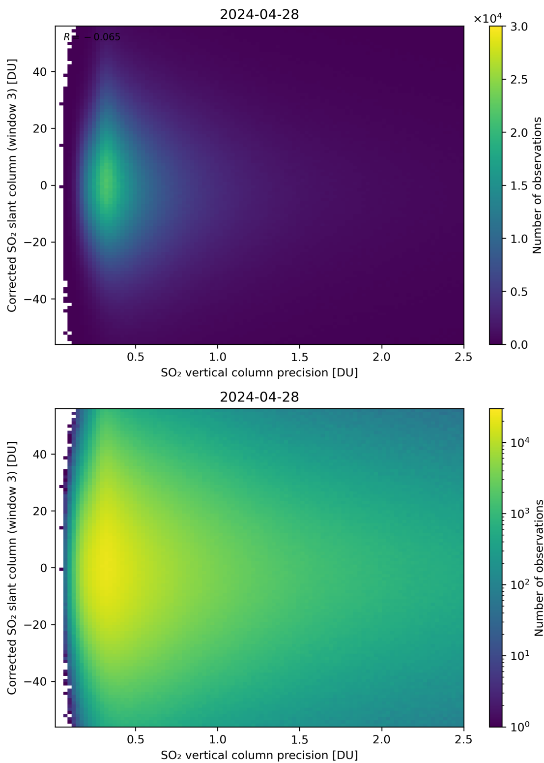
Figure 288: Scatter density plot of “SO 2 vertical column precision” against “Corrected SO 2 slant column (window 3)” for 2024-04-27 to 2024-04-29.
