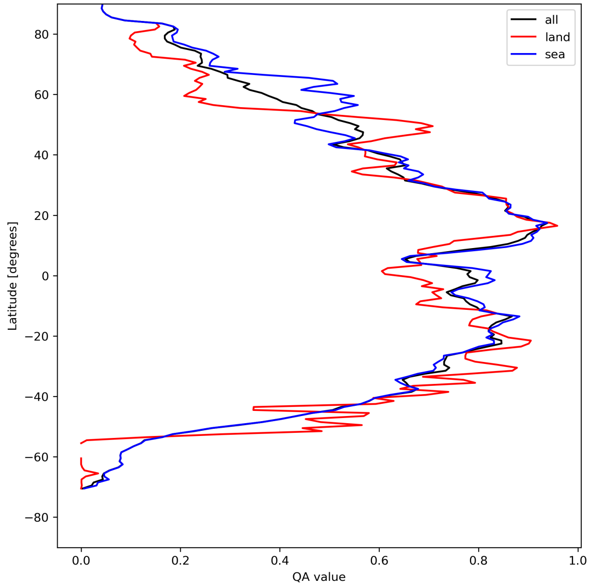
Figure 29: Zonal average of “QA value” for 2024-04-27 to 2024-04-29.
