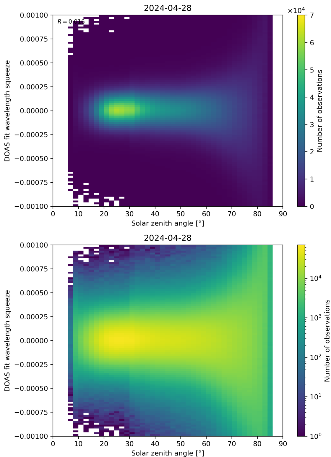
Figure 162: Scatter density plot of “Solar zenith angle” against “DOAS fit wavelength squeeze” for 2024-04-27 to 2024-04-29.
