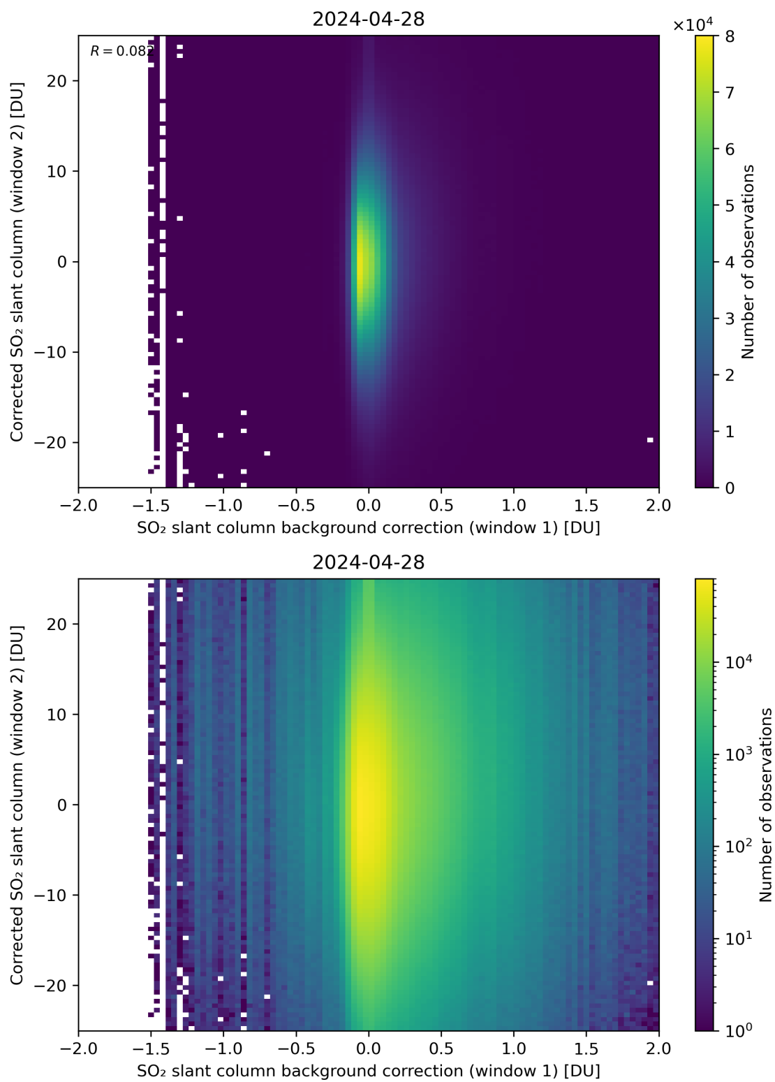
Figure 104: Scatter density plot of “SO 2 slant column background correction (window 1)” against “Corrected SO 2 slant column (window 2)” for 2024-04-27 to 2024-04-29.
