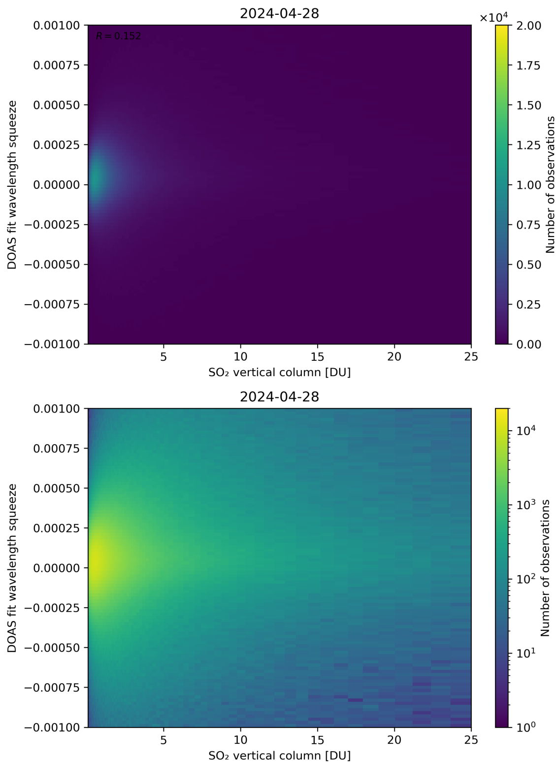
Figure 277: Scatter density plot of “SO 2 vertical column” against “DOAS fit wavelength squeeze” for 2024-04-27 to 2024-04-29.
