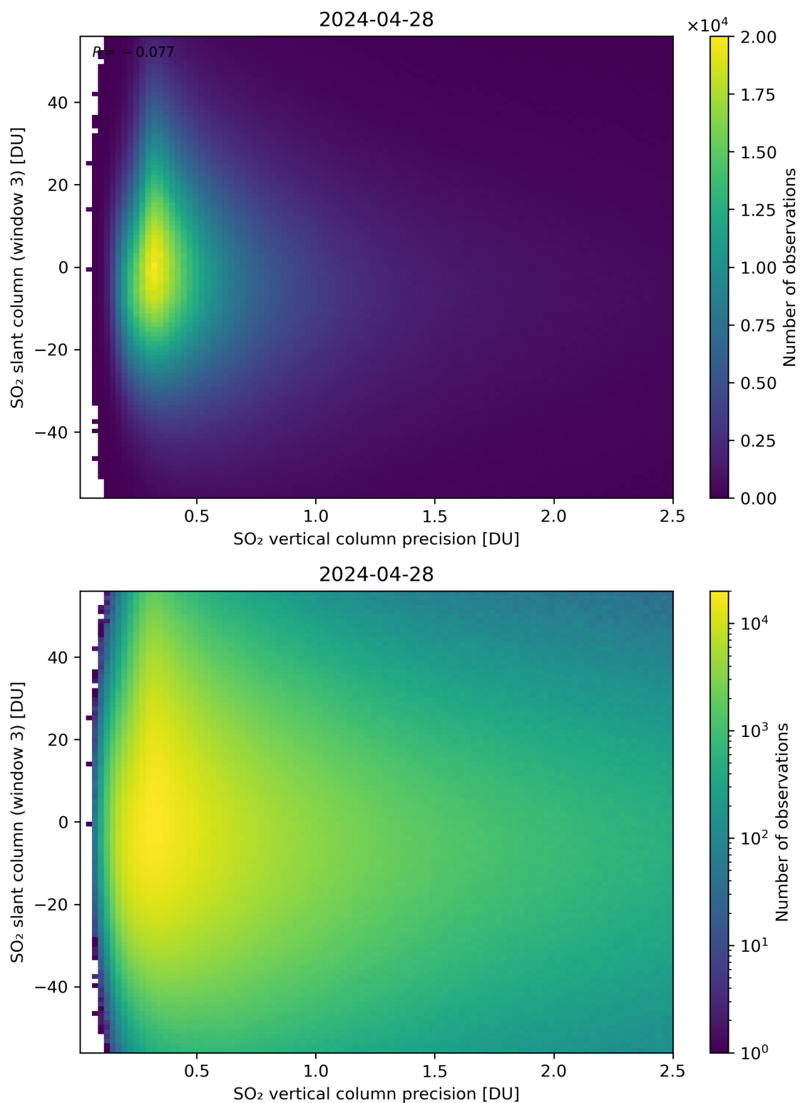
Figure 292: Scatter density plot of “SO 2 vertical column precision” against “SO 2 slant column (window 3)” for 2024-04-27 to 2024-04-29.
