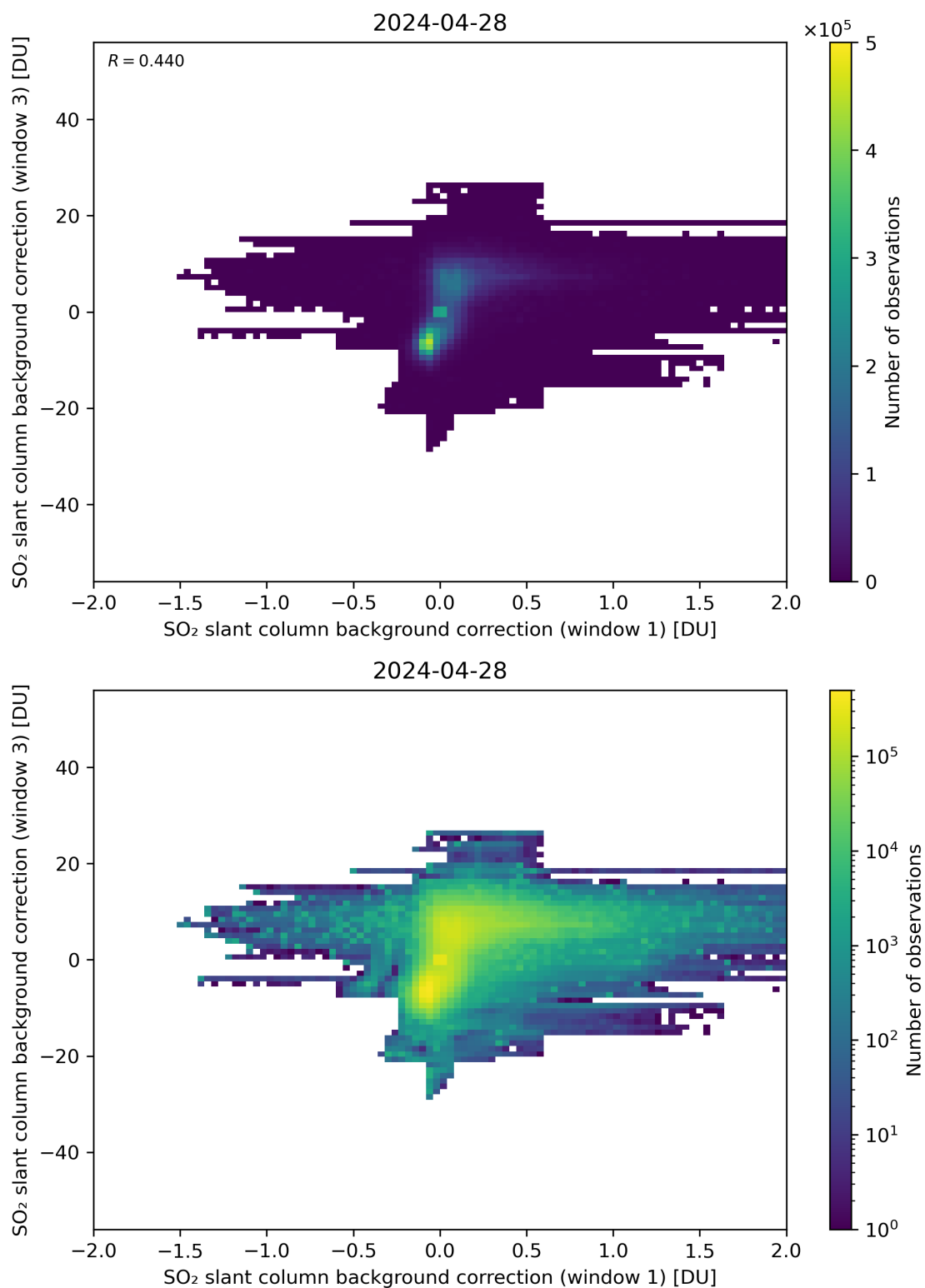
Figure 99: Scatter density plot of “SO 2 slant column background correction (window 1)” against “SO 2 slant column background correction (window 3)” for 2024-04-27 to 2024-04-29.
