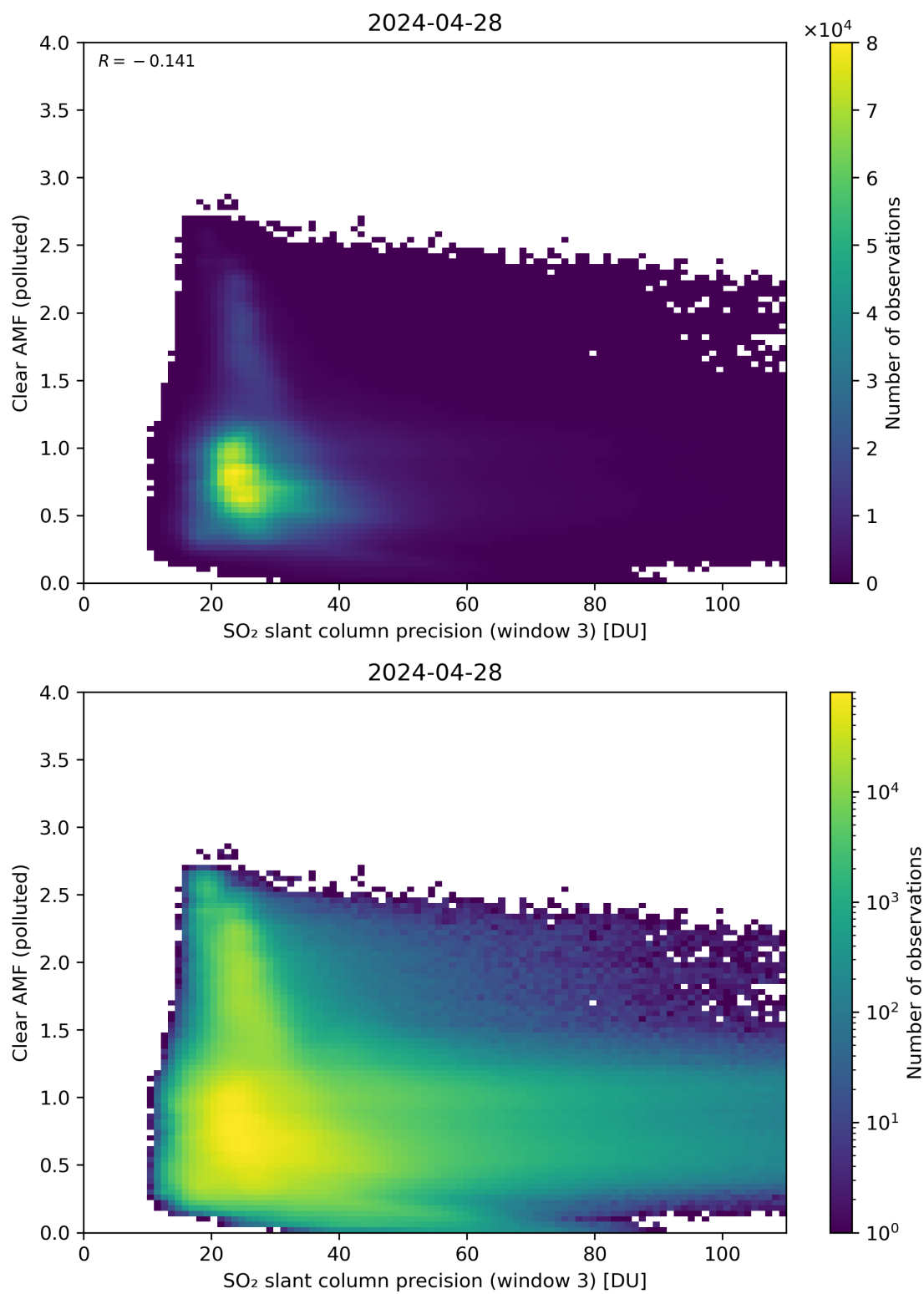
Figure 261: Scatter density plot of “SO 2 slant column precision (window 3)” against “Clear AMF (polluted)” for 2024-04-27 to 2024-04-29.
