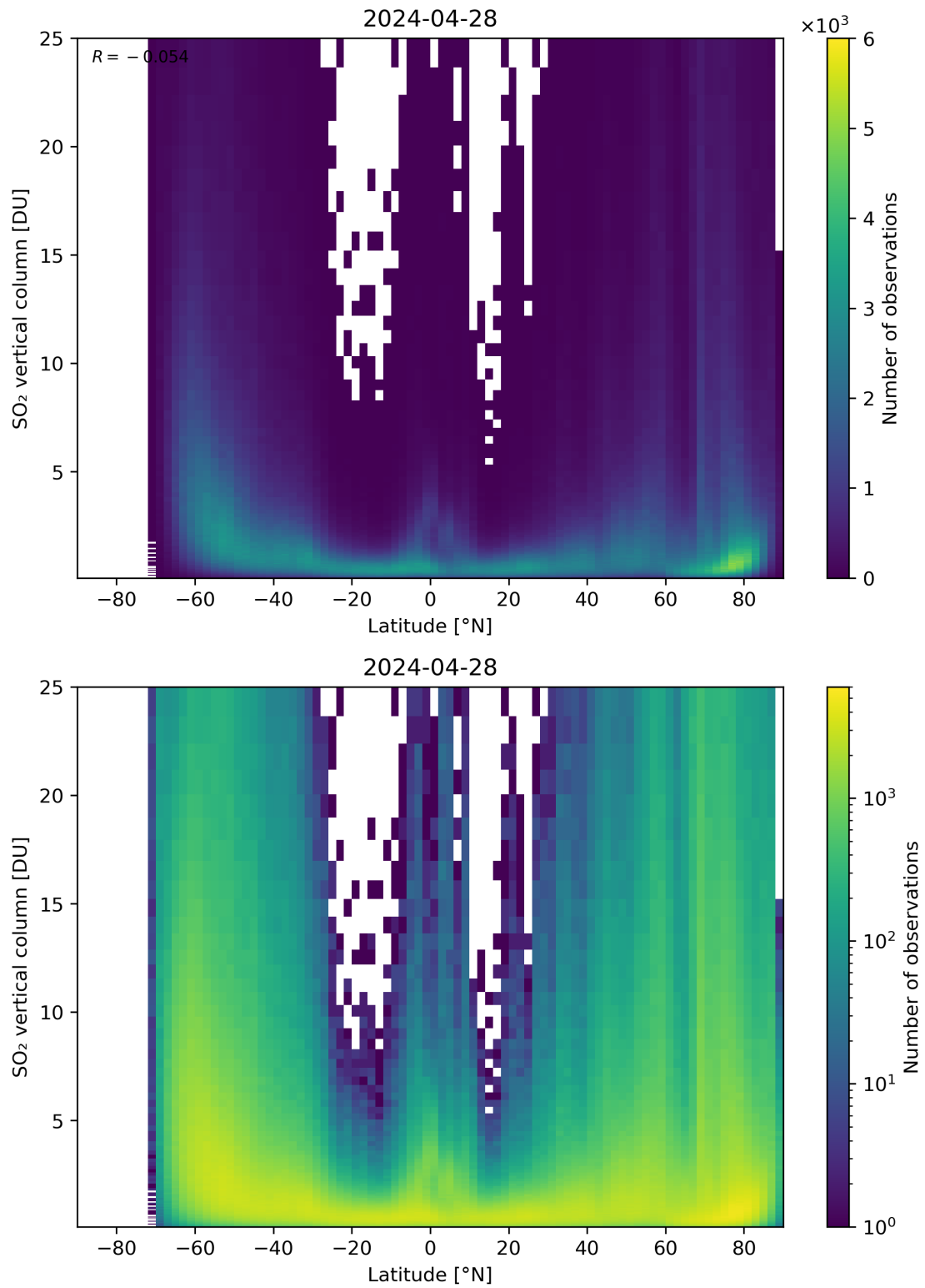
Figure 156: Scatter density plot of “Latitude” against “SO 2 vertical column” for 2024-04-27 to 2024-04-29.
