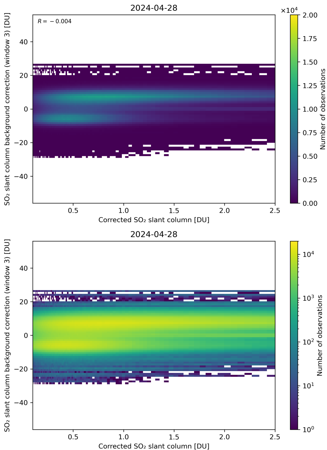
Figure 180: Scatter density plot of “Corrected SO 2 slant column” against “SO 2 slant column background correction (window 3)” for 2024-04-27 to 2024-04-29.
