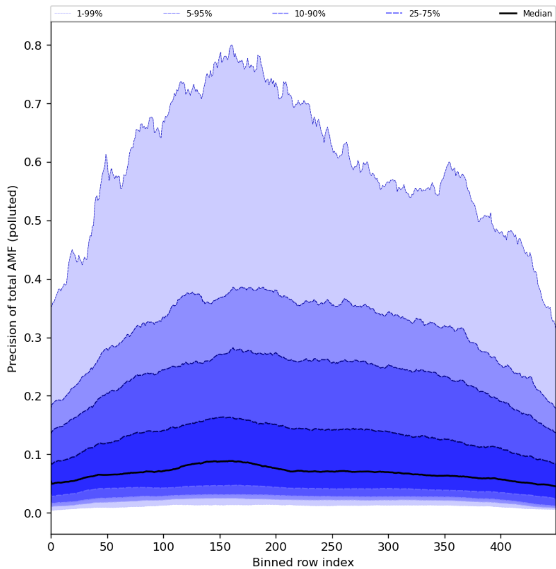
Figure 95: Along track statistics of “Precision of total AMF (polluted)” for 2024-04-27 to 2024-04-29
