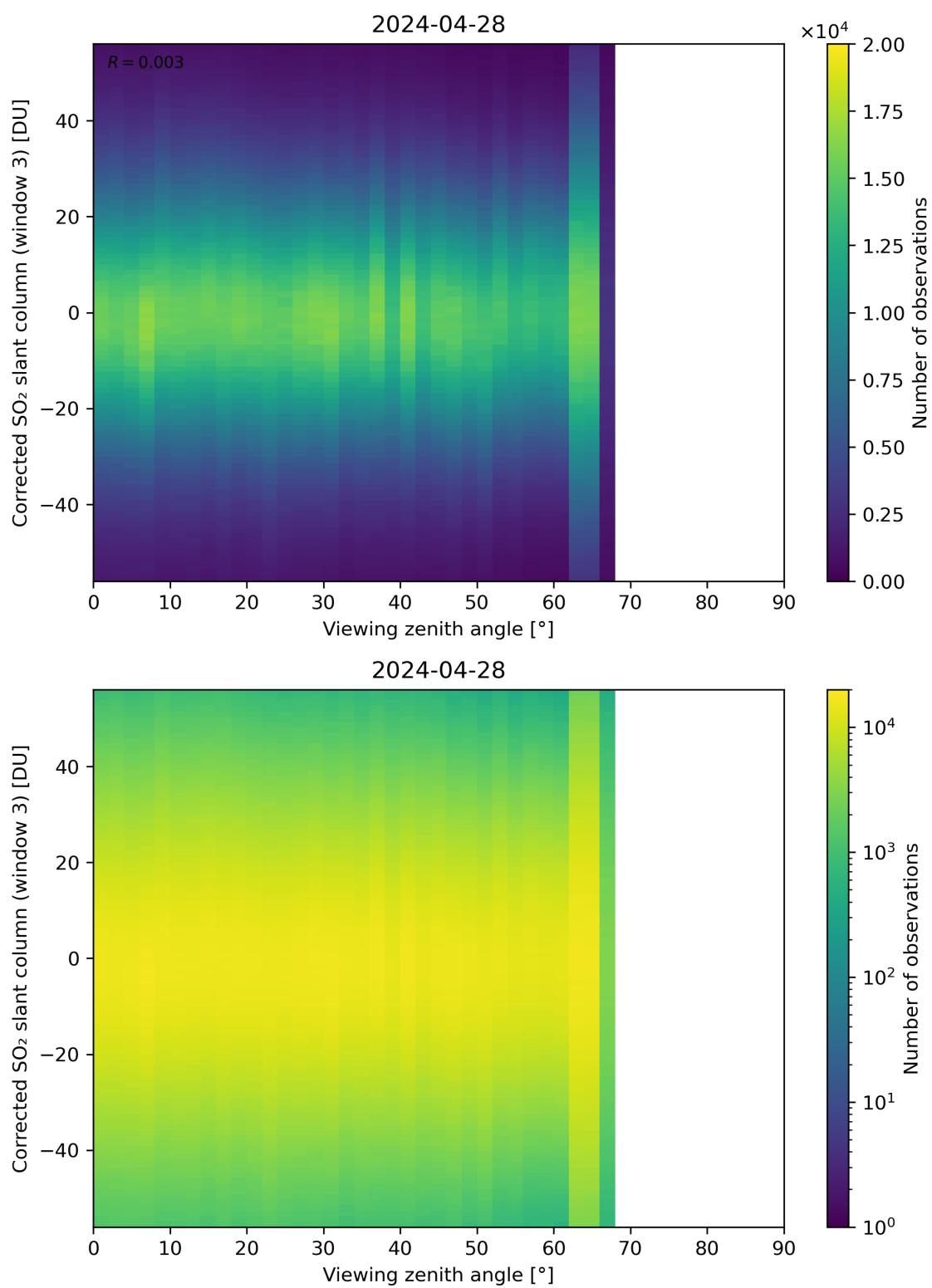
Figure 319: Scatter density plot of “Viewing zenith angle” against “Corrected SO 2 slant column (window 3)” for 2024-04-27 to 2024-04-29.
