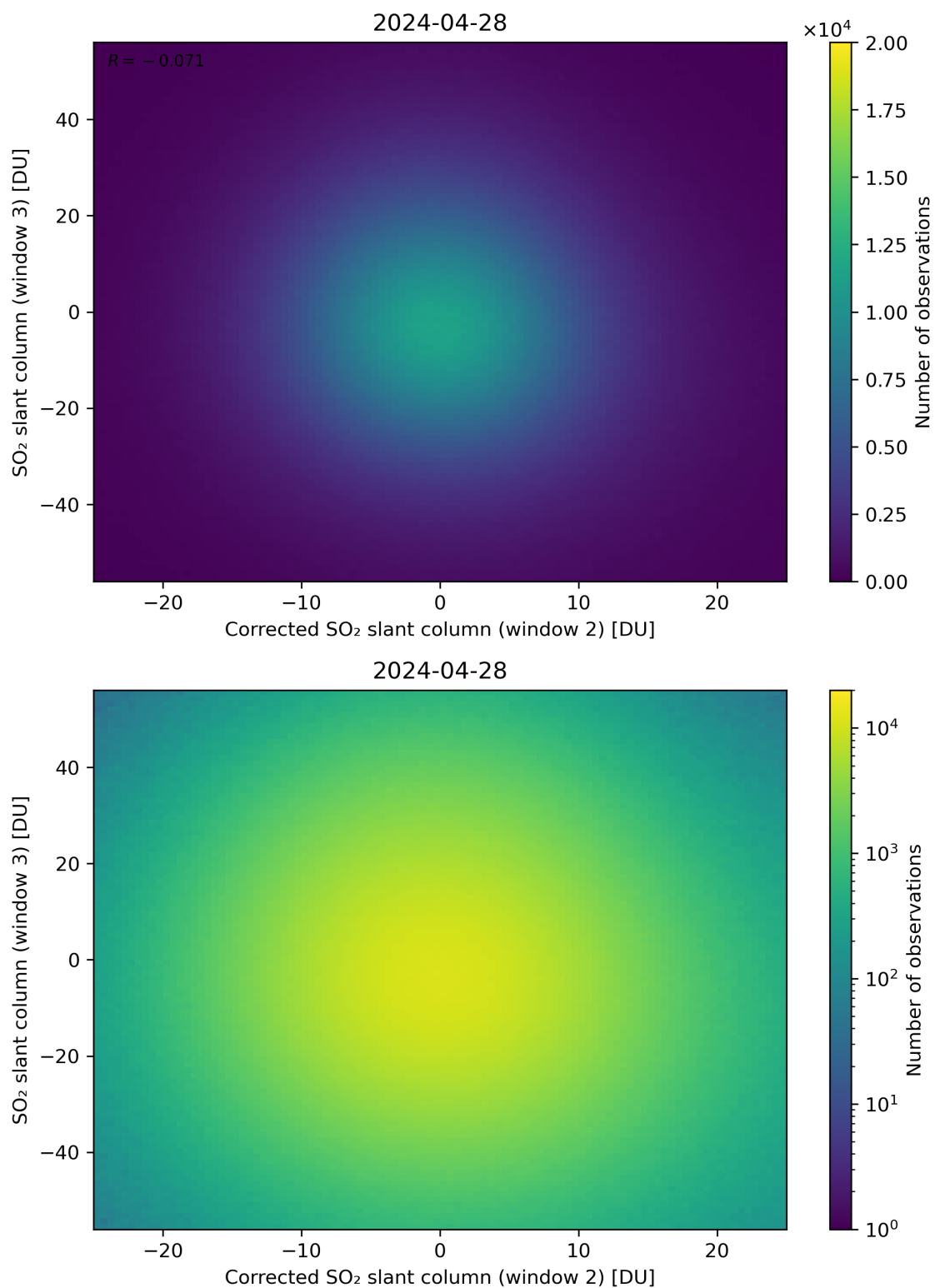
Figure 201: Scatter density plot of “Corrected SO 2 slant column (window 2)” against “SO 2 slant column (window 3)” for 2024-04-27 to 2024-04-29.
