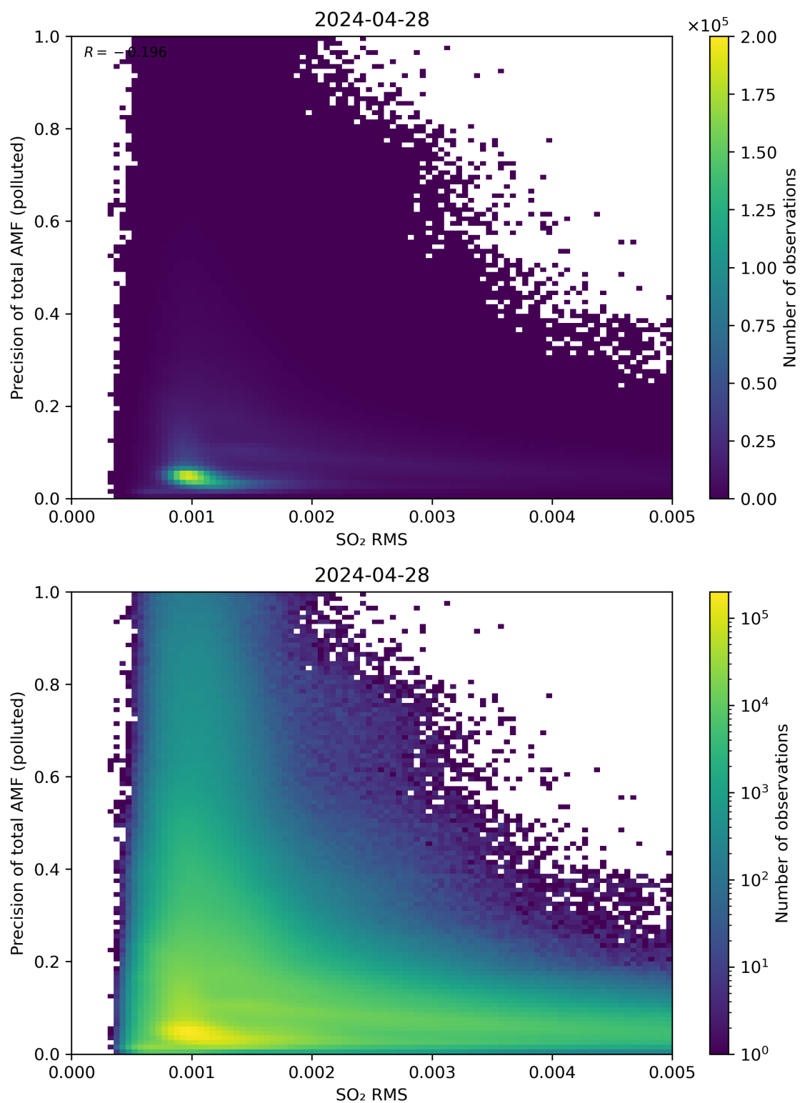
Figure 138: Scatter density plot of “SO 2 RMS” against “Precision of total AMF (polluted)” for 2024-04-27 to 2024-04-29.
