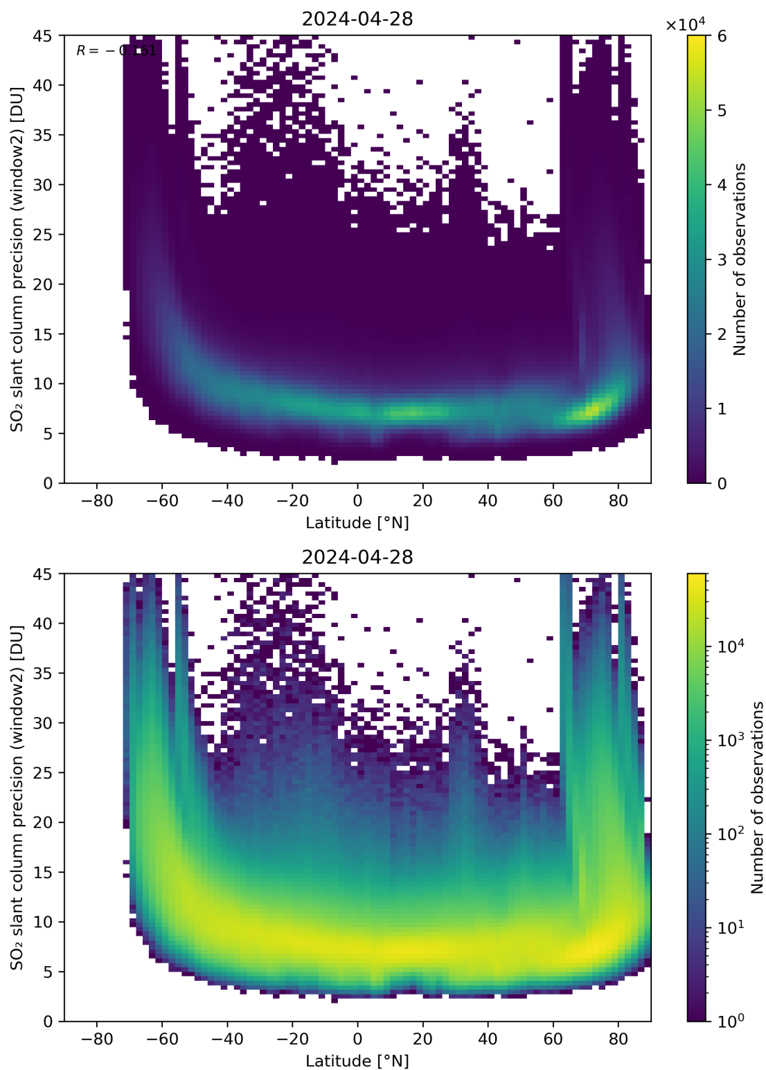
Figure 151: Scatter density plot of “Latitude” against “SO 2 slant column precision (window2)” for 2024-04-27 to 2024-04-29.
