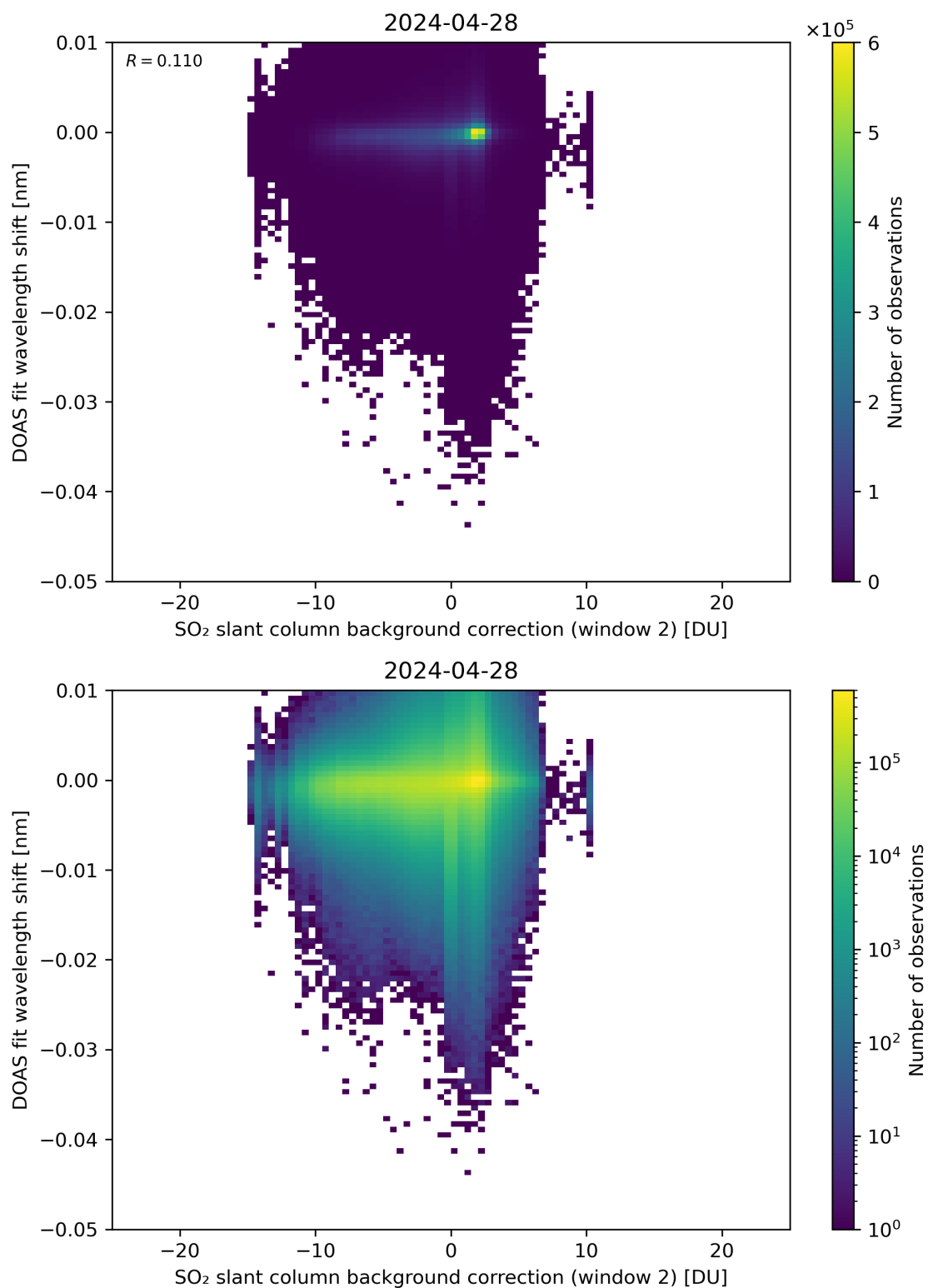
Figure 112: Scatter density plot of “SO 2 slant column background correction (window 2)” against “DOAS fit wavelength shift” for 2024-04-27 to 2024-04-29.
