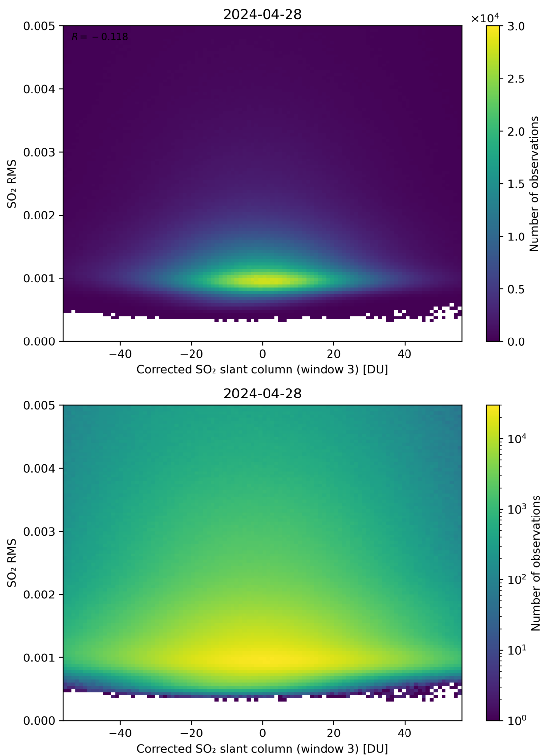
Figure 208: Scatter density plot of “Corrected SO 2 slant column (window 3)” against “SO 2 RMS” for 2024-04-27 to 2024-04-29.
