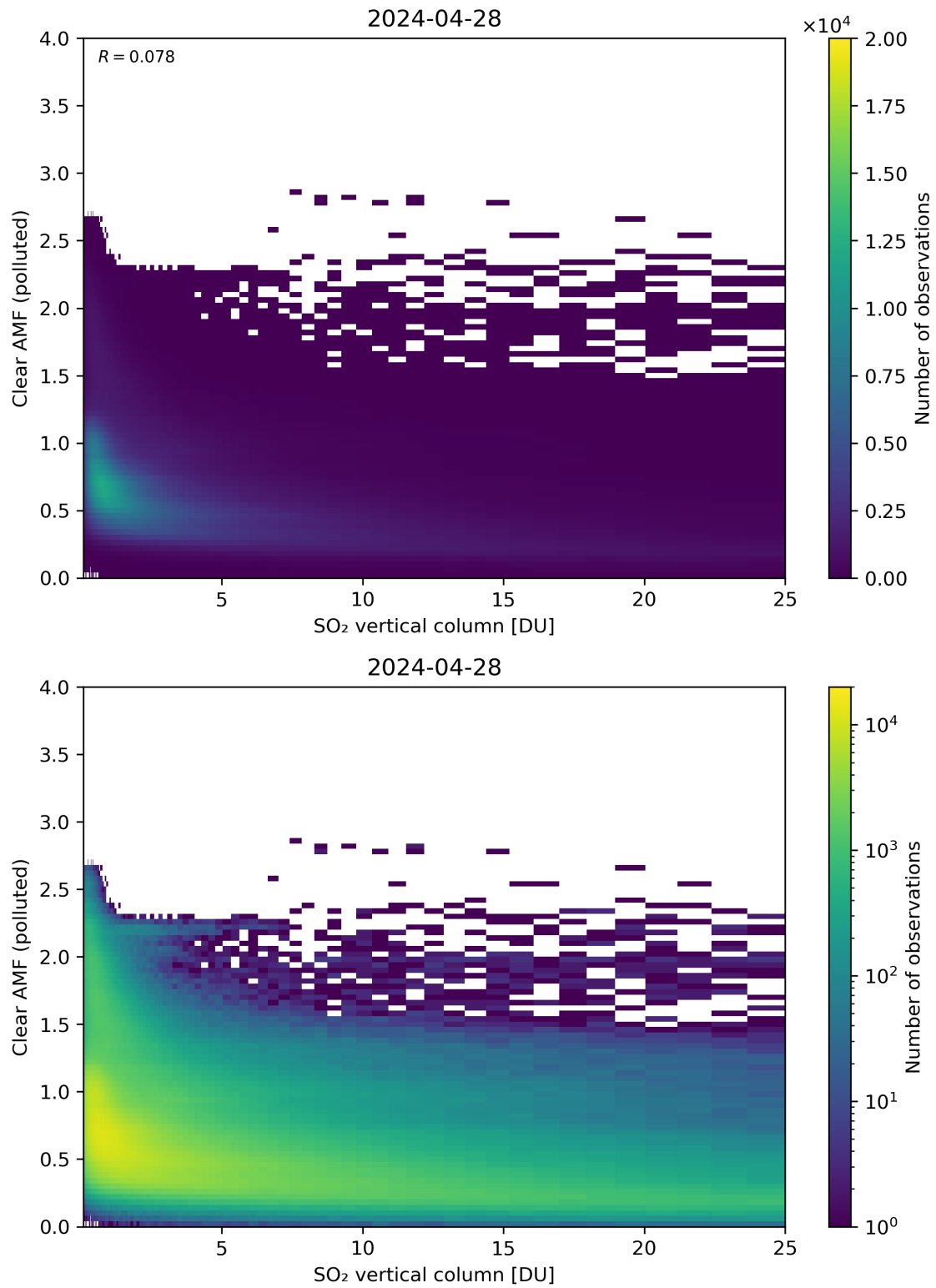
Figure 296: Scatter density plot of “SO 2 vertical column” against “Clear AMF (polluted)” for 2024-04-27 to 2024-04-29.
