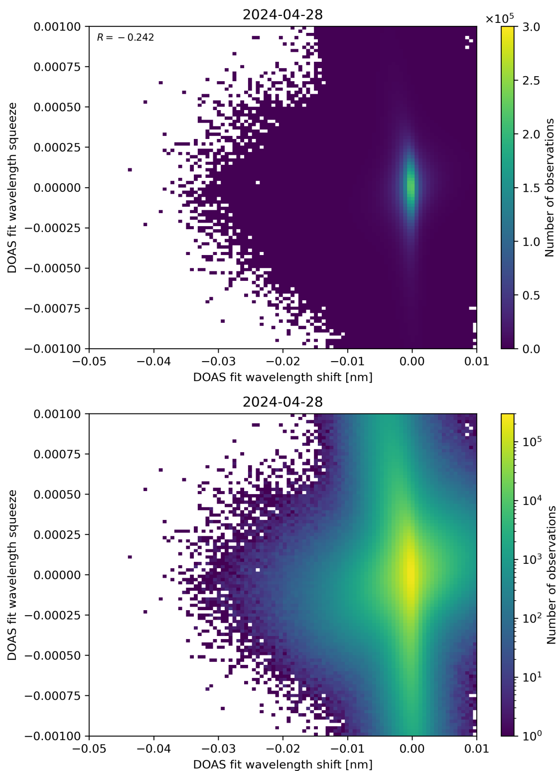
Figure 127: Scatter density plot of “DOAS fit wavelength shift” against “DOAS fit wavelength squeeze” for 2024-04-27 to 2024-04-29.
