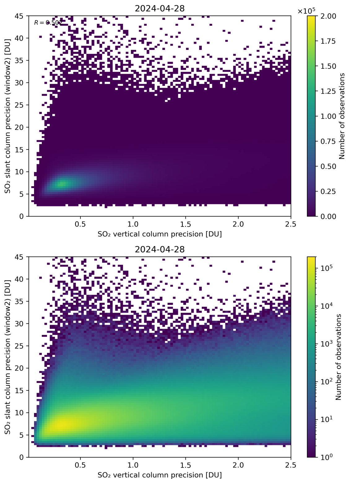
Figure 291: Scatter density plot of “SO 2 vertical column precision” against “SO 2 slant column precision (window2)” for 2024-04-27 to 2024-04-29.
