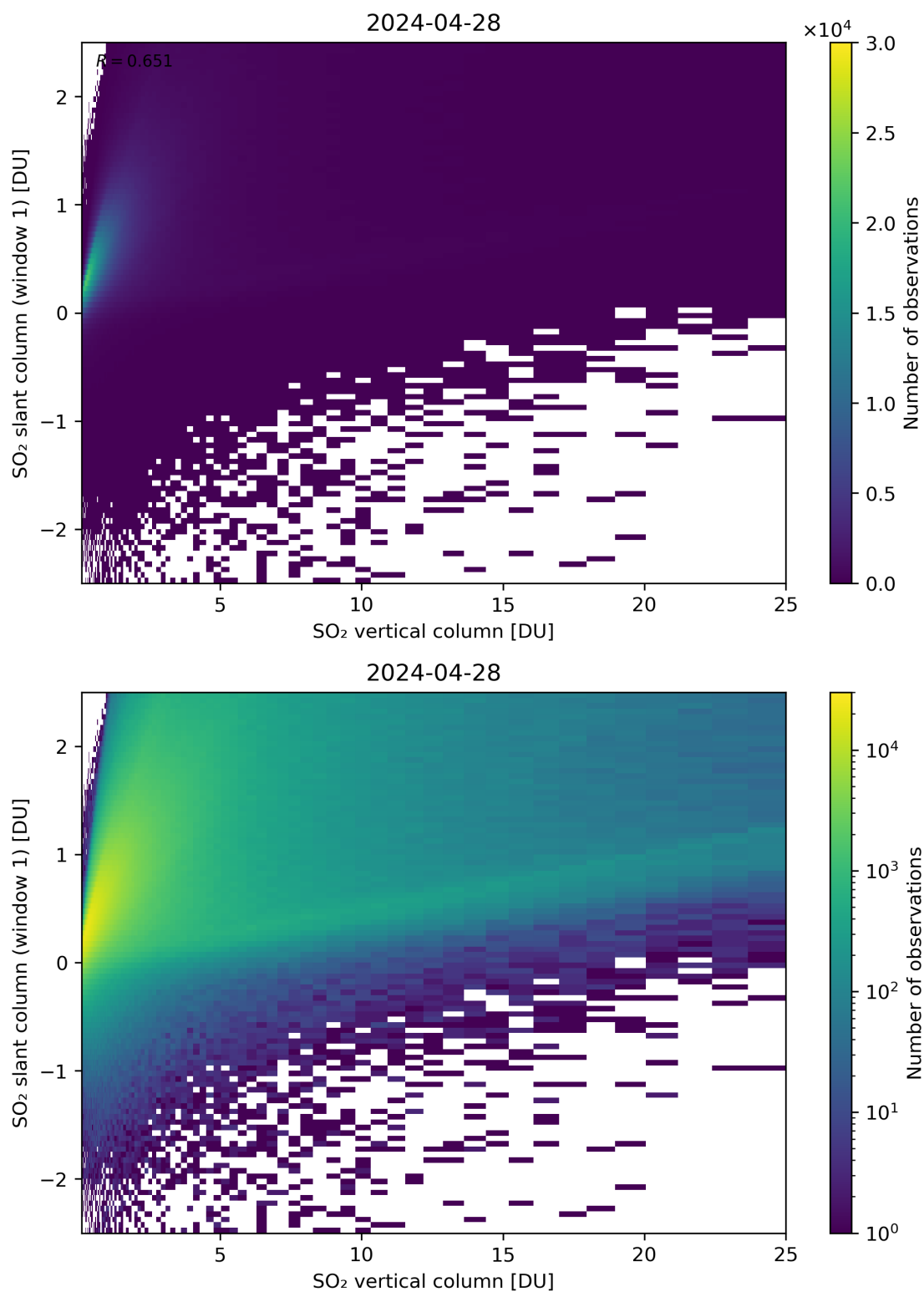
Figure 300: Scatter density plot of “SO 2 vertical column” against “SO 2 slant column (window 1)” for 2024-04-27 to 2024-04-29.
