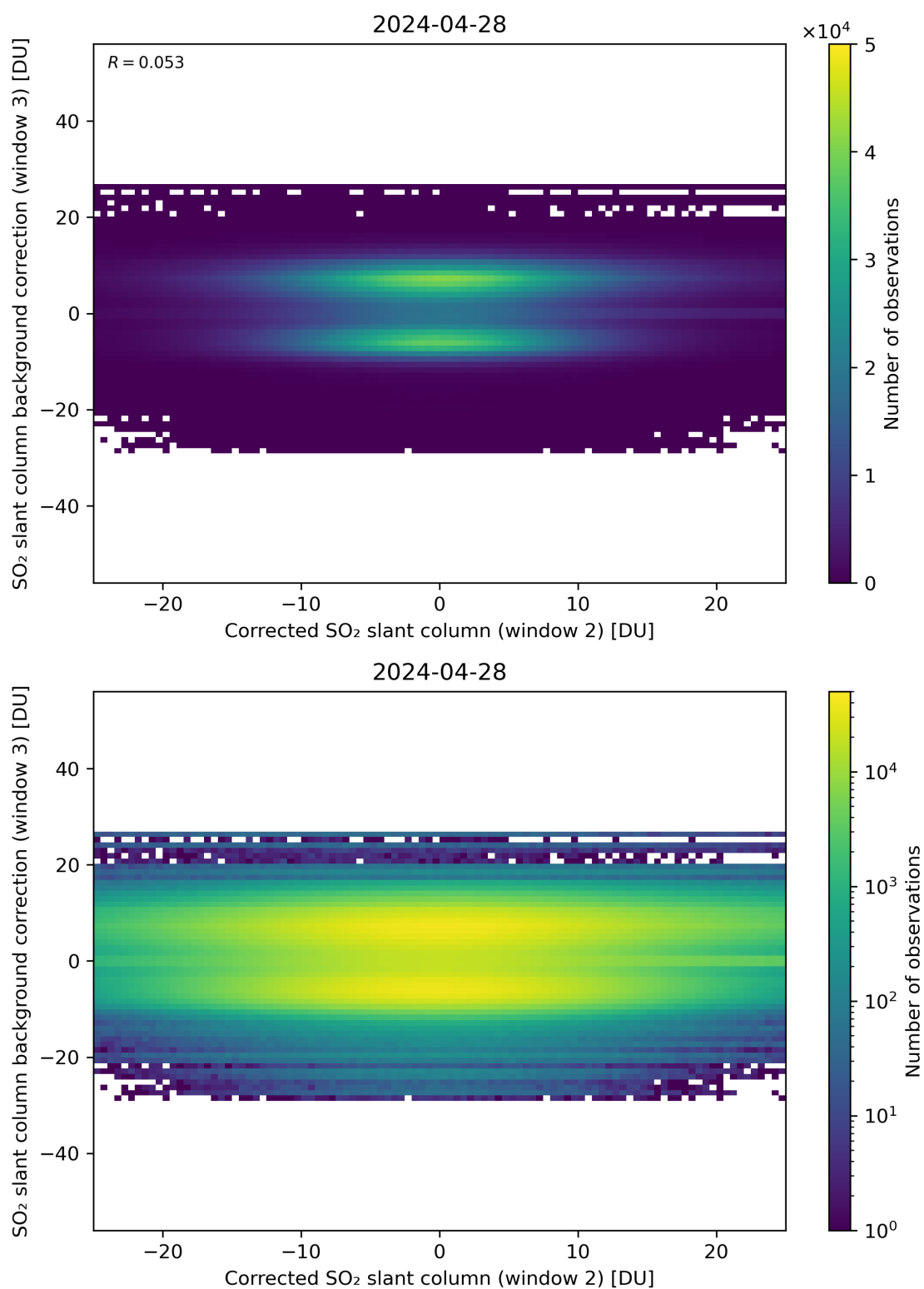
Figure 195: Scatter density plot of “Corrected SO 2 slant column (window 2)” against “SO 2 slant column background correction (window 3)” for 2024-04-27 to 2024-04-29.
