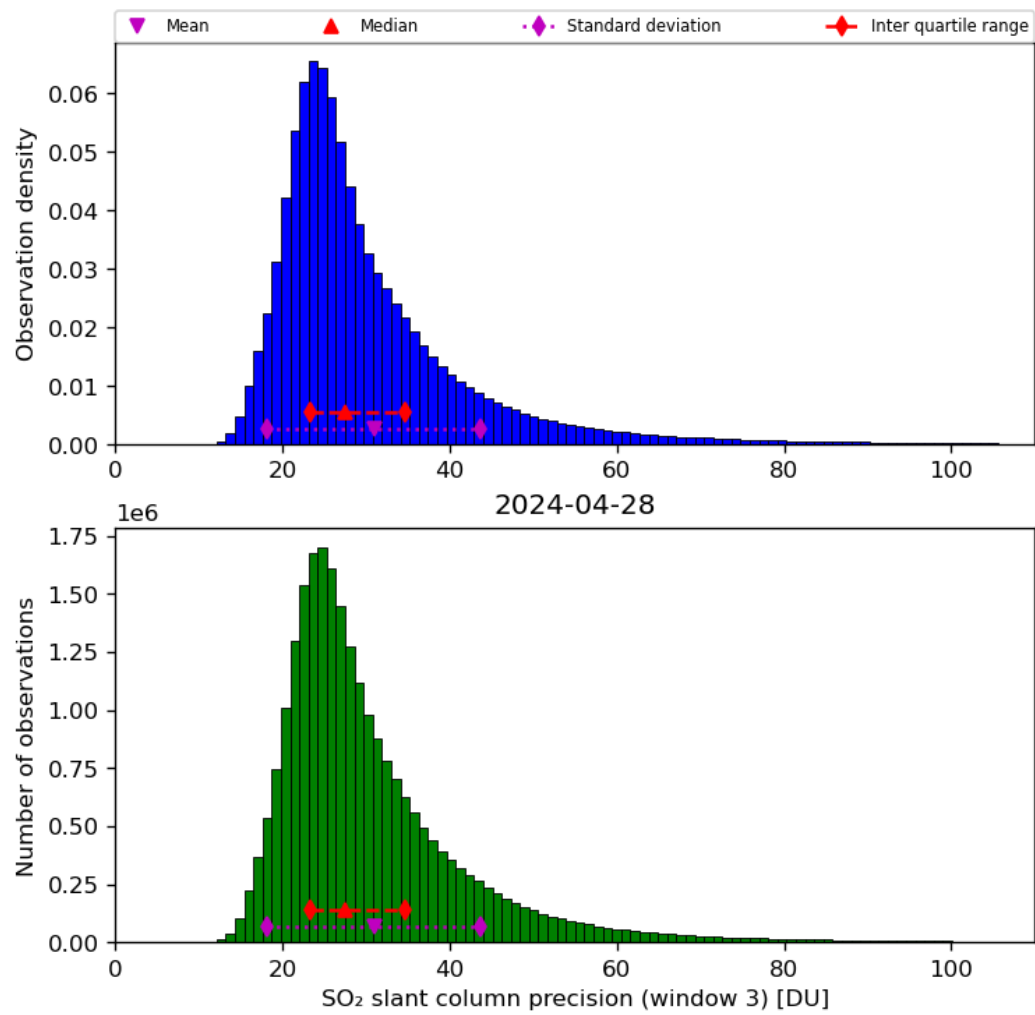
Figure 65: Histogram of “SO 2 slant column precision (window 3)” for 2024-04-27 to 2024-04-29
