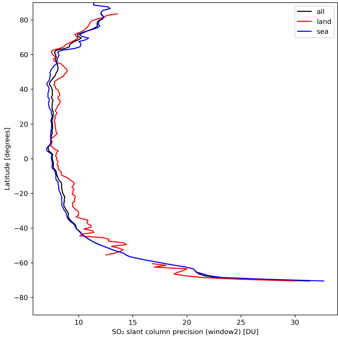
Figure 38: Zonal average of “SO 2 slant column precision (window2)” for 2024-04-27 to 2024-04-29.
