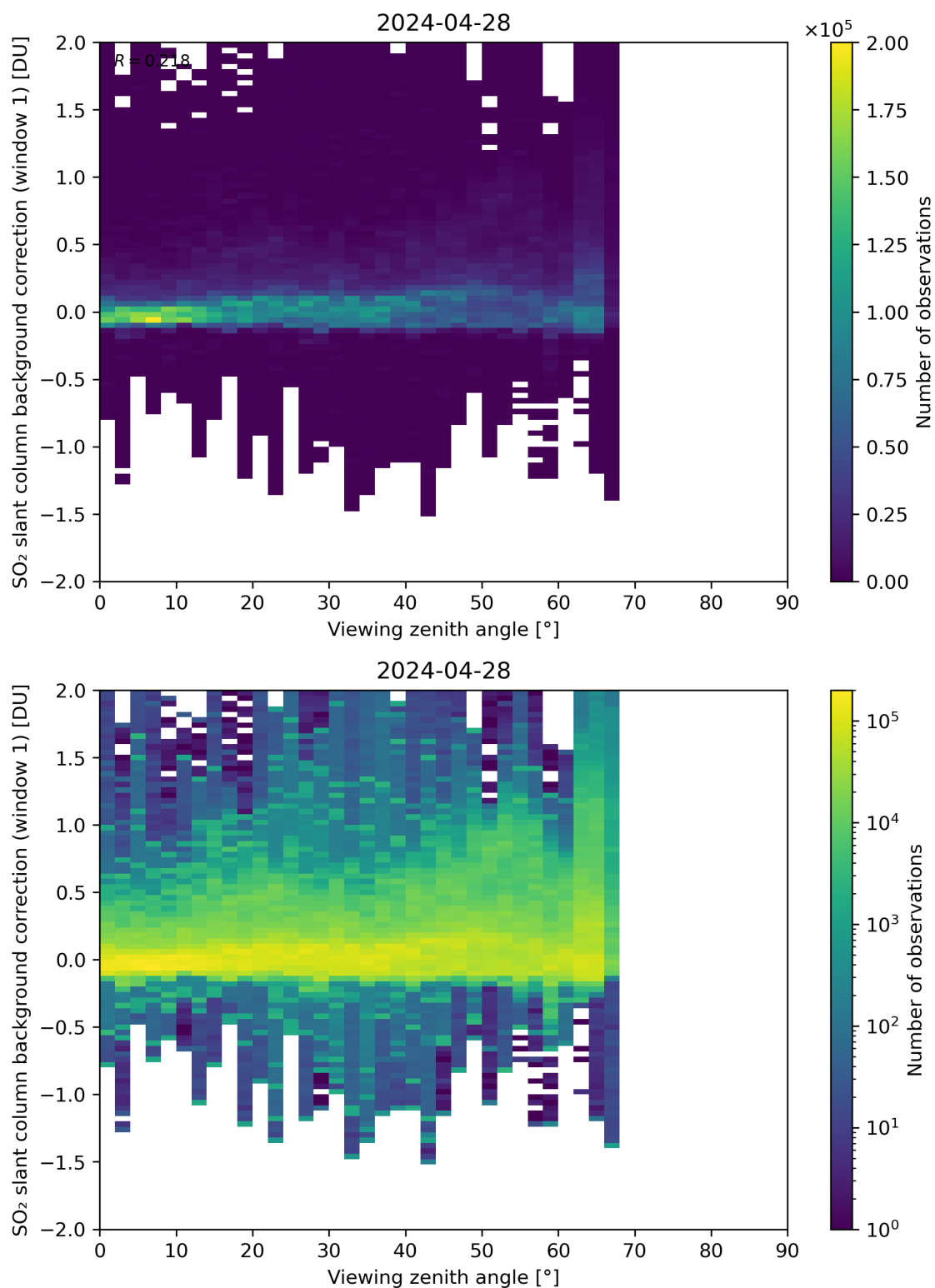
Figure 308: Scatter density plot of “Viewing zenith angle” against “SO 2 slant column background correction (window 1)” for 2024-04-27 to 2024-04-29.
