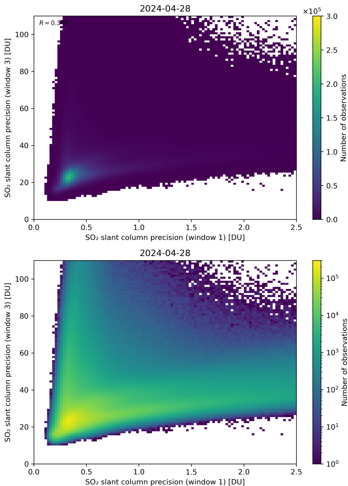
Figure 229: Scatter density plot of “SO 2 slant column precision (window 1)” against “SO 2 slant column precision (window 3)” for 2024-04-27 to 2024-04-29.
