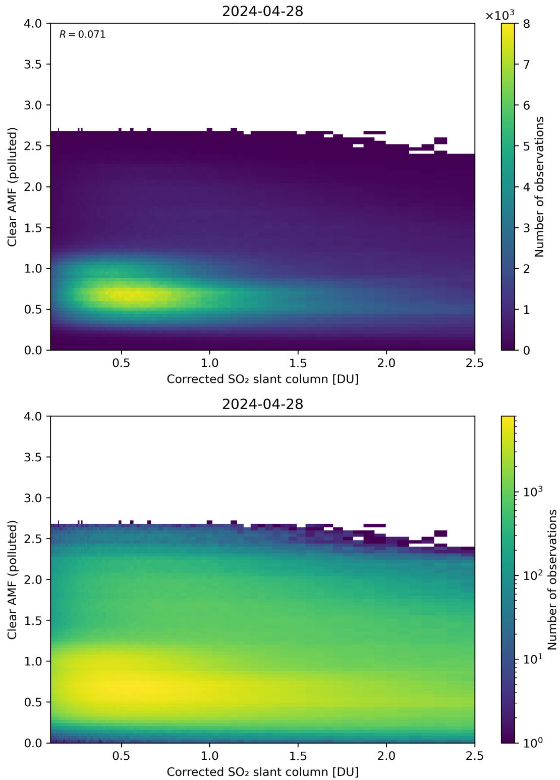
Figure 184: Scatter density plot of “Corrected SO 2 slant column” against “Clear AMF (polluted)” for 2024-04-27 to 2024-04-29.
