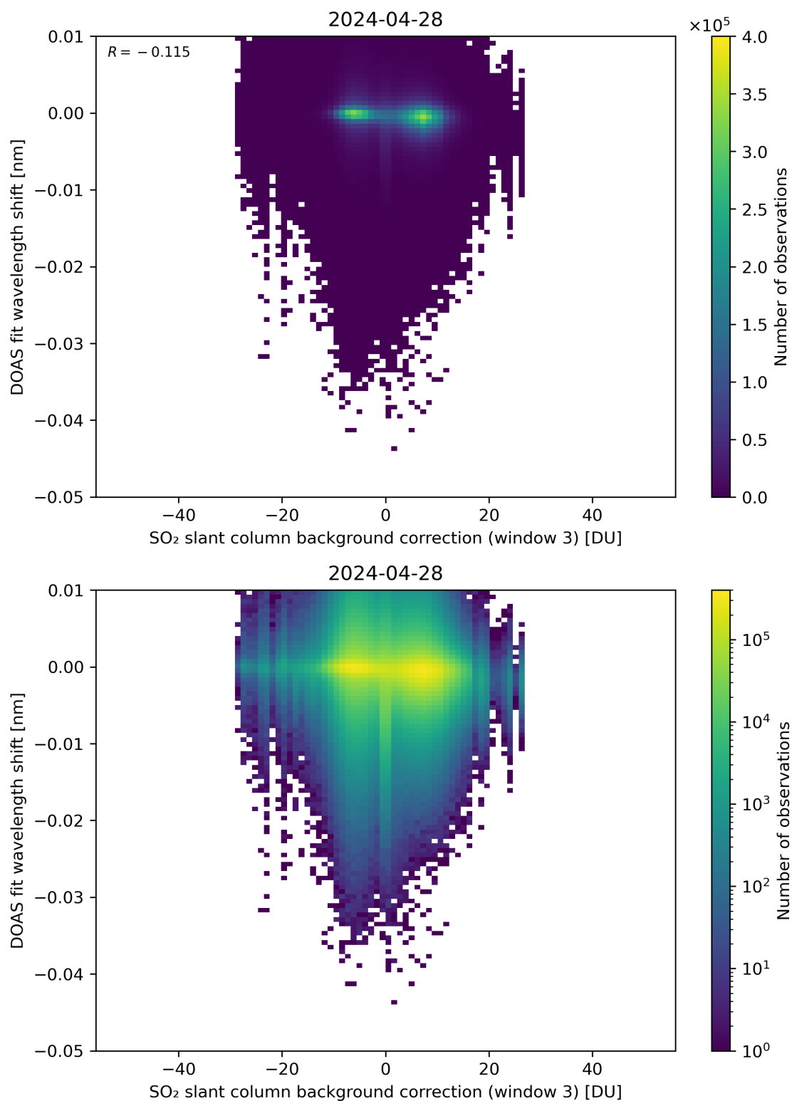
Figure 121: Scatter density plot of “SO 2 slant column background correction (window 3)” against “DOAS fit wavelength shift” for 2024-04-27 to 2024-04-29.
