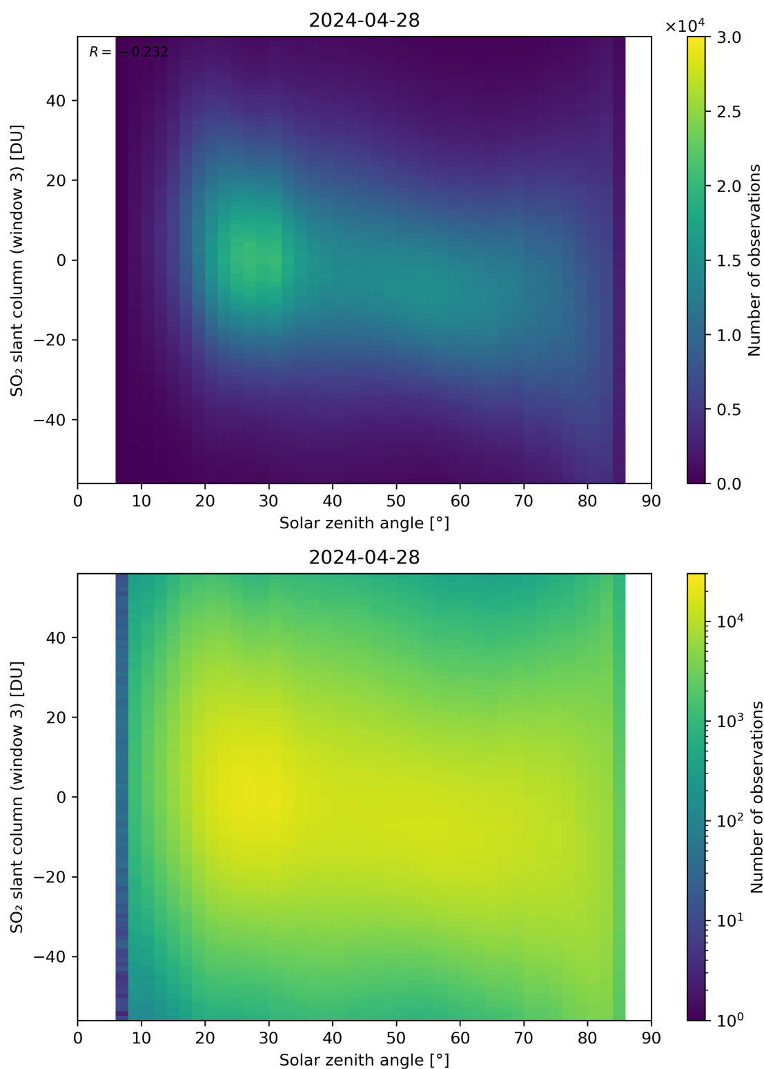
Figure 172: Scatter density plot of “Solar zenith angle” against “SO 2 slant column (window 3)” for 2024-04-27 to 2024-04-29.
