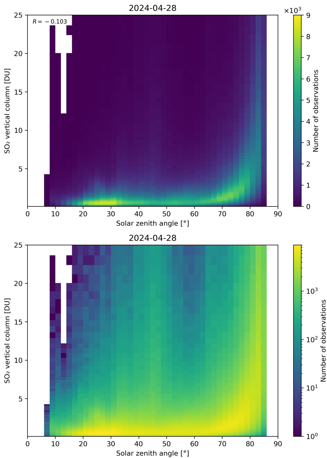
Figure 176: Scatter density plot of “Solar zenith angle” against “SO 2 vertical column” for 2024-04-27 to 2024-04-29.
