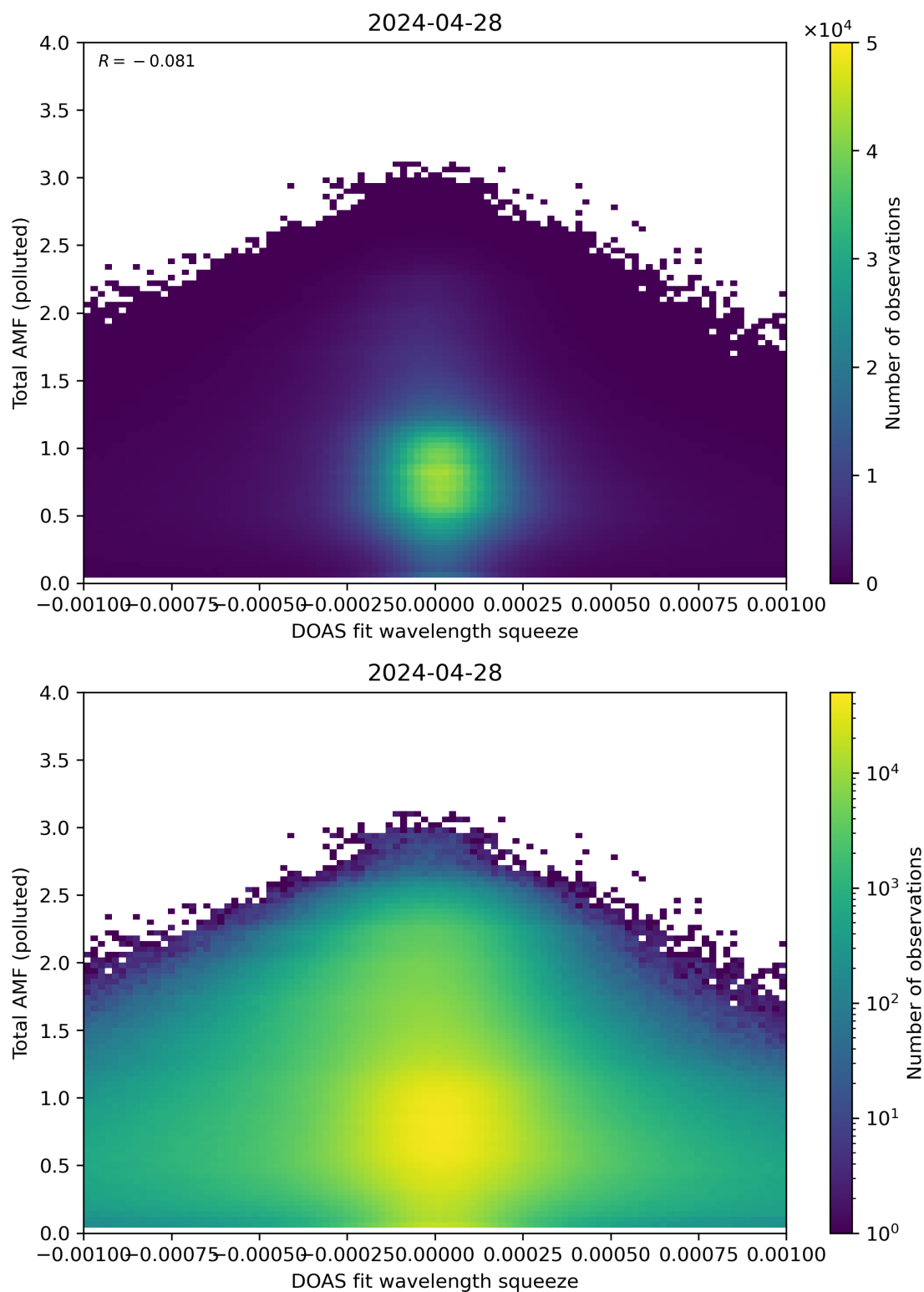
Figure 134: Scatter density plot of “DOAS fit wavelength squeeze” against “Total AMF (polluted)” for 2024-04-27 to 2024-04-29.
