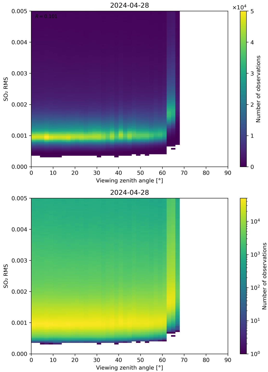
Figure 313: Scatter density plot of “Viewing zenith angle” against “SO 2 RMS” for 2024-04-27 to 2024-04-29.
