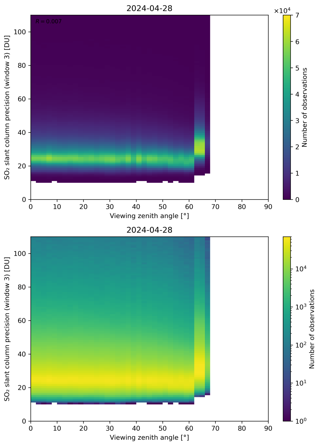
Figure 324: Scatter density plot of “Viewing zenith angle” against “SO 2 slant column precision (window 3)” for 2024-04-27 to 2024-04-29.
