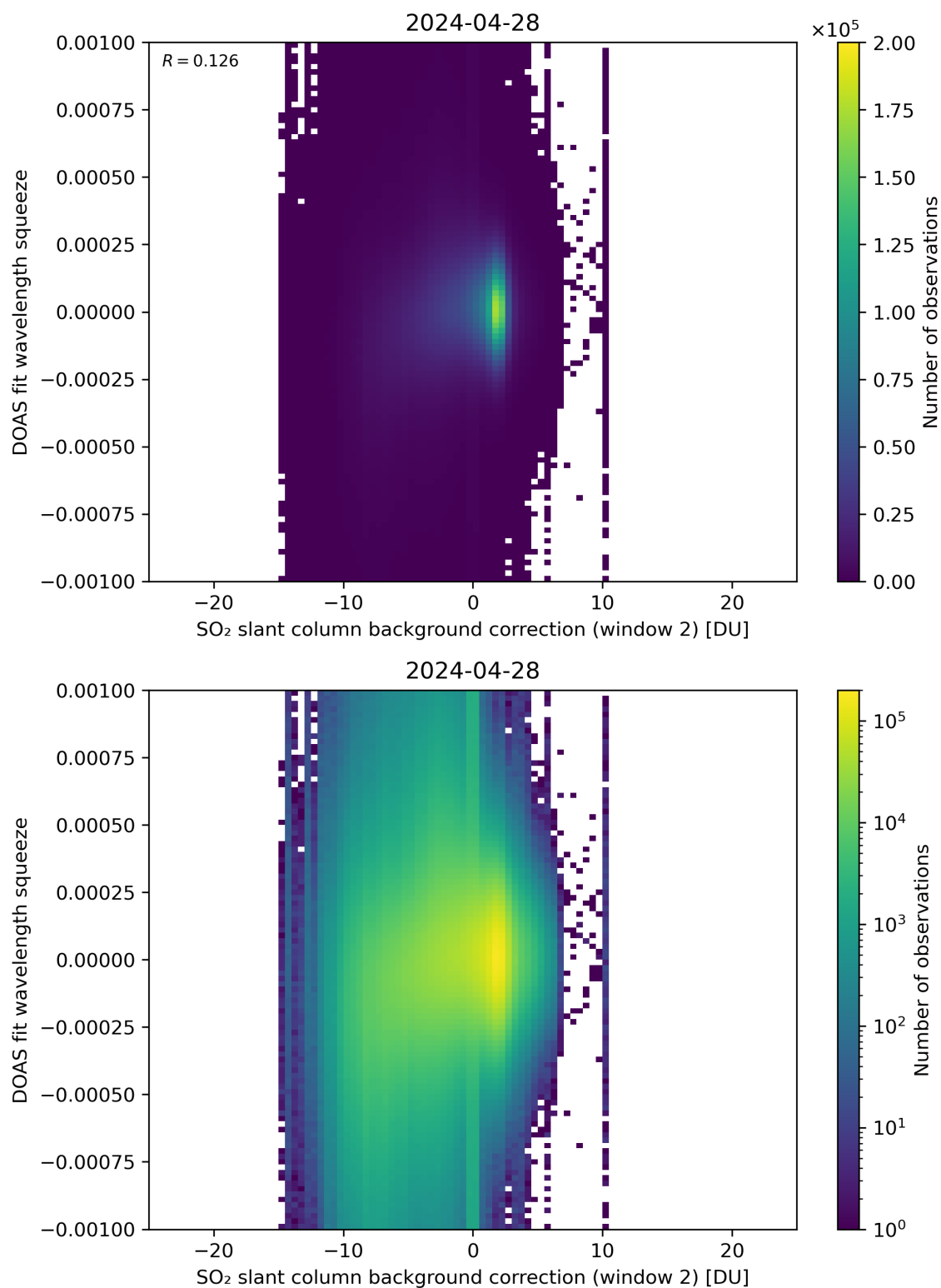
Figure 113: Scatter density plot of “SO 2 slant column background correction (window 2)” against “DOAS fit wavelength squeeze” for 2024-04-27 to 2024-04-29.
