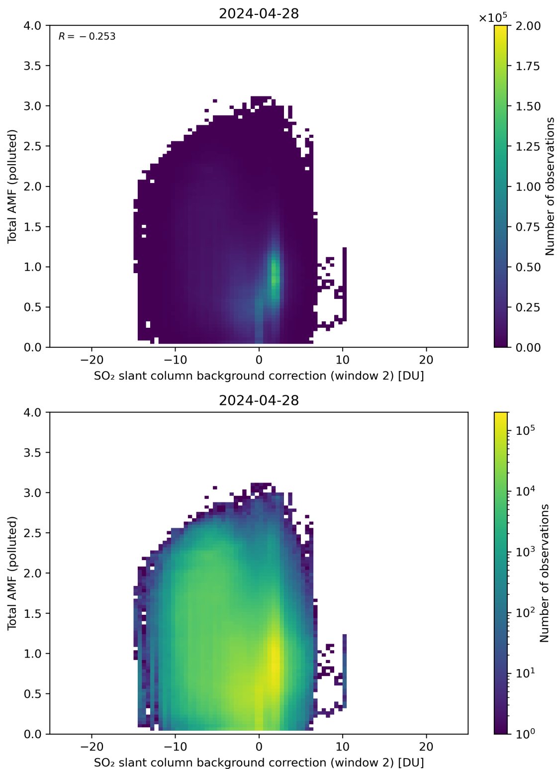
Figure 119: Scatter density plot of “SO 2 slant column background correction (window 2)” against “Total AMF (polluted)” for 2024-04-27 to 2024-04-29.
