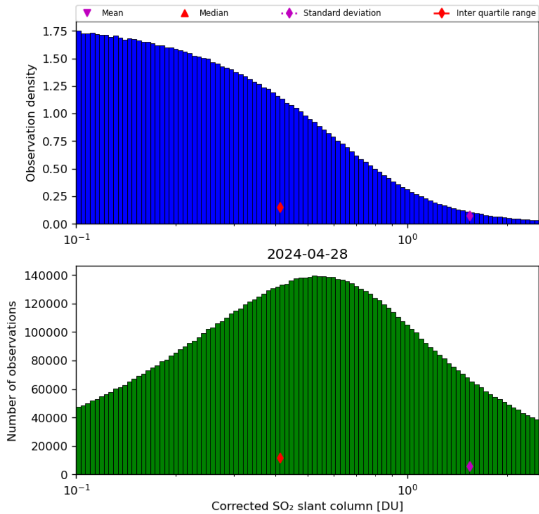
Figure 55: Histogram of “Corrected SO 2 slant column” for 2024-04-27 to 2024-04-29
