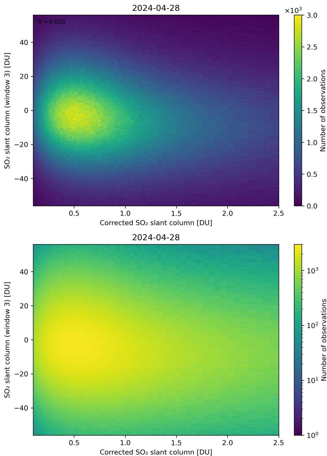
Figure 190: Scatter density plot of “Corrected SO 2 slant column” against “SO 2 slant column (window 3)” for 2024-04-27 to 2024-04-29.
