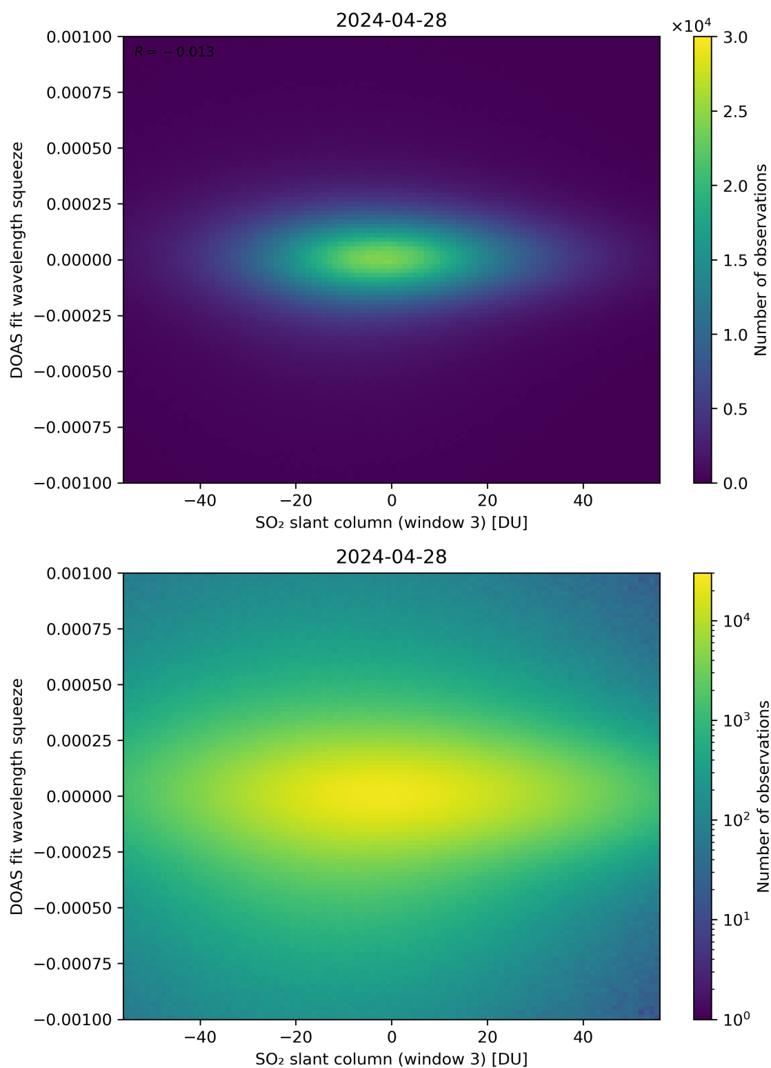
Figure 255: Scatter density plot of “SO 2 slant column (window 3)” against “DOAS fit wavelength squeeze” for 2024-04-27 to 2024-04-29.
