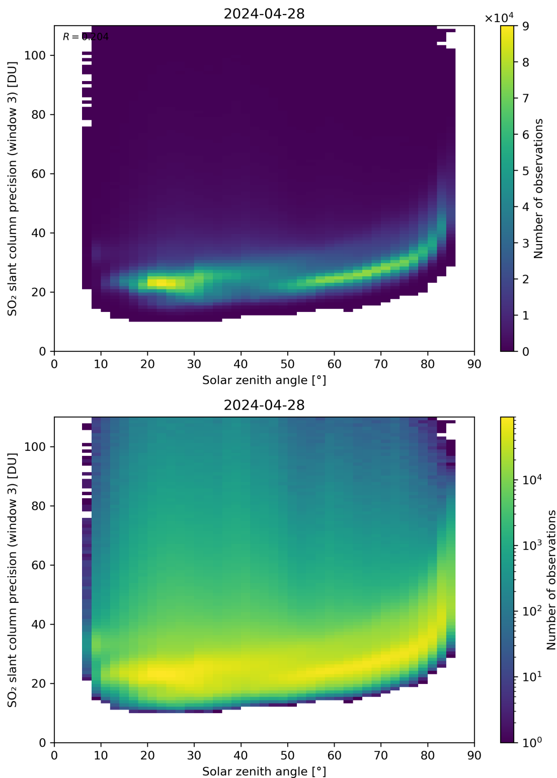
Figure 173: Scatter density plot of “Solar zenith angle” against “SO 2 slant column precision (window 3)” for 2024-04-27 to 2024-04-29.
