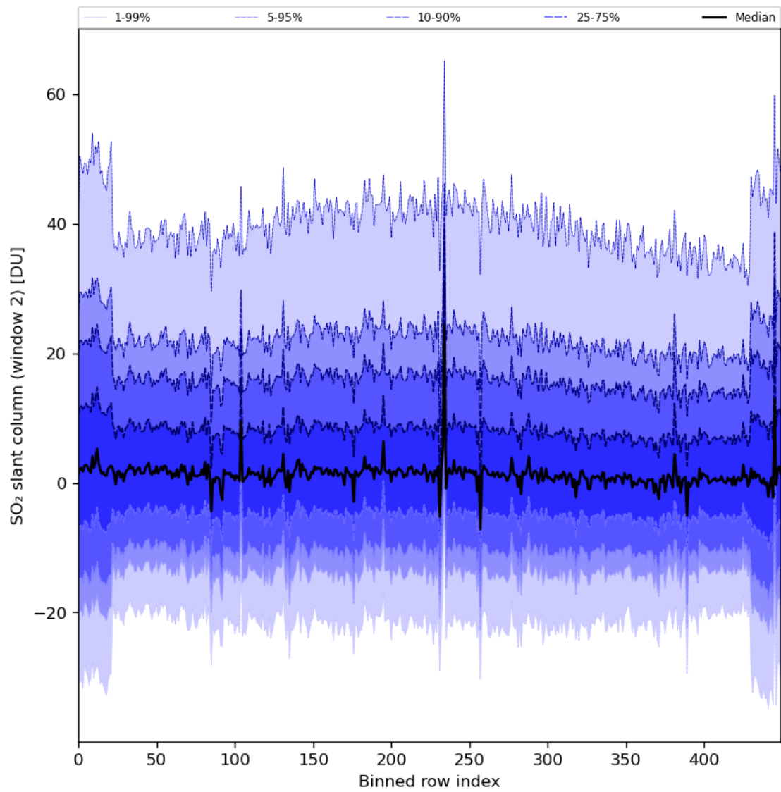
Figure 83: Along track statistics of “SO 2 slant column (window 2)” for 2024-04-27 to 2024-04-29
