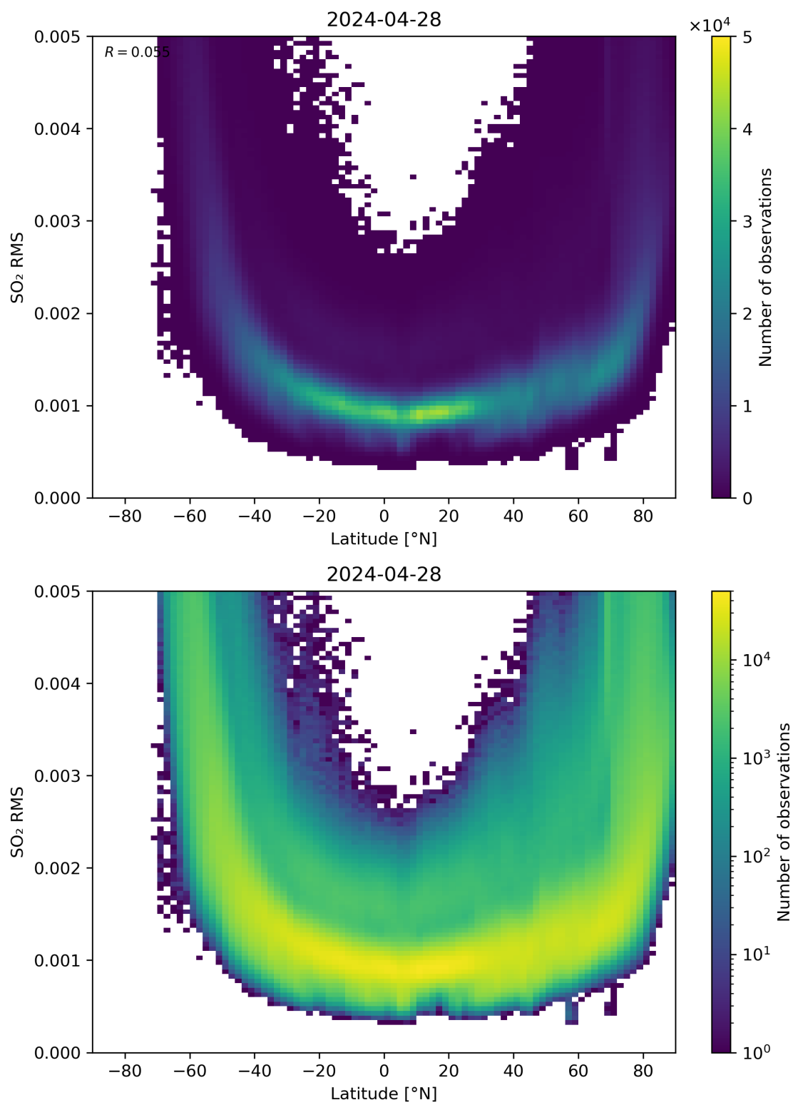
Figure 144: Scatter density plot of “Latitude” against “SO 2 RMS” for 2024-04-27 to 2024-04-29.
