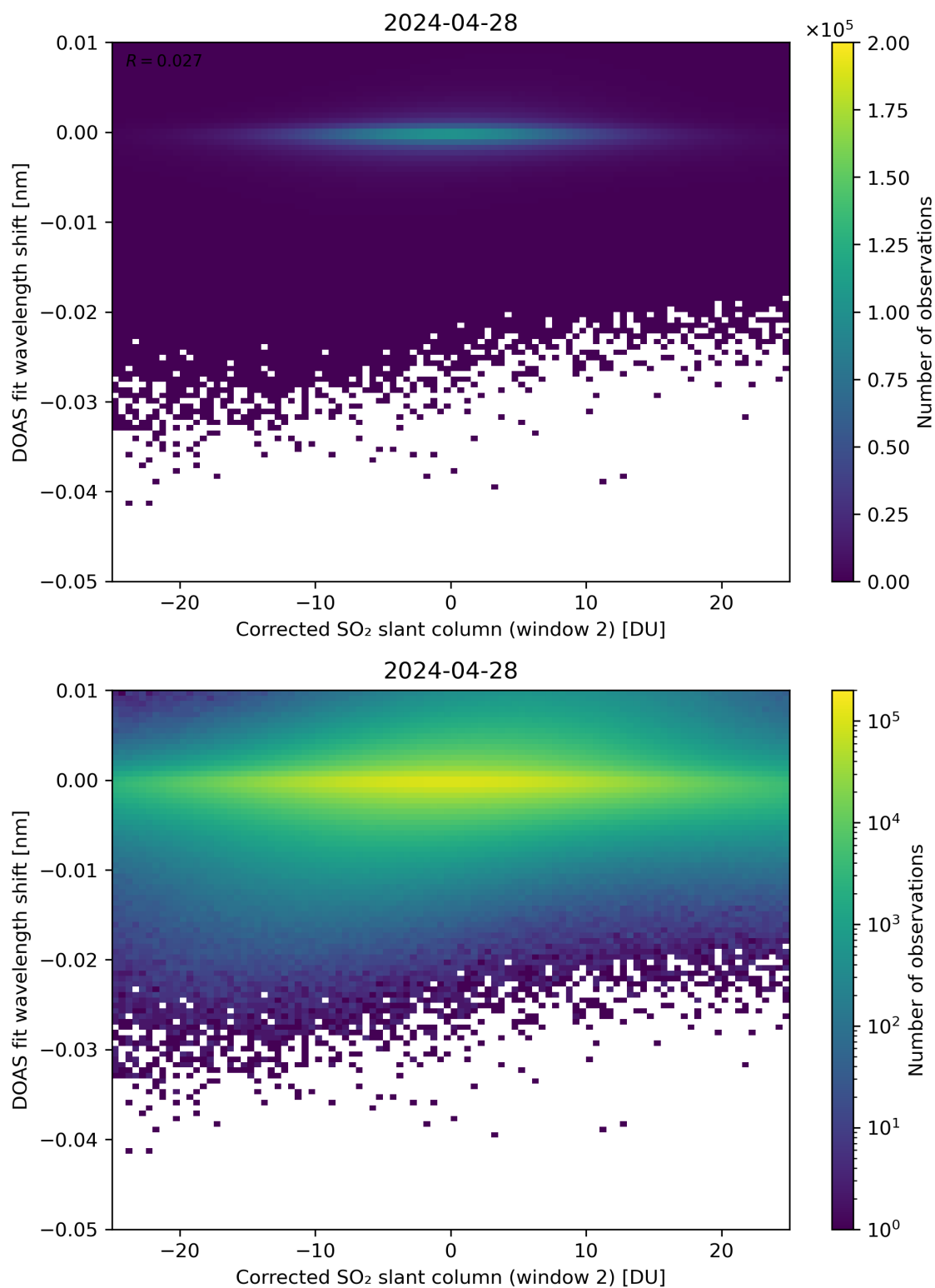
Figure 196: Scatter density plot of “Corrected SO 2 slant column (window 2)” against “DOAS fit wavelength shift” for 2024-04-27 to 2024-04-29.
