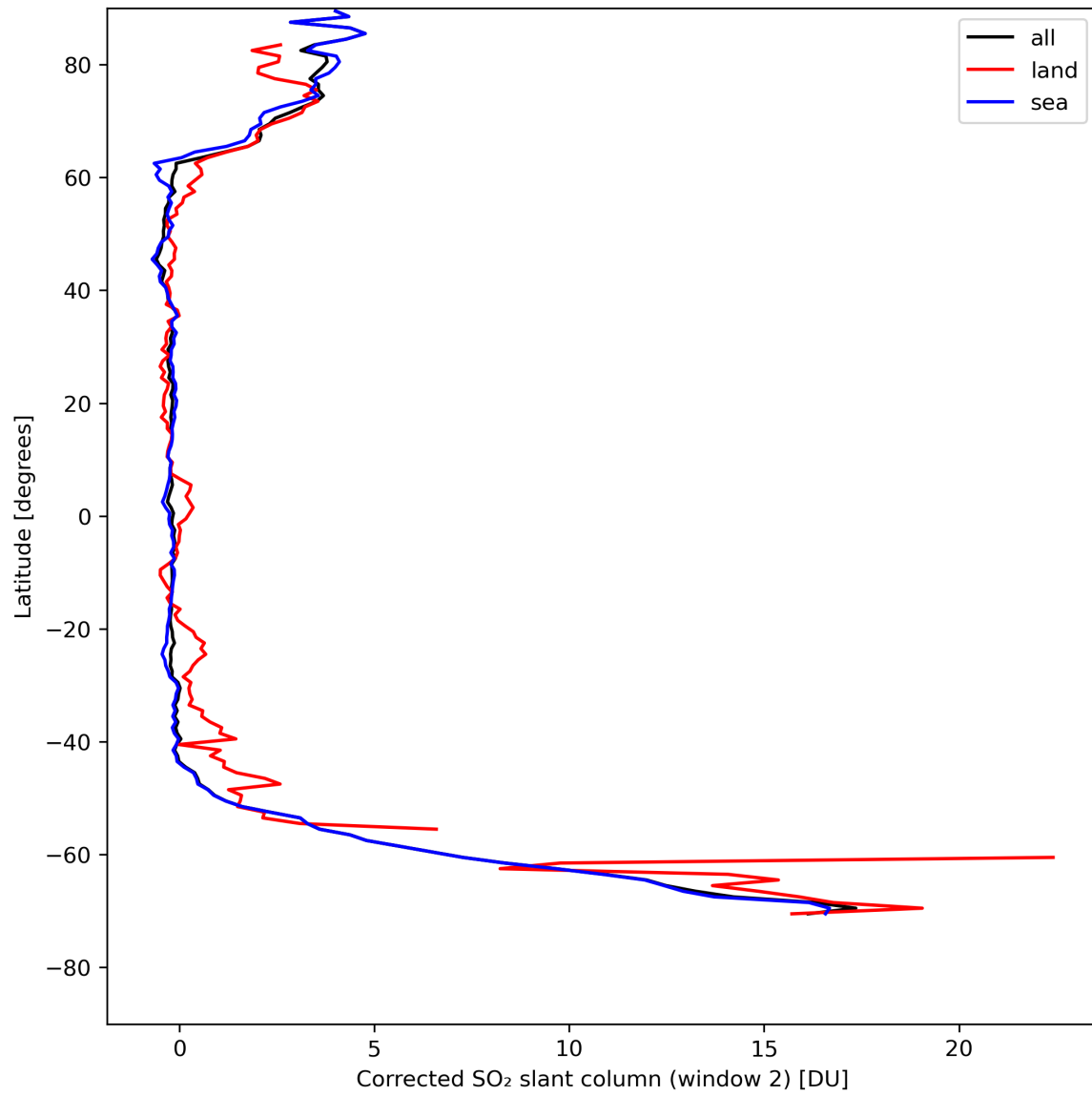
Figure 39: Zonal average of “Corrected SO 2 slant column (window 2)” for 2024-04-27 to 2024-04-29.
