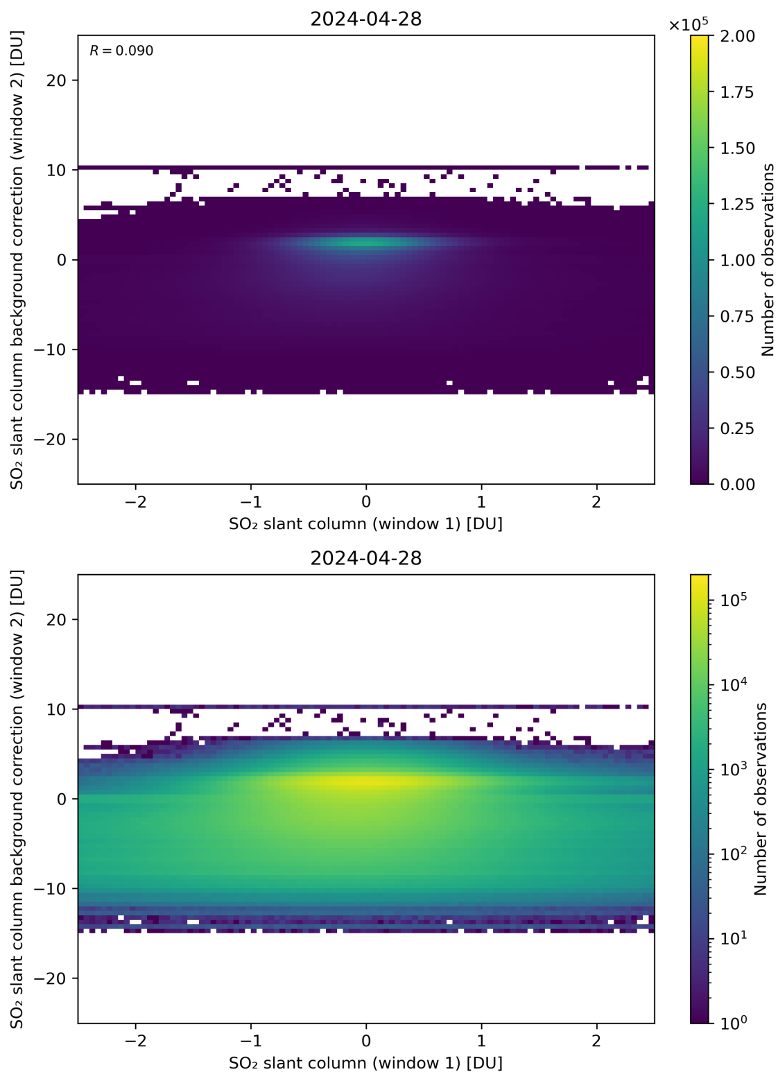
Figure 213: Scatter density plot of “SO 2 slant column (window 1)” against “SO 2 slant column background correction (window 2)” for 2024-04-27 to 2024-04-29.
