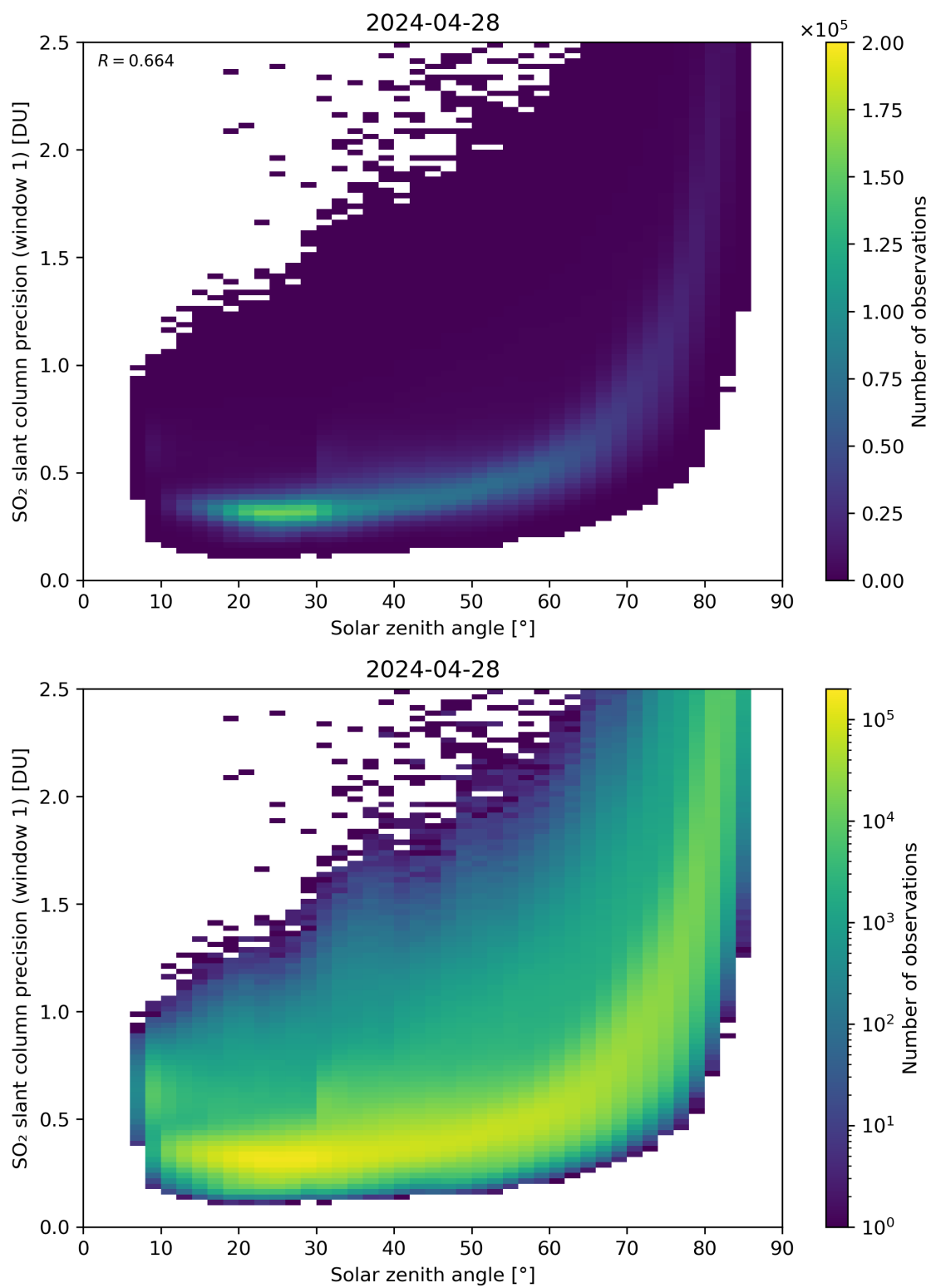
Figure 170: Scatter density plot of “Solar zenith angle” against “SO 2 slant column precision (window 1)” for 2024-04-27 to 2024-04-29.
