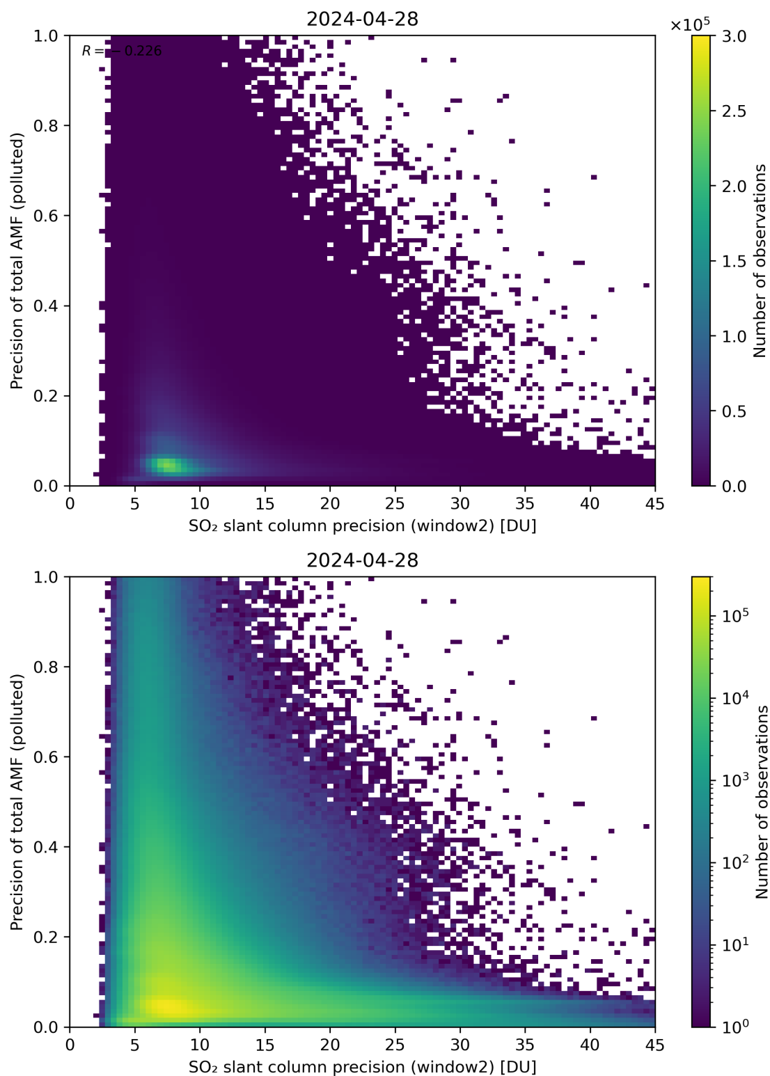
Figure 252: Scatter density plot of “SO 2 slant column precision (window2)” against “Precision of total AMF (polluted)” for 2024-04-27 to 2024-04-29.
