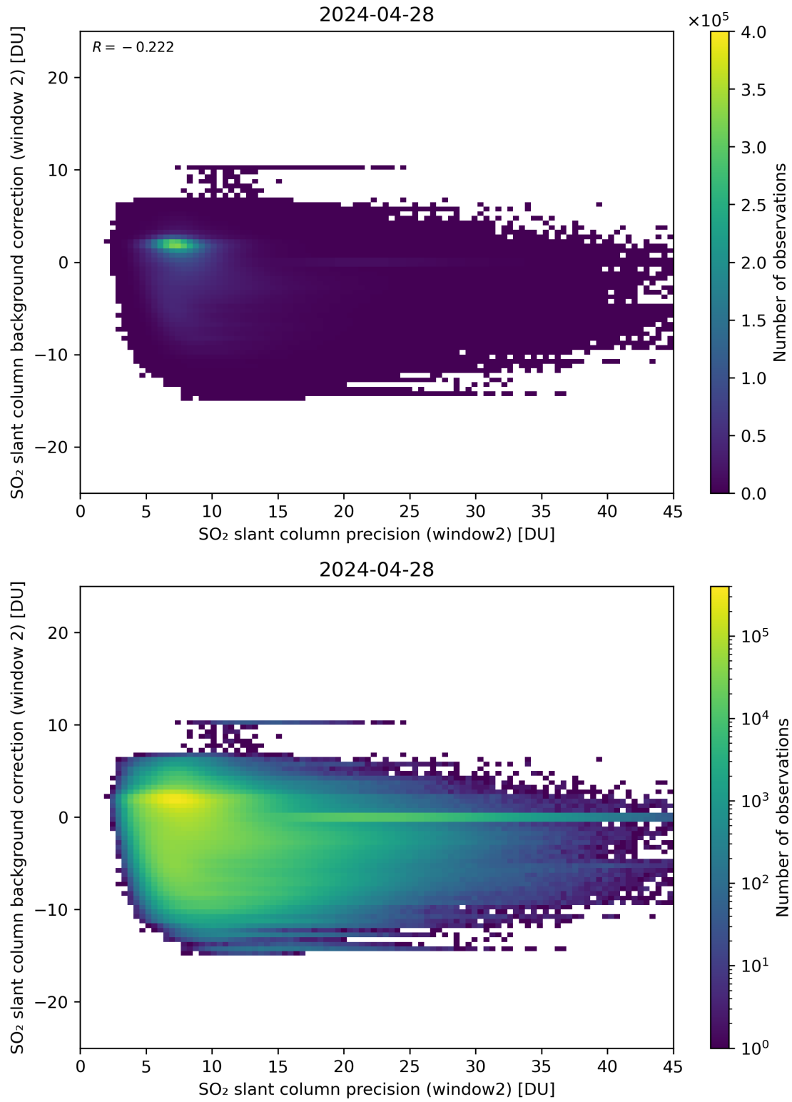
Figure 241: Scatter density plot of “SO 2 slant column precision (window2)” against “SO 2 slant column background correction (window 2)” for 2024-04-27 to 2024-04-29.
