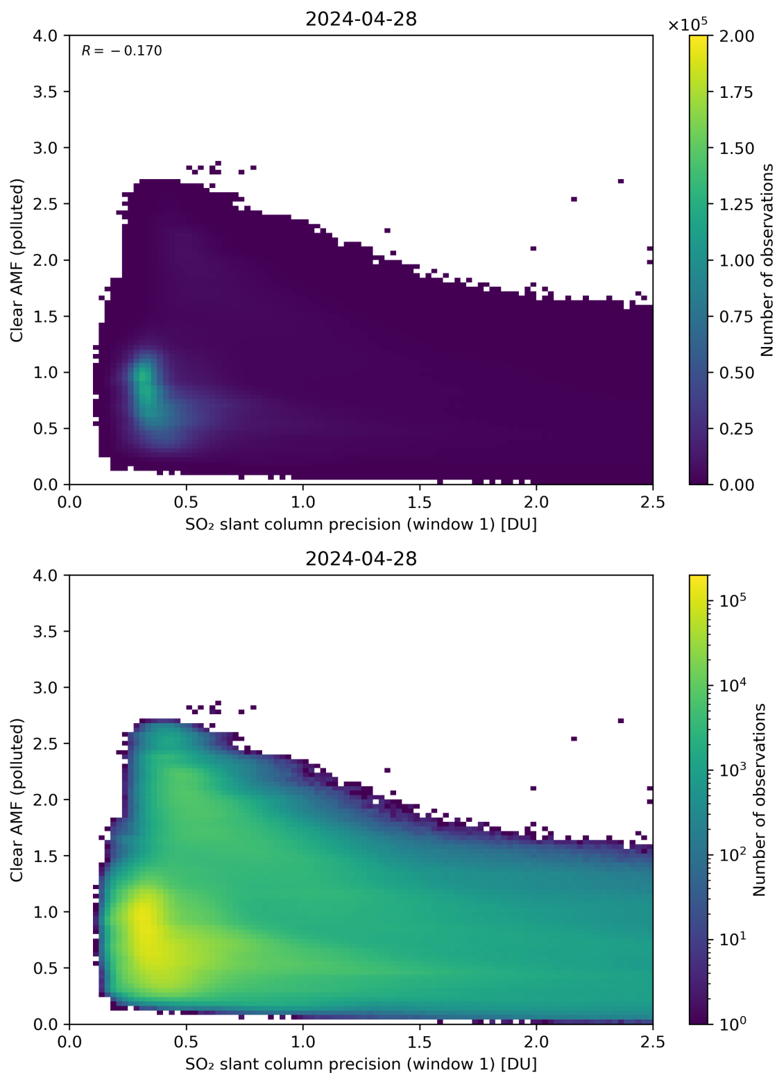
Figure 224: Scatter density plot of “SO 2 slant column precision (window 1)” against “Clear AMF (polluted)” for 2024-04-27 to 2024-04-29.
