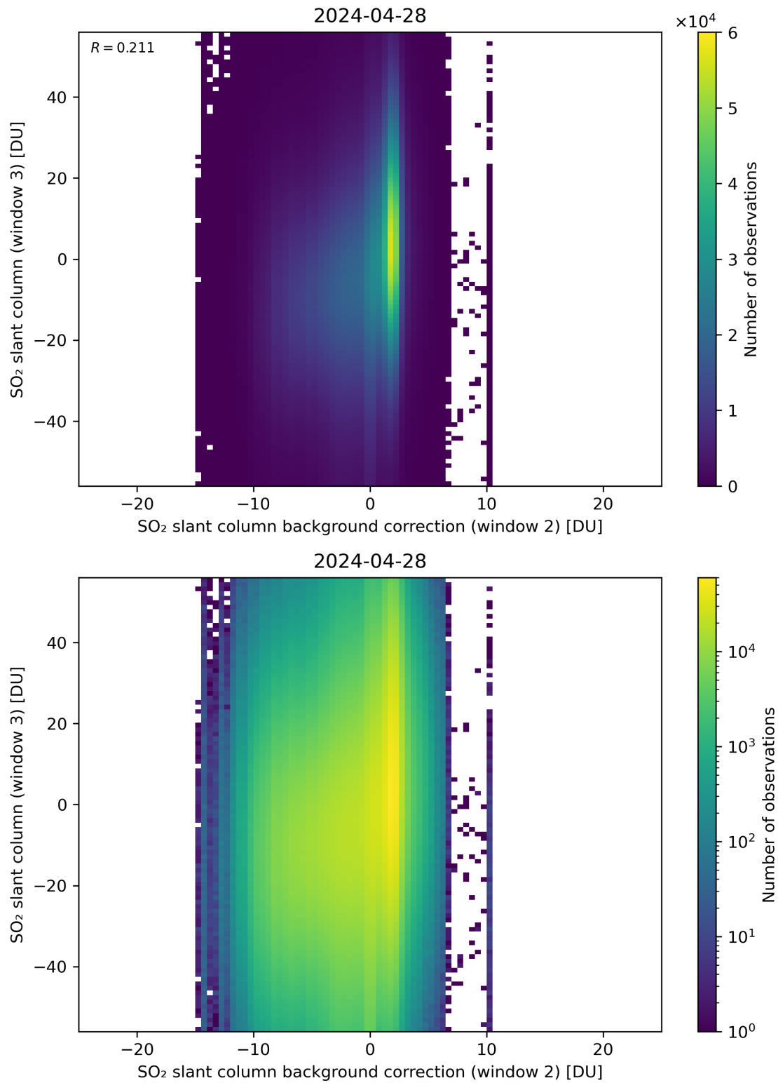
Figure 117: Scatter density plot of “SO 2 slant column background correction (window 2)” against “SO 2 slant column (window 3)” for 2024-04-27 to 2024-04-29.
