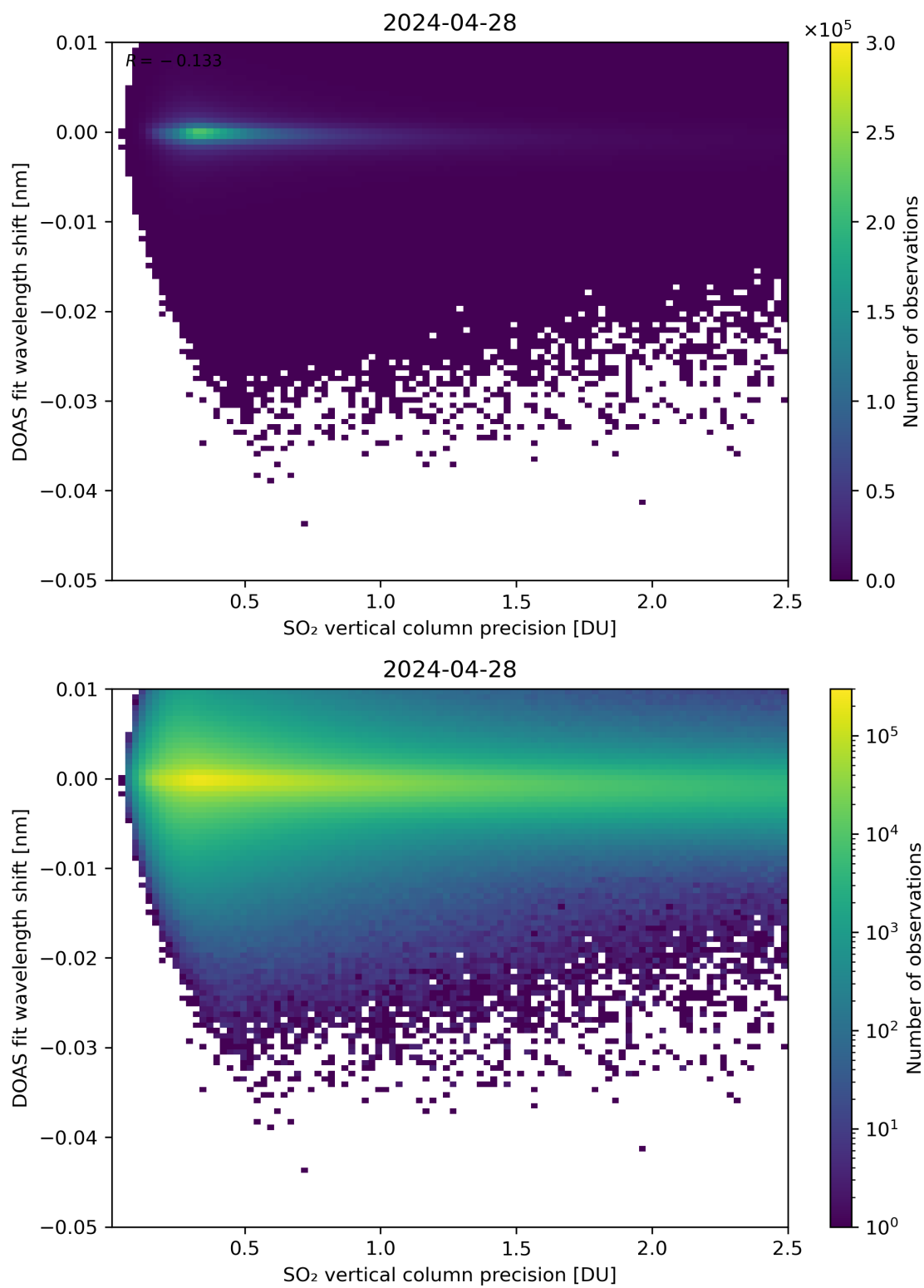
Figure 282: Scatter density plot of “SO 2 vertical column precision” against “DOAS fit wavelength shift” for 2024-04-27 to 2024-04-29.
