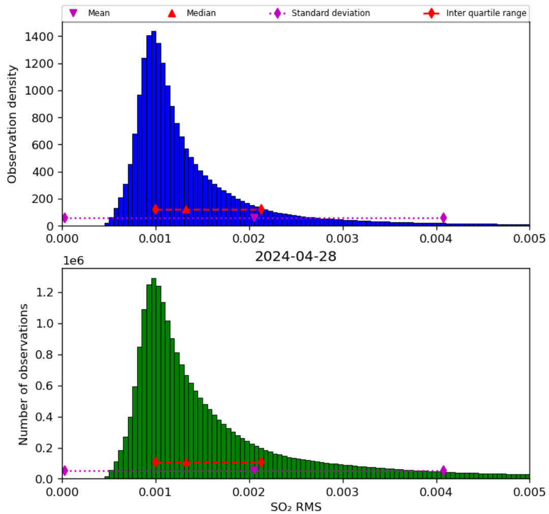
Figure 70: Histogram of “SO 2 RMS” for 2024-04-27 to 2024-04-29
