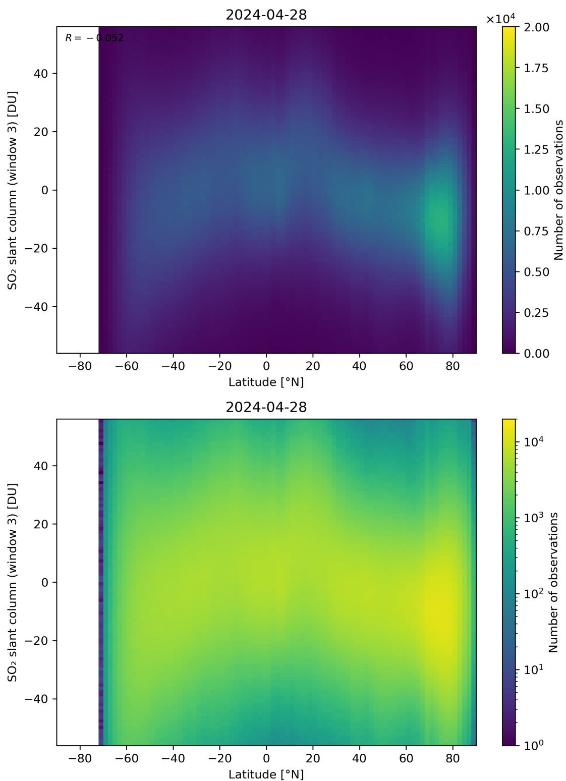
Figure 152: Scatter density plot of “Latitude” against “SO 2 slant column (window 3)” for 2024-04-27 to 2024-04-29.
