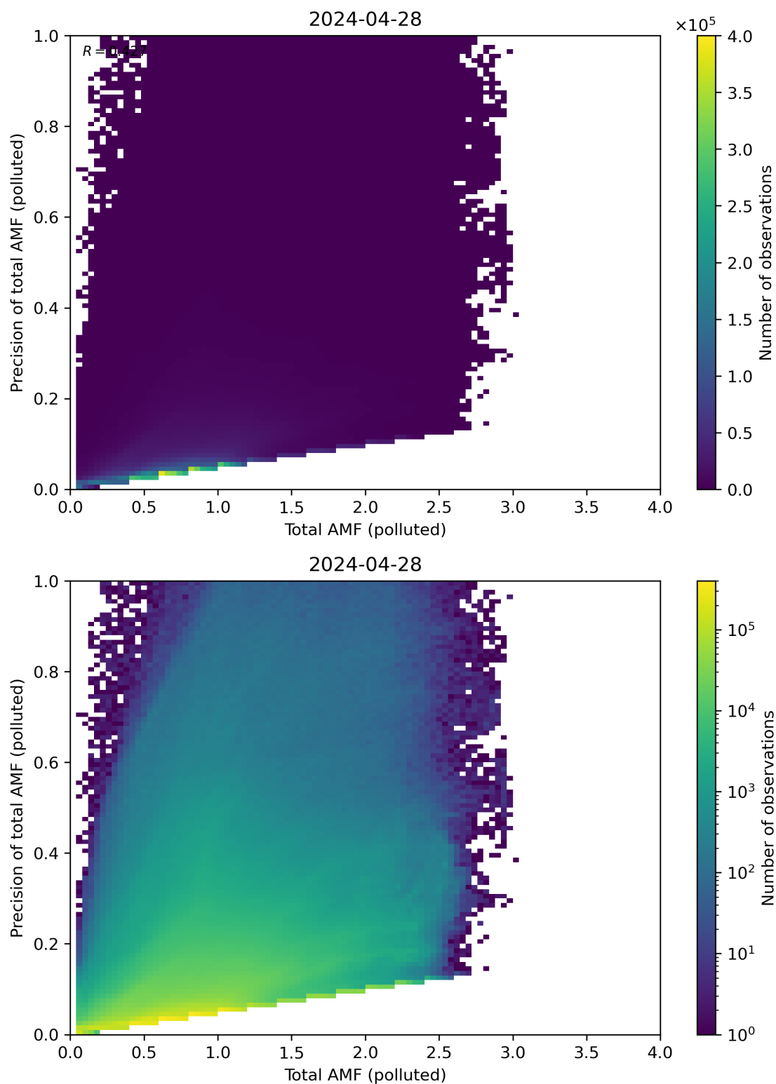
Figure 272: Scatter density plot of “Total AMF (polluted)” against “Precision of total AMF (polluted)” for 2024-04-27 to 2024-04-29.
