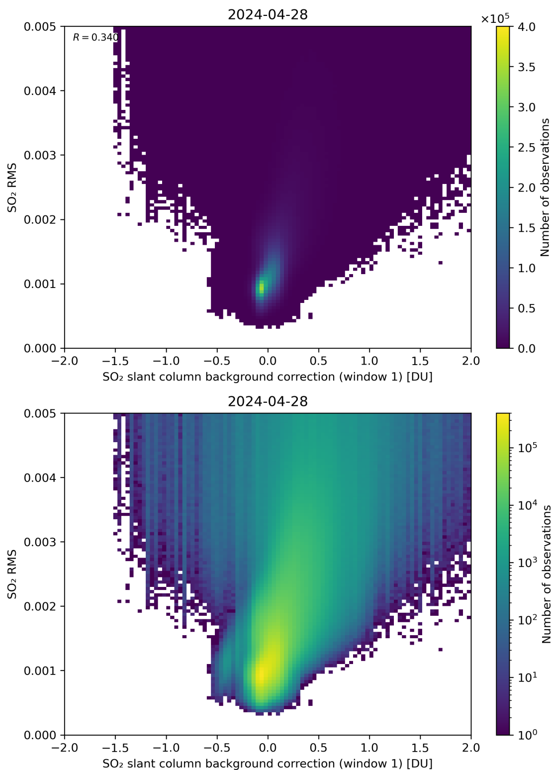
Figure 102: Scatter density plot of “SO 2 slant column background correction (window 1)” against “SO 2 RMS” for 2024-04-27 to 2024-04-29.
