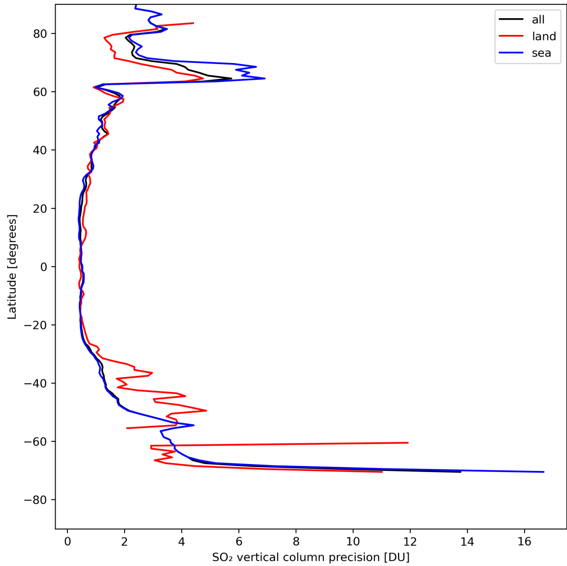
Figure 31: Zonal average of “SO 2 vertical column precision” for 2024-04-27 to 2024-04-29.
