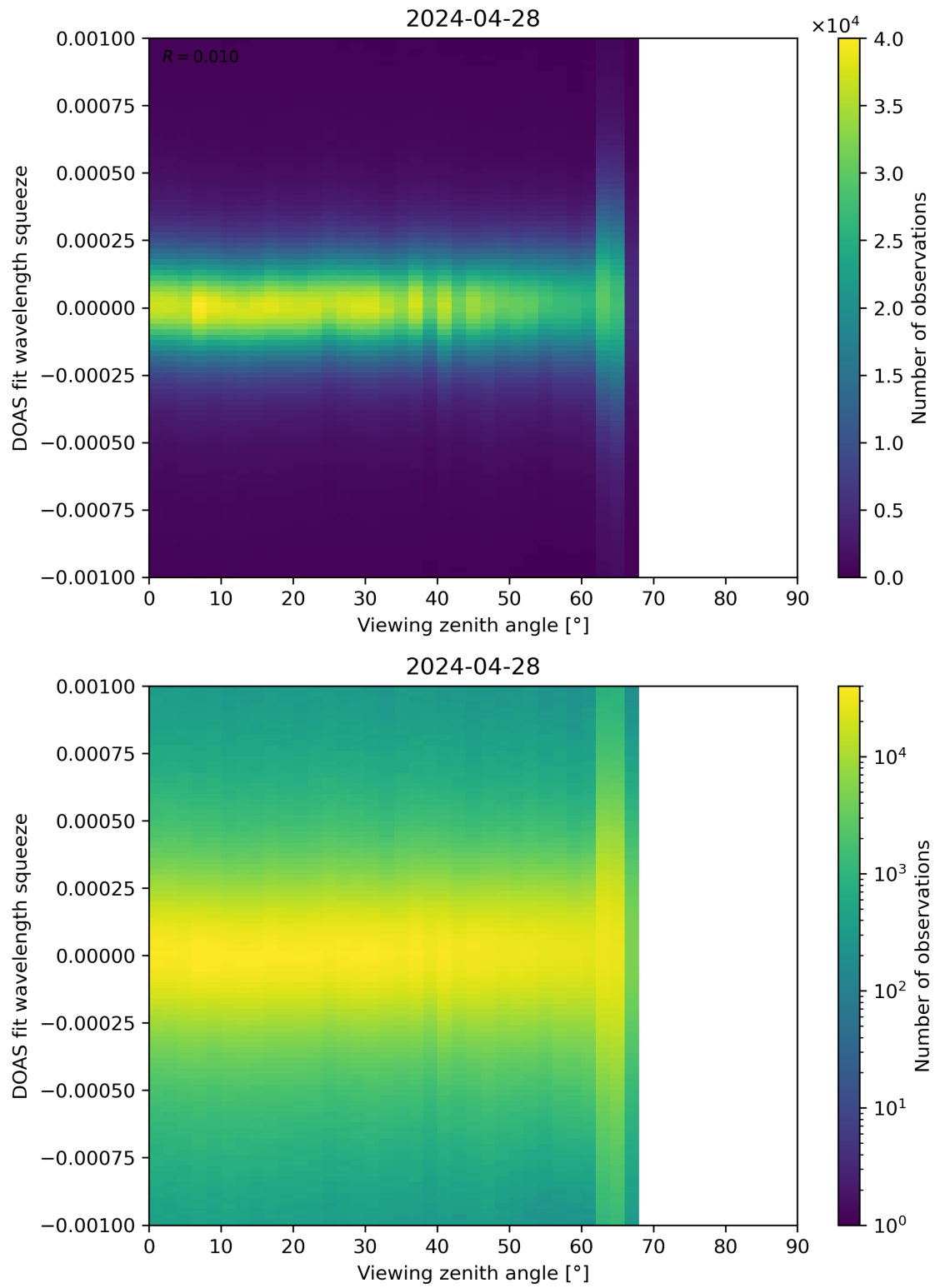
Figure 312: Scatter density plot of “Viewing zenith angle” against “DOAS fit wavelength squeeze” for 2024-04-27 to 2024-04-29.
