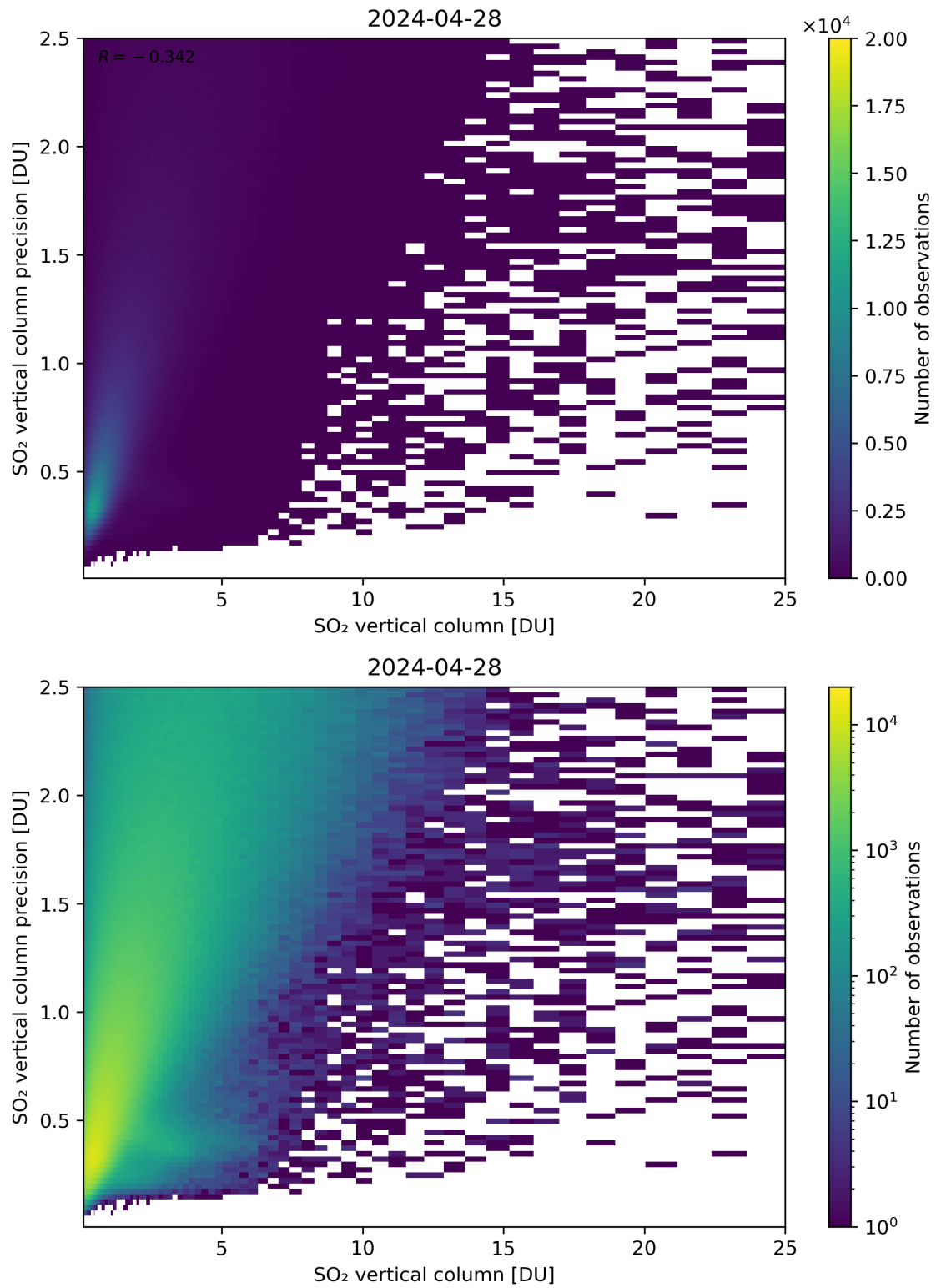
Figure 307: Scatter density plot of “SO 2 vertical column” against “SO 2 vertical column precision” for 2024-04-27 to 2024-04-29.
