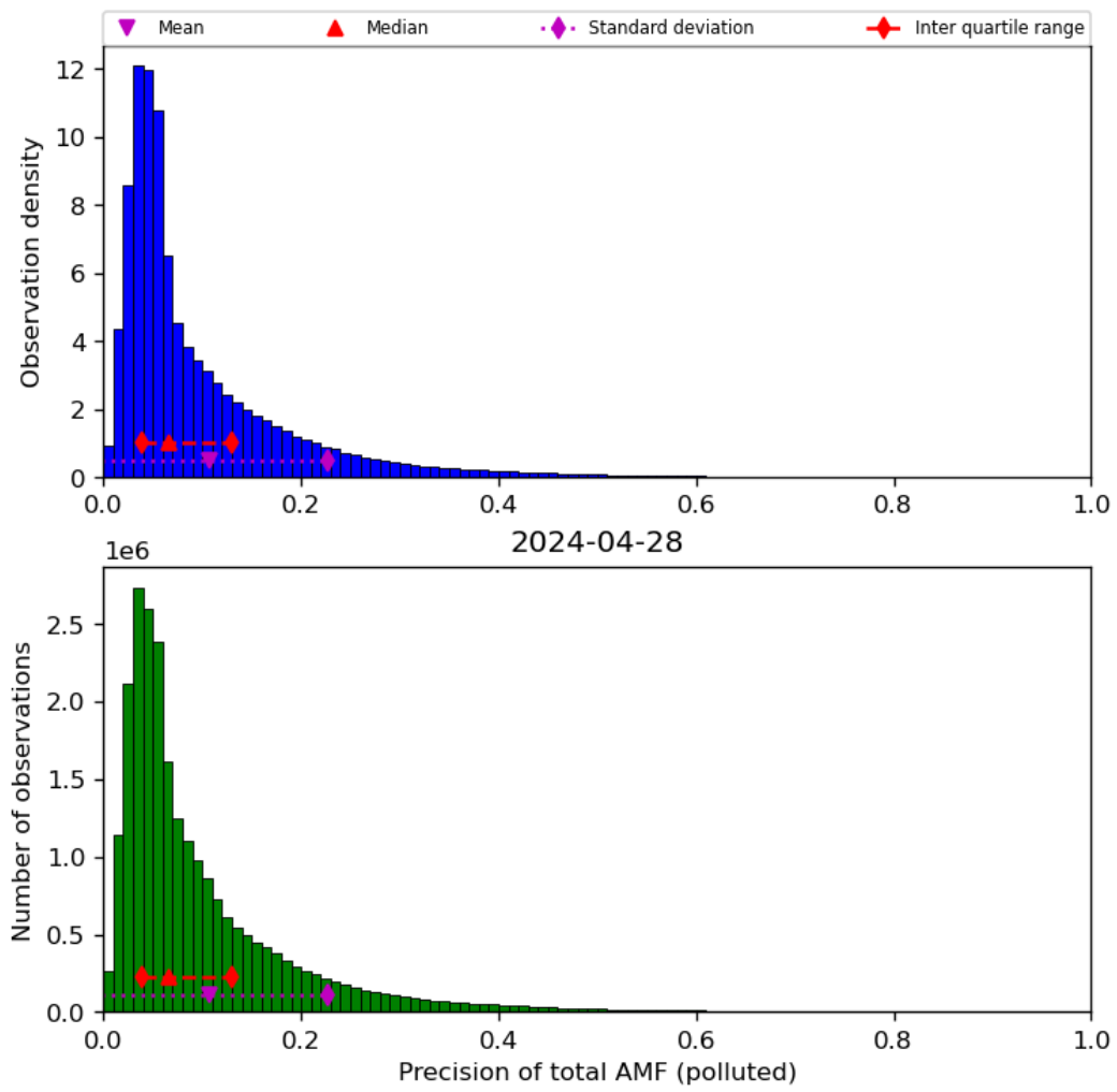
Figure 72: Histogram of “Precision of total AMF (polluted)” for 2024-04-27 to 2024-04-29
