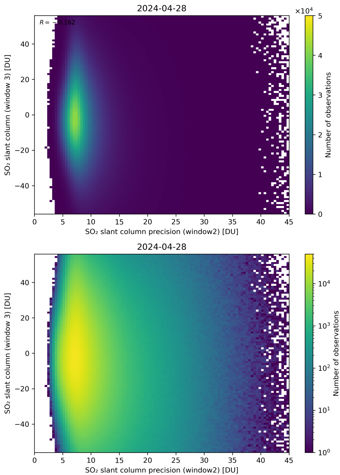
Figure 249: Scatter density plot of “SO 2 slant column precision (window2)” against “SO 2 slant column (window 3)” for 2024-04-27 to 2024-04-29.
