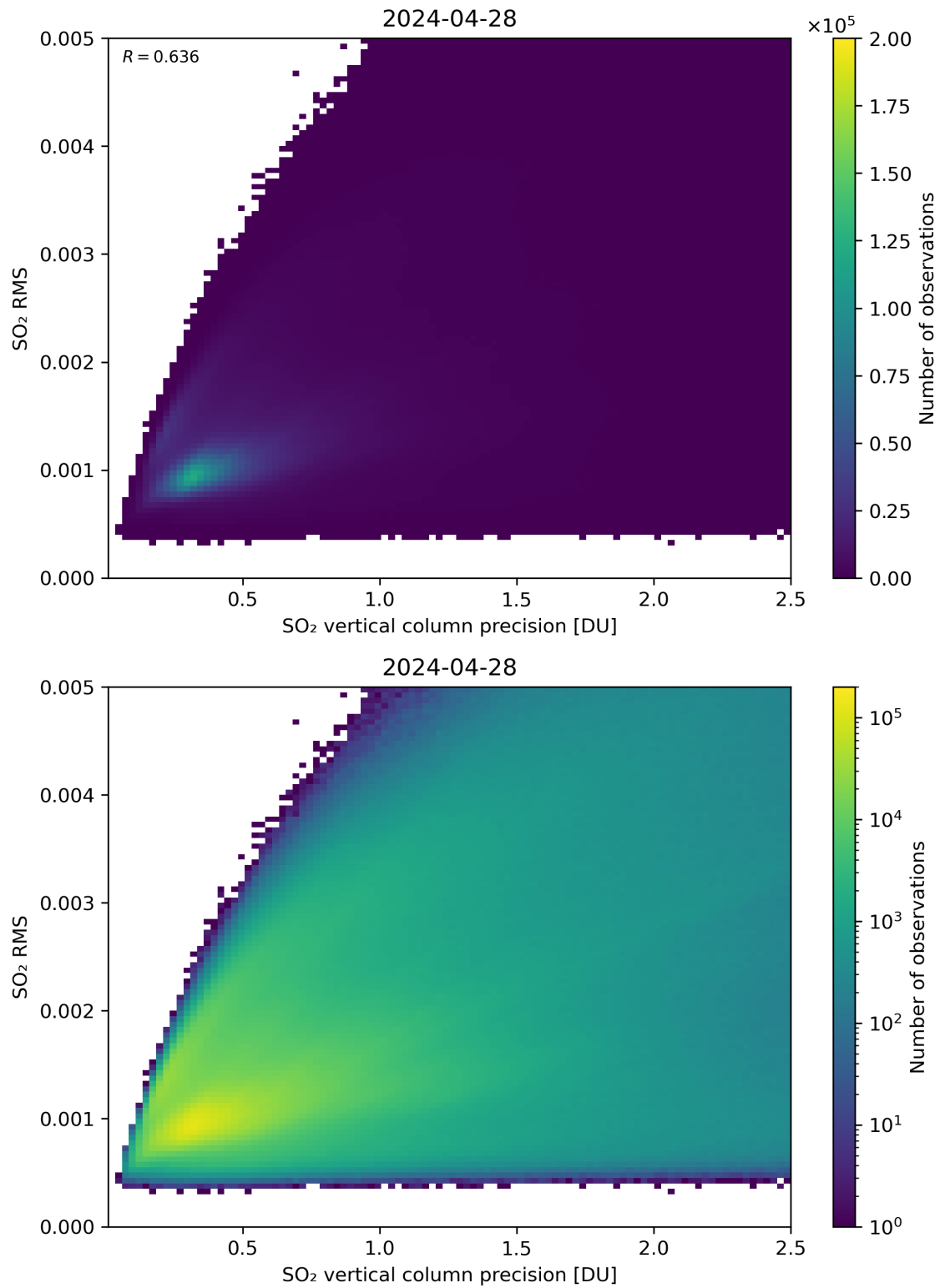
Figure 284: Scatter density plot of “SO 2 vertical column precision” against “SO 2 RMS” for 2024-04-27 to 2024-04-29.
