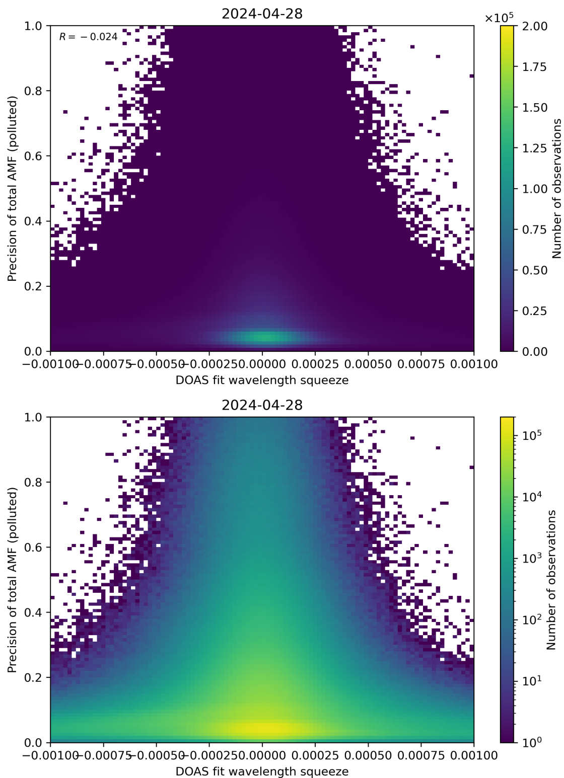
Figure 135: Scatter density plot of “DOAS fit wavelength squeeze” against “Precision of total AMF (polluted)” for 2024-04-27 to 2024-04-29.
