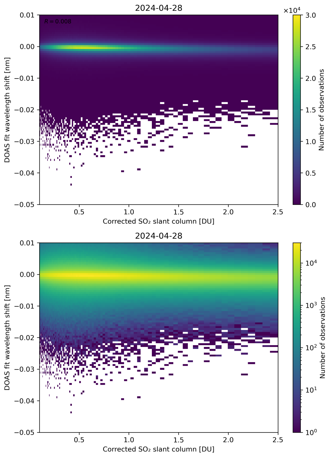
Figure 181: Scatter density plot of “Corrected SO 2 slant column” against “DOAS fit wavelength shift” for 2024-04-27 to 2024-04-29.
