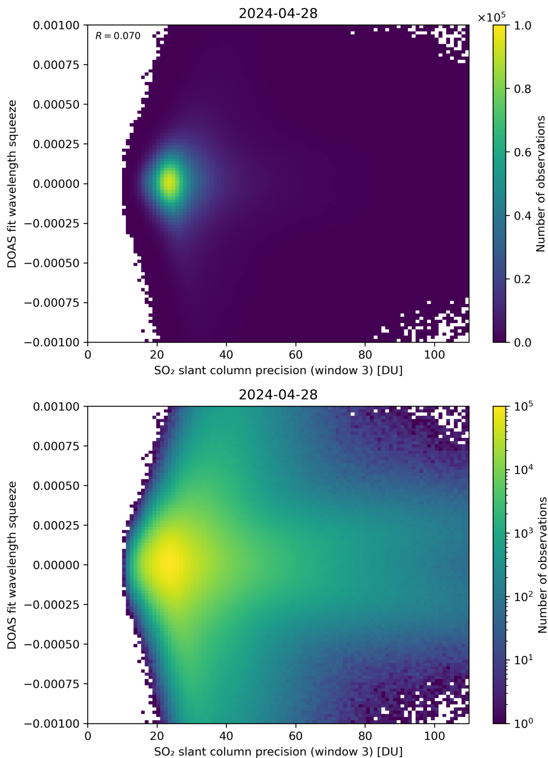
Figure 259: Scatter density plot of “SO 2 slant column precision (window 3)” against “DOAS fit wavelength squeeze” for 2024-04-27 to 2024-04-29.
