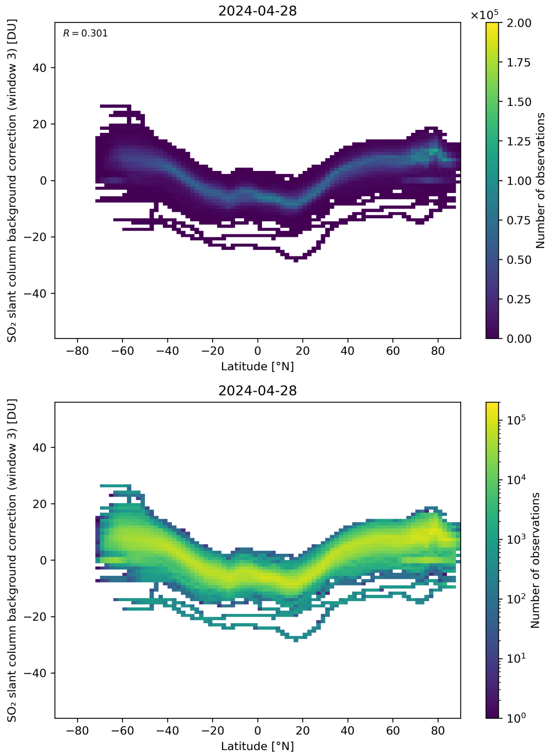
Figure 141: Scatter density plot of “Latitude” against “SO 2 slant column background correction (window 3)” for 2024-04-27 to 2024-04-29.
