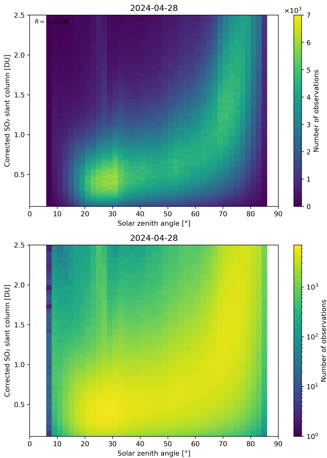
Figure 166: Scatter density plot of “Solar zenith angle” against “Corrected SO 2 slant column” for 2024-04-27 to 2024-04-29.
