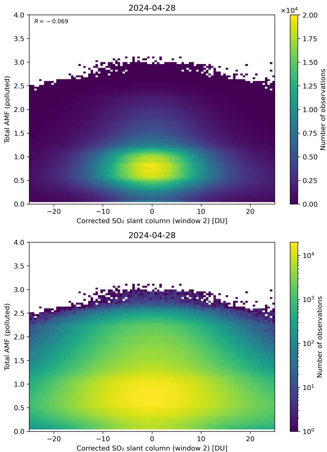
Figure 203: Scatter density plot of “Corrected SO 2 slant column (window 2)” against “Total AMF (polluted)” for 2024-04-27 to 2024-04-29.
