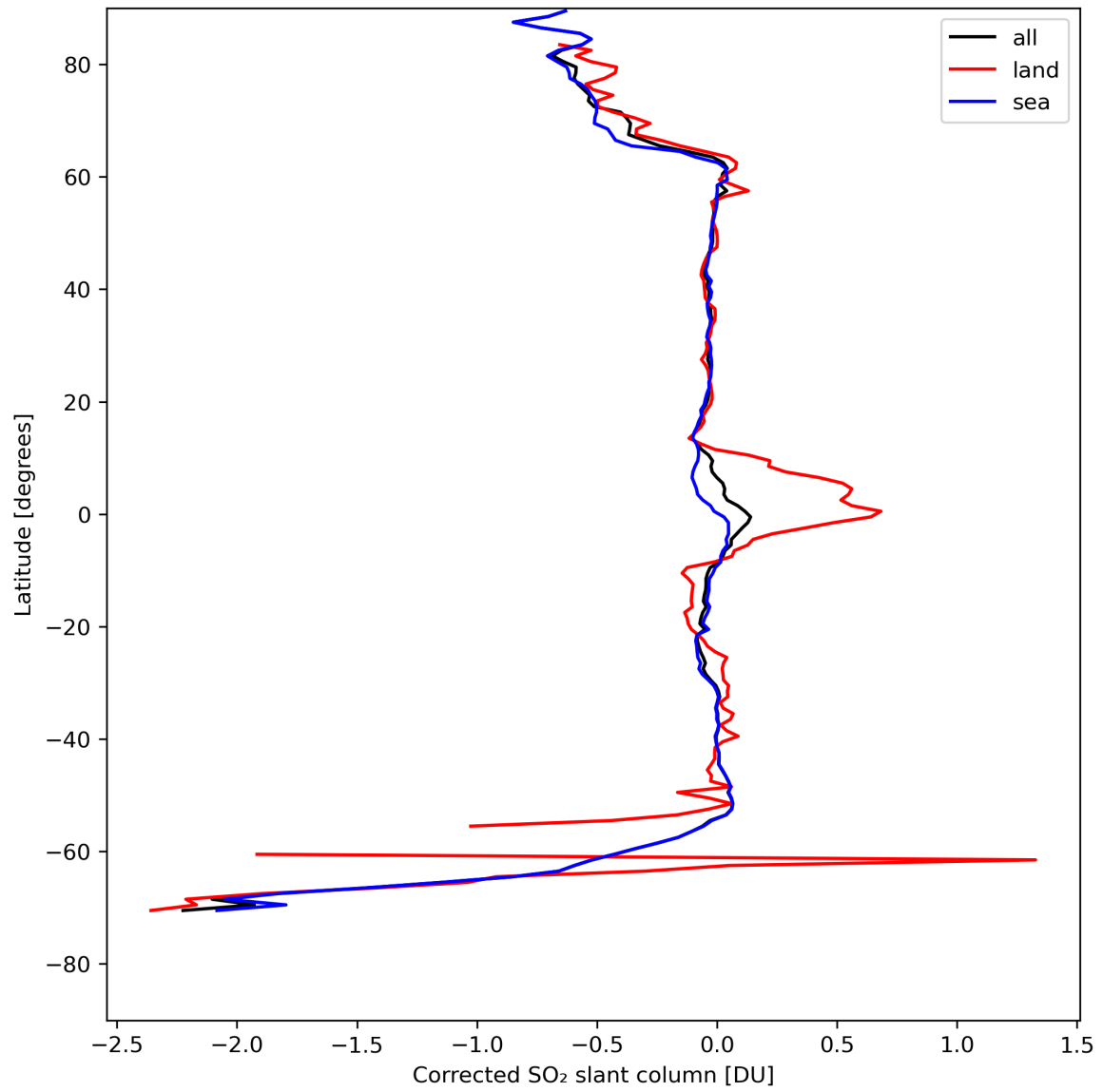
Figure 32: Zonal average of "Corrected SO 2 slant column" for 2024-04-27 to 2024-04-29.
