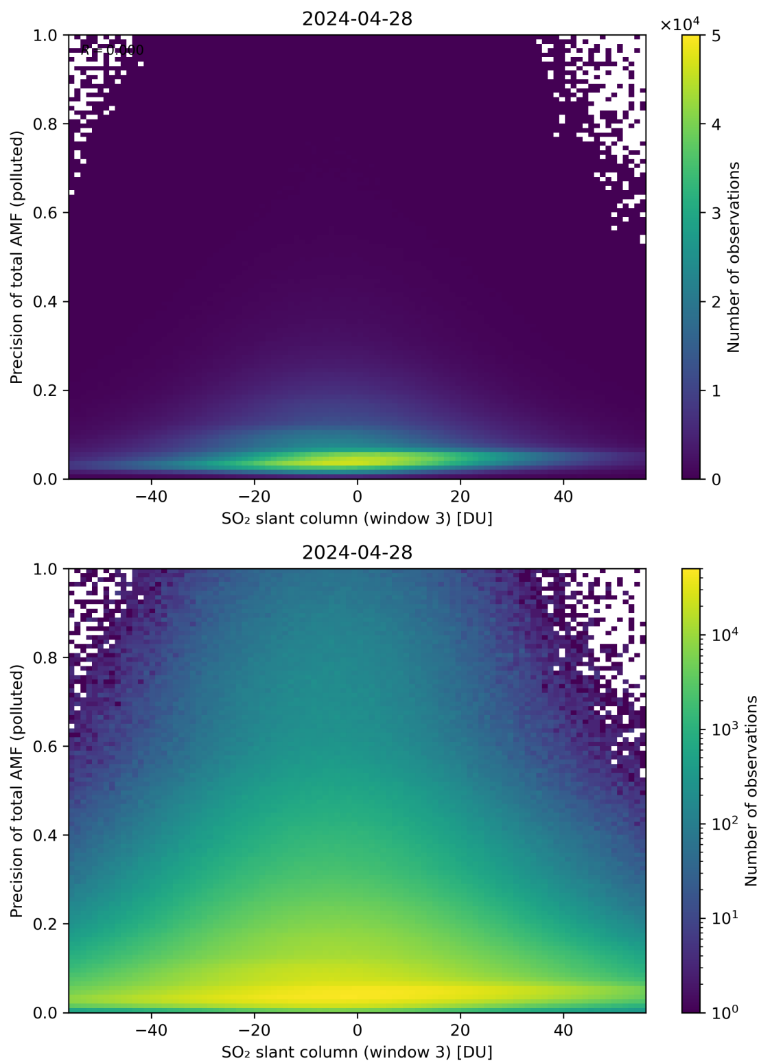
Figure 269: Scatter density plot of “SO 2 slant column (window 3)” against “Precision of total AMF (polluted)” for 2024-04-27 to 2024-04-29.
