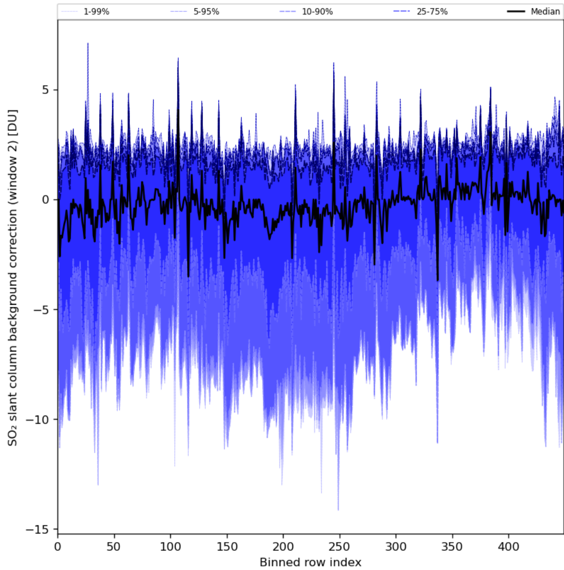
Figure 86: Along track statistics of “SO 2 slant column background correction (window 2)” for 2024-04-27 to 2024-04-29
