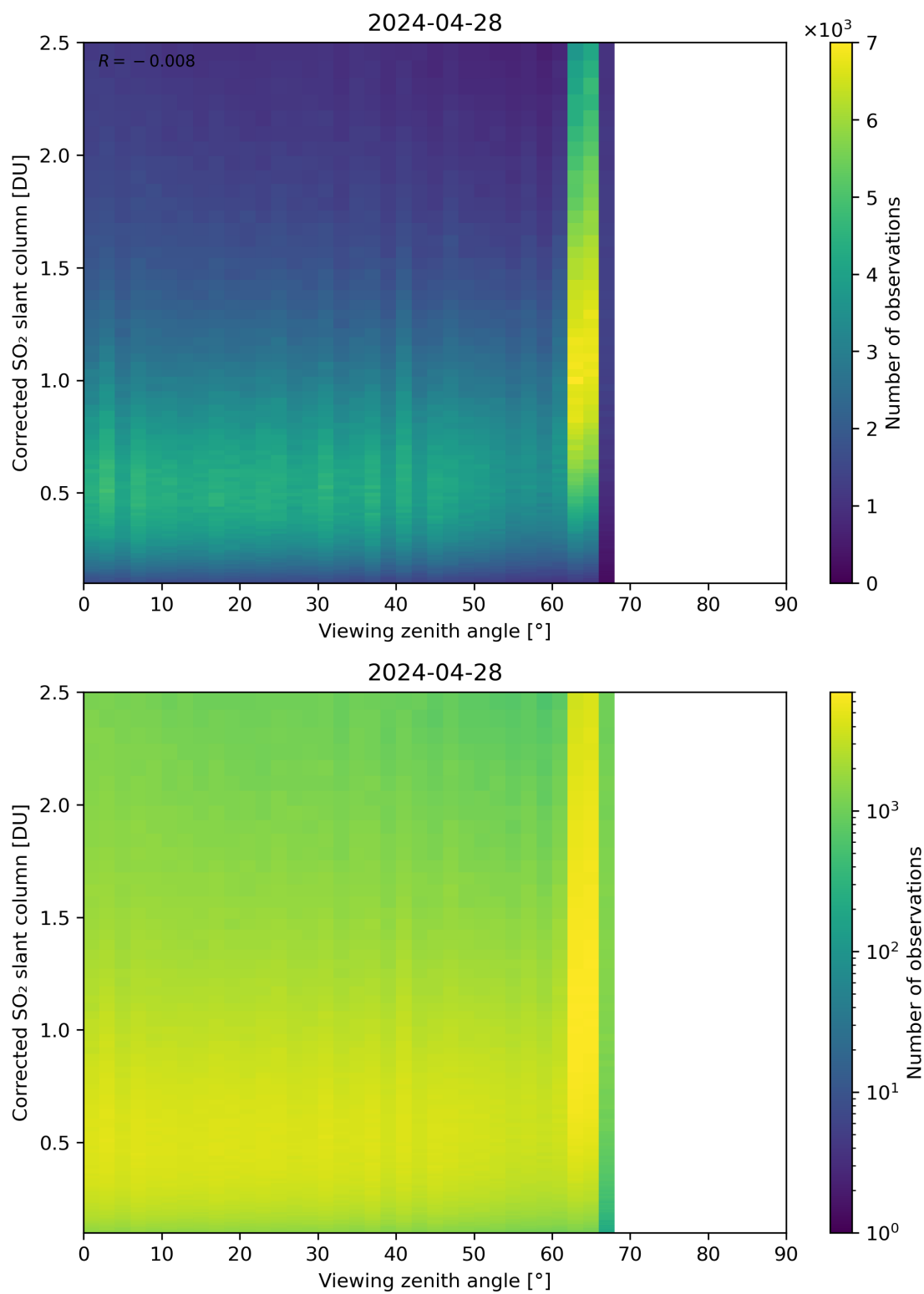
Figure 317: Scatter density plot of “Viewing zenith angle” against “Corrected SO 2 slant column” for 2024-04-27 to 2024-04-29.
