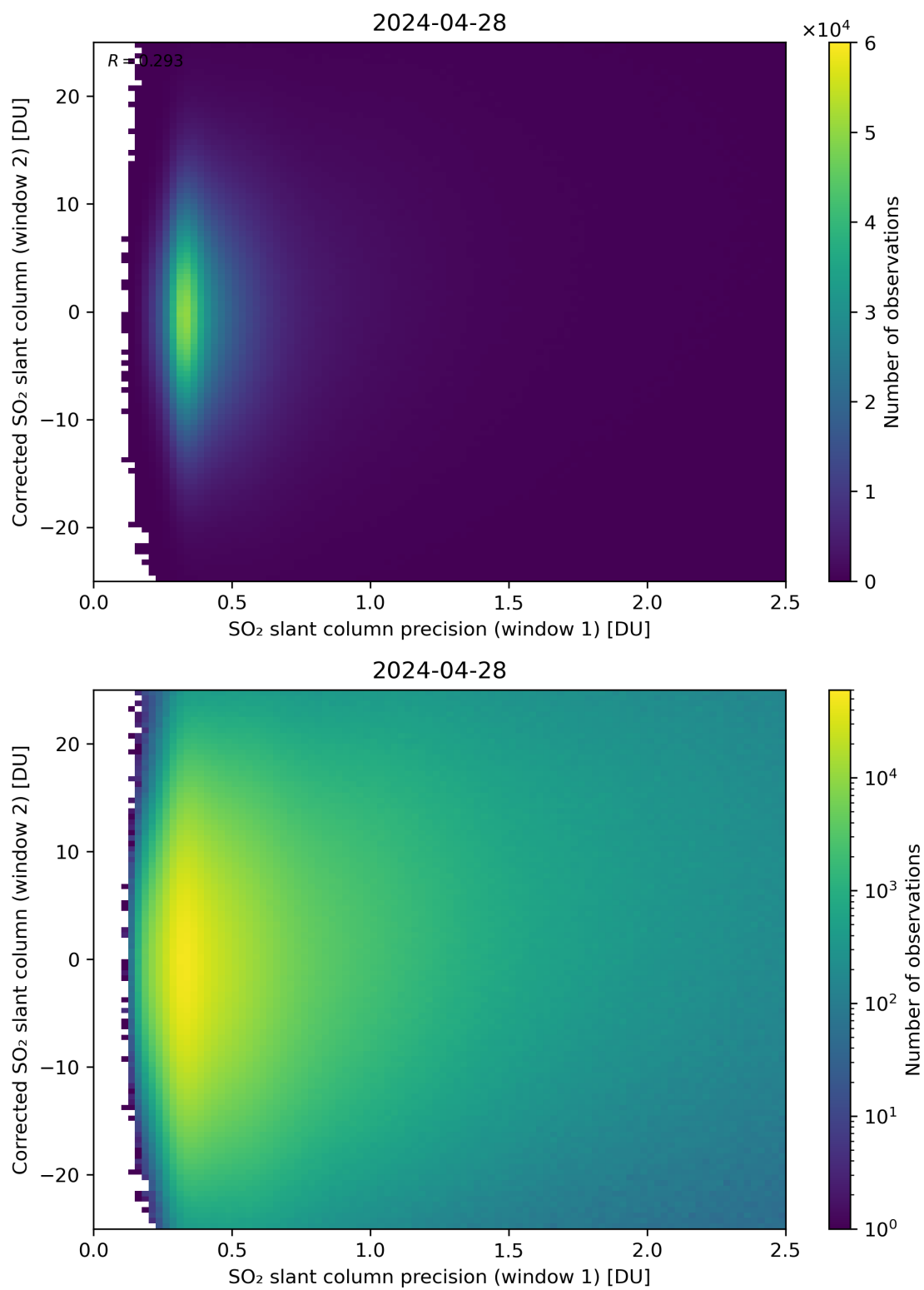
Figure 225: Scatter density plot of “SO 2 slant column precision (window 1)” against “Corrected SO 2 slant column (window 2)” for 2024-04-27 to 2024-04-29.
