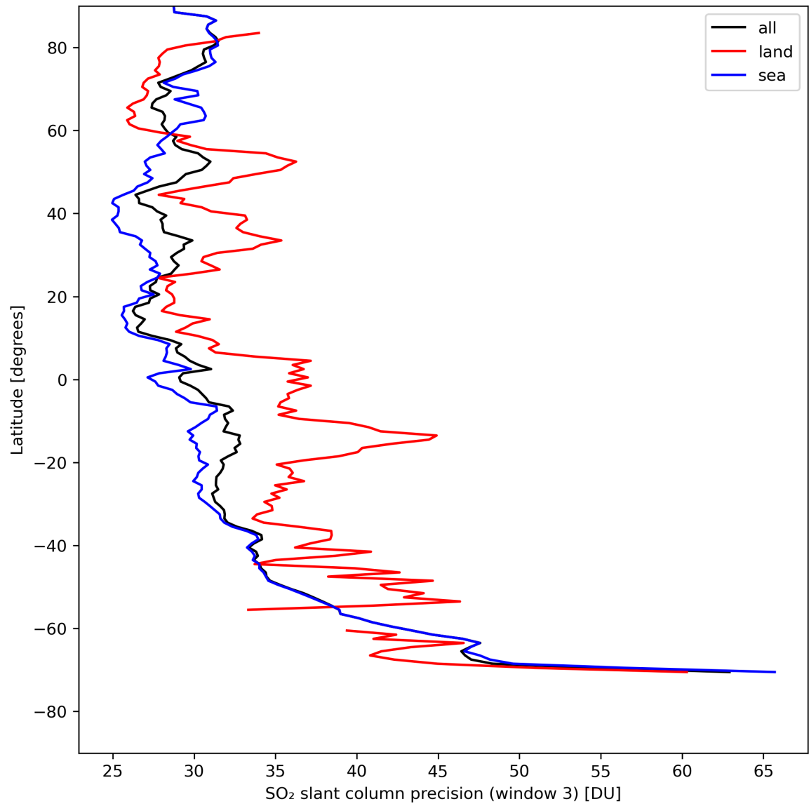
Figure 42: Zonal average of “SO 2 slant column precision (window 3)” for 2024-04-27 to 2024-04-29.
