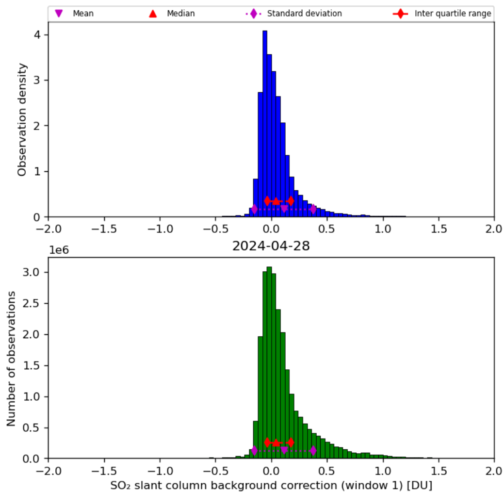
Figure 59: Histogram of “SO 2 slant column background correction (window 1)” for 2024-04-27 to 2024-04-29
