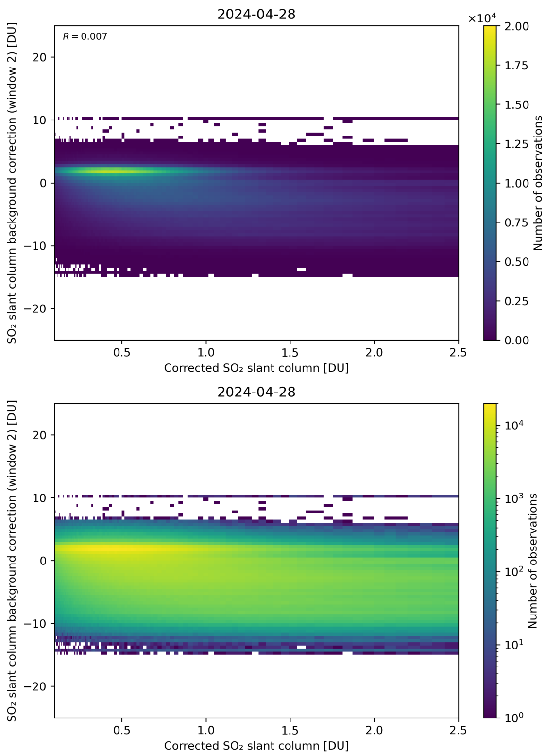
Figure 179: Scatter density plot of “Corrected SO 2 slant column” against “SO 2 slant column background correction (window 2)” for 2024-04-27 to 2024-04-29.
