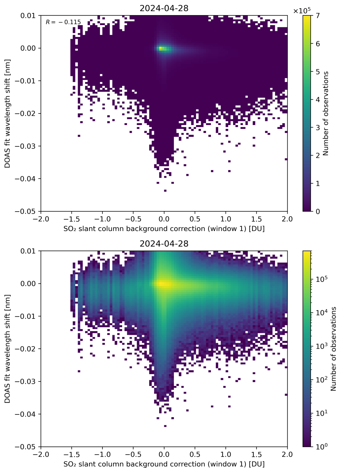
Figure 100: Scatter density plot of “SO 2 slant column background correction (window 1)” against “DOAS fit wavelength shift” for 2024-04-27 to 2024-04-29.
