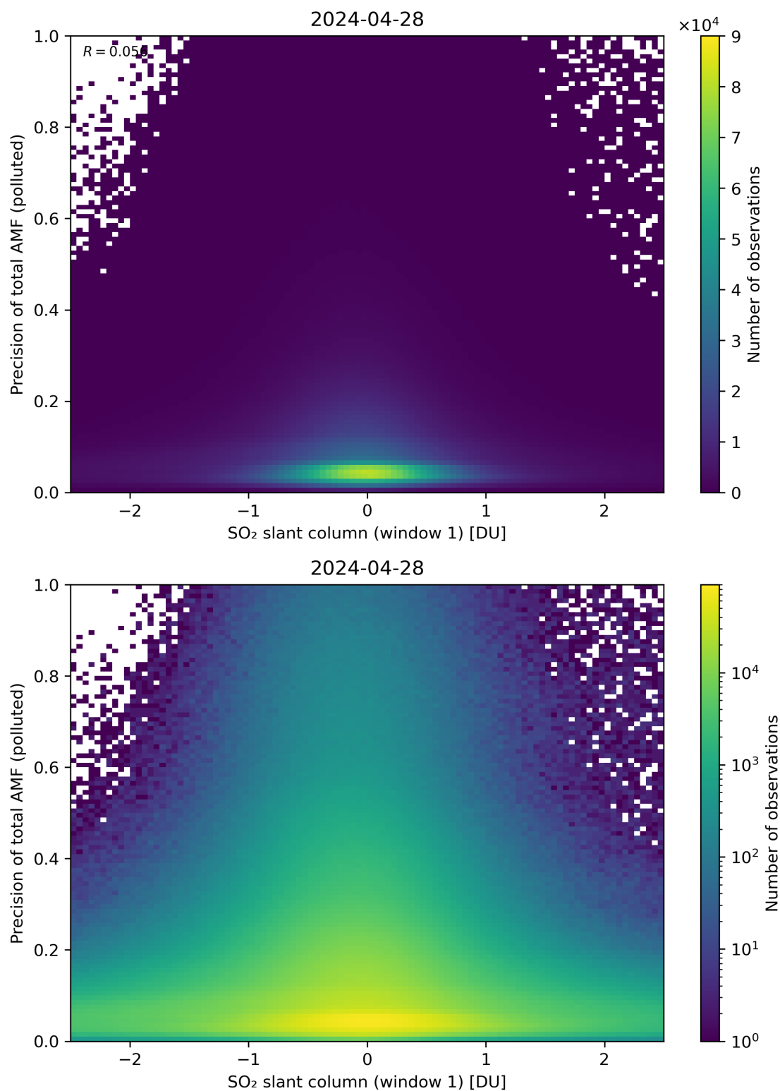
Figure 240: Scatter density plot of “SO 2 slant column (window 1)” against “Precision of total AMF (polluted)” for 2024-04-27 to 2024-04-29.
