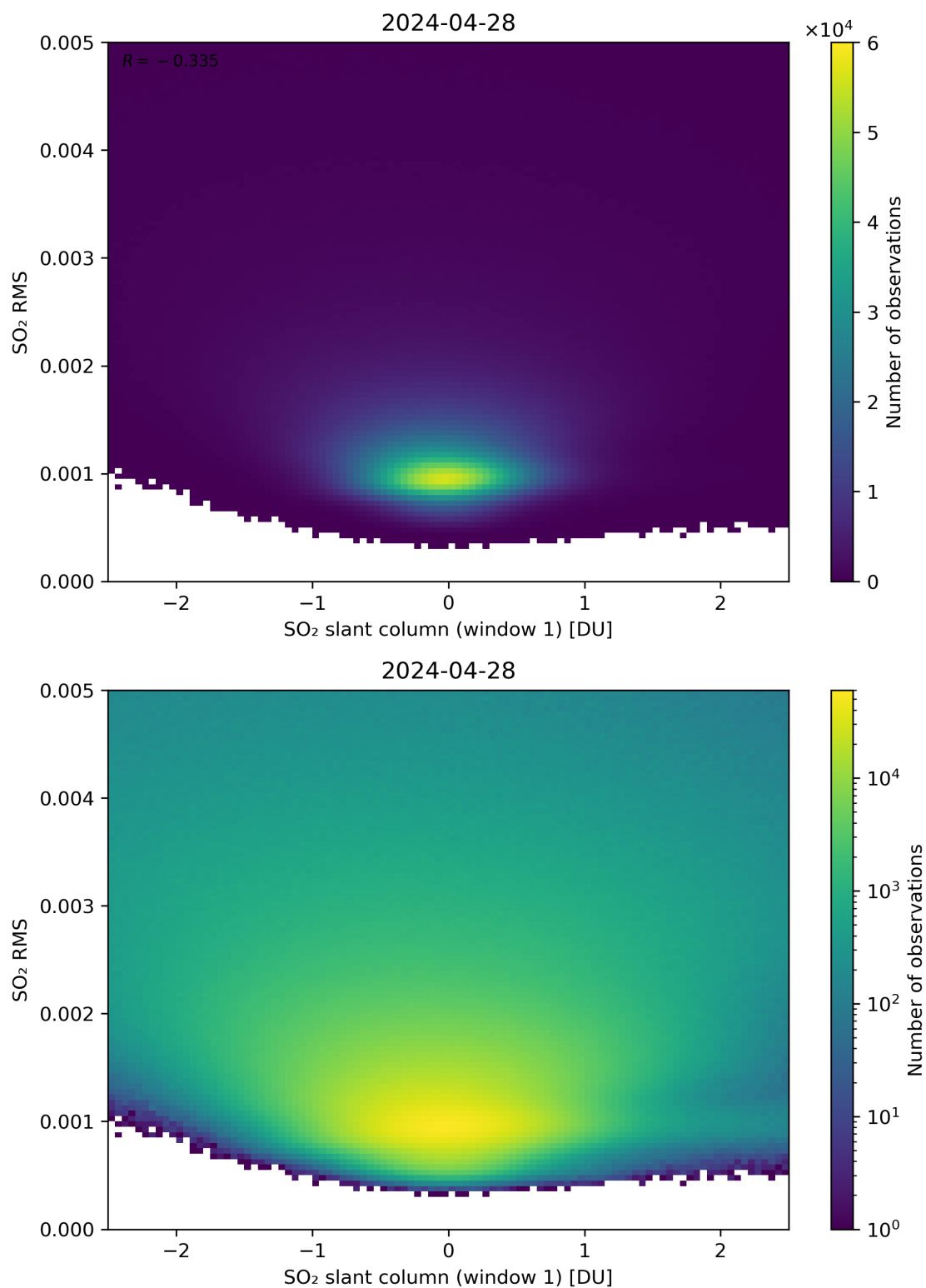
Figure 217: Scatter density plot of “SO 2 slant column (window 1)” against “SO 2 RMS” for 2024-04-27 to 2024-04-29.
