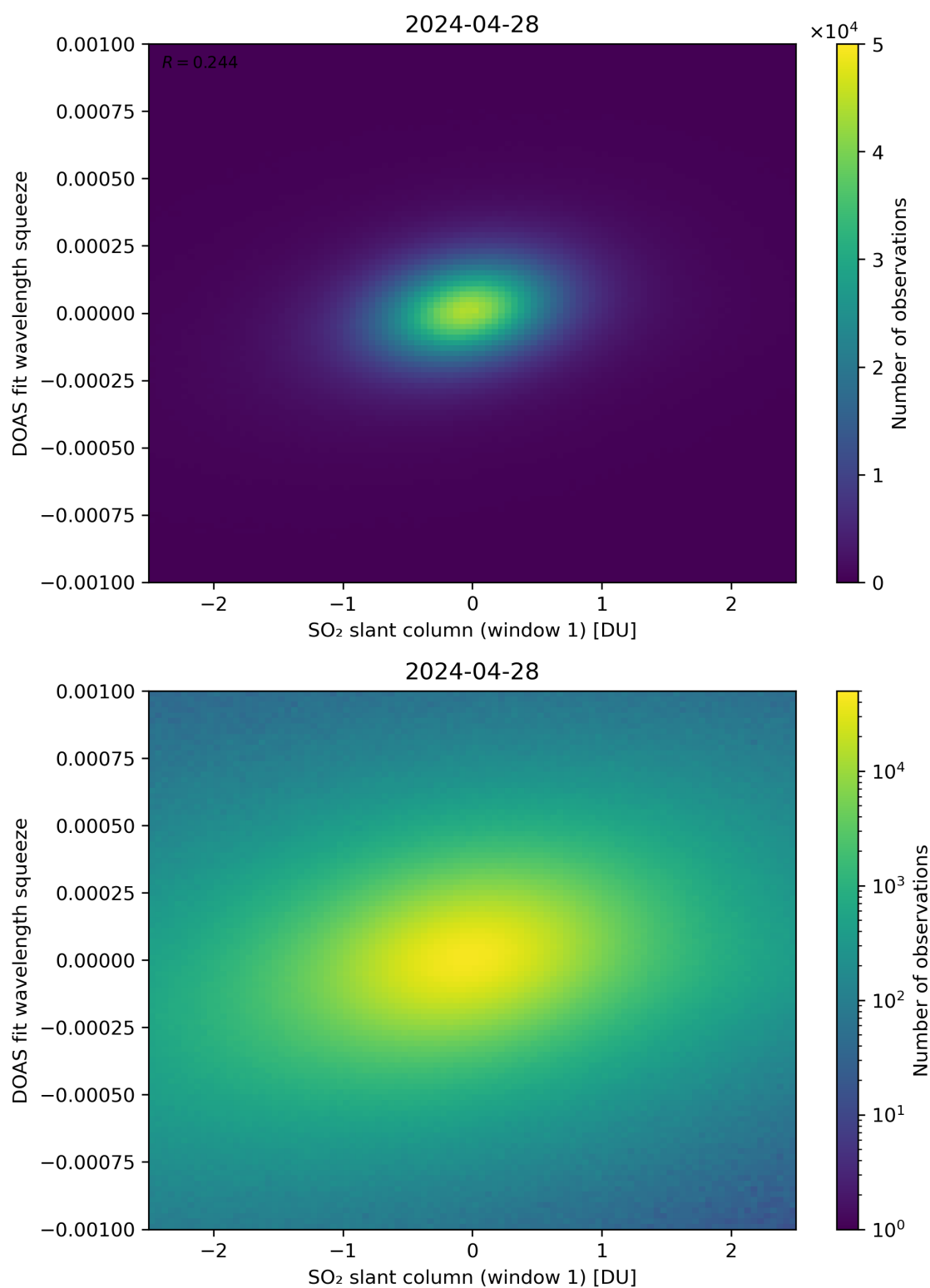
Figure 216: Scatter density plot of “SO 2 slant column (window 1)” against “DOAS fit wavelength squeeze” for 2024-04-27 to 2024-04-29.
