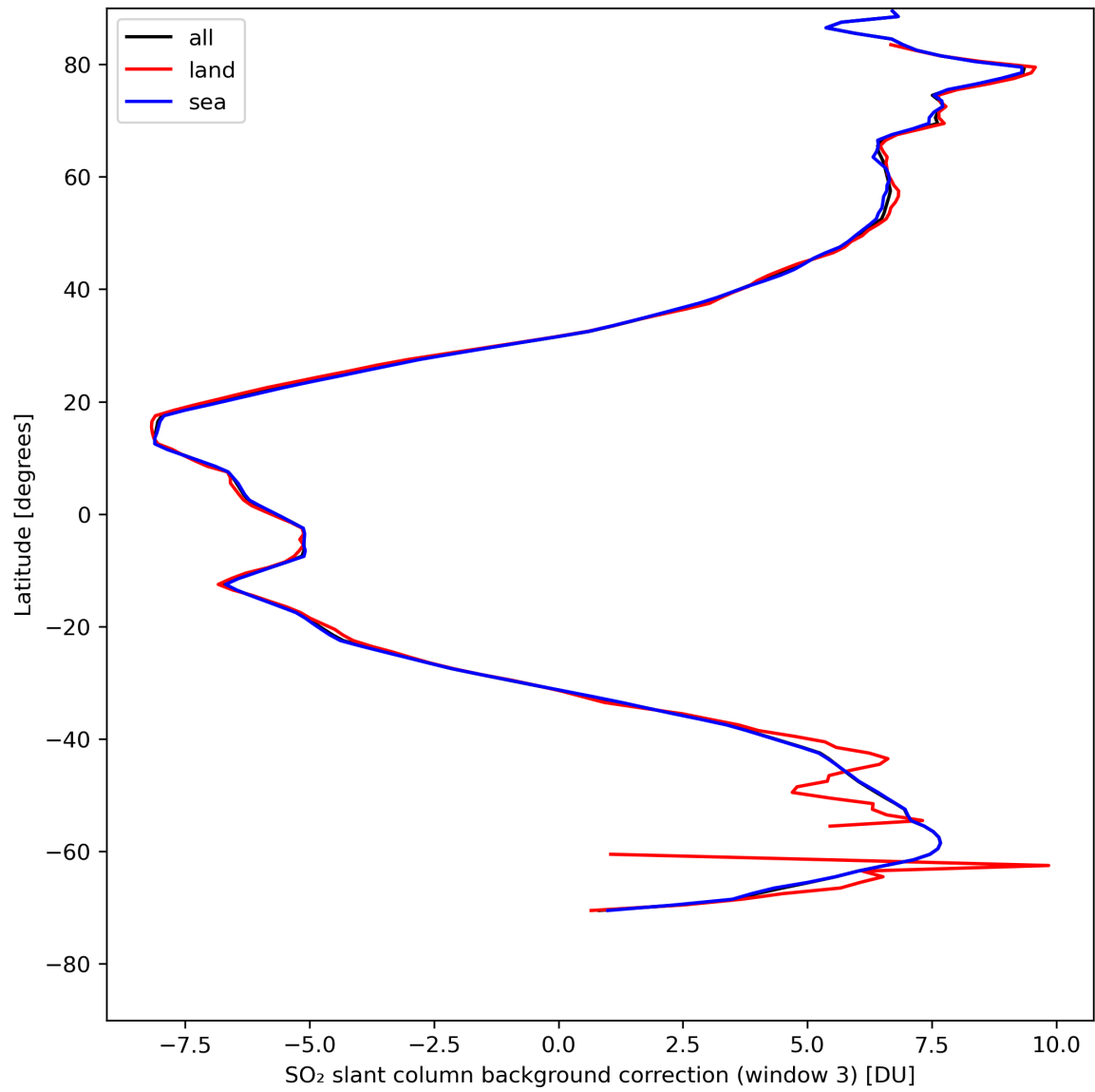
Figure 44: Zonal average of “SO 2 slant column background correction (window 3)” for 2024-04-27 to 2024-04-29.
