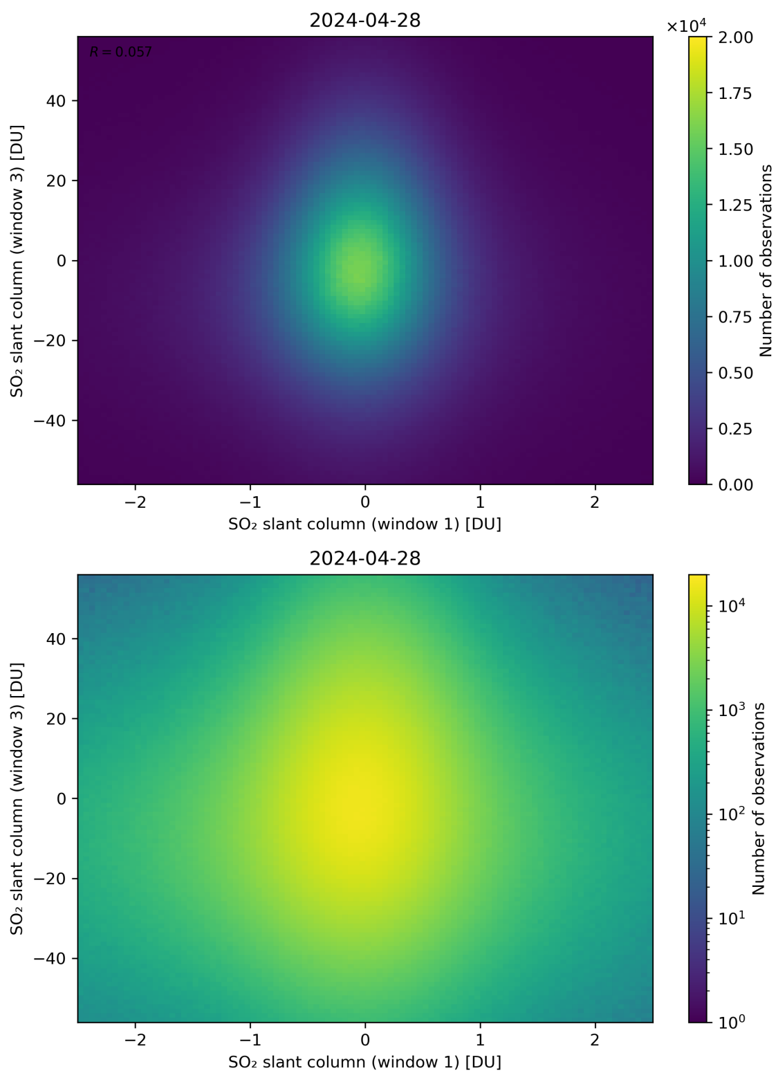
Figure 237: Scatter density plot of “SO 2 slant column (window 1)” against “SO 2 slant column (window 3)” for 2024-04-27 to 2024-04-29.
