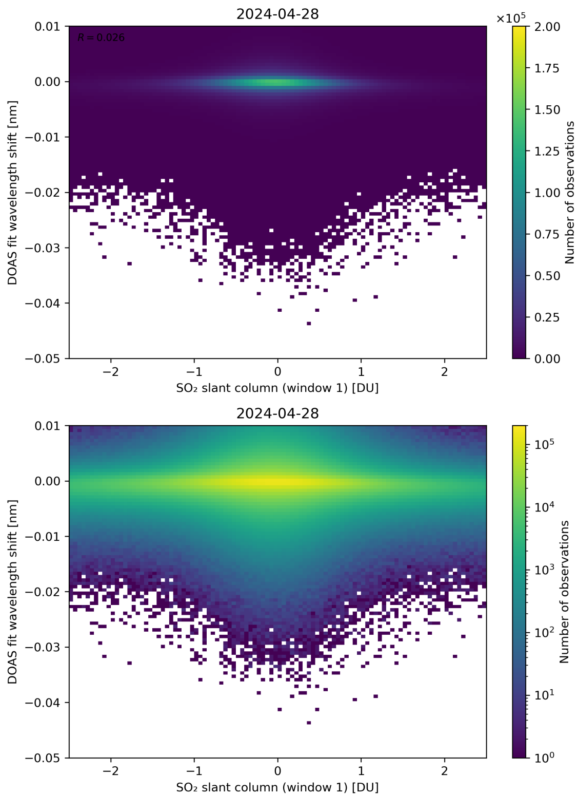
Figure 215: Scatter density plot of “SO 2 slant column (window 1)” against “DOAS fit wavelength shift” for 2024-04-27 to 2024-04-29.
