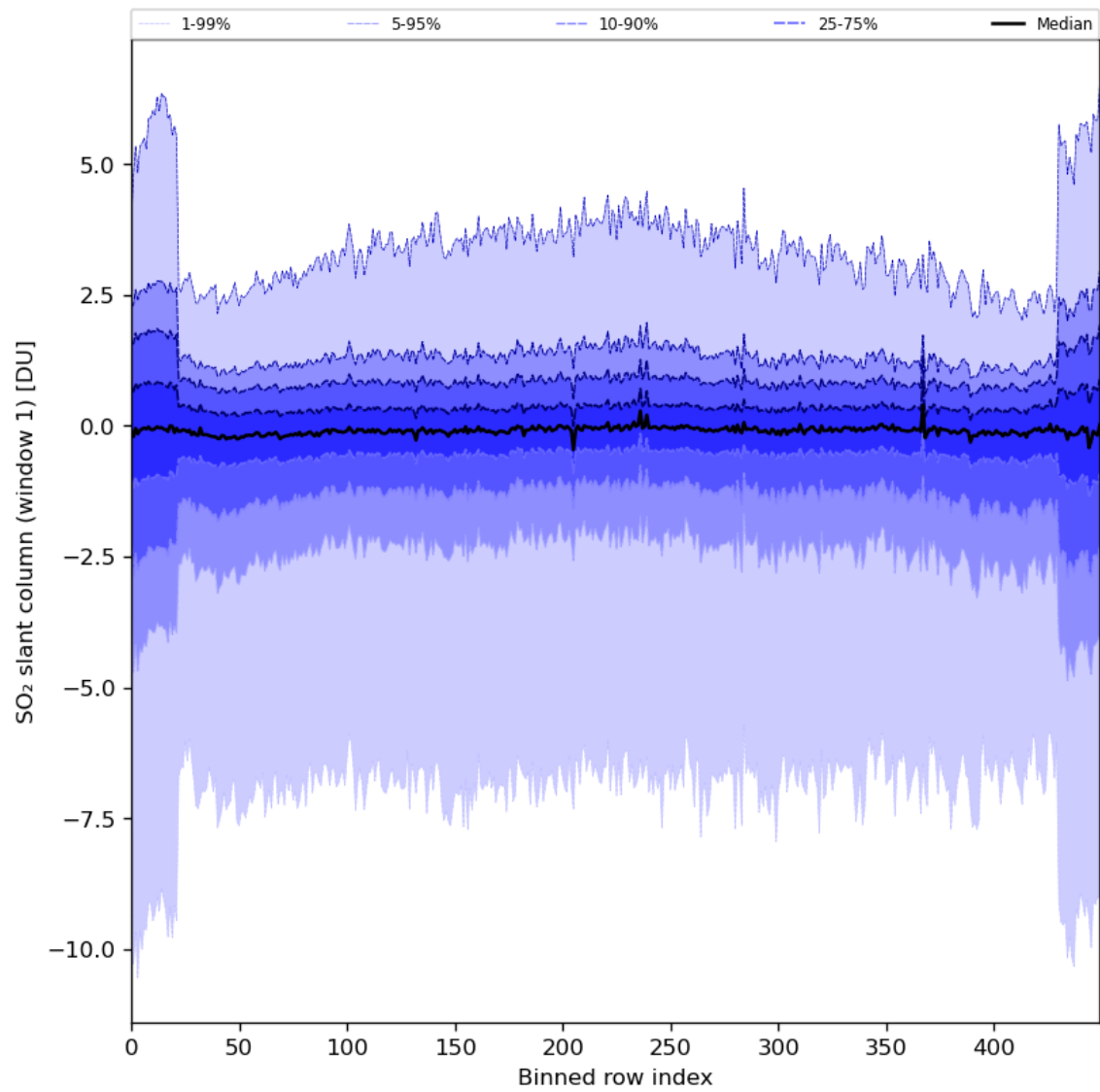
Figure 79: Along track statistics of “SO 2 slant column (window 1)” for 2024-04-27 to 2024-04-29
