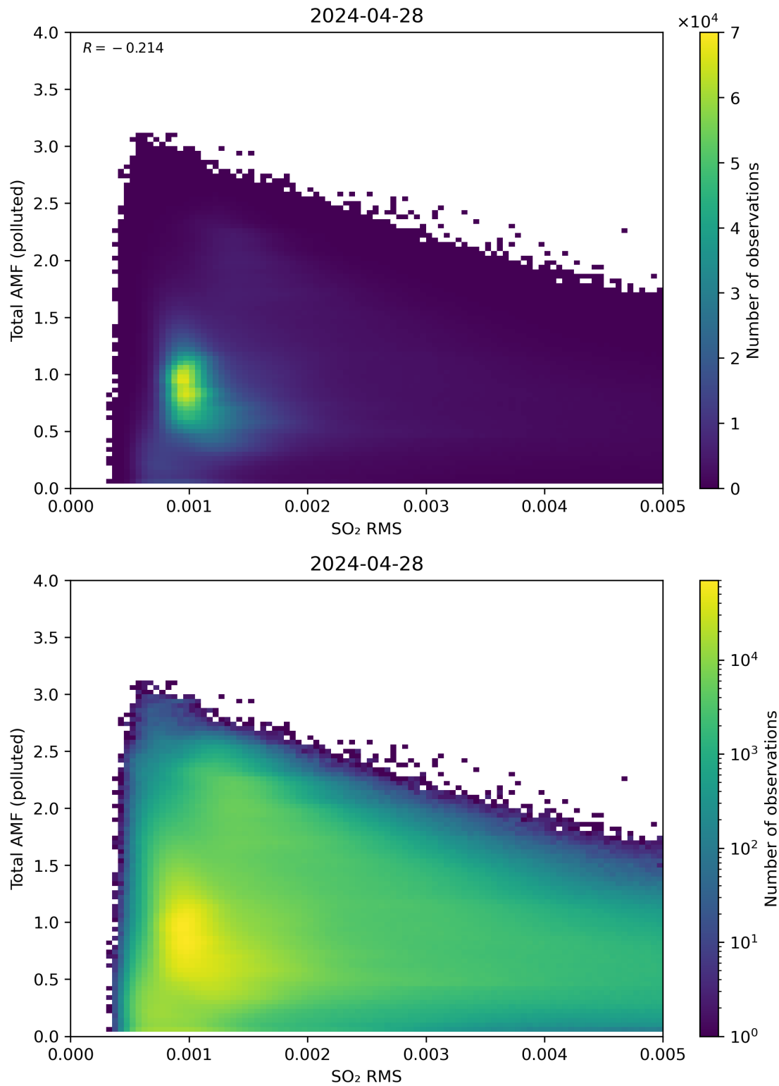
Figure 137: Scatter density plot of “SO 2 RMS” against “Total AMF (polluted)” for 2024-04-27 to 2024-04-29.
