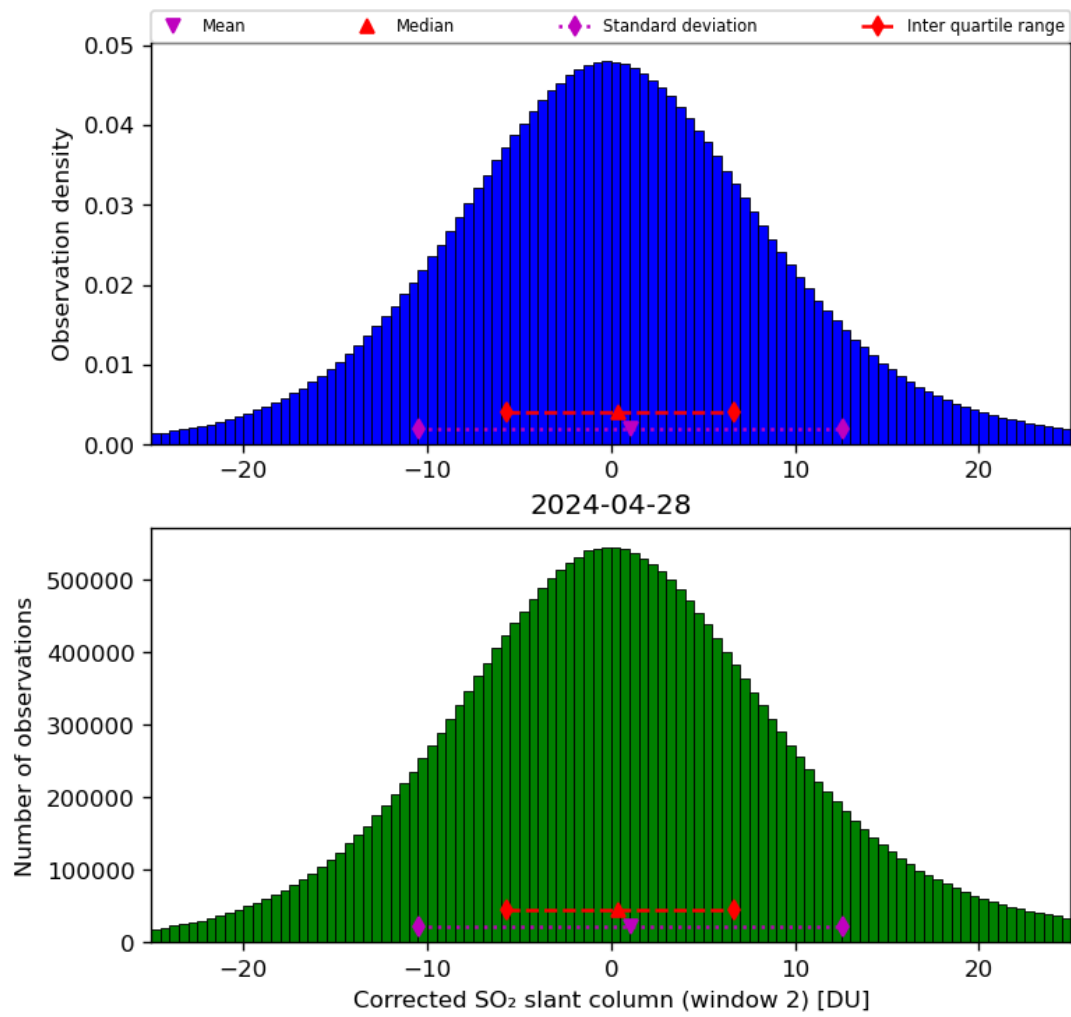
Figure 62: Histogram of “Corrected SO 2 slant column (window 2)” for 2024-04-27 to 2024-04-29
