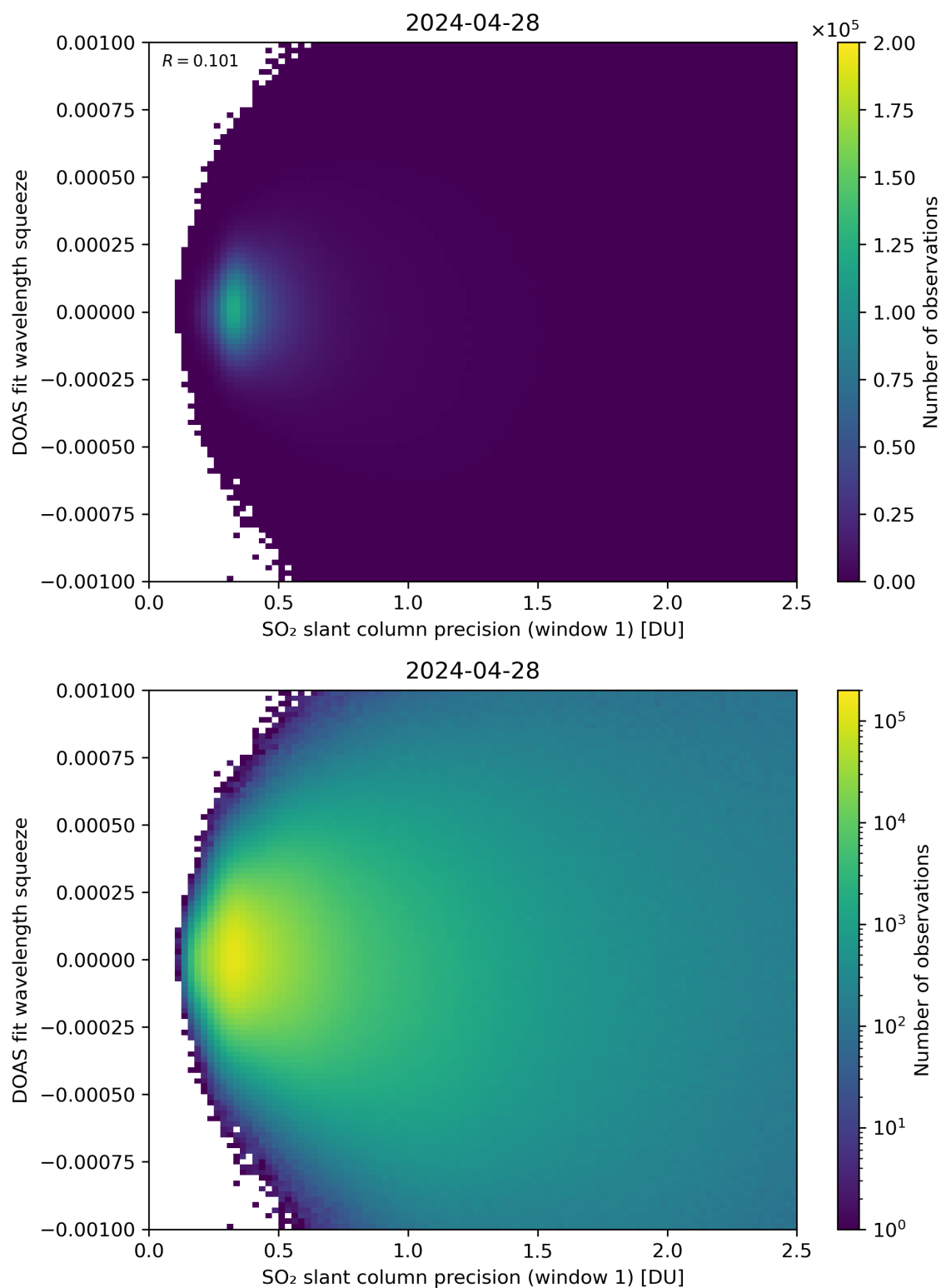
Figure 222: Scatter density plot of “SO 2 slant column precision (window 1)” against “DOAS fit wavelength squeeze” for 2024-04-27 to 2024-04-29.
