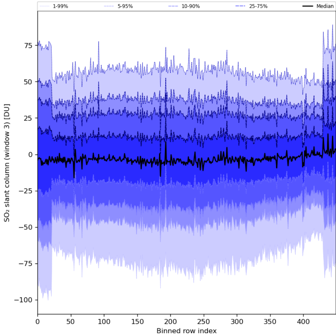
Figure 87: Along track statistics of “SO 2 slant column (window 3)” for 2024-04-27 to 2024-04-29
