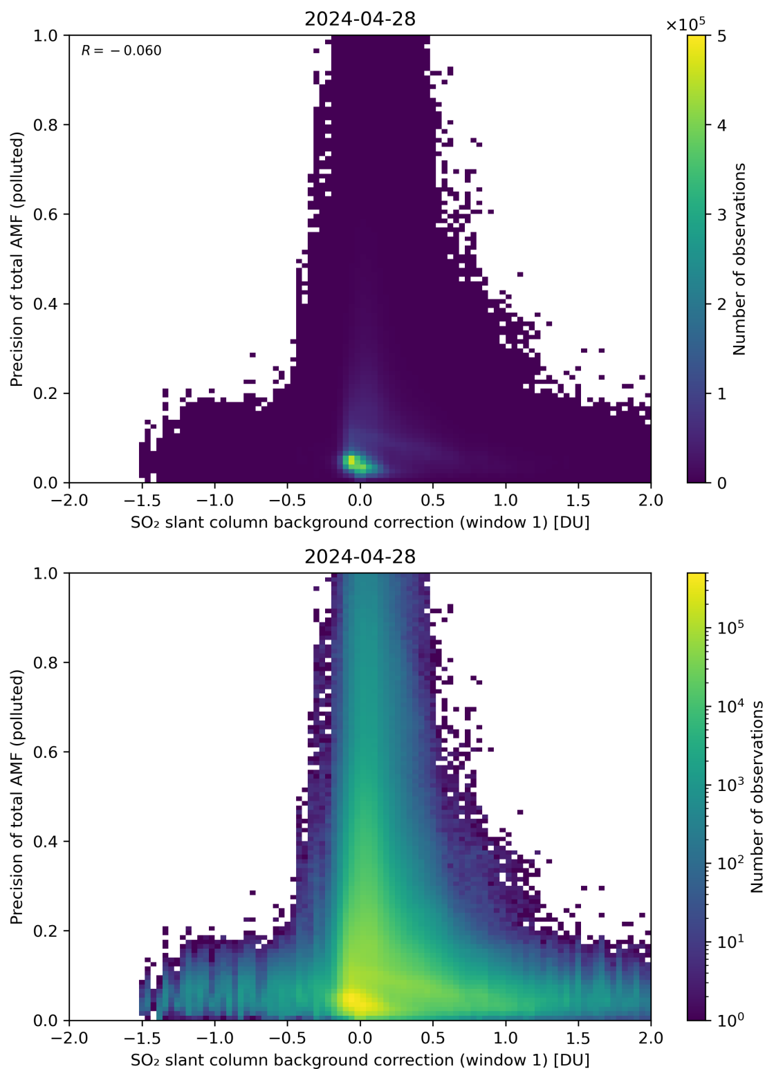
Figure 110: Scatter density plot of “SO 2 slant column background correction (window 1)” against “Precision of total AMF (polluted)” for 2024-04-27 to 2024-04-29.
