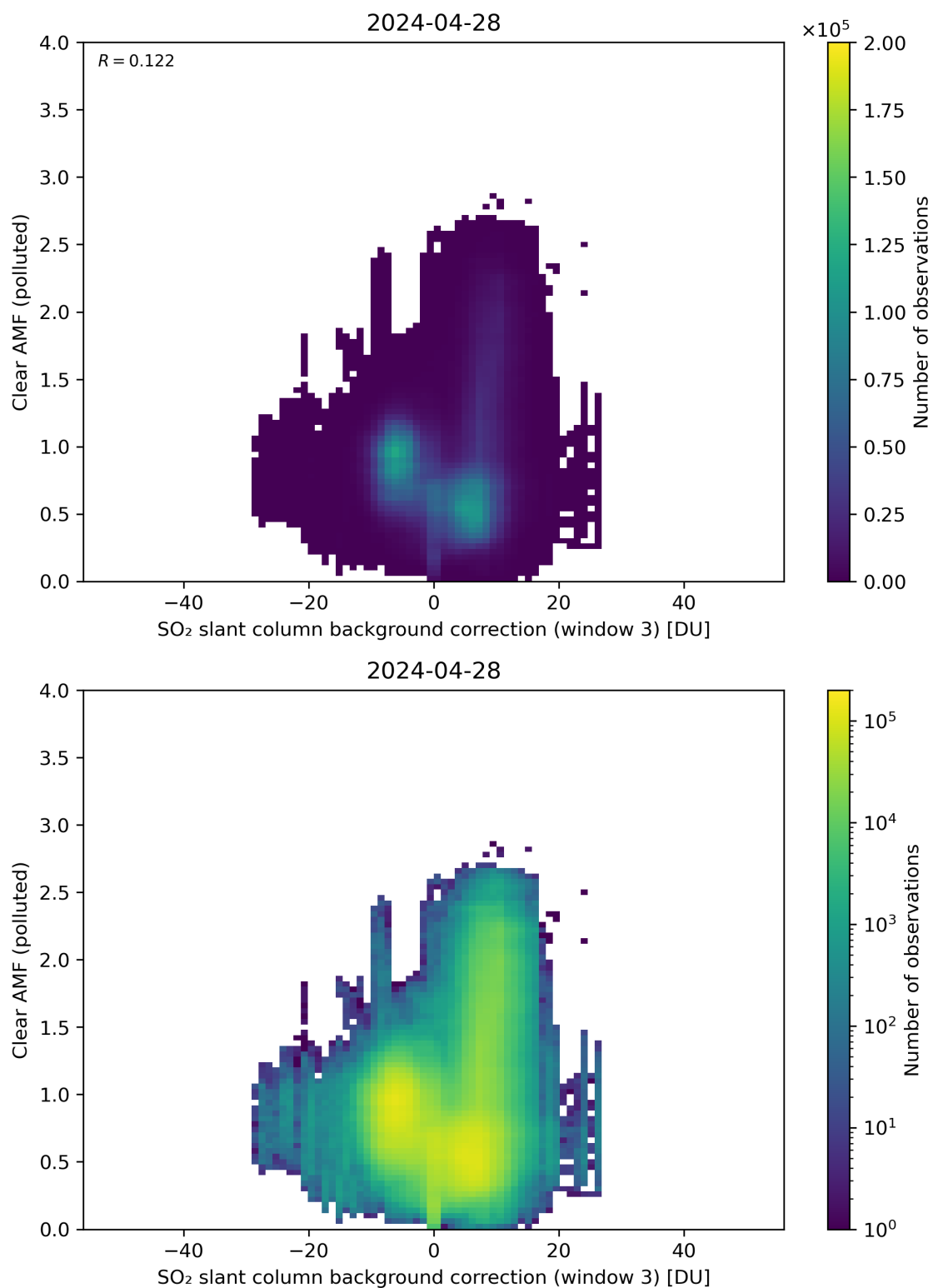
Figure 124: Scatter density plot of “SO 2 slant column background correction (window 3)” against “Clear AMF (polluted)” for 2024-04-27 to 2024-04-29.
