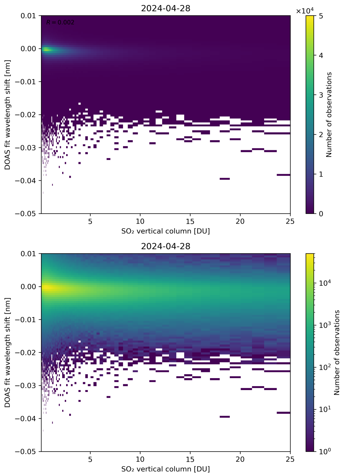
Figure 276: Scatter density plot of “SO 2 vertical column” against “DOAS fit wavelength shift” for 2024-04-27 to 2024-04-29.
