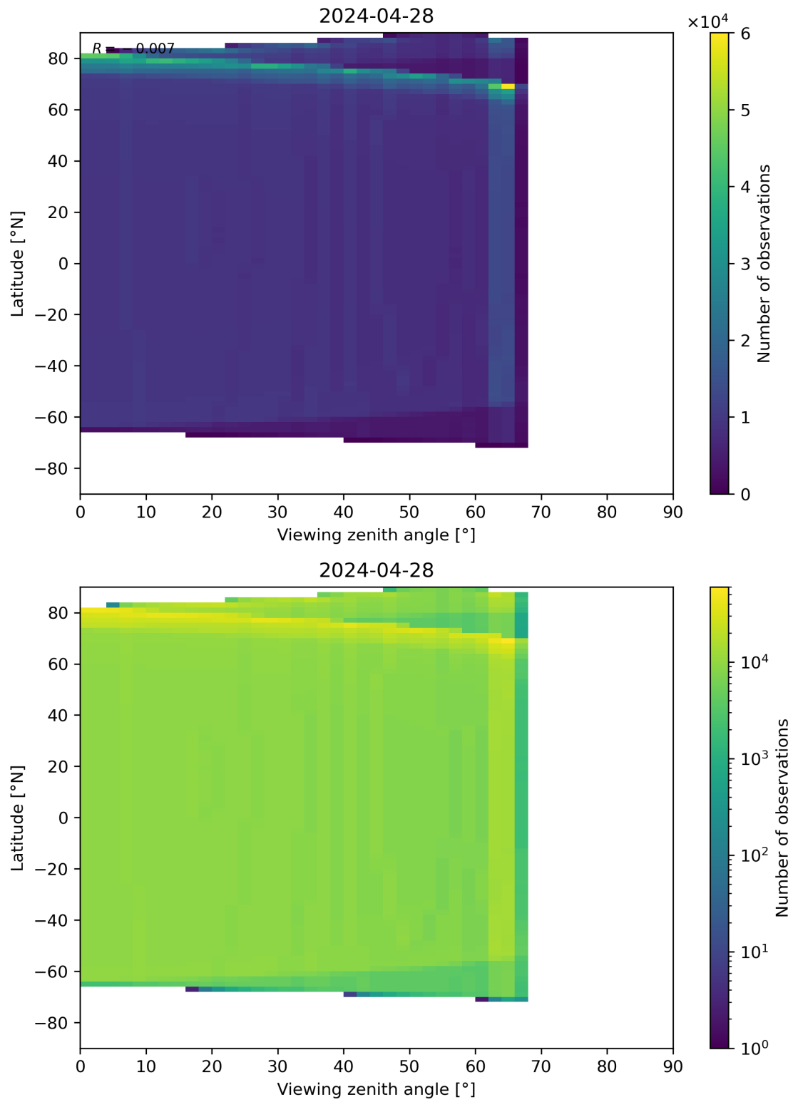
Figure 314: Scatter density plot of “Viewing zenith angle” against “Latitude” for 2024-04-27 to 2024-04-29.
