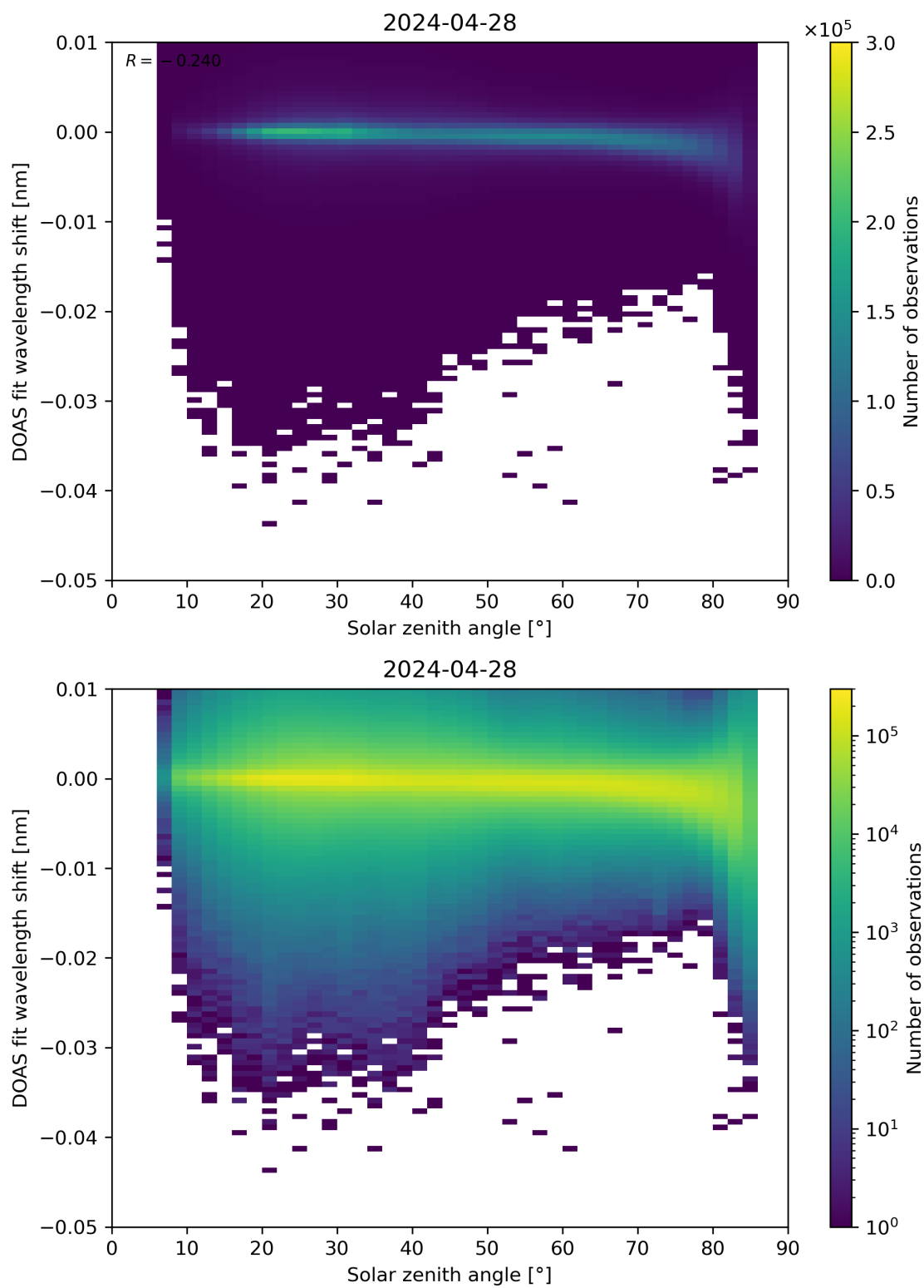
Figure 161: Scatter density plot of “Solar zenith angle” against “DOAS fit wavelength shift” for 2024-04-27 to 2024-04-29.
