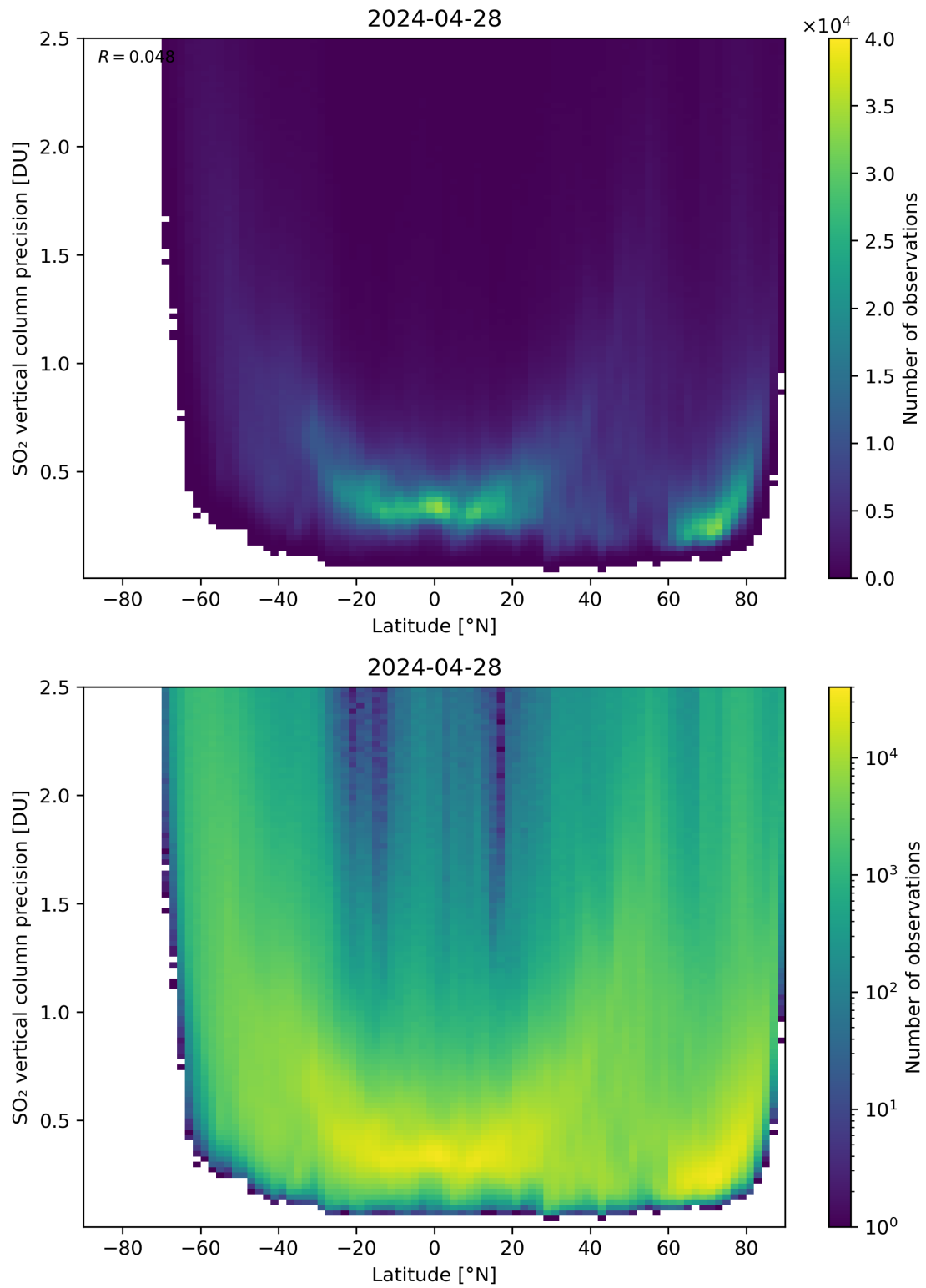
Figure 157: Scatter density plot of “Latitude” against “SO 2 vertical column precision” for 2024-04-27 to 2024-04-29.
