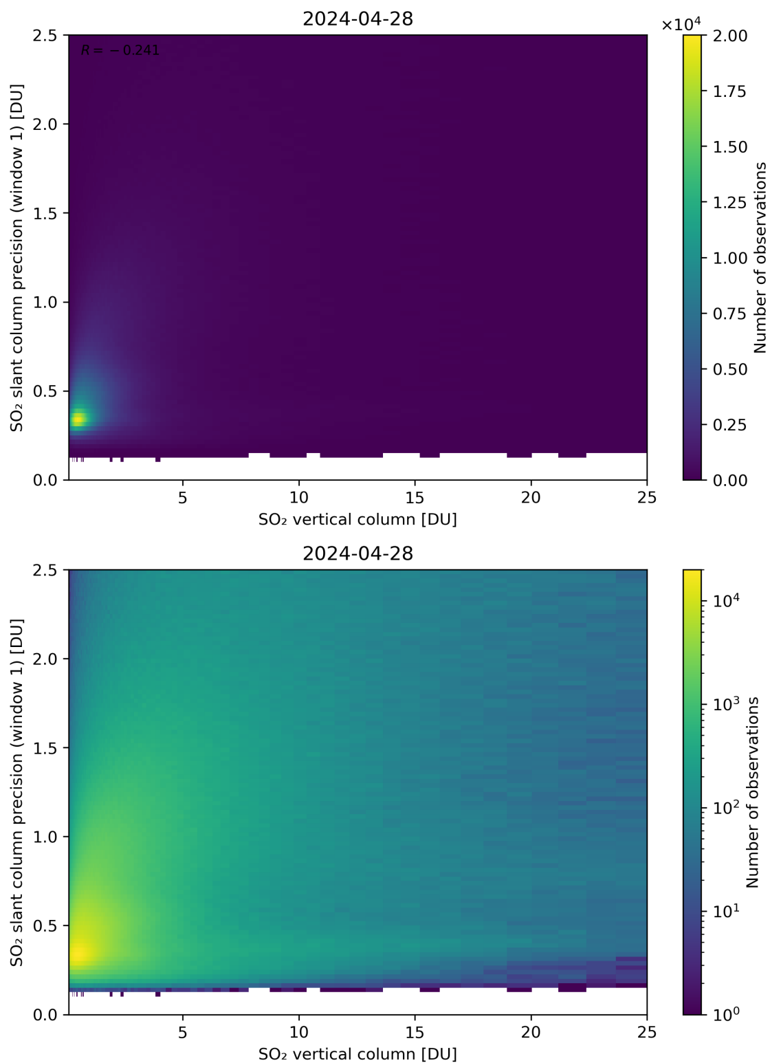
Figure 301: Scatter density plot of “SO 2 vertical column” against “SO 2 slant column precision (window 1)” for 2024-04-27 to 2024-04-29.
