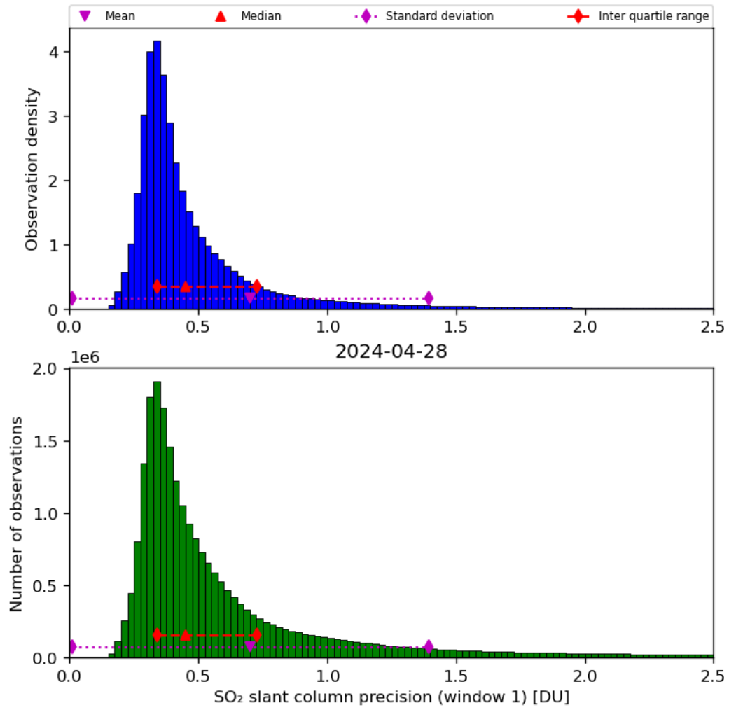
Figure 57: Histogram of “SO 2 slant column precision (window 1)” for 2024-04-27 to 2024-04-29
