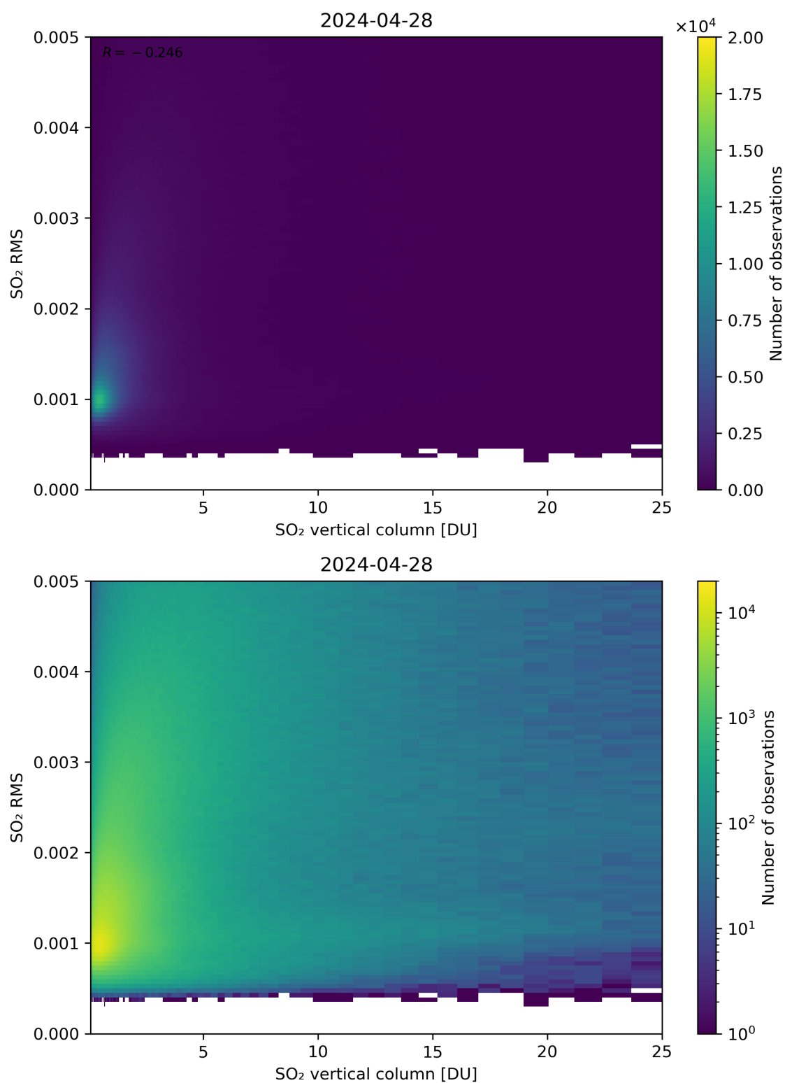
Figure 278: Scatter density plot of “SO 2 vertical column” against “SO 2 RMS” for 2024-04-27 to 2024-04-29.
