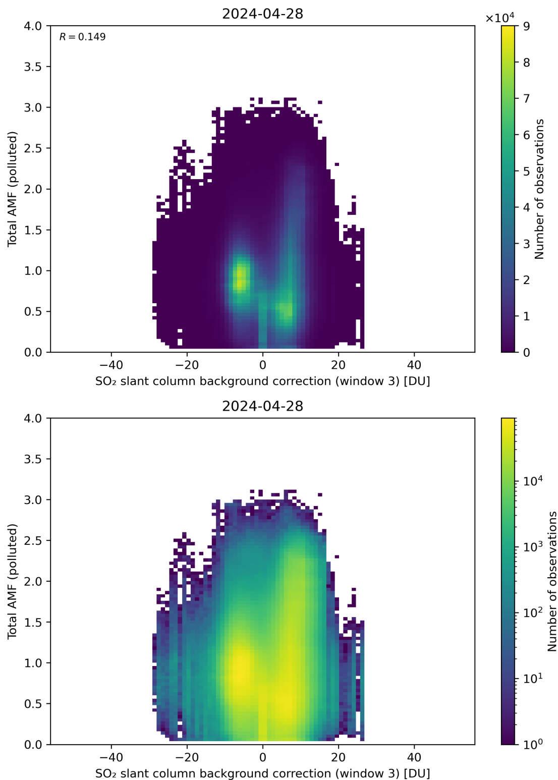
Figure 125: Scatter density plot of “SO 2 slant column background correction (window 3)” against “Total AMF (polluted)” for 2024-04-27 to 2024-04-29.
