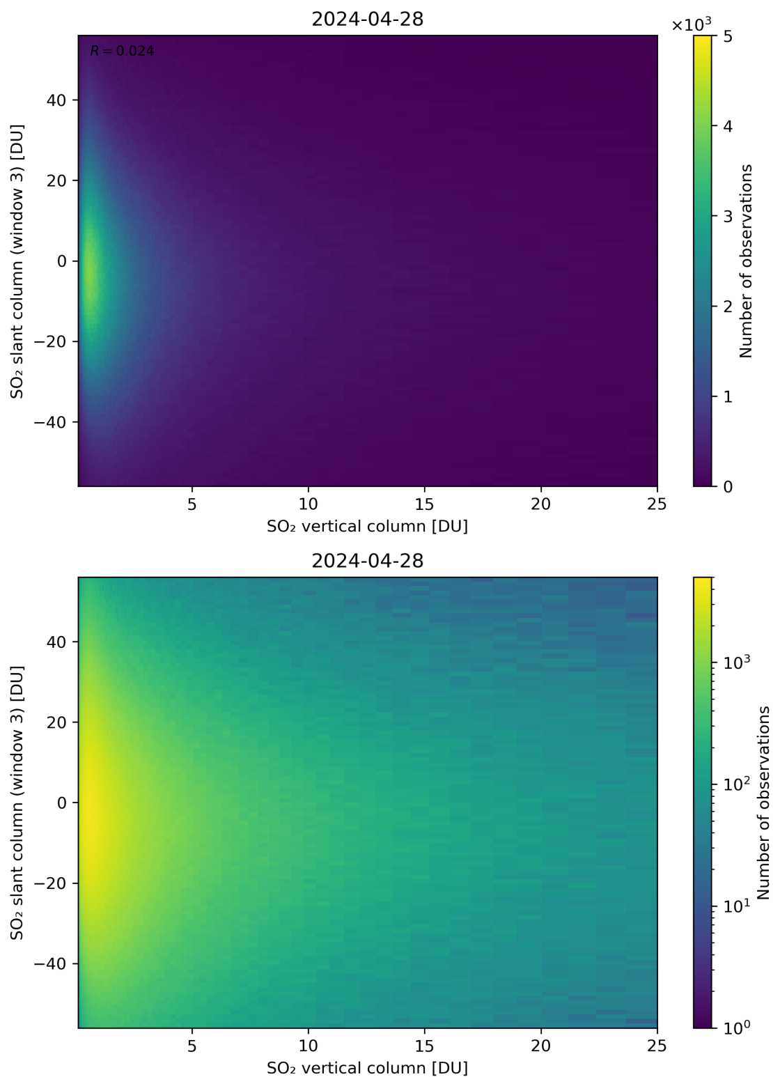
Figure 303: Scatter density plot of “SO 2 vertical column” against “SO 2 slant column (window 3)” for 2024-04-27 to 2024-04-29.
