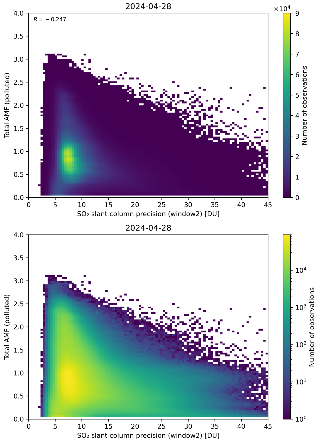
Figure 251: Scatter density plot of “SO 2 slant column precision (window2)” against “Total AMF (polluted)” for 2024-04-27 to 2024-04-29.
