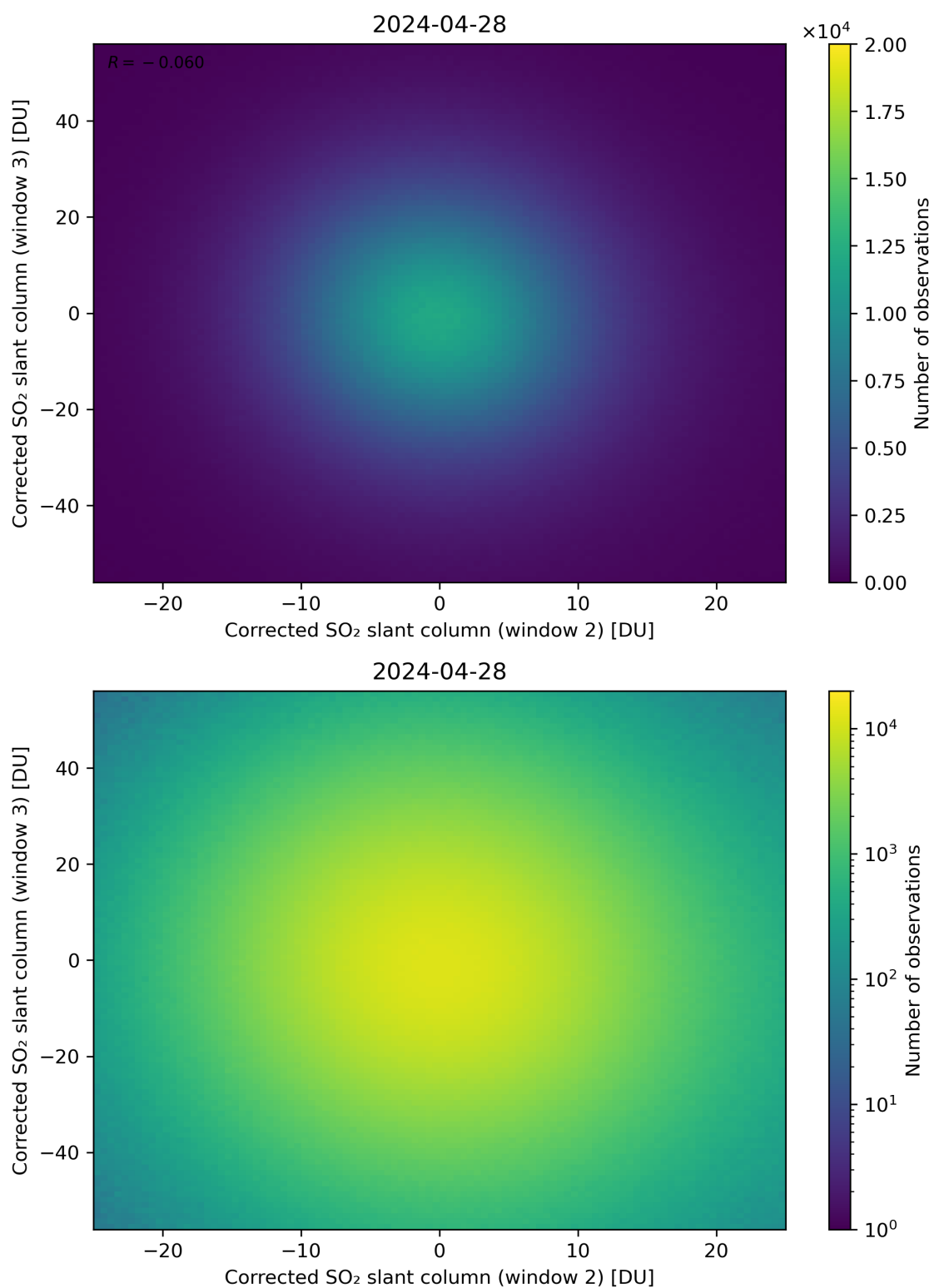
Figure 200: Scatter density plot of “Corrected SO 2 slant column (window 2)” against “Corrected SO 2 slant column (window 3)” for 2024-04-27 to 2024-04-29.
