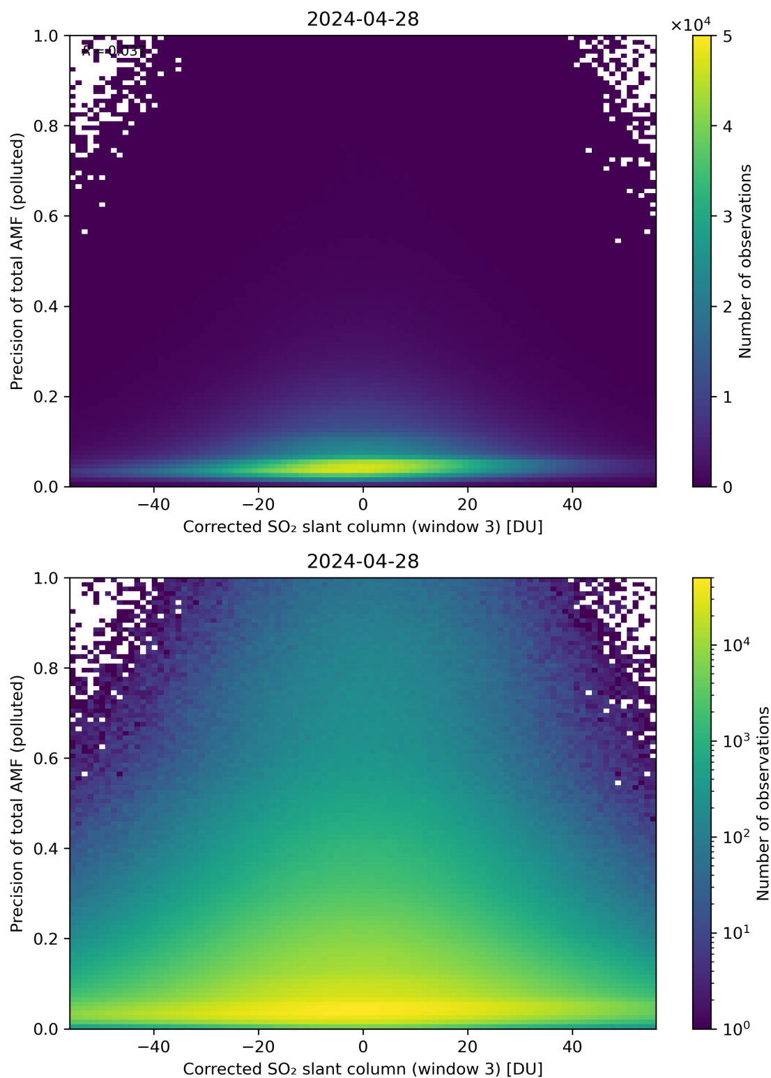
Figure 211: Scatter density plot of “Corrected SO 2 slant column (window 3)” against “Precision of total AMF (polluted)” for 2024-04-27 to 2024-04-29.
