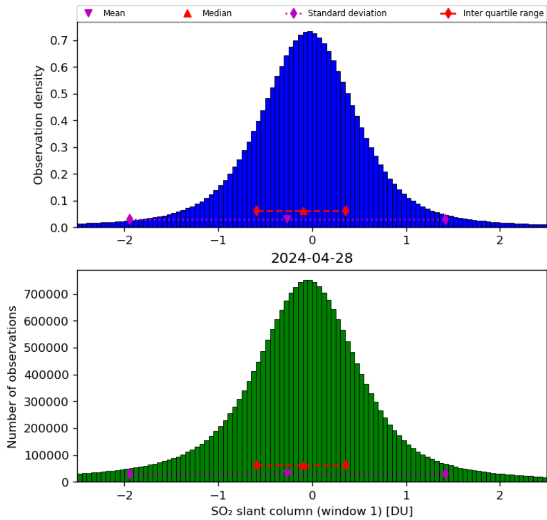
Figure 56: Histogram of “SO 2 slant column (window 1)” for 2024-04-27 to 2024-04-29
