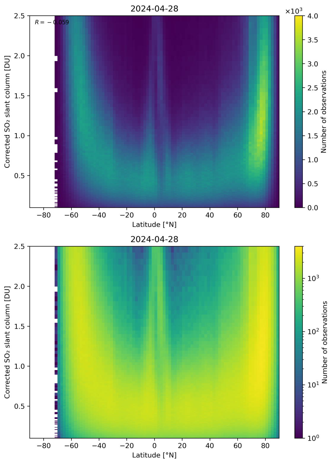
Figure 146: Scatter density plot of “Latitude” against “Corrected SO 2 slant column” for 2024-04-27 to 2024-04-29.
