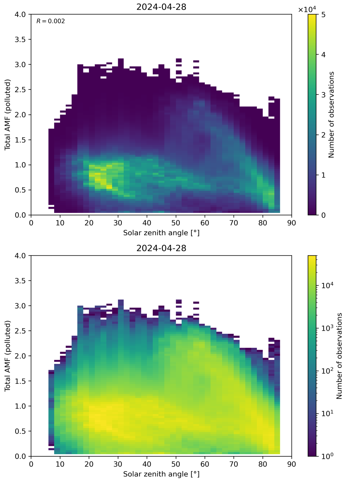
Figure 174: Scatter density plot of “Solar zenith angle” against “Total AMF (polluted)” for 2024-04-27 to 2024-04-29.
