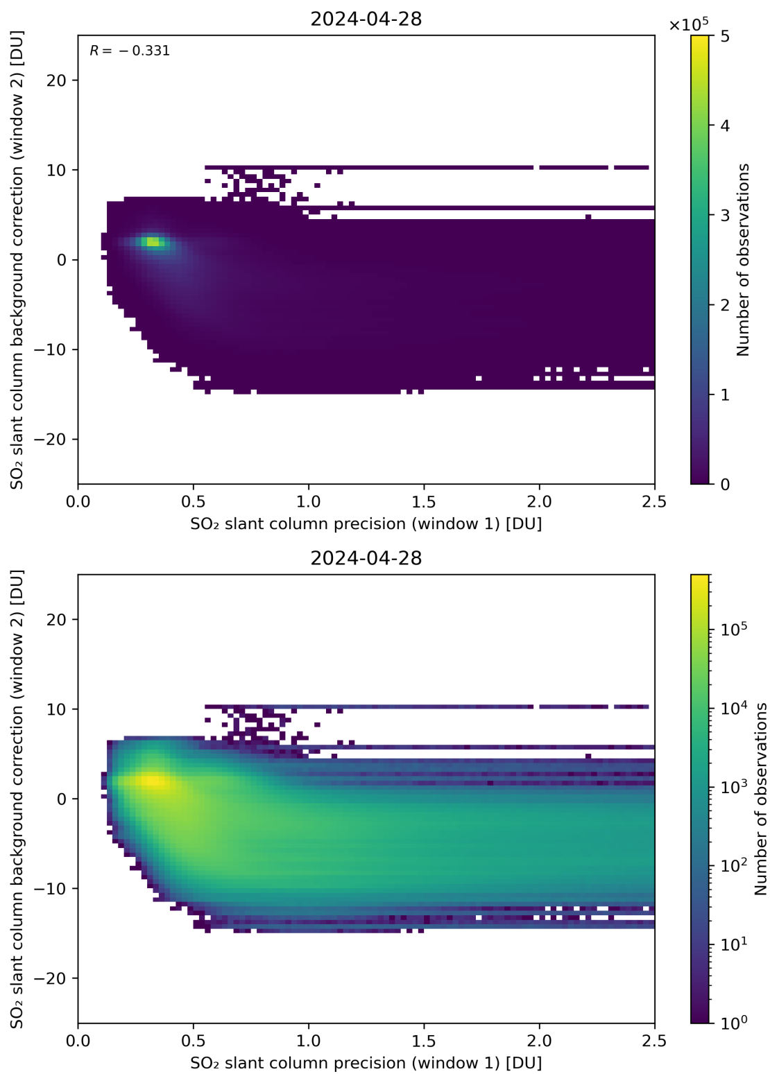
Figure 219: Scatter density plot of “SO 2 slant column precision (window 1)” against “SO 2 slant column background correction (window 2)” for 2024-04-27 to 2024-04-29.
