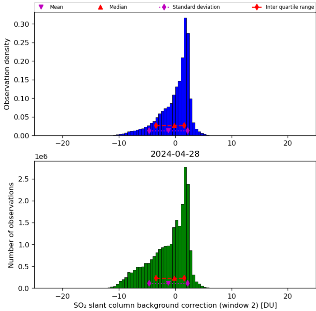
Figure 63: Histogram of “SO 2 slant column background correction (window 2)” for 2024-04-27 to 2024-04-29
