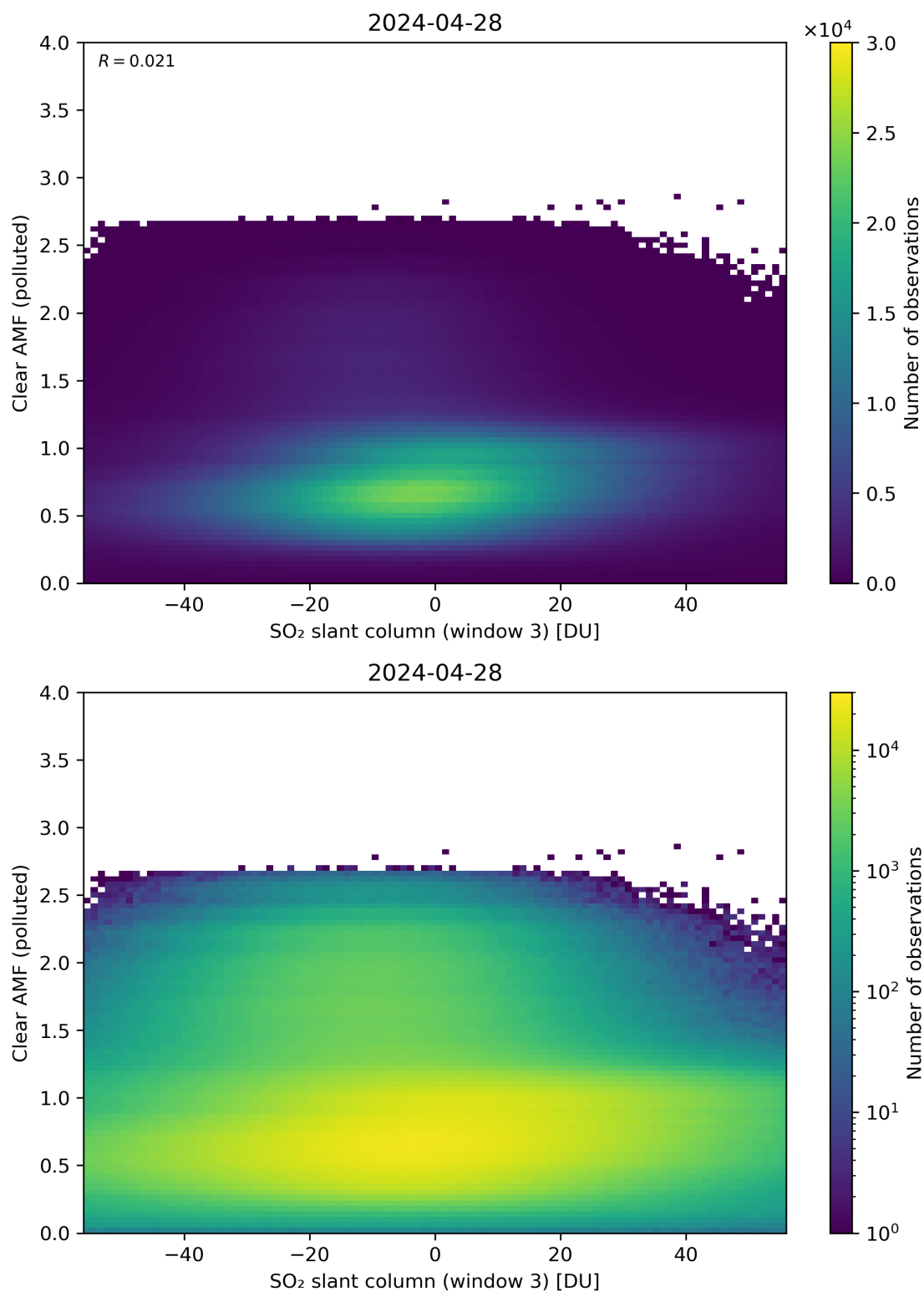
Figure 265: Scatter density plot of “SO 2 slant column (window 3)” against “Clear AMF (polluted)” for 2024-04-27 to 2024-04-29.
