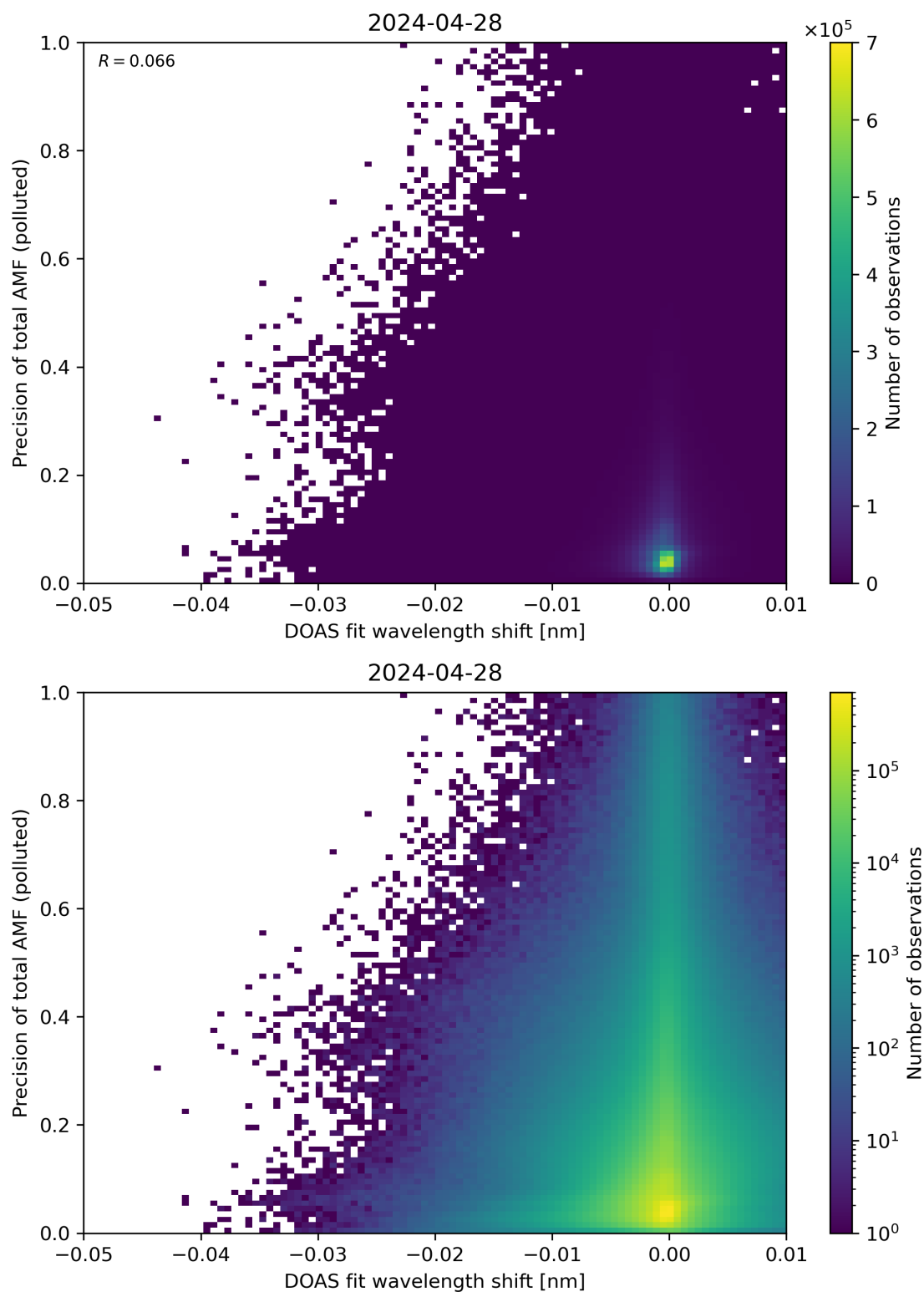
Figure 131: Scatter density plot of “DOAS fit wavelength shift” against “Precision of total AMF (polluted)” for 2024-04-27 to 2024-04-29.
