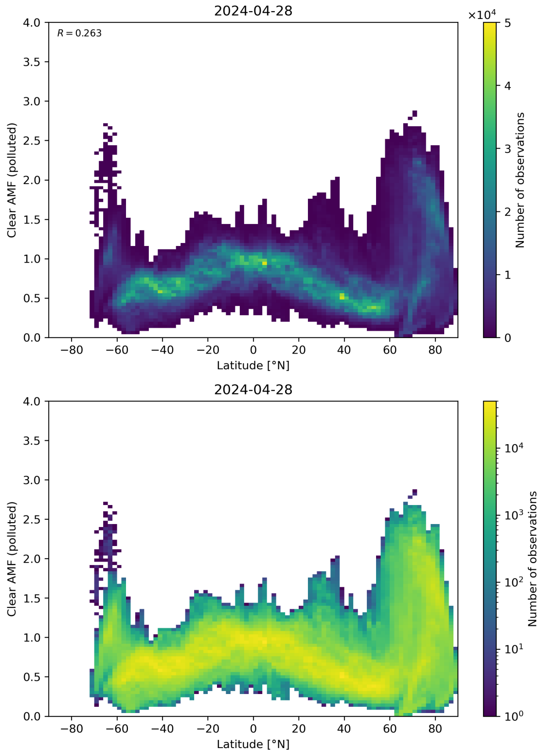
Figure 145: Scatter density plot of “Latitude” against “Clear AMF (polluted)” for 2024-04-27 to 2024-04-29.
