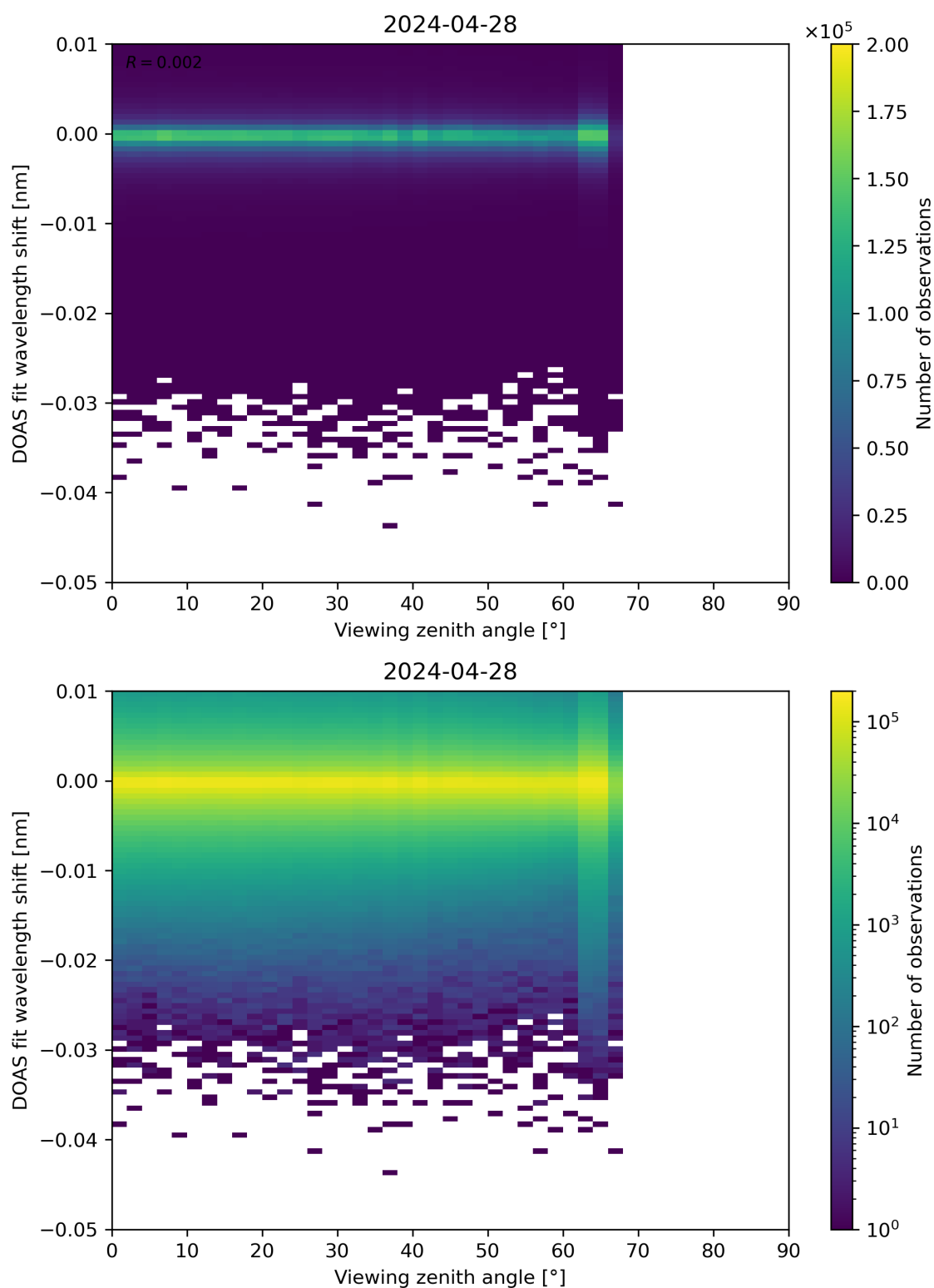
Figure 311: Scatter density plot of “Viewing zenith angle” against “DOAS fit wavelength shift” for 2024-04-27 to 2024-04-29.
