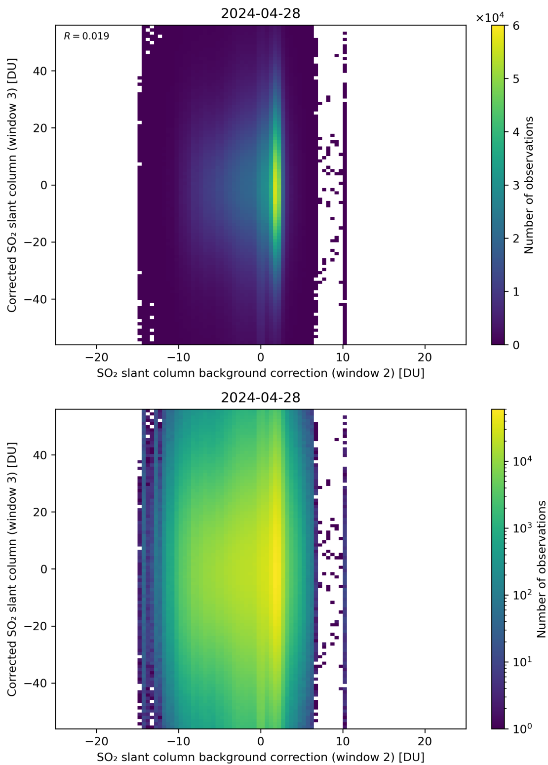
Figure 116: Scatter density plot of “SO 2 slant column background correction (window 2)” against “Corrected SO 2 slant column (window 3)” for 2024-04-27 to 2024-04-29.
