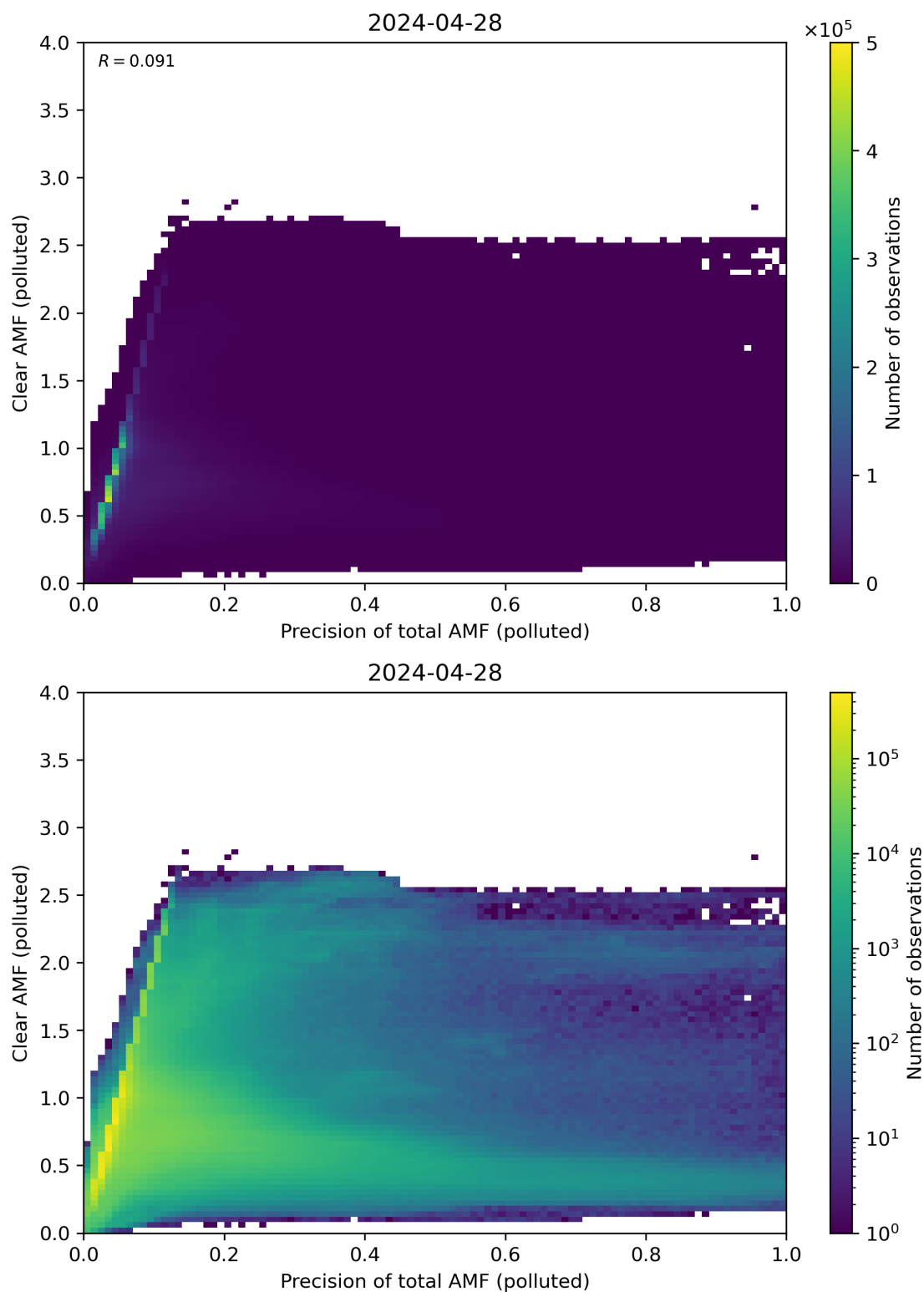
Figure 270: Scatter density plot of “Precision of total AMF (polluted)” against “Clear AMF (polluted)” for 2024-04-27 to 2024-04-29.
