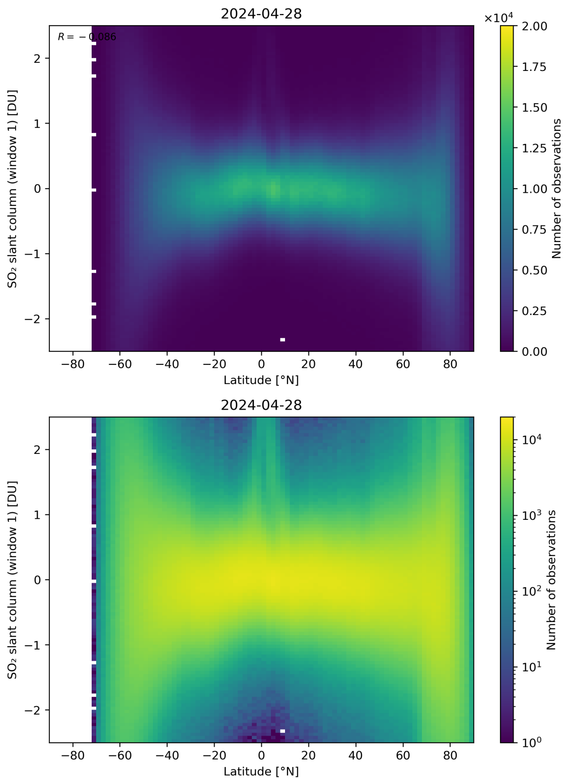
Figure 149: Scatter density plot of “Latitude” against “SO 2 slant column (window 1)” for 2024-04-27 to 2024-04-29.
