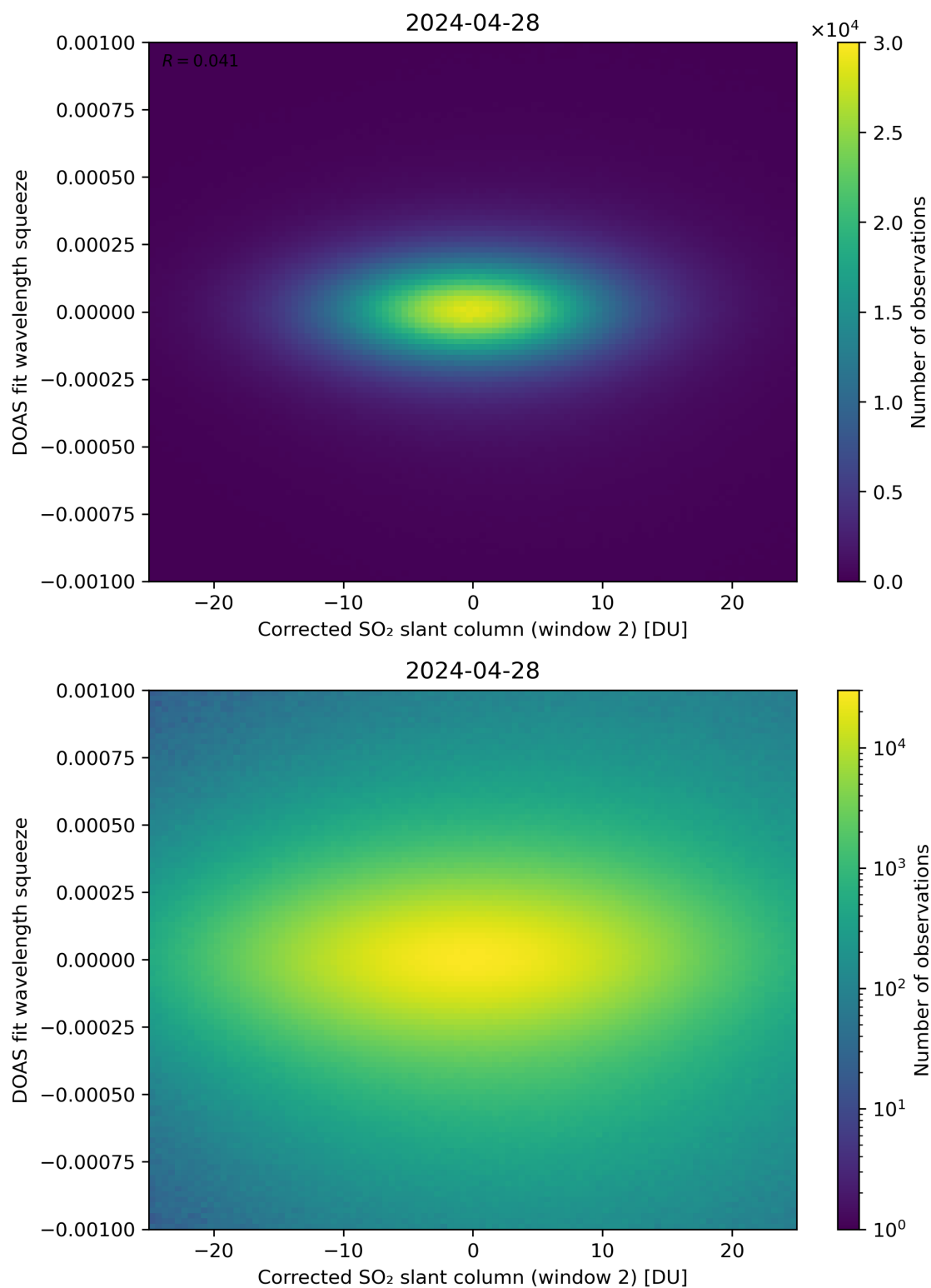
Figure 197: Scatter density plot of “Corrected SO 2 slant column (window 2)” against “DOAS fit wavelength squeeze” for 2024-04-27 to 2024-04-29.
