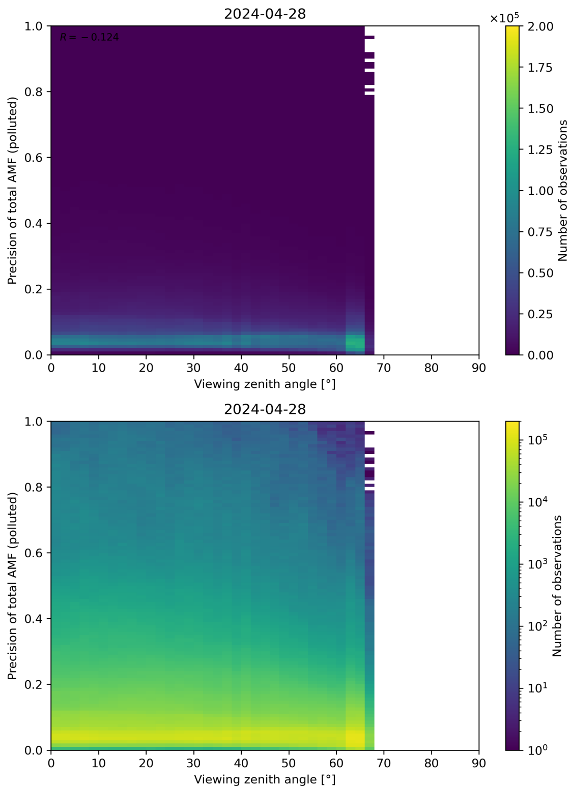
Figure 326: Scatter density plot of “Viewing zenith angle” against “Precision of total AMF (polluted)” for 2024-04-27 to 2024-04-29.
