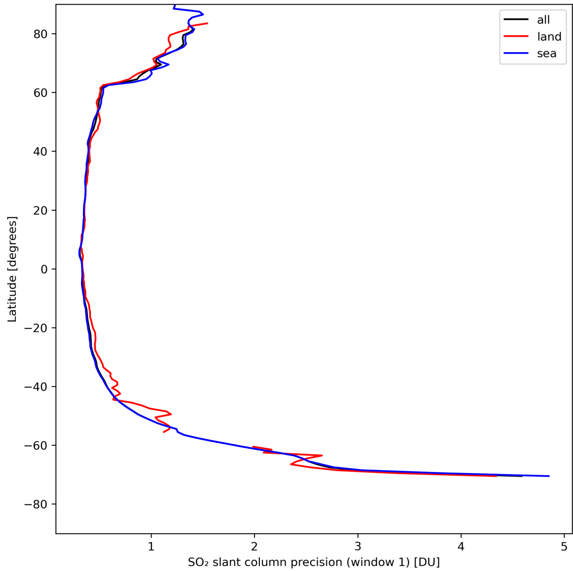
Figure 34: Zonal average of “SO 2 slant column precision (window 1)” for 2024-04-27 to 2024-04-29.
