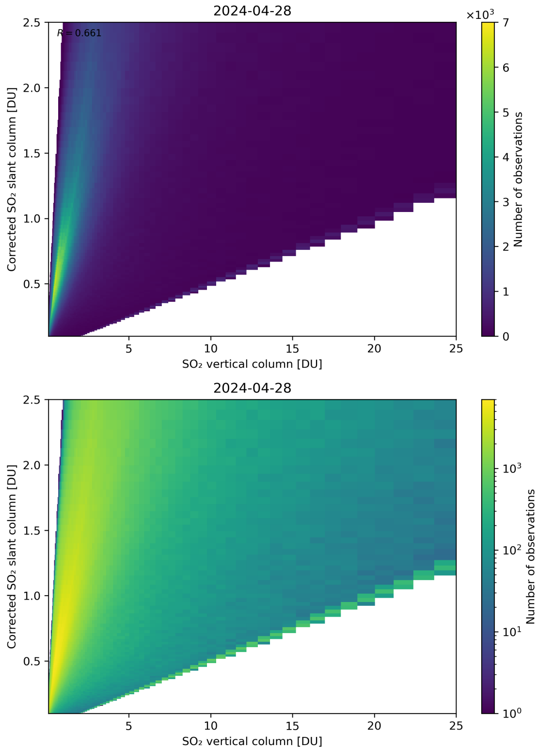
Figure 297: Scatter density plot of “SO 2 vertical column” against “Corrected SO 2 slant column” for 2024-04-27 to 2024-04-29.
