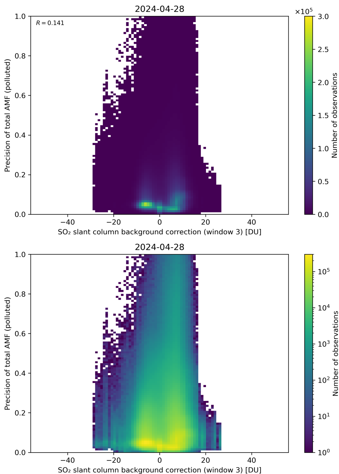
Figure 126: Scatter density plot of “SO 2 slant column background correction (window 3)” against “Precision of total AMF (polluted)” for 2024-04-27 to 2024-04-29.
