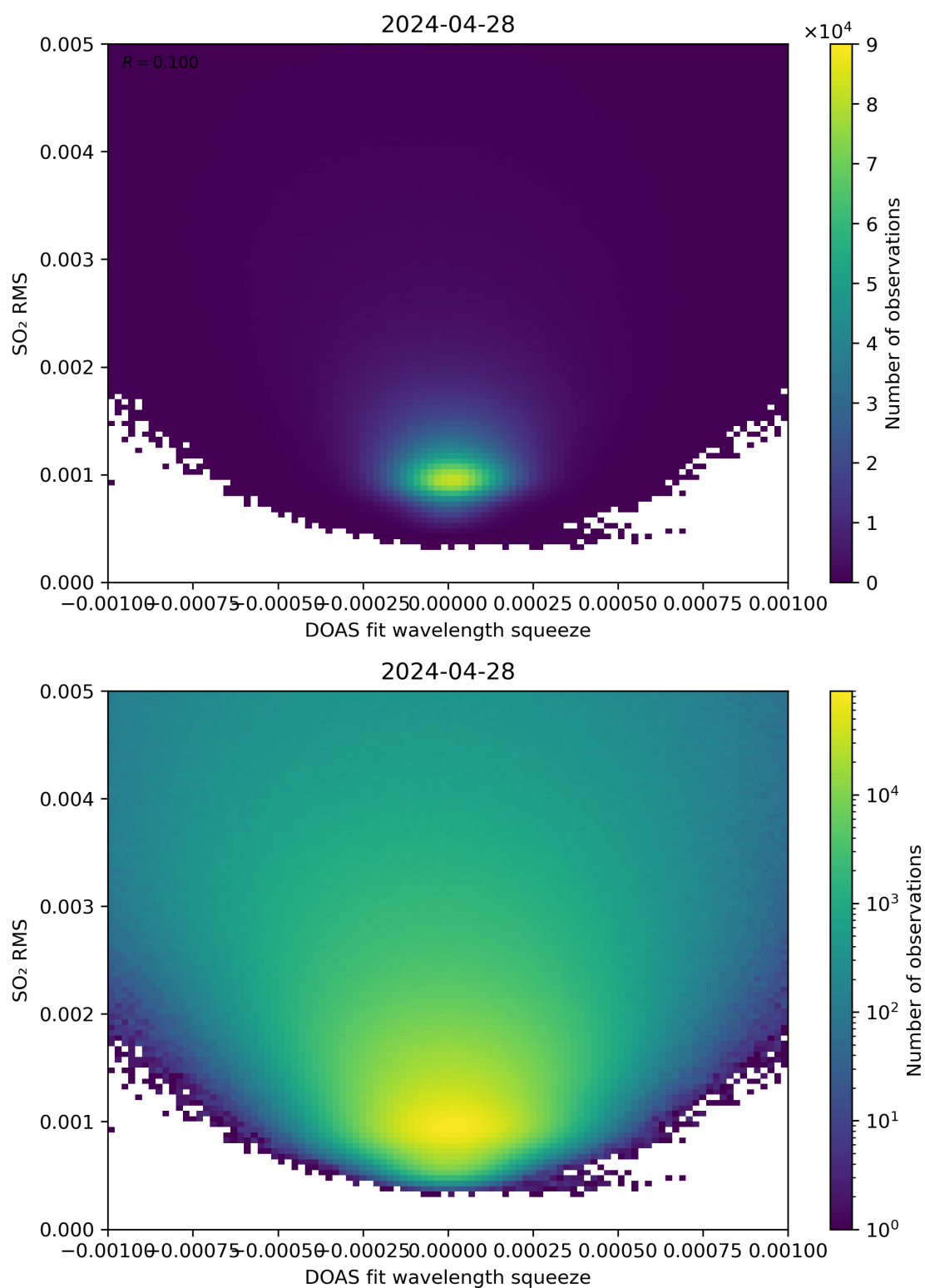
Figure 132: Scatter density plot of “DOAS fit wavelength squeeze” against “SO 2 RMS” for 2024-04-27 to 2024-04-29.
