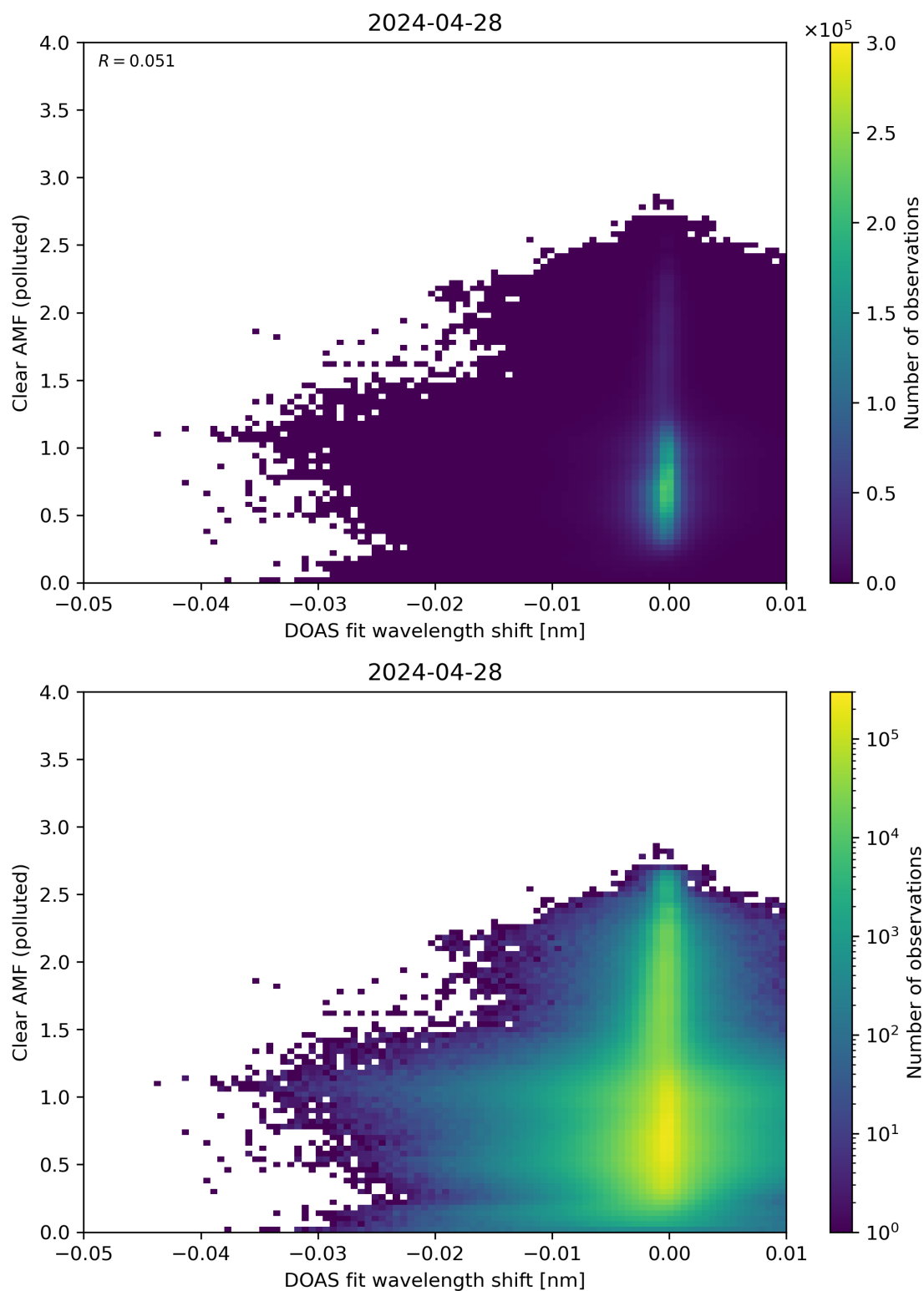
Figure 129: Scatter density plot of “DOAS fit wavelength shift” against “Clear AMF (polluted)” for 2024-04-27 to 2024-04-29.
