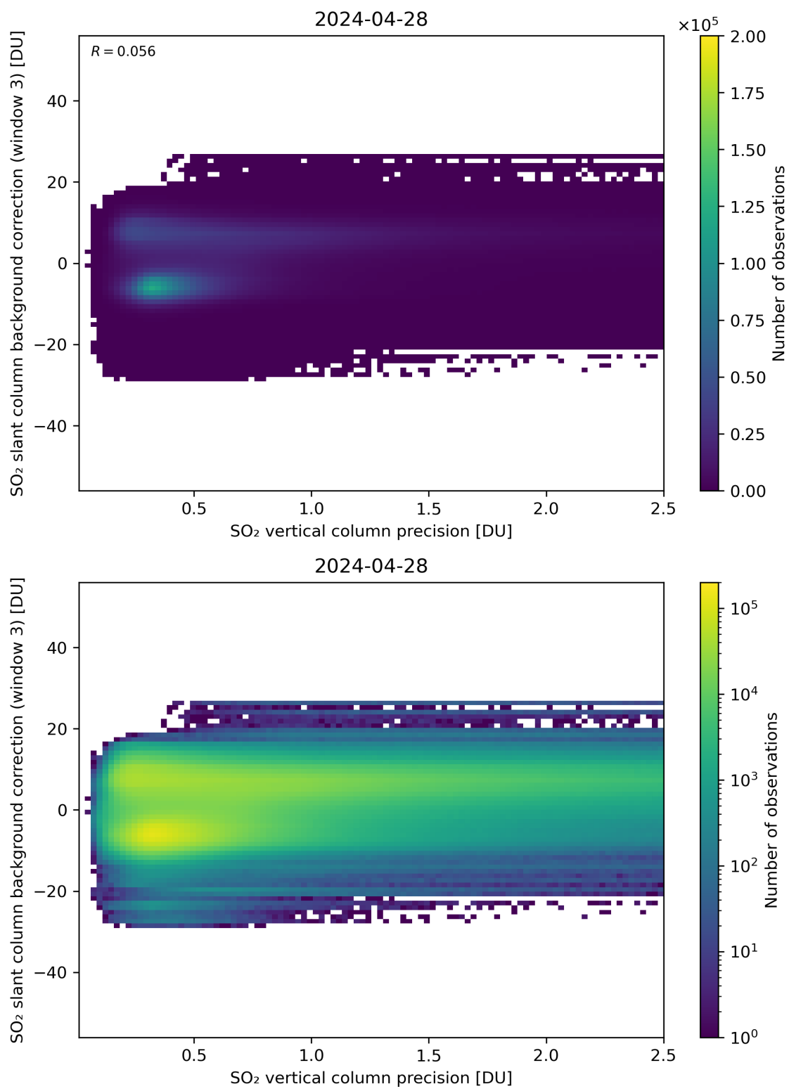
Figure 281: Scatter density plot of “SO 2 vertical column precision” against “SO 2 slant column background correction (window 3)” for 2024-04-27 to 2024-04-29.
