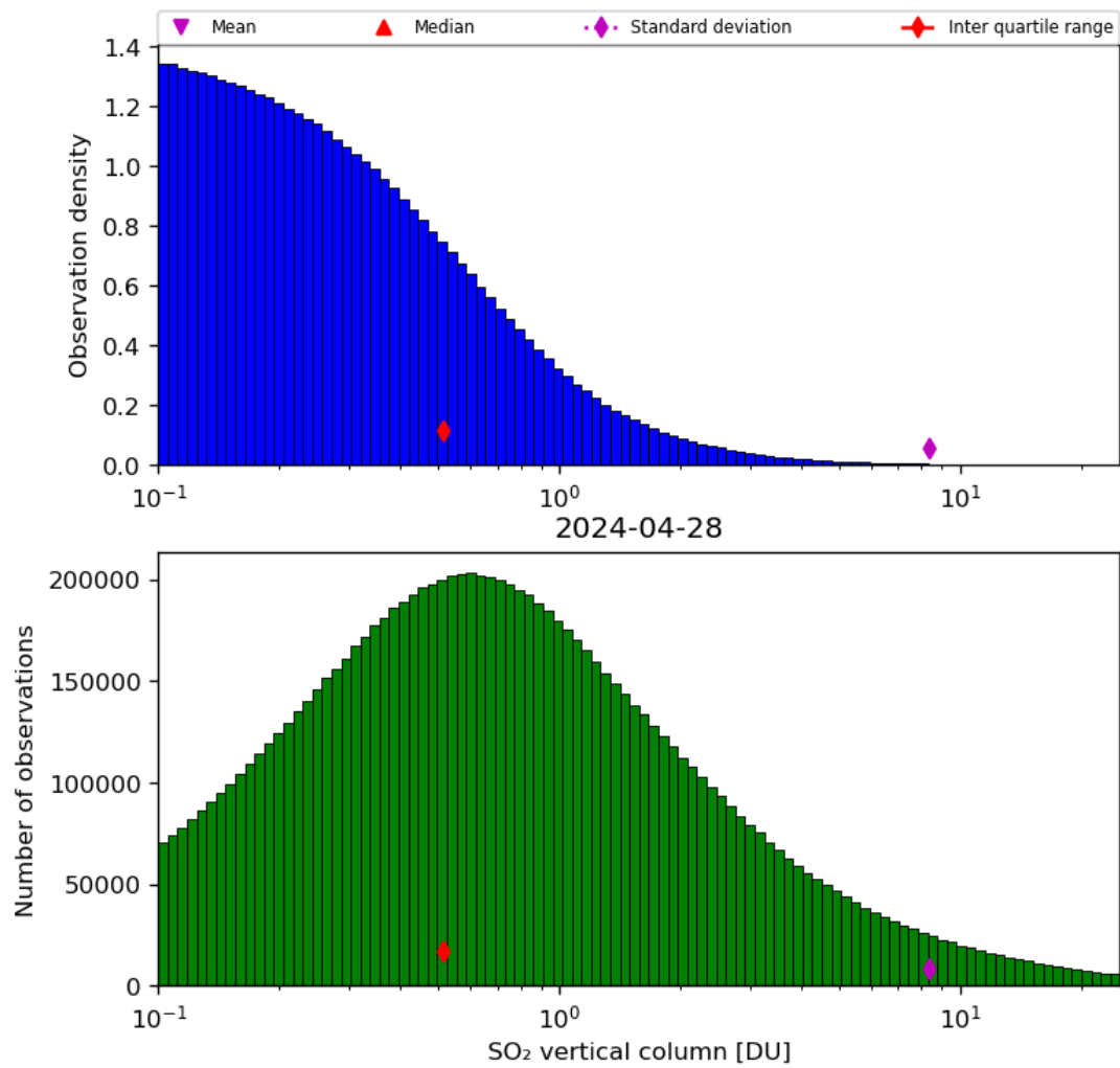
Figure 53: Histogram of “SO 2 vertical column” for 2024-04-27 to 2024-04-29
