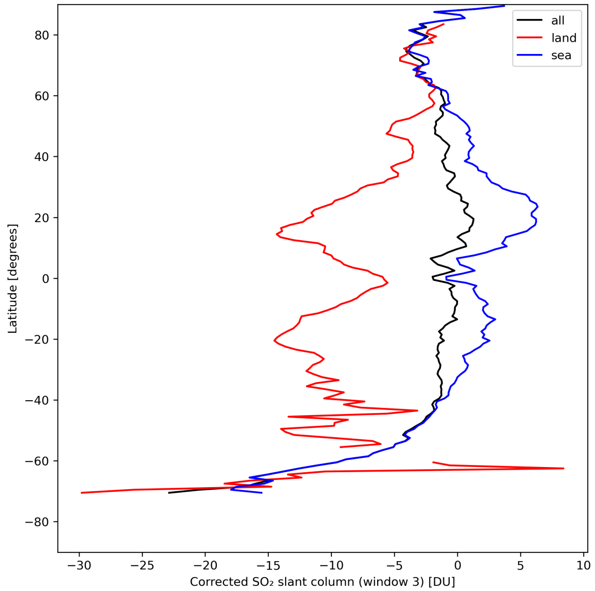
Figure 43: Zonal average of “Corrected SO 2 slant column (window 3)” for 2024-04-27 to 2024-04-29.
