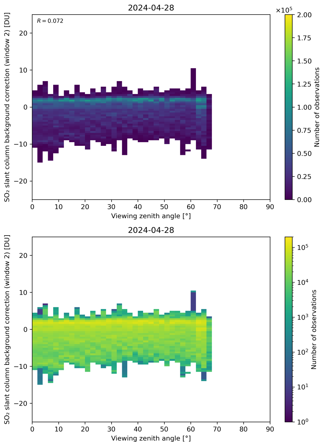
Figure 309: Scatter density plot of “Viewing zenith angle” against “SO 2 slant column background correction (window 2)” for 2024-04-27 to 2024-04-29.
