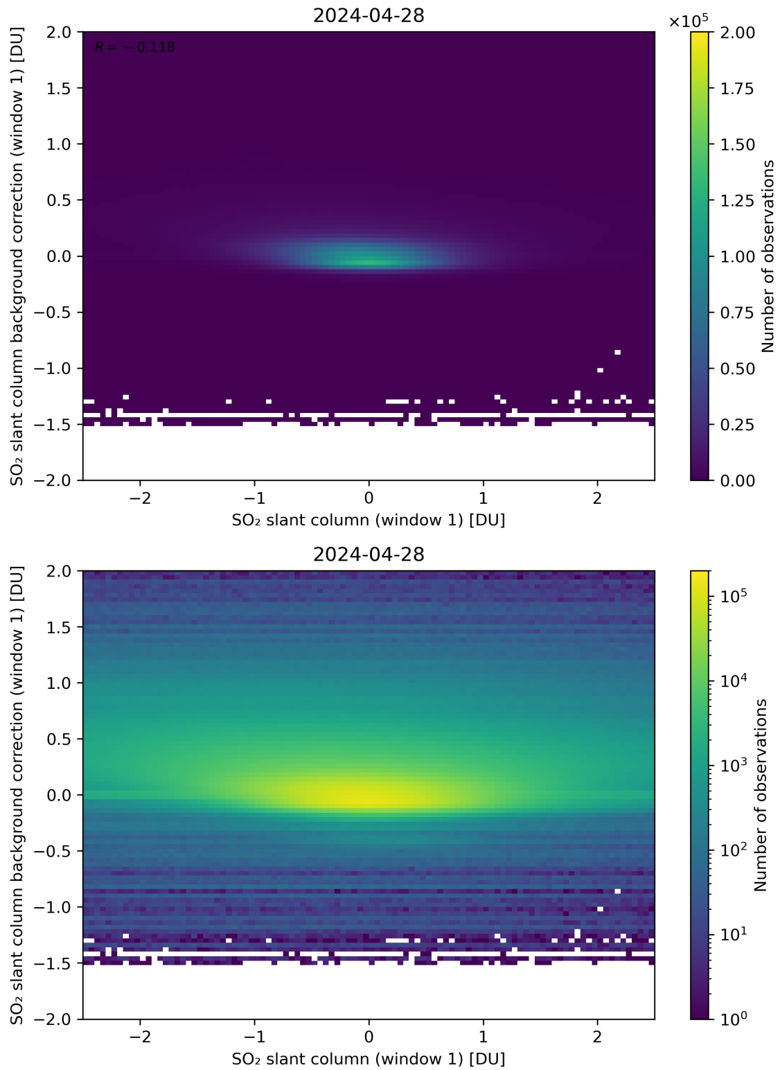
Figure 212: Scatter density plot of “SO 2 slant column (window 1)” against “SO 2 slant column background correction (window 1)” for 2024-04-27 to 2024-04-29.
