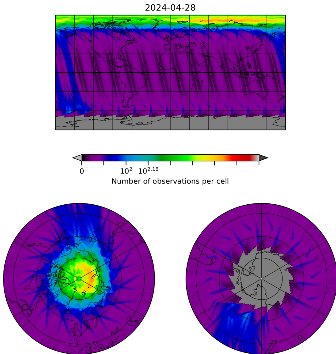
Figure 28: Map of the number of observations for 2024-04-27 to 2024-04-29
