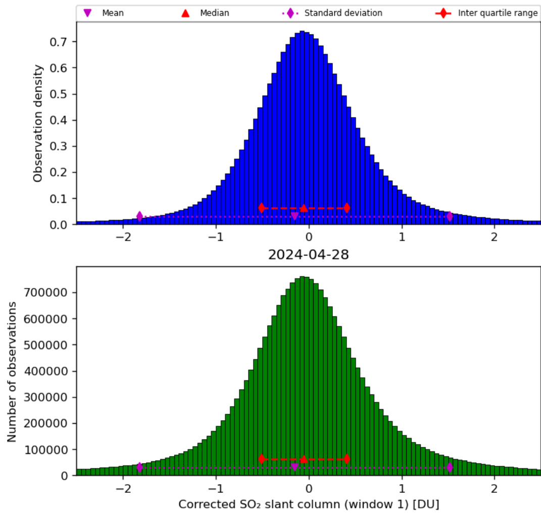
Figure 58: Histogram of “Corrected SO 2 slant column (window 1)” for 2024-04-27 to 2024-04-29
