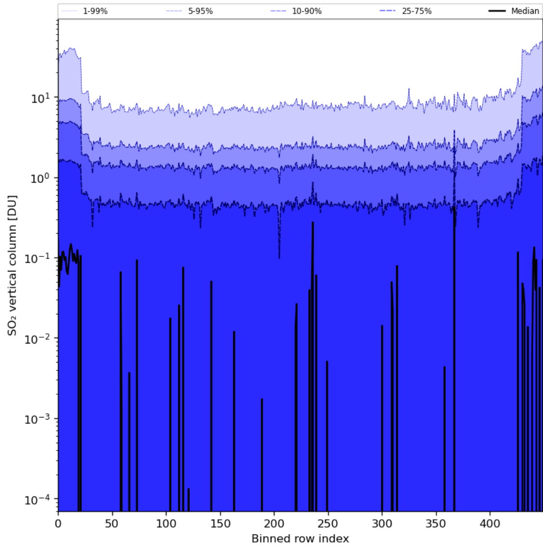
Figure 76: Along track statistics of “SO 2 vertical column” for 2024-04-27 to 2024-04-29
