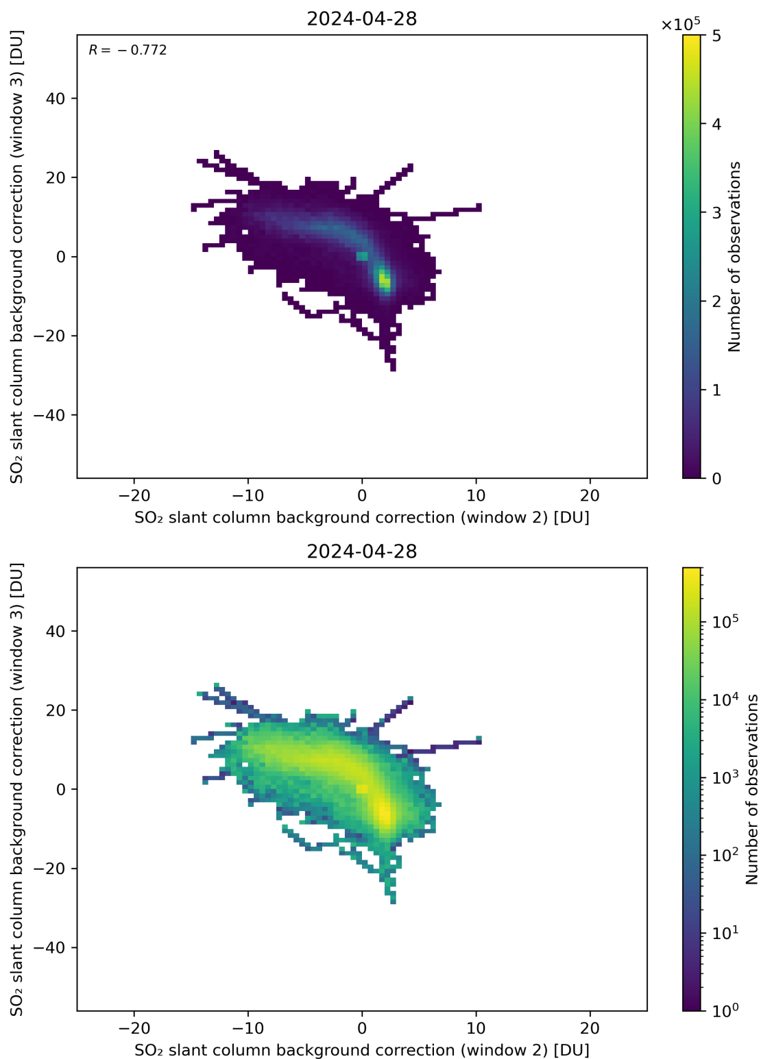
Figure 111: Scatter density plot of “SO 2 slant column background correction (window 2)” against “SO 2 slant column background correction (window 3)” for 2024-04-27 to 2024-04-29.
