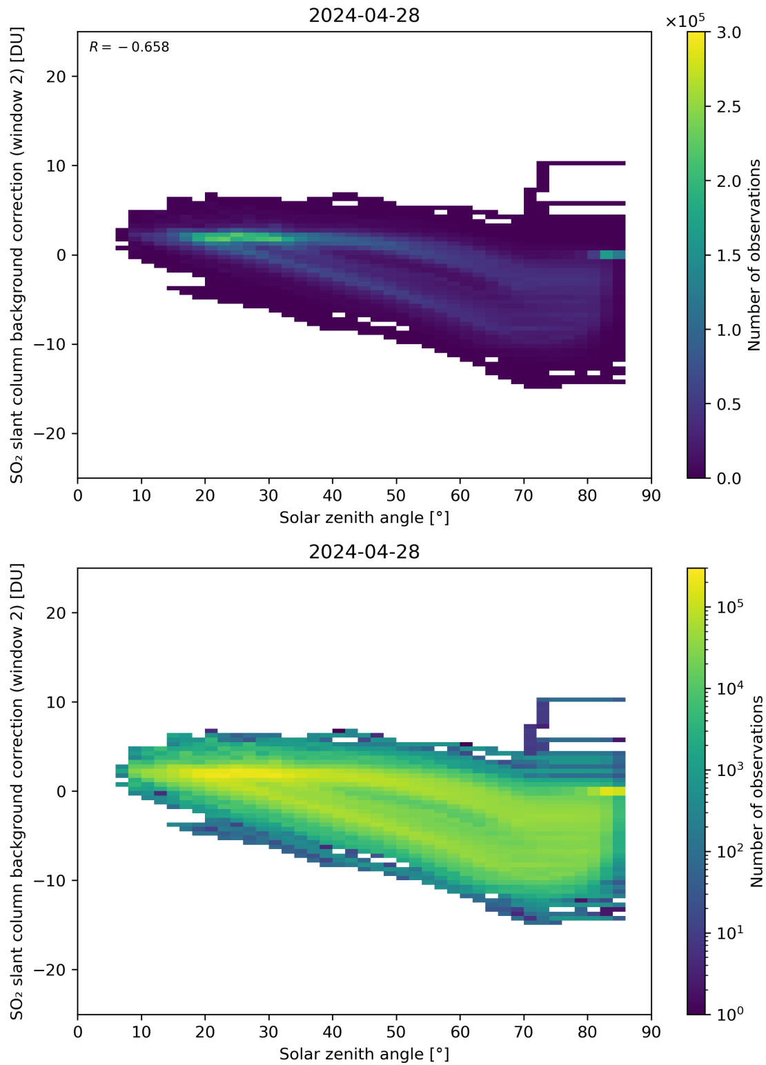
Figure 159: Scatter density plot of “Solar zenith angle” against “SO 2 slant column background correction (window 2)” for 2024-04-27 to 2024-04-29.
