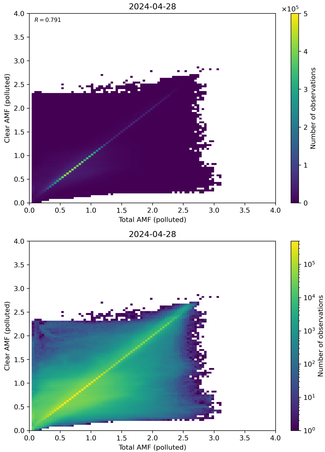
Figure 271: Scatter density plot of “Total AMF (polluted)” against “Clear AMF (polluted)” for 2024-04-27 to 2024-04-29.
