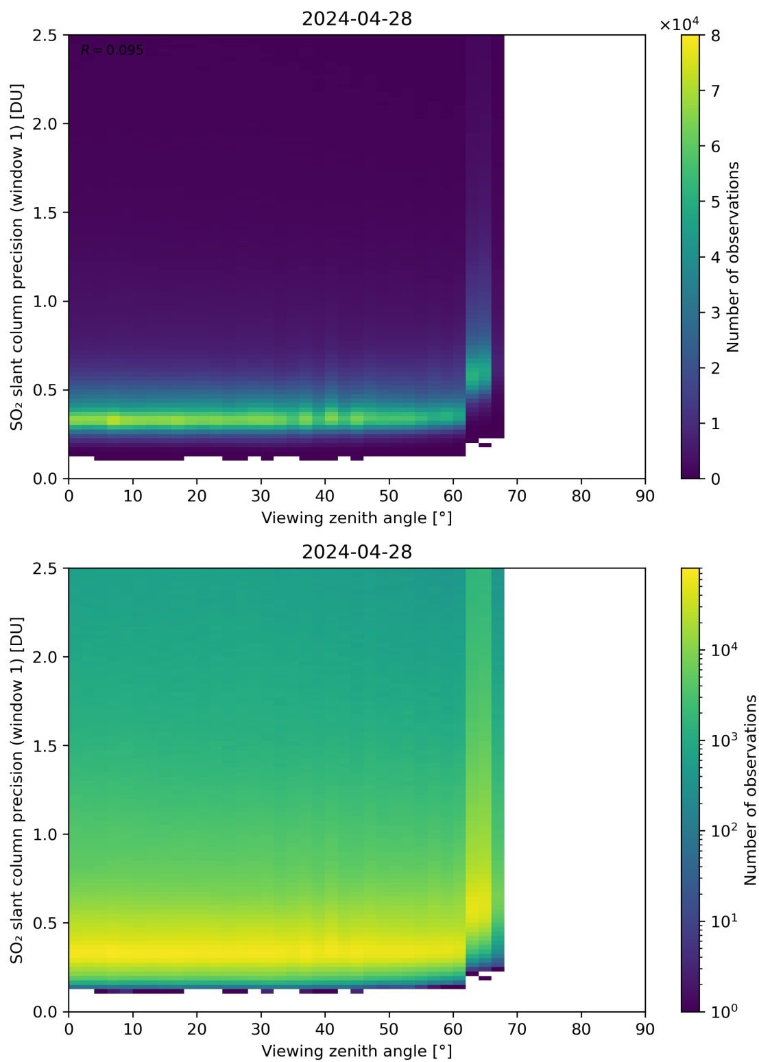
Figure 321: Scatter density plot of “Viewing zenith angle” against “SO 2 slant column precision (window 1)” for 2024-04-27 to 2024-04-29.
