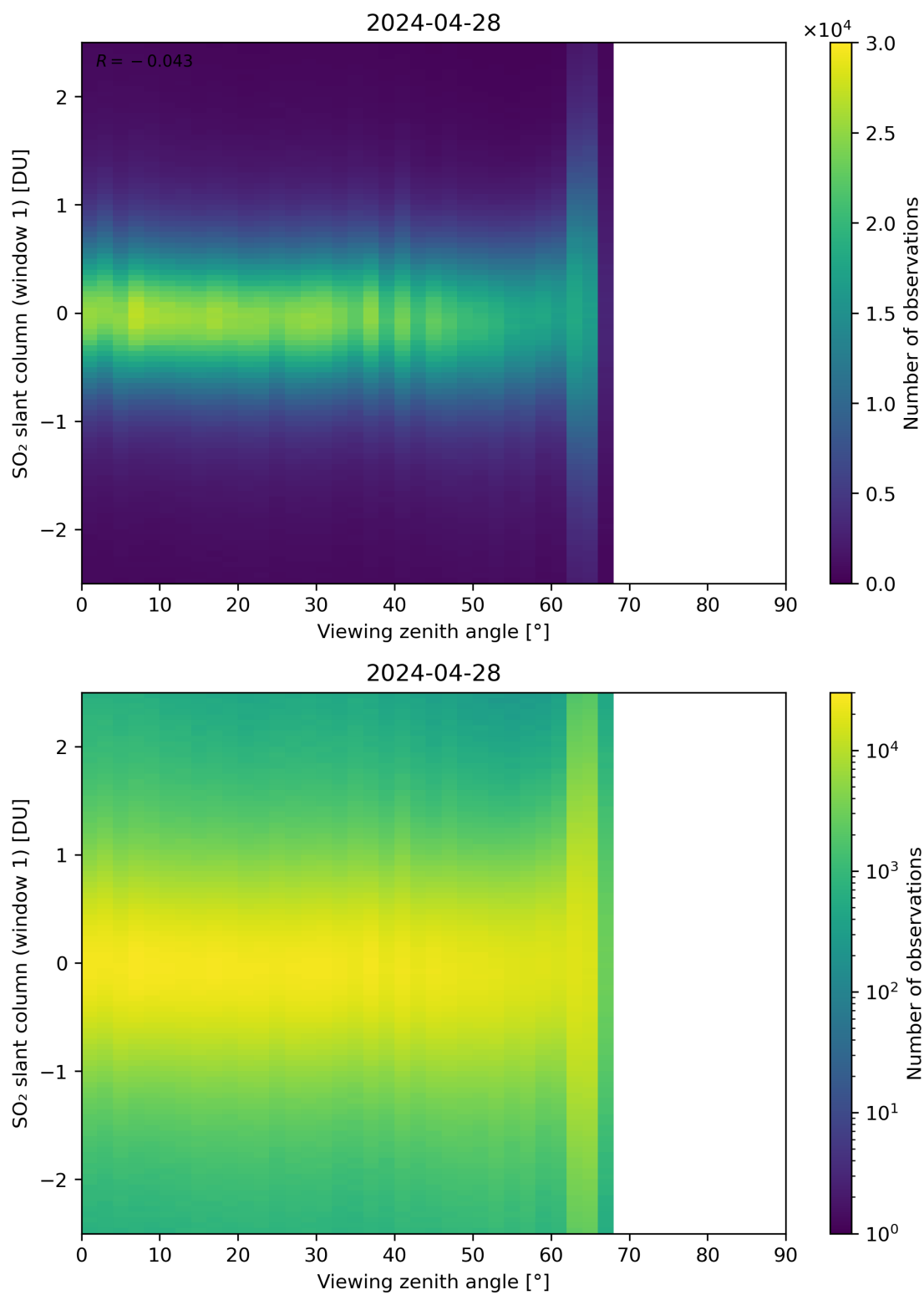
Figure 320: Scatter density plot of “Viewing zenith angle” against “SO 2 slant column (window 1)” for 2024-04-27 to 2024-04-29.
