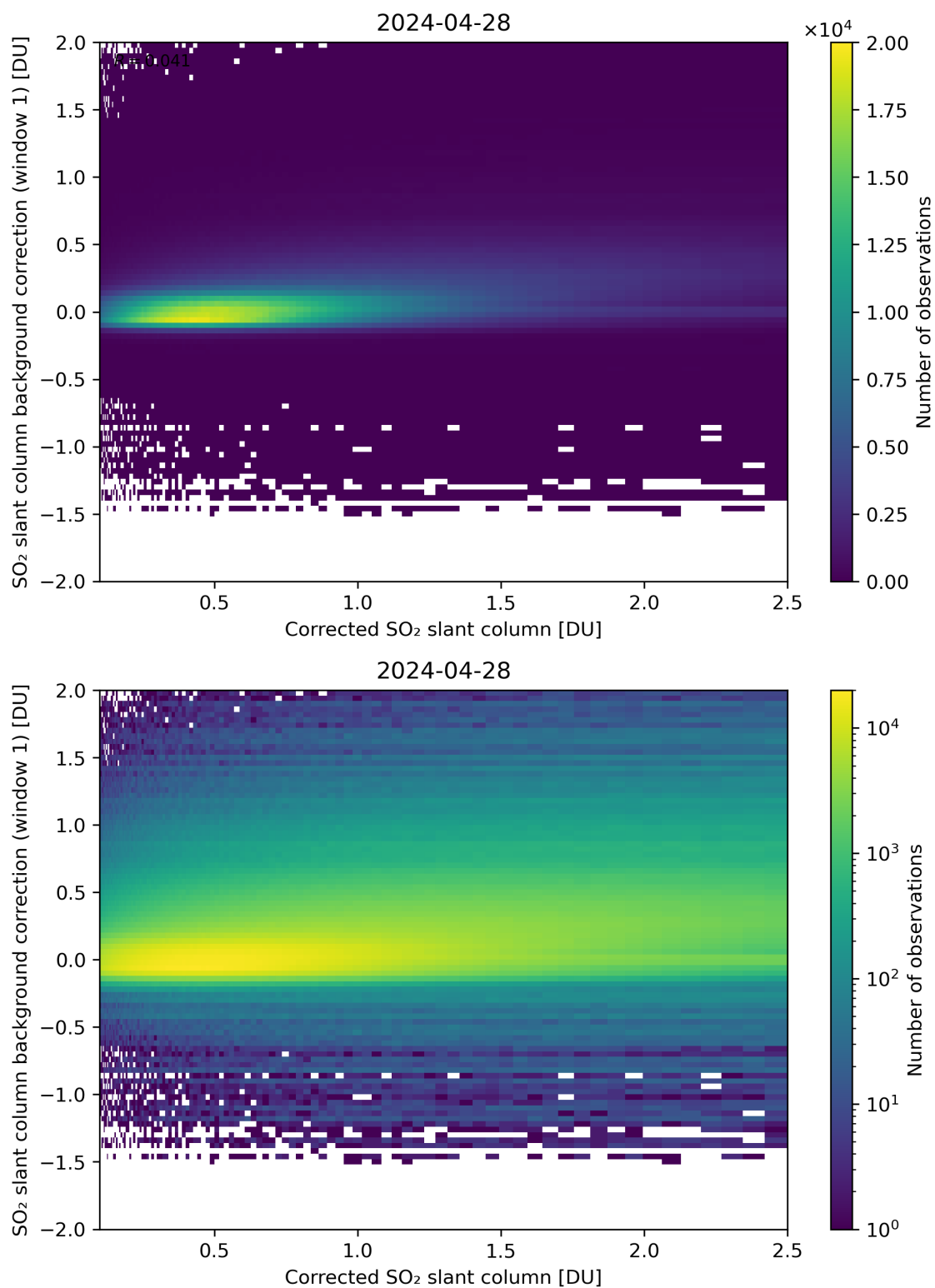
Figure 178: Scatter density plot of “Corrected SO 2 slant column” against “SO 2 slant column background correction (window 1)” for 2024-04-27 to 2024-04-29.
