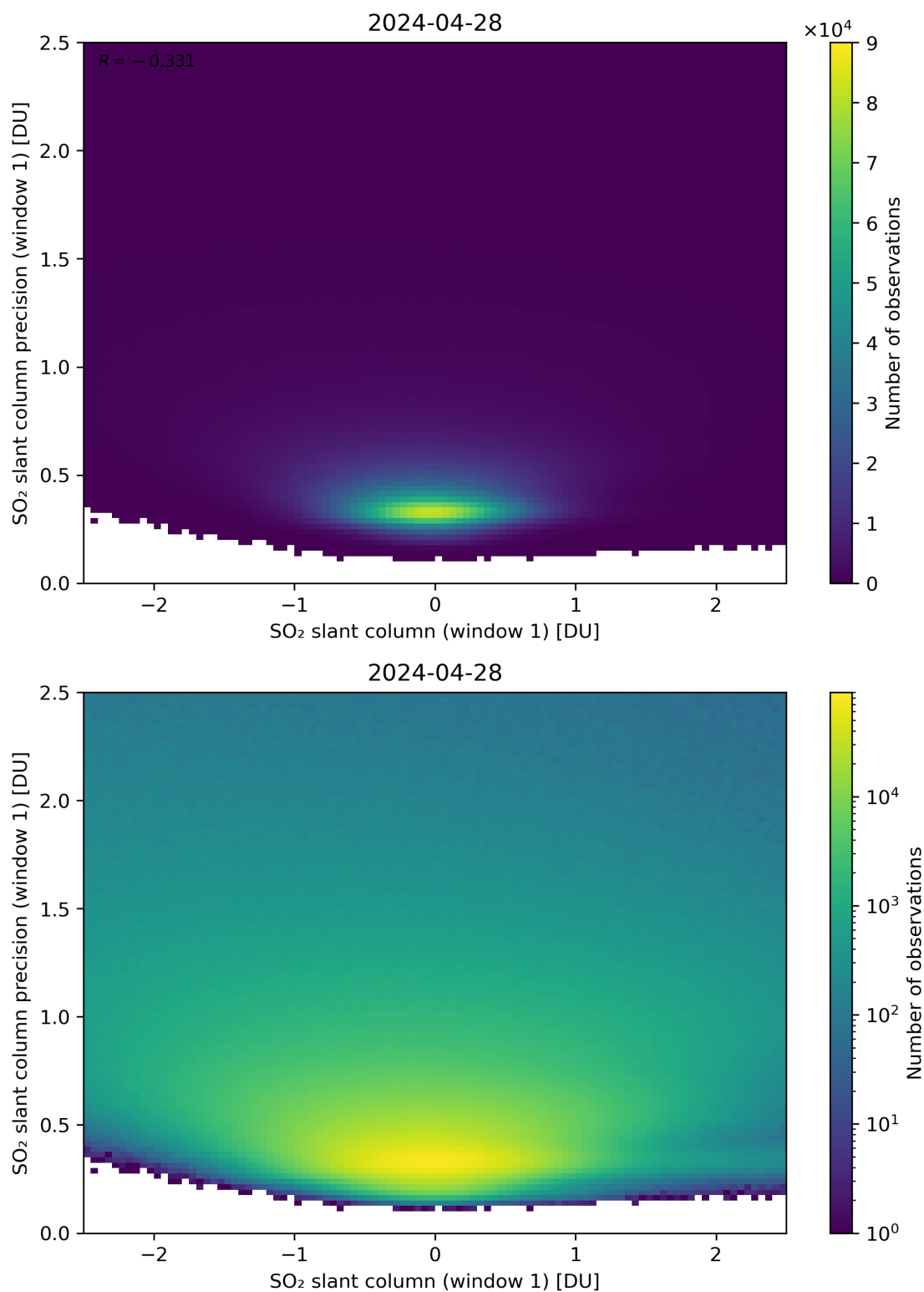
Figure 235: Scatter density plot of “SO 2 slant column (window 1)” against “SO 2 slant column precision (window 1)” for 2024-04-27 to 2024-04-29.
