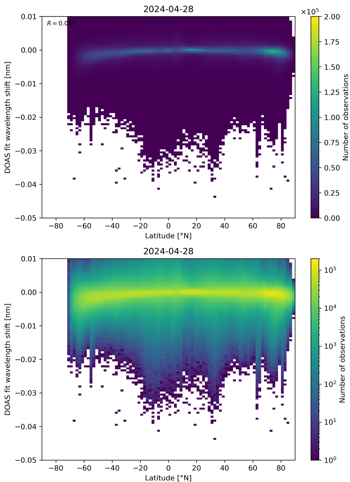
Figure 142: Scatter density plot of “Latitude” against “DOAS fit wavelength shift” for 2024-04-27 to 2024-04-29.
