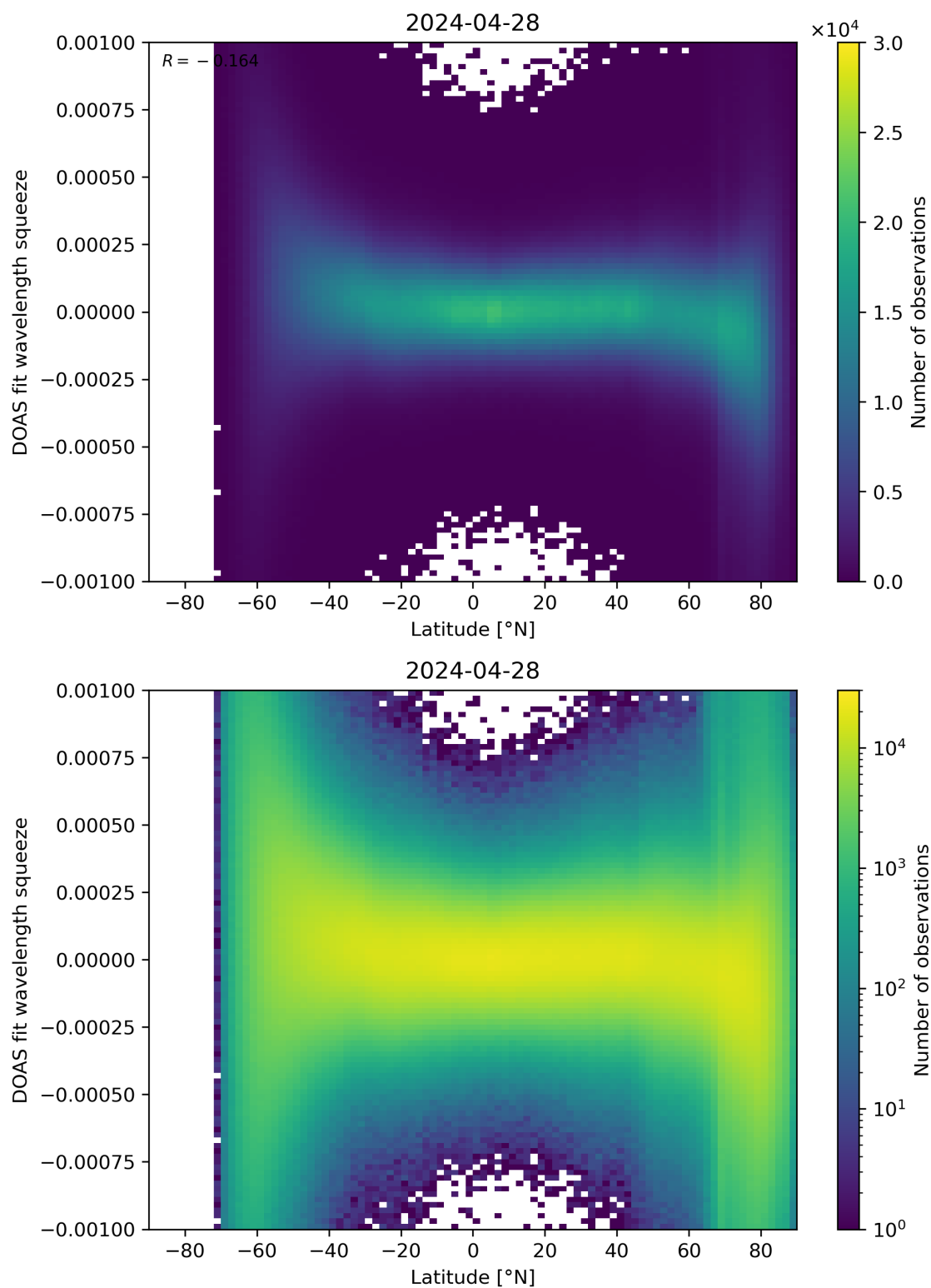
Figure 143: Scatter density plot of “Latitude” against “DOAS fit wavelength squeeze” for 2024-04-27 to 2024-04-29.
