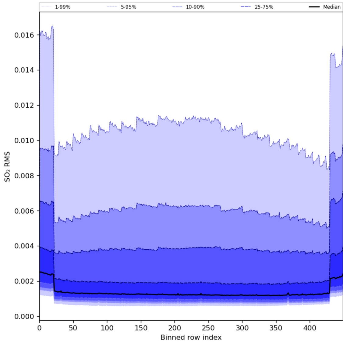
Figure 93: Along track statistics of “SO 2 RMS” for 2024-04-27 to 2024-04-29
