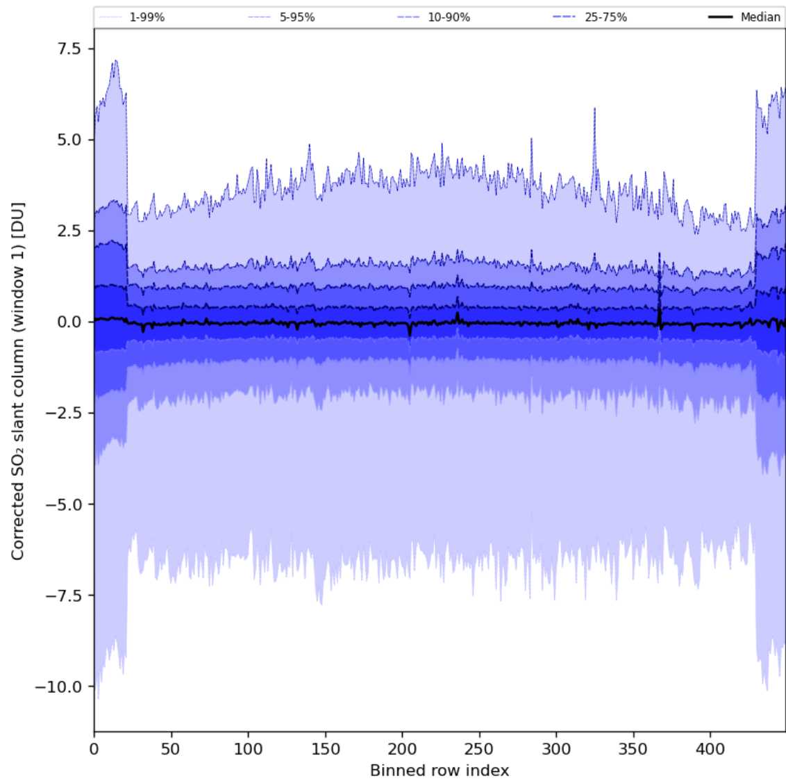
Figure 81: Along track statistics of “Corrected SO 2 slant column (window 1)” for 2024-04-27 to 2024-04-29
