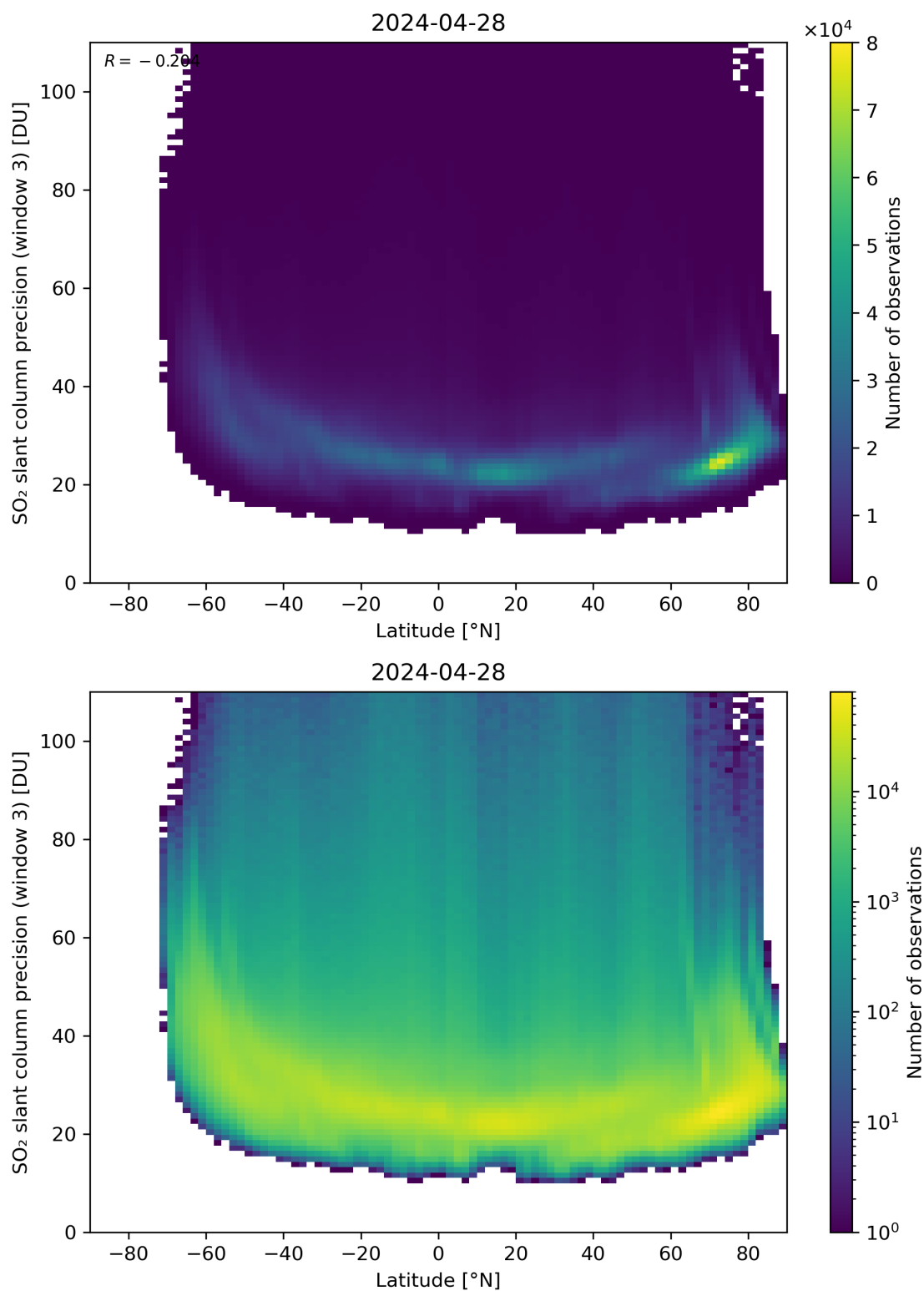
Figure 153: Scatter density plot of “Latitude” against “SO 2 slant column precision (window 3)” for 2024-04-27 to 2024-04-29.
