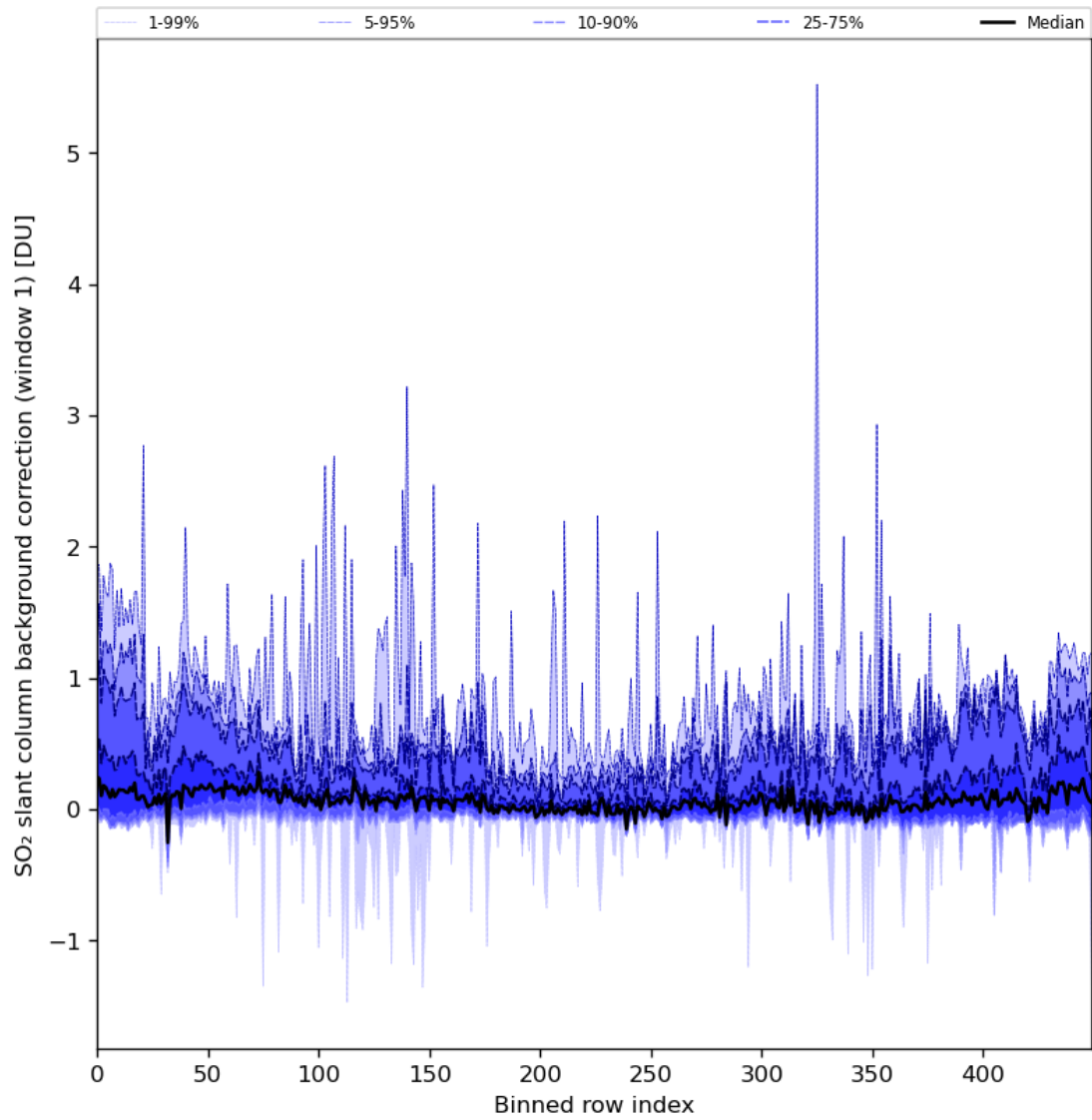
Figure 82: Along track statistics of “SO 2 slant column background correction (window 1)” for 2024-04-27 to 2024-04-29
