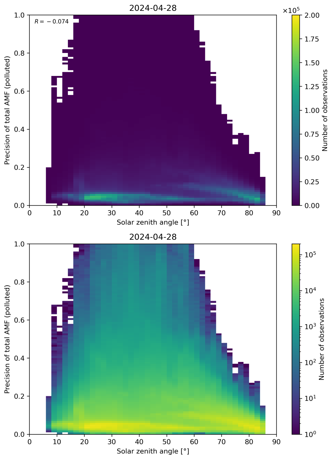
Figure 175: Scatter density plot of “Solar zenith angle” against “Precision of total AMF (polluted)” for 2024-04-27 to 2024-04-29.
