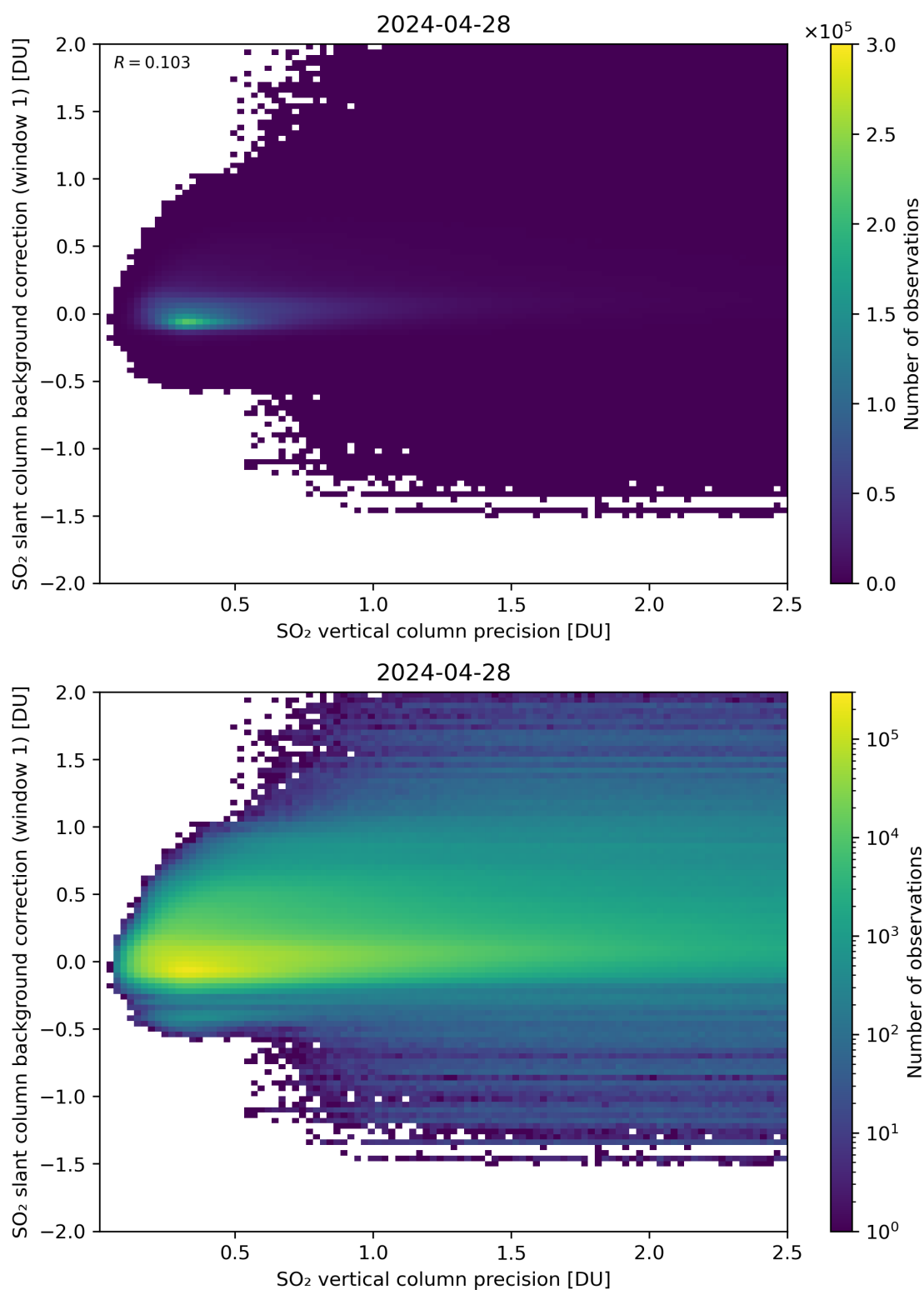
Figure 279: Scatter density plot of “SO 2 vertical column precision” against “SO 2 slant column background correction (window 1)” for 2024-04-27 to 2024-04-29.
