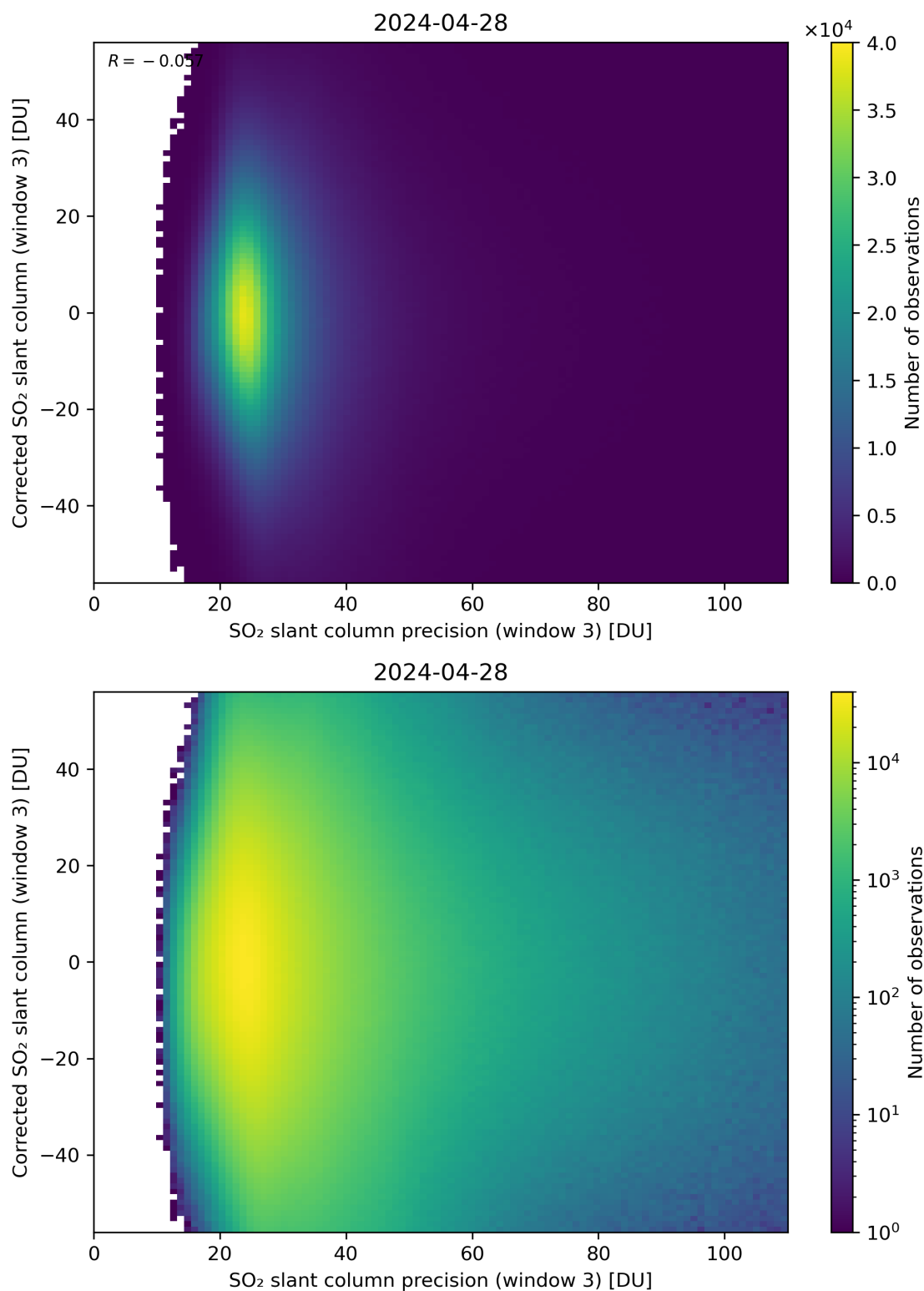
Figure 262: Scatter density plot of “SO 2 slant column precision (window 3)” against “Corrected SO 2 slant column (window 3)” for 2024-04-27 to 2024-04-29.
