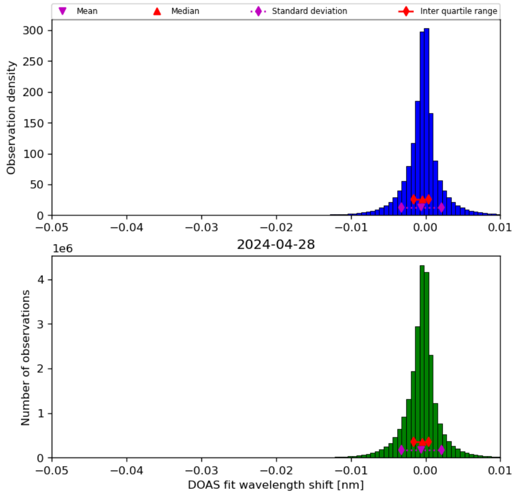
Figure 68: Histogram of “DOAS fit wavelength shift” for 2024-04-27 to 2024-04-29
