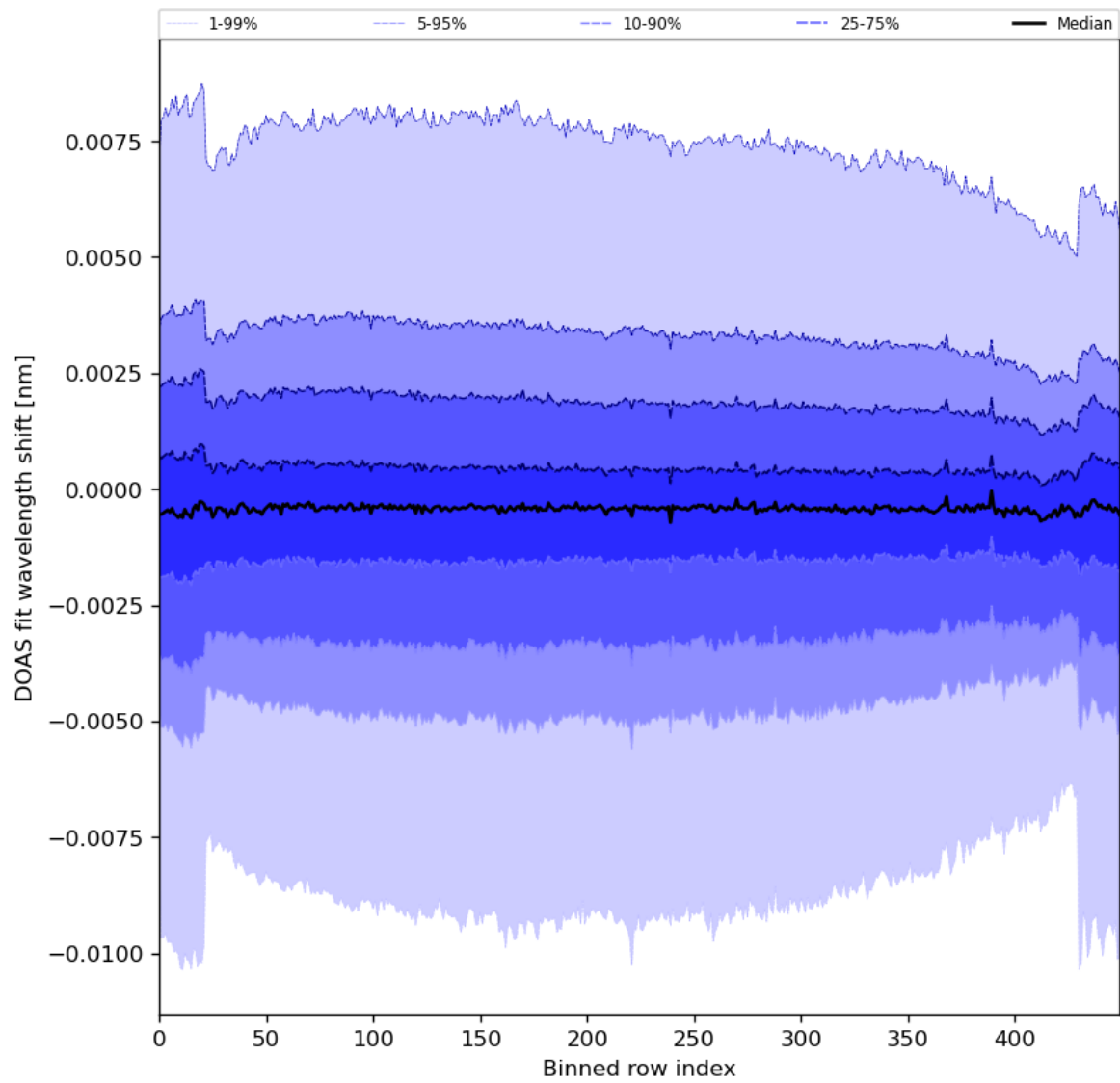
Figure 91: Along track statistics of “DOAS fit wavelength shift” for 2024-04-27 to 2024-04-29
