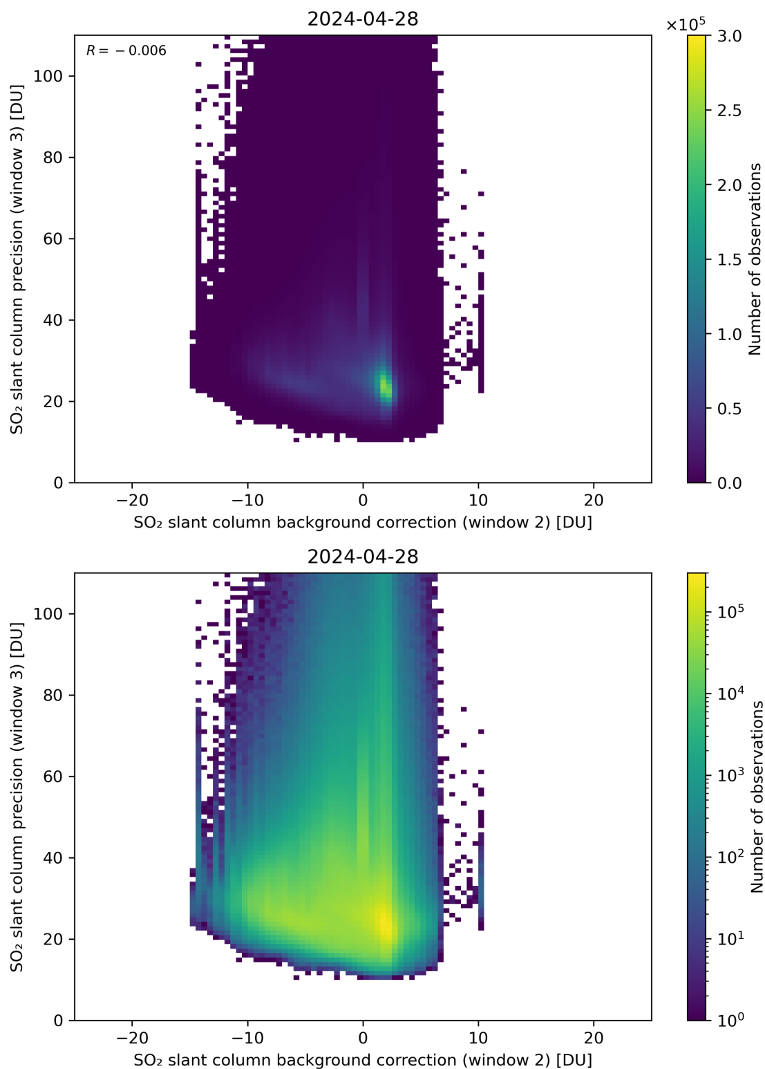
Figure 118: Scatter density plot of “SO 2 slant column background correction (window 2)” against “SO 2 slant column precision (window 3)” for 2024-04-27 to 2024-04-29.
