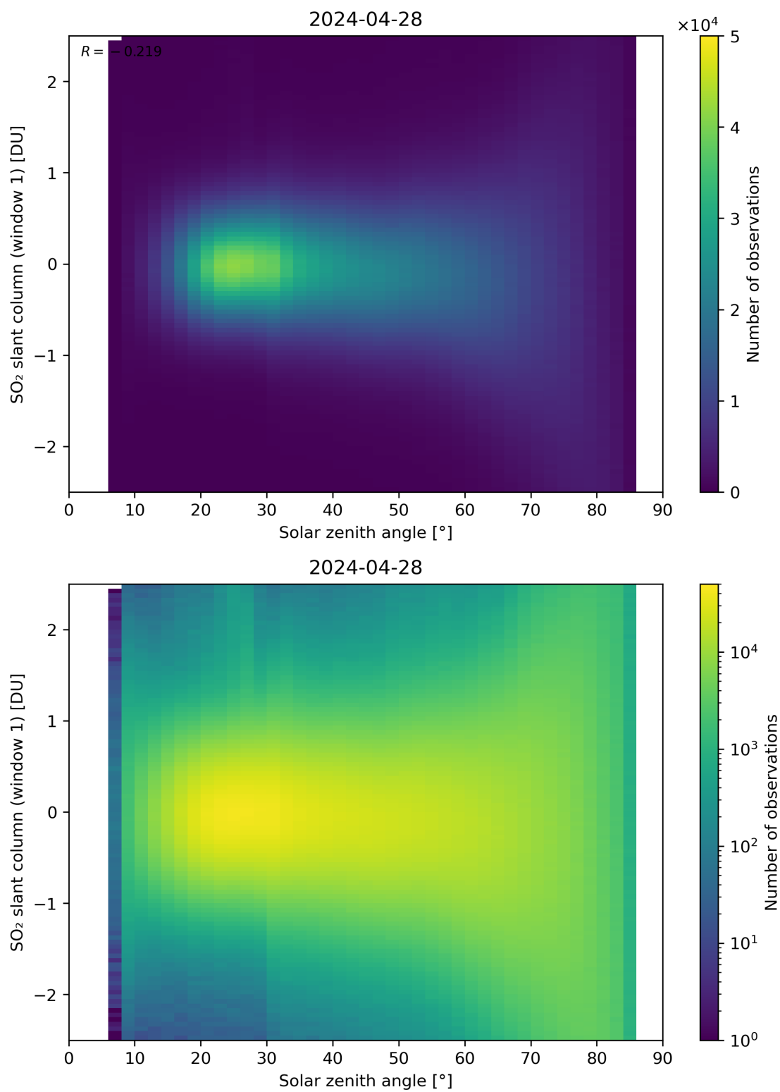
Figure 169: Scatter density plot of “Solar zenith angle” against “SO 2 slant column (window 1)” for 2024-04-27 to 2024-04-29.
