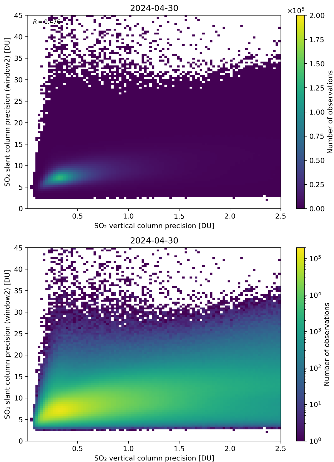
Figure 291: Scatter density plot of “SO 2 vertical column precision” against “SO 2 slant column precision (window2)” for 2024-04-29 to 2024-05-01.
