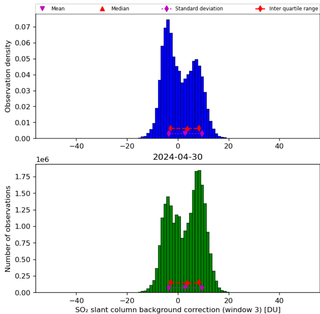
Figure 67: Histogram of "SO 2 slant column background correction (window 3)" for 2024-04-29 to 2024-05-01
