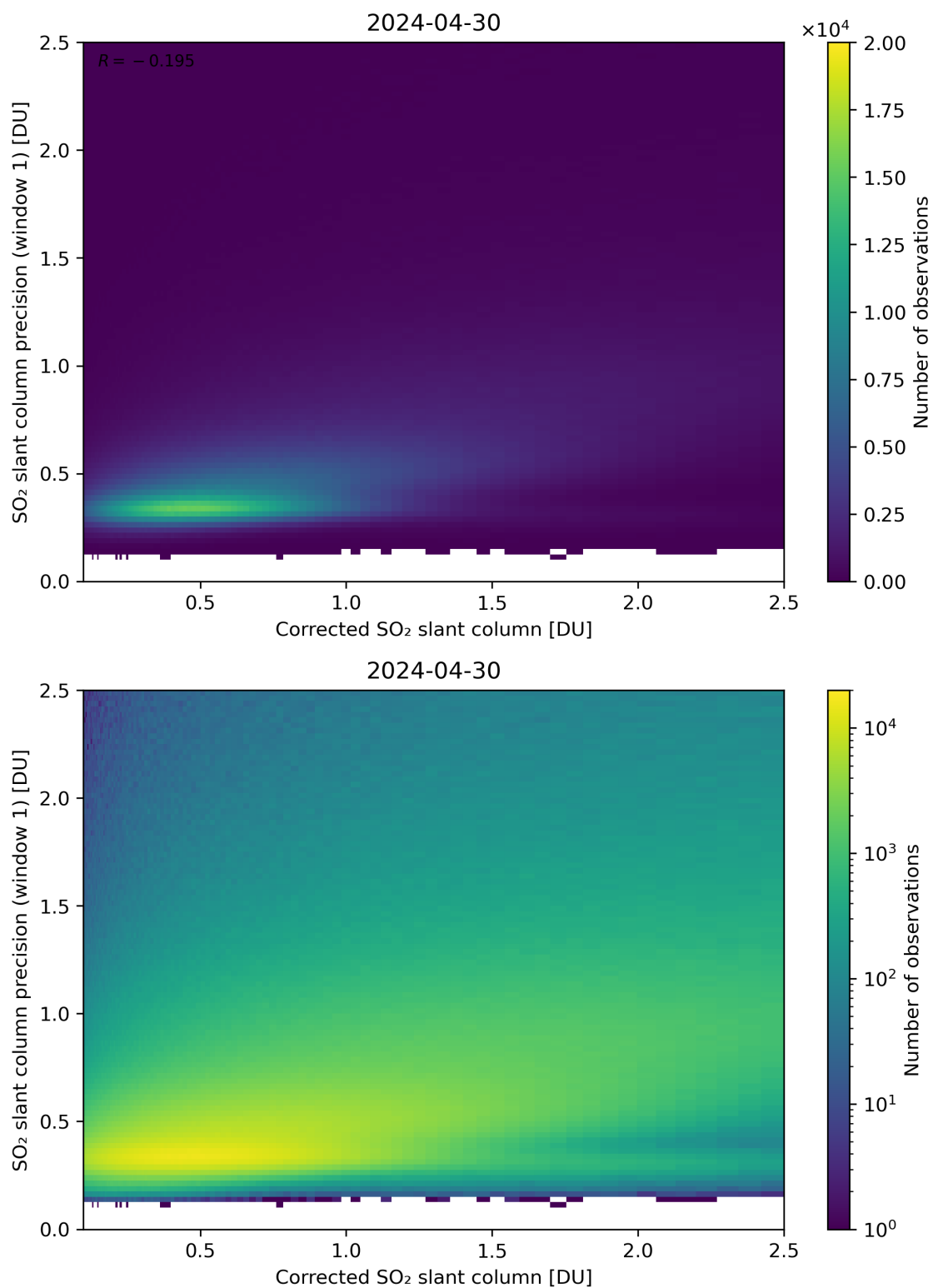
Figure 188: Scatter density plot of “Corrected SO 2 slant column” against “SO 2 slant column precision (window 1)” for 2024-04-29 to 2024-05-01.
