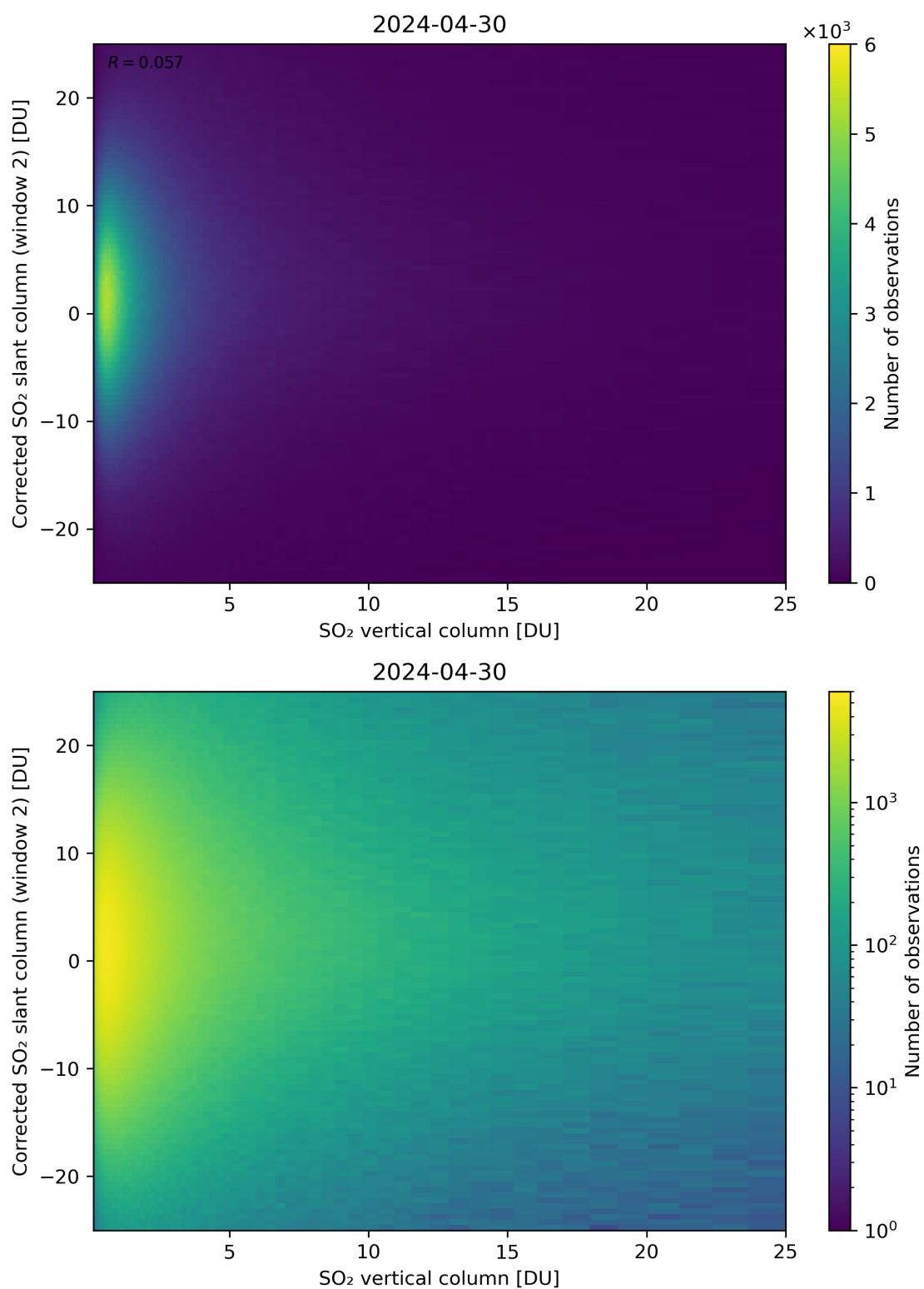
Figure 298: Scatter density plot of “SO 2 vertical column” against “Corrected SO 2 slant column (window 2)” for 2024-04-29 to 2024-05-01.
