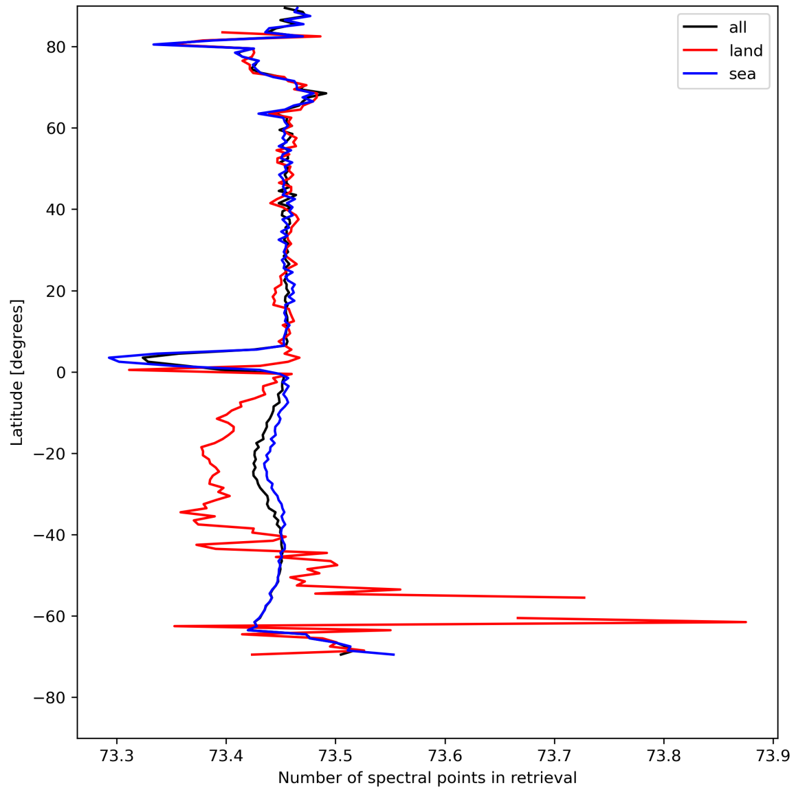
Figure 51: Zonal average of “Number of spectral points in retrieval” for 2024-04-29 to 2024-05-01.
