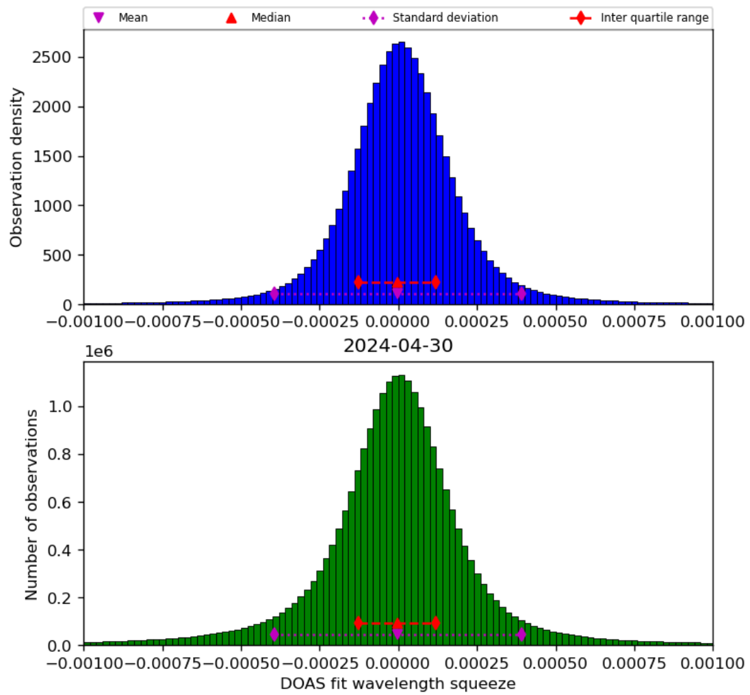
Figure 69: Histogram of “DOAS fit wavelength squeeze” for 2024-04-29 to 2024-05-01
