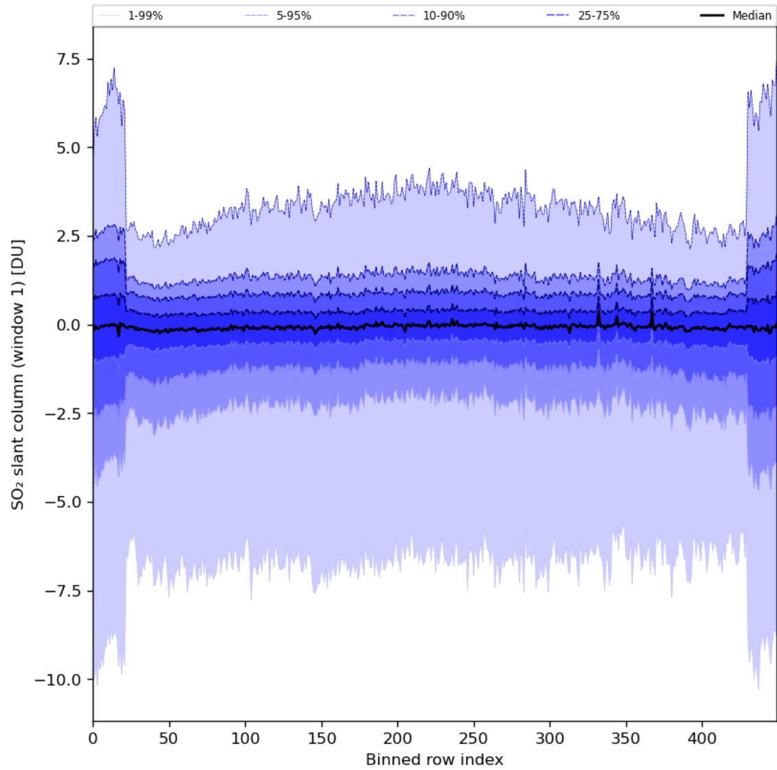
Figure 79: Along track statistics of “SO 2 slant column (window 1)” for 2024-04-29 to 2024-05-01
