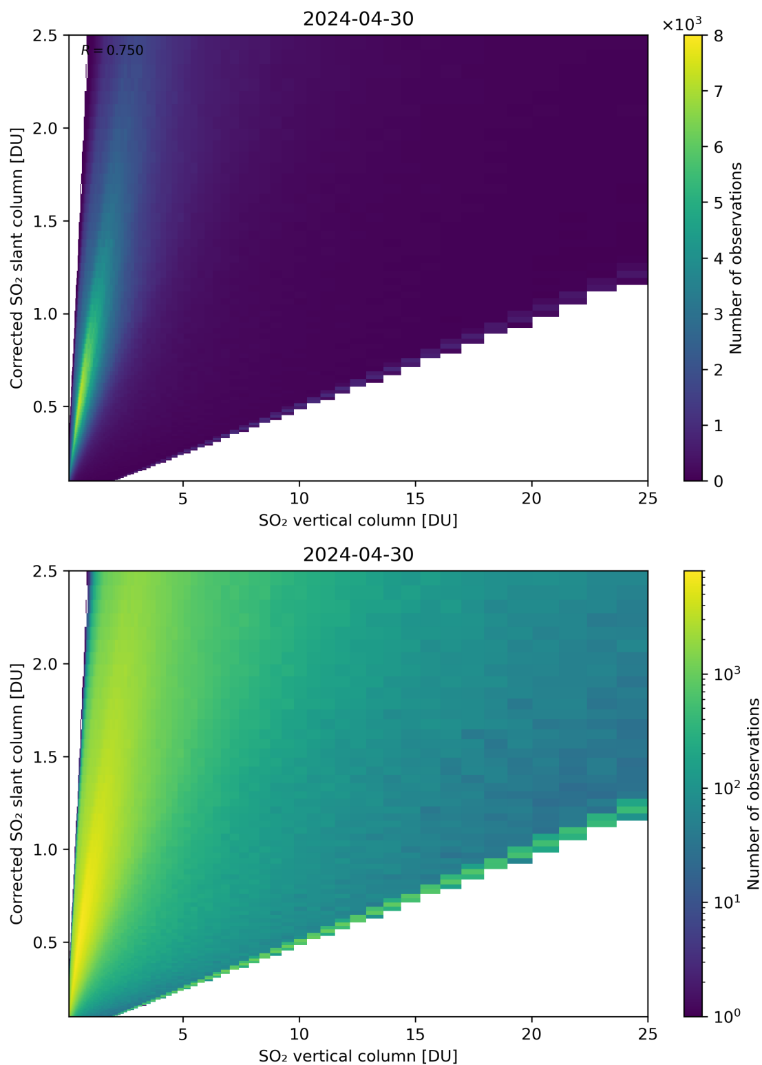
Figure 297: Scatter density plot of “SO 2 vertical column” against “Corrected SO 2 slant column” for 2024-04-29 to 2024-05-01.
