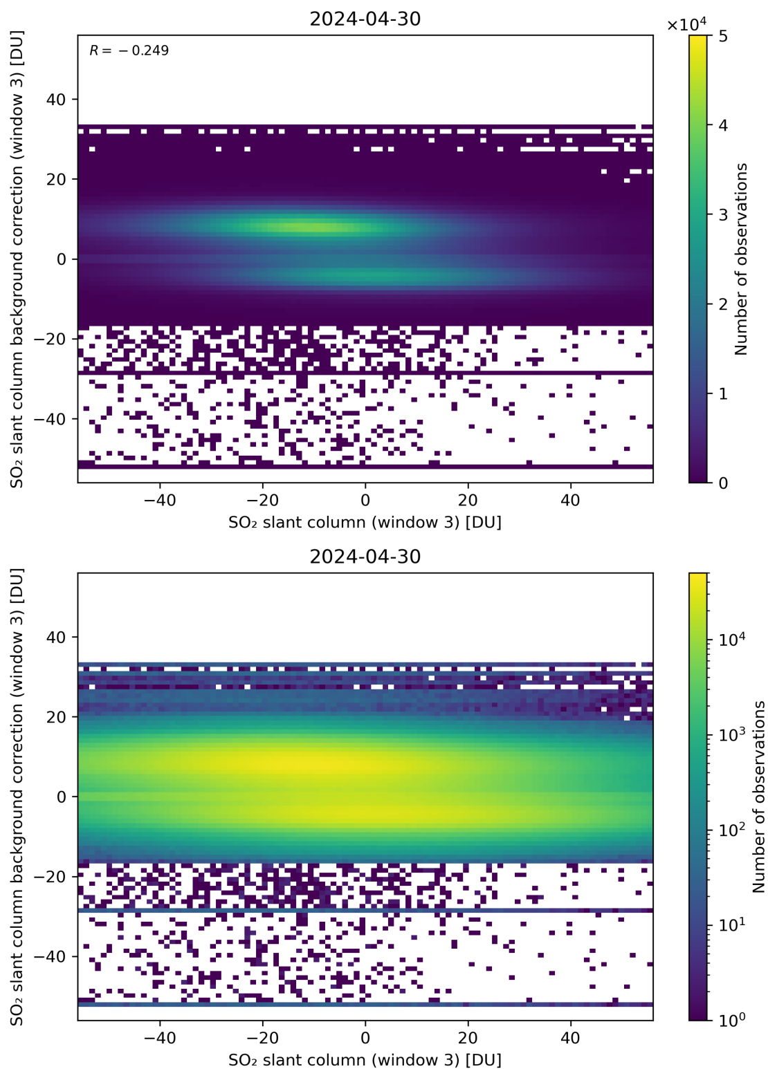
Figure 253: Scatter density plot of “SO 2 slant column (window 3)” against “SO 2 slant column background correction (window 3)” for 2024-04-29 to 2024-05-01.
