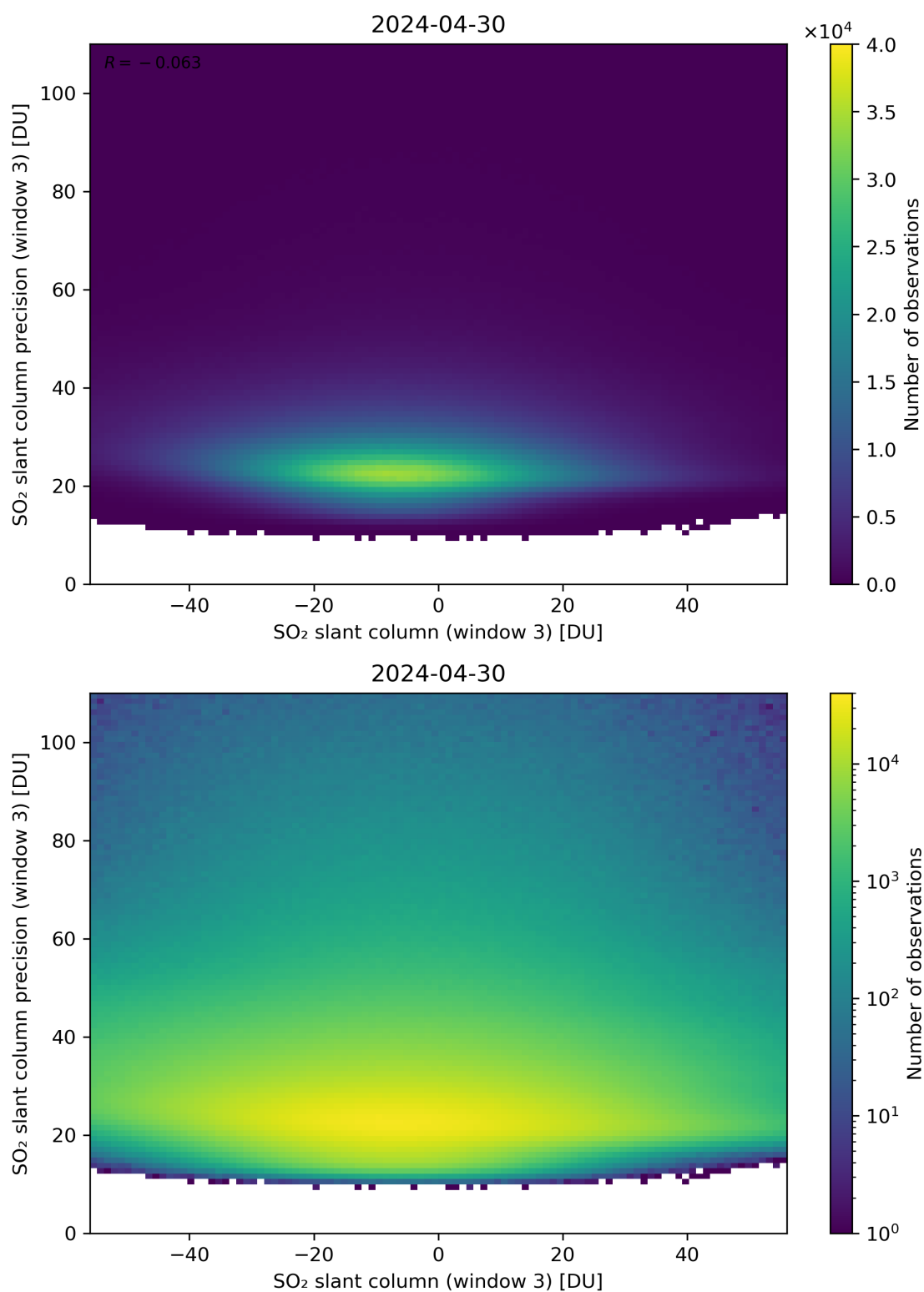
Figure 267: Scatter density plot of “SO 2 slant column (window 3)” against “SO 2 slant column precision (window 3)” for 2024-04-29 to 2024-05-01.
