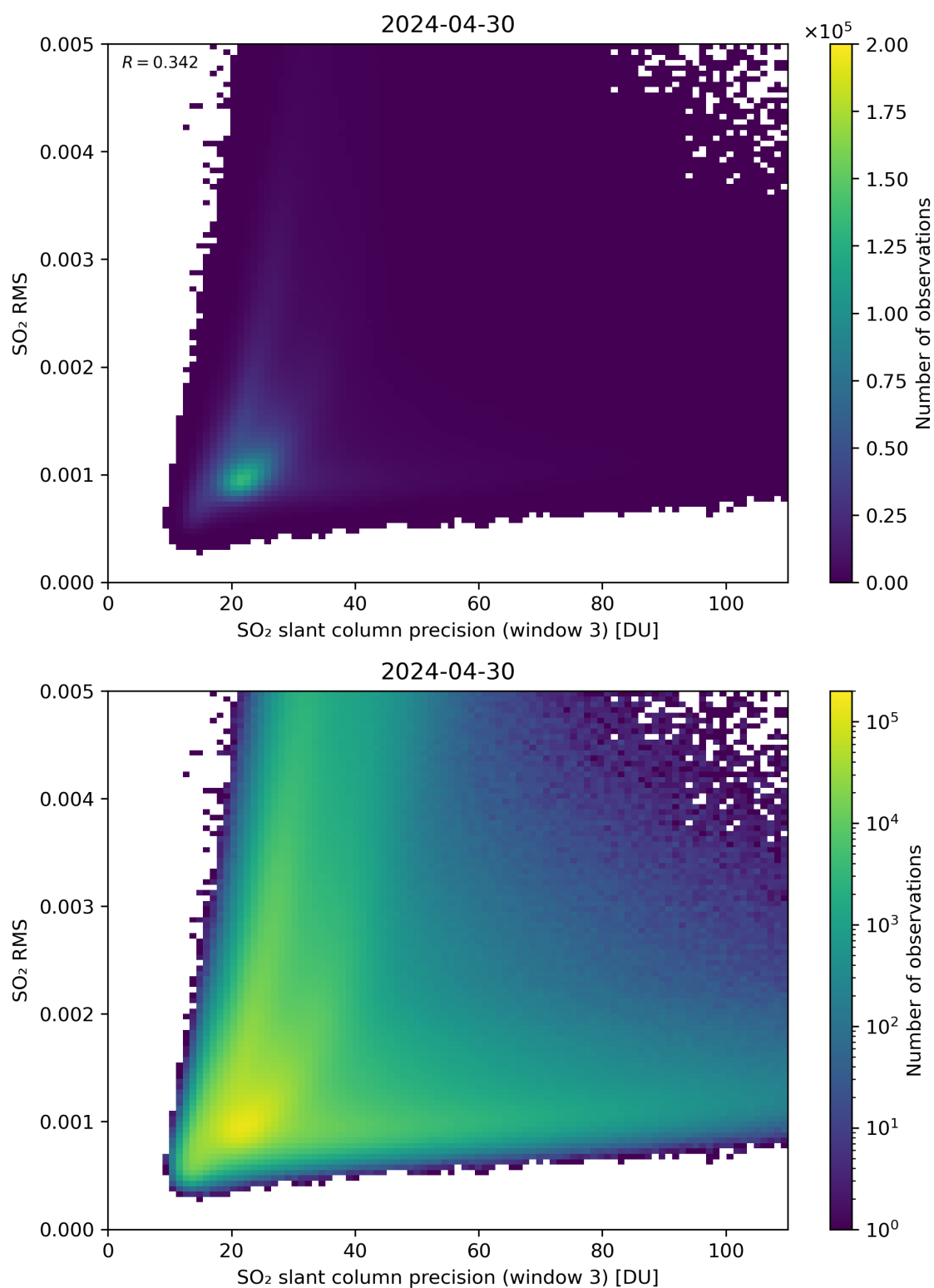
Figure 260: Scatter density plot of “SO 2 slant column precision (window 3)” against “SO 2 RMS” for 2024-04-29 to 2024-05-01.
