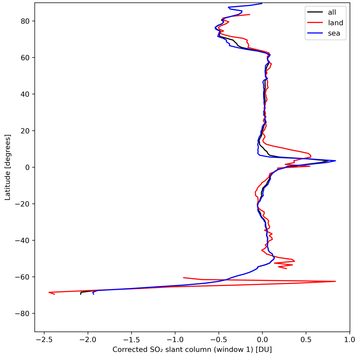
Figure 35: Zonal average of “Corrected SO 2 slant column (window 1)” for 2024-04-29 to 2024-05-01.
