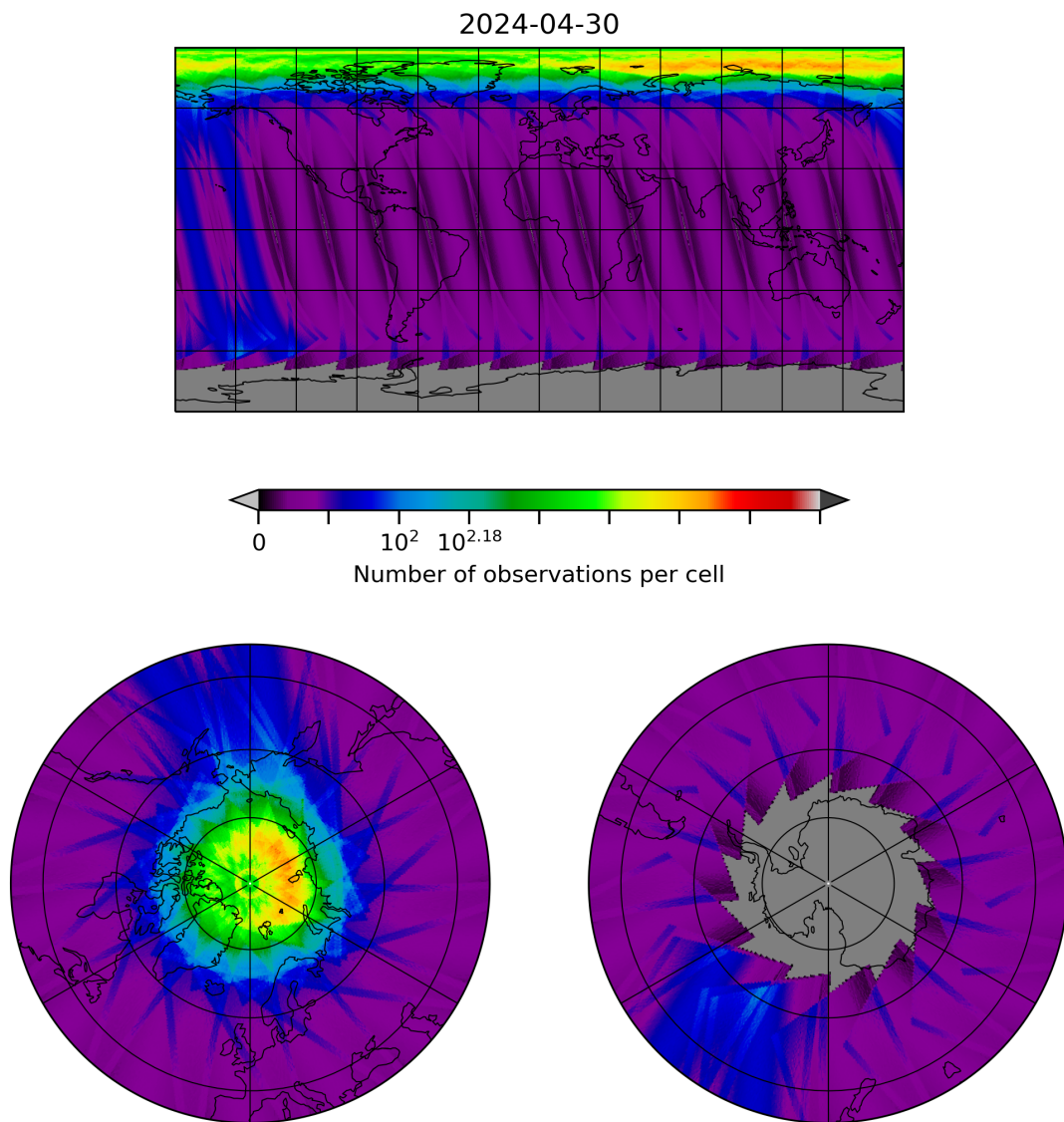
Figure 28: Map of the number of observations for 2024-04-29 to 2024-05-01
