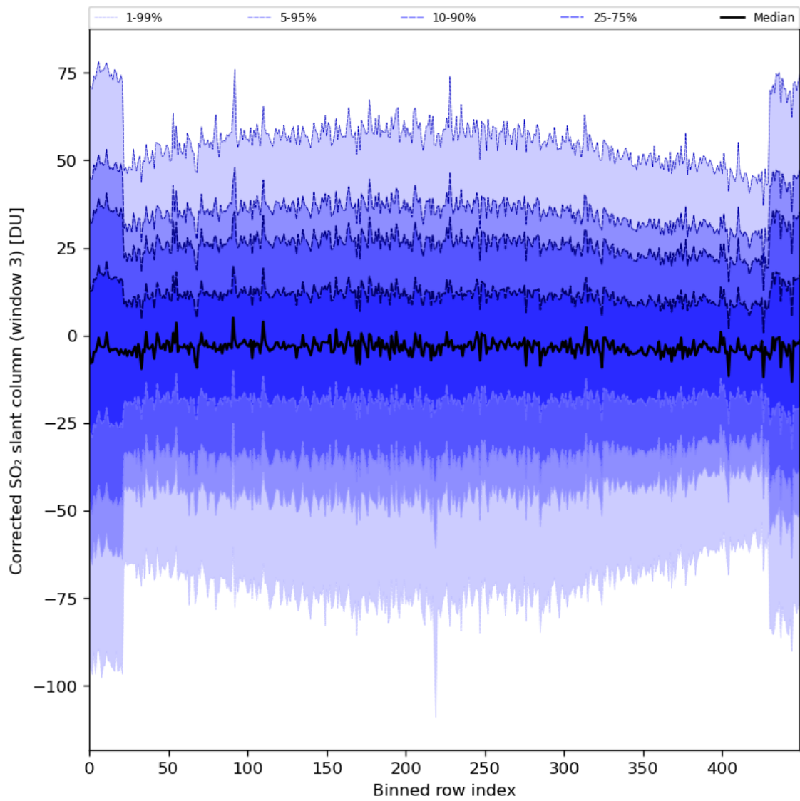
Figure 89: Along track statistics of “Corrected SO 2 slant column (window 3)” for 2024-04-29 to 2024-05-01
