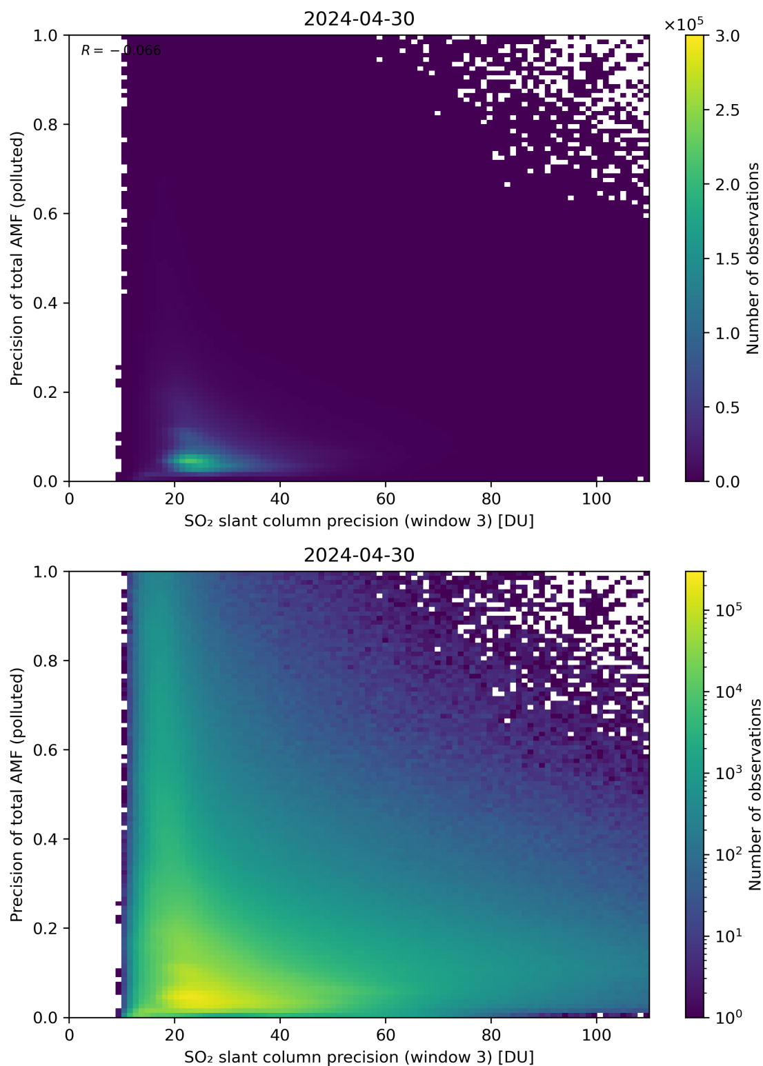
Figure 264: Scatter density plot of “SO 2 slant column precision (window 3)” against “Precision of total AMF (polluted)” for 2024-04-29 to 2024-05-01.
