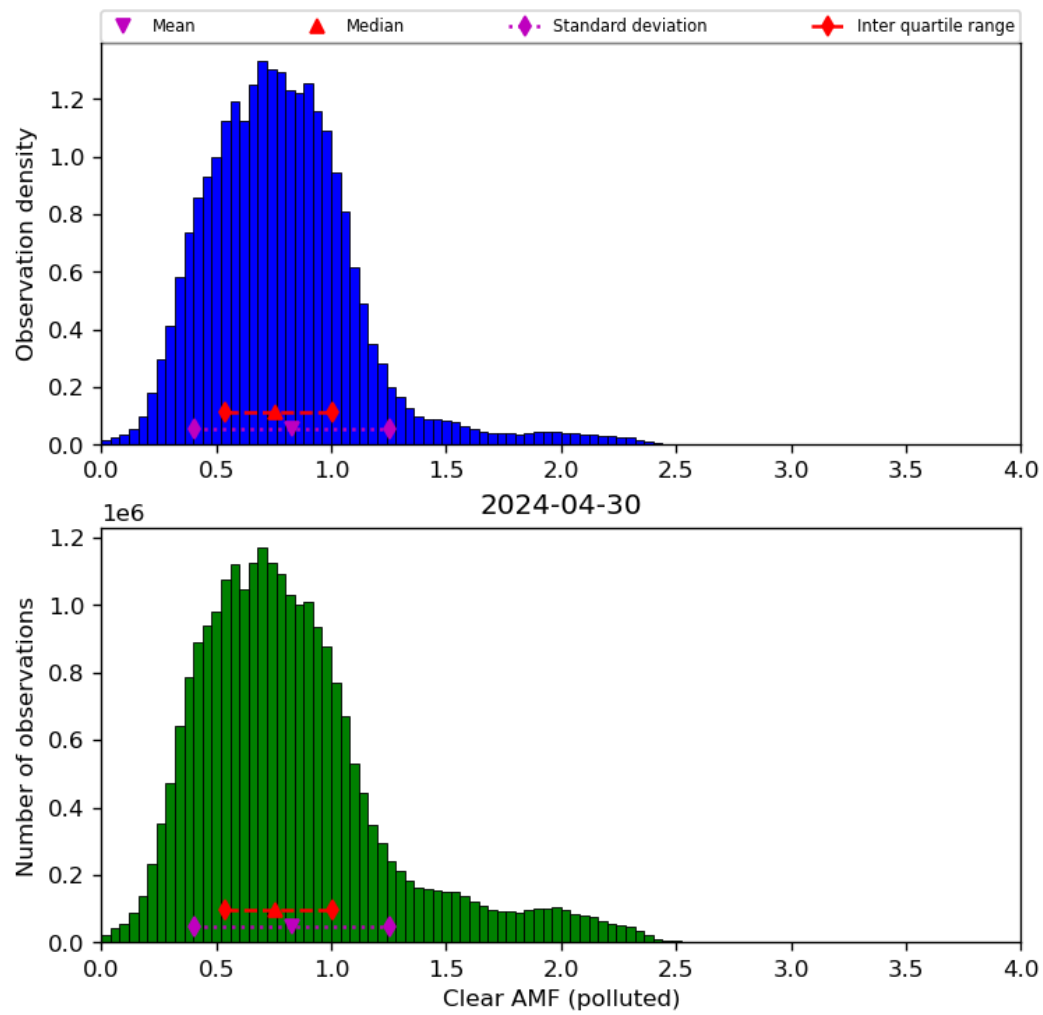
Figure 73: Histogram of “Clear AMF (polluted)” for 2024-04-29 to 2024-05-01
