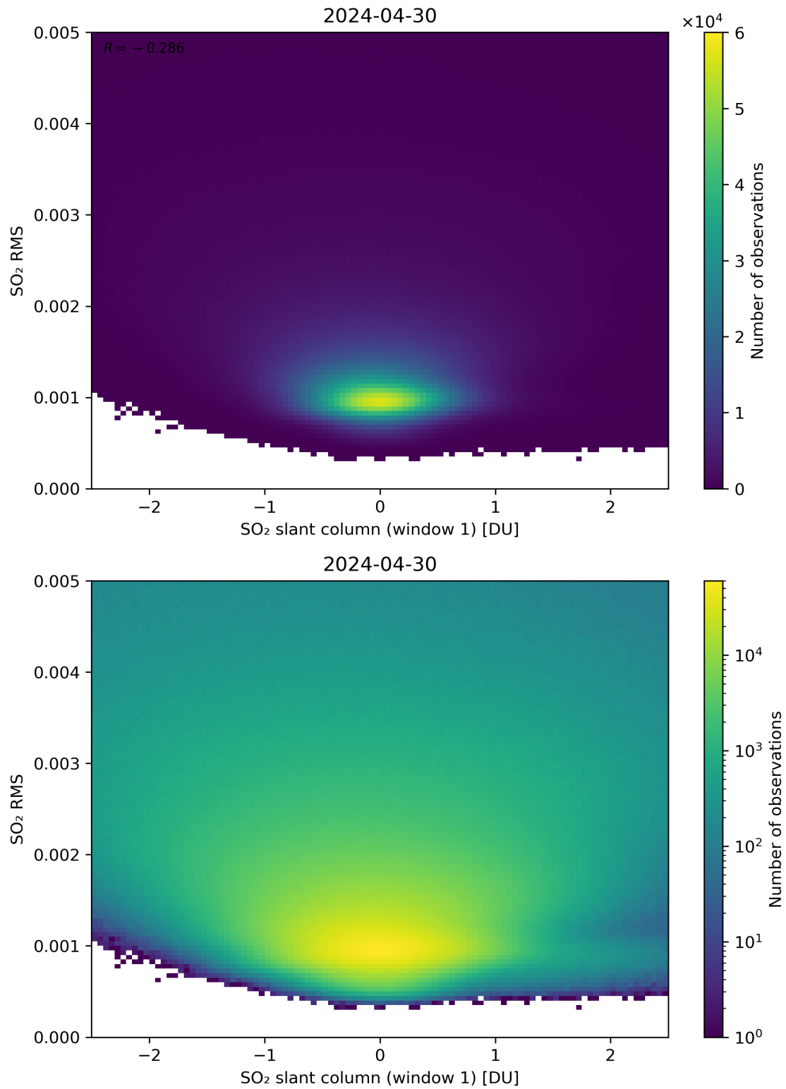
Figure 217: Scatter density plot of “SO 2 slant column (window 1)” against “SO 2 RMS” for 2024-04-29 to 2024-05-01.
