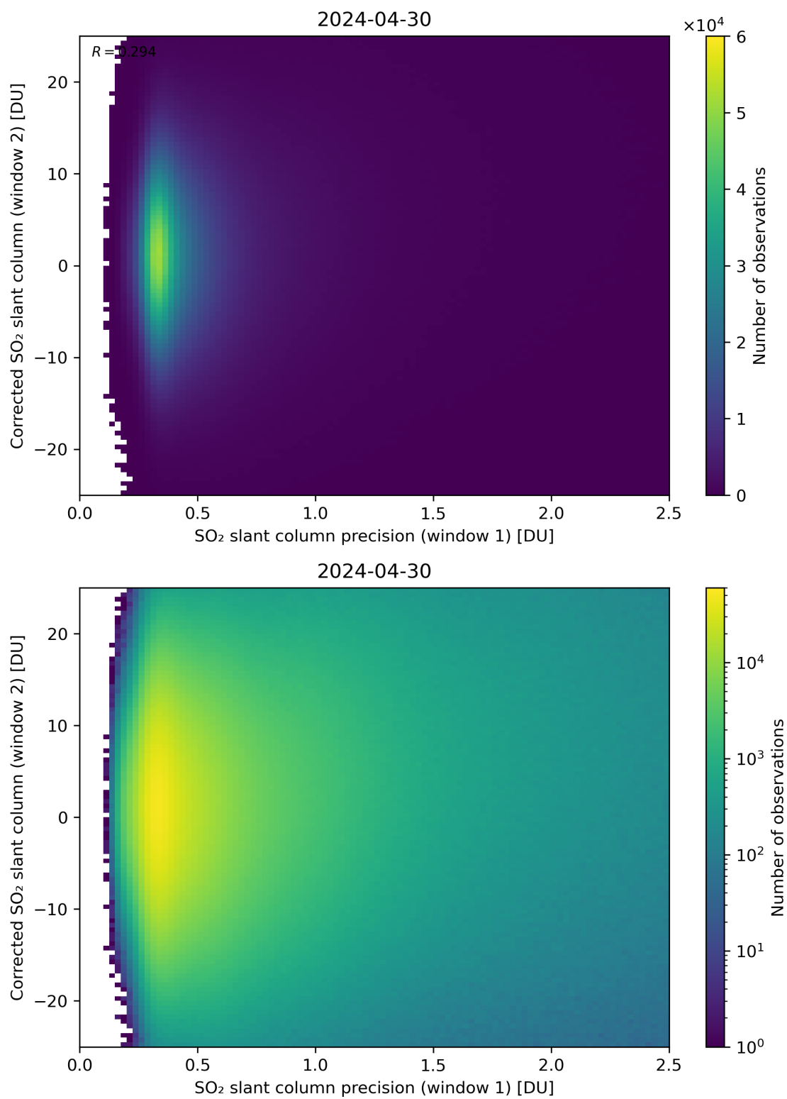
Figure 225: Scatter density plot of “SO 2 slant column precision (window 1)” against “Corrected SO 2 slant column (window 2)” for 2024-04-29 to 2024-05-01.
