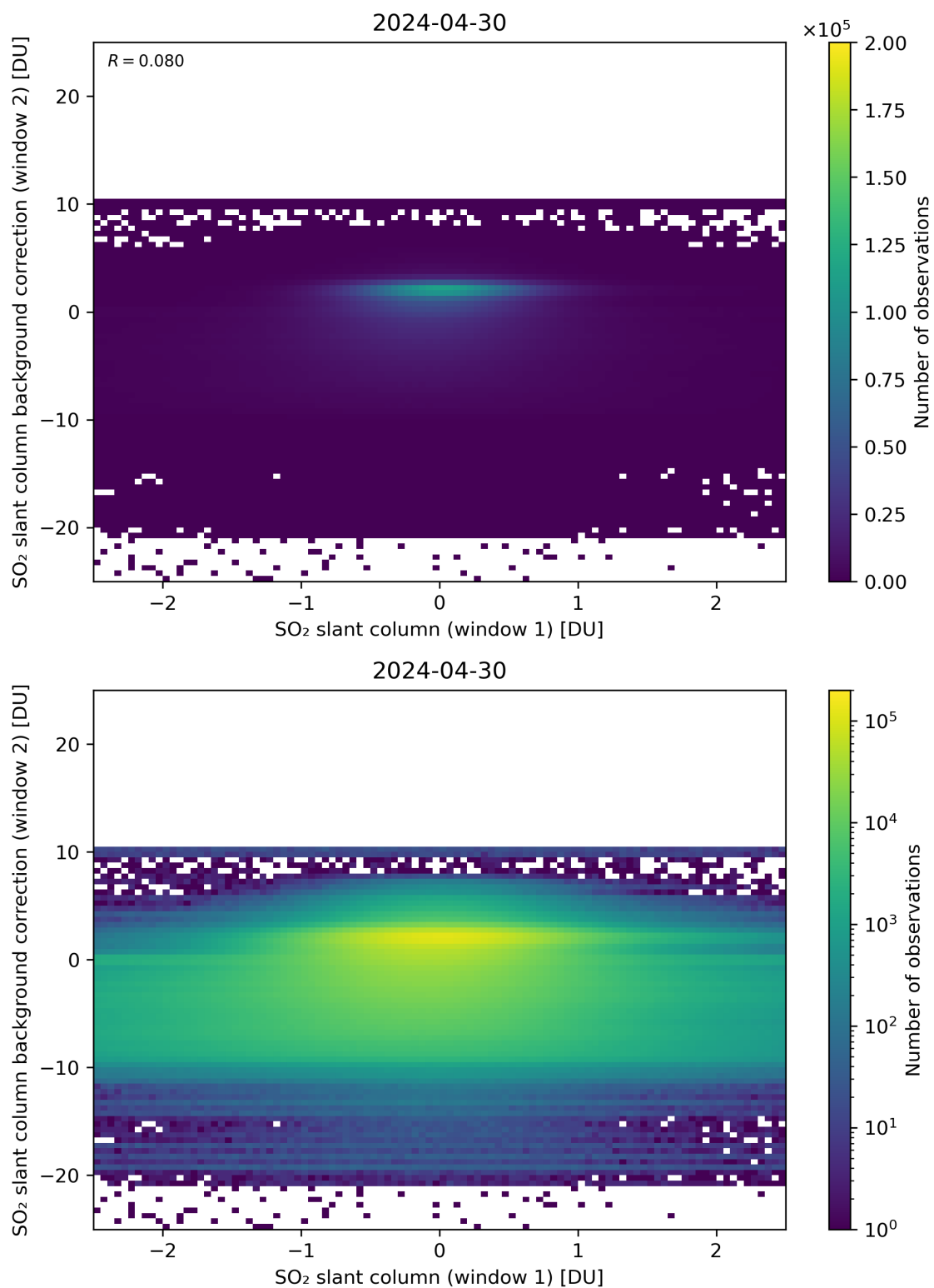
Figure 213: Scatter density plot of “SO 2 slant column (window 1)” against “SO 2 slant column background correction (window 2)” for 2024-04-29 to 2024-05-01.
