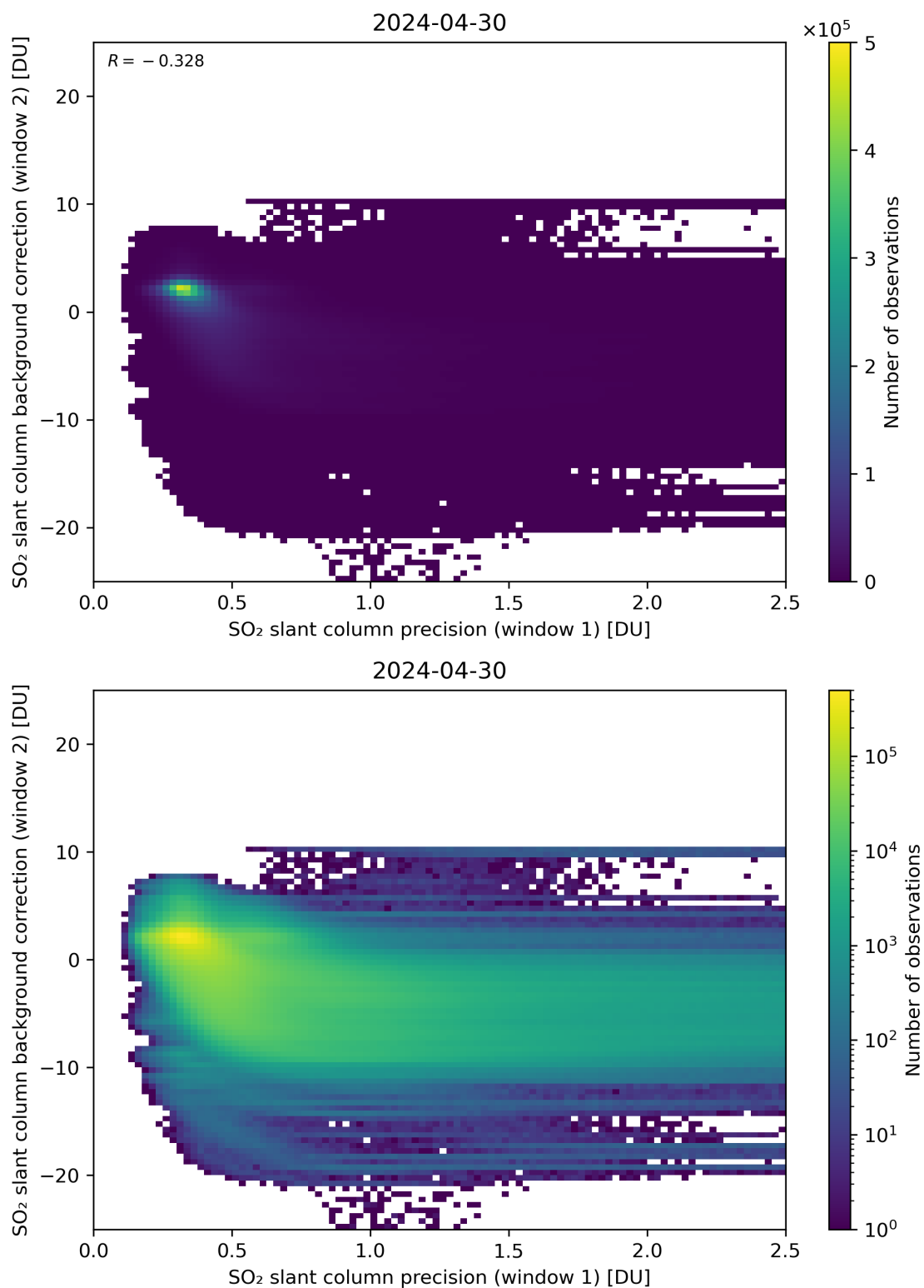
Figure 219: Scatter density plot of “SO 2 slant column precision (window 1)” against “SO 2 slant column background correction (window 2)” for 2024-04-29 to 2024-05-01.
