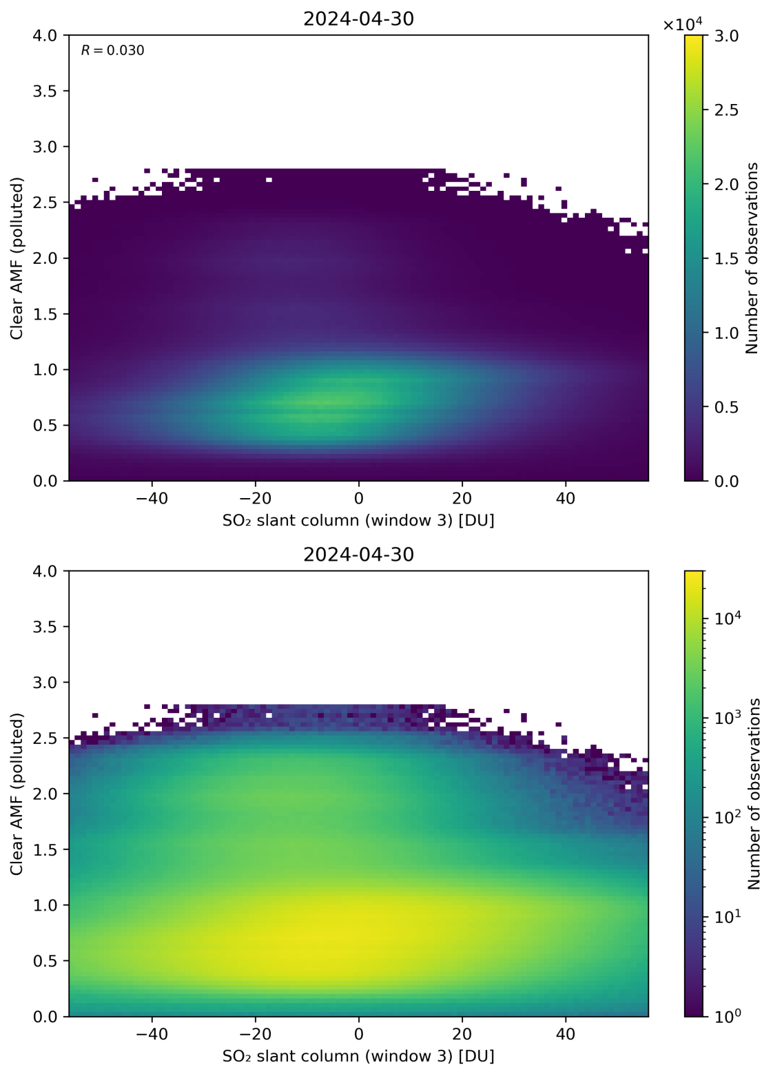
Figure 265: Scatter density plot of “SO 2 slant column (window 3)” against “Clear AMF (polluted)” for 2024-04-29 to 2024-05-01.
