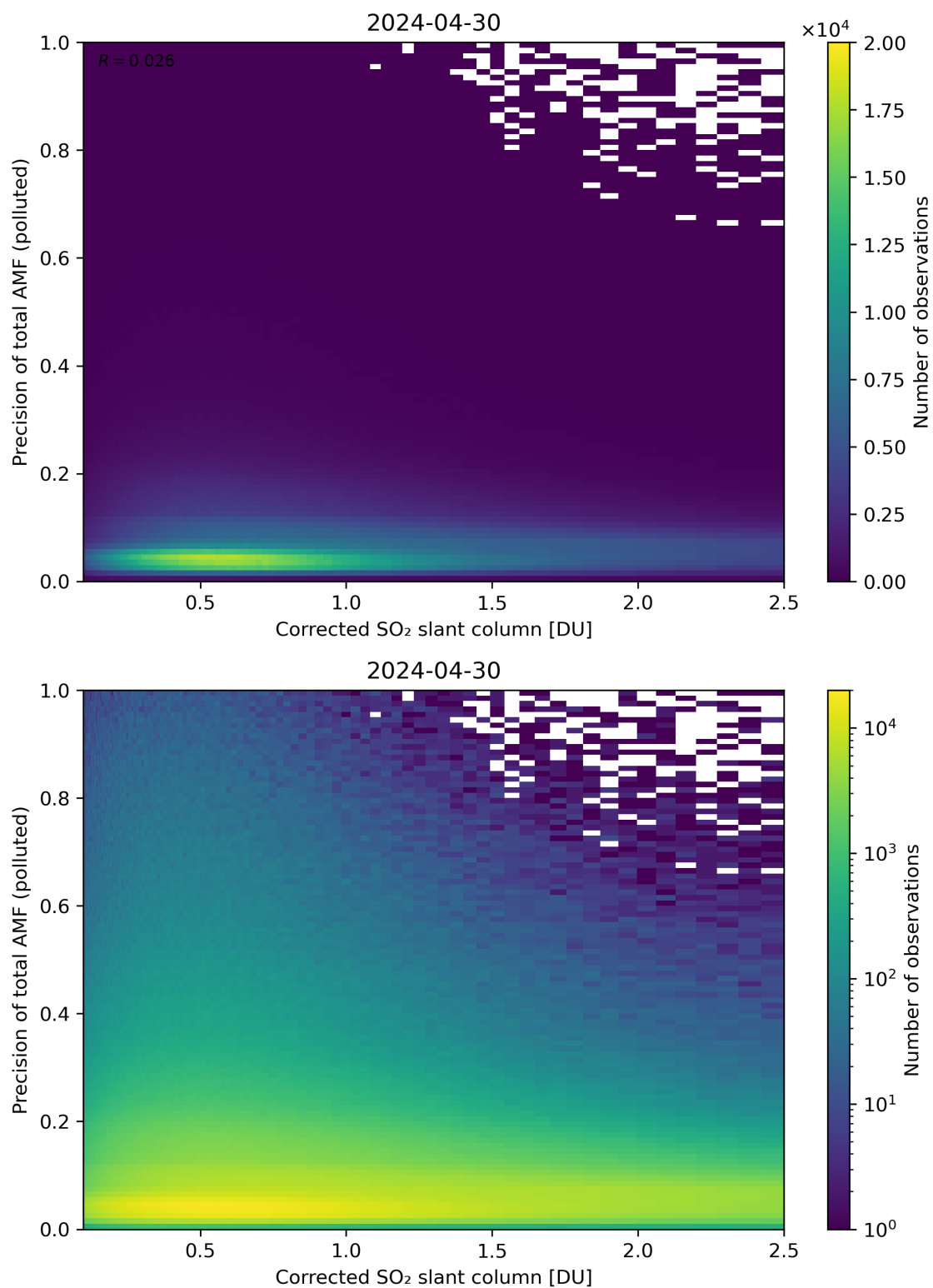
Figure 193: Scatter density plot of “Corrected SO 2 slant column” against “Precision of total AMF (polluted)” for 2024-04-29 to 2024-05-01.
