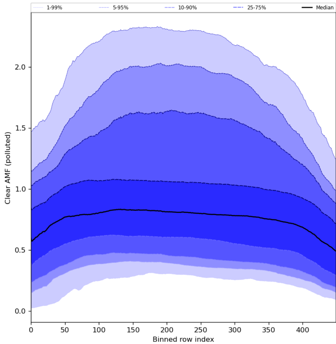
Figure 96: Along track statistics of “Clear AMF (polluted)” for 2024-04-29 to 2024-05-01
