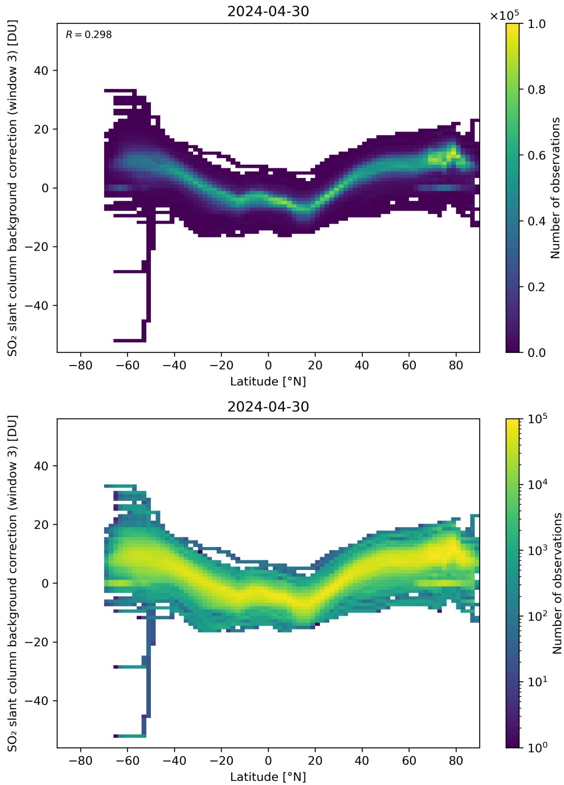
Figure 141: Scatter density plot of “Latitude” against “SO 2 slant column background correction (window 3)” for 2024-04-29 to 2024-05-01.
