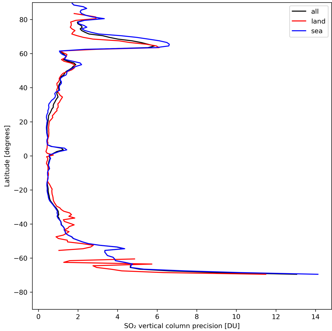
Figure 31: Zonal average of “SO 2 vertical column precision” for 2024-04-29 to 2024-05-01.
