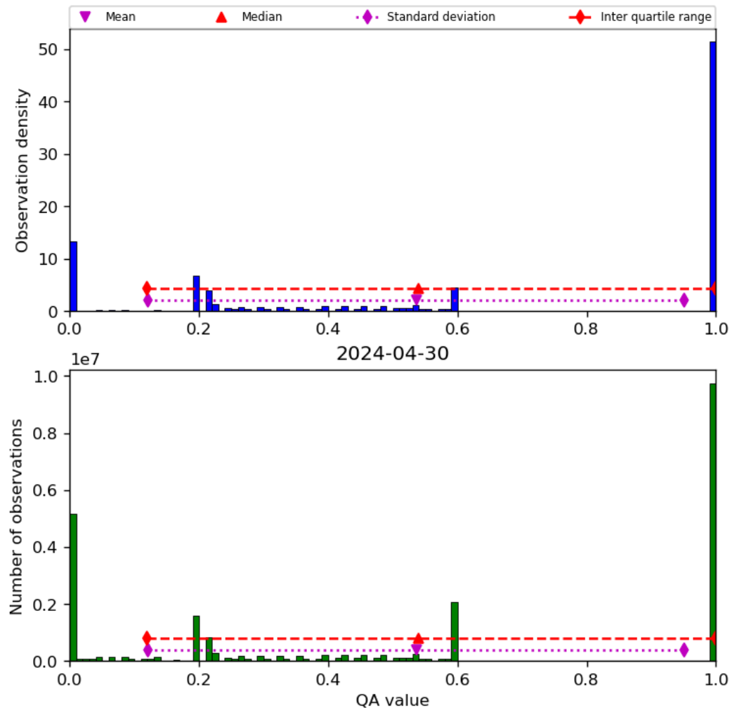
Figure 52: Histogram of “QA value” for 2024-04-29 to 2024-05-01
