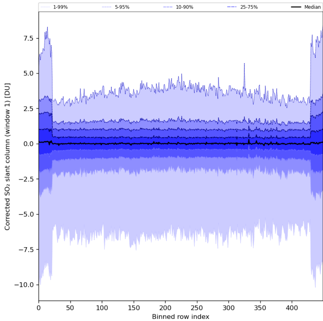
Figure 81: Along track statistics of “Corrected SO 2 slant column (window 1)” for 2024-04-29 to 2024-05-01
