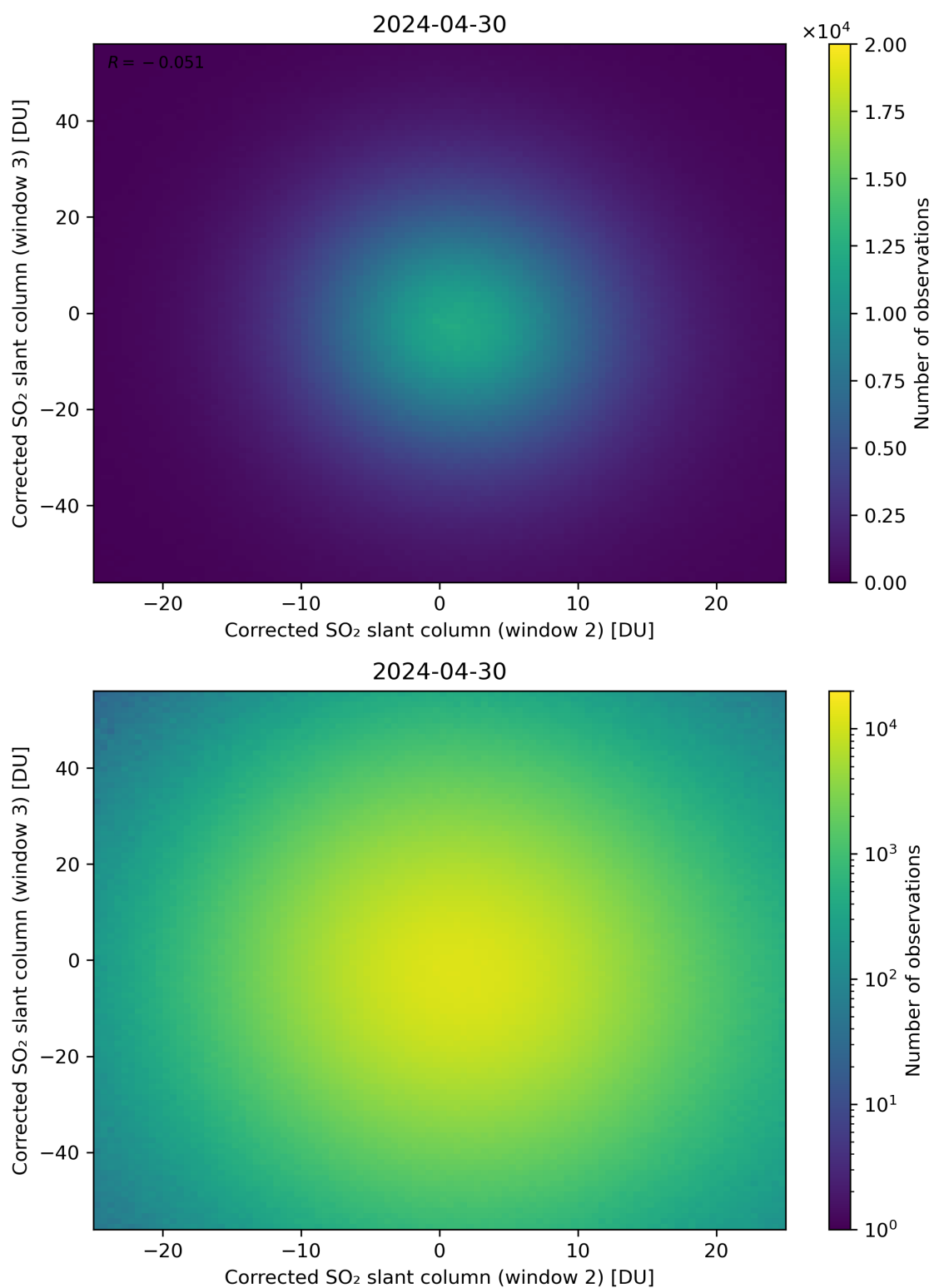
Figure 200: Scatter density plot of “Corrected SO 2 slant column (window 2)” against “Corrected SO 2 slant column (window 3)” for 2024-04-29 to 2024-05-01.
