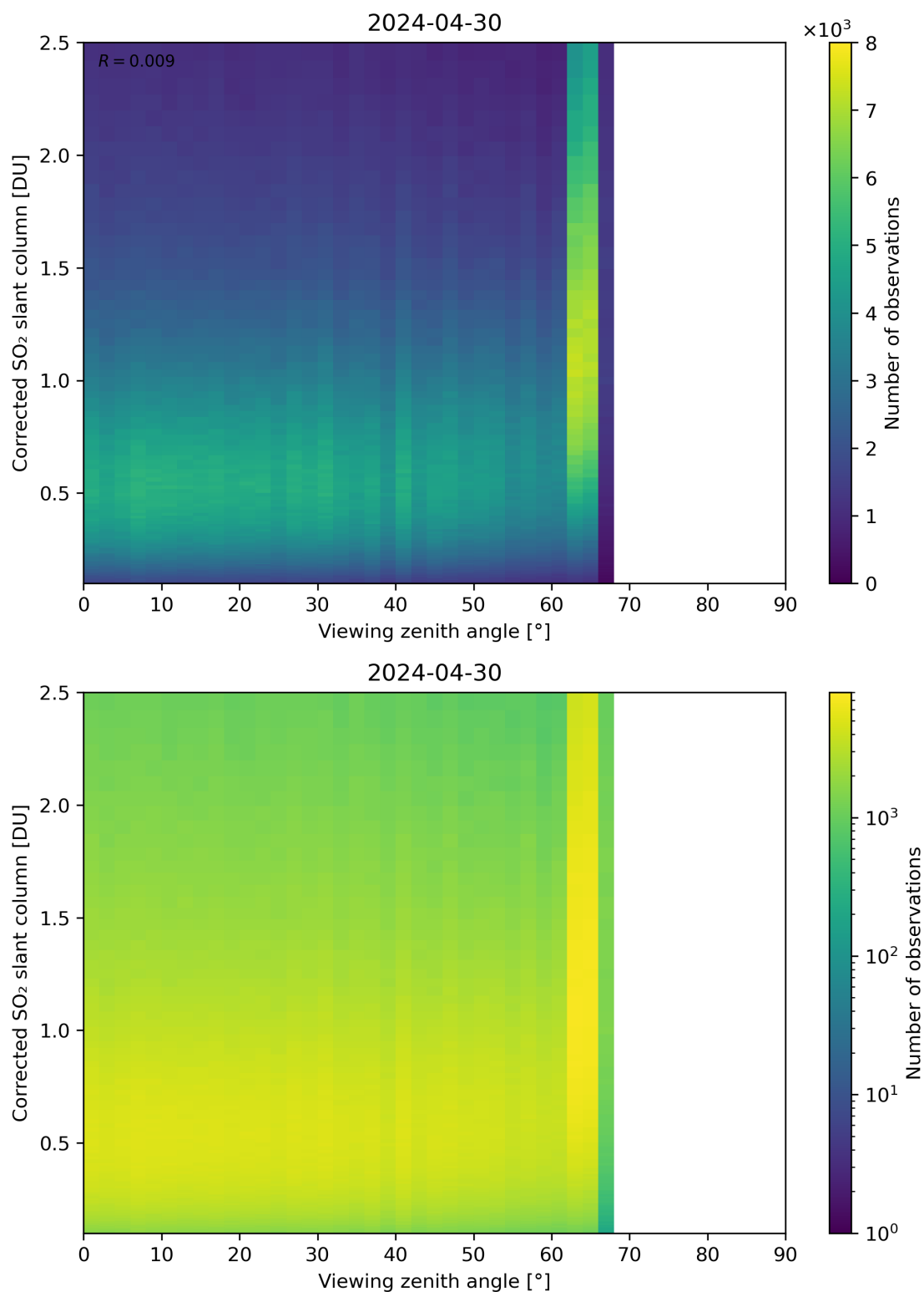
Figure 317: Scatter density plot of “Viewing zenith angle” against “Corrected SO 2 slant column” for 2024-04-29 to 2024-05-01.
