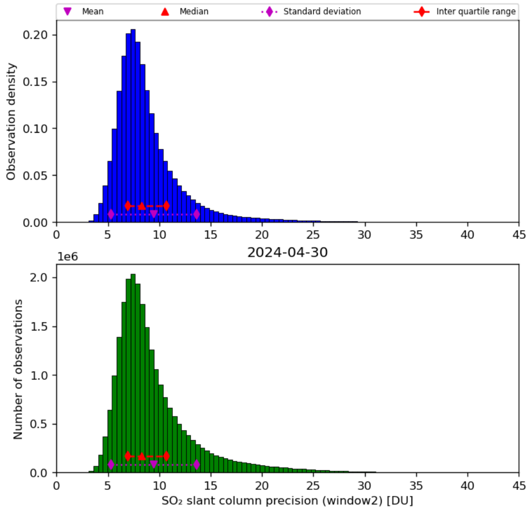
Figure 61: Histogram of “SO 2 slant column precision (window2)” for 2024-04-29 to 2024-05-01
