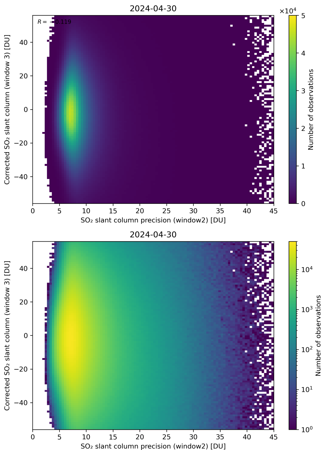
Figure 248: Scatter density plot of “SO 2 slant column precision (window2)” against “Corrected SO 2 slant column (window 3)” for 2024-04-29 to 2024-05-01.
