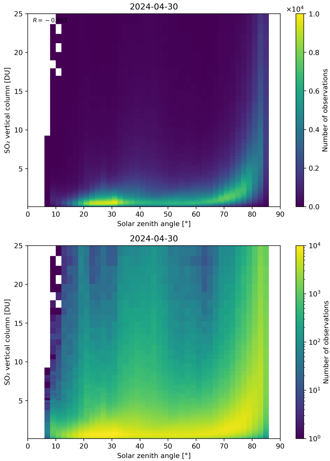
Figure 176: Scatter density plot of “Solar zenith angle” against “SO 2 vertical column” for 2024-04-29 to 2024-05-01.
