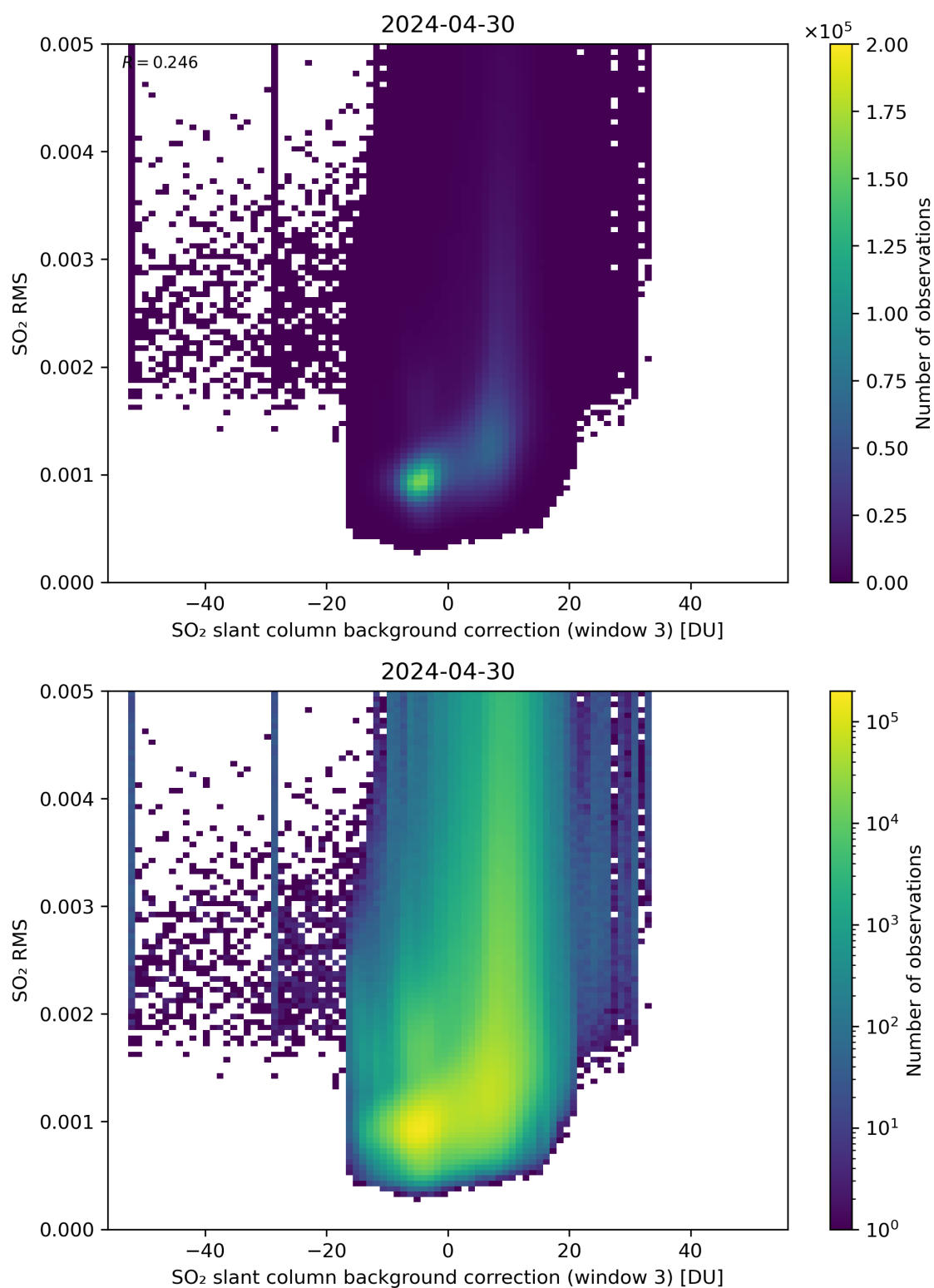
Figure 123: Scatter density plot of “SO 2 slant column background correction (window 3)” against “SO 2 RMS” for 2024-04-29 to 2024-05-01.
