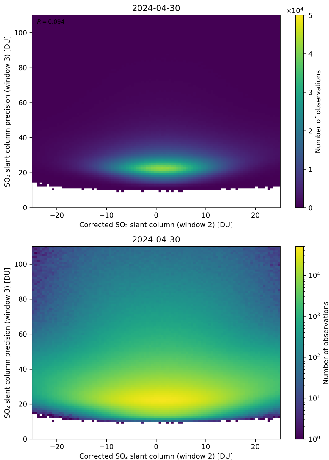
Figure 202: Scatter density plot of “Corrected SO 2 slant column (window 2)” against “SO 2 slant column precision (window 3)” for 2024-04-29 to 2024-05-01.
