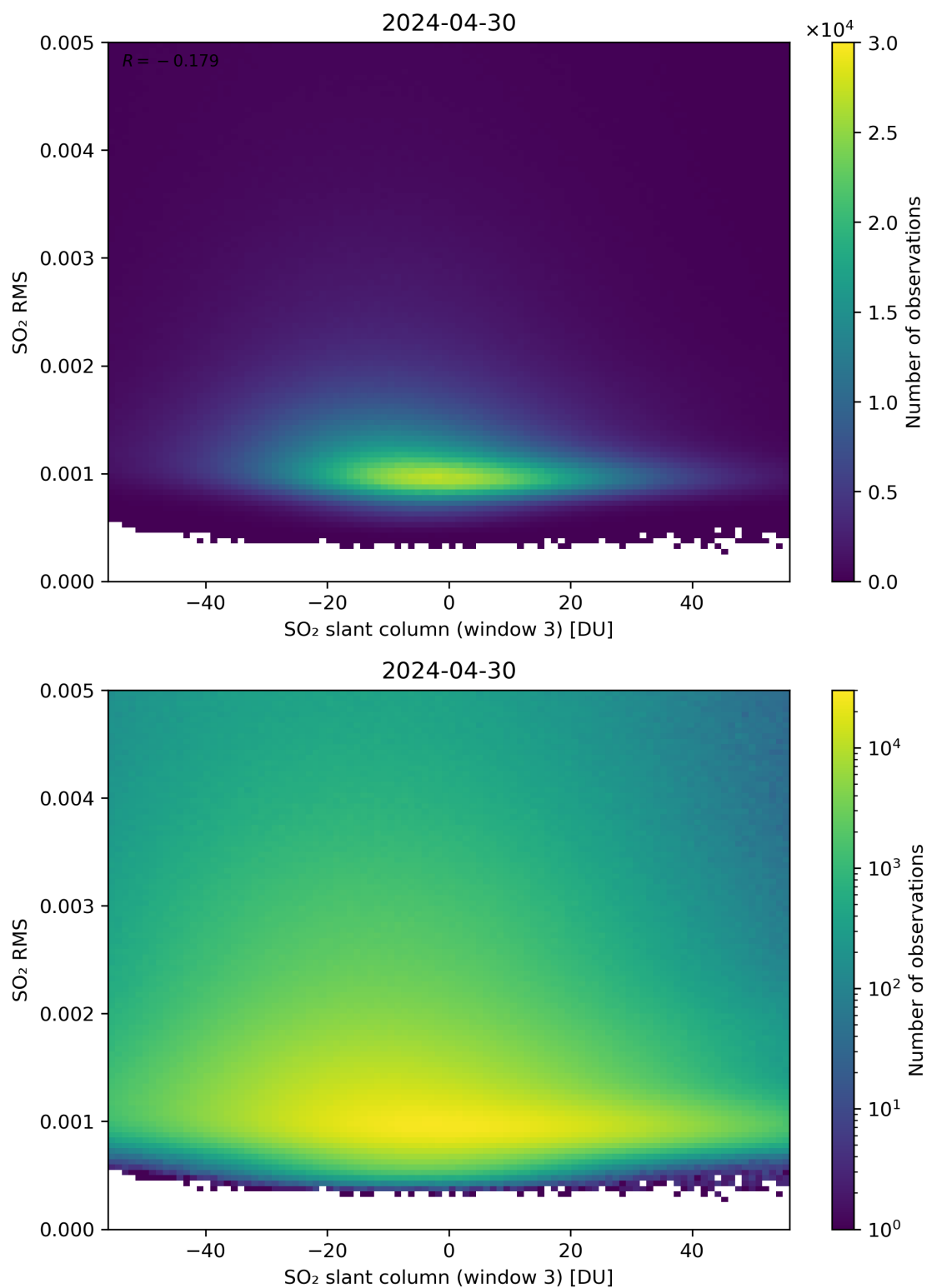
Figure 256: Scatter density plot of “SO 2 slant column (window 3)” against “SO 2 RMS” for 2024-04-29 to 2024-05-01.
