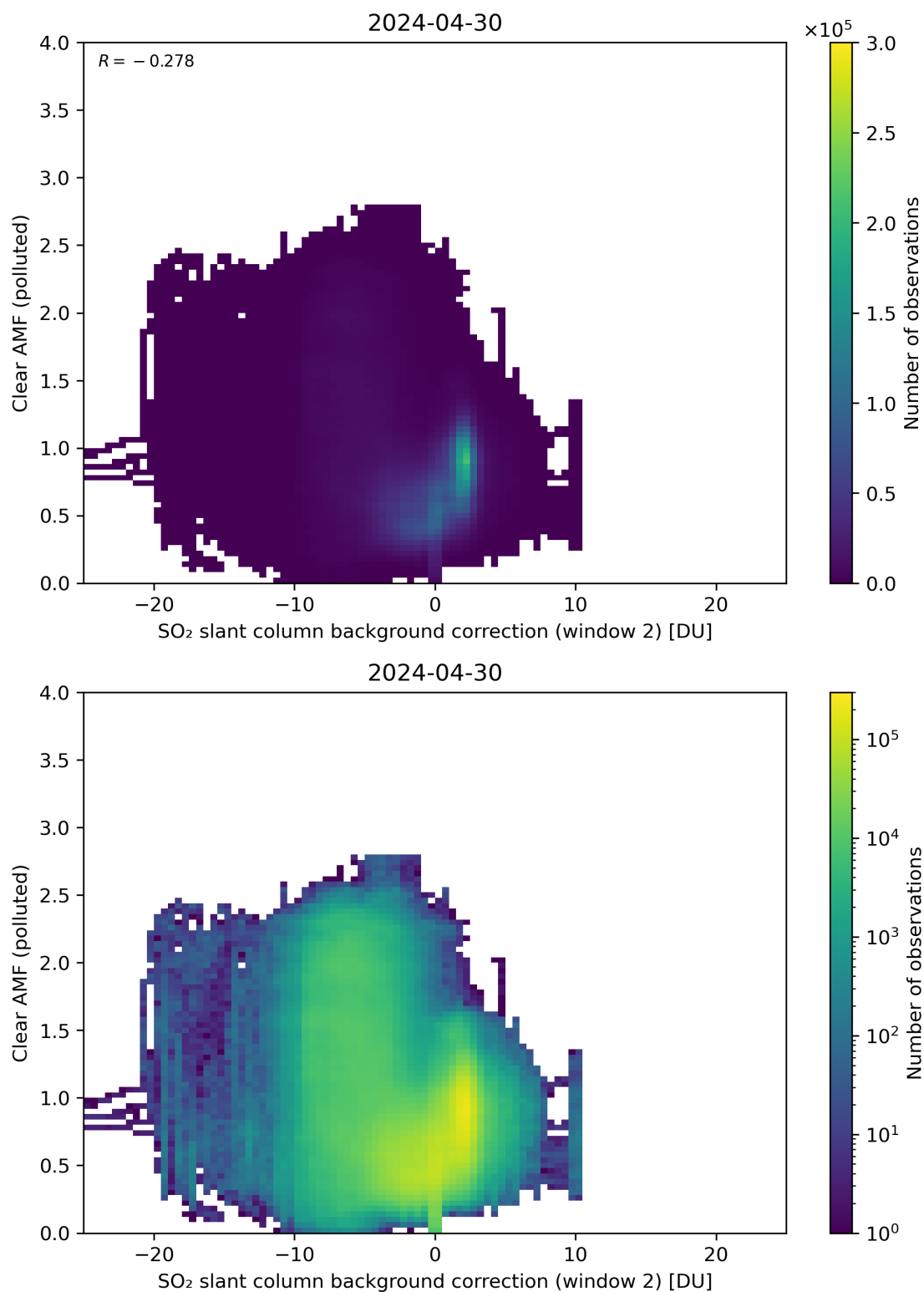
Figure 115: Scatter density plot of “SO 2 slant column background correction (window 2)” against “Clear AMF (polluted)” for 2024-04-29 to 2024-05-01.
