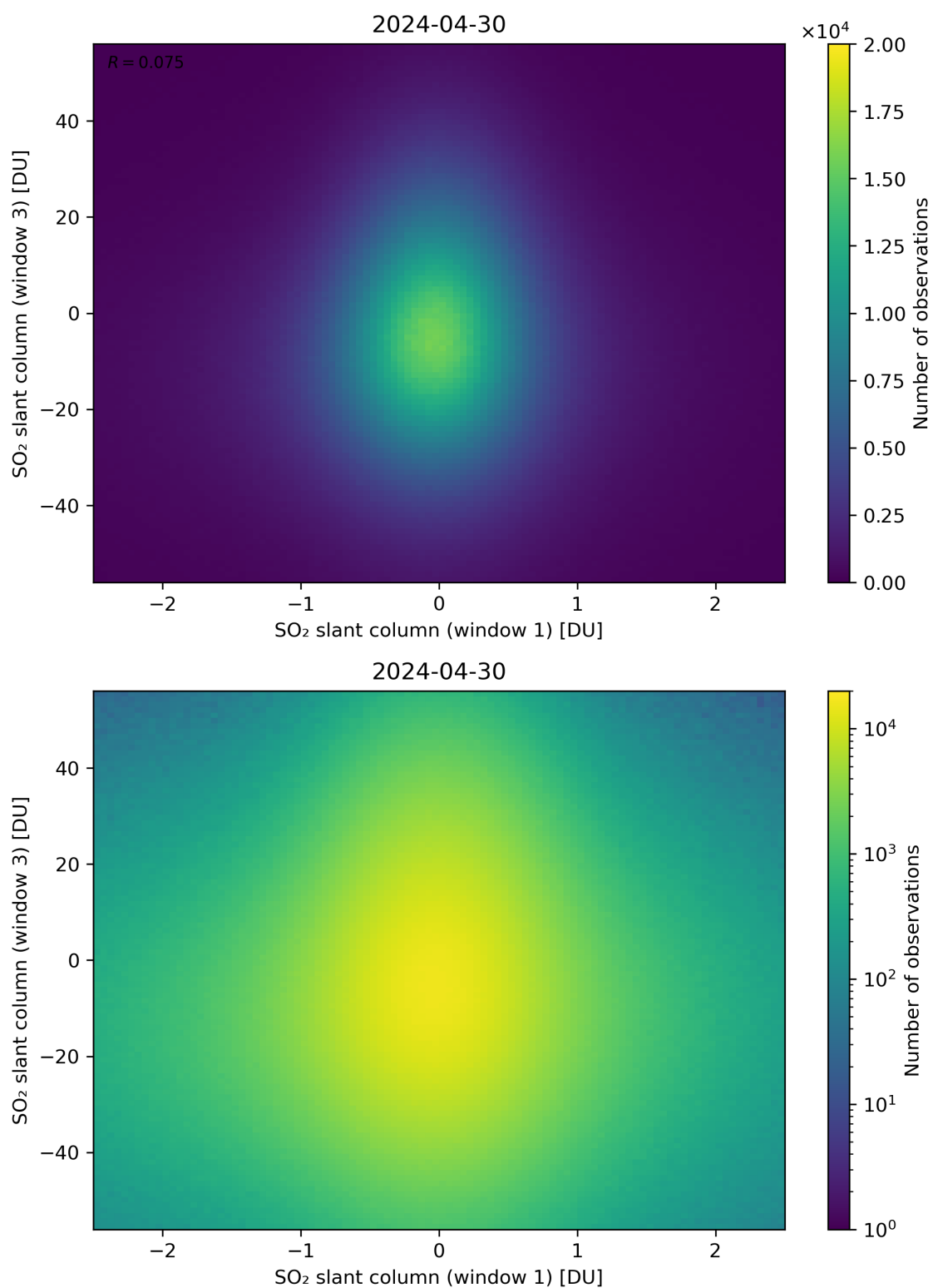
Figure 237: Scatter density plot of “SO 2 slant column (window 1)” against “SO 2 slant column (window 3)” for 2024-04-29 to 2024-05-01.
