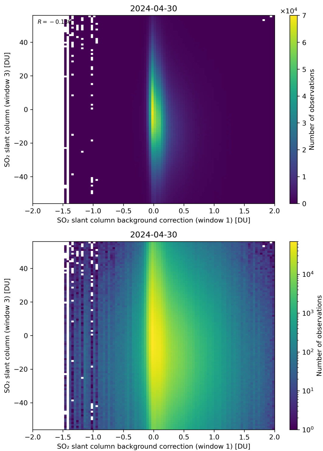
Figure 107: Scatter density plot of “SO 2 slant column background correction (window 1)” against “SO 2 slant column (window 3)” for 2024-04-29 to 2024-05-01.
