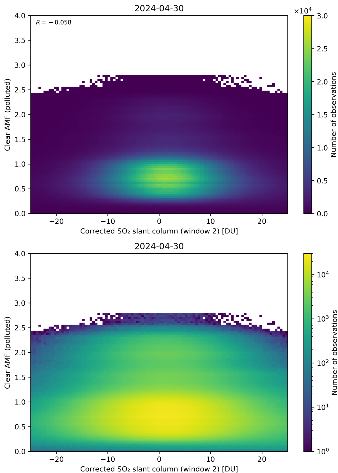
Figure 199: Scatter density plot of “Corrected SO 2 slant column (window 2)” against “Clear AMF (polluted)” for 2024-04-29 to 2024-05-01.
