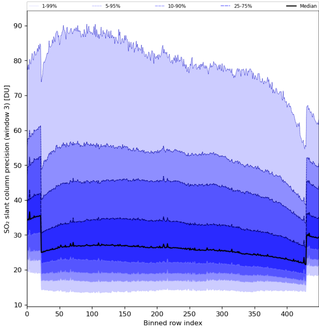
Figure 88: Along track statistics of “SO 2 slant column precision (window 3)” for 2024-04-29 to 2024-05-01
