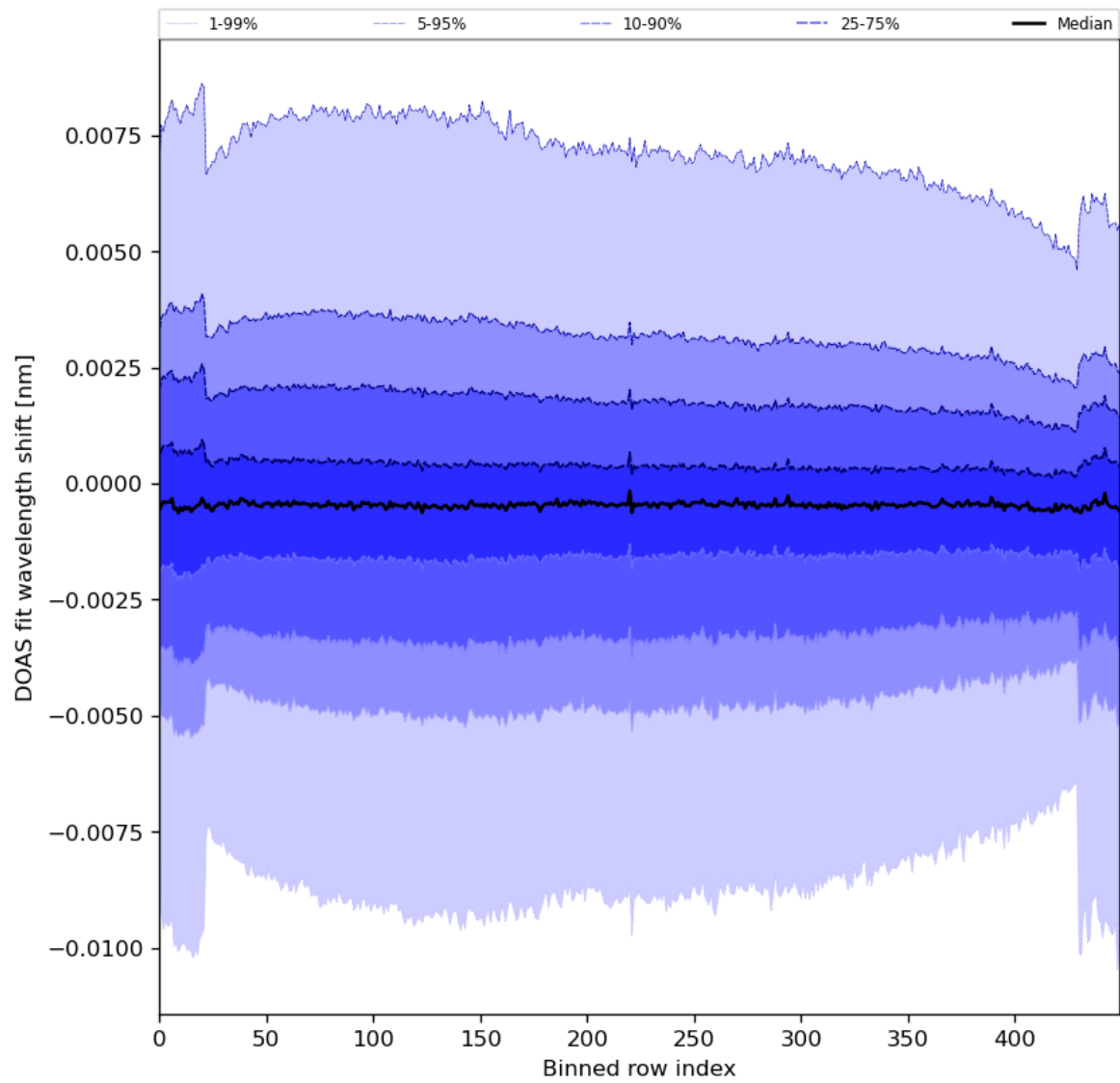
Figure 91: Along track statistics of “DOAS fit wavelength shift” for 2024-04-29 to 2024-05-01
