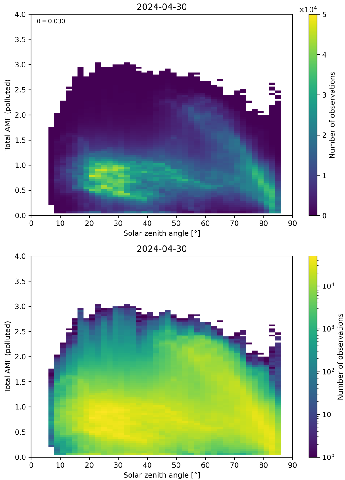
Figure 174: Scatter density plot of “Solar zenith angle” against “Total AMF (polluted)” for 2024-04-29 to 2024-05-01.
