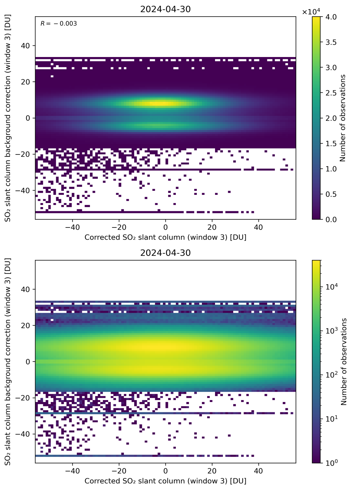
Figure 205: Scatter density plot of “Corrected SO 2 slant column (window 3)” against “SO 2 slant column background correction (window 3)” for 2024-04-29 to 2024-05-01.
