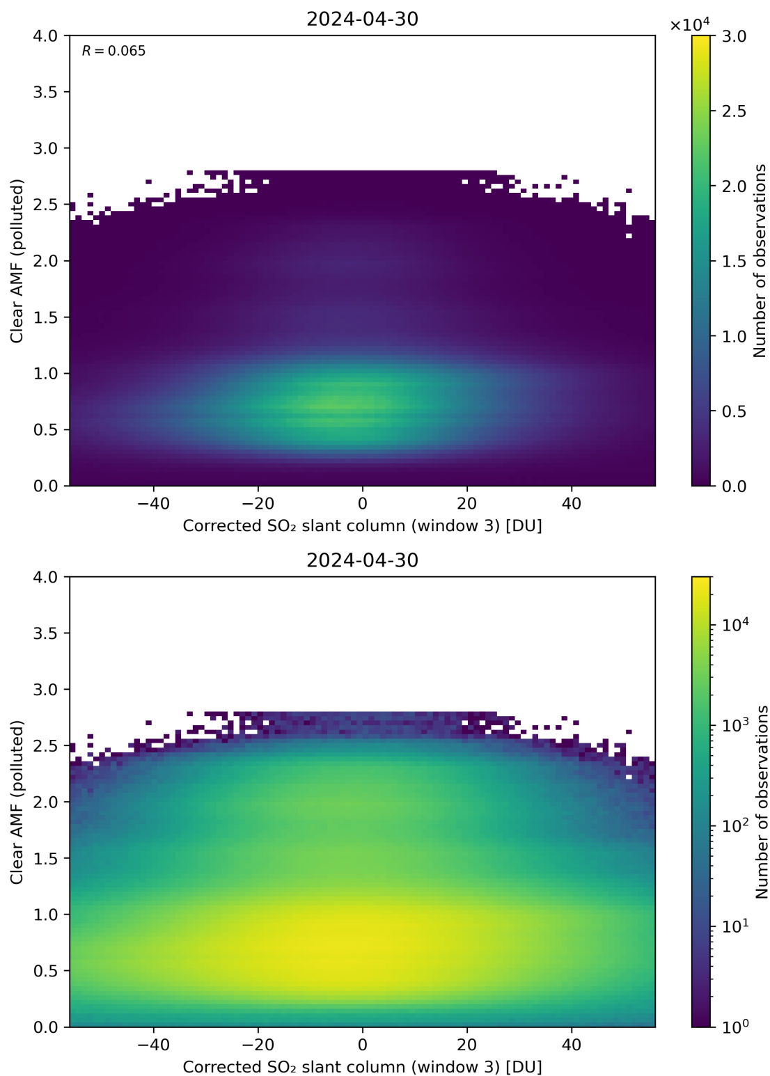
Figure 209: Scatter density plot of “Corrected SO 2 slant column (window 3)” against “Clear AMF (polluted)” for 2024-04-29 to 2024-05-01.
