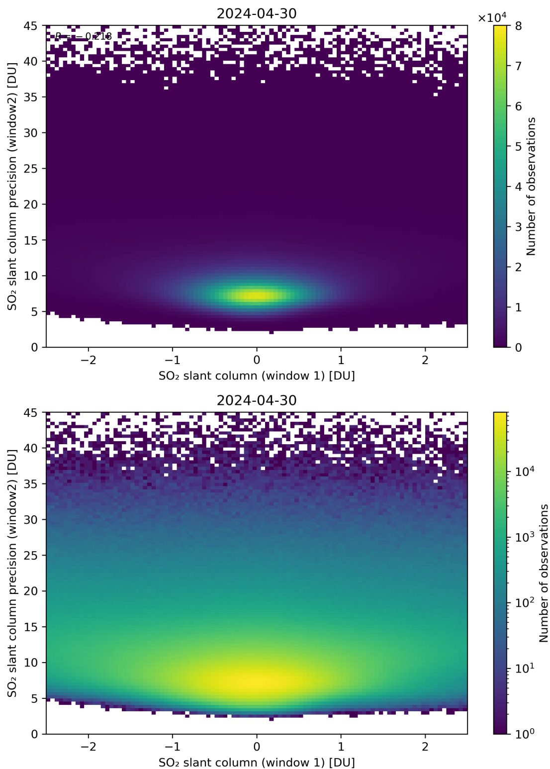
Figure 236: Scatter density plot of “SO 2 slant column (window 1)” against “SO 2 slant column precision (window2)” for 2024-04-29 to 2024-05-01.
