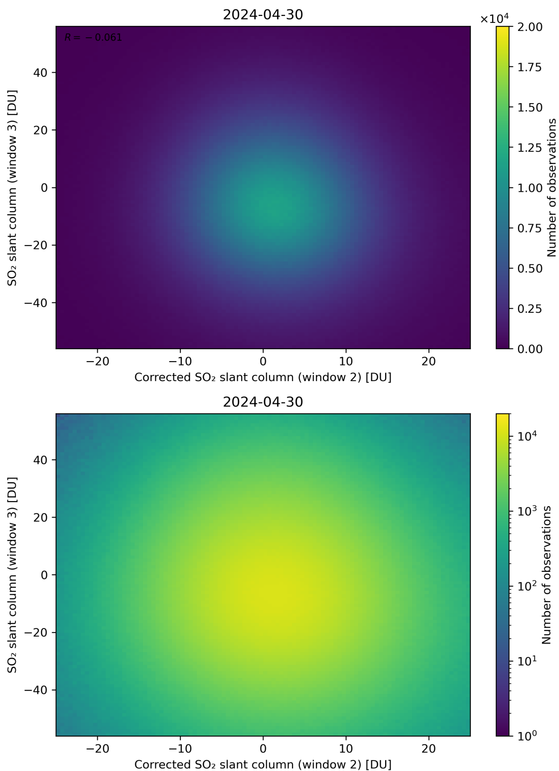
Figure 201: Scatter density plot of “Corrected SO 2 slant column (window 2)” against “SO 2 slant column (window 3)” for 2024-04-29 to 2024-05-01.
