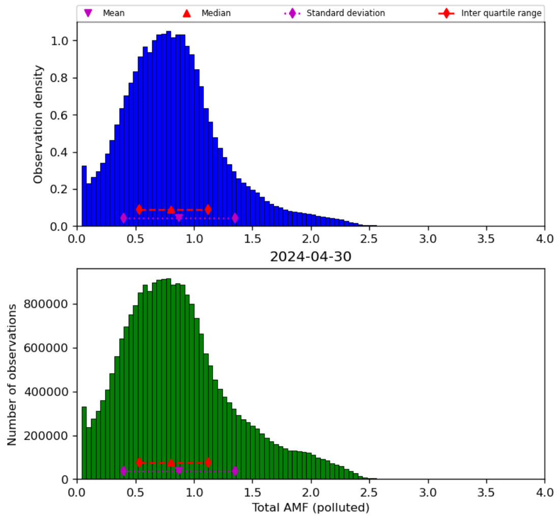
Figure 71: Histogram of “Total AMF (polluted)” for 2024-04-29 to 2024-05-01
