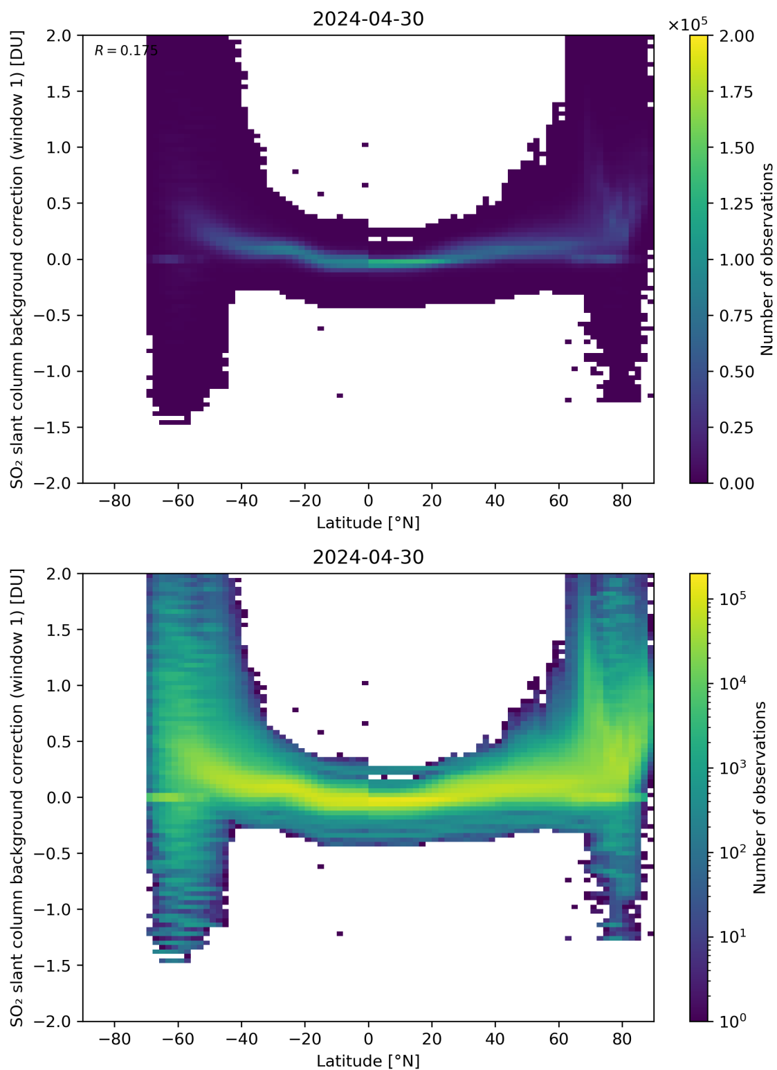
Figure 139: Scatter density plot of “Latitude” against “SO 2 slant column background correction (window 1)” for 2024-04-29 to 2024-05-01.
