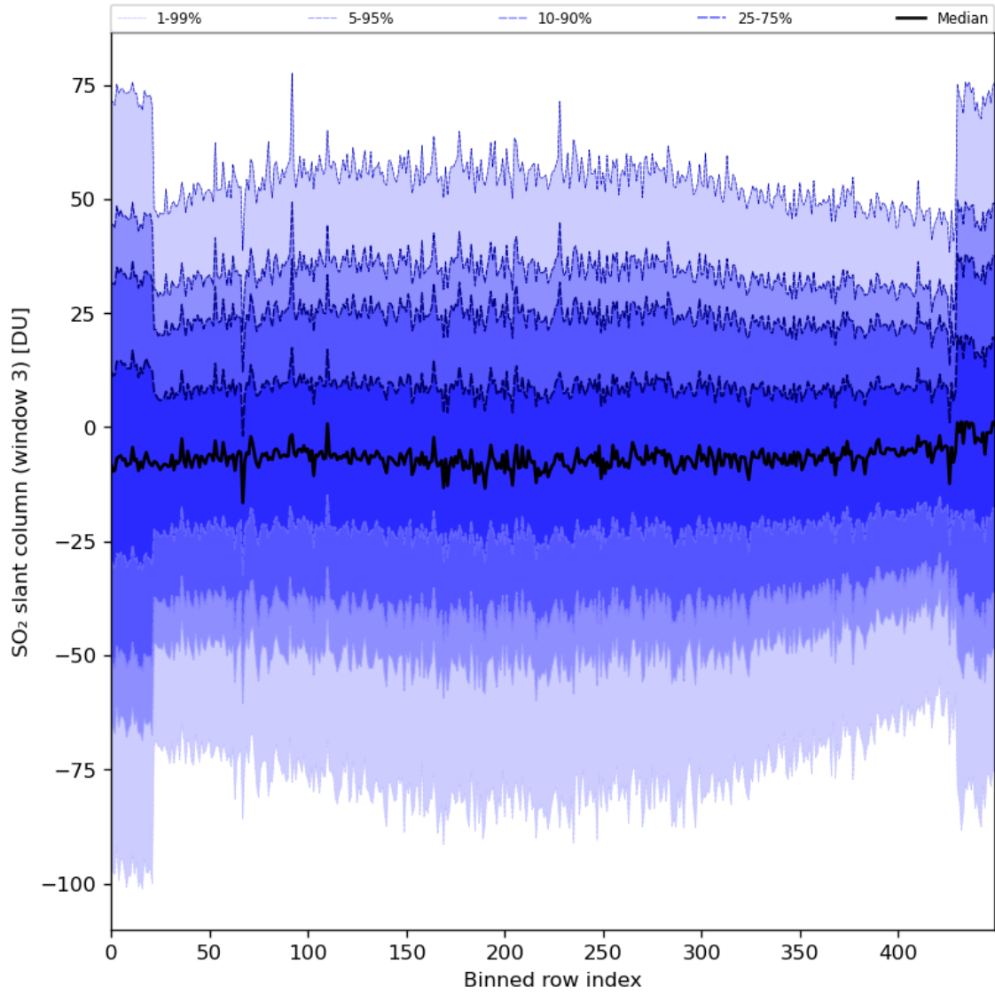
Figure 87: Along track statistics of “SO 2 slant column (window 3)” for 2024-04-29 to 2024-05-01
