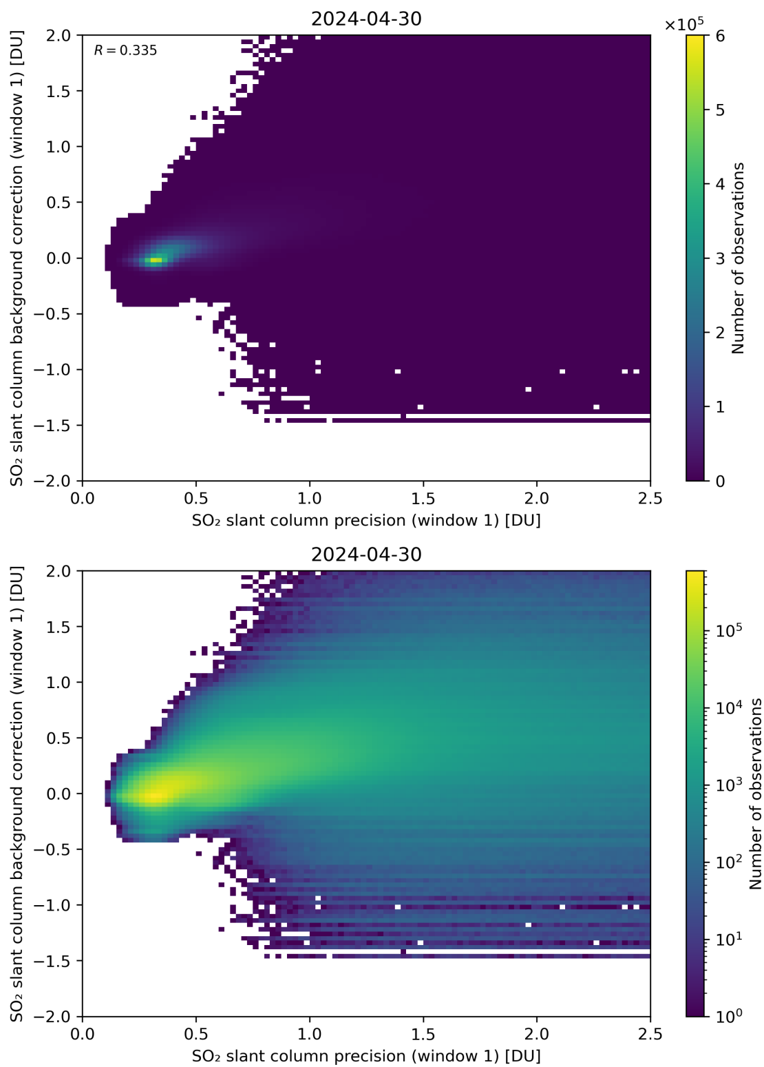
Figure 218: Scatter density plot of “SO 2 slant column precision (window 1)” against “SO 2 slant column background correction (window 1)” for 2024-04-29 to 2024-05-01.
