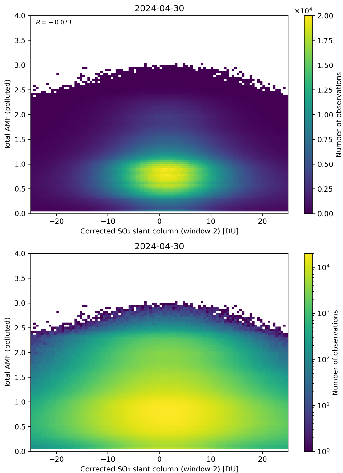
Figure 203: Scatter density plot of “Corrected SO 2 slant column (window 2)” against “Total AMF (polluted)” for 2024-04-29 to 2024-05-01.
