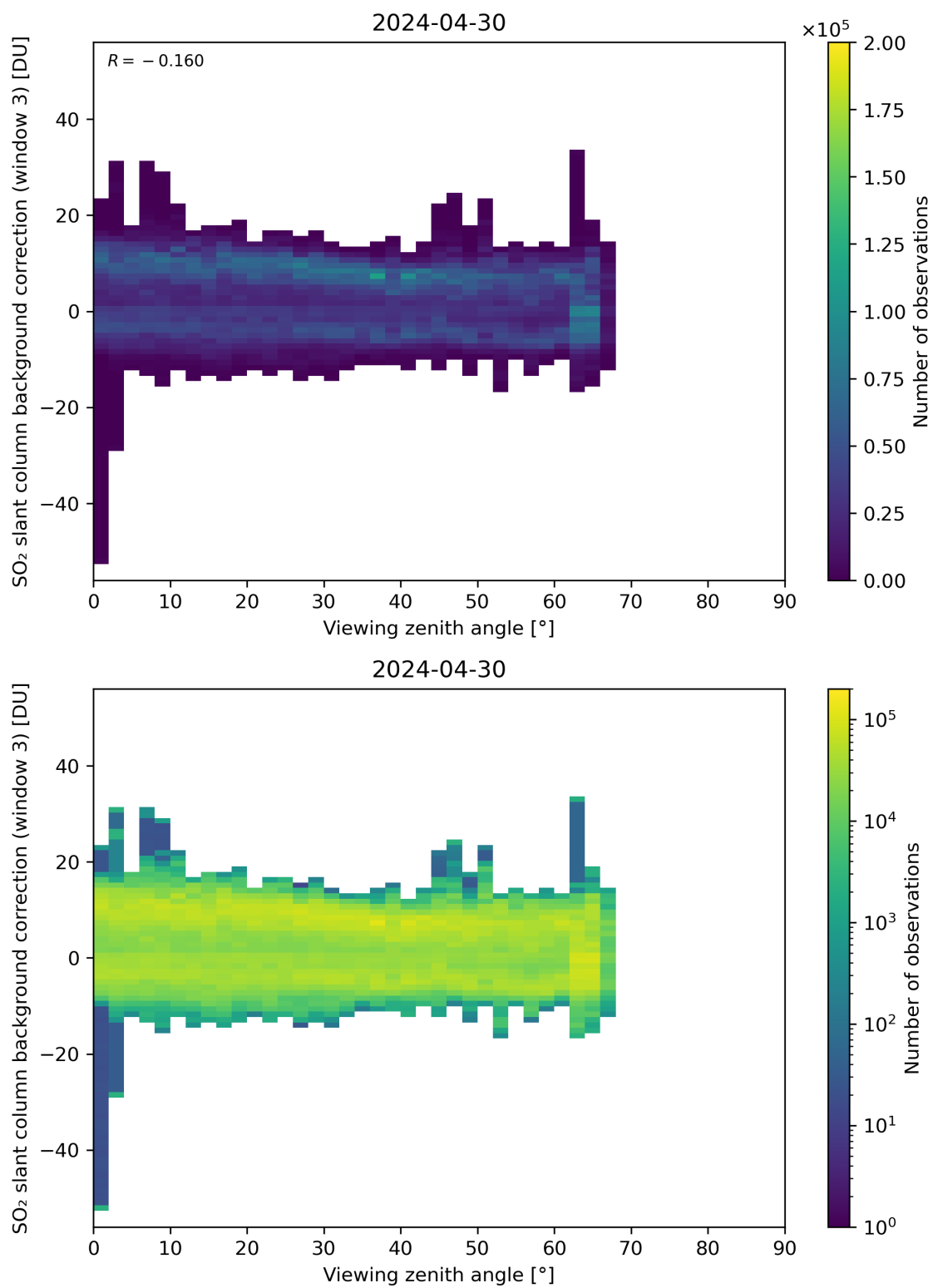
Figure 310: Scatter density plot of “Viewing zenith angle” against “SO 2 slant column background correction (window 3)” for 2024-04-29 to 2024-05-01.
