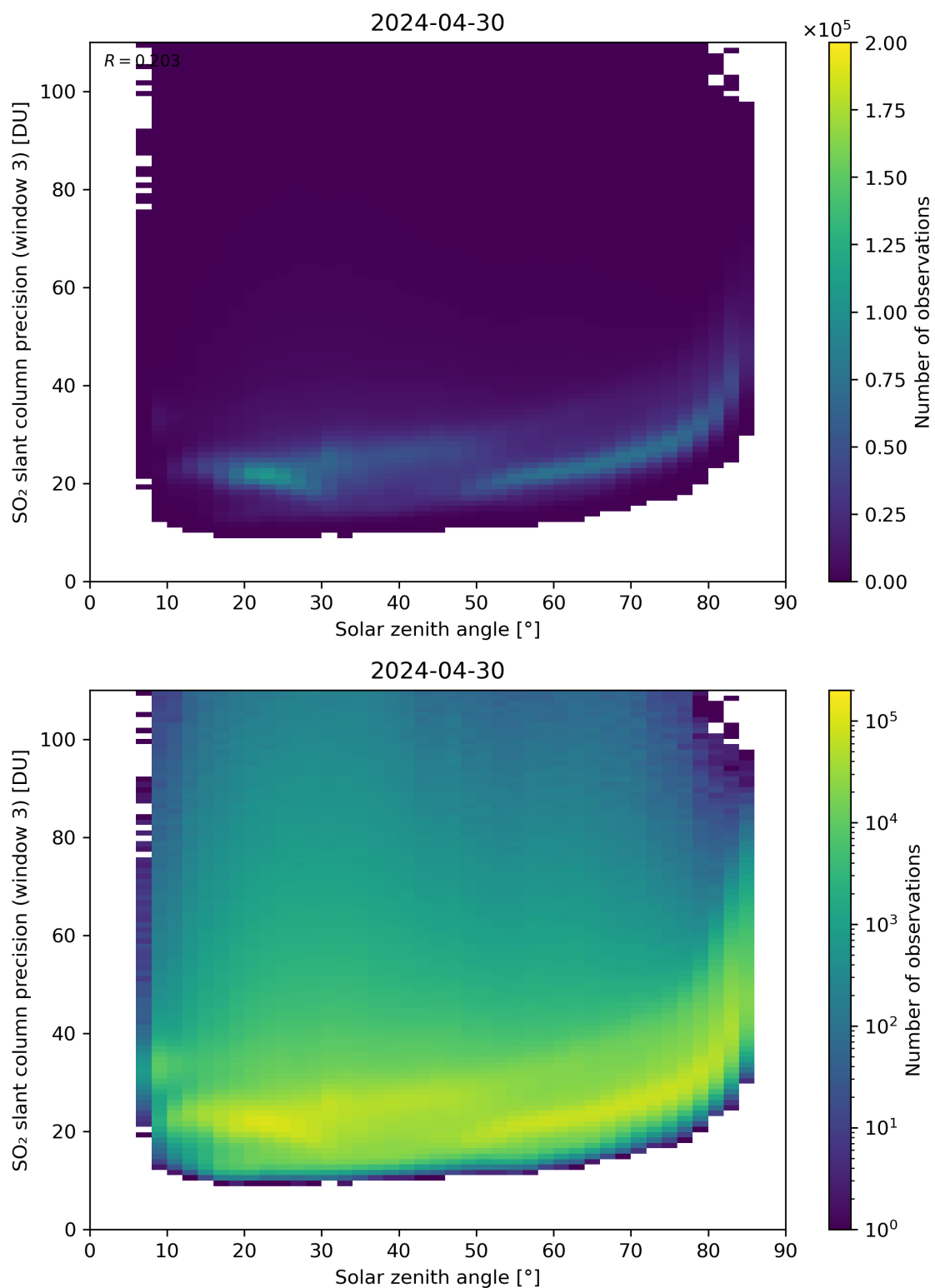
Figure 173: Scatter density plot of “Solar zenith angle” against “SO 2 slant column precision (window 3)” for 2024-04-29 to 2024-05-01.
