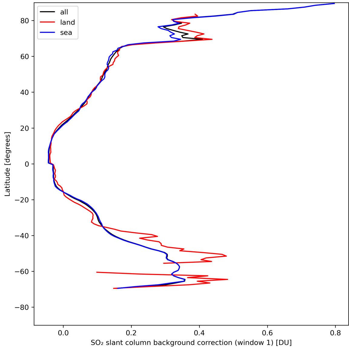
Figure 36: Zonal average of “SO 2 slant column background correction (window 1)” for 2024-04-29 to 2024-05-01.
