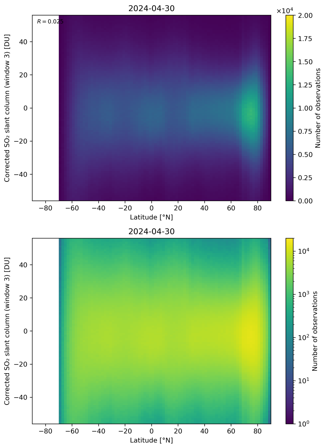
Figure 148: Scatter density plot of “Latitude” against “Corrected SO 2 slant column (window 3)” for 2024-04-29 to 2024-05-01.
