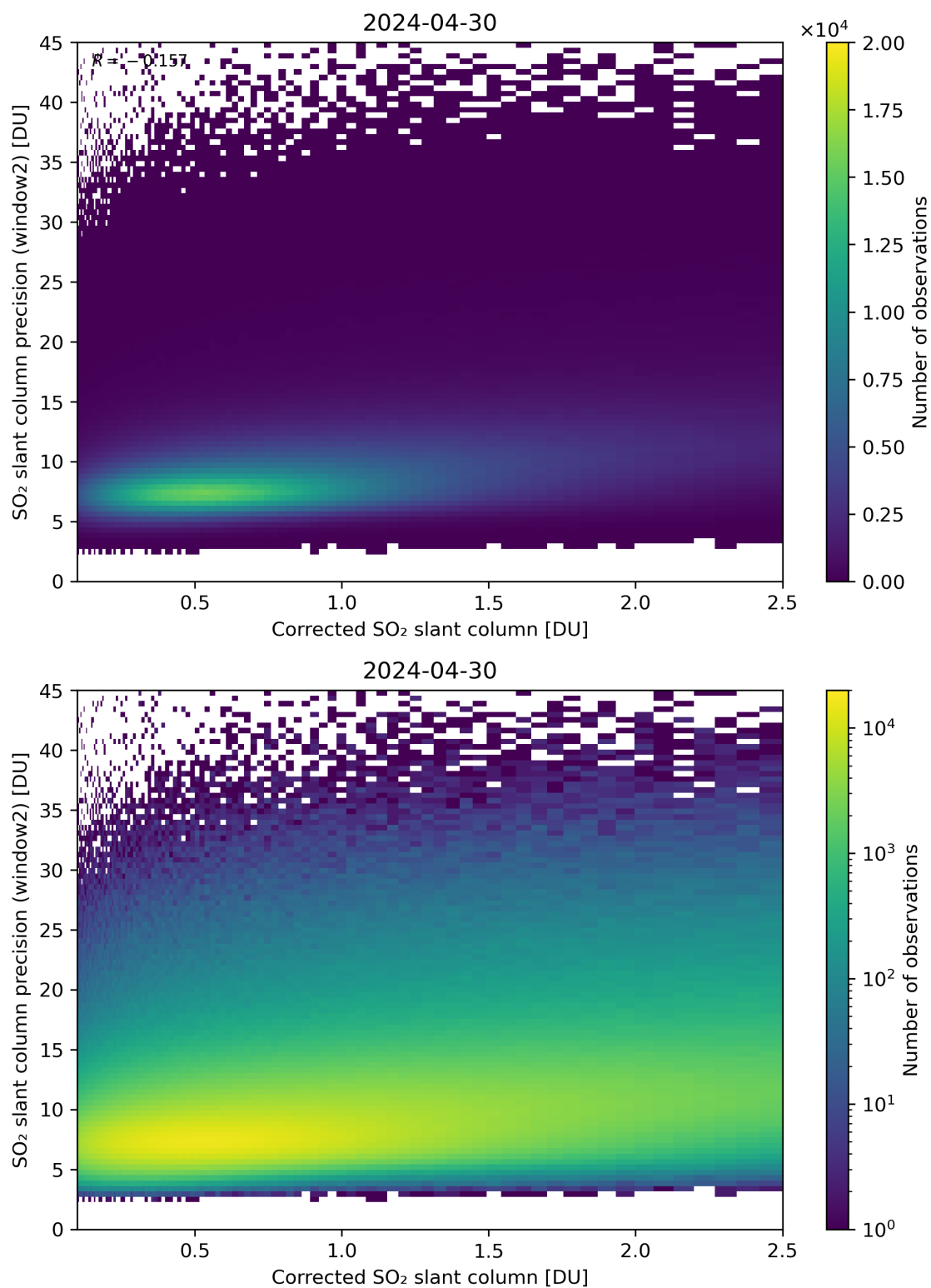
Figure 189: Scatter density plot of “Corrected SO 2 slant column” against “SO 2 slant column precision (window2)” for 2024-04-29 to 2024-05-01.
