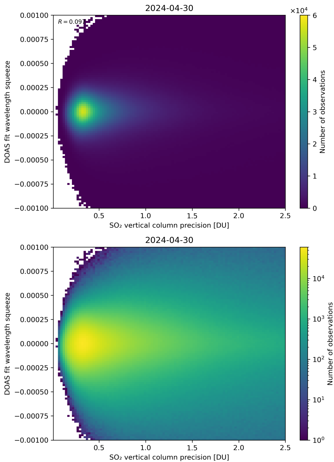
Figure 283: Scatter density plot of “SO 2 vertical column precision” against “DOAS fit wavelength squeeze” for 2024-04-29 to 2024-05-01.
