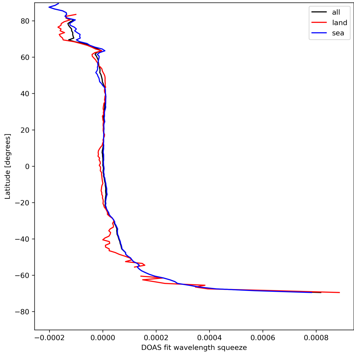
Figure 46: Zonal average of “DOAS fit wavelength squeeze” for 2024-04-29 to 2024-05-01.
