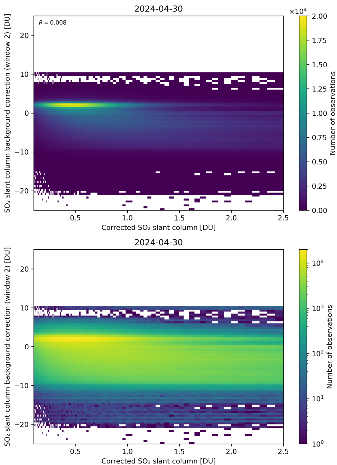
Figure 179: Scatter density plot of “Corrected SO 2 slant column” against “SO 2 slant column background correction (window 2)” for 2024-04-29 to 2024-05-01.
