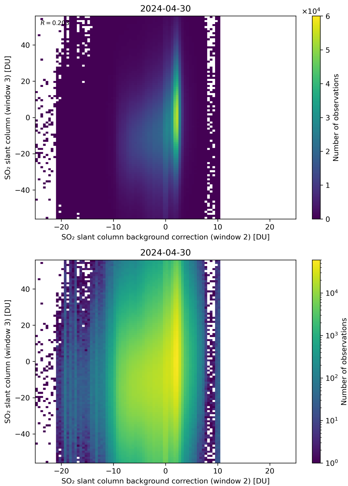
Figure 117: Scatter density plot of “SO 2 slant column background correction (window 2)” against “SO 2 slant column (window 3)” for 2024-04-29 to 2024-05-01.
