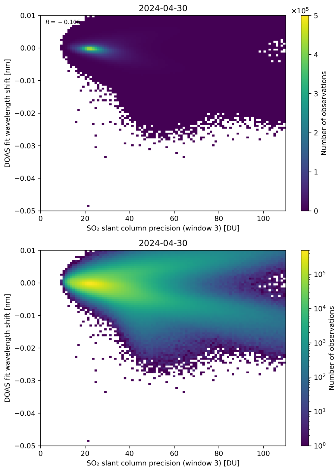
Figure 258: Scatter density plot of “SO 2 slant column precision (window 3)” against “DOAS fit wavelength shift” for 2024-04-29 to 2024-05-01.
