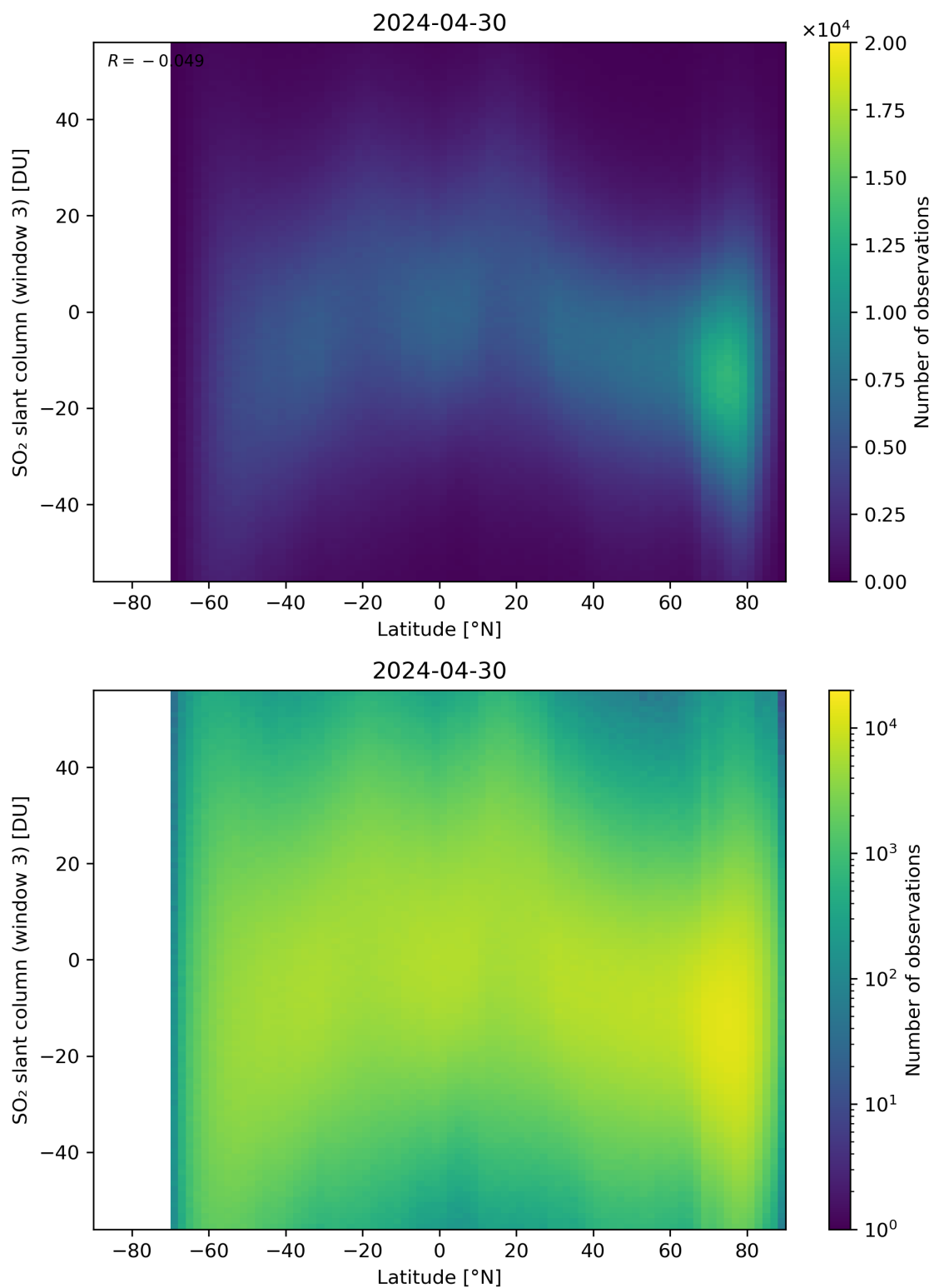
Figure 152: Scatter density plot of “Latitude” against “SO 2 slant column (window 3)” for 2024-04-29 to 2024-05-01.
