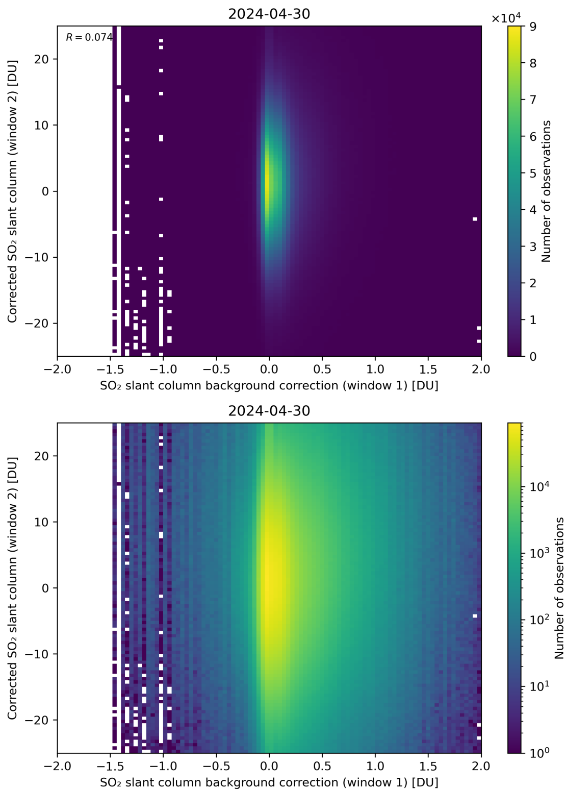
Figure 104: Scatter density plot of “SO 2 slant column background correction (window 1)” against “Corrected SO 2 slant column (window 2)” for 2024-04-29 to 2024-05-01.
