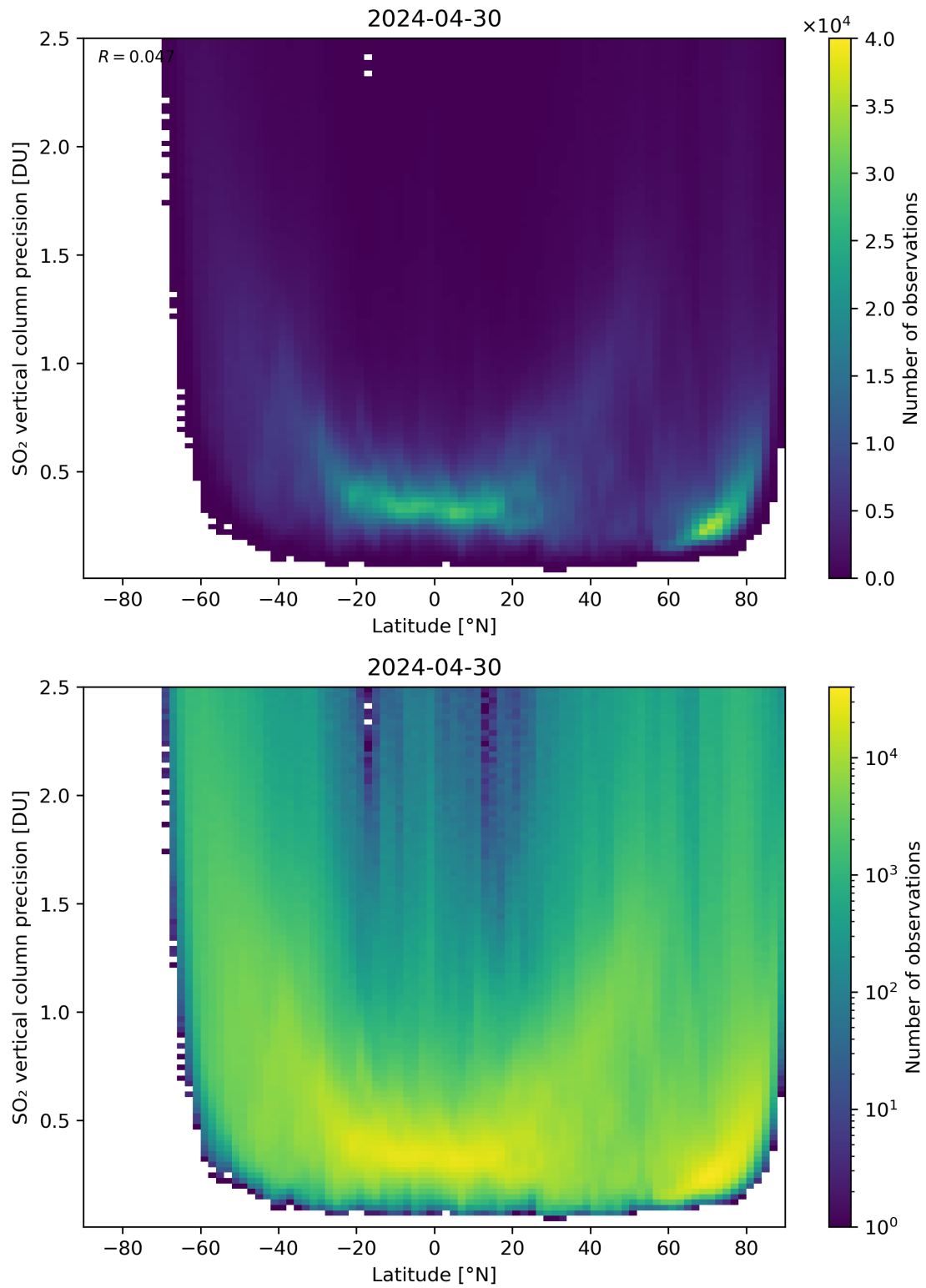
Figure 157: Scatter density plot of “Latitude” against “SO 2 vertical column precision” for 2024-04-29 to 2024-05-01.
