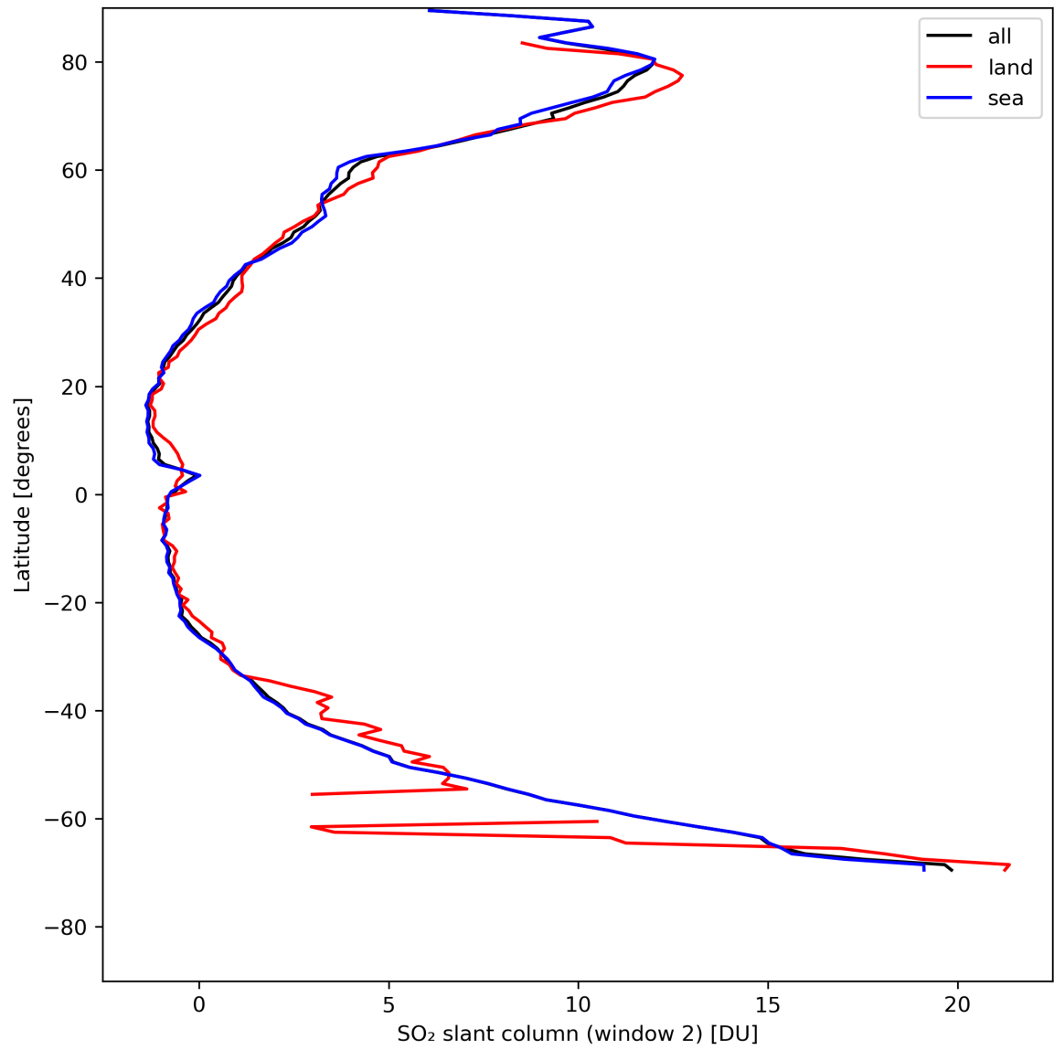
Figure 37: Zonal average of “SO 2 slant column (window 2)” for 2024-04-29 to 2024-05-01.
