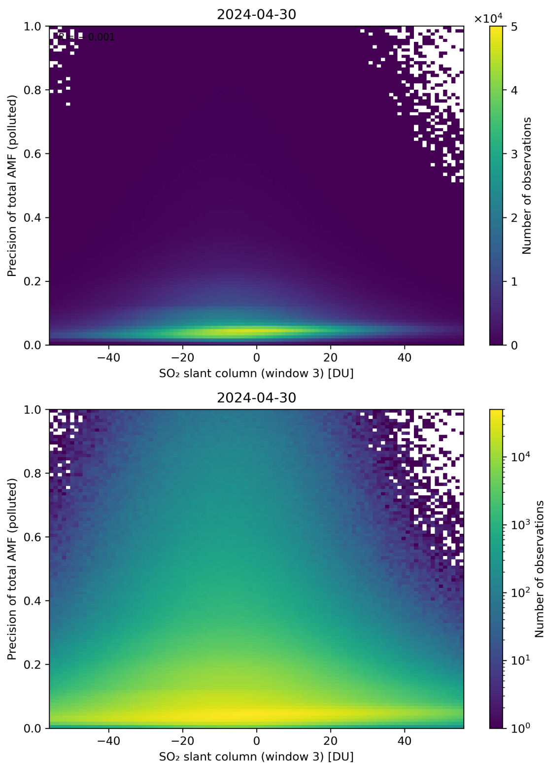
Figure 269: Scatter density plot of “SO 2 slant column (window 3)” against “Precision of total AMF (polluted)” for 2024-04-29 to 2024-05-01.
