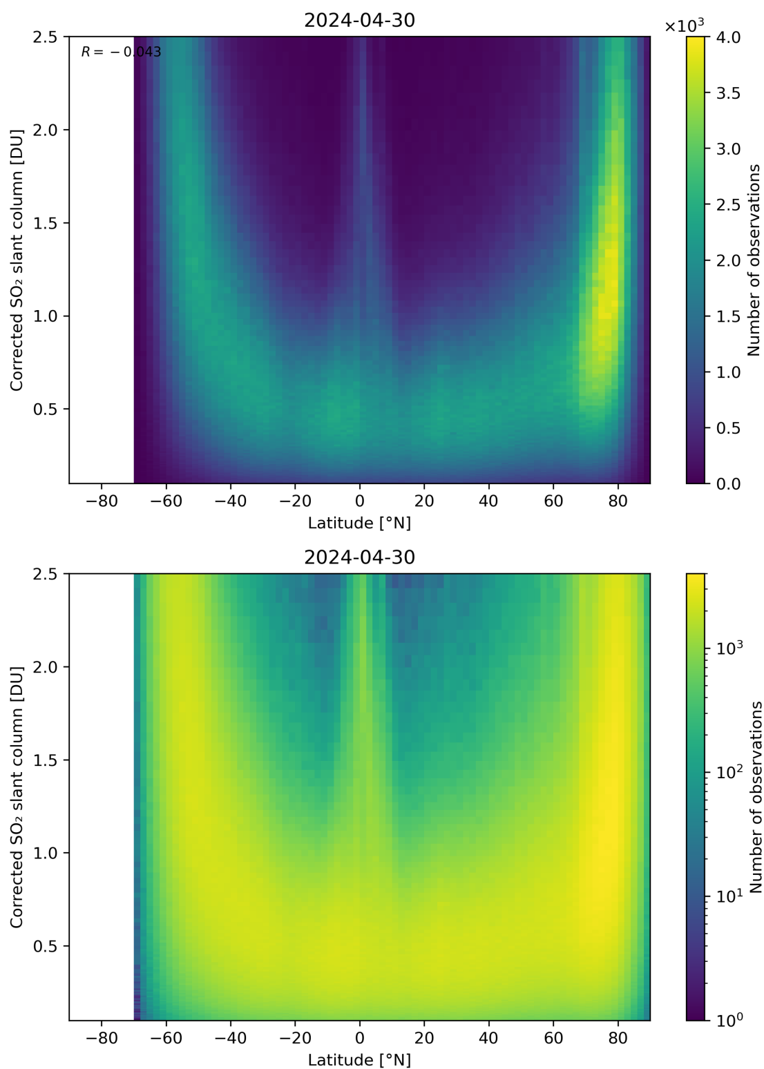
Figure 146: Scatter density plot of “Latitude” against “Corrected SO 2 slant column” for 2024-04-29 to 2024-05-01.
