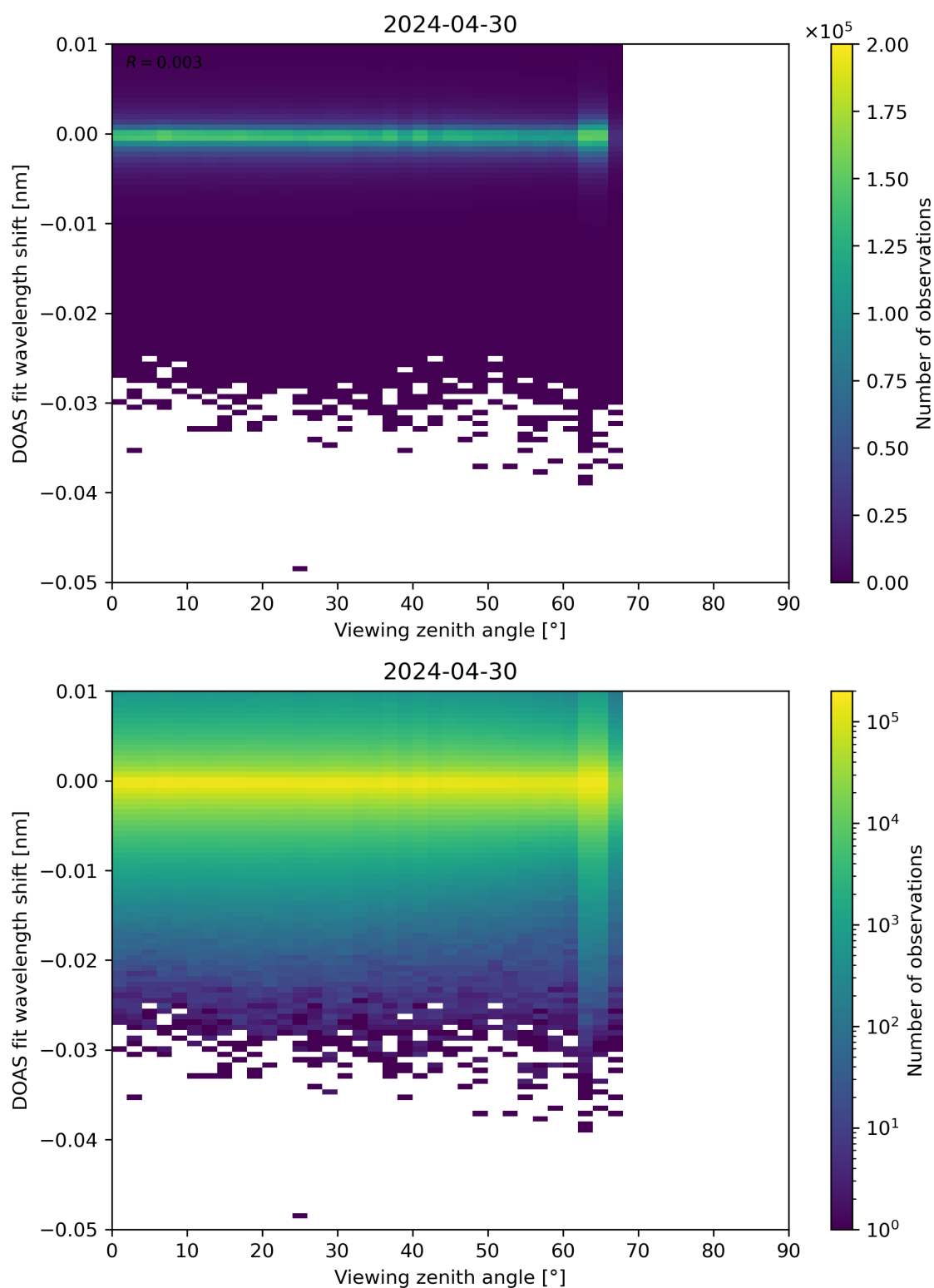
Figure 311: Scatter density plot of “Viewing zenith angle” against “DOAS fit wavelength shift” for 2024-04-29 to 2024-05-01.
