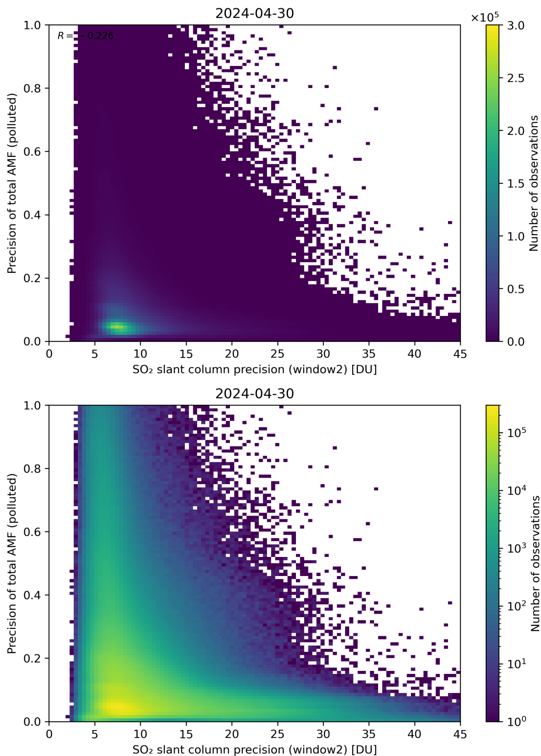
Figure 252: Scatter density plot of “SO 2 slant column precision (window2)” against “Precision of total AMF (polluted)” for 2024-04-29 to 2024-05-01.
