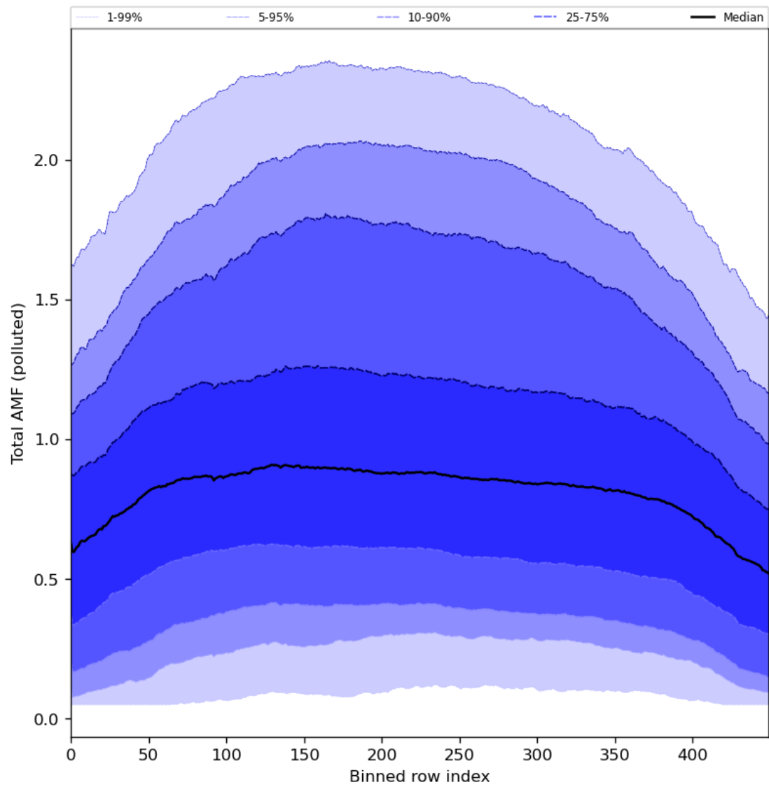
Figure 94: Along track statistics of “Total AMF (polluted)” for 2024-04-29 to 2024-05-01
