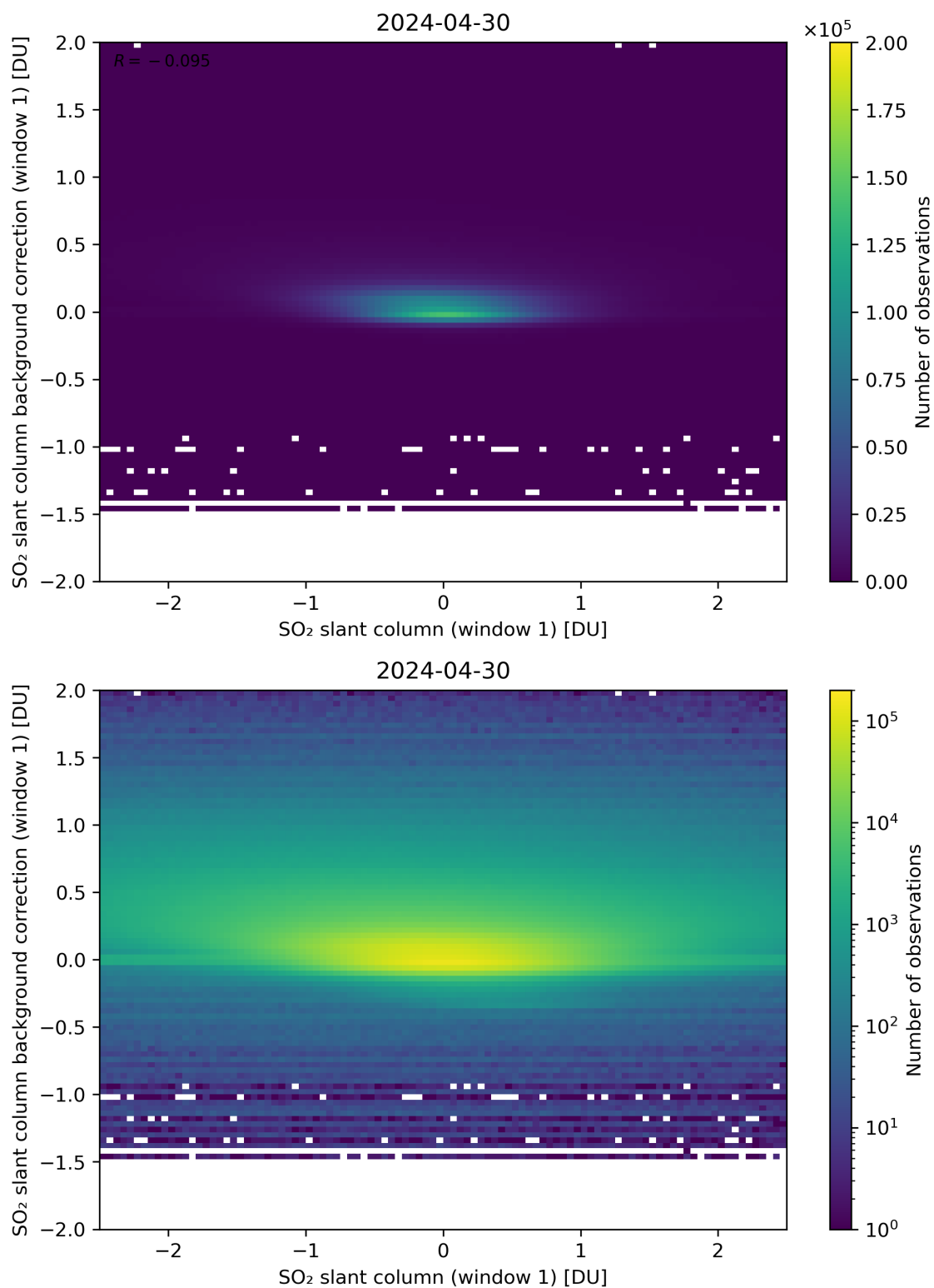
Figure 212: Scatter density plot of “SO 2 slant column (window 1)” against “SO 2 slant column background correction (window 1)” for 2024-04-29 to 2024-05-01.
