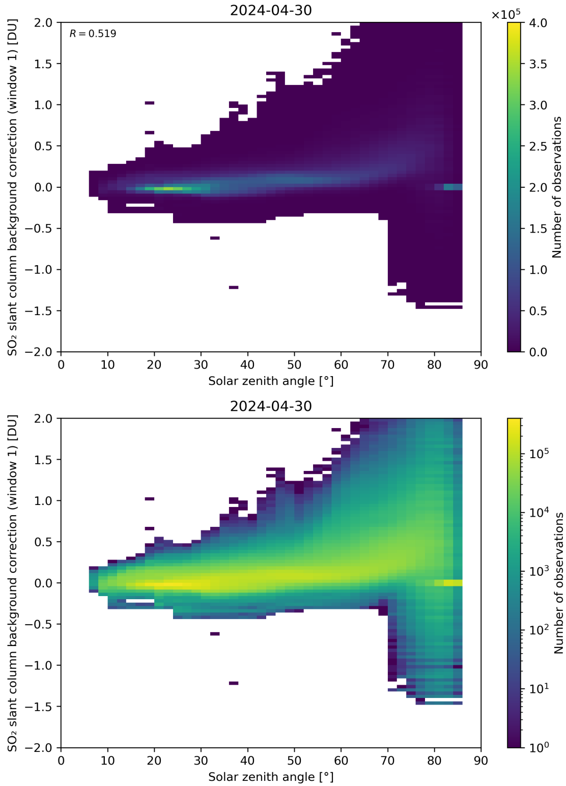
Figure 158: Scatter density plot of “Solar zenith angle” against “SO 2 slant column background correction (window 1)” for 2024-04-29 to 2024-05-01.
