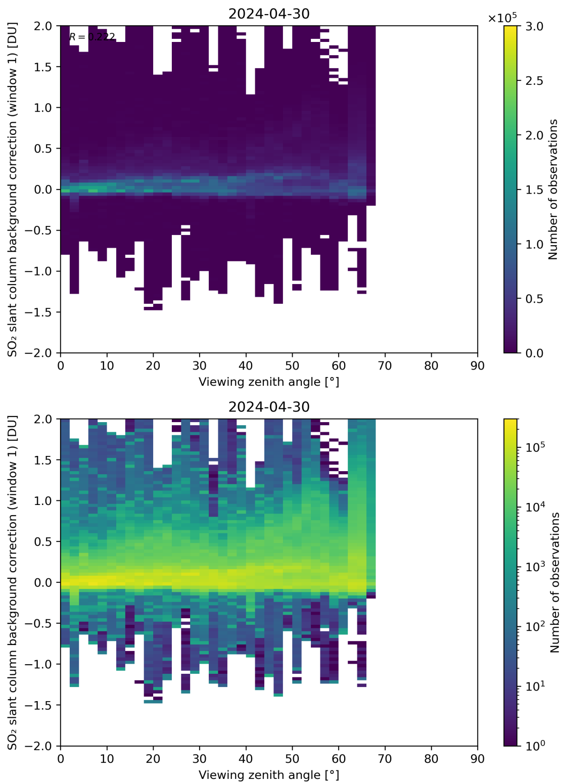
Figure 308: Scatter density plot of “Viewing zenith angle” against “SO 2 slant column background correction (window 1)” for 2024-04-29 to 2024-05-01.
