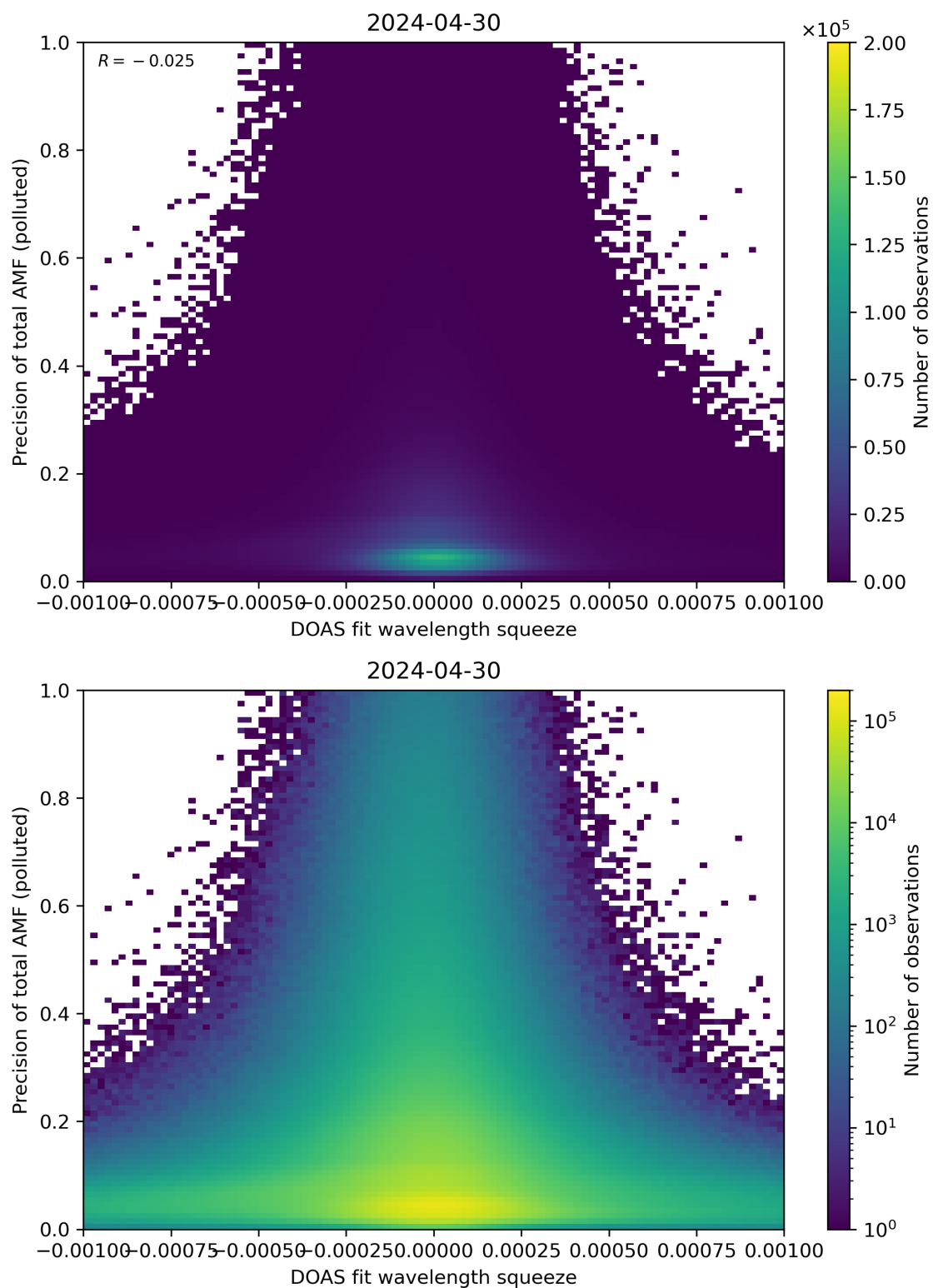
Figure 135: Scatter density plot of “DOAS fit wavelength squeeze” against “Precision of total AMF (polluted)” for 2024-04-29 to 2024-05-01.
