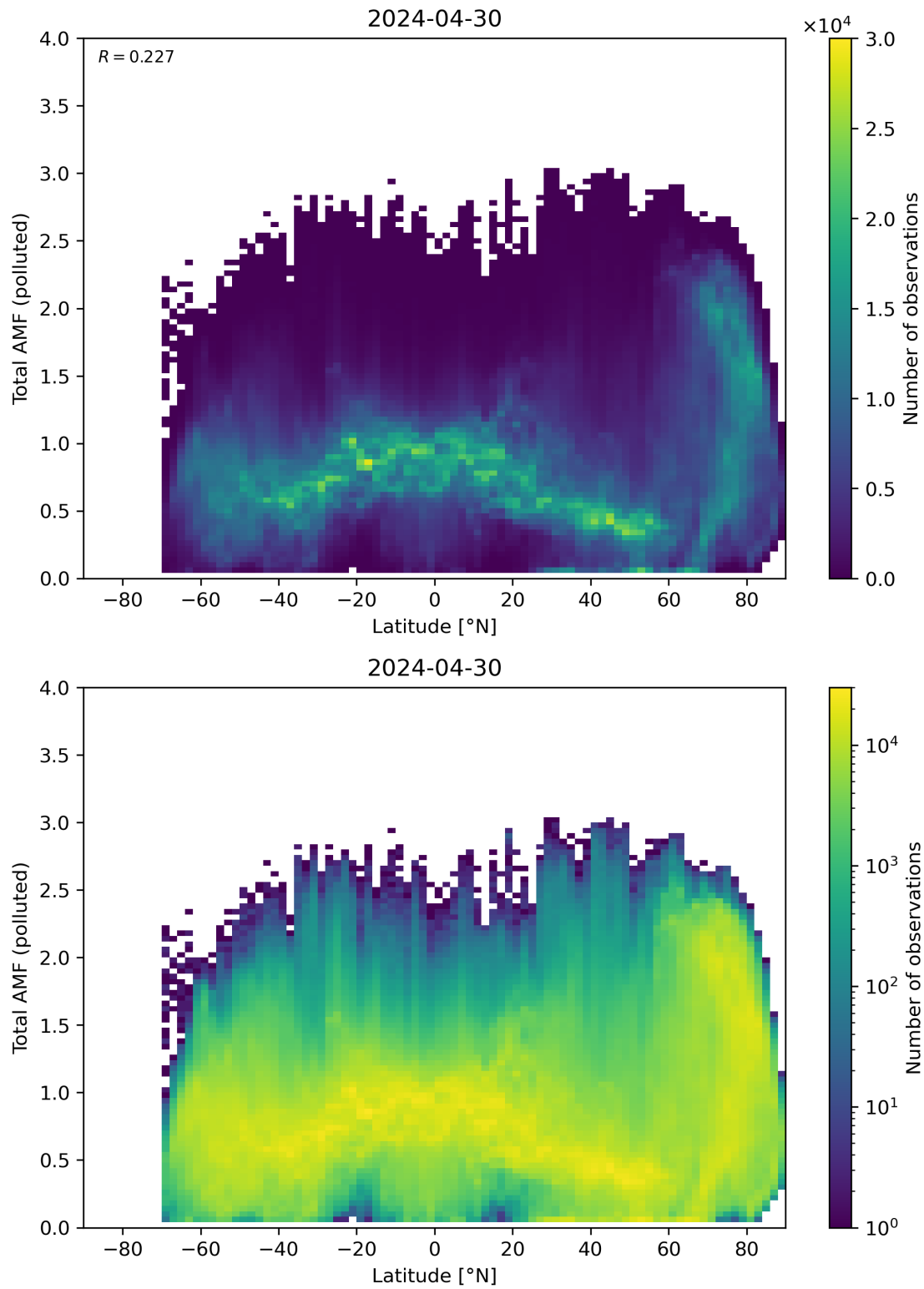
Figure 154: Scatter density plot of “Latitude” against “Total AMF (polluted)” for 2024-04-29 to 2024-05-01.
