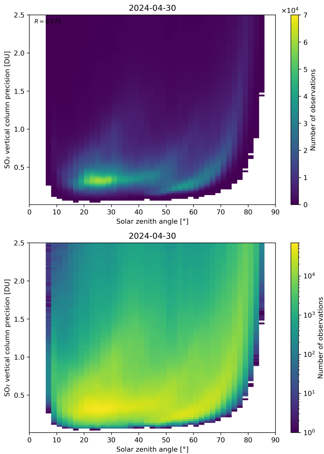
Figure 177: Scatter density plot of “Solar zenith angle” against “SO 2 vertical column precision” for 2024-04-29 to 2024-05-01.
