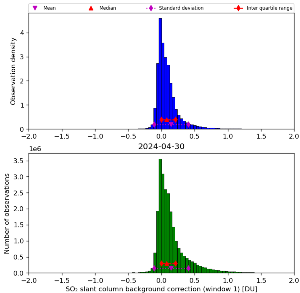
Figure 59: Histogram of “SO 2 slant column background correction (window 1)” for 2024-04-29 to 2024-05-01
