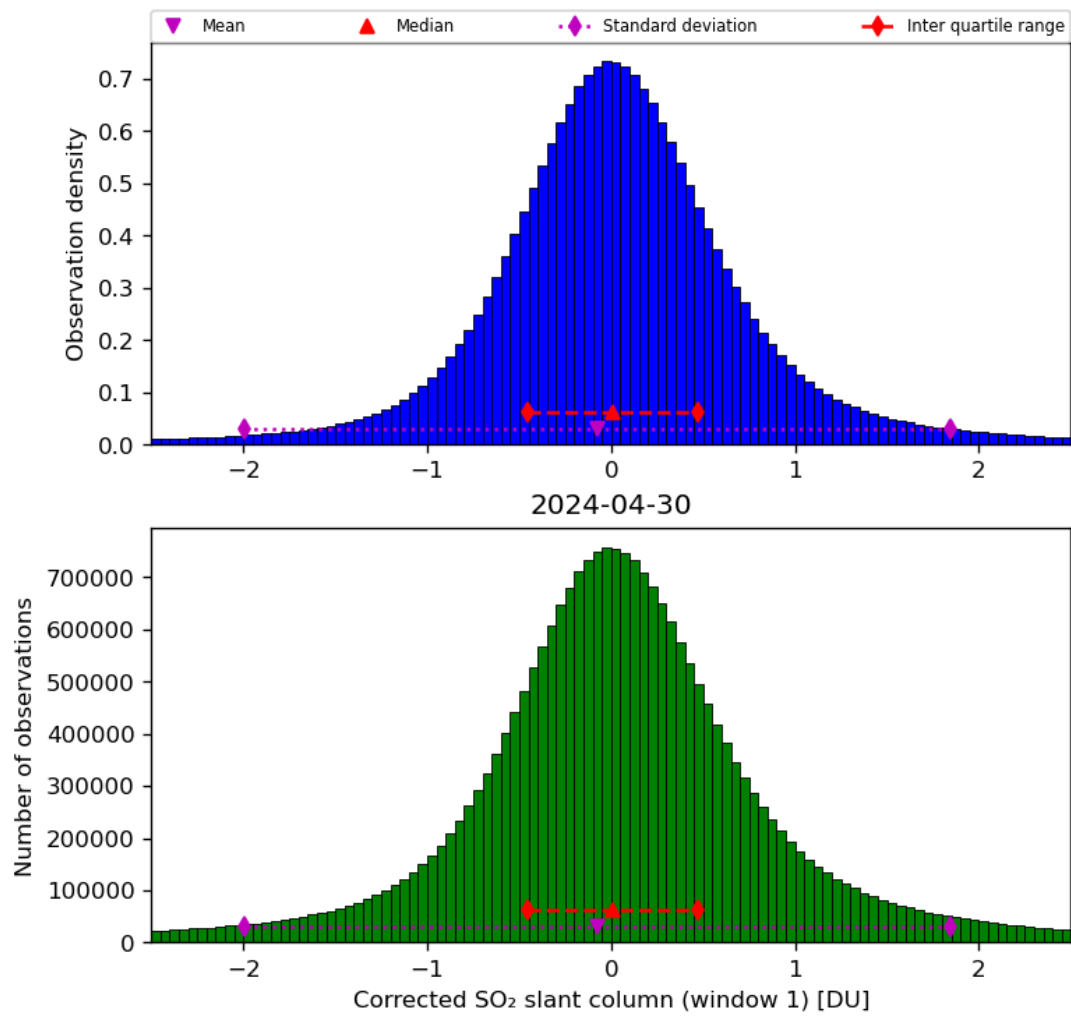
Figure 58: Histogram of “Corrected SO 2 slant column (window 1)” for 2024-04-29 to 2024-05-01
