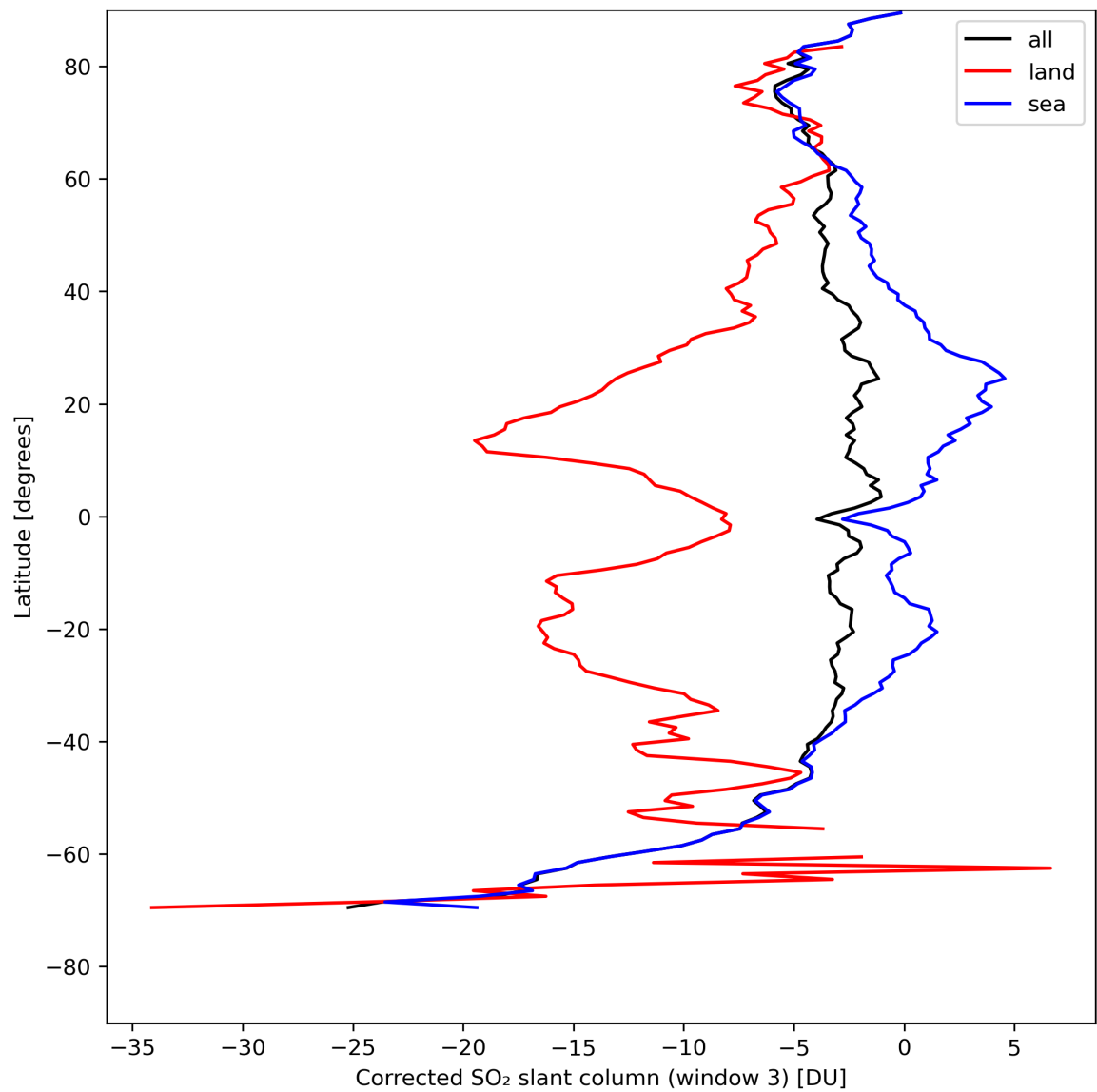
Figure 43: Zonal average of “Corrected SO 2 slant column (window 3)” for 2024-04-29 to 2024-05-01.
