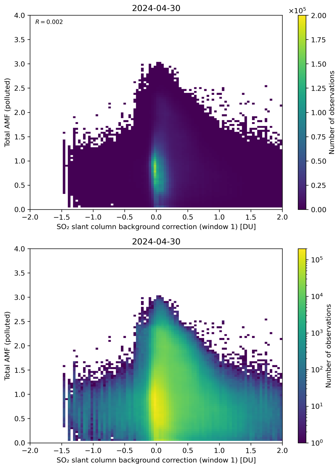
Figure 109: Scatter density plot of “SO 2 slant column background correction (window 1)” against “Total AMF (polluted)” for 2024-04-29 to 2024-05-01.
