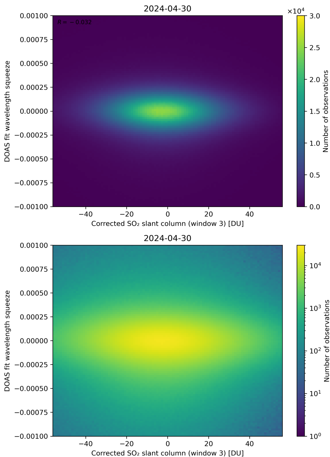
Figure 207: Scatter density plot of “Corrected SO 2 slant column (window 3)” against “DOAS fit wavelength squeeze” for 2024-04-29 to 2024-05-01.
