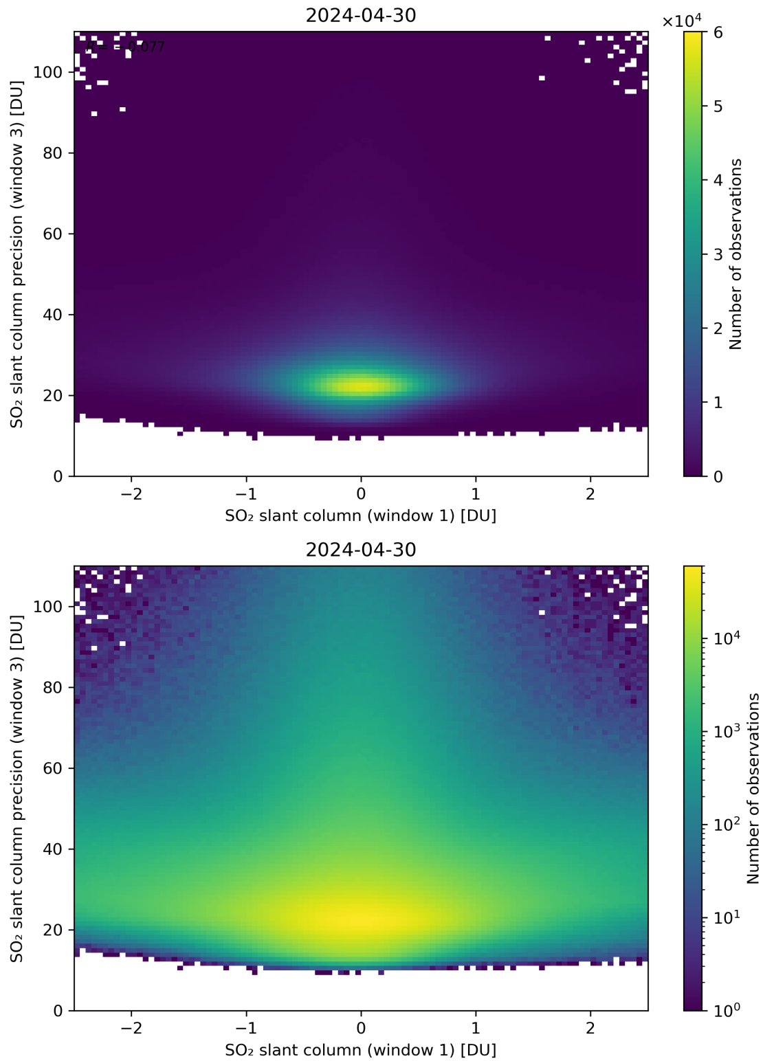
Figure 238: Scatter density plot of “SO 2 slant column (window 1)” against “SO 2 slant column precision (window 3)” for 2024-04-29 to 2024-05-01.
