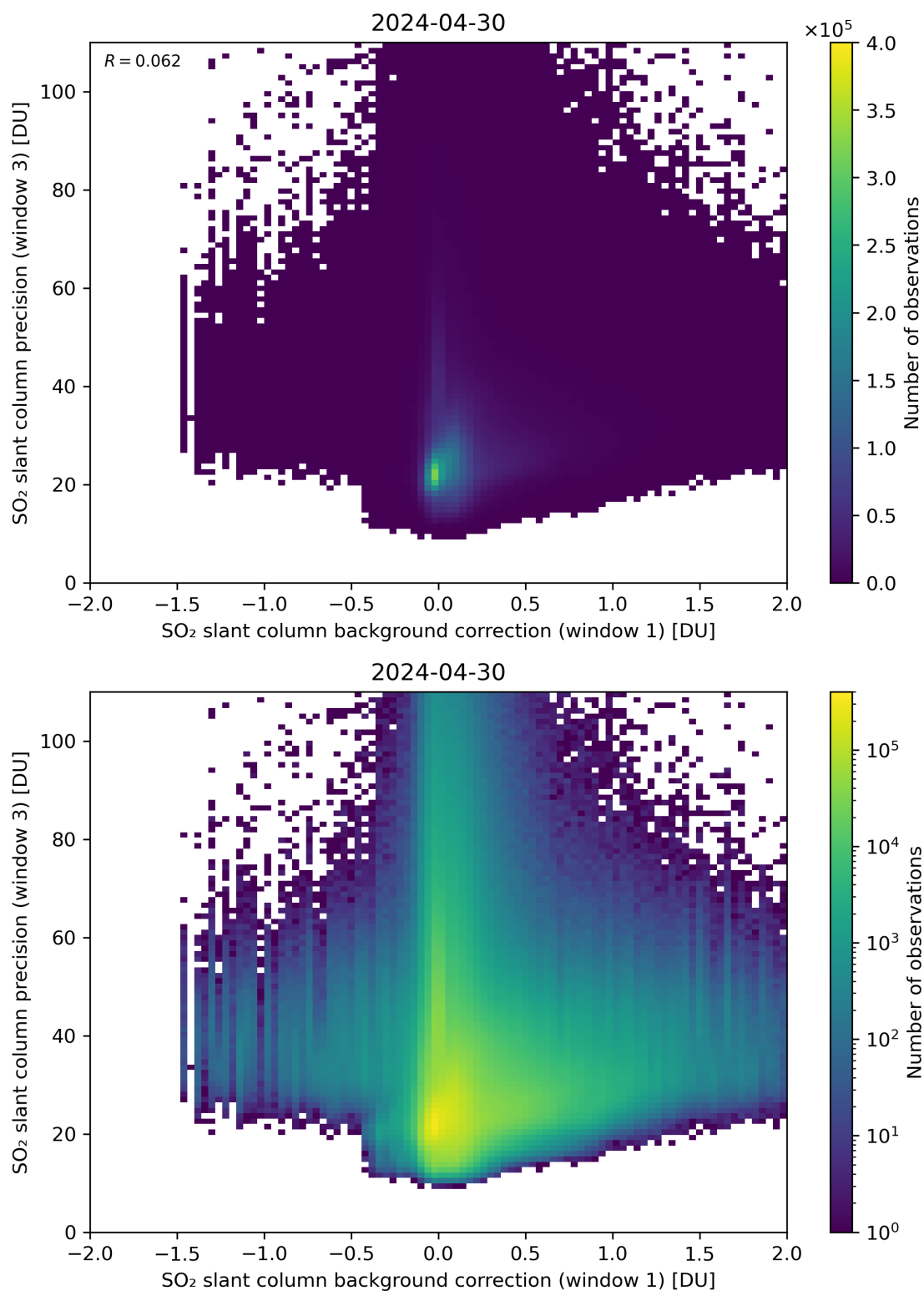
Figure 108: Scatter density plot of “SO 2 slant column background correction (window 1)” against “SO 2 slant column precision (window 3)” for 2024-04-29 to 2024-05-01.
