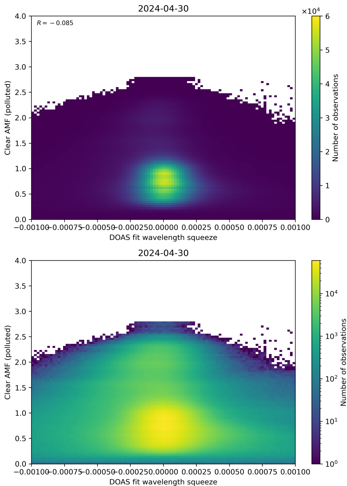
Figure 133: Scatter density plot of “DOAS fit wavelength squeeze” against “Clear AMF (polluted)” for 2024-04-29 to 2024-05-01.
