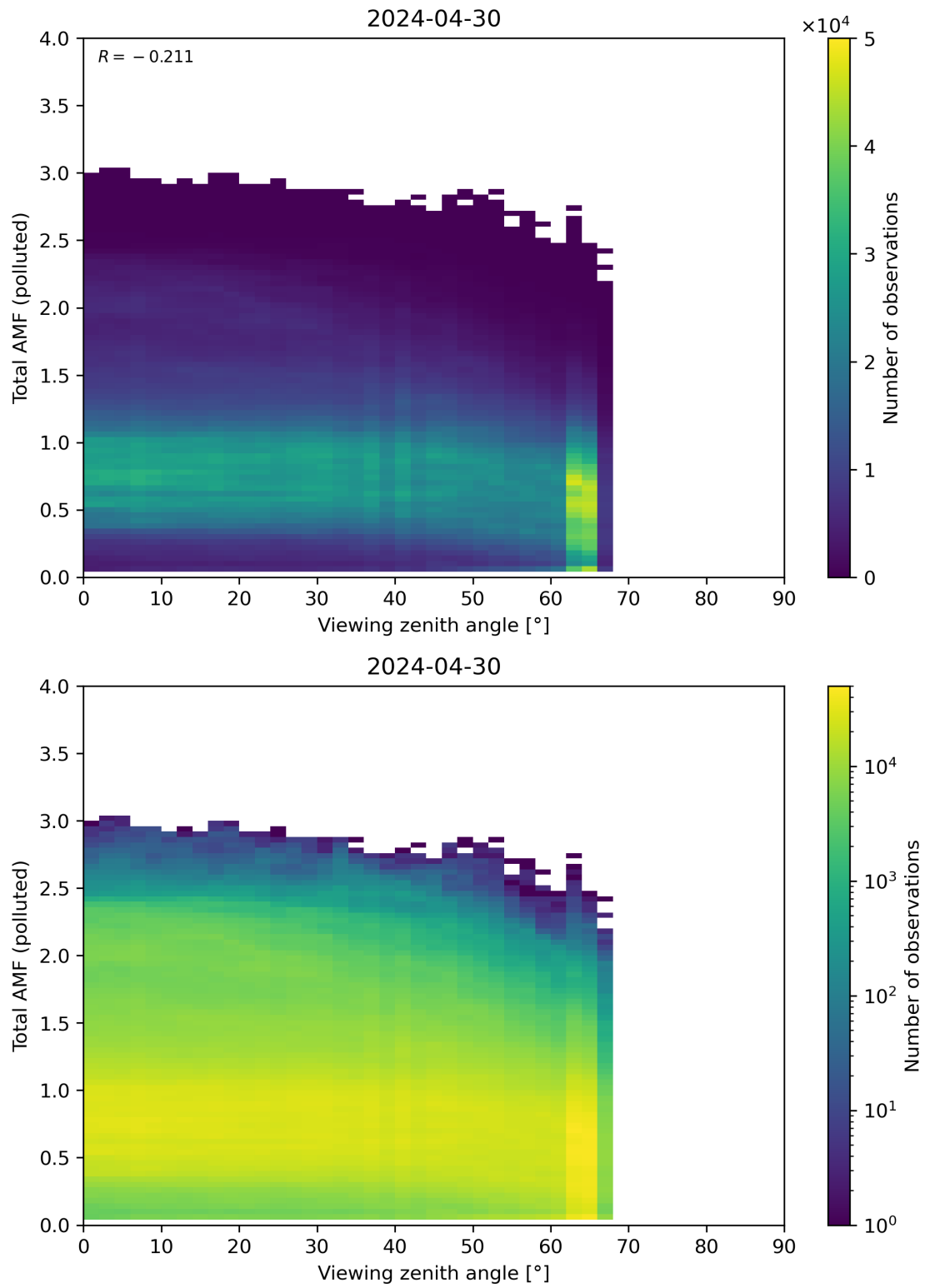
Figure 325: Scatter density plot of “Viewing zenith angle” against “Total AMF (polluted)” for 2024-04-29 to 2024-05-01.
