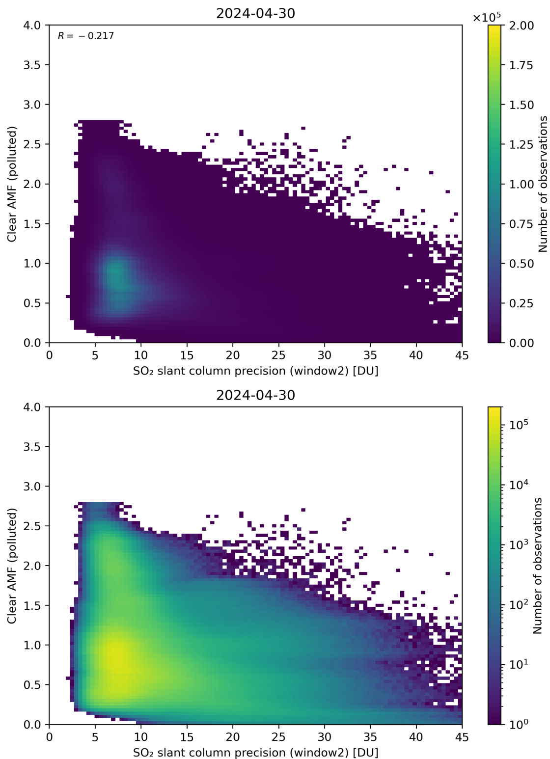
Figure 246: Scatter density plot of “SO 2 slant column precision (window2)” against “Clear AMF (polluted)” for 2024-04-29 to 2024-05-01.
