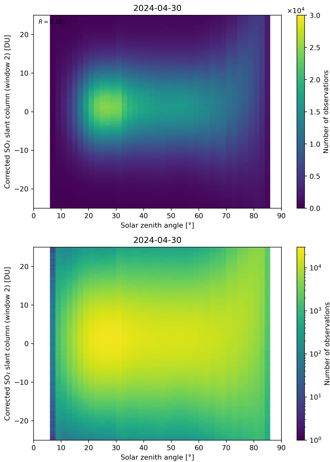
Figure 167: Scatter density plot of “Solar zenith angle” against “Corrected SO 2 slant column (window 2)” for 2024-04-29 to 2024-05-01.
