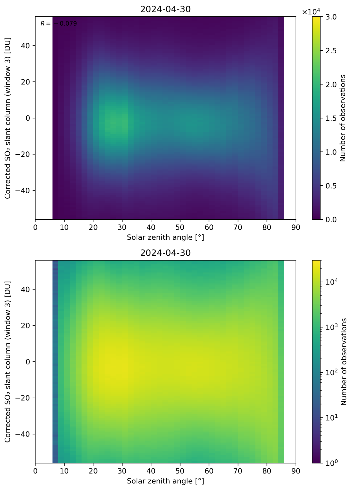
Figure 168: Scatter density plot of “Solar zenith angle” against “Corrected SO 2 slant column (window 3)” for 2024-04-29 to 2024-05-01.
