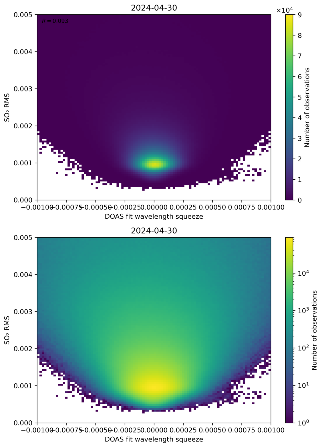
Figure 132: Scatter density plot of “DOAS fit wavelength squeeze” against “SO 2 RMS” for 2024-04-29 to 2024-05-01.
