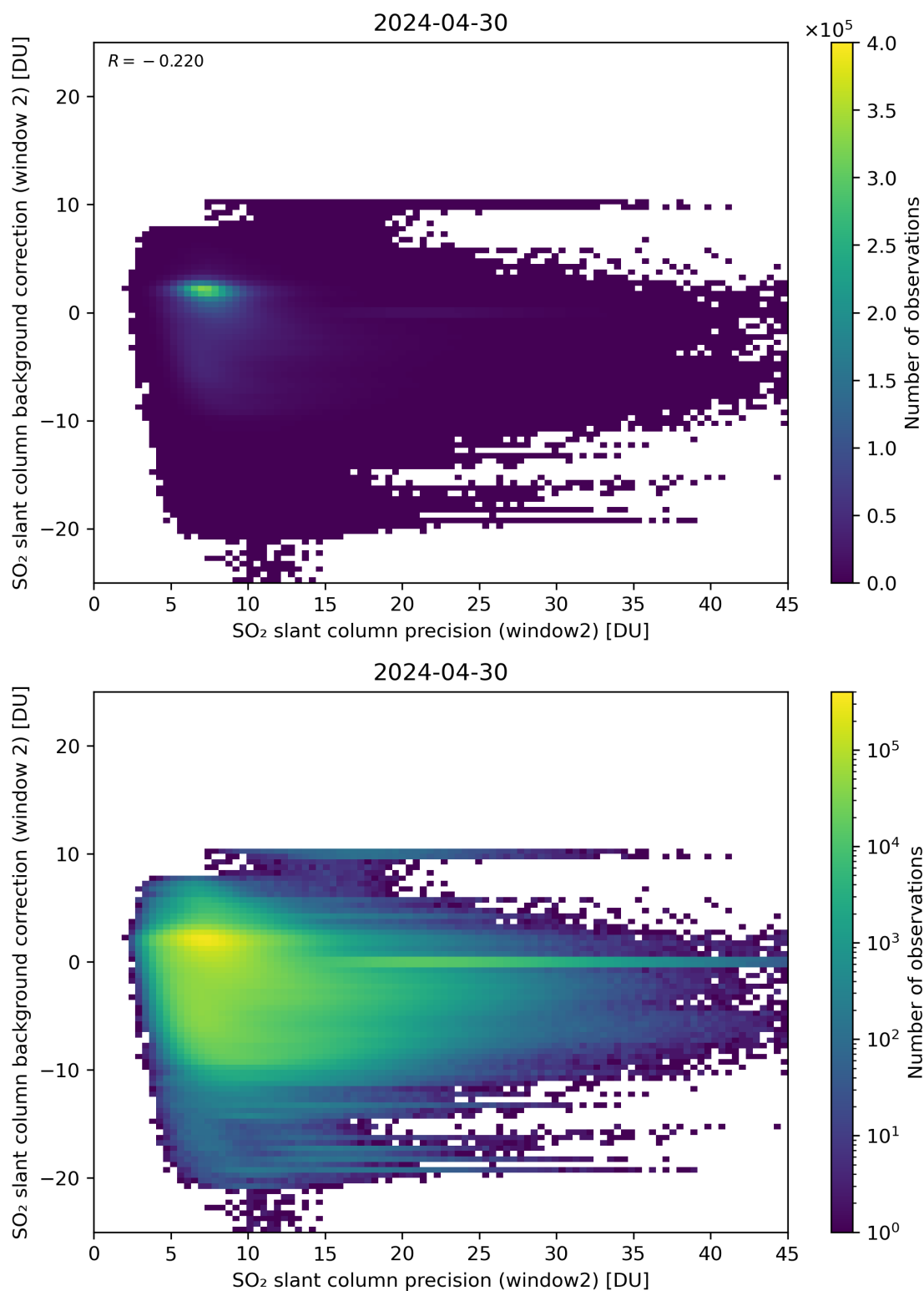
Figure 241: Scatter density plot of “SO 2 slant column precision (window2)” against “SO 2 slant column background correction (window 2)” for 2024-04-29 to 2024-05-01.
