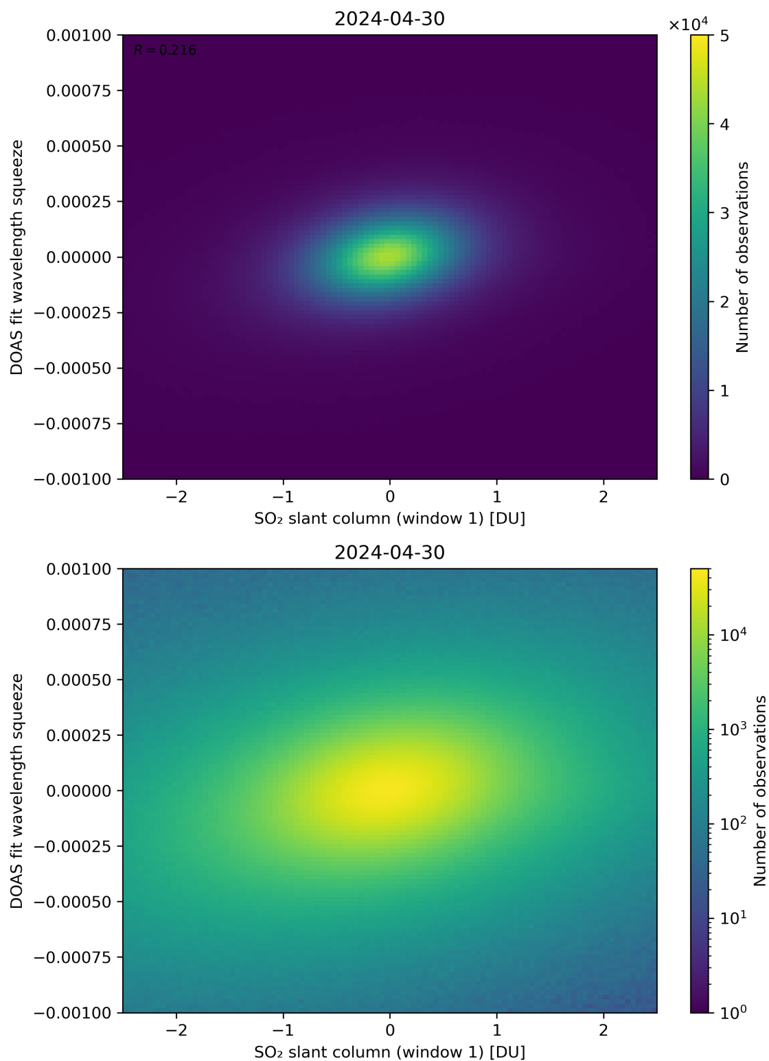
Figure 216: Scatter density plot of “SO 2 slant column (window 1)” against “DOAS fit wavelength squeeze” for 2024-04-29 to 2024-05-01.
