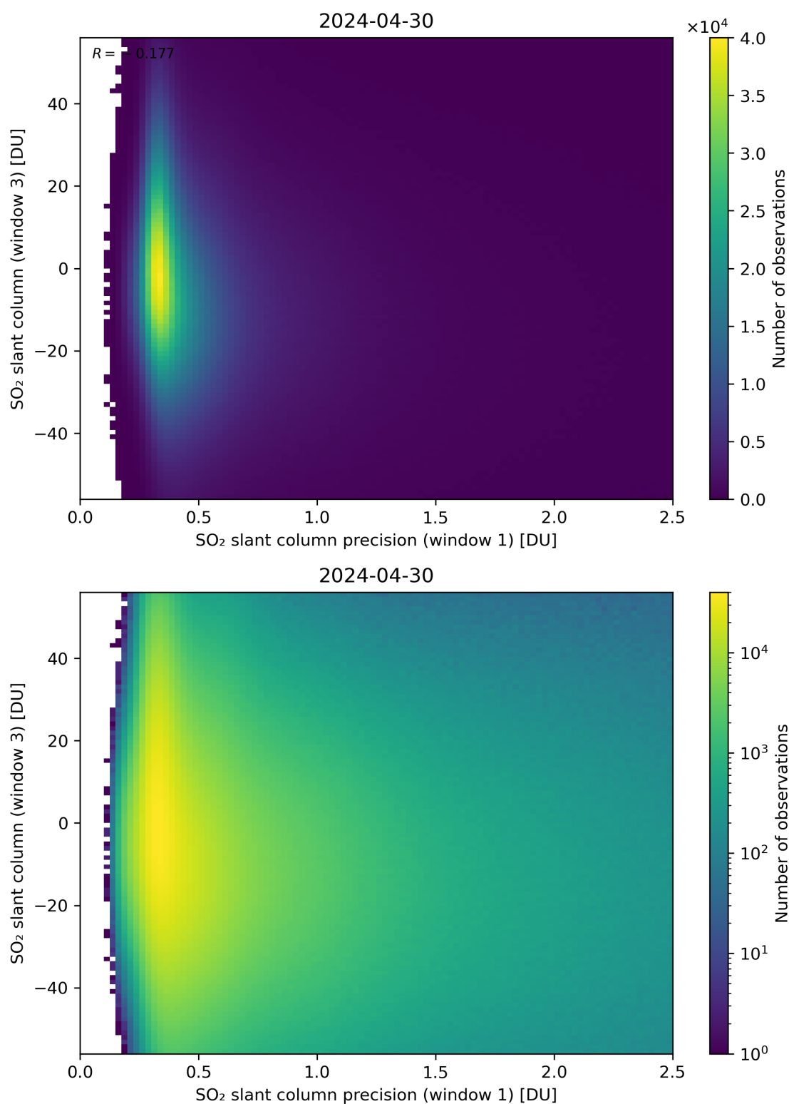
Figure 228: Scatter density plot of “SO 2 slant column precision (window 1)” against “SO 2 slant column (window 3)” for 2024-04-29 to 2024-05-01.
