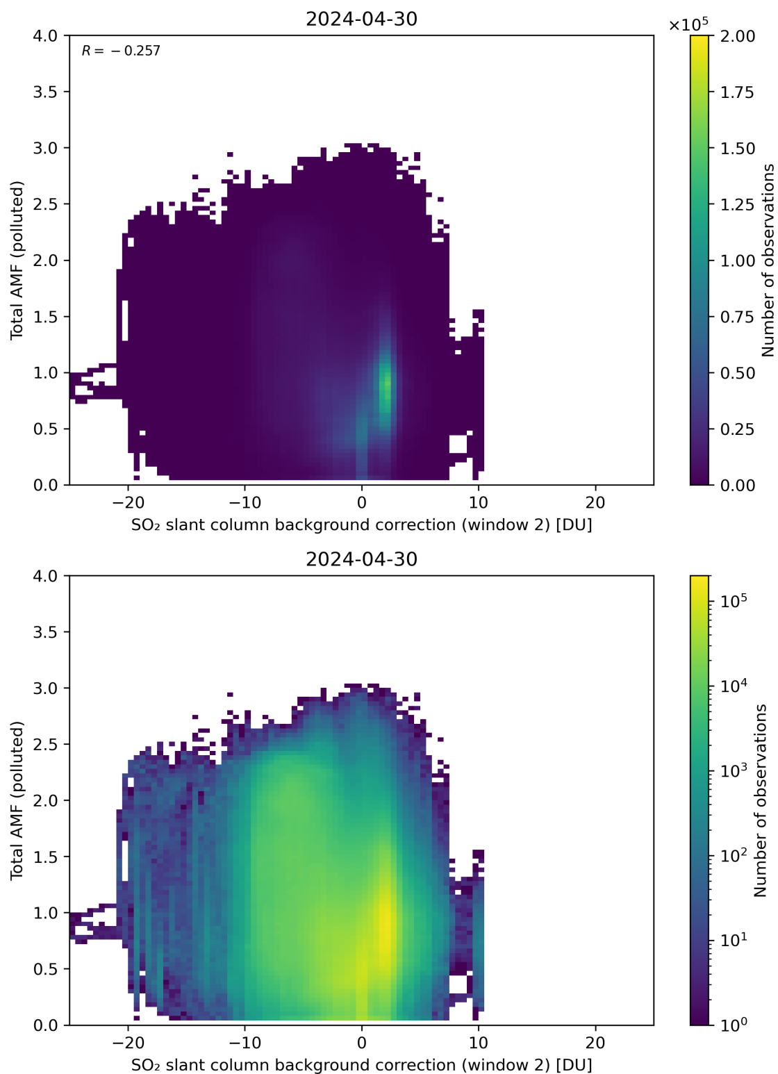
Figure 119: Scatter density plot of “SO 2 slant column background correction (window 2)” against “Total AMF (polluted)” for 2024-04-29 to 2024-05-01.
