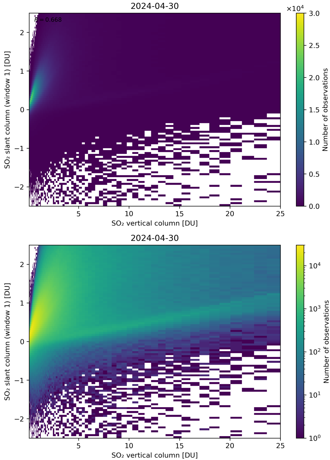
Figure 300: Scatter density plot of “SO 2 vertical column” against “SO 2 slant column (window 1)” for 2024-04-29 to 2024-05-01.
