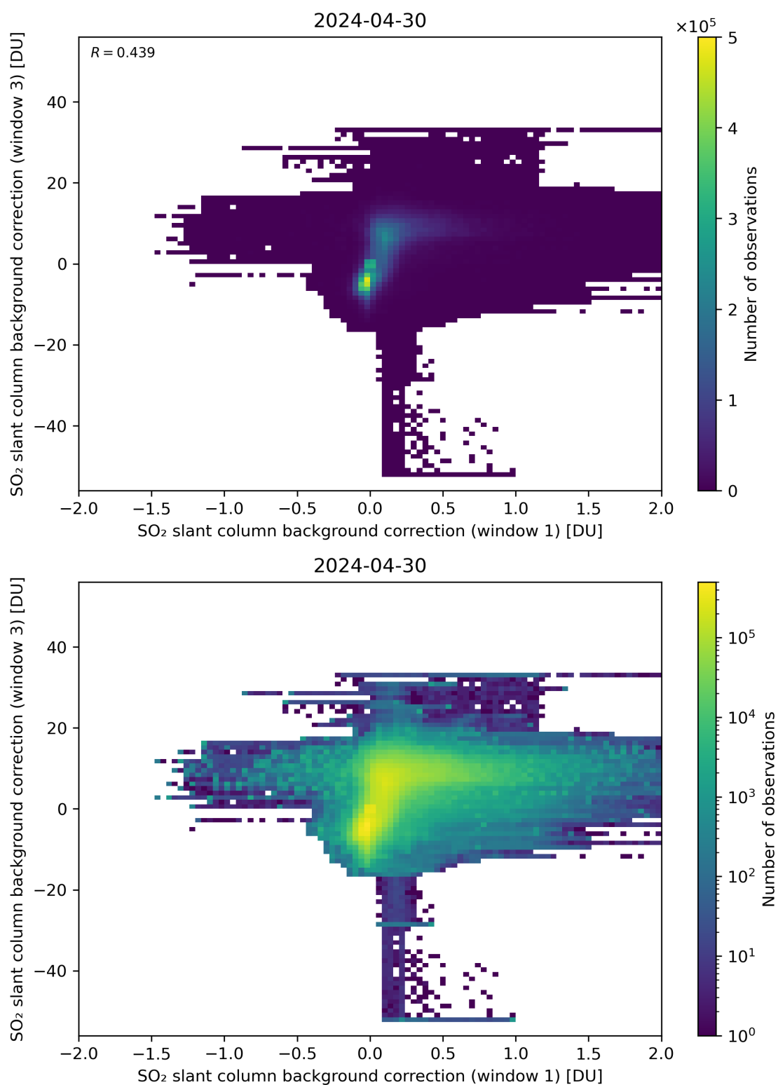
Figure 99: Scatter density plot of “SO 2 slant column background correction (window 1)” against “SO 2 slant column background correction (window 3)” for 2024-04-29 to 2024-05-01.
