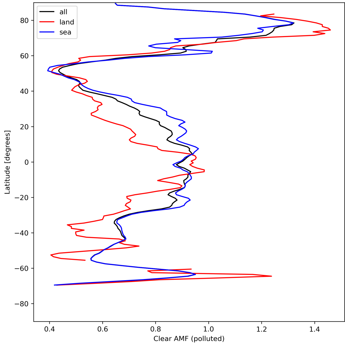
Figure 50: Zonal average of “Clear AMF (polluted)” for 2024-04-29 to 2024-05-01.
