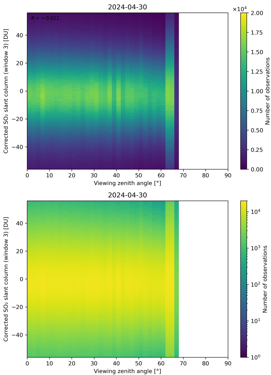
Figure 319: Scatter density plot of “Viewing zenith angle” against “Corrected SO 2 slant column (window 3)” for 2024-04-29 to 2024-05-01.
