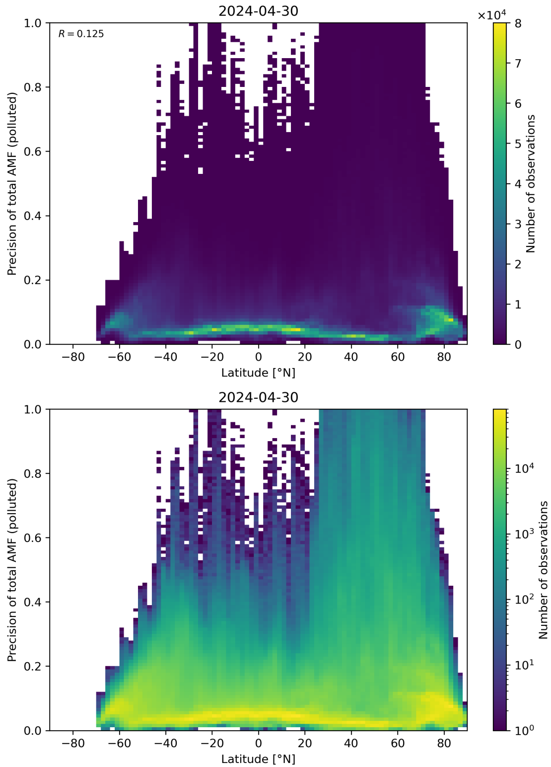
Figure 155: Scatter density plot of “Latitude” against “Precision of total AMF (polluted)” for 2024-04-29 to 2024-05-01.
