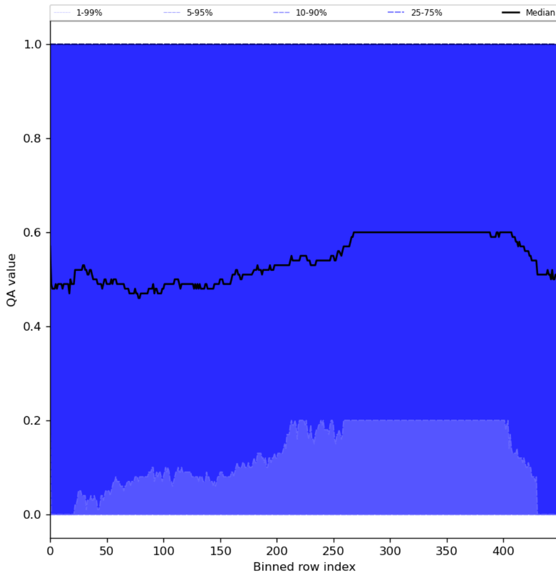
Figure 75: Along track statistics of “QA value” for 2024-04-29 to 2024-05-01
