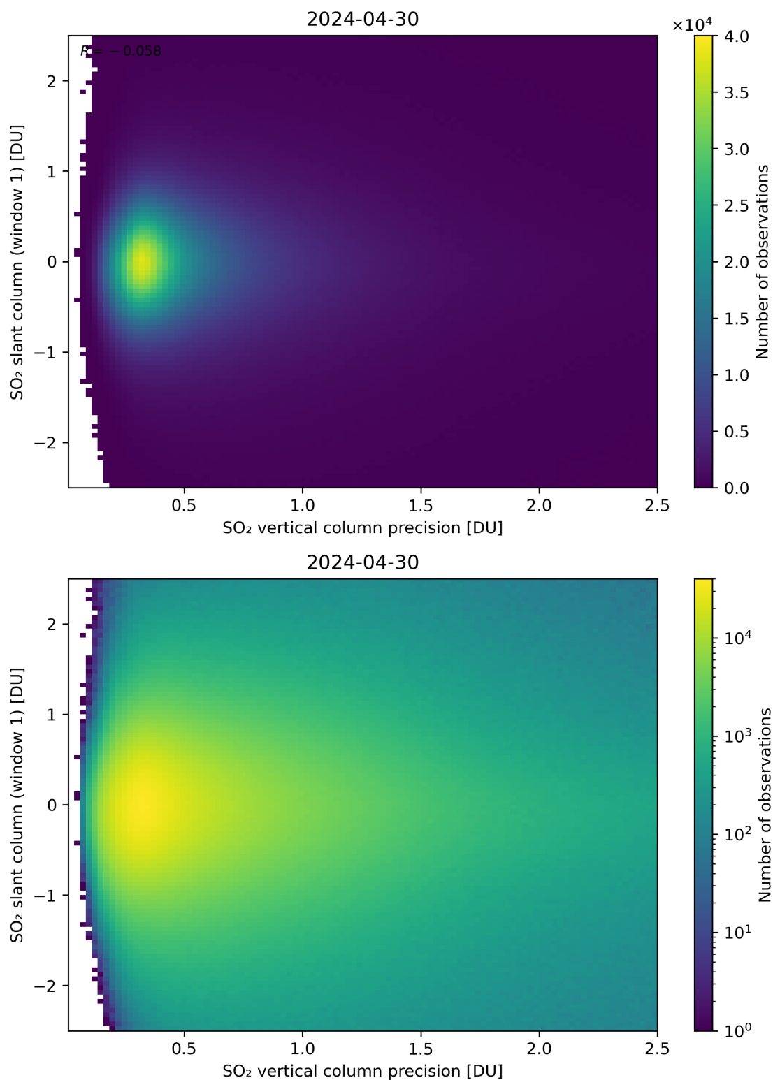
Figure 289: Scatter density plot of “SO 2 vertical column precision” against “SO 2 slant column (window 1)” for 2024-04-29 to 2024-05-01.
