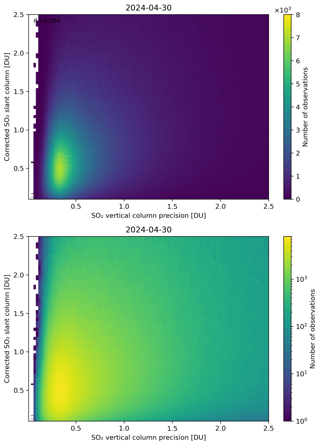
Figure 286: Scatter density plot of “SO 2 vertical column precision” against “Corrected SO 2 slant column” for 2024-04-29 to 2024-05-01.
