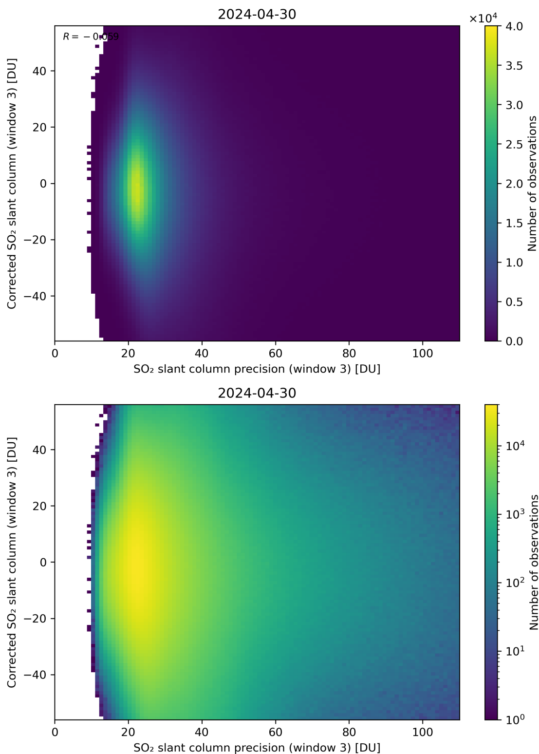
Figure 262: Scatter density plot of “SO 2 slant column precision (window 3)” against “Corrected SO 2 slant column (window 3)” for 2024-04-29 to 2024-05-01.
