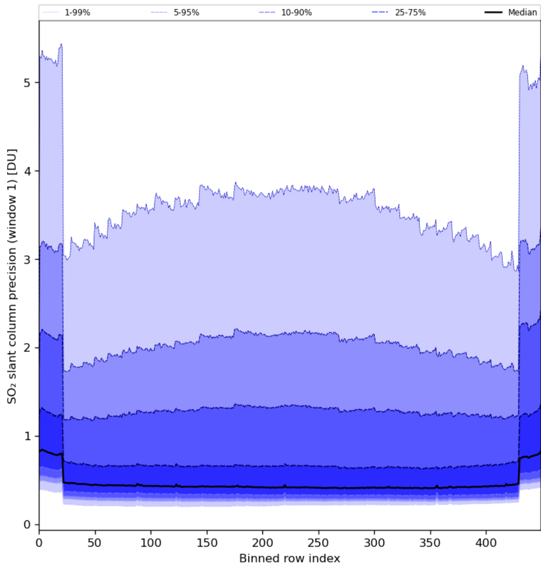
Figure 80: Along track statistics of “SO 2 slant column precision (window 1)” for 2024-04-29 to 2024-05-01
