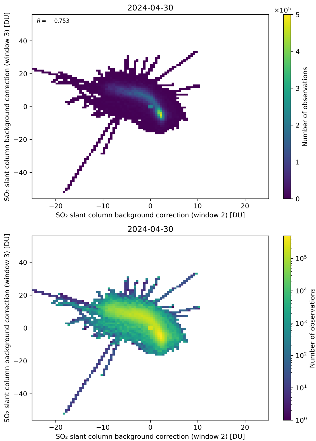
Figure 111: Scatter density plot of “SO 2 slant column background correction (window 2)” against “SO 2 slant column background correction (window 3)” for 2024-04-29 to 2024-05-01.
