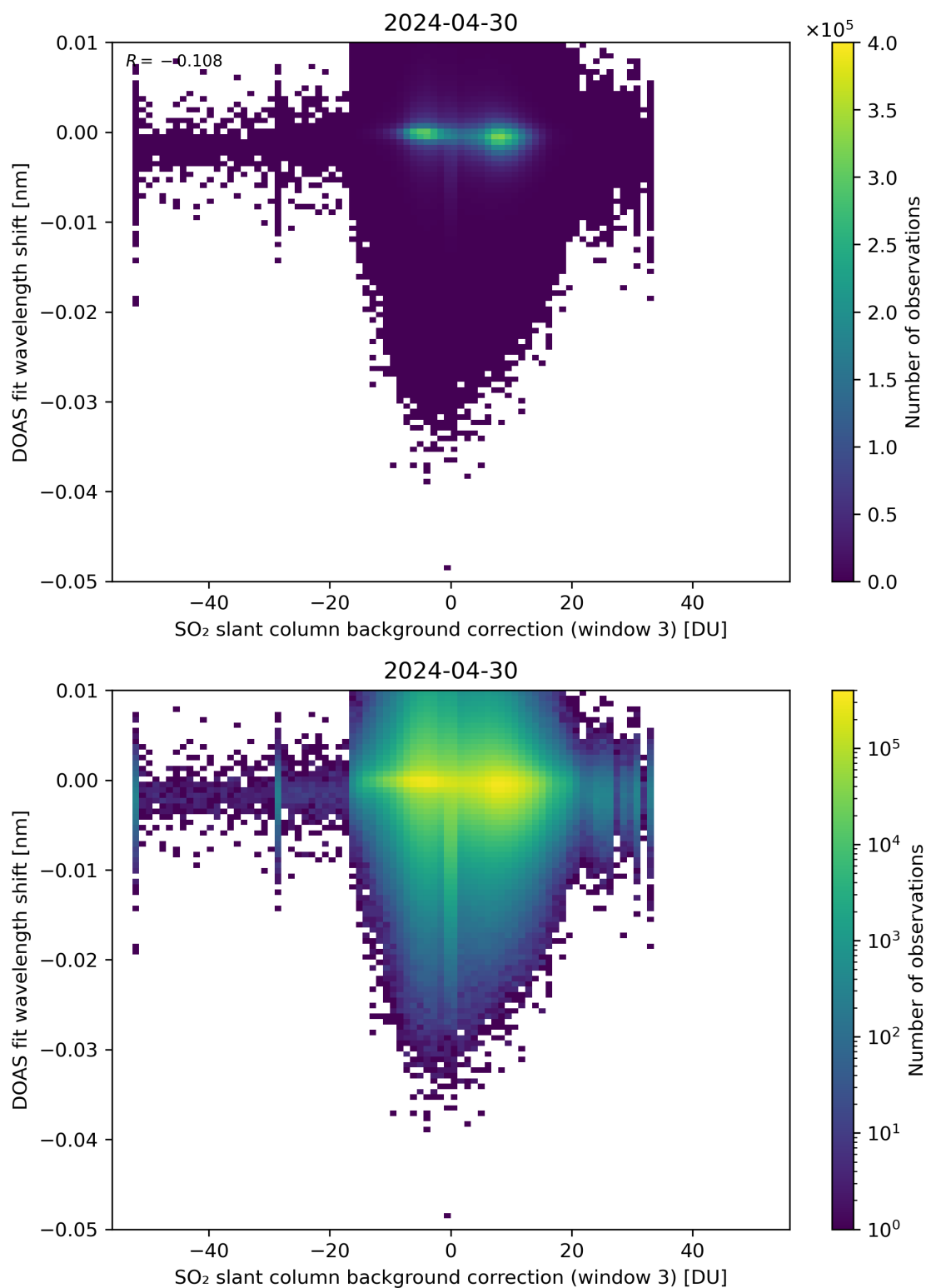
Figure 121: Scatter density plot of “SO 2 slant column background correction (window 3)” against “DOAS fit wavelength shift” for 2024-04-29 to 2024-05-01.
