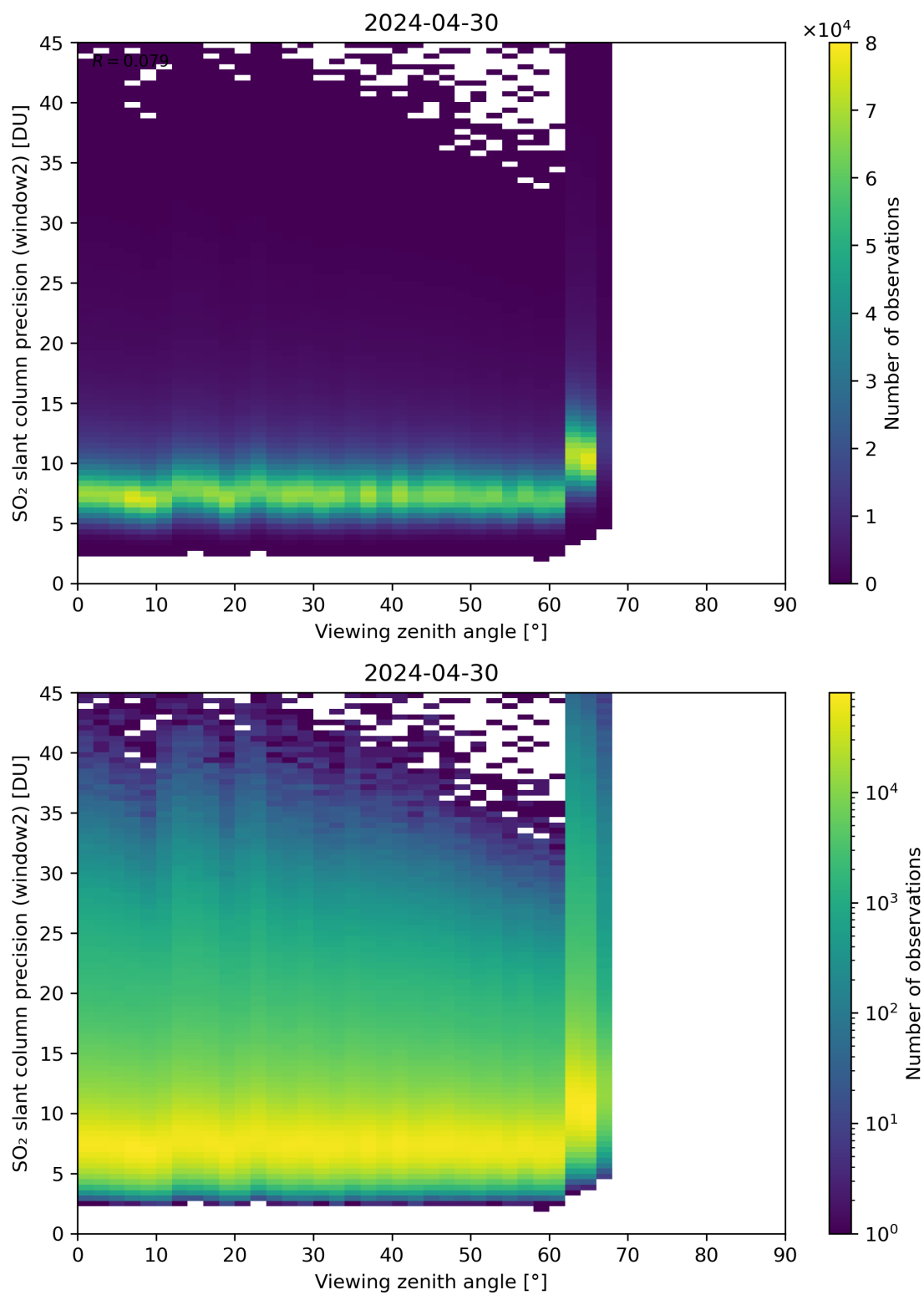
Figure 322: Scatter density plot of “Viewing zenith angle” against “SO 2 slant column precision (window2)” for 2024-04-29 to 2024-05-01.
