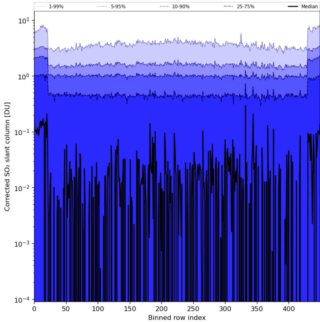
Figure 78: Along track statistics of “Corrected SO 2 slant column” for 2024-04-29 to 2024-05-01
