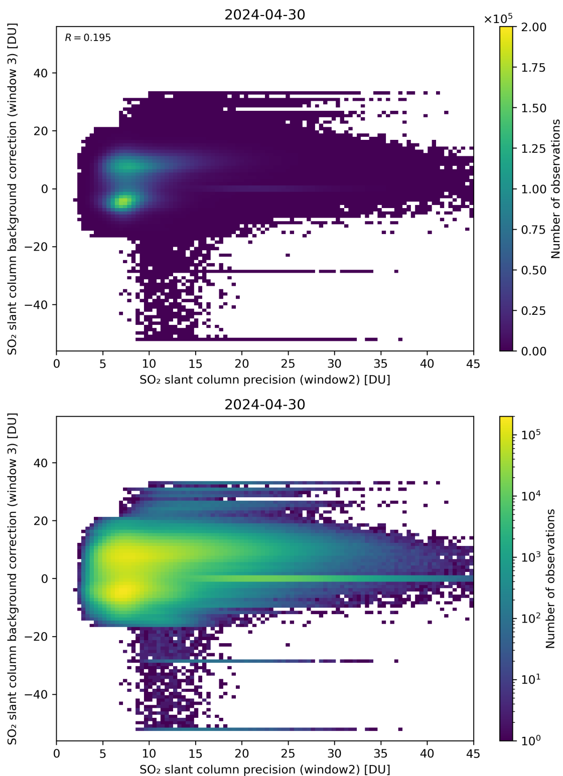
Figure 242: Scatter density plot of “SO 2 slant column precision (window2)” against “SO 2 slant column background correction (window 3)” for 2024-04-29 to 2024-05-01.
