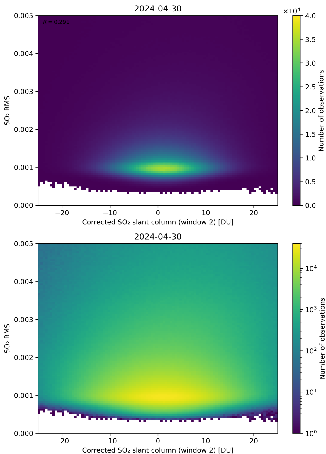
Figure 198: Scatter density plot of “Corrected SO 2 slant column (window 2)” against “SO 2 RMS” for 2024-04-29 to 2024-05-01.
