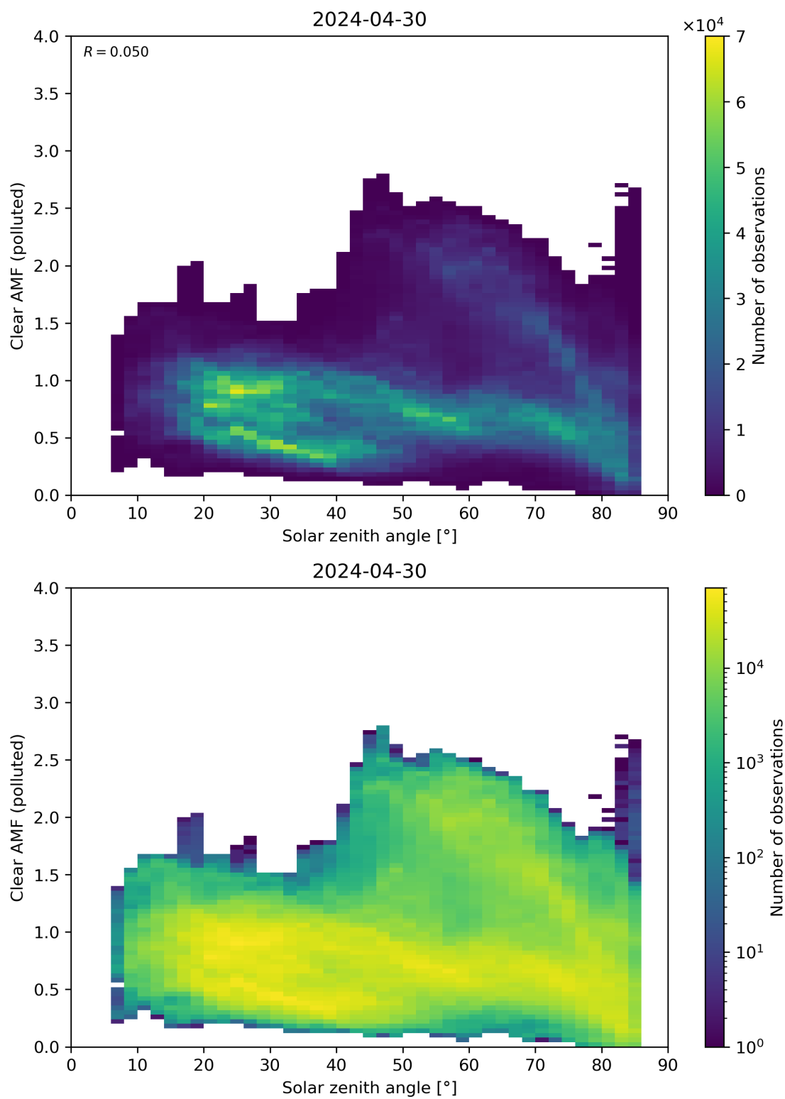
Figure 165: Scatter density plot of “Solar zenith angle” against “Clear AMF (polluted)” for 2024-04-29 to 2024-05-01.
