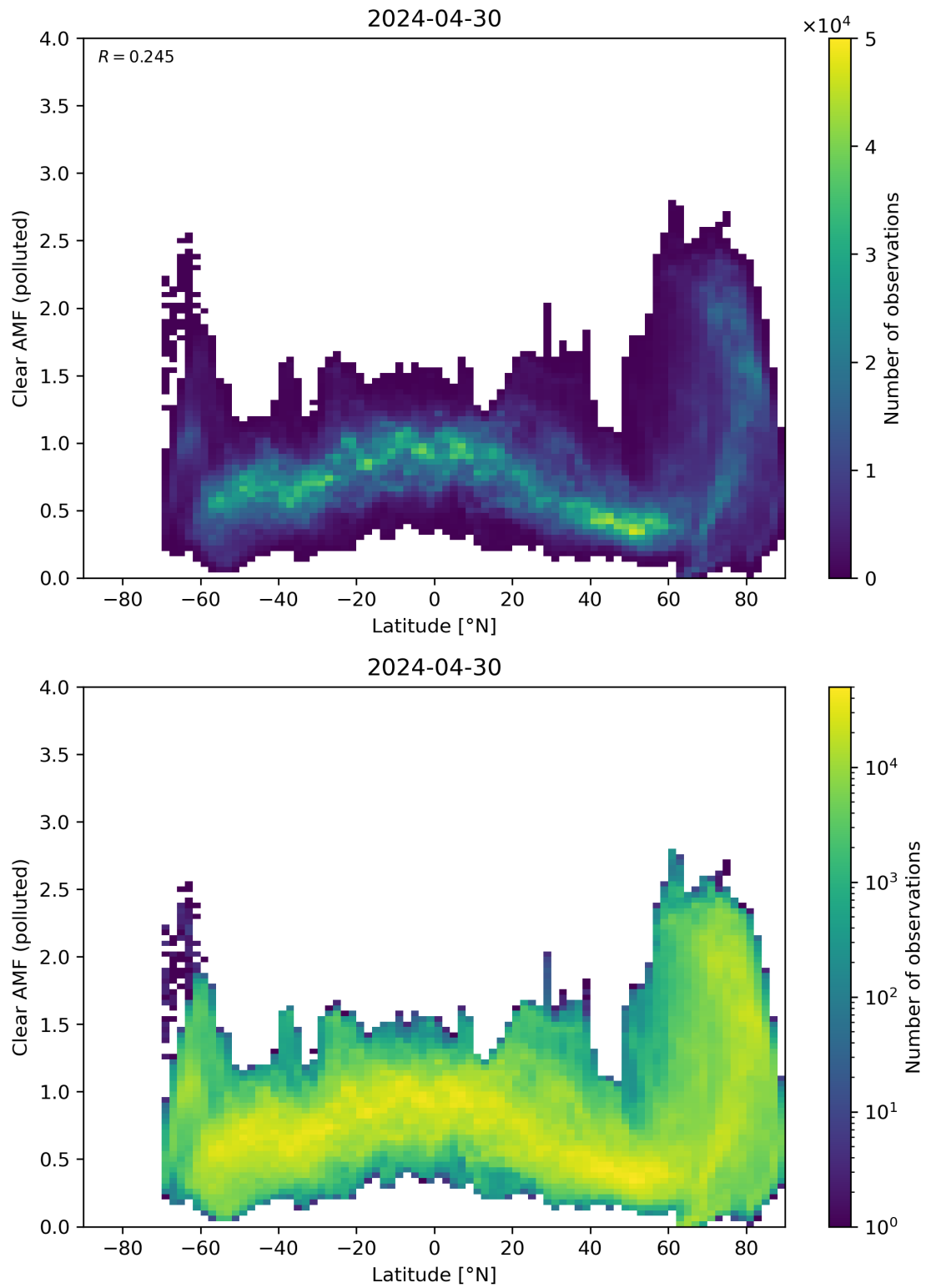
Figure 145: Scatter density plot of “Latitude” against “Clear AMF (polluted)” for 2024-04-29 to 2024-05-01.
