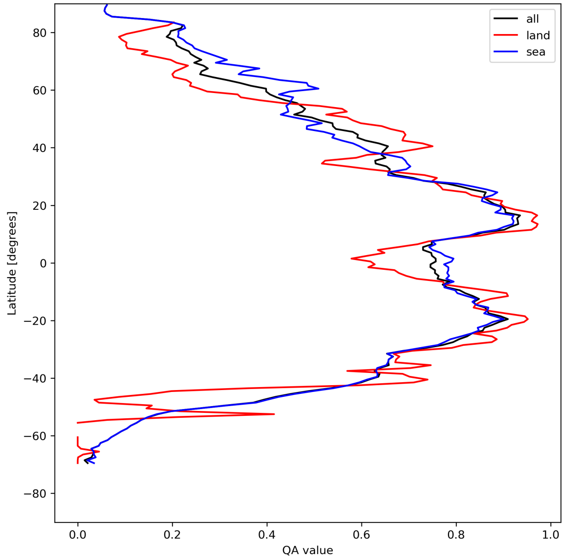
Figure 29: Zonal average of “QA value” for 2024-04-29 to 2024-05-01.
