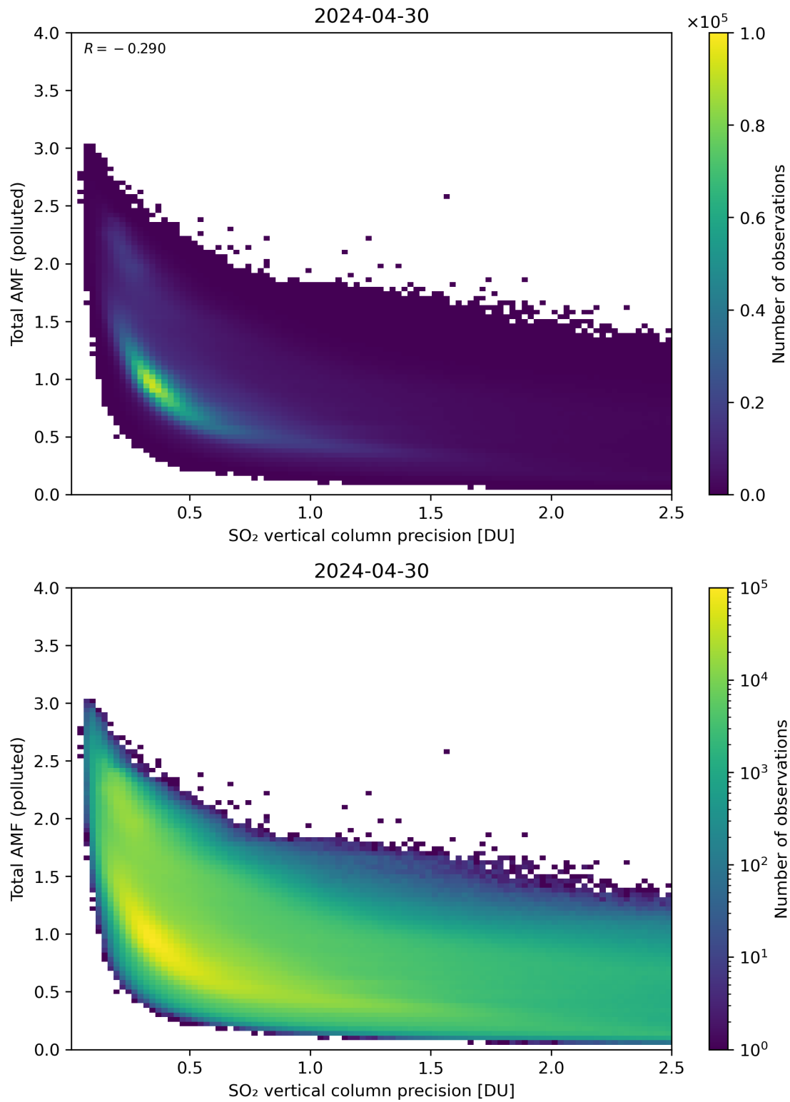
Figure 294: Scatter density plot of “SO 2 vertical column precision” against “Total AMF (polluted)” for 2024-04-29 to 2024-05-01.
