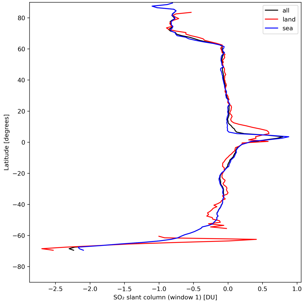
Figure 33: Zonal average of “SO 2 slant column (window 1)” for 2024-04-29 to 2024-05-01.
