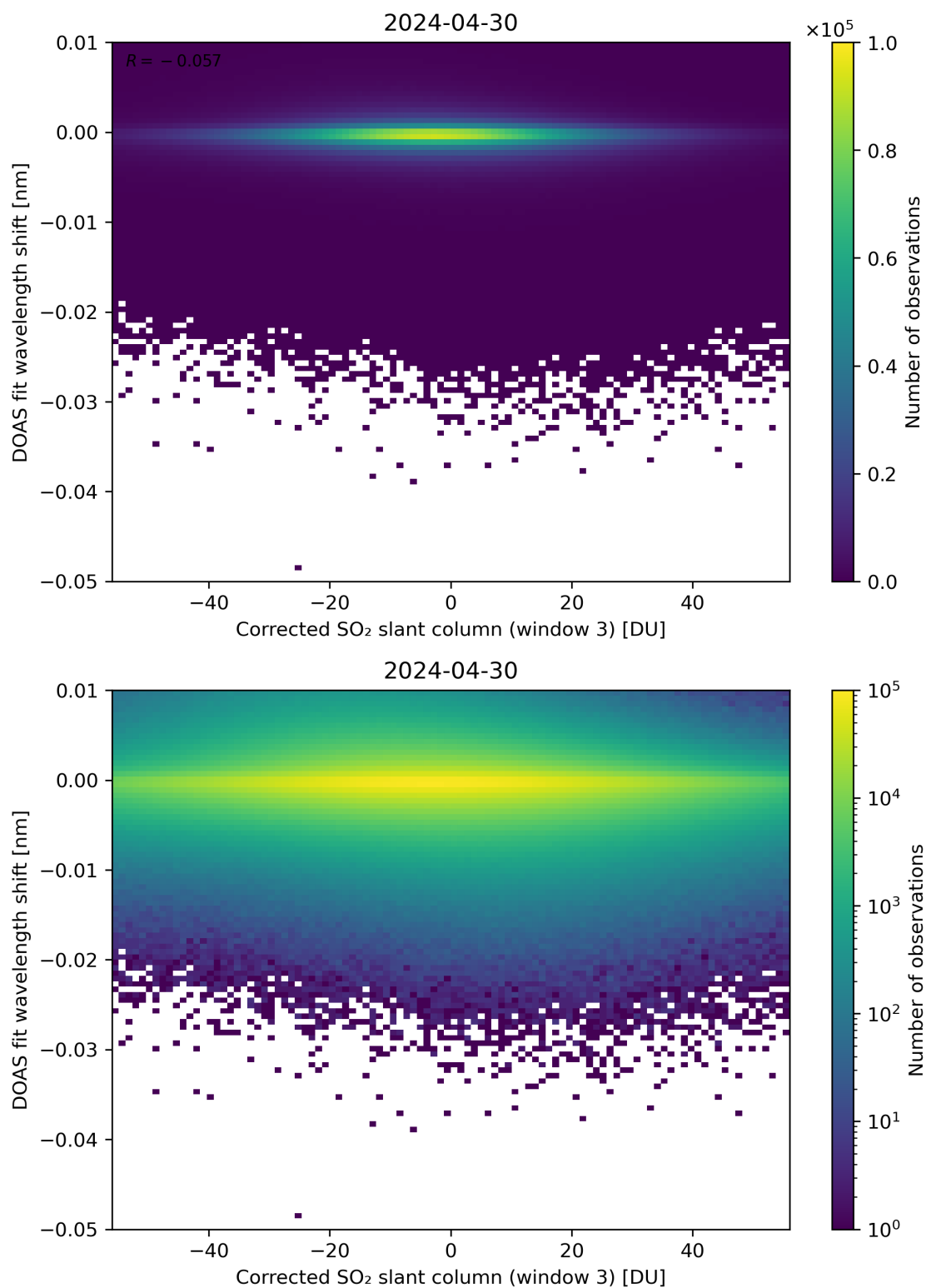
Figure 206: Scatter density plot of “Corrected SO 2 slant column (window 3)” against “DOAS fit wavelength shift” for 2024-04-29 to 2024-05-01.
