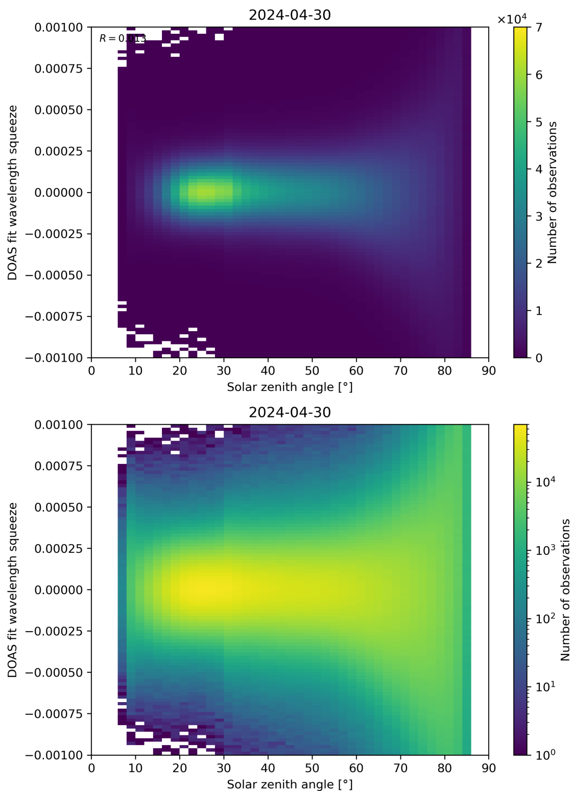
Figure 162: Scatter density plot of “Solar zenith angle” against “DOAS fit wavelength squeeze” for 2024-04-29 to 2024-05-01.
