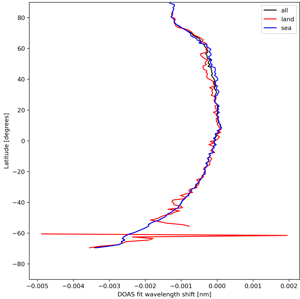
Figure 45: Zonal average of “DOAS fit wavelength shift” for 2024-04-29 to 2024-05-01.
