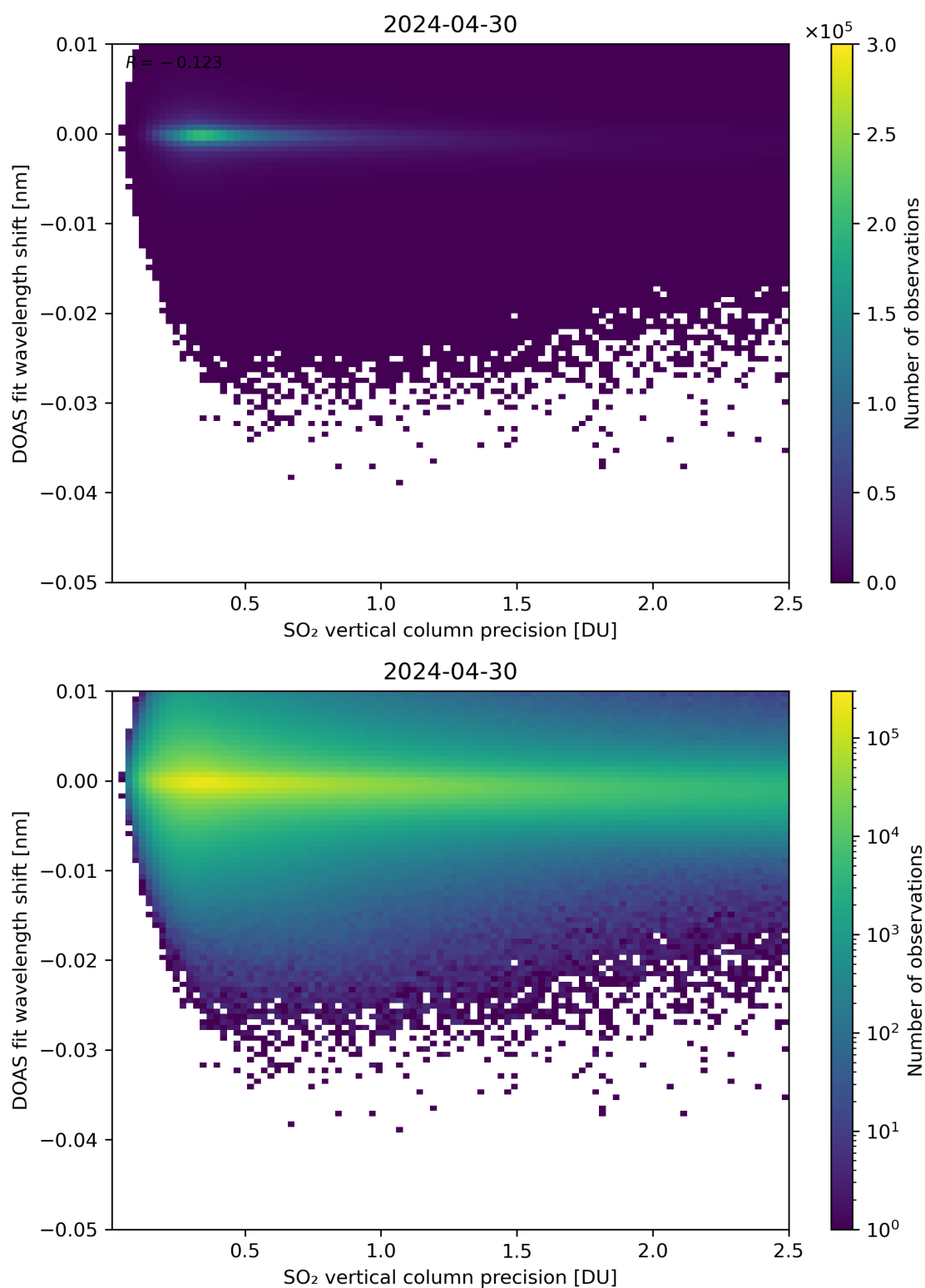
Figure 282: Scatter density plot of “SO 2 vertical column precision” against “DOAS fit wavelength shift” for 2024-04-29 to 2024-05-01.
