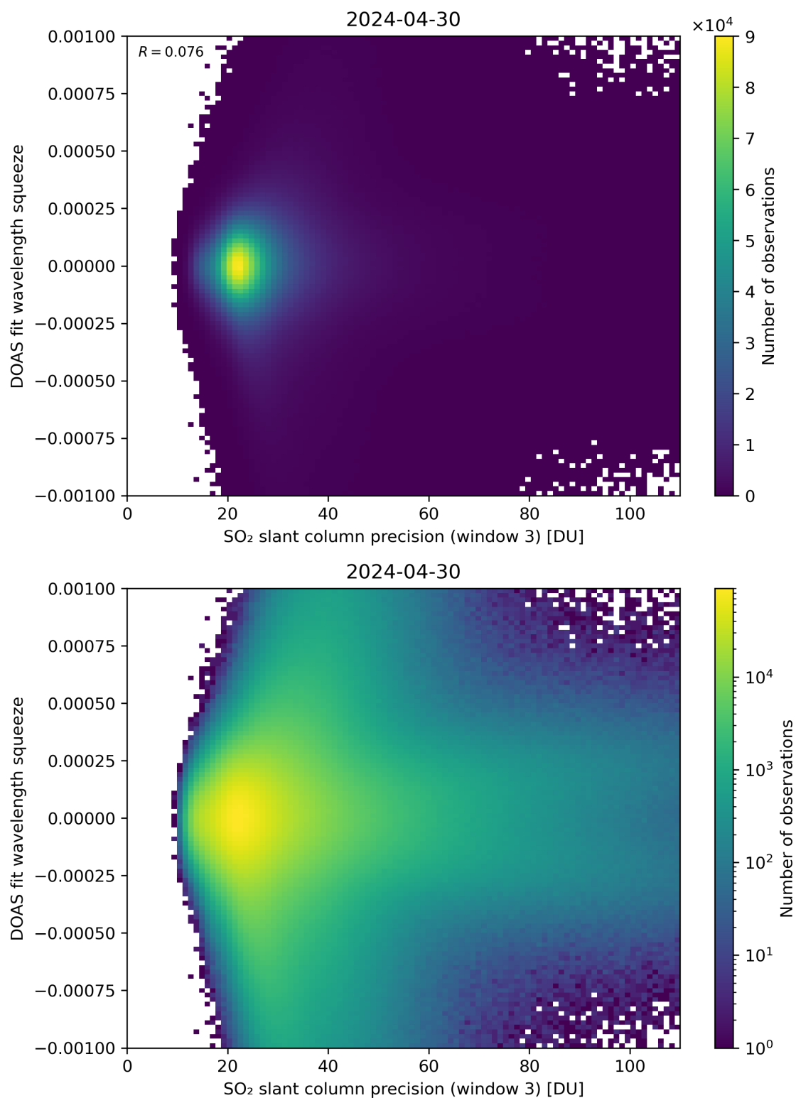
Figure 259: Scatter density plot of “SO 2 slant column precision (window 3)” against “DOAS fit wavelength squeeze” for 2024-04-29 to 2024-05-01.
