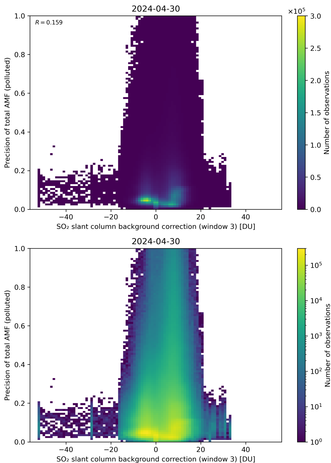
Figure 126: Scatter density plot of “SO 2 slant column background correction (window 3)” against “Precision of total AMF (polluted)” for 2024-04-29 to 2024-05-01.
