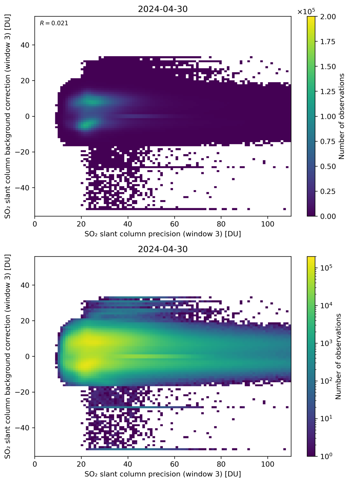
Figure 257: Scatter density plot of “SO 2 slant column precision (window 3)” against “SO 2 slant column background correction (window 3)” for 2024-04-29 to 2024-05-01.
