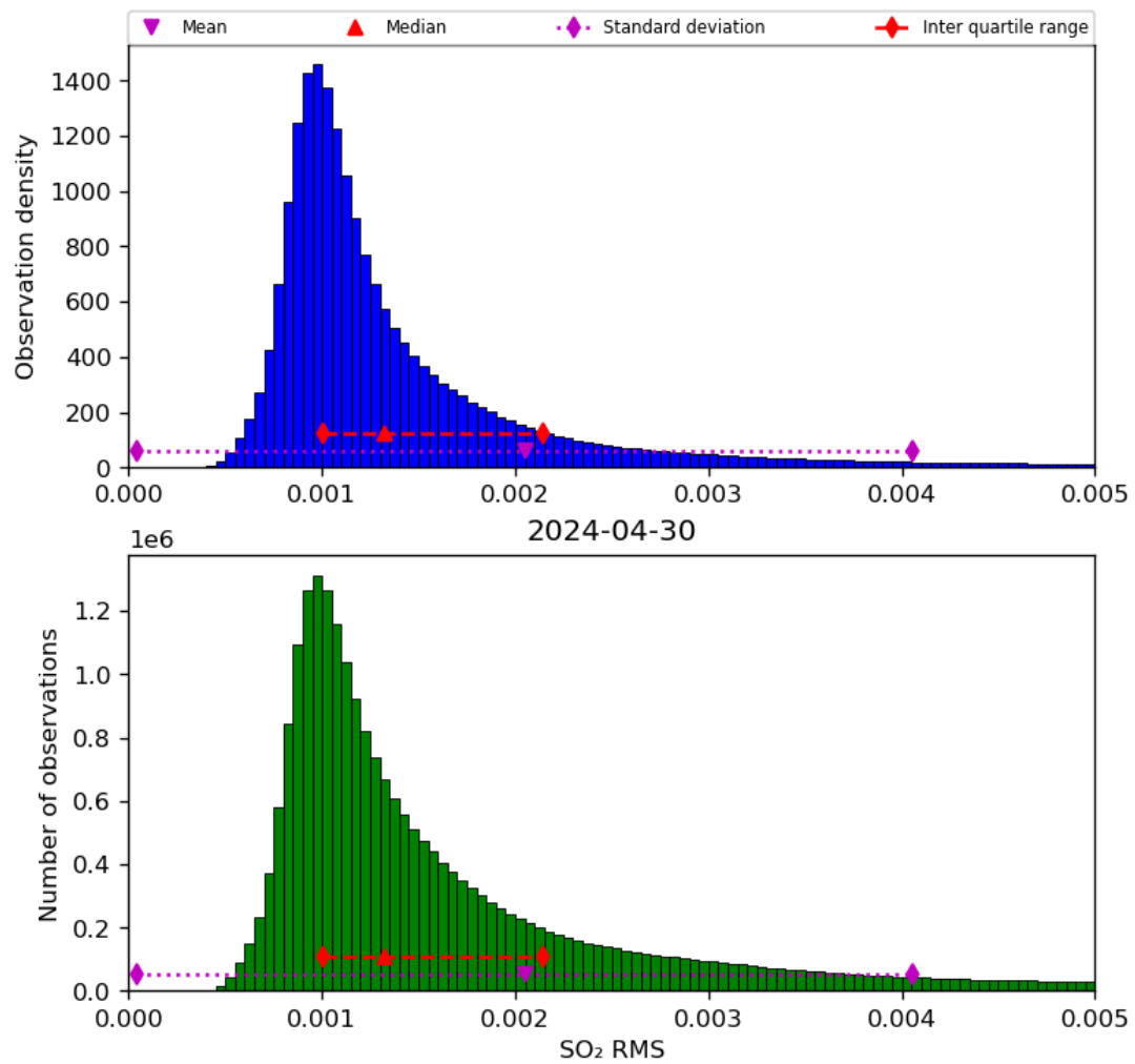
Figure 70: Histogram of “SO 2 RMS” for 2024-04-29 to 2024-05-01
