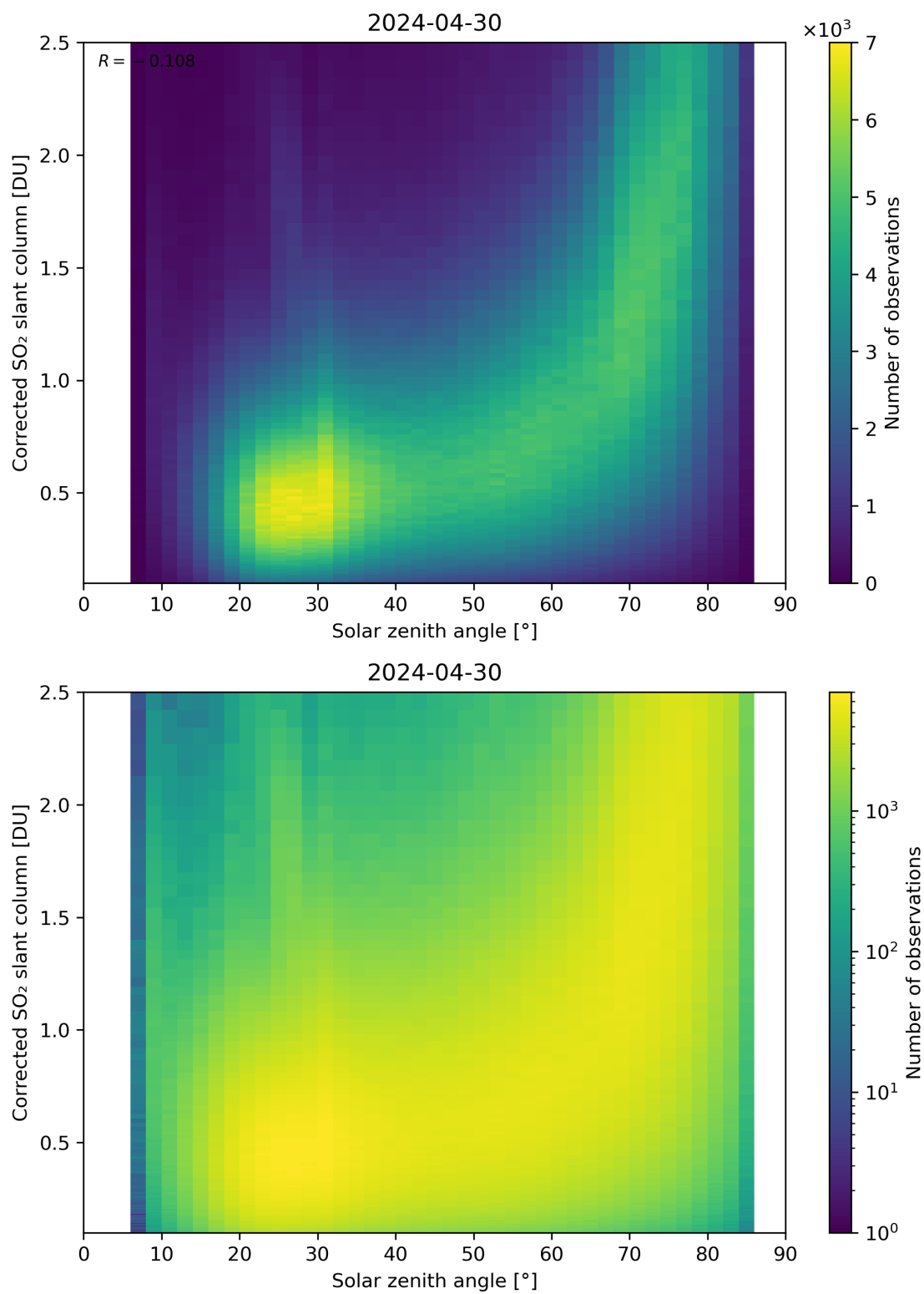
Figure 166: Scatter density plot of “Solar zenith angle” against “Corrected SO 2 slant column” for 2024-04-29 to 2024-05-01.
