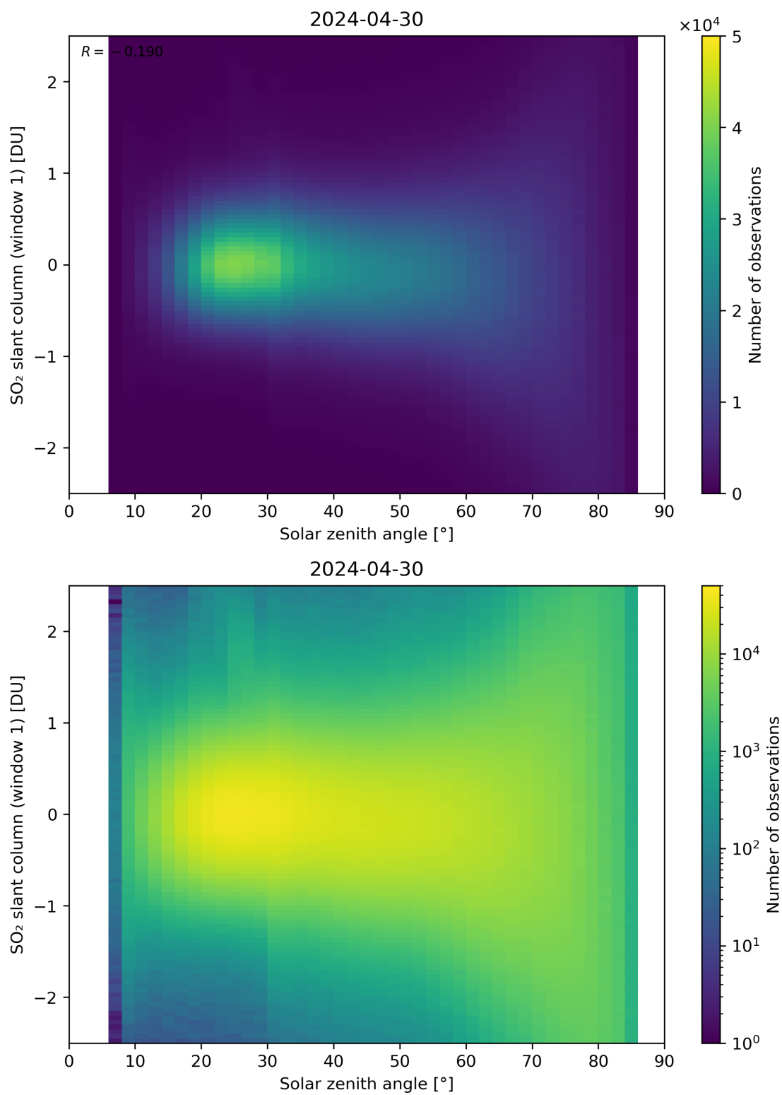
Figure 169: Scatter density plot of “Solar zenith angle” against “SO 2 slant column (window 1)” for 2024-04-29 to 2024-05-01.
