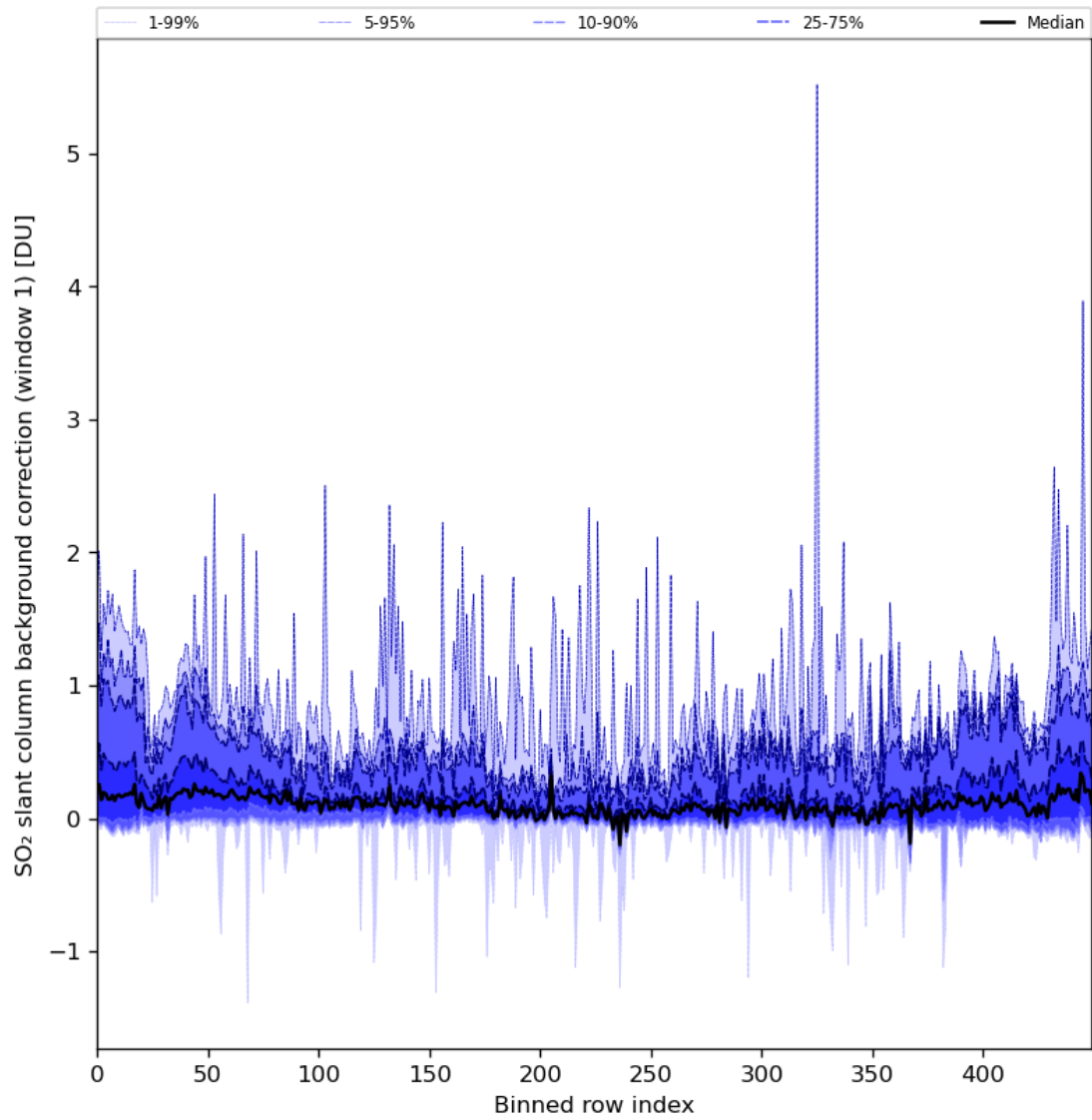
Figure 82: Along track statistics of “SO 2 slant column background correction (window 1)” for 2024-04-29 to 2024-05-01
