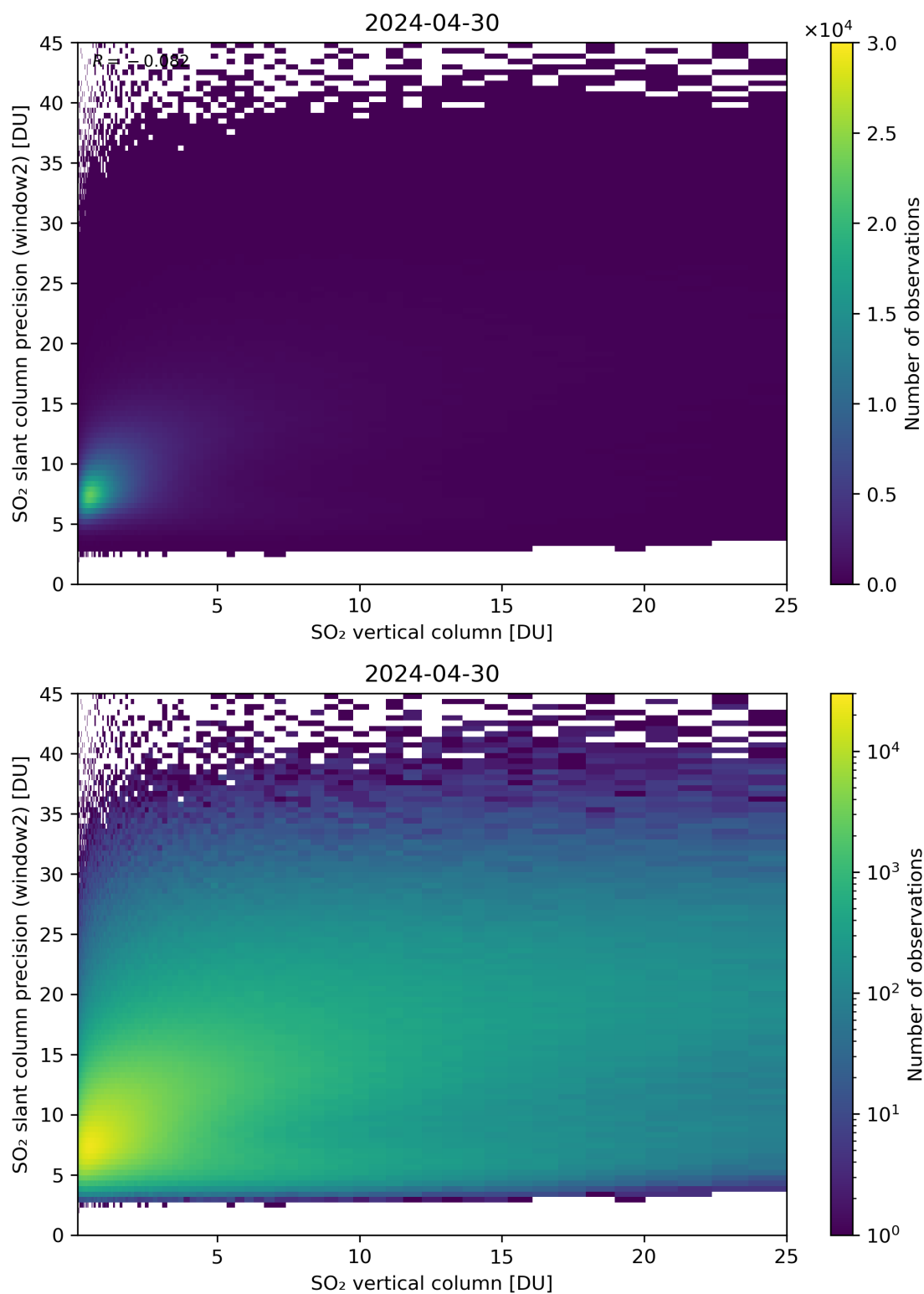
Figure 302: Scatter density plot of “SO 2 vertical column” against “SO 2 slant column precision (window2)” for 2024-04-29 to 2024-05-01.
