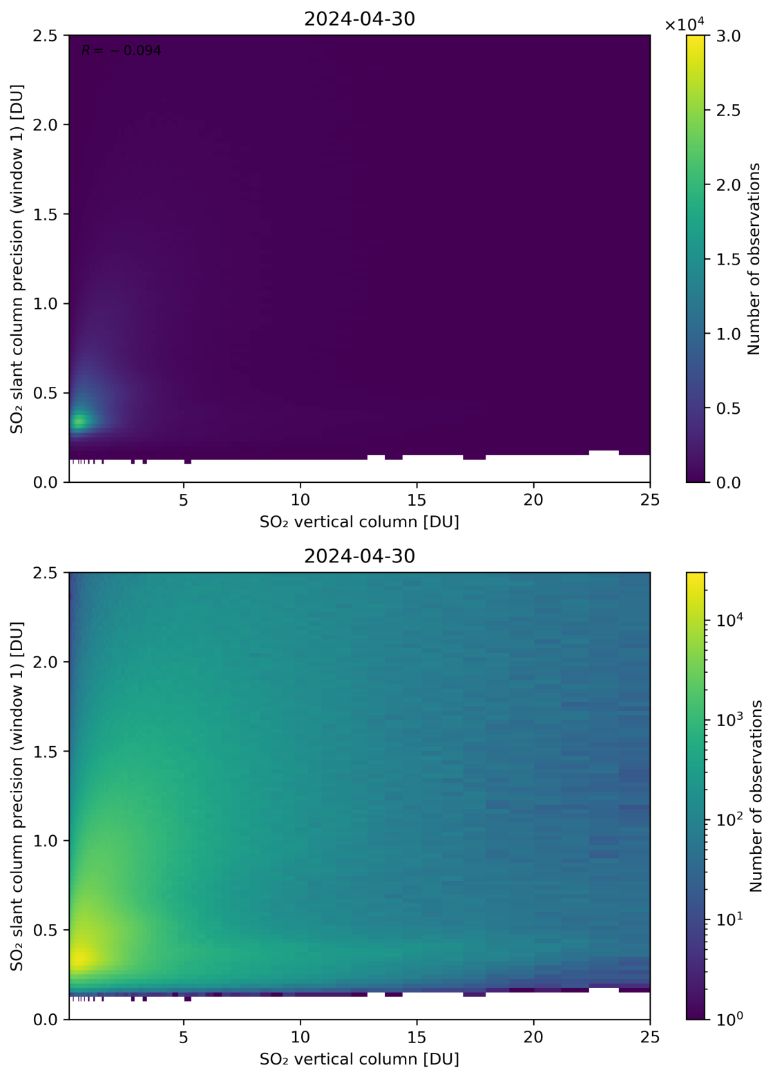
Figure 301: Scatter density plot of “SO 2 vertical column” against “SO 2 slant column precision (window 1)” for 2024-04-29 to 2024-05-01.
