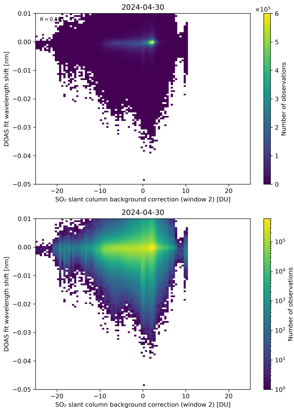
Figure 112: Scatter density plot of “SO 2 slant column background correction (window 2)” against “DOAS fit wavelength shift” for 2024-04-29 to 2024-05-01.
