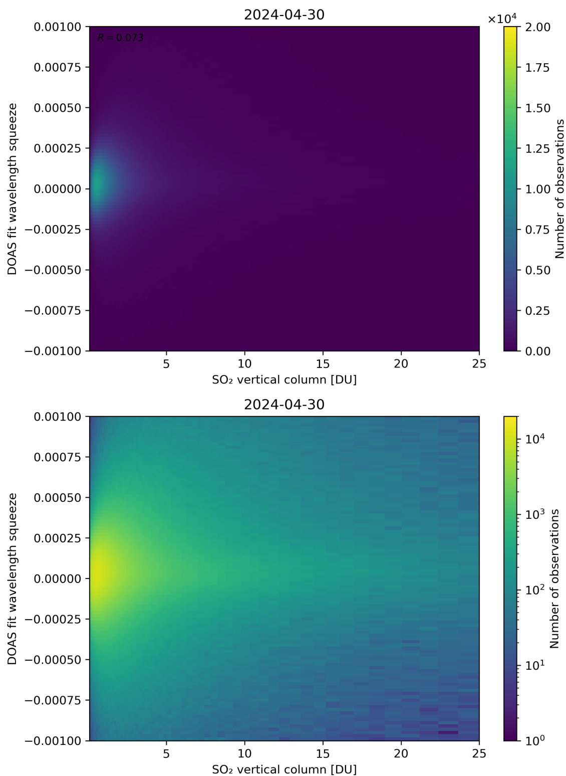
Figure 277: Scatter density plot of “SO 2 vertical column” against “DOAS fit wavelength squeeze” for 2024-04-29 to 2024-05-01.
