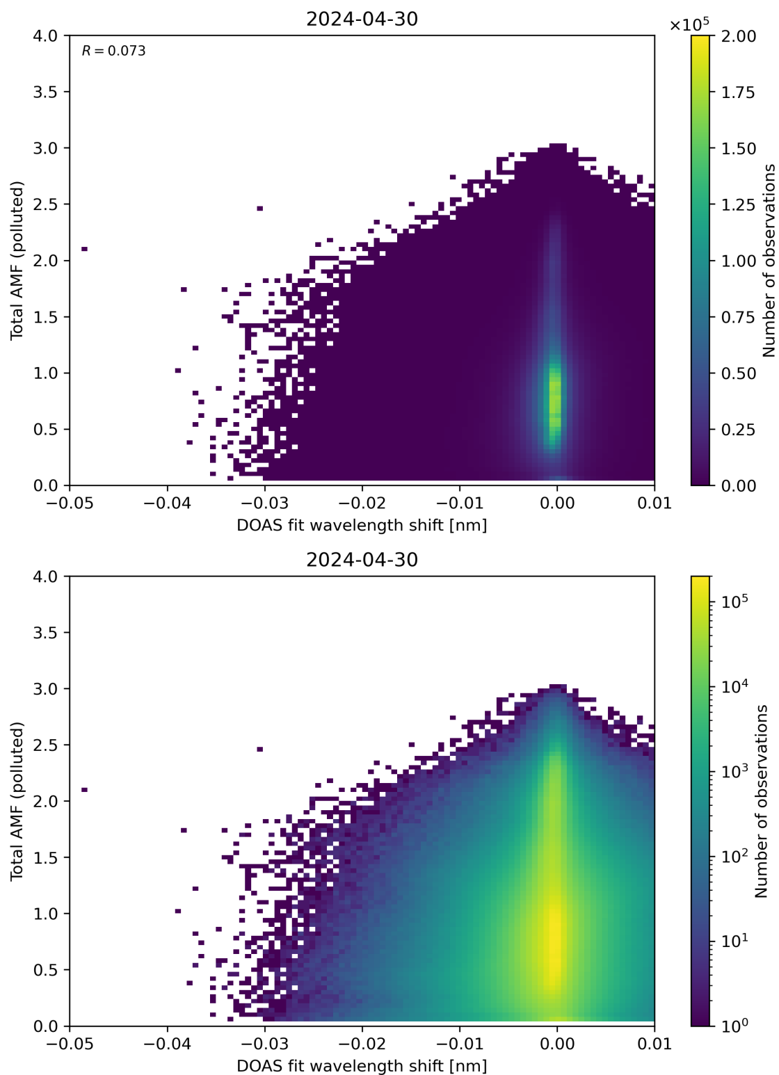
Figure 130: Scatter density plot of “DOAS fit wavelength shift” against “Total AMF (polluted)” for 2024-04-29 to 2024-05-01.
