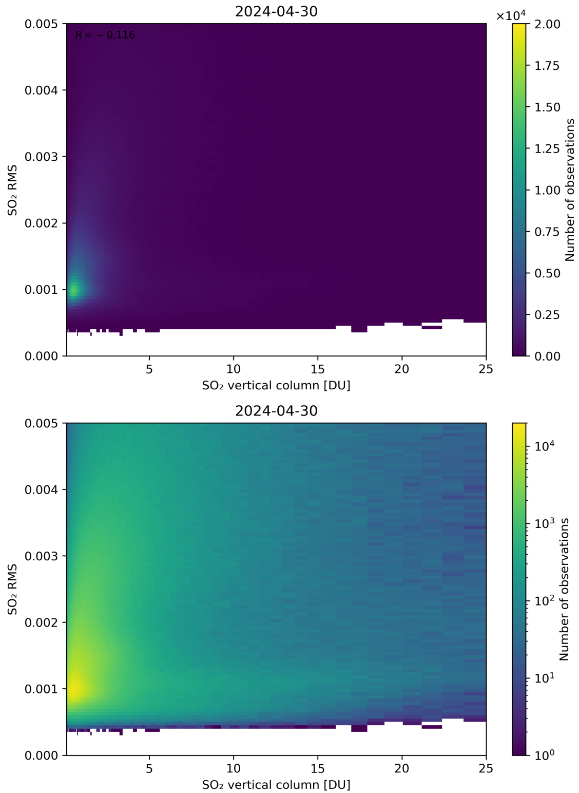
Figure 278: Scatter density plot of “SO 2 vertical column” against “SO 2 RMS” for 2024-04-29 to 2024-05-01.
