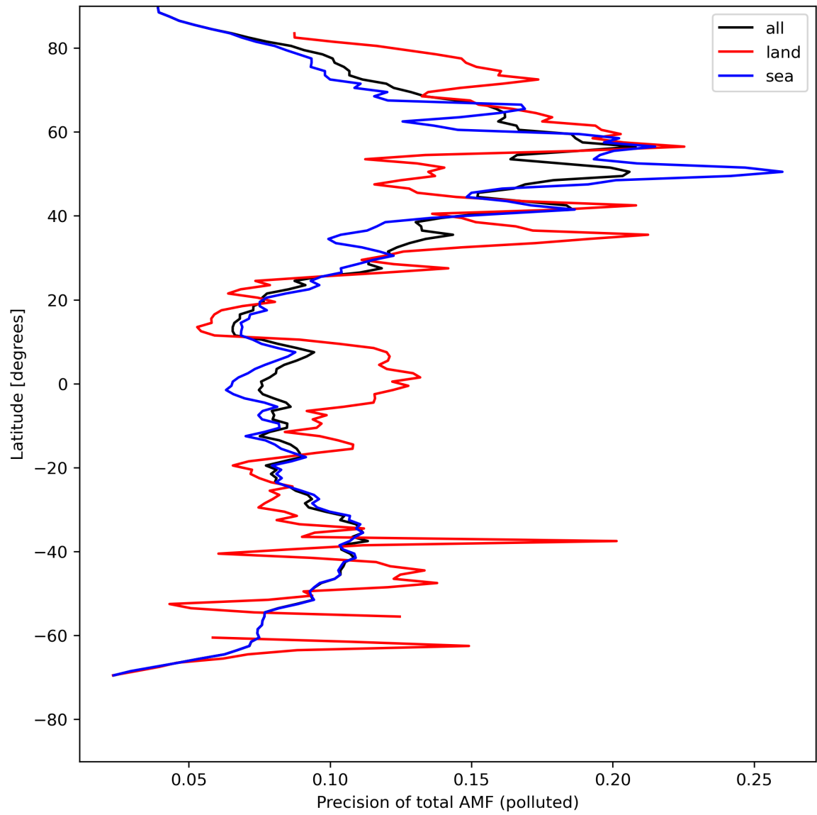
Figure 49: Zonal average of “Precision of total AMF (polluted)” for 2024-04-29 to 2024-05-01.
