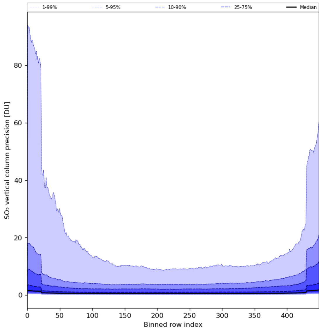
Figure 77: Along track statistics of “SO 2 vertical column precision” for 2024-04-29 to 2024-05-01
