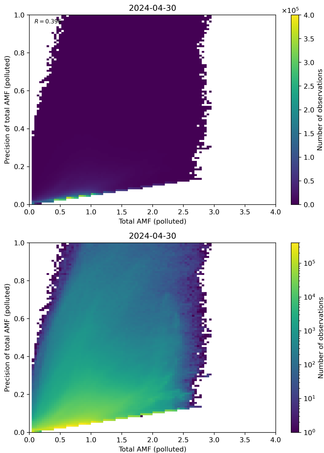
Figure 272: Scatter density plot of “Total AMF (polluted)” against “Precision of total AMF (polluted)” for 2024-04-29 to 2024-05-01.
