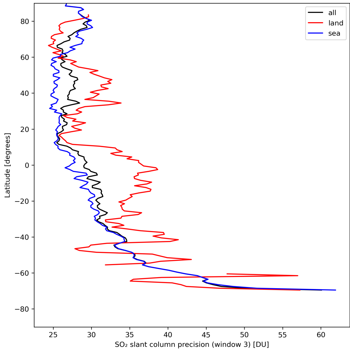
Figure 42: Zonal average of “SO 2 slant column precision (window 3)” for 2024-04-29 to 2024-05-01.
