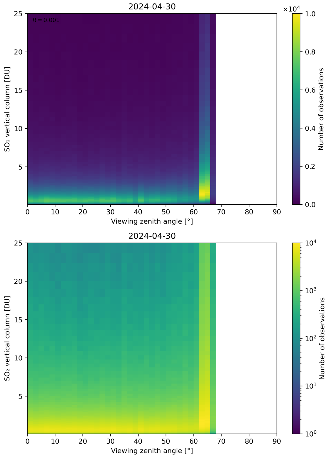
Figure 327: Scatter density plot of “Viewing zenith angle” against “SO 2 vertical column” for 2024-04-29 to 2024-05-01.
