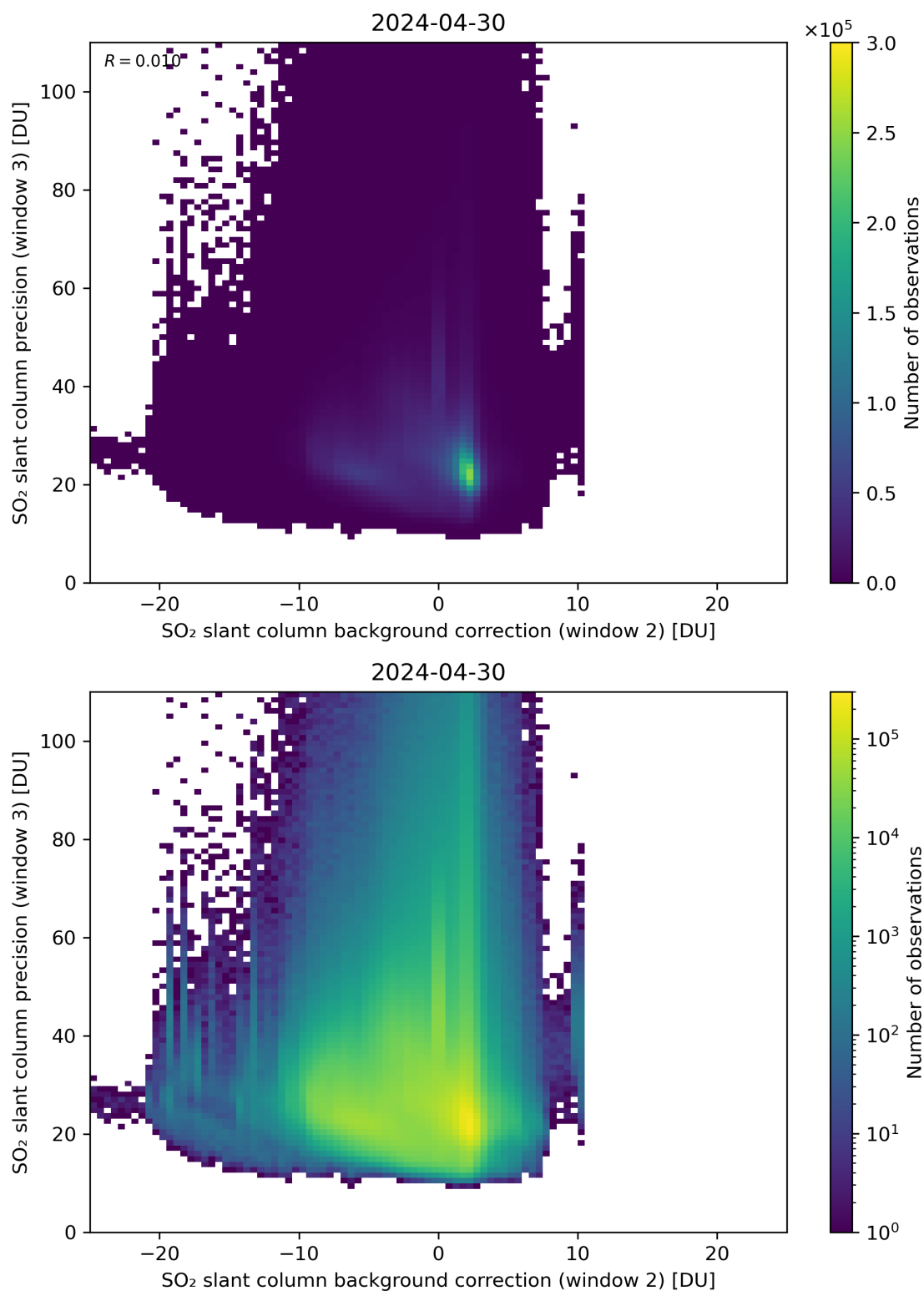
Figure 118: Scatter density plot of “SO 2 slant column background correction (window 2)” against “SO 2 slant column precision (window 3)” for 2024-04-29 to 2024-05-01.
