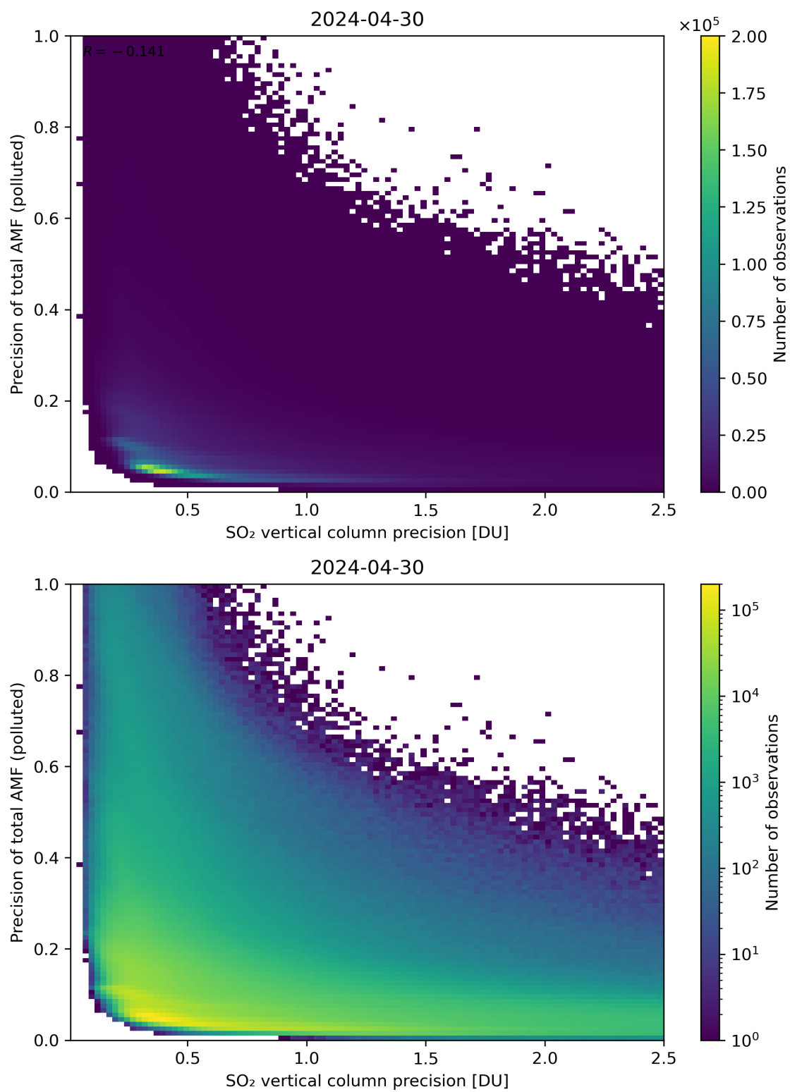
Figure 295: Scatter density plot of “SO 2 vertical column precision” against “Precision of total AMF (polluted)” for 2024-04-29 to 2024-05-01.
