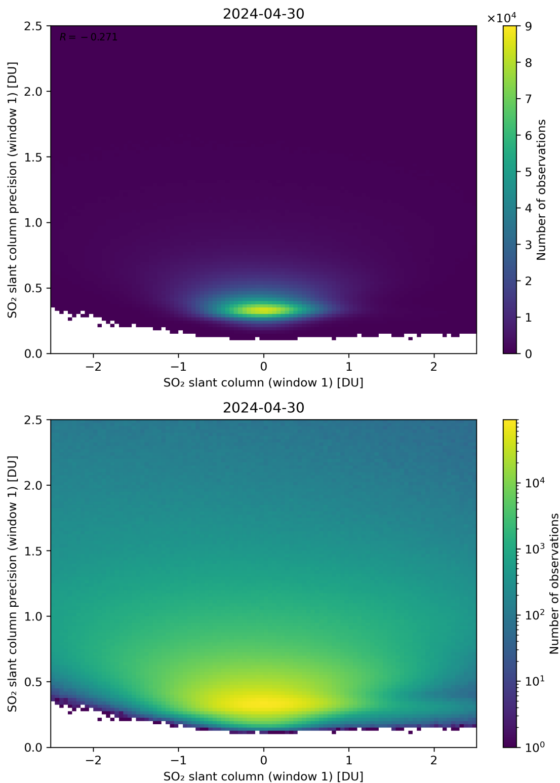
Figure 235: Scatter density plot of “SO 2 slant column (window 1)” against “SO 2 slant column precision (window 1)” for 2024-04-29 to 2024-05-01.
