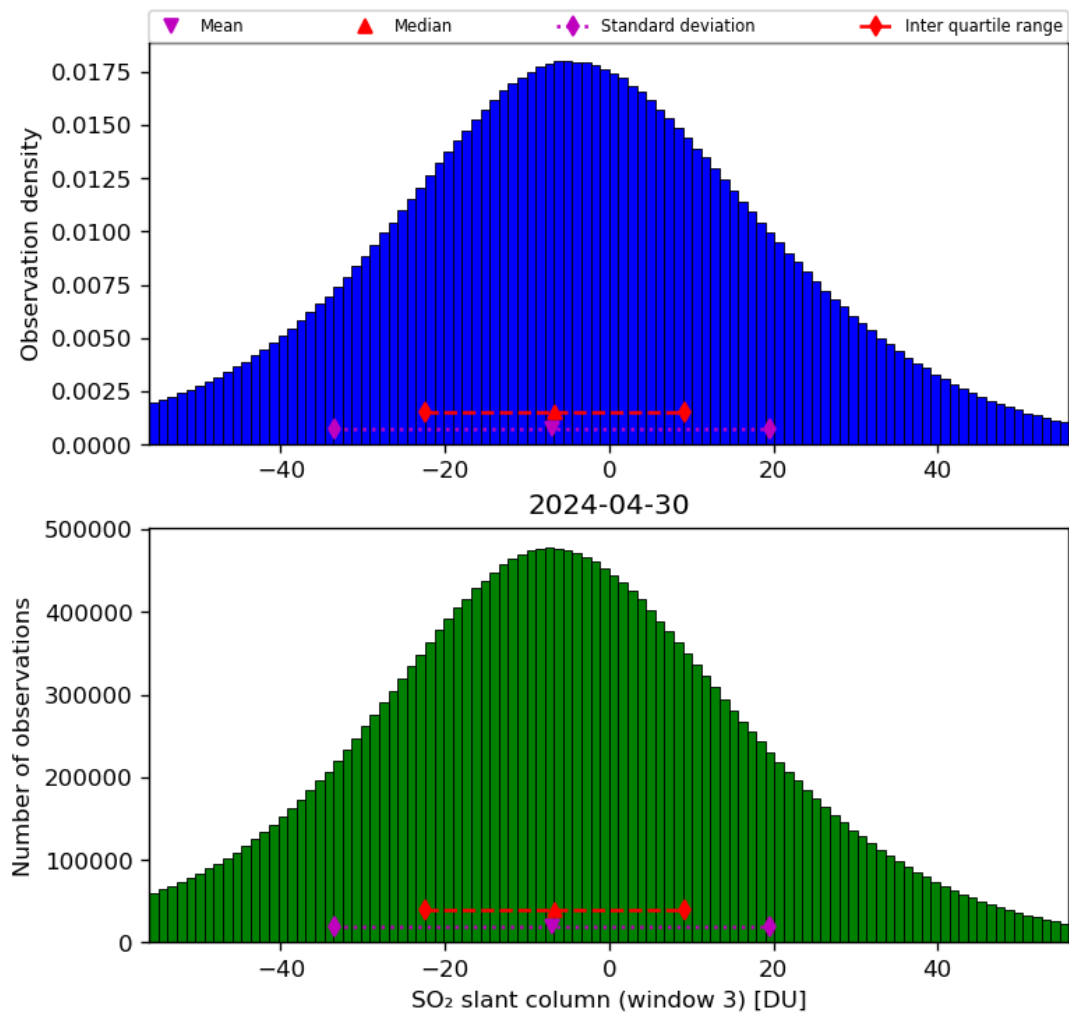
Figure 64: Histogram of “SO 2 slant column (window 3)” for 2024-04-29 to 2024-05-01
