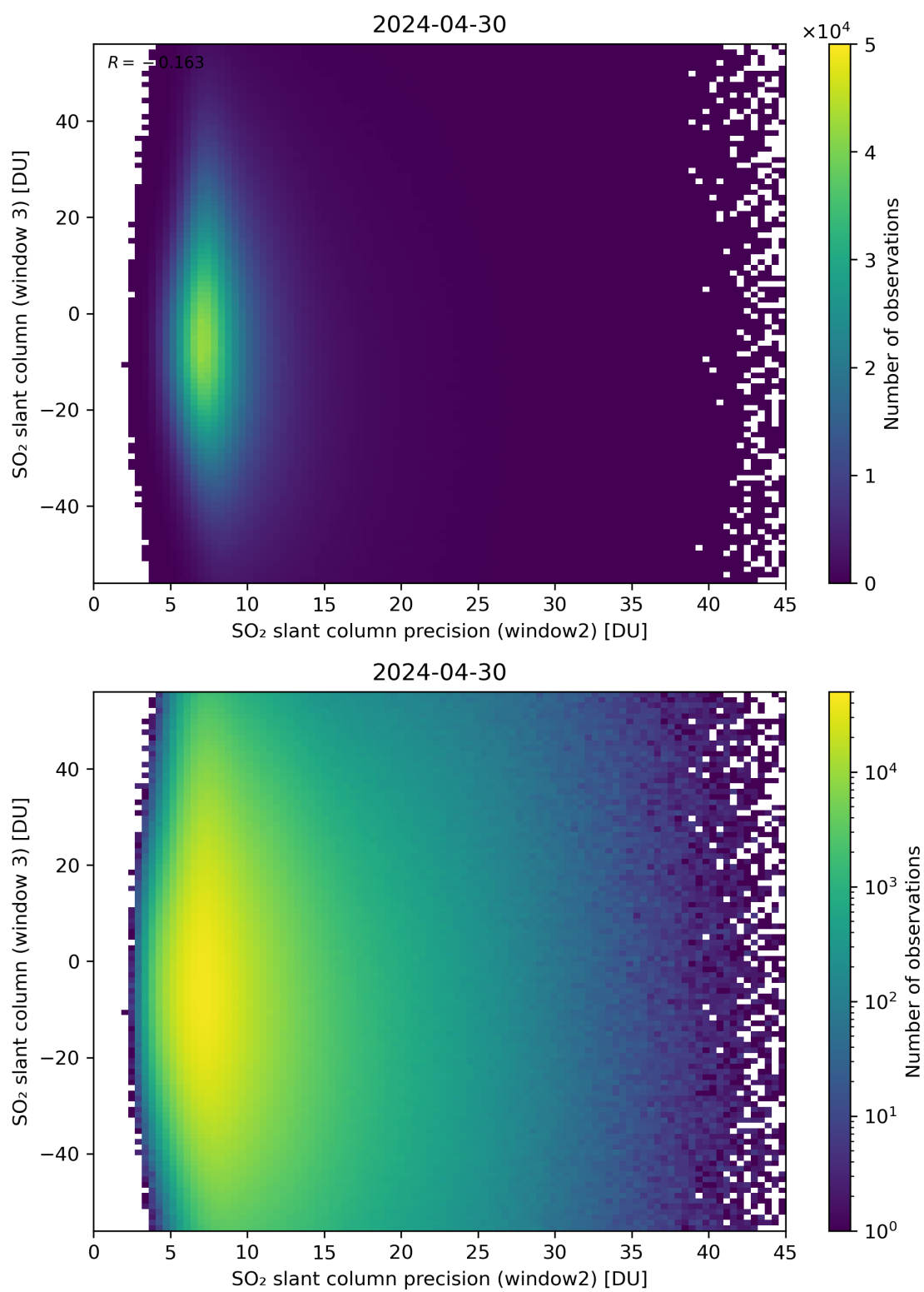
Figure 249: Scatter density plot of “SO 2 slant column precision (window2)” against “SO 2 slant column (window 3)” for 2024-04-29 to 2024-05-01.
