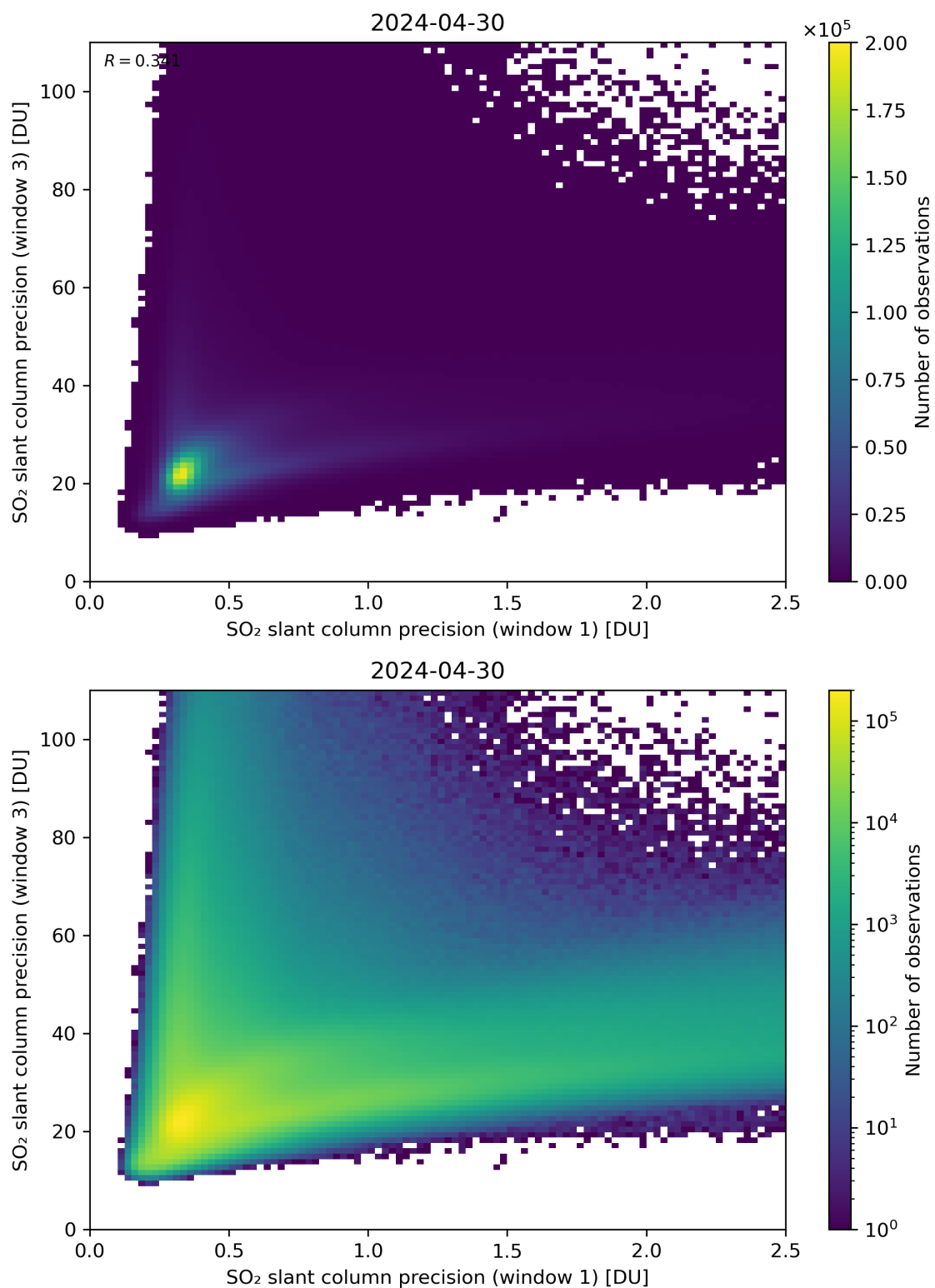
Figure 229: Scatter density plot of “SO 2 slant column precision (window 1)” against “SO 2 slant column precision (window 3)” for 2024-04-29 to 2024-05-01.
