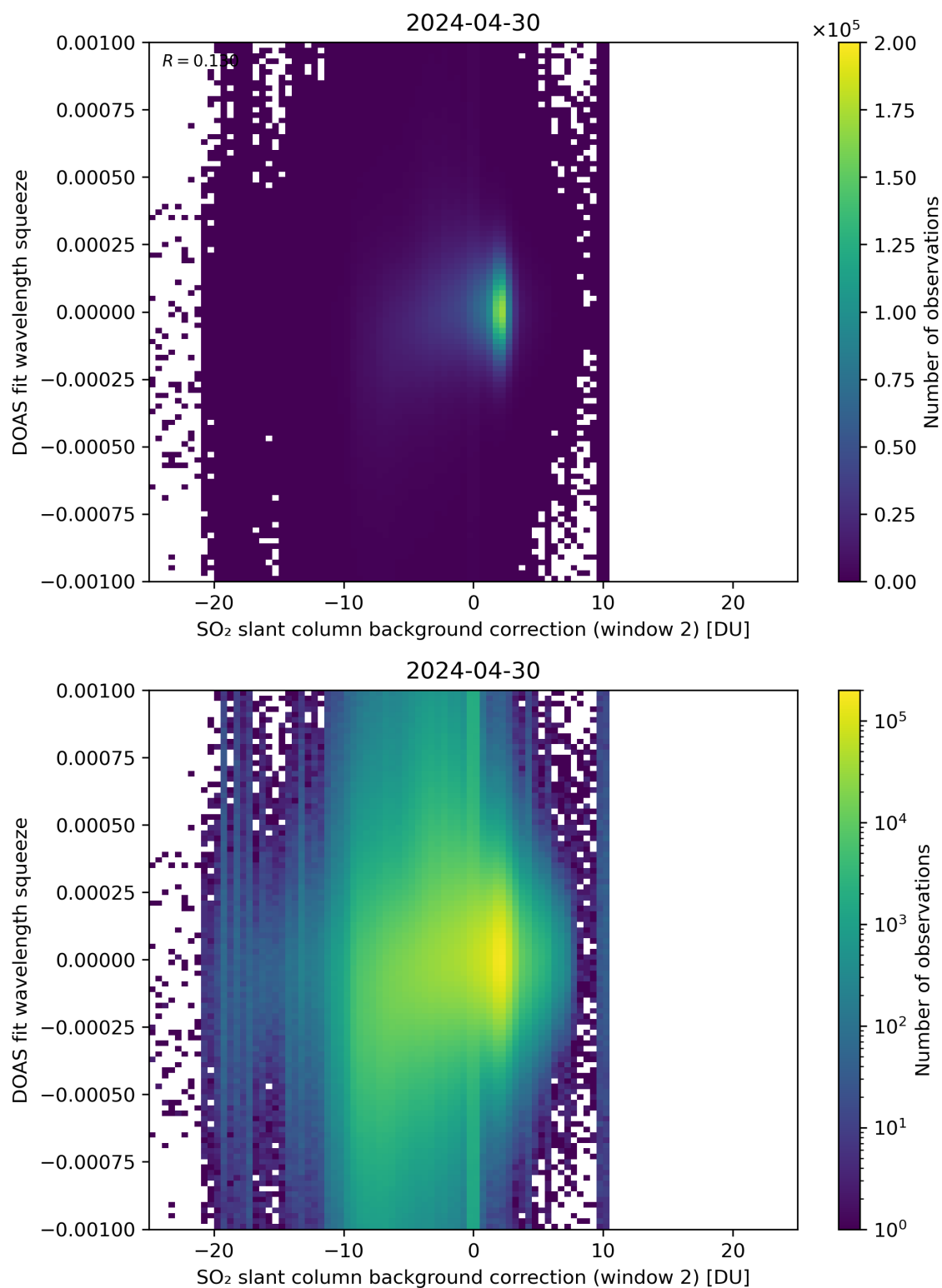
Figure 113: Scatter density plot of “SO 2 slant column background correction (window 2)” against “DOAS fit wavelength squeeze” for 2024-04-29 to 2024-05-01.
