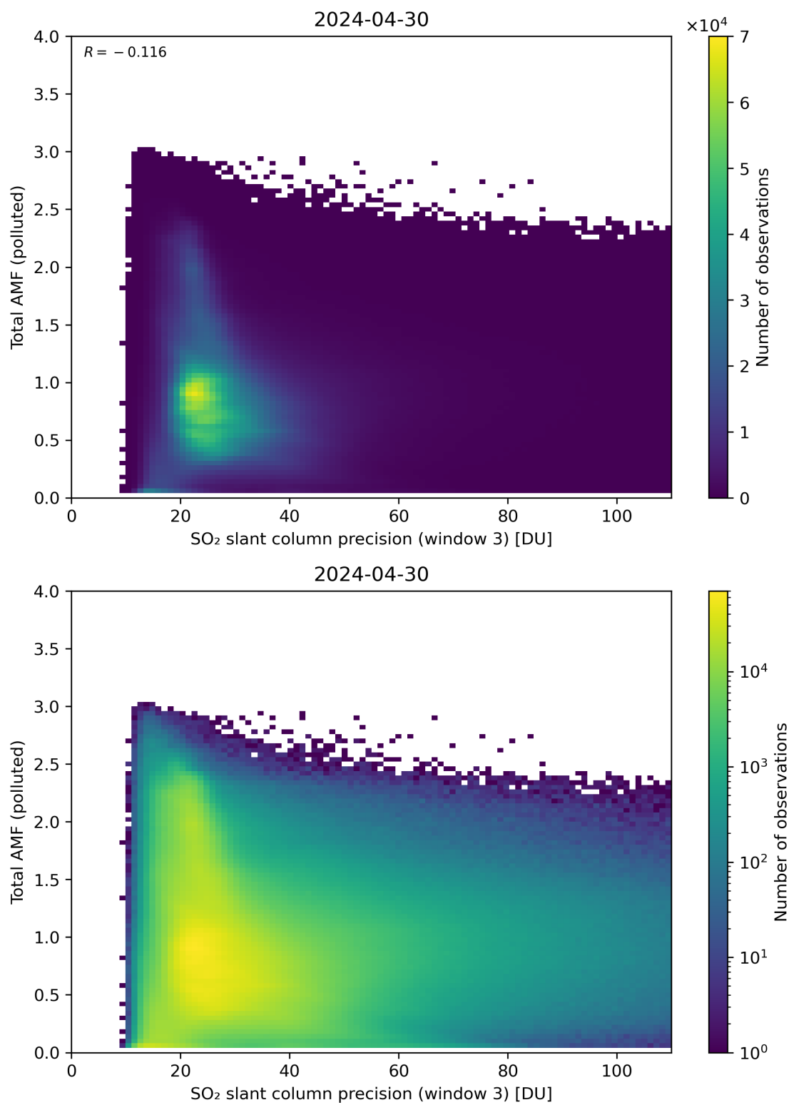
Figure 263: Scatter density plot of “SO 2 slant column precision (window 3)” against “Total AMF (polluted)” for 2024-04-29 to 2024-05-01.
