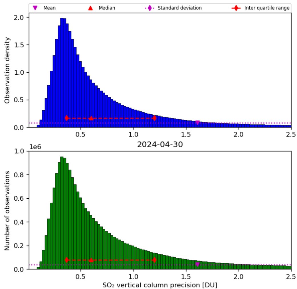
Figure 54: Histogram of “SO 2 vertical column precision” for 2024-04-29 to 2024-05-01
