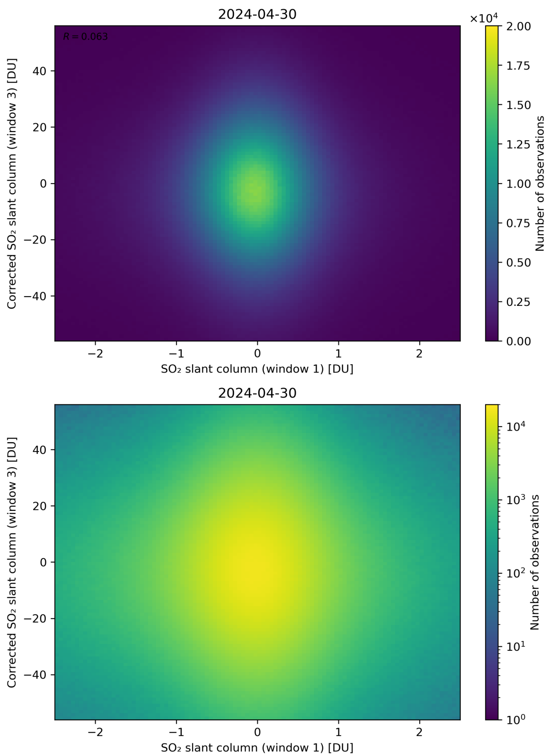
Figure 234: Scatter density plot of “SO 2 slant column (window 1)” against “Corrected SO 2 slant column (window 3)” for 2024-04-29 to 2024-05-01.
