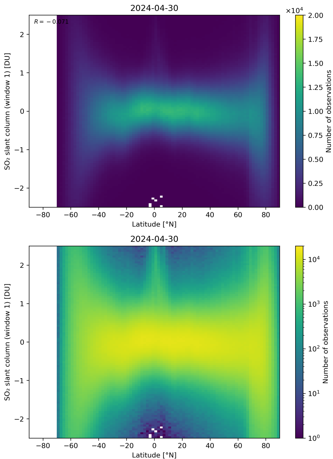
Figure 149: Scatter density plot of “Latitude” against “SO 2 slant column (window 1)” for 2024-04-29 to 2024-05-01.
