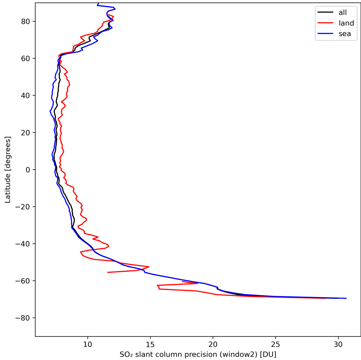
Figure 38: Zonal average of “SO 2 slant column precision (window2)” for 2024-04-29 to 2024-05-01.
