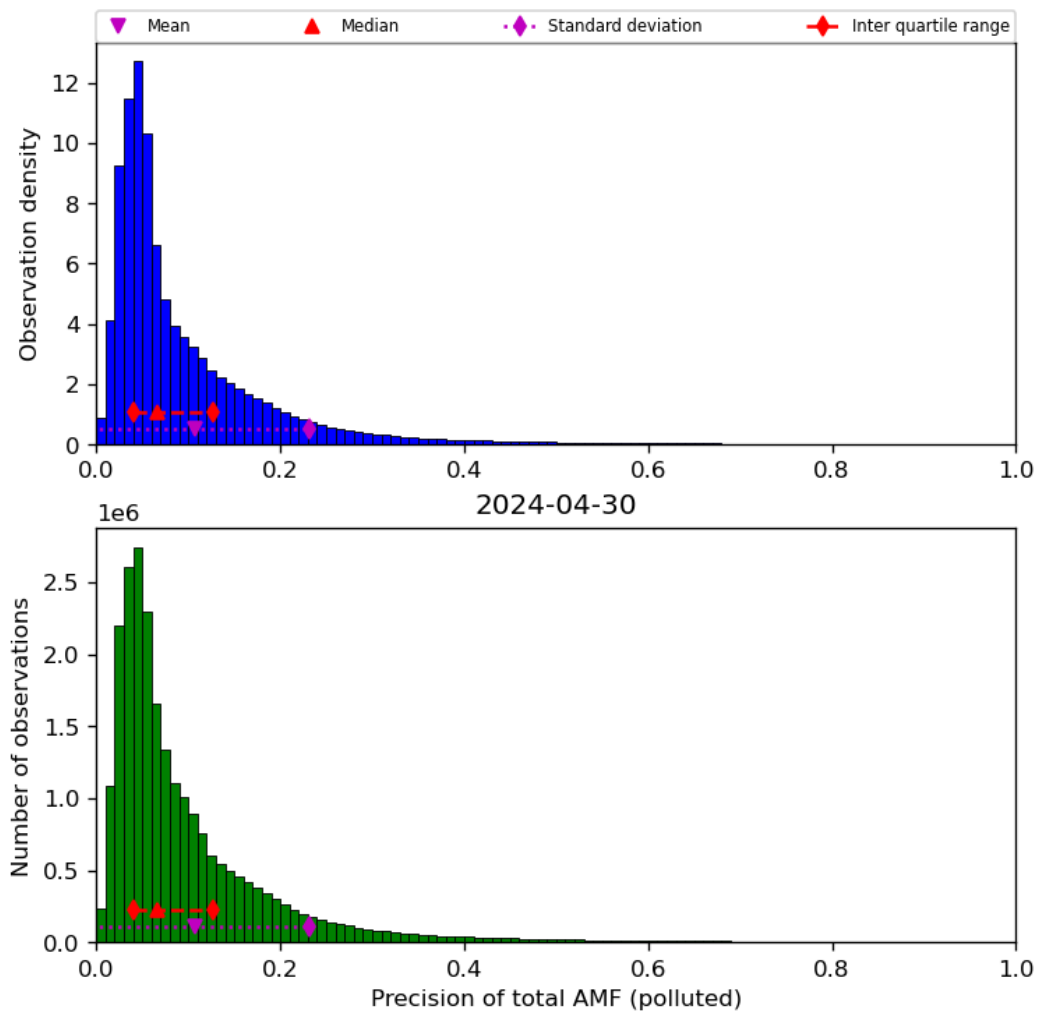
Figure 72: Histogram of “Precision of total AMF (polluted)” for 2024-04-29 to 2024-05-01
