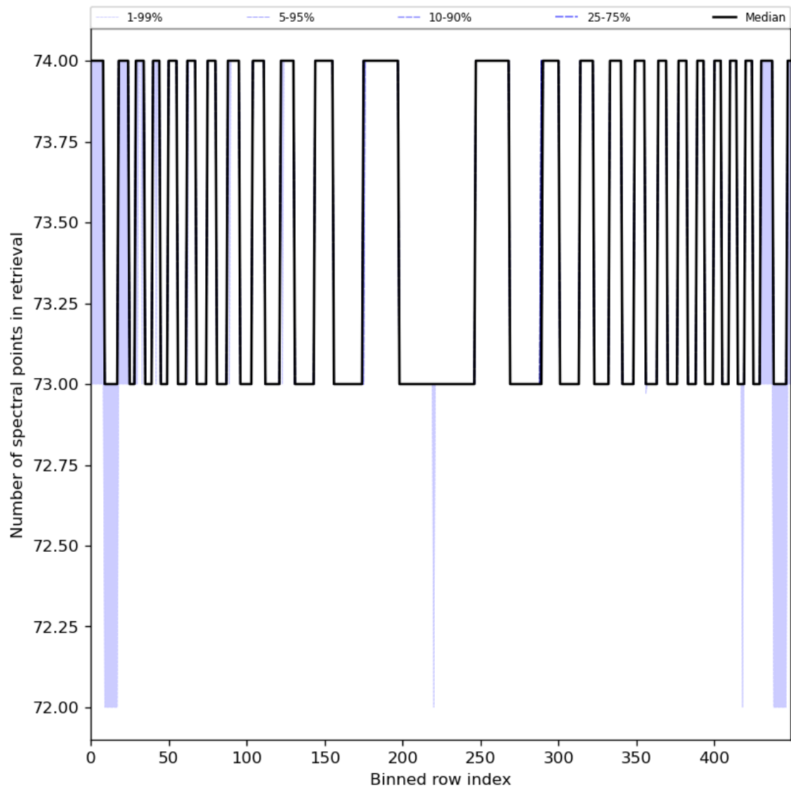
Figure 97: Along track statistics of “Number of spectral points in retrieval” for 2024-04-29 to 2024-05-01
