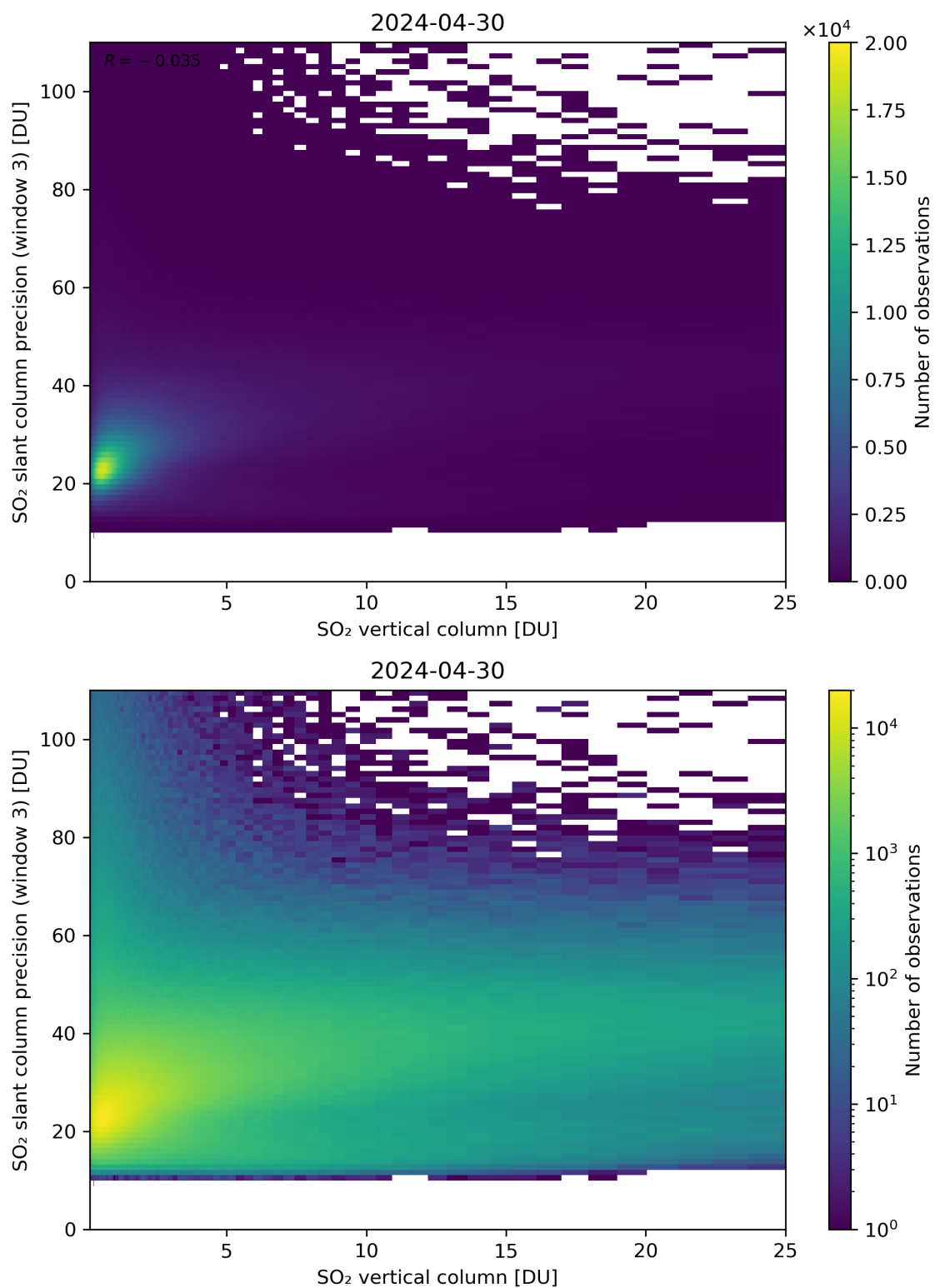
Figure 304: Scatter density plot of “SO 2 vertical column” against “SO 2 slant column precision (window 3)” for 2024-04-29 to 2024-05-01.
