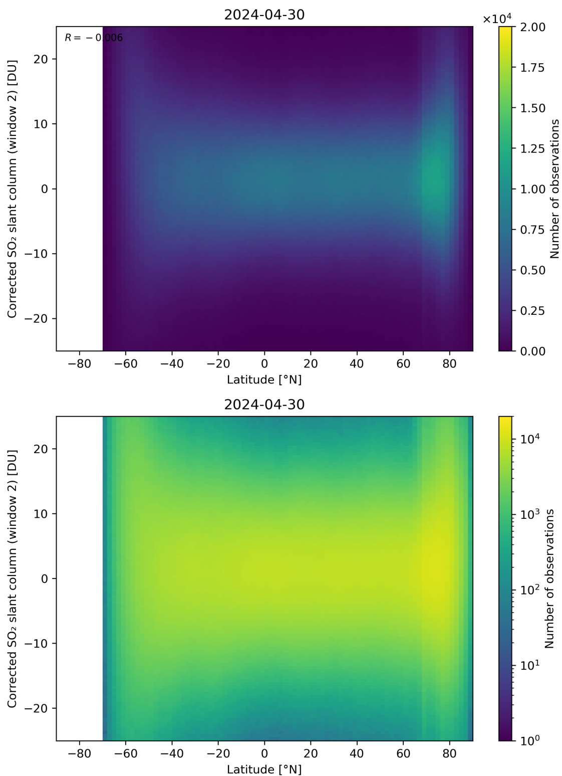
Figure 147: Scatter density plot of “Latitude” against “Corrected SO 2 slant column (window 2)” for 2024-04-29 to 2024-05-01.
