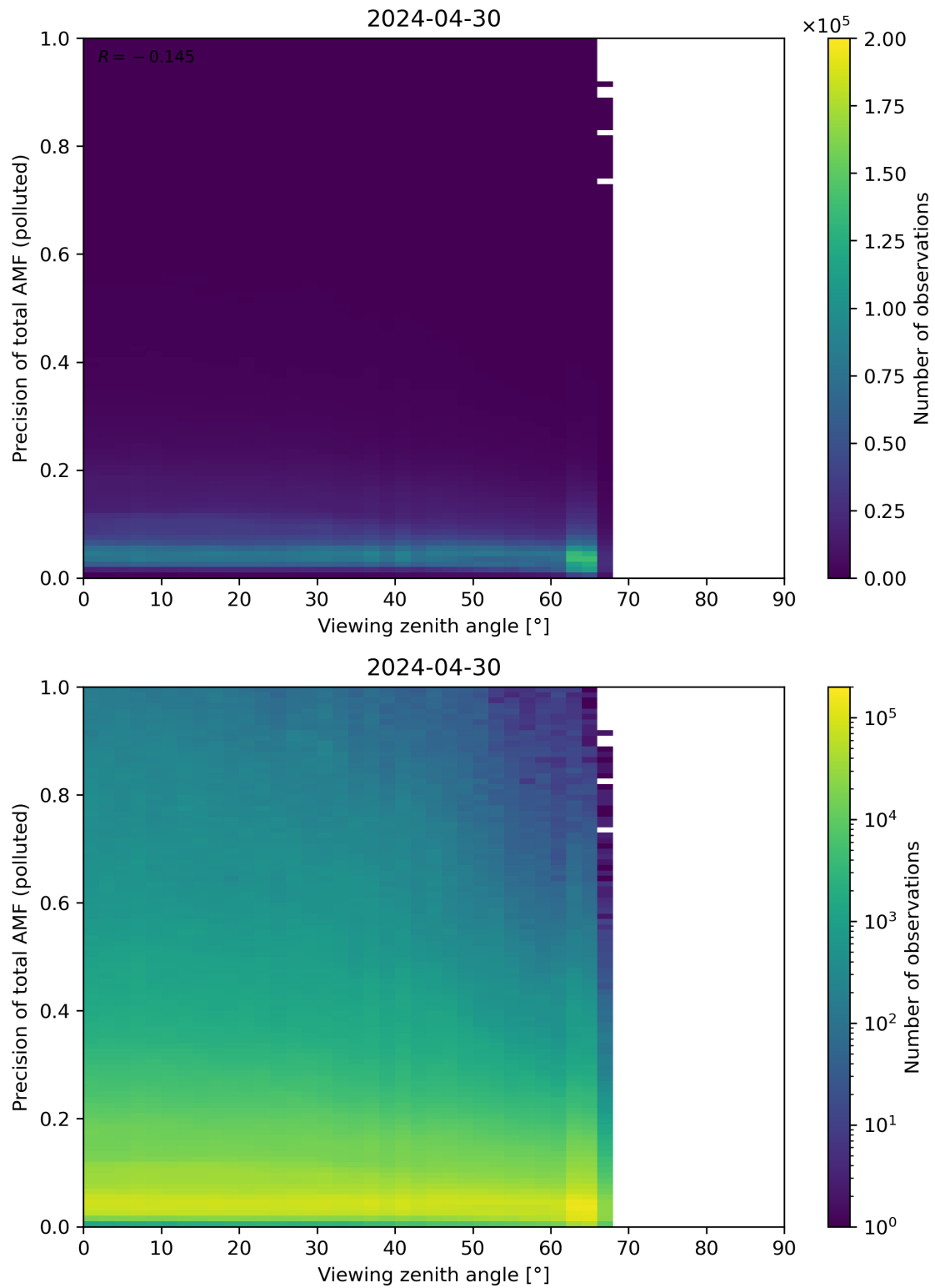
Figure 326: Scatter density plot of “Viewing zenith angle” against “Precision of total AMF (polluted)” for 2024-04-29 to 2024-05-01.
