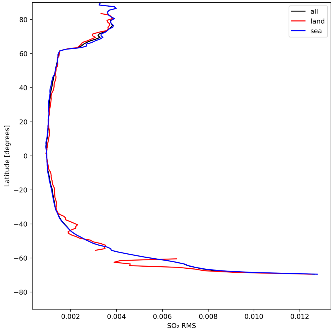
Figure 47: Zonal average of “SO 2 RMS” for 2024-04-29 to 2024-05-01.
