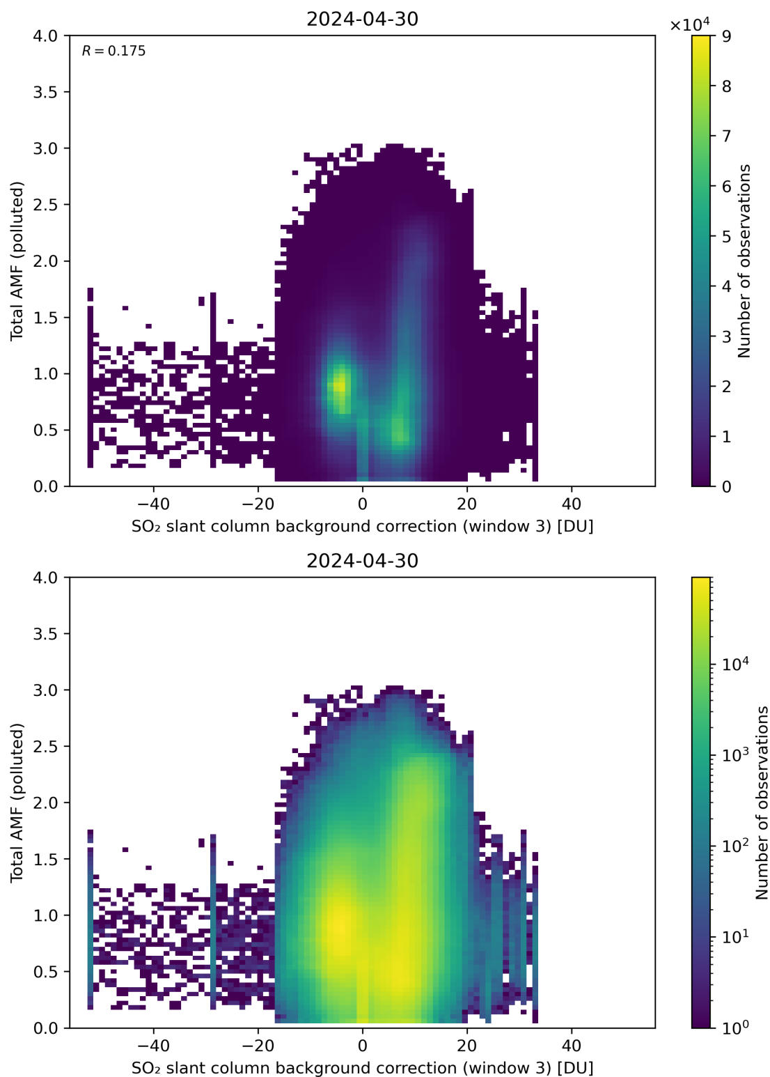
Figure 125: Scatter density plot of “SO 2 slant column background correction (window 3)” against “Total AMF (polluted)” for 2024-04-29 to 2024-05-01.
