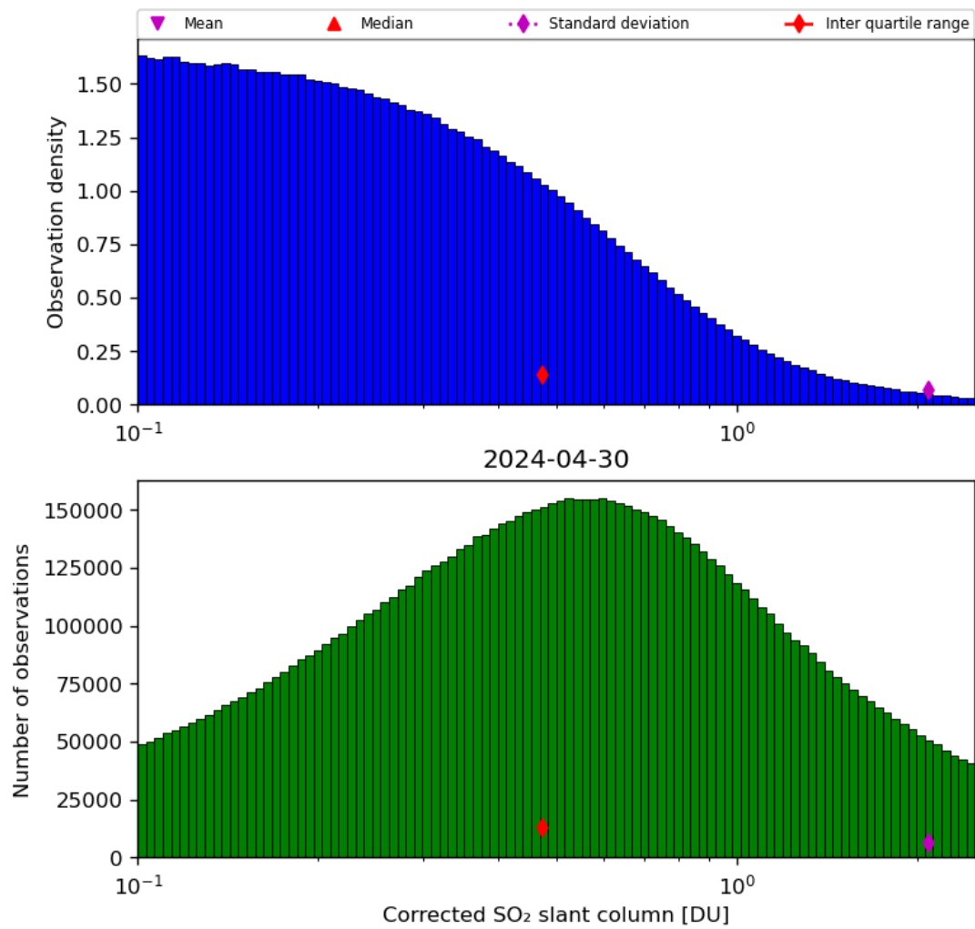
Figure 55: Histogram of “Corrected SO 2 slant column” for 2024-04-29 to 2024-05-01
