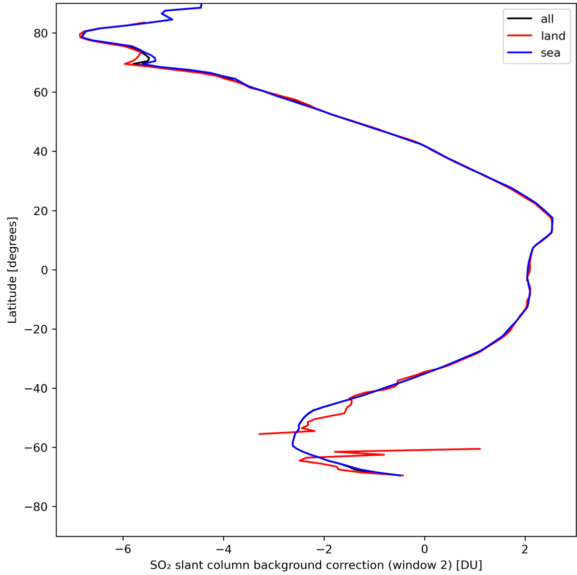
Figure 40: Zonal average of “SO 2 slant column background correction (window 2)” for 2024-04-29 to 2024-05-01.
