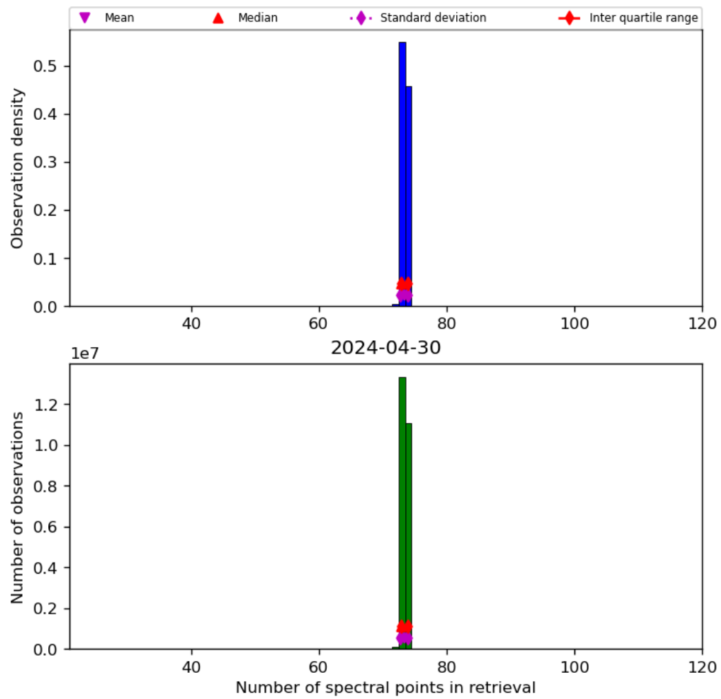
Figure 74: Histogram of “Number of spectral points in retrieval” for 2024-04-29 to 2024-05-01
