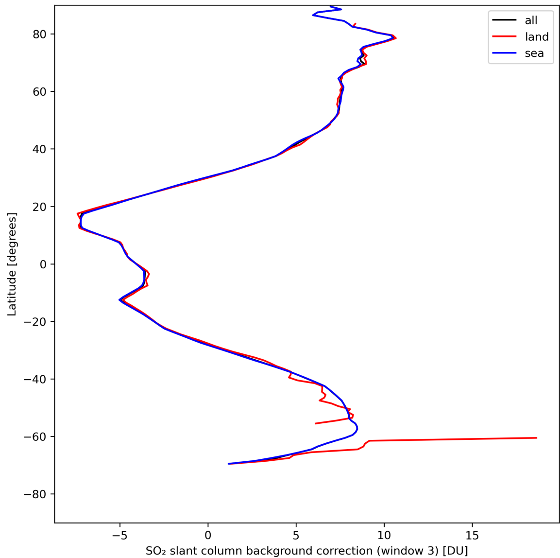
Figure 44: Zonal average of “SO 2 slant column background correction (window 3)” for 2024-04-29 to 2024-05-01.
