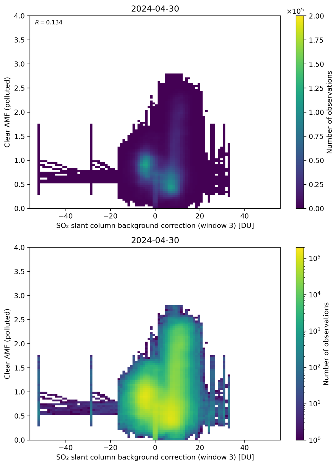
Figure 124: Scatter density plot of “SO 2 slant column background correction (window 3)” against “Clear AMF (polluted)” for 2024-04-29 to 2024-05-01.
