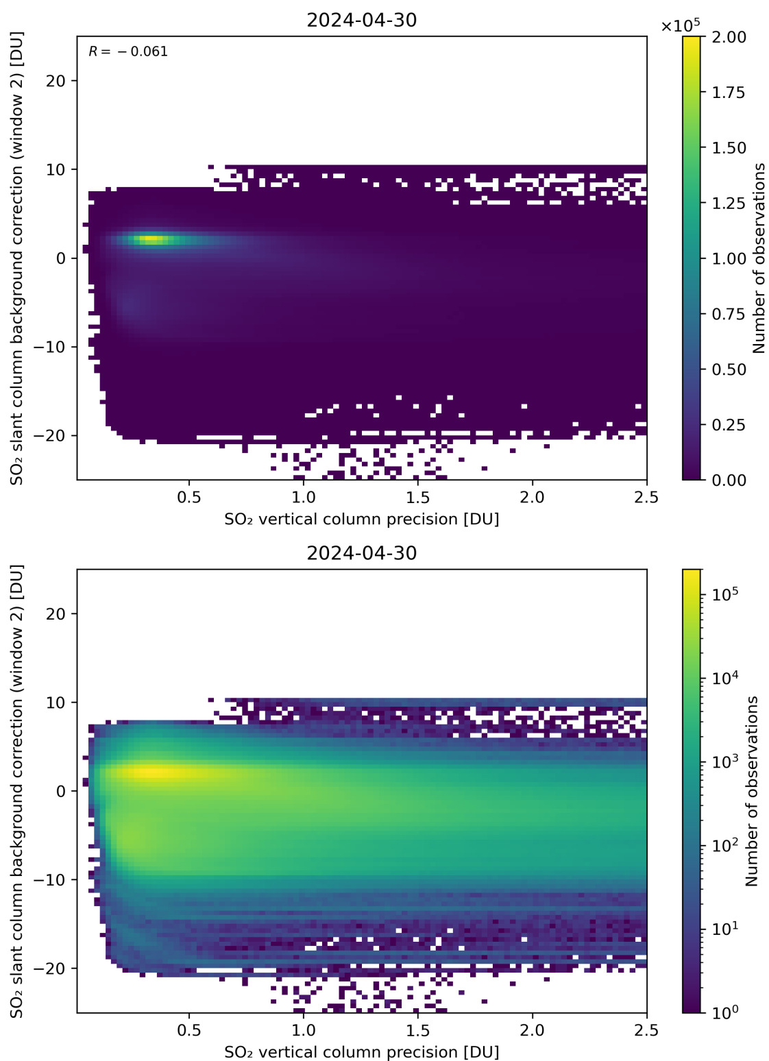
Figure 280: Scatter density plot of “SO 2 vertical column precision” against “SO 2 slant column background correction (window 2)” for 2024-04-29 to 2024-05-01.
