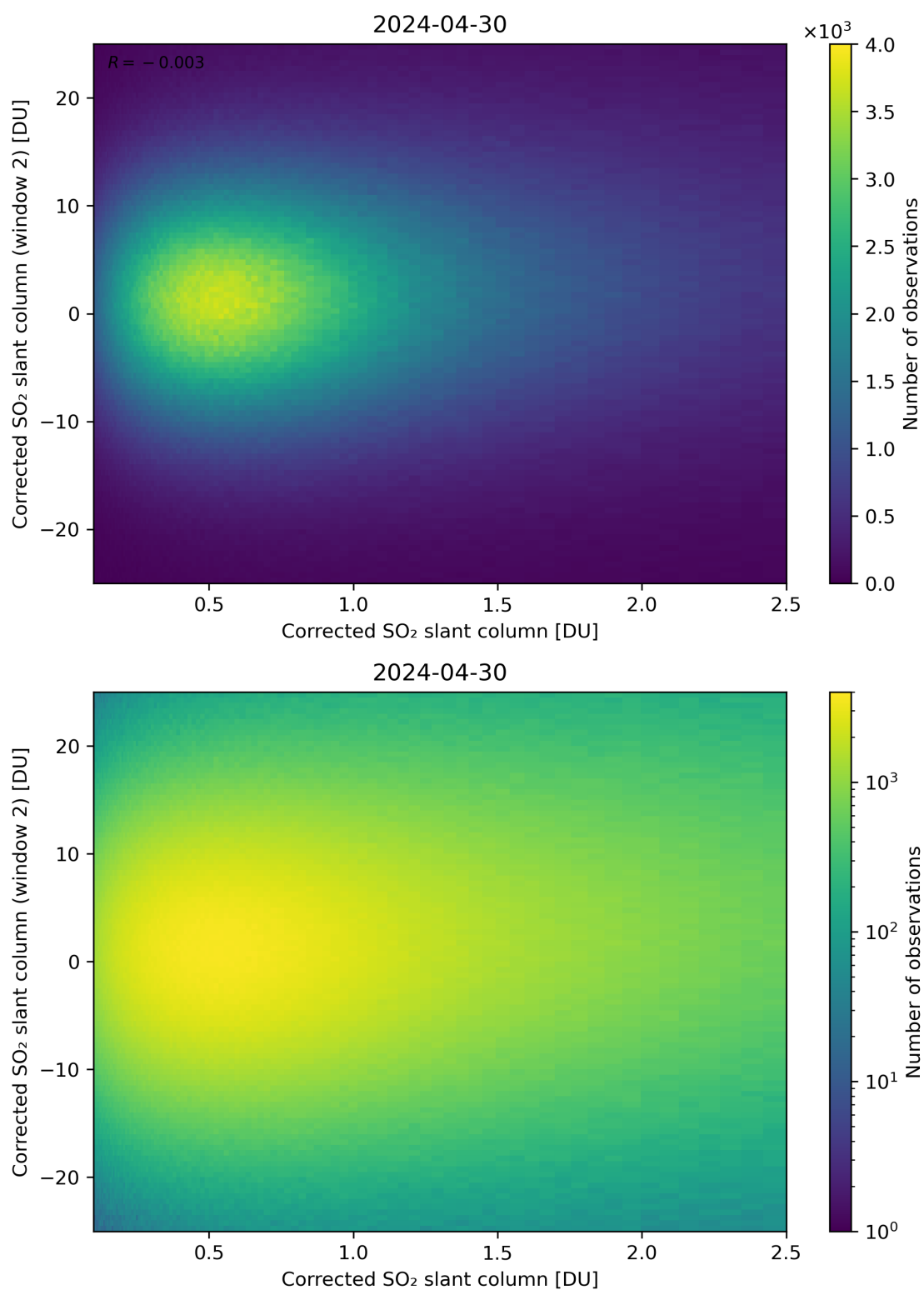
Figure 185: Scatter density plot of “Corrected SO 2 slant column” against “Corrected SO 2 slant column (window 2)” for 2024-04-29 to 2024-05-01.
