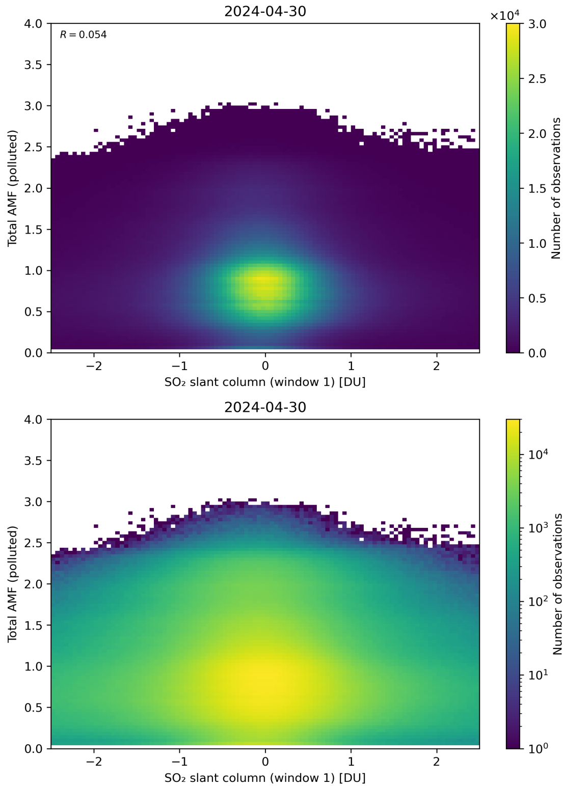
Figure 239: Scatter density plot of “SO 2 slant column (window 1)” against “Total AMF (polluted)” for 2024-04-29 to 2024-05-01.
