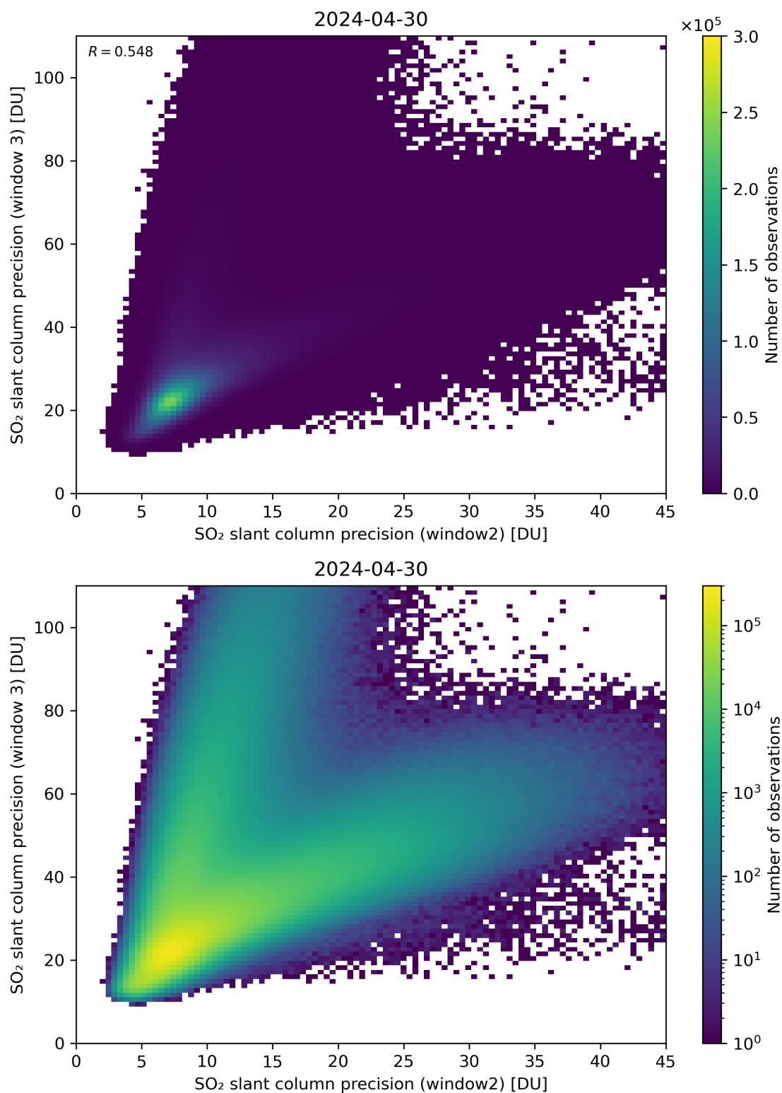
Figure 250: Scatter density plot of “SO 2 slant column precision (window2)” against “SO 2 slant column precision (window 3)” for 2024-04-29 to 2024-05-01.
