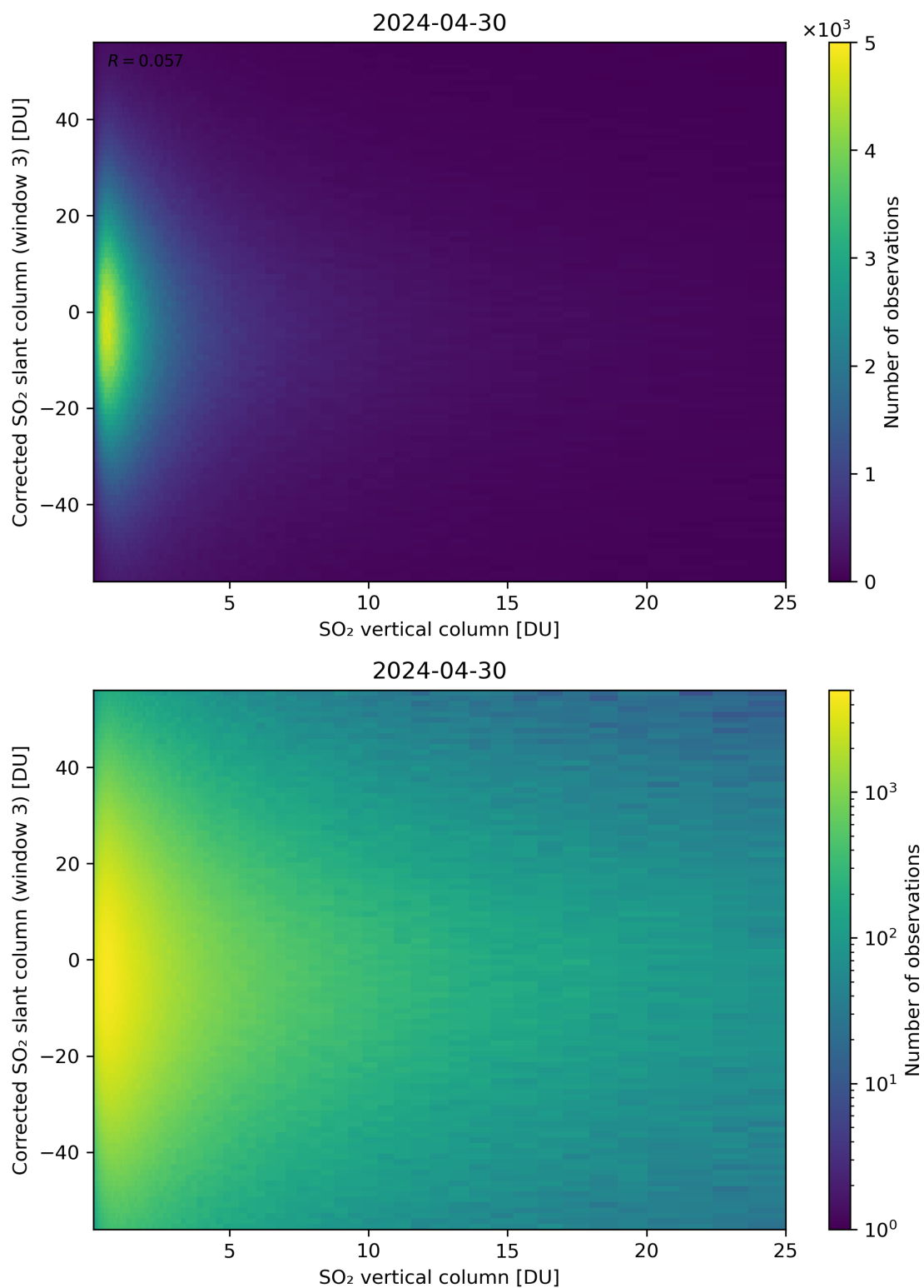
Figure 299: Scatter density plot of “SO 2 vertical column” against “Corrected SO 2 slant column (window 3)” for 2024-04-29 to 2024-05-01.
