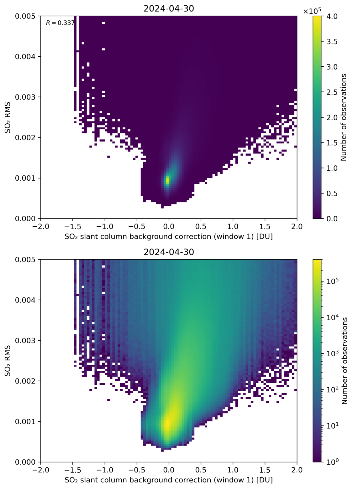
Figure 102: Scatter density plot of “SO 2 slant column background correction (window 1)” against “SO 2 RMS” for 2024-04-29 to 2024-05-01.
