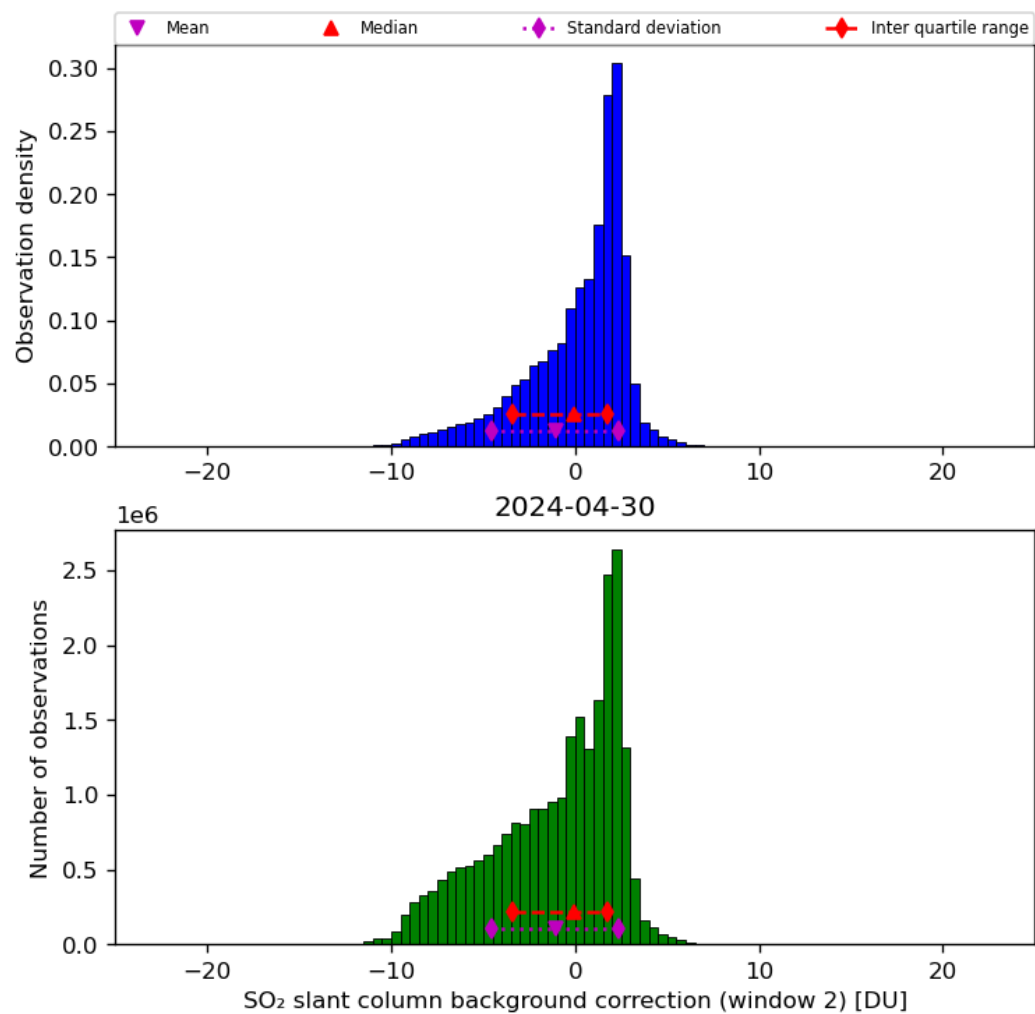
Figure 63: Histogram of “SO 2 slant column background correction (window 2)” for 2024-04-29 to 2024-05-01
