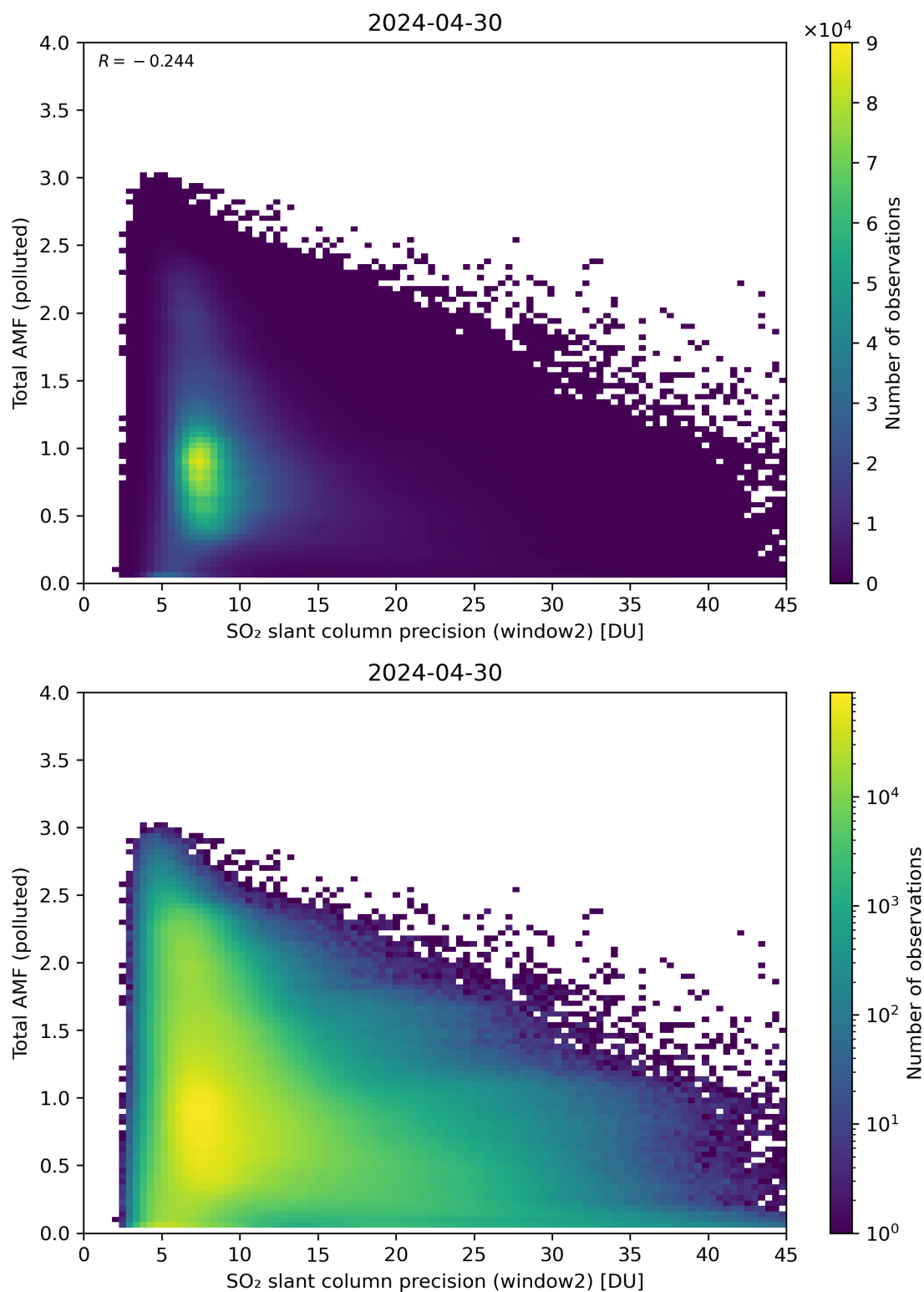
Figure 251: Scatter density plot of “SO 2 slant column precision (window2)” against “Total AMF (polluted)” for 2024-04-29 to 2024-05-01.
