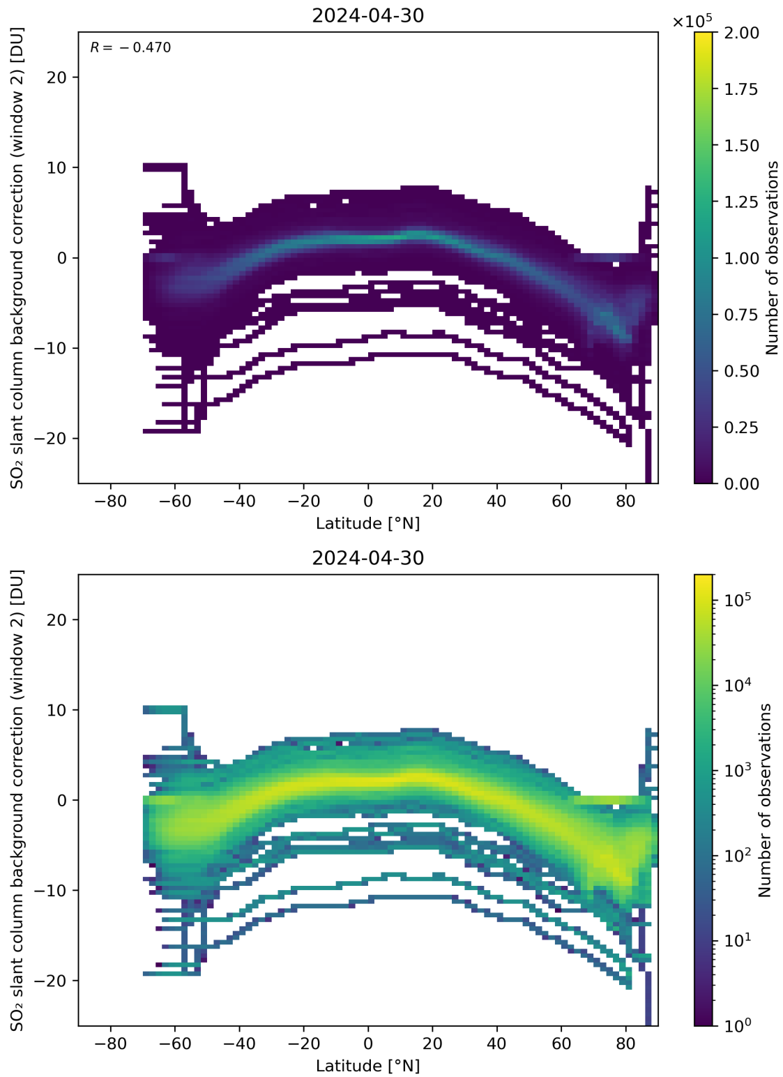
Figure 140: Scatter density plot of “Latitude” against “SO 2 slant column background correction (window 2)” for 2024-04-29 to 2024-05-01.
