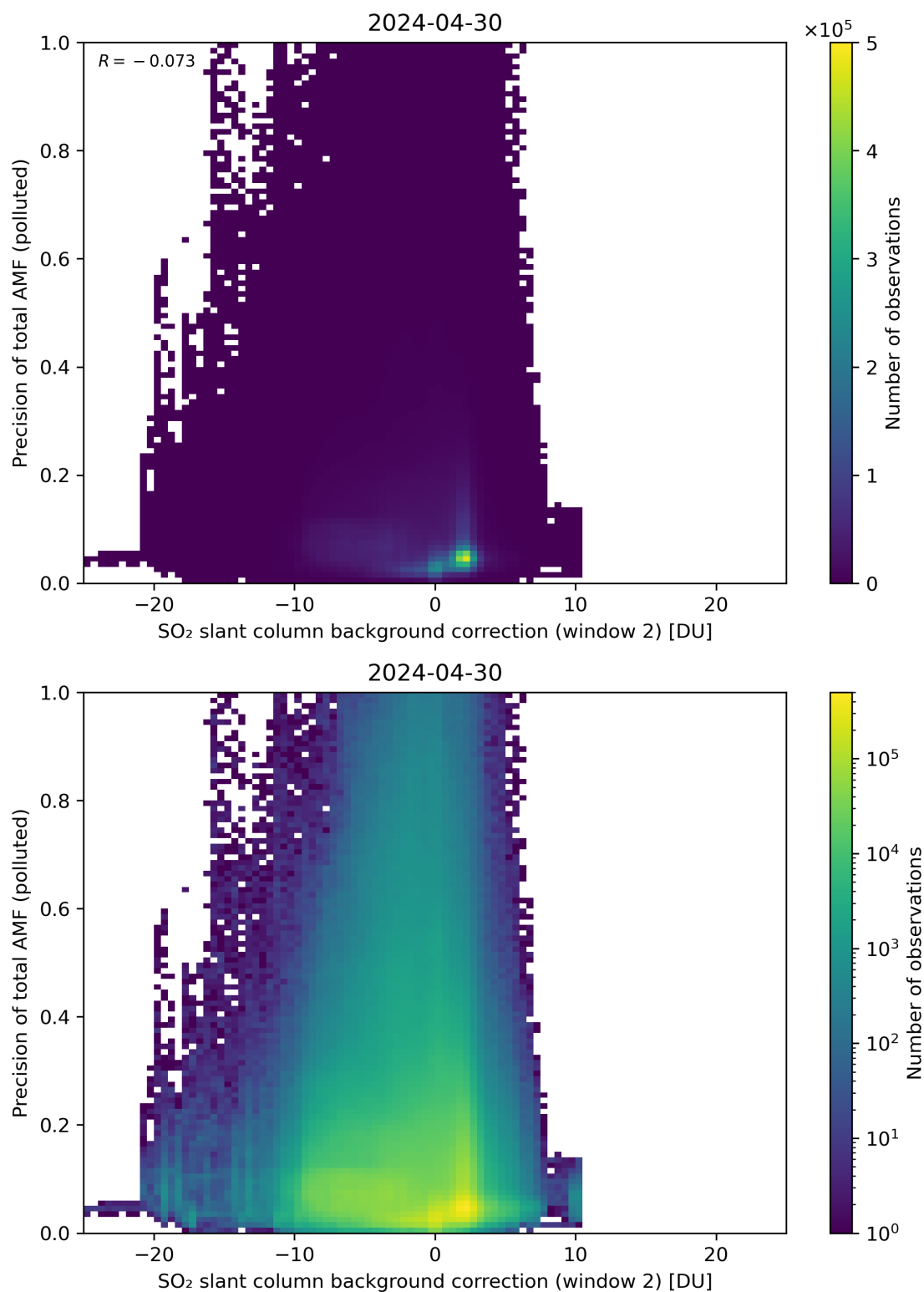
Figure 120: Scatter density plot of “SO 2 slant column background correction (window 2)” against “Precision of total AMF (polluted)” for 2024-04-29 to 2024-05-01.
