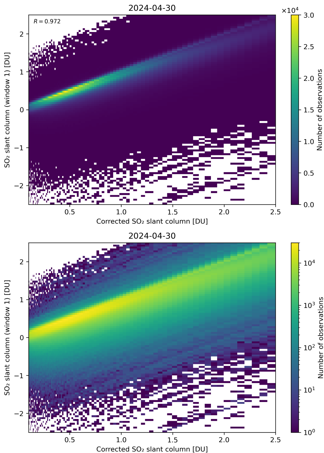
Figure 187: Scatter density plot of “Corrected SO 2 slant column” against “SO 2 slant column (window 1)” for 2024-04-29 to 2024-05-01.
