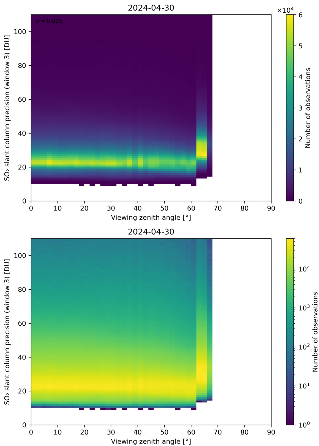
Figure 324: Scatter density plot of “Viewing zenith angle” against “SO 2 slant column precision (window 3)” for 2024-04-29 to 2024-05-01.
