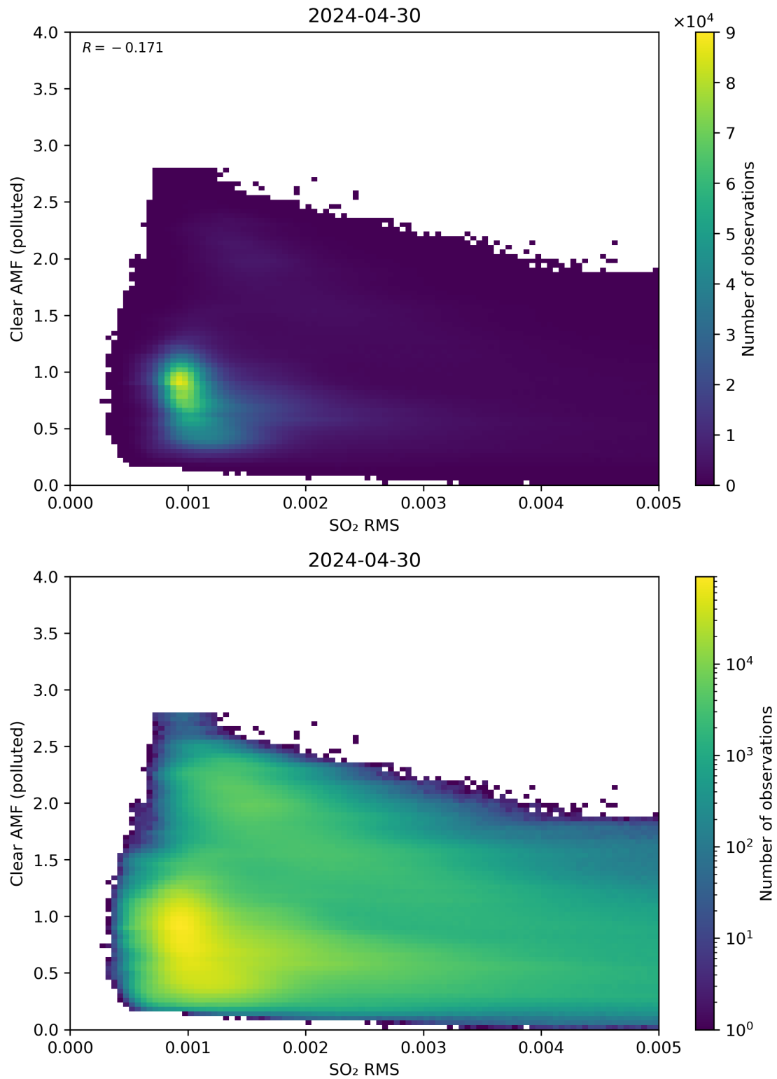
Figure 136: Scatter density plot of “SO 2 RMS” against “Clear AMF (polluted)” for 2024-04-29 to 2024-05-01.
