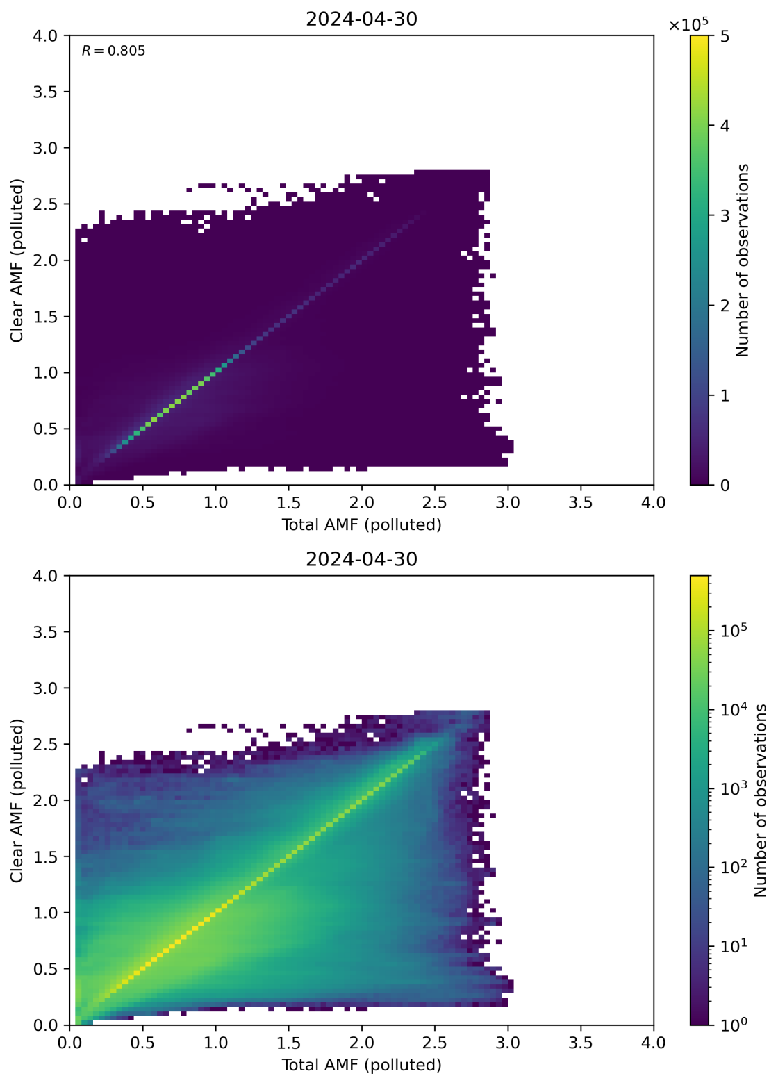
Figure 271: Scatter density plot of “Total AMF (polluted)” against “Clear AMF (polluted)” for 2024-04-29 to 2024-05-01.
