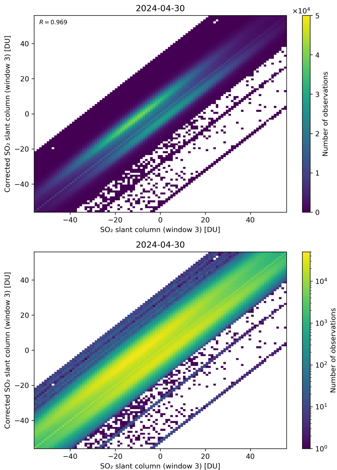
Figure 266: Scatter density plot of “SO 2 slant column (window 3)” against “Corrected SO 2 slant column (window 3)” for 2024-04-29 to 2024-05-01.
