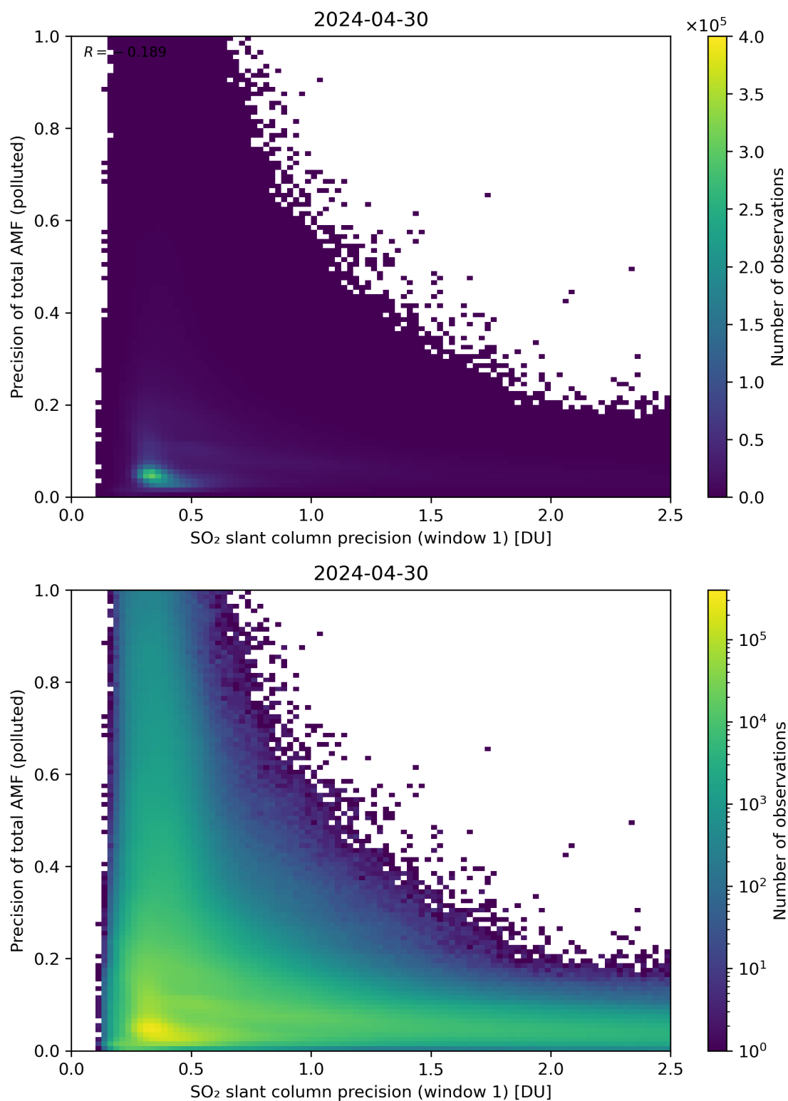
Figure 231: Scatter density plot of “SO 2 slant column precision (window 1)” against “Precision of total AMF (polluted)” for 2024-04-29 to 2024-05-01.
