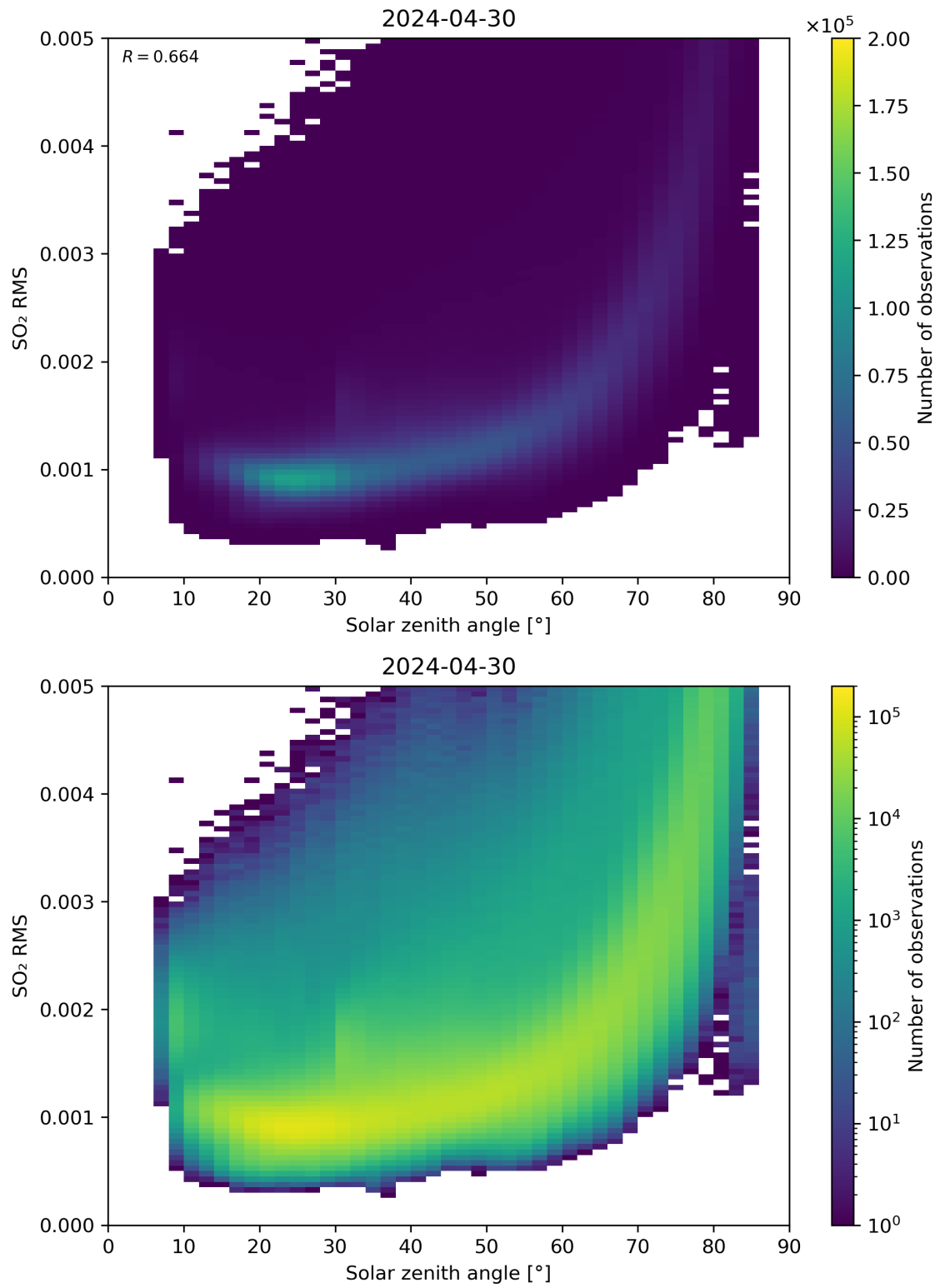
Figure 163: Scatter density plot of “Solar zenith angle” against “SO 2 RMS” for 2024-04-29 to 2024-05-01.
