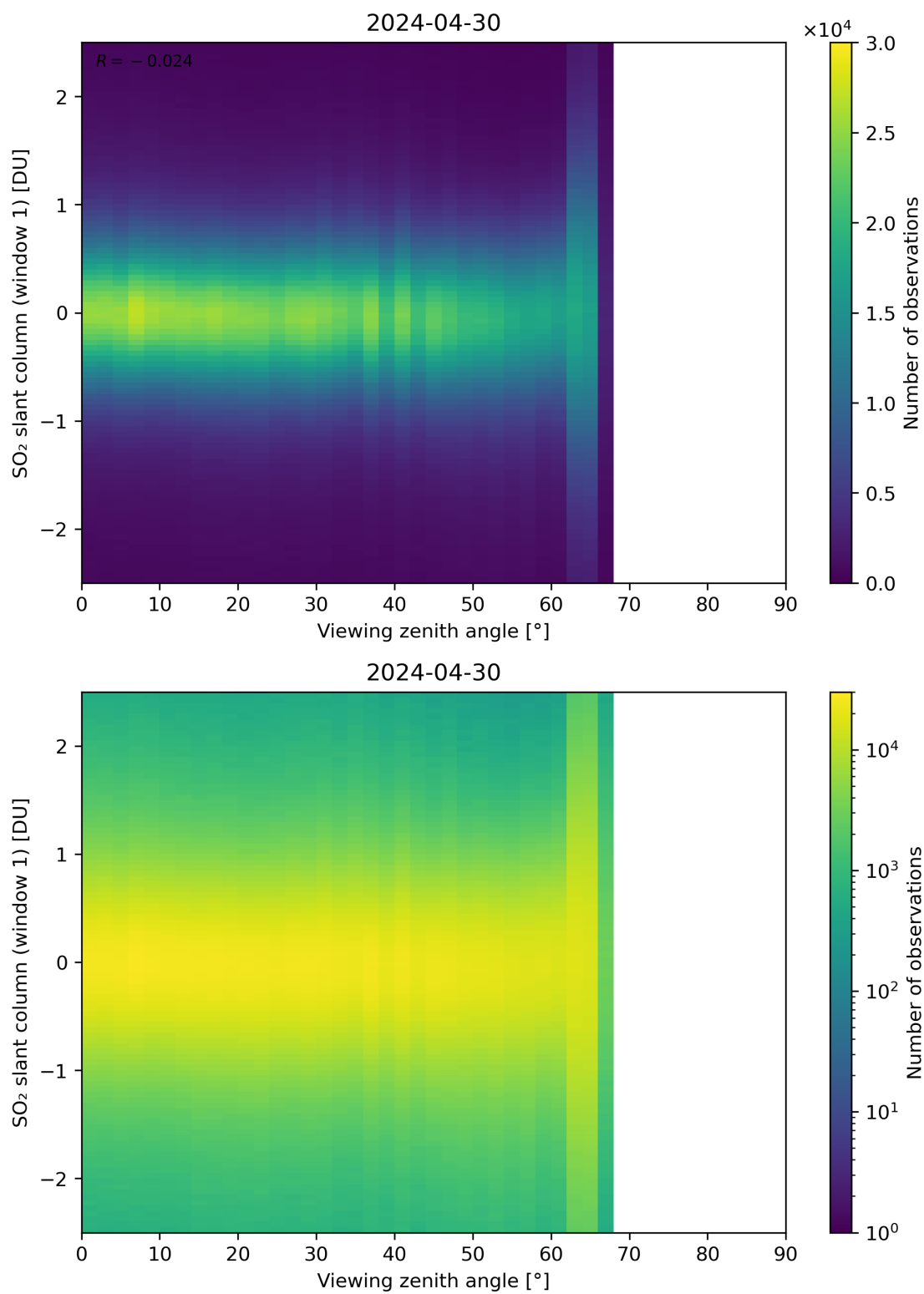
Figure 320: Scatter density plot of “Viewing zenith angle” against “SO 2 slant column (window 1)” for 2024-04-29 to 2024-05-01.
