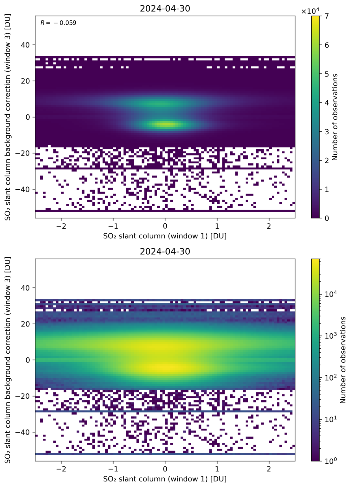
Figure 214: Scatter density plot of “SO 2 slant column (window 1)” against “SO 2 slant column background correction (window 3)” for 2024-04-29 to 2024-05-01.
