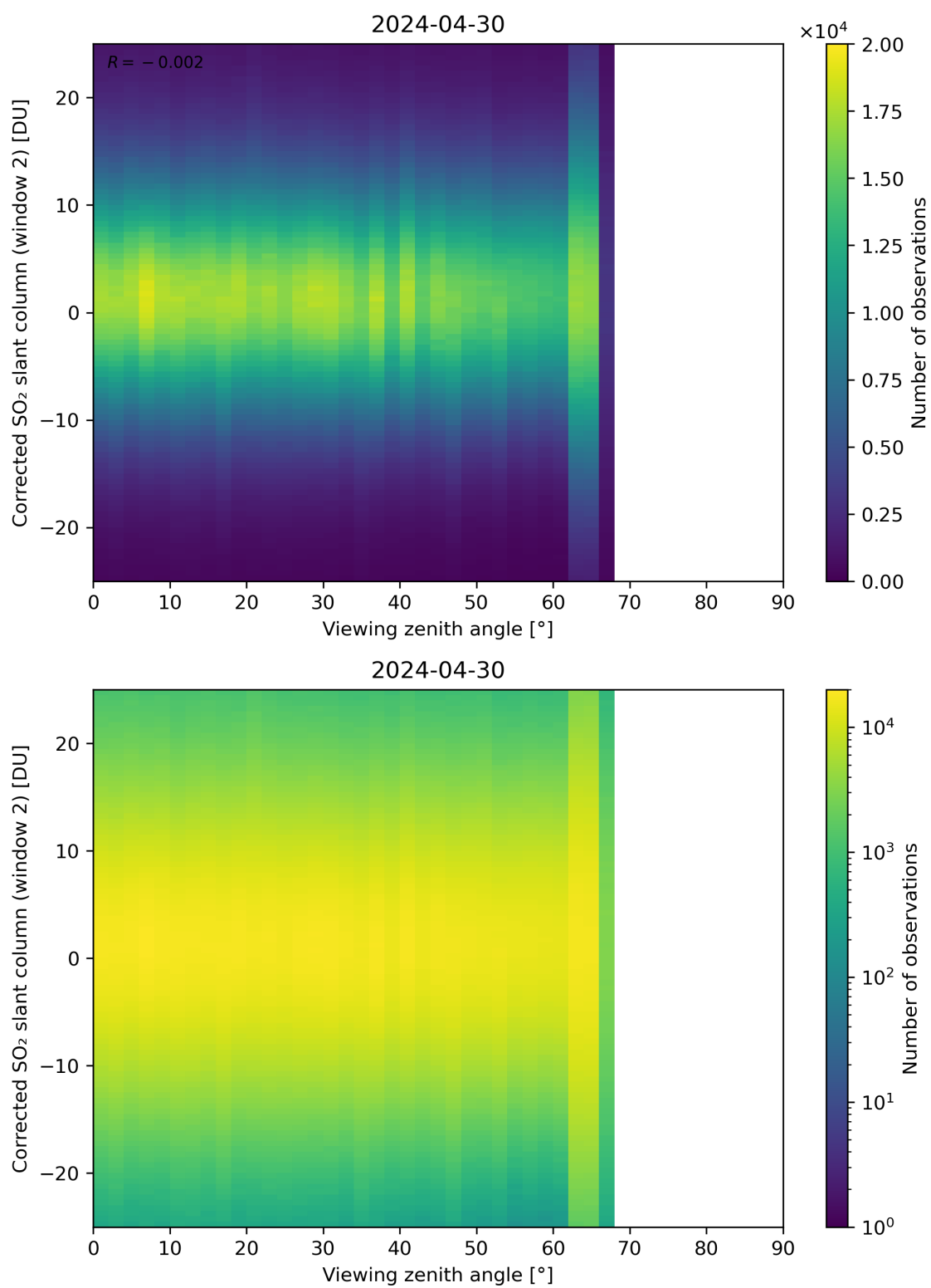
Figure 318: Scatter density plot of “Viewing zenith angle” against “Corrected SO 2 slant column (window 2)” for 2024-04-29 to 2024-05-01.
