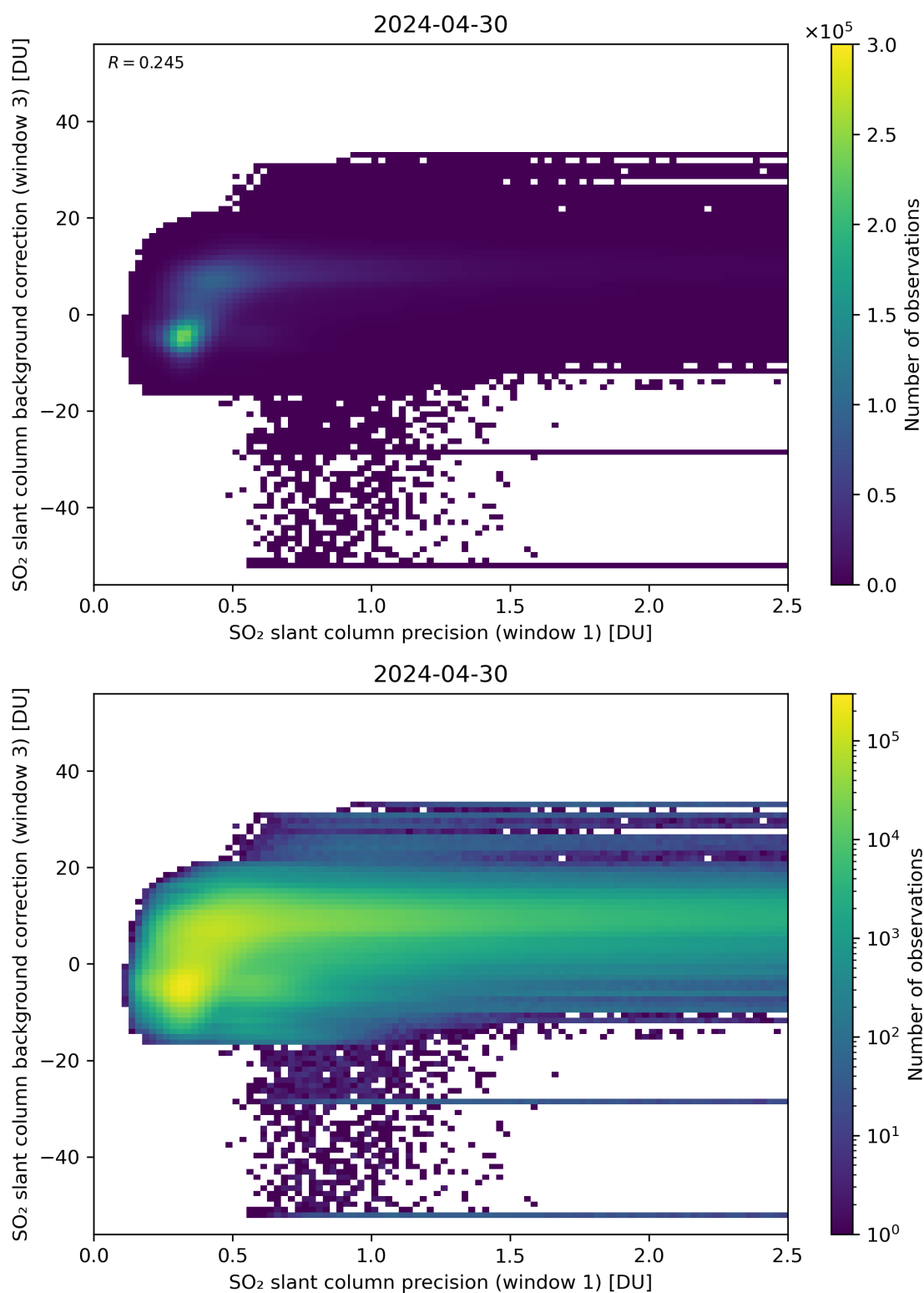
Figure 220: Scatter density plot of “SO 2 slant column precision (window 1)” against “SO 2 slant column background correction (window 3)” for 2024-04-29 to 2024-05-01.
