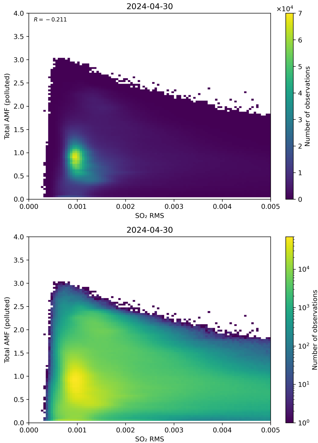
Figure 137: Scatter density plot of “SO 2 RMS” against “Total AMF (polluted)” for 2024-04-29 to 2024-05-01.
