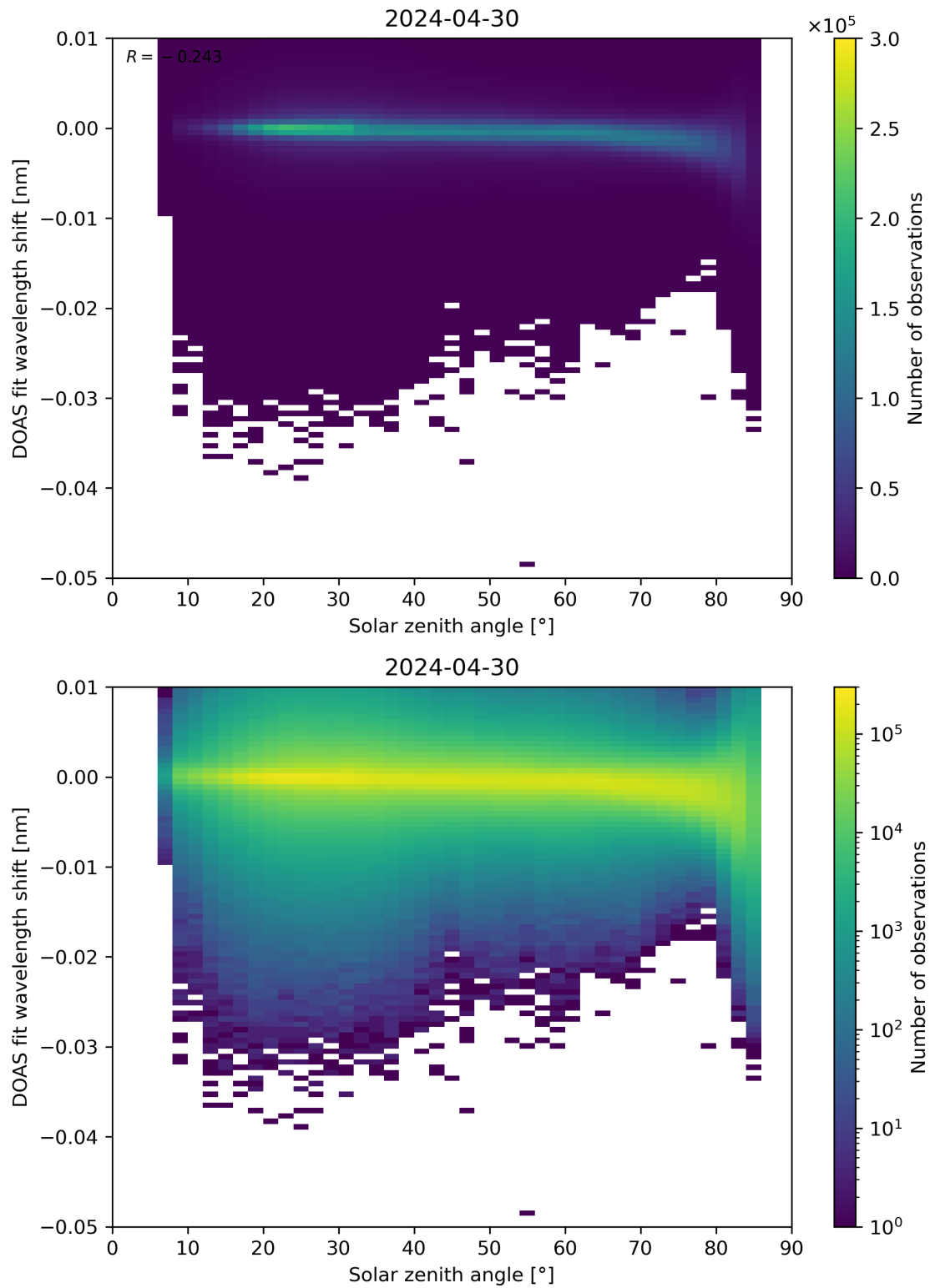
Figure 161: Scatter density plot of “Solar zenith angle” against “DOAS fit wavelength shift” for 2024-04-29 to 2024-05-01.
