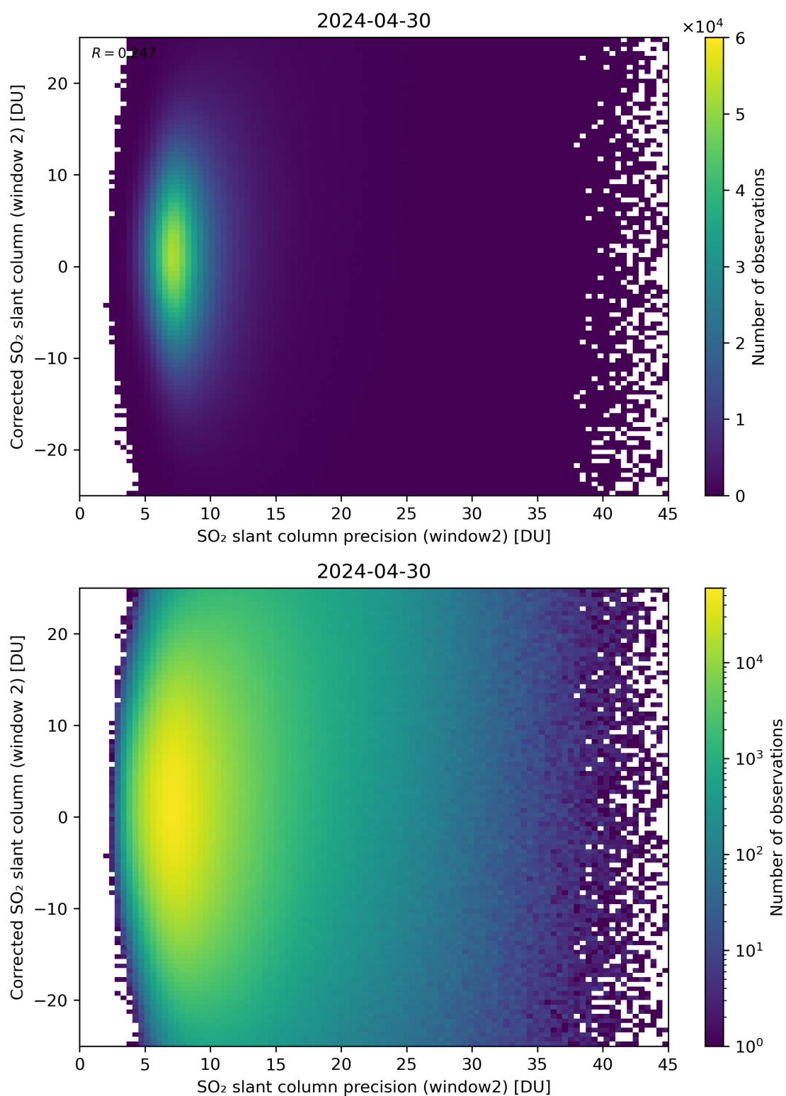
Figure 247: Scatter density plot of “SO 2 slant column precision (window2)” against “Corrected SO 2 slant column (window 2)” for 2024-04-29 to 2024-05-01.
