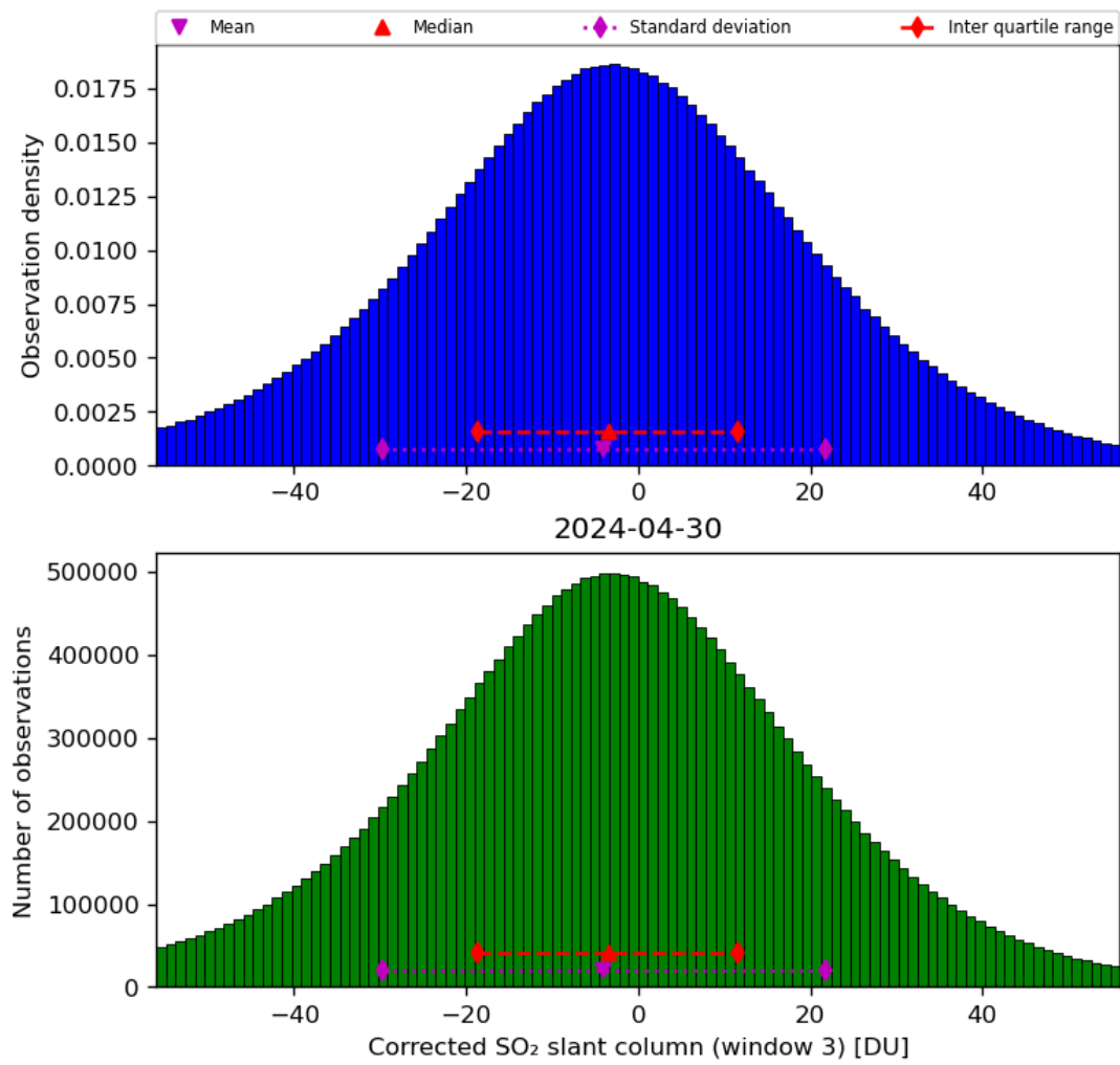
Figure 66: Histogram of “Corrected SO 2 slant column (window 3)” for 2024-04-29 to 2024-05-01
