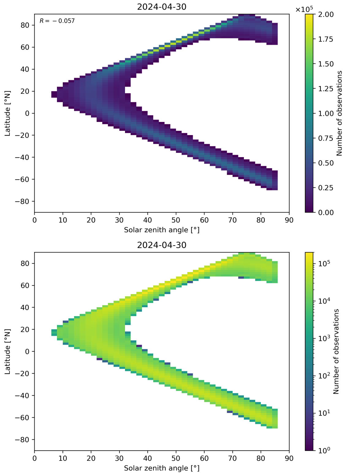
Figure 164: Scatter density plot of “Solar zenith angle” against “Latitude” for 2024-04-29 to 2024-05-01.
