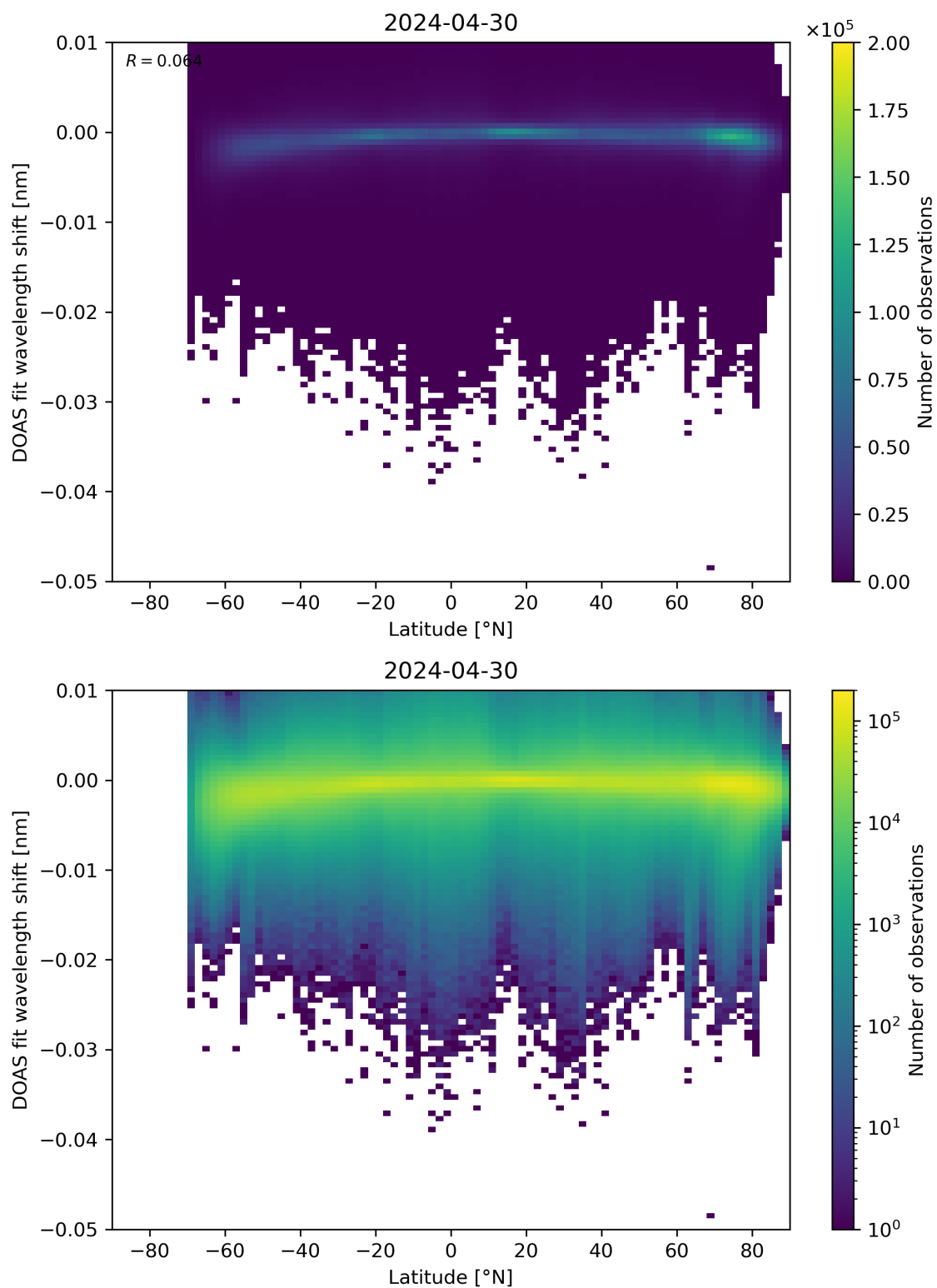
Figure 142: Scatter density plot of “Latitude” against “DOAS fit wavelength shift” for 2024-04-29 to 2024-05-01.
