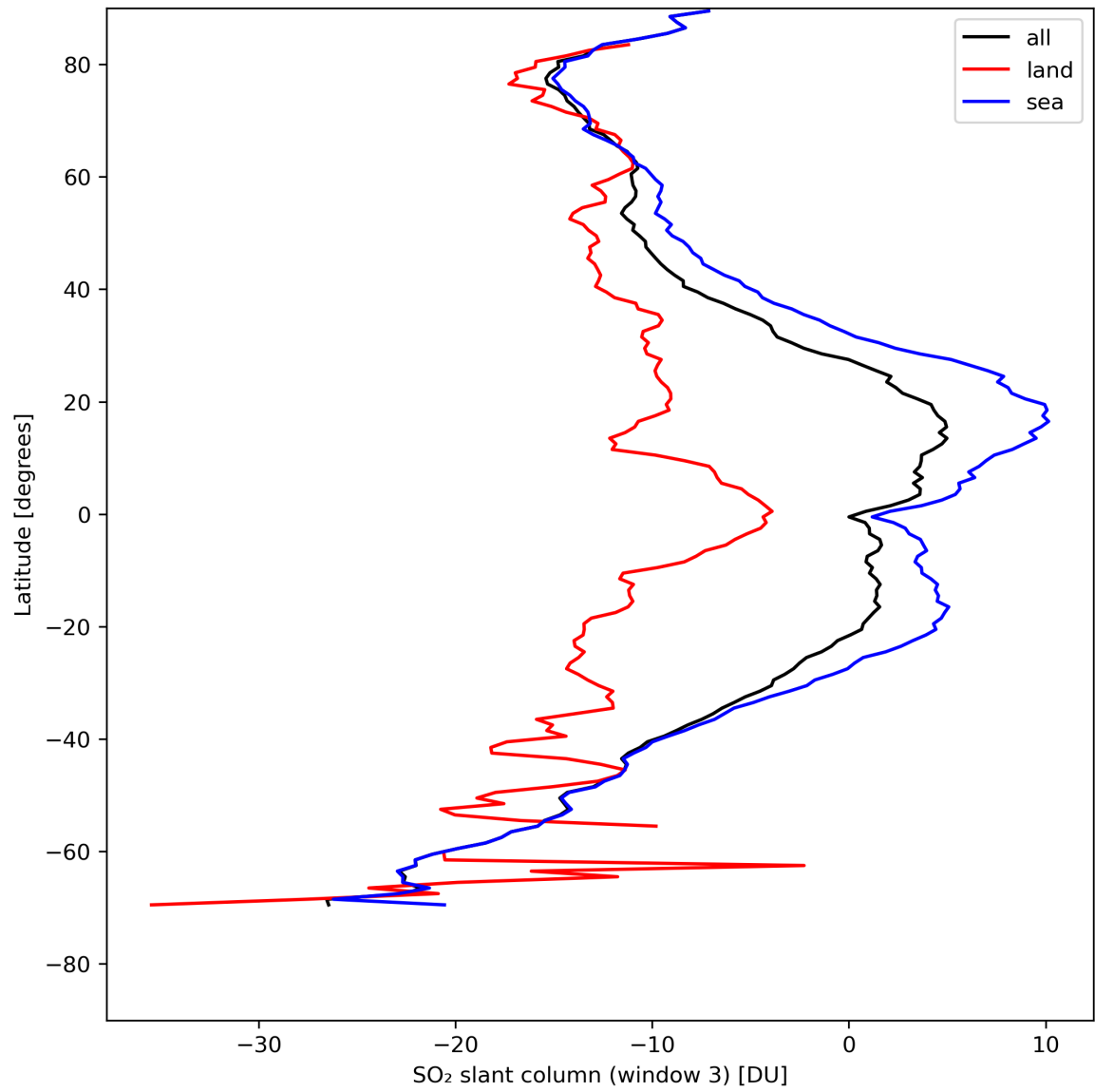
Figure 41: Zonal average of “SO 2 slant column (window 3)” for 2024-04-29 to 2024-05-01.
