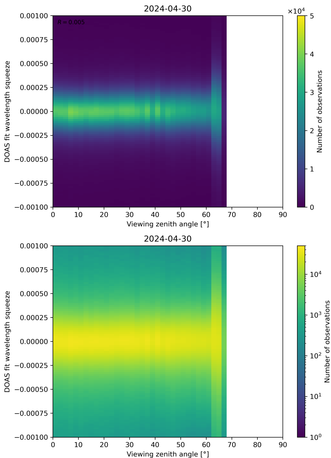
Figure 312: Scatter density plot of “Viewing zenith angle” against “DOAS fit wavelength squeeze” for 2024-04-29 to 2024-05-01.
