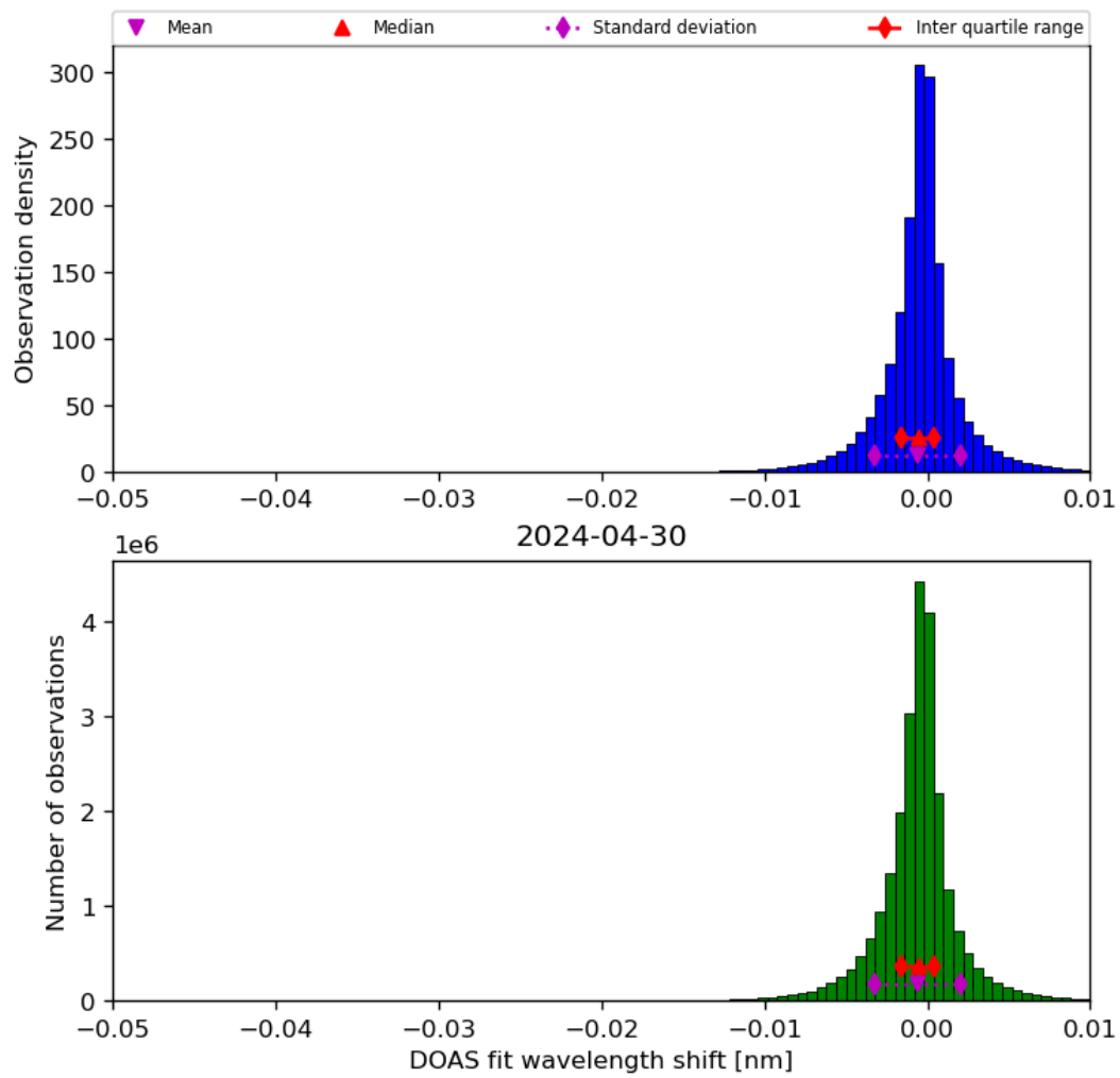
Figure 68: Histogram of “DOAS fit wavelength shift” for 2024-04-29 to 2024-05-01
