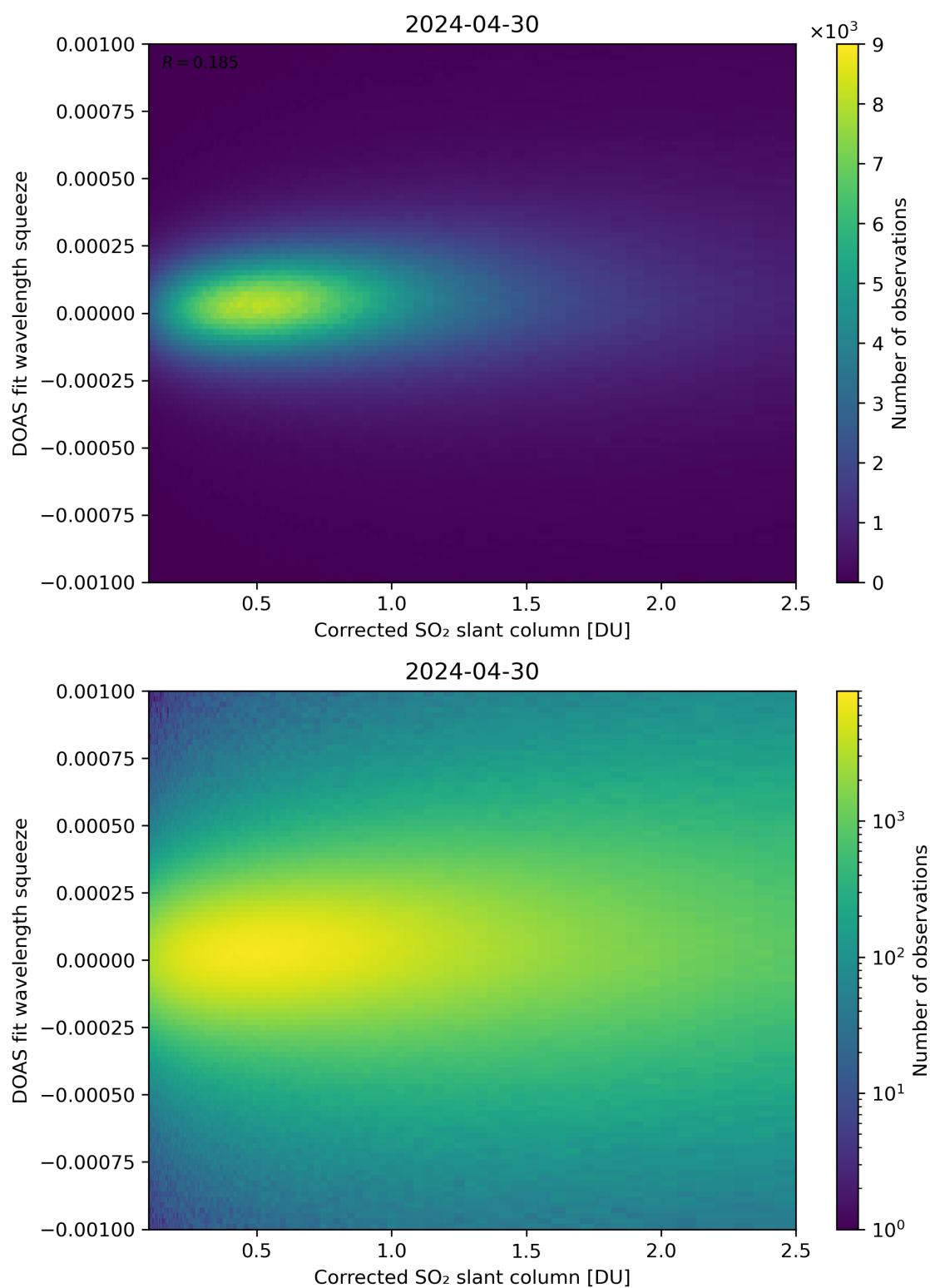
Figure 182: Scatter density plot of “Corrected SO 2 slant column” against “DOAS fit wavelength squeeze” for 2024-04-29 to 2024-05-01.
