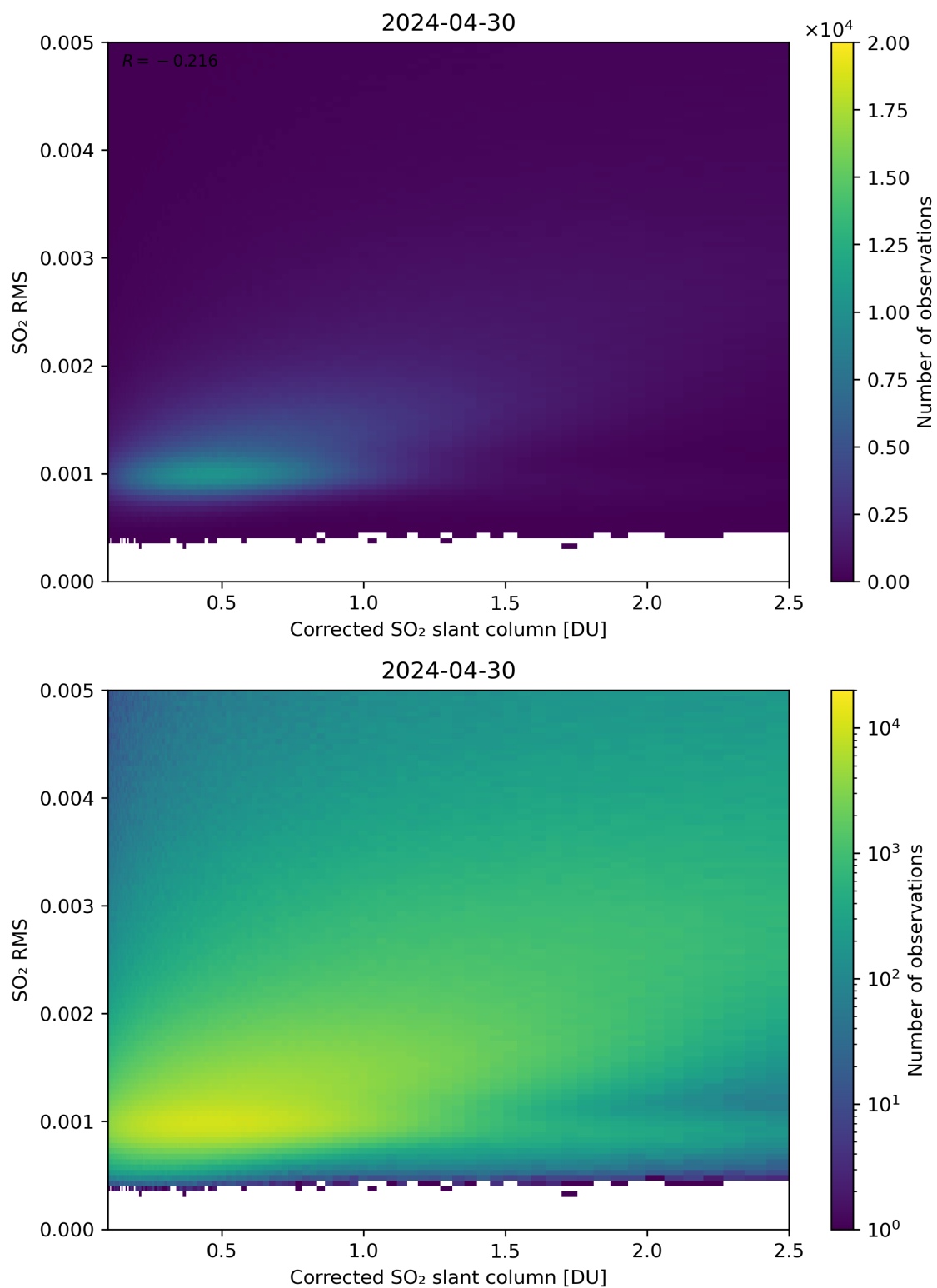
Figure 183: Scatter density plot of “Corrected SO 2 slant column” against “SO 2 RMS” for 2024-04-29 to 2024-05-01.
