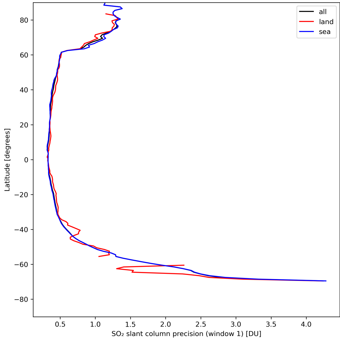
Figure 34: Zonal average of “SO 2 slant column precision (window 1)” for 2024-04-29 to 2024-05-01.
