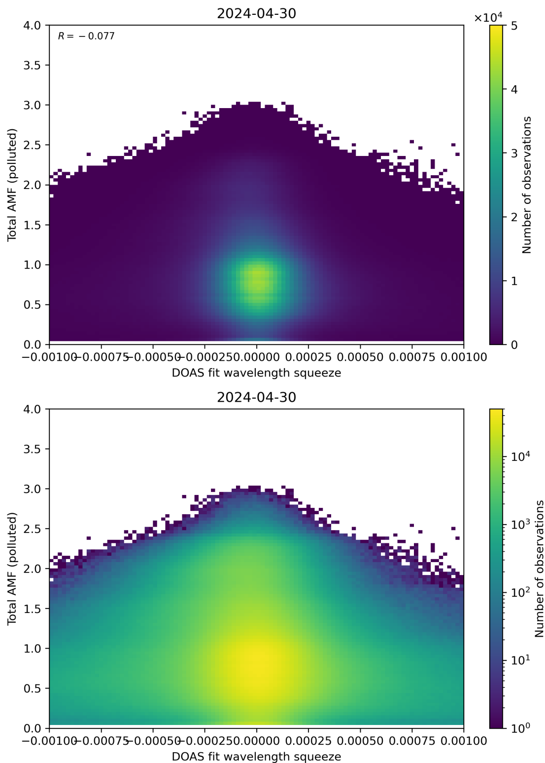
Figure 134: Scatter density plot of “DOAS fit wavelength squeeze” against “Total AMF (polluted)” for 2024-04-29 to 2024-05-01.
