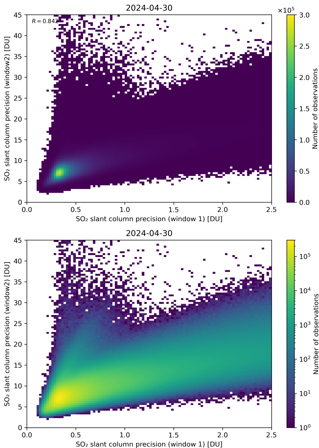
Figure 227: Scatter density plot of “SO 2 slant column precision (window 1)” against “SO 2 slant column precision (window2)” for 2024-04-29 to 2024-05-01.
