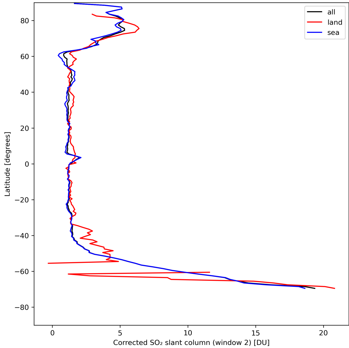
Figure 39: Zonal average of “Corrected SO 2 slant column (window 2)” for 2024-04-29 to 2024-05-01.
