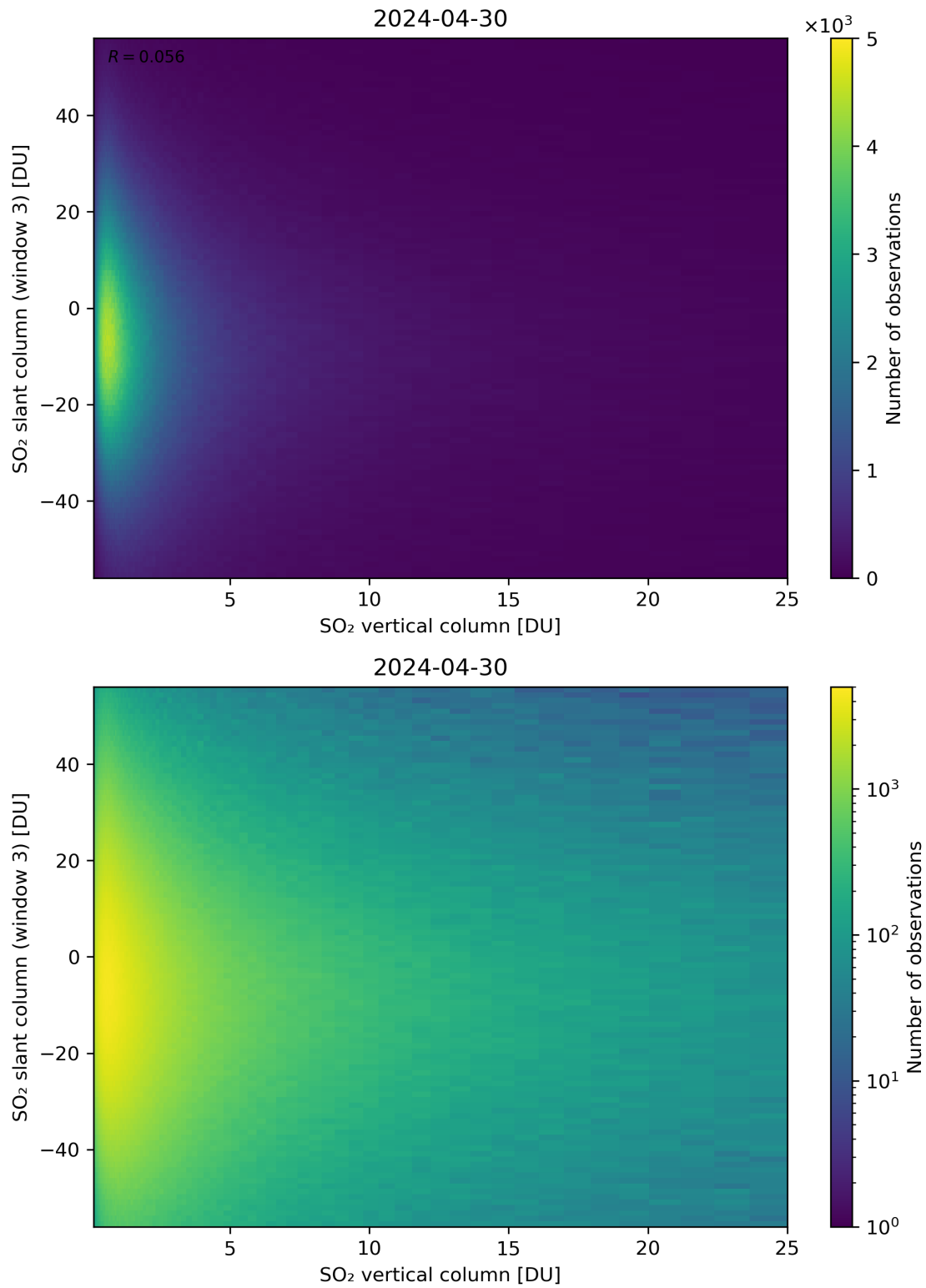
Figure 303: Scatter density plot of “SO 2 vertical column” against “SO 2 slant column (window 3)” for 2024-04-29 to 2024-05-01.
