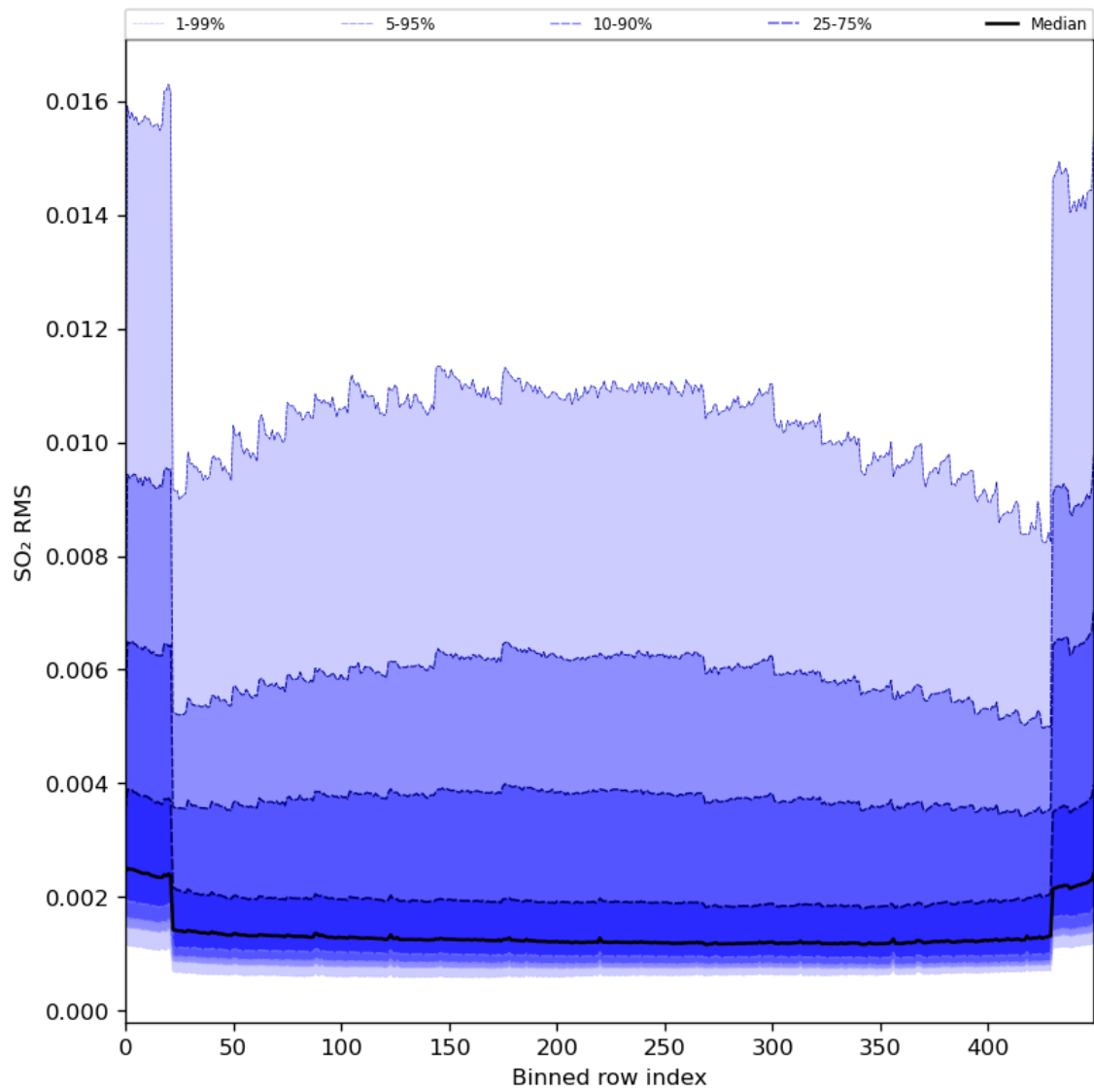
Figure 93: Along track statistics of “SO 2 RMS” for 2024-04-29 to 2024-05-01
