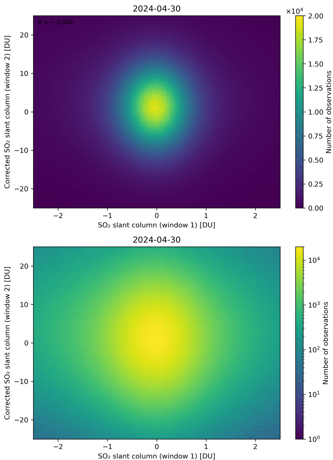
Figure 233: Scatter density plot of “SO 2 slant column (window 1)” against “Corrected SO 2 slant column (window 2)” for 2024-04-29 to 2024-05-01.
