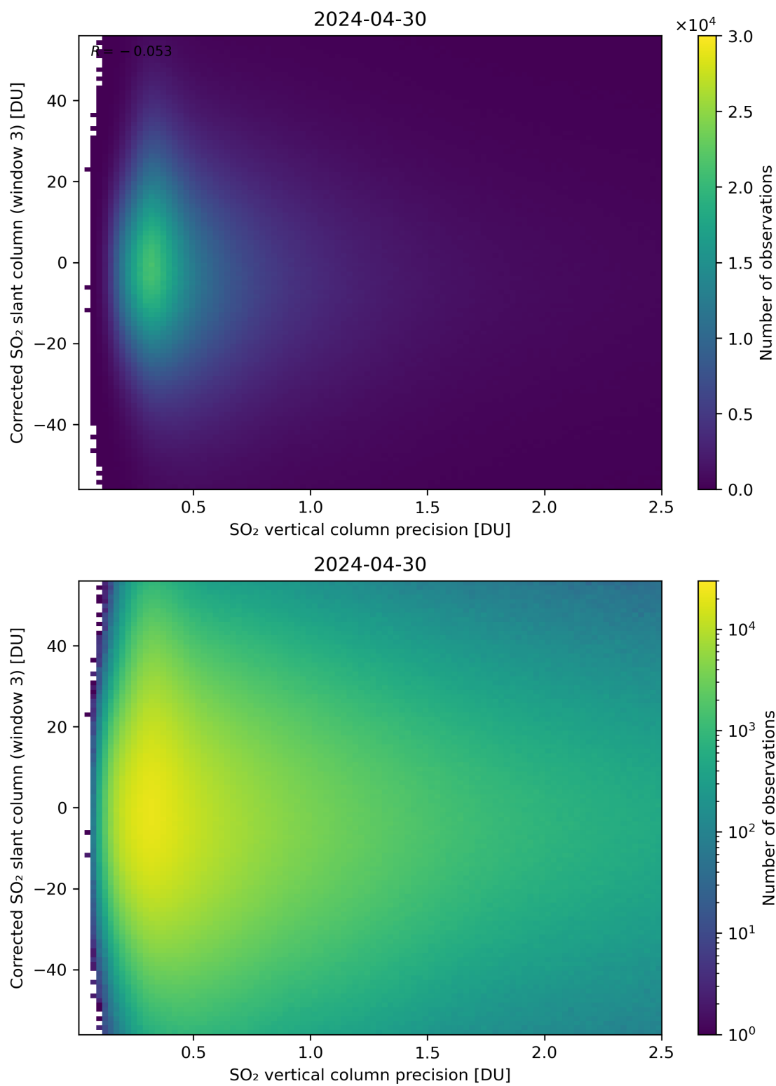
Figure 288: Scatter density plot of “SO 2 vertical column precision” against “Corrected SO 2 slant column (window 3)” for 2024-04-29 to 2024-05-01.
