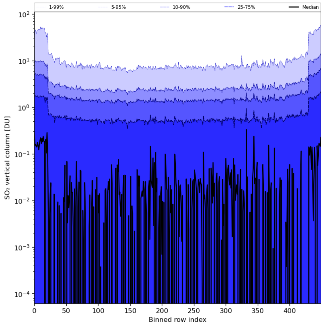
Figure 76: Along track statistics of “SO 2 vertical column” for 2024-04-29 to 2024-05-01
