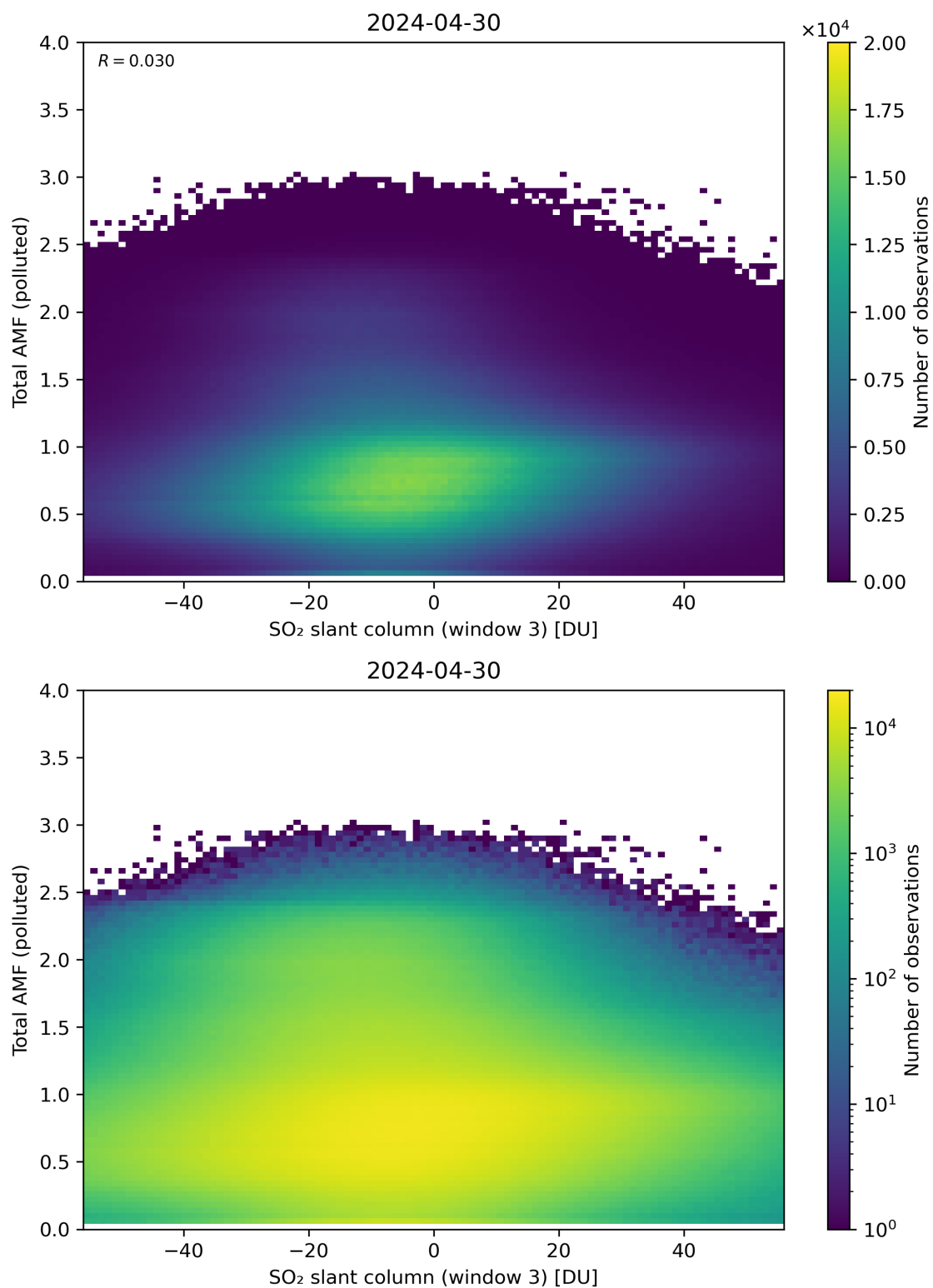
Figure 268: Scatter density plot of “SO 2 slant column (window 3)” against “Total AMF (polluted)” for 2024-04-29 to 2024-05-01.
