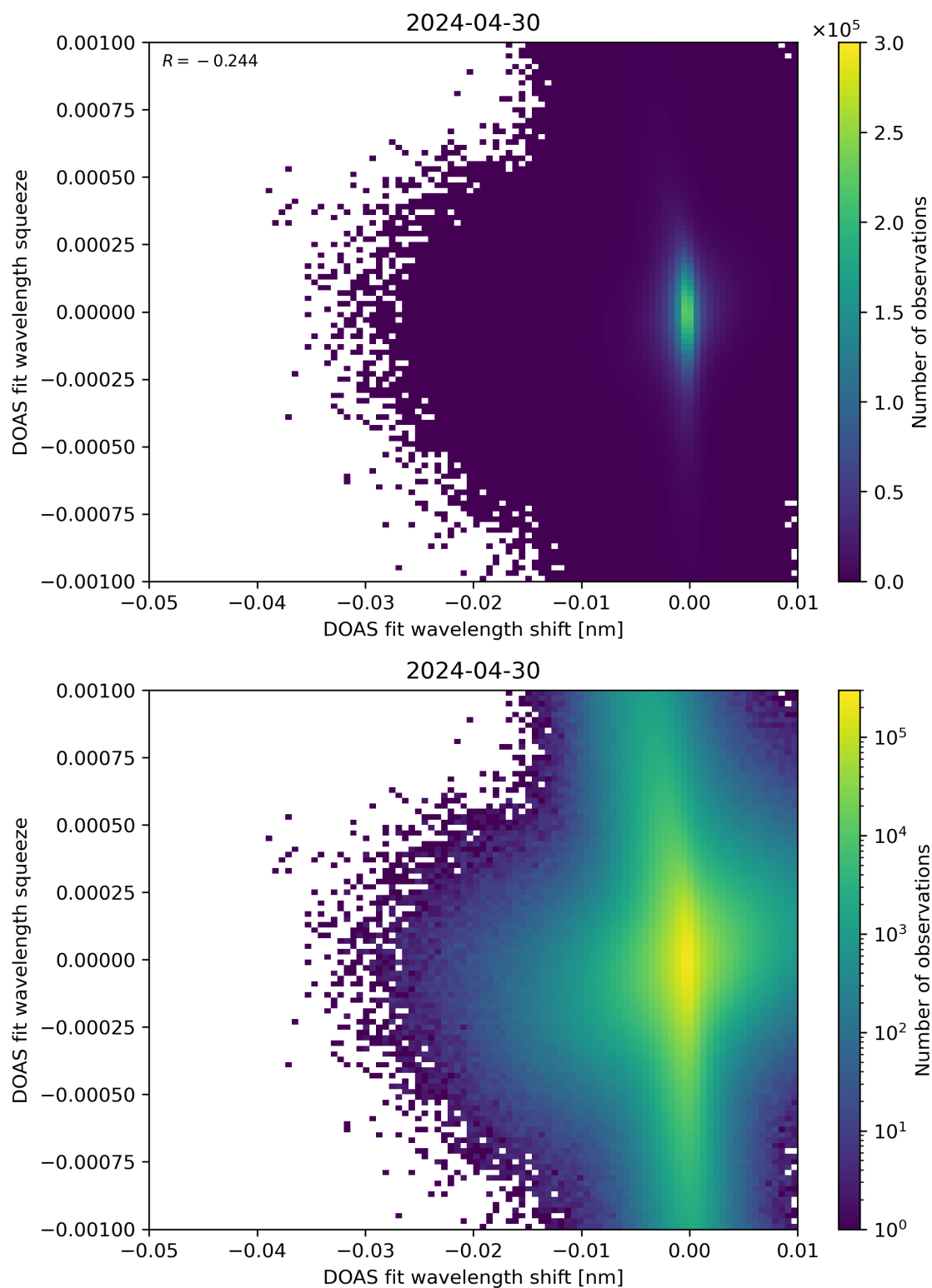
Figure 127: Scatter density plot of “DOAS fit wavelength shift” against “DOAS fit wavelength squeeze” for 2024-04-29 to 2024-05-01.
