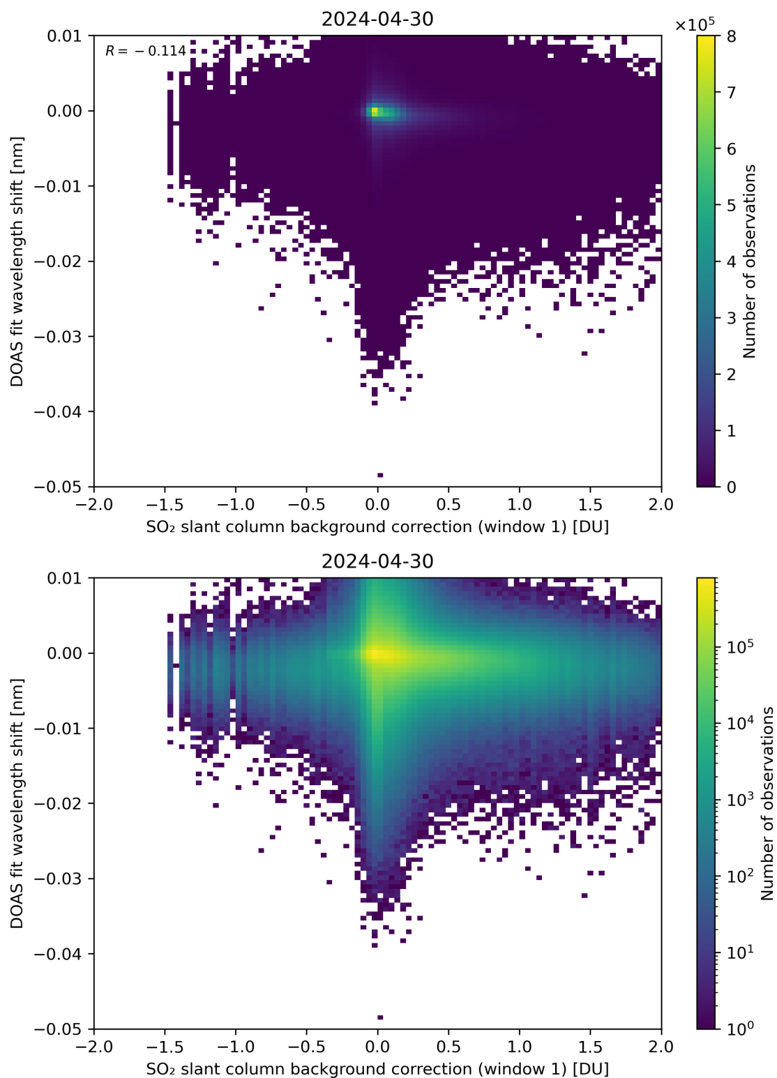
Figure 100: Scatter density plot of “SO 2 slant column background correction (window 1)” against “DOAS fit wavelength shift” for 2024-04-29 to 2024-05-01.
