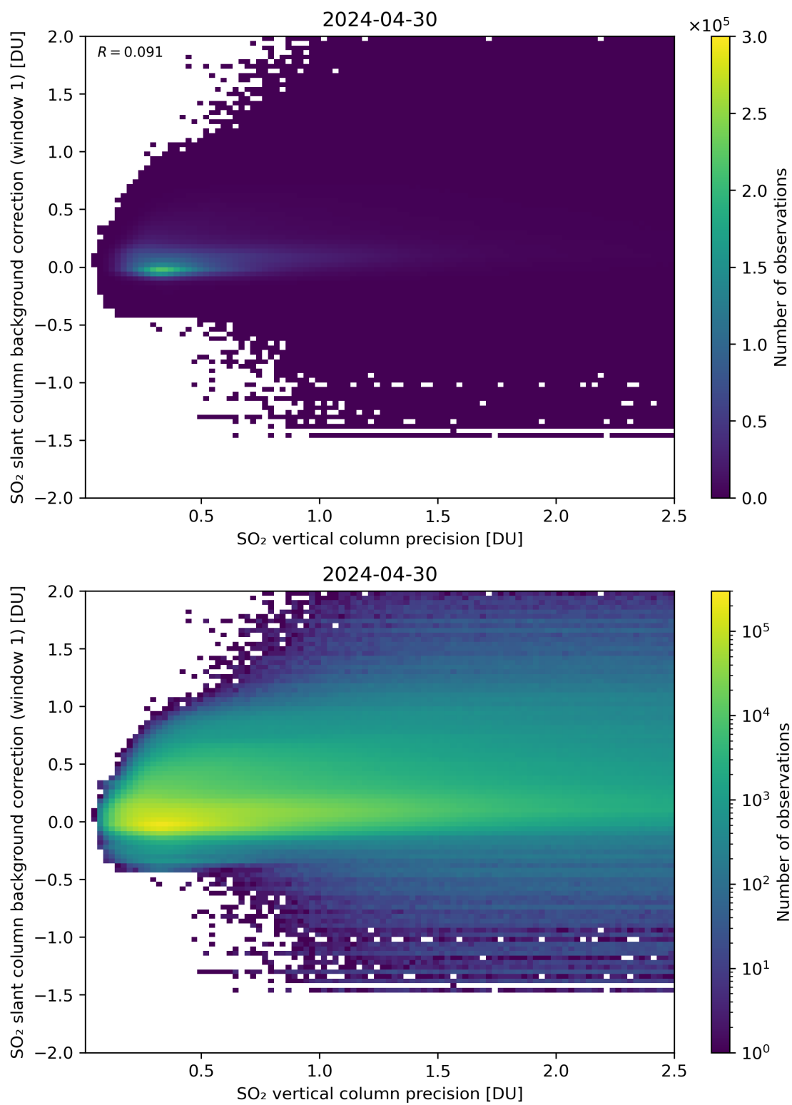
Figure 279: Scatter density plot of “SO 2 vertical column precision” against “SO 2 slant column background correction (window 1)” for 2024-04-29 to 2024-05-01.
