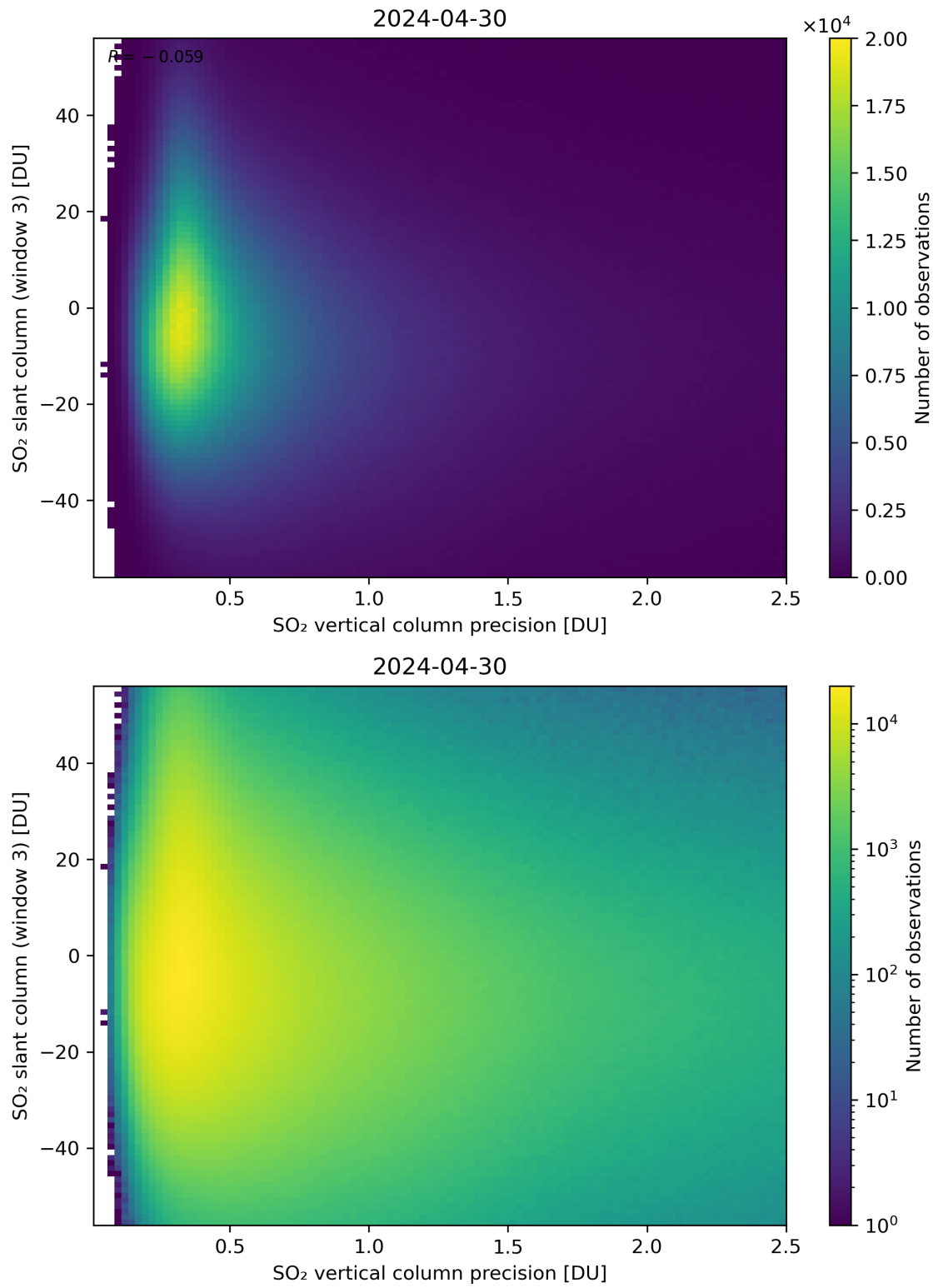
Figure 292: Scatter density plot of “SO 2 vertical column precision” against “SO 2 slant column (window 3)” for 2024-04-29 to 2024-05-01.
