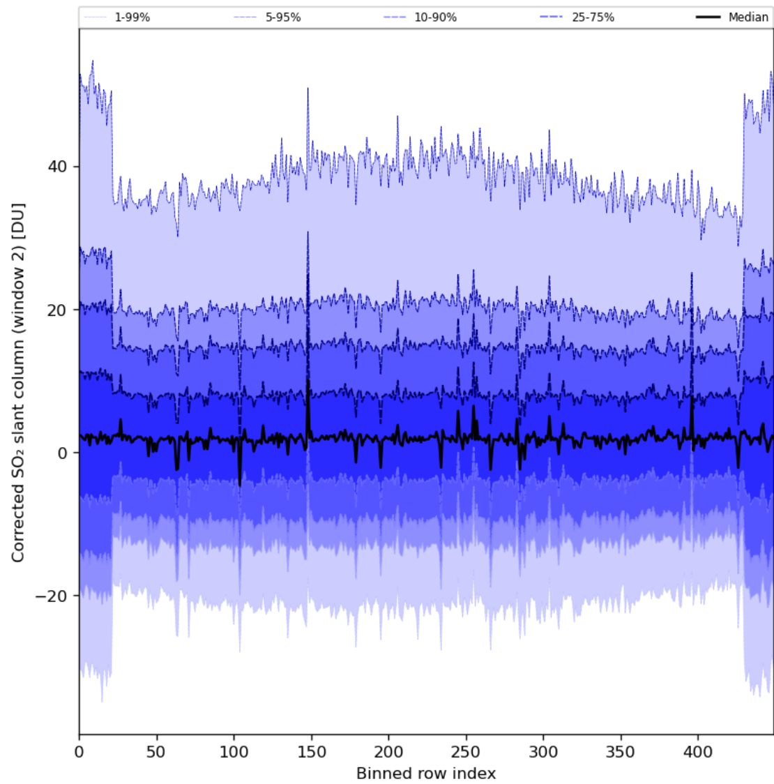
Figure 85: Along track statistics of “Corrected SO 2 slant column (window 2)” for 2024-04-29 to 2024-05-01
