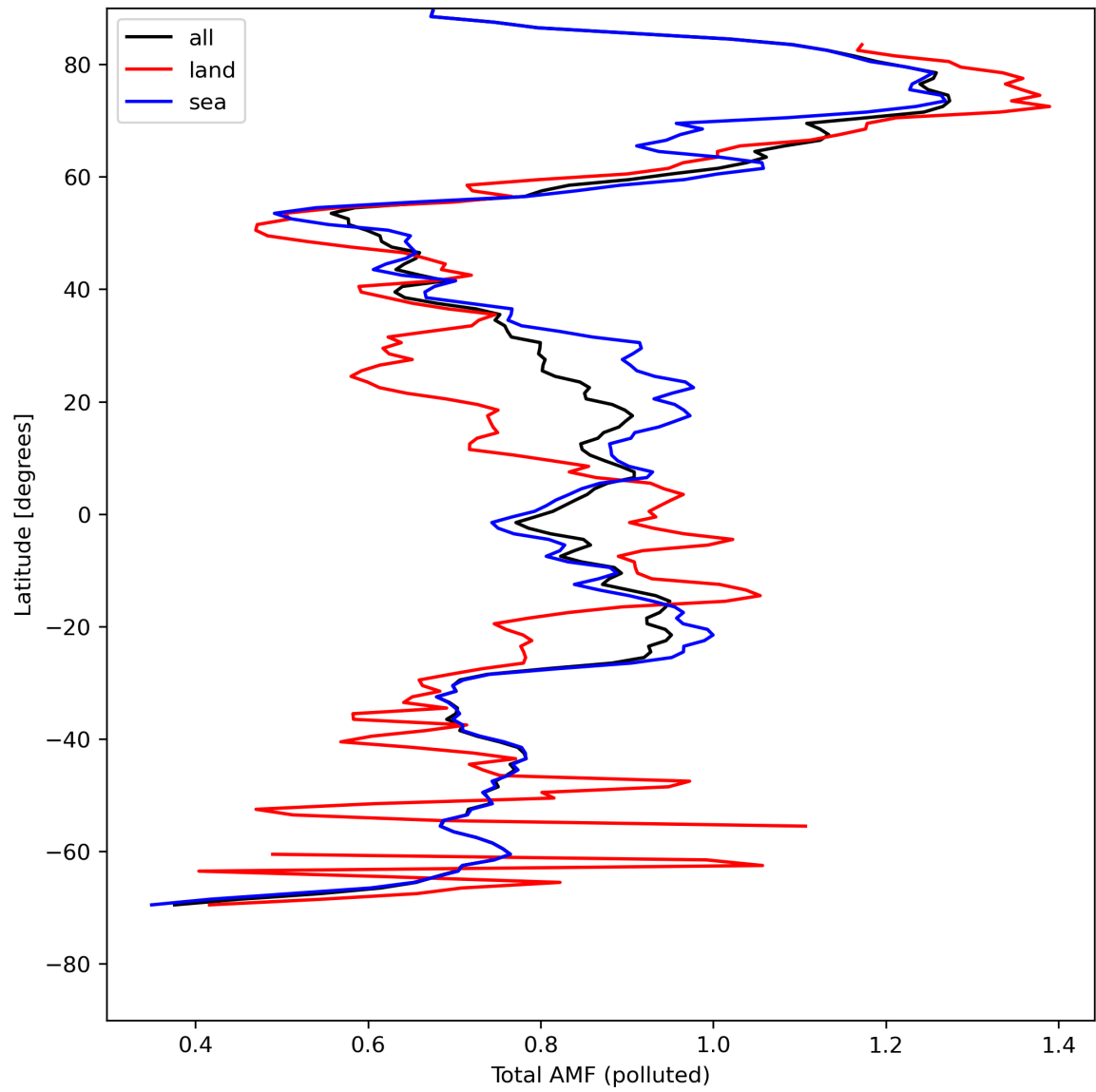
Figure 48: Zonal average of “Total AMF (polluted)” for 2024-04-29 to 2024-05-01.
