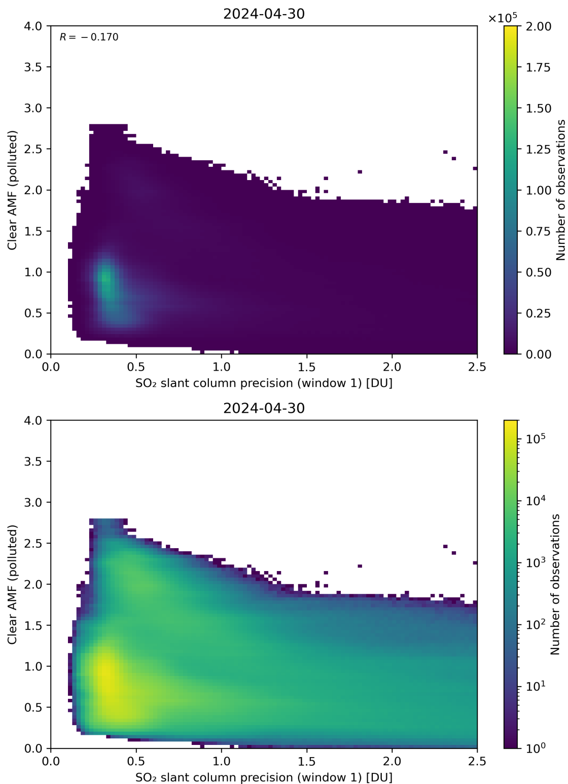
Figure 224: Scatter density plot of “SO 2 slant column precision (window 1)” against “Clear AMF (polluted)” for 2024-04-29 to 2024-05-01.
