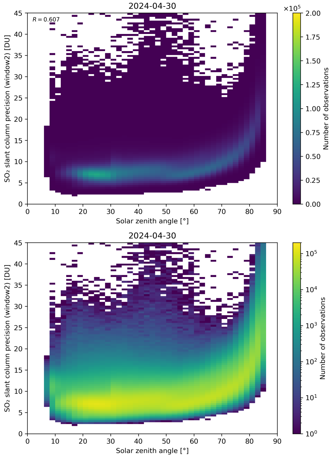
Figure 171: Scatter density plot of “Solar zenith angle” against “SO 2 slant column precision (window2)” for 2024-04-29 to 2024-05-01.
