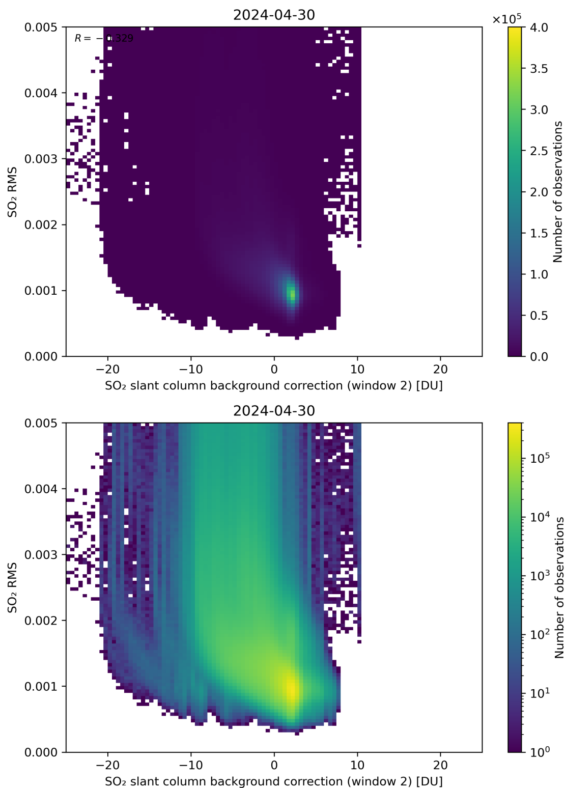
Figure 114: Scatter density plot of “SO 2 slant column background correction (window 2)” against “SO 2 RMS” for 2024-04-29 to 2024-05-01.
