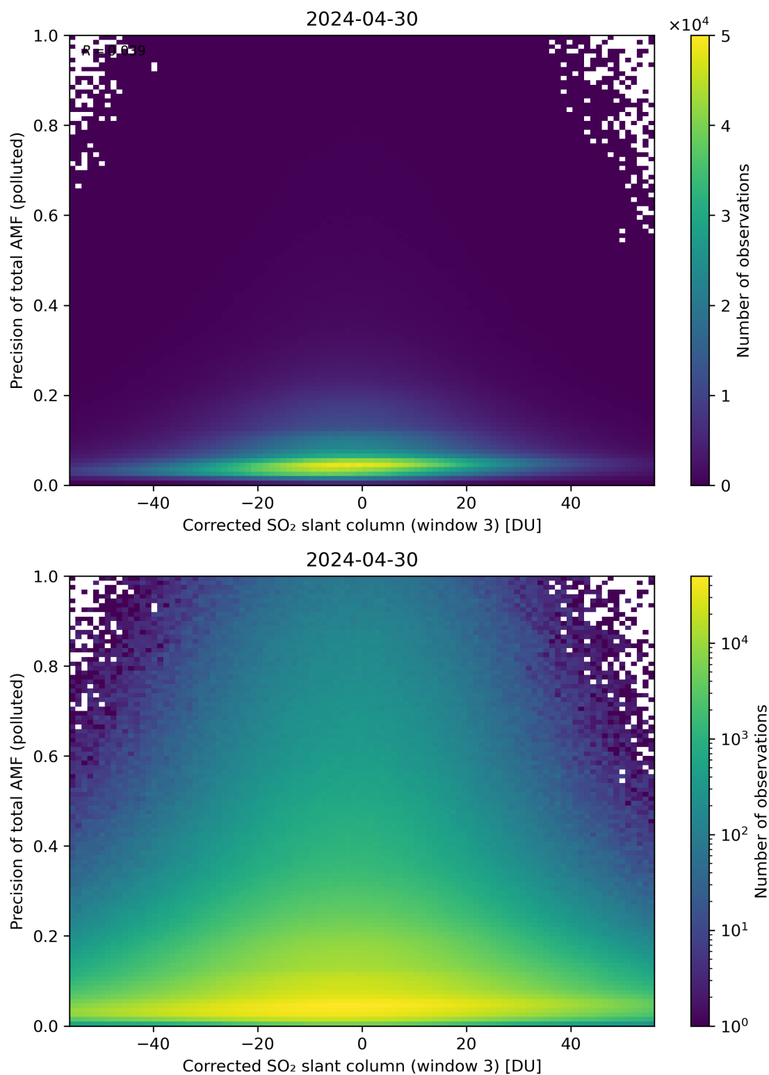
Figure 211: Scatter density plot of “Corrected SO 2 slant column (window 3)” against “Precision of total AMF (polluted)” for 2024-04-29 to 2024-05-01.
