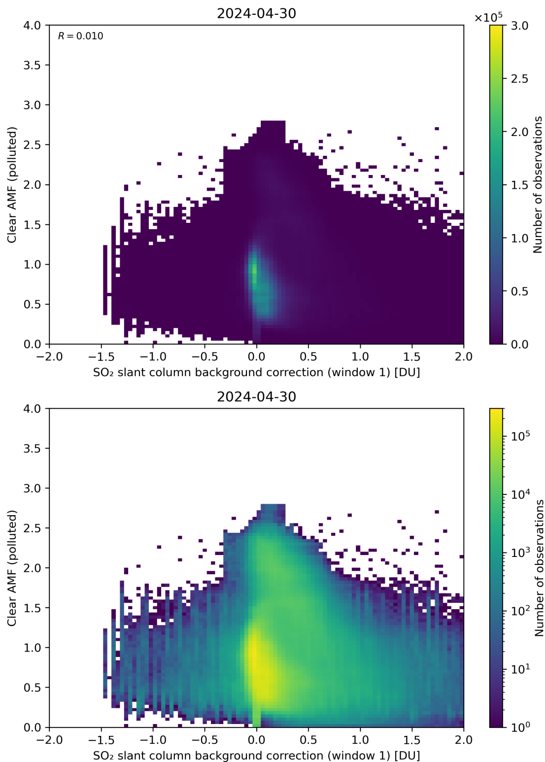
Figure 103: Scatter density plot of “SO 2 slant column background correction (window 1)” against “Clear AMF (polluted)” for 2024-04-29 to 2024-05-01.
