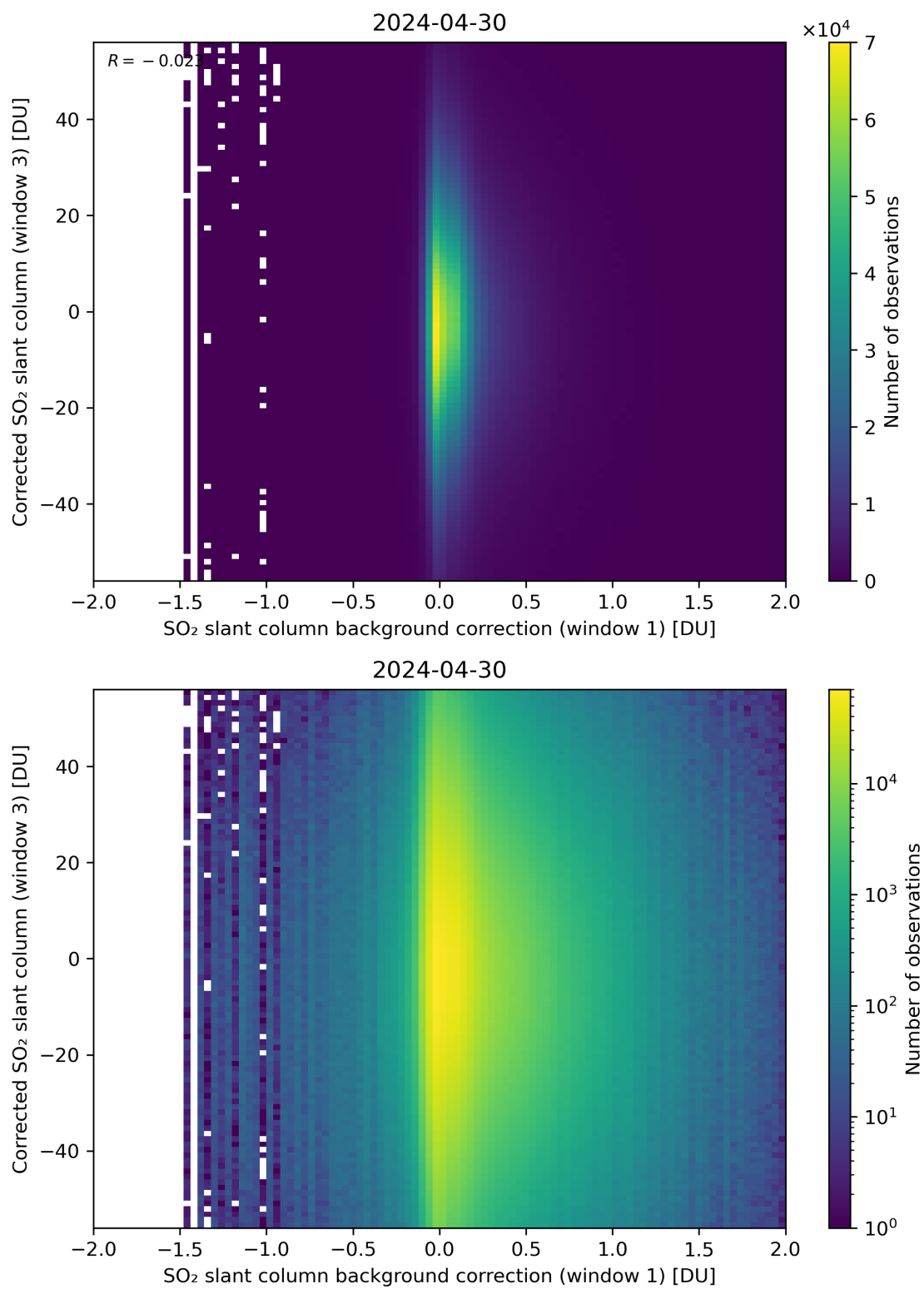
Figure 105: Scatter density plot of “SO 2 slant column background correction (window 1)” against “Corrected SO 2 slant column (window 3)” for 2024-04-29 to 2024-05-01.
