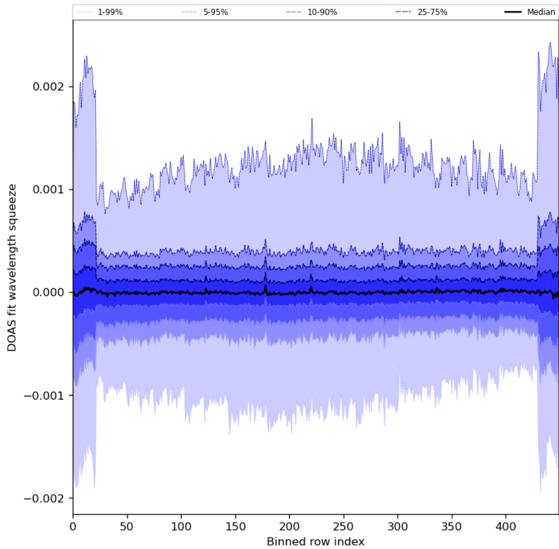
Figure 92: Along track statistics of “DOAS fit wavelength squeeze” for 2024-04-29 to 2024-05-01
