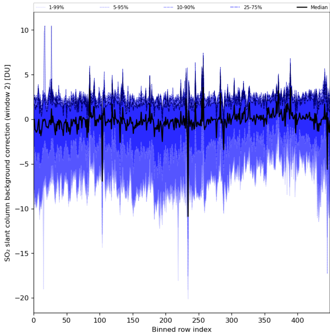
Figure 86: Along track statistics of “SO 2 slant column background correction (window 2)” for 2024-04-29 to 2024-05-01
