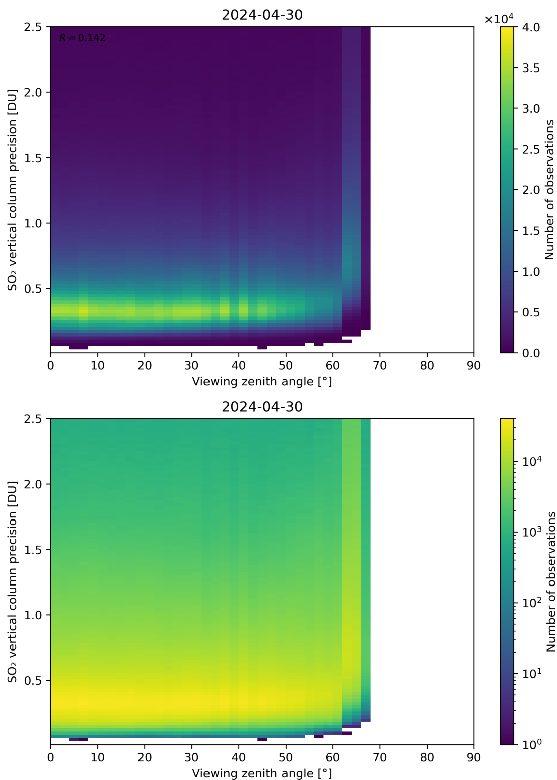
Figure 328: Scatter density plot of “Viewing zenith angle” against “SO 2 vertical column precision” for 2024-04-29 to 2024-05-01.
