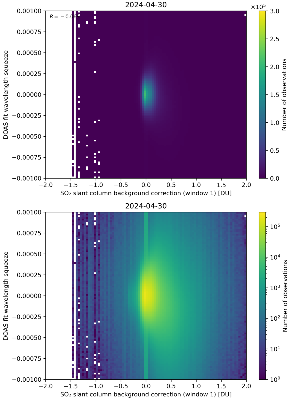
Figure 101: Scatter density plot of “SO 2 slant column background correction (window 1)” against “DOAS fit wavelength squeeze” for 2024-04-29 to 2024-05-01.
