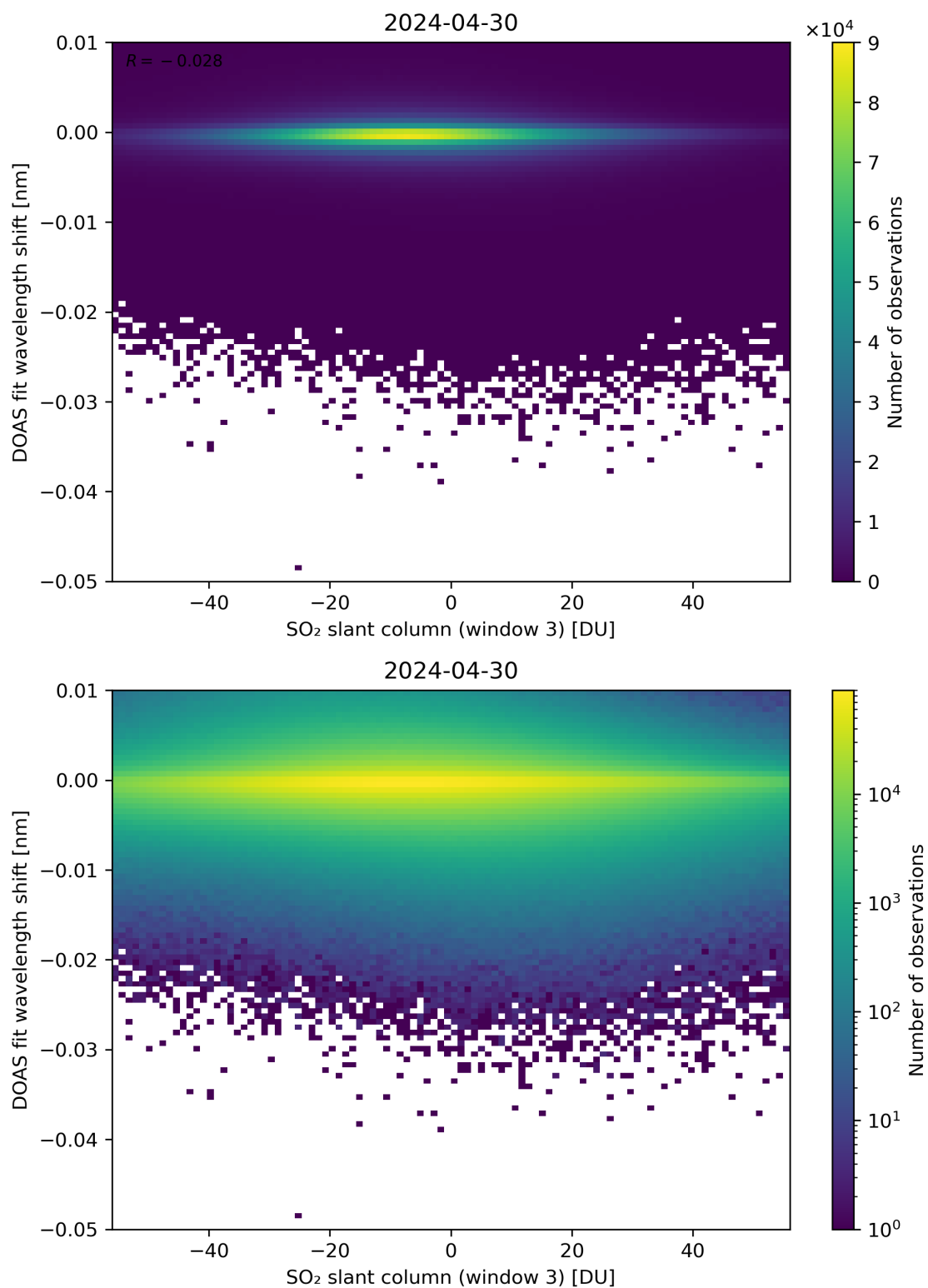
Figure 254: Scatter density plot of “SO 2 slant column (window 3)” against “DOAS fit wavelength shift” for 2024-04-29 to 2024-05-01.
