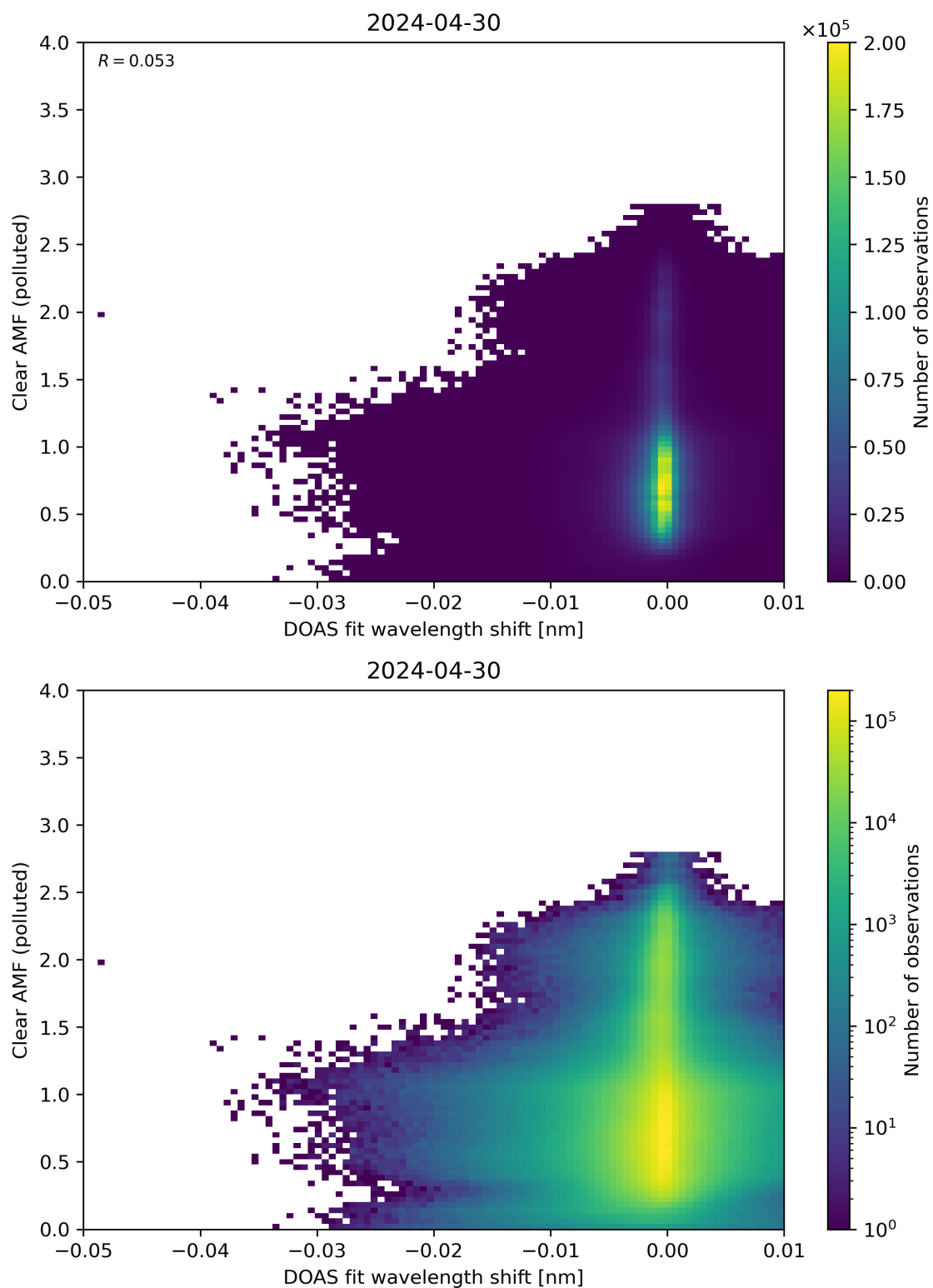
Figure 129: Scatter density plot of “DOAS fit wavelength shift” against “Clear AMF (polluted)” for 2024-04-29 to 2024-05-01.
