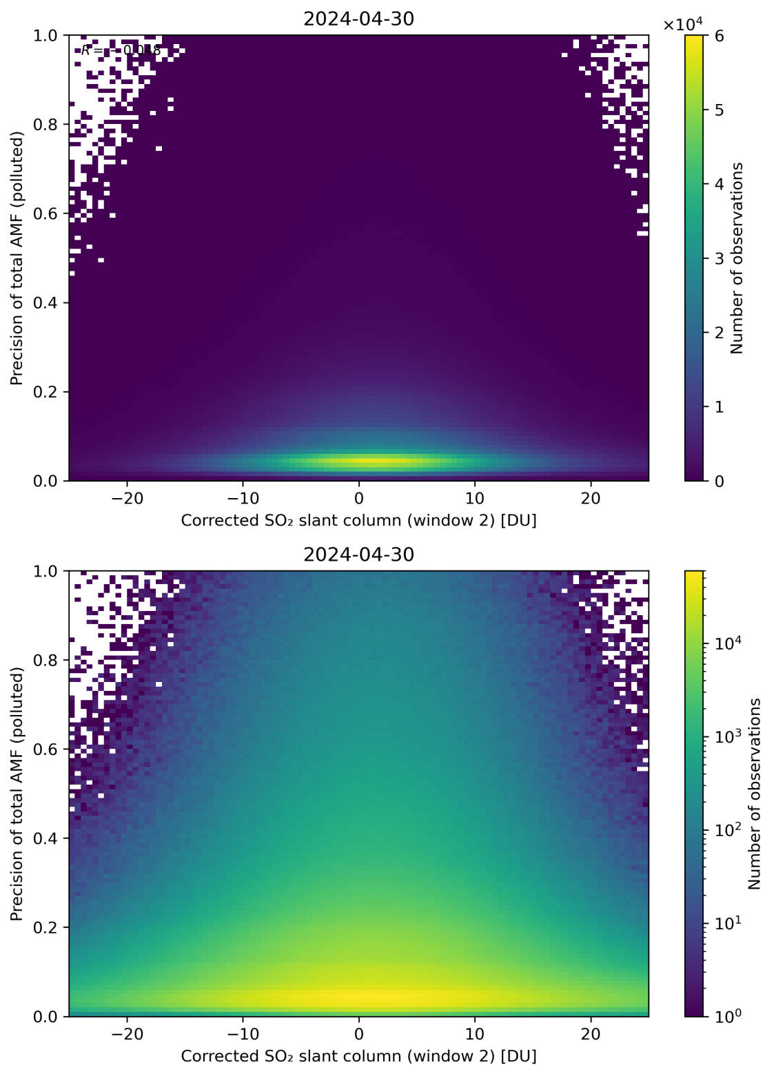
Figure 204: Scatter density plot of “Corrected SO 2 slant column (window 2)” against “Precision of total AMF (polluted)” for 2024-04-29 to 2024-05-01.
