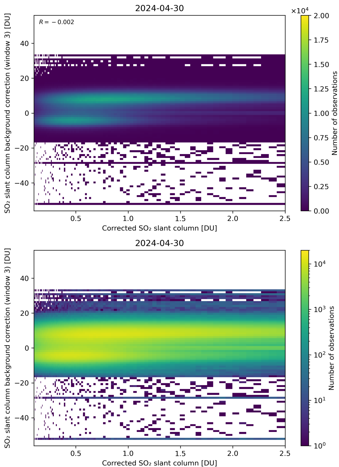
Figure 180: Scatter density plot of “Corrected SO 2 slant column” against “SO 2 slant column background correction (window 3)” for 2024-04-29 to 2024-05-01.
