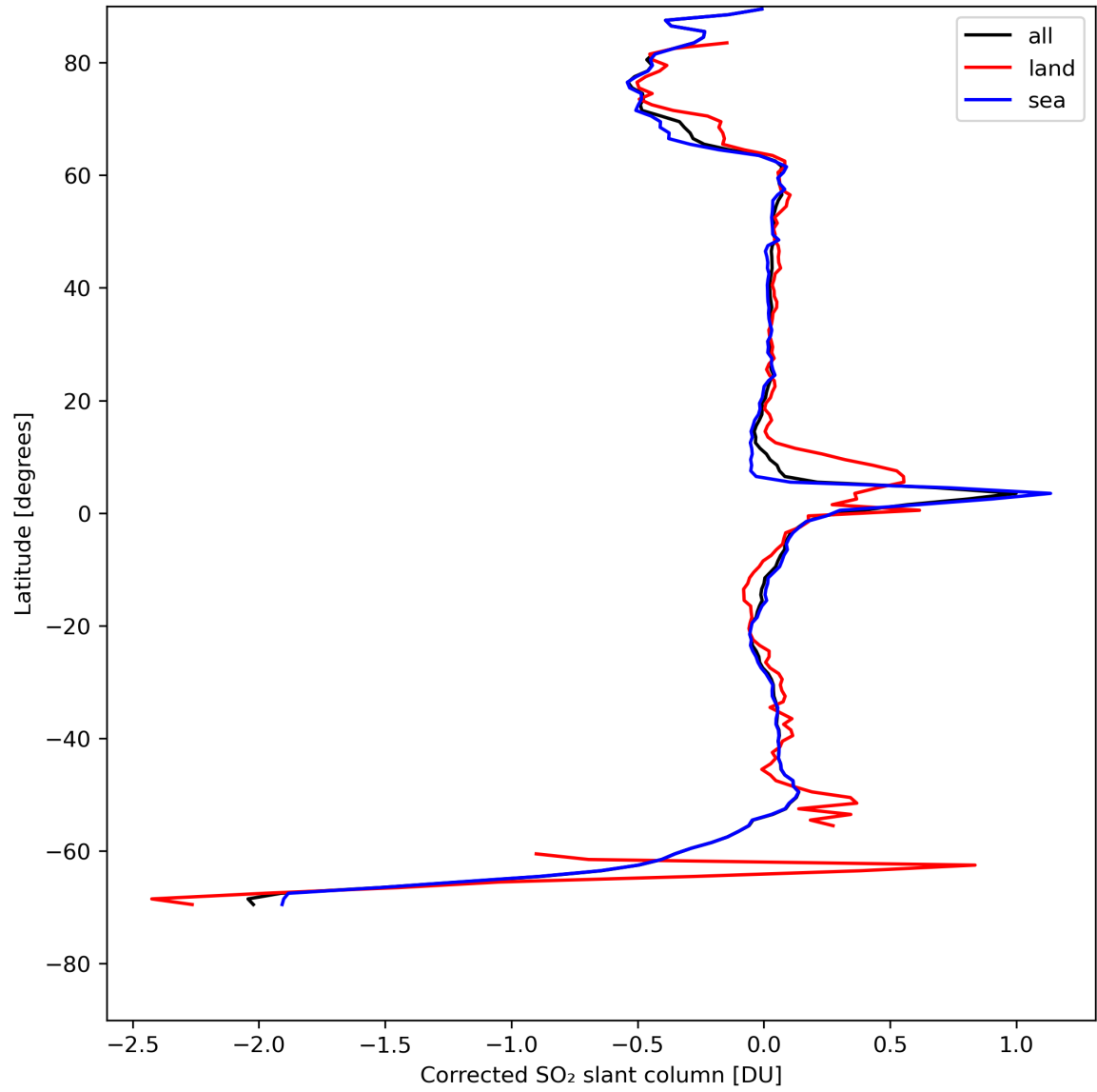
Figure 32: Zonal average of “Corrected SO 2 slant column” for 2024-04-29 to 2024-05-01.
