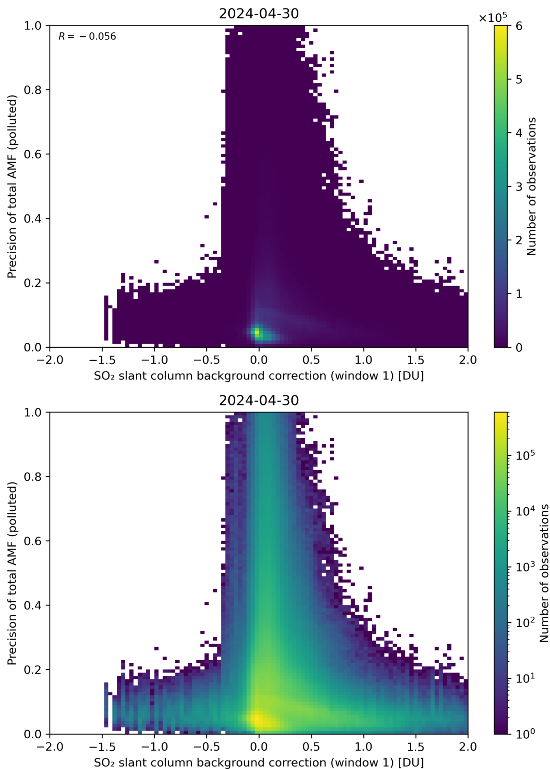
Figure 110: Scatter density plot of “SO 2 slant column background correction (window 1)” against “Precision of total AMF (polluted)” for 2024-04-29 to 2024-05-01.
