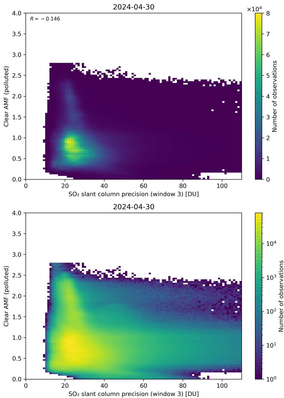
Figure 261: Scatter density plot of “SO 2 slant column precision (window 3)” against “Clear AMF (polluted)” for 2024-04-29 to 2024-05-01.
