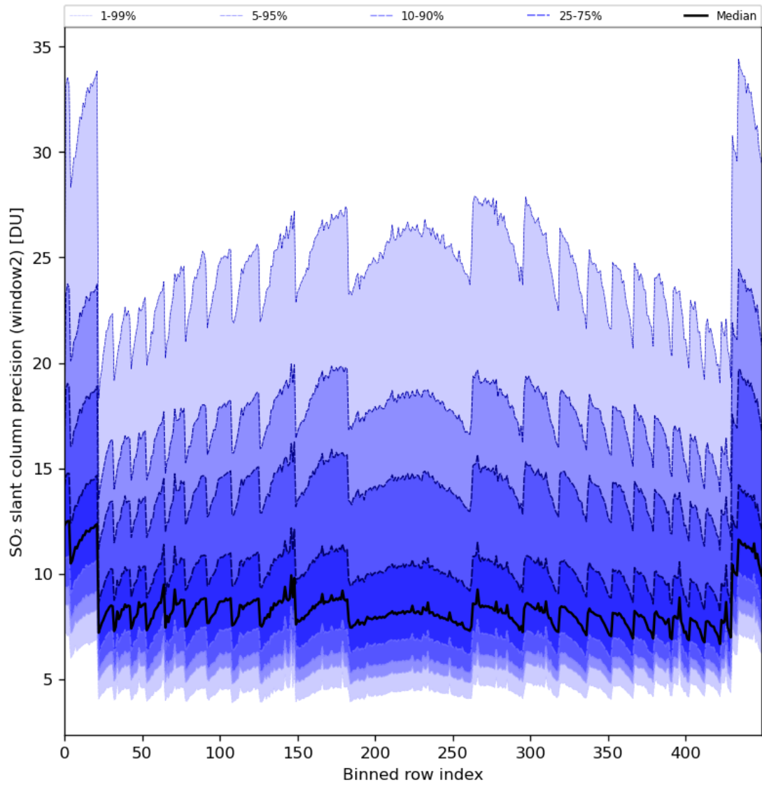
Figure 84: Along track statistics of “SO 2 slant column precision (window2)” for 2024-04-29 to 2024-05-01
