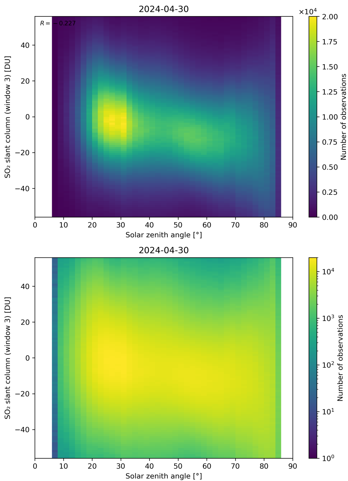
Figure 172: Scatter density plot of “Solar zenith angle” against “SO 2 slant column (window 3)” for 2024-04-29 to 2024-05-01.
