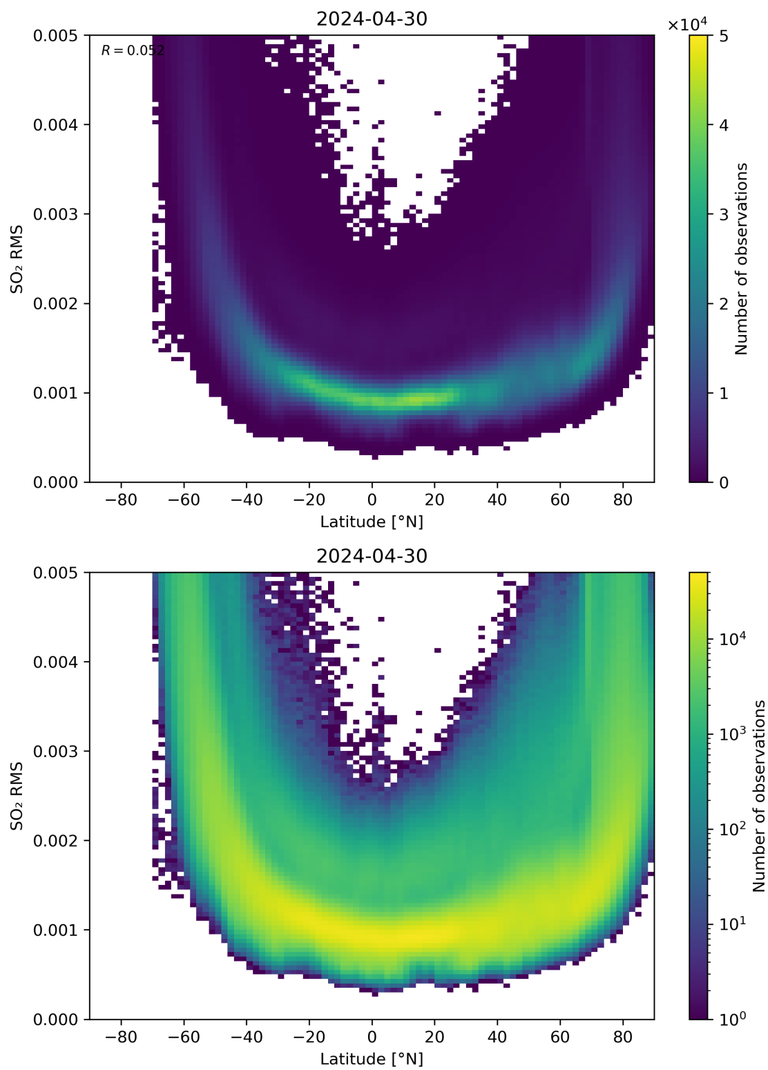
Figure 144: Scatter density plot of “Latitude” against “SO 2 RMS” for 2024-04-29 to 2024-05-01.
