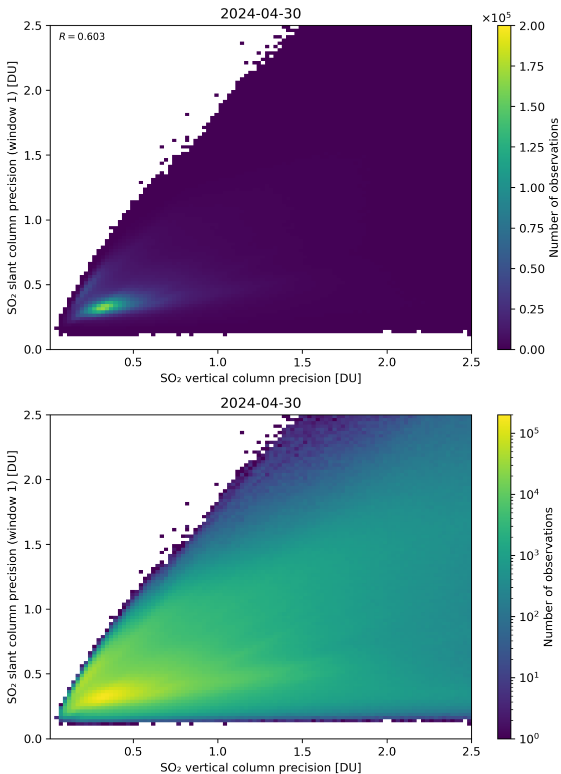
Figure 290: Scatter density plot of “SO 2 vertical column precision” against “SO 2 slant column precision (window 1)” for 2024-04-29 to 2024-05-01.
