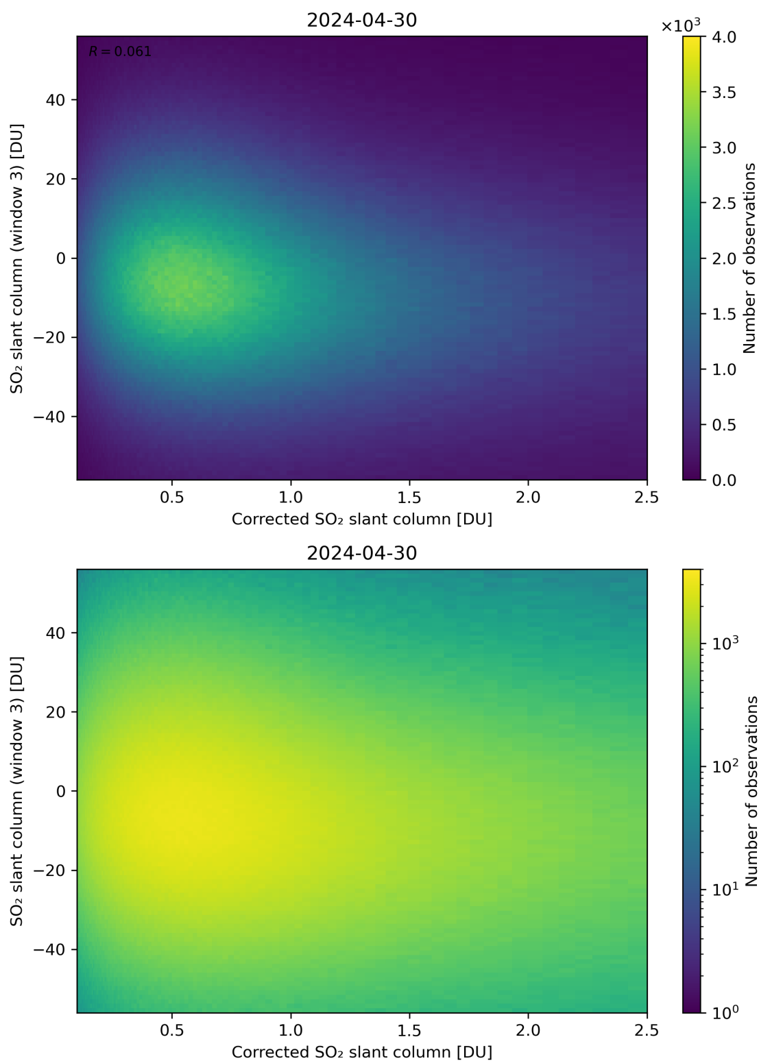
Figure 190: Scatter density plot of “Corrected SO 2 slant column” against “SO 2 slant column (window 3)” for 2024-04-29 to 2024-05-01.
