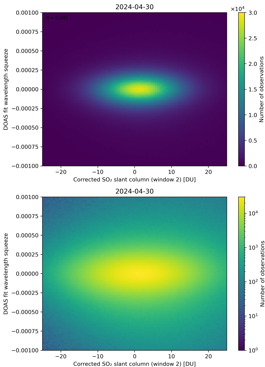
Figure 197: Scatter density plot of “Corrected SO 2 slant column (window 2)” against “DOAS fit wavelength squeeze” for 2024-04-29 to 2024-05-01.
