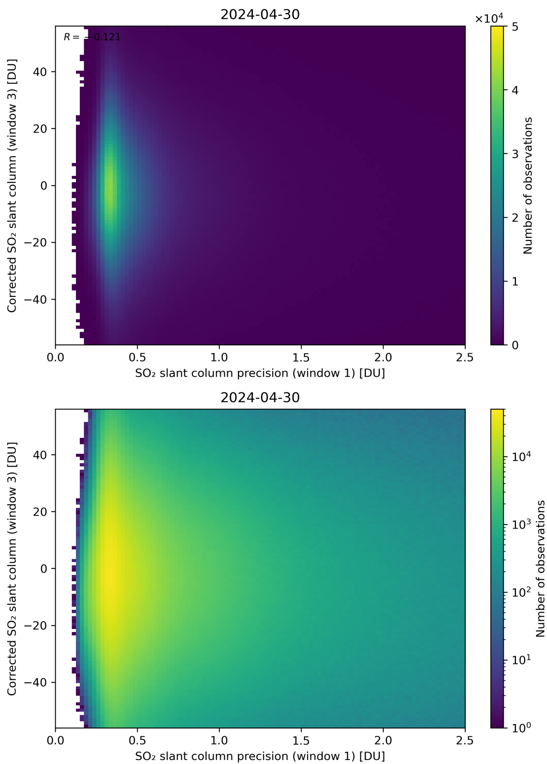
Figure 226: Scatter density plot of “SO 2 slant column precision (window 1)” against “Corrected SO 2 slant column (window 3)” for 2024-04-29 to 2024-05-01.
