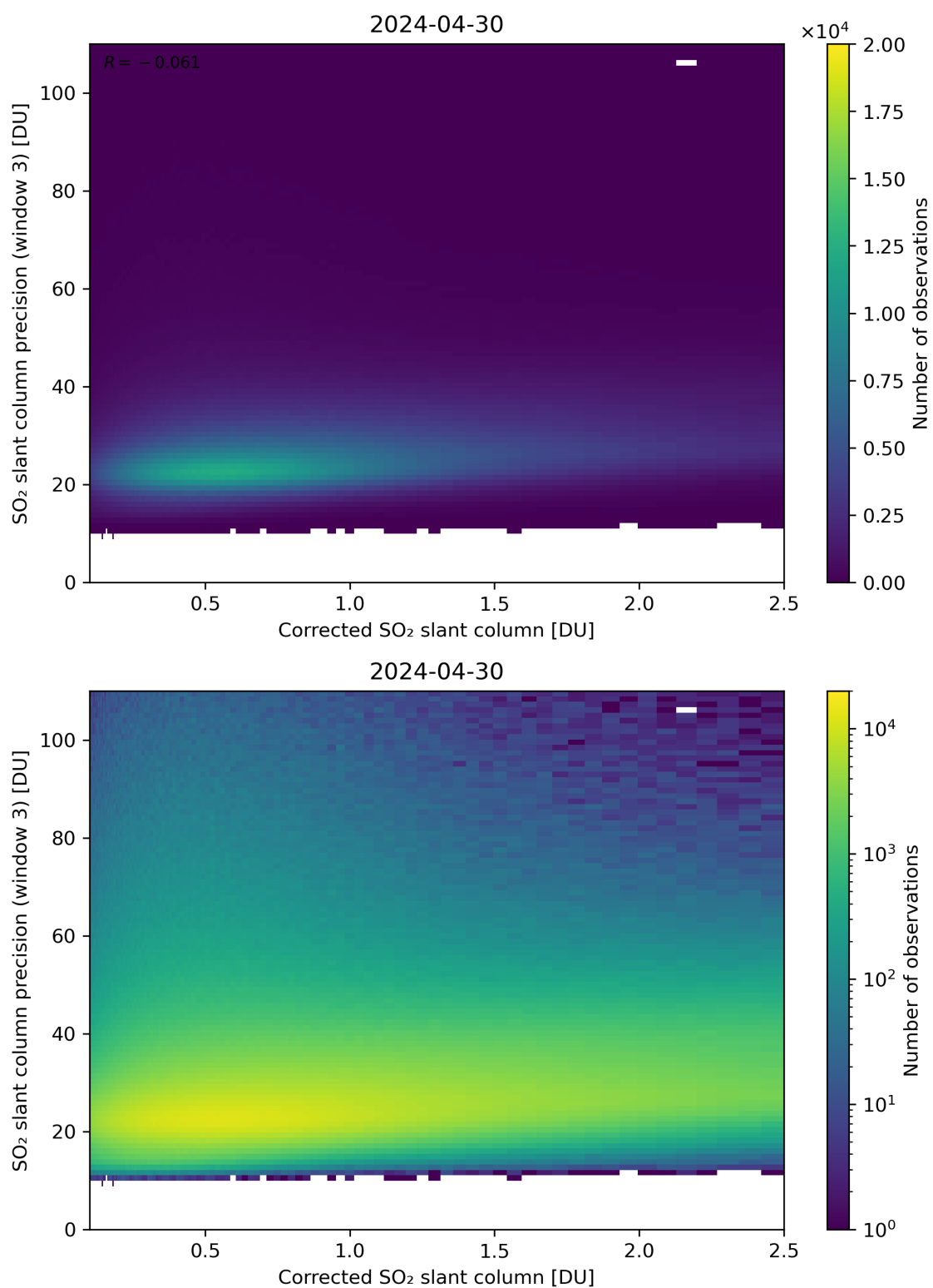
Figure 191: Scatter density plot of “Corrected SO 2 slant column” against “SO 2 slant column precision (window 3)” for 2024-04-29 to 2024-05-01.
