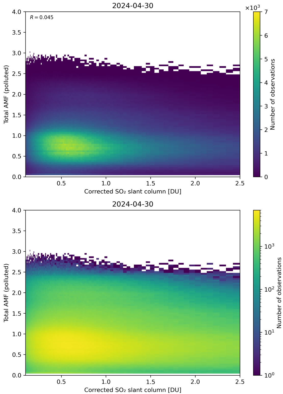
Figure 192: Scatter density plot of “Corrected SO 2 slant column” against “Total AMF (polluted)” for 2024-04-29 to 2024-05-01.
