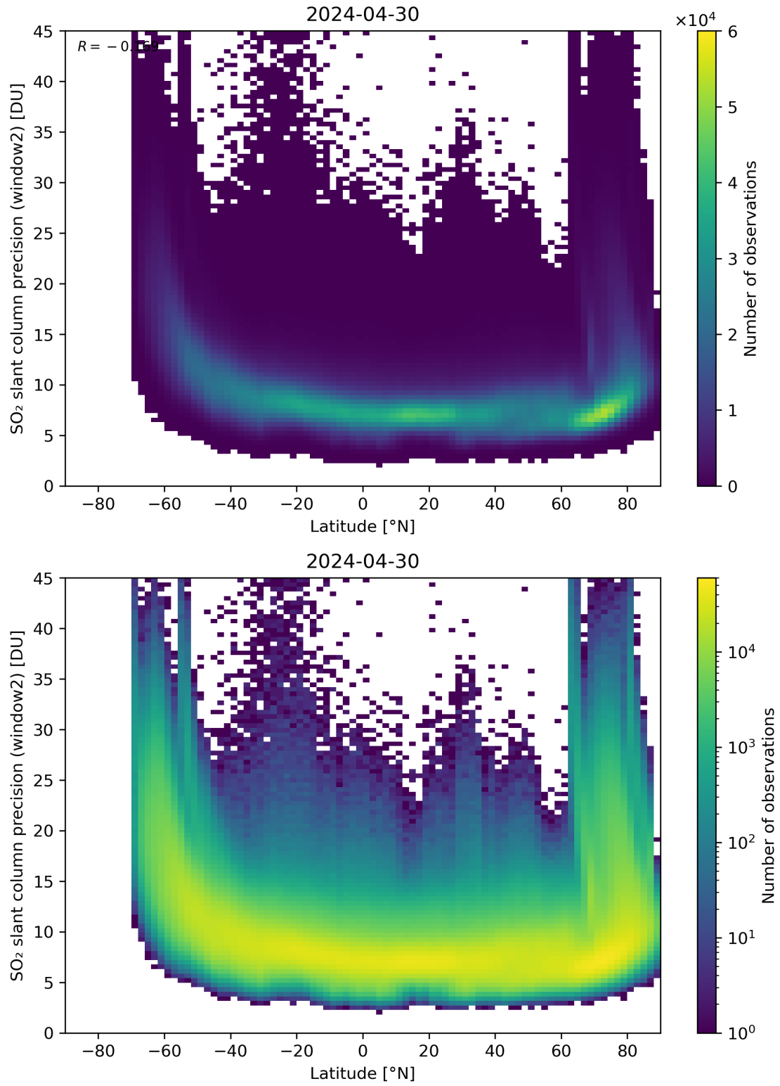
Figure 151: Scatter density plot of “Latitude” against “SO 2 slant column precision (window2)” for 2024-04-29 to 2024-05-01.
