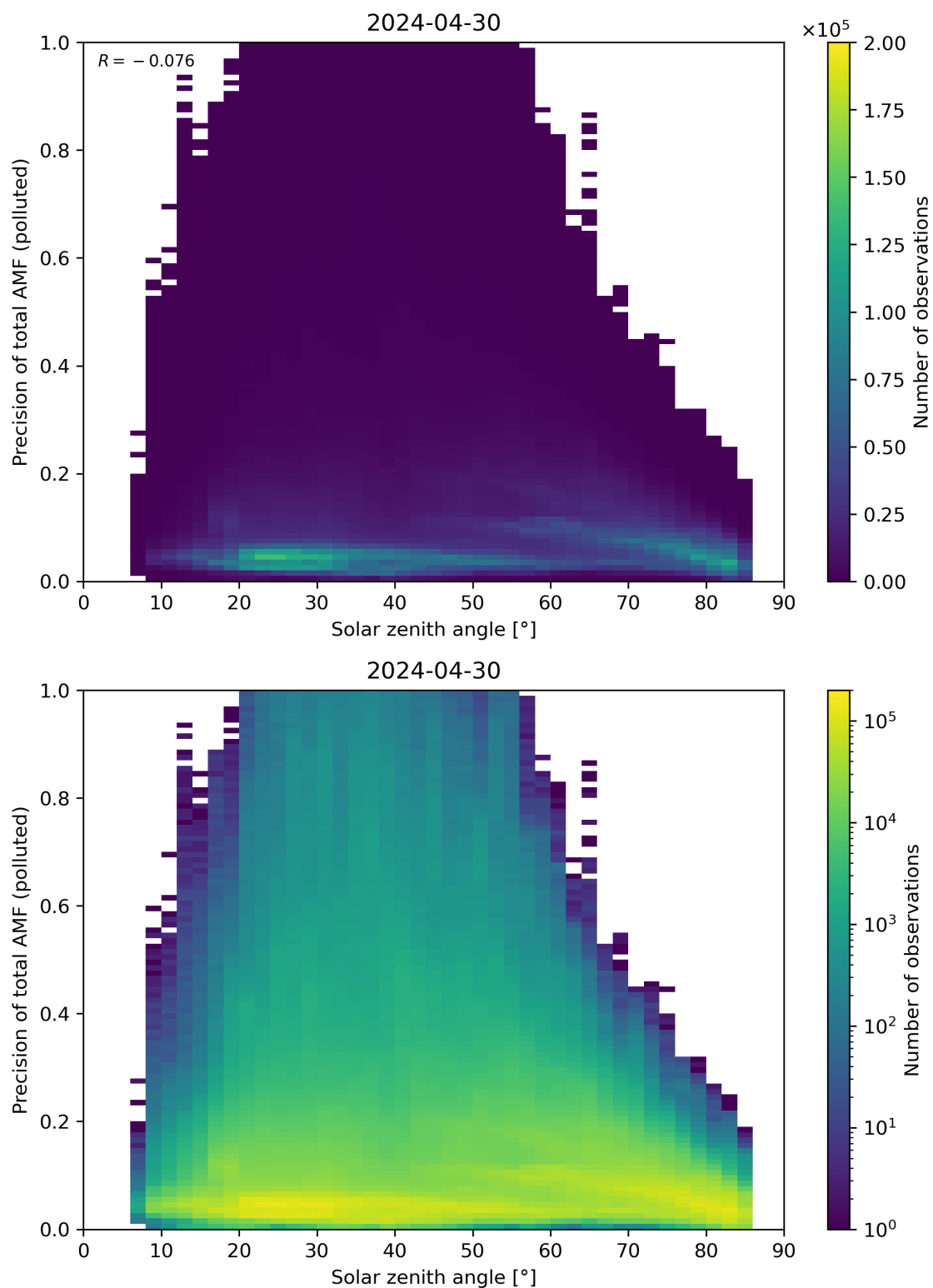
Figure 175: Scatter density plot of “Solar zenith angle” against “Precision of total AMF (polluted)” for 2024-04-29 to 2024-05-01.
