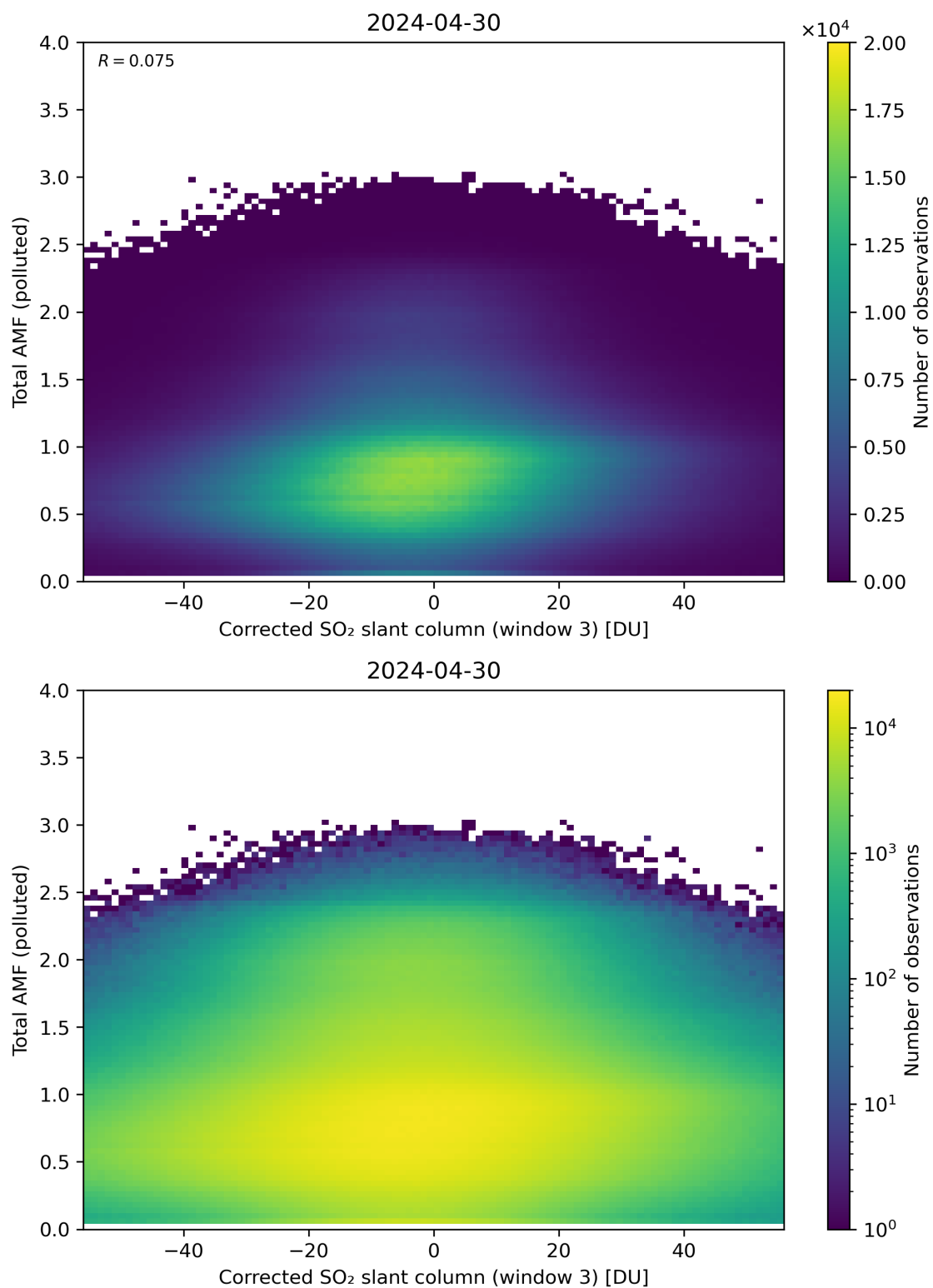
Figure 210: Scatter density plot of “Corrected SO 2 slant column (window 3)” against “Total AMF (polluted)” for 2024-04-29 to 2024-05-01.
