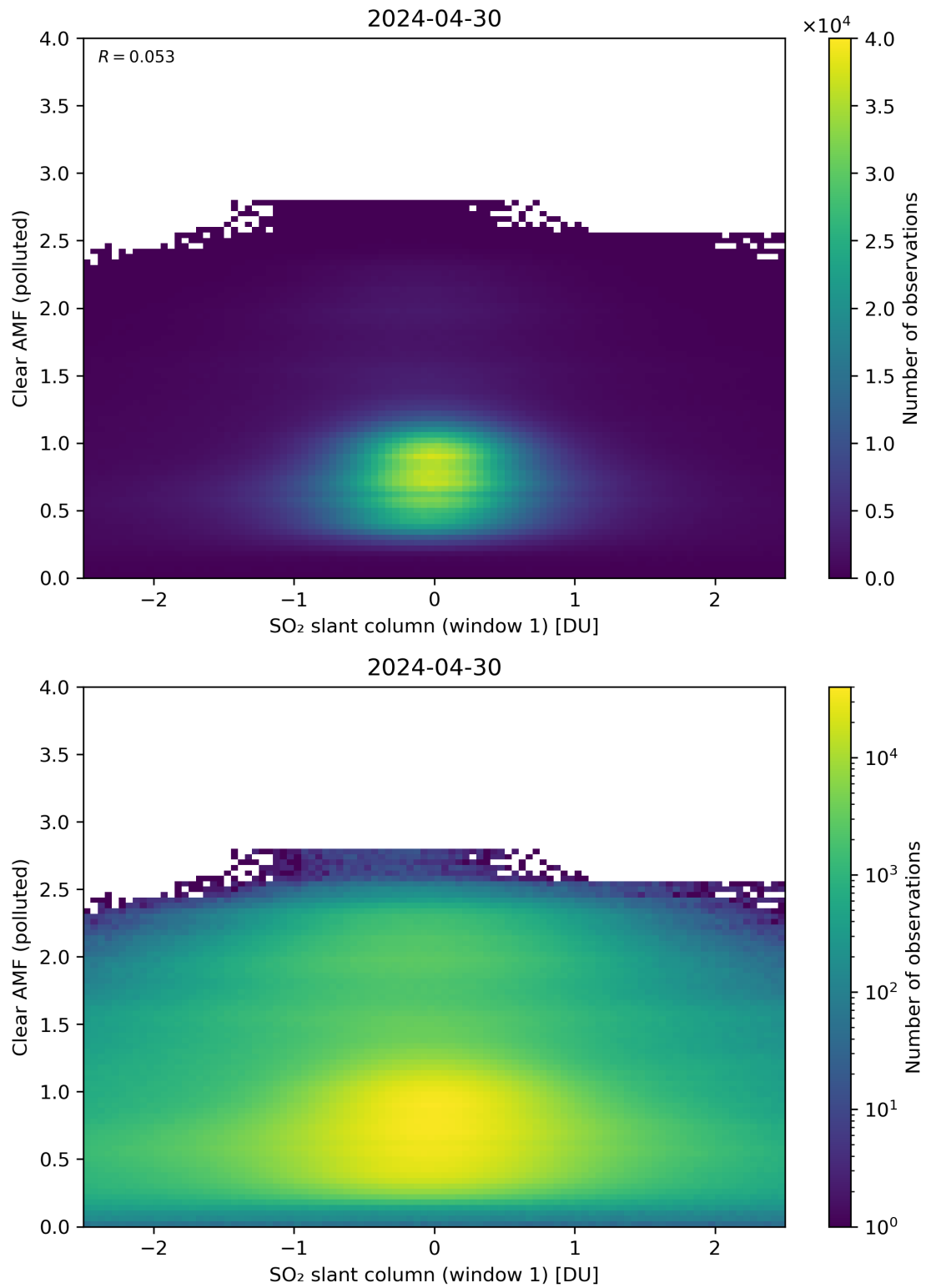
Figure 232: Scatter density plot of “SO 2 slant column (window 1)” against “Clear AMF (polluted)” for 2024-04-29 to 2024-05-01.
