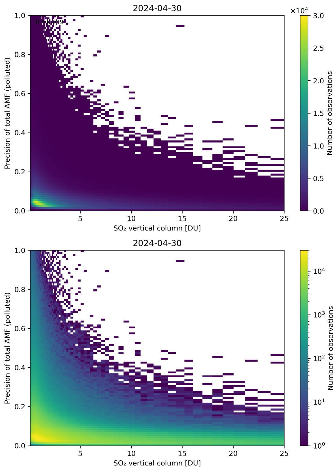
Figure 306: Scatter density plot of “SO 2 vertical column” against “Precision of total AMF (polluted)” for 2024-04-29 to 2024-05-01.
