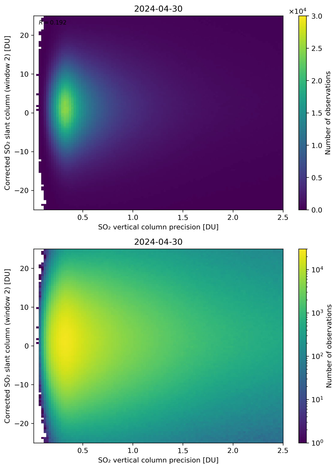
Figure 287: Scatter density plot of “SO 2 vertical column precision” against “Corrected SO 2 slant column (window 2)” for 2024-04-29 to 2024-05-01.
