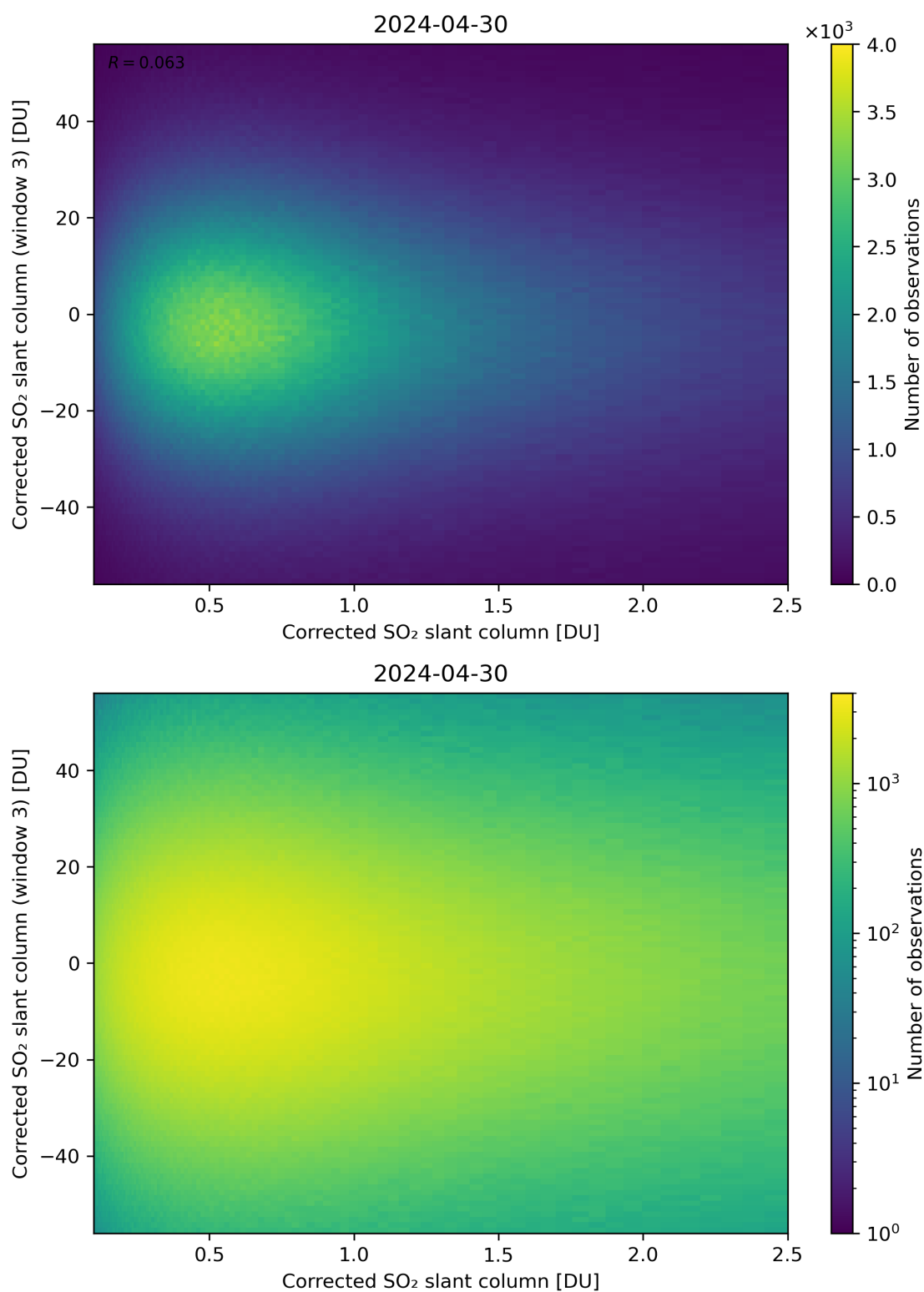
Figure 186: Scatter density plot of “Corrected SO 2 slant column” against “Corrected SO 2 slant column (window 3)” for 2024-04-29 to 2024-05-01.
