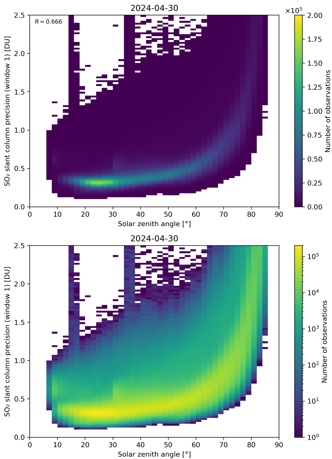
Figure 170: Scatter density plot of “Solar zenith angle” against “SO 2 slant column precision (window 1)” for 2024-04-29 to 2024-05-01.
