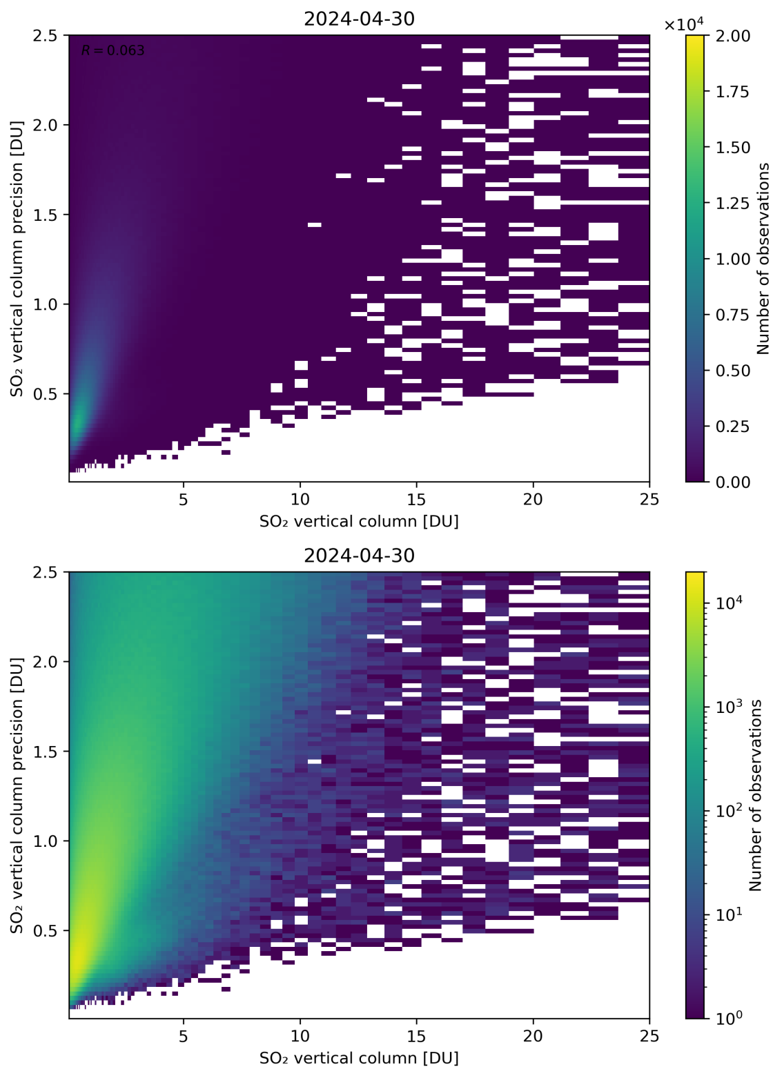
Figure 307: Scatter density plot of “SO 2 vertical column” against “SO 2 vertical column precision” for 2024-04-29 to 2024-05-01.
