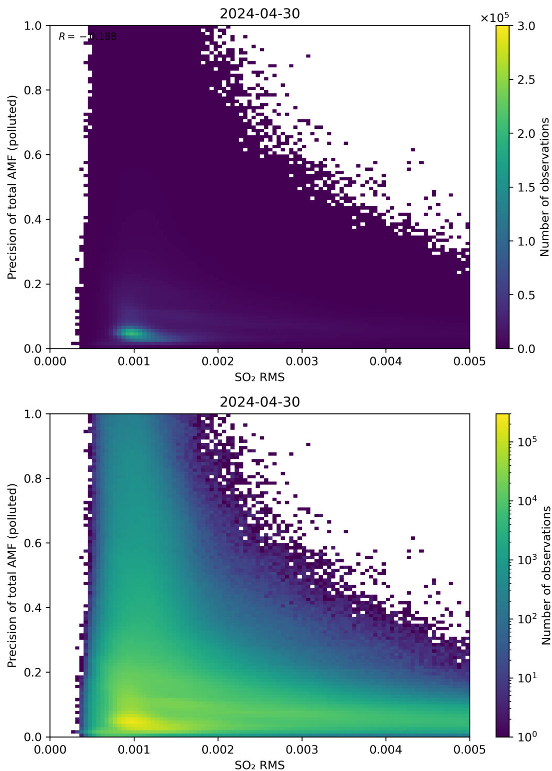
Figure 138: Scatter density plot of “SO 2 RMS” against “Precision of total AMF (polluted)” for 2024-04-29 to 2024-05-01.
