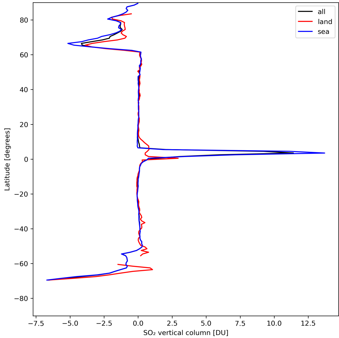
Figure 30: Zonal average of “SO 2 vertical column” for 2024-04-29 to 2024-05-01.
