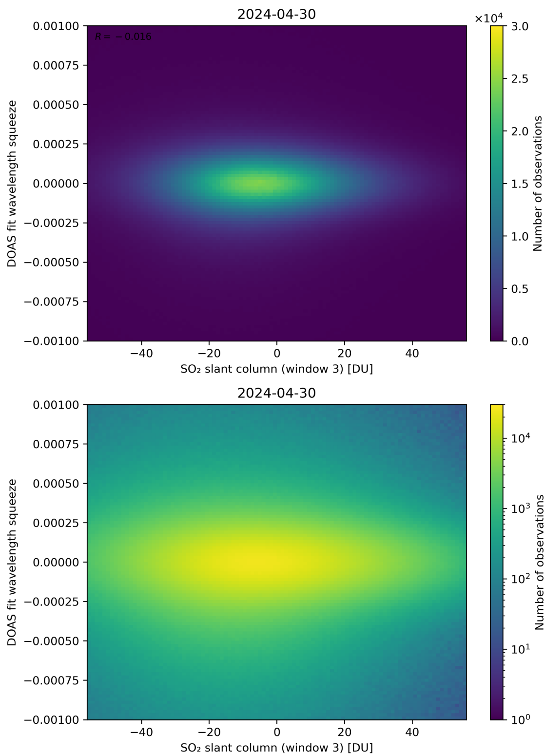
Figure 255: Scatter density plot of “SO 2 slant column (window 3)” against “DOAS fit wavelength squeeze” for 2024-04-29 to 2024-05-01.
