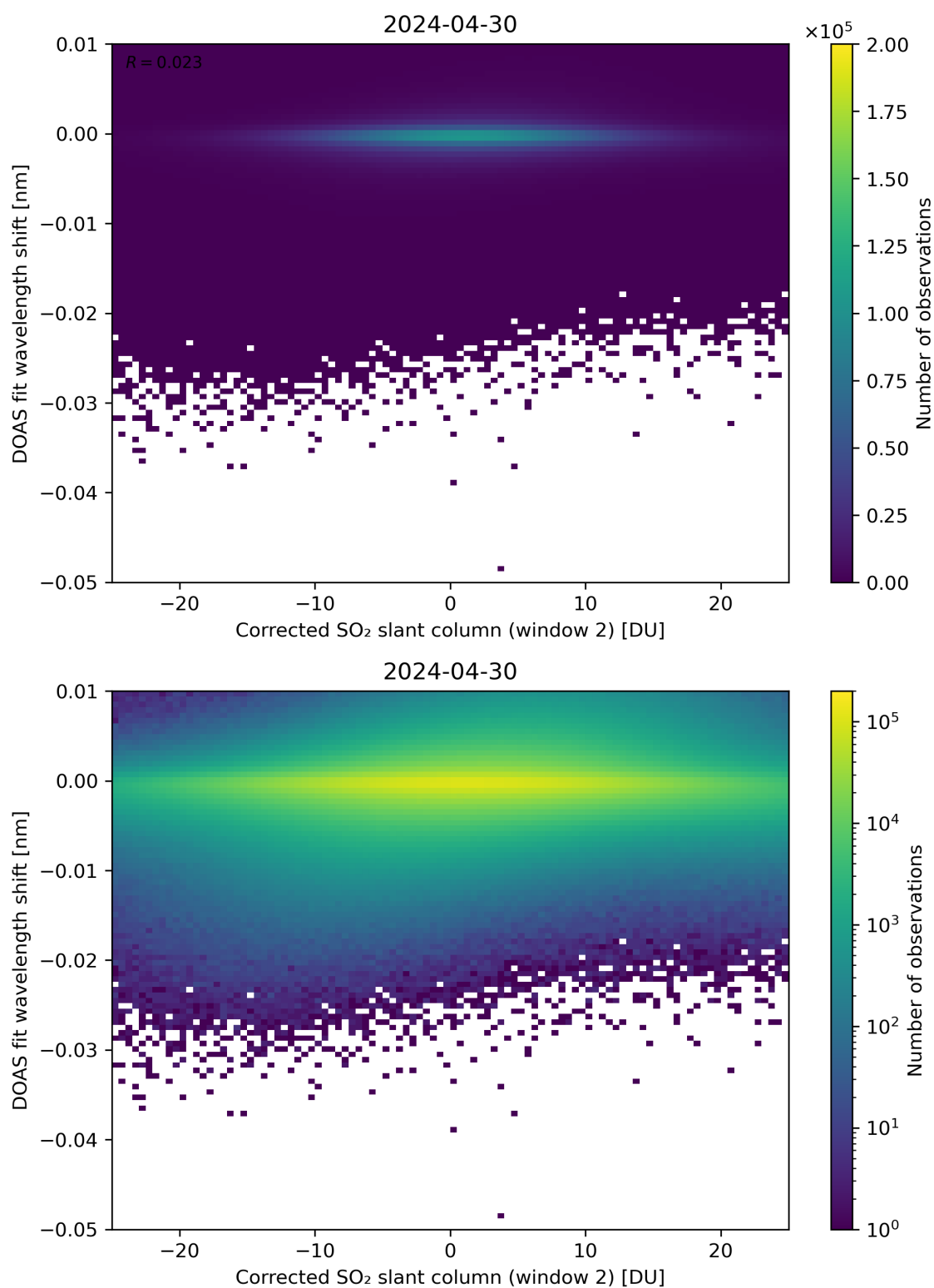
Figure 196: Scatter density plot of “Corrected SO 2 slant column (window 2)” against “DOAS fit wavelength shift” for 2024-04-29 to 2024-05-01.
