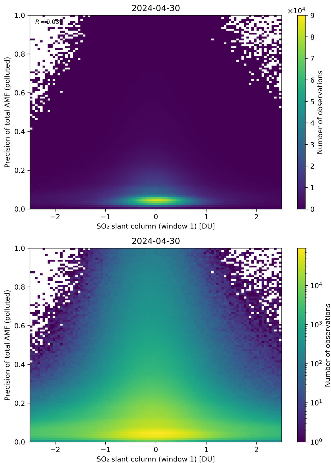
Figure 240: Scatter density plot of “SO 2 slant column (window 1)” against “Precision of total AMF (polluted)” for 2024-04-29 to 2024-05-01.
