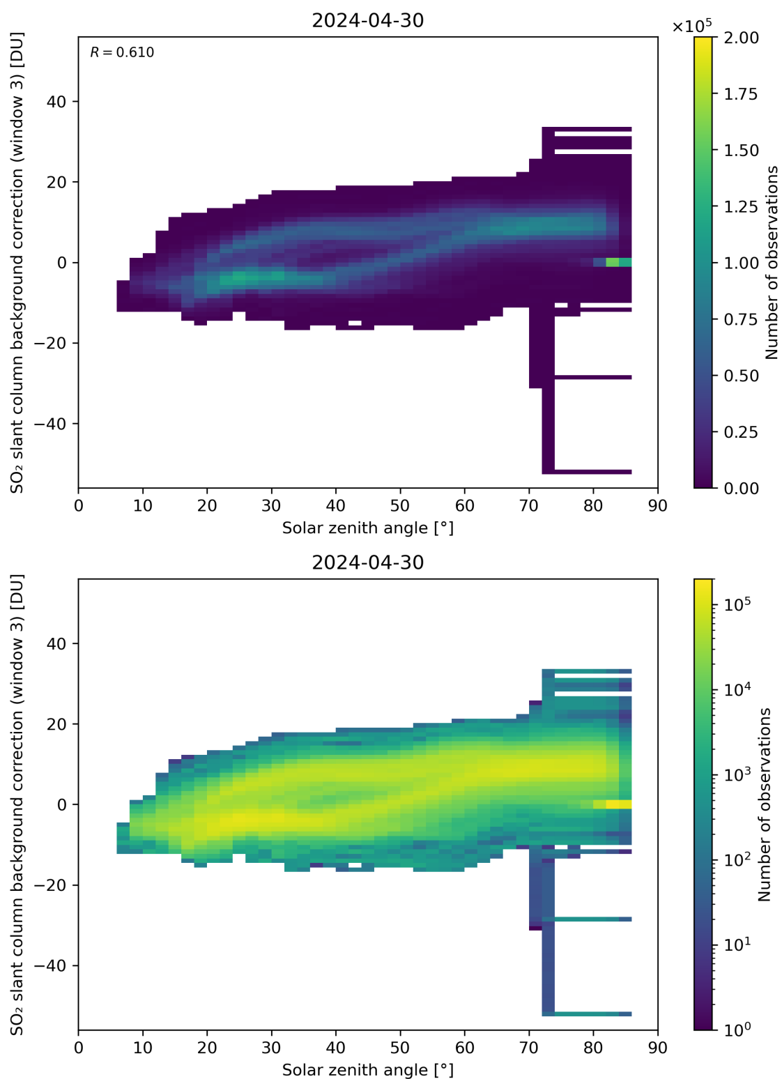
Figure 160: Scatter density plot of “Solar zenith angle” against “SO 2 slant column background correction (window 3)” for 2024-04-29 to 2024-05-01.
