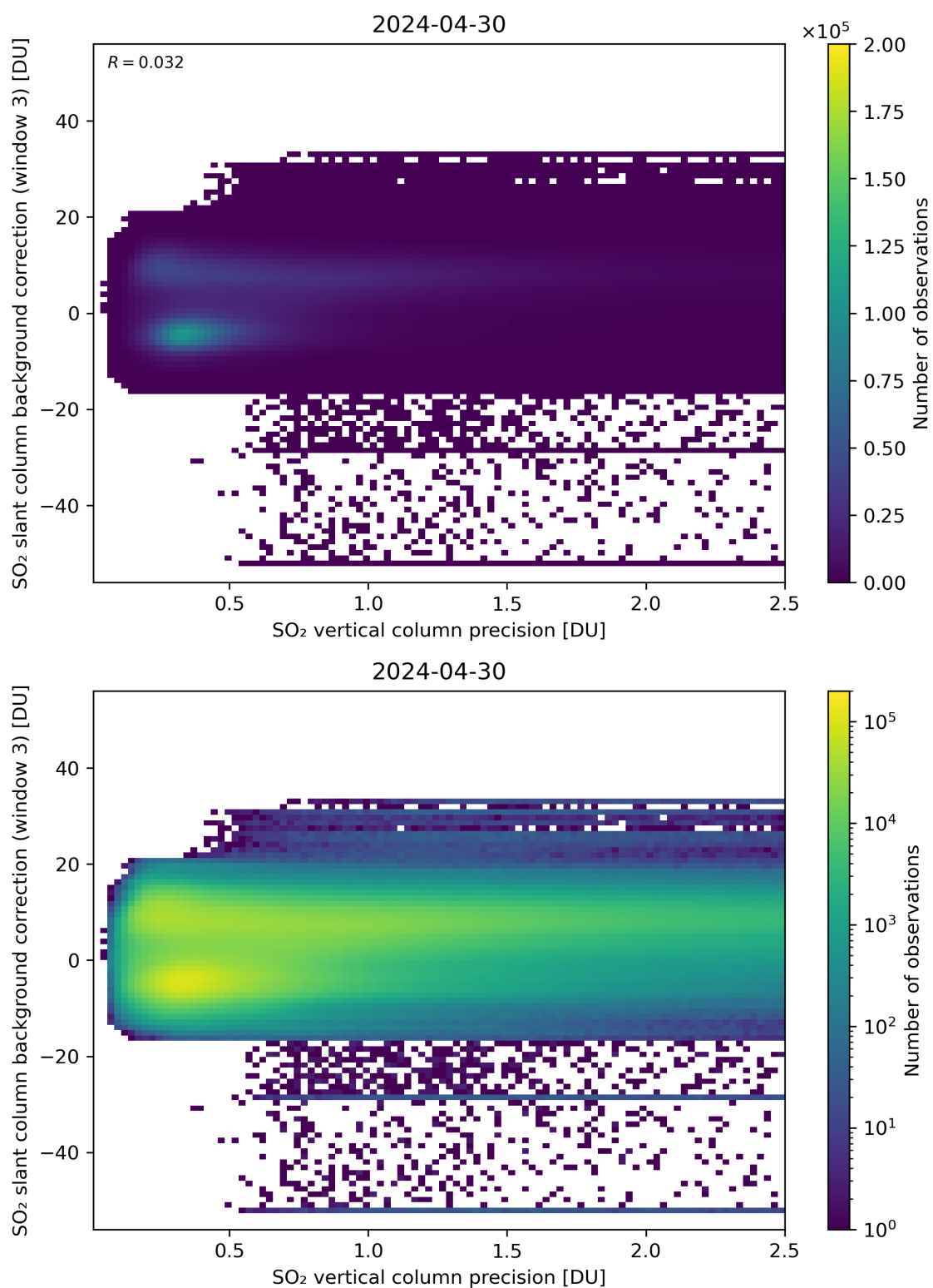
Figure 281: Scatter density plot of “SO 2 vertical column precision” against “SO 2 slant column background correction (window 3)” for 2024-04-29 to 2024-05-01.
