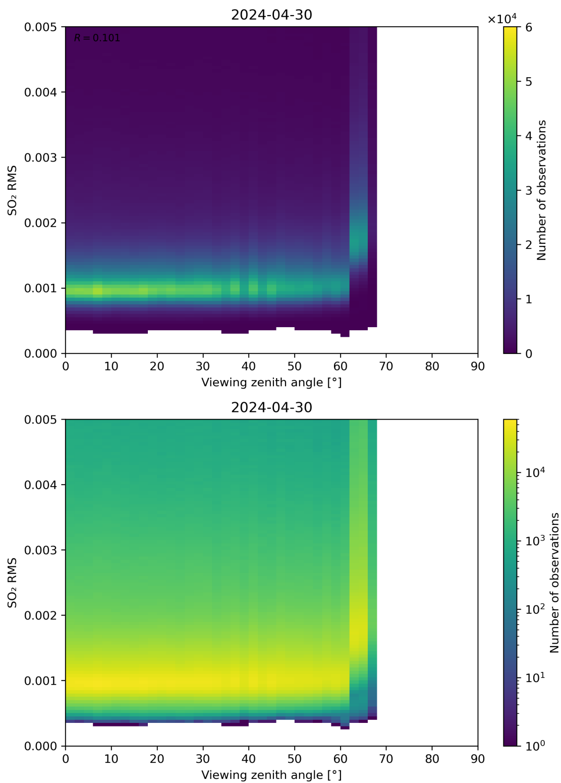
Figure 313: Scatter density plot of “Viewing zenith angle” against “SO 2 RMS” for 2024-04-29 to 2024-05-01.
