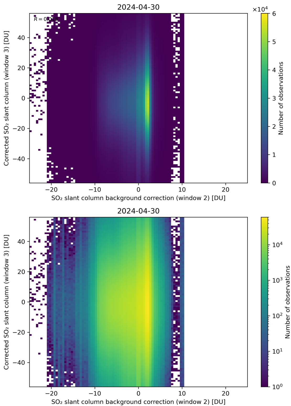
Figure 116: Scatter density plot of “SO 2 slant column background correction (window 2)” against “Corrected SO 2 slant column (window 3)” for 2024-04-29 to 2024-05-01.
