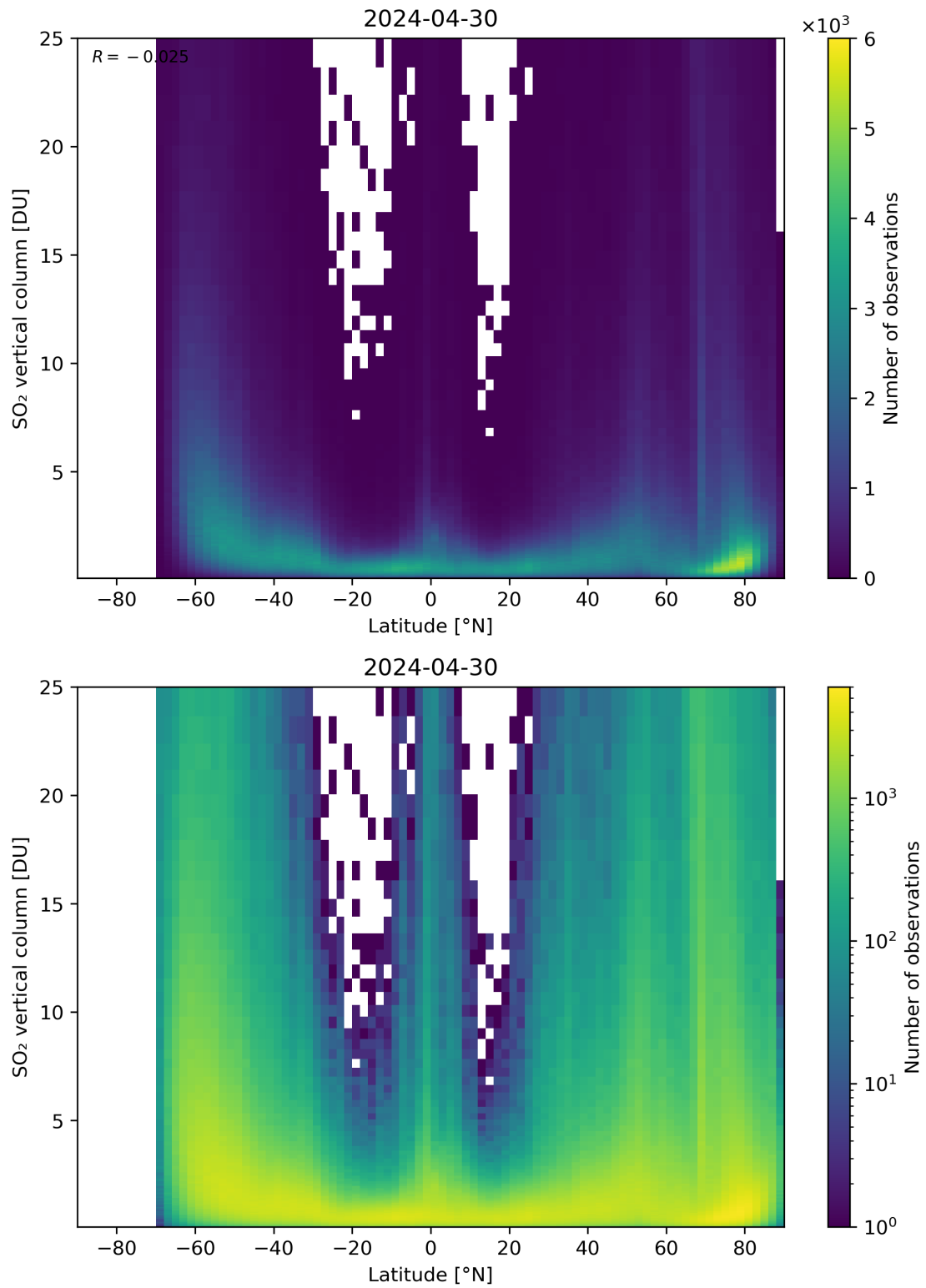
Figure 156: Scatter density plot of “Latitude” against “SO 2 vertical column” for 2024-04-29 to 2024-05-01.
