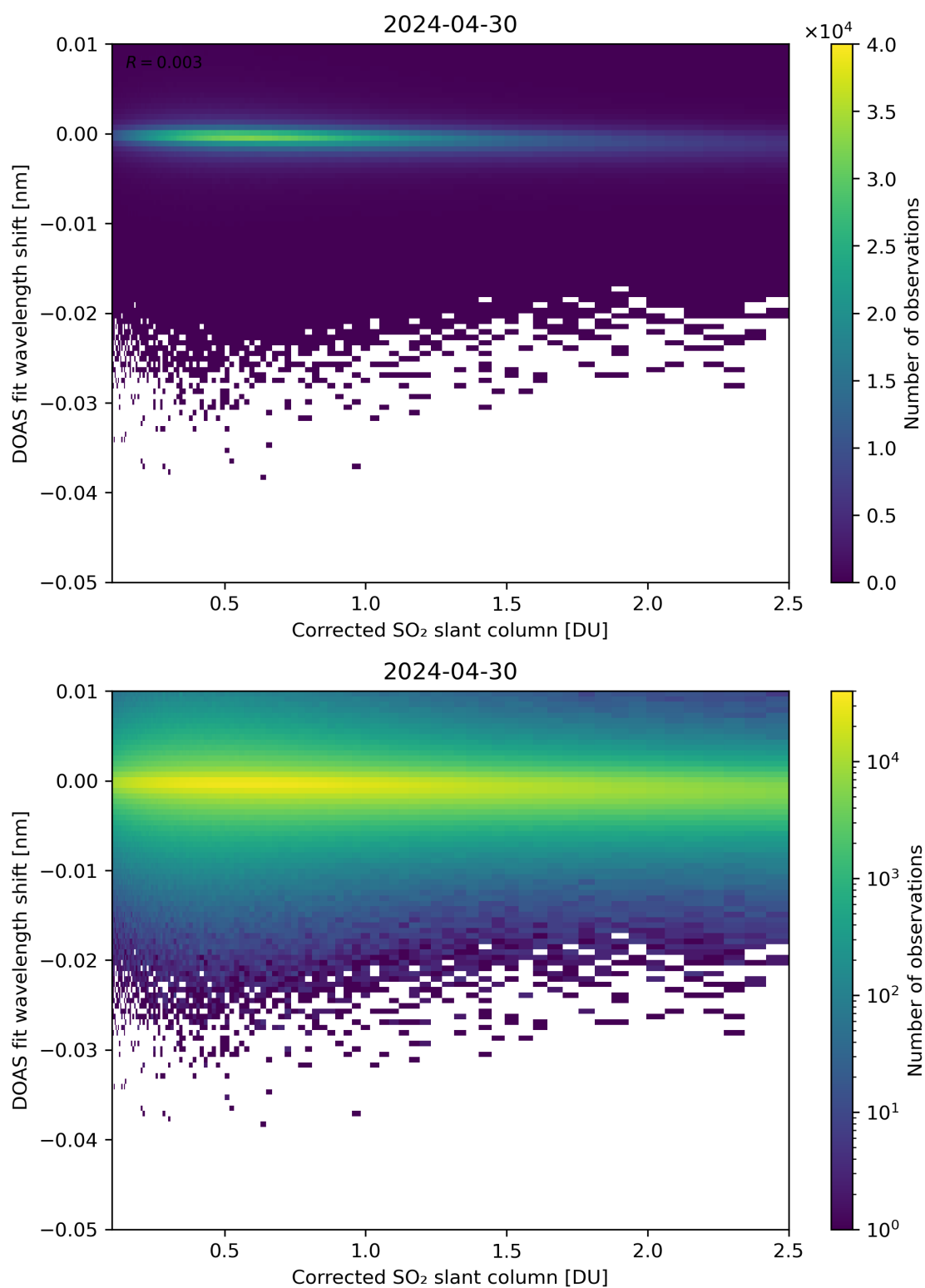
Figure 181: Scatter density plot of “Corrected SO 2 slant column” against “DOAS fit wavelength shift” for 2024-04-29 to 2024-05-01.
