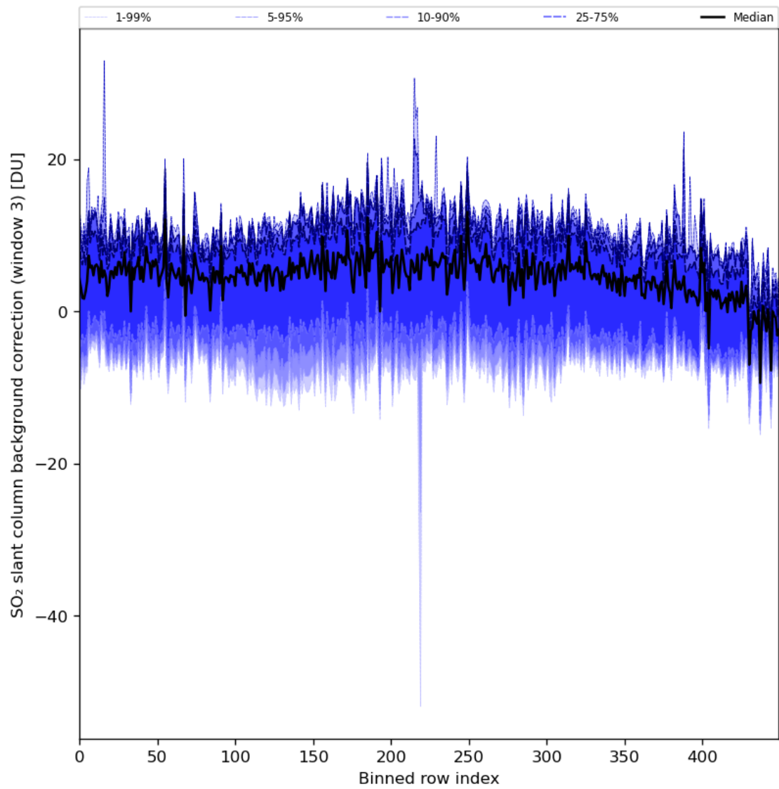
Figure 90: Along track statistics of “SO 2 slant column background correction (window 3)” for 2024-04-29 to 2024-05-01
