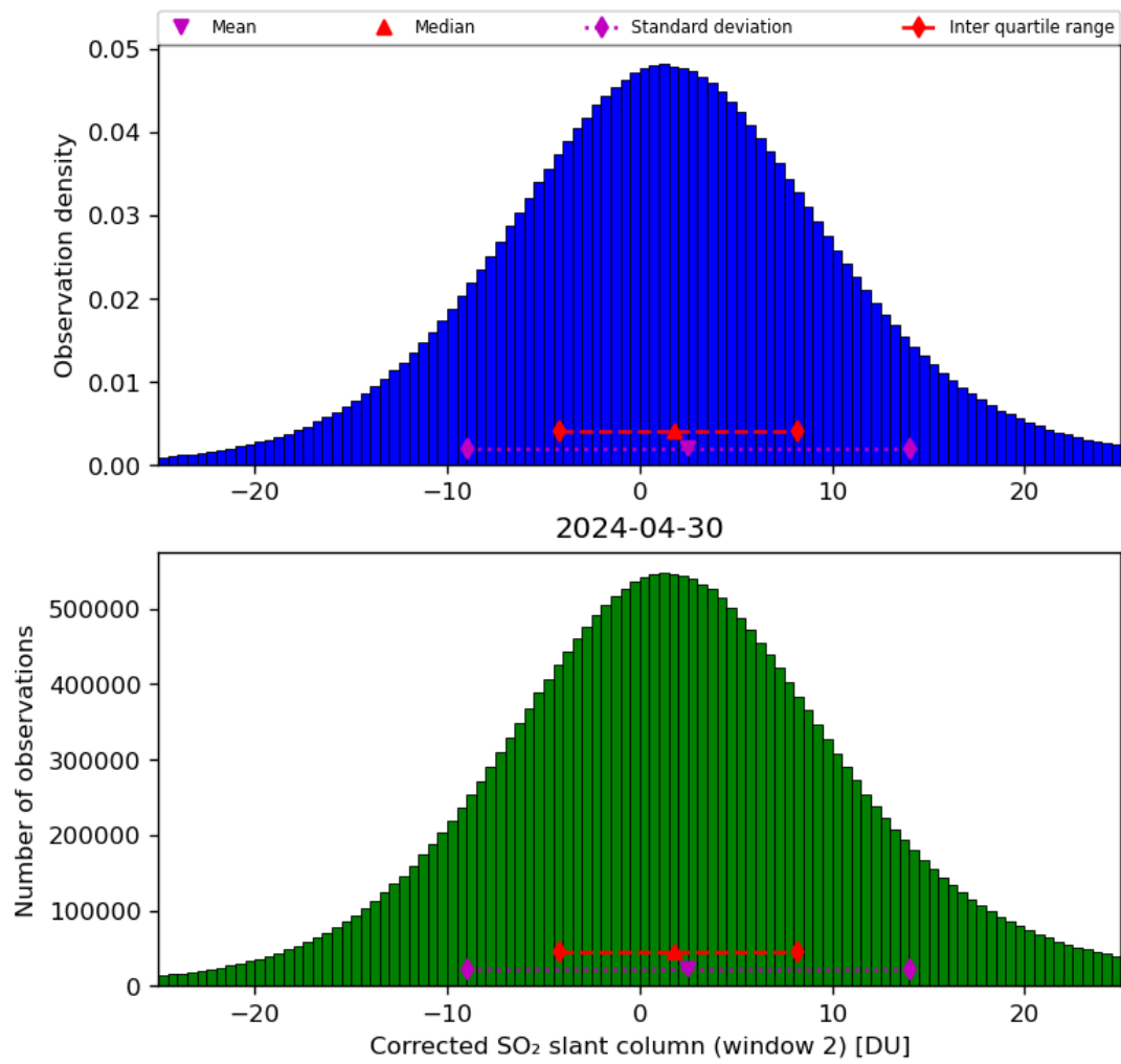
Figure 62: Histogram of “Corrected SO 2 slant column (window 2)” for 2024-04-29 to 2024-05-01
