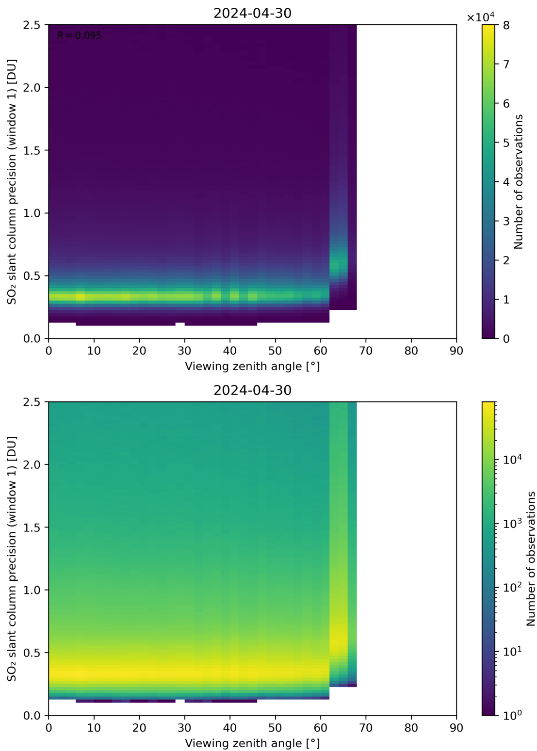
Figure 321: Scatter density plot of “Viewing zenith angle” against “SO 2 slant column precision (window 1)” for 2024-04-29 to 2024-05-01.
