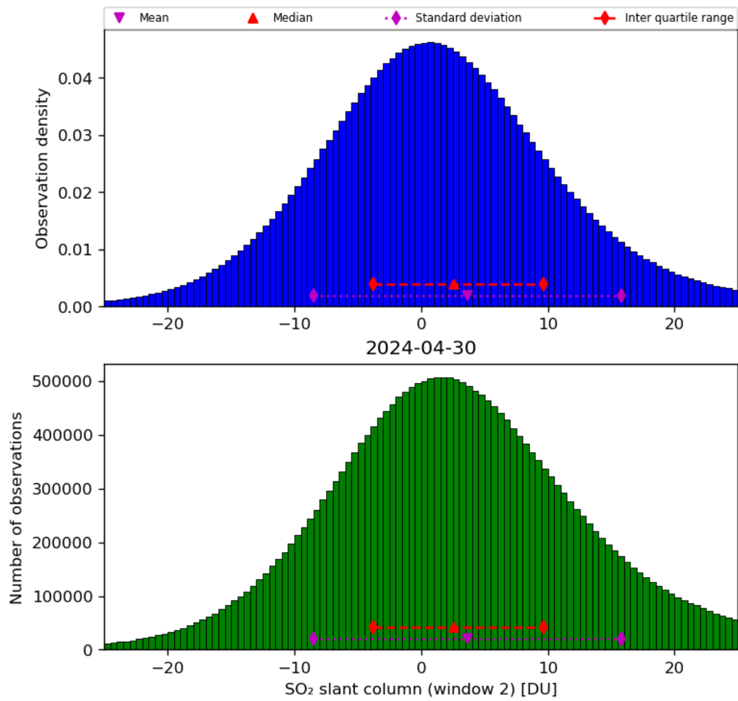
Figure 60: Histogram of “SO 2 slant column (window 2)” for 2024-04-29 to 2024-05-01
