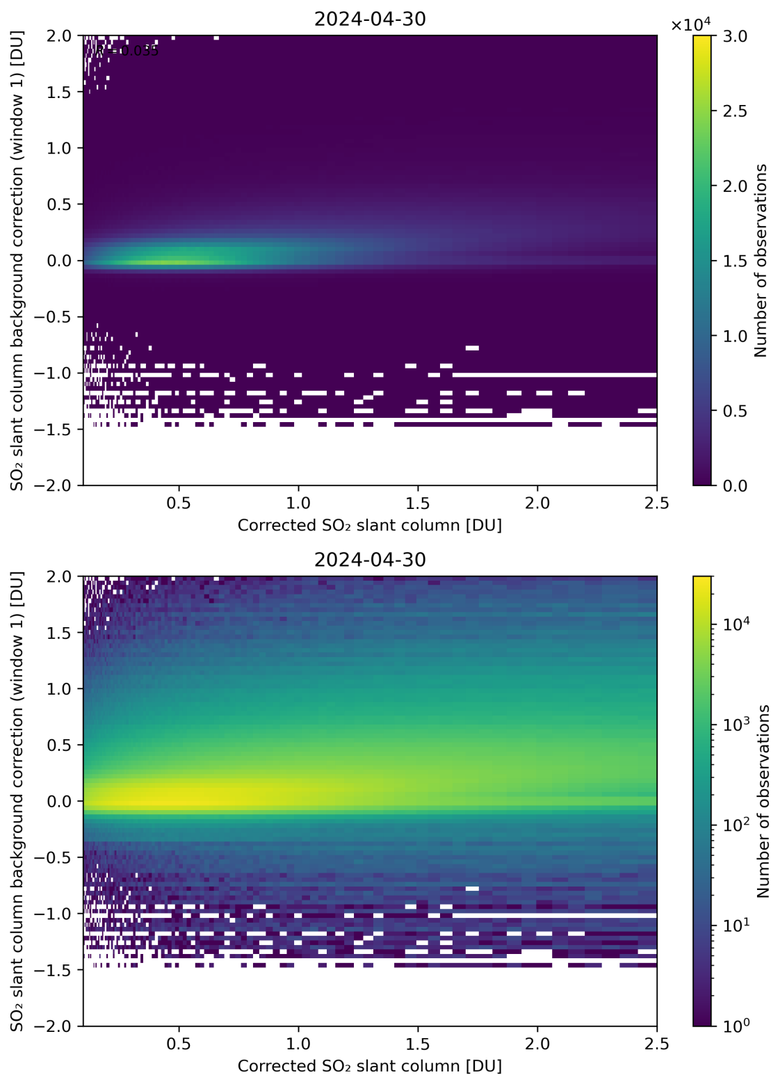
Figure 178: Scatter density plot of “Corrected SO 2 slant column” against “SO 2 slant column background correction (window 1)” for 2024-04-29 to 2024-05-01.
