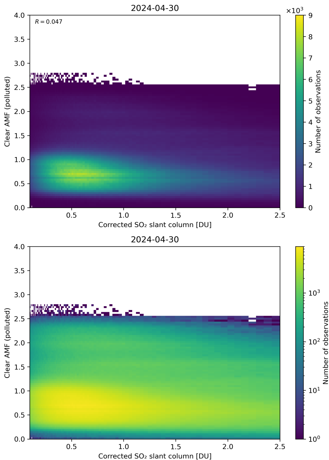
Figure 184: Scatter density plot of “Corrected SO 2 slant column” against “Clear AMF (polluted)” for 2024-04-29 to 2024-05-01.
