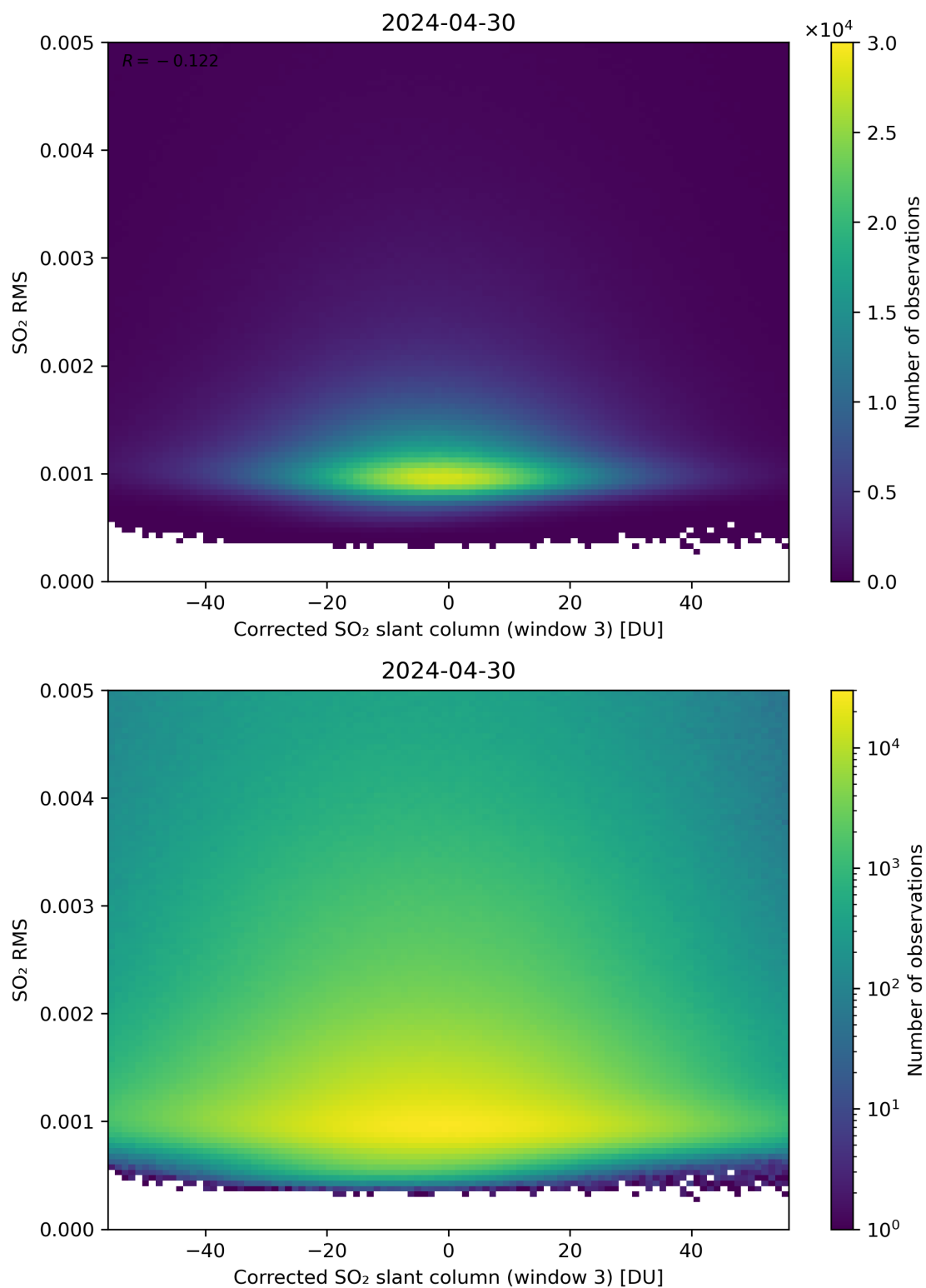
Figure 208: Scatter density plot of “Corrected SO 2 slant column (window 3)” against “SO 2 RMS” for 2024-04-29 to 2024-05-01.
