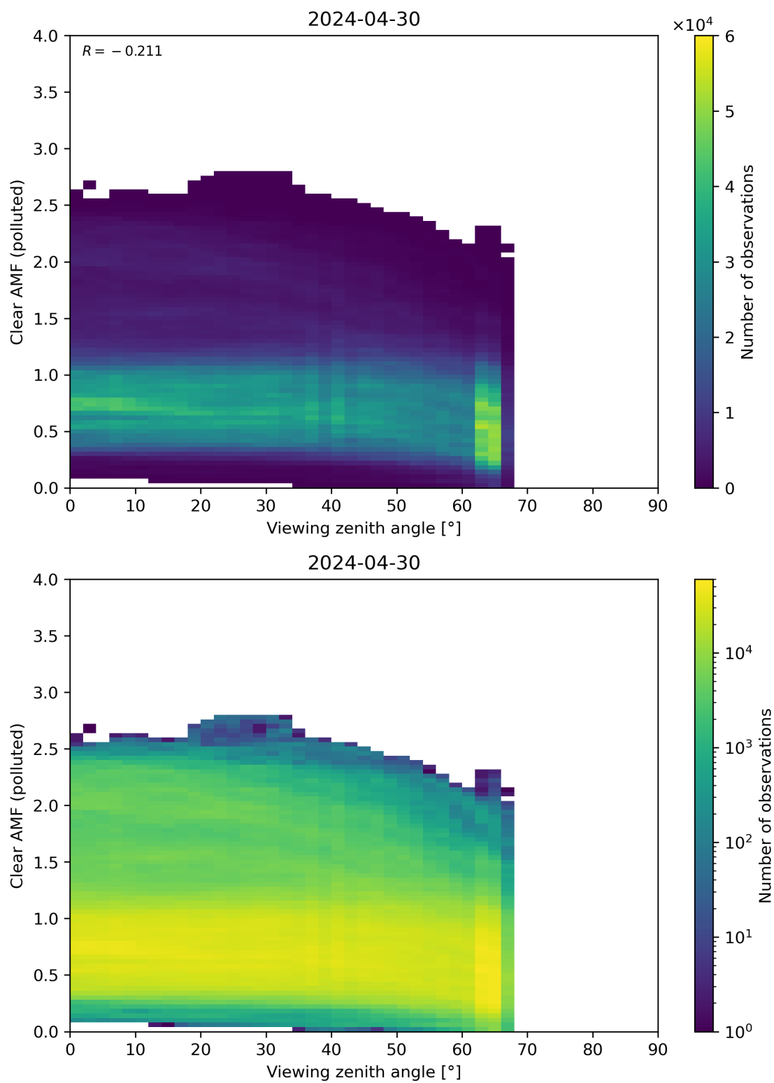
Figure 316: Scatter density plot of “Viewing zenith angle” against “Clear AMF (polluted)” for 2024-04-29 to 2024-05-01.
