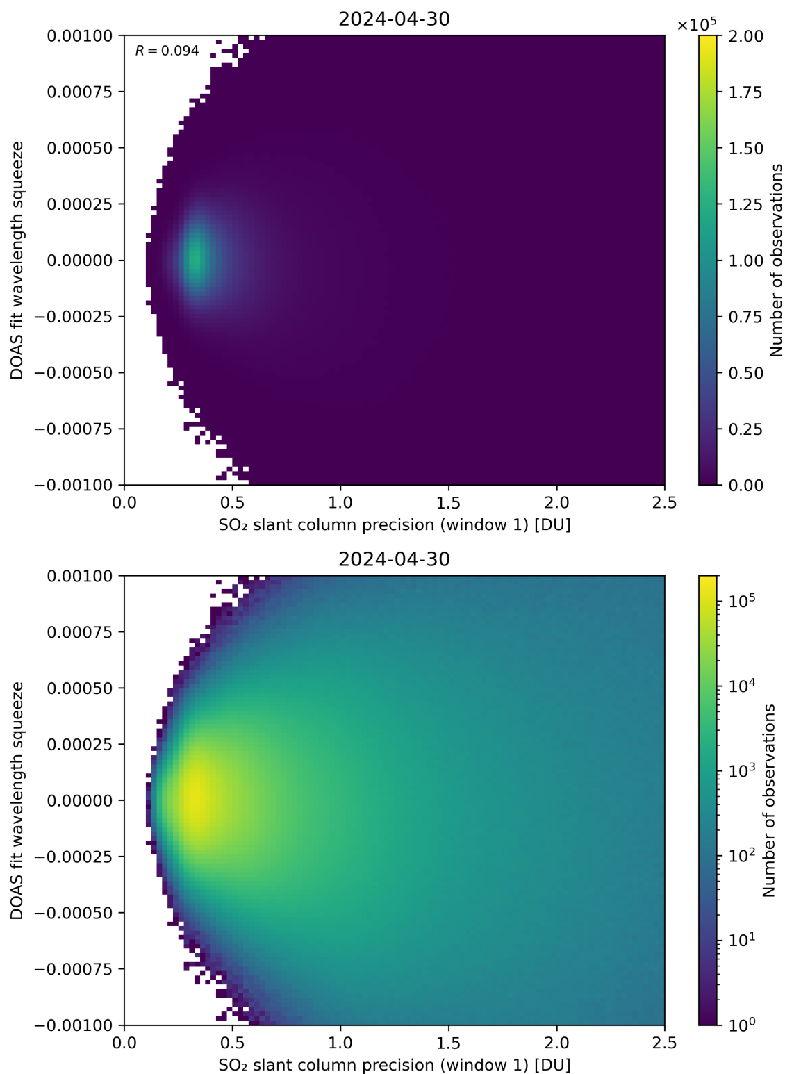
Figure 222: Scatter density plot of “SO 2 slant column precision (window 1)” against “DOAS fit wavelength squeeze” for 2024-04-29 to 2024-05-01.
