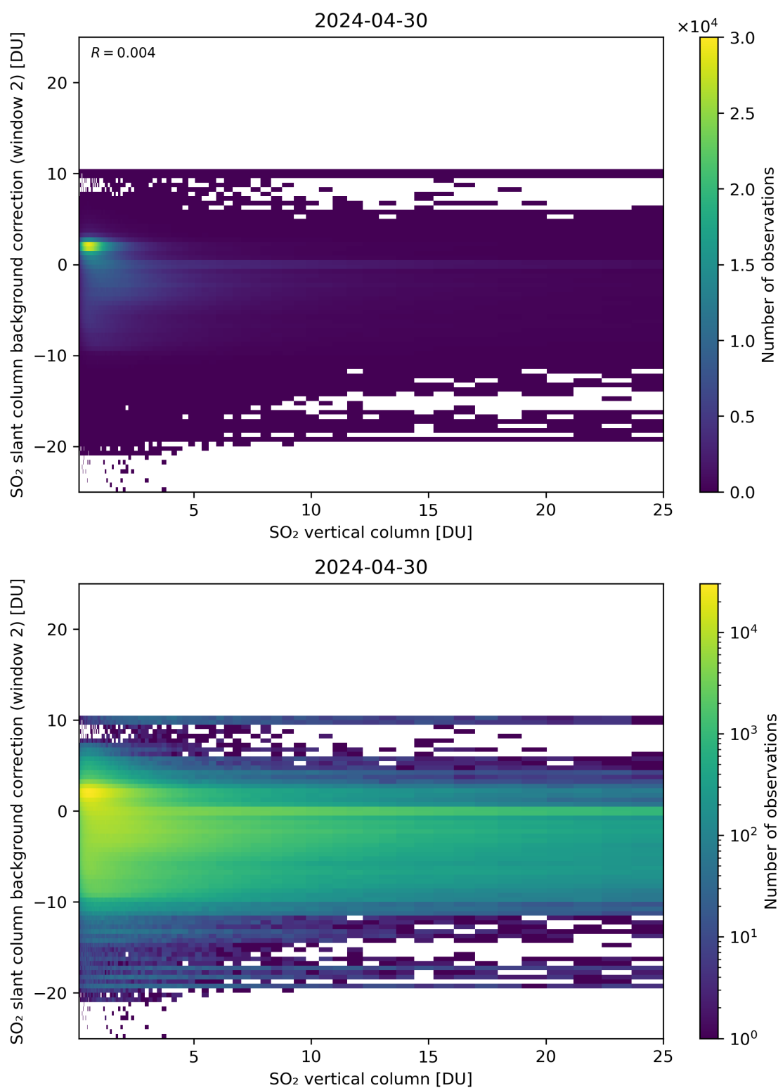
Figure 274: Scatter density plot of “SO 2 vertical column” against “SO 2 slant column background correction (window 2)” for 2024-04-29 to 2024-05-01.
