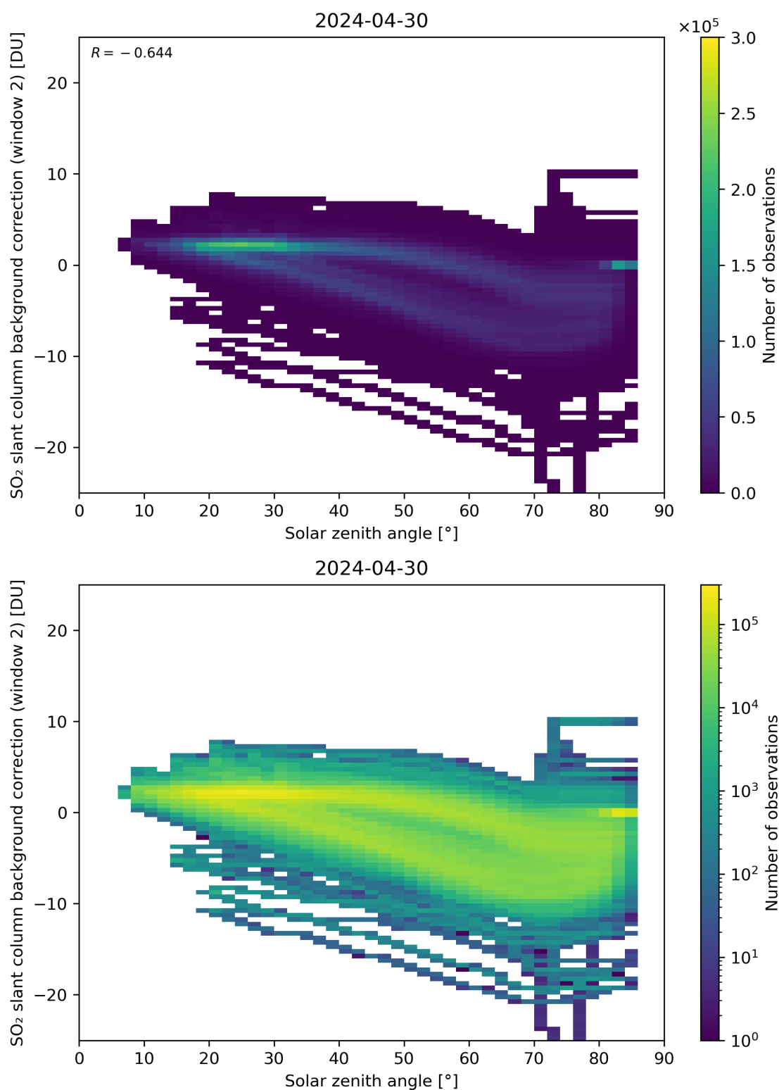
Figure 159: Scatter density plot of “Solar zenith angle” against “SO 2 slant column background correction (window 2)” for 2024-04-29 to 2024-05-01.
