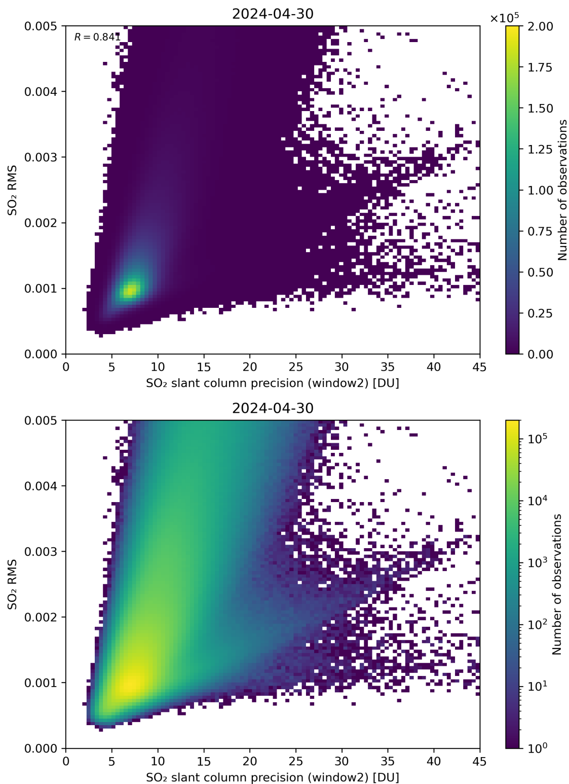
Figure 245: Scatter density plot of “SO 2 slant column precision (window2)” against “SO 2 RMS” for 2024-04-29 to 2024-05-01.
