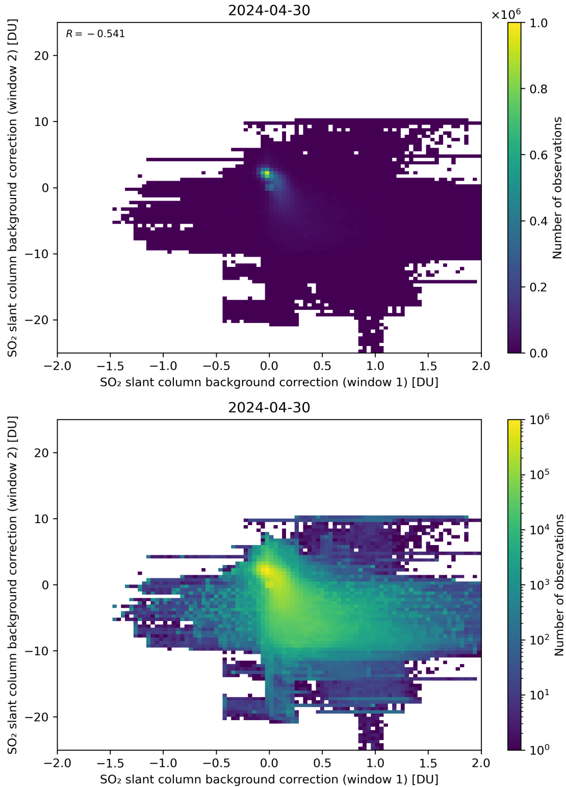
Figure 98: Scatter density plot of “SO 2 slant column background correction (window 1)” against “SO 2 slant column background correction (window 2)” for 2024-04-29 to 2024-05-01.
