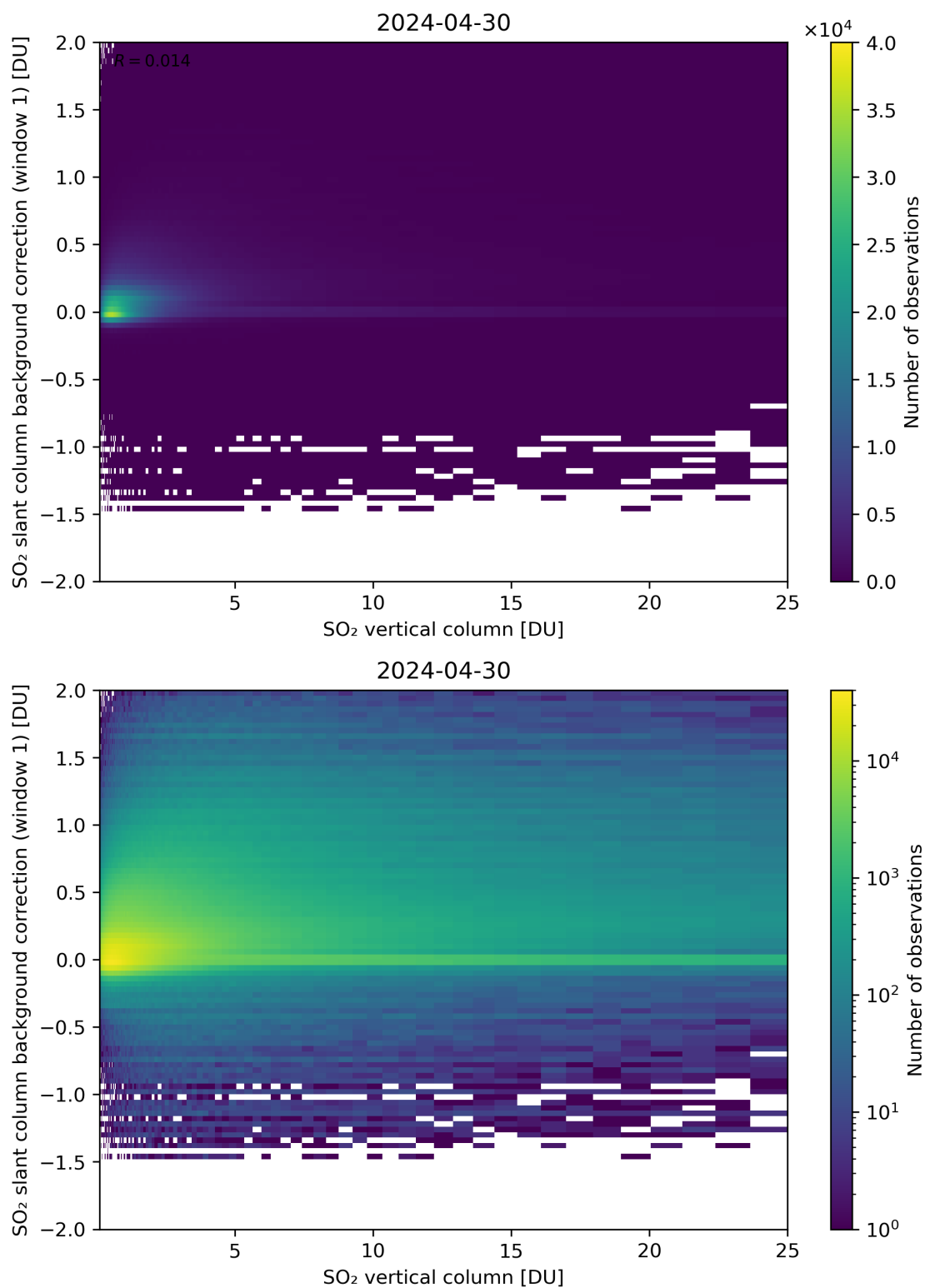
Figure 273: Scatter density plot of “SO 2 vertical column” against “SO 2 slant column background correction (window 1)” for 2024-04-29 to 2024-05-01.
