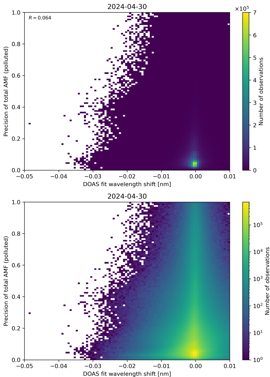
Figure 131: Scatter density plot of “DOAS fit wavelength shift” against “Precision of total AMF (polluted)” for 2024-04-29 to 2024-05-01.
