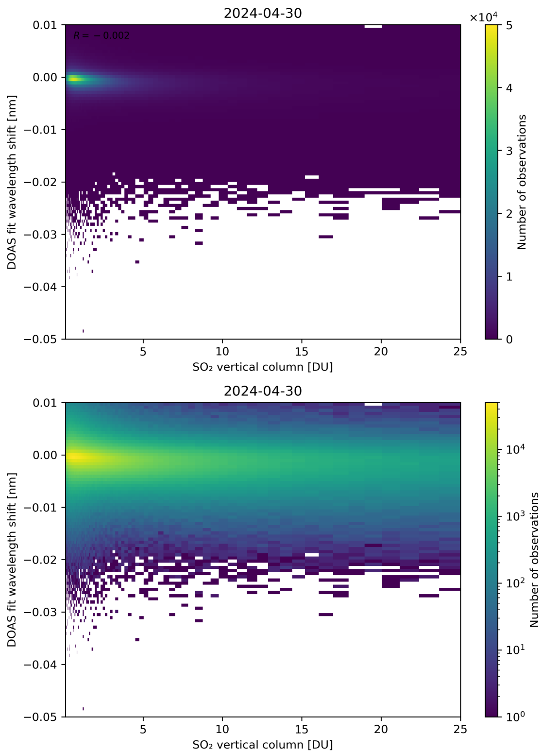
Figure 276: Scatter density plot of “SO 2 vertical column” against “DOAS fit wavelength shift” for 2024-04-29 to 2024-05-01.
