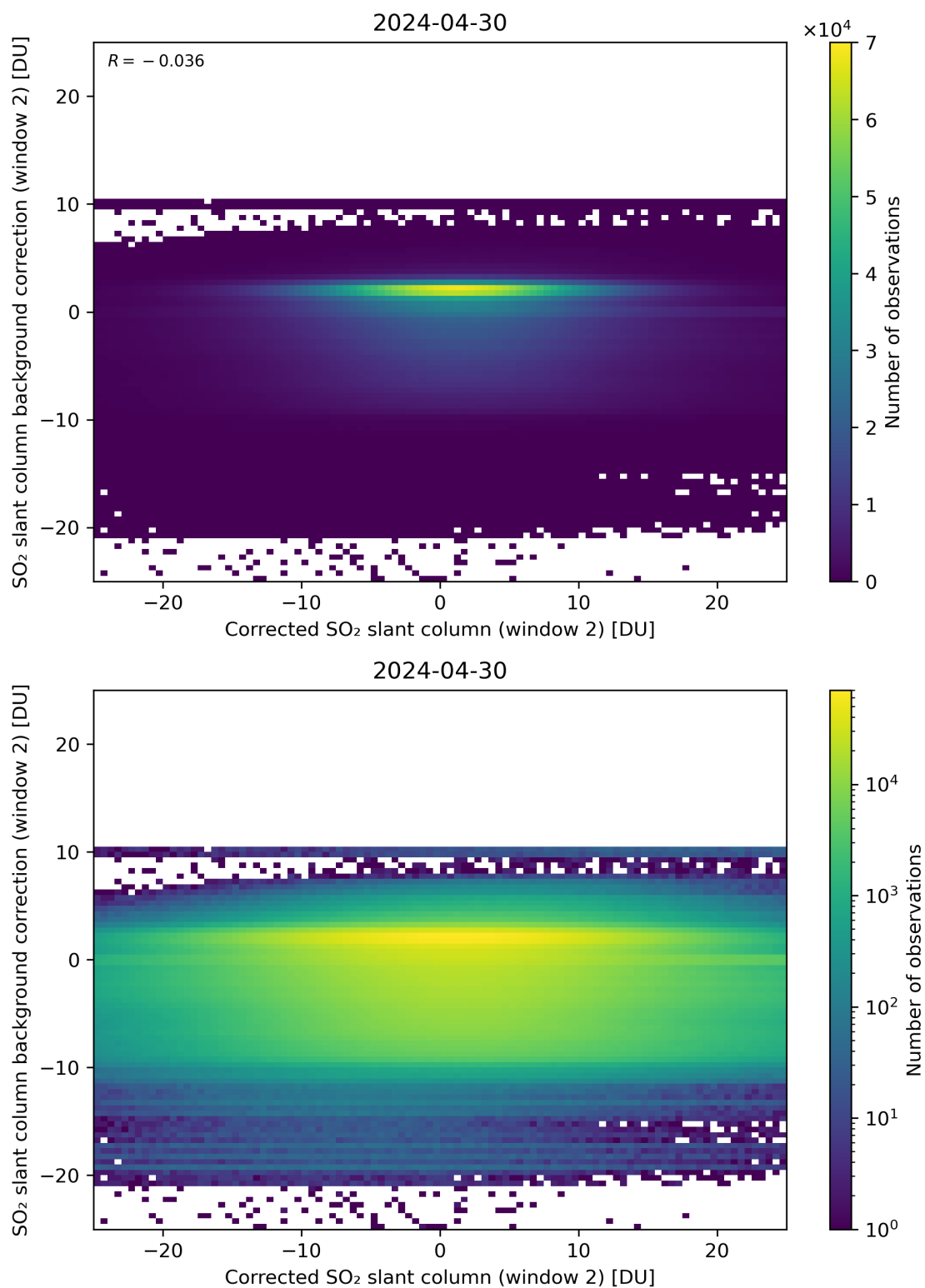
Figure 194: Scatter density plot of “Corrected SO 2 slant column (window 2)” against “SO 2 slant column background correction (window 2)” for 2024-04-29 to 2024-05-01.
