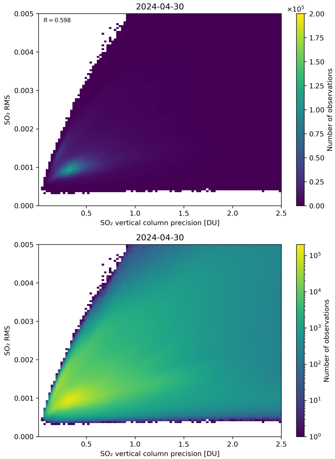
Figure 284: Scatter density plot of “SO 2 vertical column precision” against “SO 2 RMS” for 2024-04-29 to 2024-05-01.
