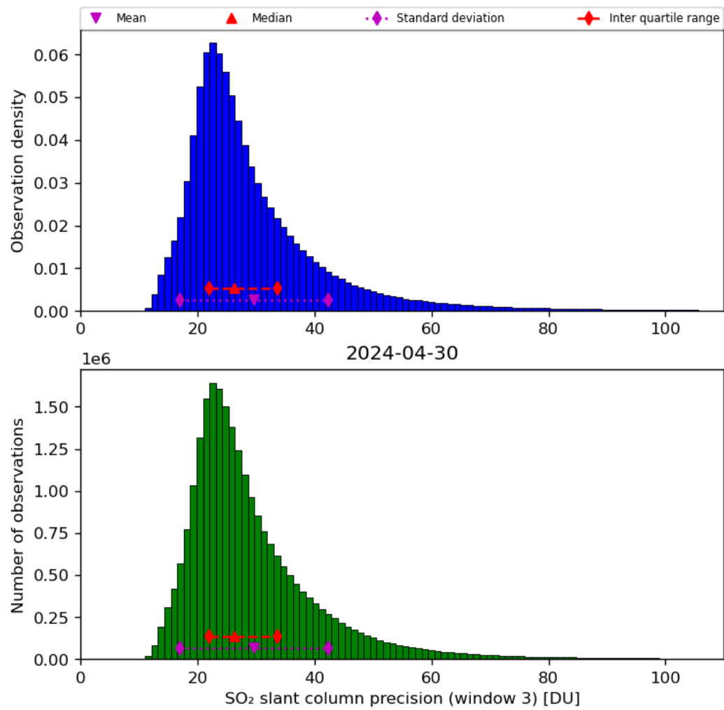
Figure 65: Histogram of “SO 2 slant column precision (window 3)” for 2024-04-29 to 2024-05-01
