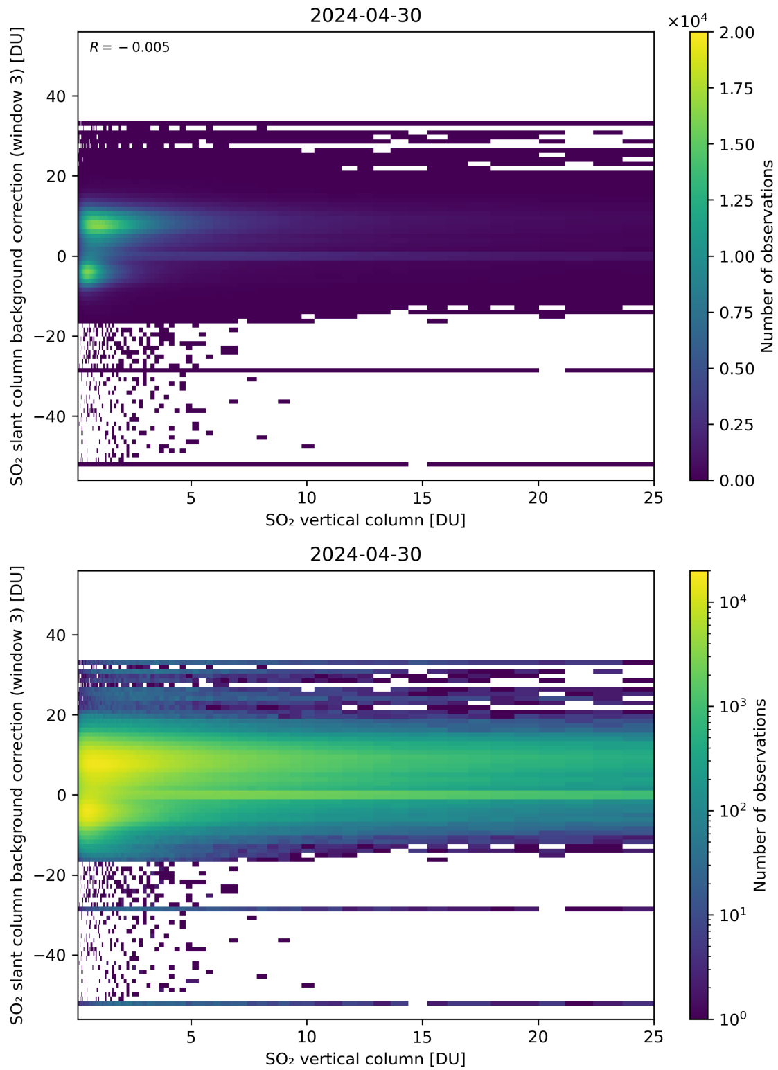
Figure 275: Scatter density plot of “SO 2 vertical column” against “SO 2 slant column background correction (window 3)” for 2024-04-29 to 2024-05-01.
