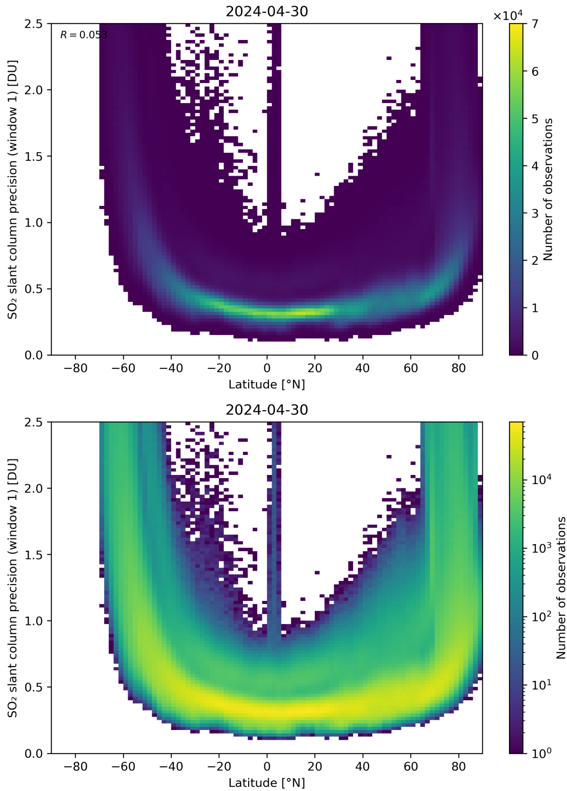
Figure 150: Scatter density plot of “Latitude” against “SO 2 slant column precision (window 1)” for 2024-04-29 to 2024-05-01.
