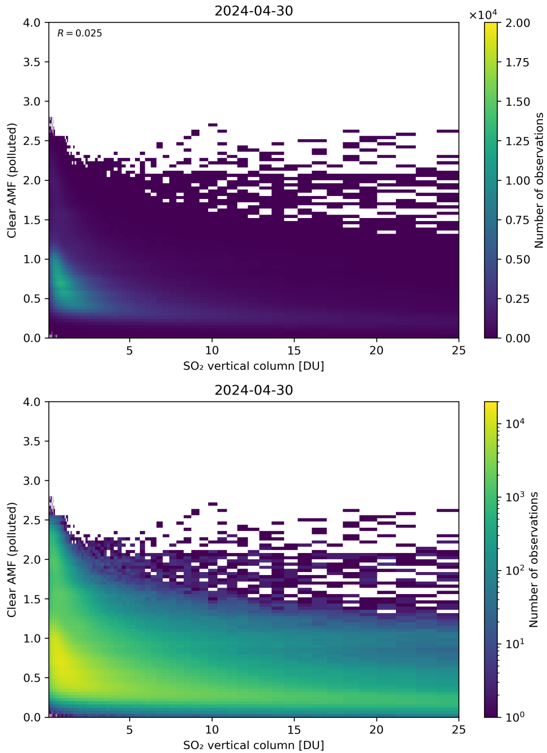
Figure 296: Scatter density plot of “SO 2 vertical column” against “Clear AMF (polluted)” for 2024-04-29 to 2024-05-01.
