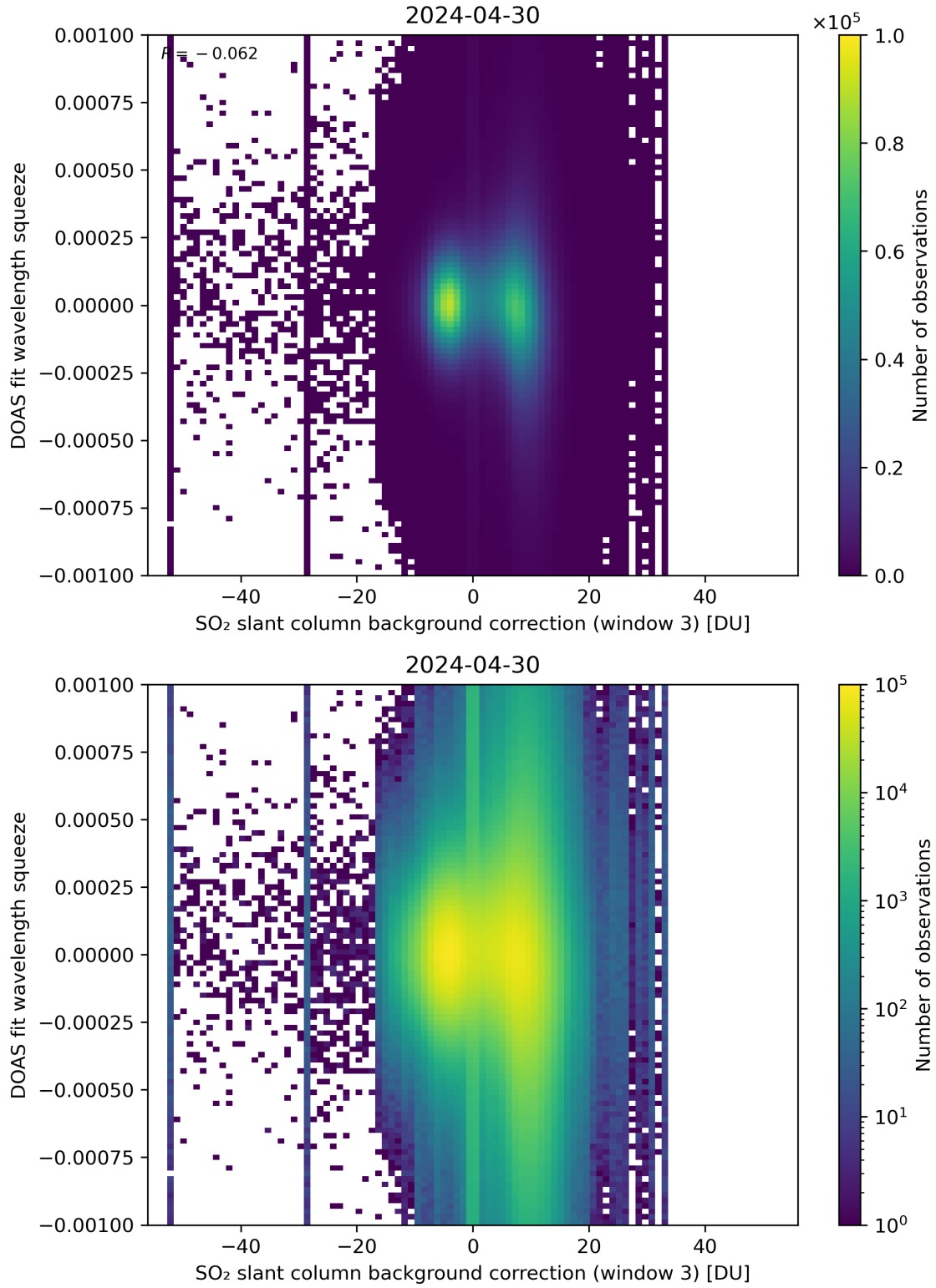
Figure 122: Scatter density plot of “SO 2 slant column background correction (window 3)” against “DOAS fit wavelength squeeze” for 2024-04-29 to 2024-05-01.
