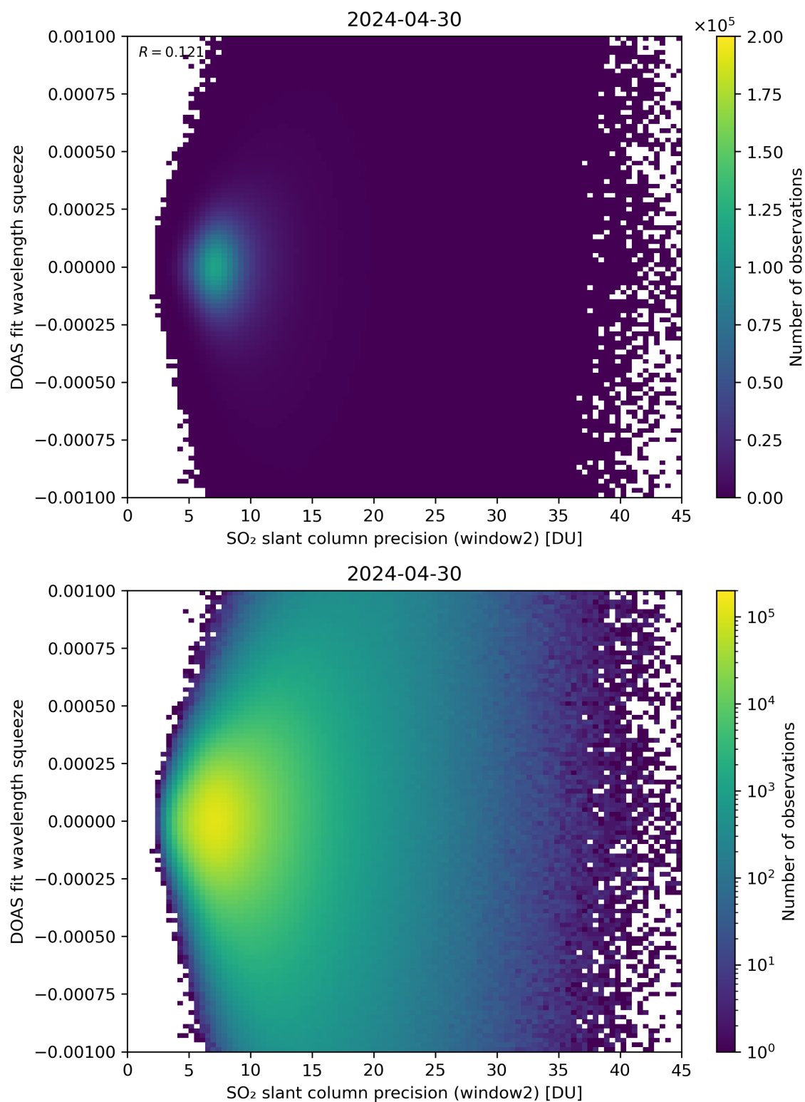
Figure 244: Scatter density plot of “SO 2 slant column precision (window2)” against “DOAS fit wavelength squeeze” for 2024-04-29 to 2024-05-01.
