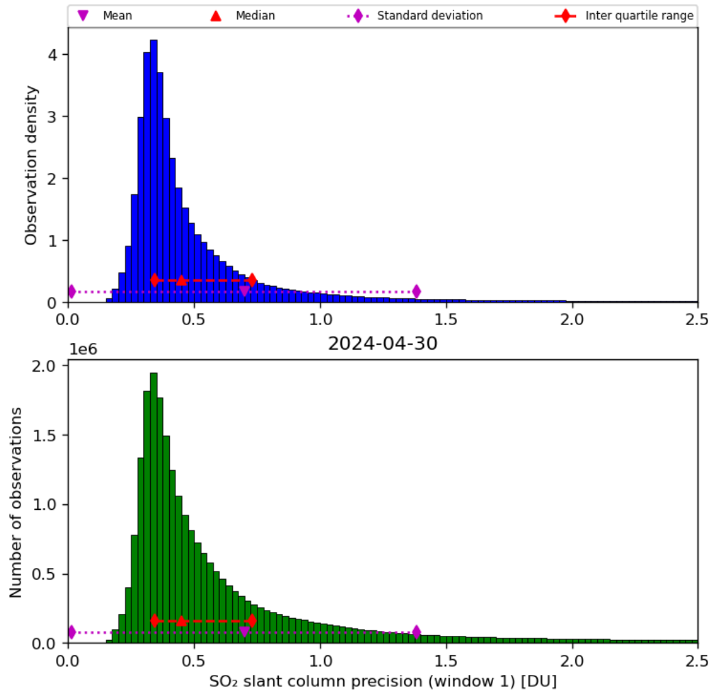
Figure 57: Histogram of “SO 2 slant column precision (window 1)” for 2024-04-29 to 2024-05-01
