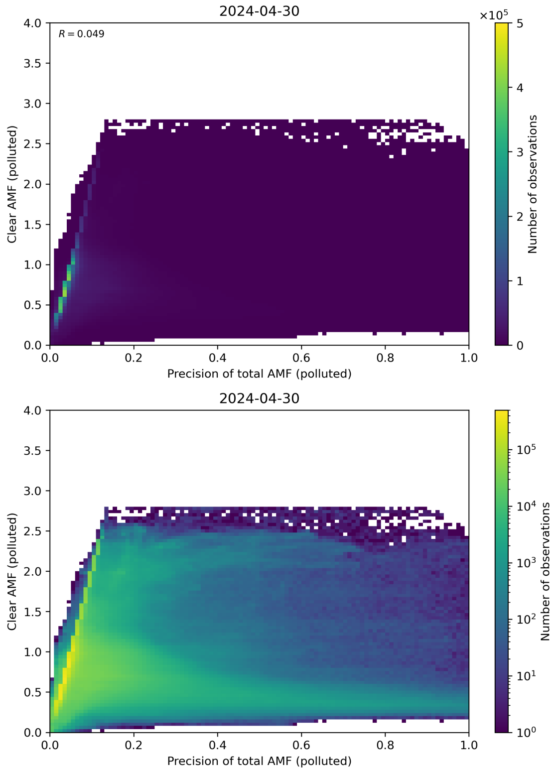
Figure 270: Scatter density plot of “Precision of total AMF (polluted)” against “Clear AMF (polluted)” for 2024-04-29 to 2024-05-01.
