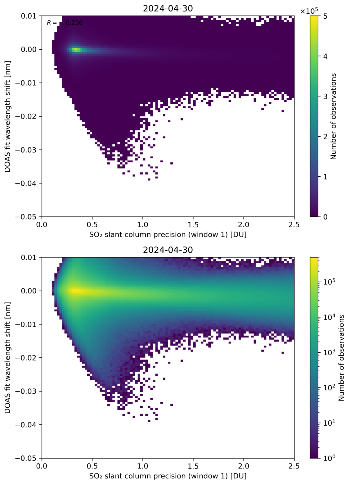
Figure 221: Scatter density plot of “SO 2 slant column precision (window 1)” against “DOAS fit wavelength shift” for 2024-04-29 to 2024-05-01.
