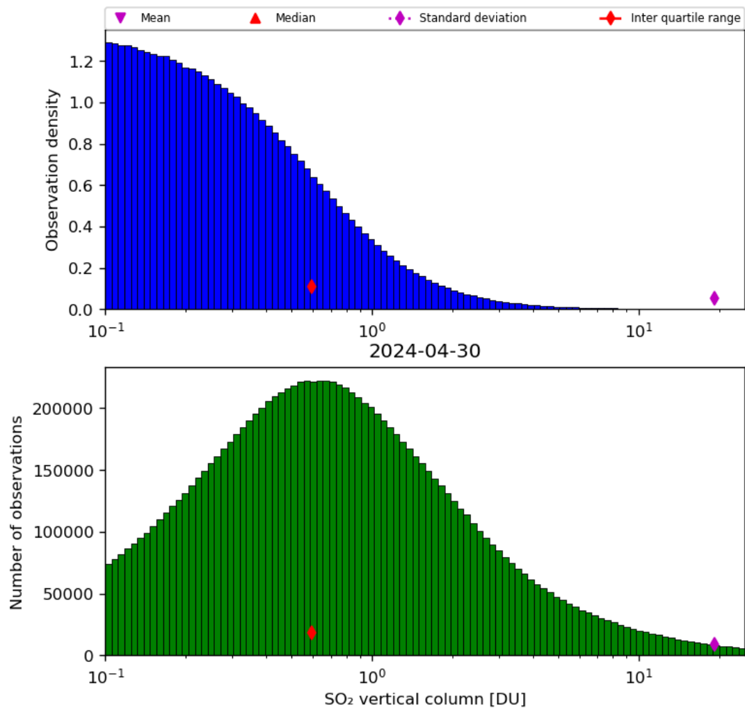
Figure 53: Histogram of “SO 2 vertical column” for 2024-04-29 to 2024-05-01
