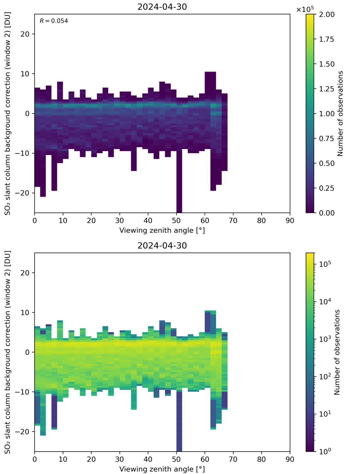
Figure 309: Scatter density plot of “Viewing zenith angle” against “SO 2 slant column background correction (window 2)” for 2024-04-29 to 2024-05-01.
