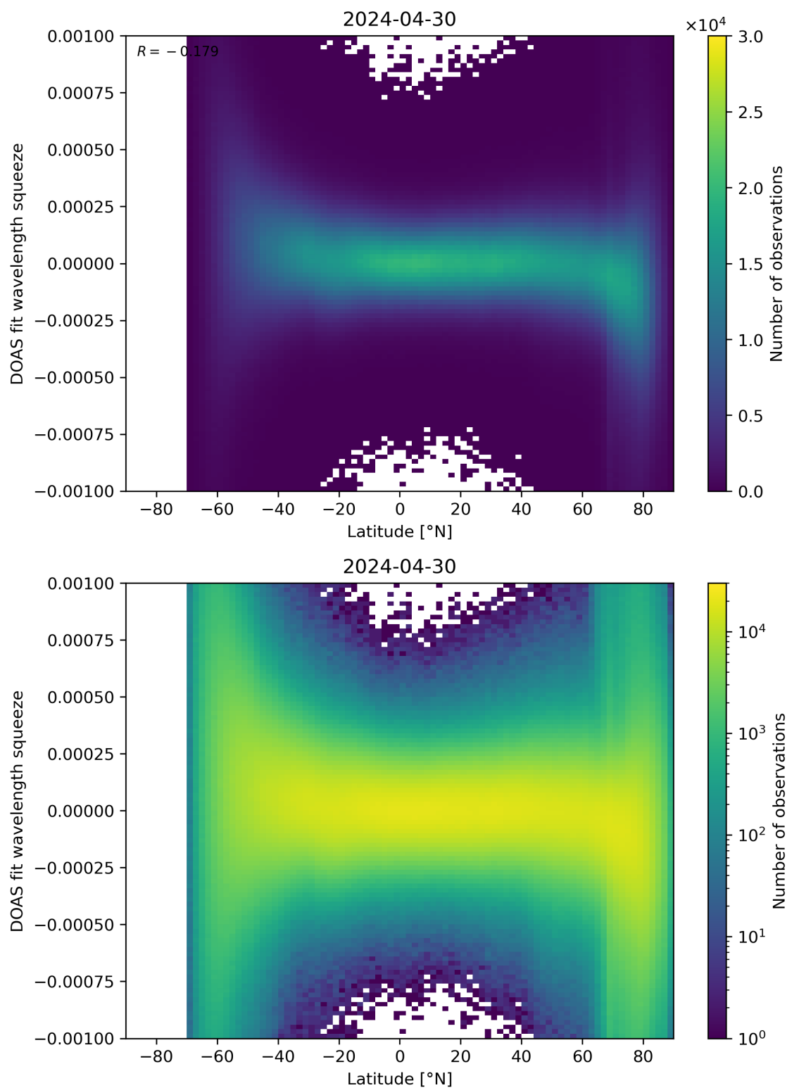
Figure 143: Scatter density plot of “Latitude” against “DOAS fit wavelength squeeze” for 2024-04-29 to 2024-05-01.
