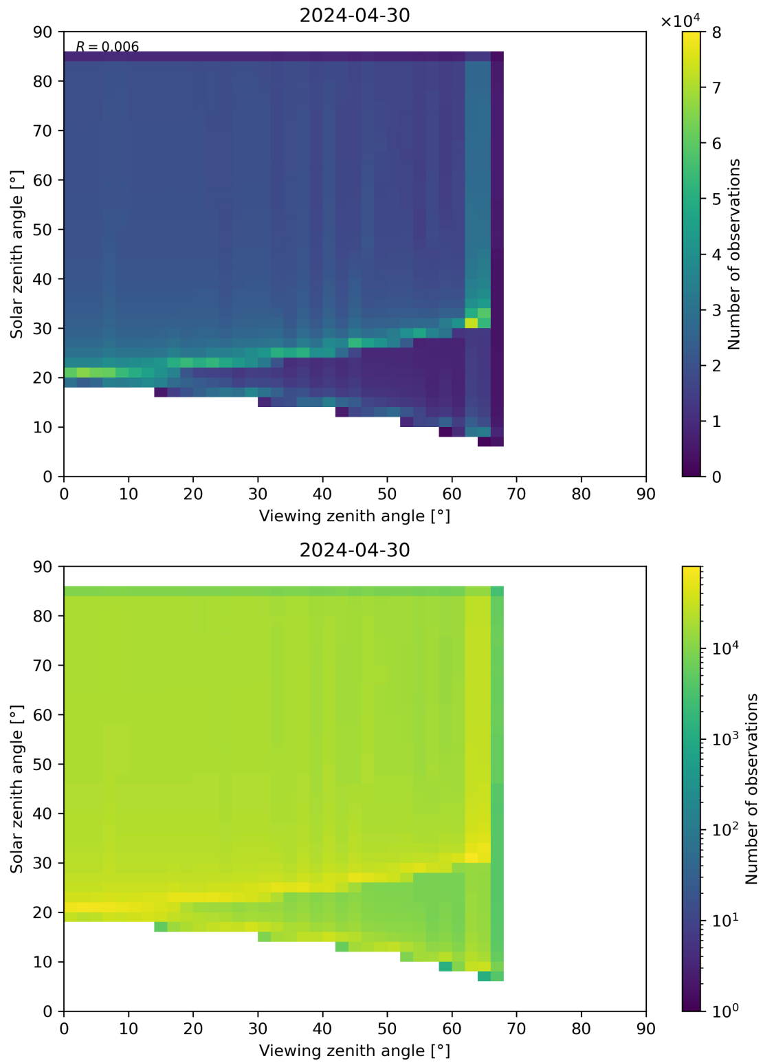
Figure 315: Scatter density plot of “Viewing zenith angle” against “Solar zenith angle” for 2024-04-29 to 2024-05-01.
