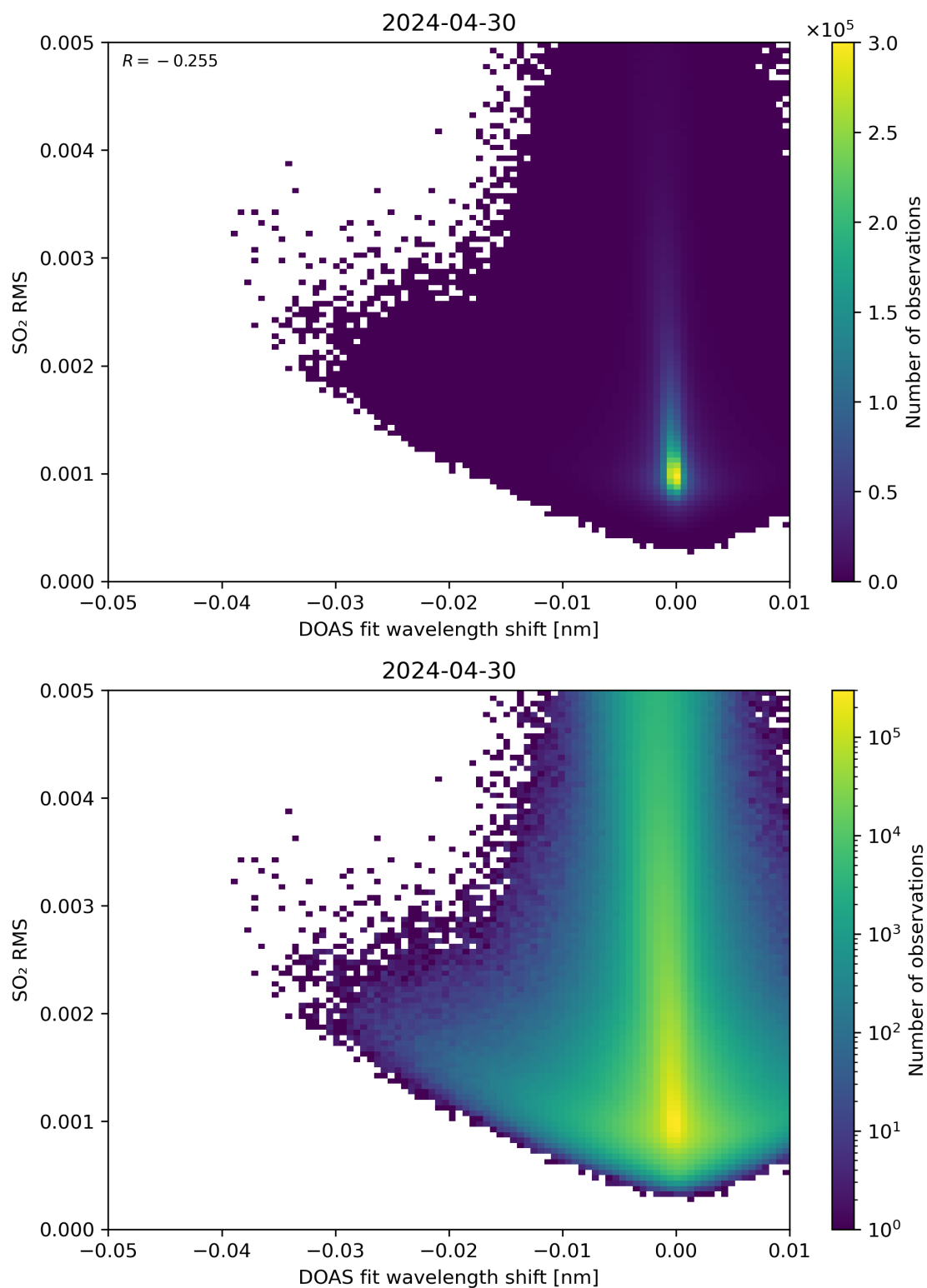
Figure 128: Scatter density plot of “DOAS fit wavelength shift” against “SO 2 RMS” for 2024-04-29 to 2024-05-01.
