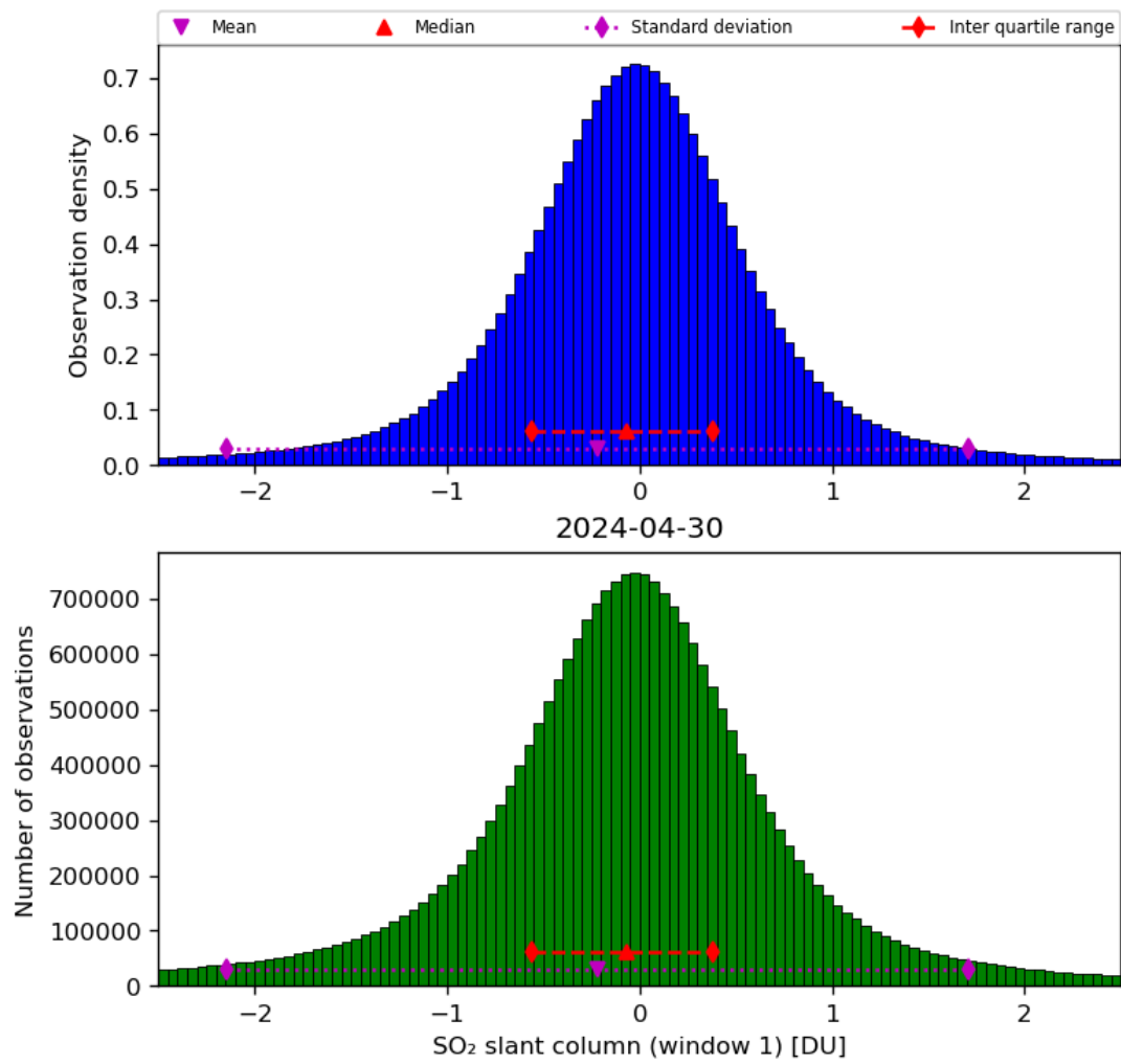
Figure 56: Histogram of “SO 2 slant column (window 1)” for 2024-04-29 to 2024-05-01
