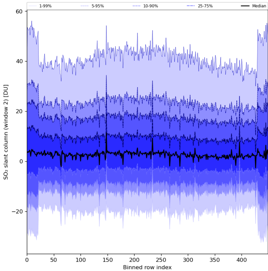
Figure 83: Along track statistics of “SO 2 slant column (window 2)” for 2024-04-29 to 2024-05-01
