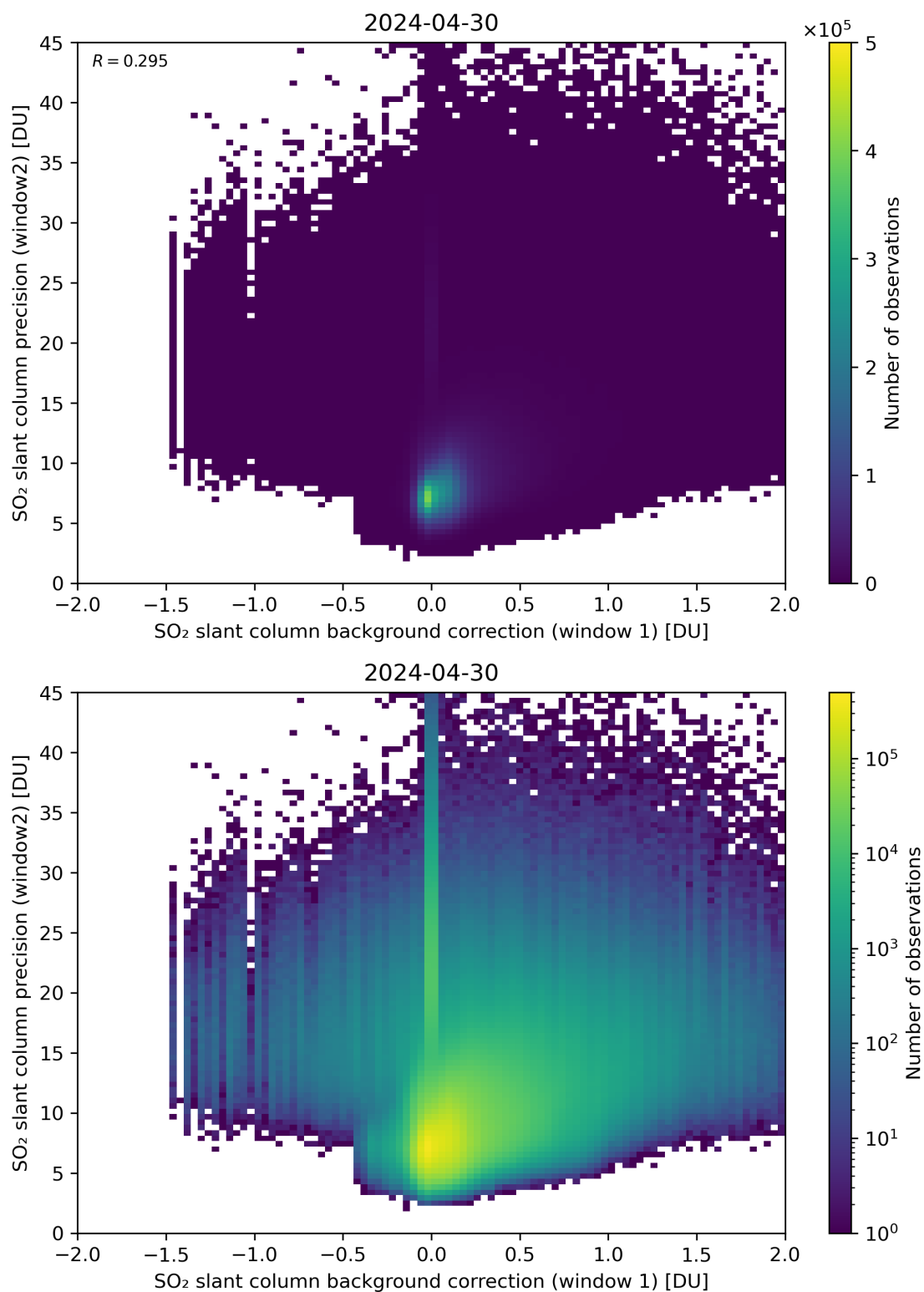
Figure 106: Scatter density plot of “SO 2 slant column background correction (window 1)” against “SO 2 slant column precision (window2)” for 2024-04-29 to 2024-05-01.
