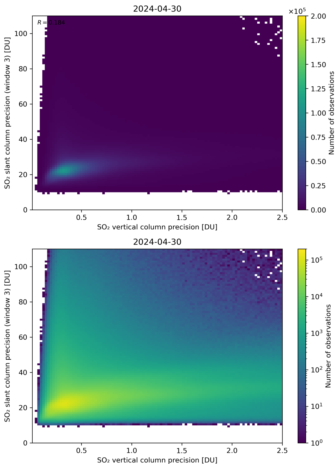
Figure 293: Scatter density plot of “SO 2 vertical column precision” against “SO 2 slant column precision (window 3)” for 2024-04-29 to 2024-05-01.
