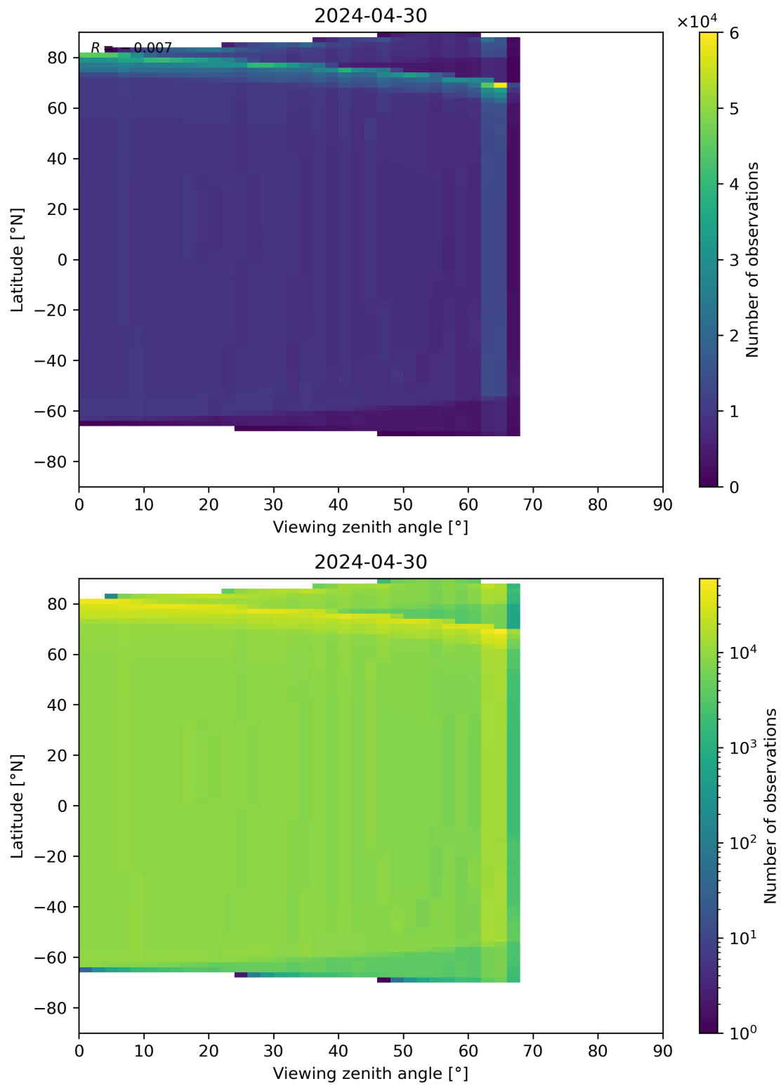
Figure 314: Scatter density plot of “Viewing zenith angle” against “Latitude” for 2024-04-29 to 2024-05-01.
