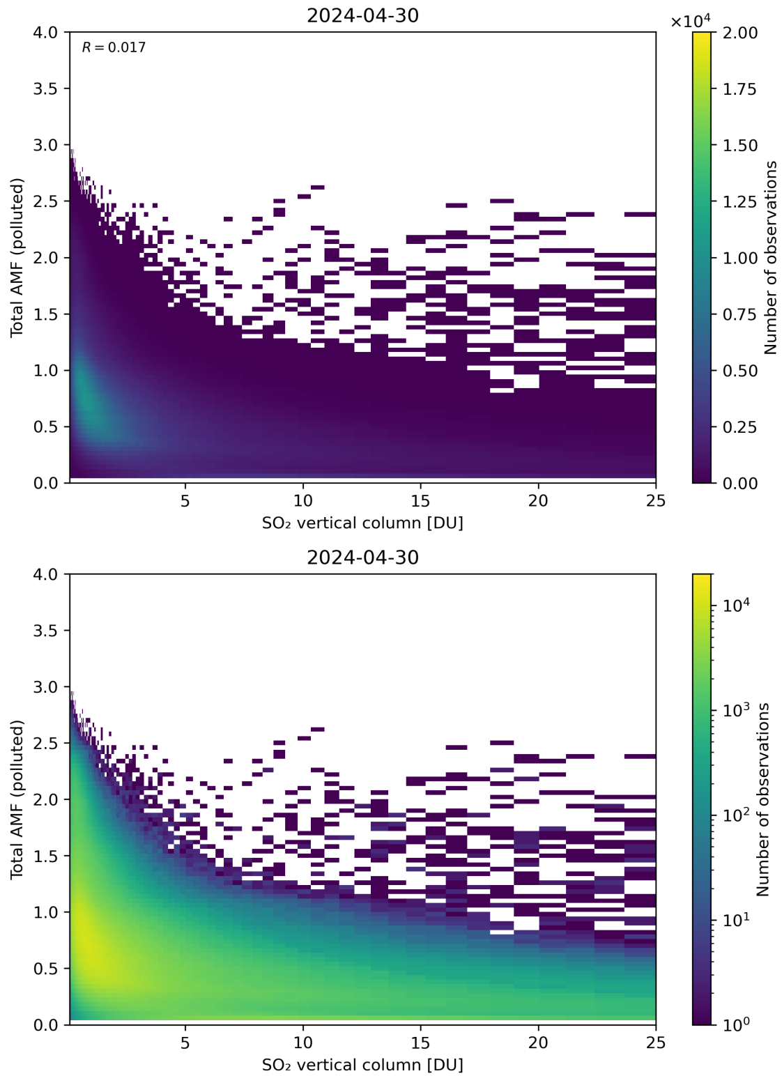
Figure 305: Scatter density plot of “SO 2 vertical column” against “Total AMF (polluted)” for 2024-04-29 to 2024-05-01.
