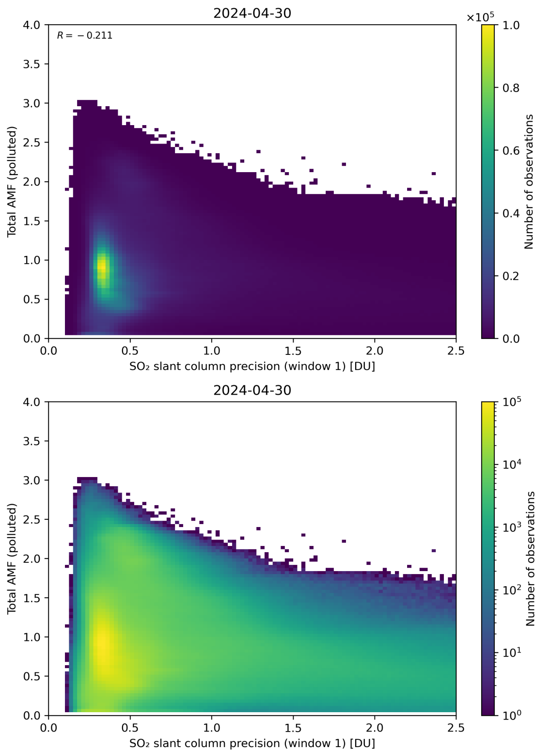
Figure 230: Scatter density plot of “SO 2 slant column precision (window 1)” against “Total AMF (polluted)” for 2024-04-29 to 2024-05-01.
