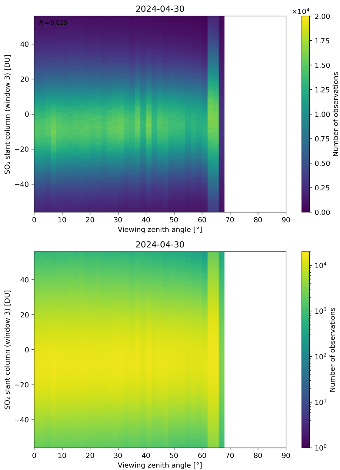
Figure 323: Scatter density plot of “Viewing zenith angle” against “SO 2 slant column (window 3)” for 2024-04-29 to 2024-05-01.
