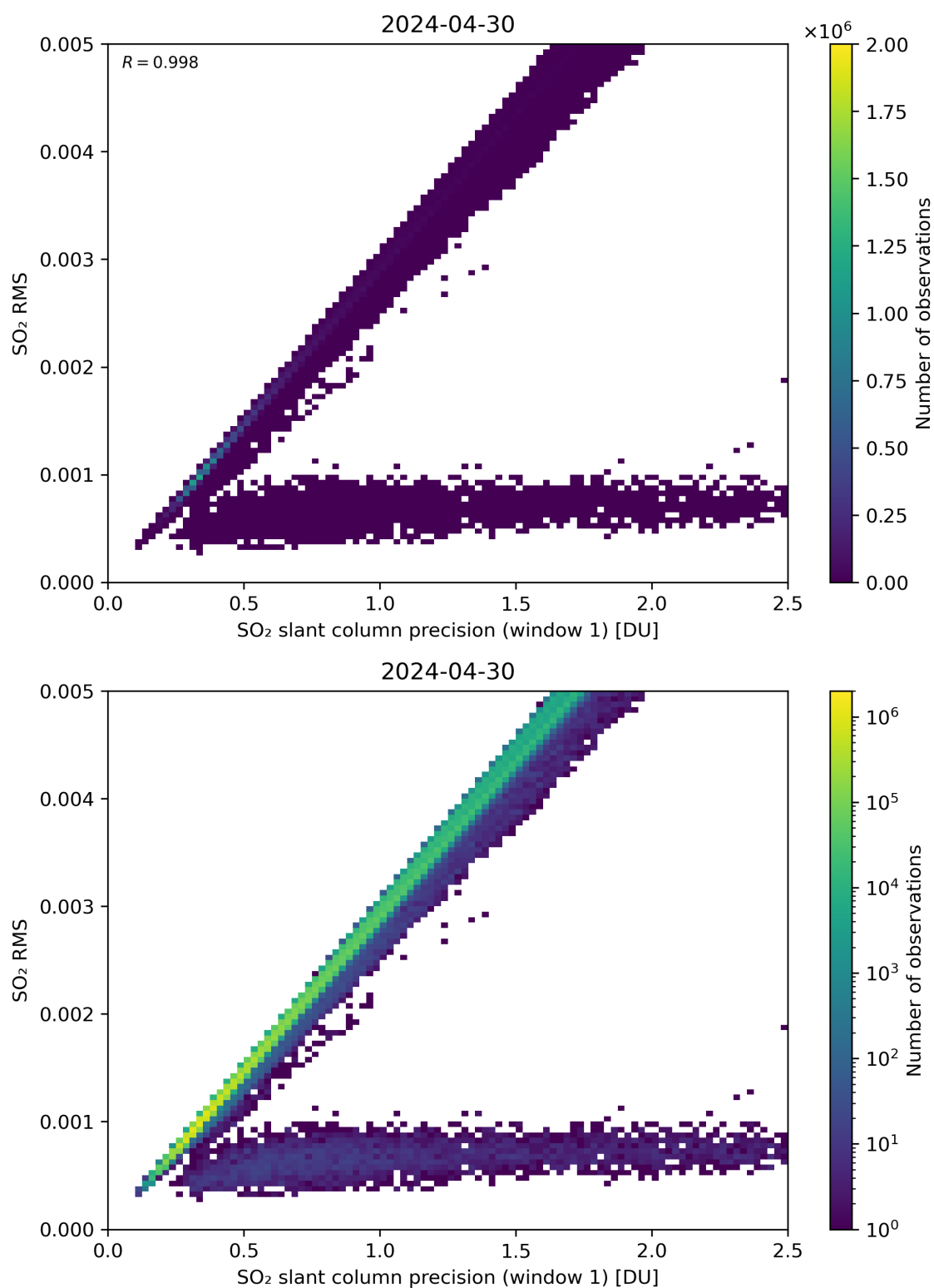
Figure 223: Scatter density plot of “SO 2 slant column precision (window 1)” against “SO 2 RMS” for 2024-04-29 to 2024-05-01.
