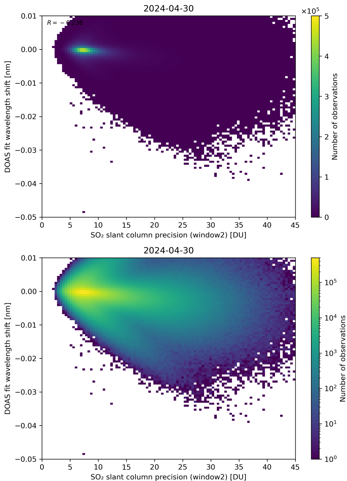
Figure 243: Scatter density plot of “SO 2 slant column precision (window2)” against “DOAS fit wavelength shift” for 2024-04-29 to 2024-05-01.
