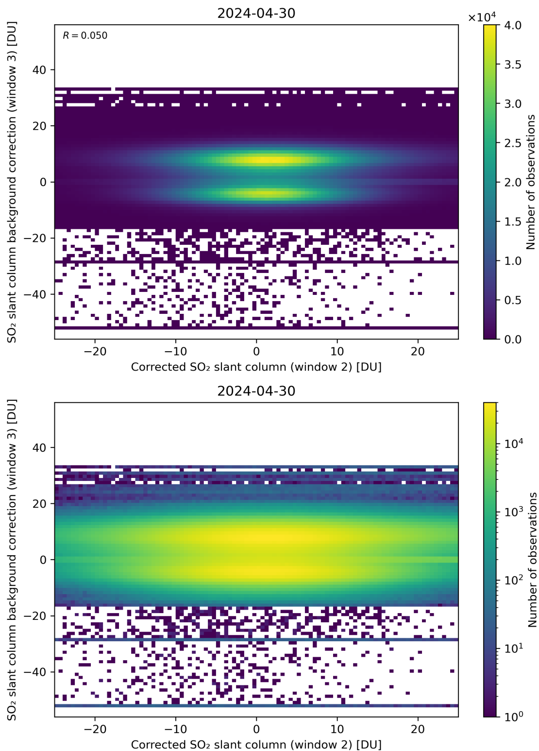
Figure 195: Scatter density plot of “Corrected SO 2 slant column (window 2)” against “SO 2 slant column background correction (window 3)” for 2024-04-29 to 2024-05-01.
