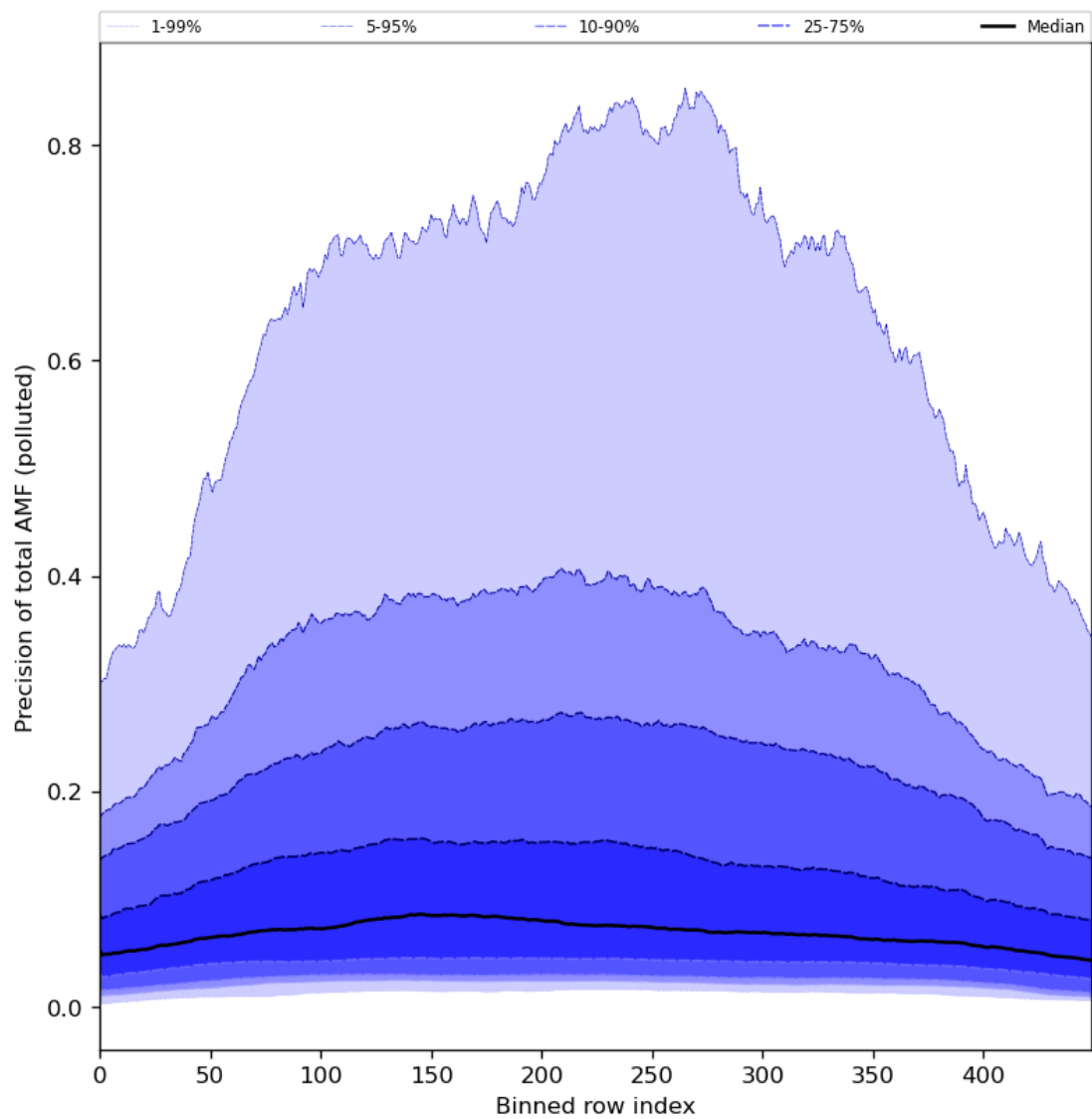
Figure 95: Along track statistics of “Precision of total AMF (polluted)” for 2024-04-29 to 2024-05-01
