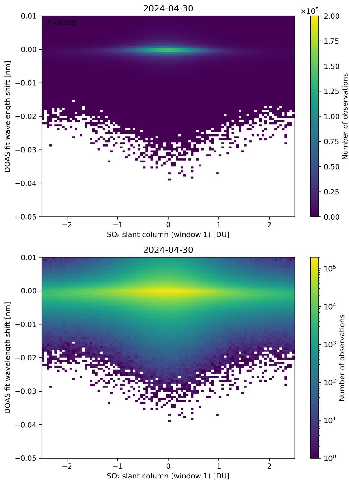
Figure 215: Scatter density plot of “SO 2 slant column (window 1)” against “DOAS fit wavelength shift” for 2024-04-29 to 2024-05-01.
