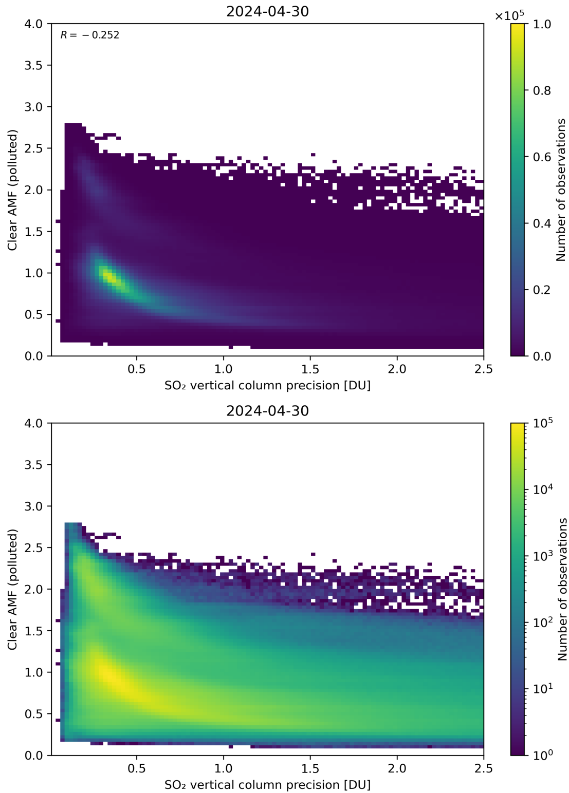
Figure 285: Scatter density plot of “SO 2 vertical column precision” against “Clear AMF (polluted)” for 2024-04-29 to 2024-05-01.
