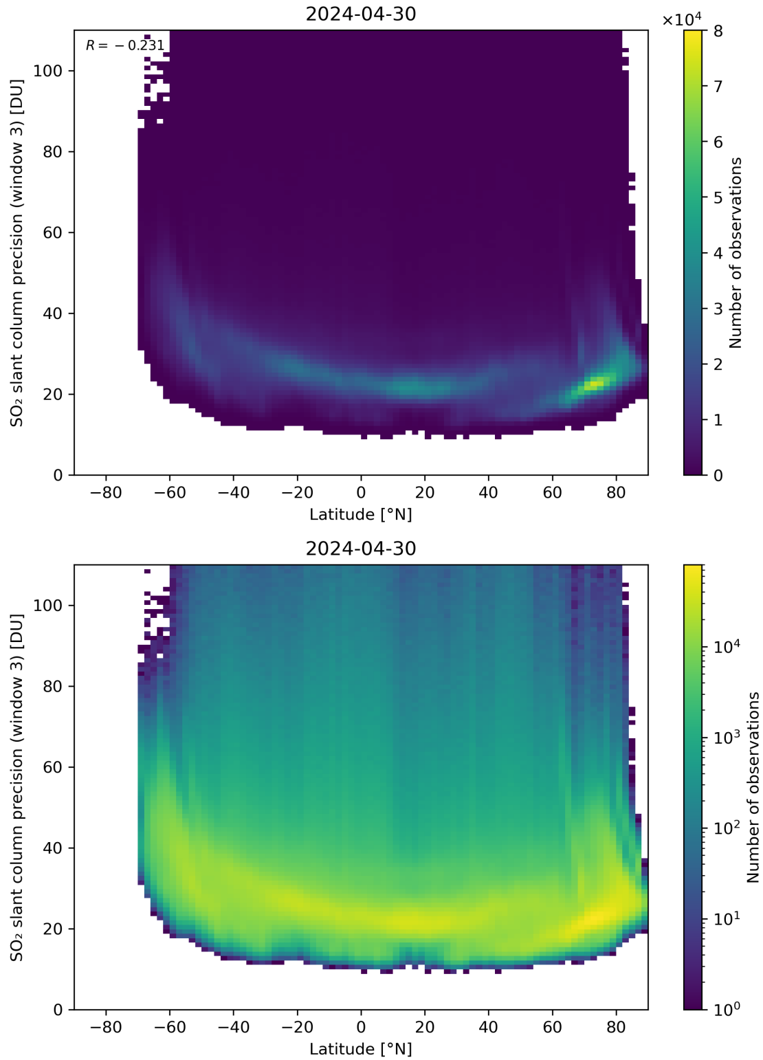
Figure 153: Scatter density plot of “Latitude” against “SO 2 slant column precision (window 3)” for 2024-04-29 to 2024-05-01.
