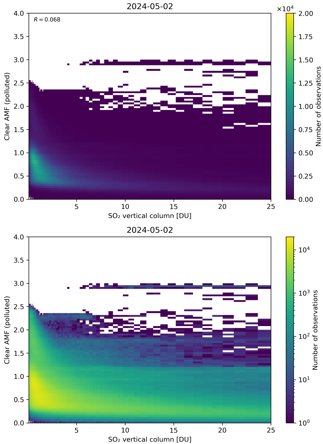
Figure 296: Scatter density plot of “SO 2 vertical column” against “Clear AMF (polluted)” for 2024-05-02 to 2024-05-03.
