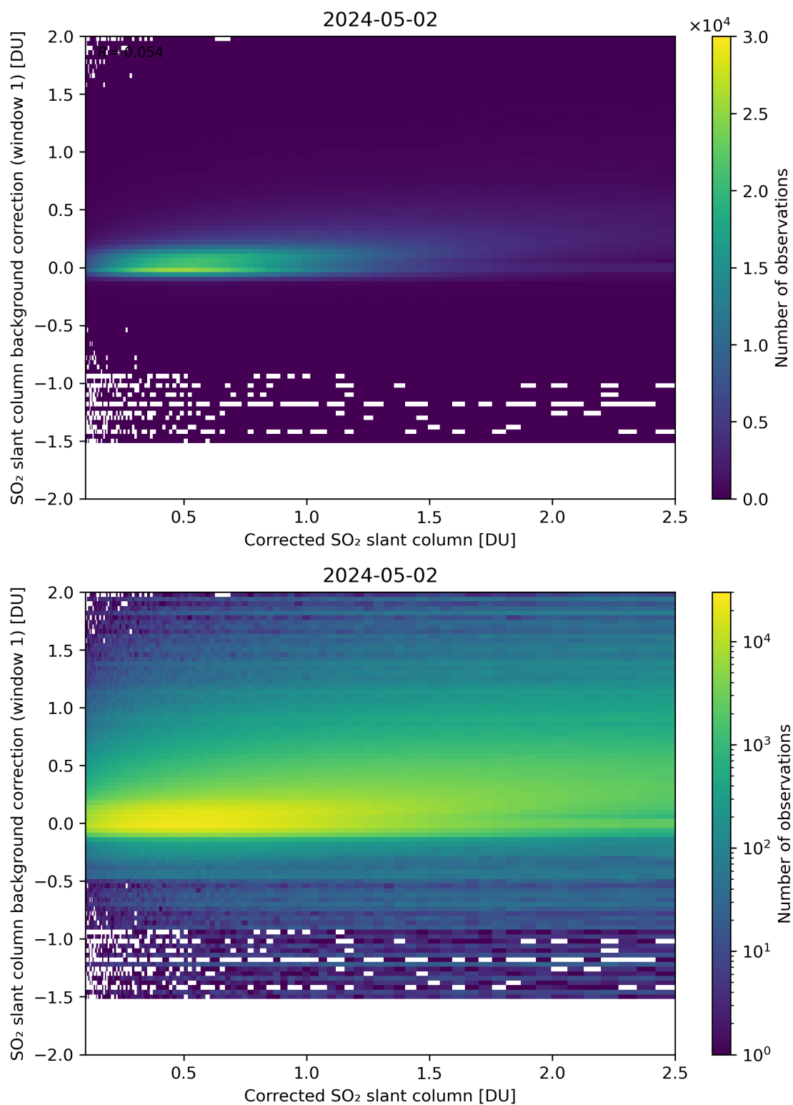
Figure 178: Scatter density plot of “Corrected SO 2 slant column” against “SO 2 slant column background correction (window 1)” for 2024-05-02 to 2024-05-03.
