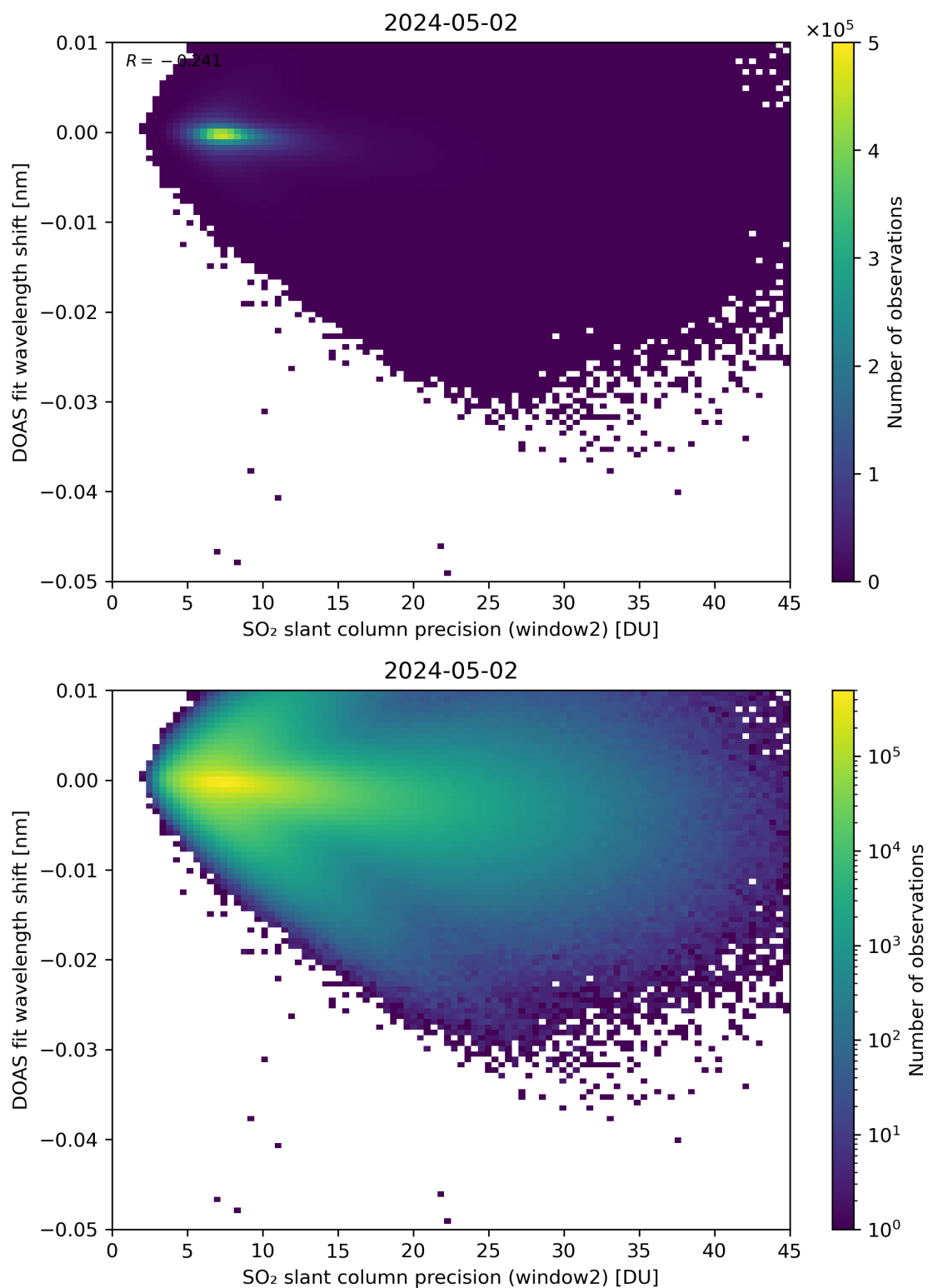
Figure 243: Scatter density plot of “SO 2 slant column precision (window2)” against “DOAS fit wavelength shift” for 2024-05-02 to 2024-05-03.
