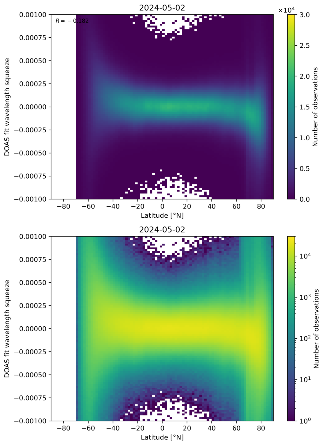
Figure 143: Scatter density plot of “Latitude” against “DOAS fit wavelength squeeze” for 2024-05-02 to 2024-05-03.
