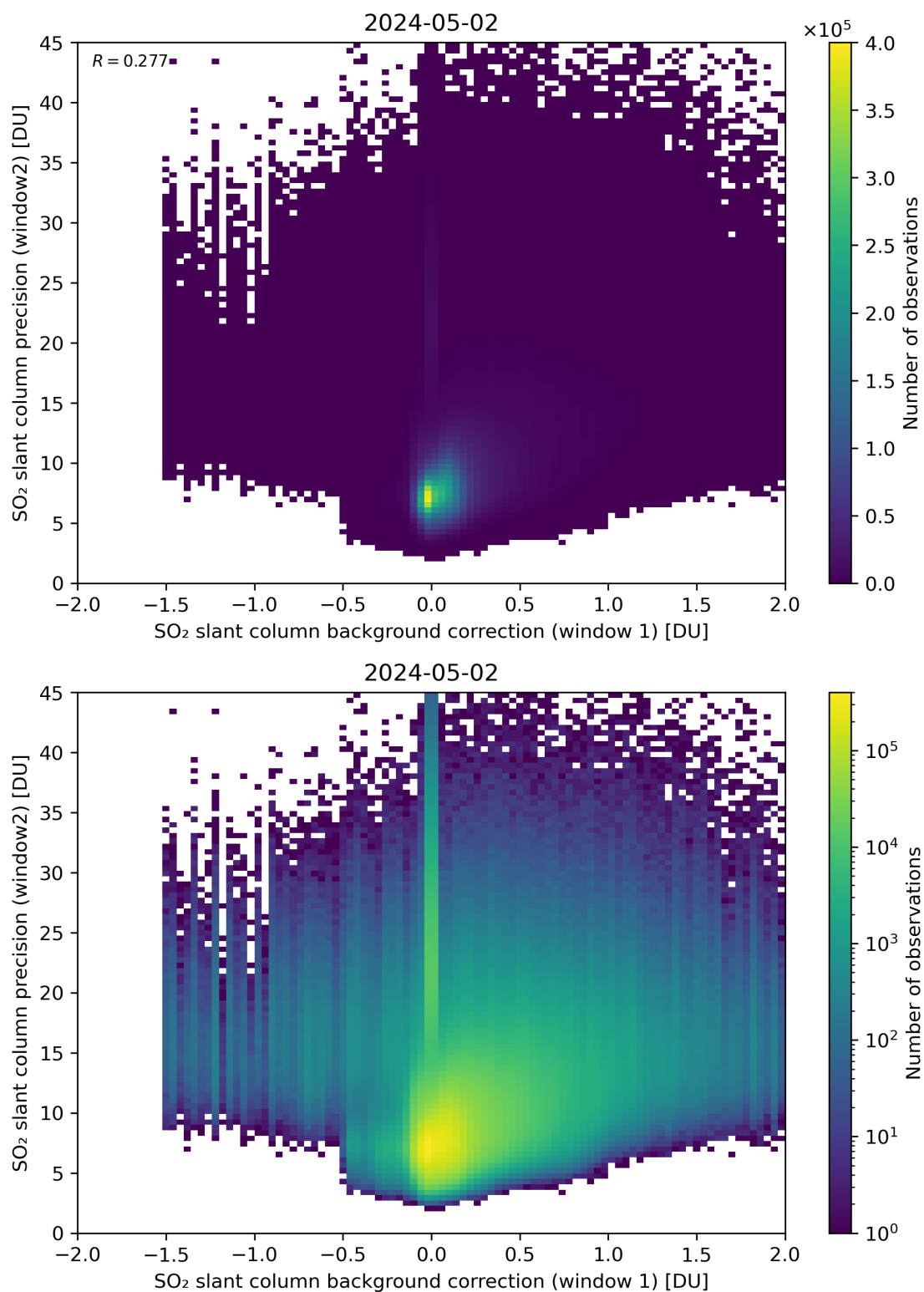
Figure 106: Scatter density plot of “SO 2 slant column background correction (window 1)” against “SO 2 slant column precision (window2)” for 2024-05-02 to 2024-05-03.
