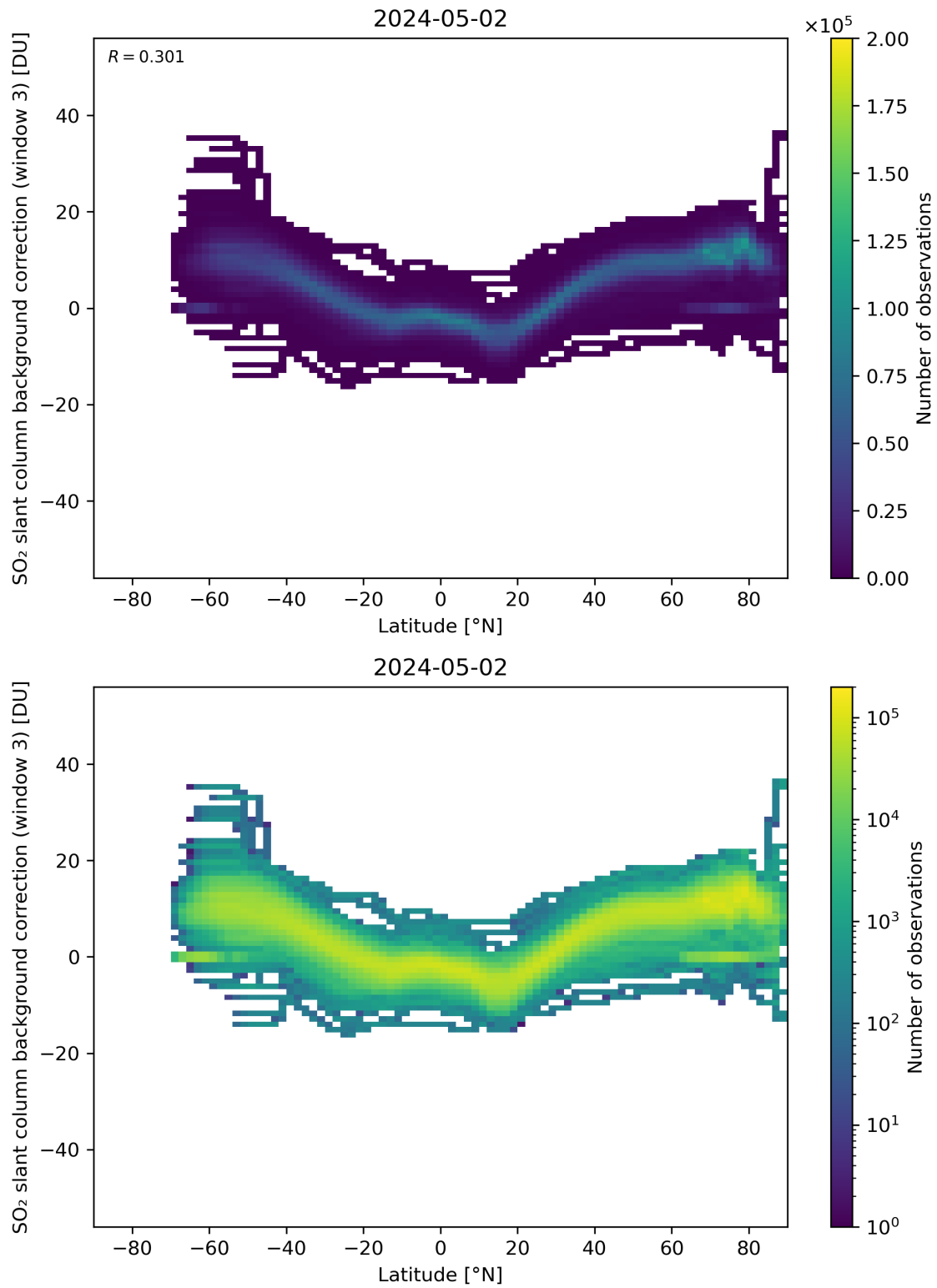
Figure 141: Scatter density plot of “Latitude” against “SO 2 slant column background correction (window 3)” for 2024-05-02 to 2024-05-03.
