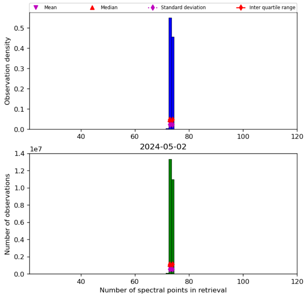
Figure 74: Histogram of “Number of spectral points in retrieval” for 2024-05-02 to 2024-05-03
