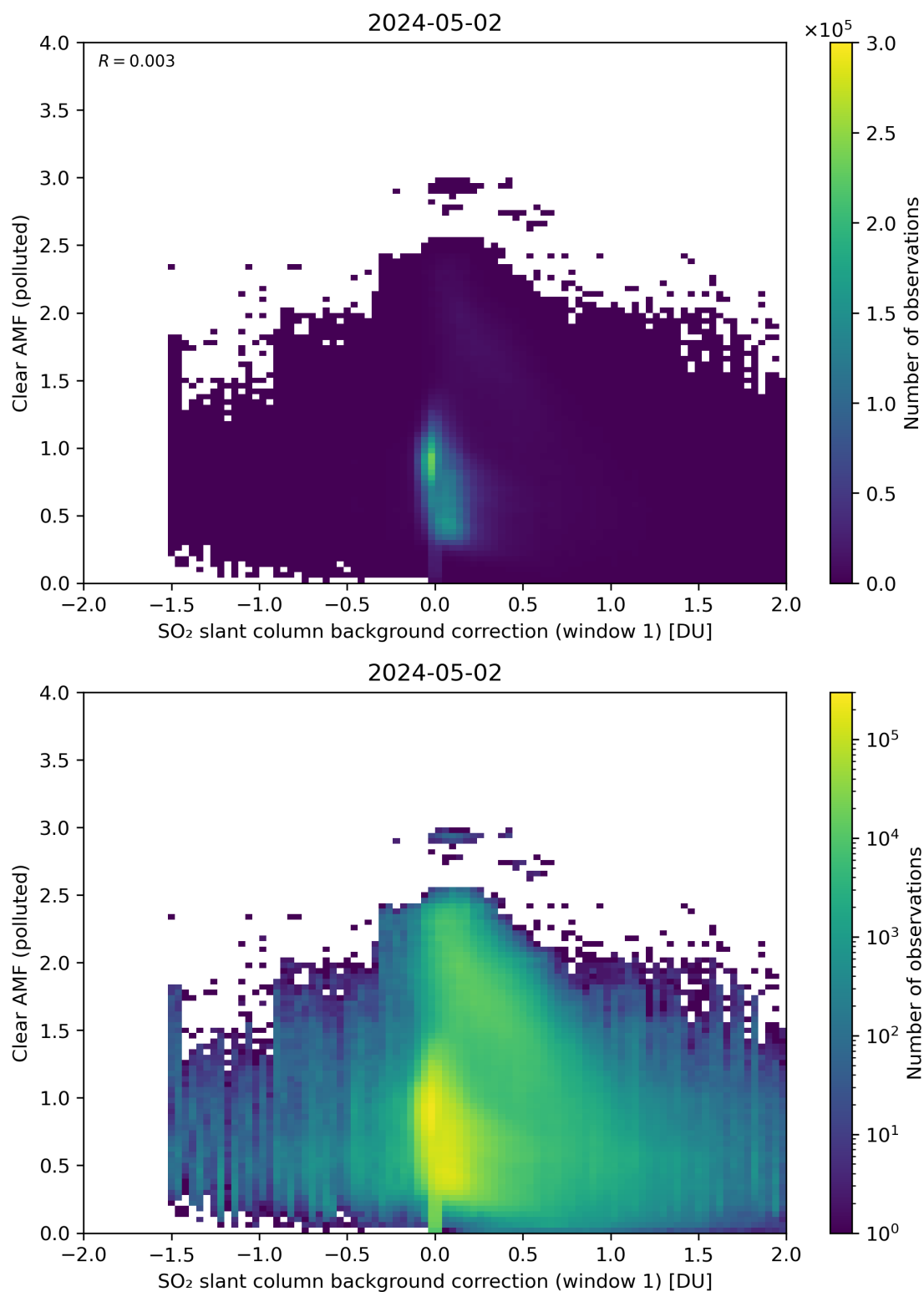
Figure 103: Scatter density plot of “SO 2 slant column background correction (window 1)” against “Clear AMF (polluted)” for 2024-05-02 to 2024-05-03.
