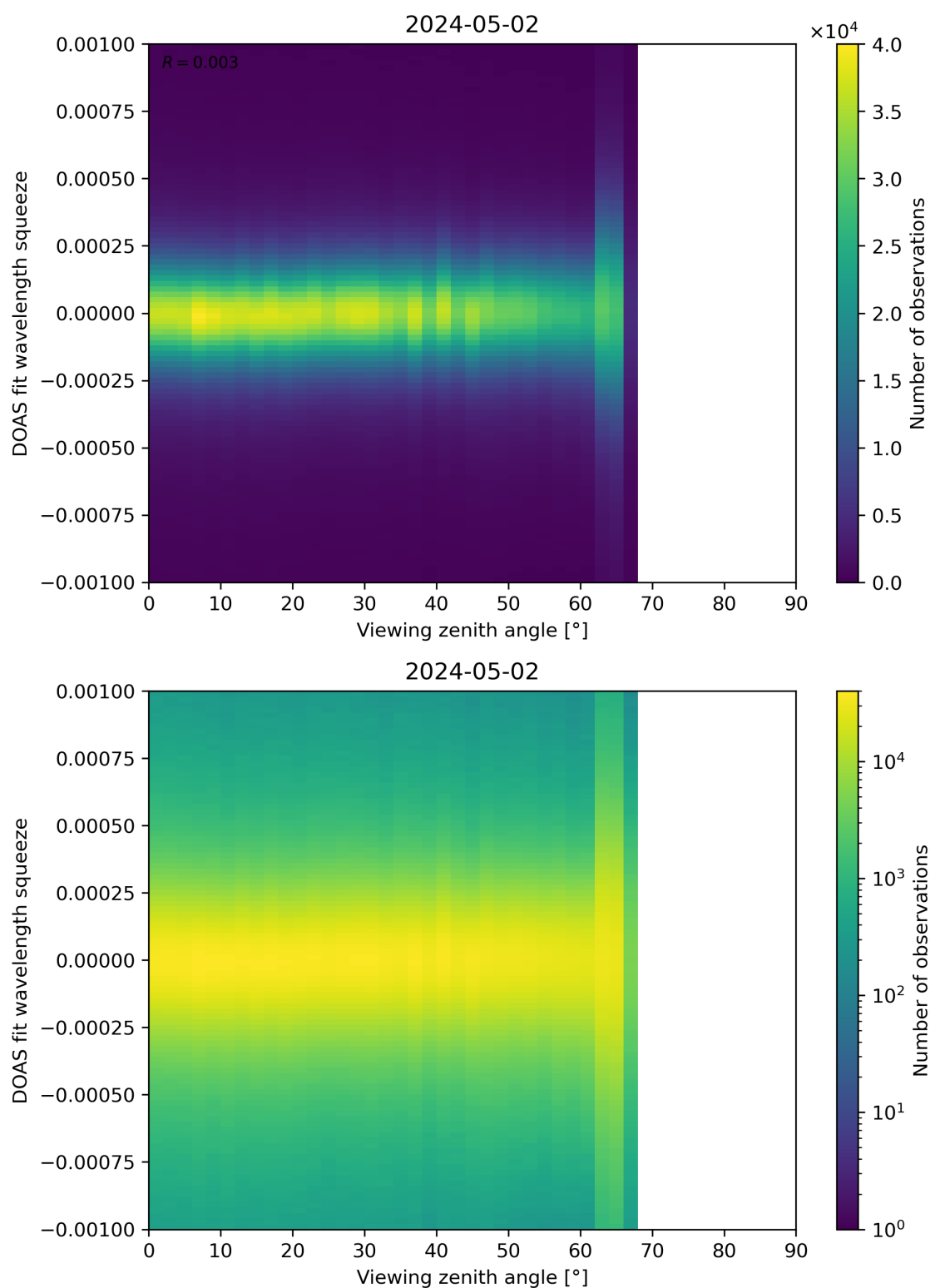
Figure 312: Scatter density plot of “Viewing zenith angle” against “DOAS fit wavelength squeeze” for 2024-05-02 to 2024-05-03.
