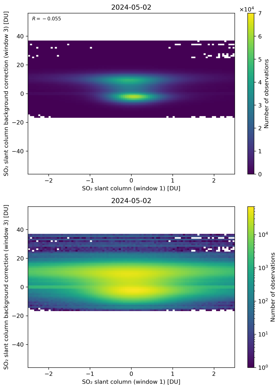
Figure 214: Scatter density plot of “SO 2 slant column (window 1)” against “SO 2 slant column background correction (window 3)” for 2024-05-02 to 2024-05-03.
