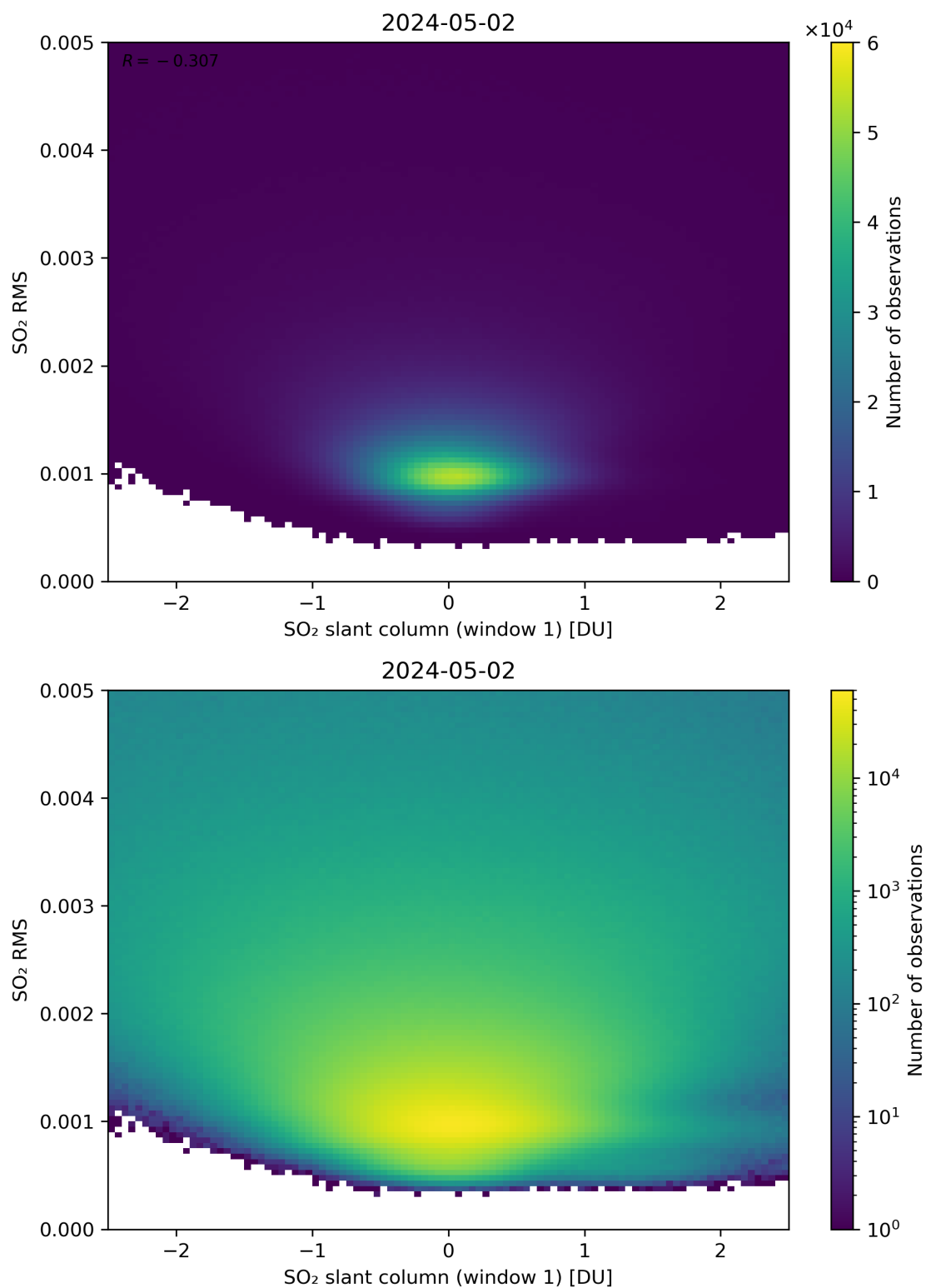
Figure 217: Scatter density plot of “SO 2 slant column (window 1)” against “SO 2 RMS” for 2024-05-02 to 2024-05-03.
