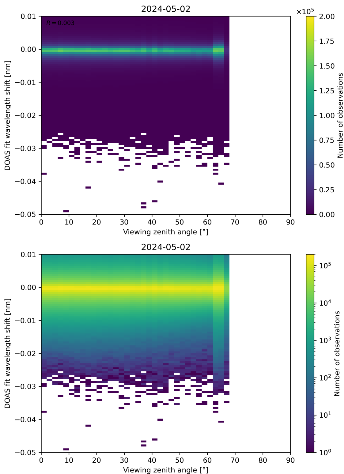
Figure 311: Scatter density plot of “Viewing zenith angle” against “DOAS fit wavelength shift” for 2024-05-02 to 2024-05-03.
