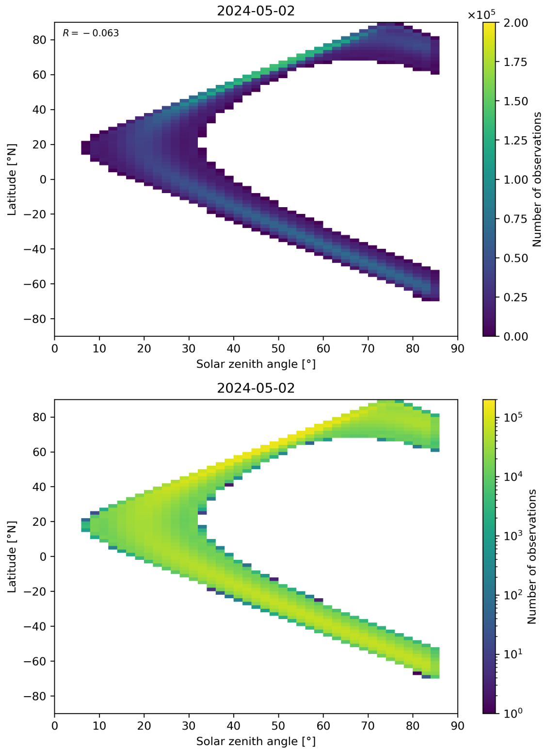
Figure 164: Scatter density plot of “Solar zenith angle” against “Latitude” for 2024-05-02 to 2024-05-03.
