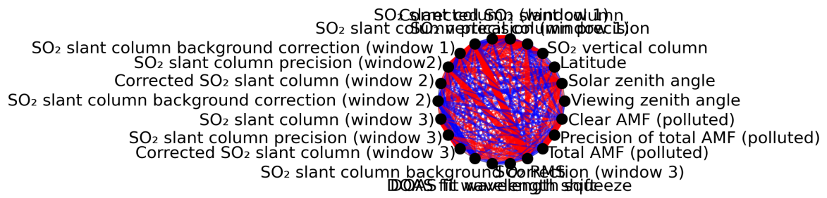
Figure 1: Map of correlation graph for 2024-05-02 to 2024-05-03.
