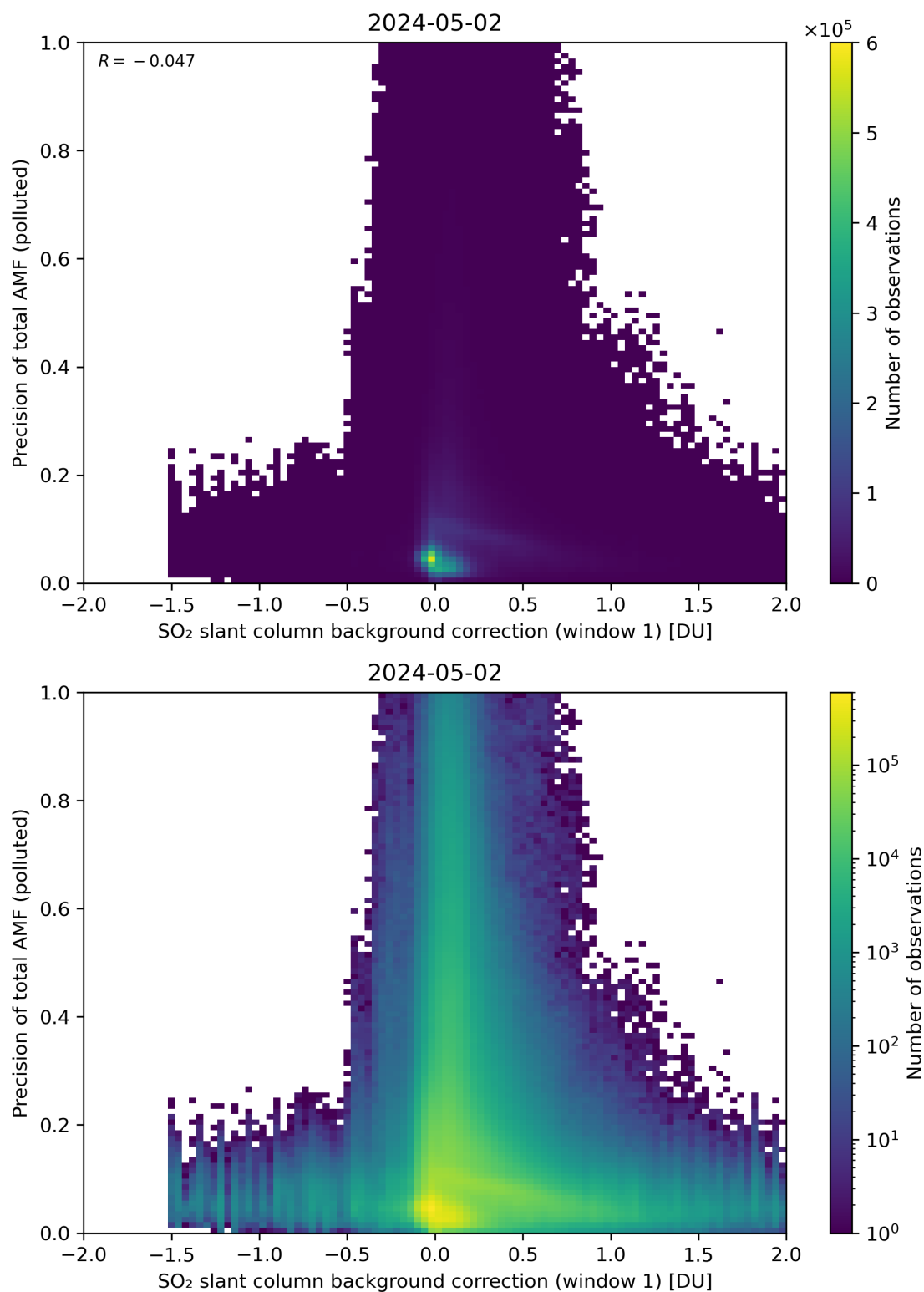
Figure 110: Scatter density plot of “SO 2 slant column background correction (window 1)” against “Precision of total AMF (polluted)” for 2024-05-02 to 2024-05-03.
