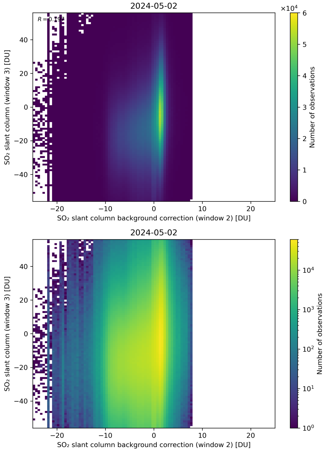
Figure 117: Scatter density plot of “SO 2 slant column background correction (window 2)” against “SO 2 slant column (window 3)” for 2024-05-02 to 2024-05-03.
