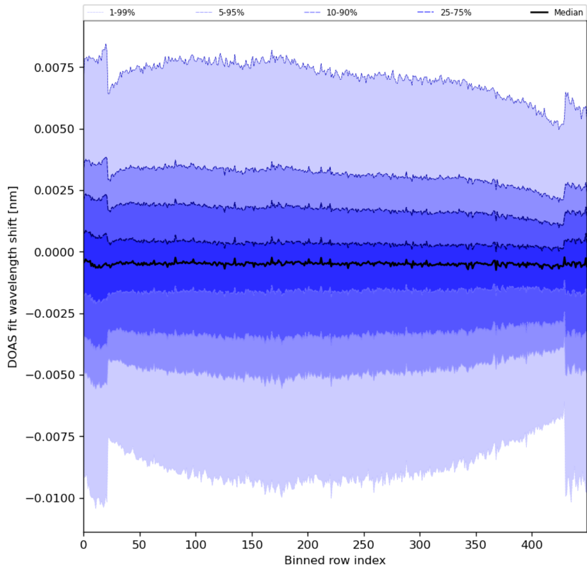
Figure 91: Along track statistics of “DOAS fit wavelength shift” for 2024-05-02 to 2024-05-03
