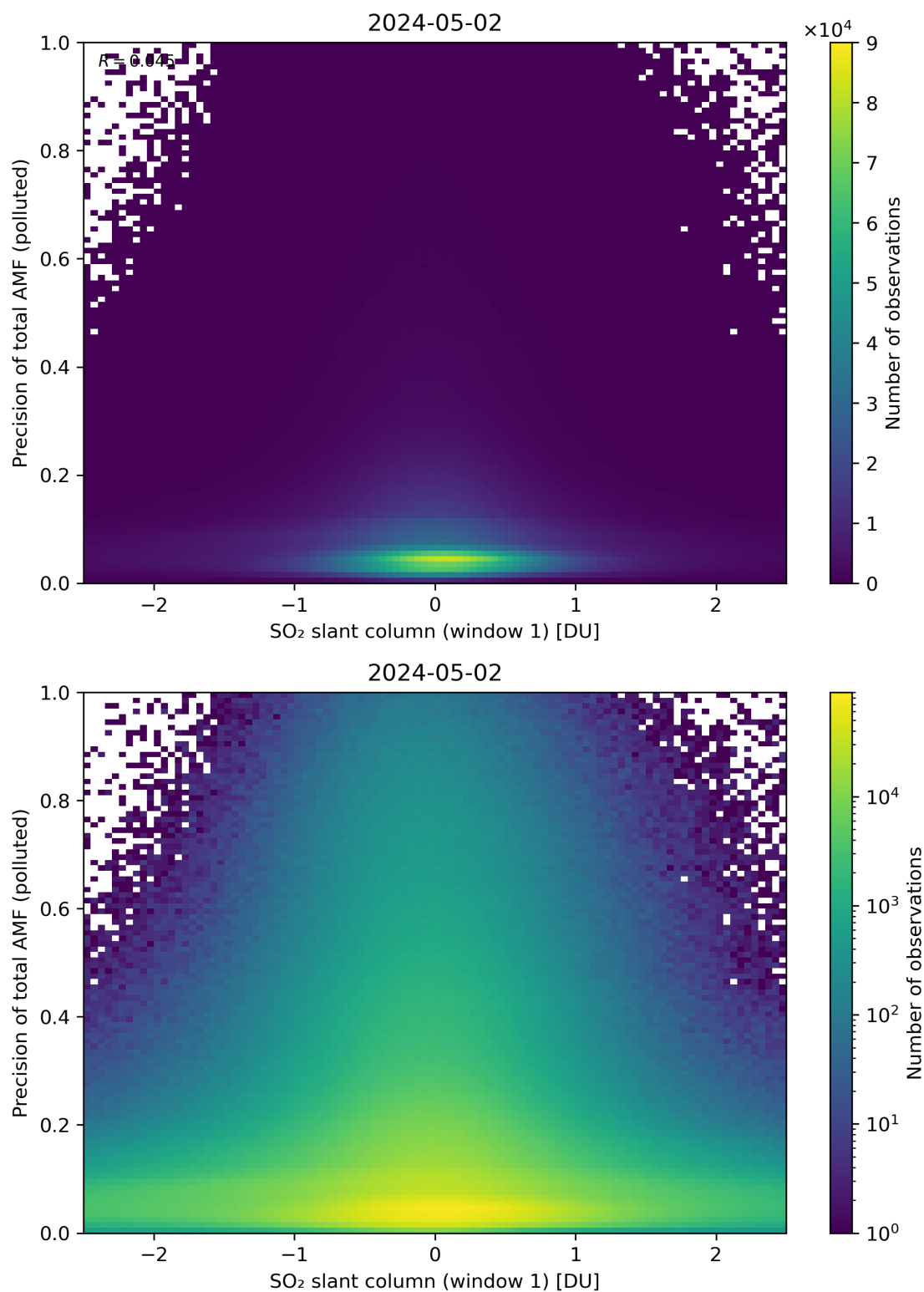
Figure 240: Scatter density plot of “SO 2 slant column (window 1)” against “Precision of total AMF (polluted)” for 2024-05-02 to 2024-05-03.
