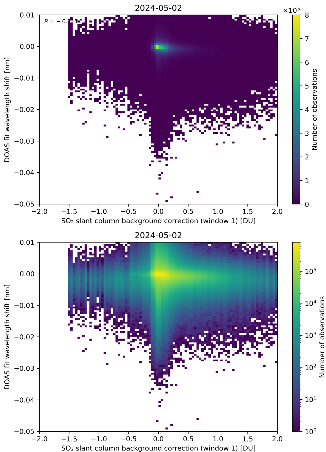
Figure 100: Scatter density plot of “SO 2 slant column background correction (window 1)” against “DOAS fit wavelength shift” for 2024-05-02 to 2024-05-03.
