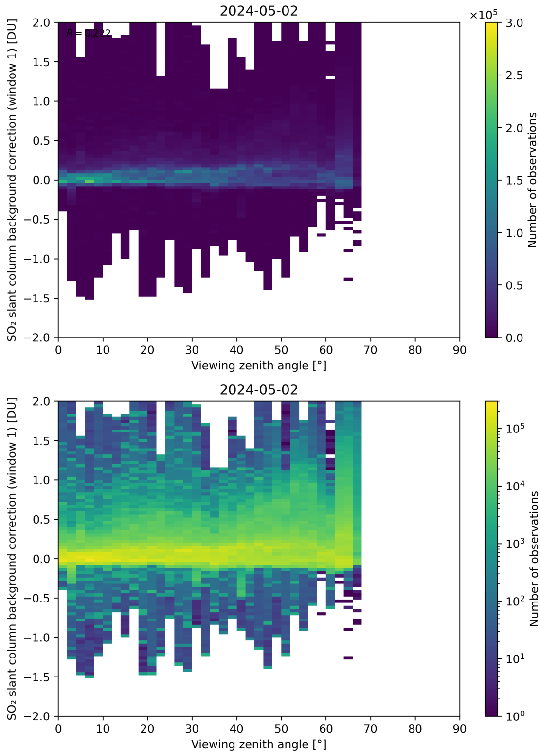
Figure 308: Scatter density plot of “Viewing zenith angle” against “SO 2 slant column background correction (window 1)” for 2024-05-02 to 2024-05-03.
