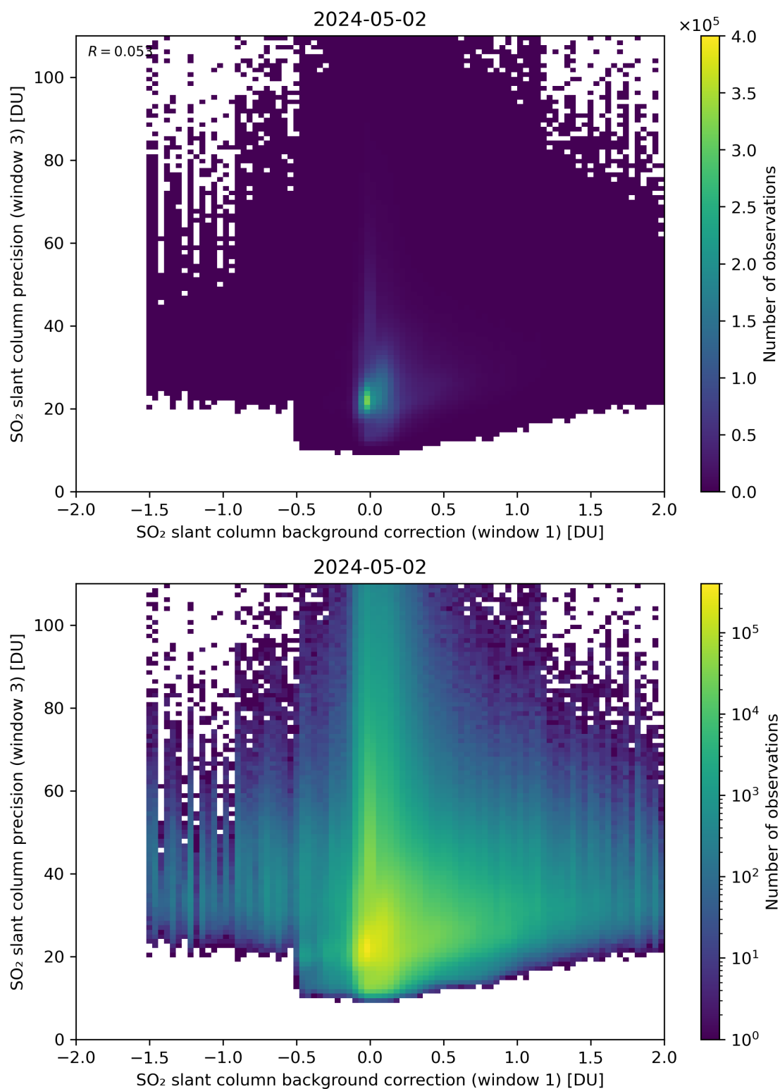
Figure 108: Scatter density plot of “SO 2 slant column background correction (window 1)” against “SO 2 slant column precision (window 3)” for 2024-05-02 to 2024-05-03.
