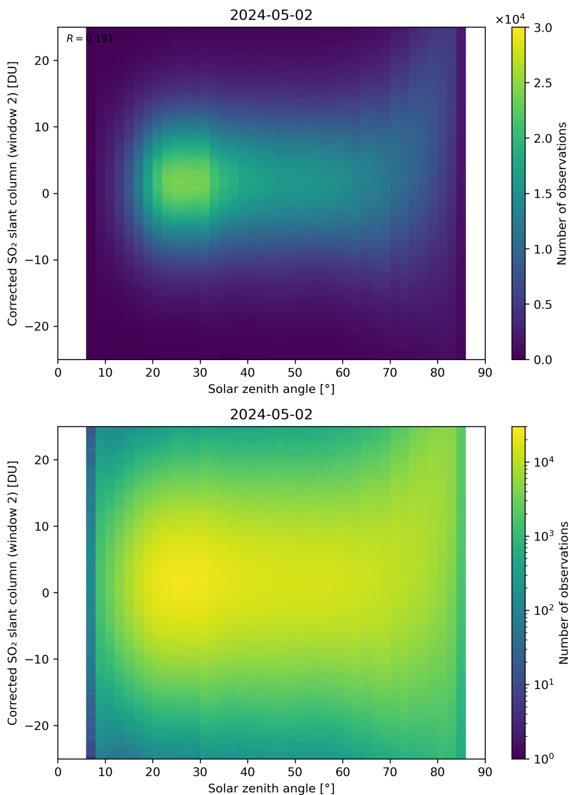
Figure 167: Scatter density plot of “Solar zenith angle” against “Corrected SO 2 slant column (window 2)” for 2024-05-02 to 2024-05-03.
