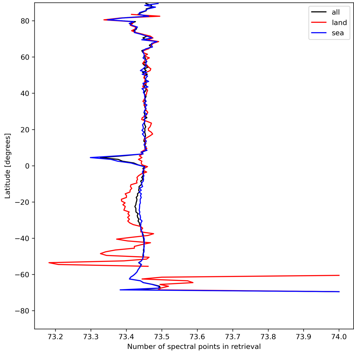
Figure 51: Zonal average of “Number of spectral points in retrieval” for 2024-05-02 to 2024-05-03.
