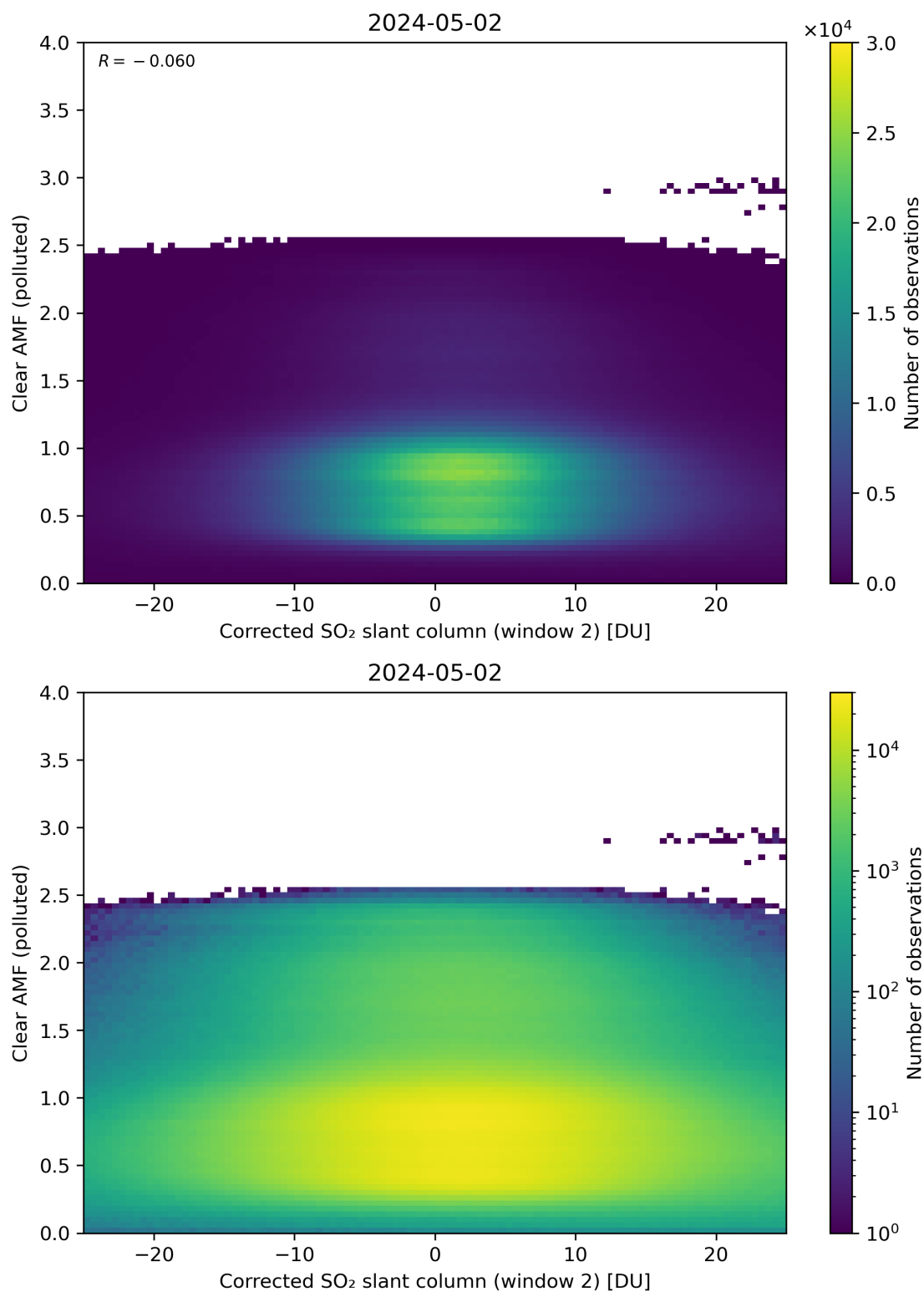
Figure 199: Scatter density plot of “Corrected SO 2 slant column (window 2)” against “Clear AMF (polluted)” for 2024-05-02 to 2024-05-03.
