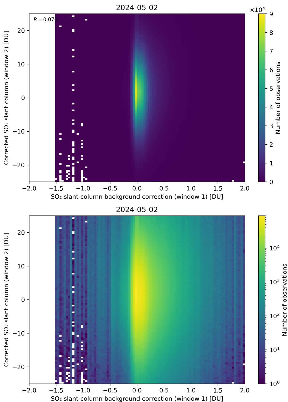
Figure 104: Scatter density plot of “SO 2 slant column background correction (window 1)” against “Corrected SO 2 slant column (window 2)” for 2024-05-02 to 2024-05-03.
