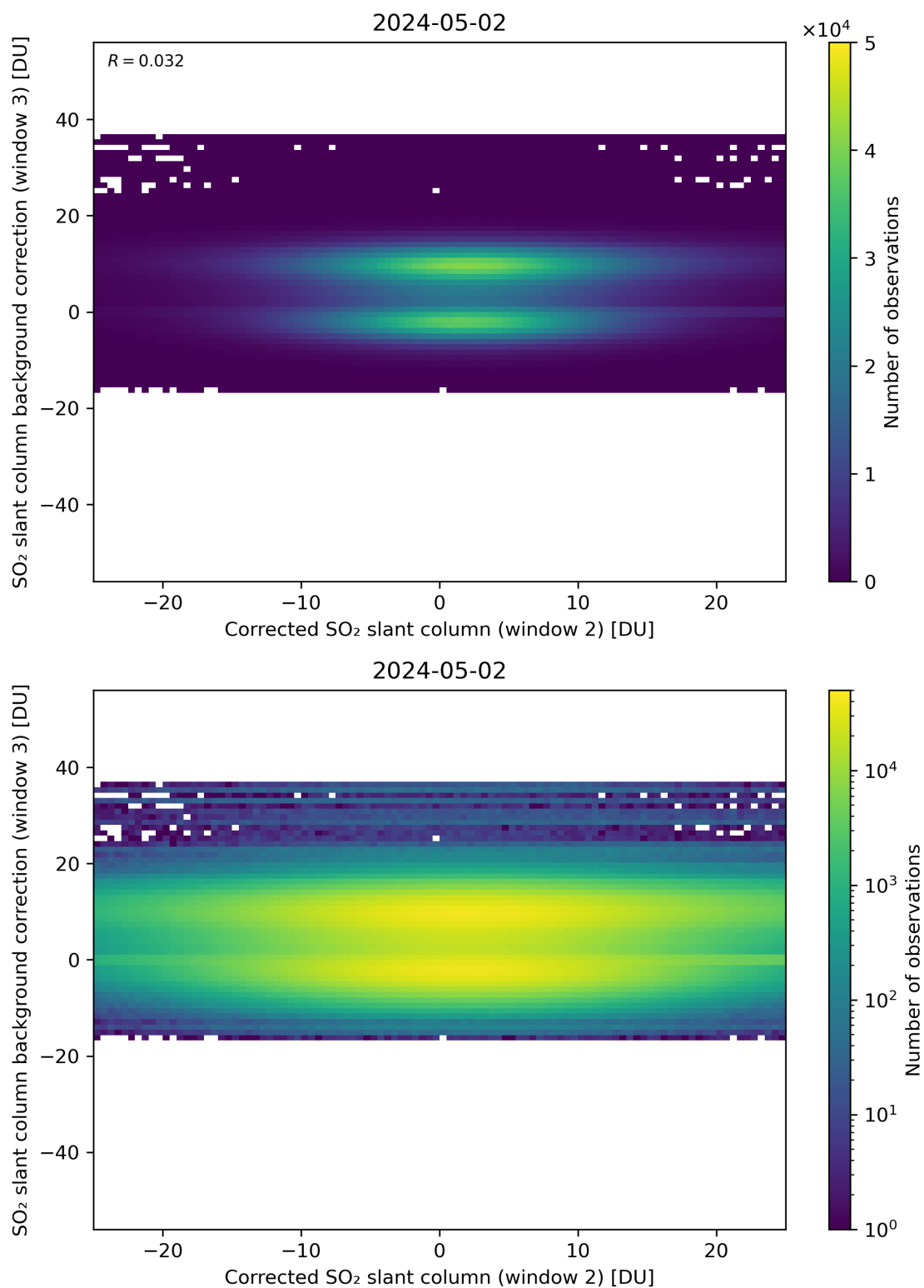
Figure 195: Scatter density plot of “Corrected SO 2 slant column (window 2)” against “SO 2 slant column background correction (window 3)” for 2024-05-02 to 2024-05-03.
