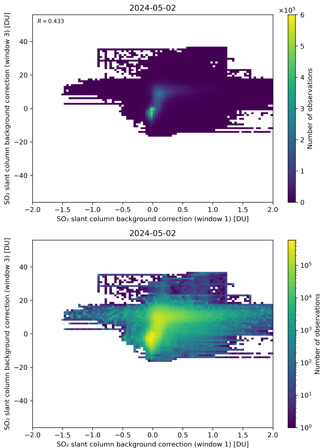
Figure 99: Scatter density plot of “SO 2 slant column background correction (window 1)” against “SO 2 slant column background correction (window 3)” for 2024-05-02 to 2024-05-03.
