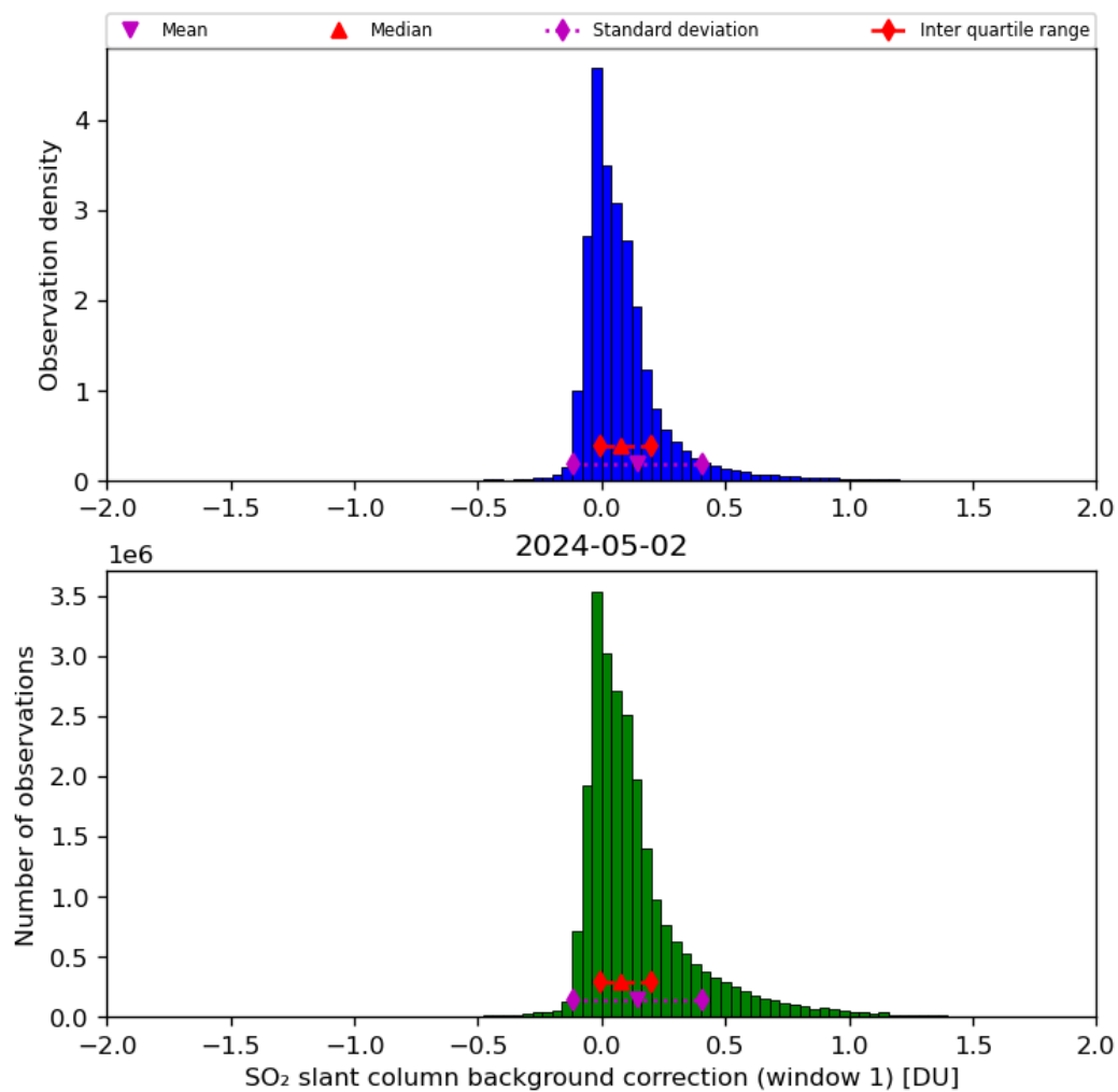
Figure 59: Histogram of “SO 2 slant column background correction (window 1)” for 2024-05-02 to 2024-05-03
