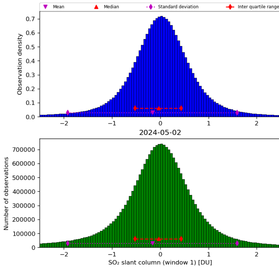
Figure 56: Histogram of “SO 2 slant column (window 1)” for 2024-05-02 to 2024-05-03
