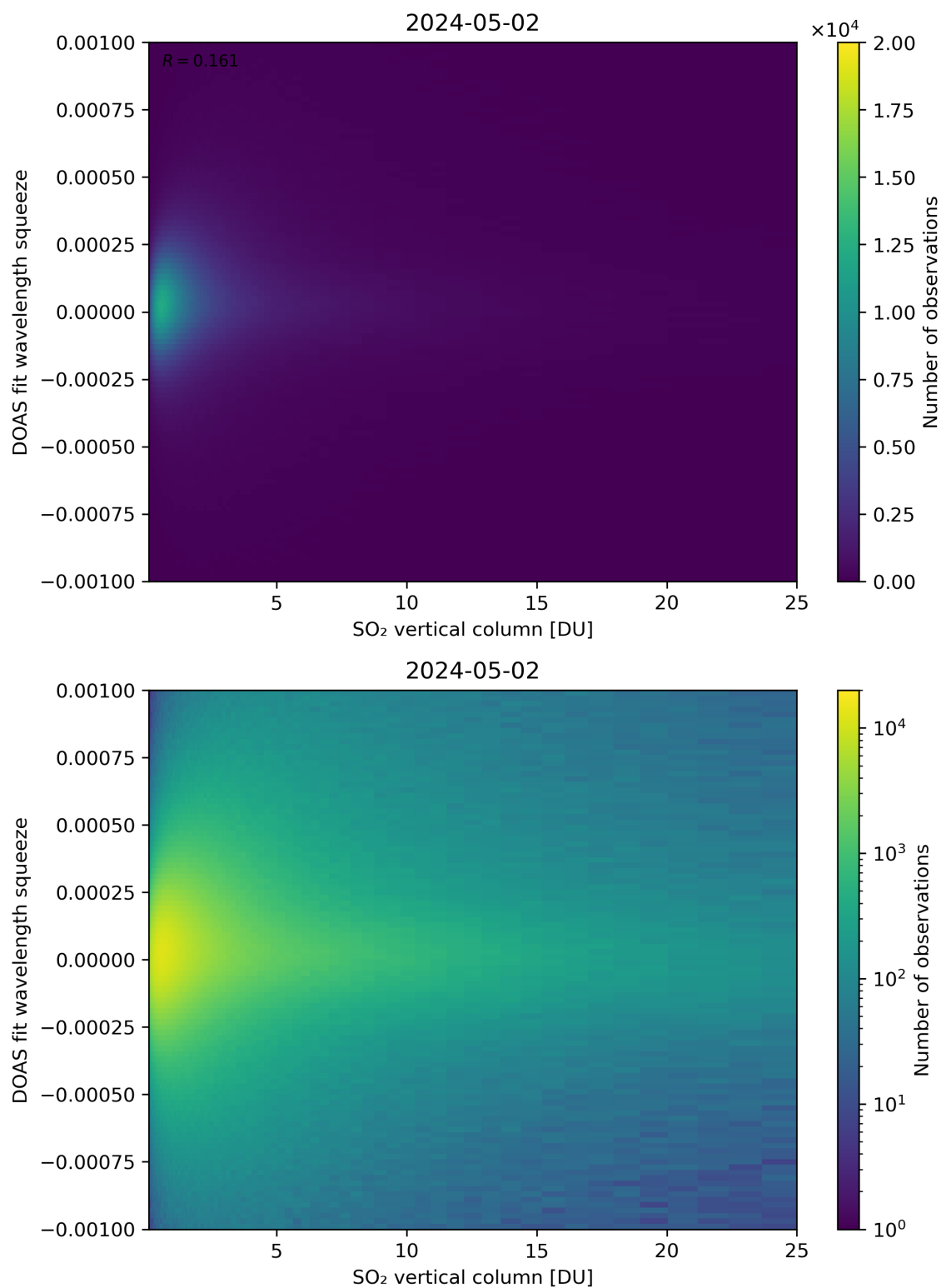
Figure 277: Scatter density plot of “SO 2 vertical column” against “DOAS fit wavelength squeeze” for 2024-05-02 to 2024-05-03.
