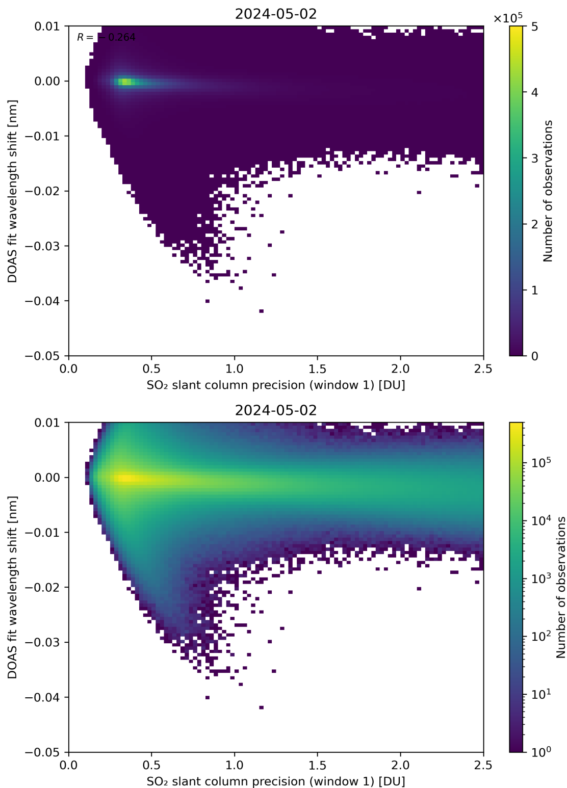
Figure 221: Scatter density plot of “SO 2 slant column precision (window 1)” against “DOAS fit wavelength shift” for 2024-05-02 to 2024-05-03.
