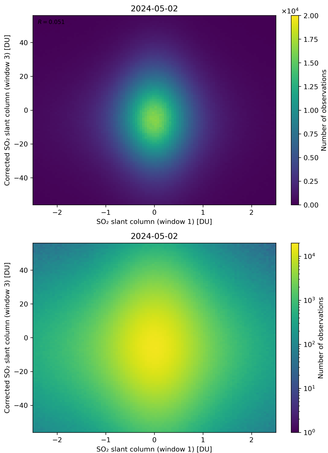
Figure 234: Scatter density plot of “SO 2 slant column (window 1)” against “Corrected SO 2 slant column (window 3)” for 2024-05-02 to 2024-05-03.
