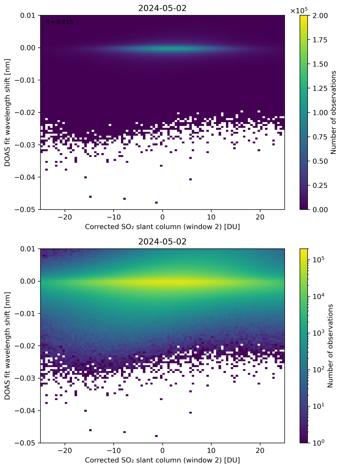
Figure 196: Scatter density plot of “Corrected SO 2 slant column (window 2)” against “DOAS fit wavelength shift” for 2024-05-02 to 2024-05-03.
