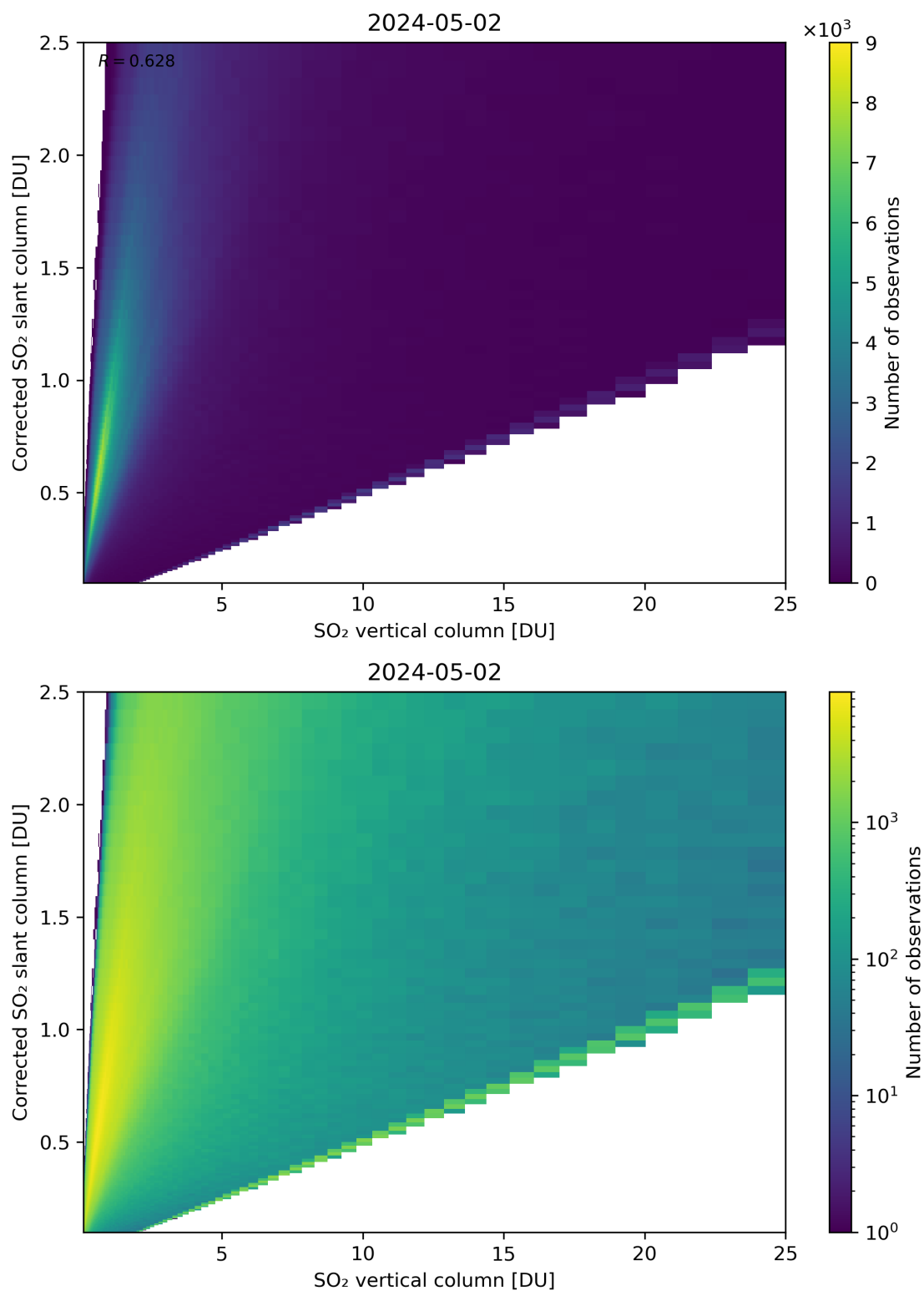
Figure 297: Scatter density plot of “SO 2 vertical column” against “Corrected SO 2 slant column” for 2024-05-02 to 2024-05-03.
