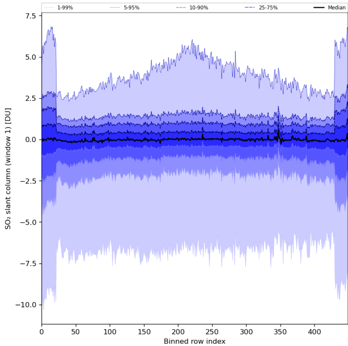
Figure 79: Along track statistics of “SO 2 slant column (window 1)” for 2024-05-02 to 2024-05-03
