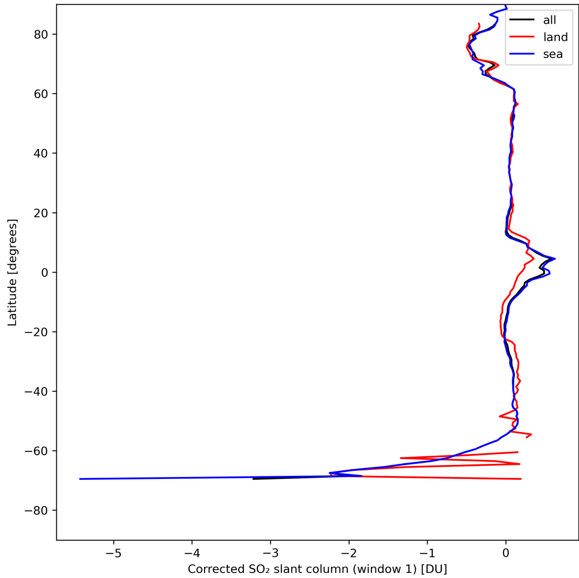
Figure 35: Zonal average of “Corrected SO 2 slant column (window 1)” for 2024-05-02 to 2024-05-03.
