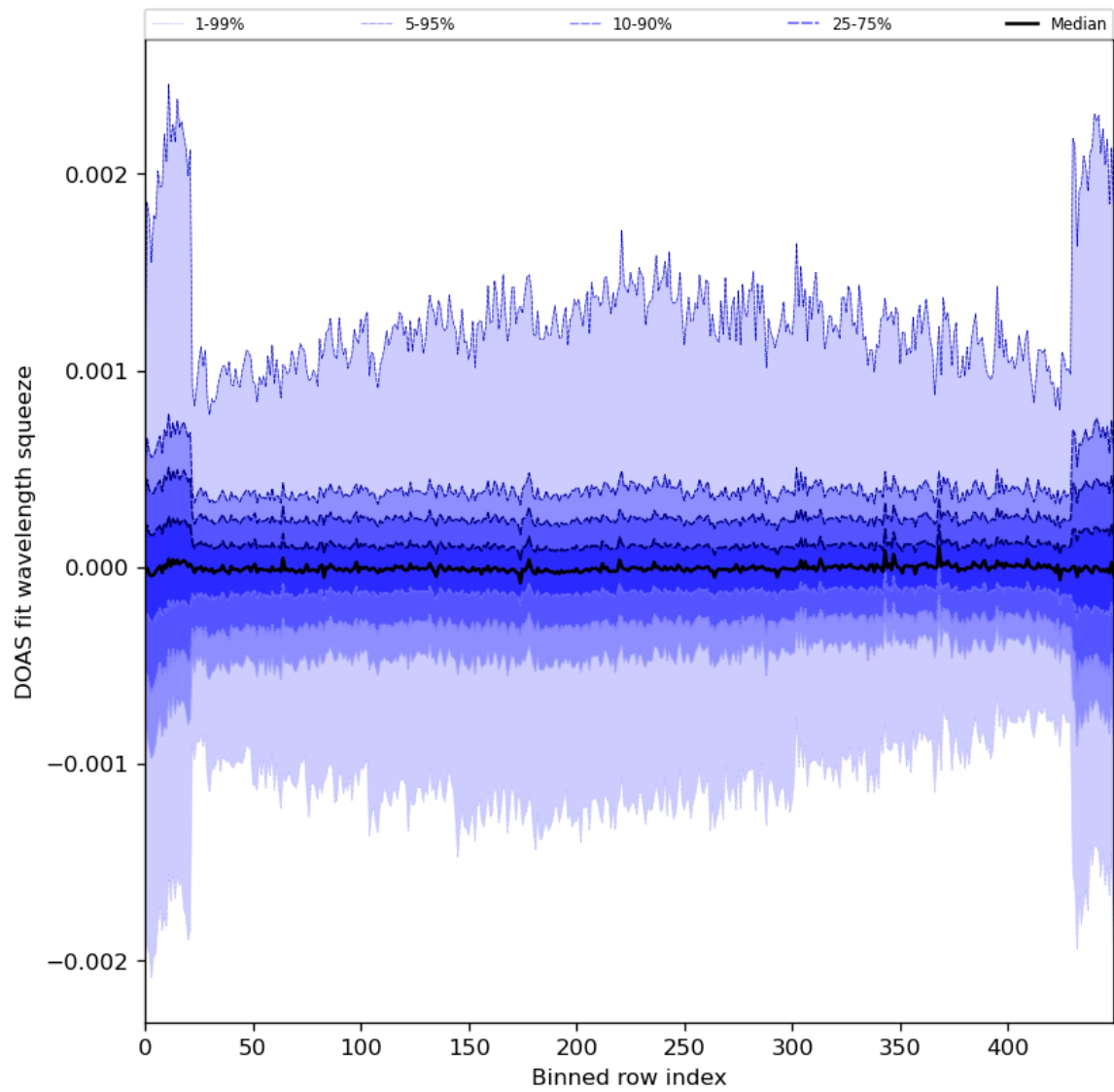
Figure 92: Along track statistics of “DOAS fit wavelength squeeze” for 2024-05-02 to 2024-05-03
