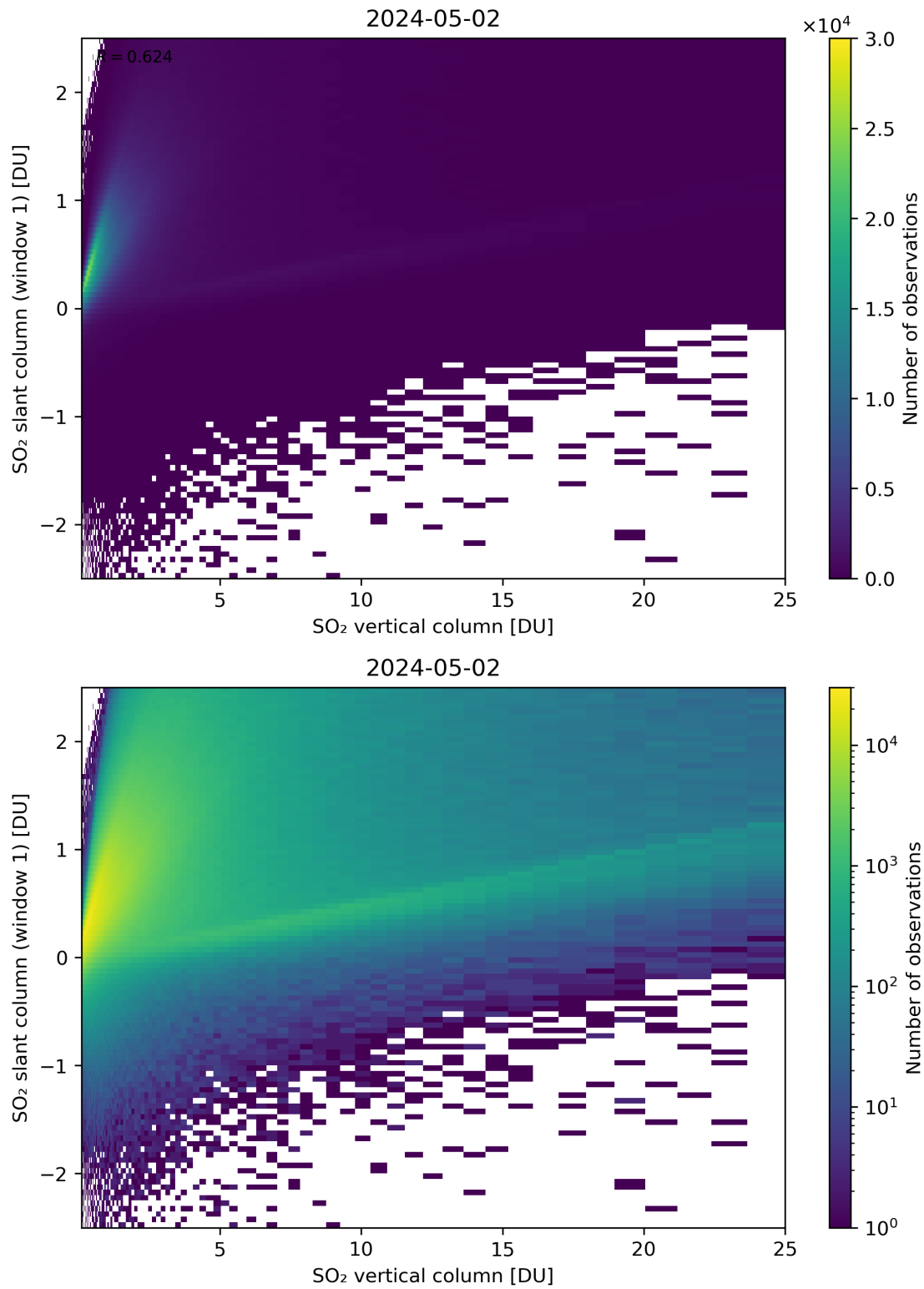
Figure 300: Scatter density plot of “SO 2 vertical column” against “SO 2 slant column (window 1)” for 2024-05-02 to 2024-05-03.
