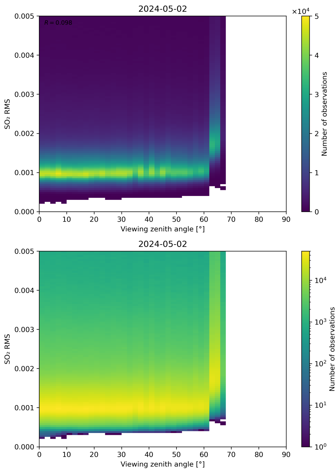
Figure 313: Scatter density plot of “Viewing zenith angle” against “SO 2 RMS” for 2024-05-02 to 2024-05-03.
