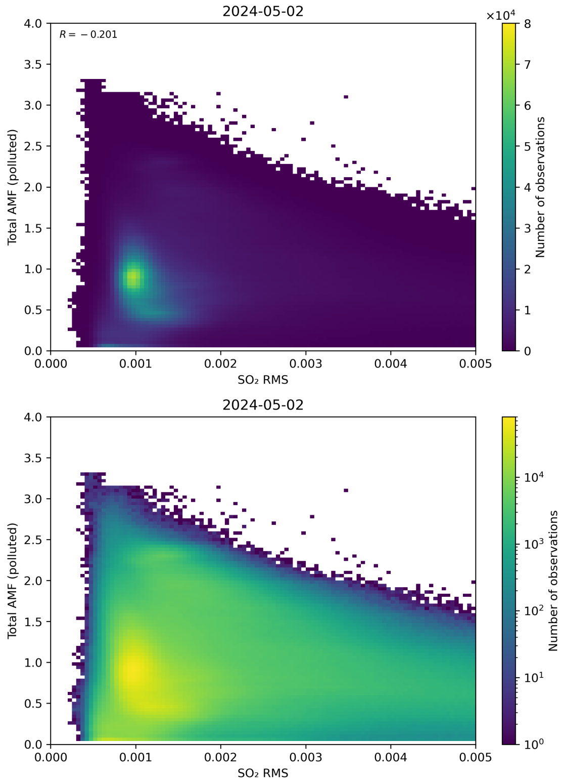
Figure 137: Scatter density plot of “SO 2 RMS” against “Total AMF (polluted)” for 2024-05-02 to 2024-05-03.
