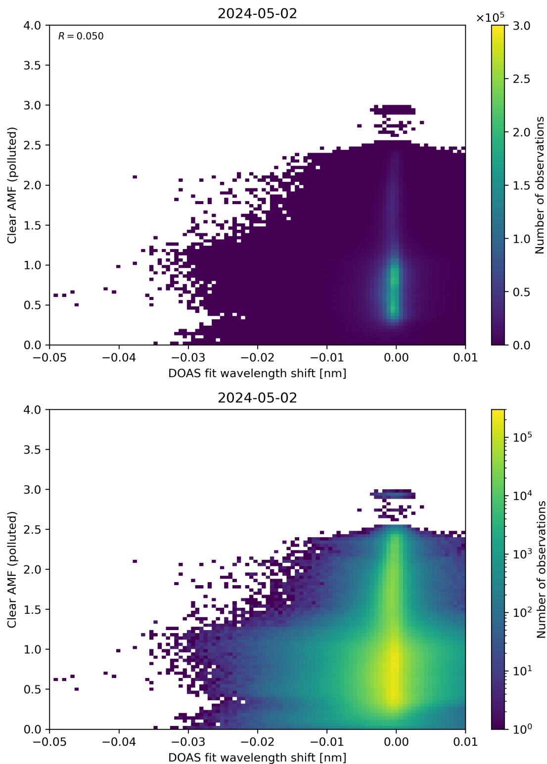
Figure 129: Scatter density plot of “DOAS fit wavelength shift” against “Clear AMF (polluted)” for 2024-05-02 to 2024-05-03.
