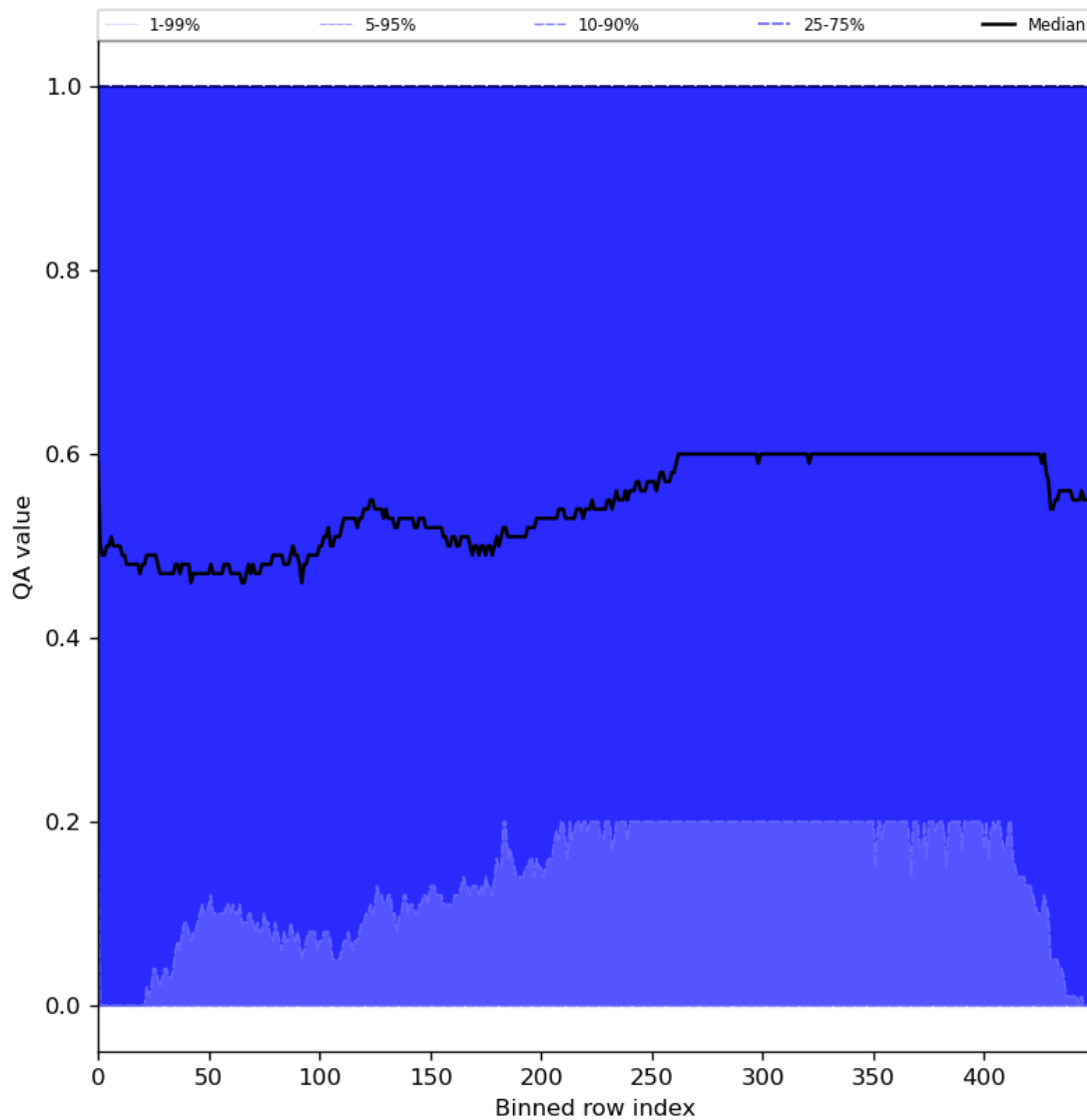
Figure 75: Along track statistics of “QA value” for 2024-05-02 to 2024-05-03
