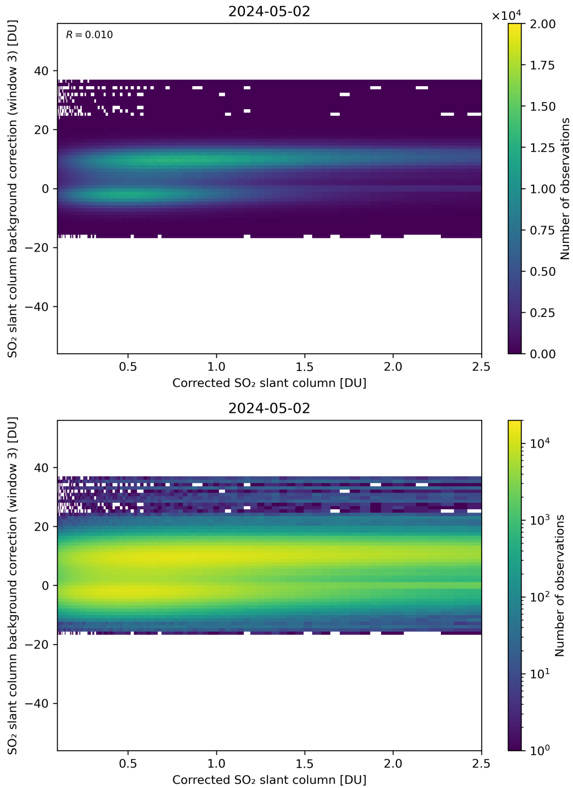
Figure 180: Scatter density plot of “Corrected SO 2 slant column” against “SO 2 slant column background correction (window 3)” for 2024-05-02 to 2024-05-03.
