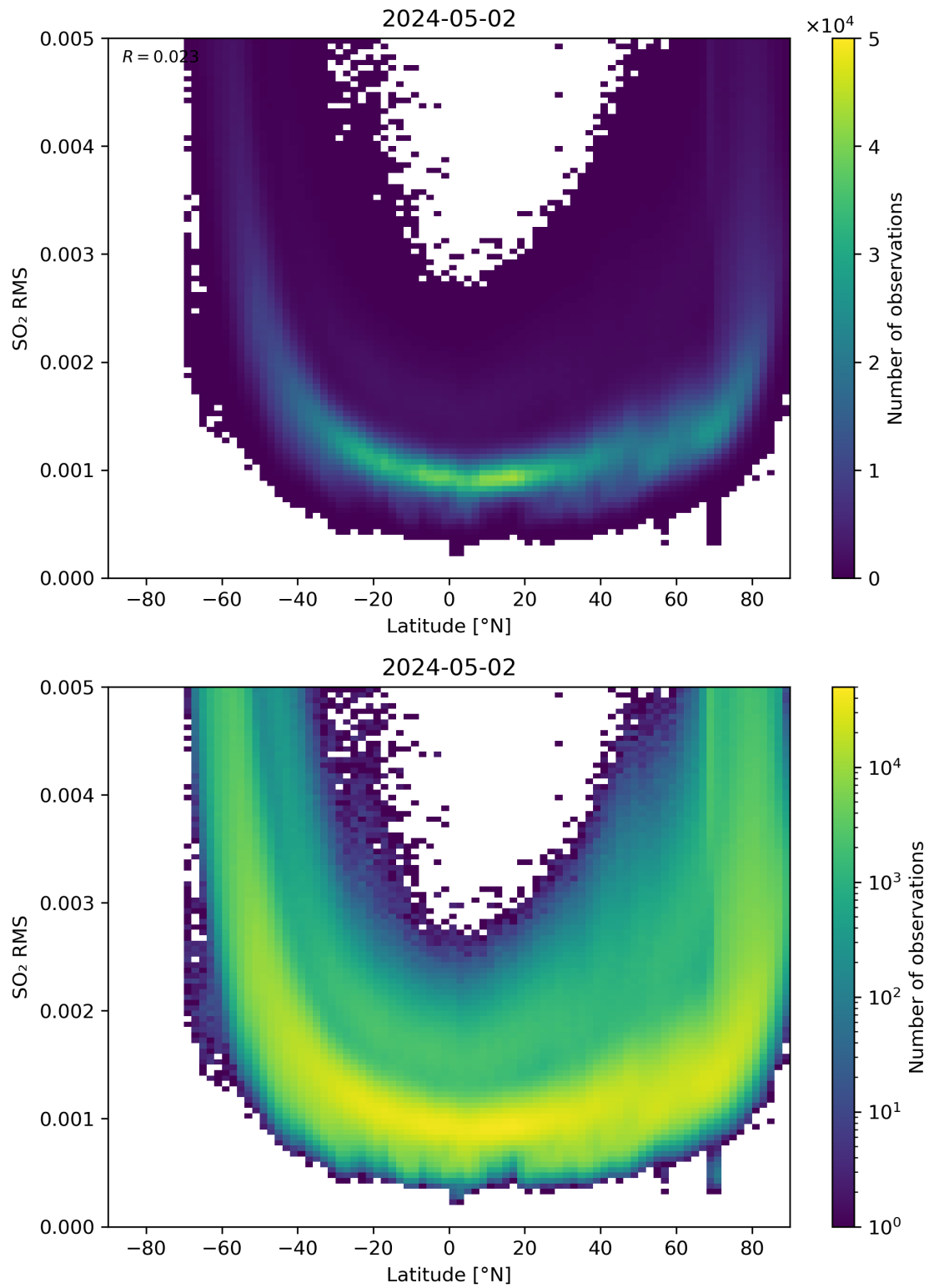
Figure 144: Scatter density plot of “Latitude” against “SO 2 RMS” for 2024-05-02 to 2024-05-03.
