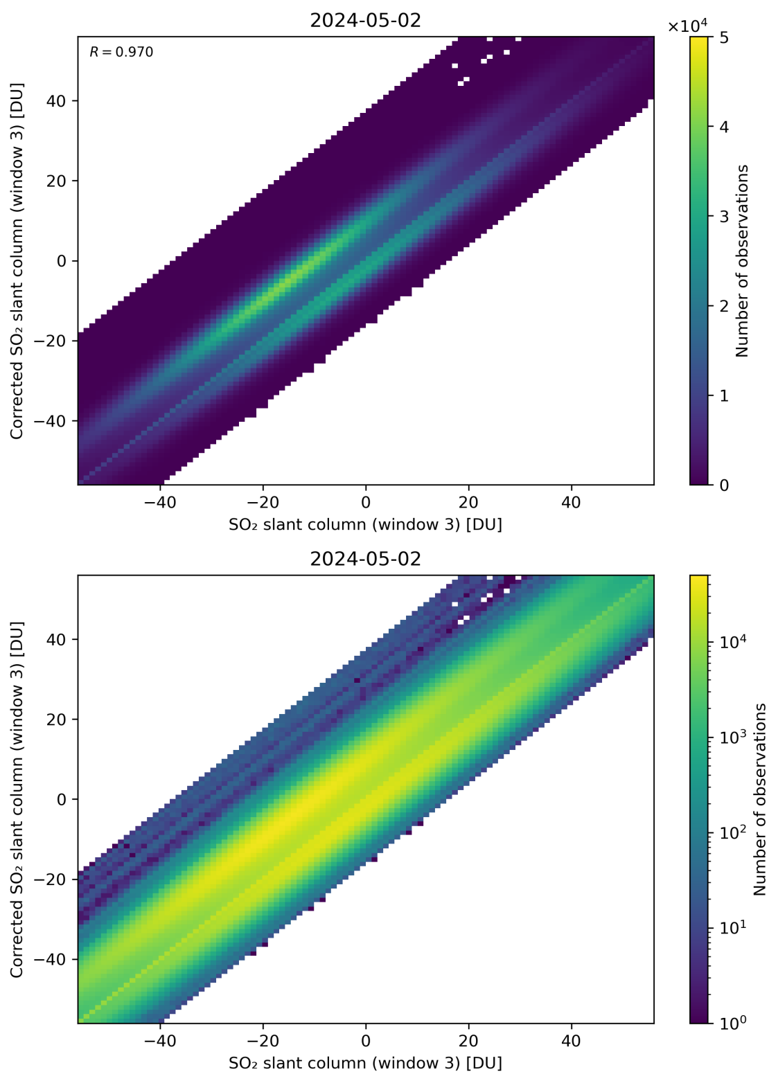
Figure 266: Scatter density plot of “SO 2 slant column (window 3)” against “Corrected SO 2 slant column (window 3)” for 2024-05-02 to 2024-05-03.
