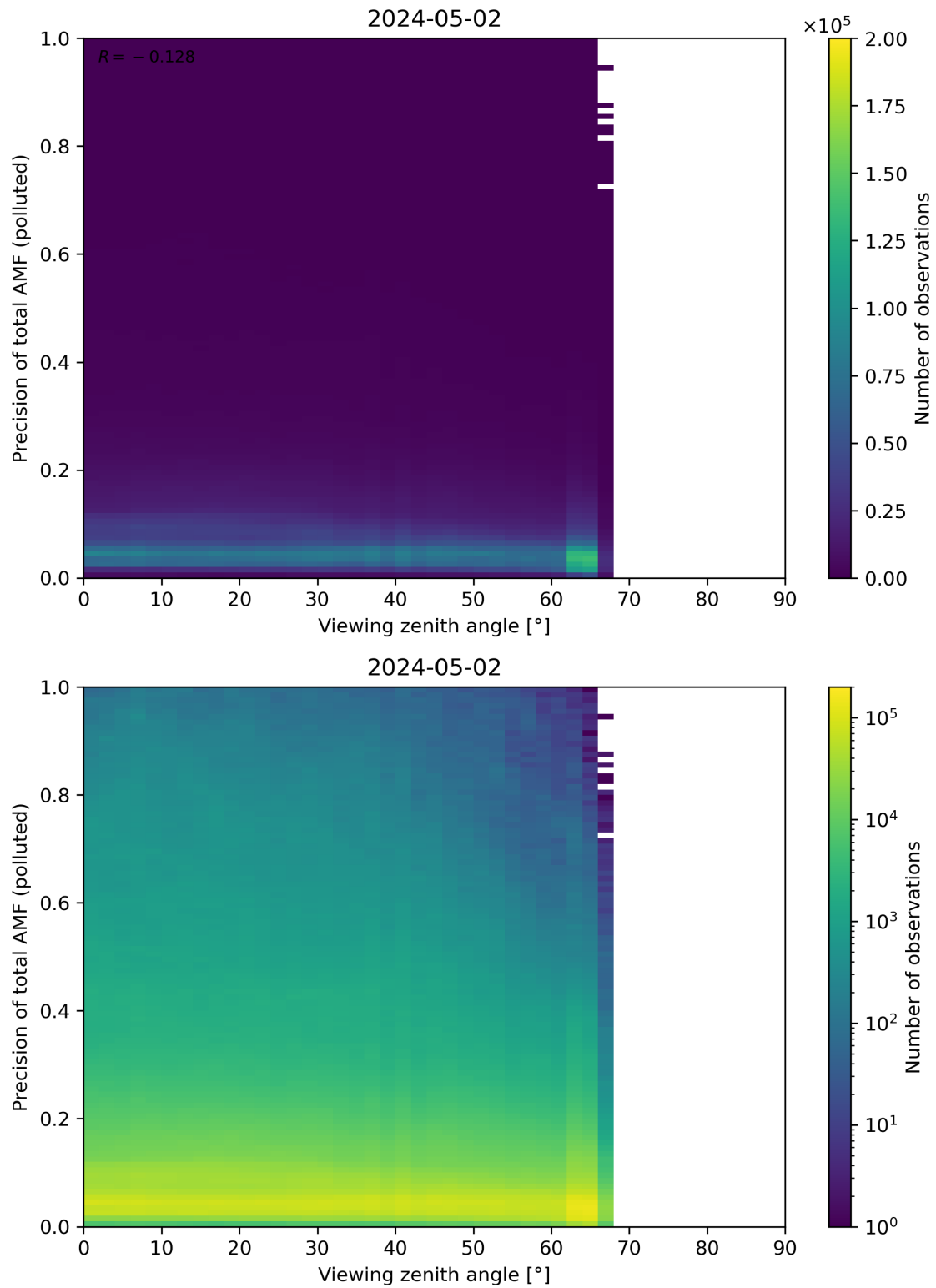
Figure 326: Scatter density plot of “Viewing zenith angle” against “Precision of total AMF (polluted)” for 2024-05-02 to 2024-05-03.
