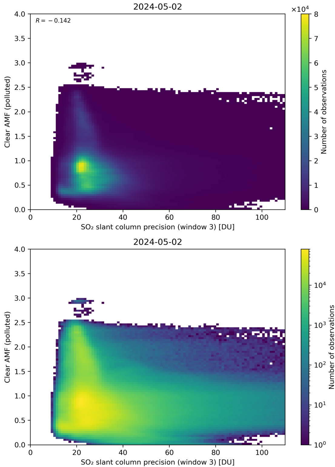
Figure 261: Scatter density plot of “SO 2 slant column precision (window 3)” against “Clear AMF (polluted)” for 2024-05-02 to 2024-05-03.
