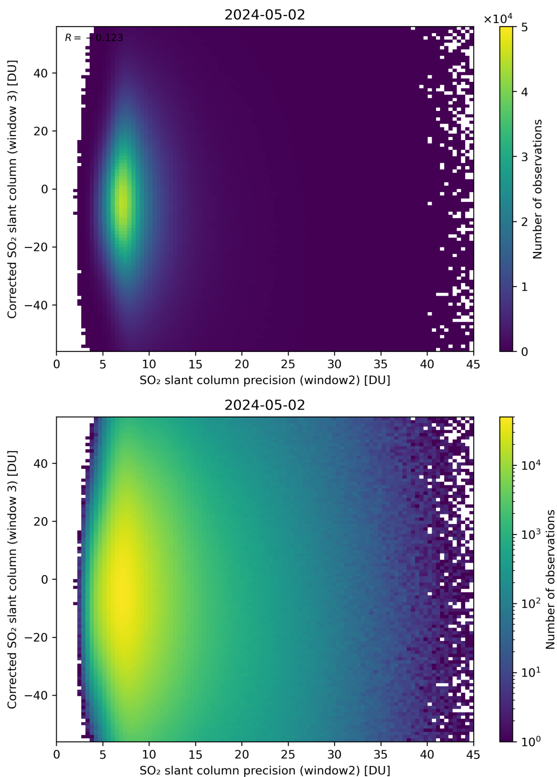
Figure 248: Scatter density plot of “SO 2 slant column precision (window2)” against “Corrected SO 2 slant column (window 3)” for 2024-05-02 to 2024-05-03.
