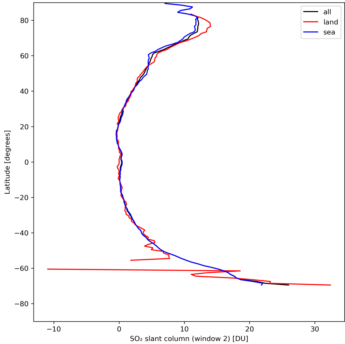
Figure 37: Zonal average of “SO 2 slant column (window 2)” for 2024-05-02 to 2024-05-03.
