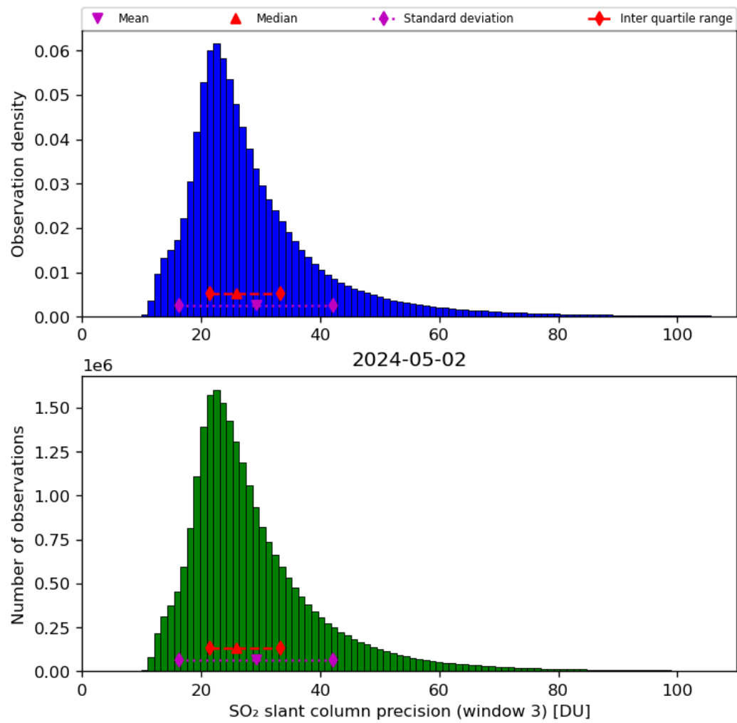
Figure 65: Histogram of “SO 2 slant column precision (window 3)” for 2024-05-02 to 2024-05-03
