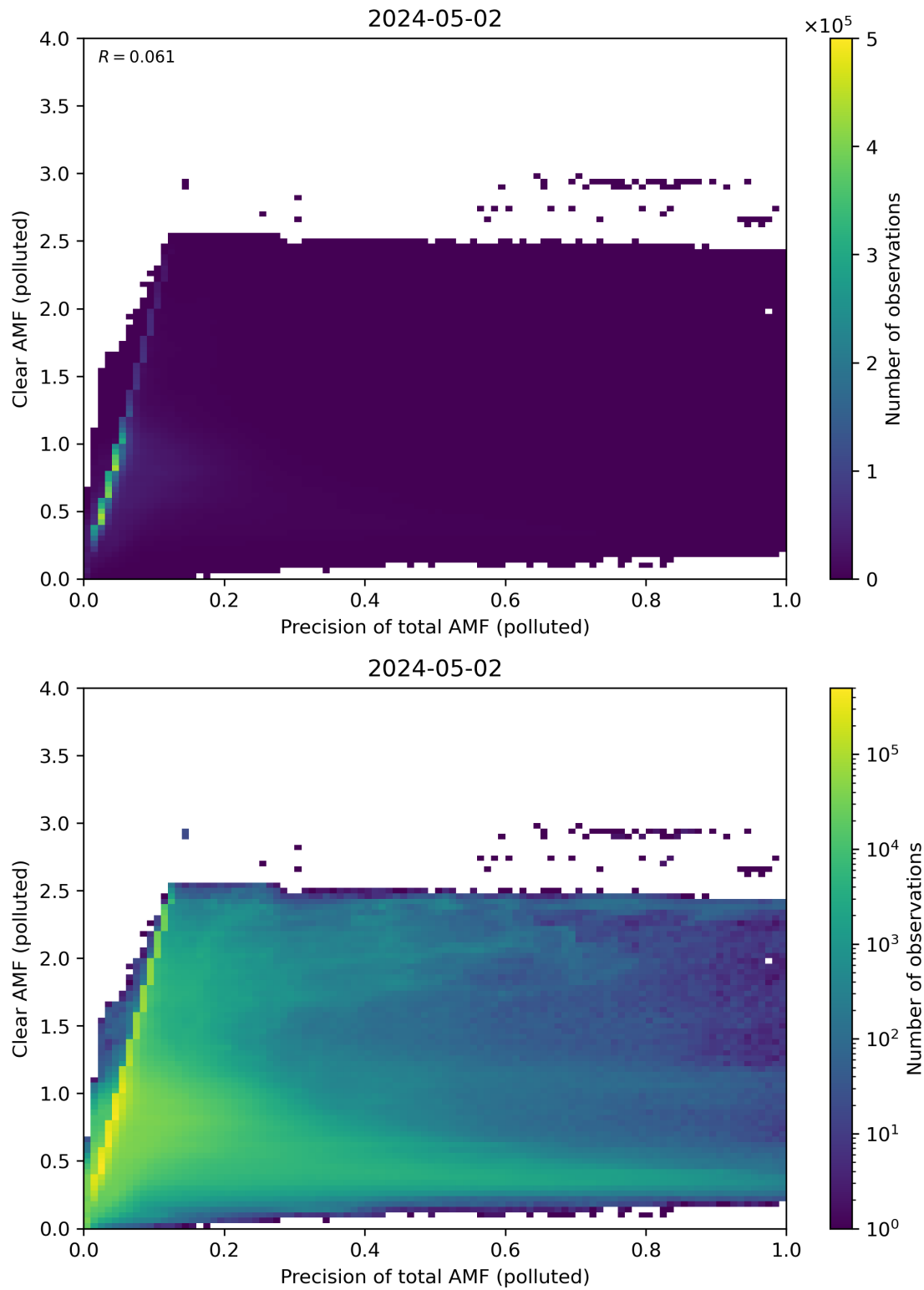
Figure 270: Scatter density plot of “Precision of total AMF (polluted)” against “Clear AMF (polluted)” for 2024-05-02 to 2024-05-03.
