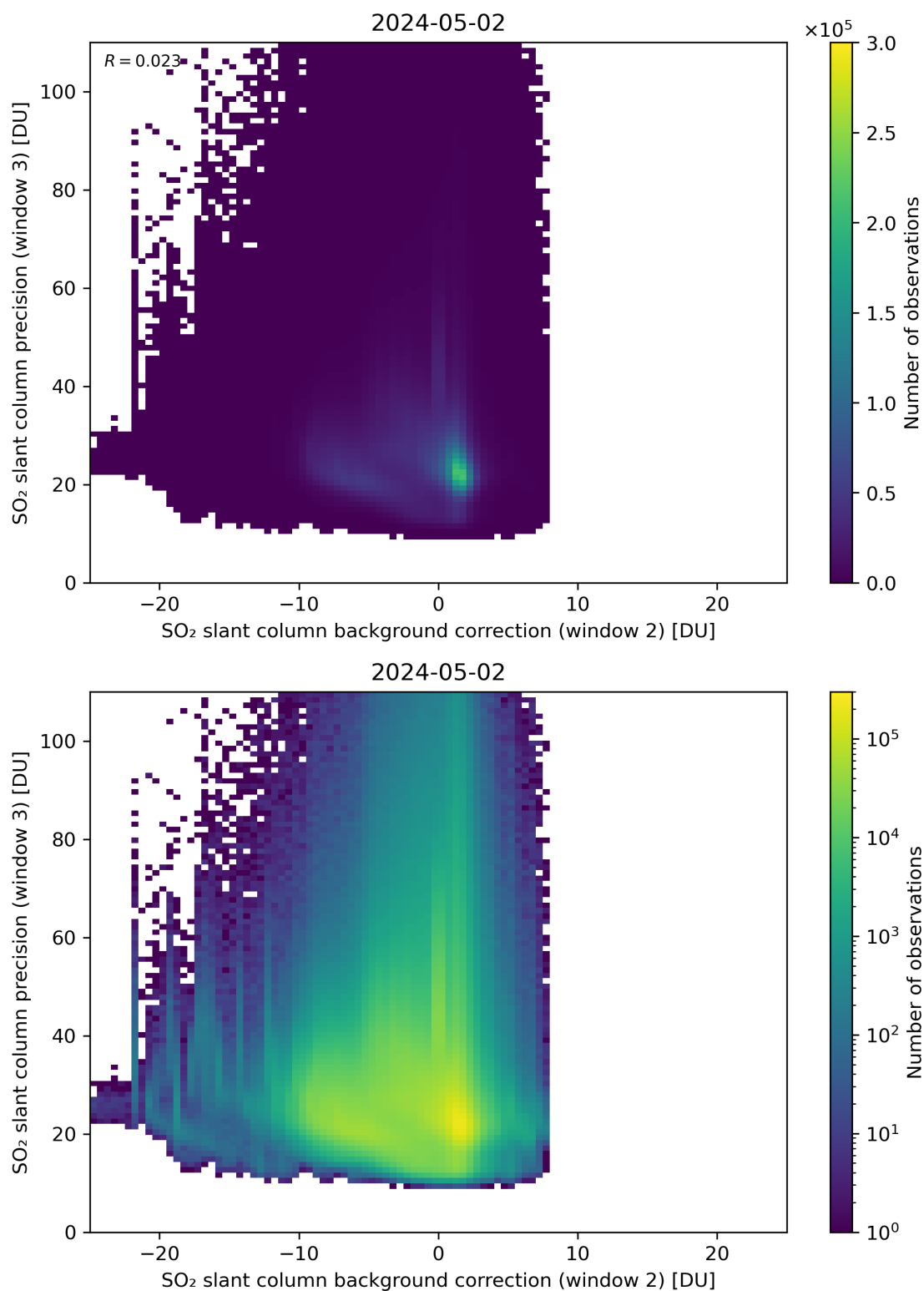
Figure 118: Scatter density plot of “SO 2 slant column background correction (window 2)” against “SO 2 slant column precision (window 3)” for 2024-05-02 to 2024-05-03.
