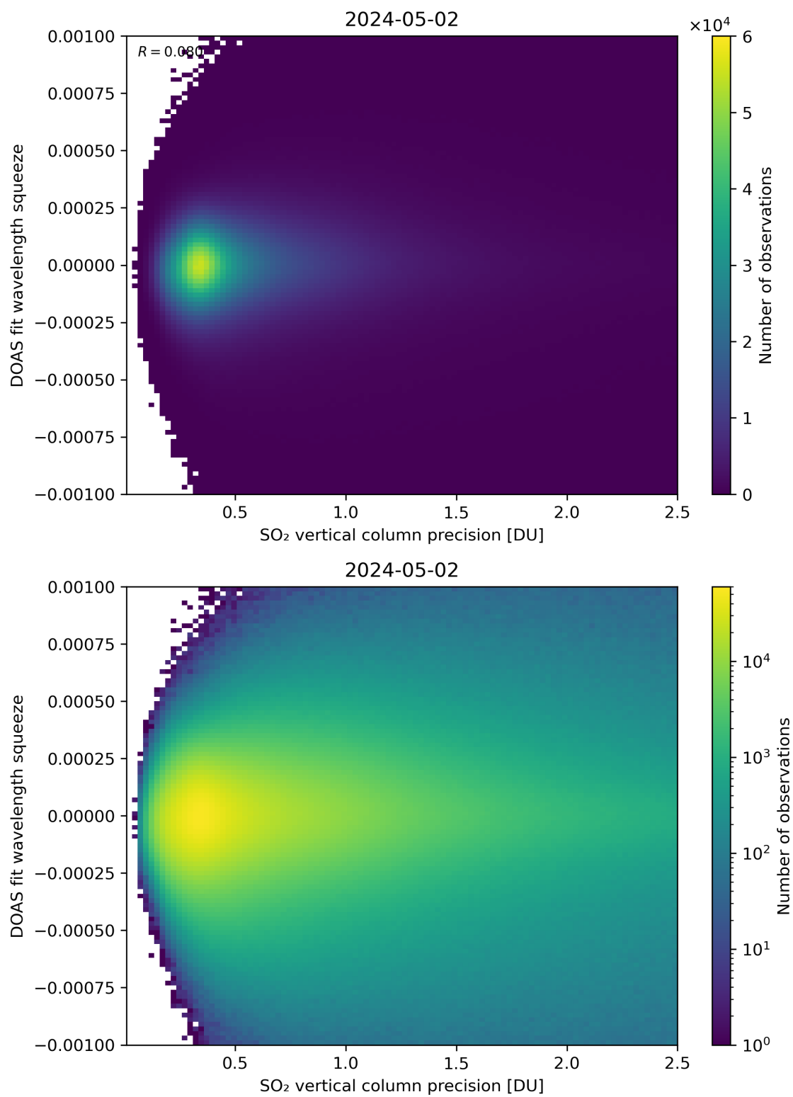
Figure 283: Scatter density plot of “SO 2 vertical column precision” against “DOAS fit wavelength squeeze” for 2024-05-02 to 2024-05-03.
