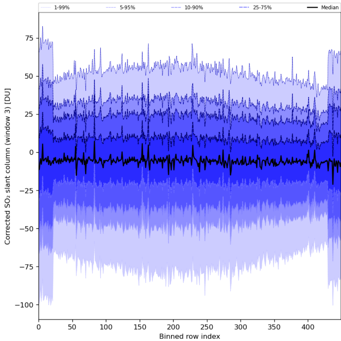
Figure 89: Along track statistics of “Corrected SO 2 slant column (window 3)” for 2024-05-02 to 2024-05-03
