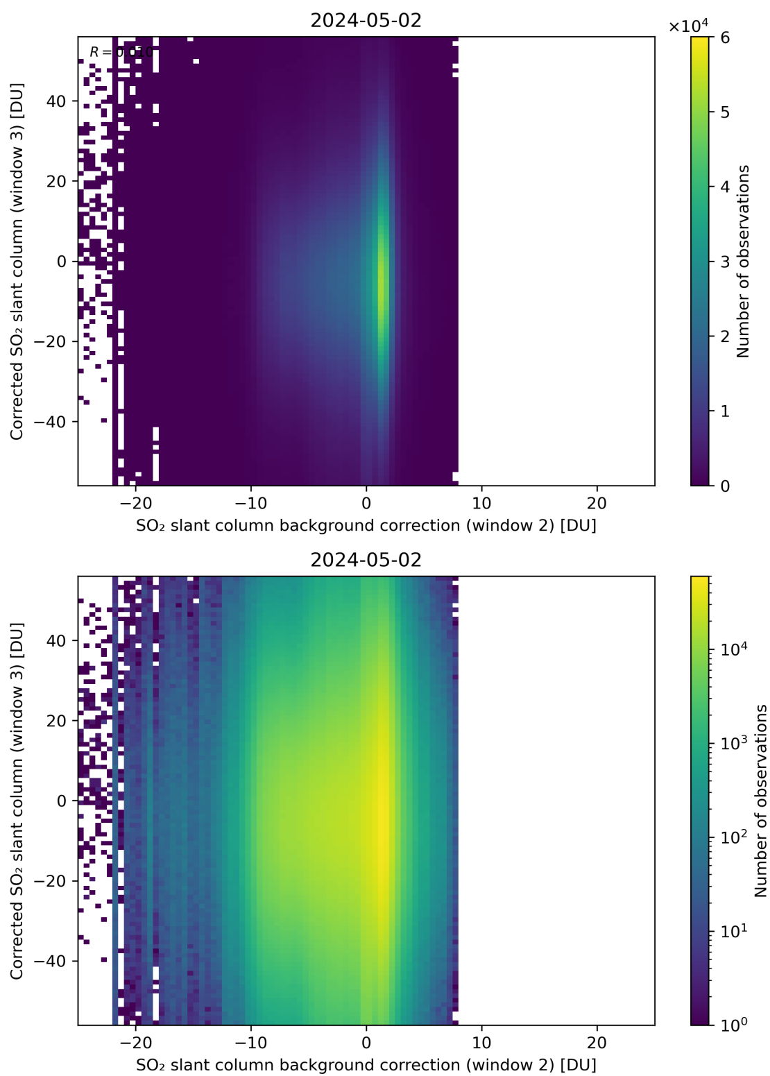
Figure 116: Scatter density plot of “SO 2 slant column background correction (window 2)” against “Corrected SO 2 slant column (window 3)” for 2024-05-02 to 2024-05-03.
