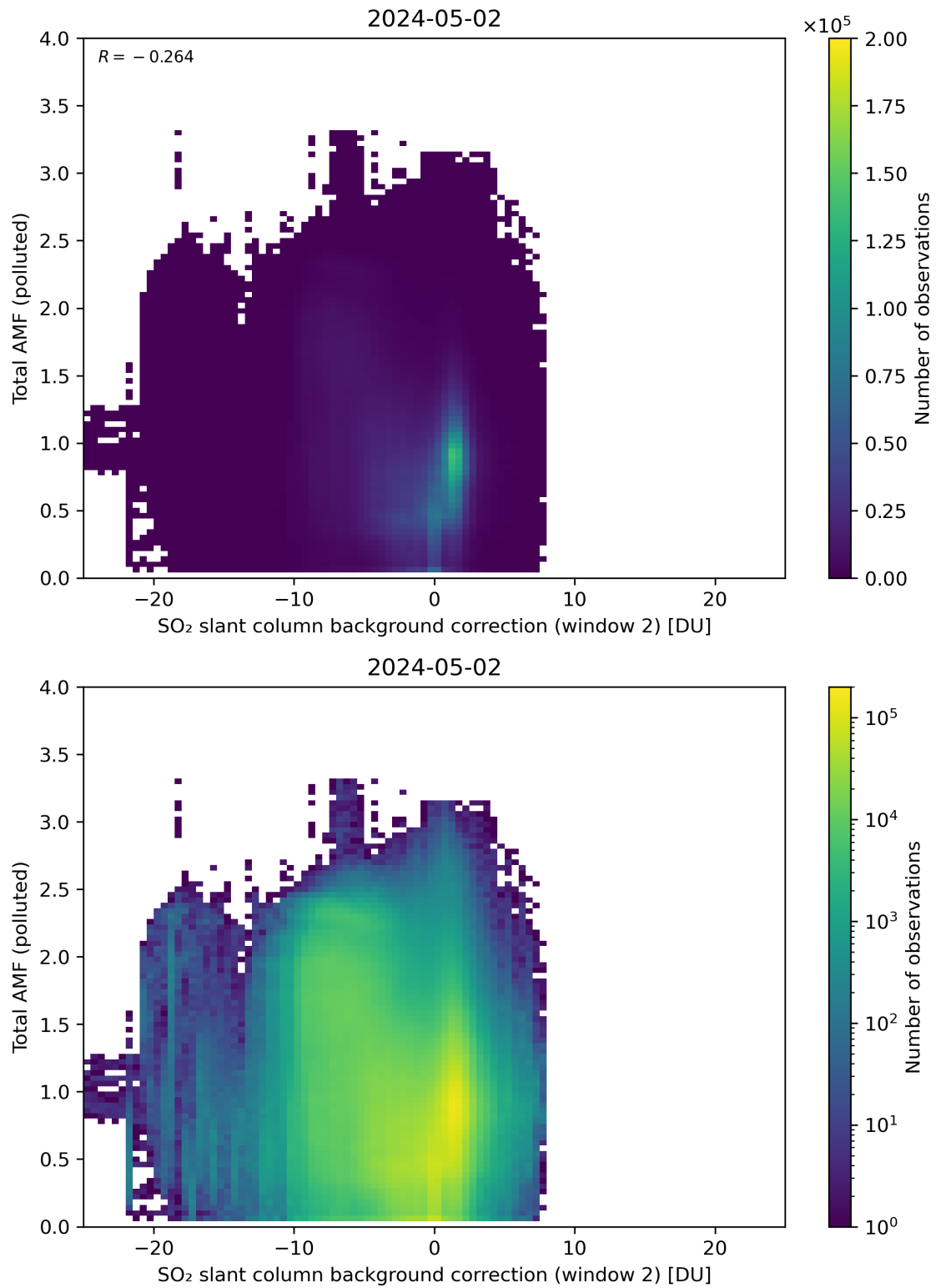
Figure 119: Scatter density plot of “SO 2 slant column background correction (window 2)” against “Total AMF (polluted)” for 2024-05-02 to 2024-05-03.
