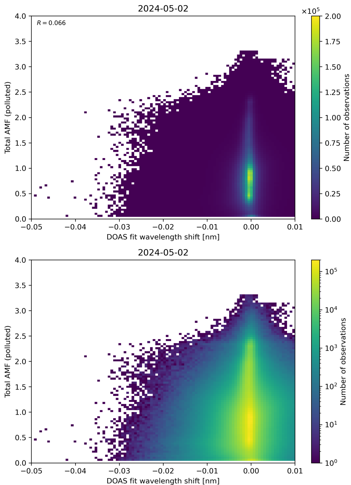
Figure 130: Scatter density plot of “DOAS fit wavelength shift” against “Total AMF (polluted)” for 2024-05-02 to 2024-05-03.
