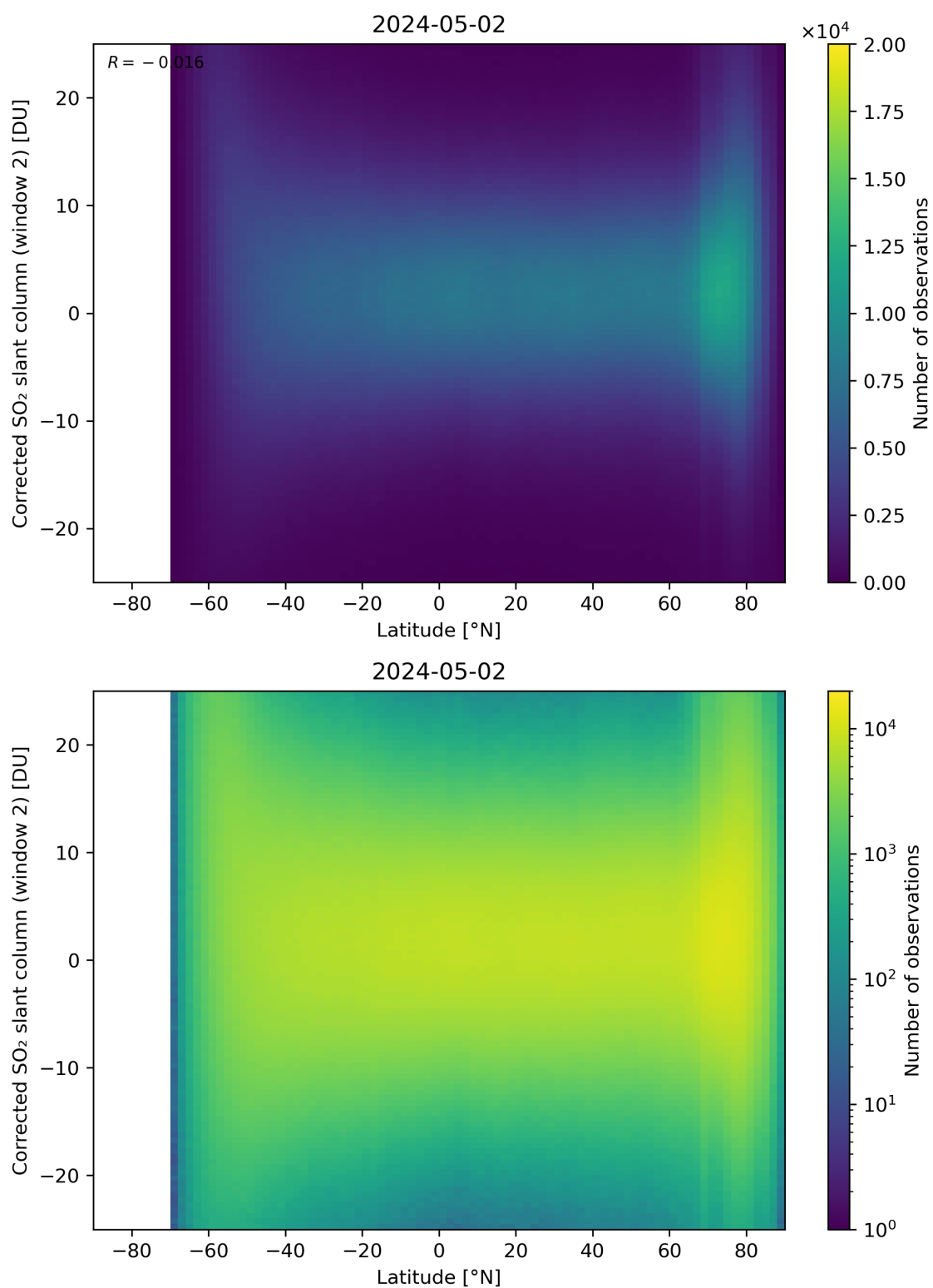
Figure 147: Scatter density plot of “Latitude” against “Corrected SO 2 slant column (window 2)” for 2024-05-02 to 2024-05-03.
