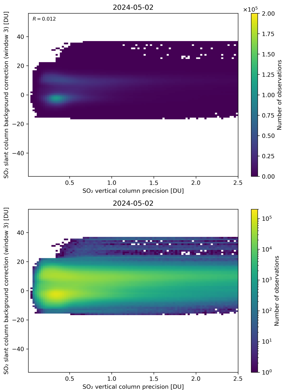
Figure 281: Scatter density plot of “SO 2 vertical column precision” against “SO 2 slant column background correction (window 3)” for 2024-05-02 to 2024-05-03.
