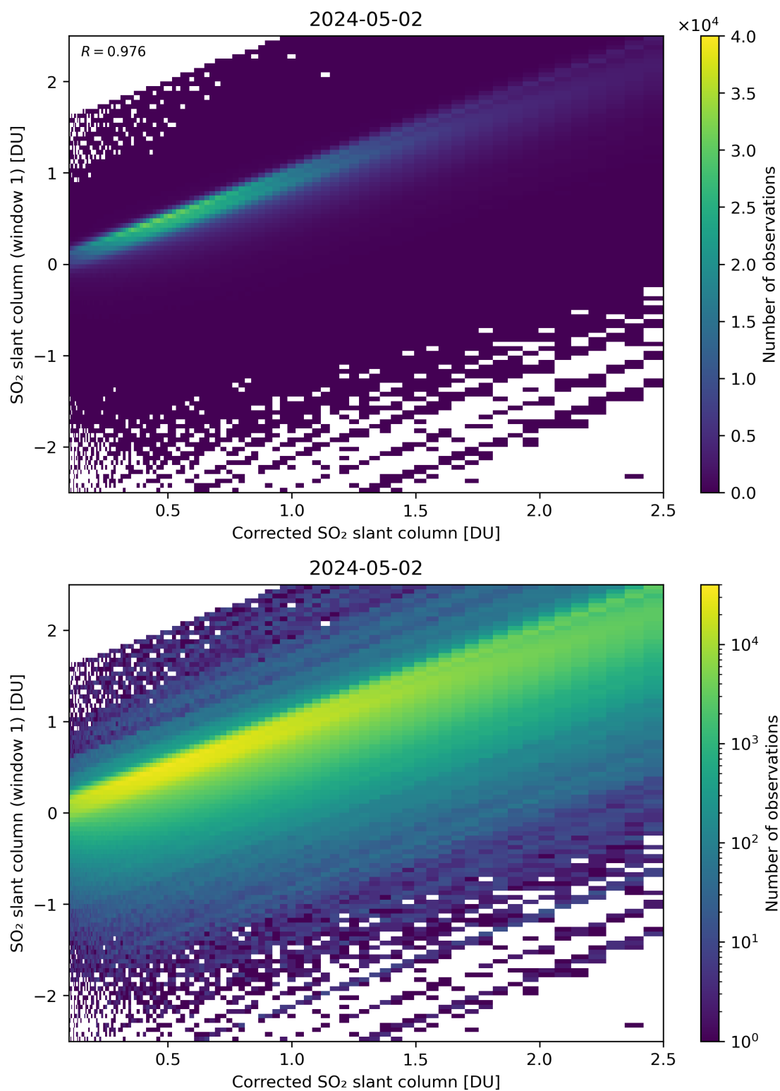
Figure 187: Scatter density plot of “Corrected SO 2 slant column” against “SO 2 slant column (window 1)” for 2024-05-02 to 2024-05-03.
