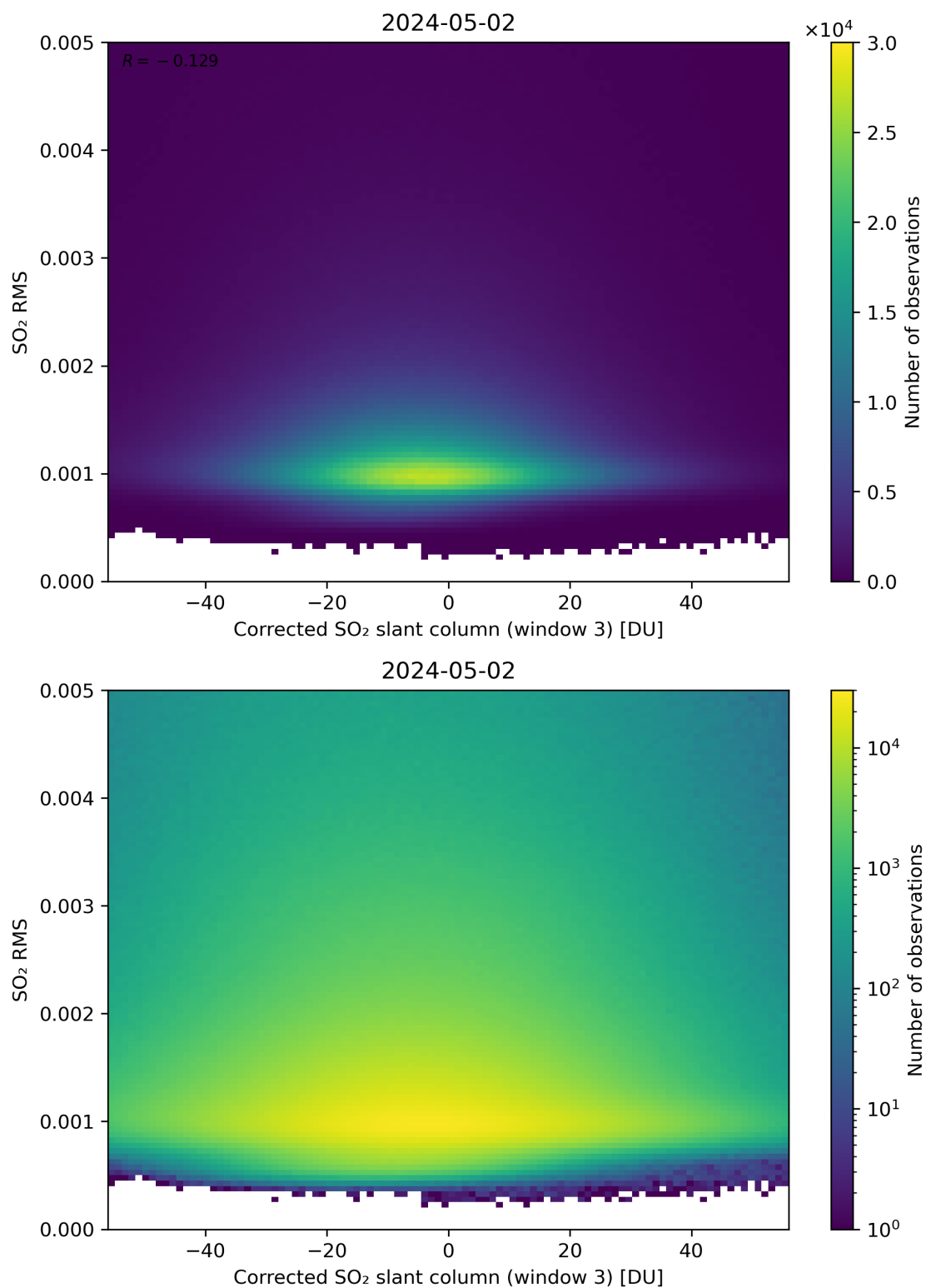
Figure 208: Scatter density plot of “Corrected SO 2 slant column (window 3)” against “SO 2 RMS” for 2024-05-02 to 2024-05-03.
