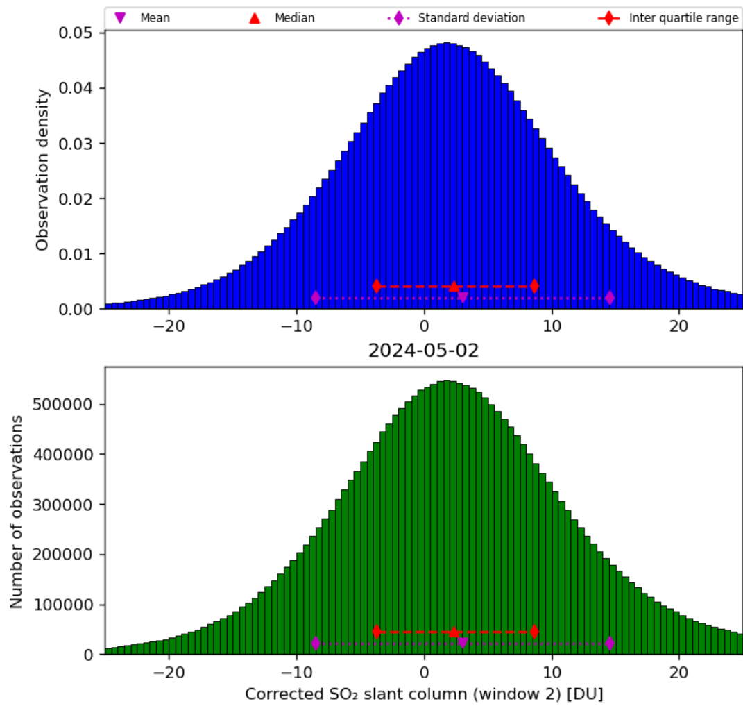
Figure 62: Histogram of “Corrected SO 2 slant column (window 2)” for 2024-05-02 to 2024-05-03
