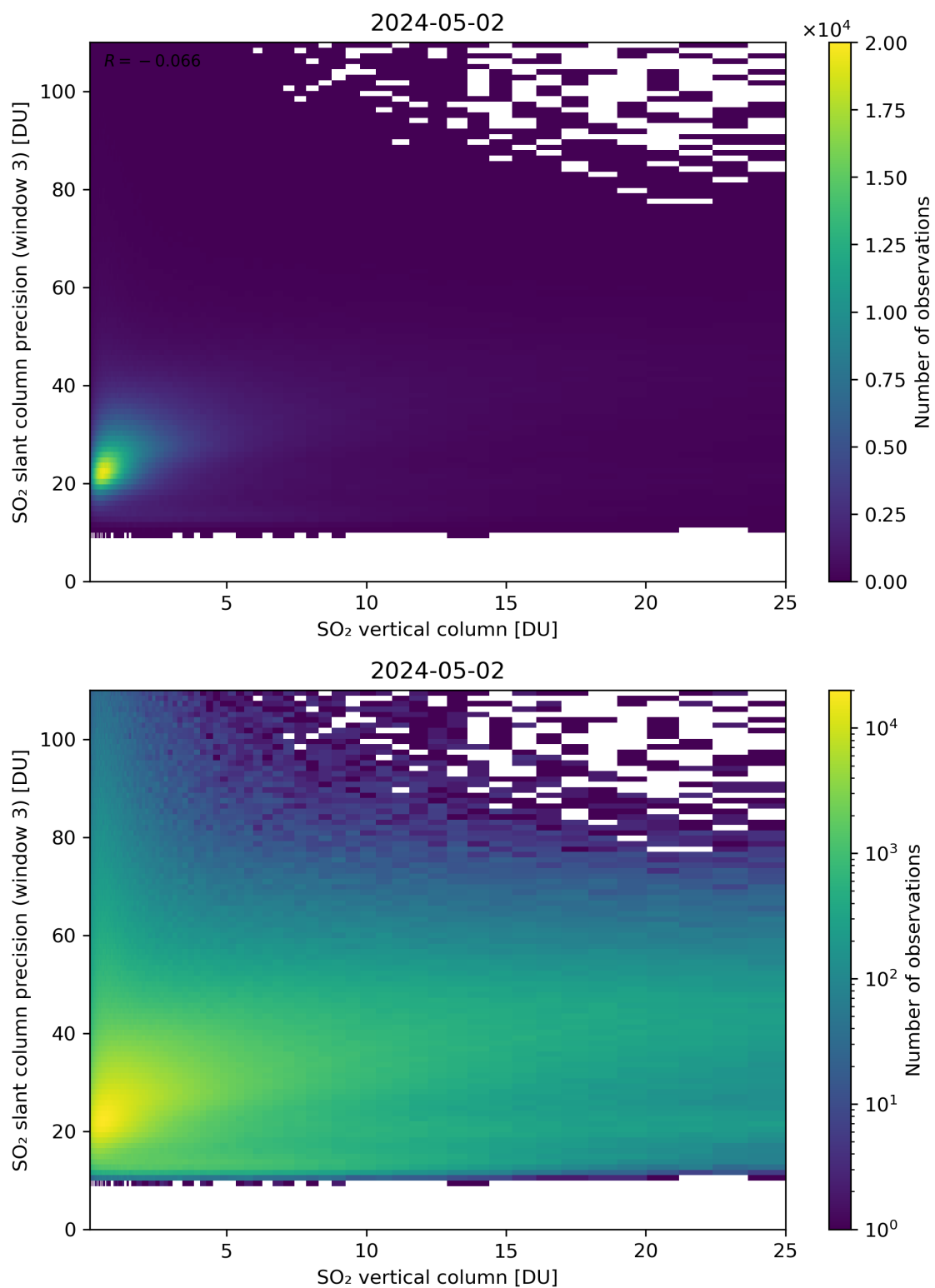
Figure 304: Scatter density plot of “SO 2 vertical column” against “SO 2 slant column precision (window 3)” for 2024-05-02 to 2024-05-03.
