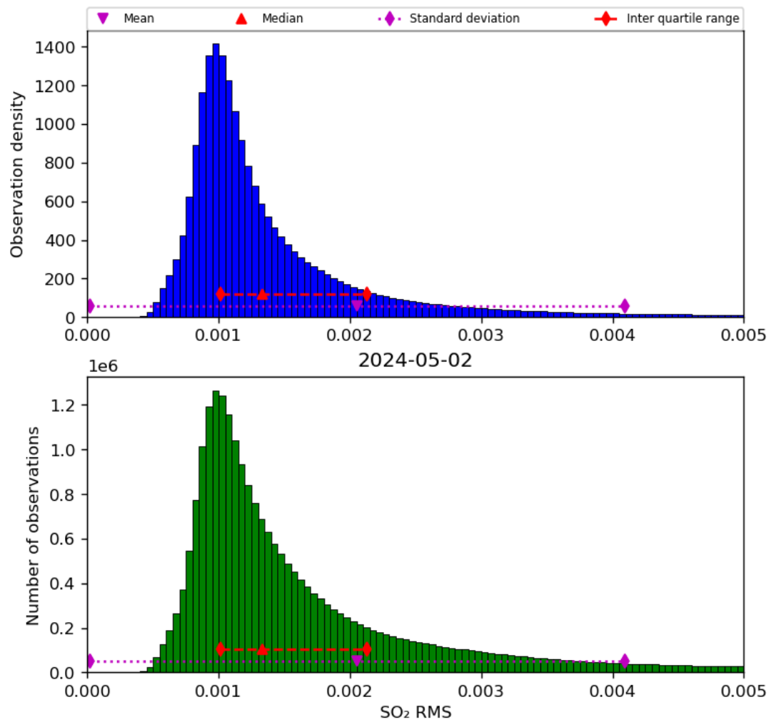
Figure 70: Histogram of “SO 2 RMS” for 2024-05-02 to 2024-05-03
