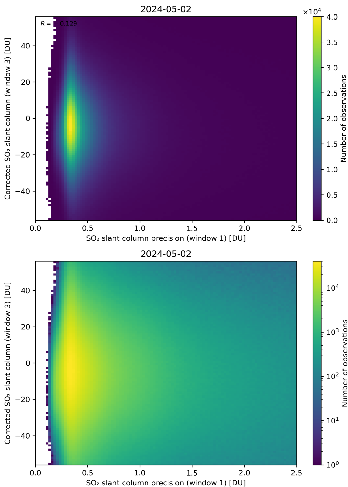
Figure 226: Scatter density plot of “SO 2 slant column precision (window 1)” against “Corrected SO 2 slant column (window 3)” for 2024-05-02 to 2024-05-03.
