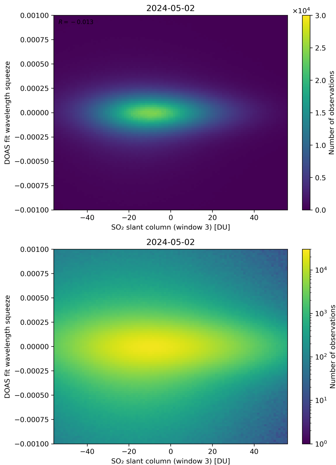
Figure 255: Scatter density plot of “SO 2 slant column (window 3)” against “DOAS fit wavelength squeeze” for 2024-05-02 to 2024-05-03.
