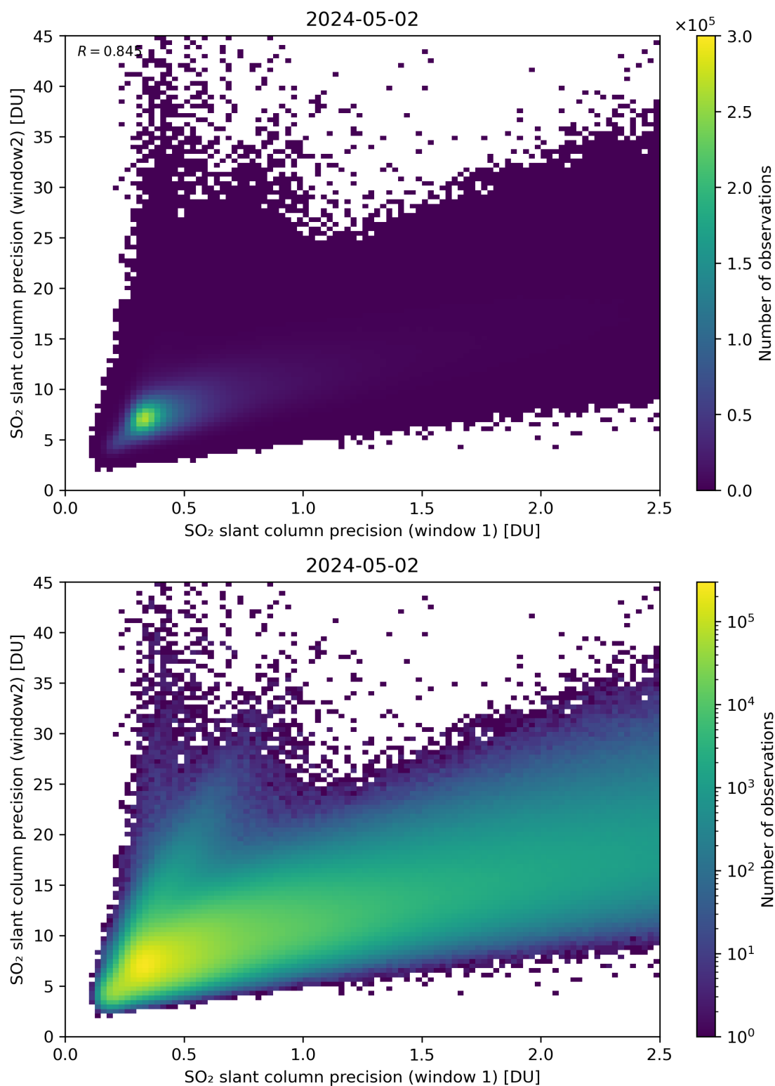
Figure 227: Scatter density plot of “SO 2 slant column precision (window 1)” against “SO 2 slant column precision (window2)” for 2024-05-02 to 2024-05-03.
