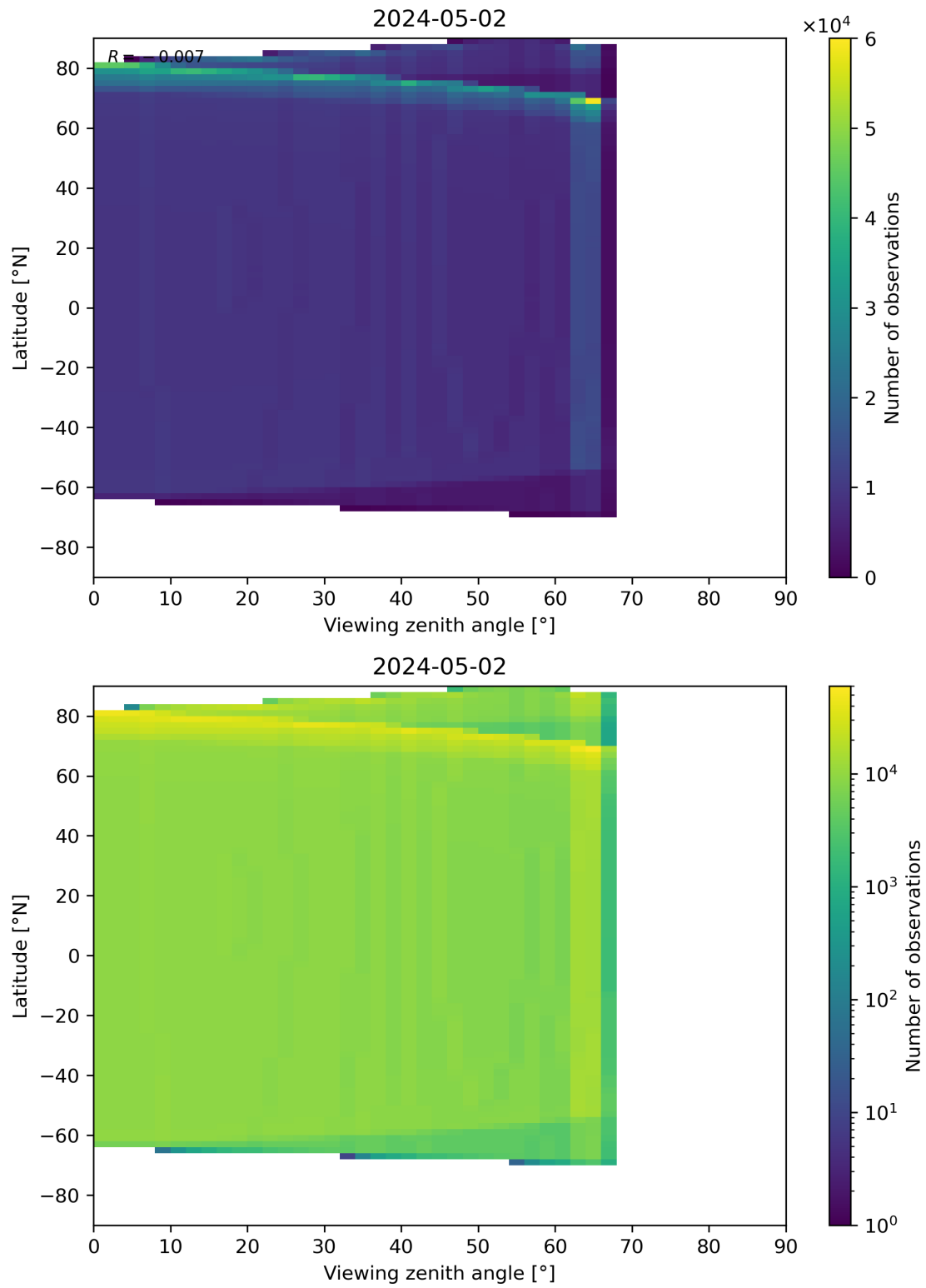
Figure 314: Scatter density plot of “Viewing zenith angle” against “Latitude” for 2024-05-02 to 2024-05-03.
