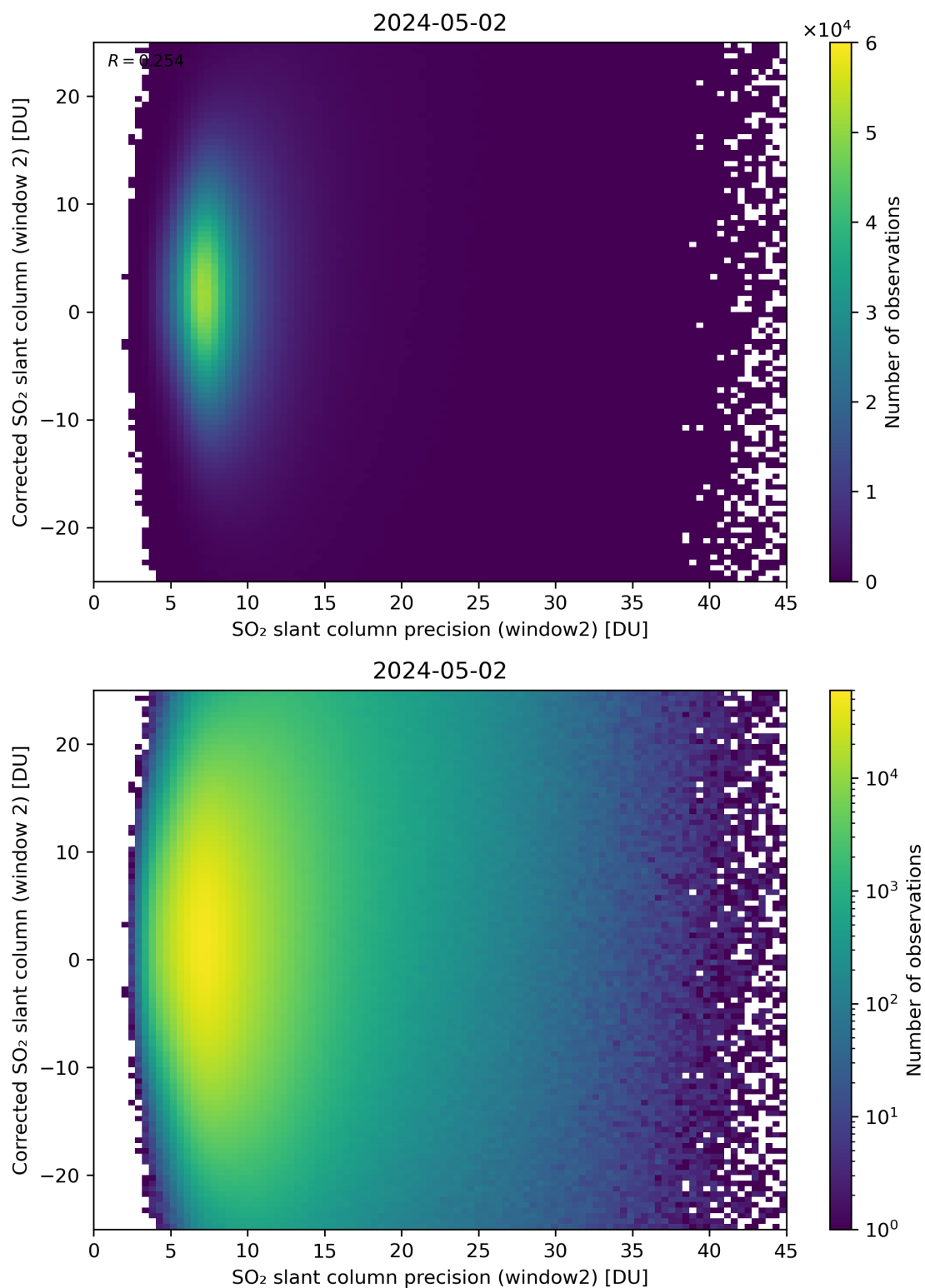
Figure 247: Scatter density plot of “SO 2 slant column precision (window2)” against “Corrected SO 2 slant column (window 2)” for 2024-05-02 to 2024-05-03.
