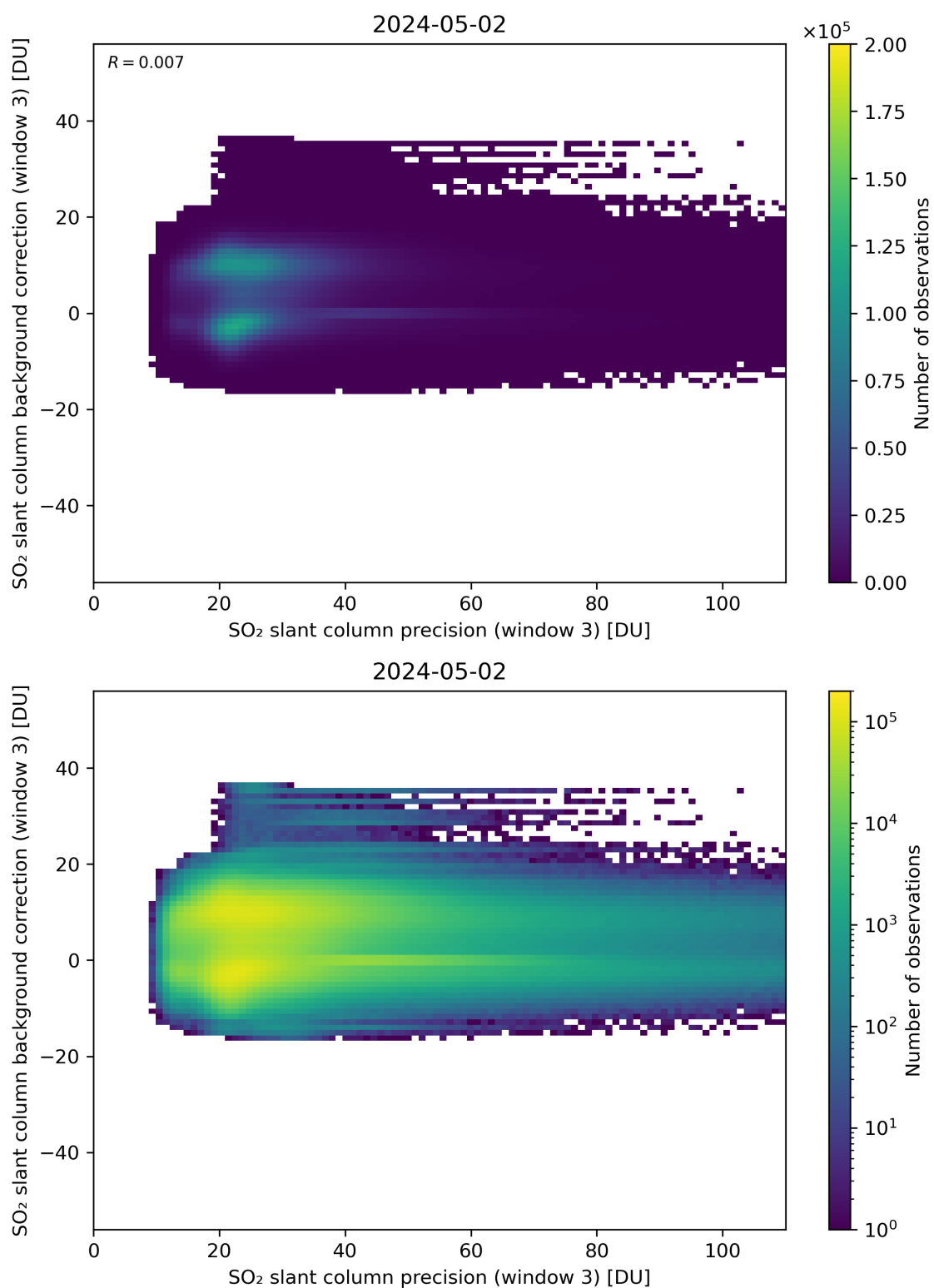
Figure 257: Scatter density plot of “SO 2 slant column precision (window 3)” against “SO 2 slant column background correction (window 3)” for 2024-05-02 to 2024-05-03.
