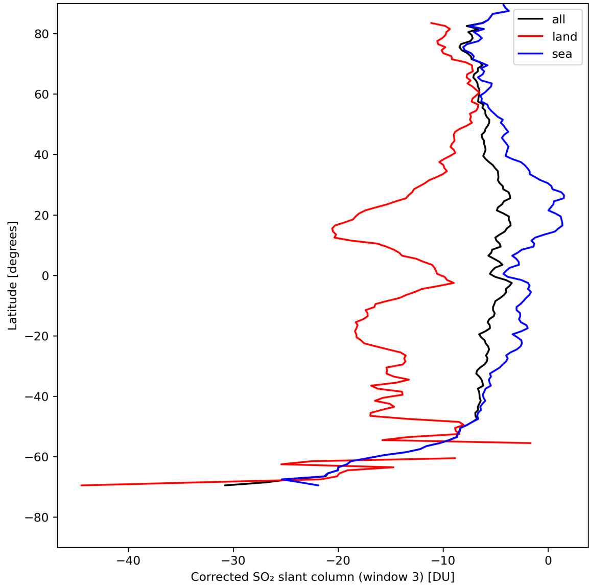
Figure 43: Zonal average of “Corrected SO 2 slant column (window 3)” for 2024-05-02 to 2024-05-03.
