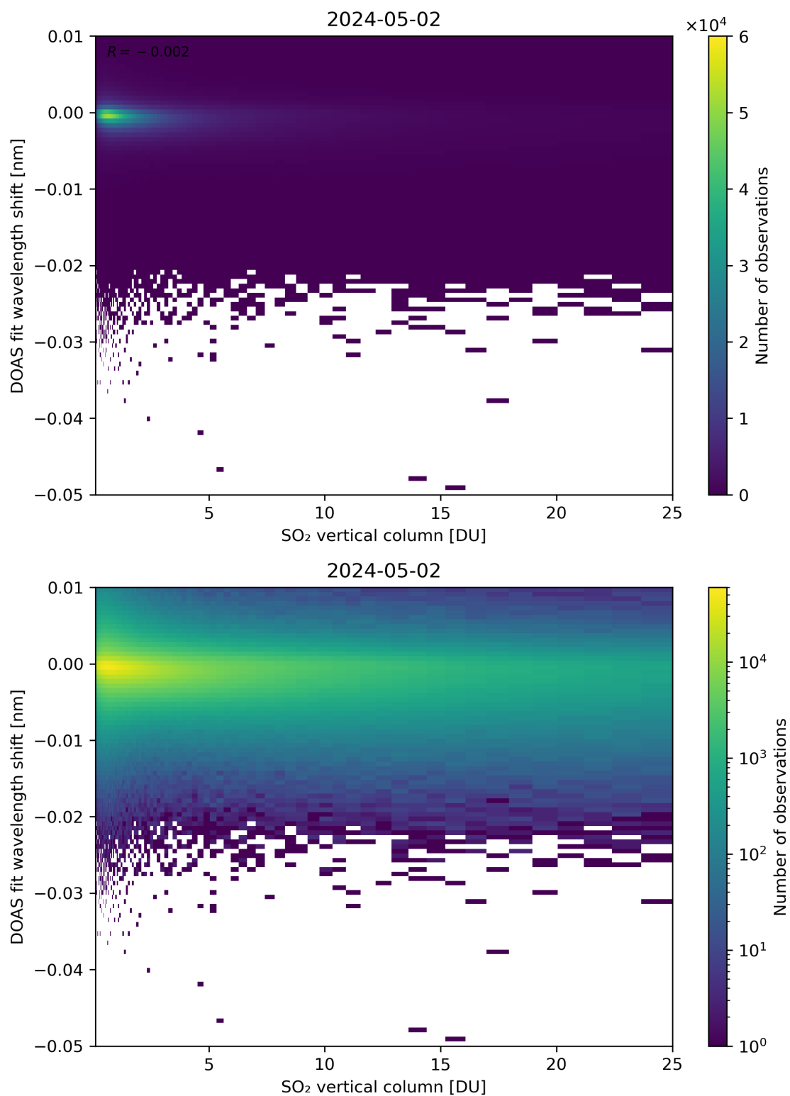
Figure 276: Scatter density plot of “SO 2 vertical column” against “DOAS fit wavelength shift” for 2024-05-02 to 2024-05-03.
