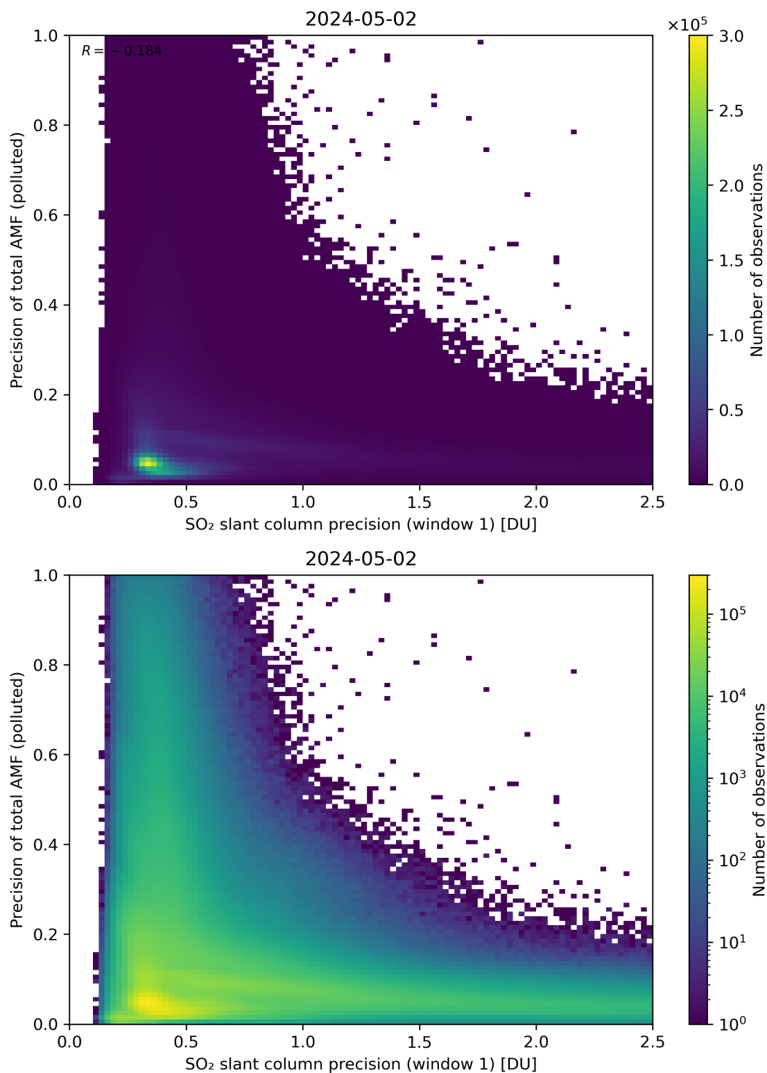
Figure 231: Scatter density plot of “SO 2 slant column precision (window 1)” against “Precision of total AMF (polluted)” for 2024-05-02 to 2024-05-03.
