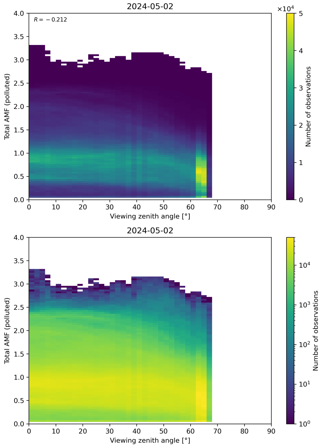
Figure 325: Scatter density plot of “Viewing zenith angle” against “Total AMF (polluted)” for 2024-05-02 to 2024-05-03.
