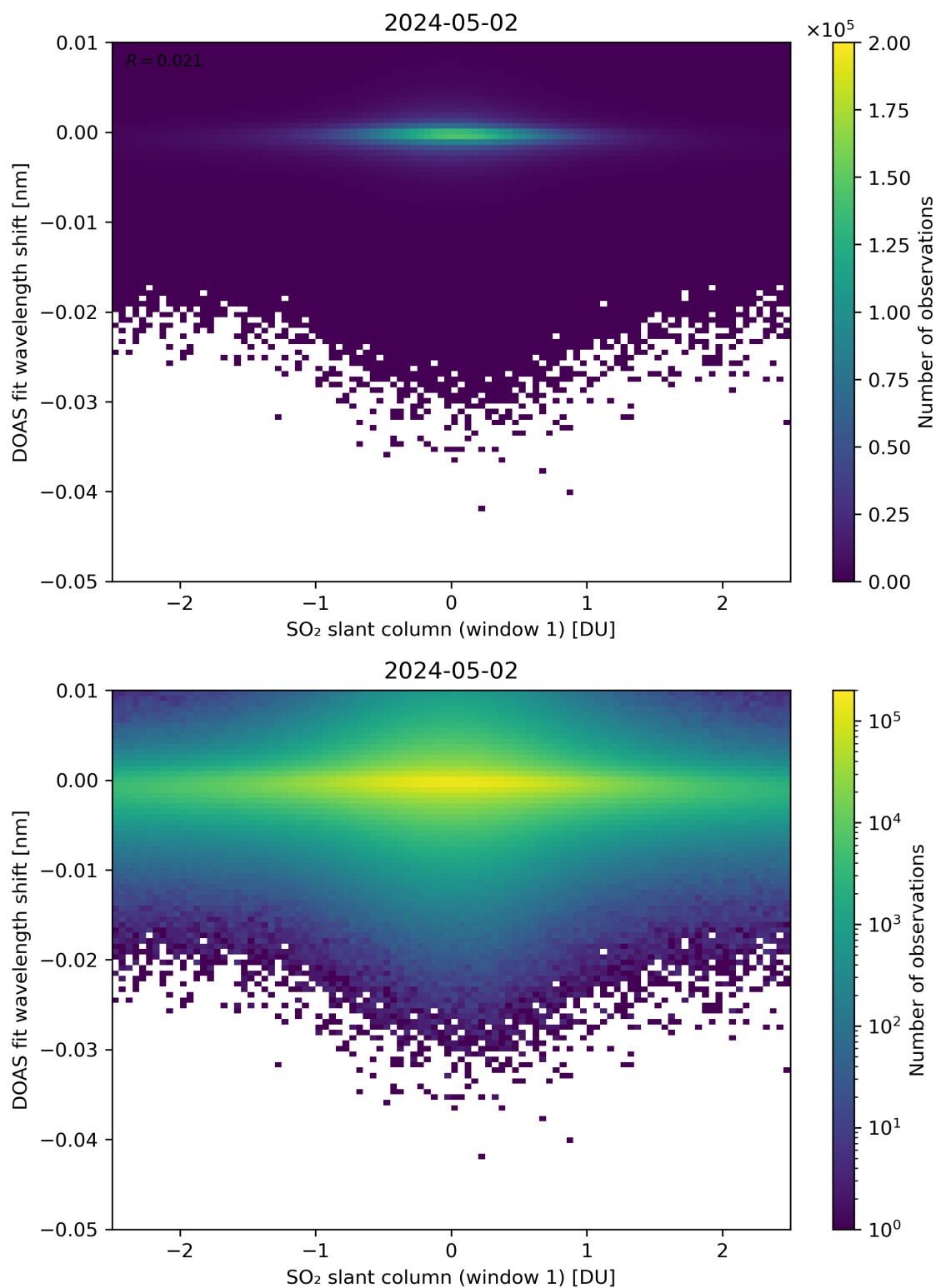
Figure 215: Scatter density plot of “SO 2 slant column (window 1)” against “DOAS fit wavelength shift” for 2024-05-02 to 2024-05-03.
