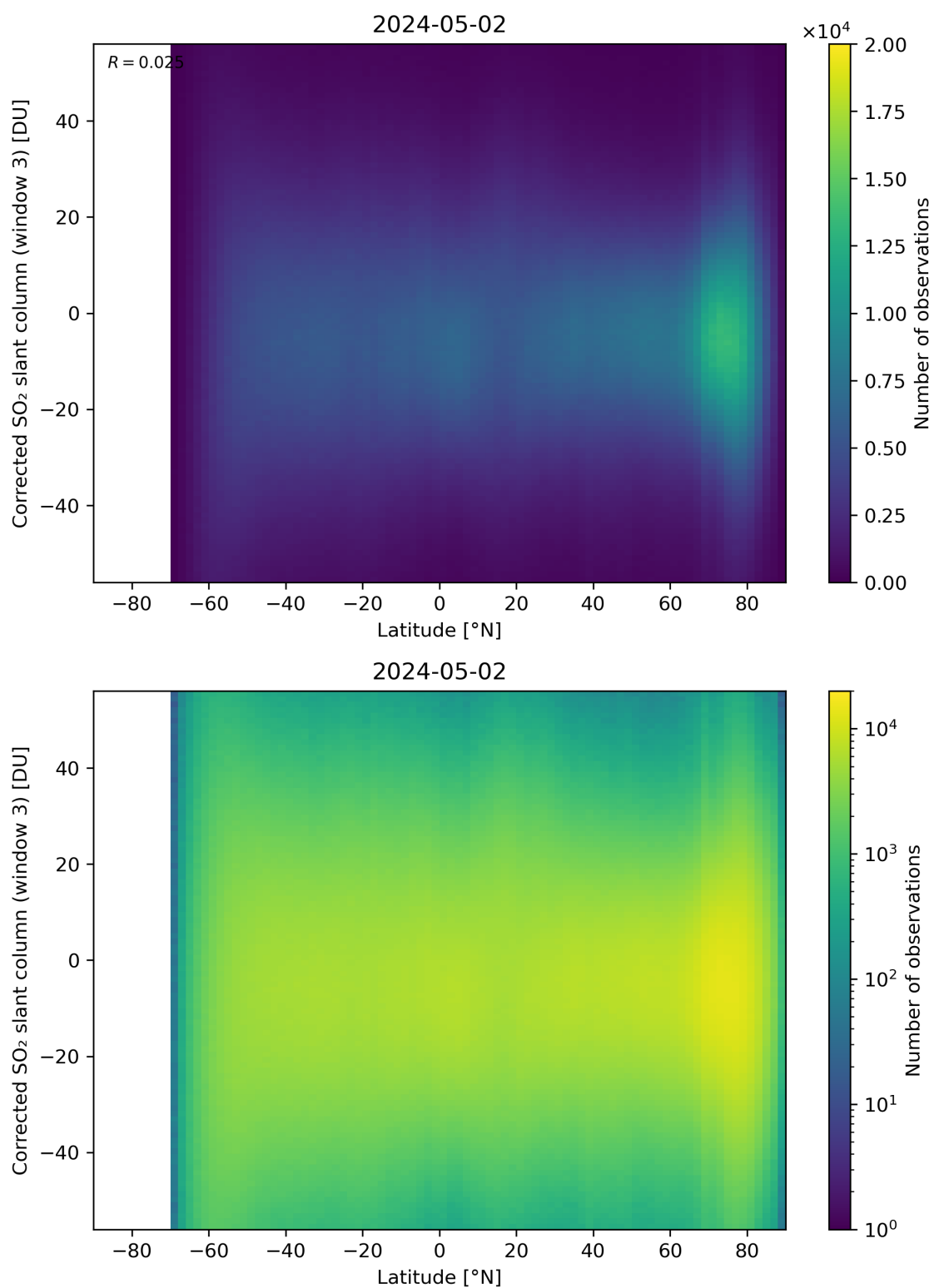
Figure 148: Scatter density plot of “Latitude” against “Corrected SO 2 slant column (window 3)” for 2024-05-02 to 2024-05-03.
