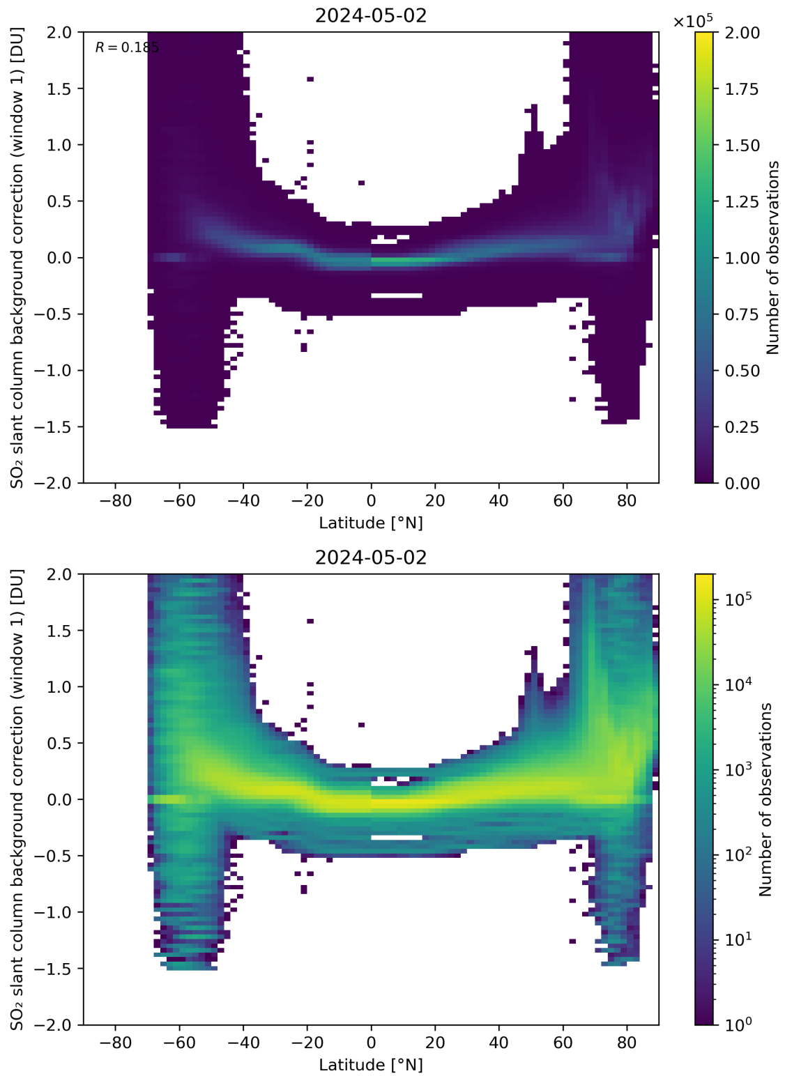
Figure 139: Scatter density plot of “Latitude” against “SO 2 slant column background correction (window 1)” for 2024-05-02 to 2024-05-03.
