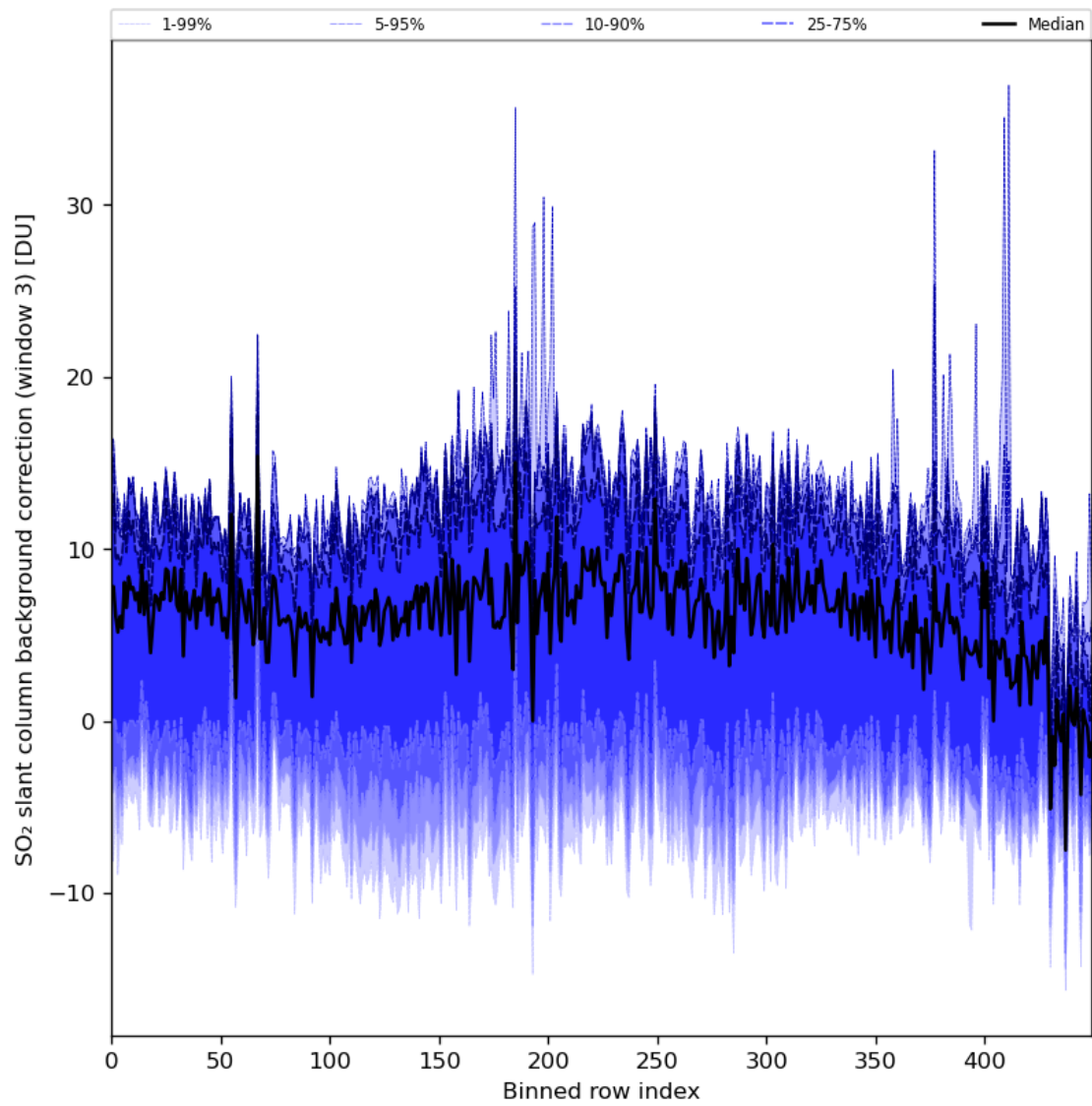
Figure 90: Along track statistics of “SO 2 slant column background correction (window 3)” for 2024-05-02 to 2024-05-03
