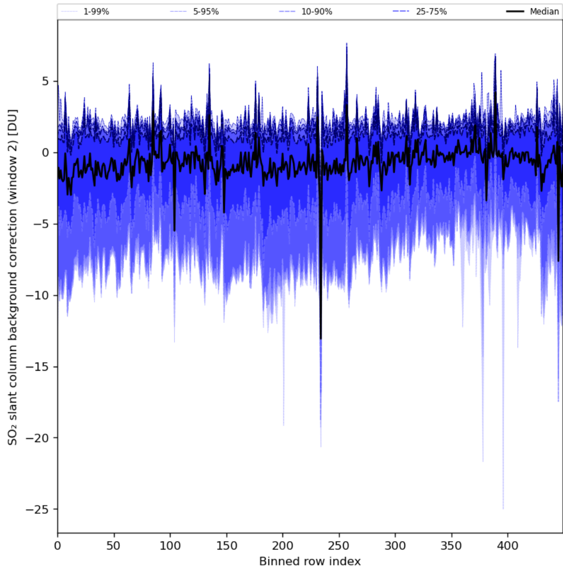
Figure 86: Along track statistics of “SO 2 slant column background correction (window 2)” for 2024-05-02 to 2024-05-03
