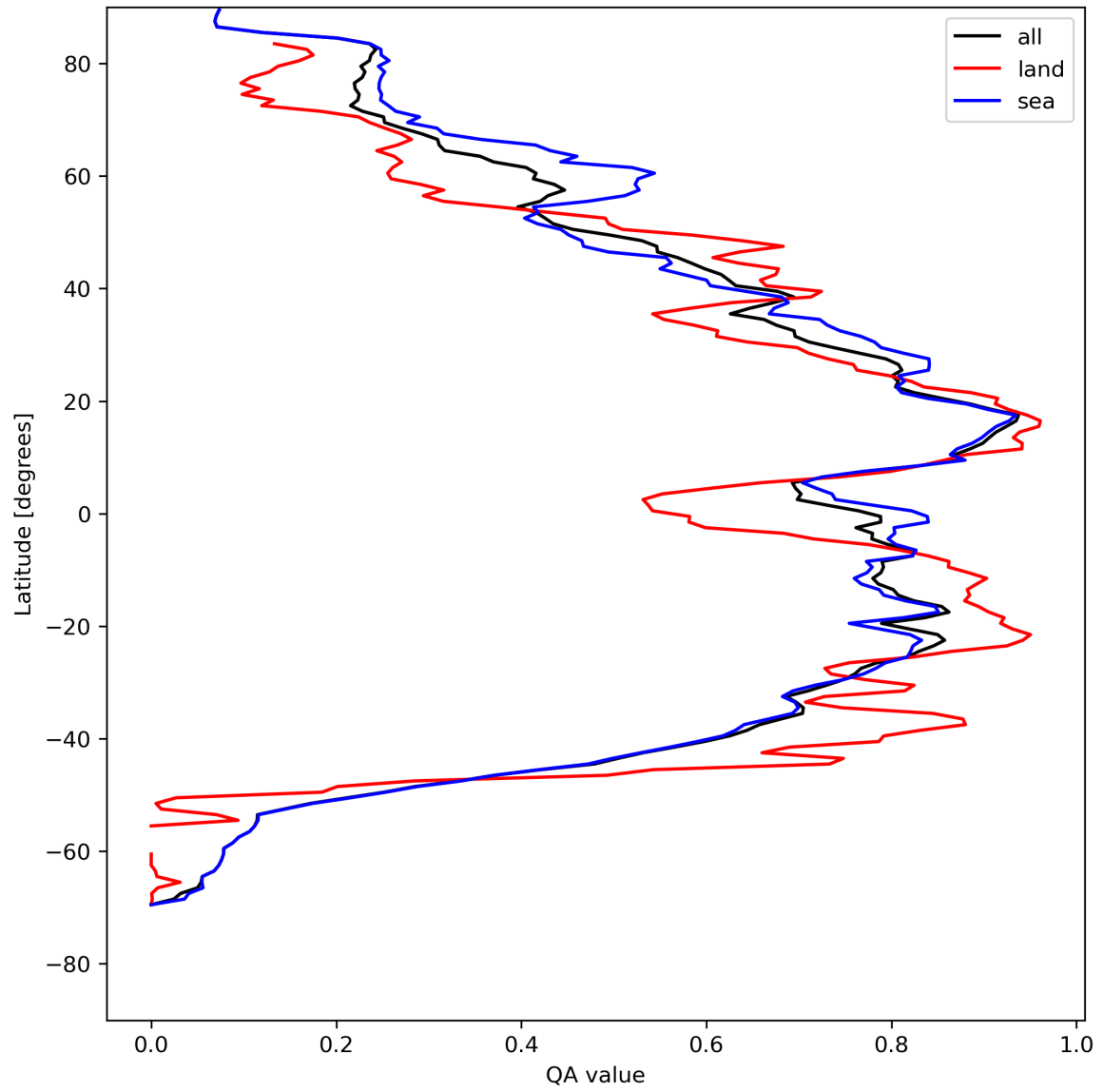
Figure 29: Zonal average of “QA value” for 2024-05-02 to 2024-05-03.
