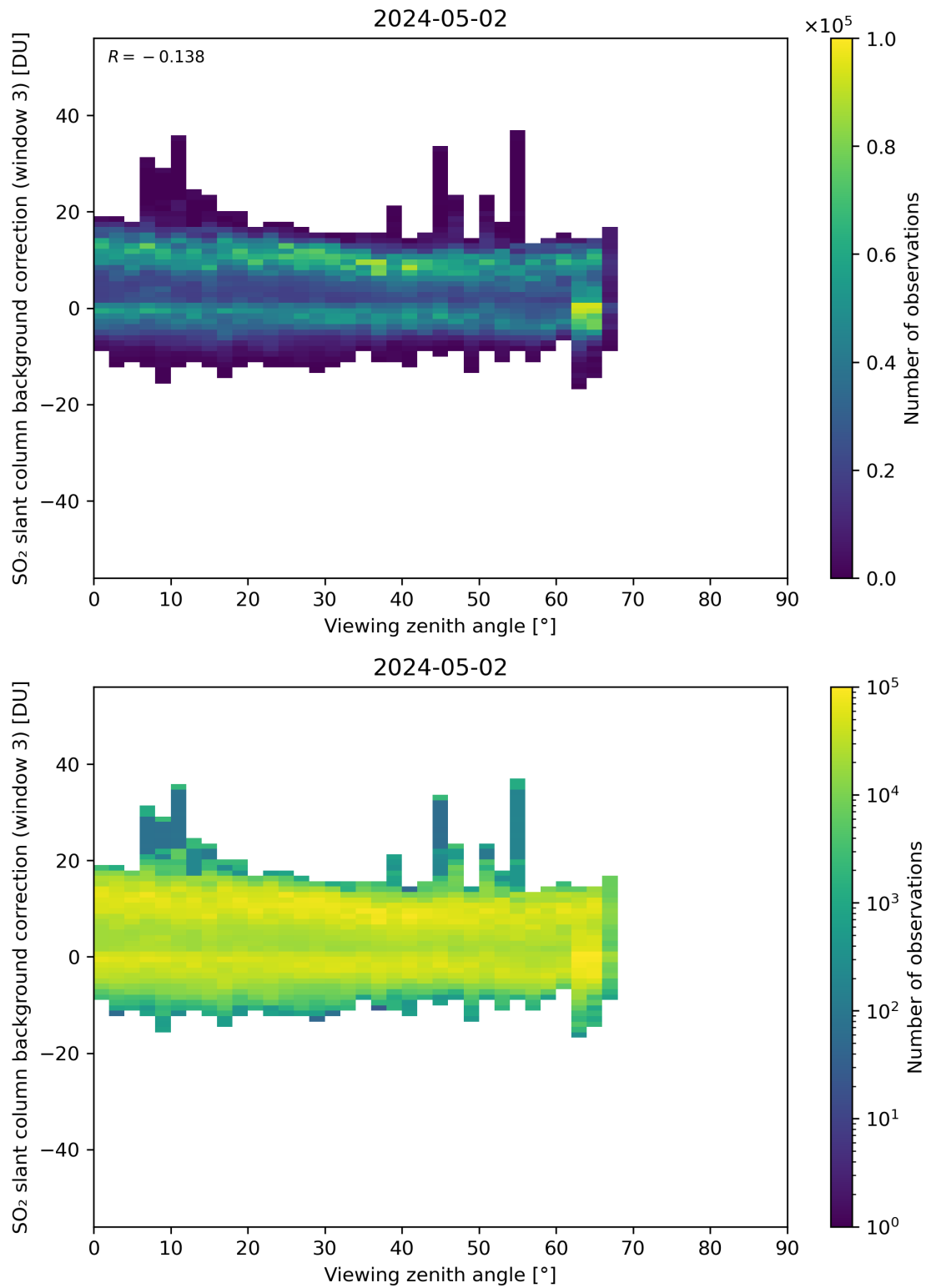
Figure 310: Scatter density plot of “Viewing zenith angle” against “SO 2 slant column background correction (window 3)” for 2024-05-02 to 2024-05-03.
