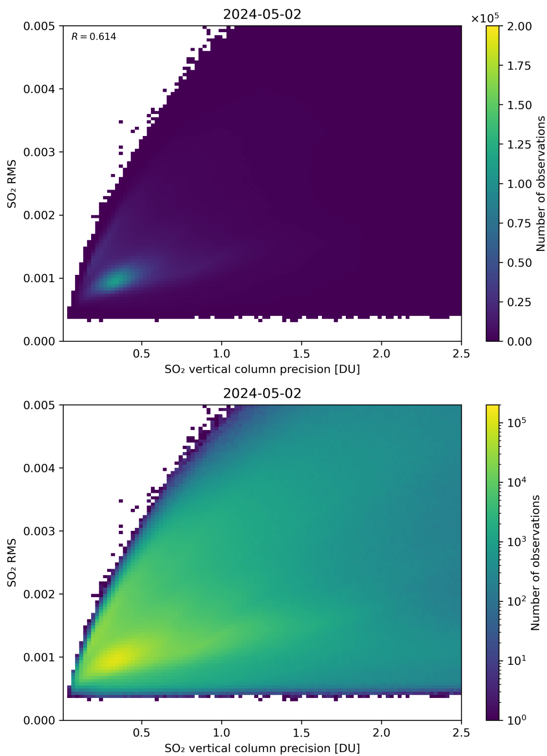
Figure 284: Scatter density plot of “SO 2 vertical column precision” against “SO 2 RMS” for 2024-05-02 to 2024-05-03.
