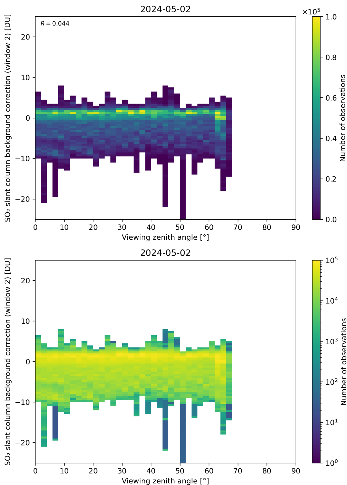
Figure 309: Scatter density plot of “Viewing zenith angle” against “SO 2 slant column background correction (window 2)” for 2024-05-02 to 2024-05-03.
