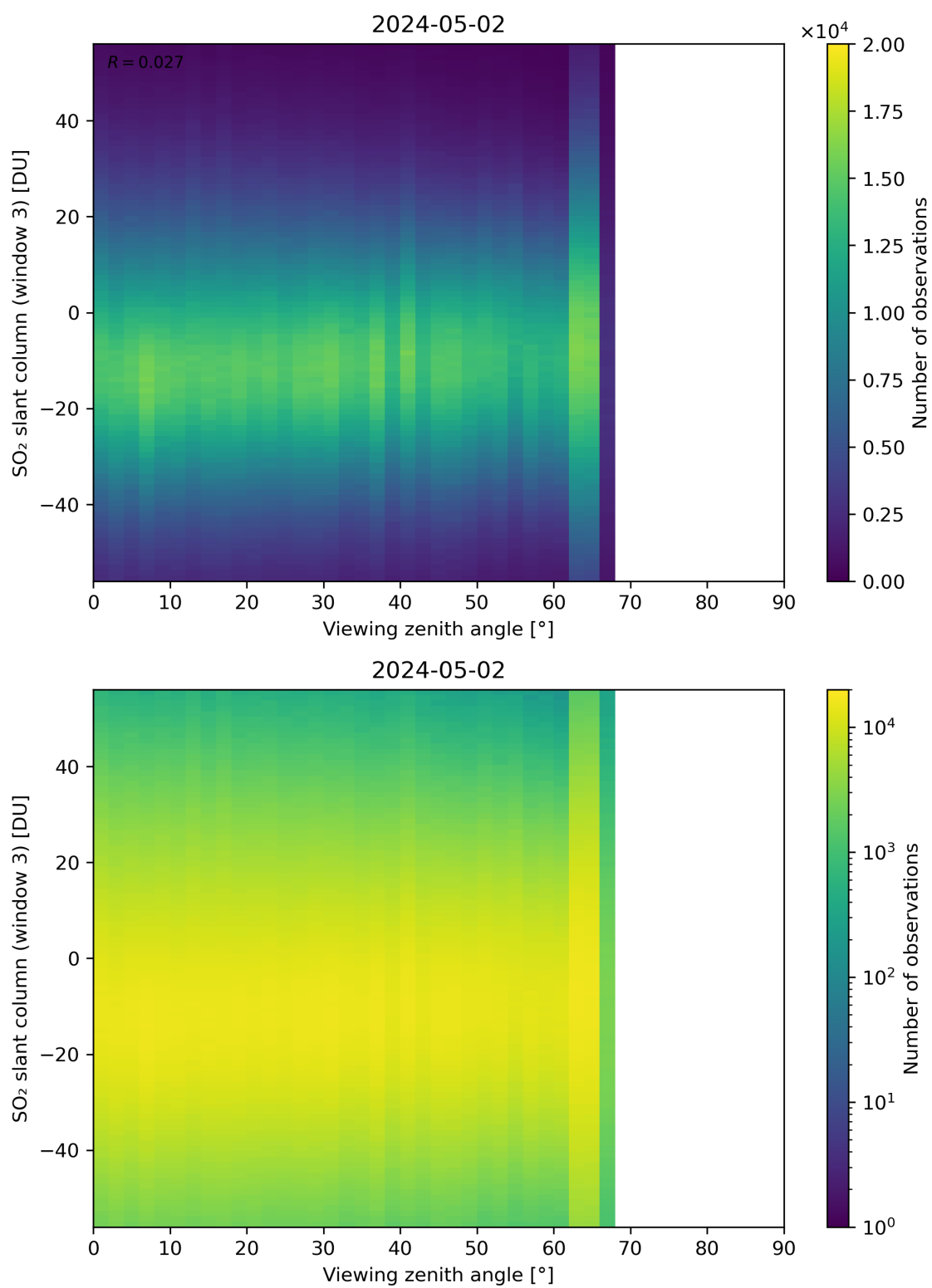
Figure 323: Scatter density plot of “Viewing zenith angle” against “SO 2 slant column (window 3)” for 2024-05-02 to 2024-05-03.
