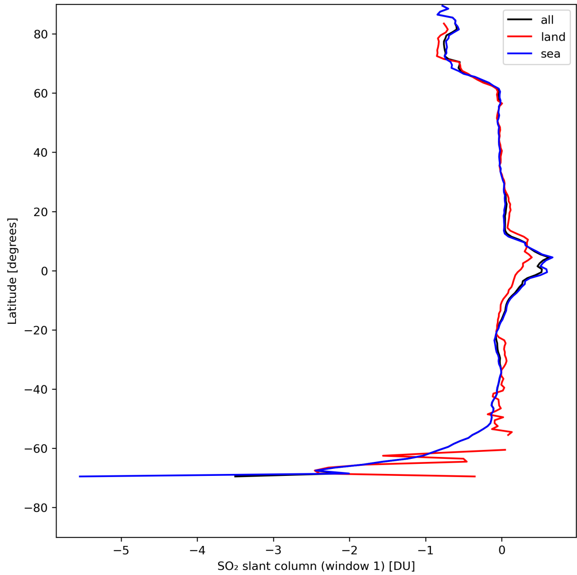
Figure 33: Zonal average of “SO 2 slant column (window 1)” for 2024-05-02 to 2024-05-03.
