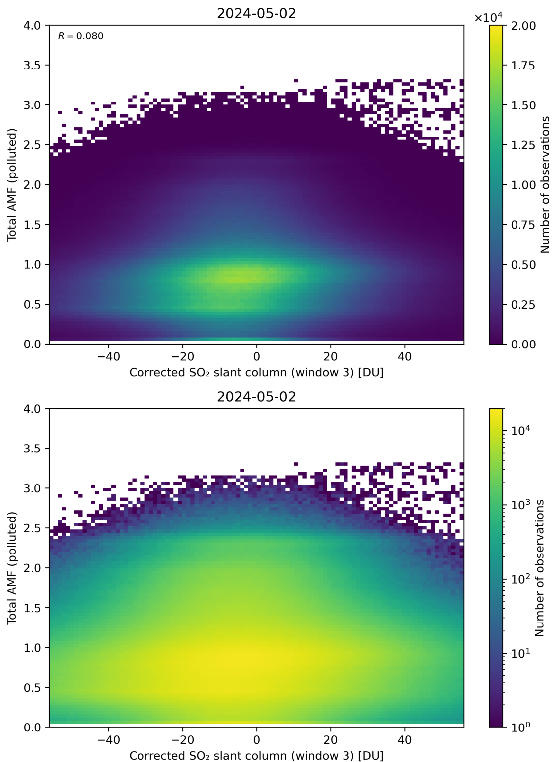
Figure 210: Scatter density plot of “Corrected SO 2 slant column (window 3)” against “Total AMF (polluted)” for 2024-05-02 to 2024-05-03.
