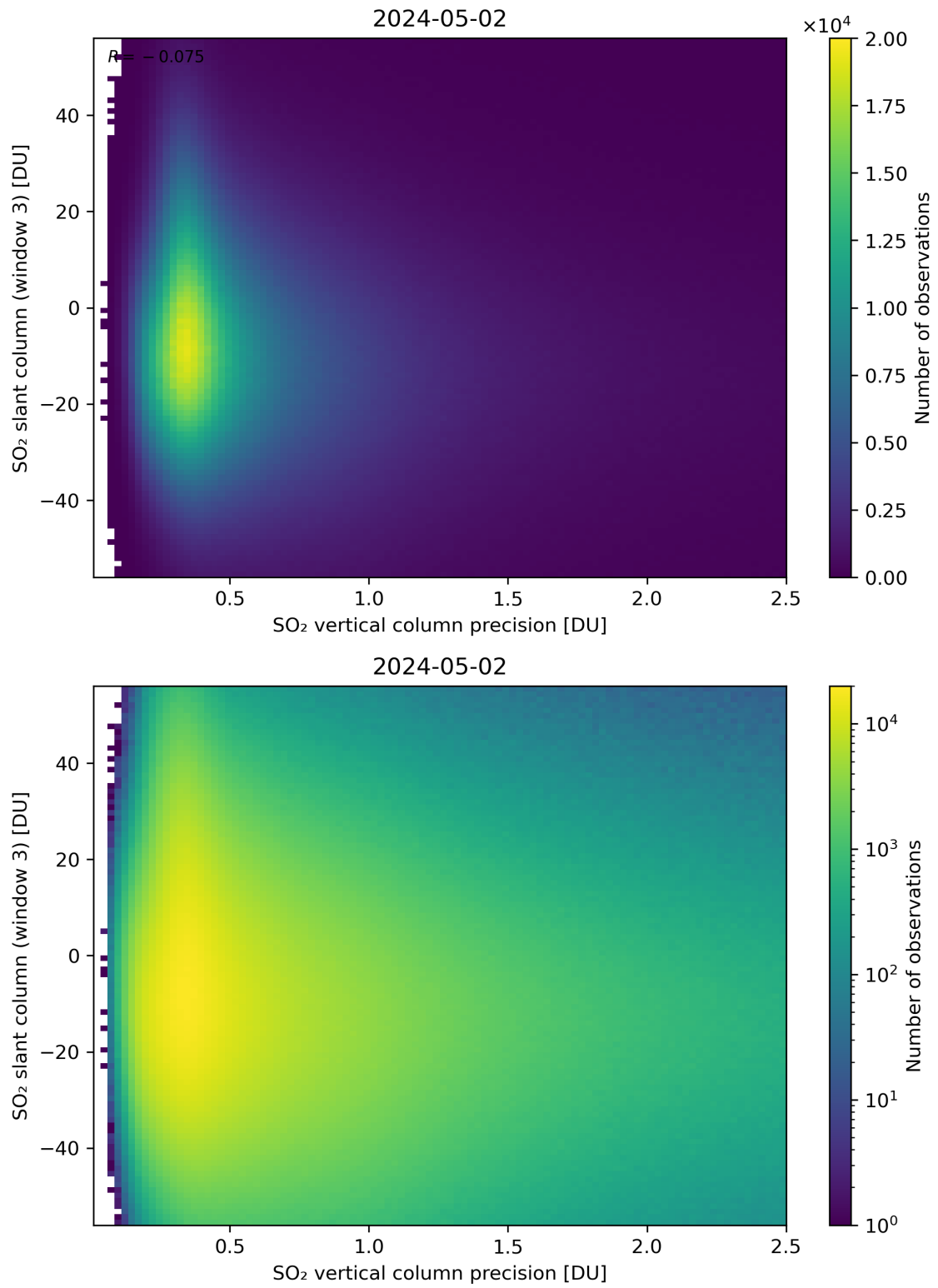
Figure 292: Scatter density plot of “SO 2 vertical column precision” against “SO 2 slant column (window 3)” for 2024-05-02 to 2024-05-03.
