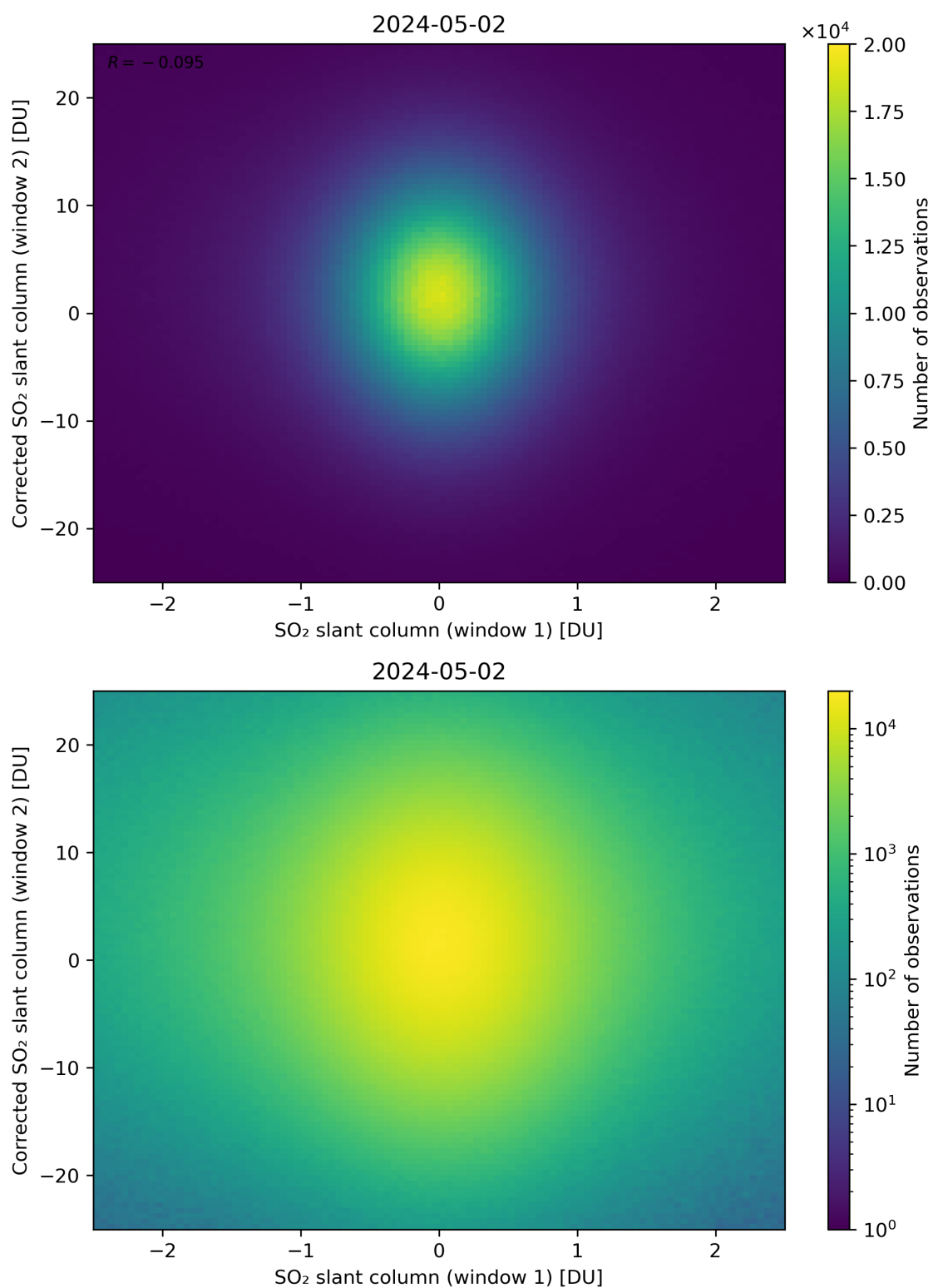
Figure 233: Scatter density plot of “SO 2 slant column (window 1)” against “Corrected SO 2 slant column (window 2)” for 2024-05-02 to 2024-05-03.
