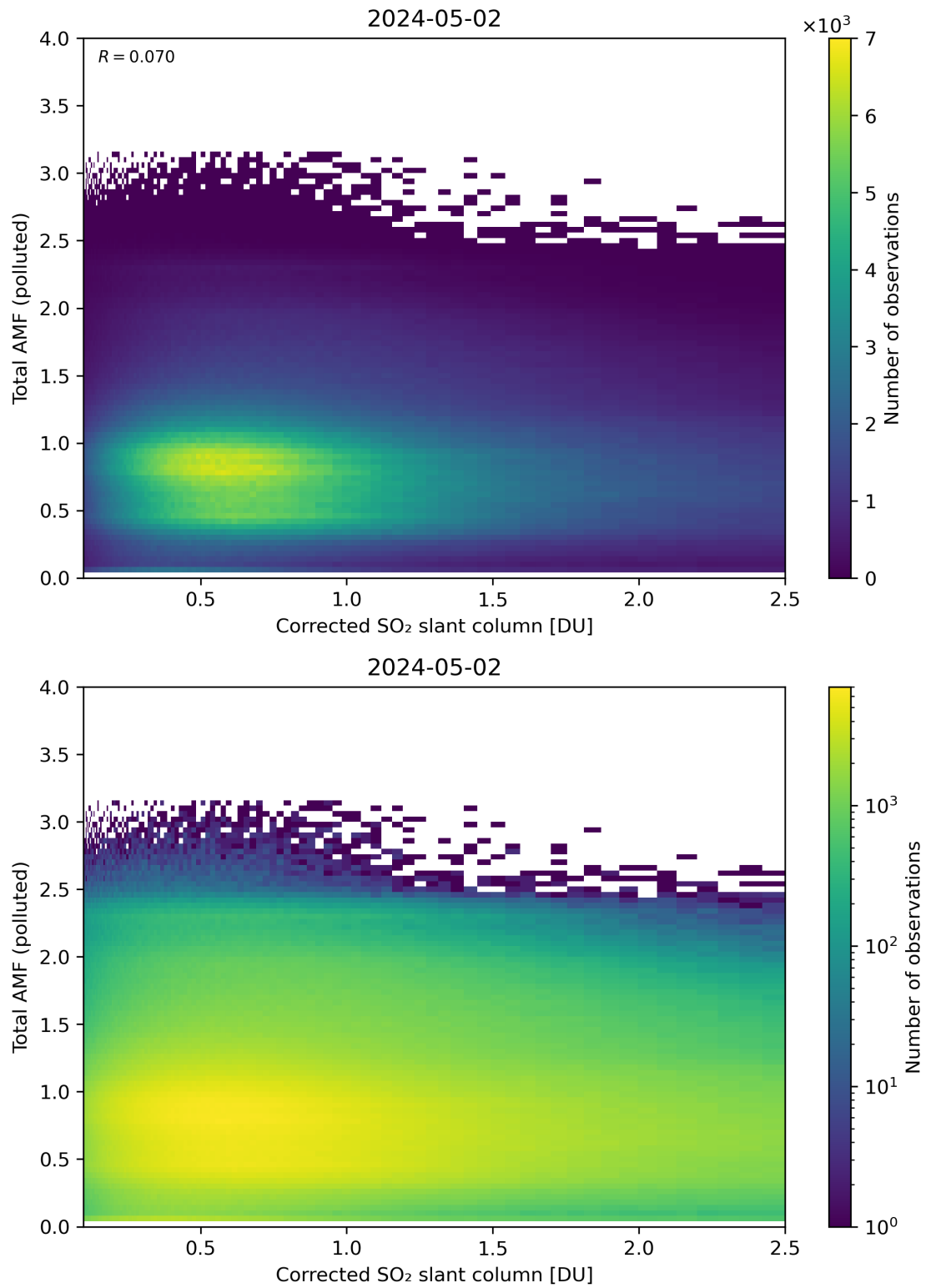
Figure 192: Scatter density plot of “Corrected SO 2 slant column” against “Total AMF (polluted)” for 2024-05-02 to 2024-05-03.
