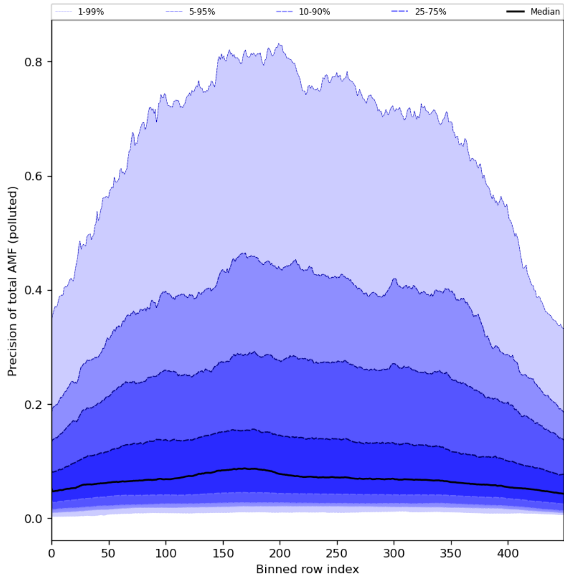
Figure 95: Along track statistics of “Precision of total AMF (polluted)” for 2024-05-02 to 2024-05-03
