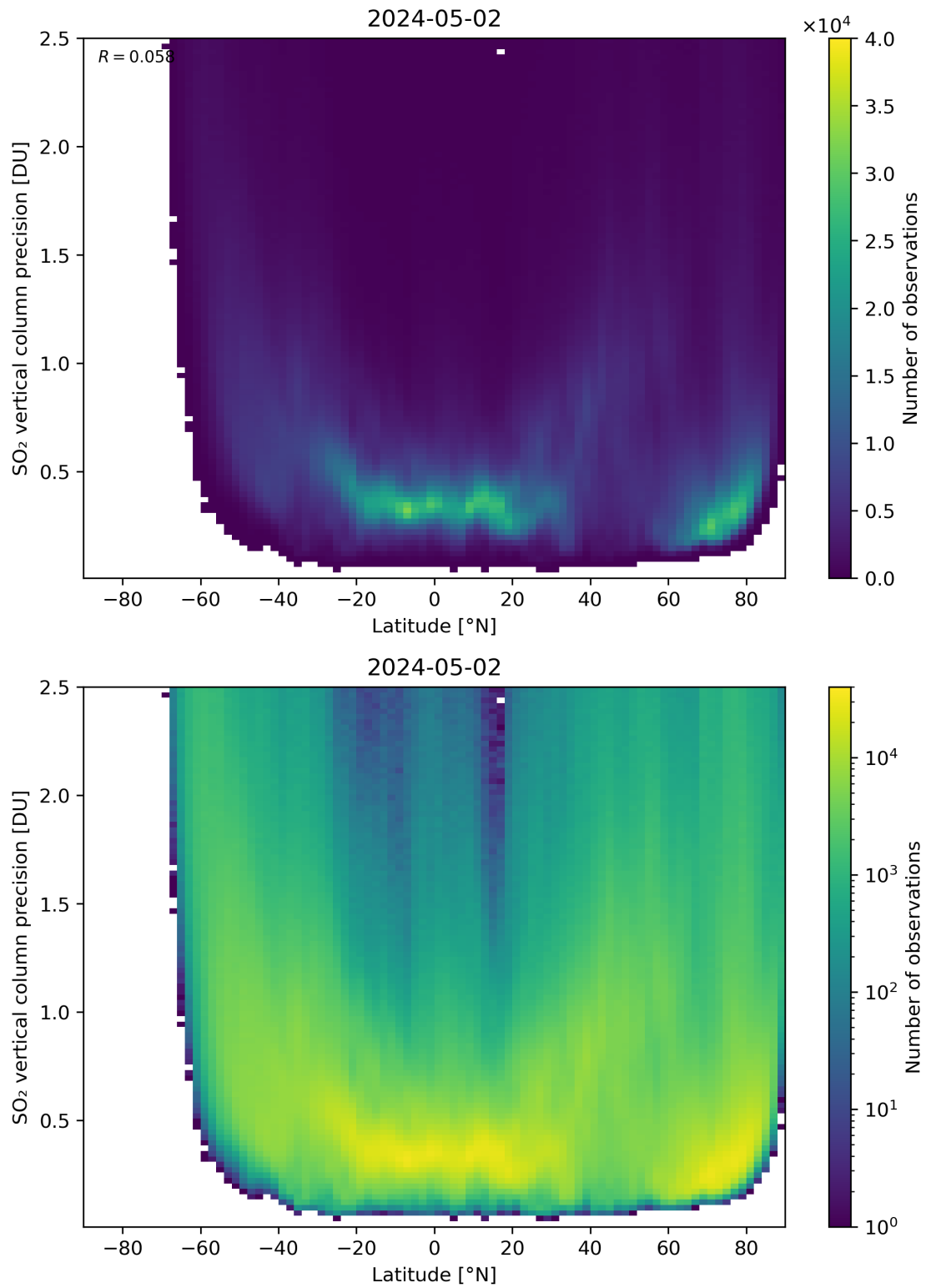
Figure 157: Scatter density plot of “Latitude” against “SO 2 vertical column precision” for 2024-05-02 to 2024-05-03.
