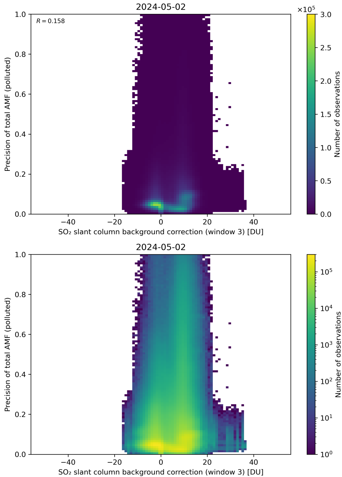
Figure 126: Scatter density plot of “SO 2 slant column background correction (window 3)” against “Precision of total AMF (polluted)” for 2024-05-02 to 2024-05-03.
