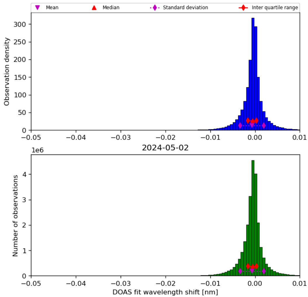
Figure 68: Histogram of “DOAS fit wavelength shift” for 2024-05-02 to 2024-05-03
