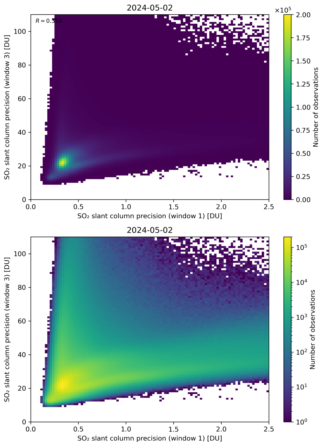
Figure 229: Scatter density plot of “SO 2 slant column precision (window 1)” against “SO 2 slant column precision (window 3)” for 2024-05-02 to 2024-05-03.
