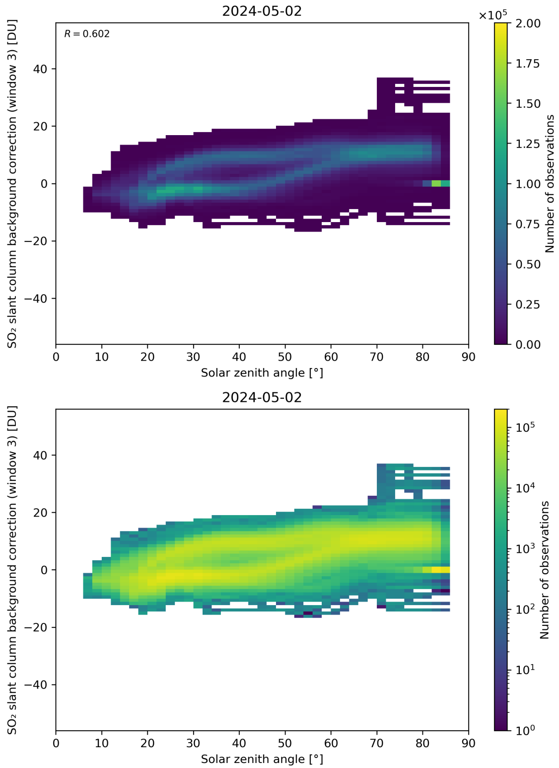
Figure 160: Scatter density plot of “Solar zenith angle” against “SO 2 slant column background correction (window 3)” for 2024-05-02 to 2024-05-03.
