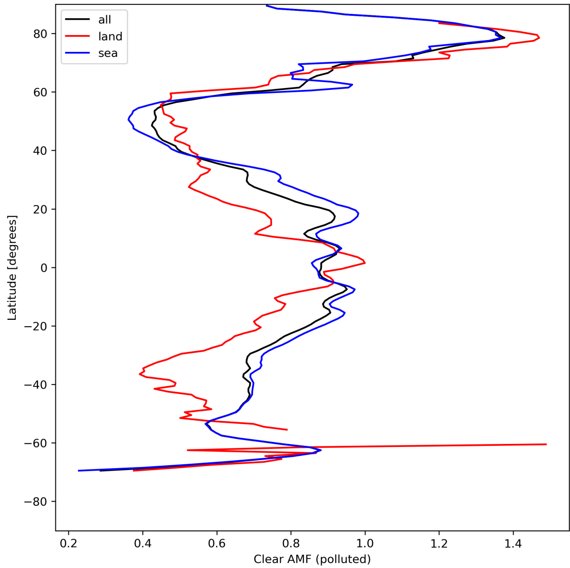
Figure 50: Zonal average of “Clear AMF (polluted)” for 2024-05-02 to 2024-05-03.
