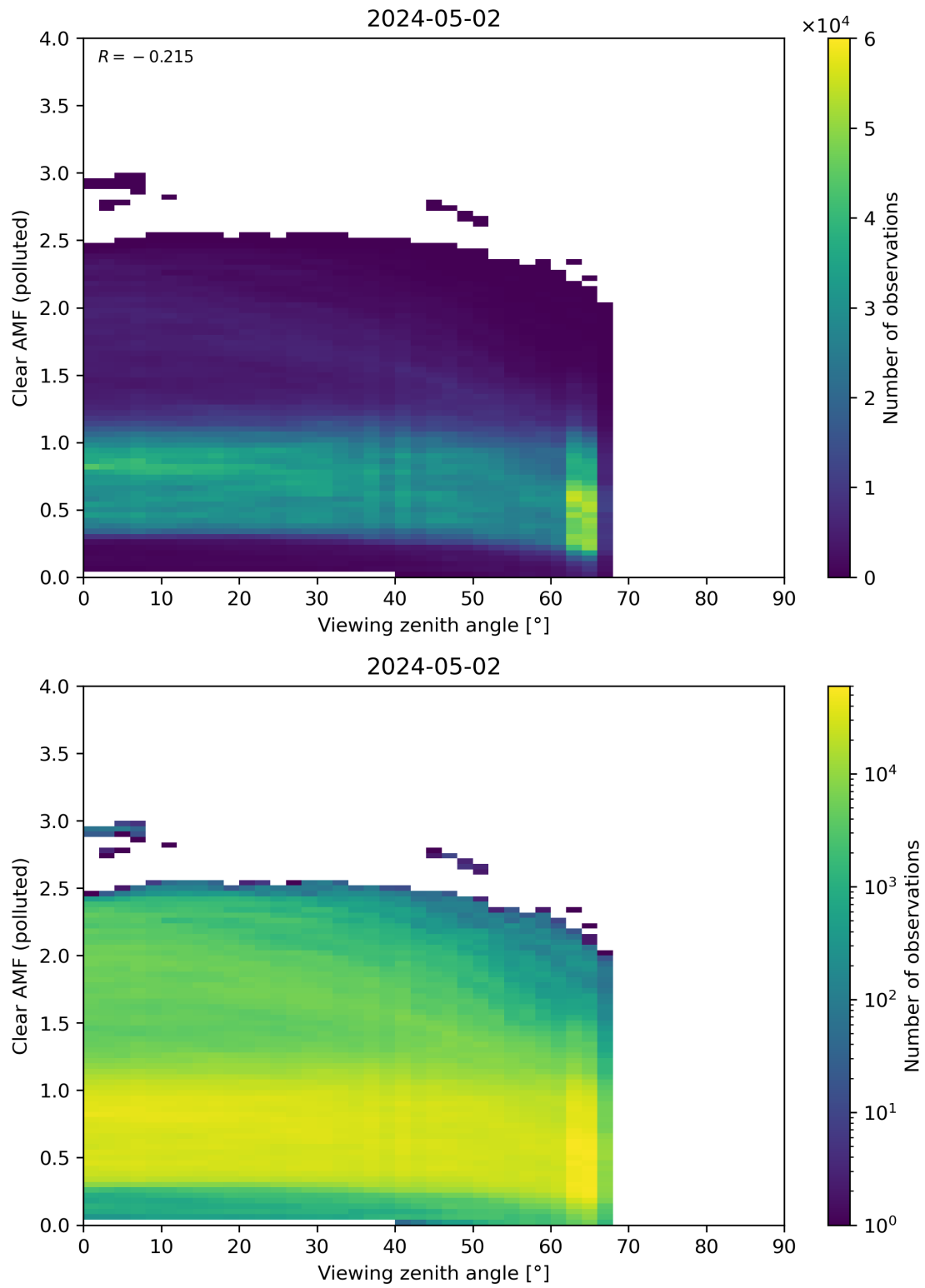
Figure 316: Scatter density plot of “Viewing zenith angle” against “Clear AMF (polluted)” for 2024-05-02 to 2024-05-03.
