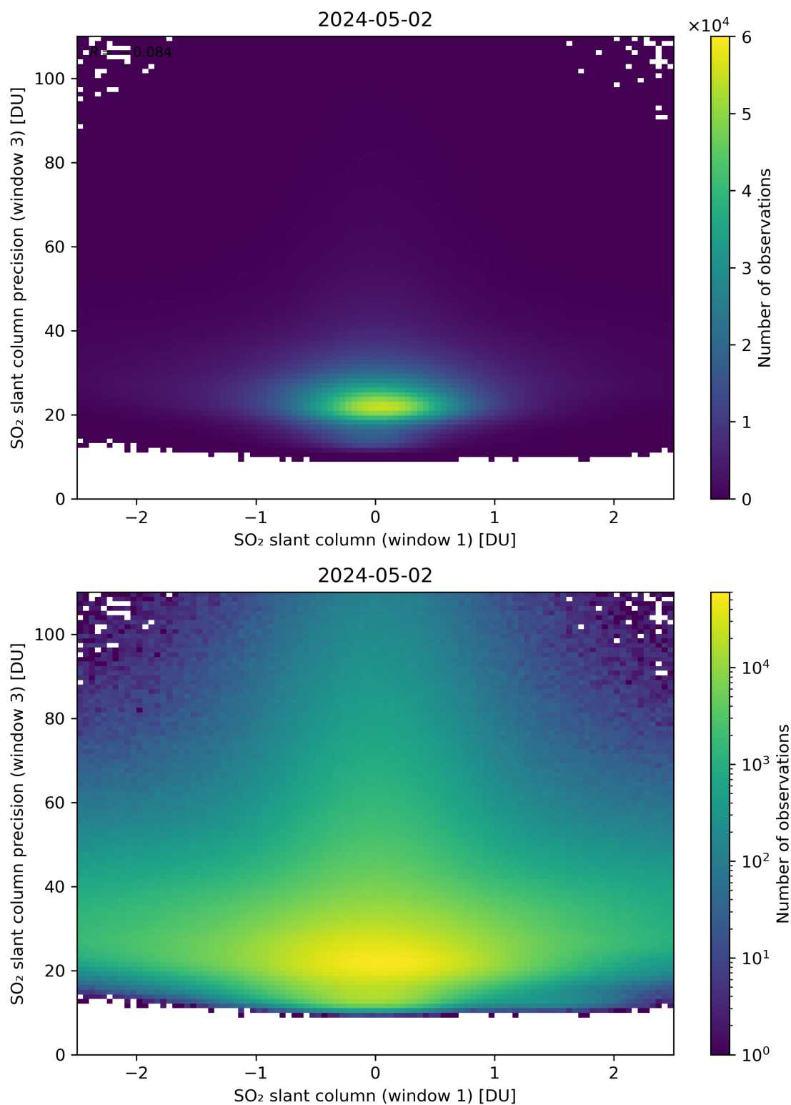
Figure 238: Scatter density plot of “SO 2 slant column (window 1)” against “SO 2 slant column precision (window 3)” for 2024-05-02 to 2024-05-03.
