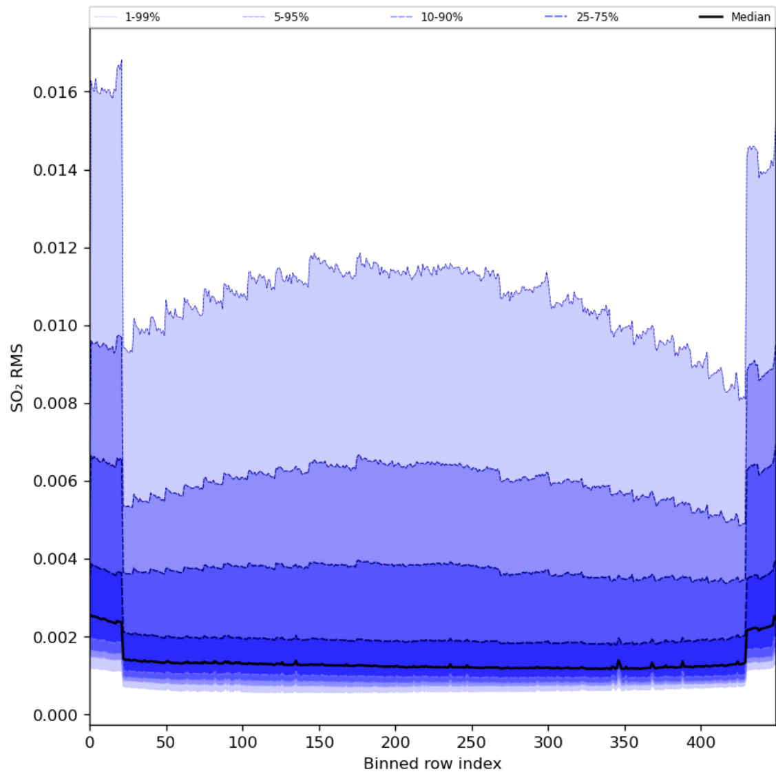
Figure 93: Along track statistics of “SO 2 RMS” for 2024-05-02 to 2024-05-03
