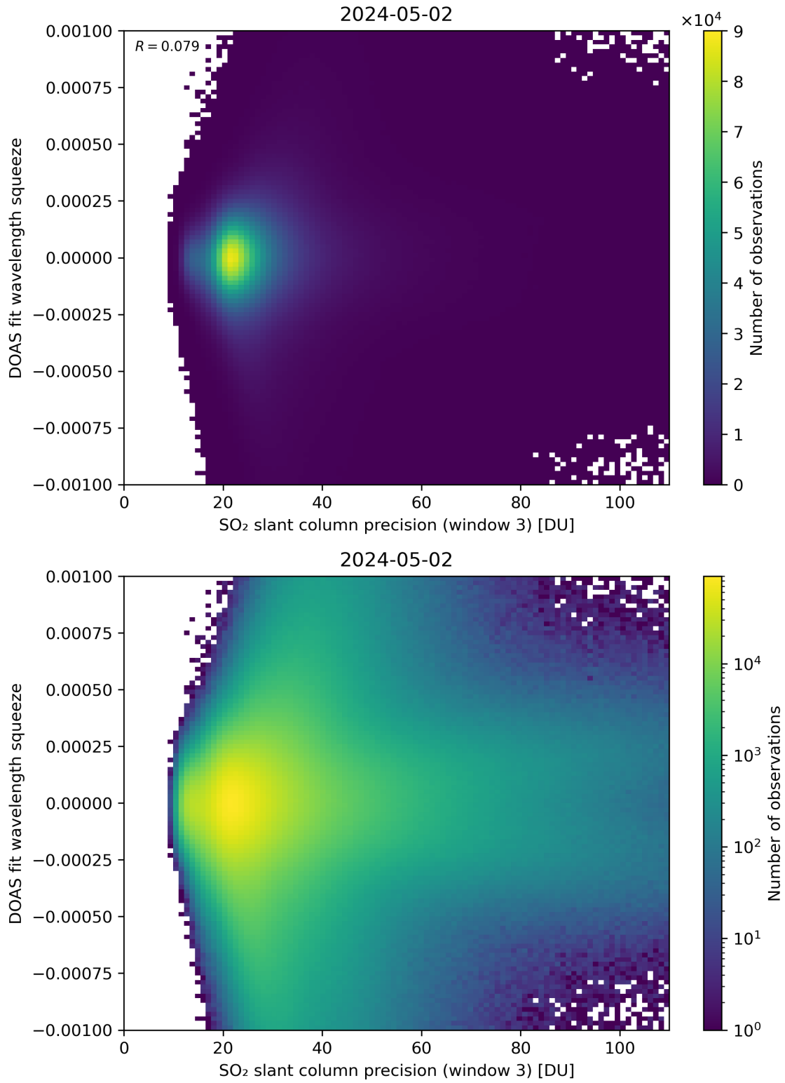
Figure 259: Scatter density plot of “SO 2 slant column precision (window 3)” against “DOAS fit wavelength squeeze” for 2024-05-02 to 2024-05-03.
