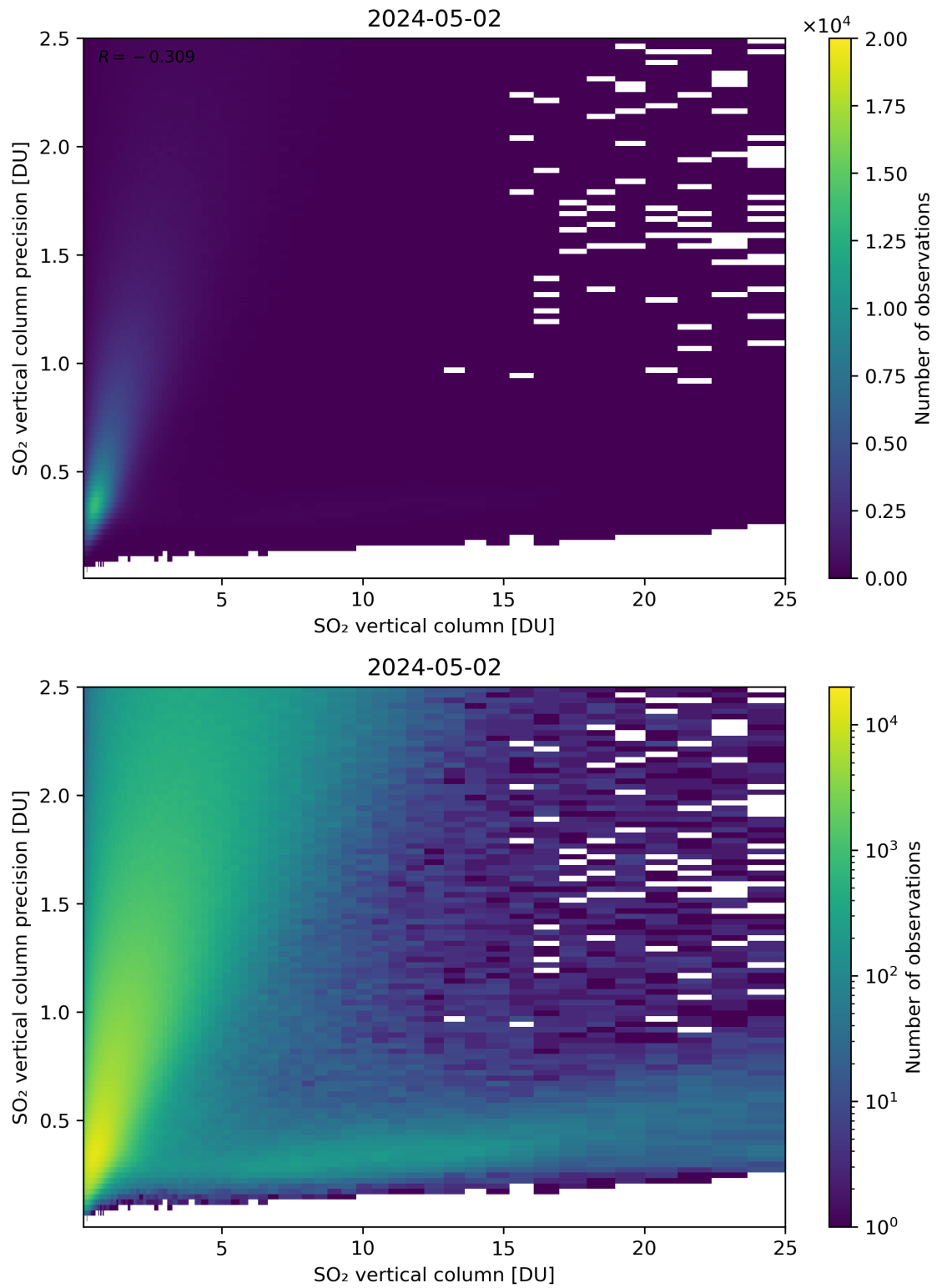
Figure 307: Scatter density plot of “SO 2 vertical column” against “SO 2 vertical column precision” for 2024-05-02 to 2024-05-03.
