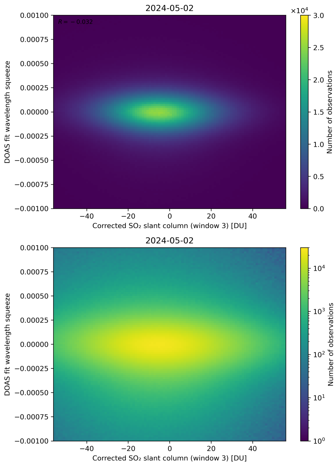
Figure 207: Scatter density plot of “Corrected SO 2 slant column (window 3)” against “DOAS fit wavelength squeeze” for 2024-05-02 to 2024-05-03.
