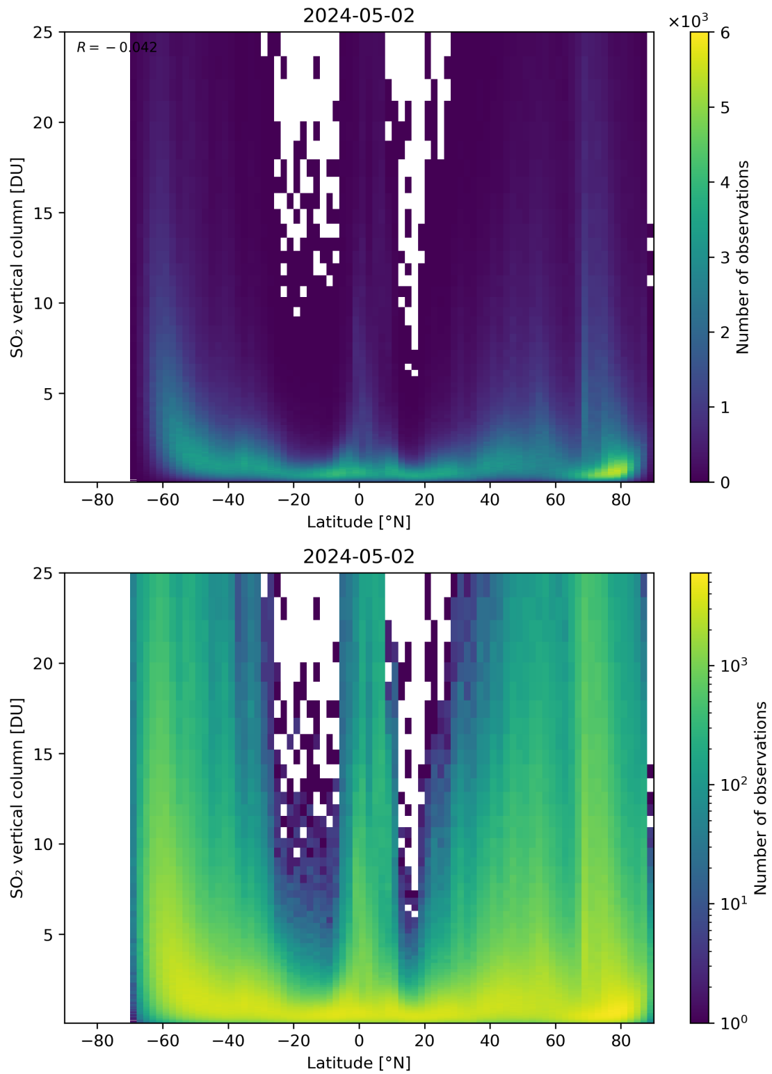
Figure 156: Scatter density plot of “Latitude” against “SO 2 vertical column” for 2024-05-02 to 2024-05-03.
