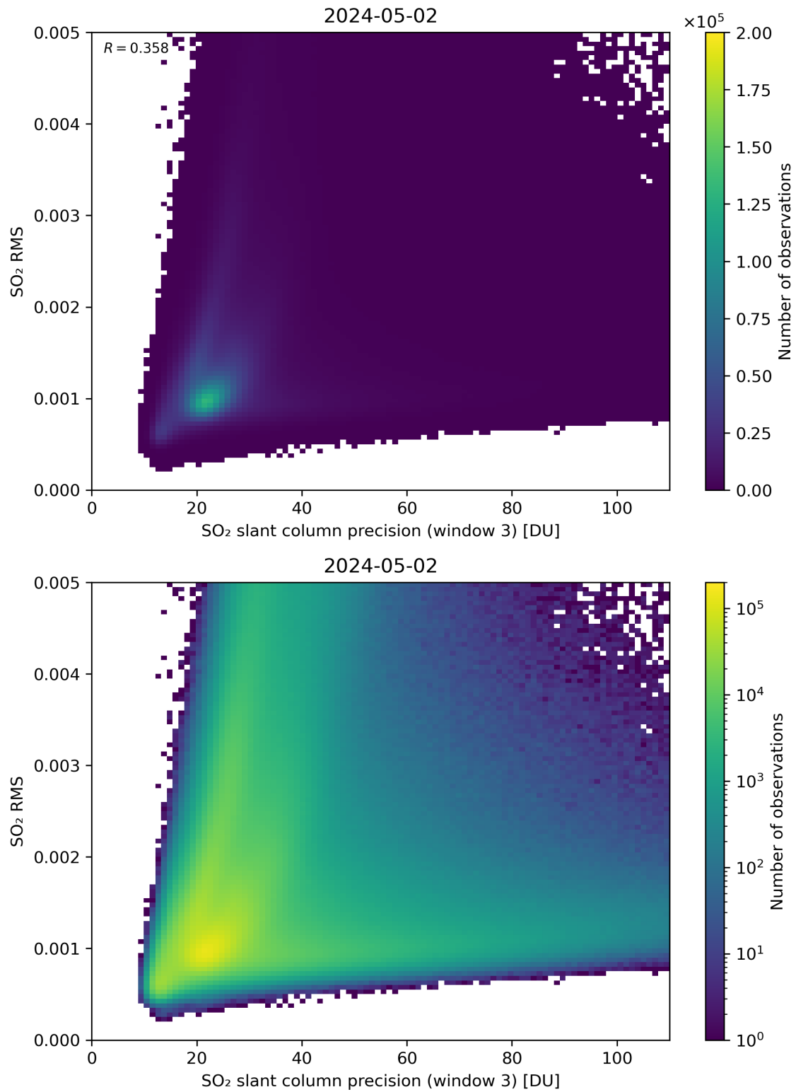
Figure 260: Scatter density plot of “SO 2 slant column precision (window 3)” against “SO 2 RMS” for 2024-05-02 to 2024-05-03.
