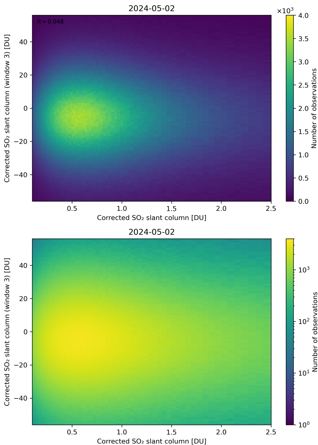
Figure 186: Scatter density plot of “Corrected SO 2 slant column” against “Corrected SO 2 slant column (window 3)” for 2024-05-02 to 2024-05-03.
