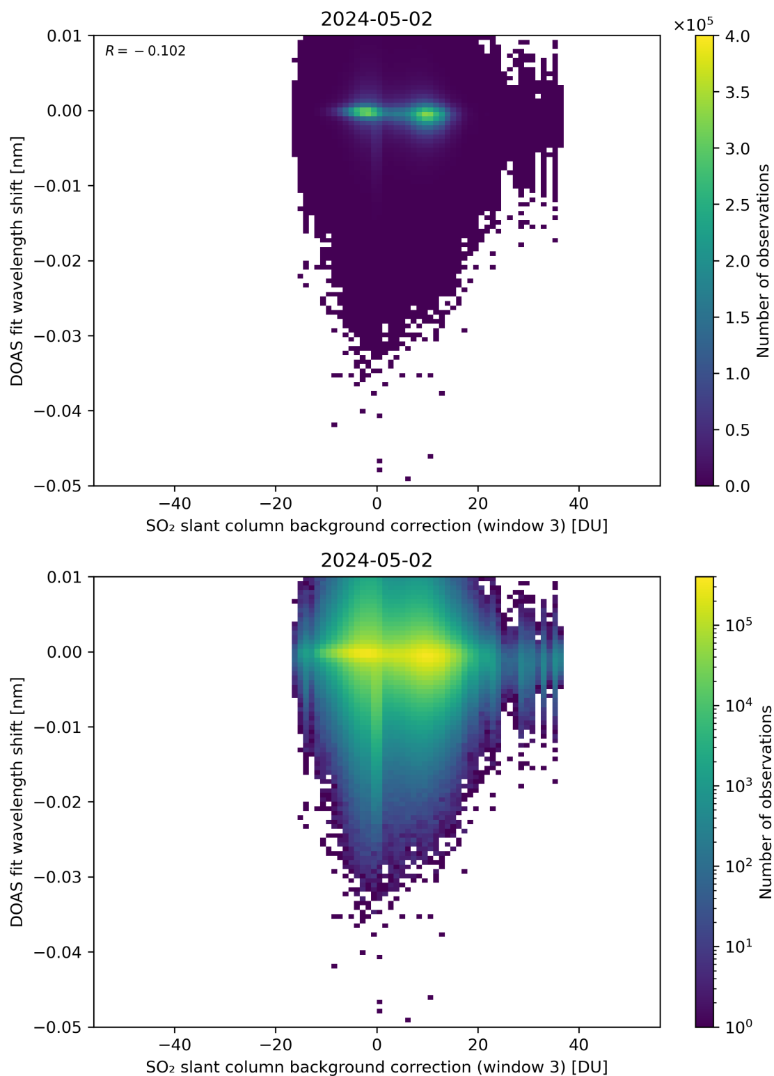
Figure 121: Scatter density plot of “SO 2 slant column background correction (window 3)” against “DOAS fit wavelength shift” for 2024-05-02 to 2024-05-03.
