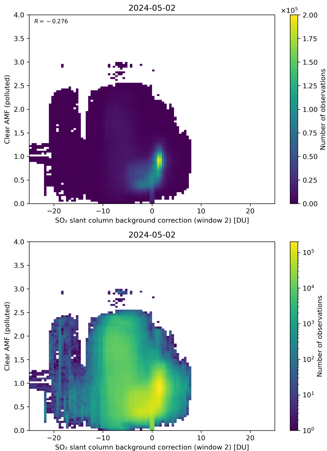
Figure 115: Scatter density plot of “SO 2 slant column background correction (window 2)” against “Clear AMF (polluted)” for 2024-05-02 to 2024-05-03.
