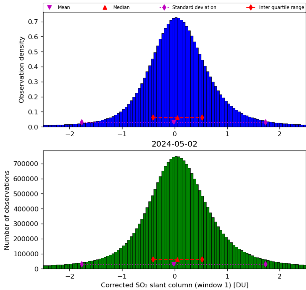
Figure 58: Histogram of “Corrected SO 2 slant column (window 1)” for 2024-05-02 to 2024-05-03
