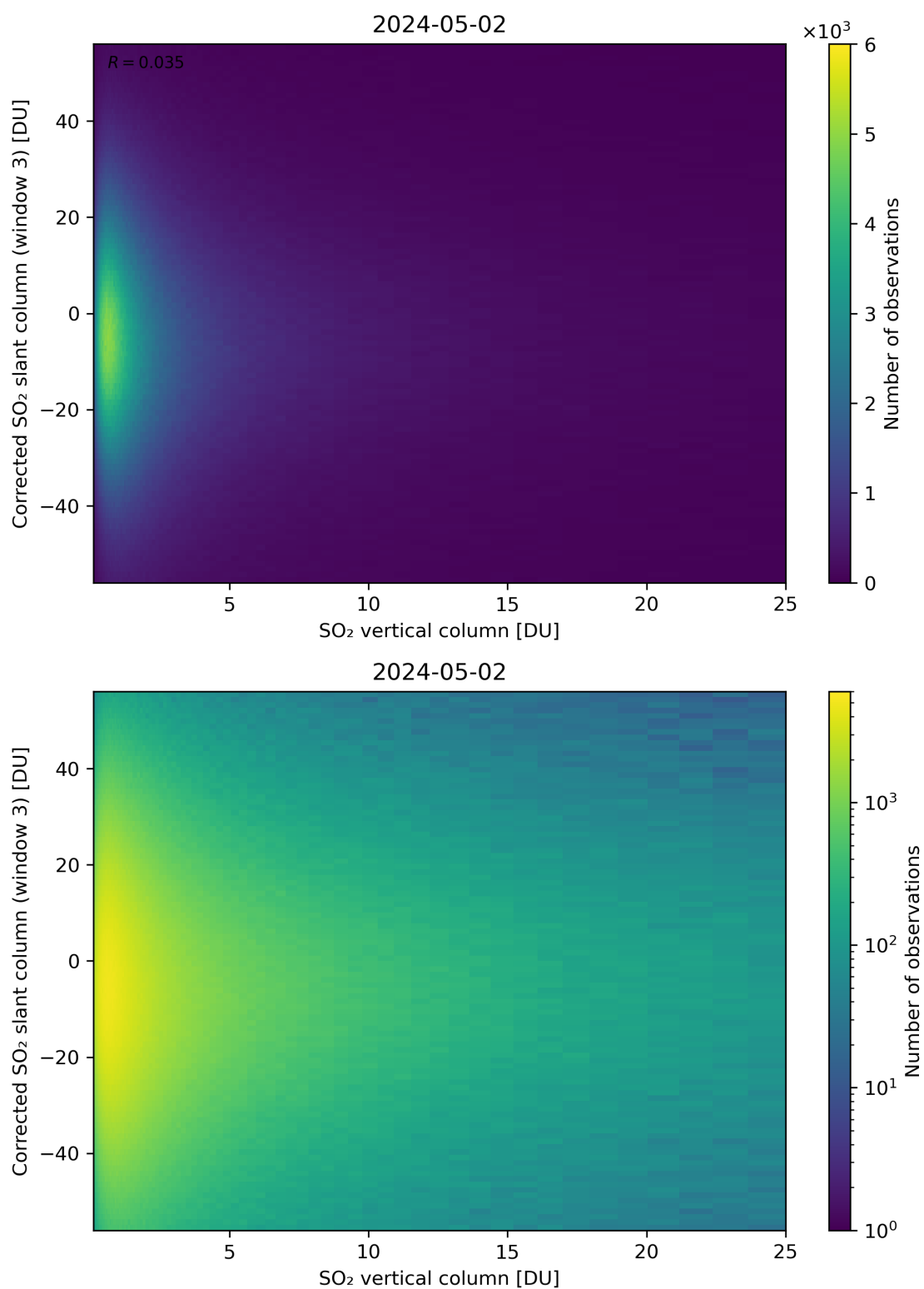
Figure 299: Scatter density plot of “SO 2 vertical column” against “Corrected SO 2 slant column (window 3)” for 2024-05-02 to 2024-05-03.
