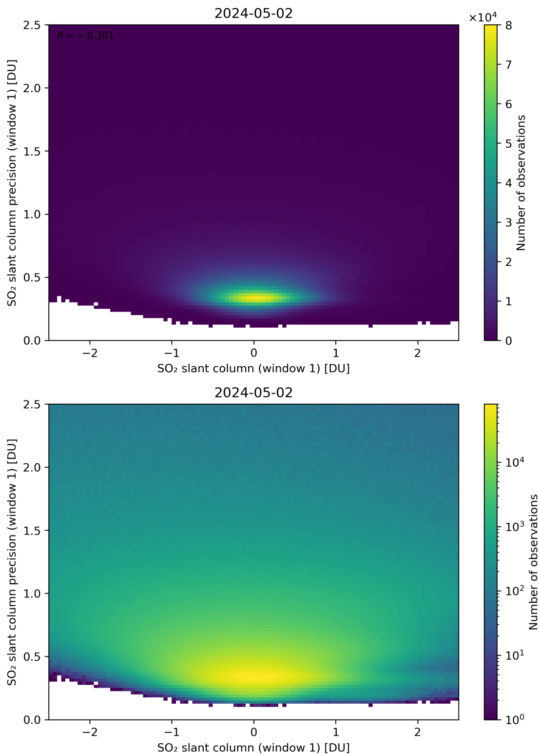
Figure 235: Scatter density plot of “SO 2 slant column (window 1)” against “SO 2 slant column precision (window 1)” for 2024-05-02 to 2024-05-03.
