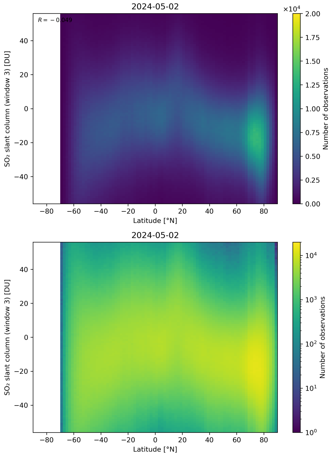
Figure 152: Scatter density plot of “Latitude” against “SO 2 slant column (window 3)” for 2024-05-02 to 2024-05-03.
