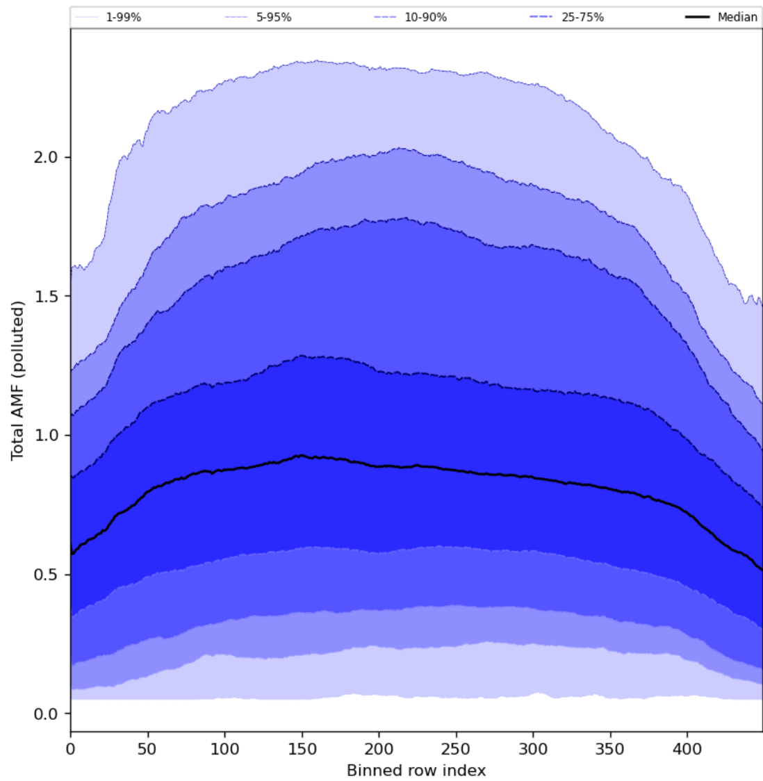
Figure 94: Along track statistics of “Total AMF (polluted)” for 2024-05-02 to 2024-05-03
