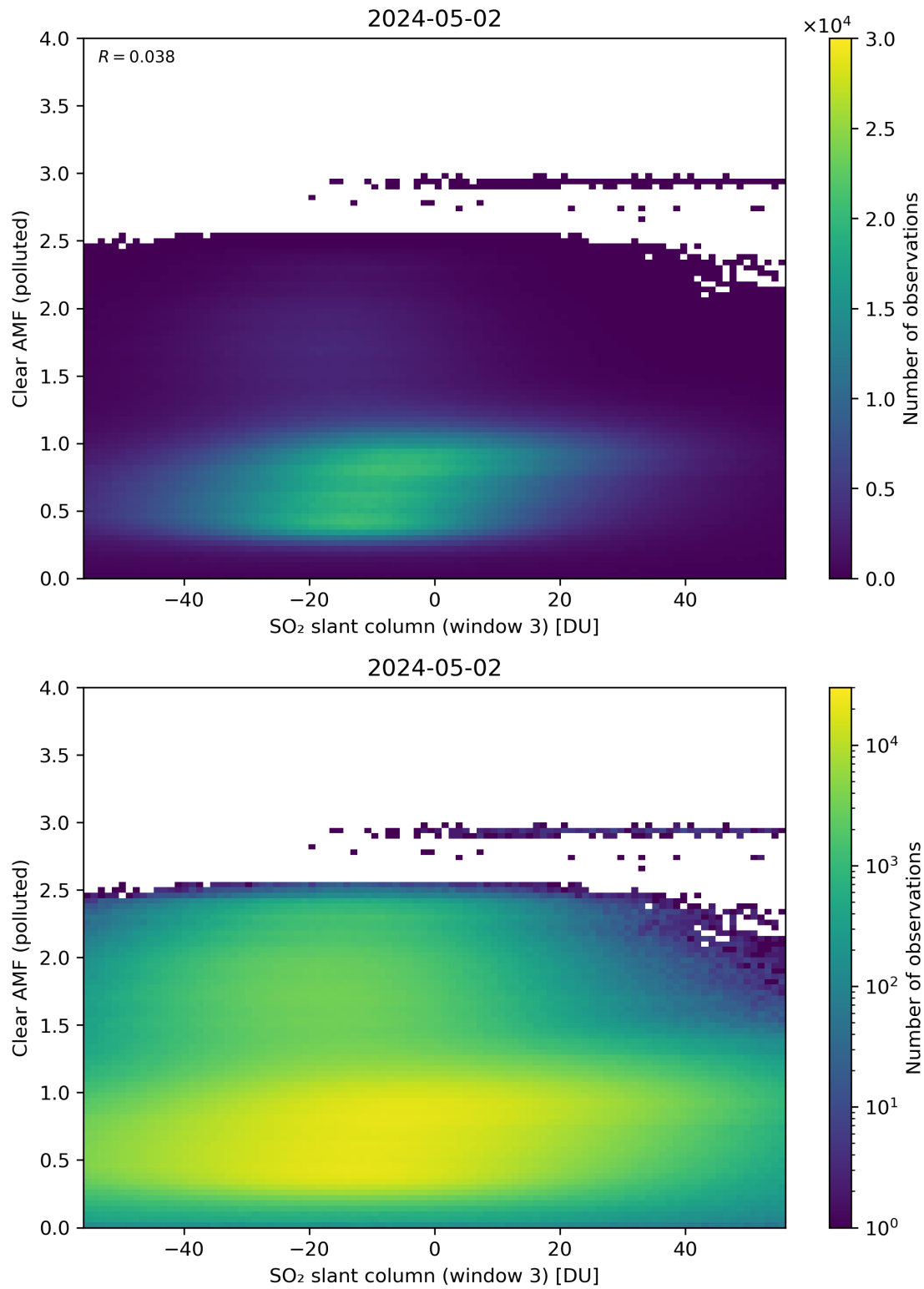
Figure 265: Scatter density plot of “SO 2 slant column (window 3)” against “Clear AMF (polluted)” for 2024-05-02 to 2024-05-03.
