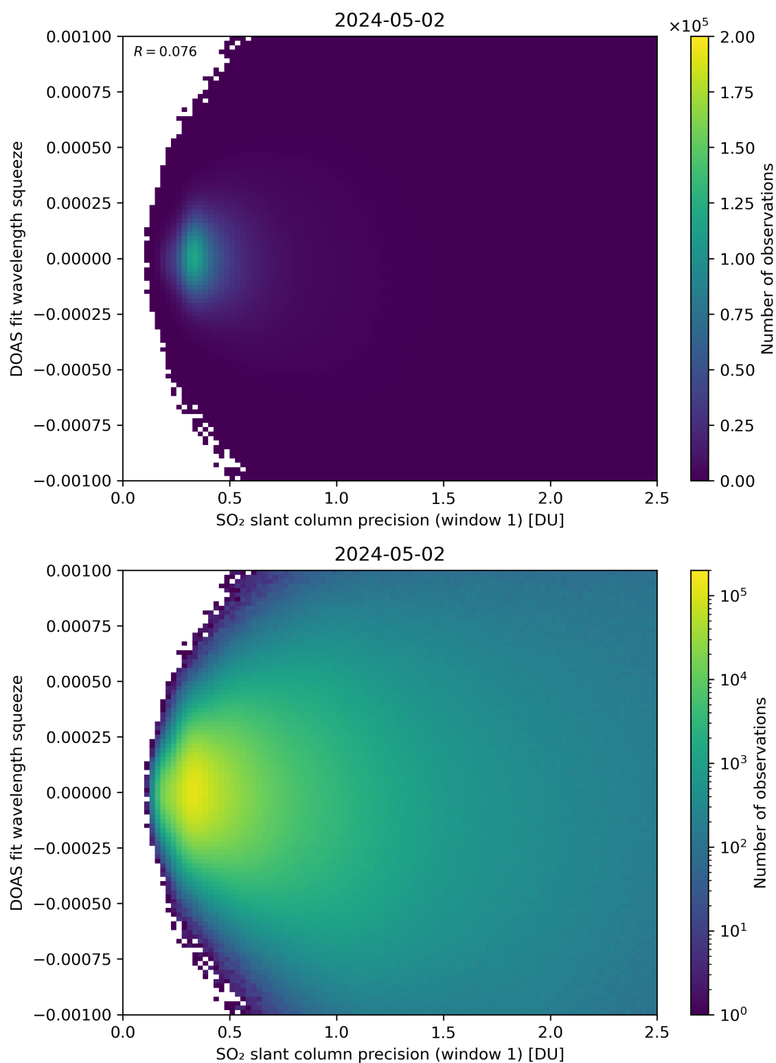
Figure 222: Scatter density plot of “SO 2 slant column precision (window 1)” against “DOAS fit wavelength squeeze” for 2024-05-02 to 2024-05-03.
