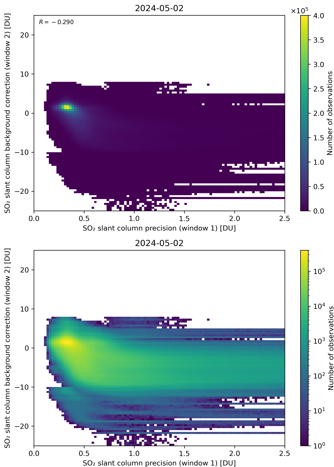
Figure 219: Scatter density plot of “SO 2 slant column precision (window 1)” against “SO 2 slant column background correction (window 2)” for 2024-05-02 to 2024-05-03.
