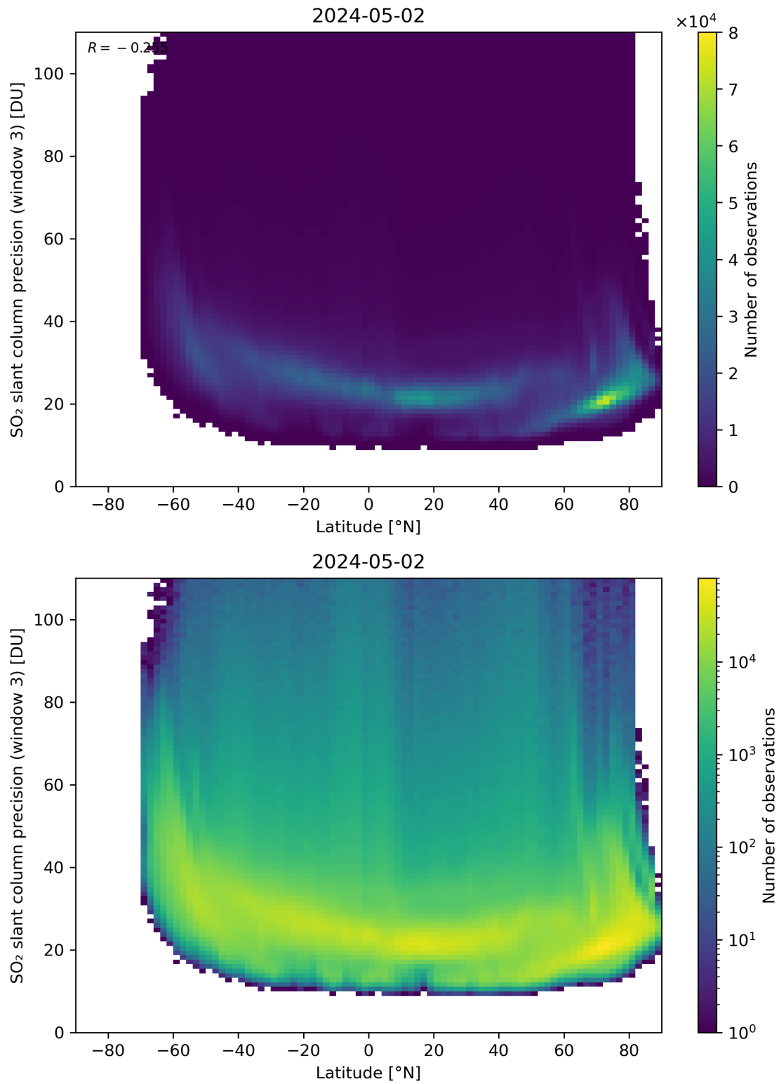
Figure 153: Scatter density plot of “Latitude” against “SO 2 slant column precision (window 3)” for 2024-05-02 to 2024-05-03.
