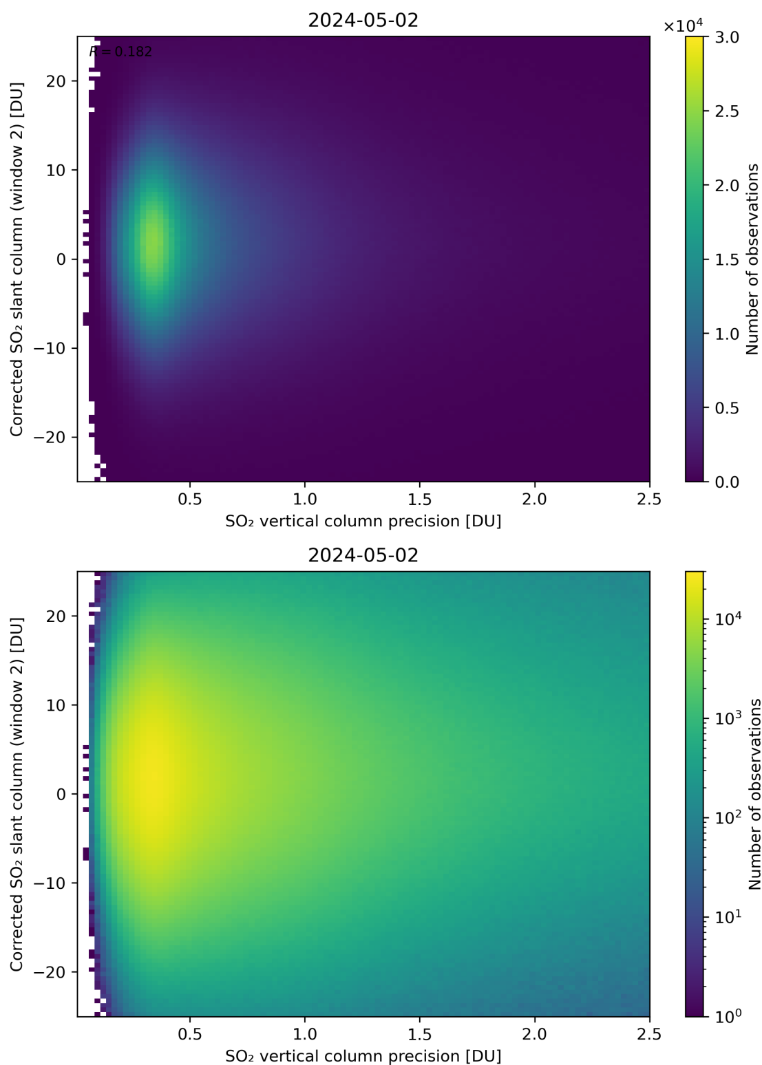
Figure 287: Scatter density plot of “SO 2 vertical column precision” against “Corrected SO 2 slant column (window 2)” for 2024-05-02 to 2024-05-03.
