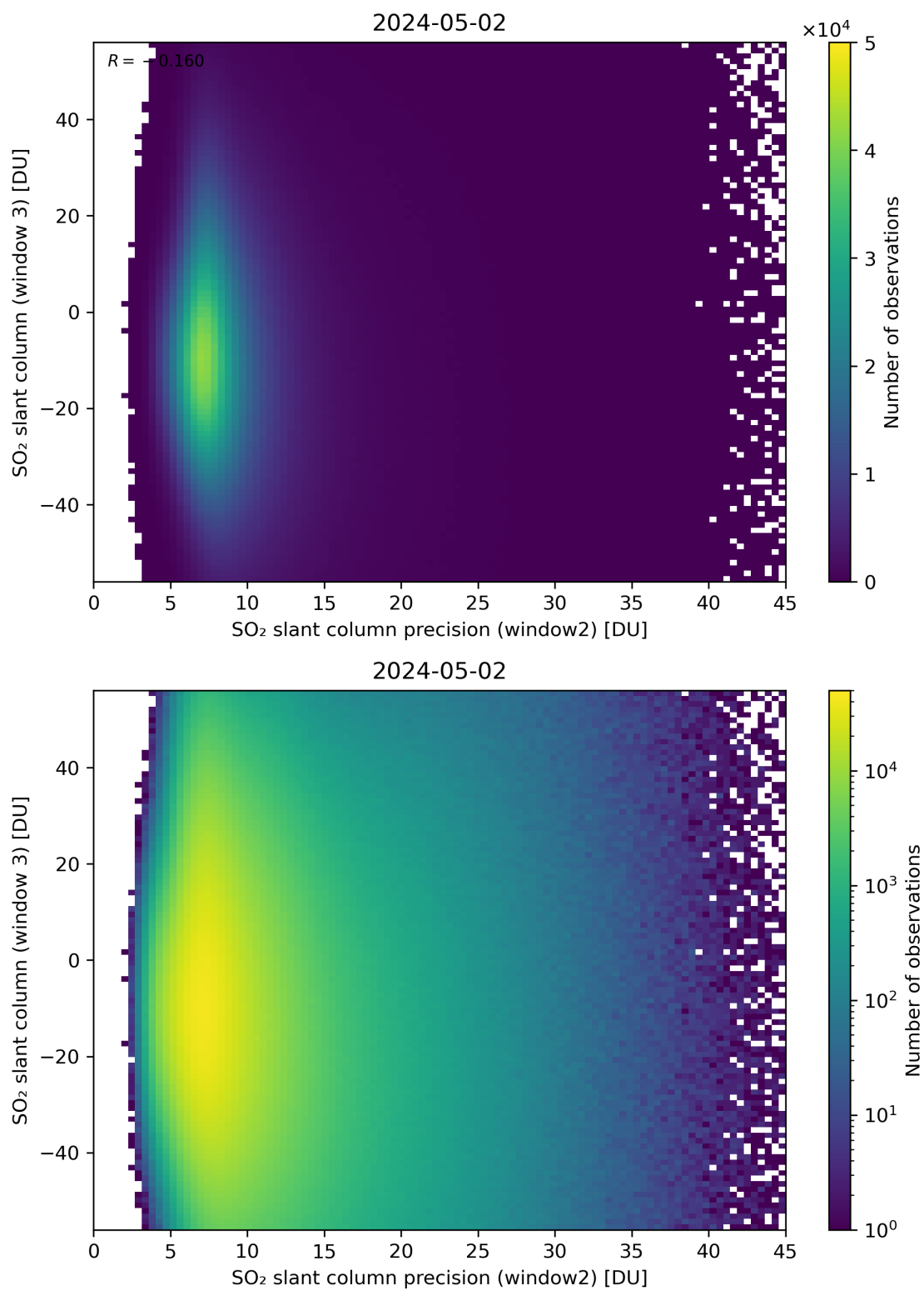
Figure 249: Scatter density plot of “SO 2 slant column precision (window2)” against “SO 2 slant column (window 3)” for 2024-05-02 to 2024-05-03.
