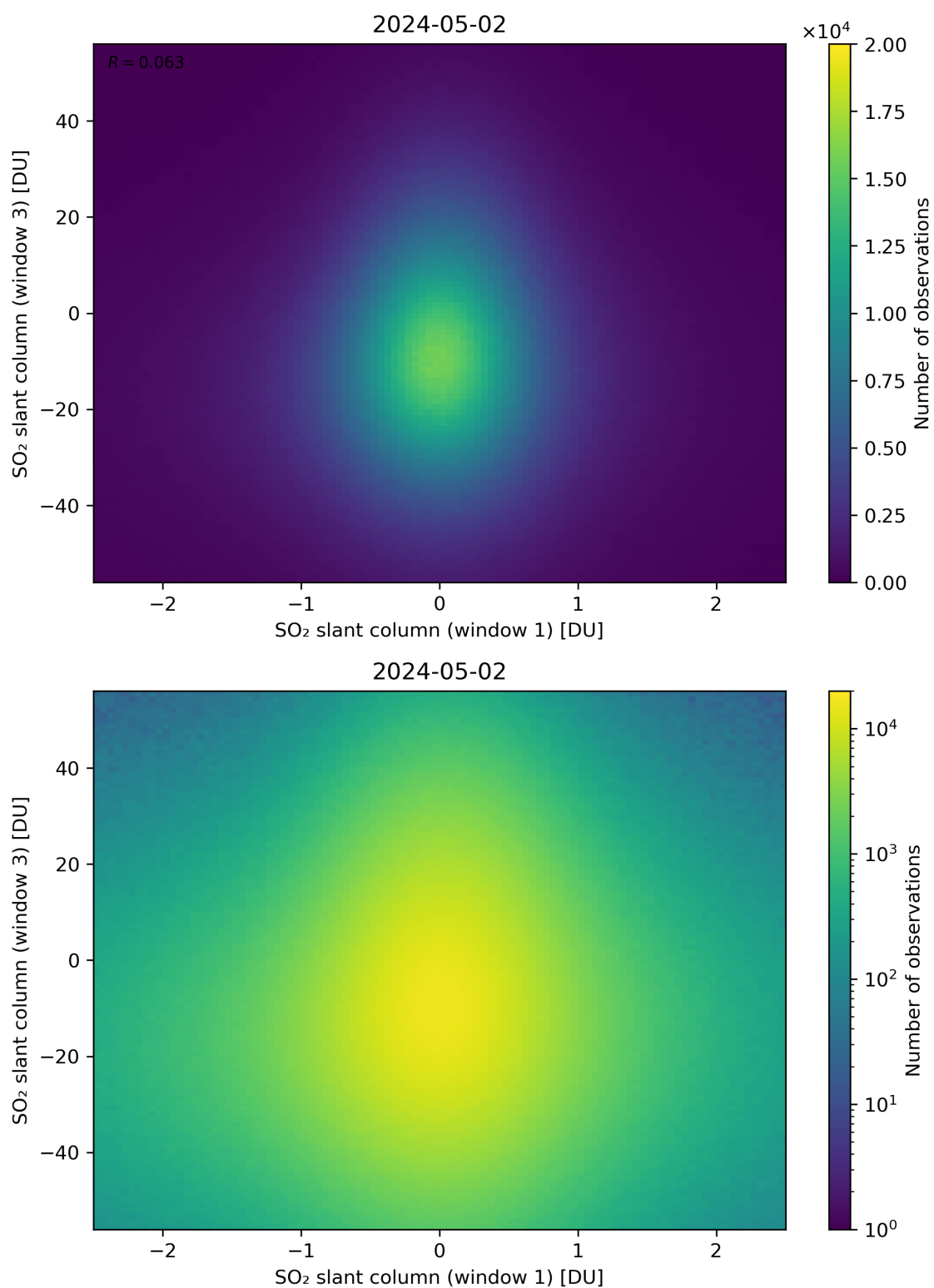
Figure 237: Scatter density plot of “SO 2 slant column (window 1)” against “SO 2 slant column (window 3)” for 2024-05-02 to 2024-05-03.
