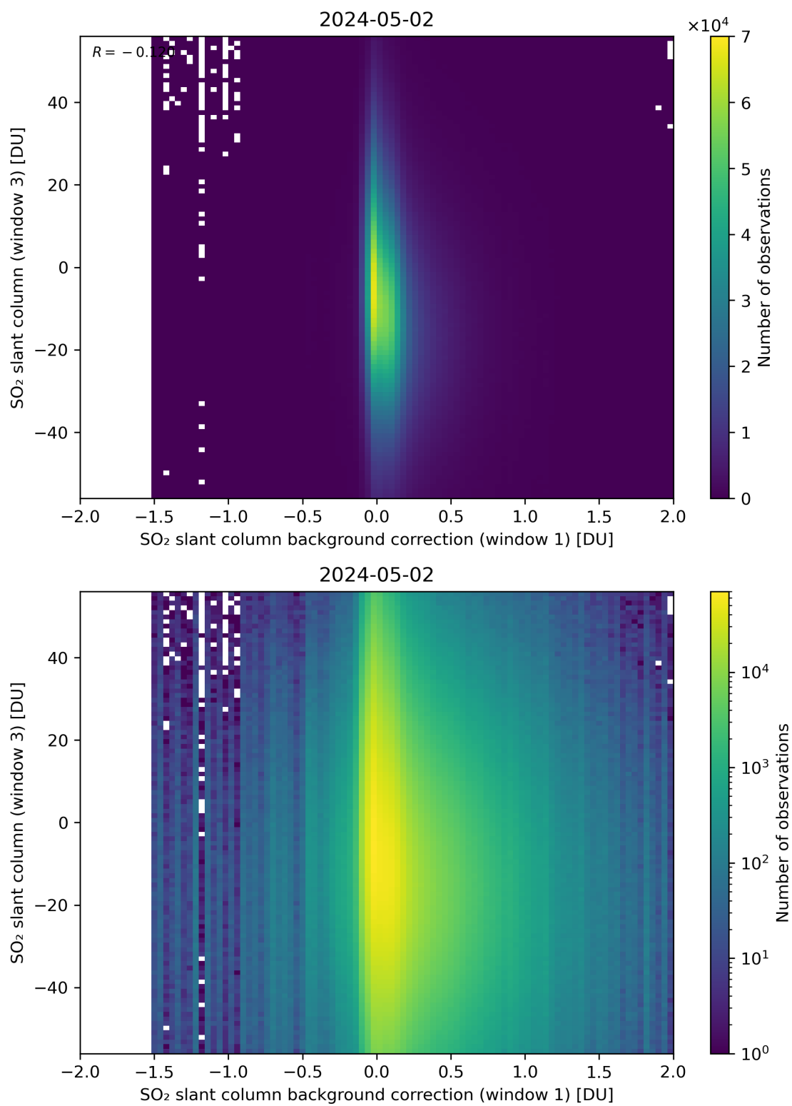
Figure 107: Scatter density plot of “SO 2 slant column background correction (window 1)” against “SO 2 slant column (window 3)” for 2024-05-02 to 2024-05-03.
