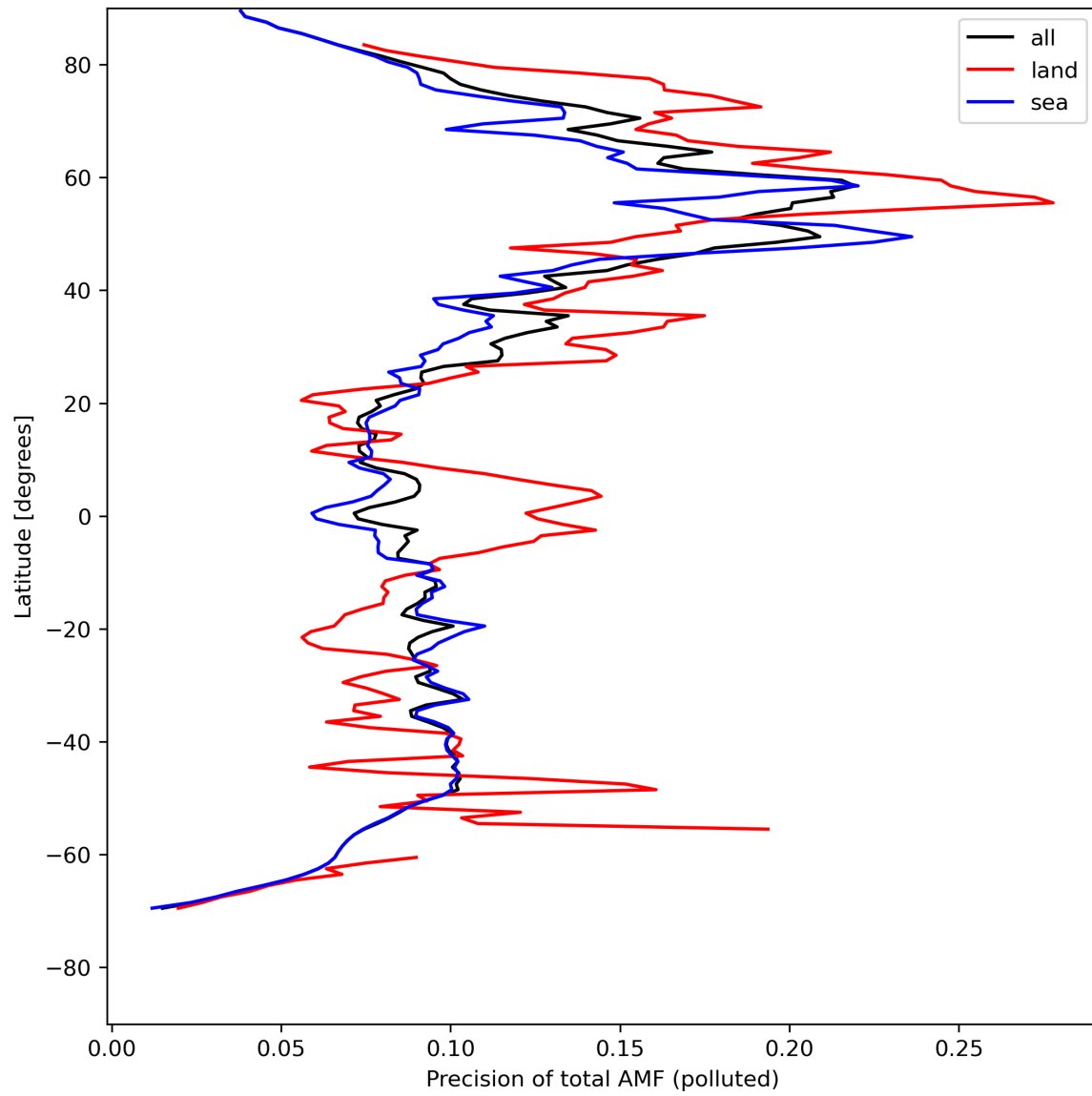
Figure 49: Zonal average of “Precision of total AMF (polluted)” for 2024-05-02 to 2024-05-03.
