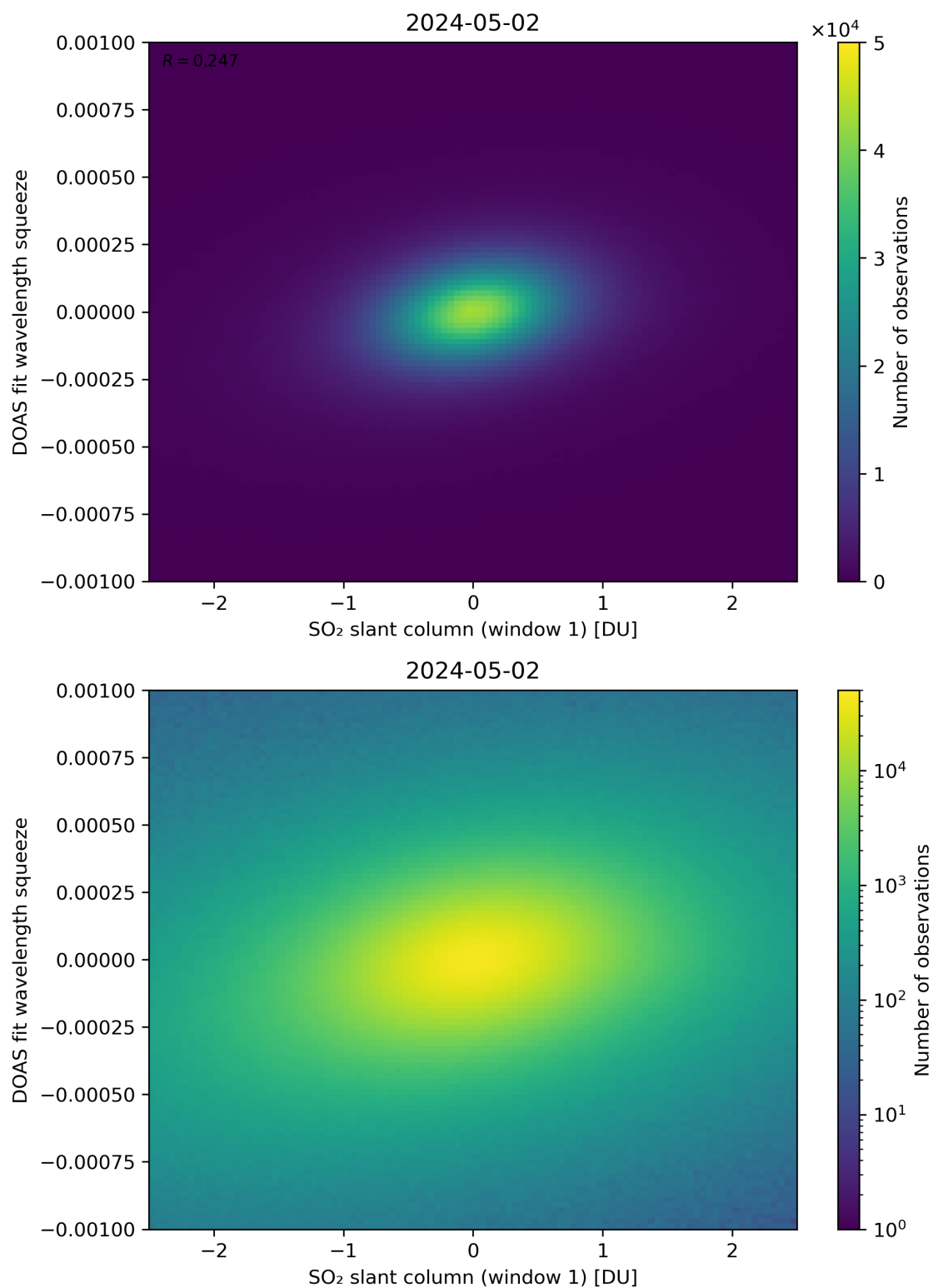
Figure 216: Scatter density plot of “SO 2 slant column (window 1)” against “DOAS fit wavelength squeeze” for 2024-05-02 to 2024-05-03.
