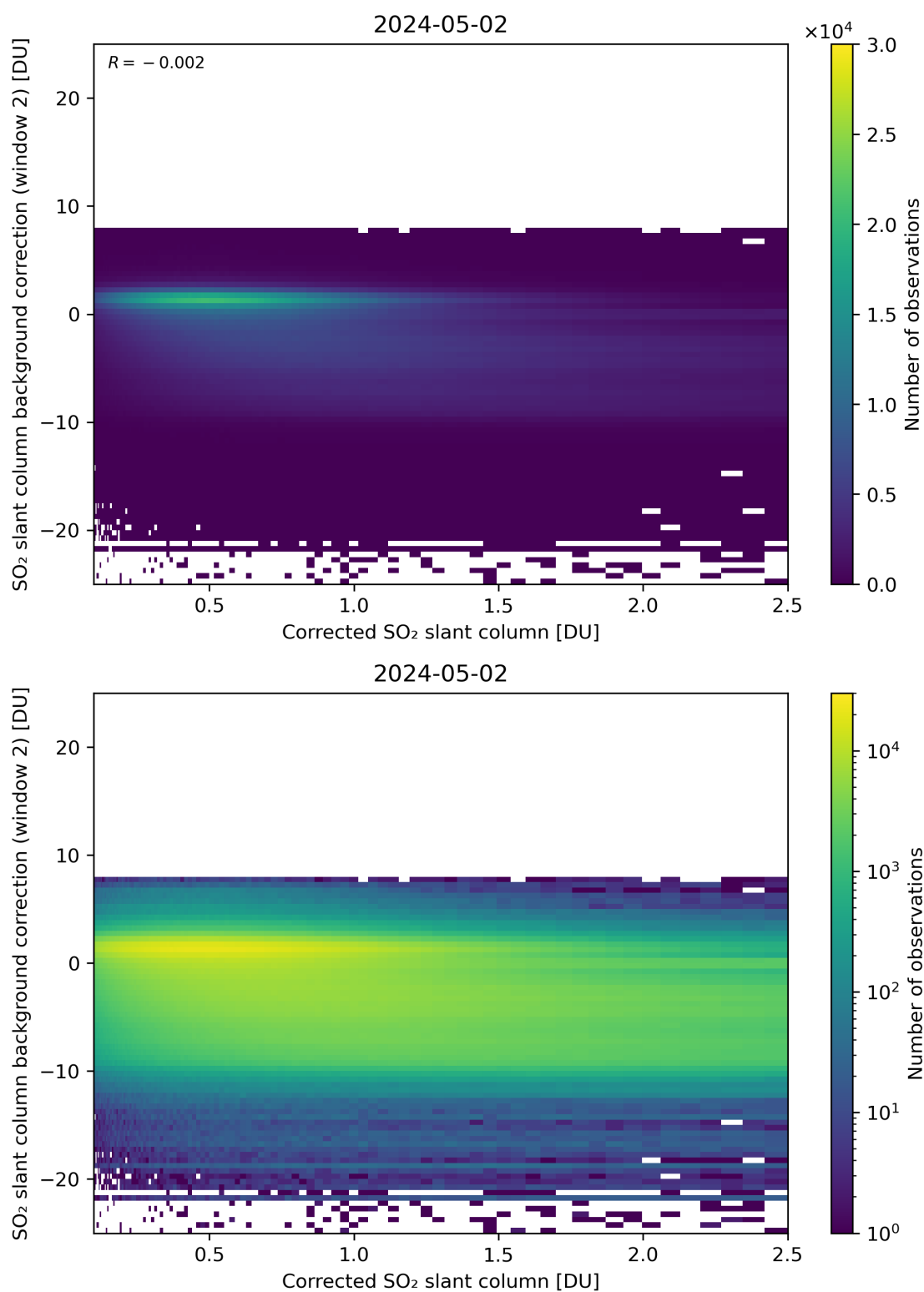
Figure 179: Scatter density plot of “Corrected SO 2 slant column” against “SO 2 slant column background correction (window 2)” for 2024-05-02 to 2024-05-03.
