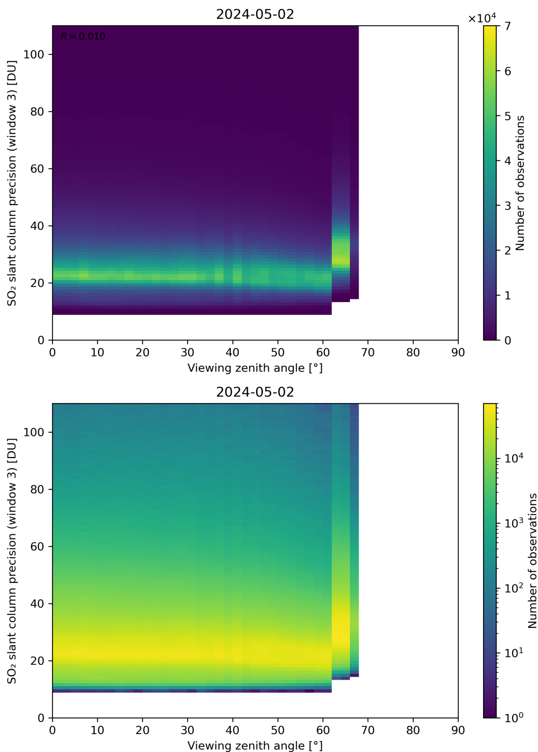
Figure 324: Scatter density plot of “Viewing zenith angle” against “SO 2 slant column precision (window 3)” for 2024-05-02 to 2024-05-03.
