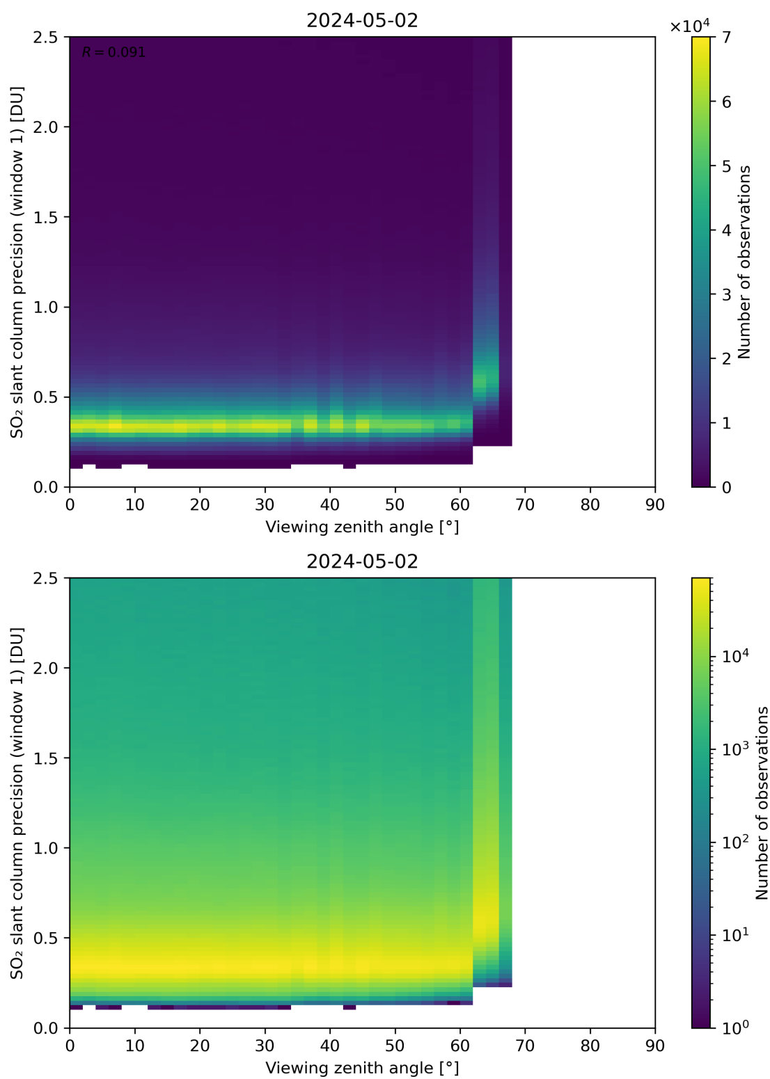
Figure 321: Scatter density plot of “Viewing zenith angle” against “SO 2 slant column precision (window 1)” for 2024-05-02 to 2024-05-03.
