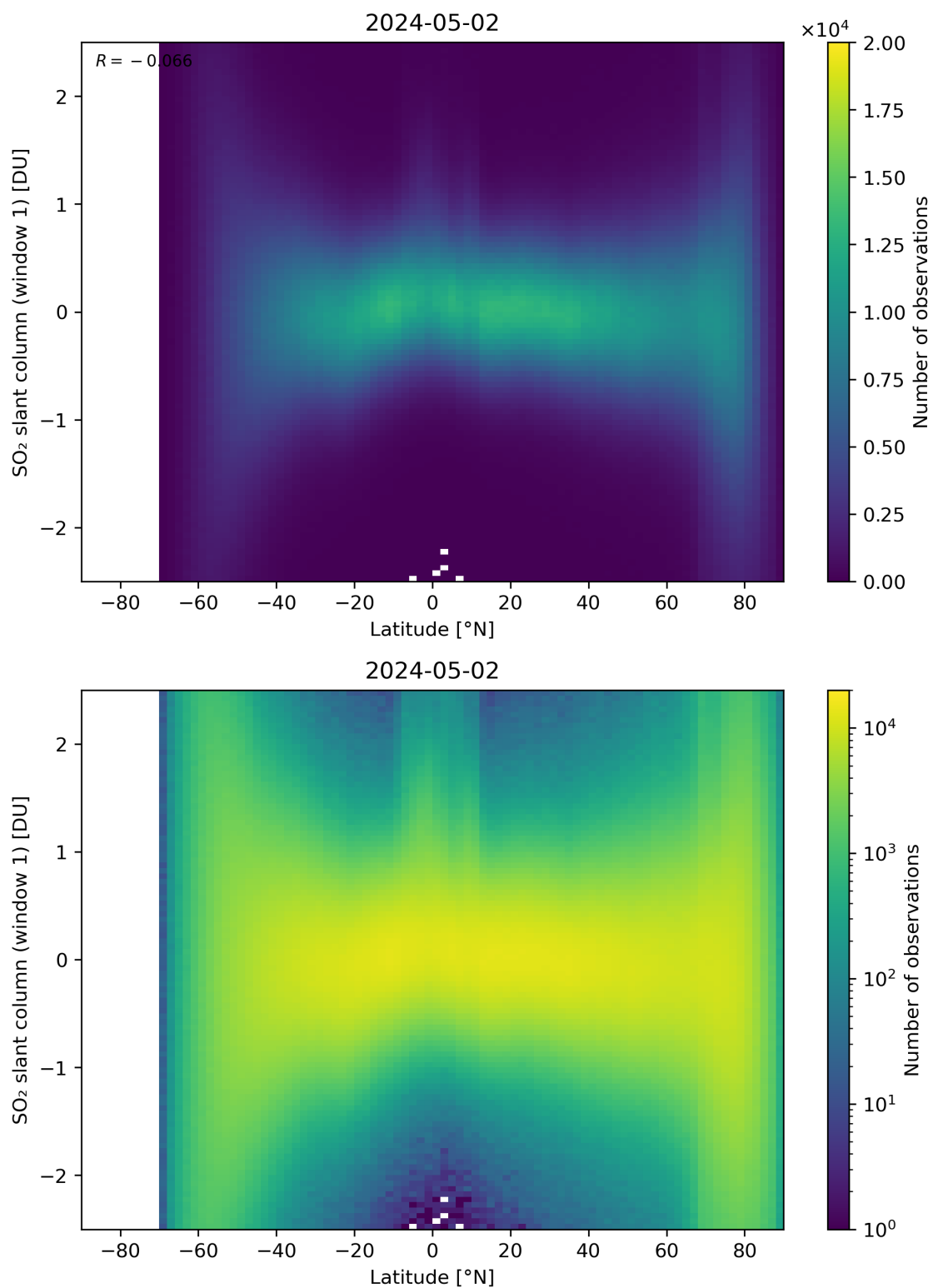
Figure 149: Scatter density plot of “Latitude” against “SO 2 slant column (window 1)” for 2024-05-02 to 2024-05-03.
