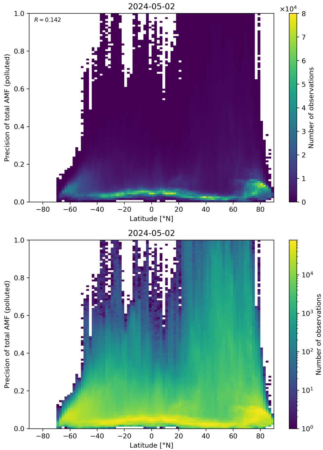
Figure 155: Scatter density plot of “Latitude” against “Precision of total AMF (polluted)” for 2024-05-02 to 2024-05-03.
