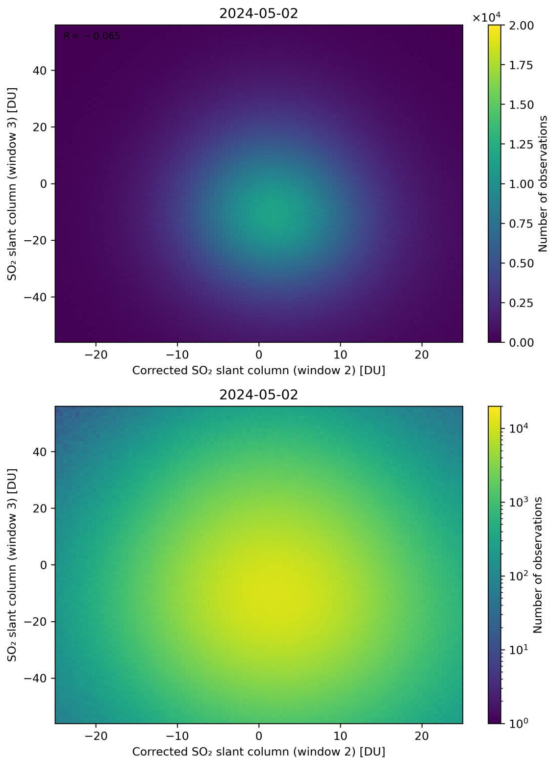
Figure 201: Scatter density plot of “Corrected SO 2 slant column (window 2)” against “SO 2 slant column (window 3)” for 2024-05-02 to 2024-05-03.
