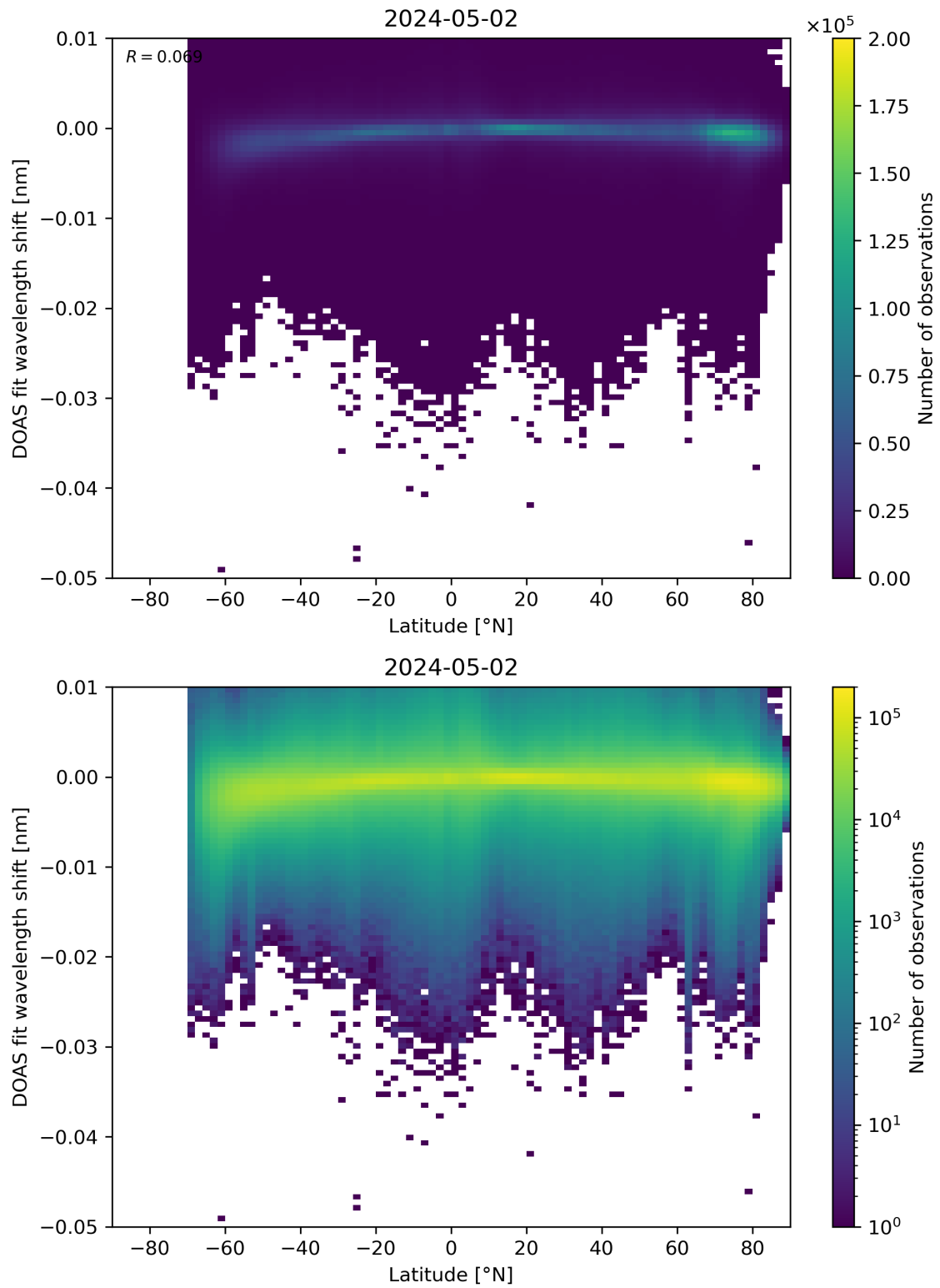
Figure 142: Scatter density plot of “Latitude” against “DOAS fit wavelength shift” for 2024-05-02 to 2024-05-03.
