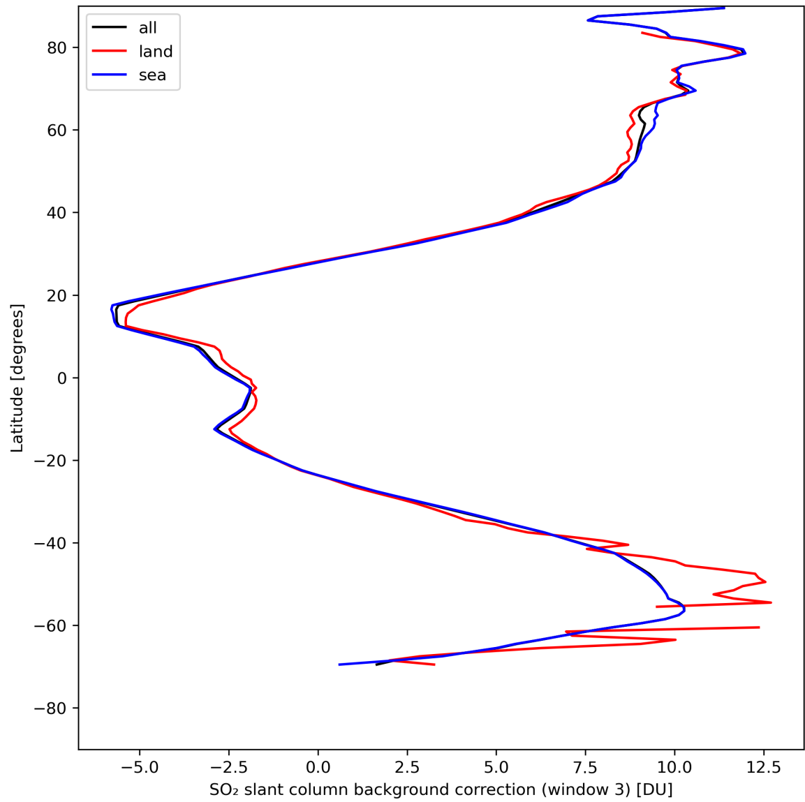
Figure 44: Zonal average of “SO 2 slant column background correction (window 3)” for 2024-05-02 to 2024-05-03.
