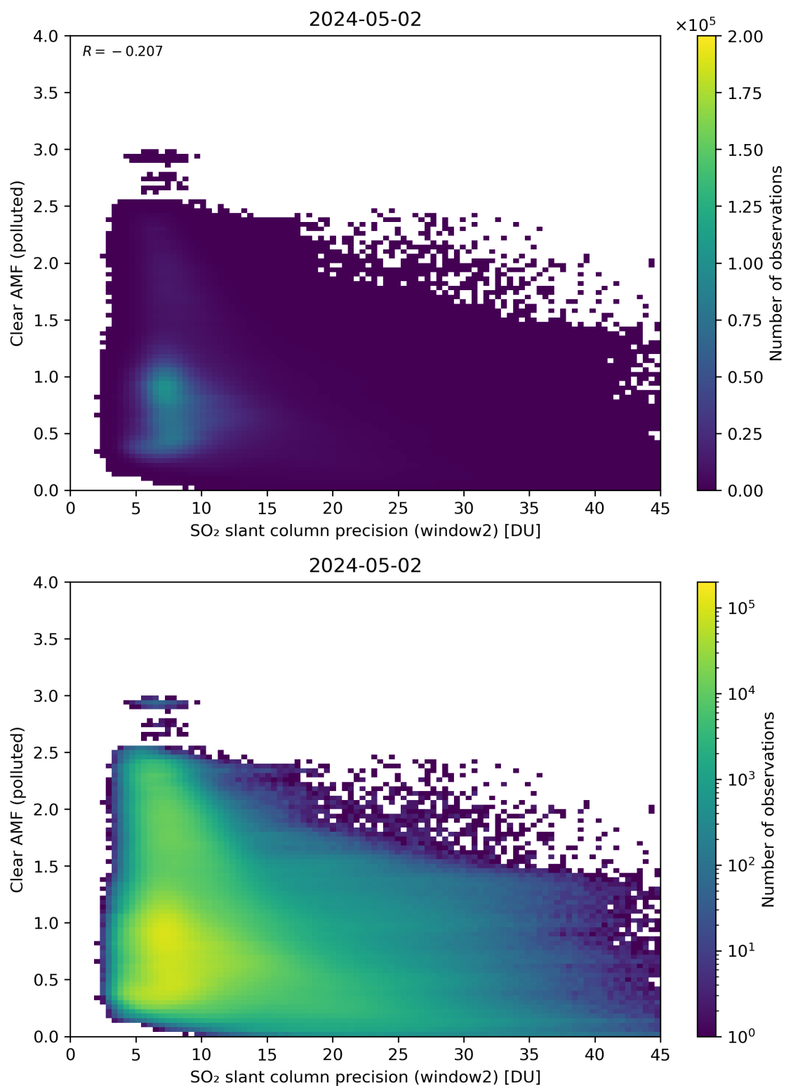
Figure 246: Scatter density plot of “SO 2 slant column precision (window2)” against “Clear AMF (polluted)” for 2024-05-02 to 2024-05-03.
