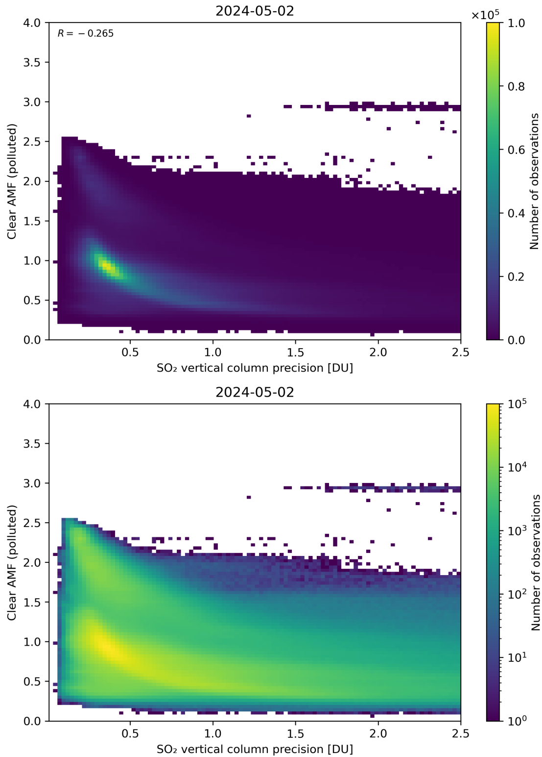
Figure 285: Scatter density plot of “SO 2 vertical column precision” against “Clear AMF (polluted)” for 2024-05-02 to 2024-05-03.
