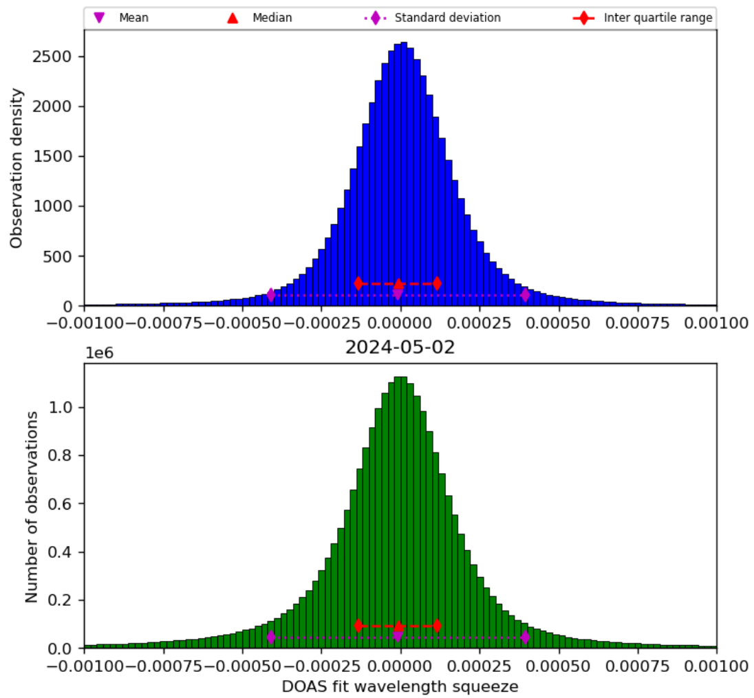
Figure 69: Histogram of “DOAS fit wavelength squeeze” for 2024-05-02 to 2024-05-03
