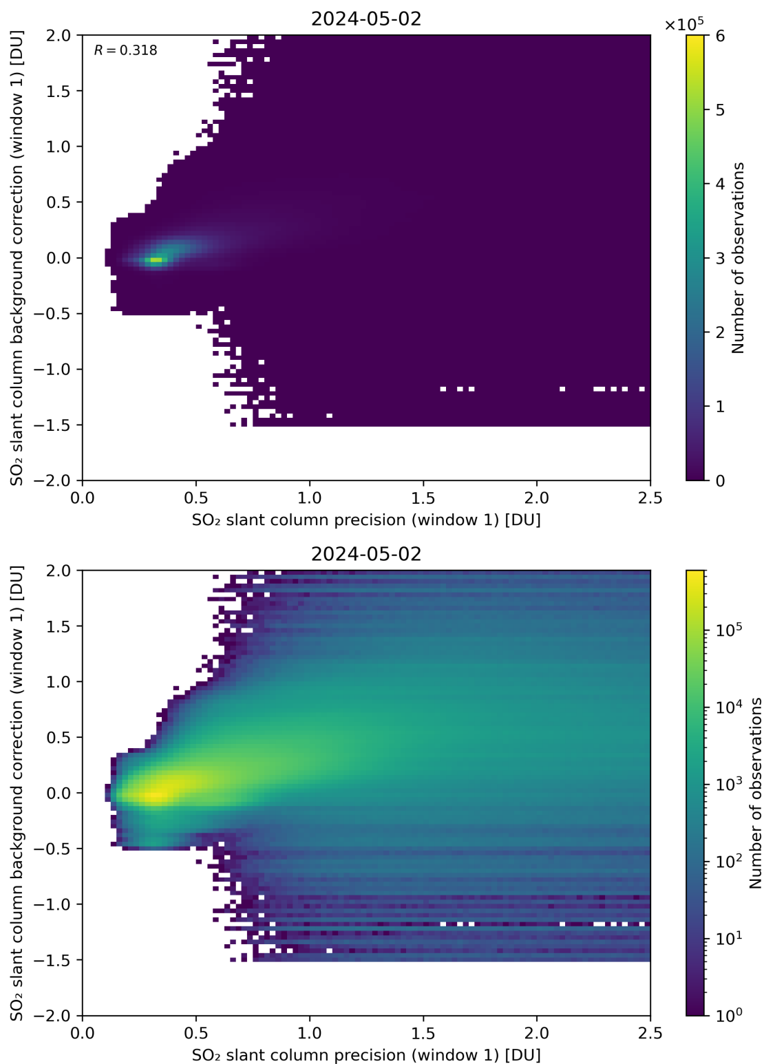
Figure 218: Scatter density plot of “SO 2 slant column precision (window 1)” against “SO 2 slant column background correction (window 1)” for 2024-05-02 to 2024-05-03.
