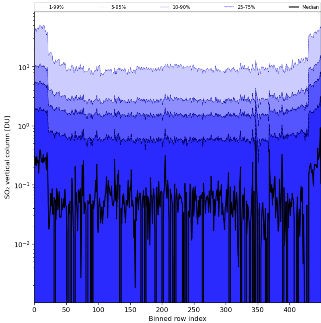
Figure 76: Along track statistics of “SO 2 vertical column” for 2024-05-02 to 2024-05-03
