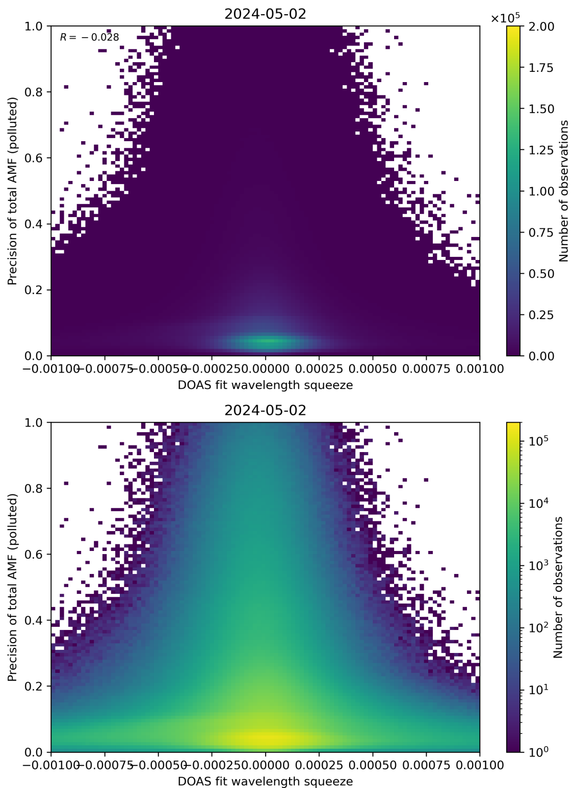
Figure 135: Scatter density plot of “DOAS fit wavelength squeeze” against “Precision of total AMF (polluted)” for 2024-05-02 to 2024-05-03.
