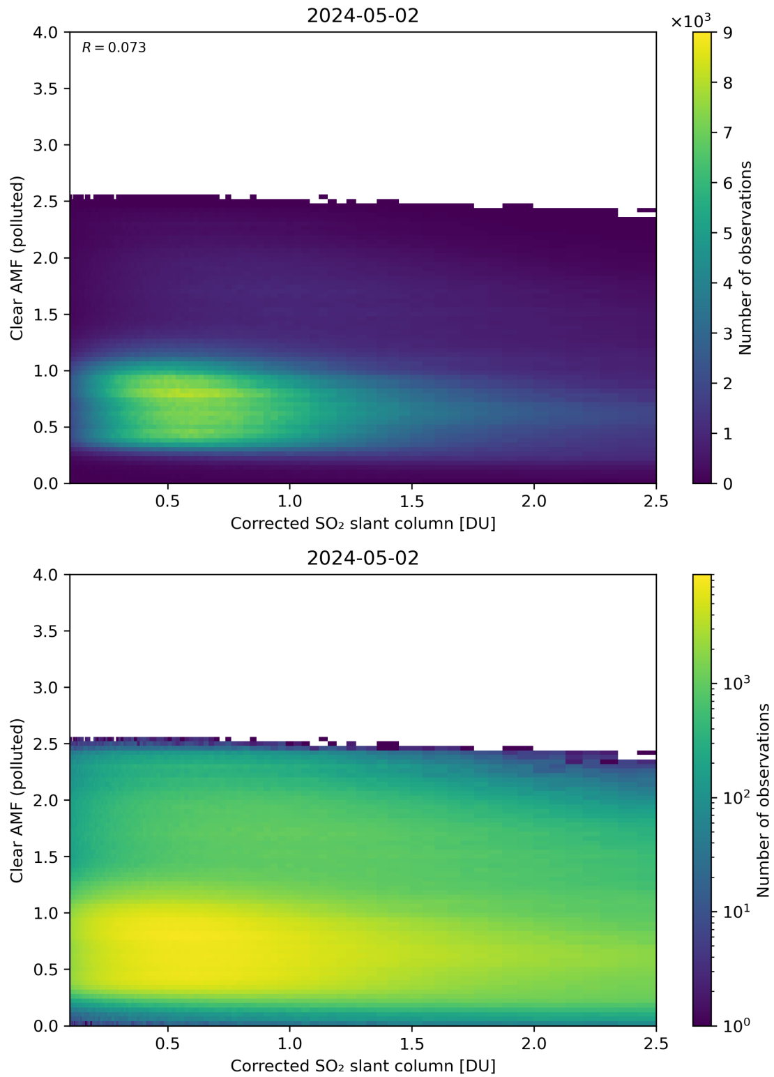
Figure 184: Scatter density plot of “Corrected SO 2 slant column” against “Clear AMF (polluted)” for 2024-05-02 to 2024-05-03.
