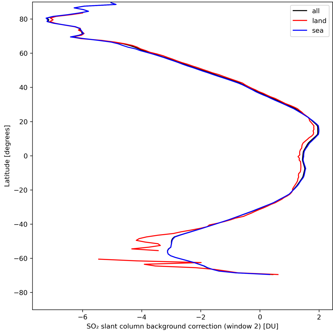
Figure 40: Zonal average of “SO 2 slant column background correction (window 2)” for 2024-05-02 to 2024-05-03.
