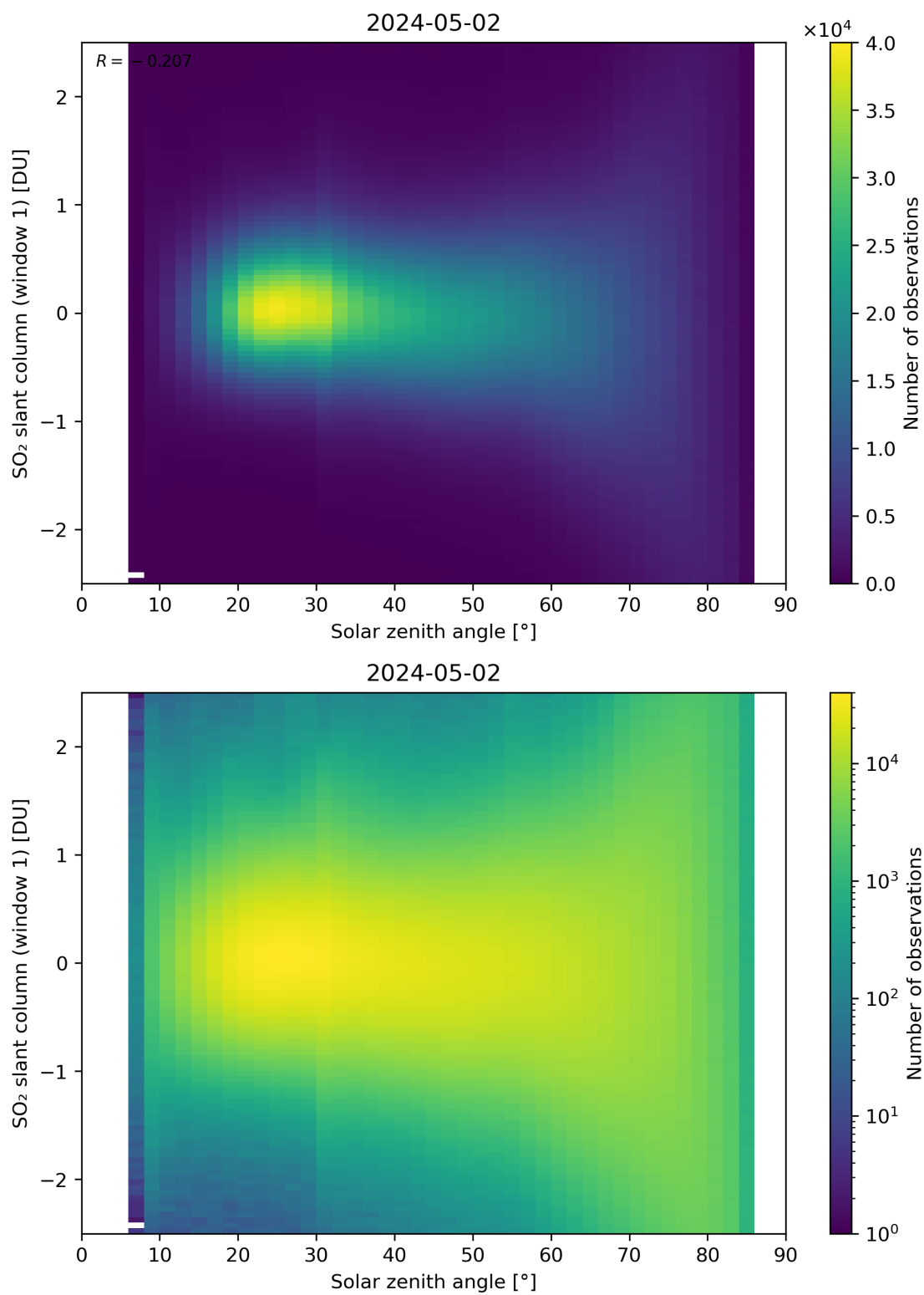
Figure 169: Scatter density plot of “Solar zenith angle” against “SO 2 slant column (window 1)” for 2024-05-02 to 2024-05-03.
