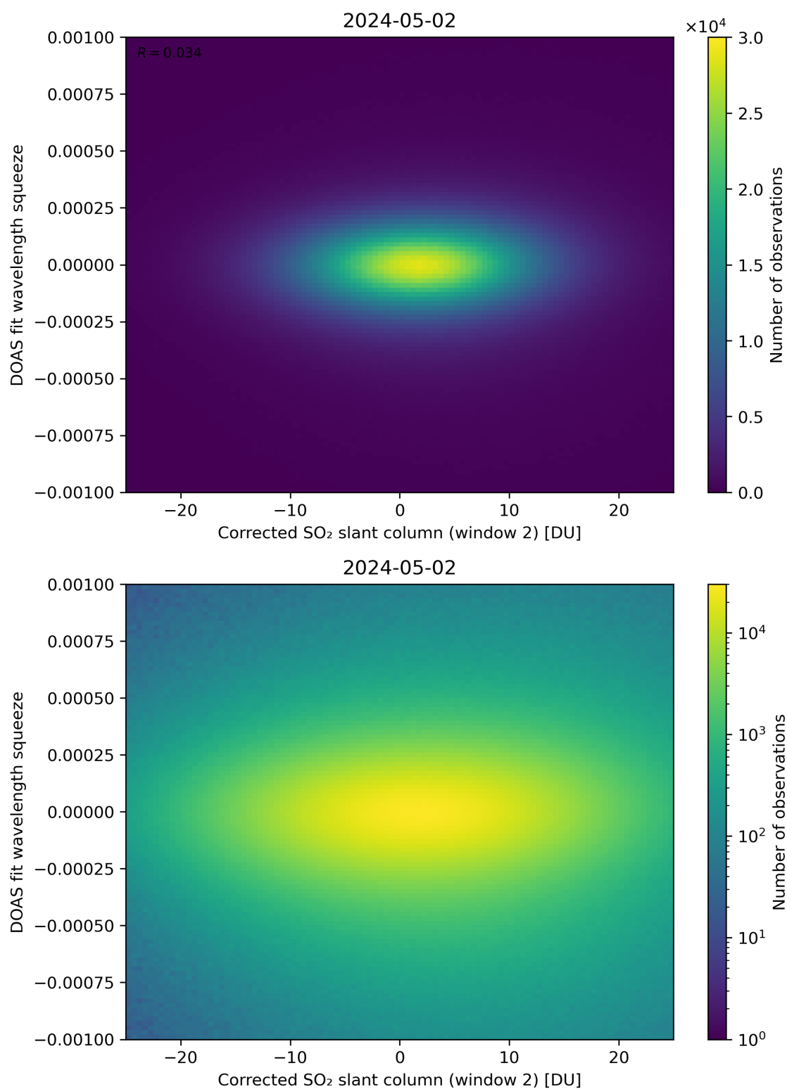
Figure 197: Scatter density plot of “Corrected SO 2 slant column (window 2)” against “DOAS fit wavelength squeeze” for 2024-05-02 to 2024-05-03.
