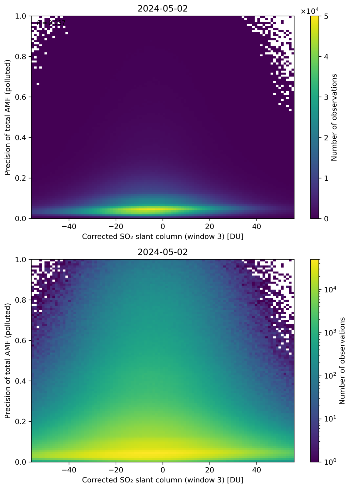
Figure 211: Scatter density plot of “Corrected SO 2 slant column (window 3)” against “Precision of total AMF (polluted)” for 2024-05-02 to 2024-05-03.
