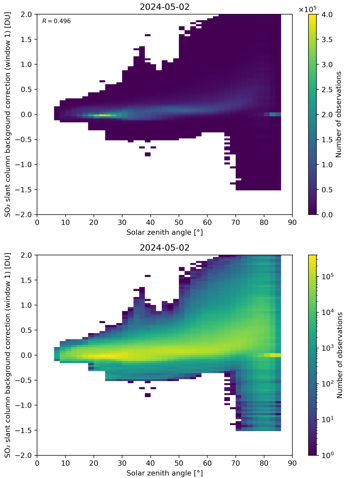
Figure 158: Scatter density plot of “Solar zenith angle” against “SO 2 slant column background correction (window 1)” for 2024-05-02 to 2024-05-03.
