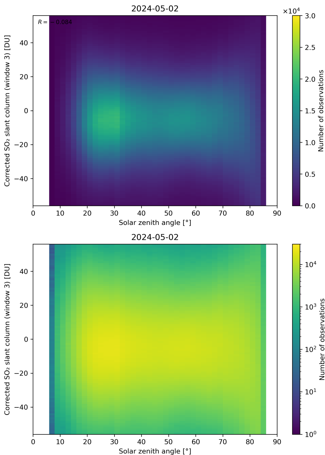
Figure 168: Scatter density plot of “Solar zenith angle” against “Corrected SO 2 slant column (window 3)” for 2024-05-02 to 2024-05-03.
