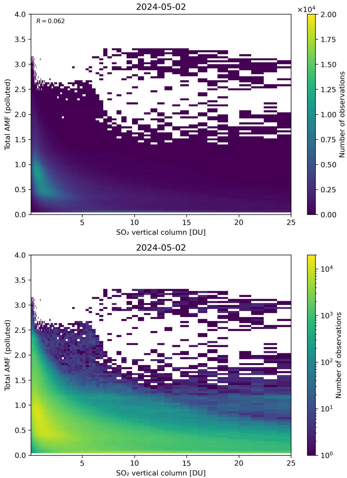
Figure 305: Scatter density plot of “SO 2 vertical column” against “Total AMF (polluted)” for 2024-05-02 to 2024-05-03.
