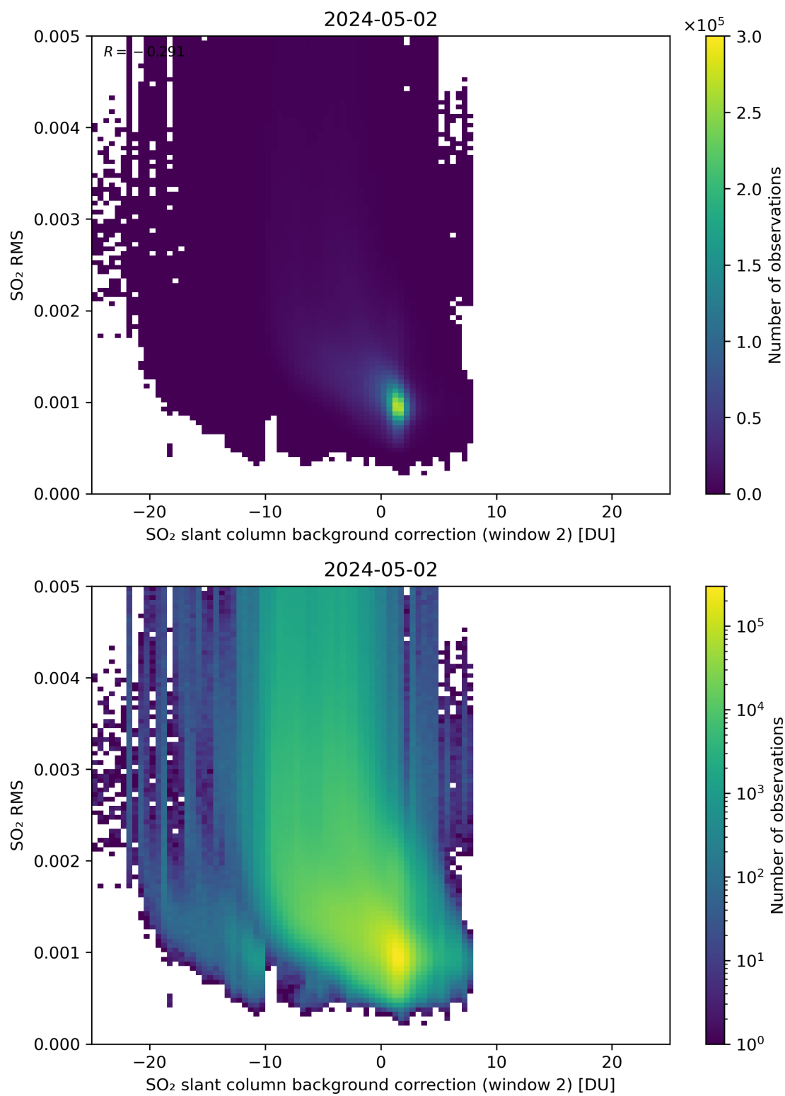
Figure 114: Scatter density plot of “SO 2 slant column background correction (window 2)” against “SO 2 RMS” for 2024-05-02 to 2024-05-03.
