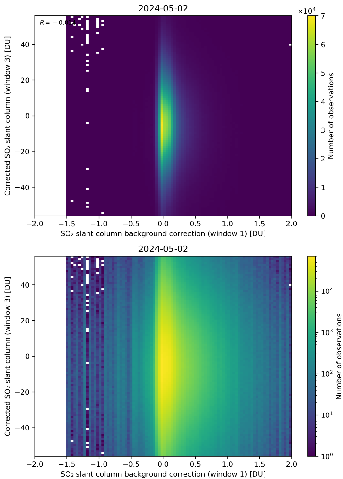
Figure 105: Scatter density plot of “SO 2 slant column background correction (window 1)” against “Corrected SO 2 slant column (window 3)” for 2024-05-02 to 2024-05-03.
