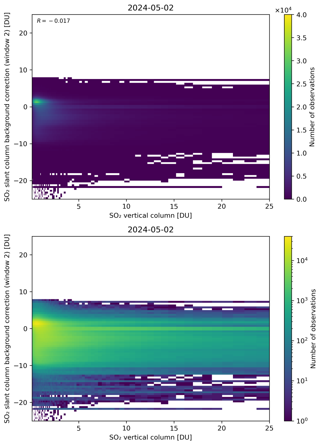
Figure 274: Scatter density plot of “SO 2 vertical column” against “SO 2 slant column background correction (window 2)” for 2024-05-02 to 2024-05-03.
