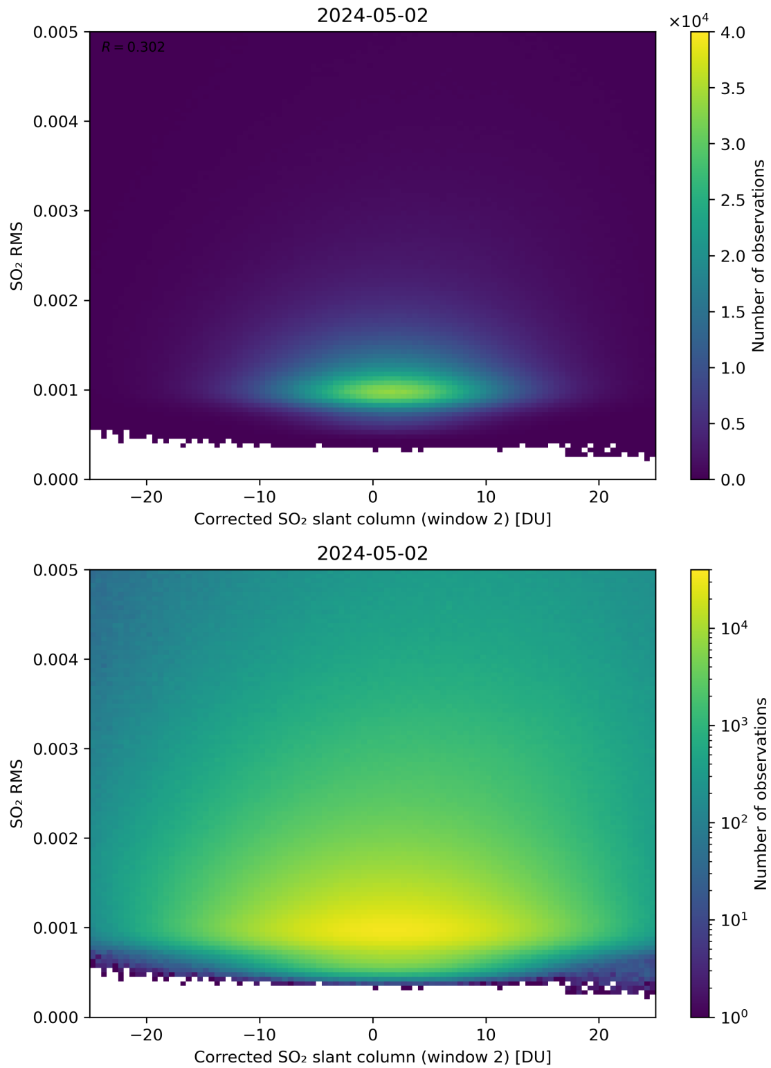
Figure 198: Scatter density plot of “Corrected SO 2 slant column (window 2)” against “SO 2 RMS” for 2024-05-02 to 2024-05-03.
