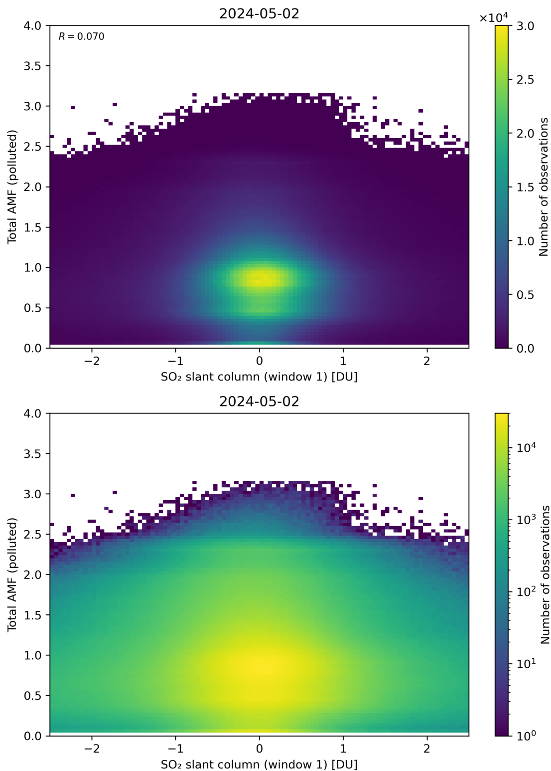
Figure 239: Scatter density plot of “SO 2 slant column (window 1)” against “Total AMF (polluted)” for 2024-05-02 to 2024-05-03.
