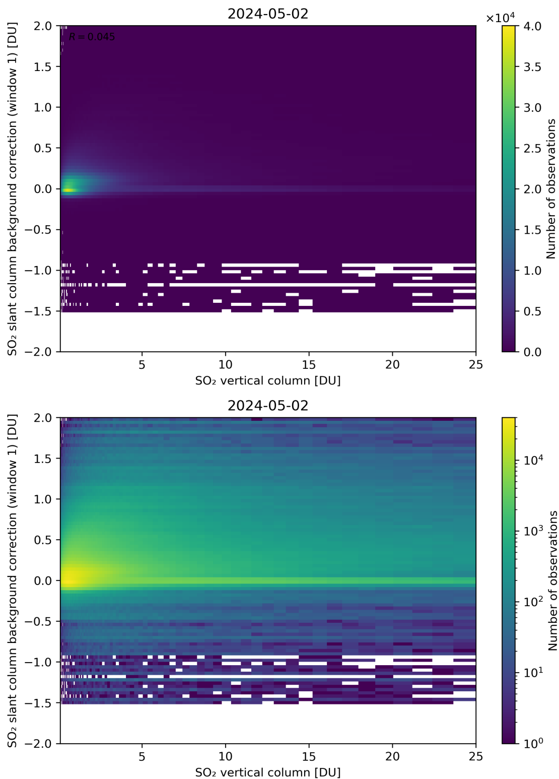
Figure 273: Scatter density plot of “SO 2 vertical column” against “SO 2 slant column background correction (window 1)” for 2024-05-02 to 2024-05-03.
