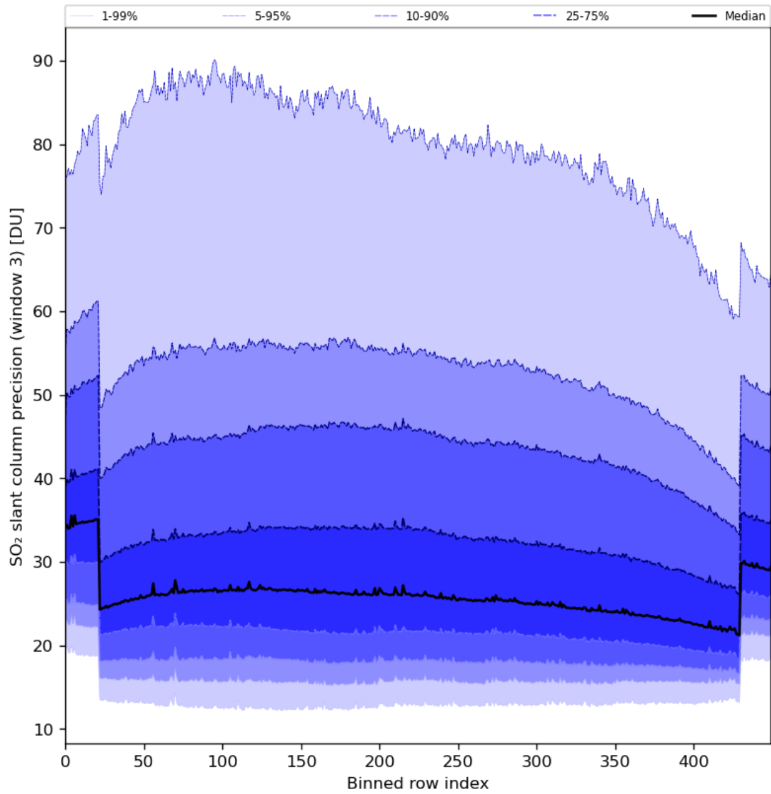
Figure 88: Along track statistics of “SO 2 slant column precision (window 3)” for 2024-05-02 to 2024-05-03
