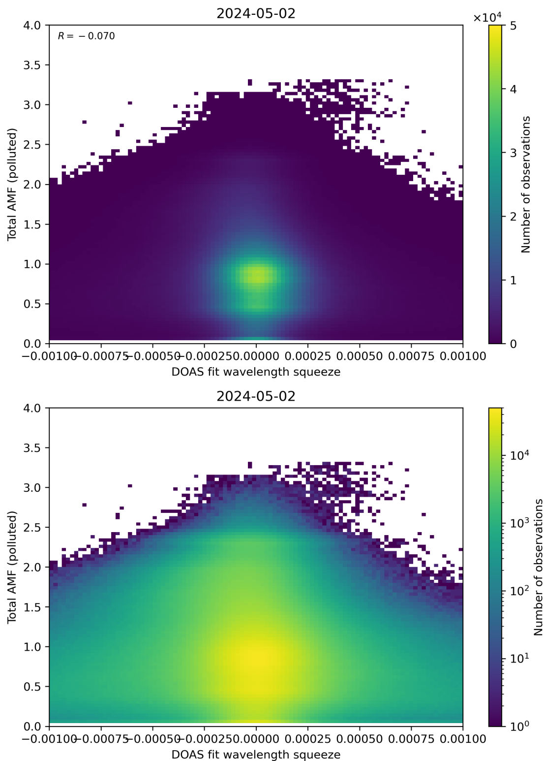
Figure 134: Scatter density plot of “DOAS fit wavelength squeeze” against “Total AMF (polluted)” for 2024-05-02 to 2024-05-03.
