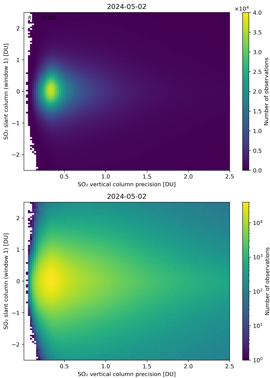
Figure 289: Scatter density plot of “SO 2 vertical column precision” against “SO 2 slant column (window 1)” for 2024-05-02 to 2024-05-03.
