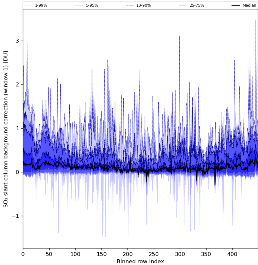
Figure 82: Along track statistics of “SO 2 slant column background correction (window 1)” for 2024-05-02 to 2024-05-03
