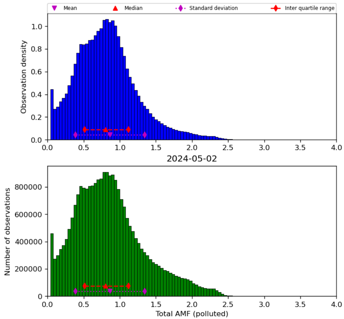
Figure 71: Histogram of “Total AMF (polluted)” for 2024-05-02 to 2024-05-03
