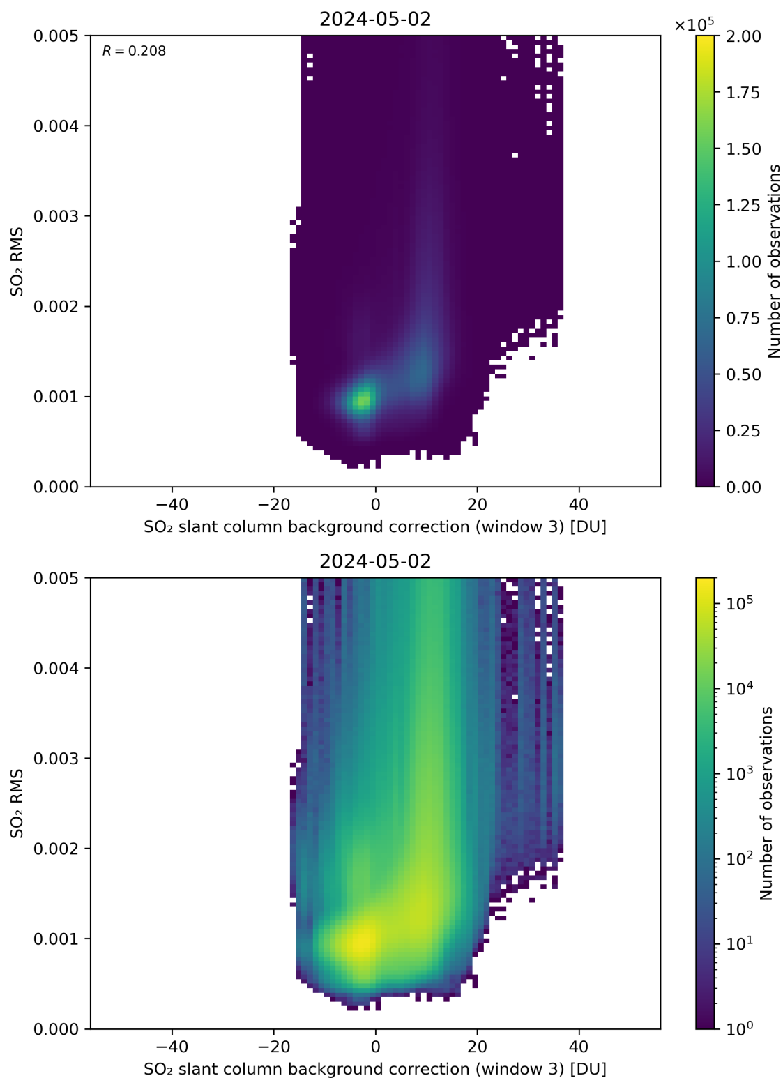
Figure 123: Scatter density plot of “SO 2 slant column background correction (window 3)” against “SO 2 RMS” for 2024-05-02 to 2024-05-03.
