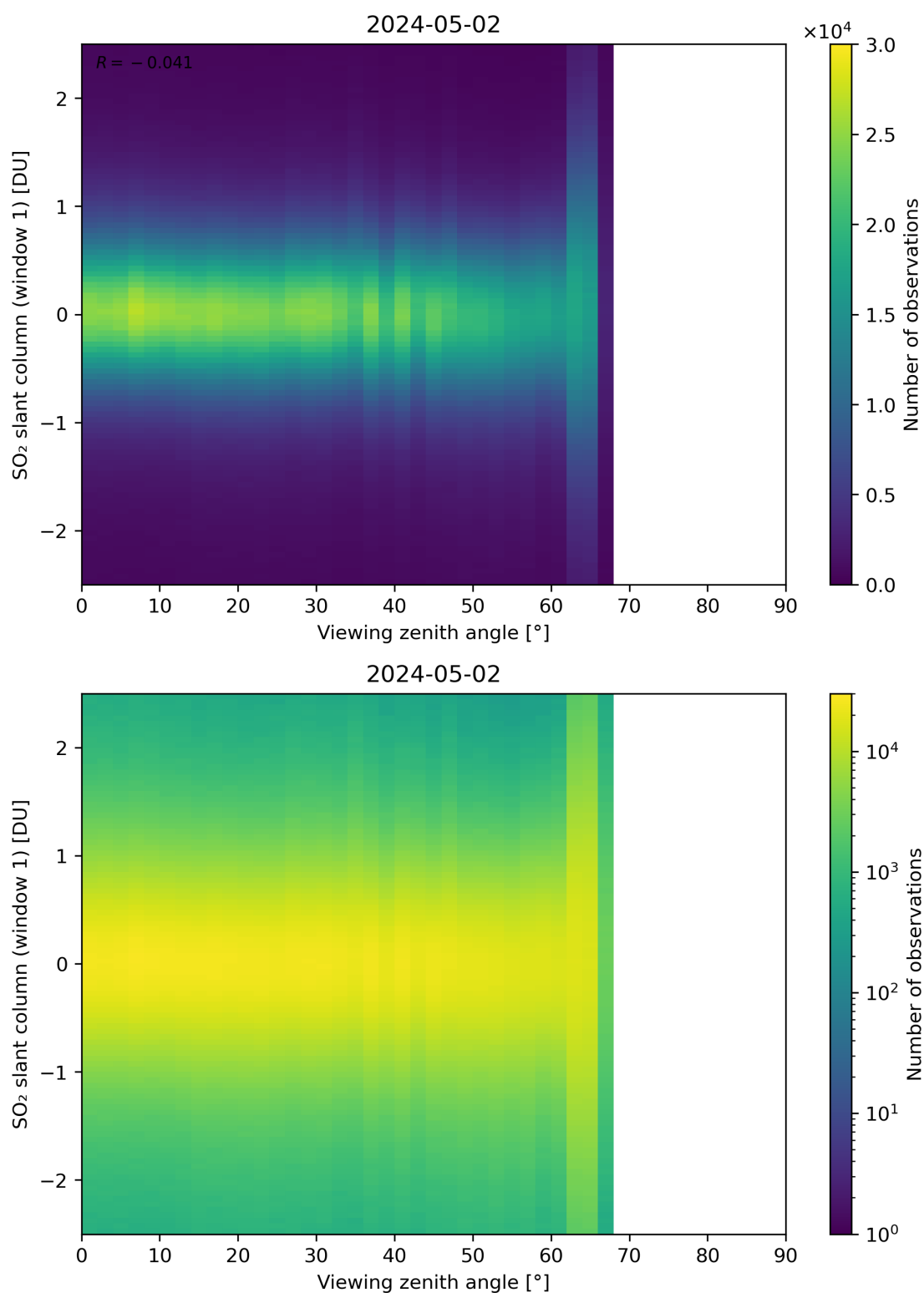
Figure 320: Scatter density plot of “Viewing zenith angle” against “SO 2 slant column (window 1)” for 2024-05-02 to 2024-05-03.
