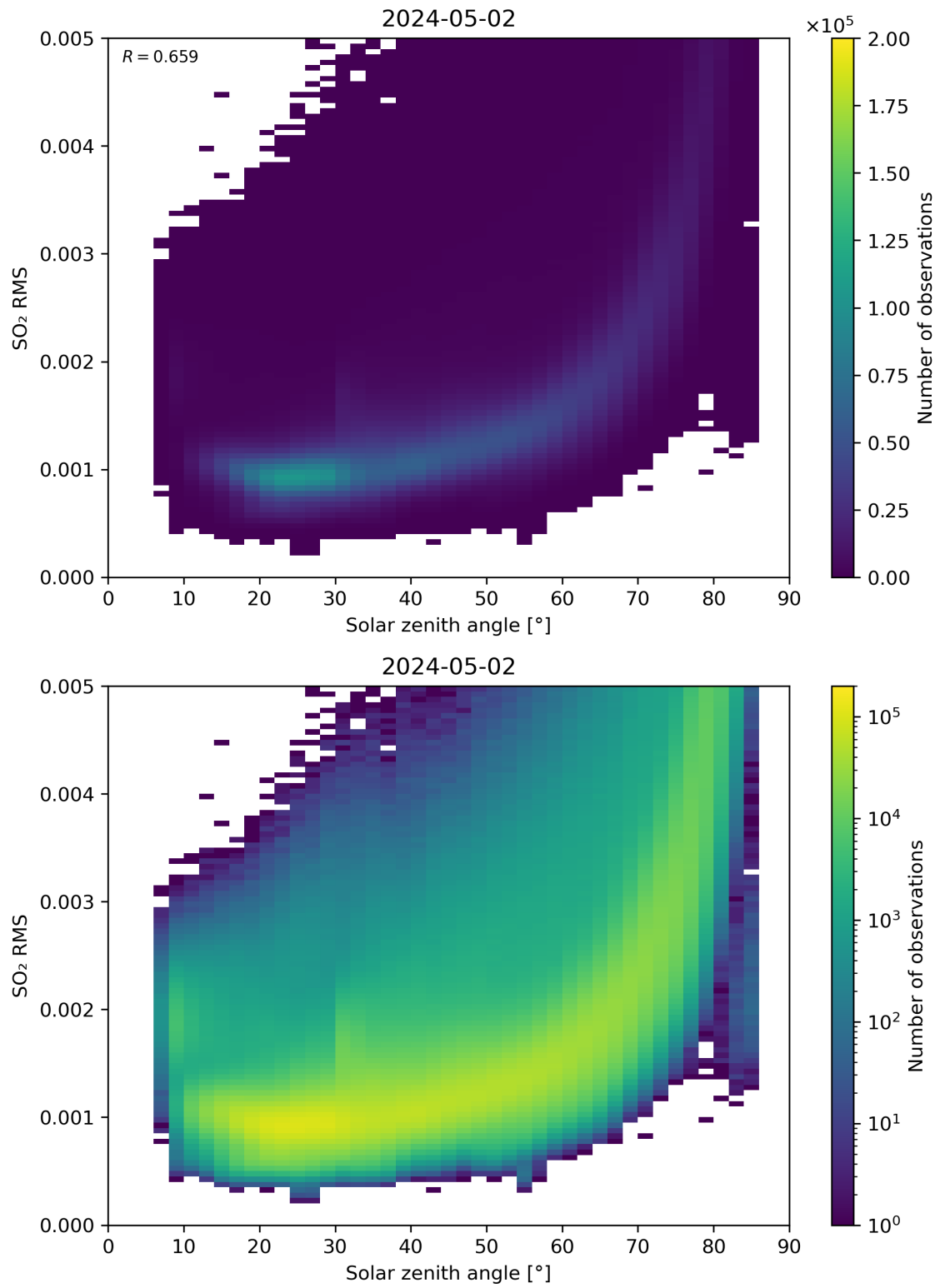
Figure 163: Scatter density plot of “Solar zenith angle” against “SO 2 RMS” for 2024-05-02 to 2024-05-03.
