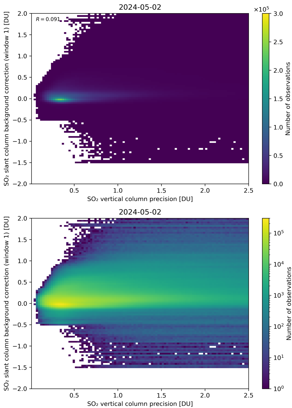
Figure 279: Scatter density plot of “SO 2 vertical column precision” against “SO 2 slant column background correction (window 1)” for 2024-05-02 to 2024-05-03.
