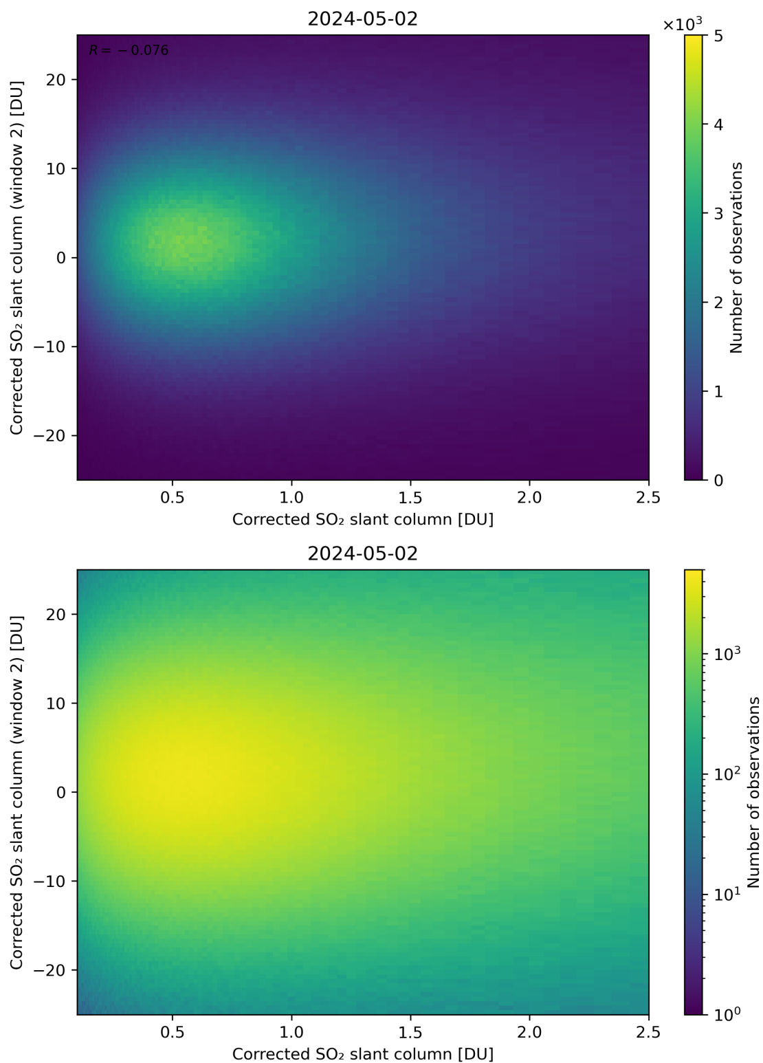
Figure 185: Scatter density plot of “Corrected SO 2 slant column” against “Corrected SO 2 slant column (window 2)” for 2024-05-02 to 2024-05-03.
