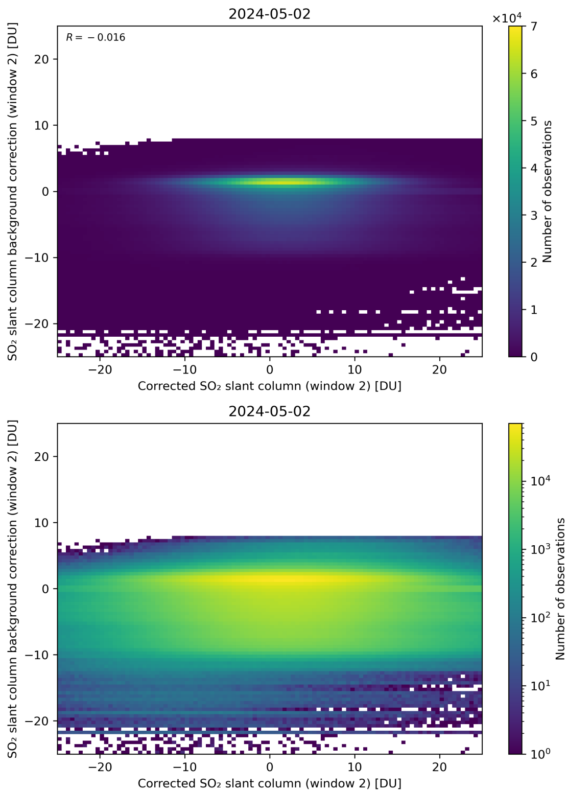
Figure 194: Scatter density plot of “Corrected SO 2 slant column (window 2)” against “SO 2 slant column background correction (window 2)” for 2024-05-02 to 2024-05-03.
