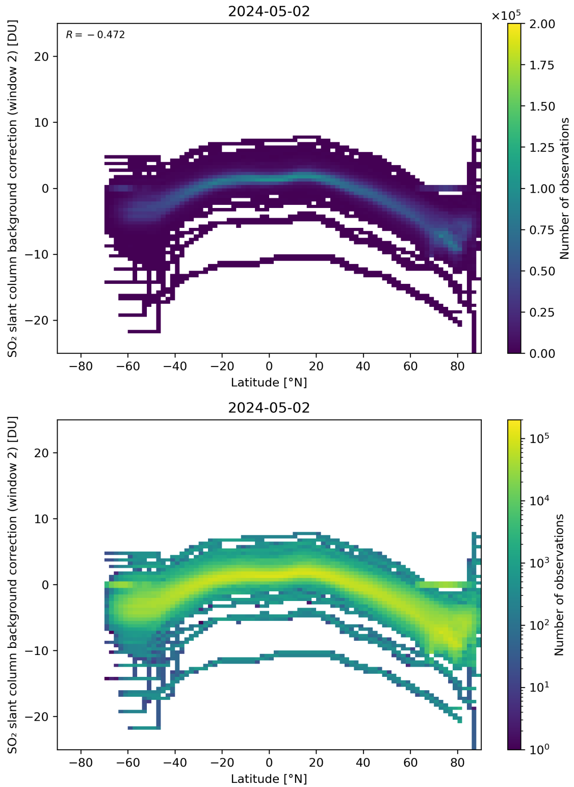
Figure 140: Scatter density plot of “Latitude” against “SO 2 slant column background correction (window 2)” for 2024-05-02 to 2024-05-03.
