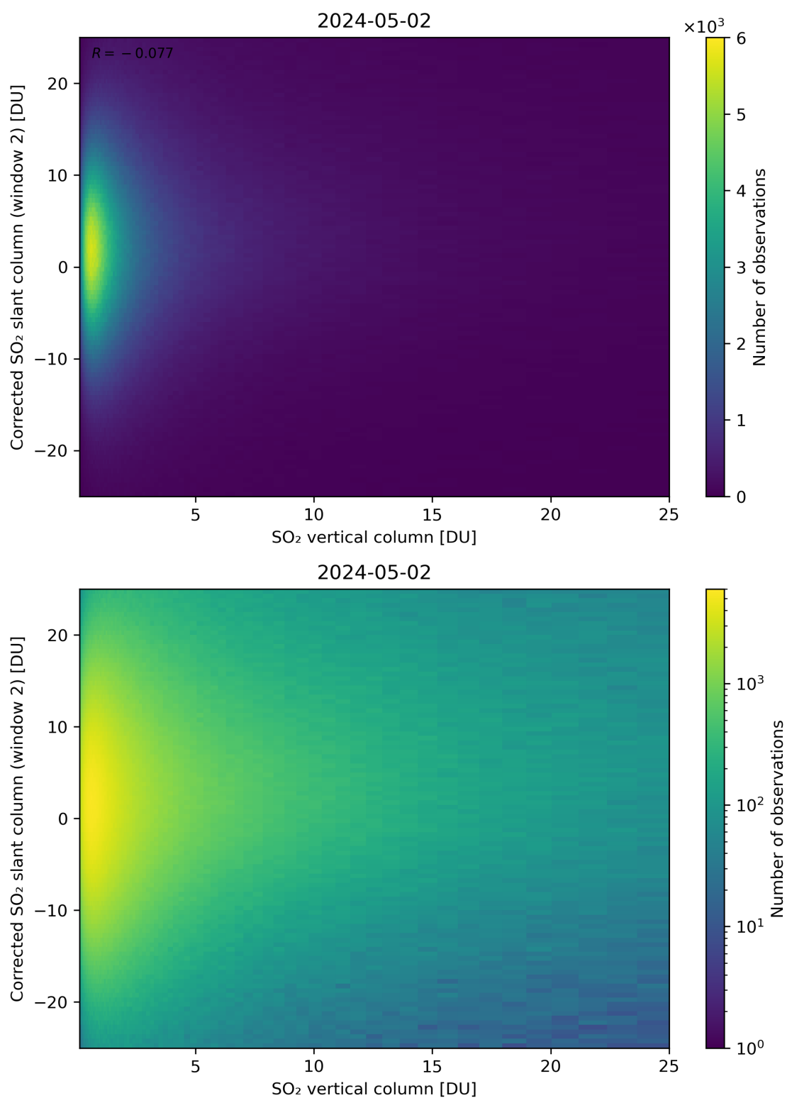
Figure 298: Scatter density plot of “SO 2 vertical column” against “Corrected SO 2 slant column (window 2)” for 2024-05-02 to 2024-05-03.
