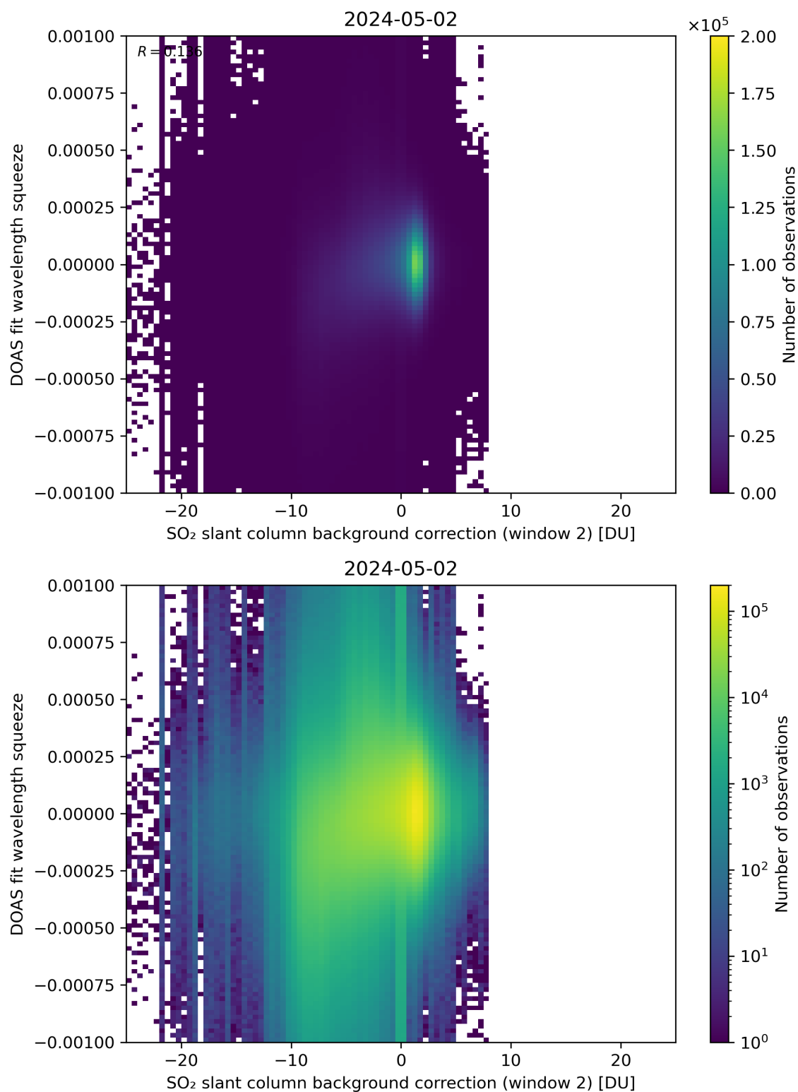
Figure 113: Scatter density plot of “SO 2 slant column background correction (window 2)” against “DOAS fit wavelength squeeze” for 2024-05-02 to 2024-05-03.
