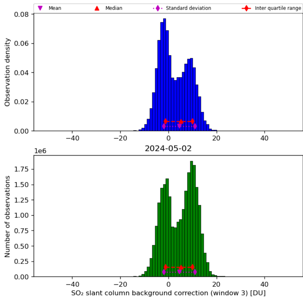
Figure 67: Histogram of "SO 2 slant column background correction (window 3)" for 2024-05-02 to 2024-05-03
