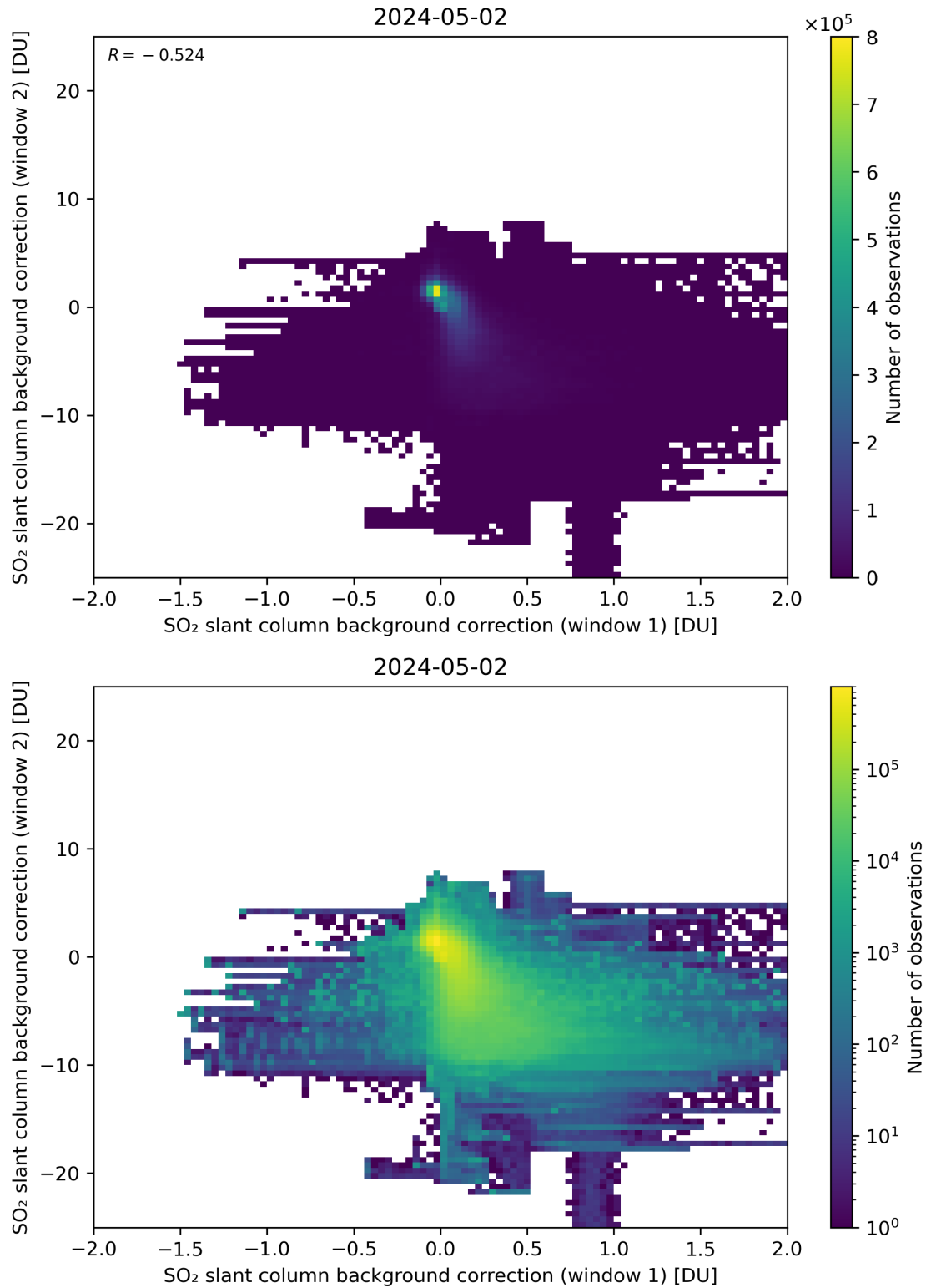
Figure 98: Scatter density plot of “SO 2 slant column background correction (window 1)” against “SO 2 slant column background correction (window 2)” for 2024-05-02 to 2024-05-03.
