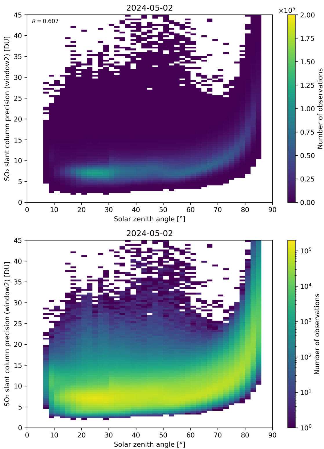
Figure 171: Scatter density plot of “Solar zenith angle” against “SO 2 slant column precision (window2)” for 2024-05-02 to 2024-05-03.
