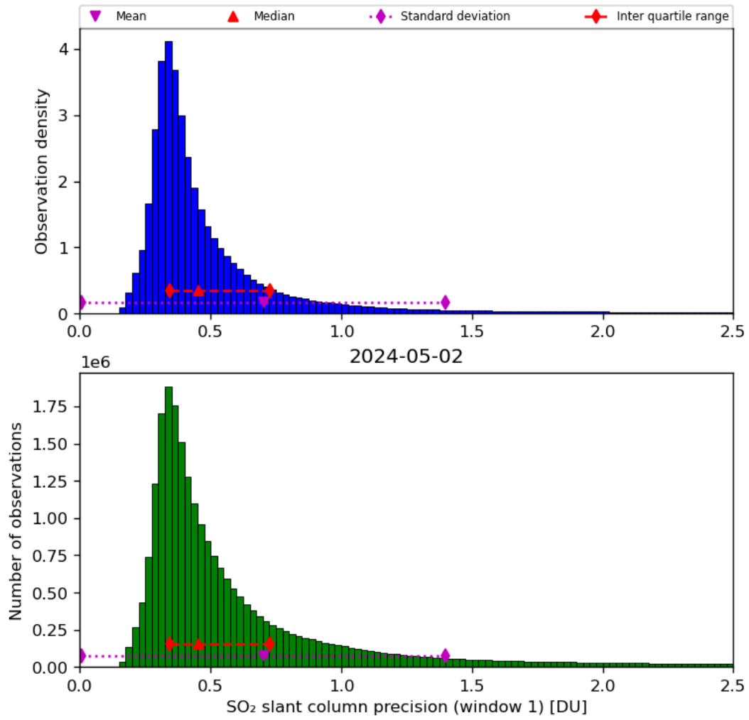
Figure 57: Histogram of “SO 2 slant column precision (window 1)” for 2024-05-02 to 2024-05-03
