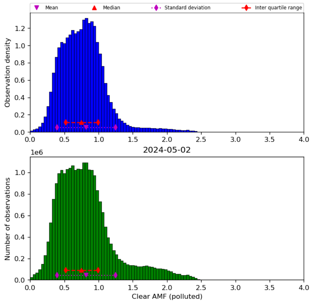
Figure 73: Histogram of “Clear AMF (polluted)” for 2024-05-02 to 2024-05-03
