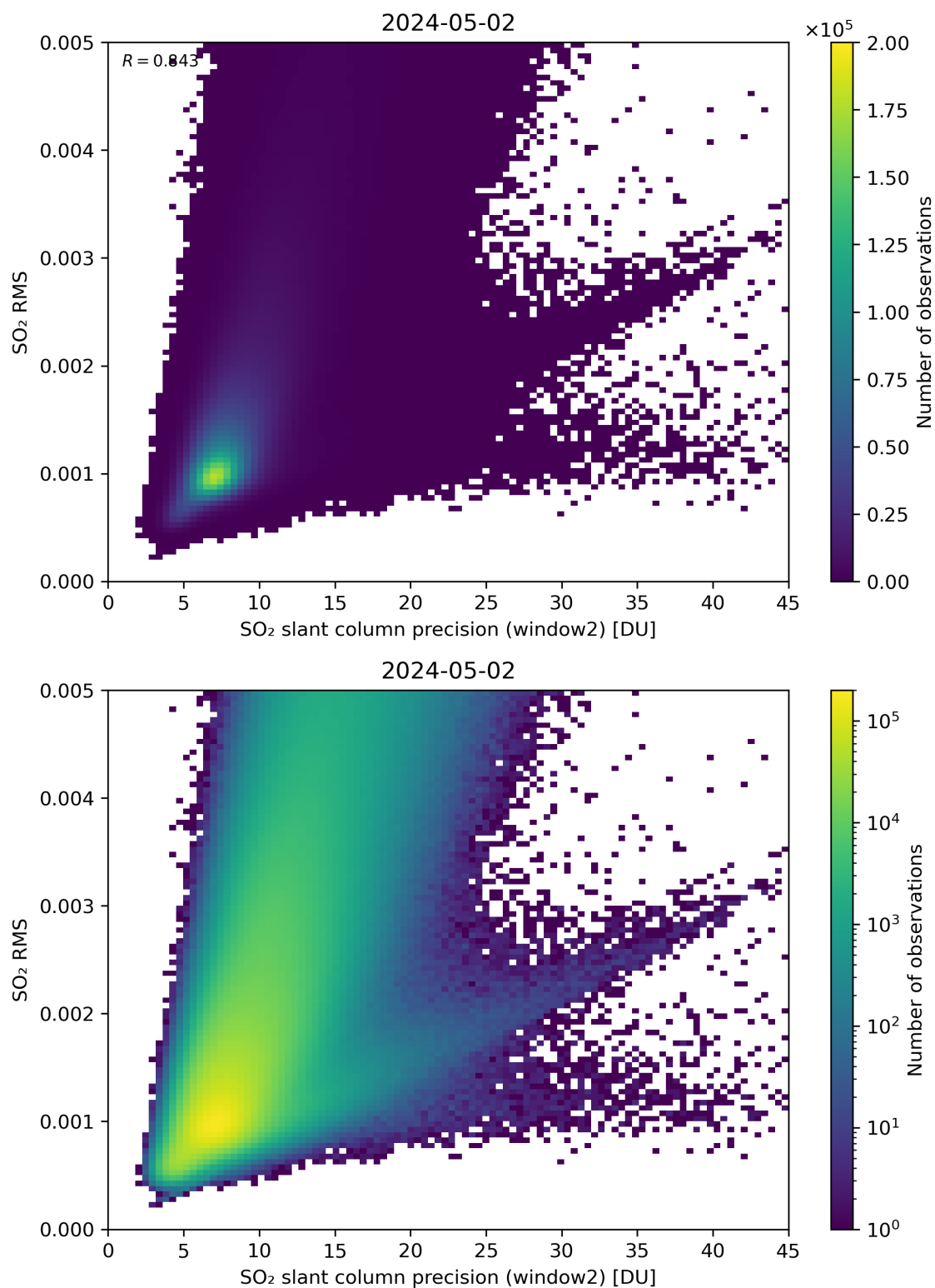
Figure 245: Scatter density plot of “SO 2 slant column precision (window2)” against “SO 2 RMS” for 2024-05-02 to 2024-05-03.
