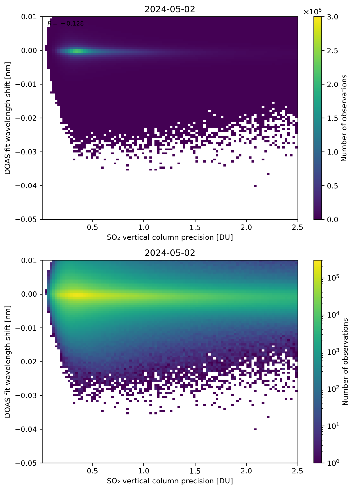
Figure 282: Scatter density plot of “SO 2 vertical column precision” against “DOAS fit wavelength shift” for 2024-05-02 to 2024-05-03.
