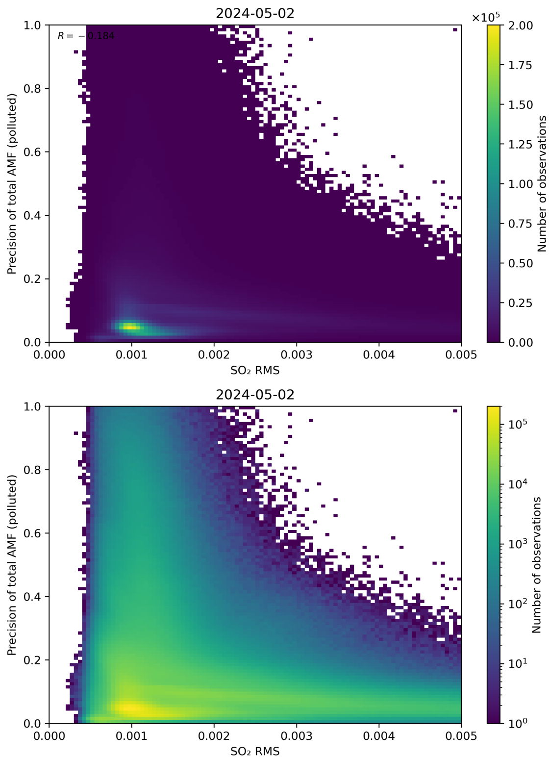
Figure 138: Scatter density plot of “SO 2 RMS” against “Precision of total AMF (polluted)” for 2024-05-02 to 2024-05-03.
