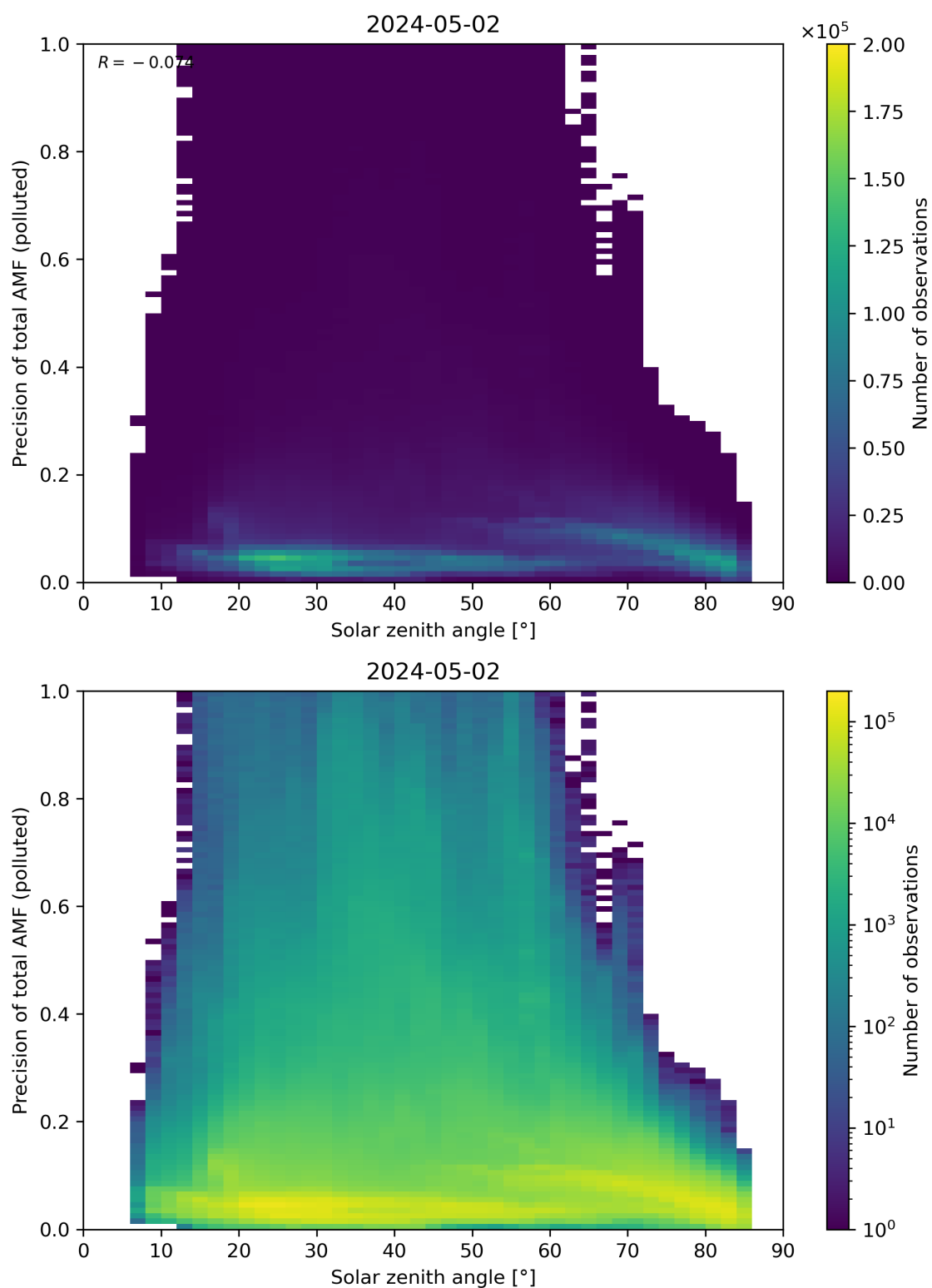
Figure 175: Scatter density plot of “Solar zenith angle” against “Precision of total AMF (polluted)” for 2024-05-02 to 2024-05-03.
