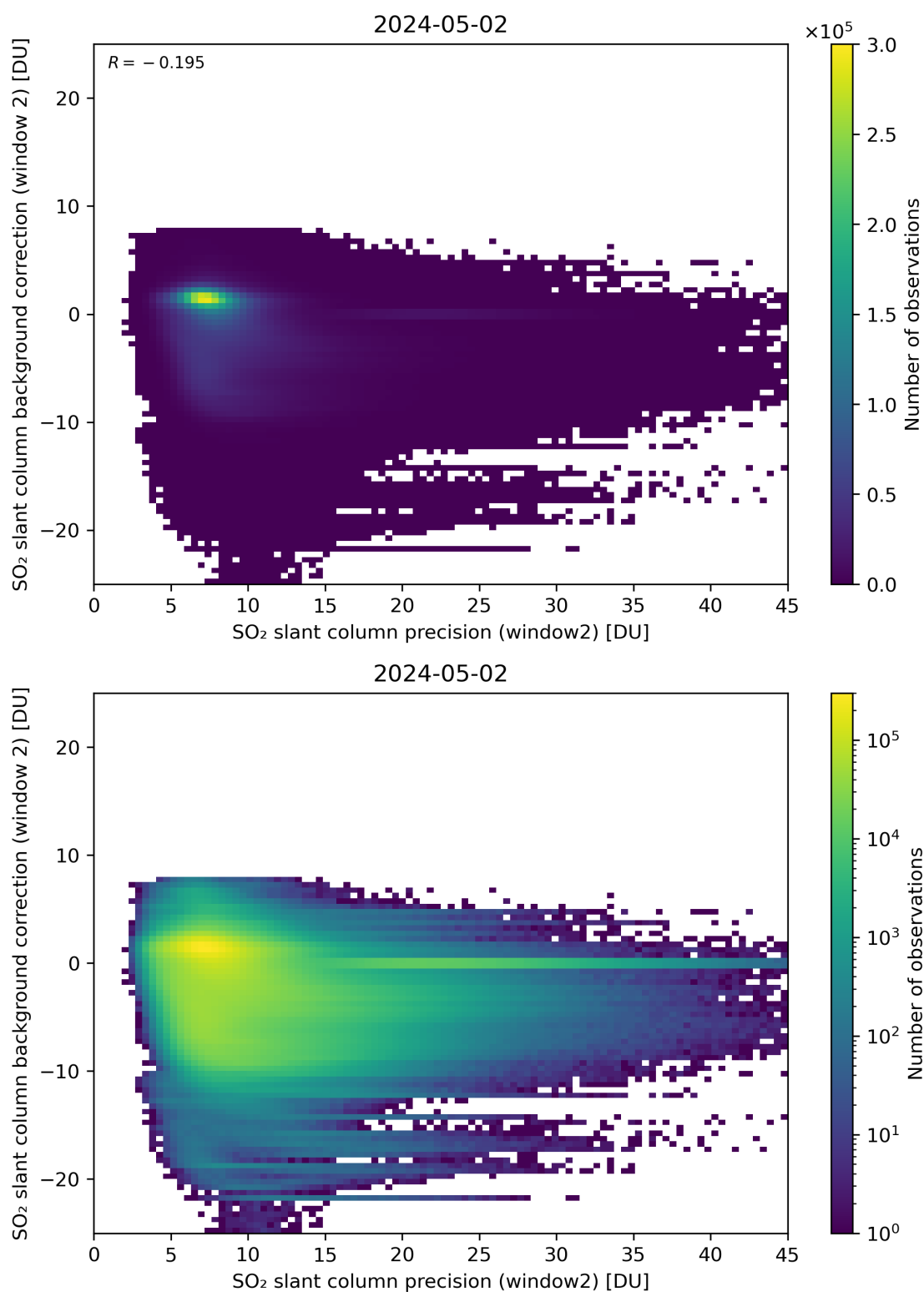
Figure 241: Scatter density plot of “SO 2 slant column precision (window2)” against “SO 2 slant column background correction (window 2)” for 2024-05-02 to 2024-05-03.
