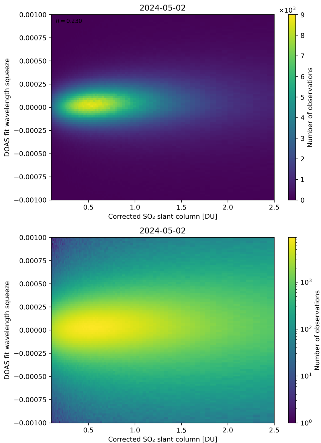
Figure 182: Scatter density plot of “Corrected SO 2 slant column” against “DOAS fit wavelength squeeze” for 2024-05-02 to 2024-05-03.
