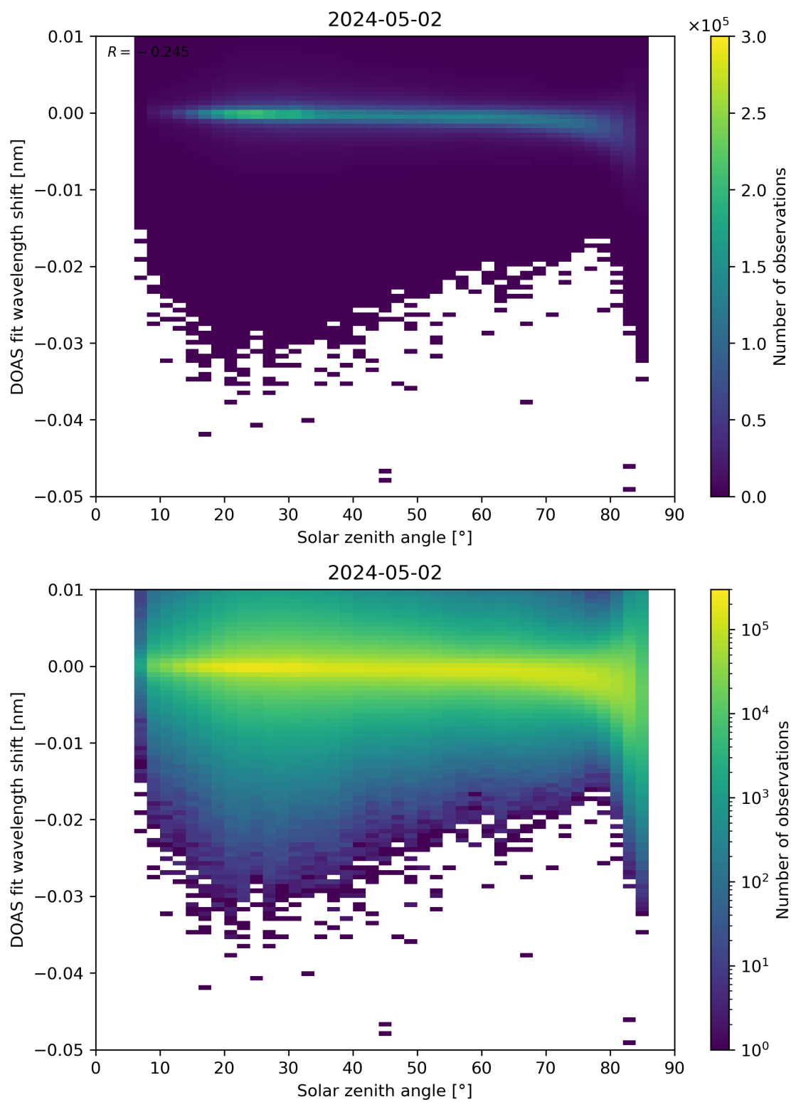
Figure 161: Scatter density plot of “Solar zenith angle” against “DOAS fit wavelength shift” for 2024-05-02 to 2024-05-03.
