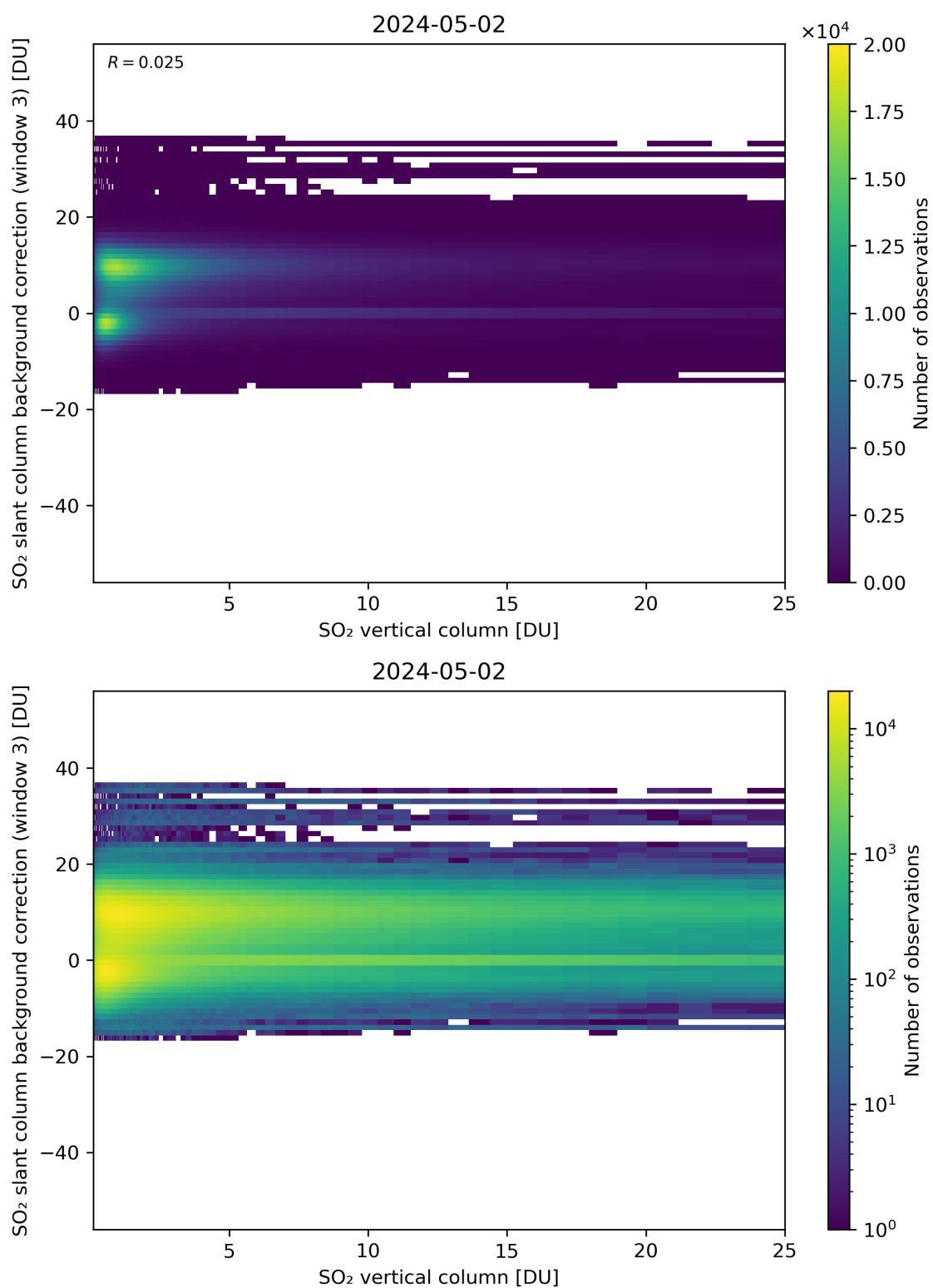
Figure 275: Scatter density plot of “SO 2 vertical column” against “SO 2 slant column background correction (window 3)” for 2024-05-02 to 2024-05-03.
