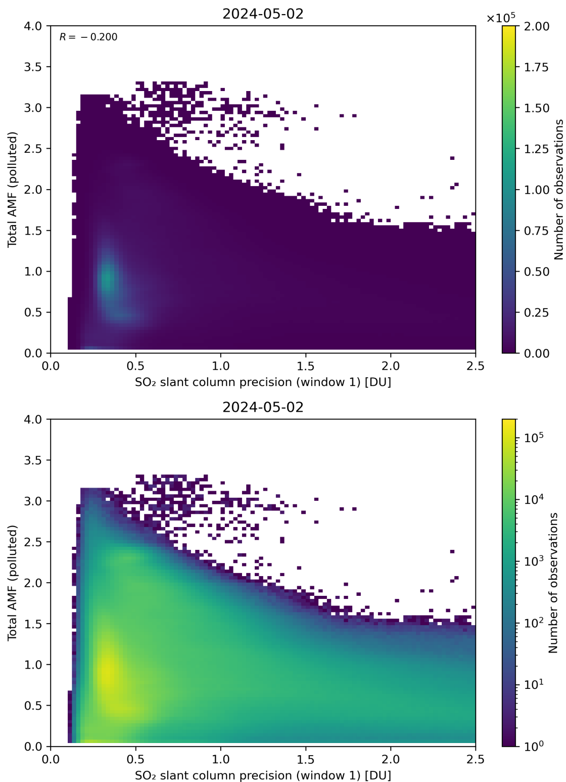
Figure 230: Scatter density plot of “SO 2 slant column precision (window 1)” against “Total AMF (polluted)” for 2024-05-02 to 2024-05-03.
