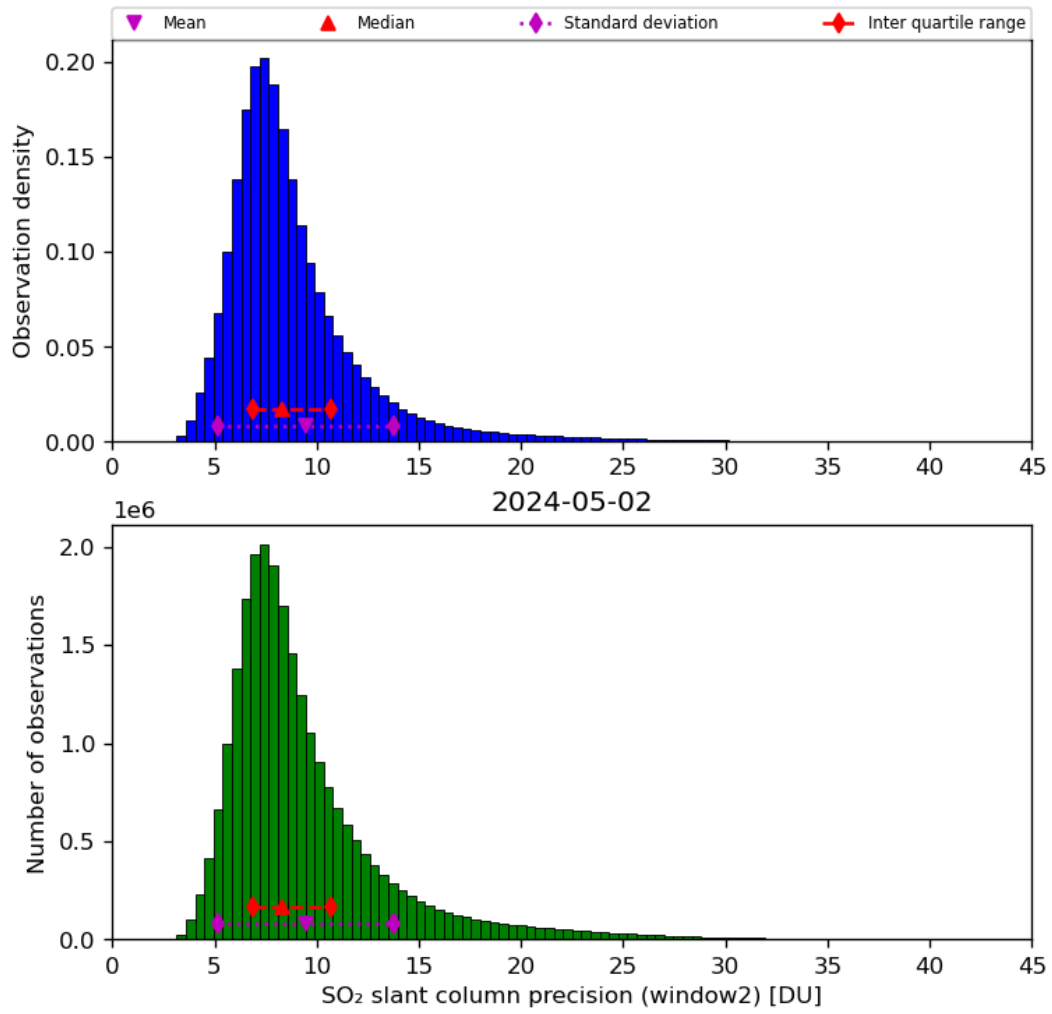
Figure 61: Histogram of “SO 2 slant column precision (window2)” for 2024-05-02 to 2024-05-03
