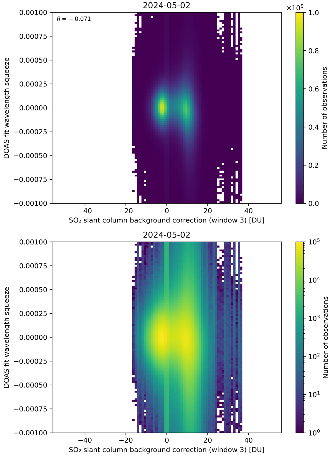
Figure 122: Scatter density plot of “SO 2 slant column background correction (window 3)” against “DOAS fit wavelength squeeze” for 2024-05-02 to 2024-05-03.
