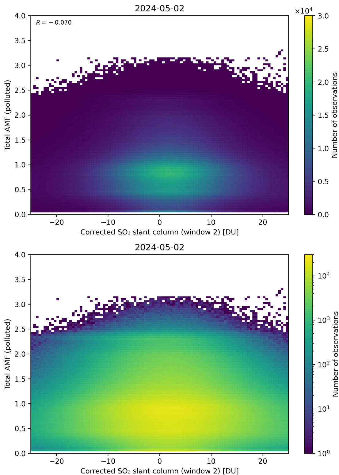
Figure 203: Scatter density plot of “Corrected SO 2 slant column (window 2)” against “Total AMF (polluted)” for 2024-05-02 to 2024-05-03.
