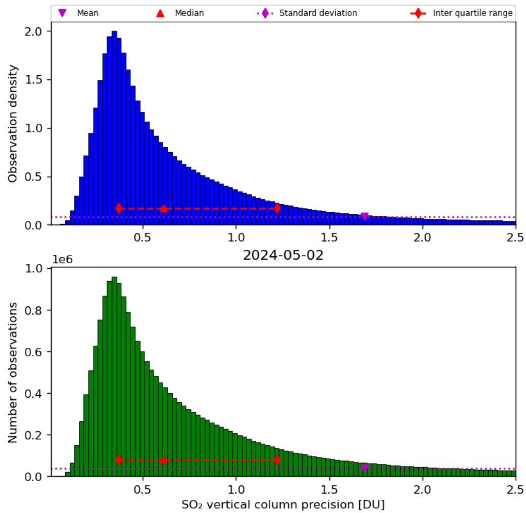
Figure 54: Histogram of “SO 2 vertical column precision” for 2024-05-02 to 2024-05-03
