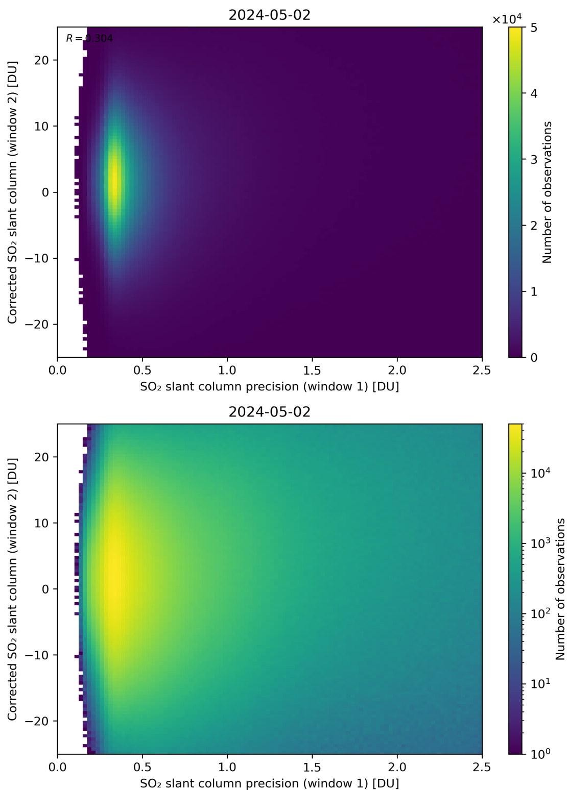
Figure 225: Scatter density plot of “SO 2 slant column precision (window 1)” against “Corrected SO 2 slant column (window 2)” for 2024-05-02 to 2024-05-03.
