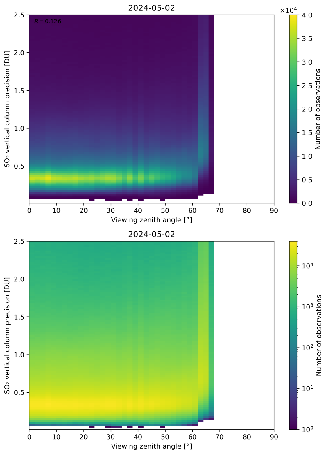
Figure 328: Scatter density plot of “Viewing zenith angle” against “SO 2 vertical column precision” for 2024-05-02 to 2024-05-03.
