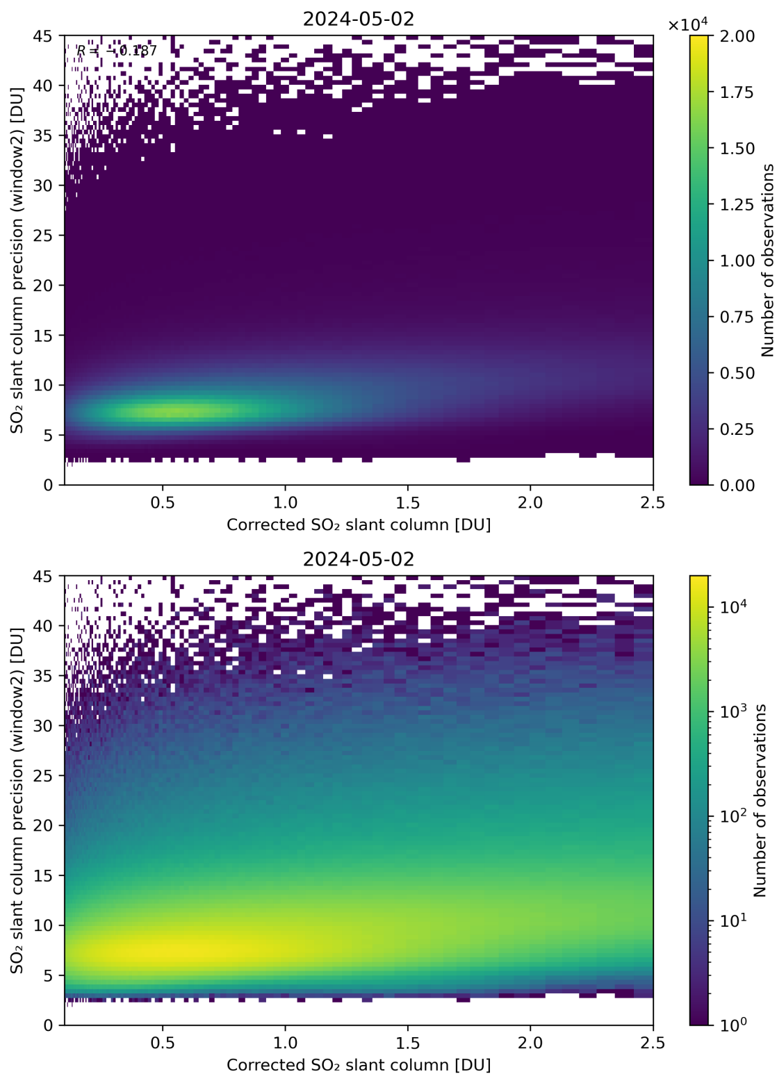
Figure 189: Scatter density plot of “Corrected SO 2 slant column” against “SO 2 slant column precision (window2)” for 2024-05-02 to 2024-05-03.
