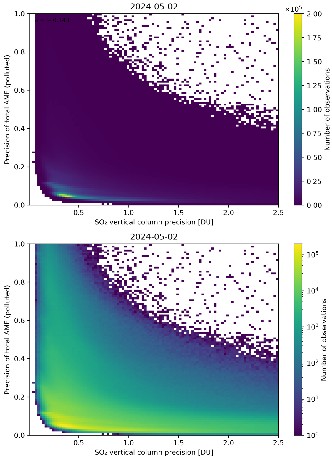
Figure 295: Scatter density plot of “SO 2 vertical column precision” against “Precision of total AMF (polluted)” for 2024-05-02 to 2024-05-03.
