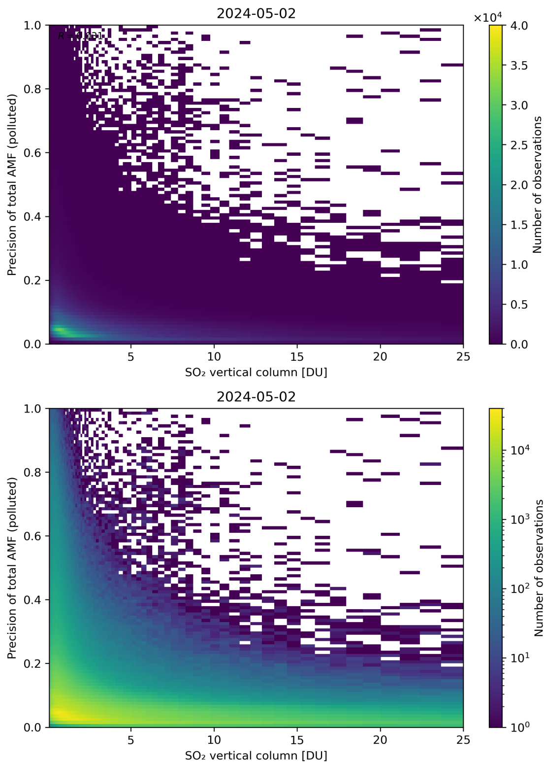
Figure 306: Scatter density plot of “SO 2 vertical column” against “Precision of total AMF (polluted)” for 2024-05-02 to 2024-05-03.
