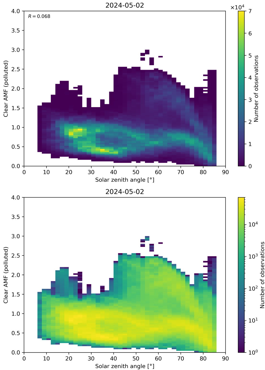
Figure 165: Scatter density plot of “Solar zenith angle” against “Clear AMF (polluted)” for 2024-05-02 to 2024-05-03.
