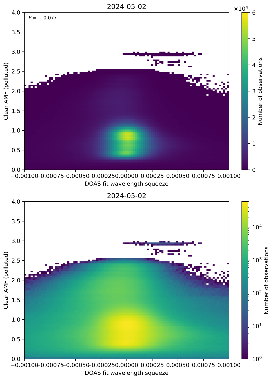
Figure 133: Scatter density plot of “DOAS fit wavelength squeeze” against “Clear AMF (polluted)” for 2024-05-02 to 2024-05-03.
