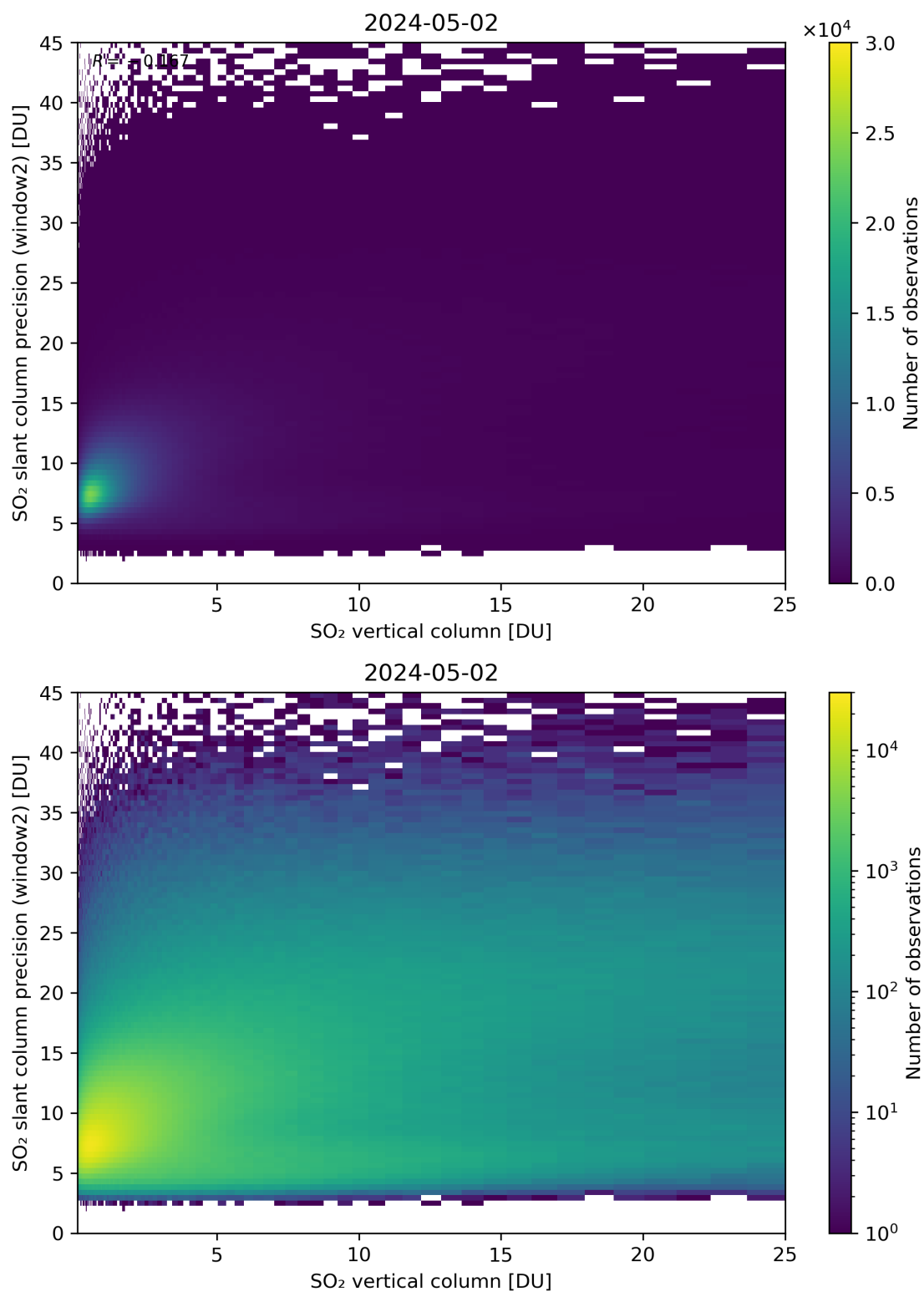
Figure 302: Scatter density plot of “SO 2 vertical column” against “SO 2 slant column precision (window2)” for 2024-05-02 to 2024-05-03.
