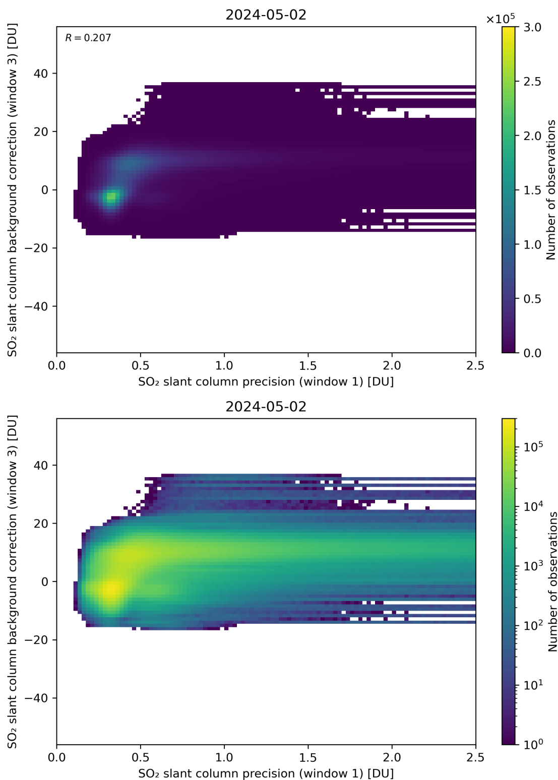
Figure 220: Scatter density plot of “SO 2 slant column precision (window 1)” against “SO 2 slant column background correction (window 3)” for 2024-05-02 to 2024-05-03.
