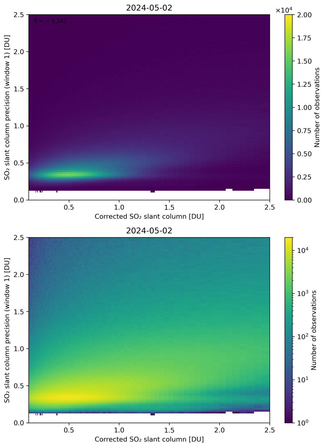
Figure 188: Scatter density plot of “Corrected SO 2 slant column” against “SO 2 slant column precision (window 1)” for 2024-05-02 to 2024-05-03.
