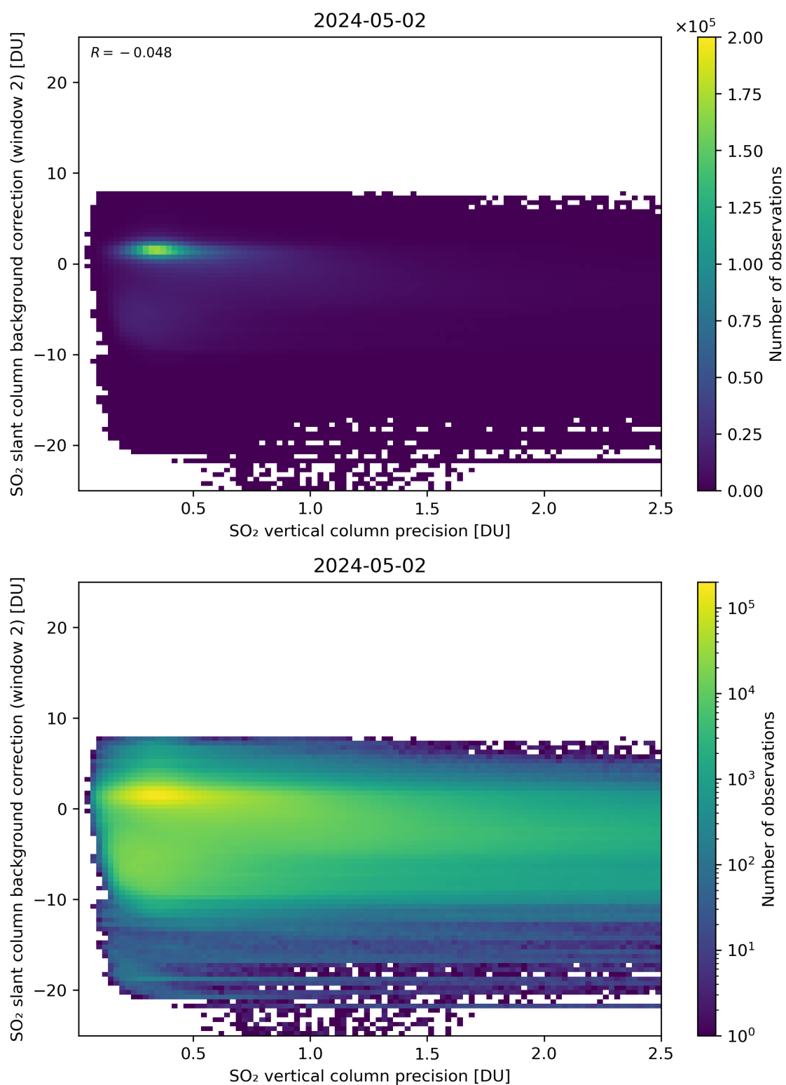
Figure 280: Scatter density plot of “SO 2 vertical column precision” against “SO 2 slant column background correction (window 2)” for 2024-05-02 to 2024-05-03.
