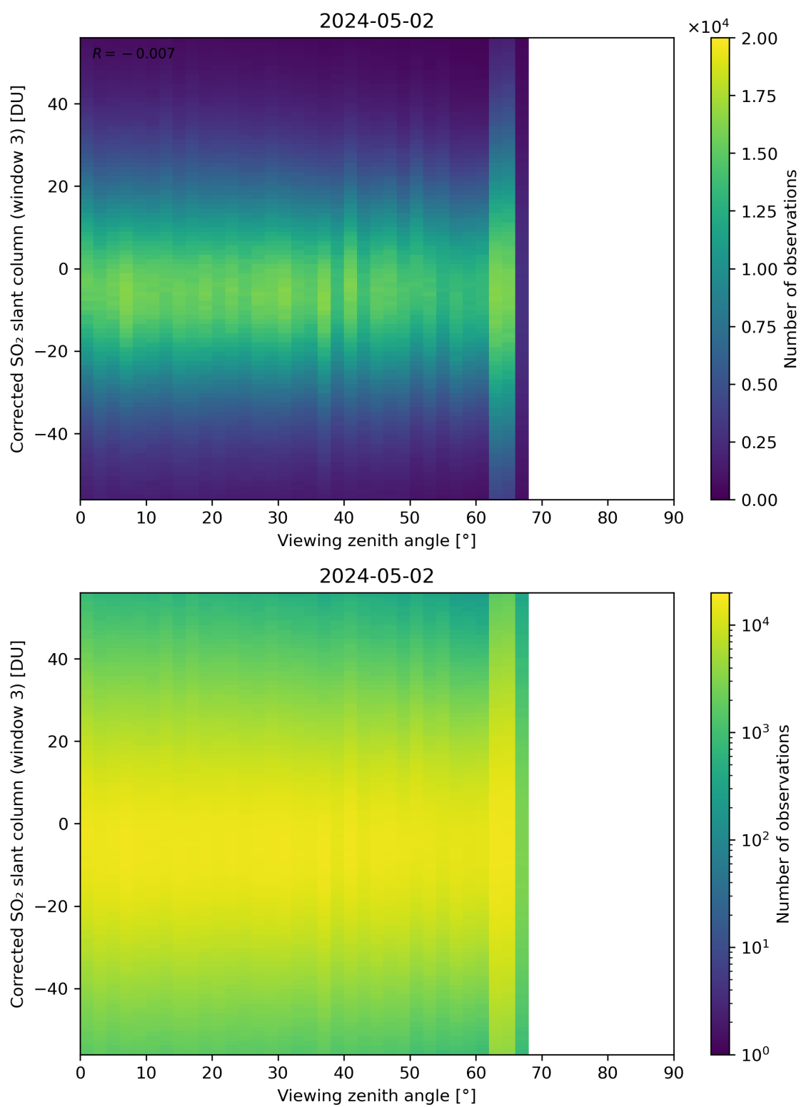
Figure 319: Scatter density plot of “Viewing zenith angle” against “Corrected SO 2 slant column (window 3)” for 2024-05-02 to 2024-05-03.
