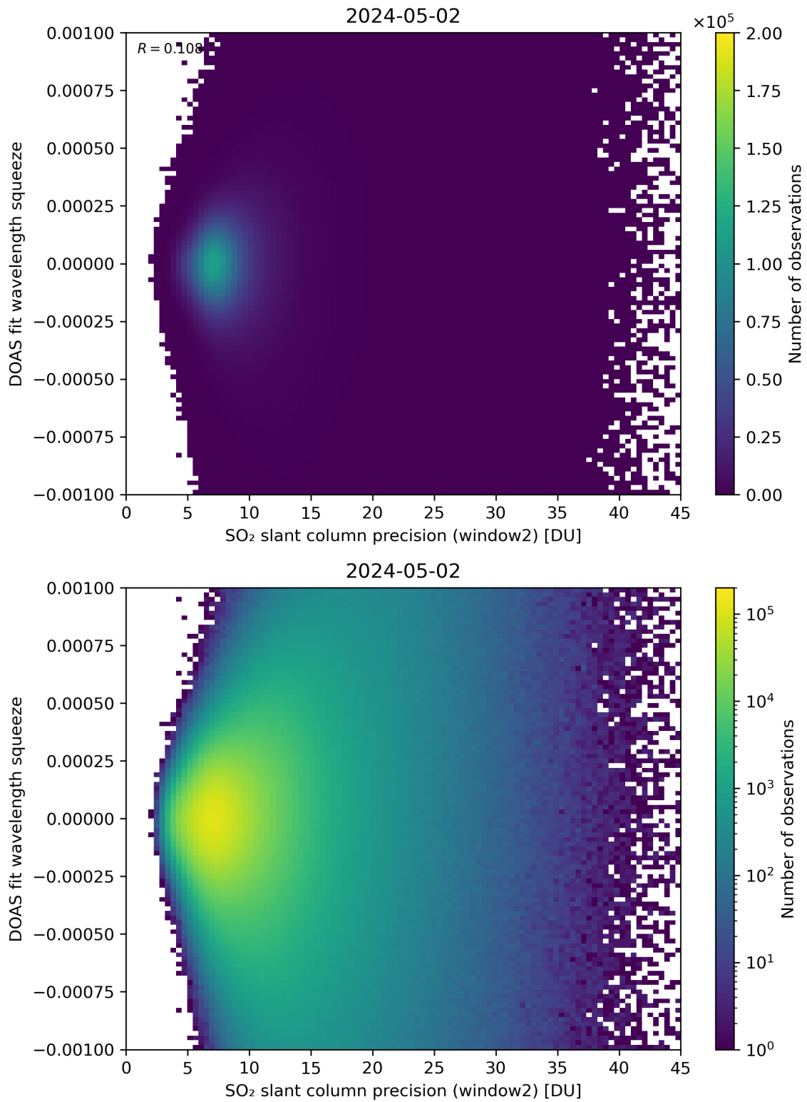
Figure 244: Scatter density plot of “SO 2 slant column precision (window2)” against “DOAS fit wavelength squeeze” for 2024-05-02 to 2024-05-03.
