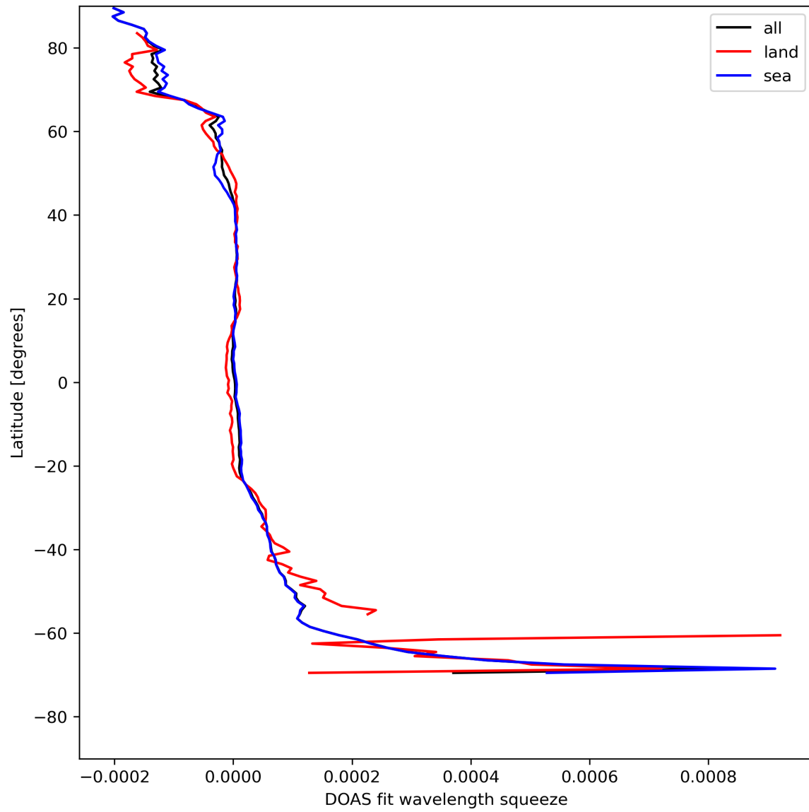
Figure 46: Zonal average of “DOAS fit wavelength squeeze” for 2024-05-02 to 2024-05-03.
