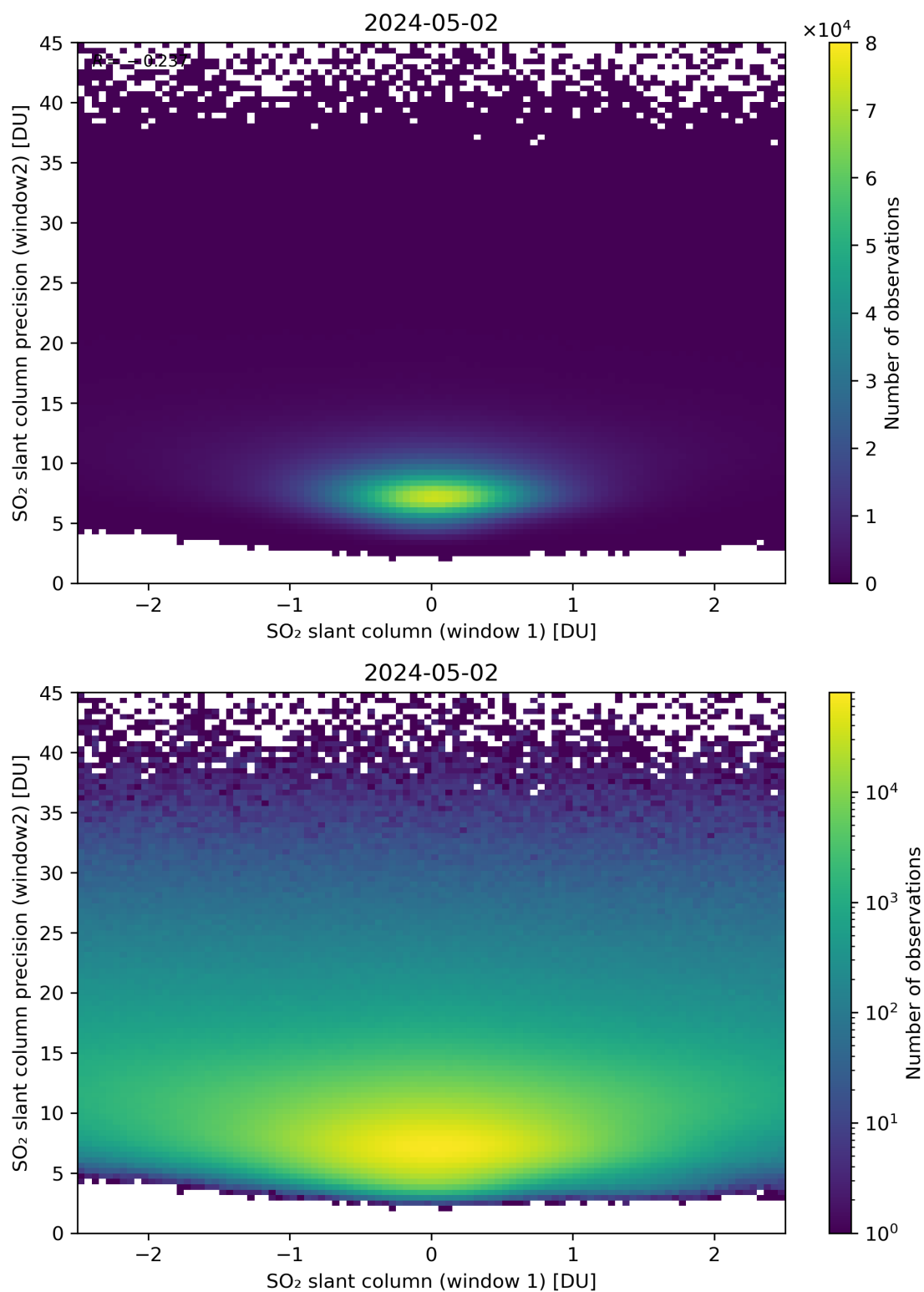
Figure 236: Scatter density plot of “SO 2 slant column (window 1)” against “SO 2 slant column precision (window2)” for 2024-05-02 to 2024-05-03.
