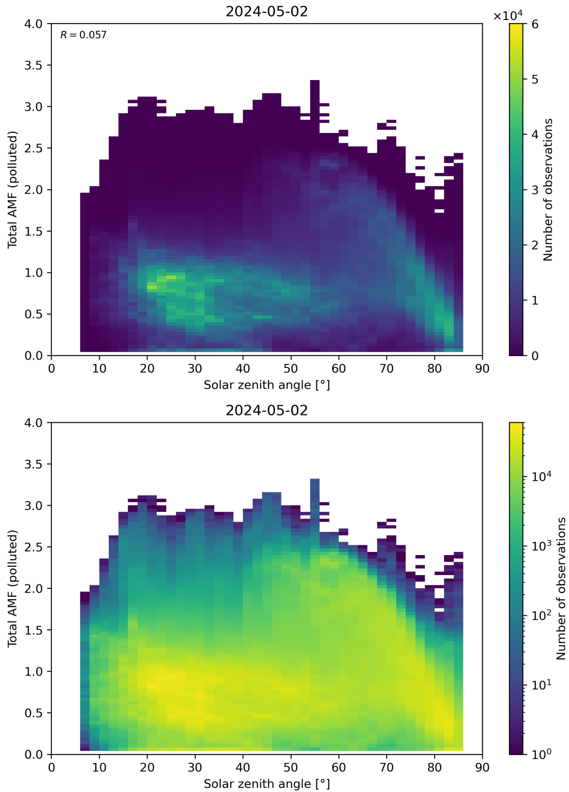
Figure 174: Scatter density plot of “Solar zenith angle” against “Total AMF (polluted)” for 2024-05-02 to 2024-05-03.
