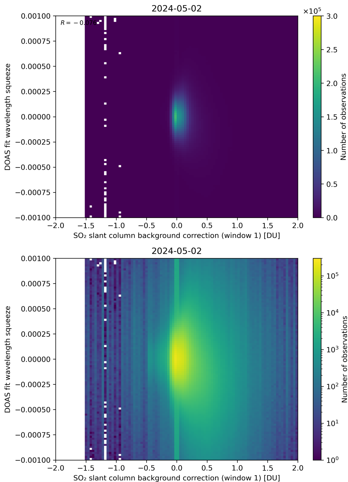
Figure 101: Scatter density plot of “SO 2 slant column background correction (window 1)” against “DOAS fit wavelength squeeze” for 2024-05-02 to 2024-05-03.
