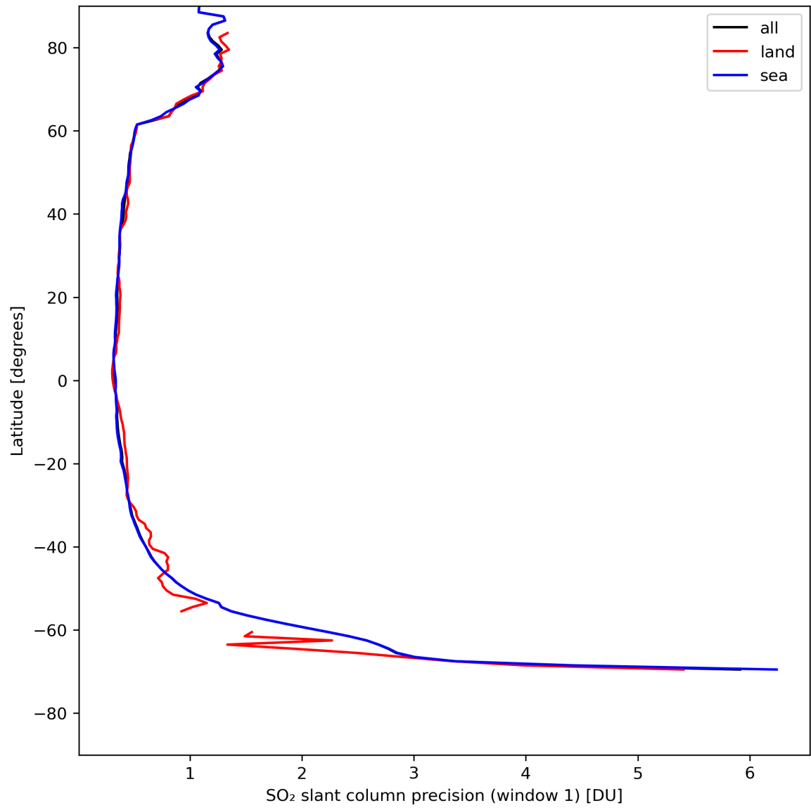
Figure 34: Zonal average of “SO 2 slant column precision (window 1)” for 2024-05-02 to 2024-05-03.
