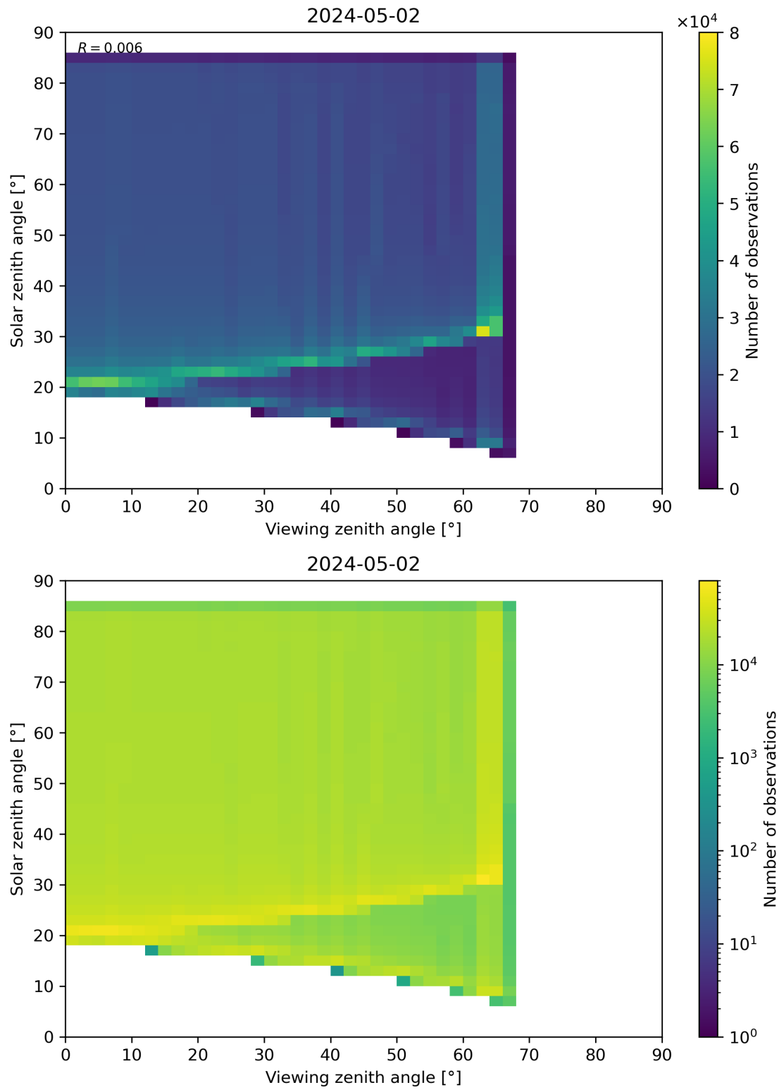
Figure 315: Scatter density plot of “Viewing zenith angle” against “Solar zenith angle” for 2024-05-02 to 2024-05-03.
