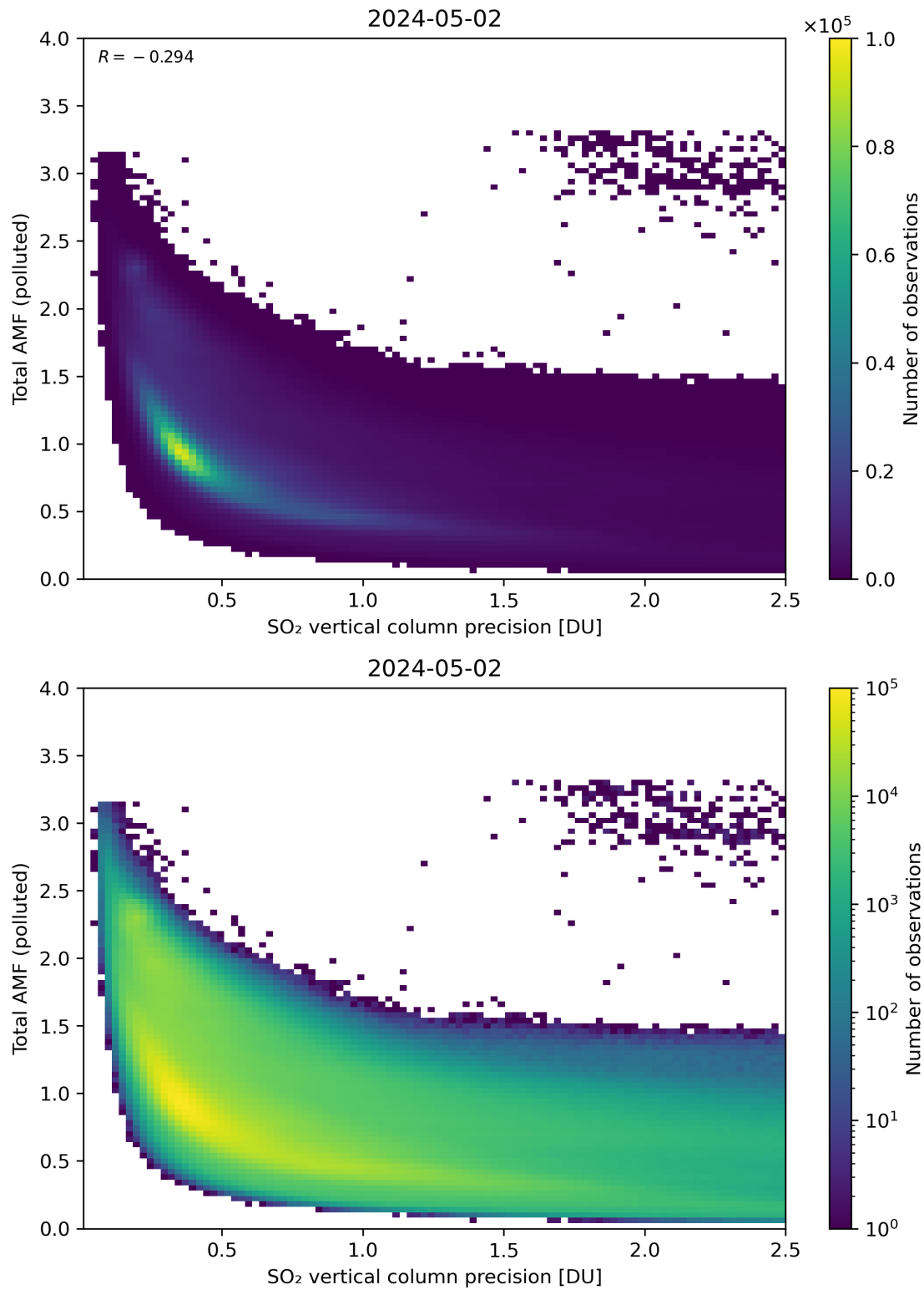
Figure 294: Scatter density plot of “SO 2 vertical column precision” against “Total AMF (polluted)” for 2024-05-02 to 2024-05-03.
