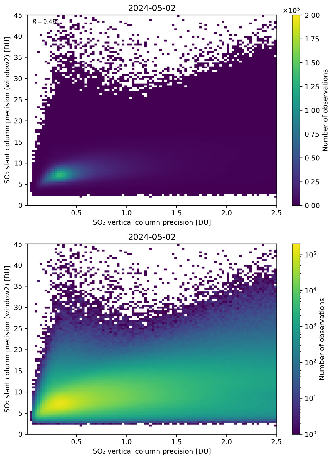
Figure 291: Scatter density plot of “SO 2 vertical column precision” against “SO 2 slant column precision (window2)” for 2024-05-02 to 2024-05-03.
