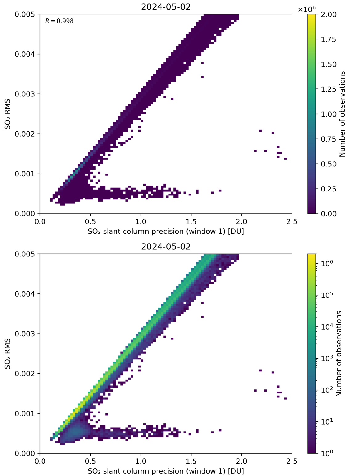
Figure 223: Scatter density plot of “SO 2 slant column precision (window 1)” against “SO 2 RMS” for 2024-05-02 to 2024-05-03.
