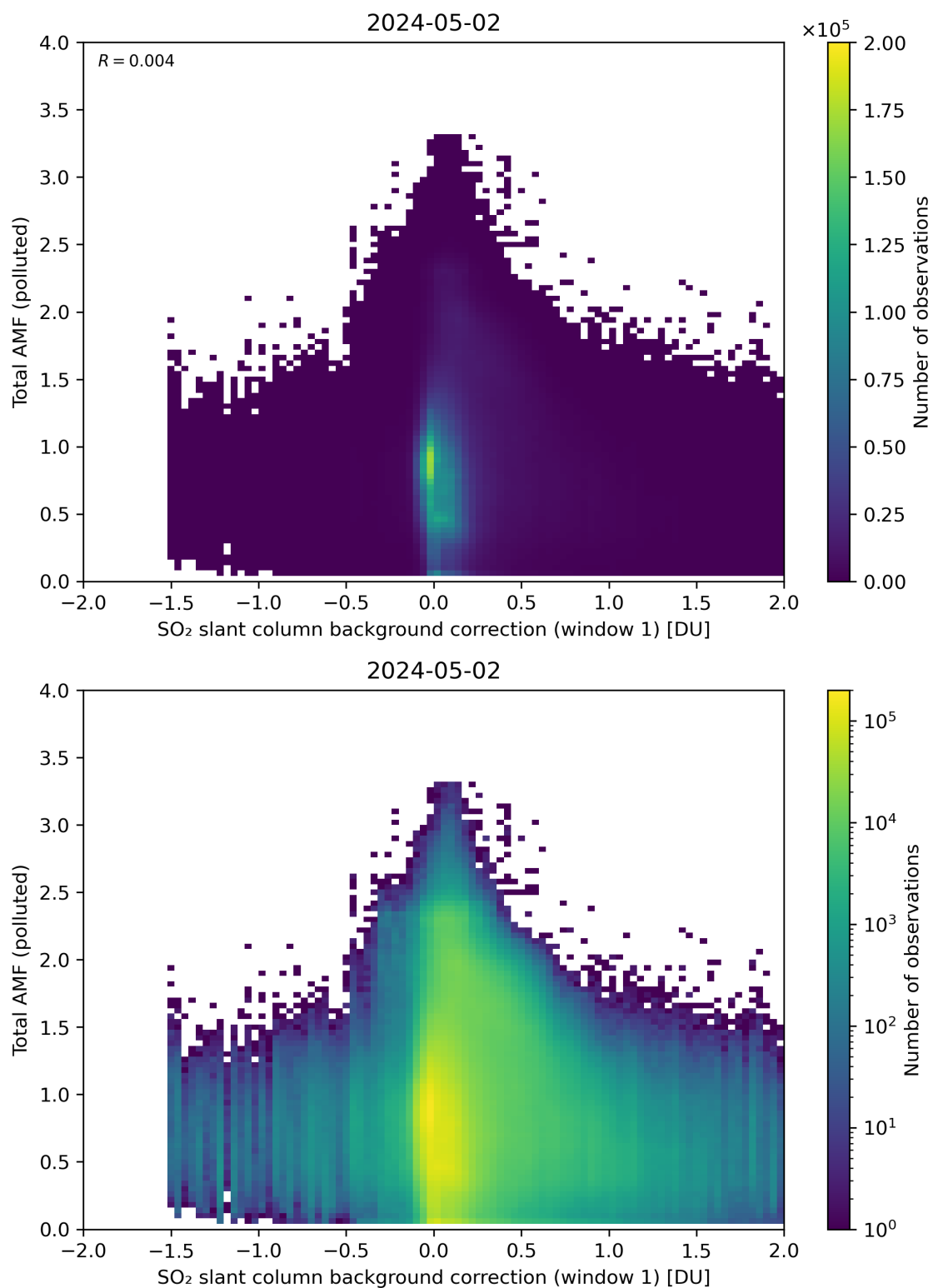
Figure 109: Scatter density plot of “SO 2 slant column background correction (window 1)” against “Total AMF (polluted)” for 2024-05-02 to 2024-05-03.
