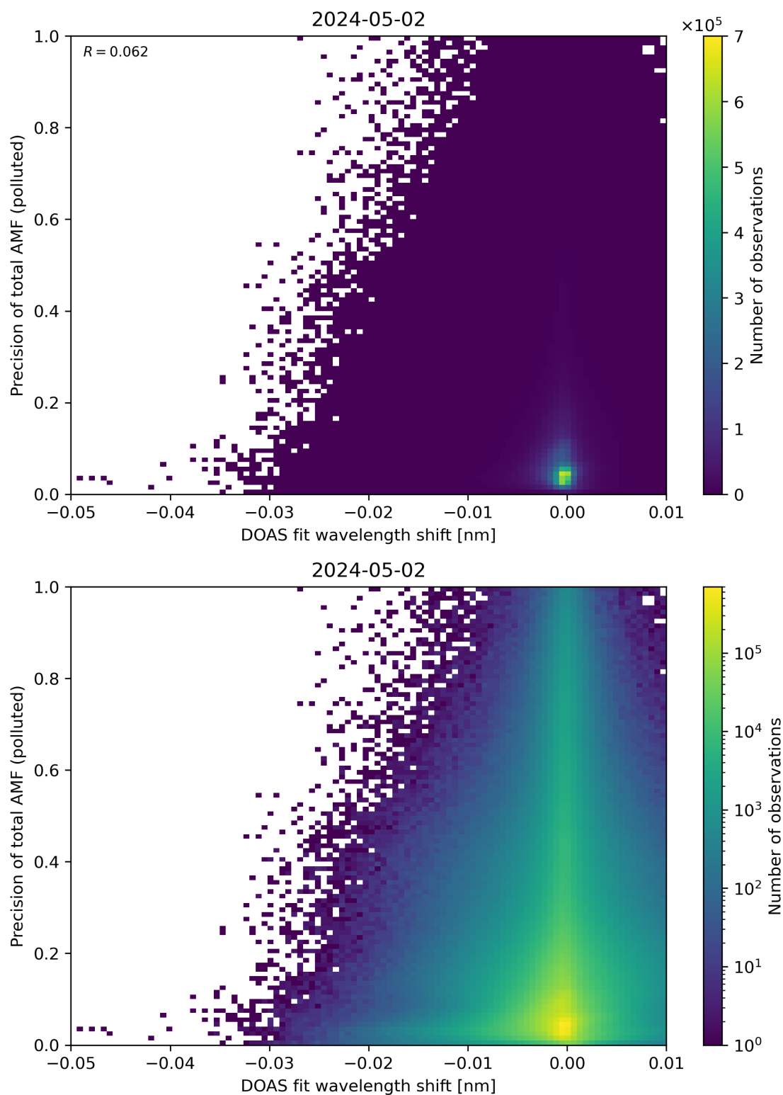
Figure 131: Scatter density plot of “DOAS fit wavelength shift” against “Precision of total AMF (polluted)” for 2024-05-02 to 2024-05-03.
