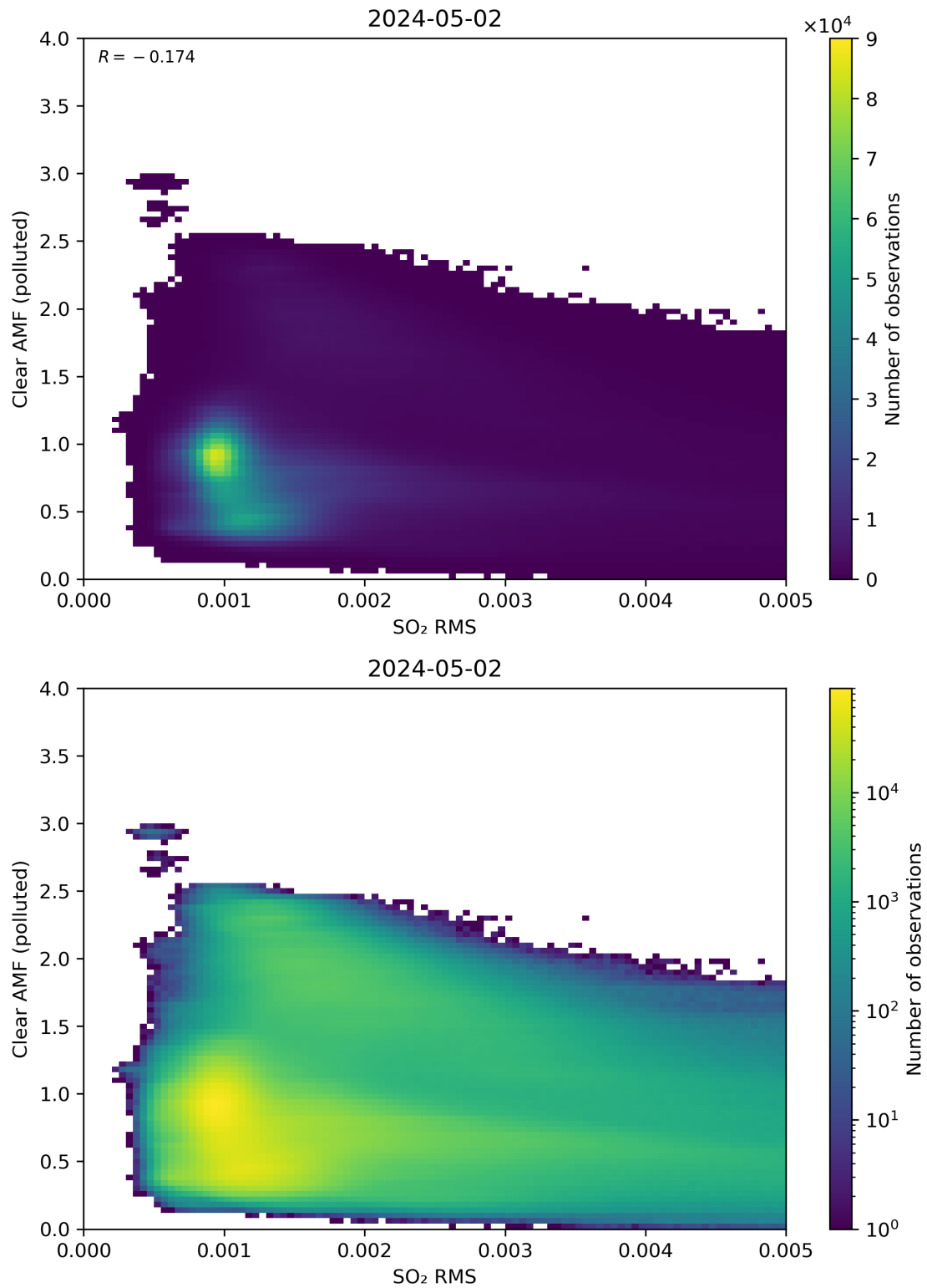
Figure 136: Scatter density plot of “SO 2 RMS” against “Clear AMF (polluted)” for 2024-05-02 to 2024-05-03.
