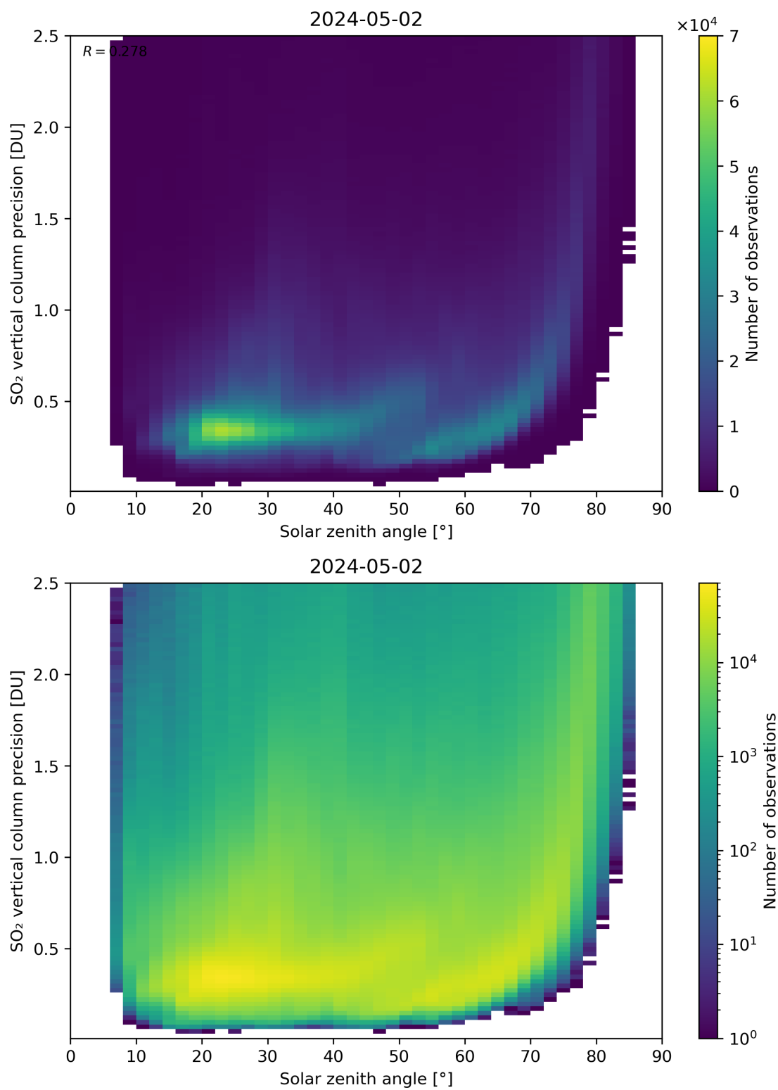
Figure 177: Scatter density plot of “Solar zenith angle” against “SO 2 vertical column precision” for 2024-05-02 to 2024-05-03.
