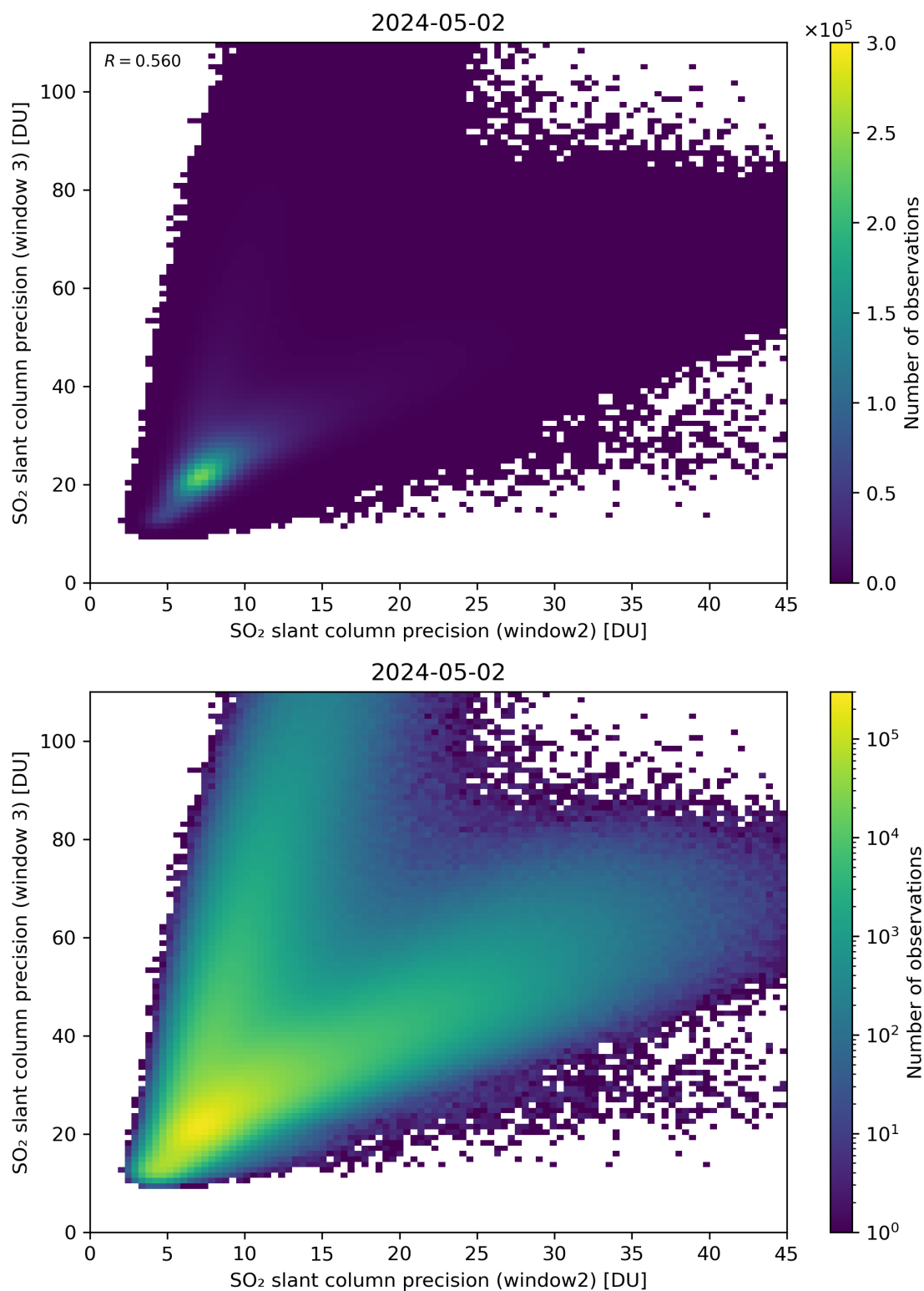
Figure 250: Scatter density plot of “SO 2 slant column precision (window2)” against “SO 2 slant column precision (window 3)” for 2024-05-02 to 2024-05-03.
