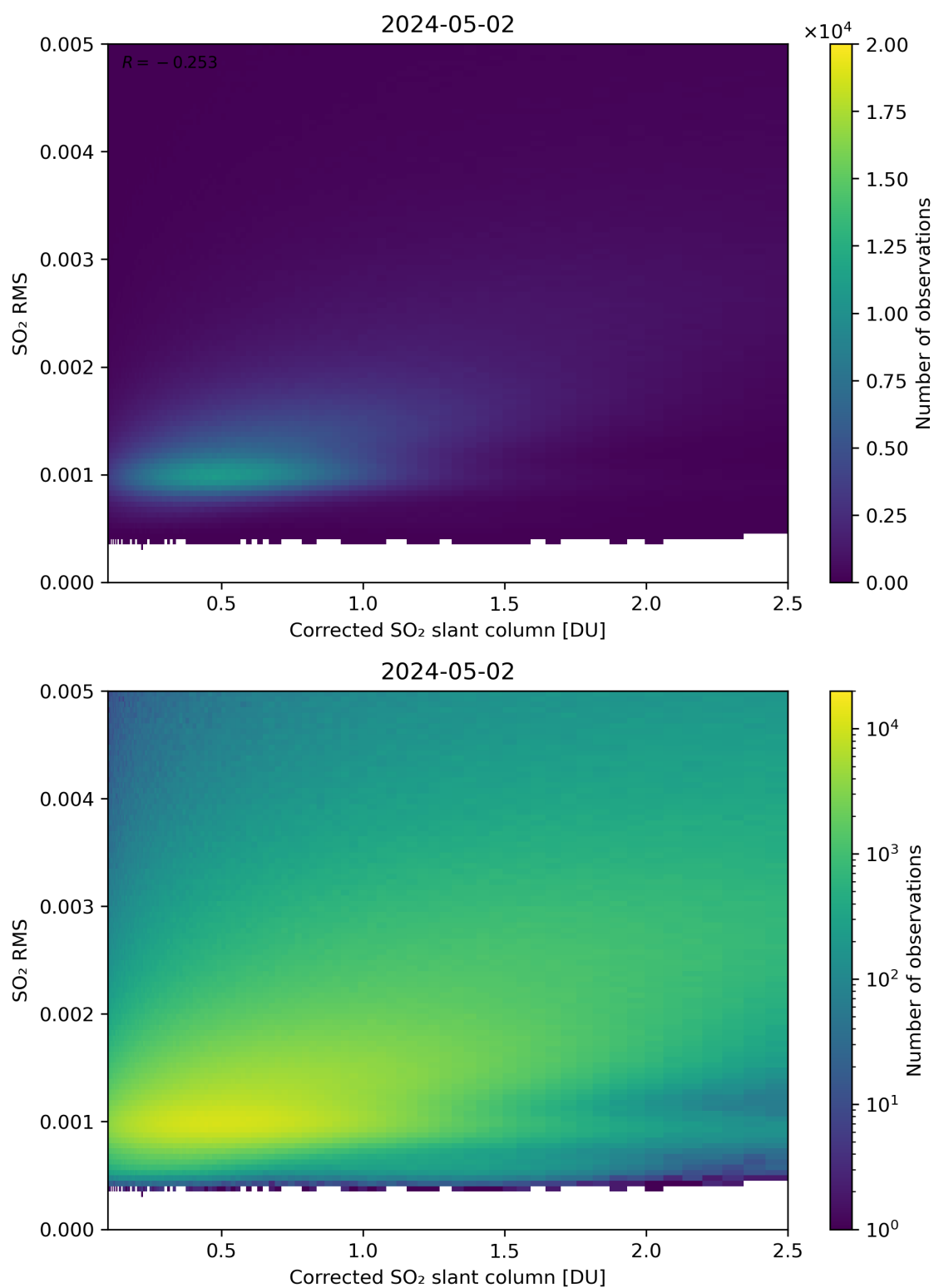
Figure 183: Scatter density plot of “Corrected SO 2 slant column” against “SO 2 RMS” for 2024-05-02 to 2024-05-03.
