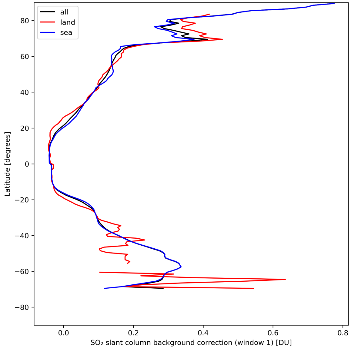
Figure 36: Zonal average of “SO 2 slant column background correction (window 1)” for 2024-05-02 to 2024-05-03.
