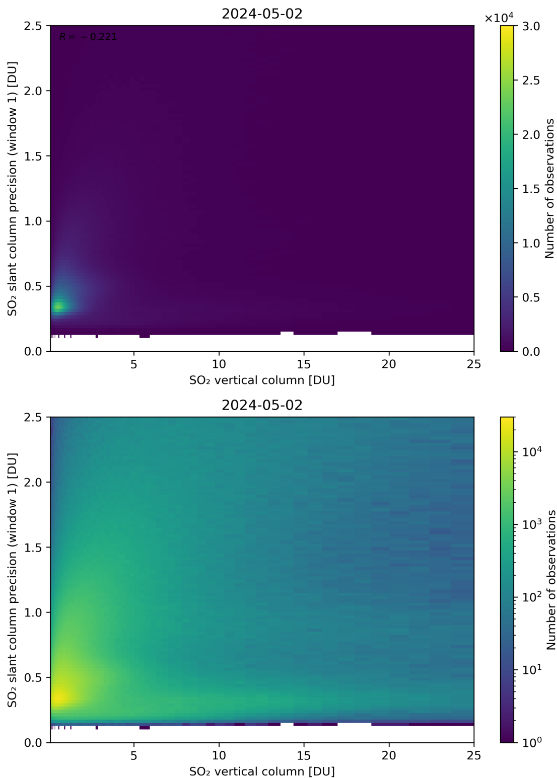
Figure 301: Scatter density plot of “SO 2 vertical column” against “SO 2 slant column precision (window 1)” for 2024-05-02 to 2024-05-03.
