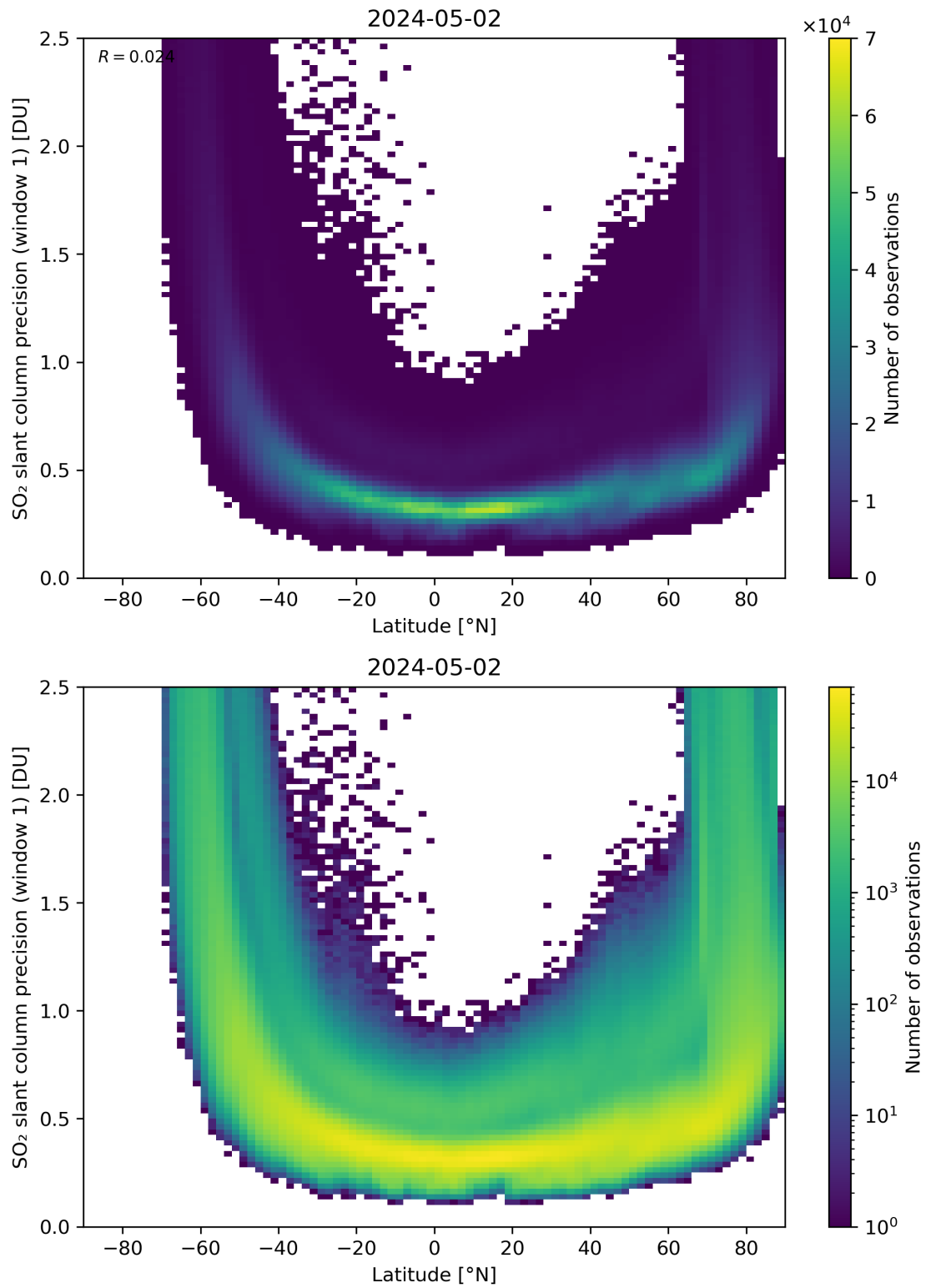
Figure 150: Scatter density plot of “Latitude” against “SO 2 slant column precision (window 1)” for 2024-05-02 to 2024-05-03.
