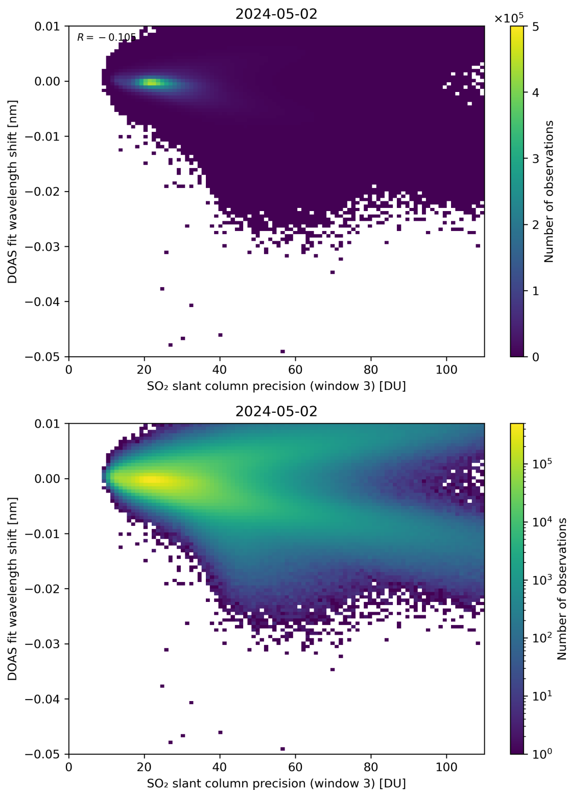
Figure 258: Scatter density plot of “SO 2 slant column precision (window 3)” against “DOAS fit wavelength shift” for 2024-05-02 to 2024-05-03.
