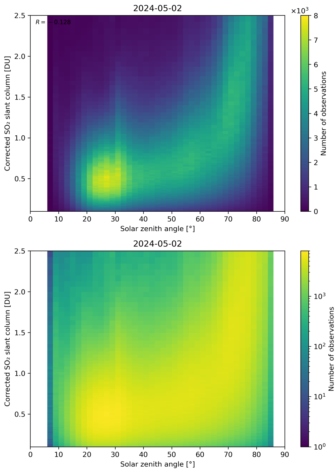
Figure 166: Scatter density plot of “Solar zenith angle” against “Corrected SO 2 slant column” for 2024-05-02 to 2024-05-03.
