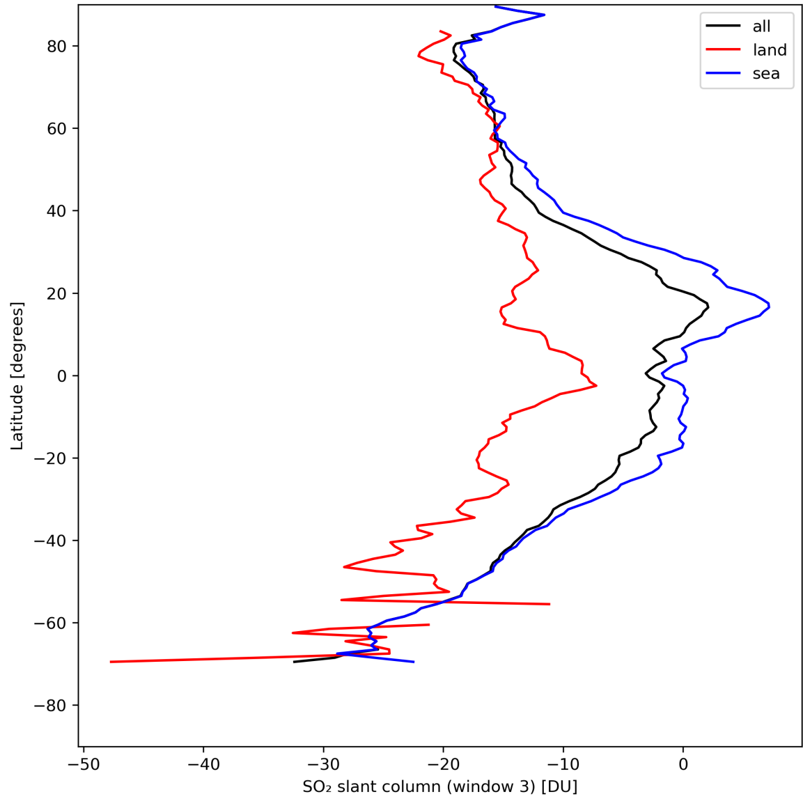
Figure 41: Zonal average of “SO 2 slant column (window 3)” for 2024-05-02 to 2024-05-03.
