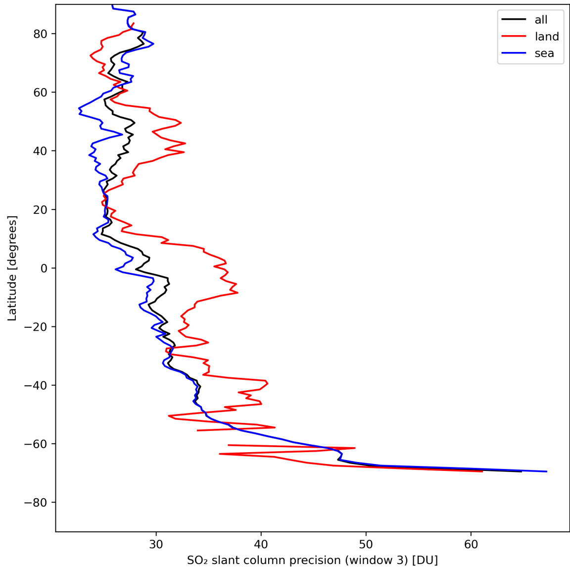
Figure 42: Zonal average of “SO 2 slant column precision (window 3)” for 2024-05-02 to 2024-05-03.
