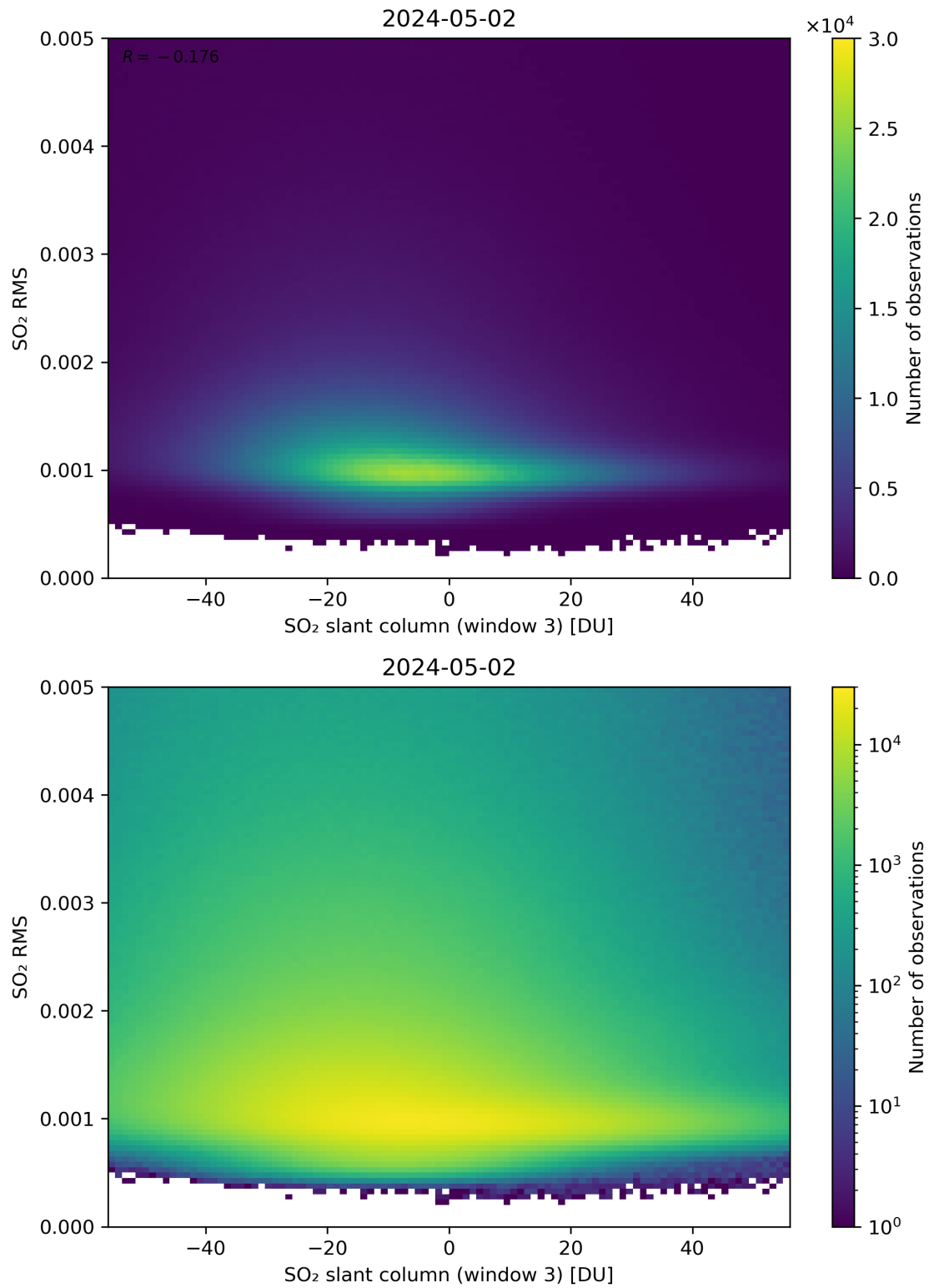
Figure 256: Scatter density plot of “SO 2 slant column (window 3)” against “SO 2 RMS” for 2024-05-02 to 2024-05-03.
