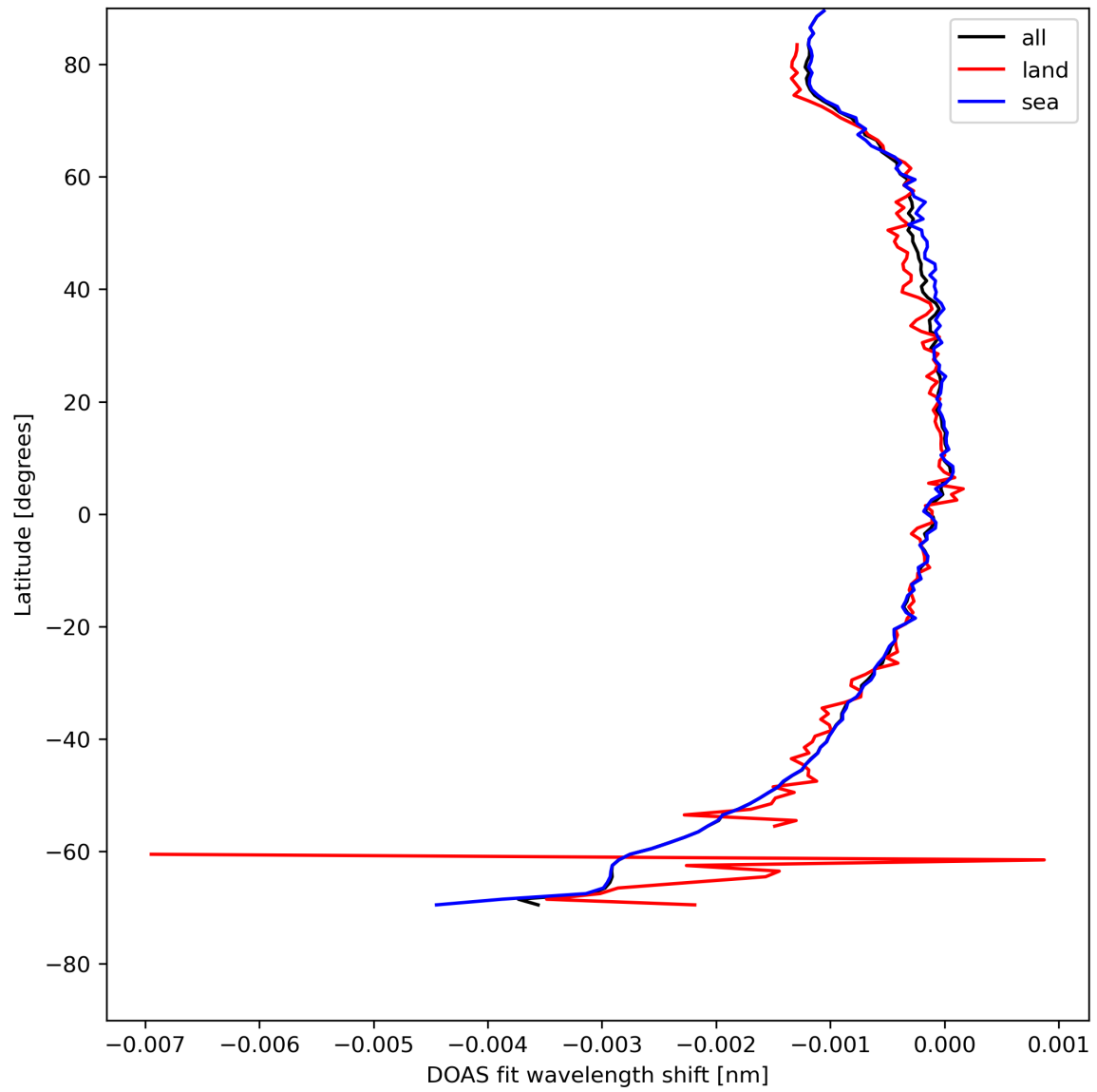
Figure 45: Zonal average of “DOAS fit wavelength shift” for 2024-05-02 to 2024-05-03.
