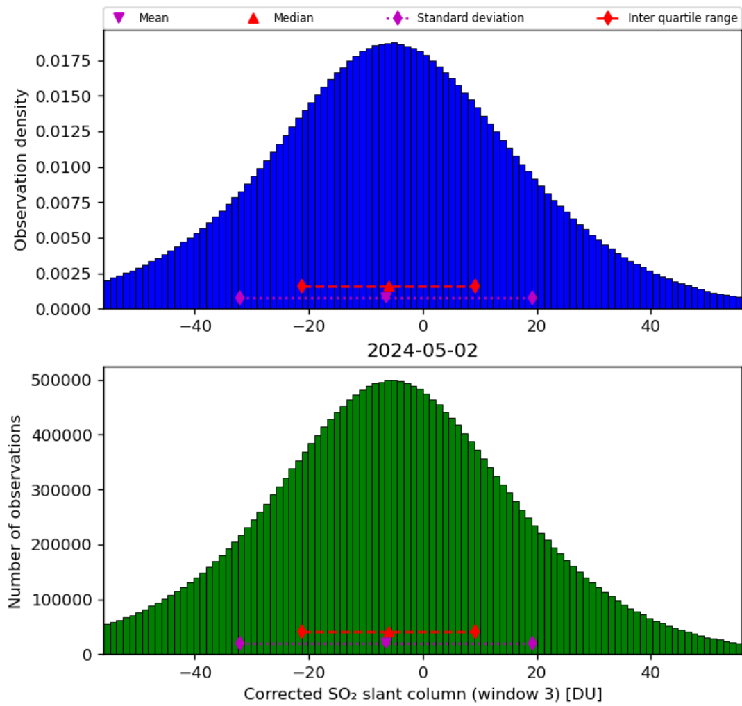
Figure 66: Histogram of “Corrected SO 2 slant column (window 3)” for 2024-05-02 to 2024-05-03
