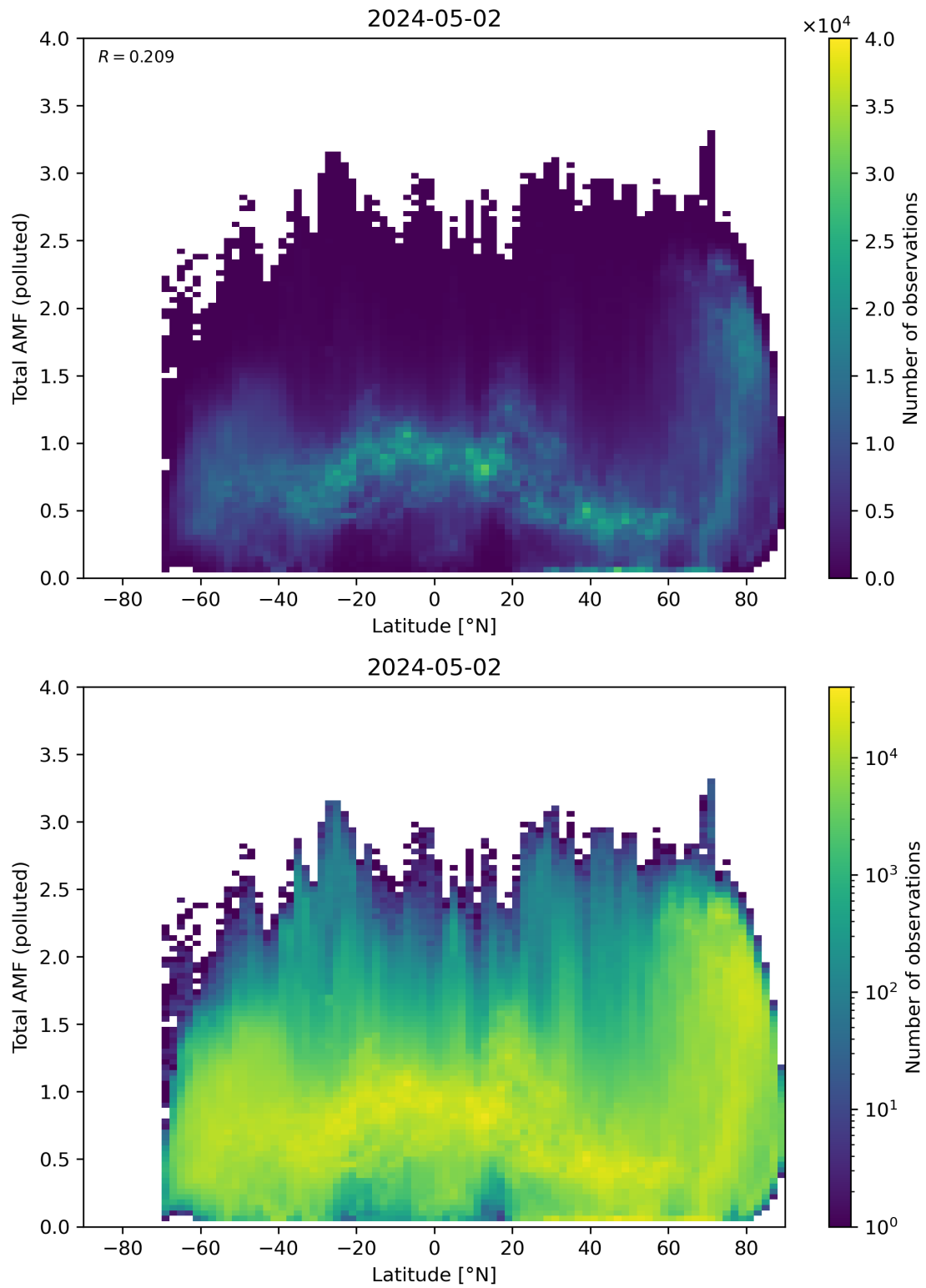
Figure 154: Scatter density plot of “Latitude” against “Total AMF (polluted)” for 2024-05-02 to 2024-05-03.
