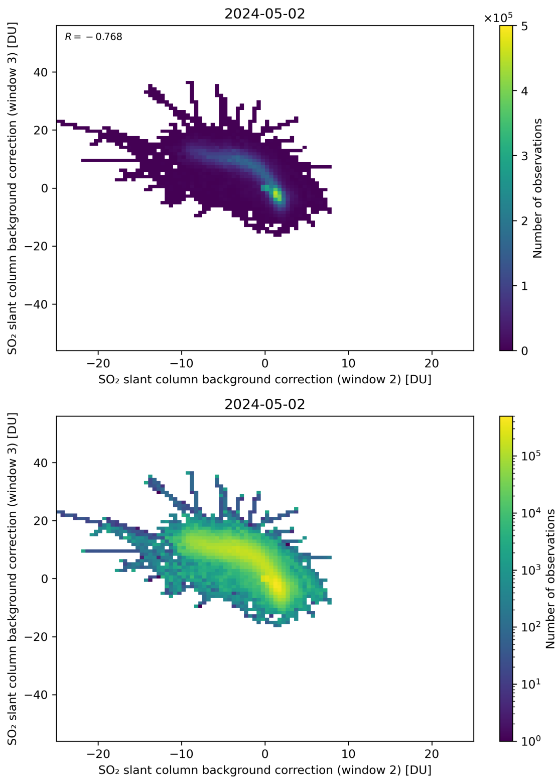
Figure 111: Scatter density plot of “SO 2 slant column background correction (window 2)” against “SO 2 slant column background correction (window 3)” for 2024-05-02 to 2024-05-03.
