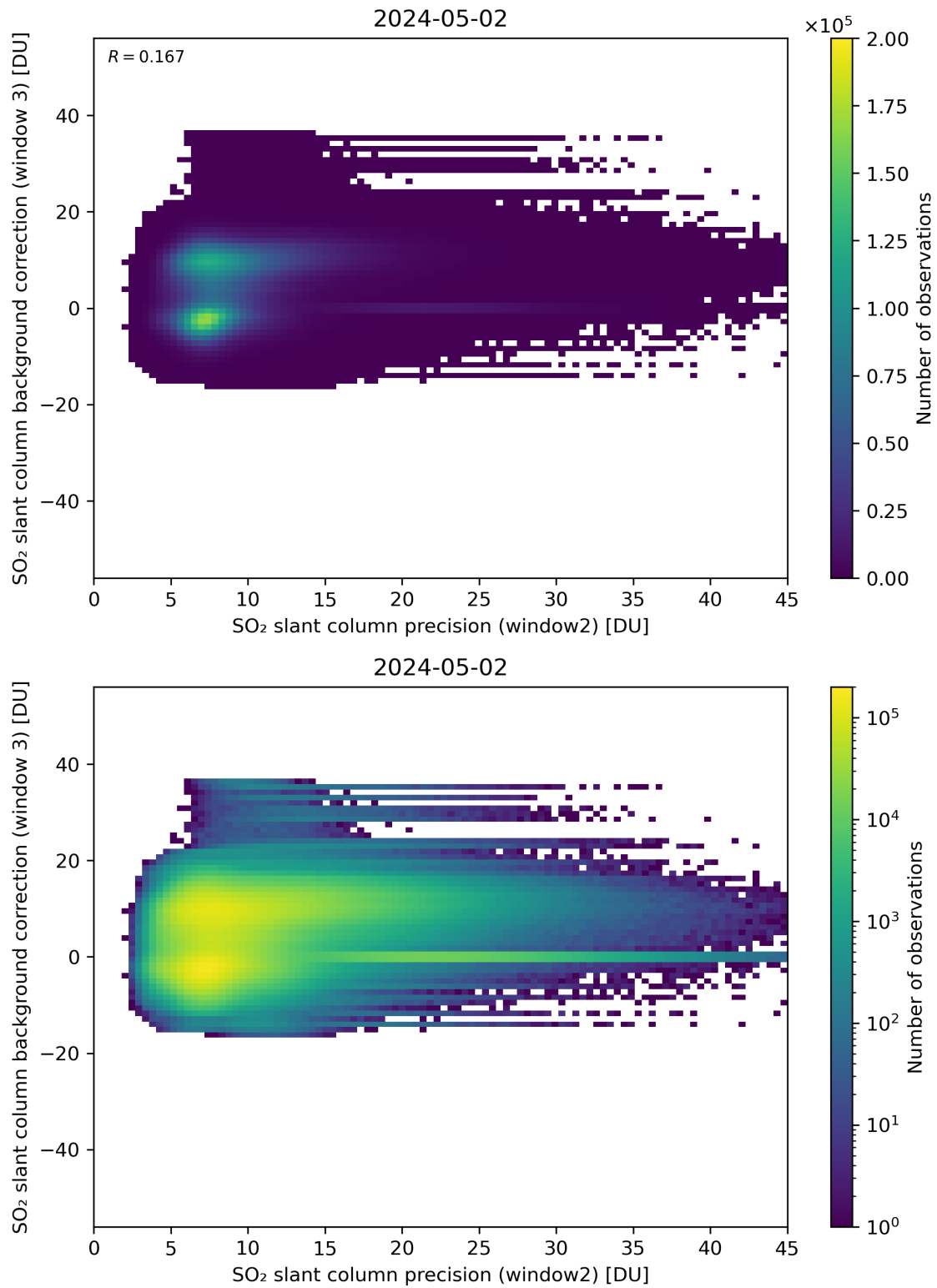
Figure 242: Scatter density plot of “SO 2 slant column precision (window2)” against “SO 2 slant column background correction (window 3)” for 2024-05-02 to 2024-05-03.
