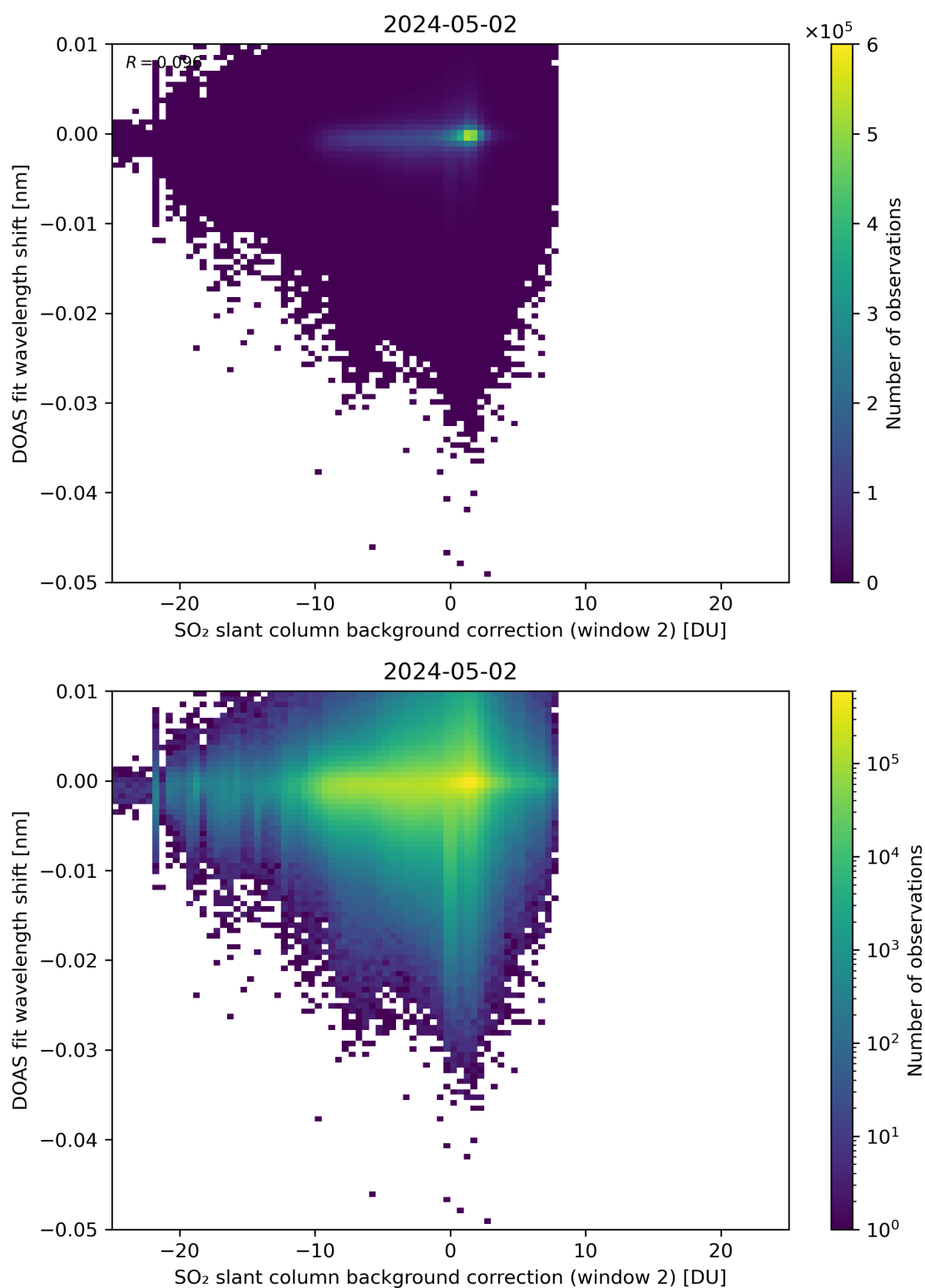
Figure 112: Scatter density plot of “SO 2 slant column background correction (window 2)” against “DOAS fit wavelength shift” for 2024-05-02 to 2024-05-03.
