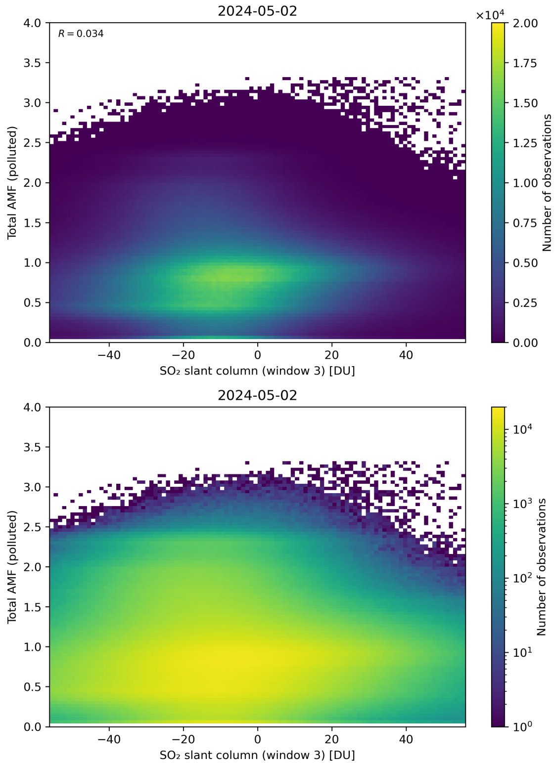
Figure 268: Scatter density plot of “SO 2 slant column (window 3)” against “Total AMF (polluted)” for 2024-05-02 to 2024-05-03.
