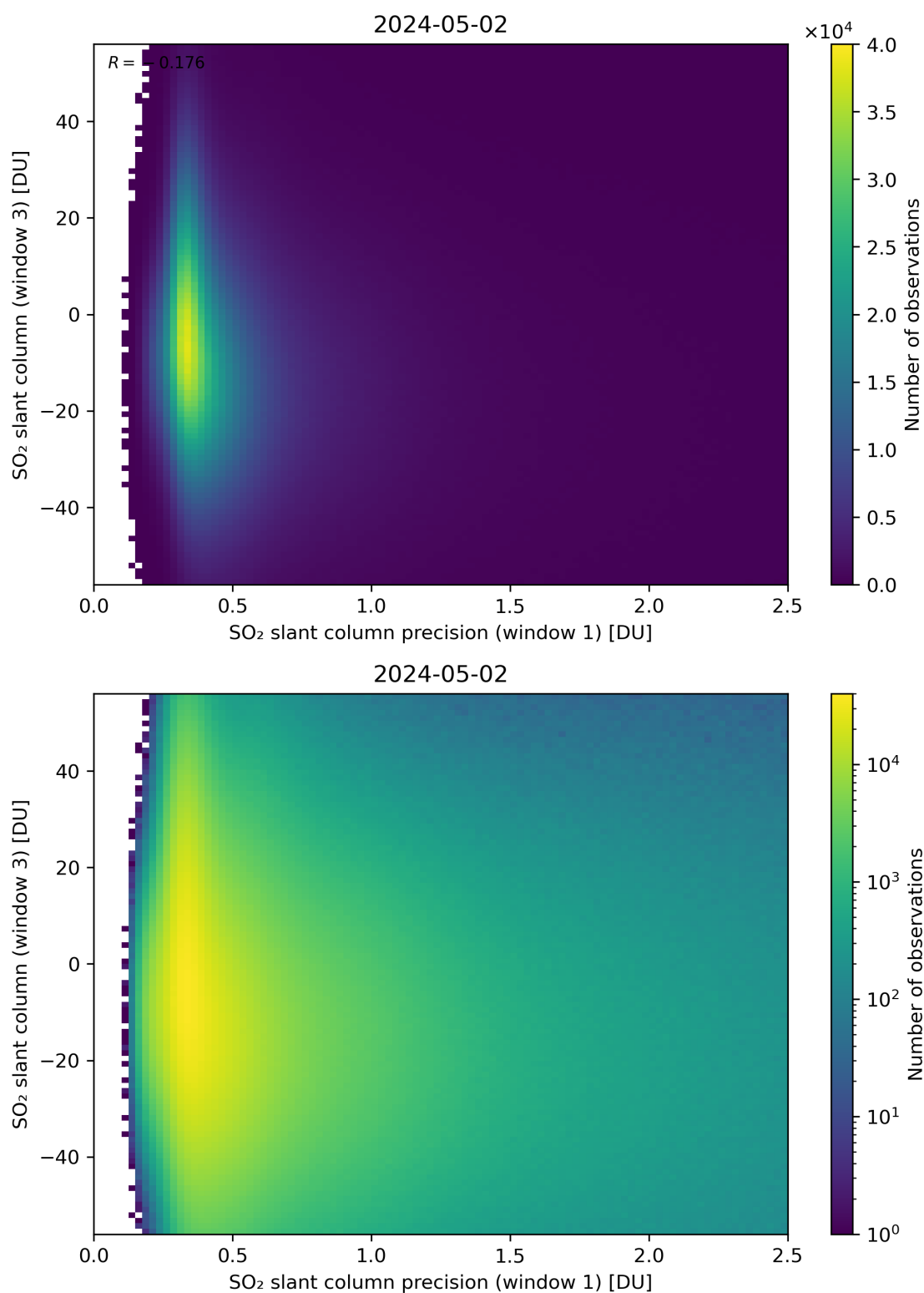
Figure 228: Scatter density plot of “SO 2 slant column precision (window 1)” against “SO 2 slant column (window 3)” for 2024-05-02 to 2024-05-03.
