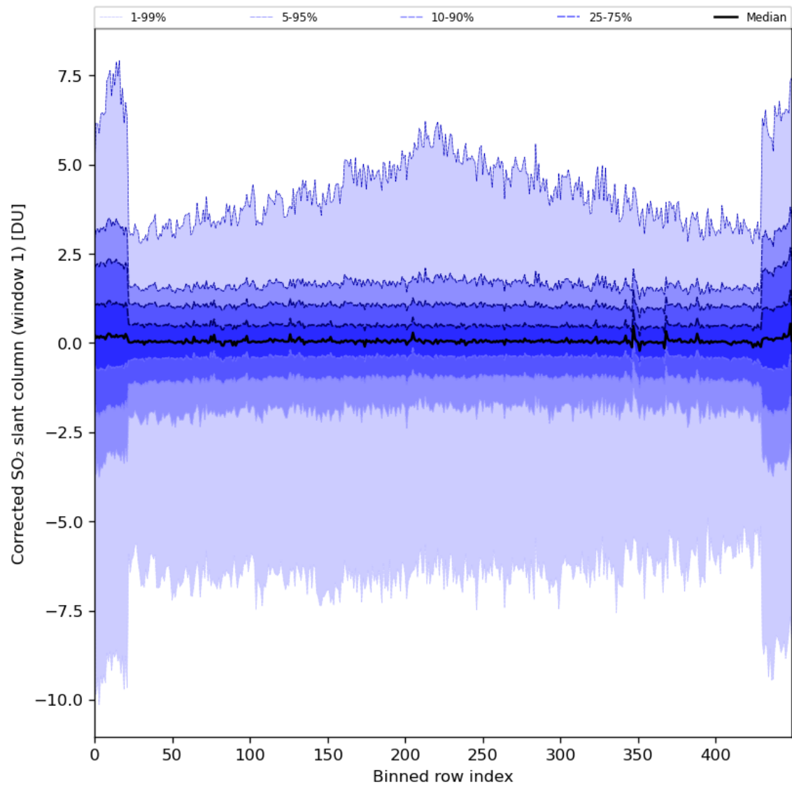
Figure 81: Along track statistics of “Corrected SO 2 slant column (window 1)” for 2024-05-02 to 2024-05-03
