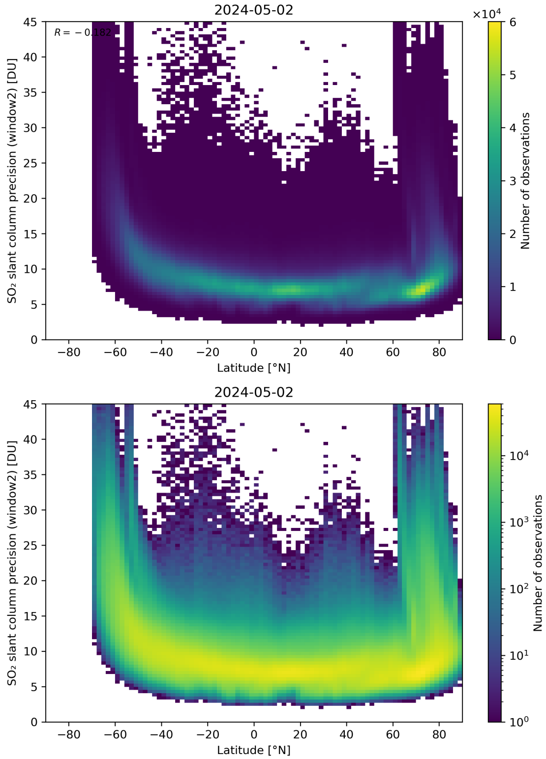
Figure 151: Scatter density plot of “Latitude” against “SO 2 slant column precision (window2)” for 2024-05-02 to 2024-05-03.
