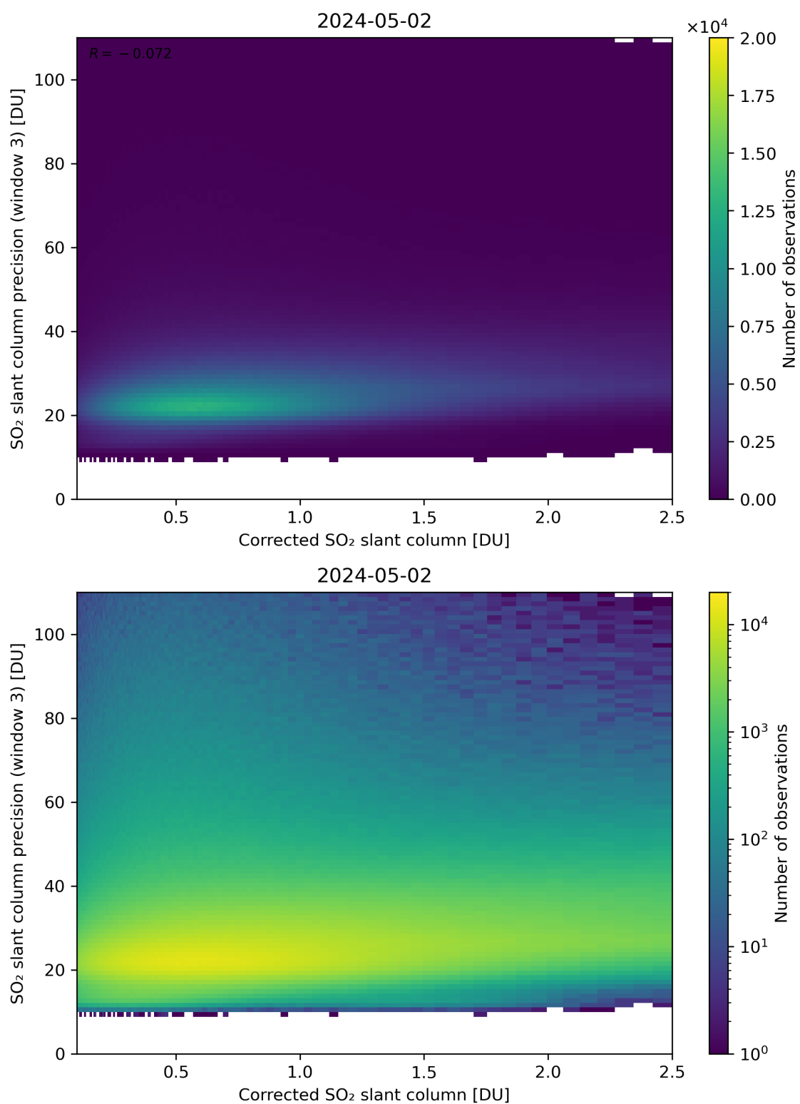
Figure 191: Scatter density plot of “Corrected SO 2 slant column” against “SO 2 slant column precision (window 3)” for 2024-05-02 to 2024-05-03.
