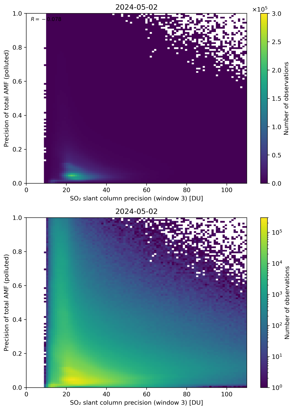
Figure 264: Scatter density plot of “SO 2 slant column precision (window 3)” against “Precision of total AMF (polluted)” for 2024-05-02 to 2024-05-03.
