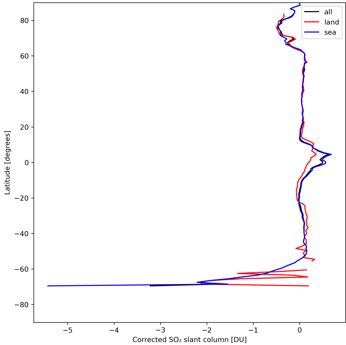
Figure 32: Zonal average of “Corrected SO 2 slant column” for 2024-05-02 to 2024-05-03.
