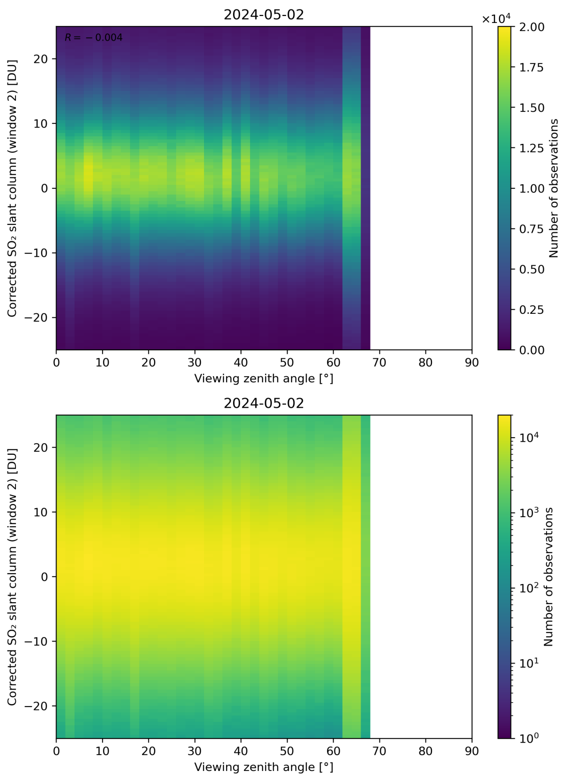
Figure 318: Scatter density plot of “Viewing zenith angle” against “Corrected SO 2 slant column (window 2)” for 2024-05-02 to 2024-05-03.
