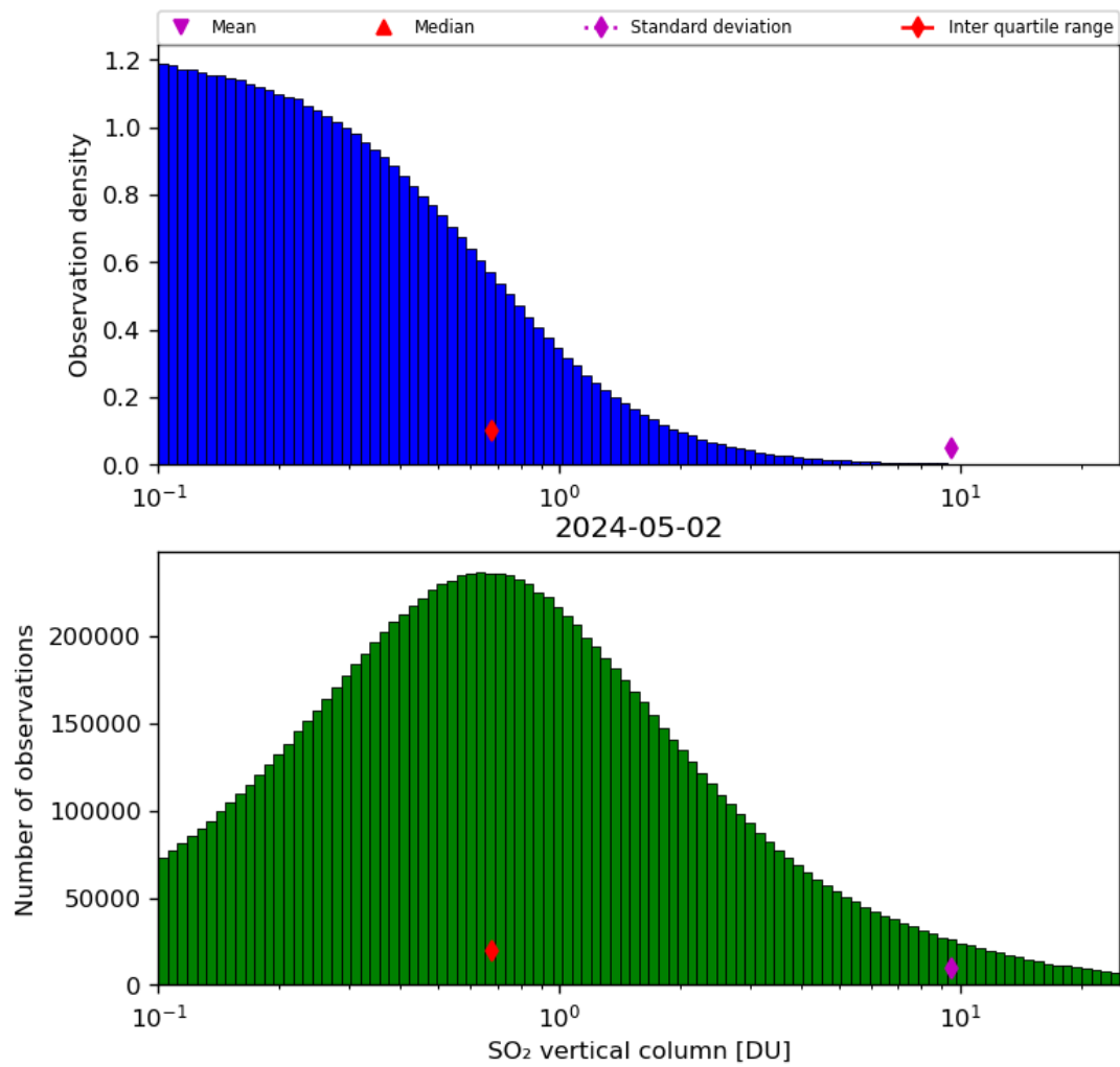
Figure 53: Histogram of “SO 2 vertical column” for 2024-05-02 to 2024-05-03
