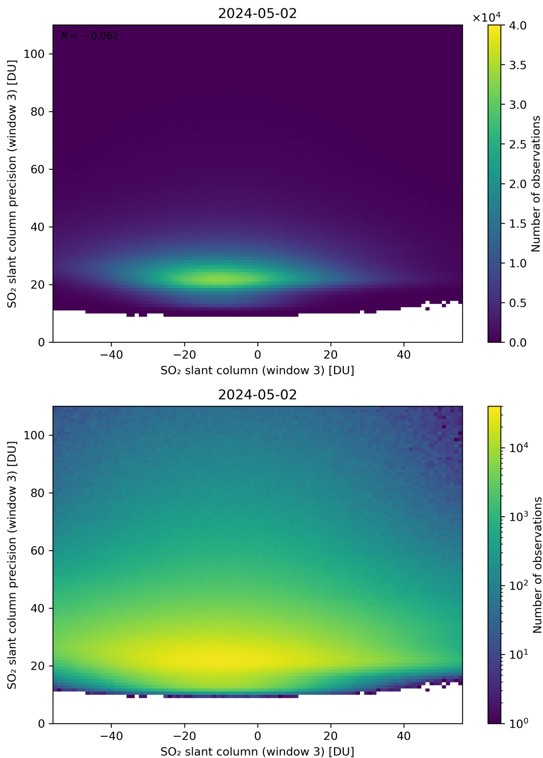
Figure 267: Scatter density plot of “SO 2 slant column (window 3)” against “SO 2 slant column precision (window 3)” for 2024-05-02 to 2024-05-03.
