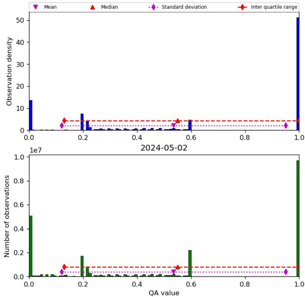
Figure 52: Histogram of “QA value” for 2024-05-02 to 2024-05-03
