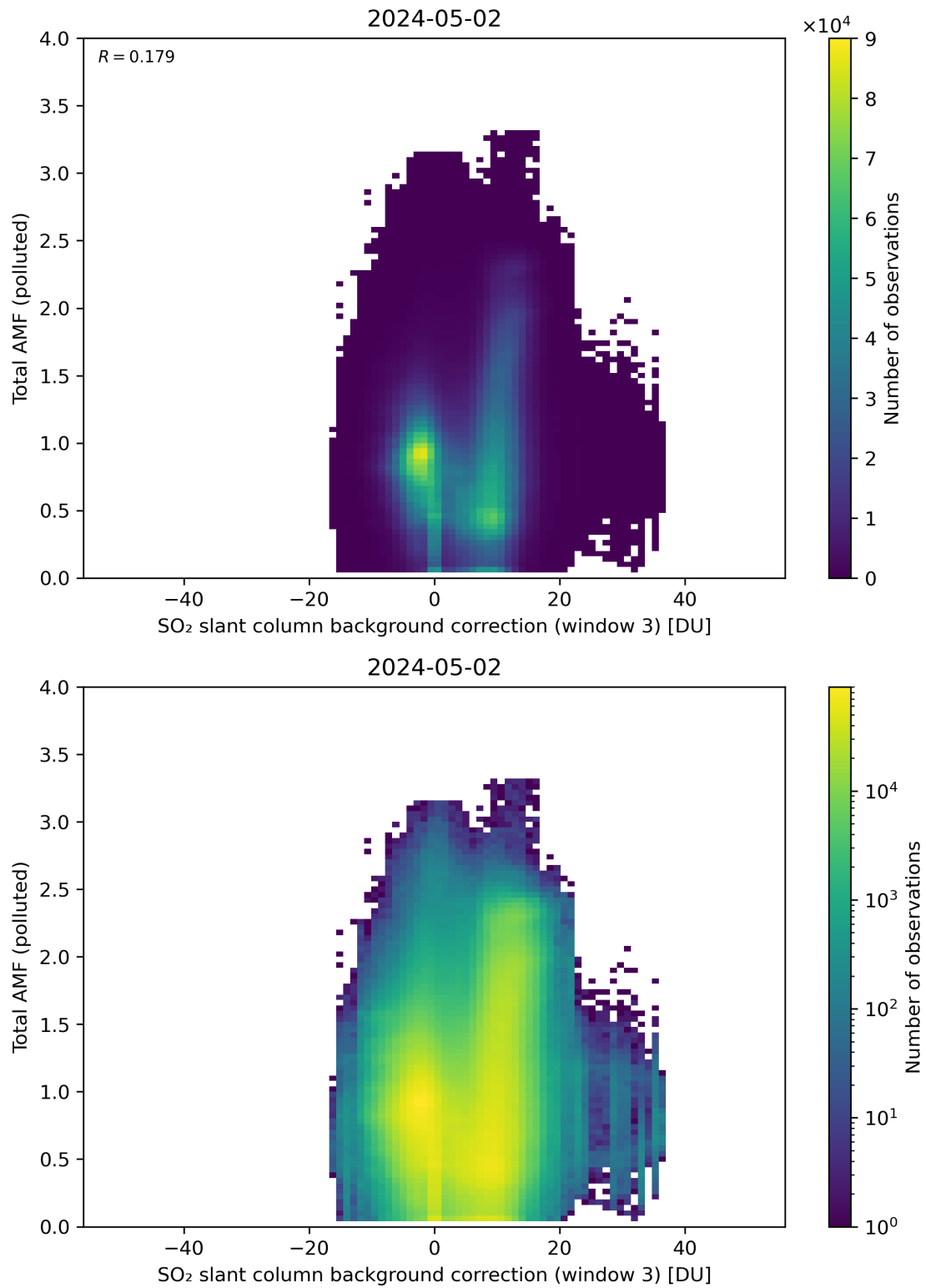
Figure 125: Scatter density plot of “SO 2 slant column background correction (window 3)” against “Total AMF (polluted)” for 2024-05-02 to 2024-05-03.
