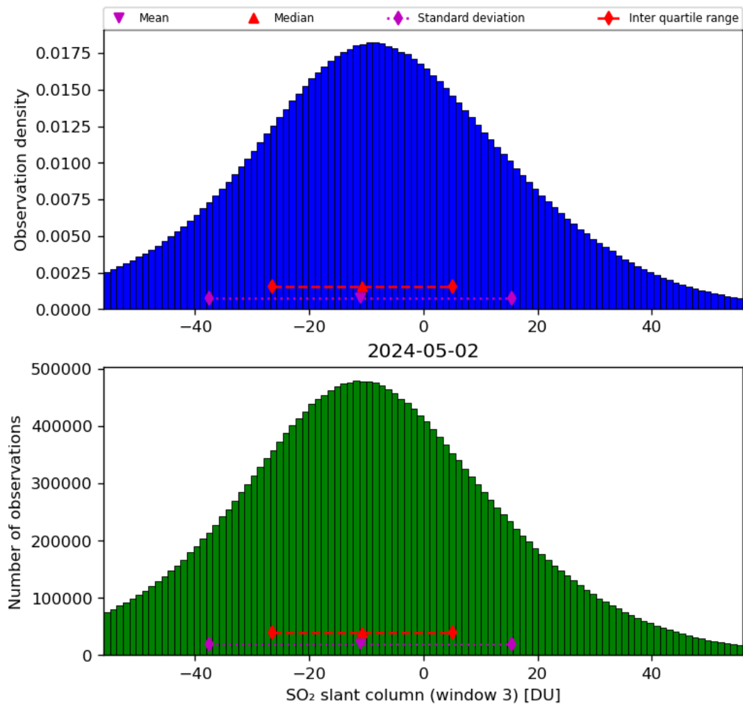
Figure 64: Histogram of “SO 2 slant column (window 3)” for 2024-05-02 to 2024-05-03
