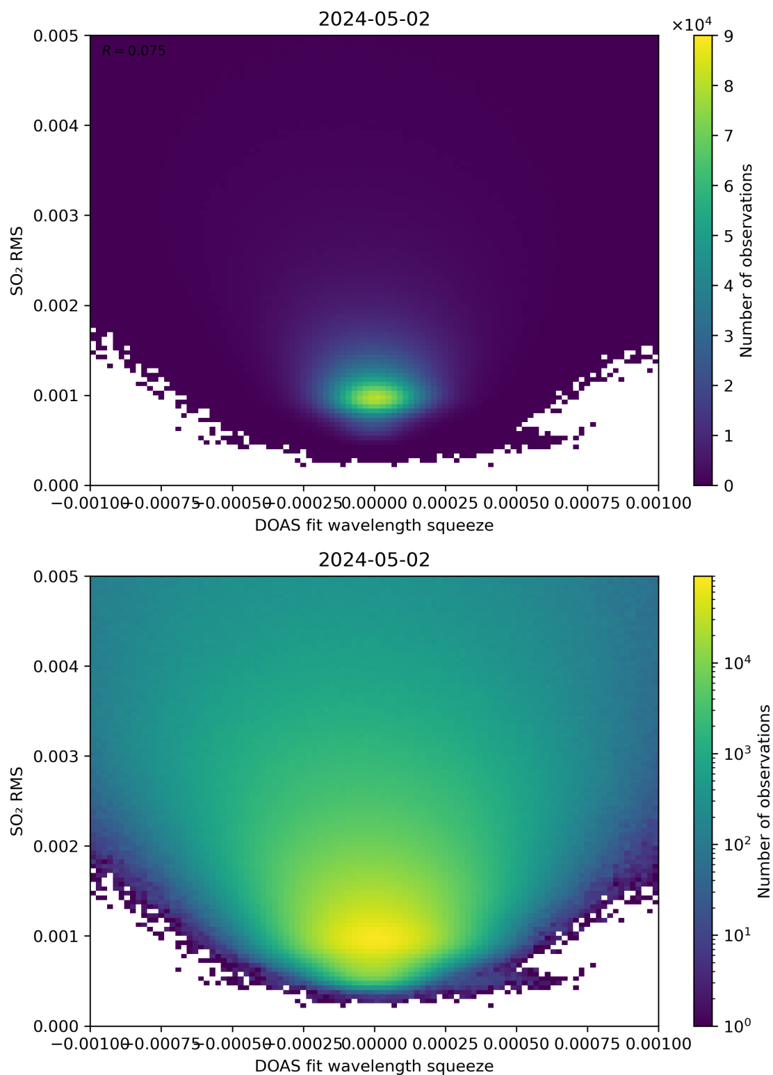
Figure 132: Scatter density plot of “DOAS fit wavelength squeeze” against “SO 2 RMS” for 2024-05-02 to 2024-05-03.
