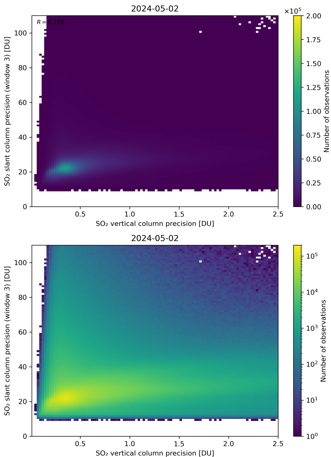
Figure 293: Scatter density plot of “SO 2 vertical column precision” against “SO 2 slant column precision (window 3)” for 2024-05-02 to 2024-05-03.
