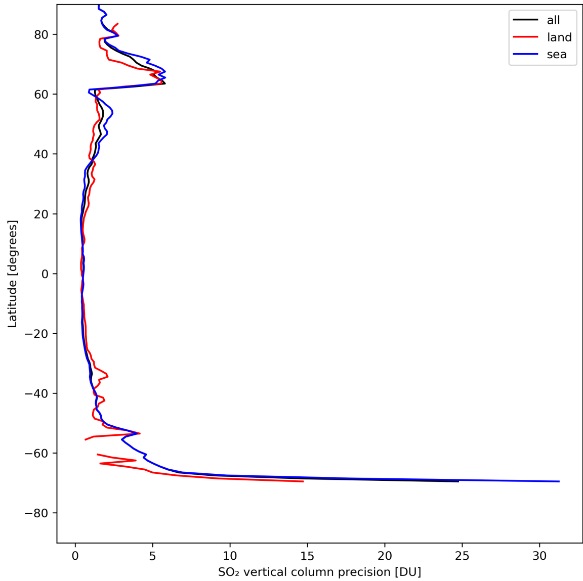
Figure 31: Zonal average of “SO 2 vertical column precision” for 2024-05-02 to 2024-05-03.
