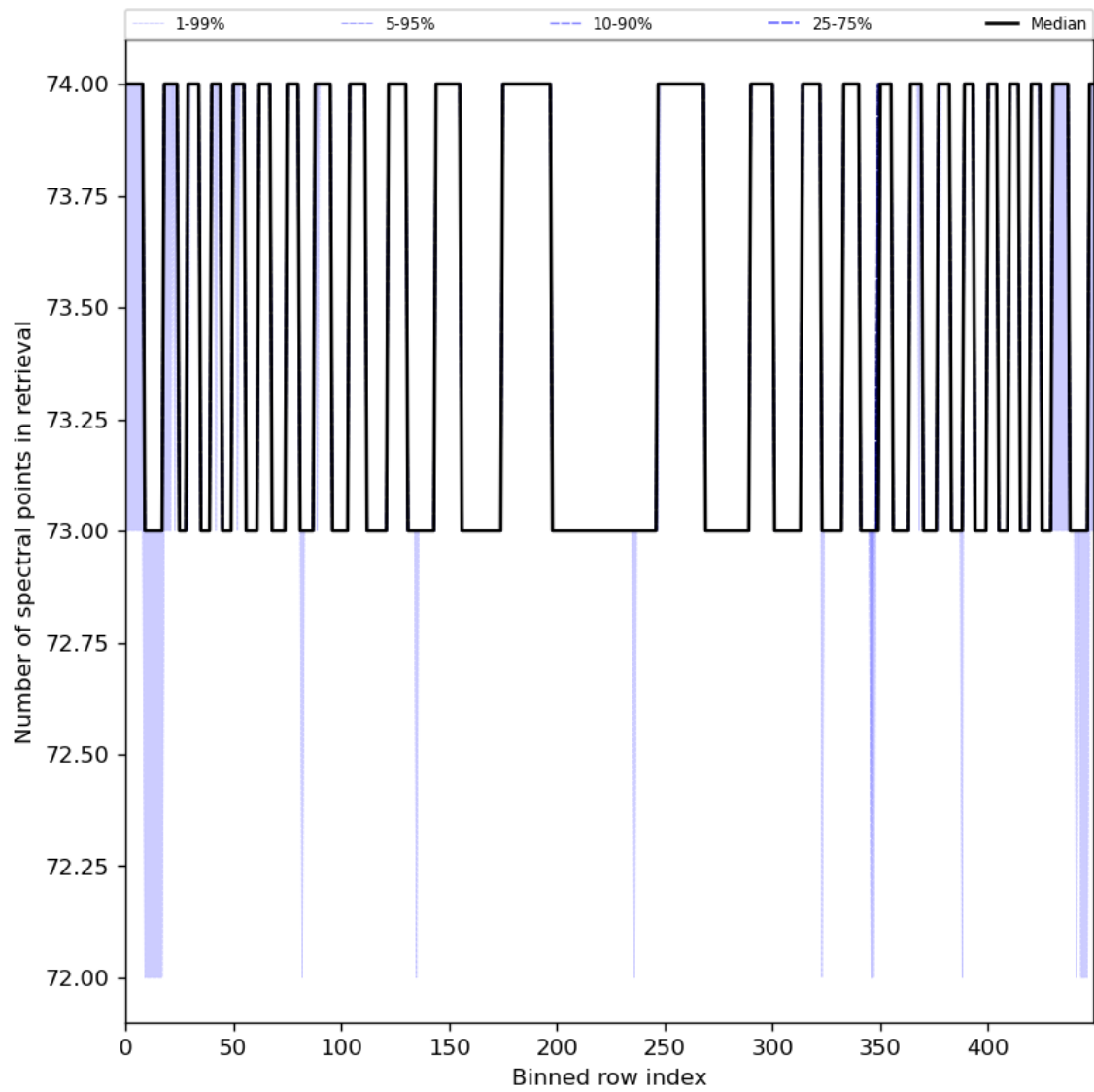
Figure 97: Along track statistics of “Number of spectral points in retrieval” for 2024-05-02 to 2024-05-03
