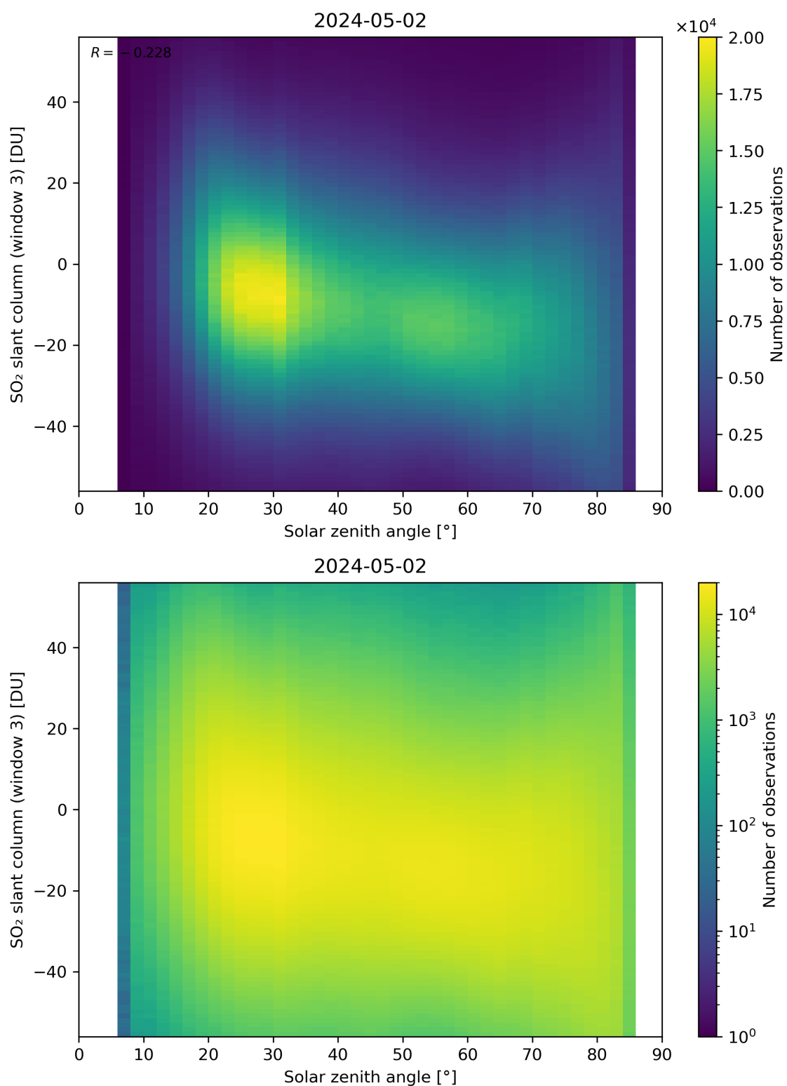
Figure 172: Scatter density plot of “Solar zenith angle” against “SO 2 slant column (window 3)” for 2024-05-02 to 2024-05-03.
