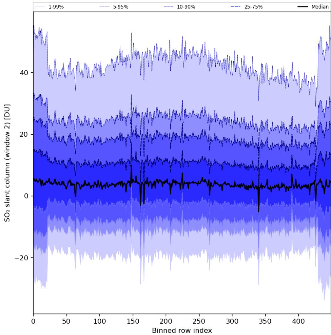
Figure 83: Along track statistics of “SO 2 slant column (window 2)” for 2024-05-02 to 2024-05-03
