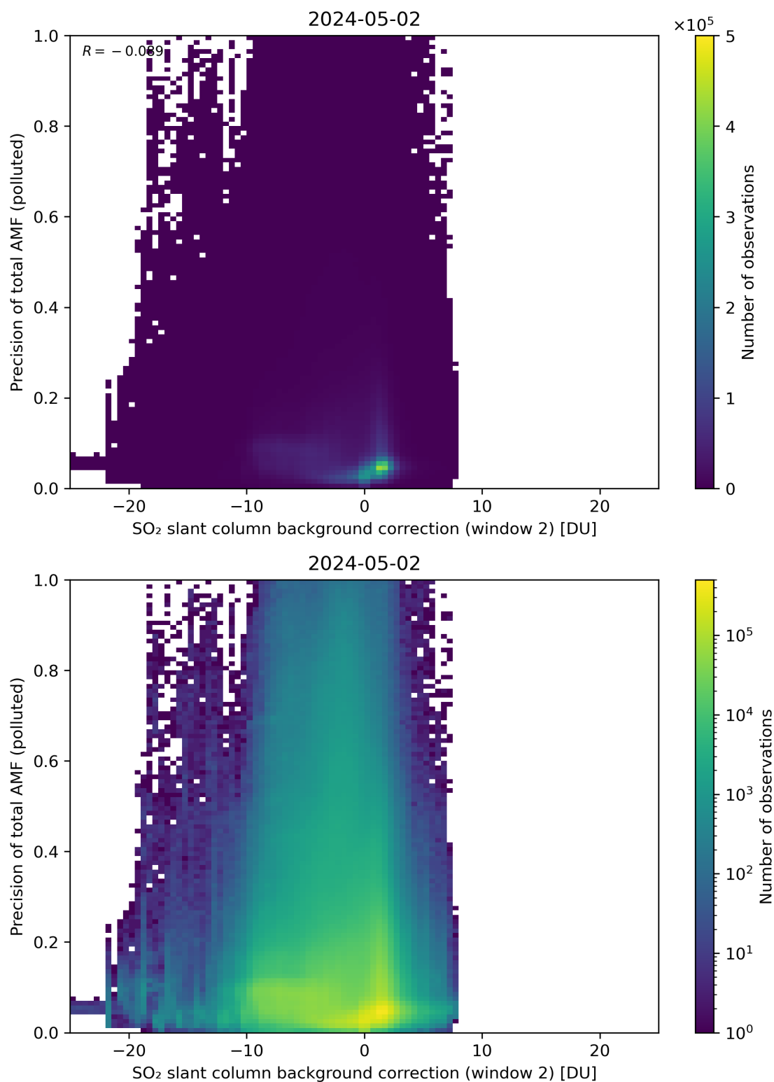
Figure 120: Scatter density plot of “SO 2 slant column background correction (window 2)” against “Precision of total AMF (polluted)” for 2024-05-02 to 2024-05-03.
