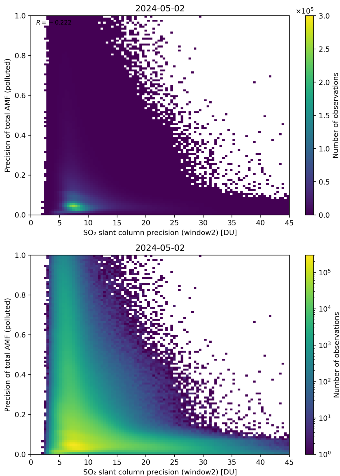
Figure 252: Scatter density plot of “SO 2 slant column precision (window2)” against “Precision of total AMF (polluted)” for 2024-05-02 to 2024-05-03.
