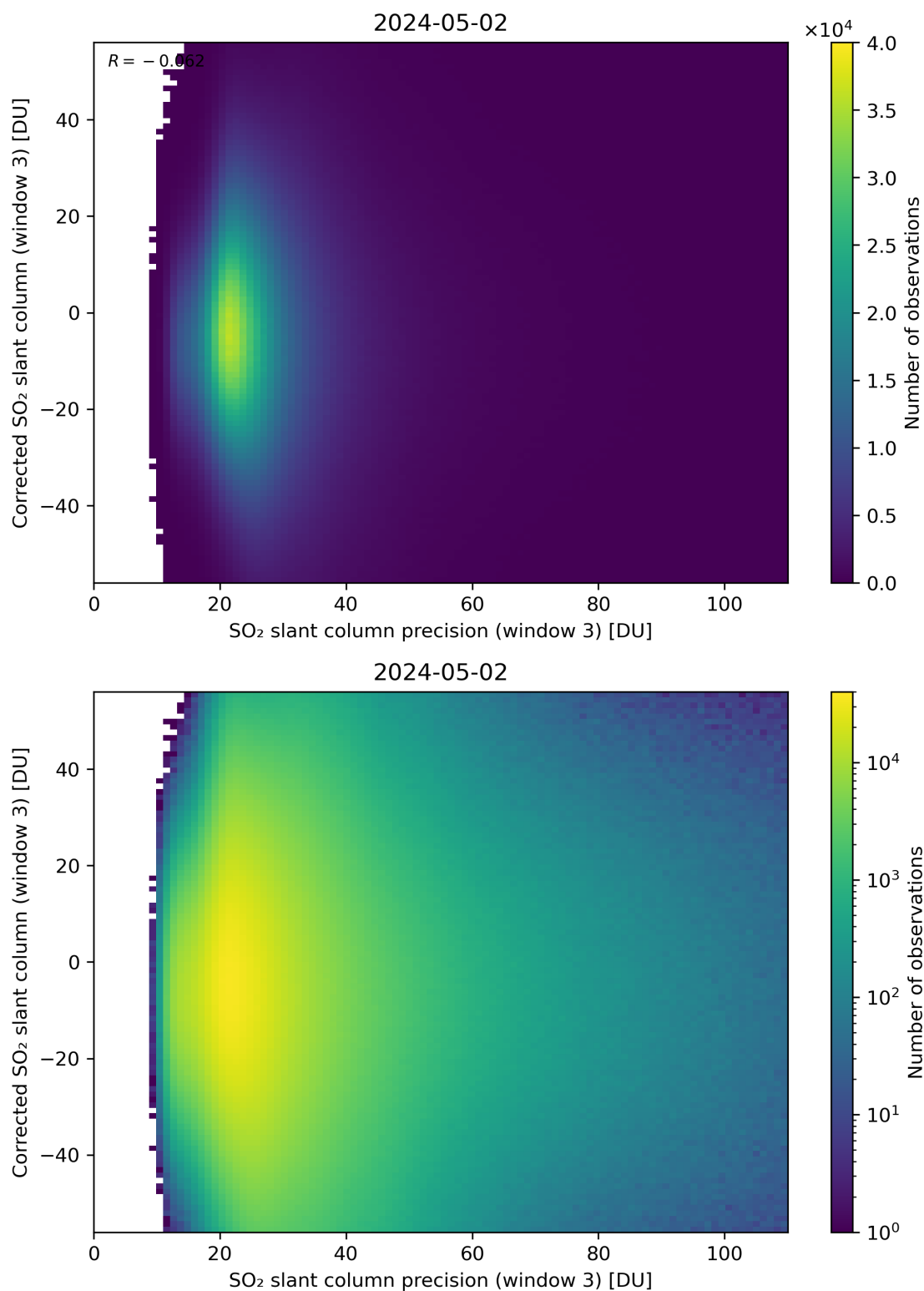
Figure 262: Scatter density plot of “SO 2 slant column precision (window 3)” against “Corrected SO 2 slant column (window 3)” for 2024-05-02 to 2024-05-03.
