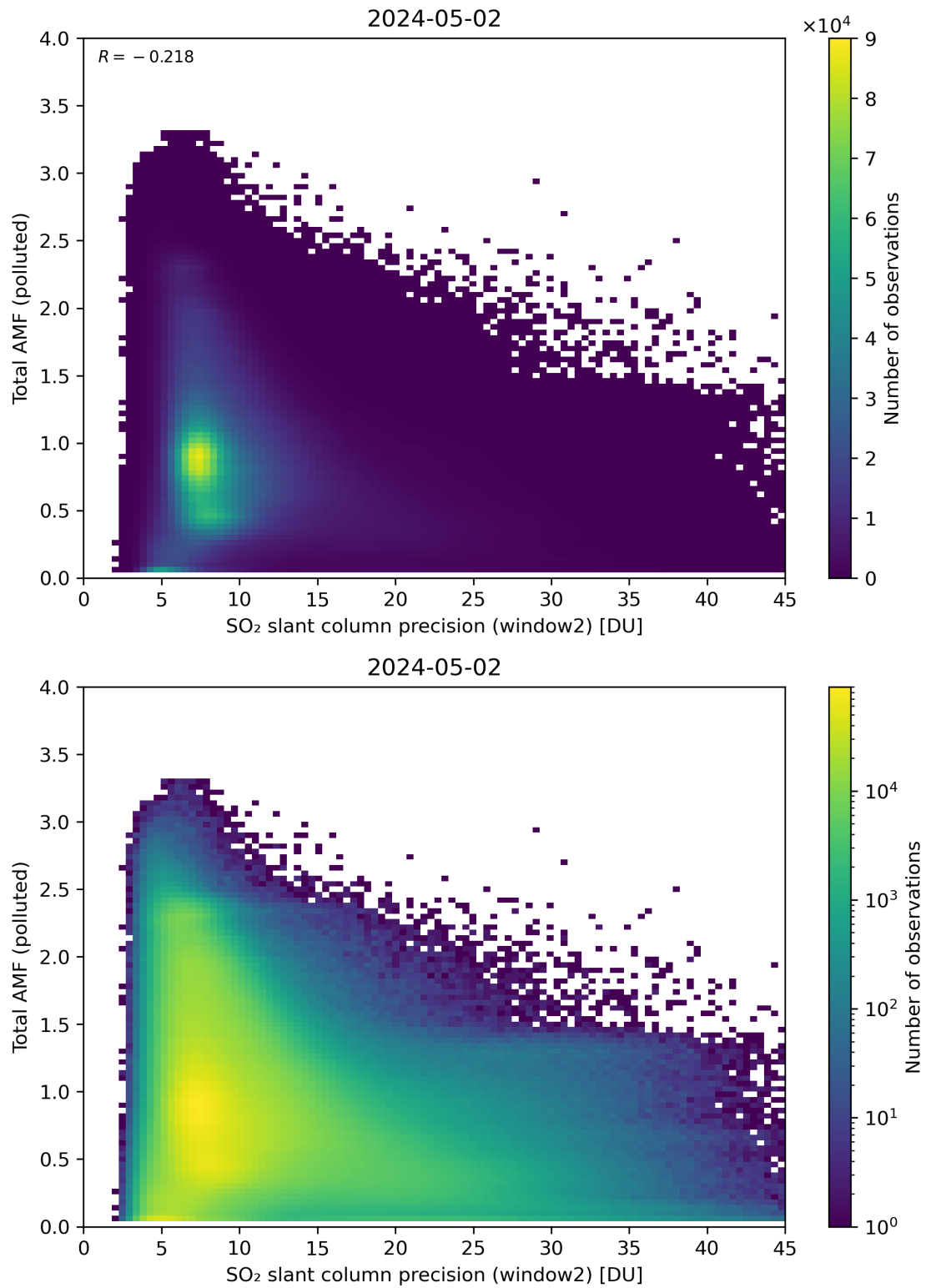
Figure 251: Scatter density plot of “SO 2 slant column precision (window2)” against “Total AMF (polluted)” for 2024-05-02 to 2024-05-03.
