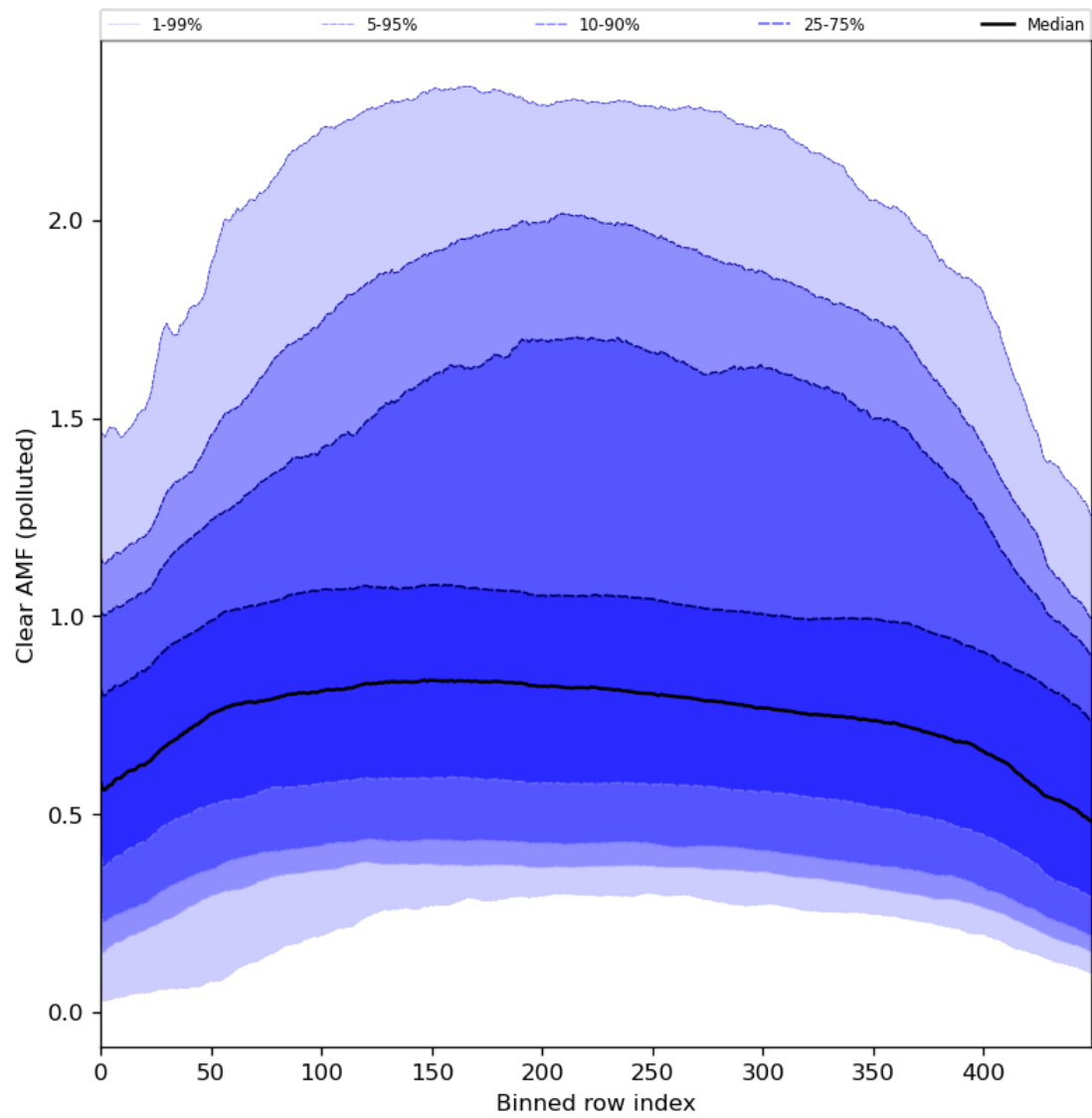
Figure 96: Along track statistics of “Clear AMF (polluted)” for 2024-05-02 to 2024-05-03
