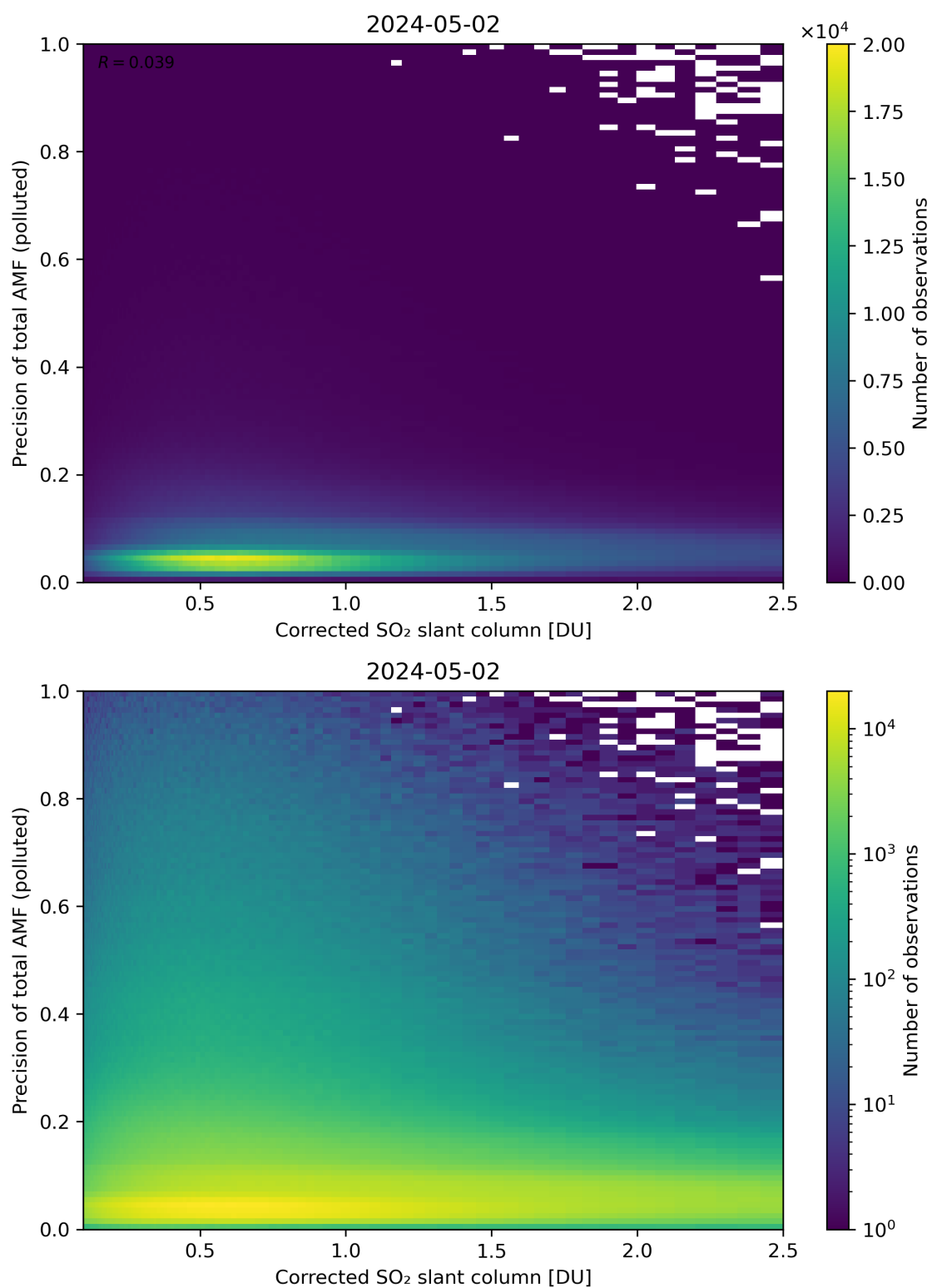
Figure 193: Scatter density plot of “Corrected SO 2 slant column” against “Precision of total AMF (polluted)” for 2024-05-02 to 2024-05-03.
