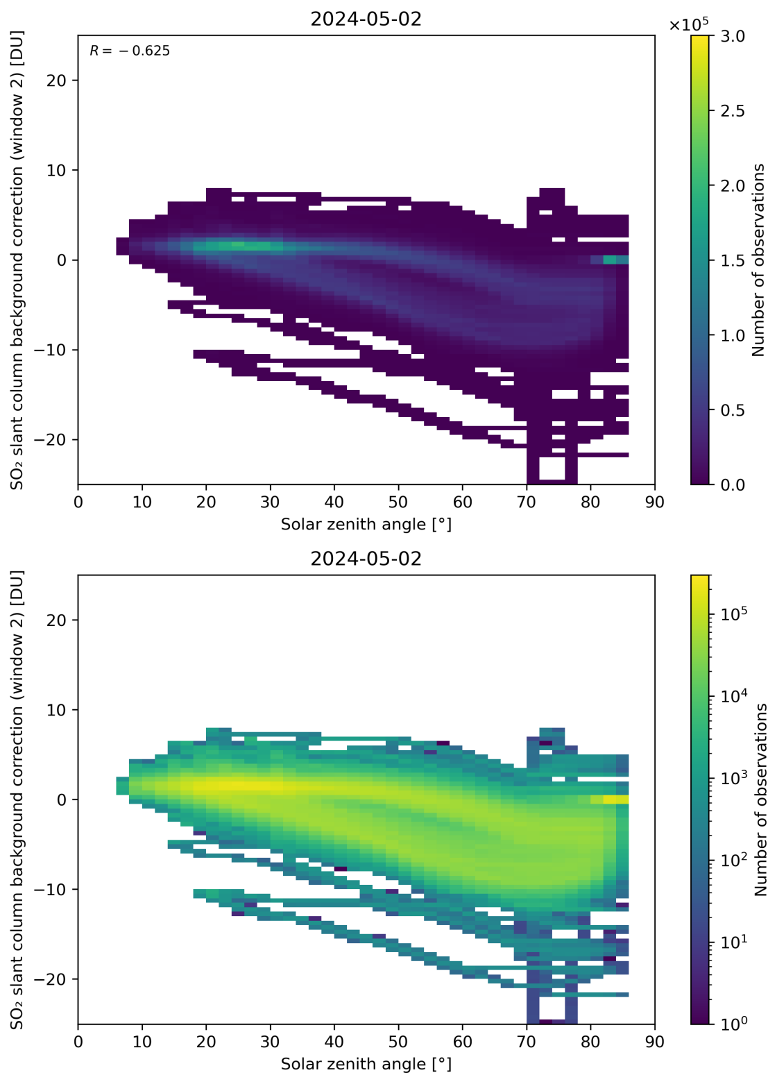
Figure 159: Scatter density plot of “Solar zenith angle” against “SO 2 slant column background correction (window 2)” for 2024-05-02 to 2024-05-03.
