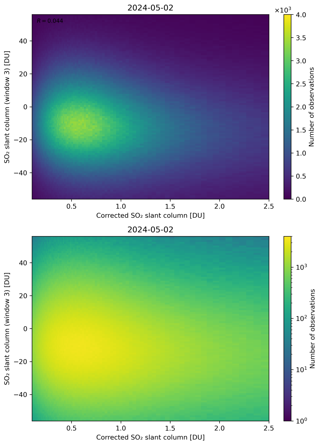
Figure 190: Scatter density plot of “Corrected SO 2 slant column” against “SO 2 slant column (window 3)” for 2024-05-02 to 2024-05-03.
