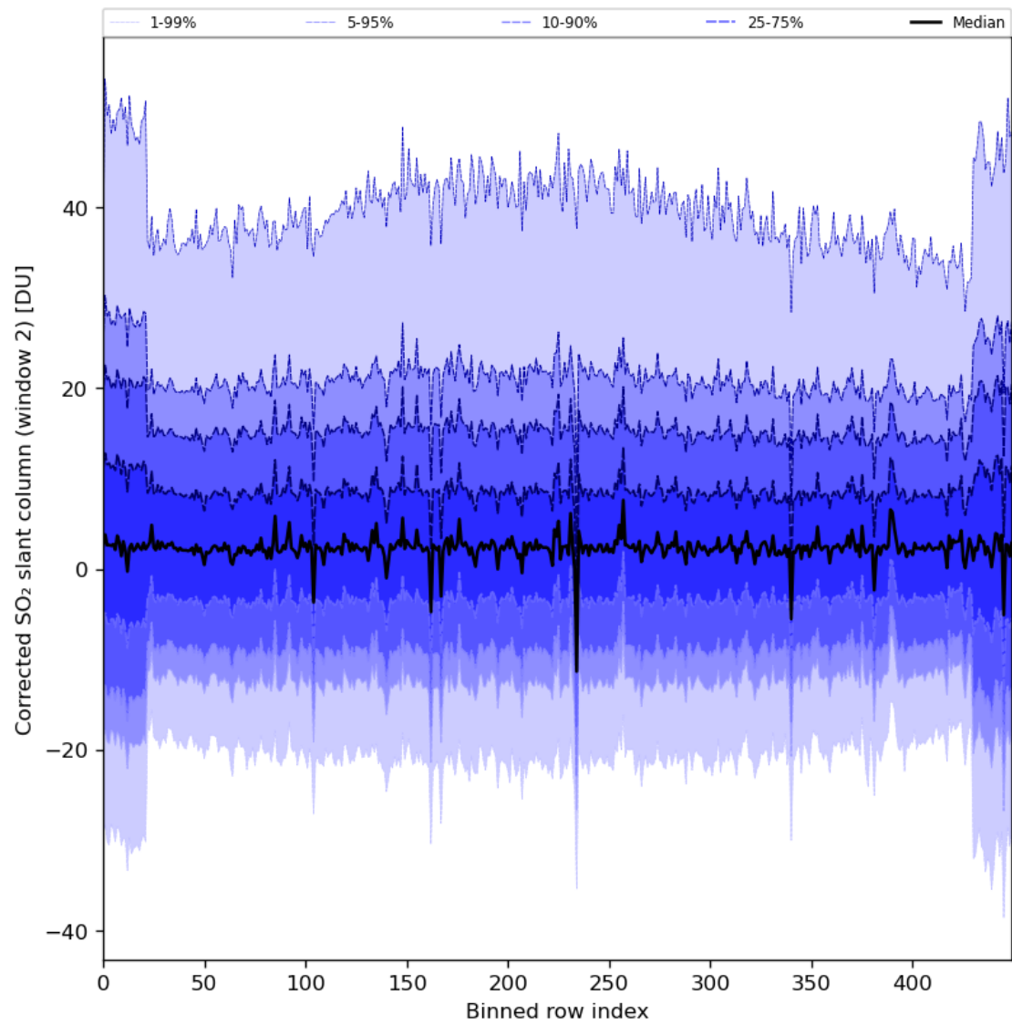
Figure 85: Along track statistics of “Corrected SO 2 slant column (window 2)” for 2024-05-02 to 2024-05-03
