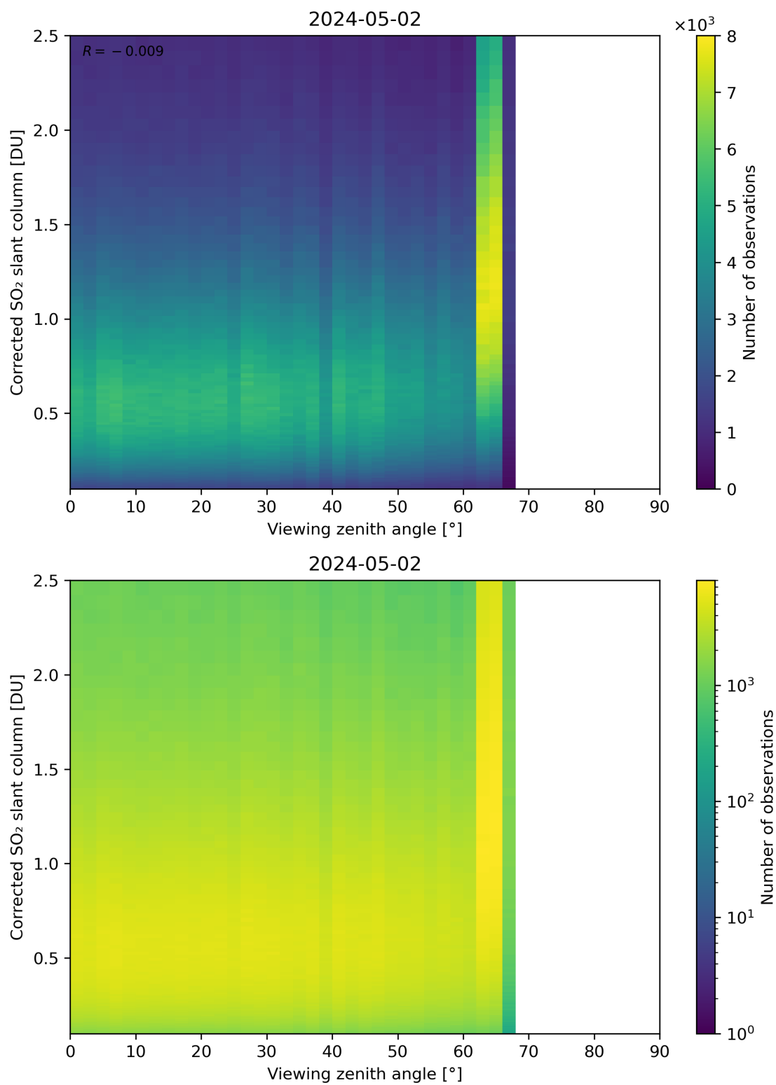
Figure 317: Scatter density plot of “Viewing zenith angle” against “Corrected SO 2 slant column” for 2024-05-02 to 2024-05-03.
