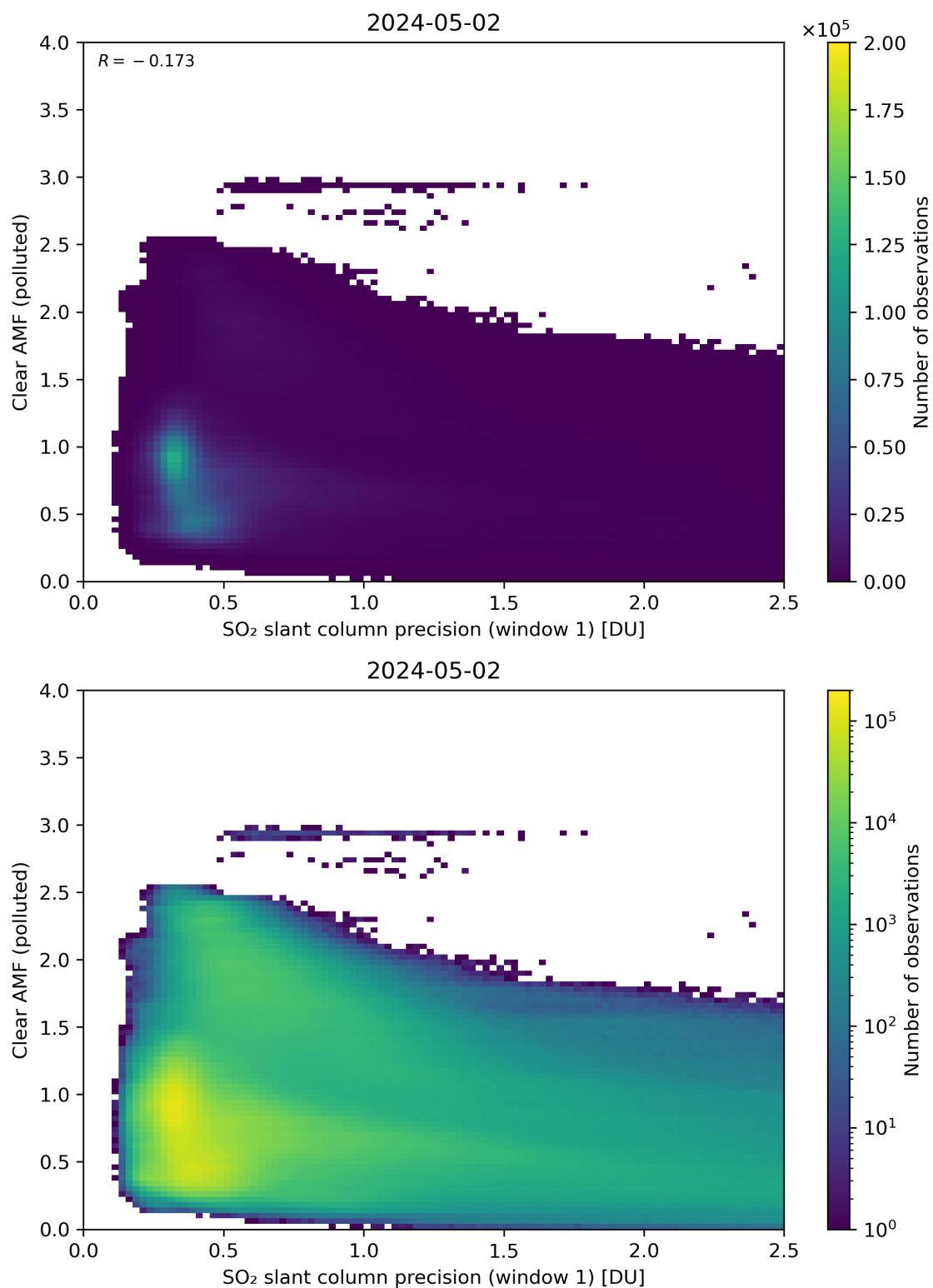
Figure 224: Scatter density plot of “SO 2 slant column precision (window 1)” against “Clear AMF (polluted)” for 2024-05-02 to 2024-05-03.
