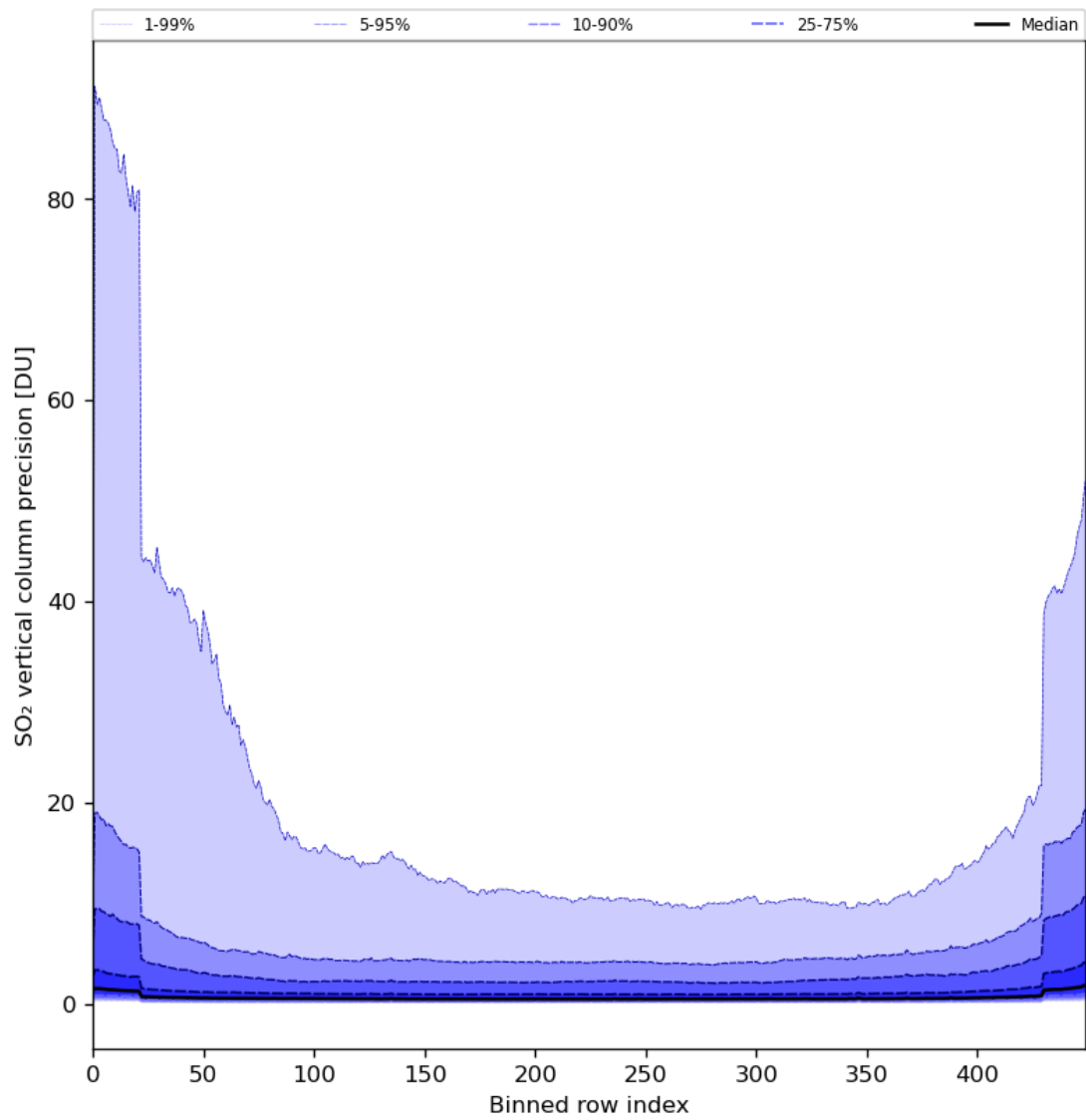
Figure 77: Along track statistics of “SO 2 vertical column precision” for 2024-05-02 to 2024-05-03
