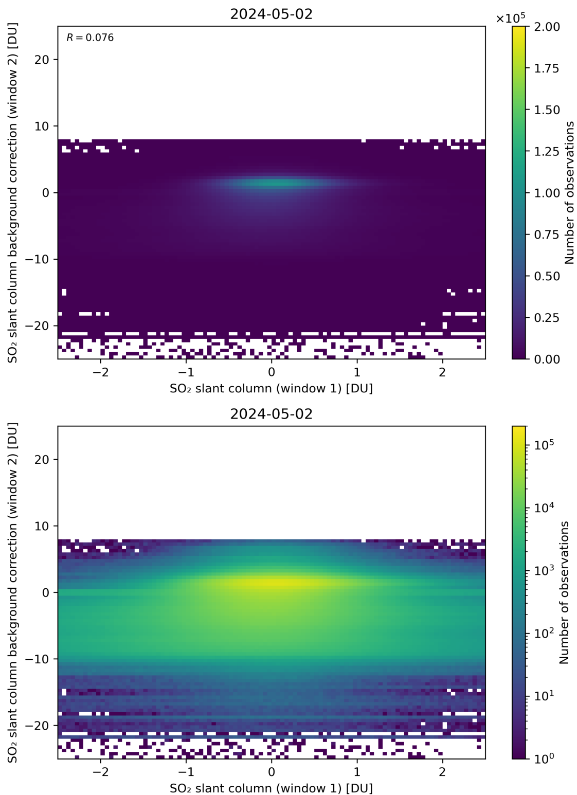
Figure 213: Scatter density plot of “SO 2 slant column (window 1)” against “SO 2 slant column background correction (window 2)” for 2024-05-02 to 2024-05-03.
