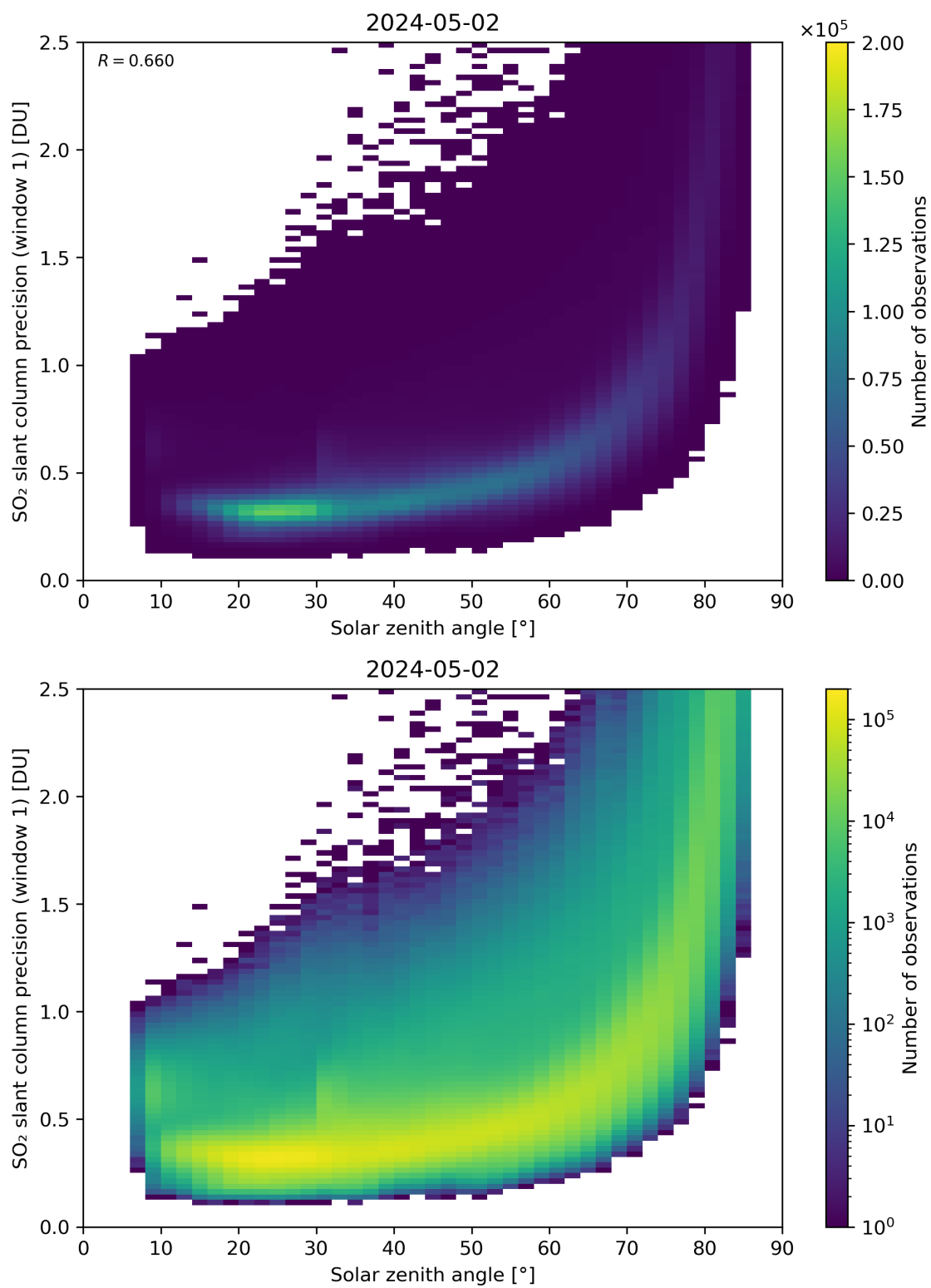
Figure 170: Scatter density plot of “Solar zenith angle” against “SO 2 slant column precision (window 1)” for 2024-05-02 to 2024-05-03.
