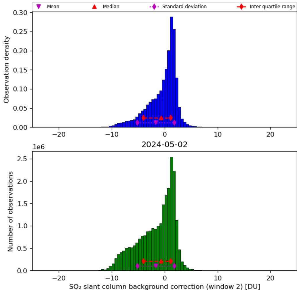
Figure 63: Histogram of “SO 2 slant column background correction (window 2)” for 2024-05-02 to 2024-05-03
