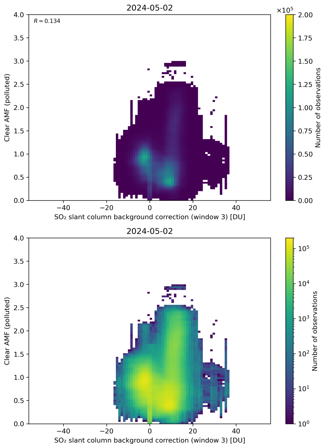
Figure 124: Scatter density plot of “SO 2 slant column background correction (window 3)” against “Clear AMF (polluted)” for 2024-05-02 to 2024-05-03.
