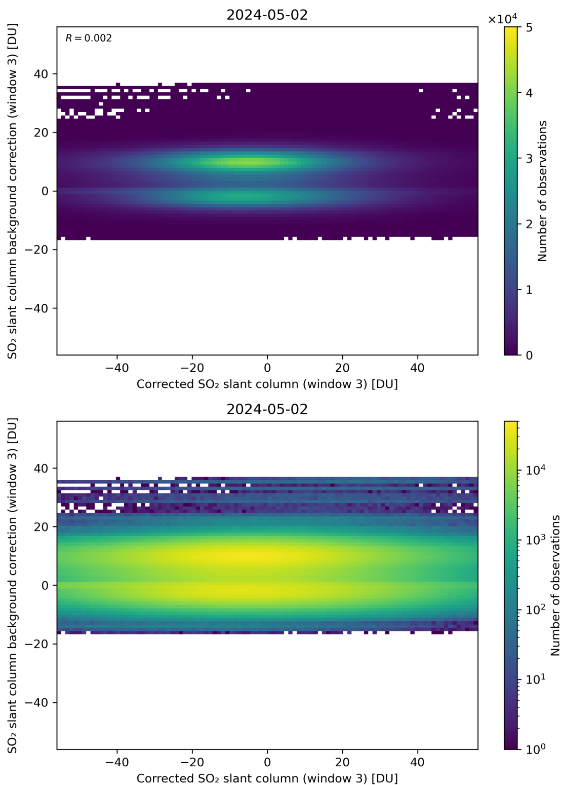
Figure 205: Scatter density plot of “Corrected SO 2 slant column (window 3)” against “SO 2 slant column background correction (window 3)” for 2024-05-02 to 2024-05-03.
