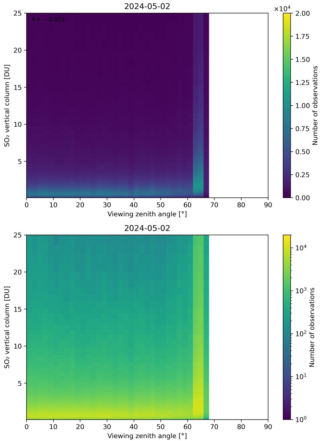
Figure 327: Scatter density plot of “Viewing zenith angle” against “SO 2 vertical column” for 2024-05-02 to 2024-05-03.
