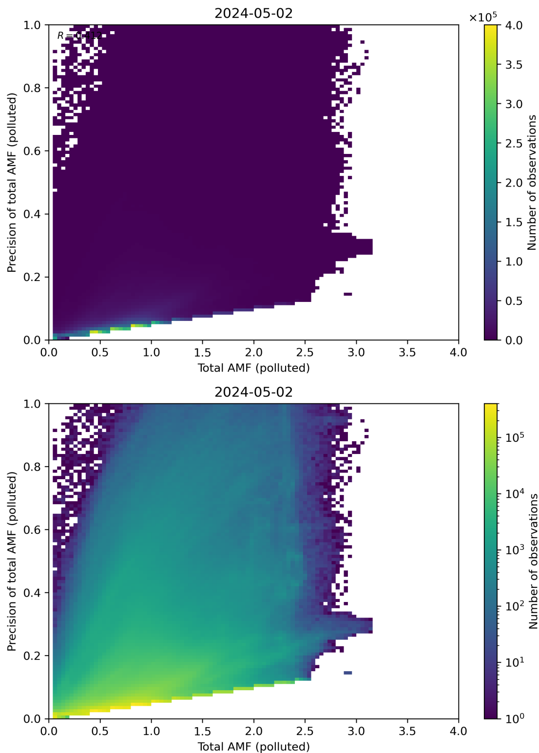
Figure 272: Scatter density plot of “Total AMF (polluted)” against “Precision of total AMF (polluted)” for 2024-05-02 to 2024-05-03.
