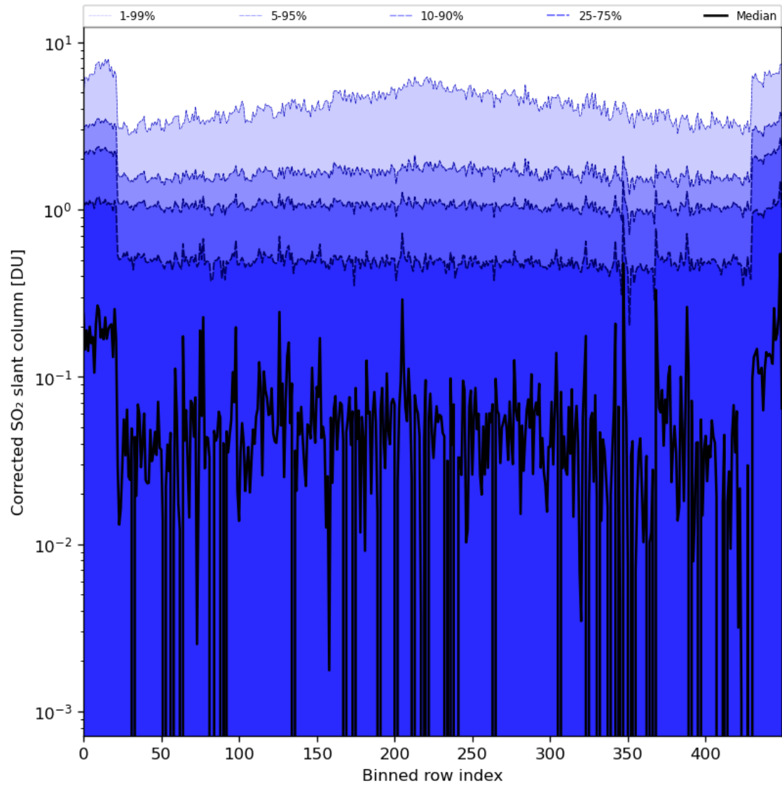
Figure 78: Along track statistics of “Corrected SO 2 slant column” for 2024-05-02 to 2024-05-03
