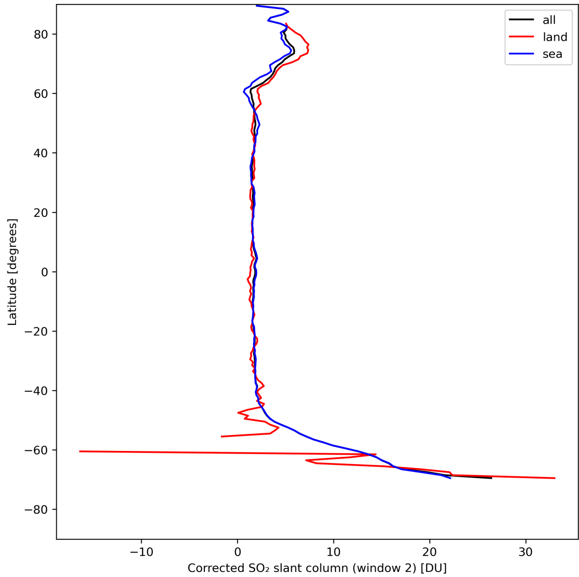
Figure 39: Zonal average of “Corrected SO 2 slant column (window 2)” for 2024-05-02 to 2024-05-03.
