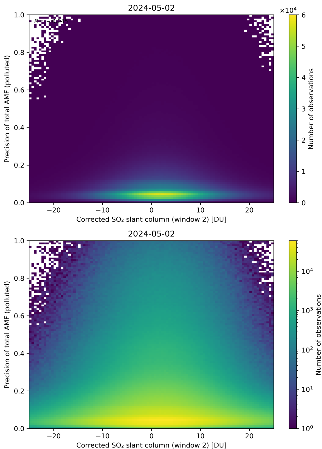
Figure 204: Scatter density plot of “Corrected SO 2 slant column (window 2)” against “Precision of total AMF (polluted)” for 2024-05-02 to 2024-05-03.
