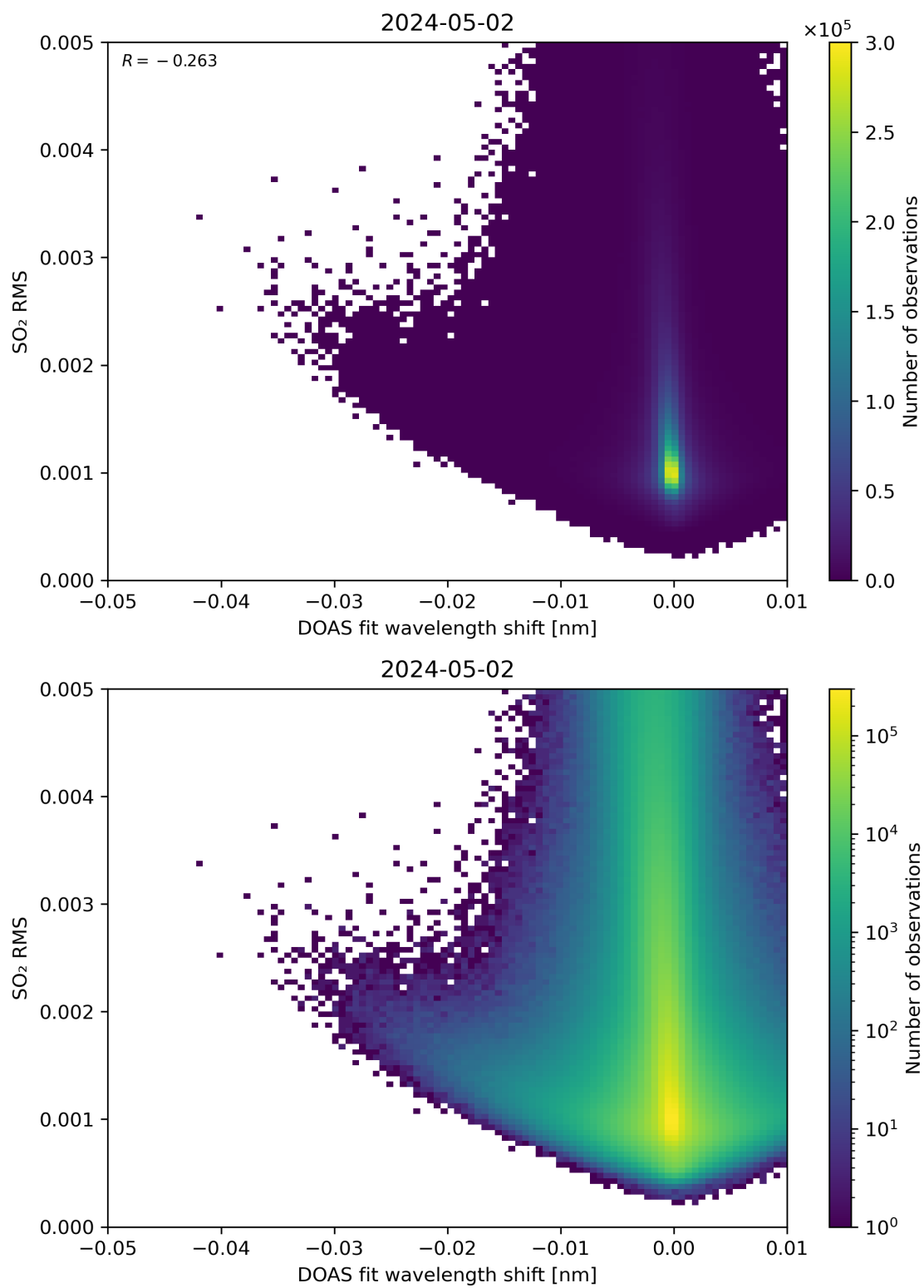
Figure 128: Scatter density plot of “DOAS fit wavelength shift” against “SO 2 RMS” for 2024-05-02 to 2024-05-03.
