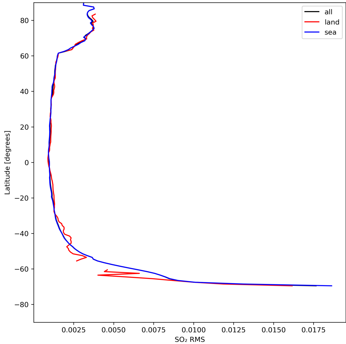
Figure 47: Zonal average of “SO 2 RMS” for 2024-05-02 to 2024-05-03.
