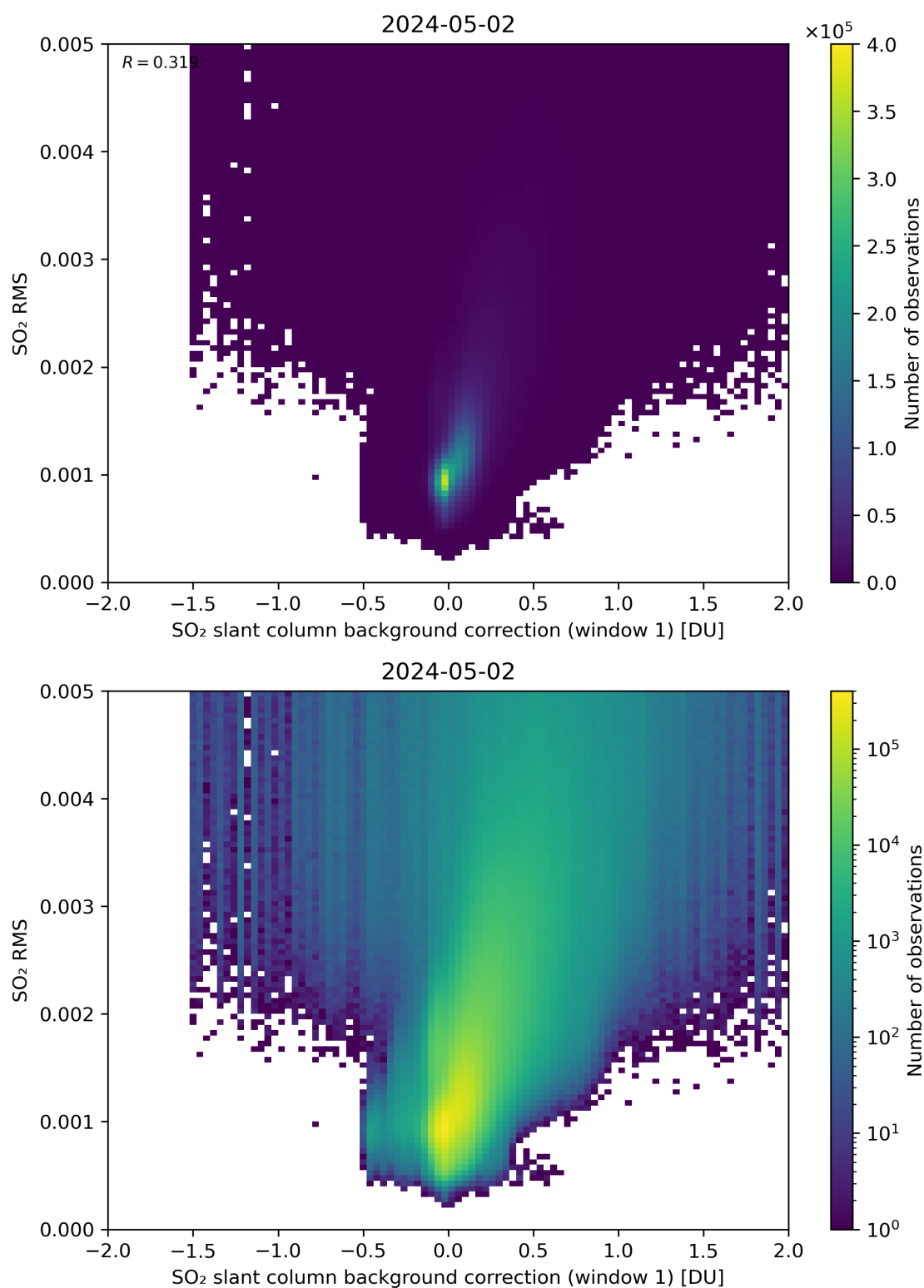
Figure 102: Scatter density plot of “SO 2 slant column background correction (window 1)” against “SO 2 RMS” for 2024-05-02 to 2024-05-03.
