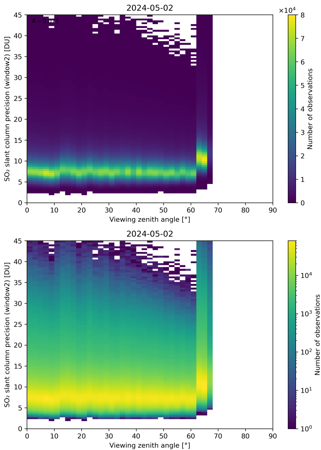
Figure 322: Scatter density plot of “Viewing zenith angle” against “SO 2 slant column precision (window2)” for 2024-05-02 to 2024-05-03.
