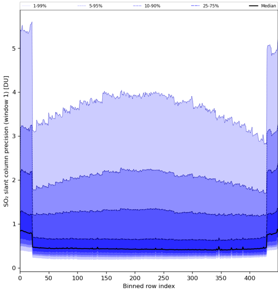
Figure 80: Along track statistics of “SO 2 slant column precision (window 1)” for 2024-05-02 to 2024-05-03
