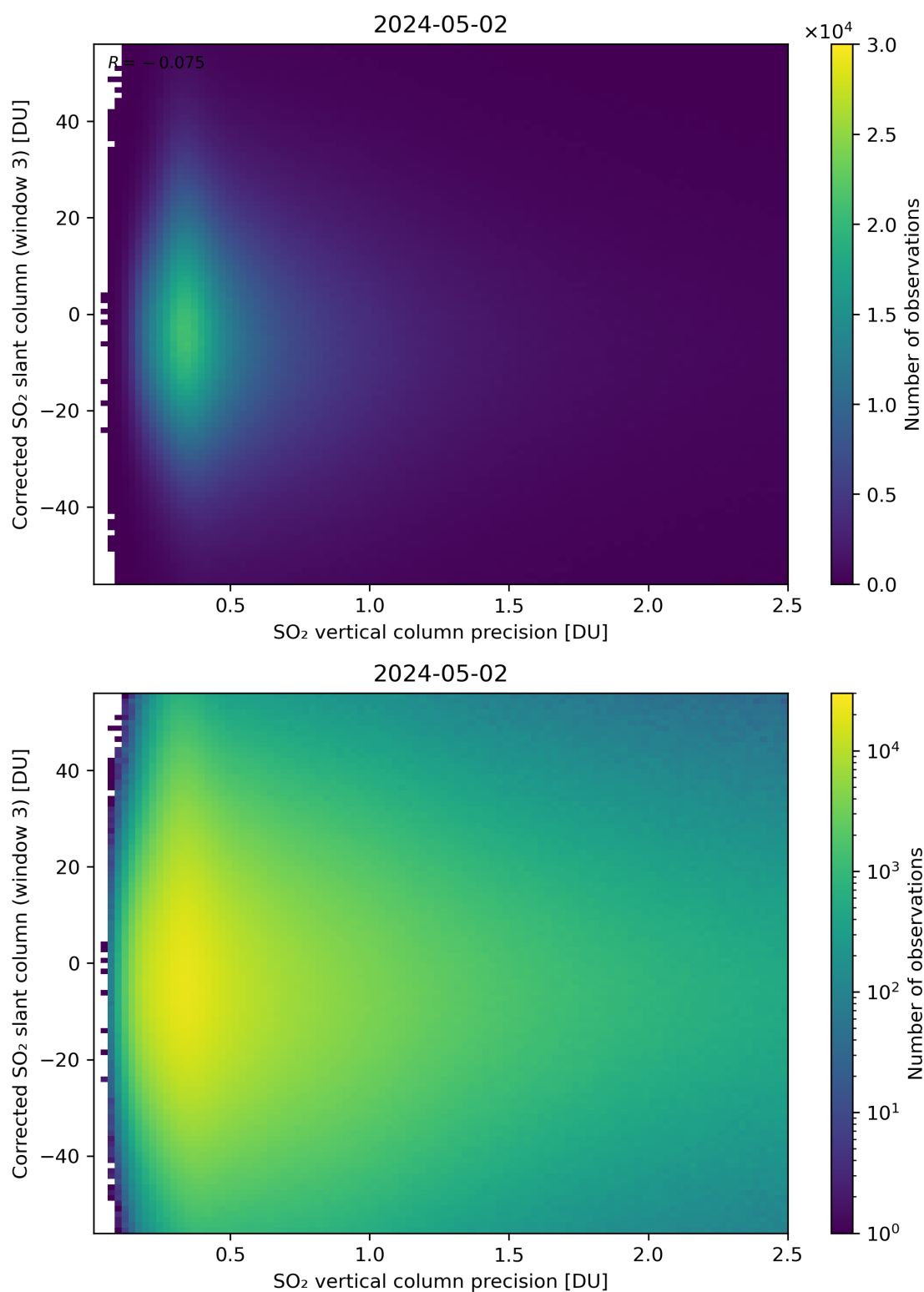
Figure 288: Scatter density plot of “SO 2 vertical column precision” against “Corrected SO 2 slant column (window 3)” for 2024-05-02 to 2024-05-03.
