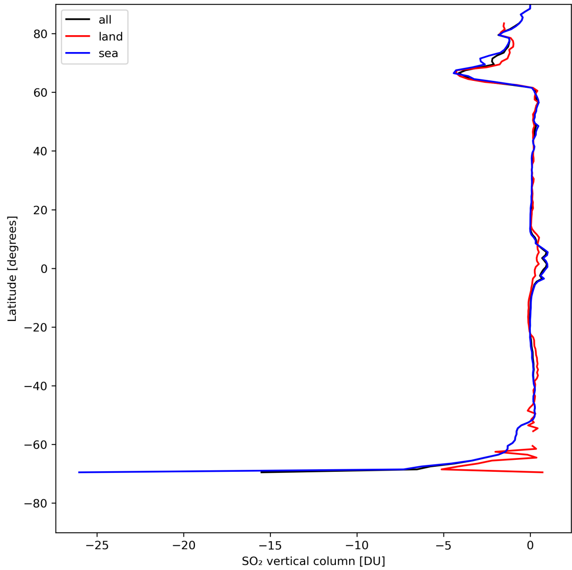
Figure 30: Zonal average of “SO 2 vertical column” for 2024-05-02 to 2024-05-03.
