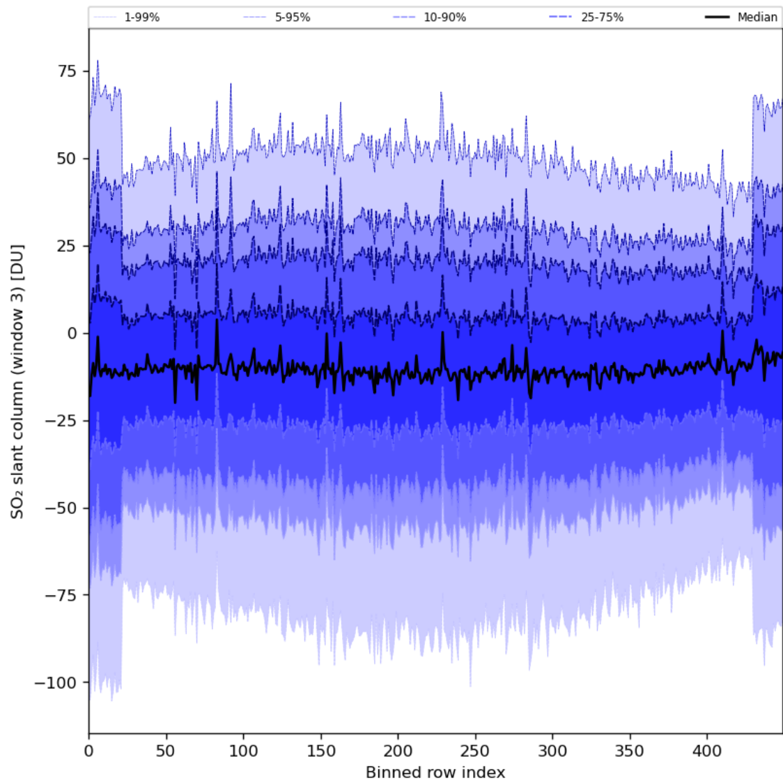
Figure 87: Along track statistics of “SO 2 slant column (window 3)” for 2024-05-02 to 2024-05-03
