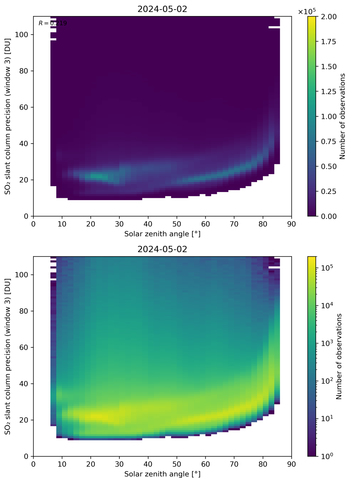
Figure 173: Scatter density plot of “Solar zenith angle” against “SO 2 slant column precision (window 3)” for 2024-05-02 to 2024-05-03.
