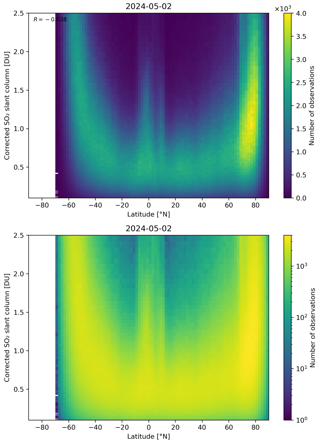
Figure 146: Scatter density plot of “Latitude” against “Corrected SO 2 slant column” for 2024-05-02 to 2024-05-03.
