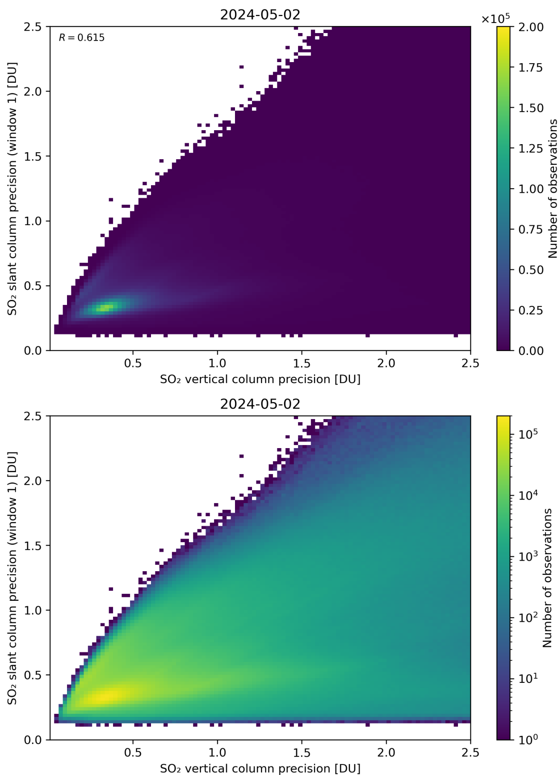
Figure 290: Scatter density plot of “SO 2 vertical column precision” against “SO 2 slant column precision (window 1)” for 2024-05-02 to 2024-05-03.
