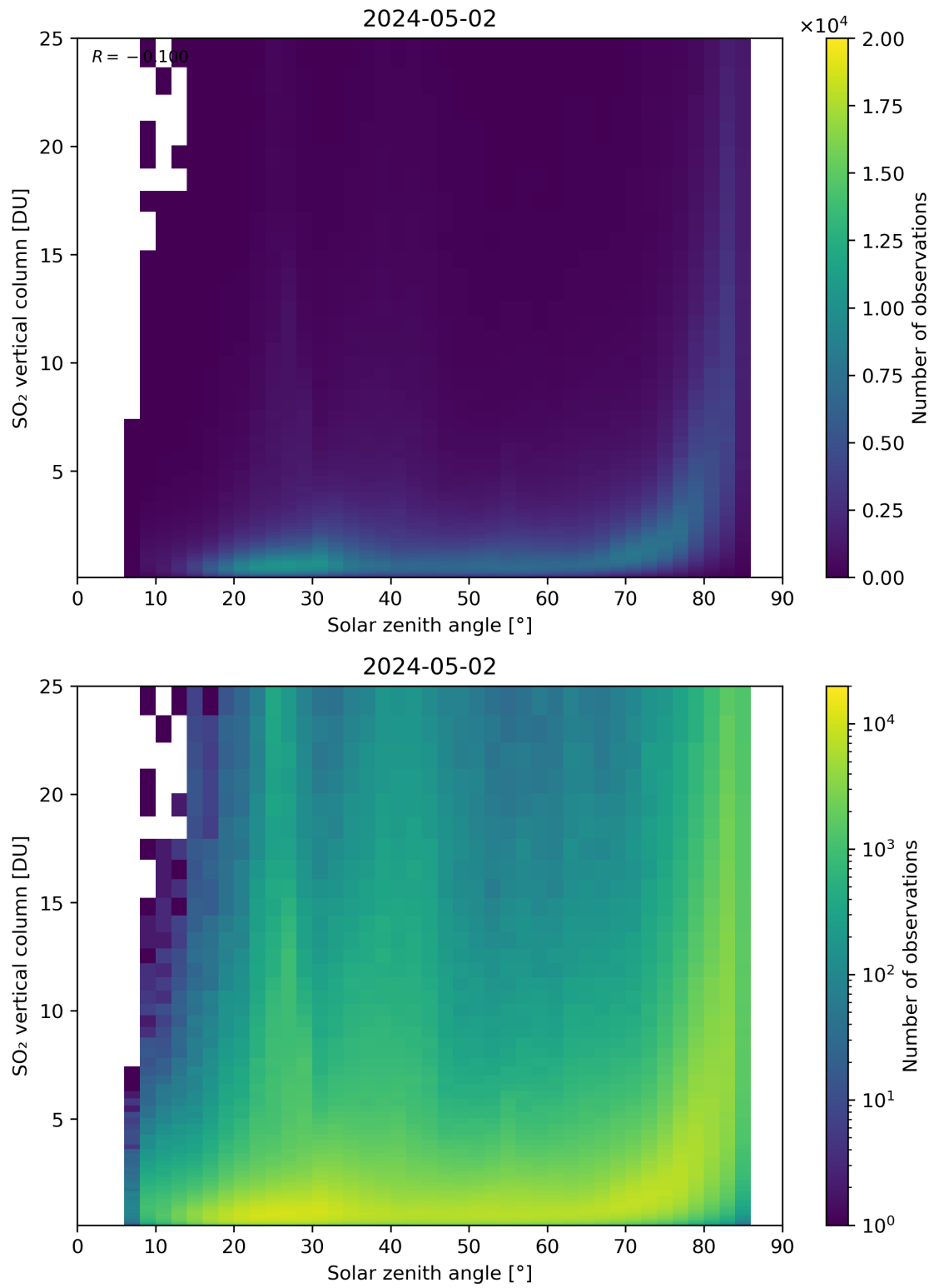
Figure 176: Scatter density plot of “Solar zenith angle” against “SO 2 vertical column” for 2024-05-02 to 2024-05-03.
