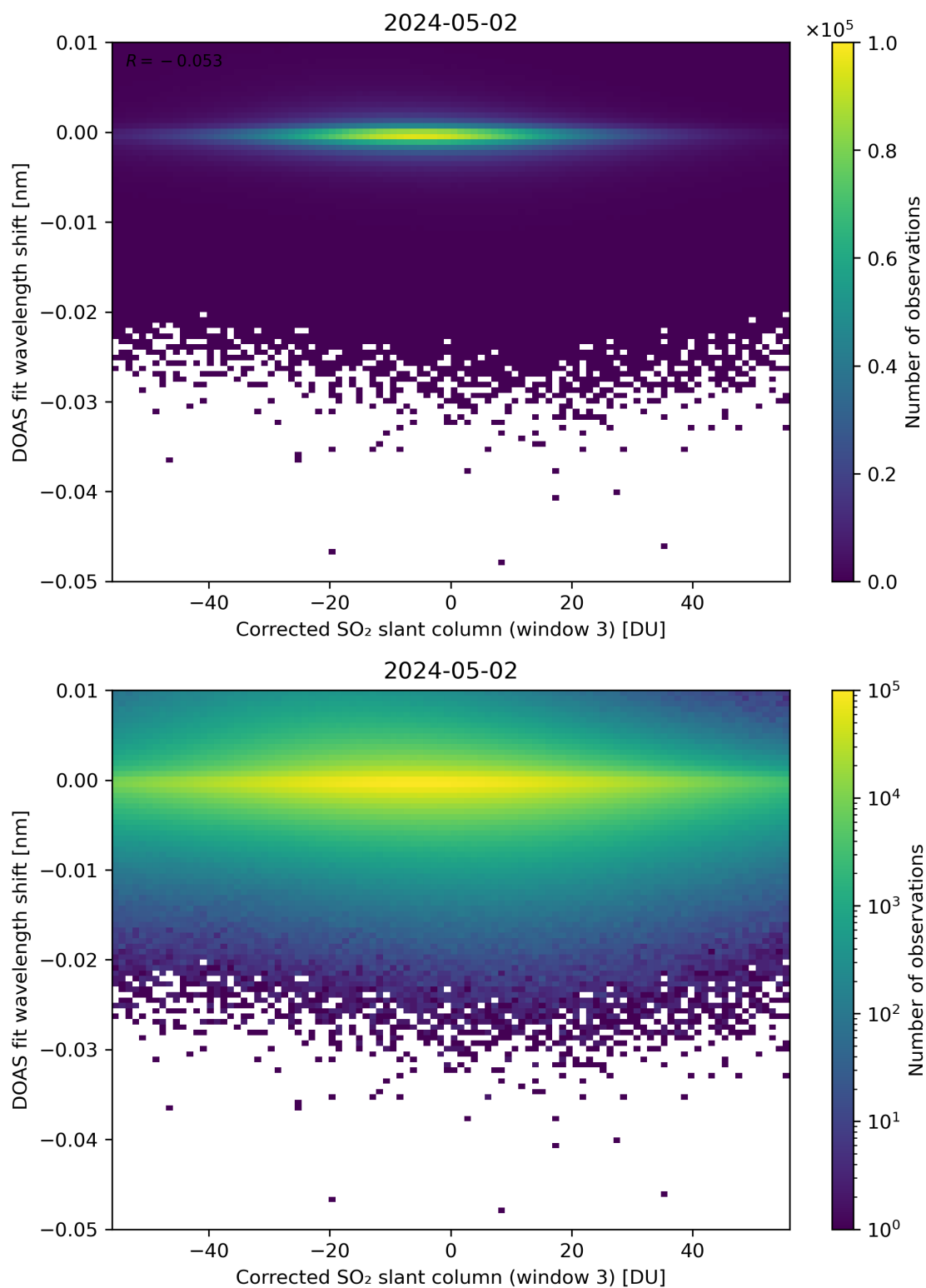
Figure 206: Scatter density plot of “Corrected SO 2 slant column (window 3)” against “DOAS fit wavelength shift” for 2024-05-02 to 2024-05-03.
