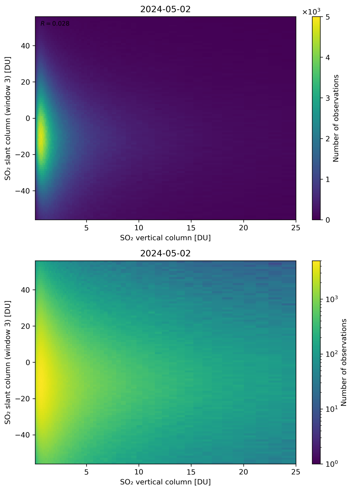
Figure 303: Scatter density plot of “SO 2 vertical column” against “SO 2 slant column (window 3)” for 2024-05-02 to 2024-05-03.
