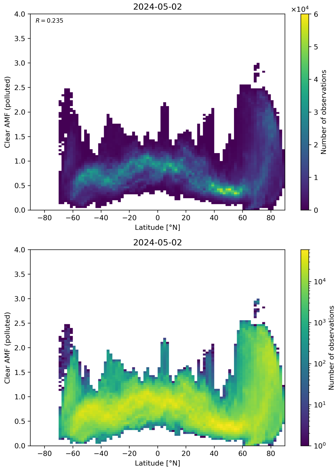
Figure 145: Scatter density plot of “Latitude” against “Clear AMF (polluted)” for 2024-05-02 to 2024-05-03.
