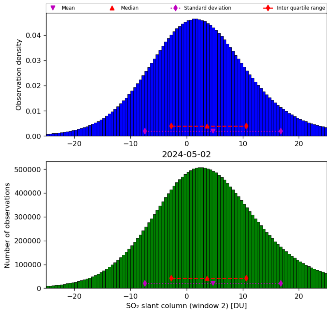
Figure 60: Histogram of “SO 2 slant column (window 2)” for 2024-05-02 to 2024-05-03
