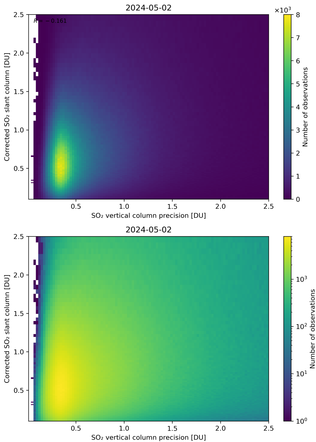
Figure 286: Scatter density plot of “SO 2 vertical column precision” against “Corrected SO 2 slant column” for 2024-05-02 to 2024-05-03.
