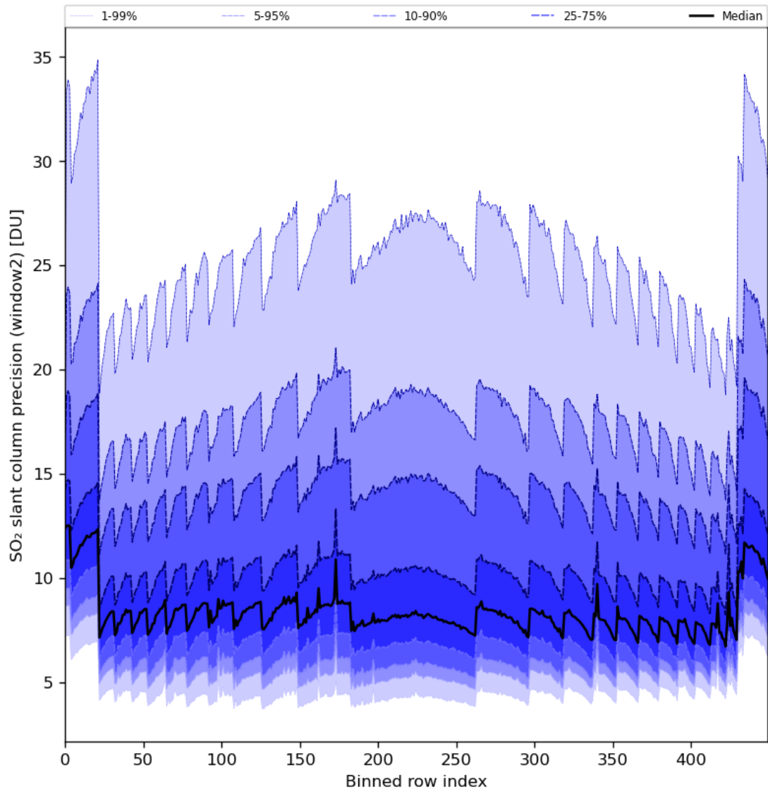
Figure 84: Along track statistics of “SO 2 slant column precision (window2)” for 2024-05-02 to 2024-05-03
