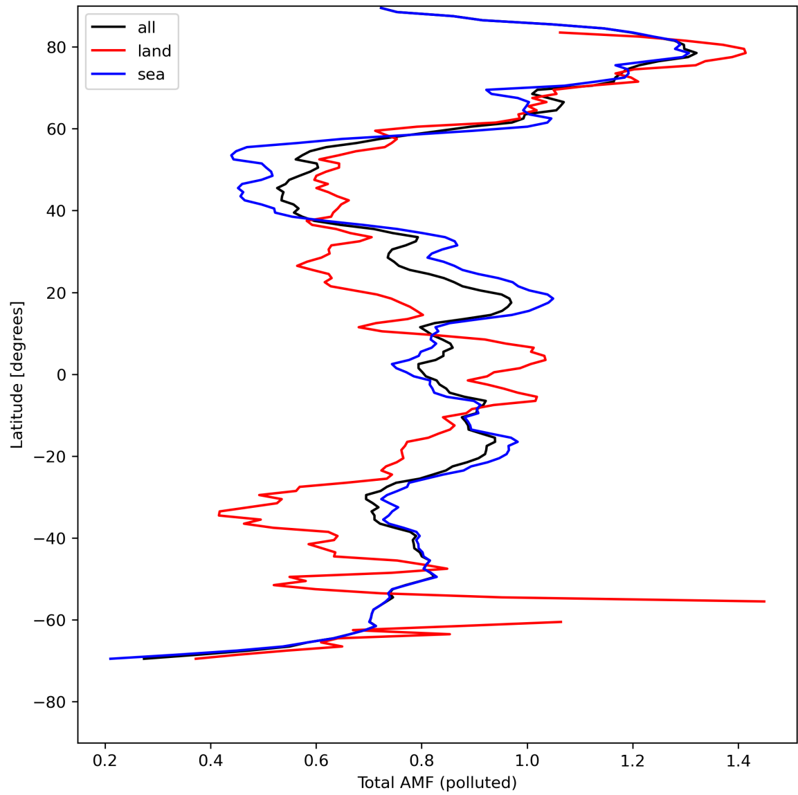
Figure 48: Zonal average of “Total AMF (polluted)” for 2024-05-02 to 2024-05-03.
