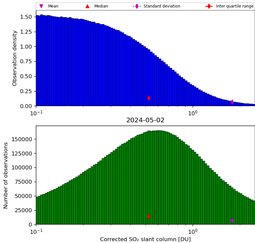
Figure 55: Histogram of “Corrected SO 2 slant column” for 2024-05-02 to 2024-05-03
