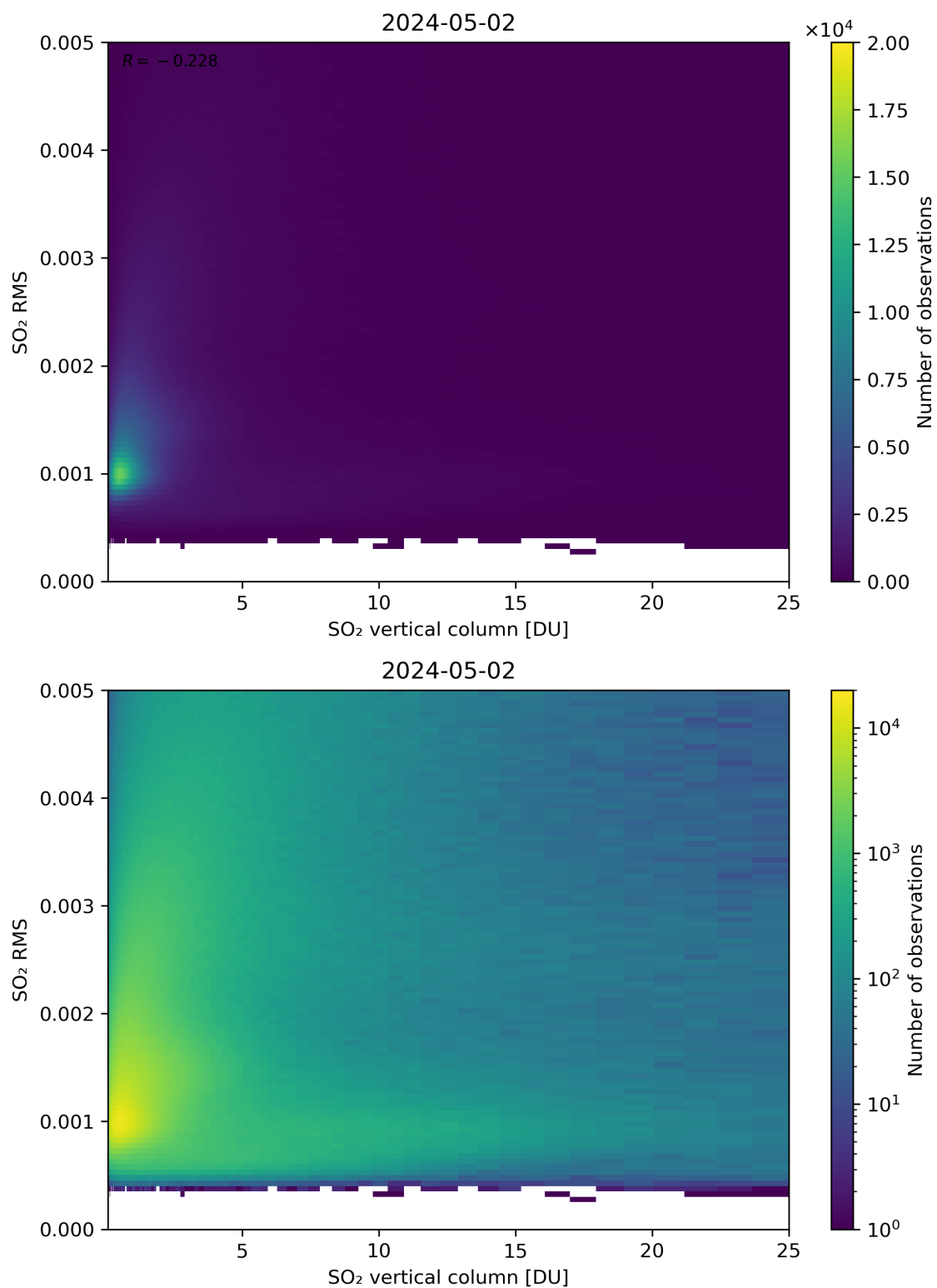
Figure 278: Scatter density plot of “SO 2 vertical column” against “SO 2 RMS” for 2024-05-02 to 2024-05-03.
