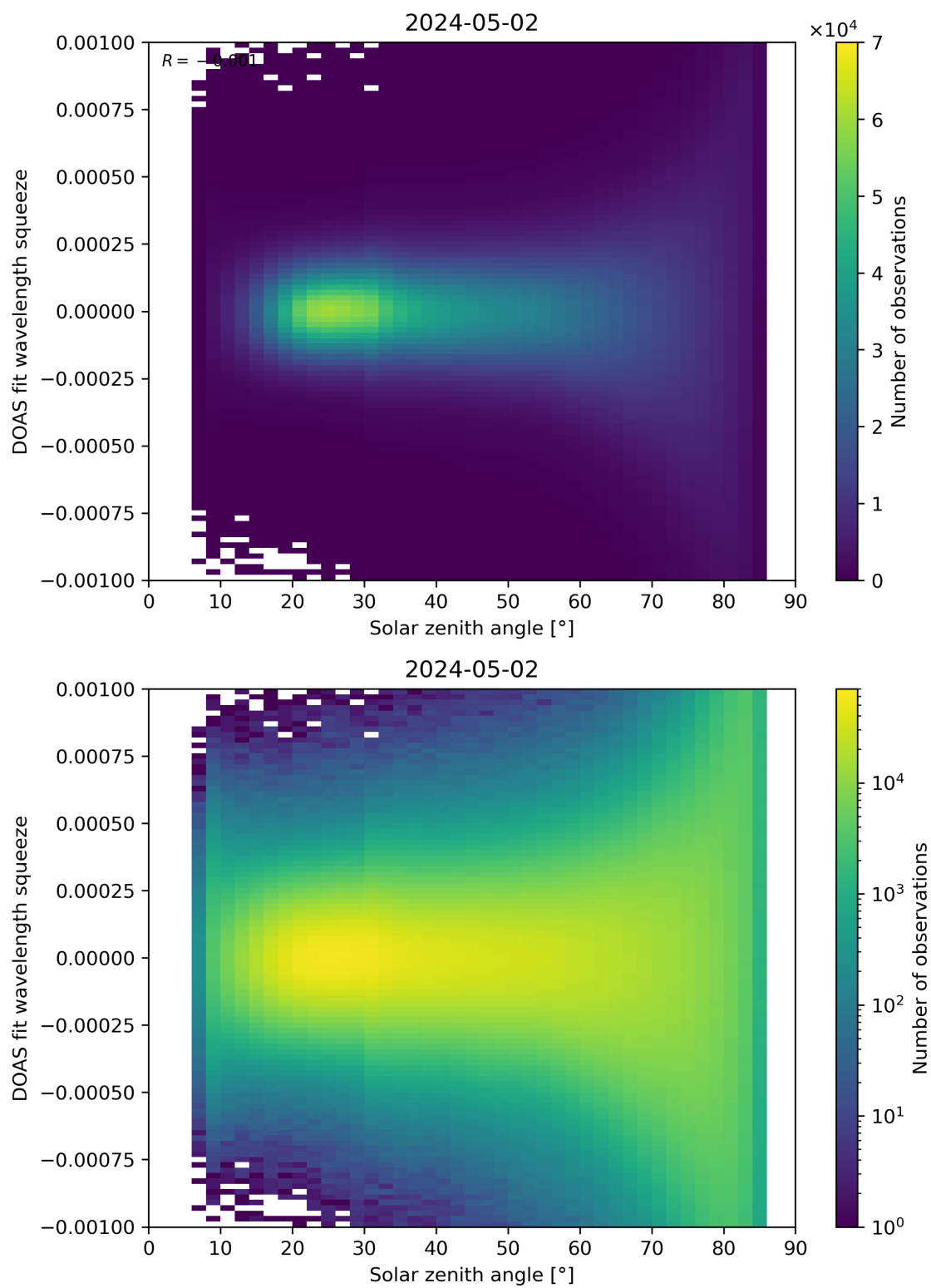
Figure 162: Scatter density plot of “Solar zenith angle” against “DOAS fit wavelength squeeze” for 2024-05-02 to 2024-05-03.
