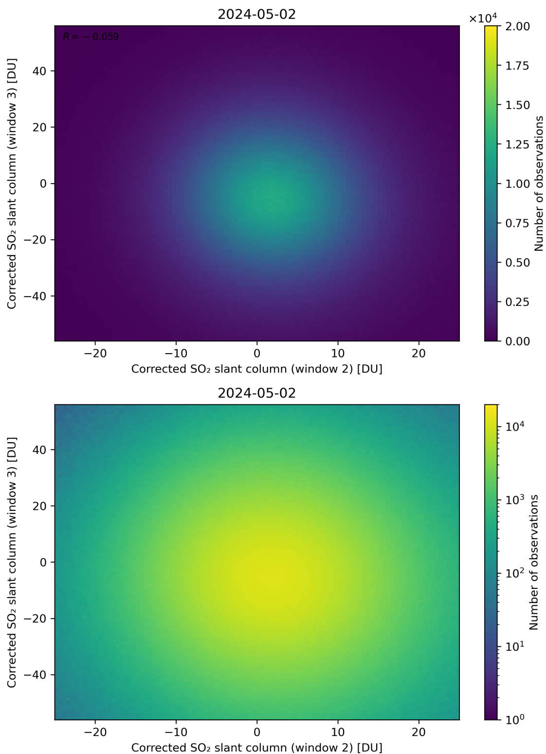
Figure 200: Scatter density plot of “Corrected SO 2 slant column (window 2)” against “Corrected SO 2 slant column (window 3)” for 2024-05-02 to 2024-05-03.
