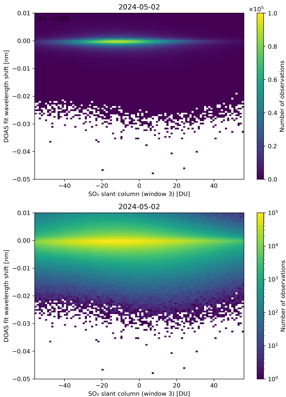
Figure 254: Scatter density plot of “SO 2 slant column (window 3)” against “DOAS fit wavelength shift” for 2024-05-02 to 2024-05-03.
