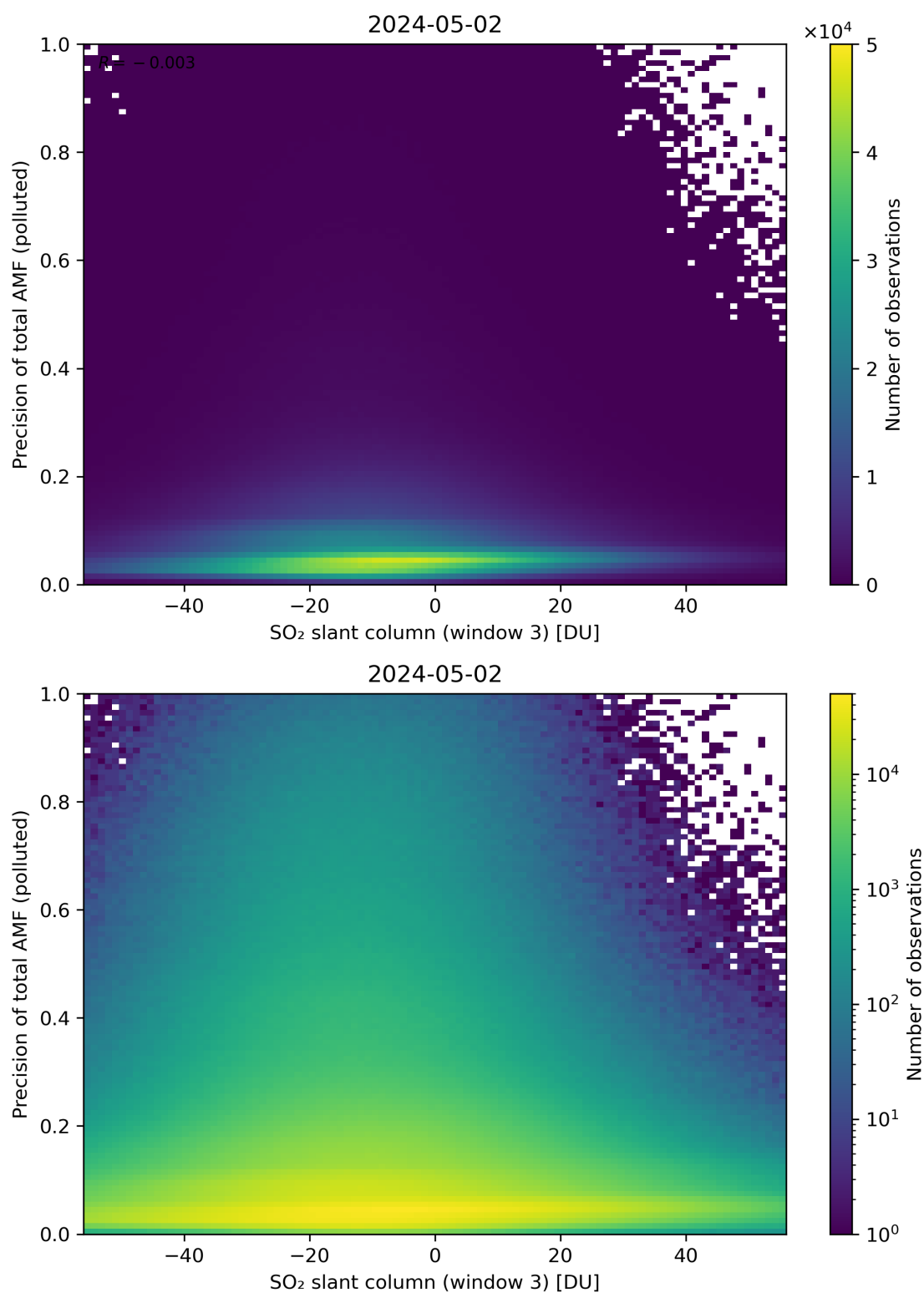
Figure 269: Scatter density plot of “SO 2 slant column (window 3)” against “Precision of total AMF (polluted)” for 2024-05-02 to 2024-05-03.
