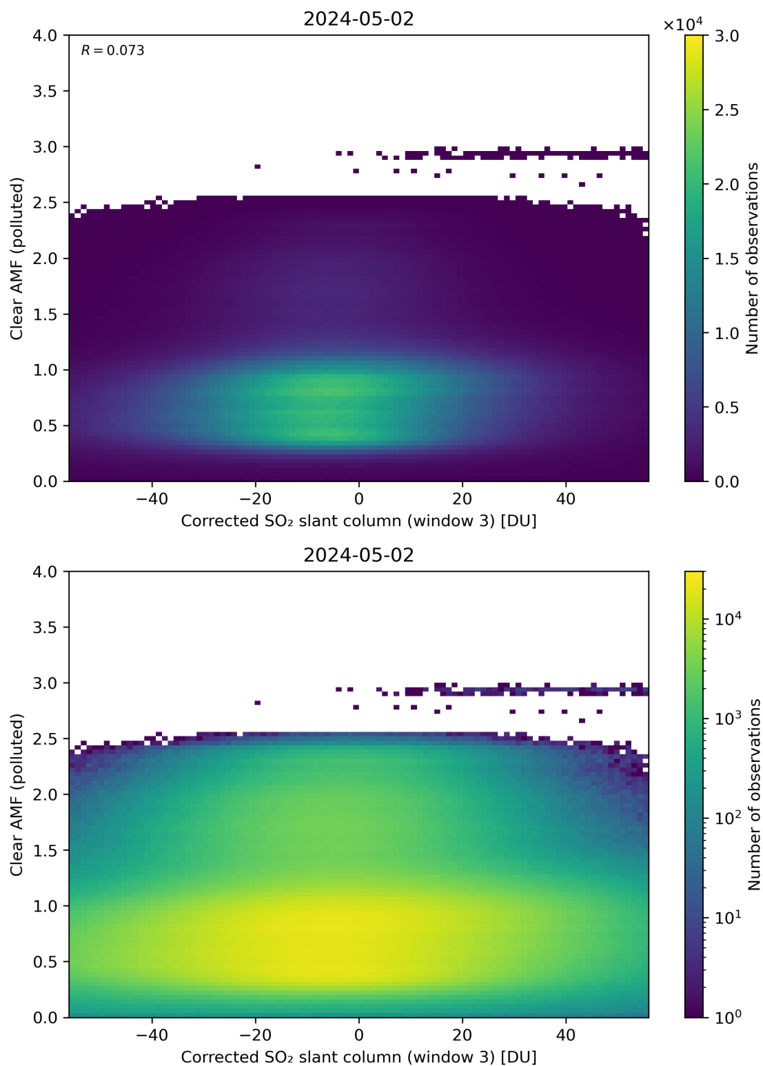
Figure 209: Scatter density plot of “Corrected SO 2 slant column (window 3)” against “Clear AMF (polluted)” for 2024-05-02 to 2024-05-03.
