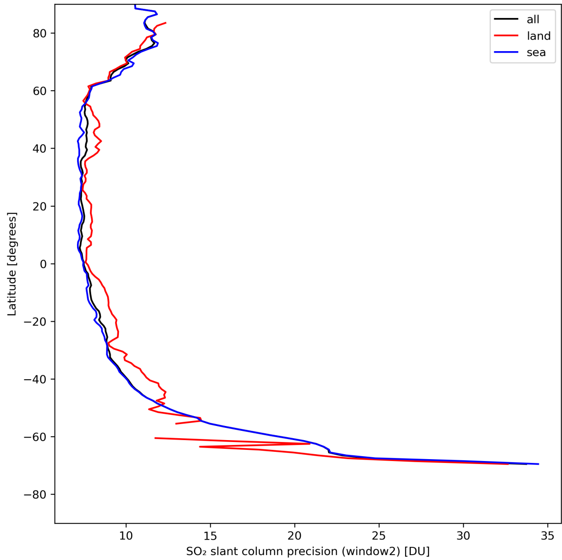
Figure 38: Zonal average of “SO 2 slant column precision (window2)” for 2024-05-02 to 2024-05-03.
