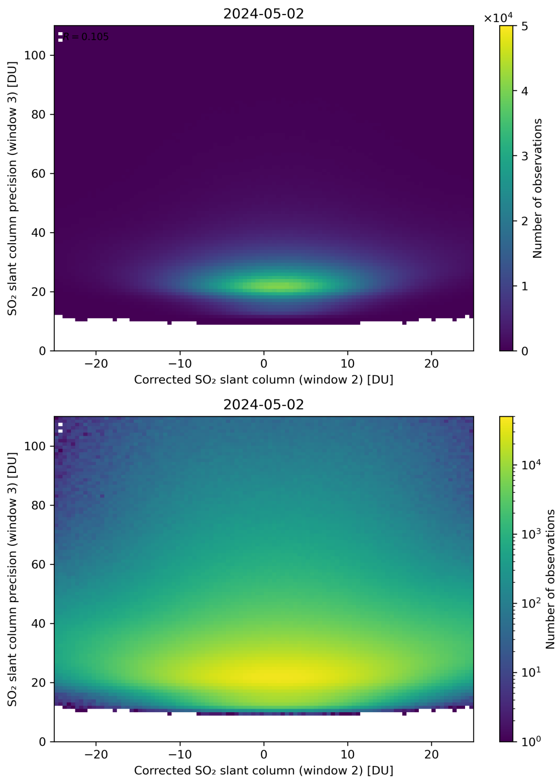
Figure 202: Scatter density plot of “Corrected SO 2 slant column (window 2)” against “SO 2 slant column precision (window 3)” for 2024-05-02 to 2024-05-03.
