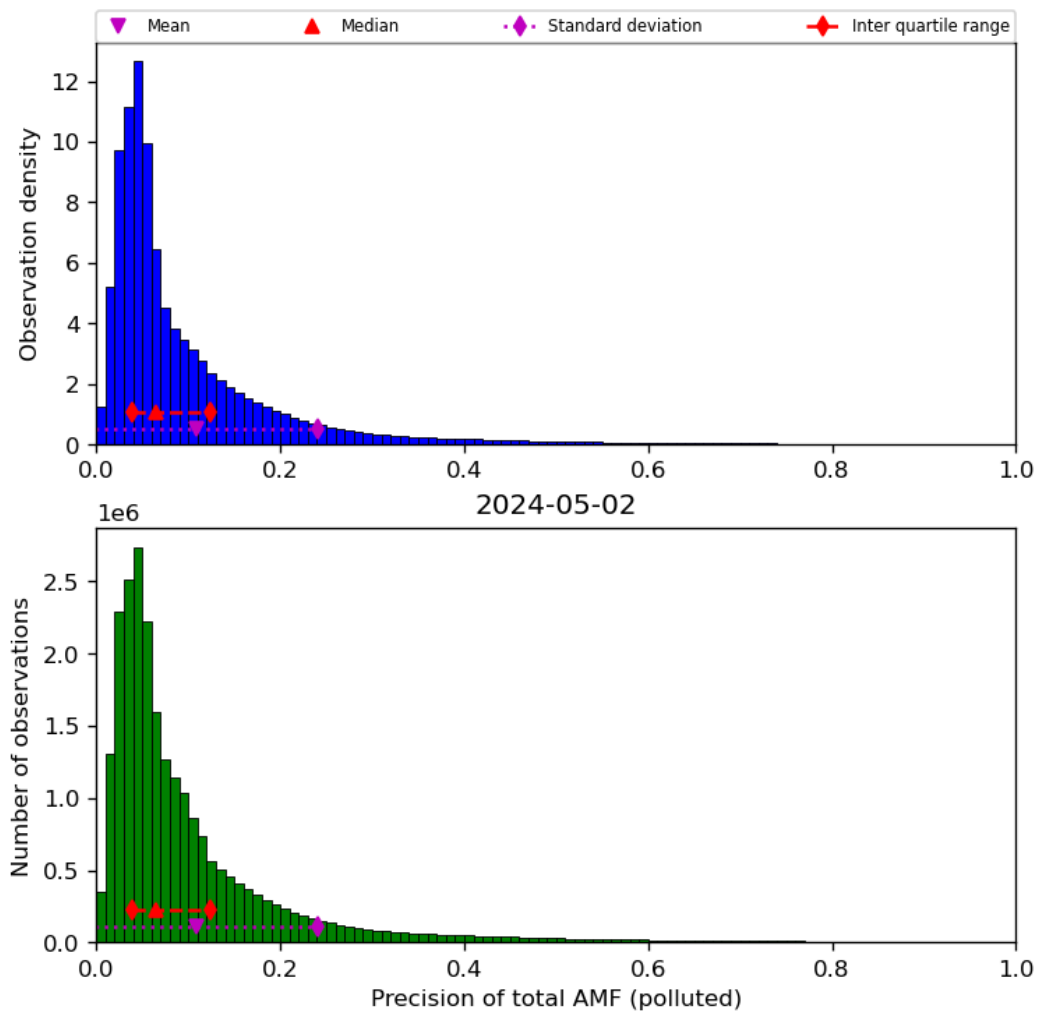
Figure 72: Histogram of “Precision of total AMF (polluted)” for 2024-05-02 to 2024-05-03
