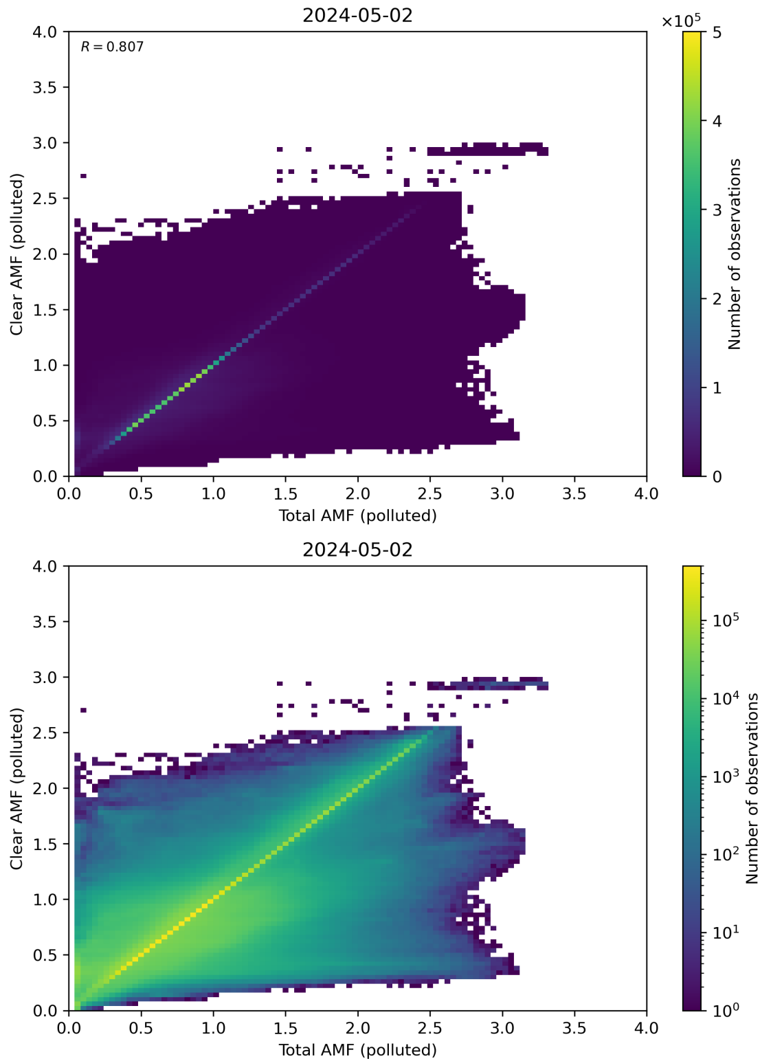
Figure 271: Scatter density plot of “Total AMF (polluted)” against “Clear AMF (polluted)” for 2024-05-02 to 2024-05-03.
