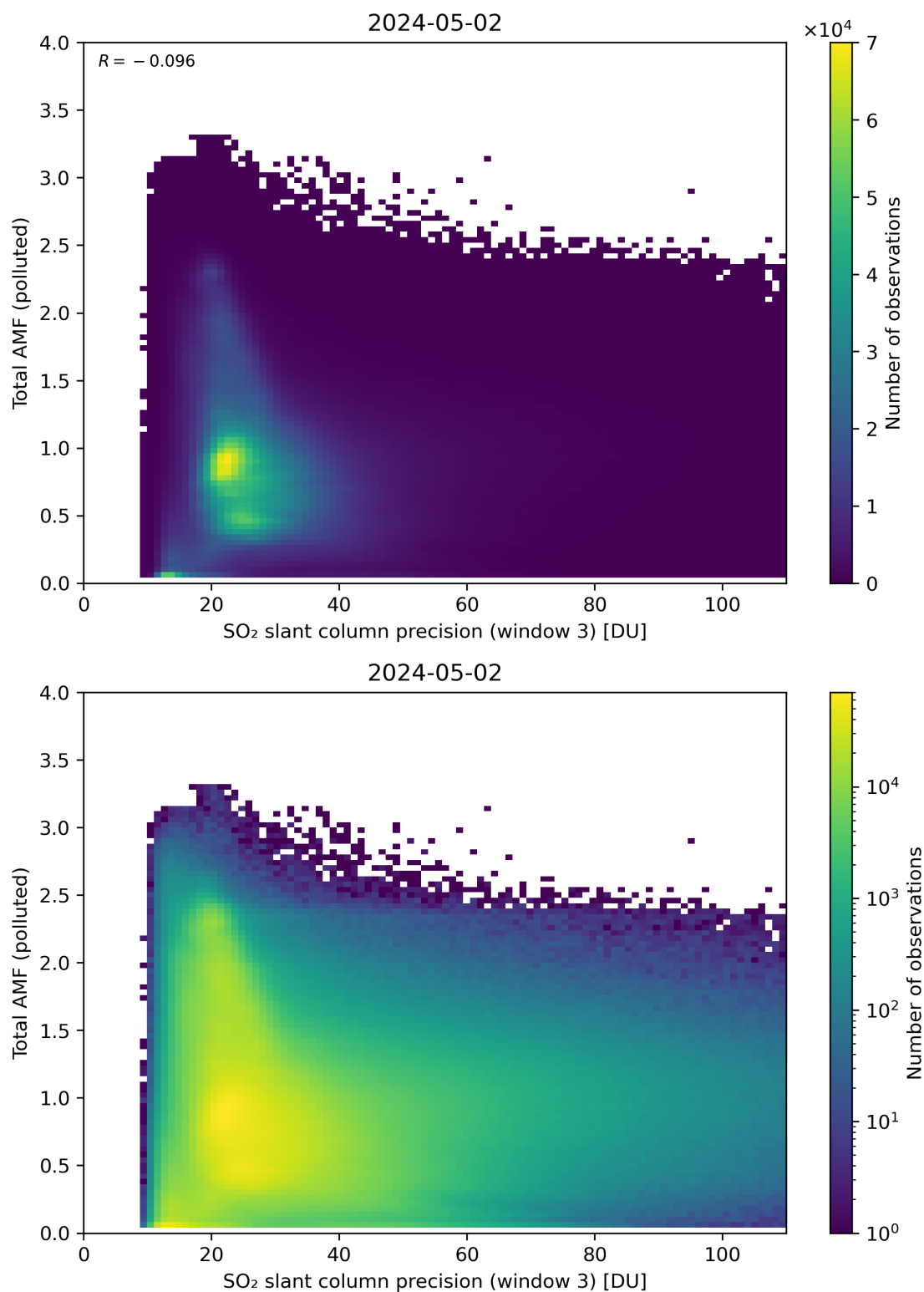
Figure 263: Scatter density plot of “SO 2 slant column precision (window 3)” against “Total AMF (polluted)” for 2024-05-02 to 2024-05-03.
