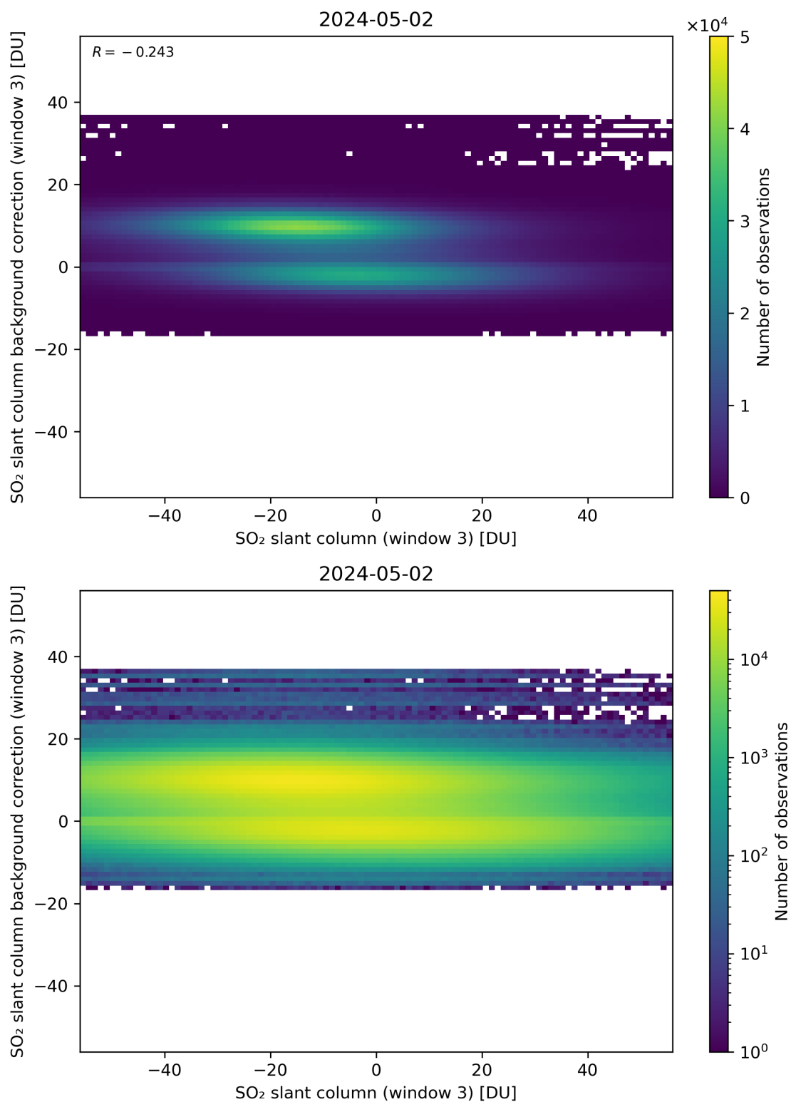
Figure 253: Scatter density plot of “SO 2 slant column (window 3)” against “SO 2 slant column background correction (window 3)” for 2024-05-02 to 2024-05-03.
