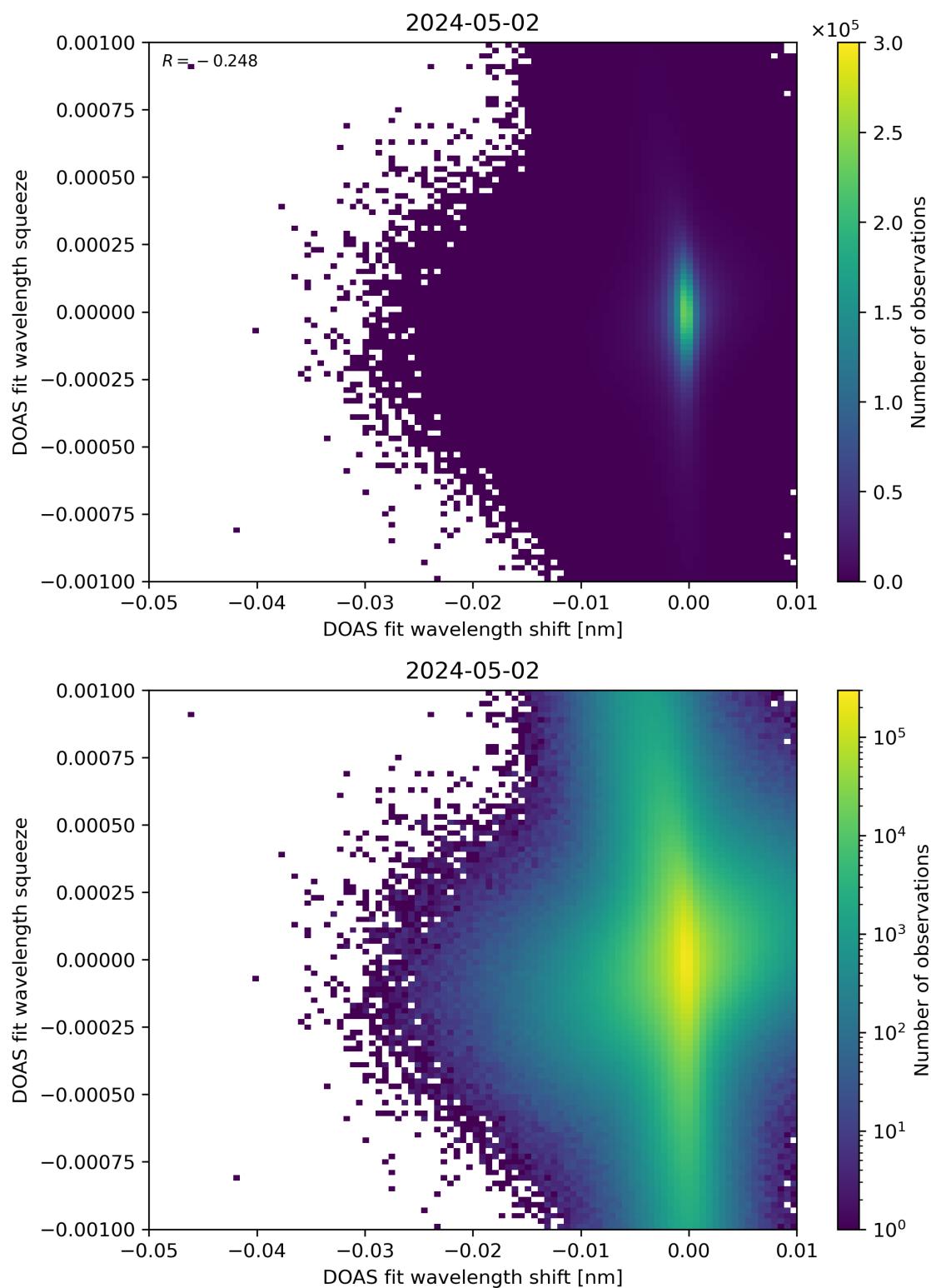
Figure 127: Scatter density plot of “DOAS fit wavelength shift” against “DOAS fit wavelength squeeze” for 2024-05-02 to 2024-05-03.
