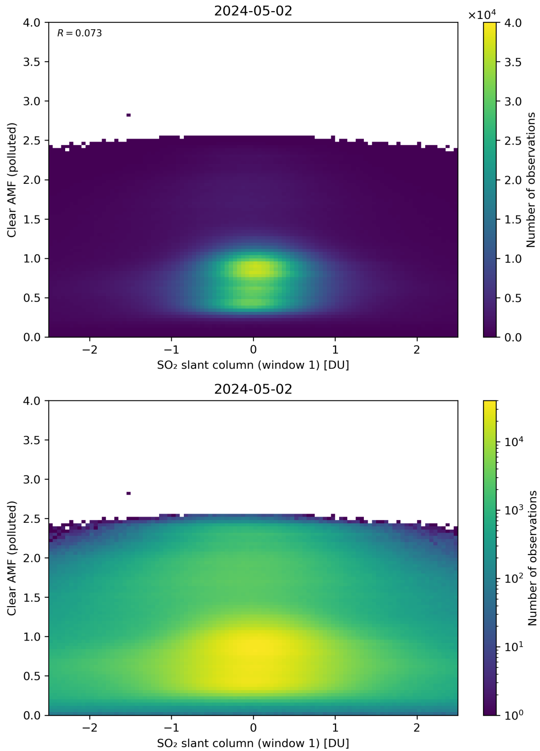
Figure 232: Scatter density plot of “SO 2 slant column (window 1)” against “Clear AMF (polluted)” for 2024-05-02 to 2024-05-03.
