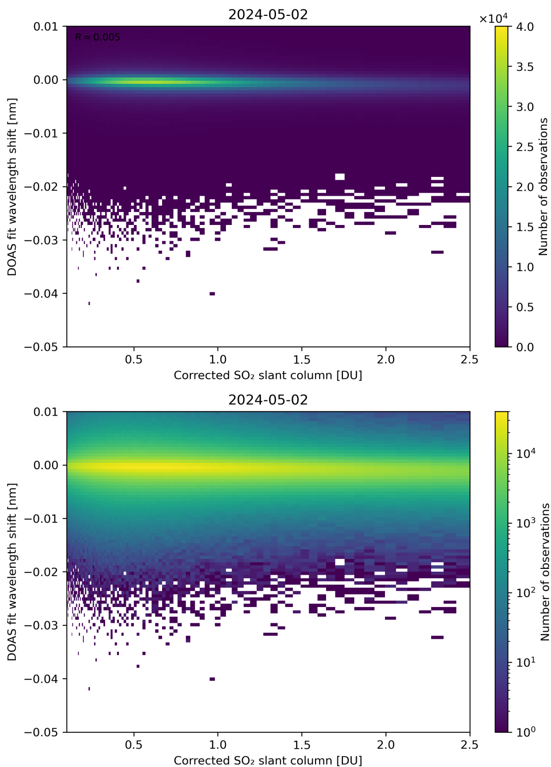
Figure 181: Scatter density plot of “Corrected SO 2 slant column” against “DOAS fit wavelength shift” for 2024-05-02 to 2024-05-03.
