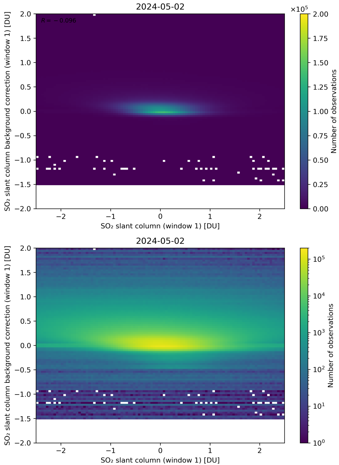
Figure 212: Scatter density plot of “SO 2 slant column (window 1)” against “SO 2 slant column background correction (window 1)” for 2024-05-02 to 2024-05-03.
