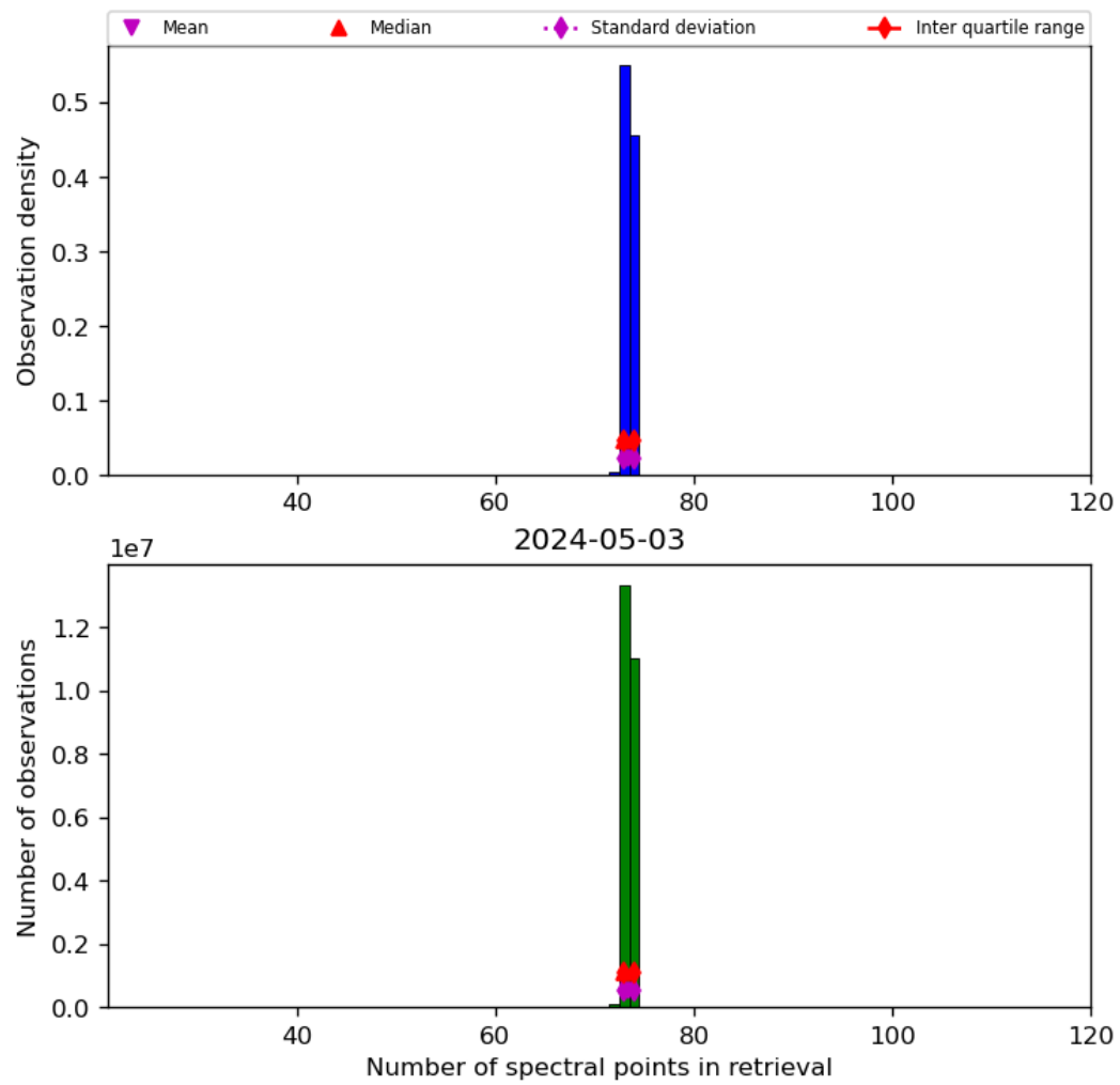
Figure 74: Histogram of “Number of spectral points in retrieval” for 2024-05-02 to 2024-05-04
