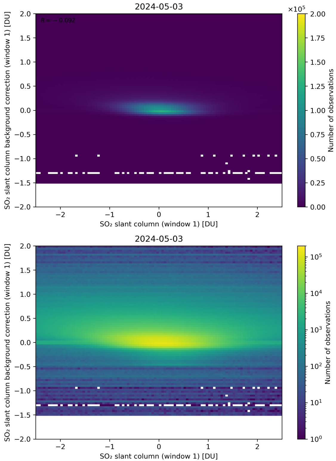
Figure 212: Scatter density plot of “SO 2 slant column (window 1)” against “SO 2 slant column background correction (window 1)” for 2024-05-02 to 2024-05-04.
