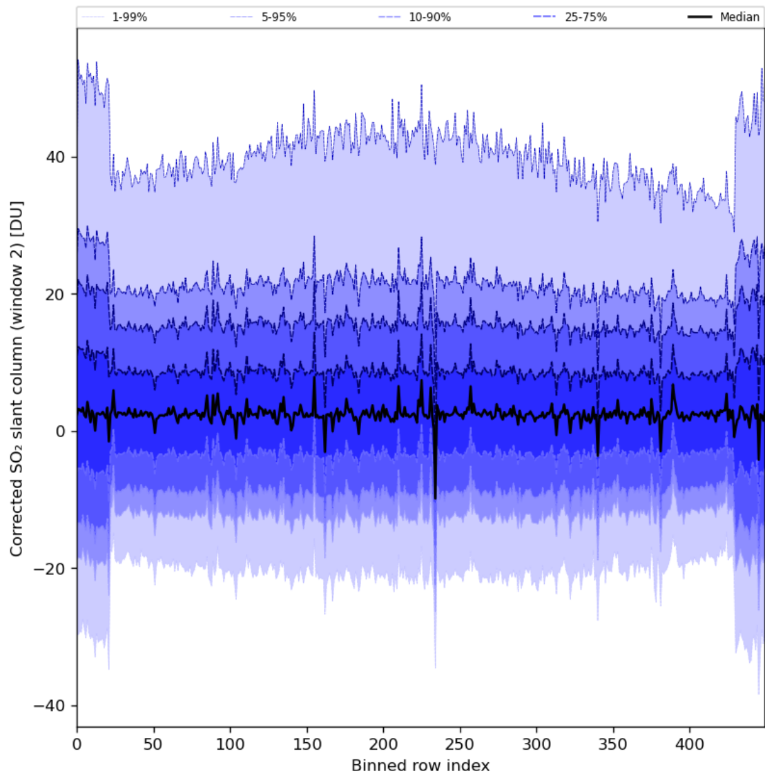
Figure 85: Along track statistics of “Corrected SO 2 slant column (window 2)” for 2024-05-02 to 2024-05-04
