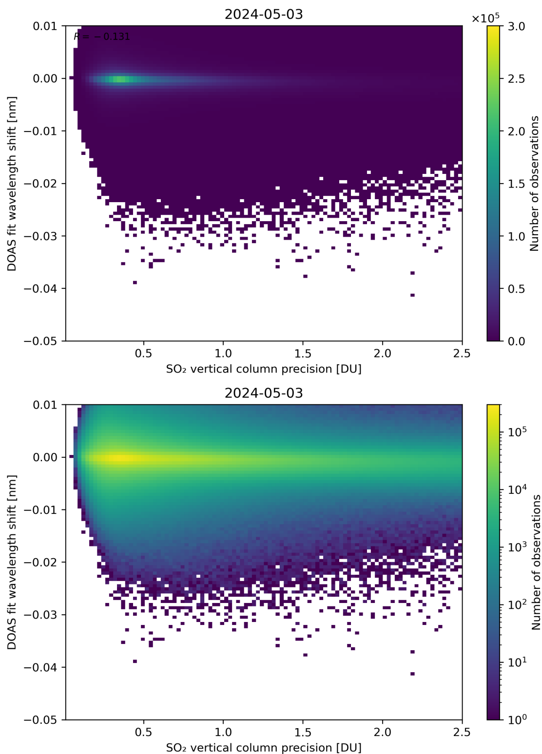
Figure 282: Scatter density plot of “SO 2 vertical column precision” against “DOAS fit wavelength shift” for 2024-05-02 to 2024-05-04.
