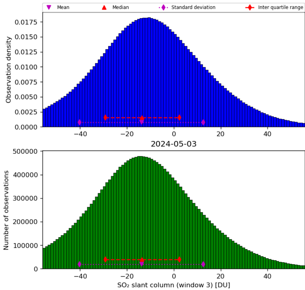
Figure 64: Histogram of “SO 2 slant column (window 3)” for 2024-05-02 to 2024-05-04
