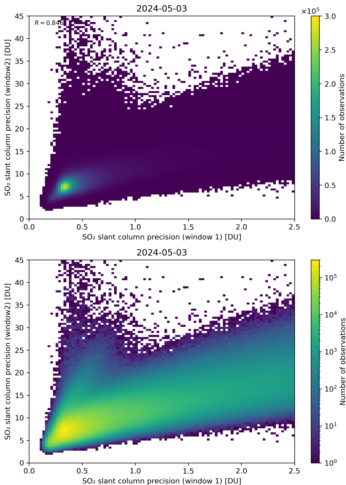
Figure 227: Scatter density plot of “SO 2 slant column precision (window 1)” against “SO 2 slant column precision (window 2)” for 2024-05-02 to 2024-05-04.
