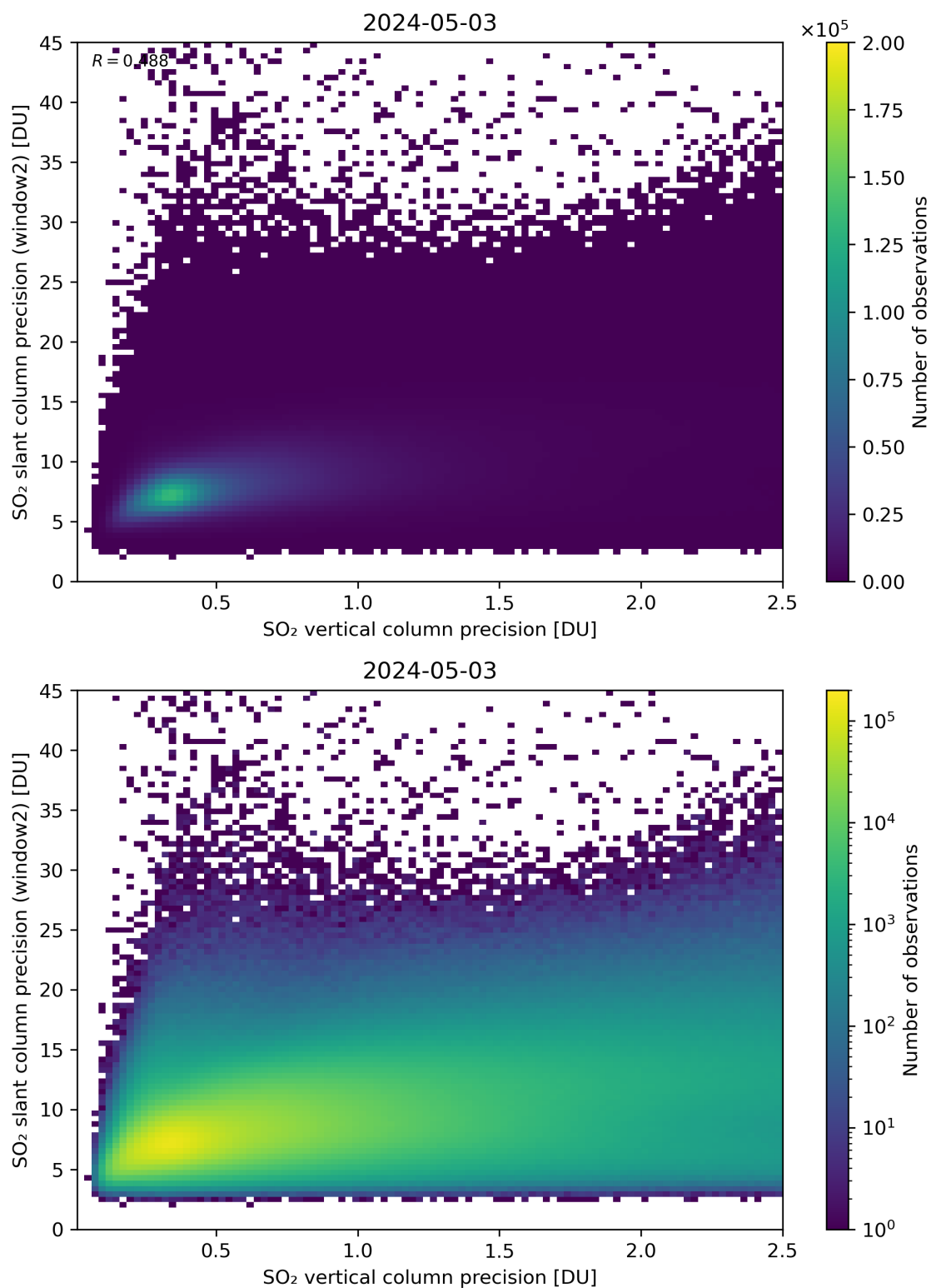
Figure 291: Scatter density plot of “SO 2 vertical column precision” against “SO 2 slant column precision (window2)” for 2024-05-02 to 2024-05-04.
