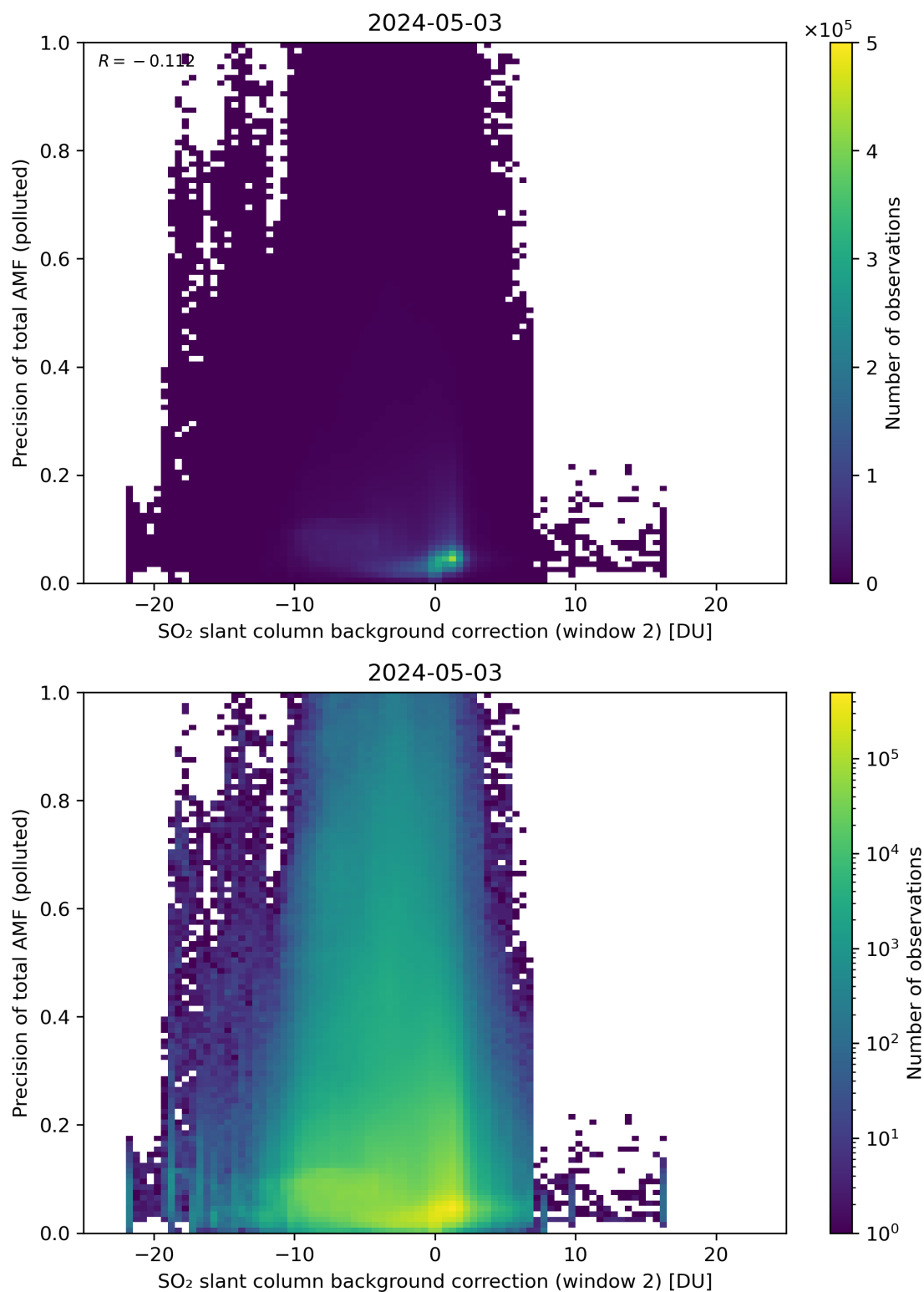
Figure 120: Scatter density plot of “SO 2 slant column background correction (window 2)” against “Precision of total AMF (polluted)” for 2024-05-02 to 2024-05-04.
