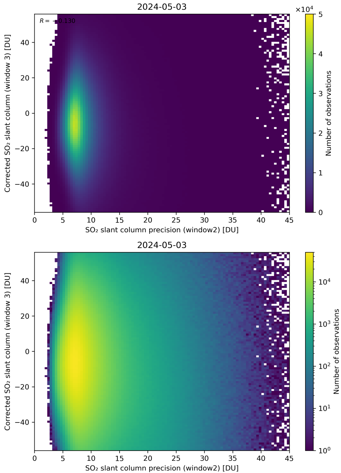
Figure 248: Scatter density plot of “SO 2 slant column precision (window2)” against “Corrected SO 2 slant column (window 3)” for 2024-05-02 to 2024-05-04.
