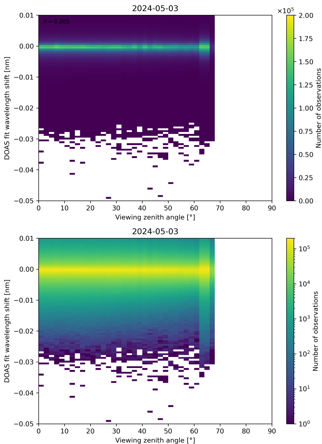
Figure 311: Scatter density plot of “Viewing zenith angle” against “DOAS fit wavelength shift” for 2024-05-02 to 2024-05-04.
