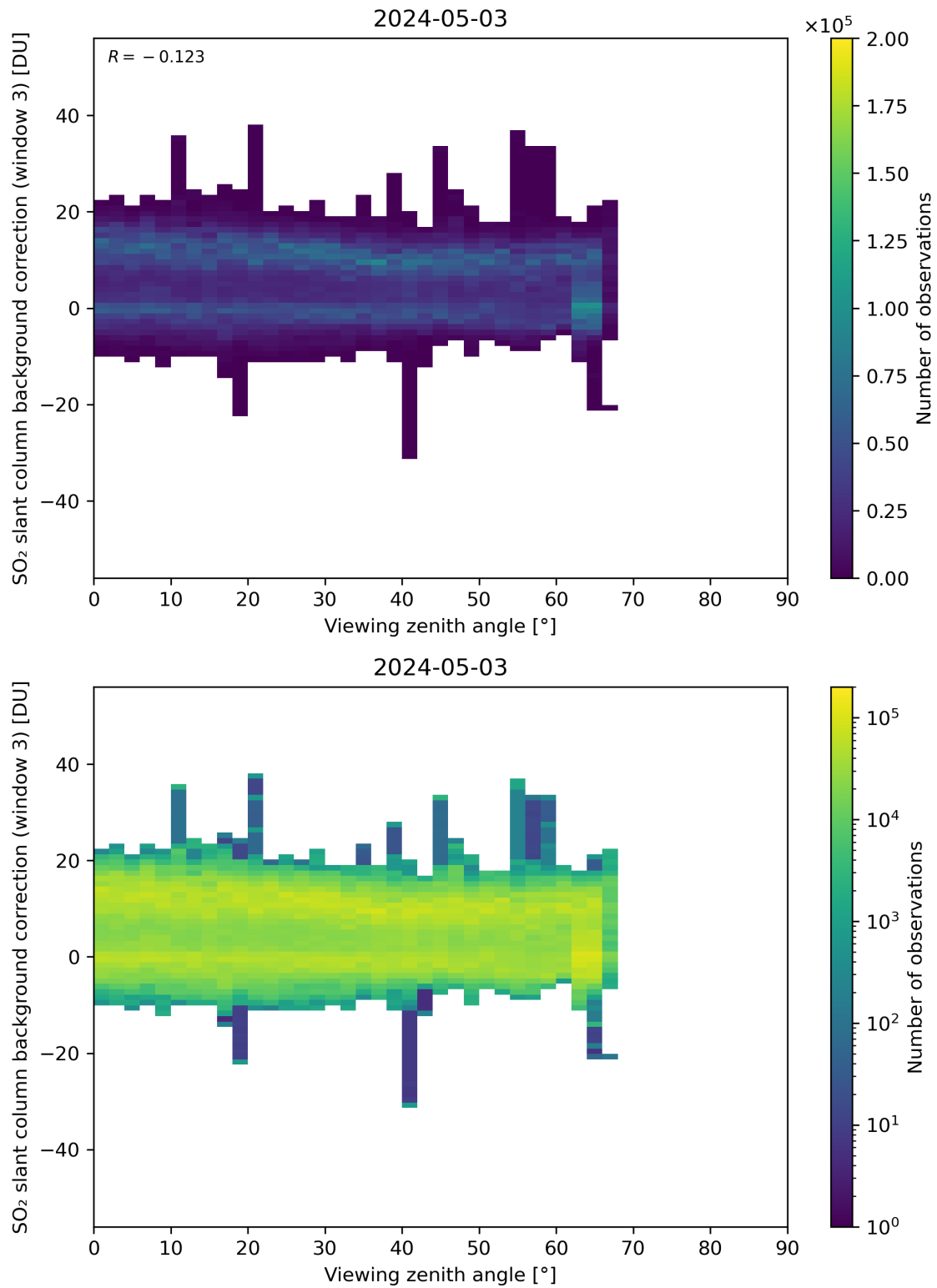
Figure 310: Scatter density plot of “Viewing zenith angle” against “SO 2 slant column background correction (window 3)” for 2024-05-02 to 2024-05-04.
