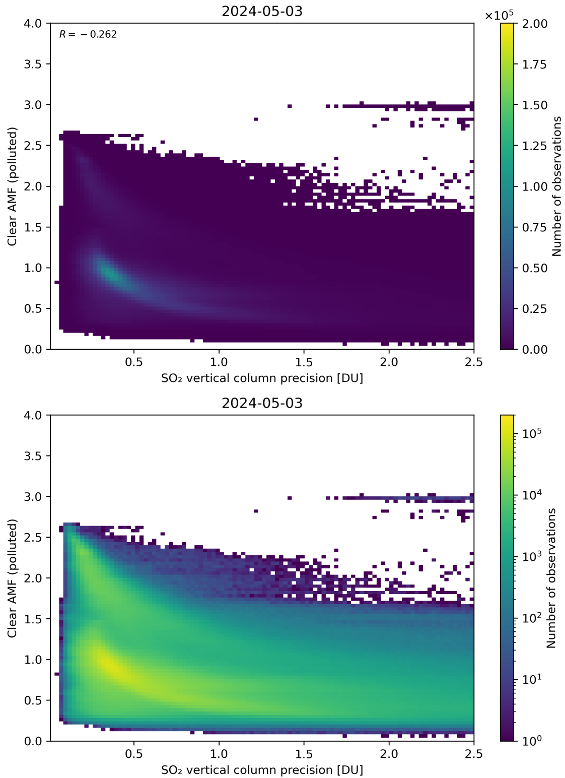
Figure 285: Scatter density plot of “SO 2 vertical column precision” against “Clear AMF (polluted)” for 2024-05-02 to 2024-05-04.
