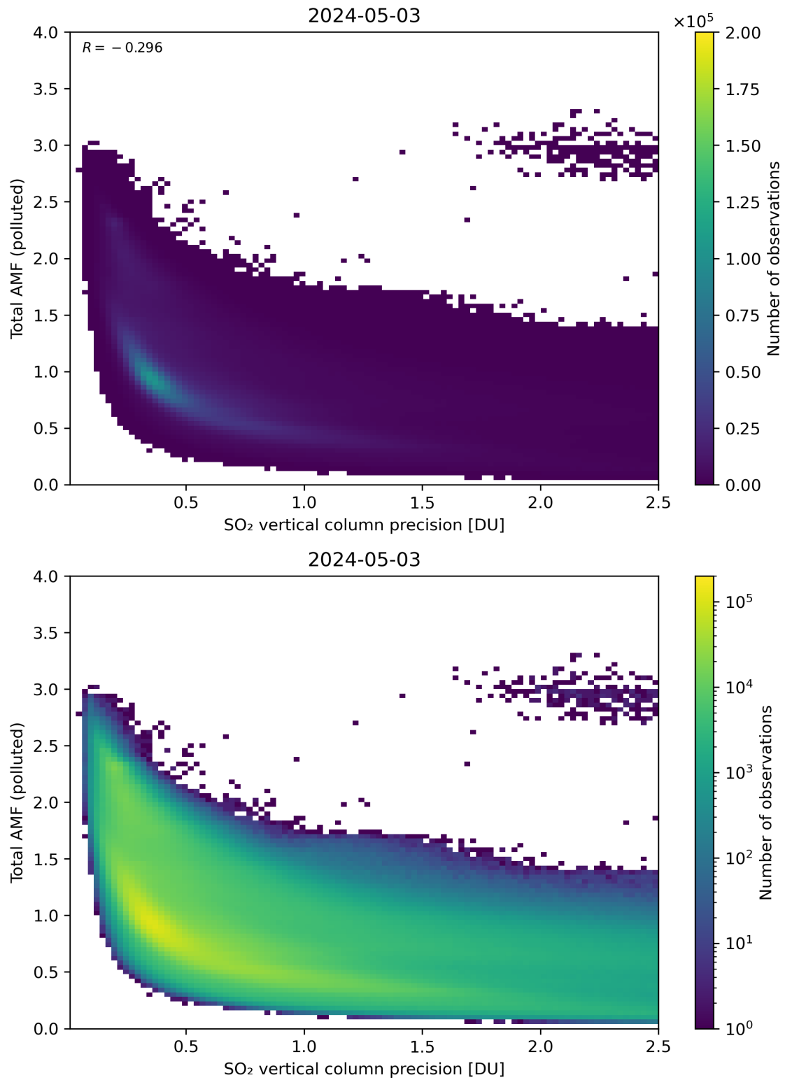
Figure 294: Scatter density plot of “SO 2 vertical column precision” against “Total AMF (polluted)” for 2024-05-02 to 2024-05-04.
