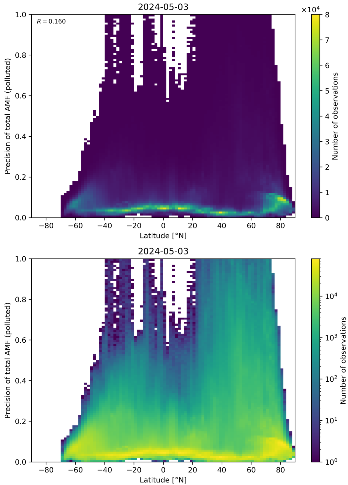
Figure 155: Scatter density plot of “Latitude” against “Precision of total AMF (polluted)” for 2024-05-02 to 2024-05-04.
