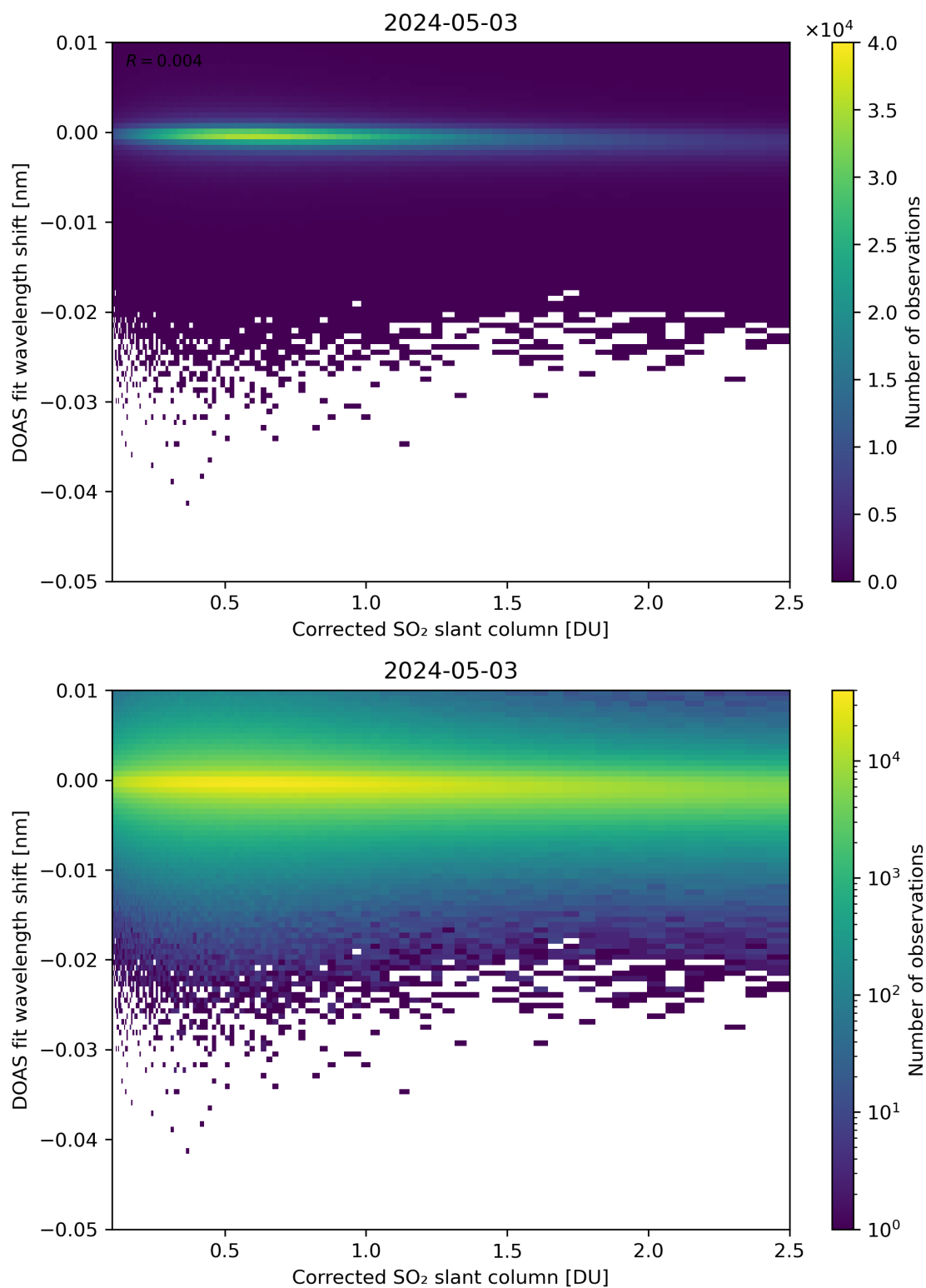
Figure 181: Scatter density plot of “Corrected SO 2 slant column” against “DOAS fit wavelength shift” for 2024-05-02 to 2024-05-04.
