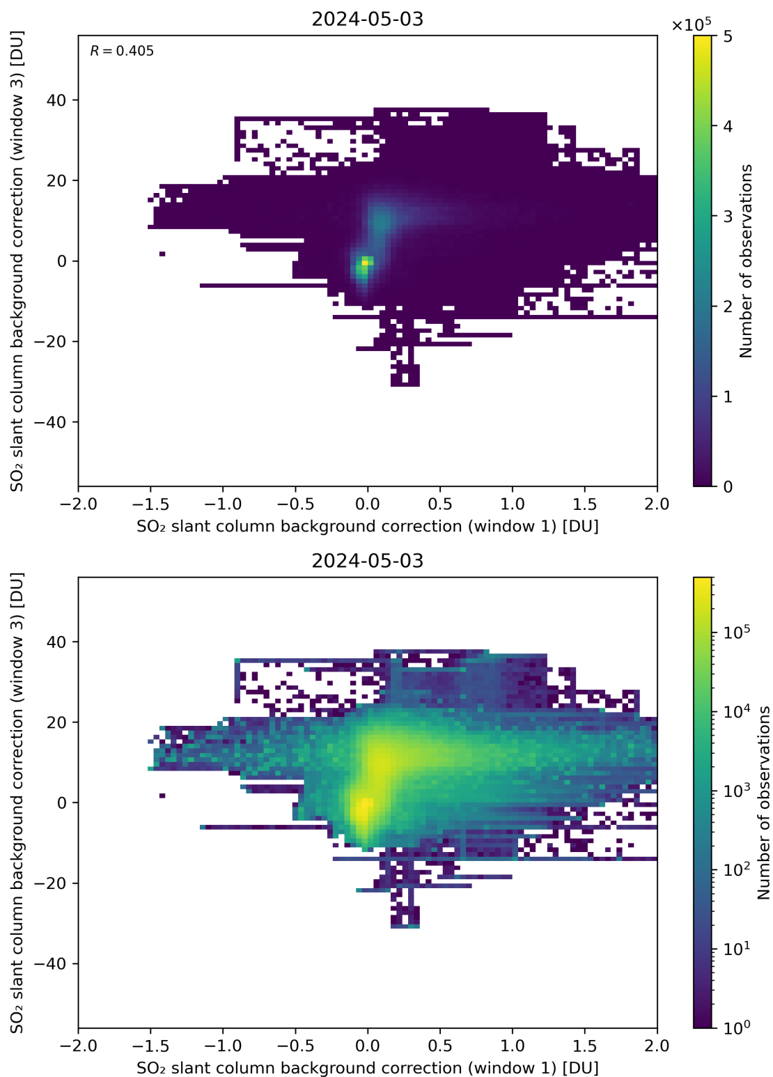
Figure 99: Scatter density plot of “SO 2 slant column background correction (window 1)” against “SO 2 slant column background correction (window 3)” for 2024-05-02 to 2024-05-04.
