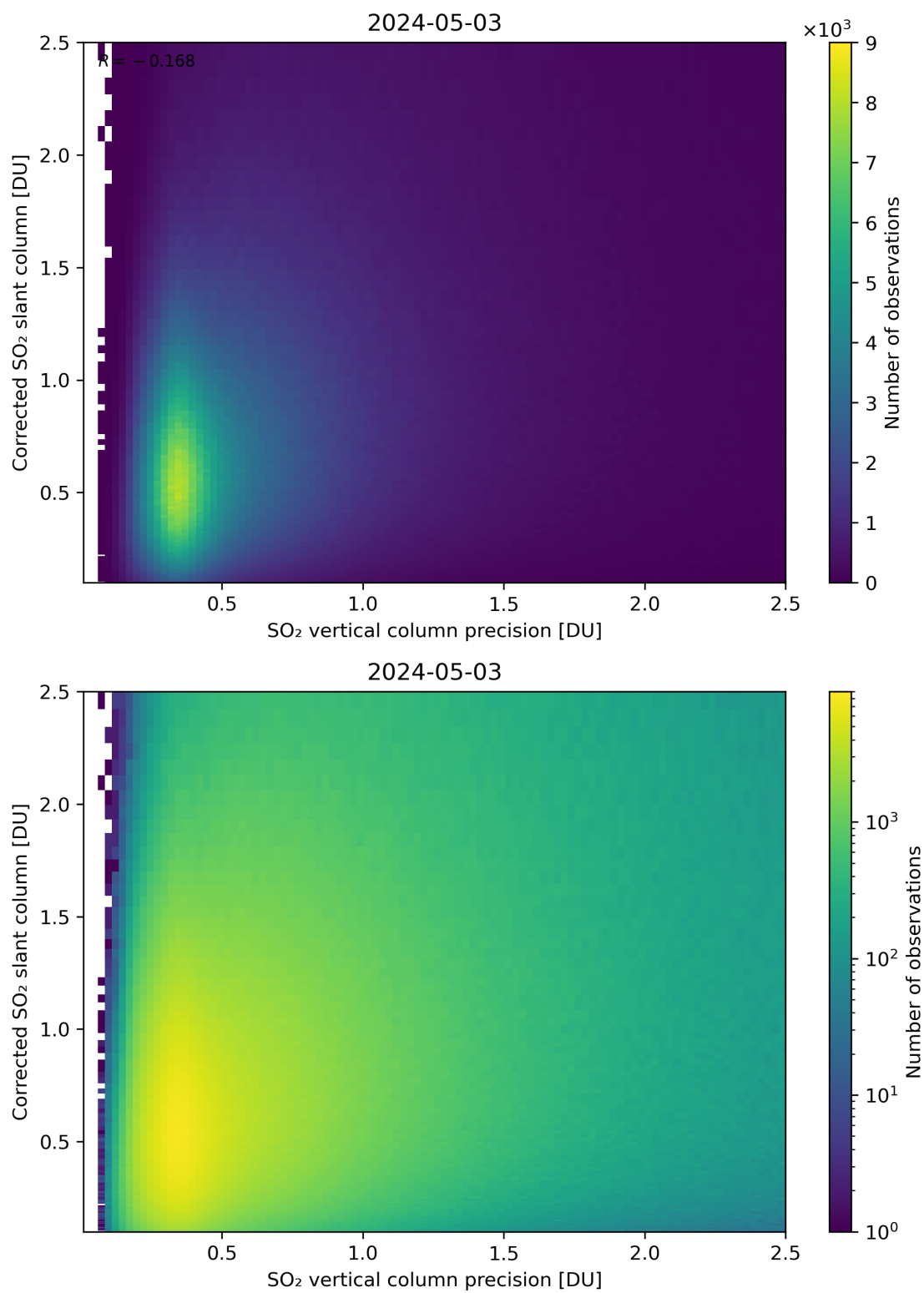
Figure 286: Scatter density plot of “SO 2 vertical column precision” against “Corrected SO 2 slant column” for 2024-05-02 to 2024-05-04.
