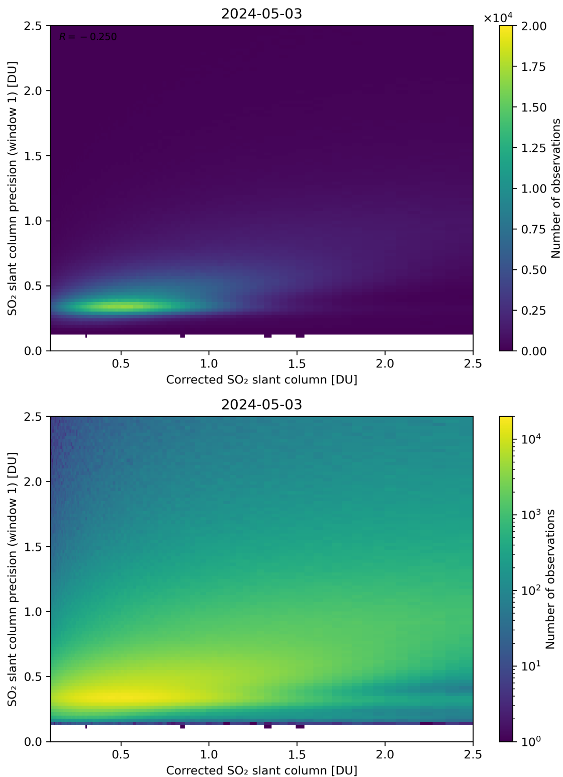
Figure 188: Scatter density plot of “Corrected SO 2 slant column” against “SO 2 slant column precision (window 1)” for 2024-05-02 to 2024-05-04.
