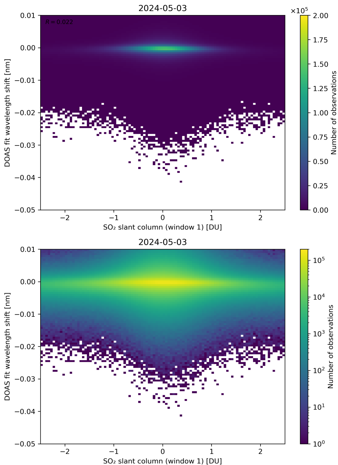
Figure 215: Scatter density plot of “SO 2 slant column (window 1)” against “DOAS fit wavelength shift” for 2024-05-02 to 2024-05-04.
