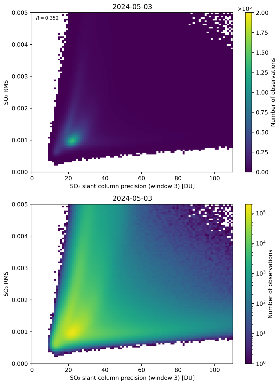
Figure 260: Scatter density plot of “SO 2 slant column precision (window 3)” against “SO 2 RMS” for 2024-05-02 to 2024-05-04.
