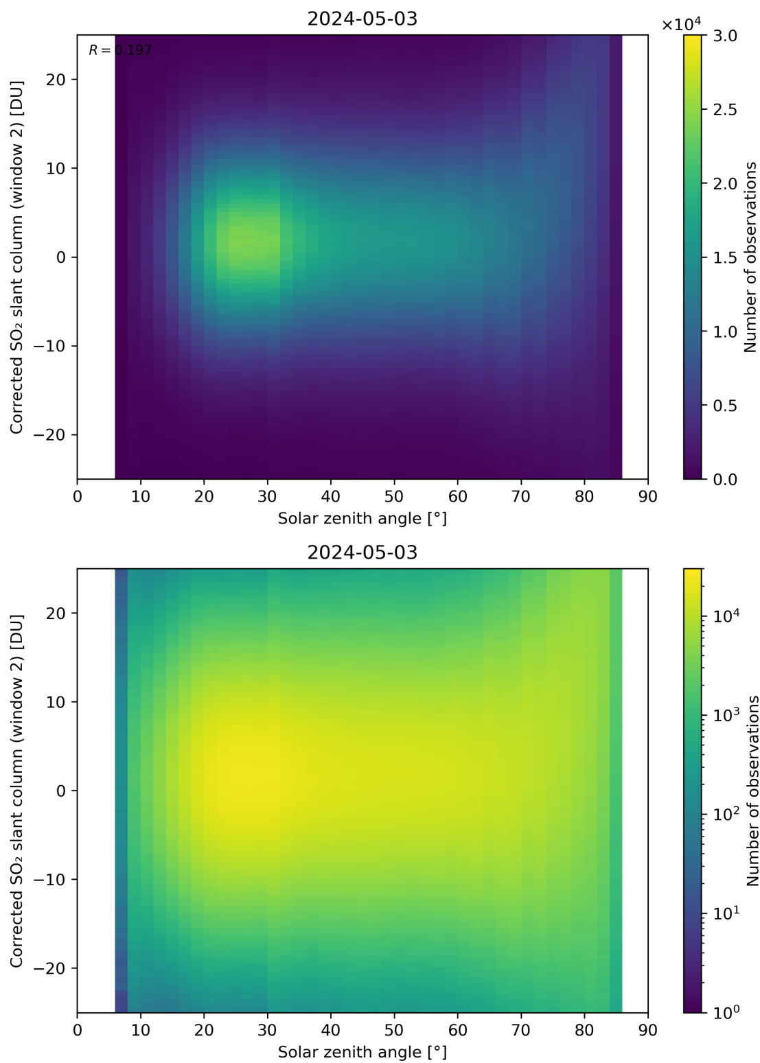
Figure 167: Scatter density plot of “Solar zenith angle” against “Corrected SO 2 slant column (window 2)” for 2024-05-02 to 2024-05-04.
