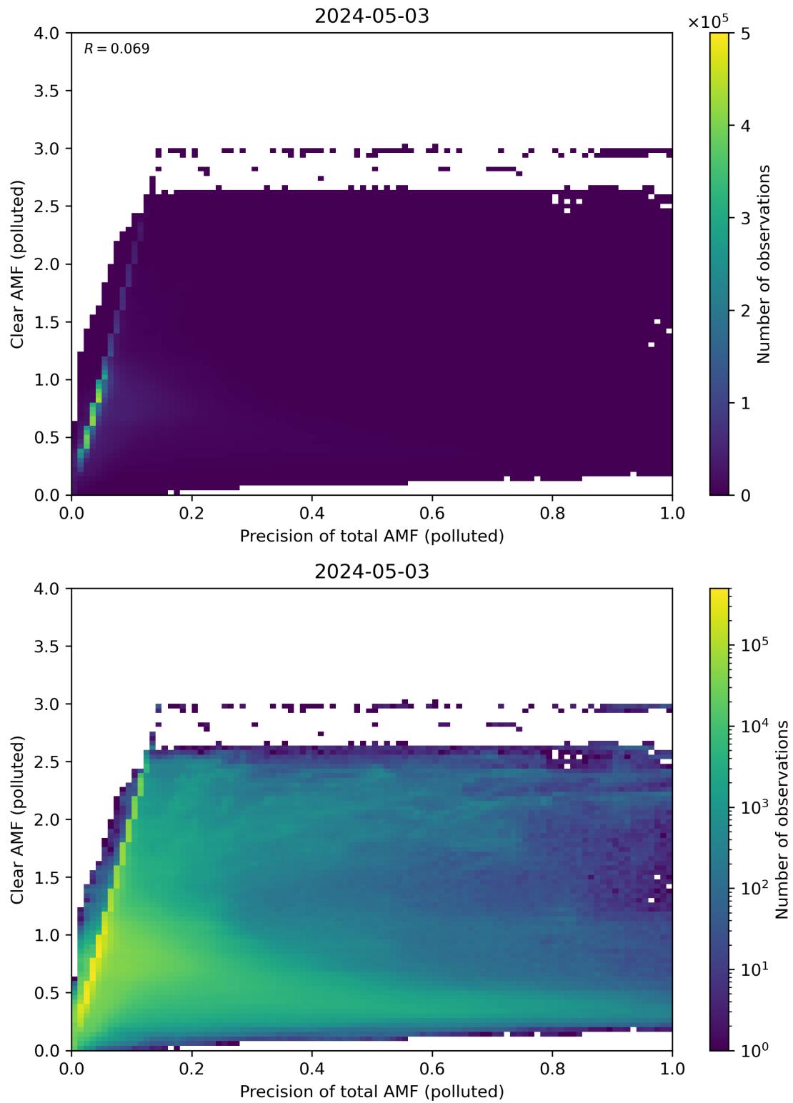
Figure 270: Scatter density plot of “Precision of total AMF (polluted)” against “Clear AMF (polluted)” for 2024-05-02 to 2024-05-04.
