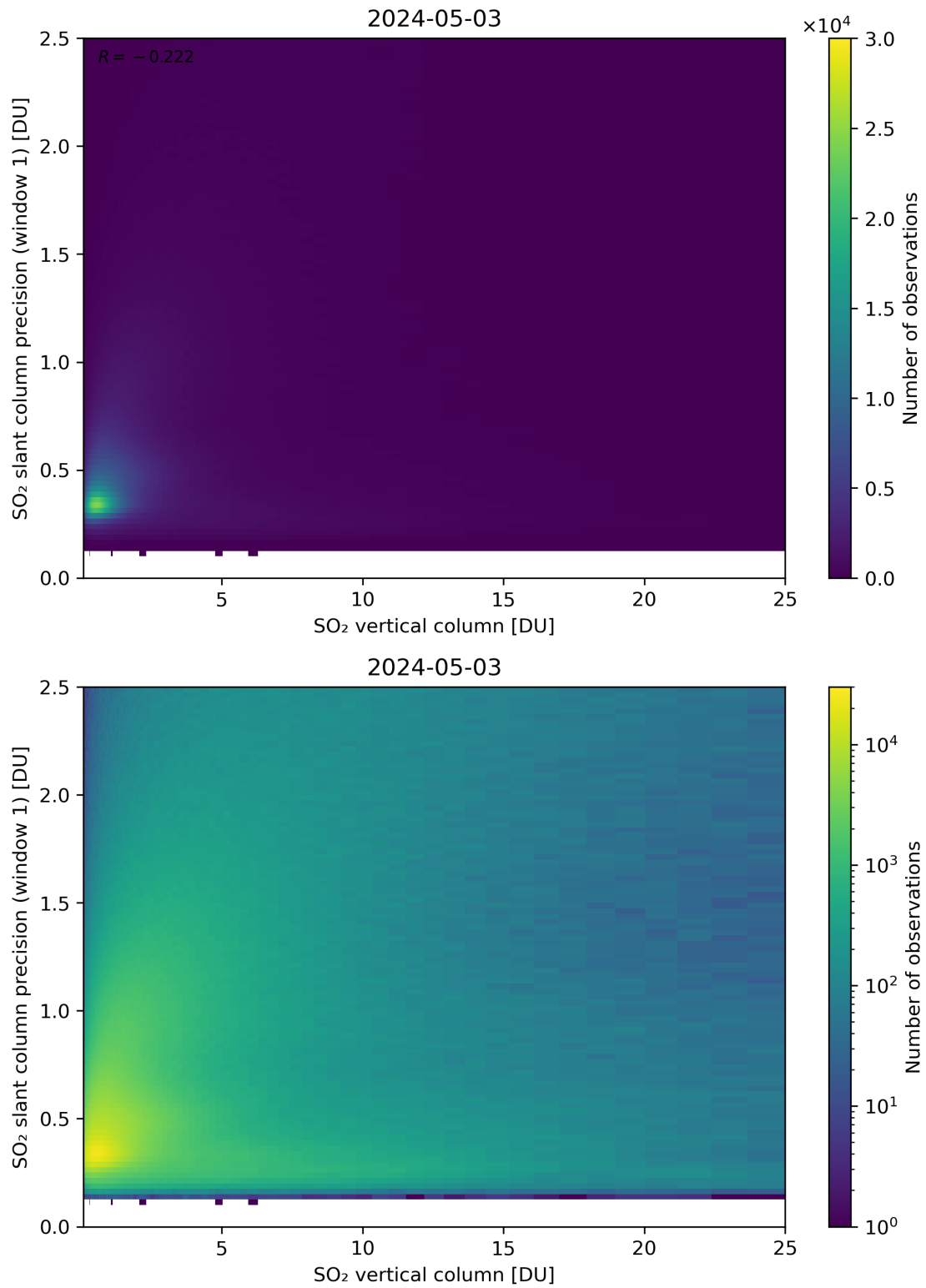
Figure 301: Scatter density plot of “SO 2 vertical column” against “SO 2 slant column precision (window 1)” for 2024-05-02 to 2024-05-04.
