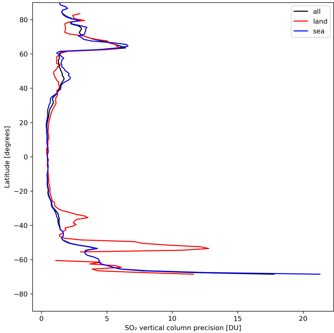
Figure 31: Zonal average of “SO 2 vertical column precision” for 2024-05-02 to 2024-05-04.
