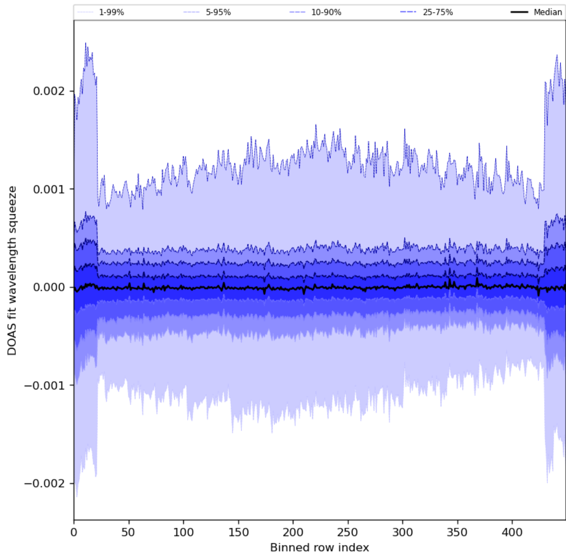
Figure 92: Along track statistics of “DOAS fit wavelength squeeze” for 2024-05-02 to 2024-05-04
