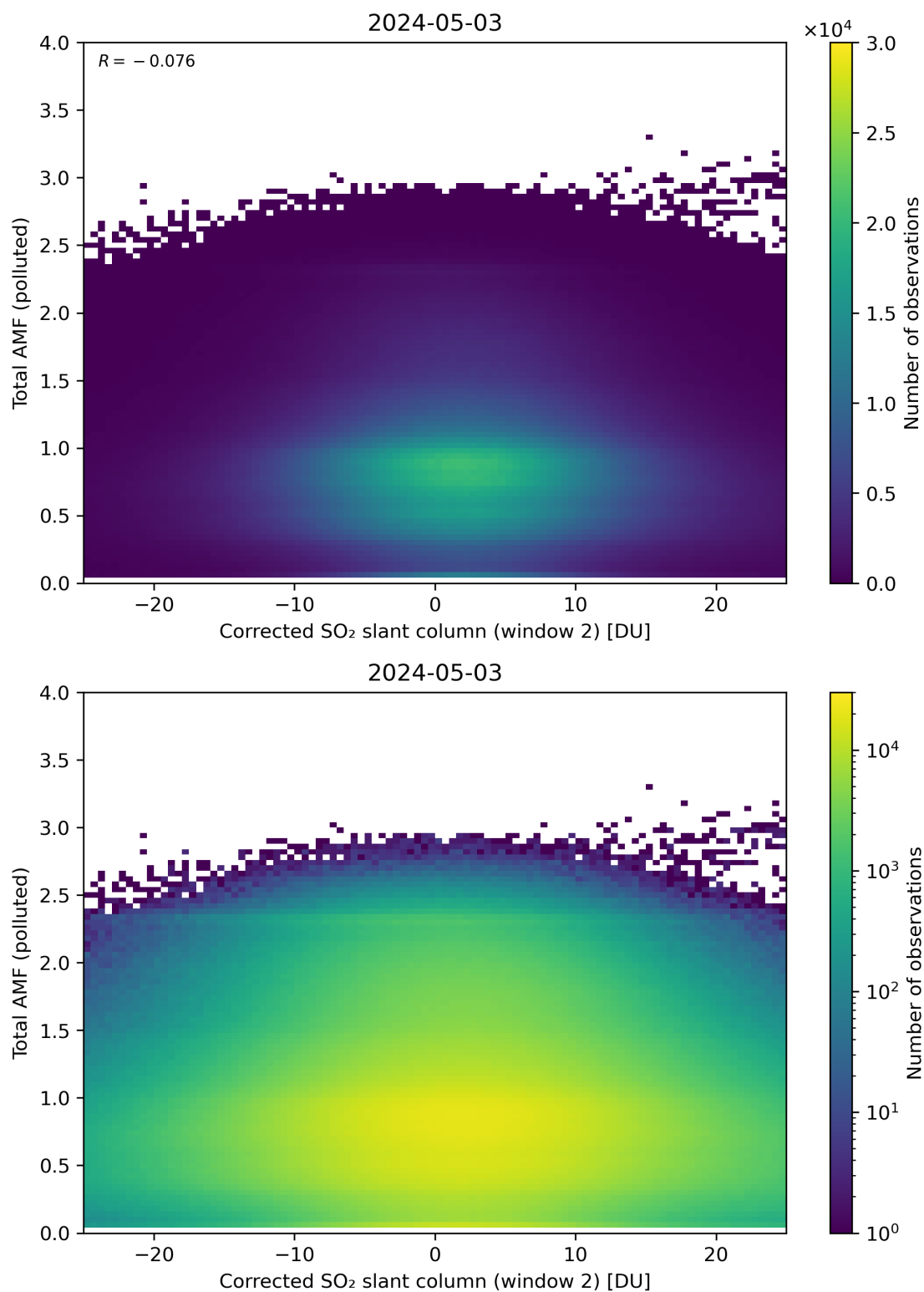
Figure 203: Scatter density plot of “Corrected SO 2 slant column (window 2)” against “Total AMF (polluted)” for 2024-05-02 to 2024-05-04.
