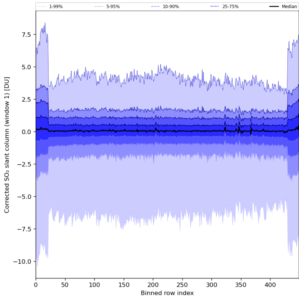
Figure 81: Along track statistics of “Corrected SO 2 slant column (window 1)” for 2024-05-02 to 2024-05-04
