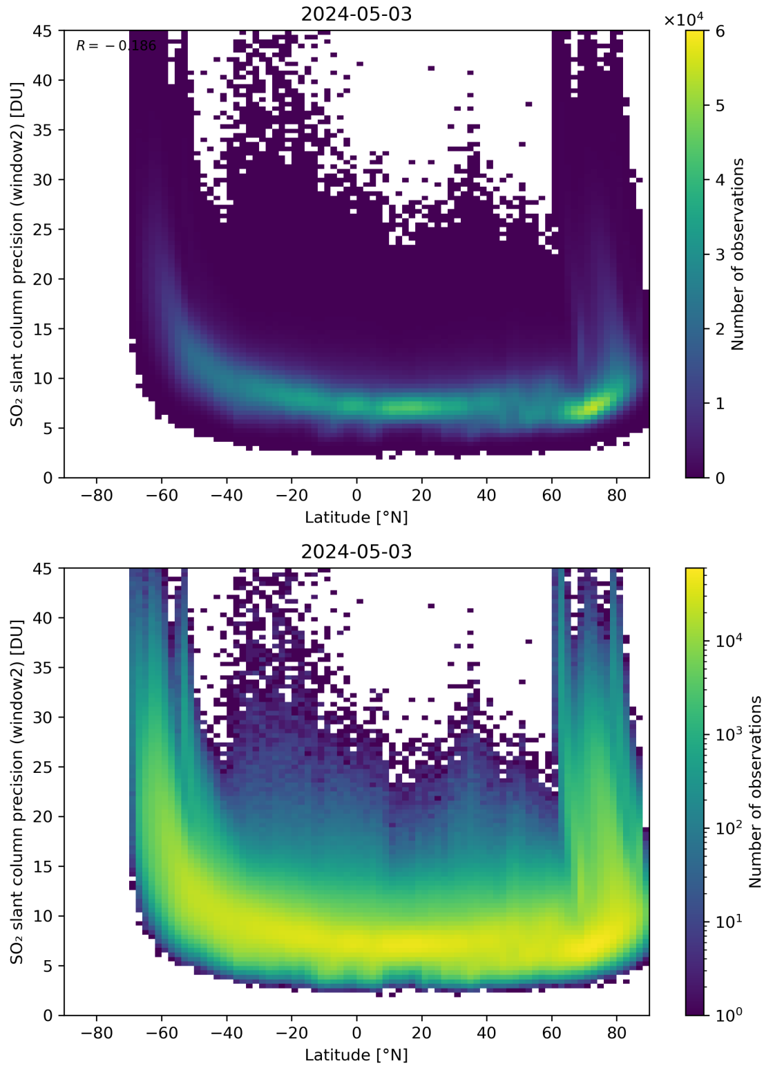
Figure 151: Scatter density plot of “Latitude” against “SO 2 slant column precision (window2)” for 2024-05-02 to 2024-05-04.
