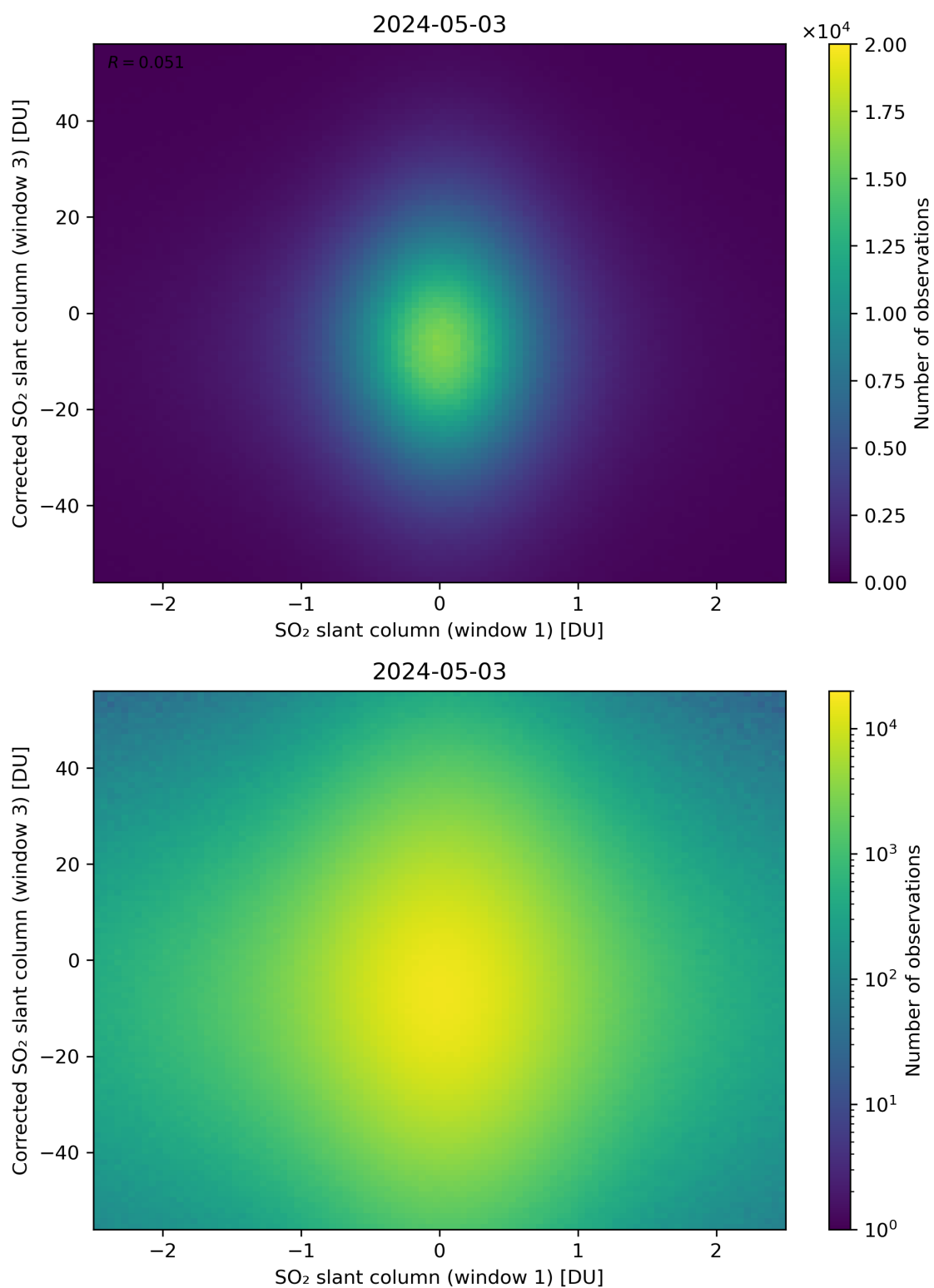
Figure 234: Scatter density plot of “SO 2 slant column (window 1)” against “Corrected SO 2 slant column (window 3)” for 2024-05-02 to 2024-05-04.
