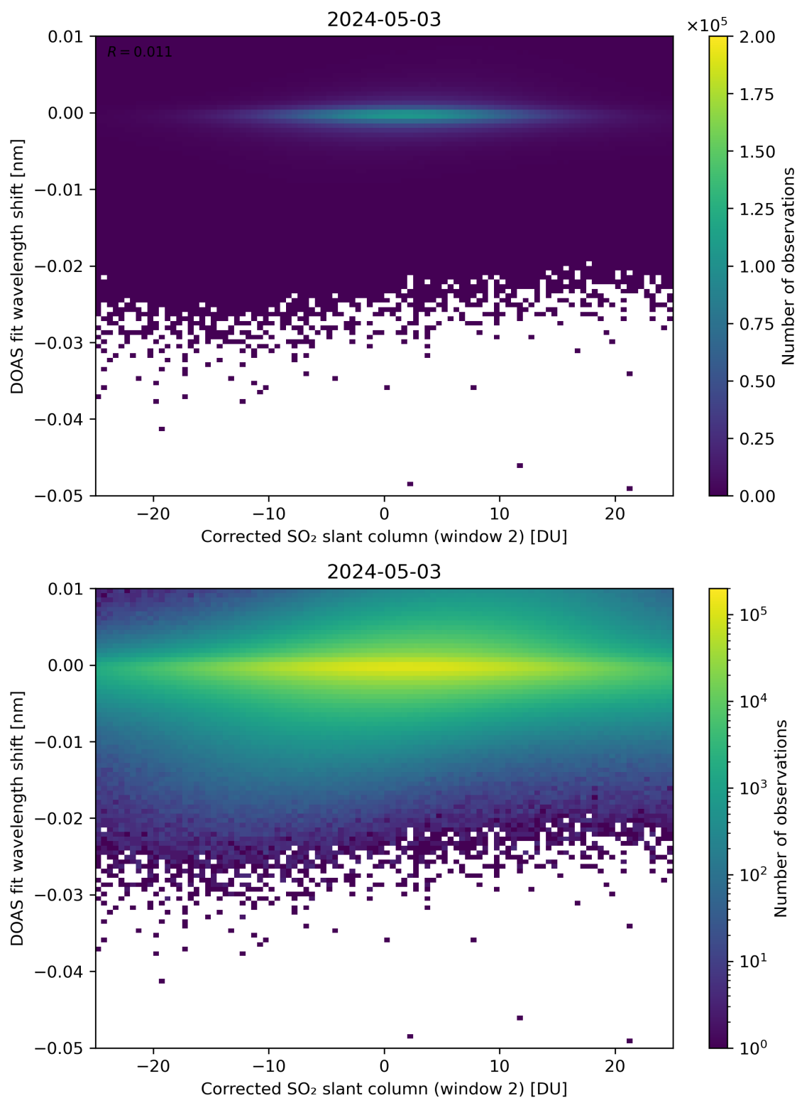
Figure 196: Scatter density plot of “Corrected SO 2 slant column (window 2)” against “DOAS fit wavelength shift” for 2024-05-02 to 2024-05-04.
