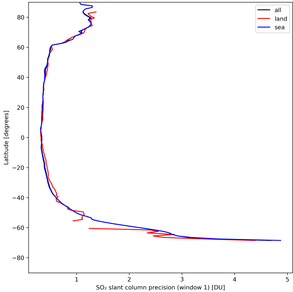
Figure 34: Zonal average of “SO 2 slant column precision (window 1)” for 2024-05-02 to 2024-05-04.
