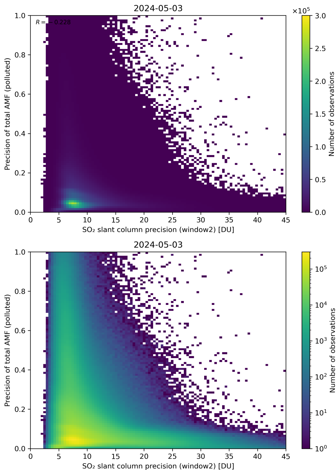
Figure 252: Scatter density plot of “SO 2 slant column precision (window2)” against “Precision of total AMF (polluted)” for 2024-05-02 to 2024-05-04.
