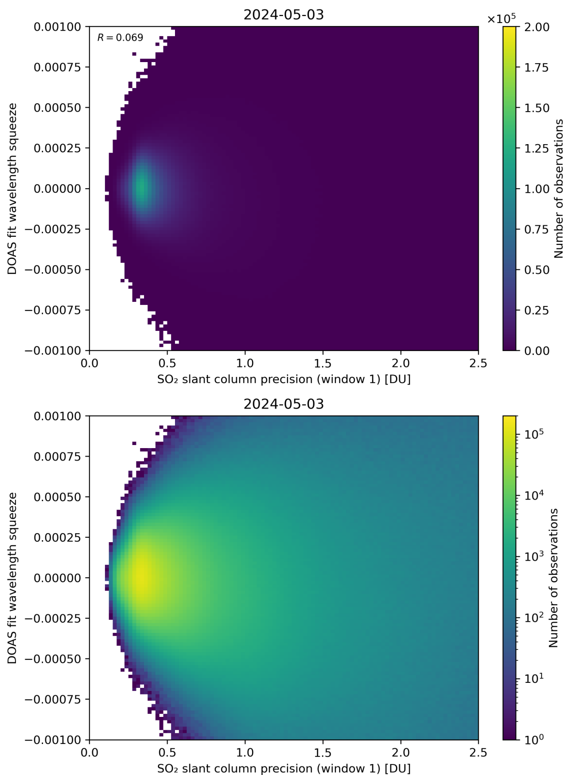
Figure 222: Scatter density plot of “SO 2 slant column precision (window 1)” against “DOAS fit wavelength squeeze” for 2024-05-02 to 2024-05-04.
