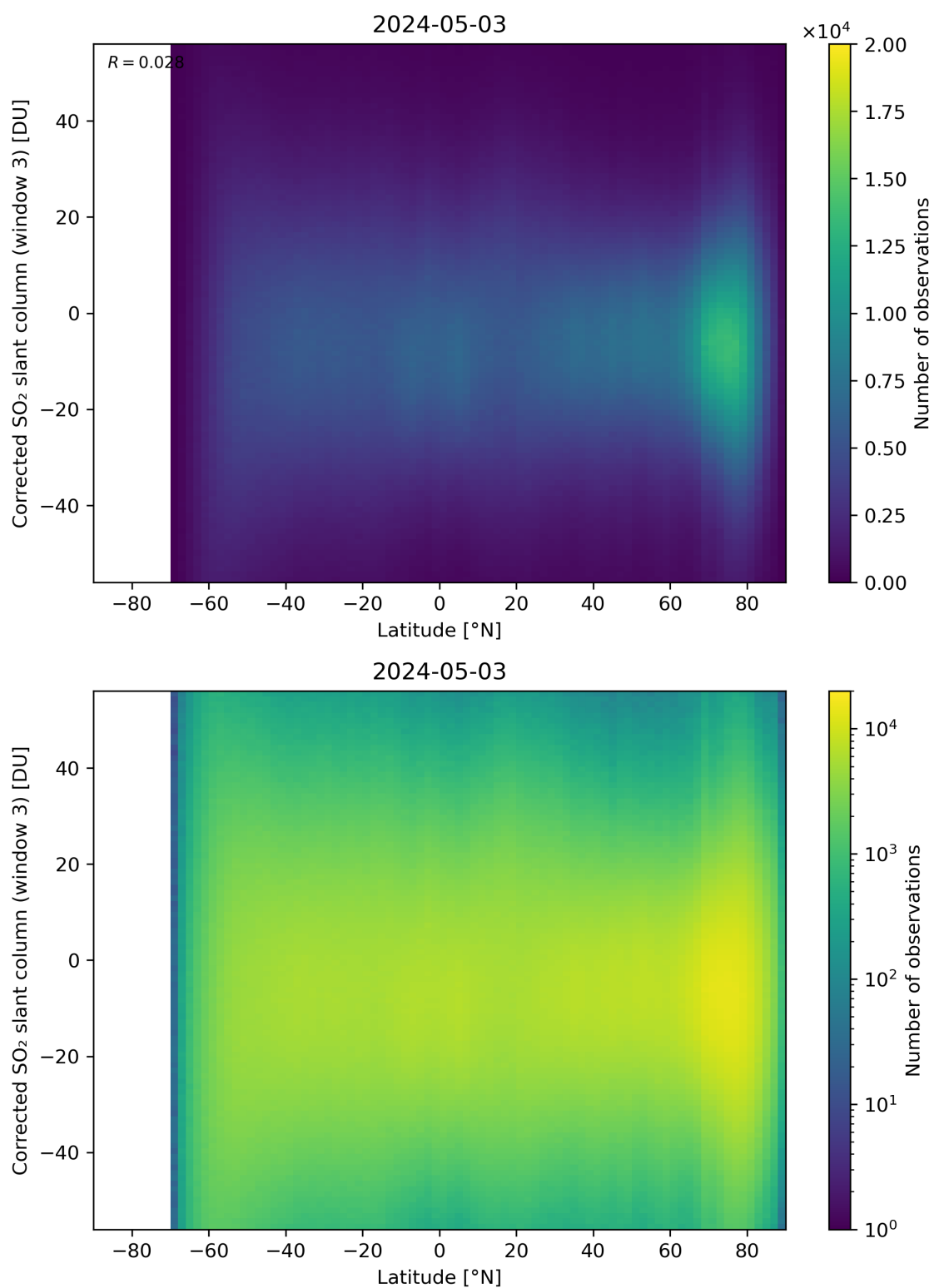
Figure 148: Scatter density plot of “Latitude” against “Corrected SO 2 slant column (window 3)” for 2024-05-02 to 2024-05-04.
