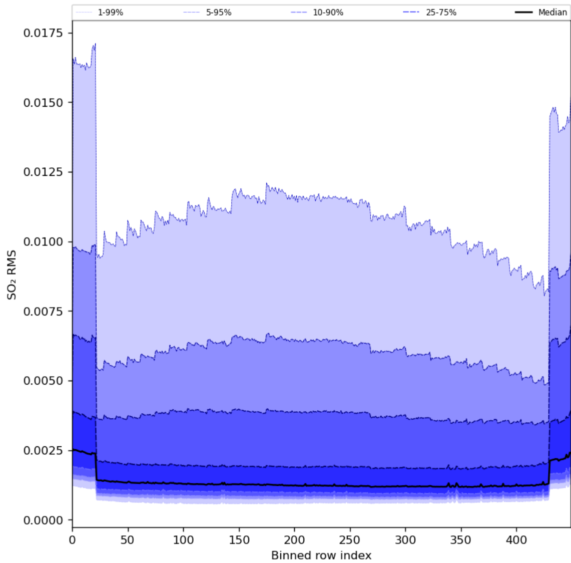
Figure 93: Along track statistics of “SO 2 RMS” for 2024-05-02 to 2024-05-04
