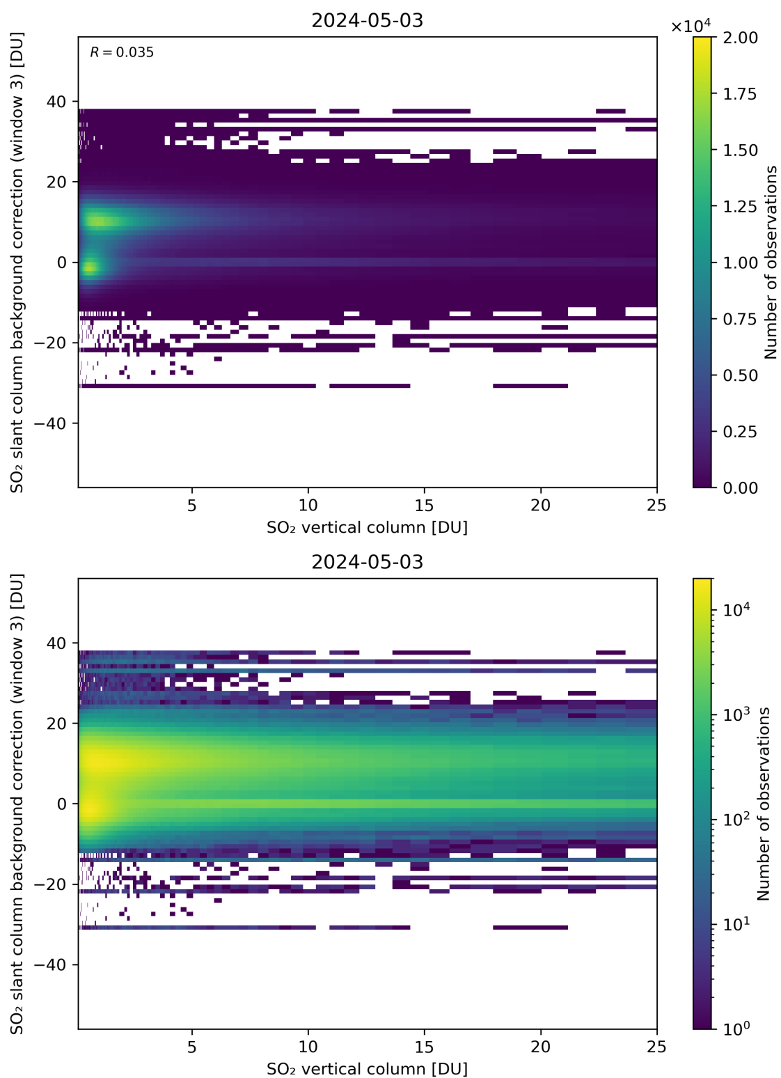
Figure 275: Scatter density plot of “SO 2 vertical column” against “SO 2 slant column background correction (window 3)” for 2024-05-02 to 2024-05-04.
