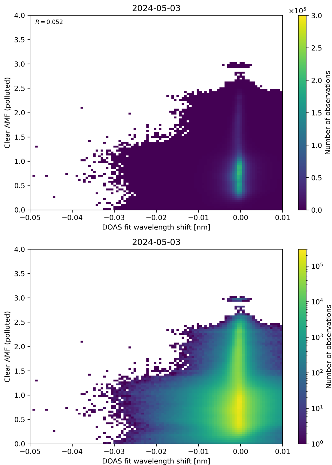
Figure 129: Scatter density plot of “DOAS fit wavelength shift” against “Clear AMF (polluted)” for 2024-05-02 to 2024-05-04.
