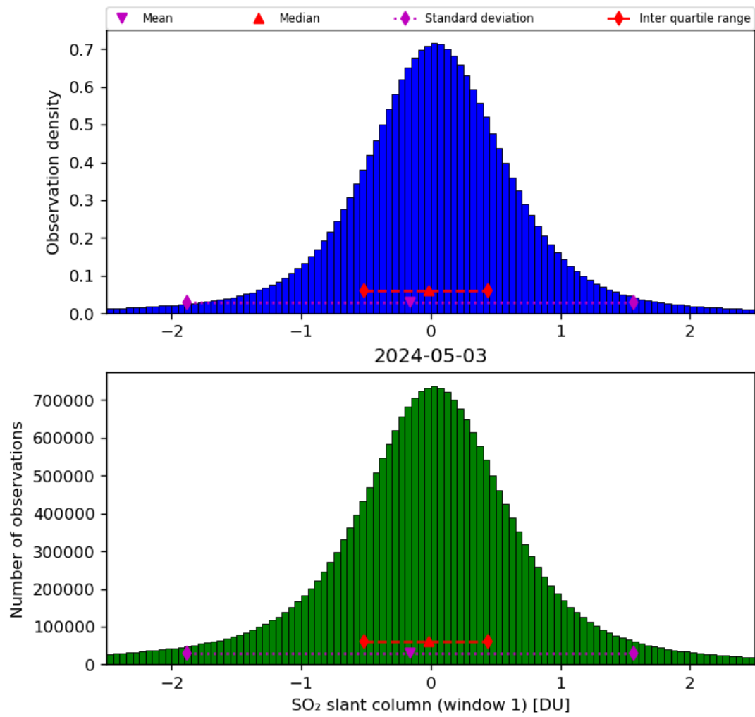
Figure 56: Histogram of “SO 2 slant column (window 1)” for 2024-05-02 to 2024-05-04
