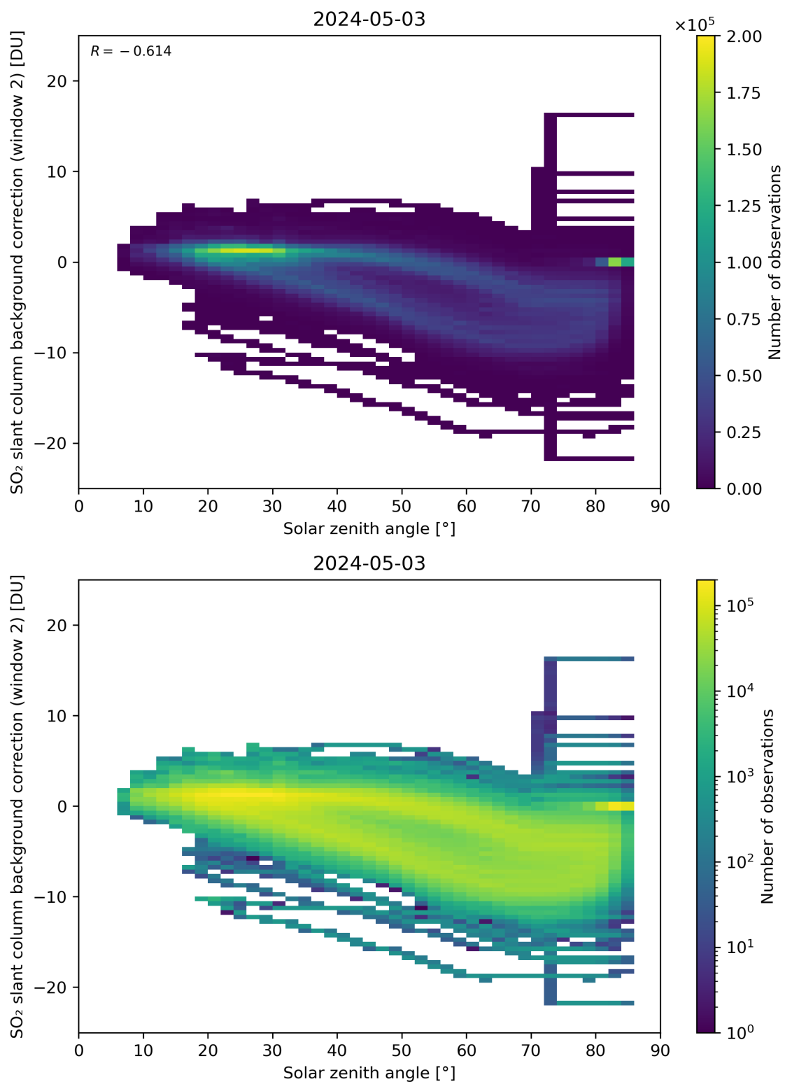
Figure 159: Scatter density plot of “Solar zenith angle” against “SO 2 slant column background correction (window 2)” for 2024-05-02 to 2024-05-04.
