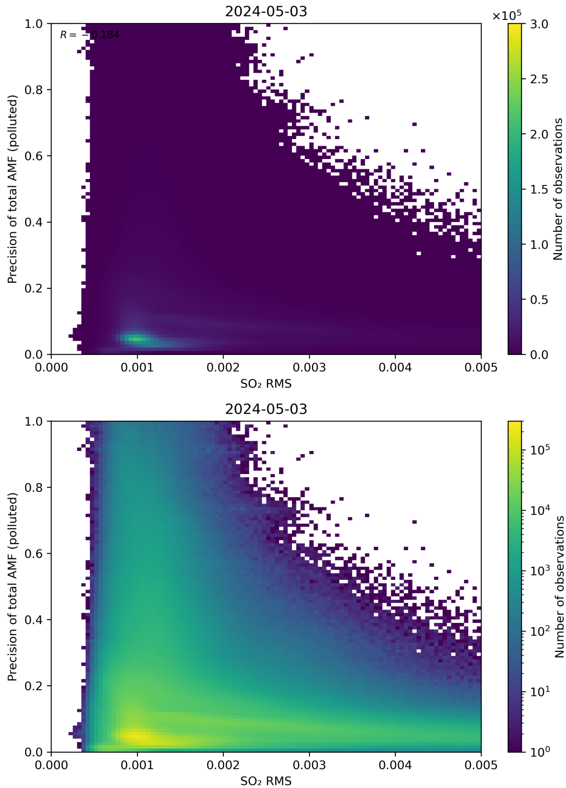
Figure 138: Scatter density plot of “SO 2 RMS” against “Precision of total AMF (polluted)” for 2024-05-02 to 2024-05-04.
