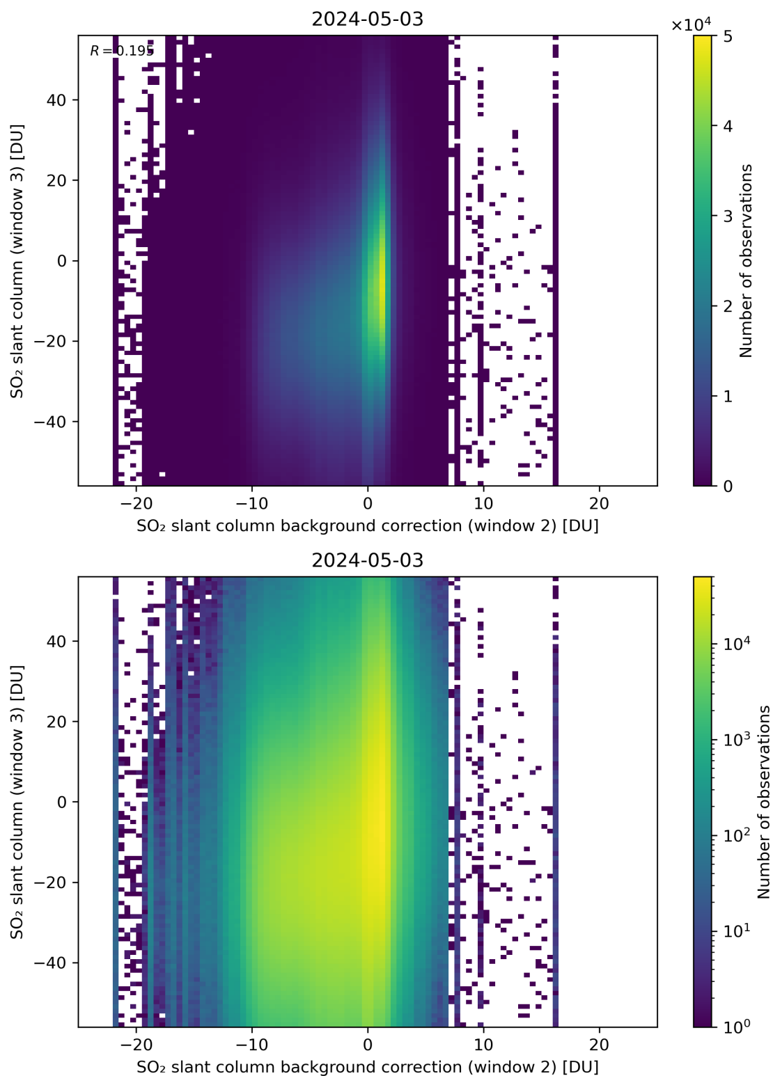
Figure 117: Scatter density plot of “SO 2 slant column background correction (window 2)” against “SO 2 slant column (window 3)” for 2024-05-02 to 2024-05-04.
