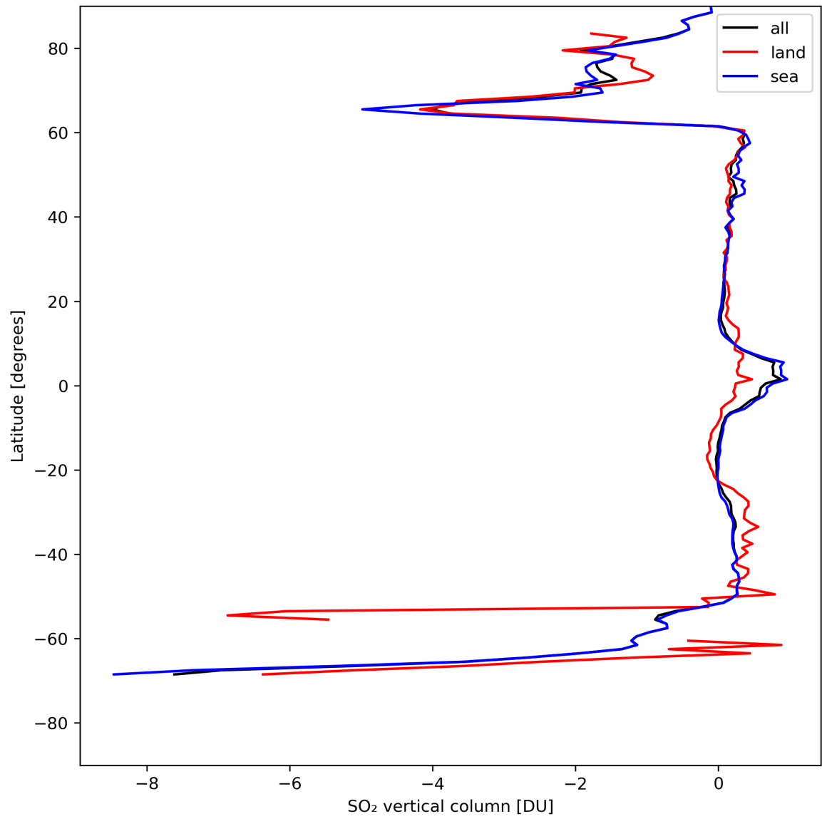
Figure 30: Zonal average of “SO 2 vertical column” for 2024-05-02 to 2024-05-04.
