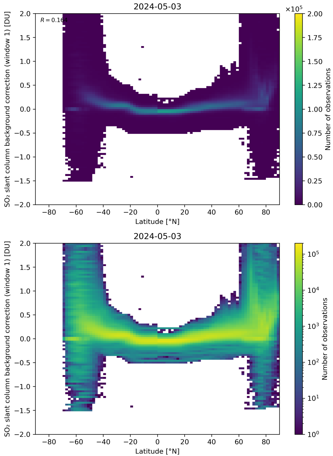
Figure 139: Scatter density plot of “Latitude” against “SO 2 slant column background correction (window 1)” for 2024-05-02 to 2024-05-04.
