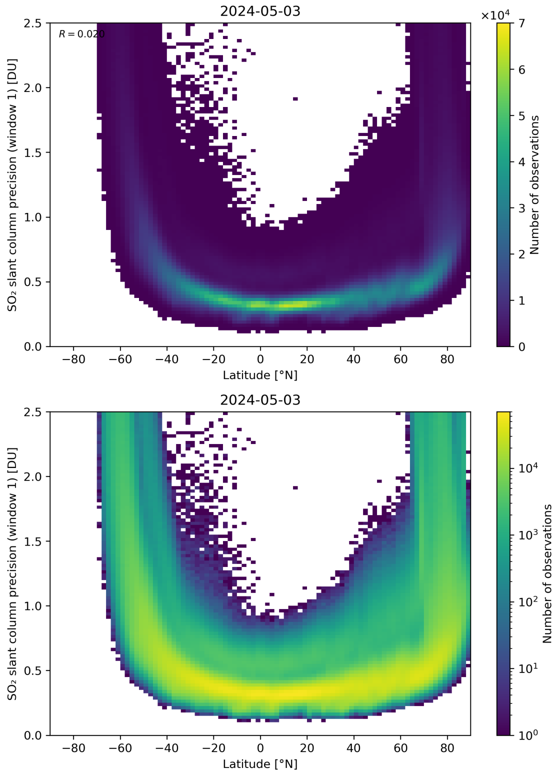
Figure 150: Scatter density plot of “Latitude” against “SO 2 slant column precision (window 1)” for 2024-05-02 to 2024-05-04.
