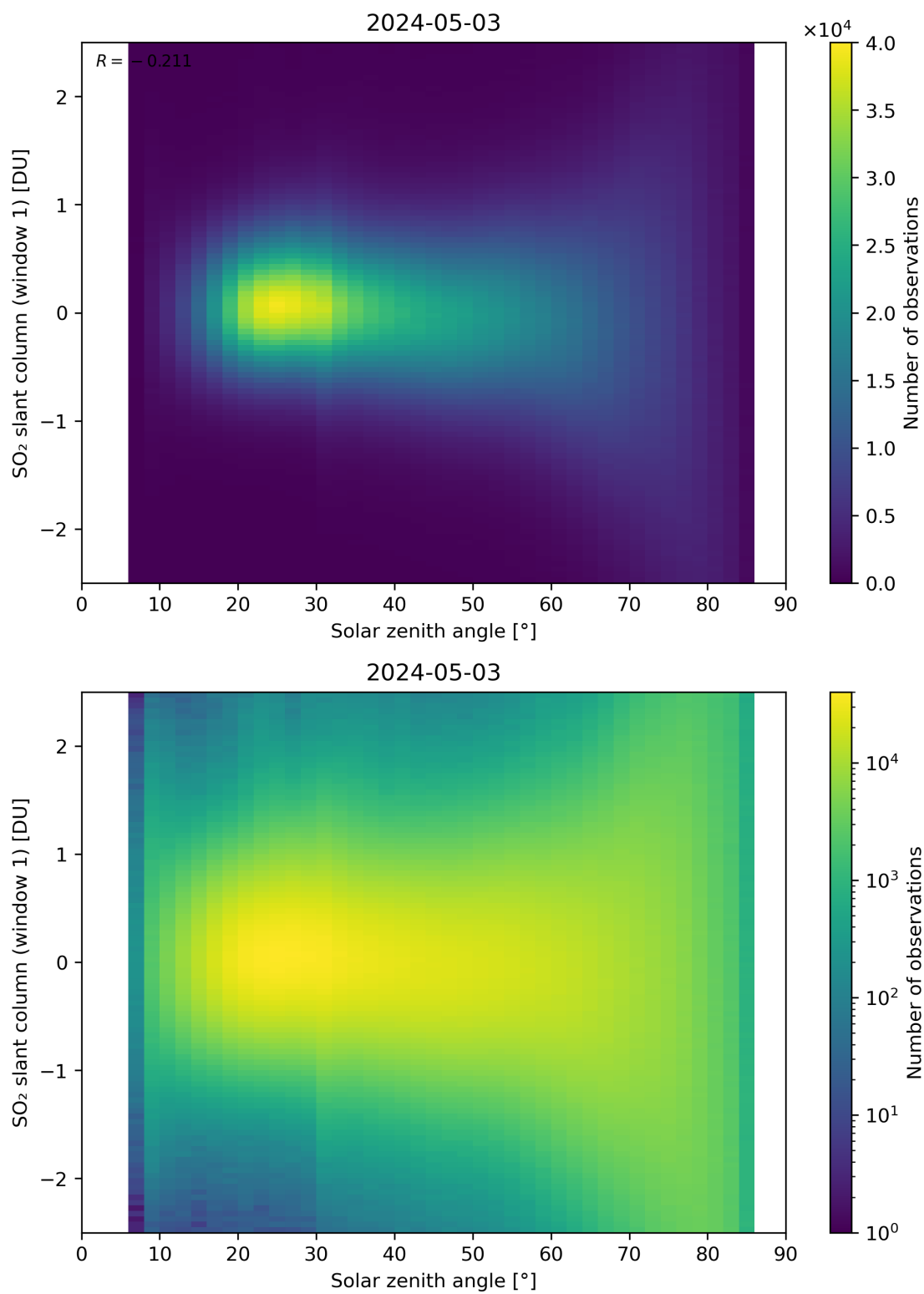
Figure 169: Scatter density plot of “Solar zenith angle” against “SO 2 slant column (window 1)” for 2024-05-02 to 2024-05-04.
