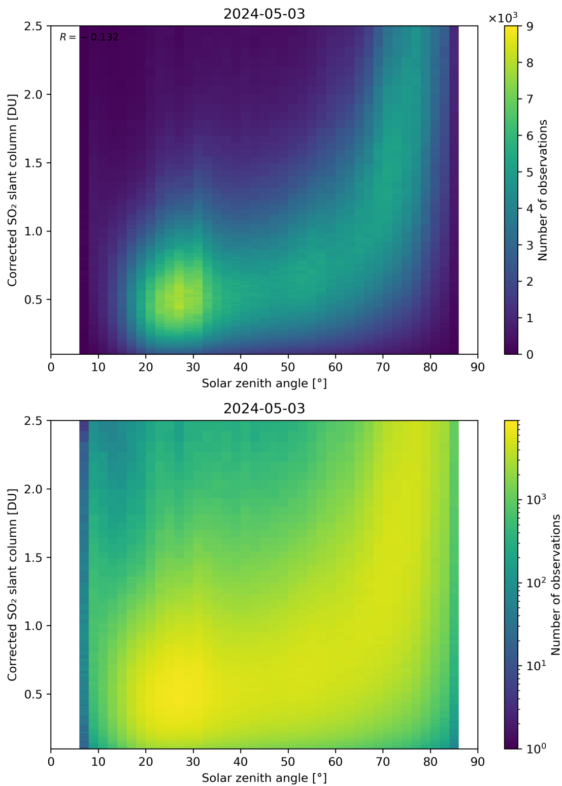
Figure 166: Scatter density plot of “Solar zenith angle” against “Corrected SO 2 slant column” for 2024-05-02 to 2024-05-04.
