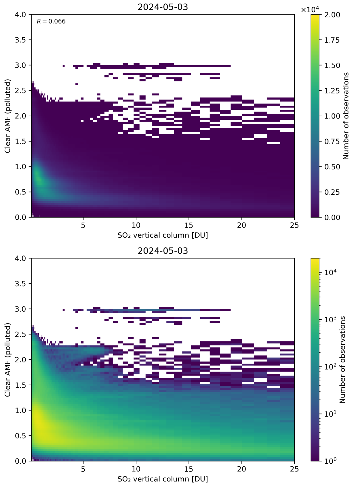
Figure 296: Scatter density plot of “SO 2 vertical column” against “Clear AMF (polluted)” for 2024-05-02 to 2024-05-04.
