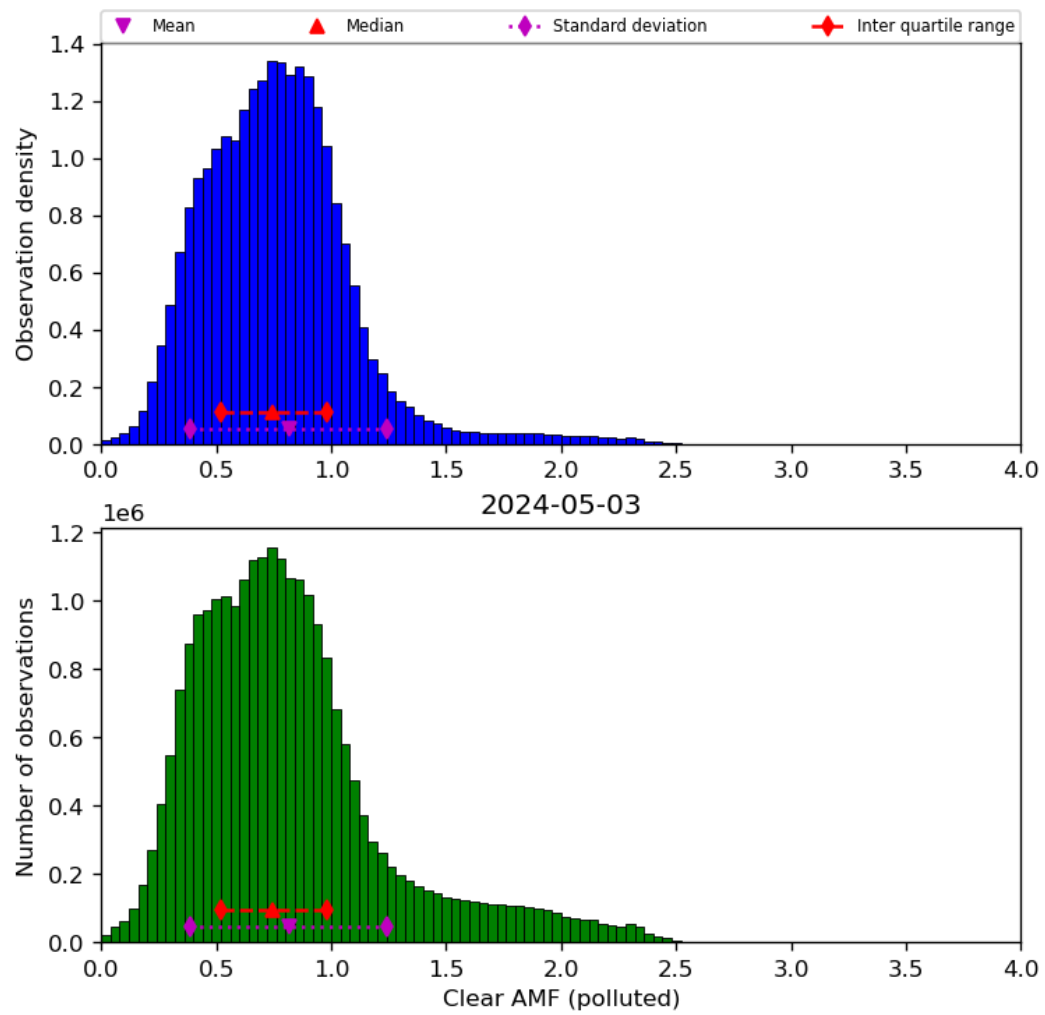
Figure 73: Histogram of “Clear AMF (polluted)” for 2024-05-02 to 2024-05-04
