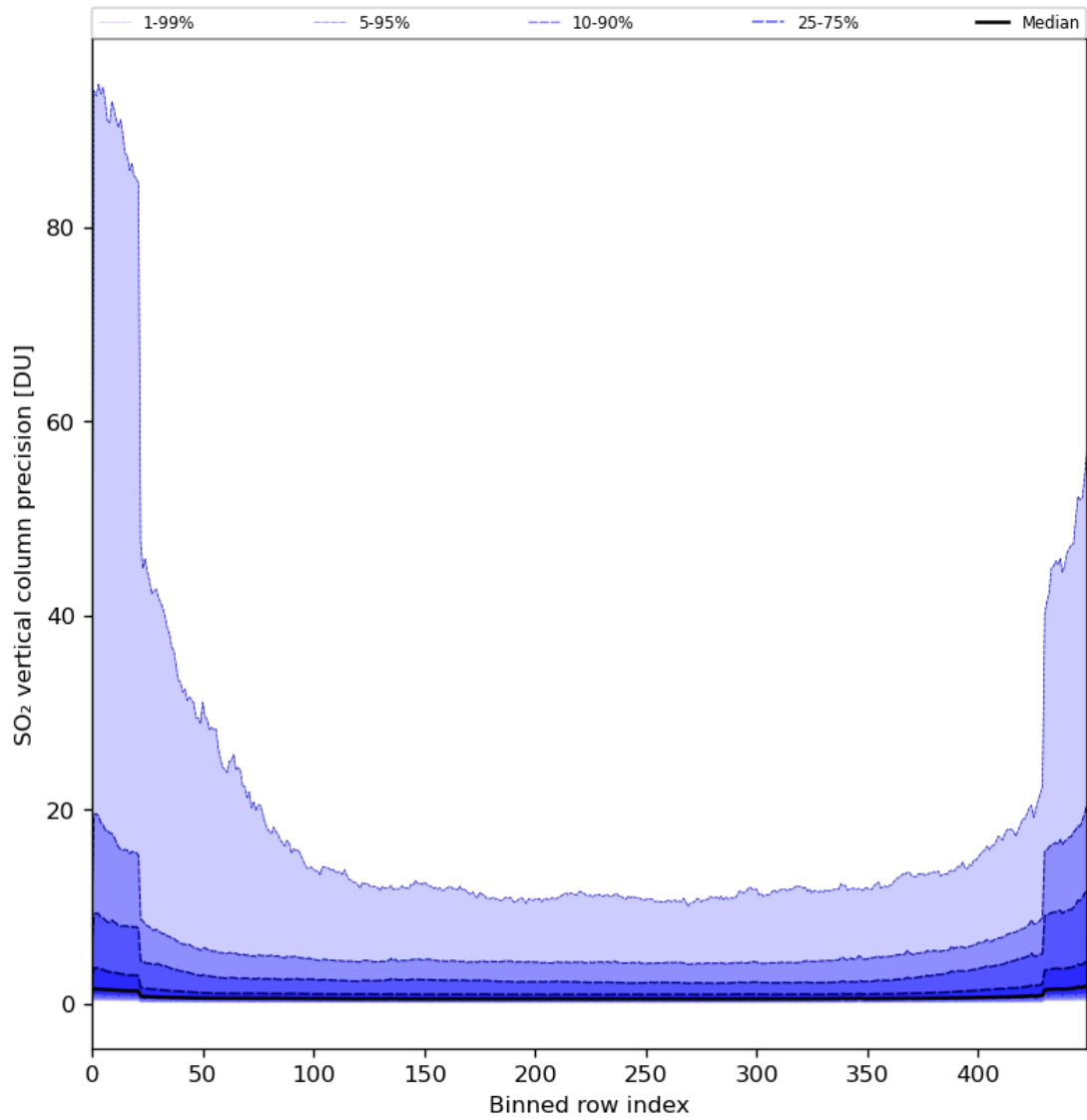
Figure 77: Along track statistics of “SO 2 vertical column precision” for 2024-05-02 to 2024-05-04
