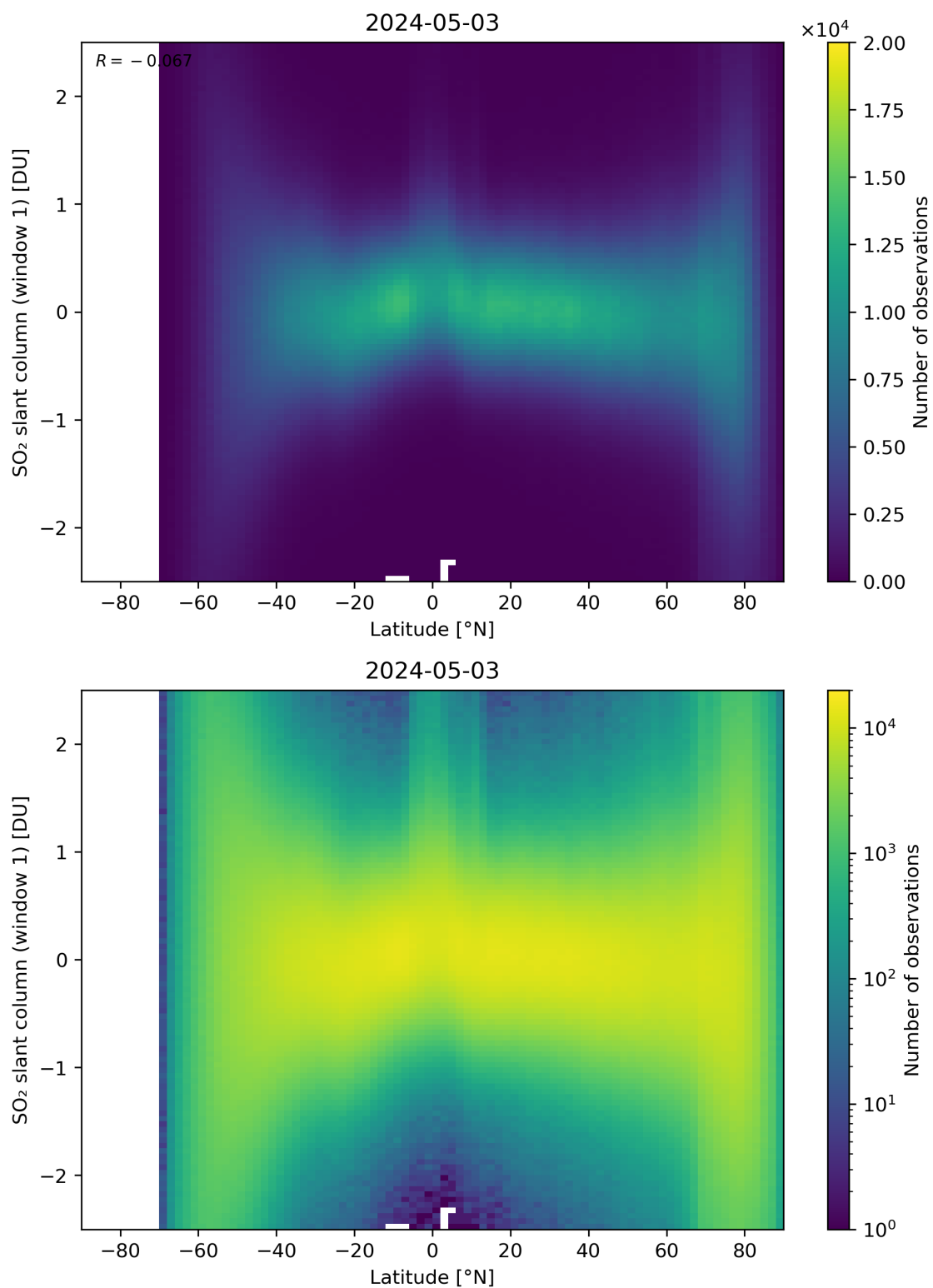
Figure 149: Scatter density plot of “Latitude” against “SO 2 slant column (window 1)” for 2024-05-02 to 2024-05-04.
