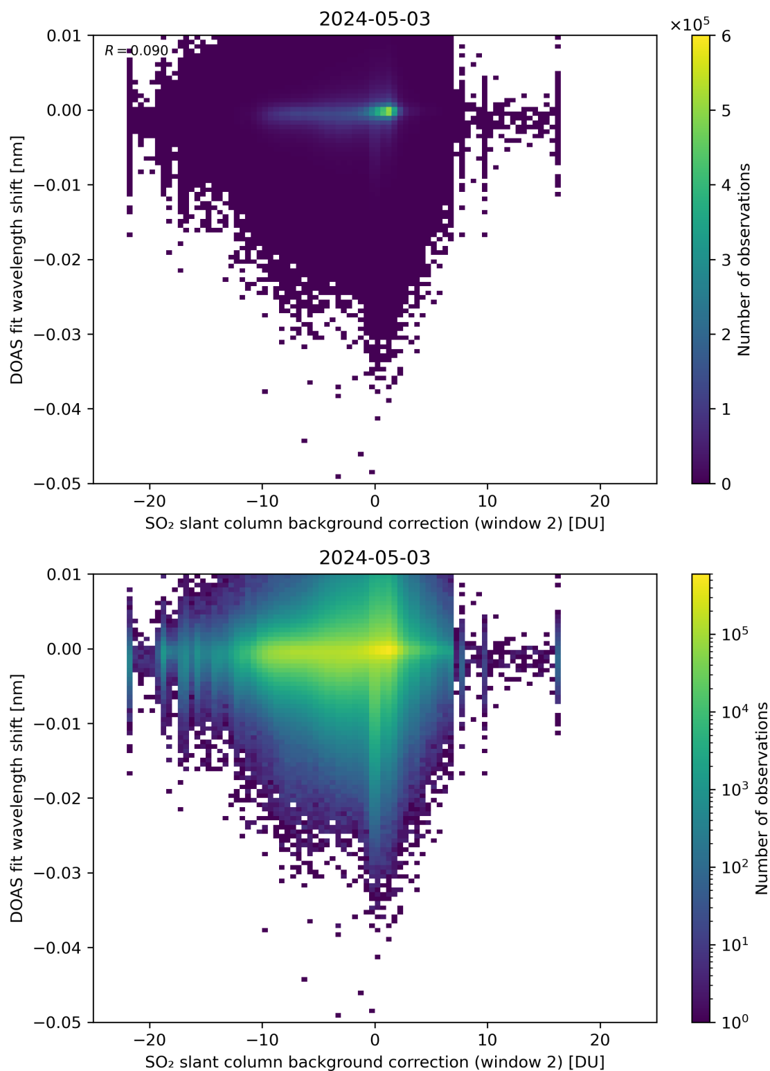
Figure 112: Scatter density plot of “SO 2 slant column background correction (window 2)” against “DOAS fit wavelength shift” for 2024-05-02 to 2024-05-04.
