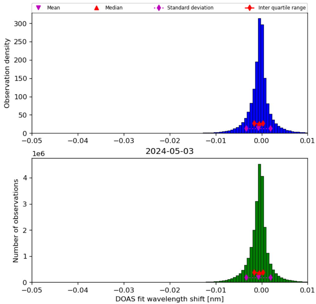
Figure 68: Histogram of “DOAS fit wavelength shift” for 2024-05-02 to 2024-05-04
