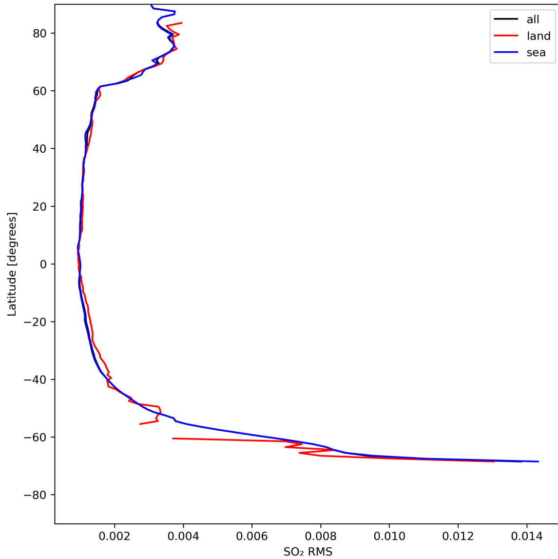
Figure 47: Zonal average of “SO 2 RMS” for 2024-05-02 to 2024-05-04.
