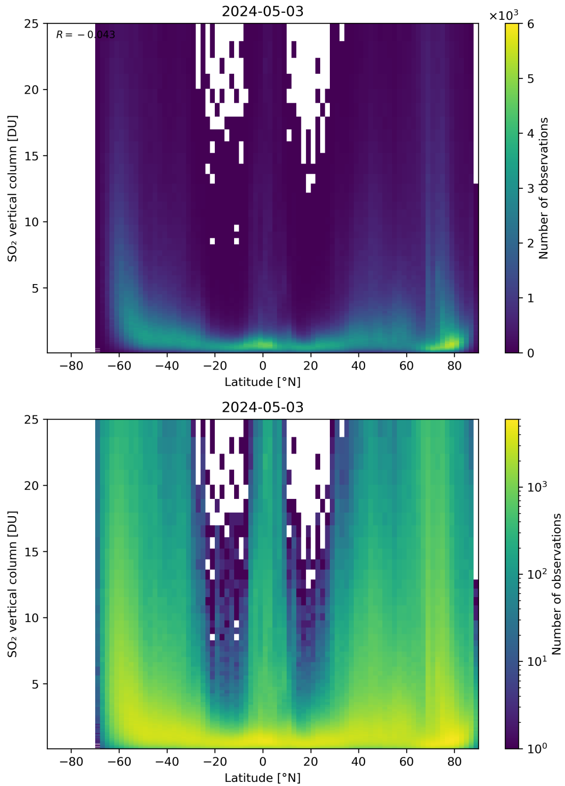
Figure 156: Scatter density plot of “Latitude” against “SO 2 vertical column” for 2024-05-02 to 2024-05-04.
