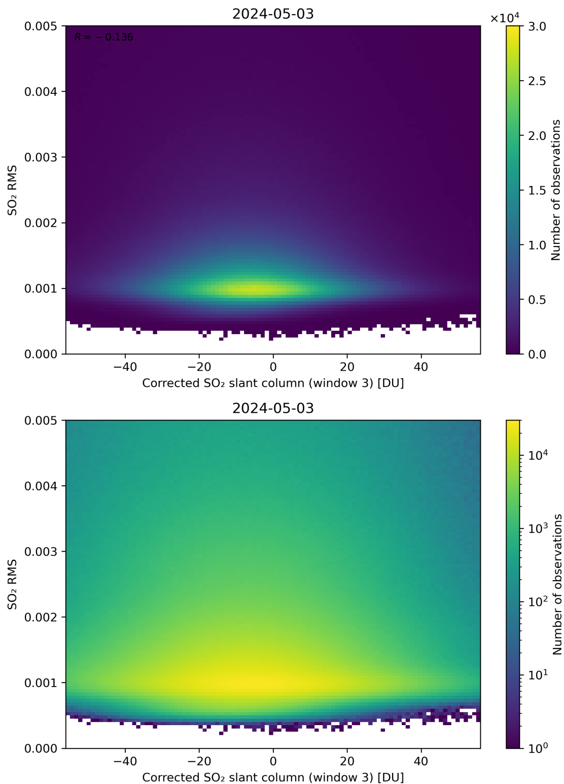
Figure 208: Scatter density plot of “Corrected SO 2 slant column (window 3)” against “SO 2 RMS” for 2024-05-02 to 2024-05-04.
