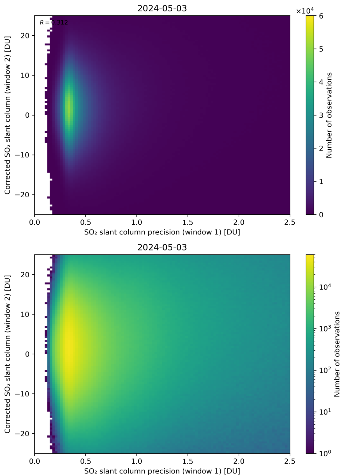
Figure 225: Scatter density plot of “SO 2 slant column precision (window 1)” against “Corrected SO 2 slant column (window 2)” for 2024-05-02 to 2024-05-04.
