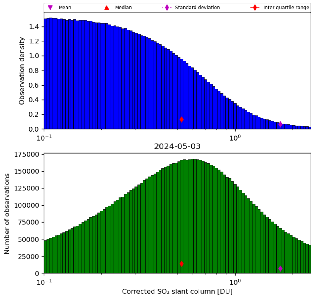
Figure 55: Histogram of “Corrected SO 2 slant column” for 2024-05-02 to 2024-05-04
