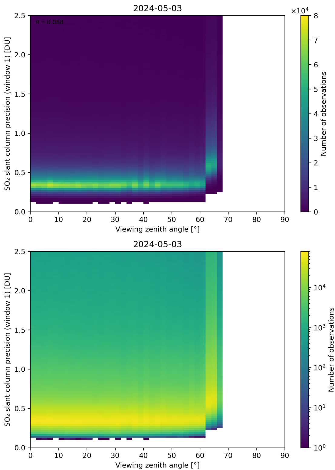
Figure 321: Scatter density plot of “Viewing zenith angle” against “SO 2 slant column precision (window 1)” for 2024-05-02 to 2024-05-04.
