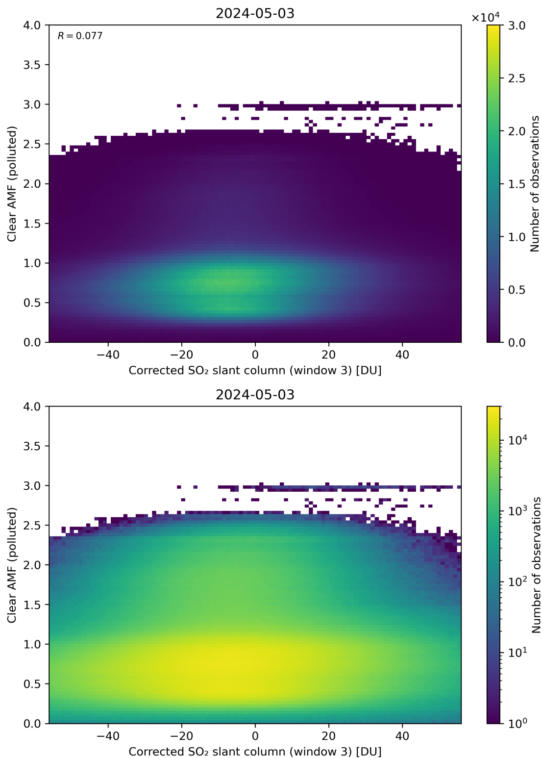
Figure 209: Scatter density plot of “Corrected SO 2 slant column (window 3)” against “Clear AMF (polluted)” for 2024-05-02 to 2024-05-04.
