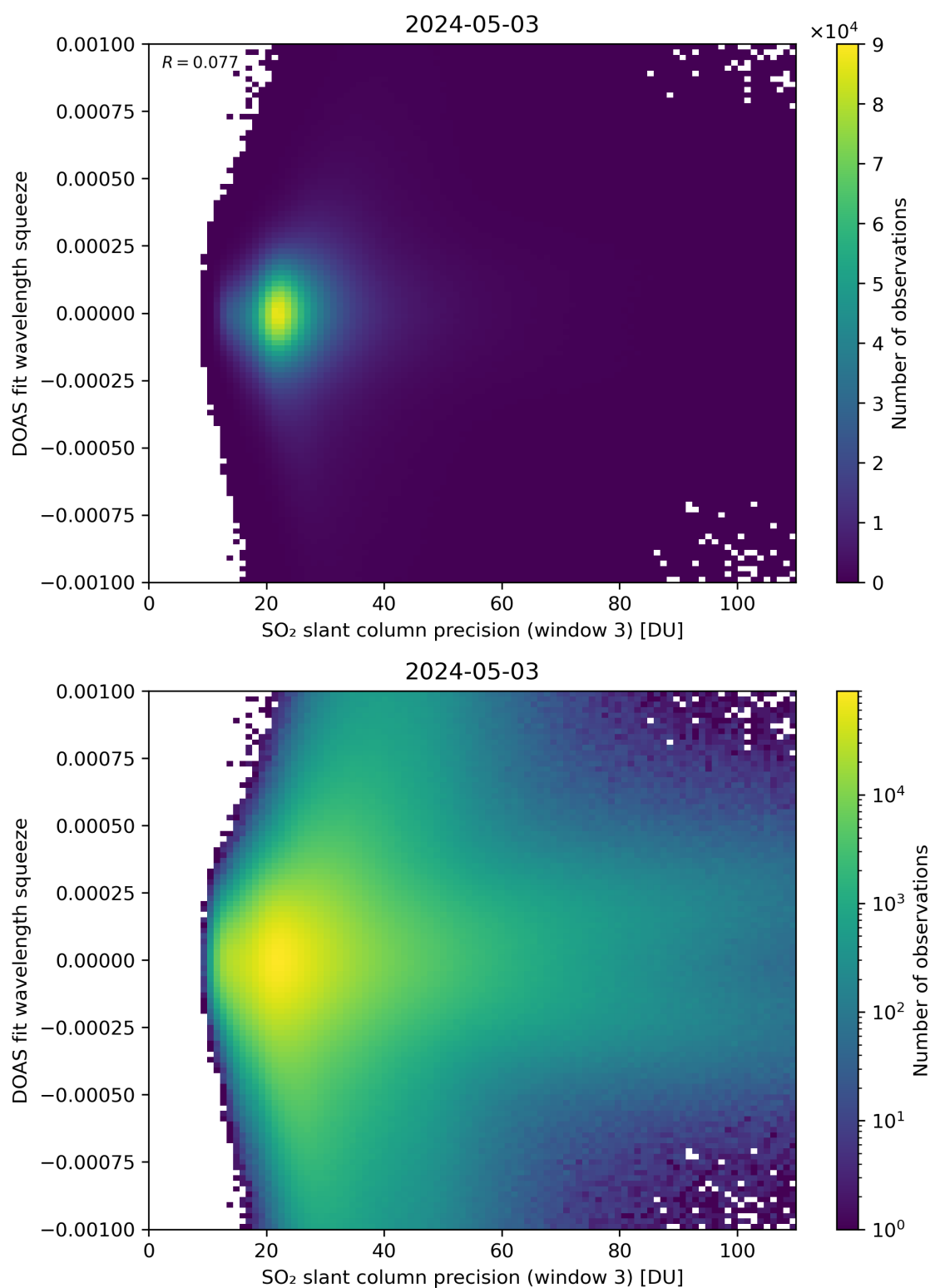
Figure 259: Scatter density plot of “SO 2 slant column precision (window 3)” against “DOAS fit wavelength squeeze” for 2024-05-02 to 2024-05-04.
