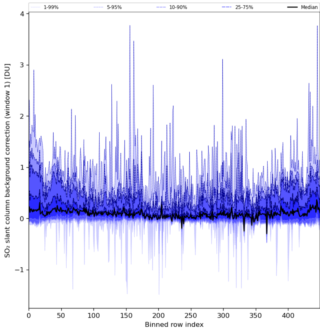
Figure 82: Along track statistics of “SO 2 slant column background correction (window 1)” for 2024-05-02 to 2024-05-04
