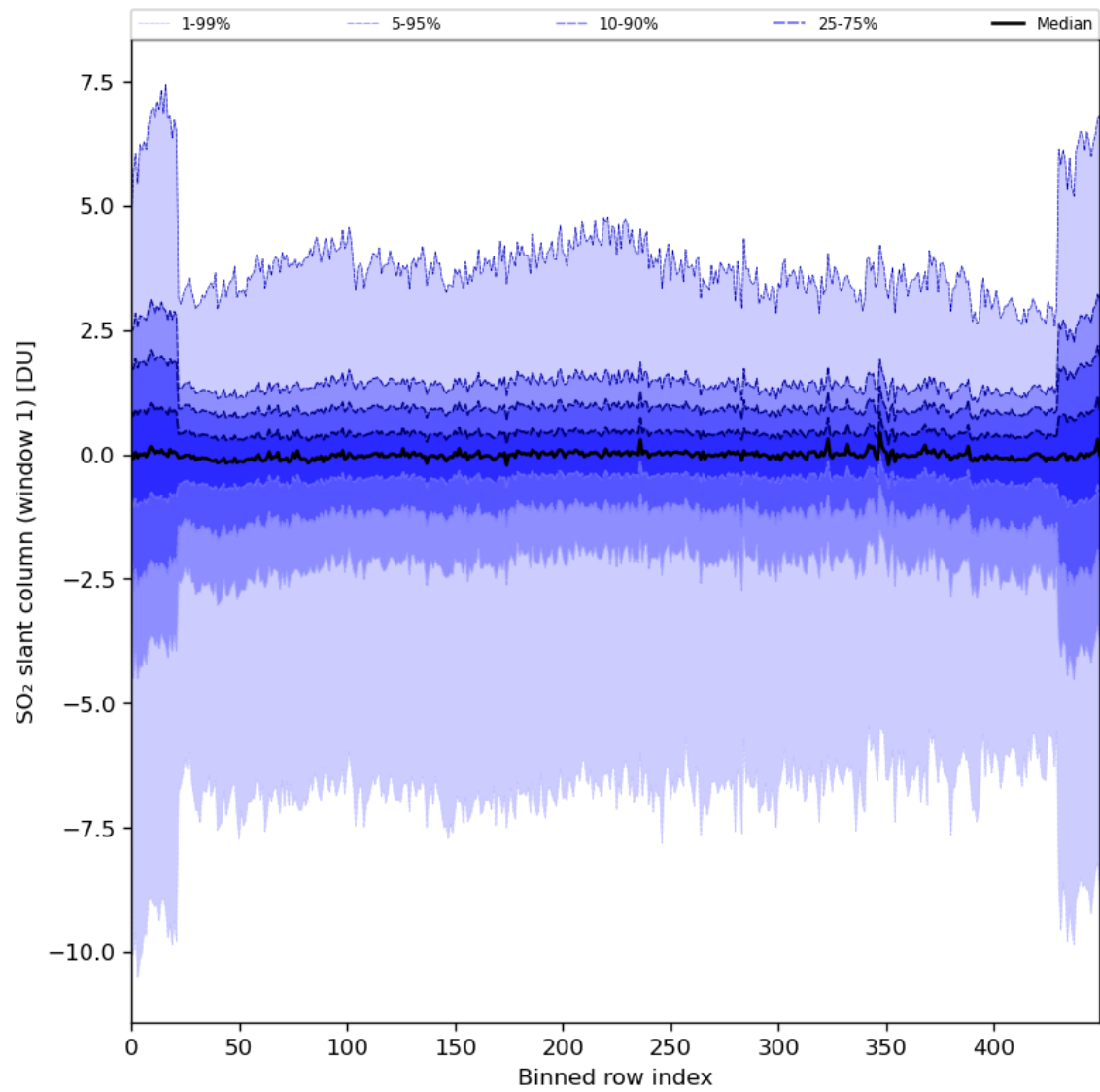
Figure 79: Along track statistics of “SO 2 slant column (window 1)” for 2024-05-02 to 2024-05-04
