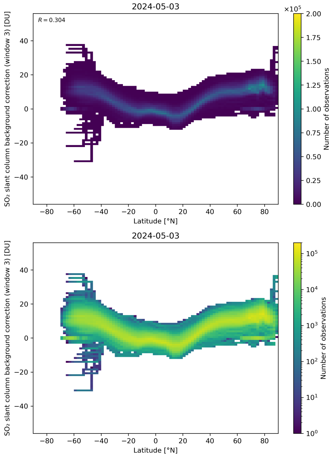
Figure 141: Scatter density plot of “Latitude” against “SO 2 slant column background correction (window 3)” for 2024-05-02 to 2024-05-04.
