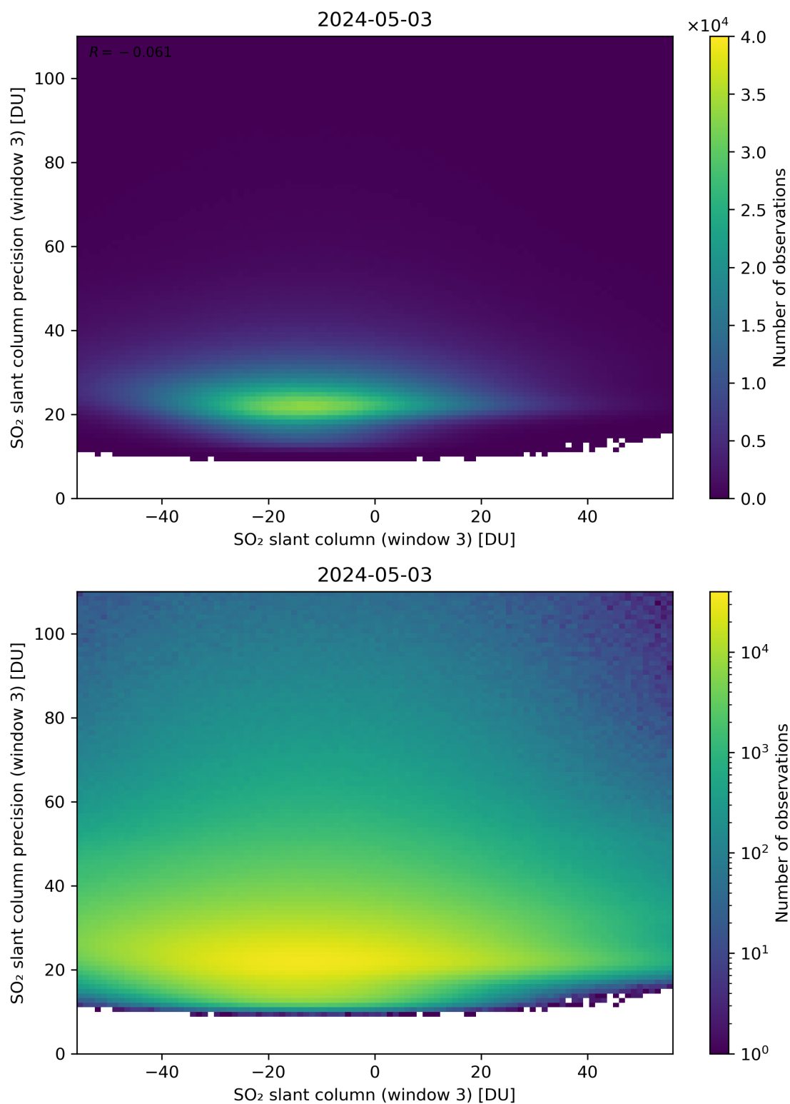
Figure 267: Scatter density plot of “SO 2 slant column (window 3)” against “SO 2 slant column precision (window 3)” for 2024-05-02 to 2024-05-04.
