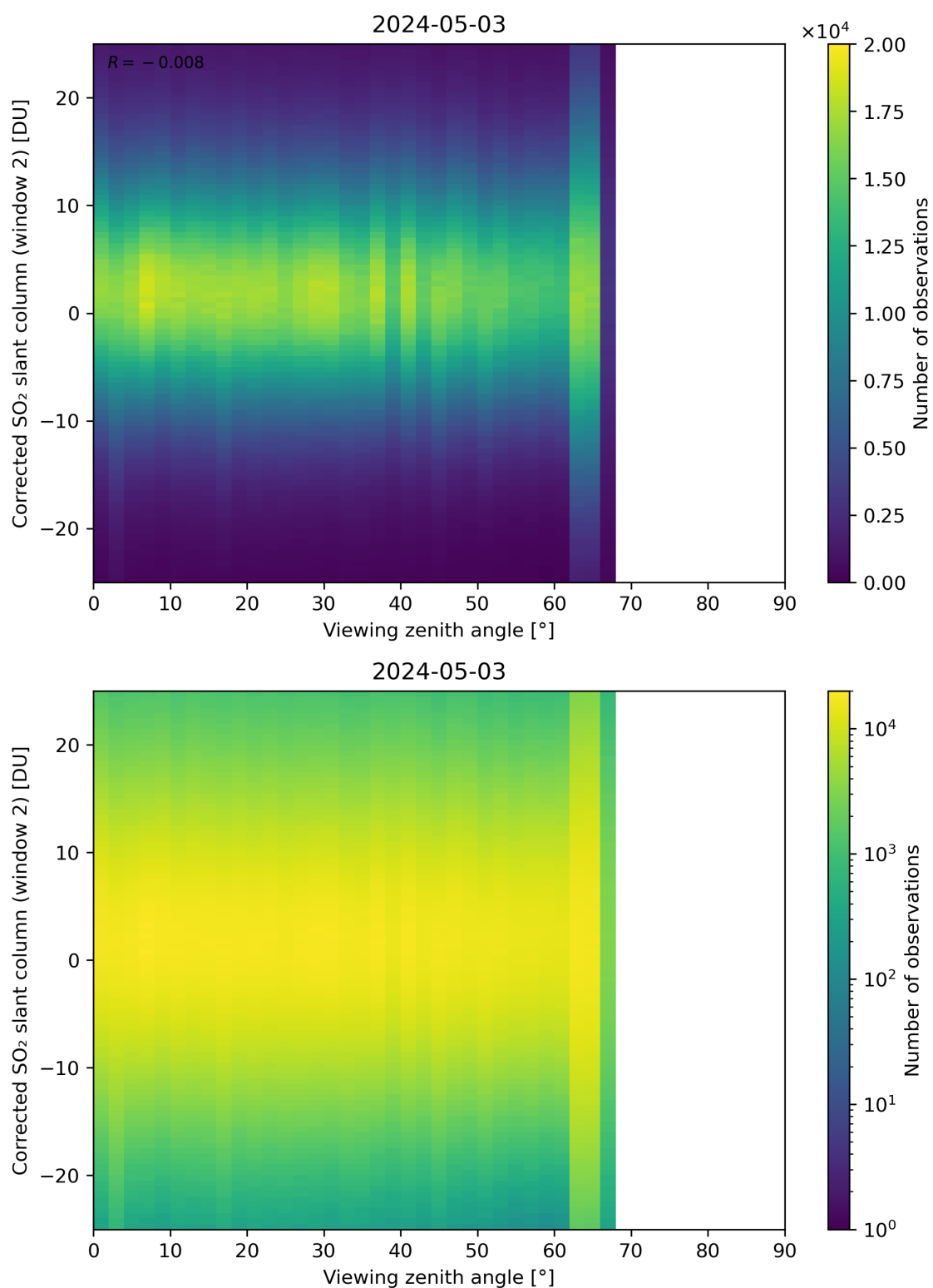
Figure 318: Scatter density plot of “Viewing zenith angle” against “Corrected SO 2 slant column (window 2)” for 2024-05-02 to 2024-05-04.
