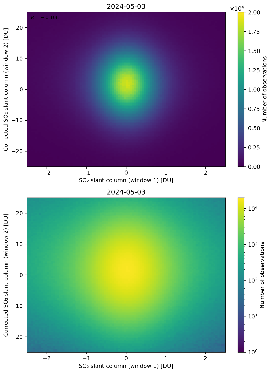
Figure 233: Scatter density plot of “SO 2 slant column (window 1)” against “Corrected SO 2 slant column (window 2)” for 2024-05-02 to 2024-05-04.
