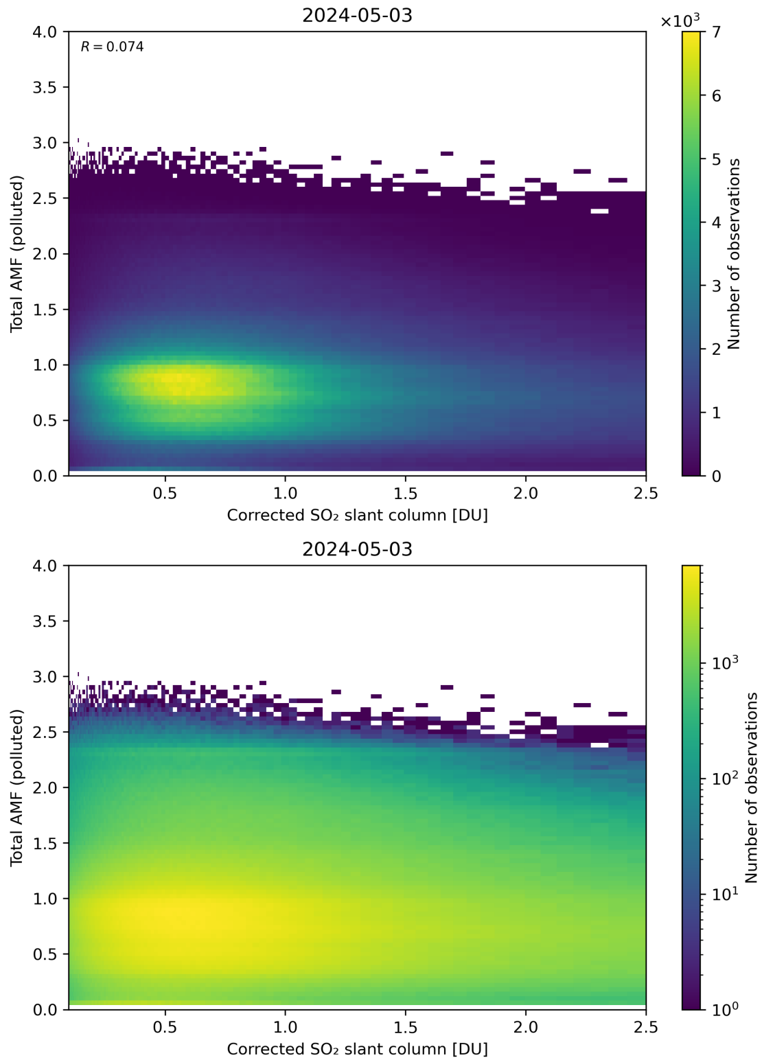
Figure 192: Scatter density plot of “Corrected SO 2 slant column” against “Total AMF (polluted)” for 2024-05-02 to 2024-05-04.
