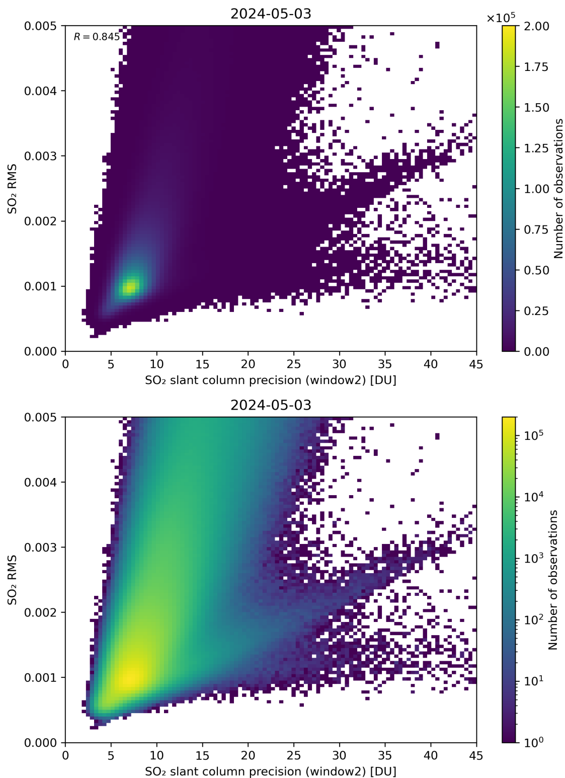
Figure 245: Scatter density plot of “SO 2 slant column precision (window2)” against “SO 2 RMS” for 2024-05-02 to 2024-05-04.
