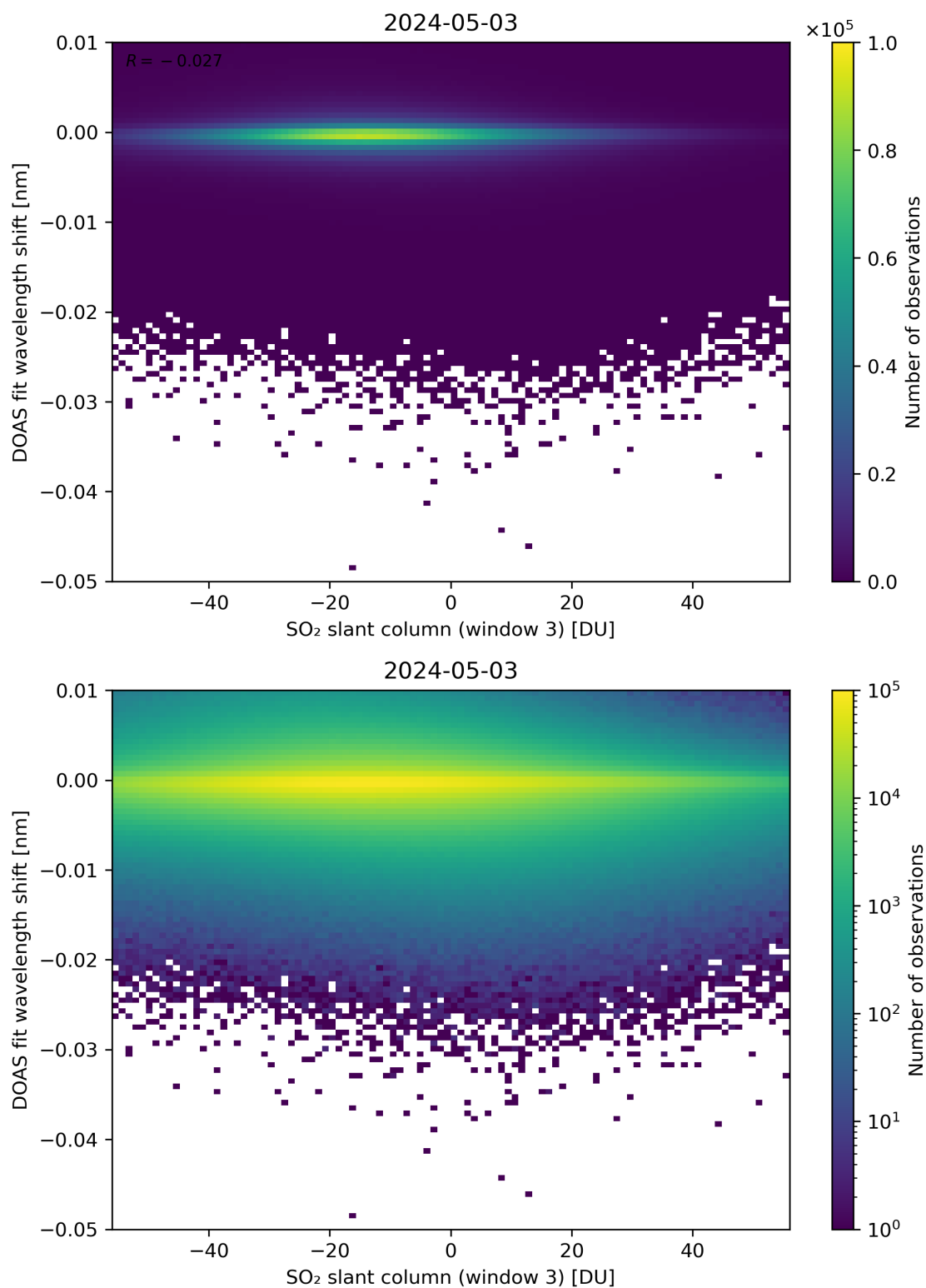
Figure 254: Scatter density plot of “SO 2 slant column (window 3)” against “DOAS fit wavelength shift” for 2024-05-02 to 2024-05-04.
