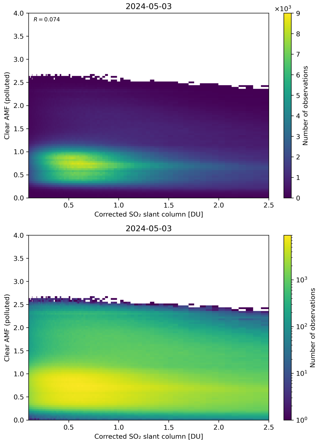
Figure 184: Scatter density plot of “Corrected SO 2 slant column” against “Clear AMF (polluted)” for 2024-05-02 to 2024-05-04.
