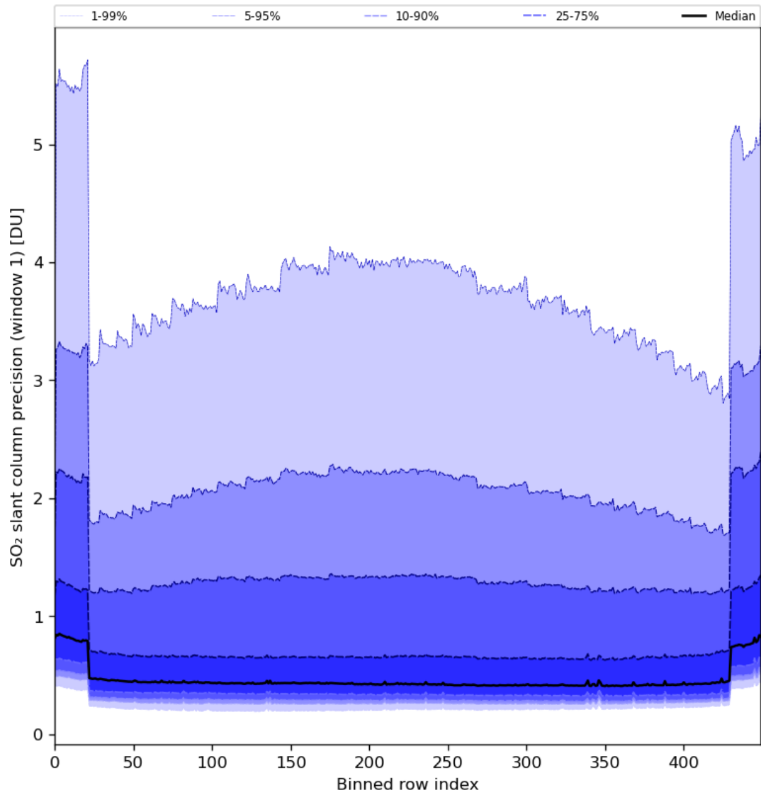
Figure 80: Along track statistics of “SO 2 slant column precision (window 1)” for 2024-05-02 to 2024-05-04
