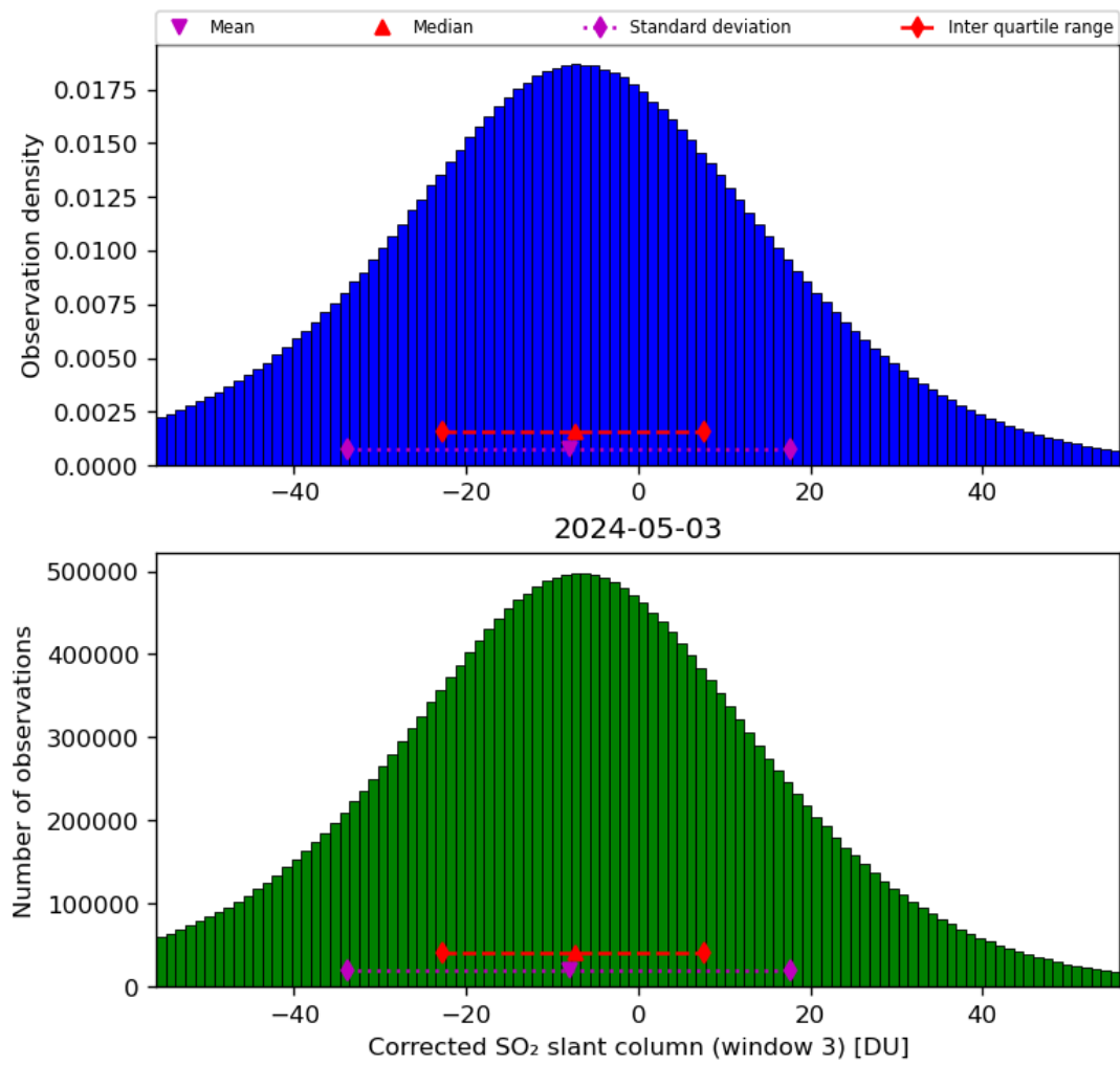
Figure 66: Histogram of “Corrected SO 2 slant column (window 3)” for 2024-05-02 to 2024-05-04
