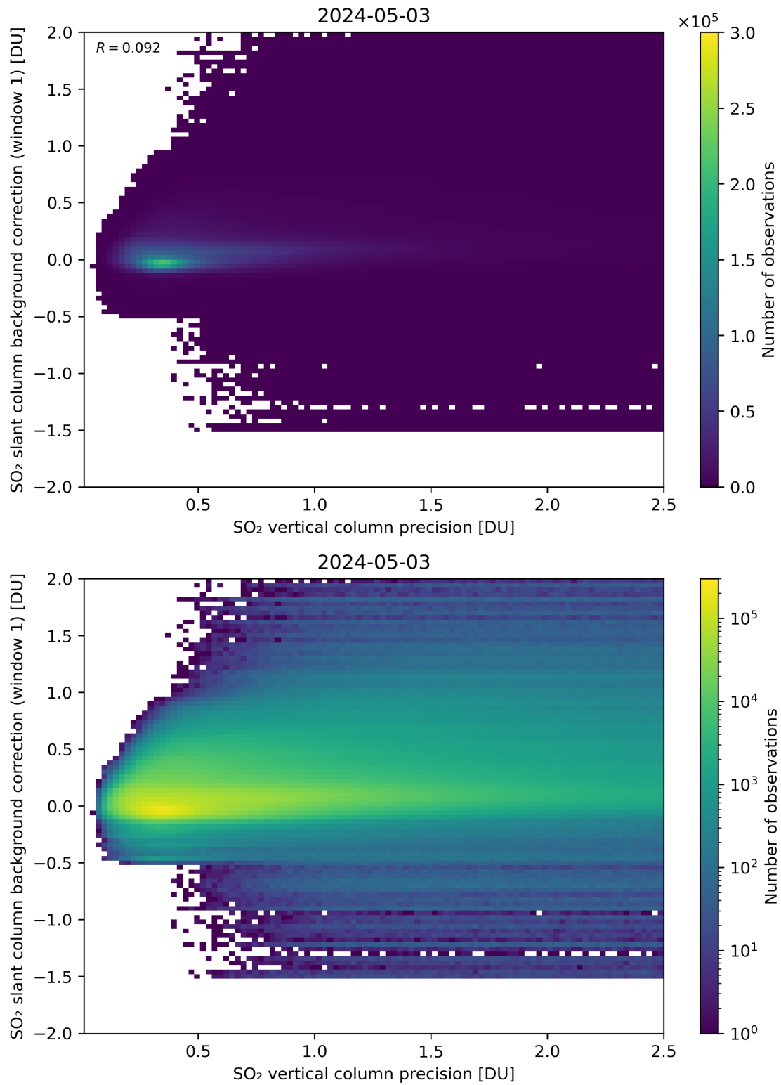
Figure 279: Scatter density plot of “SO 2 vertical column precision” against “SO 2 slant column background correction (window 1)” for 2024-05-02 to 2024-05-04.
