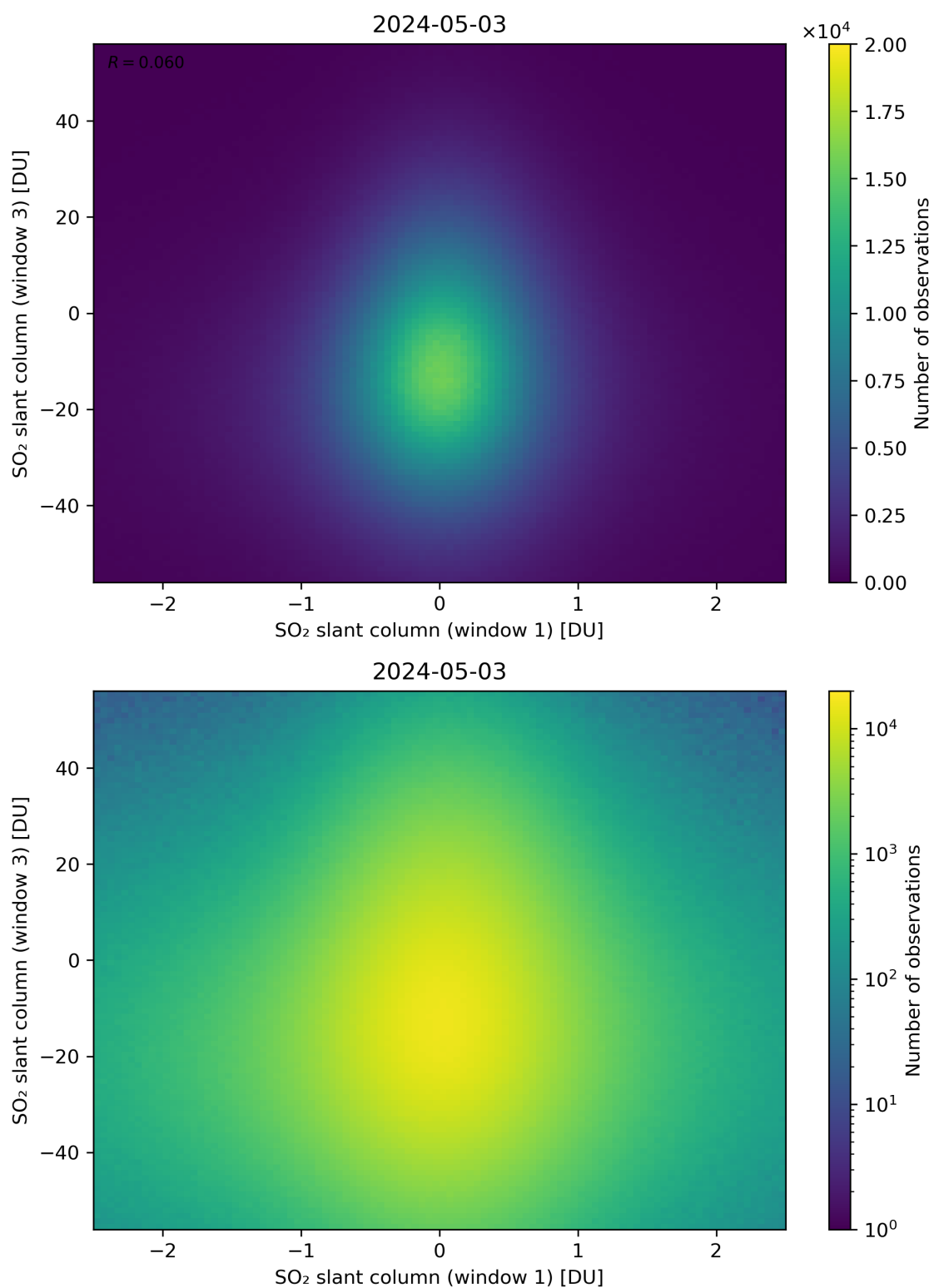
Figure 237: Scatter density plot of “SO 2 slant column (window 1)” against “SO 2 slant column (window 3)” for 2024-05-02 to 2024-05-04.
