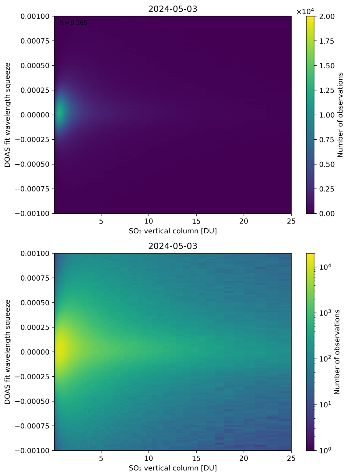
Figure 277: Scatter density plot of “SO 2 vertical column” against “DOAS fit wavelength squeeze” for 2024-05-02 to 2024-05-04.
