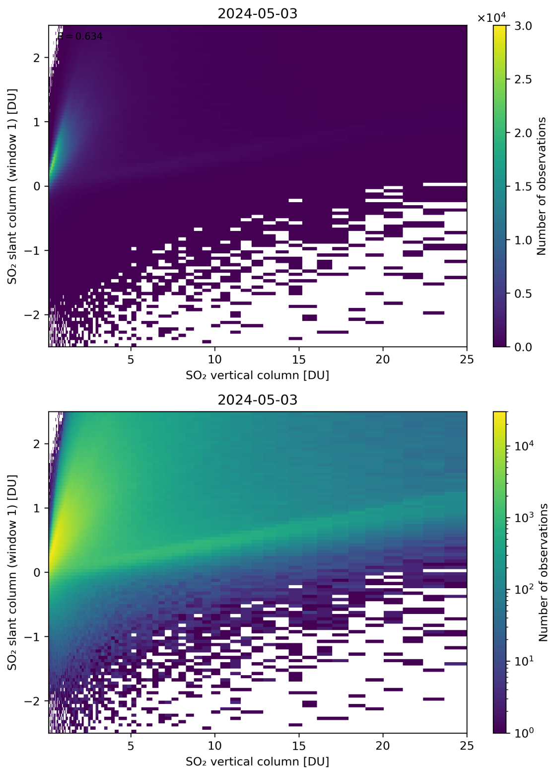
Figure 300: Scatter density plot of “SO 2 vertical column” against “SO 2 slant column (window 1)” for 2024-05-02 to 2024-05-04.
