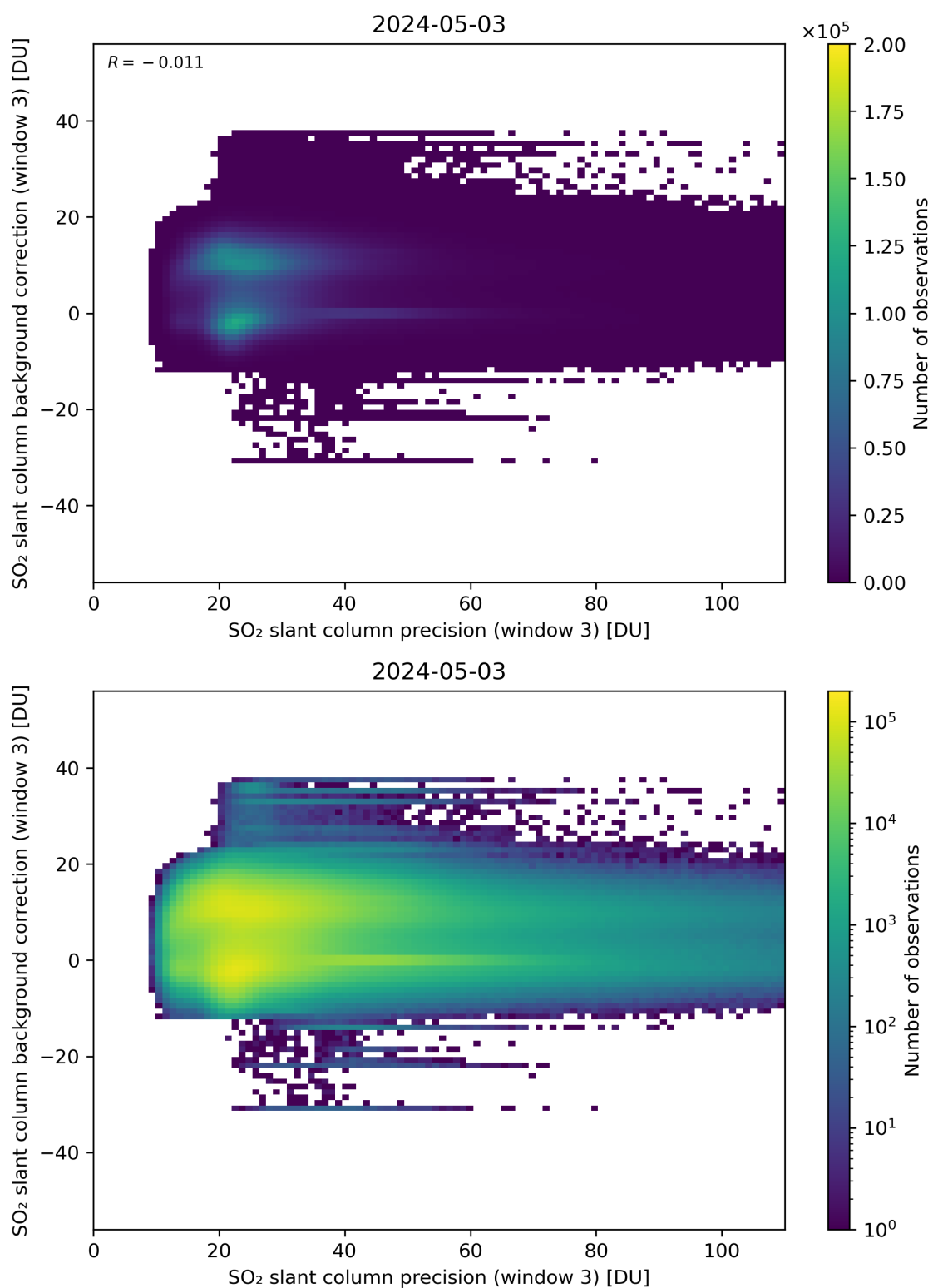
Figure 257: Scatter density plot of “SO 2 slant column precision (window 3)” against “SO 2 slant column background correction (window 3)” for 2024-05-02 to 2024-05-04.
