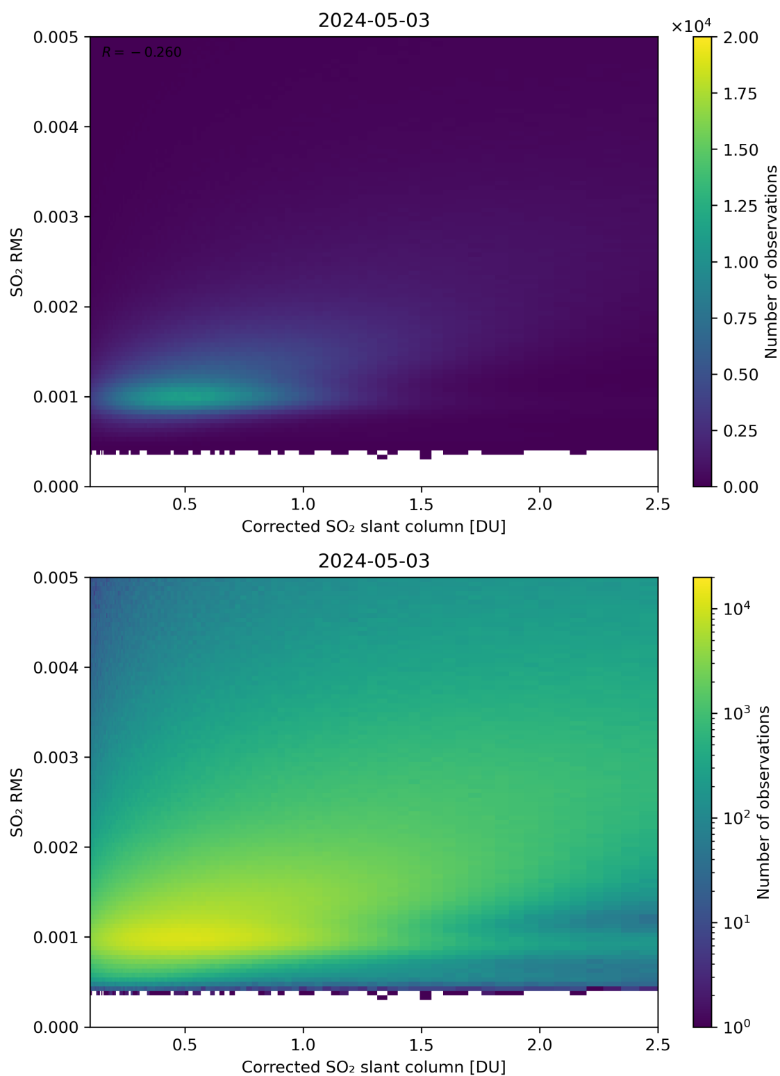
Figure 183: Scatter density plot of “Corrected SO 2 slant column” against “SO 2 RMS” for 2024-05-02 to 2024-05-04.
