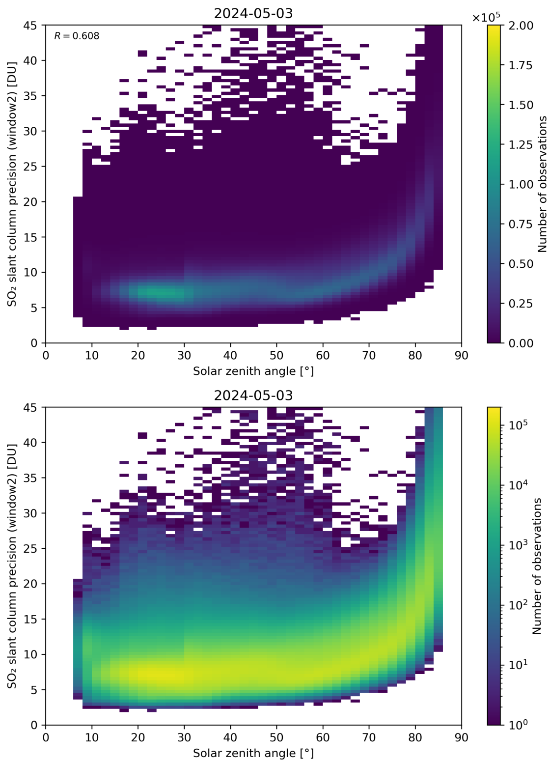
Figure 171: Scatter density plot of “Solar zenith angle” against “SO 2 slant column precision (window2)” for 2024-05-02 to 2024-05-04.
