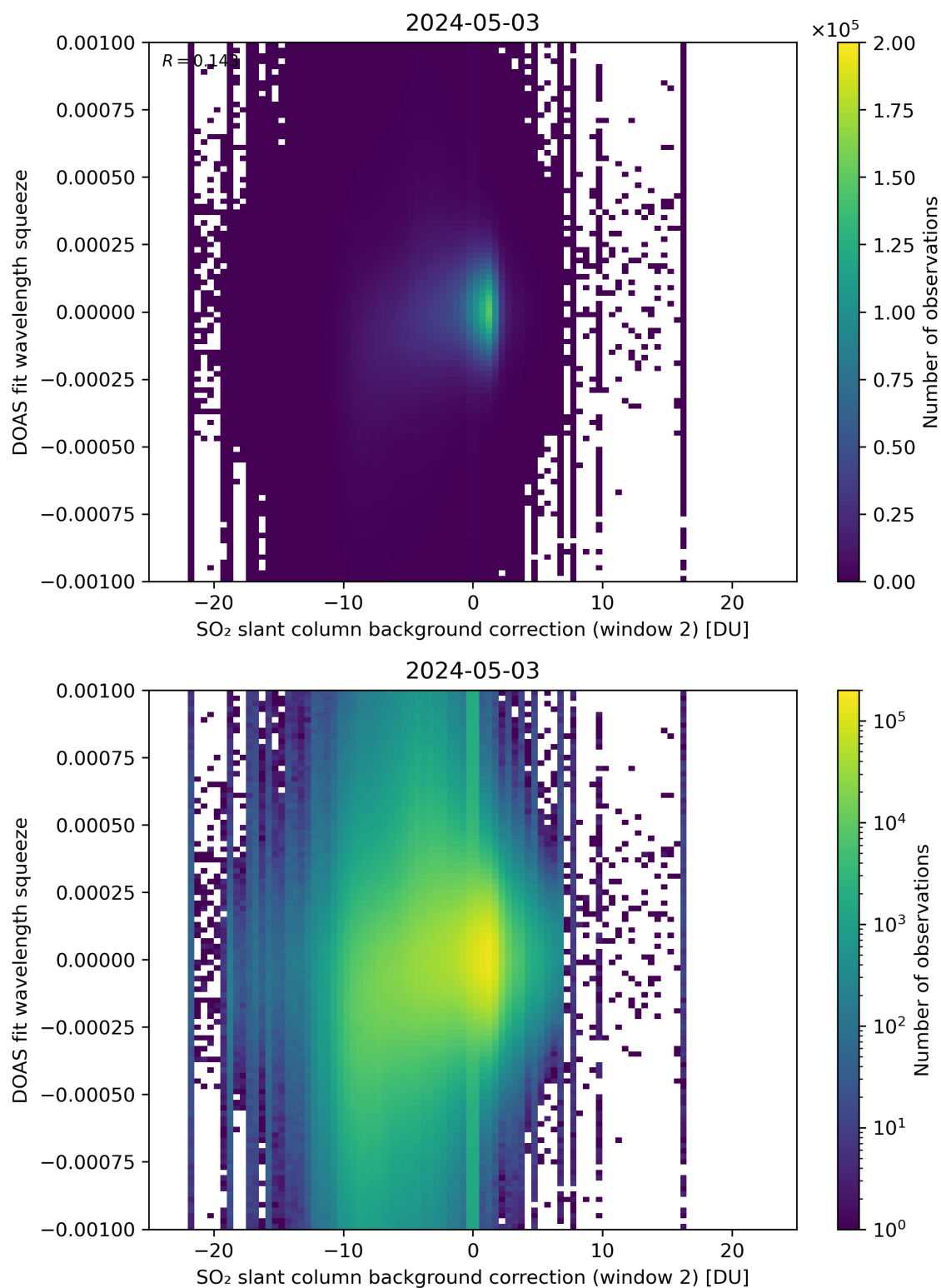
Figure 113: Scatter density plot of “SO 2 slant column background correction (window 2)” against “DOAS fit wavelength squeeze” for 2024-05-02 to 2024-05-04.
