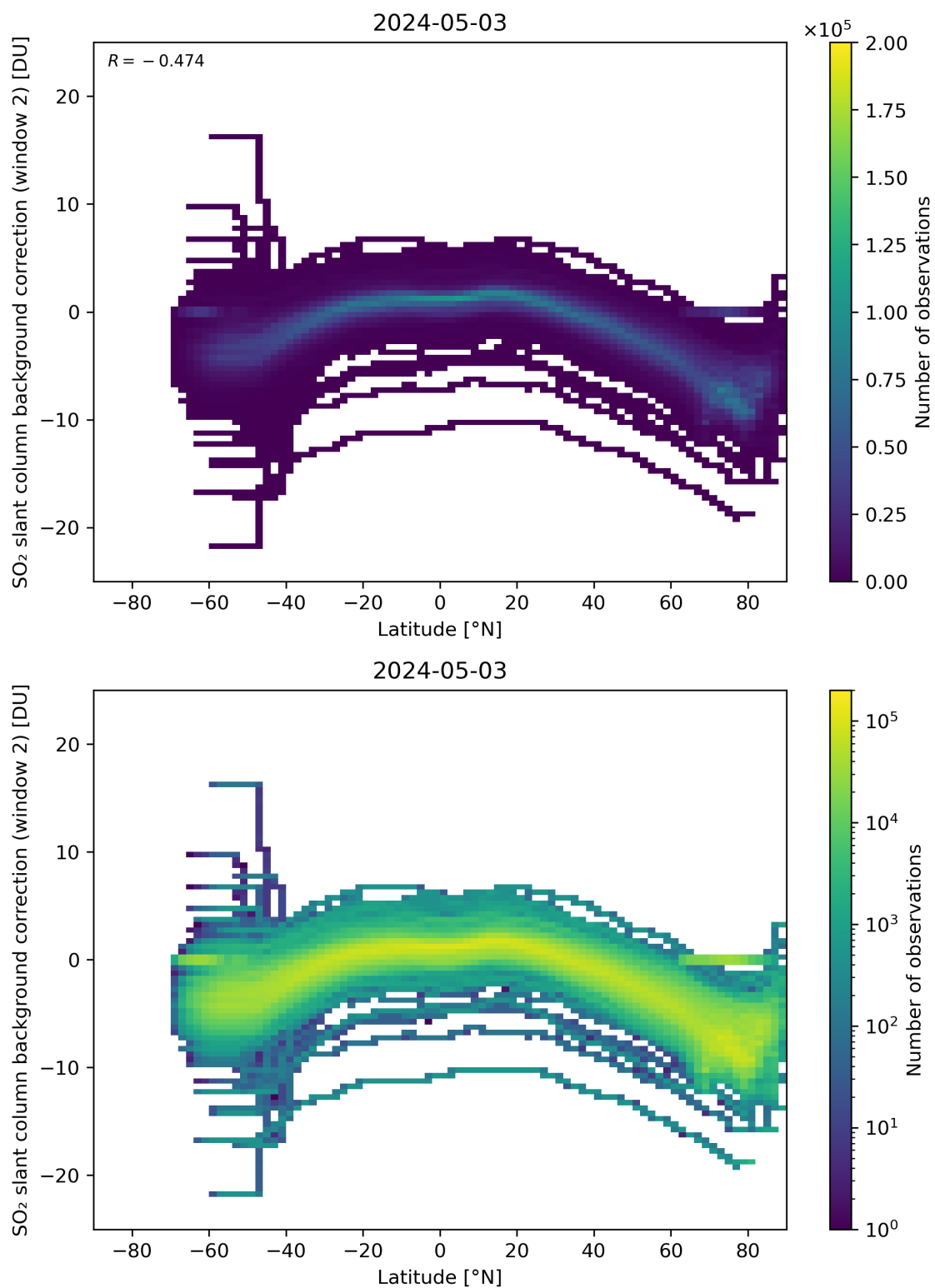
Figure 140: Scatter density plot of “Latitude” against “SO 2 slant column background correction (window 2)” for 2024-05-02 to 2024-05-04.
