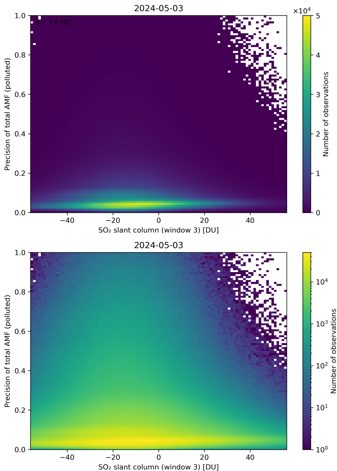
Figure 269: Scatter density plot of “SO 2 slant column (window 3)” against “Precision of total AMF (polluted)” for 2024-05-02 to 2024-05-04.
