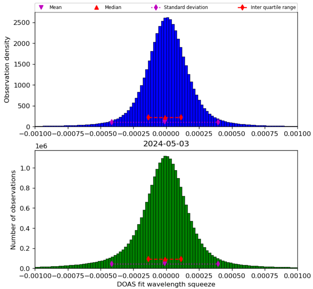
Figure 69: Histogram of “DOAS fit wavelength squeeze” for 2024-05-02 to 2024-05-04
