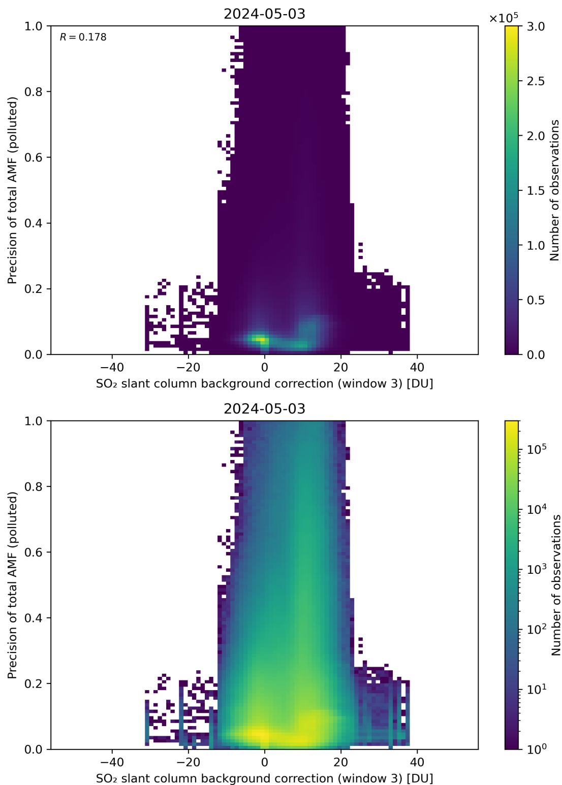
Figure 126: Scatter density plot of “SO 2 slant column background correction (window 3)” against “Precision of total AMF (polluted)” for 2024-05-02 to 2024-05-04.
