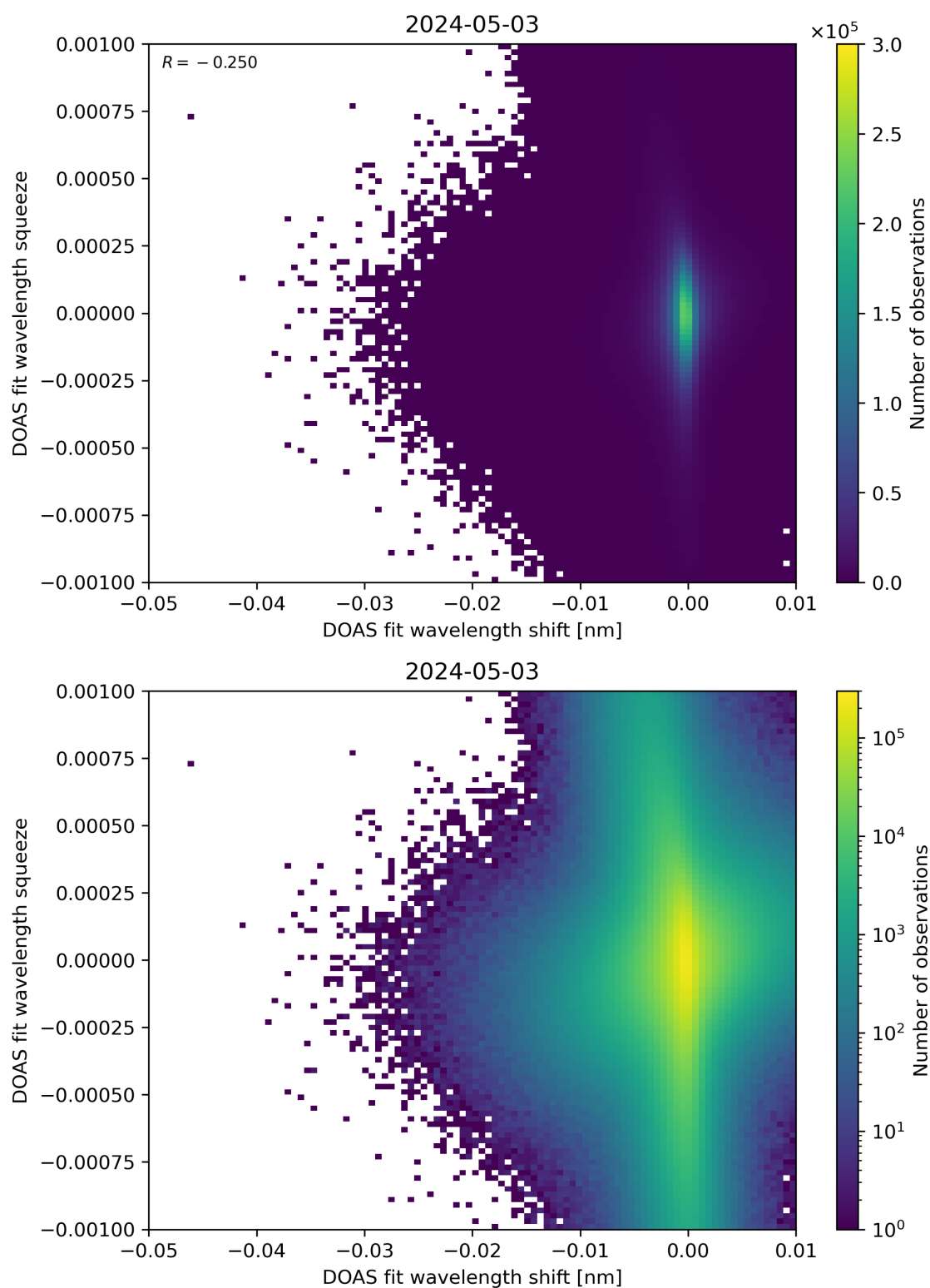
Figure 127: Scatter density plot of “DOAS fit wavelength shift” against “DOAS fit wavelength squeeze” for 2024-05-02 to 2024-05-04.
