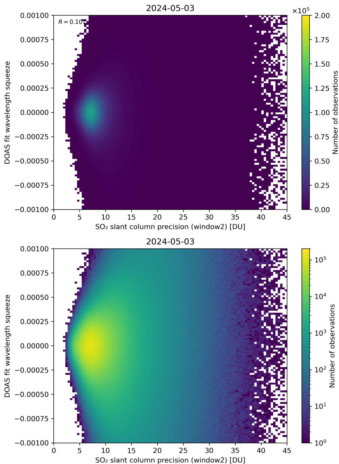
Figure 244: Scatter density plot of “SO 2 slant column precision (window2)” against “DOAS fit wavelength squeeze” for 2024-05-02 to 2024-05-04.
