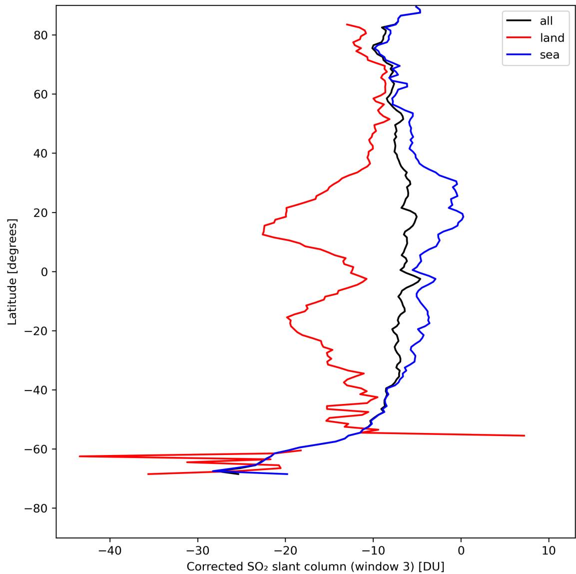
Figure 43: Zonal average of “Corrected SO 2 slant column (window 3)” for 2024-05-02 to 2024-05-04.
