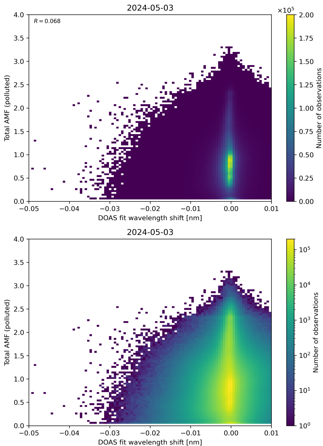
Figure 130: Scatter density plot of “DOAS fit wavelength shift” against “Total AMF (polluted)” for 2024-05-02 to 2024-05-04.
