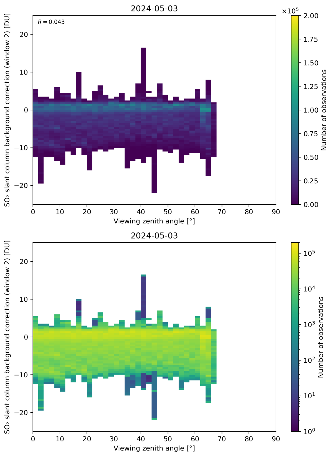
Figure 309: Scatter density plot of “Viewing zenith angle” against “SO 2 slant column background correction (window 2)” for 2024-05-02 to 2024-05-04.
