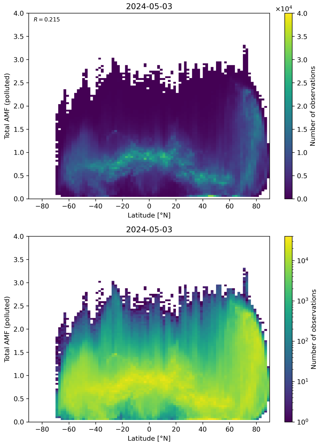
Figure 154: Scatter density plot of “Latitude” against “Total AMF (polluted)” for 2024-05-02 to 2024-05-04.
