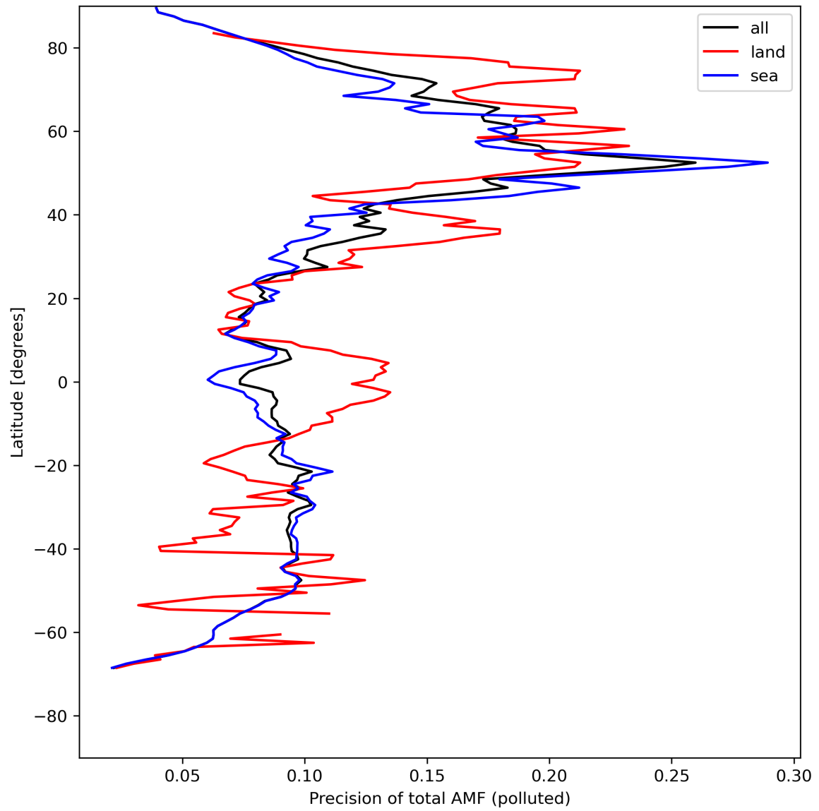
Figure 49: Zonal average of “Precision of total AMF (polluted)” for 2024-05-02 to 2024-05-04.
