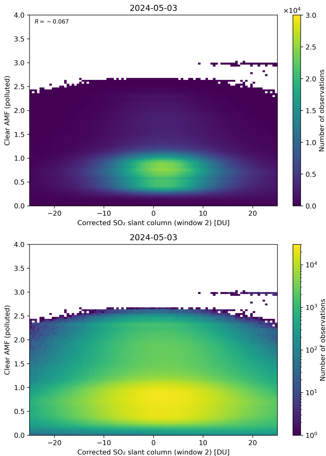
Figure 199: Scatter density plot of “Corrected SO 2 slant column (window 2)” against “Clear AMF (polluted)” for 2024-05-02 to 2024-05-04.
