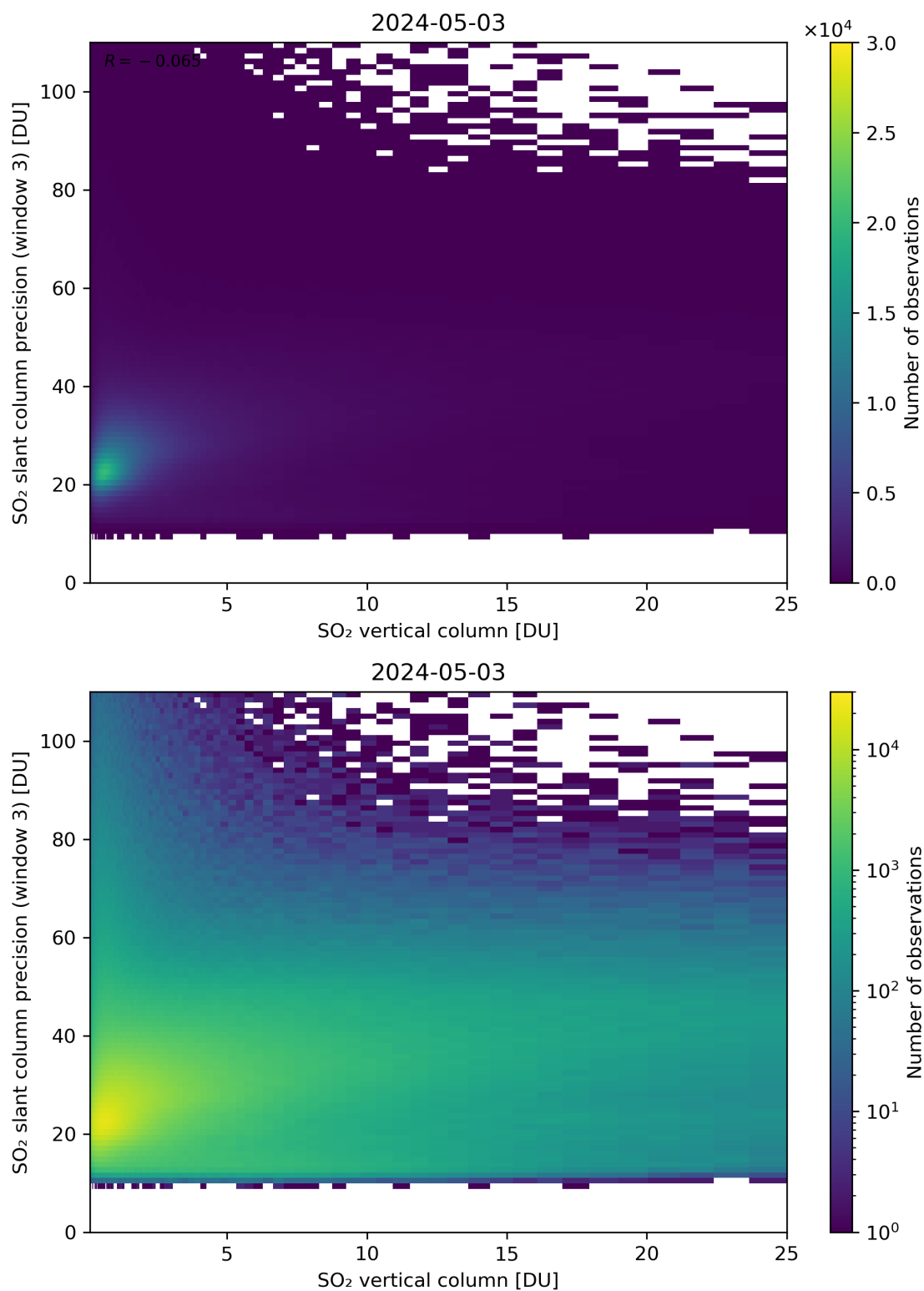
Figure 304: Scatter density plot of “SO 2 vertical column” against “SO 2 slant column precision (window 3)” for 2024-05-02 to 2024-05-04.
