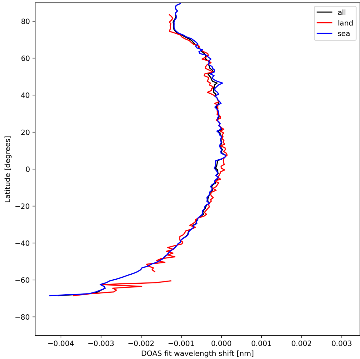
Figure 45: Zonal average of “DOAS fit wavelength shift” for 2024-05-02 to 2024-05-04.
