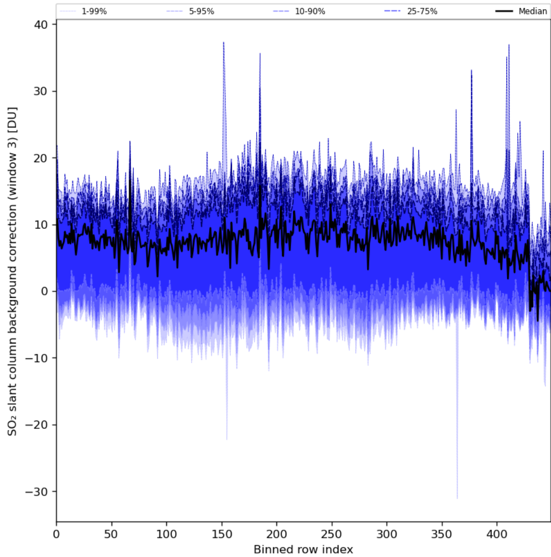
Figure 90: Along track statistics of “SO 2 slant column background correction (window 3)” for 2024-05-02 to 2024-05-04
