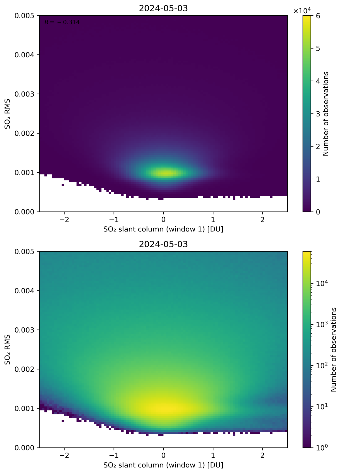
Figure 217: Scatter density plot of “SO 2 slant column (window 1)” against “SO 2 RMS” for 2024-05-02 to 2024-05-04.
