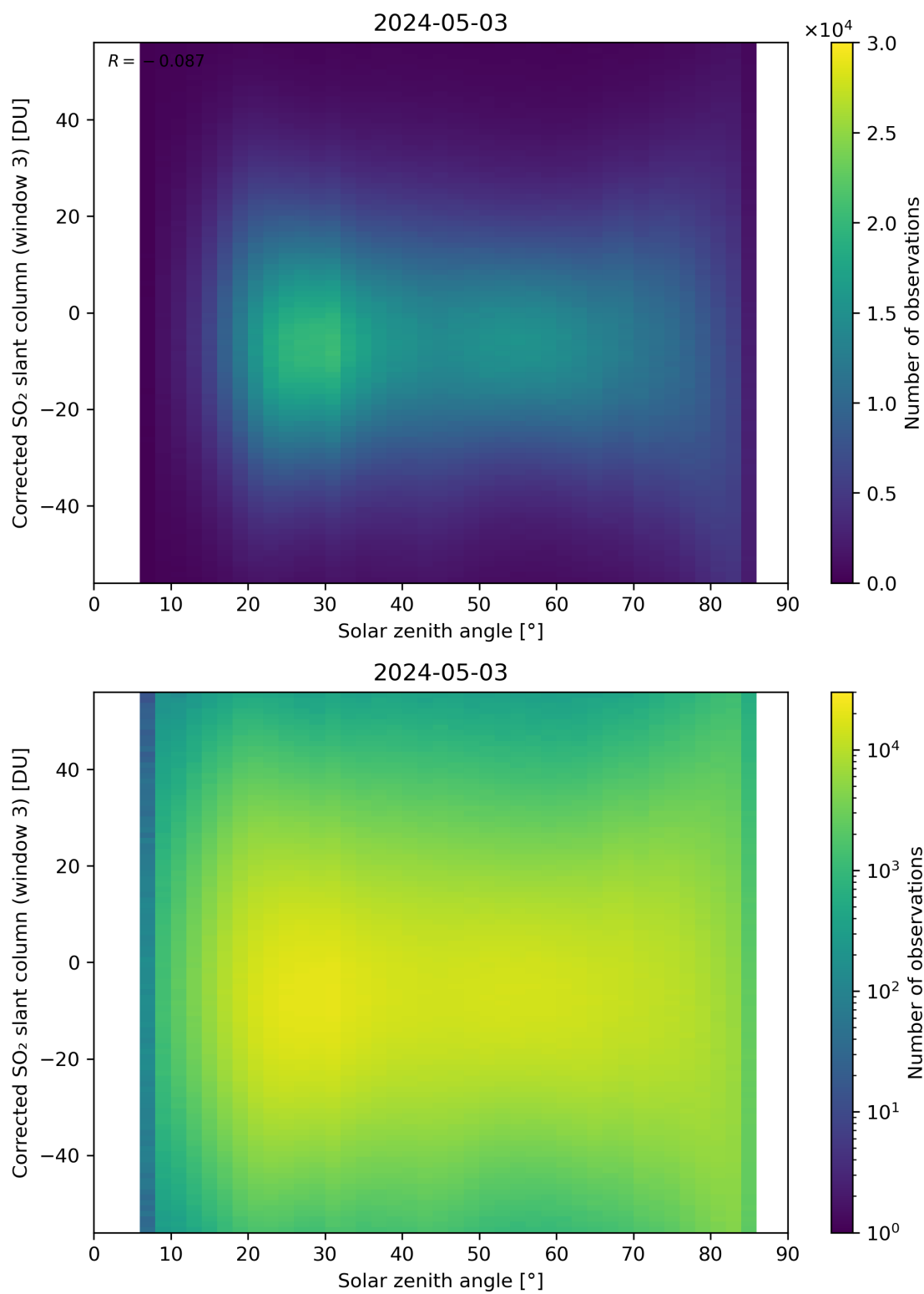
Figure 168: Scatter density plot of “Solar zenith angle” against “Corrected SO 2 slant column (window 3)” for 2024-05-02 to 2024-05-04.
