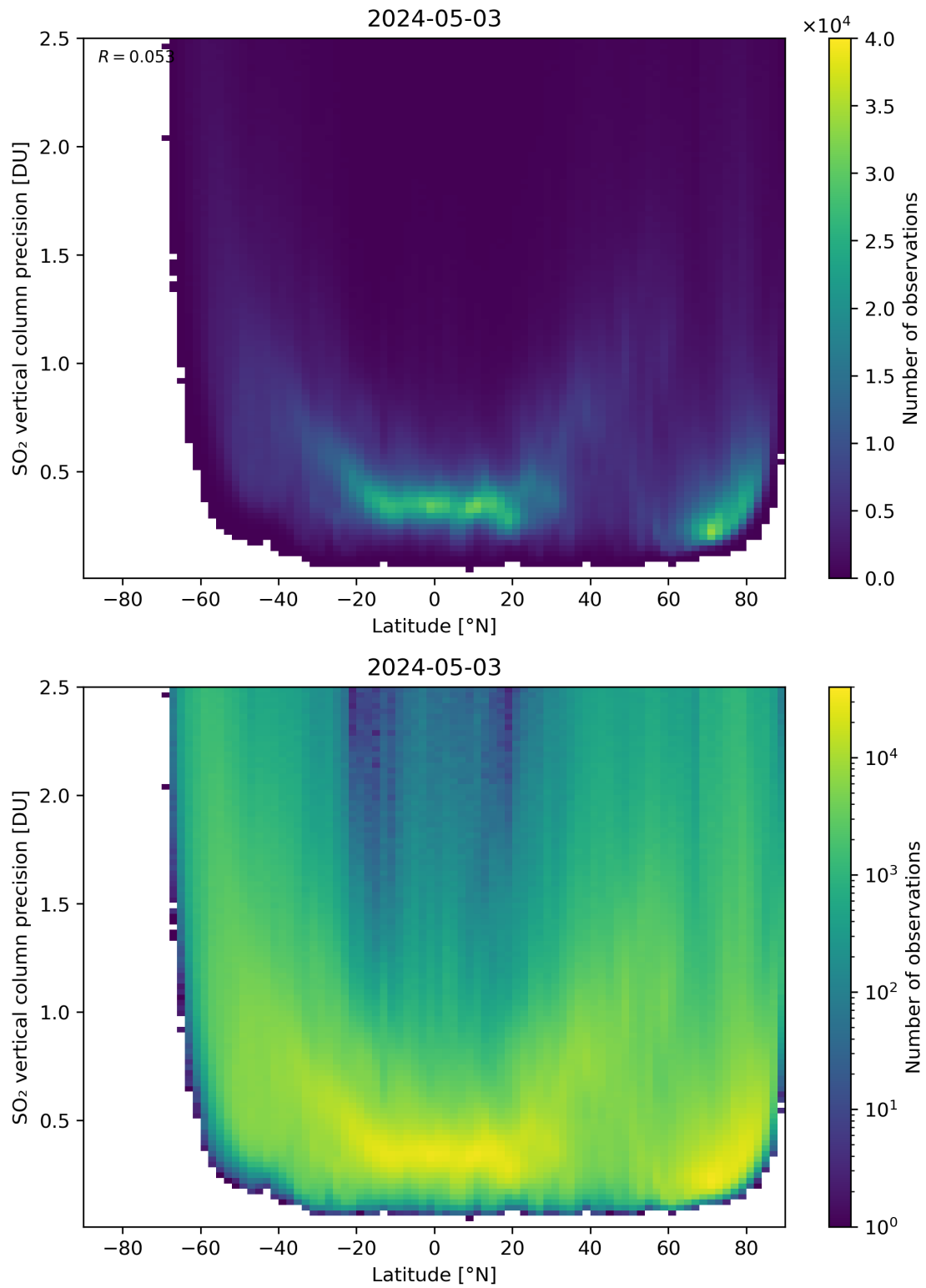
Figure 157: Scatter density plot of “Latitude” against “SO 2 vertical column precision” for 2024-05-02 to 2024-05-04.
