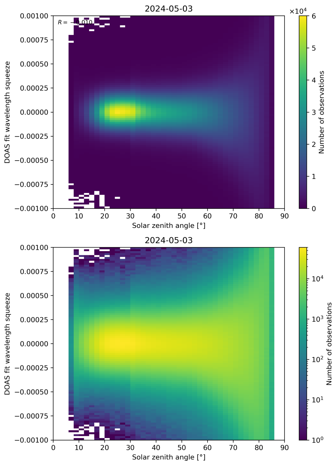
Figure 162: Scatter density plot of “Solar zenith angle” against “DOAS fit wavelength squeeze” for 2024-05-02 to 2024-05-04.
