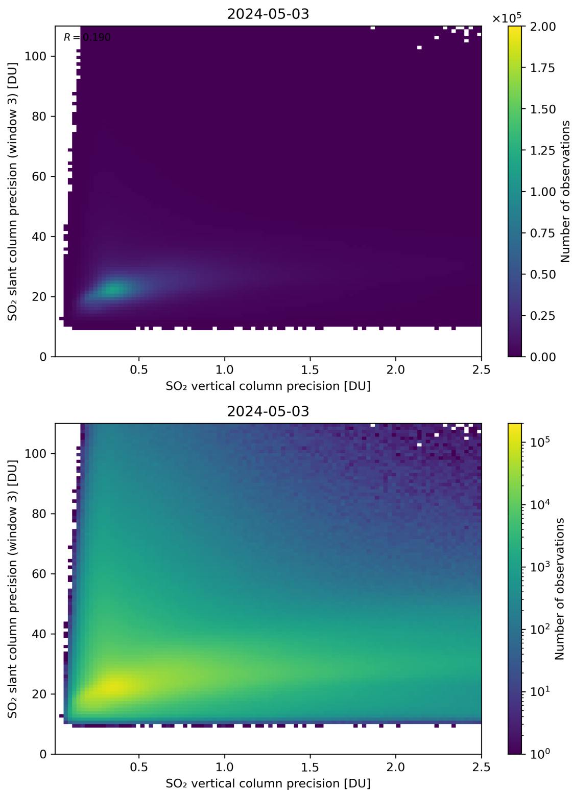
Figure 293: Scatter density plot of “SO 2 vertical column precision” against “SO 2 slant column precision (window 3)” for 2024-05-02 to 2024-05-04.
