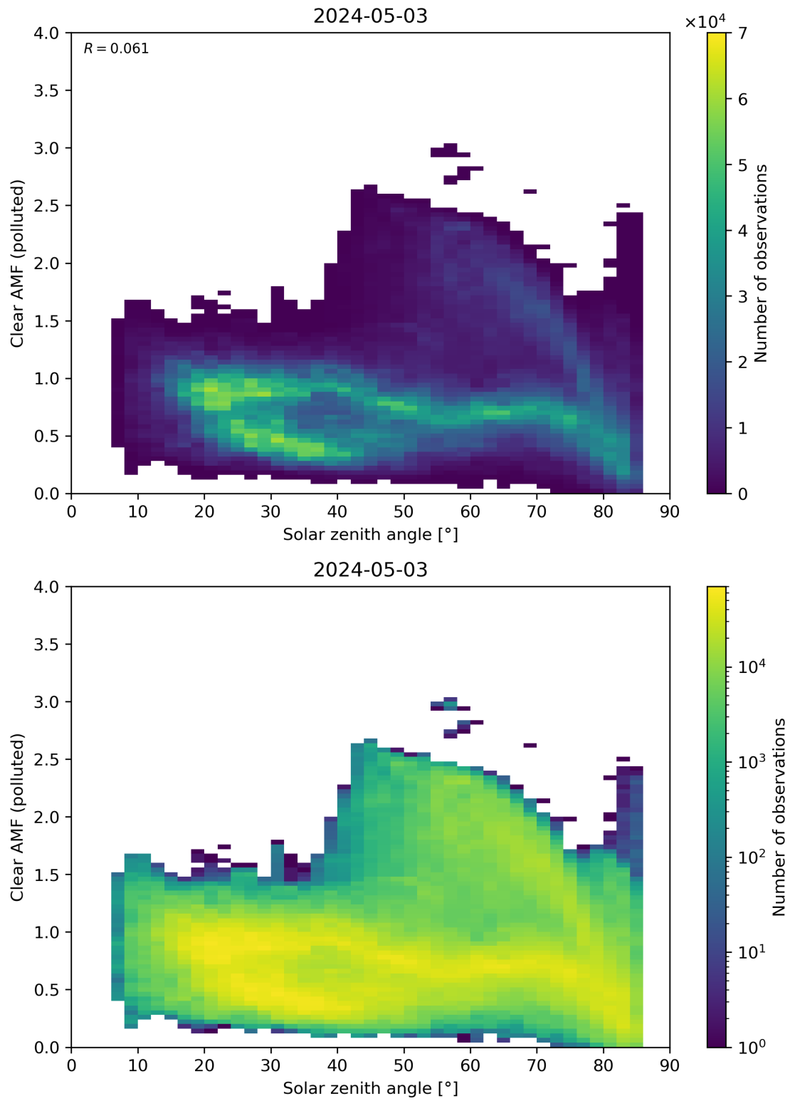
Figure 165: Scatter density plot of “Solar zenith angle” against “Clear AMF (polluted)” for 2024-05-02 to 2024-05-04.
