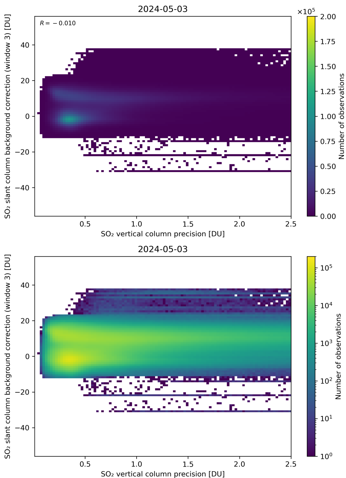
Figure 281: Scatter density plot of “SO 2 vertical column precision” against “SO 2 slant column background correction (window 3)” for 2024-05-02 to 2024-05-04.
