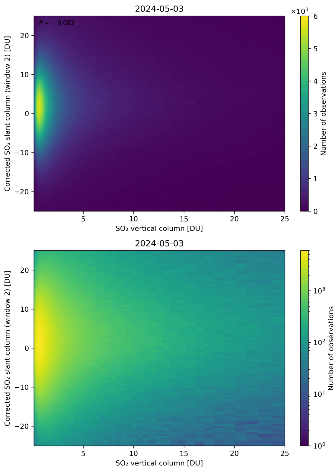
Figure 298: Scatter density plot of “SO 2 vertical column” against “Corrected SO 2 slant column (window 2)” for 2024-05-02 to 2024-05-04.
