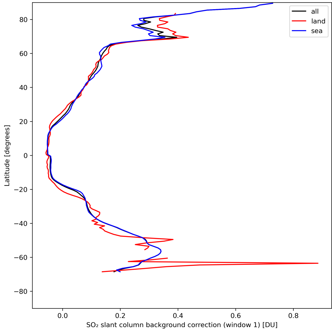
Figure 36: Zonal average of "SO 2 slant column background correction (window 1)" for 2024-05-02 to 2024-05-04.
