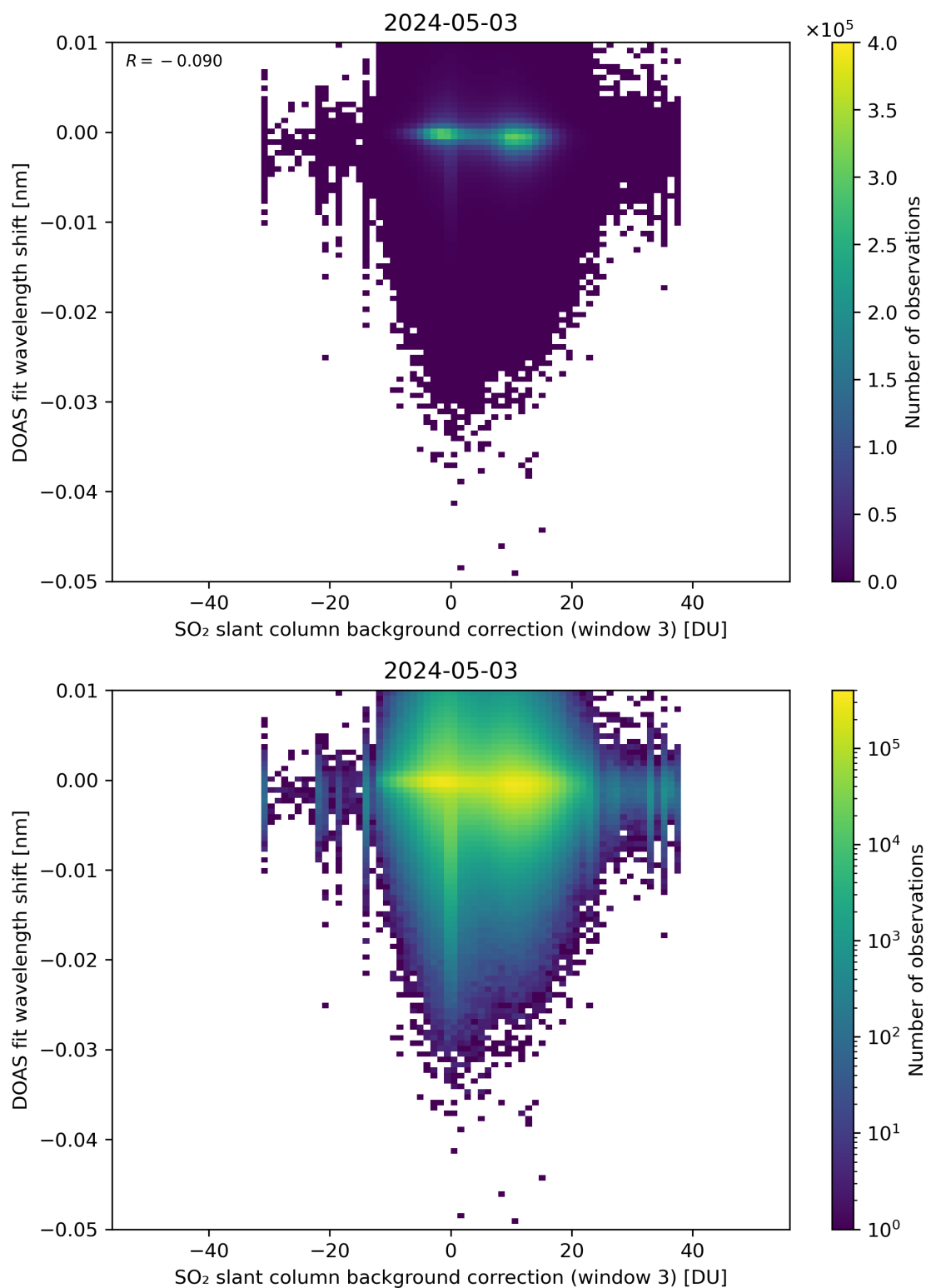
Figure 121: Scatter density plot of “SO 2 slant column background correction (window 3)” against “DOAS fit wavelength shift” for 2024-05-02 to 2024-05-04.
