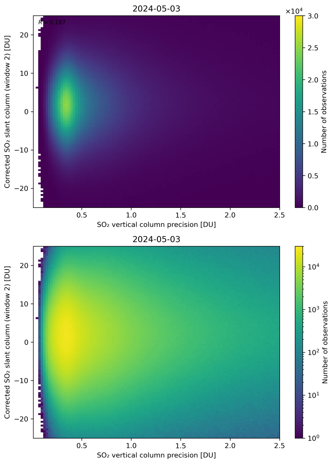
Figure 287: Scatter density plot of “SO 2 vertical column precision” against “Corrected SO 2 slant column (window 2)” for 2024-05-02 to 2024-05-04.
