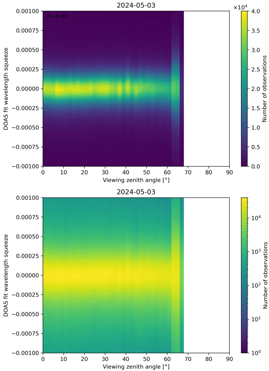
Figure 312: Scatter density plot of “Viewing zenith angle” against “DOAS fit wavelength squeeze” for 2024-05-02 to 2024-05-04.
