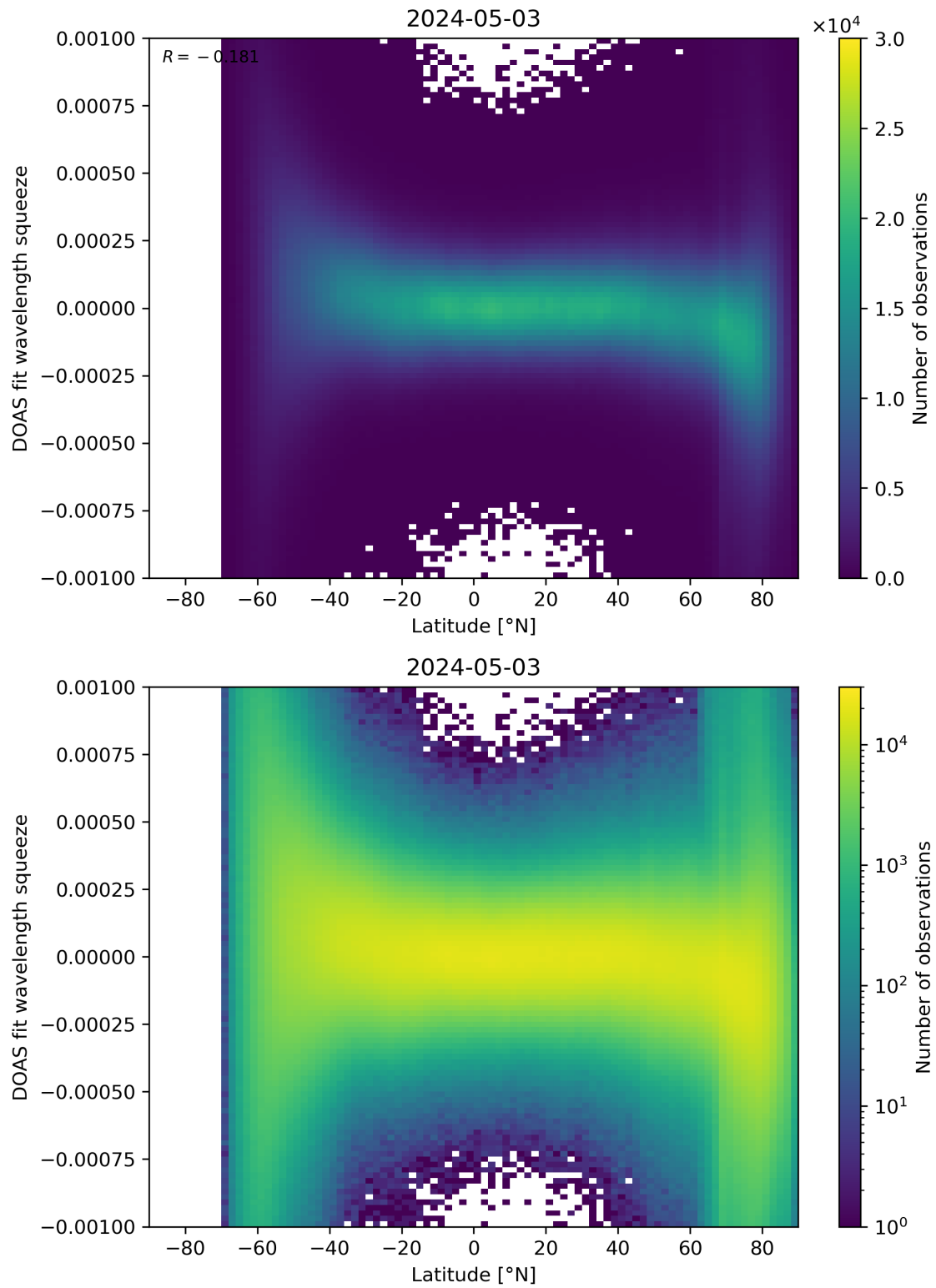
Figure 143: Scatter density plot of “Latitude” against “DOAS fit wavelength squeeze” for 2024-05-02 to 2024-05-04.
