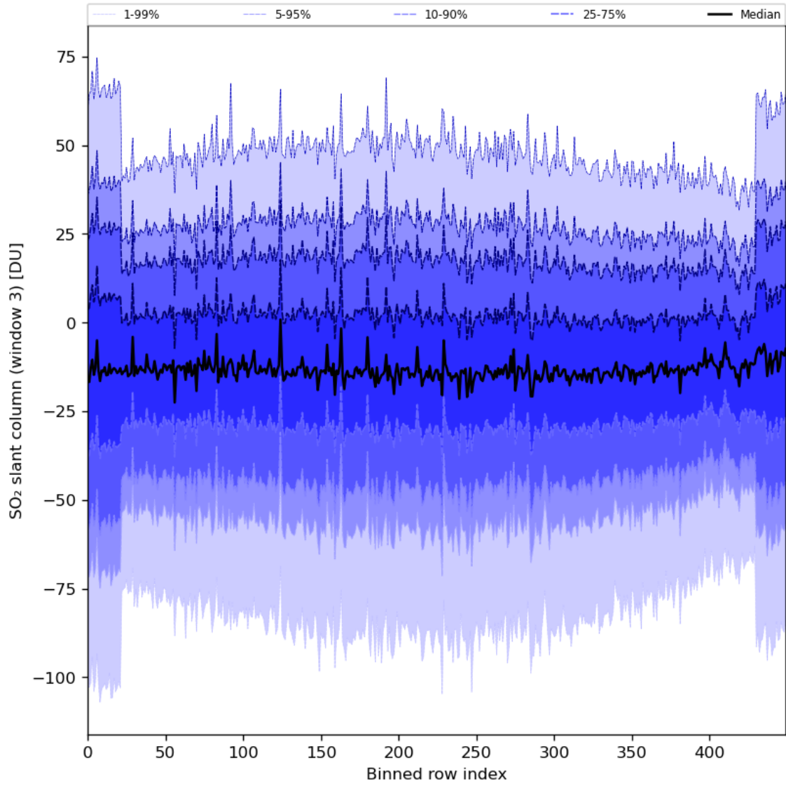
Figure 87: Along track statistics of “SO 2 slant column (window 3)” for 2024-05-02 to 2024-05-04
