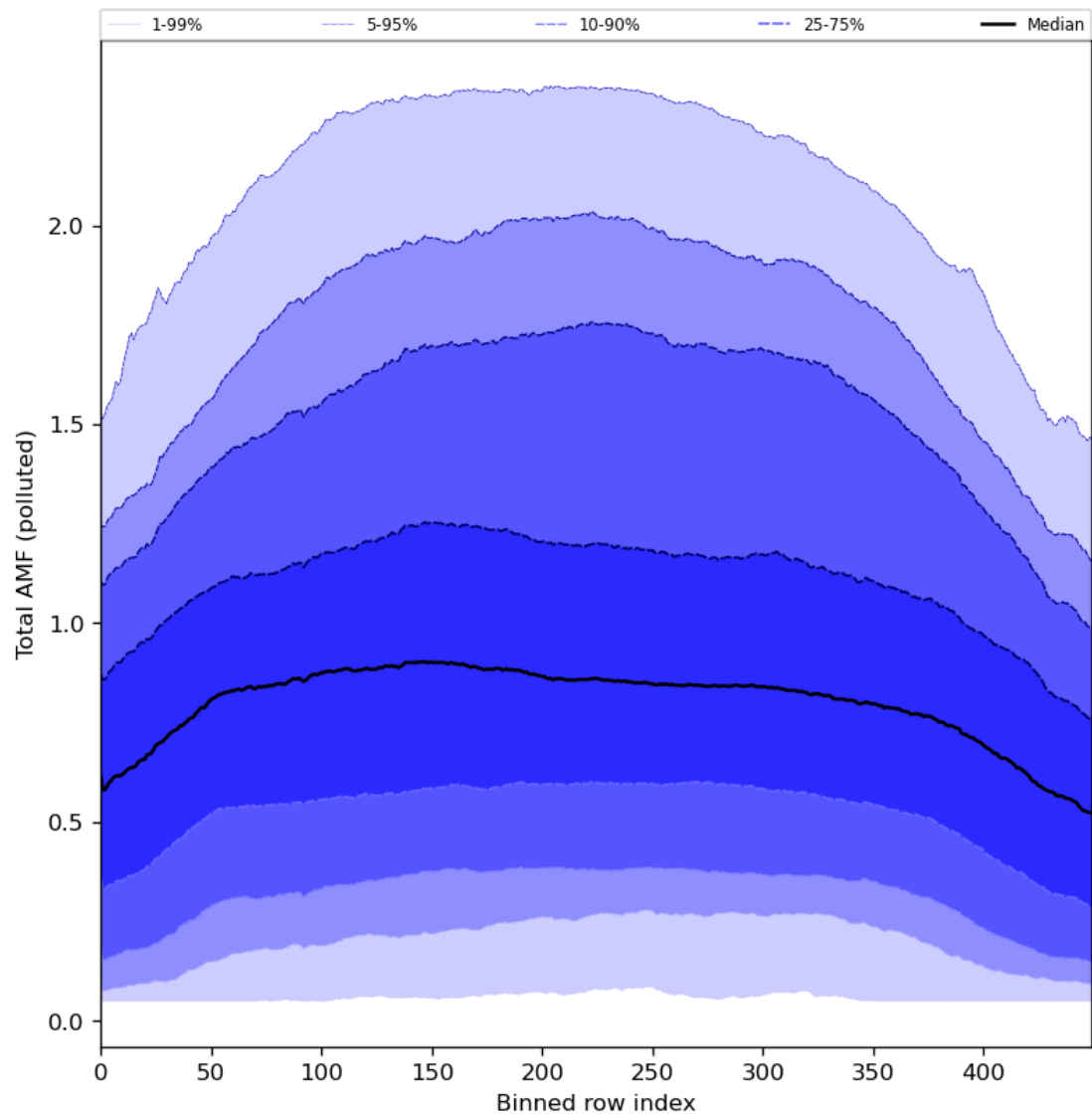
Figure 94: Along track statistics of “Total AMF (polluted)” for 2024-05-02 to 2024-05-04
