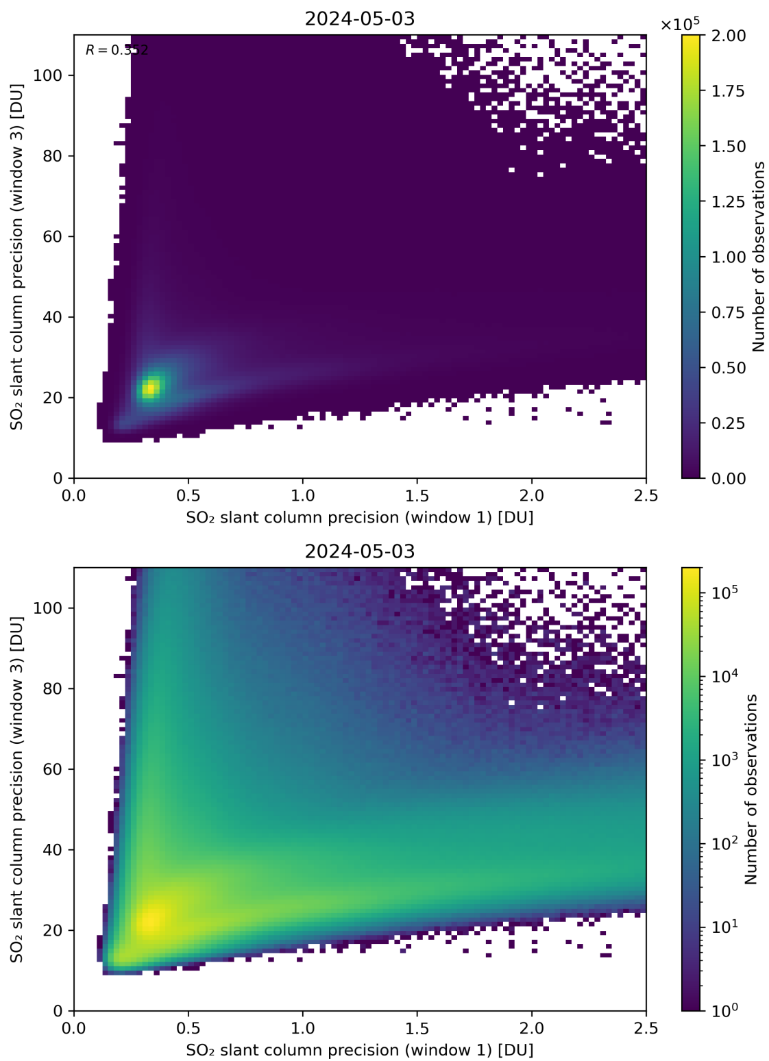
Figure 229: Scatter density plot of “SO 2 slant column precision (window 1)” against “SO 2 slant column precision (window 3)” for 2024-05-02 to 2024-05-04.
