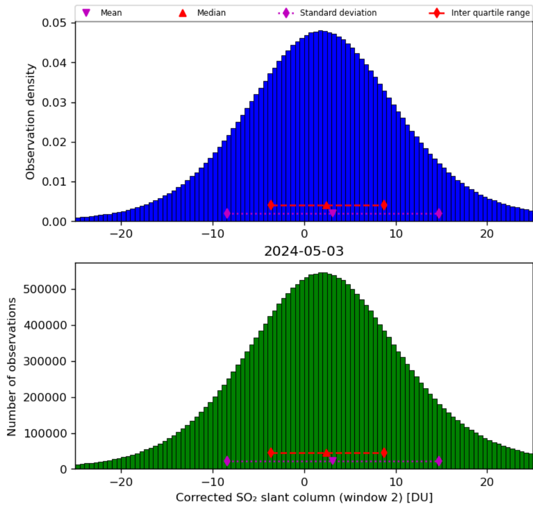
Figure 62: Histogram of “Corrected SO 2 slant column (window 2)” for 2024-05-02 to 2024-05-04
