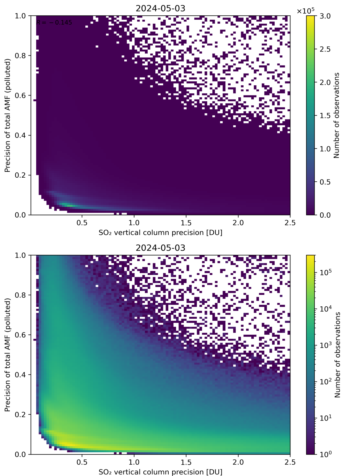
Figure 295: Scatter density plot of “SO 2 vertical column precision” against “Precision of total AMF (polluted)” for 2024-05-02 to 2024-05-04.
