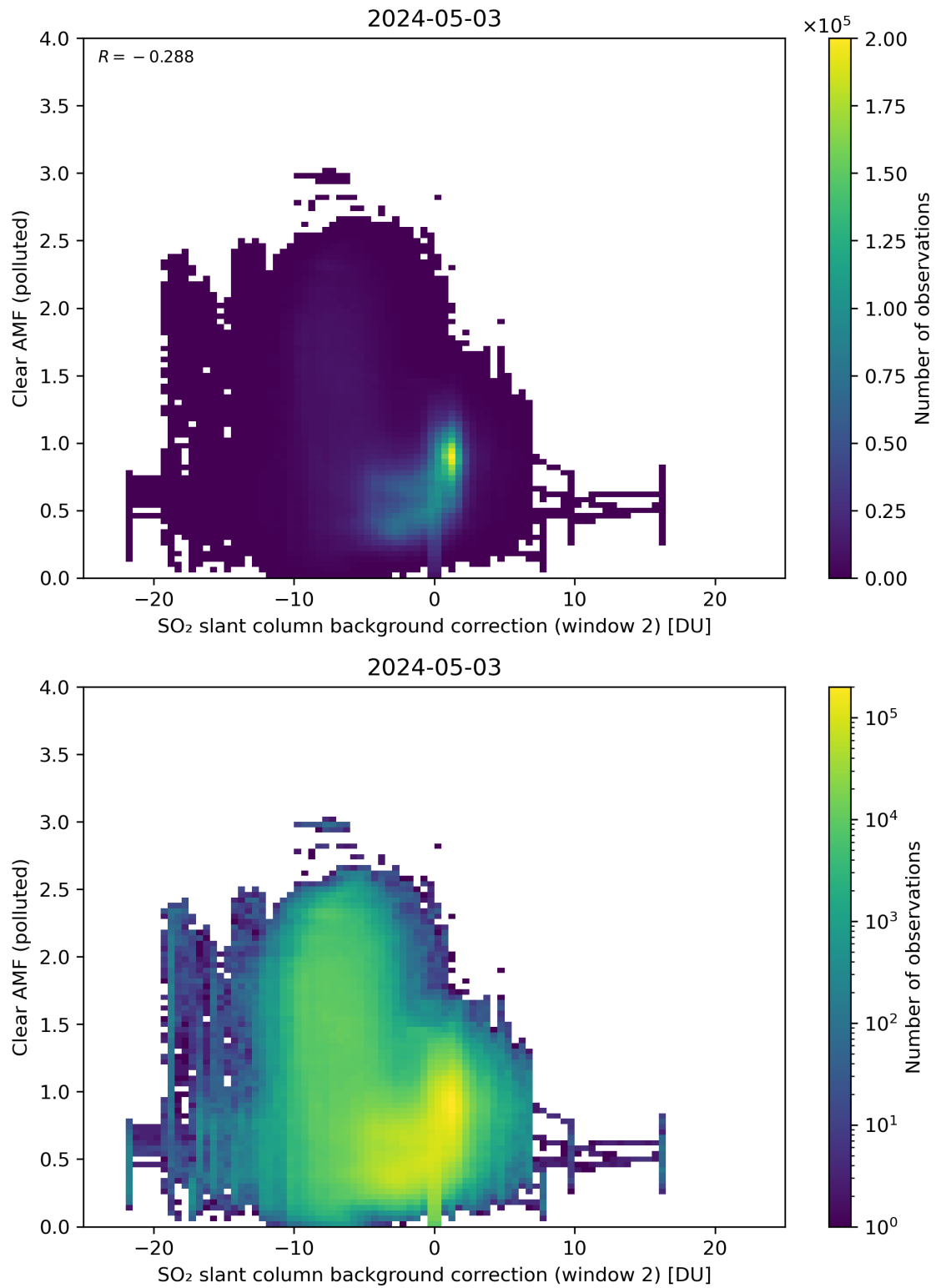
Figure 115: Scatter density plot of “SO 2 slant column background correction (window 2)” against “Clear AMF (polluted)” for 2024-05-02 to 2024-05-04.
