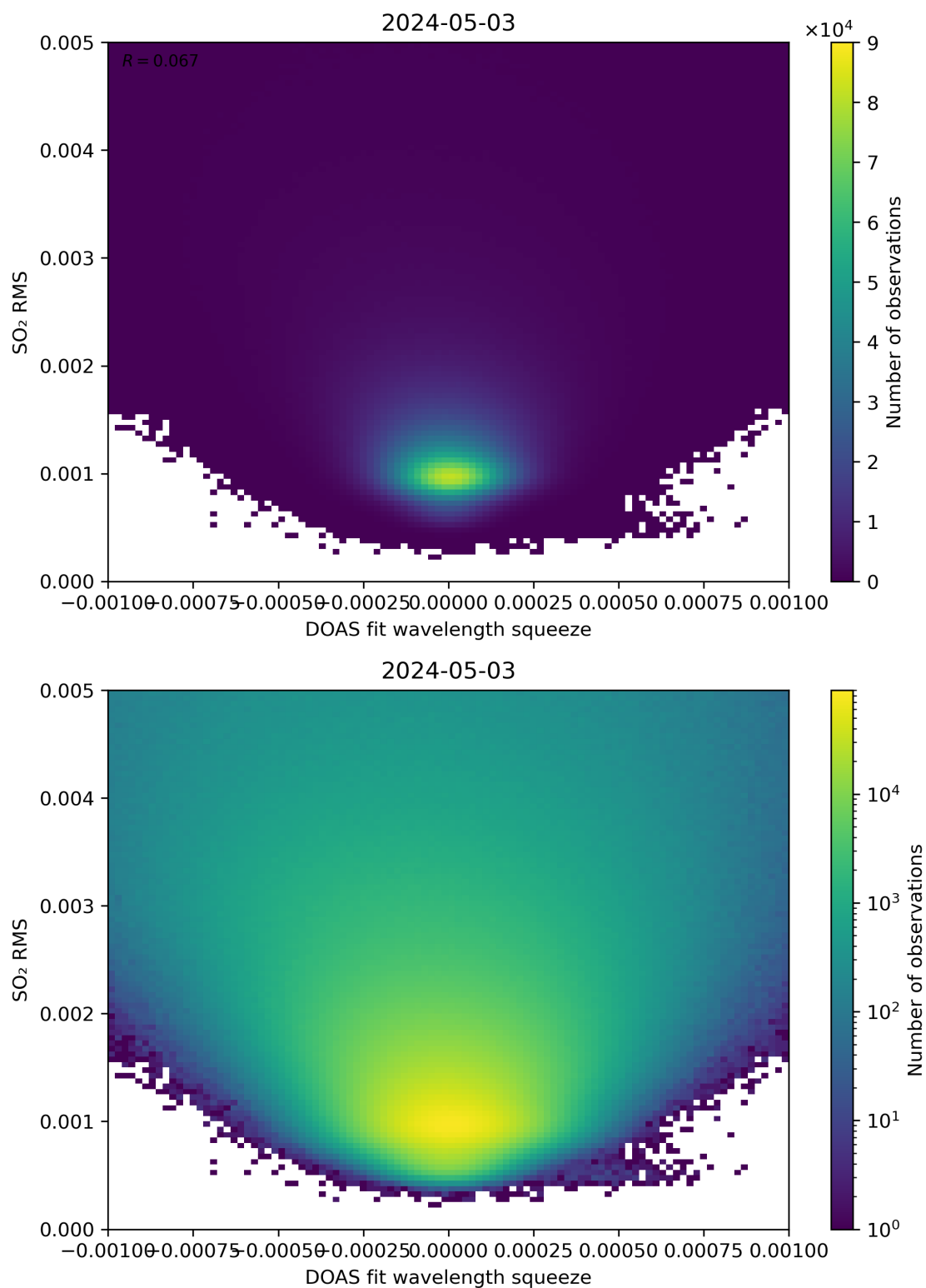
Figure 132: Scatter density plot of “DOAS fit wavelength squeeze” against “SO 2 RMS” for 2024-05-02 to 2024-05-04.
