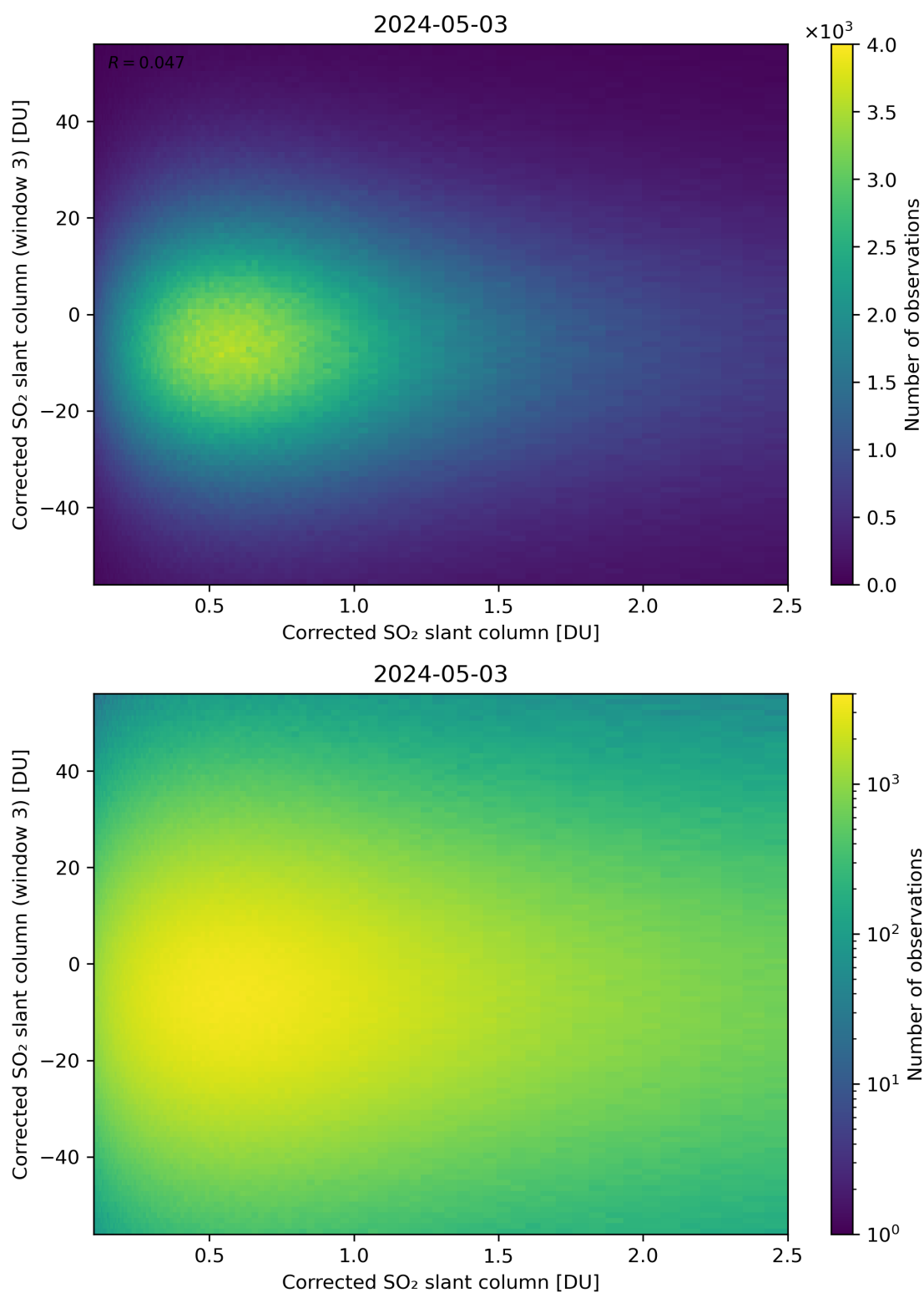
Figure 186: Scatter density plot of “Corrected SO 2 slant column” against “Corrected SO 2 slant column (window 3)” for 2024-05-02 to 2024-05-04.
