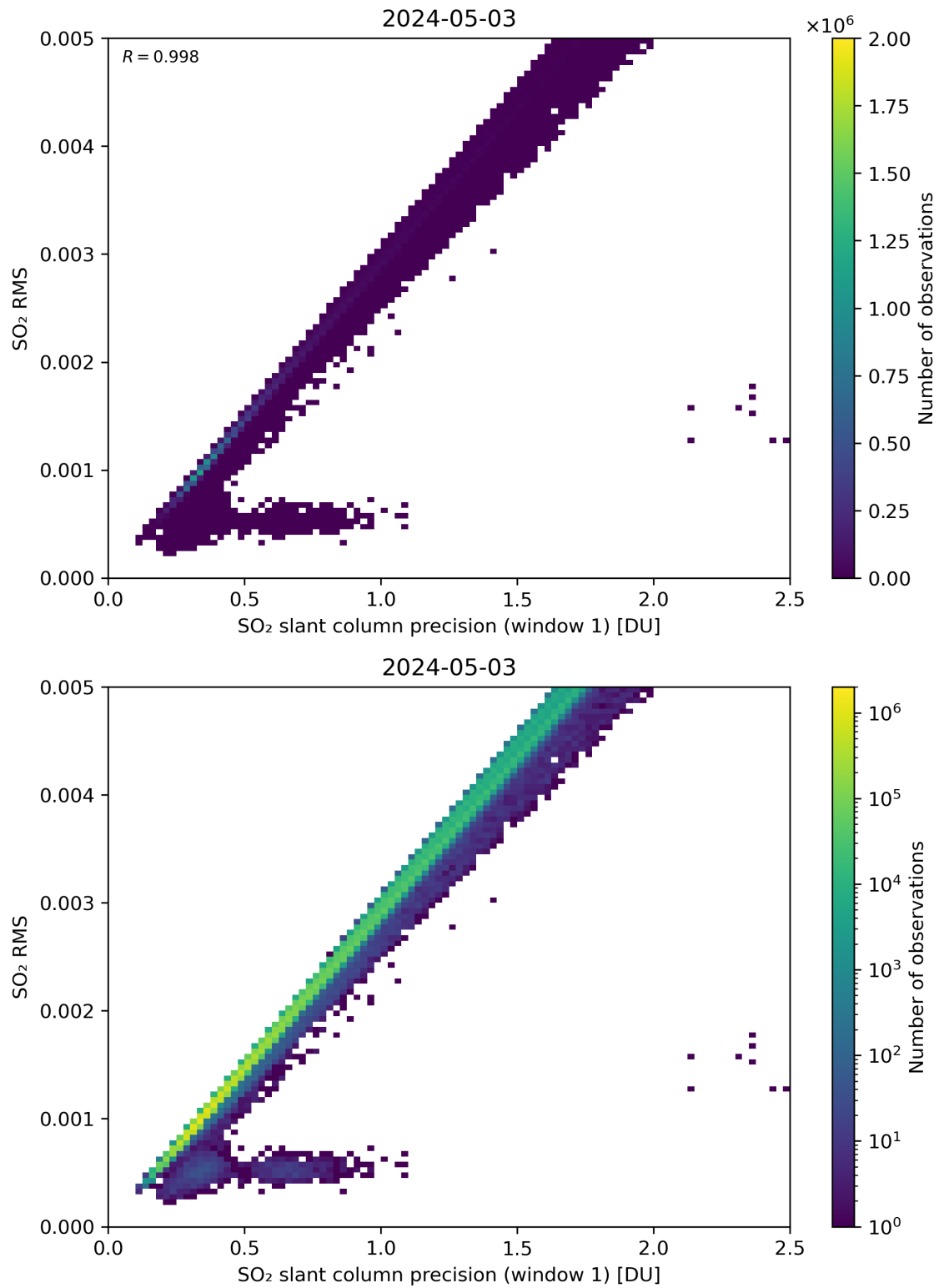
Figure 223: Scatter density plot of “SO 2 slant column precision (window 1)” against “SO 2 RMS” for 2024-05-02 to 2024-05-04.
