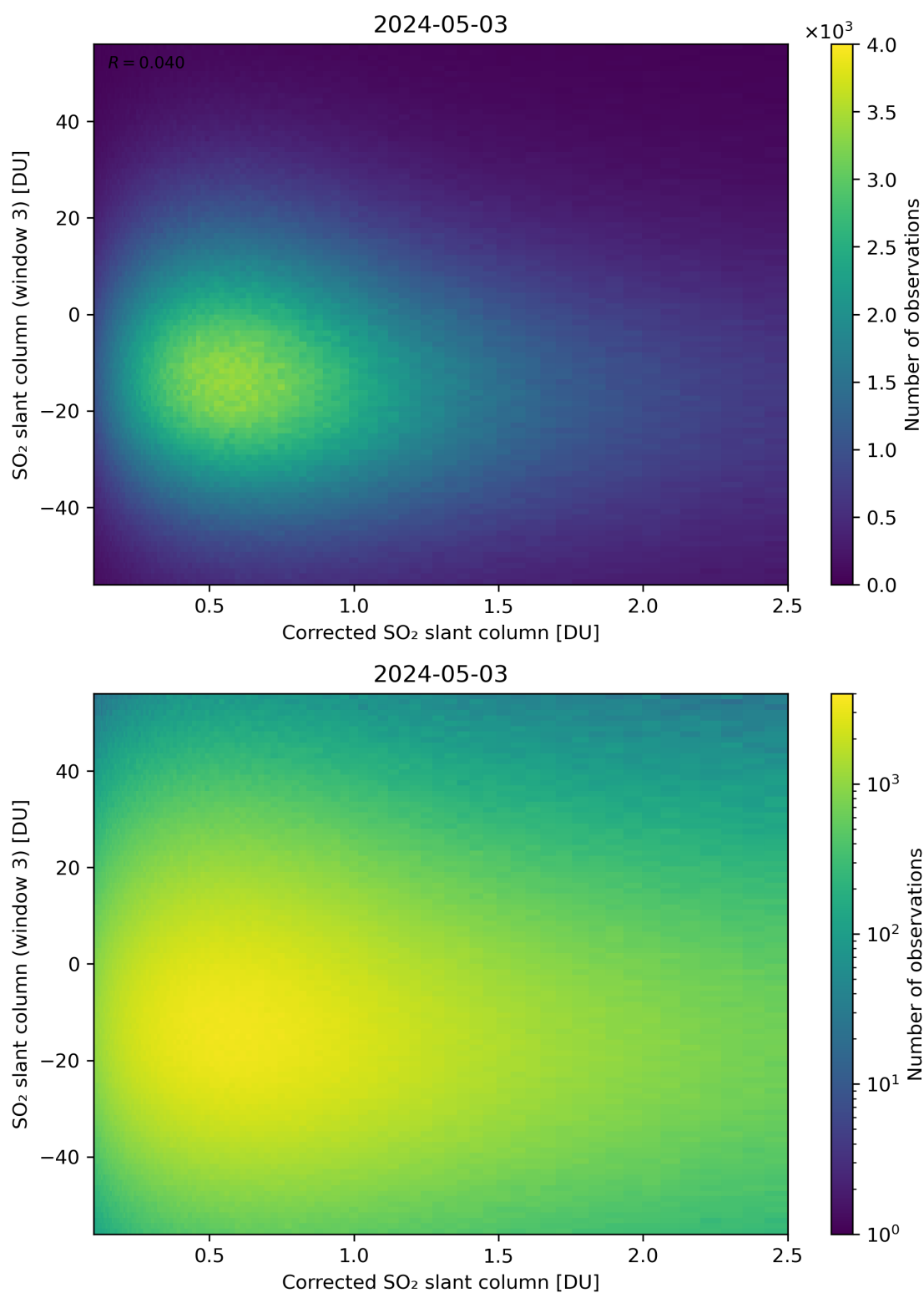
Figure 190: Scatter density plot of “Corrected SO 2 slant column” against “SO 2 slant column (window 3)” for 2024-05-02 to 2024-05-04.
