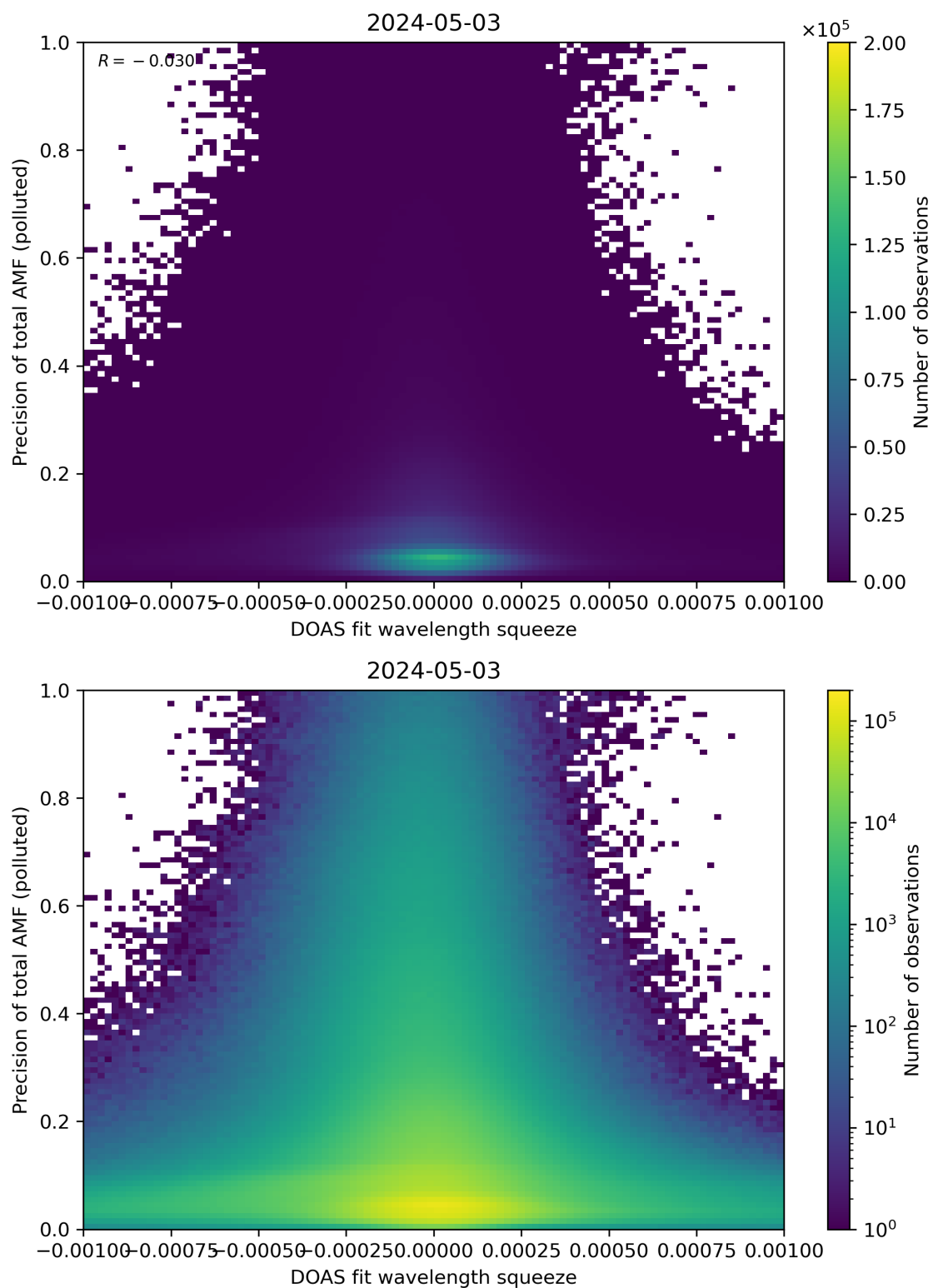
Figure 135: Scatter density plot of “DOAS fit wavelength squeeze” against “Precision of total AMF (polluted)” for 2024-05-02 to 2024-05-04.
