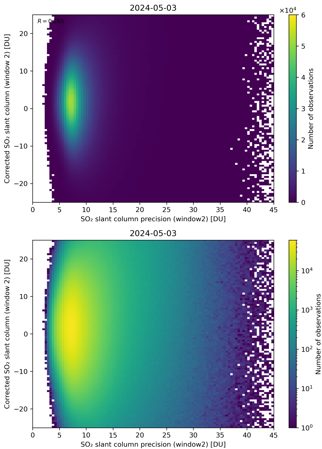
Figure 247: Scatter density plot of “SO 2 slant column precision (window2)” against “Corrected SO 2 slant column (window 2)” for 2024-05-02 to 2024-05-04.
