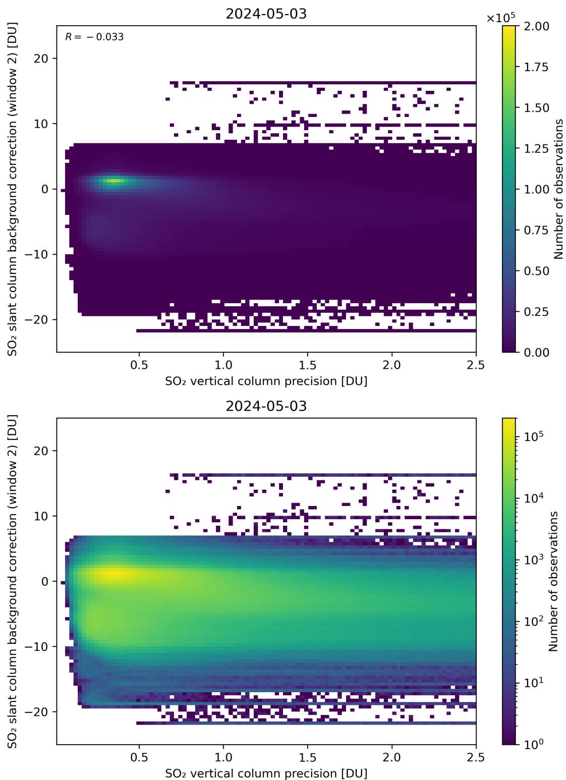
Figure 280: Scatter density plot of “SO 2 vertical column precision” against “SO 2 slant column background correction (window 2)” for 2024-05-02 to 2024-05-04.
