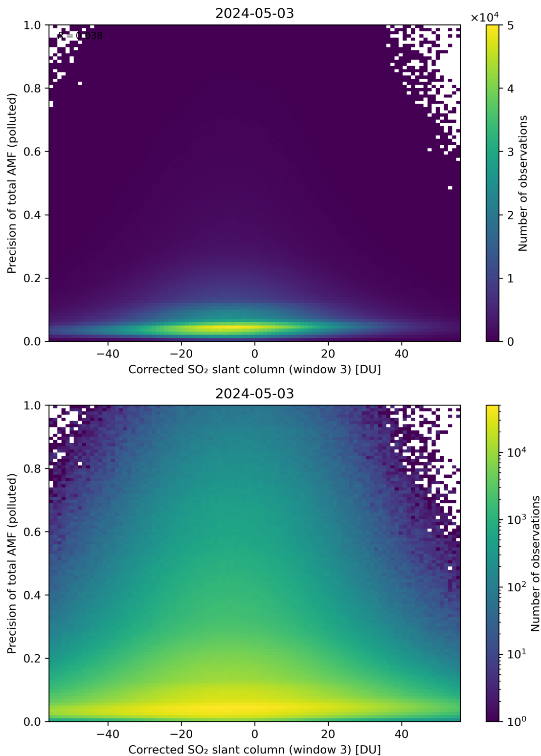
Figure 211: Scatter density plot of “Corrected SO 2 slant column (window 3)” against “Precision of total AMF (polluted)” for 2024-05-02 to 2024-05-04.
