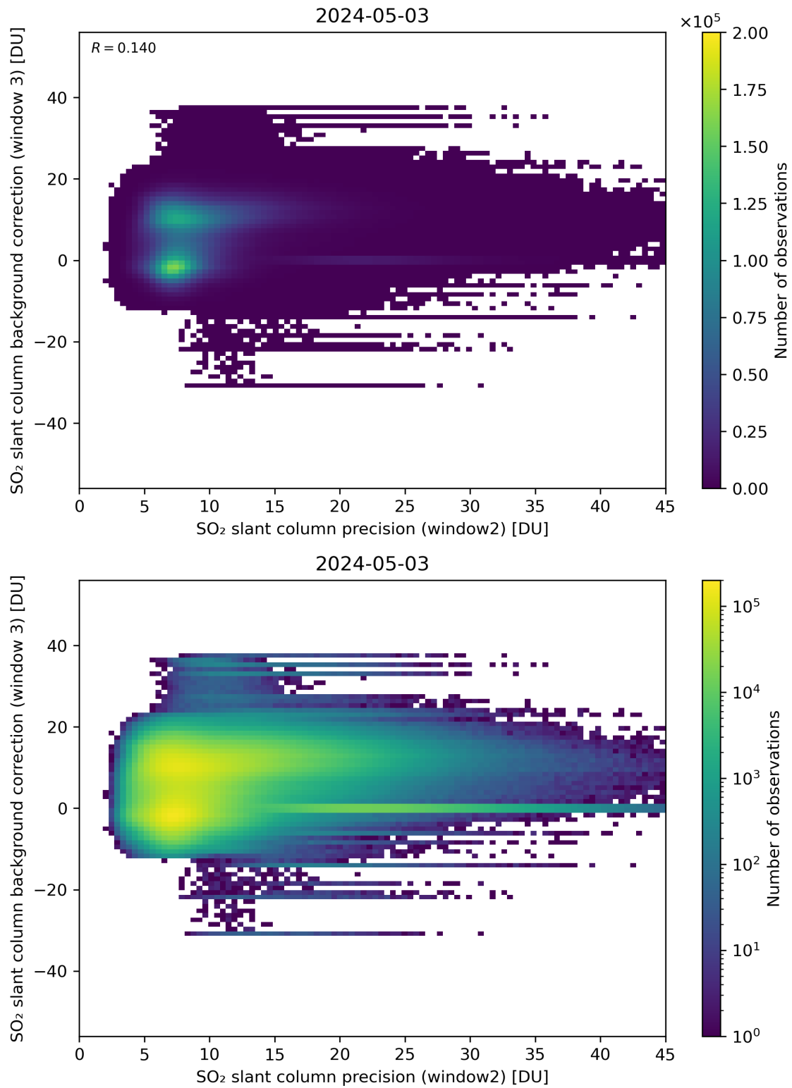
Figure 242: Scatter density plot of “SO 2 slant column precision (window2)” against “SO 2 slant column background correction (window 3)” for 2024-05-02 to 2024-05-04.
