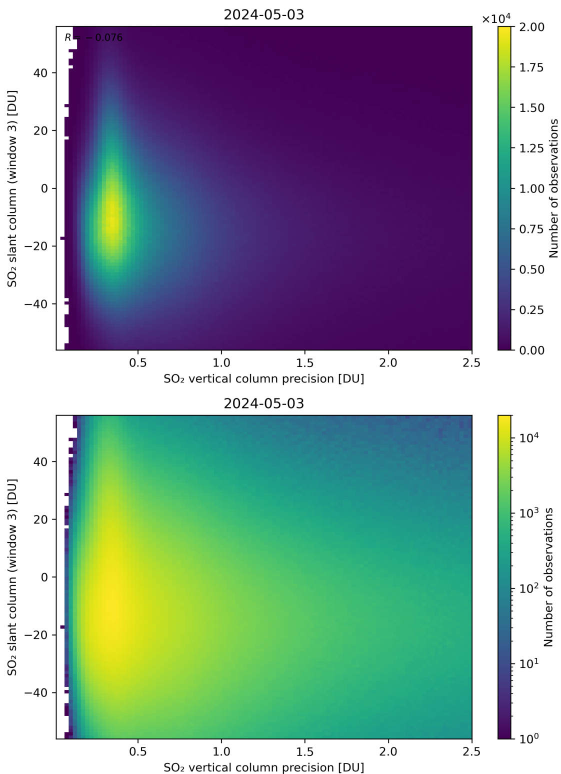
Figure 292: Scatter density plot of “SO 2 vertical column precision” against “SO 2 slant column (window 3)” for 2024-05-02 to 2024-05-04.
