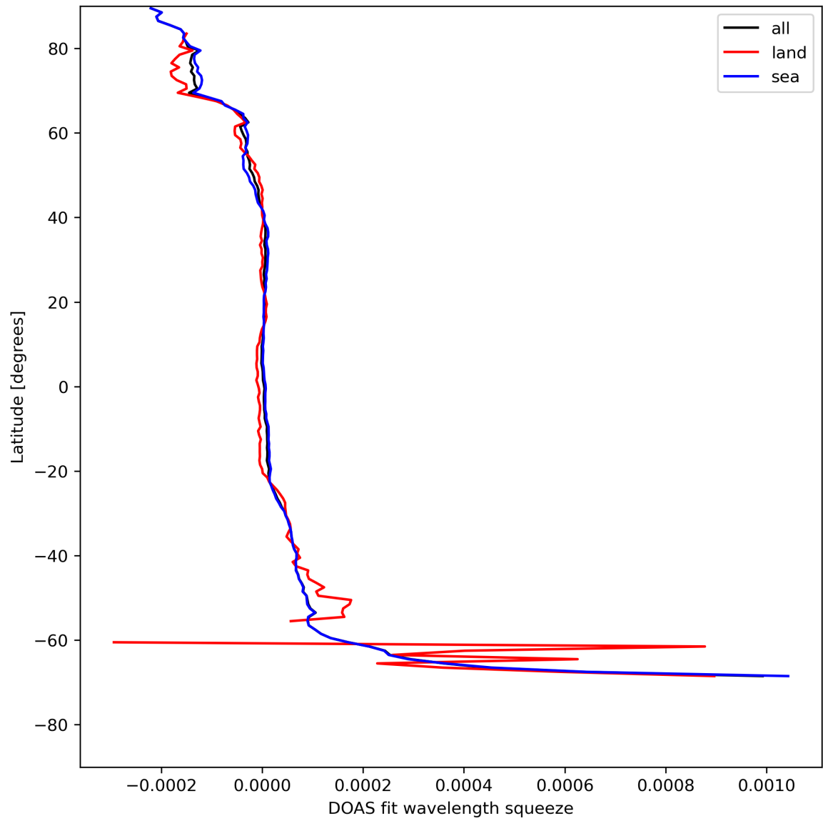
Figure 46: Zonal average of “DOAS fit wavelength squeeze” for 2024-05-02 to 2024-05-04.
