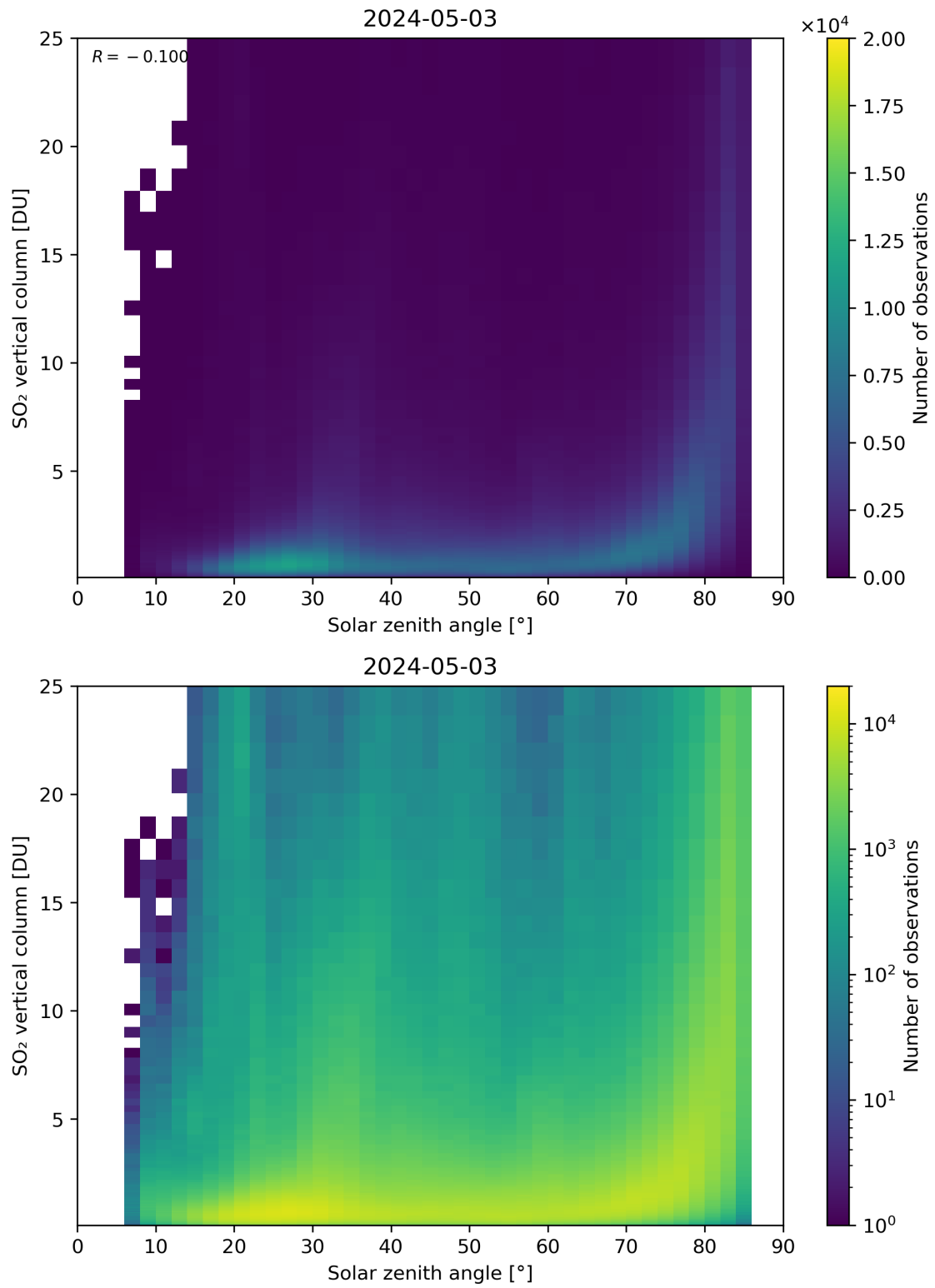
Figure 176: Scatter density plot of “Solar zenith angle” against “SO 2 vertical column” for 2024-05-02 to 2024-05-04.
