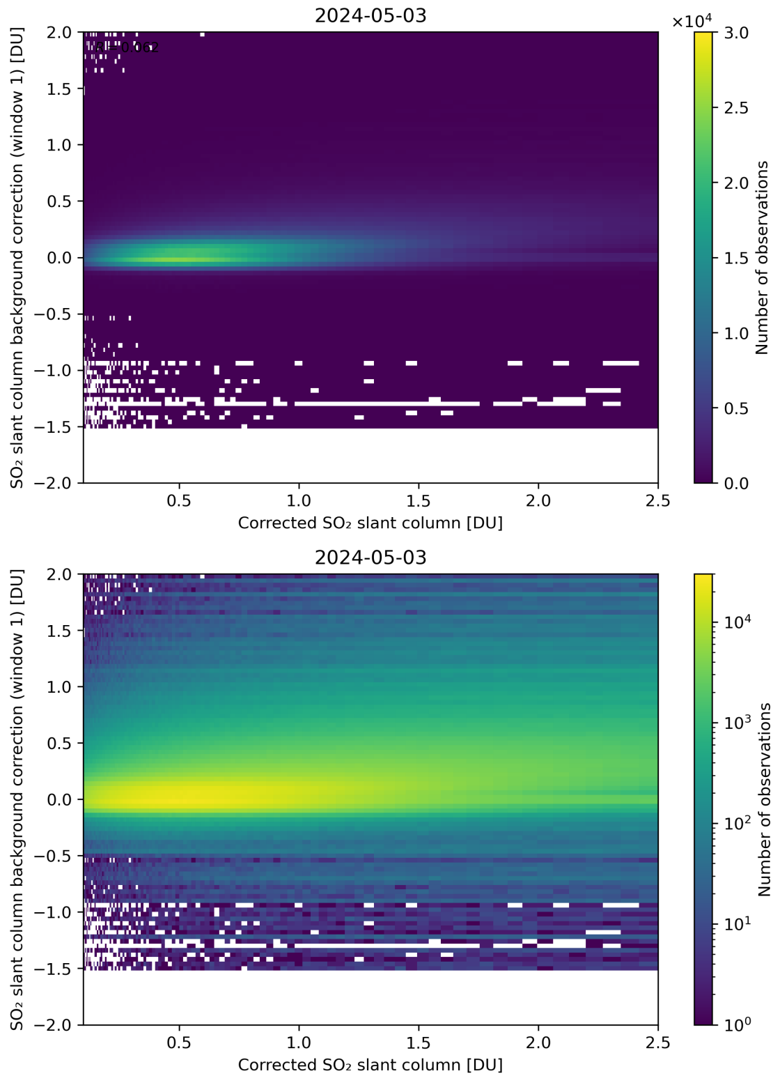
Figure 178: Scatter density plot of “Corrected SO 2 slant column” against “SO 2 slant column background correction (window 1)” for 2024-05-02 to 2024-05-04.
