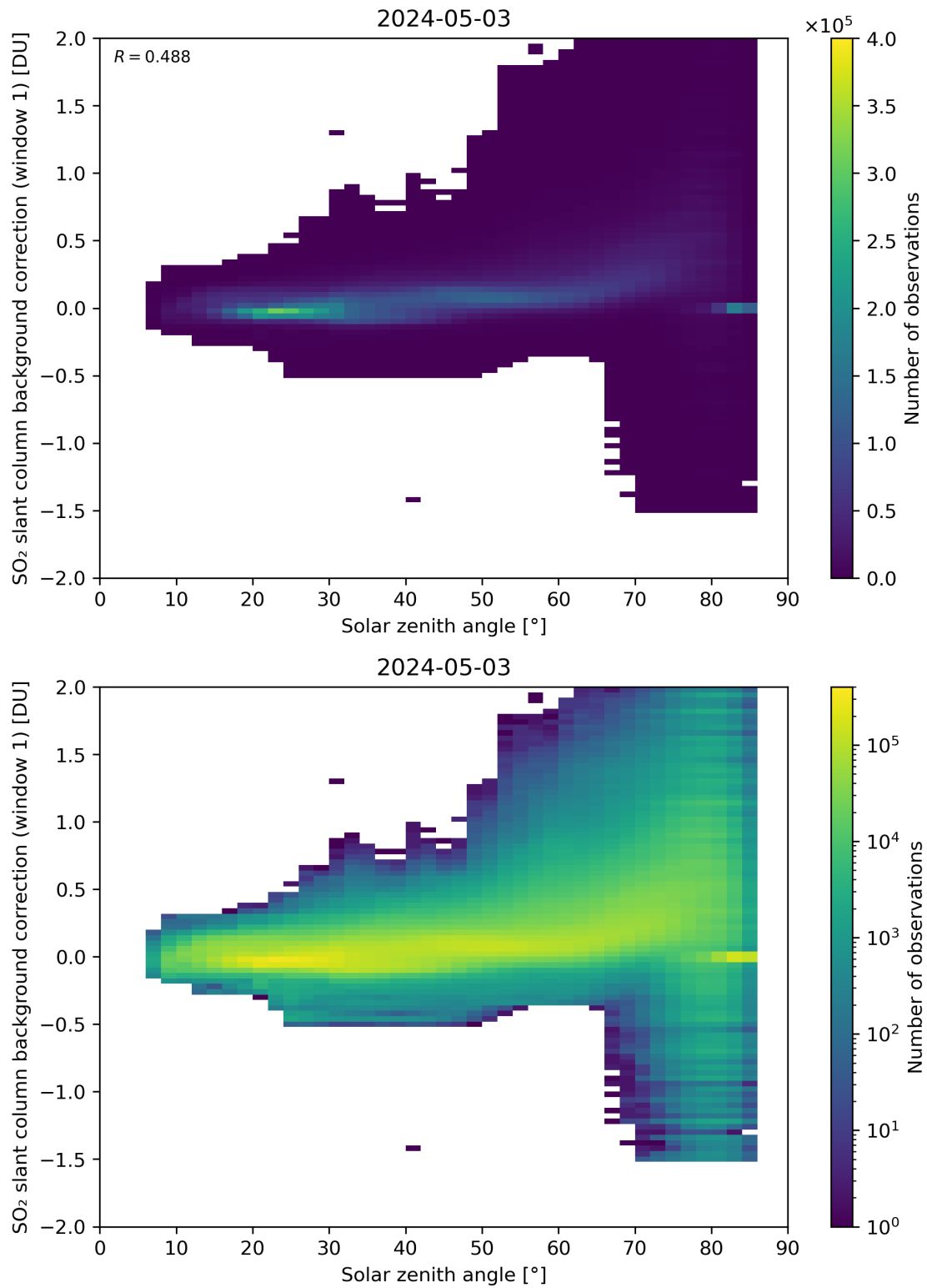
Figure 158: Scatter density plot of “Solar zenith angle” against “SO 2 slant column background correction (window 1)” for 2024-05-02 to 2024-05-04.
