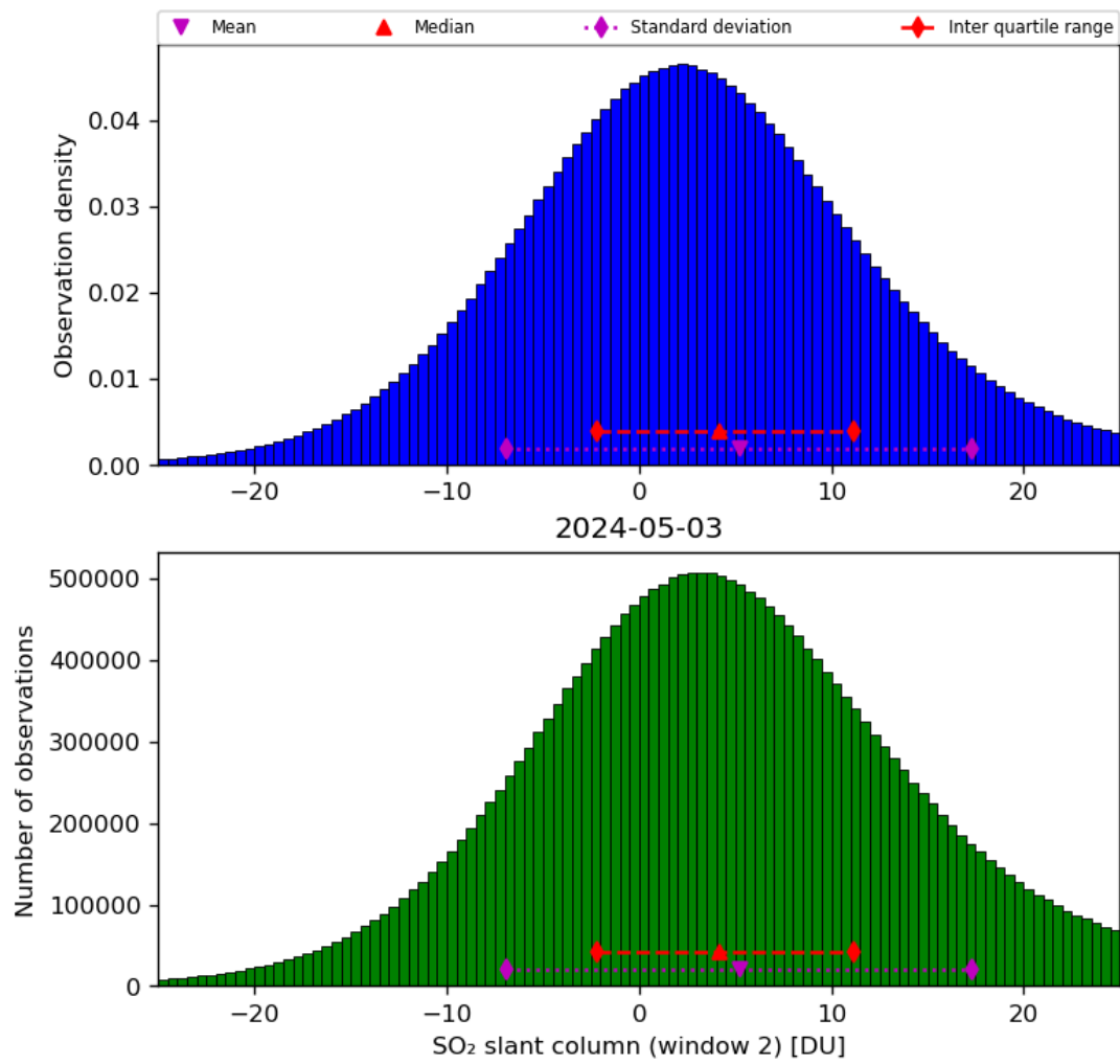
Figure 60: Histogram of “SO 2 slant column (window 2)” for 2024-05-02 to 2024-05-04
