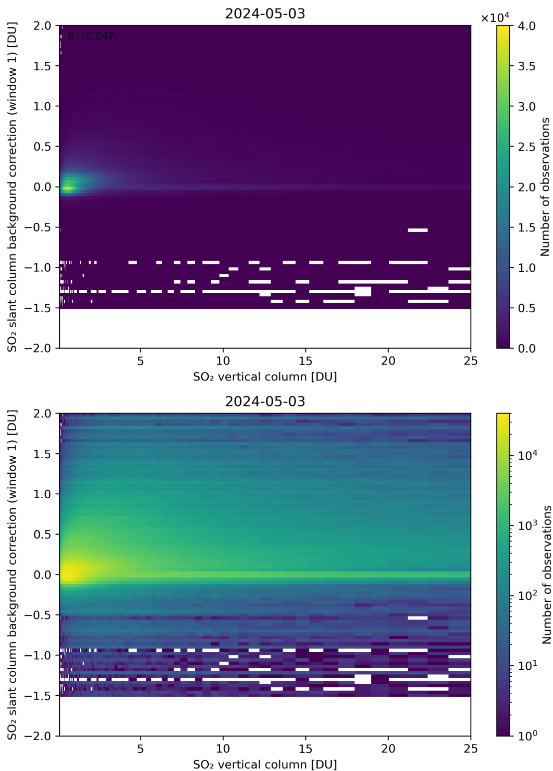
Figure 273: Scatter density plot of “SO 2 vertical column” against “SO 2 slant column background correction (window 1)” for 2024-05-02 to 2024-05-04.
