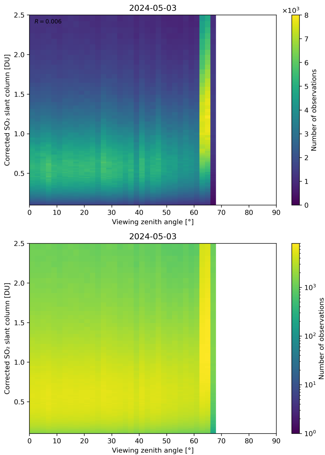
Figure 317: Scatter density plot of “Viewing zenith angle” against “Corrected SO 2 slant column” for 2024-05-02 to 2024-05-04.
