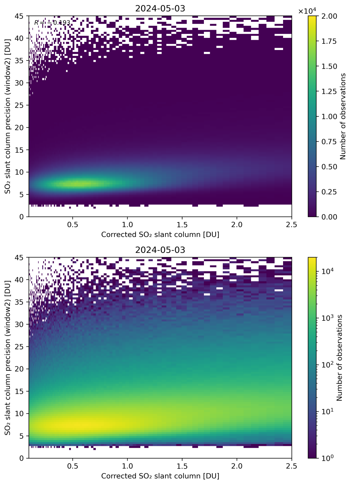
Figure 189: Scatter density plot of “Corrected SO 2 slant column” against “SO 2 slant column precision (window2)” for 2024-05-02 to 2024-05-04.
