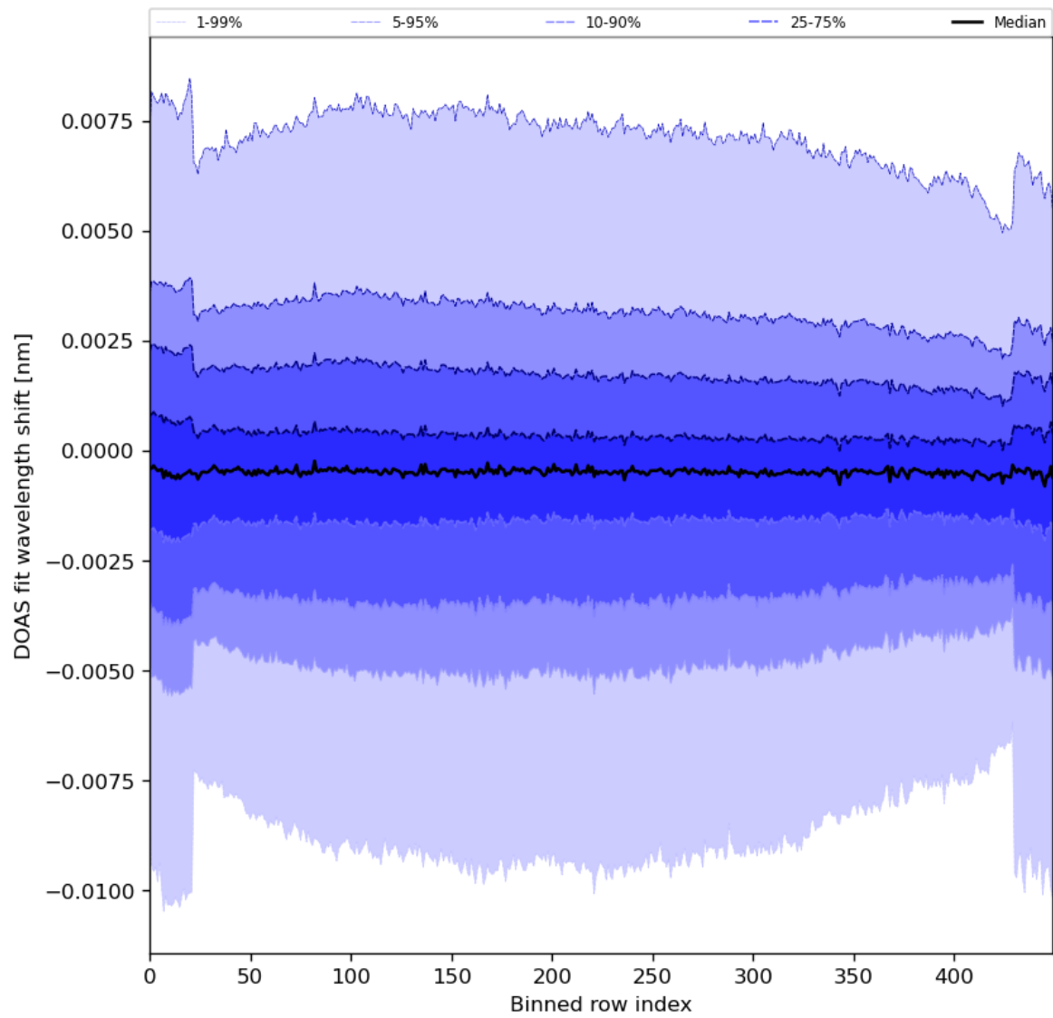
Figure 91: Along track statistics of “DOAS fit wavelength shift” for 2024-05-02 to 2024-05-04
