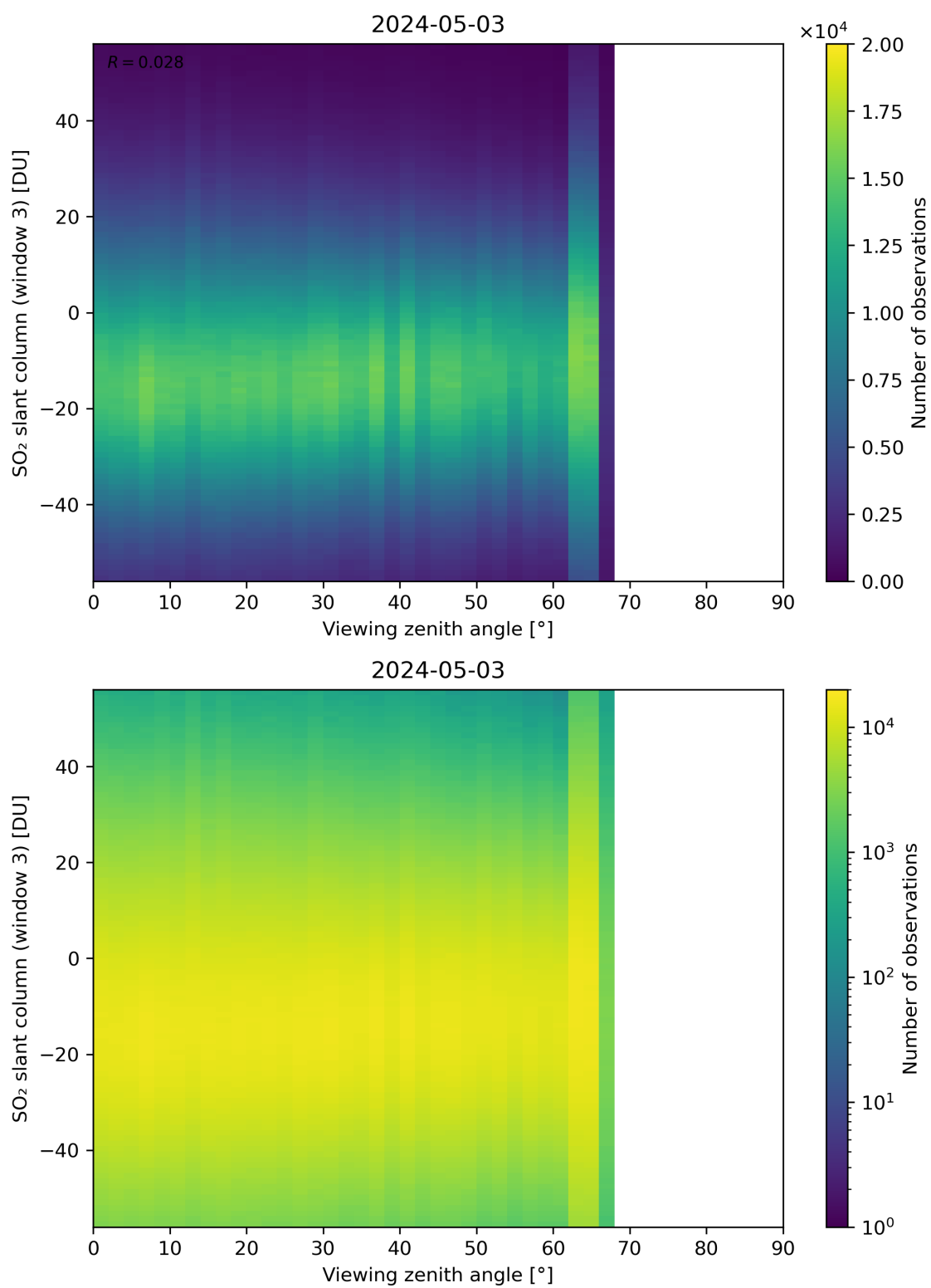
Figure 323: Scatter density plot of “Viewing zenith angle” against “SO 2 slant column (window 3)” for 2024-05-02 to 2024-05-04.
