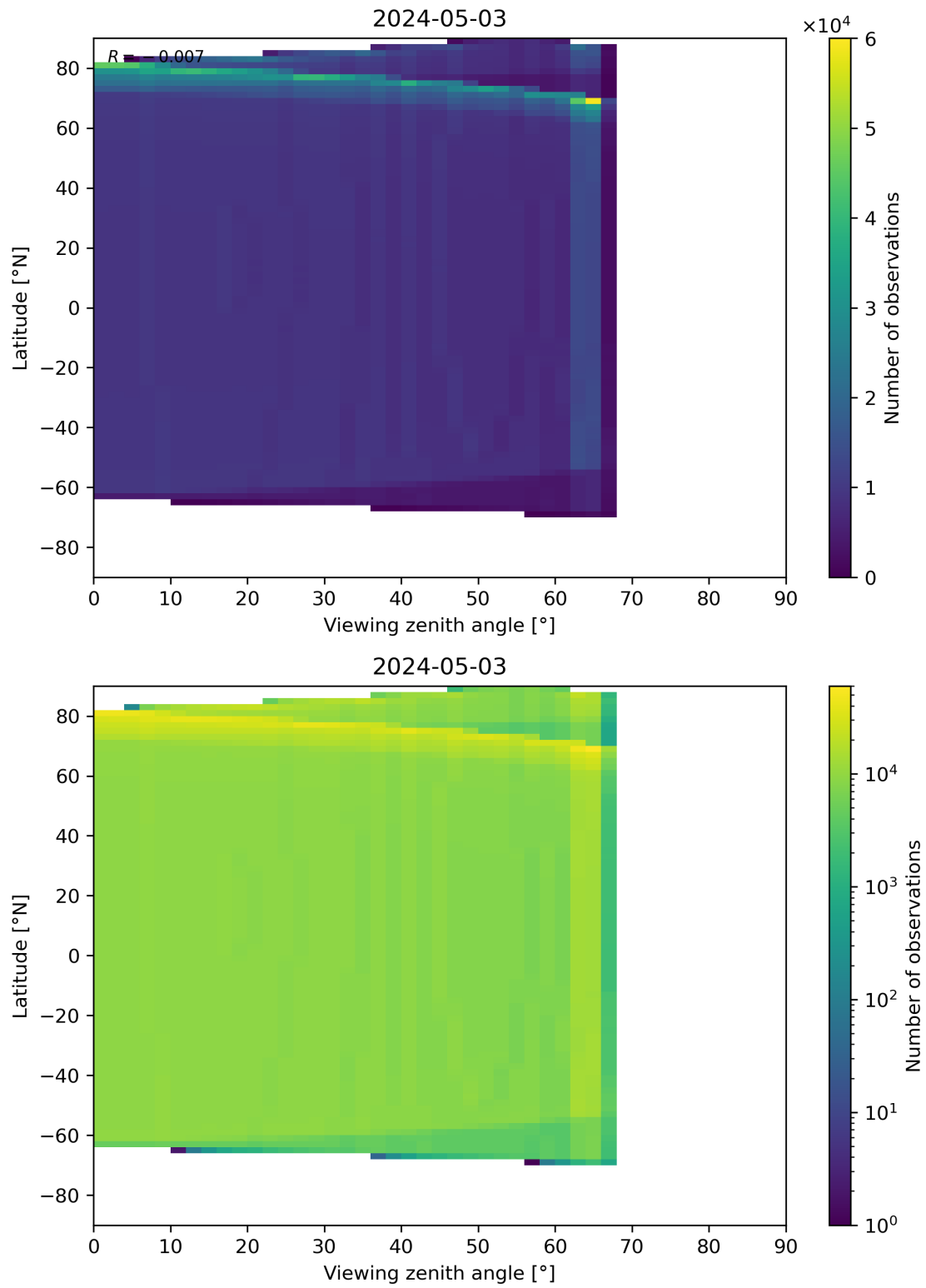
Figure 314: Scatter density plot of “Viewing zenith angle” against “Latitude” for 2024-05-02 to 2024-05-04.
