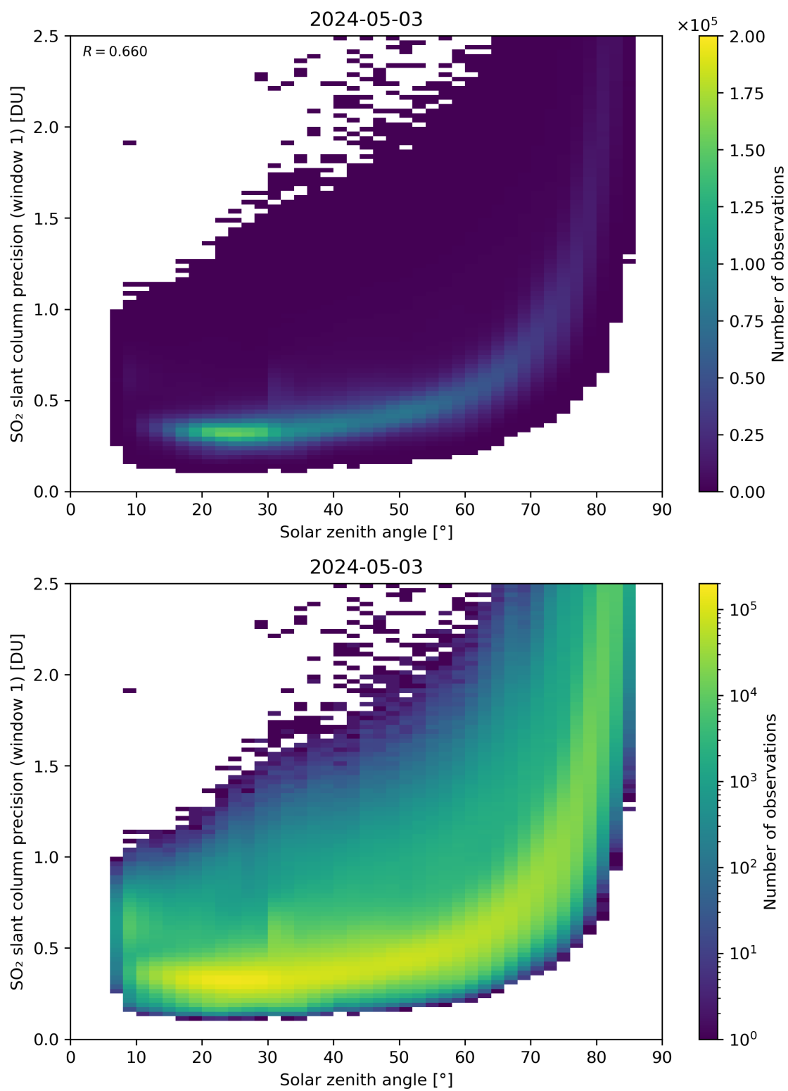
Figure 170: Scatter density plot of “Solar zenith angle” against “SO 2 slant column precision (window 1)” for 2024-05-02 to 2024-05-04.
