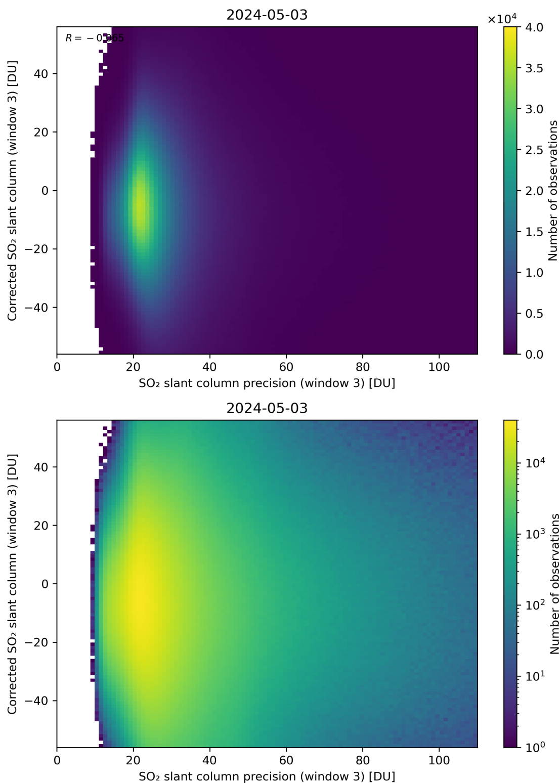
Figure 262: Scatter density plot of “SO 2 slant column precision (window 3)” against “Corrected SO 2 slant column (window 3)” for 2024-05-02 to 2024-05-04.
