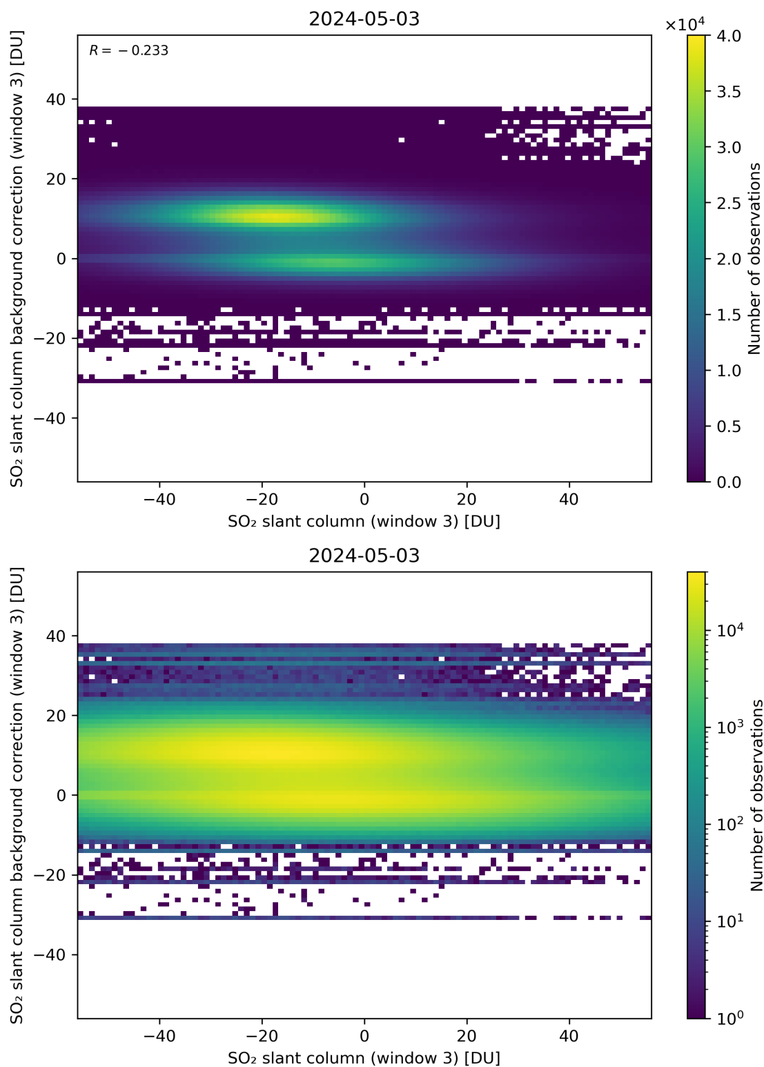
Figure 253: Scatter density plot of “SO 2 slant column (window 3)” against “SO 2 slant column background correction (window 3)” for 2024-05-02 to 2024-05-04.
