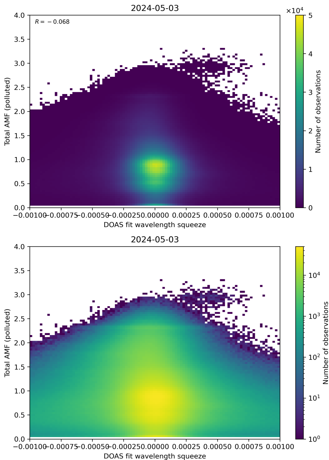
Figure 134: Scatter density plot of “DOAS fit wavelength squeeze” against “Total AMF (polluted)” for 2024-05-02 to 2024-05-04.
