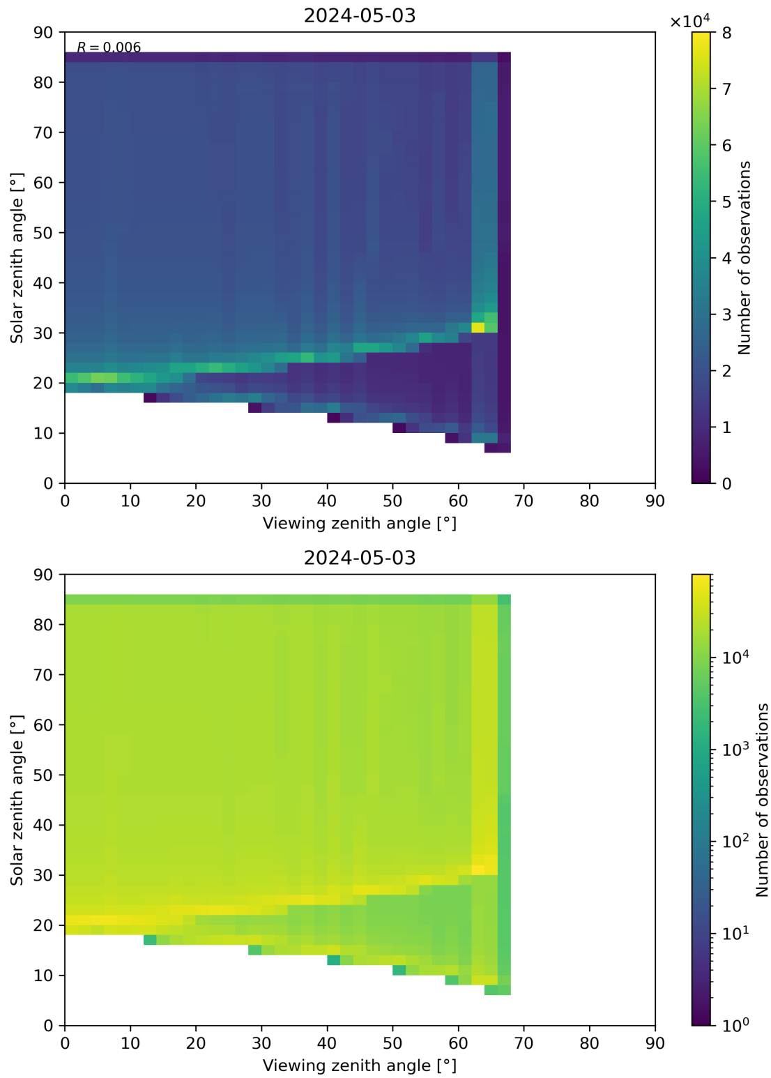
Figure 315: Scatter density plot of “Viewing zenith angle” against “Solar zenith angle” for 2024-05-02 to 2024-05-04.
