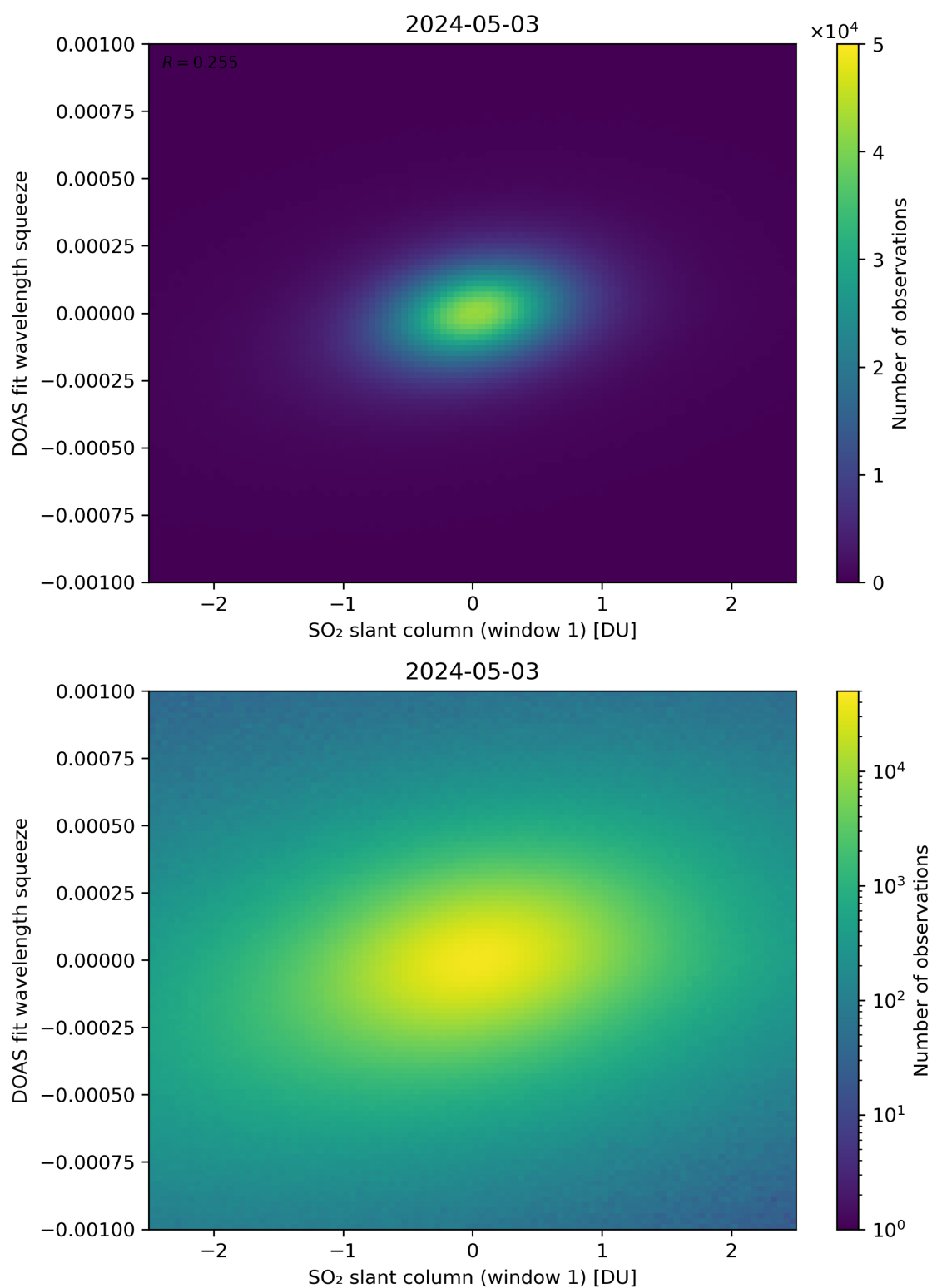
Figure 216: Scatter density plot of “SO 2 slant column (window 1)” against “DOAS fit wavelength squeeze” for 2024-05-02 to 2024-05-04.
