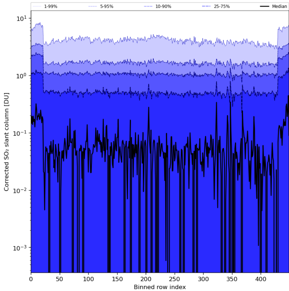
Figure 78: Along track statistics of “Corrected SO 2 slant column” for 2024-05-02 to 2024-05-04
