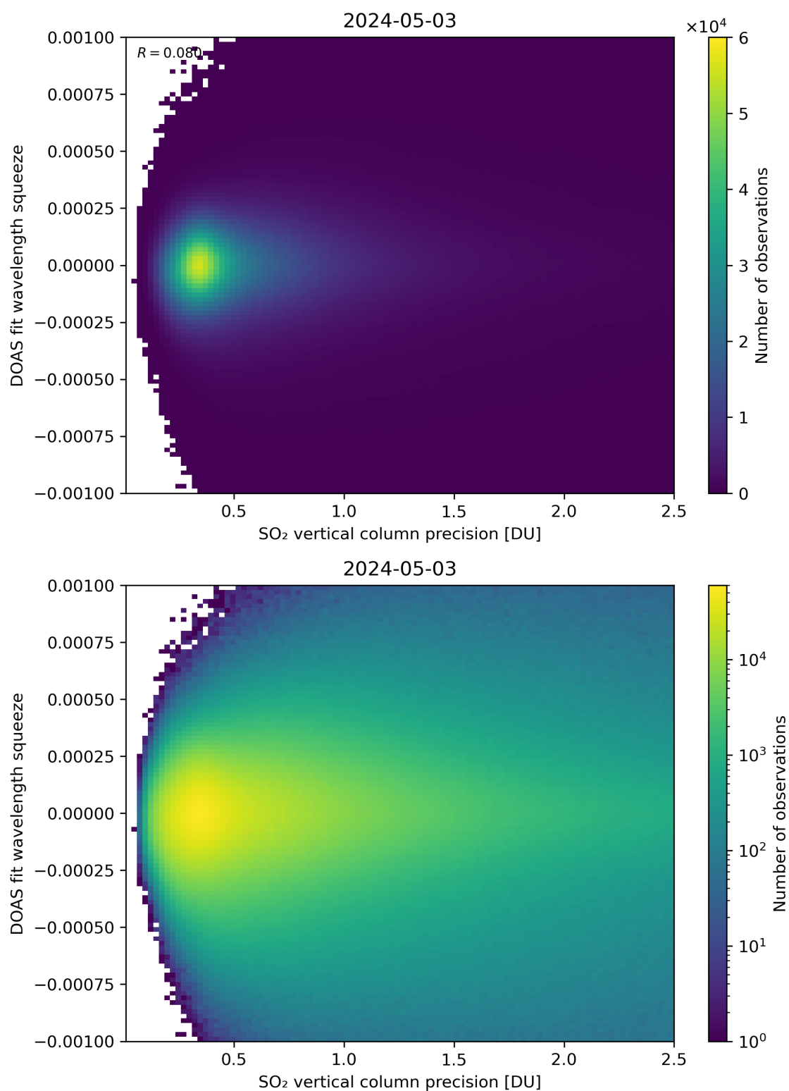
Figure 283: Scatter density plot of “SO 2 vertical column precision” against “DOAS fit wavelength squeeze” for 2024-05-02 to 2024-05-04.
