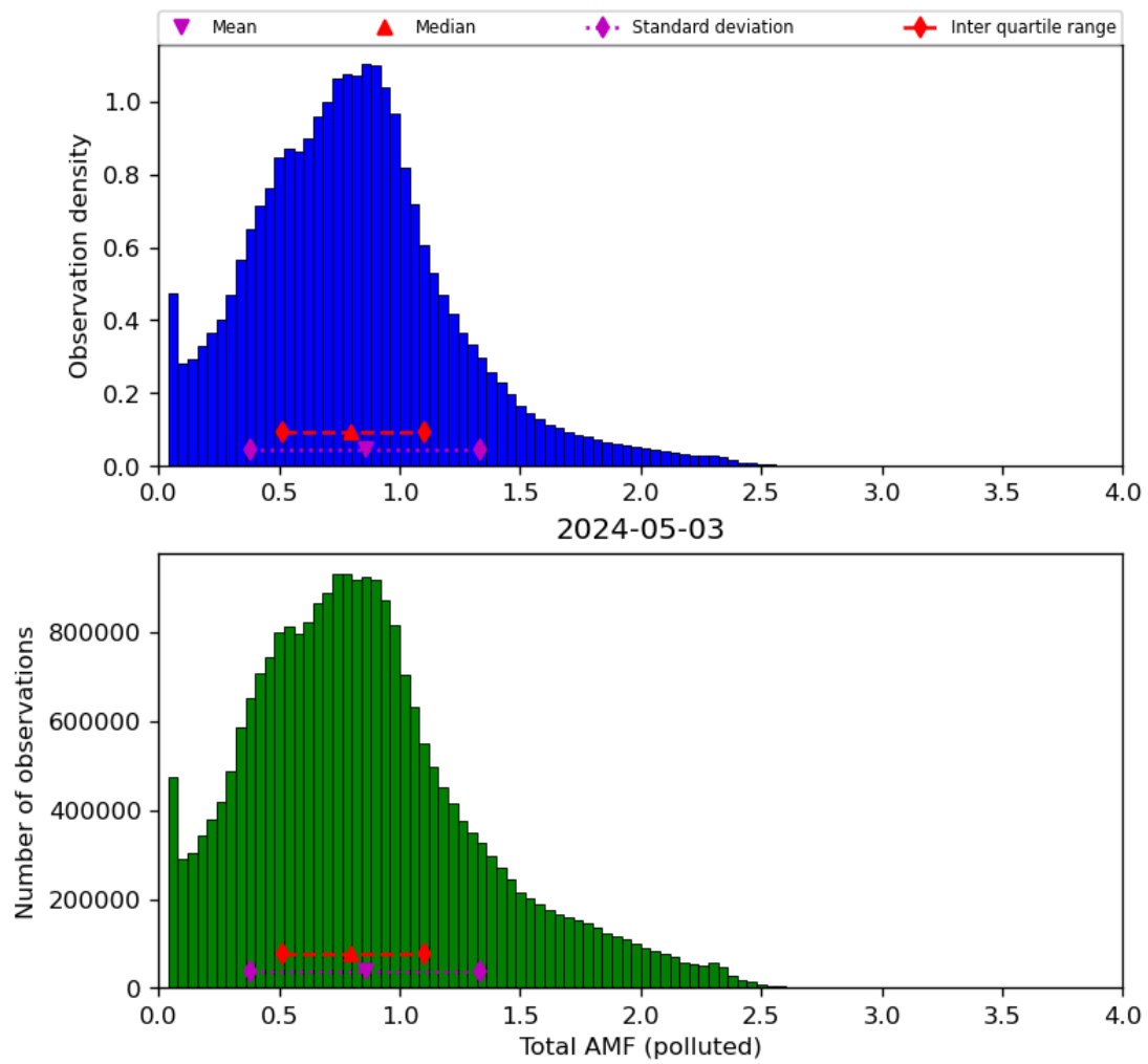
Figure 71: Histogram of “Total AMF (polluted)” for 2024-05-02 to 2024-05-04
