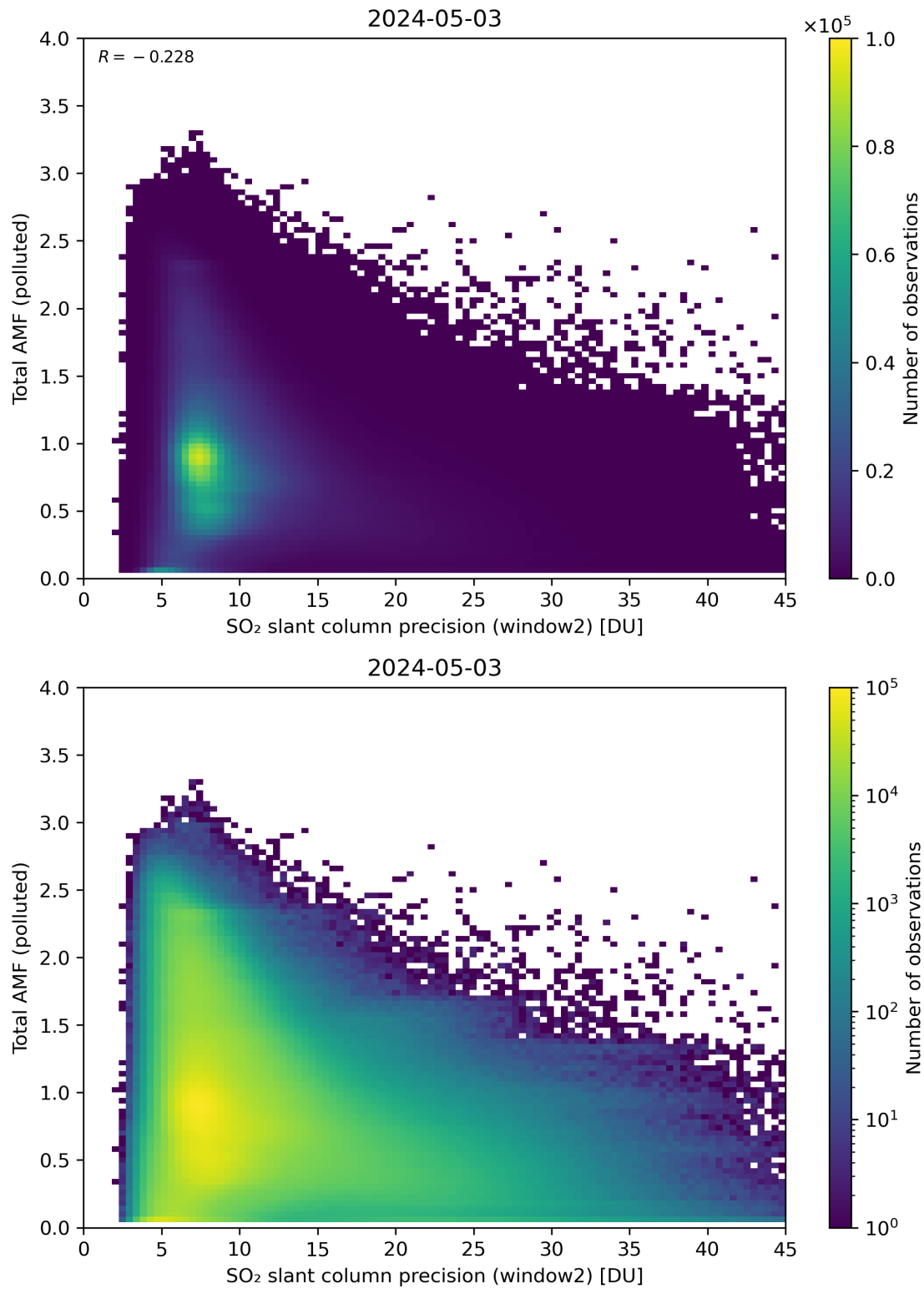
Figure 251: Scatter density plot of “SO 2 slant column precision (window2)” against “Total AMF (polluted)” for 2024-05-02 to 2024-05-04.
