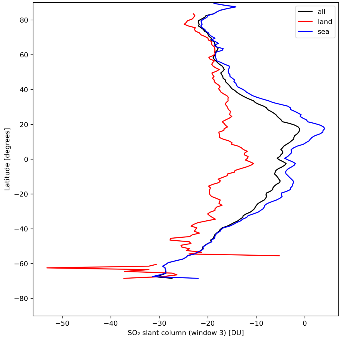
Figure 41: Zonal average of “SO 2 slant column (window 3)” for 2024-05-02 to 2024-05-04.
