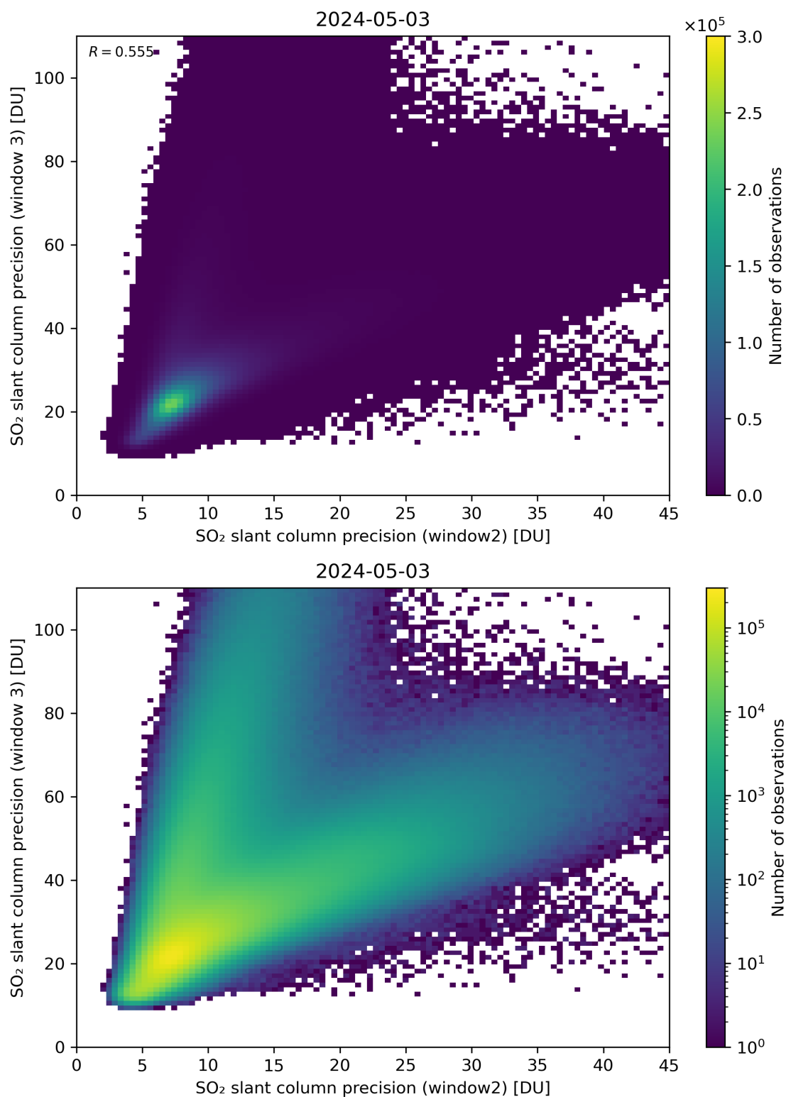
Figure 250: Scatter density plot of “SO 2 slant column precision (window2)” against “SO 2 slant column precision (window 3)” for 2024-05-02 to 2024-05-04.
