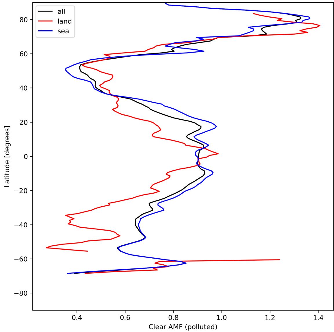
Figure 50: Zonal average of “Clear AMF (polluted)” for 2024-05-02 to 2024-05-04.
