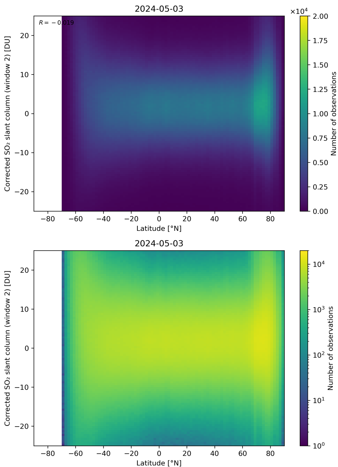
Figure 147: Scatter density plot of “Latitude” against “Corrected SO 2 slant column (window 2)” for 2024-05-02 to 2024-05-04.
