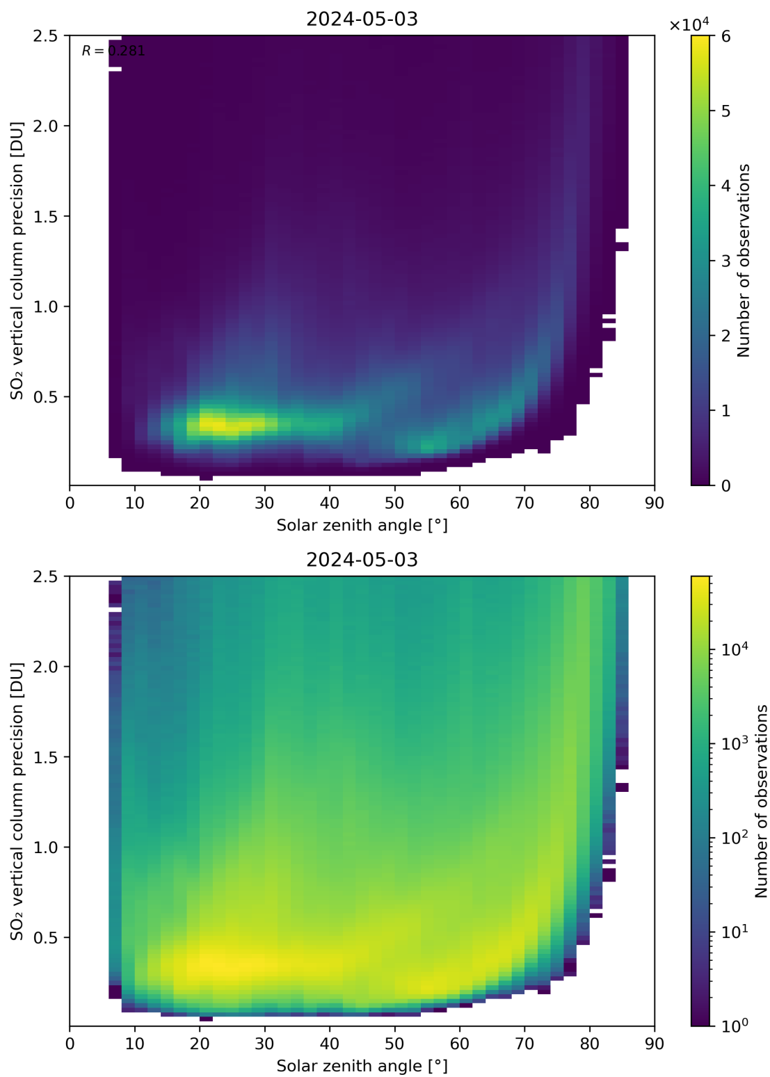
Figure 177: Scatter density plot of “Solar zenith angle” against “SO 2 vertical column precision” for 2024-05-02 to 2024-05-04.
