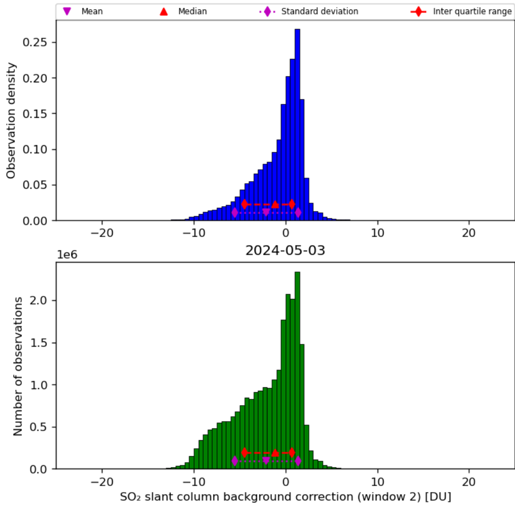
Figure 63: Histogram of “SO 2 slant column background correction (window 2)” for 2024-05-02 to 2024-05-04
