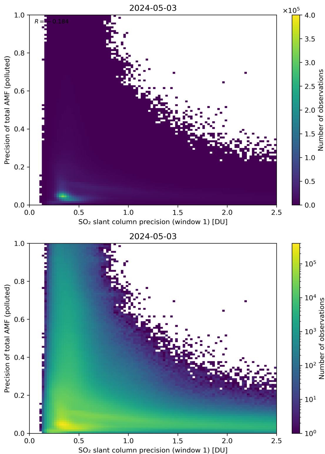
Figure 231: Scatter density plot of “SO 2 slant column precision (window 1)” against “Precision of total AMF (polluted)” for 2024-05-02 to 2024-05-04.
