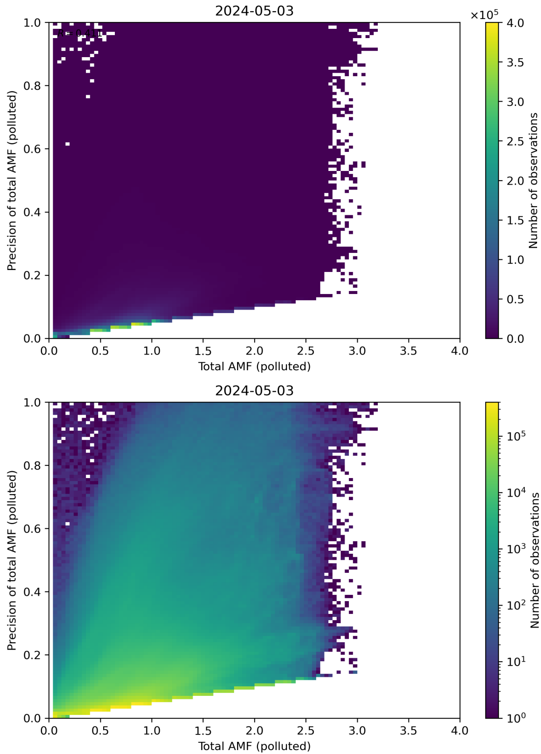
Figure 272: Scatter density plot of “Total AMF (polluted)” against “Precision of total AMF (polluted)” for 2024-05-02 to 2024-05-04.
