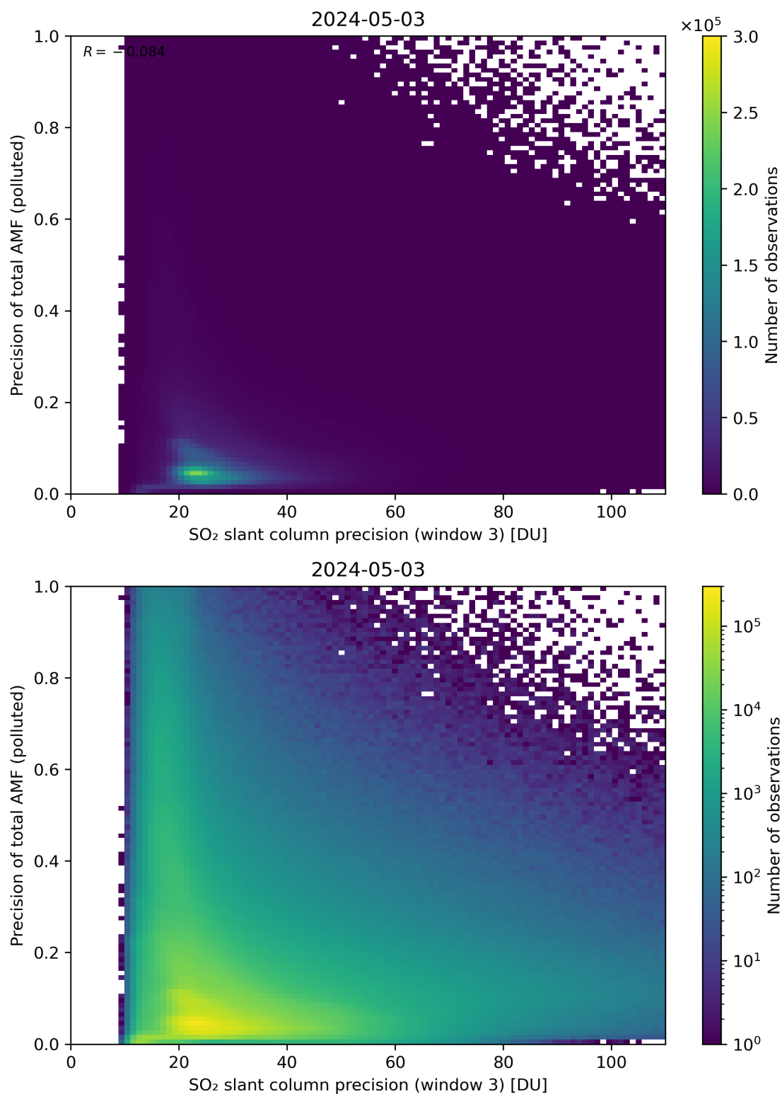
Figure 264: Scatter density plot of “SO 2 slant column precision (window 3)” against “Precision of total AMF (polluted)” for 2024-05-02 to 2024-05-04.
