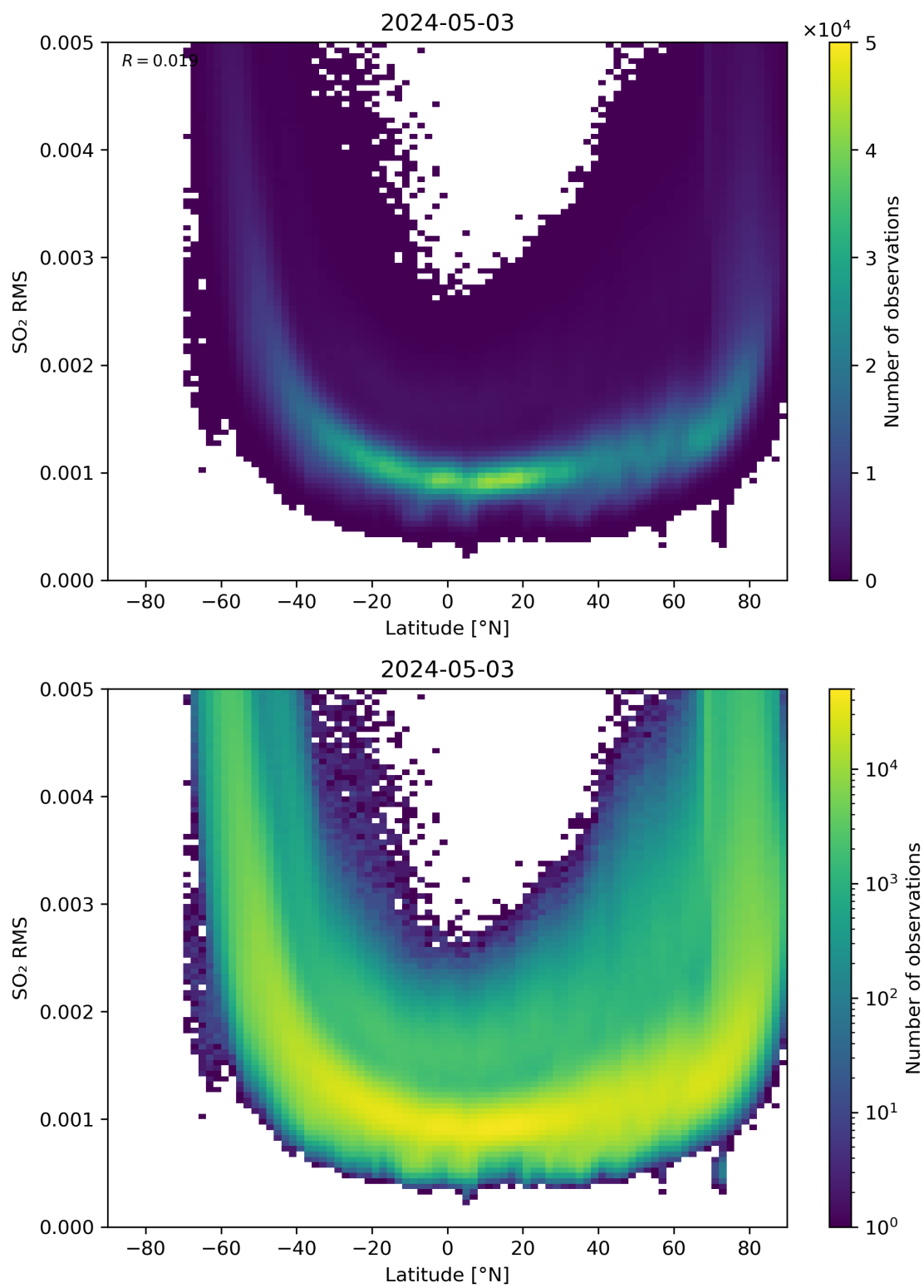
Figure 144: Scatter density plot of “Latitude” against “SO 2 RMS” for 2024-05-02 to 2024-05-04.
