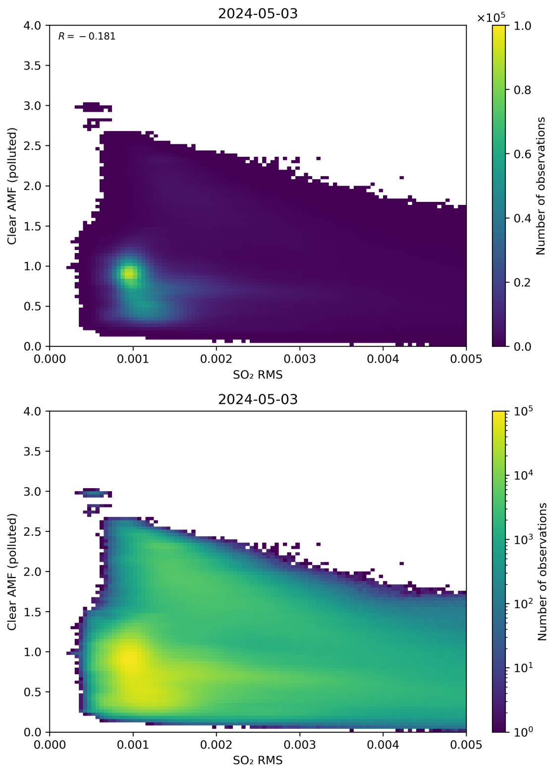
Figure 136: Scatter density plot of “SO 2 RMS” against “Clear AMF (polluted)” for 2024-05-02 to 2024-05-04.
