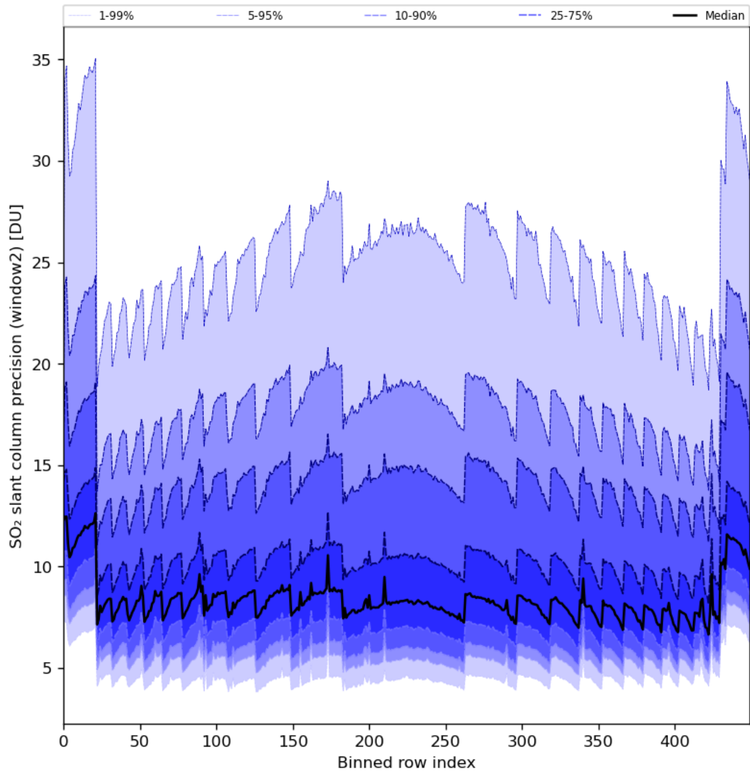
Figure 84: Along track statistics of “SO 2 slant column precision (window2)” for 2024-05-02 to 2024-05-04
