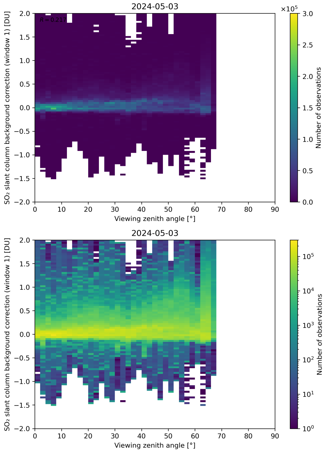
Figure 308: Scatter density plot of “Viewing zenith angle” against “SO 2 slant column background correction (window 1)” for 2024-05-02 to 2024-05-04.
