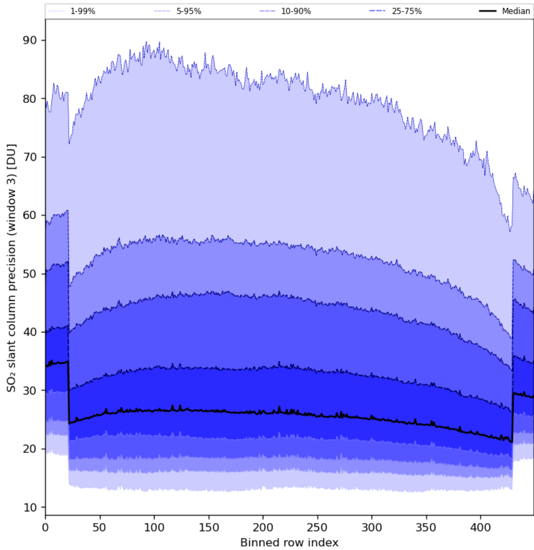
Figure 88: Along track statistics of “SO 2 slant column precision (window 3)” for 2024-05-02 to 2024-05-04
