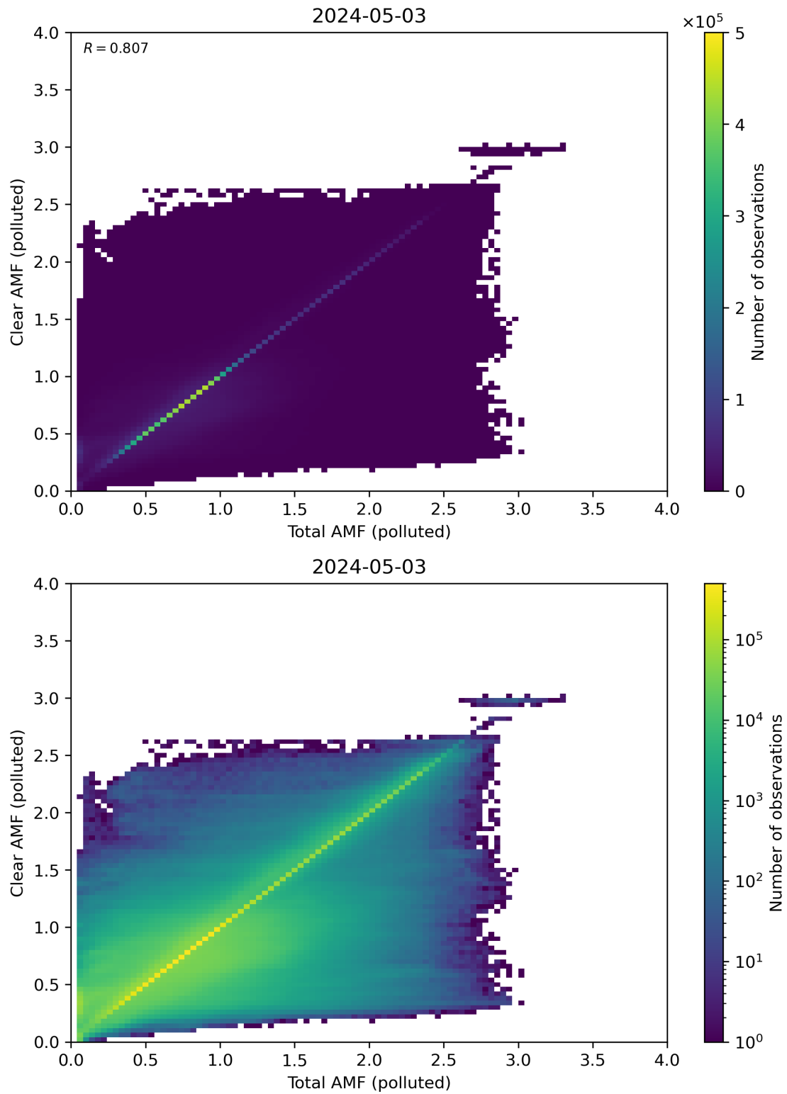
Figure 271: Scatter density plot of “Total AMF (polluted)” against “Clear AMF (polluted)” for 2024-05-02 to 2024-05-04.
