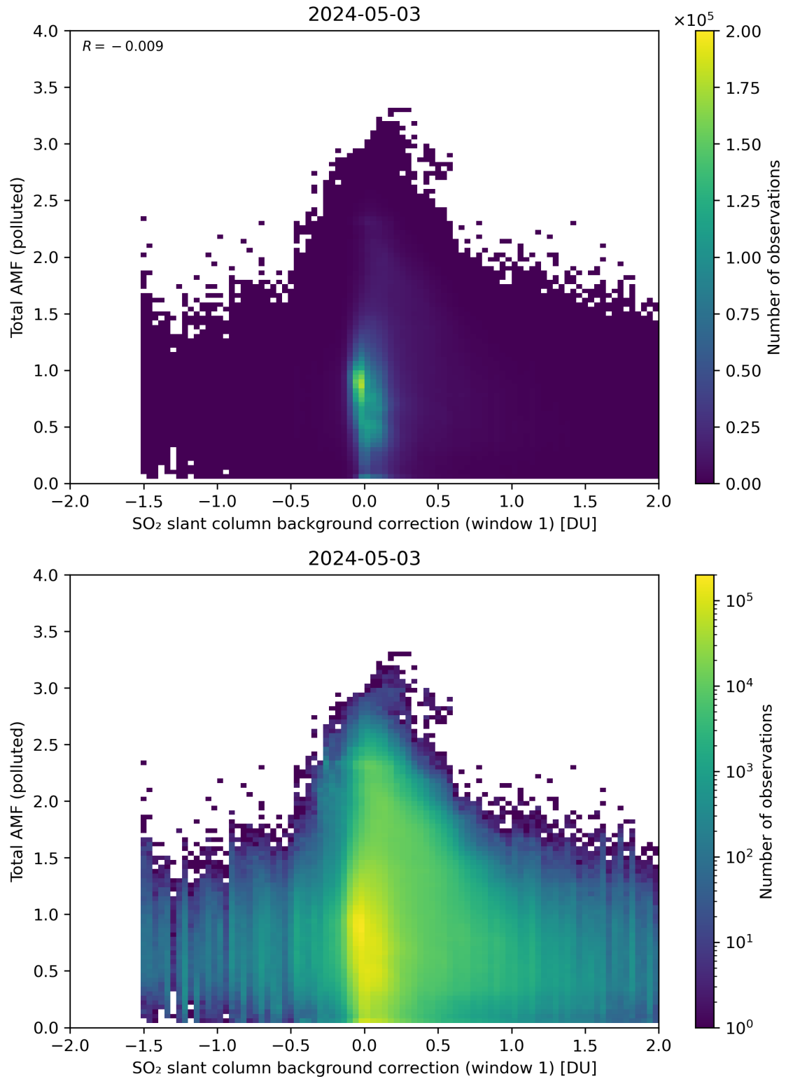
Figure 109: Scatter density plot of “SO 2 slant column background correction (window 1)” against “Total AMF (polluted)” for 2024-05-02 to 2024-05-04.
