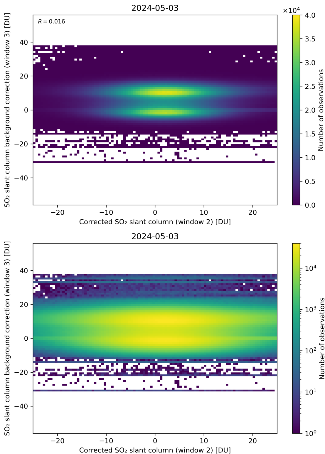
Figure 195: Scatter density plot of “Corrected SO 2 slant column (window 2)” against “SO 2 slant column background correction (window 3)” for 2024-05-02 to 2024-05-04.
