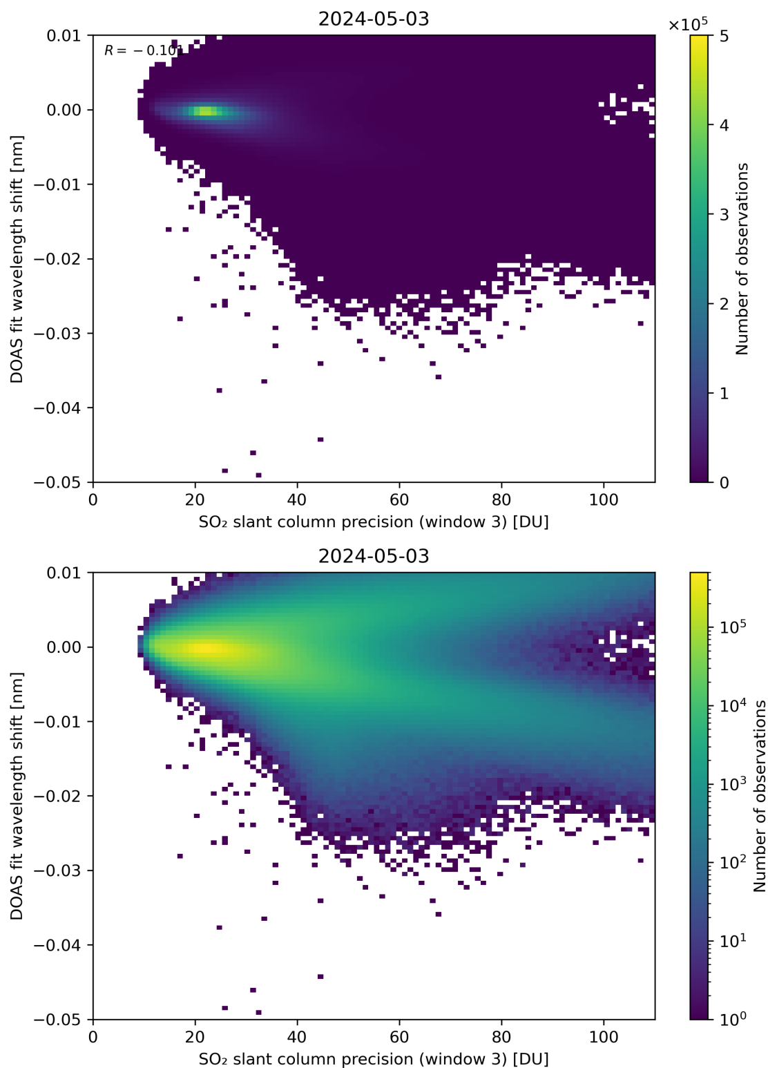
Figure 258: Scatter density plot of “SO 2 slant column precision (window 3)” against “DOAS fit wavelength shift” for 2024-05-02 to 2024-05-04.
