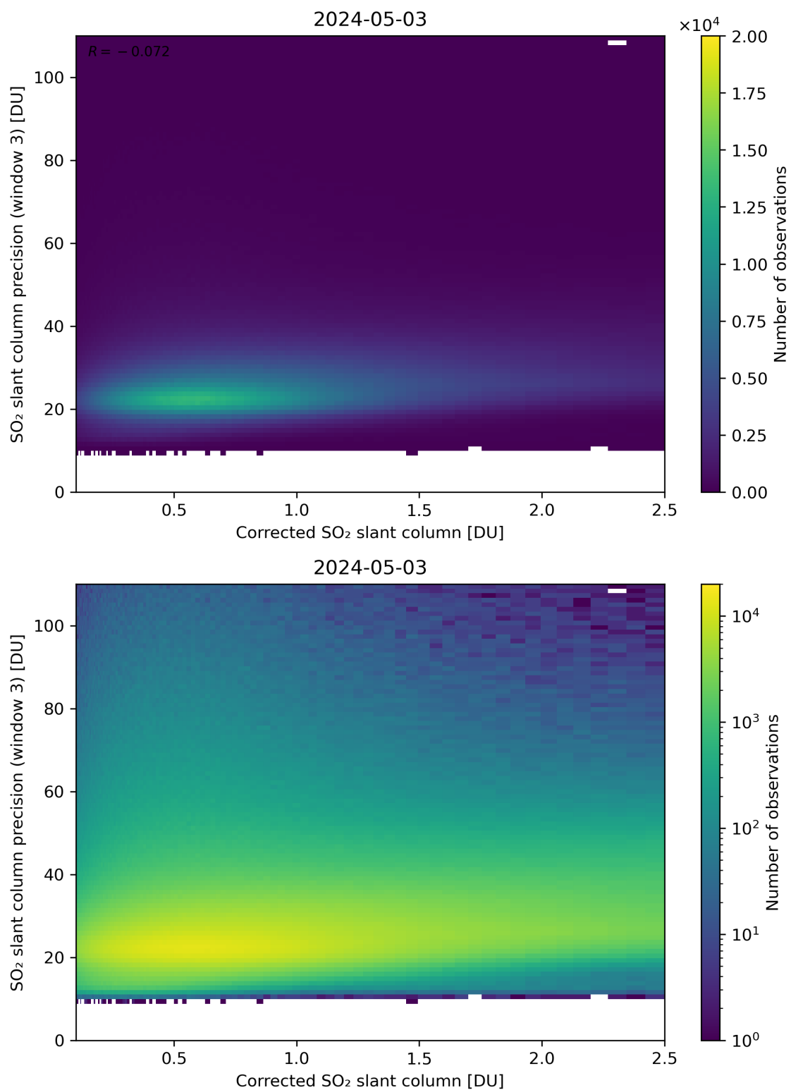
Figure 191: Scatter density plot of “Corrected SO 2 slant column” against “SO 2 slant column precision (window 3)” for 2024-05-02 to 2024-05-04.
