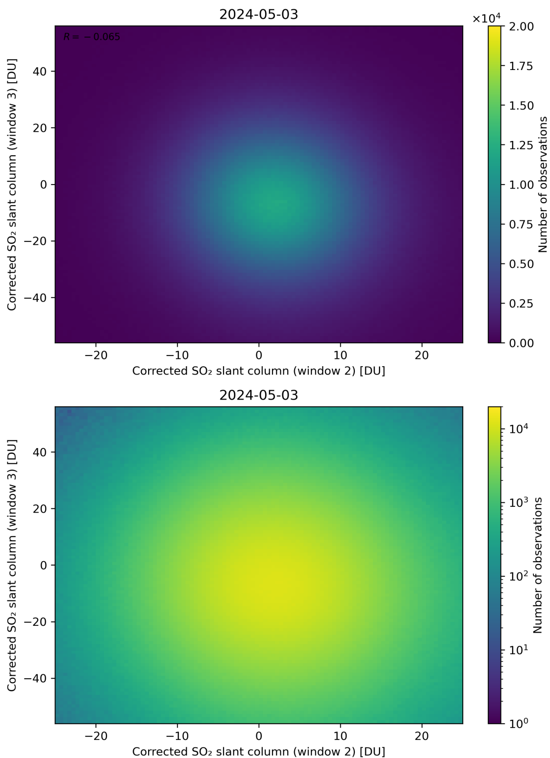
Figure 200: Scatter density plot of “Corrected SO 2 slant column (window 2)” against “Corrected SO 2 slant column (window 3)” for 2024-05-02 to 2024-05-04.
