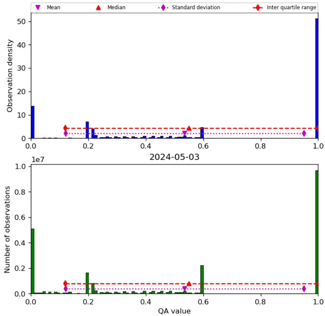
Figure 52: Histogram of “QA value” for 2024-05-02 to 2024-05-04
