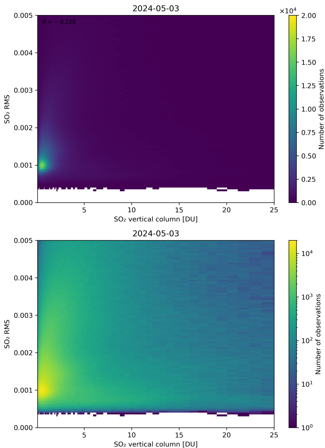
Figure 278: Scatter density plot of “SO 2 vertical column” against “SO 2 RMS” for 2024-05-02 to 2024-05-04.
