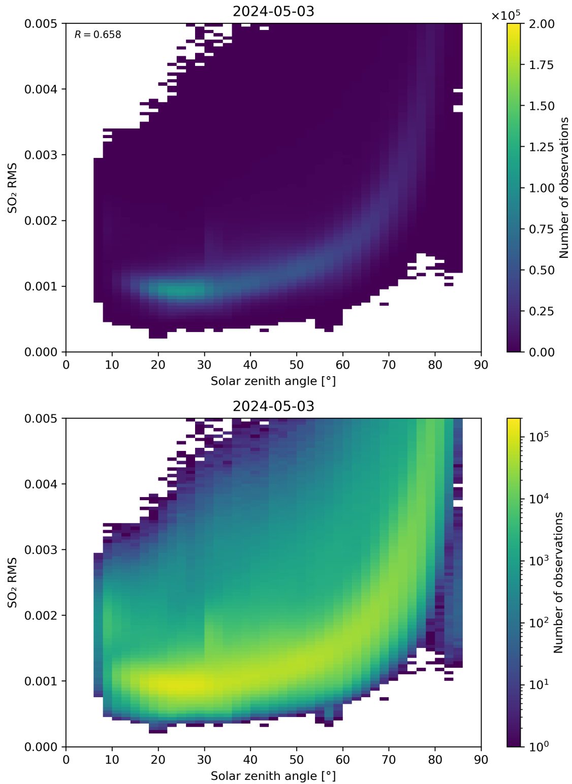
Figure 163: Scatter density plot of “Solar zenith angle” against “SO 2 RMS” for 2024-05-02 to 2024-05-04.
