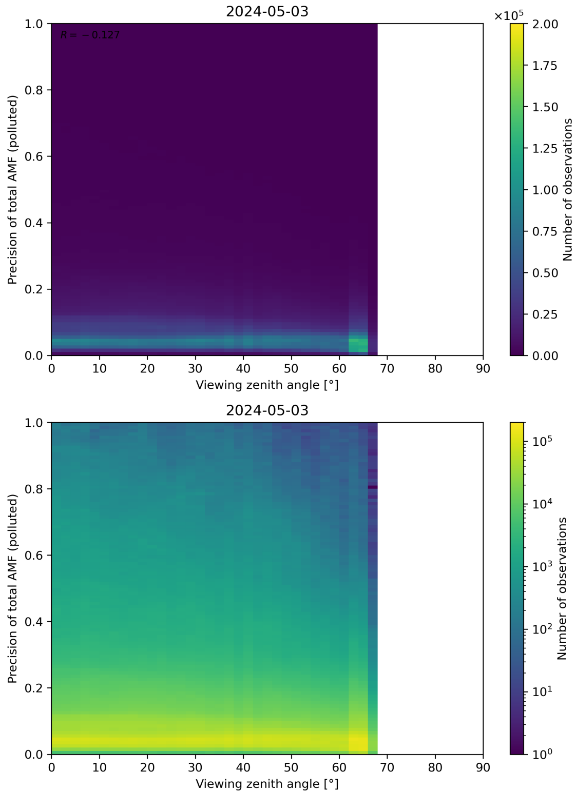
Figure 326: Scatter density plot of “Viewing zenith angle” against “Precision of total AMF (polluted)” for 2024-05-02 to 2024-05-04.
