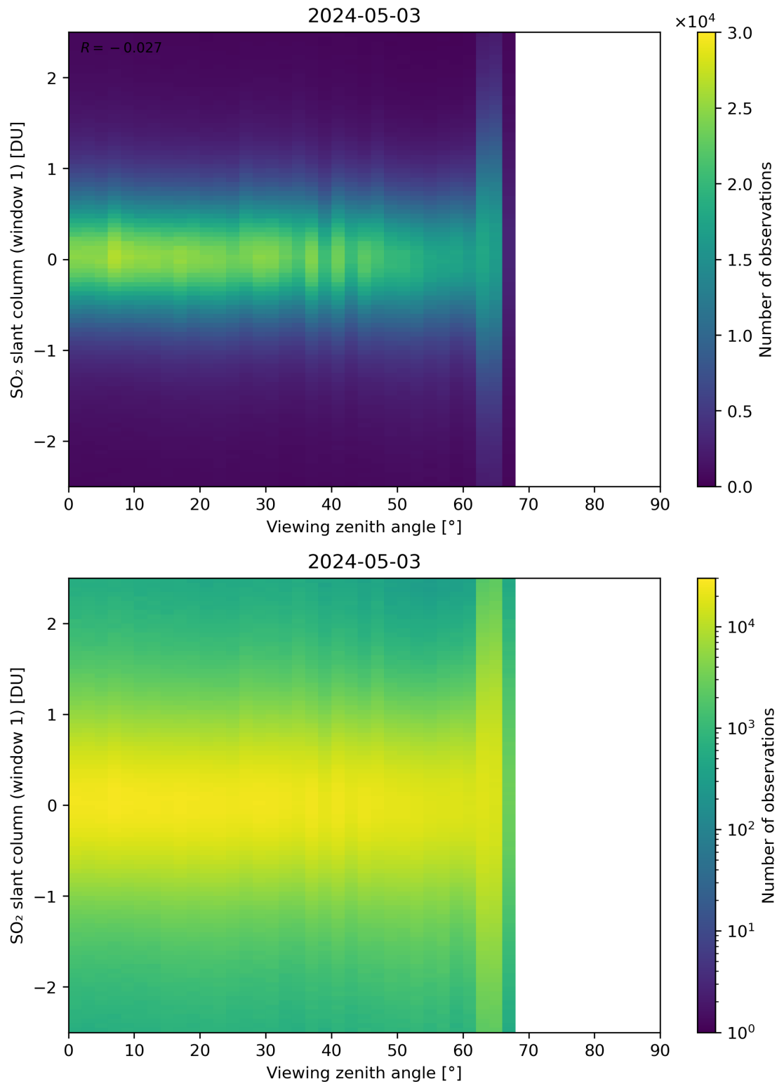
Figure 320: Scatter density plot of “Viewing zenith angle” against “SO 2 slant column (window 1)” for 2024-05-02 to 2024-05-04.
