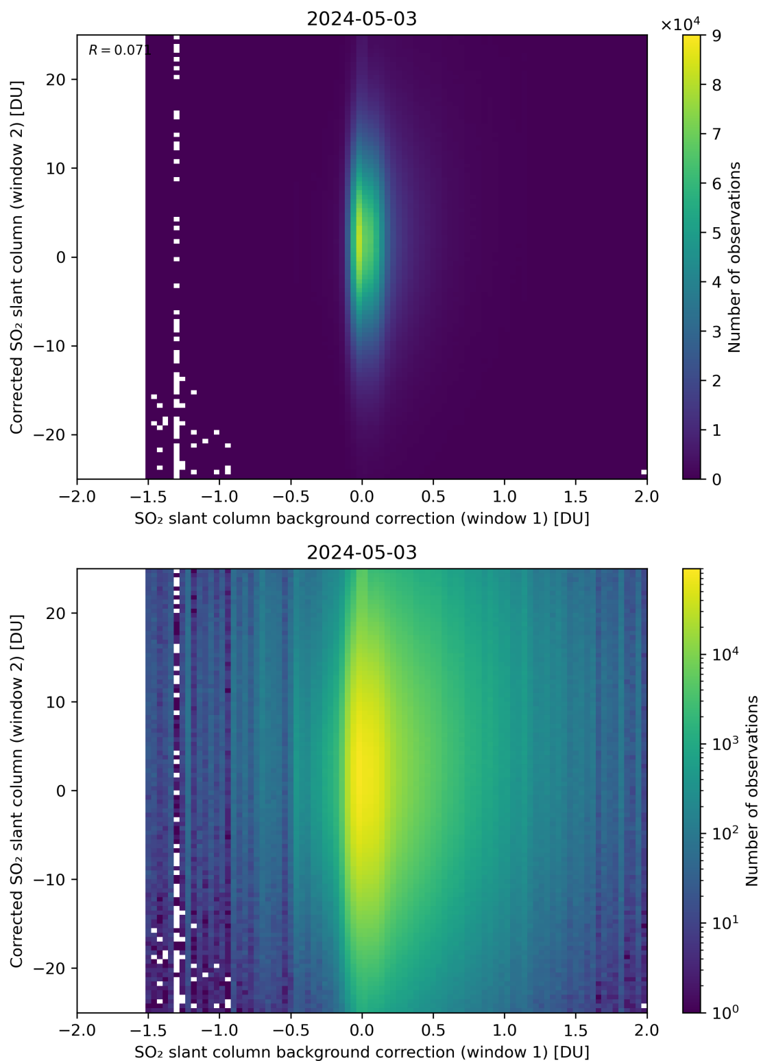
Figure 104: Scatter density plot of “SO 2 slant column background correction (window 1)” against “Corrected SO 2 slant column (window 2)” for 2024-05-02 to 2024-05-04.
