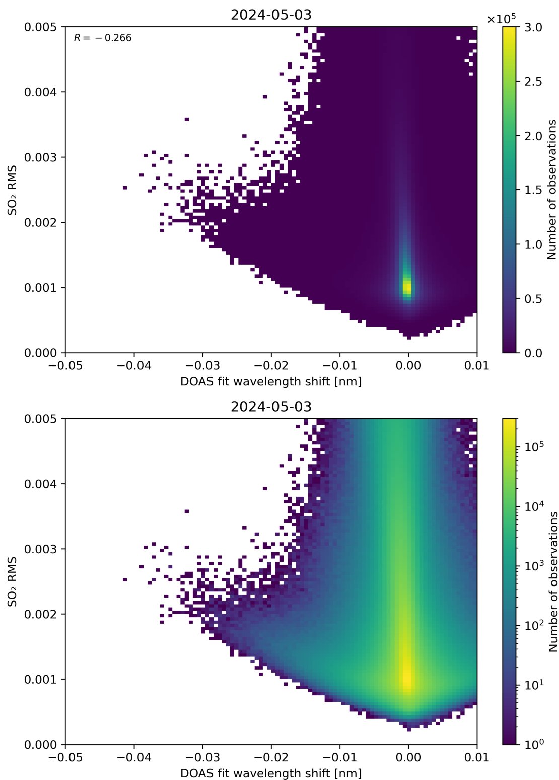
Figure 128: Scatter density plot of “DOAS fit wavelength shift” against “SO 2 RMS” for 2024-05-02 to 2024-05-04.
