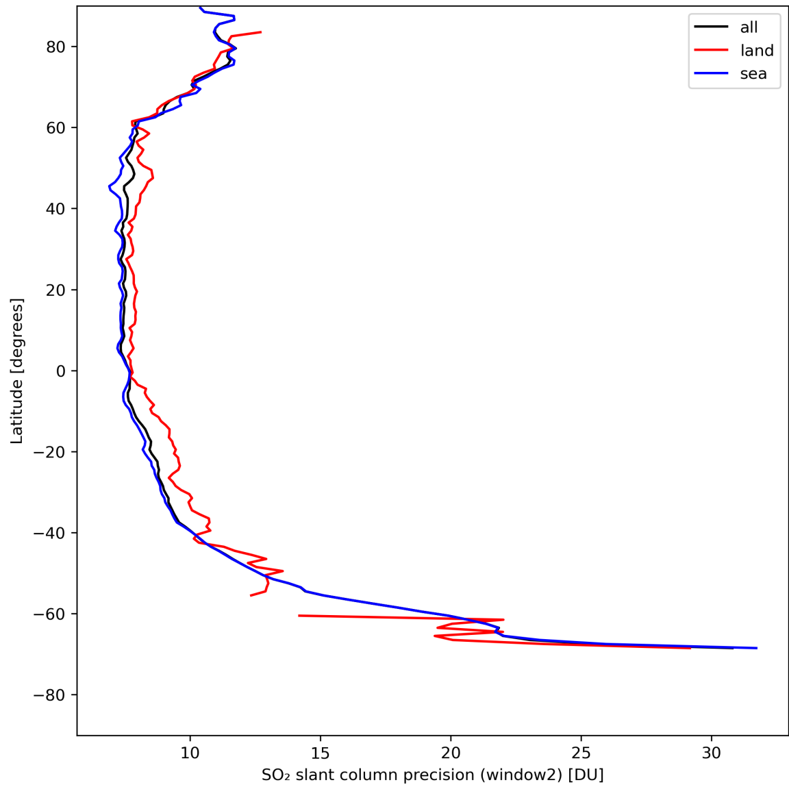
Figure 38: Zonal average of “SO 2 slant column precision (window2)” for 2024-05-02 to 2024-05-04.
