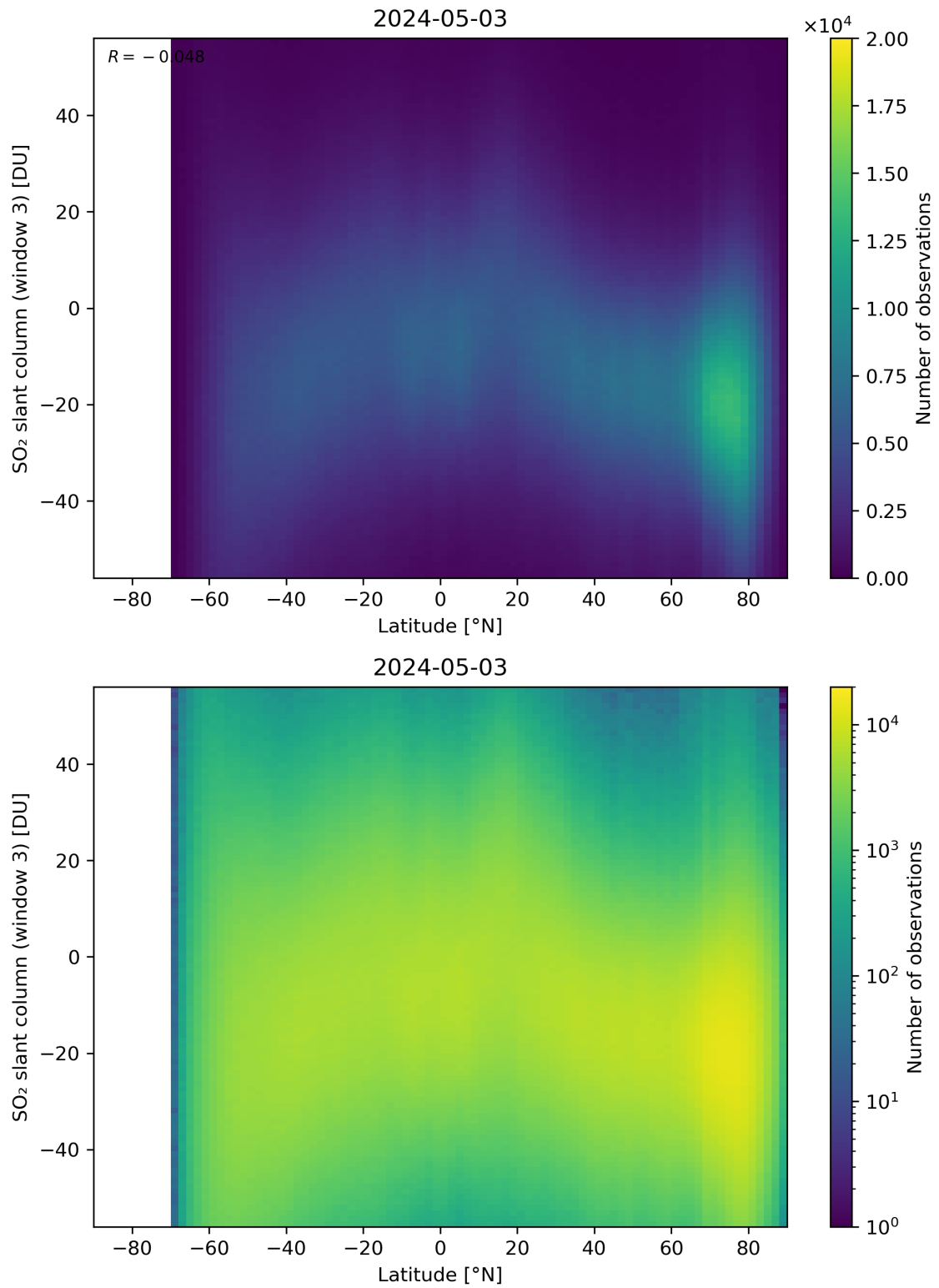
Figure 152: Scatter density plot of “Latitude” against “SO 2 slant column (window 3)” for 2024-05-02 to 2024-05-04.
