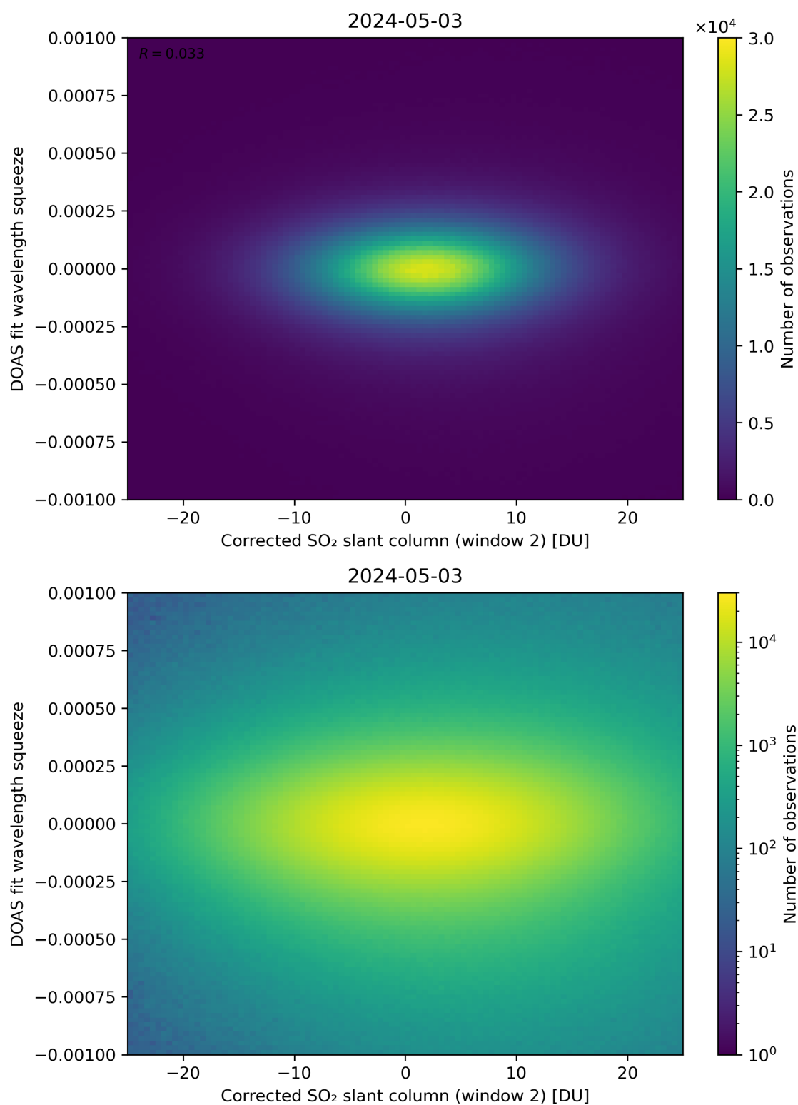
Figure 197: Scatter density plot of “Corrected SO 2 slant column (window 2)” against “DOAS fit wavelength squeeze” for 2024-05-02 to 2024-05-04.
