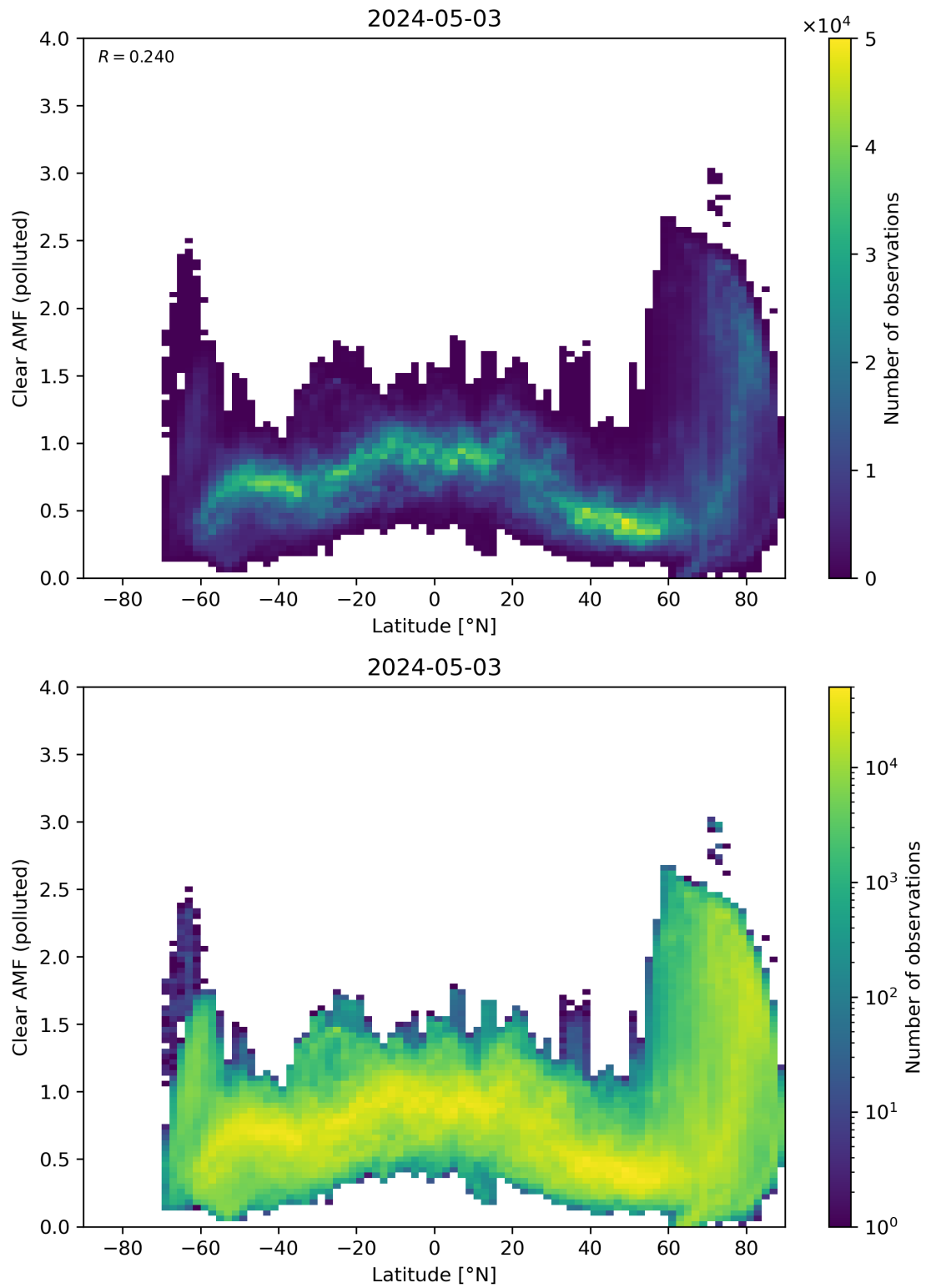
Figure 145: Scatter density plot of “Latitude” against “Clear AMF (polluted)” for 2024-05-02 to 2024-05-04.
