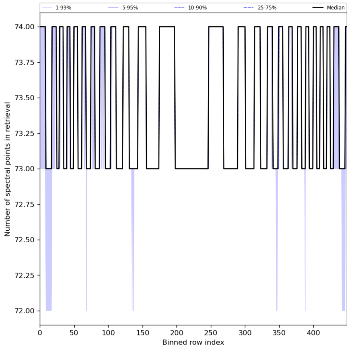
Figure 97: Along track statistics of “Number of spectral points in retrieval” for 2024-05-02 to 2024-05-04
