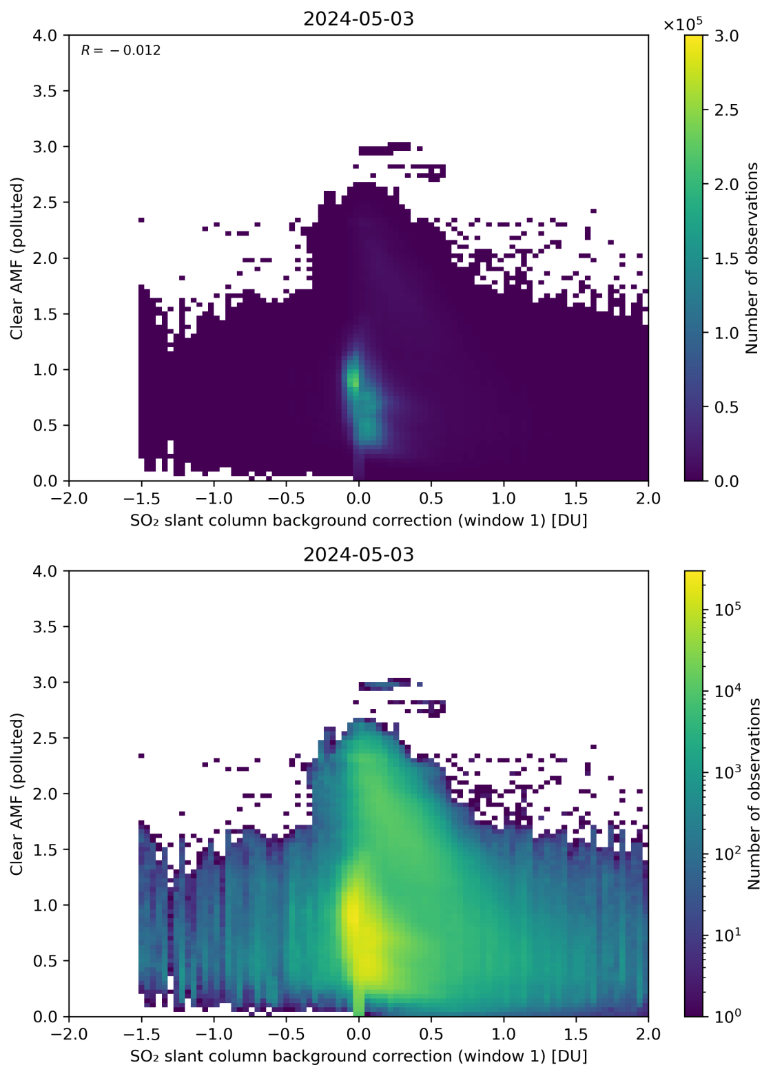
Figure 103: Scatter density plot of “SO 2 slant column background correction (window 1)” against “Clear AMF (polluted)” for 2024-05-02 to 2024-05-04.
