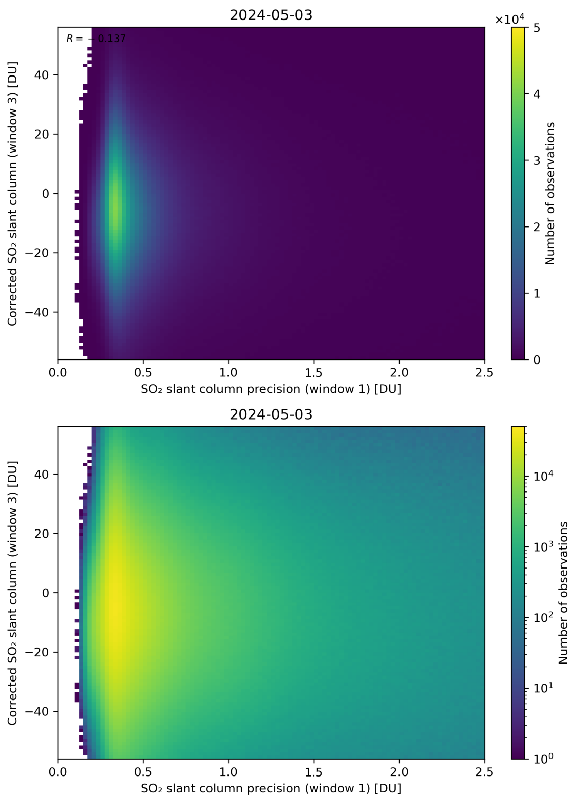
Figure 226: Scatter density plot of “SO 2 slant column precision (window 1)” against “Corrected SO 2 slant column (window 3)” for 2024-05-02 to 2024-05-04.
