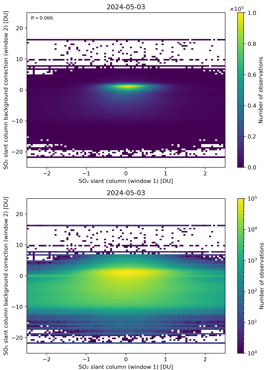
Figure 213: Scatter density plot of “SO 2 slant column (window 1)” against “SO 2 slant column background correction (window 2)” for 2024-05-02 to 2024-05-04.
