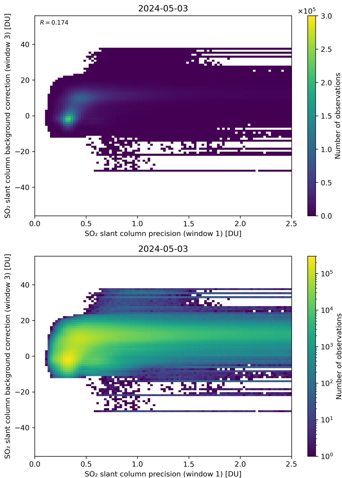
Figure 220: Scatter density plot of “SO 2 slant column precision (window 1)” against “SO 2 slant column background correction (window 3)” for 2024-05-02 to 2024-05-04.
