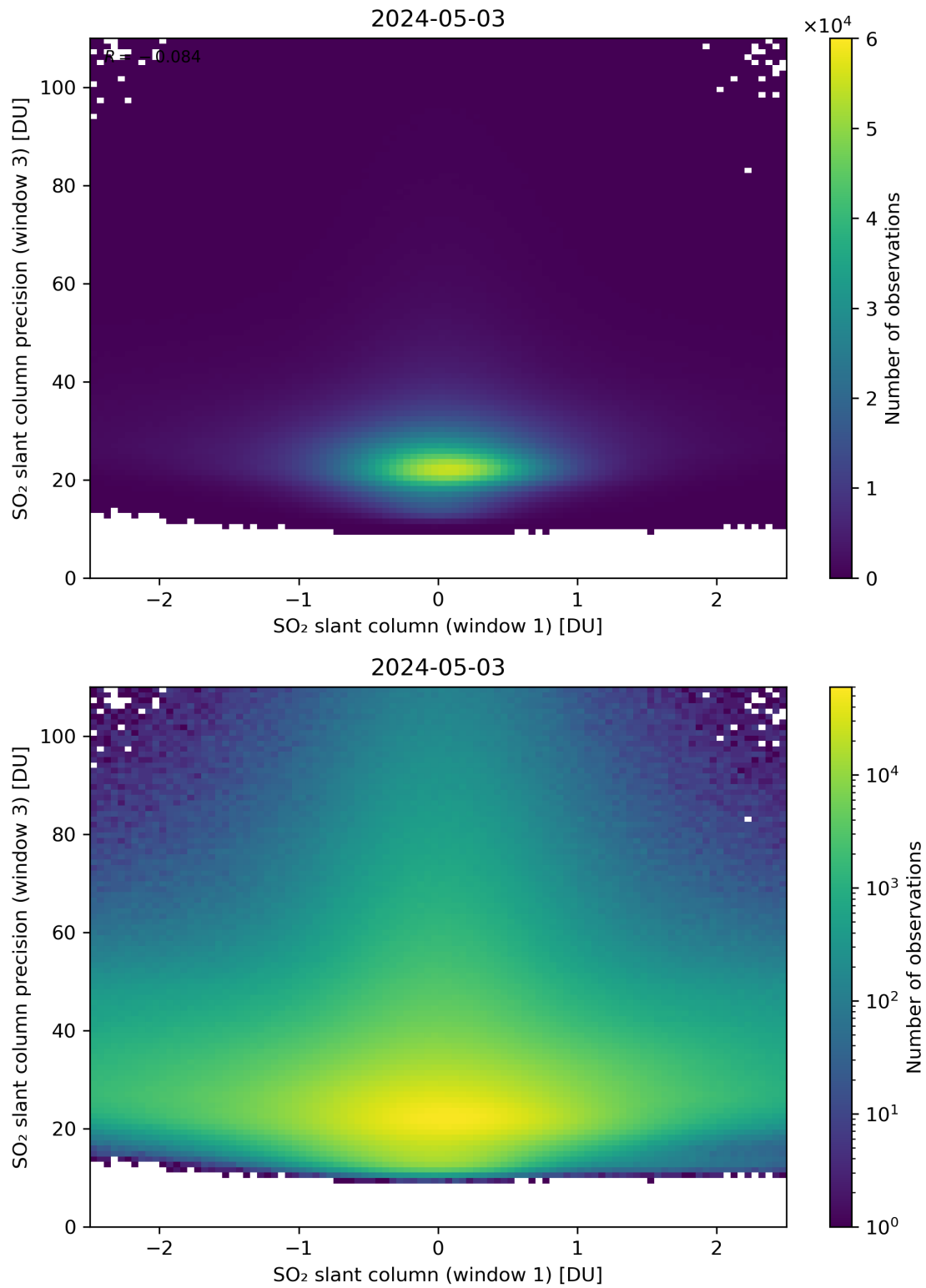
Figure 238: Scatter density plot of “SO 2 slant column (window 1)” against “SO 2 slant column precision (window 3)” for 2024-05-02 to 2024-05-04.
