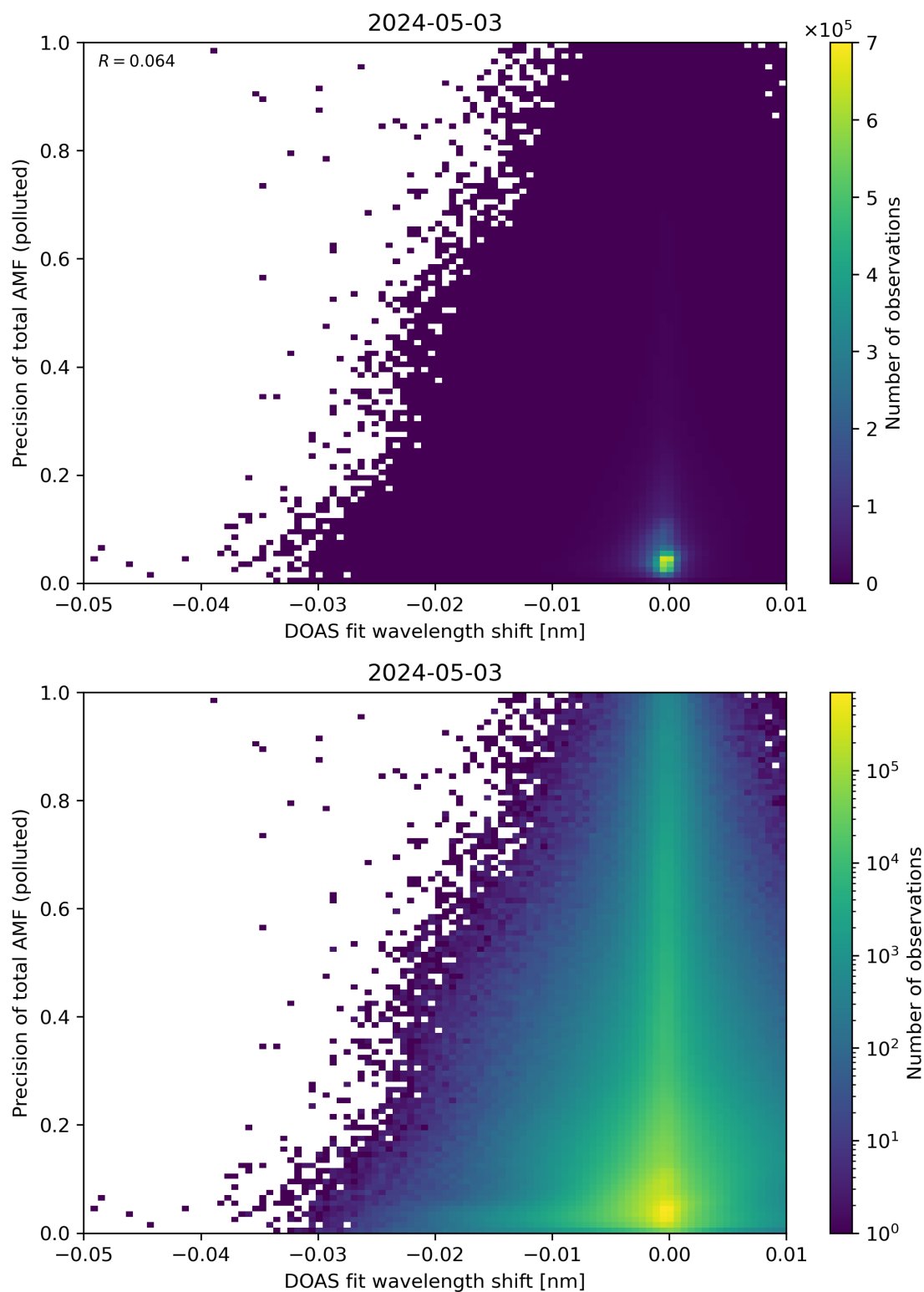
Figure 131: Scatter density plot of “DOAS fit wavelength shift” against “Precision of total AMF (polluted)” for 2024-05-02 to 2024-05-04.
