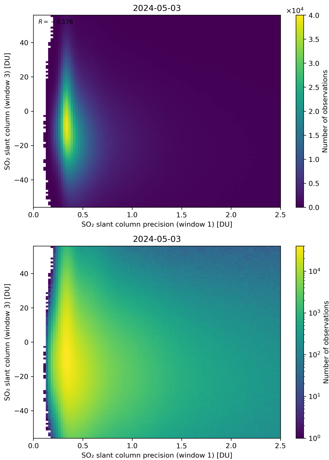
Figure 228: Scatter density plot of “SO 2 slant column precision (window 1)” against “SO 2 slant column (window 3)” for 2024-05-02 to 2024-05-04.
