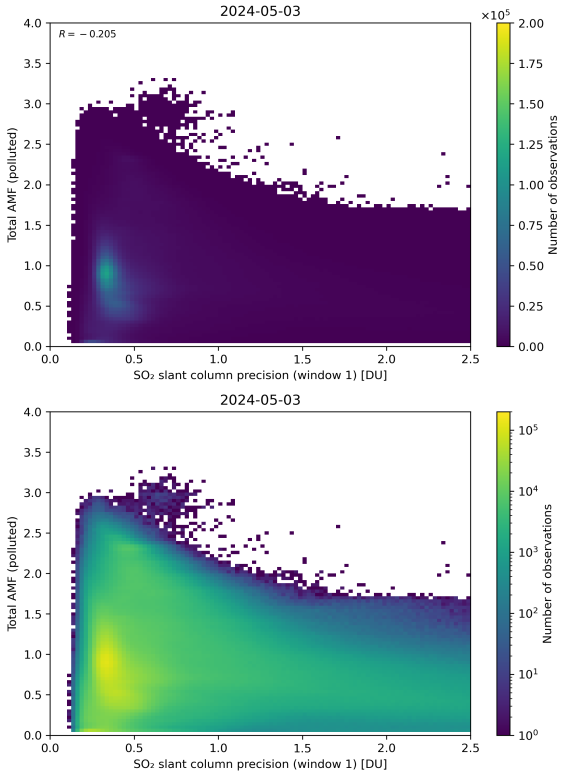
Figure 230: Scatter density plot of “SO 2 slant column precision (window 1)” against “Total AMF (polluted)” for 2024-05-02 to 2024-05-04.
