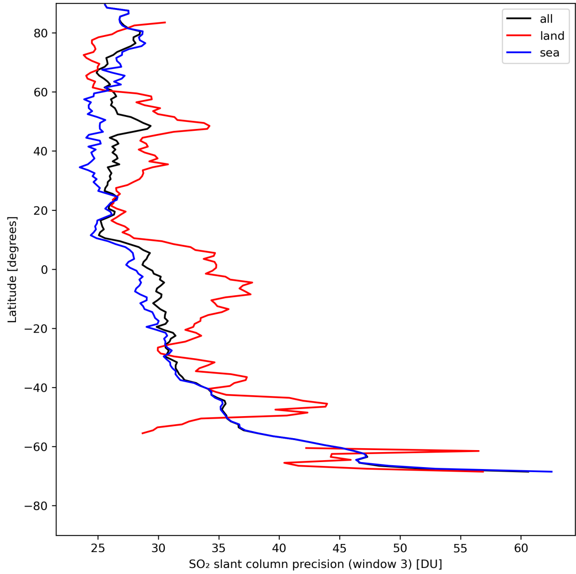
Figure 42: Zonal average of “SO 2 slant column precision (window 3)” for 2024-05-02 to 2024-05-04.
