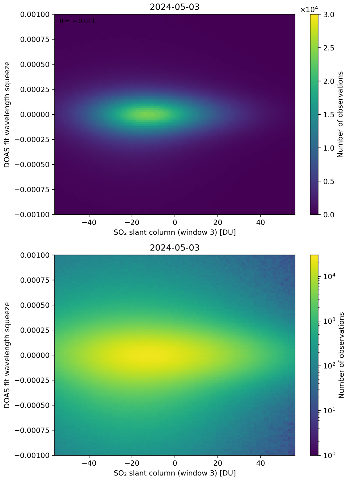
Figure 255: Scatter density plot of “SO 2 slant column (window 3)” against “DOAS fit wavelength squeeze” for 2024-05-02 to 2024-05-04.
