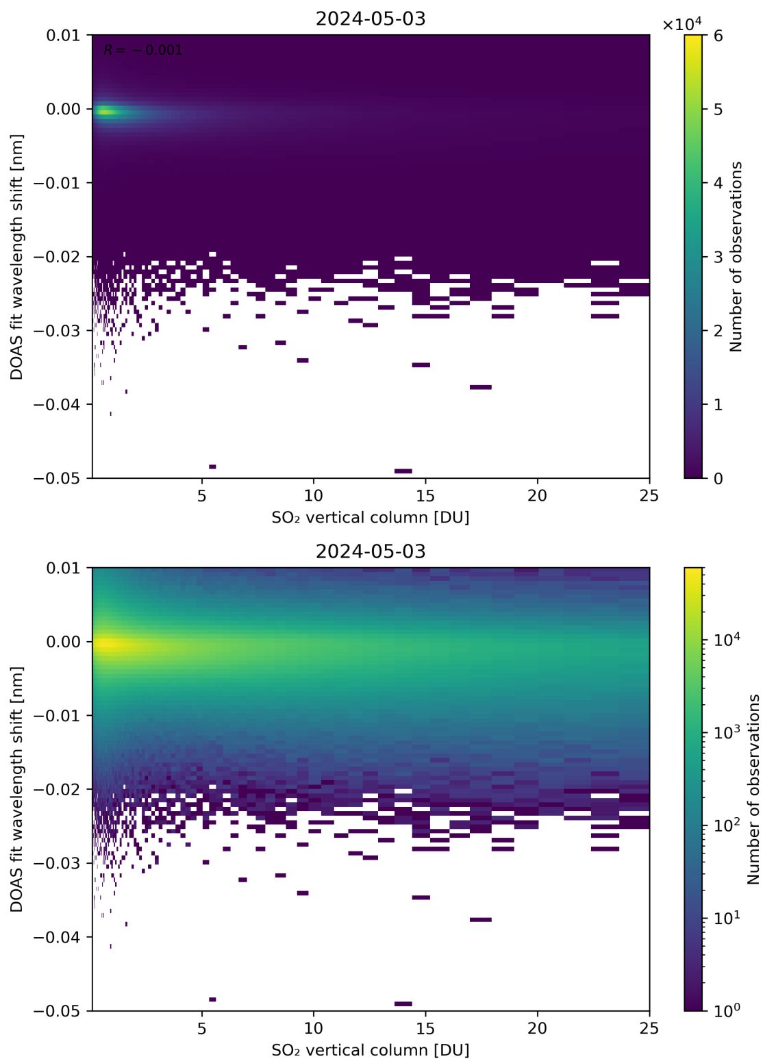
Figure 276: Scatter density plot of “SO 2 vertical column” against “DOAS fit wavelength shift” for 2024-05-02 to 2024-05-04.
