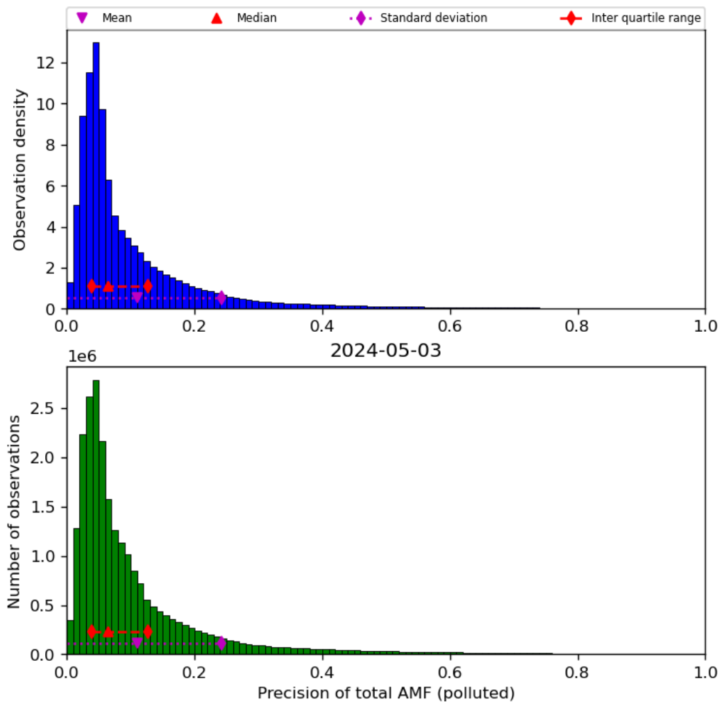
Figure 72: Histogram of “Precision of total AMF (polluted)” for 2024-05-02 to 2024-05-04
