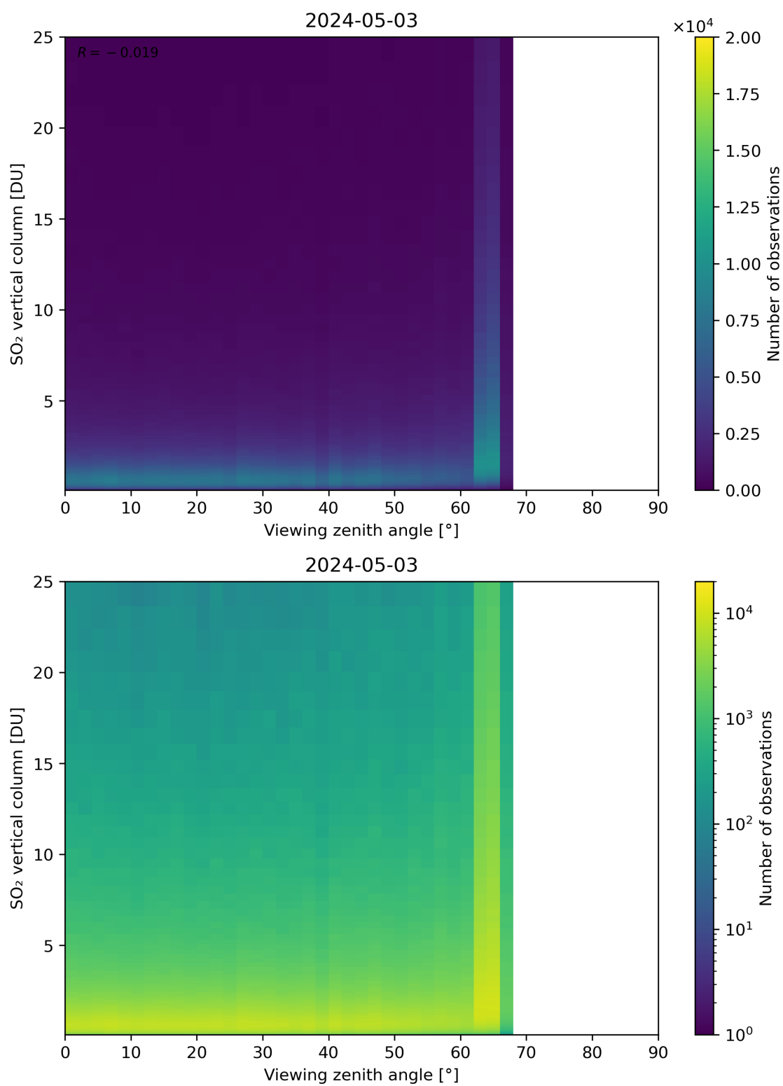
Figure 327: Scatter density plot of “Viewing zenith angle” against “SO 2 vertical column” for 2024-05-02 to 2024-05-04.
