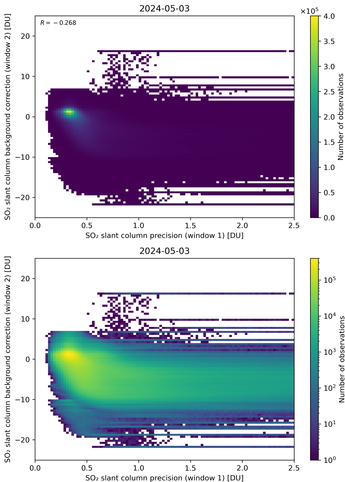
Figure 219: Scatter density plot of “SO 2 slant column precision (window 1)” against “SO 2 slant column background correction (window 2)” for 2024-05-02 to 2024-05-04.
