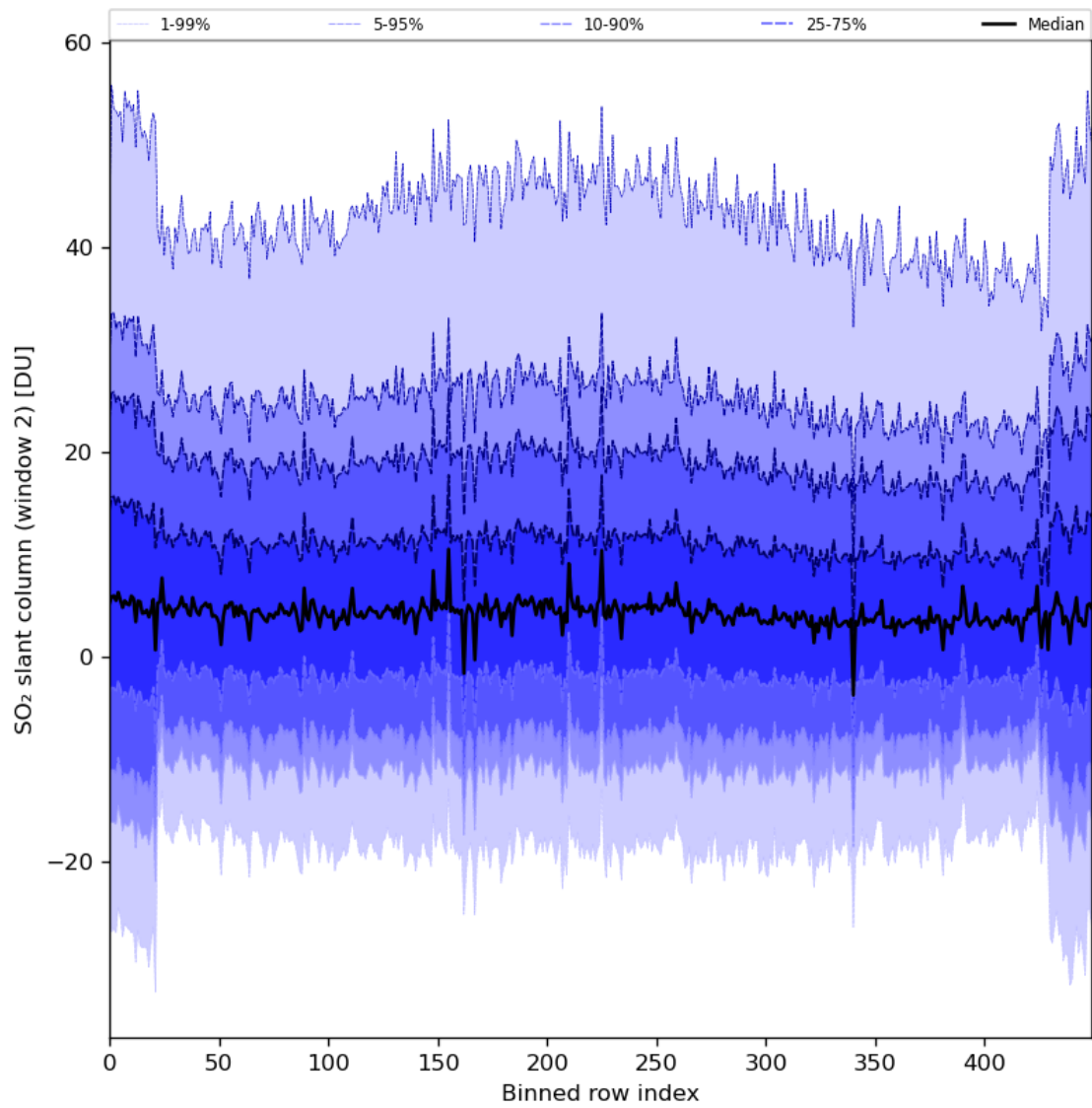
Figure 83: Along track statistics of “SO 2 slant column (window 2)” for 2024-05-02 to 2024-05-04
