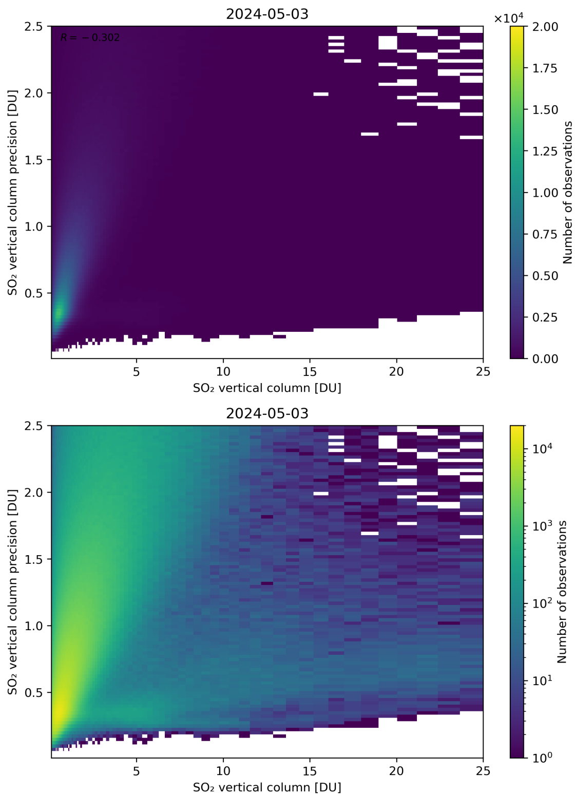
Figure 307: Scatter density plot of “SO 2 vertical column” against “SO 2 vertical column precision” for 2024-05-02 to 2024-05-04.
