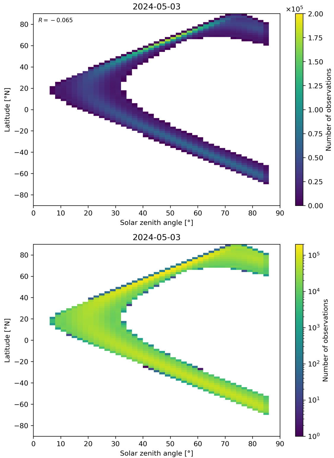
Figure 164: Scatter density plot of “Solar zenith angle” against “Latitude” for 2024-05-02 to 2024-05-04.
