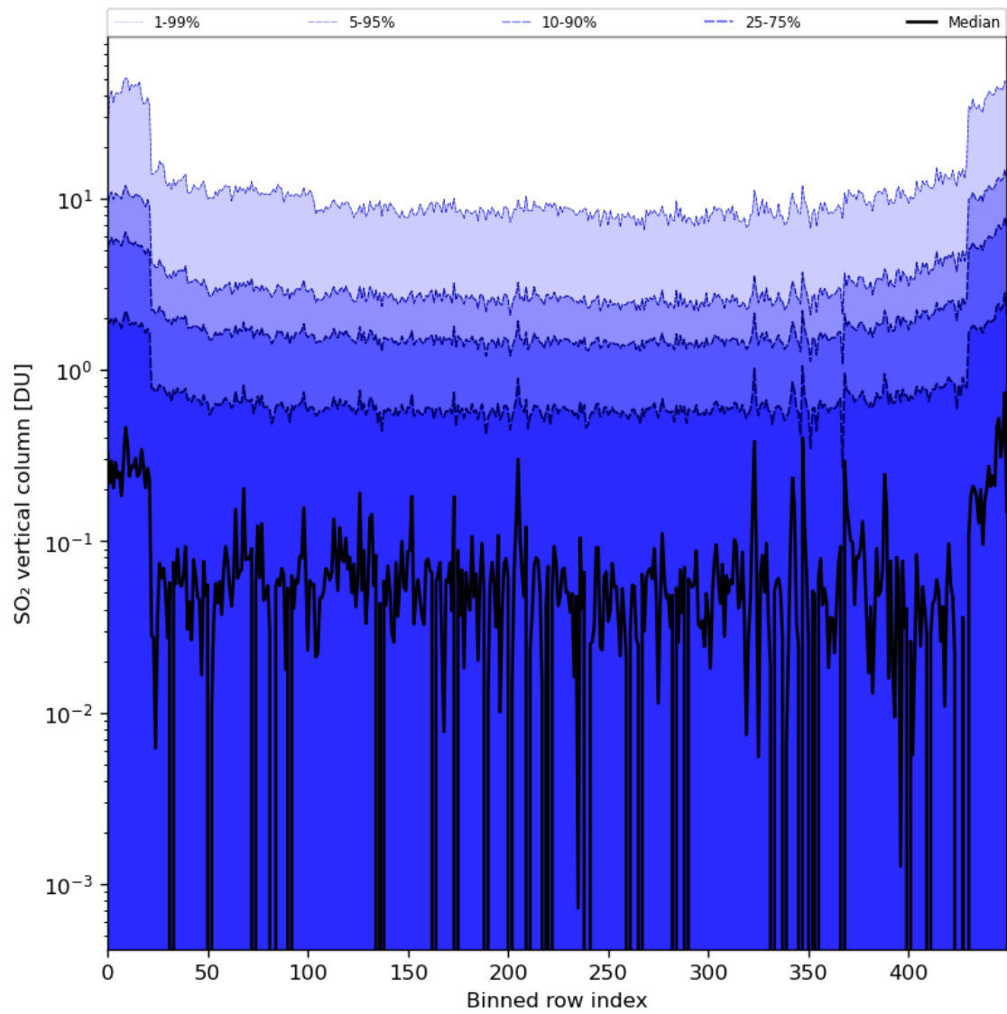
Figure 76: Along track statistics of “SO 2 vertical column” for 2024-05-02 to 2024-05-04
