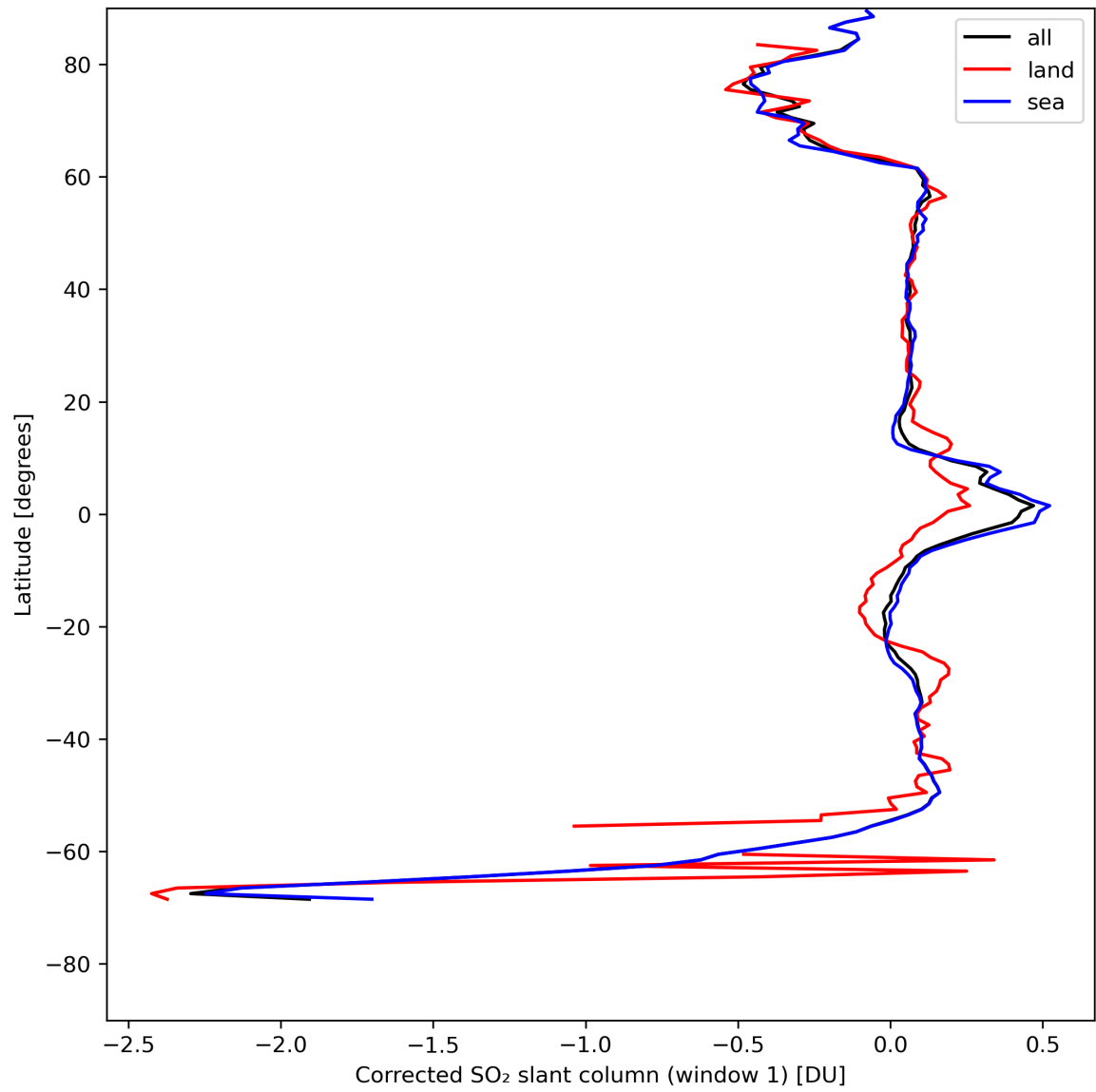
Figure 35: Zonal average of “Corrected SO 2 slant column (window 1)” for 2024-05-02 to 2024-05-04.
