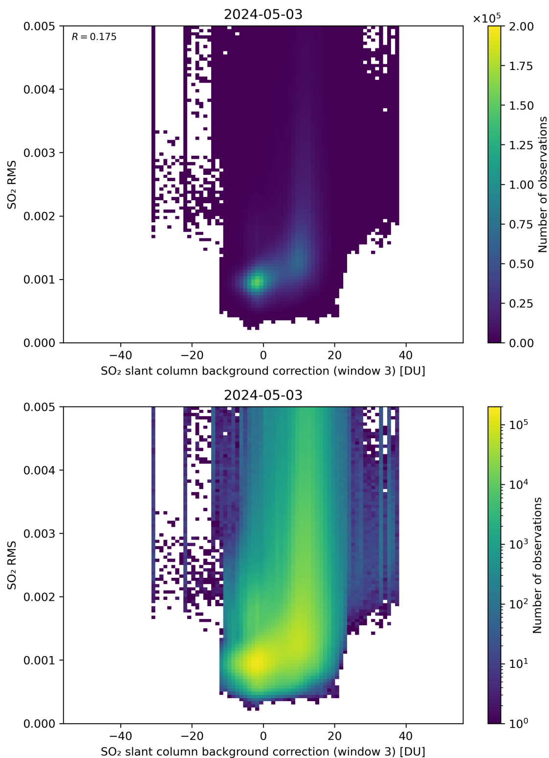
Figure 123: Scatter density plot of “SO 2 slant column background correction (window 3)” against “SO 2 RMS” for 2024-05-02 to 2024-05-04.
