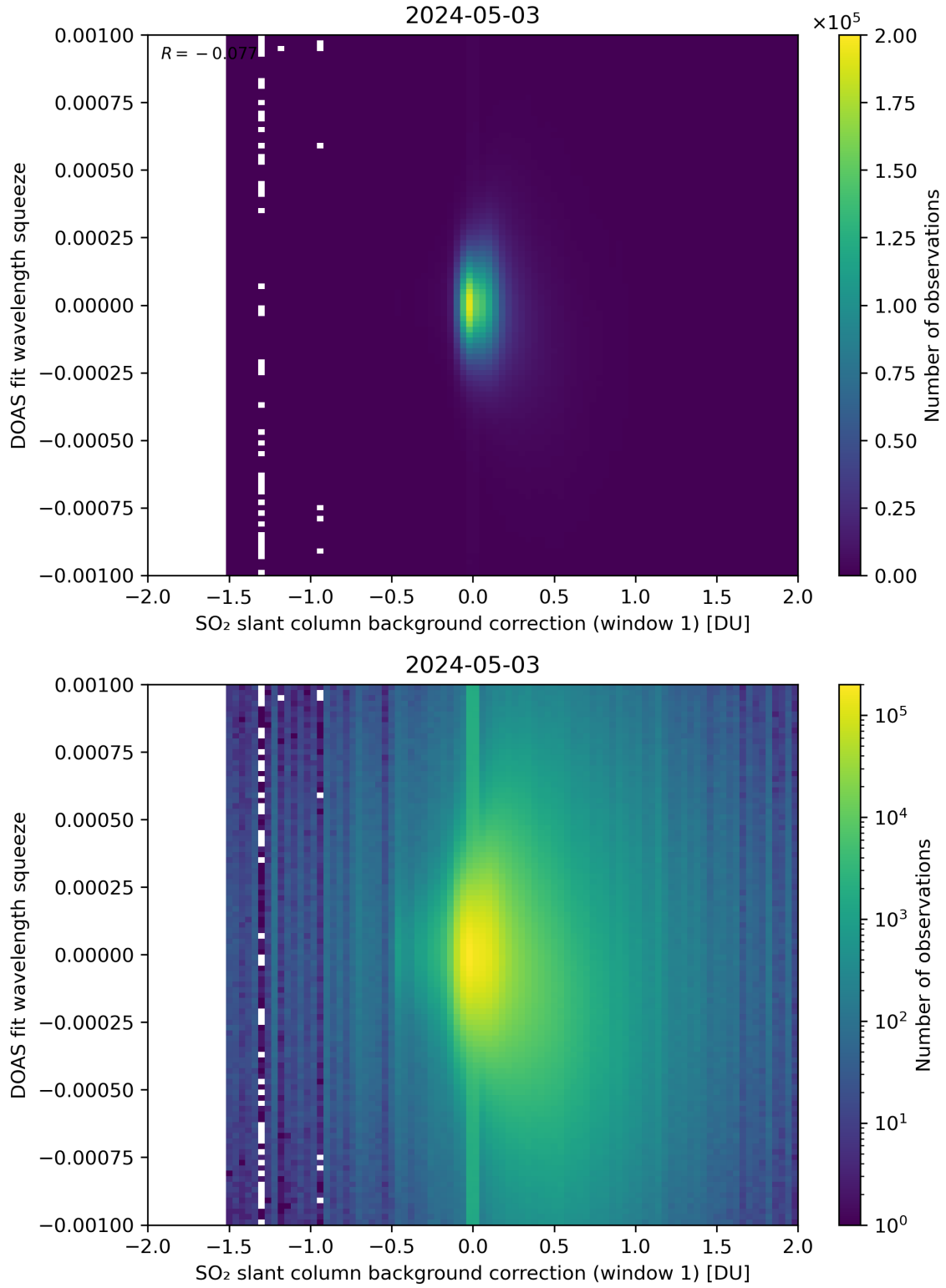
Figure 101: Scatter density plot of “SO 2 slant column background correction (window 1)” against “DOAS fit wavelength squeeze” for 2024-05-02 to 2024-05-04.
