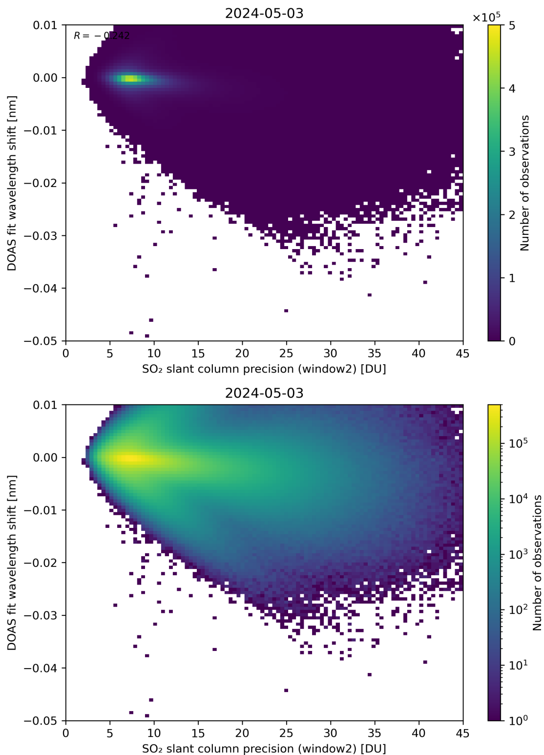
Figure 243: Scatter density plot of “SO 2 slant column precision (window2)” against “DOAS fit wavelength shift” for 2024-05-02 to 2024-05-04.
