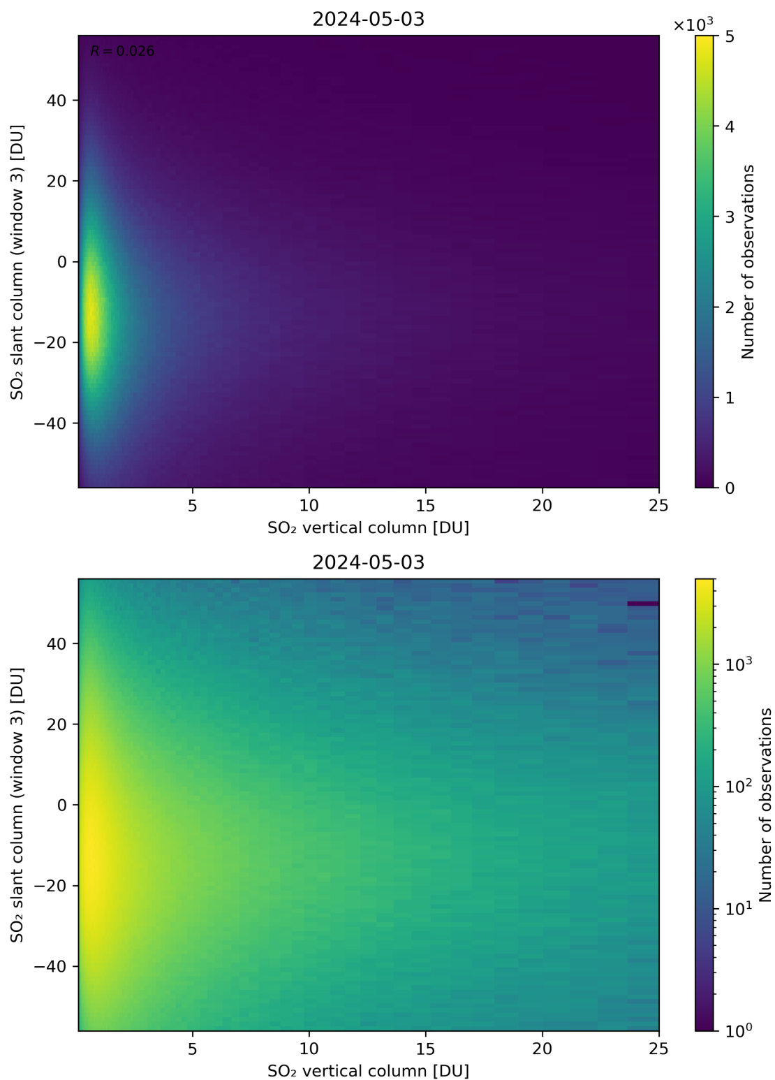
Figure 303: Scatter density plot of “SO 2 vertical column” against “SO 2 slant column (window 3)” for 2024-05-02 to 2024-05-04.
