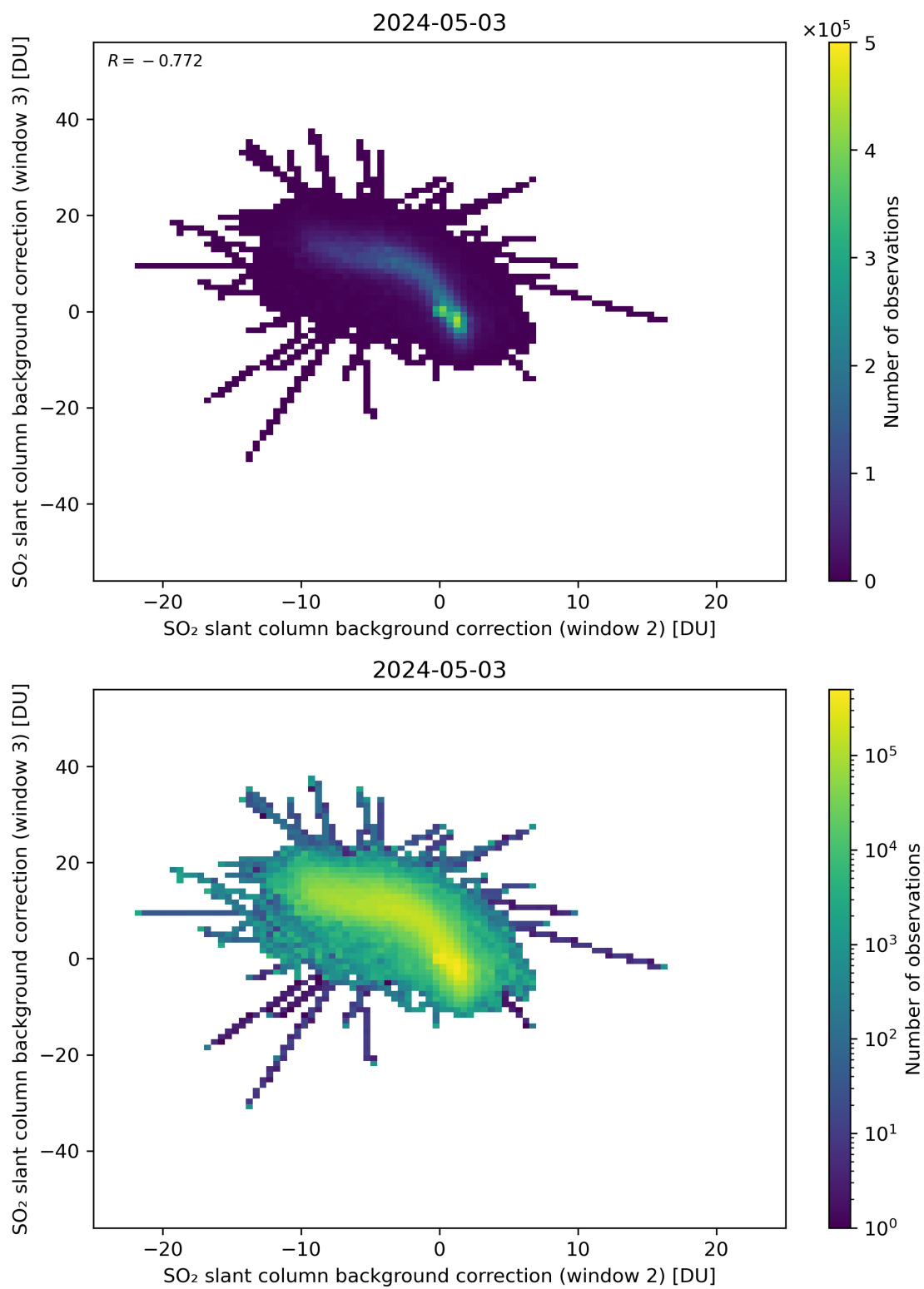
Figure 111: Scatter density plot of “SO 2 slant column background correction (window 2)” against “SO 2 slant column background correction (window 3)” for 2024-05-02 to 2024-05-04.
