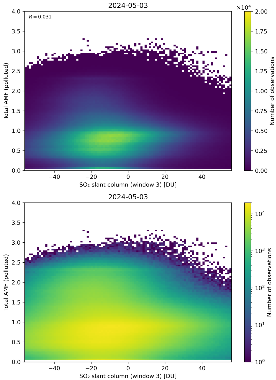
Figure 268: Scatter density plot of “SO 2 slant column (window 3)” against “Total AMF (polluted)” for 2024-05-02 to 2024-05-04.
