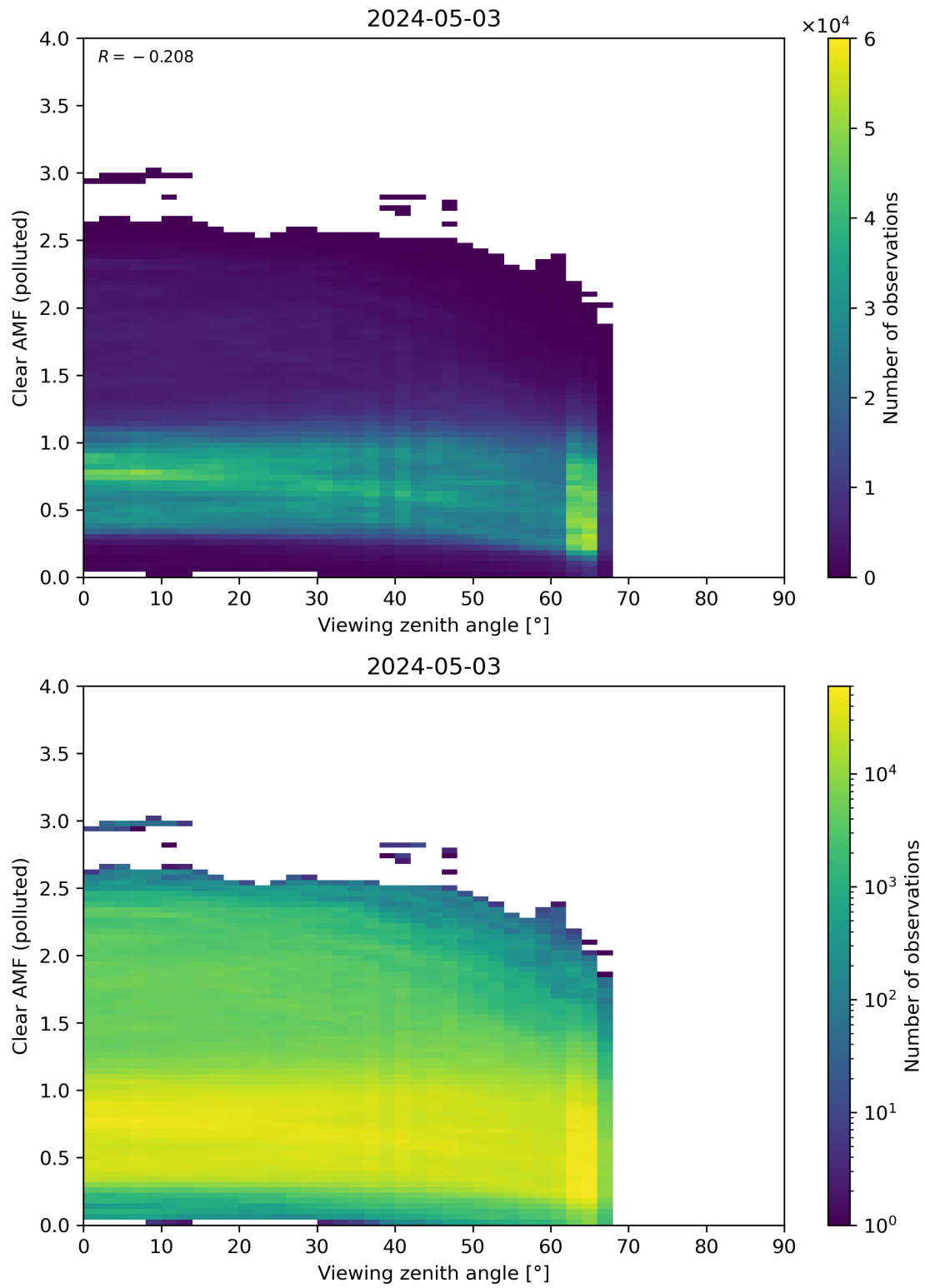
Figure 316: Scatter density plot of “Viewing zenith angle” against “Clear AMF (polluted)” for 2024-05-02 to 2024-05-04.
