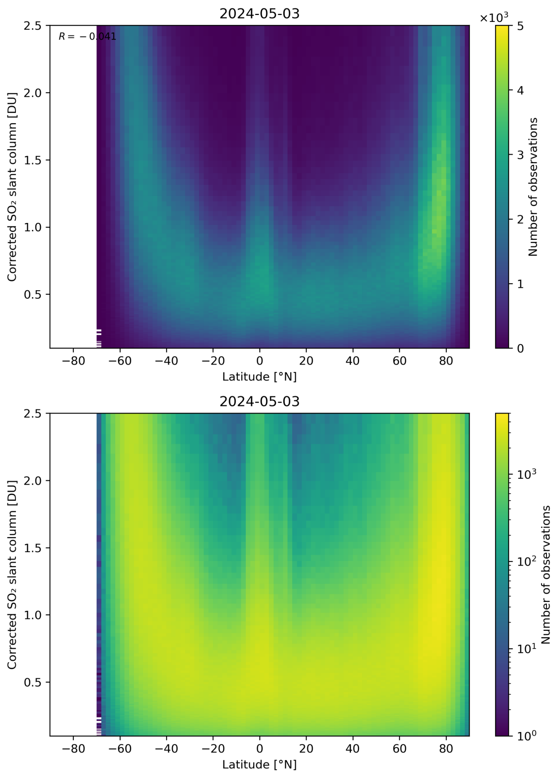
Figure 146: Scatter density plot of “Latitude” against “Corrected SO 2 slant column” for 2024-05-02 to 2024-05-04.
