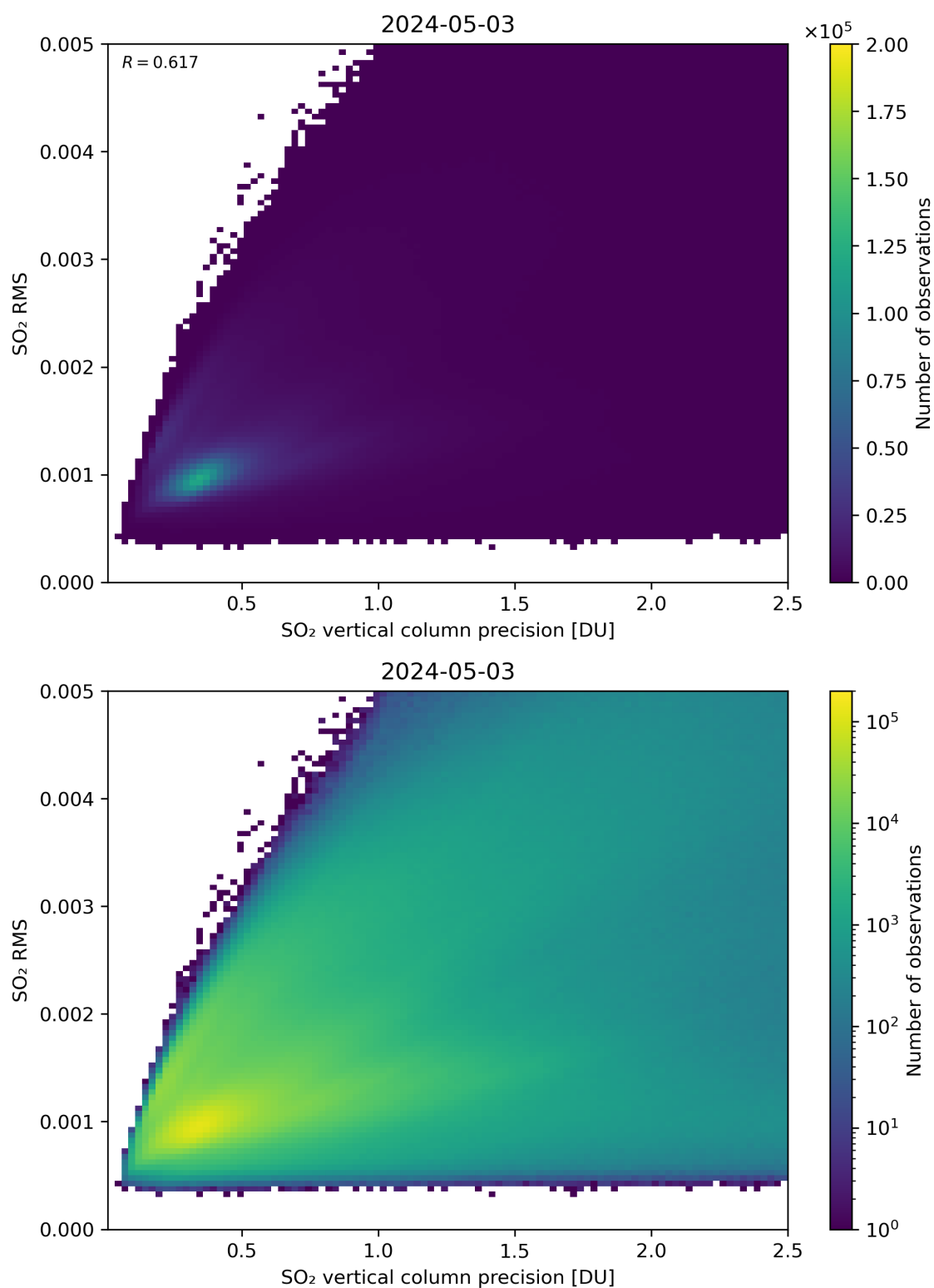
Figure 284: Scatter density plot of “SO 2 vertical column precision” against “SO 2 RMS” for 2024-05-02 to 2024-05-04.
