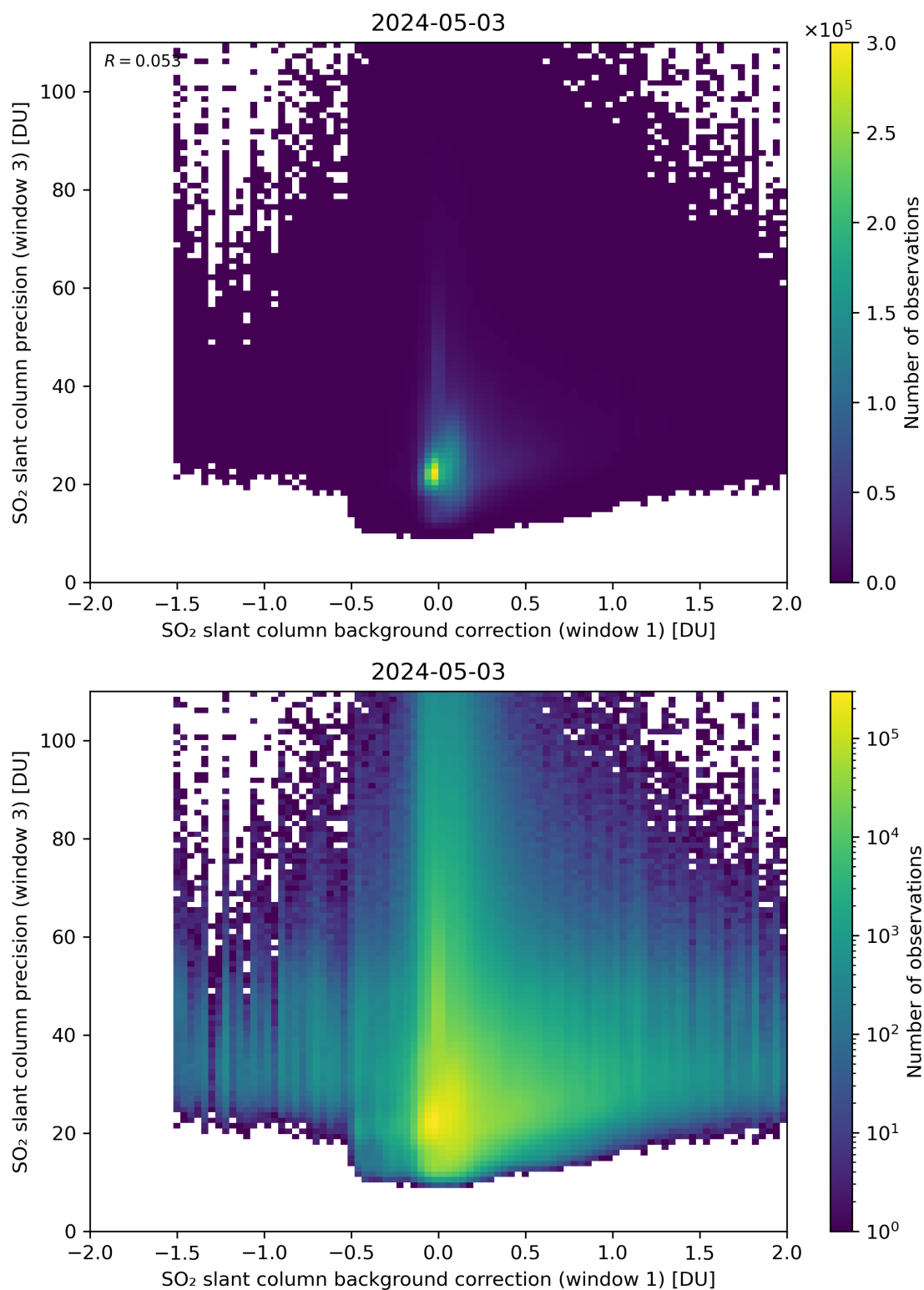
Figure 108: Scatter density plot of “SO 2 slant column background correction (window 1)” against “SO 2 slant column precision (window 3)” for 2024-05-02 to 2024-05-04.
