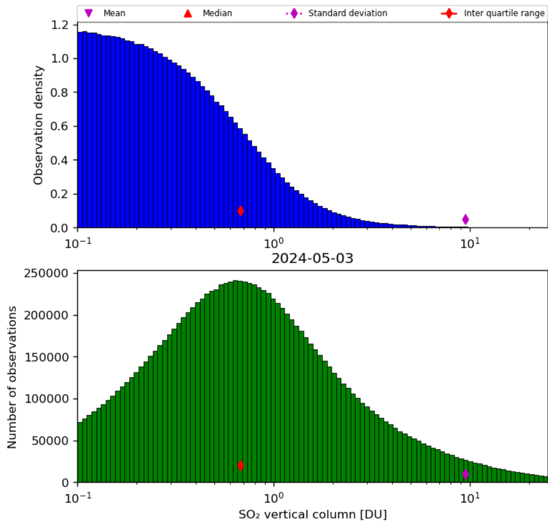
Figure 53: Histogram of “SO 2 vertical column” for 2024-05-02 to 2024-05-04
