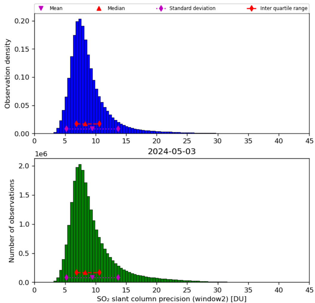
Figure 61: Histogram of “SO 2 slant column precision (window2)” for 2024-05-02 to 2024-05-04
