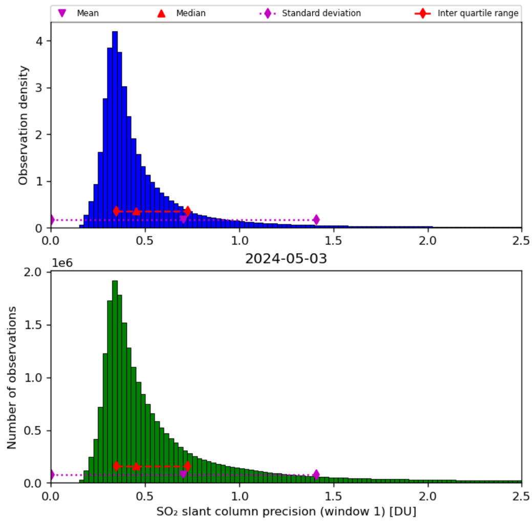
Figure 57: Histogram of “SO 2 slant column precision (window 1)” for 2024-05-02 to 2024-05-04
