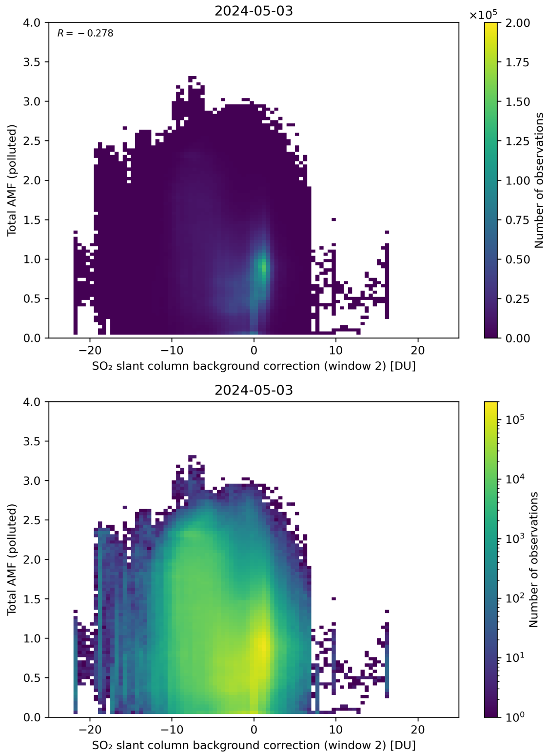
Figure 119: Scatter density plot of “SO 2 slant column background correction (window 2)” against “Total AMF (polluted)” for 2024-05-02 to 2024-05-04.
