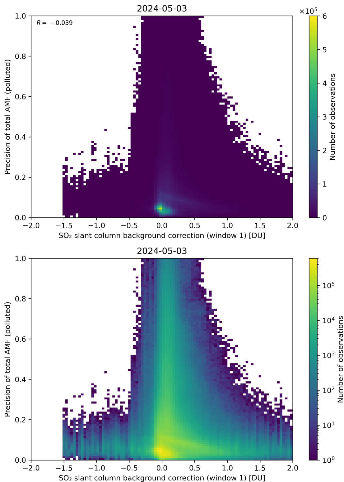
Figure 110: Scatter density plot of “SO 2 slant column background correction (window 1)” against “Precision of total AMF (polluted)” for 2024-05-02 to 2024-05-04.
