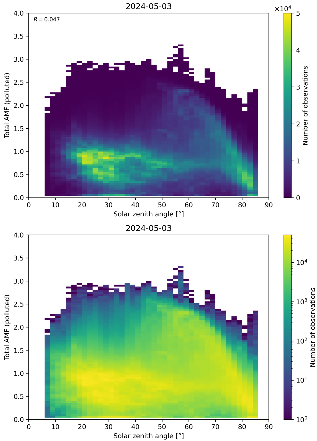
Figure 174: Scatter density plot of “Solar zenith angle” against “Total AMF (polluted)” for 2024-05-02 to 2024-05-04.
