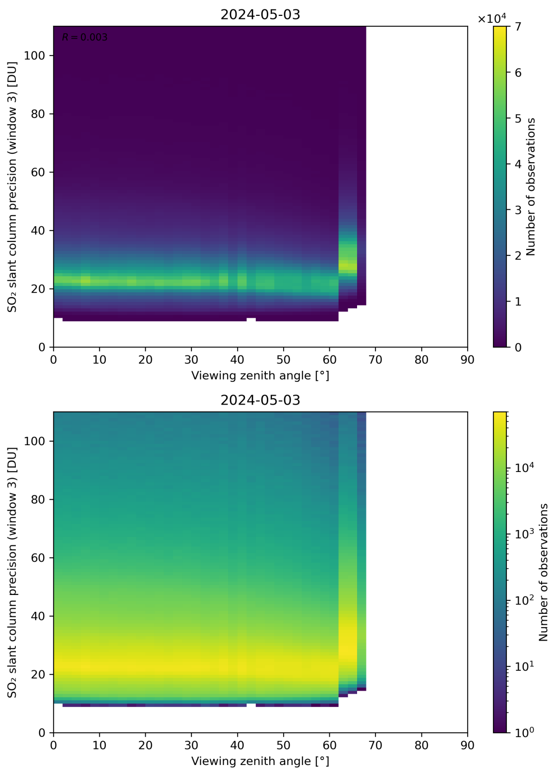
Figure 324: Scatter density plot of “Viewing zenith angle” against “SO 2 slant column precision (window 3)” for 2024-05-02 to 2024-05-04.
