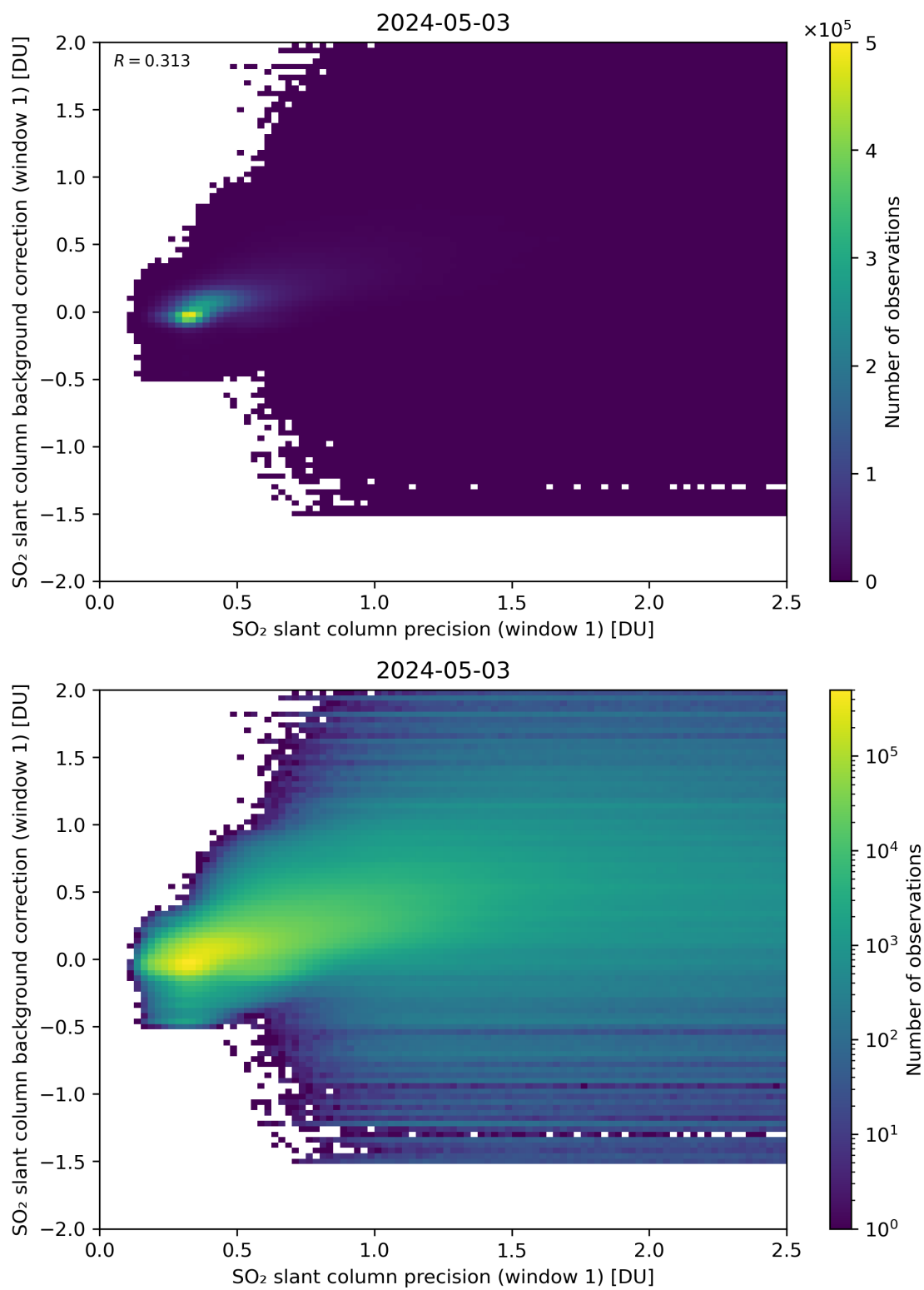
Figure 218: Scatter density plot of “SO 2 slant column precision (window 1)” against “SO 2 slant column background correction (window 1)” for 2024-05-02 to 2024-05-04.
