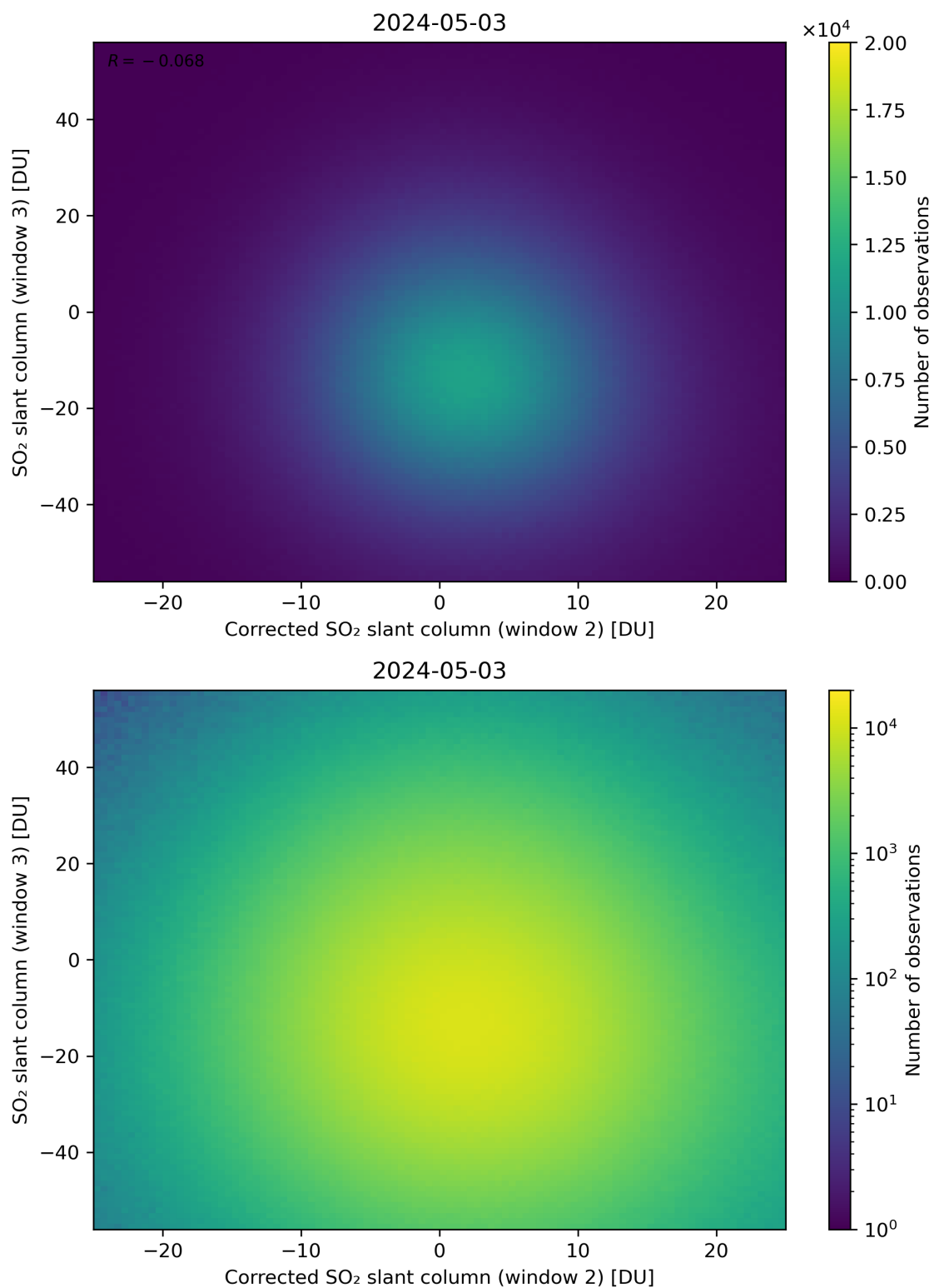
Figure 201: Scatter density plot of “Corrected SO 2 slant column (window 2)” against “SO 2 slant column (window 3)” for 2024-05-02 to 2024-05-04.
