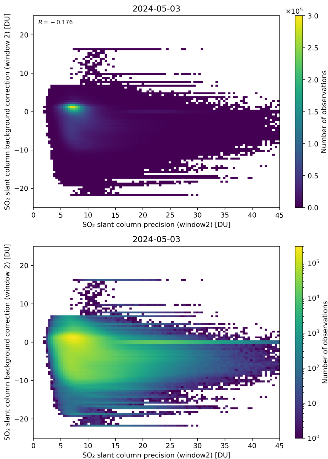
Figure 241: Scatter density plot of “SO 2 slant column precision (window2)” against “SO 2 slant column background correction (window 2)” for 2024-05-02 to 2024-05-04.
