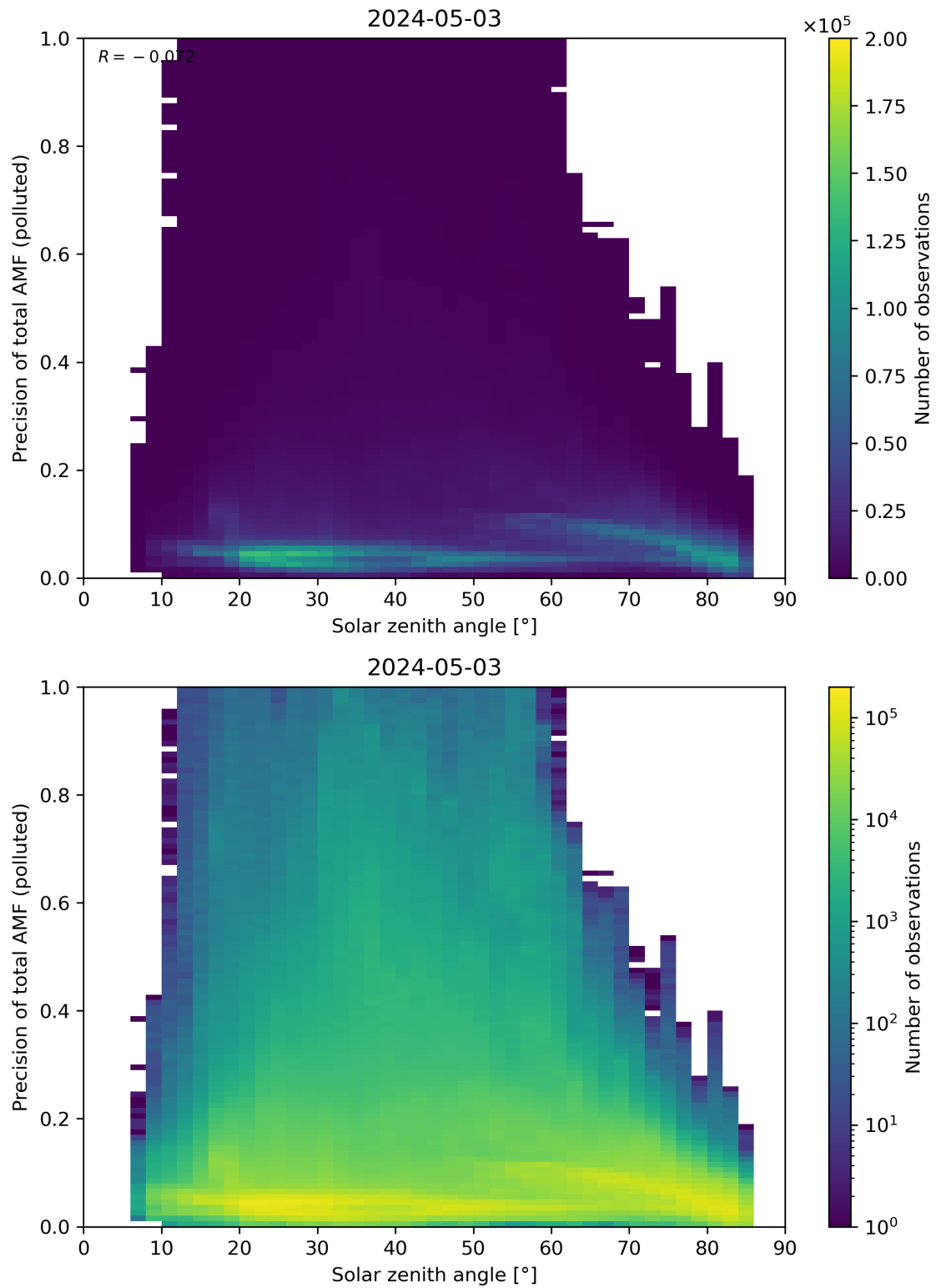
Figure 175: Scatter density plot of “Solar zenith angle” against “Precision of total AMF (polluted)” for 2024-05-02 to 2024-05-04.
