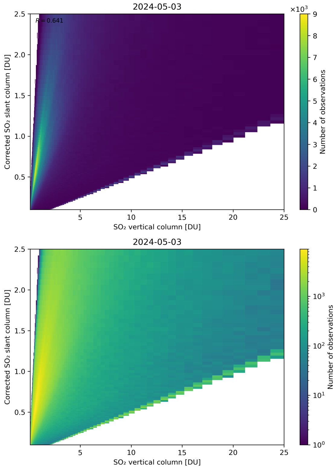
Figure 297: Scatter density plot of “SO 2 vertical column” against “Corrected SO 2 slant column” for 2024-05-02 to 2024-05-04.
