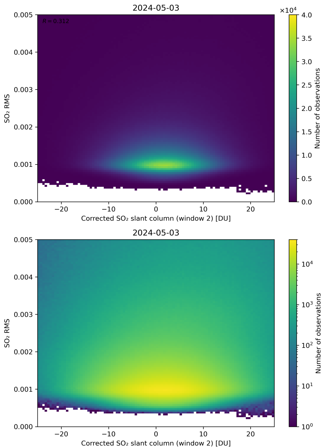
Figure 198: Scatter density plot of “Corrected SO 2 slant column (window 2)” against “SO 2 RMS” for 2024-05-02 to 2024-05-04.
