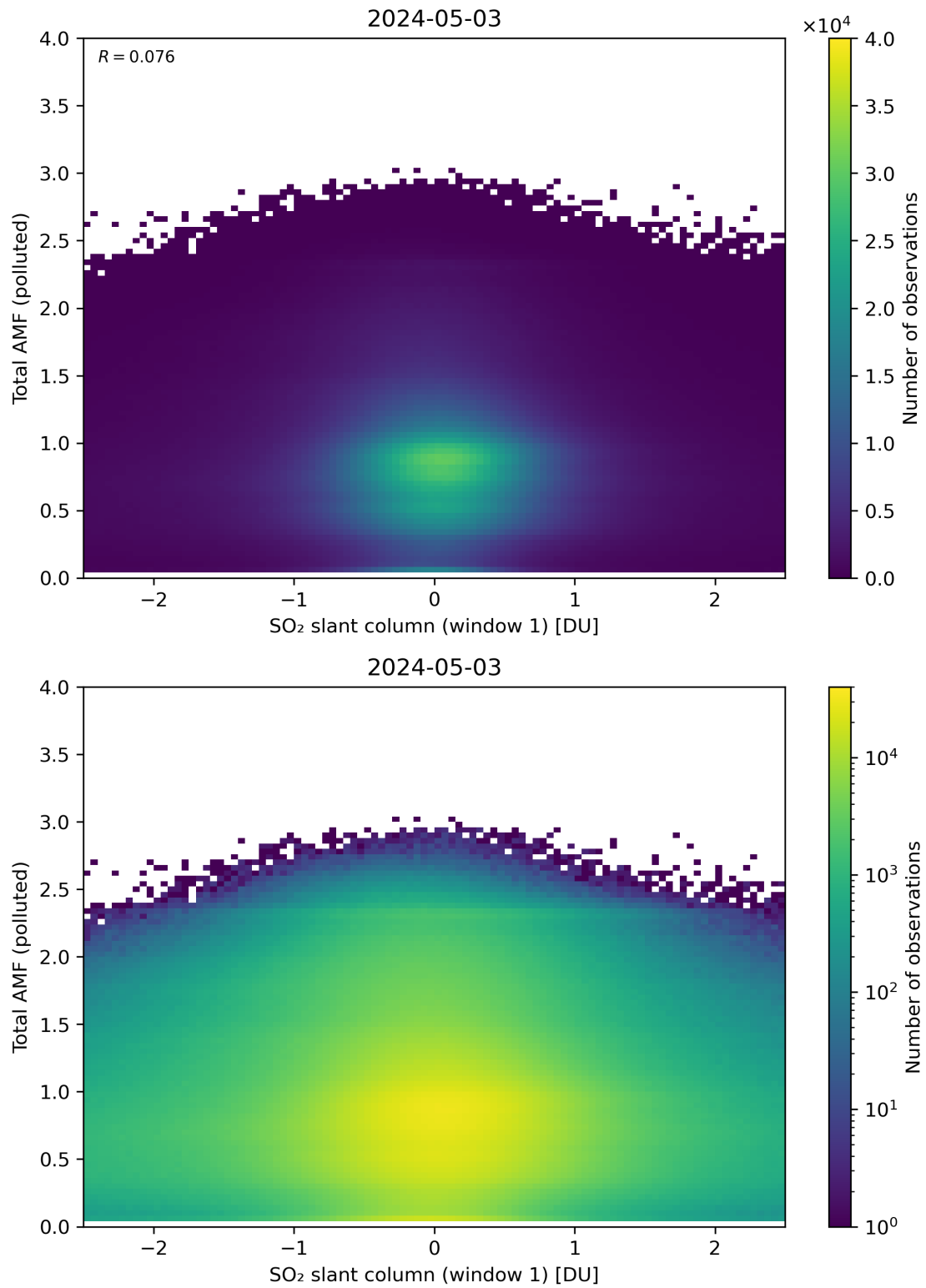
Figure 239: Scatter density plot of “SO 2 slant column (window 1)” against “Total AMF (polluted)” for 2024-05-02 to 2024-05-04.
