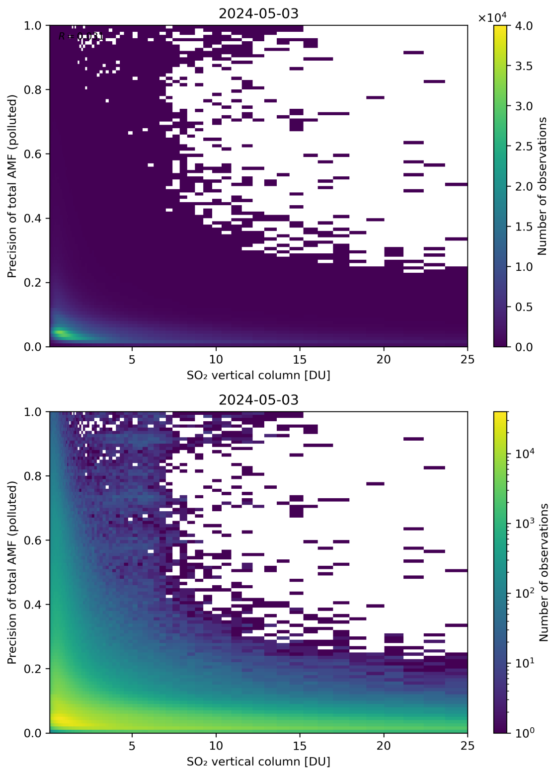
Figure 306: Scatter density plot of “SO 2 vertical column” against “Precision of total AMF (polluted)” for 2024-05-02 to 2024-05-04.
