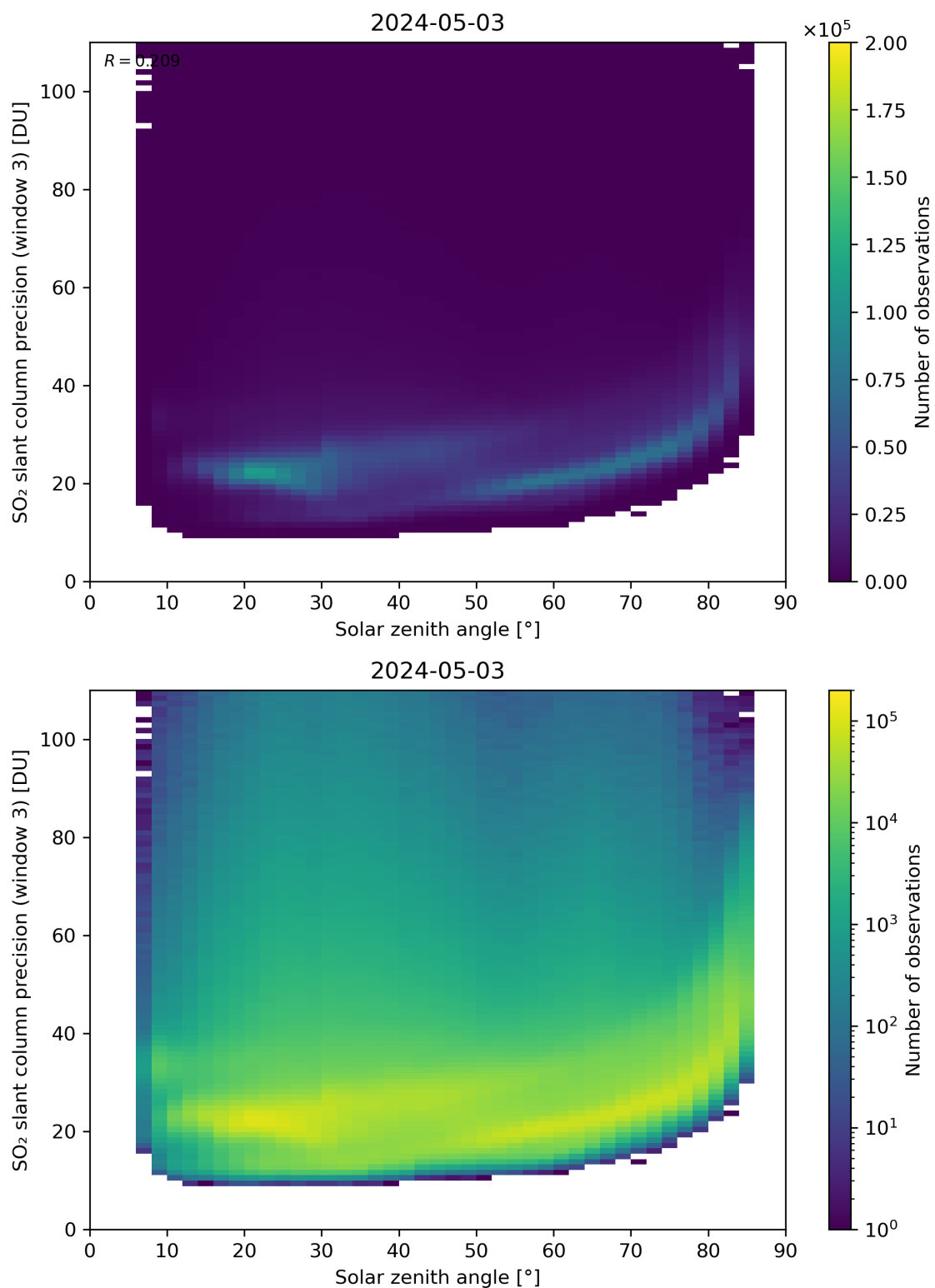
Figure 173: Scatter density plot of “Solar zenith angle” against “SO 2 slant column precision (window 3)” for 2024-05-02 to 2024-05-04.
