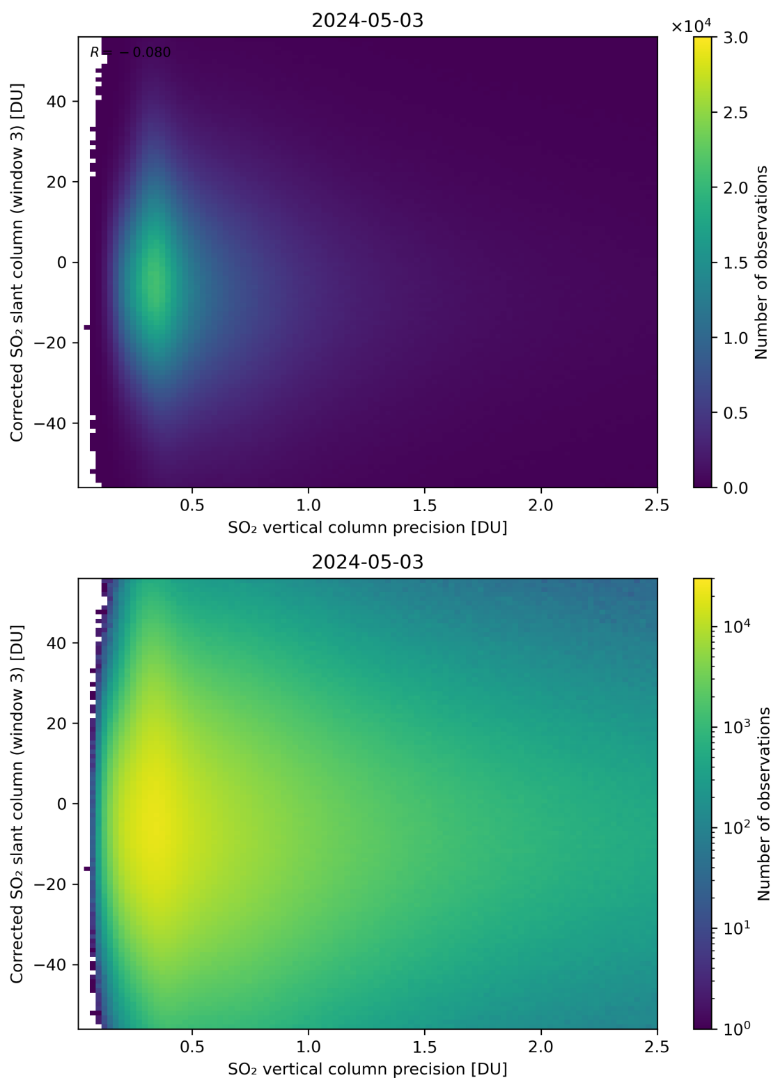
Figure 288: Scatter density plot of “SO 2 vertical column precision” against “Corrected SO 2 slant column (window 3)” for 2024-05-02 to 2024-05-04.
