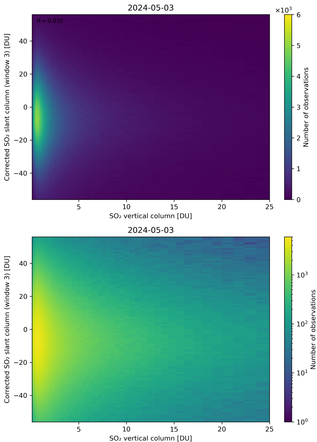
Figure 299: Scatter density plot of “SO 2 vertical column” against “Corrected SO 2 slant column (window 3)” for 2024-05-02 to 2024-05-04.
