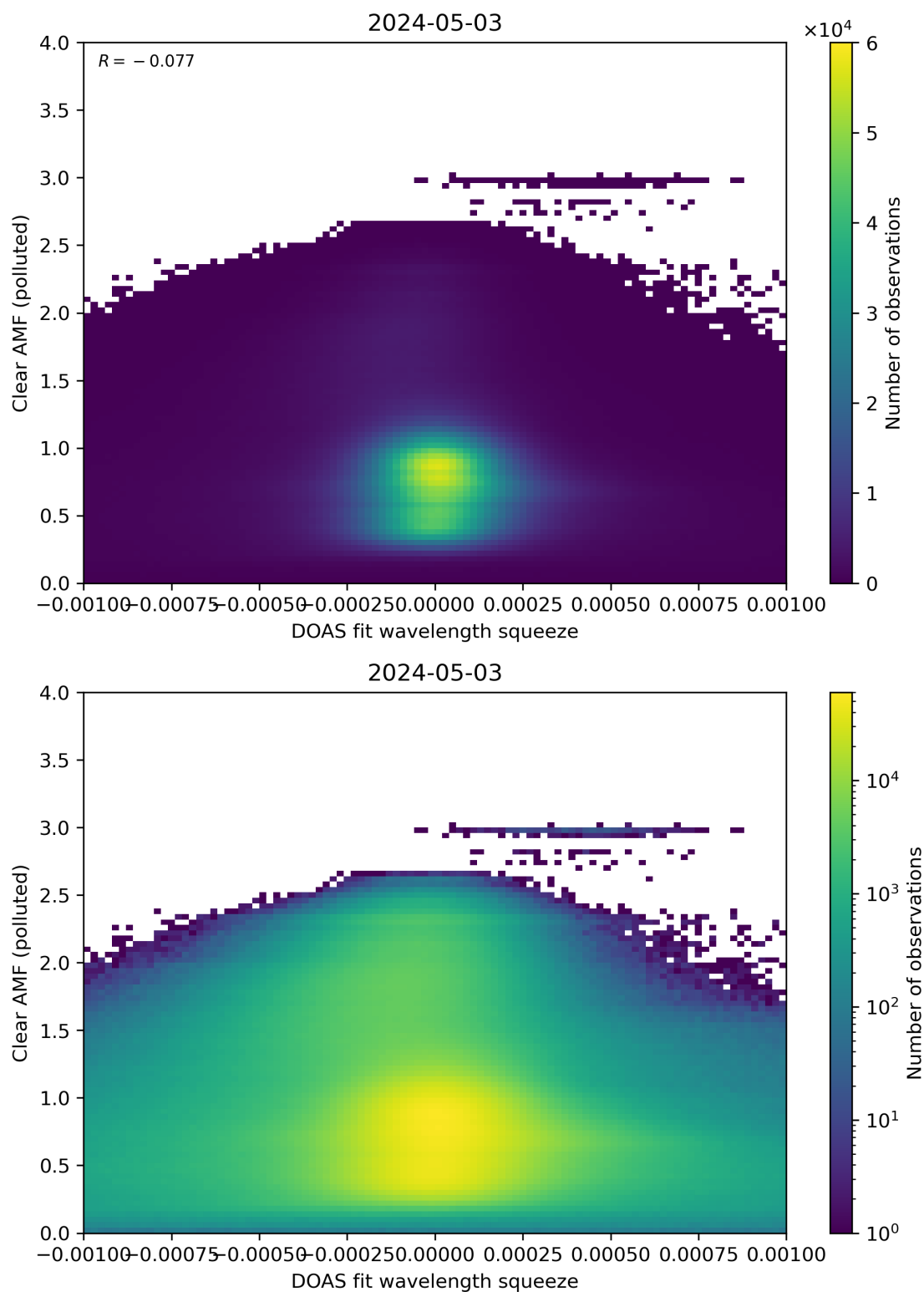
Figure 133: Scatter density plot of “DOAS fit wavelength squeeze” against “Clear AMF (polluted)” for 2024-05-02 to 2024-05-04.
