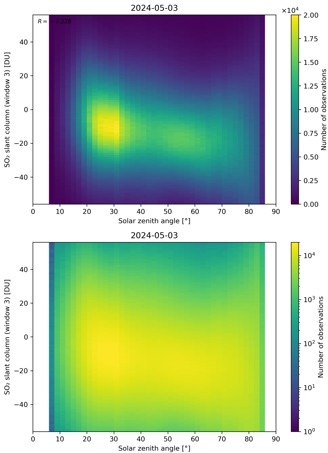
Figure 172: Scatter density plot of “Solar zenith angle” against “SO 2 slant column (window 3)” for 2024-05-02 to 2024-05-04.
