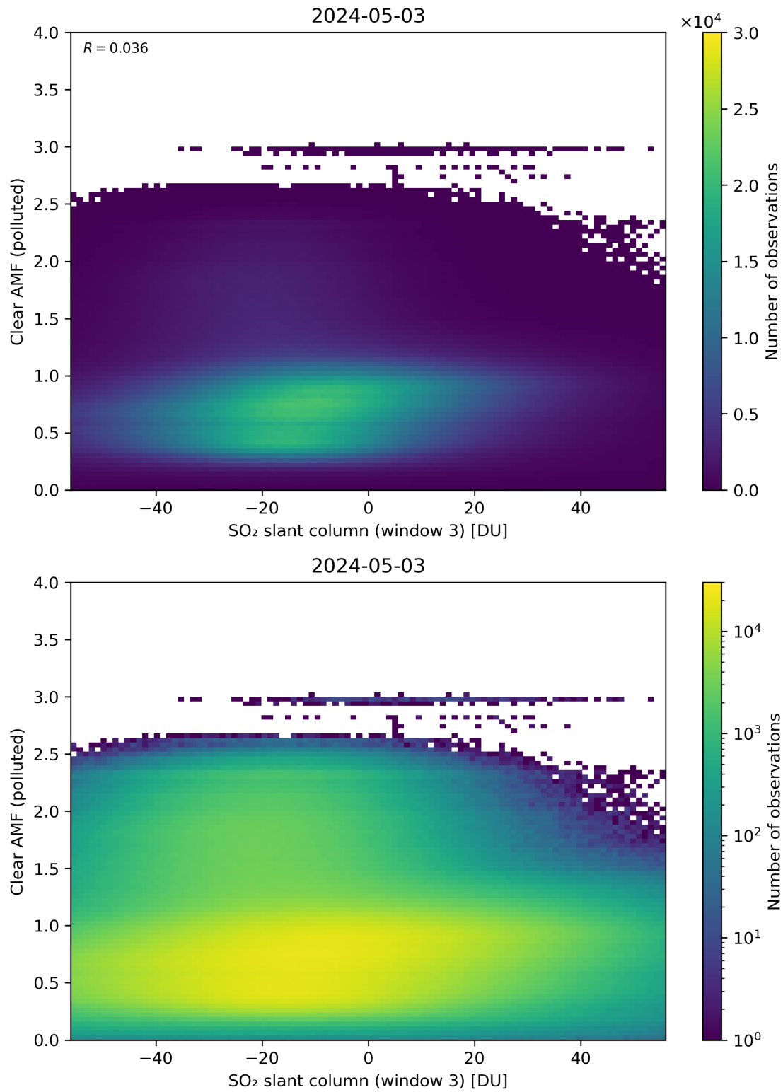
Figure 265: Scatter density plot of “SO 2 slant column (window 3)” against “Clear AMF (polluted)” for 2024-05-02 to 2024-05-04.
