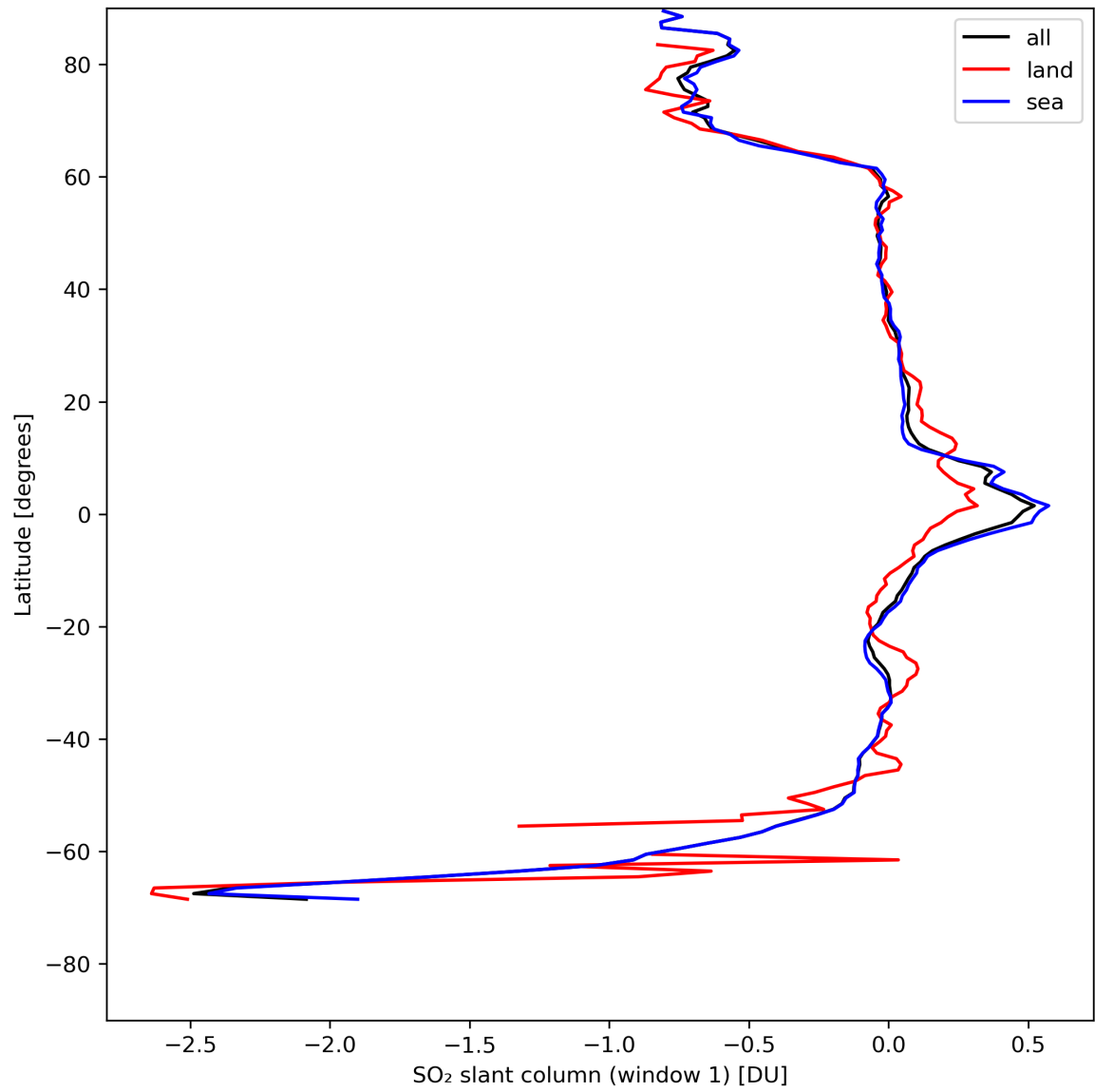
Figure 33: Zonal average of “SO 2 slant column (window 1)” for 2024-05-02 to 2024-05-04.
