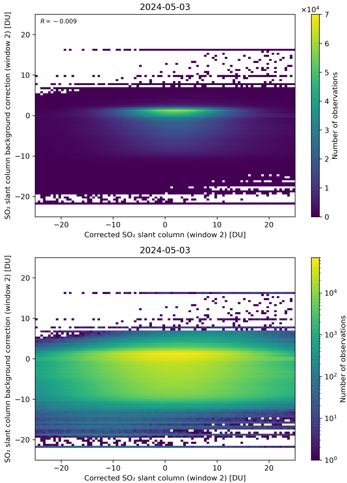
Figure 194: Scatter density plot of “Corrected SO 2 slant column (window 2)” against “SO 2 slant column background correction (window 2)” for 2024-05-02 to 2024-05-04.
