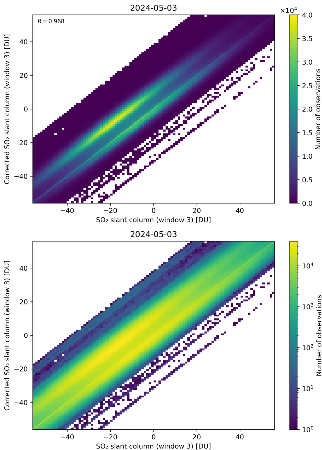
Figure 266: Scatter density plot of “SO 2 slant column (window 3)” against “Corrected SO 2 slant column (window 3)” for 2024-05-02 to 2024-05-04.
