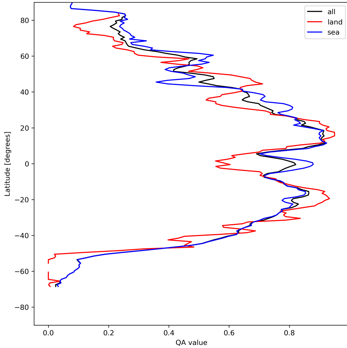
Figure 29: Zonal average of “QA value” for 2024-05-02 to 2024-05-04.
