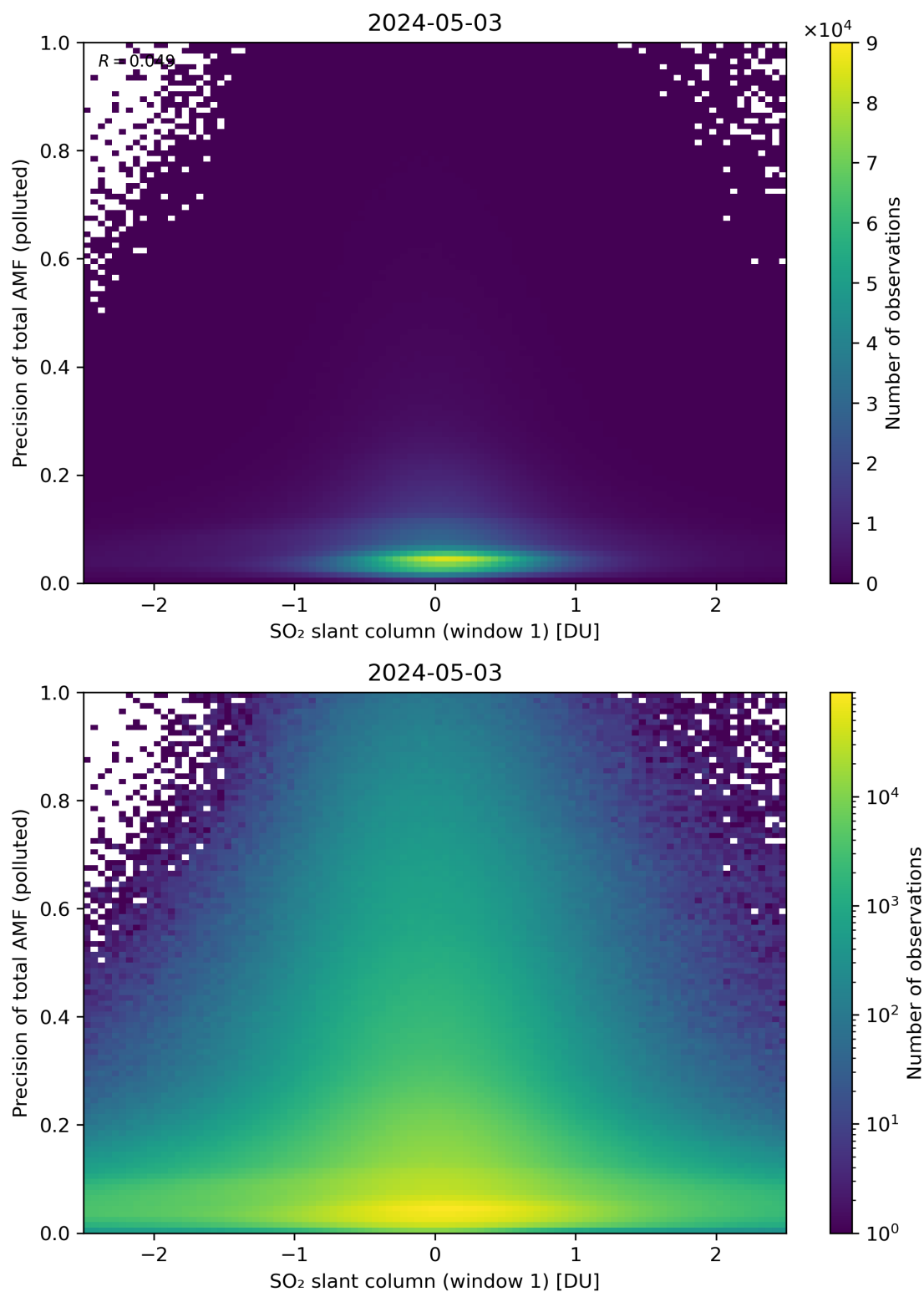
Figure 240: Scatter density plot of “SO 2 slant column (window 1)” against “Precision of total AMF (polluted)” for 2024-05-02 to 2024-05-04.
