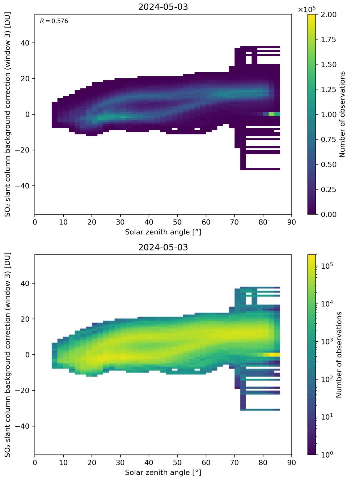
Figure 160: Scatter density plot of “Solar zenith angle” against “SO 2 slant column background correction (window 3)” for 2024-05-02 to 2024-05-04.
