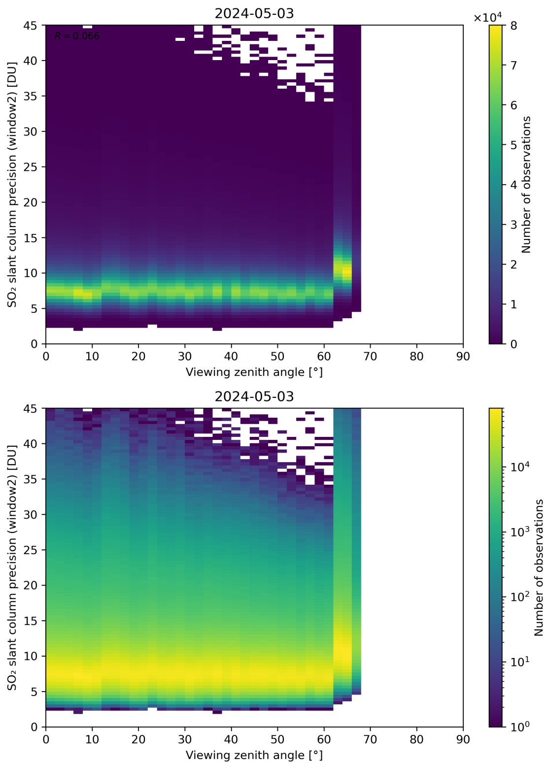
Figure 322: Scatter density plot of “Viewing zenith angle” against “SO 2 slant column precision (window2)” for 2024-05-02 to 2024-05-04.
