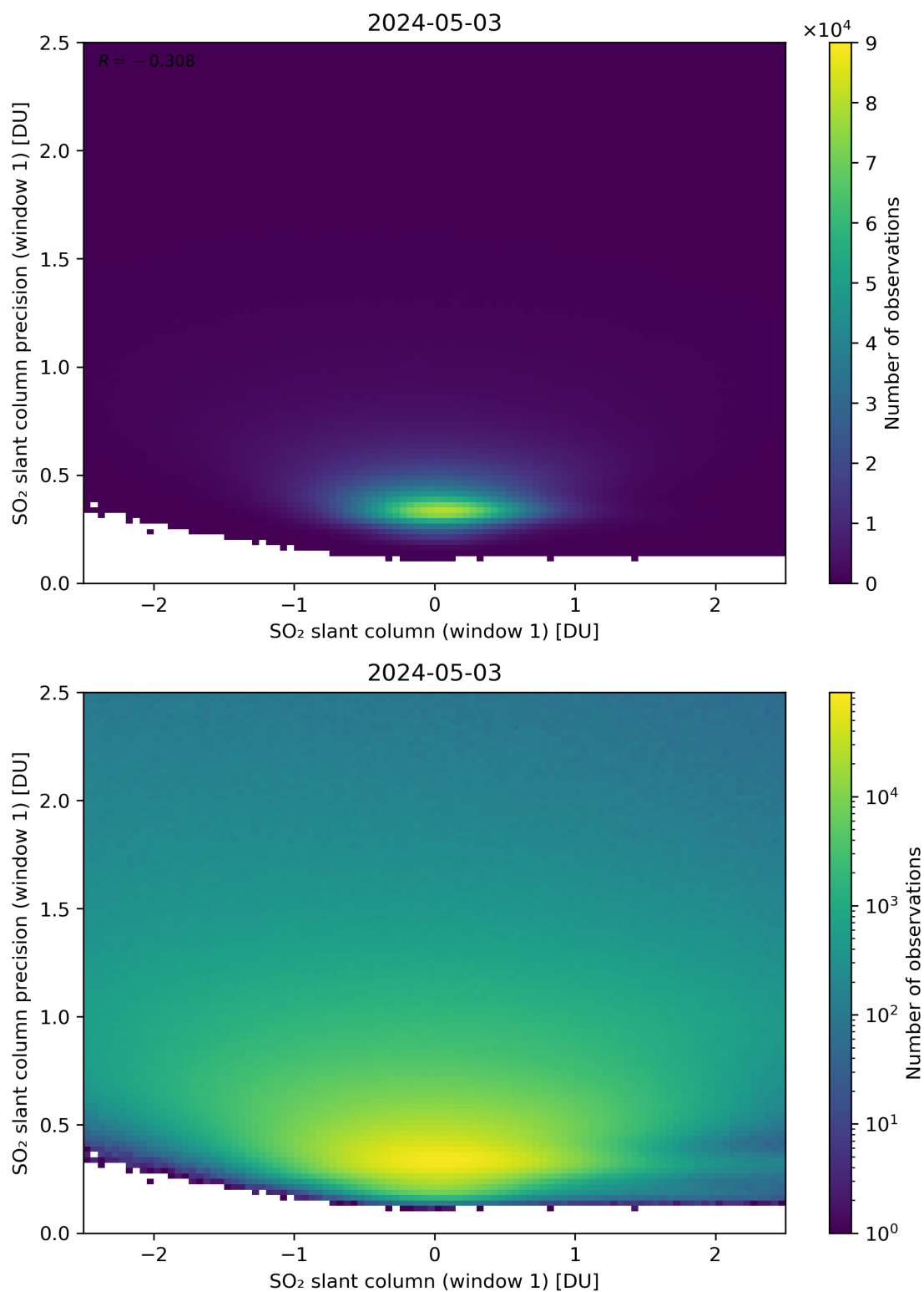
Figure 235: Scatter density plot of “SO 2 slant column (window 1)” against “SO 2 slant column precision (window 1)” for 2024-05-02 to 2024-05-04.
