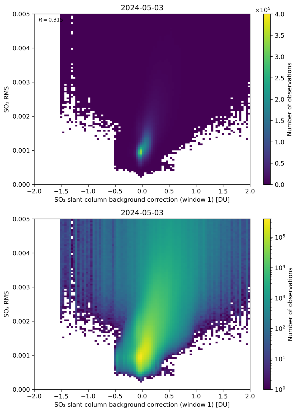
Figure 102: Scatter density plot of “SO 2 slant column background correction (window 1)” against “SO 2 RMS” for 2024-05-02 to 2024-05-04.
