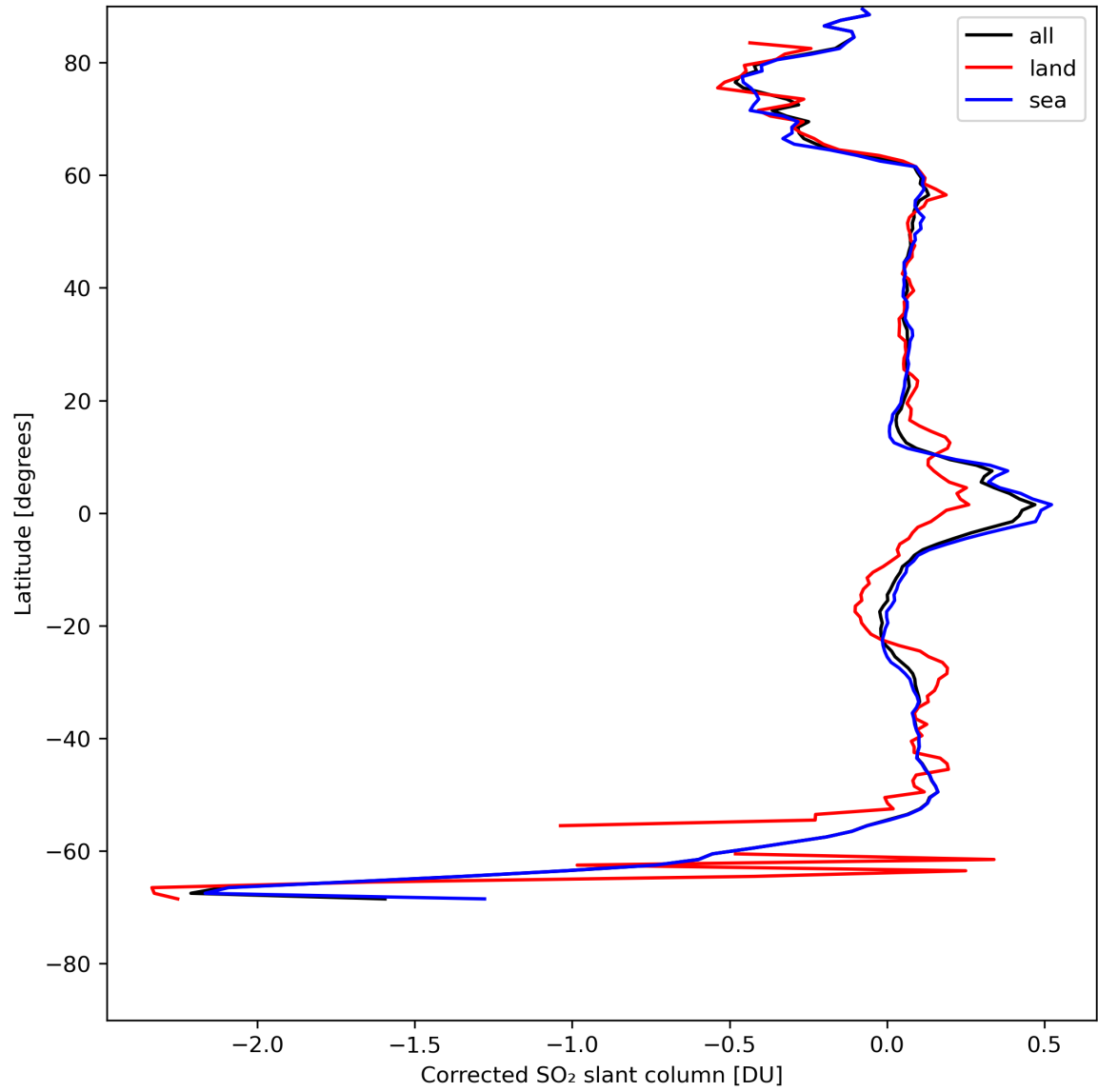
Figure 32: Zonal average of “Corrected SO 2 slant column” for 2024-05-02 to 2024-05-04.
