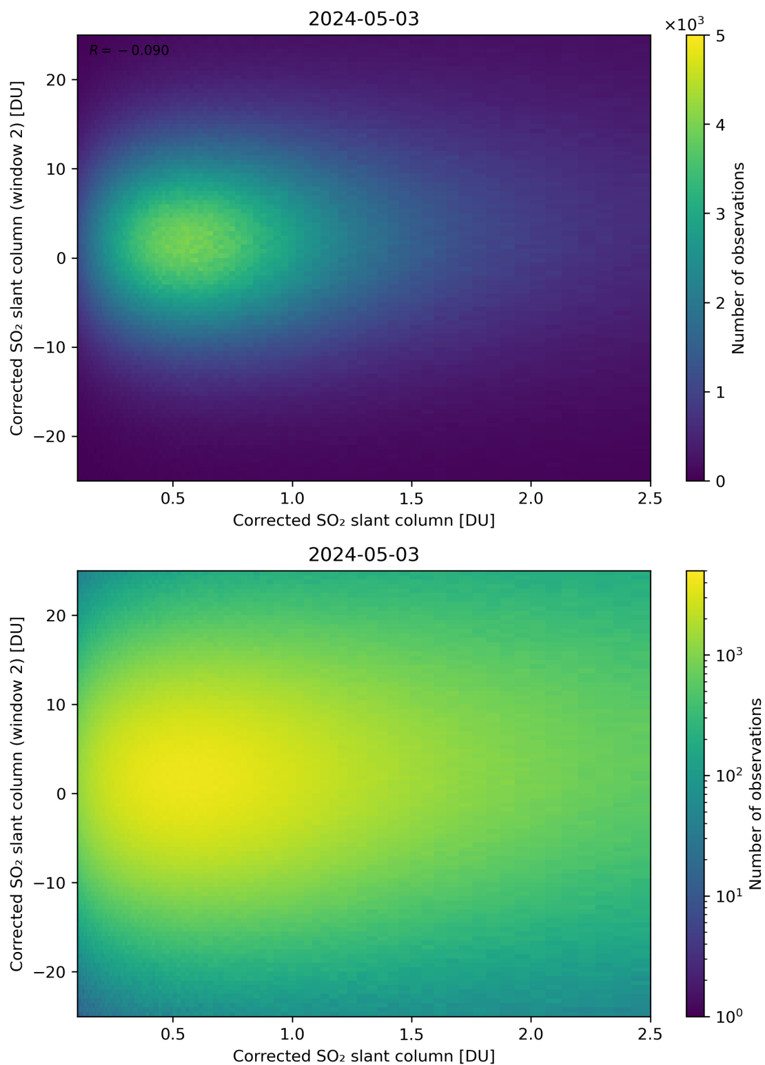
Figure 185: Scatter density plot of “Corrected SO 2 slant column” against “Corrected SO 2 slant column (window 2)” for 2024-05-02 to 2024-05-04.
