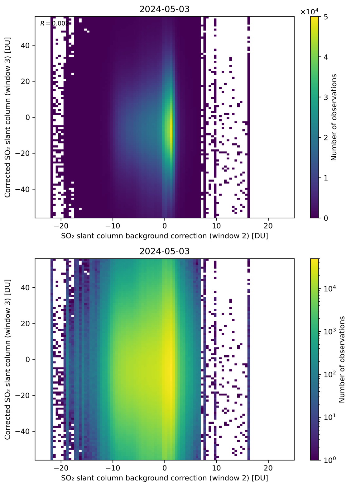
Figure 116: Scatter density plot of “SO 2 slant column background correction (window 2)” against “Corrected SO 2 slant column (window 3)” for 2024-05-02 to 2024-05-04.
