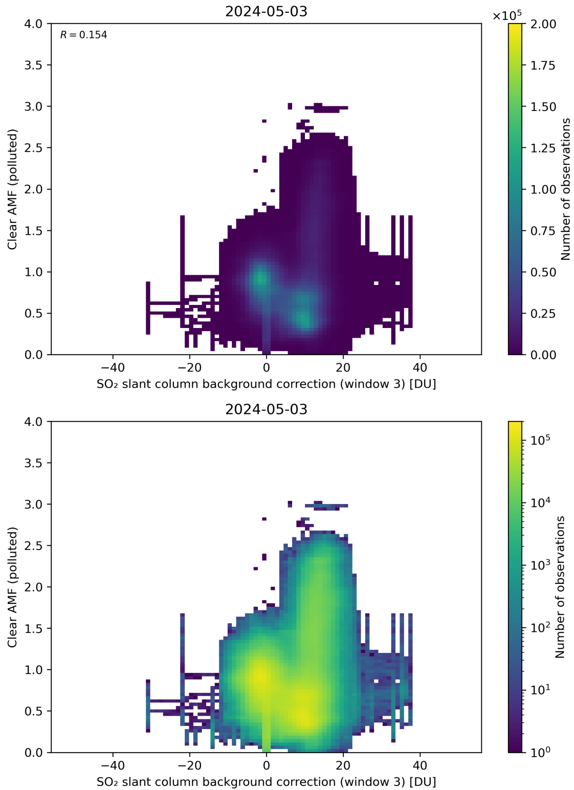
Figure 124: Scatter density plot of “SO 2 slant column background correction (window 3)” against “Clear AMF (polluted)” for 2024-05-02 to 2024-05-04.
