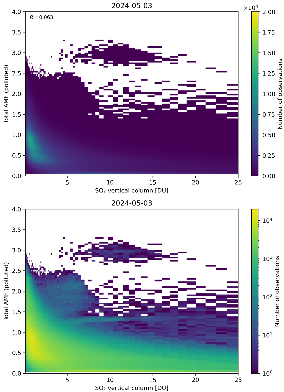
Figure 305: Scatter density plot of “SO 2 vertical column” against “Total AMF (polluted)” for 2024-05-02 to 2024-05-04.
