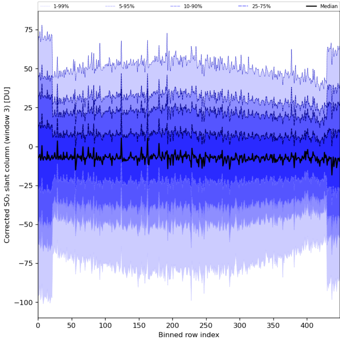
Figure 89: Along track statistics of “Corrected SO 2 slant column (window 3)” for 2024-05-02 to 2024-05-04
