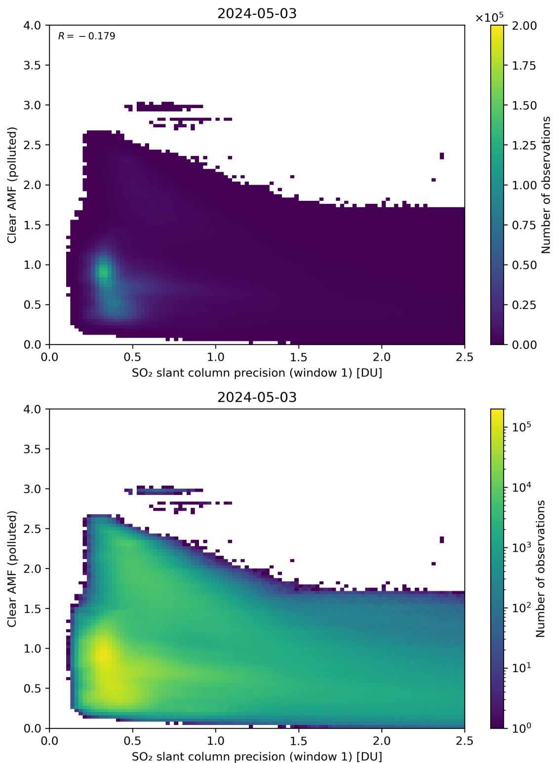
Figure 224: Scatter density plot of “SO 2 slant column precision (window 1)” against “Clear AMF (polluted)” for 2024-05-02 to 2024-05-04.
