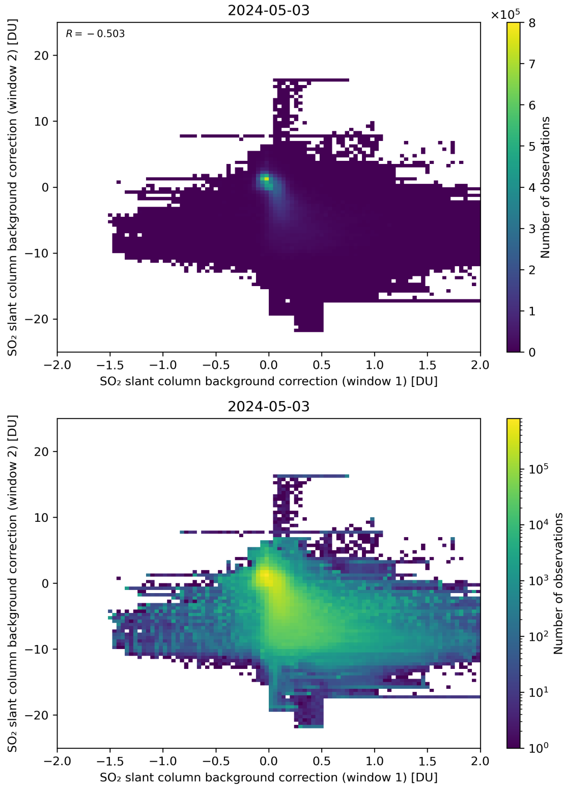
Figure 98: Scatter density plot of “SO 2 slant column background correction (window 1)” against “SO 2 slant column background correction (window 2)” for 2024-05-02 to 2024-05-04.
