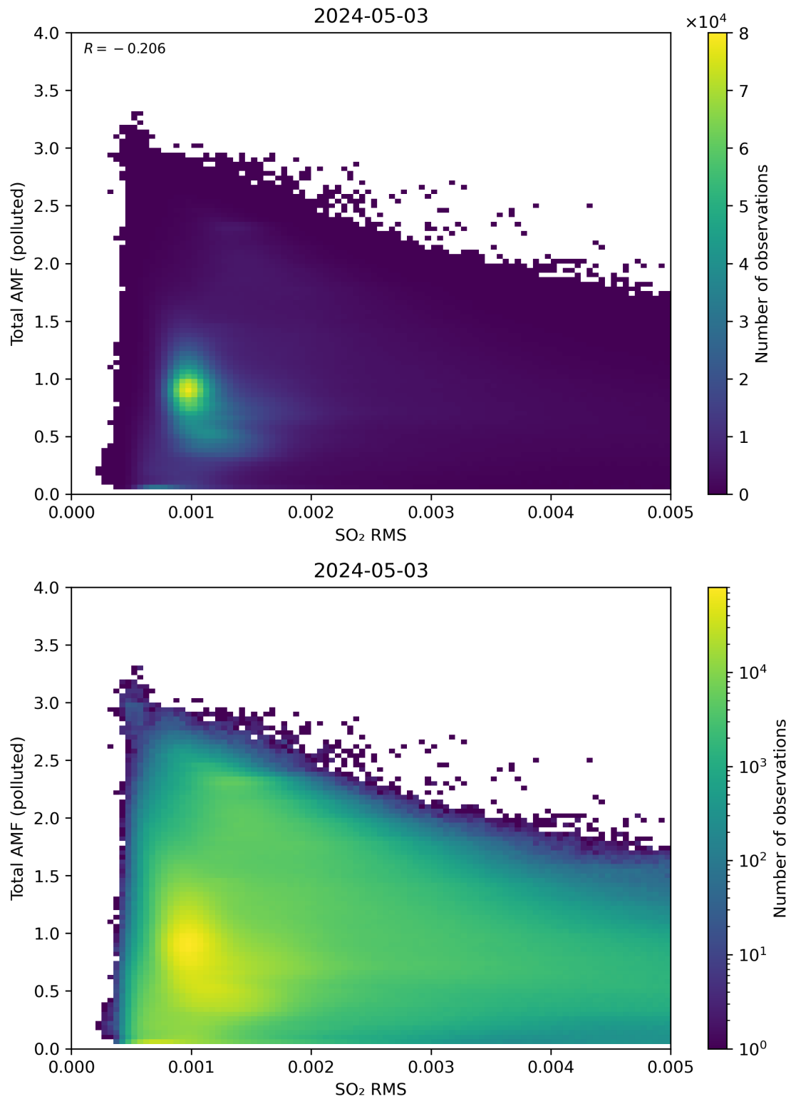
Figure 137: Scatter density plot of “SO 2 RMS” against “Total AMF (polluted)” for 2024-05-02 to 2024-05-04.
