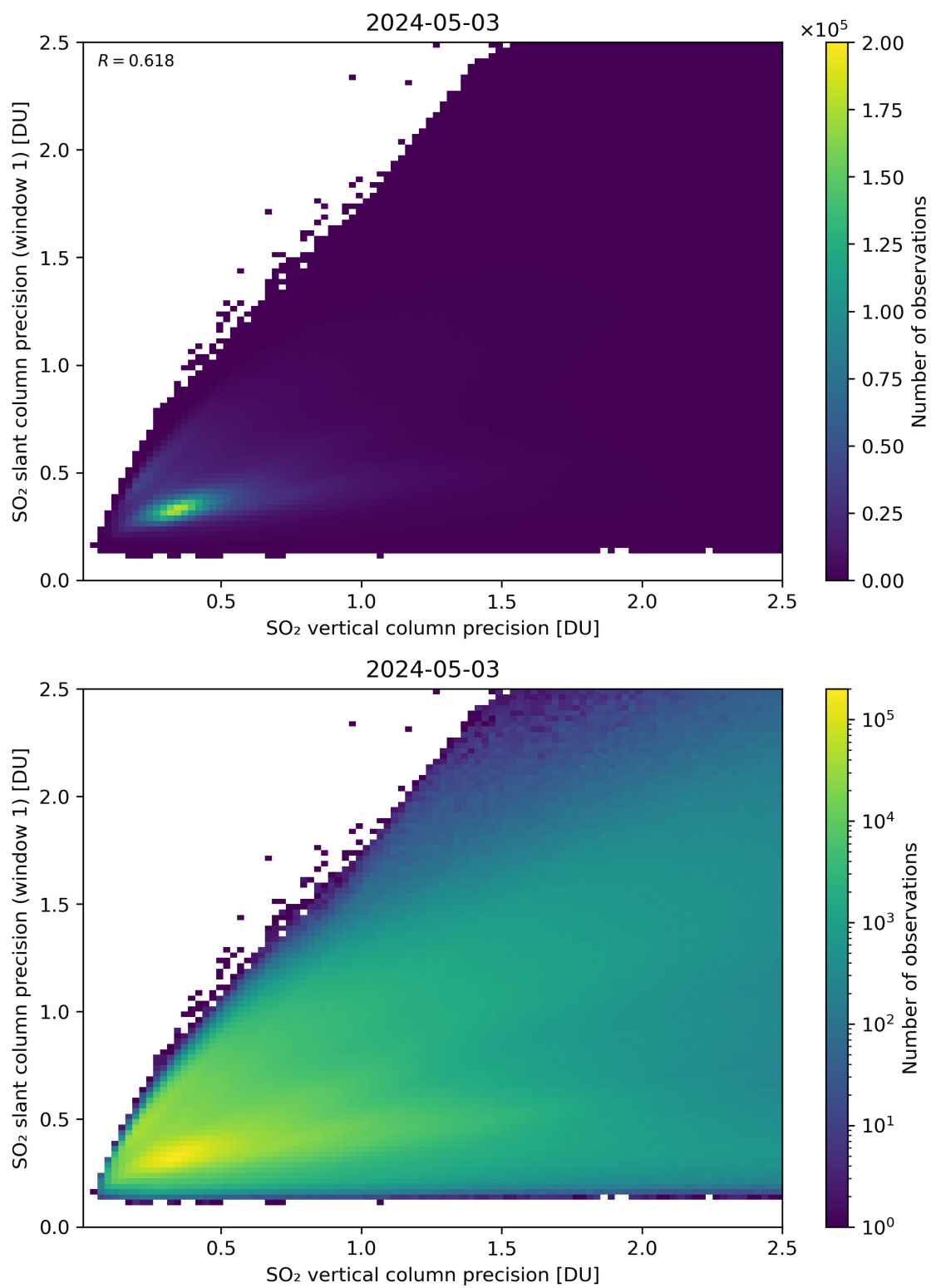
Figure 290: Scatter density plot of “SO 2 vertical column precision” against “SO 2 slant column precision (window 1)” for 2024-05-02 to 2024-05-04.
