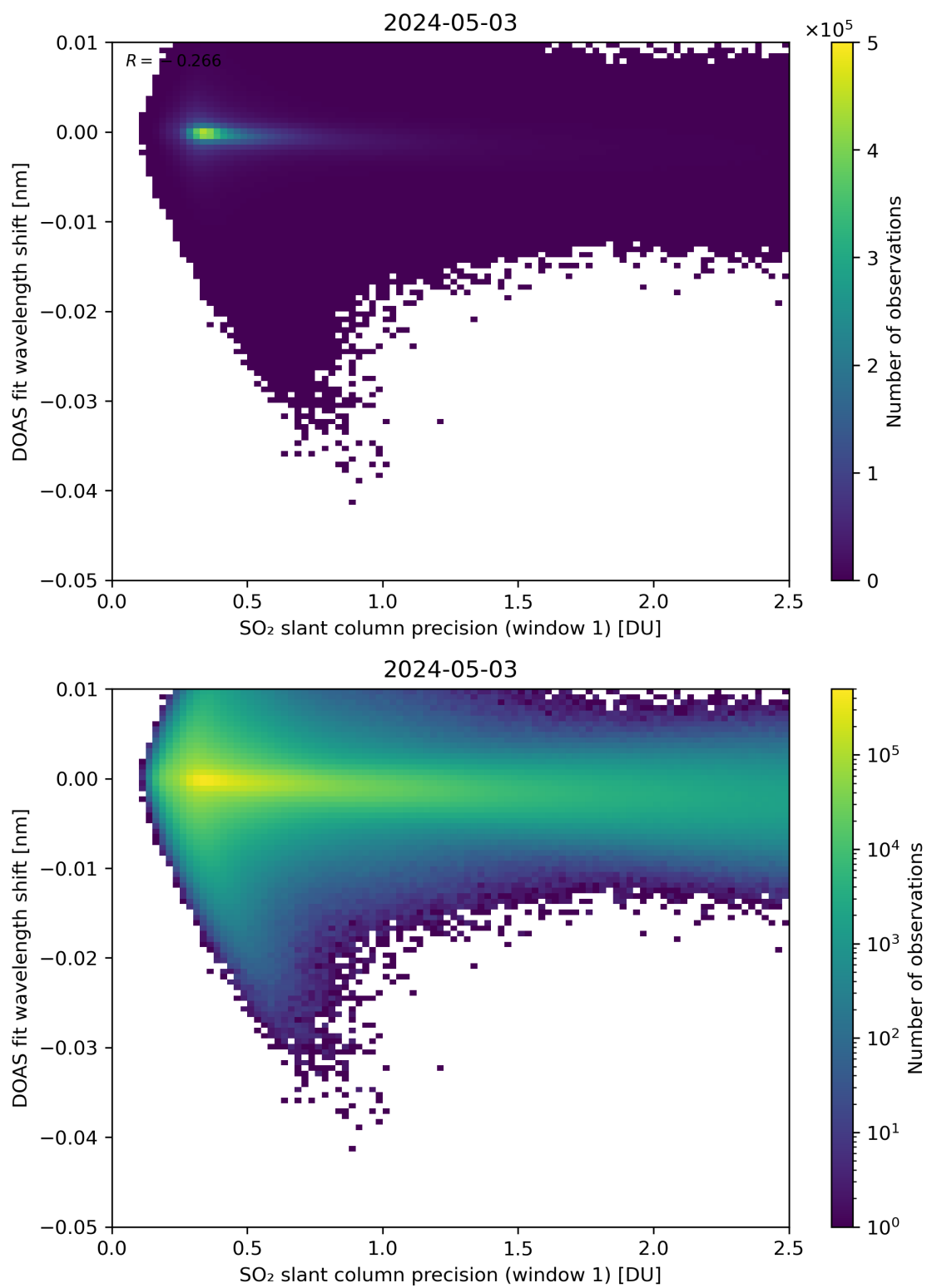
Figure 221: Scatter density plot of “SO 2 slant column precision (window 1)” against “DOAS fit wavelength shift” for 2024-05-02 to 2024-05-04.
