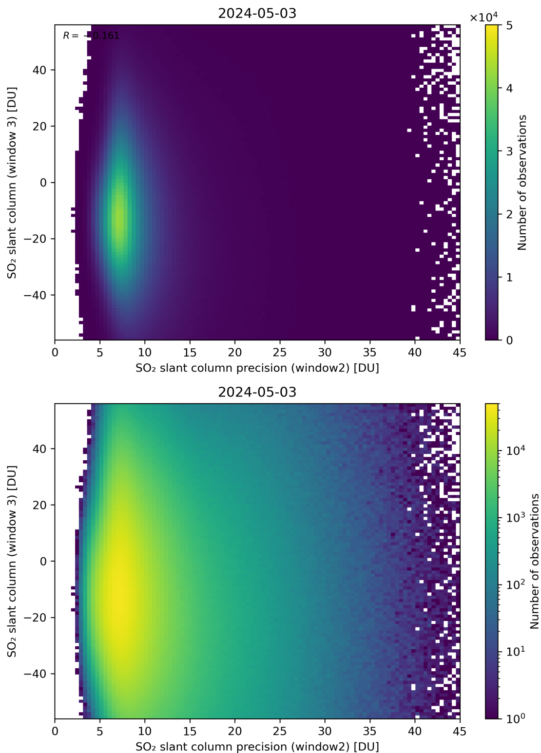
Figure 249: Scatter density plot of “SO 2 slant column precision (window2)” against “SO 2 slant column (window 3)” for 2024-05-02 to 2024-05-04.
