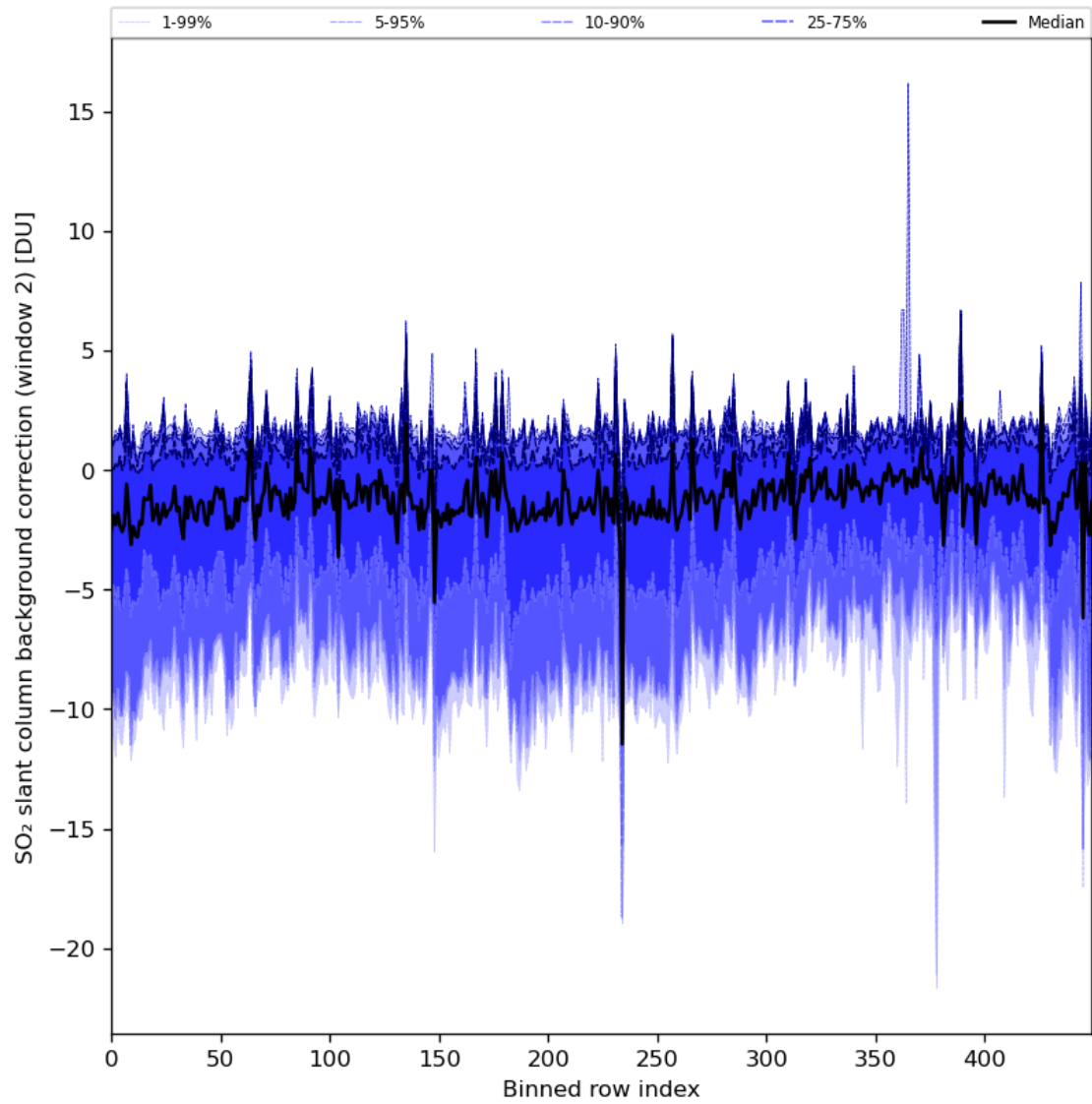
Figure 86: Along track statistics of “SO 2 slant column background correction (window 2)” for 2024-05-02 to 2024-05-04
