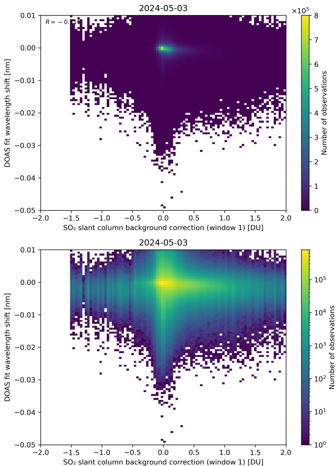
Figure 100: Scatter density plot of “SO 2 slant column background correction (window 1)” against “DOAS fit wavelength shift” for 2024-05-02 to 2024-05-04.
