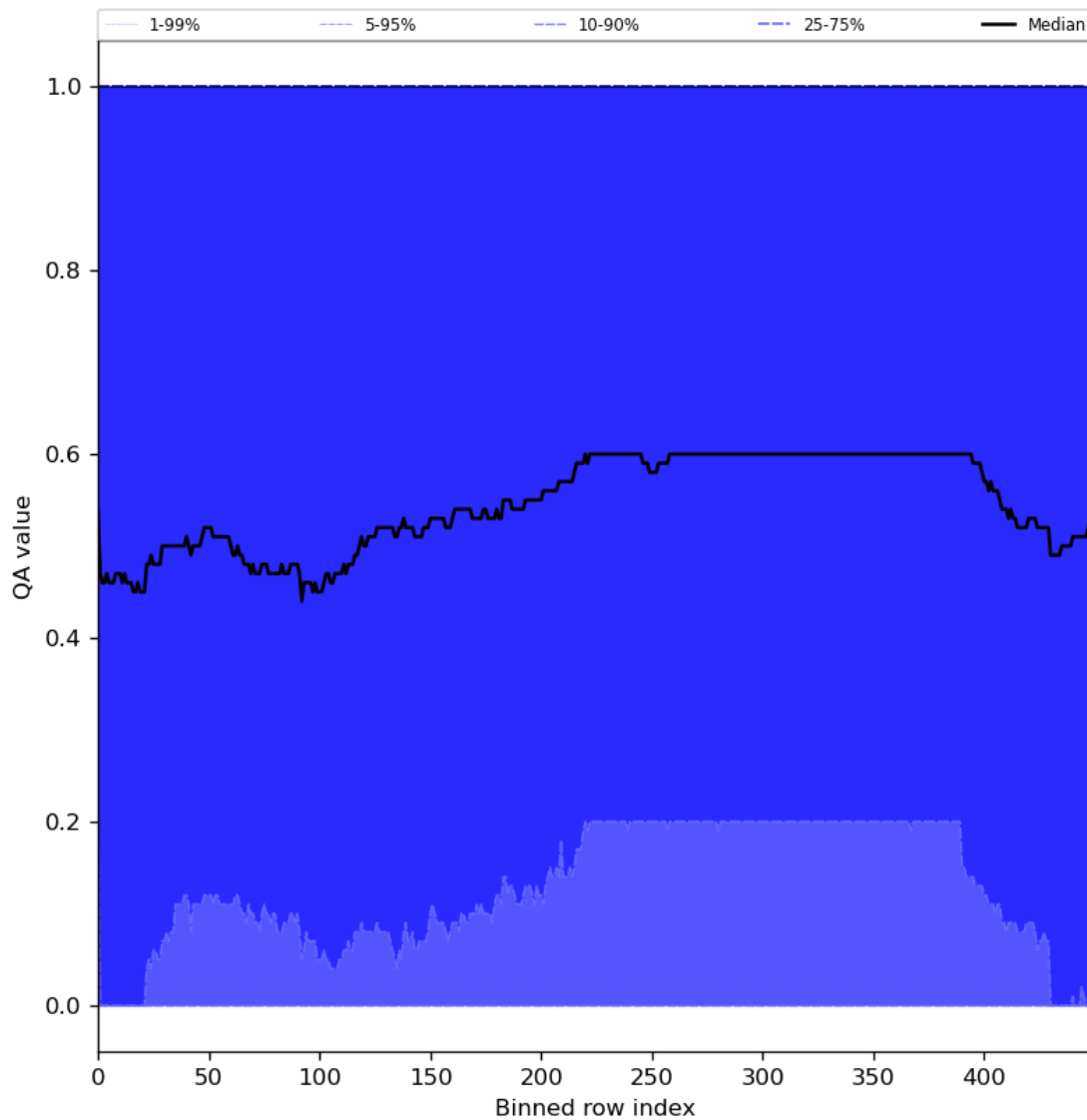
Figure 75: Along track statistics of “QA value” for 2024-05-02 to 2024-05-04
