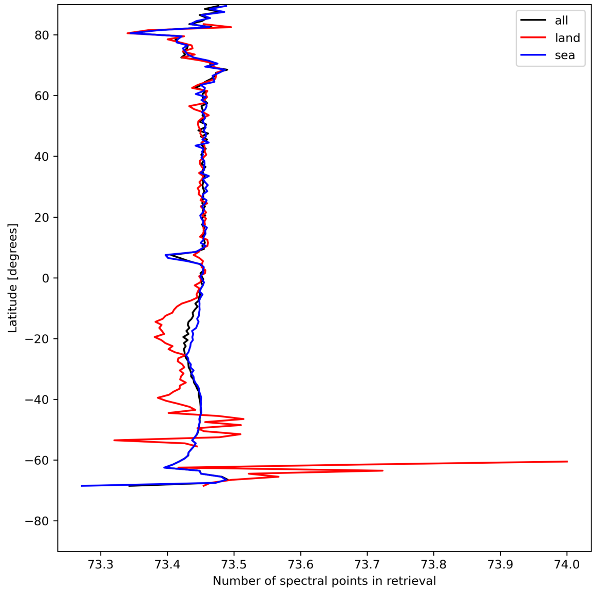
Figure 51: Zonal average of “Number of spectral points in retrieval” for 2024-05-02 to 2024-05-04.
