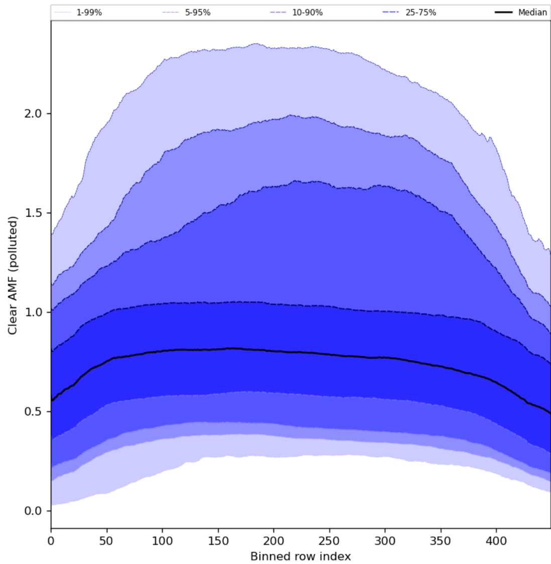
Figure 96: Along track statistics of “Clear AMF (polluted)” for 2024-05-02 to 2024-05-04
