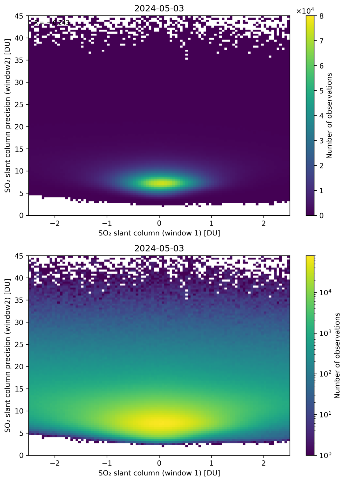
Figure 236: Scatter density plot of “SO 2 slant column (window 1)” against “SO 2 slant column precision (window2)” for 2024-05-02 to 2024-05-04.
