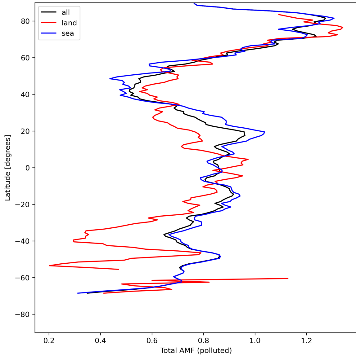
Figure 48: Zonal average of “Total AMF (polluted)” for 2024-05-02 to 2024-05-04.
