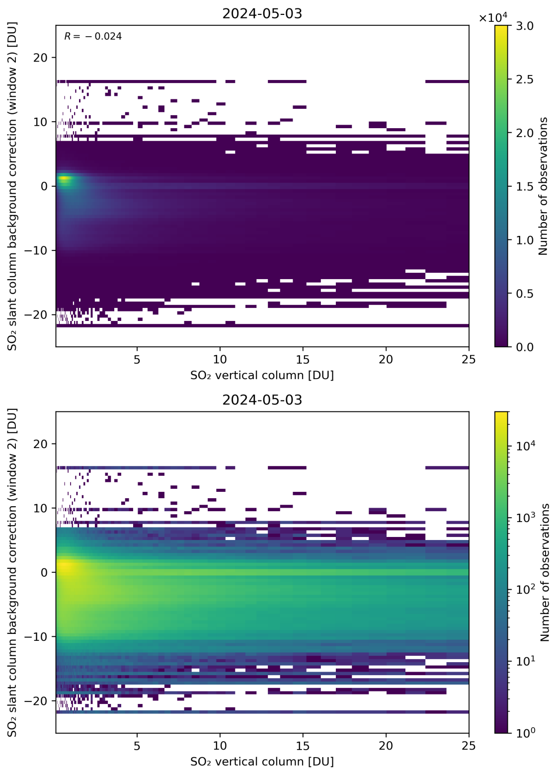
Figure 274: Scatter density plot of “SO 2 vertical column” against “SO 2 slant column background correction (window 2)” for 2024-05-02 to 2024-05-04.
