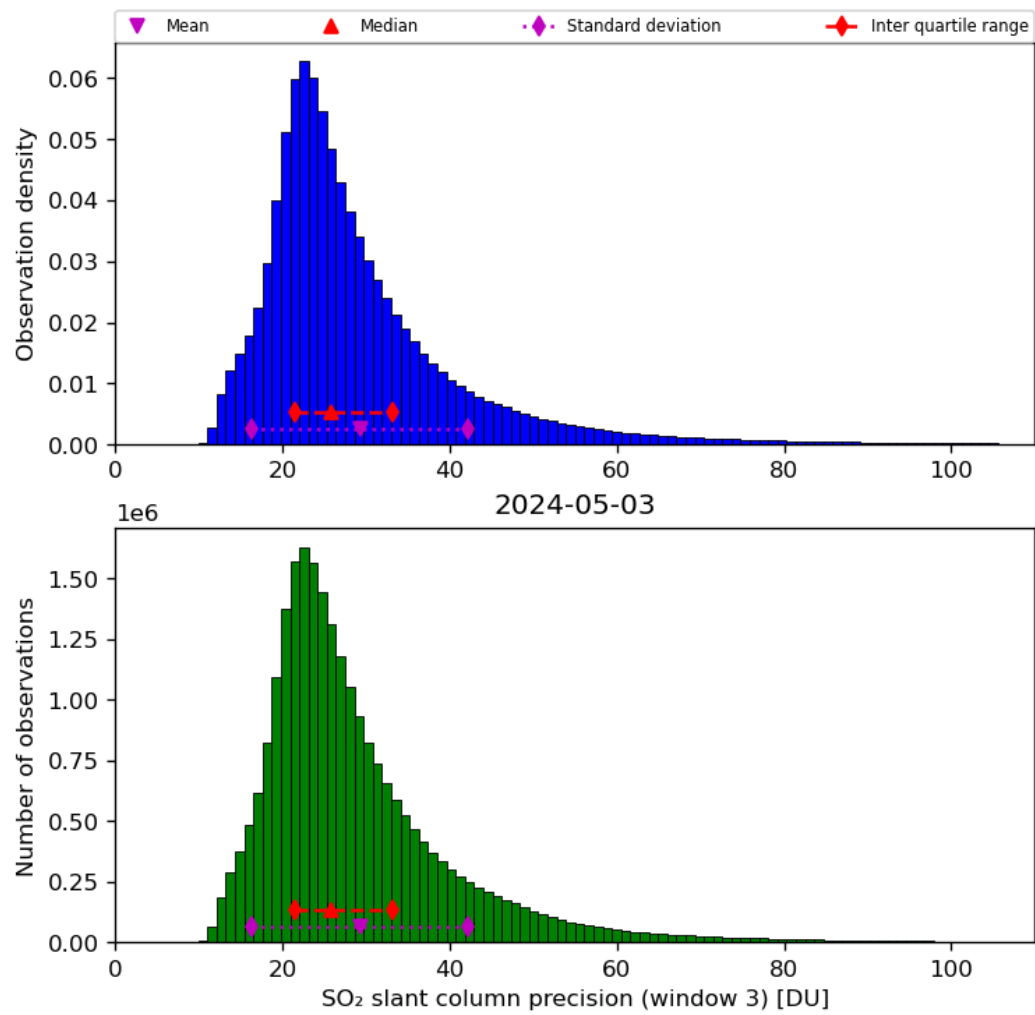
Figure 65: Histogram of “SO 2 slant column precision (window 3)” for 2024-05-02 to 2024-05-04
