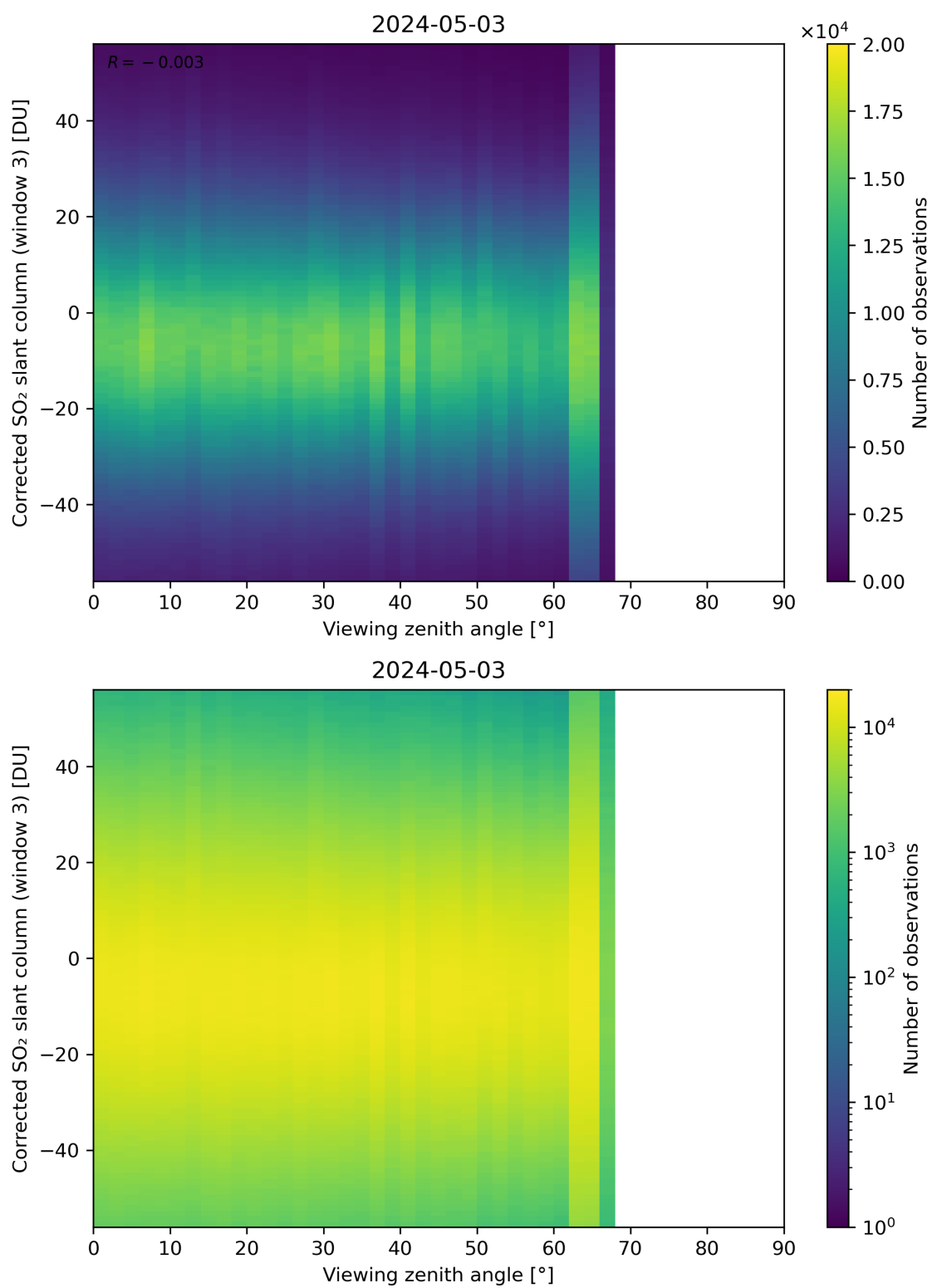
Figure 319: Scatter density plot of “Viewing zenith angle” against “Corrected SO 2 slant column (window 3)” for 2024-05-02 to 2024-05-04.
