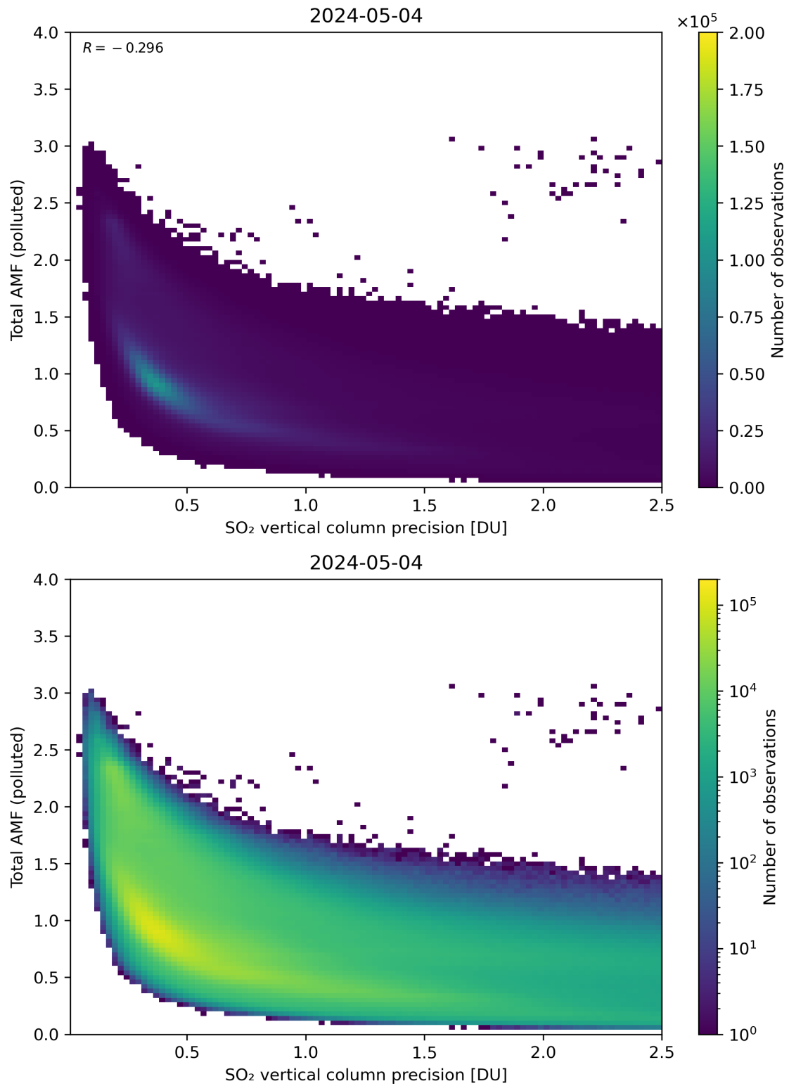
Figure 294: Scatter density plot of “SO 2 vertical column precision” against “Total AMF (polluted)” for 2024-05-03 to 2024-05-05.
