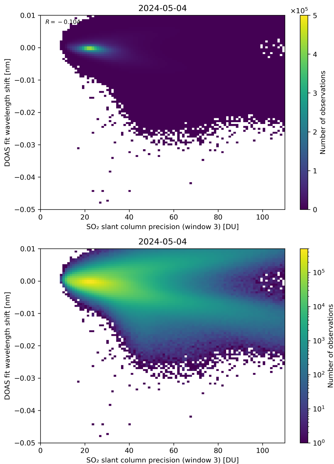
Figure 258: Scatter density plot of “SO 2 slant column precision (window 3)” against “DOAS fit wavelength shift” for 2024-05-03 to 2024-05-05.
