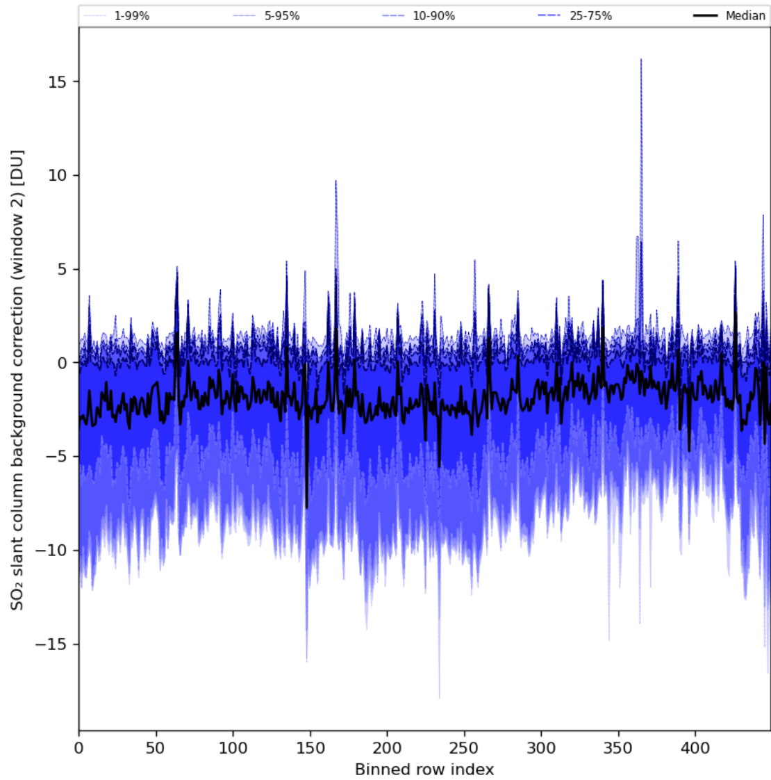
Figure 86: Along track statistics of “SO 2 slant column background correction (window 2)” for 2024-05-03 to 2024-05-05
