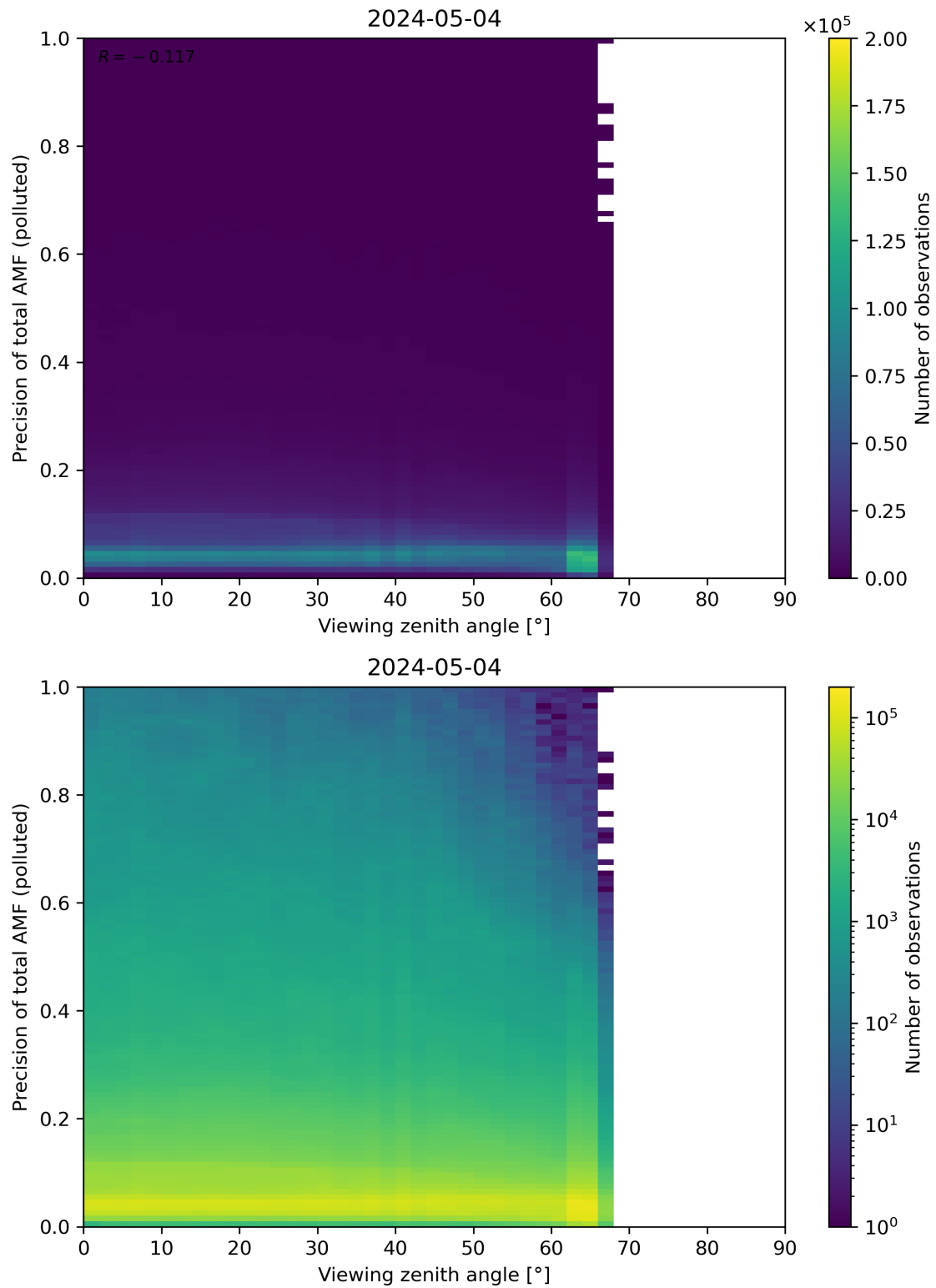
Figure 326: Scatter density plot of “Viewing zenith angle” against “Precision of total AMF (polluted)” for 2024-05-03 to 2024-05-05.
