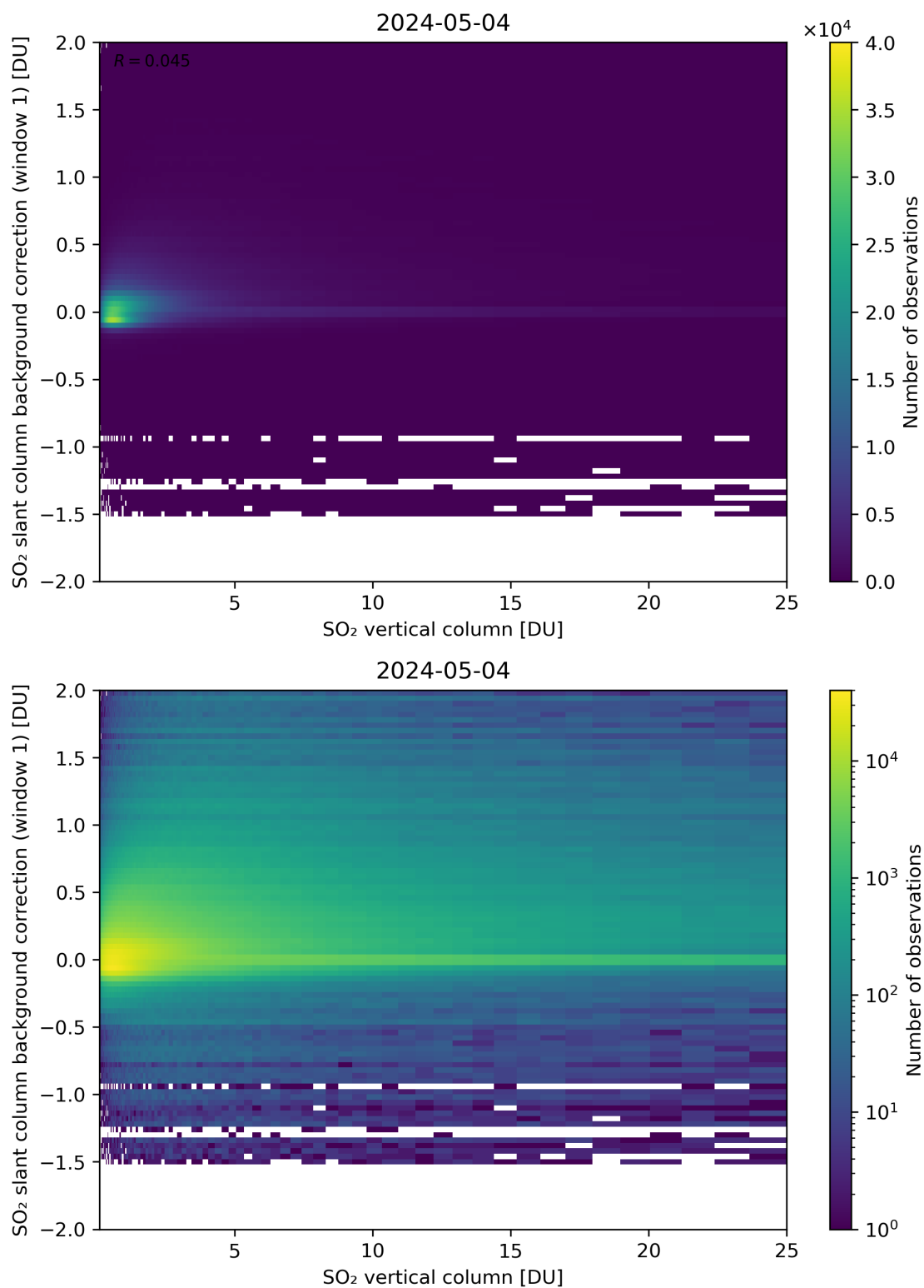
Figure 273: Scatter density plot of “SO 2 vertical column” against “SO 2 slant column background correction (window 1)” for 2024-05-03 to 2024-05-05.
