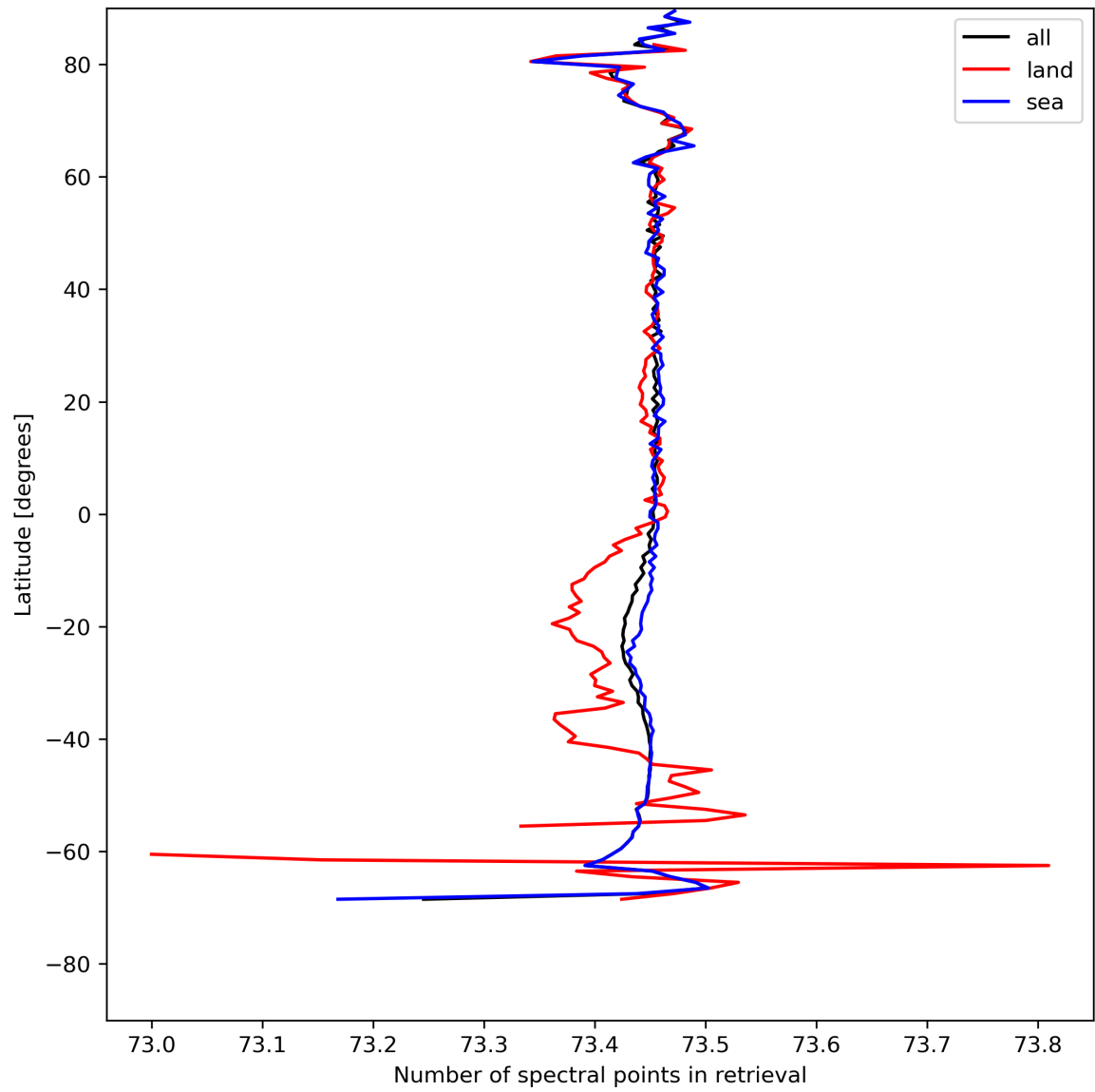
Figure 51: Zonal average of “Number of spectral points in retrieval” for 2024-05-03 to 2024-05-05.
