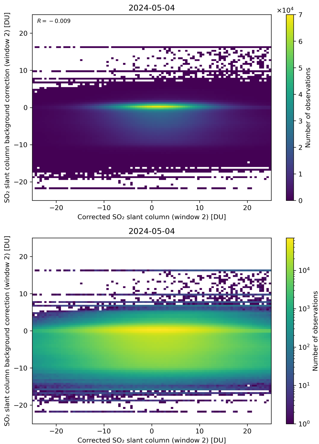
Figure 194: Scatter density plot of “Corrected SO 2 slant column (window 2)” against “SO 2 slant column background correction (window 2)” for 2024-05-03 to 2024-05-05.
