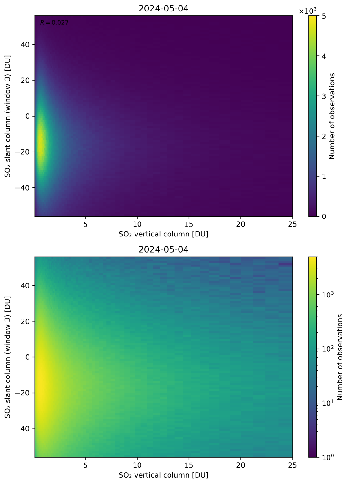
Figure 303: Scatter density plot of “SO 2 vertical column” against “SO 2 slant column (window 3)” for 2024-05-03 to 2024-05-05.
