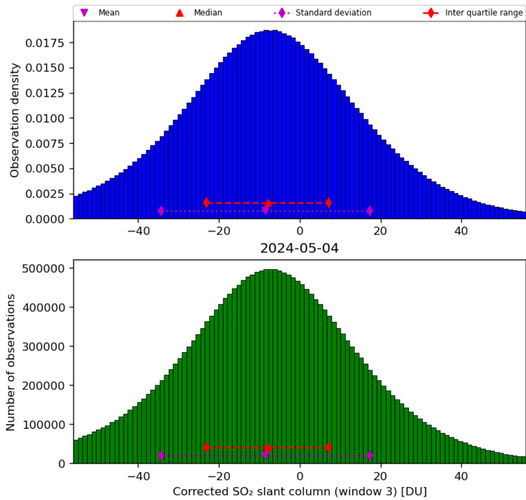
Figure 66: Histogram of “Corrected SO 2 slant column (window 3)” for 2024-05-03 to 2024-05-05
