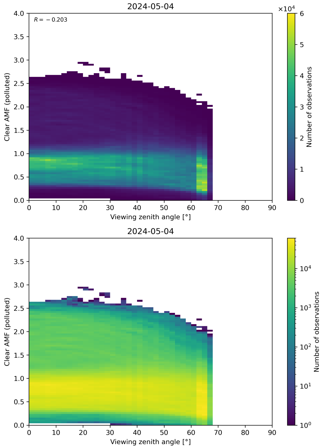
Figure 316: Scatter density plot of “Viewing zenith angle” against “Clear AMF (polluted)” for 2024-05-03 to 2024-05-05.
