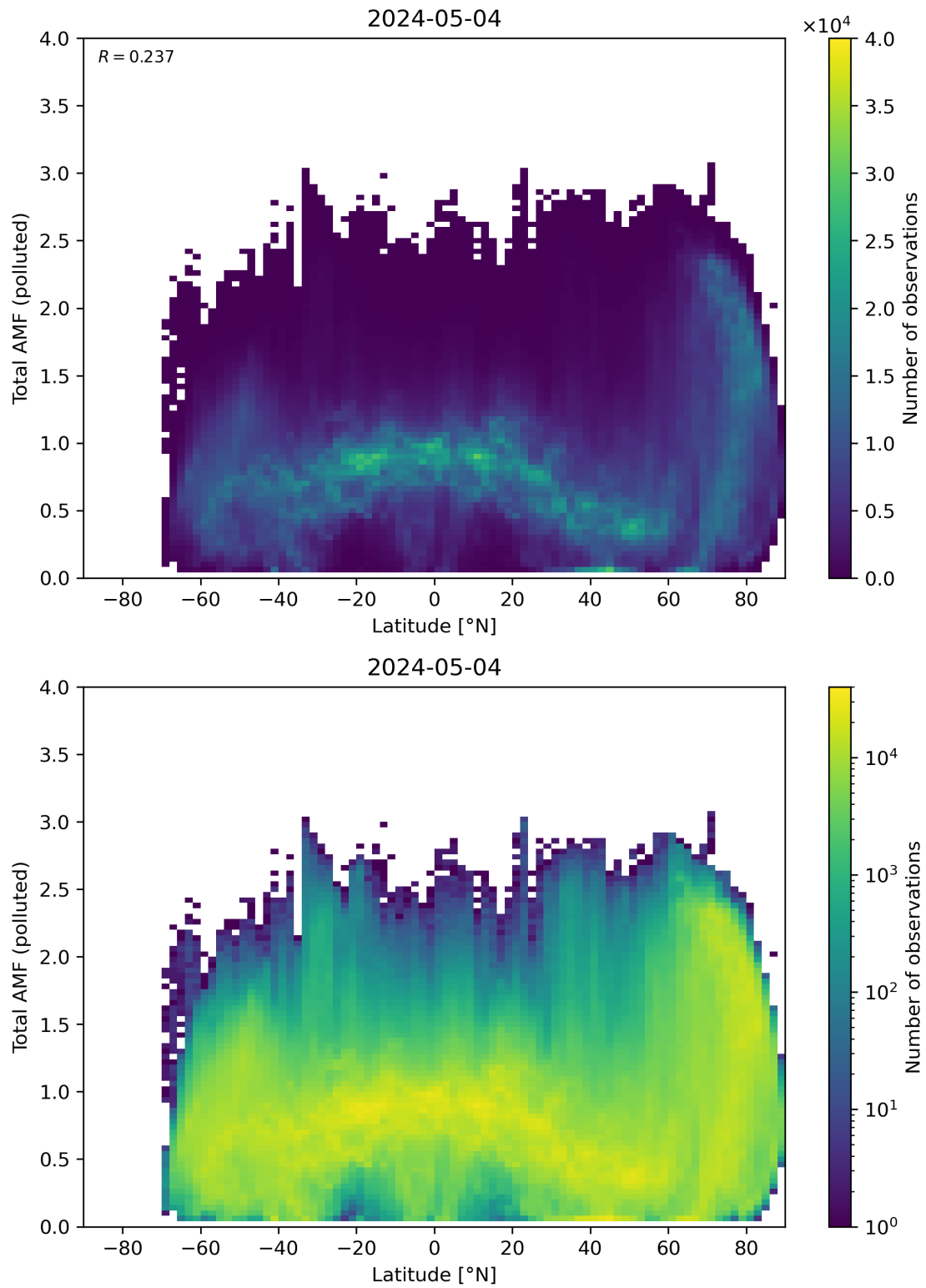
Figure 154: Scatter density plot of “Latitude” against “Total AMF (polluted)” for 2024-05-03 to 2024-05-05.
