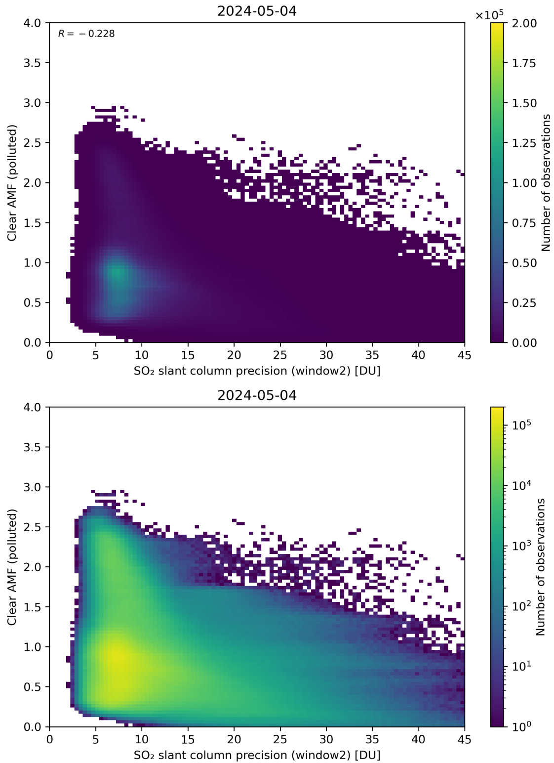
Figure 246: Scatter density plot of “SO 2 slant column precision (window2)” against “Clear AMF (polluted)” for 2024-05-03 to 2024-05-05.
