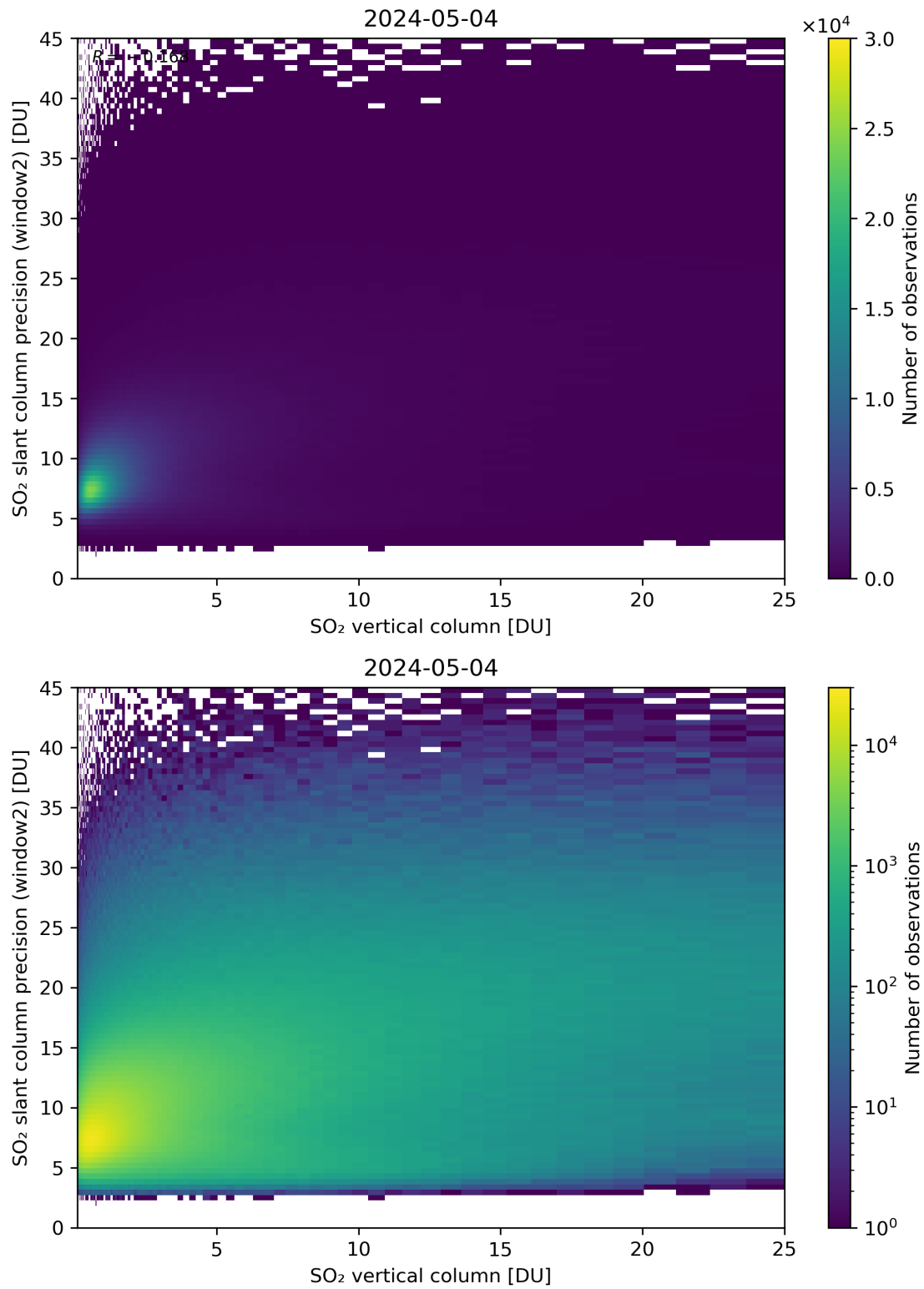
Figure 302: Scatter density plot of “SO 2 vertical column” against “SO 2 slant column precision (window2)” for 2024-05-03 to 2024-05-05.
