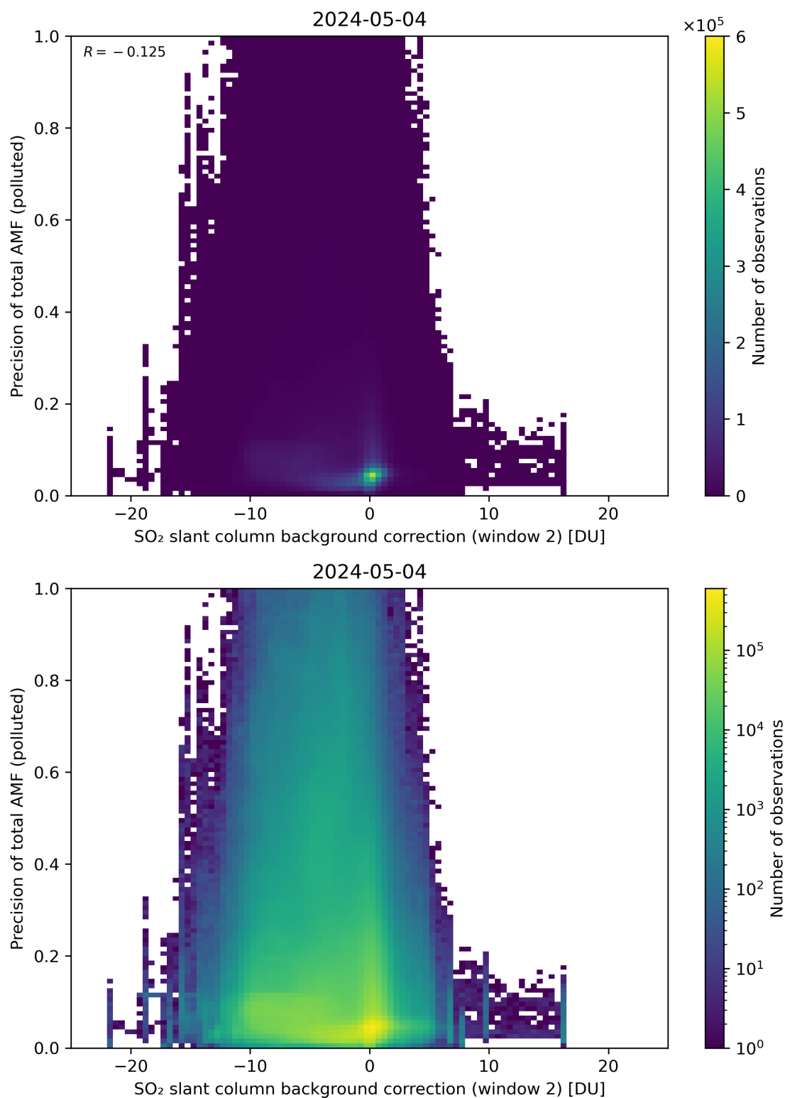
Figure 120: Scatter density plot of “SO 2 slant column background correction (window 2)” against “Precision of total AMF (polluted)” for 2024-05-03 to 2024-05-05.
