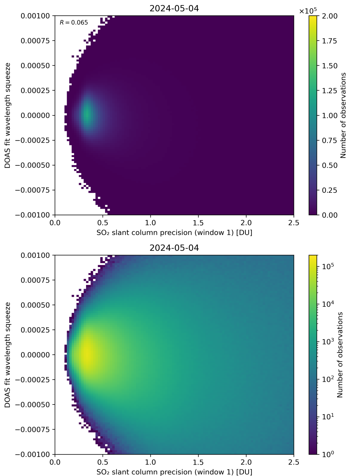
Figure 222: Scatter density plot of “SO 2 slant column precision (window 1)” against “DOAS fit wavelength squeeze” for 2024-05-03 to 2024-05-05.
