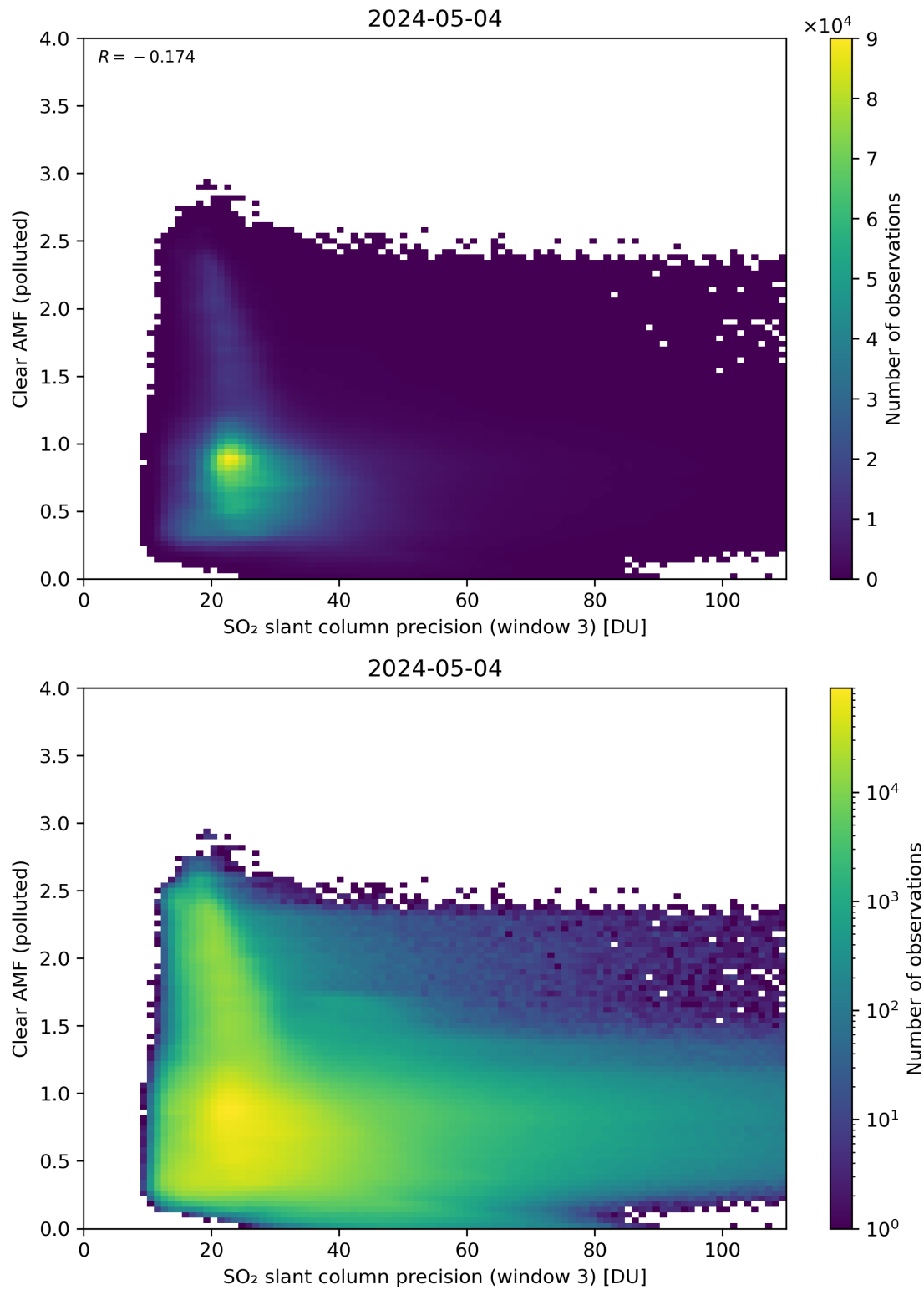
Figure 261: Scatter density plot of “SO 2 slant column precision (window 3)” against “Clear AMF (polluted)” for 2024-05-03 to 2024-05-05.
