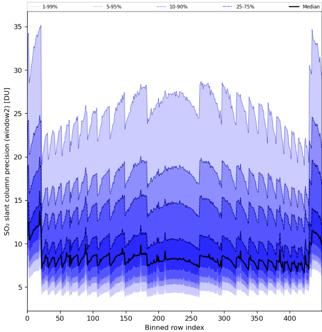
Figure 84: Along track statistics of “SO 2 slant column precision (window2)” for 2024-05-03 to 2024-05-05
