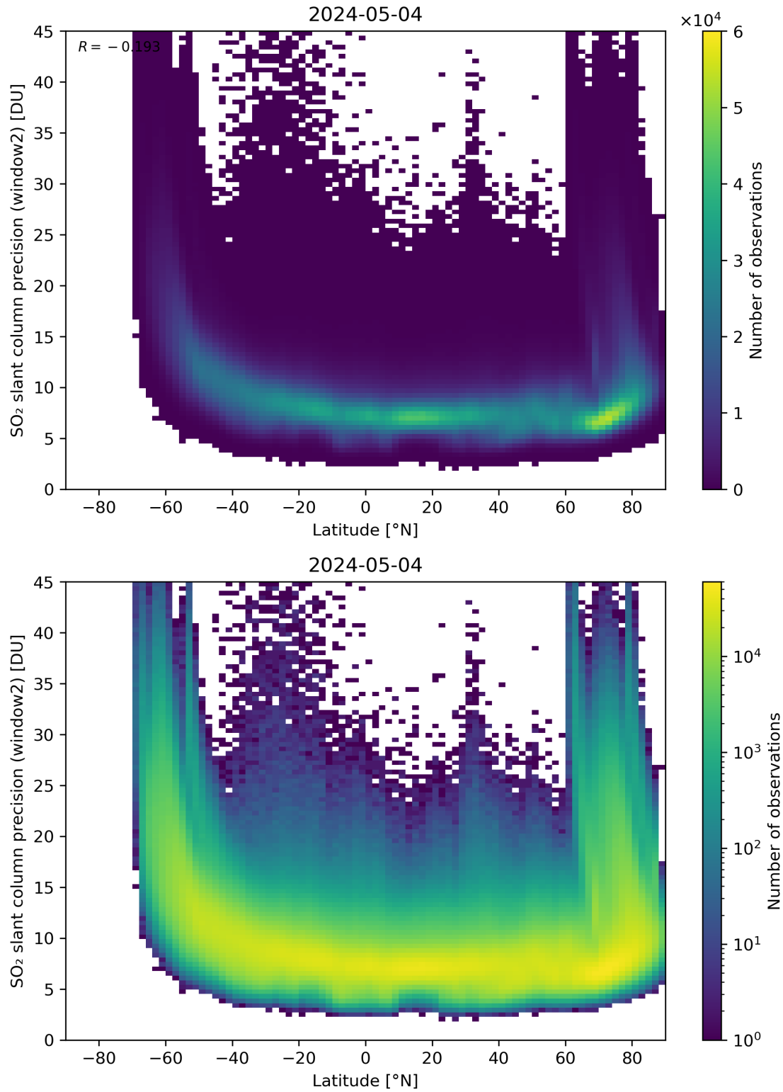
Figure 151: Scatter density plot of “Latitude” against “SO 2 slant column precision (window2)” for 2024-05-03 to 2024-05-05.
