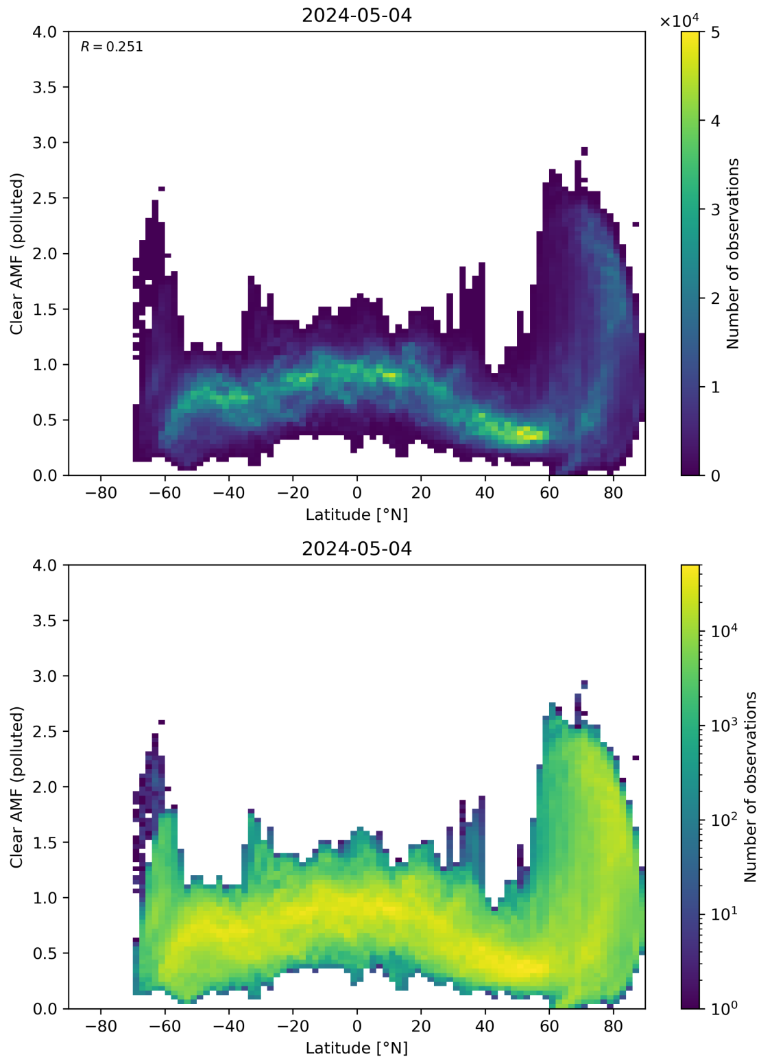
Figure 145: Scatter density plot of “Latitude” against “Clear AMF (polluted)” for 2024-05-03 to 2024-05-05.
