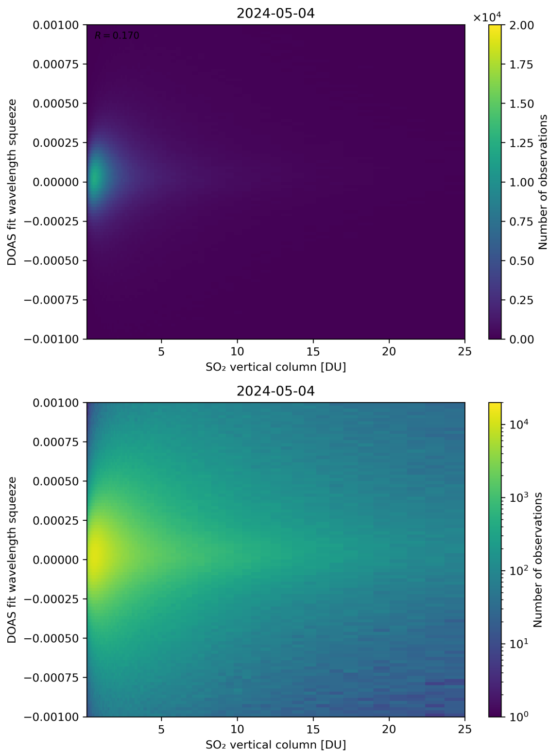
Figure 277: Scatter density plot of “SO 2 vertical column” against “DOAS fit wavelength squeeze” for 2024-05-03 to 2024-05-05.
