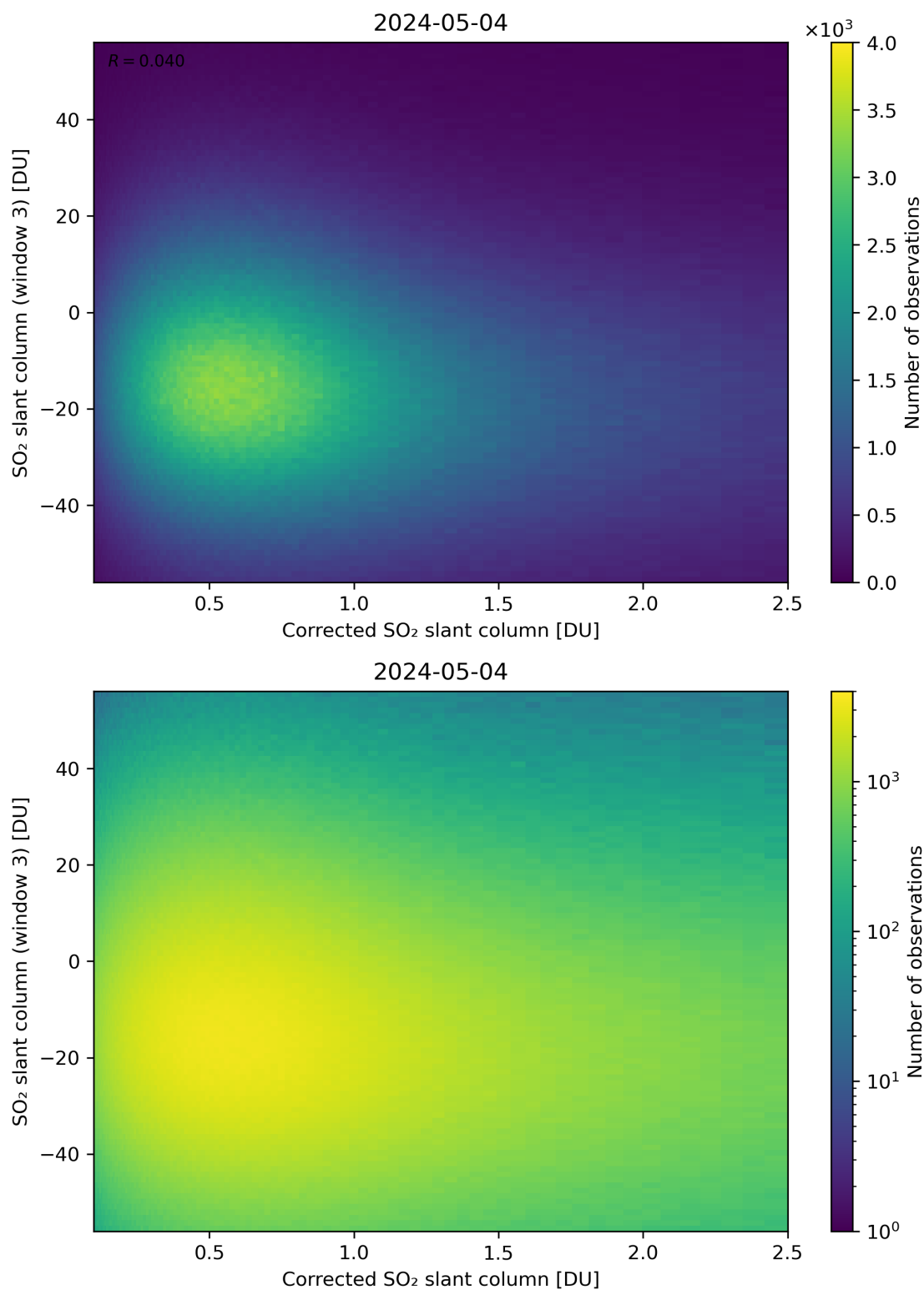
Figure 190: Scatter density plot of “Corrected SO 2 slant column” against “SO 2 slant column (window 3)” for 2024-05-03 to 2024-05-05.
