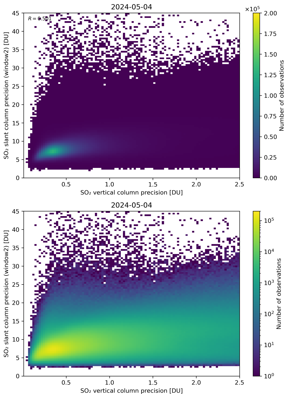
Figure 291: Scatter density plot of “SO 2 vertical column precision” against “SO 2 slant column precision (window2)” for 2024-05-03 to 2024-05-05.
