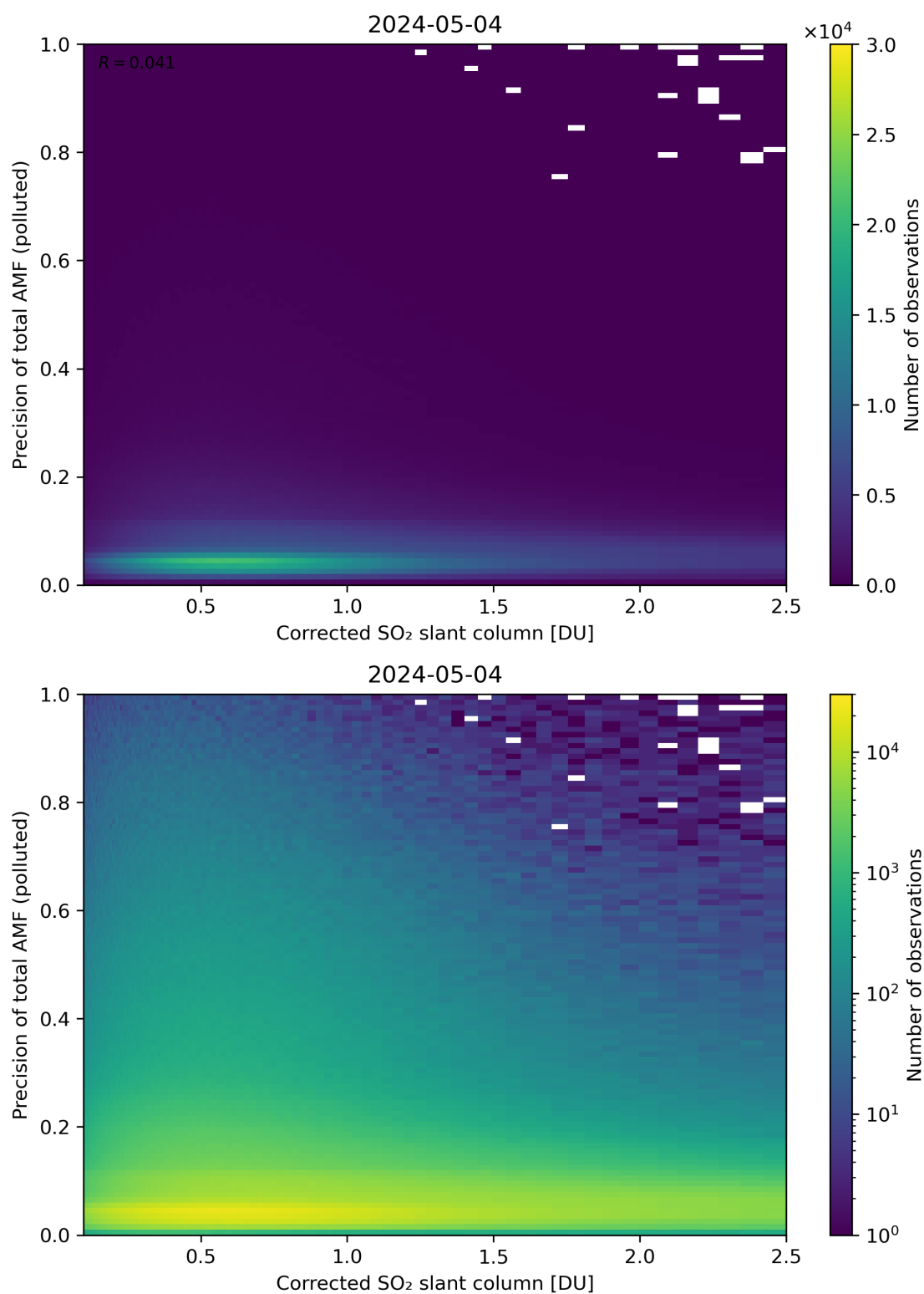
Figure 193: Scatter density plot of “Corrected SO 2 slant column” against “Precision of total AMF (polluted)” for 2024-05-03 to 2024-05-05.
