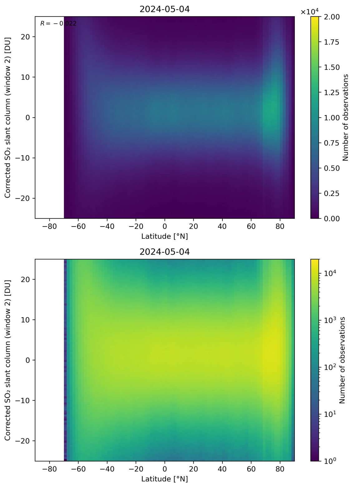
Figure 147: Scatter density plot of “Latitude” against “Corrected SO 2 slant column (window 2)” for 2024-05-03 to 2024-05-05.
