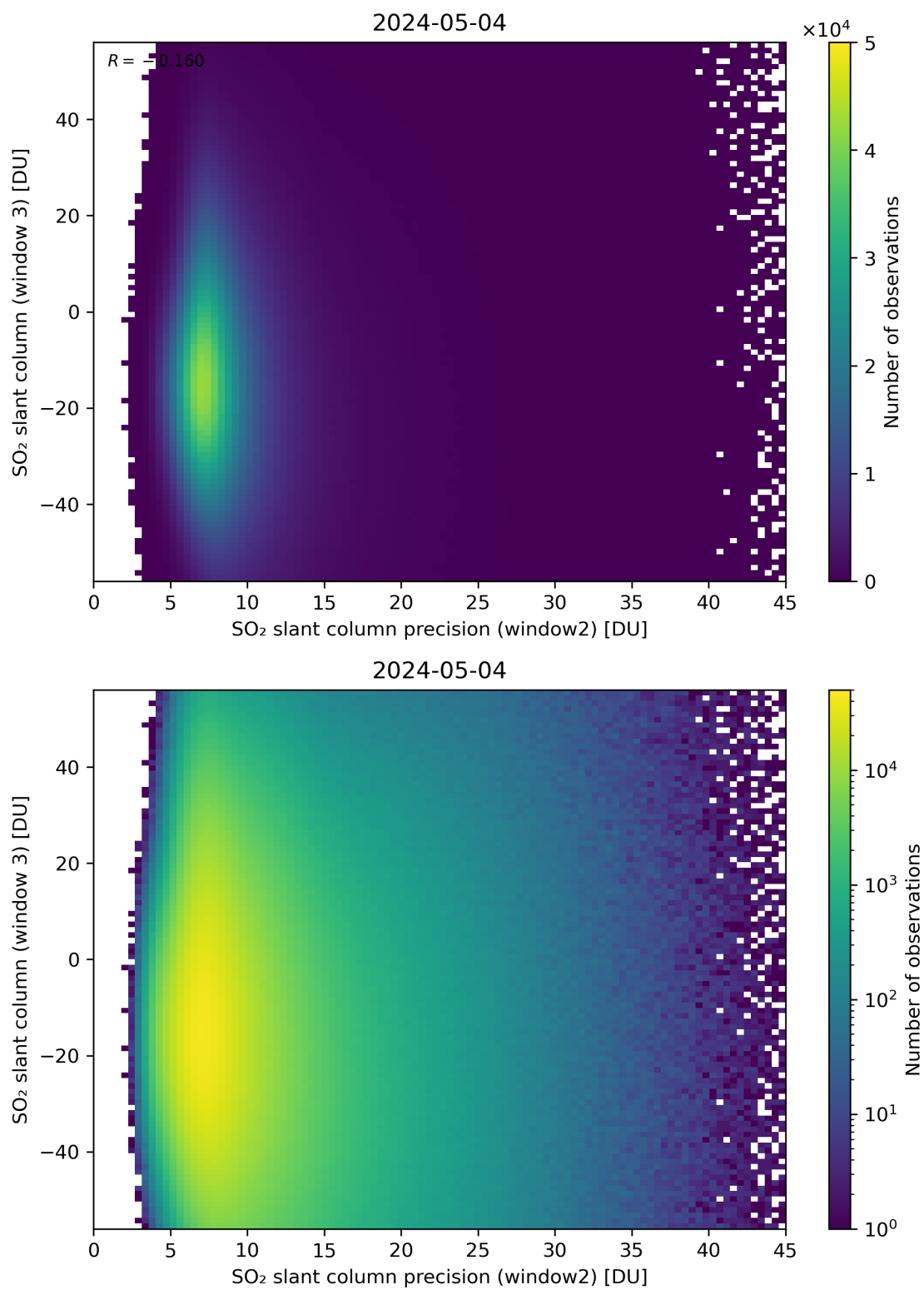
Figure 249: Scatter density plot of “SO 2 slant column precision (window2)” against “SO 2 slant column (window 3)” for 2024-05-03 to 2024-05-05.
