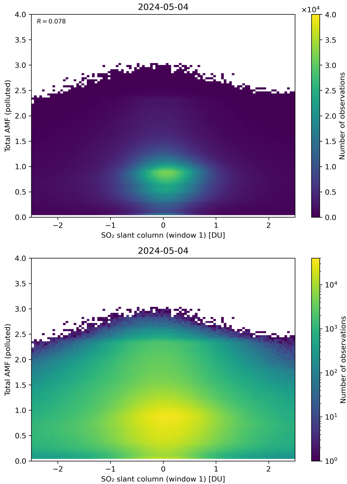
Figure 239: Scatter density plot of “SO 2 slant column (window 1)” against “Total AMF (polluted)” for 2024-05-03 to 2024-05-05.
