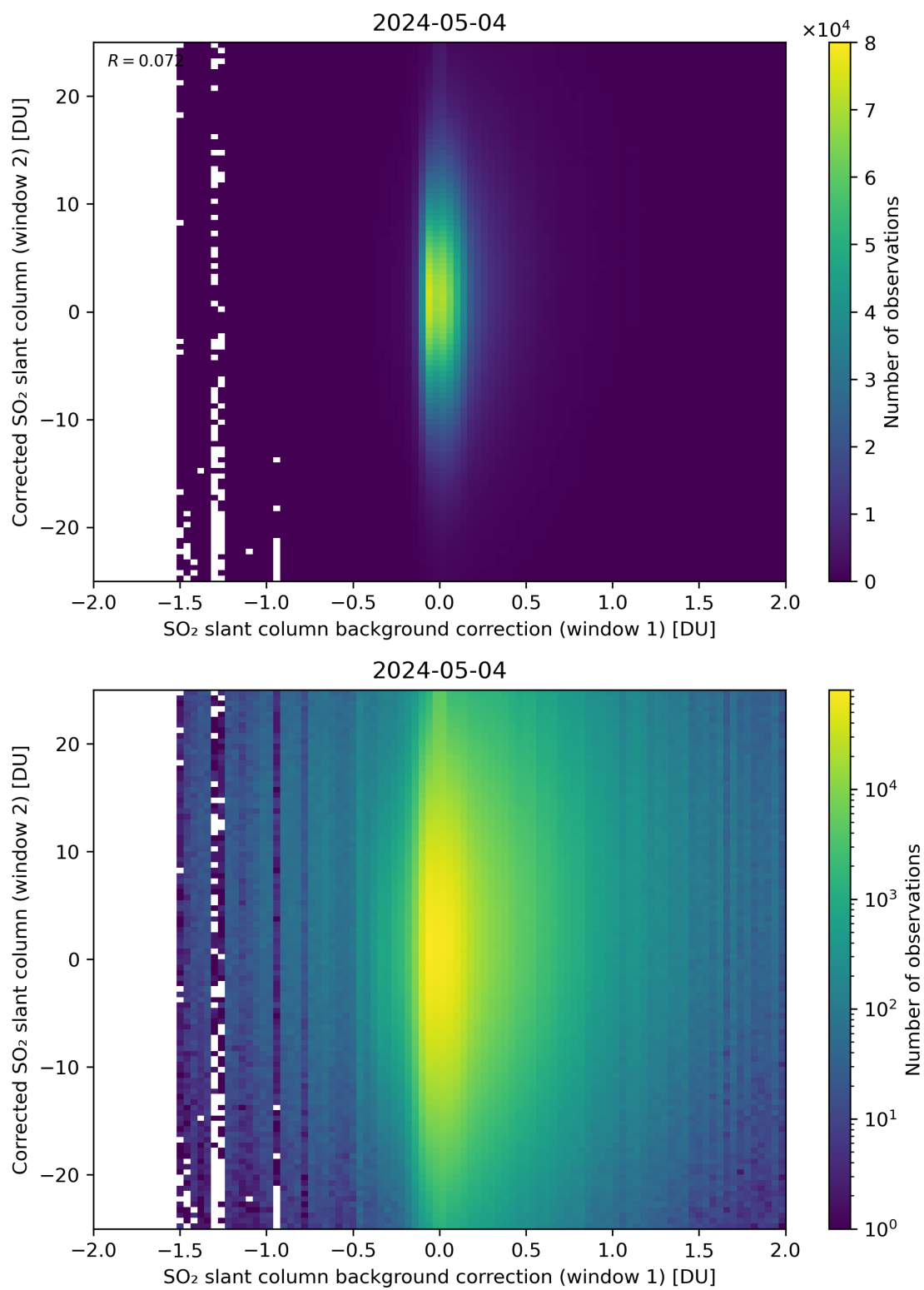
Figure 104: Scatter density plot of “SO 2 slant column background correction (window 1)” against “Corrected SO 2 slant column (window 2)” for 2024-05-03 to 2024-05-05.
