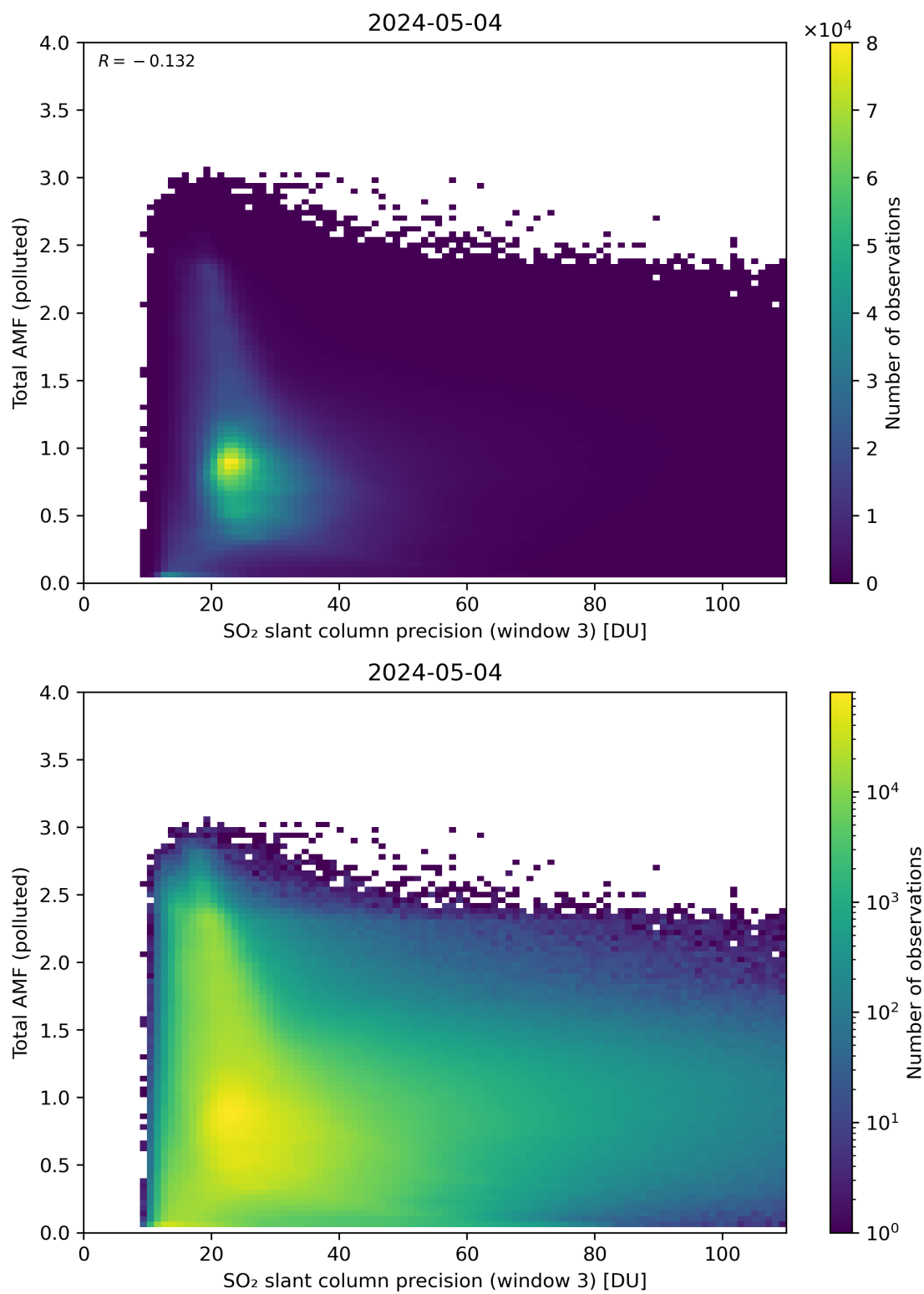
Figure 263: Scatter density plot of “SO 2 slant column precision (window 3)” against “Total AMF (polluted)” for 2024-05-03 to 2024-05-05.
