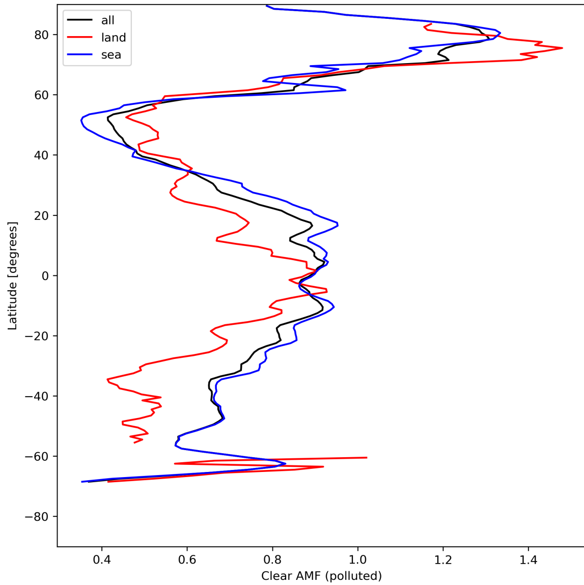
Figure 50: Zonal average of “Clear AMF (polluted)” for 2024-05-03 to 2024-05-05.
