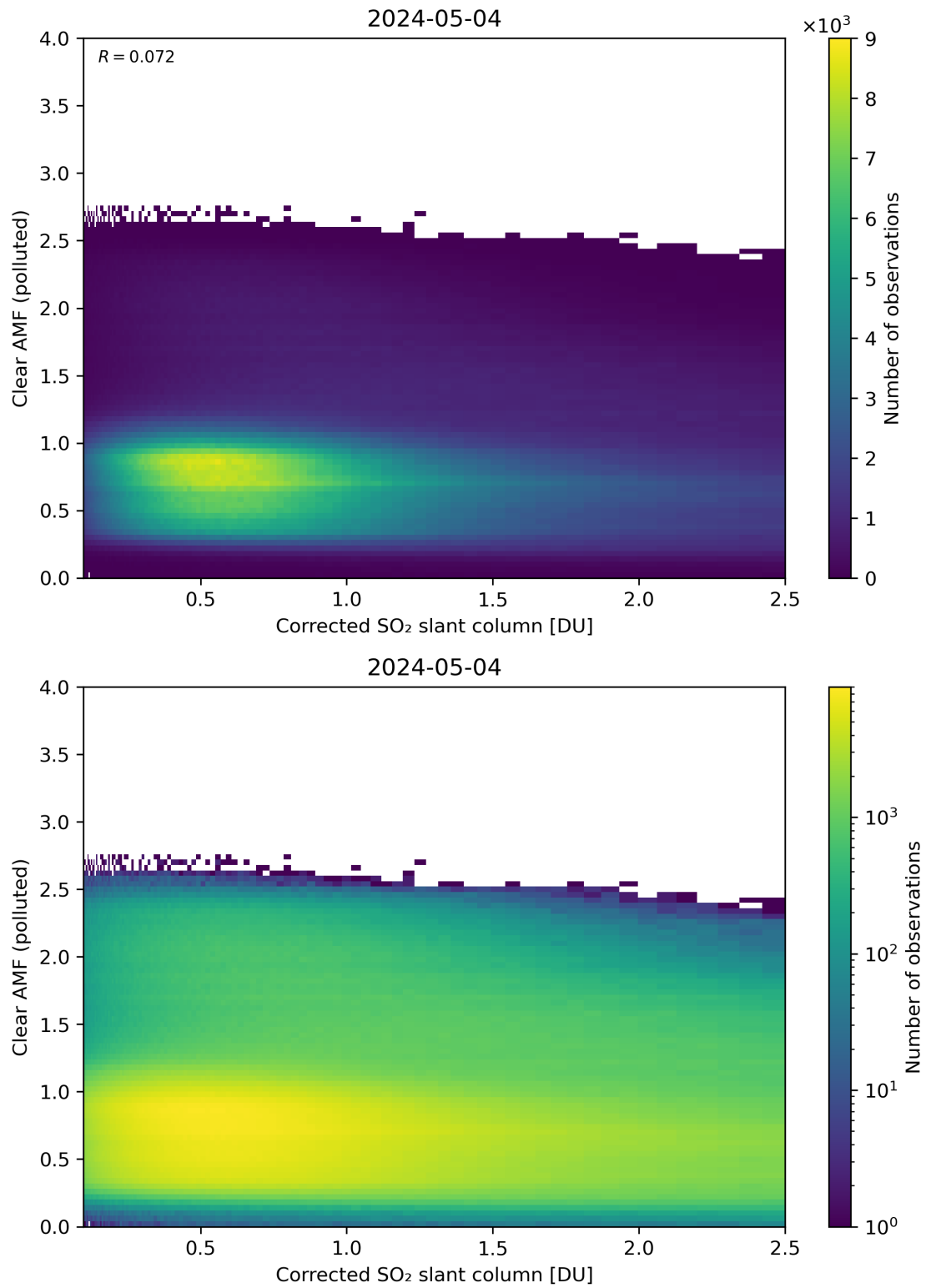
Figure 184: Scatter density plot of “Corrected SO 2 slant column” against “Clear AMF (polluted)” for 2024-05-03 to 2024-05-05.
