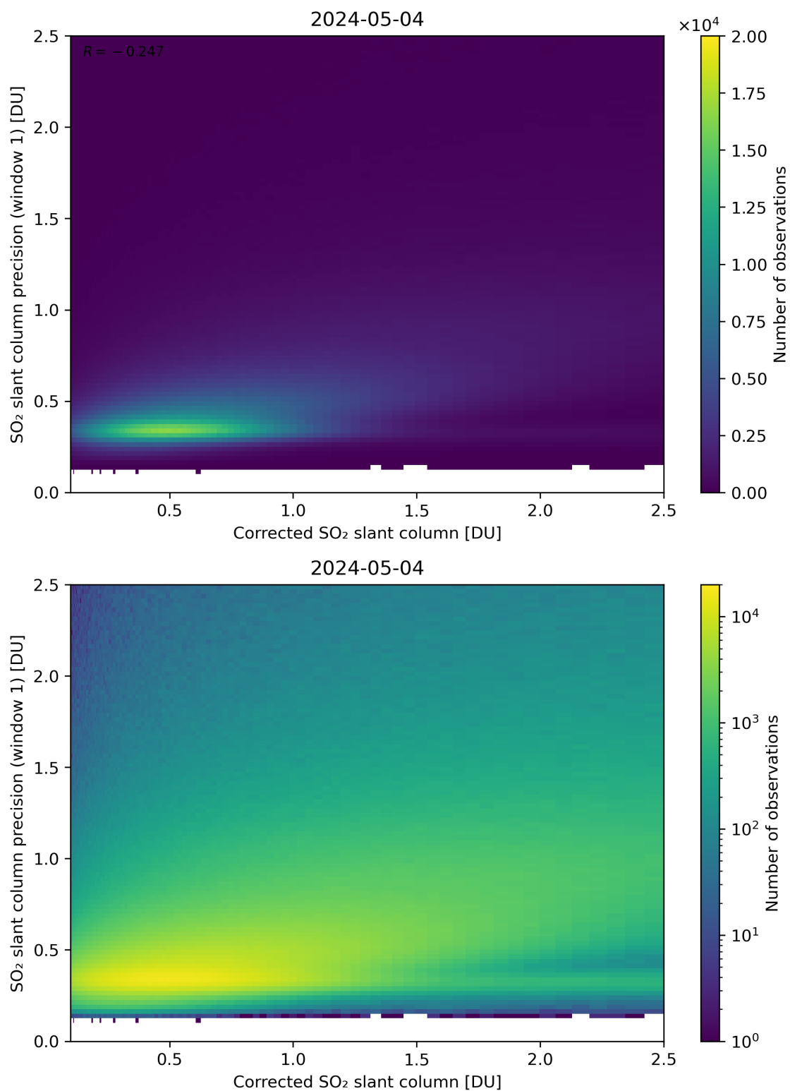
Figure 188: Scatter density plot of “Corrected SO 2 slant column” against “SO 2 slant column precision (window 1)” for 2024-05-03 to 2024-05-05.
