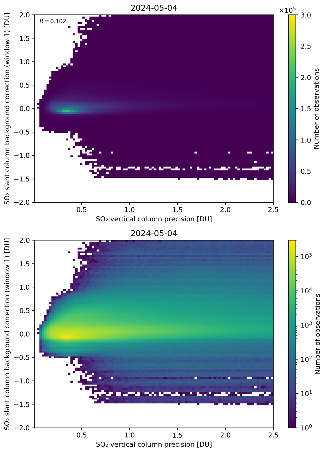
Figure 279: Scatter density plot of “SO 2 vertical column precision” against “SO 2 slant column background correction (window 1)” for 2024-05-03 to 2024-05-05.
