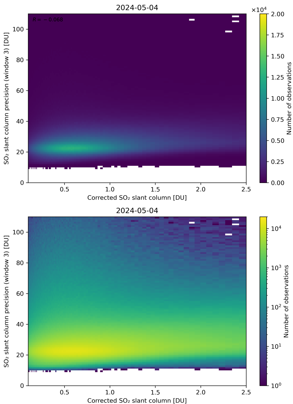
Figure 191: Scatter density plot of “Corrected SO 2 slant column” against “SO 2 slant column precision (window 3)” for 2024-05-03 to 2024-05-05.
