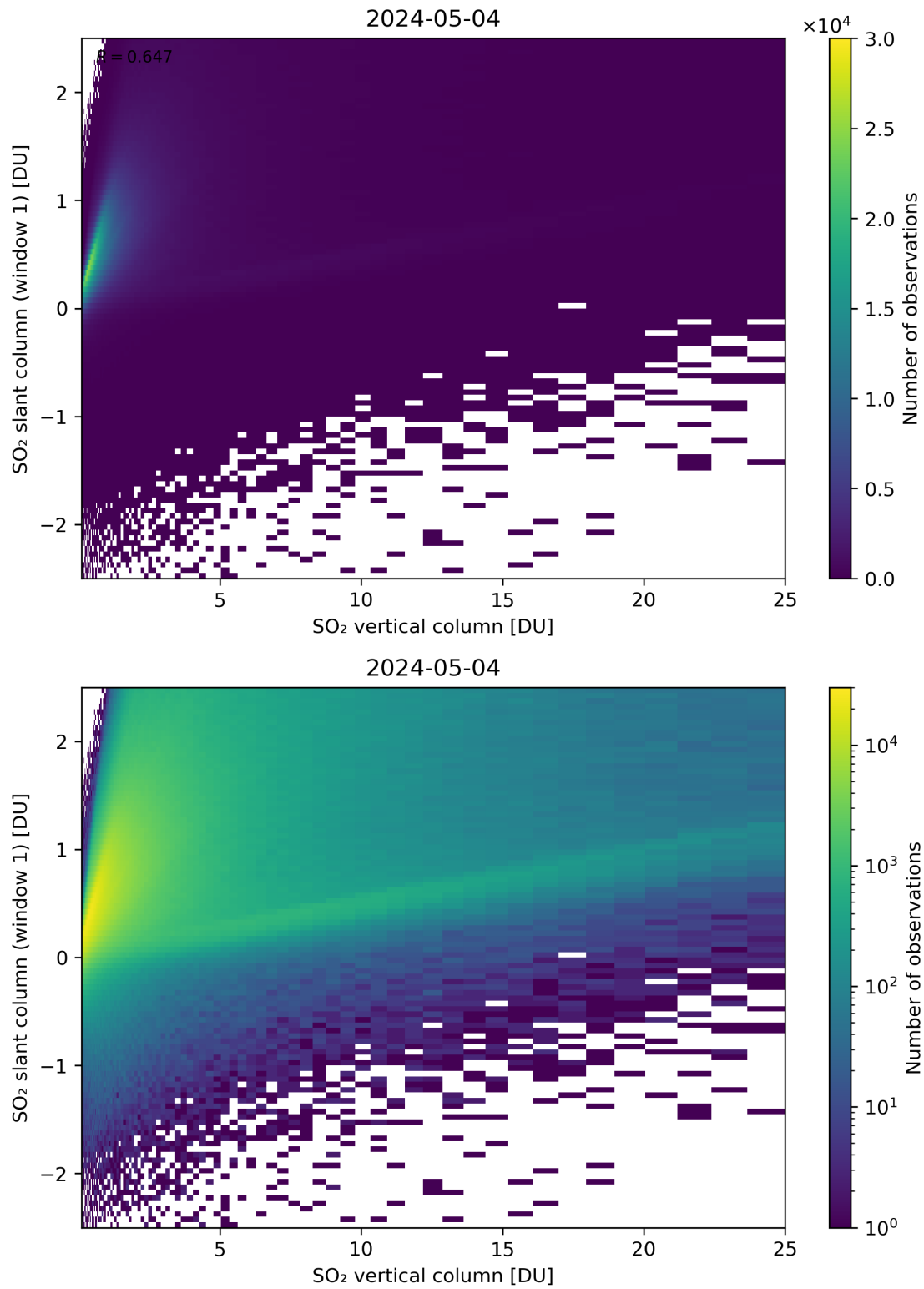
Figure 300: Scatter density plot of “SO 2 vertical column” against “SO 2 slant column (window 1)” for 2024-05-03 to 2024-05-05.
