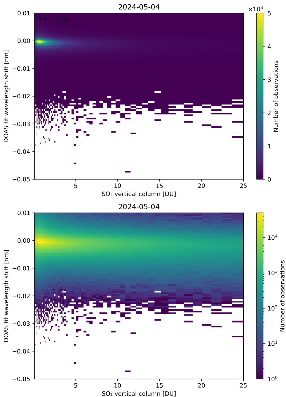
Figure 276: Scatter density plot of “SO 2 vertical column” against “DOAS fit wavelength shift” for 2024-05-03 to 2024-05-05.
