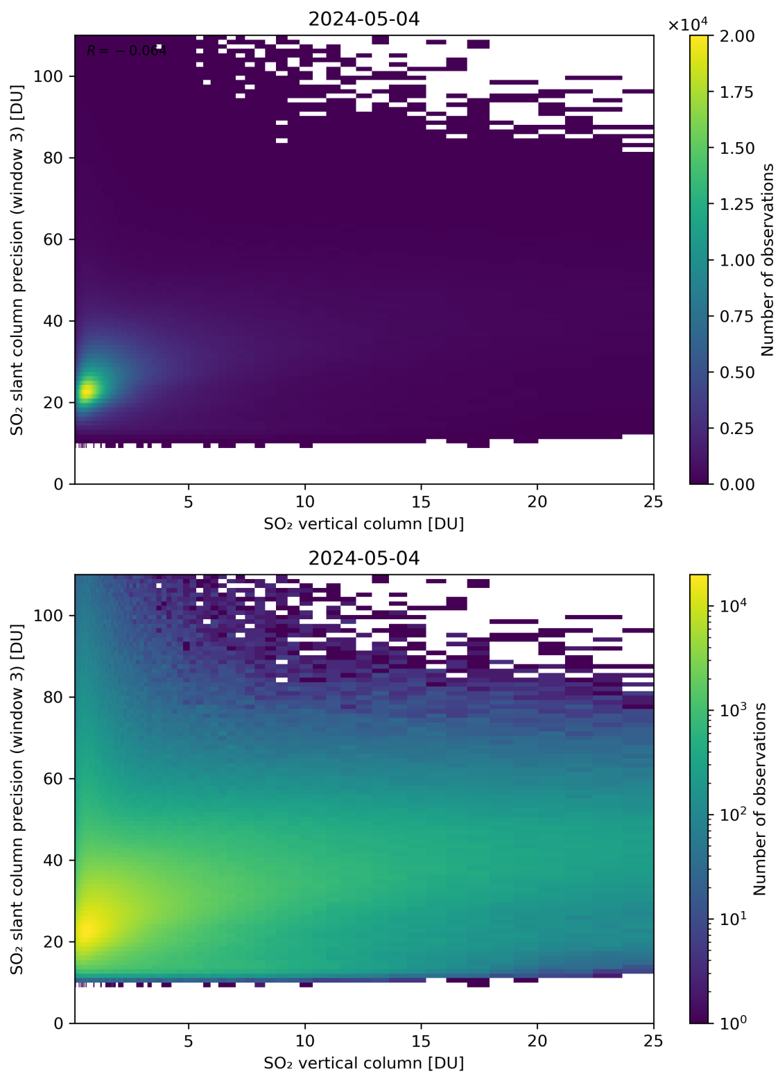
Figure 304: Scatter density plot of “SO 2 vertical column” against “SO 2 slant column precision (window 3)” for 2024-05-03 to 2024-05-05.
