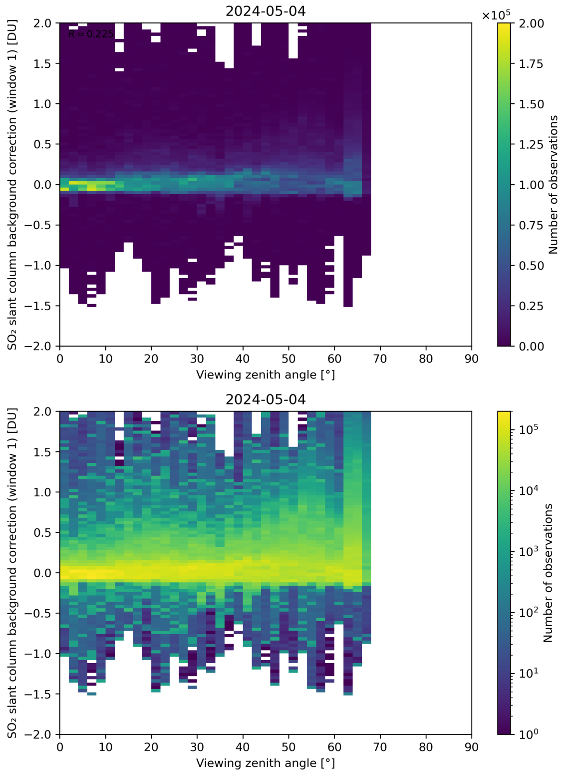
Figure 308: Scatter density plot of “Viewing zenith angle” against “SO 2 slant column background correction (window 1)” for 2024-05-03 to 2024-05-05.
