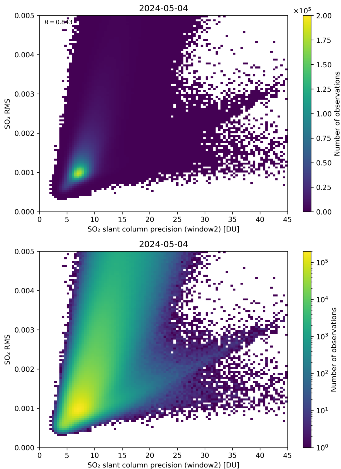
Figure 245: Scatter density plot of “SO 2 slant column precision (window2)” against “SO 2 RMS” for 2024-05-03 to 2024-05-05.
