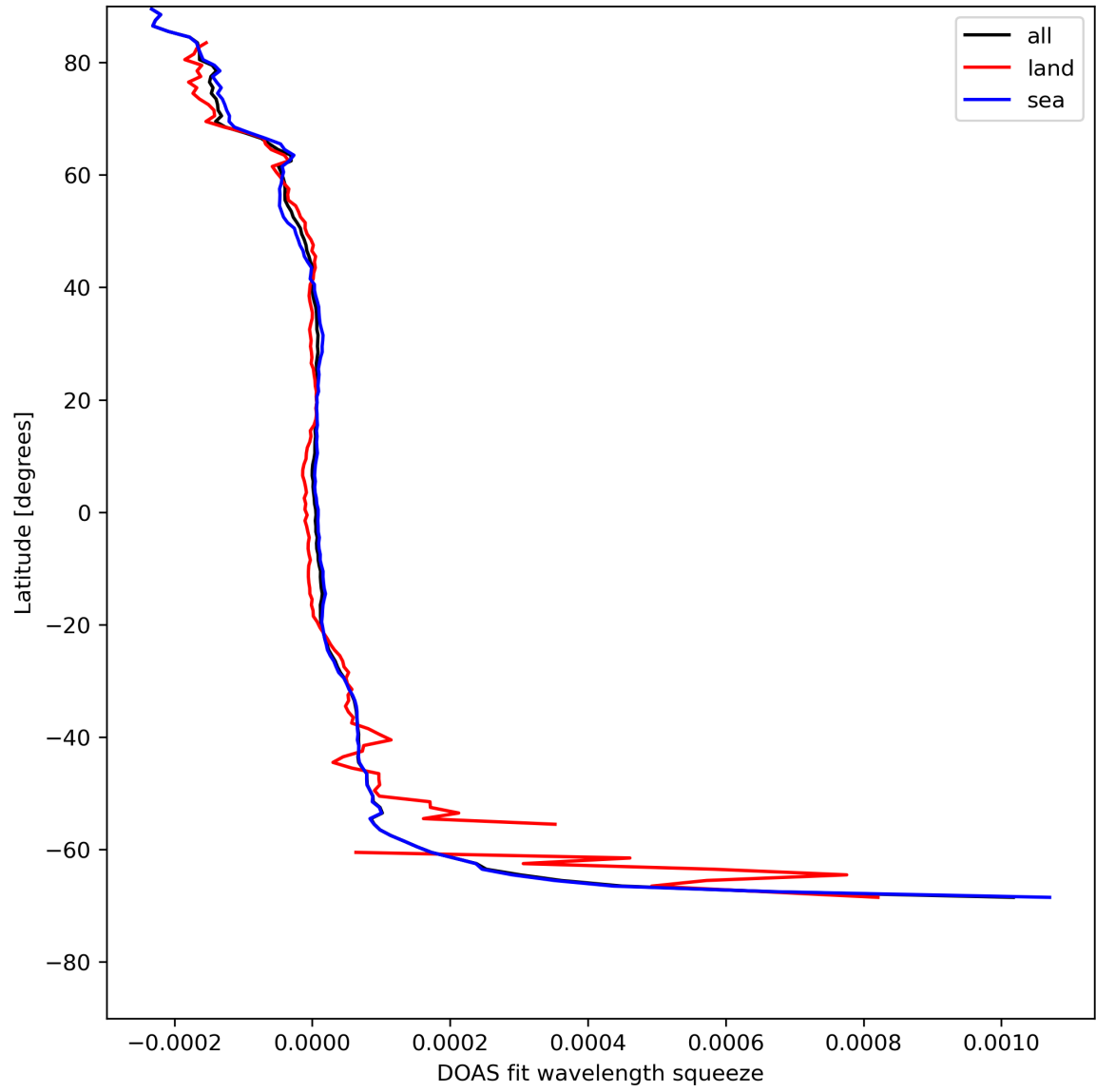
Figure 46: Zonal average of “DOAS fit wavelength squeeze” for 2024-05-03 to 2024-05-05.
