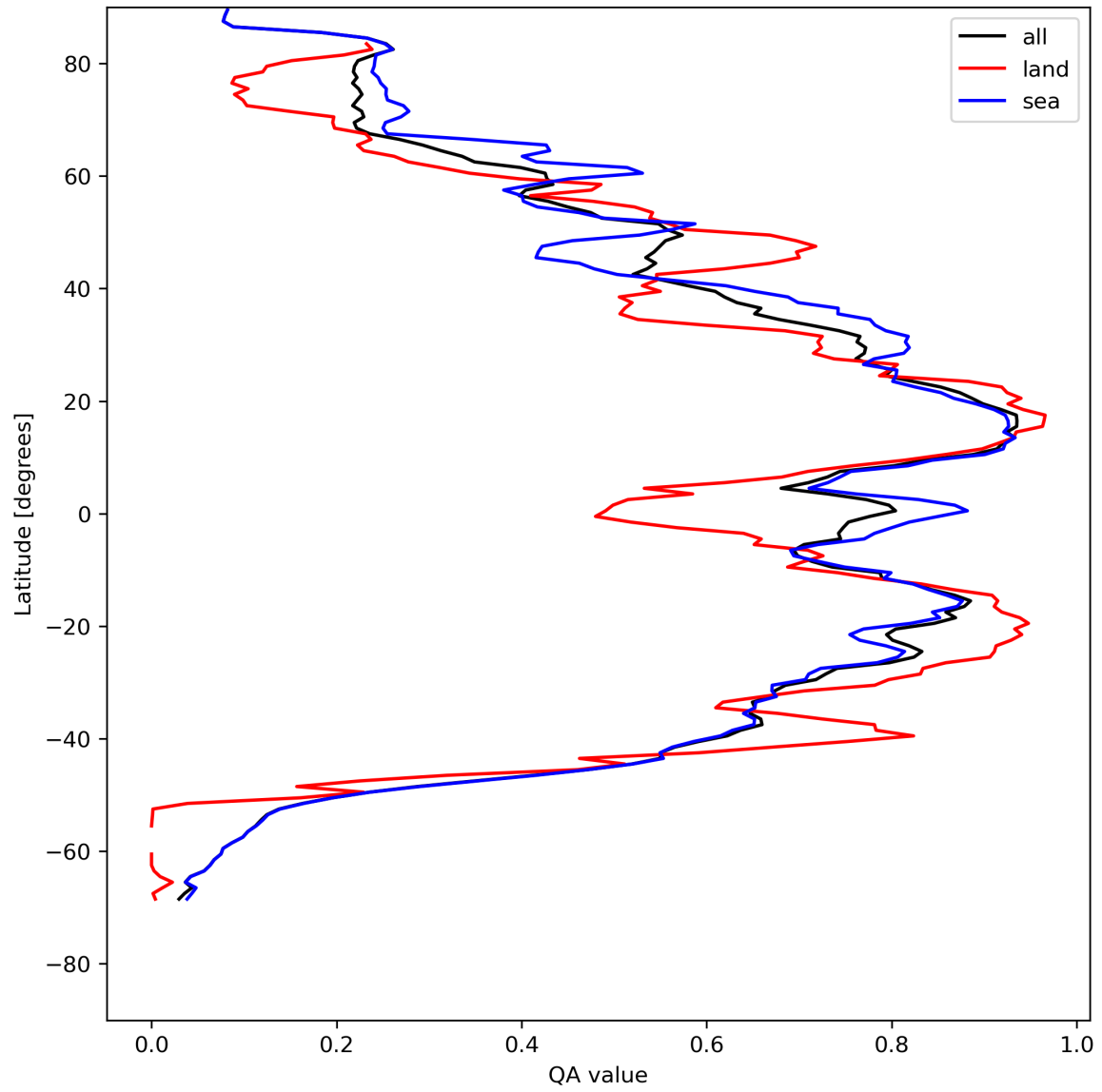
Figure 29: Zonal average of “QA value” for 2024-05-03 to 2024-05-05.
