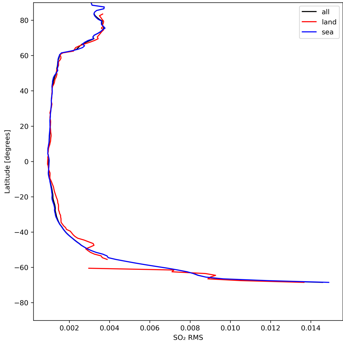
Figure 47: Zonal average of “SO 2 RMS” for 2024-05-03 to 2024-05-05.
