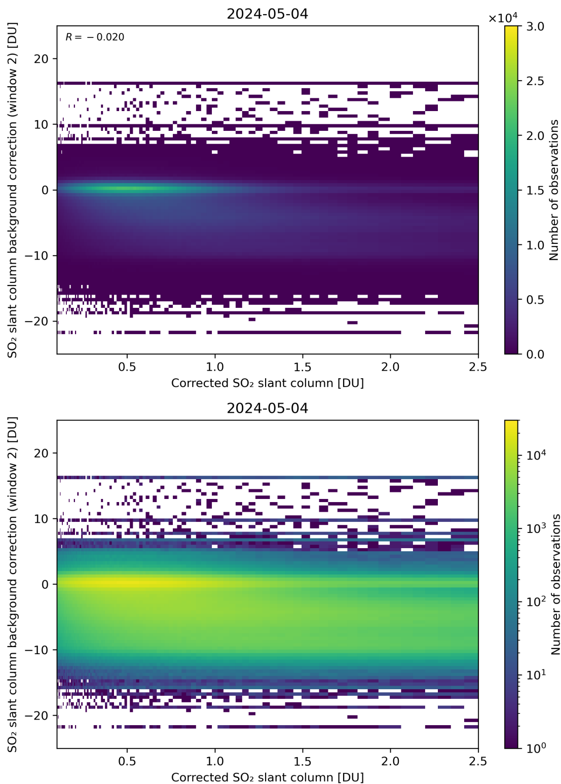
Figure 179: Scatter density plot of “Corrected SO 2 slant column” against “SO 2 slant column background correction (window 2)” for 2024-05-03 to 2024-05-05.
