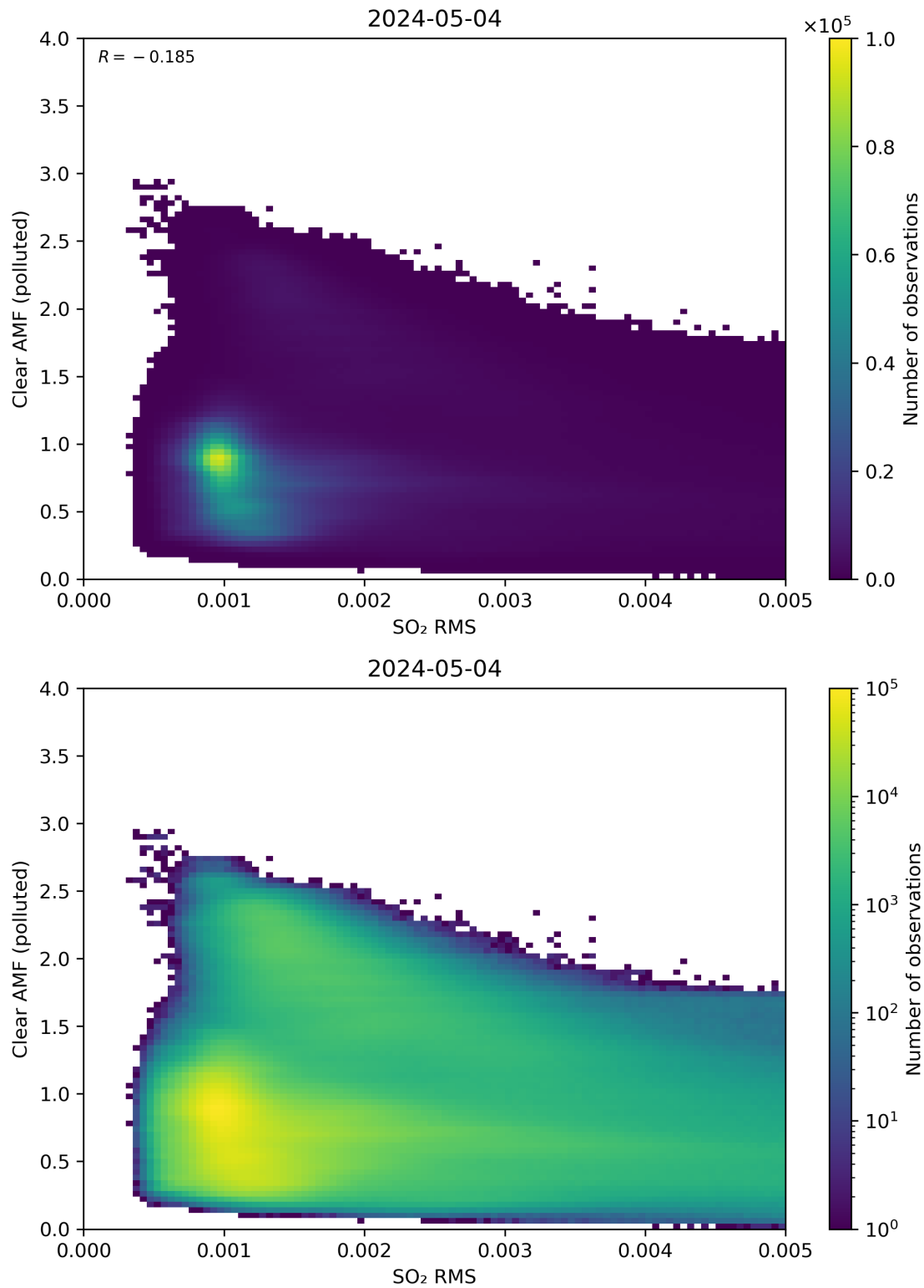
Figure 136: Scatter density plot of “SO 2 RMS” against “Clear AMF (polluted)” for 2024-05-03 to 2024-05-05.
