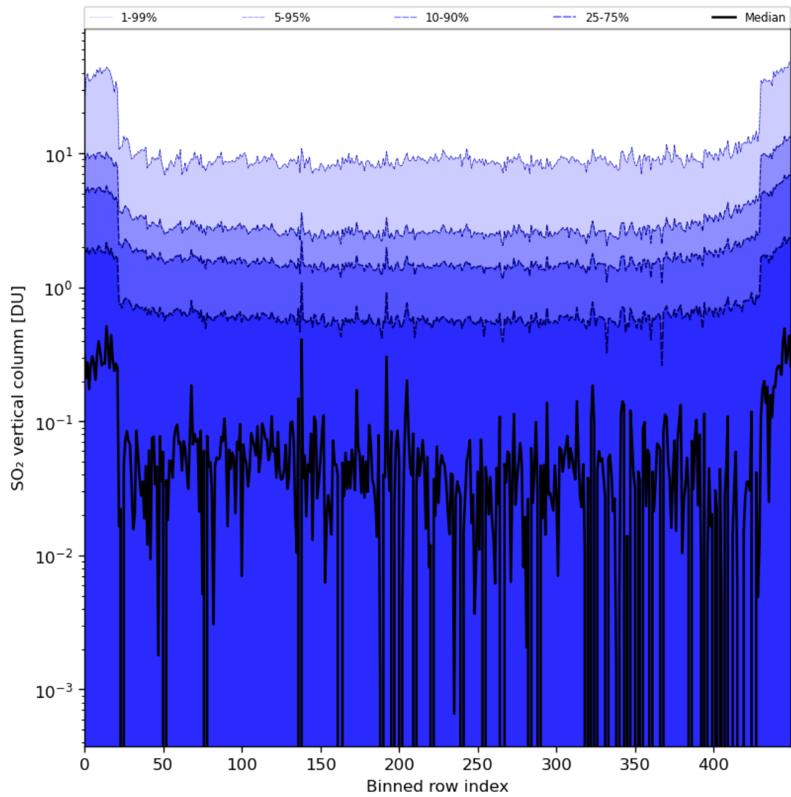
Figure 76: Along track statistics of “SO 2 vertical column” for 2024-05-03 to 2024-05-05
