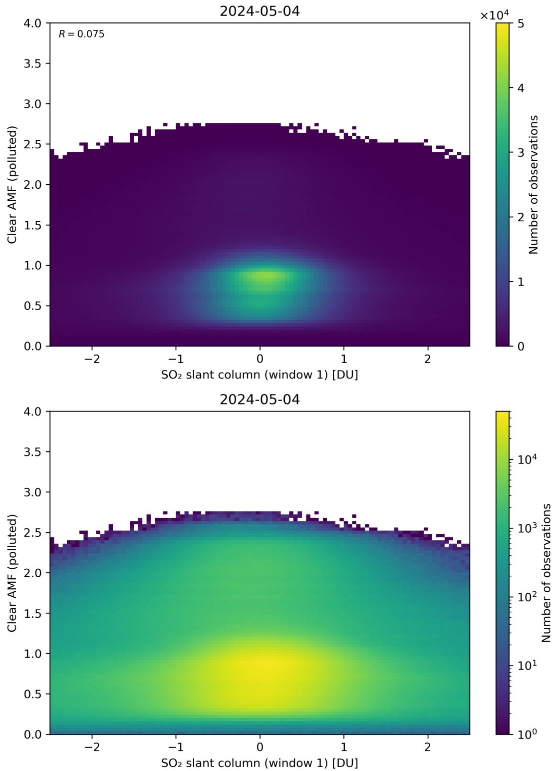
Figure 232: Scatter density plot of “SO 2 slant column (window 1)” against “Clear AMF (polluted)” for 2024-05-03 to 2024-05-05.
