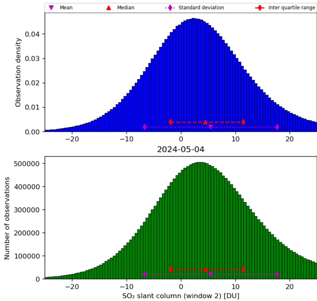
Figure 60: Histogram of “SO 2 slant column (window 2)” for 2024-05-03 to 2024-05-05
