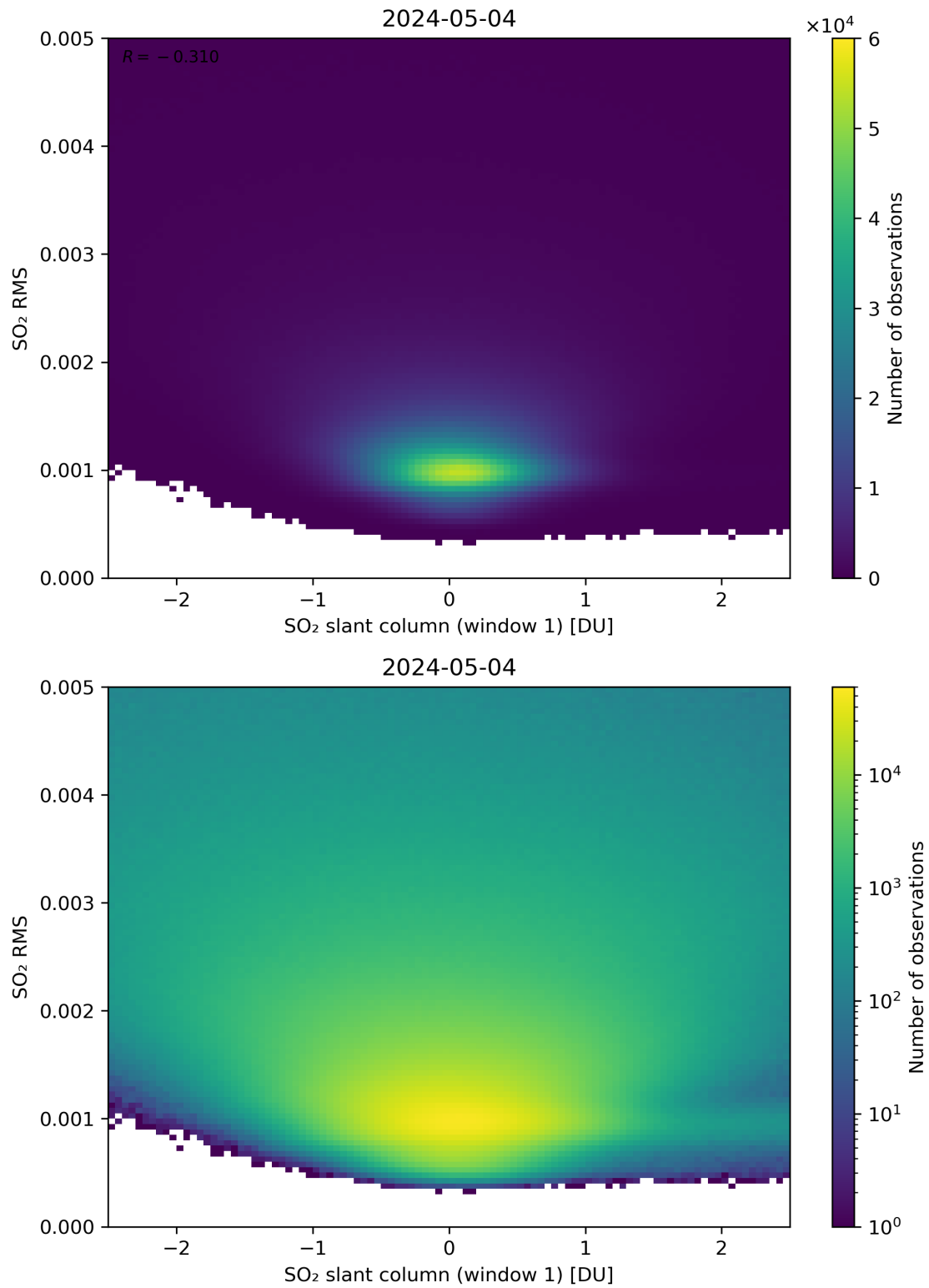
Figure 217: Scatter density plot of “SO 2 slant column (window 1)” against “SO 2 RMS” for 2024-05-03 to 2024-05-05.
