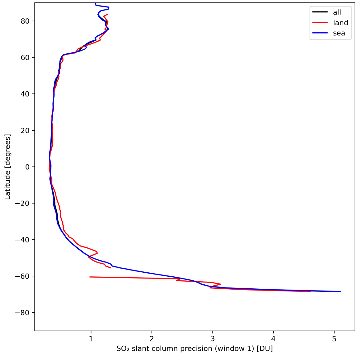
Figure 34: Zonal average of “SO 2 slant column precision (window 1)” for 2024-05-03 to 2024-05-05.
