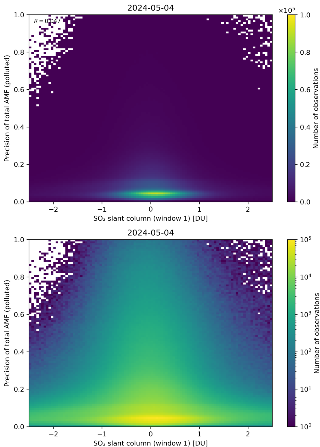
Figure 240: Scatter density plot of “SO 2 slant column (window 1)” against “Precision of total AMF (polluted)” for 2024-05-03 to 2024-05-05.
