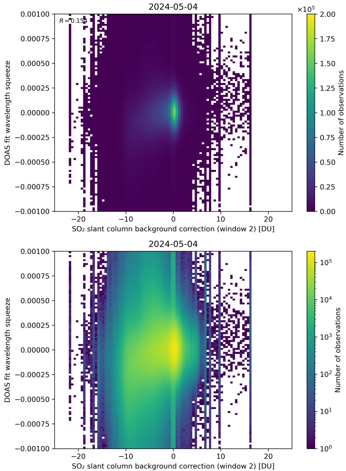
Figure 113: Scatter density plot of “SO 2 slant column background correction (window 2)” against “DOAS fit wavelength squeeze” for 2024-05-03 to 2024-05-05.
