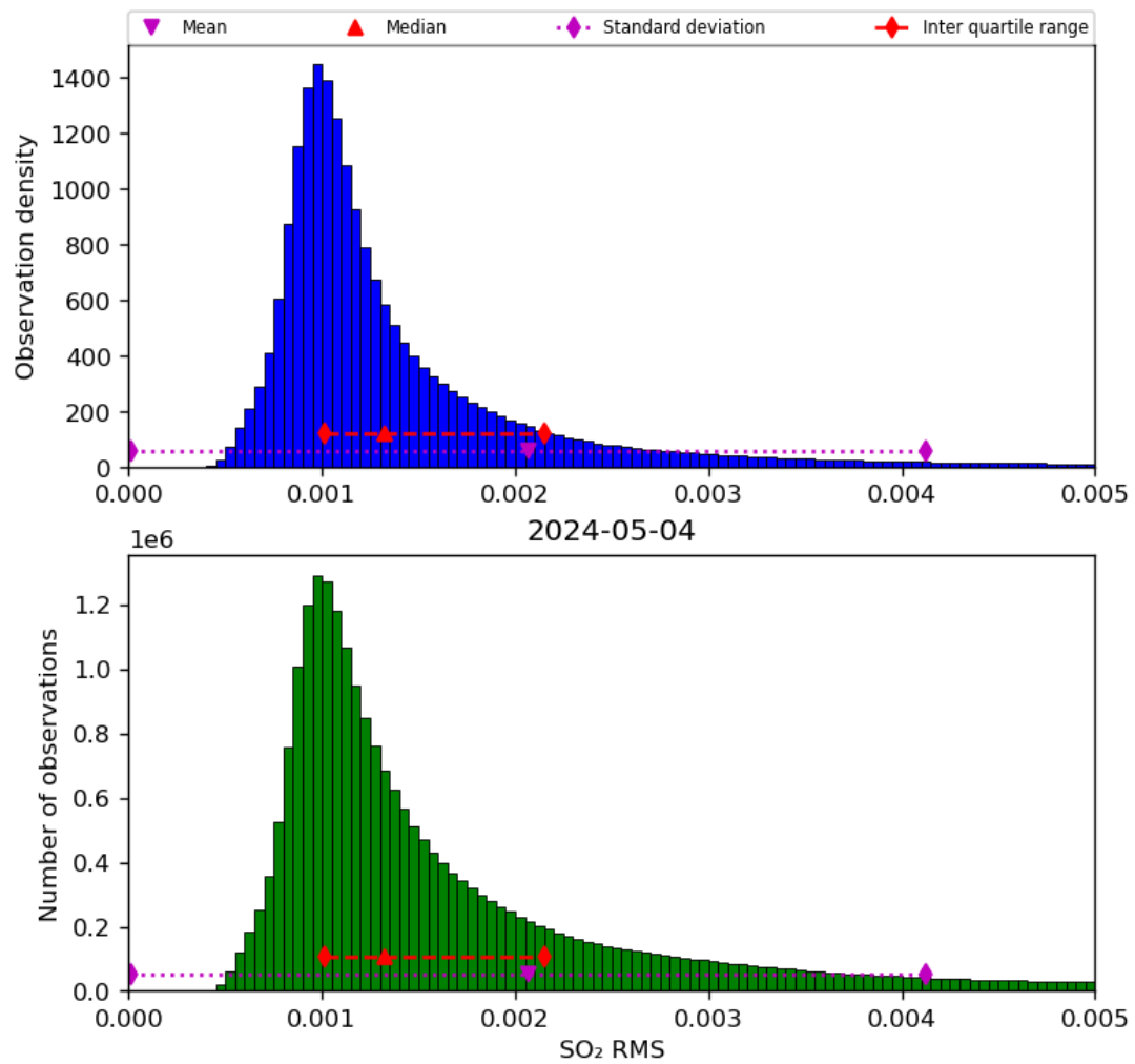
Figure 70: Histogram of “SO 2 RMS” for 2024-05-03 to 2024-05-05
