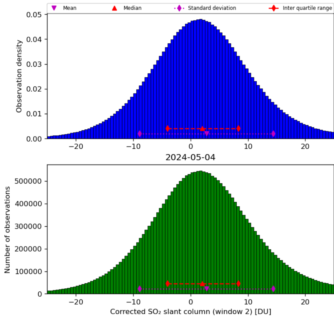
Figure 62: Histogram of “Corrected SO 2 slant column (window 2)” for 2024-05-03 to 2024-05-05
