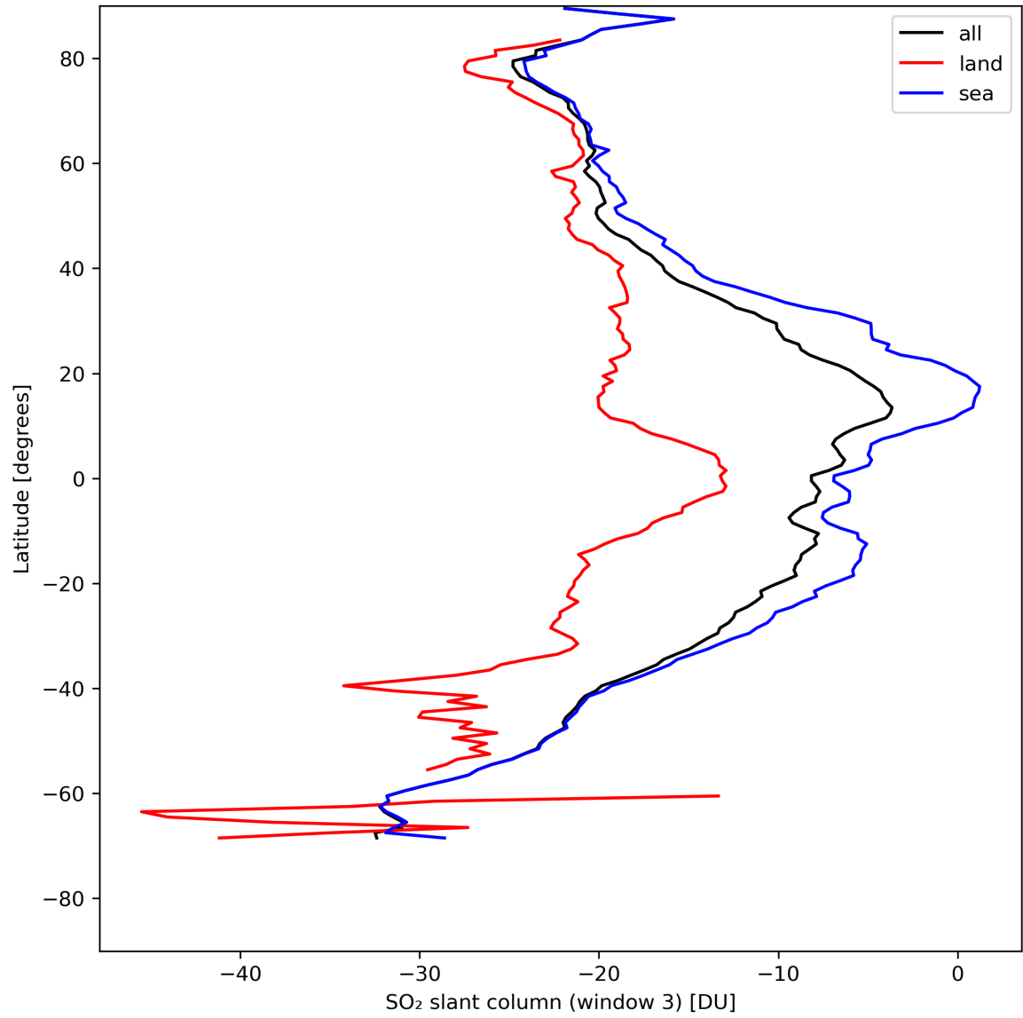
Figure 41: Zonal average of “SO 2 slant column (window 3)” for 2024-05-03 to 2024-05-05.
