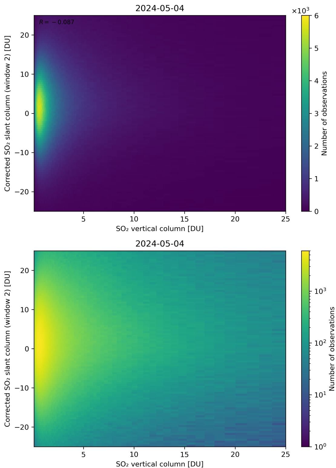
Figure 298: Scatter density plot of “SO 2 vertical column” against “Corrected SO 2 slant column (window 2)” for 2024-05-03 to 2024-05-05.
