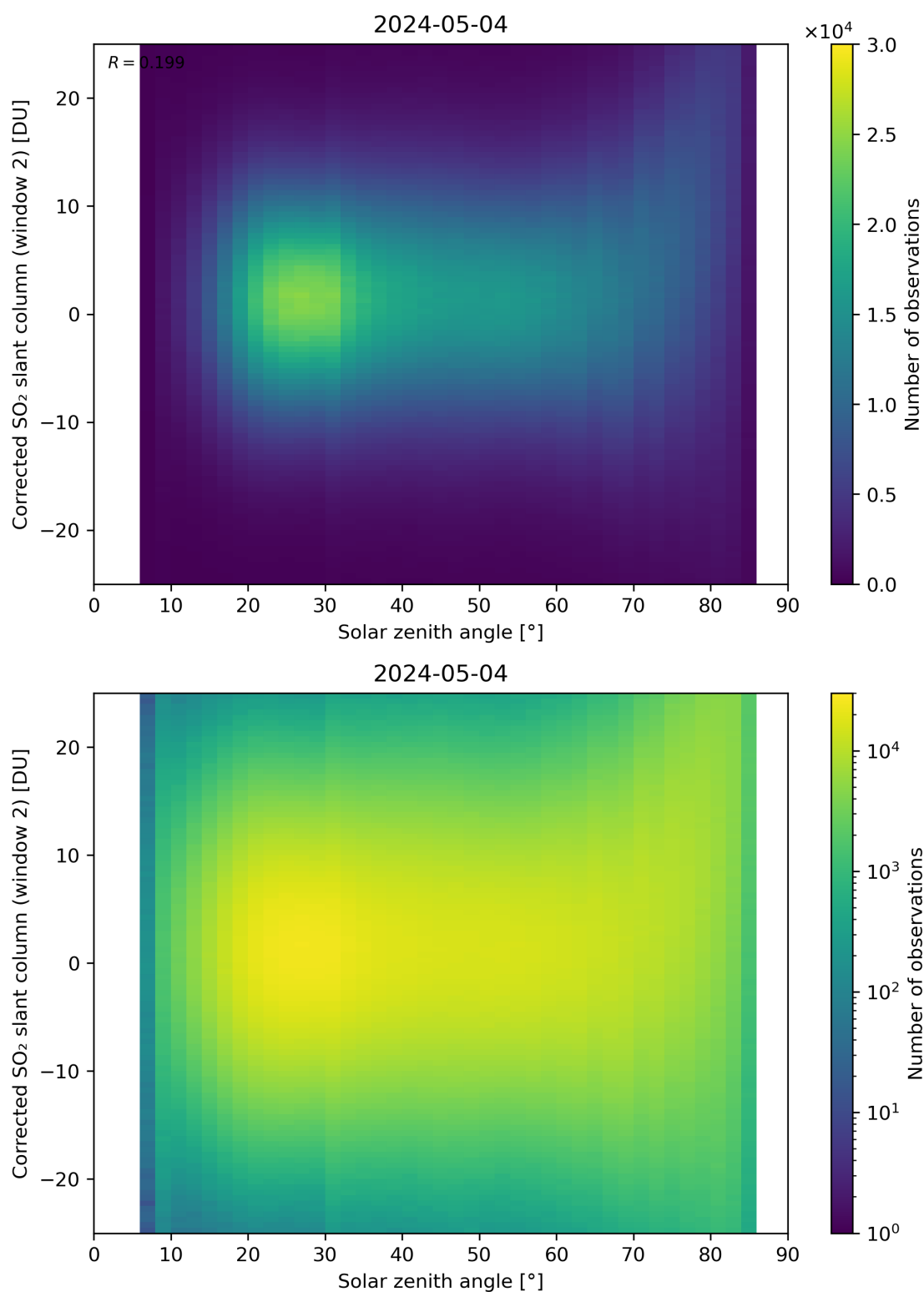
Figure 167: Scatter density plot of “Solar zenith angle” against “Corrected SO 2 slant column (window 2)” for 2024-05-03 to 2024-05-05.
