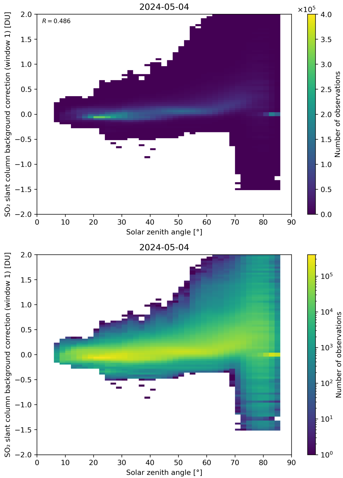
Figure 158: Scatter density plot of “Solar zenith angle” against “SO 2 slant column background correction (window 1)” for 2024-05-03 to 2024-05-05.
