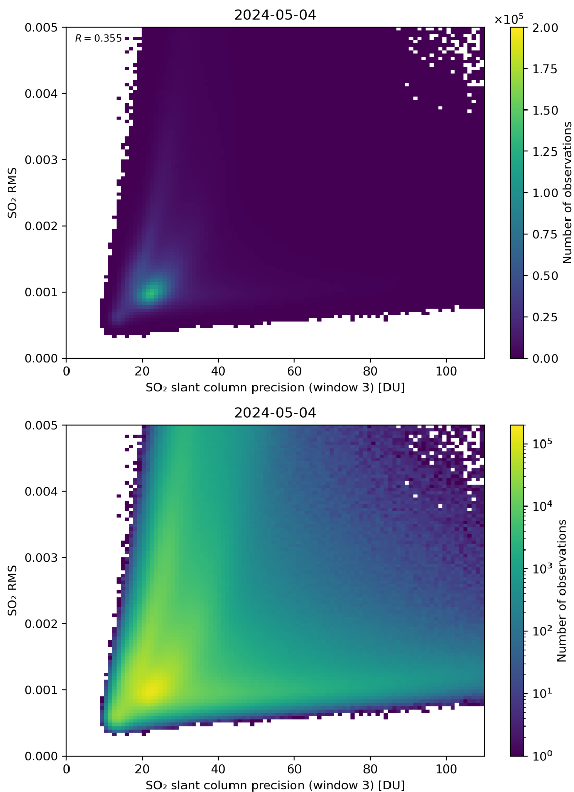
Figure 260: Scatter density plot of “SO 2 slant column precision (window 3)” against “SO 2 RMS” for 2024-05-03 to 2024-05-05.
