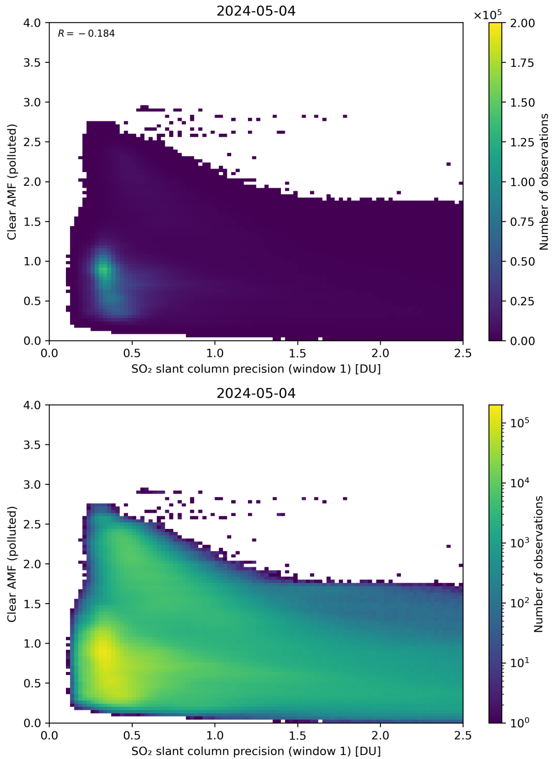
Figure 224: Scatter density plot of “SO 2 slant column precision (window 1)” against “Clear AMF (polluted)” for 2024-05-03 to 2024-05-05.
