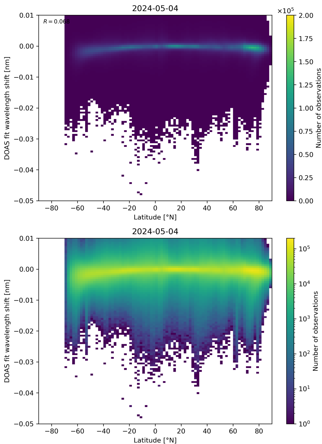
Figure 142: Scatter density plot of “Latitude” against “DOAS fit wavelength shift” for 2024-05-03 to 2024-05-05.
