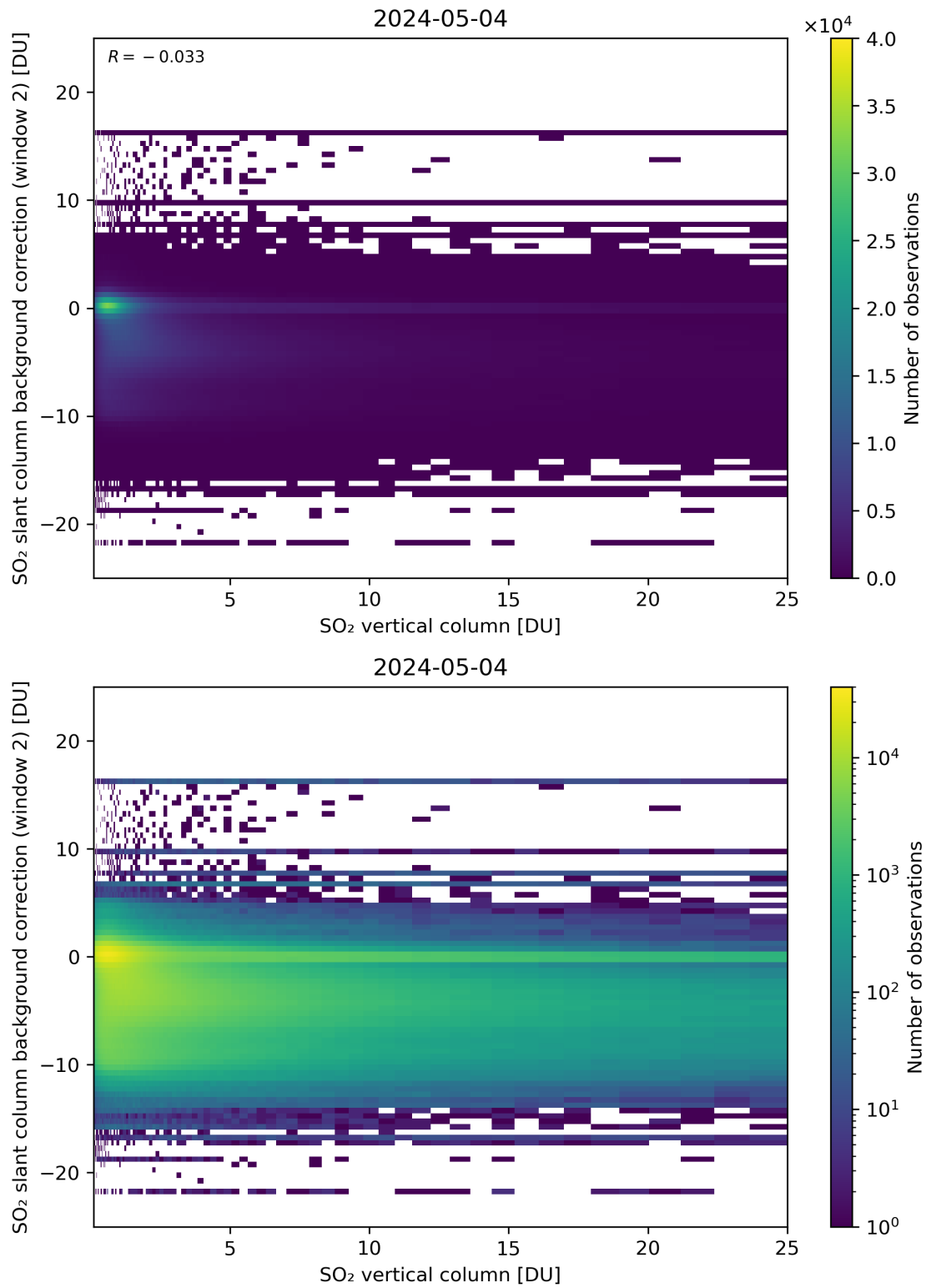
Figure 274: Scatter density plot of “SO 2 vertical column” against “SO 2 slant column background correction (window 2)” for 2024-05-03 to 2024-05-05.
