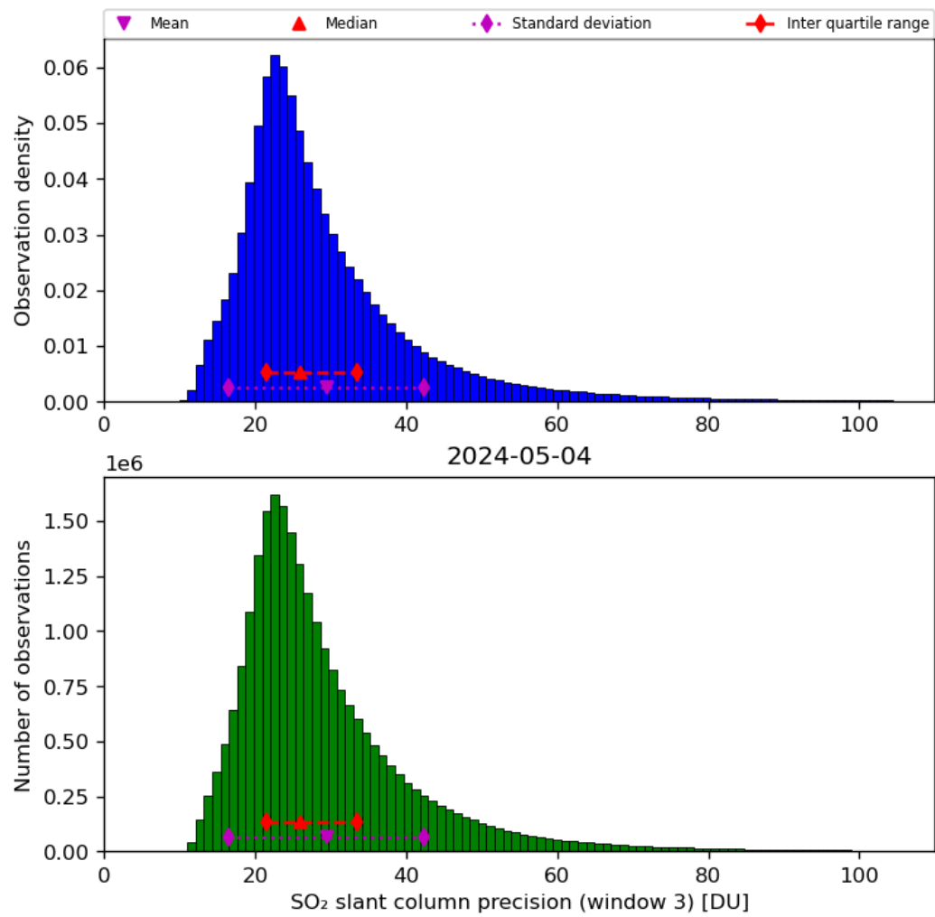
Figure 65: Histogram of “SO 2 slant column precision (window 3)” for 2024-05-03 to 2024-05-05
