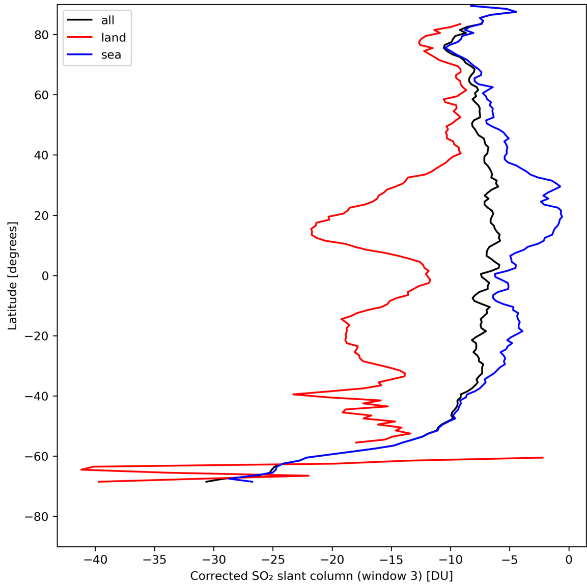
Figure 43: Zonal average of “Corrected SO 2 slant column (window 3)” for 2024-05-03 to 2024-05-05.
