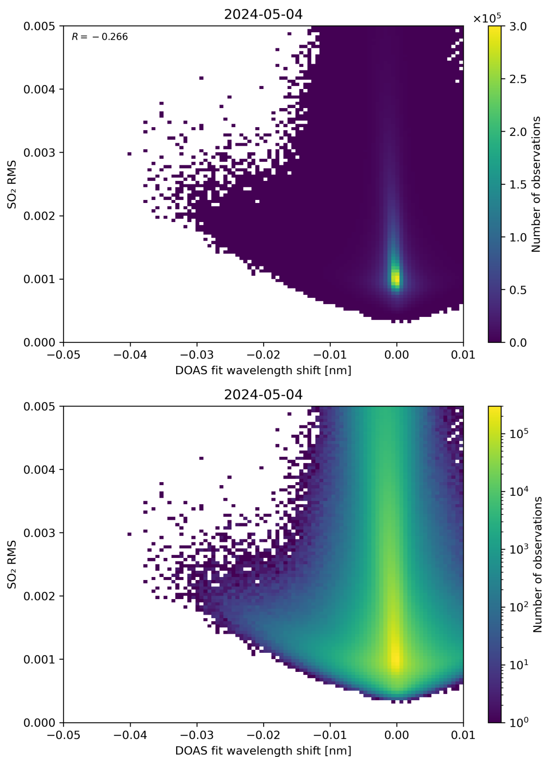
Figure 128: Scatter density plot of “DOAS fit wavelength shift” against “SO 2 RMS” for 2024-05-03 to 2024-05-05.
