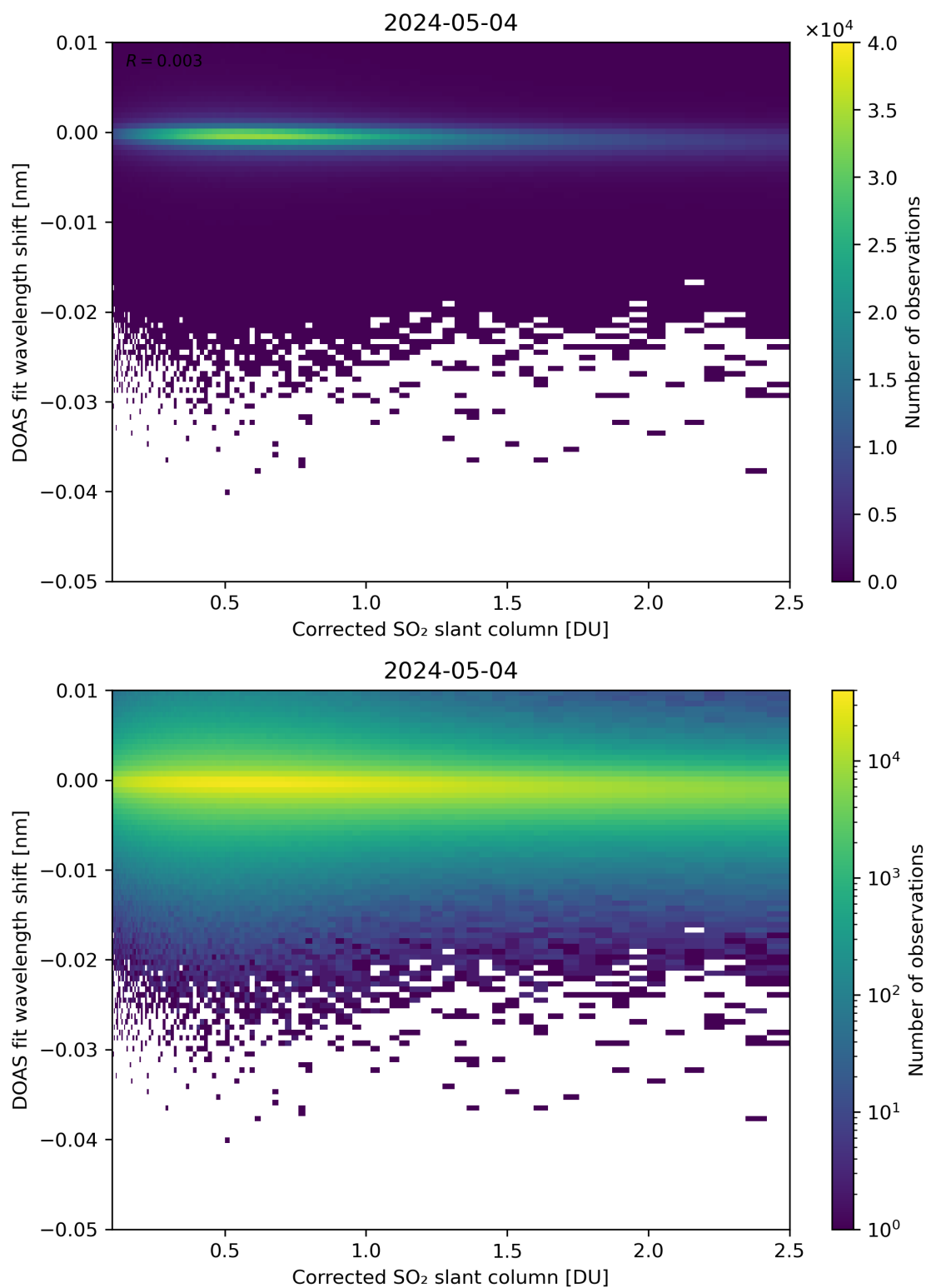
Figure 181: Scatter density plot of “Corrected SO 2 slant column” against “DOAS fit wavelength shift” for 2024-05-03 to 2024-05-05.
