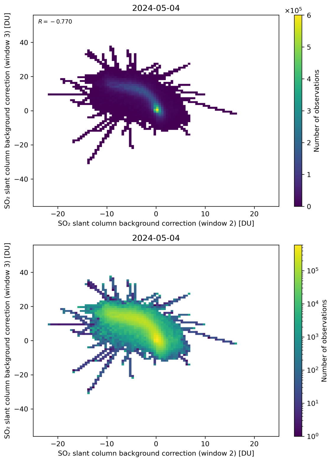
Figure 111: Scatter density plot of “SO 2 slant column background correction (window 2)” against “SO 2 slant column background correction (window 3)” for 2024-05-03 to 2024-05-05.
