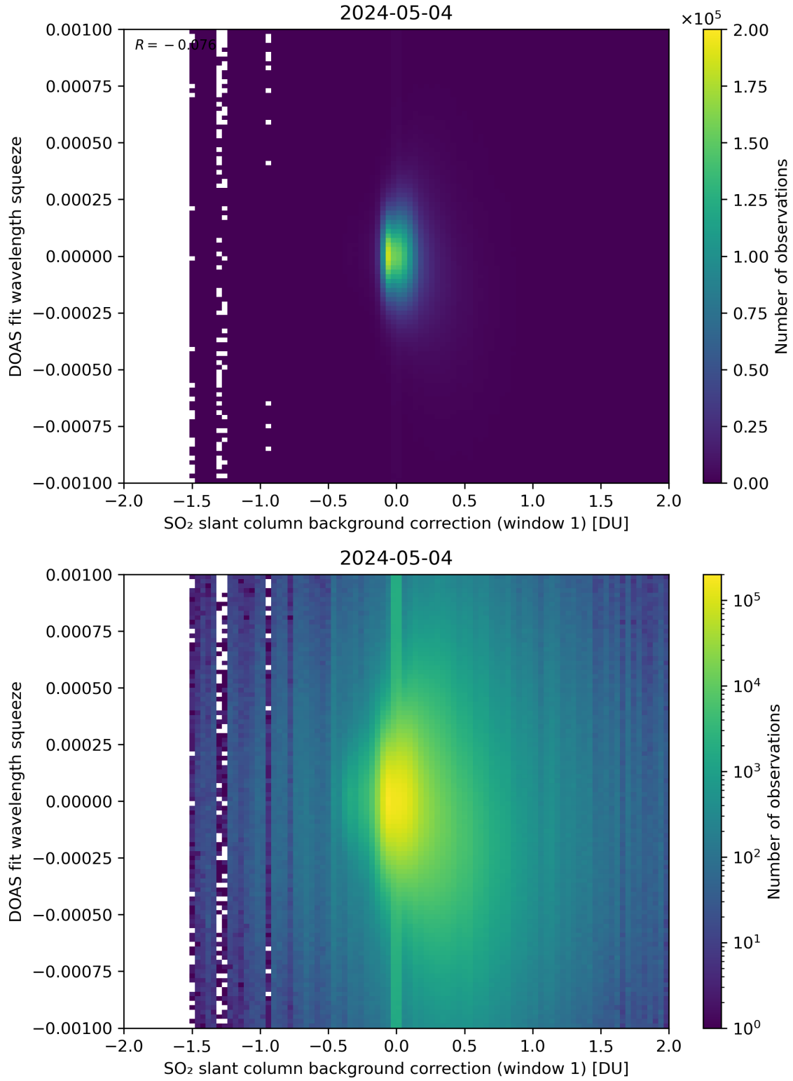
Figure 101: Scatter density plot of “SO 2 slant column background correction (window 1)” against “DOAS fit wavelength squeeze” for 2024-05-03 to 2024-05-05.
