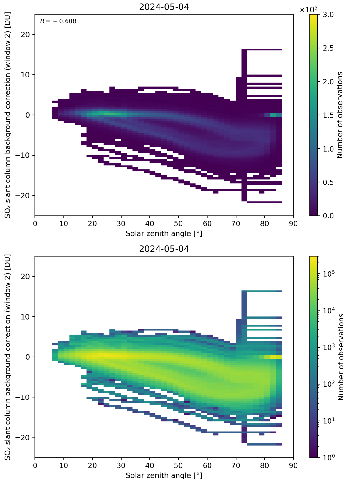
Figure 159: Scatter density plot of “Solar zenith angle” against “SO 2 slant column background correction (window 2)” for 2024-05-03 to 2024-05-05.
