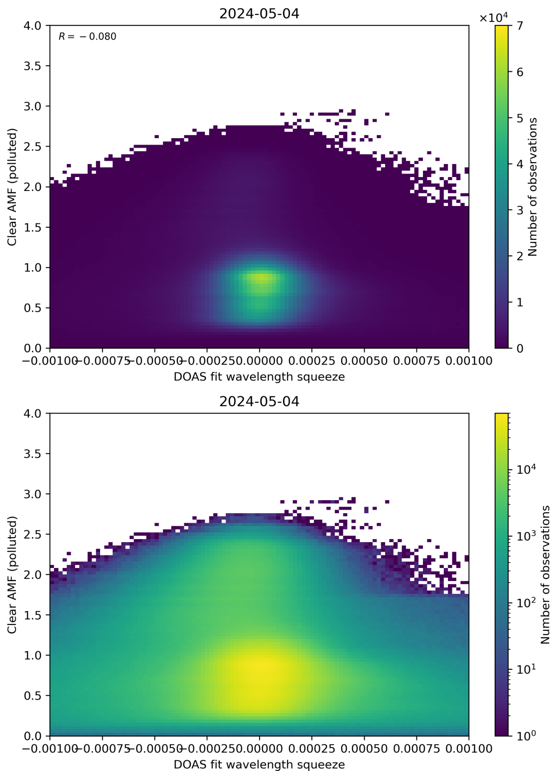
Figure 133: Scatter density plot of “DOAS fit wavelength squeeze” against “Clear AMF (polluted)” for 2024-05-03 to 2024-05-05.
