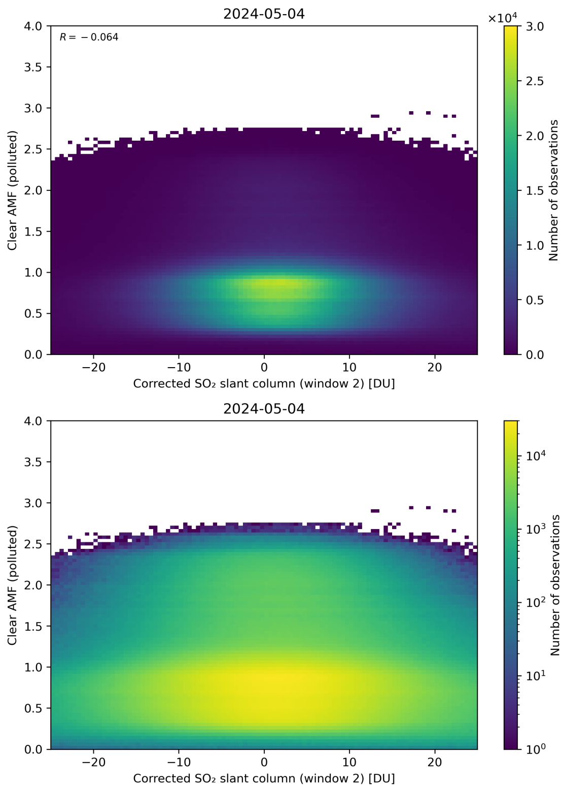
Figure 199: Scatter density plot of “Corrected SO 2 slant column (window 2)” against “Clear AMF (polluted)” for 2024-05-03 to 2024-05-05.
