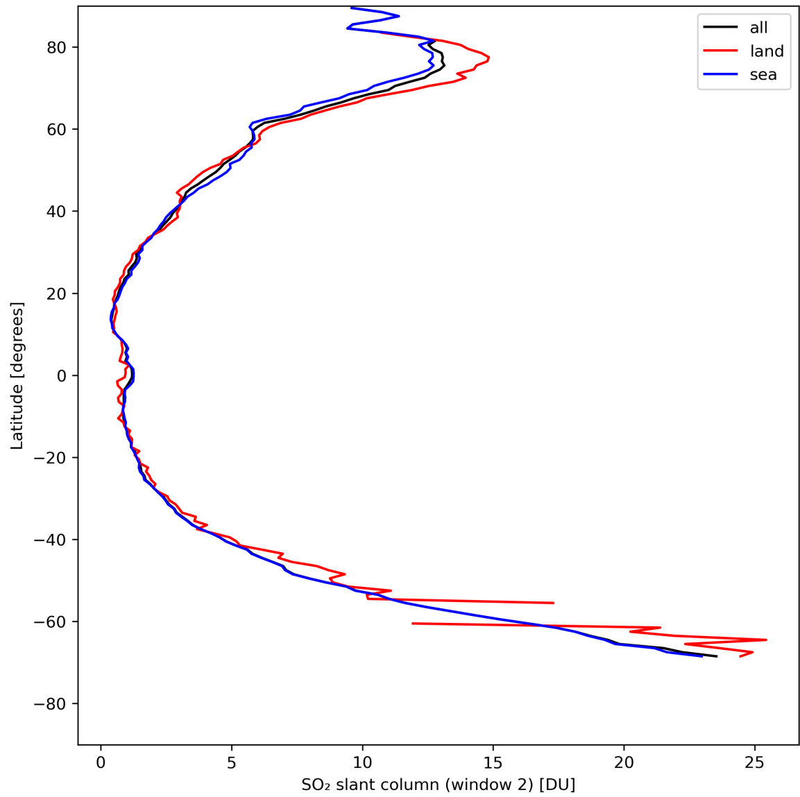
Figure 37: Zonal average of “SO 2 slant column (window 2)” for 2024-05-03 to 2024-05-05.
