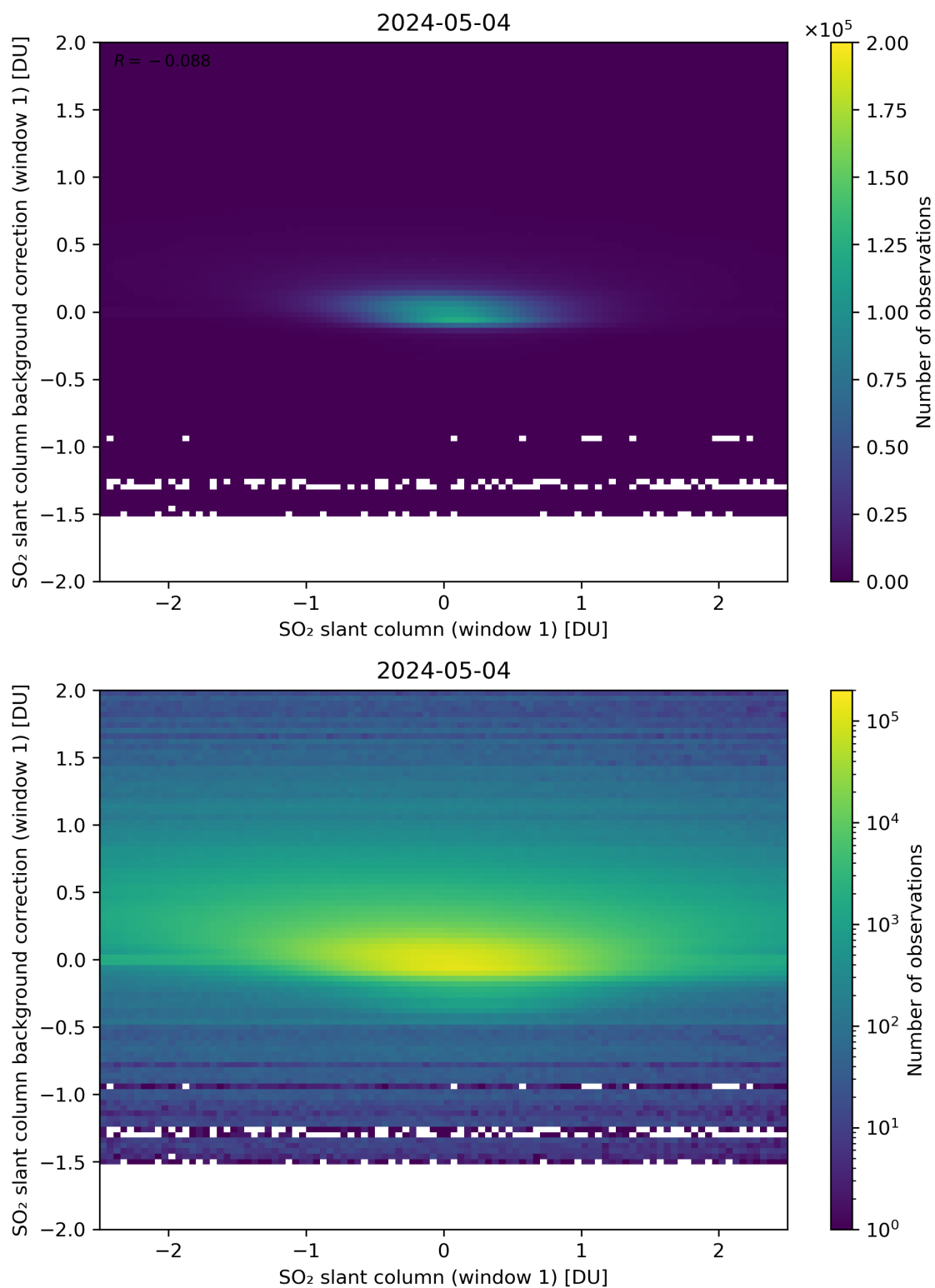
Figure 212: Scatter density plot of “SO 2 slant column (window 1)” against “SO 2 slant column background correction (window 1)” for 2024-05-03 to 2024-05-05.
