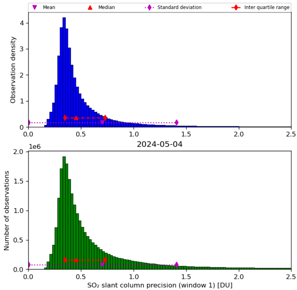
Figure 57: Histogram of “SO 2 slant column precision (window 1)” for 2024-05-03 to 2024-05-05
