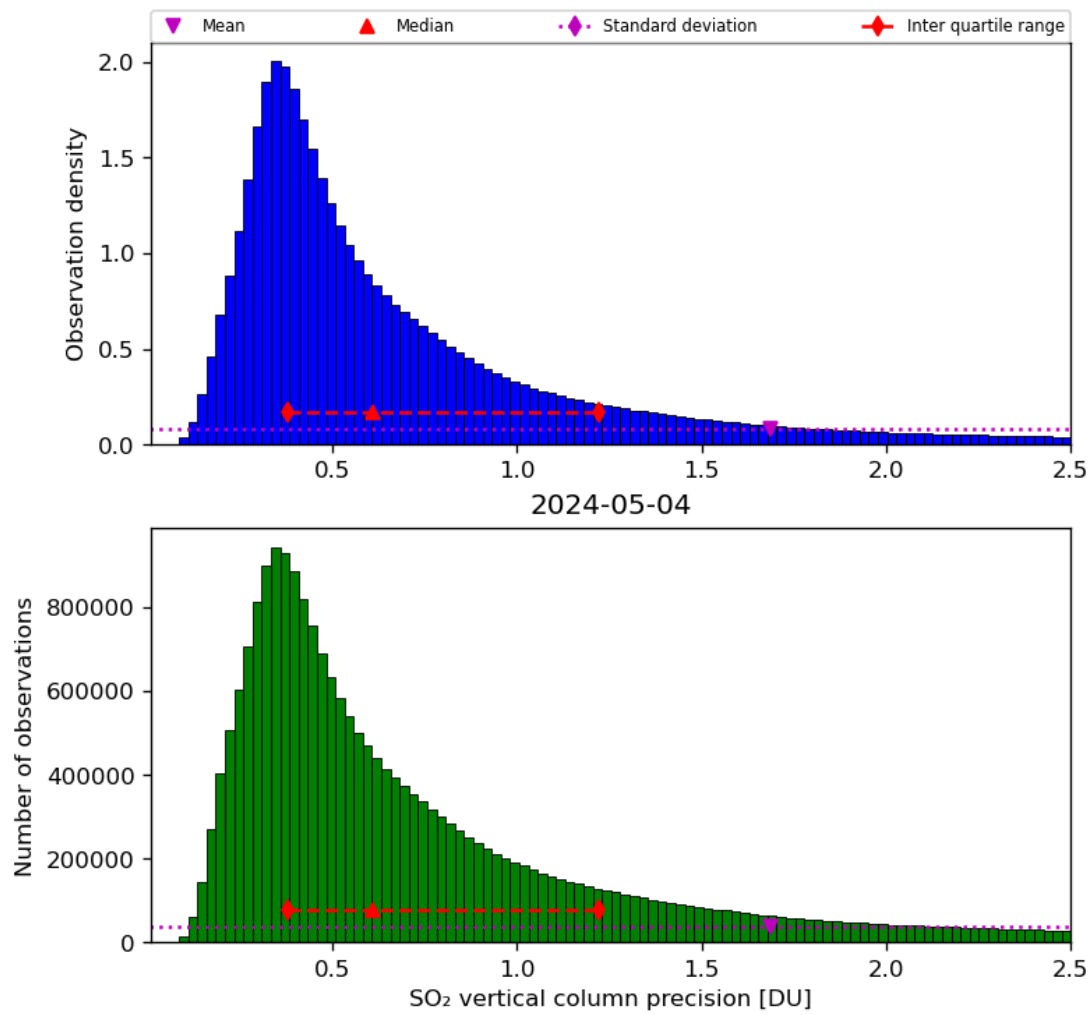
Figure 54: Histogram of “SO 2 vertical column precision” for 2024-05-03 to 2024-05-05
