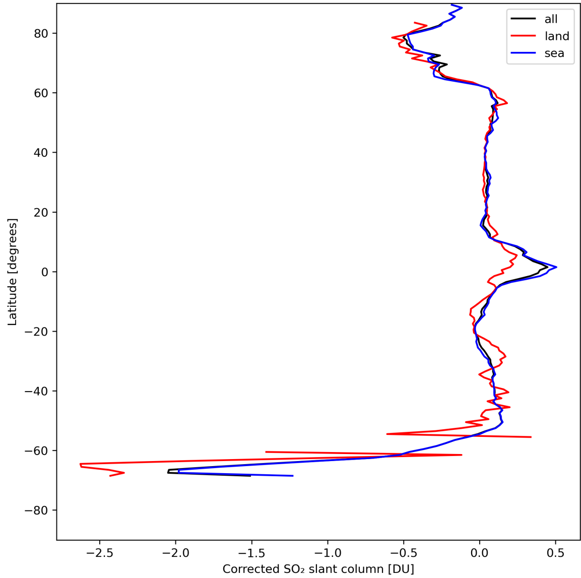
Figure 32: Zonal average of “Corrected SO 2 slant column” for 2024-05-03 to 2024-05-05.
