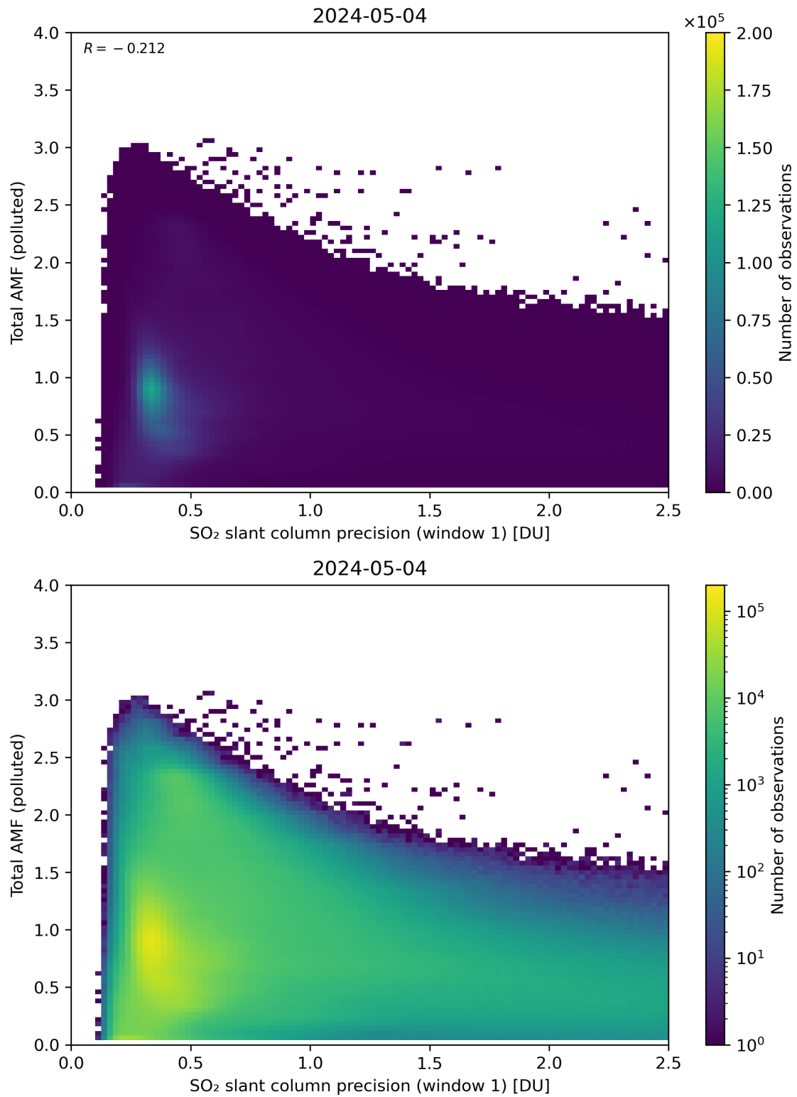
Figure 230: Scatter density plot of “SO 2 slant column precision (window 1)” against “Total AMF (polluted)” for 2024-05-03 to 2024-05-05.
