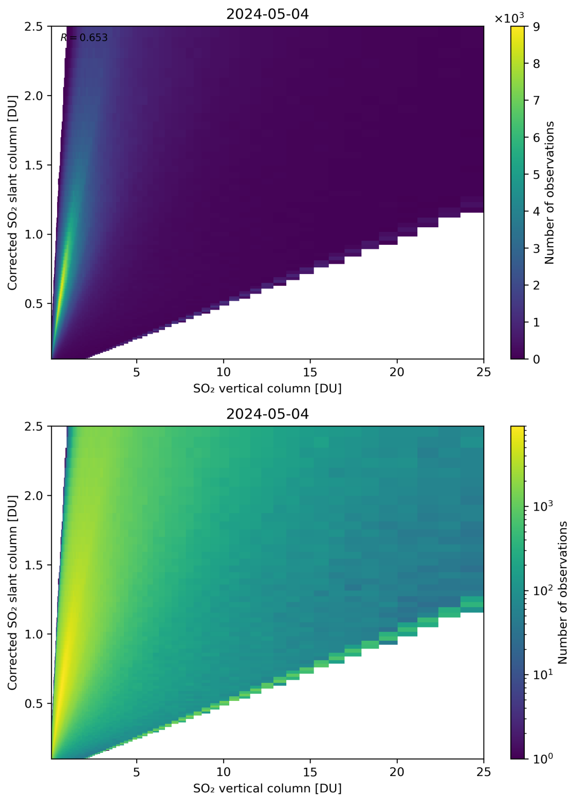
Figure 297: Scatter density plot of “SO 2 vertical column” against “Corrected SO 2 slant column” for 2024-05-03 to 2024-05-05.
