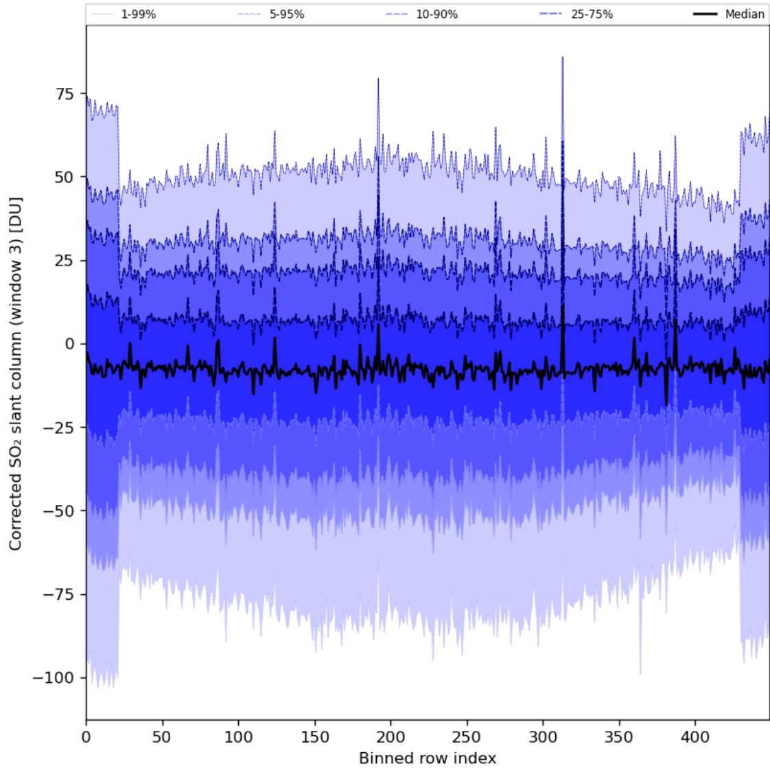
Figure 89: Along track statistics of “Corrected SO 2 slant column (window 3)” for 2024-05-03 to 2024-05-05
