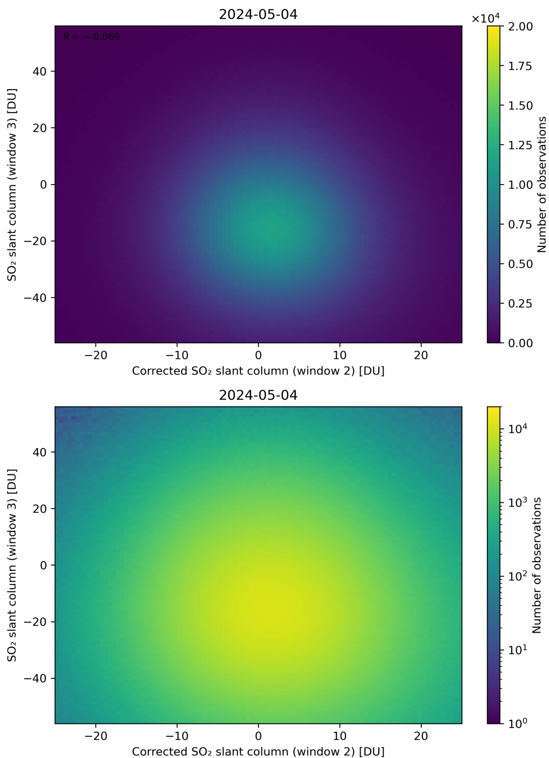
Figure 201: Scatter density plot of “Corrected SO 2 slant column (window 2)” against “SO 2 slant column (window 3)” for 2024-05-03 to 2024-05-05.
