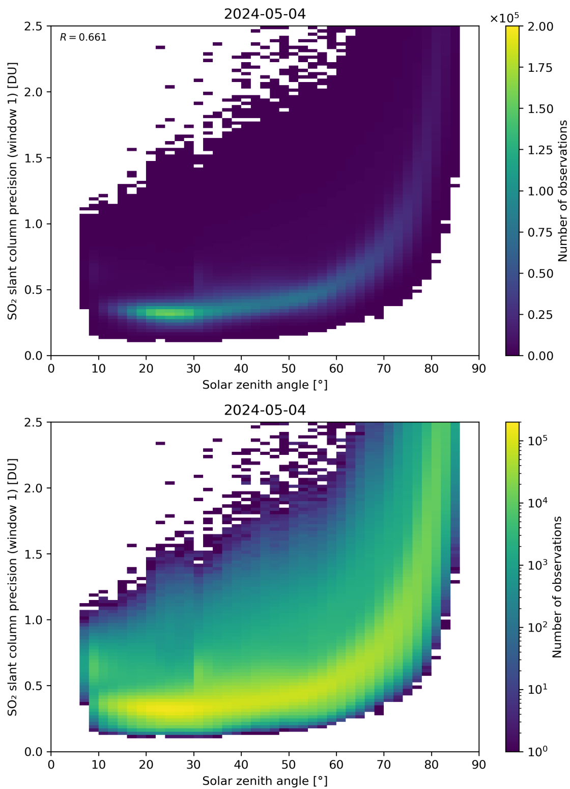
Figure 170: Scatter density plot of “Solar zenith angle” against “SO 2 slant column precision (window 1)” for 2024-05-03 to 2024-05-05.
