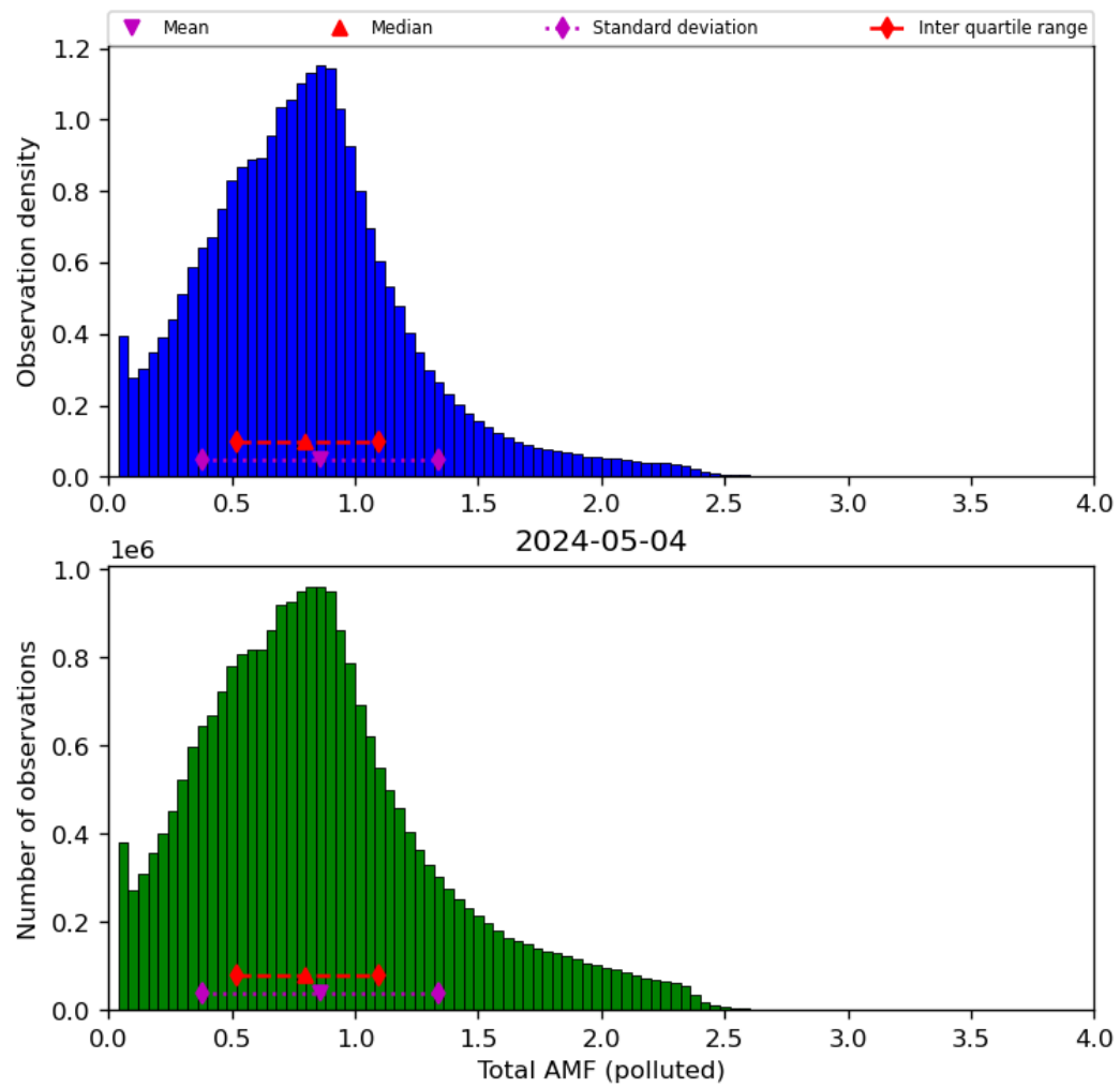
Figure 71: Histogram of “Total AMF (polluted)” for 2024-05-03 to 2024-05-05
