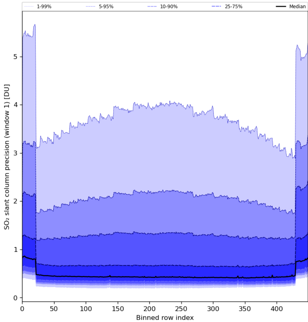
Figure 80: Along track statistics of “SO 2 slant column precision (window 1)” for 2024-05-03 to 2024-05-05
