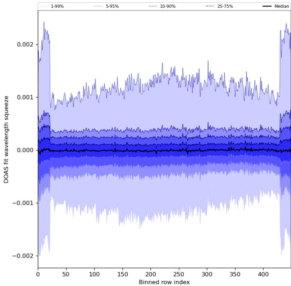
Figure 92: Along track statistics of “DOAS fit wavelength squeeze” for 2024-05-03 to 2024-05-05
