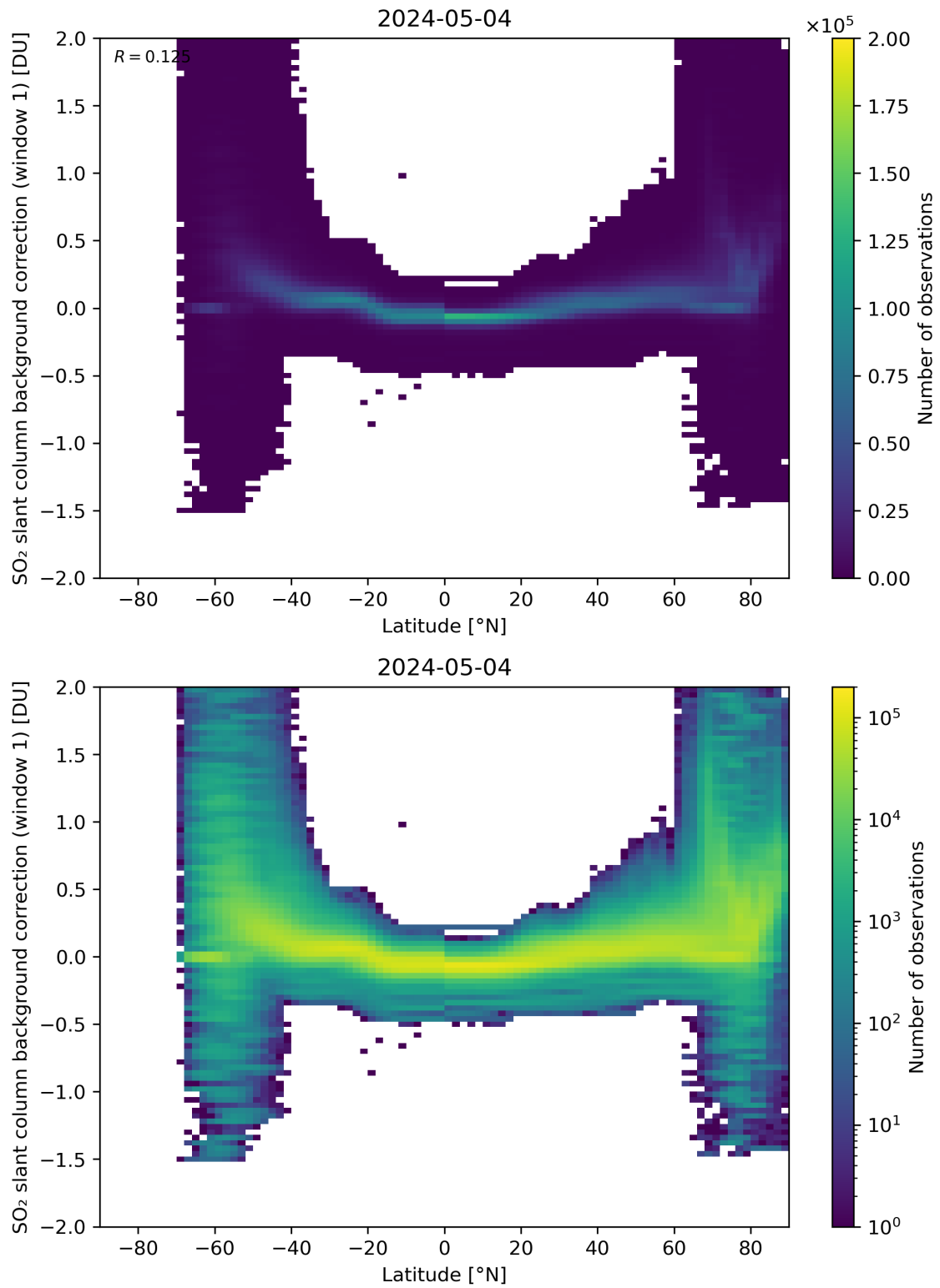
Figure 139: Scatter density plot of “Latitude” against “SO 2 slant column background correction (window 1)” for 2024-05-03 to 2024-05-05.
