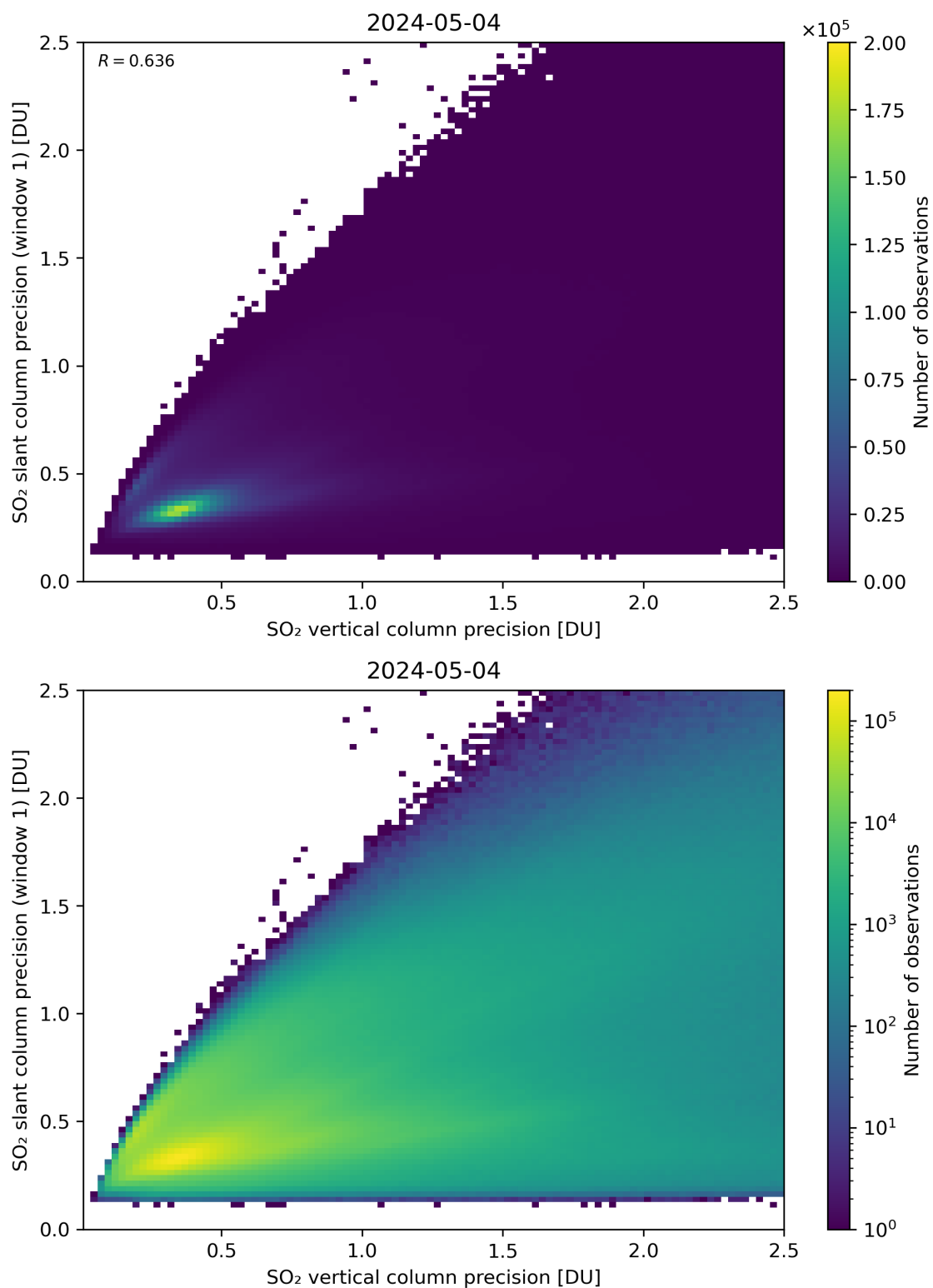
Figure 290: Scatter density plot of “SO 2 vertical column precision” against “SO 2 slant column precision (window 1)” for 2024-05-03 to 2024-05-05.
