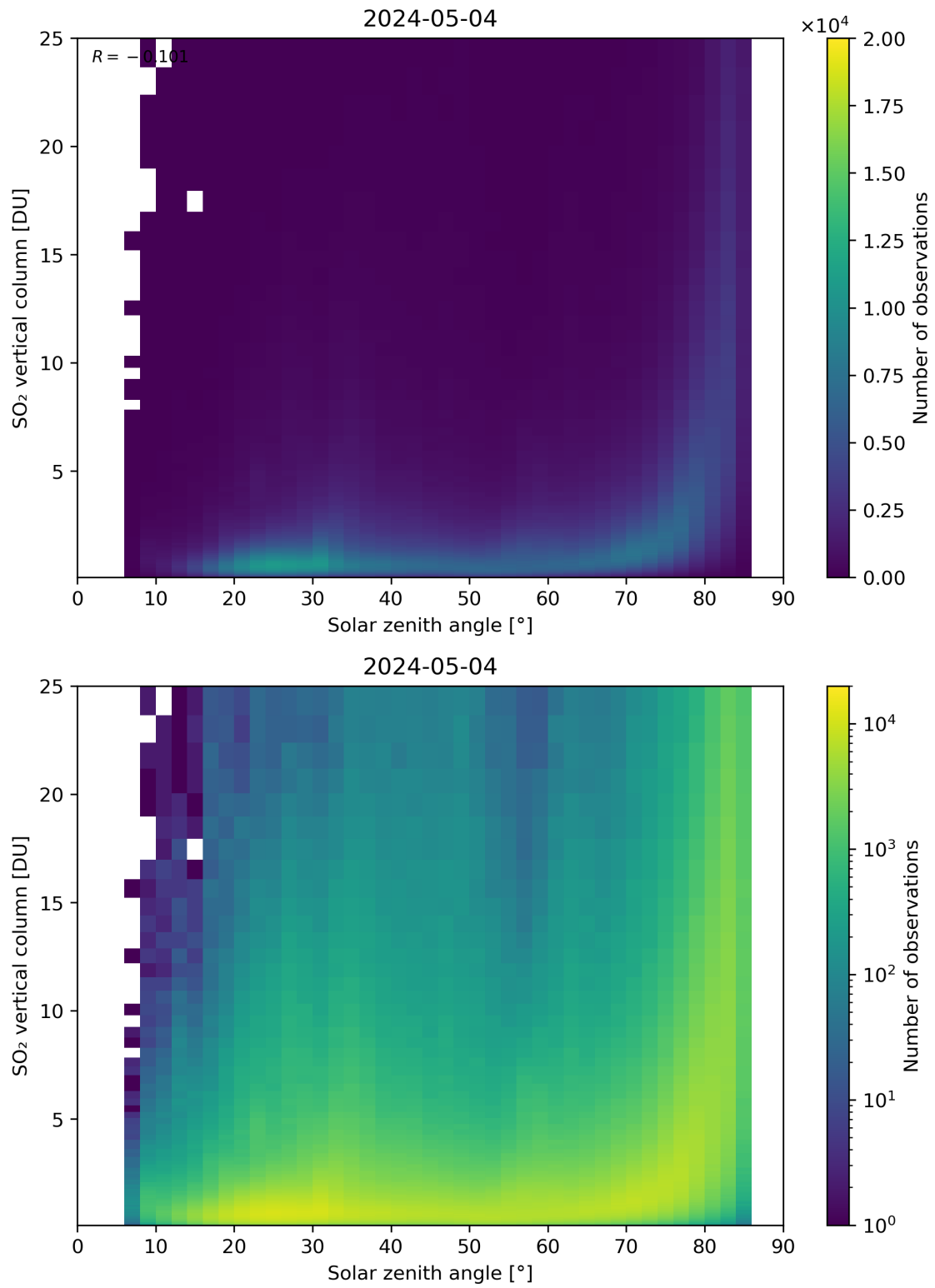
Figure 176: Scatter density plot of “Solar zenith angle” against “SO 2 vertical column” for 2024-05-03 to 2024-05-05.
