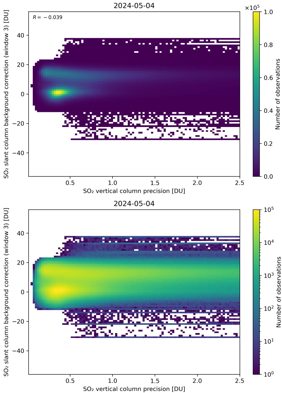
Figure 281: Scatter density plot of “SO 2 vertical column precision” against “SO 2 slant column background correction (window 3)” for 2024-05-03 to 2024-05-05.
