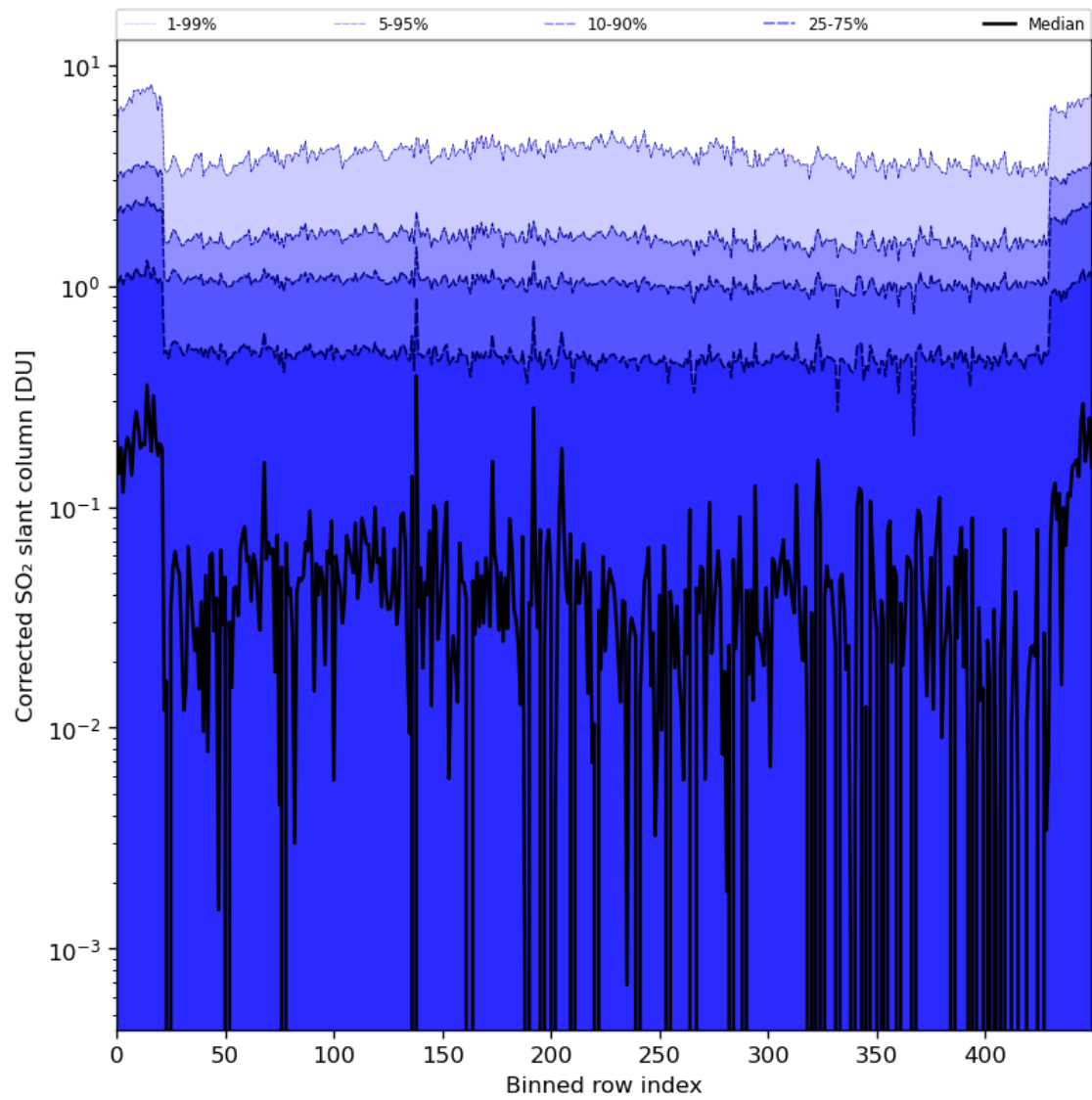
Figure 78: Along track statistics of “Corrected SO 2 slant column” for 2024-05-03 to 2024-05-05
