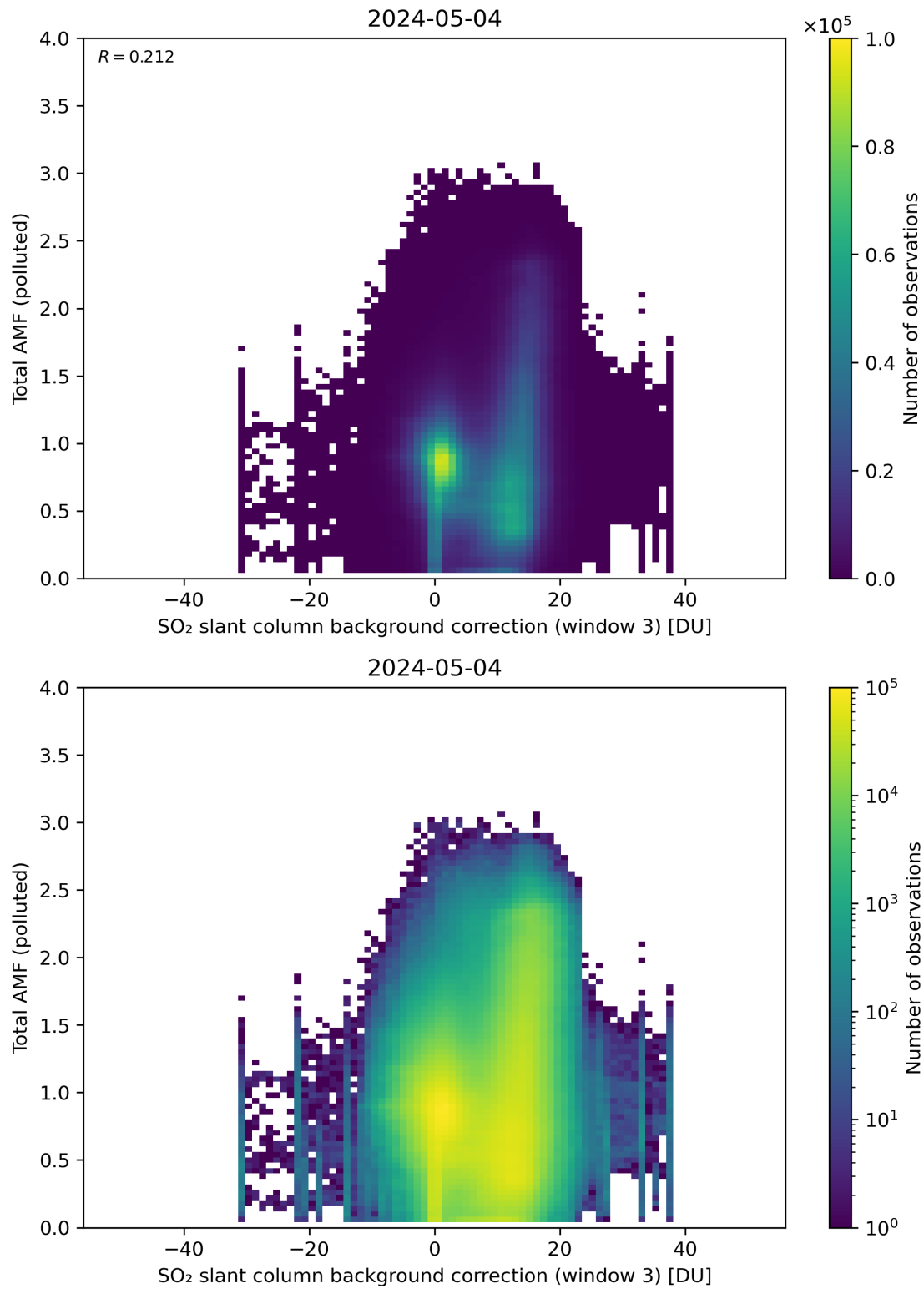
Figure 125: Scatter density plot of “SO 2 slant column background correction (window 3)” against “Total AMF (polluted)” for 2024-05-03 to 2024-05-05.
