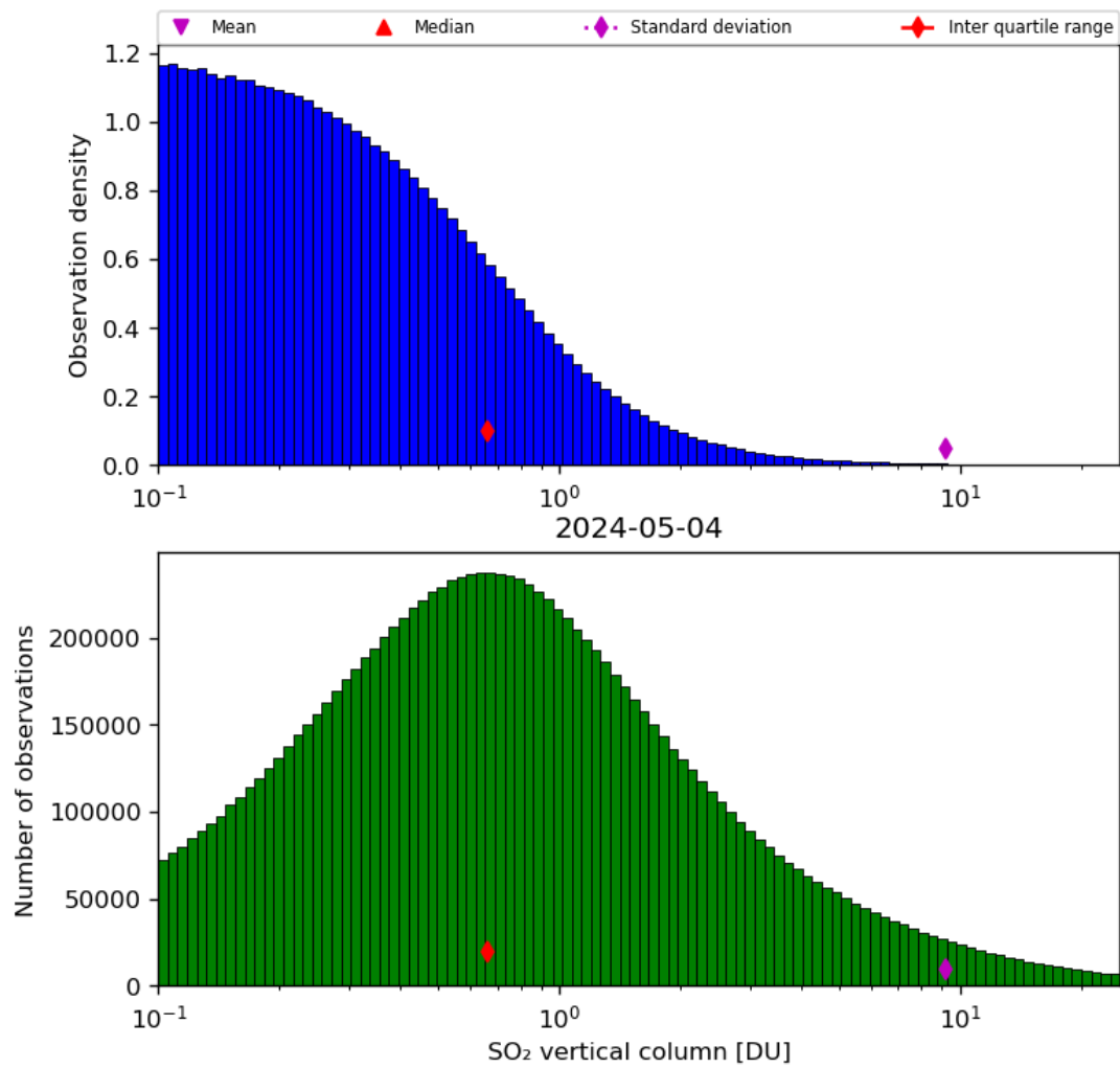
Figure 53: Histogram of “SO 2 vertical column” for 2024-05-03 to 2024-05-05
