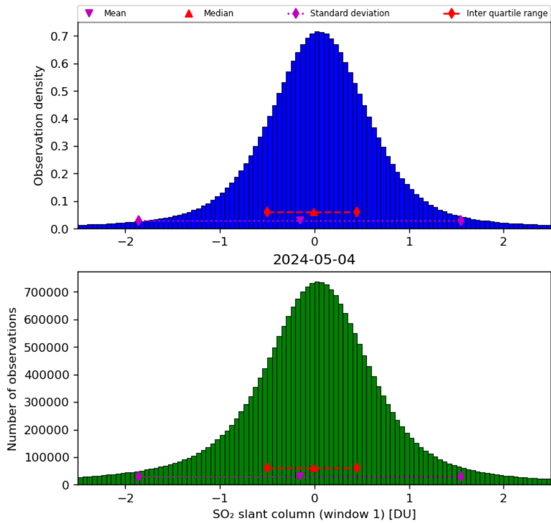
Figure 56: Histogram of “SO 2 slant column (window 1)” for 2024-05-03 to 2024-05-05
