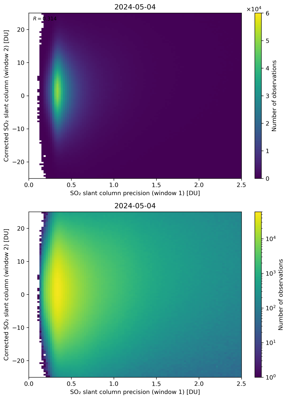
Figure 225: Scatter density plot of “SO 2 slant column precision (window 1)” against “Corrected SO 2 slant column (window 2)” for 2024-05-03 to 2024-05-05.
