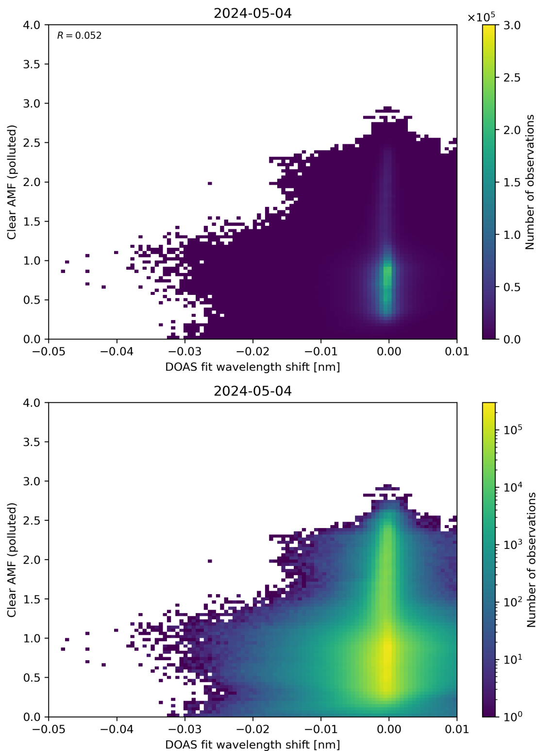
Figure 129: Scatter density plot of “DOAS fit wavelength shift” against “Clear AMF (polluted)” for 2024-05-03 to 2024-05-05.
