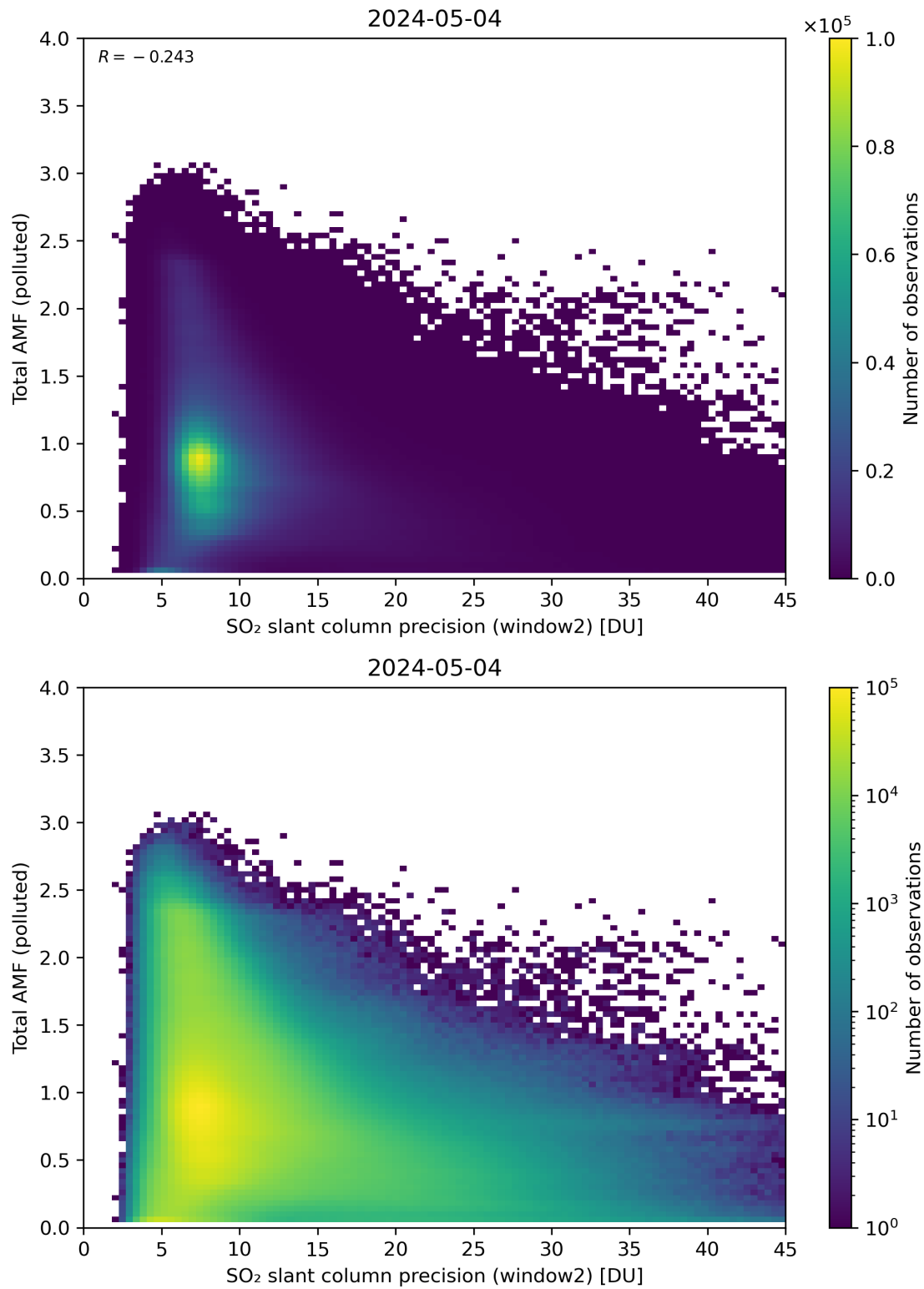
Figure 251: Scatter density plot of “SO 2 slant column precision (window2)” against “Total AMF (polluted)” for 2024-05-03 to 2024-05-05.
