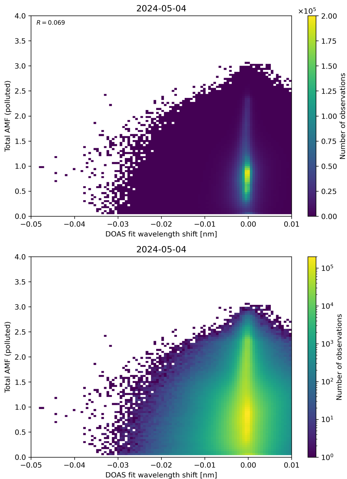
Figure 130: Scatter density plot of “DOAS fit wavelength shift” against “Total AMF (polluted)” for 2024-05-03 to 2024-05-05.
