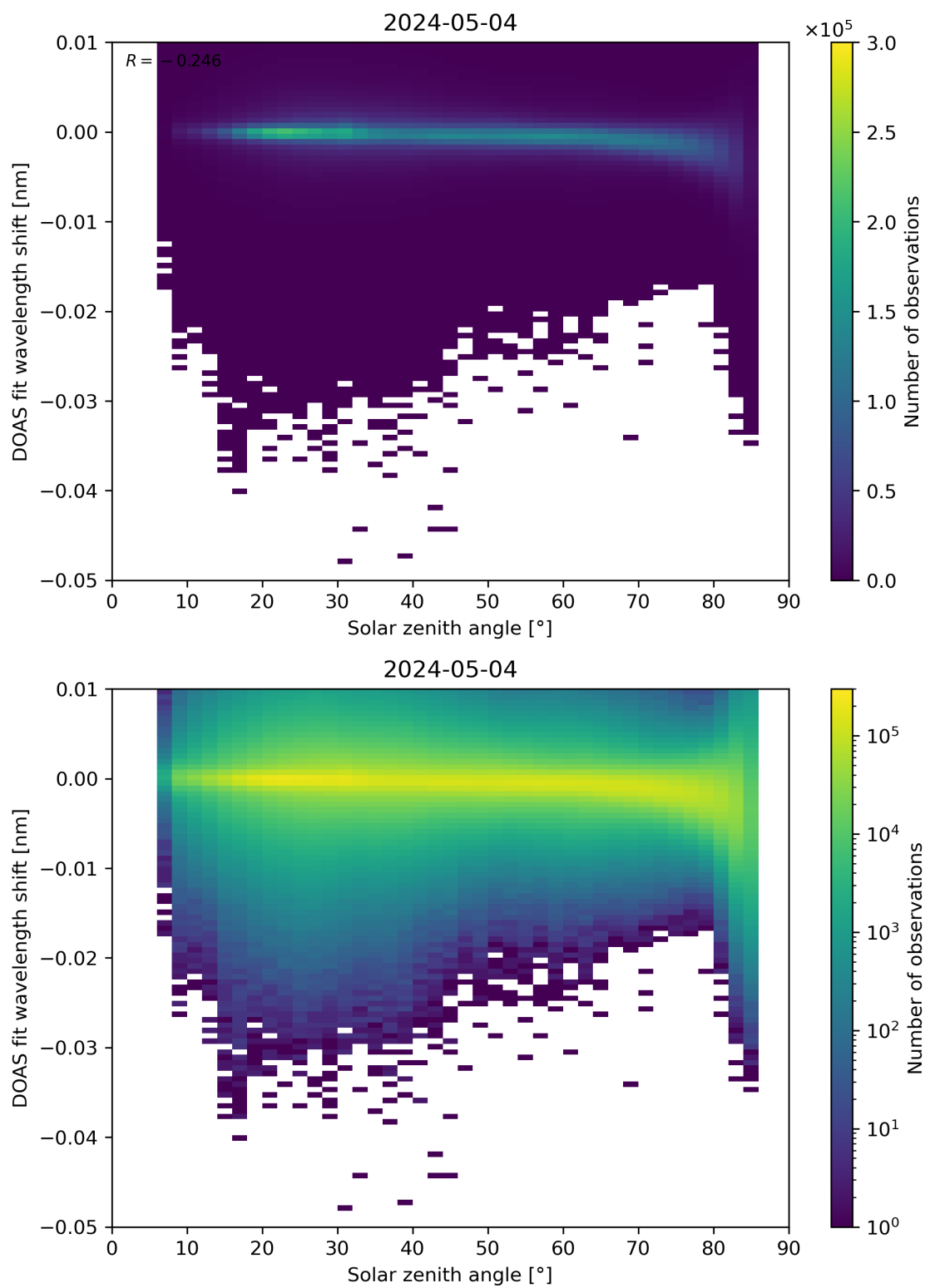
Figure 161: Scatter density plot of “Solar zenith angle” against “DOAS fit wavelength shift” for 2024-05-03 to 2024-05-05.
