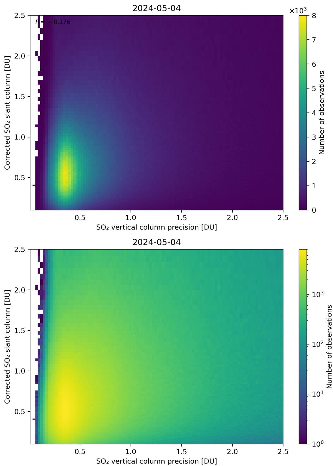
Figure 286: Scatter density plot of “SO 2 vertical column precision” against “Corrected SO 2 slant column” for 2024-05-03 to 2024-05-05.
