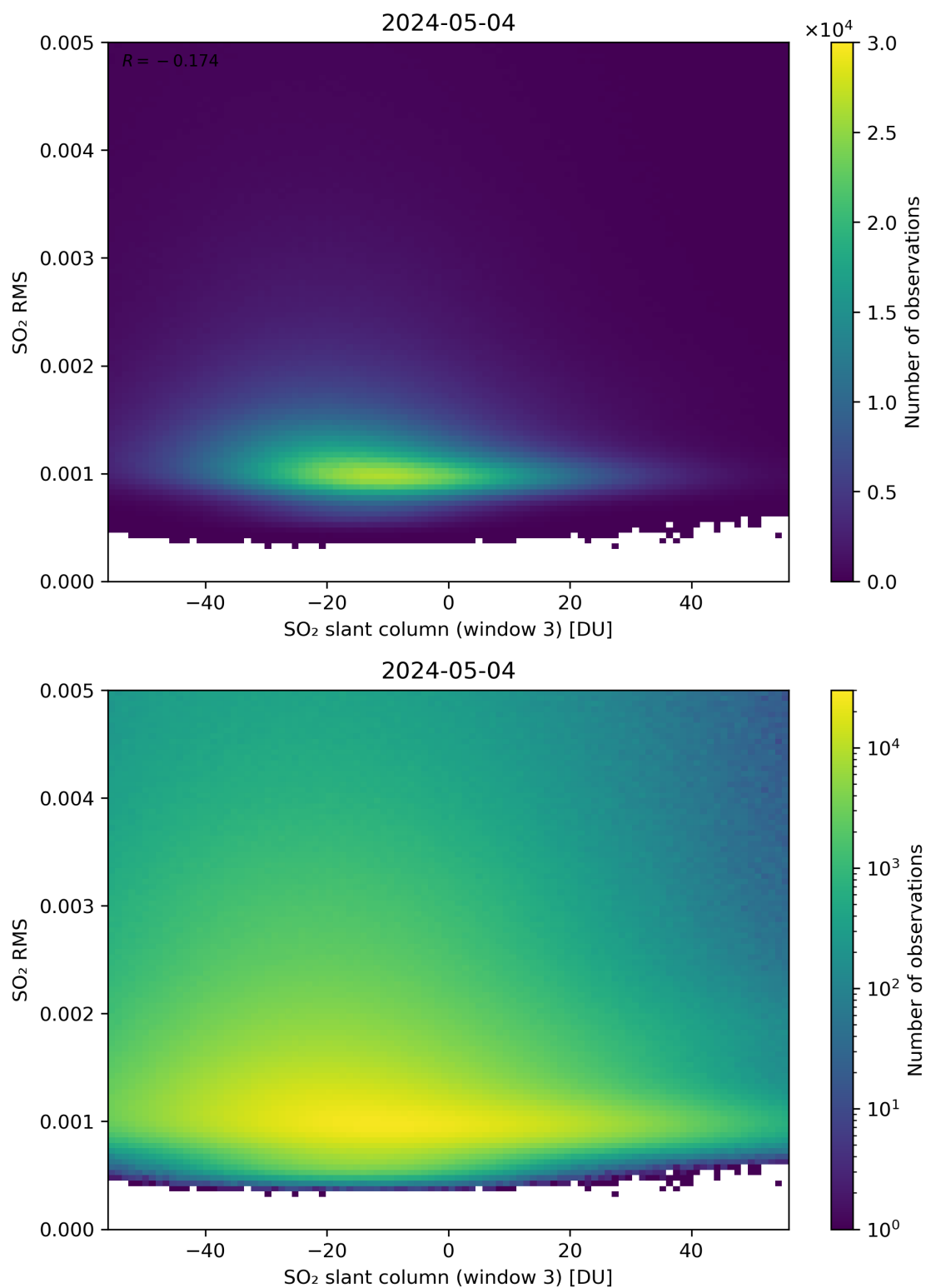
Figure 256: Scatter density plot of “SO 2 slant column (window 3)” against “SO 2 RMS” for 2024-05-03 to 2024-05-05.
