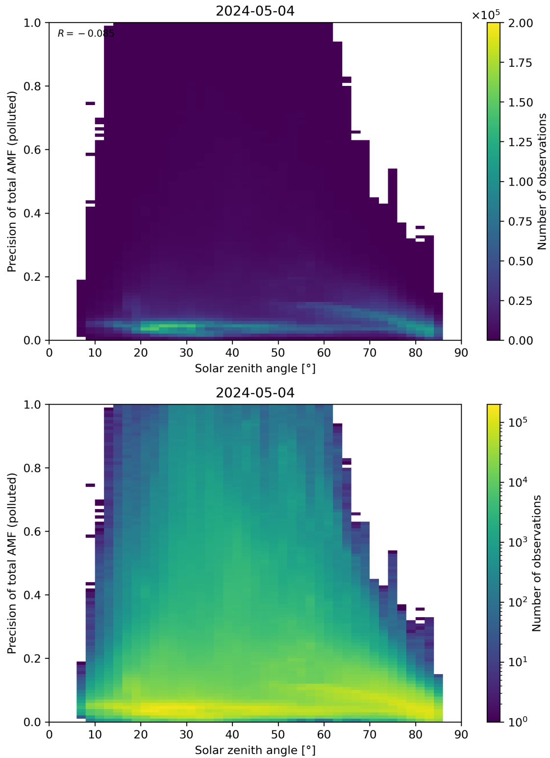
Figure 175: Scatter density plot of “Solar zenith angle” against “Precision of total AMF (polluted)” for 2024-05-03 to 2024-05-05.
