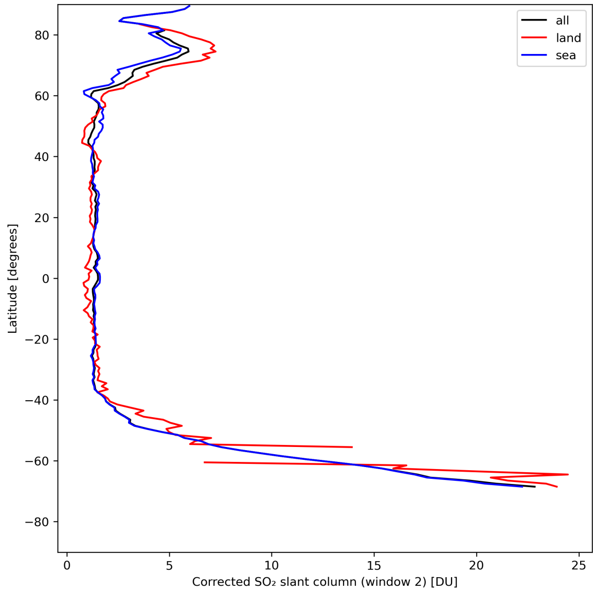
Figure 39: Zonal average of “Corrected SO 2 slant column (window 2)” for 2024-05-03 to 2024-05-05.
