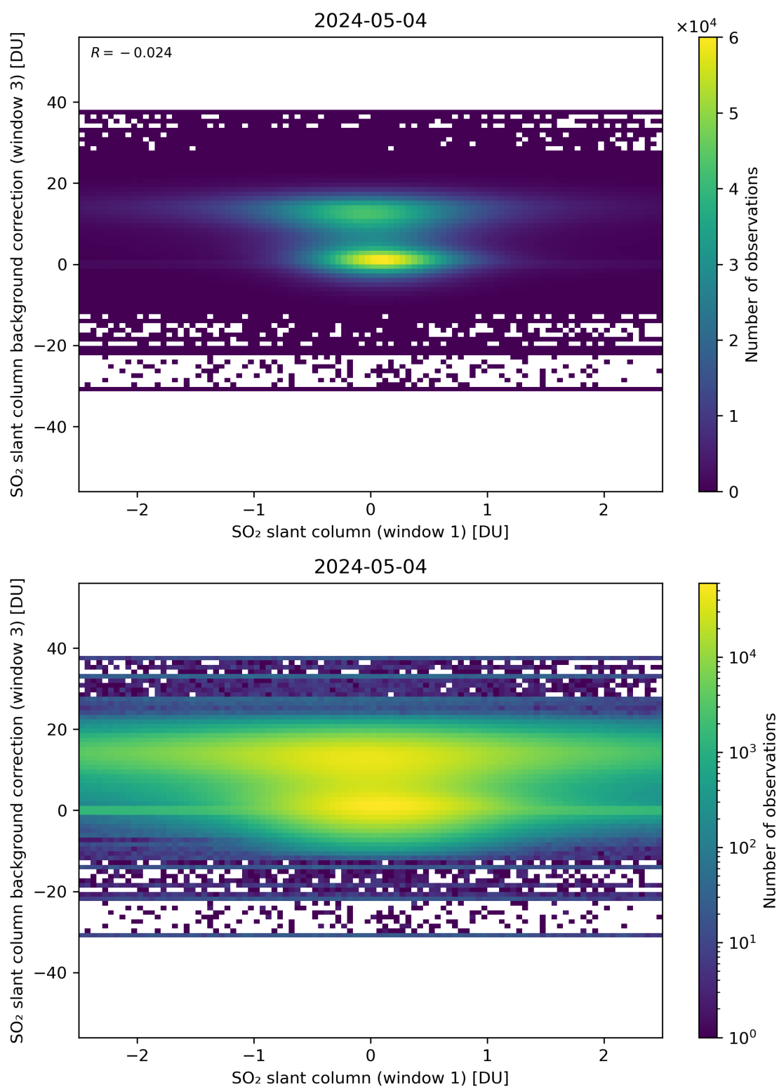
Figure 214: Scatter density plot of “SO 2 slant column (window 1)” against “SO 2 slant column background correction (window 3)” for 2024-05-03 to 2024-05-05.
