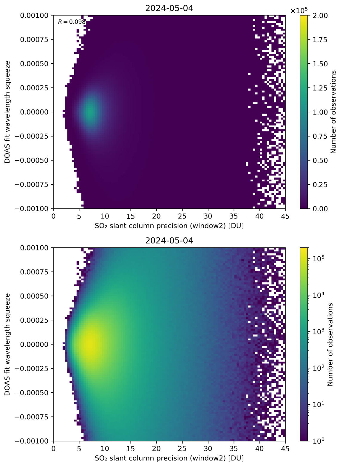
Figure 244: Scatter density plot of “SO 2 slant column precision (window2)” against “DOAS fit wavelength squeeze” for 2024-05-03 to 2024-05-05.
