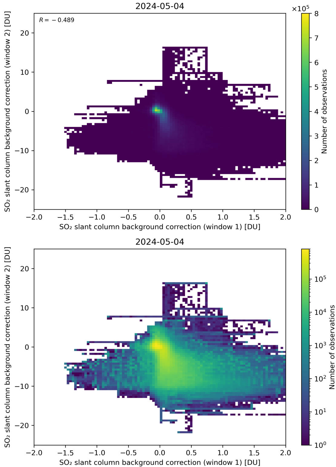
Figure 98: Scatter density plot of “SO 2 slant column background correction (window 1)” against “SO 2 slant column background correction (window 2)” for 2024-05-03 to 2024-05-05.
