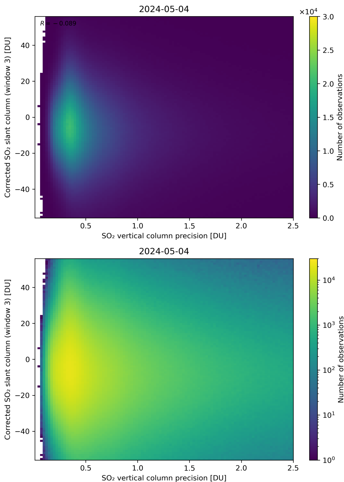
Figure 288: Scatter density plot of “SO 2 vertical column precision” against “Corrected SO 2 slant column (window 3)” for 2024-05-03 to 2024-05-05.
