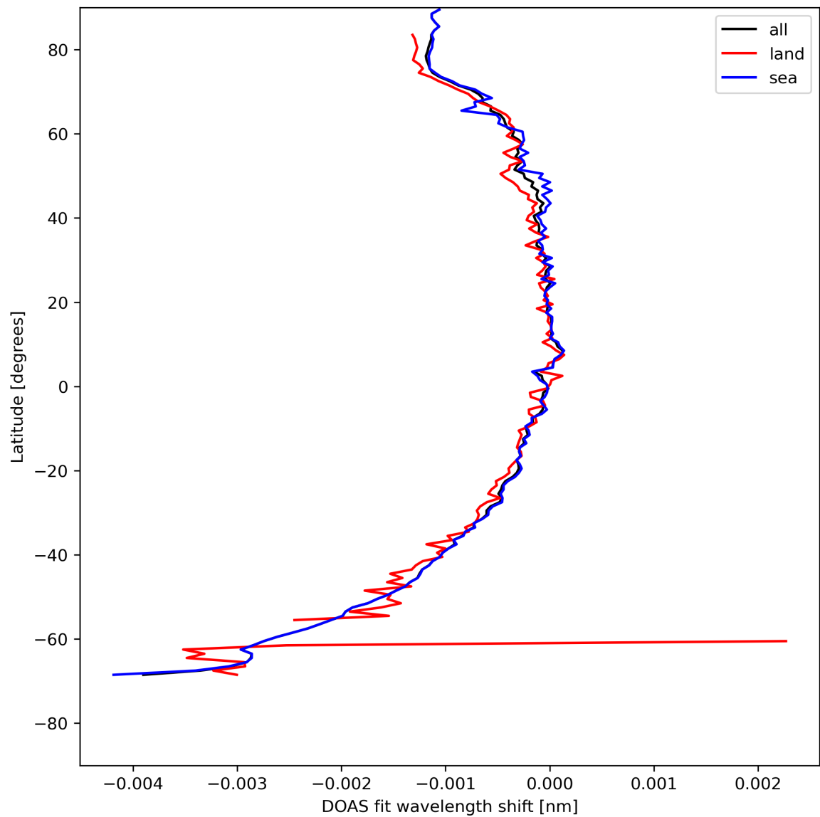
Figure 45: Zonal average of “DOAS fit wavelength shift” for 2024-05-03 to 2024-05-05.
