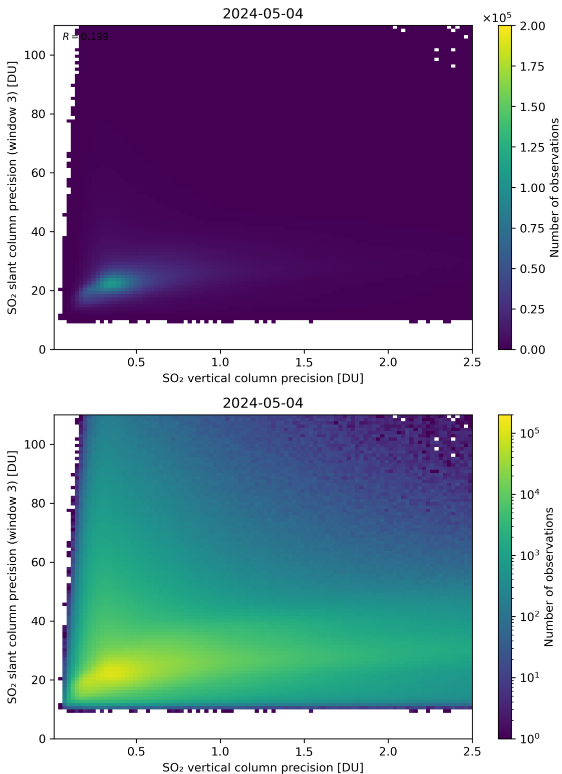
Figure 293: Scatter density plot of “SO 2 vertical column precision” against “SO 2 slant column precision (window 3)” for 2024-05-03 to 2024-05-05.
