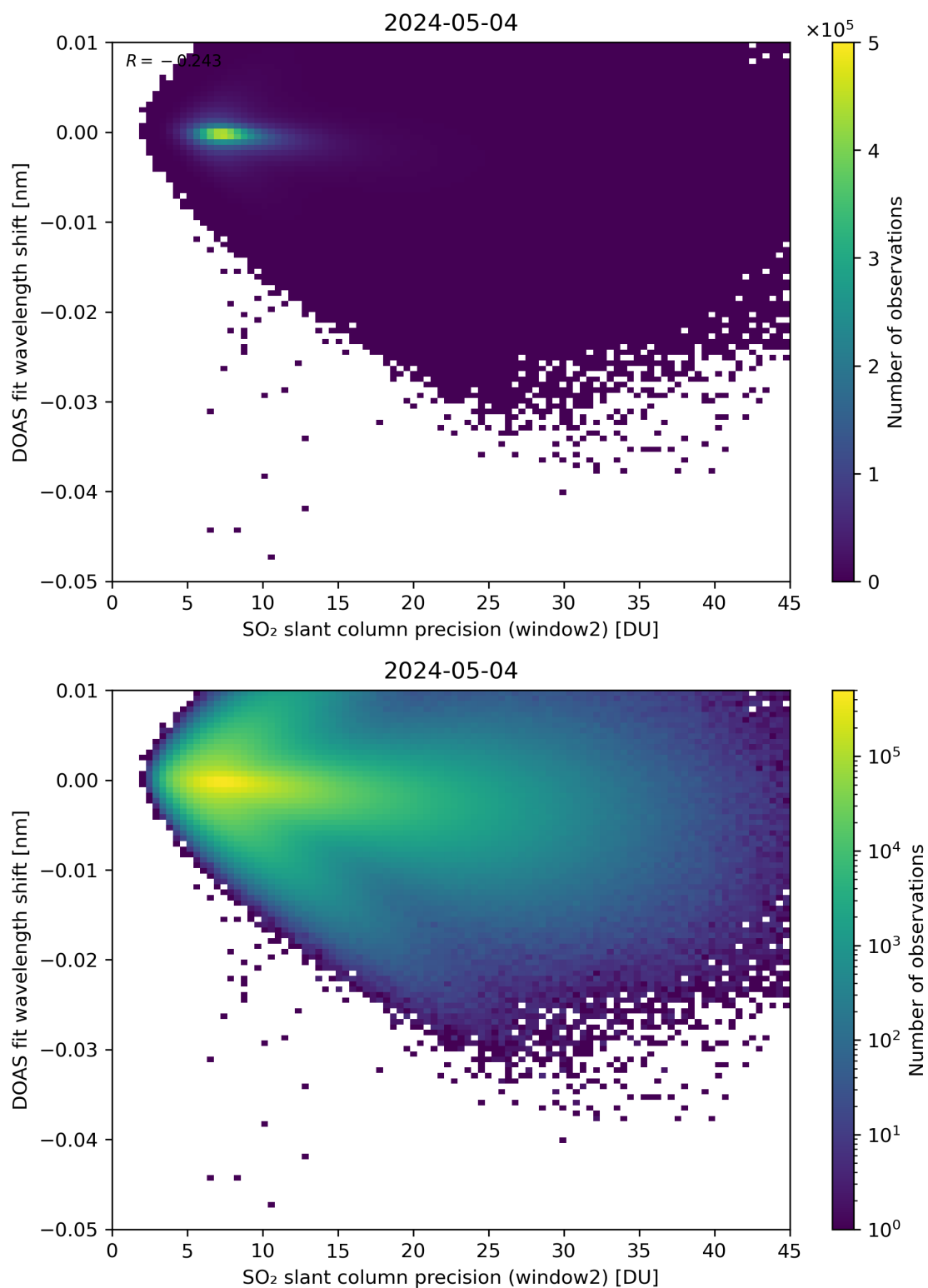
Figure 243: Scatter density plot of “SO 2 slant column precision (window2)” against “DOAS fit wavelength shift” for 2024-05-03 to 2024-05-05.
