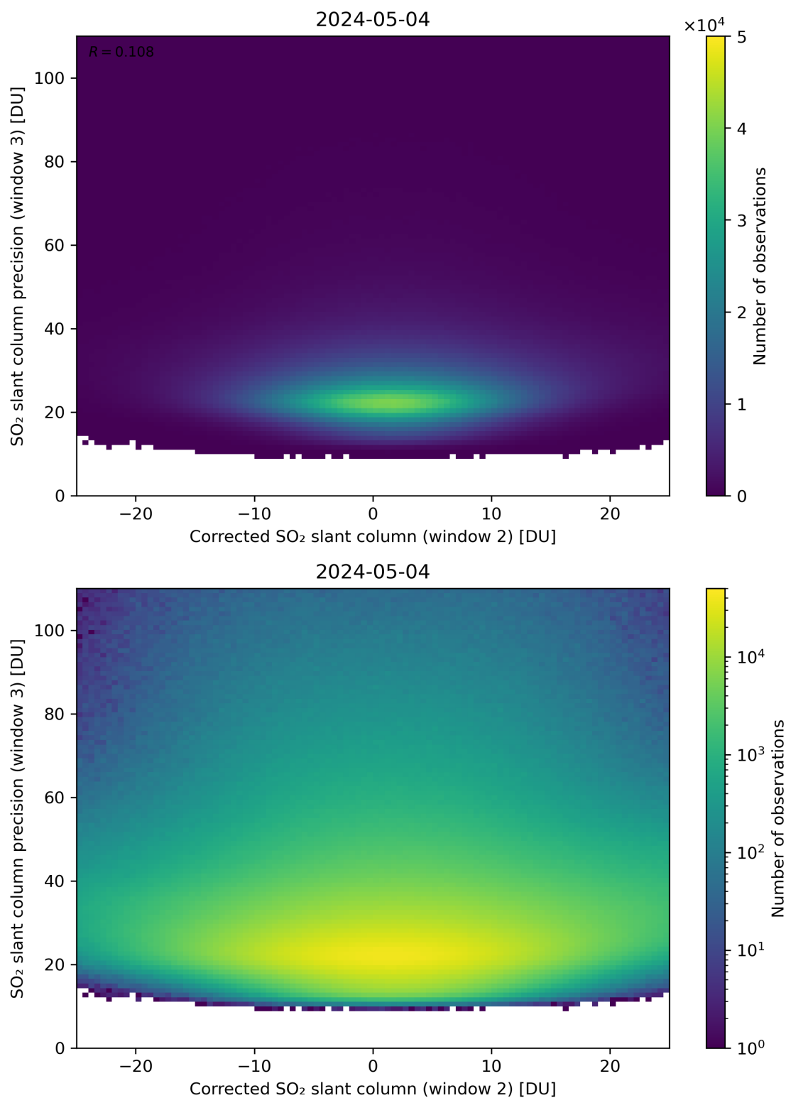
Figure 202: Scatter density plot of “Corrected SO 2 slant column (window 2)” against “SO 2 slant column precision (window 3)” for 2024-05-03 to 2024-05-05.
