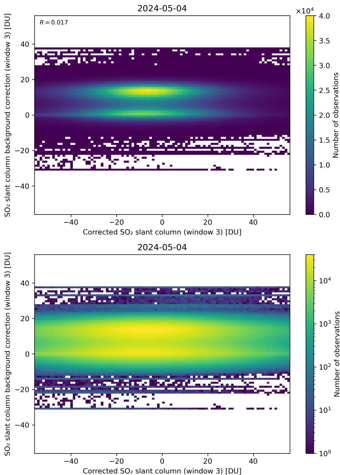
Figure 205: Scatter density plot of “Corrected SO 2 slant column (window 3)” against “SO 2 slant column background correction (window 3)” for 2024-05-03 to 2024-05-05.
