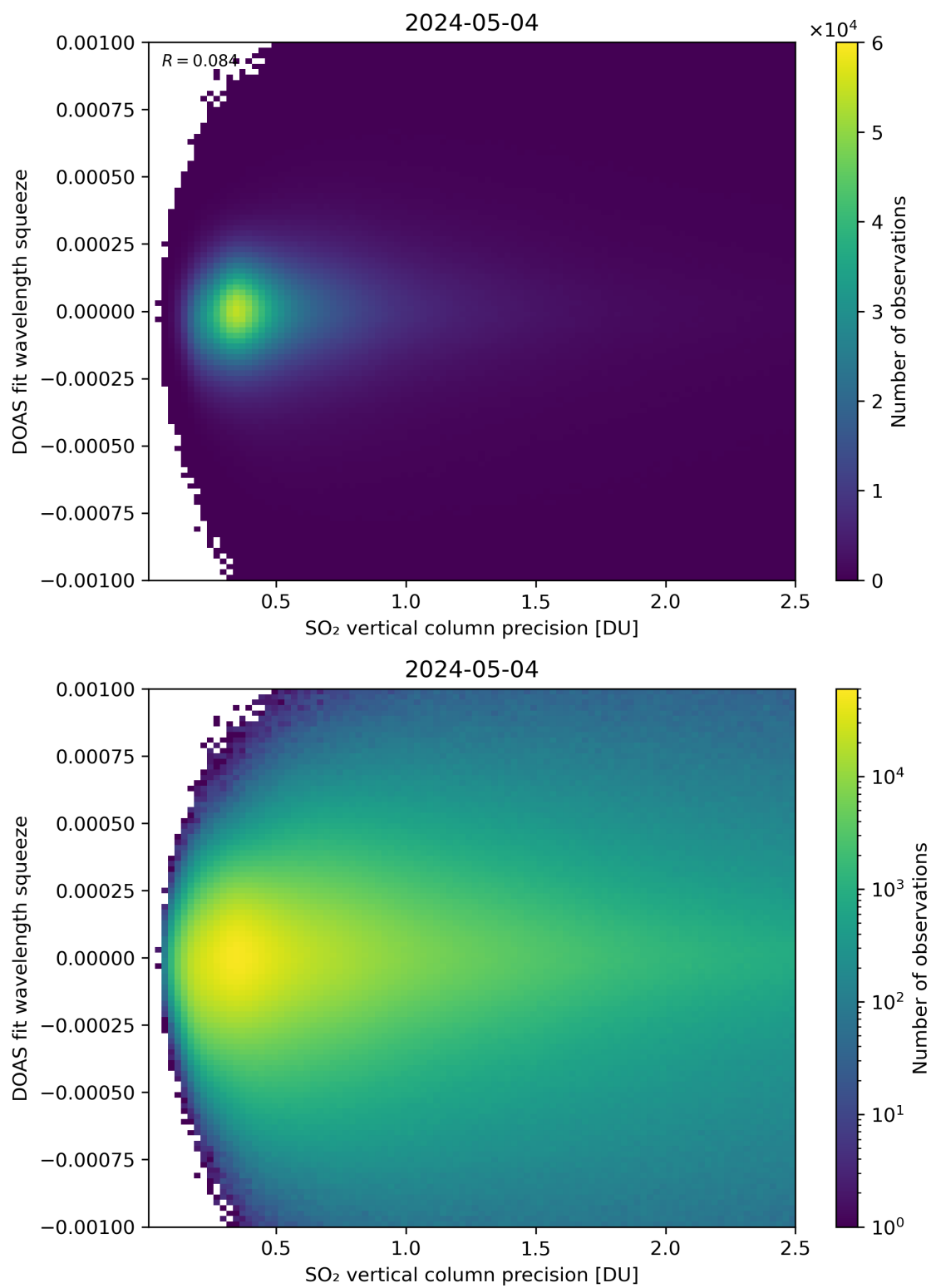
Figure 283: Scatter density plot of “SO 2 vertical column precision” against “DOAS fit wavelength squeeze” for 2024-05-03 to 2024-05-05.
