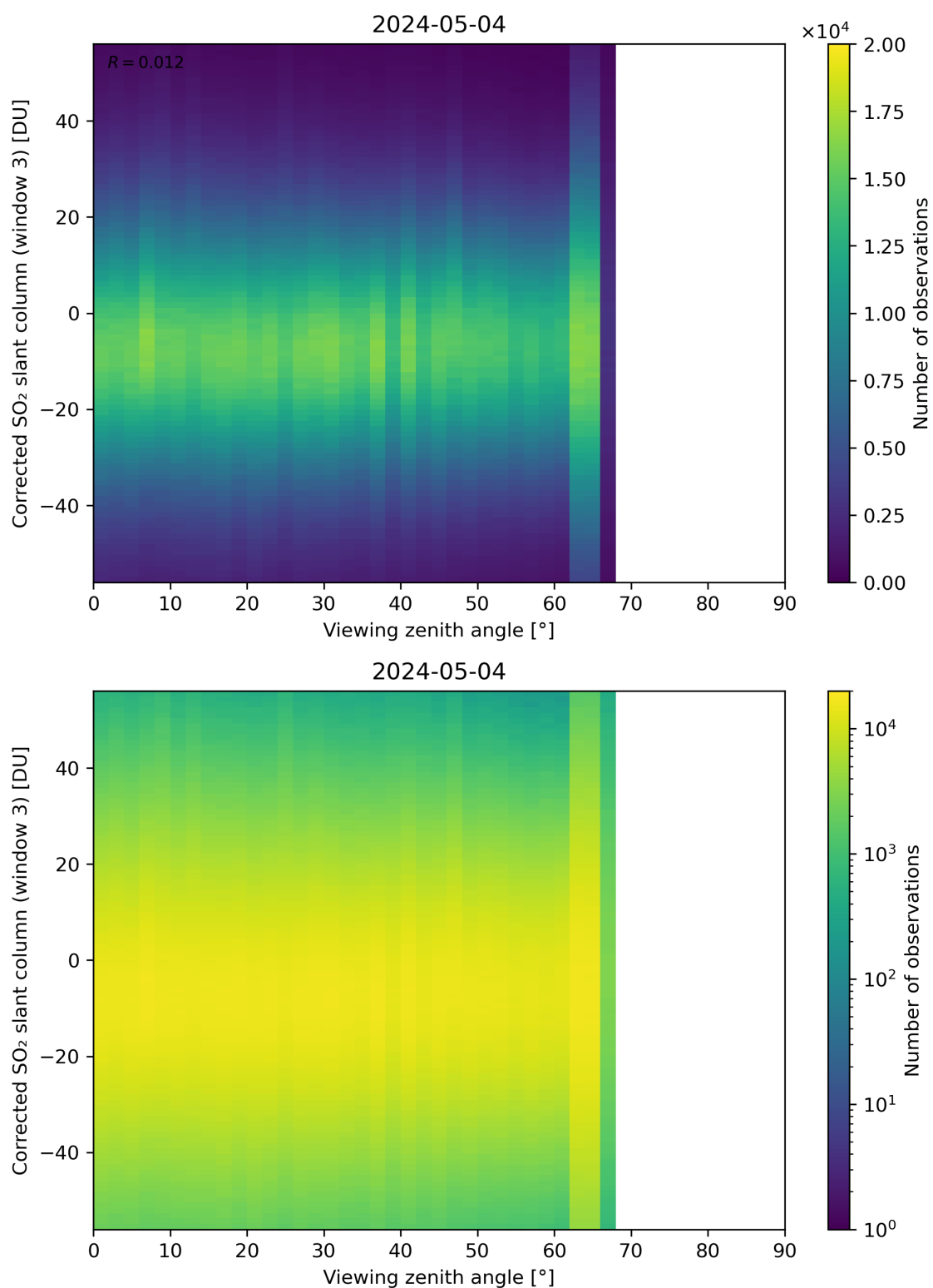
Figure 319: Scatter density plot of “Viewing zenith angle” against “Corrected SO 2 slant column (window 3)” for 2024-05-03 to 2024-05-05.
