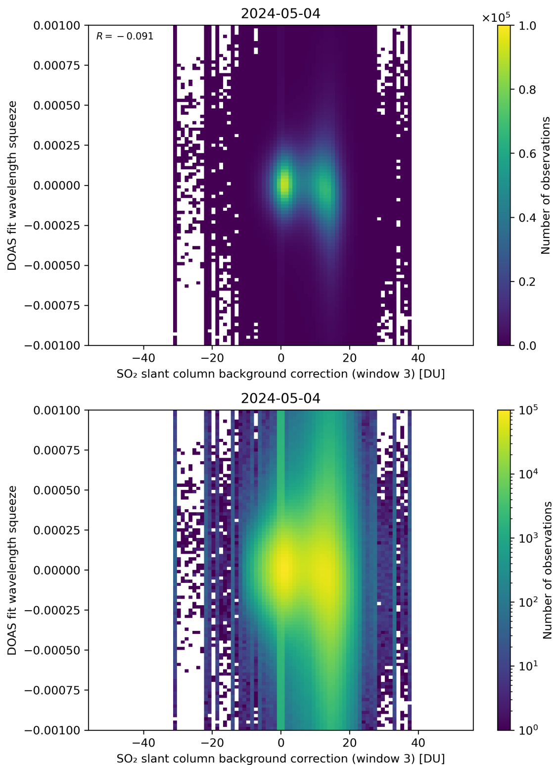
Figure 122: Scatter density plot of “SO 2 slant column background correction (window 3)” against “DOAS fit wavelength squeeze” for 2024-05-03 to 2024-05-05.
