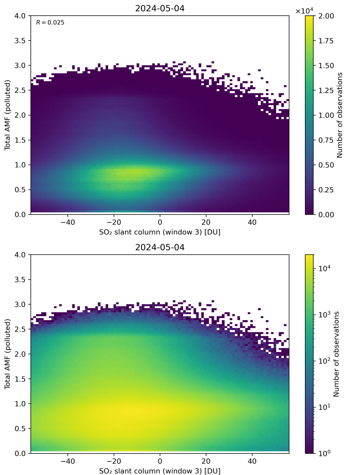
Figure 268: Scatter density plot of “SO 2 slant column (window 3)” against “Total AMF (polluted)” for 2024-05-03 to 2024-05-05.
