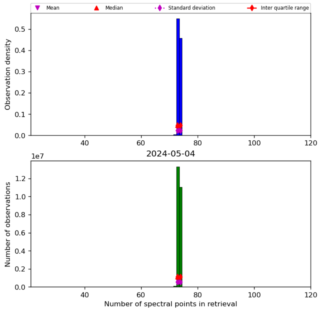
Figure 74: Histogram of “Number of spectral points in retrieval” for 2024-05-03 to 2024-05-05
