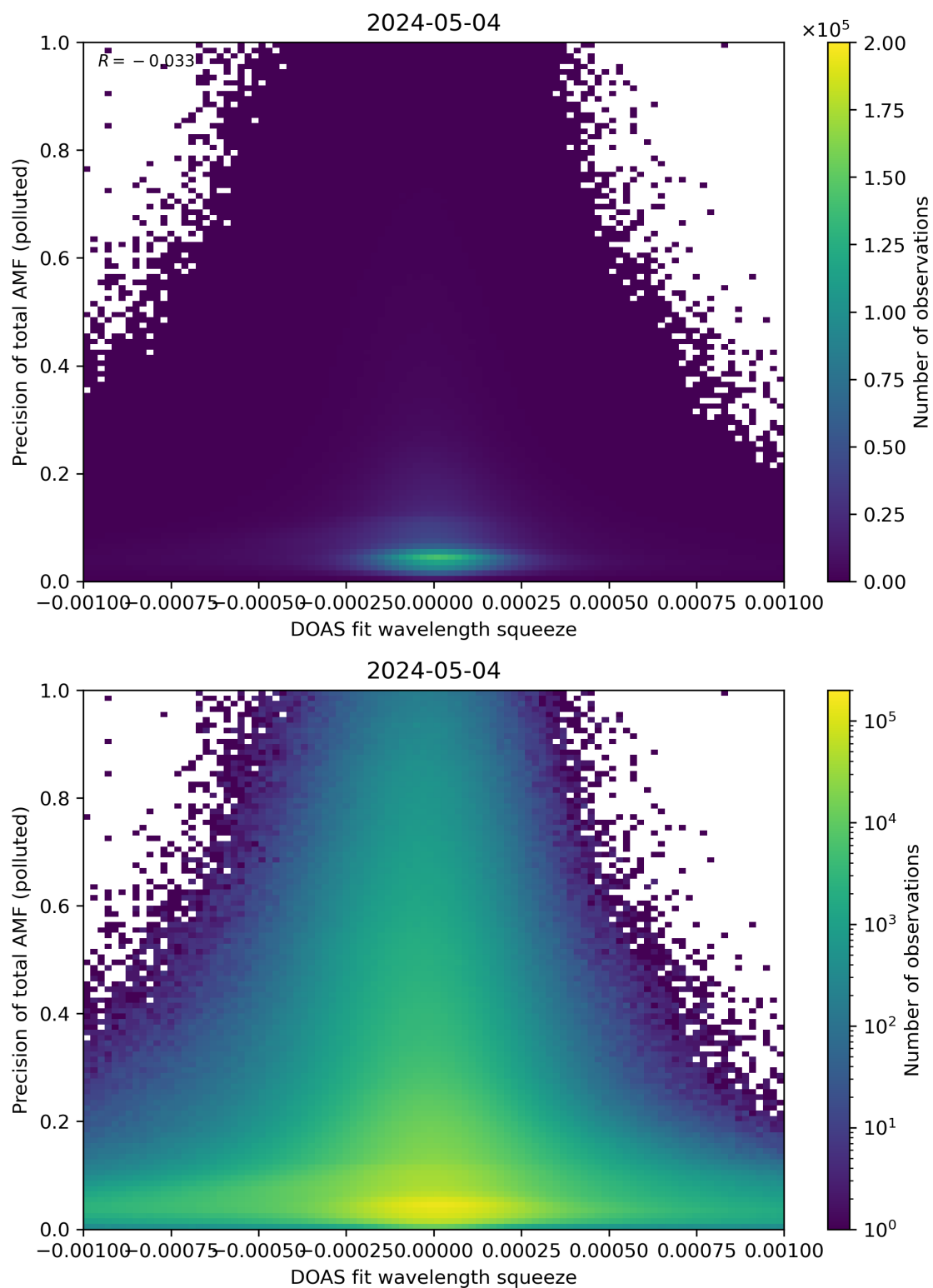
Figure 135: Scatter density plot of “DOAS fit wavelength squeeze” against “Precision of total AMF (polluted)” for 2024-05-03 to 2024-05-05.
