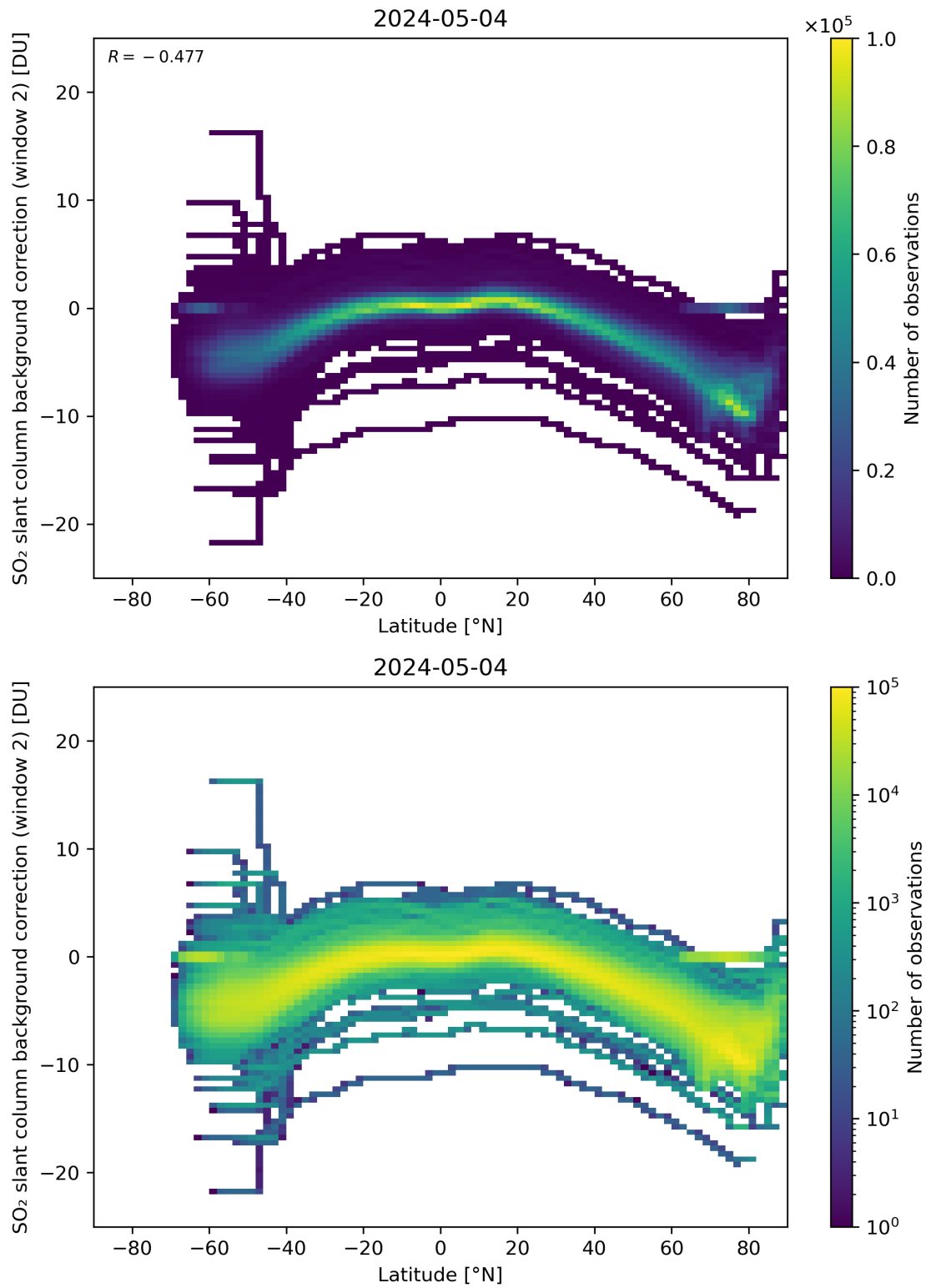
Figure 140: Scatter density plot of “Latitude” against “SO 2 slant column background correction (window 2)” for 2024-05-03 to 2024-05-05.
