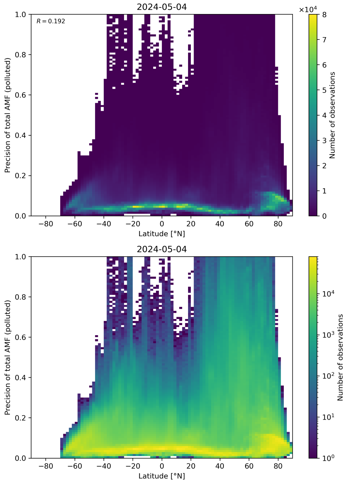
Figure 155: Scatter density plot of “Latitude” against “Precision of total AMF (polluted)” for 2024-05-03 to 2024-05-05.
