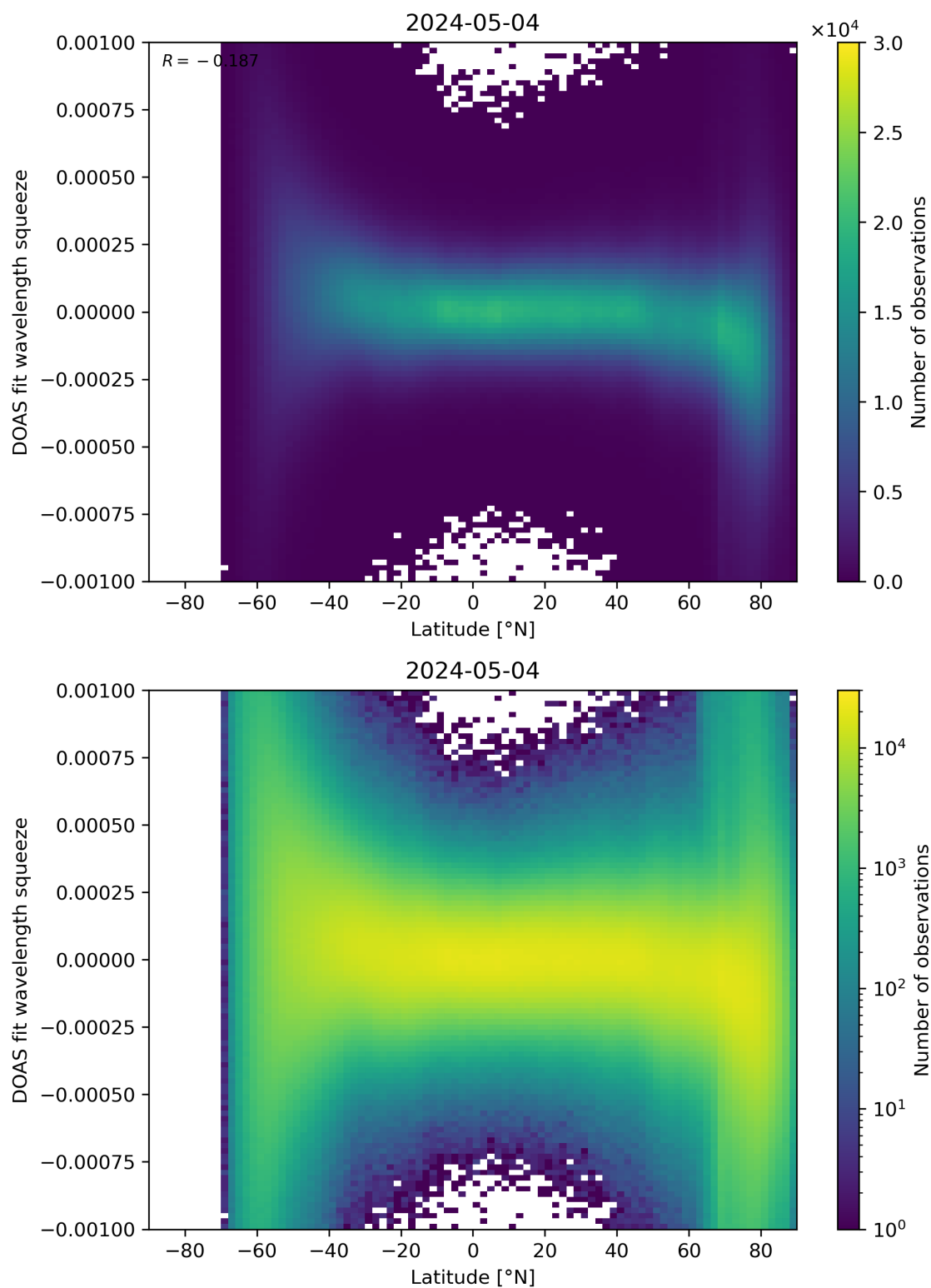
Figure 143: Scatter density plot of “Latitude” against “DOAS fit wavelength squeeze” for 2024-05-03 to 2024-05-05.
