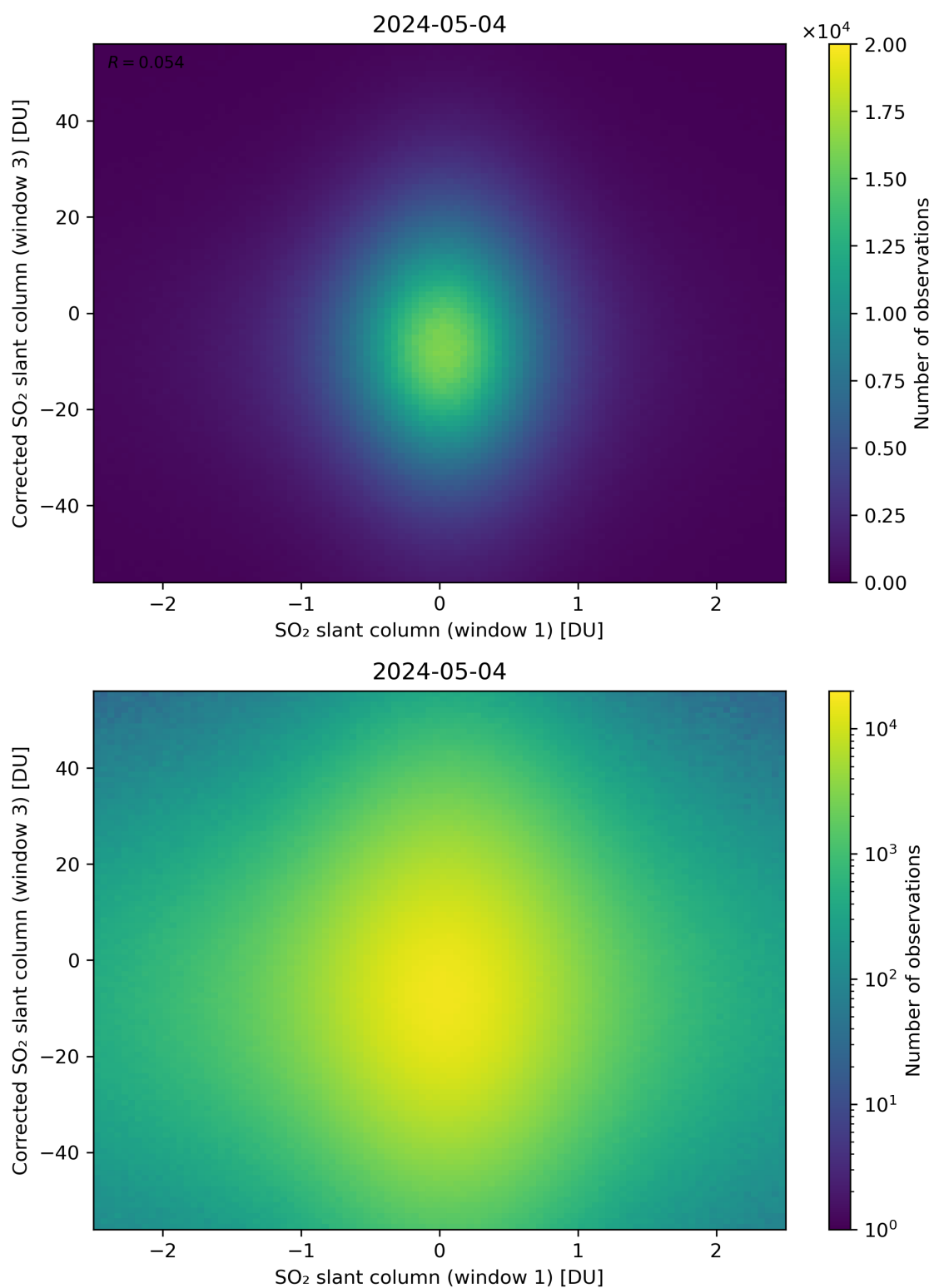
Figure 234: Scatter density plot of “SO 2 slant column (window 1)” against “Corrected SO 2 slant column (window 3)” for 2024-05-03 to 2024-05-05.
