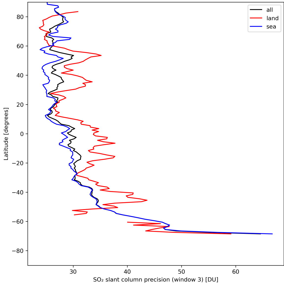
Figure 42: Zonal average of “SO 2 slant column precision (window 3)” for 2024-05-03 to 2024-05-05.
