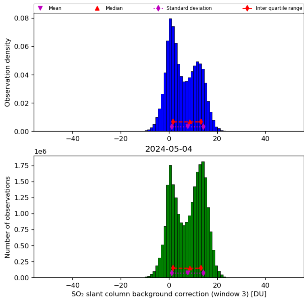
Figure 67: Histogram of “SO 2 slant column background correction (window 3)” for 2024-05-03 to 2024-05-05
