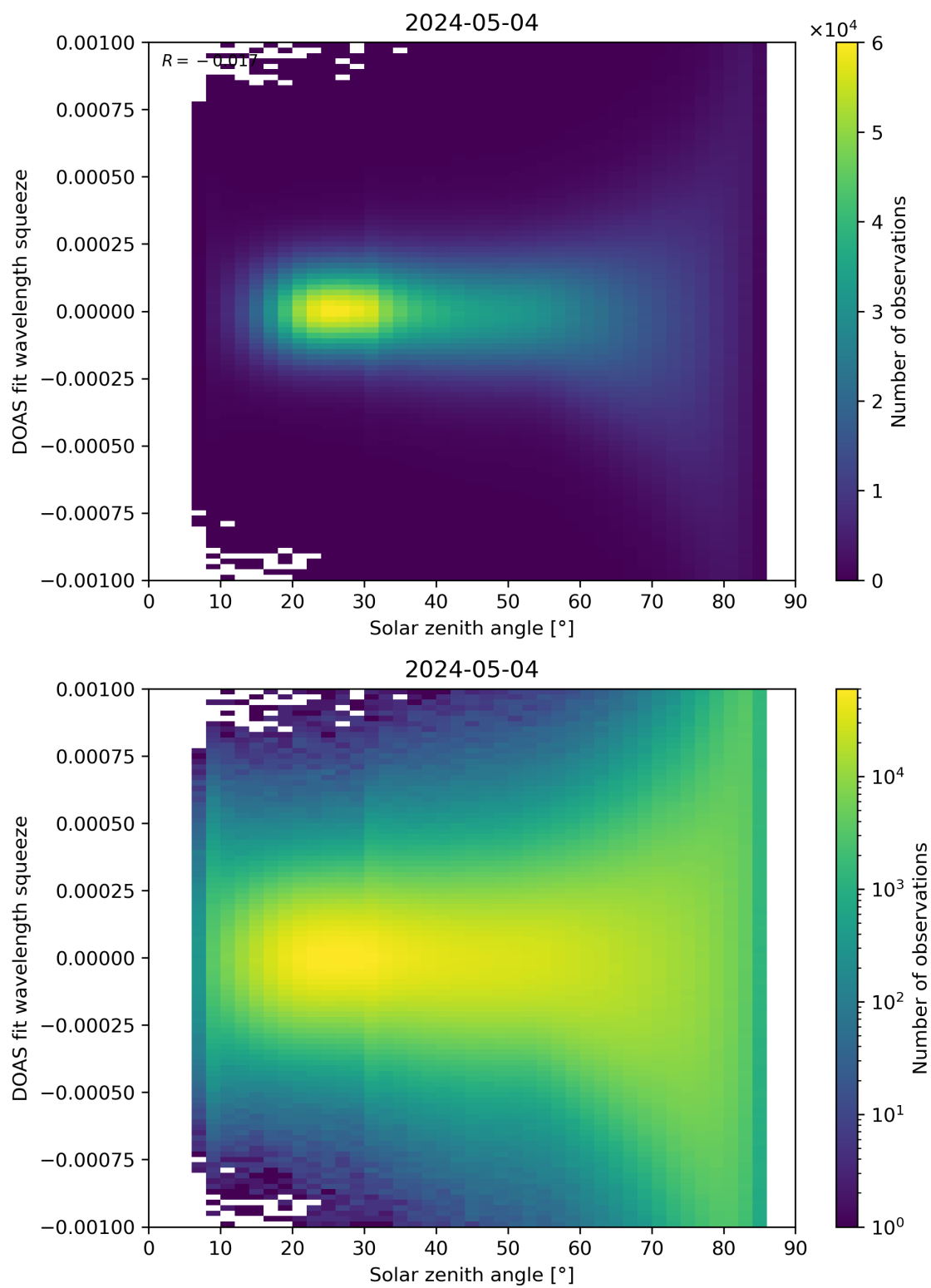
Figure 162: Scatter density plot of “Solar zenith angle” against “DOAS fit wavelength squeeze” for 2024-05-03 to 2024-05-05.
