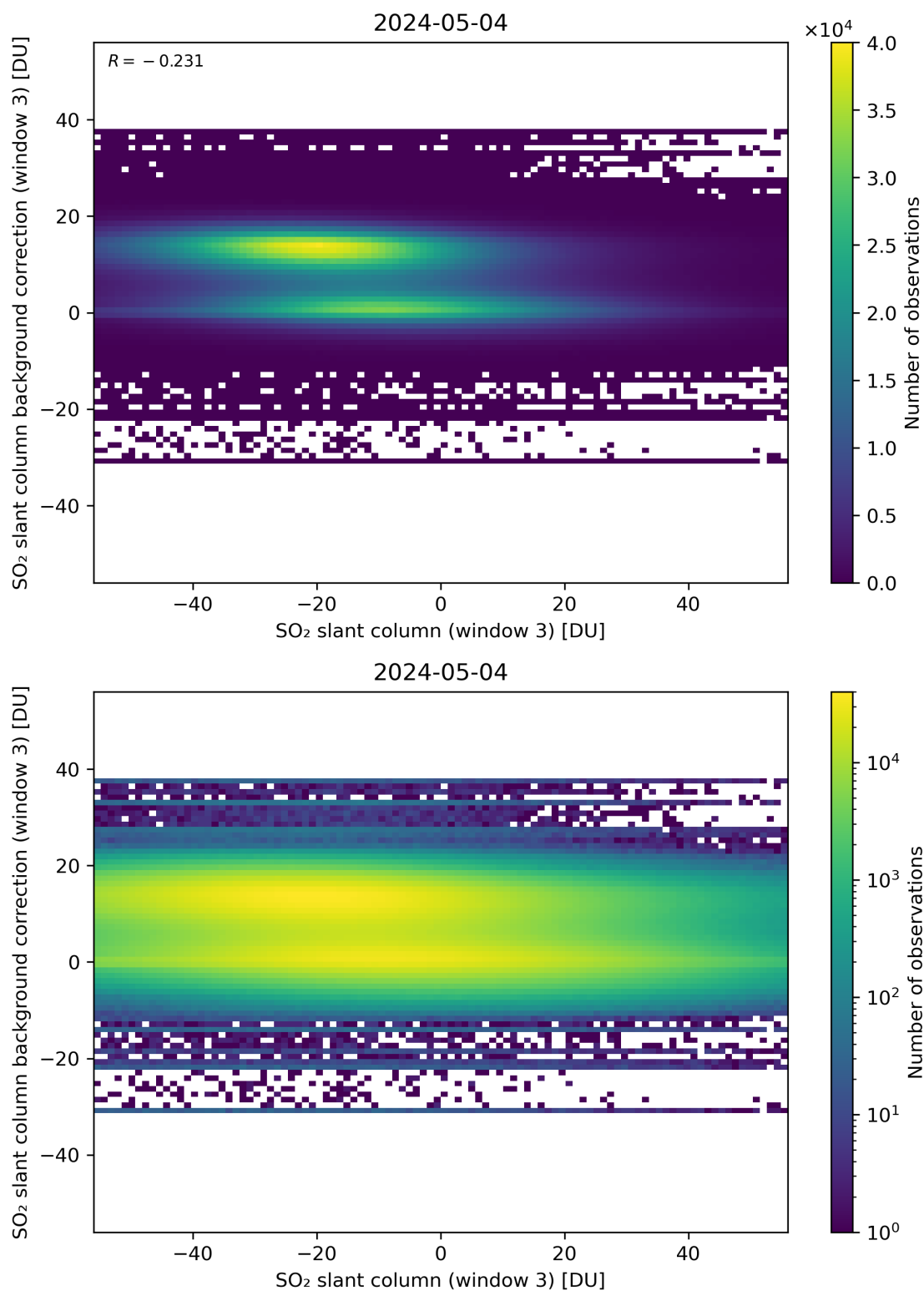
Figure 253: Scatter density plot of “SO 2 slant column (window 3)” against “SO 2 slant column background correction (window 3)” for 2024-05-03 to 2024-05-05.
