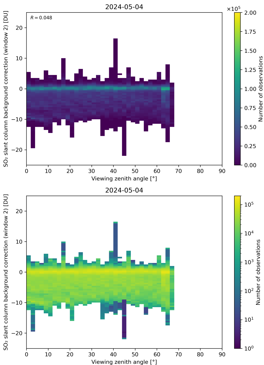
Figure 309: Scatter density plot of “Viewing zenith angle” against “SO 2 slant column background correction (window 2)” for 2024-05-03 to 2024-05-05.
