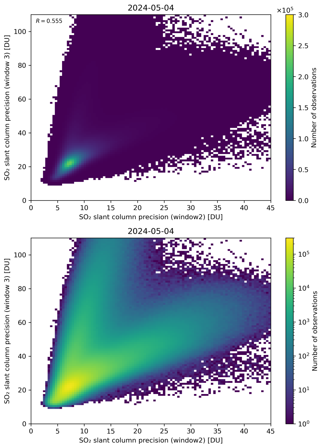
Figure 250: Scatter density plot of “SO 2 slant column precision (window2)” against “SO 2 slant column precision (window 3)” for 2024-05-03 to 2024-05-05.
