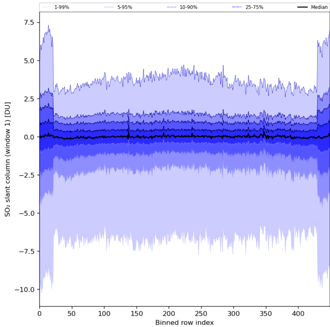
Figure 79: Along track statistics of “SO 2 slant column (window 1)” for 2024-05-03 to 2024-05-05
