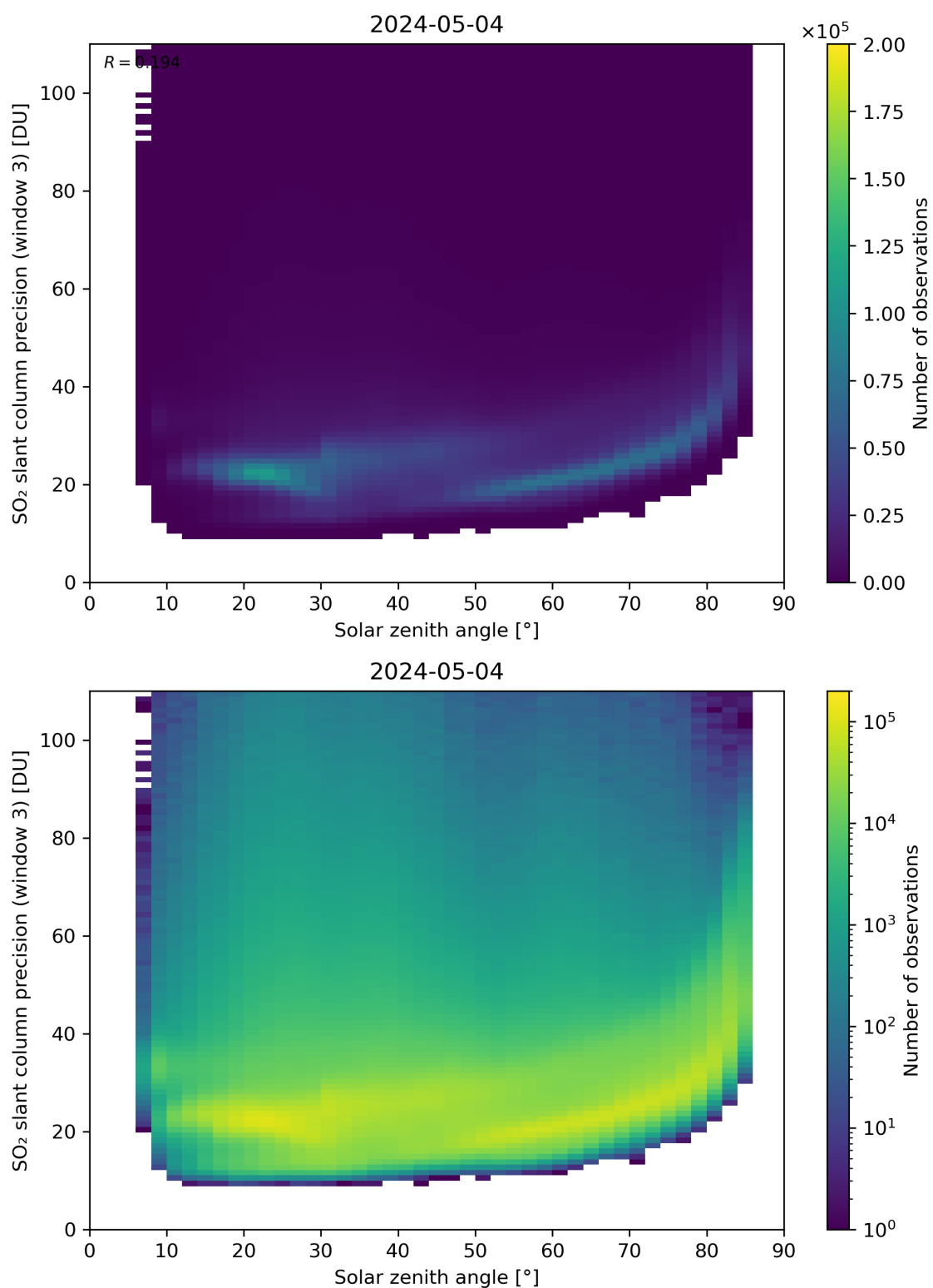
Figure 173: Scatter density plot of “Solar zenith angle” against “SO 2 slant column precision (window 3)” for 2024-05-03 to 2024-05-05.
