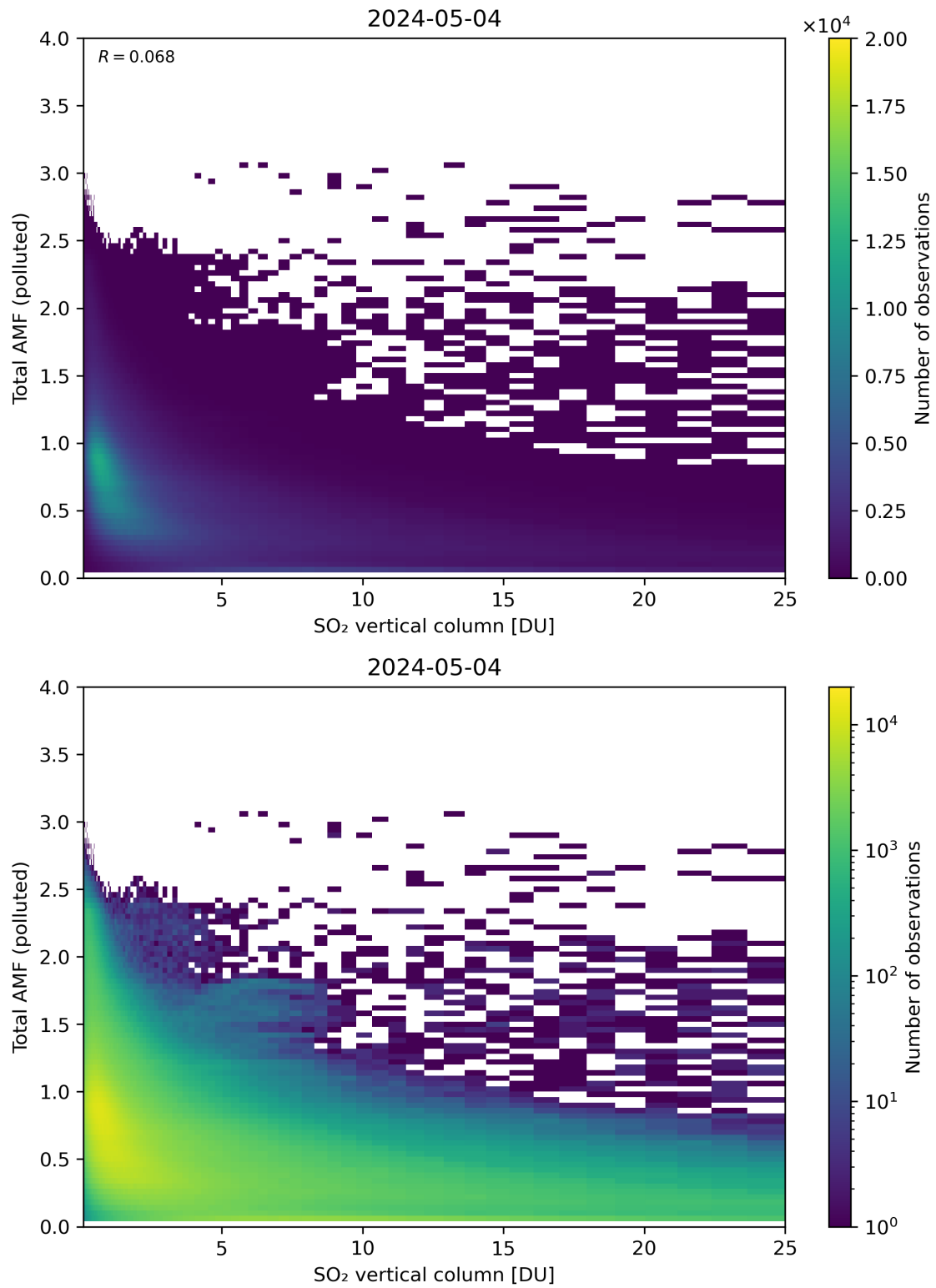
Figure 305: Scatter density plot of “SO 2 vertical column” against “Total AMF (polluted)” for 2024-05-03 to 2024-05-05.
