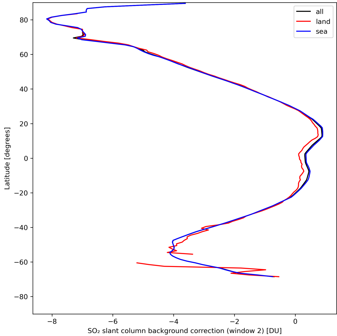
Figure 40: Zonal average of “SO 2 slant column background correction (window 2)” for 2024-05-03 to 2024-05-05.
