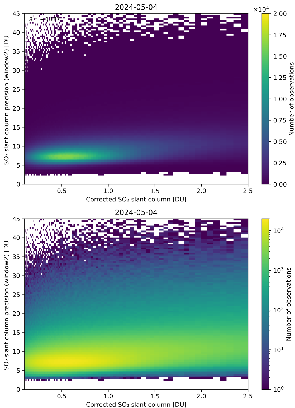
Figure 189: Scatter density plot of “Corrected SO 2 slant column” against “SO 2 slant column precision (window2)” for 2024-05-03 to 2024-05-05.
