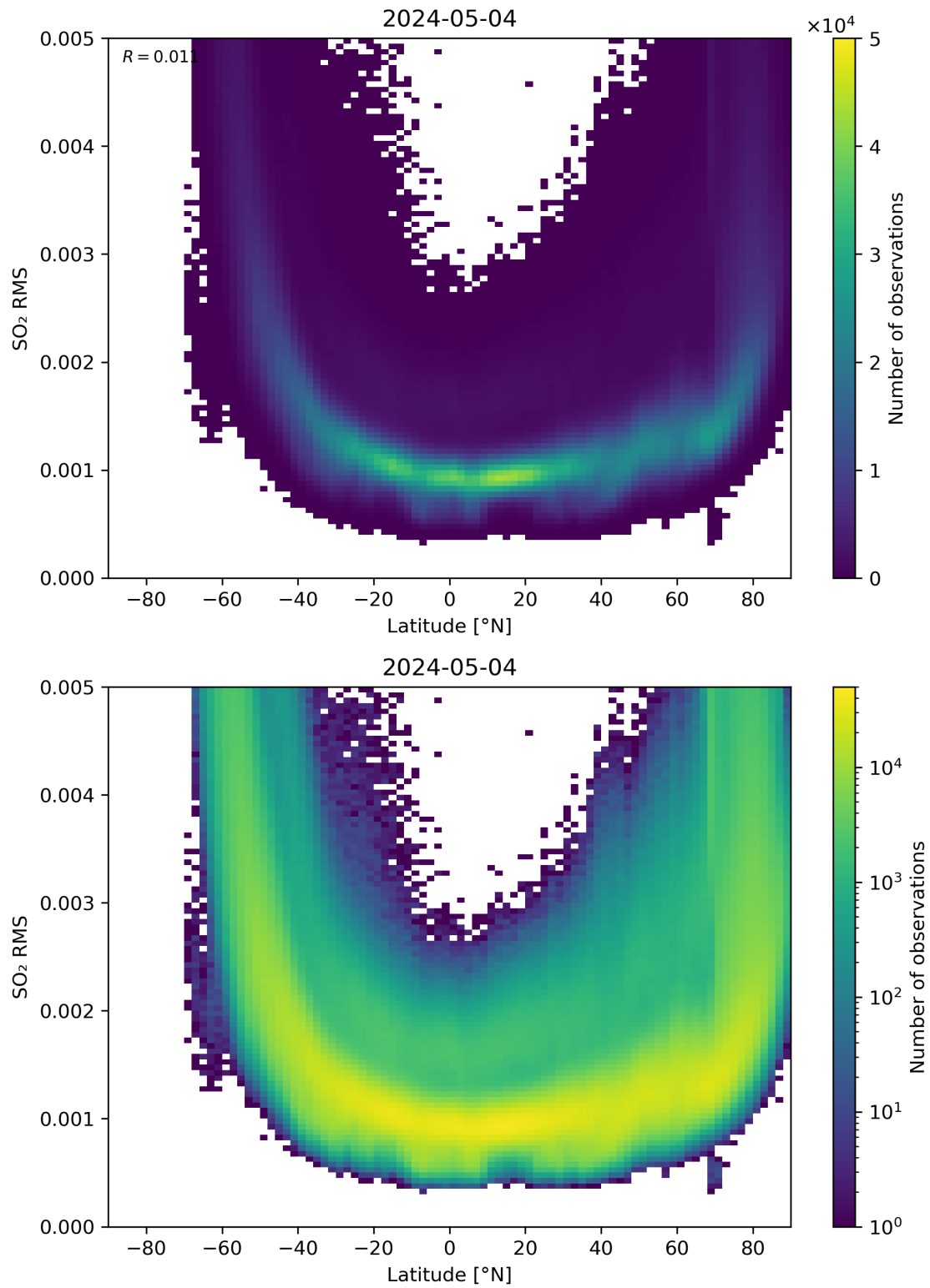
Figure 144: Scatter density plot of “Latitude” against “SO 2 RMS” for 2024-05-03 to 2024-05-05.
