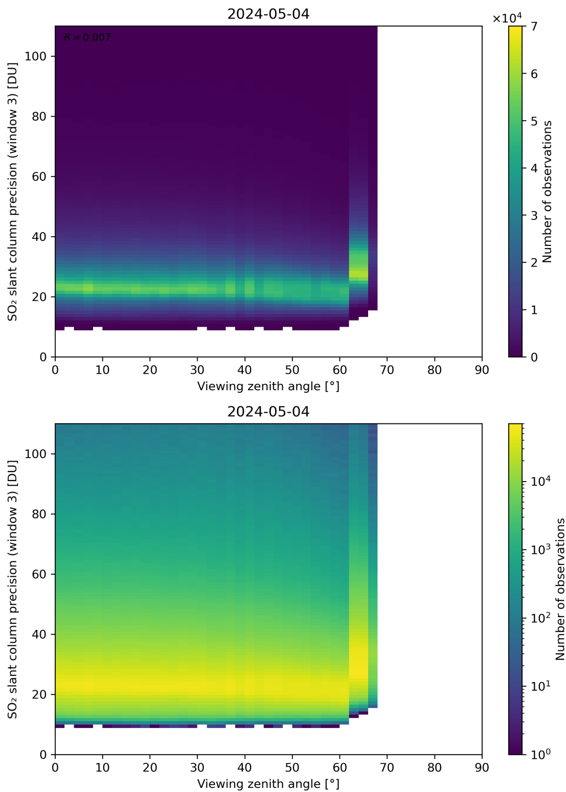
Figure 324: Scatter density plot of “Viewing zenith angle” against “SO 2 slant column precision (window 3)” for 2024-05-03 to 2024-05-05.
