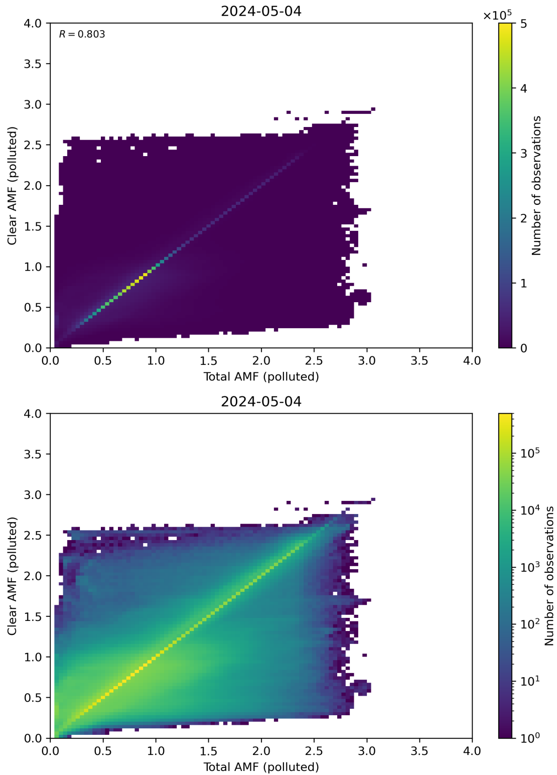
Figure 271: Scatter density plot of “Total AMF (polluted)” against “Clear AMF (polluted)” for 2024-05-03 to 2024-05-05.
