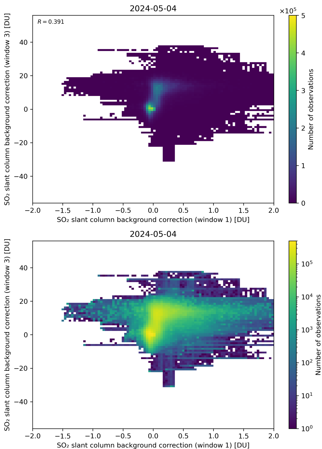
Figure 99: Scatter density plot of “SO 2 slant column background correction (window 1)” against “SO 2 slant column background correction (window 3)” for 2024-05-03 to 2024-05-05.
