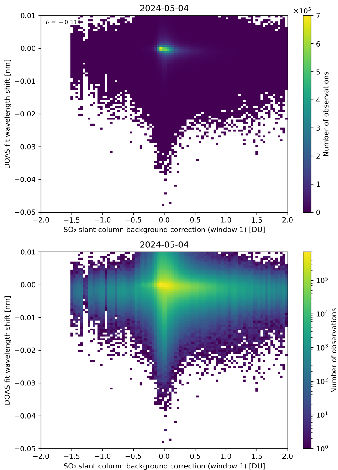
Figure 100: Scatter density plot of “SO 2 slant column background correction (window 1)” against “DOAS fit wavelength shift” for 2024-05-03 to 2024-05-05.
