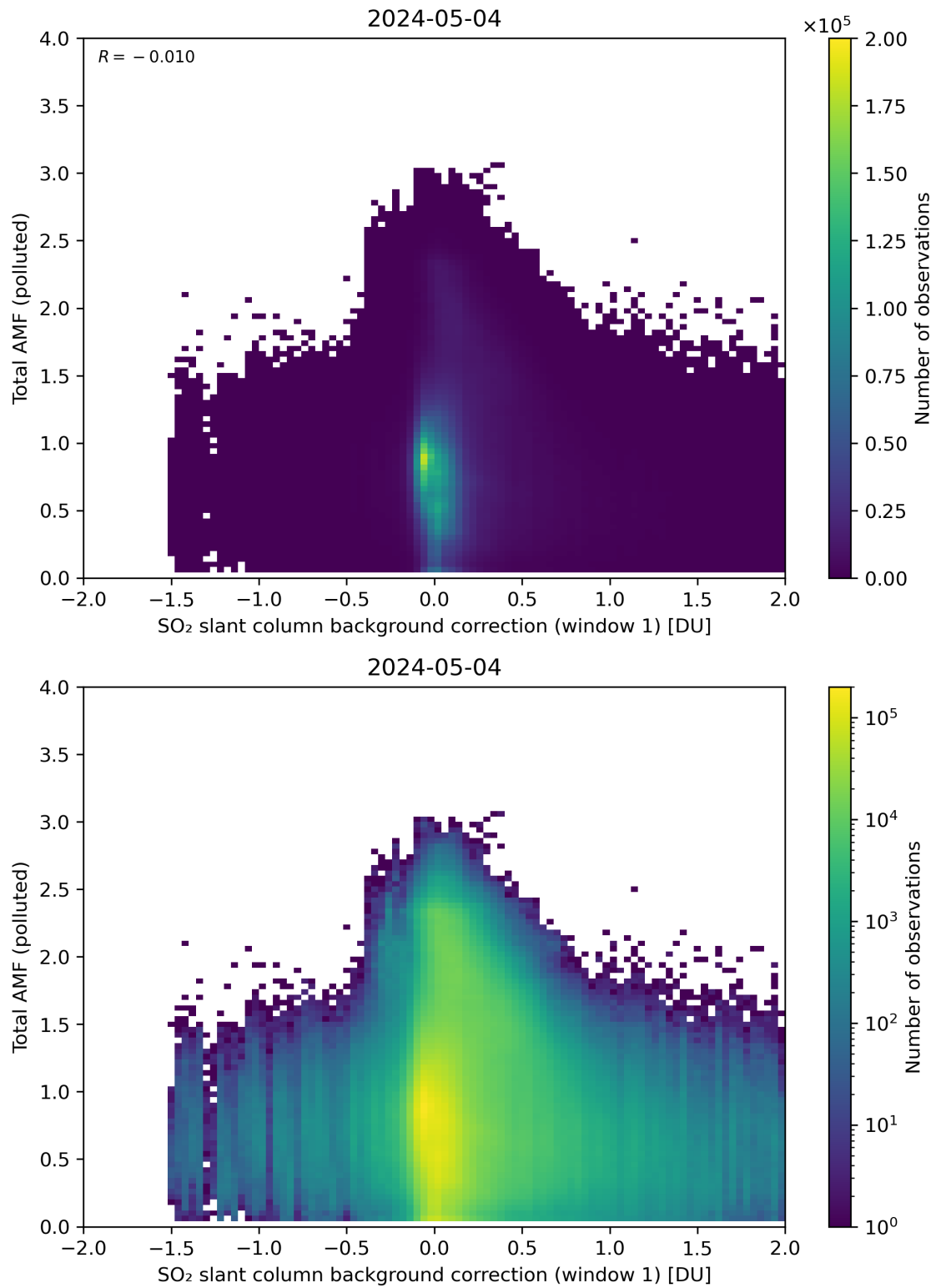
Figure 109: Scatter density plot of “SO 2 slant column background correction (window 1)” against “Total AMF (polluted)” for 2024-05-03 to 2024-05-05.
