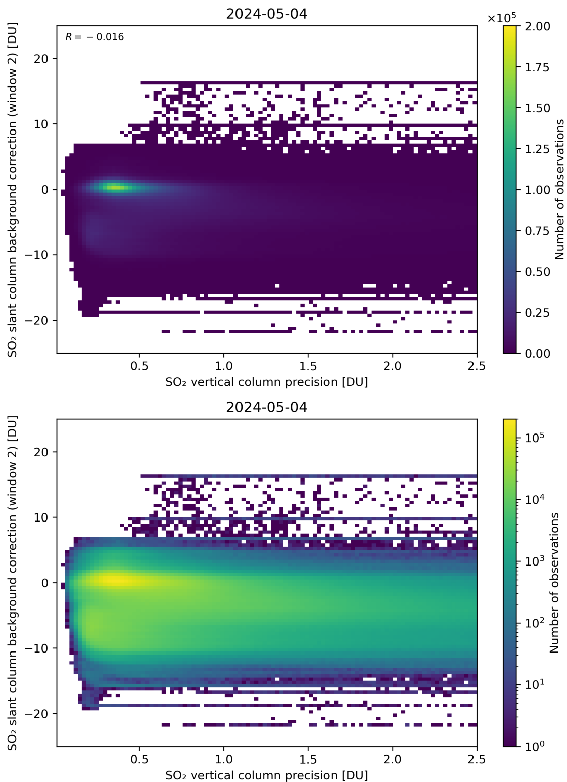
Figure 280: Scatter density plot of “SO 2 vertical column precision” against “SO 2 slant column background correction (window 2)” for 2024-05-03 to 2024-05-05.
