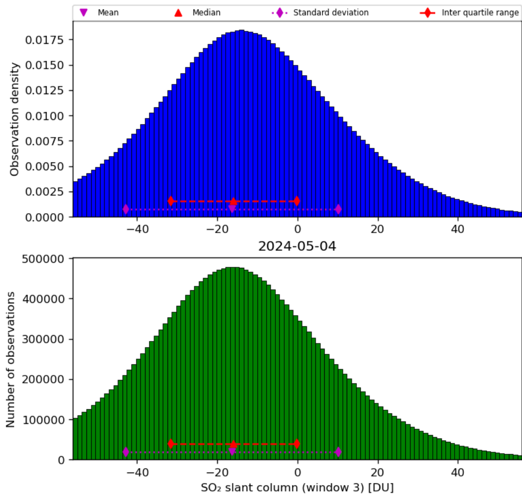
Figure 64: Histogram of “SO 2 slant column (window 3)” for 2024-05-03 to 2024-05-05
