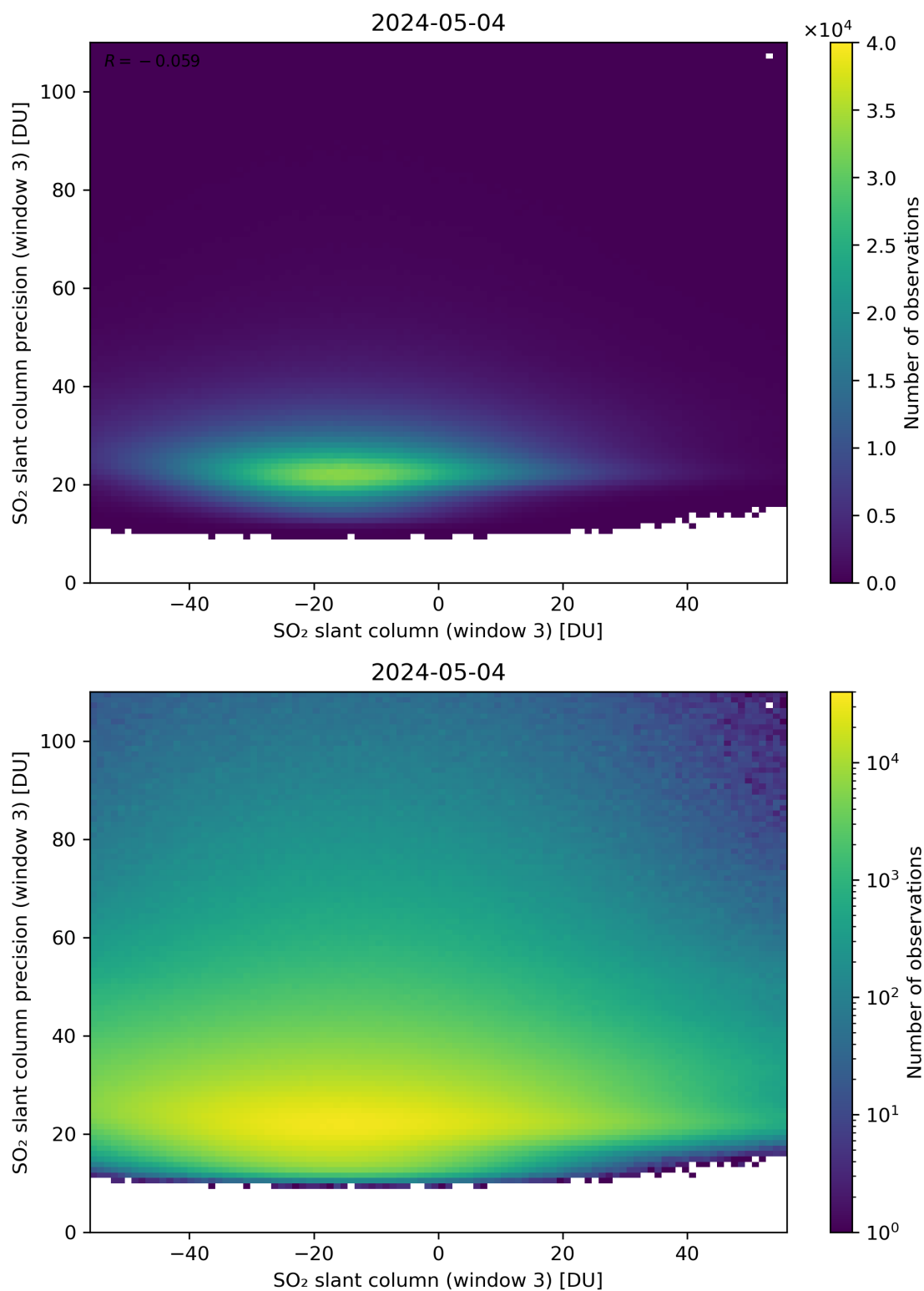
Figure 267: Scatter density plot of “SO 2 slant column (window 3)” against “SO 2 slant column precision (window 3)” for 2024-05-03 to 2024-05-05.
