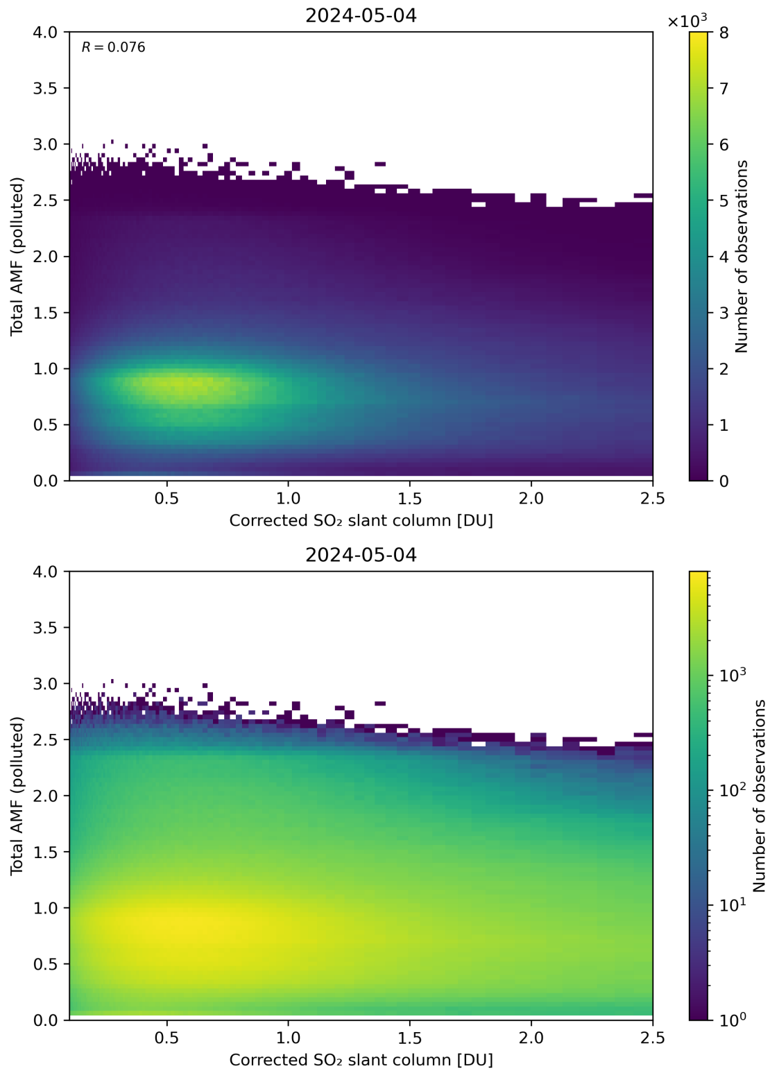
Figure 192: Scatter density plot of “Corrected SO 2 slant column” against “Total AMF (polluted)” for 2024-05-03 to 2024-05-05.
