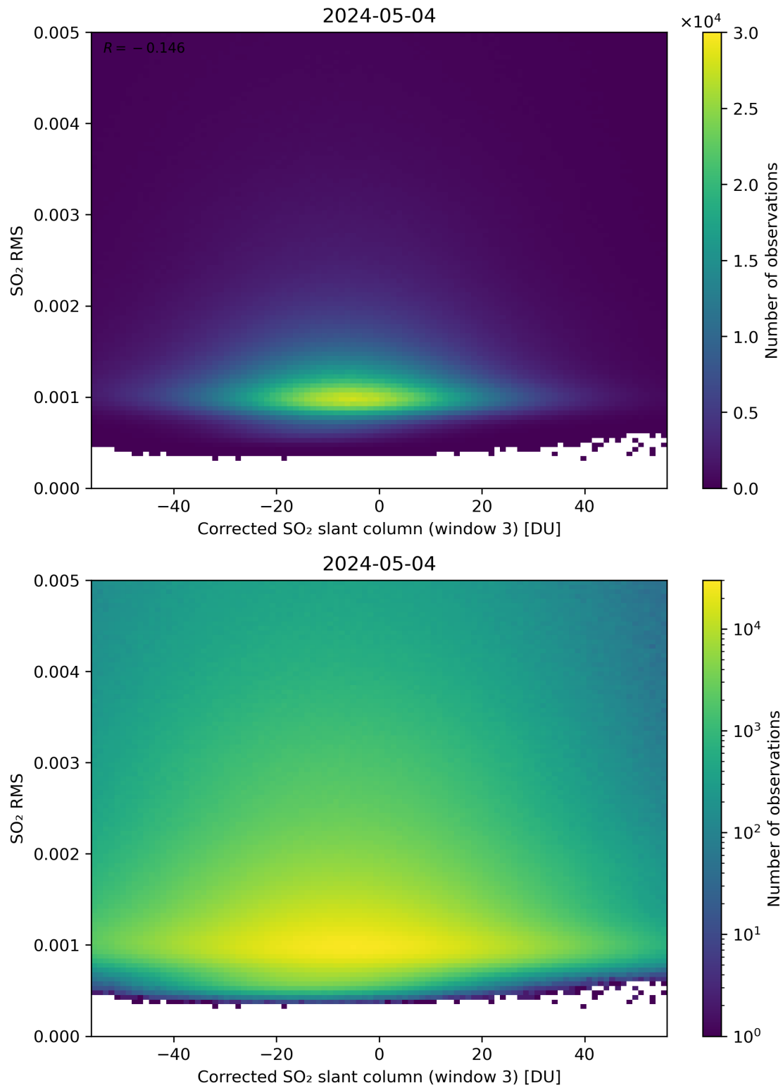
Figure 208: Scatter density plot of “Corrected SO 2 slant column (window 3)” against “SO 2 RMS” for 2024-05-03 to 2024-05-05.
