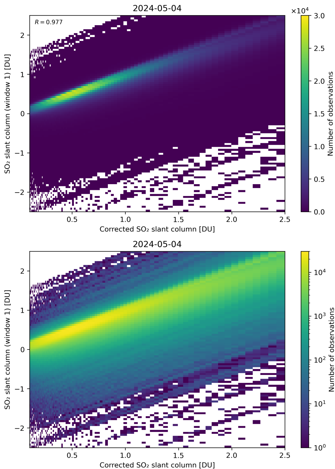
Figure 187: Scatter density plot of “Corrected SO 2 slant column” against “SO 2 slant column (window 1)” for 2024-05-03 to 2024-05-05.
