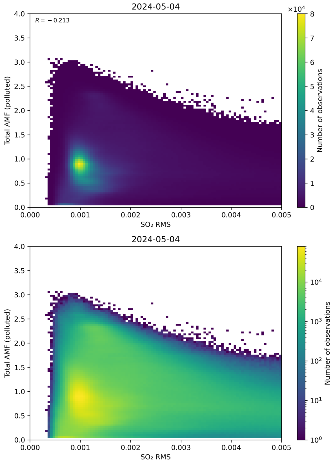
Figure 137: Scatter density plot of “SO 2 RMS” against “Total AMF (polluted)” for 2024-05-03 to 2024-05-05.
