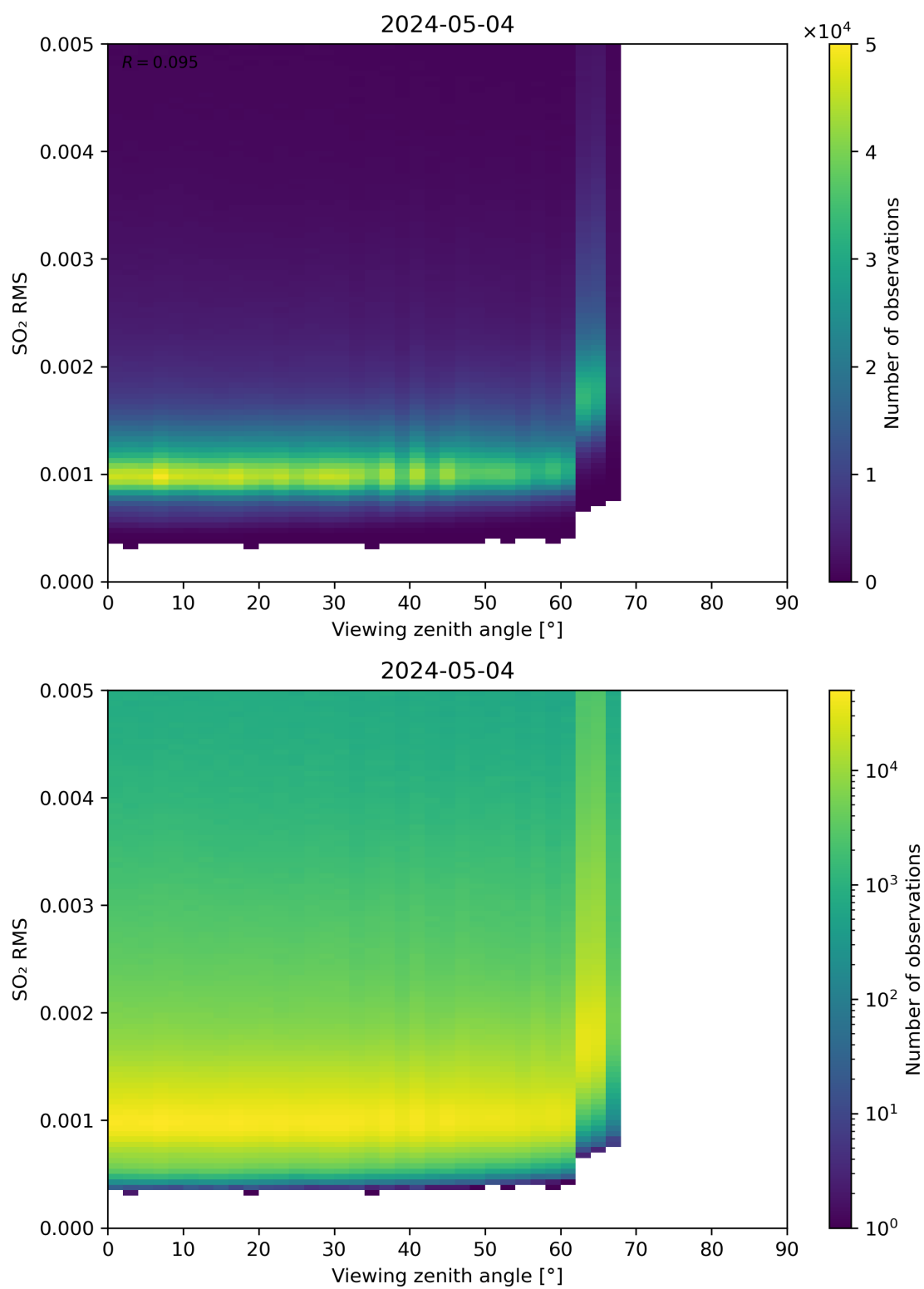
Figure 313: Scatter density plot of “Viewing zenith angle” against “SO 2 RMS” for 2024-05-03 to 2024-05-05.
