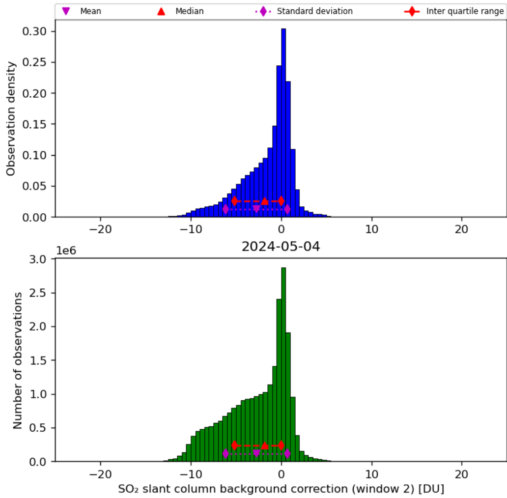
Figure 63: Histogram of “SO 2 slant column background correction (window 2)” for 2024-05-03 to 2024-05-05
