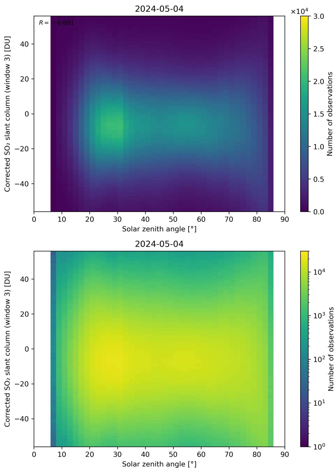
Figure 168: Scatter density plot of “Solar zenith angle” against “Corrected SO 2 slant column (window 3)” for 2024-05-03 to 2024-05-05.
