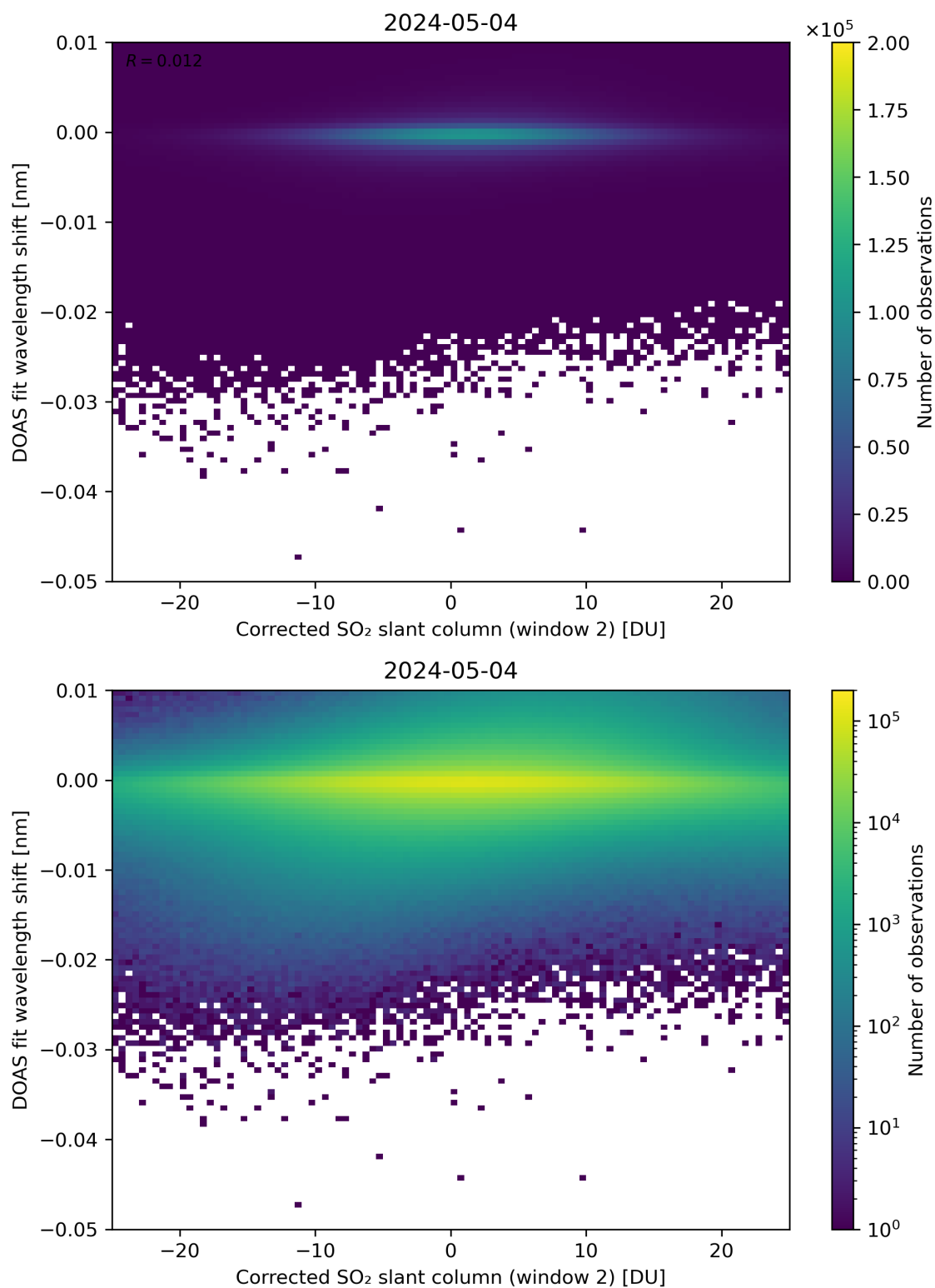
Figure 196: Scatter density plot of “Corrected SO 2 slant column (window 2)” against “DOAS fit wavelength shift” for 2024-05-03 to 2024-05-05.
