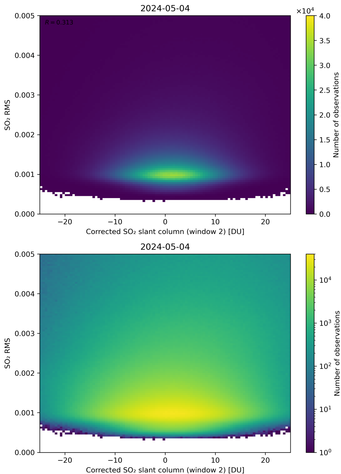
Figure 198: Scatter density plot of “Corrected SO 2 slant column (window 2)” against “SO 2 RMS” for 2024-05-03 to 2024-05-05.
