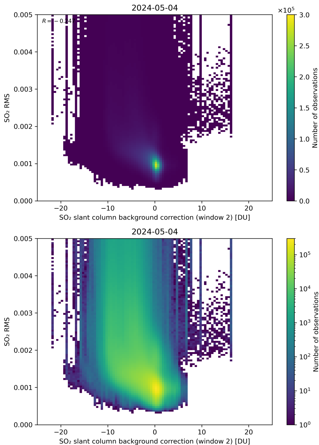
Figure 114: Scatter density plot of “SO 2 slant column background correction (window 2)” against “SO 2 RMS” for 2024-05-03 to 2024-05-05.
