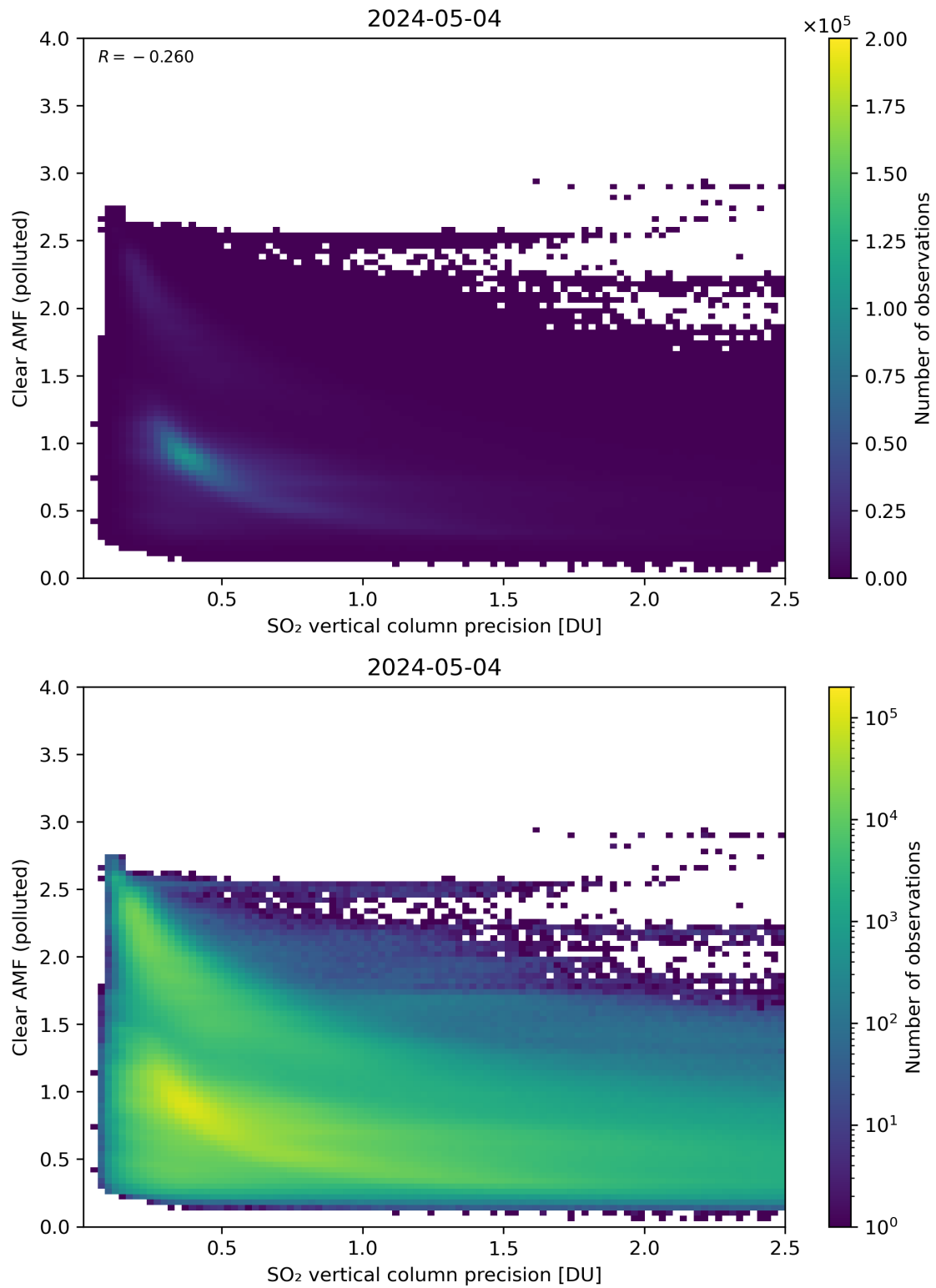
Figure 285: Scatter density plot of “SO 2 vertical column precision” against “Clear AMF (polluted)” for 2024-05-03 to 2024-05-05.
