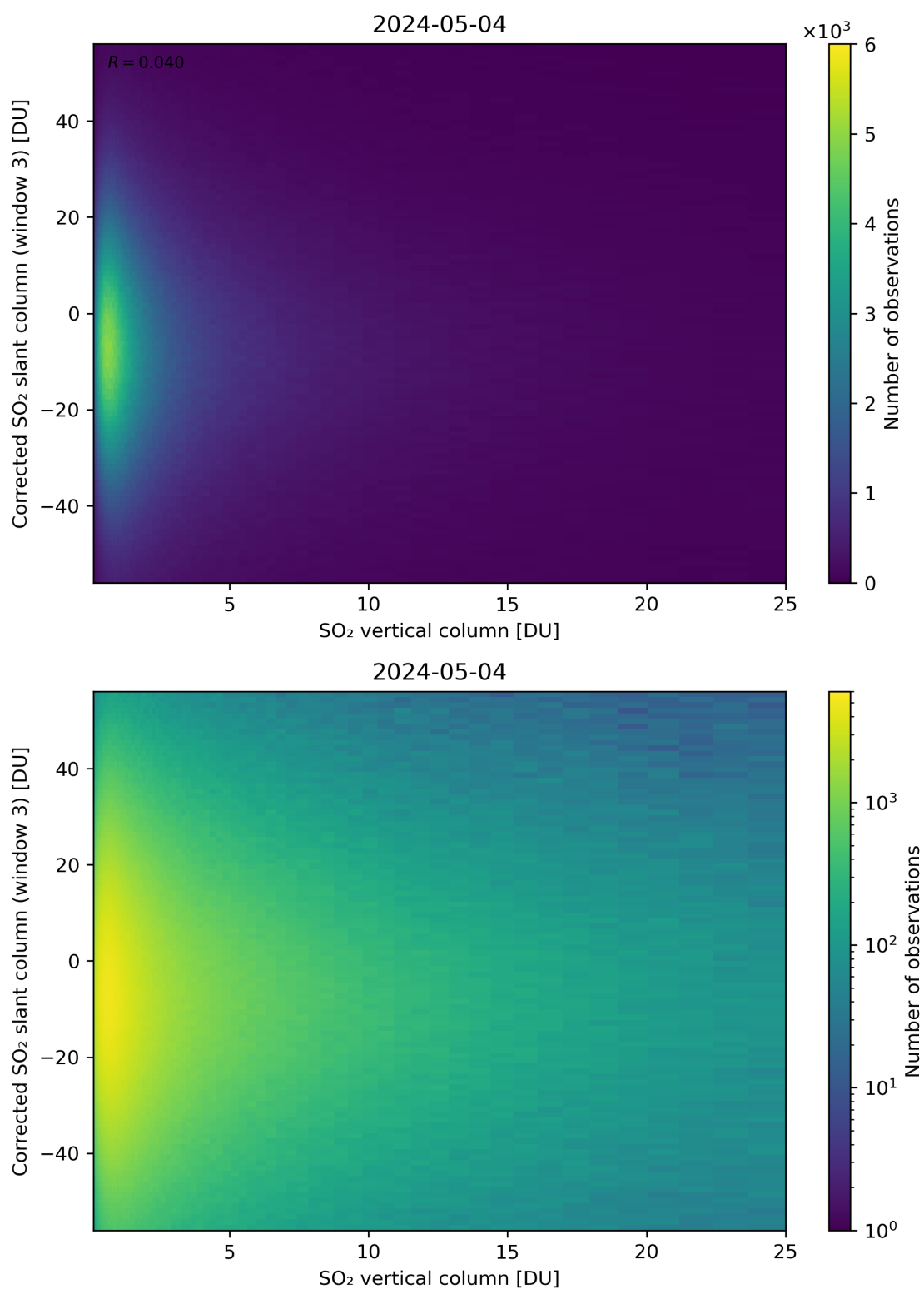
Figure 299: Scatter density plot of “SO 2 vertical column” against “Corrected SO 2 slant column (window 3)” for 2024-05-03 to 2024-05-05.
