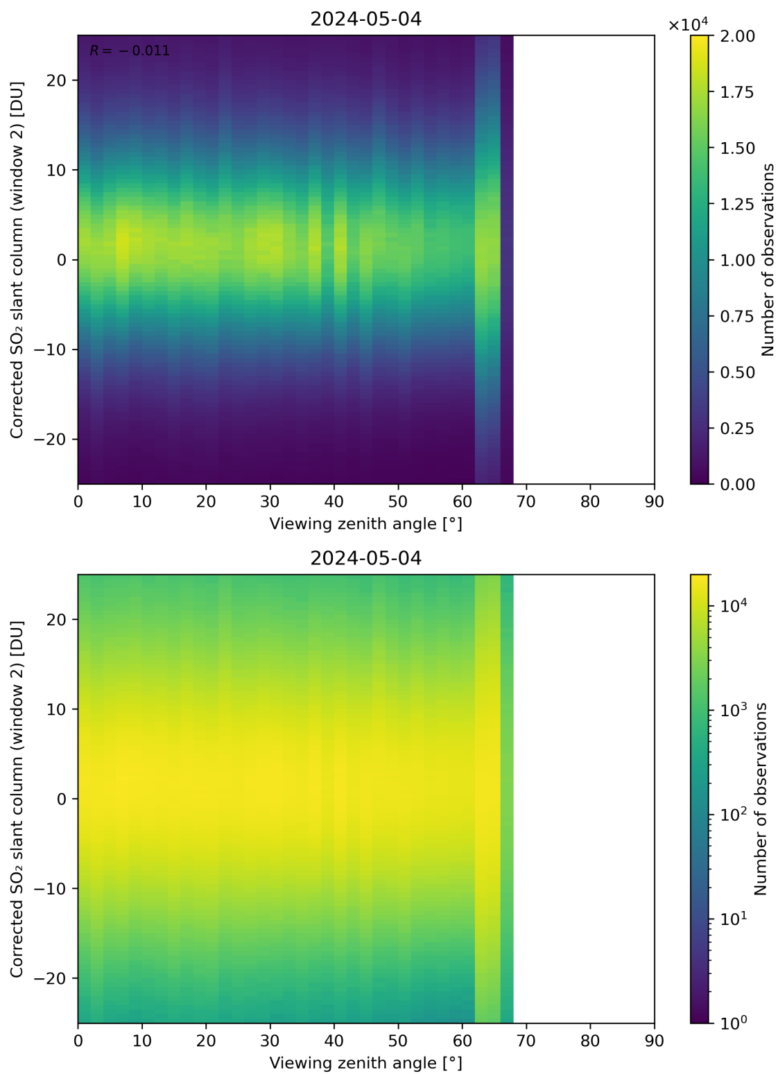
Figure 318: Scatter density plot of “Viewing zenith angle” against “Corrected SO 2 slant column (window 2)” for 2024-05-03 to 2024-05-05.
