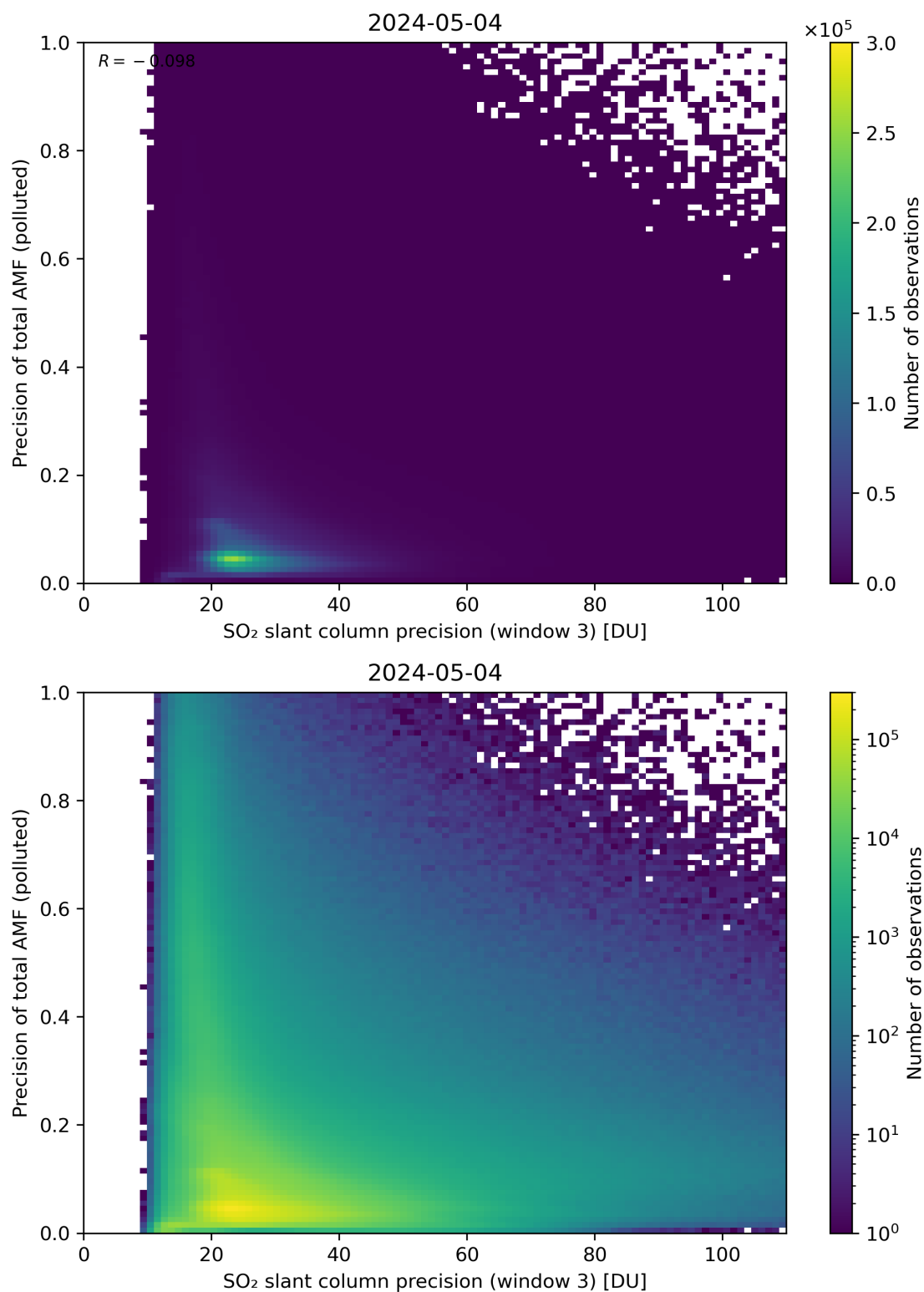
Figure 264: Scatter density plot of “SO 2 slant column precision (window 3)” against “Precision of total AMF (polluted)” for 2024-05-03 to 2024-05-05.
