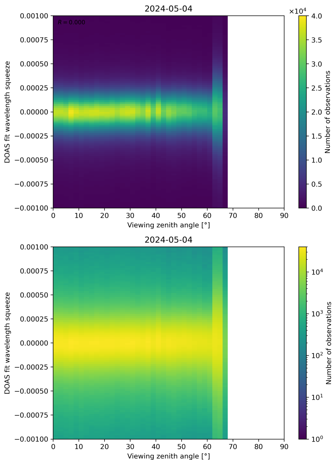
Figure 312: Scatter density plot of “Viewing zenith angle” against “DOAS fit wavelength squeeze” for 2024-05-03 to 2024-05-05.
