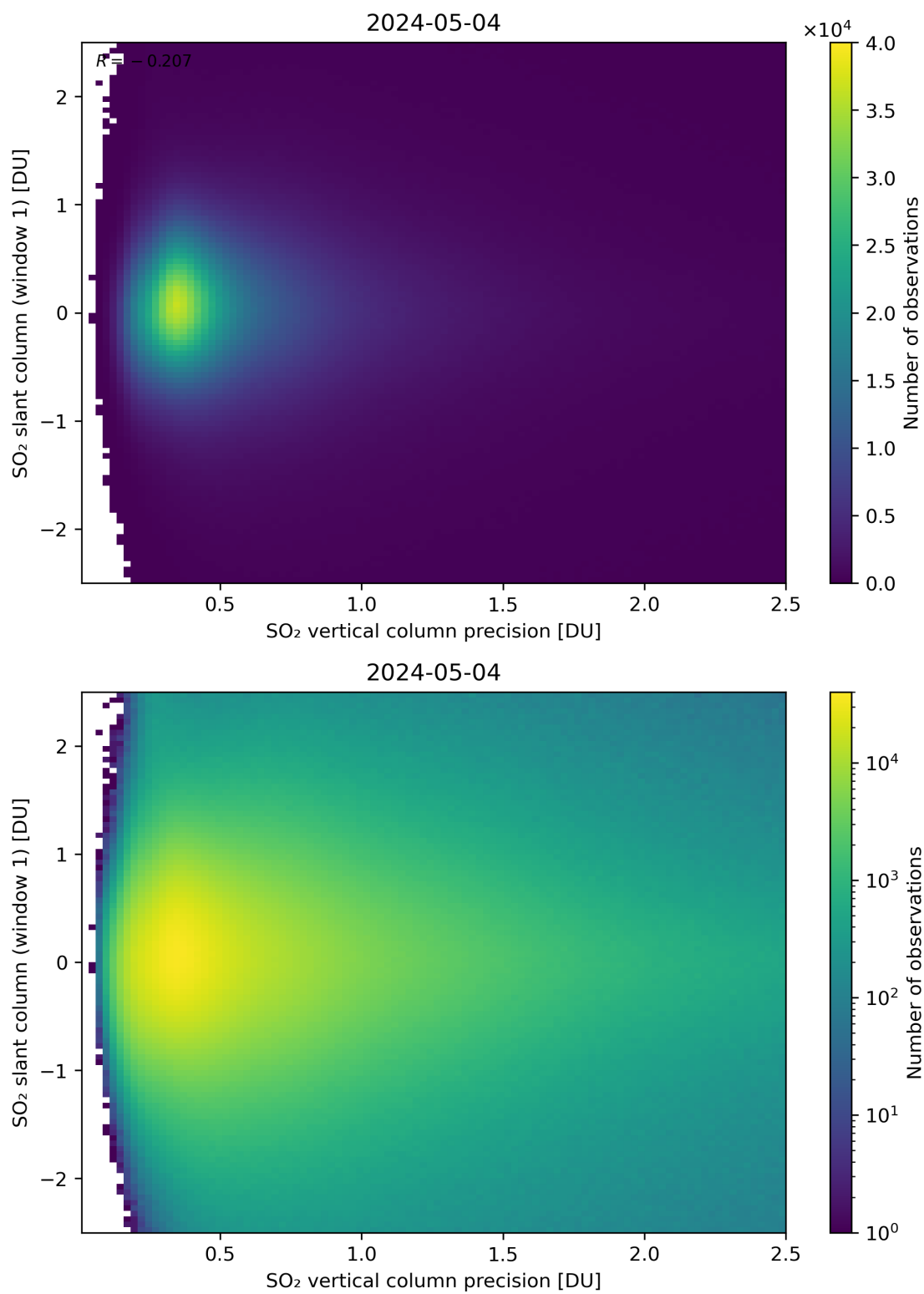
Figure 289: Scatter density plot of “SO 2 vertical column precision” against “SO 2 slant column (window 1)” for 2024-05-03 to 2024-05-05.
