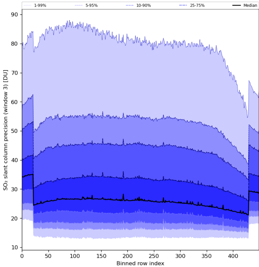
Figure 88: Along track statistics of “SO 2 slant column precision (window 3)” for 2024-05-03 to 2024-05-05
