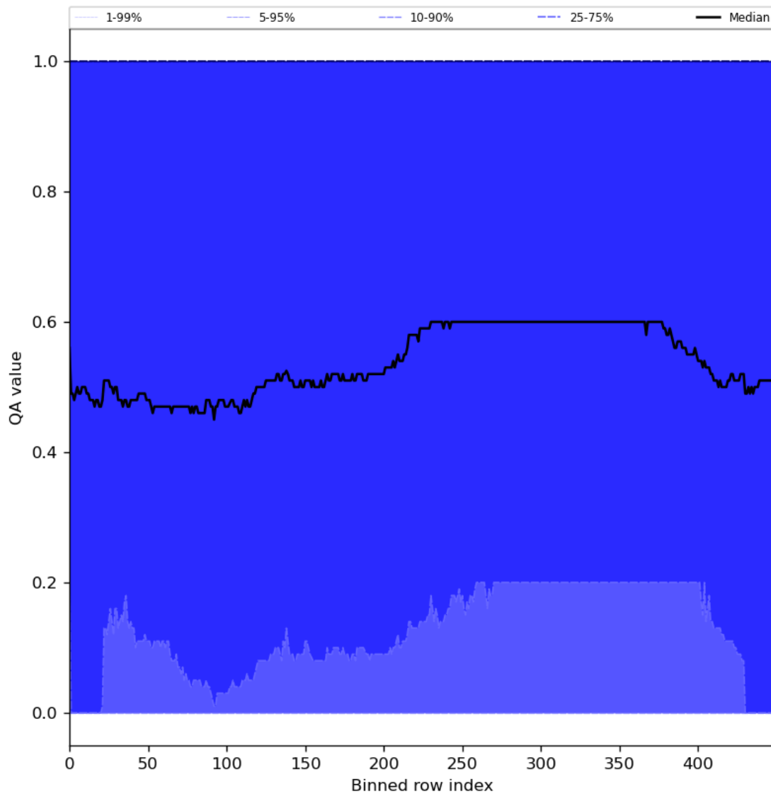
Figure 75: Along track statistics of “QA value” for 2024-05-03 to 2024-05-05
