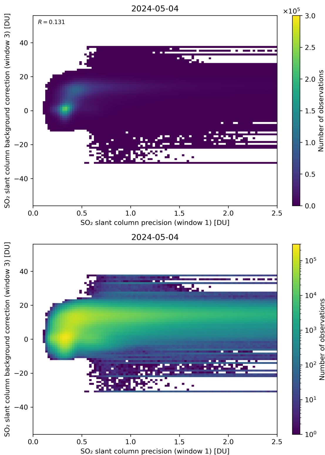
Figure 220: Scatter density plot of “SO 2 slant column precision (window 1)” against “SO 2 slant column background correction (window 3)” for 2024-05-03 to 2024-05-05.
