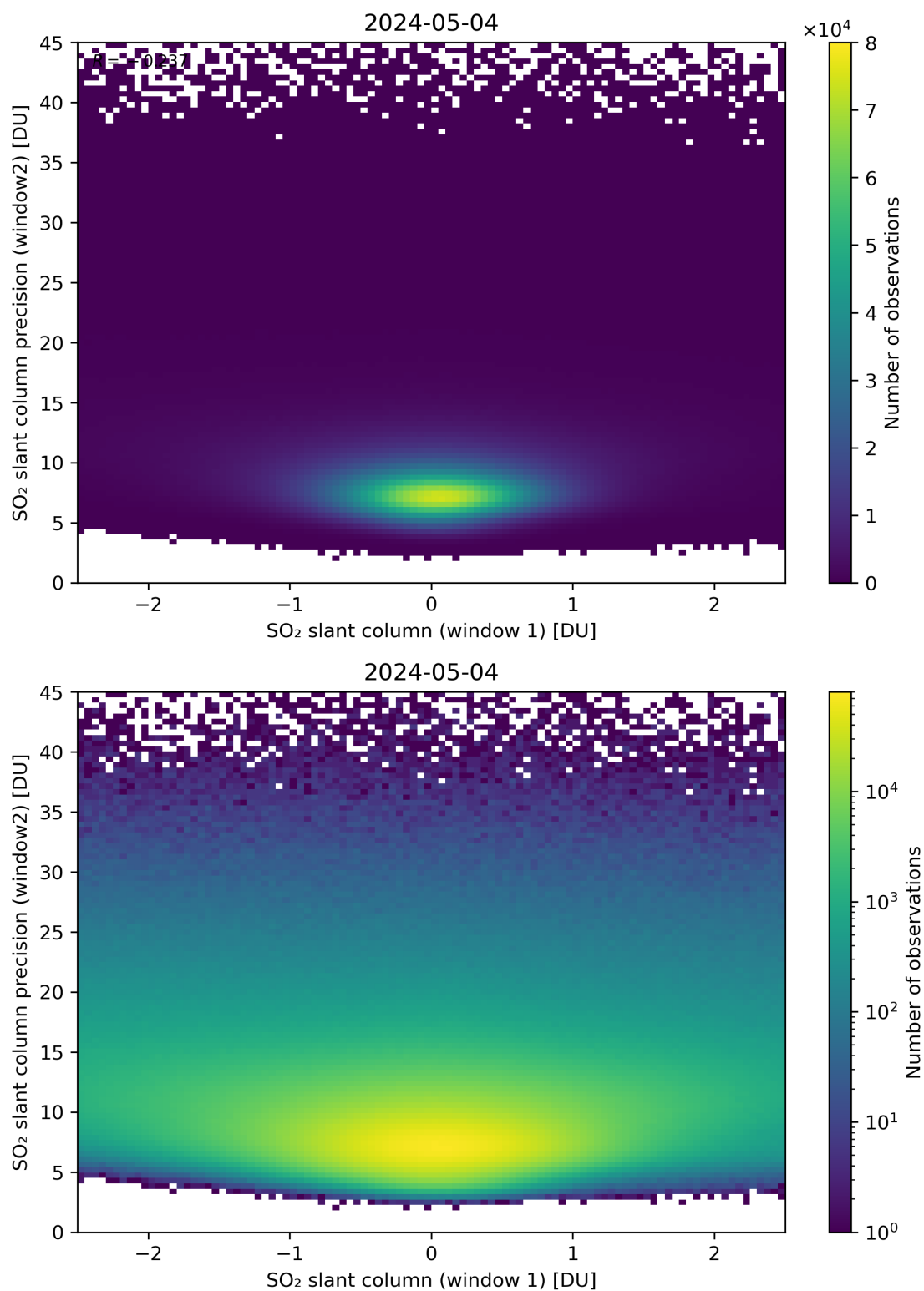
Figure 236: Scatter density plot of “SO 2 slant column (window 1)” against “SO 2 slant column precision (window2)” for 2024-05-03 to 2024-05-05.
