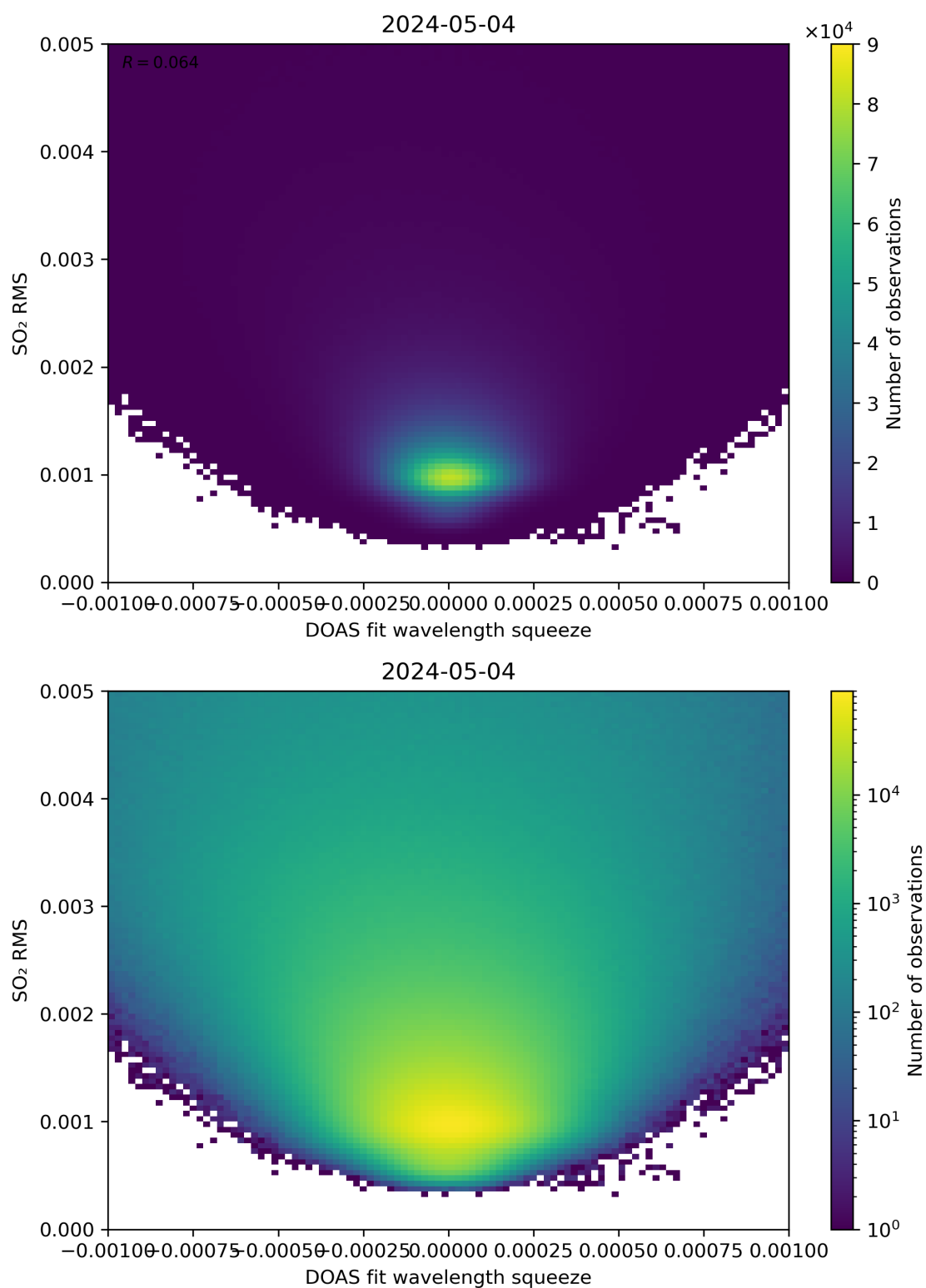
Figure 132: Scatter density plot of “DOAS fit wavelength squeeze” against “SO 2 RMS” for 2024-05-03 to 2024-05-05.
