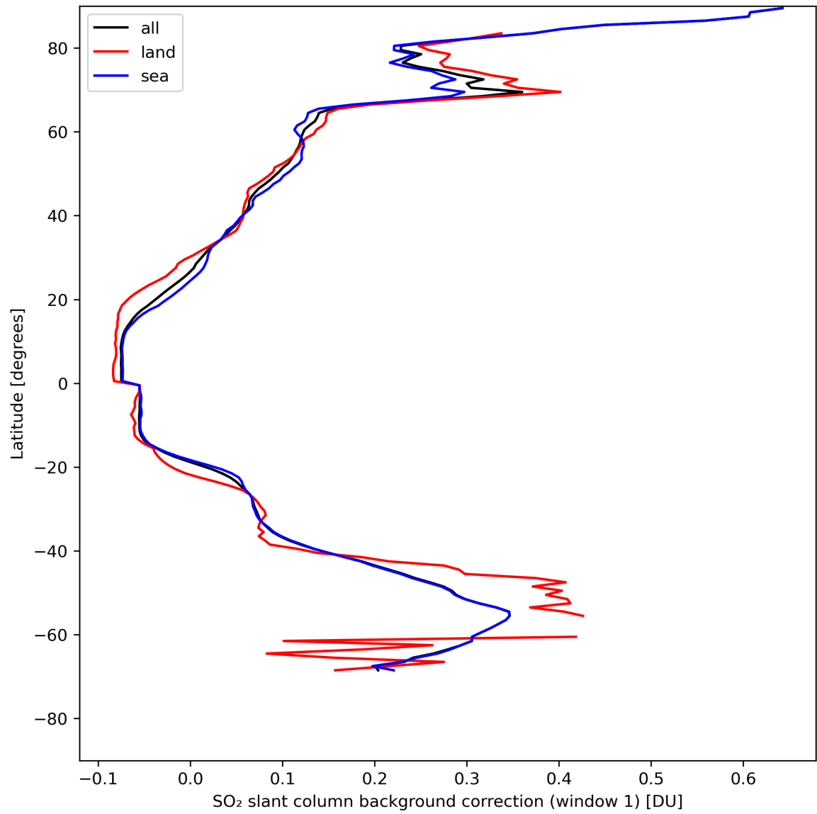
Figure 36: Zonal average of “SO 2 slant column background correction (window 1)” for 2024-05-03 to 2024-05-05.
