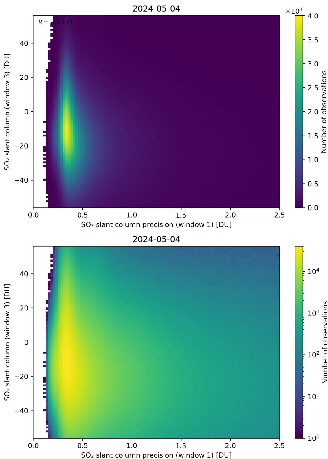
Figure 228: Scatter density plot of “SO 2 slant column precision (window 1)” against “SO 2 slant column (window 3)” for 2024-05-03 to 2024-05-05.
