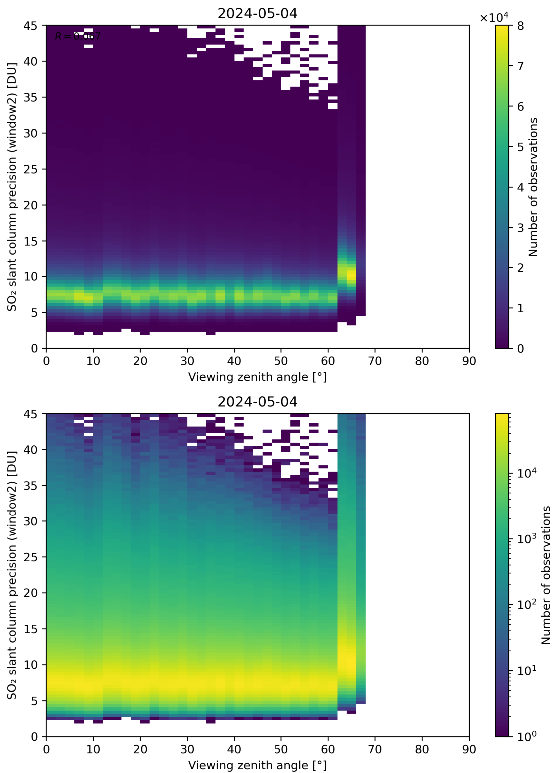
Figure 322: Scatter density plot of “Viewing zenith angle” against “SO 2 slant column precision (window2)” for 2024-05-03 to 2024-05-05.
