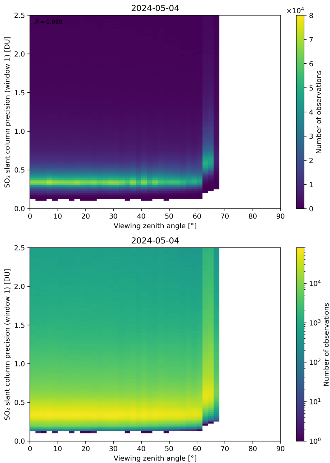
Figure 321: Scatter density plot of “Viewing zenith angle” against “SO 2 slant column precision (window 1)” for 2024-05-03 to 2024-05-05.
