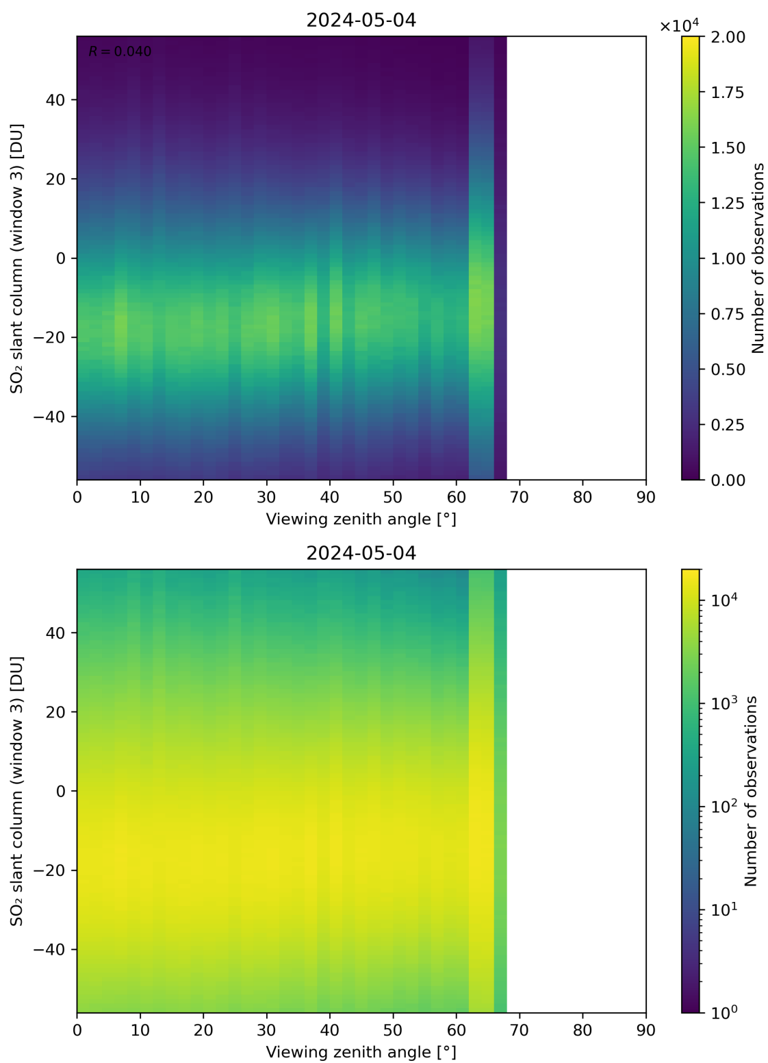
Figure 323: Scatter density plot of “Viewing zenith angle” against “SO 2 slant column (window 3)” for 2024-05-03 to 2024-05-05.
