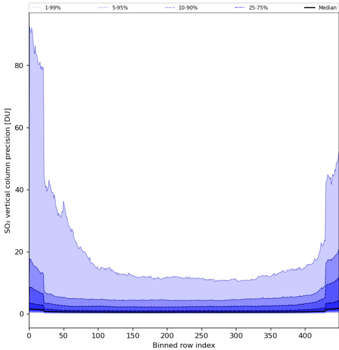
Figure 77: Along track statistics of “SO 2 vertical column precision” for 2024-05-03 to 2024-05-05
