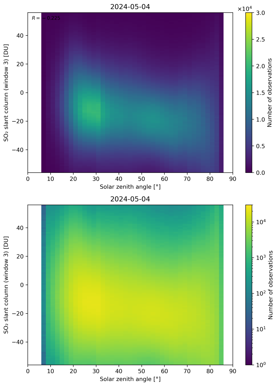
Figure 172: Scatter density plot of “Solar zenith angle” against “SO 2 slant column (window 3)” for 2024-05-03 to 2024-05-05.
