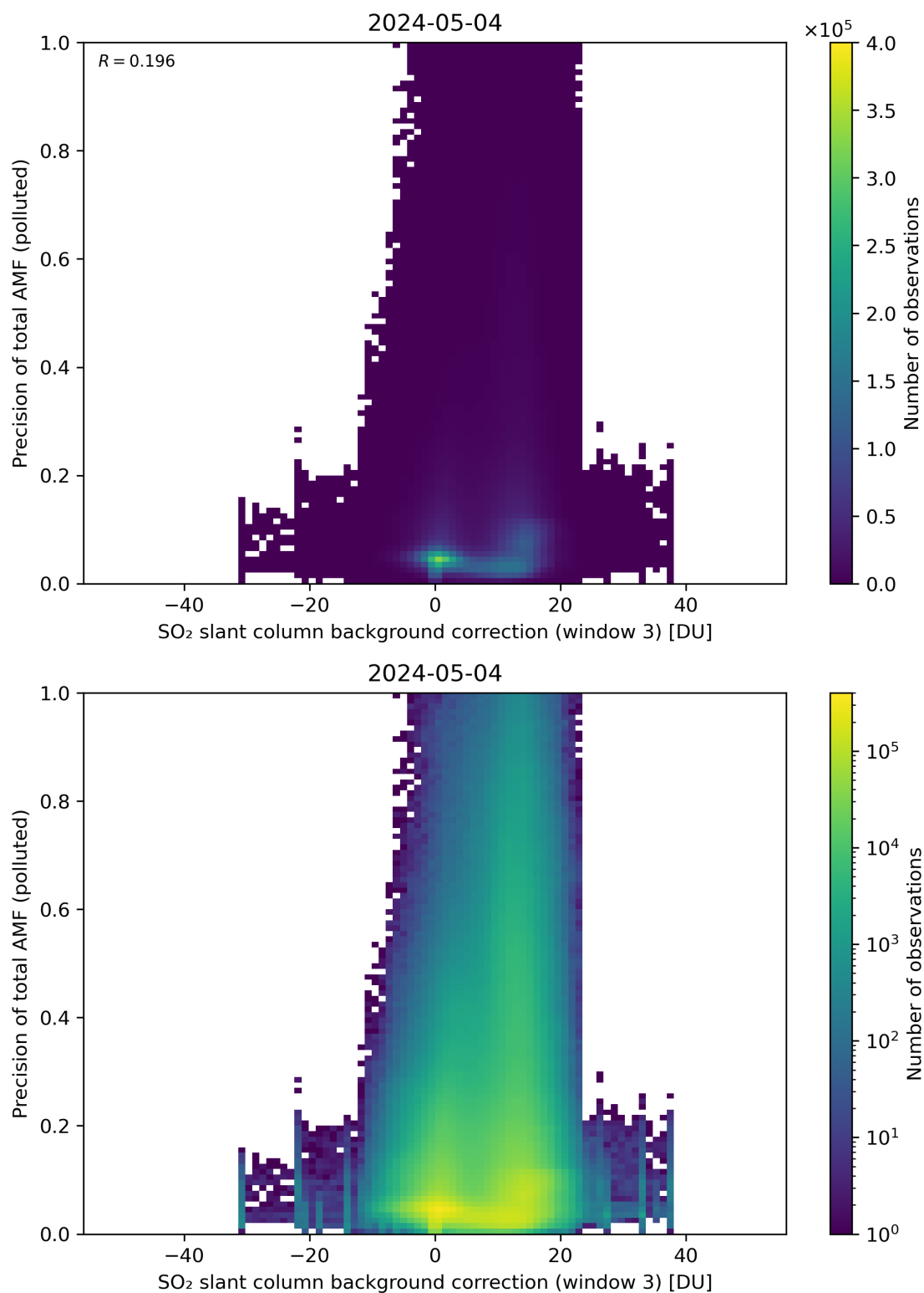
Figure 126: Scatter density plot of “SO 2 slant column background correction (window 3)” against “Precision of total AMF (polluted)” for 2024-05-03 to 2024-05-05.
