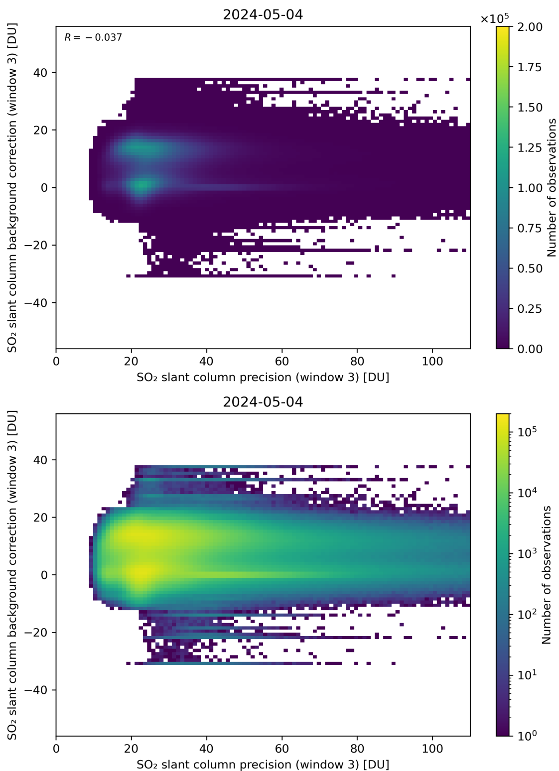
Figure 257: Scatter density plot of “SO 2 slant column precision (window 3)” against “SO 2 slant column background correction (window 3)” for 2024-05-03 to 2024-05-05.
