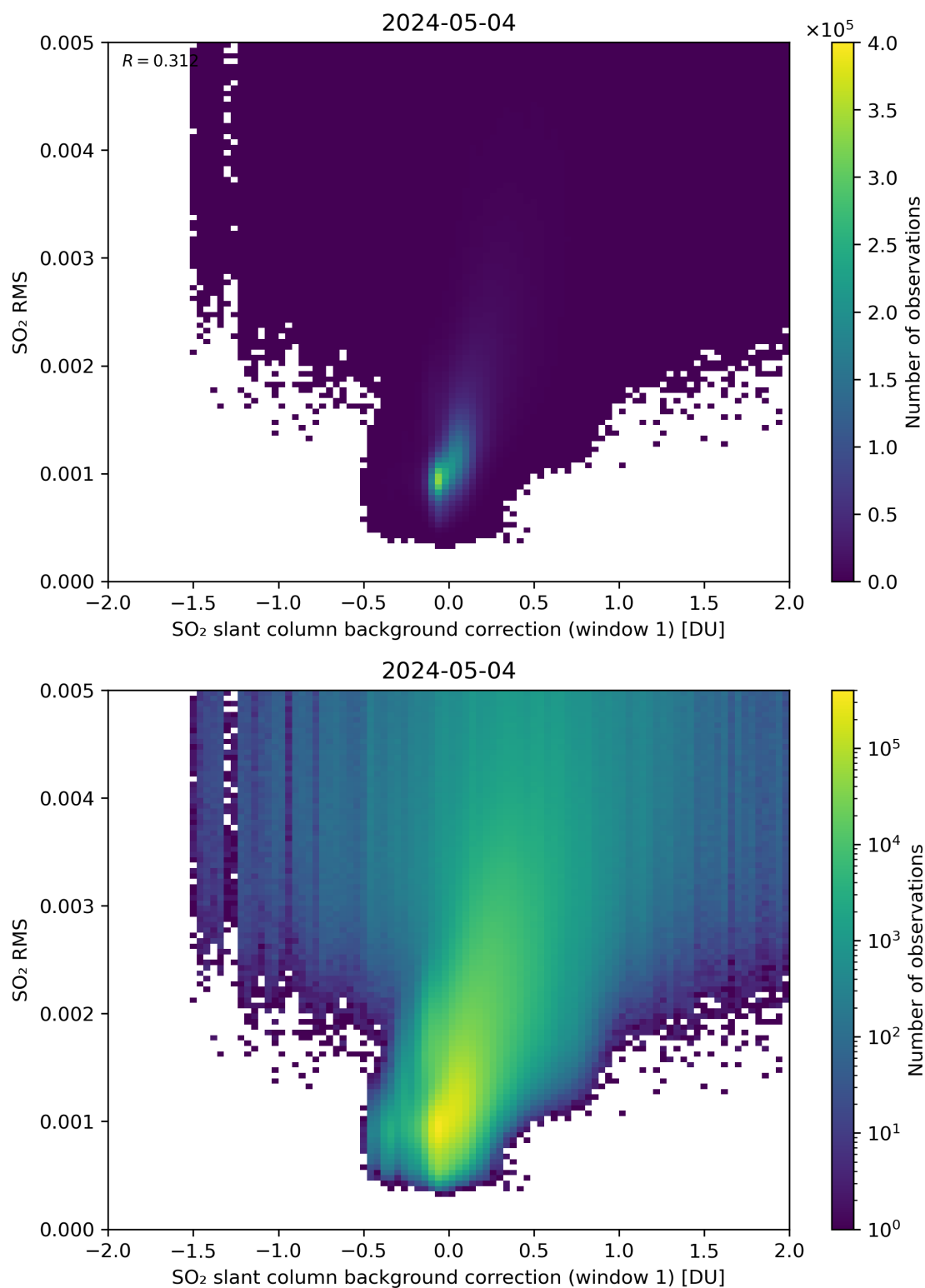
Figure 102: Scatter density plot of “SO 2 slant column background correction (window 1)” against “SO 2 RMS” for 2024-05-03 to 2024-05-05.
