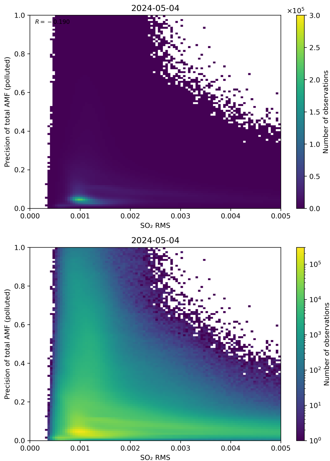
Figure 138: Scatter density plot of “SO 2 RMS” against “Precision of total AMF (polluted)” for 2024-05-03 to 2024-05-05.
