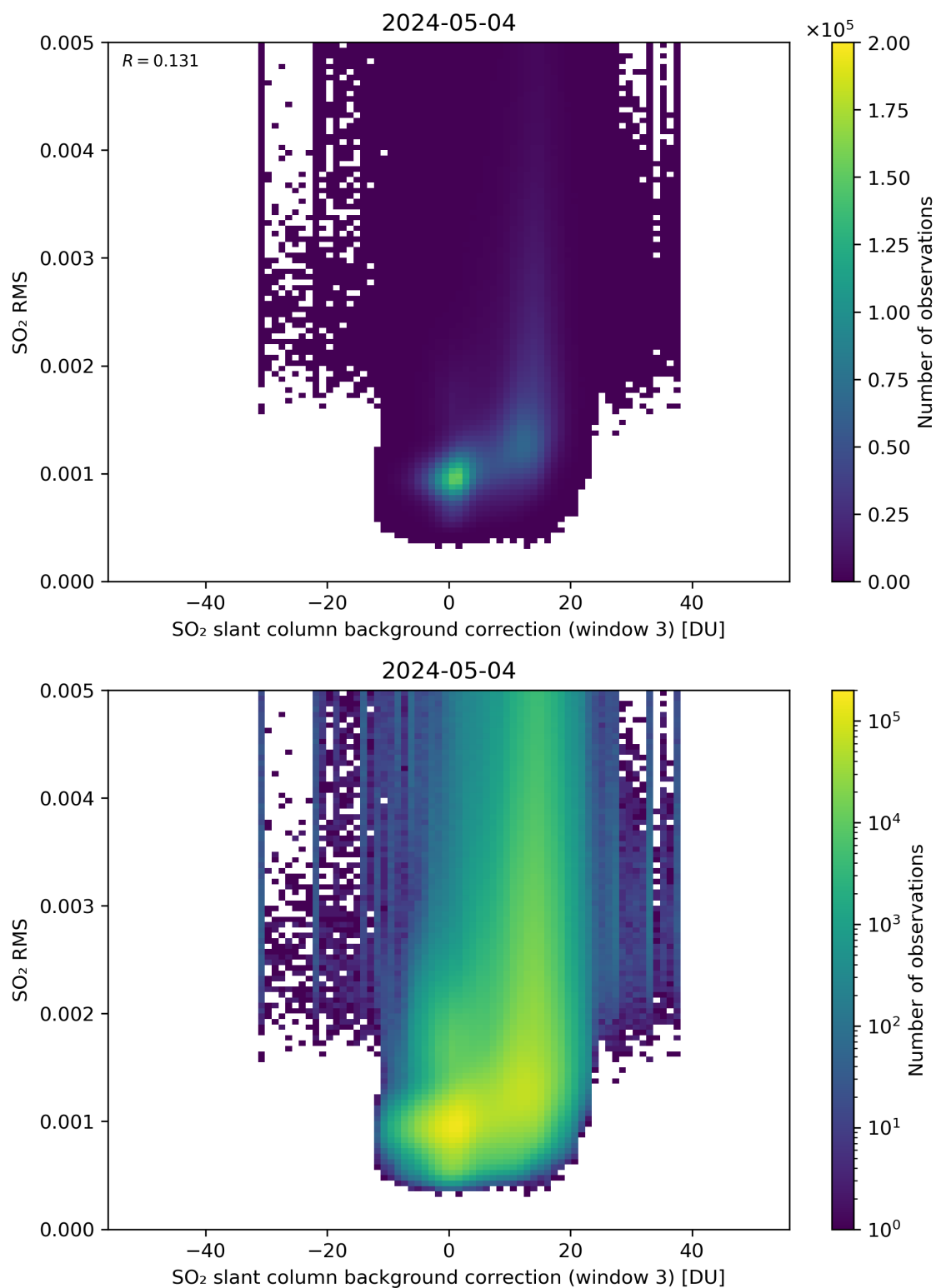
Figure 123: Scatter density plot of “SO 2 slant column background correction (window 3)” against “SO 2 RMS” for 2024-05-03 to 2024-05-05.
