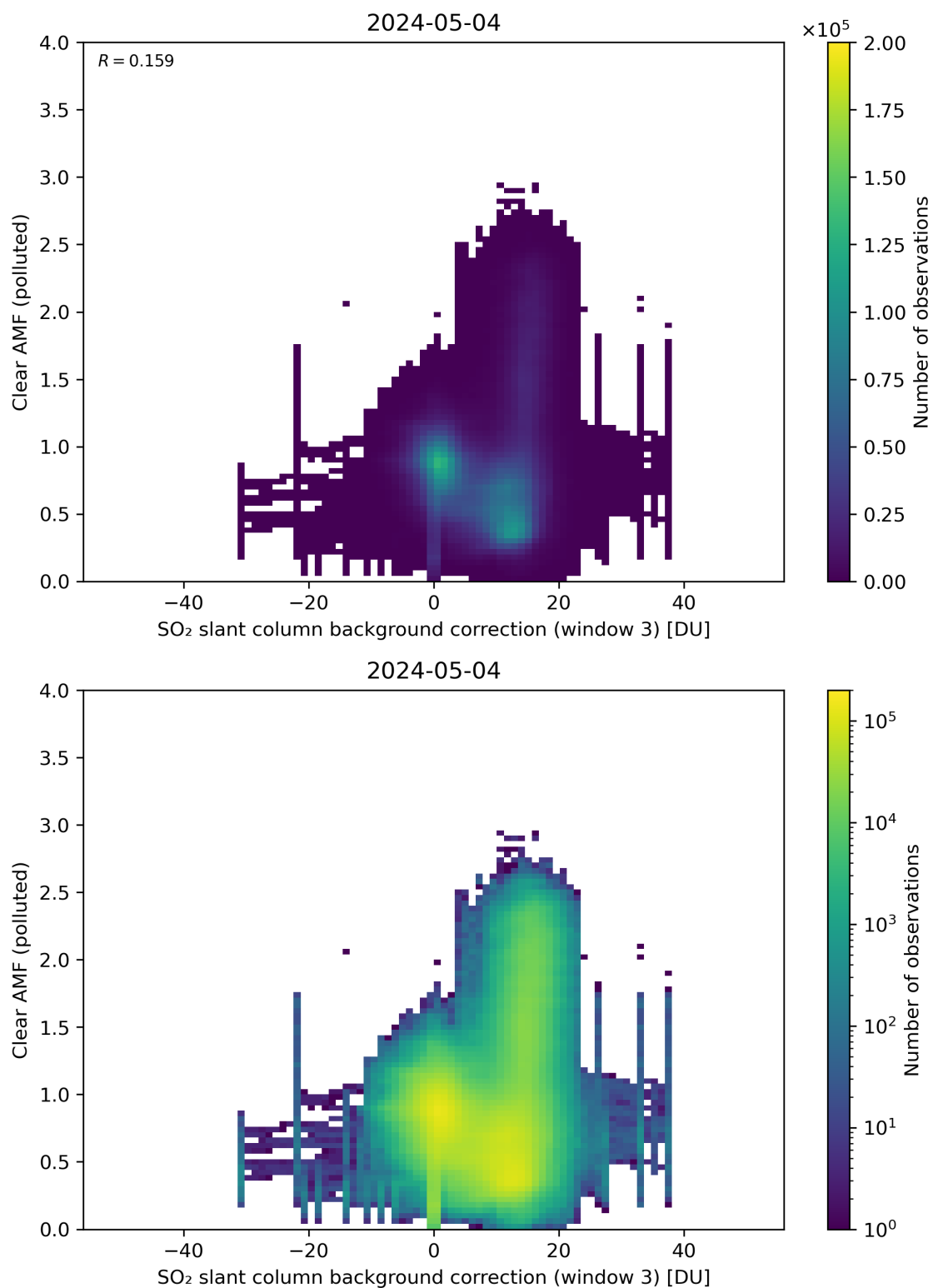
Figure 124: Scatter density plot of “SO 2 slant column background correction (window 3)” against “Clear AMF (polluted)” for 2024-05-03 to 2024-05-05.
