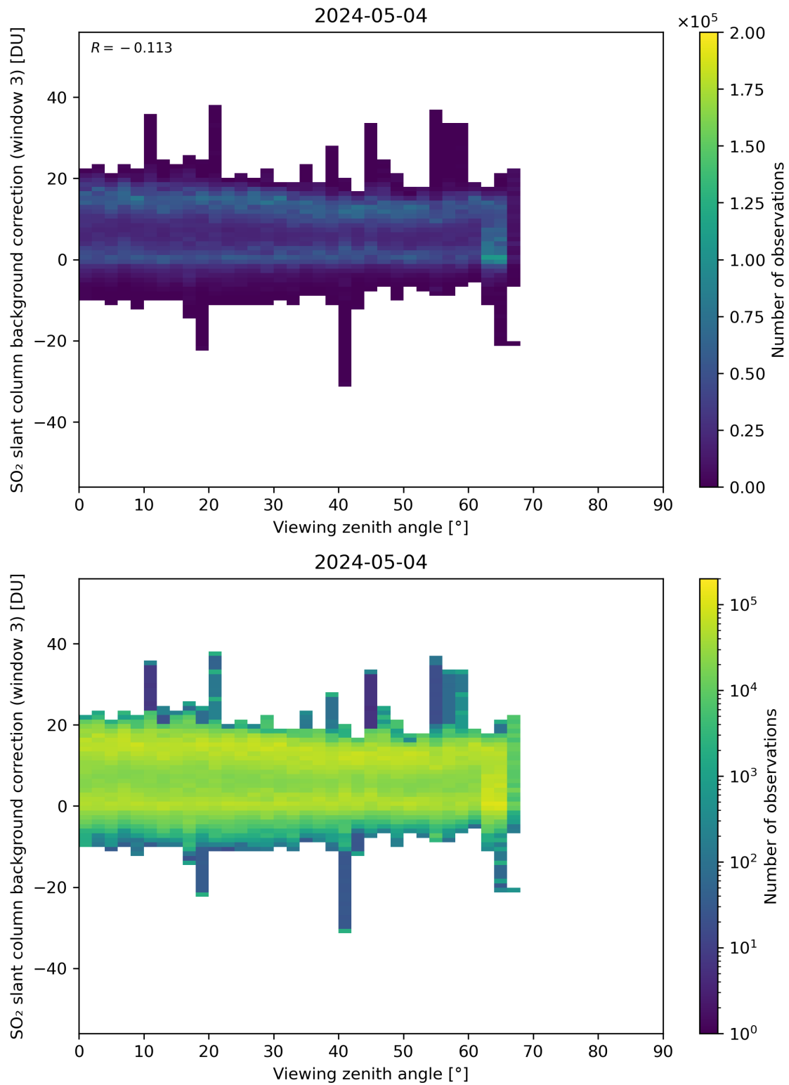
Figure 310: Scatter density plot of “Viewing zenith angle” against “SO 2 slant column background correction (window 3)” for 2024-05-03 to 2024-05-05.
