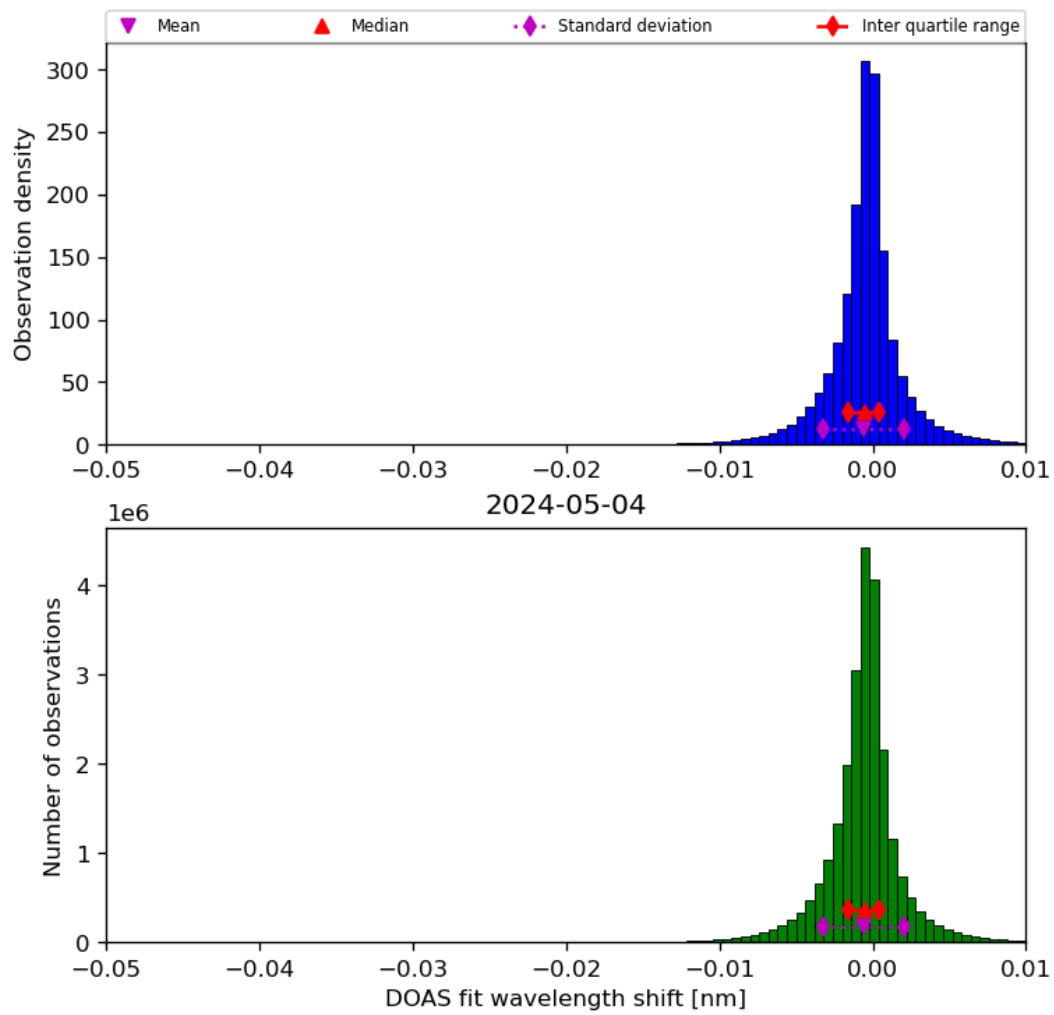
Figure 68: Histogram of “DOAS fit wavelength shift” for 2024-05-03 to 2024-05-05
