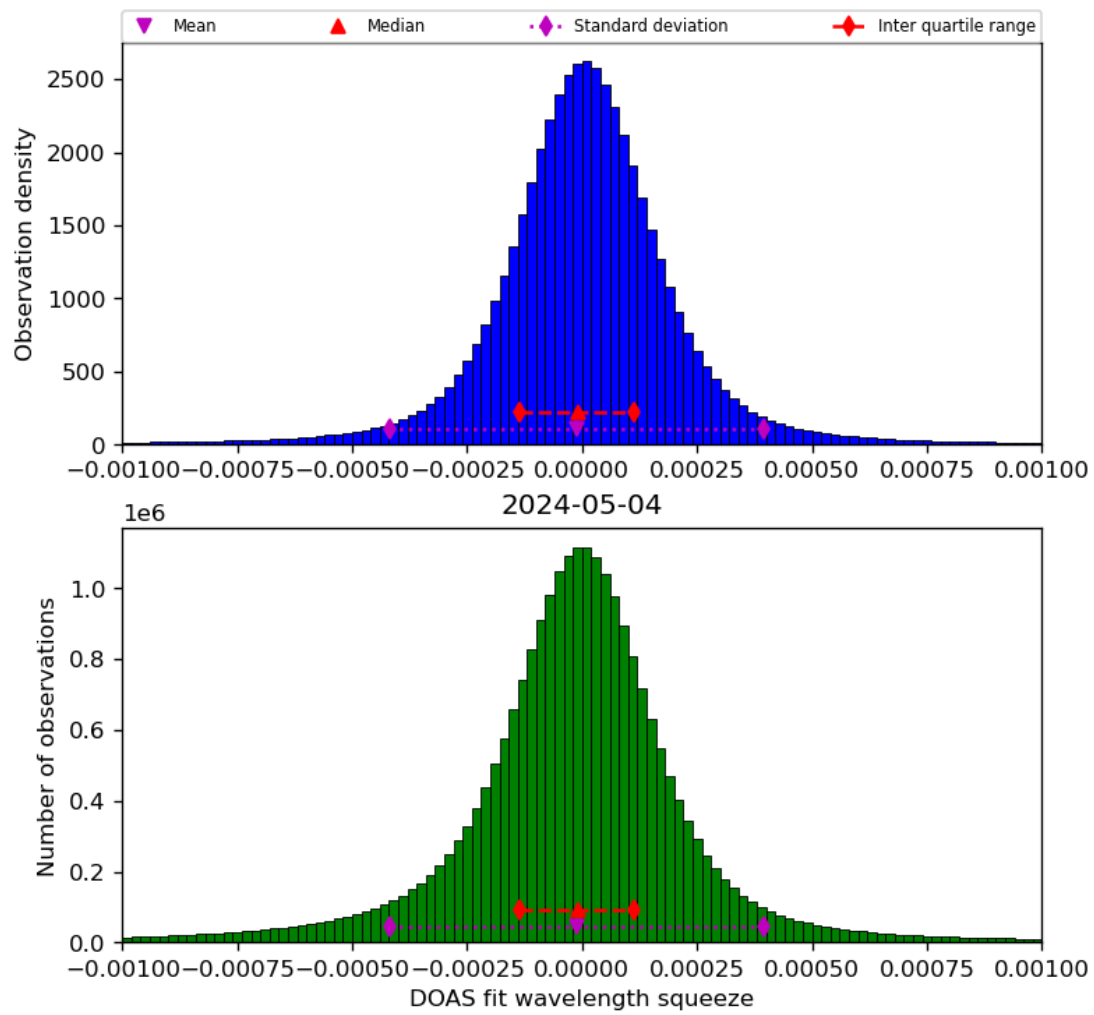
Figure 69: Histogram of “DOAS fit wavelength squeeze” for 2024-05-03 to 2024-05-05
