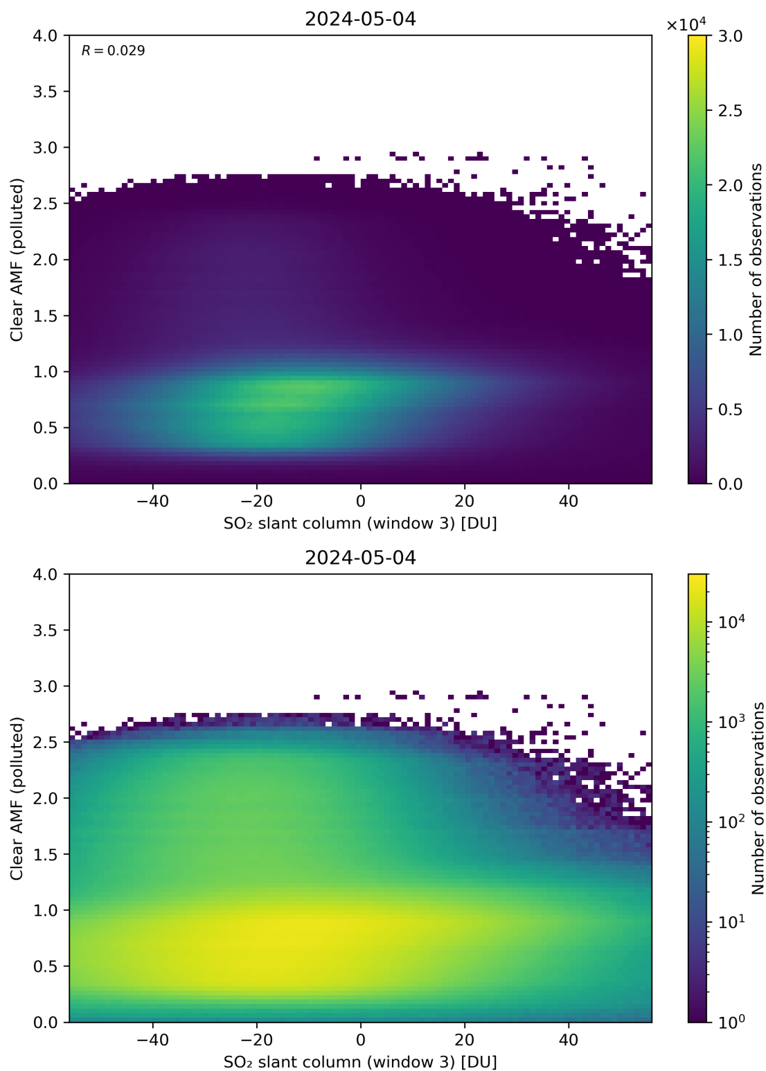
Figure 265: Scatter density plot of “SO 2 slant column (window 3)” against “Clear AMF (polluted)” for 2024-05-03 to 2024-05-05.
