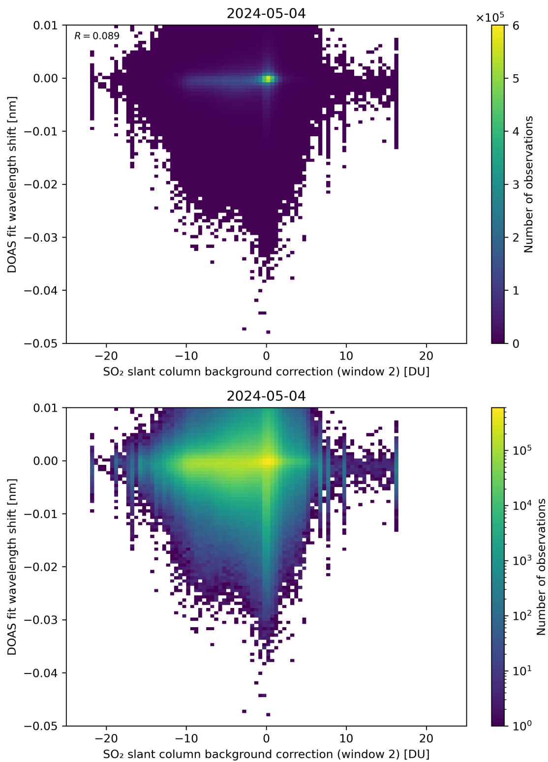
Figure 112: Scatter density plot of “SO 2 slant column background correction (window 2)” against “DOAS fit wavelength shift” for 2024-05-03 to 2024-05-05.
