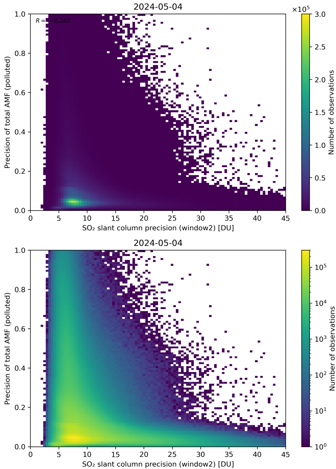
Figure 252: Scatter density plot of “SO 2 slant column precision (window2)” against “Precision of total AMF (polluted)” for 2024-05-03 to 2024-05-05.
