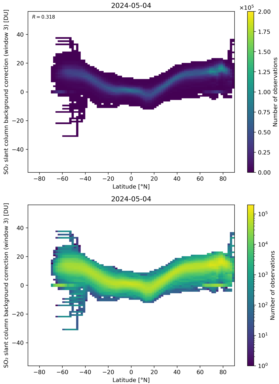
Figure 141: Scatter density plot of “Latitude” against “SO 2 slant column background correction (window 3)” for 2024-05-03 to 2024-05-05.
