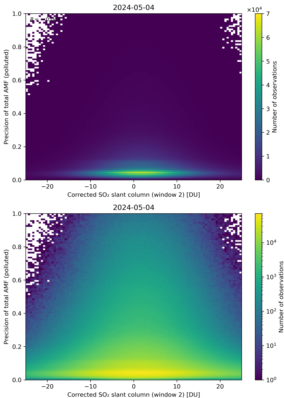
Figure 204: Scatter density plot of “Corrected SO 2 slant column (window 2)” against “Precision of total AMF (polluted)” for 2024-05-03 to 2024-05-05.
