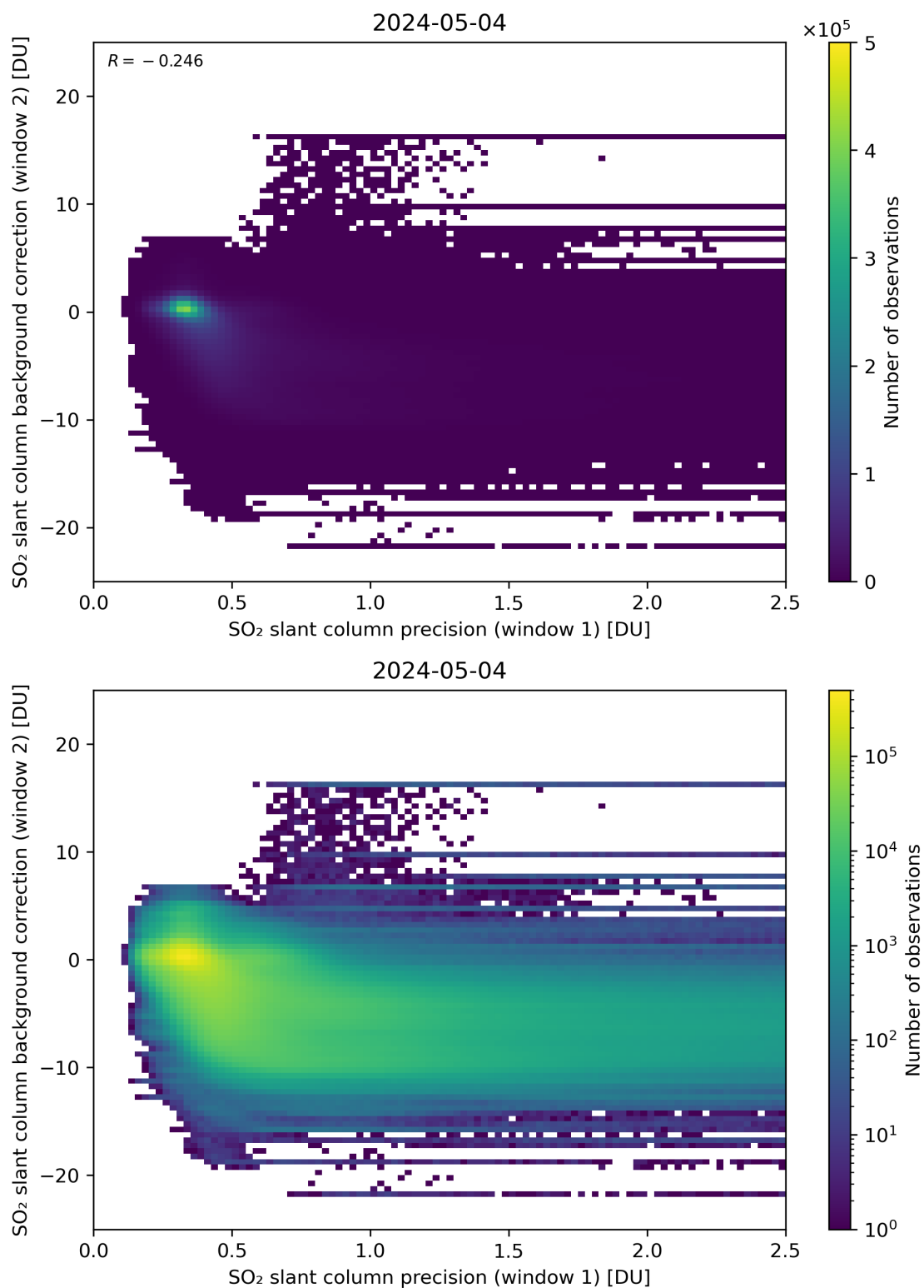
Figure 219: Scatter density plot of “SO 2 slant column precision (window 1)” against “SO 2 slant column background correction (window 2)” for 2024-05-03 to 2024-05-05.
