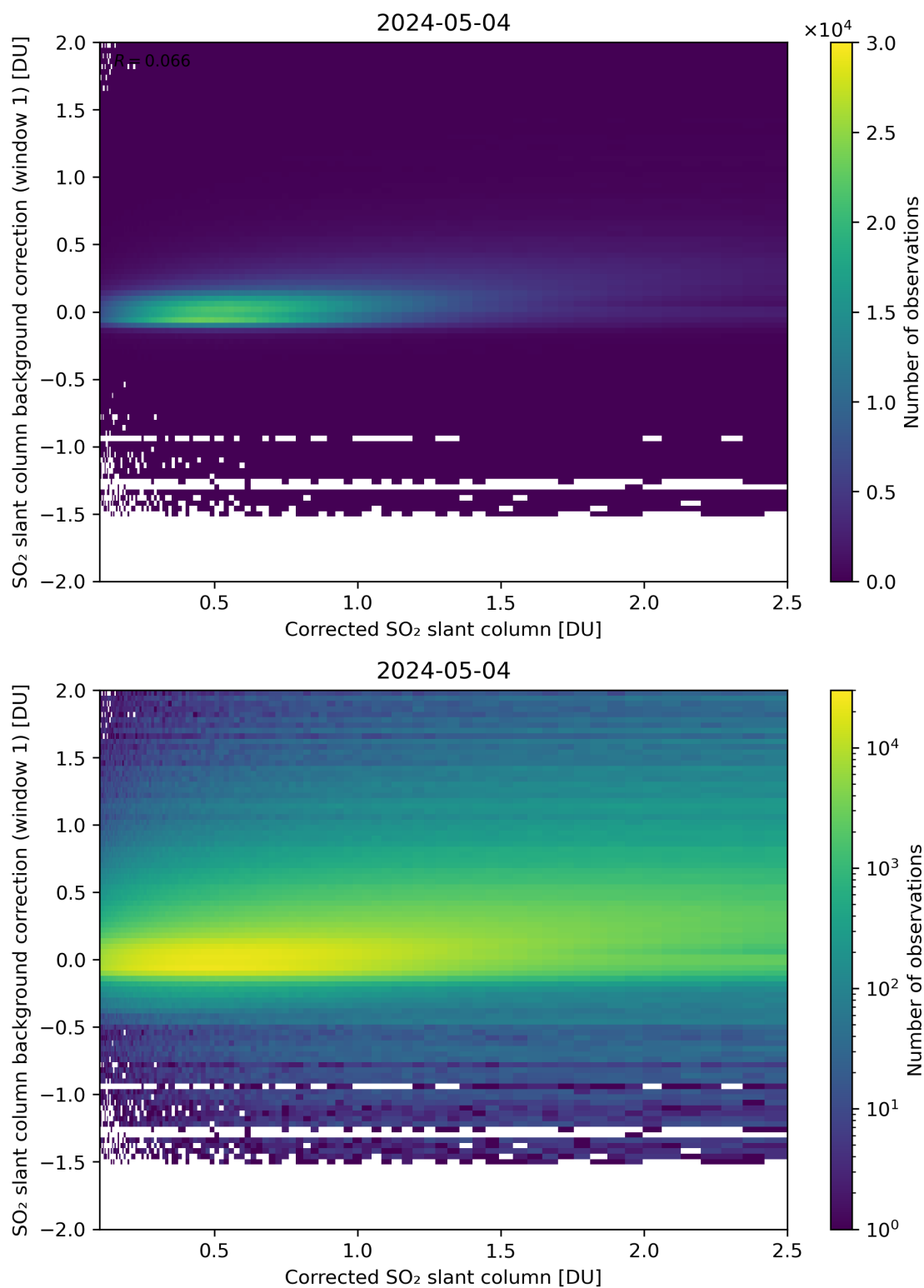
Figure 178: Scatter density plot of “Corrected SO 2 slant column” against “SO 2 slant column background correction (window 1)” for 2024-05-03 to 2024-05-05.
