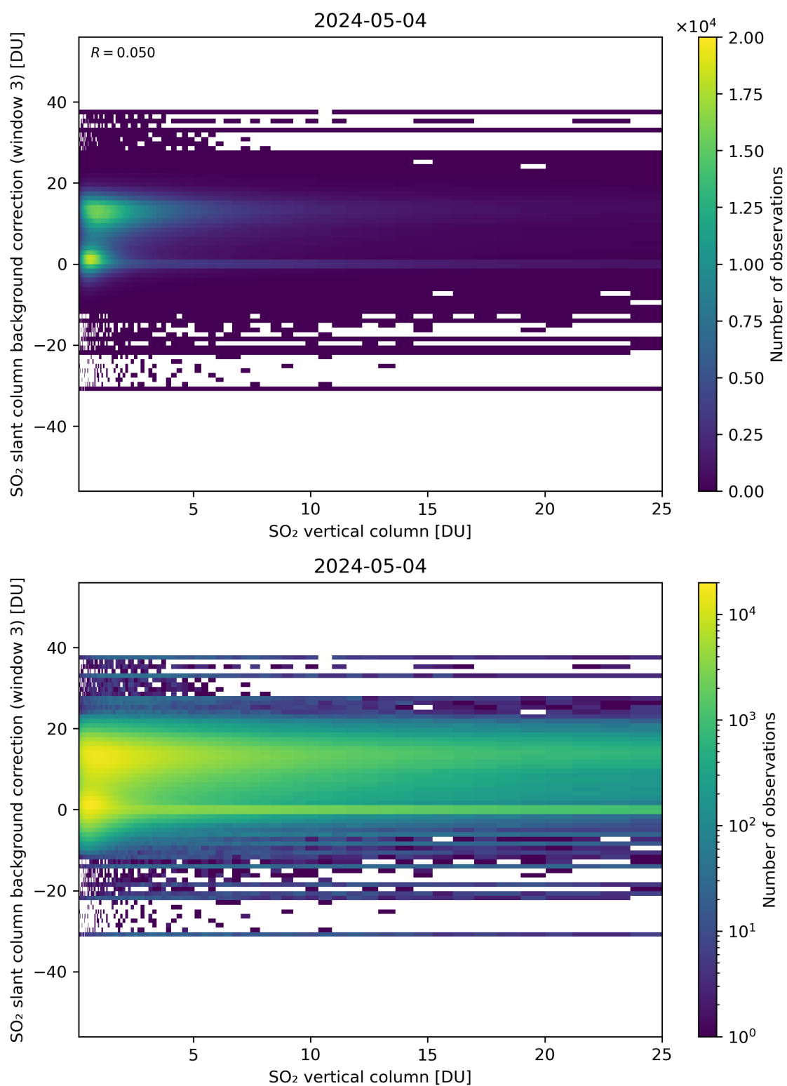
Figure 275: Scatter density plot of “SO 2 vertical column” against “SO 2 slant column background correction (window 3)” for 2024-05-03 to 2024-05-05.
