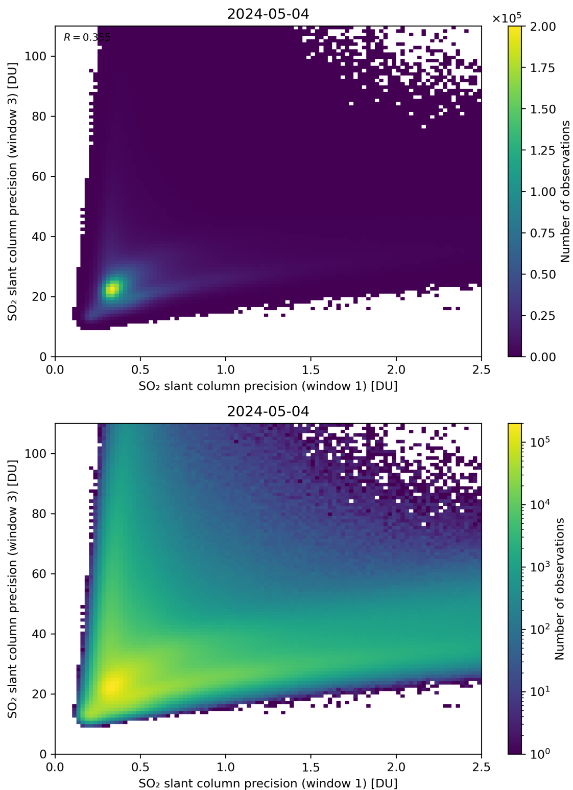
Figure 229: Scatter density plot of “SO 2 slant column precision (window 1)” against “SO 2 slant column precision (window 3)” for 2024-05-03 to 2024-05-05.
