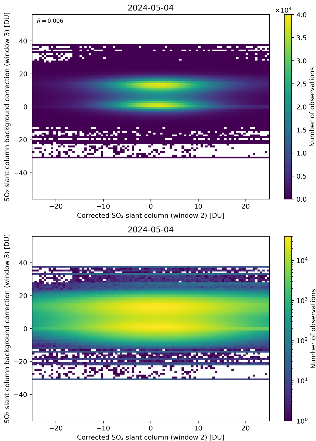
Figure 195: Scatter density plot of “Corrected SO 2 slant column (window 2)” against “SO 2 slant column background correction (window 3)” for 2024-05-03 to 2024-05-05.
