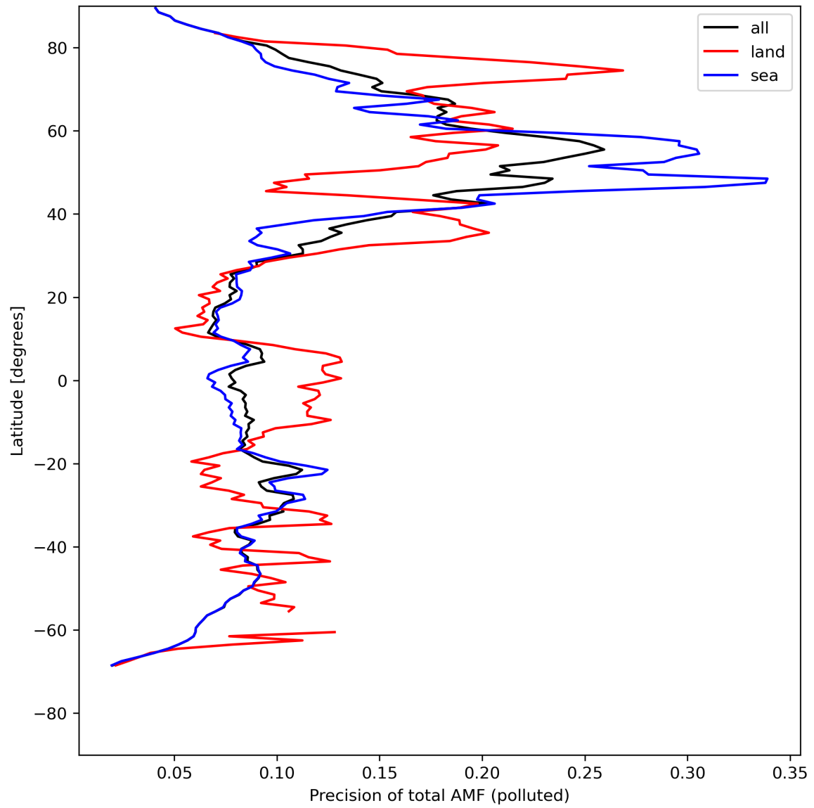
Figure 49: Zonal average of “Precision of total AMF (polluted)” for 2024-05-03 to 2024-05-05.
