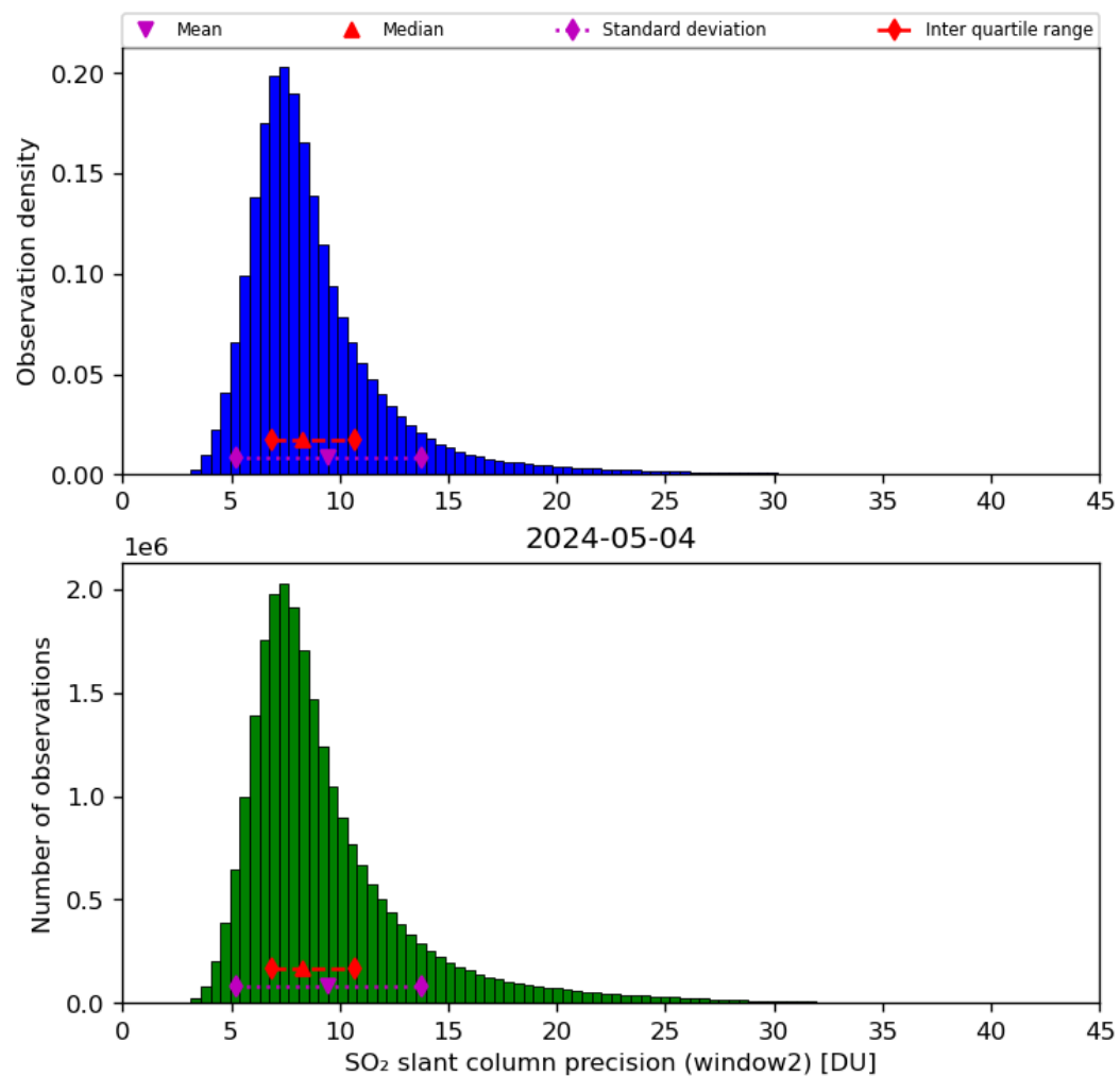
Figure 61: Histogram of “SO 2 slant column precision (window2)” for 2024-05-03 to 2024-05-05
