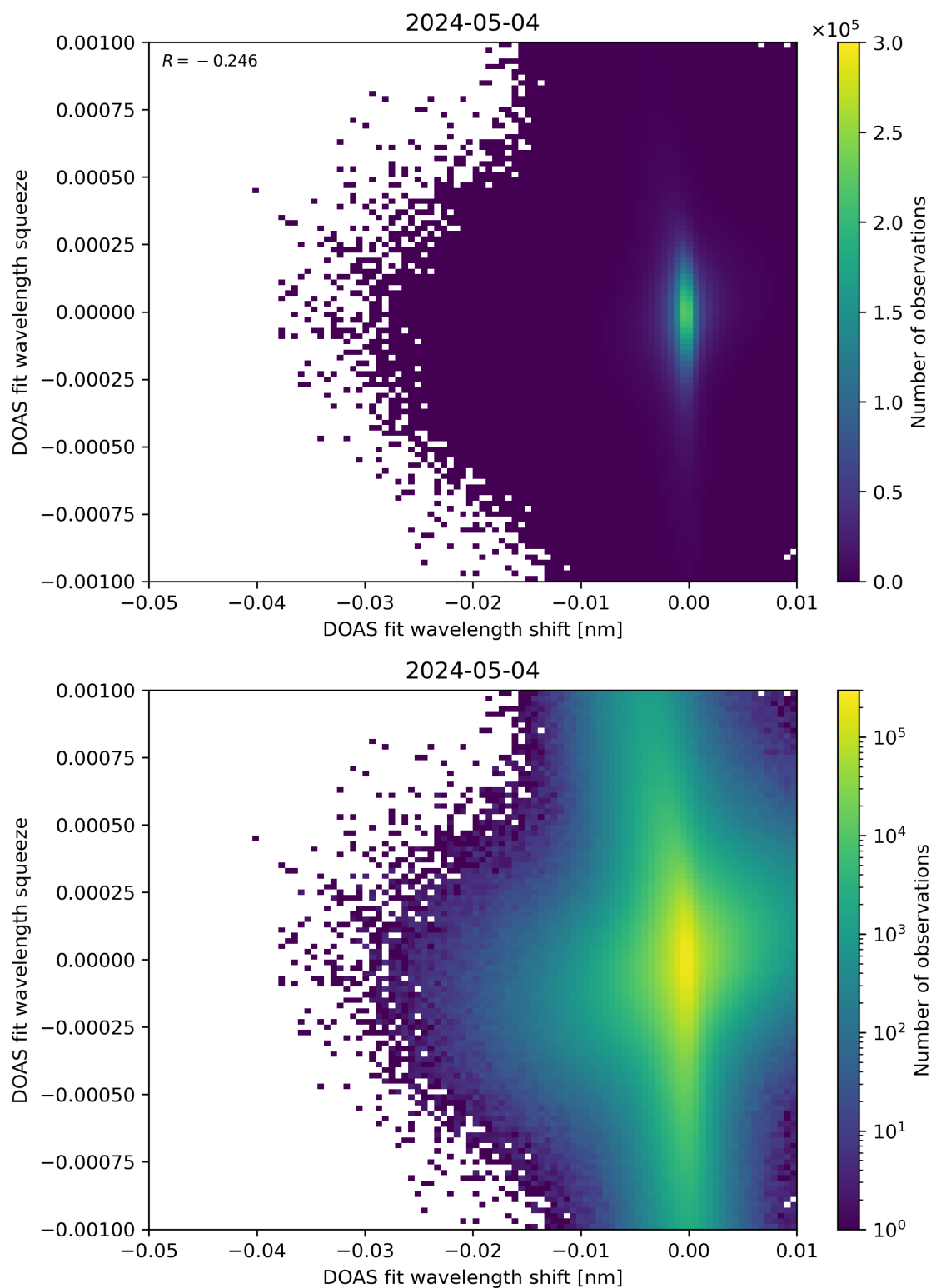
Figure 127: Scatter density plot of “DOAS fit wavelength shift” against “DOAS fit wavelength squeeze” for 2024-05-03 to 2024-05-05.
