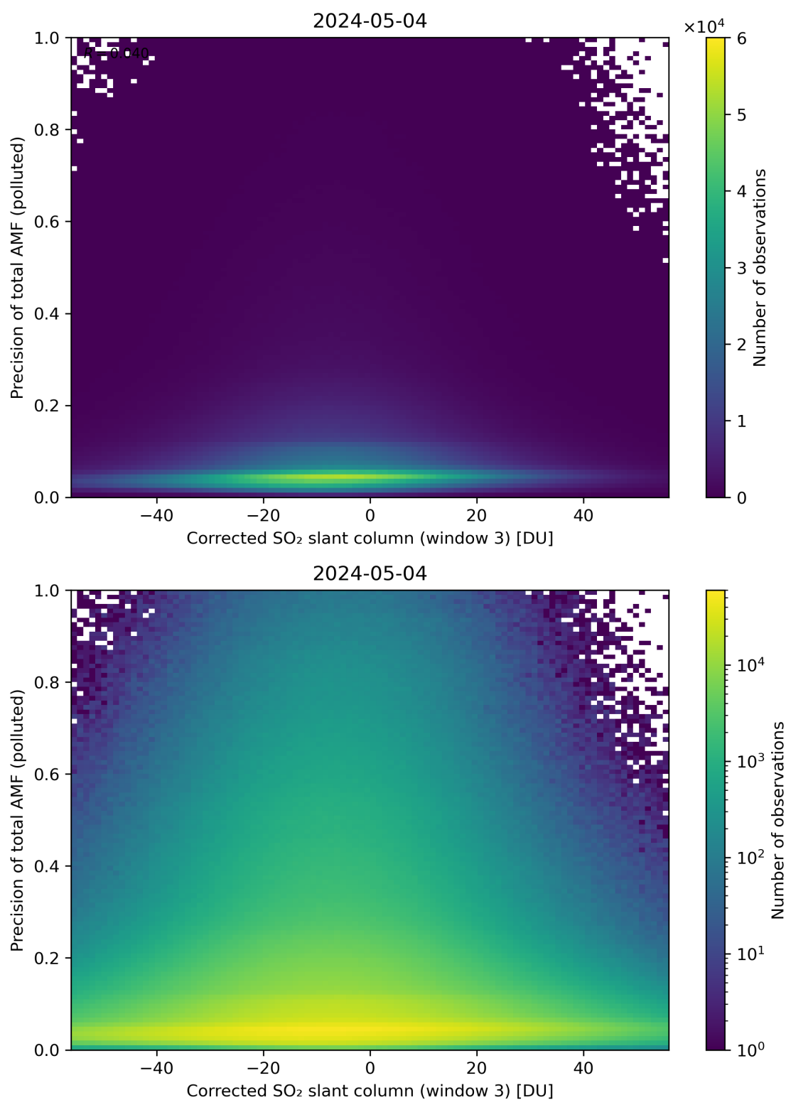
Figure 211: Scatter density plot of “Corrected SO 2 slant column (window 3)” against “Precision of total AMF (polluted)” for 2024-05-03 to 2024-05-05.
