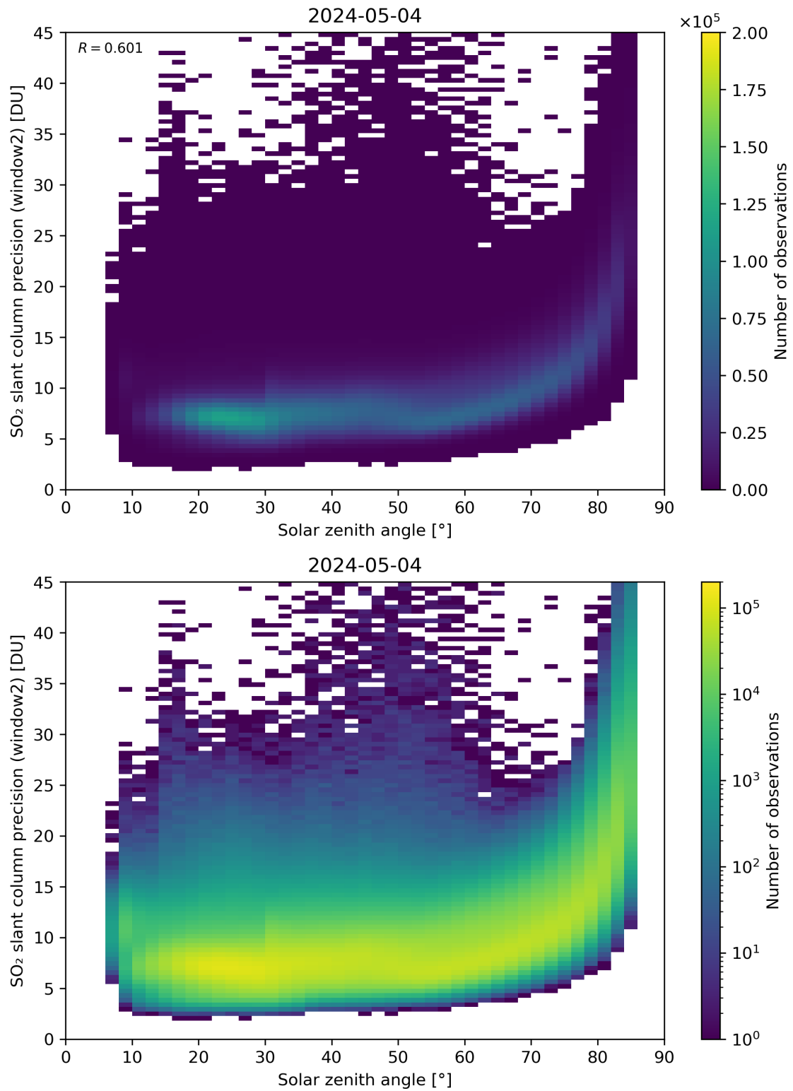
Figure 171: Scatter density plot of “Solar zenith angle” against “SO 2 slant column precision (window2)” for 2024-05-03 to 2024-05-05.
