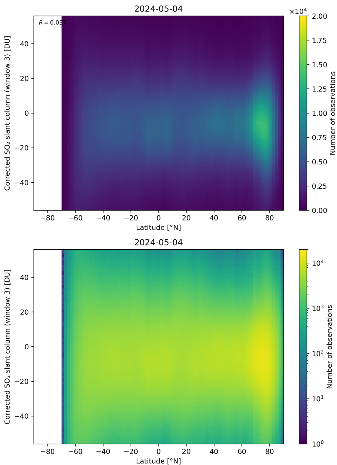
Figure 148: Scatter density plot of “Latitude” against “Corrected SO 2 slant column (window 3)” for 2024-05-03 to 2024-05-05.
