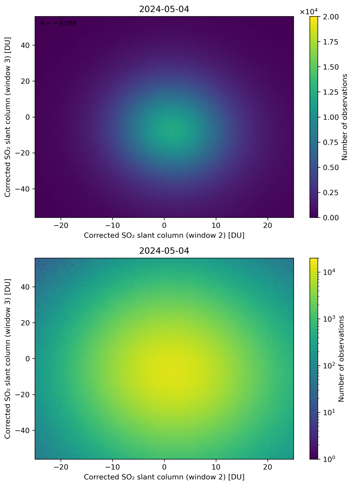
Figure 200: Scatter density plot of “Corrected SO 2 slant column (window 2)” against “Corrected SO 2 slant column (window 3)” for 2024-05-03 to 2024-05-05.
