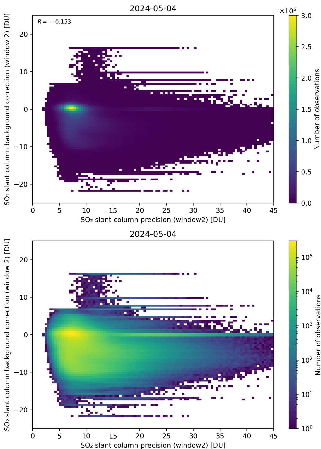
Figure 241: Scatter density plot of “SO 2 slant column precision (window2)” against “SO 2 slant column background correction (window 2)” for 2024-05-03 to 2024-05-05.
