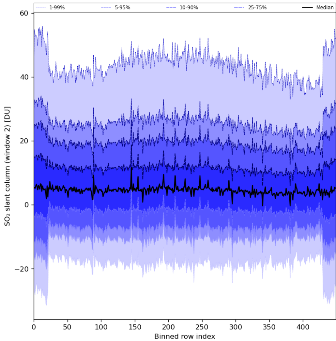
Figure 83: Along track statistics of “SO 2 slant column (window 2)” for 2024-05-03 to 2024-05-05
