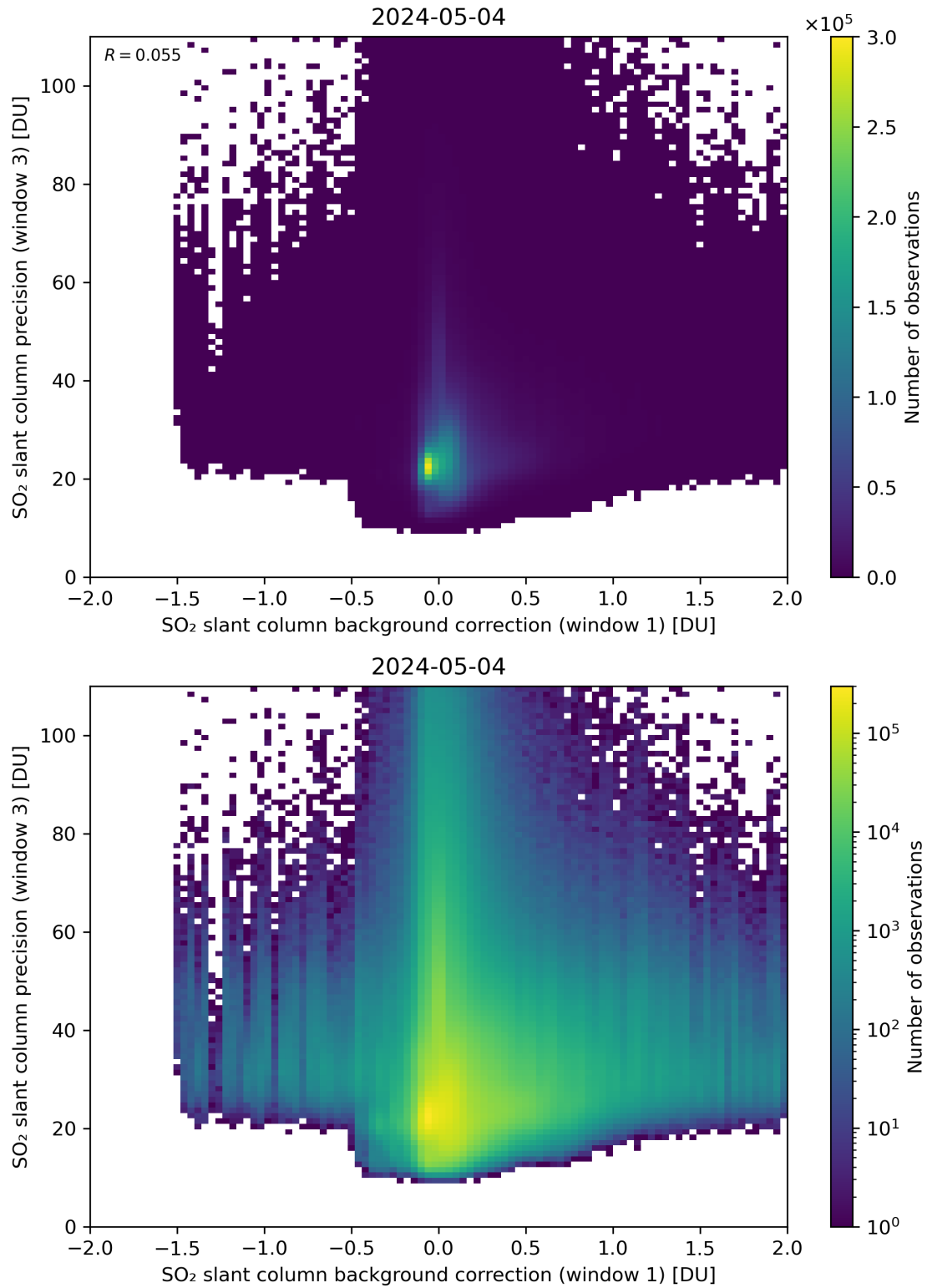
Figure 108: Scatter density plot of “SO 2 slant column background correction (window 1)” against “SO 2 slant column precision (window 3)” for 2024-05-03 to 2024-05-05.
