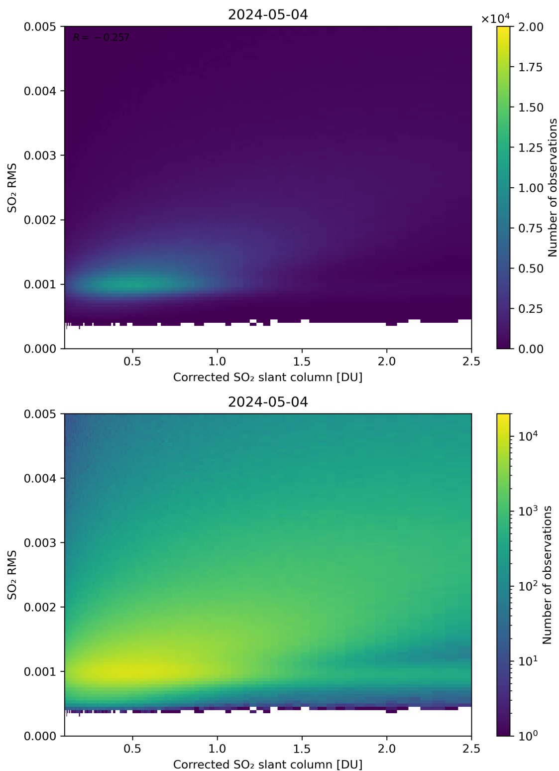
Figure 183: Scatter density plot of “Corrected SO 2 slant column” against “SO 2 RMS” for 2024-05-03 to 2024-05-05.
