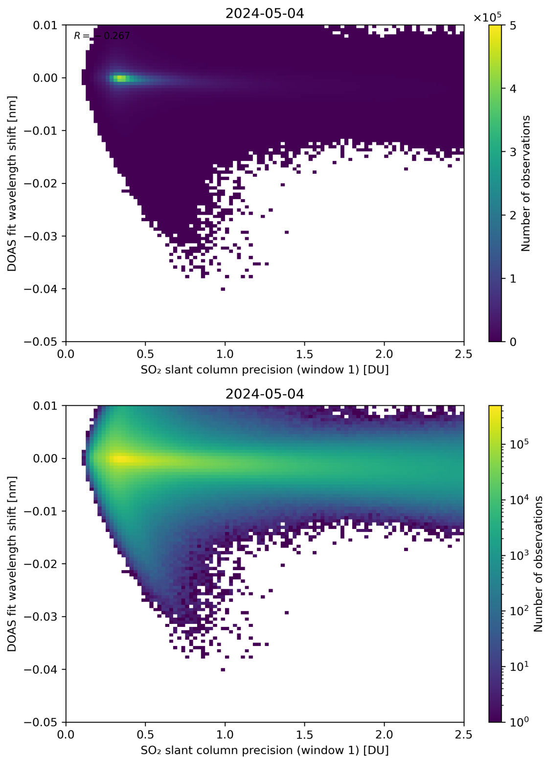
Figure 221: Scatter density plot of “SO 2 slant column precision (window 1)” against “DOAS fit wavelength shift” for 2024-05-03 to 2024-05-05.
