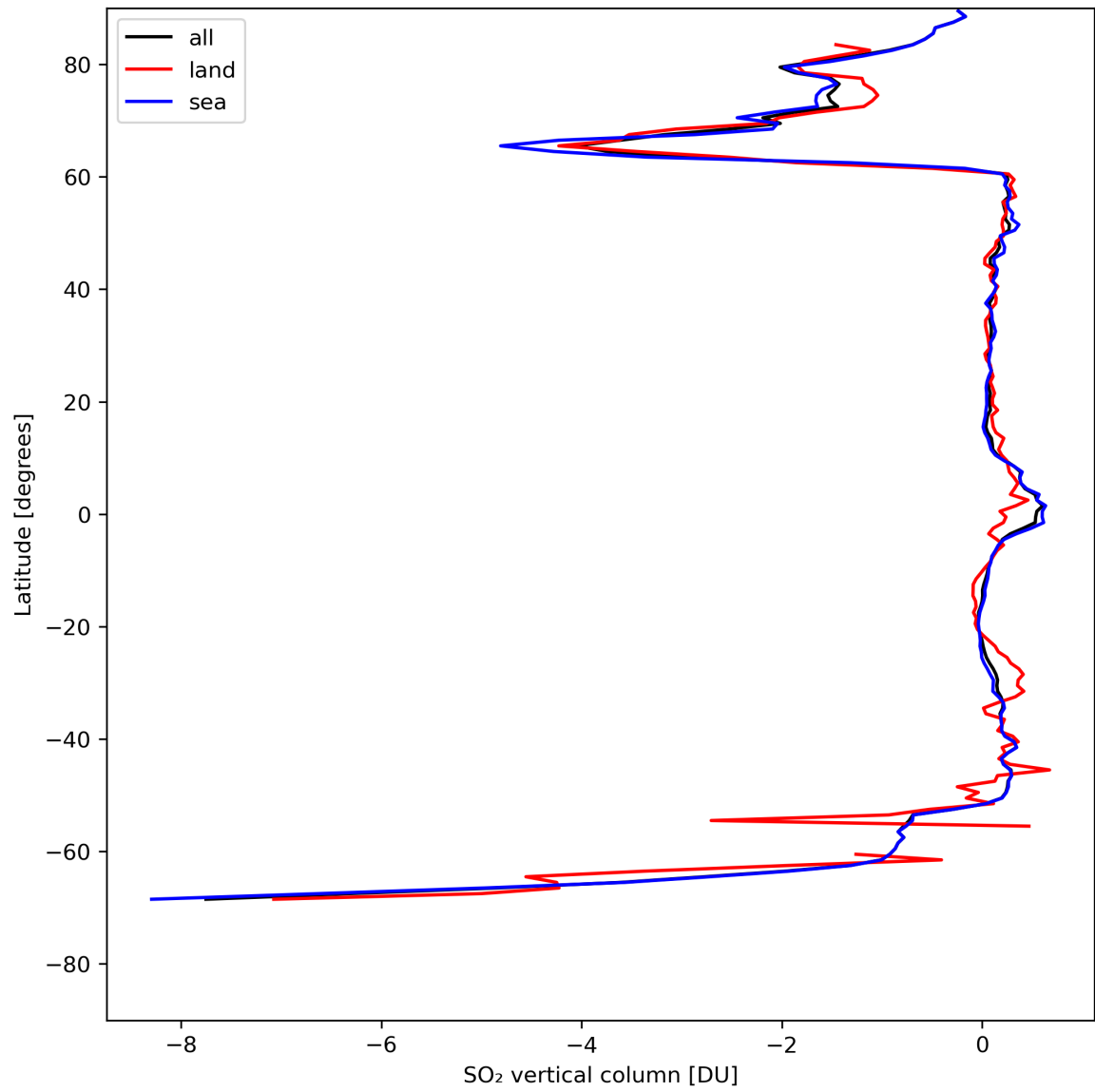
Figure 30: Zonal average of “SO 2 vertical column” for 2024-05-03 to 2024-05-05.
