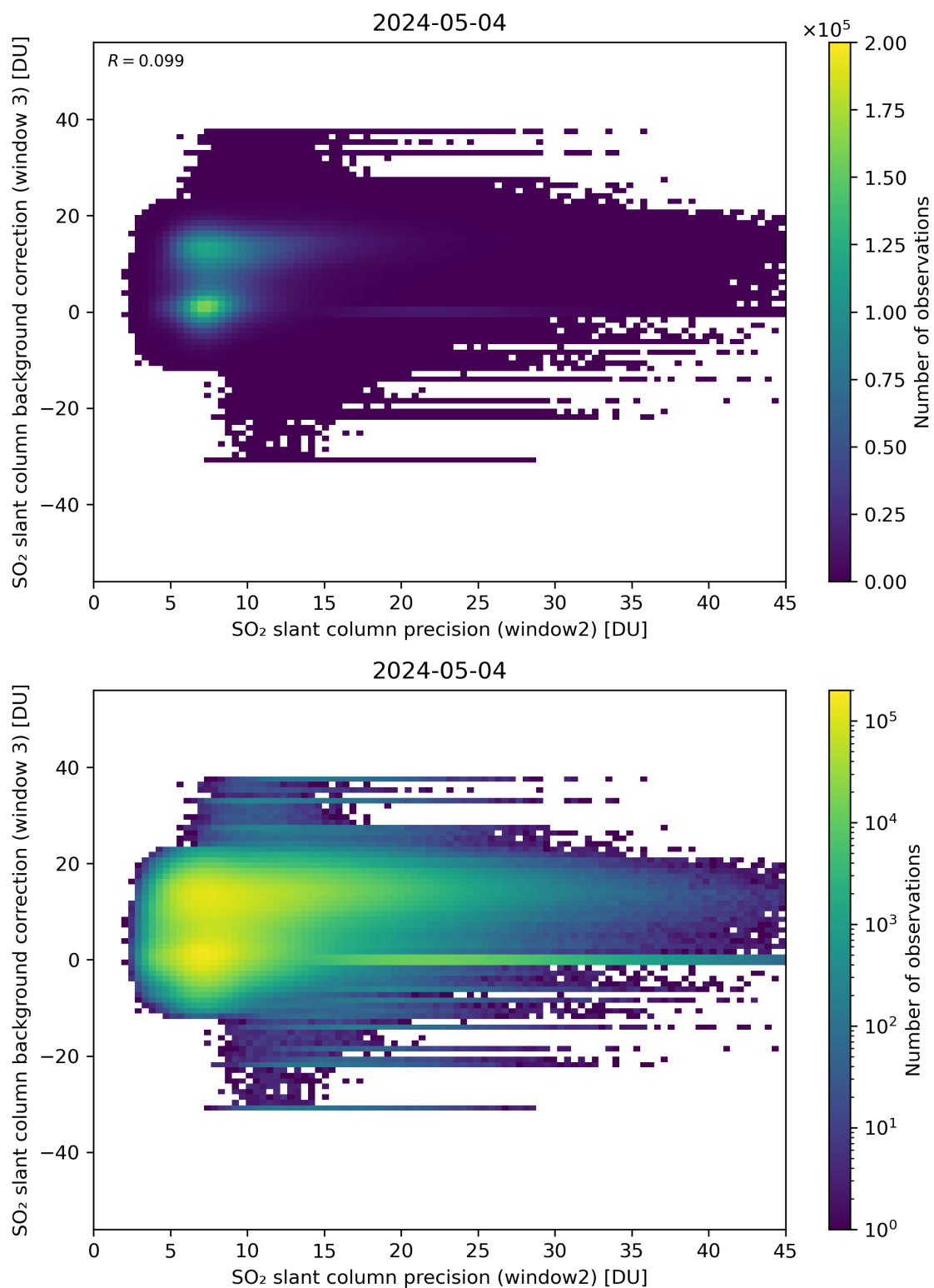
Figure 242: Scatter density plot of “SO 2 slant column precision (window2)” against “SO 2 slant column background correction (window 3)” for 2024-05-03 to 2024-05-05.
