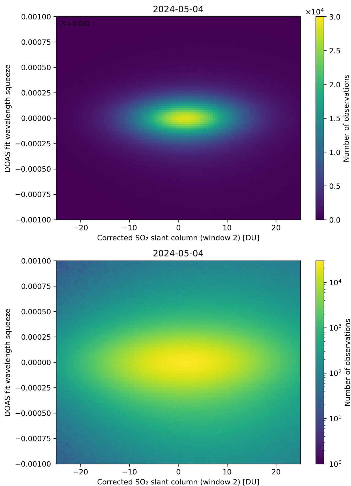
Figure 197: Scatter density plot of “Corrected SO 2 slant column (window 2)” against “DOAS fit wavelength squeeze” for 2024-05-03 to 2024-05-05.
