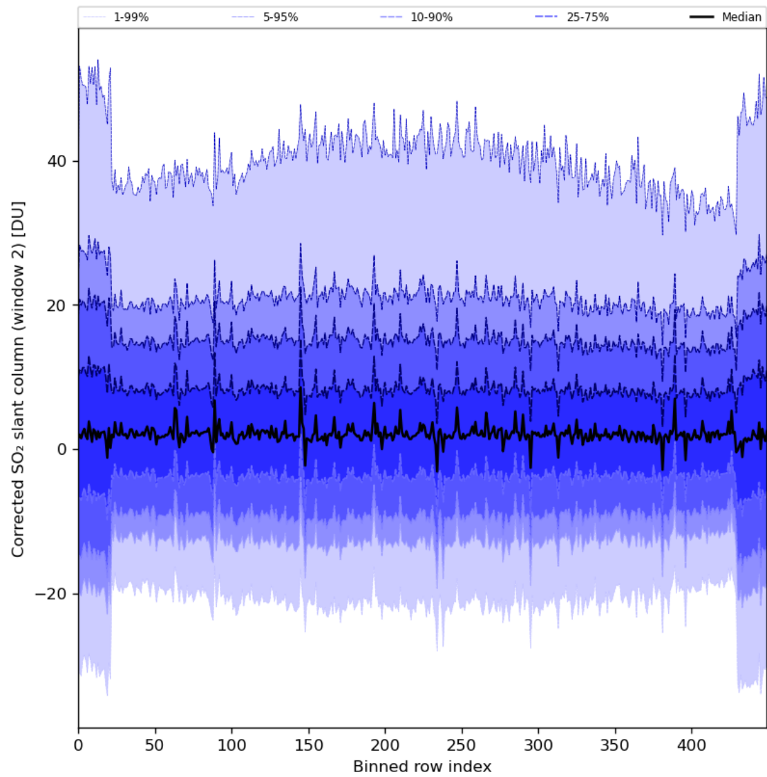
Figure 85: Along track statistics of “Corrected SO 2 slant column (window 2)” for 2024-05-03 to 2024-05-05
