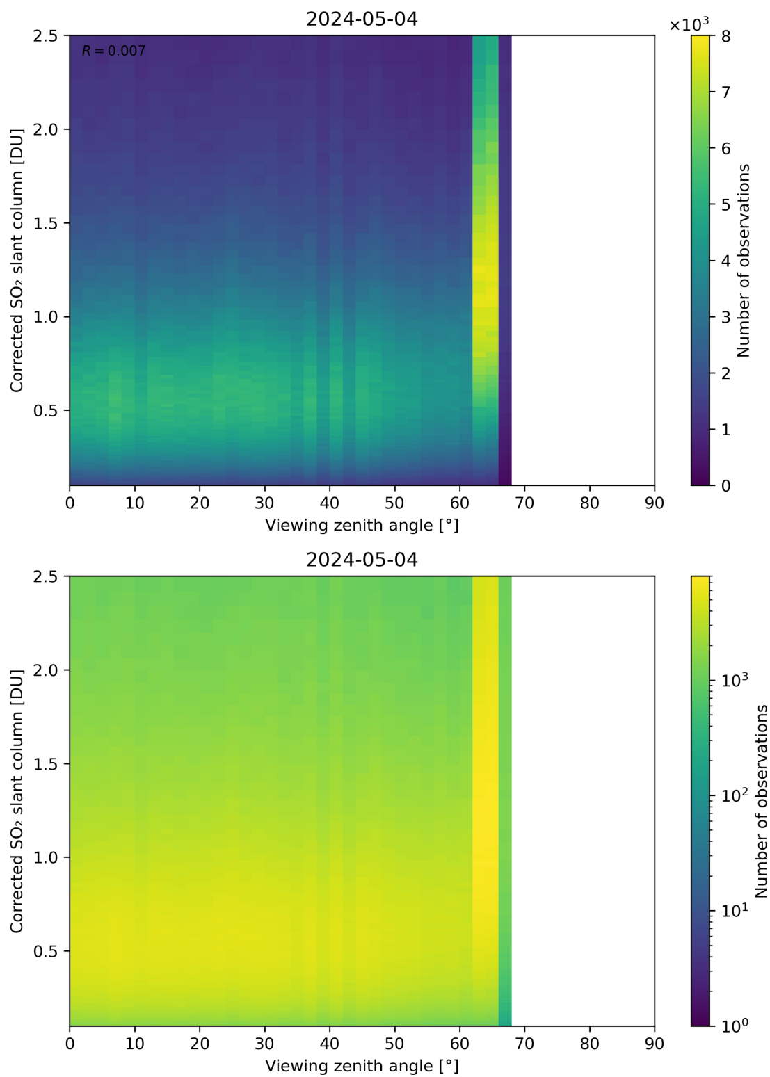
Figure 317: Scatter density plot of “Viewing zenith angle” against “Corrected SO 2 slant column” for 2024-05-03 to 2024-05-05.
