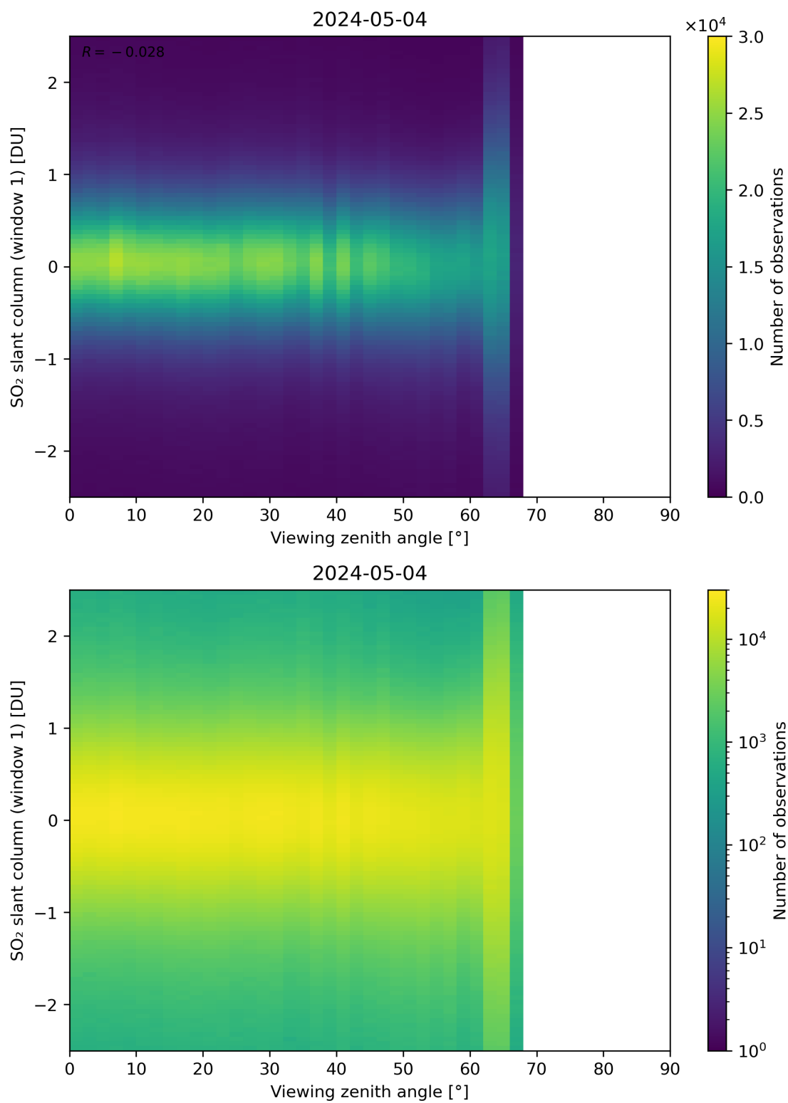
Figure 320: Scatter density plot of “Viewing zenith angle” against “SO 2 slant column (window 1)” for 2024-05-03 to 2024-05-05.
