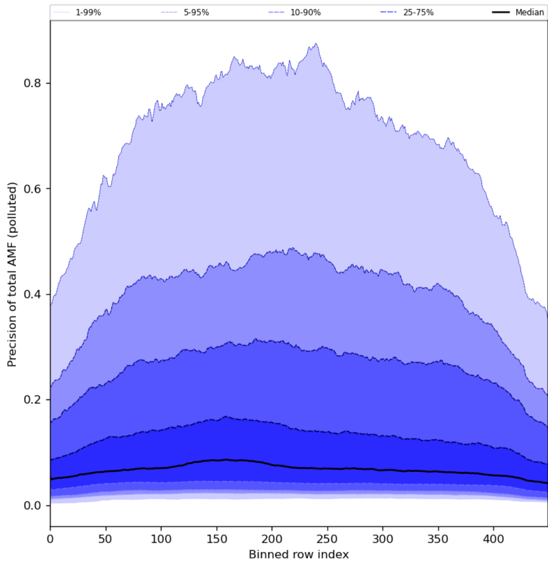
Figure 95: Along track statistics of “Precision of total AMF (polluted)” for 2024-05-03 to 2024-05-05
