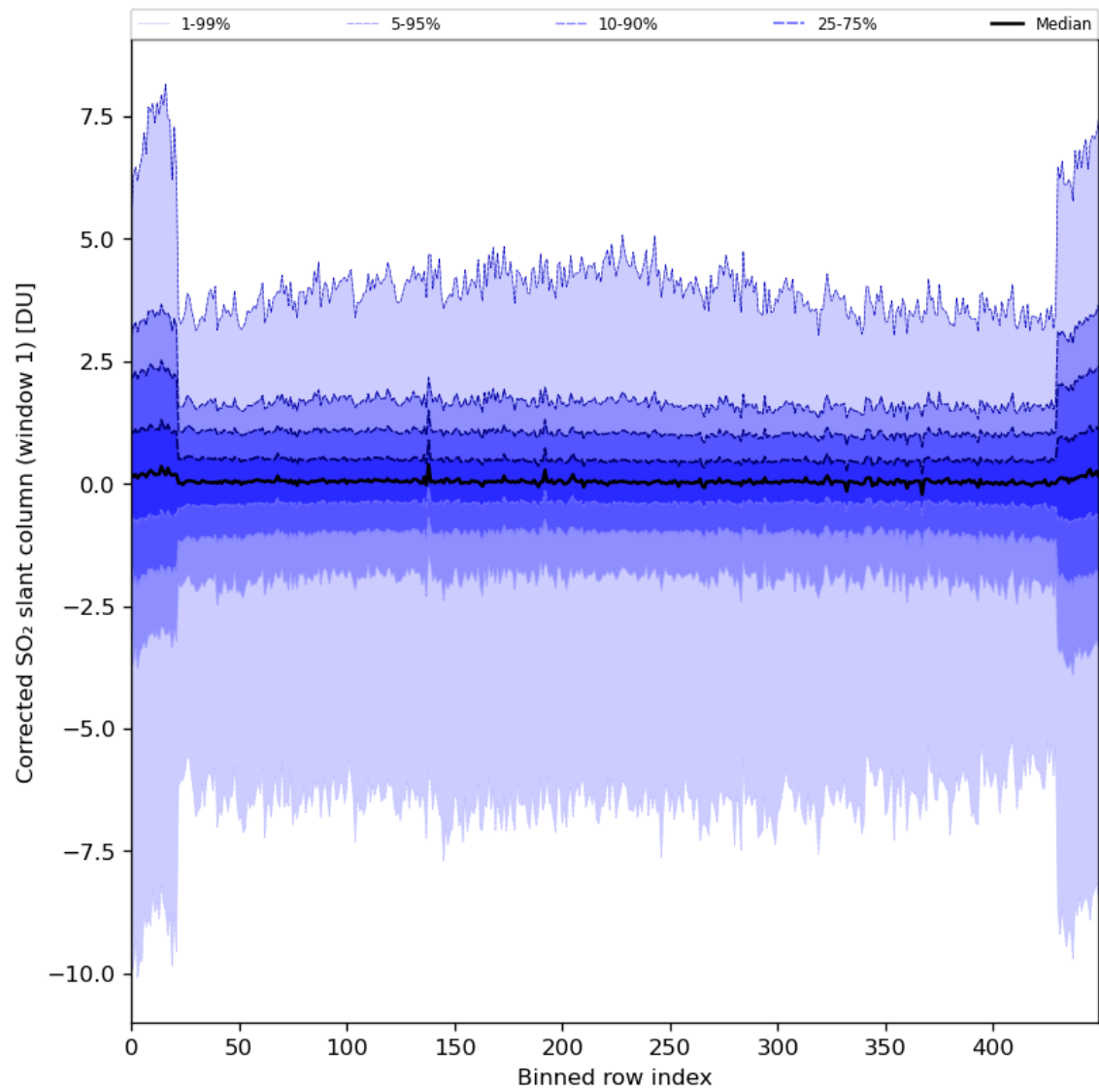
Figure 81: Along track statistics of “Corrected SO 2 slant column (window 1)” for 2024-05-03 to 2024-05-05
