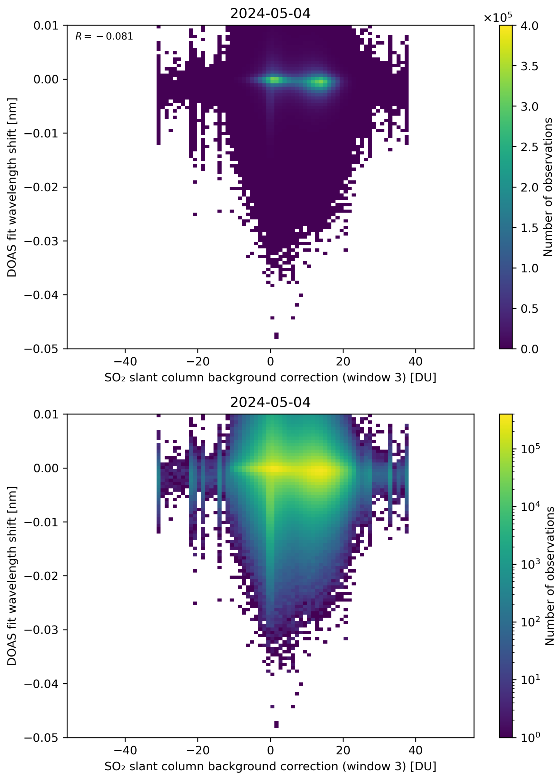
Figure 121: Scatter density plot of “SO 2 slant column background correction (window 3)” against “DOAS fit wavelength shift” for 2024-05-03 to 2024-05-05.
