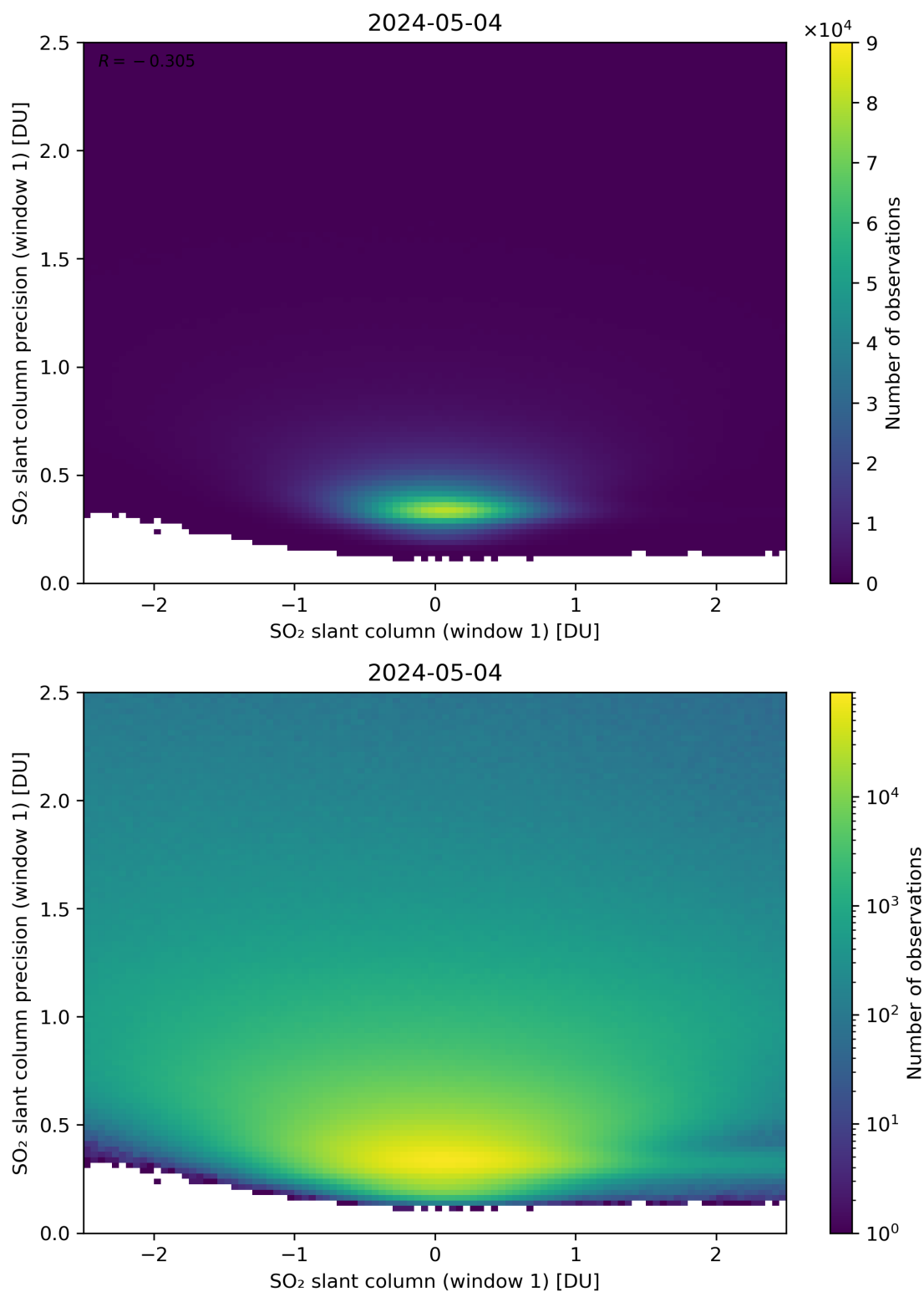
Figure 235: Scatter density plot of “SO 2 slant column (window 1)” against “SO 2 slant column precision (window 1)” for 2024-05-03 to 2024-05-05.
