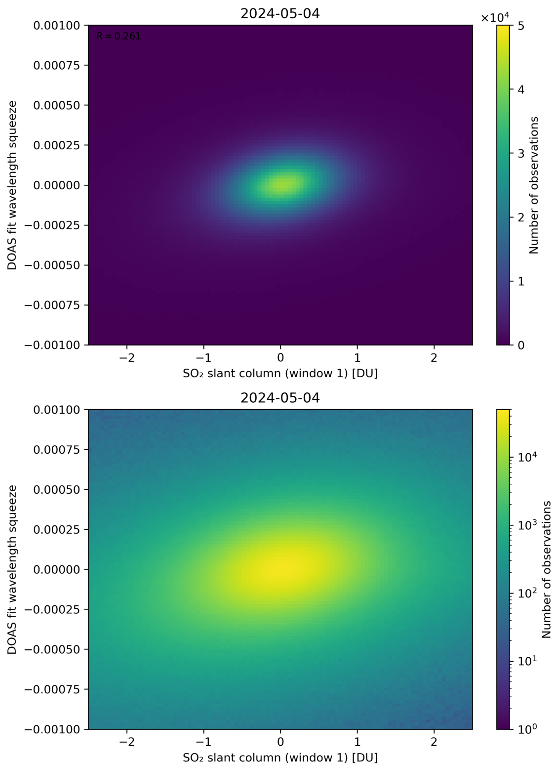
Figure 216: Scatter density plot of “SO 2 slant column (window 1)” against “DOAS fit wavelength squeeze” for 2024-05-03 to 2024-05-05.
