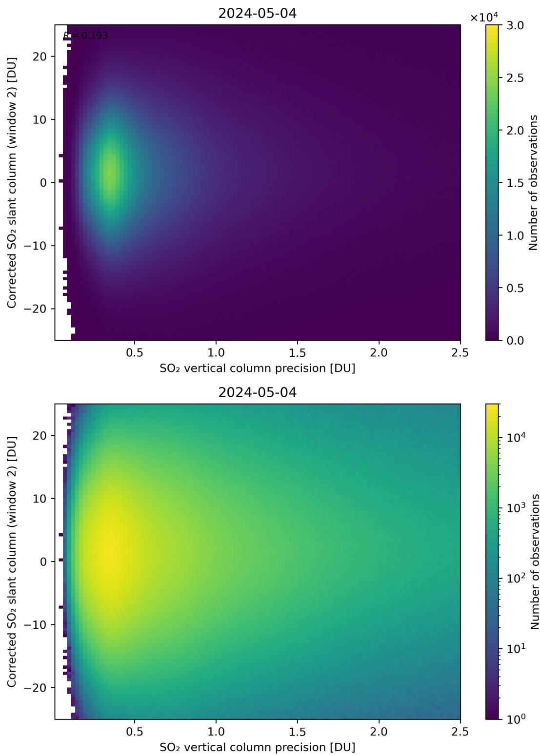
Figure 287: Scatter density plot of “SO 2 vertical column precision” against “Corrected SO 2 slant column (window 2)” for 2024-05-03 to 2024-05-05.
