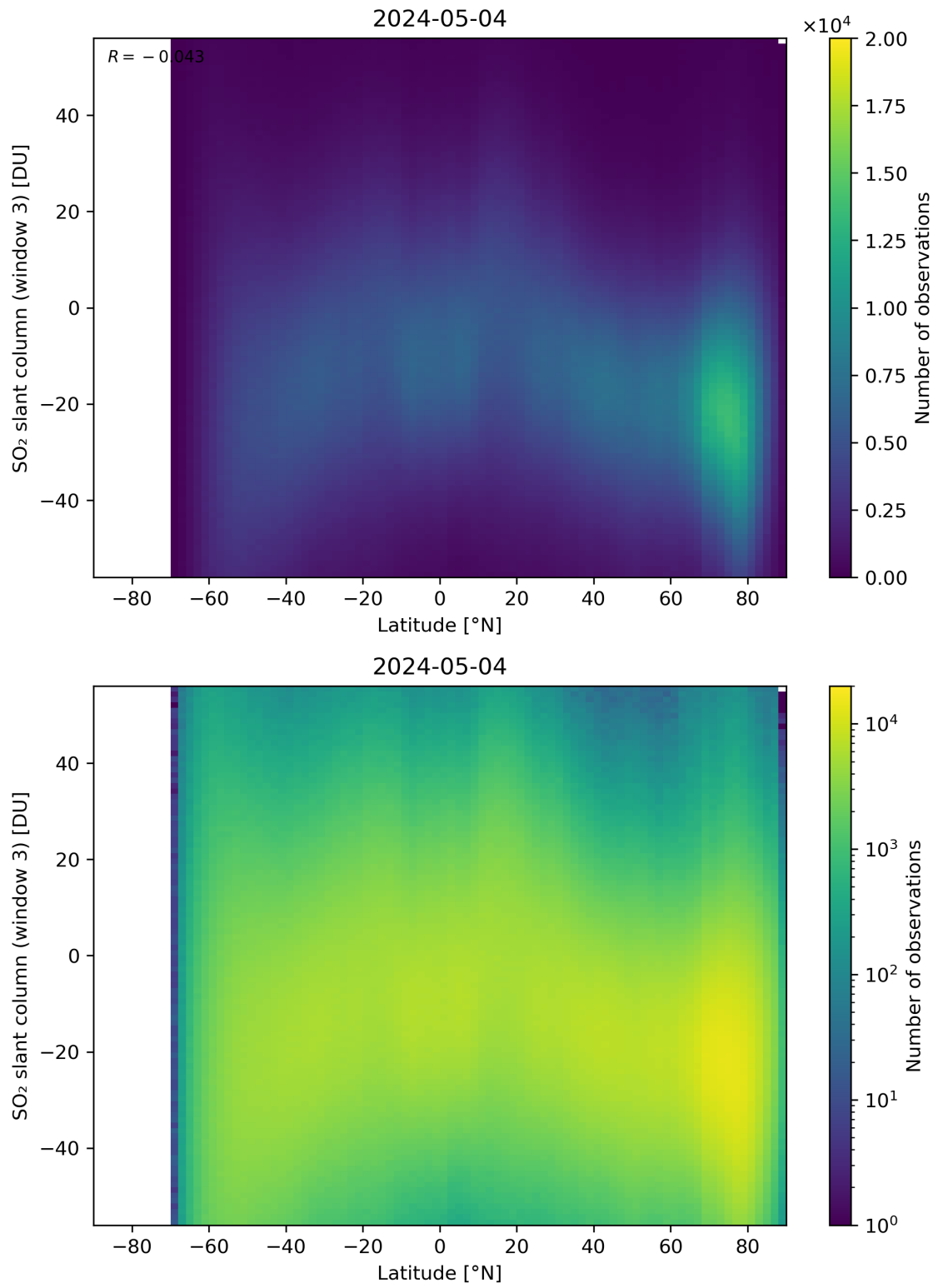
Figure 152: Scatter density plot of “Latitude” against “SO 2 slant column (window 3)” for 2024-05-03 to 2024-05-05.
