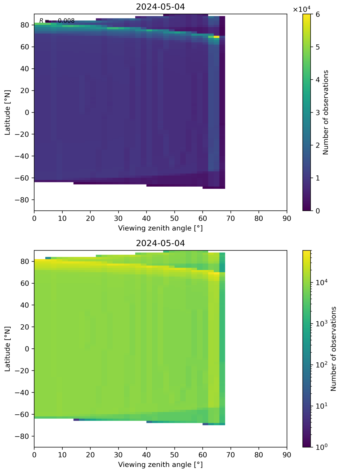
Figure 314: Scatter density plot of “Viewing zenith angle” against “Latitude” for 2024-05-03 to 2024-05-05.
