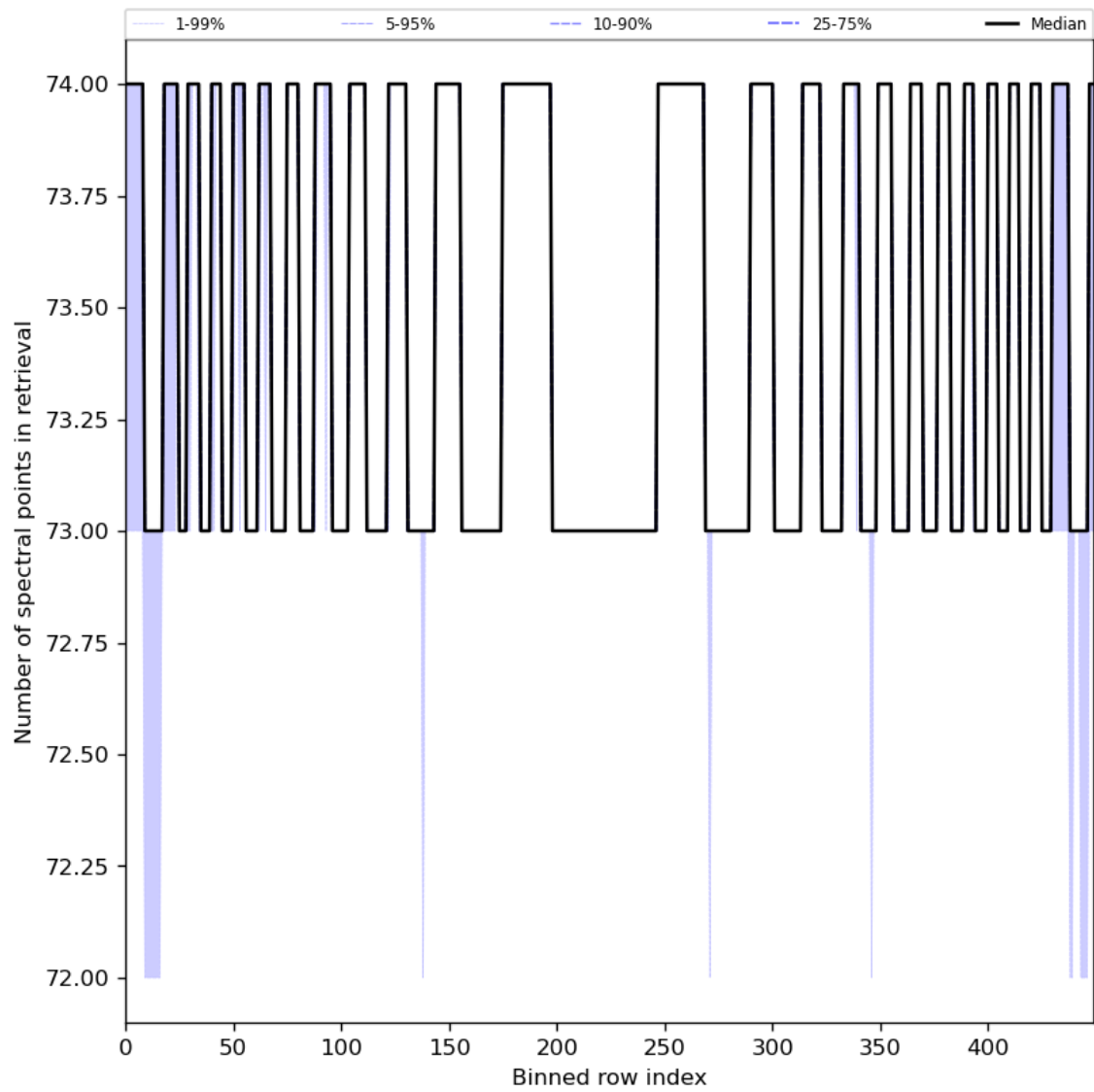
Figure 97: Along track statistics of “Number of spectral points in retrieval” for 2024-05-03 to 2024-05-05
