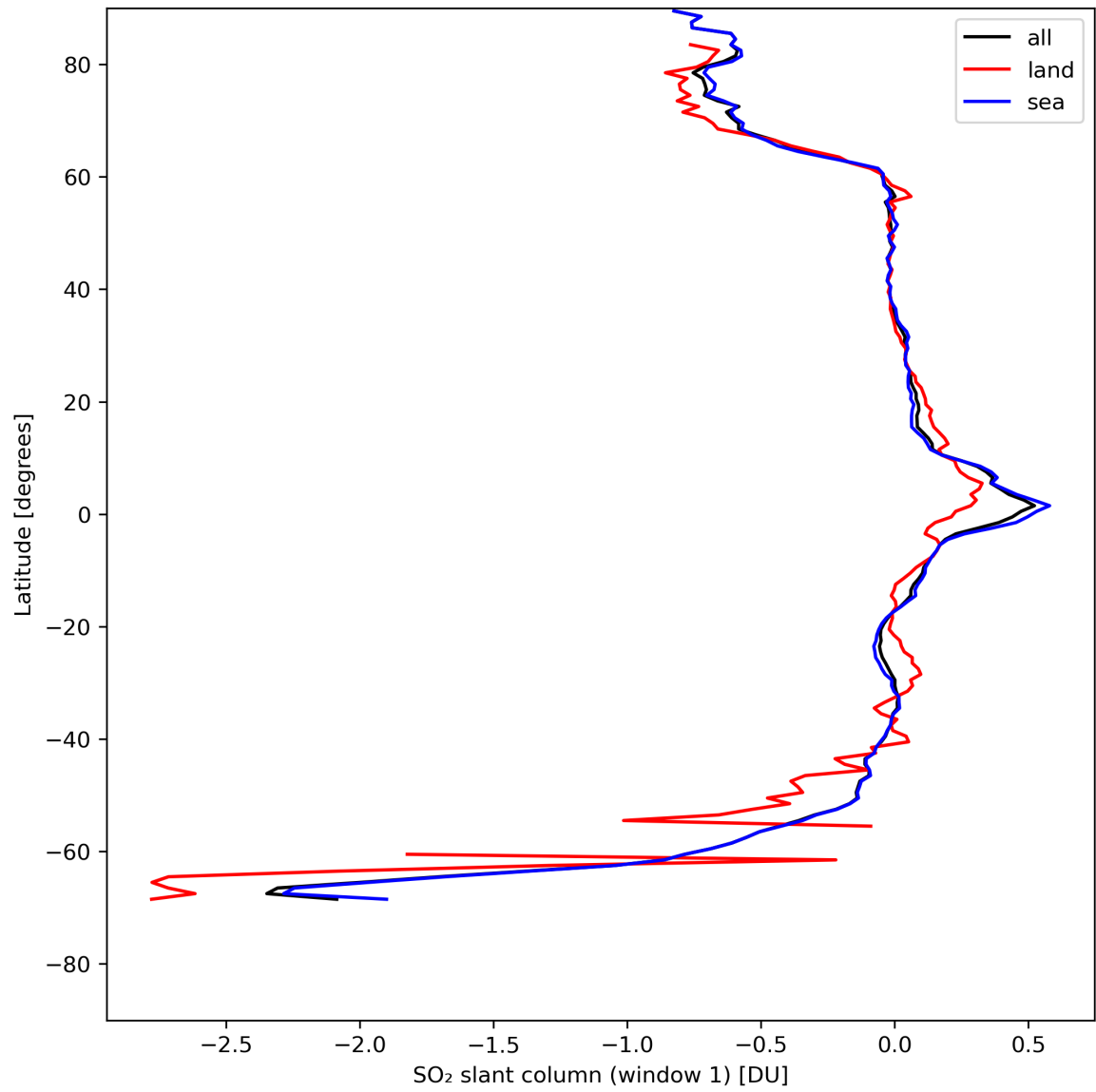
Figure 33: Zonal average of “SO 2 slant column (window 1)” for 2024-05-03 to 2024-05-05.
