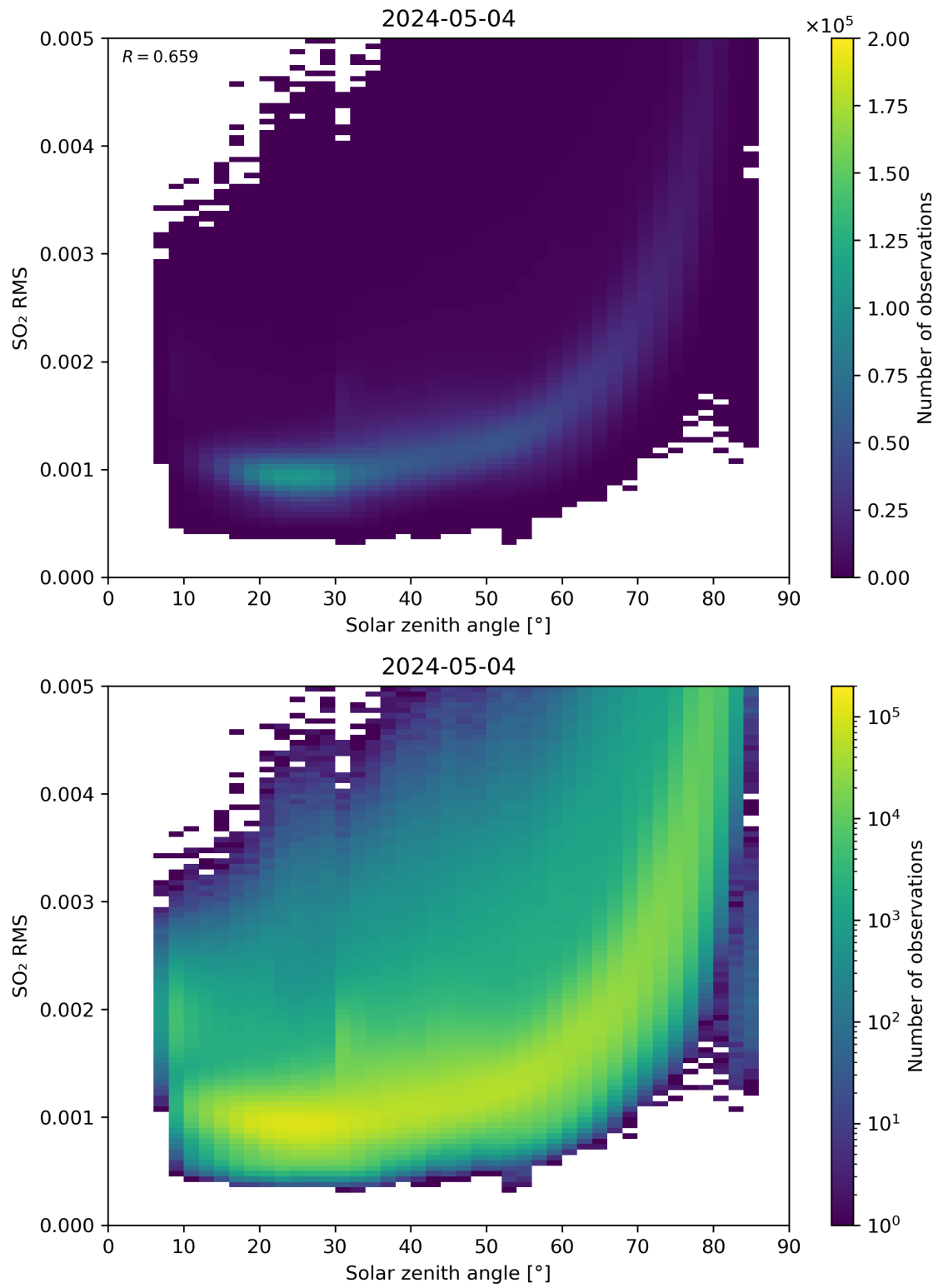
Figure 163: Scatter density plot of “Solar zenith angle” against “SO 2 RMS” for 2024-05-03 to 2024-05-05.
