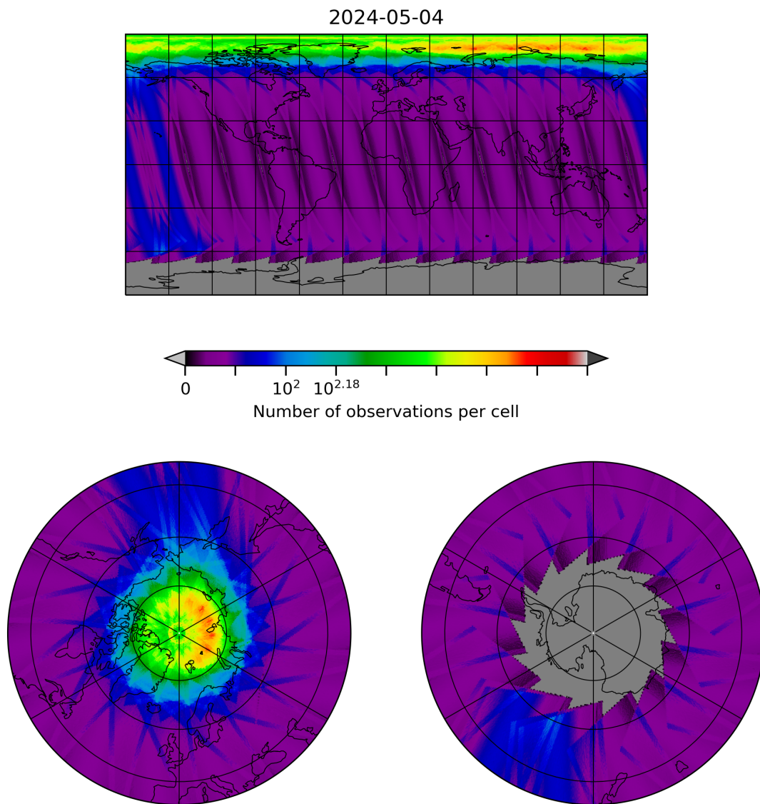
Figure 28: Map of the number of observations for 2024-05-03 to 2024-05-05
