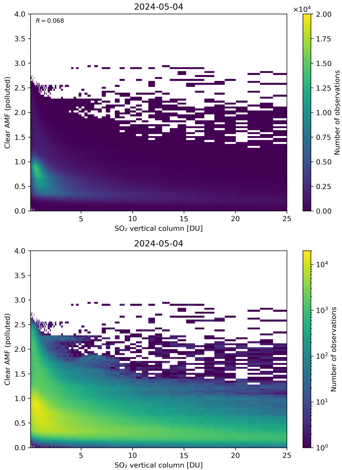
Figure 296: Scatter density plot of “SO 2 vertical column” against “Clear AMF (polluted)” for 2024-05-03 to 2024-05-05.
