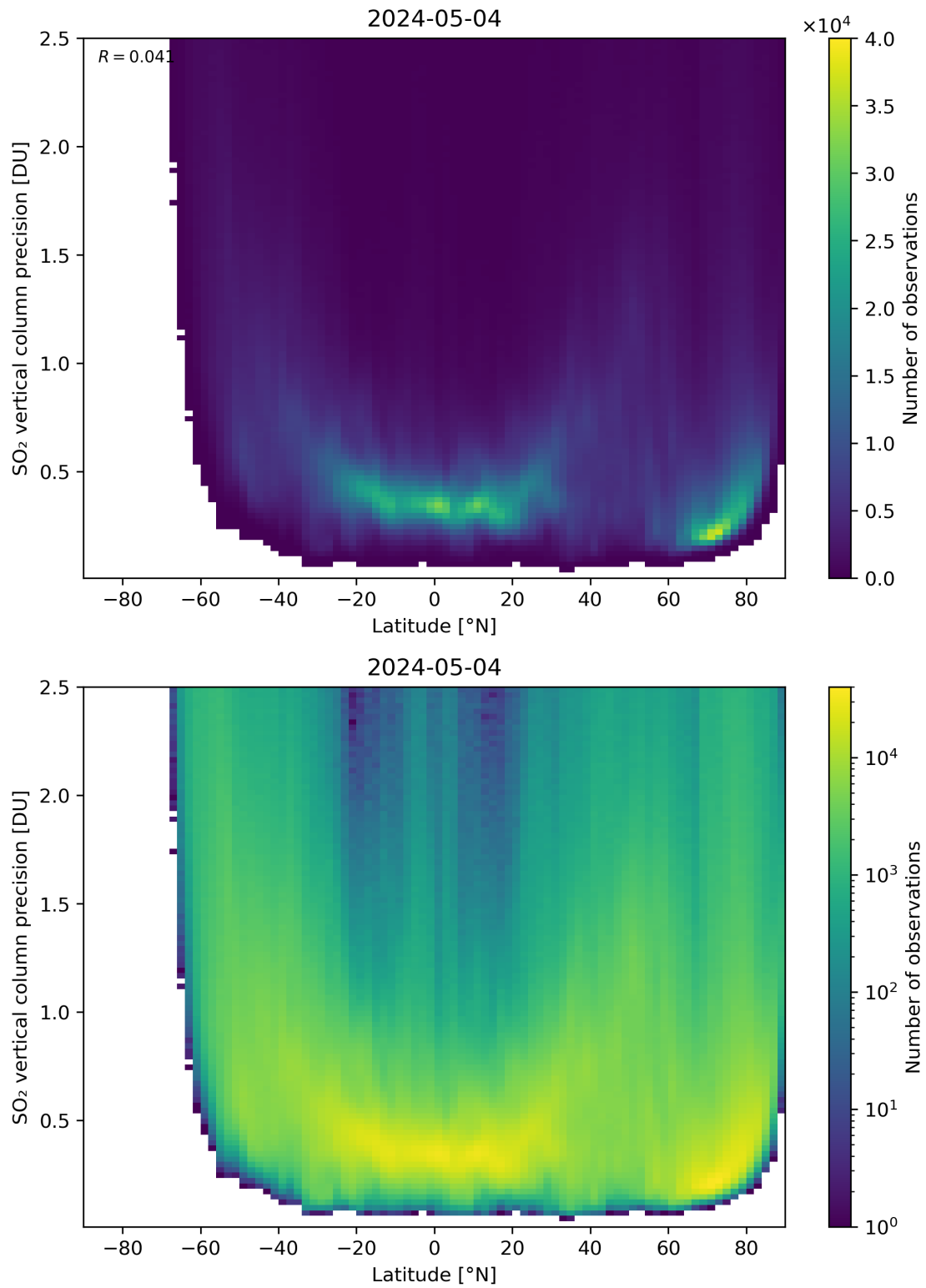
Figure 157: Scatter density plot of “Latitude” against “SO 2 vertical column precision” for 2024-05-03 to 2024-05-05.
