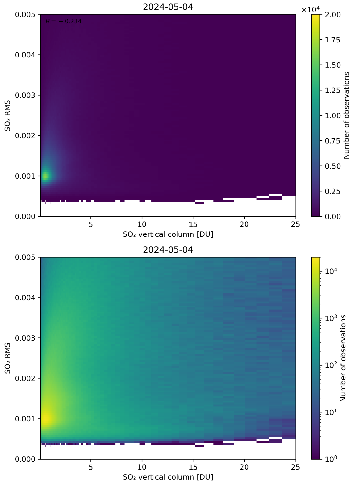
Figure 278: Scatter density plot of “SO 2 vertical column” against “SO 2 RMS” for 2024-05-03 to 2024-05-05.
