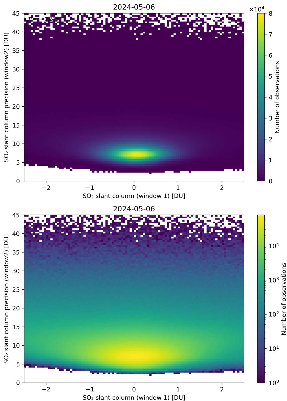
Figure 236: Scatter density plot of “SO 2 slant column (window 1)” against “SO 2 slant column precision (window2)” for 2024-05-05 to 2024-05-07.
