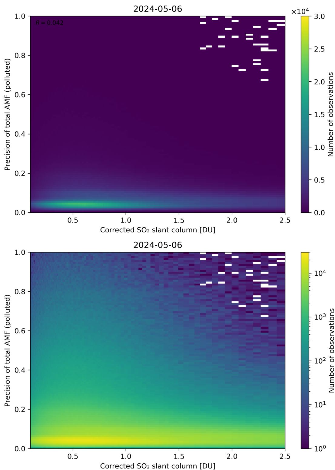
Figure 193: Scatter density plot of “Corrected SO 2 slant column” against “Precision of total AMF (polluted)” for 2024-05-05 to 2024-05-07.
