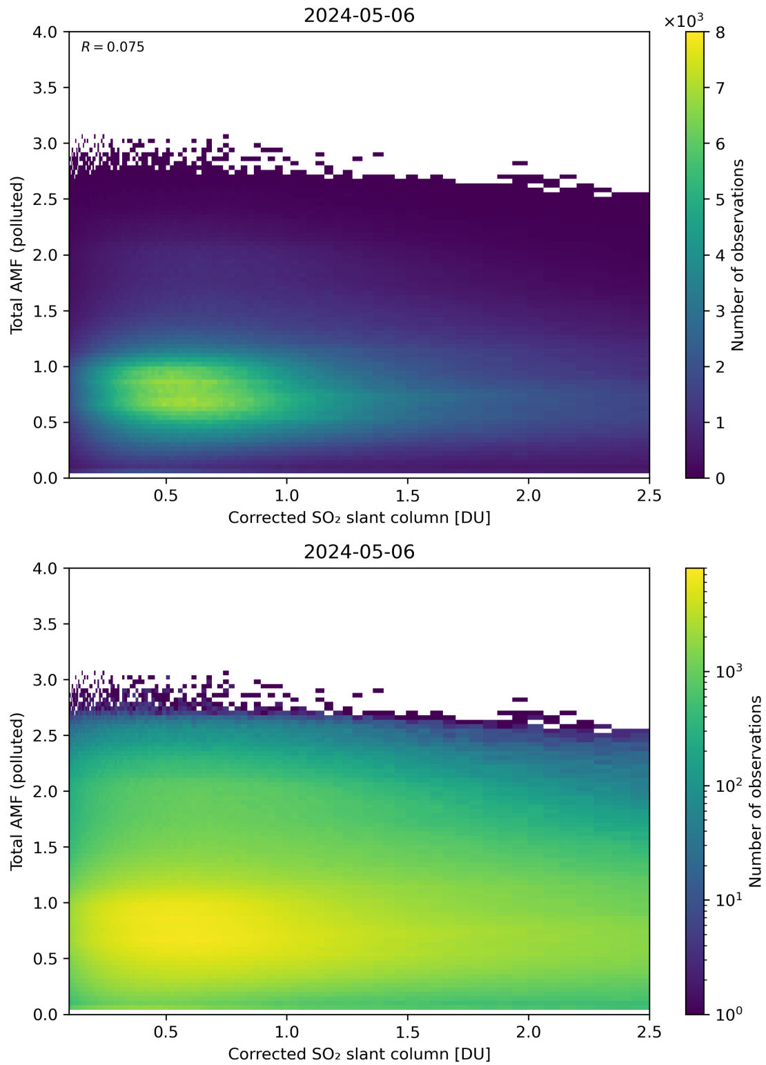
Figure 192: Scatter density plot of “Corrected SO 2 slant column” against “Total AMF (polluted)” for 2024-05-05 to 2024-05-07.
