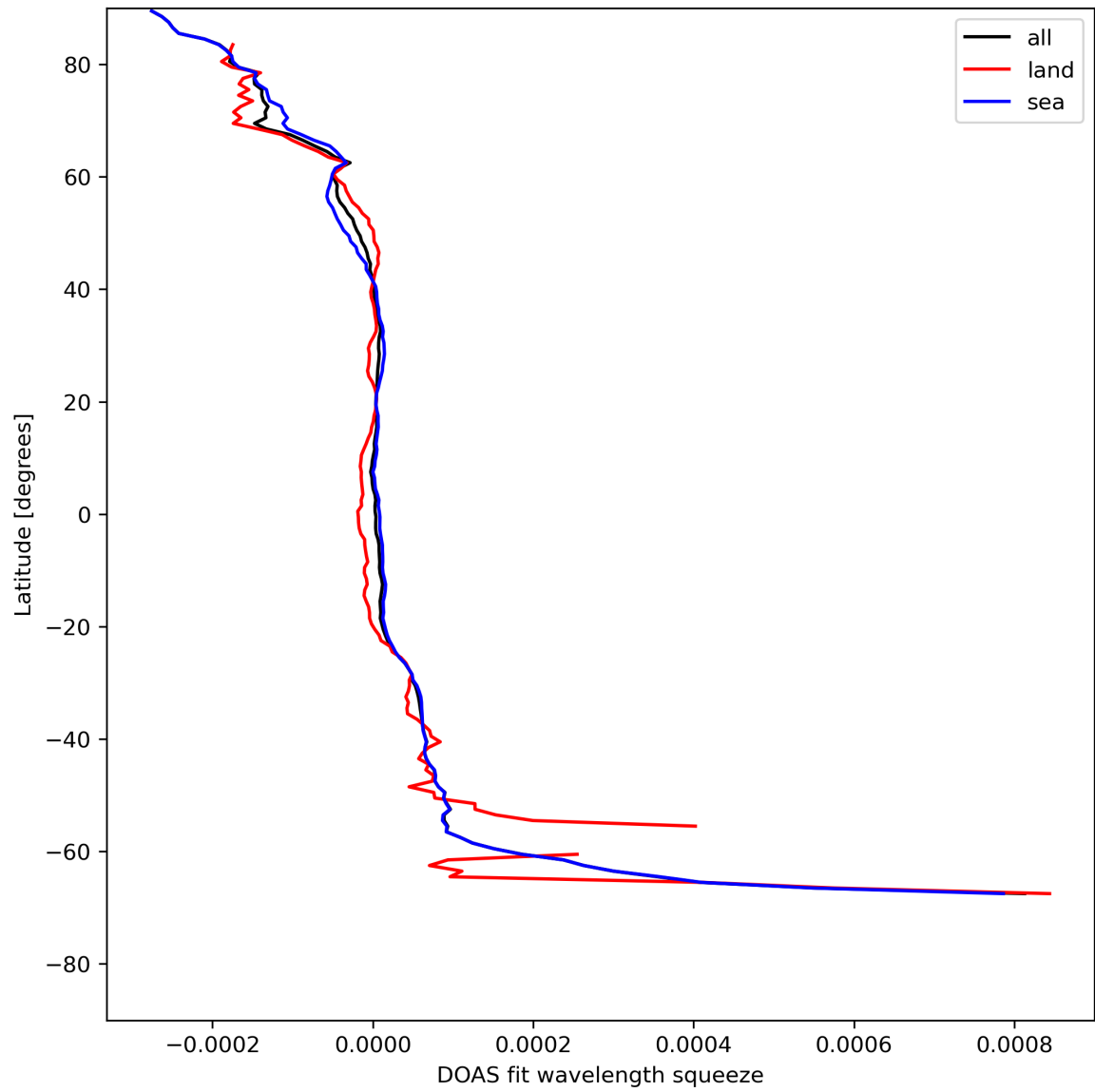
Figure 46: Zonal average of “DOAS fit wavelength squeeze” for 2024-05-05 to 2024-05-07.
