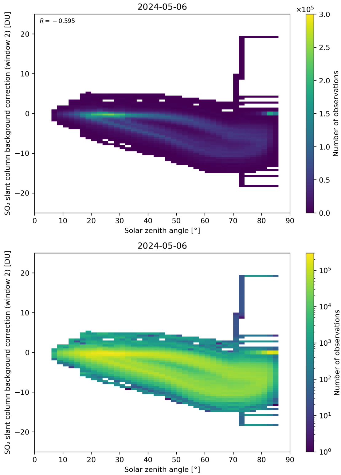
Figure 159: Scatter density plot of “Solar zenith angle” against “SO 2 slant column background correction (window 2)” for 2024-05-05 to 2024-05-07.
