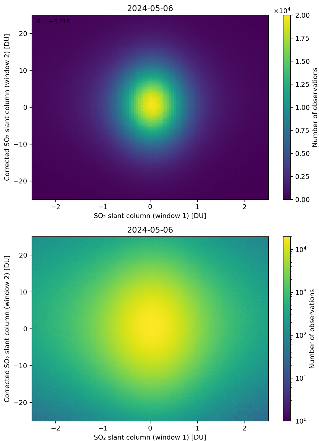
Figure 233: Scatter density plot of “SO 2 slant column (window 1)” against “Corrected SO 2 slant column (window 2)” for 2024-05-05 to 2024-05-07.
