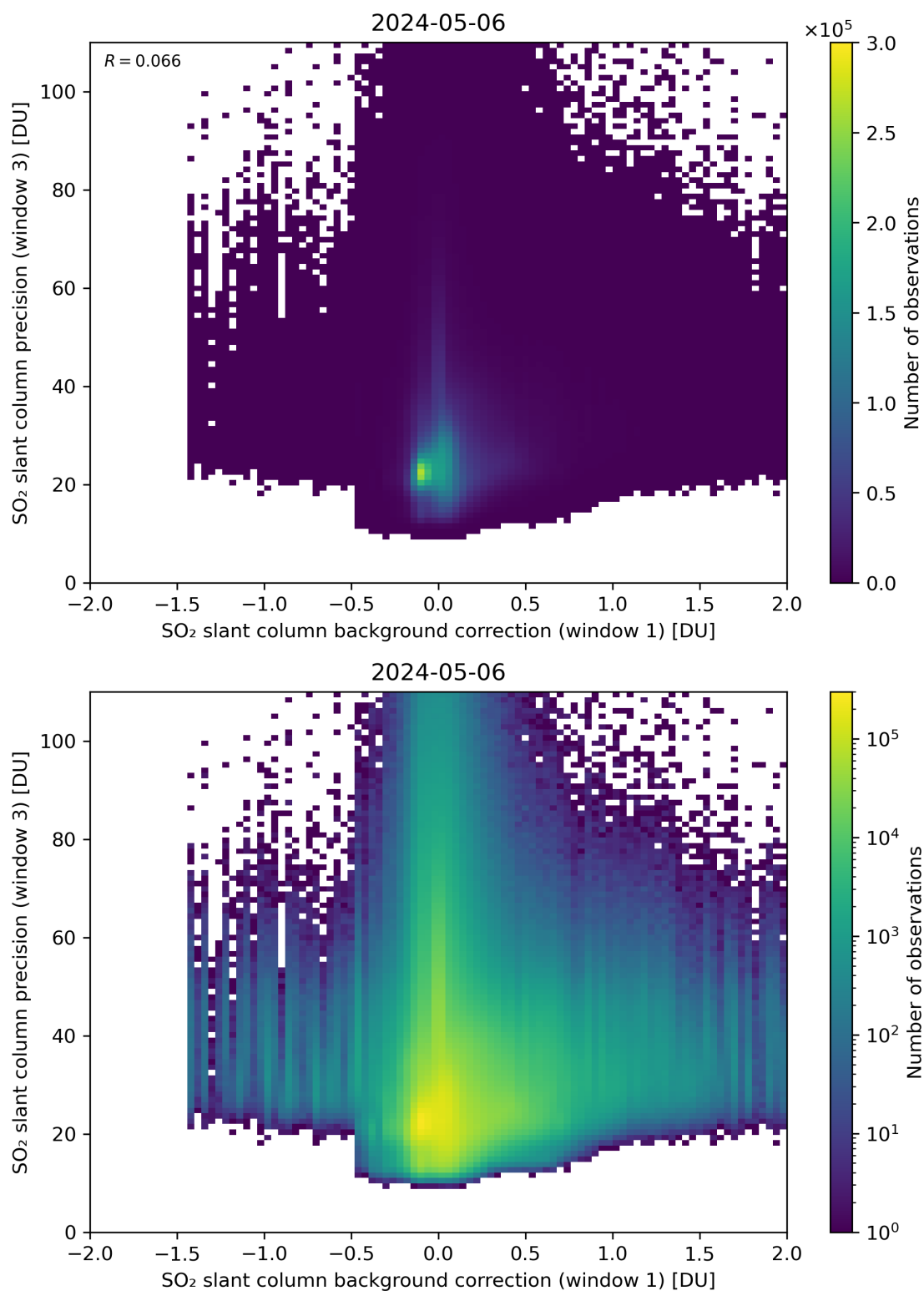
Figure 108: Scatter density plot of “SO 2 slant column background correction (window 1)” against “SO 2 slant column precision (window 3)” for 2024-05-05 to 2024-05-07.
