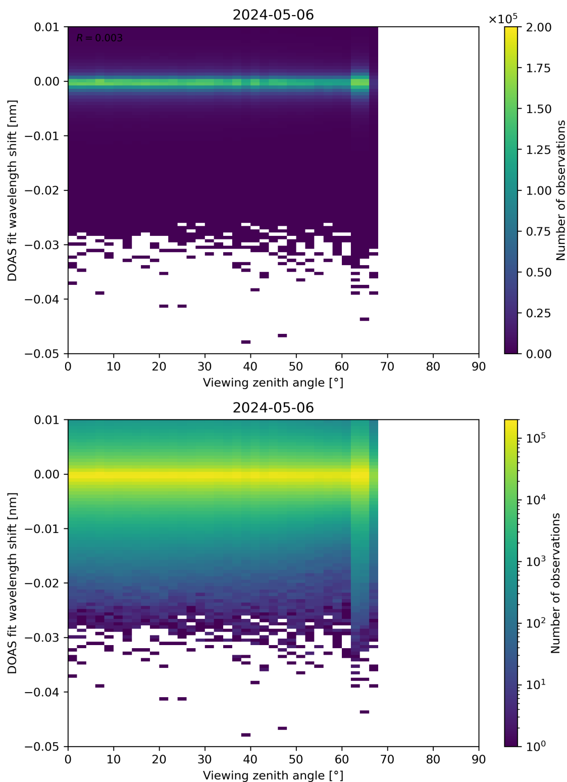
Figure 311: Scatter density plot of “Viewing zenith angle” against “DOAS fit wavelength shift” for 2024-05-05 to 2024-05-07.
