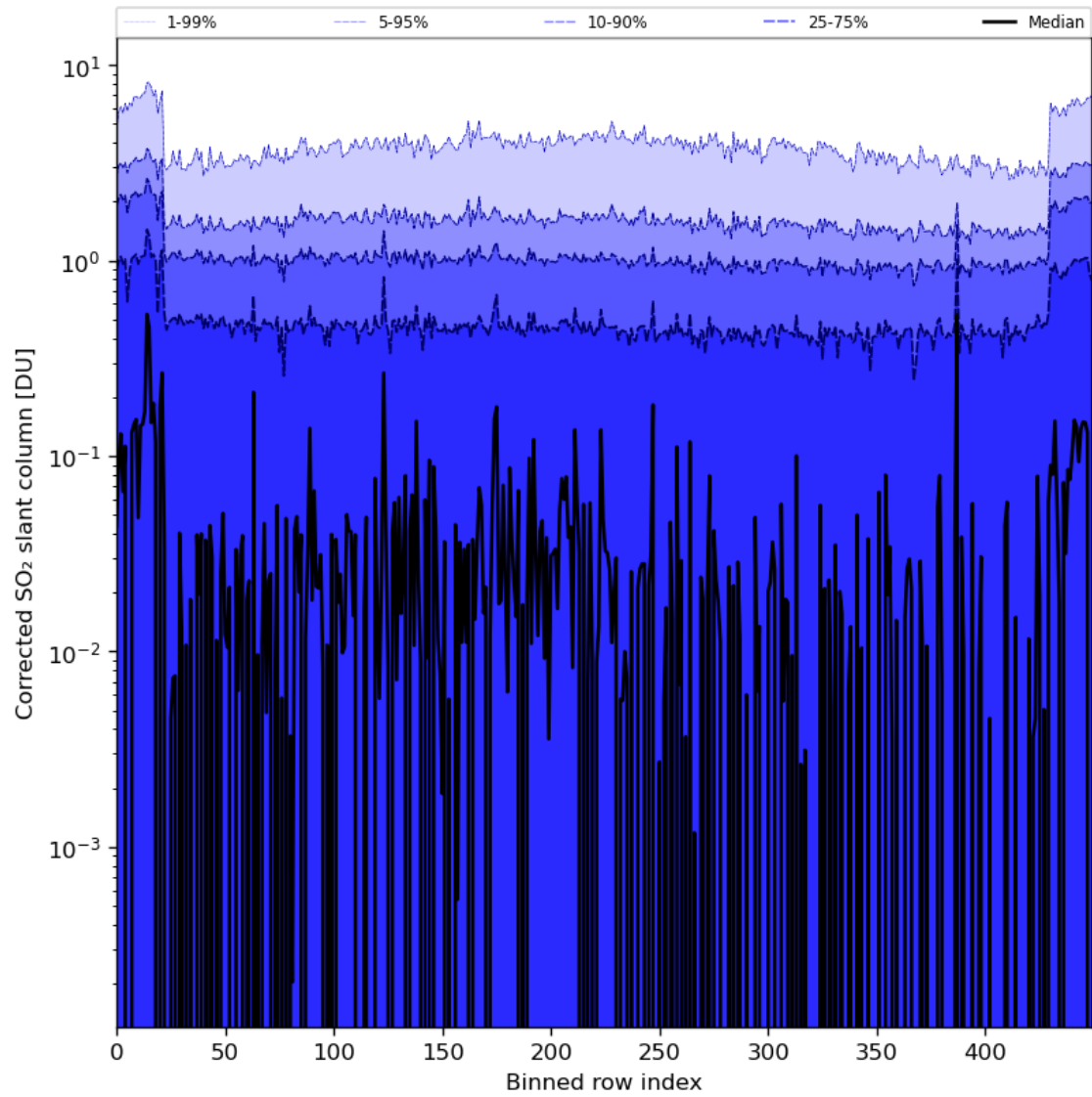
Figure 78: Along track statistics of “Corrected SO 2 slant column” for 2024-05-05 to 2024-05-07
