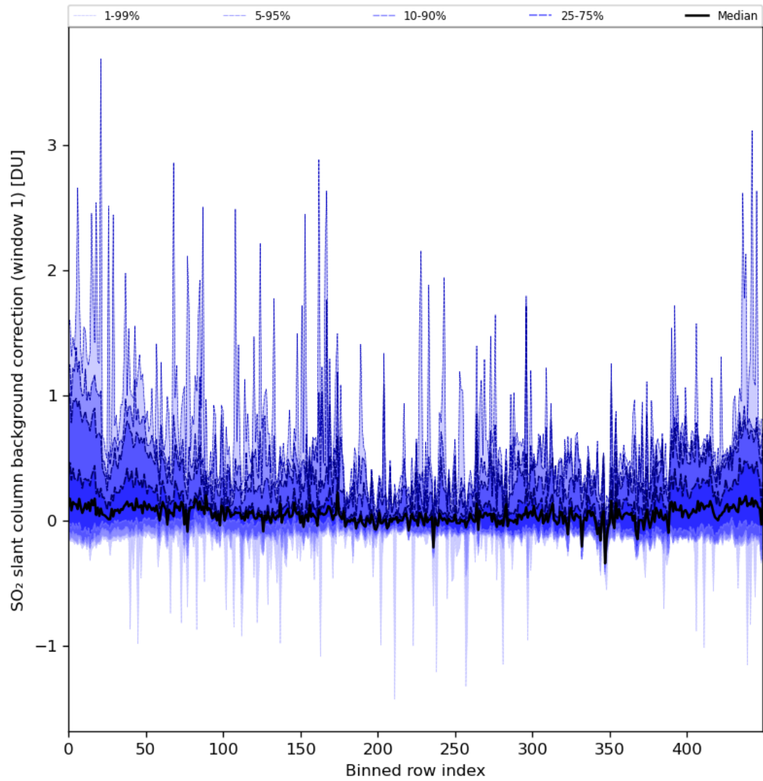
Figure 82: Along track statistics of “SO 2 slant column background correction (window 1)” for 2024-05-05 to 2024-05-07
