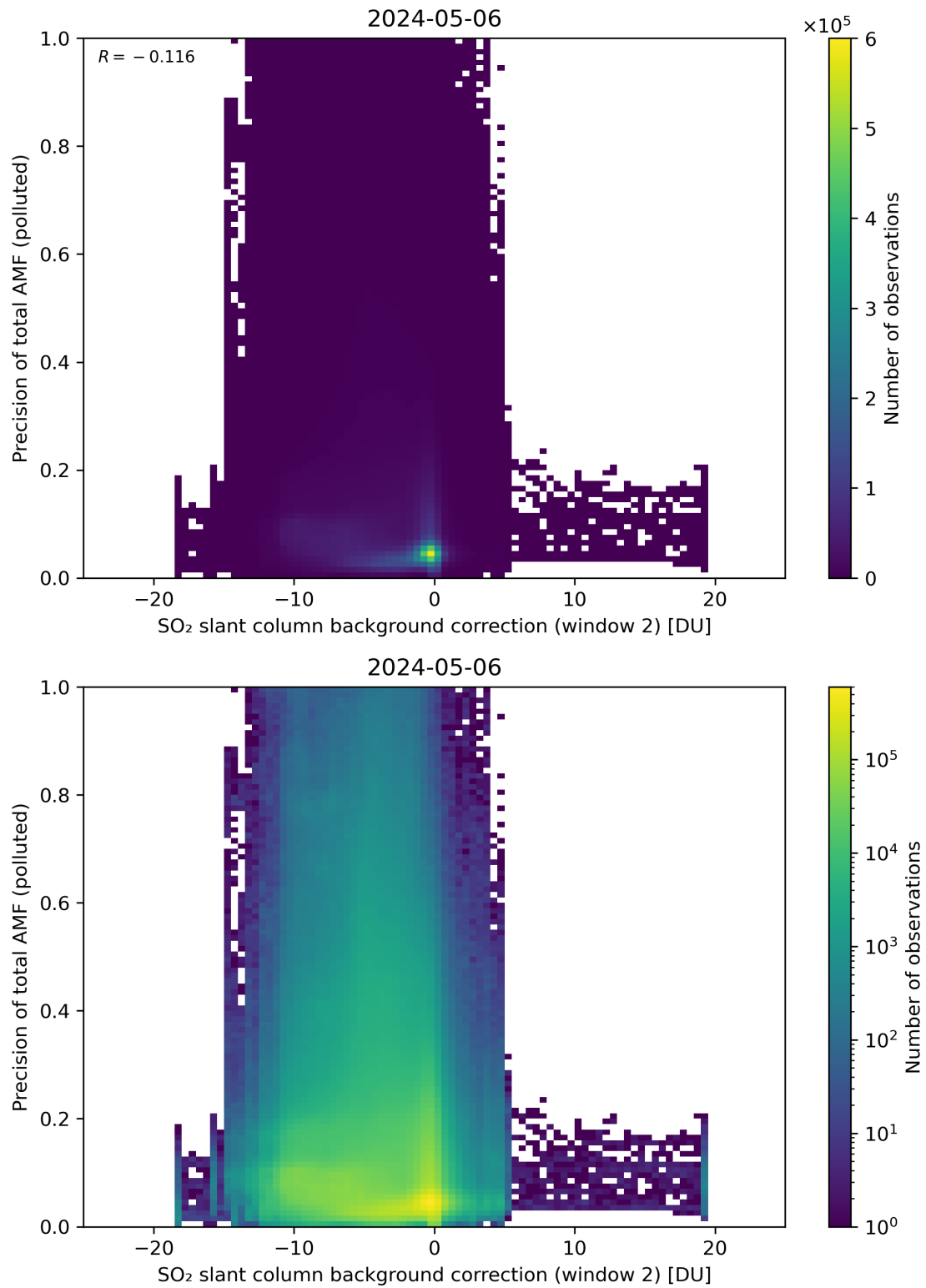
Figure 120: Scatter density plot of “SO 2 slant column background correction (window 2)” against “Precision of total AMF (polluted)” for 2024-05-05 to 2024-05-07.
