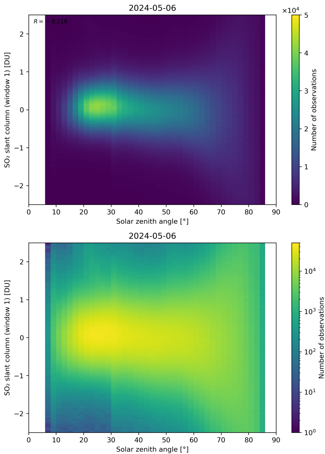
Figure 169: Scatter density plot of “Solar zenith angle” against “SO 2 slant column (window 1)” for 2024-05-05 to 2024-05-07.
