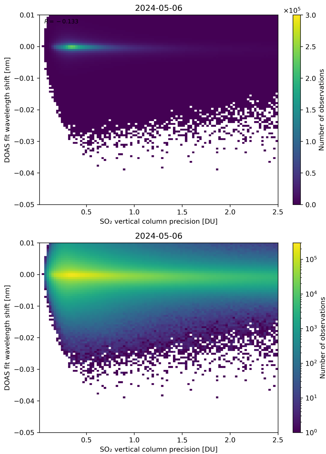
Figure 282: Scatter density plot of “SO 2 vertical column precision” against “DOAS fit wavelength shift” for 2024-05-05 to 2024-05-07.
