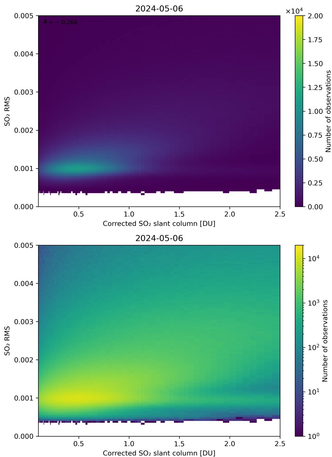
Figure 183: Scatter density plot of “Corrected SO 2 slant column” against “SO 2 RMS” for 2024-05-05 to 2024-05-07.
