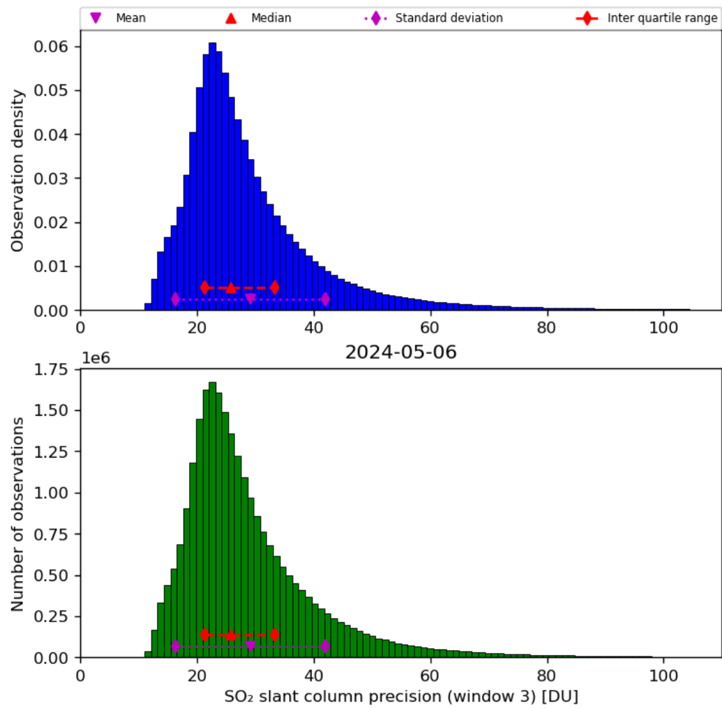
Figure 65: Histogram of “SO 2 slant column precision (window 3)” for 2024-05-05 to 2024-05-07
