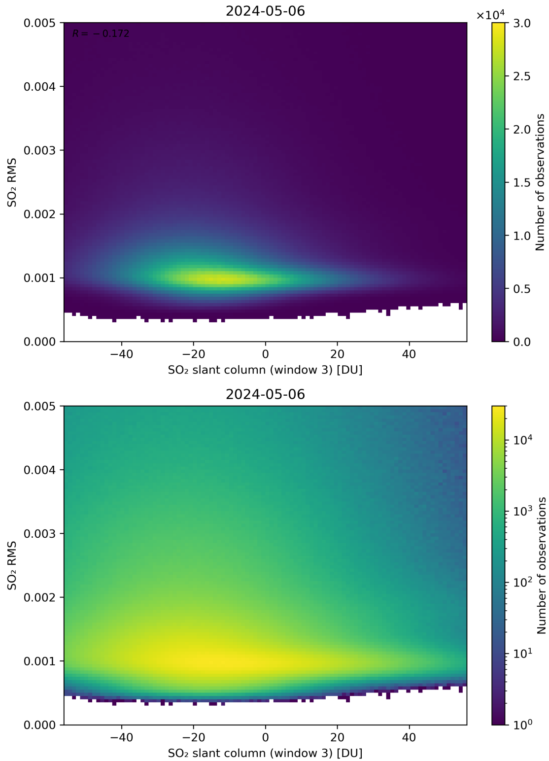
Figure 256: Scatter density plot of “SO 2 slant column (window 3)” against “SO 2 RMS” for 2024-05-05 to 2024-05-07.
