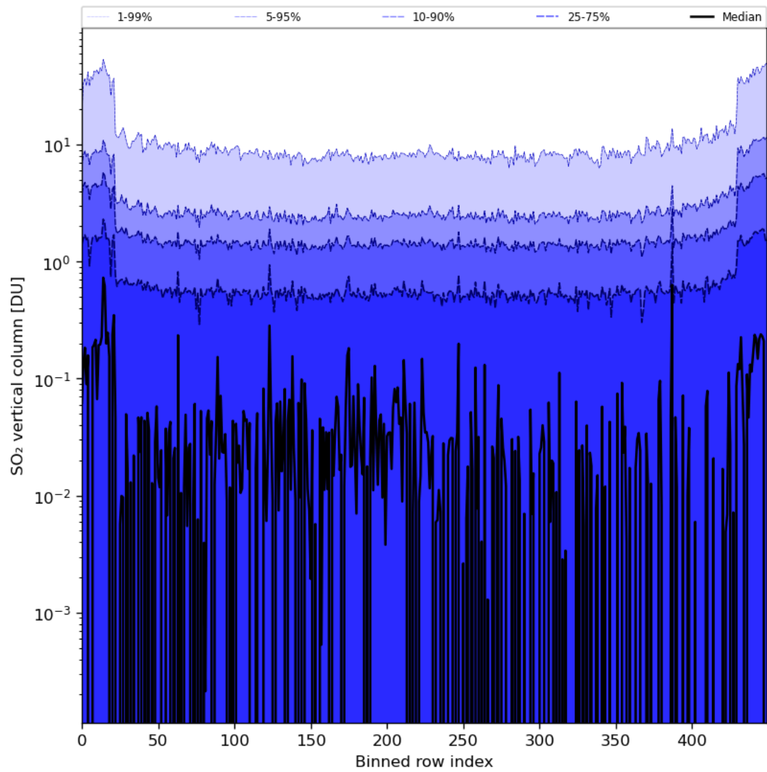
Figure 76: Along track statistics of “SO 2 vertical column” for 2024-05-05 to 2024-05-07
