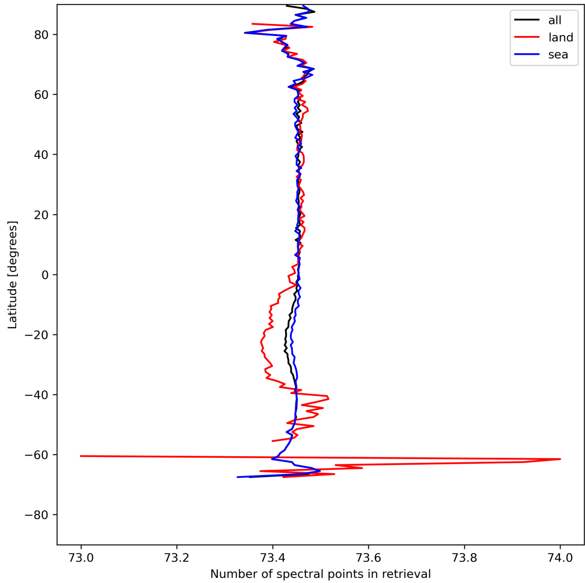
Figure 51: Zonal average of “Number of spectral points in retrieval” for 2024-05-05 to 2024-05-07.
