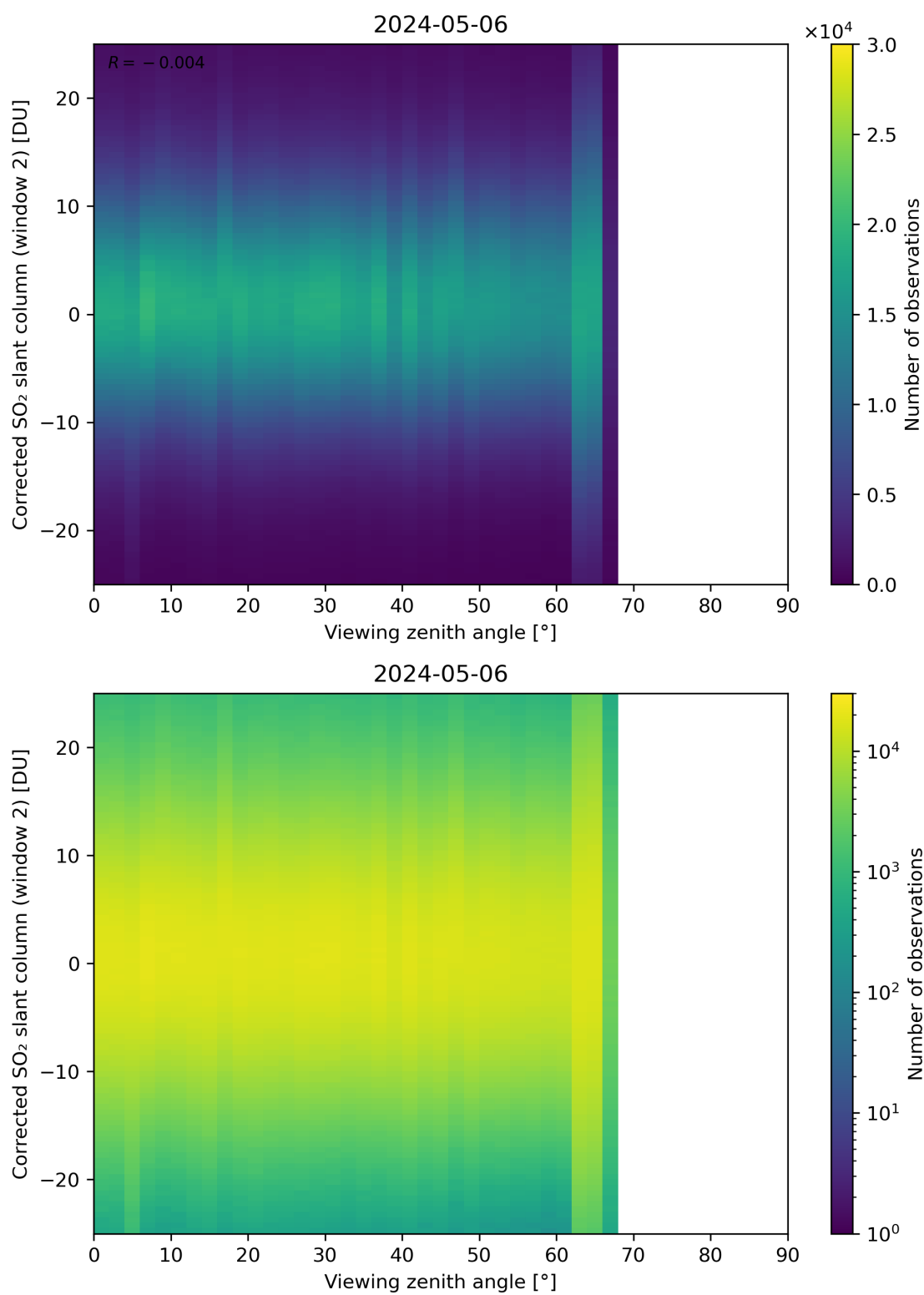
Figure 318: Scatter density plot of “Viewing zenith angle” against “Corrected SO 2 slant column (window 2)” for 2024-05-05 to 2024-05-07.
