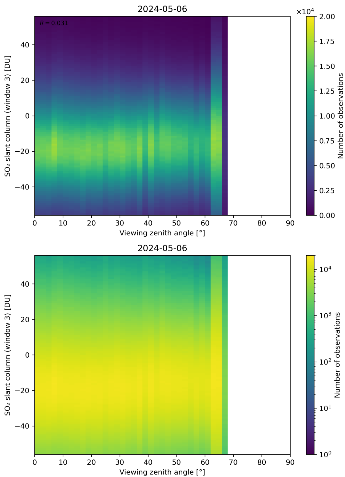
Figure 323: Scatter density plot of “Viewing zenith angle” against “SO 2 slant column (window 3)” for 2024-05-05 to 2024-05-07.
