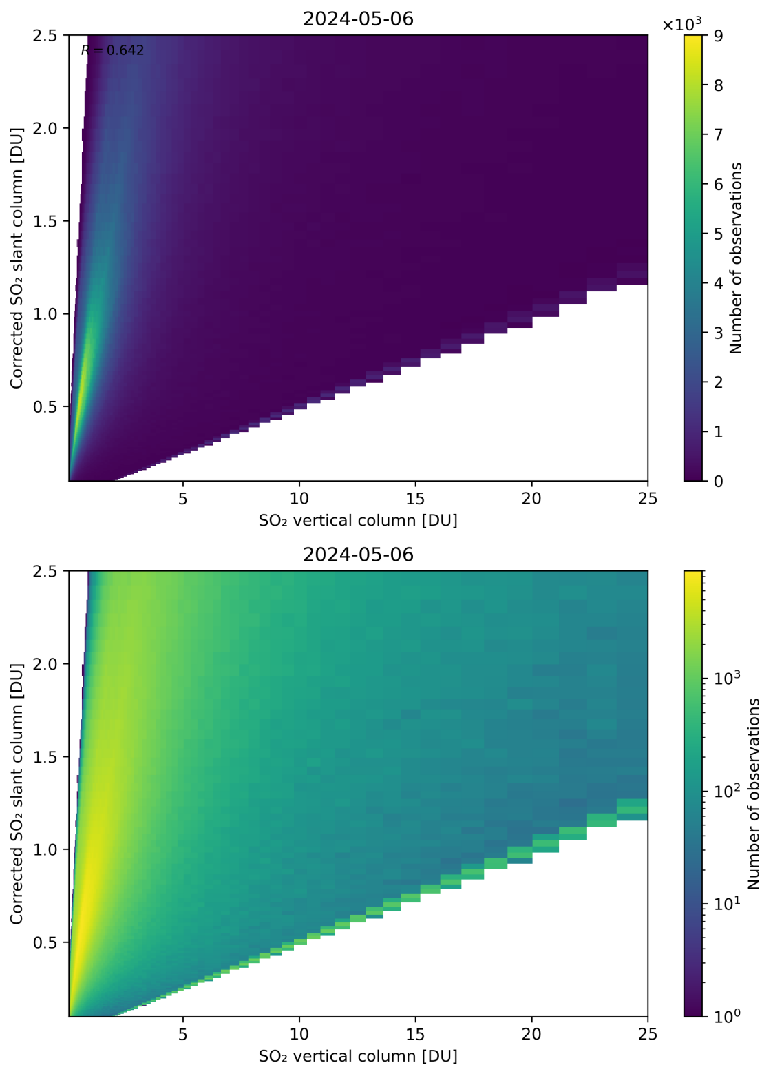
Figure 297: Scatter density plot of “SO 2 vertical column” against “Corrected SO 2 slant column” for 2024-05-05 to 2024-05-07.
