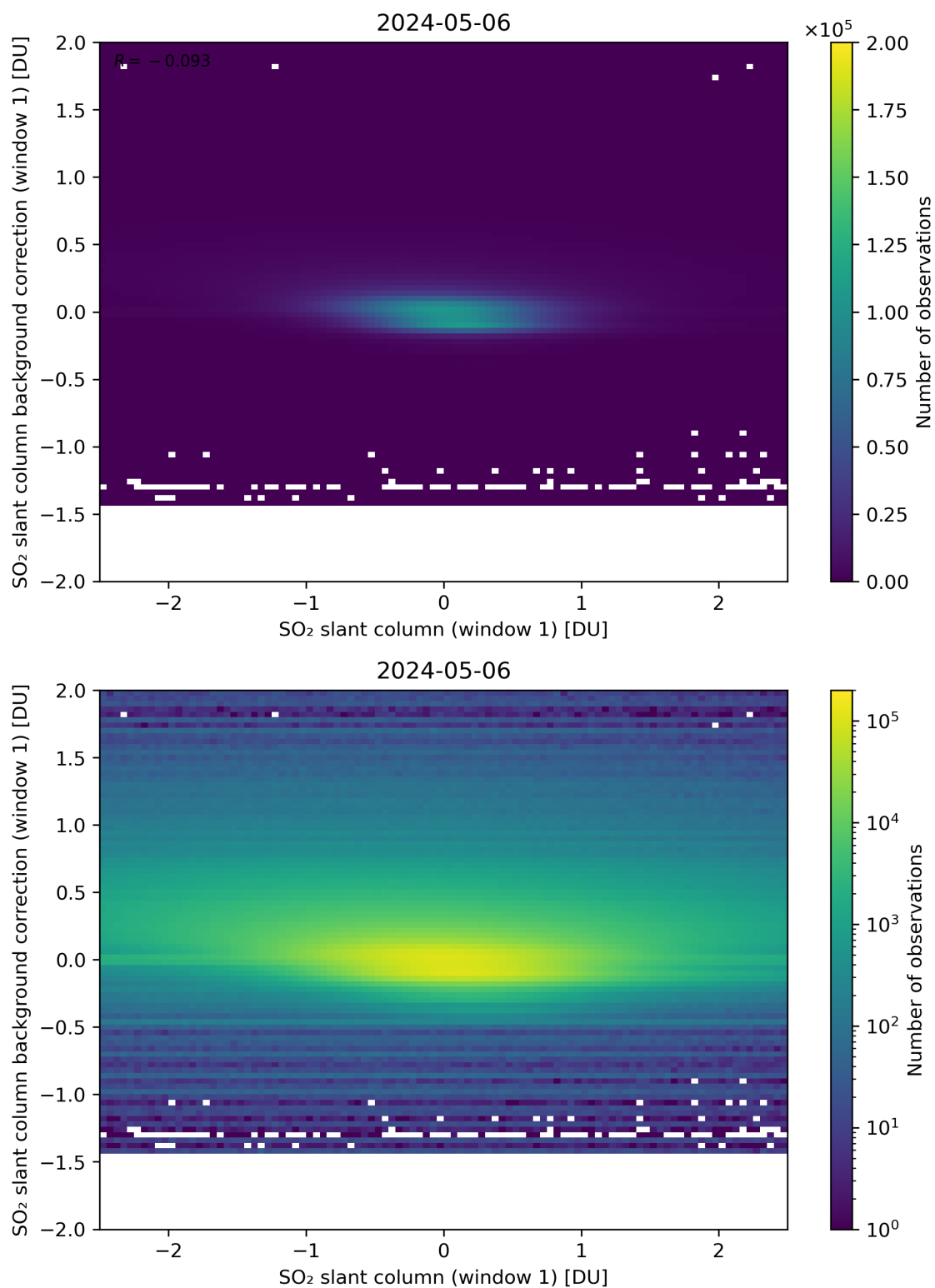
Figure 212: Scatter density plot of “SO 2 slant column (window 1)” against “SO 2 slant column background correction (window 1)” for 2024-05-05 to 2024-05-07.
