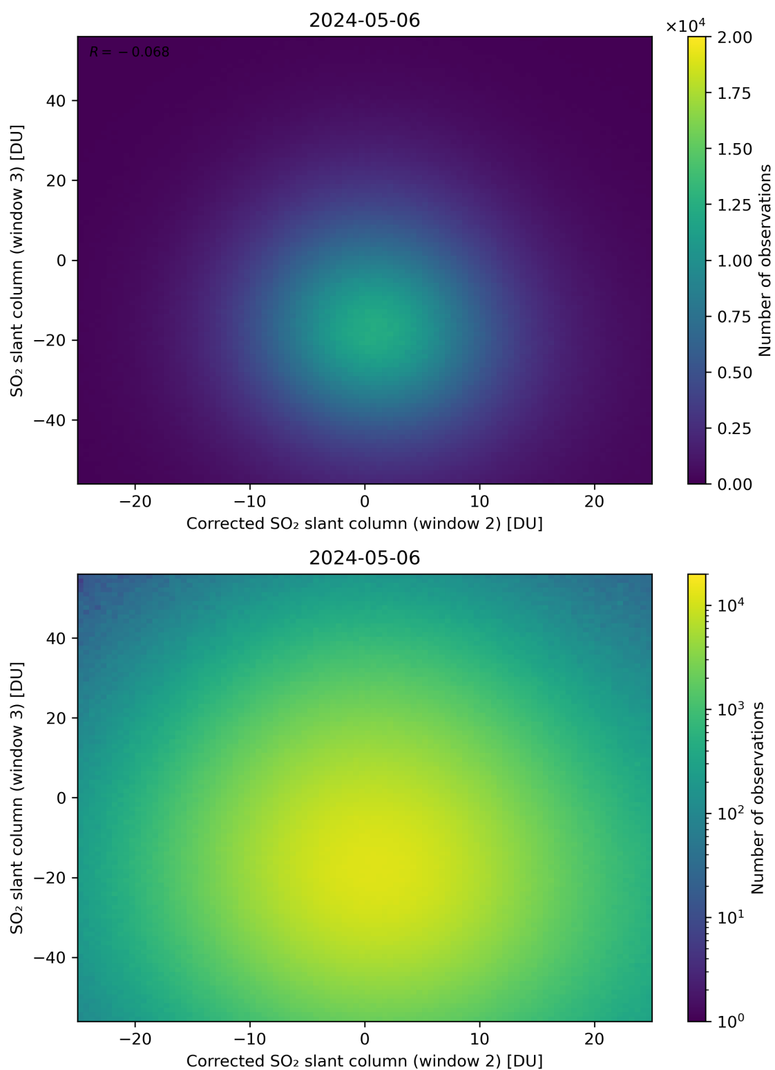
Figure 201: Scatter density plot of “Corrected SO 2 slant column (window 2)” against “SO 2 slant column (window 3)” for 2024-05-05 to 2024-05-07.
