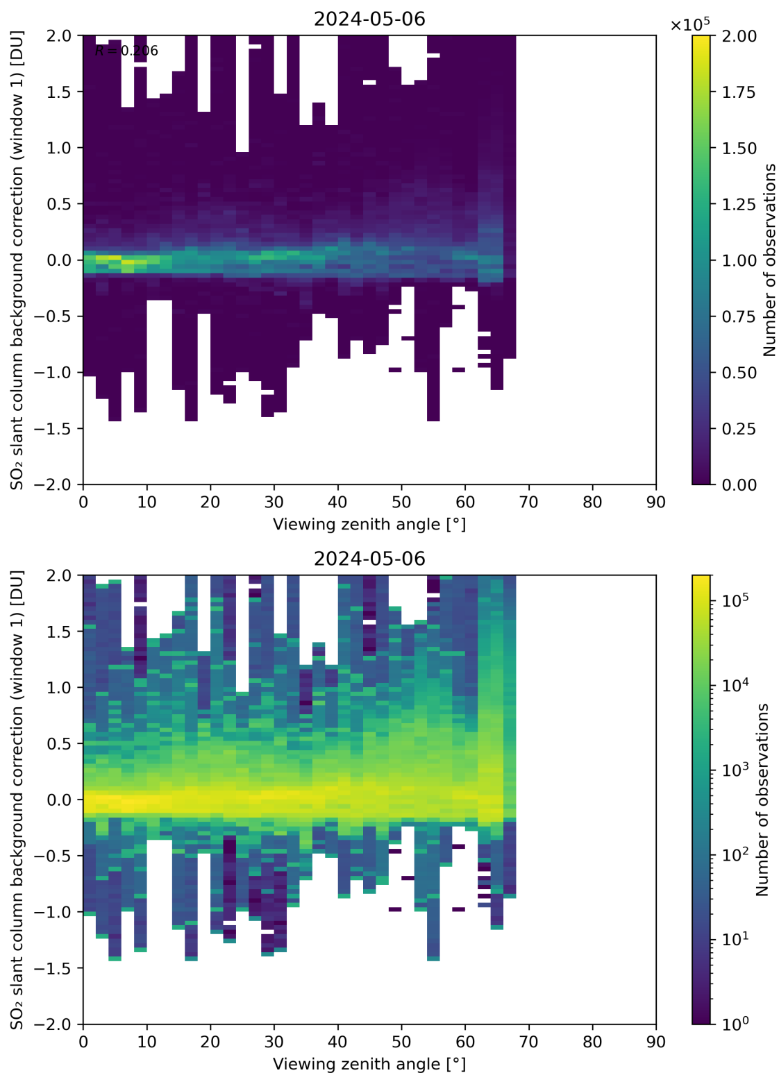
Figure 308: Scatter density plot of “Viewing zenith angle” against “SO 2 slant column background correction (window 1)” for 2024-05-05 to 2024-05-07.
