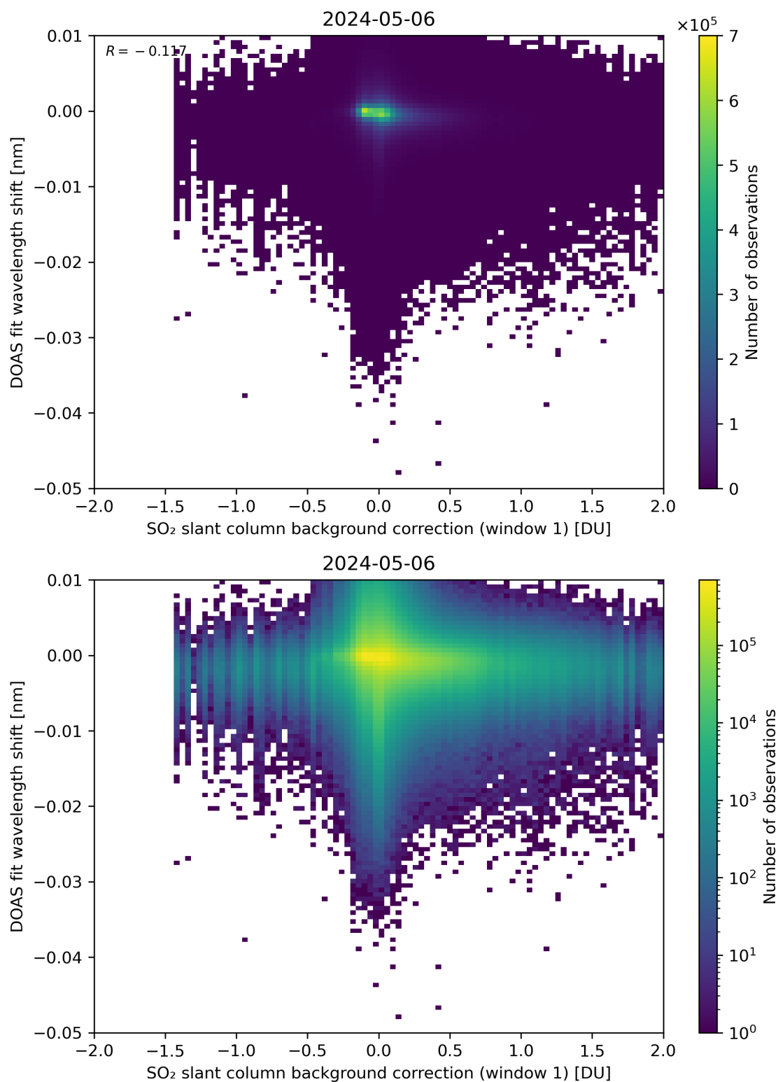
Figure 100: Scatter density plot of “SO 2 slant column background correction (window 1)” against “DOAS fit wavelength shift” for 2024-05-05 to 2024-05-07.
