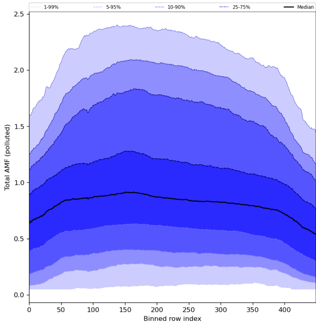
Figure 94: Along track statistics of “Total AMF (polluted)” for 2024-05-05 to 2024-05-07
