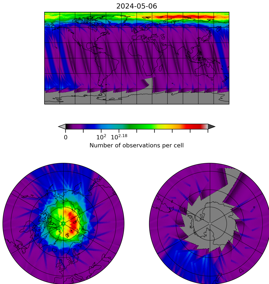
Figure 28: Map of the number of observations for 2024-05-05 to 2024-05-07
