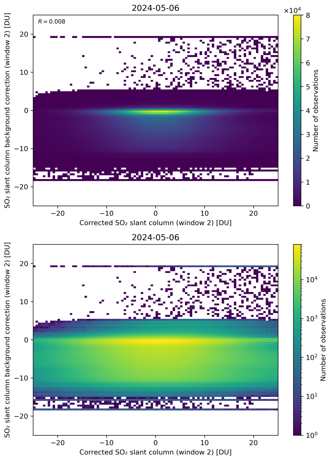
Figure 194: Scatter density plot of “Corrected SO 2 slant column (window 2)” against “SO 2 slant column background correction (window 2)” for 2024-05-05 to 2024-05-07.
