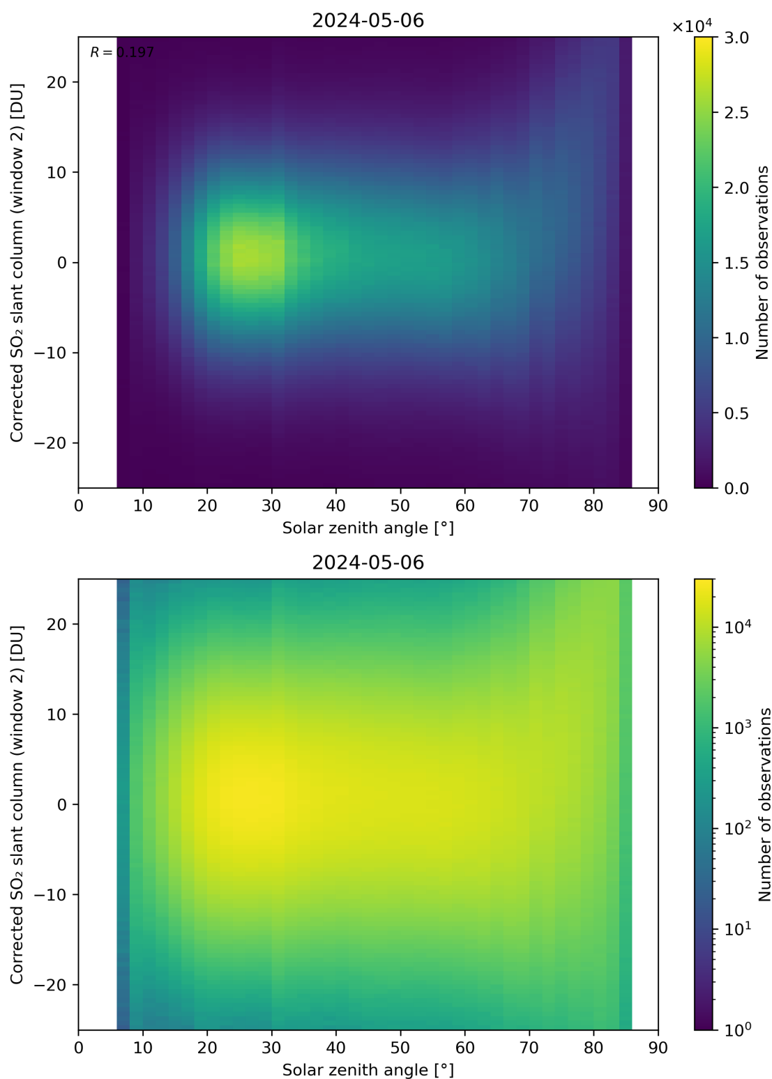
Figure 167: Scatter density plot of “Solar zenith angle” against “Corrected SO 2 slant column (window 2)” for 2024-05-05 to 2024-05-07.
