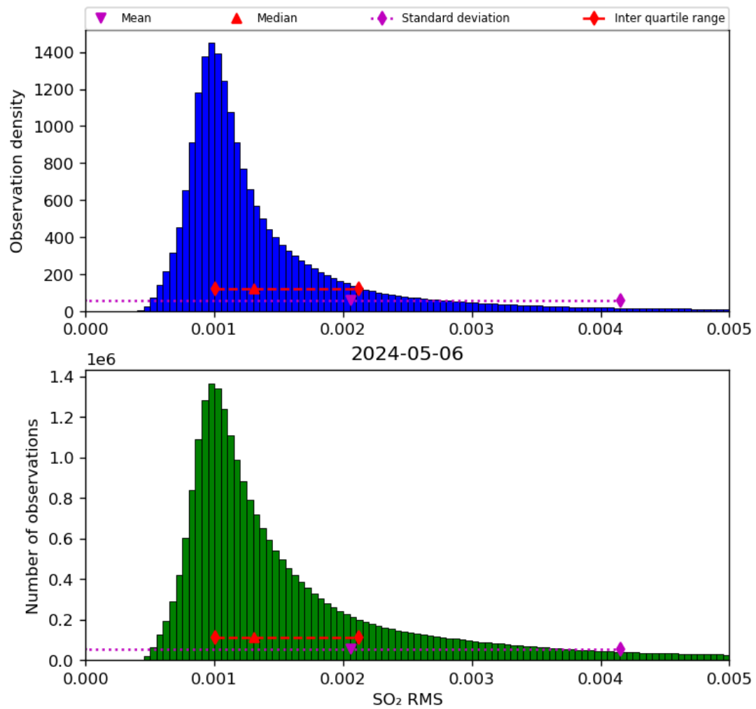
Figure 70: Histogram of “SO 2 RMS” for 2024-05-05 to 2024-05-07
