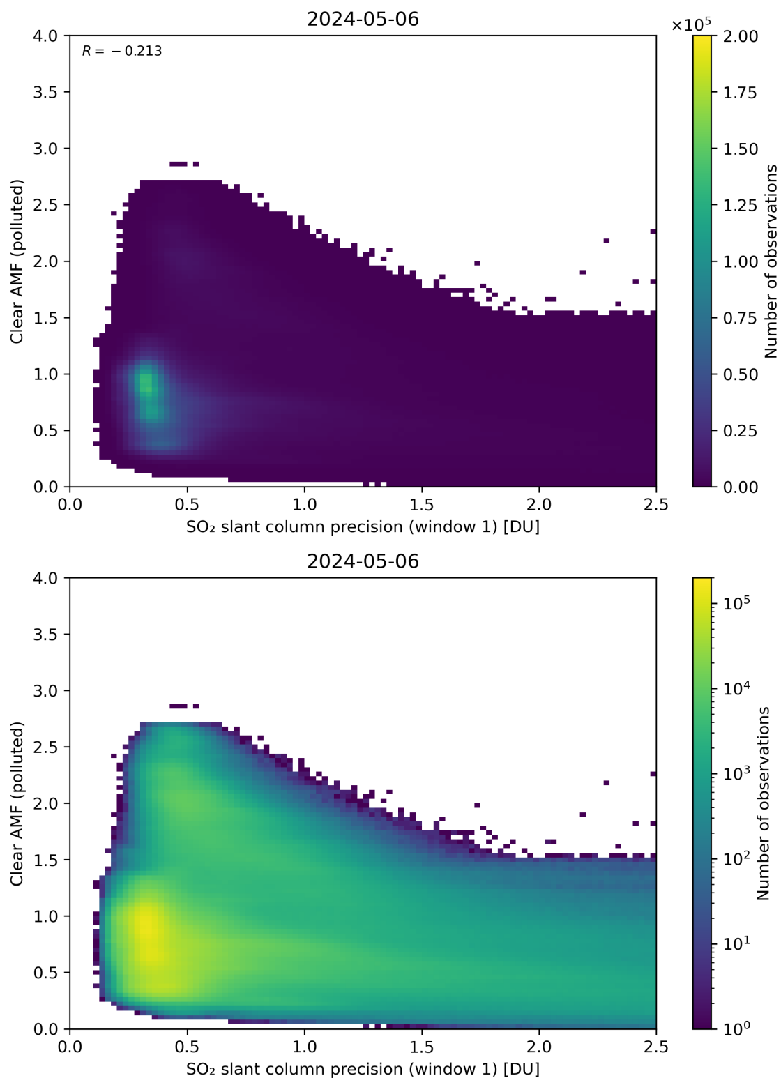
Figure 224: Scatter density plot of “SO 2 slant column precision (window 1)” against “Clear AMF (polluted)” for 2024-05-05 to 2024-05-07.
