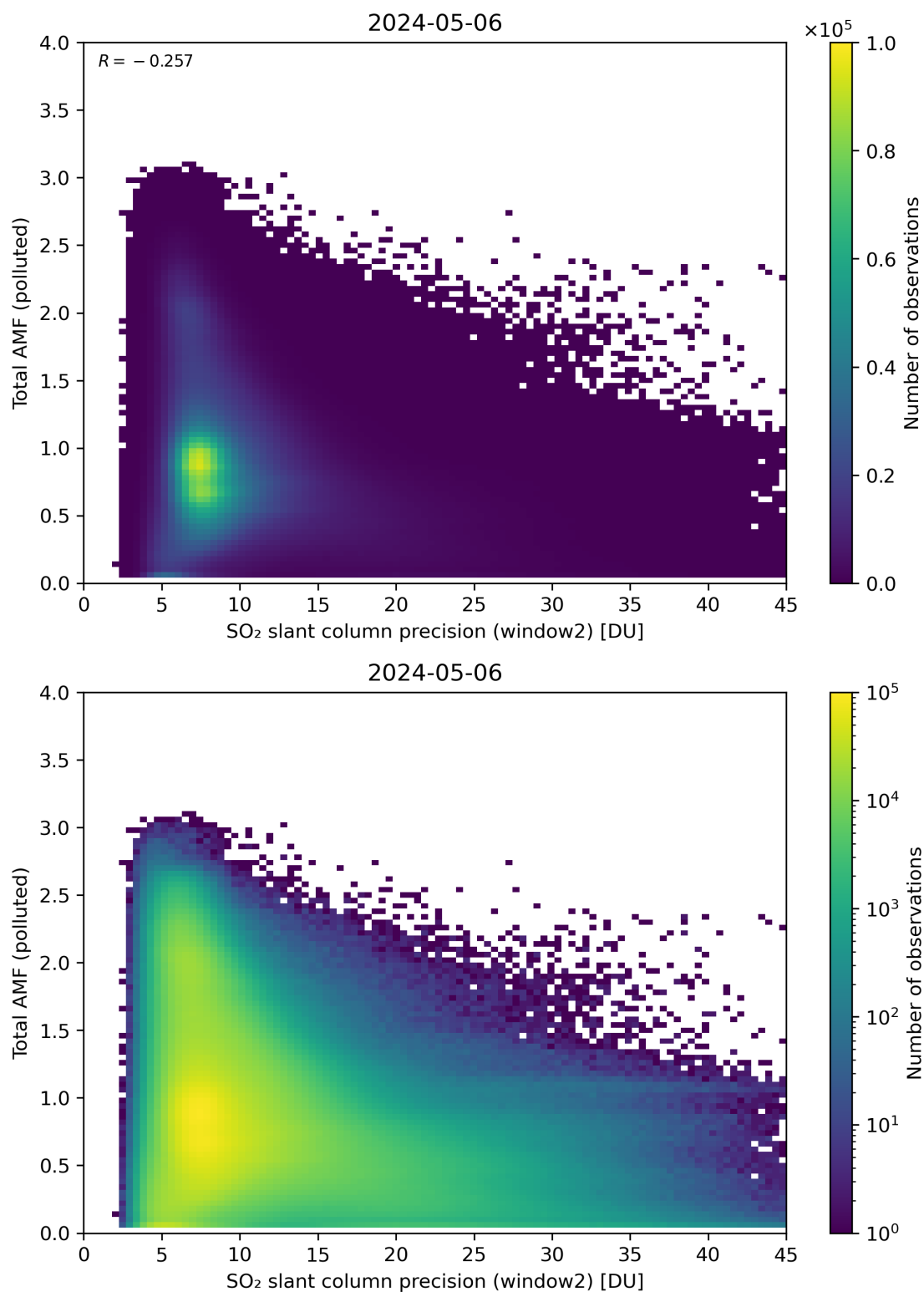
Figure 251: Scatter density plot of “SO 2 slant column precision (window2)” against “Total AMF (polluted)” for 2024-05-05 to 2024-05-07.
