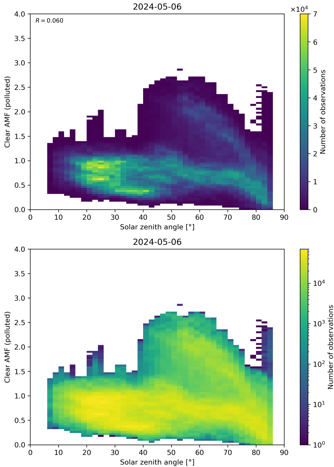
Figure 165: Scatter density plot of “Solar zenith angle” against “Clear AMF (polluted)” for 2024-05-05 to 2024-05-07.
