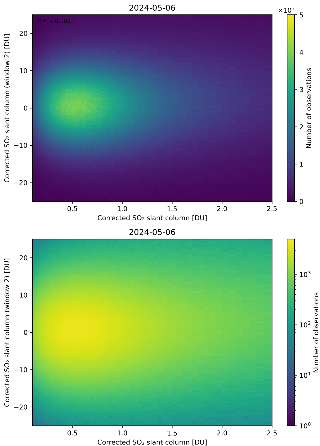
Figure 185: Scatter density plot of “Corrected SO 2 slant column” against “Corrected SO 2 slant column (window 2)” for 2024-05-05 to 2024-05-07.
