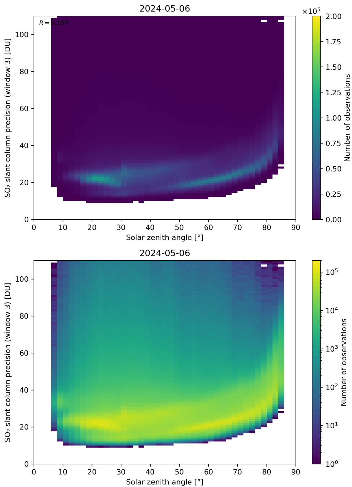
Figure 173: Scatter density plot of “Solar zenith angle” against “SO 2 slant column precision (window 3)” for 2024-05-05 to 2024-05-07.
