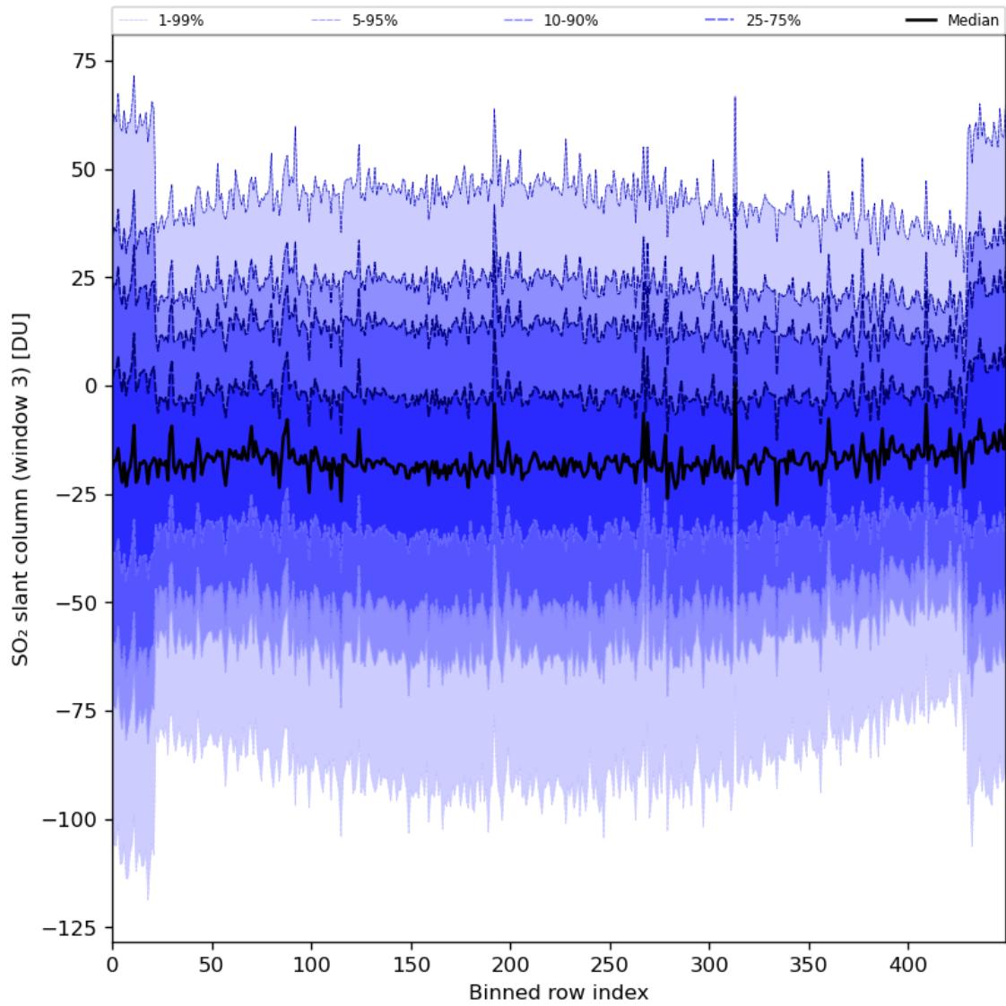
Figure 87: Along track statistics of “SO 2 slant column (window 3)” for 2024-05-05 to 2024-05-07
