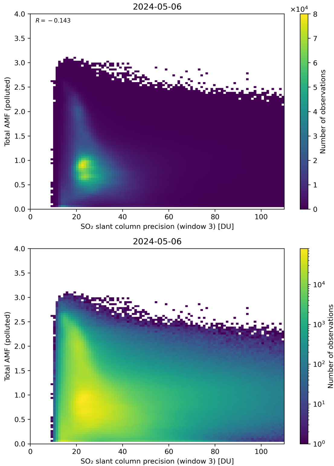
Figure 263: Scatter density plot of “SO 2 slant column precision (window 3)” against “Total AMF (polluted)” for 2024-05-05 to 2024-05-07.
