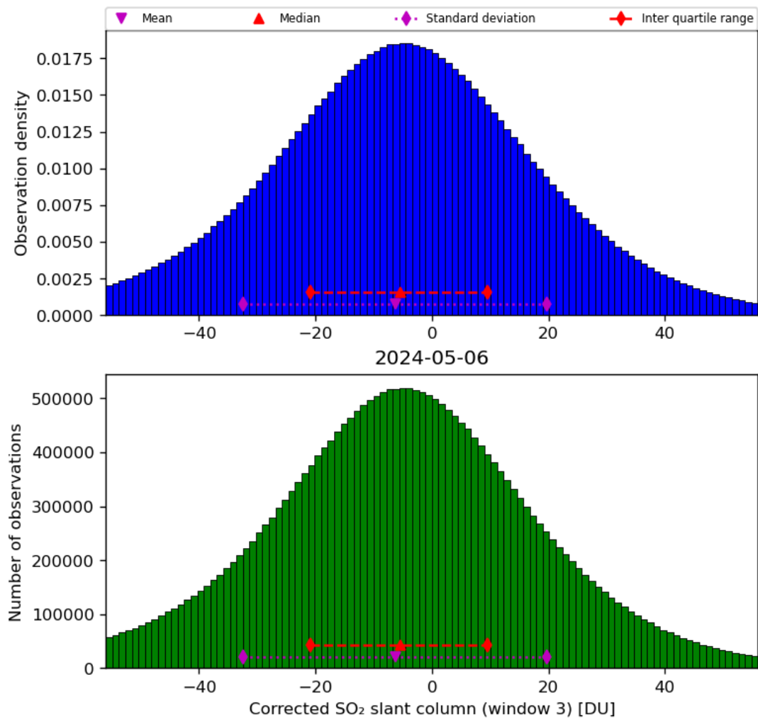
Figure 66: Histogram of “Corrected SO 2 slant column (window 3)” for 2024-05-05 to 2024-05-07
