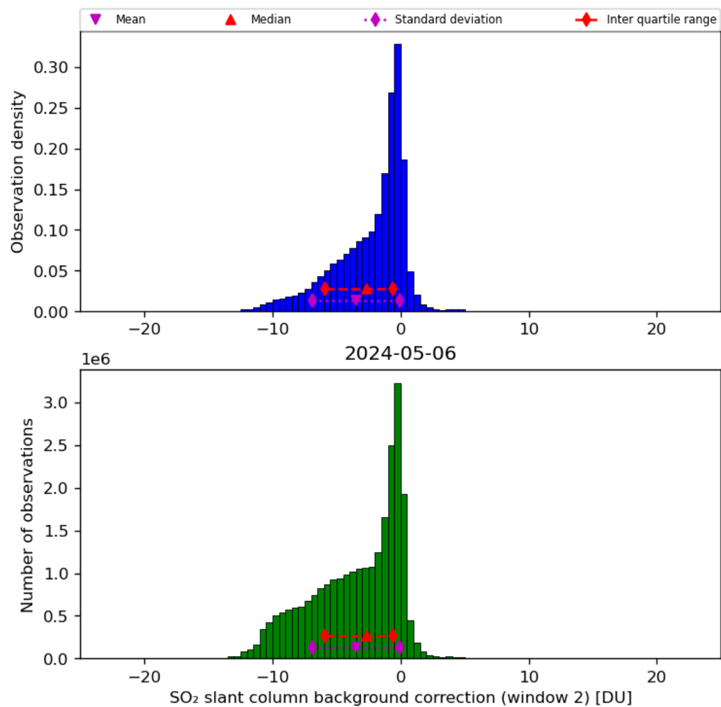
Figure 63: Histogram of “SO 2 slant column background correction (window 2)” for 2024-05-05 to 2024-05-07
