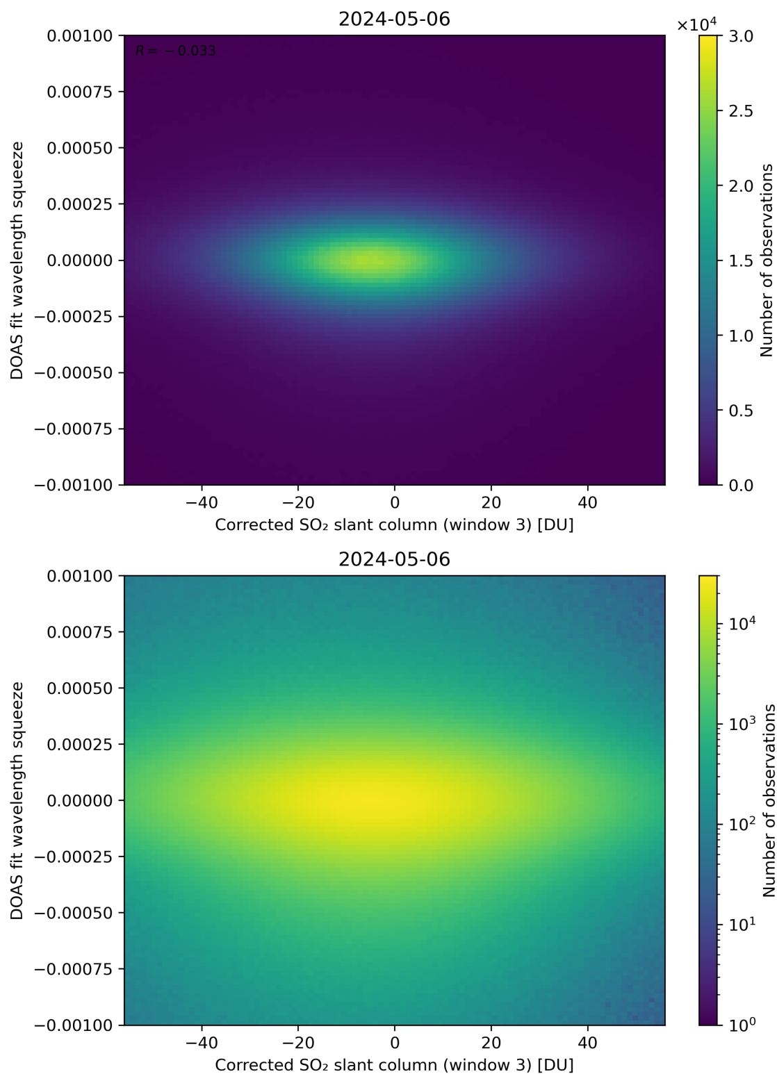
Figure 207: Scatter density plot of “Corrected SO 2 slant column (window 3)” against “DOAS fit wavelength squeeze” for 2024-05-05 to 2024-05-07.
