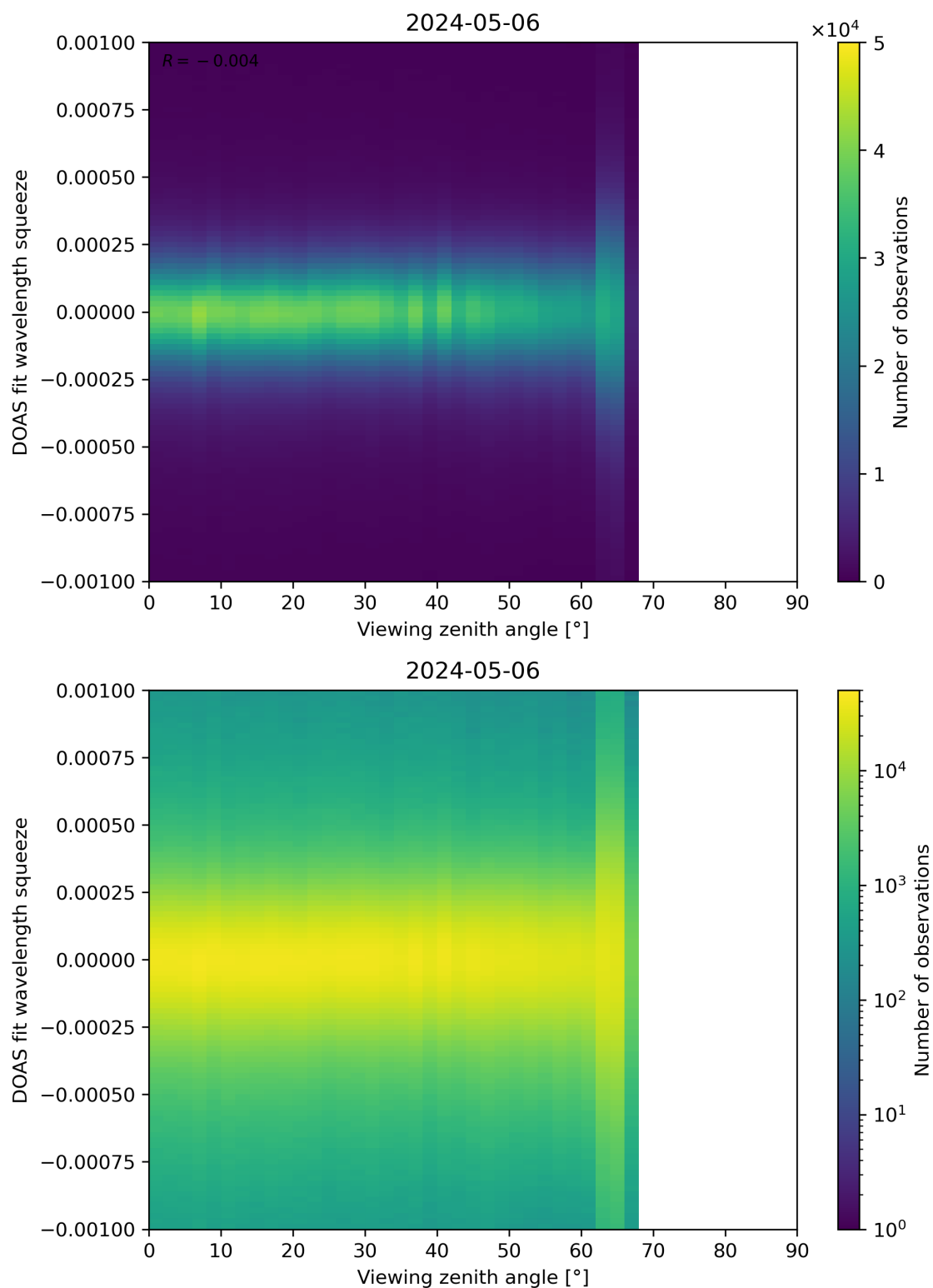
Figure 312: Scatter density plot of “Viewing zenith angle” against “DOAS fit wavelength squeeze” for 2024-05-05 to 2024-05-07.
