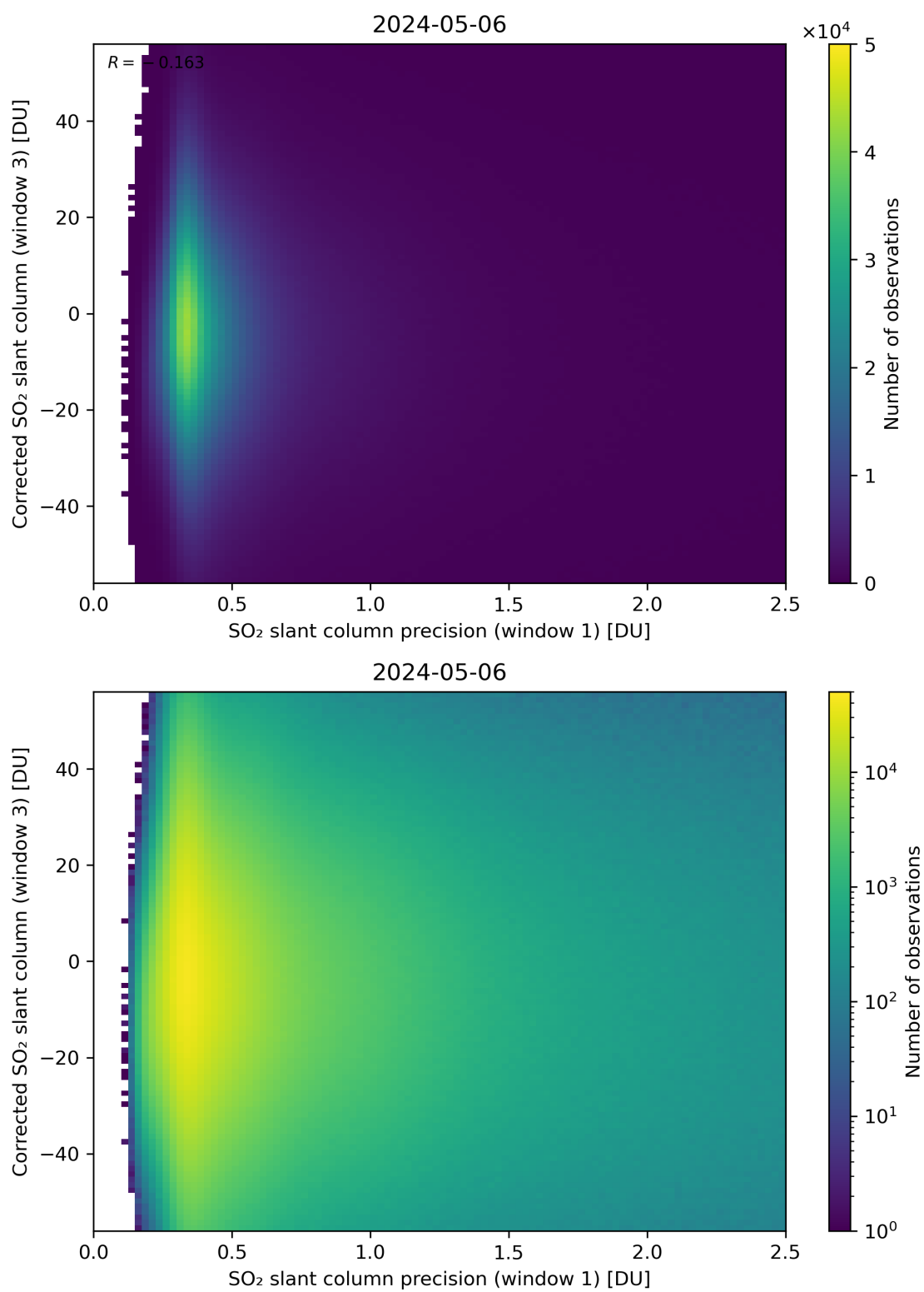
Figure 226: Scatter density plot of “SO 2 slant column precision (window 1)” against “Corrected SO 2 slant column (window 3)” for 2024-05-05 to 2024-05-07.
