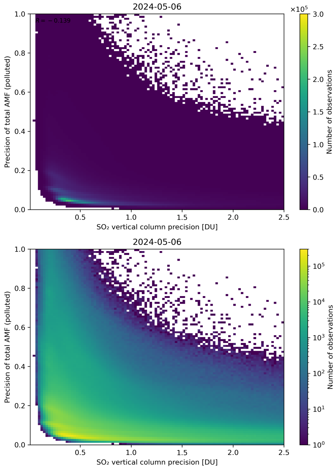
Figure 295: Scatter density plot of “SO 2 vertical column precision” against “Precision of total AMF (polluted)” for 2024-05-05 to 2024-05-07.
