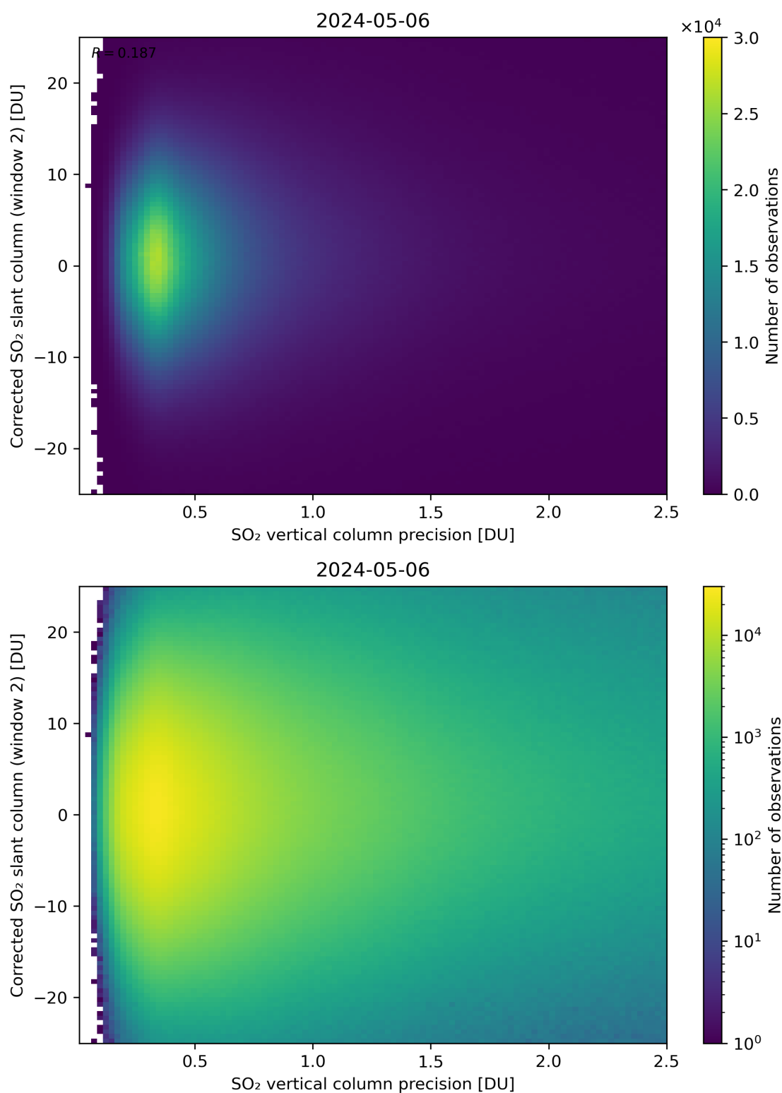
Figure 287: Scatter density plot of “SO 2 vertical column precision” against “Corrected SO 2 slant column (window 2)” for 2024-05-05 to 2024-05-07.
