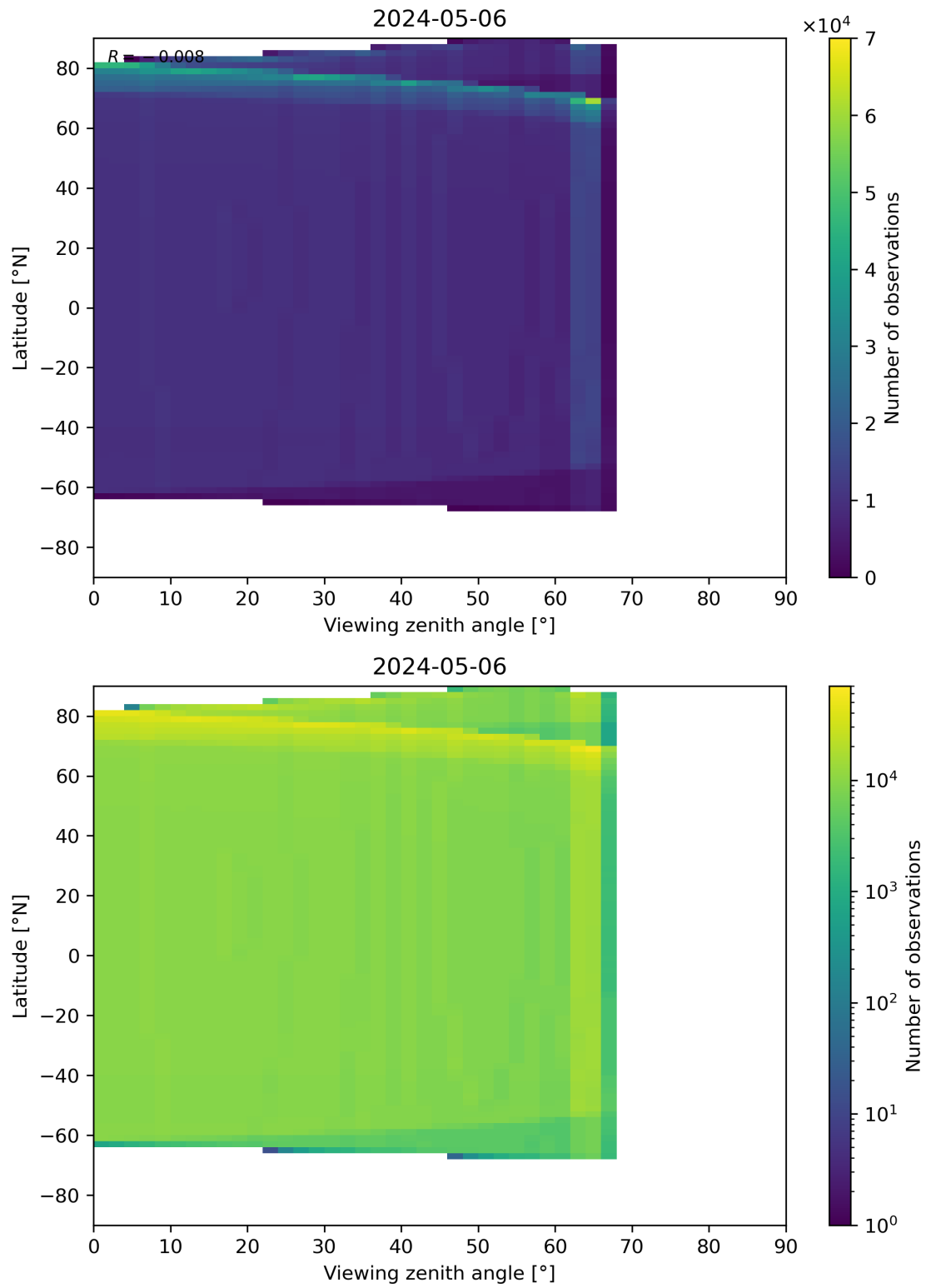
Figure 314: Scatter density plot of “Viewing zenith angle” against “Latitude” for 2024-05-05 to 2024-05-07.
