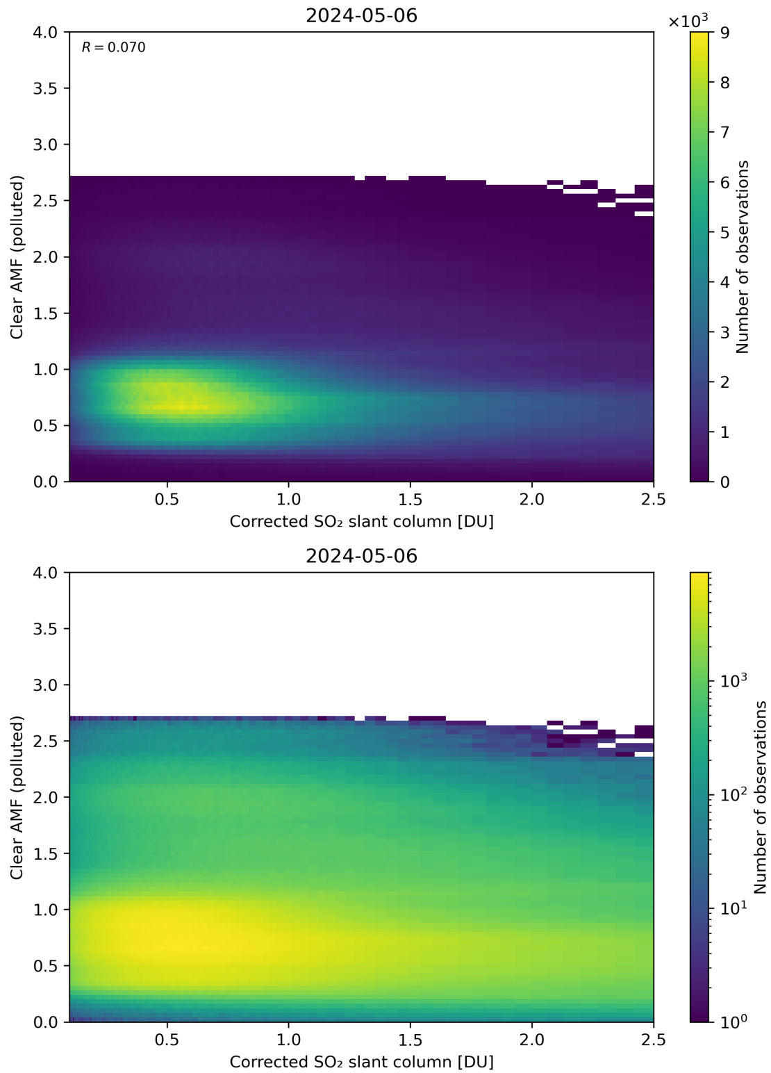
Figure 184: Scatter density plot of “Corrected SO 2 slant column” against “Clear AMF (polluted)” for 2024-05-05 to 2024-05-07.
