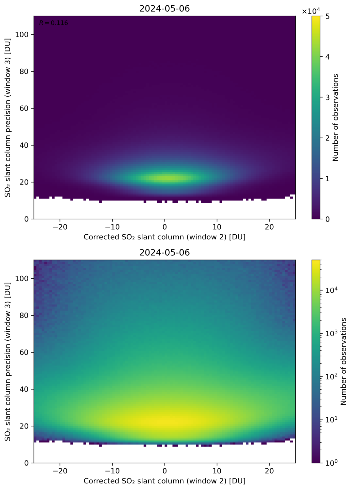
Figure 202: Scatter density plot of “Corrected SO 2 slant column (window 2)” against “SO 2 slant column precision (window 3)” for 2024-05-05 to 2024-05-07.
