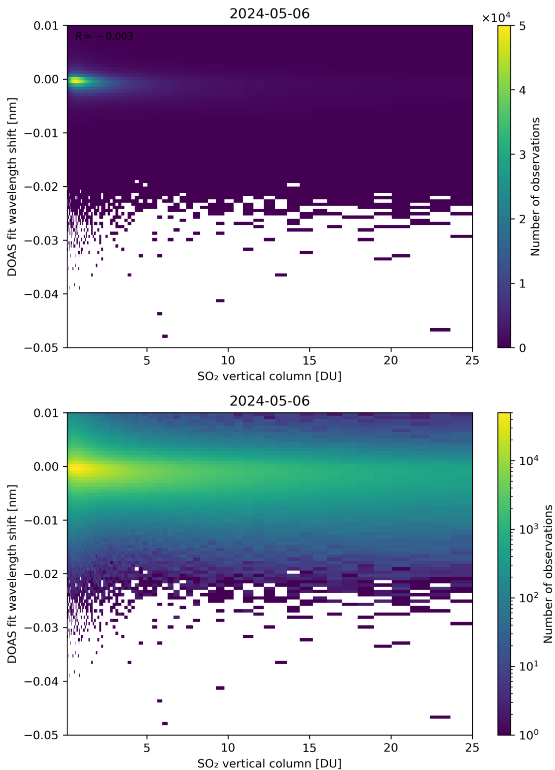
Figure 276: Scatter density plot of “SO 2 vertical column” against “DOAS fit wavelength shift” for 2024-05-05 to 2024-05-07.
