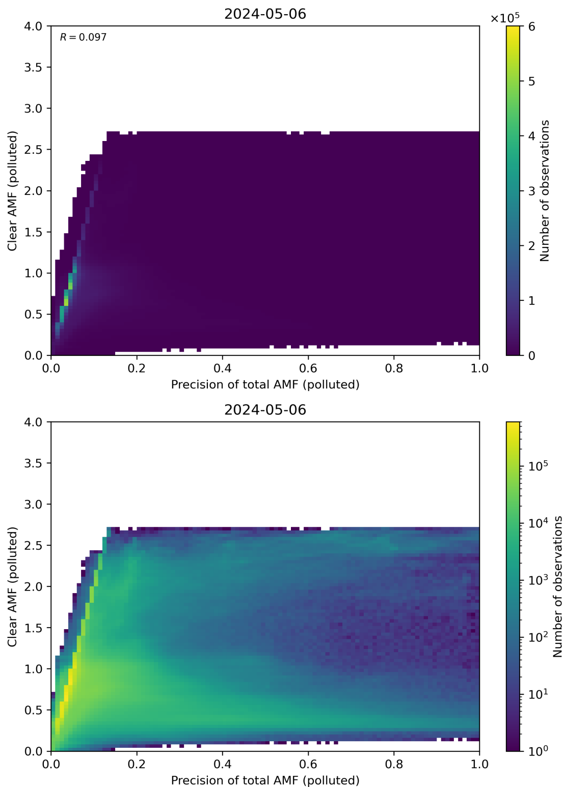
Figure 270: Scatter density plot of “Precision of total AMF (polluted)” against “Clear AMF (polluted)” for 2024-05-05 to 2024-05-07.
