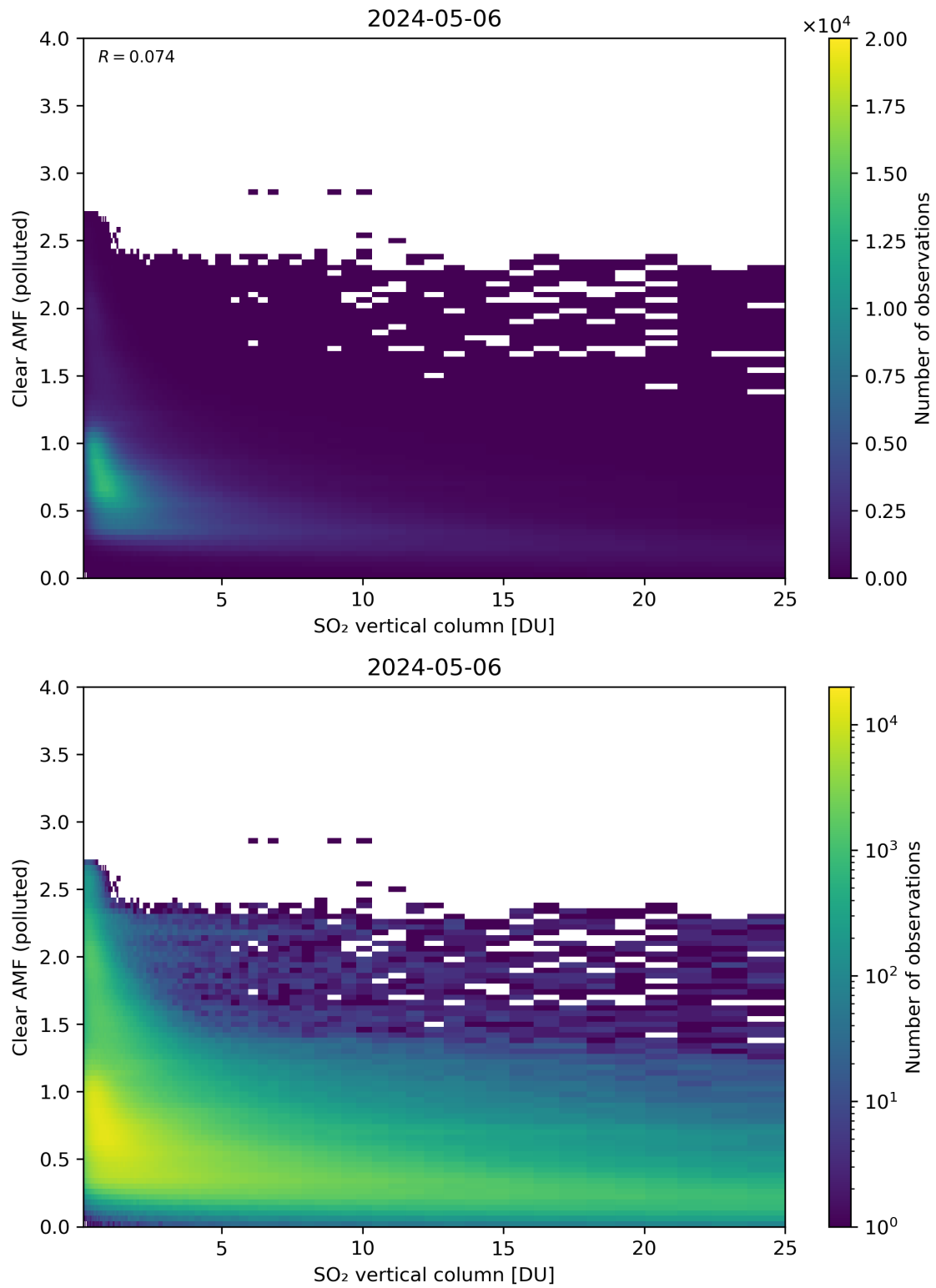
Figure 296: Scatter density plot of “SO 2 vertical column” against “Clear AMF (polluted)” for 2024-05-05 to 2024-05-07.
