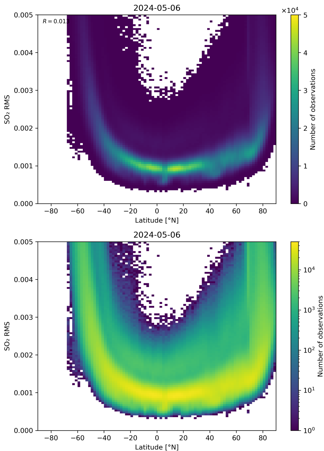
Figure 144: Scatter density plot of “Latitude” against “SO 2 RMS” for 2024-05-05 to 2024-05-07.
