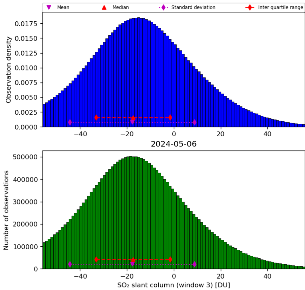
Figure 64: Histogram of “SO 2 slant column (window 3)” for 2024-05-05 to 2024-05-07
