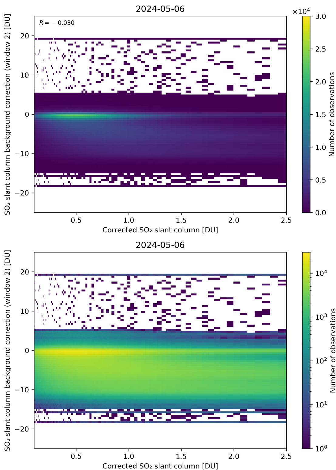
Figure 179: Scatter density plot of “Corrected SO 2 slant column” against “SO 2 slant column background correction (window 2)” for 2024-05-05 to 2024-05-07.
