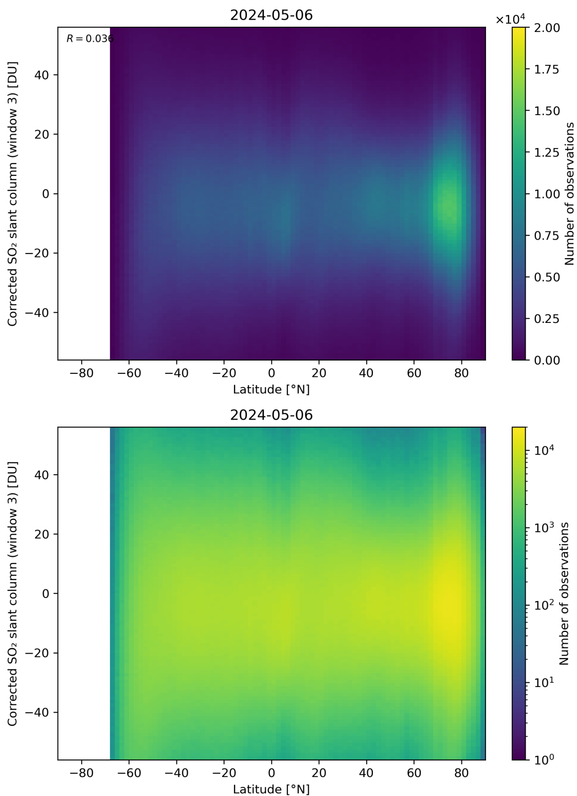
Figure 148: Scatter density plot of “Latitude” against “Corrected SO 2 slant column (window 3)” for 2024-05-05 to 2024-05-07.
