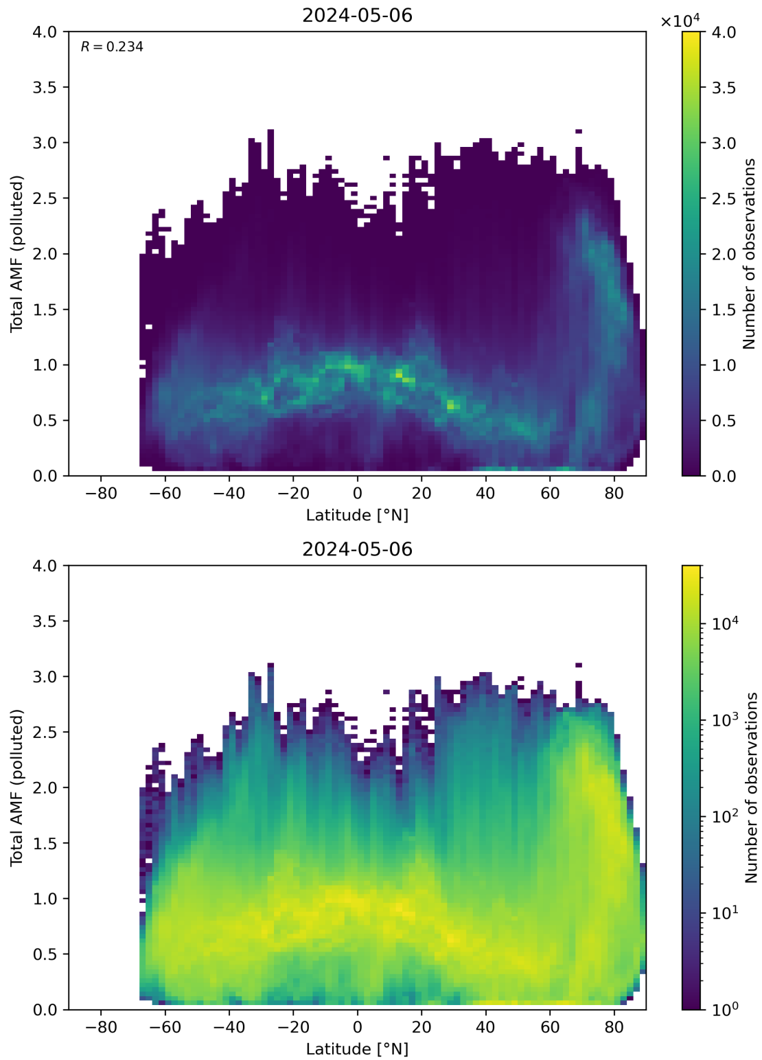
Figure 154: Scatter density plot of “Latitude” against “Total AMF (polluted)” for 2024-05-05 to 2024-05-07.
