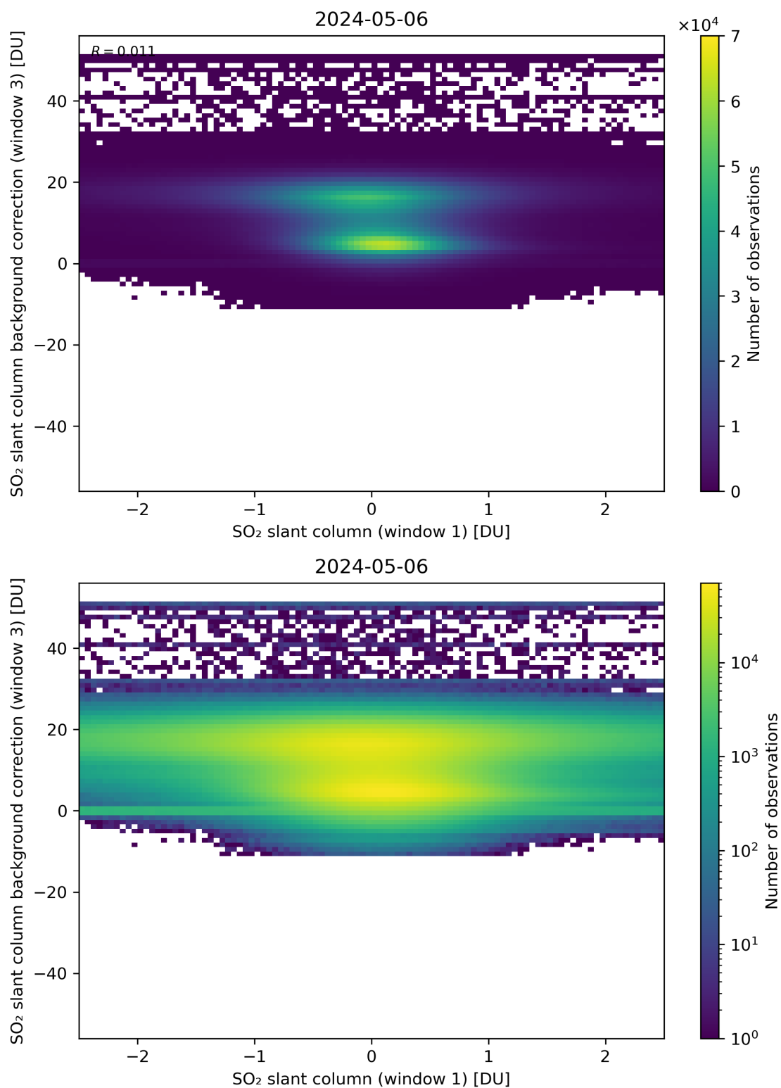
Figure 214: Scatter density plot of “SO 2 slant column (window 1)” against “SO 2 slant column background correction (window 3)” for 2024-05-05 to 2024-05-07.
