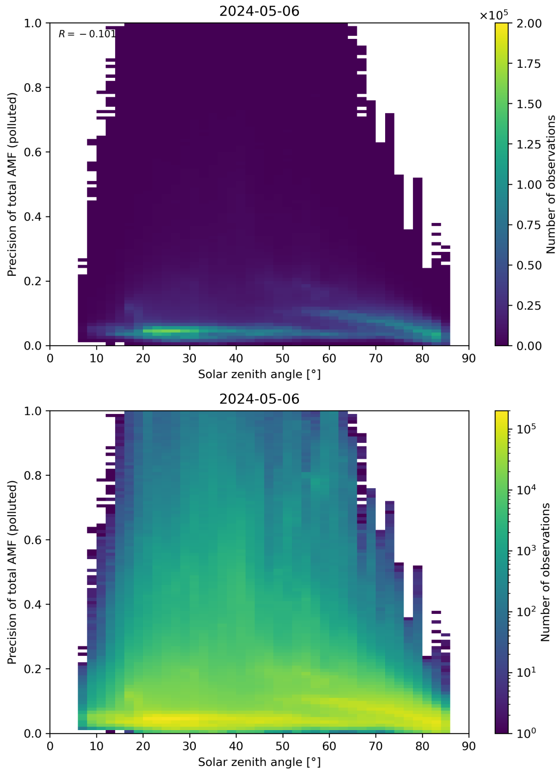
Figure 175: Scatter density plot of “Solar zenith angle” against “Precision of total AMF (polluted)” for 2024-05-05 to 2024-05-07.
