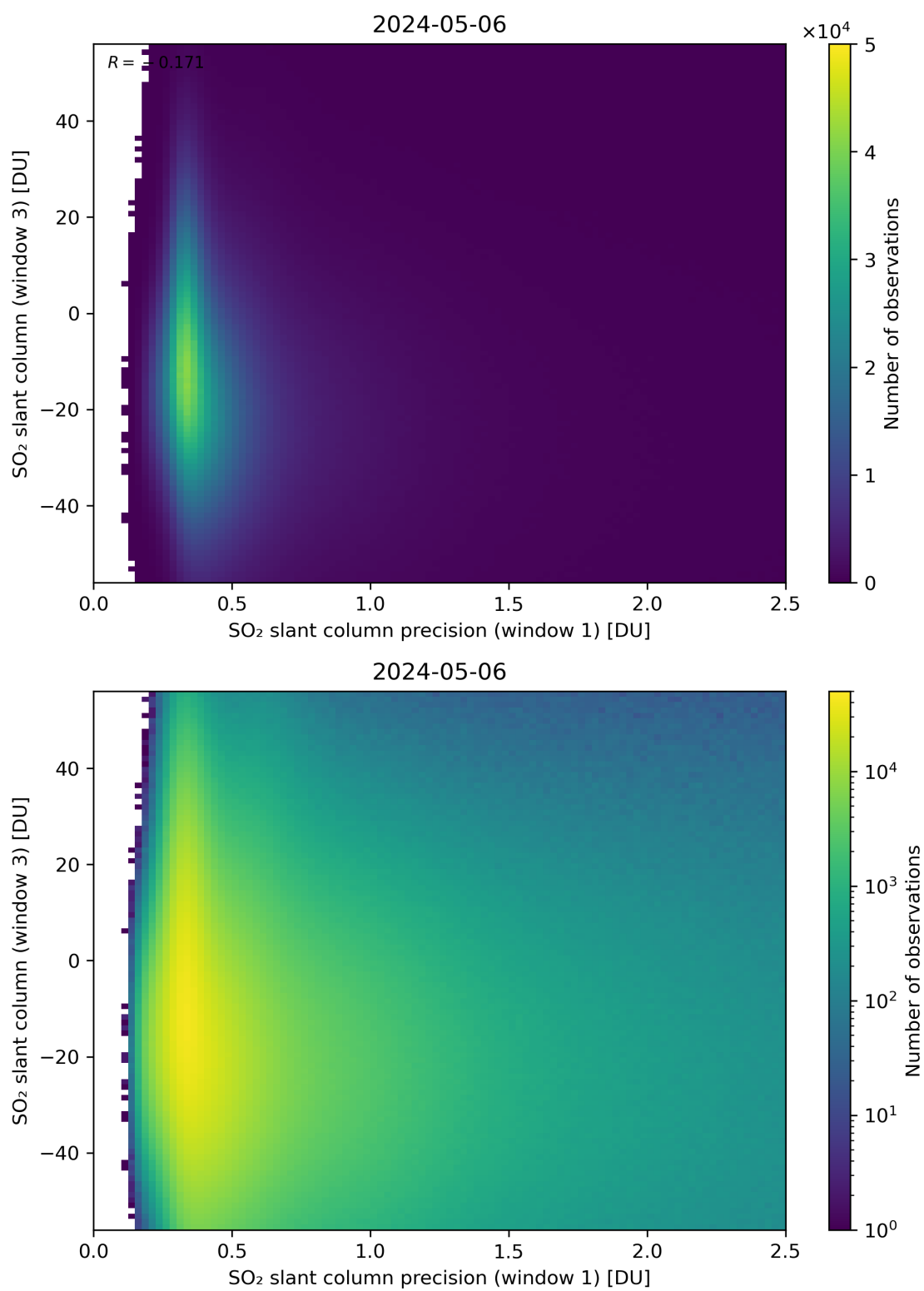
Figure 228: Scatter density plot of “SO 2 slant column precision (window 1)” against “SO 2 slant column (window 3)” for 2024-05-05 to 2024-05-07.
