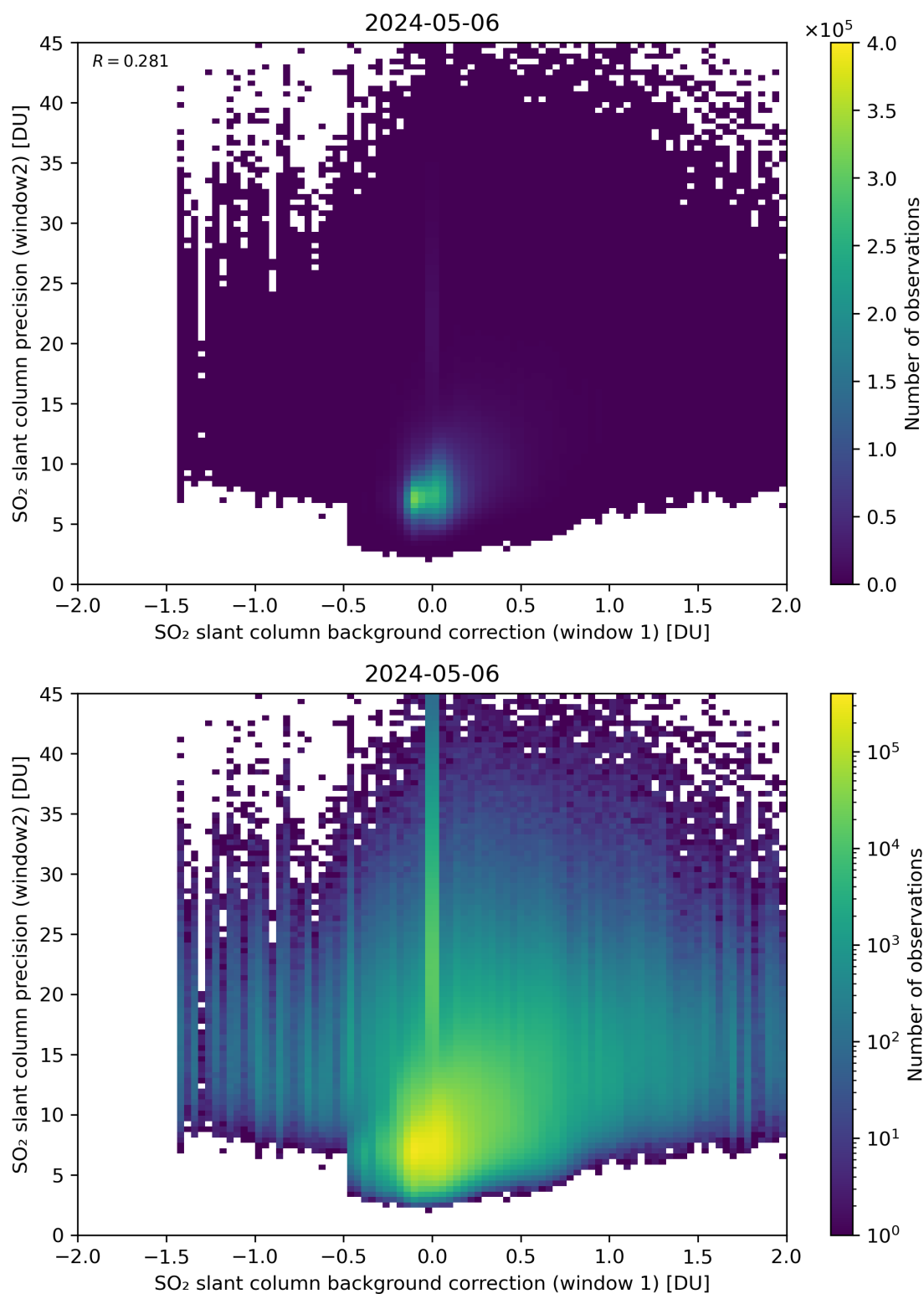
Figure 106: Scatter density plot of “SO 2 slant column background correction (window 1)” against “SO 2 slant column precision (window2)” for 2024-05-05 to 2024-05-07.
