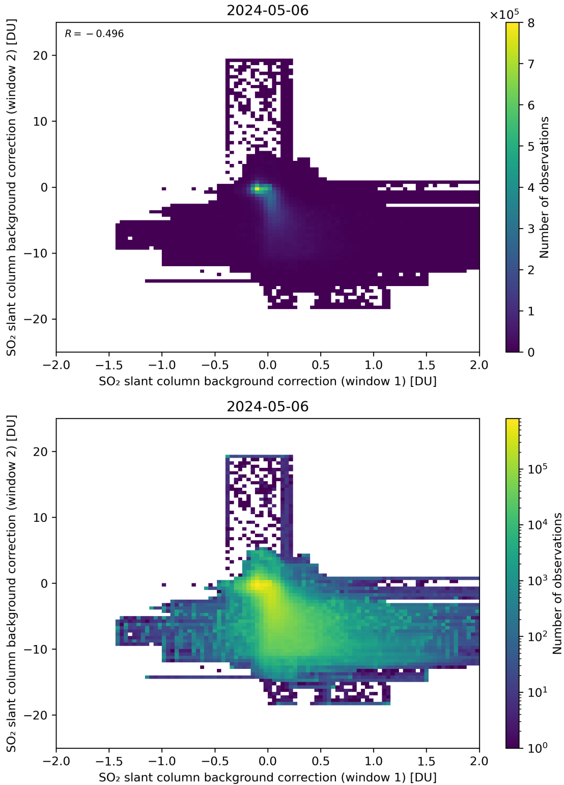
Figure 98: Scatter density plot of “SO 2 slant column background correction (window 1)” against “SO 2 slant column background correction (window 2)” for 2024-05-05 to 2024-05-07.
