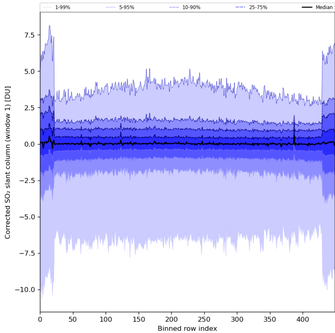
Figure 81: Along track statistics of “Corrected SO 2 slant column (window 1)” for 2024-05-05 to 2024-05-07
