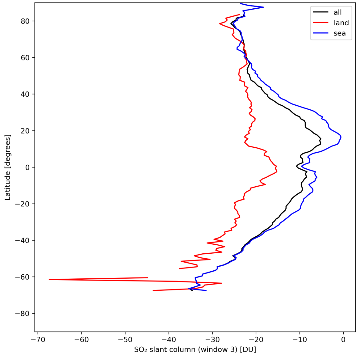
Figure 41: Zonal average of “SO 2 slant column (window 3)” for 2024-05-05 to 2024-05-07.
