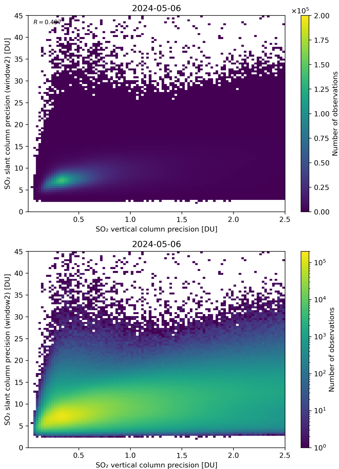
Figure 291: Scatter density plot of “SO 2 vertical column precision” against “SO 2 slant column precision (window2)” for 2024-05-05 to 2024-05-07.
