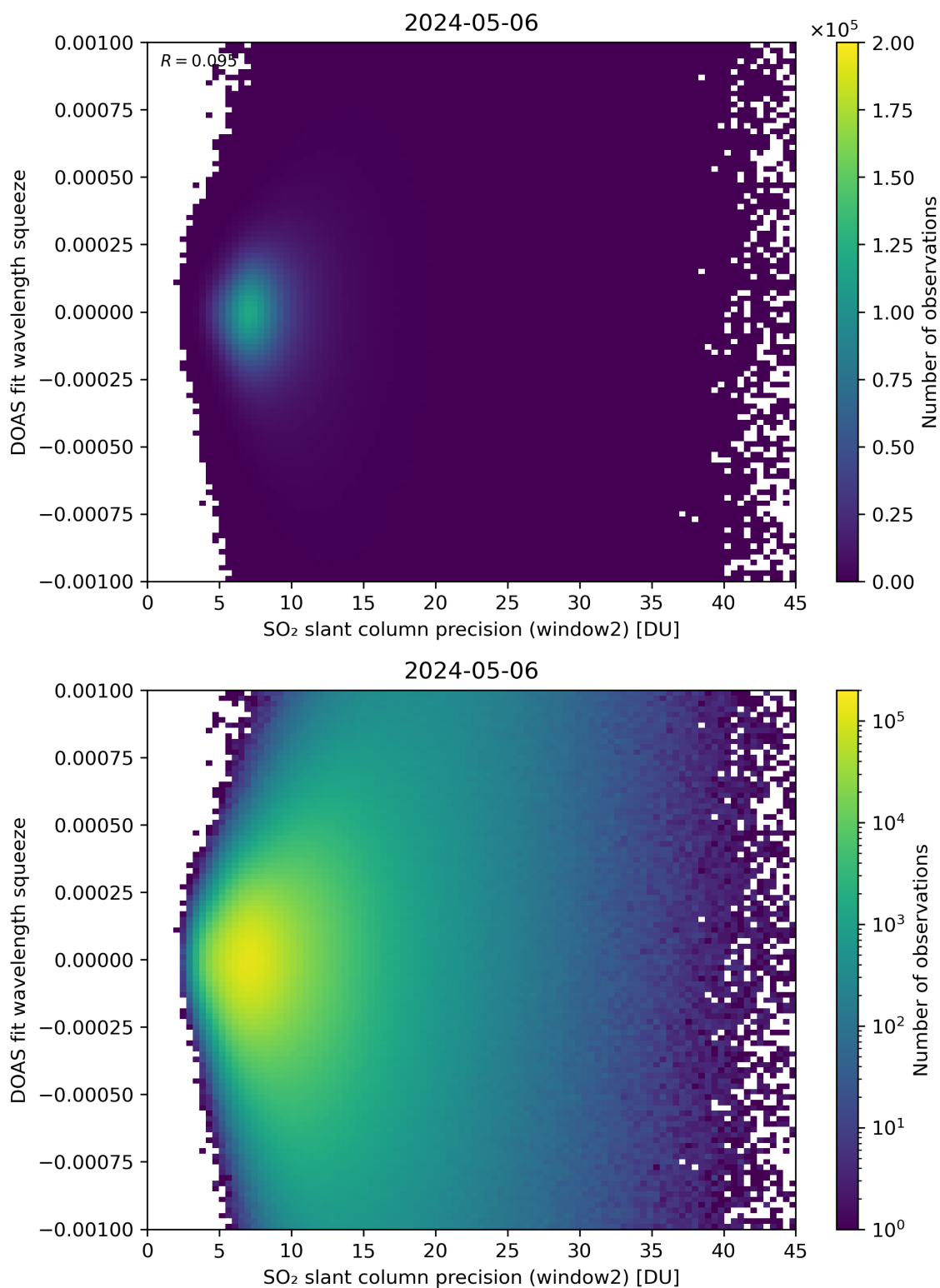
Figure 244: Scatter density plot of “SO 2 slant column precision (window2)” against “DOAS fit wavelength squeeze” for 2024-05-05 to 2024-05-07.
