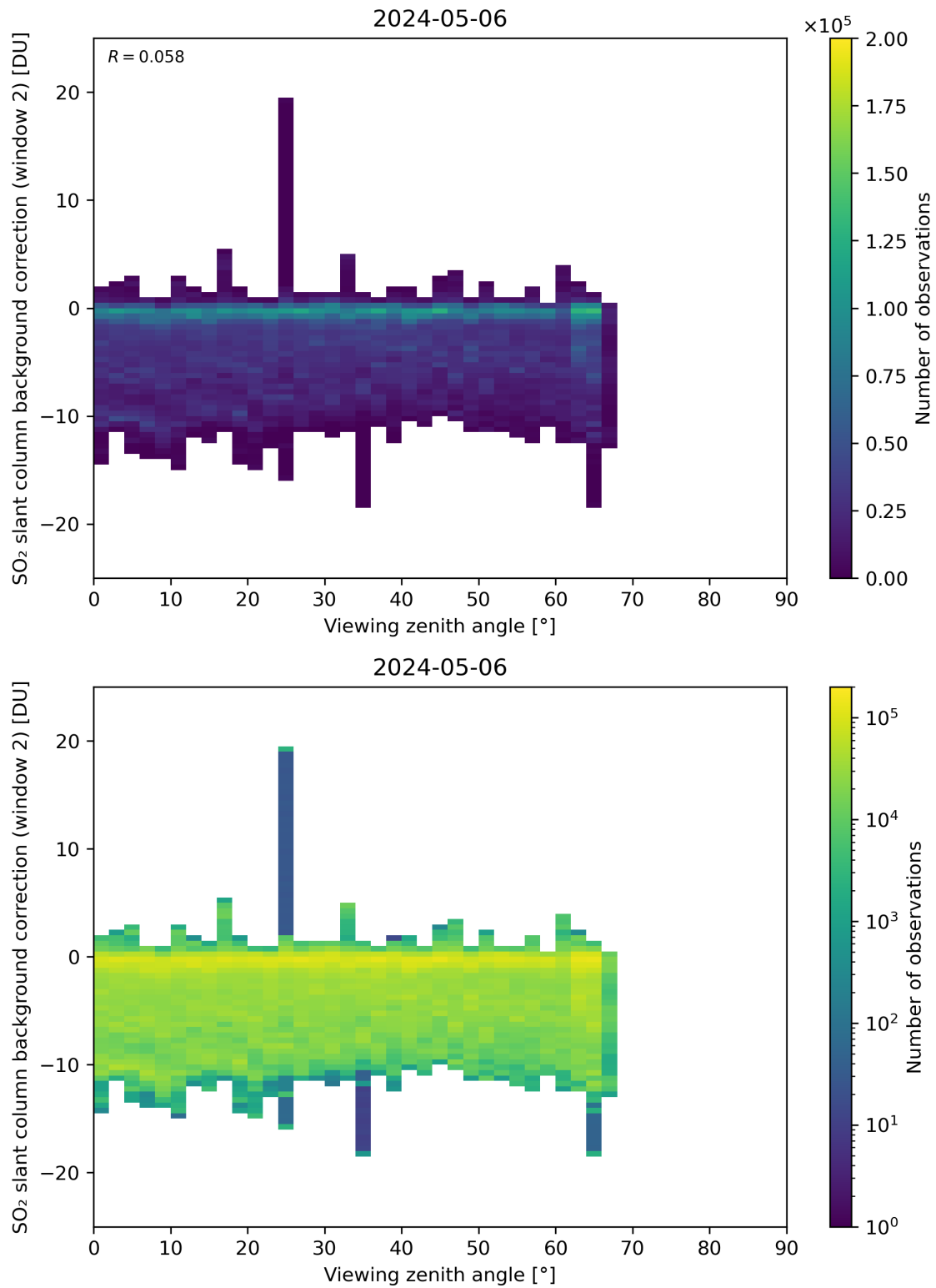
Figure 309: Scatter density plot of “Viewing zenith angle” against “SO 2 slant column background correction (window 2)” for 2024-05-05 to 2024-05-07.
