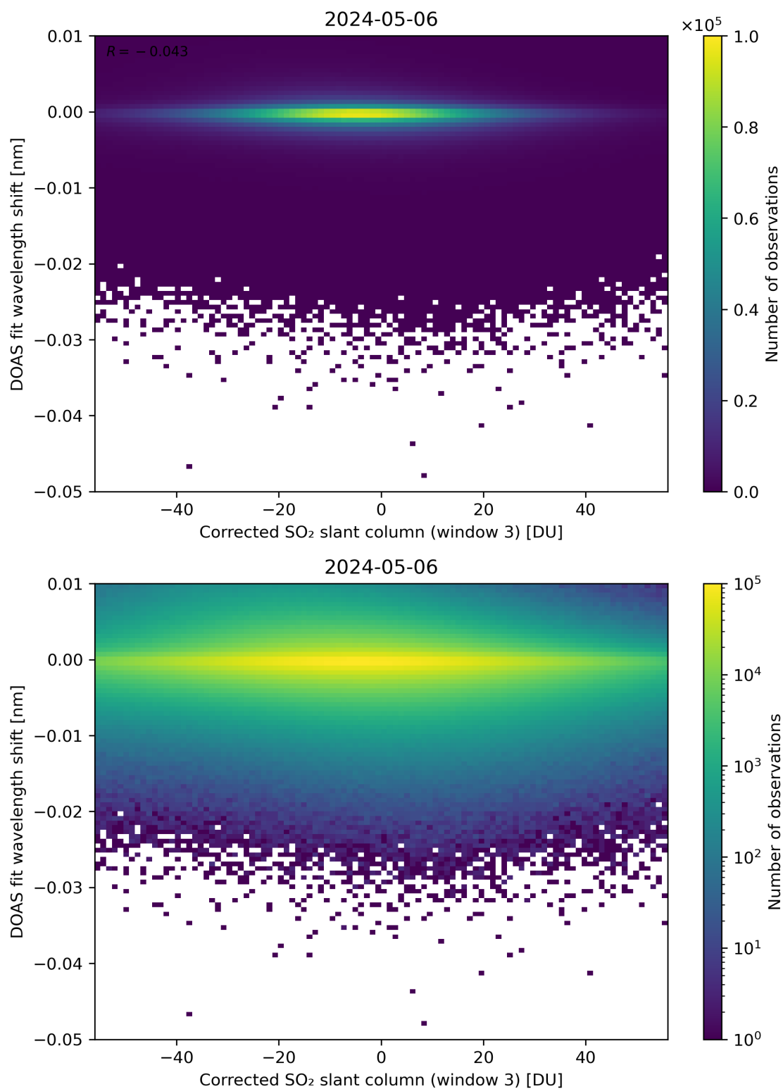
Figure 206: Scatter density plot of “Corrected SO 2 slant column (window 3)” against “DOAS fit wavelength shift” for 2024-05-05 to 2024-05-07.
