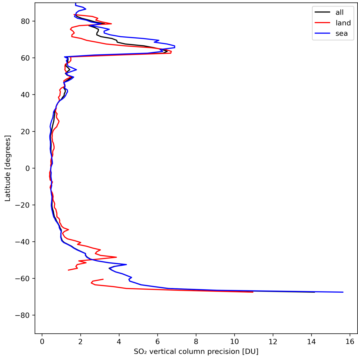
Figure 31: Zonal average of “SO 2 vertical column precision” for 2024-05-05 to 2024-05-07.
