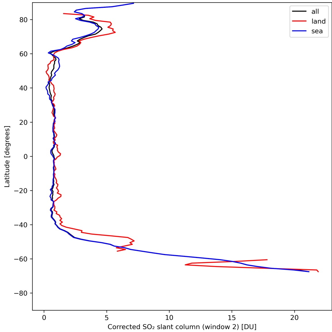
Figure 39: Zonal average of “Corrected SO 2 slant column (window 2)” for 2024-05-05 to 2024-05-07.
