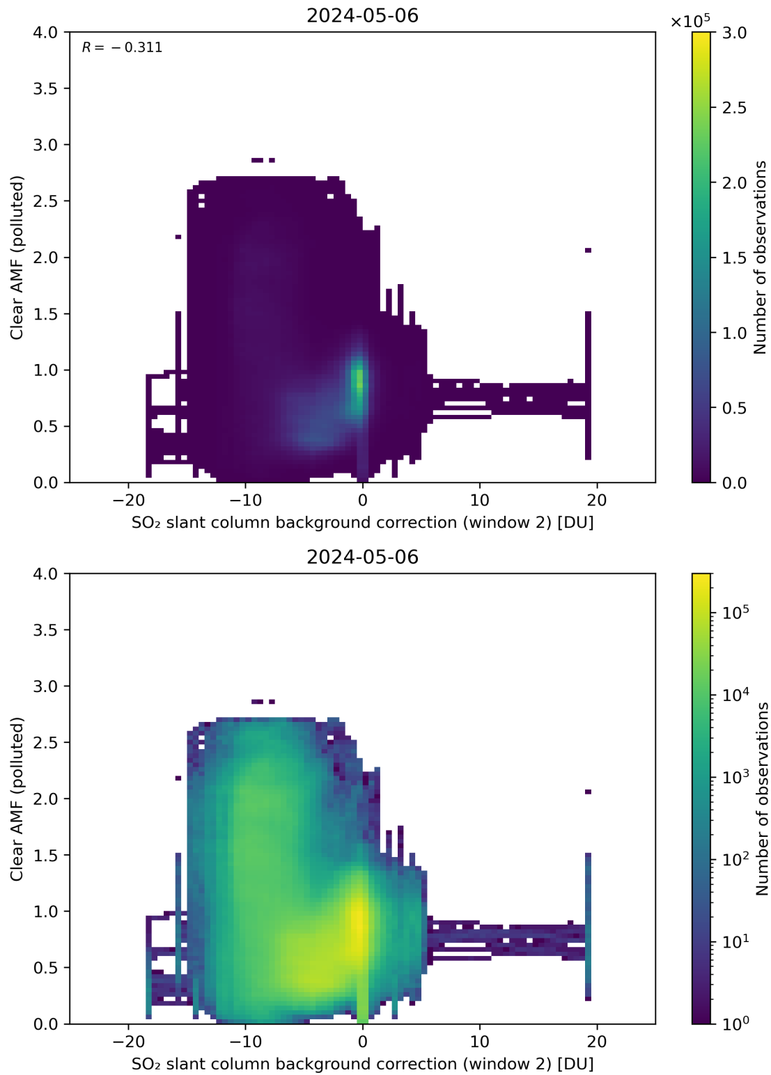
Figure 115: Scatter density plot of “SO 2 slant column background correction (window 2)” against “Clear AMF (polluted)” for 2024-05-05 to 2024-05-07.
