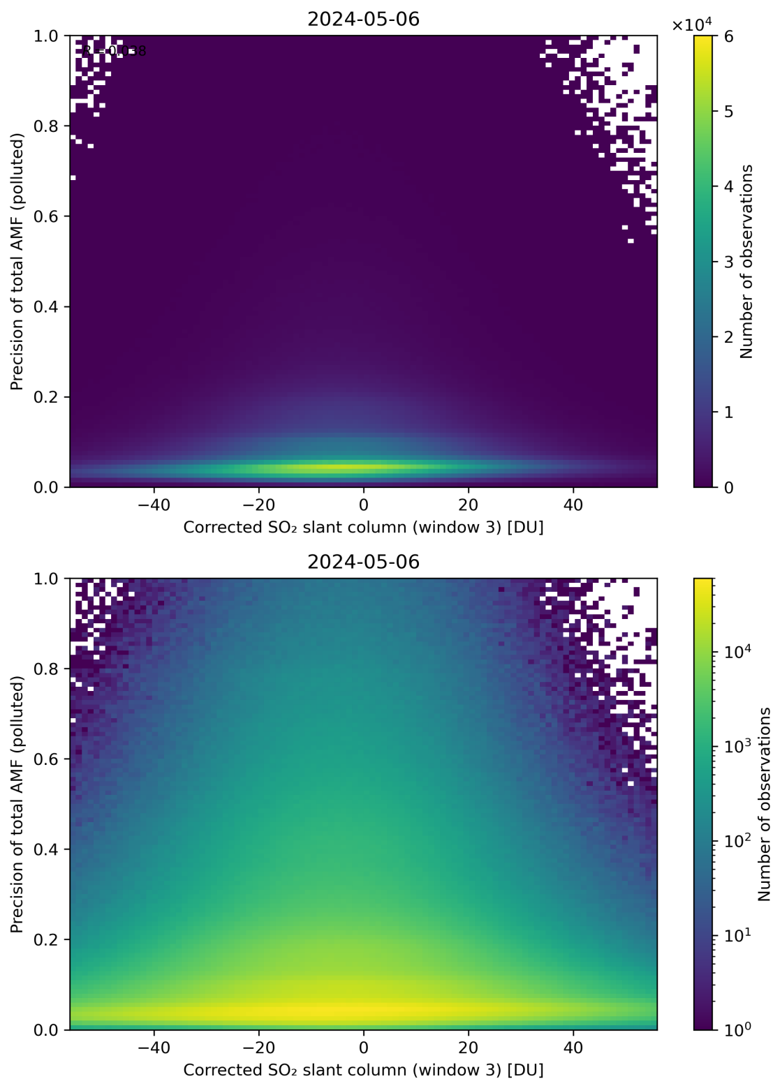
Figure 211: Scatter density plot of “Corrected SO 2 slant column (window 3)” against “Precision of total AMF (polluted)” for 2024-05-05 to 2024-05-07.
