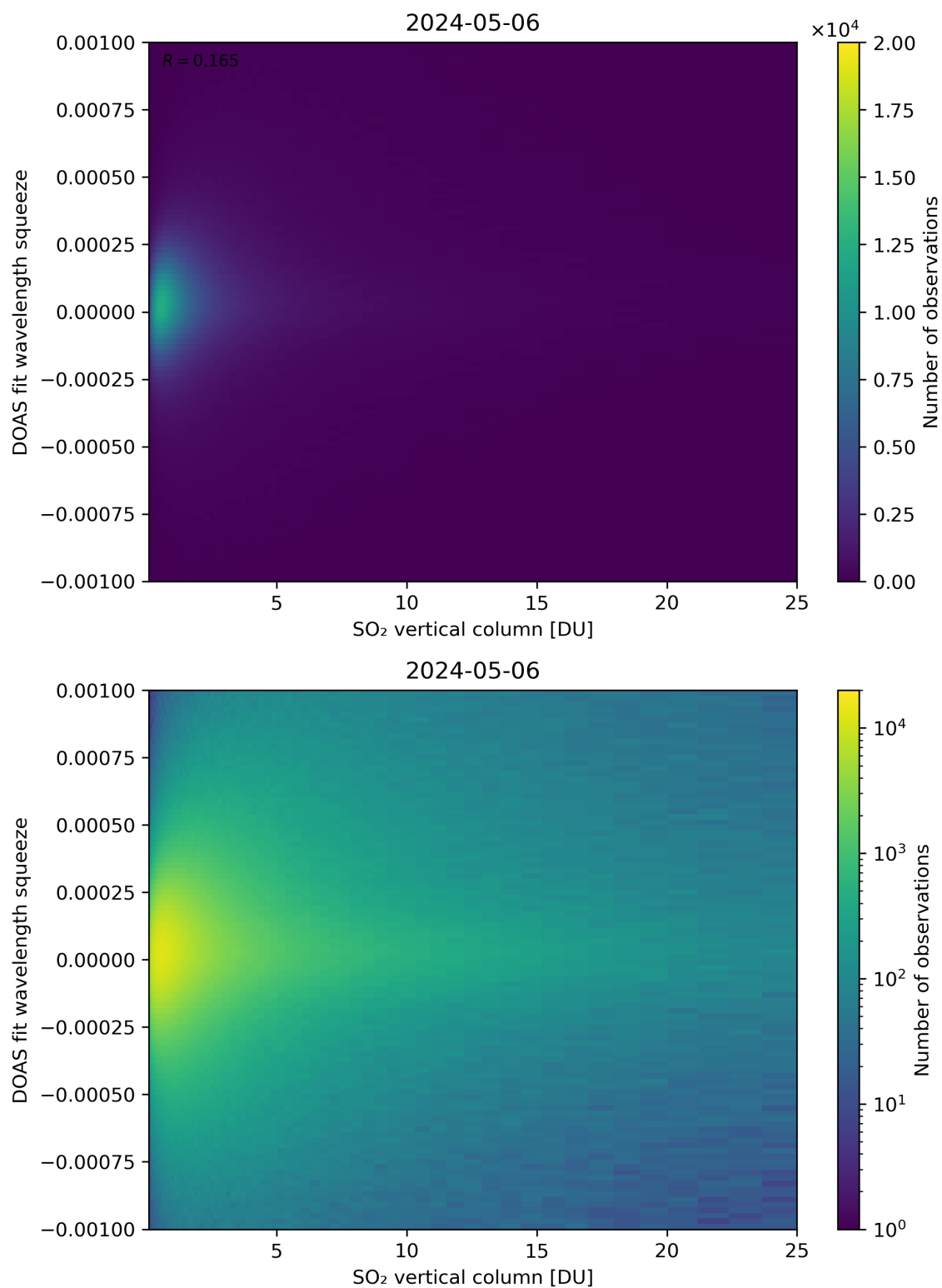
Figure 277: Scatter density plot of “SO 2 vertical column” against “DOAS fit wavelength squeeze” for 2024-05-05 to 2024-05-07.
