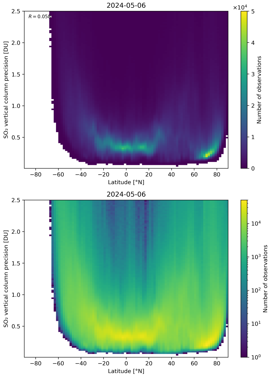
Figure 157: Scatter density plot of “Latitude” against “SO 2 vertical column precision” for 2024-05-05 to 2024-05-07.
