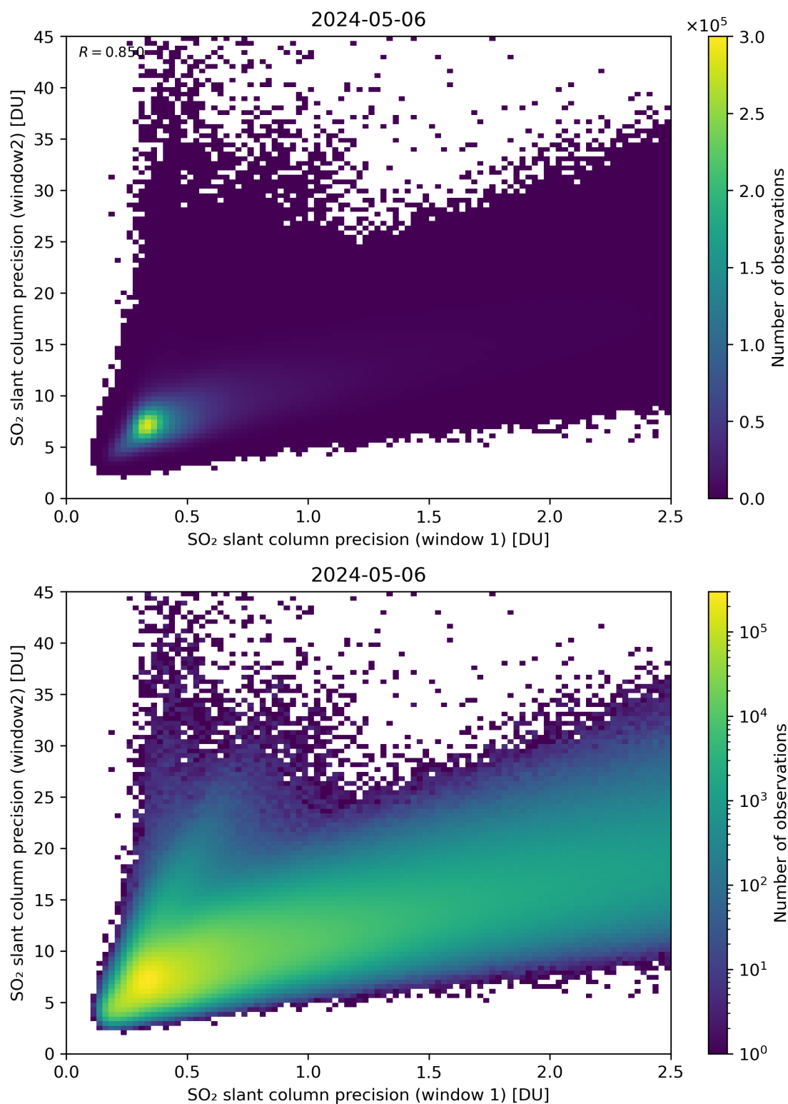
Figure 227: Scatter density plot of “SO 2 slant column precision (window 1)” against “SO 2 slant column precision (window2)” for 2024-05-05 to 2024-05-07.
