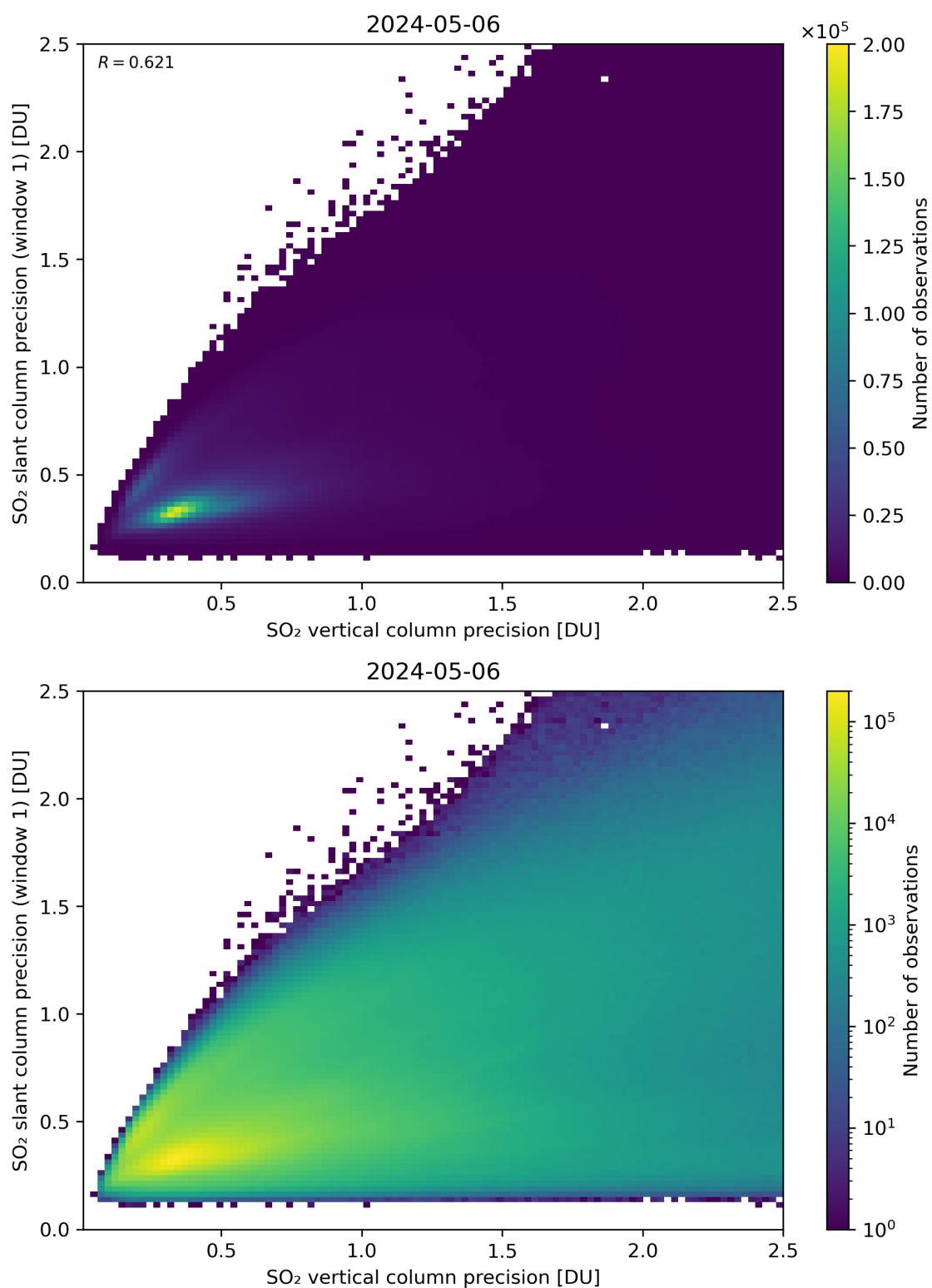
Figure 290: Scatter density plot of “SO 2 vertical column precision” against “SO 2 slant column precision (window 1)” for 2024-05-05 to 2024-05-07.
