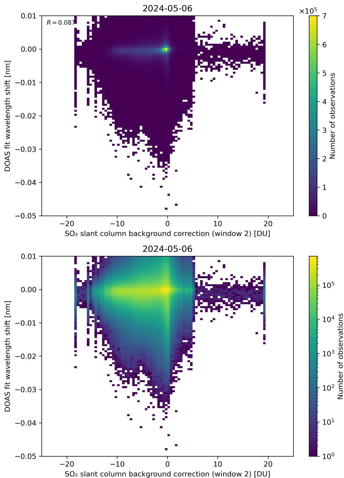
Figure 112: Scatter density plot of “SO 2 slant column background correction (window 2)” against “DOAS fit wavelength shift” for 2024-05-05 to 2024-05-07.
