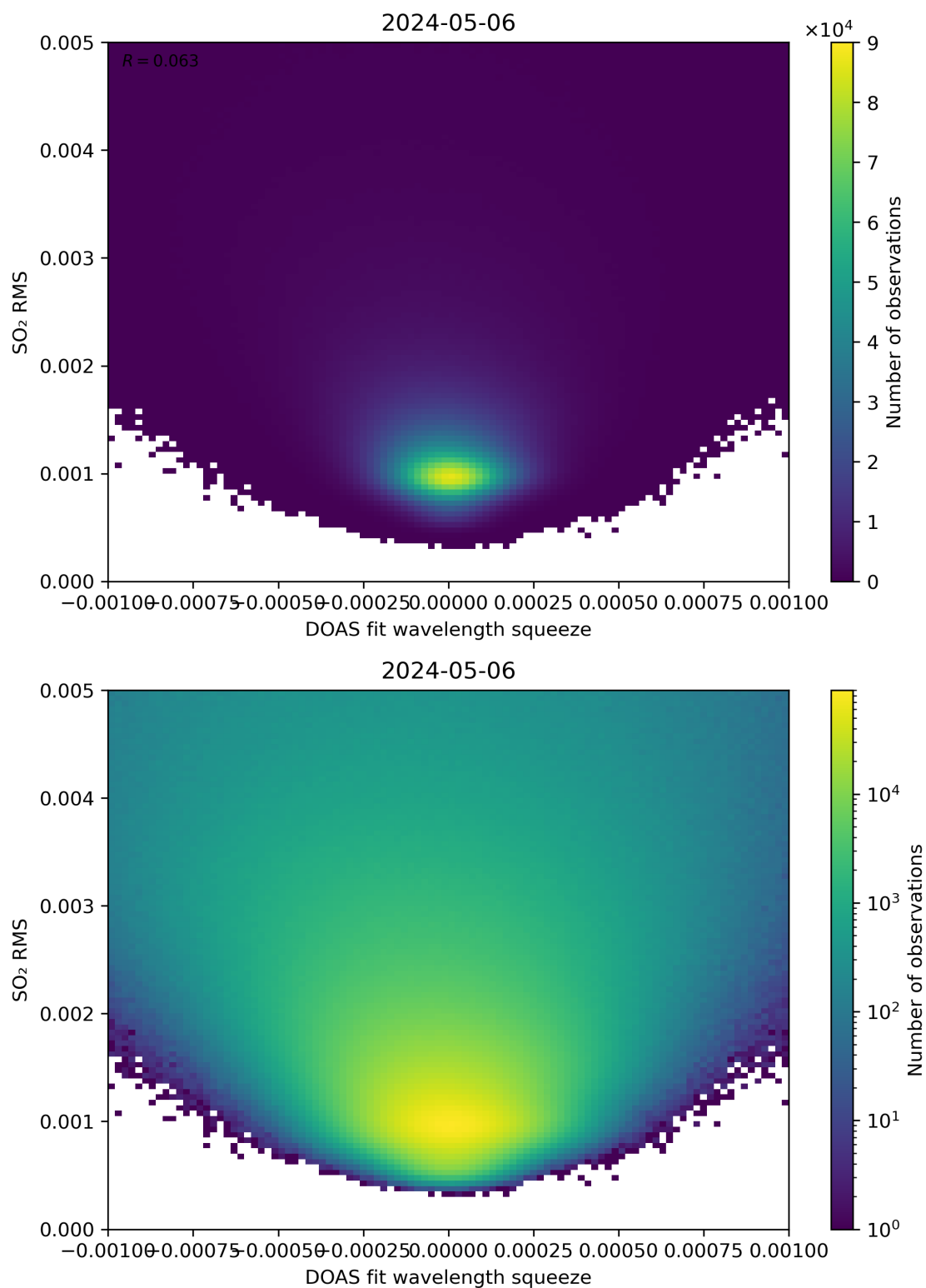
Figure 132: Scatter density plot of “DOAS fit wavelength squeeze” against “SO 2 RMS” for 2024-05-05 to 2024-05-07.
