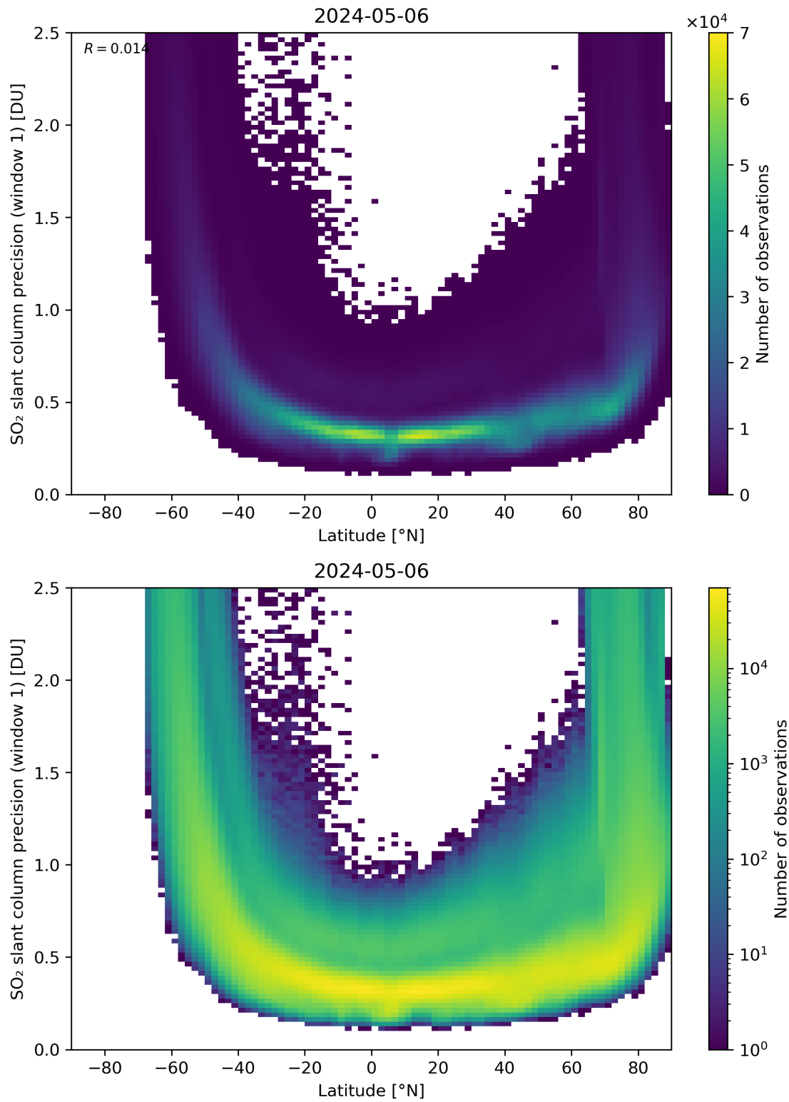
Figure 150: Scatter density plot of “Latitude” against “SO 2 slant column precision (window 1)” for 2024-05-05 to 2024-05-07.
