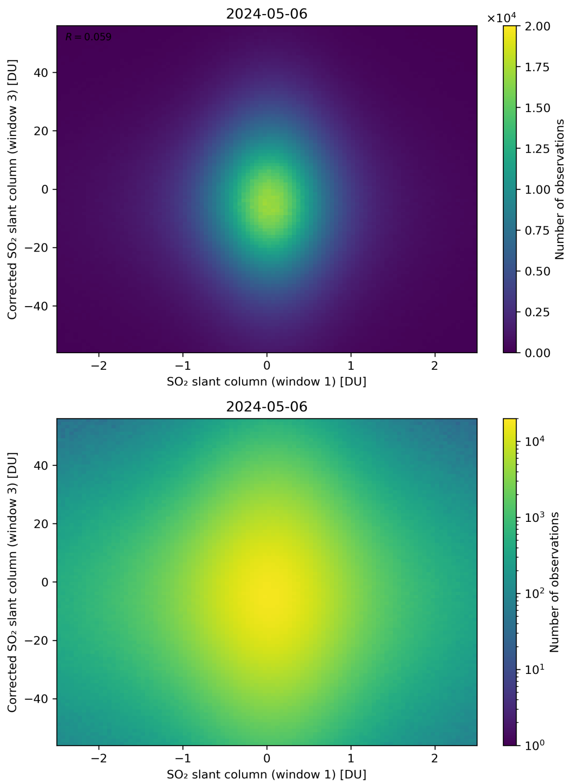
Figure 234: Scatter density plot of “SO 2 slant column (window 1)” against “Corrected SO 2 slant column (window 3)” for 2024-05-05 to 2024-05-07.
