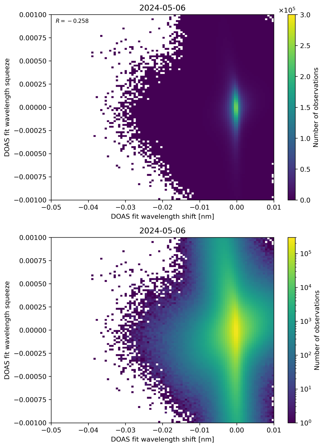
Figure 127: Scatter density plot of “DOAS fit wavelength shift” against “DOAS fit wavelength squeeze” for 2024-05-05 to 2024-05-07.
