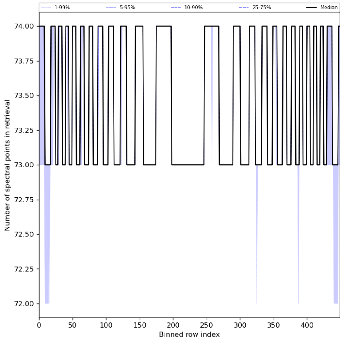
Figure 97: Along track statistics of “Number of spectral points in retrieval” for 2024-05-05 to 2024-05-07
