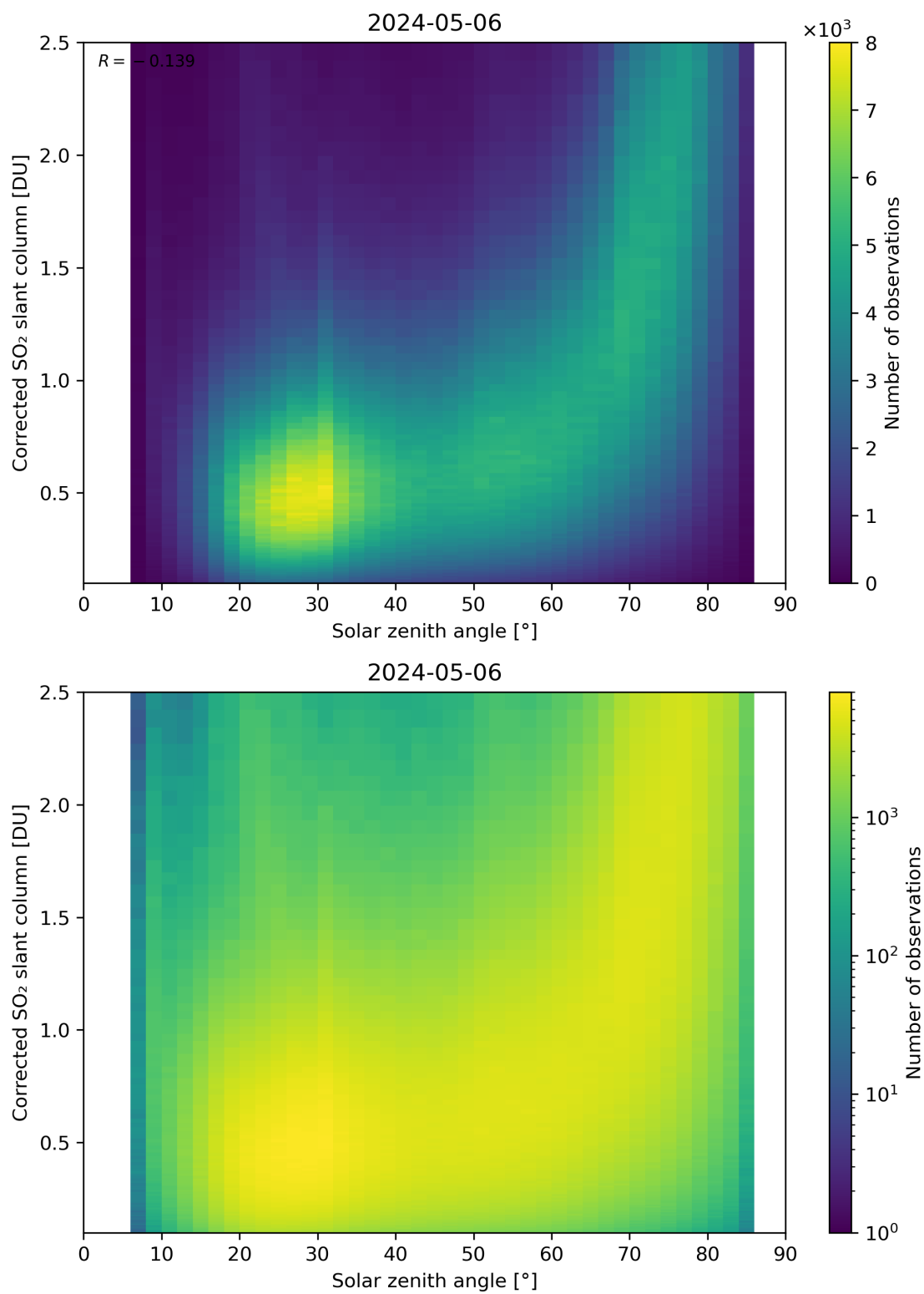
Figure 166: Scatter density plot of “Solar zenith angle” against “Corrected SO 2 slant column” for 2024-05-05 to 2024-05-07.
