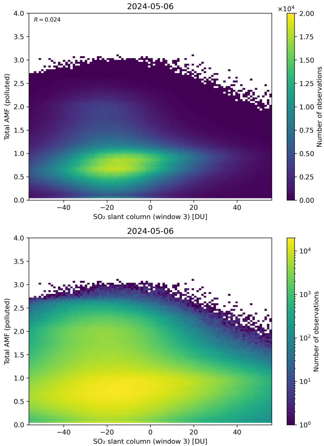
Figure 268: Scatter density plot of “SO 2 slant column (window 3)” against “Total AMF (polluted)” for 2024-05-05 to 2024-05-07.
