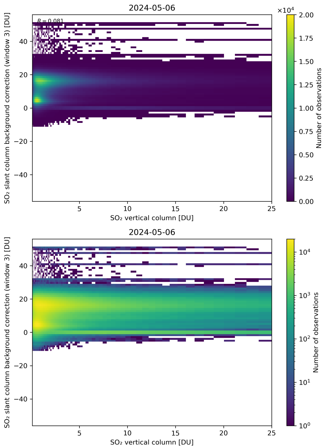
Figure 275: Scatter density plot of “SO 2 vertical column” against “SO 2 slant column background correction (window 3)” for 2024-05-05 to 2024-05-07.
