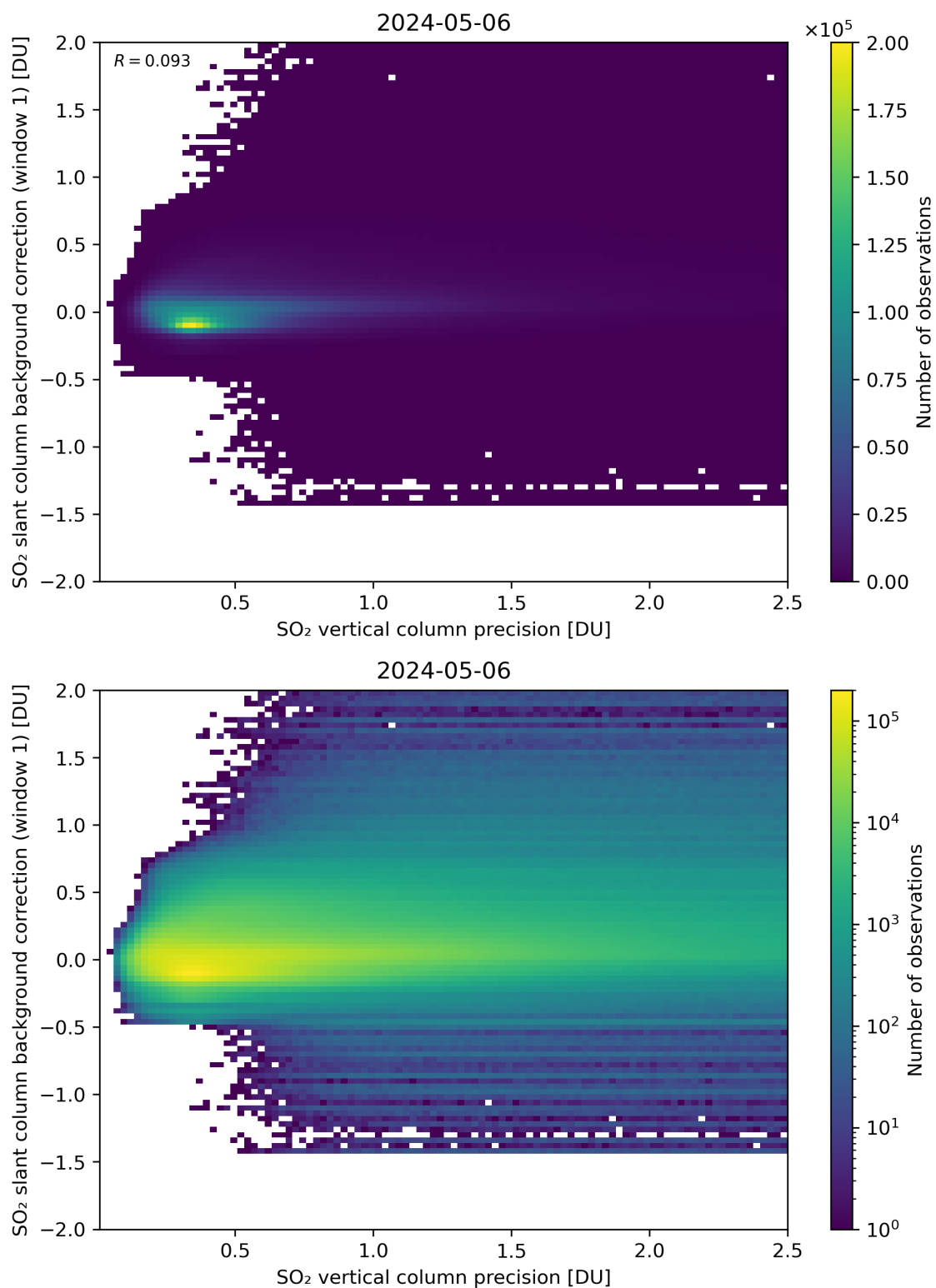
Figure 279: Scatter density plot of “SO 2 vertical column precision” against “SO 2 slant column background correction (window 1)” for 2024-05-05 to 2024-05-07.
