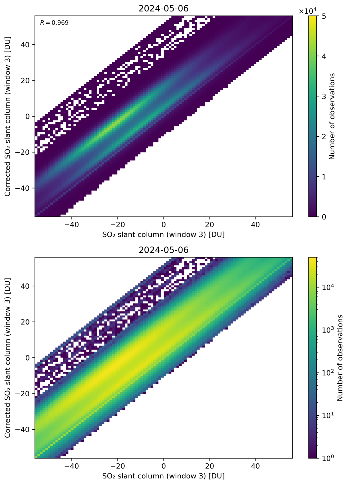
Figure 266: Scatter density plot of “SO 2 slant column (window 3)” against “Corrected SO 2 slant column (window 3)” for 2024-05-05 to 2024-05-07.
