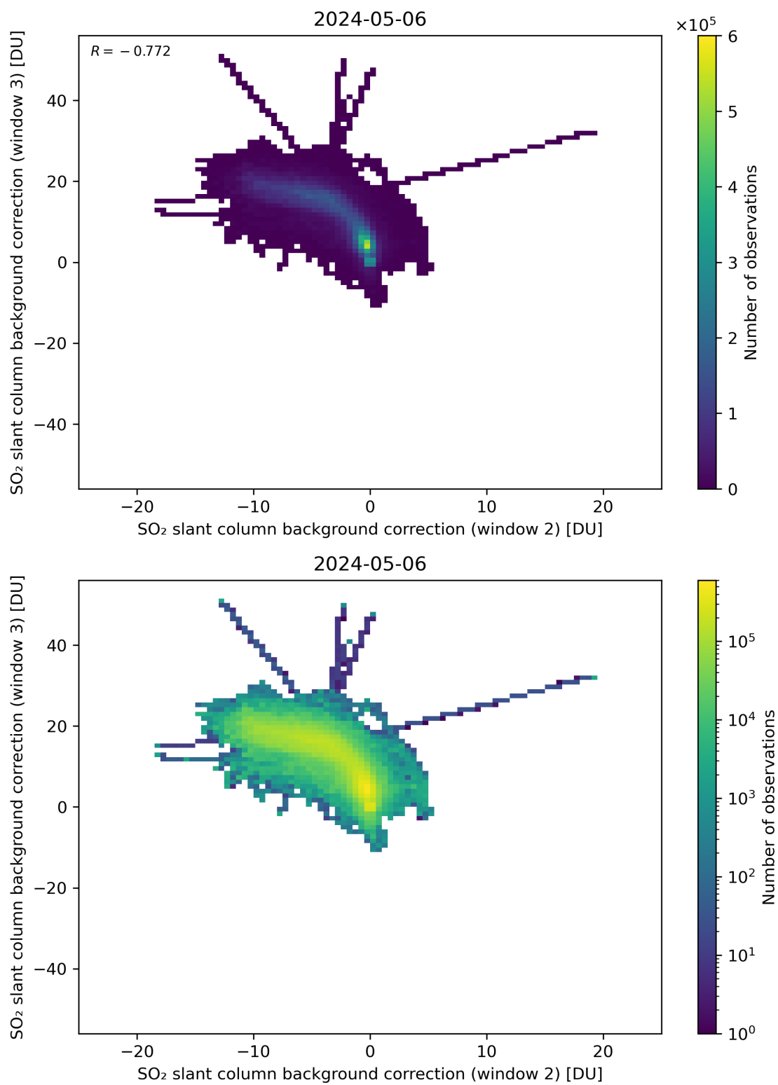
Figure 111: Scatter density plot of “SO 2 slant column background correction (window 2)” against “SO 2 slant column background correction (window 3)” for 2024-05-05 to 2024-05-07.
