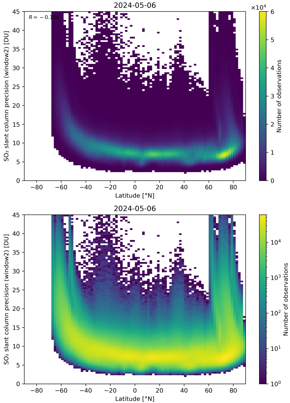
Figure 151: Scatter density plot of “Latitude” against “SO 2 slant column precision (window2)” for 2024-05-05 to 2024-05-07.
