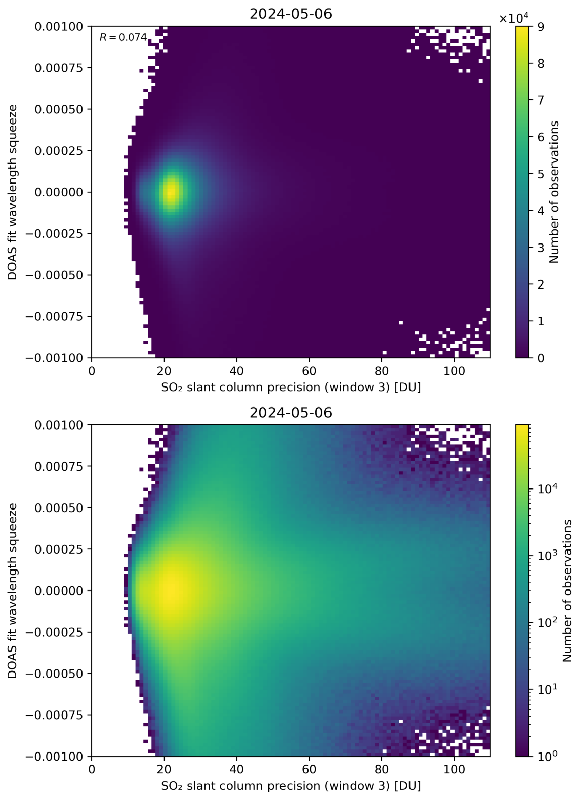
Figure 259: Scatter density plot of “SO 2 slant column precision (window 3)” against “DOAS fit wavelength squeeze” for 2024-05-05 to 2024-05-07.
