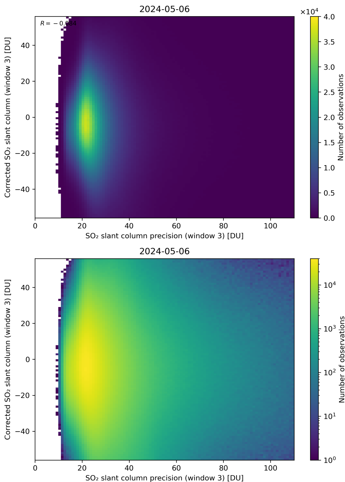
Figure 262: Scatter density plot of “SO 2 slant column precision (window 3)” against “Corrected SO 2 slant column (window 3)” for 2024-05-05 to 2024-05-07.
