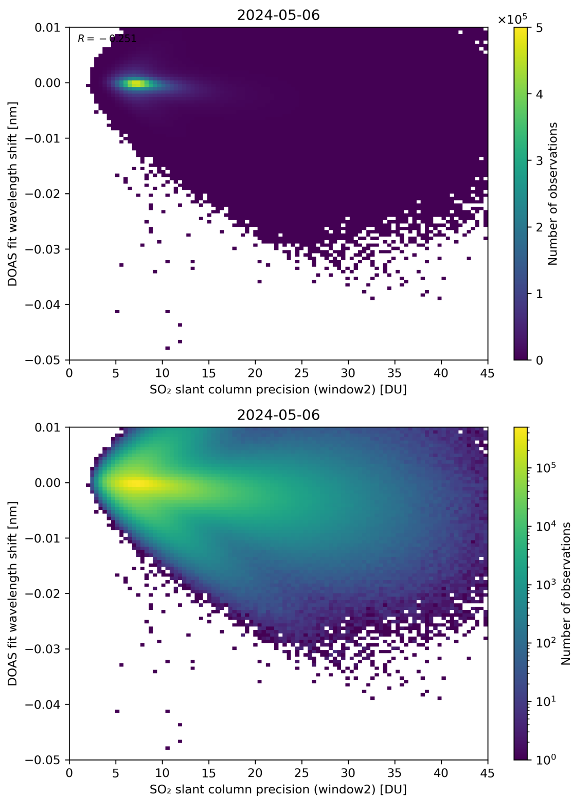
Figure 243: Scatter density plot of “SO 2 slant column precision (window2)” against “DOAS fit wavelength shift” for 2024-05-05 to 2024-05-07.
