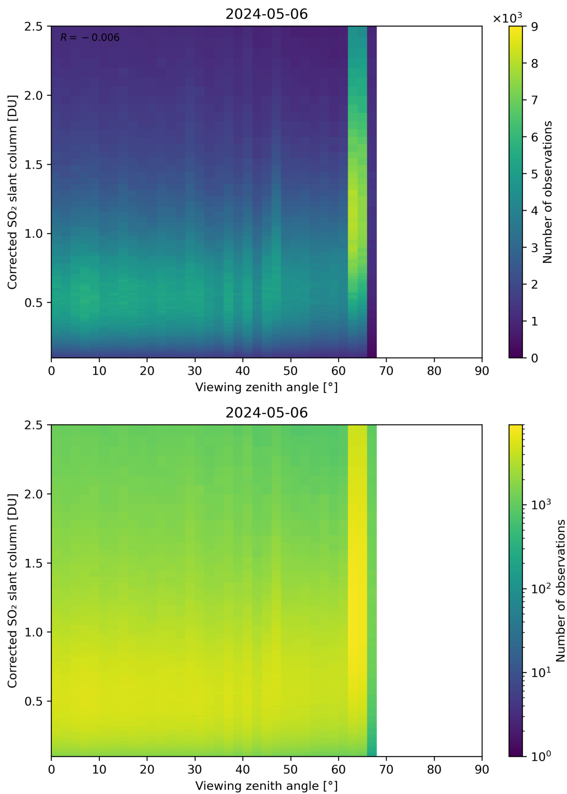
Figure 317: Scatter density plot of “Viewing zenith angle” against “Corrected SO 2 slant column” for 2024-05-05 to 2024-05-07.
