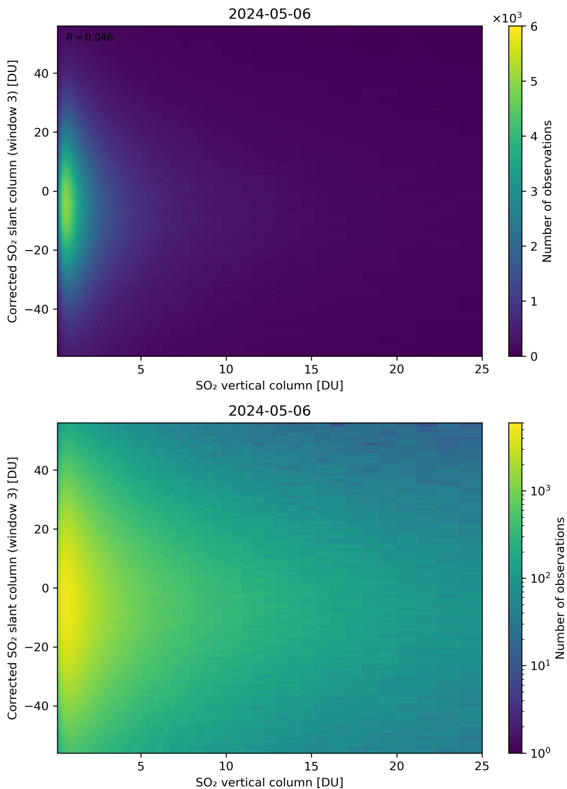
Figure 299: Scatter density plot of “SO 2 vertical column” against “Corrected SO 2 slant column (window 3)” for 2024-05-05 to 2024-05-07.
