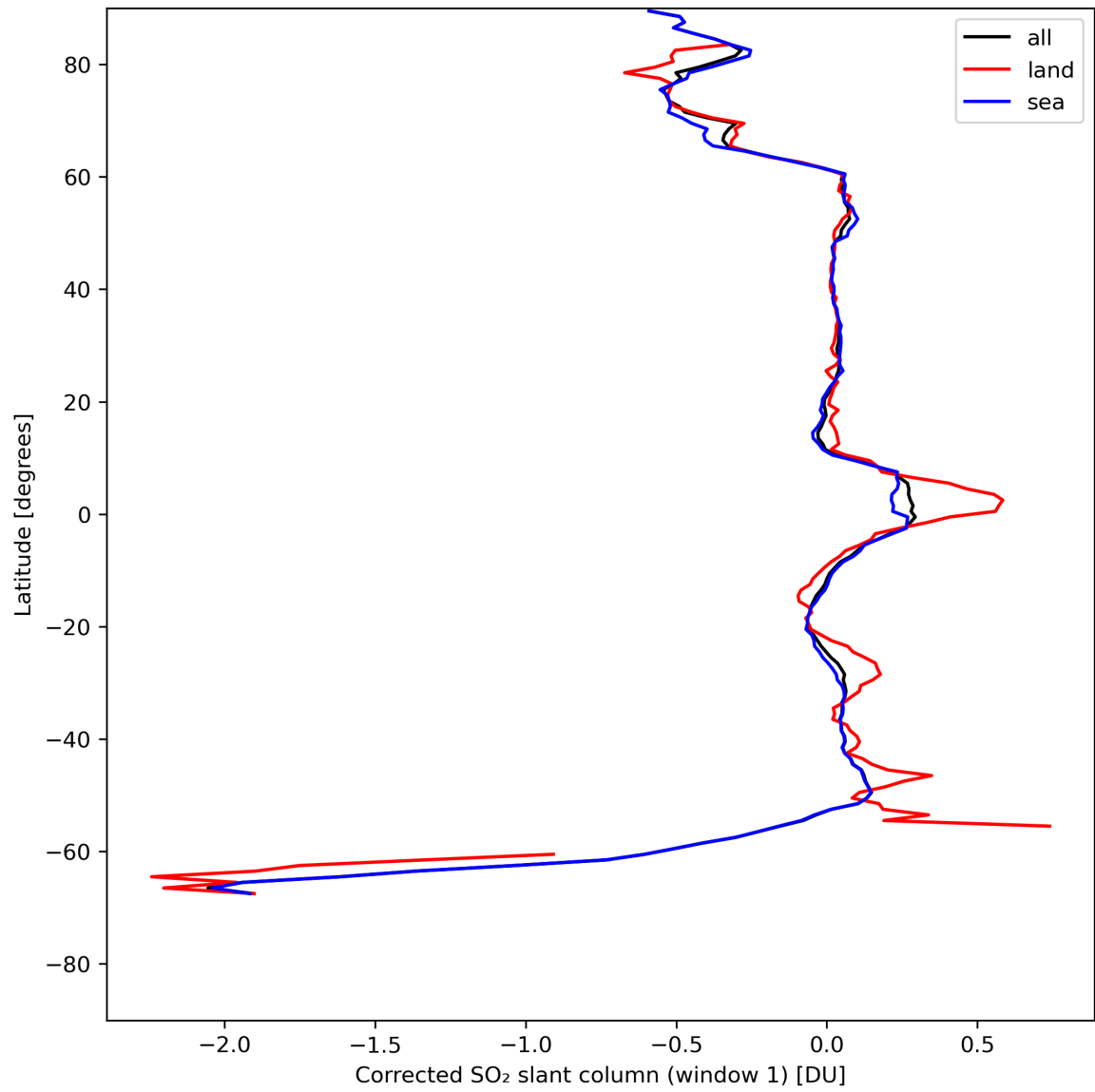
Figure 35: Zonal average of “Corrected SO 2 slant column (window 1)” for 2024-05-05 to 2024-05-07.
