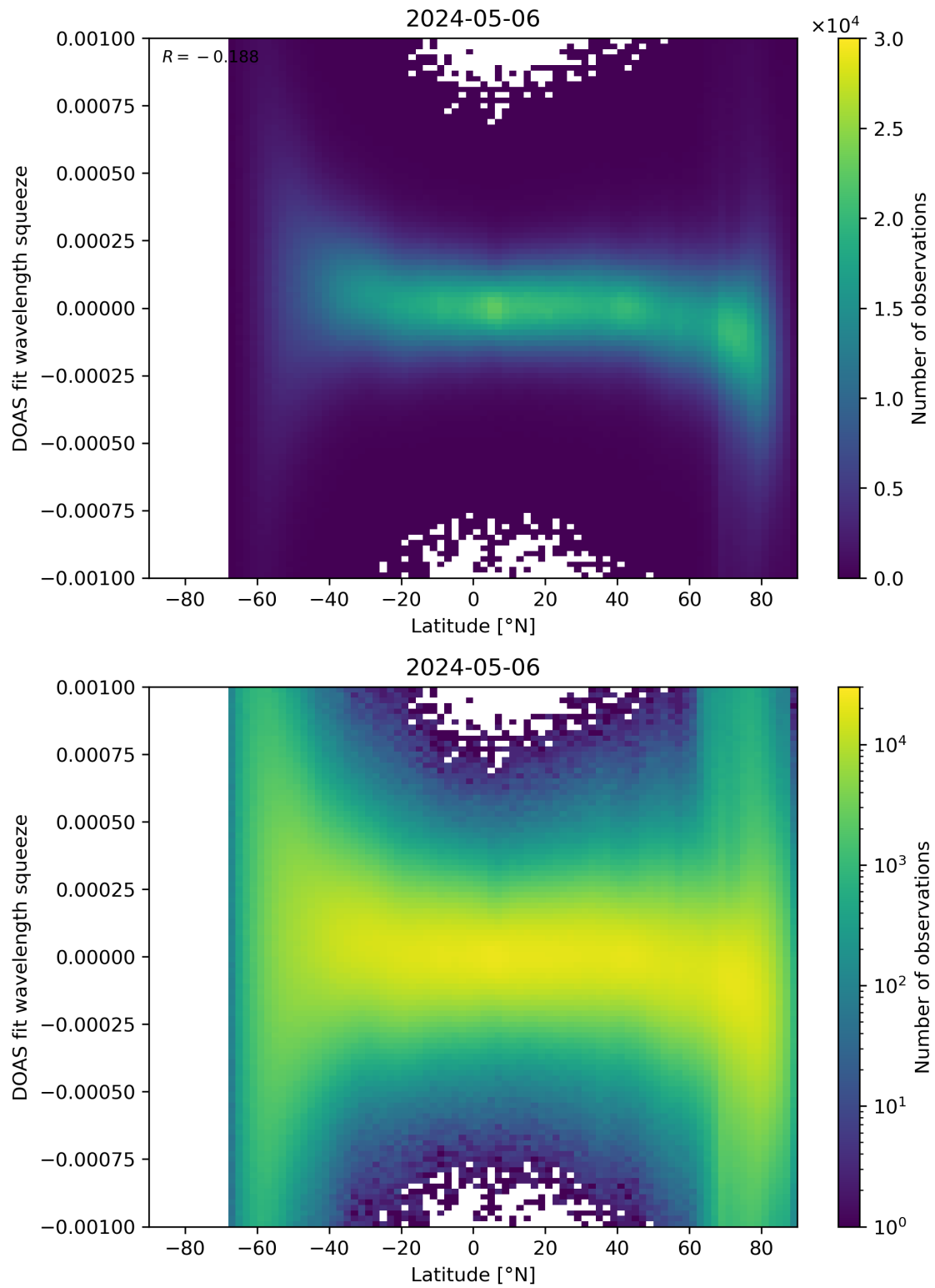
Figure 143: Scatter density plot of “Latitude” against “DOAS fit wavelength squeeze” for 2024-05-05 to 2024-05-07.
