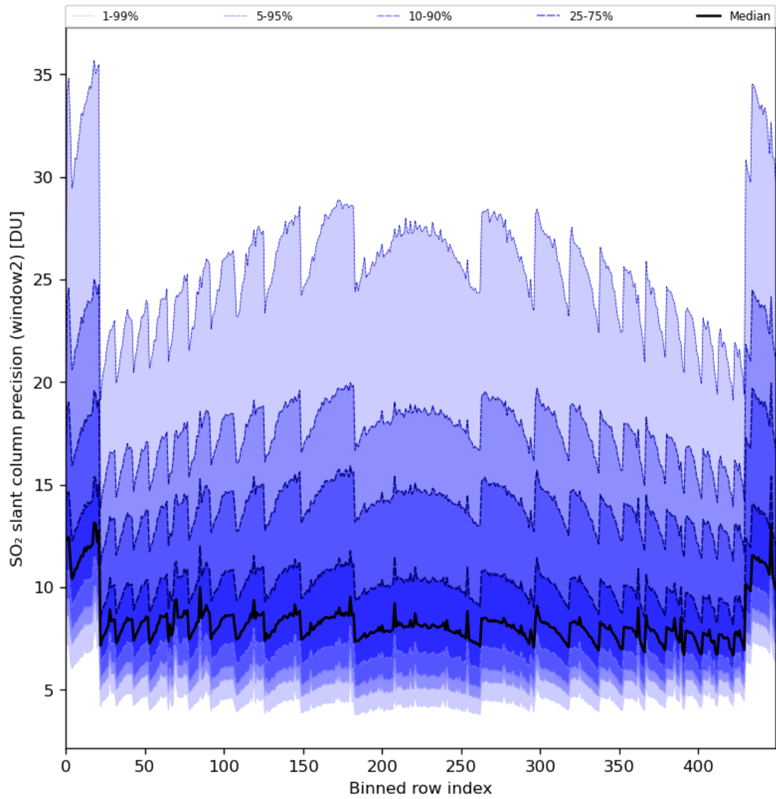
Figure 84: Along track statistics of “SO 2 slant column precision (window2)” for 2024-05-05 to 2024-05-07
