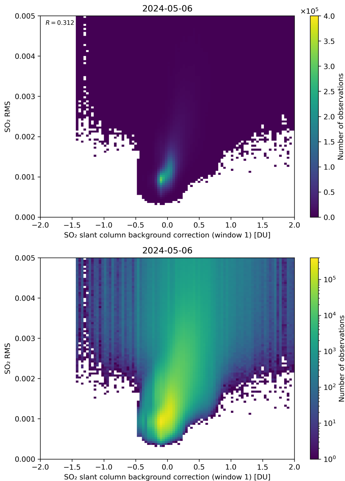
Figure 102: Scatter density plot of “SO 2 slant column background correction (window 1)” against “SO 2 RMS” for 2024-05-05 to 2024-05-07.
