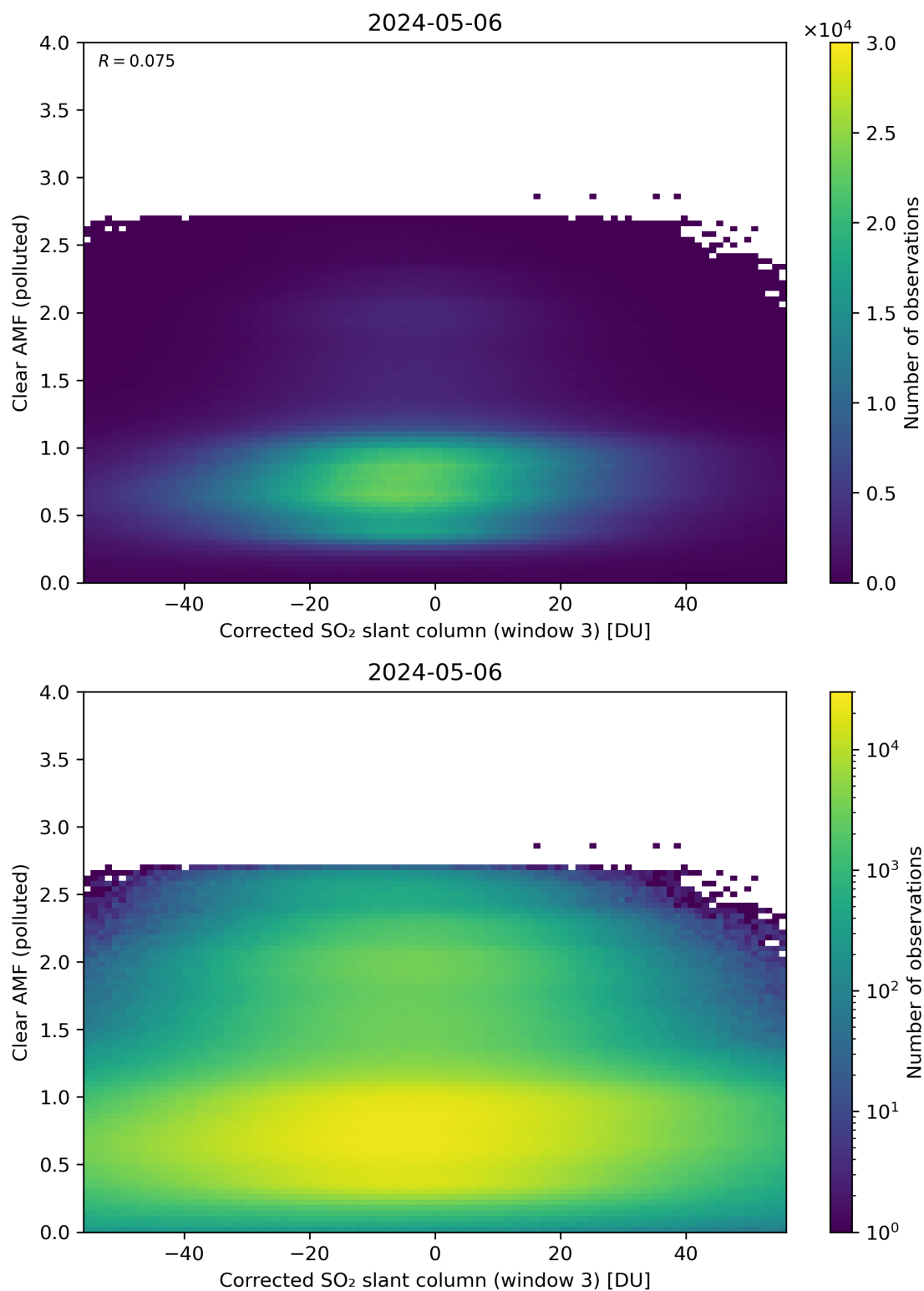
Figure 209: Scatter density plot of “Corrected SO 2 slant column (window 3)” against “Clear AMF (polluted)” for 2024-05-05 to 2024-05-07.
