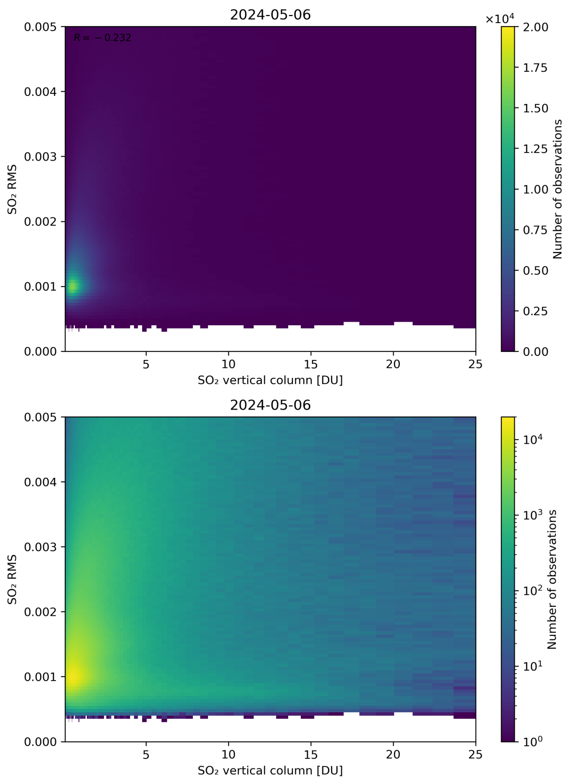
Figure 278: Scatter density plot of “SO 2 vertical column” against “SO 2 RMS” for 2024-05-05 to 2024-05-07.
