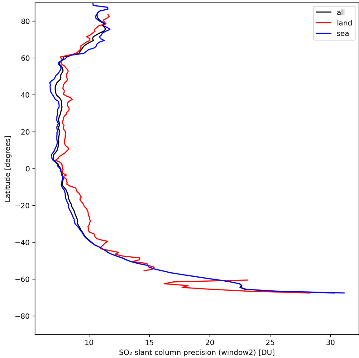
Figure 38: Zonal average of “SO 2 slant column precision (window2)” for 2024-05-05 to 2024-05-07.
