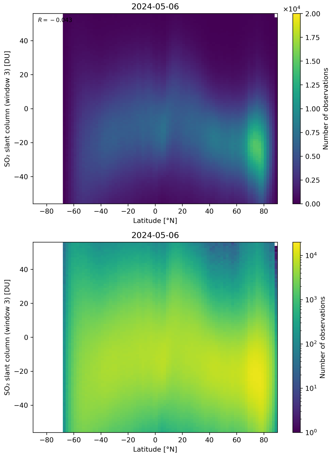
Figure 152: Scatter density plot of “Latitude” against “SO 2 slant column (window 3)” for 2024-05-05 to 2024-05-07.
