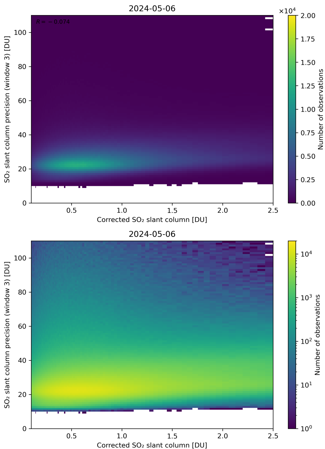
Figure 191: Scatter density plot of “Corrected SO 2 slant column” against “SO 2 slant column precision (window 3)” for 2024-05-05 to 2024-05-07.
