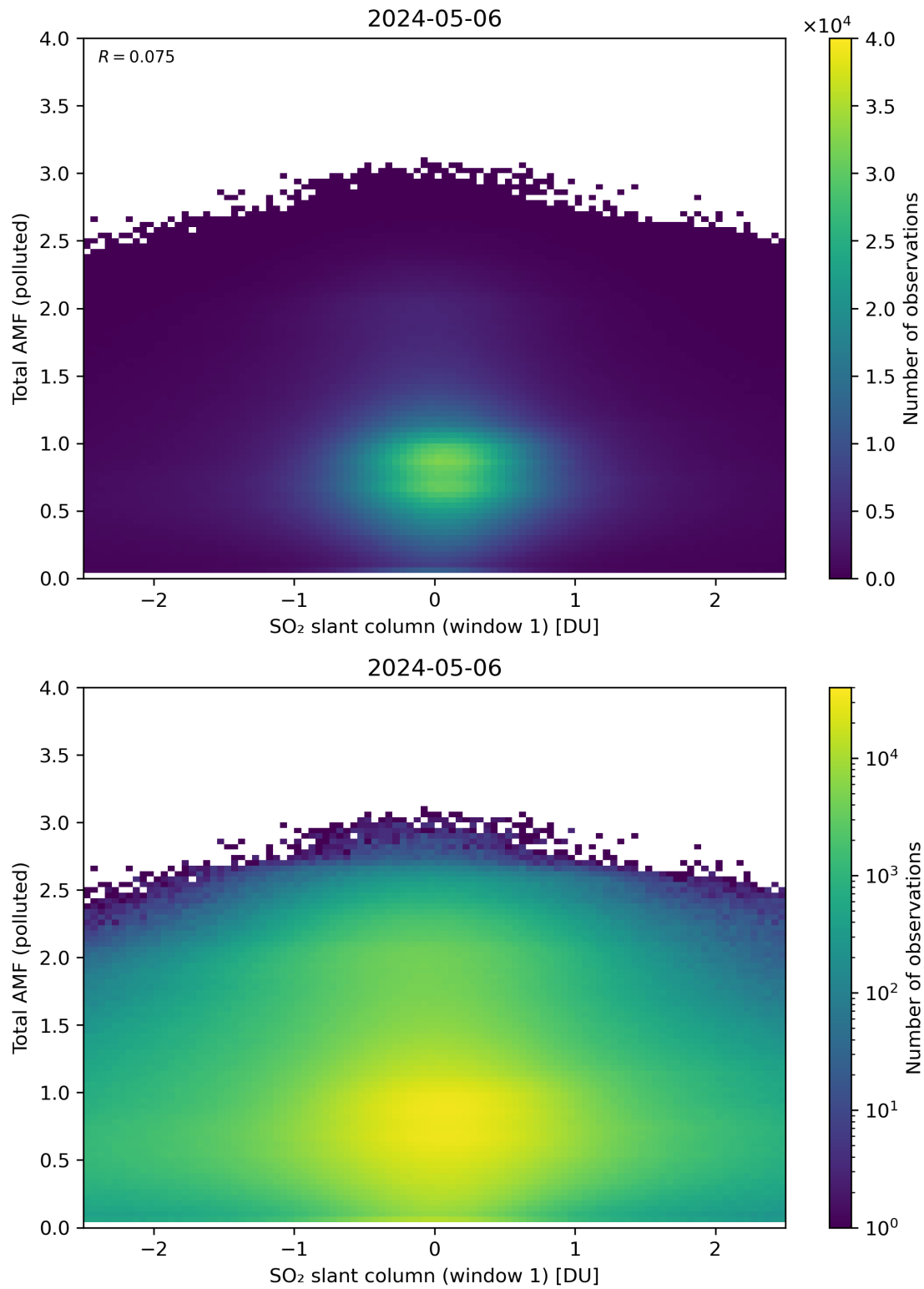
Figure 239: Scatter density plot of “SO 2 slant column (window 1)” against “Total AMF (polluted)” for 2024-05-05 to 2024-05-07.
