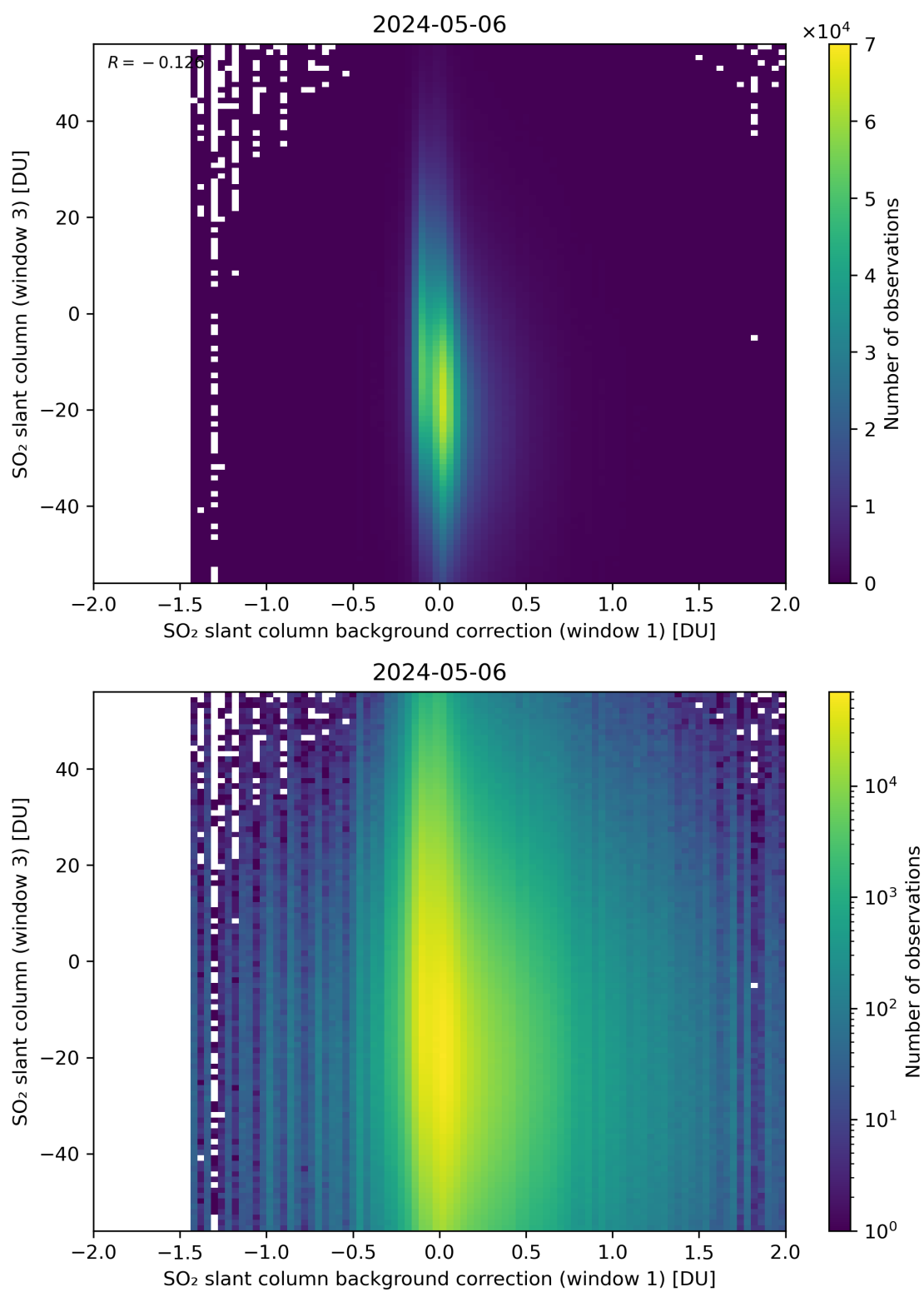
Figure 107: Scatter density plot of “SO 2 slant column background correction (window 1)” against “SO 2 slant column (window 3)” for 2024-05-05 to 2024-05-07.
