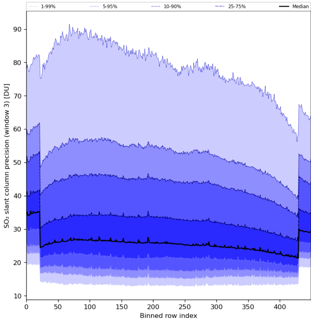
Figure 88: Along track statistics of “SO 2 slant column precision (window 3)” for 2024-05-05 to 2024-05-07
