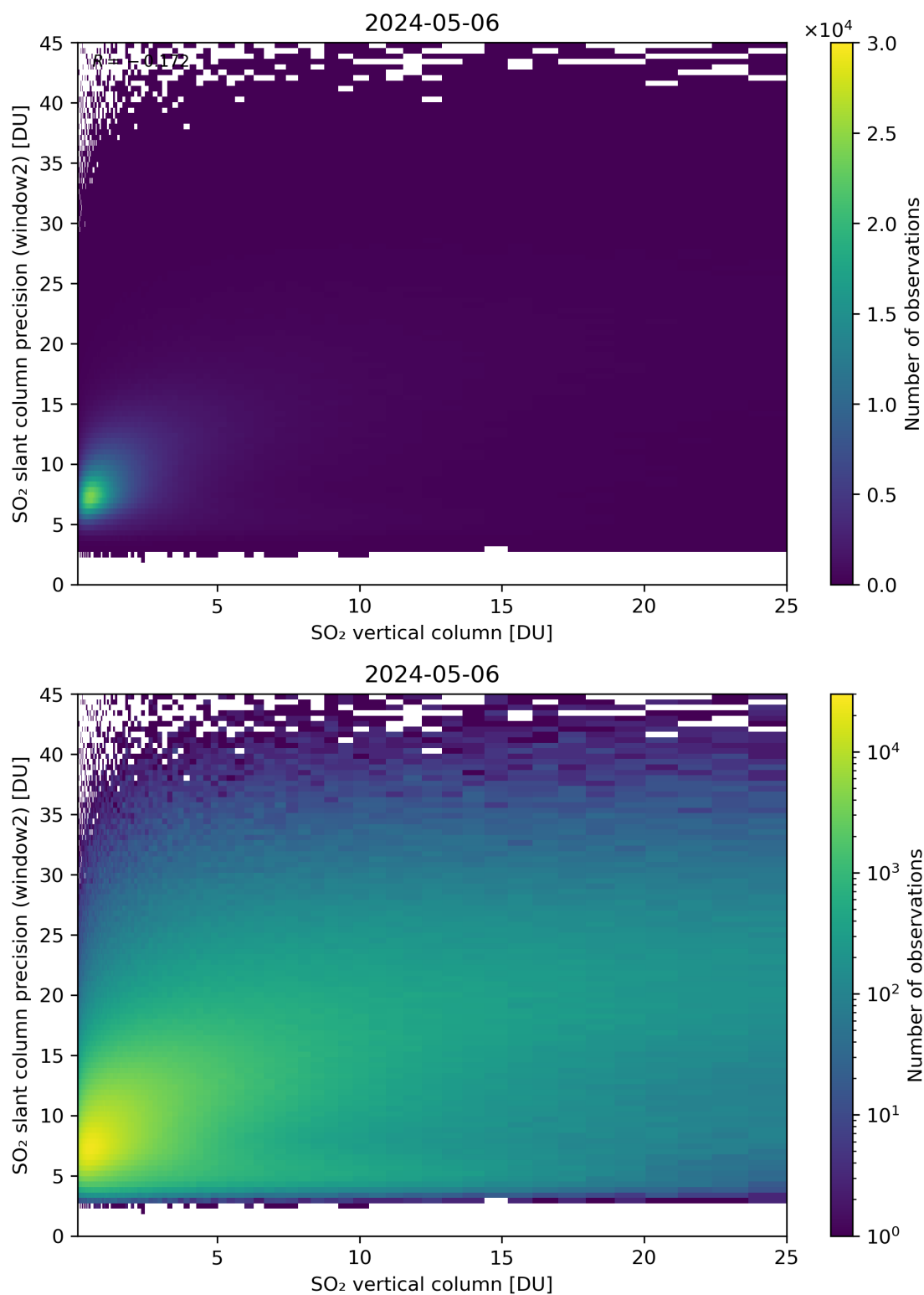
Figure 302: Scatter density plot of “SO 2 vertical column” against “SO 2 slant column precision (window2)” for 2024-05-05 to 2024-05-07.
