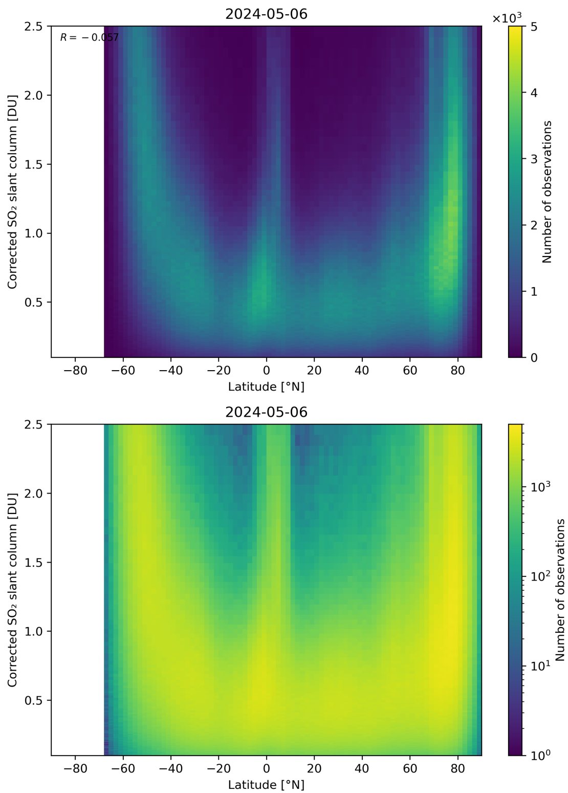
Figure 146: Scatter density plot of “Latitude” against “Corrected SO 2 slant column” for 2024-05-05 to 2024-05-07.
