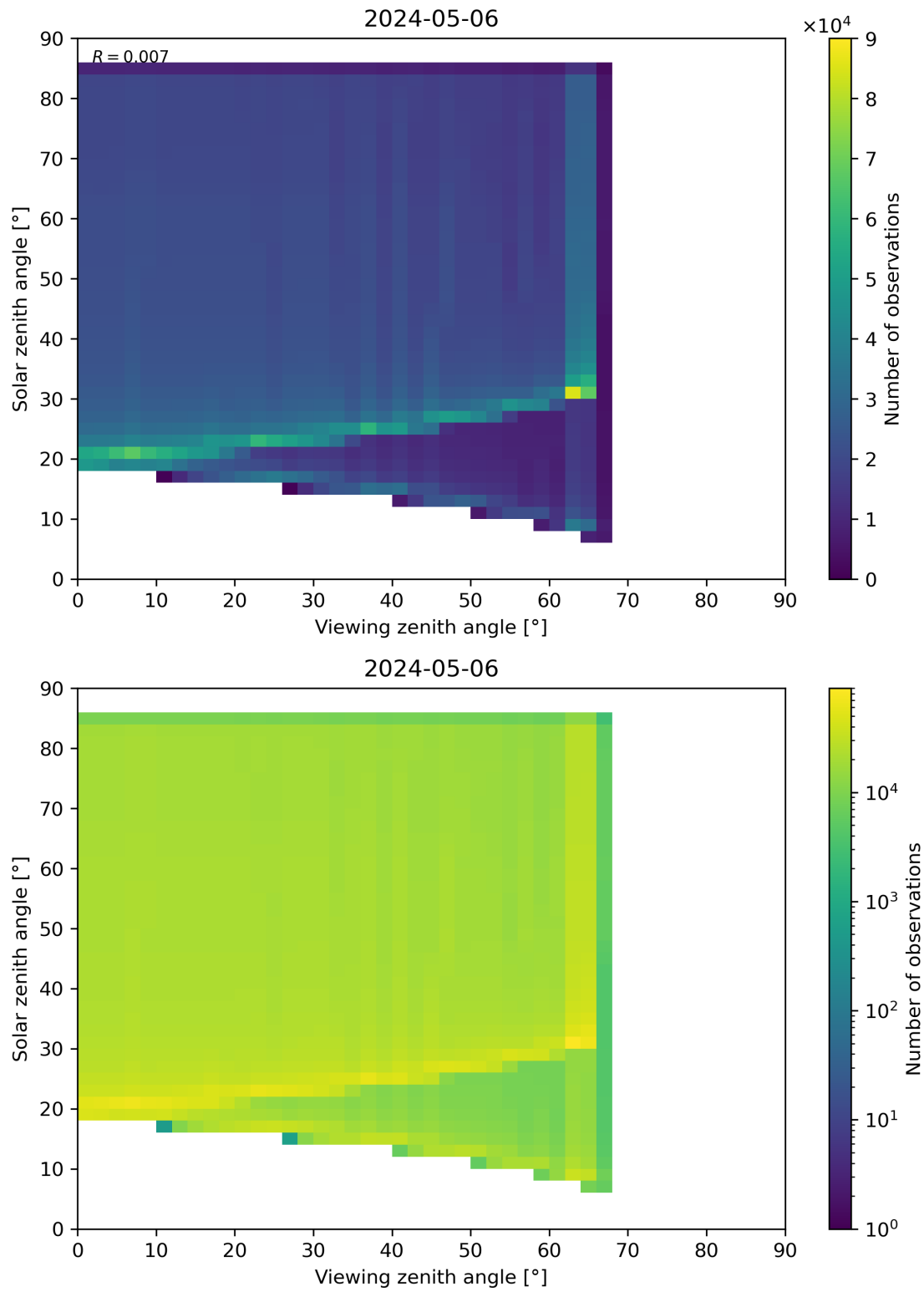
Figure 315: Scatter density plot of “Viewing zenith angle” against “Solar zenith angle” for 2024-05-05 to 2024-05-07.
