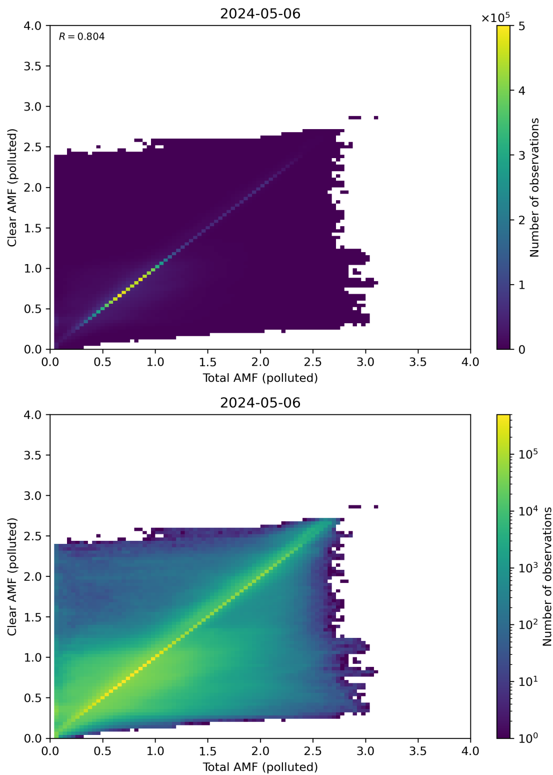
Figure 271: Scatter density plot of “Total AMF (polluted)” against “Clear AMF (polluted)” for 2024-05-05 to 2024-05-07.
