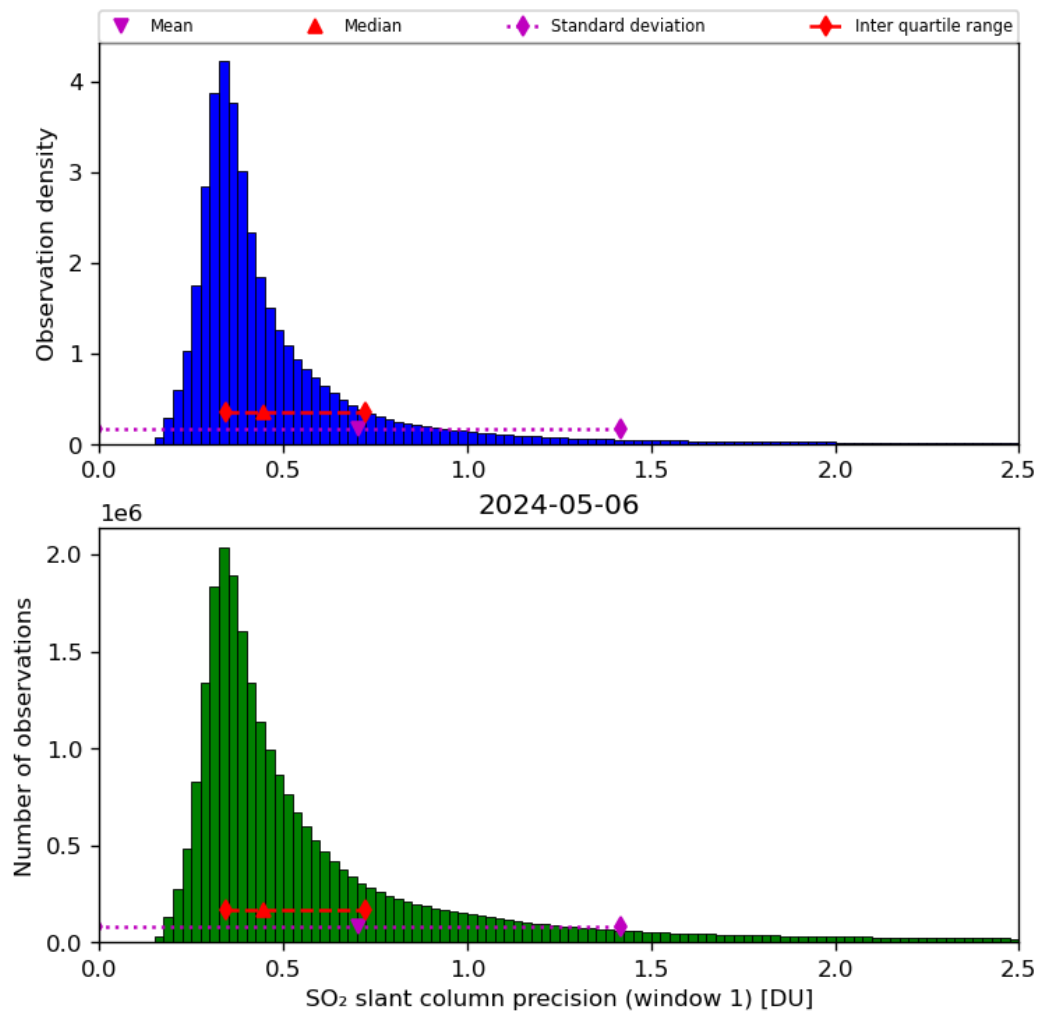
Figure 57: Histogram of “SO 2 slant column precision (window 1)” for 2024-05-05 to 2024-05-07
