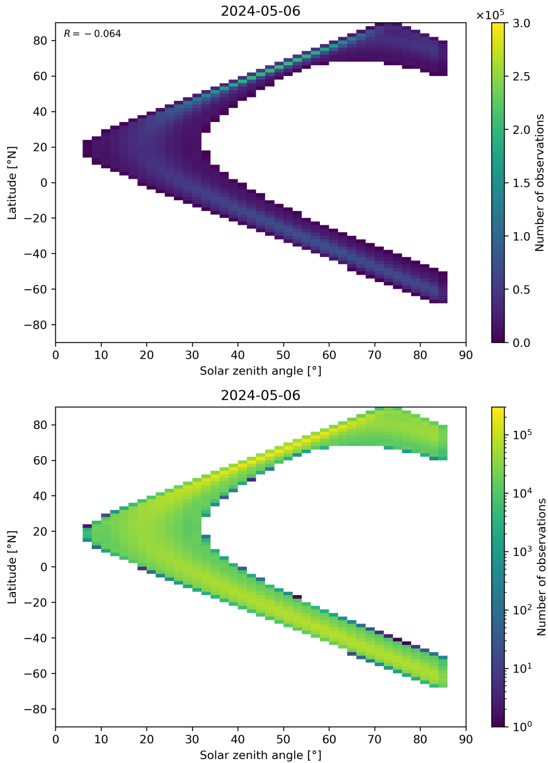
Figure 164: Scatter density plot of “Solar zenith angle” against “Latitude” for 2024-05-05 to 2024-05-07.
