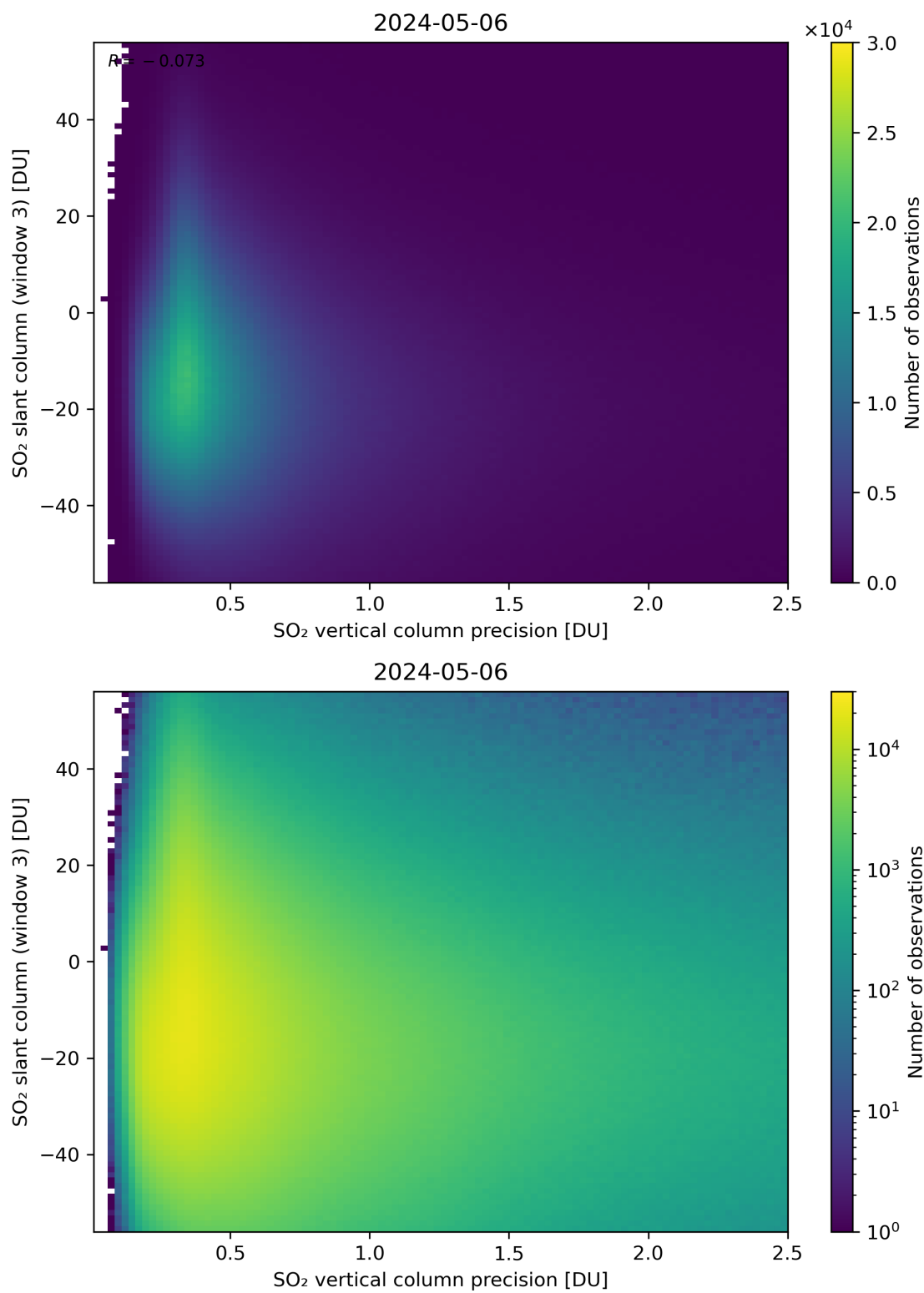
Figure 292: Scatter density plot of “SO 2 vertical column precision” against “SO 2 slant column (window 3)” for 2024-05-05 to 2024-05-07.
