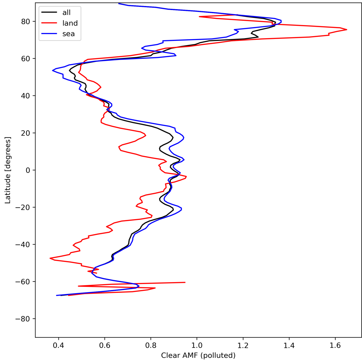
Figure 50: Zonal average of “Clear AMF (polluted)” for 2024-05-05 to 2024-05-07.
