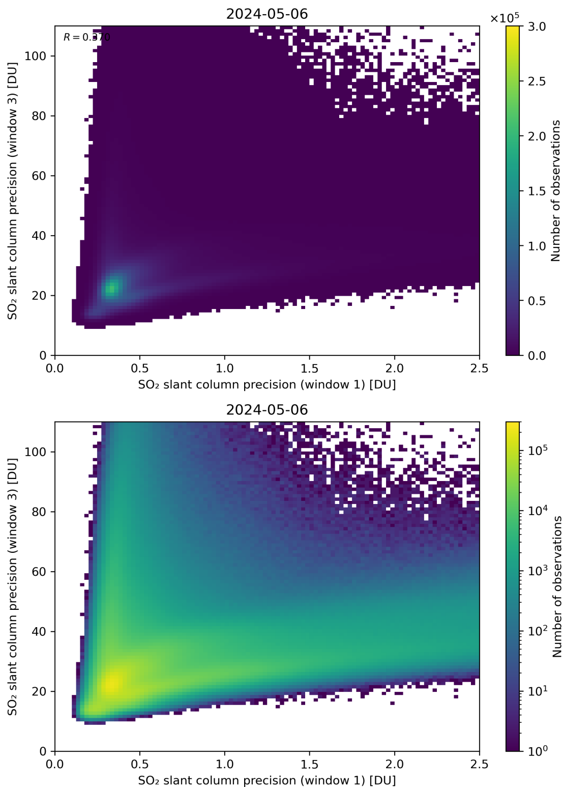
Figure 229: Scatter density plot of “SO 2 slant column precision (window 1)” against “SO 2 slant column precision (window 3)” for 2024-05-05 to 2024-05-07.
