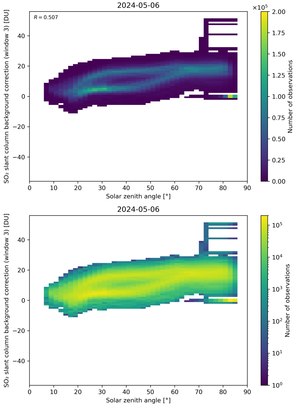
Figure 160: Scatter density plot of “Solar zenith angle” against “SO 2 slant column background correction (window 3)” for 2024-05-05 to 2024-05-07.
