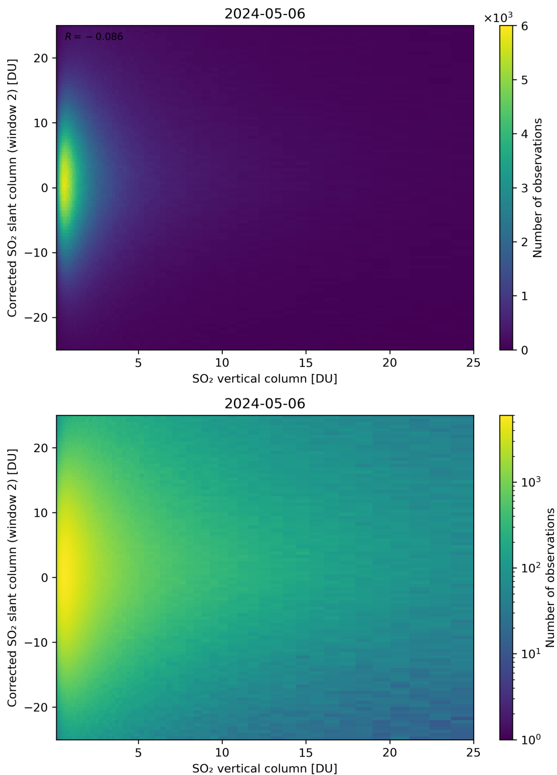
Figure 298: Scatter density plot of “SO 2 vertical column” against “Corrected SO 2 slant column (window 2)” for 2024-05-05 to 2024-05-07.
