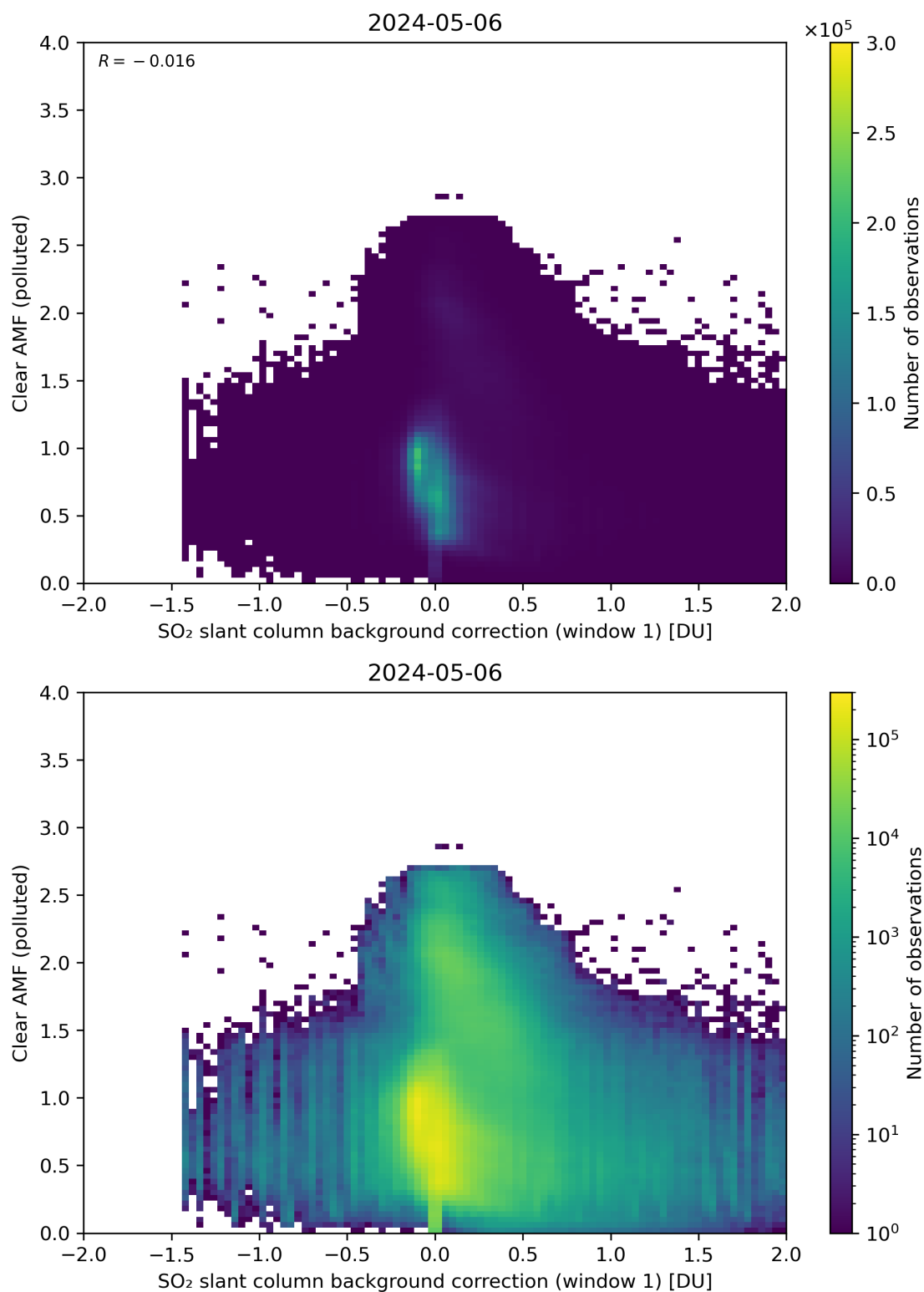
Figure 103: Scatter density plot of “SO 2 slant column background correction (window 1)” against “Clear AMF (polluted)” for 2024-05-05 to 2024-05-07.
