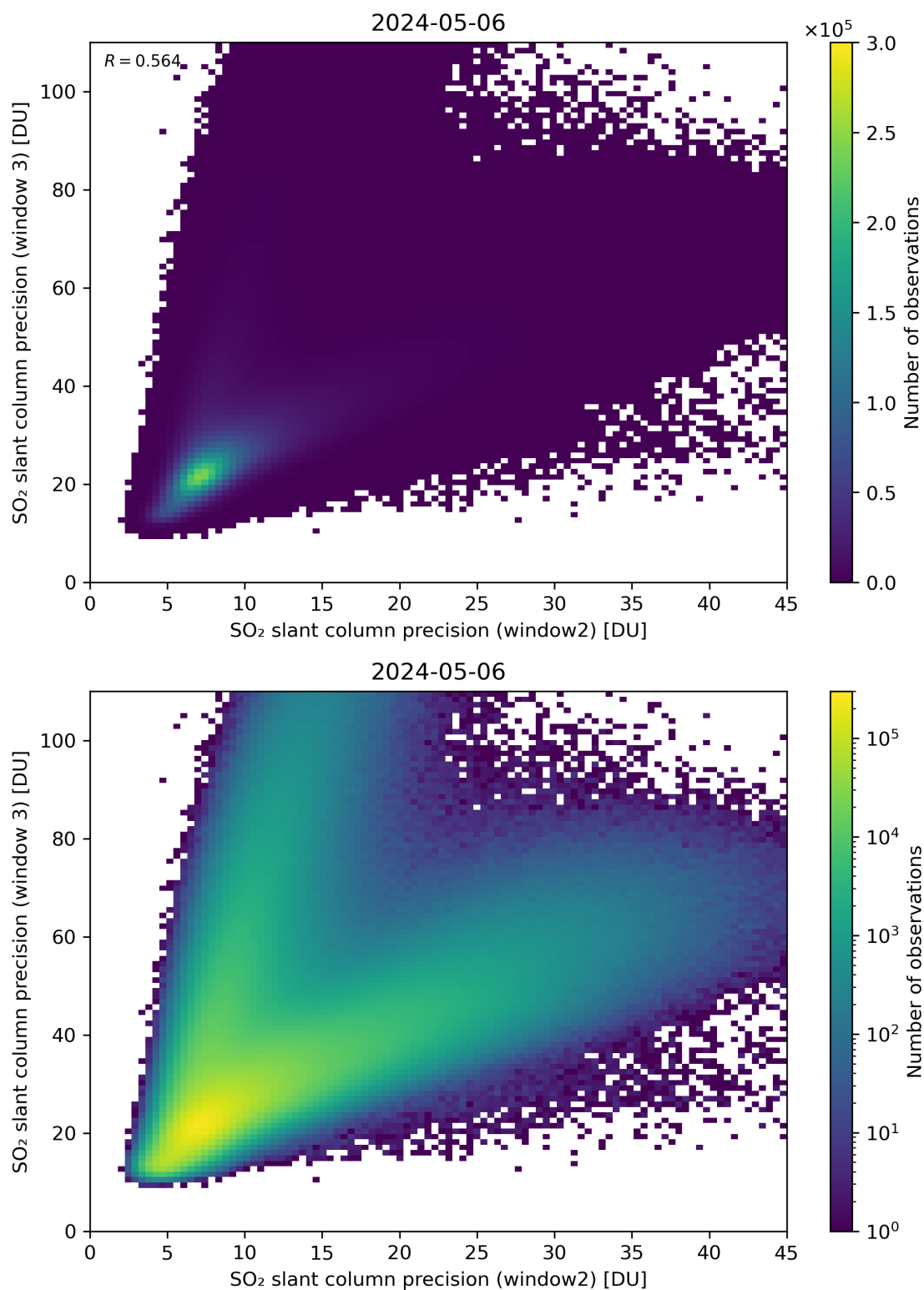
Figure 250: Scatter density plot of “SO 2 slant column precision (window2)” against “SO 2 slant column precision (window 3)” for 2024-05-05 to 2024-05-07.
