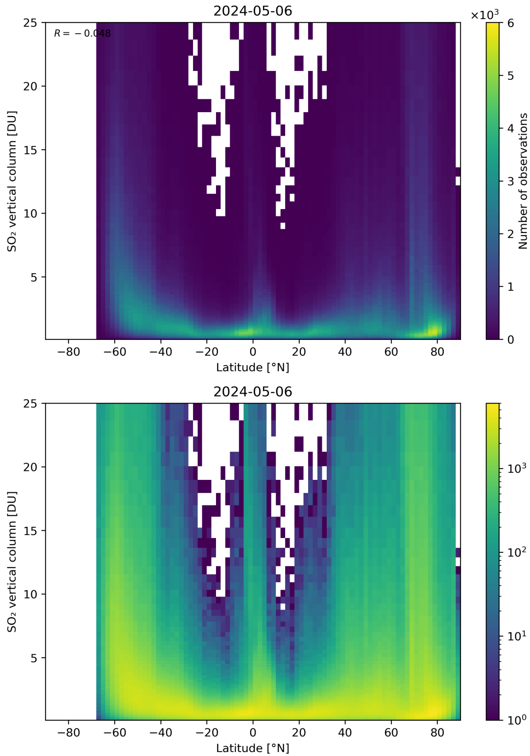
Figure 156: Scatter density plot of “Latitude” against “SO 2 vertical column” for 2024-05-05 to 2024-05-07.
