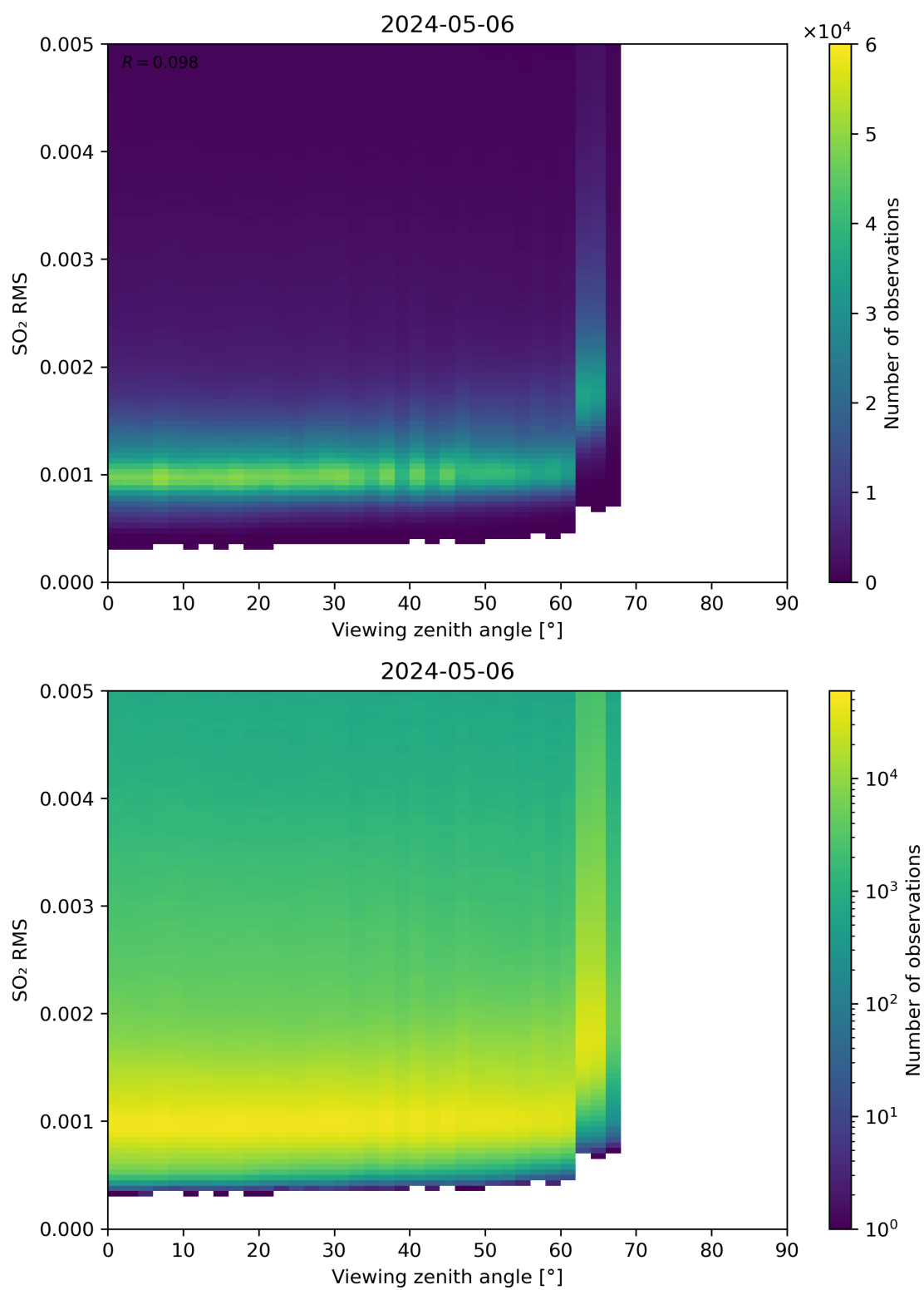
Figure 313: Scatter density plot of “Viewing zenith angle” against “SO 2 RMS” for 2024-05-05 to 2024-05-07.
