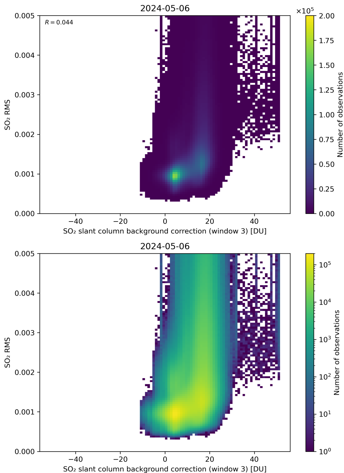
Figure 123: Scatter density plot of “SO 2 slant column background correction (window 3)” against “SO 2 RMS” for 2024-05-05 to 2024-05-07.
