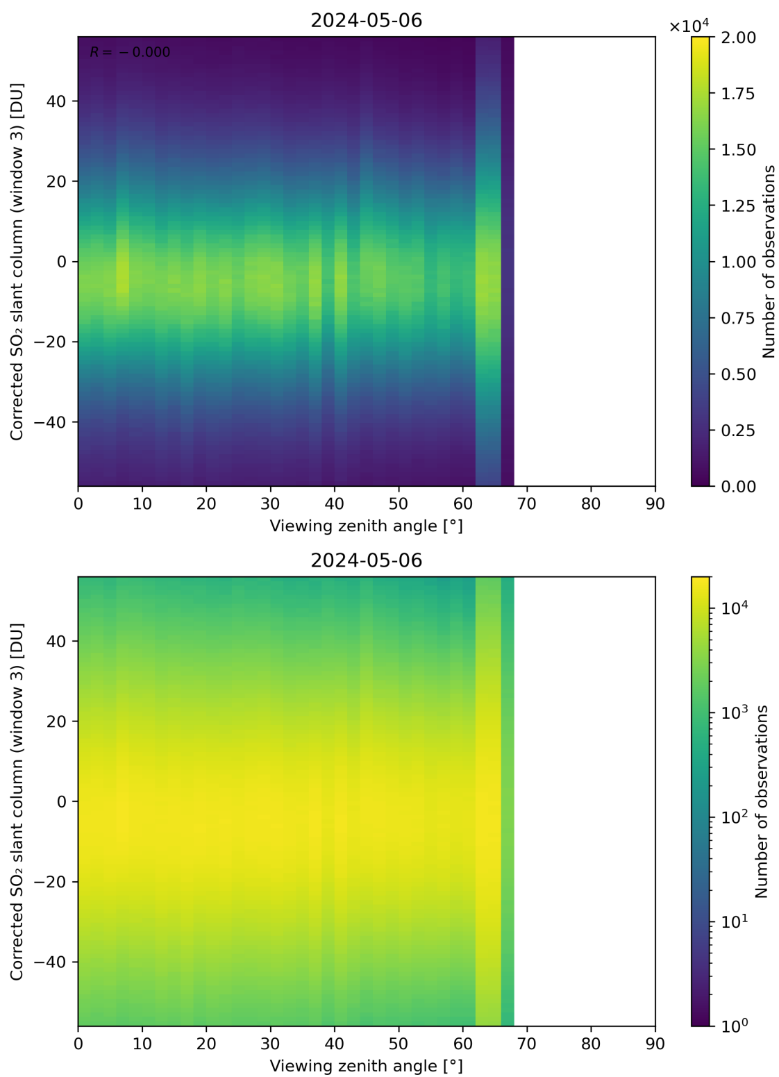
Figure 319: Scatter density plot of “Viewing zenith angle” against “Corrected SO 2 slant column (window 3)” for 2024-05-05 to 2024-05-07.
