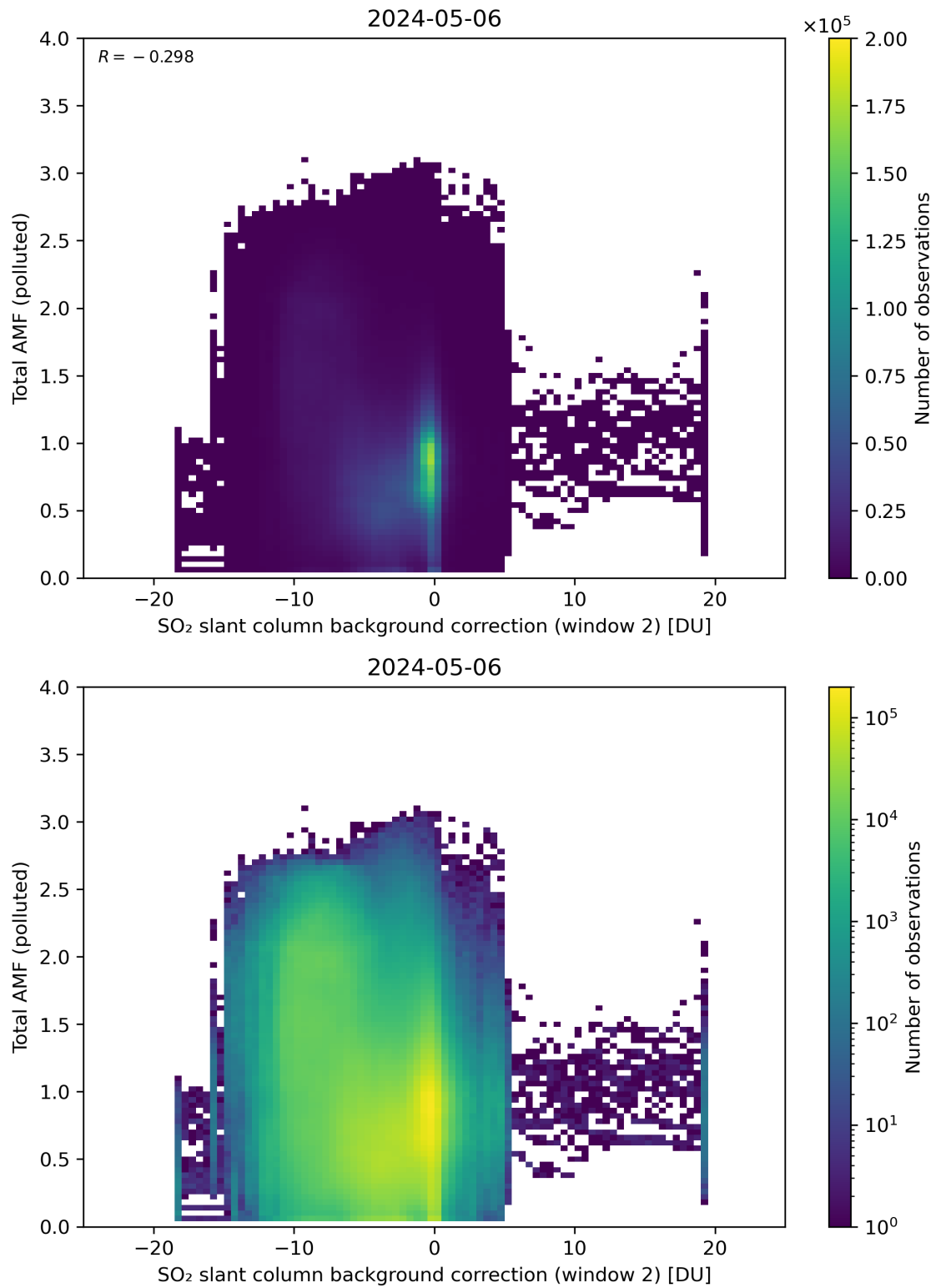
Figure 119: Scatter density plot of “SO 2 slant column background correction (window 2)” against “Total AMF (polluted)” for 2024-05-05 to 2024-05-07.
