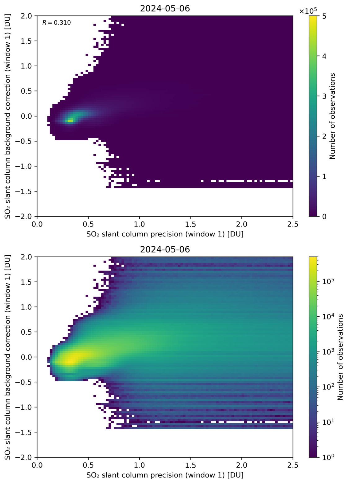
Figure 218: Scatter density plot of “SO 2 slant column precision (window 1)” against “SO 2 slant column background correction (window 1)” for 2024-05-05 to 2024-05-07.
