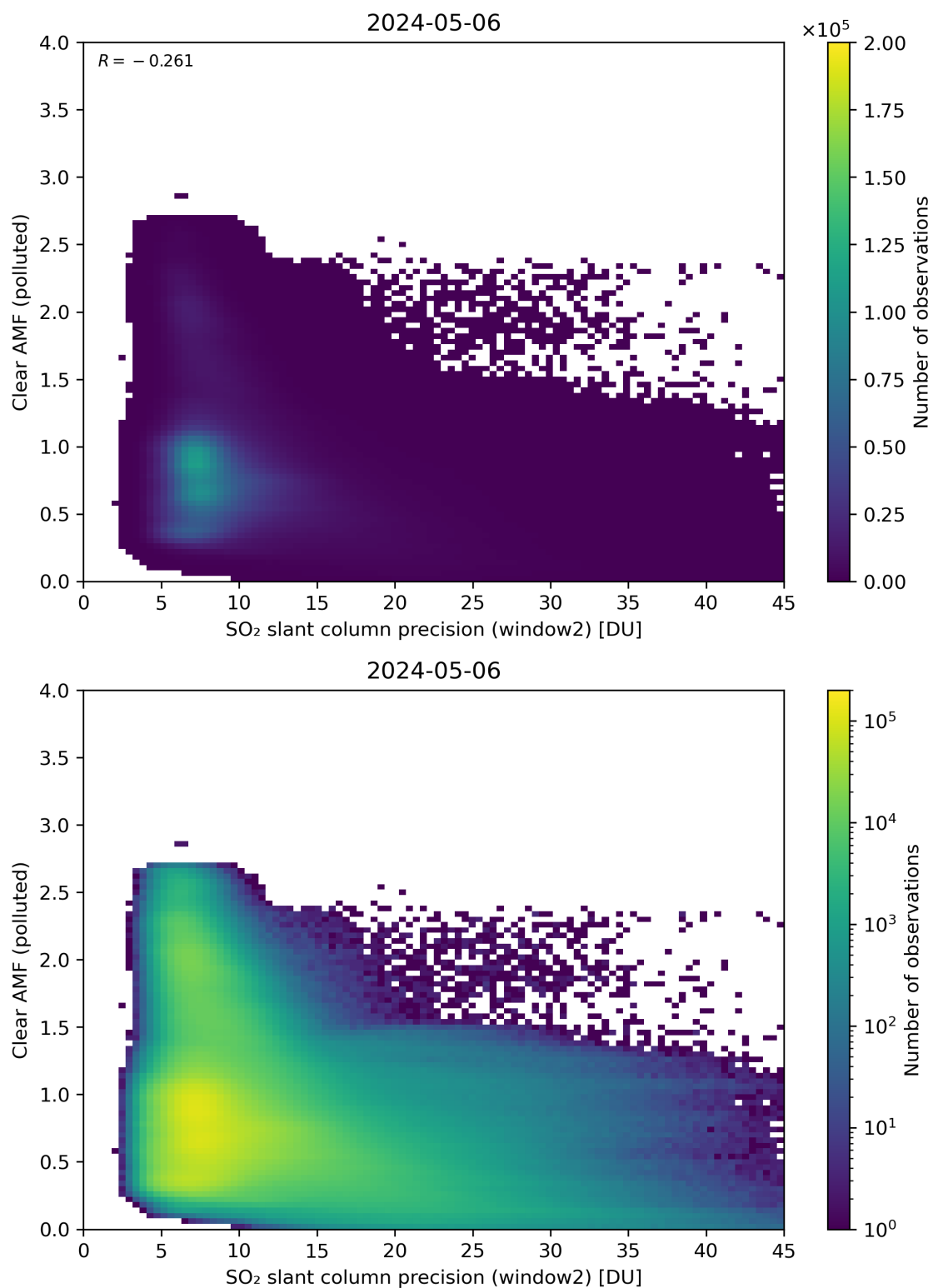
Figure 246: Scatter density plot of “SO 2 slant column precision (window2)” against “Clear AMF (polluted)” for 2024-05-05 to 2024-05-07.
