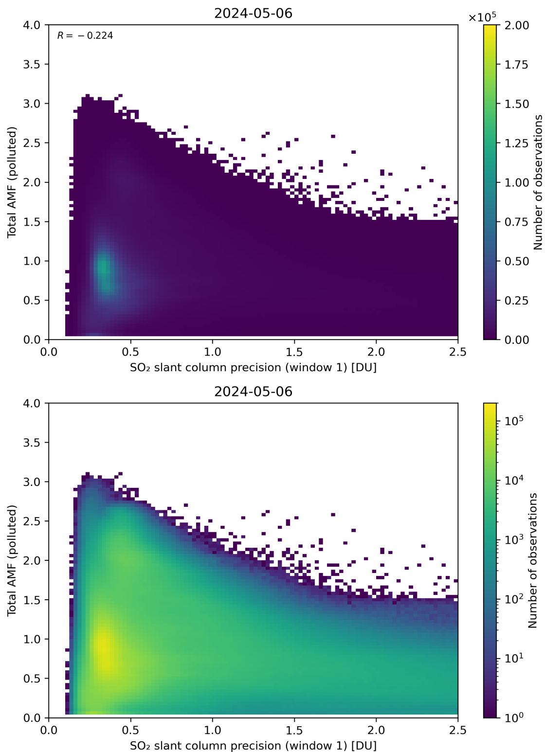
Figure 230: Scatter density plot of “SO 2 slant column precision (window 1)” against “Total AMF (polluted)” for 2024-05-05 to 2024-05-07.
