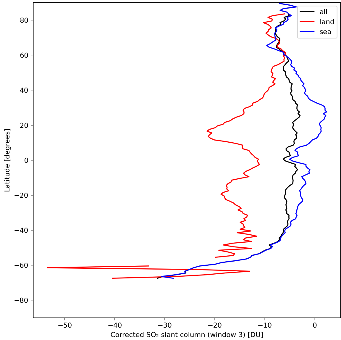
Figure 43: Zonal average of “Corrected SO 2 slant column (window 3)” for 2024-05-05 to 2024-05-07.
