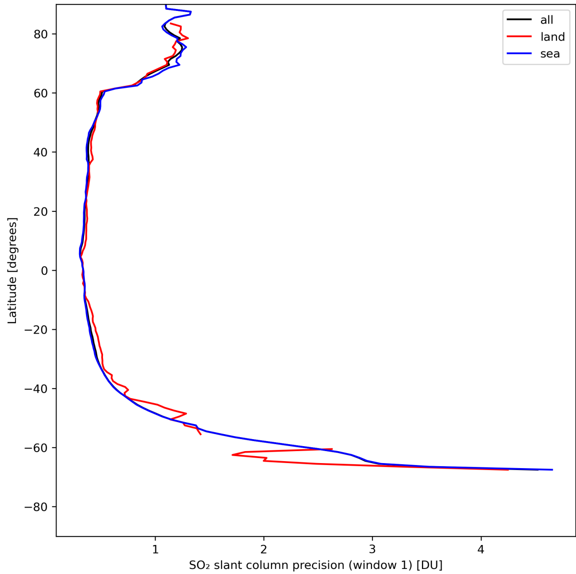
Figure 34: Zonal average of “SO 2 slant column precision (window 1)” for 2024-05-05 to 2024-05-07.
