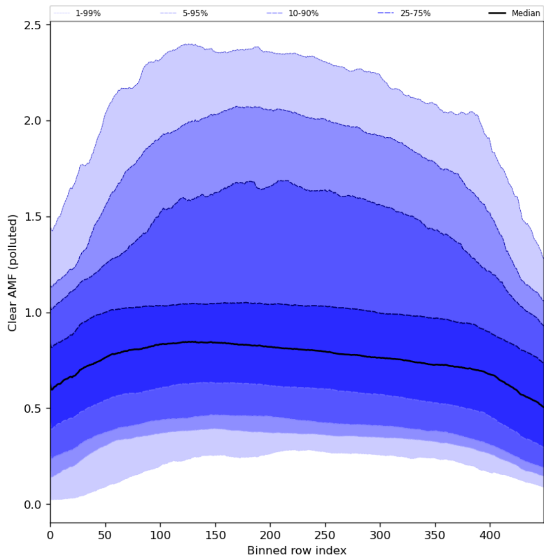
Figure 96: Along track statistics of “Clear AMF (polluted)” for 2024-05-05 to 2024-05-07
