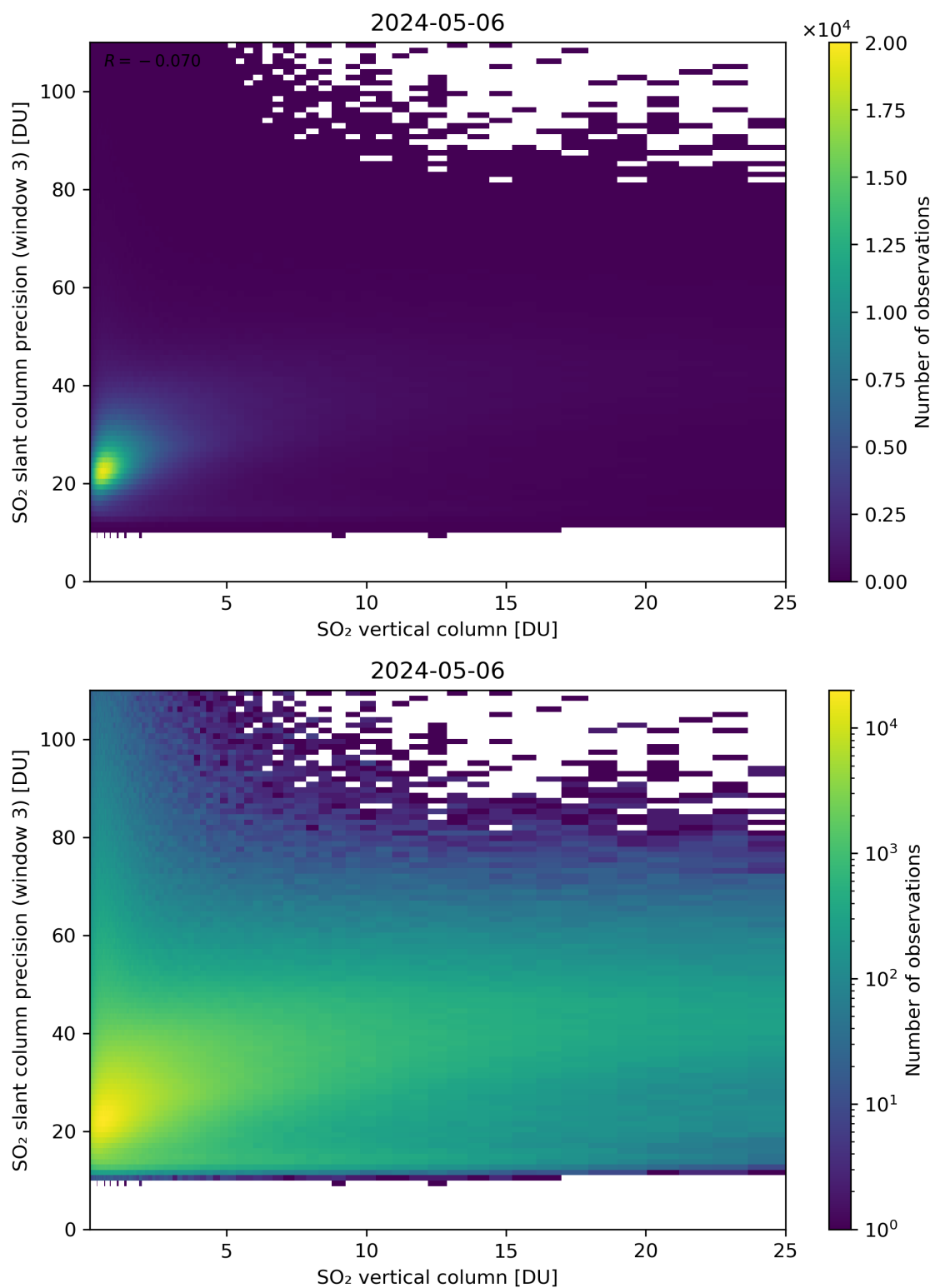
Figure 304: Scatter density plot of “SO 2 vertical column” against “SO 2 slant column precision (window 3)” for 2024-05-05 to 2024-05-07.
