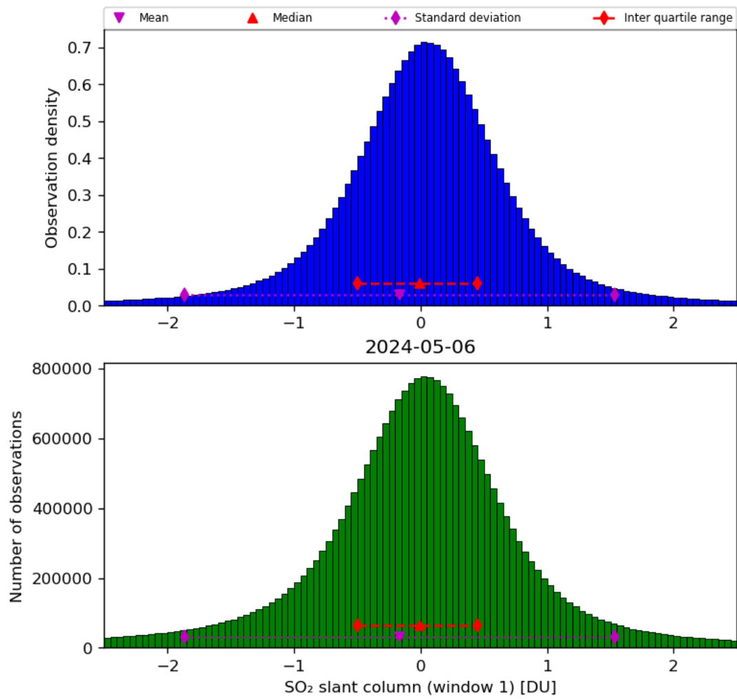
Figure 56: Histogram of “SO 2 slant column (window 1)” for 2024-05-05 to 2024-05-07
