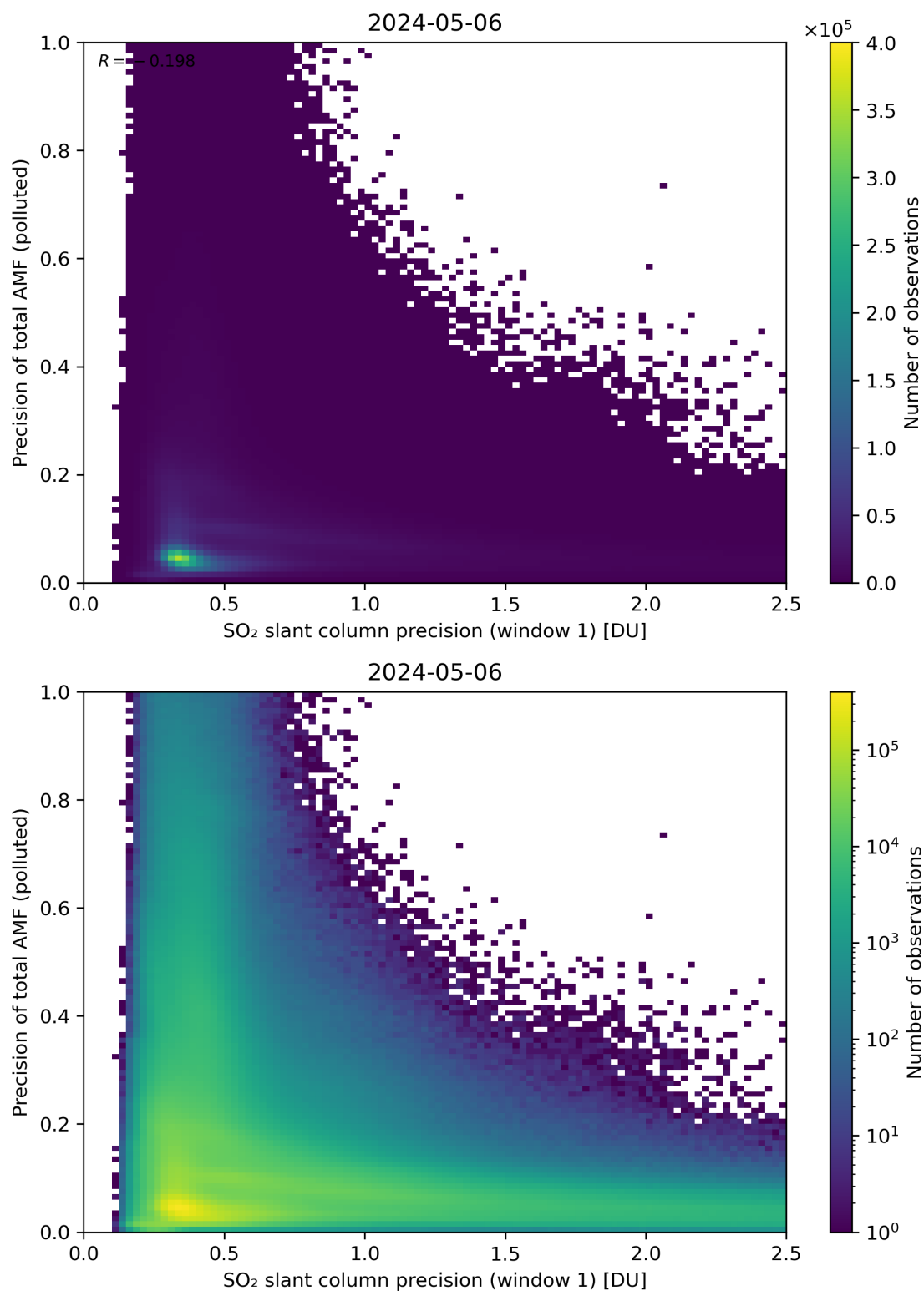
Figure 231: Scatter density plot of “SO 2 slant column precision (window 1)” against “Precision of total AMF (polluted)” for 2024-05-05 to 2024-05-07.
