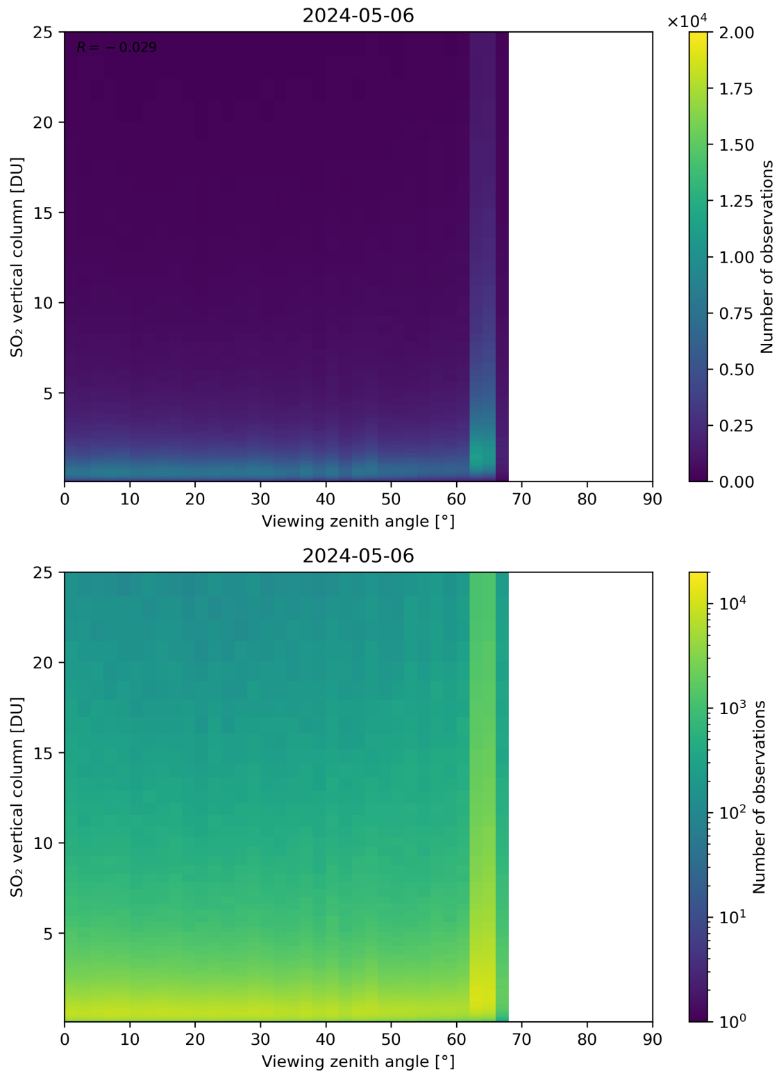
Figure 327: Scatter density plot of “Viewing zenith angle” against “SO 2 vertical column” for 2024-05-05 to 2024-05-07.
