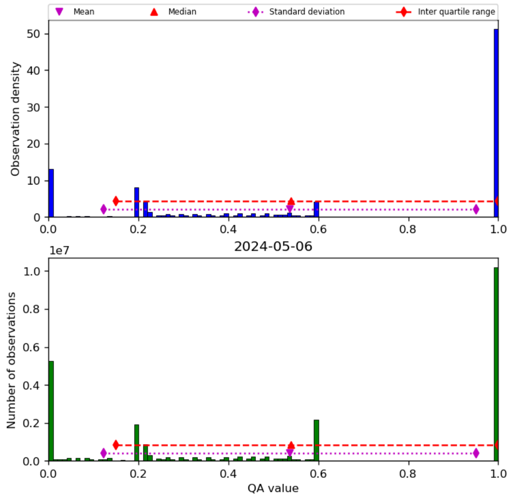
Figure 52: Histogram of “QA value” for 2024-05-05 to 2024-05-07
