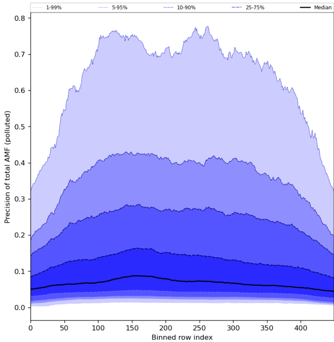
Figure 95: Along track statistics of “Precision of total AMF (polluted)” for 2024-05-05 to 2024-05-07
