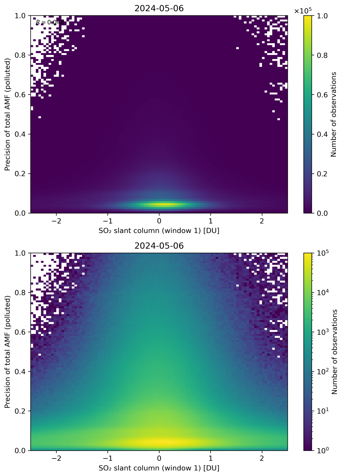
Figure 240: Scatter density plot of “SO 2 slant column (window 1)” against “Precision of total AMF (polluted)” for 2024-05-05 to 2024-05-07.
