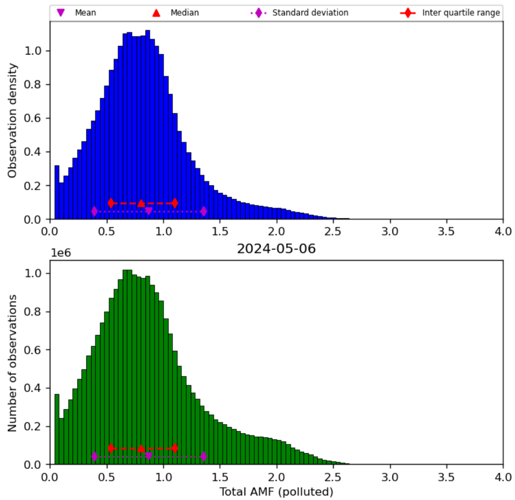
Figure 71: Histogram of “Total AMF (polluted)” for 2024-05-05 to 2024-05-07
