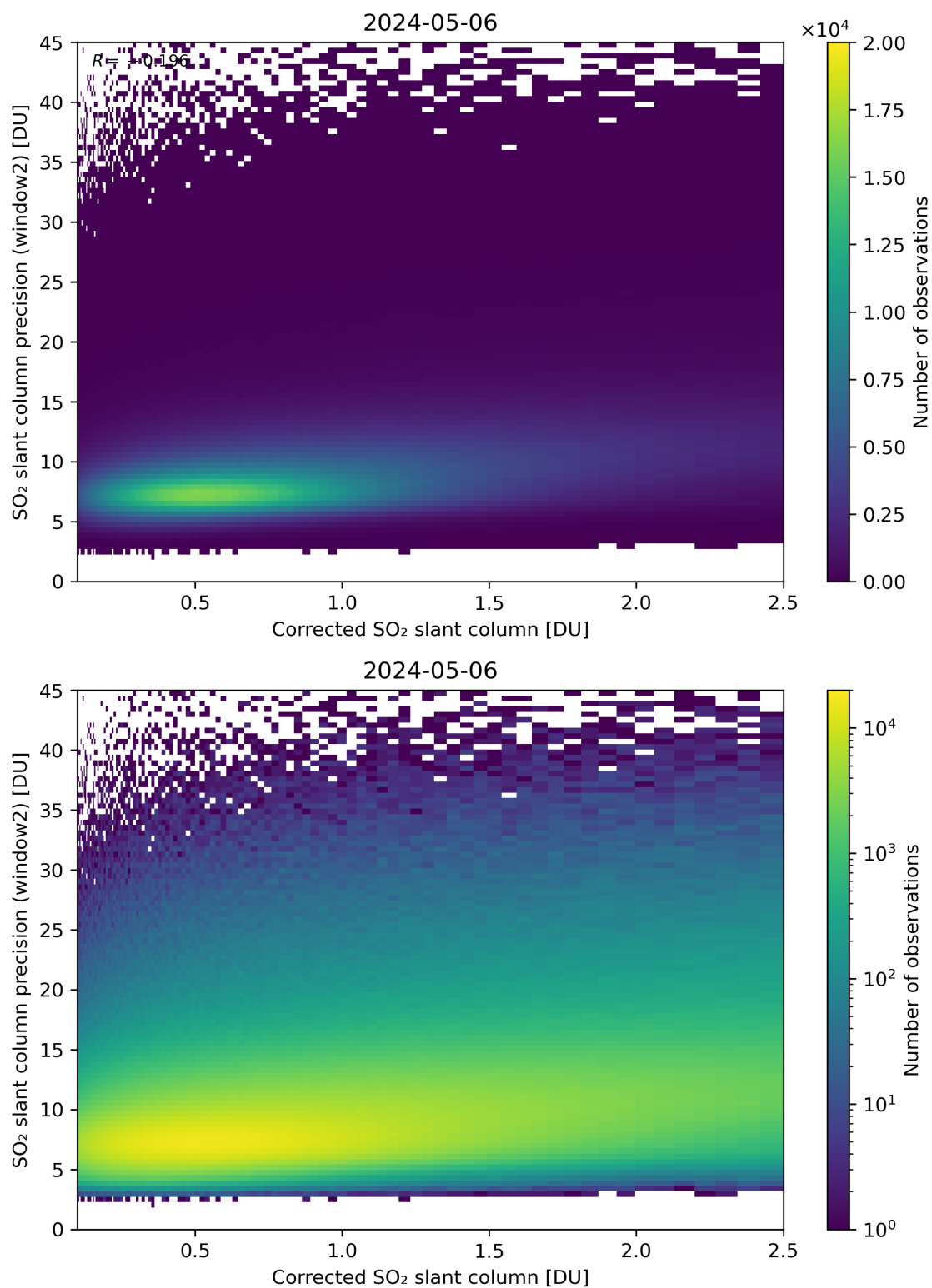
Figure 189: Scatter density plot of “Corrected SO 2 slant column” against “SO 2 slant column precision (window2)” for 2024-05-05 to 2024-05-07.
