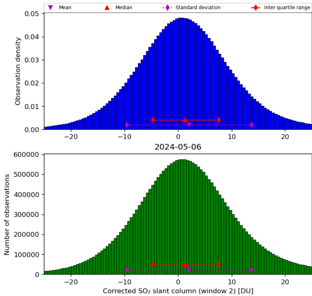
Figure 62: Histogram of “Corrected SO 2 slant column (window 2)” for 2024-05-05 to 2024-05-07
