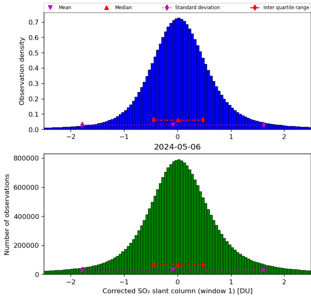
Figure 58: Histogram of “Corrected SO 2 slant column (window 1)” for 2024-05-05 to 2024-05-07
