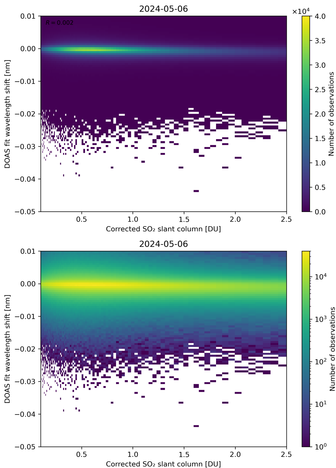
Figure 181: Scatter density plot of “Corrected SO 2 slant column” against “DOAS fit wavelength shift” for 2024-05-05 to 2024-05-07.
