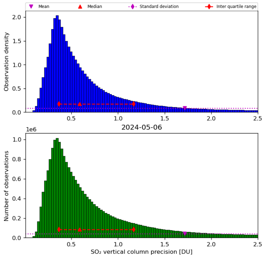
Figure 54: Histogram of “SO 2 vertical column precision” for 2024-05-05 to 2024-05-07
