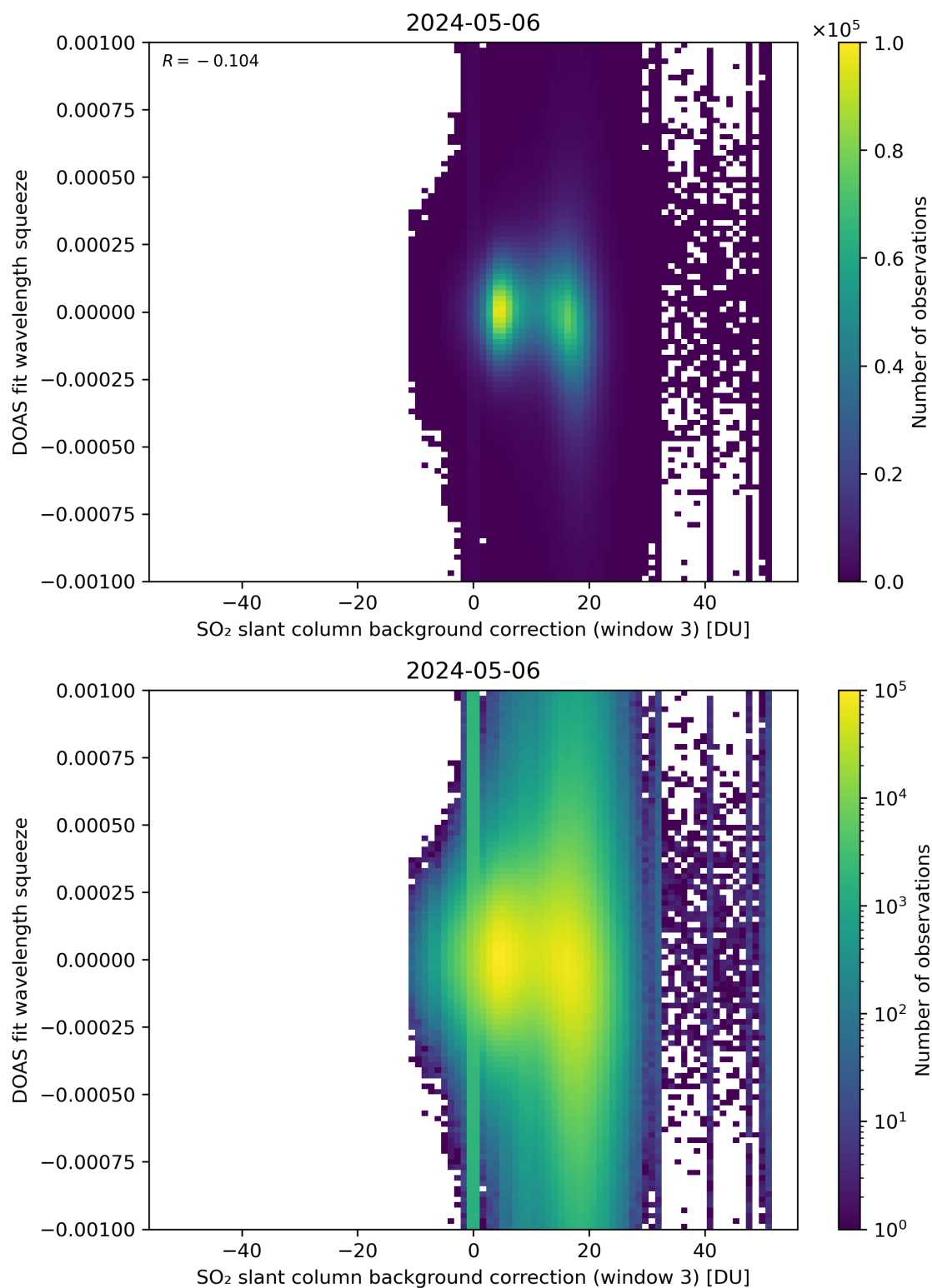
Figure 122: Scatter density plot of “SO 2 slant column background correction (window 3)” against “DOAS fit wavelength squeeze” for 2024-05-05 to 2024-05-07.
