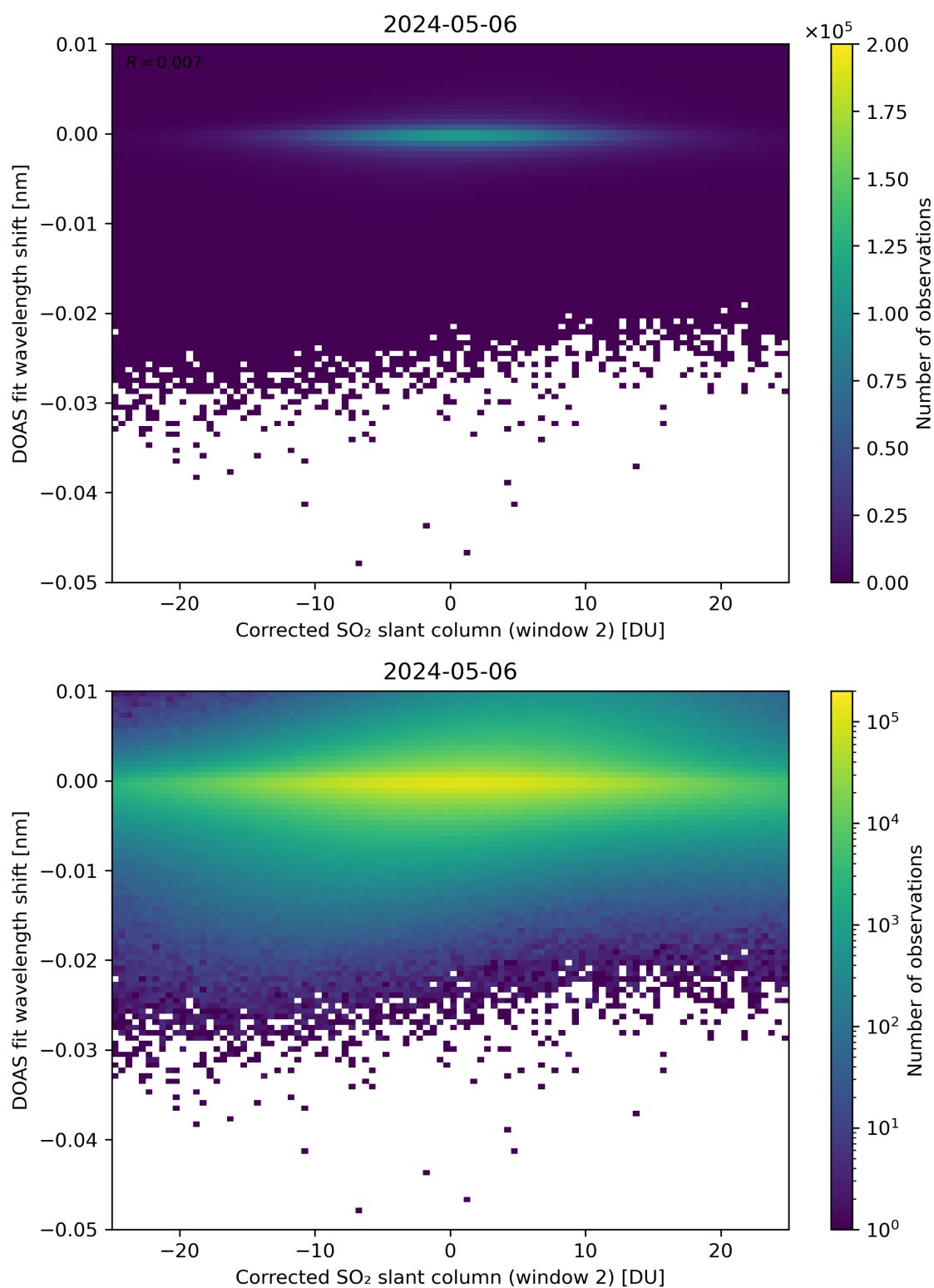
Figure 196: Scatter density plot of “Corrected SO 2 slant column (window 2)” against “DOAS fit wavelength shift” for 2024-05-05 to 2024-05-07.
