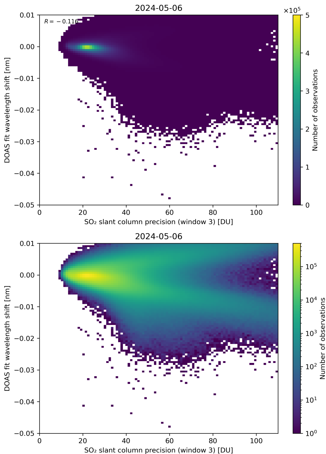
Figure 258: Scatter density plot of “SO 2 slant column precision (window 3)” against “DOAS fit wavelength shift” for 2024-05-05 to 2024-05-07.
