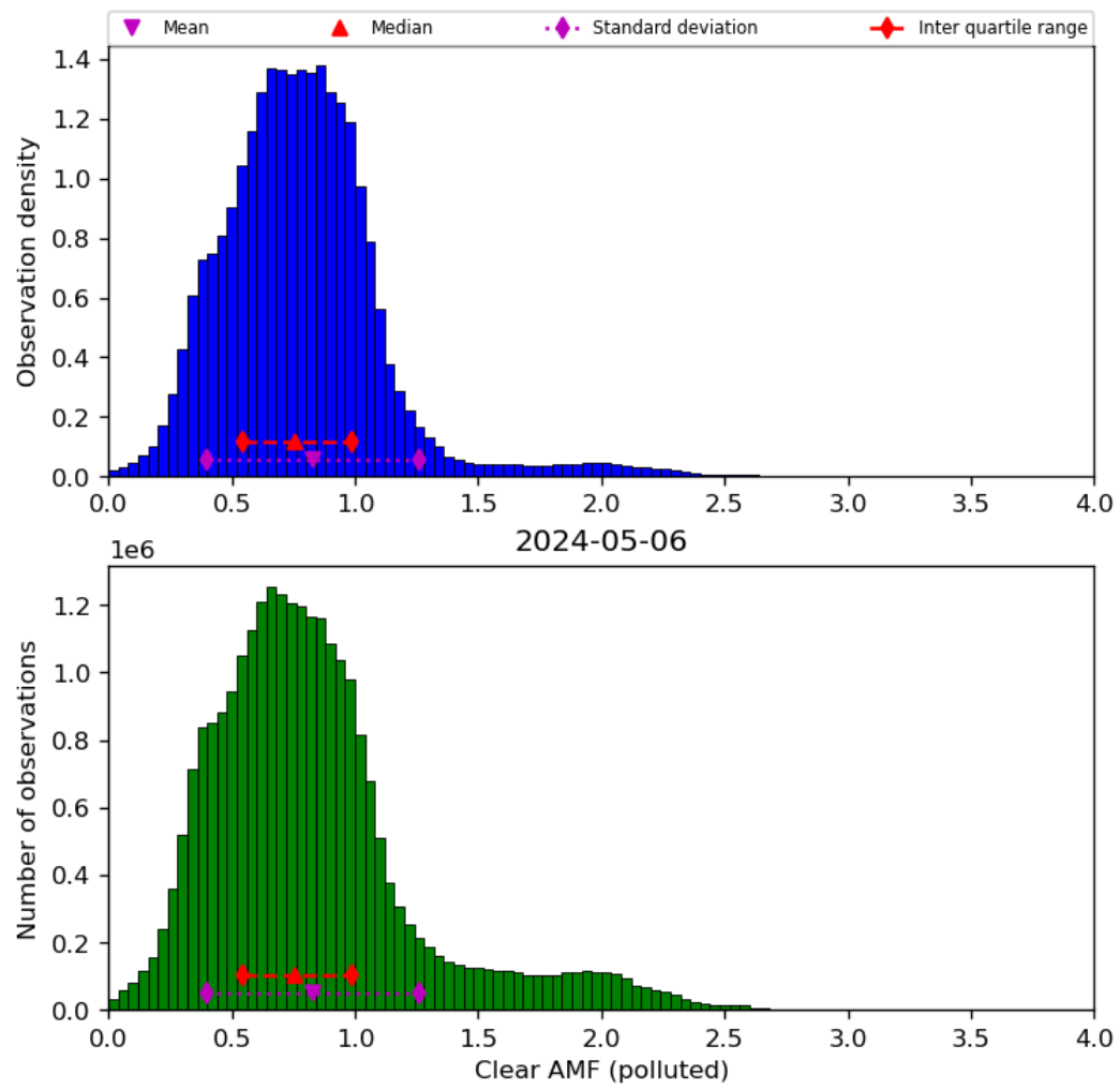
Figure 73: Histogram of “Clear AMF (polluted)” for 2024-05-05 to 2024-05-07
