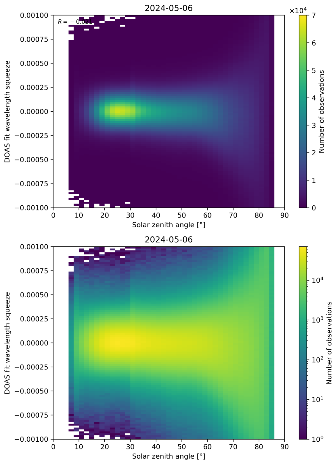
Figure 162: Scatter density plot of “Solar zenith angle” against “DOAS fit wavelength squeeze” for 2024-05-05 to 2024-05-07.
