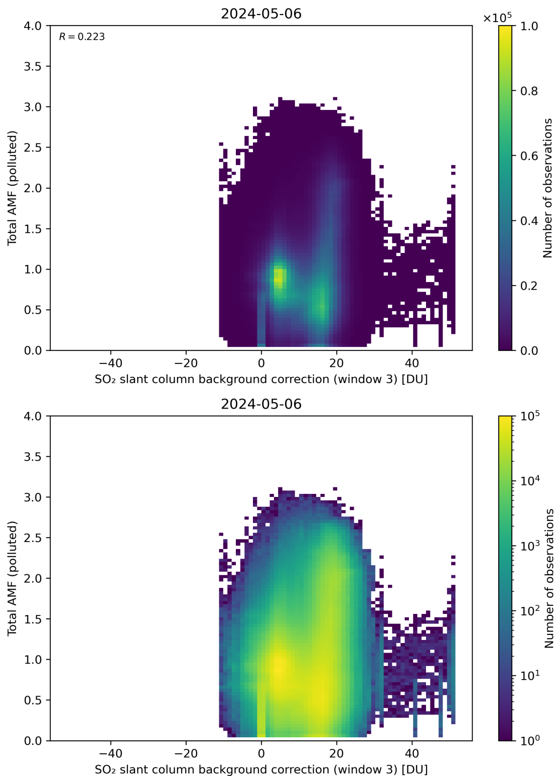
Figure 125: Scatter density plot of “SO 2 slant column background correction (window 3)” against “Total AMF (polluted)” for 2024-05-05 to 2024-05-07.
