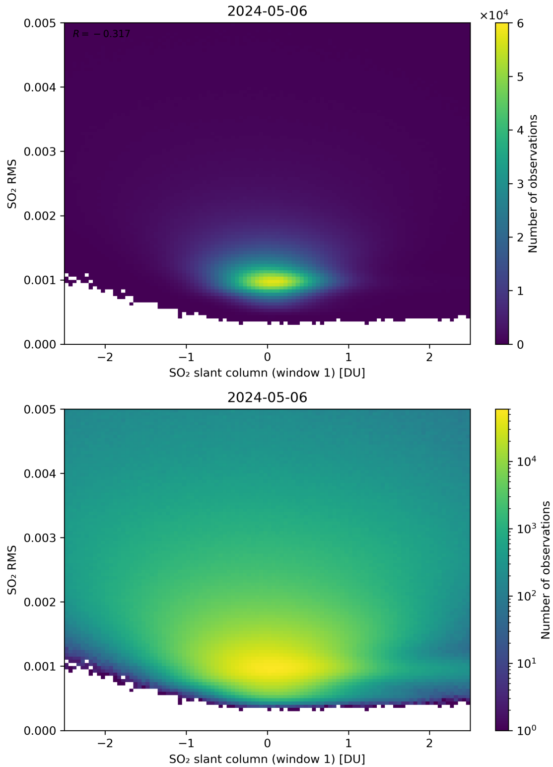
Figure 217: Scatter density plot of “SO 2 slant column (window 1)” against “SO 2 RMS” for 2024-05-05 to 2024-05-07.
