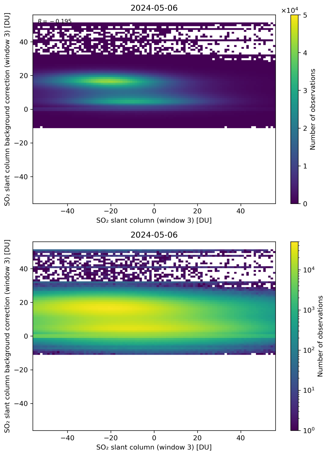
Figure 253: Scatter density plot of “SO 2 slant column (window 3)” against “SO 2 slant column background correction (window 3)” for 2024-05-05 to 2024-05-07.
