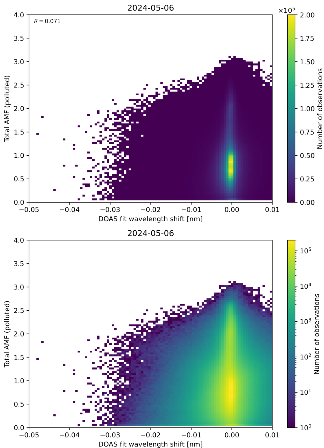
Figure 130: Scatter density plot of “DOAS fit wavelength shift” against “Total AMF (polluted)” for 2024-05-05 to 2024-05-07.
