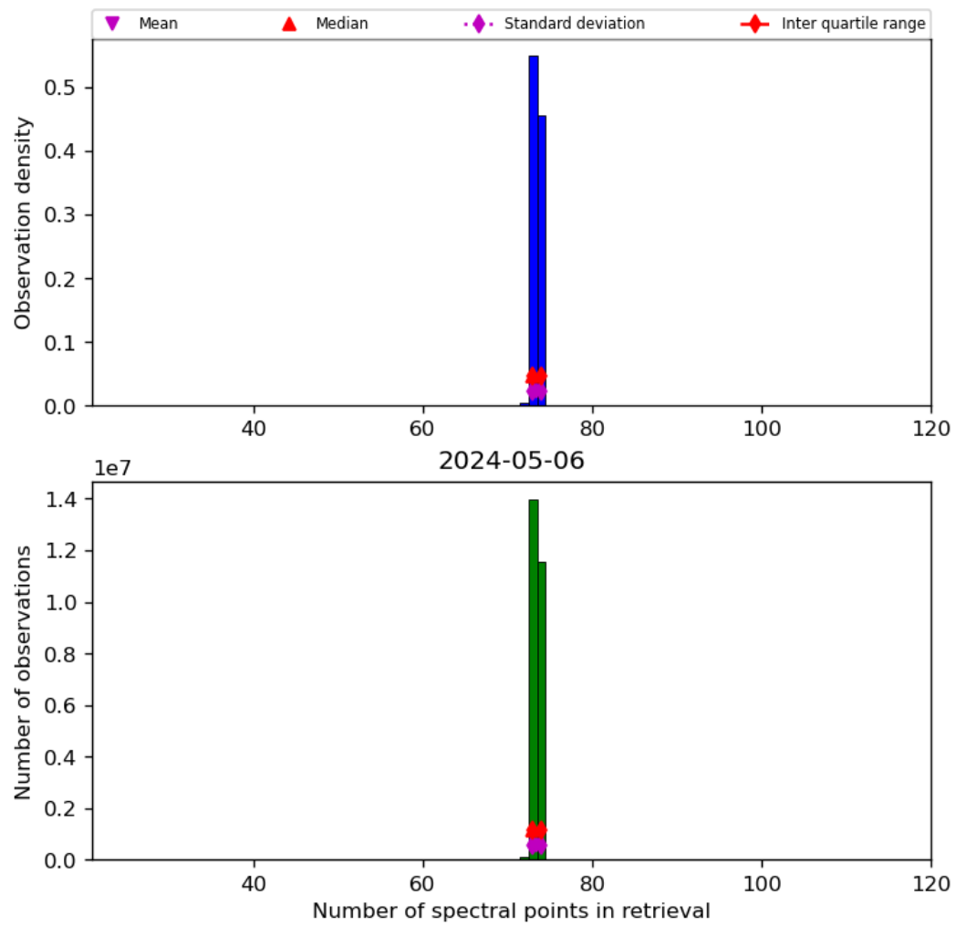
Figure 74: Histogram of “Number of spectral points in retrieval” for 2024-05-05 to 2024-05-07
