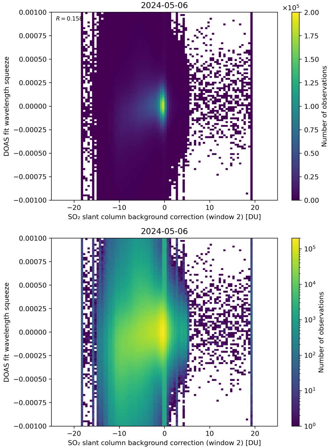
Figure 113: Scatter density plot of “SO 2 slant column background correction (window 2)” against “DOAS fit wavelength squeeze” for 2024-05-05 to 2024-05-07.
