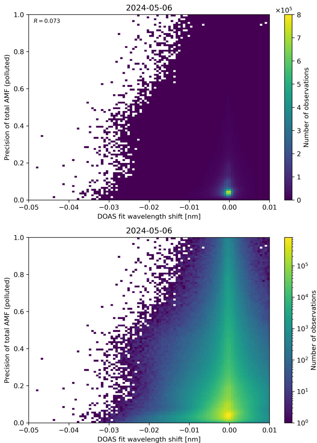
Figure 131: Scatter density plot of “DOAS fit wavelength shift” against “Precision of total AMF (polluted)” for 2024-05-05 to 2024-05-07.
