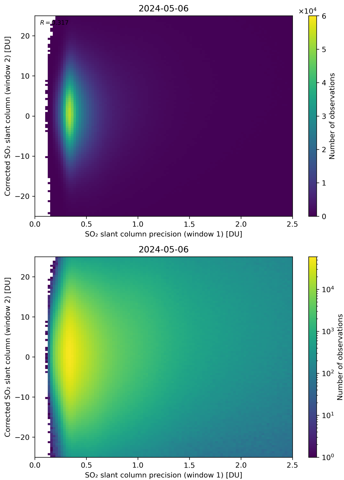
Figure 225: Scatter density plot of “SO 2 slant column precision (window 1)” against “Corrected SO 2 slant column (window 2)” for 2024-05-05 to 2024-05-07.
