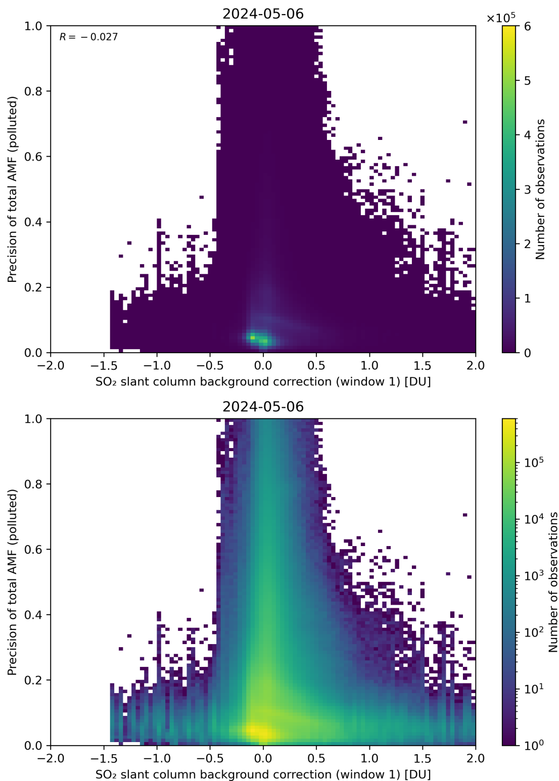
Figure 110: Scatter density plot of “SO 2 slant column background correction (window 1)” against “Precision of total AMF (polluted)” for 2024-05-05 to 2024-05-07.
