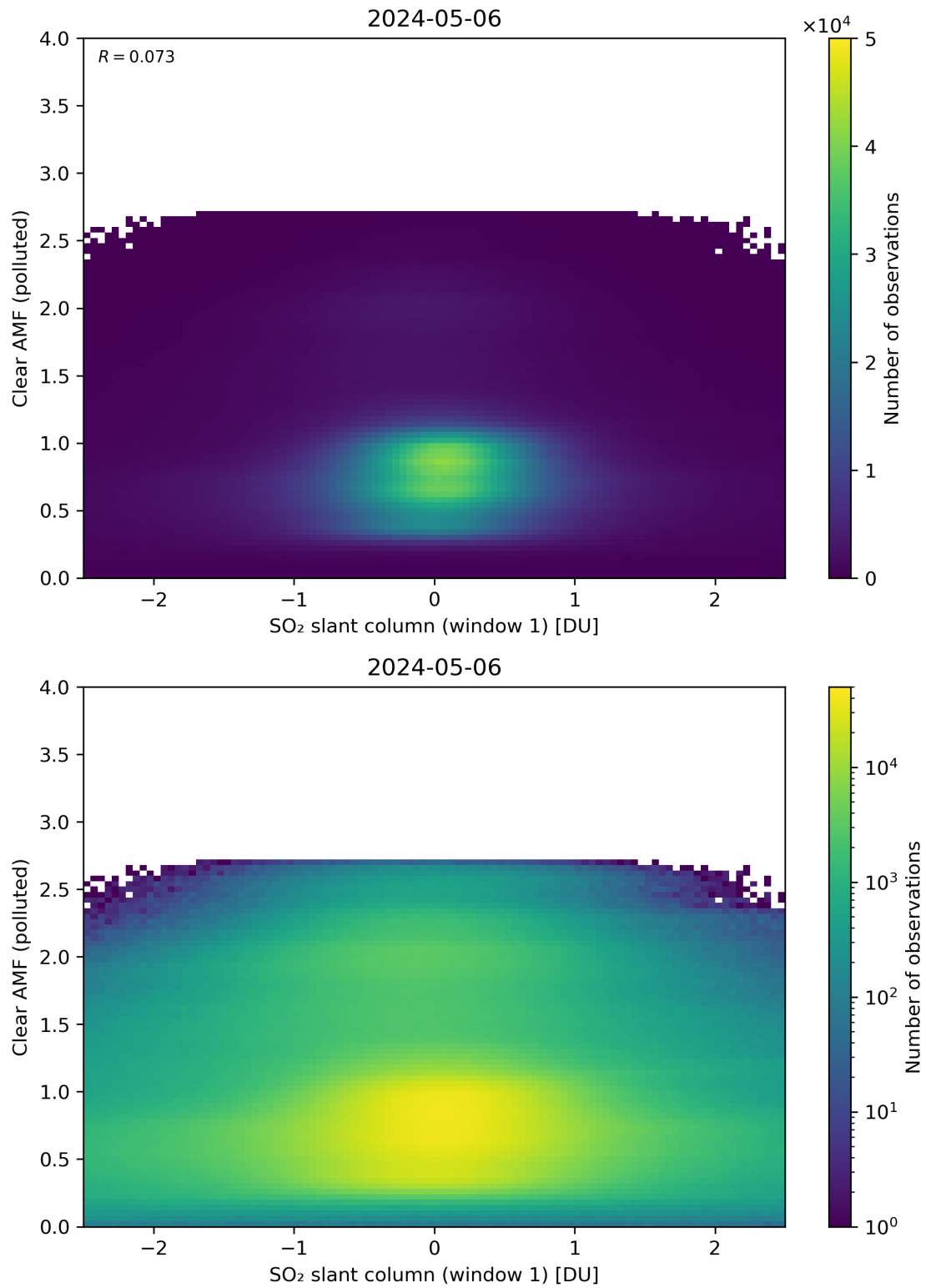
Figure 232: Scatter density plot of “SO 2 slant column (window 1)” against “Clear AMF (polluted)” for 2024-05-05 to 2024-05-07.
