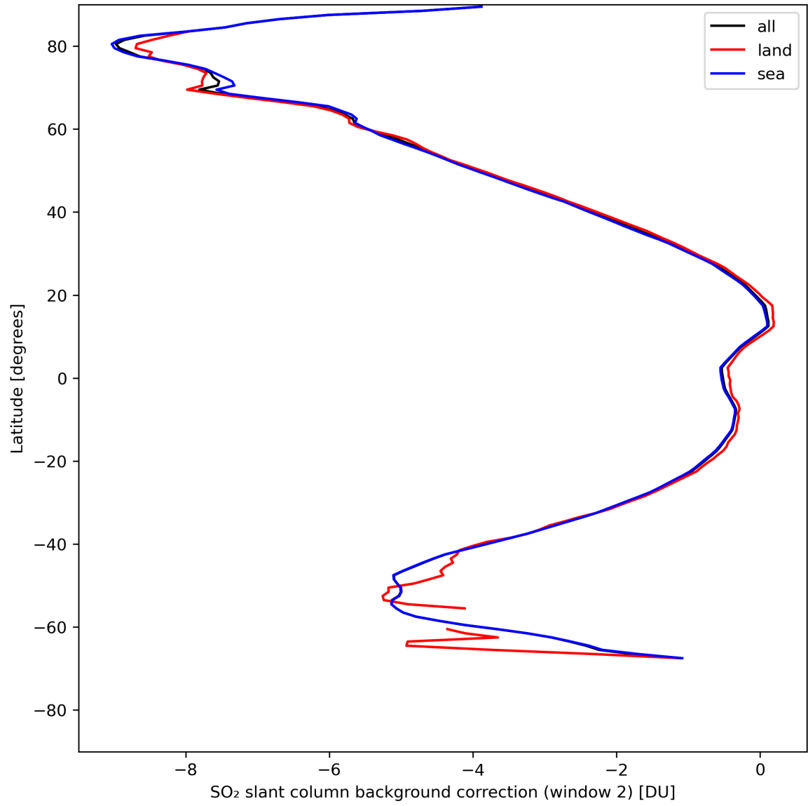
Figure 40: Zonal average of “SO 2 slant column background correction (window 2)” for 2024-05-05 to 2024-05-07.
