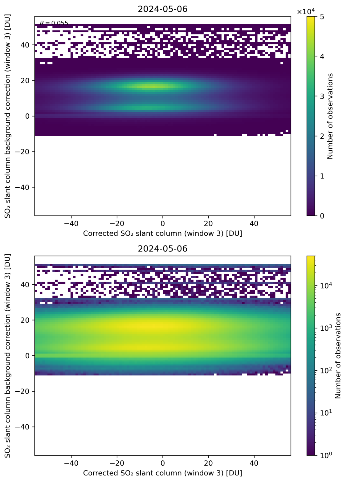
Figure 205: Scatter density plot of “Corrected SO 2 slant column (window 3)” against “SO 2 slant column background correction (window 3)” for 2024-05-05 to 2024-05-07.
