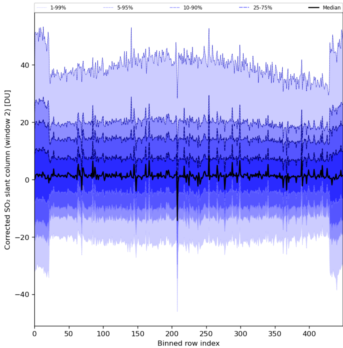
Figure 85: Along track statistics of “Corrected SO 2 slant column (window 2)” for 2024-05-05 to 2024-05-07
