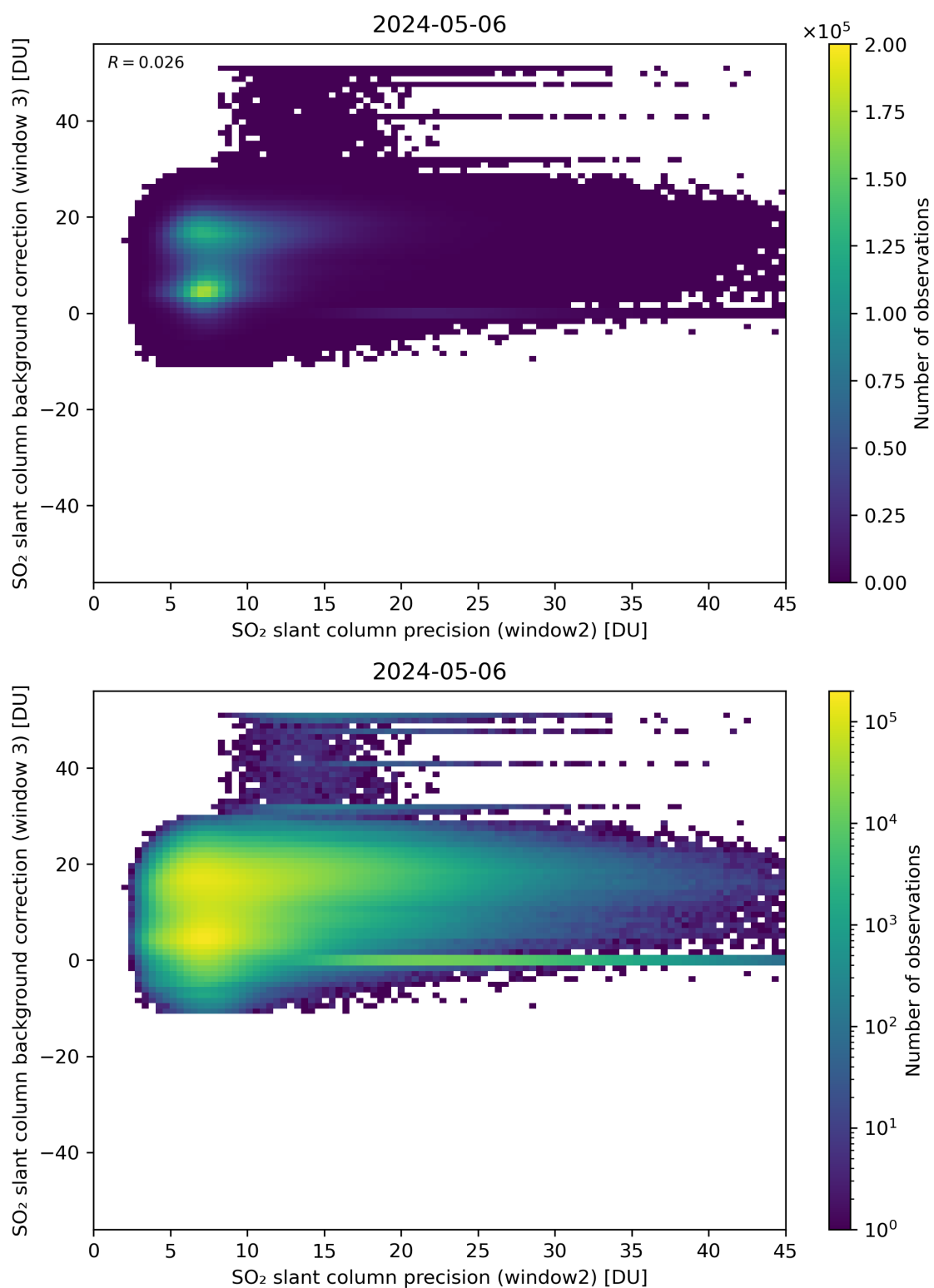
Figure 242: Scatter density plot of “SO 2 slant column precision (window2)” against “SO 2 slant column background correction (window 3)” for 2024-05-05 to 2024-05-07.
