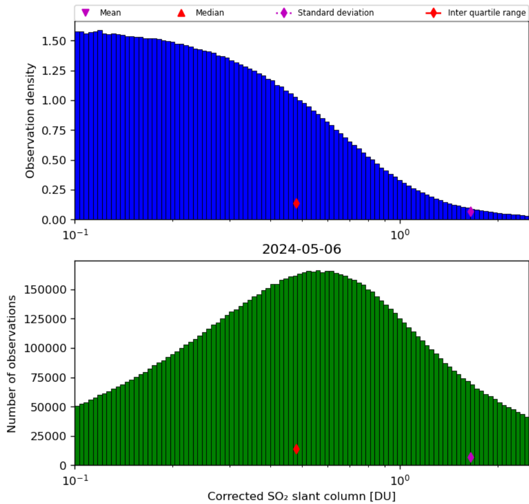
Figure 55: Histogram of “Corrected SO 2 slant column” for 2024-05-05 to 2024-05-07
