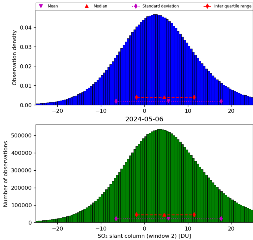
Figure 60: Histogram of “SO 2 slant column (window 2)” for 2024-05-05 to 2024-05-07
