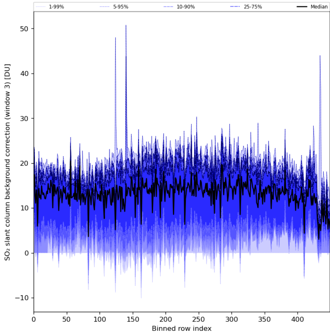
Figure 90: Along track statistics of “SO 2 slant column background correction (window 3)” for 2024-05-05 to 2024-05-07
