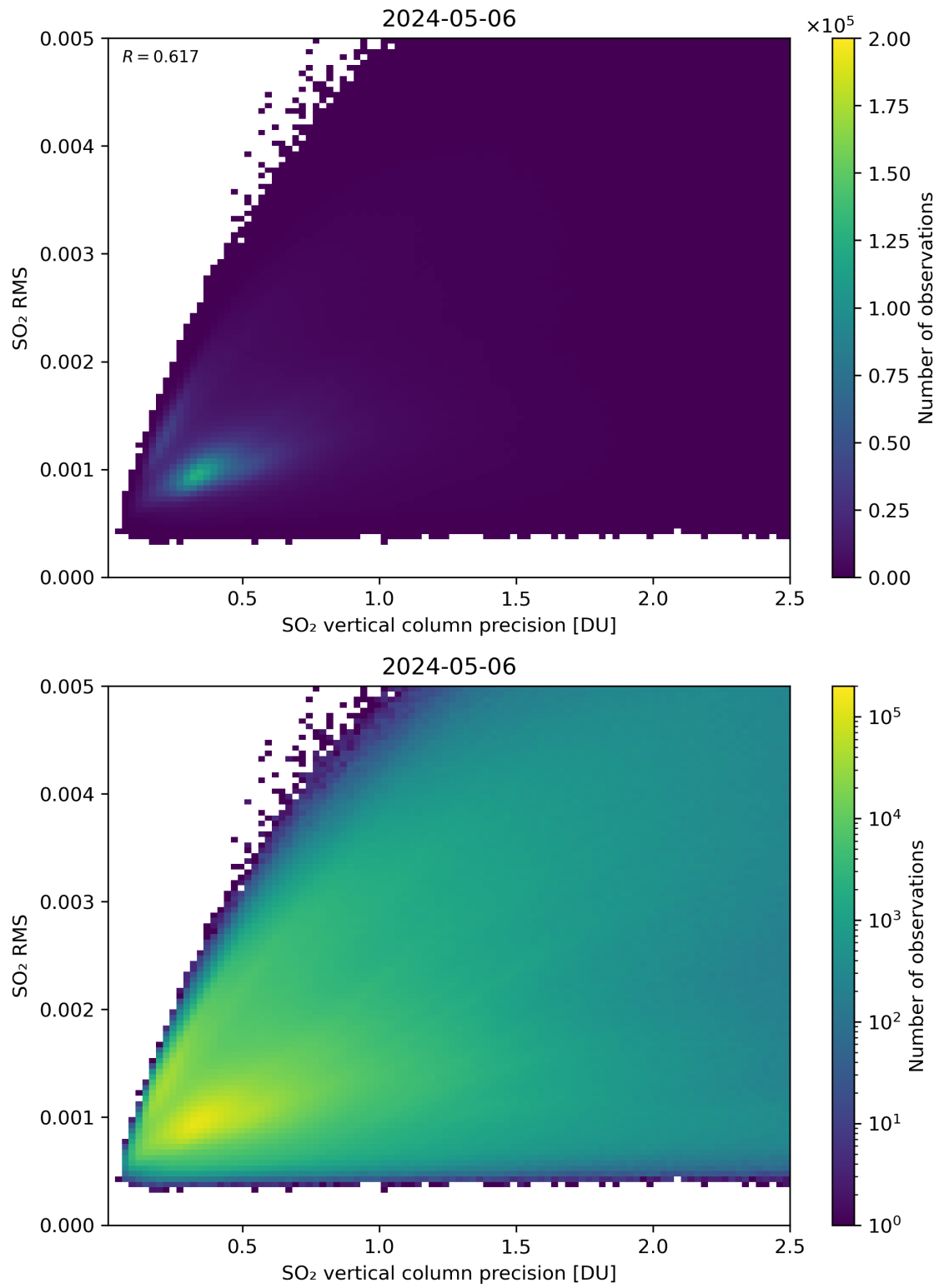
Figure 284: Scatter density plot of “SO 2 vertical column precision” against “SO 2 RMS” for 2024-05-05 to 2024-05-07.
