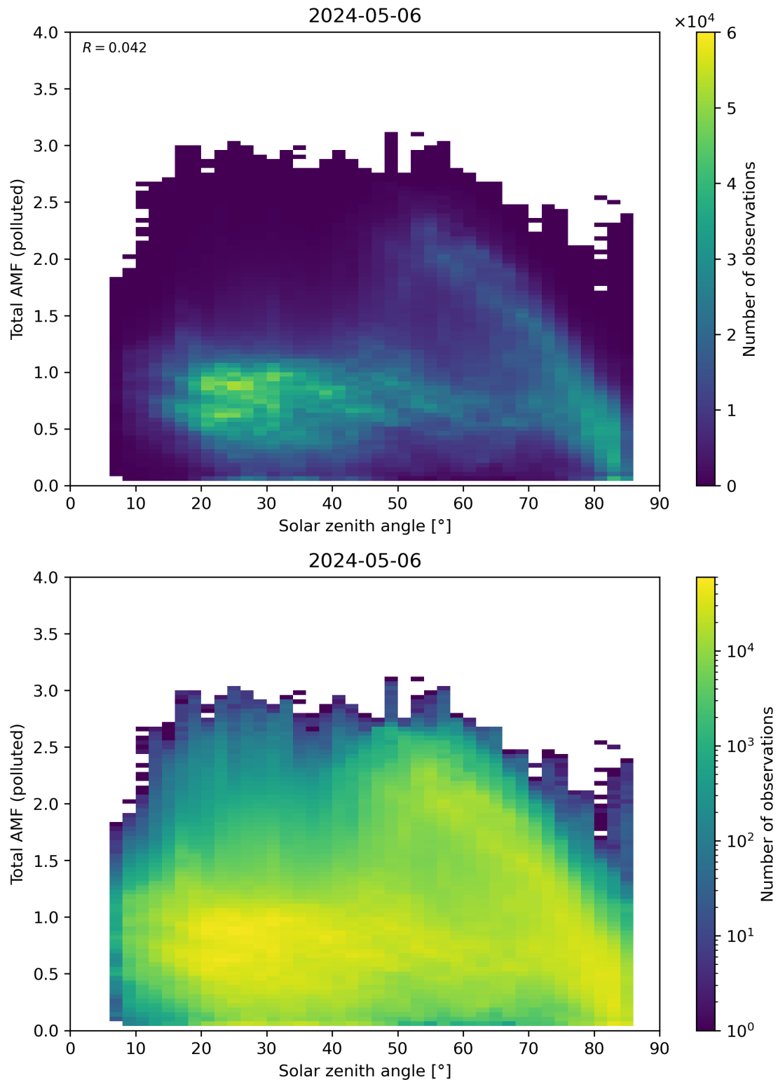
Figure 174: Scatter density plot of “Solar zenith angle” against “Total AMF (polluted)” for 2024-05-05 to 2024-05-07.
