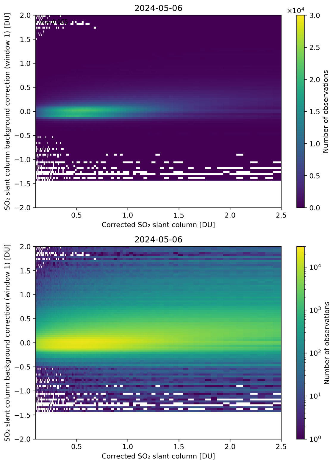
Figure 178: Scatter density plot of “Corrected SO 2 slant column” against “SO 2 slant column background correction (window 1)” for 2024-05-05 to 2024-05-07.
