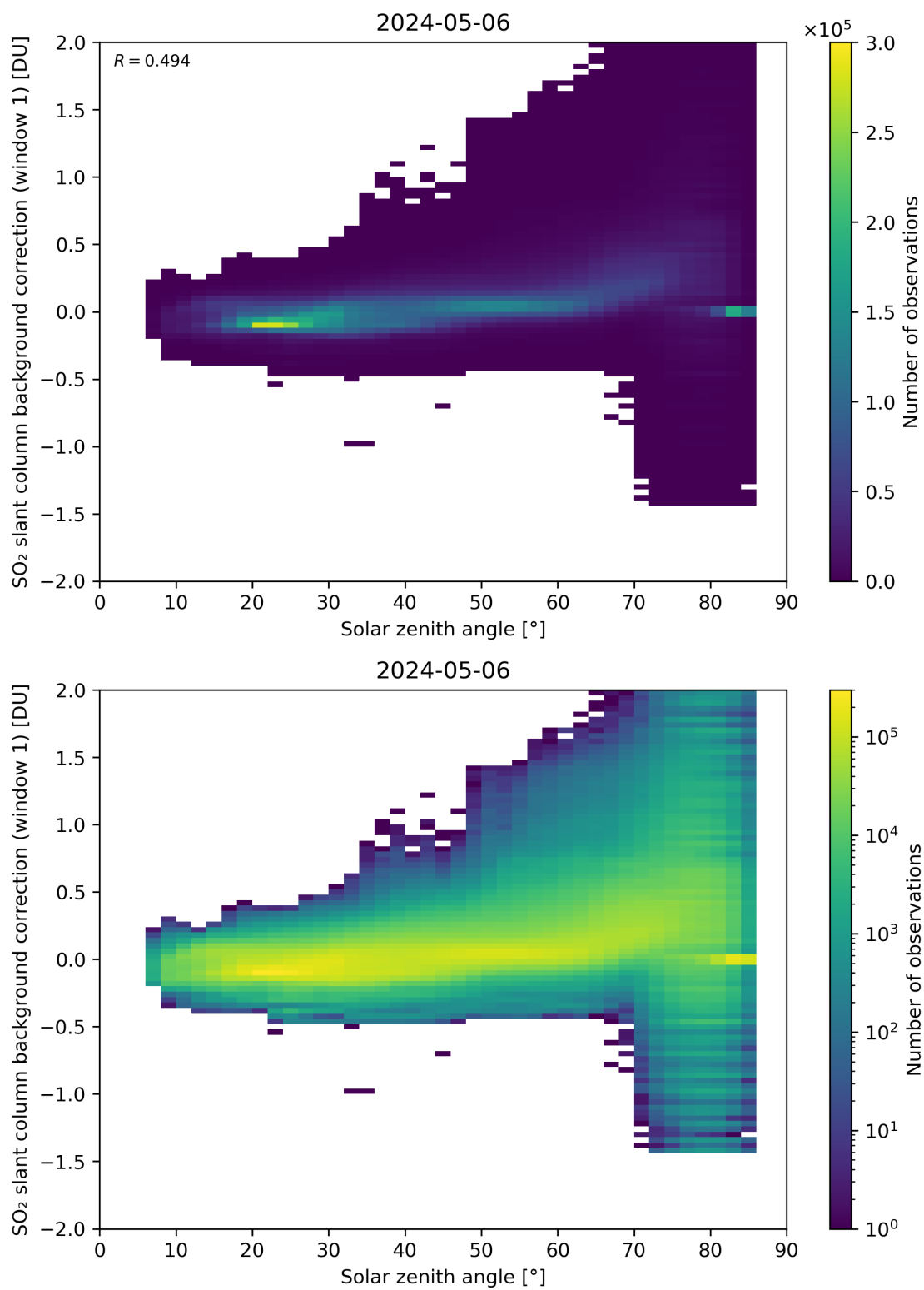
Figure 158: Scatter density plot of “Solar zenith angle” against “SO 2 slant column background correction (window 1)” for 2024-05-05 to 2024-05-07.
