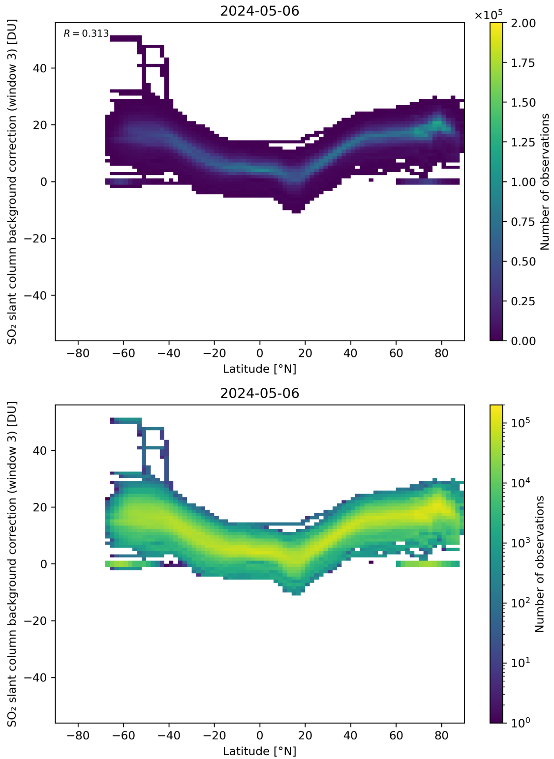
Figure 141: Scatter density plot of “Latitude” against “SO 2 slant column background correction (window 3)” for 2024-05-05 to 2024-05-07.
