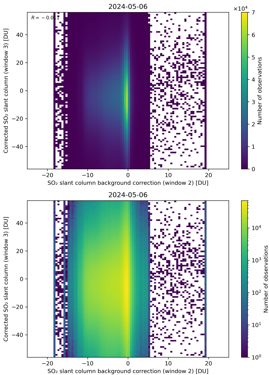
Figure 116: Scatter density plot of “SO 2 slant column background correction (window 2)” against “Corrected SO 2 slant column (window 3)” for 2024-05-05 to 2024-05-07.
