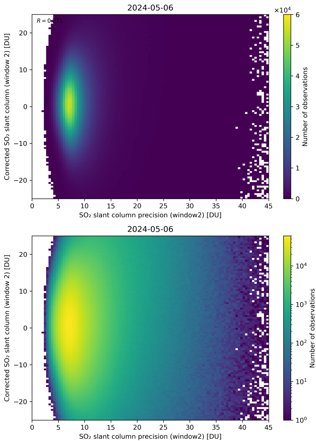
Figure 247: Scatter density plot of “SO 2 slant column precision (window2)” against “Corrected SO 2 slant column (window 2)” for 2024-05-05 to 2024-05-07.
