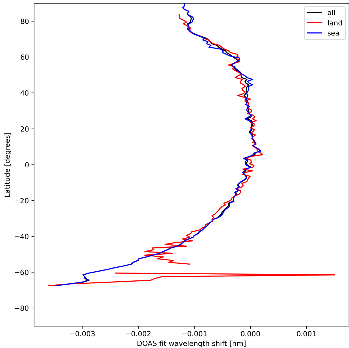
Figure 45: Zonal average of “DOAS fit wavelength shift” for 2024-05-05 to 2024-05-07.
