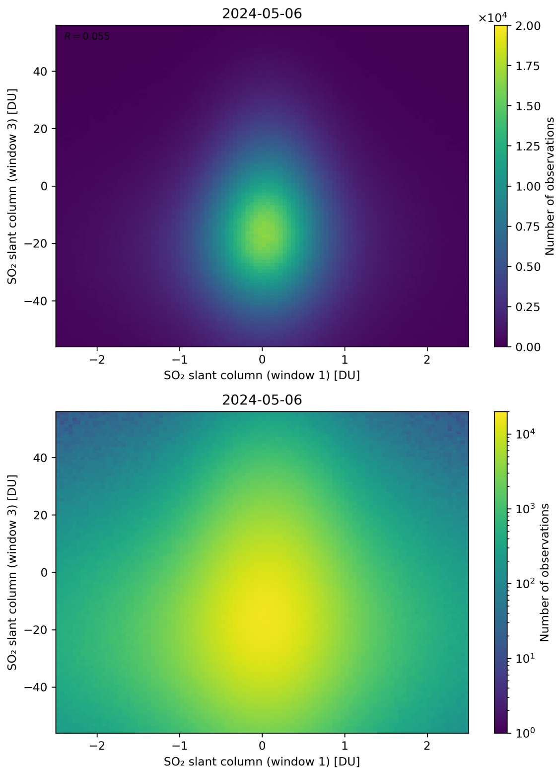
Figure 237: Scatter density plot of “SO 2 slant column (window 1)” against “SO 2 slant column (window 3)” for 2024-05-05 to 2024-05-07.
