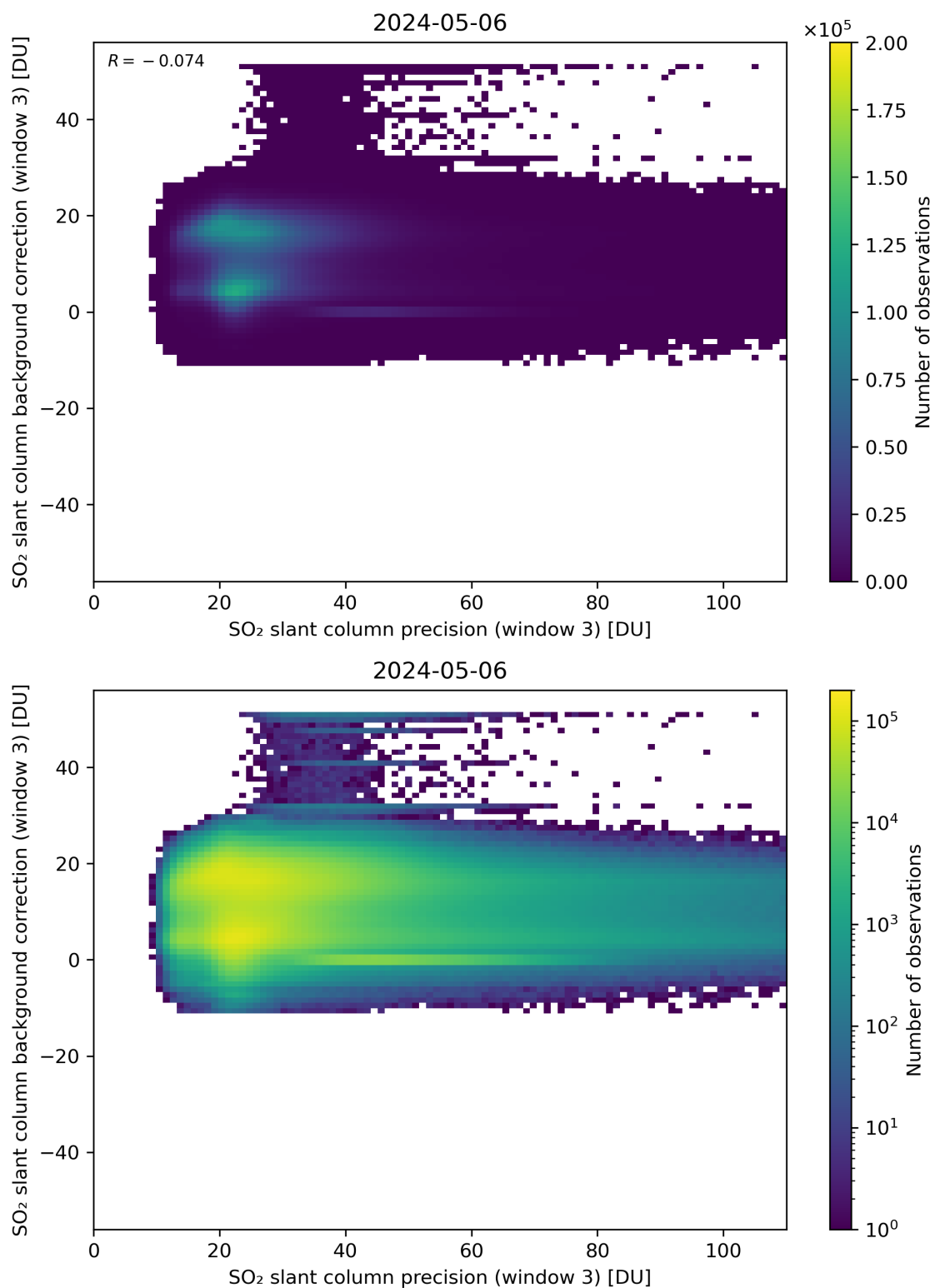
Figure 257: Scatter density plot of “SO 2 slant column precision (window 3)” against “SO 2 slant column background correction (window 3)” for 2024-05-05 to 2024-05-07.
