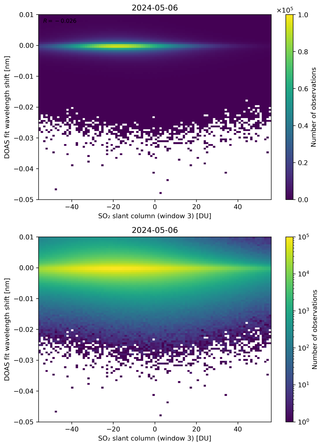
Figure 254: Scatter density plot of “SO 2 slant column (window 3)” against “DOAS fit wavelength shift” for 2024-05-05 to 2024-05-07.
