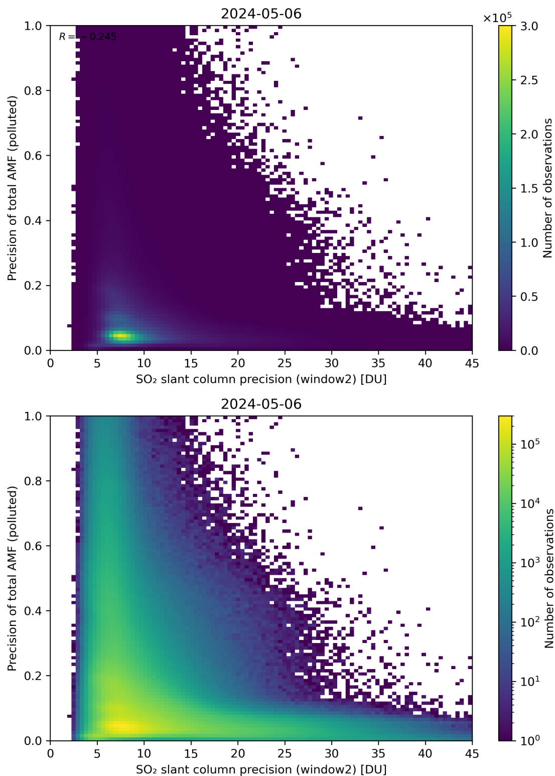
Figure 252: Scatter density plot of “SO 2 slant column precision (window2)” against “Precision of total AMF (polluted)” for 2024-05-05 to 2024-05-07.
