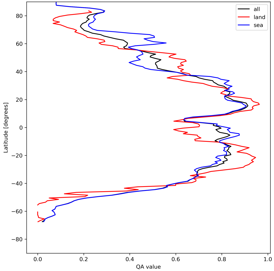
Figure 29: Zonal average of “QA value” for 2024-05-05 to 2024-05-07.
