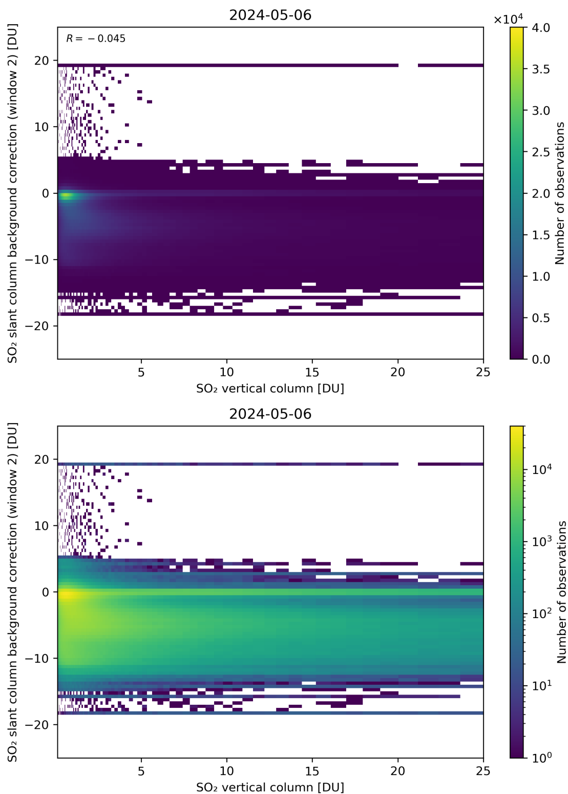
Figure 274: Scatter density plot of “SO 2 vertical column” against “SO 2 slant column background correction (window 2)” for 2024-05-05 to 2024-05-07.
