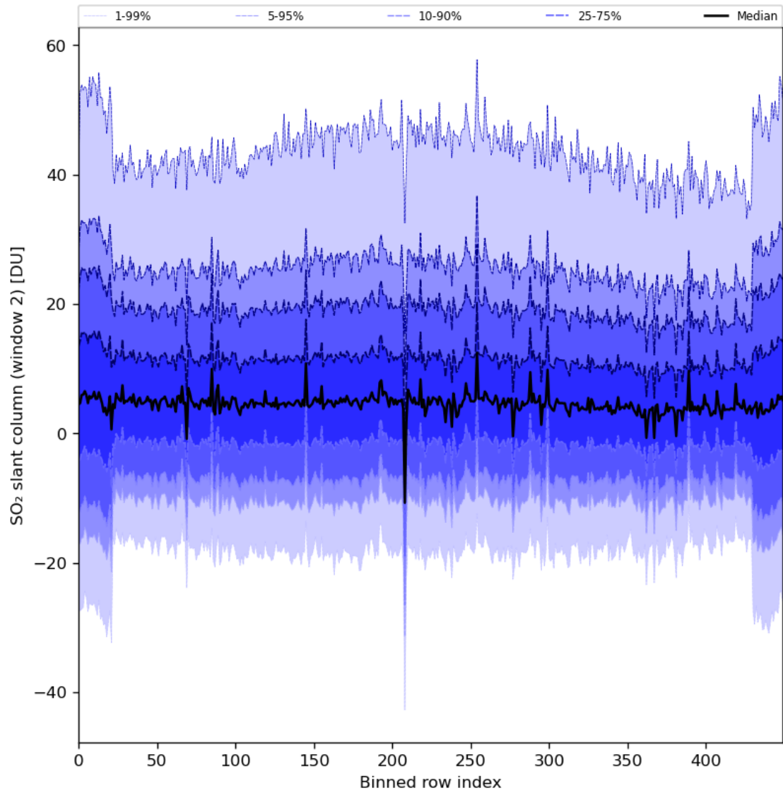
Figure 83: Along track statistics of “SO 2 slant column (window 2)” for 2024-05-05 to 2024-05-07
