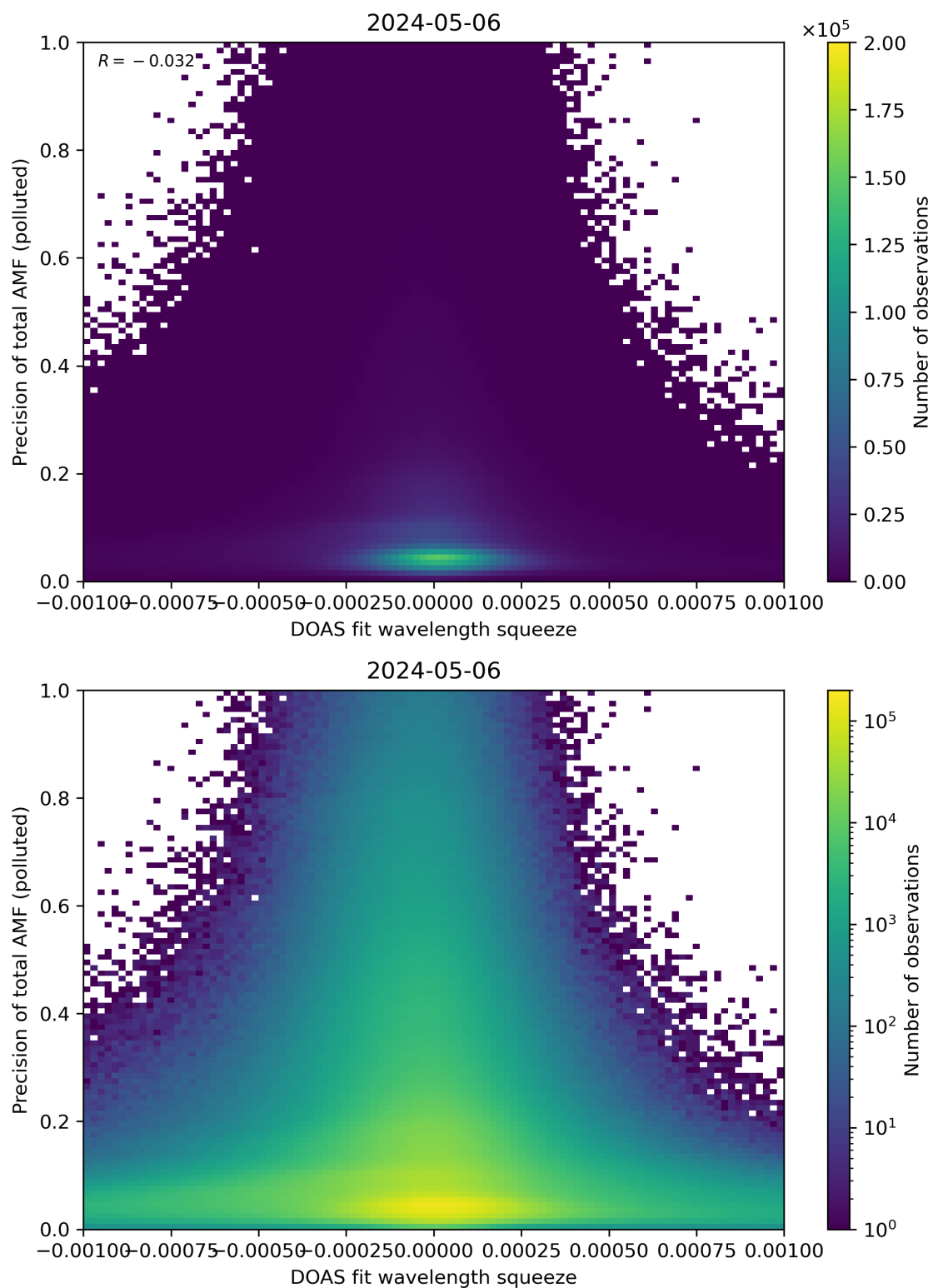
Figure 135: Scatter density plot of “DOAS fit wavelength squeeze” against “Precision of total AMF (polluted)” for 2024-05-05 to 2024-05-07.
