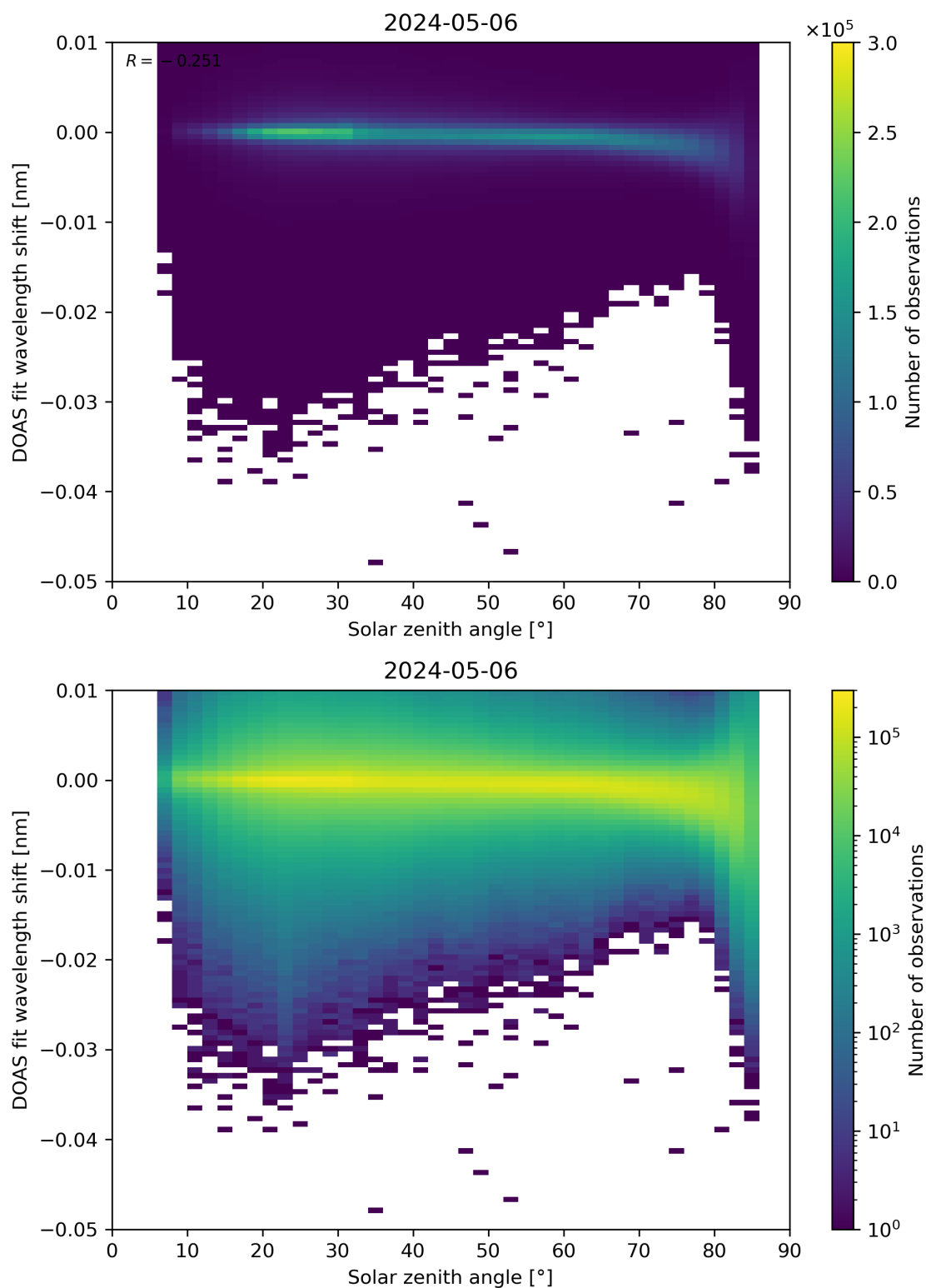
Figure 161: Scatter density plot of “Solar zenith angle” against “DOAS fit wavelength shift” for 2024-05-05 to 2024-05-07.
