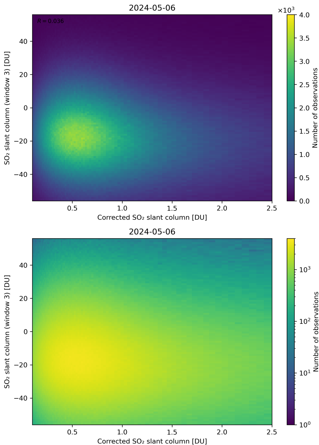
Figure 190: Scatter density plot of “Corrected SO 2 slant column” against “SO 2 slant column (window 3)” for 2024-05-05 to 2024-05-07.
