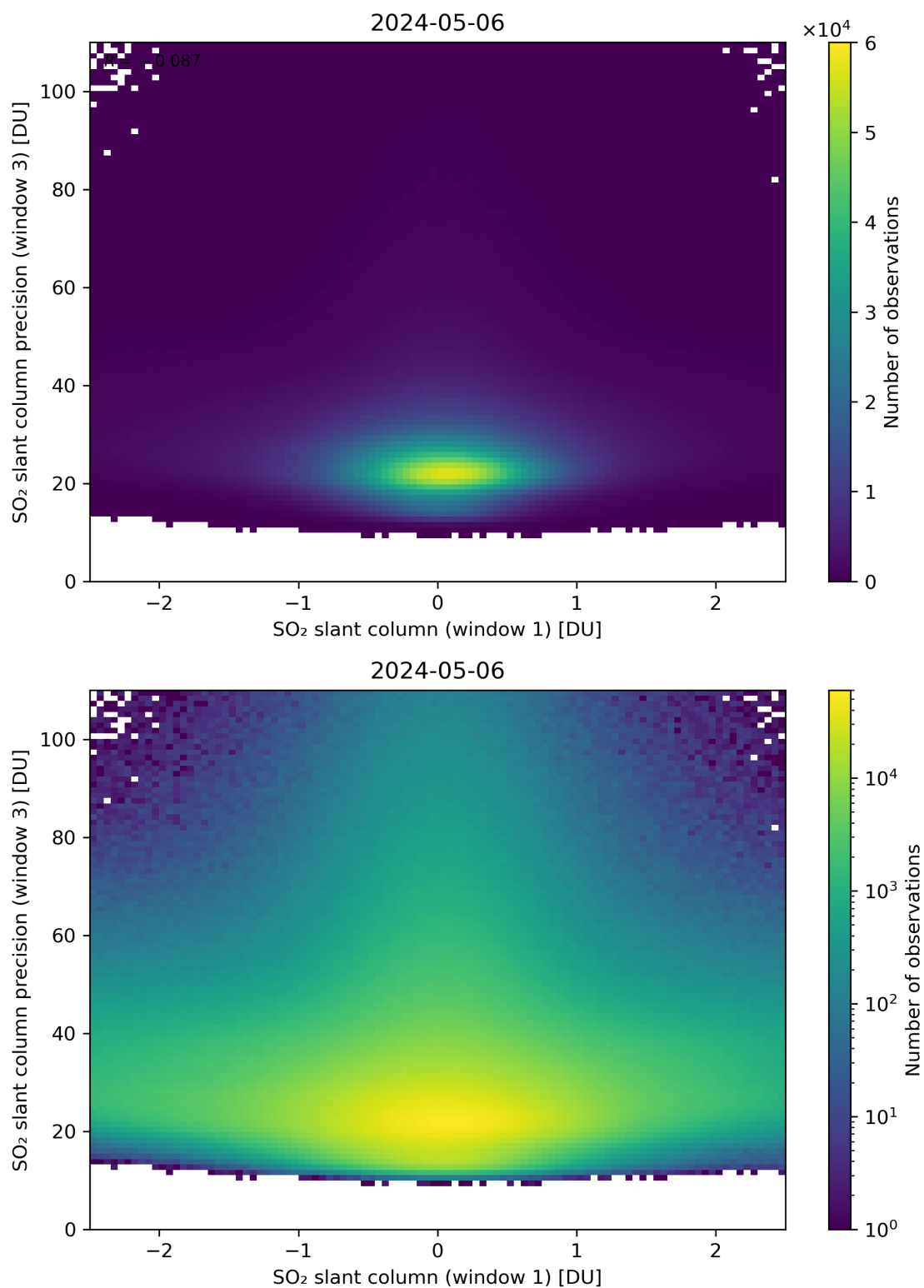
Figure 238: Scatter density plot of “SO 2 slant column (window 1)” against “SO 2 slant column precision (window 3)” for 2024-05-05 to 2024-05-07.
