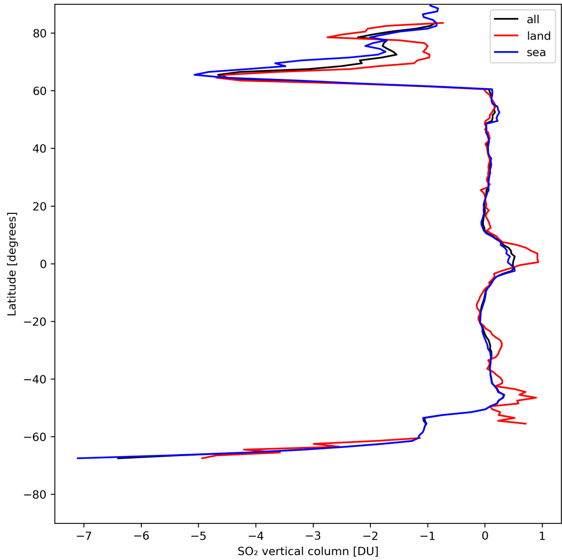
Figure 30: Zonal average of “SO 2 vertical column” for 2024-05-05 to 2024-05-07.
