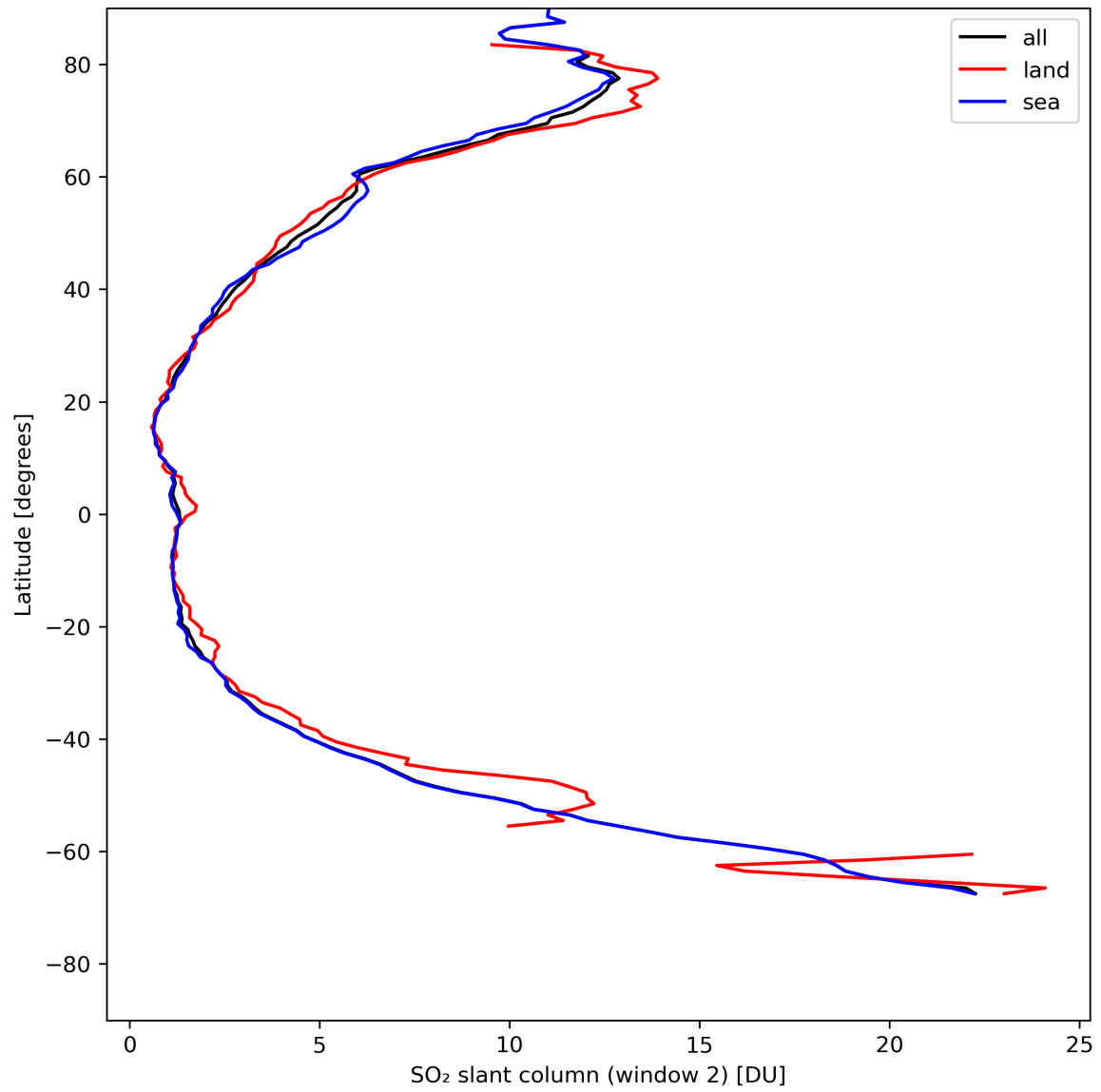
Figure 37: Zonal average of “SO 2 slant column (window 2)” for 2024-05-05 to 2024-05-07.
