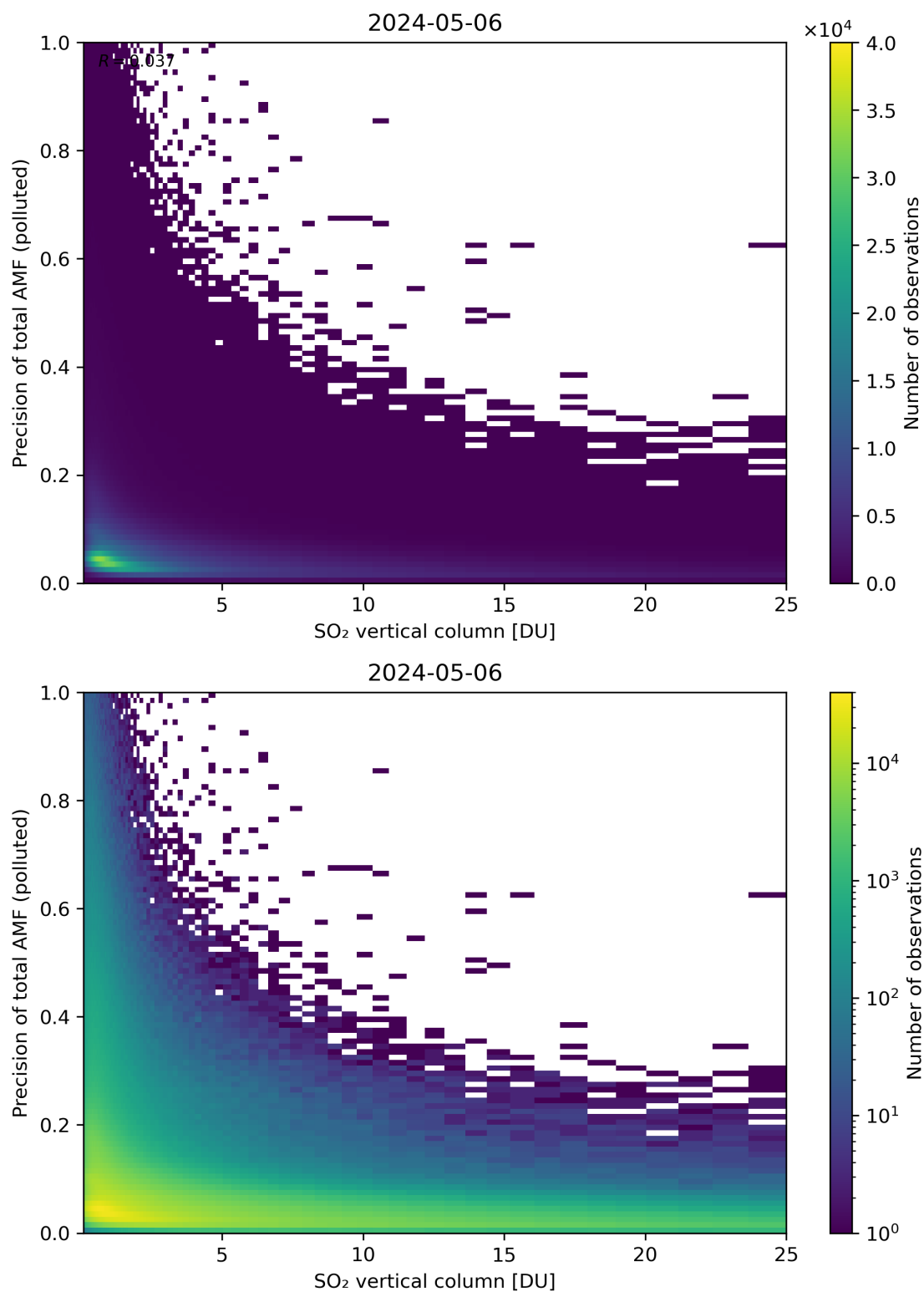
Figure 306: Scatter density plot of “SO 2 vertical column” against “Precision of total AMF (polluted)” for 2024-05-05 to 2024-05-07.
