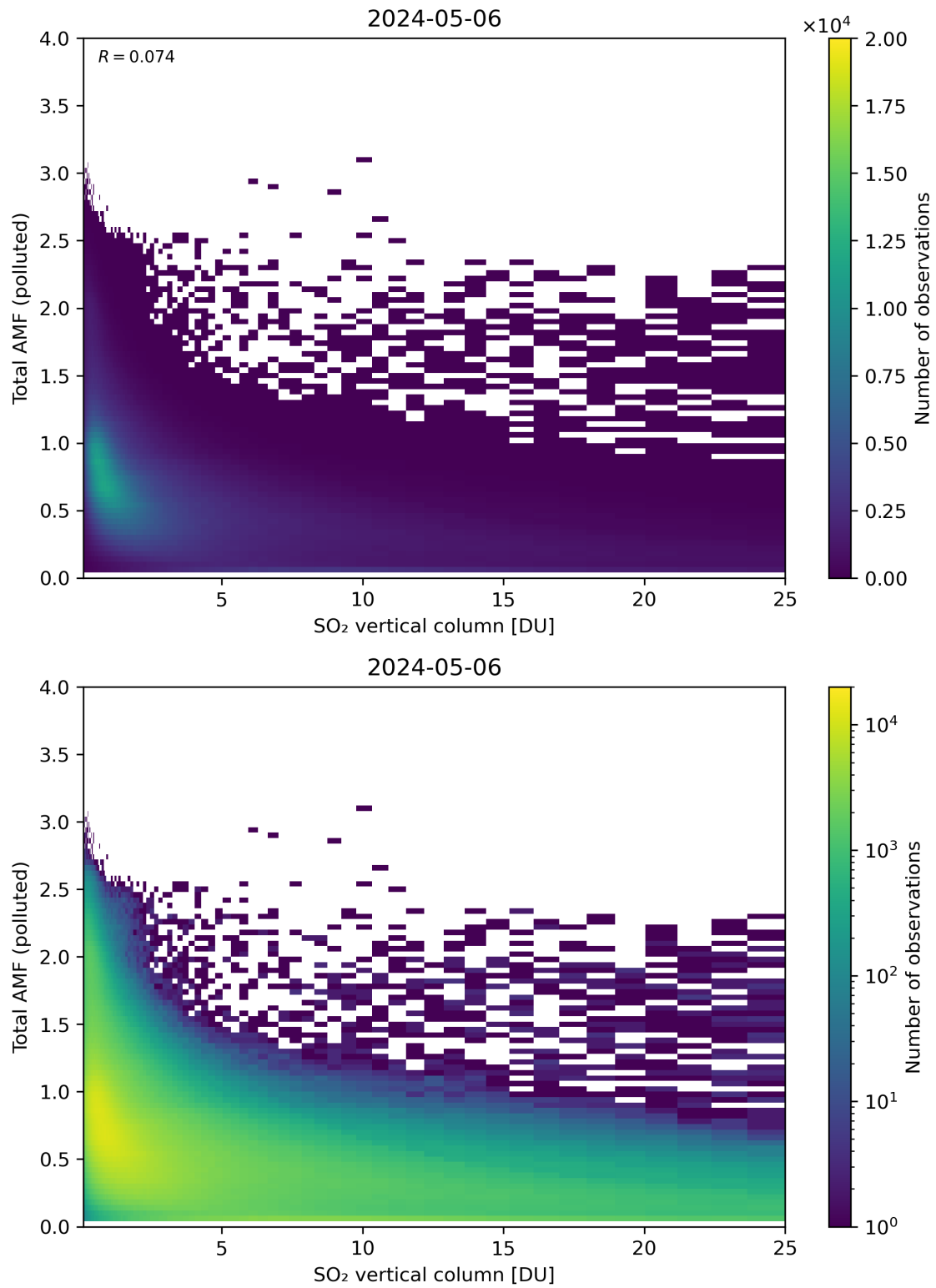
Figure 305: Scatter density plot of “SO 2 vertical column” against “Total AMF (polluted)” for 2024-05-05 to 2024-05-07.
