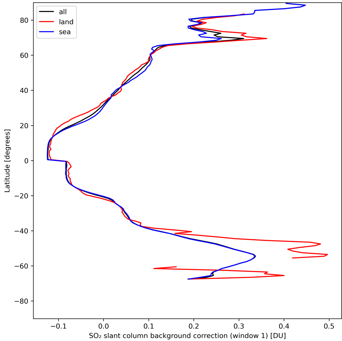
Figure 36: Zonal average of “SO 2 slant column background correction (window 1)” for 2024-05-05 to 2024-05-07.
