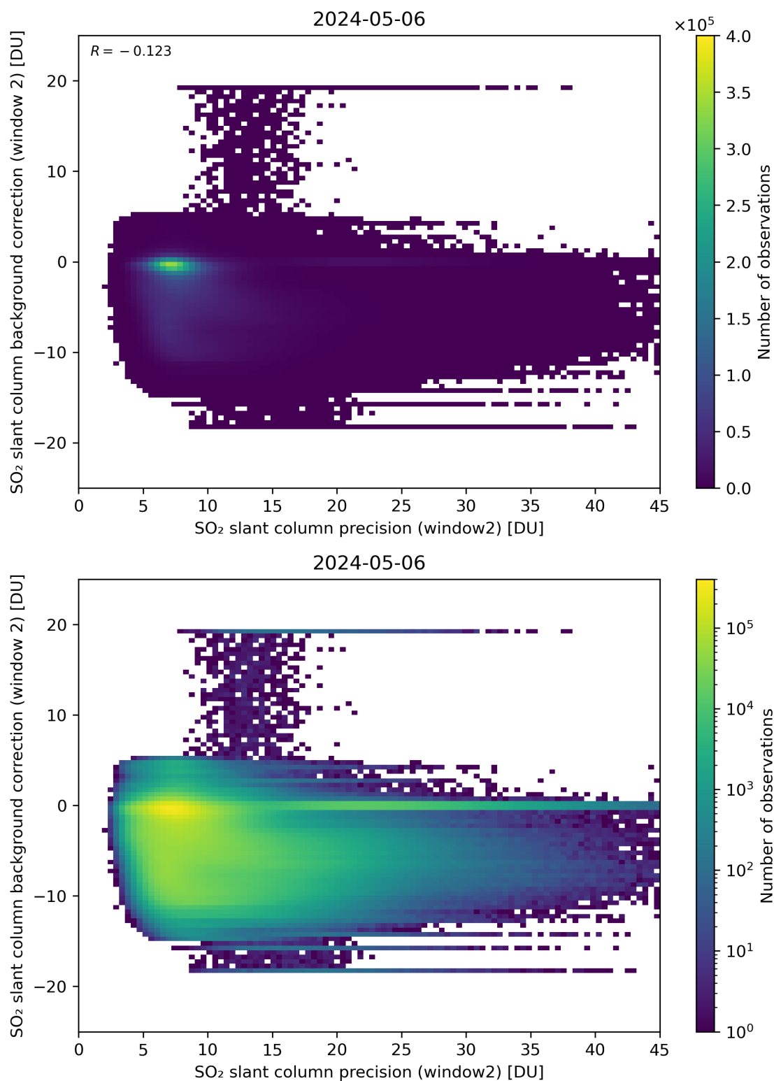
Figure 241: Scatter density plot of “SO 2 slant column precision (window2)” against “SO 2 slant column background correction (window 2)” for 2024-05-05 to 2024-05-07.
