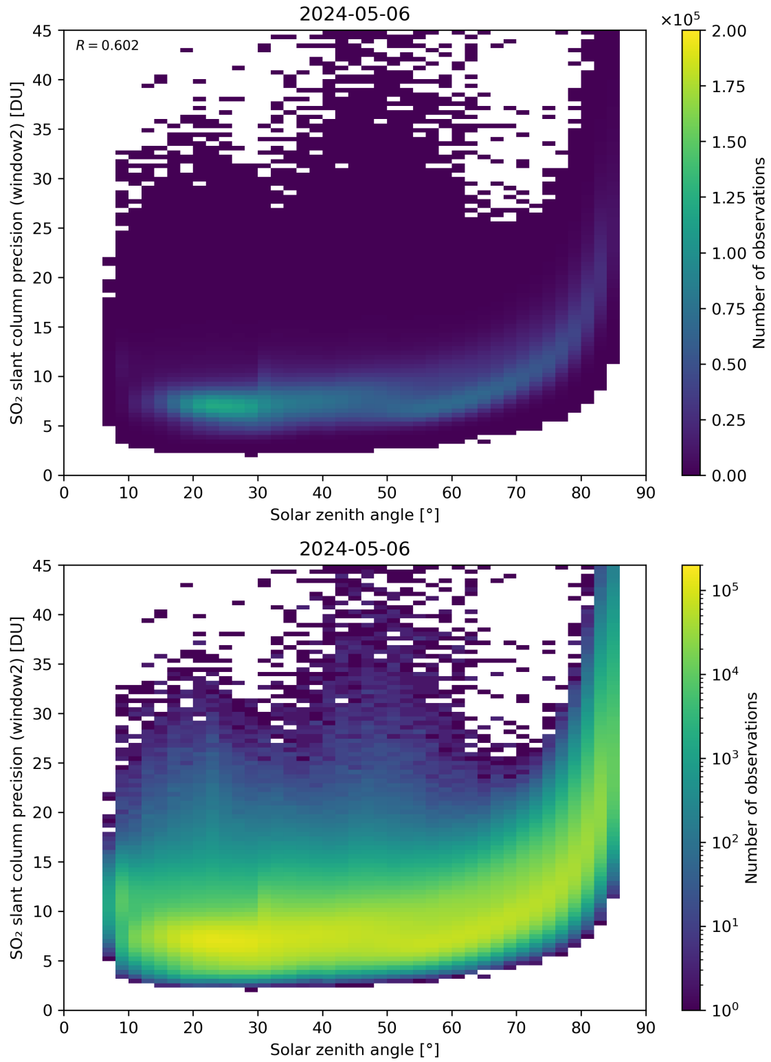
Figure 171: Scatter density plot of “Solar zenith angle” against “SO 2 slant column precision (window2)” for 2024-05-05 to 2024-05-07.
