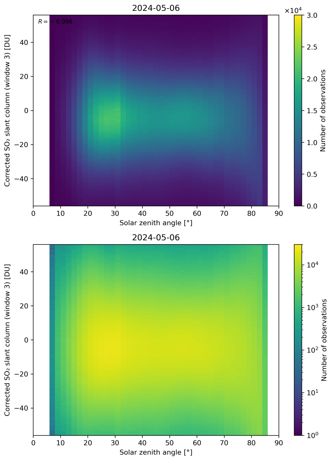
Figure 168: Scatter density plot of “Solar zenith angle” against “Corrected SO 2 slant column (window 3)” for 2024-05-05 to 2024-05-07.
