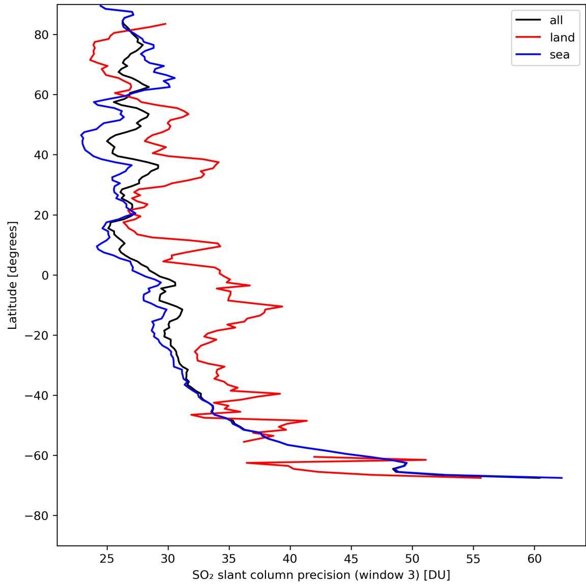
Figure 42: Zonal average of “SO 2 slant column precision (window 3)” for 2024-05-05 to 2024-05-07.
