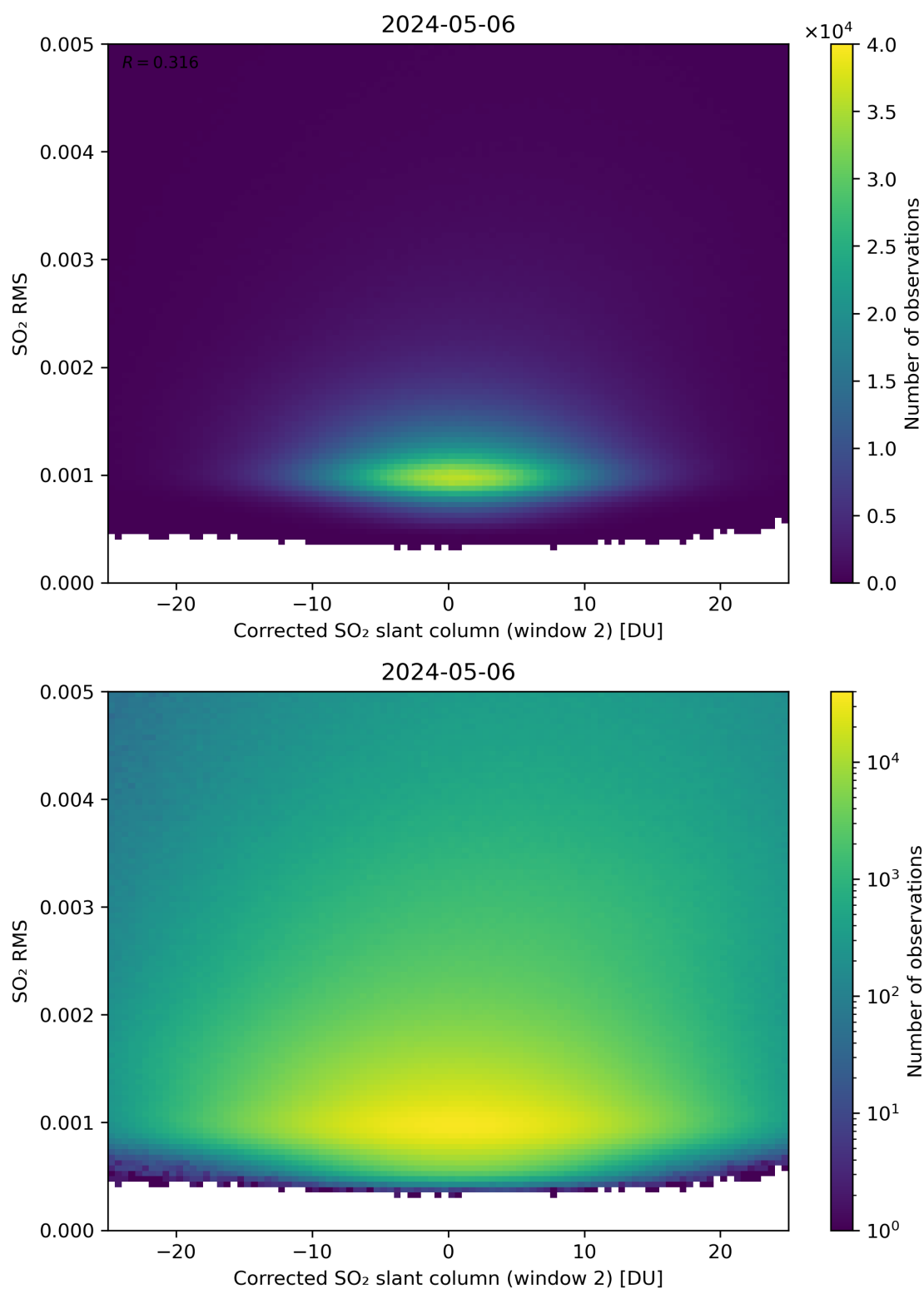
Figure 198: Scatter density plot of “Corrected SO 2 slant column (window 2)” against “SO 2 RMS” for 2024-05-05 to 2024-05-07.
