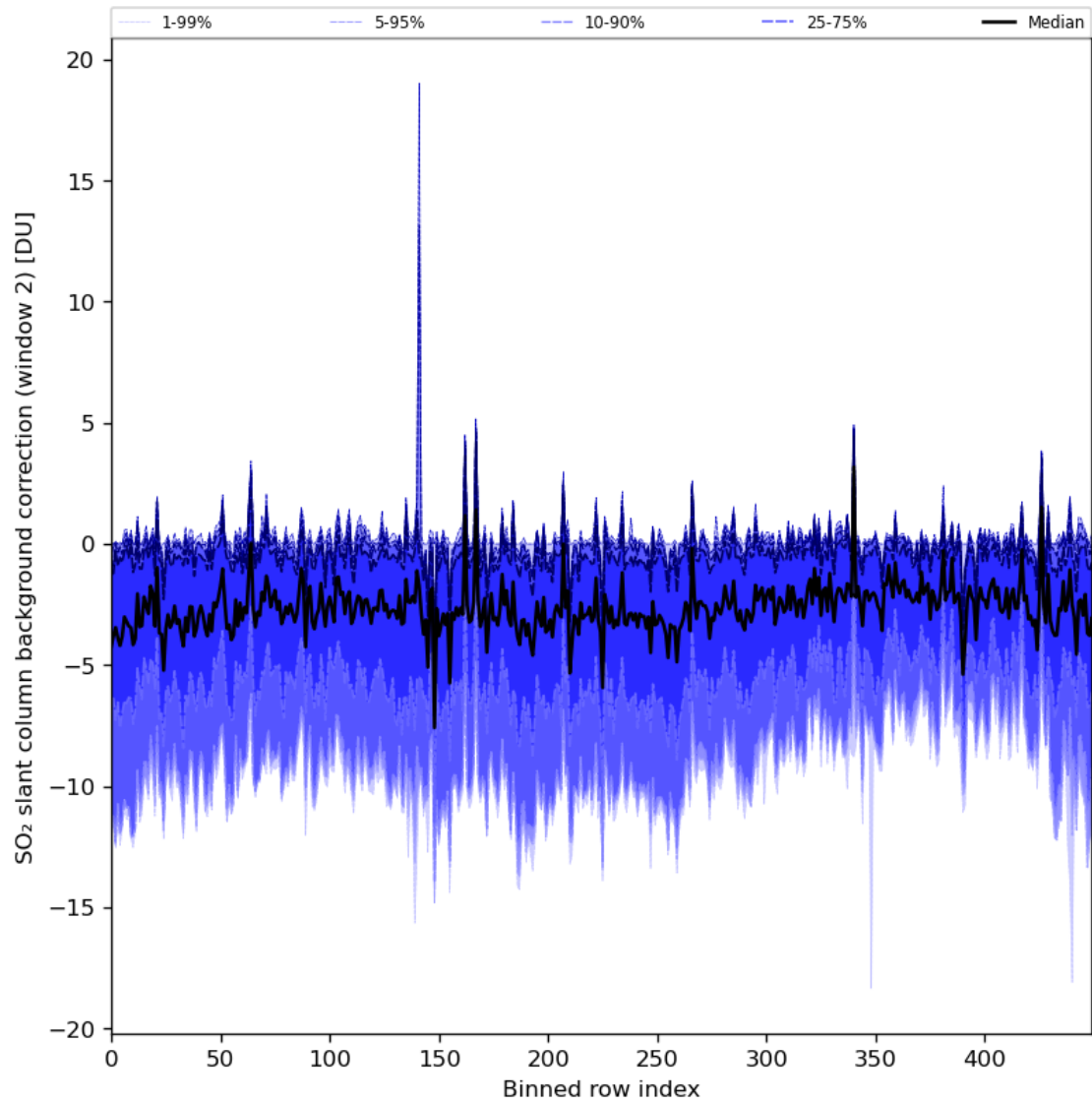
Figure 86: Along track statistics of “SO 2 slant column background correction (window 2)” for 2024-05-05 to 2024-05-07
