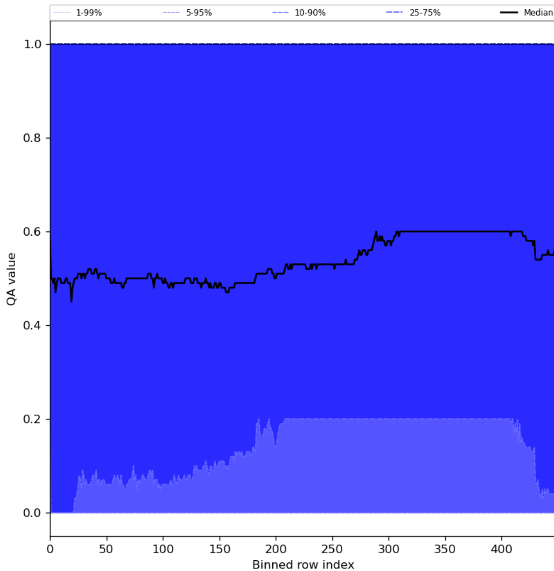
Figure 75: Along track statistics of “QA value” for 2024-05-05 to 2024-05-07
