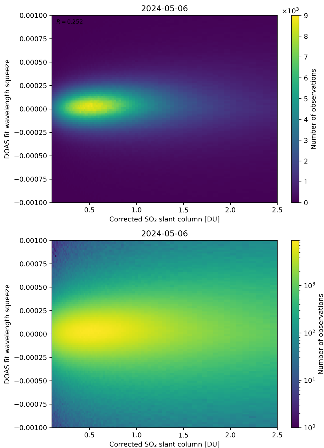
Figure 182: Scatter density plot of “Corrected SO 2 slant column” against “DOAS fit wavelength squeeze” for 2024-05-05 to 2024-05-07.
