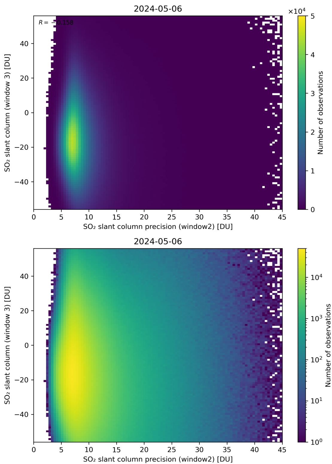
Figure 249: Scatter density plot of “SO 2 slant column precision (window2)” against “SO 2 slant column (window 3)” for 2024-05-05 to 2024-05-07.
