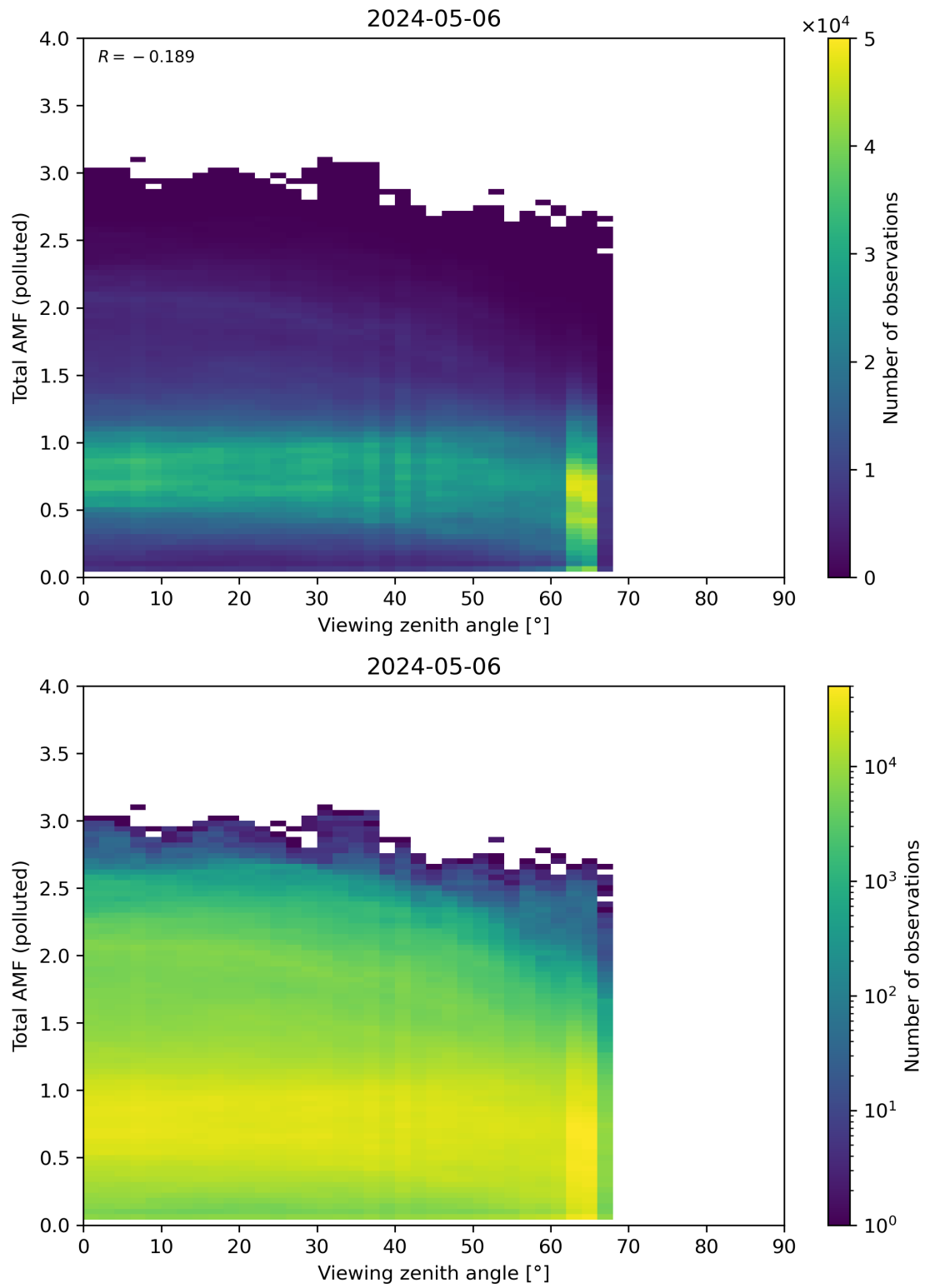
Figure 325: Scatter density plot of “Viewing zenith angle” against “Total AMF (polluted)” for 2024-05-05 to 2024-05-07.
