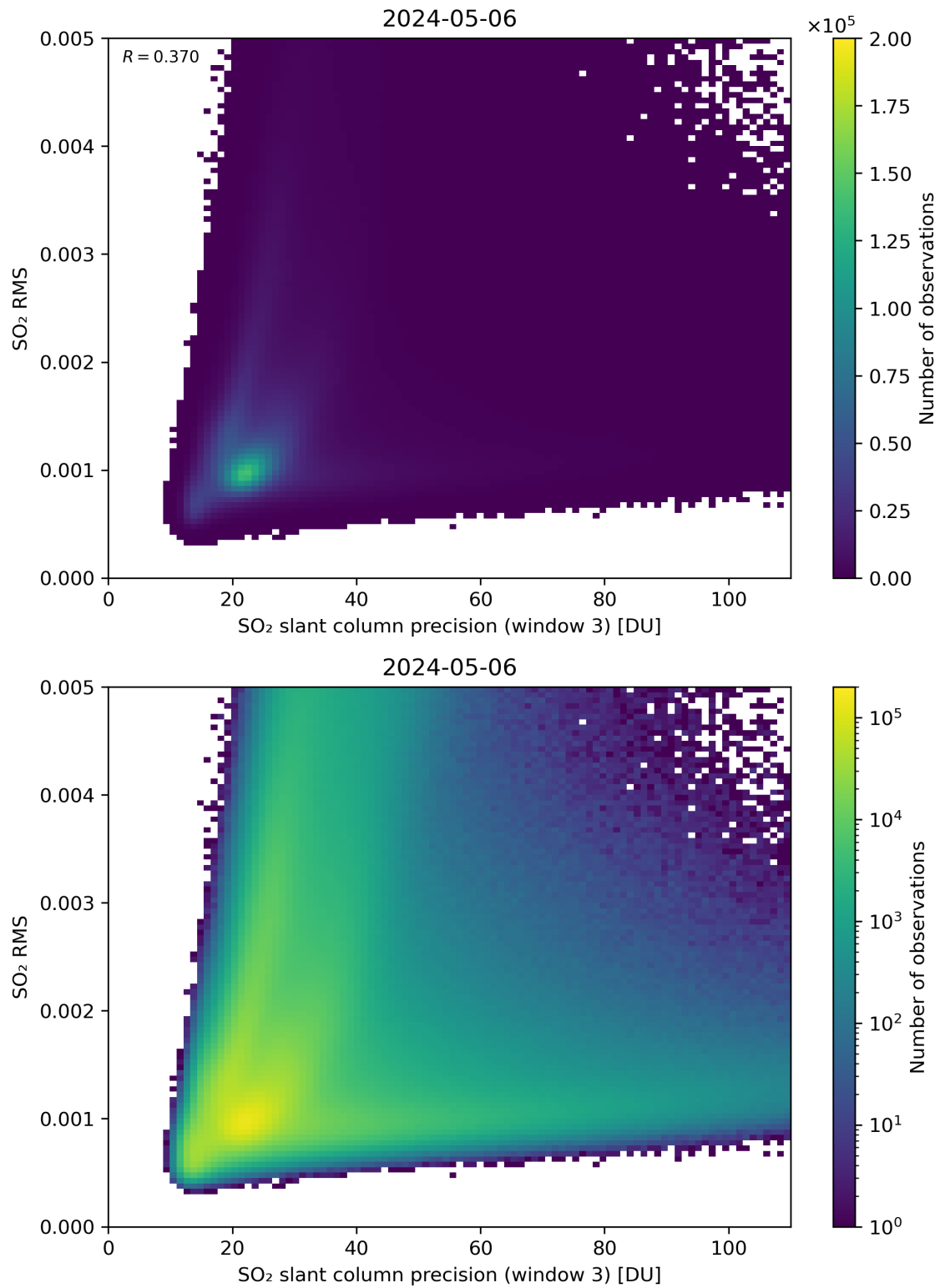
Figure 260: Scatter density plot of “SO 2 slant column precision (window 3)” against “SO 2 RMS” for 2024-05-05 to 2024-05-07.
