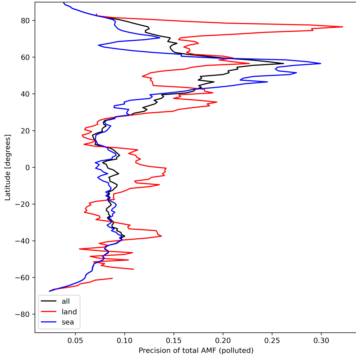
Figure 49: Zonal average of “Precision of total AMF (polluted)” for 2024-05-05 to 2024-05-07.
