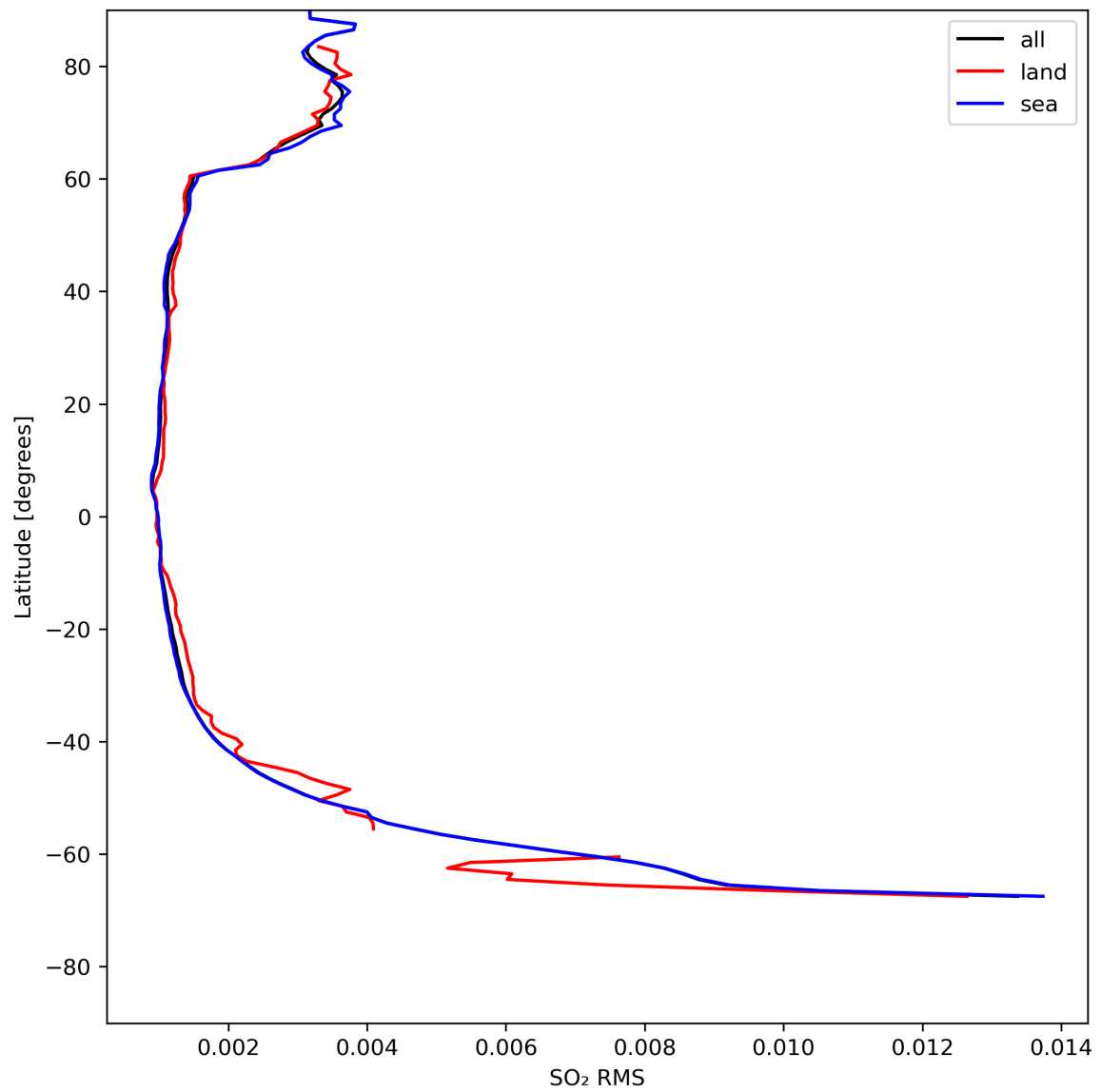
Figure 47: Zonal average of “SO 2 RMS” for 2024-05-05 to 2024-05-07.
