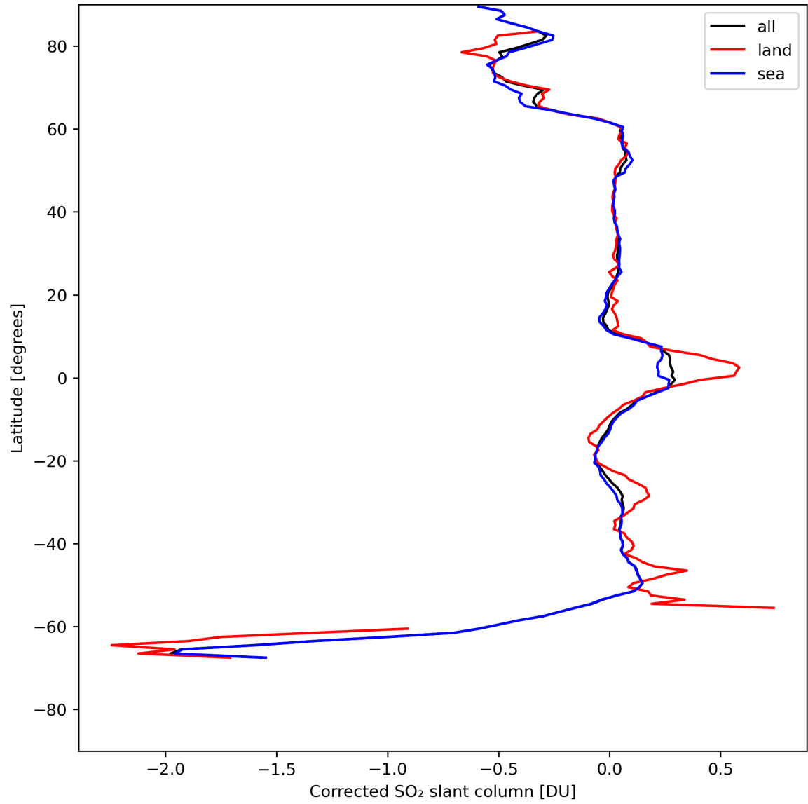
Figure 32: Zonal average of “Corrected SO 2 slant column” for 2024-05-05 to 2024-05-07.
