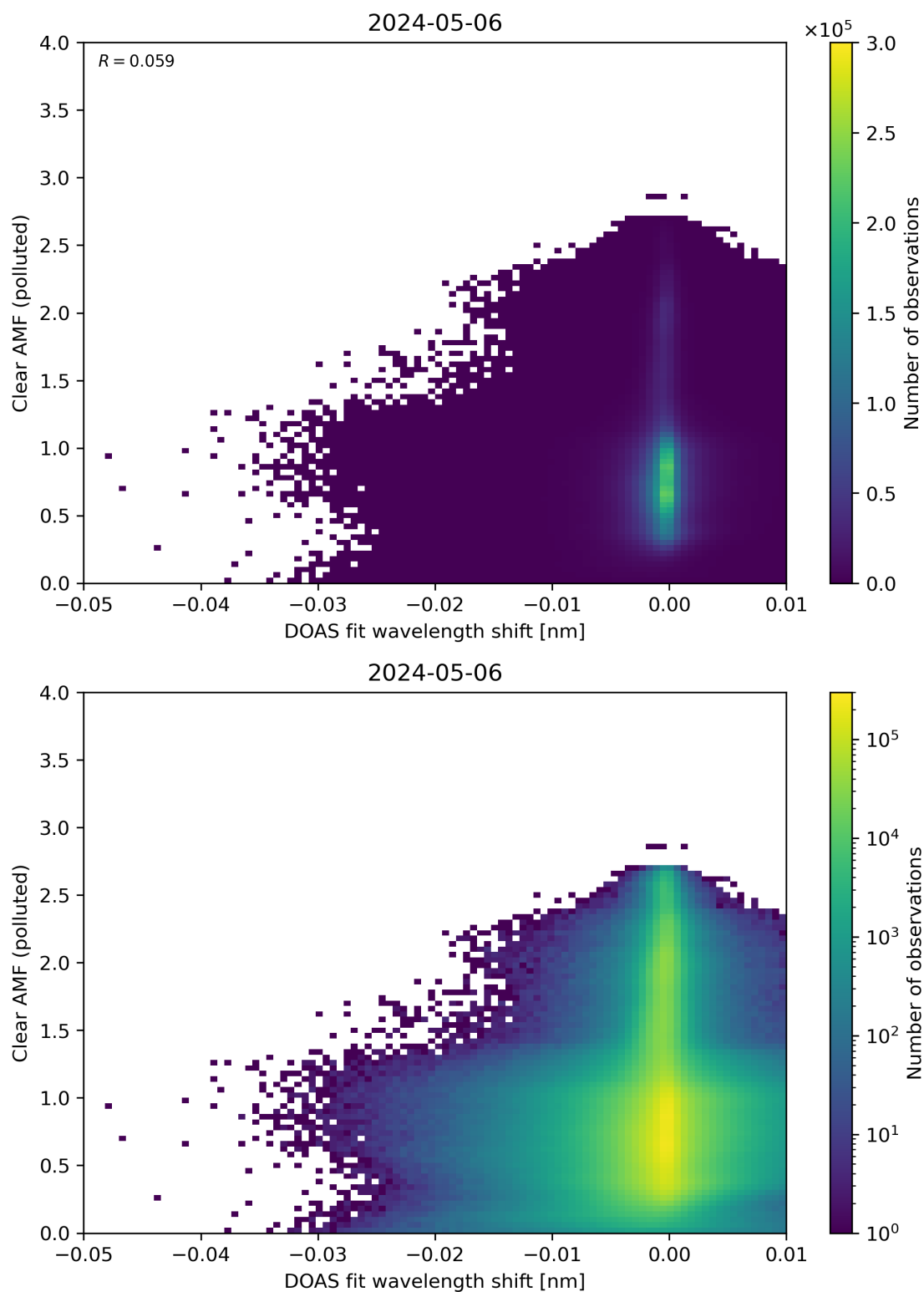
Figure 129: Scatter density plot of “DOAS fit wavelength shift” against “Clear AMF (polluted)” for 2024-05-05 to 2024-05-07.
