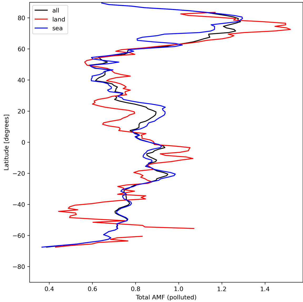
Figure 48: Zonal average of “Total AMF (polluted)” for 2024-05-05 to 2024-05-07.
