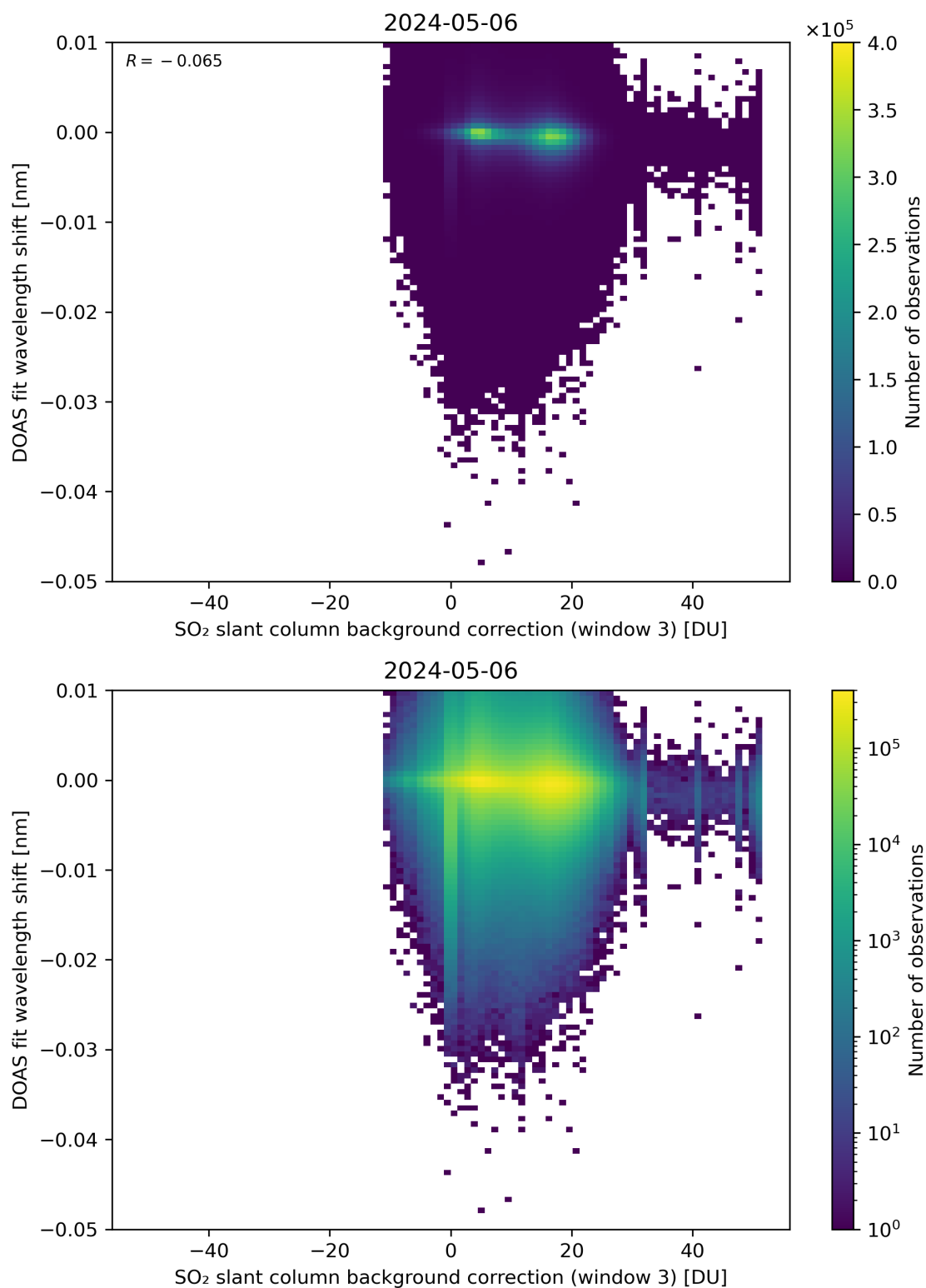
Figure 121: Scatter density plot of “SO 2 slant column background correction (window 3)” against “DOAS fit wavelength shift” for 2024-05-05 to 2024-05-07.
