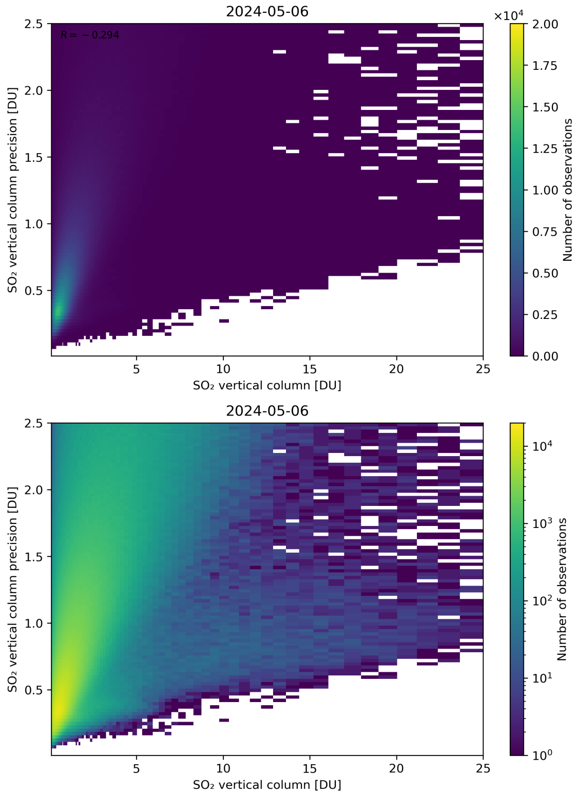
Figure 307: Scatter density plot of “SO 2 vertical column” against “SO 2 vertical column precision” for 2024-05-05 to 2024-05-07.
