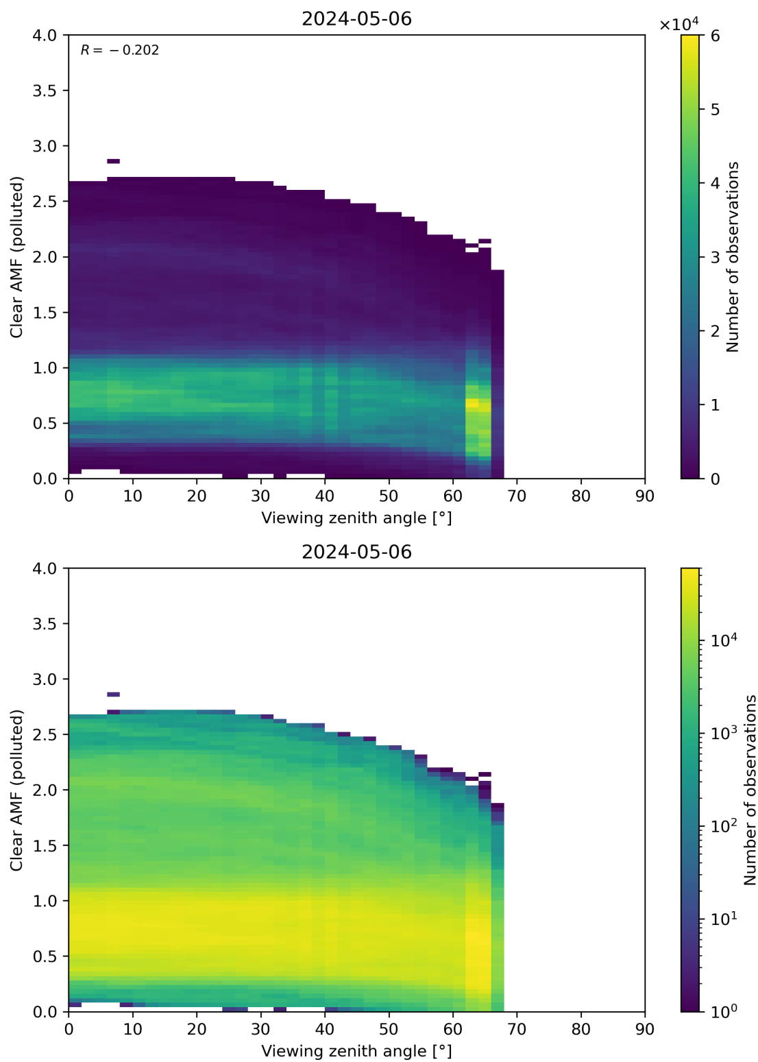
Figure 316: Scatter density plot of “Viewing zenith angle” against “Clear AMF (polluted)” for 2024-05-05 to 2024-05-07.
