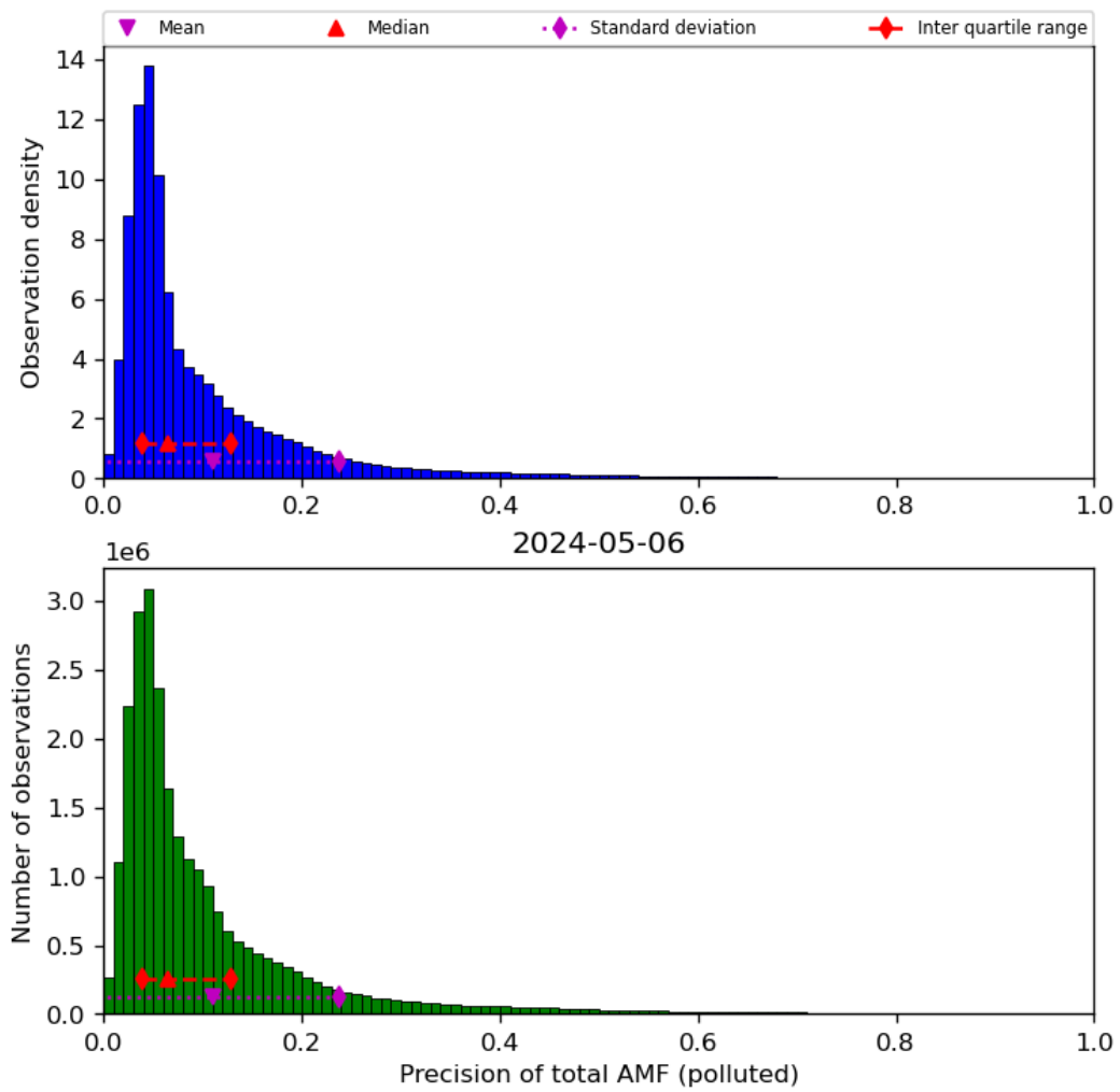
Figure 72: Histogram of “Precision of total AMF (polluted)” for 2024-05-05 to 2024-05-07
