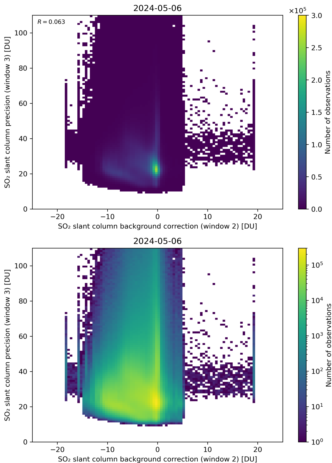
Figure 118: Scatter density plot of “SO 2 slant column background correction (window 2)” against “SO 2 slant column precision (window 3)” for 2024-05-05 to 2024-05-07.
