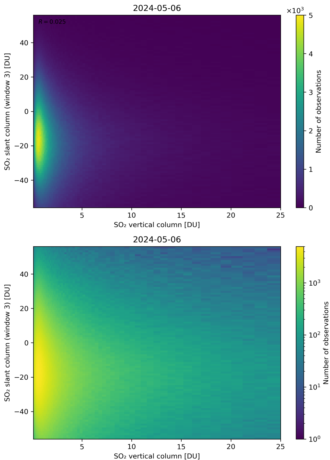
Figure 303: Scatter density plot of “SO 2 vertical column” against “SO 2 slant column (window 3)” for 2024-05-05 to 2024-05-07.
