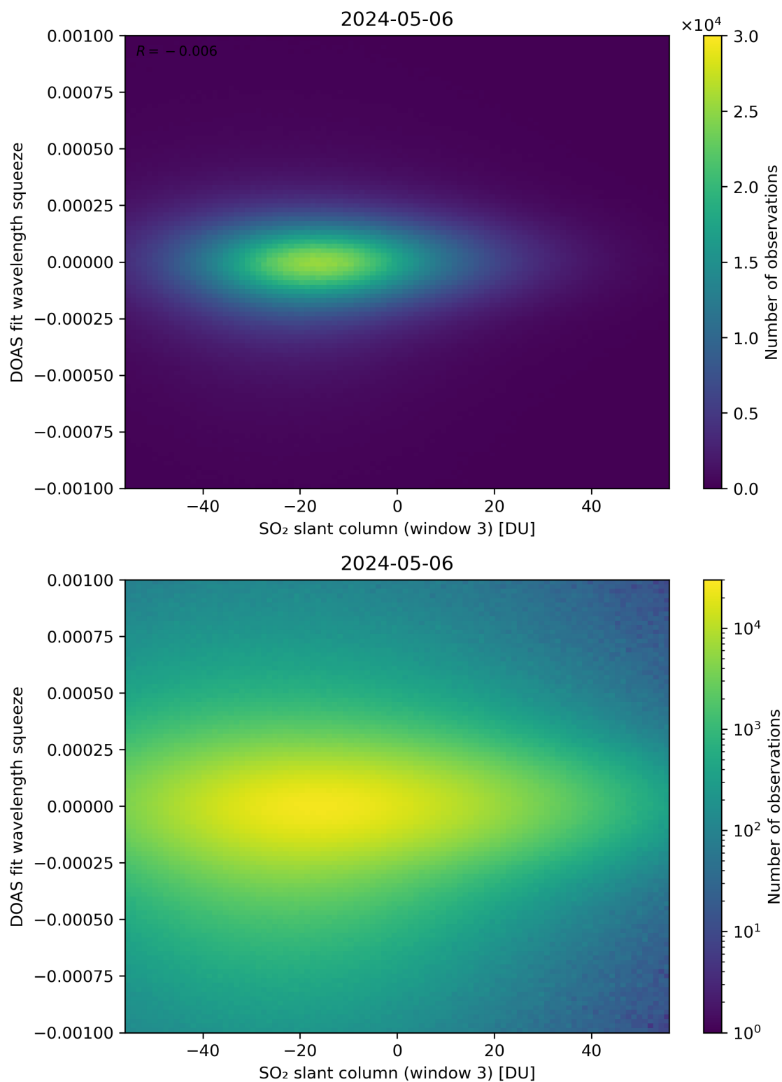
Figure 255: Scatter density plot of “SO 2 slant column (window 3)” against “DOAS fit wavelength squeeze” for 2024-05-05 to 2024-05-07.
