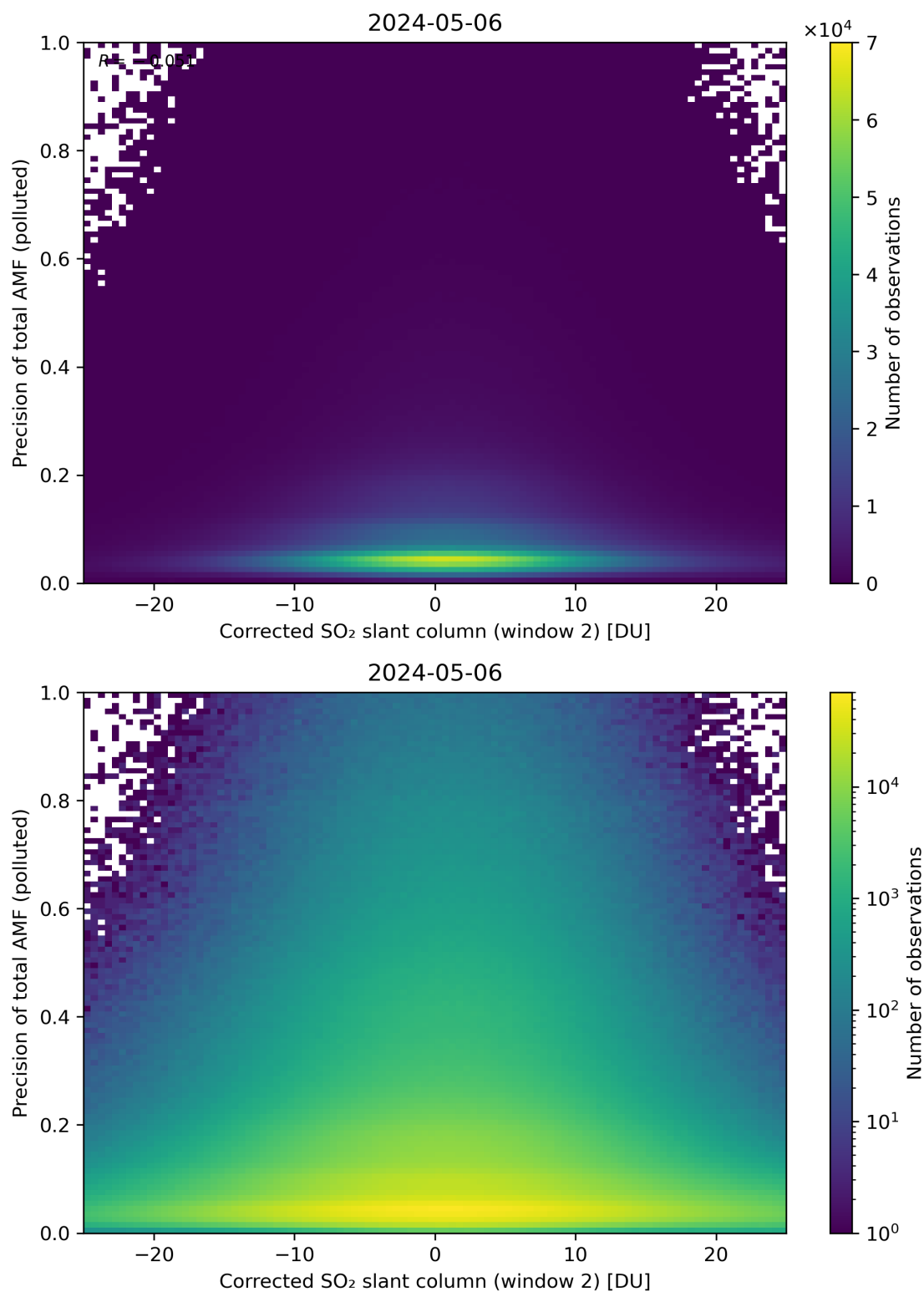
Figure 204: Scatter density plot of “Corrected SO 2 slant column (window 2)” against “Precision of total AMF (polluted)” for 2024-05-05 to 2024-05-07.
