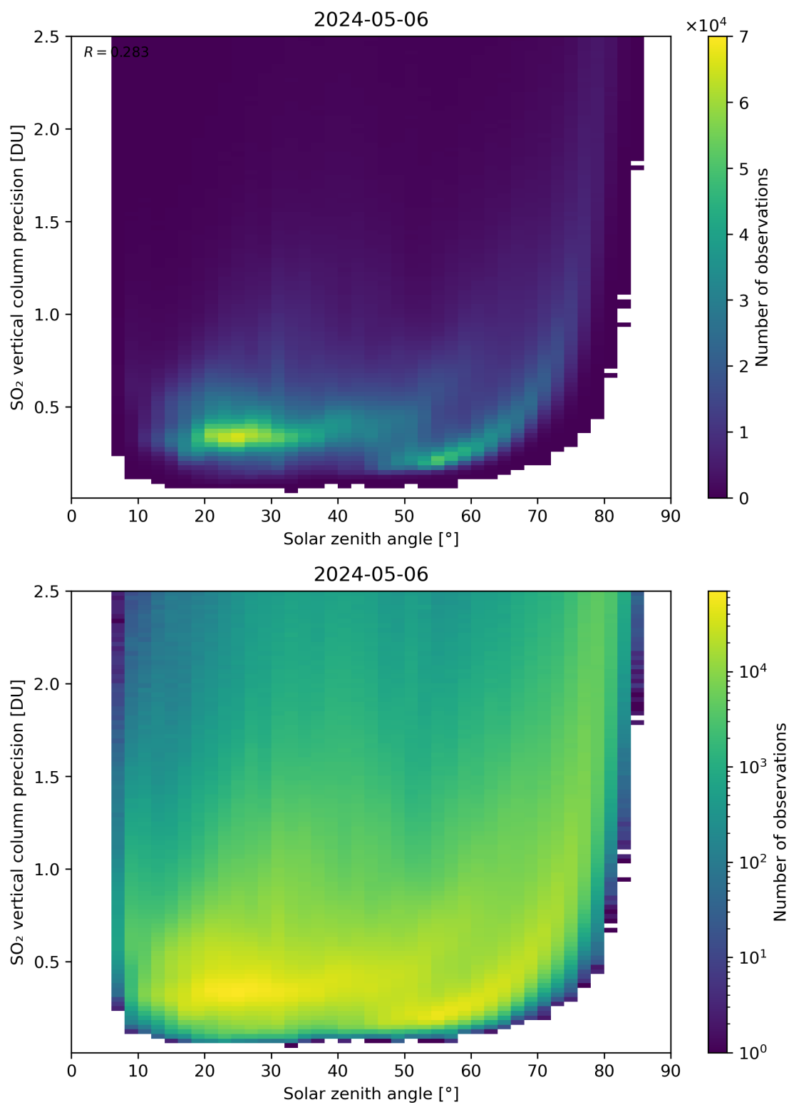
Figure 177: Scatter density plot of “Solar zenith angle” against “SO 2 vertical column precision” for 2024-05-05 to 2024-05-07.
