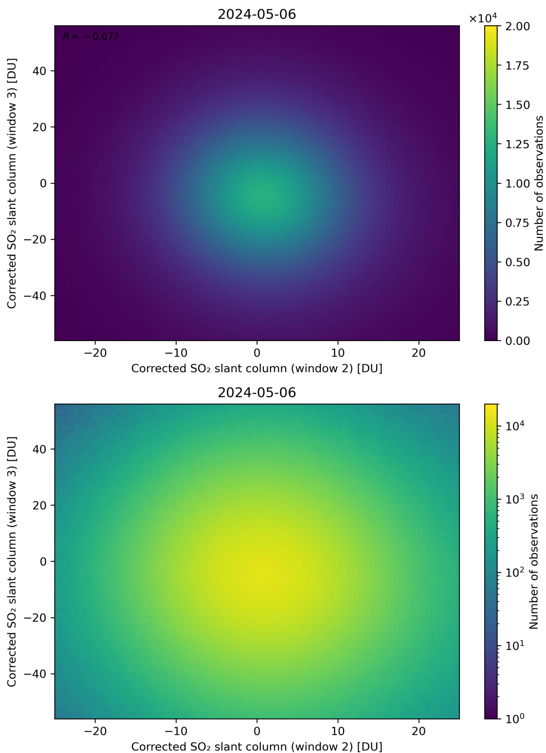
Figure 200: Scatter density plot of “Corrected SO 2 slant column (window 2)” against “Corrected SO 2 slant column (window 3)” for 2024-05-05 to 2024-05-07.
