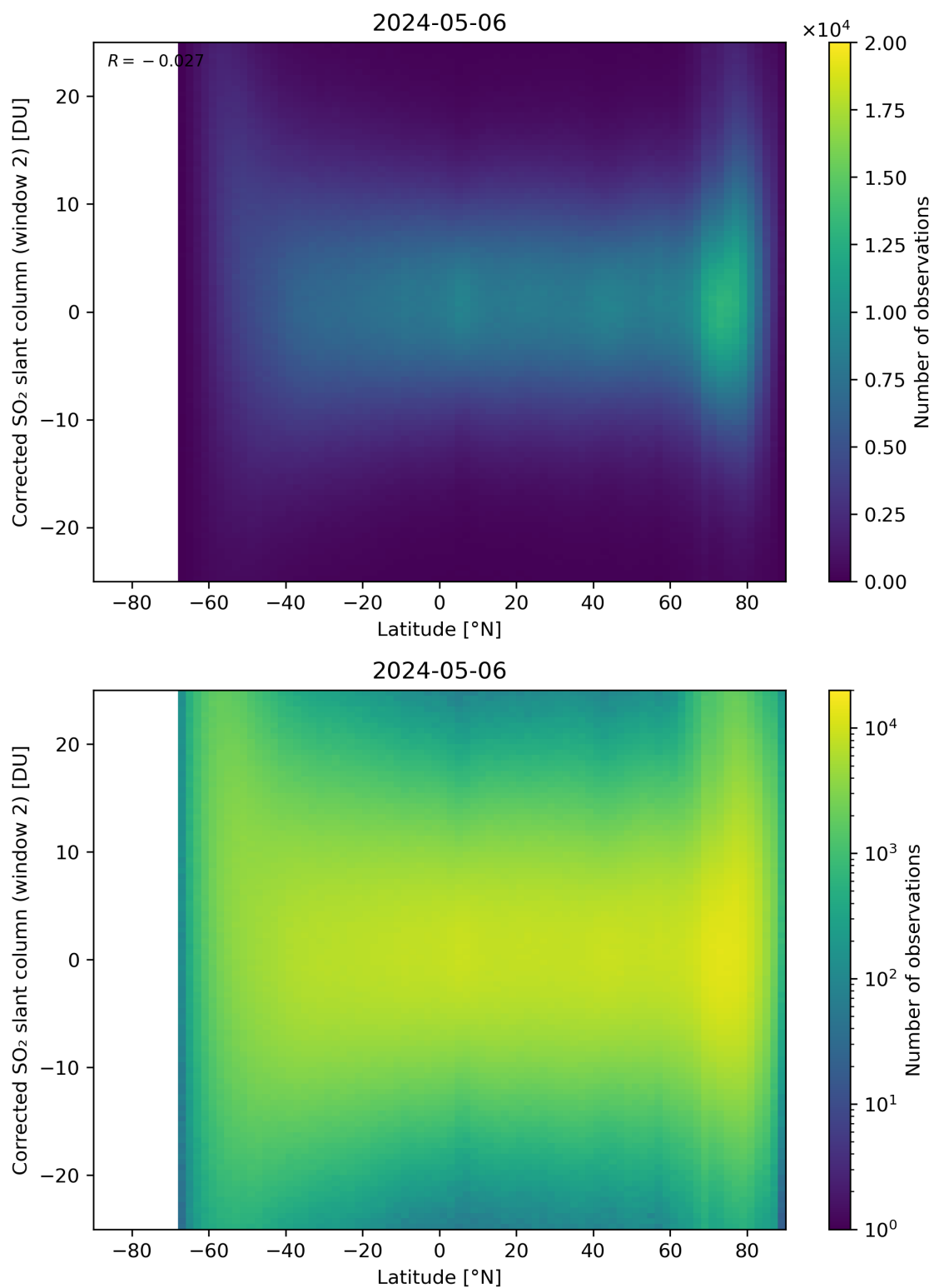
Figure 147: Scatter density plot of “Latitude” against “Corrected SO 2 slant column (window 2)” for 2024-05-05 to 2024-05-07.
