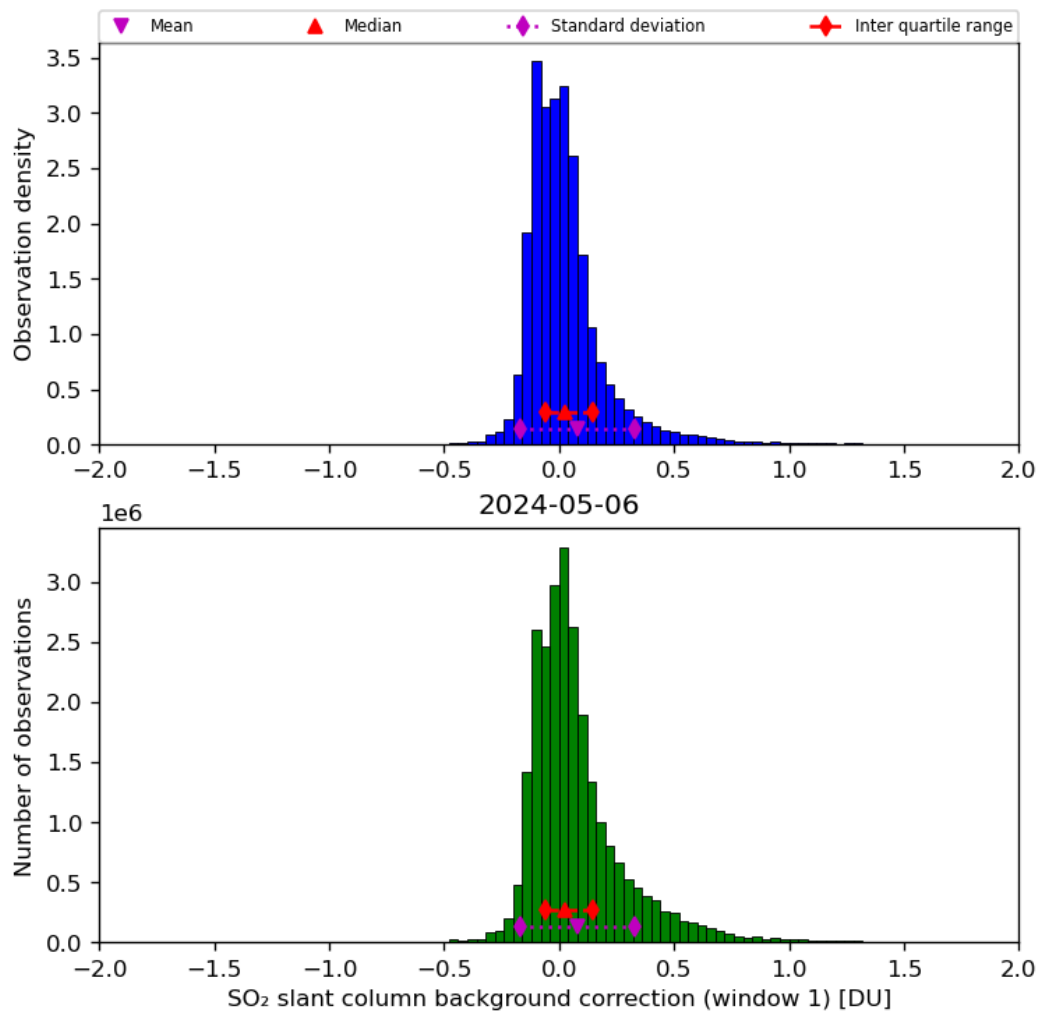
Figure 59: Histogram of “SO 2 slant column background correction (window 1)” for 2024-05-05 to 2024-05-07
