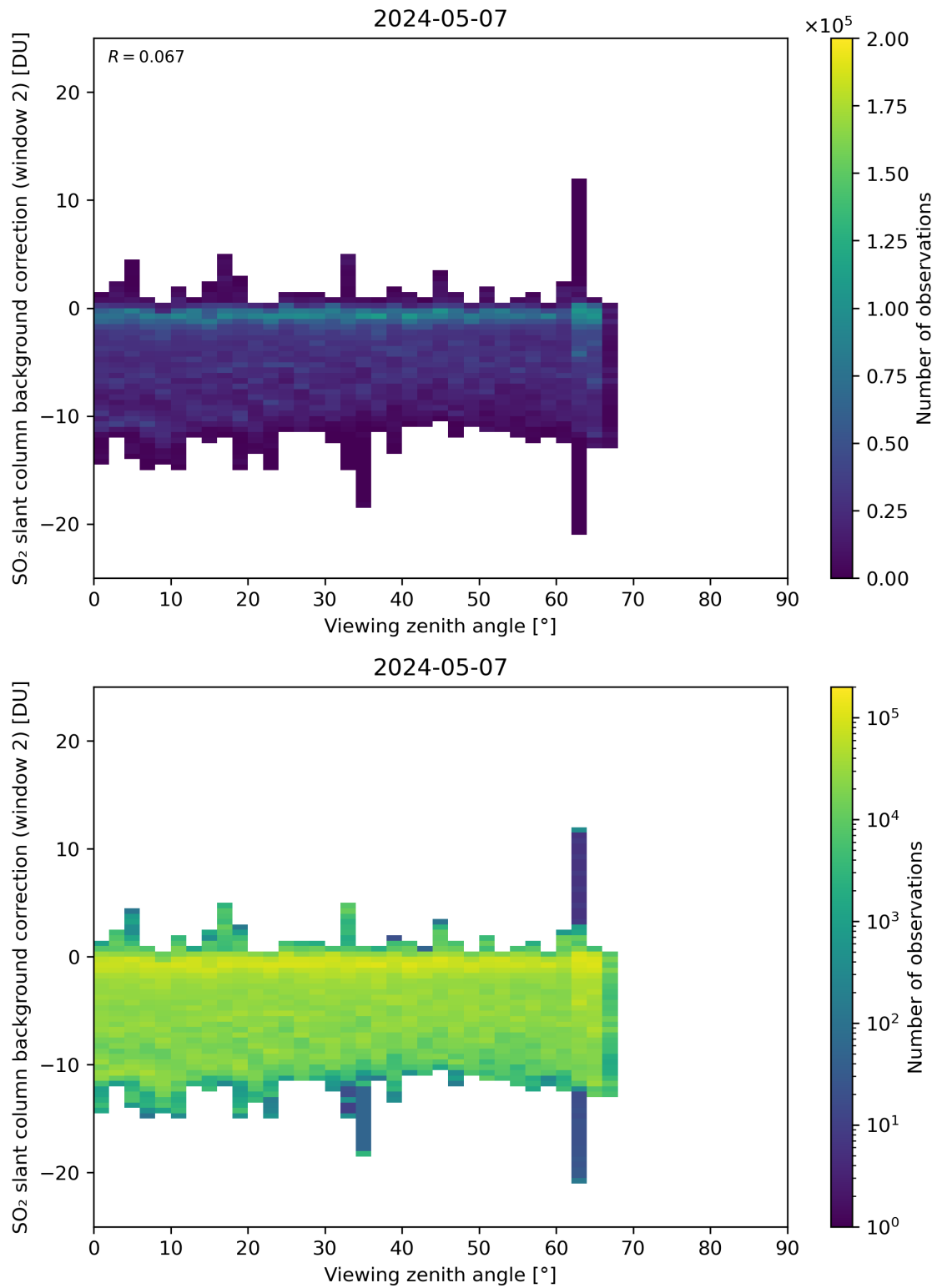
Figure 309: Scatter density plot of “Viewing zenith angle” against “SO 2 slant column background correction (window 2)” for 2024-05-07 to 2024-05-08.
