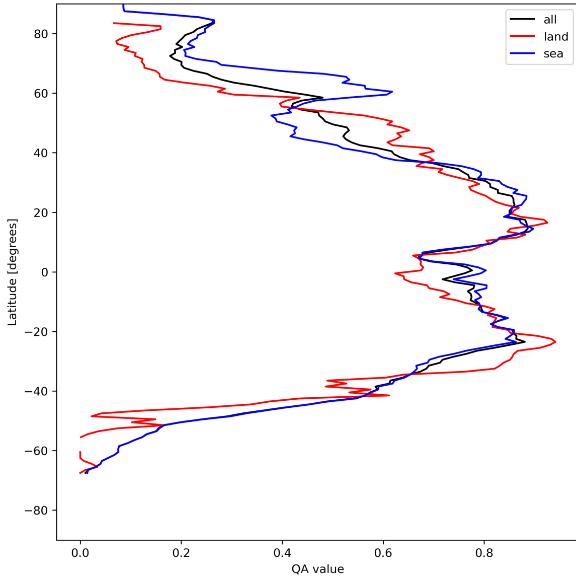
Figure 29: Zonal average of “QA value” for 2024-05-07 to 2024-05-08.
