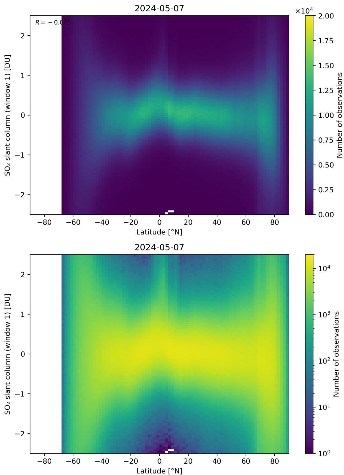
Figure 149: Scatter density plot of “Latitude” against “SO 2 slant column (window 1)” for 2024-05-07 to 2024-05-08.
