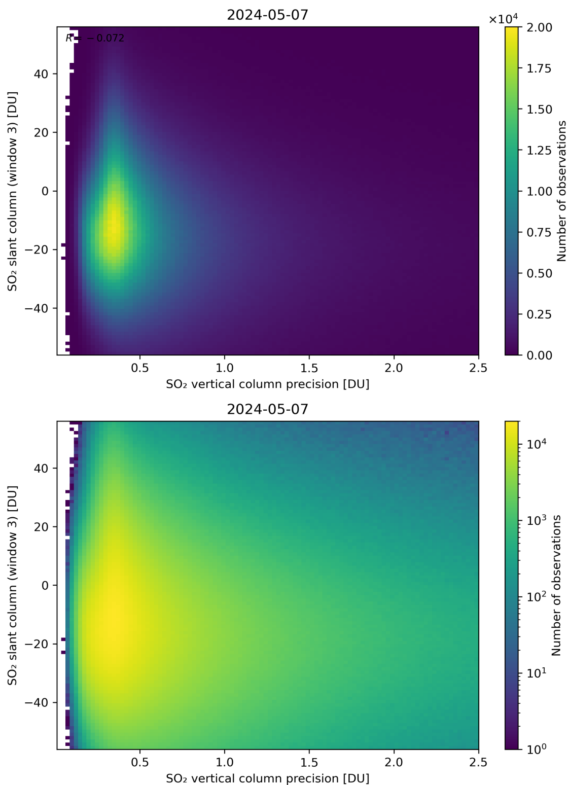
Figure 292: Scatter density plot of “SO 2 vertical column precision” against “SO 2 slant column (window 3)” for 2024-05-07 to 2024-05-08.
