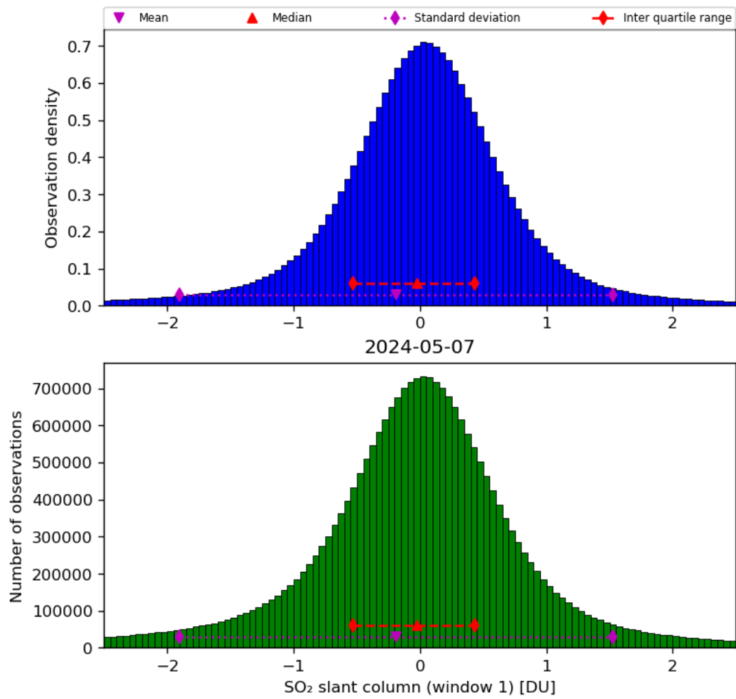
Figure 56: Histogram of “SO 2 slant column (window 1)” for 2024-05-07 to 2024-05-08
