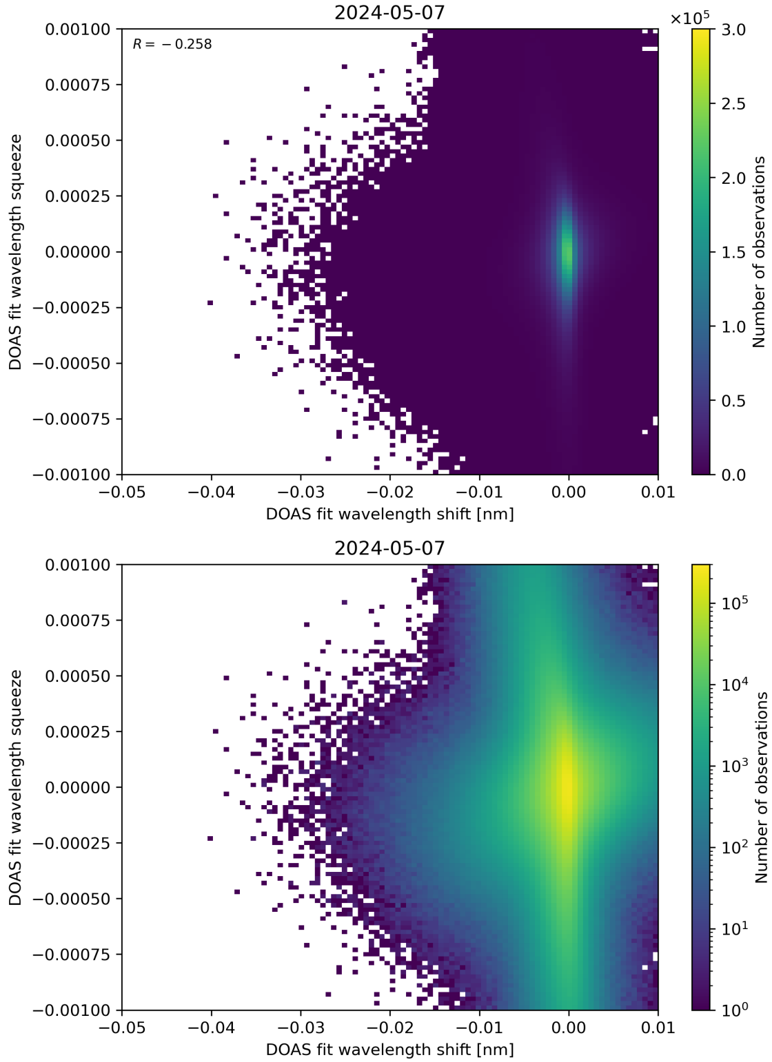
Figure 127: Scatter density plot of “DOAS fit wavelength shift” against “DOAS fit wavelength squeeze” for 2024-05-07 to 2024-05-08.
