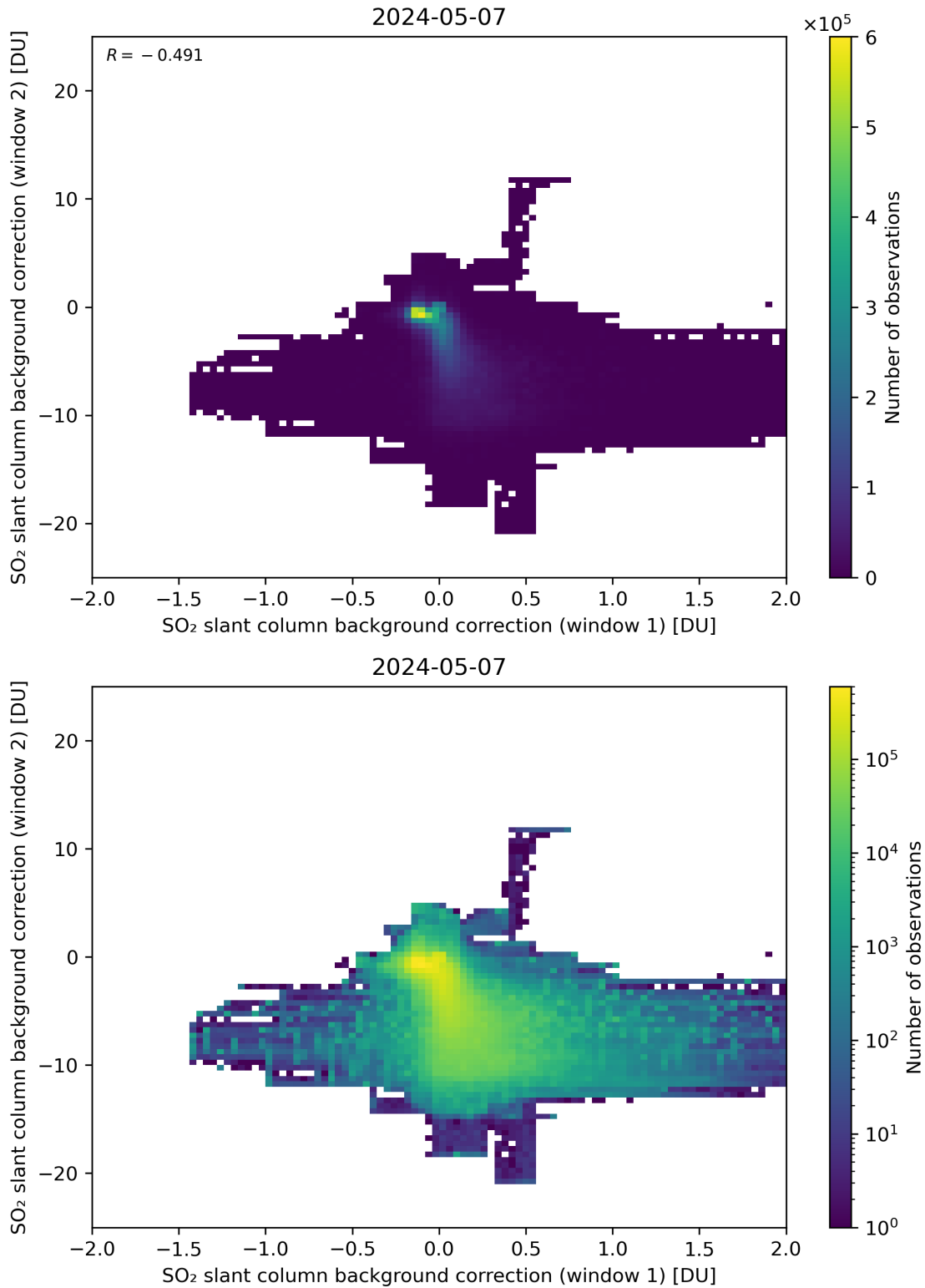
Figure 98: Scatter density plot of “SO 2 slant column background correction (window 1)” against “SO 2 slant column background correction (window 2)” for 2024-05-07 to 2024-05-08.
