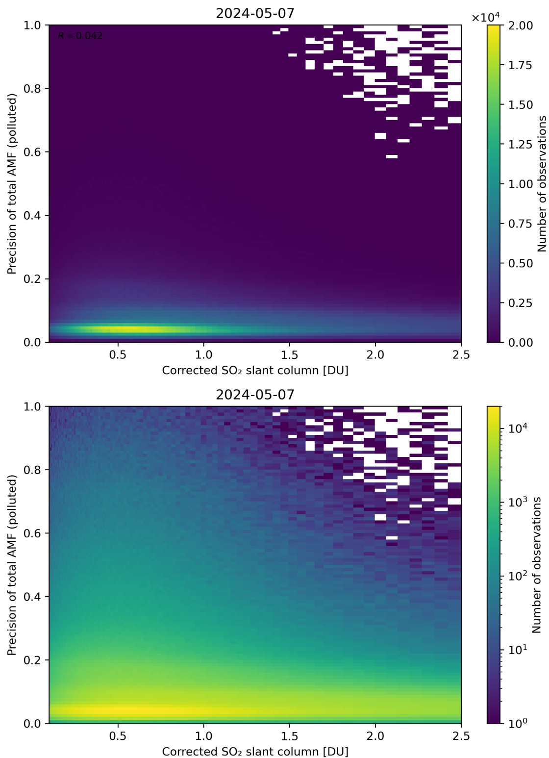
Figure 193: Scatter density plot of “Corrected SO 2 slant column” against “Precision of total AMF (polluted)” for 2024-05-07 to 2024-05-08.
