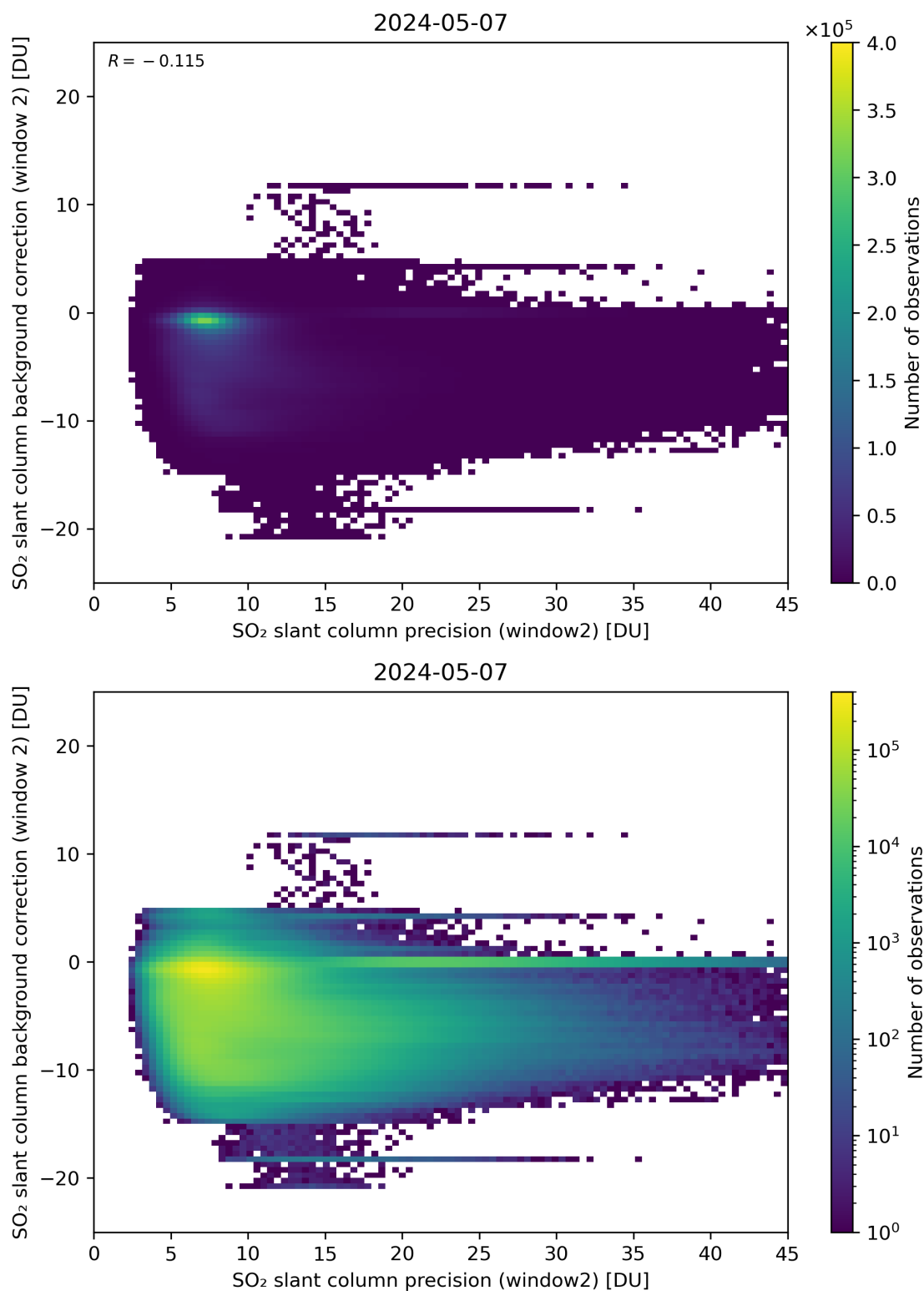
Figure 241: Scatter density plot of “SO 2 slant column precision (window2)” against “SO 2 slant column background correction (window 2)” for 2024-05-07 to 2024-05-08.
