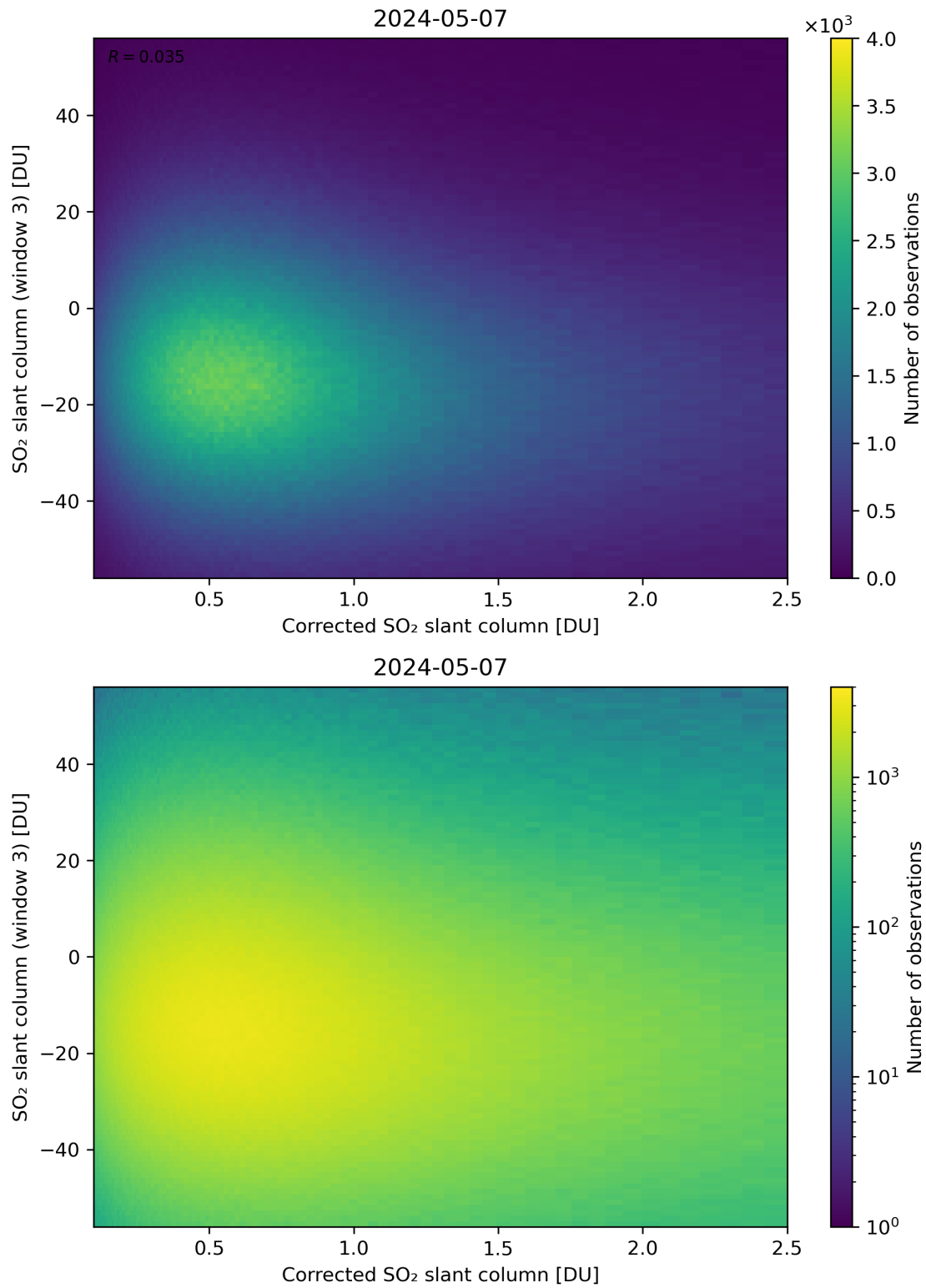
Figure 190: Scatter density plot of “Corrected SO 2 slant column” against “SO 2 slant column (window 3)” for 2024-05-07 to 2024-05-08.
