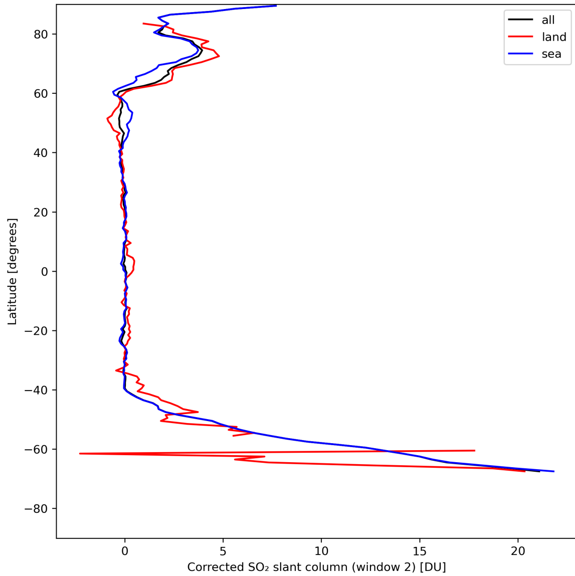
Figure 39: Zonal average of “Corrected SO 2 slant column (window 2)” for 2024-05-07 to 2024-05-08.
