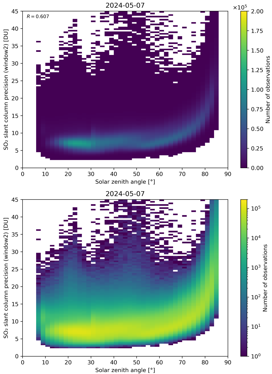
Figure 171: Scatter density plot of “Solar zenith angle” against “SO 2 slant column precision (window2)” for 2024-05-07 to 2024-05-08.
