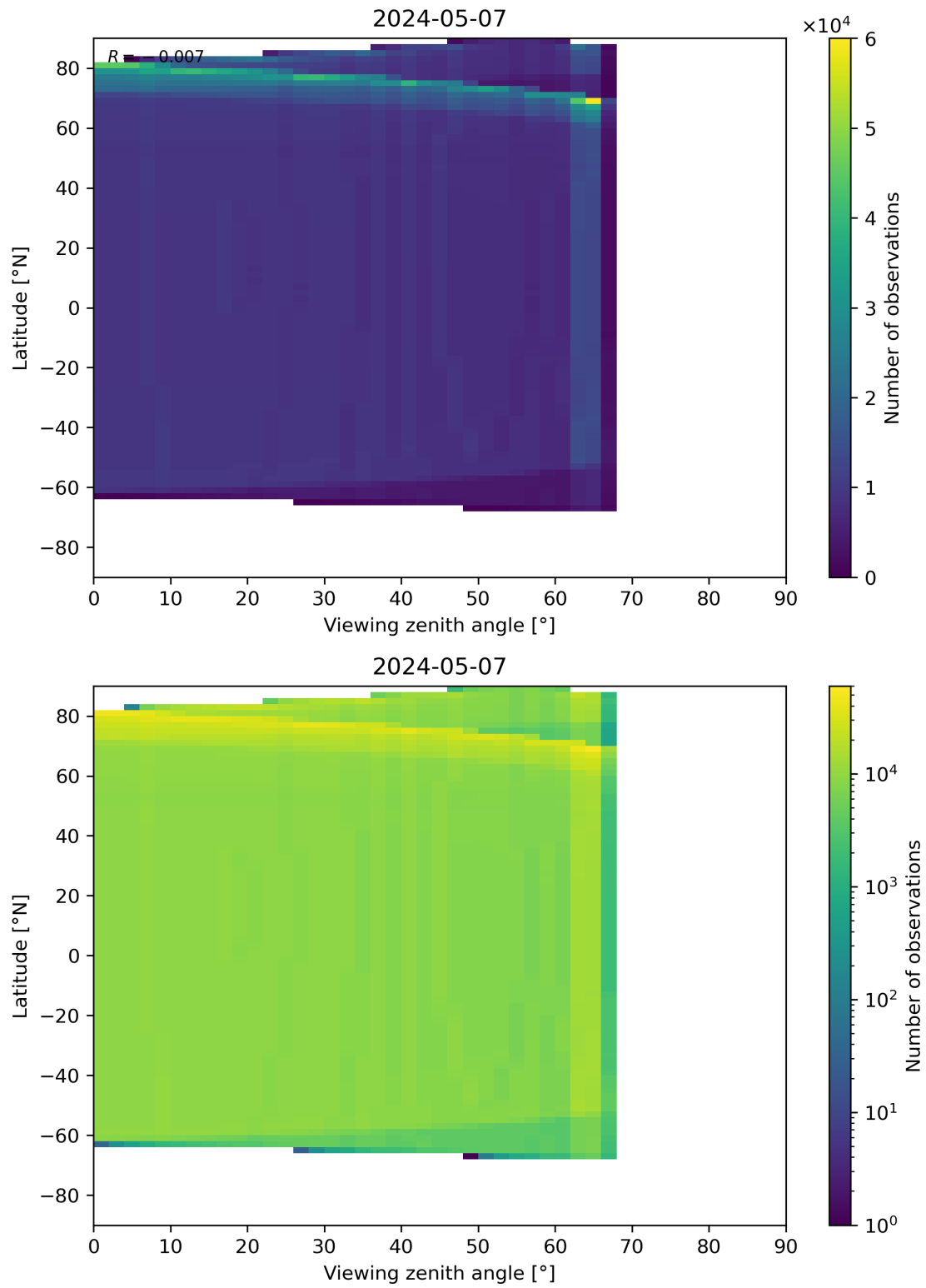
Figure 314: Scatter density plot of “Viewing zenith angle” against “Latitude” for 2024-05-07 to 2024-05-08.
