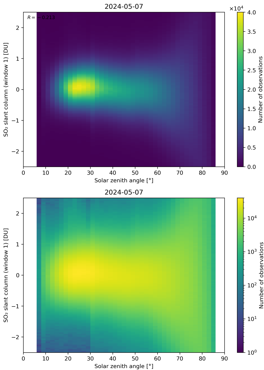
Figure 169: Scatter density plot of “Solar zenith angle” against “SO 2 slant column (window 1)” for 2024-05-07 to 2024-05-08.
