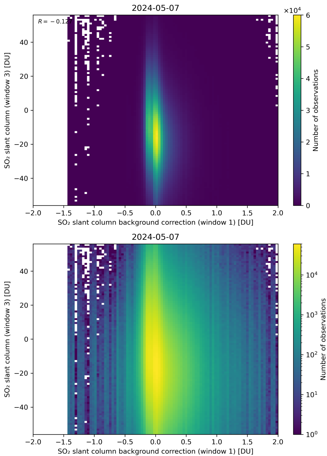
Figure 107: Scatter density plot of “SO 2 slant column background correction (window 1)” against “SO 2 slant column (window 3)” for 2024-05-07 to 2024-05-08.
