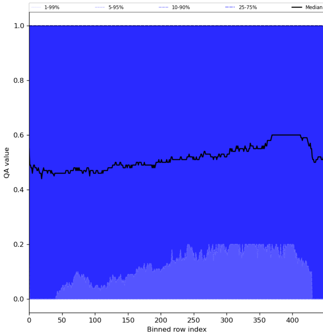
Figure 75: Along track statistics of “QA value” for 2024-05-07 to 2024-05-08
