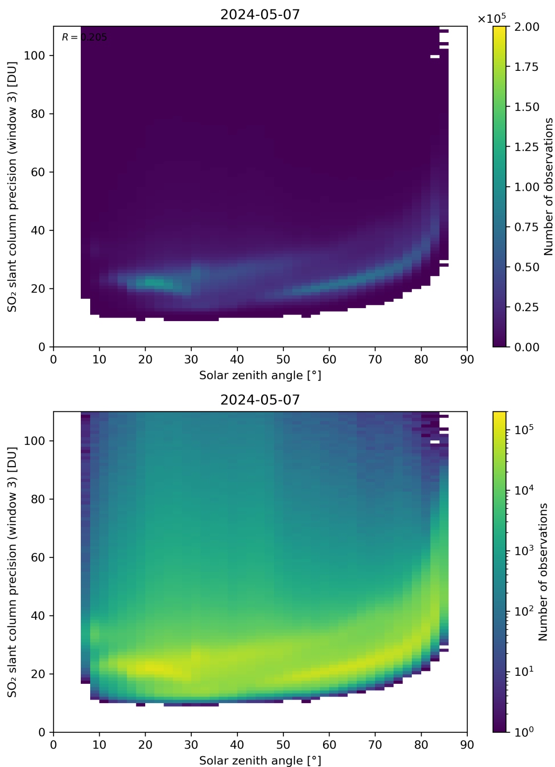
Figure 173: Scatter density plot of “Solar zenith angle” against “SO 2 slant column precision (window 3)” for 2024-05-07 to 2024-05-08.
