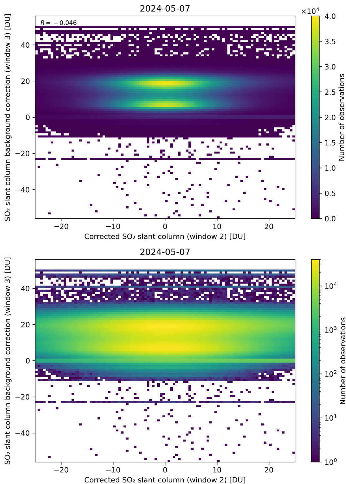
Figure 195: Scatter density plot of “Corrected SO 2 slant column (window 2)” against “SO 2 slant column background correction (window 3)” for 2024-05-07 to 2024-05-08.
