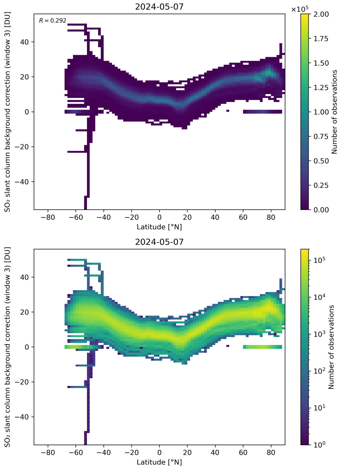
Figure 141: Scatter density plot of “Latitude” against “SO 2 slant column background correction (window 3)” for 2024-05-07 to 2024-05-08.
