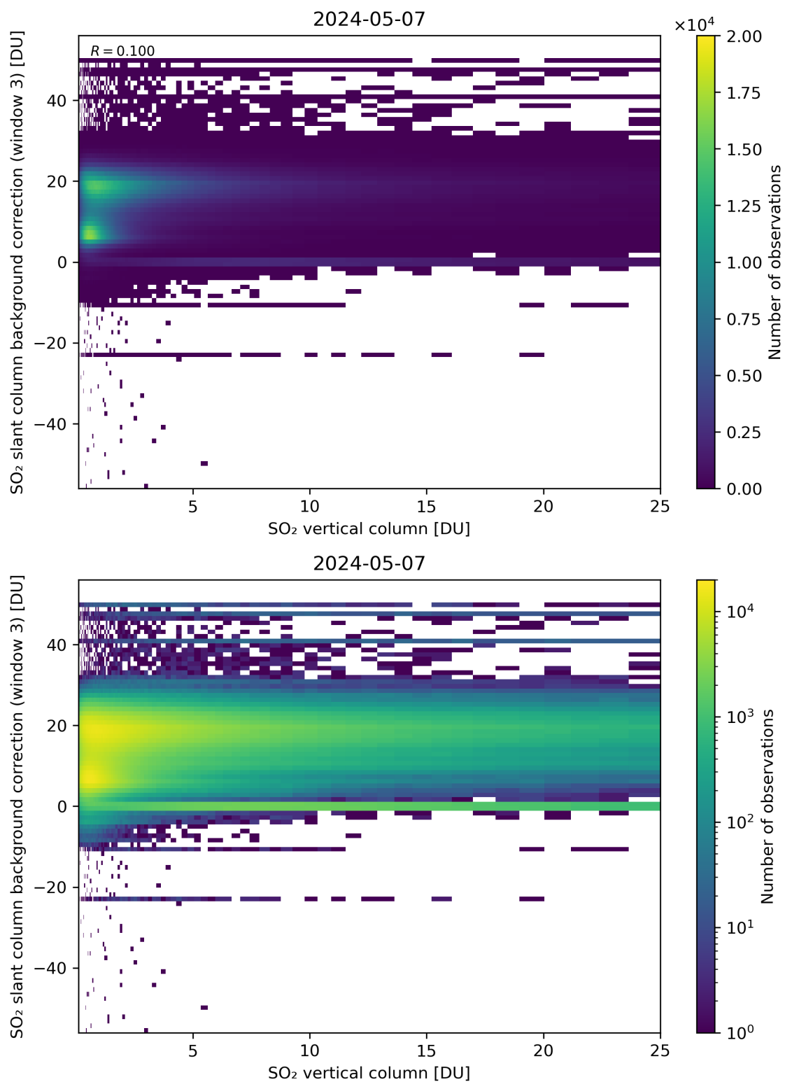
Figure 275: Scatter density plot of “SO 2 vertical column” against “SO 2 slant column background correction (window 3)” for 2024-05-07 to 2024-05-08.
