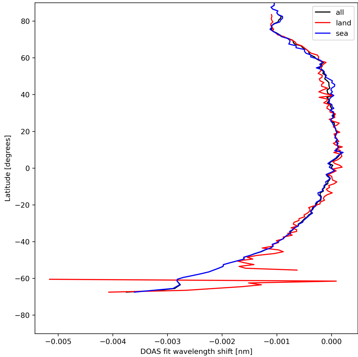
Figure 45: Zonal average of “DOAS fit wavelength shift” for 2024-05-07 to 2024-05-08.
