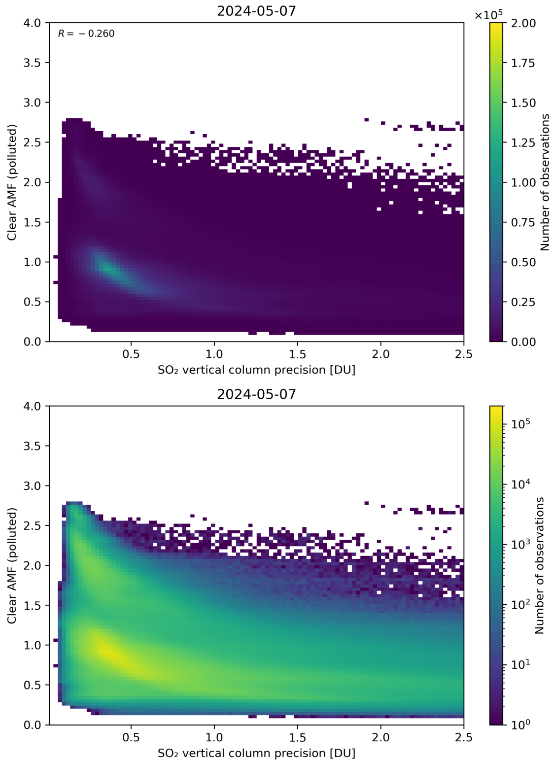
Figure 285: Scatter density plot of “SO 2 vertical column precision” against “Clear AMF (polluted)” for 2024-05-07 to 2024-05-08.
