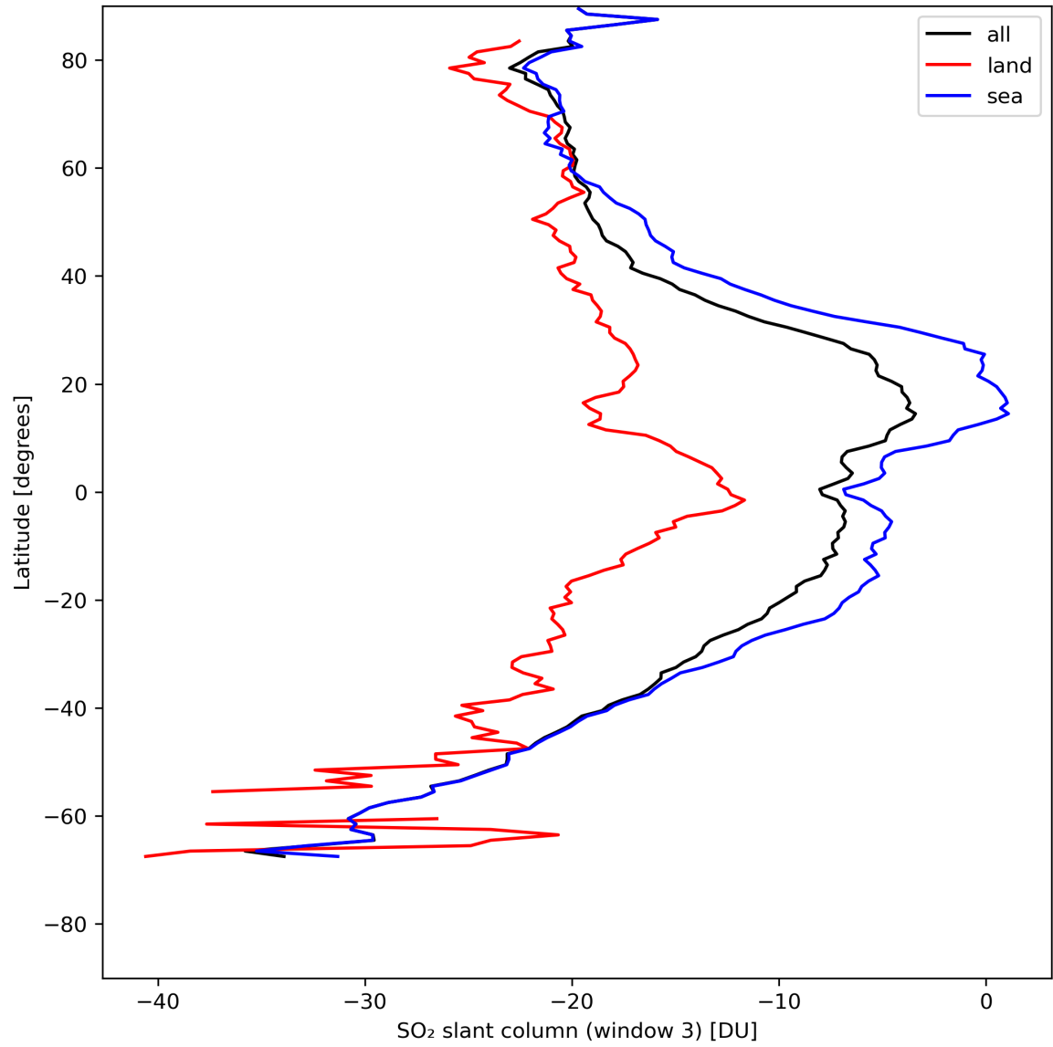
Figure 41: Zonal average of “SO 2 slant column (window 3)” for 2024-05-07 to 2024-05-08.
