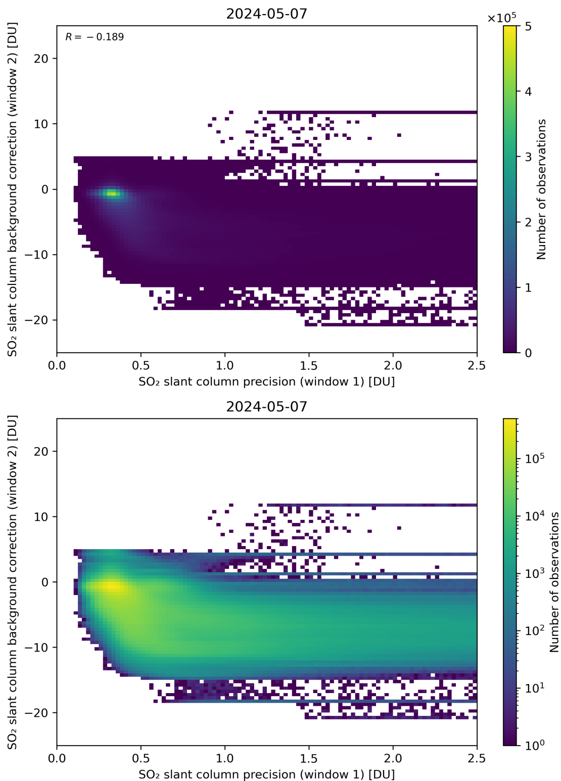
Figure 219: Scatter density plot of “SO 2 slant column precision (window 1)” against “SO 2 slant column background correction (window 2)” for 2024-05-07 to 2024-05-08.
