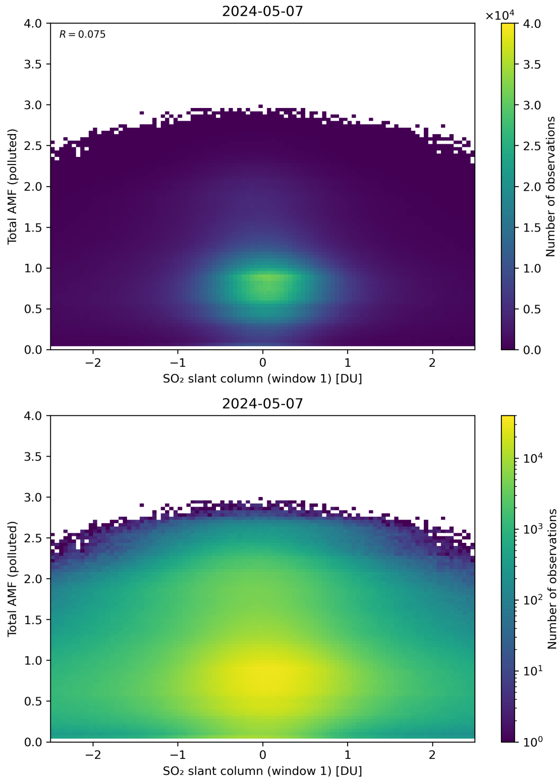
Figure 239: Scatter density plot of “SO 2 slant column (window 1)” against “Total AMF (polluted)” for 2024-05-07 to 2024-05-08.
