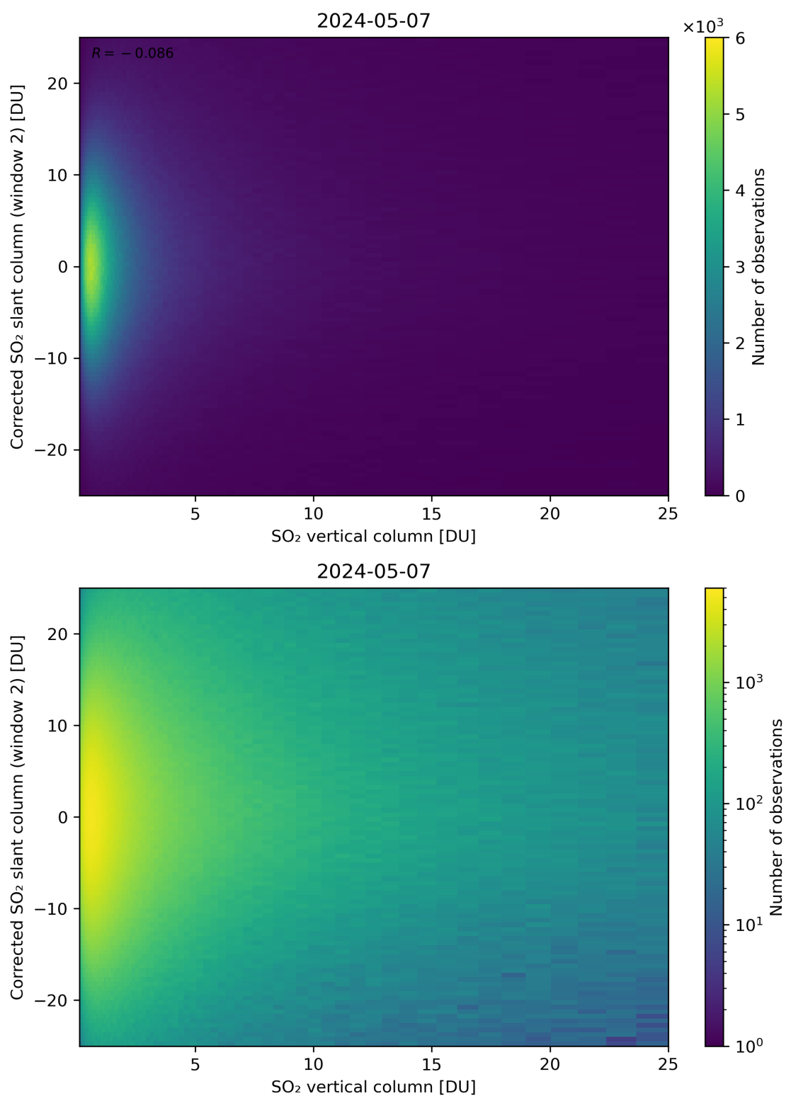
Figure 298: Scatter density plot of “SO 2 vertical column” against “Corrected SO 2 slant column (window 2)” for 2024-05-07 to 2024-05-08.
