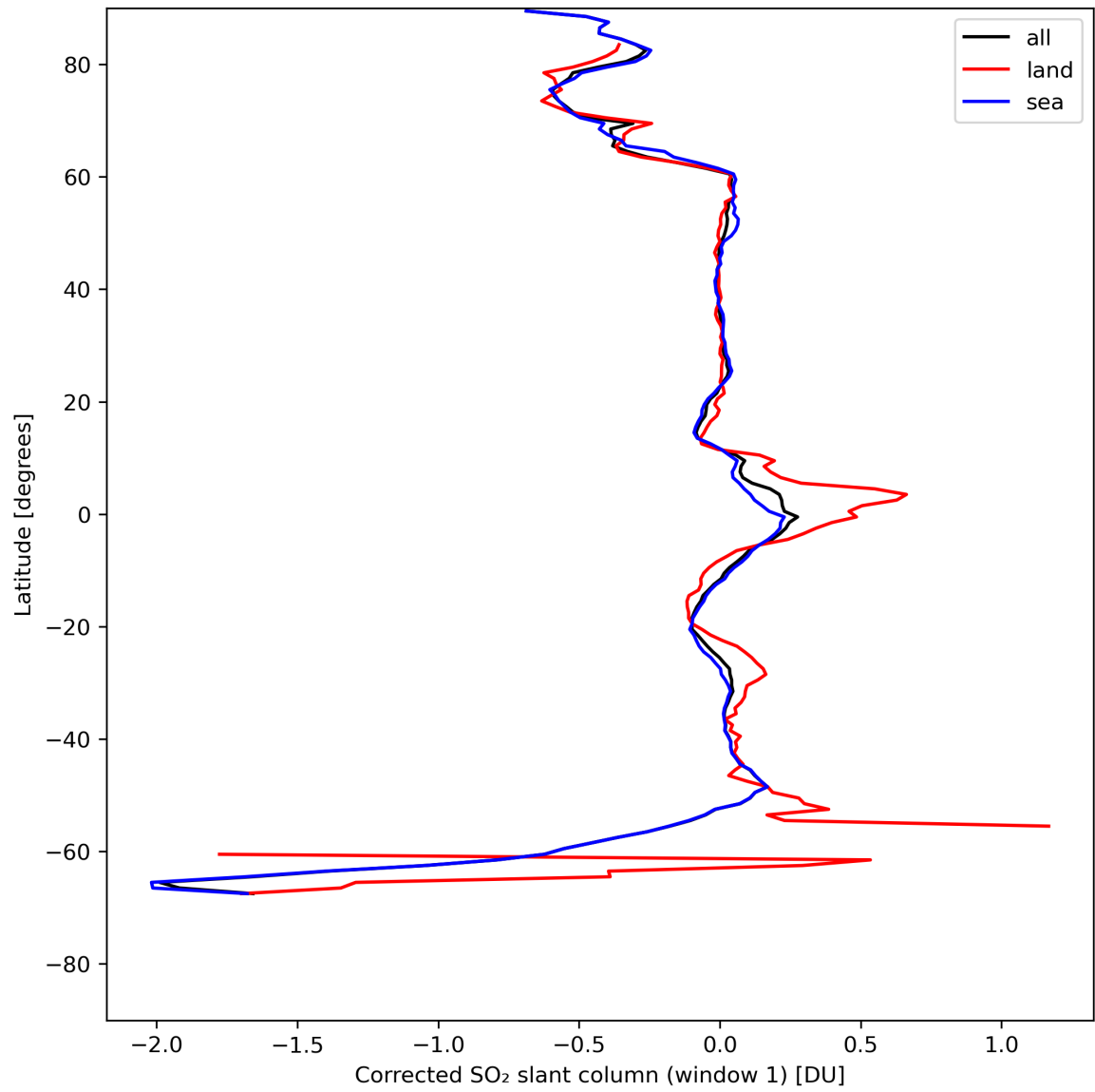
Figure 35: Zonal average of “Corrected SO 2 slant column (window 1)” for 2024-05-07 to 2024-05-08.
