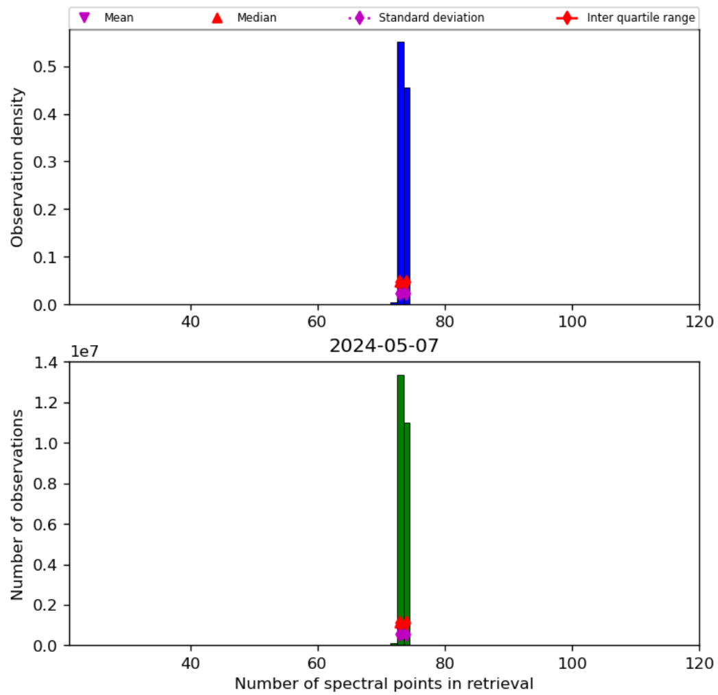
Figure 74: Histogram of “Number of spectral points in retrieval” for 2024-05-07 to 2024-05-08
