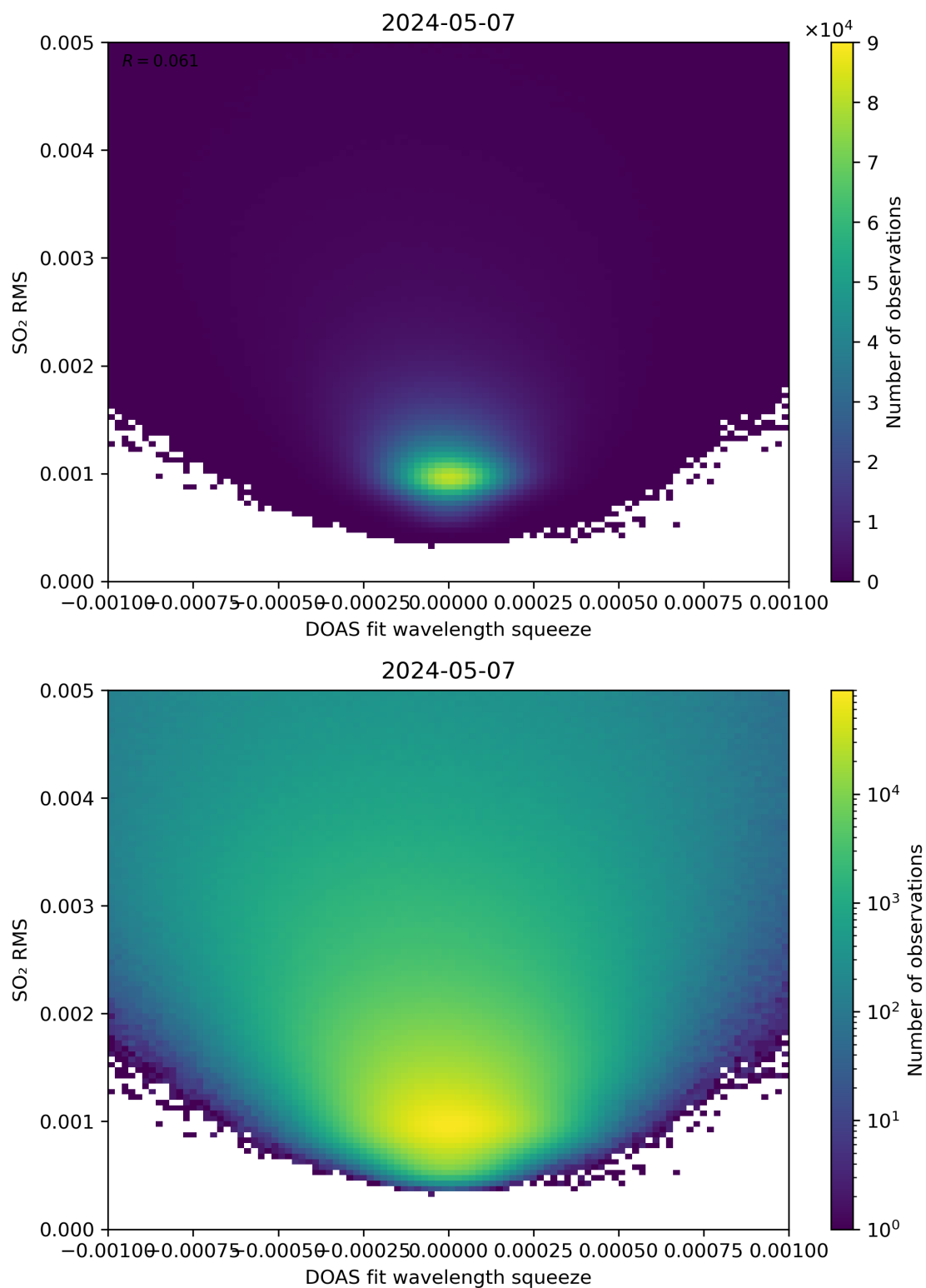
Figure 132: Scatter density plot of “DOAS fit wavelength squeeze” against “SO 2 RMS” for 2024-05-07 to 2024-05-08.
