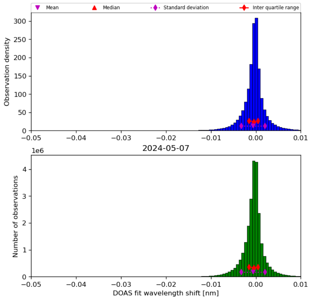
Figure 68: Histogram of “DOAS fit wavelength shift” for 2024-05-07 to 2024-05-08
