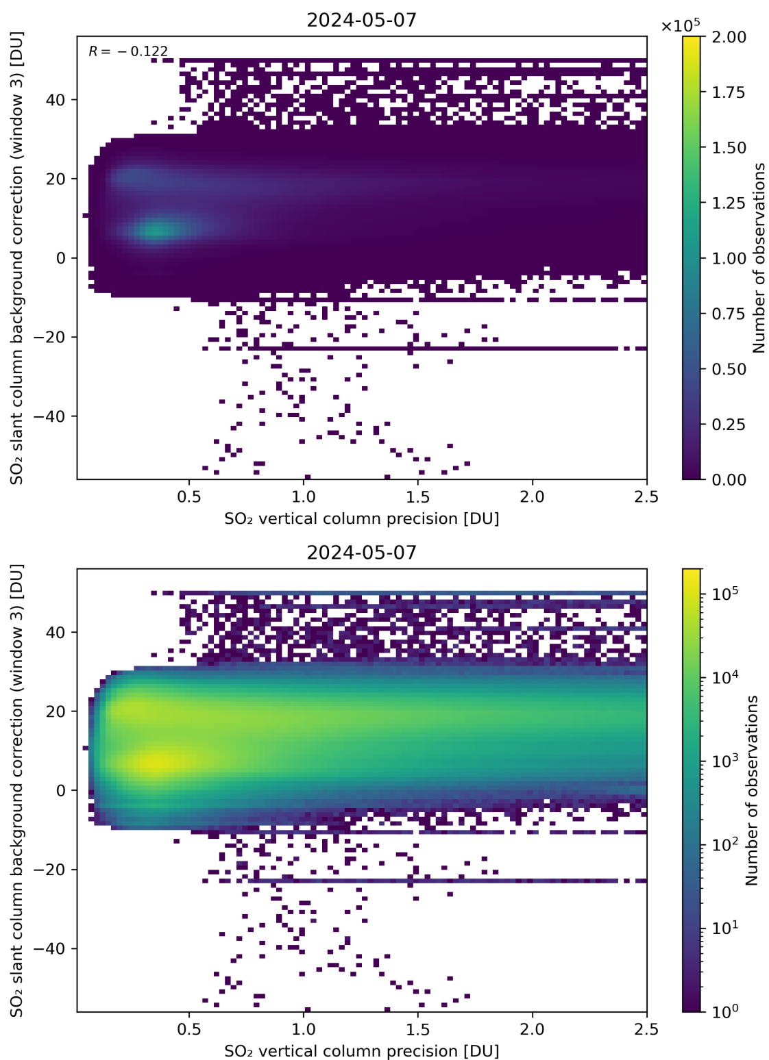
Figure 281: Scatter density plot of “SO 2 vertical column precision” against “SO 2 slant column background correction (window 3)” for 2024-05-07 to 2024-05-08.
