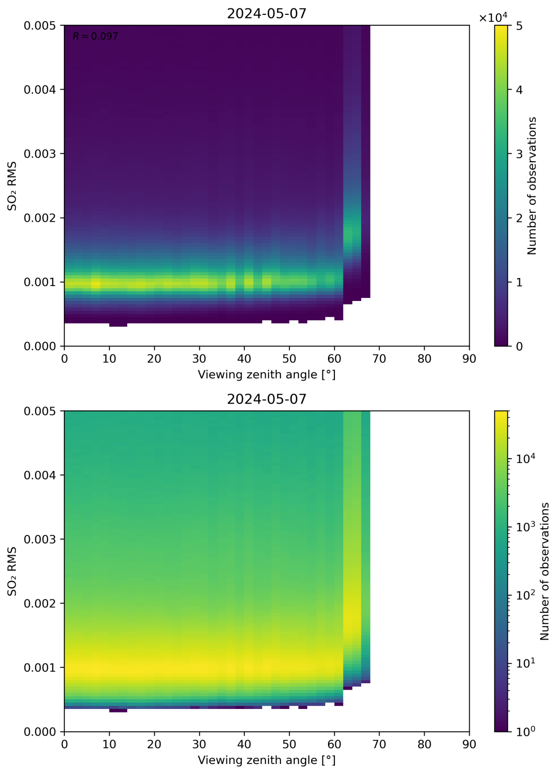
Figure 313: Scatter density plot of “Viewing zenith angle” against “SO 2 RMS” for 2024-05-07 to 2024-05-08.
