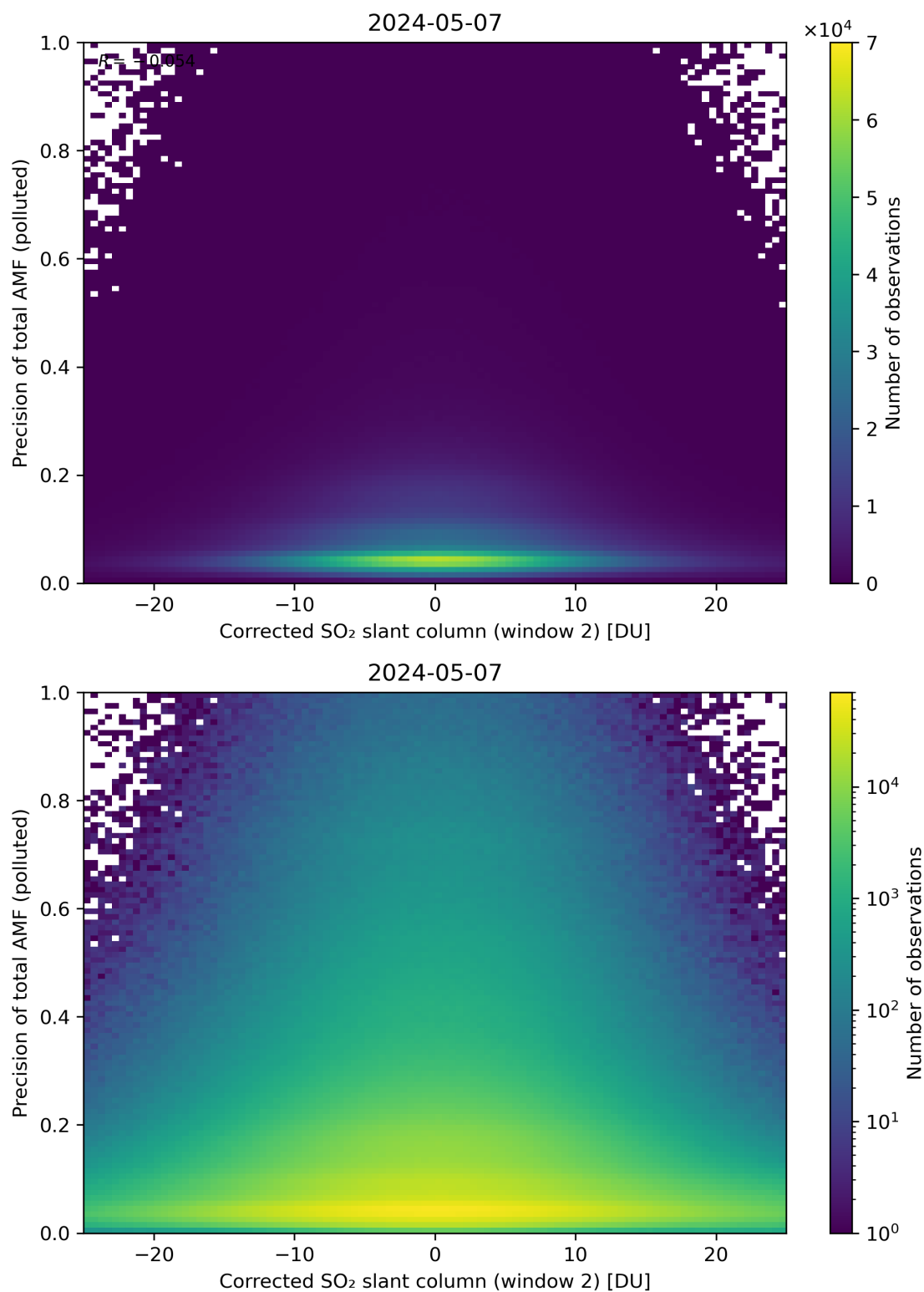
Figure 204: Scatter density plot of “Corrected SO 2 slant column (window 2)” against “Precision of total AMF (polluted)” for 2024-05-07 to 2024-05-08.
