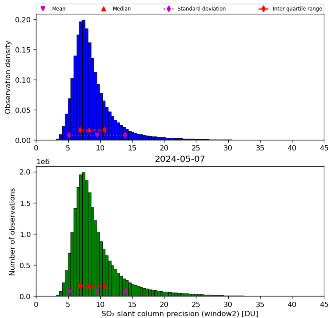
Figure 61: Histogram of “SO 2 slant column precision (window2)” for 2024-05-07 to 2024-05-08
