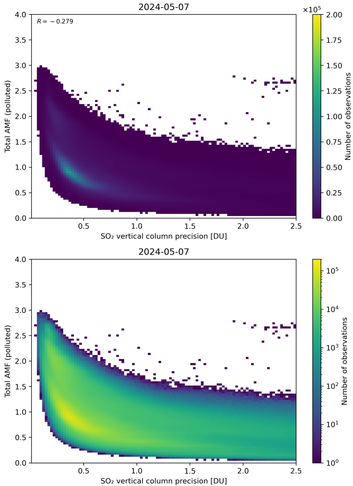
Figure 294: Scatter density plot of “SO 2 vertical column precision” against “Total AMF (polluted)” for 2024-05-07 to 2024-05-08.
