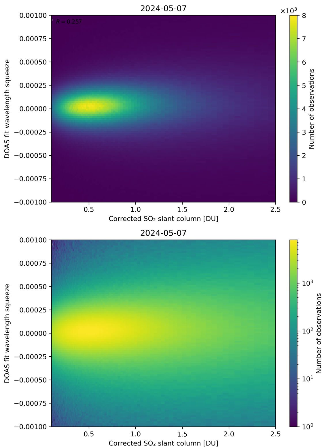
Figure 182: Scatter density plot of “Corrected SO 2 slant column” against “DOAS fit wavelength squeeze” for 2024-05-07 to 2024-05-08.
