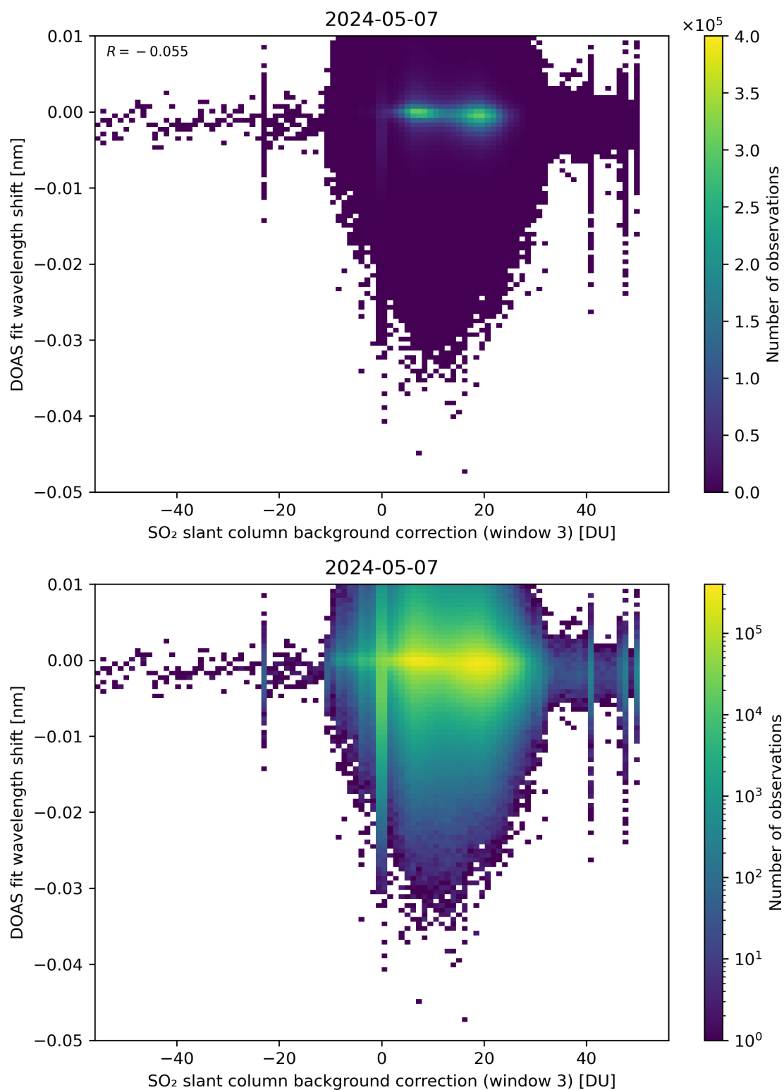
Figure 121: Scatter density plot of “SO 2 slant column background correction (window 3)” against “DOAS fit wavelength shift” for 2024-05-07 to 2024-05-08.
