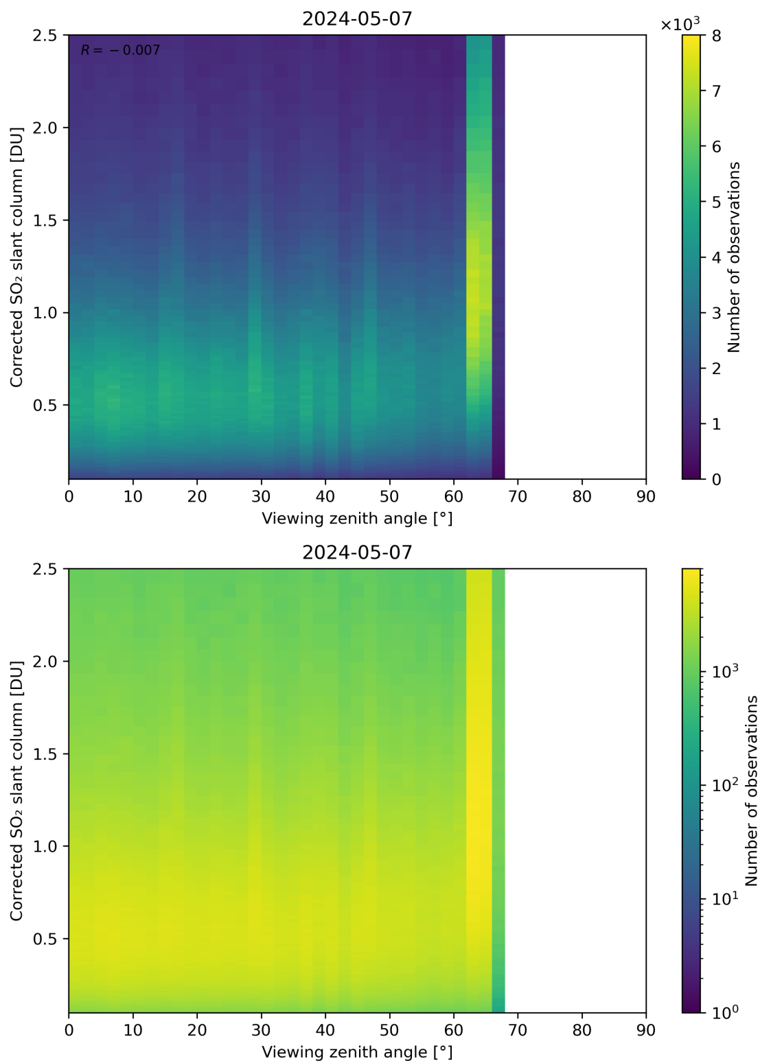
Figure 317: Scatter density plot of “Viewing zenith angle” against “Corrected SO 2 slant column” for 2024-05-07 to 2024-05-08.
