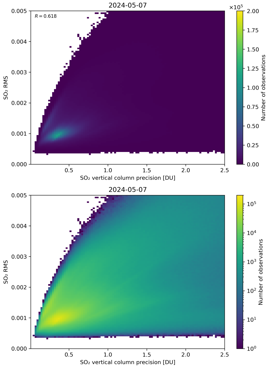
Figure 284: Scatter density plot of “SO 2 vertical column precision” against “SO 2 RMS” for 2024-05-07 to 2024-05-08.
