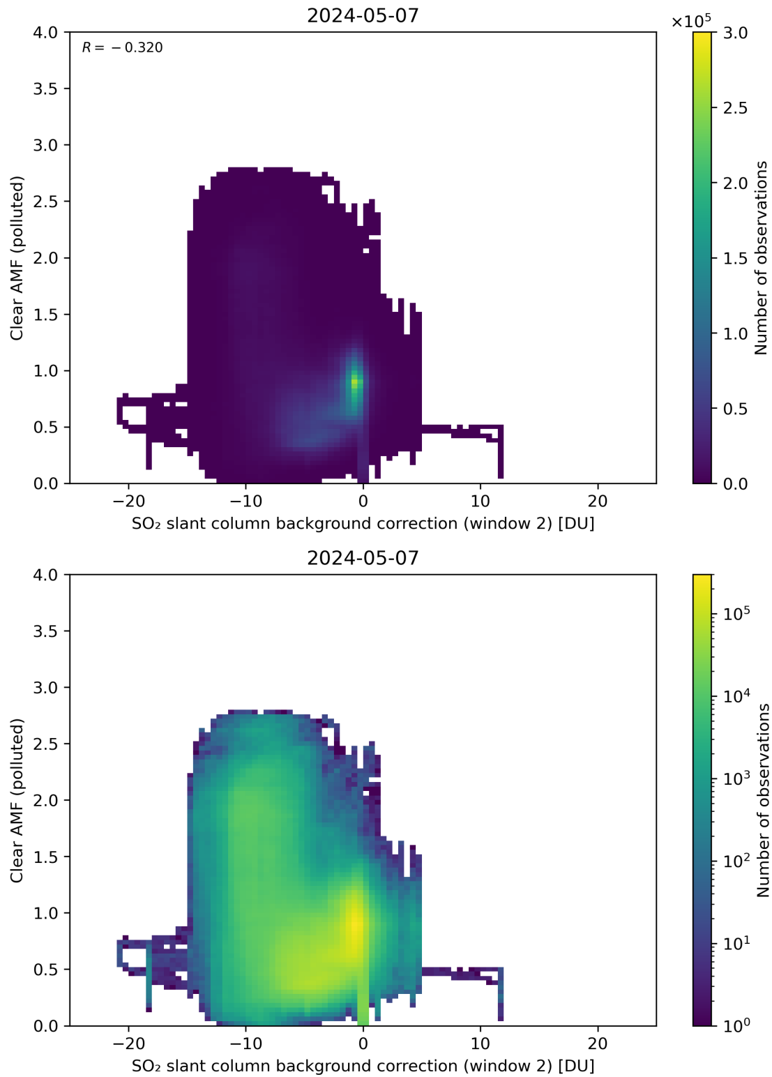
Figure 115: Scatter density plot of “SO 2 slant column background correction (window 2)” against “Clear AMF (polluted)” for 2024-05-07 to 2024-05-08.
