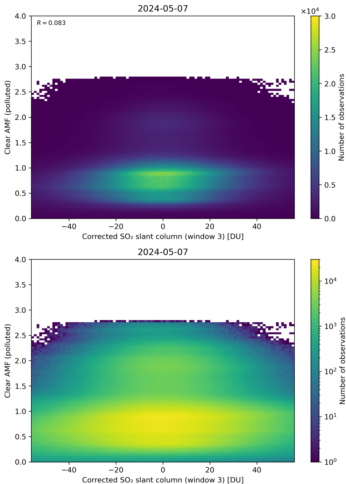
Figure 209: Scatter density plot of “Corrected SO 2 slant column (window 3)” against “Clear AMF (polluted)” for 2024-05-07 to 2024-05-08.
