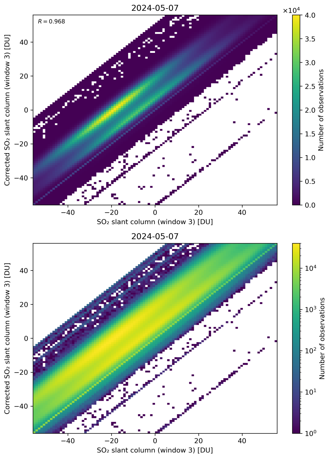
Figure 266: Scatter density plot of “SO 2 slant column (window 3)” against “Corrected SO 2 slant column (window 3)” for 2024-05-07 to 2024-05-08.
