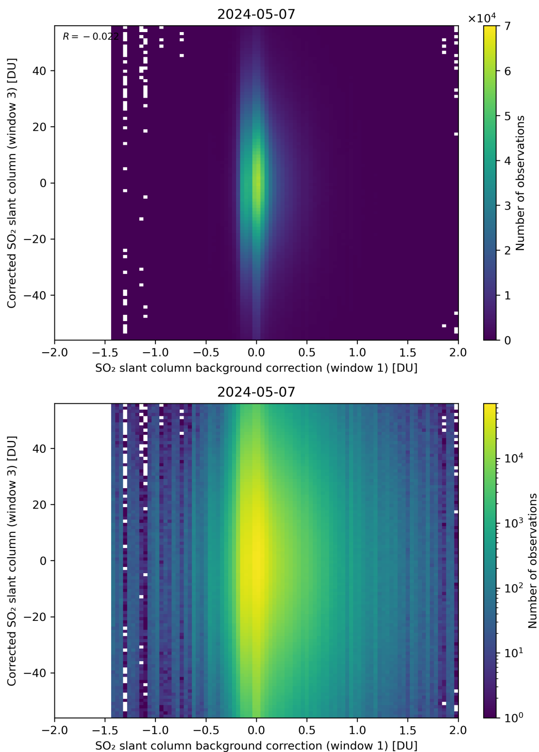
Figure 105: Scatter density plot of “SO 2 slant column background correction (window 1)” against “Corrected SO 2 slant column (window 3)” for 2024-05-07 to 2024-05-08.
