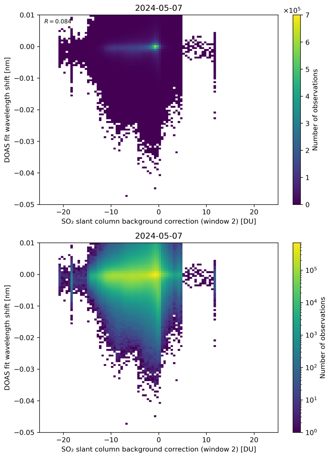
Figure 112: Scatter density plot of “SO 2 slant column background correction (window 2)” against “DOAS fit wavelength shift” for 2024-05-07 to 2024-05-08.
