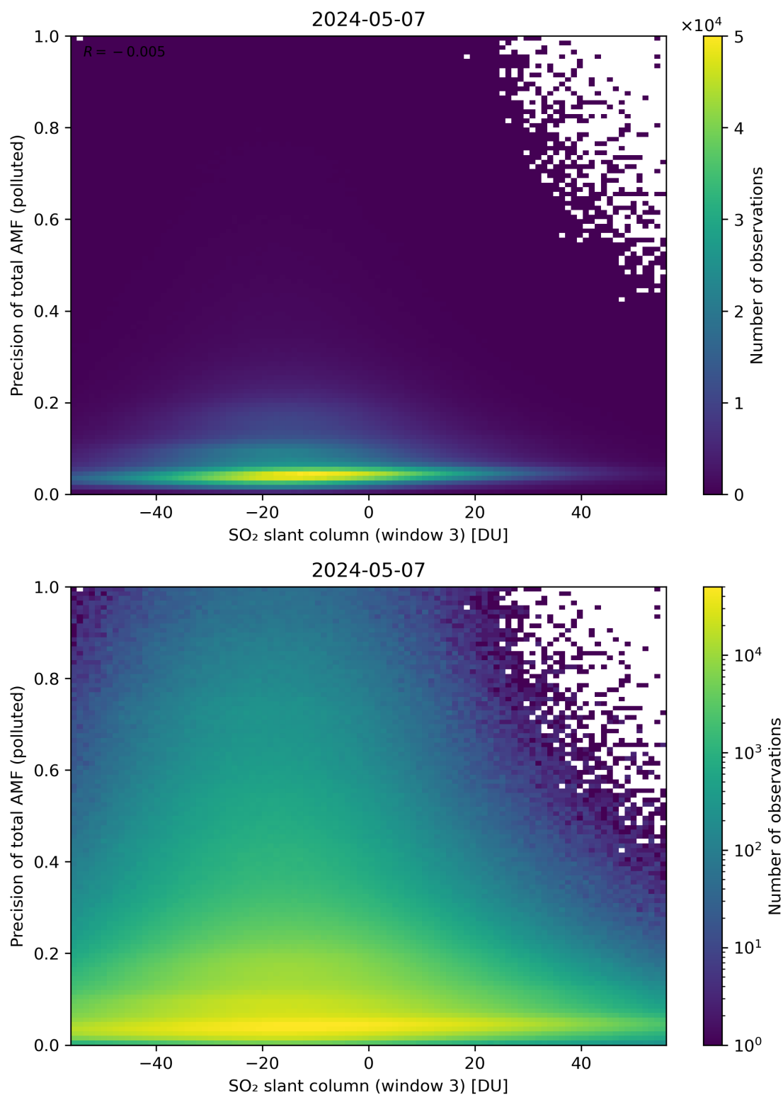
Figure 269: Scatter density plot of “SO 2 slant column (window 3)” against “Precision of total AMF (polluted)” for 2024-05-07 to 2024-05-08.
