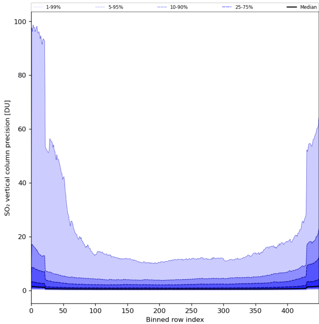
Figure 77: Along track statistics of “SO 2 vertical column precision” for 2024-05-07 to 2024-05-08
