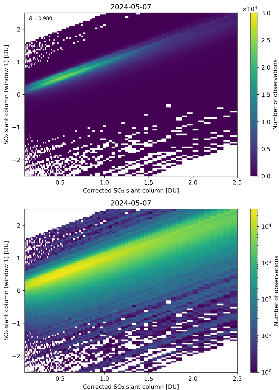
Figure 187: Scatter density plot of “Corrected SO 2 slant column” against “SO 2 slant column (window 1)” for 2024-05-07 to 2024-05-08.
