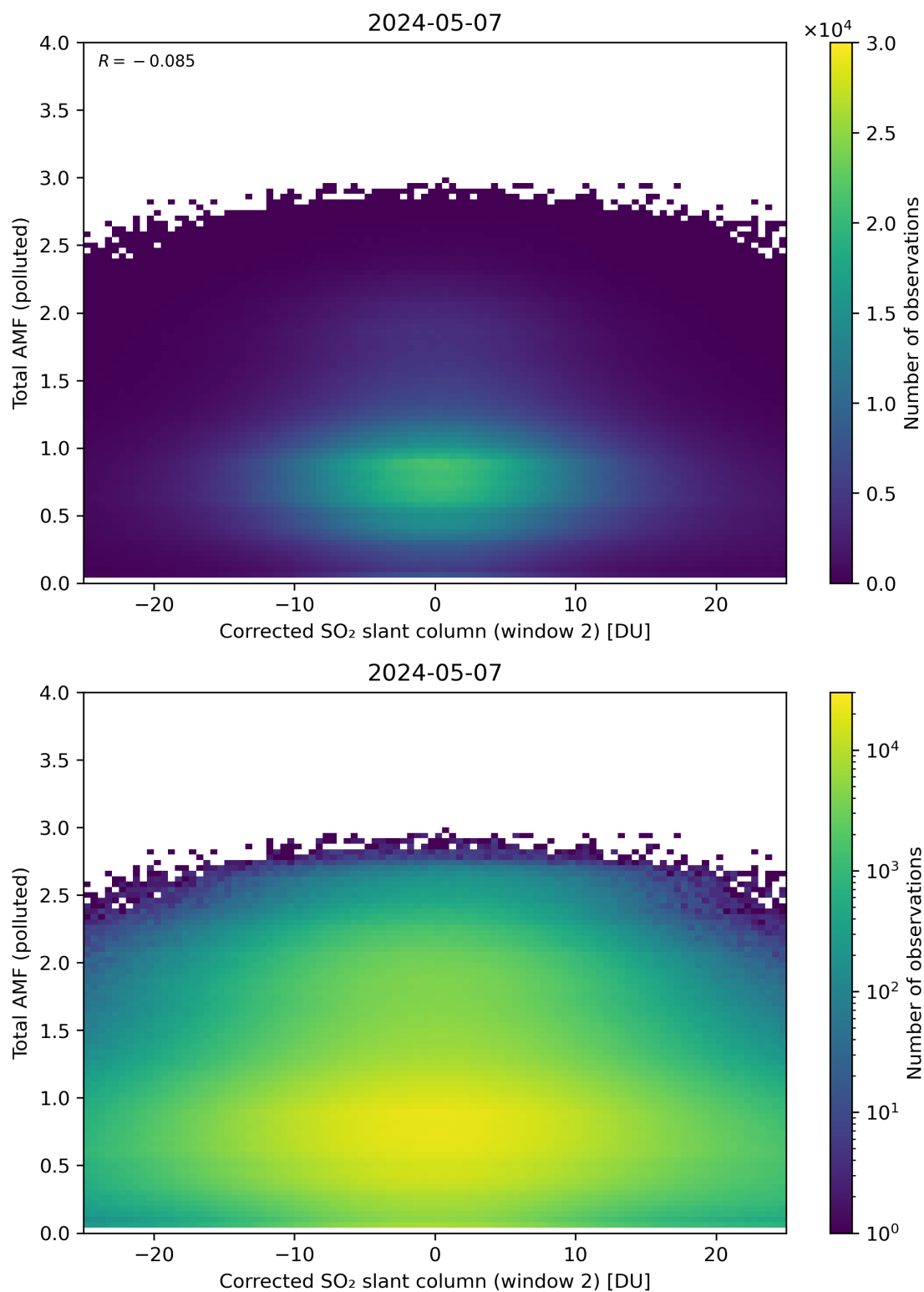
Figure 203: Scatter density plot of “Corrected SO 2 slant column (window 2)” against “Total AMF (polluted)” for 2024-05-07 to 2024-05-08.
