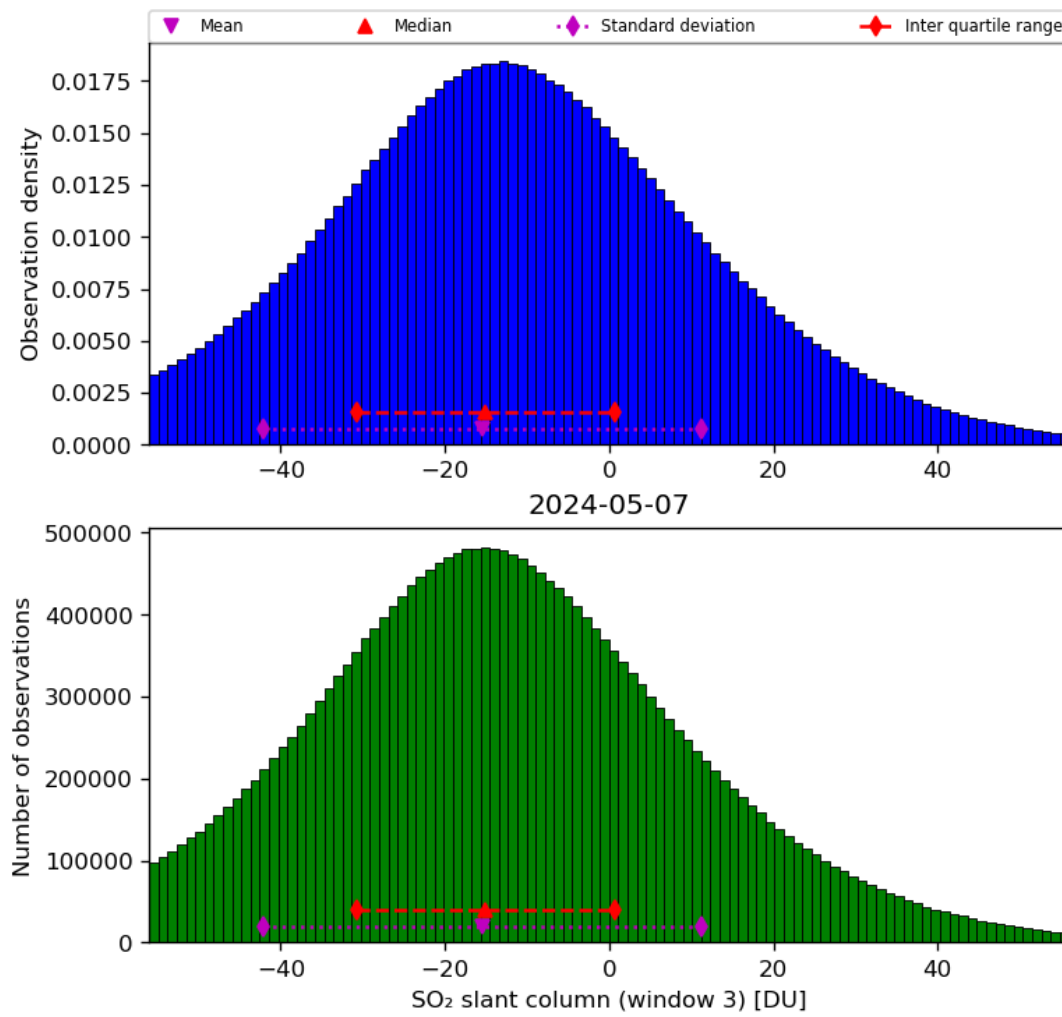
Figure 64: Histogram of “SO 2 slant column (window 3)” for 2024-05-07 to 2024-05-08
