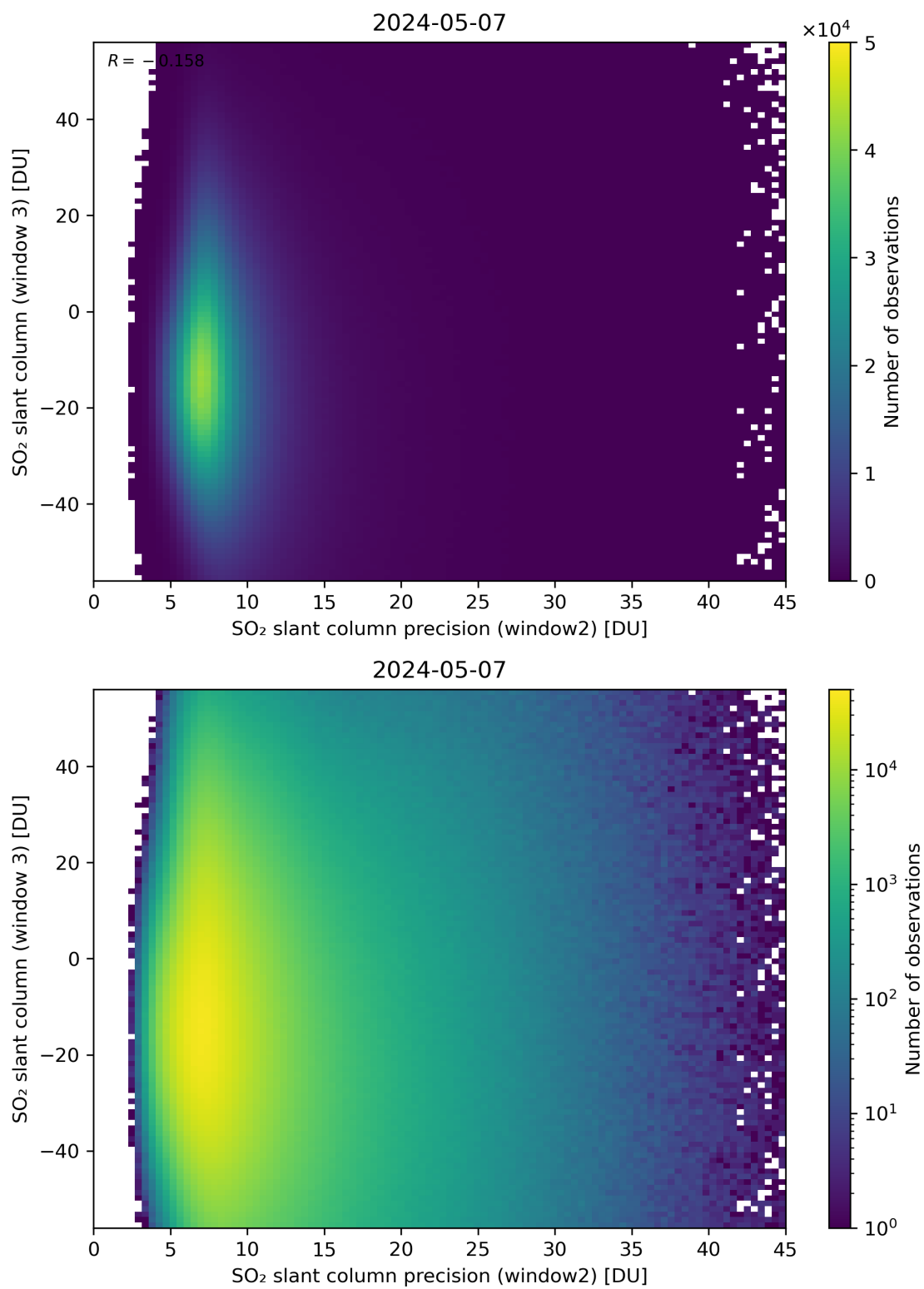
Figure 249: Scatter density plot of “SO 2 slant column precision (window2)” against “SO 2 slant column (window 3)” for 2024-05-07 to 2024-05-08.
