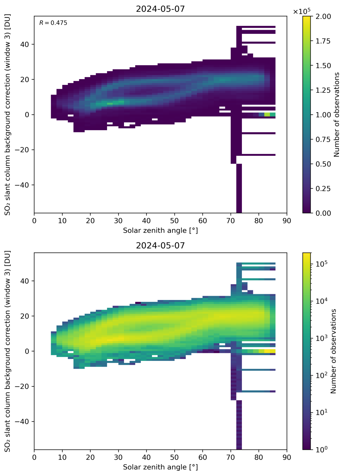
Figure 160: Scatter density plot of “Solar zenith angle” against “SO 2 slant column background correction (window 3)” for 2024-05-07 to 2024-05-08.
