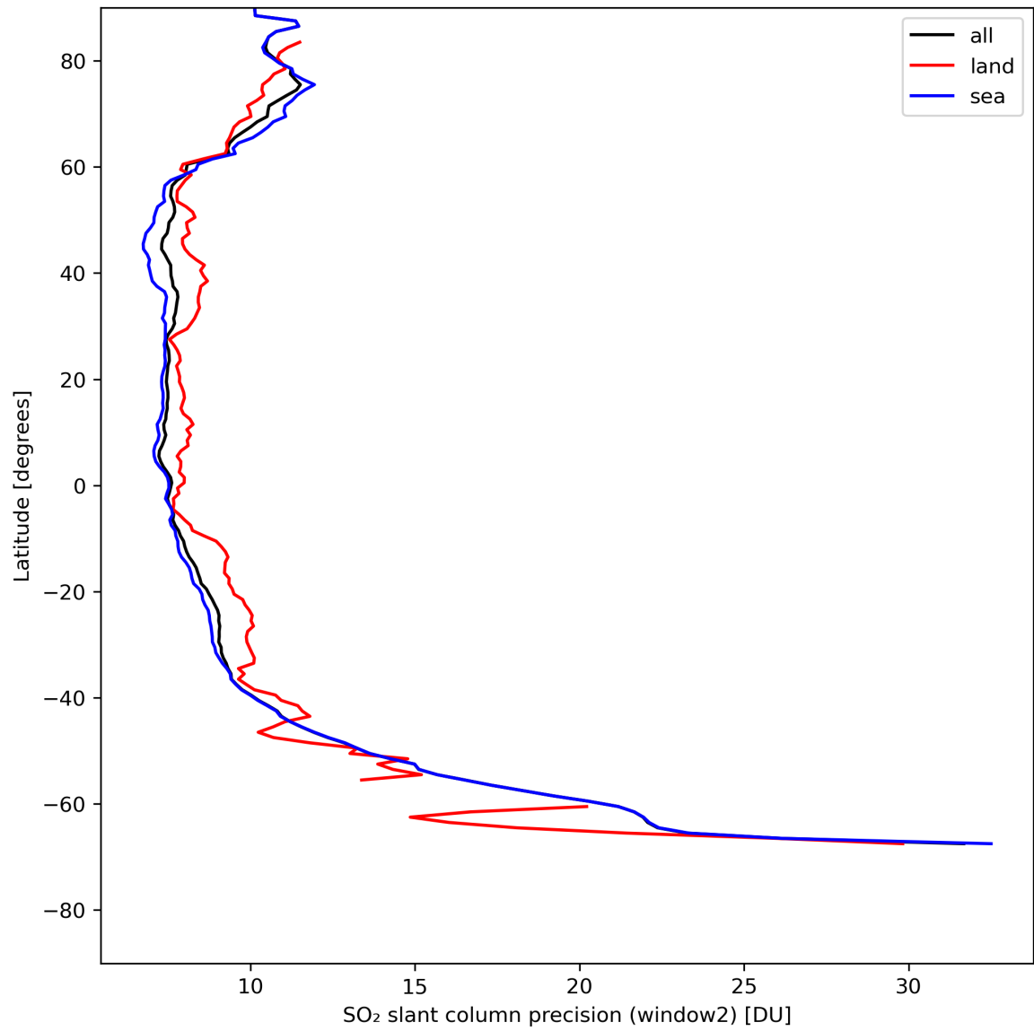
Figure 38: Zonal average of “SO 2 slant column precision (window2)” for 2024-05-07 to 2024-05-08.
