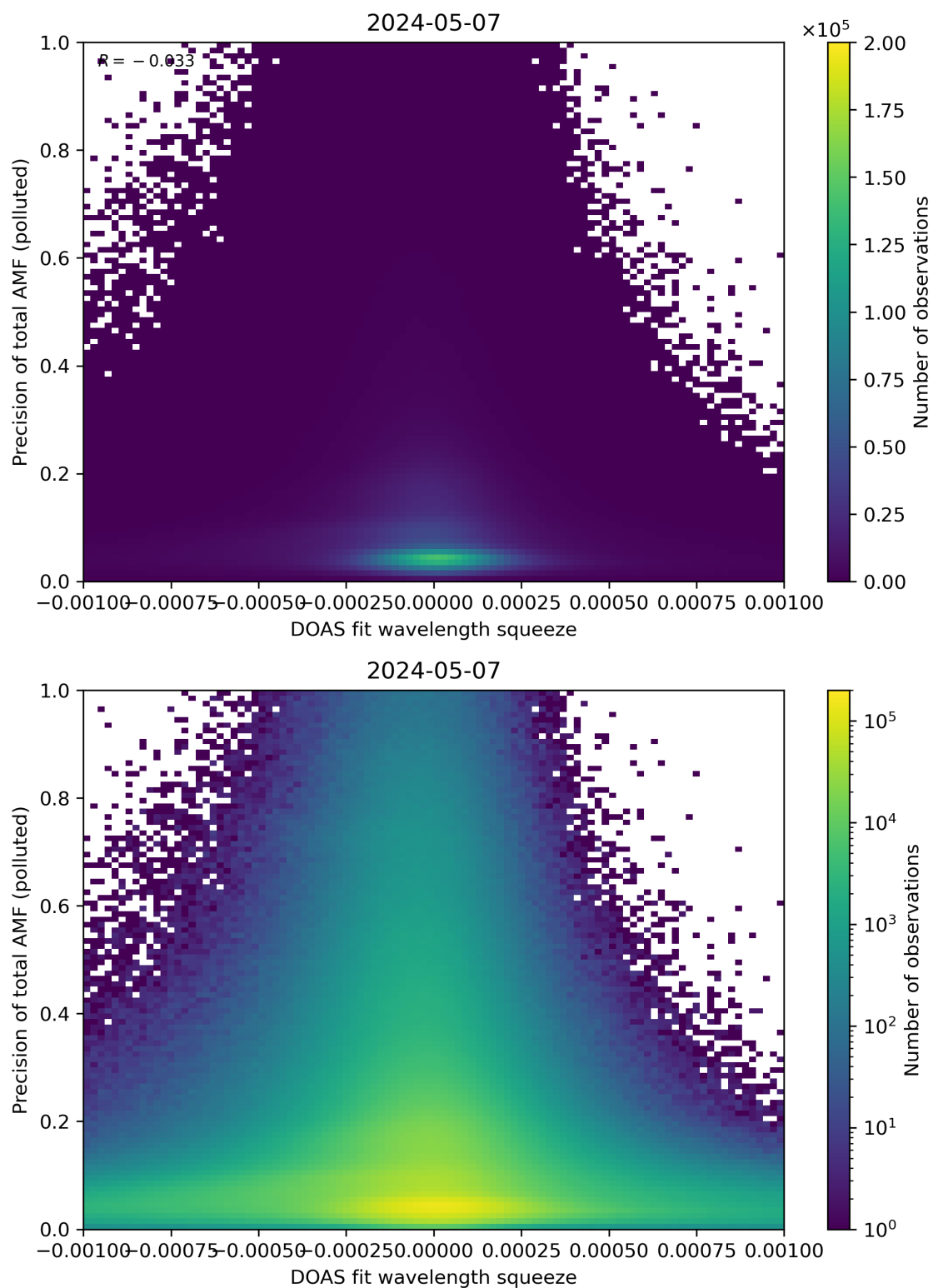
Figure 135: Scatter density plot of “DOAS fit wavelength squeeze” against “Precision of total AMF (polluted)” for 2024-05-07 to 2024-05-08.
