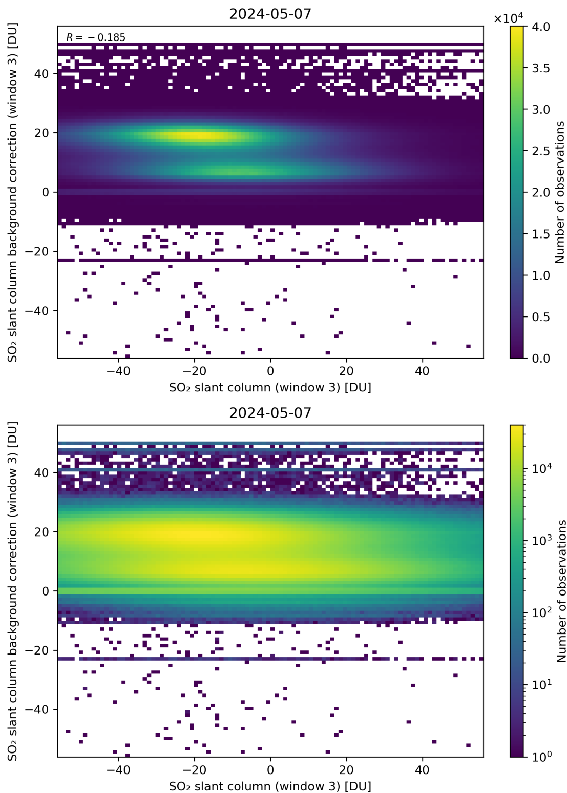
Figure 253: Scatter density plot of “SO 2 slant column (window 3)” against “SO 2 slant column background correction (window 3)” for 2024-05-07 to 2024-05-08.
