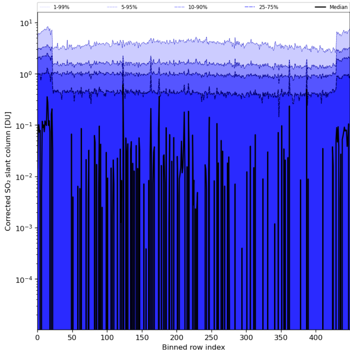
Figure 78: Along track statistics of “Corrected SO 2 slant column” for 2024-05-07 to 2024-05-08
