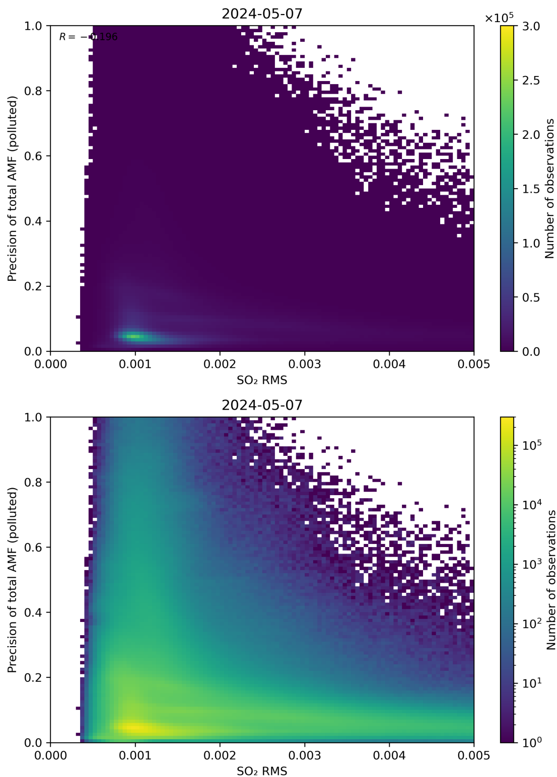
Figure 138: Scatter density plot of “SO 2 RMS” against “Precision of total AMF (polluted)” for 2024-05-07 to 2024-05-08.
