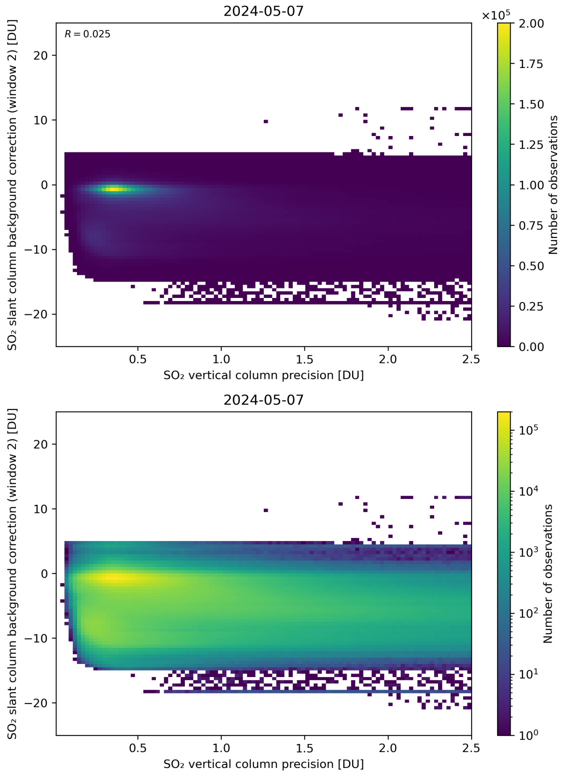
Figure 280: Scatter density plot of “SO 2 vertical column precision” against “SO 2 slant column background correction (window 2)” for 2024-05-07 to 2024-05-08.
