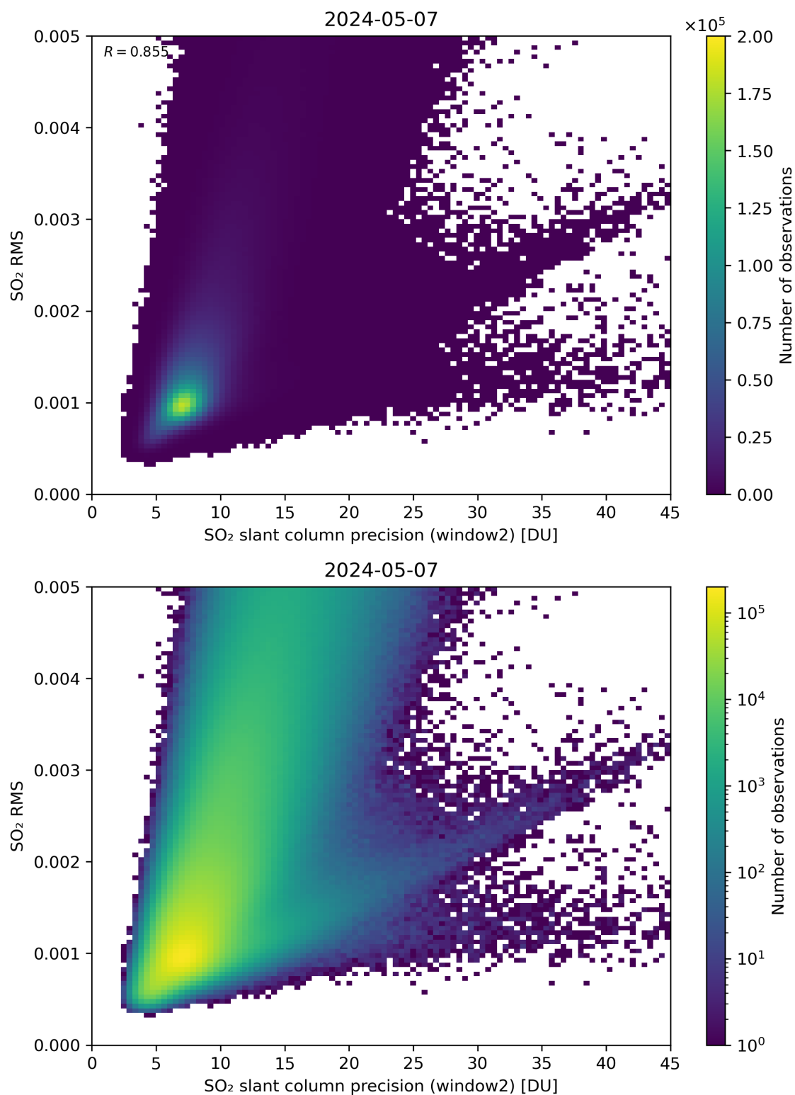
Figure 245: Scatter density plot of “SO 2 slant column precision (window2)” against “SO 2 RMS” for 2024-05-07 to 2024-05-08.
