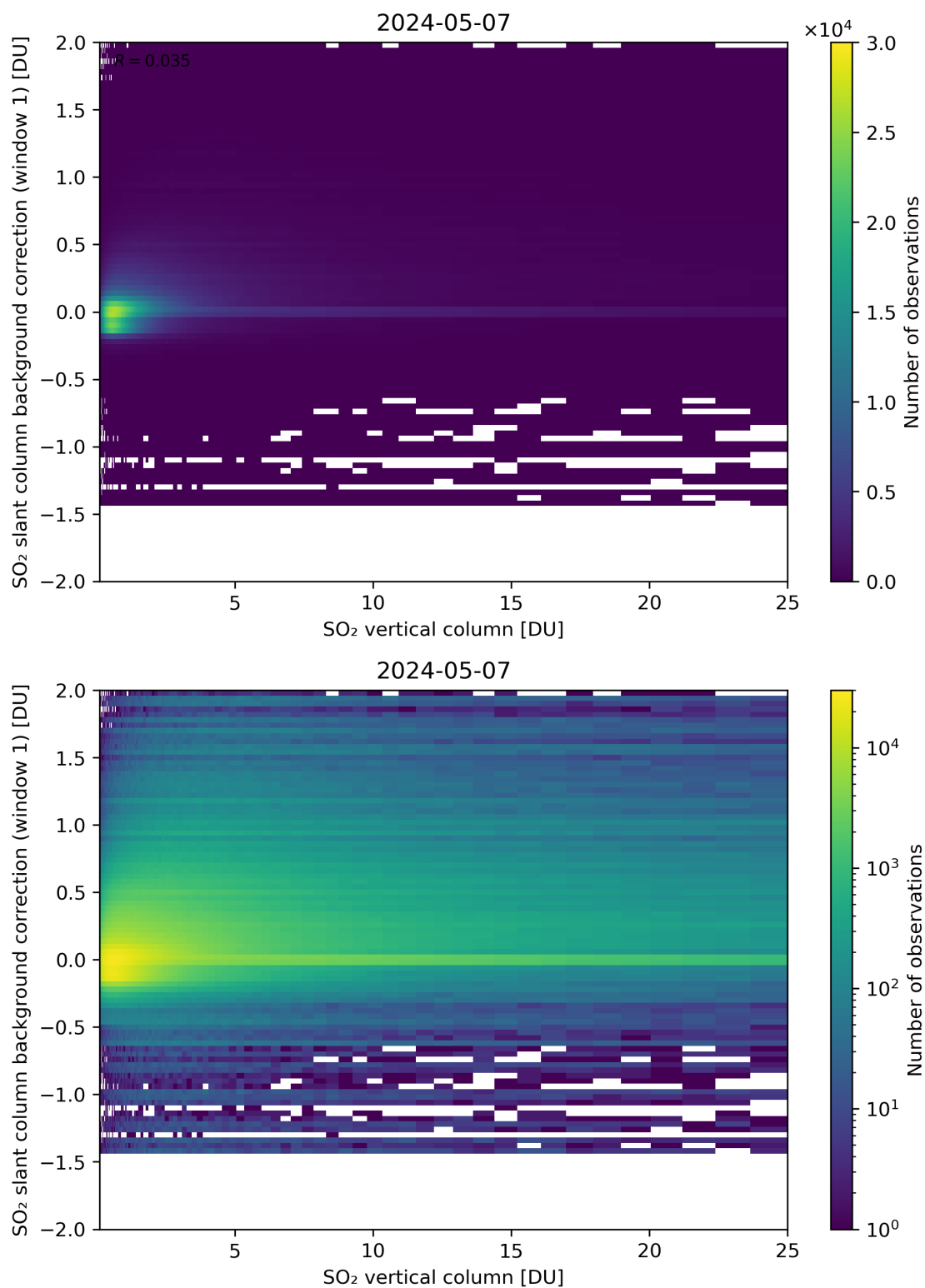
Figure 273: Scatter density plot of “SO 2 vertical column” against “SO 2 slant column background correction (window 1)” for 2024-05-07 to 2024-05-08.
