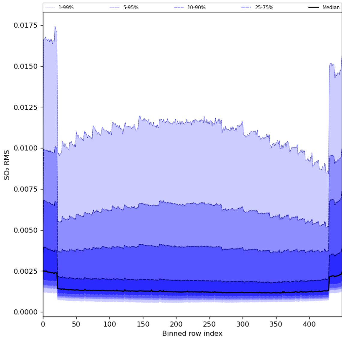
Figure 93: Along track statistics of “SO 2 RMS” for 2024-05-07 to 2024-05-08
