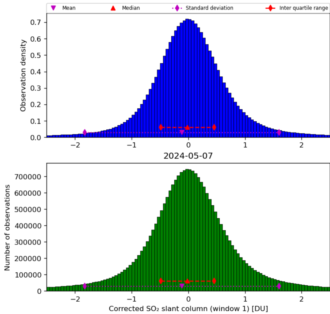
Figure 58: Histogram of “Corrected SO 2 slant column (window 1)” for 2024-05-07 to 2024-05-08
