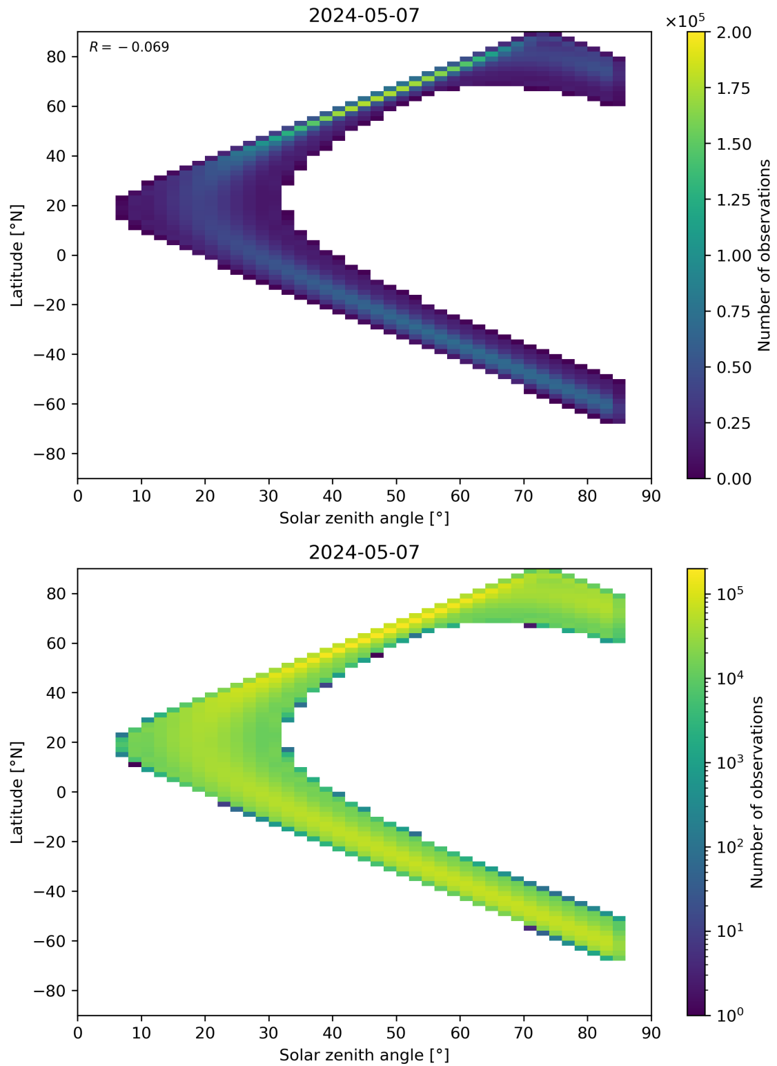
Figure 164: Scatter density plot of “Solar zenith angle” against “Latitude” for 2024-05-07 to 2024-05-08.
