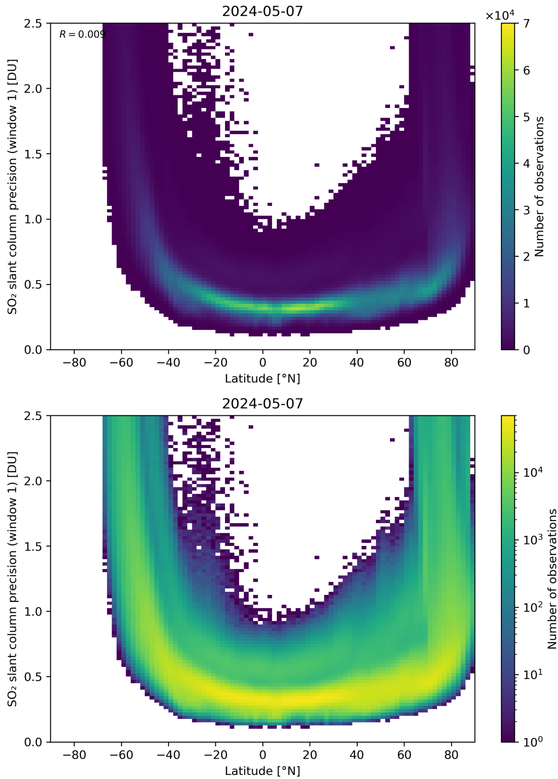
Figure 150: Scatter density plot of “Latitude” against “SO 2 slant column precision (window 1)” for 2024-05-07 to 2024-05-08.
