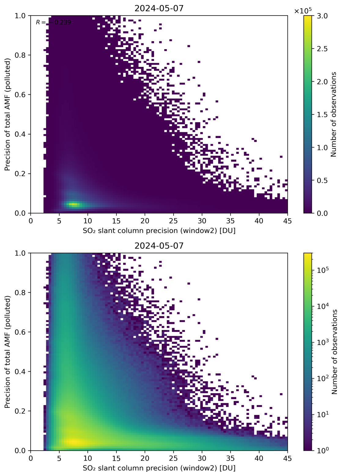
Figure 252: Scatter density plot of “SO 2 slant column precision (window2)” against “Precision of total AMF (polluted)” for 2024-05-07 to 2024-05-08.
