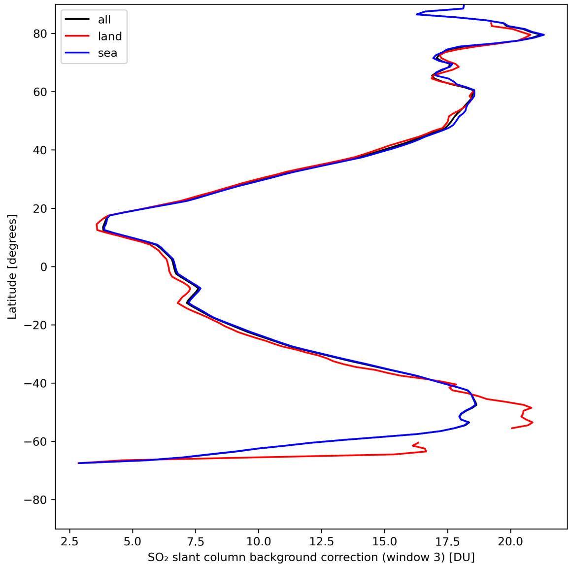
Figure 44: Zonal average of “SO 2 slant column background correction (window 3)” for 2024-05-07 to 2024-05-08.
