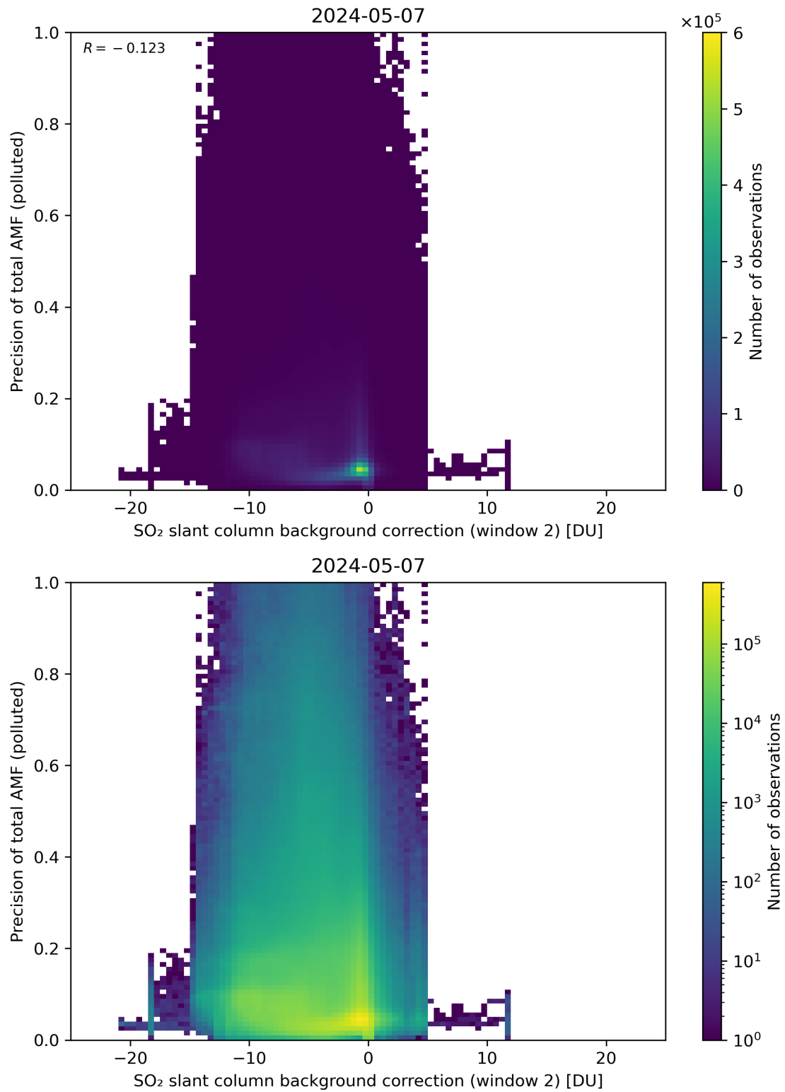
Figure 120: Scatter density plot of “SO 2 slant column background correction (window 2)” against “Precision of total AMF (polluted)” for 2024-05-07 to 2024-05-08.
