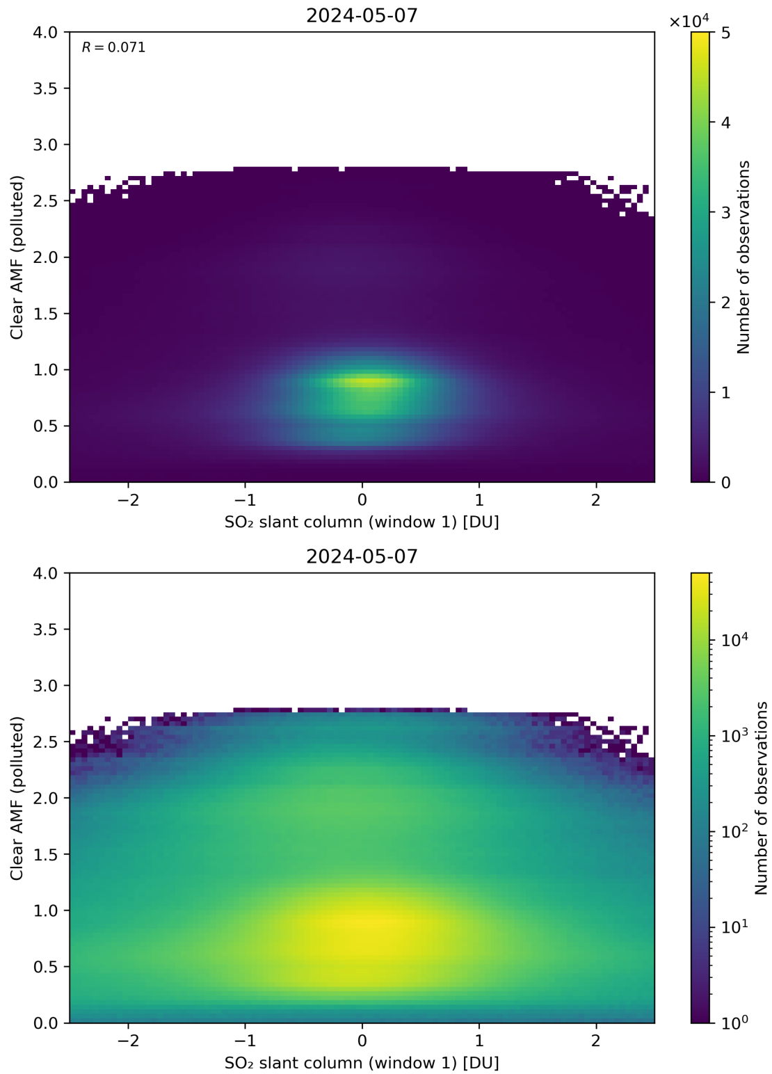
Figure 232: Scatter density plot of “SO 2 slant column (window 1)” against “Clear AMF (polluted)” for 2024-05-07 to 2024-05-08.
