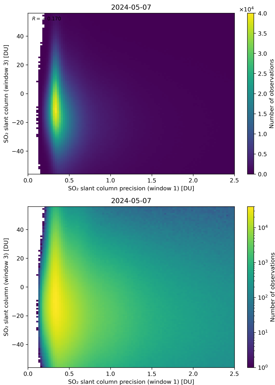
Figure 228: Scatter density plot of “SO 2 slant column precision (window 1)” against “SO 2 slant column (window 3)” for 2024-05-07 to 2024-05-08.
