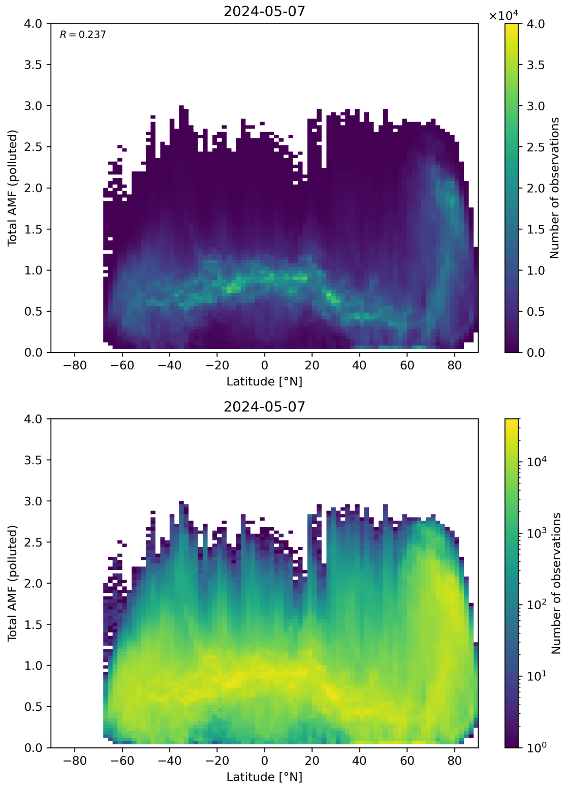
Figure 154: Scatter density plot of “Latitude” against “Total AMF (polluted)” for 2024-05-07 to 2024-05-08.
