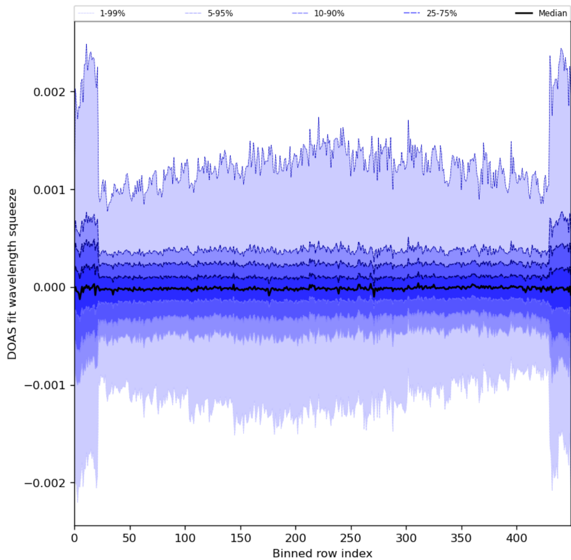
Figure 92: Along track statistics of “DOAS fit wavelength squeeze” for 2024-05-07 to 2024-05-08
