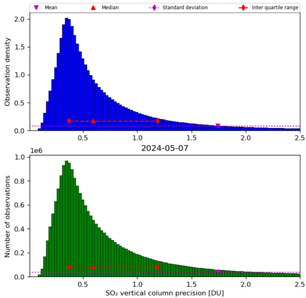
Figure 54: Histogram of “SO 2 vertical column precision” for 2024-05-07 to 2024-05-08
