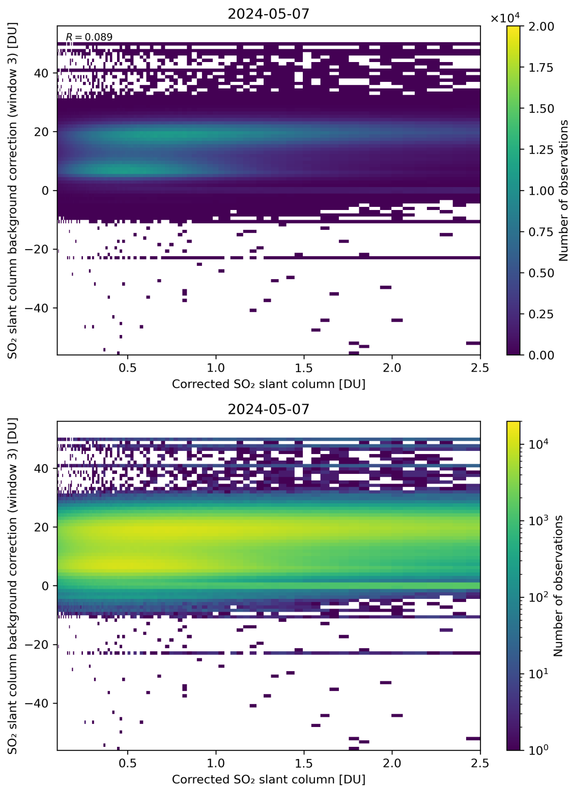
Figure 180: Scatter density plot of “Corrected SO 2 slant column” against “SO 2 slant column background correction (window 3)” for 2024-05-07 to 2024-05-08.
