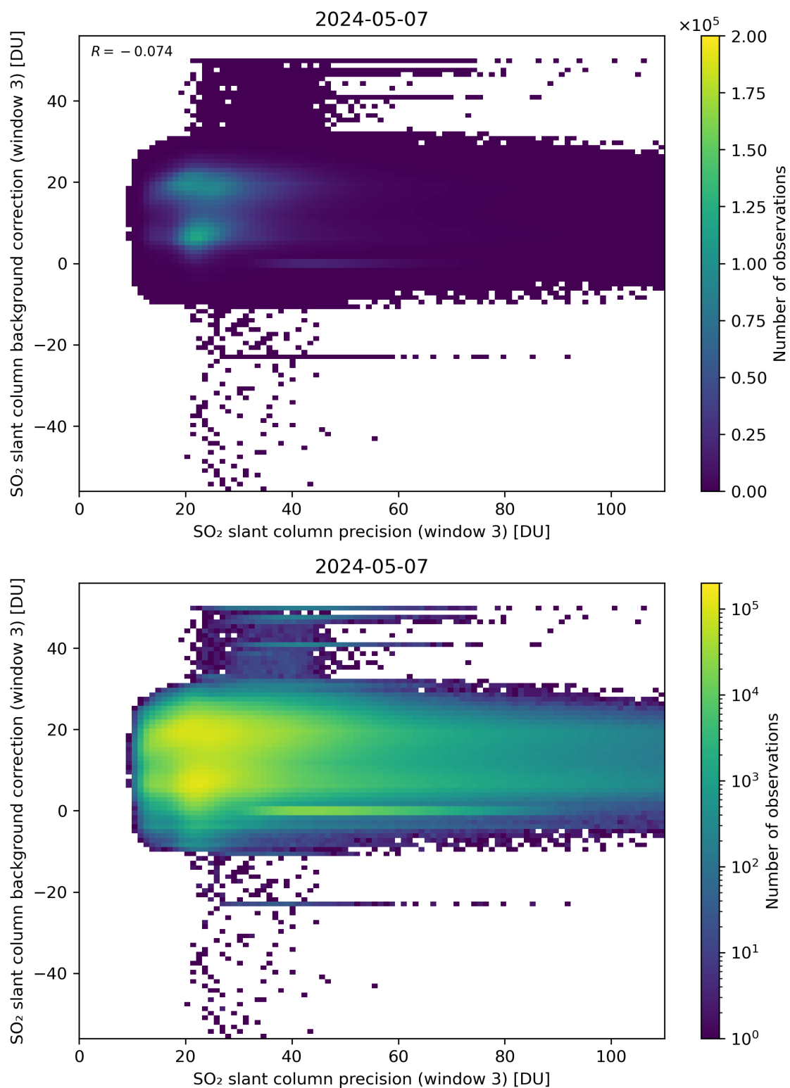
Figure 257: Scatter density plot of “SO 2 slant column precision (window 3)” against “SO 2 slant column background correction (window 3)” for 2024-05-07 to 2024-05-08.
