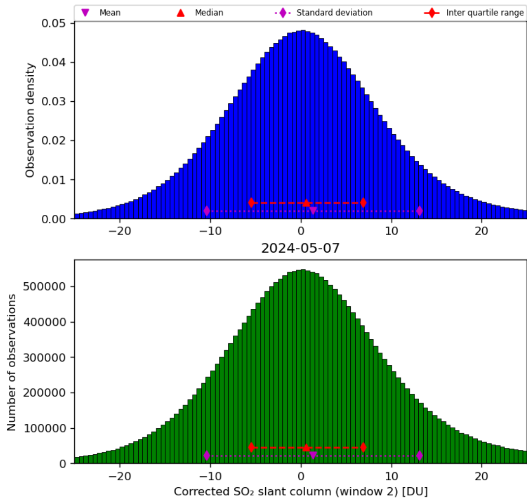
Figure 62: Histogram of “Corrected SO 2 slant column (window 2)” for 2024-05-07 to 2024-05-08
