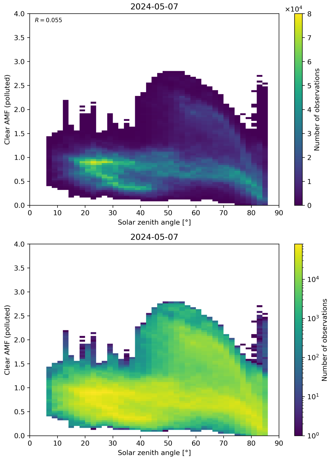
Figure 165: Scatter density plot of “Solar zenith angle” against “Clear AMF (polluted)” for 2024-05-07 to 2024-05-08.
