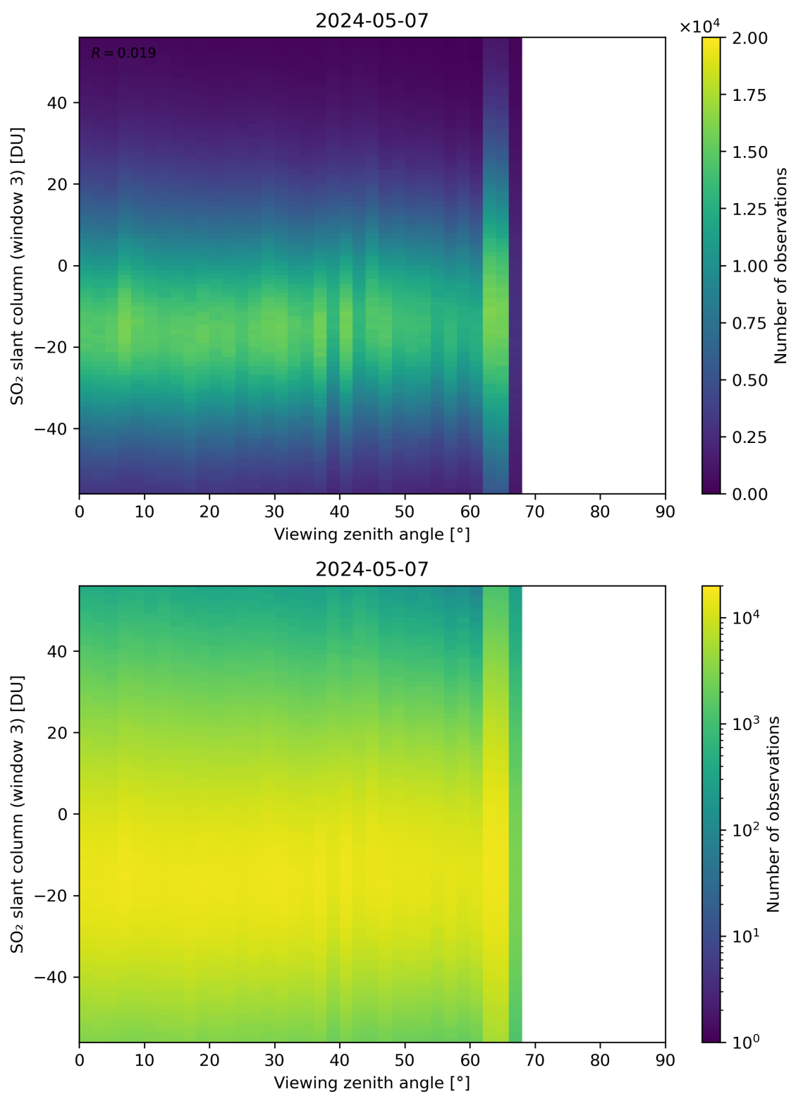
Figure 323: Scatter density plot of “Viewing zenith angle” against “SO 2 slant column (window 3)” for 2024-05-07 to 2024-05-08.
