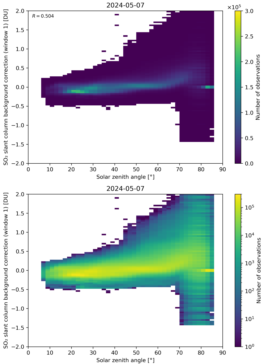
Figure 158: Scatter density plot of “Solar zenith angle” against “SO 2 slant column background correction (window 1)” for 2024-05-07 to 2024-05-08.
