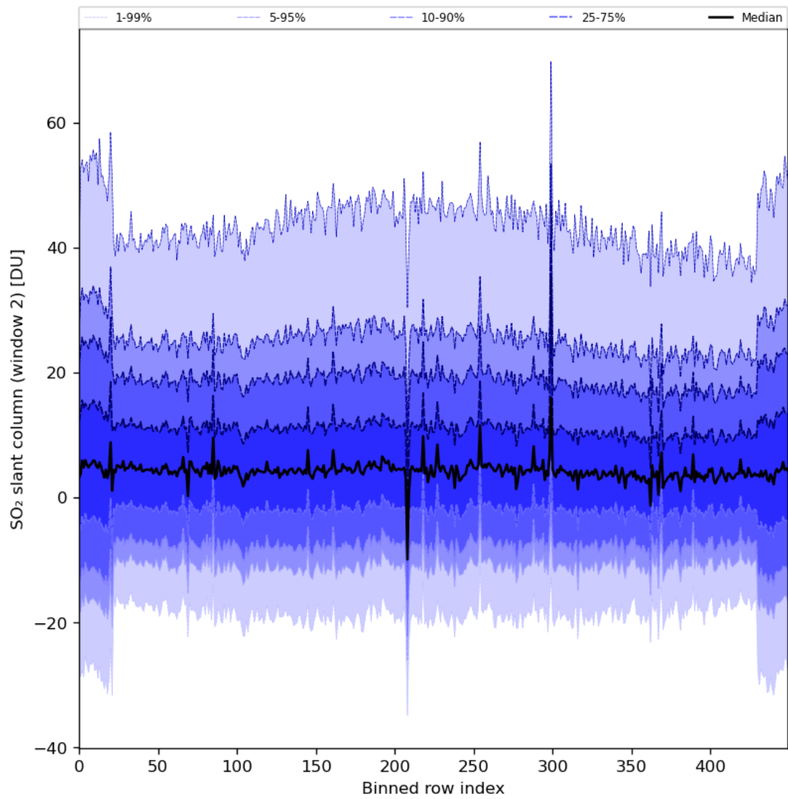
Figure 83: Along track statistics of “SO 2 slant column (window 2)” for 2024-05-07 to 2024-05-08
