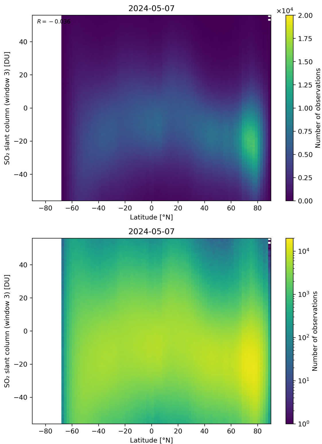
Figure 152: Scatter density plot of “Latitude” against “SO 2 slant column (window 3)” for 2024-05-07 to 2024-05-08.
