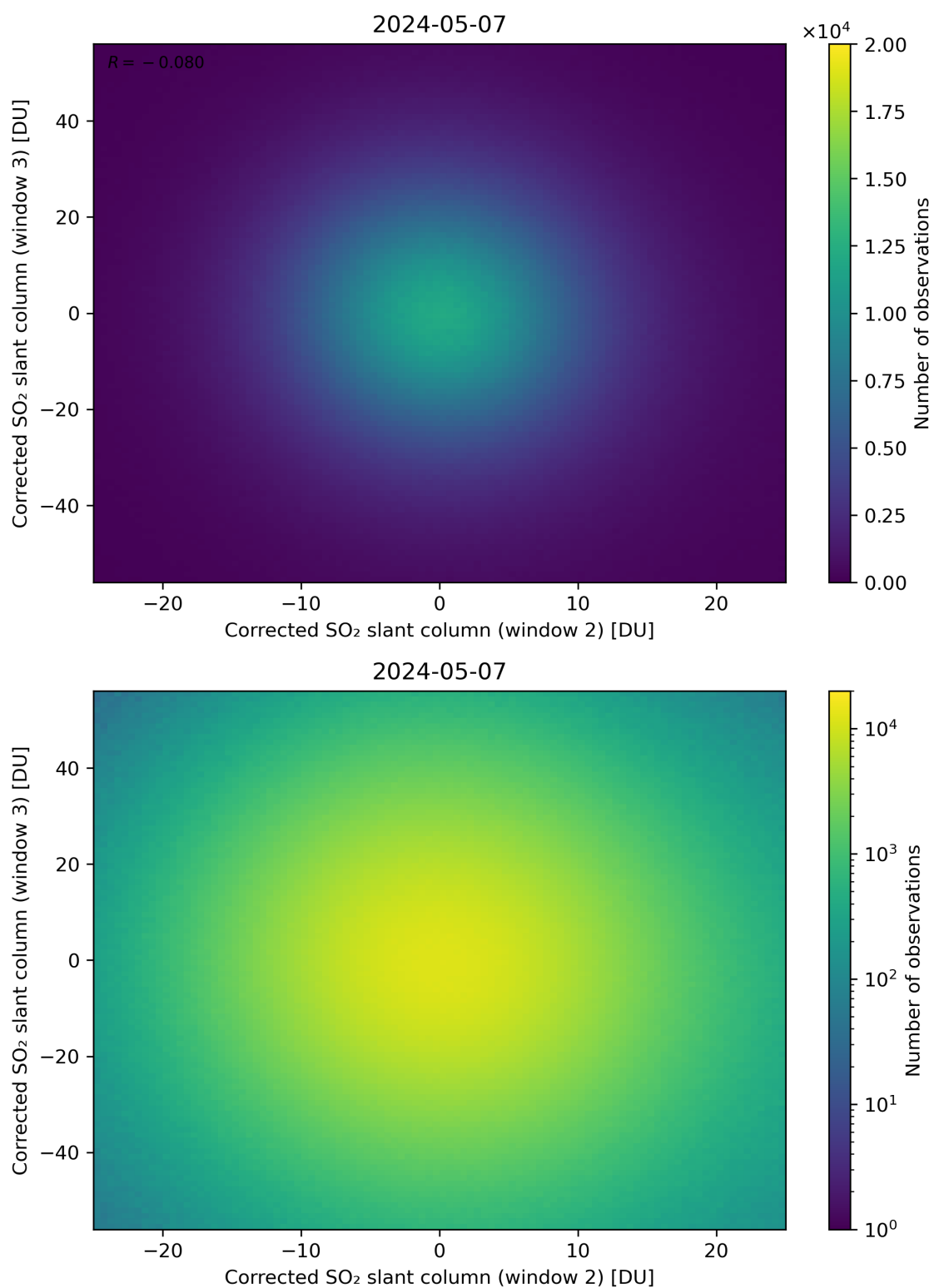
Figure 200: Scatter density plot of “Corrected SO 2 slant column (window 2)” against “Corrected SO 2 slant column (window 3)” for 2024-05-07 to 2024-05-08.
