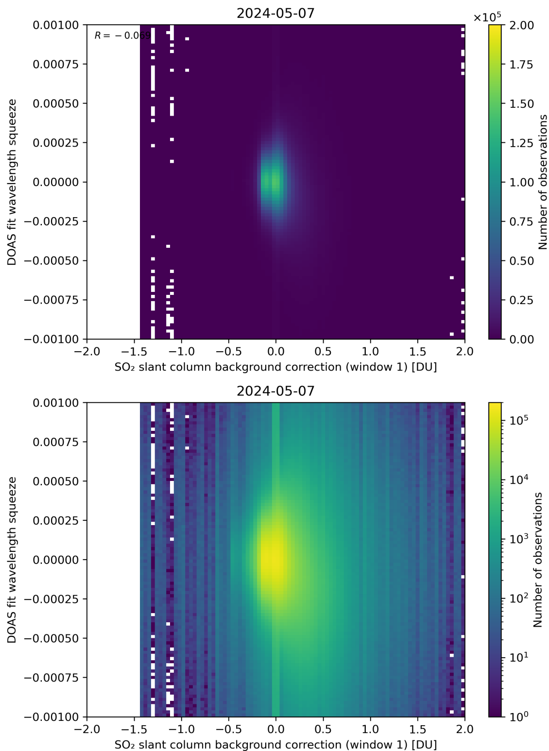
Figure 101: Scatter density plot of “SO 2 slant column background correction (window 1)” against “DOAS fit wavelength squeeze” for 2024-05-07 to 2024-05-08.
