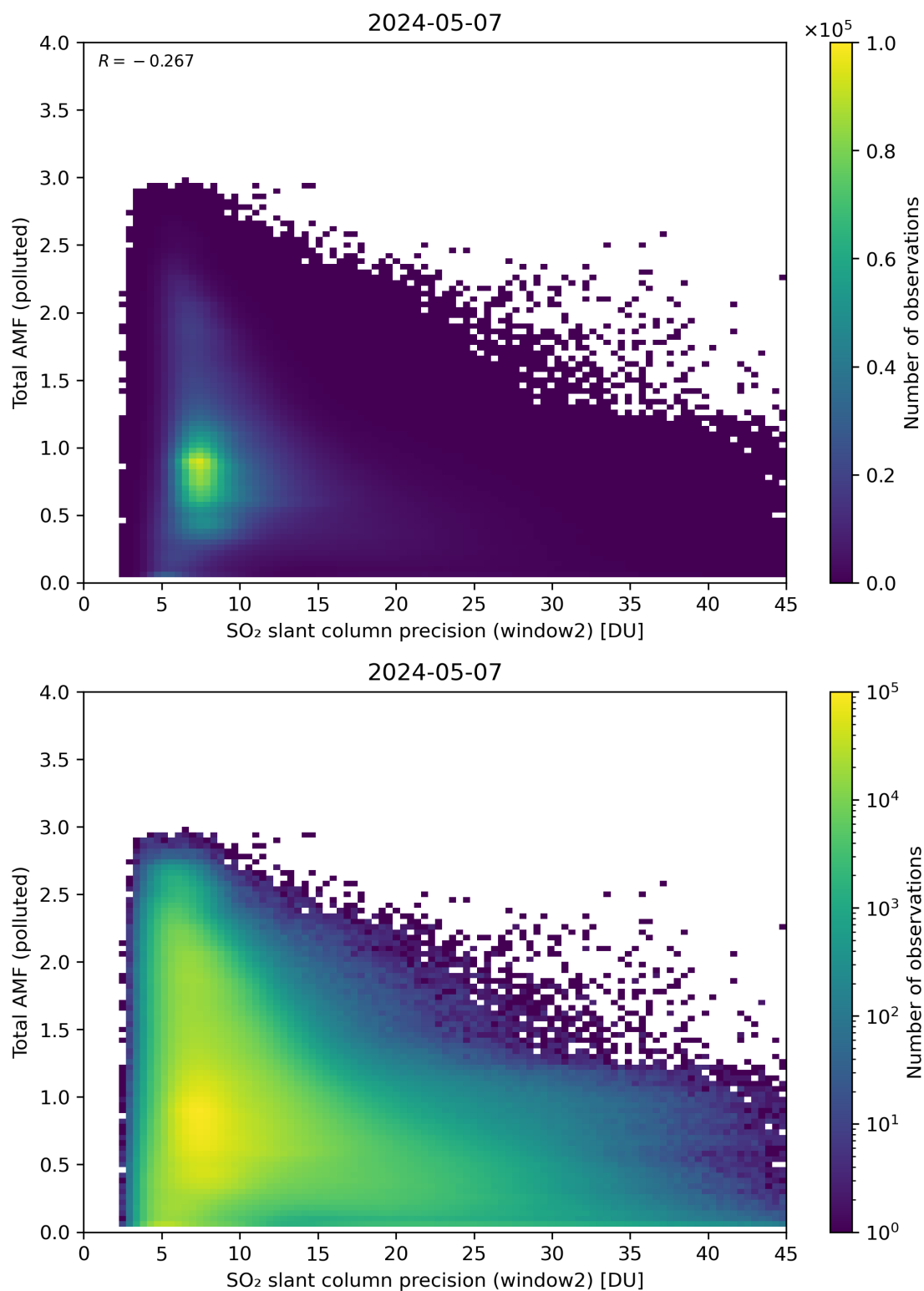
Figure 251: Scatter density plot of “SO 2 slant column precision (window2)” against “Total AMF (polluted)” for 2024-05-07 to 2024-05-08.
