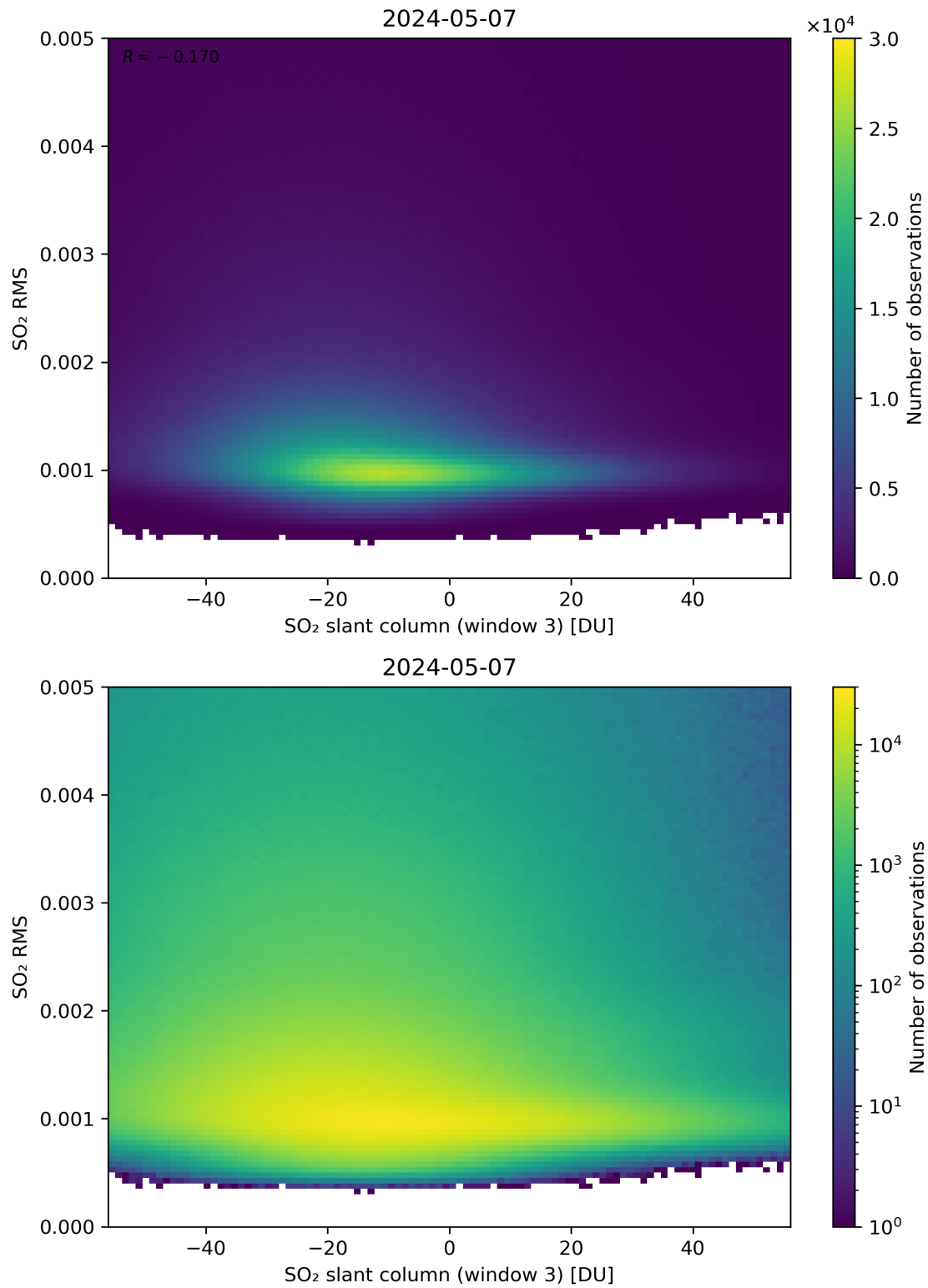
Figure 256: Scatter density plot of “SO 2 slant column (window 3)” against “SO 2 RMS” for 2024-05-07 to 2024-05-08.
