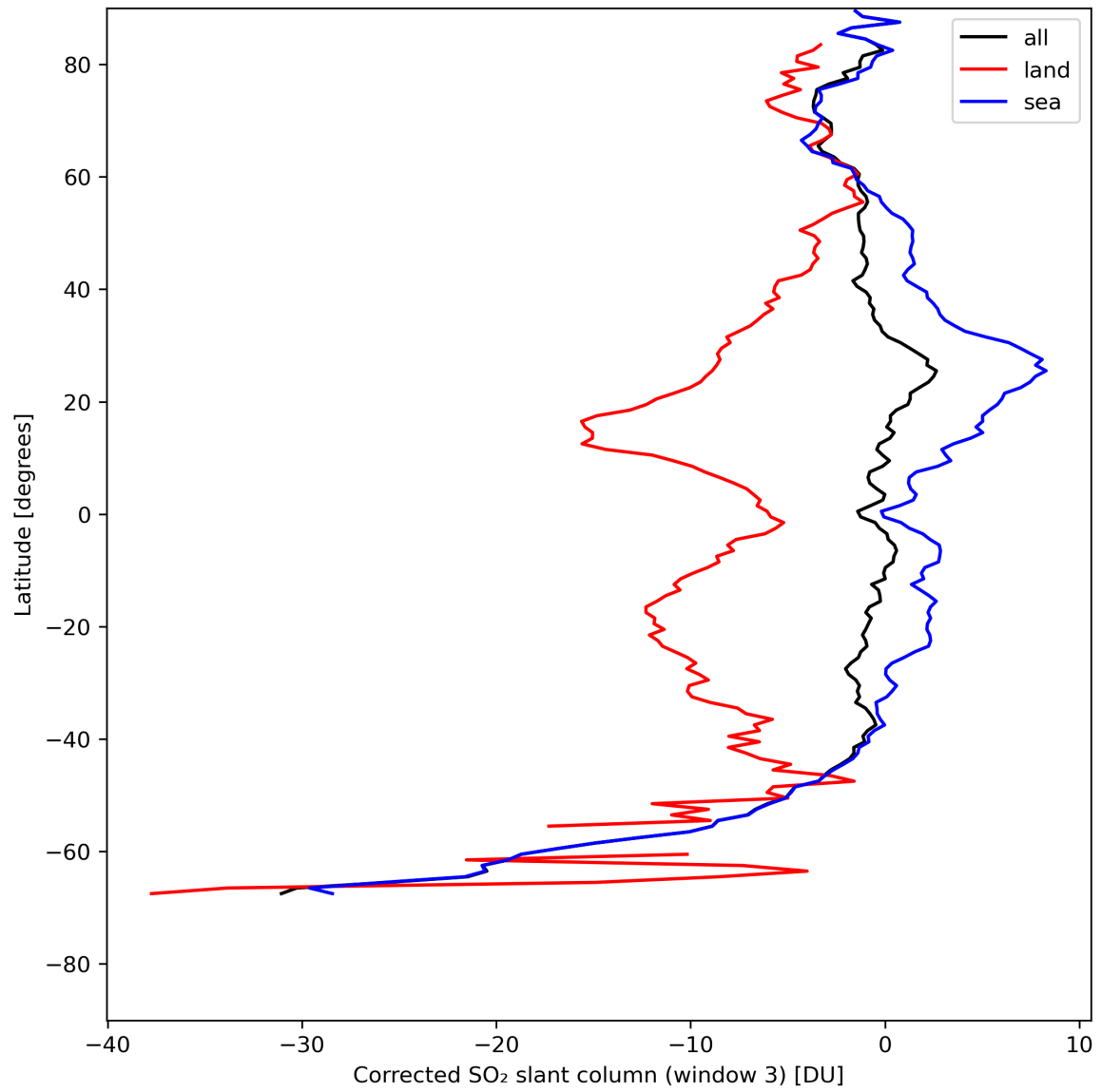
Figure 43: Zonal average of “Corrected SO 2 slant column (window 3)” for 2024-05-07 to 2024-05-08.
