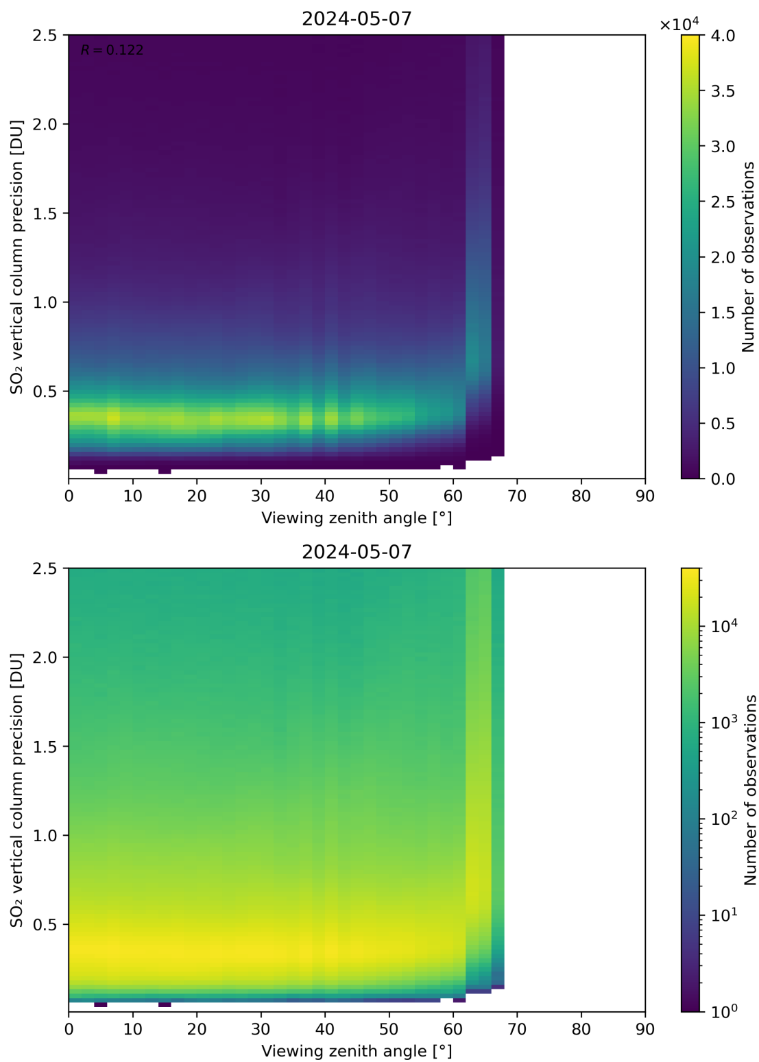
Figure 328: Scatter density plot of “Viewing zenith angle” against “SO 2 vertical column precision” for 2024-05-07 to 2024-05-08.
