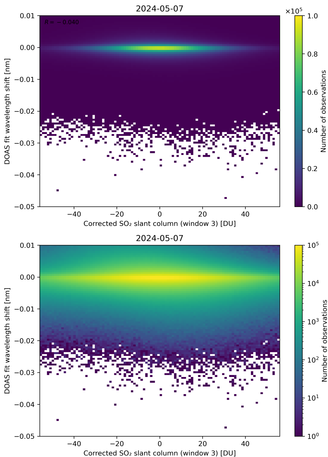
Figure 206: Scatter density plot of “Corrected SO 2 slant column (window 3)” against “DOAS fit wavelength shift” for 2024-05-07 to 2024-05-08.
