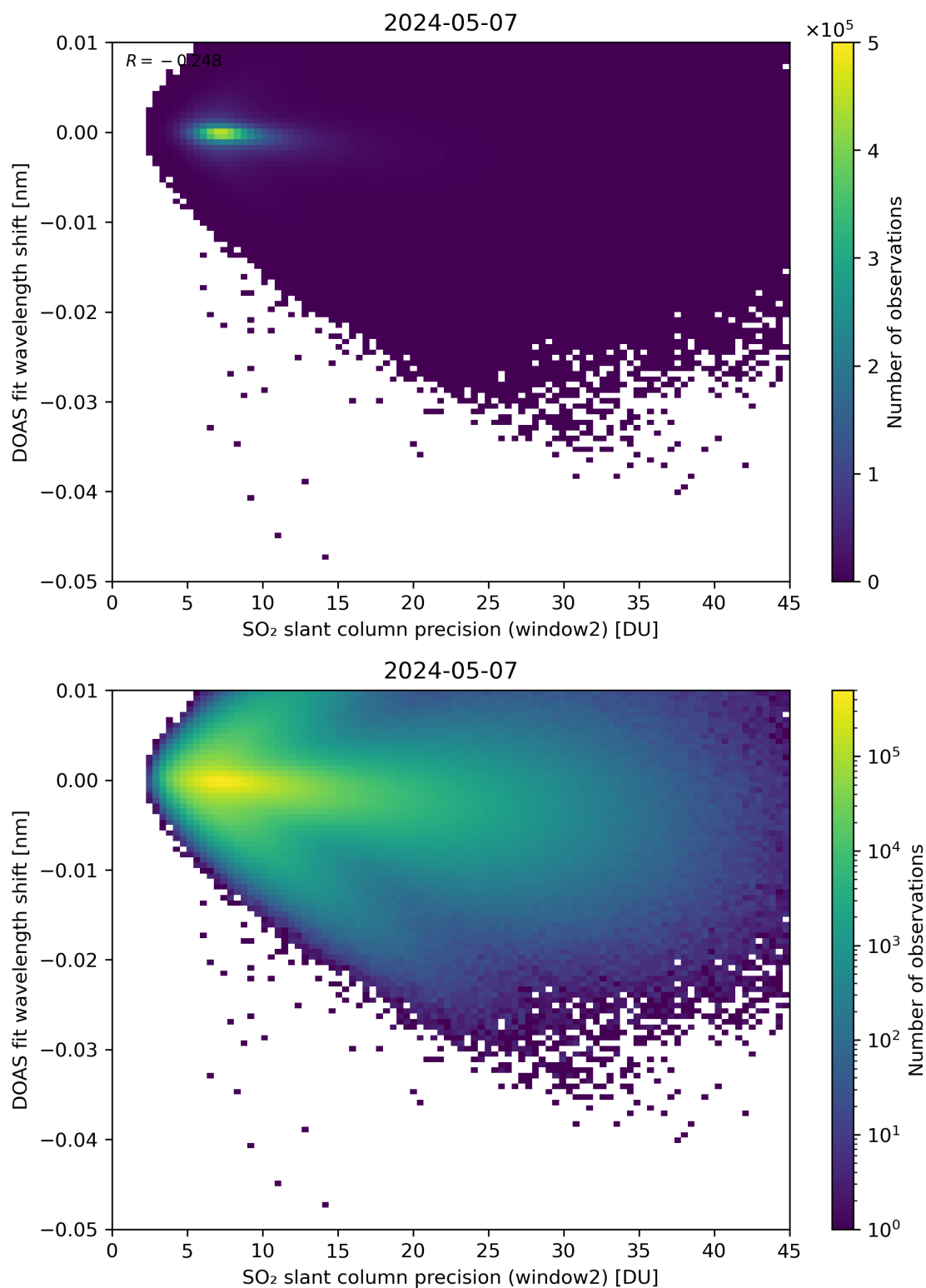
Figure 243: Scatter density plot of “SO 2 slant column precision (window2)” against “DOAS fit wavelength shift” for 2024-05-07 to 2024-05-08.
