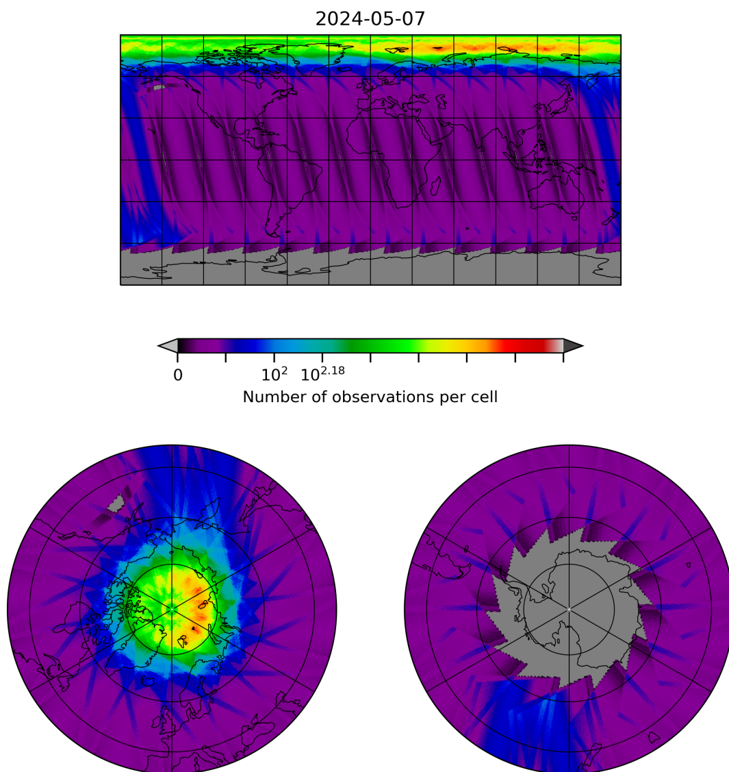
Figure 28: Map of the number of observations for 2024-05-07 to 2024-05-08
