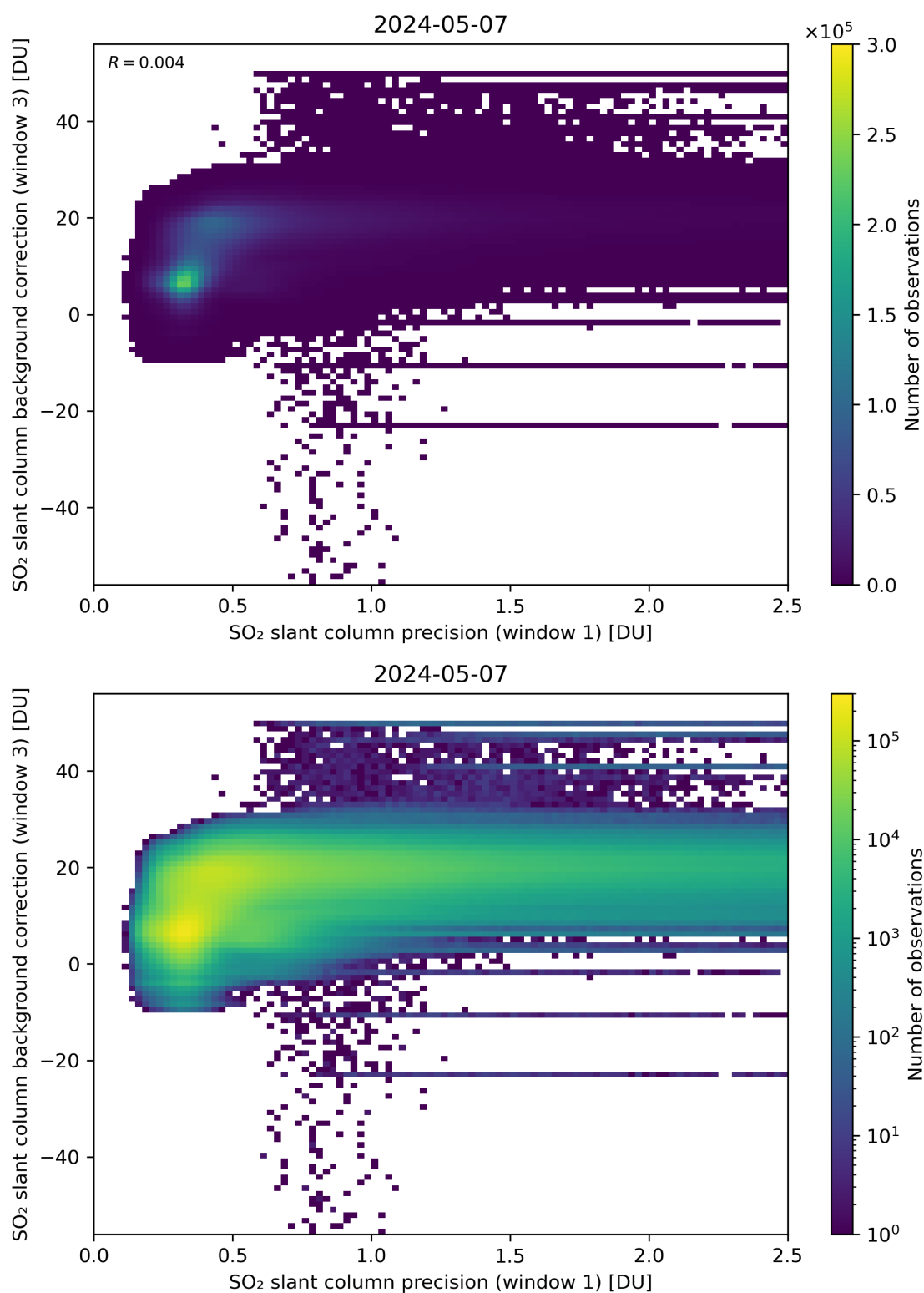
Figure 220: Scatter density plot of “SO 2 slant column precision (window 1)” against “SO 2 slant column background correction (window 3)” for 2024-05-07 to 2024-05-08.
