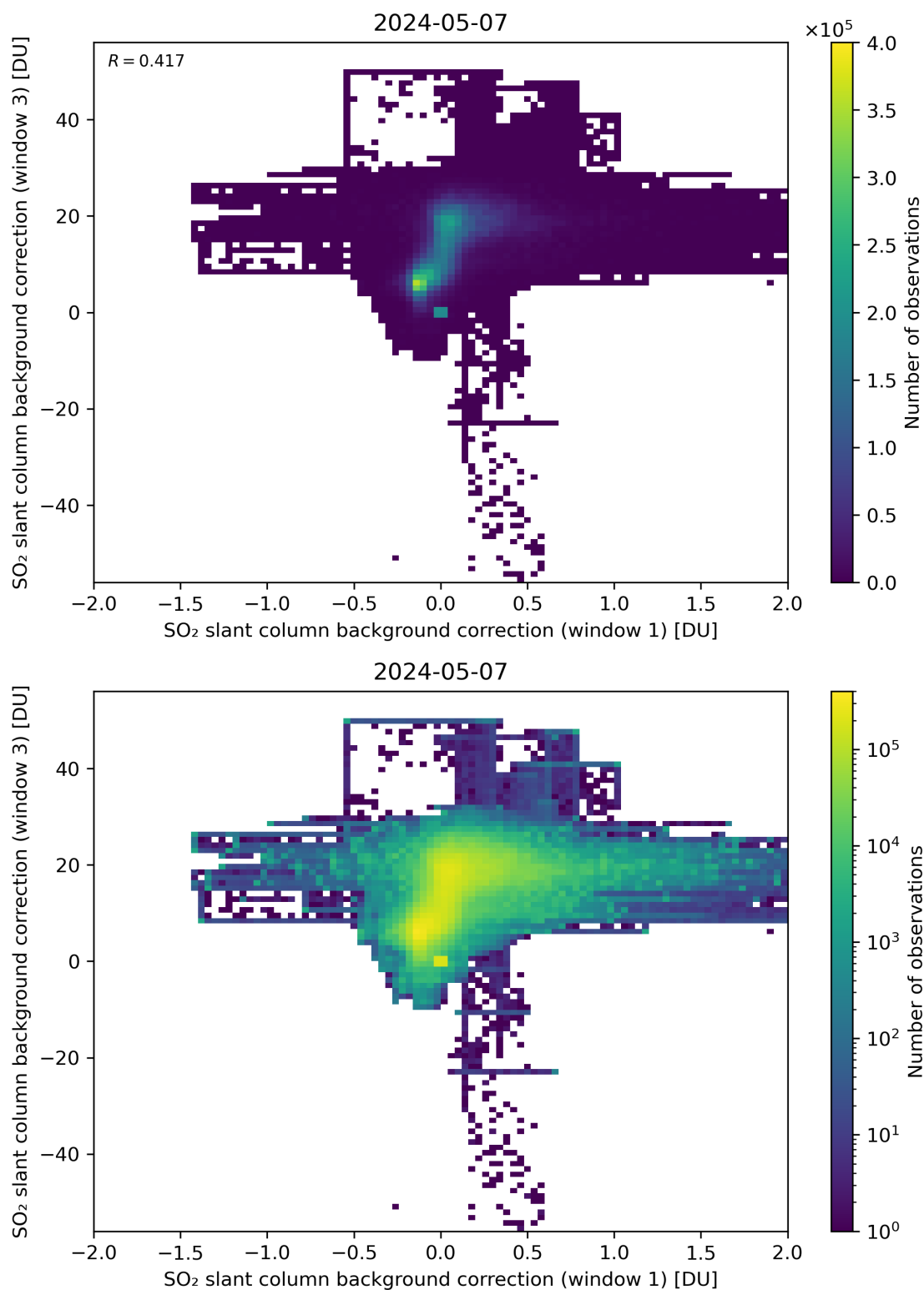
Figure 99: Scatter density plot of “SO 2 slant column background correction (window 1)” against “SO 2 slant column background correction (window 3)” for 2024-05-07 to 2024-05-08.
