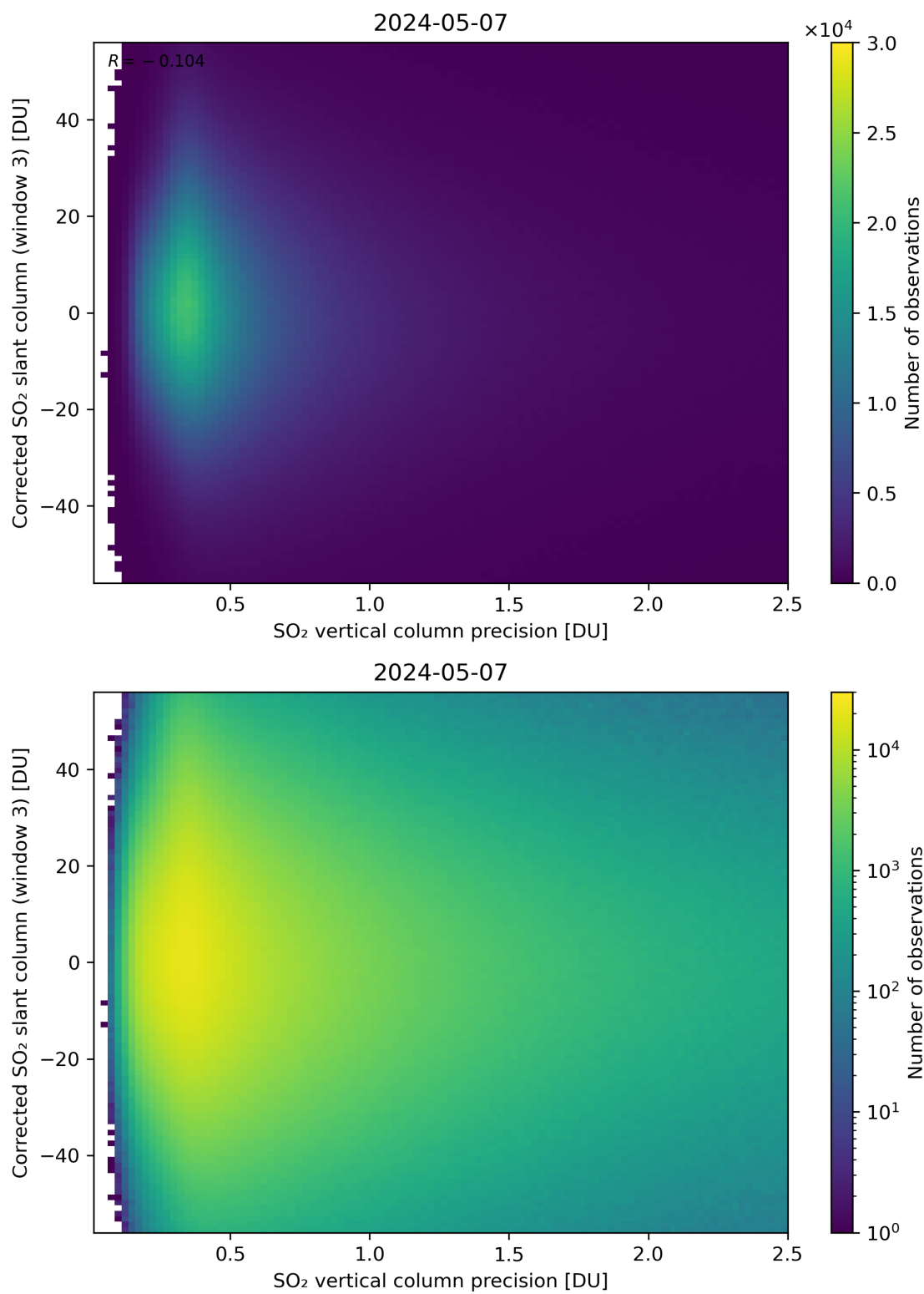
Figure 288: Scatter density plot of “SO 2 vertical column precision” against “Corrected SO 2 slant column (window 3)” for 2024-05-07 to 2024-05-08.
