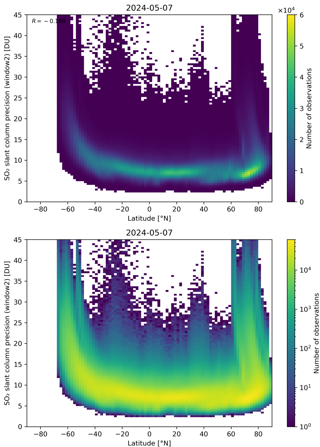
Figure 151: Scatter density plot of “Latitude” against “SO 2 slant column precision (window2)” for 2024-05-07 to 2024-05-08.
