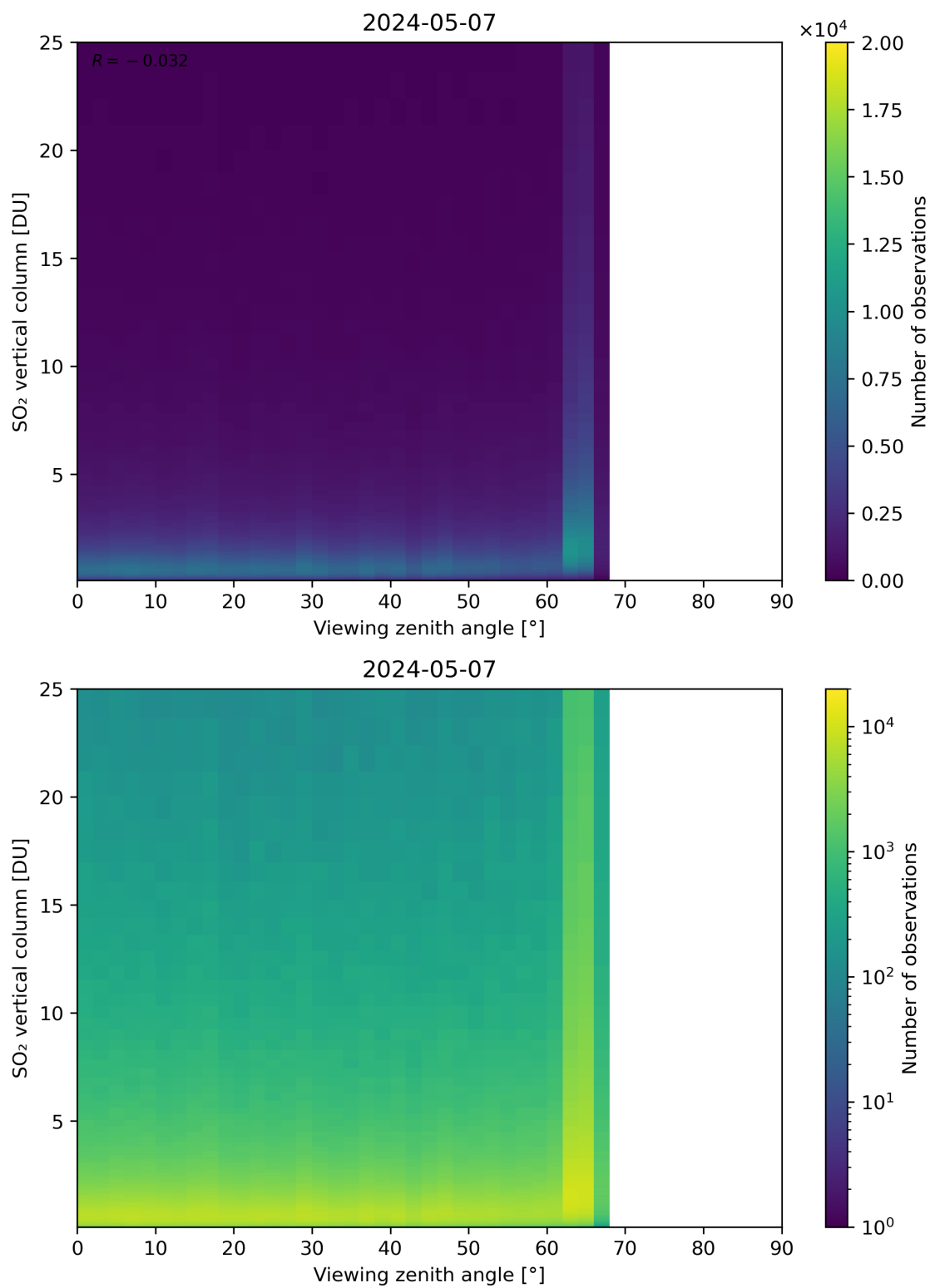
Figure 327: Scatter density plot of “Viewing zenith angle” against “SO 2 vertical column” for 2024-05-07 to 2024-05-08.
