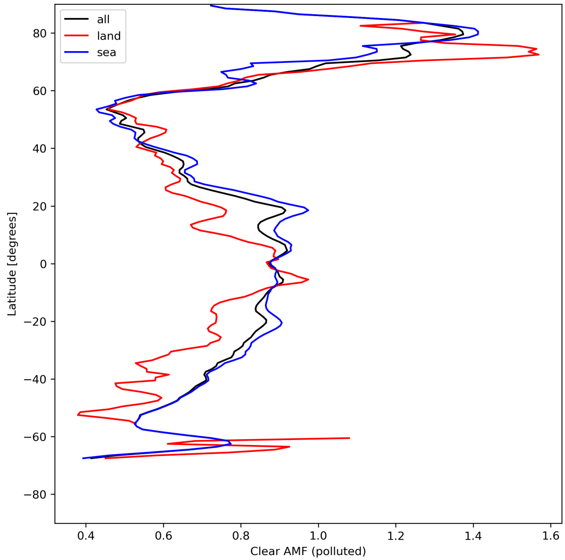
Figure 50: Zonal average of “Clear AMF (polluted)” for 2024-05-07 to 2024-05-08.
