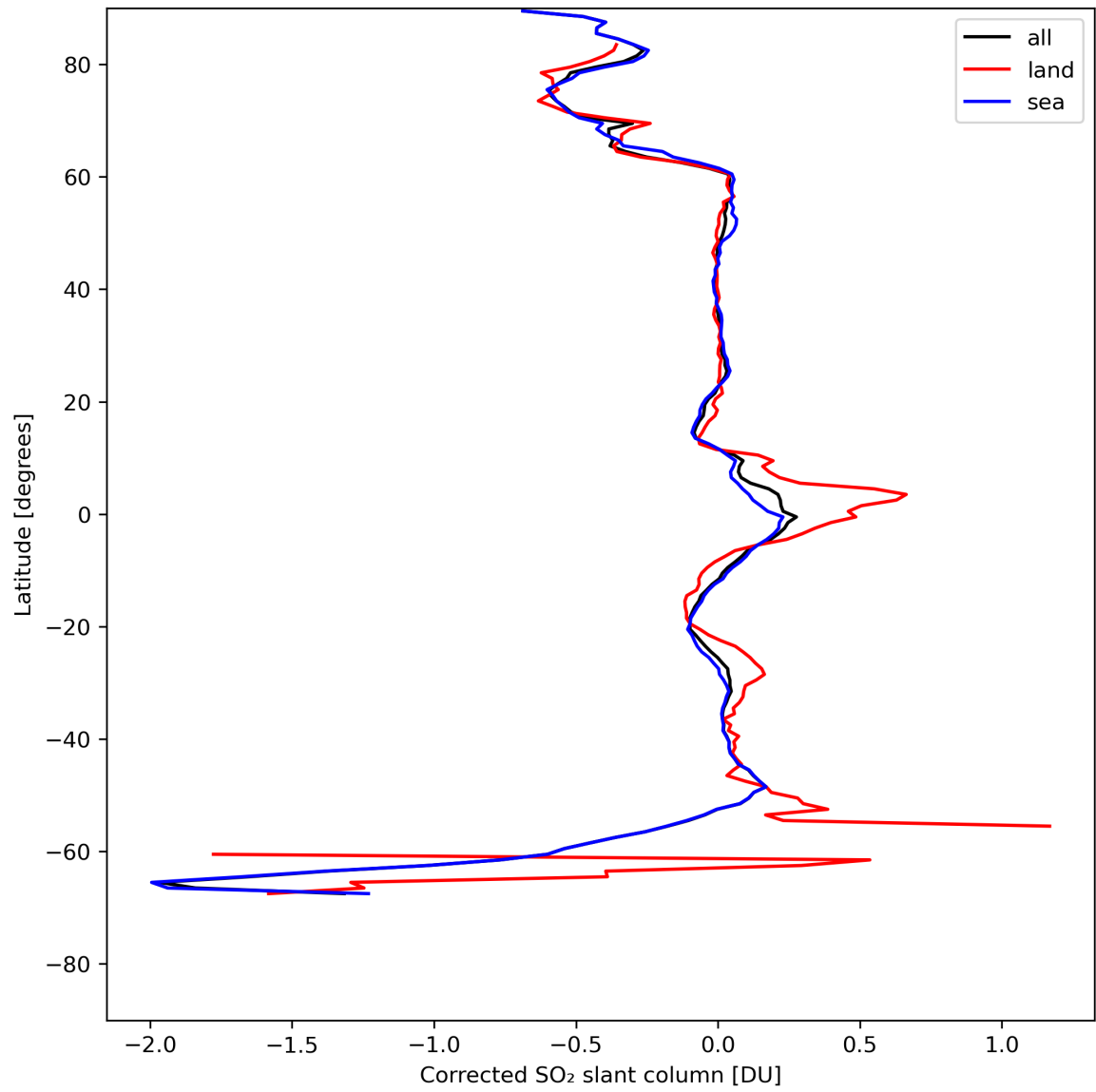
Figure 32: Zonal average of “Corrected SO 2 slant column” for 2024-05-07 to 2024-05-08.
