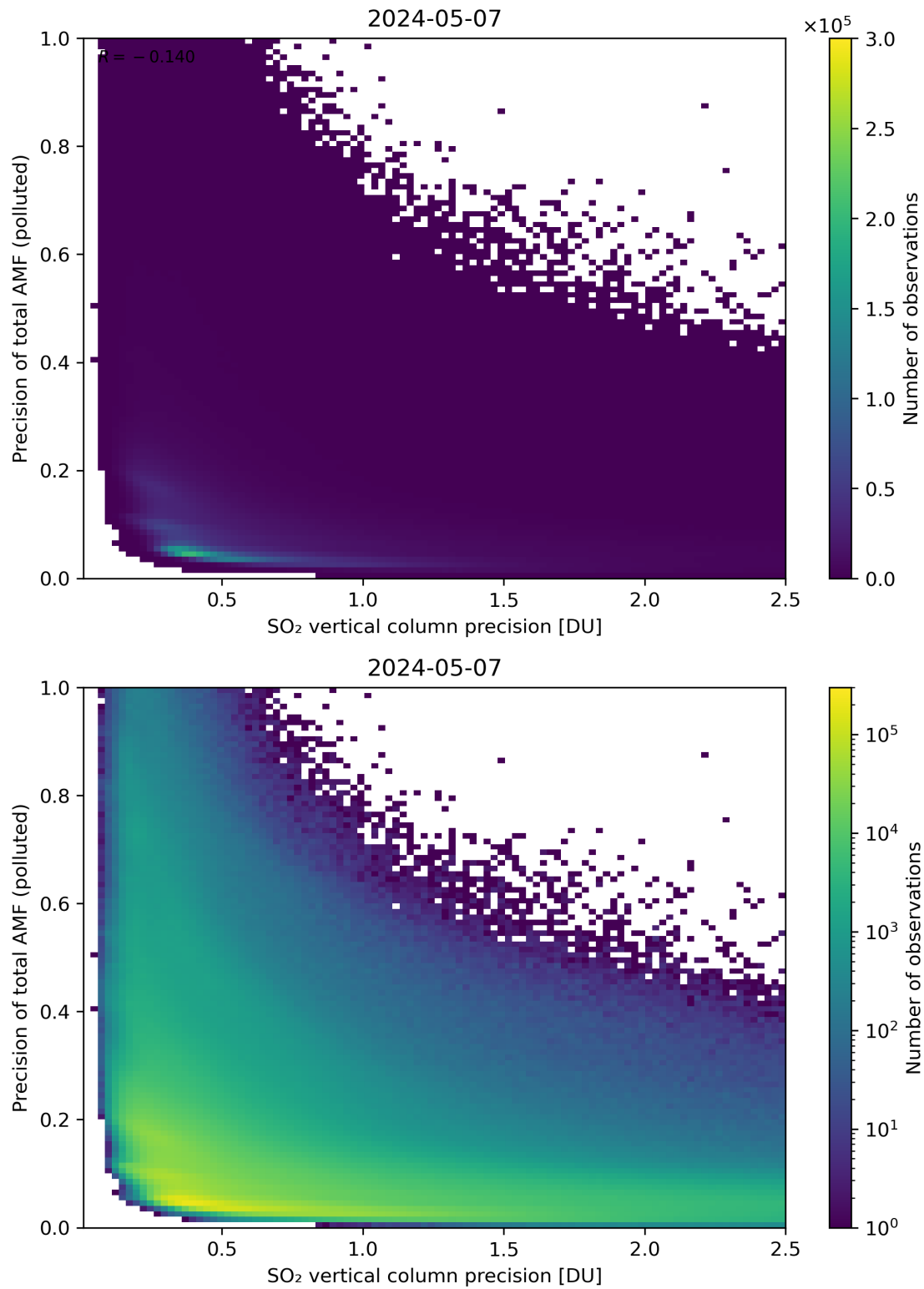
Figure 295: Scatter density plot of “SO 2 vertical column precision” against “Precision of total AMF (polluted)” for 2024-05-07 to 2024-05-08.
