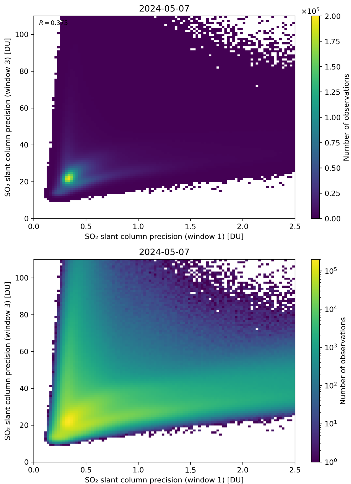
Figure 229: Scatter density plot of “SO 2 slant column precision (window 1)” against “SO 2 slant column precision (window 3)” for 2024-05-07 to 2024-05-08.
