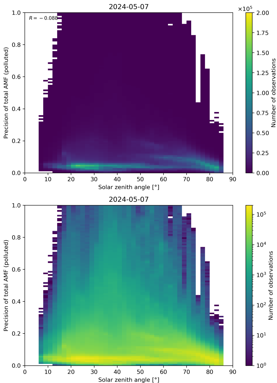
Figure 175: Scatter density plot of “Solar zenith angle” against “Precision of total AMF (polluted)” for 2024-05-07 to 2024-05-08.
