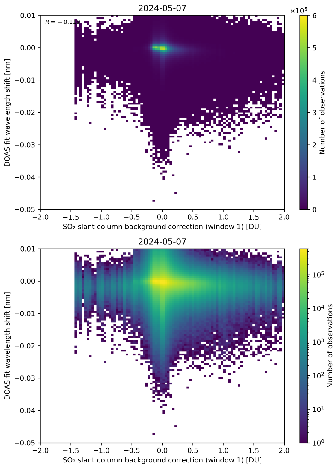
Figure 100: Scatter density plot of “SO 2 slant column background correction (window 1)” against “DOAS fit wavelength shift” for 2024-05-07 to 2024-05-08.
