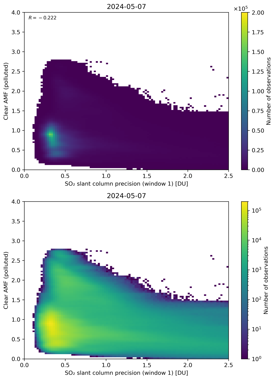
Figure 224: Scatter density plot of “SO 2 slant column precision (window 1)” against “Clear AMF (polluted)” for 2024-05-07 to 2024-05-08.
