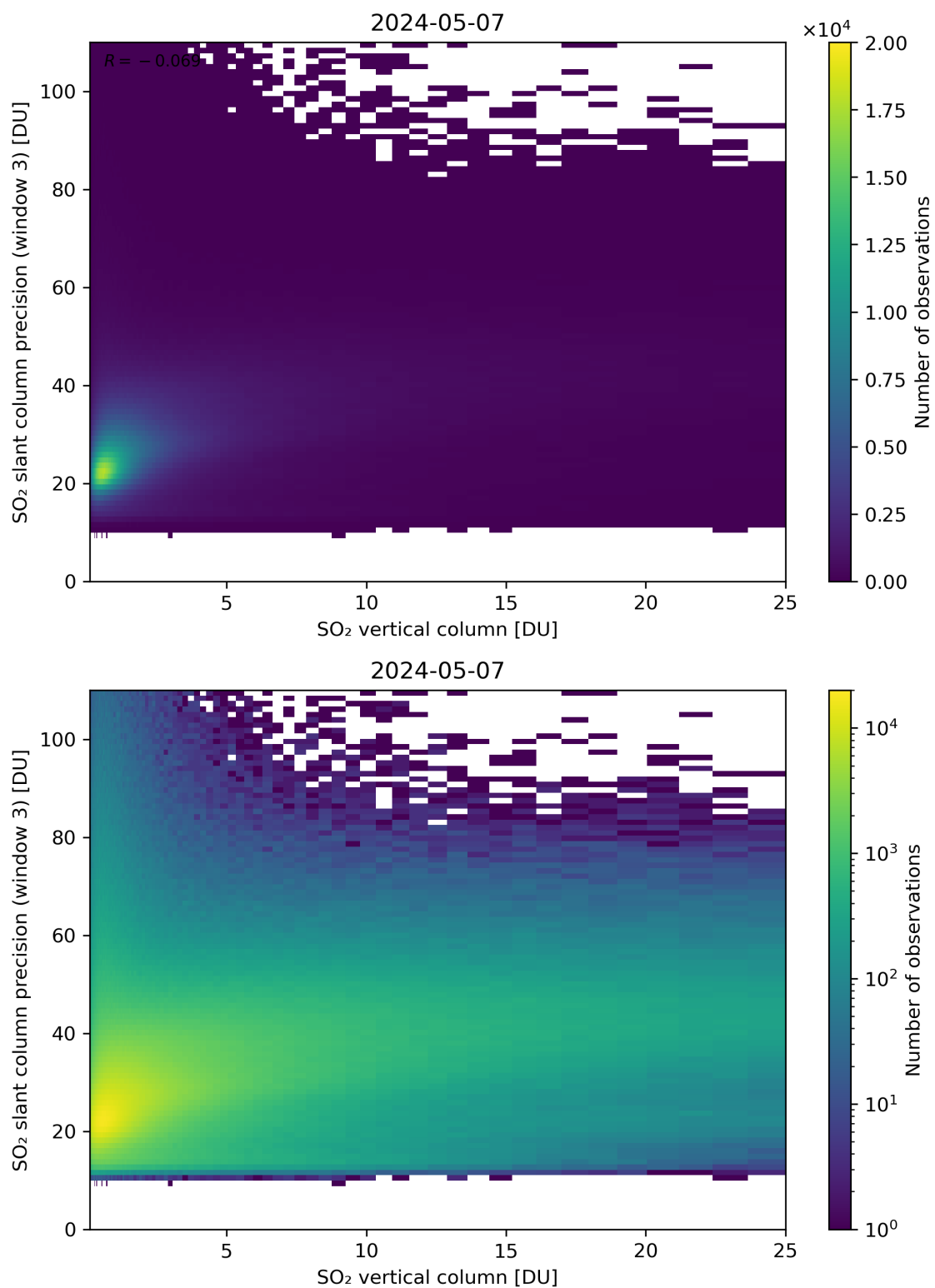
Figure 304: Scatter density plot of “SO 2 vertical column” against “SO 2 slant column precision (window 3)” for 2024-05-07 to 2024-05-08.
