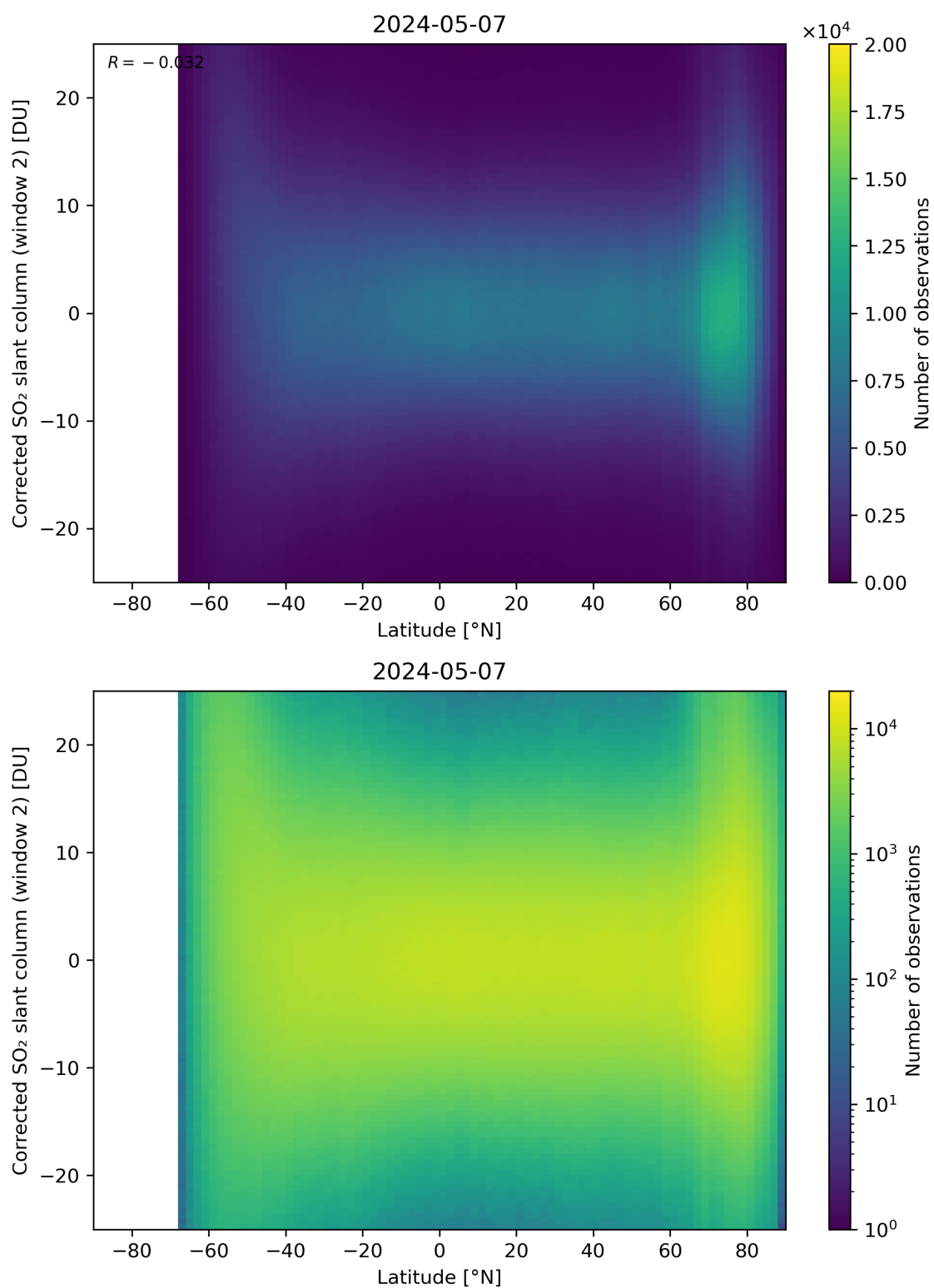
Figure 147: Scatter density plot of “Latitude” against “Corrected SO 2 slant column (window 2)” for 2024-05-07 to 2024-05-08.
