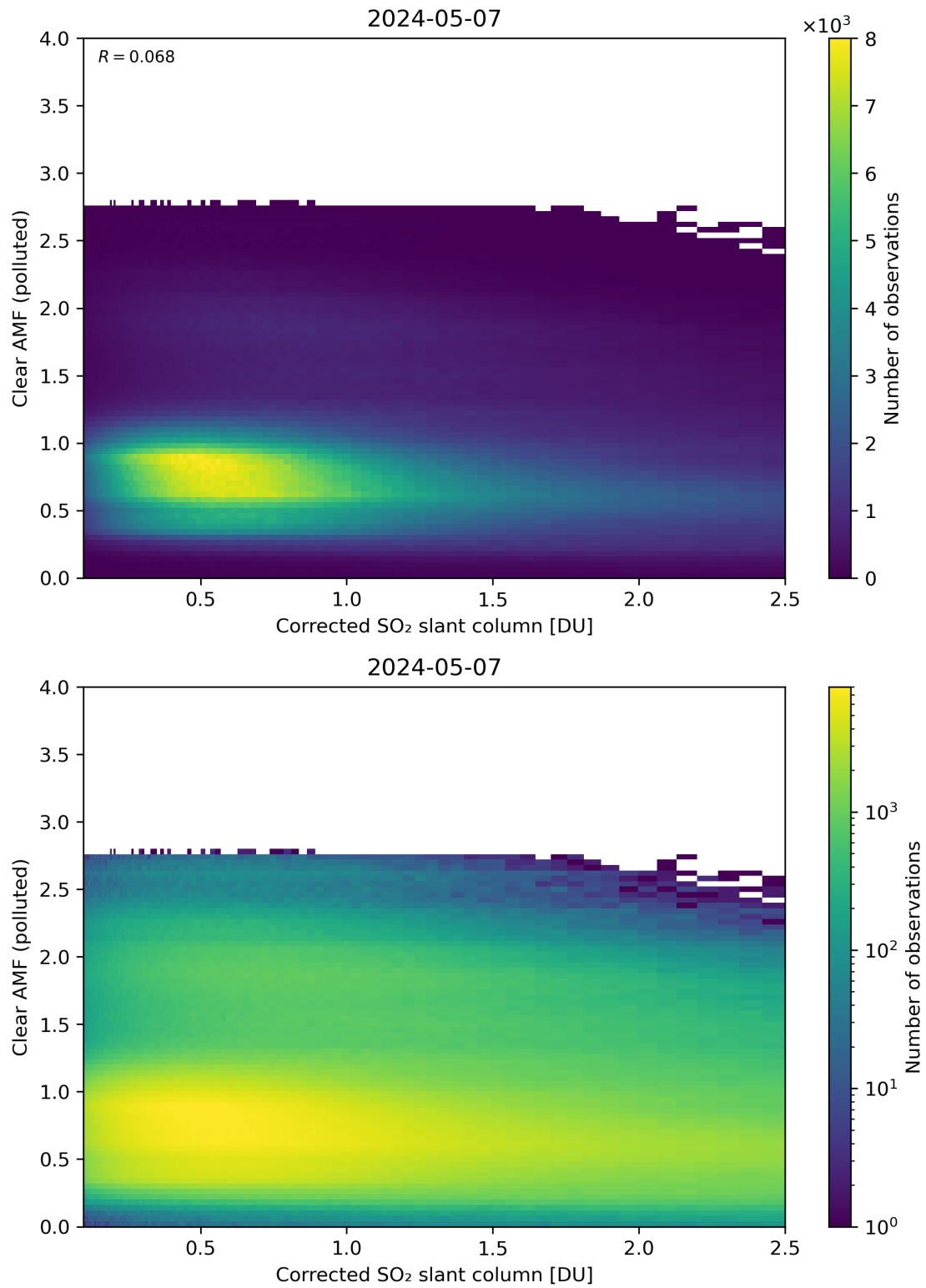
Figure 184: Scatter density plot of “Corrected SO 2 slant column” against “Clear AMF (polluted)” for 2024-05-07 to 2024-05-08.
