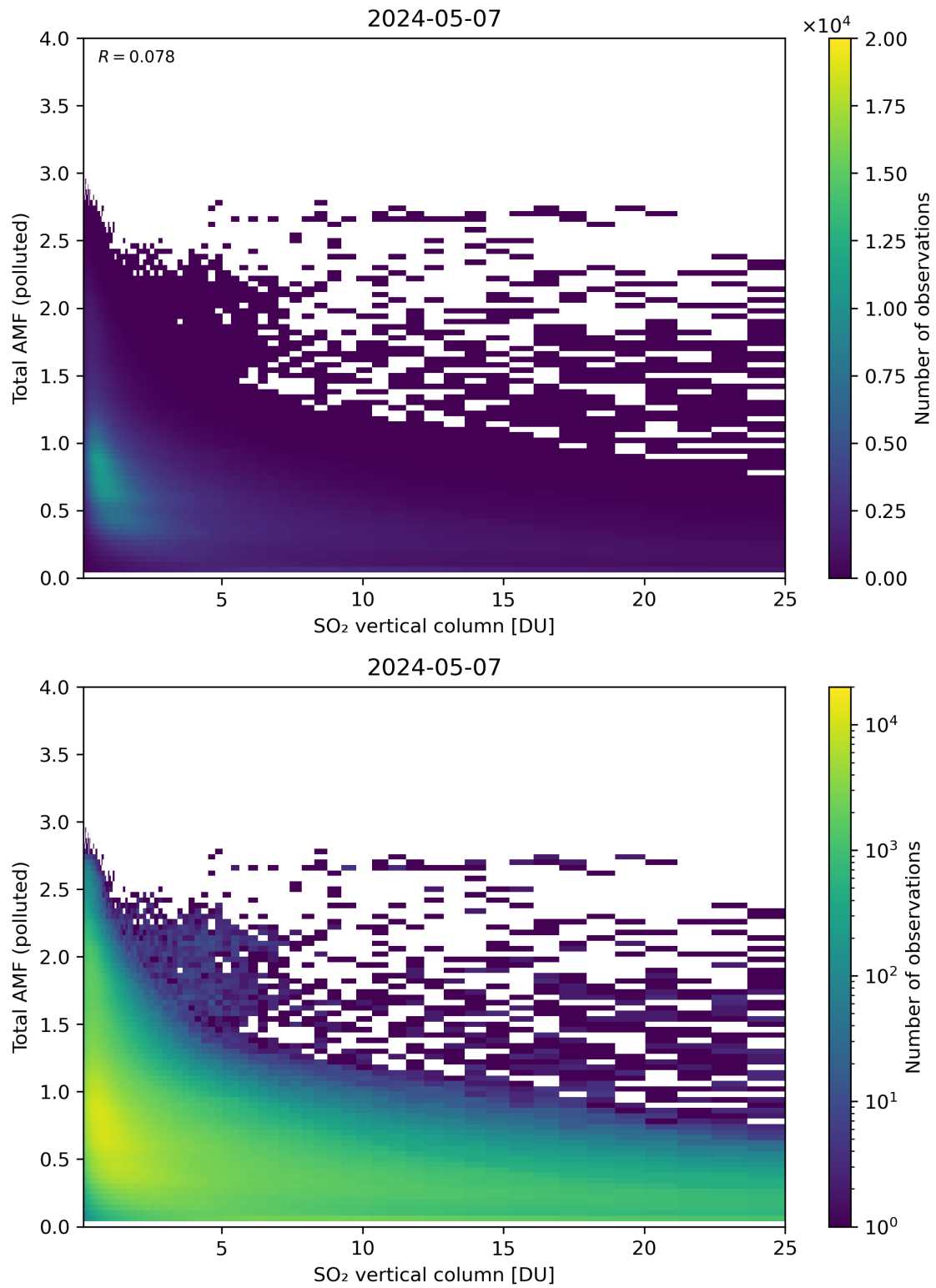
Figure 305: Scatter density plot of “SO 2 vertical column” against “Total AMF (polluted)” for 2024-05-07 to 2024-05-08.
