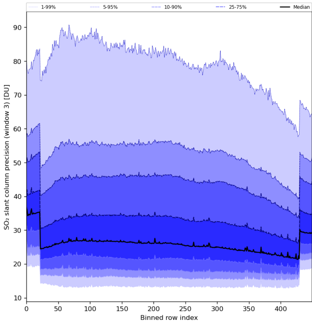
Figure 88: Along track statistics of “SO 2 slant column precision (window 3)” for 2024-05-07 to 2024-05-08
