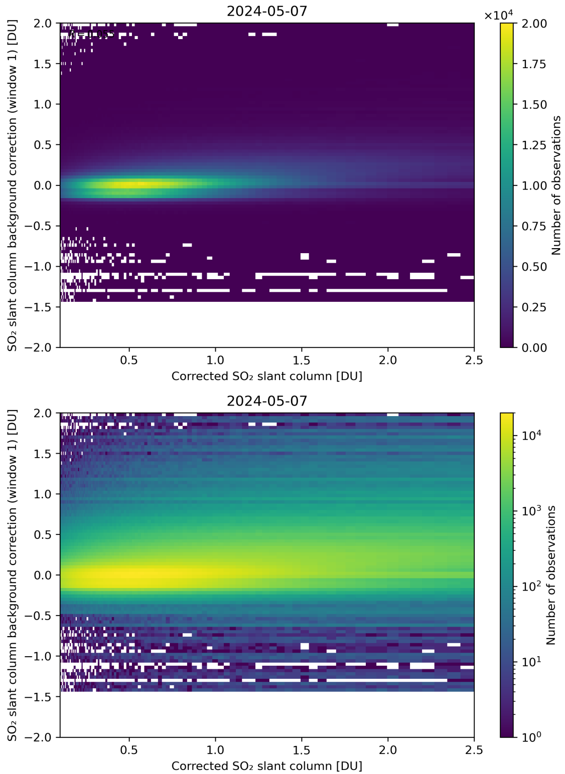
Figure 178: Scatter density plot of “Corrected SO 2 slant column” against “SO 2 slant column background correction (window 1)” for 2024-05-07 to 2024-05-08.
