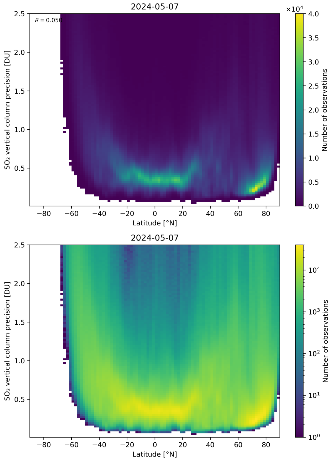
Figure 157: Scatter density plot of “Latitude” against “SO 2 vertical column precision” for 2024-05-07 to 2024-05-08.
