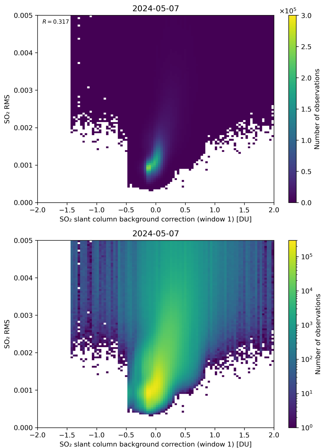
Figure 102: Scatter density plot of “SO 2 slant column background correction (window 1)” against “SO 2 RMS” for 2024-05-07 to 2024-05-08.
