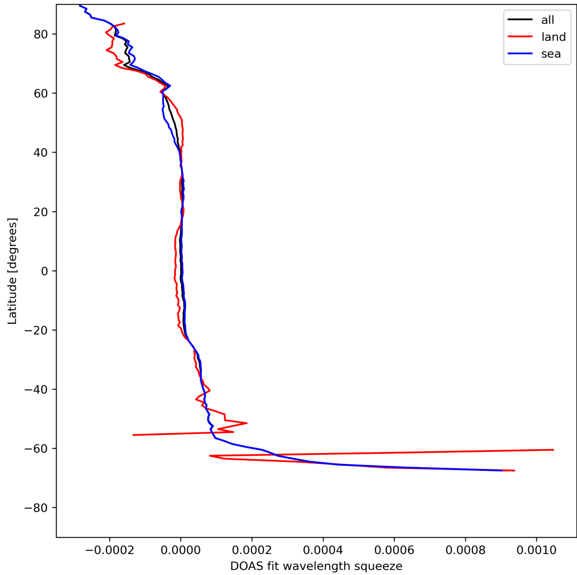
Figure 46: Zonal average of “DOAS fit wavelength squeeze” for 2024-05-07 to 2024-05-08.
