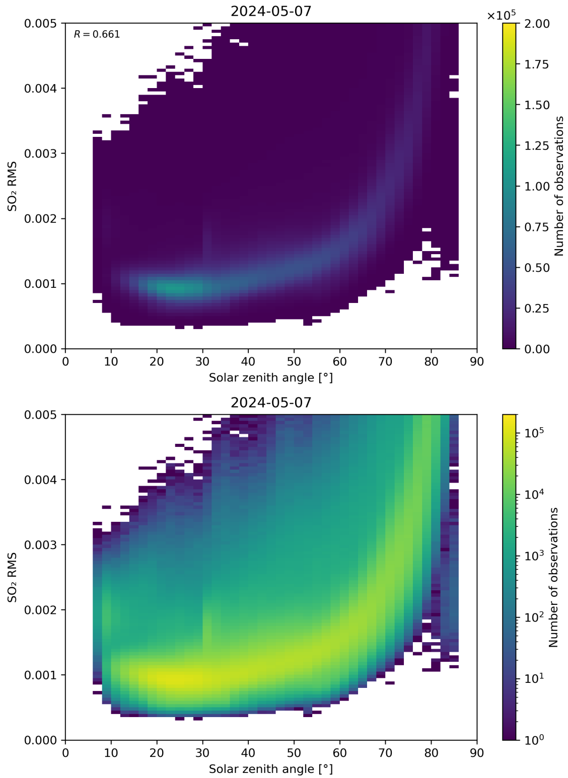
Figure 163: Scatter density plot of “Solar zenith angle” against “SO 2 RMS” for 2024-05-07 to 2024-05-08.
