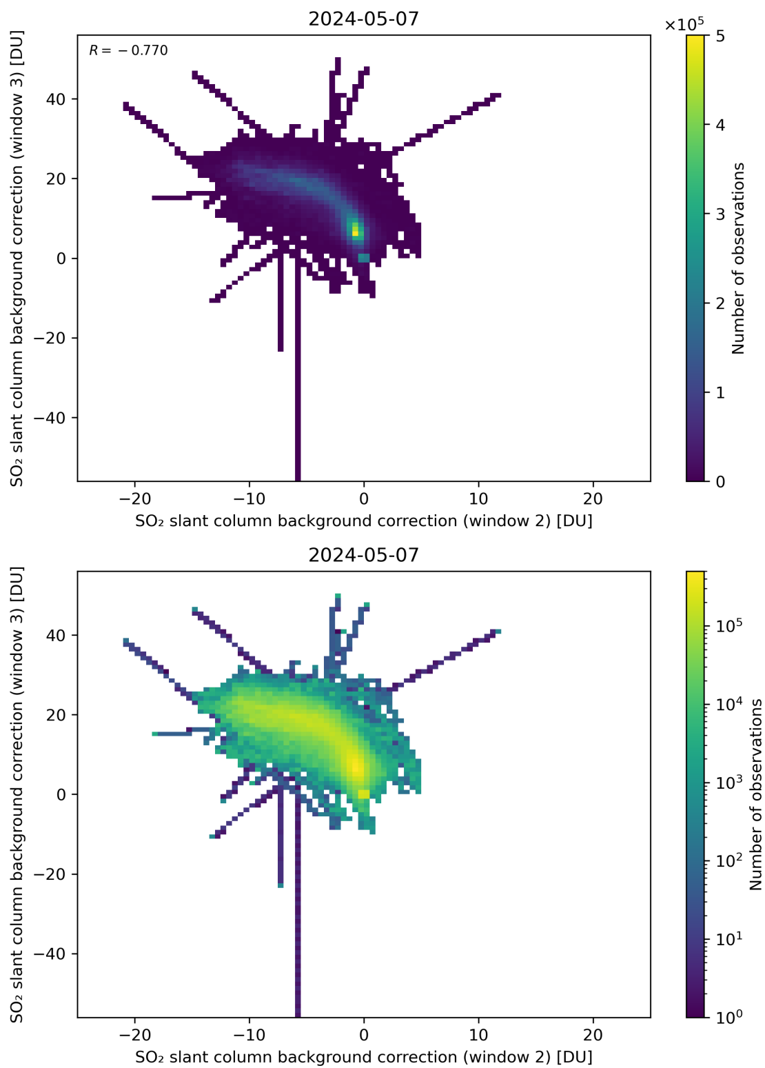
Figure 111: Scatter density plot of “SO 2 slant column background correction (window 2)” against “SO 2 slant column background correction (window 3)” for 2024-05-07 to 2024-05-08.
