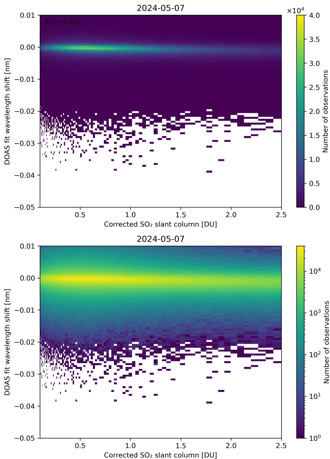
Figure 181: Scatter density plot of “Corrected SO 2 slant column” against “DOAS fit wavelength shift” for 2024-05-07 to 2024-05-08.
