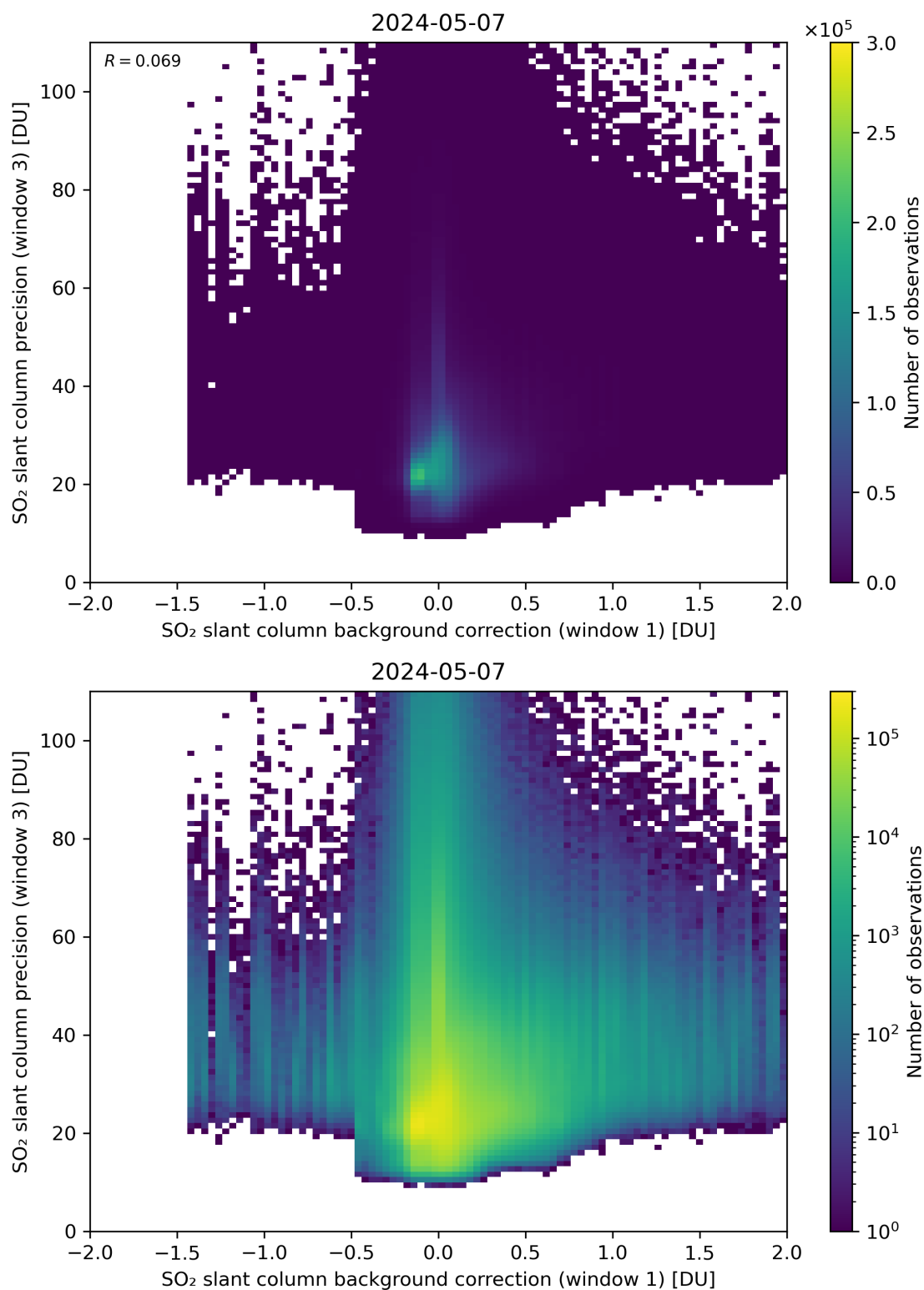
Figure 108: Scatter density plot of “SO 2 slant column background correction (window 1)” against “SO 2 slant column precision (window 3)” for 2024-05-07 to 2024-05-08.
