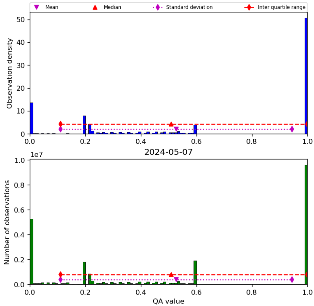
Figure 52: Histogram of “QA value” for 2024-05-07 to 2024-05-08
