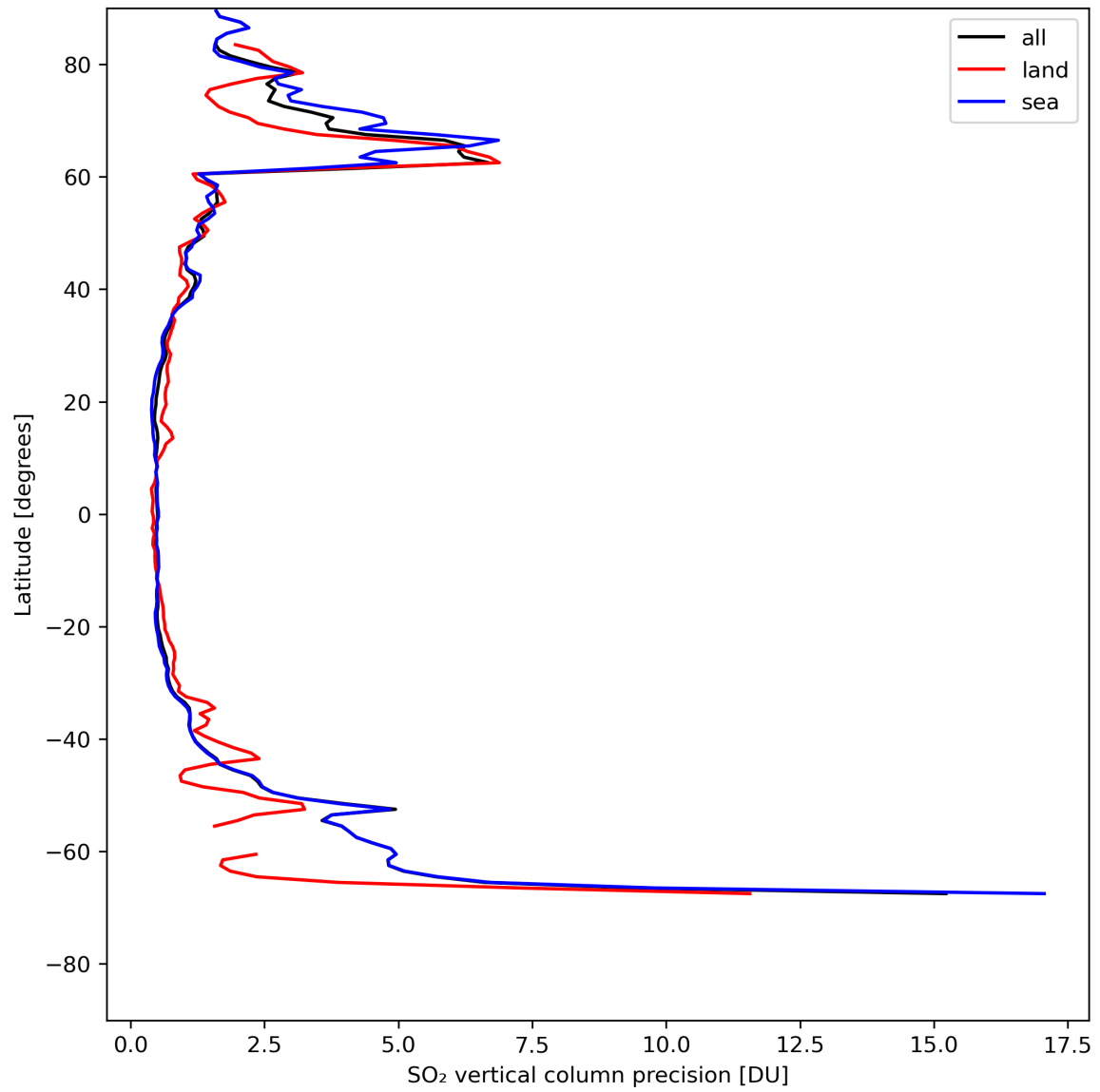
Figure 31: Zonal average of “SO 2 vertical column precision” for 2024-05-07 to 2024-05-08.
