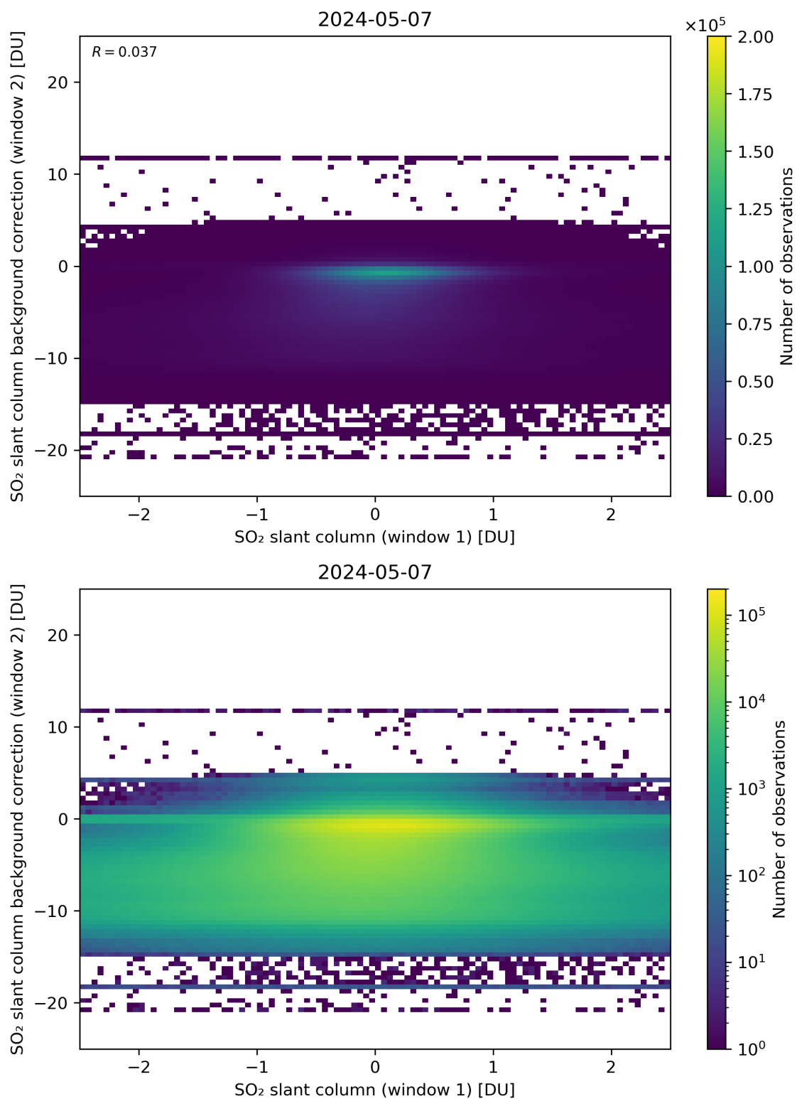
Figure 213: Scatter density plot of “SO 2 slant column (window 1)” against “SO 2 slant column background correction (window 2)” for 2024-05-07 to 2024-05-08.
