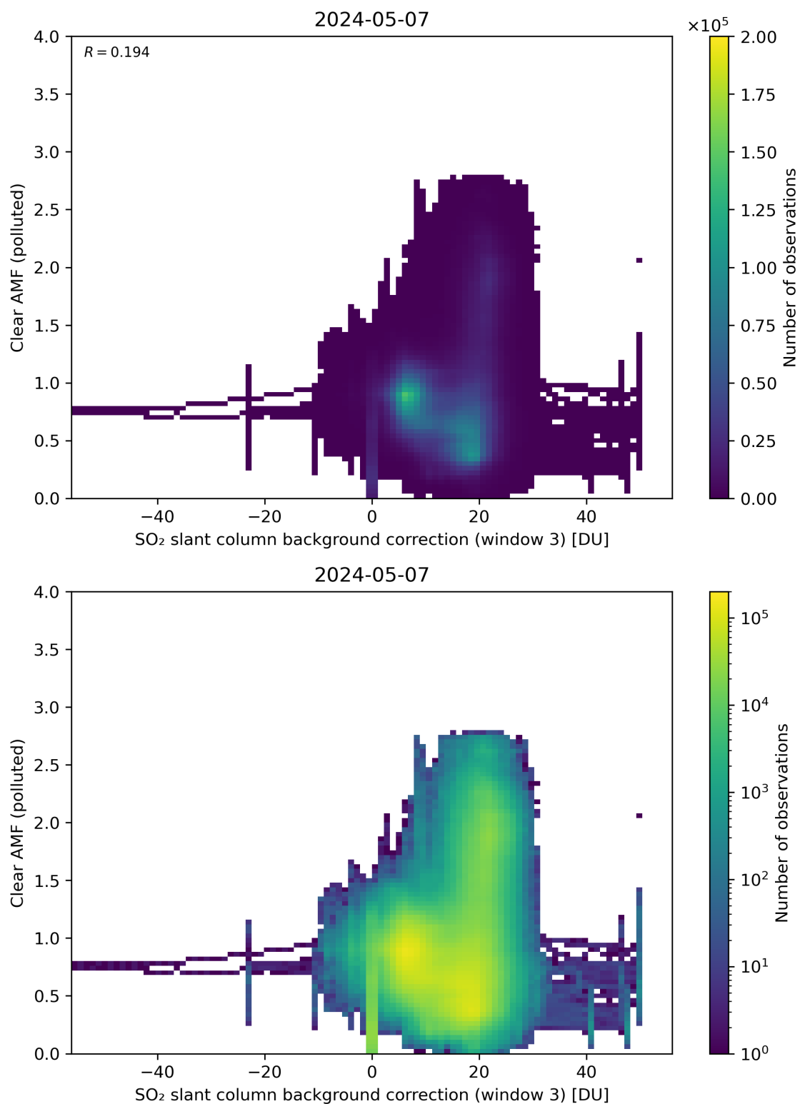
Figure 124: Scatter density plot of “SO 2 slant column background correction (window 3)” against “Clear AMF (polluted)” for 2024-05-07 to 2024-05-08.
