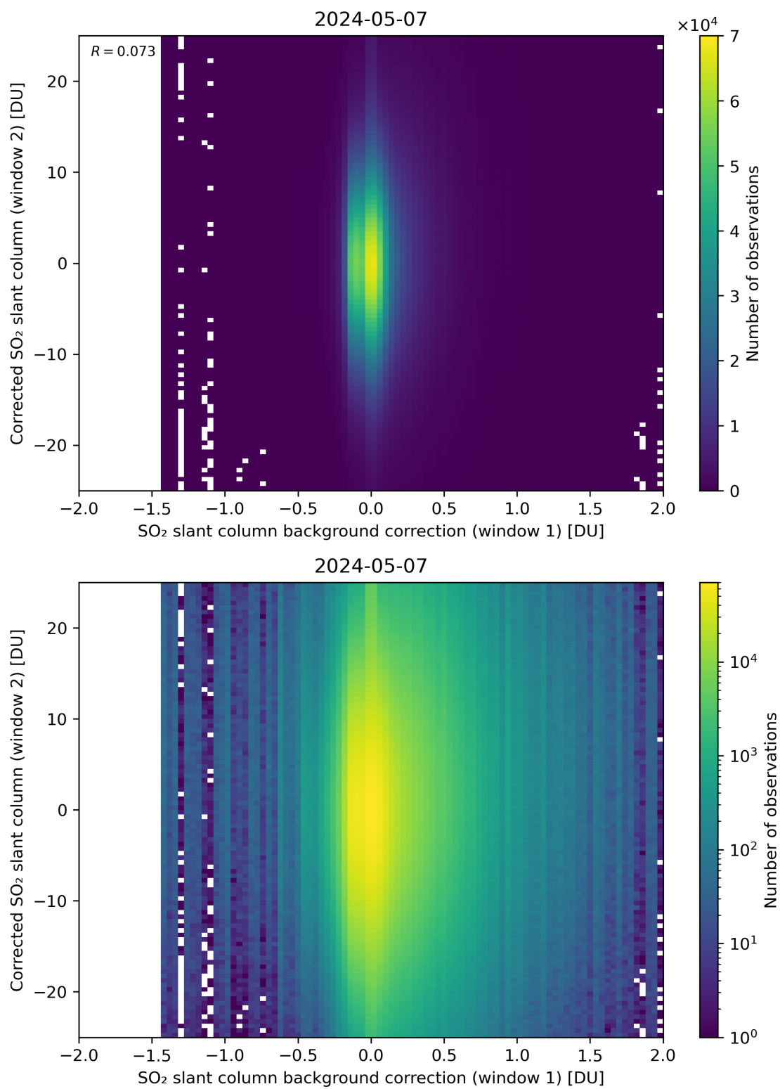
Figure 104: Scatter density plot of “SO 2 slant column background correction (window 1)” against “Corrected SO 2 slant column (window 2)” for 2024-05-07 to 2024-05-08.
