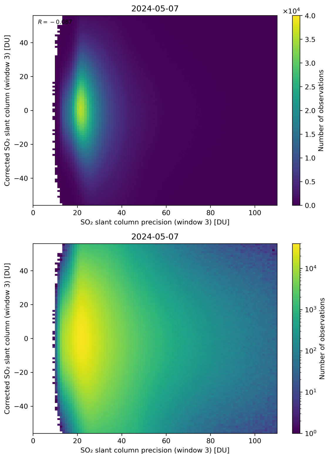
Figure 262: Scatter density plot of “SO 2 slant column precision (window 3)” against “Corrected SO 2 slant column (window 3)” for 2024-05-07 to 2024-05-08.
