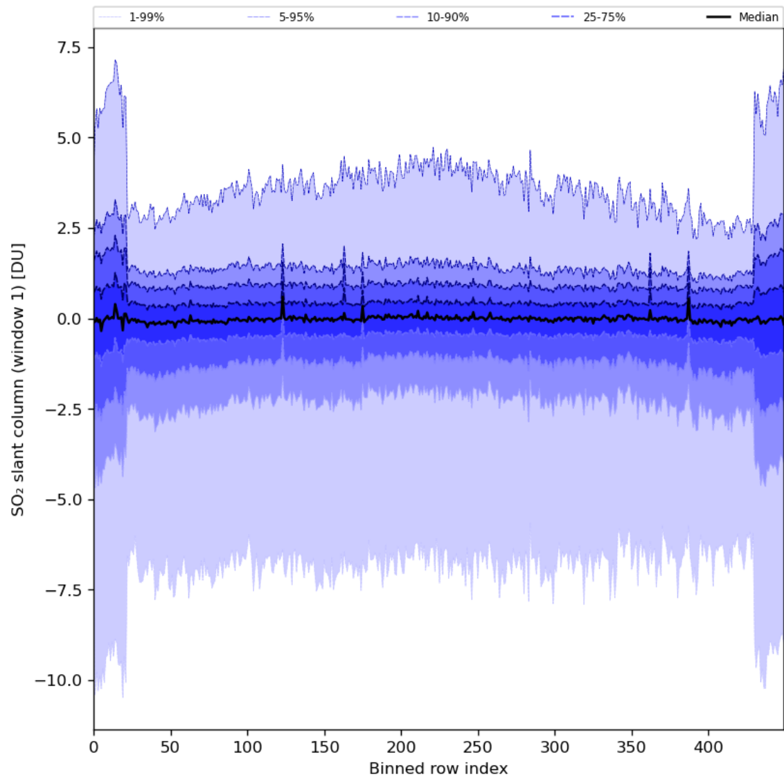
Figure 79: Along track statistics of "SO 2 slant column (window 1)" for 2024-05-07 to 2024-05-08
