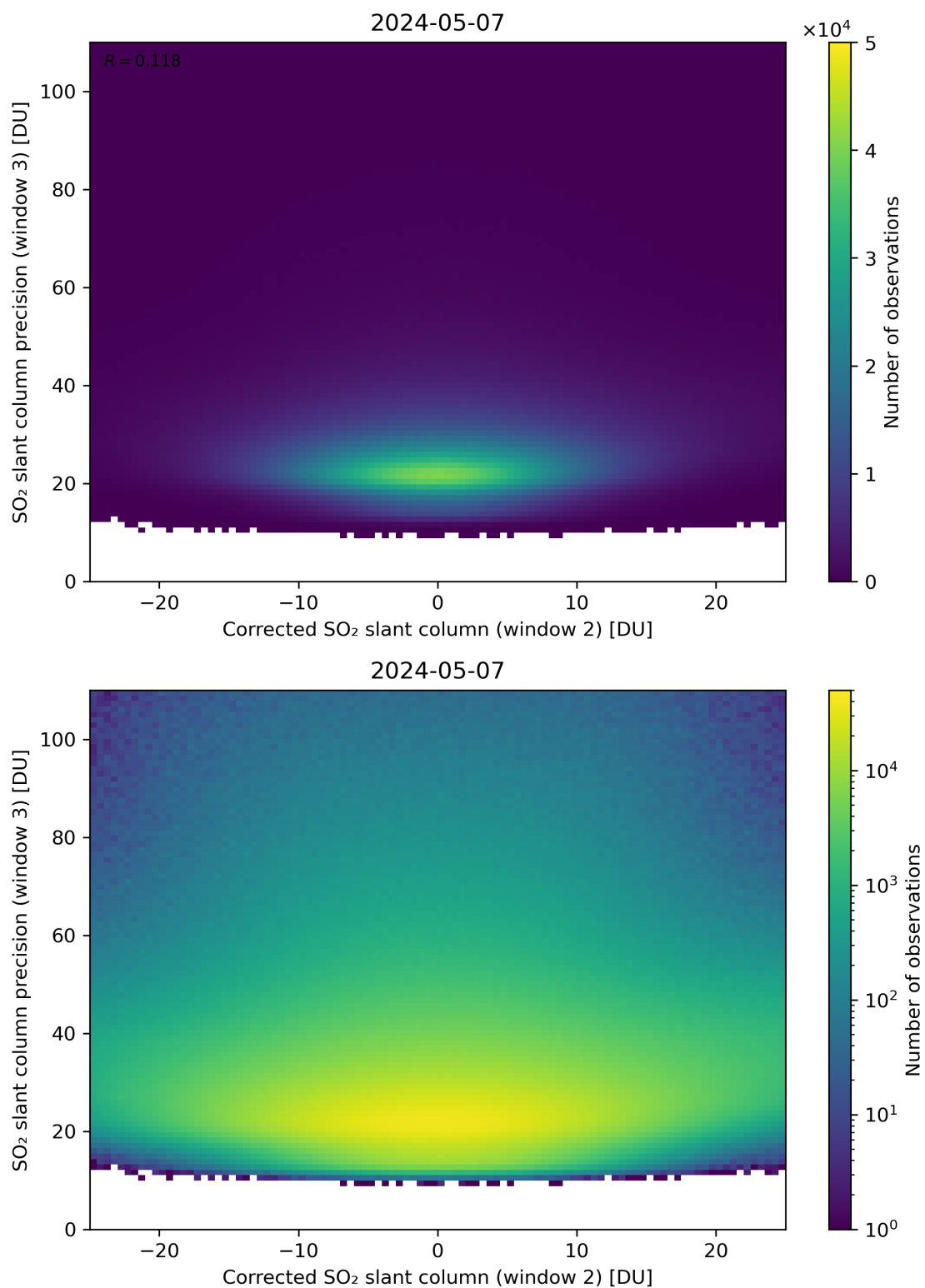
Figure 202: Scatter density plot of “Corrected SO 2 slant column (window 2)” against “SO 2 slant column precision (window 3)” for 2024-05-07 to 2024-05-08.
