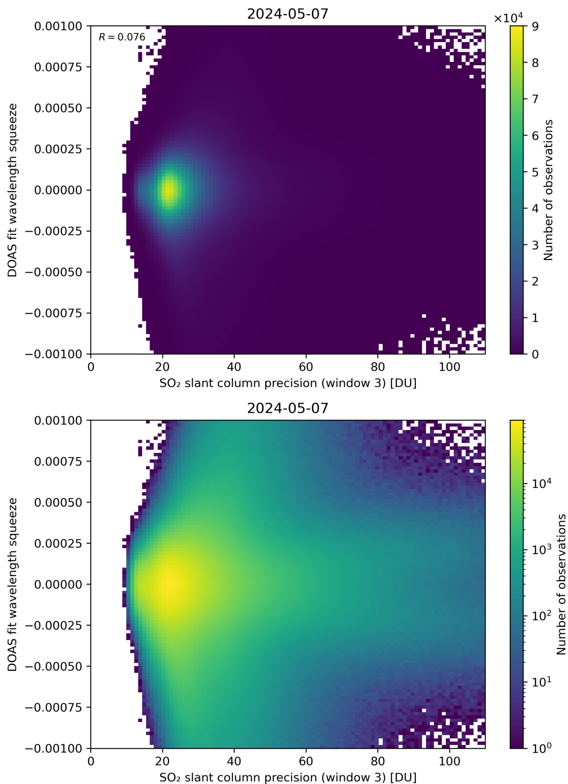
Figure 259: Scatter density plot of “SO 2 slant column precision (window 3)” against “DOAS fit wavelength squeeze” for 2024-05-07 to 2024-05-08.
