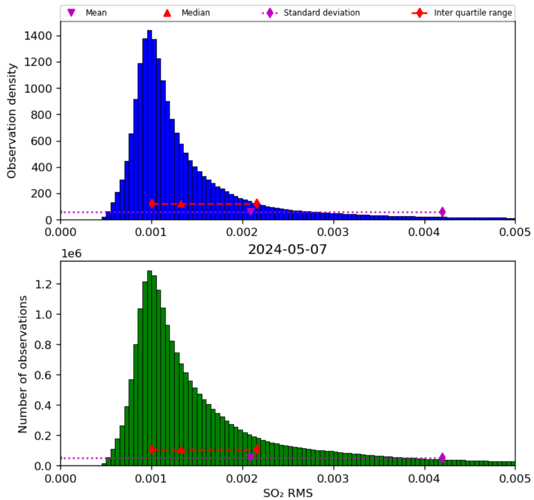
Figure 70: Histogram of “SO 2 RMS” for 2024-05-07 to 2024-05-08
