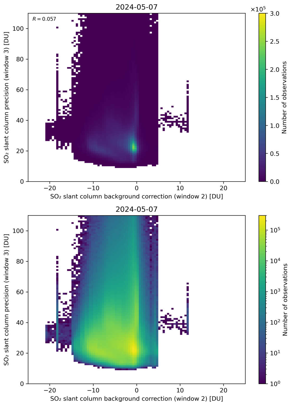
Figure 118: Scatter density plot of “SO 2 slant column background correction (window 2)” against “SO 2 slant column precision (window 3)” for 2024-05-07 to 2024-05-08.
