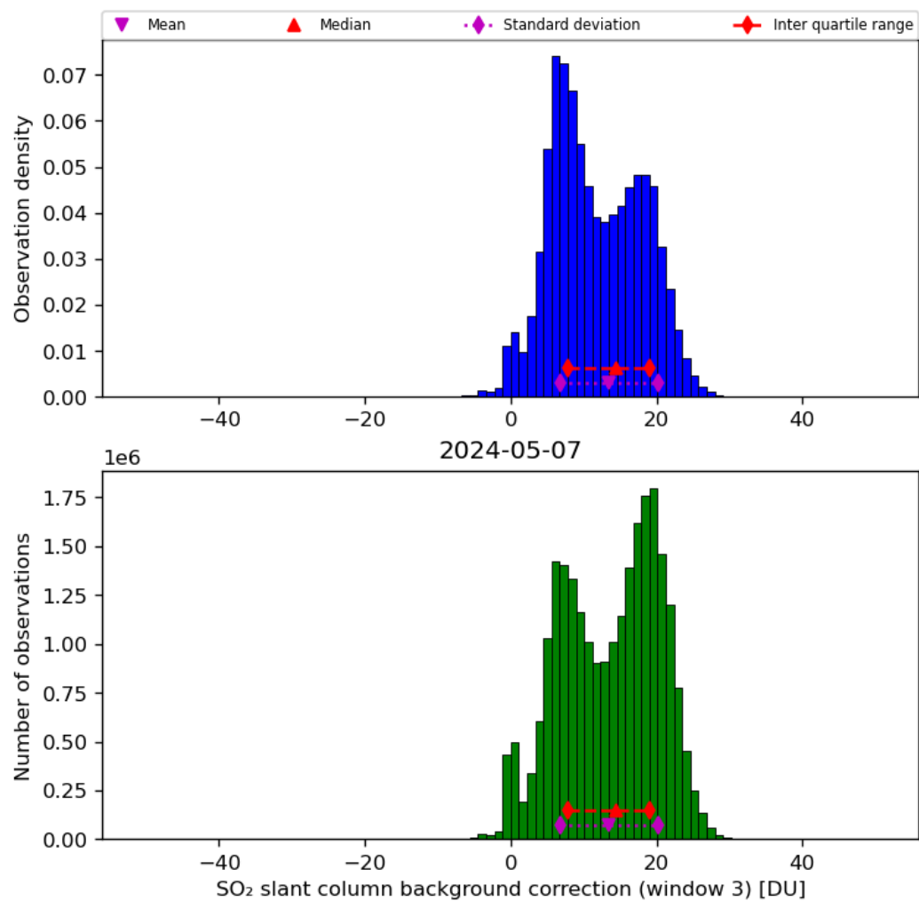
Figure 67: Histogram of “SO 2 slant column background correction (window 3)” for 2024-05-07 to 2024-05-08
