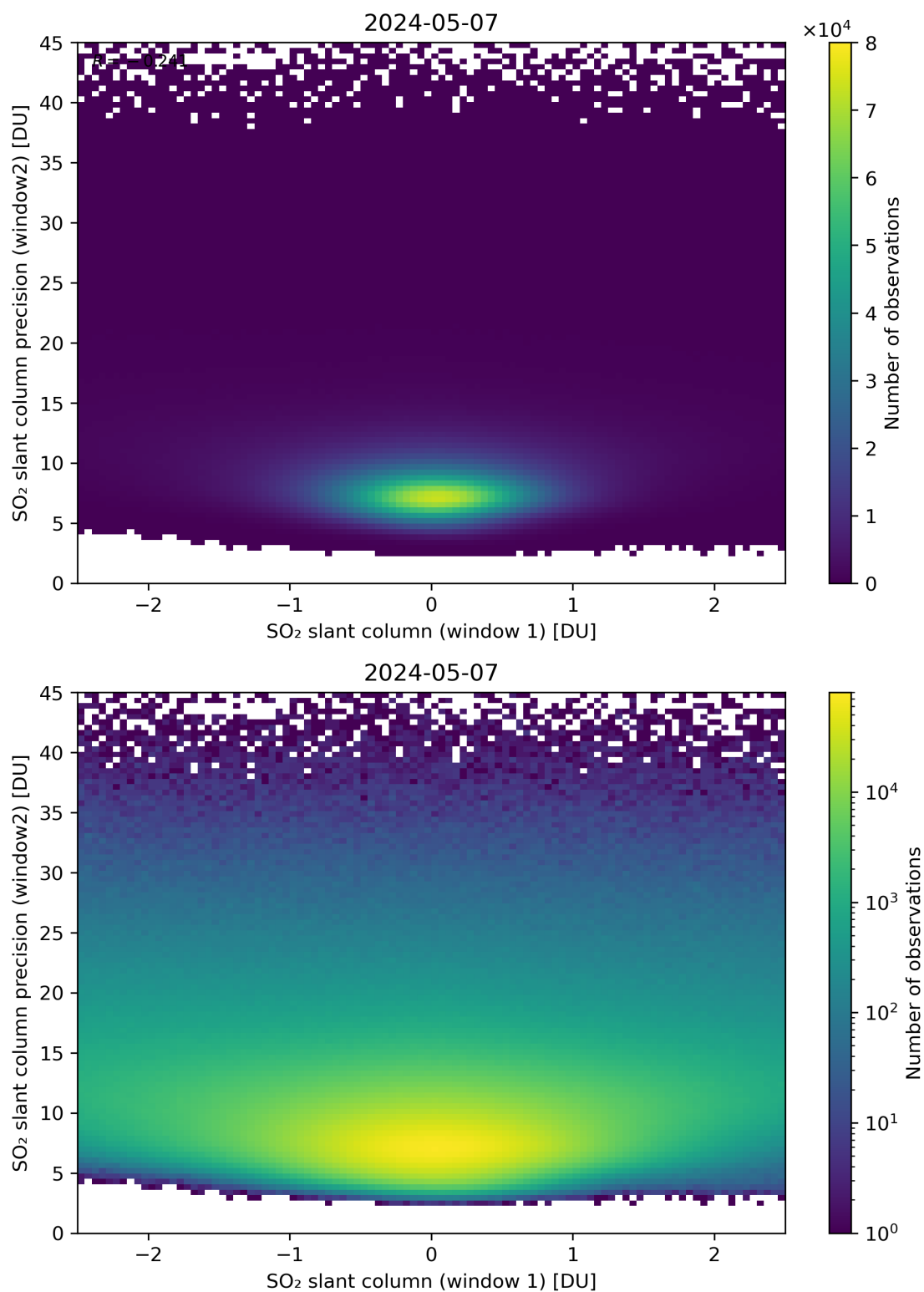
Figure 236: Scatter density plot of “SO 2 slant column (window 1)” against “SO 2 slant column precision (window2)” for 2024-05-07 to 2024-05-08.
