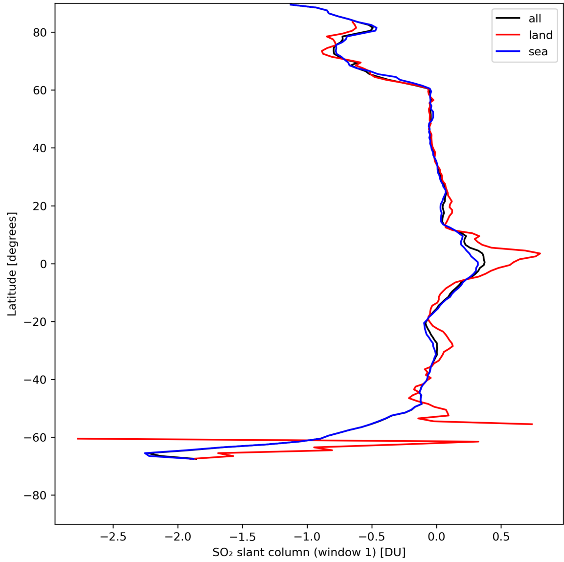
Figure 33: Zonal average of “SO 2 slant column (window 1)” for 2024-05-07 to 2024-05-08.
