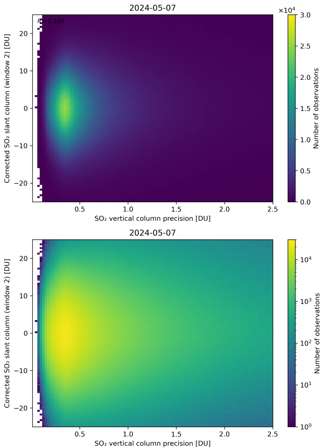
Figure 287: Scatter density plot of “SO 2 vertical column precision” against “Corrected SO 2 slant column (window 2)” for 2024-05-07 to 2024-05-08.
