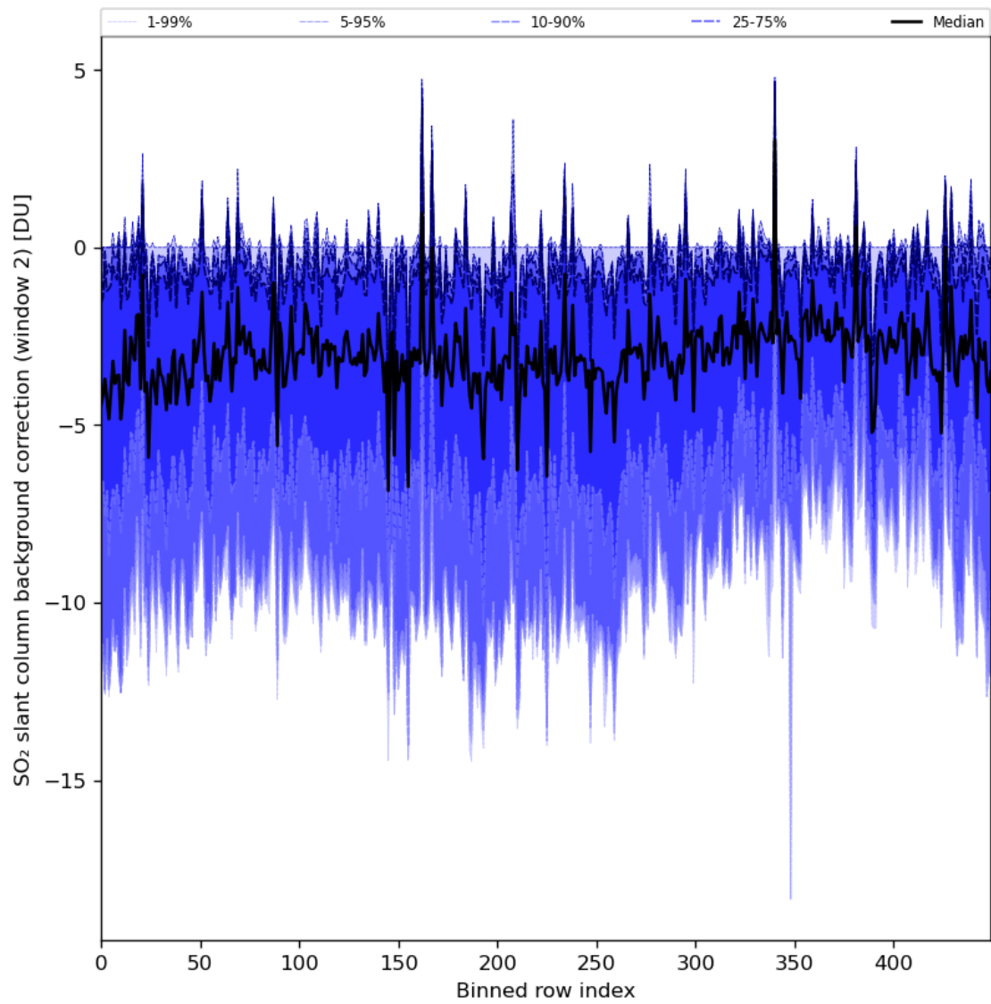
Figure 86: Along track statistics of “SO 2 slant column background correction (window 2)” for 2024-05-07 to 2024-05-08
