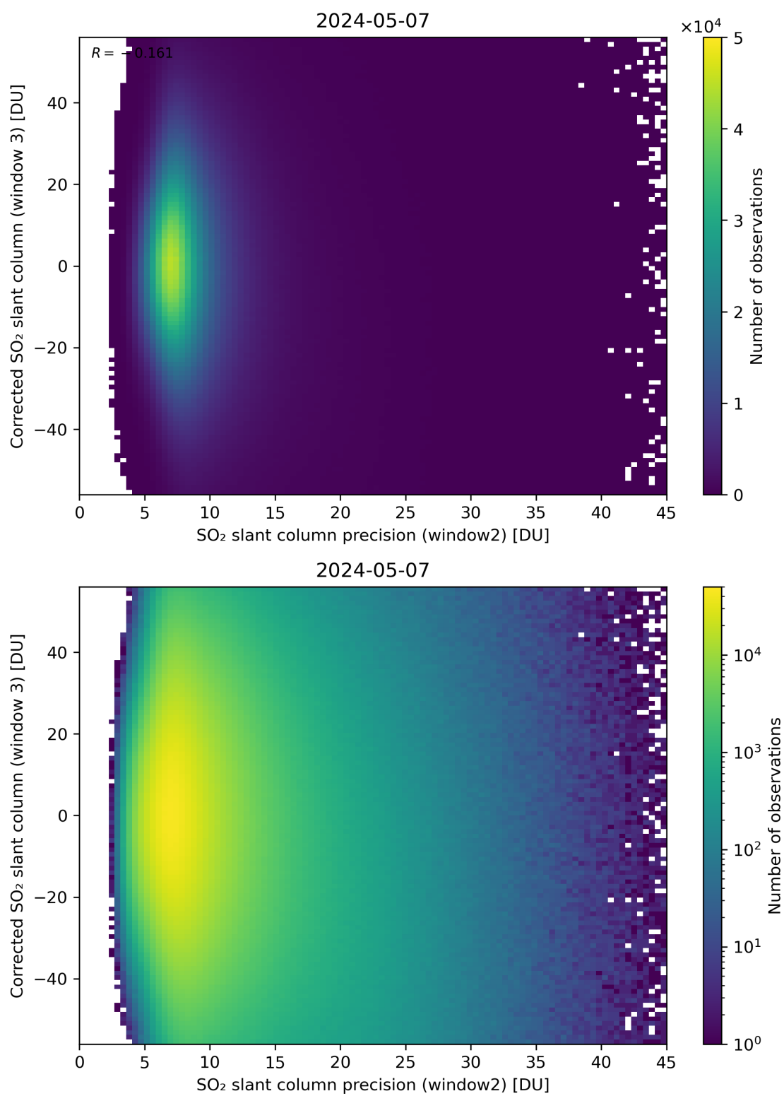
Figure 248: Scatter density plot of “SO 2 slant column precision (window2)” against “Corrected SO 2 slant column (window 3)” for 2024-05-07 to 2024-05-08.
