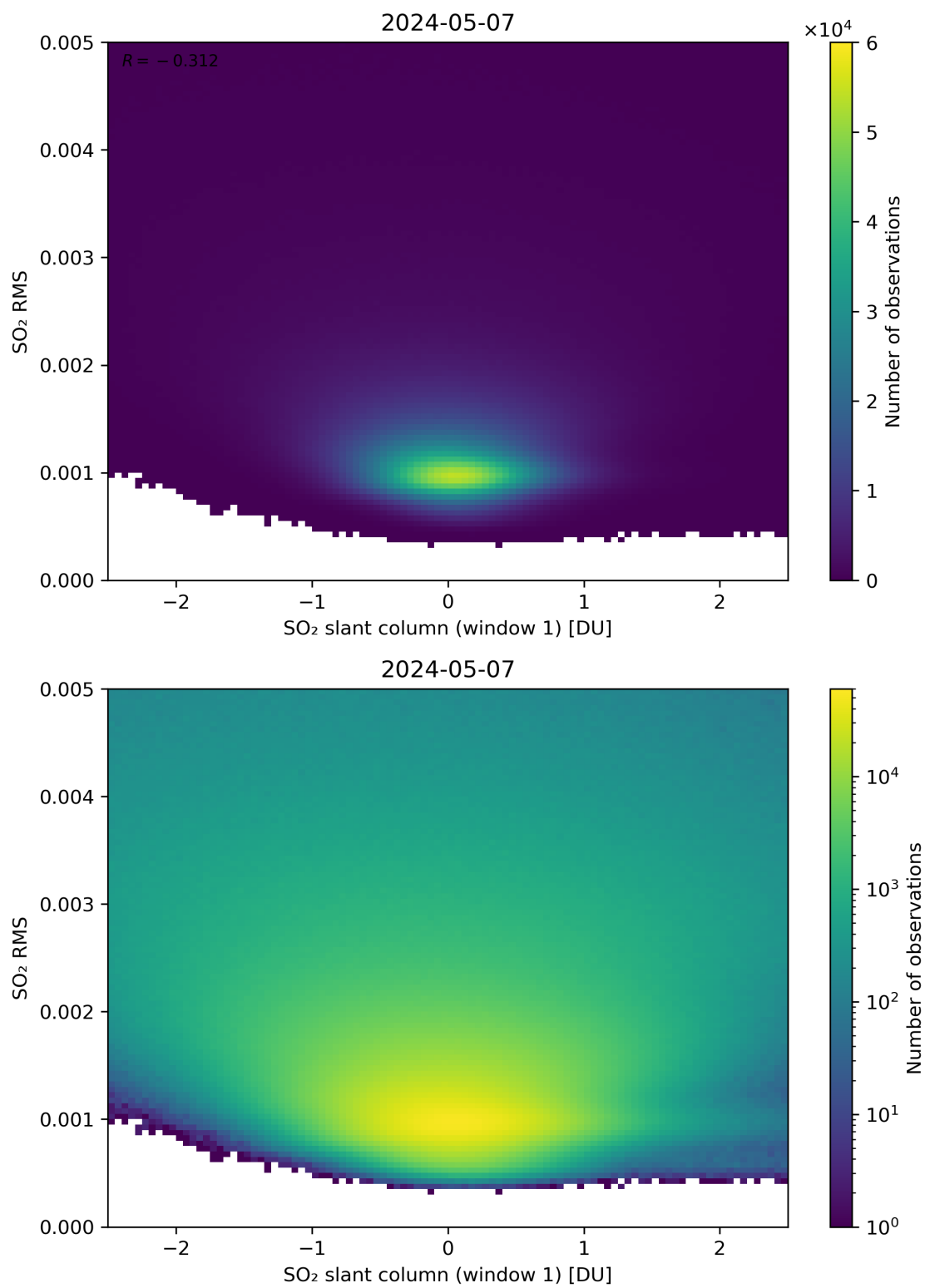
Figure 217: Scatter density plot of “SO 2 slant column (window 1)” against “SO 2 RMS” for 2024-05-07 to 2024-05-08.
