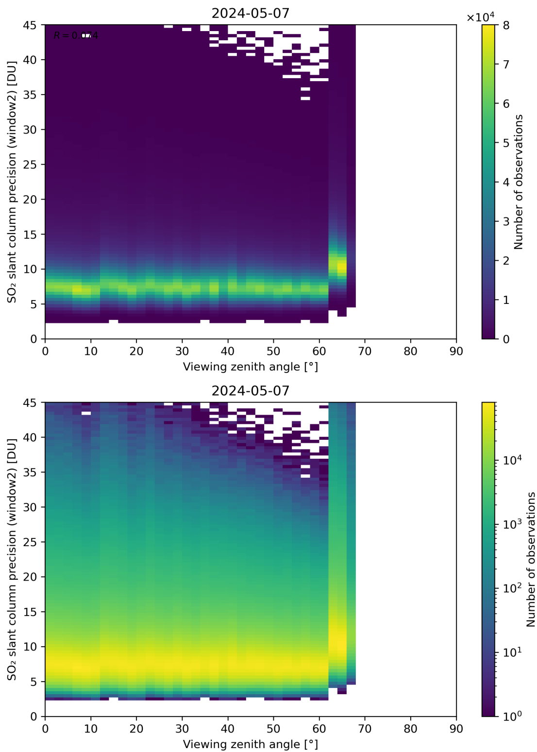
Figure 322: Scatter density plot of “Viewing zenith angle” against “SO 2 slant column precision (window2)” for 2024-05-07 to 2024-05-08.
