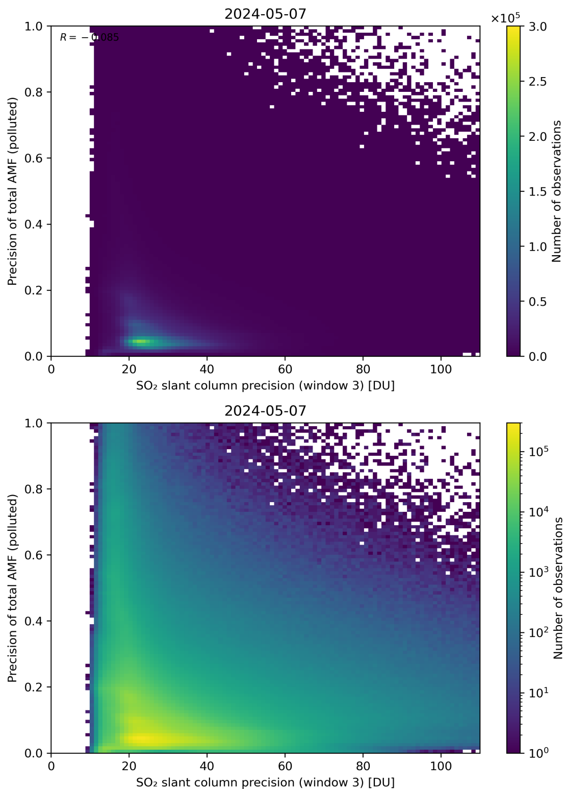
Figure 264: Scatter density plot of “SO 2 slant column precision (window 3)” against “Precision of total AMF (polluted)” for 2024-05-07 to 2024-05-08.
