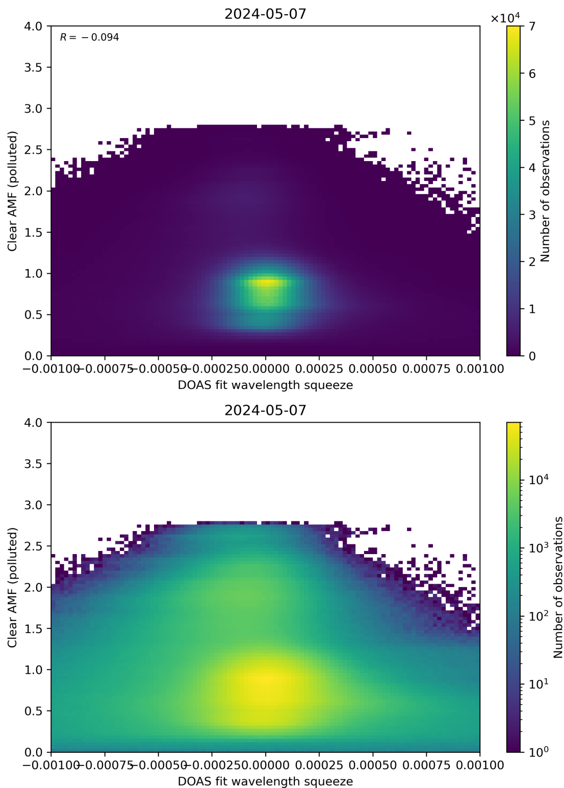
Figure 133: Scatter density plot of “DOAS fit wavelength squeeze” against “Clear AMF (polluted)” for 2024-05-07 to 2024-05-08.
