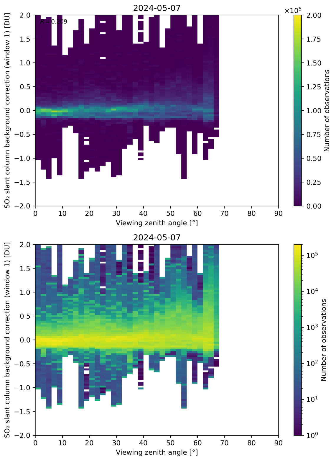
Figure 308: Scatter density plot of “Viewing zenith angle” against “SO 2 slant column background correction (window 1)” for 2024-05-07 to 2024-05-08.
