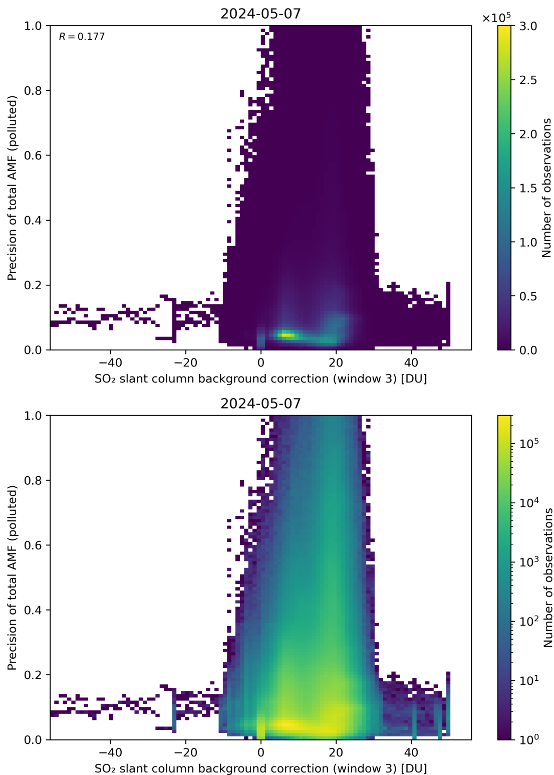
Figure 126: Scatter density plot of “SO 2 slant column background correction (window 3)” against “Precision of total AMF (polluted)” for 2024-05-07 to 2024-05-08.
