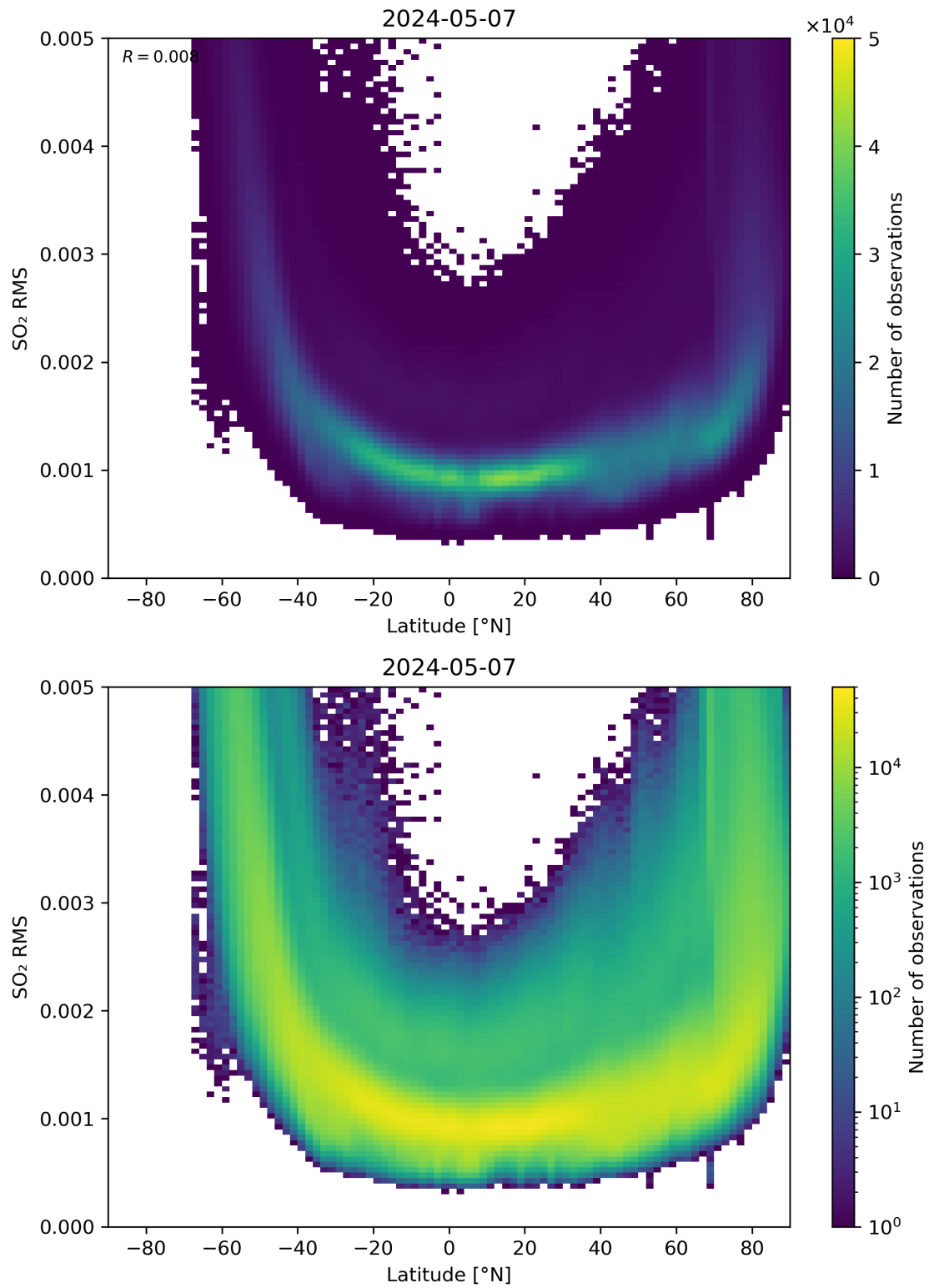
Figure 144: Scatter density plot of “Latitude” against “SO 2 RMS” for 2024-05-07 to 2024-05-08.
