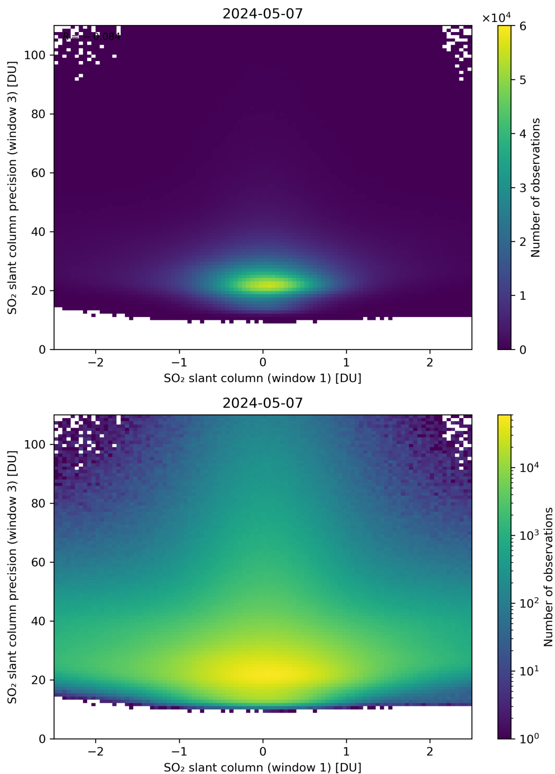
Figure 238: Scatter density plot of “SO 2 slant column (window 1)” against “SO 2 slant column precision (window 3)” for 2024-05-07 to 2024-05-08.
