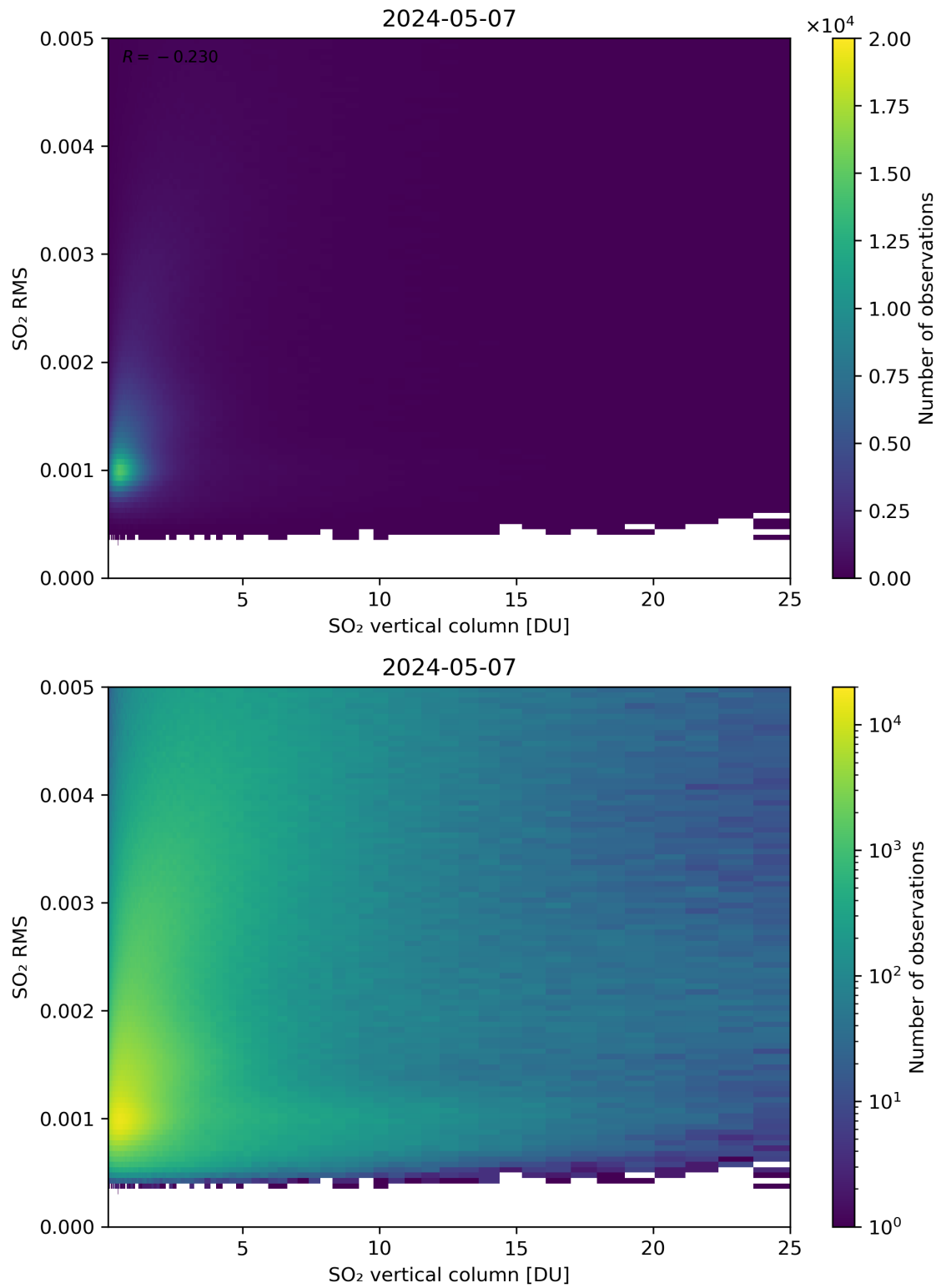
Figure 278: Scatter density plot of “SO 2 vertical column” against “SO 2 RMS” for 2024-05-07 to 2024-05-08.
