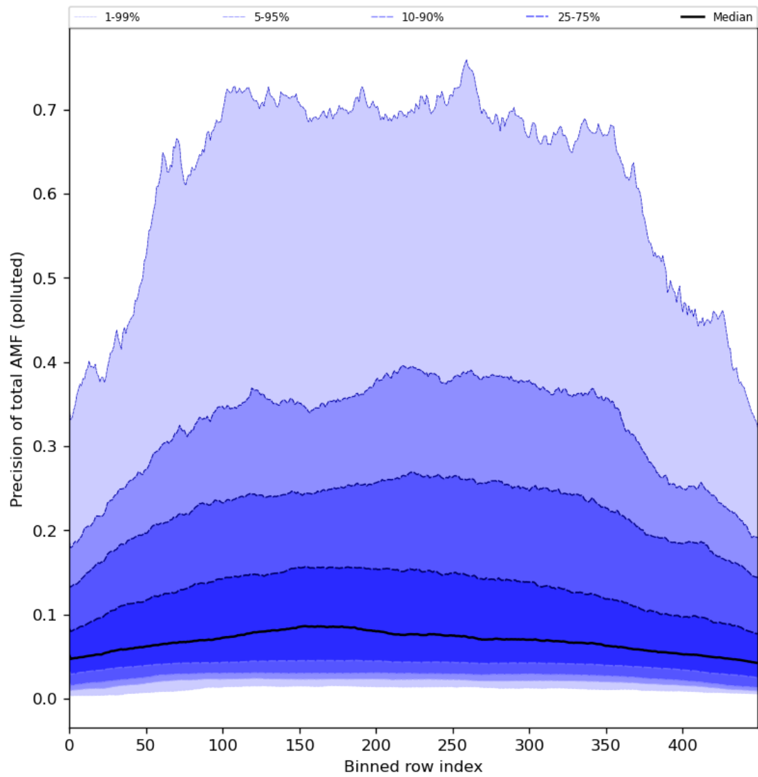
Figure 95: Along track statistics of “Precision of total AMF (polluted)” for 2024-05-07 to 2024-05-08
