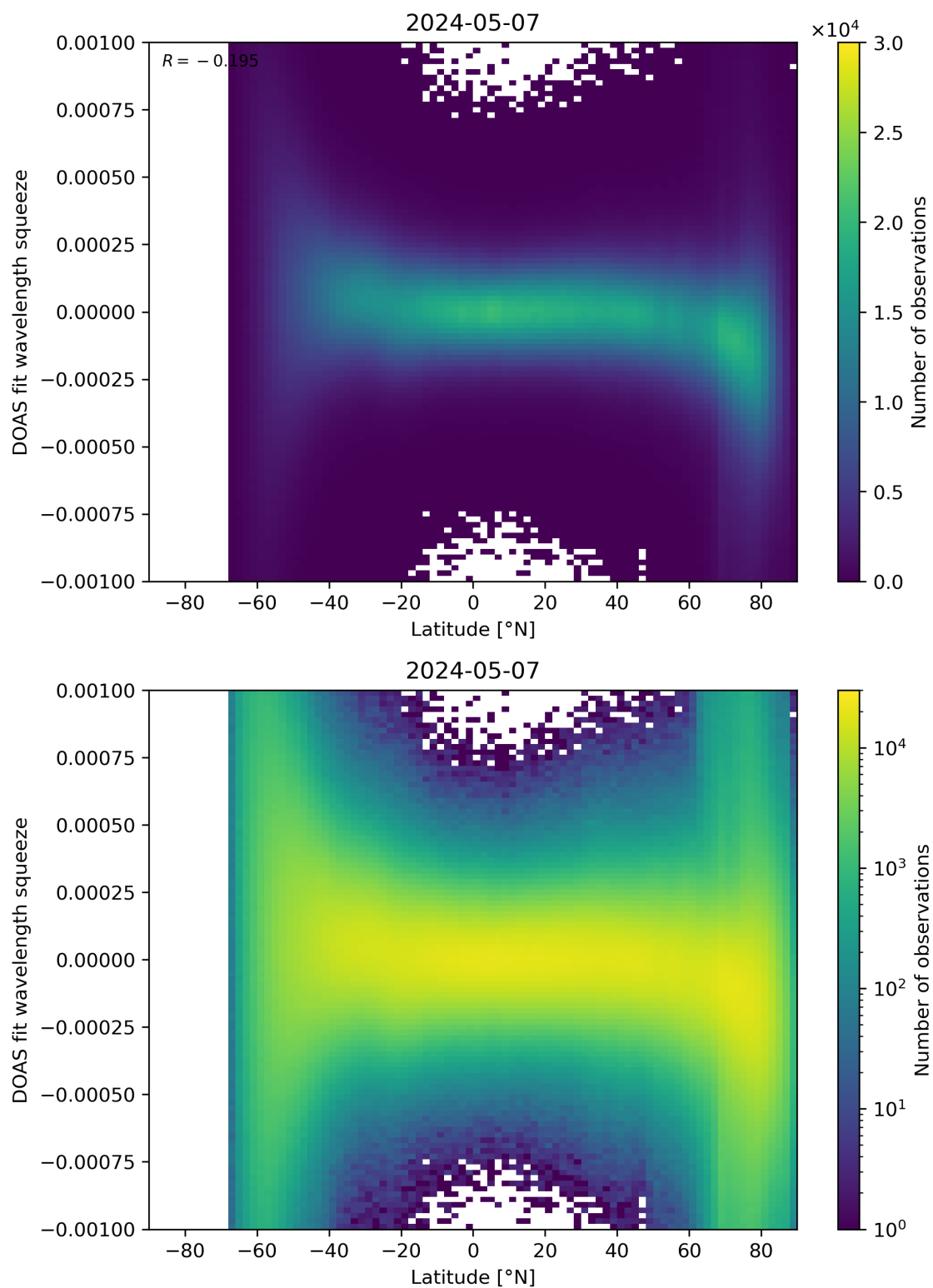
Figure 143: Scatter density plot of “Latitude” against “DOAS fit wavelength squeeze” for 2024-05-07 to 2024-05-08.
