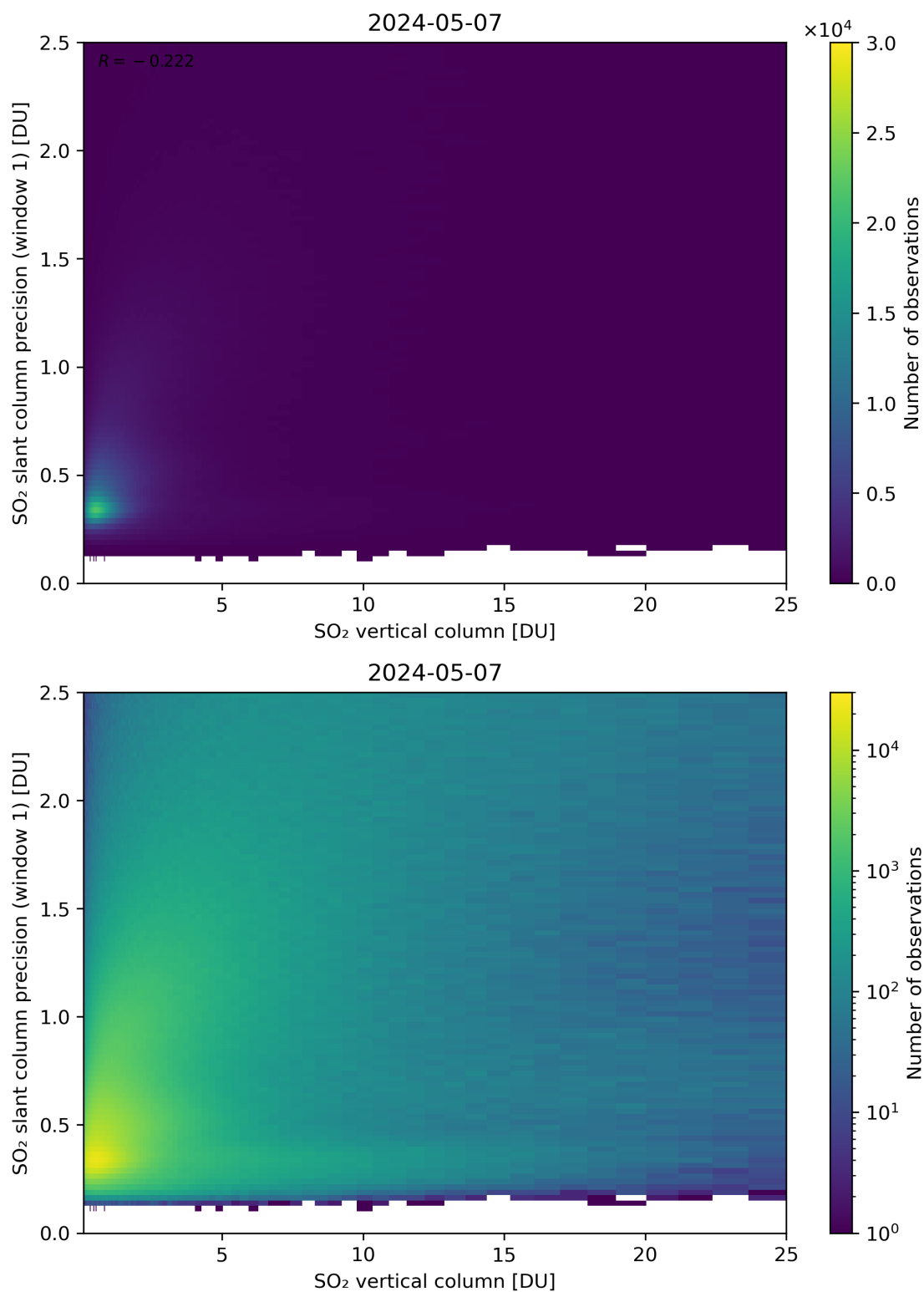
Figure 301: Scatter density plot of “SO 2 vertical column” against “SO 2 slant column precision (window 1)” for 2024-05-07 to 2024-05-08.
