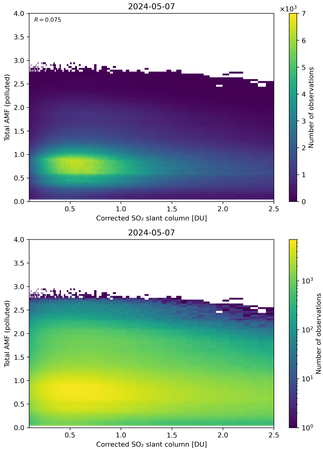
Figure 192: Scatter density plot of “Corrected SO 2 slant column” against “Total AMF (polluted)” for 2024-05-07 to 2024-05-08.
