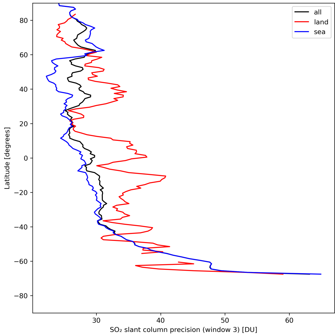
Figure 42: Zonal average of “SO 2 slant column precision (window 3)” for 2024-05-07 to 2024-05-08.
