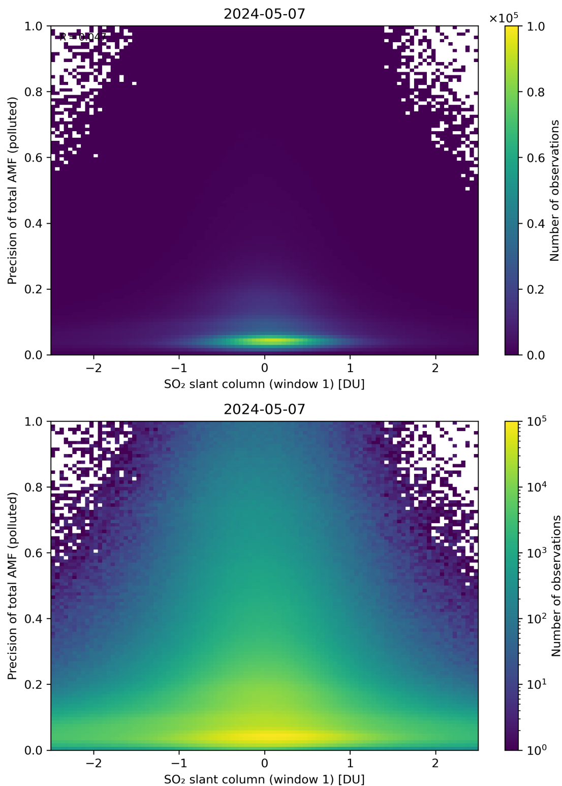
Figure 240: Scatter density plot of “SO 2 slant column (window 1)” against “Precision of total AMF (polluted)” for 2024-05-07 to 2024-05-08.
