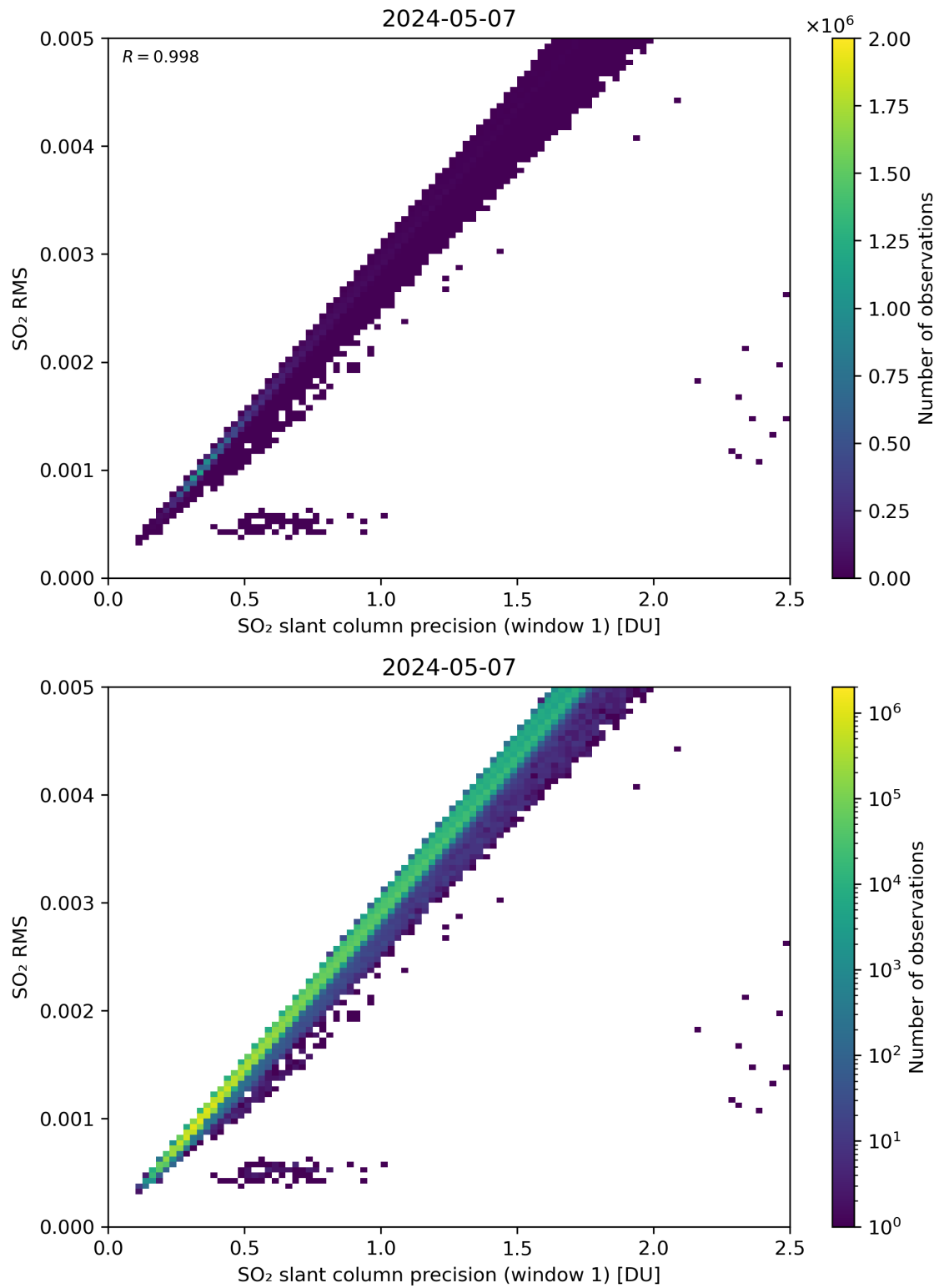
Figure 223: Scatter density plot of “SO 2 slant column precision (window 1)” against “SO 2 RMS” for 2024-05-07 to 2024-05-08.
