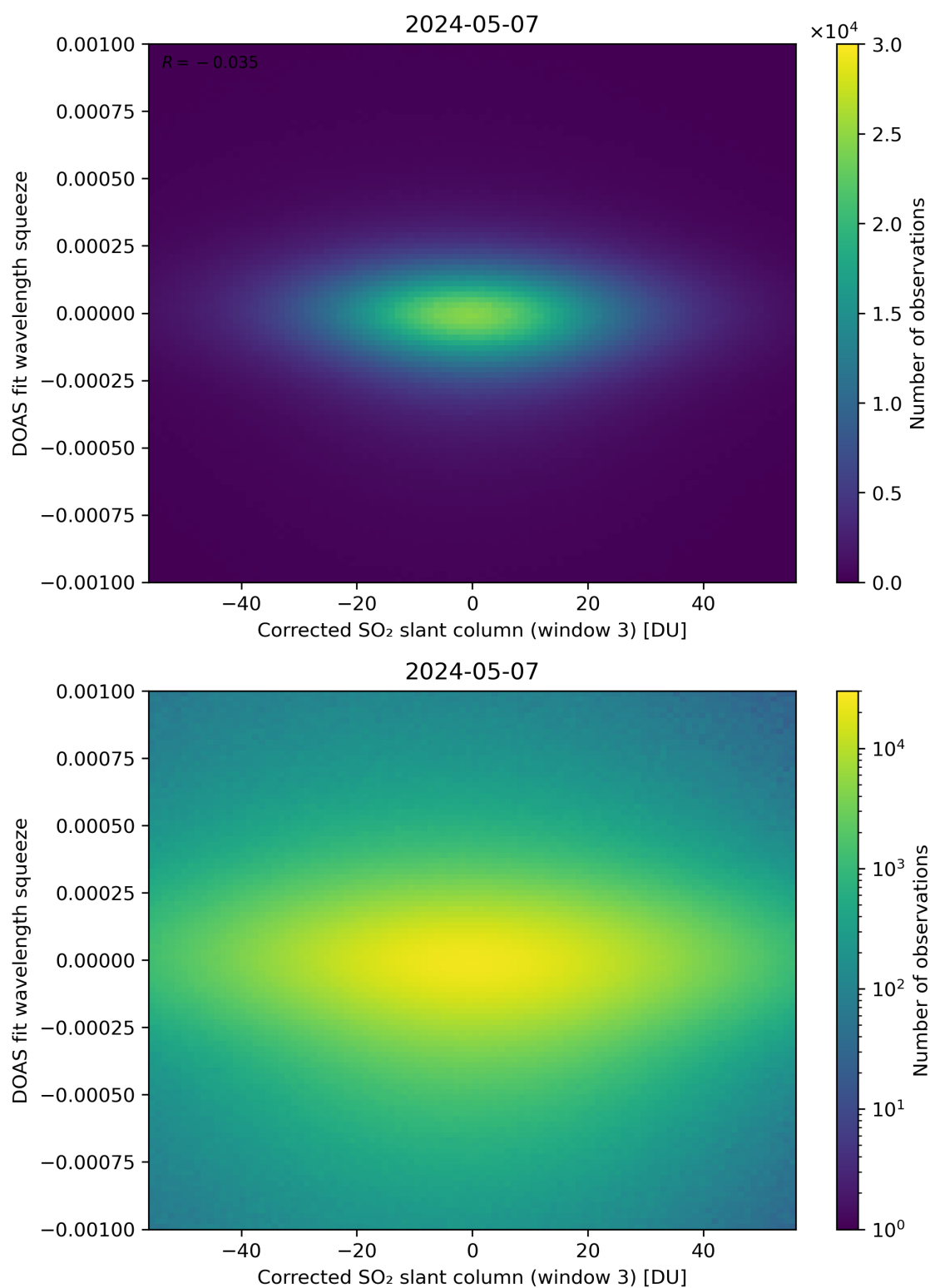
Figure 207: Scatter density plot of “Corrected SO 2 slant column (window 3)” against “DOAS fit wavelength squeeze” for 2024-05-07 to 2024-05-08.
