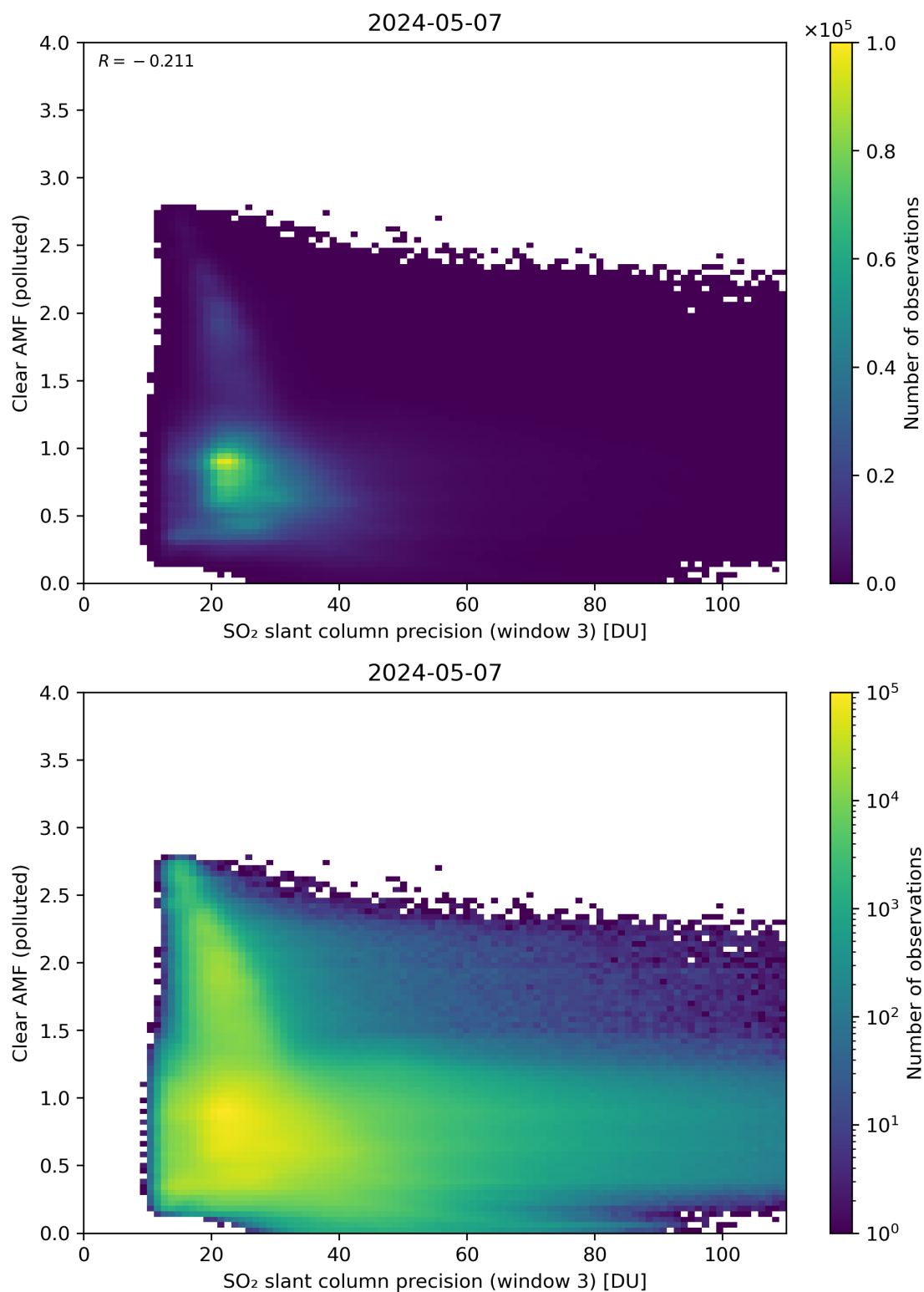
Figure 261: Scatter density plot of “SO 2 slant column precision (window 3)” against “Clear AMF (polluted)” for 2024-05-07 to 2024-05-08.
