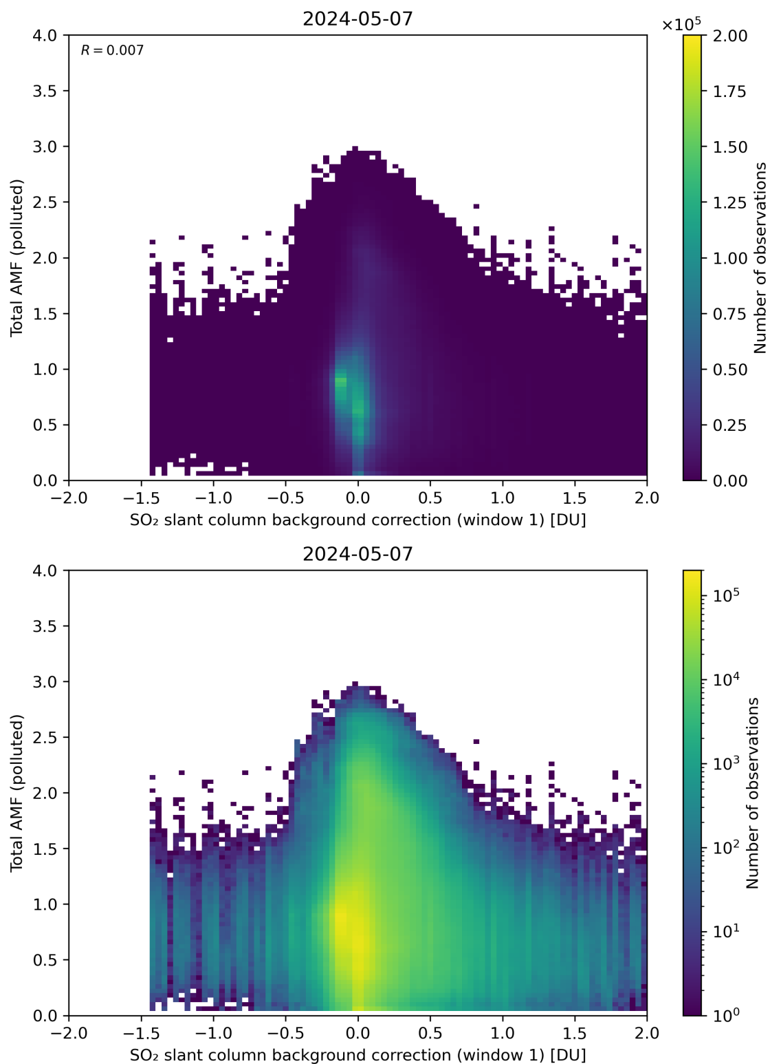
Figure 109: Scatter density plot of “SO 2 slant column background correction (window 1)” against “Total AMF (polluted)” for 2024-05-07 to 2024-05-08.
