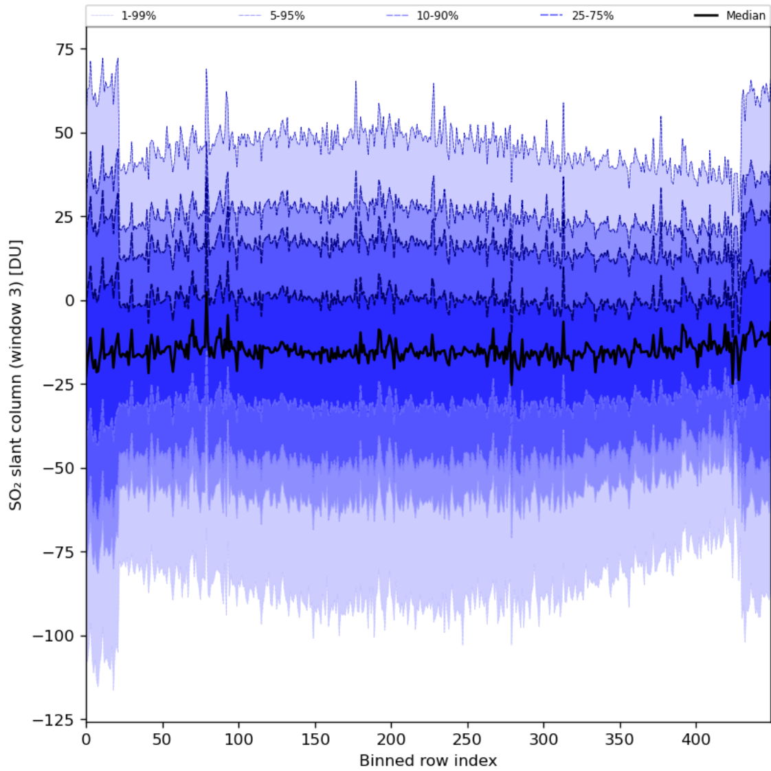
Figure 87: Along track statistics of “SO 2 slant column (window 3)” for 2024-05-07 to 2024-05-08
