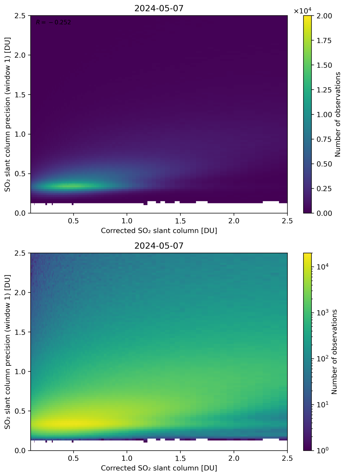
Figure 188: Scatter density plot of “Corrected SO 2 slant column” against “SO 2 slant column precision (window 1)” for 2024-05-07 to 2024-05-08.
