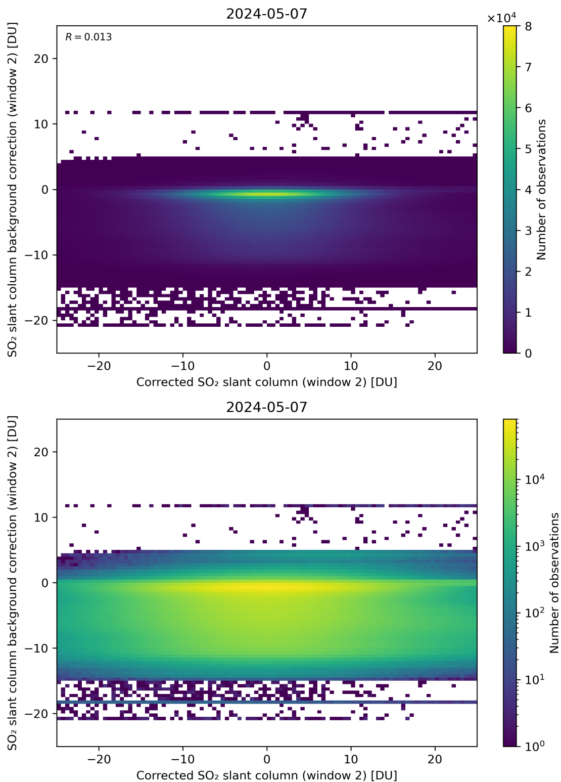
Figure 194: Scatter density plot of “Corrected SO 2 slant column (window 2)” against “SO 2 slant column background correction (window 2)” for 2024-05-07 to 2024-05-08.
