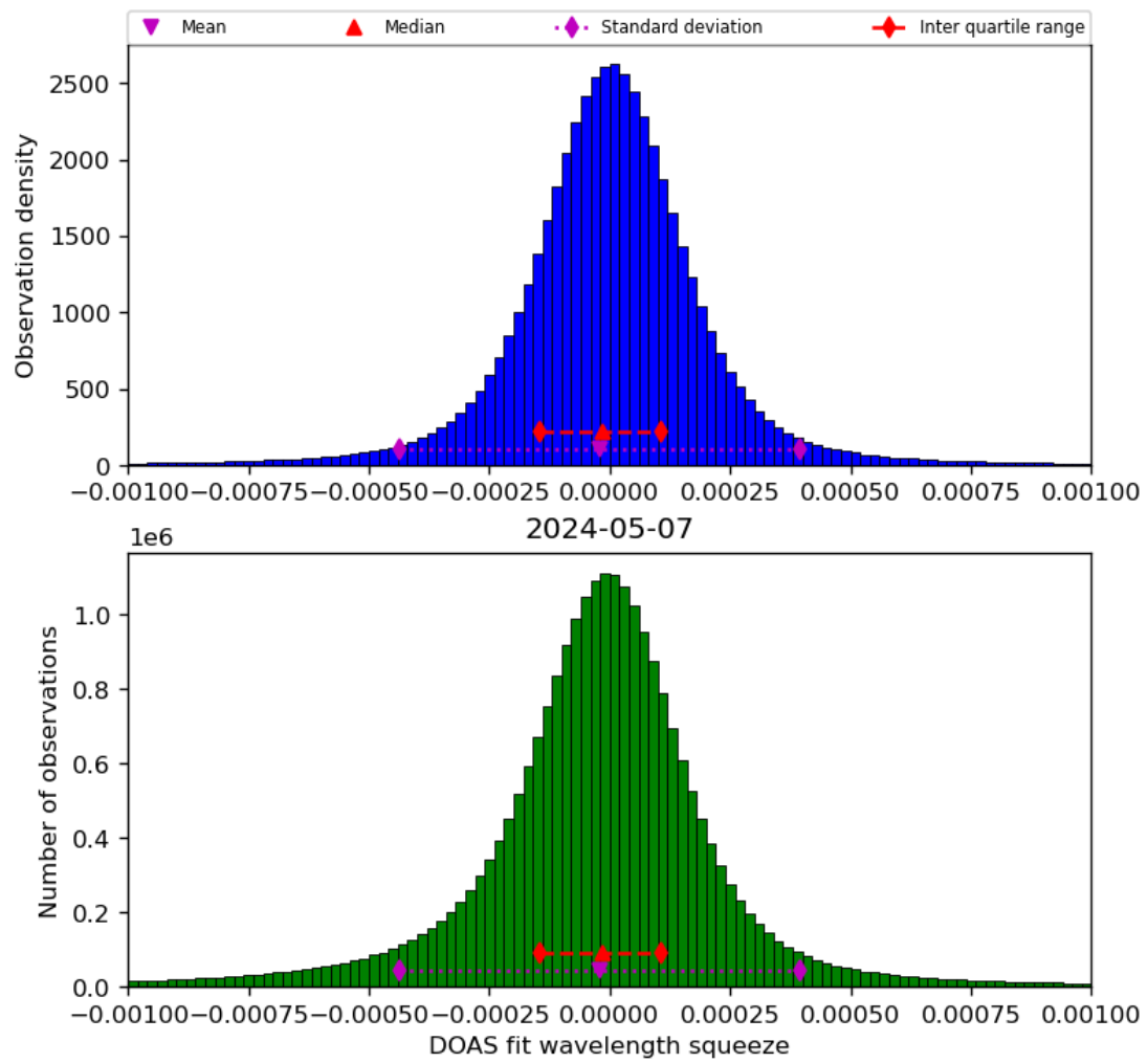
Figure 69: Histogram of “DOAS fit wavelength squeeze” for 2024-05-07 to 2024-05-08
