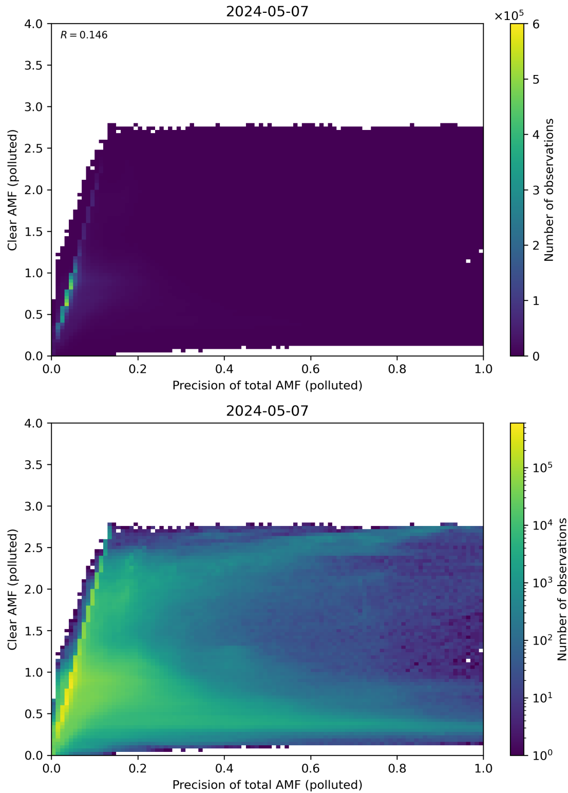
Figure 270: Scatter density plot of “Precision of total AMF (polluted)” against “Clear AMF (polluted)” for 2024-05-07 to 2024-05-08.
