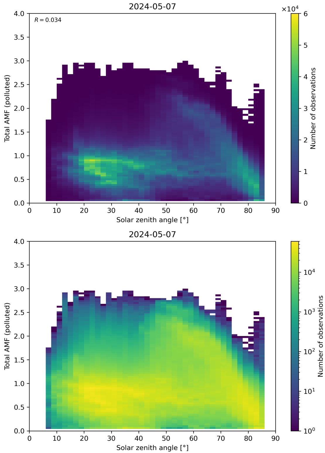
Figure 174: Scatter density plot of “Solar zenith angle” against “Total AMF (polluted)” for 2024-05-07 to 2024-05-08.
