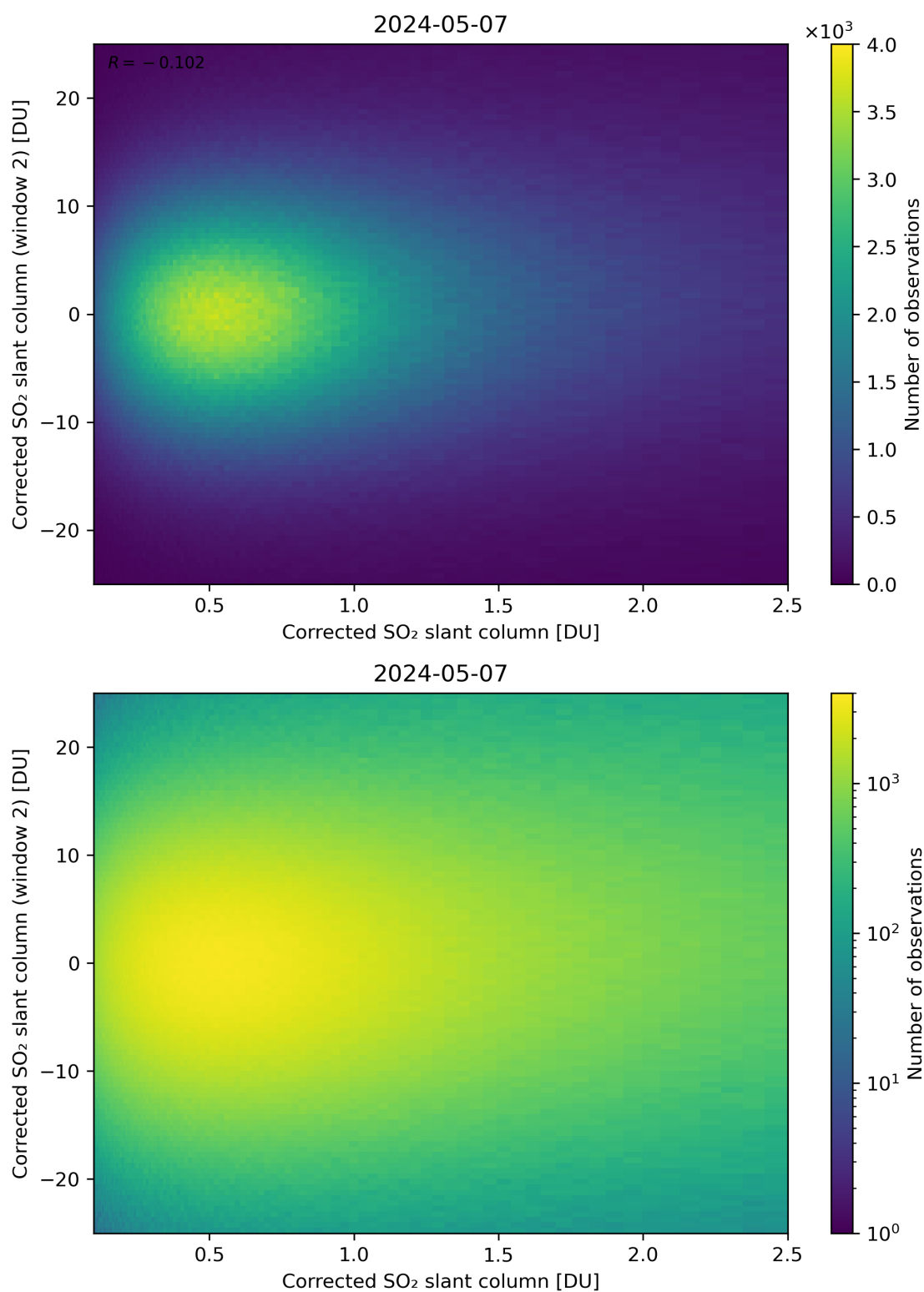
Figure 185: Scatter density plot of “Corrected SO 2 slant column” against “Corrected SO 2 slant column (window 2)” for 2024-05-07 to 2024-05-08.
