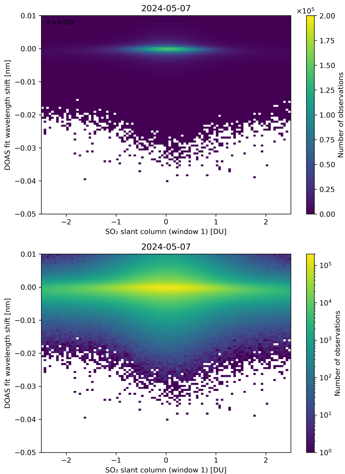
Figure 215: Scatter density plot of “SO 2 slant column (window 1)” against “DOAS fit wavelength shift” for 2024-05-07 to 2024-05-08.
