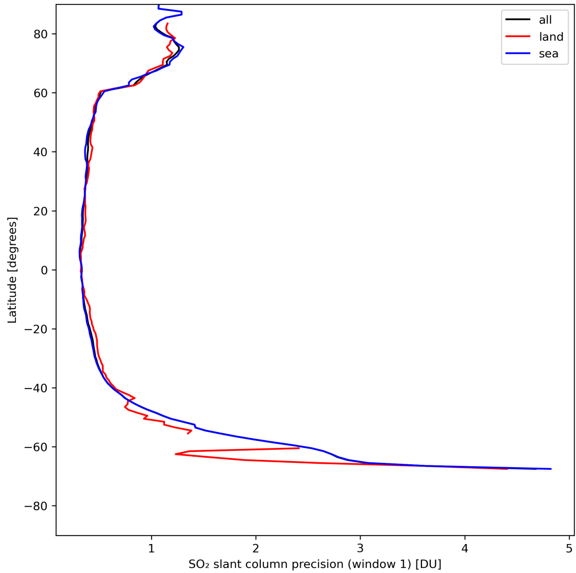
Figure 34: Zonal average of “SO 2 slant column precision (window 1)” for 2024-05-07 to 2024-05-08.
