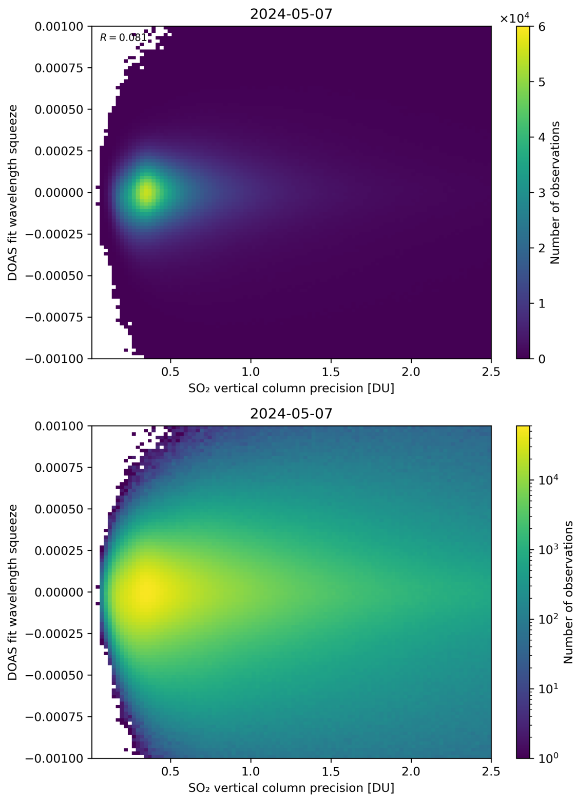
Figure 283: Scatter density plot of “SO 2 vertical column precision” against “DOAS fit wavelength squeeze” for 2024-05-07 to 2024-05-08.
