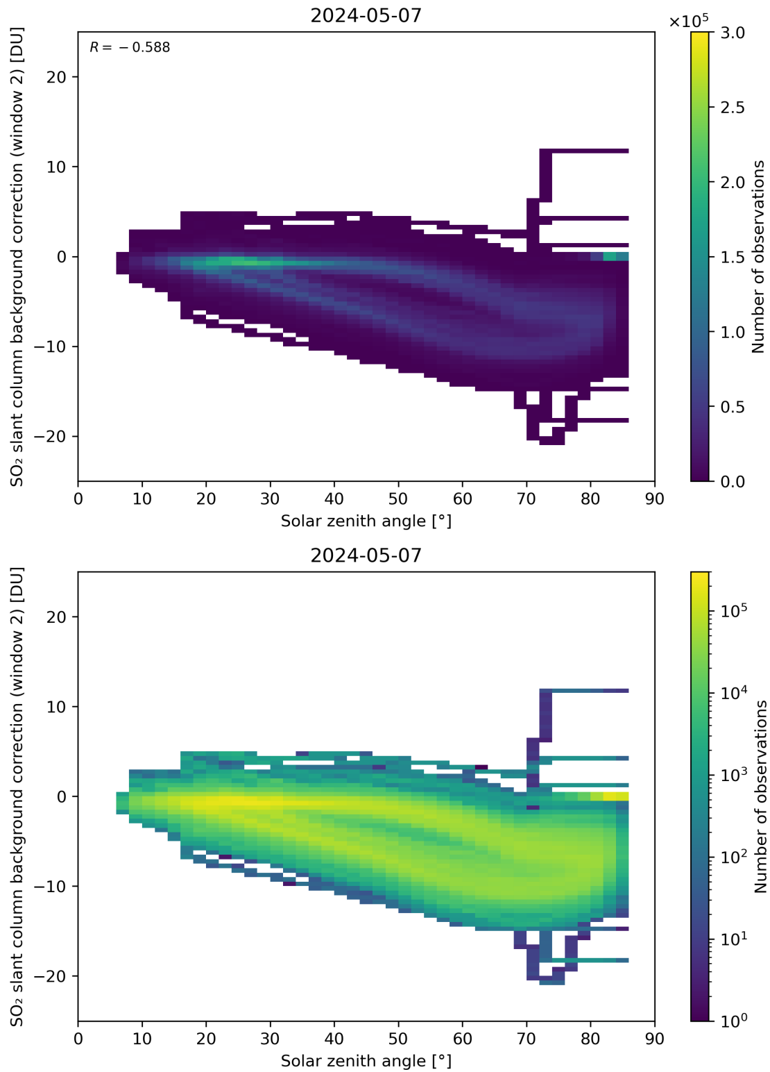
Figure 159: Scatter density plot of “Solar zenith angle” against “SO 2 slant column background correction (window 2)” for 2024-05-07 to 2024-05-08.
