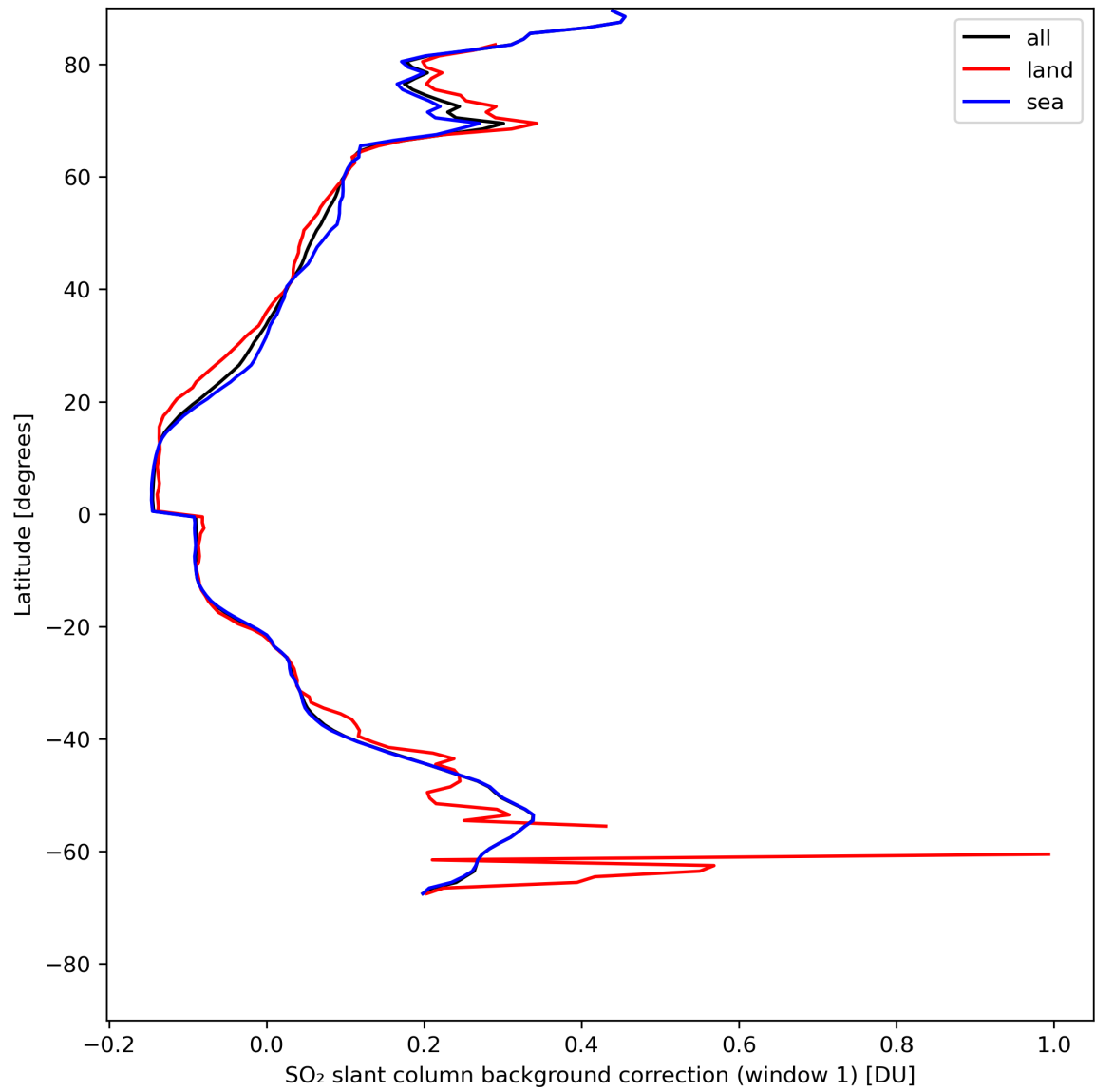
Figure 36: Zonal average of “SO 2 slant column background correction (window 1)” for 2024-05-07 to 2024-05-08.
