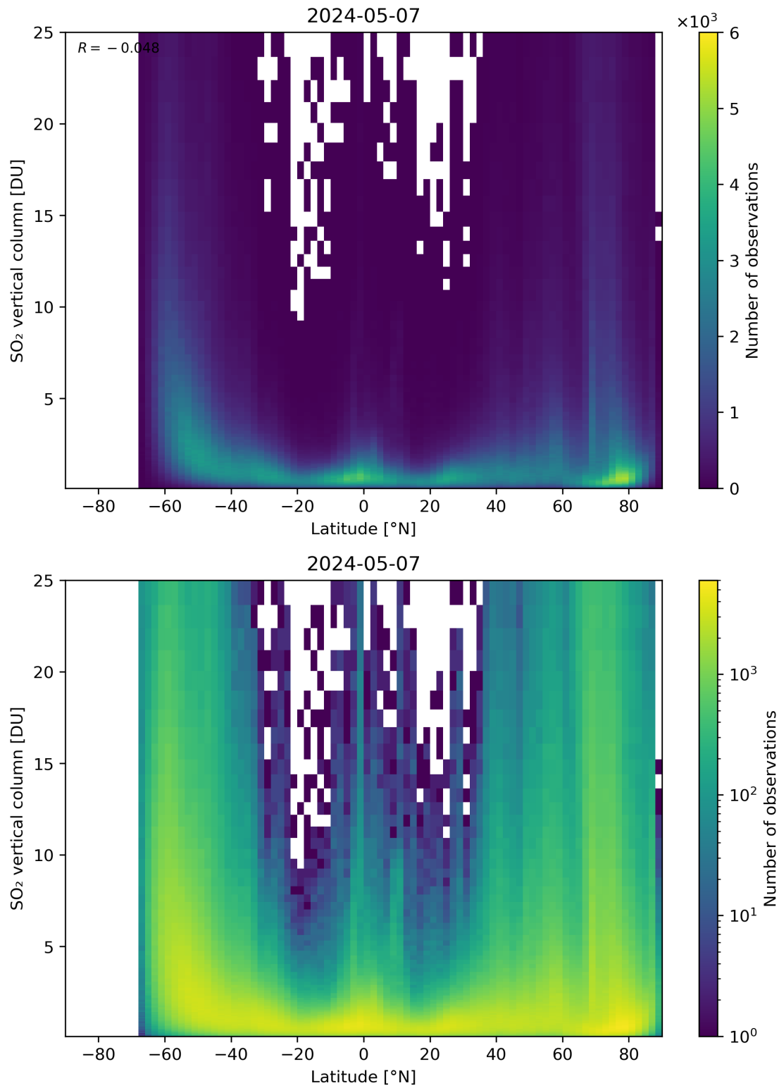
Figure 156: Scatter density plot of “Latitude” against “SO 2 vertical column” for 2024-05-07 to 2024-05-08.
