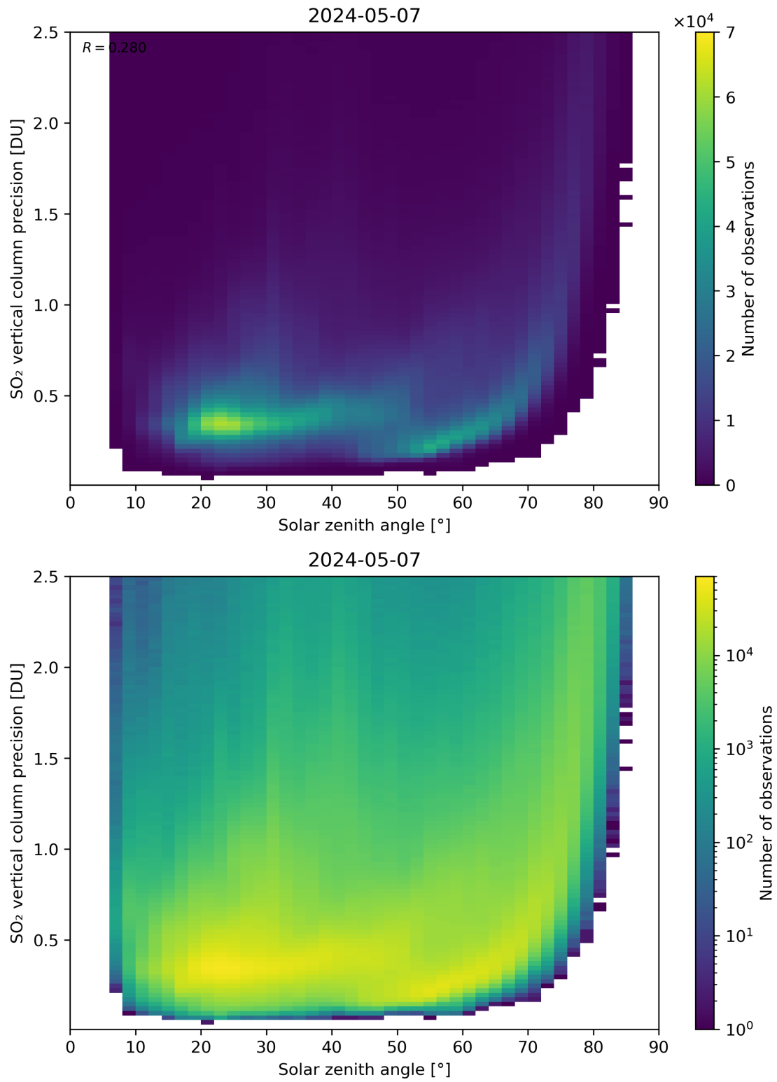
Figure 177: Scatter density plot of “Solar zenith angle” against “SO 2 vertical column precision” for 2024-05-07 to 2024-05-08.
