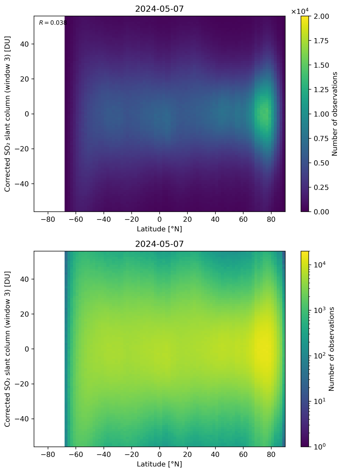
Figure 148: Scatter density plot of “Latitude” against “Corrected SO 2 slant column (window 3)” for 2024-05-07 to 2024-05-08.
