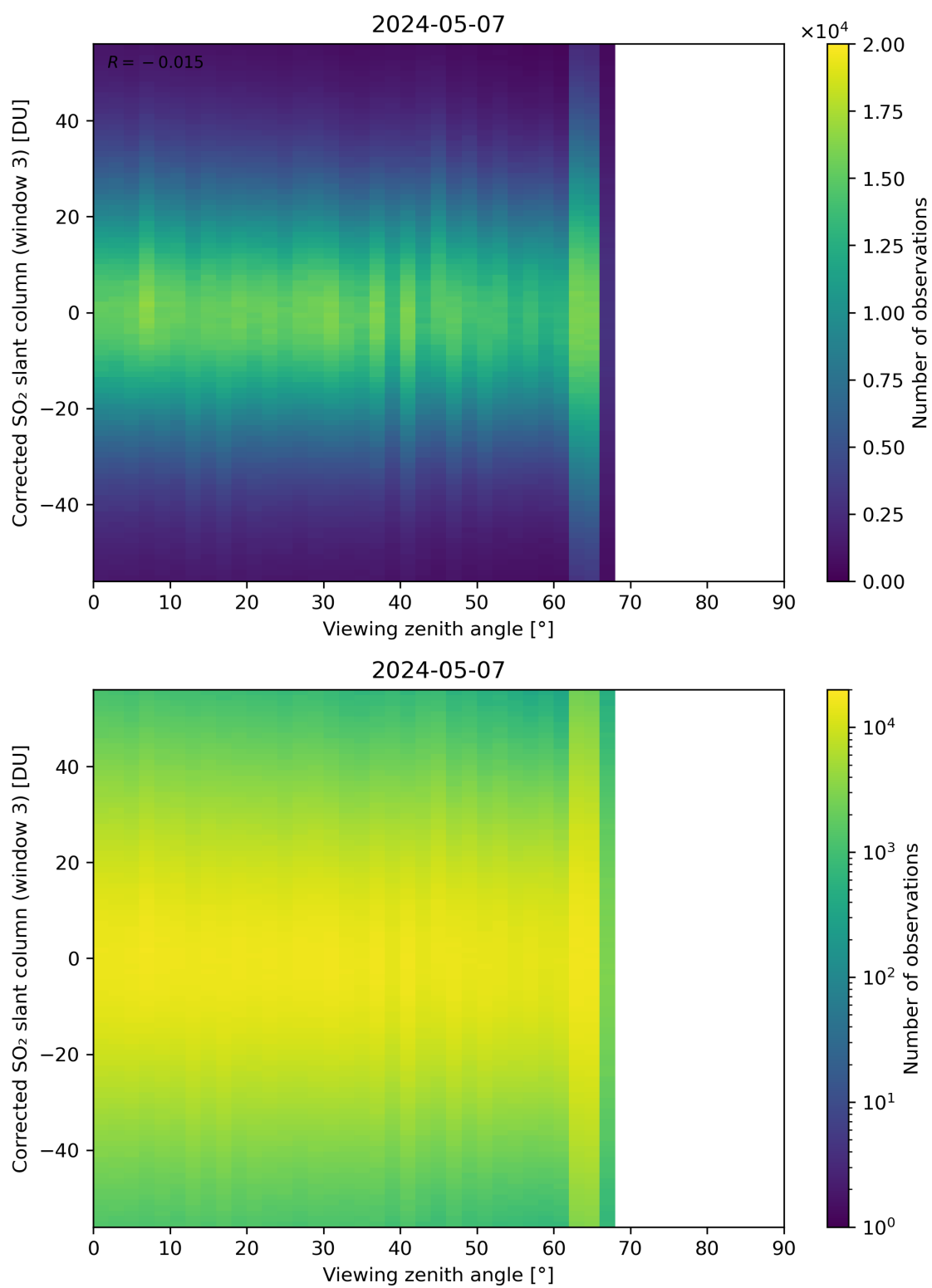
Figure 319: Scatter density plot of “Viewing zenith angle” against “Corrected SO 2 slant column (window 3)” for 2024-05-07 to 2024-05-08.
