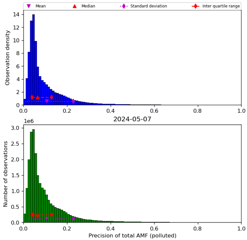
Figure 72: Histogram of “Precision of total AMF (polluted)” for 2024-05-07 to 2024-05-08
