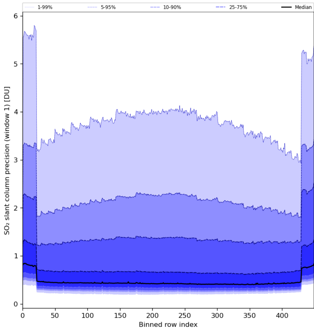
Figure 80: Along track statistics of "SO 2 slant column precision (window 1)" for 2024-05-07 to 2024-05-08
