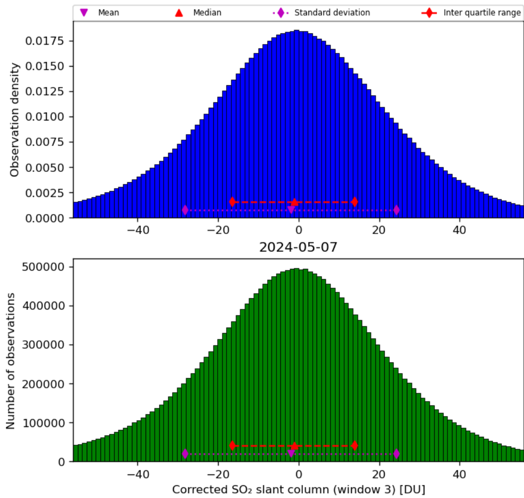
Figure 66: Histogram of “Corrected SO 2 slant column (window 3)” for 2024-05-07 to 2024-05-08
