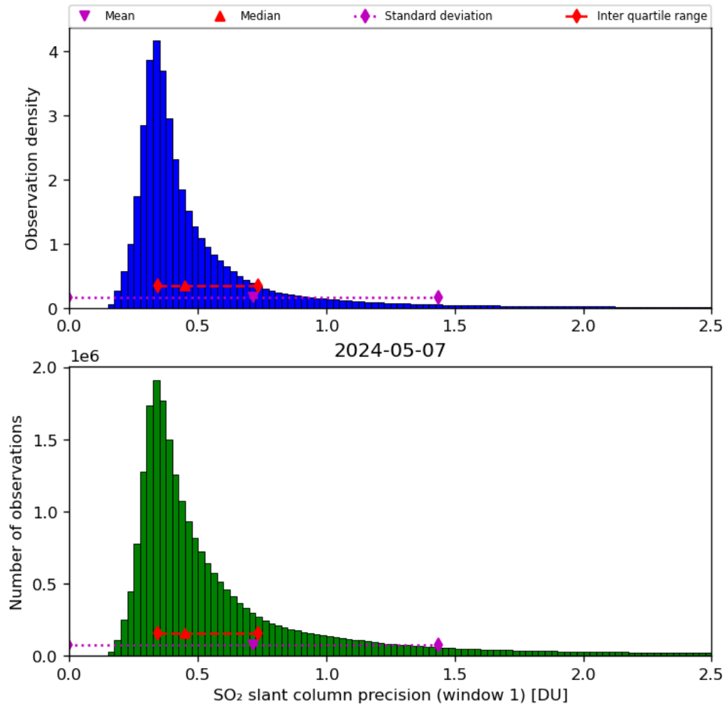
Figure 57: Histogram of “SO 2 slant column precision (window 1)” for 2024-05-07 to 2024-05-08
