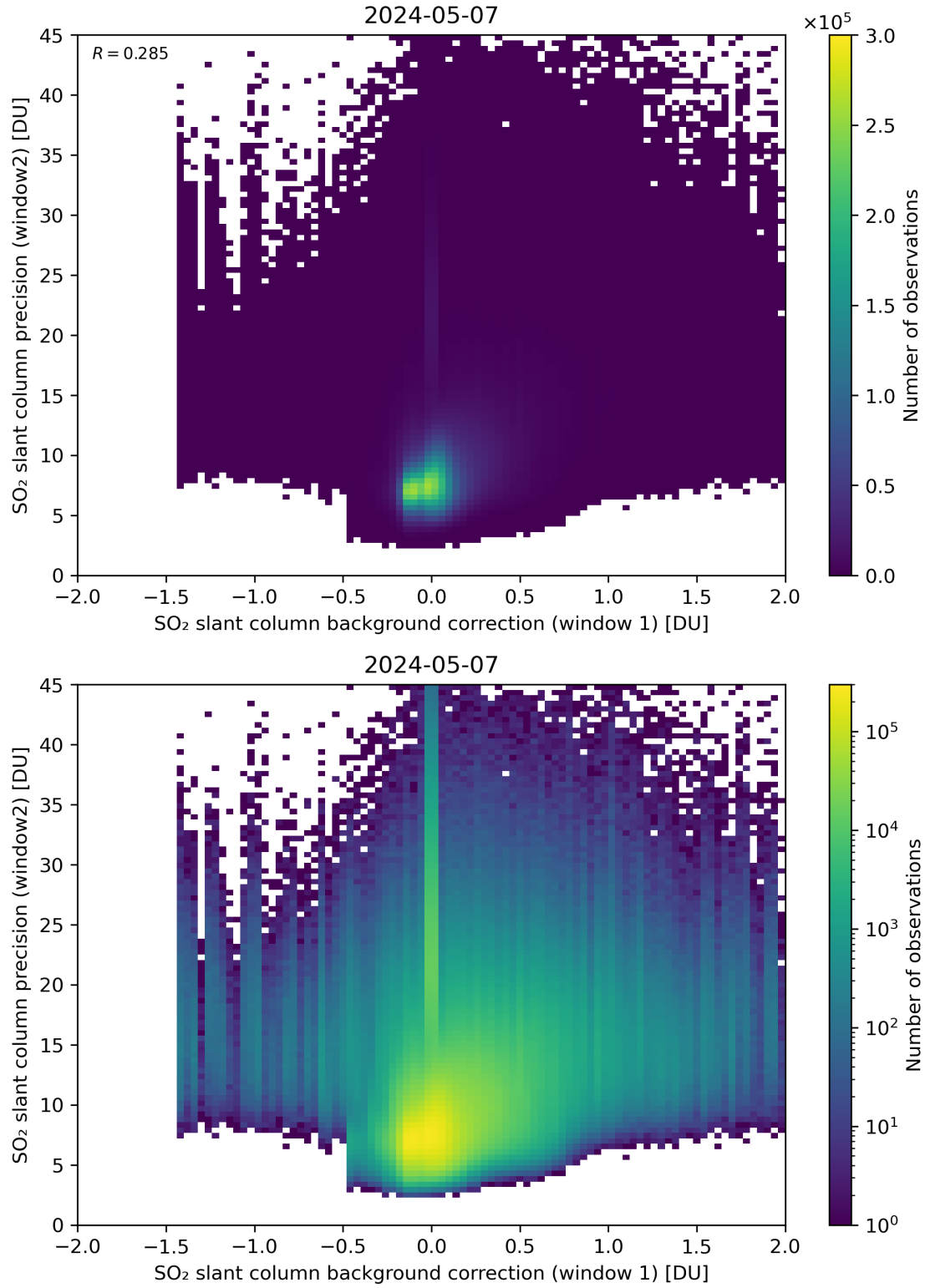
Figure 106: Scatter density plot of “SO 2 slant column background correction (window 1)” against “SO 2 slant column precision (window2)” for 2024-05-07 to 2024-05-08.
