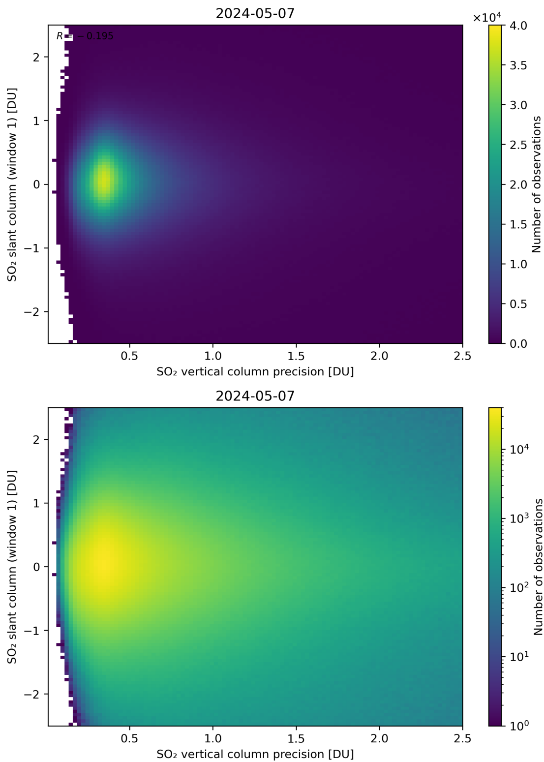
Figure 289: Scatter density plot of “SO 2 vertical column precision” against “SO 2 slant column (window 1)” for 2024-05-07 to 2024-05-08.
