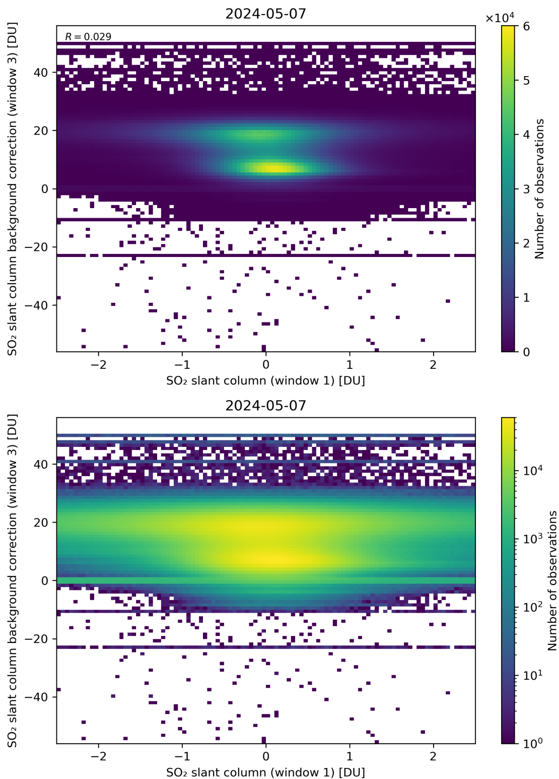
Figure 214: Scatter density plot of “SO 2 slant column (window 1)” against “SO 2 slant column background correction (window 3)” for 2024-05-07 to 2024-05-08.
