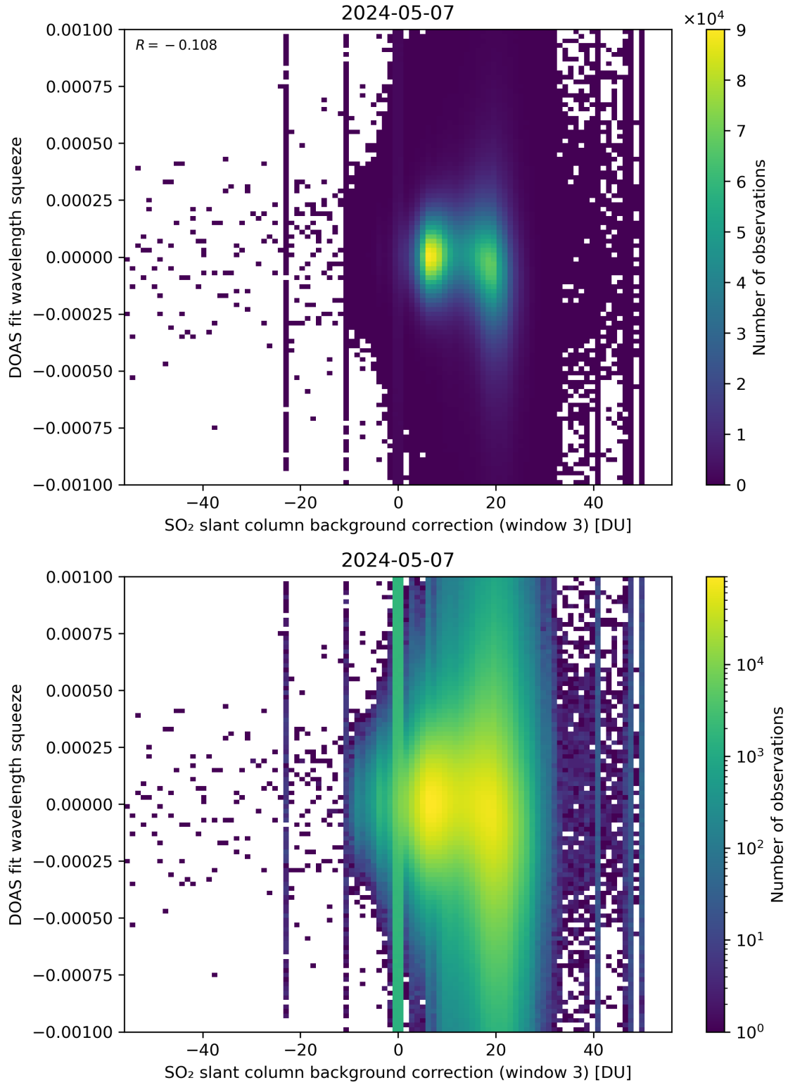
Figure 122: Scatter density plot of “SO 2 slant column background correction (window 3)” against “DOAS fit wavelength squeeze” for 2024-05-07 to 2024-05-08.
