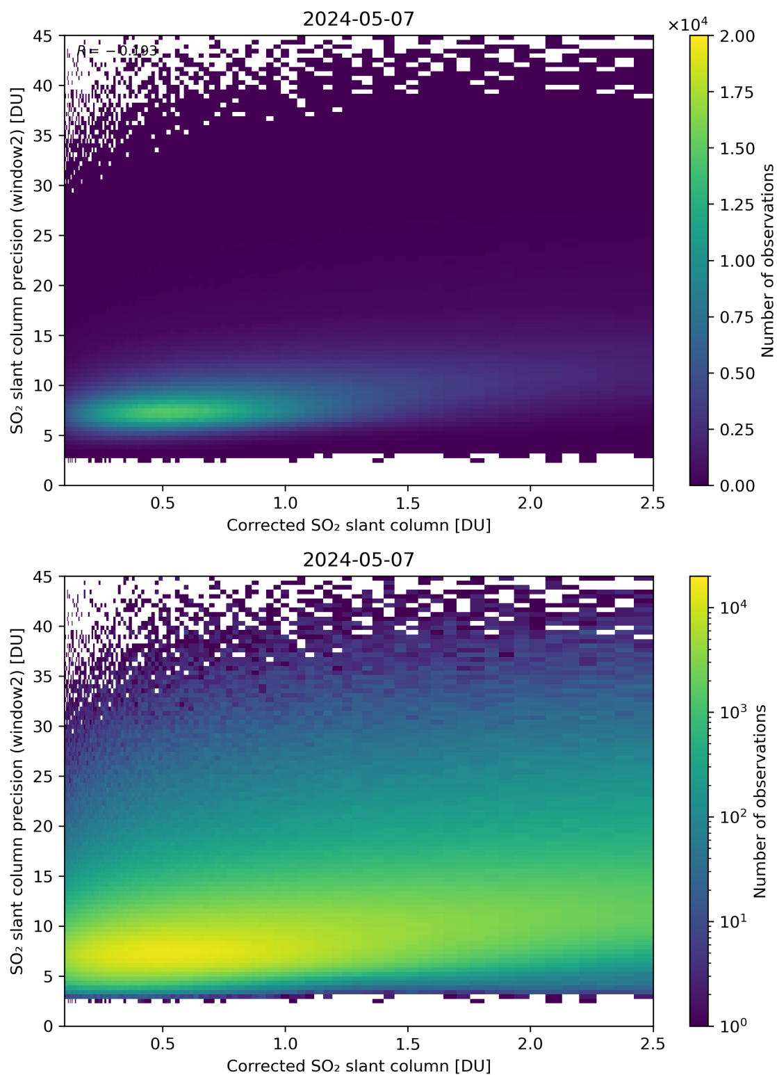
Figure 189: Scatter density plot of “Corrected SO 2 slant column” against “SO 2 slant column precision (window2)” for 2024-05-07 to 2024-05-08.
