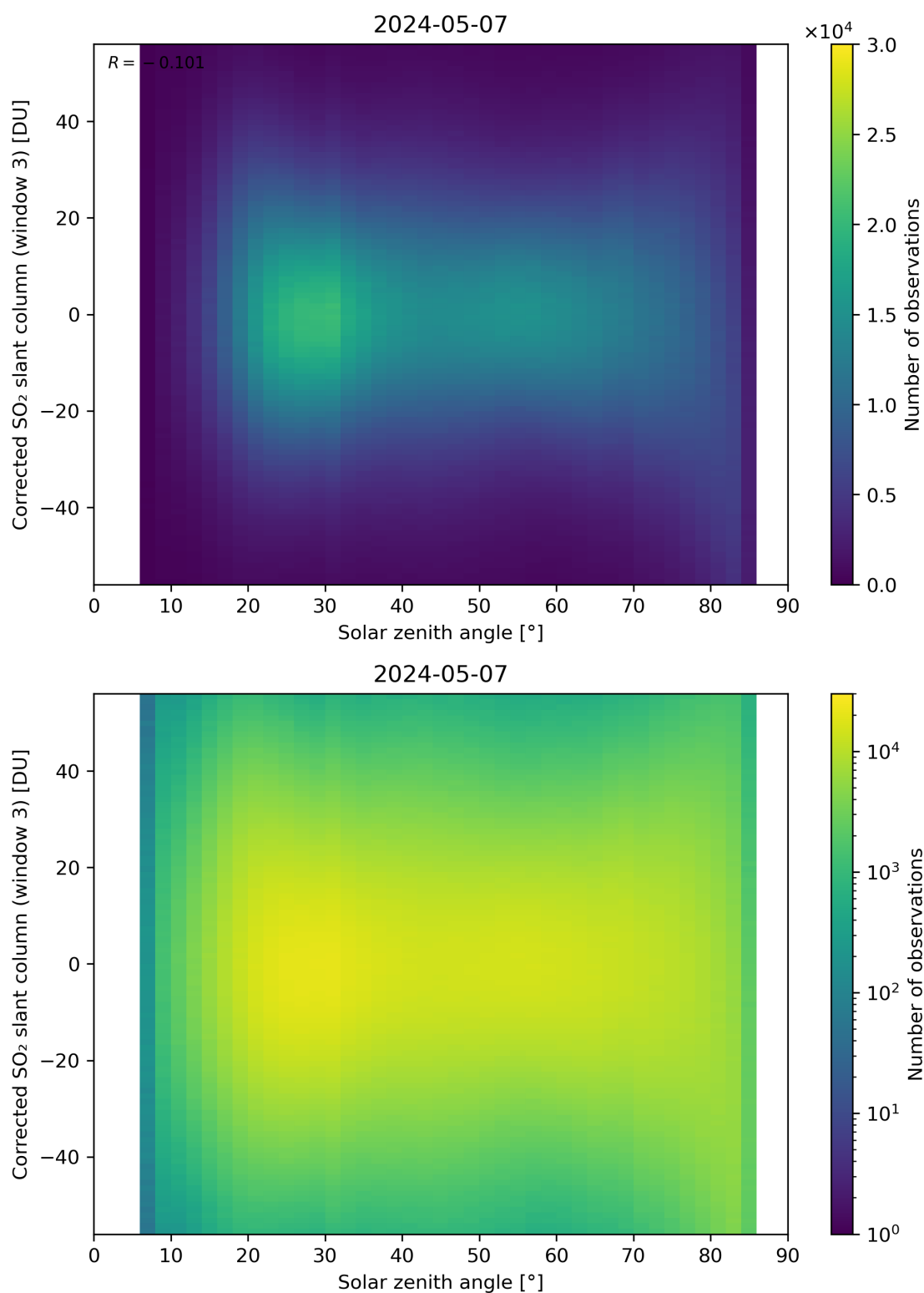
Figure 168: Scatter density plot of “Solar zenith angle” against “Corrected SO 2 slant column (window 3)” for 2024-05-07 to 2024-05-08.
