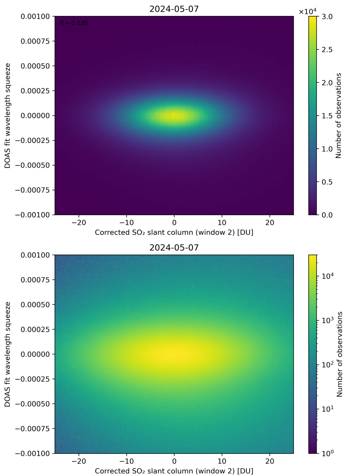
Figure 197: Scatter density plot of “Corrected SO 2 slant column (window 2)” against “DOAS fit wavelength squeeze” for 2024-05-07 to 2024-05-08.
