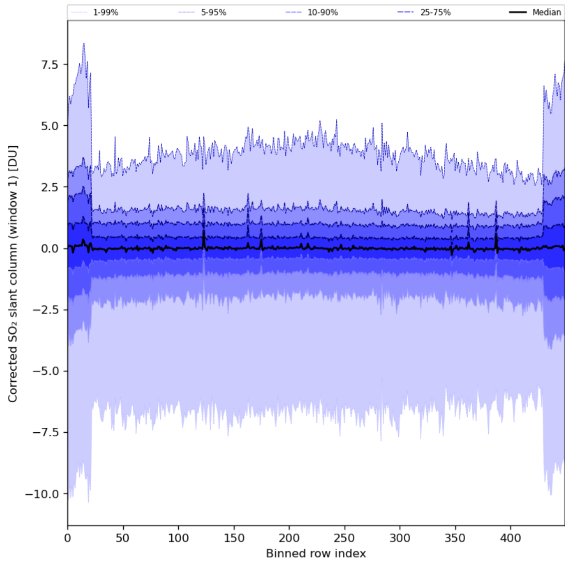
Figure 81: Along track statistics of “Corrected SO 2 slant column (window 1)” for 2024-05-07 to 2024-05-08
