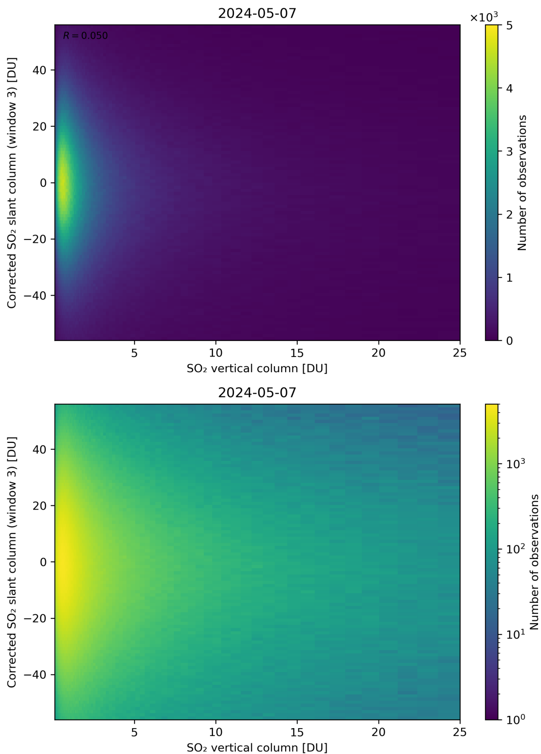
Figure 299: Scatter density plot of “SO 2 vertical column” against “Corrected SO 2 slant column (window 3)” for 2024-05-07 to 2024-05-08.
