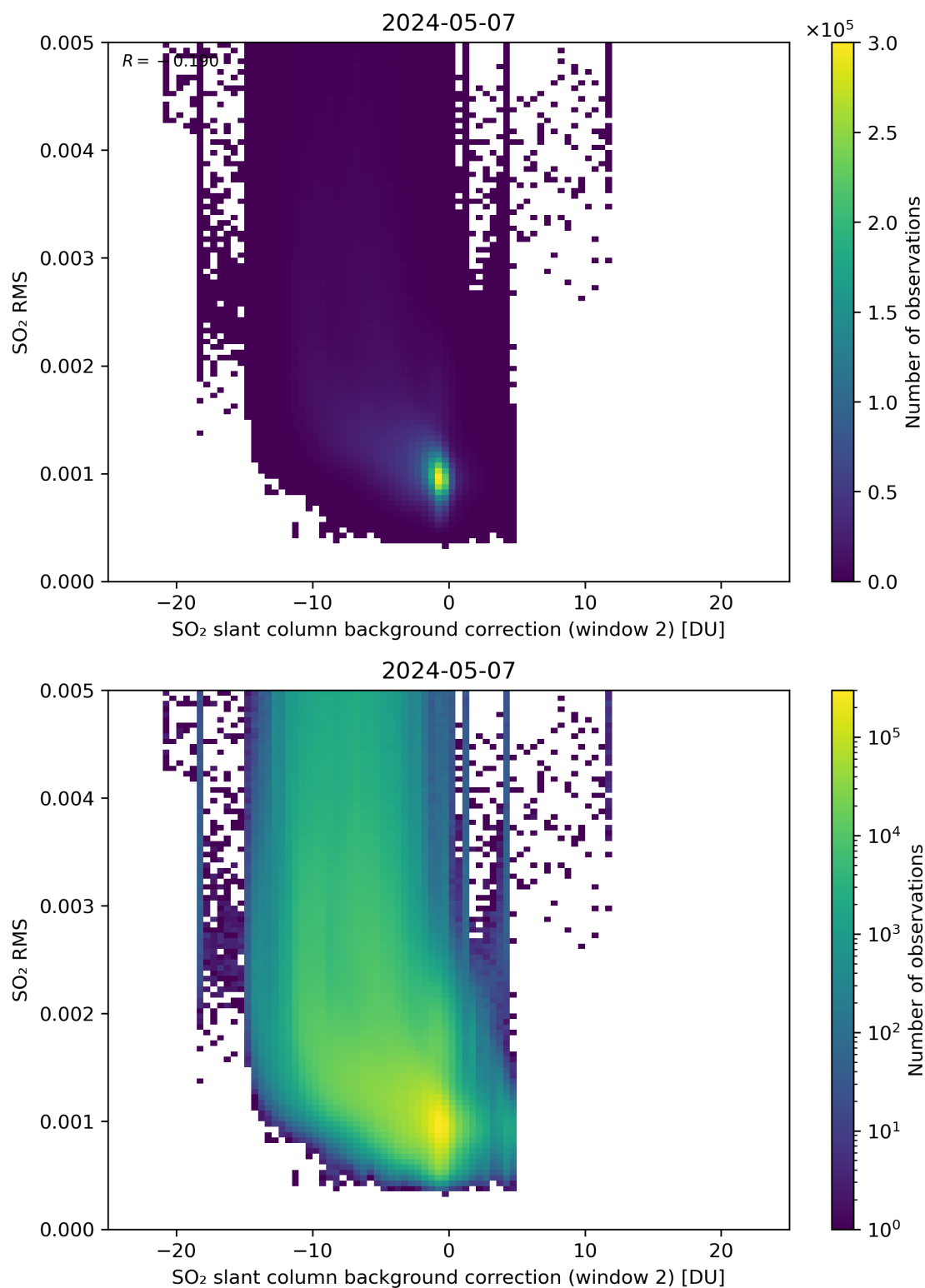
Figure 114: Scatter density plot of “SO 2 slant column background correction (window 2)” against “SO 2 RMS” for 2024-05-07 to 2024-05-08.
