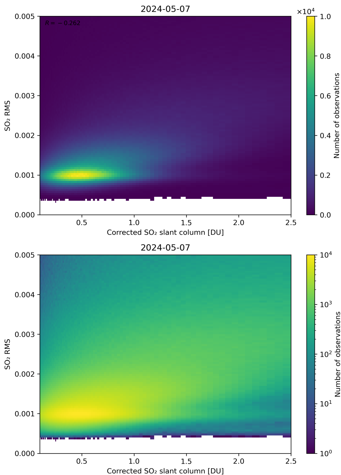
Figure 183: Scatter density plot of “Corrected SO 2 slant column” against “SO 2 RMS” for 2024-05-07 to 2024-05-08.
