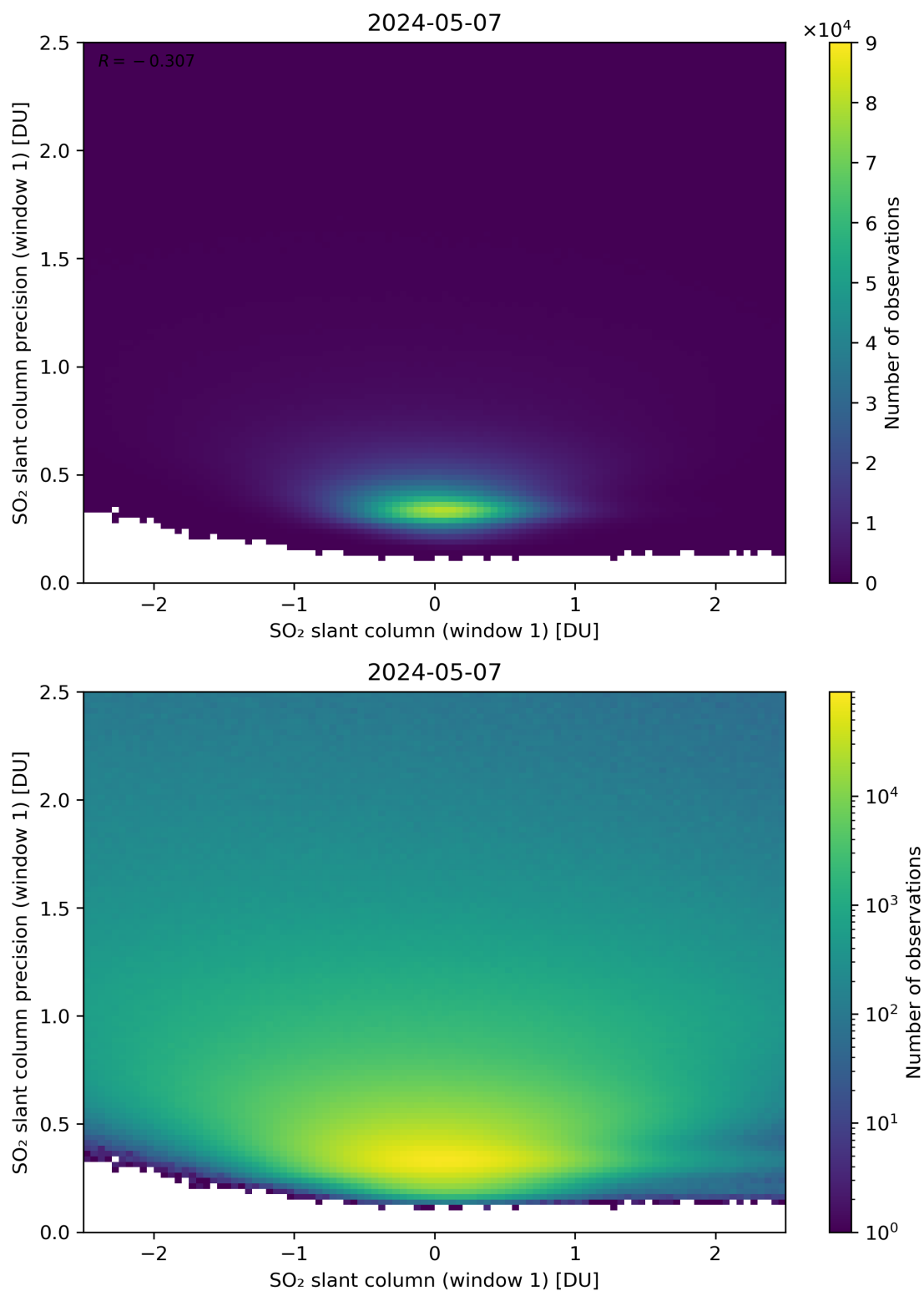
Figure 235: Scatter density plot of “SO 2 slant column (window 1)” against “SO 2 slant column precision (window 1)” for 2024-05-07 to 2024-05-08.
