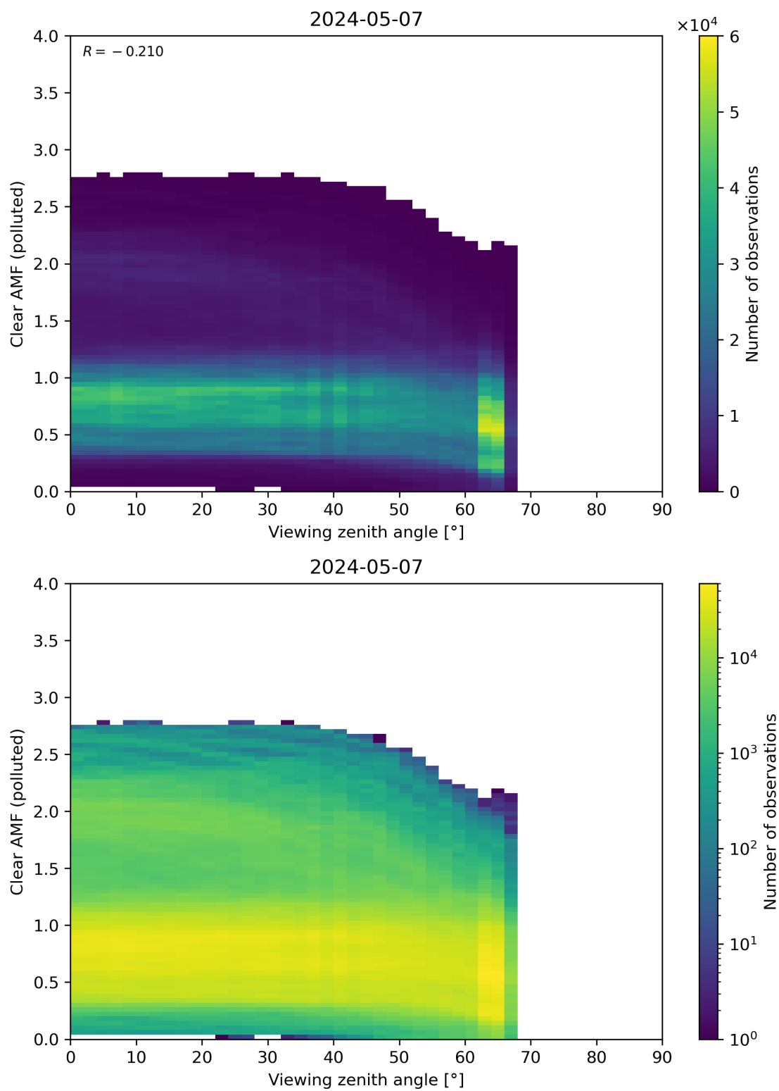
Figure 316: Scatter density plot of “Viewing zenith angle” against “Clear AMF (polluted)” for 2024-05-07 to 2024-05-08.
