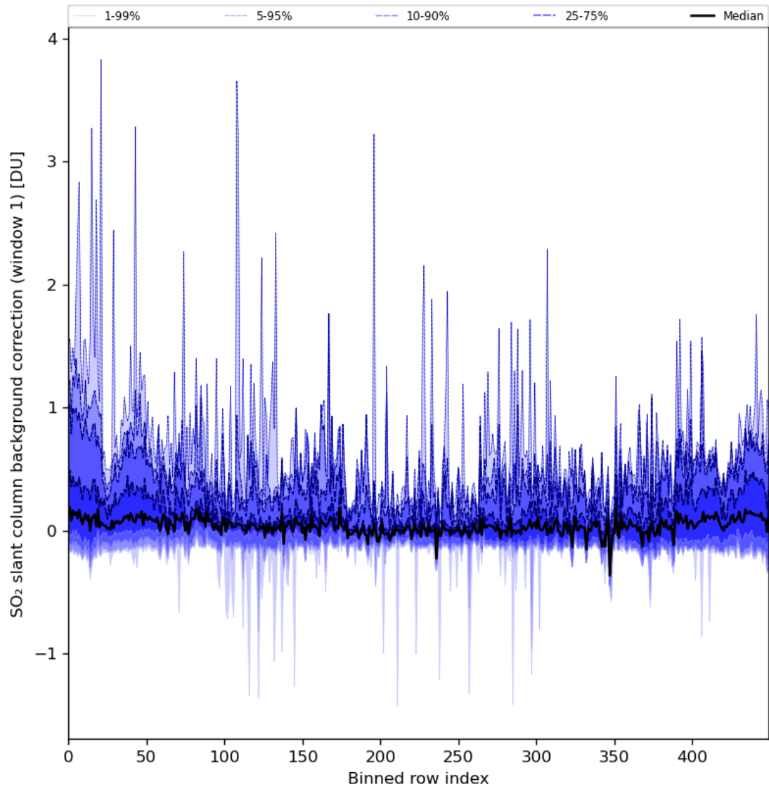
Figure 82: Along track statistics of “SO 2 slant column background correction (window 1)” for 2024-05-07 to 2024-05-08
