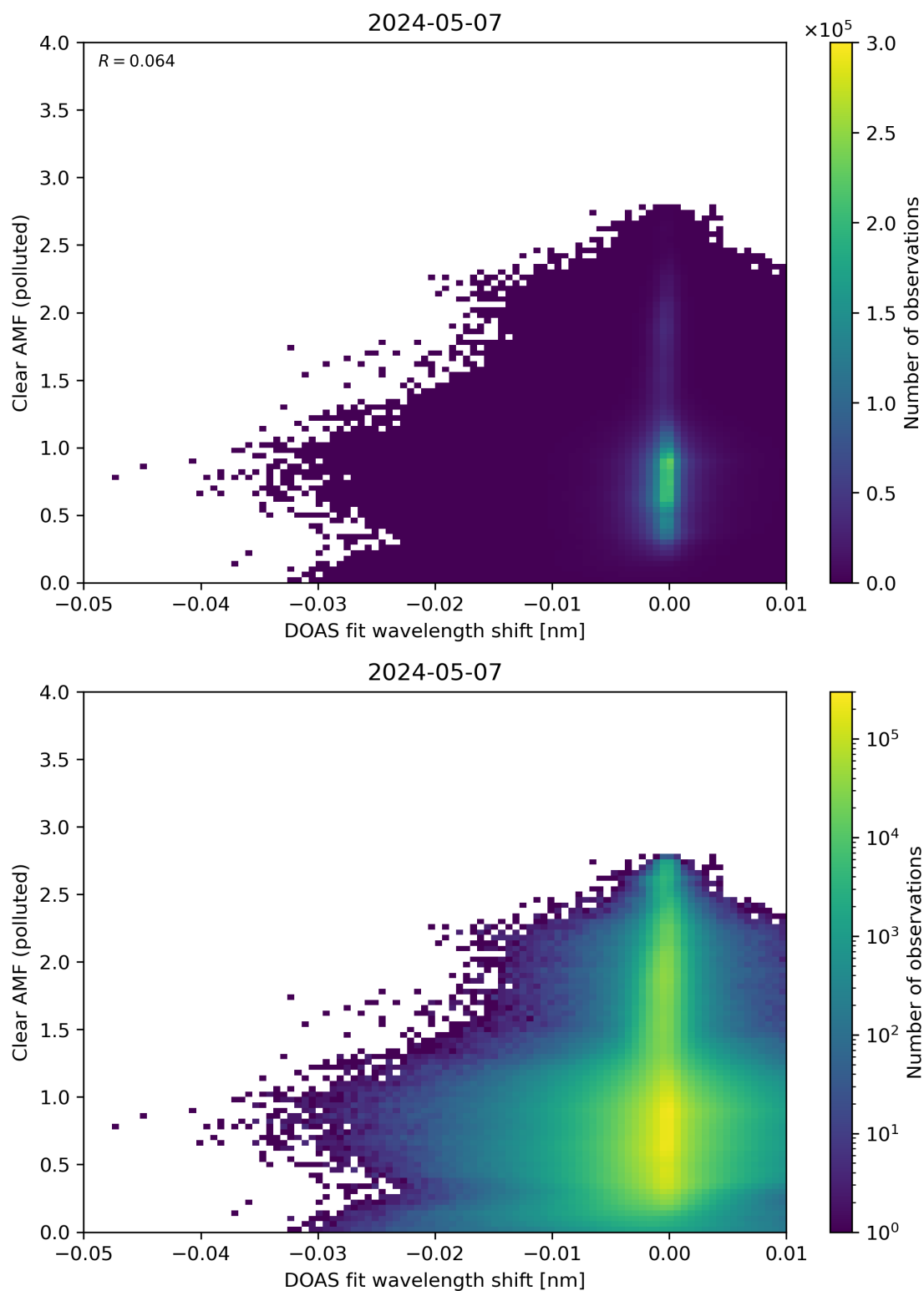
Figure 129: Scatter density plot of “DOAS fit wavelength shift” against “Clear AMF (polluted)” for 2024-05-07 to 2024-05-08.
