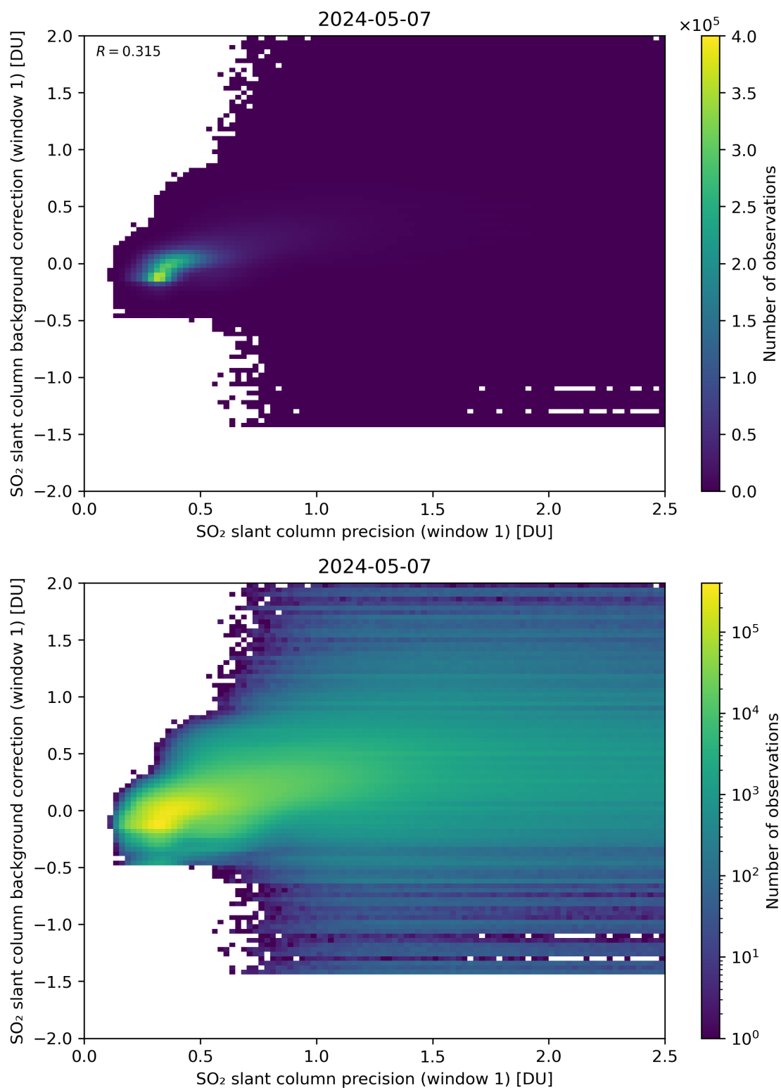
Figure 218: Scatter density plot of “SO 2 slant column precision (window 1)” against “SO 2 slant column background correction (window 1)” for 2024-05-07 to 2024-05-08.
