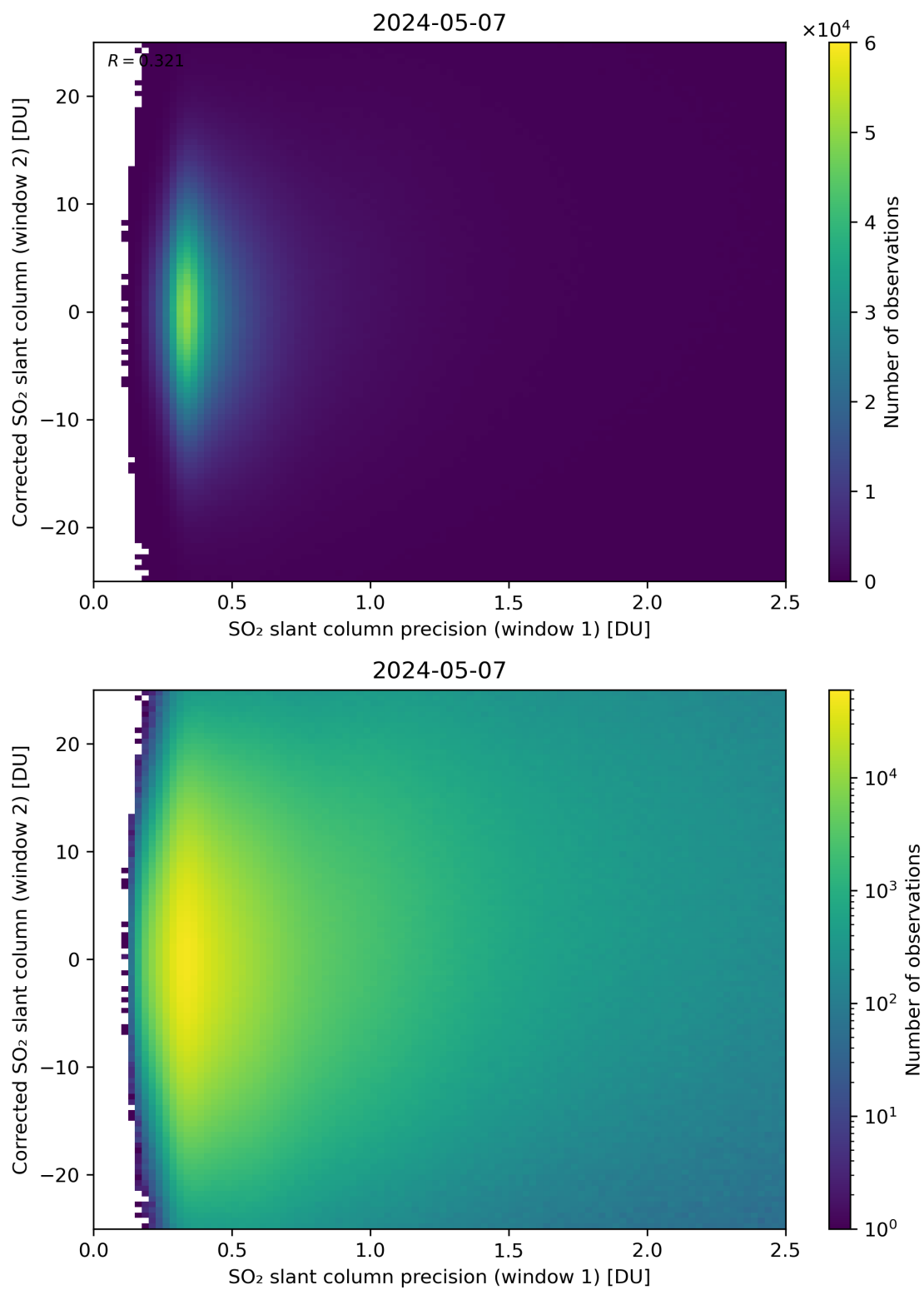
Figure 225: Scatter density plot of “SO 2 slant column precision (window 1)” against “Corrected SO 2 slant column (window 2)” for 2024-05-07 to 2024-05-08.
