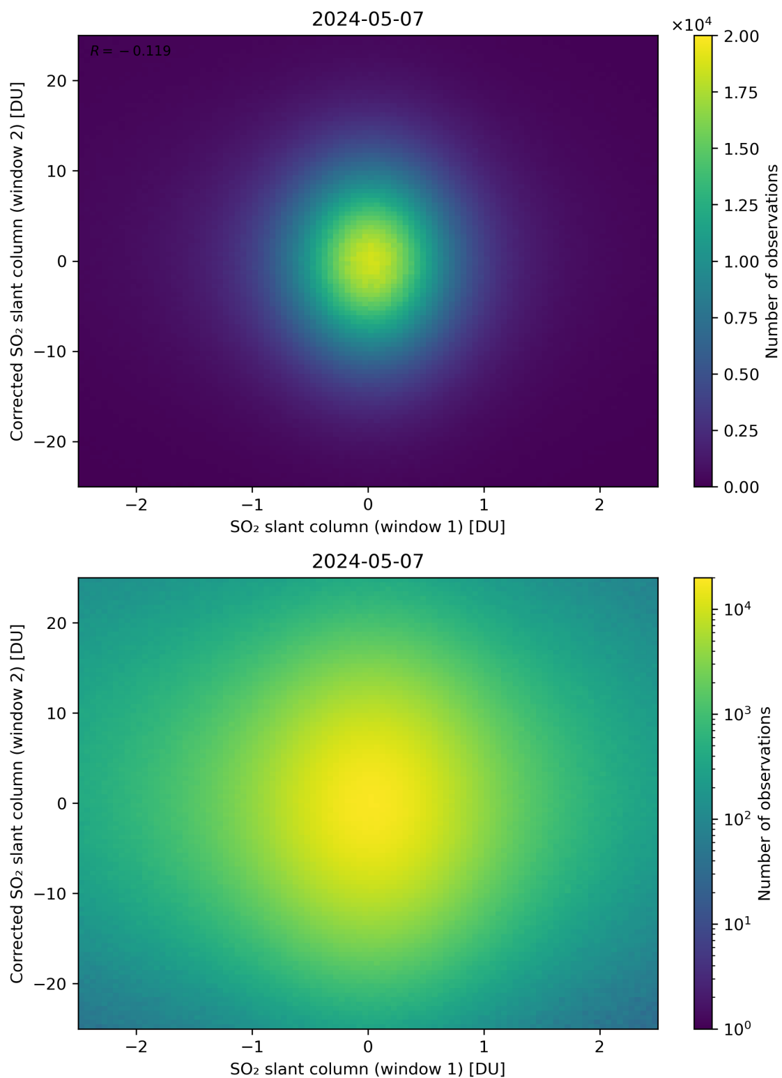
Figure 233: Scatter density plot of “SO 2 slant column (window 1)” against “Corrected SO 2 slant column (window 2)” for 2024-05-07 to 2024-05-08.
