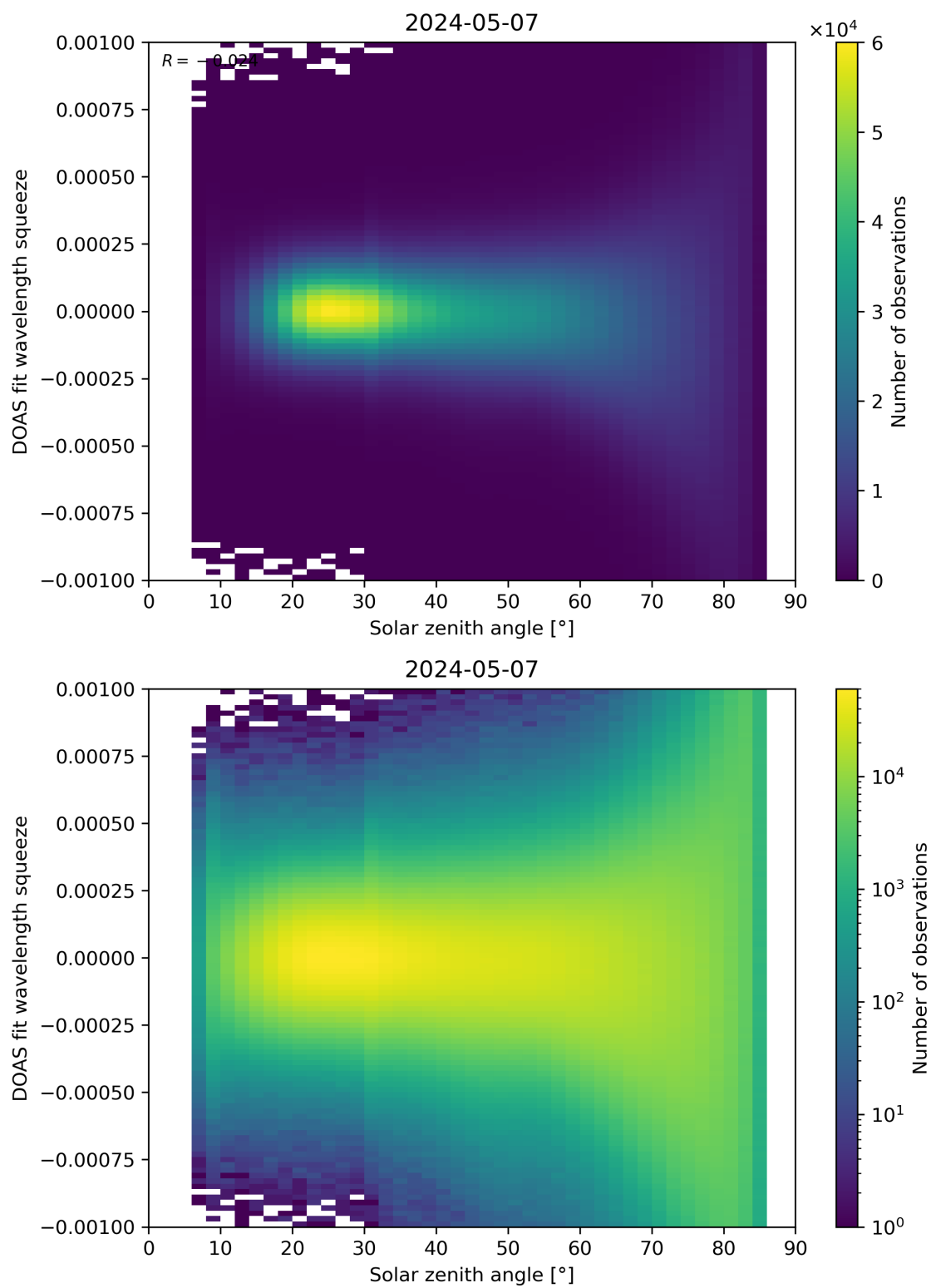
Figure 162: Scatter density plot of “Solar zenith angle” against “DOAS fit wavelength squeeze” for 2024-05-07 to 2024-05-08.
