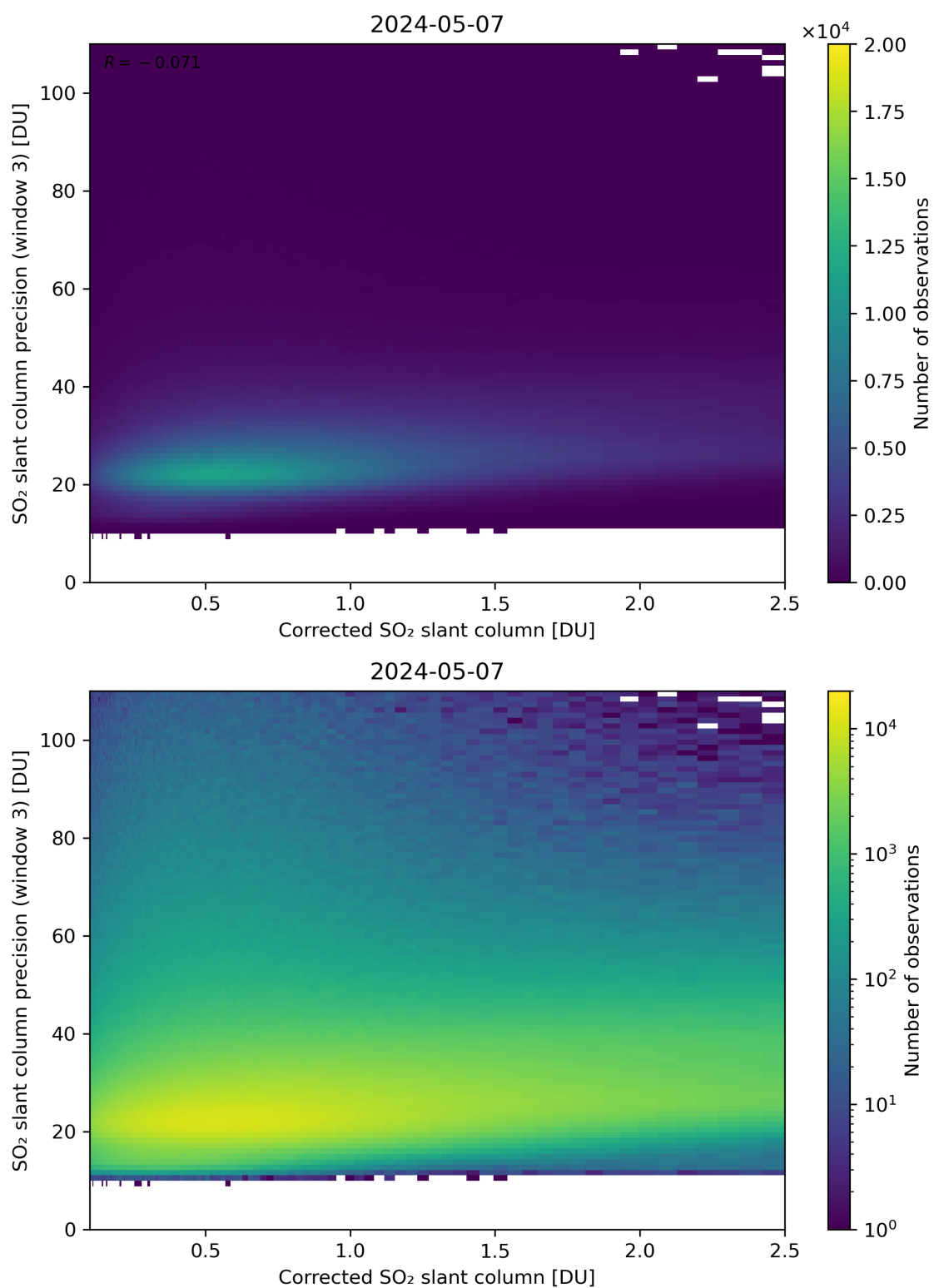
Figure 191: Scatter density plot of “Corrected SO 2 slant column” against “SO 2 slant column precision (window 3)” for 2024-05-07 to 2024-05-08.
