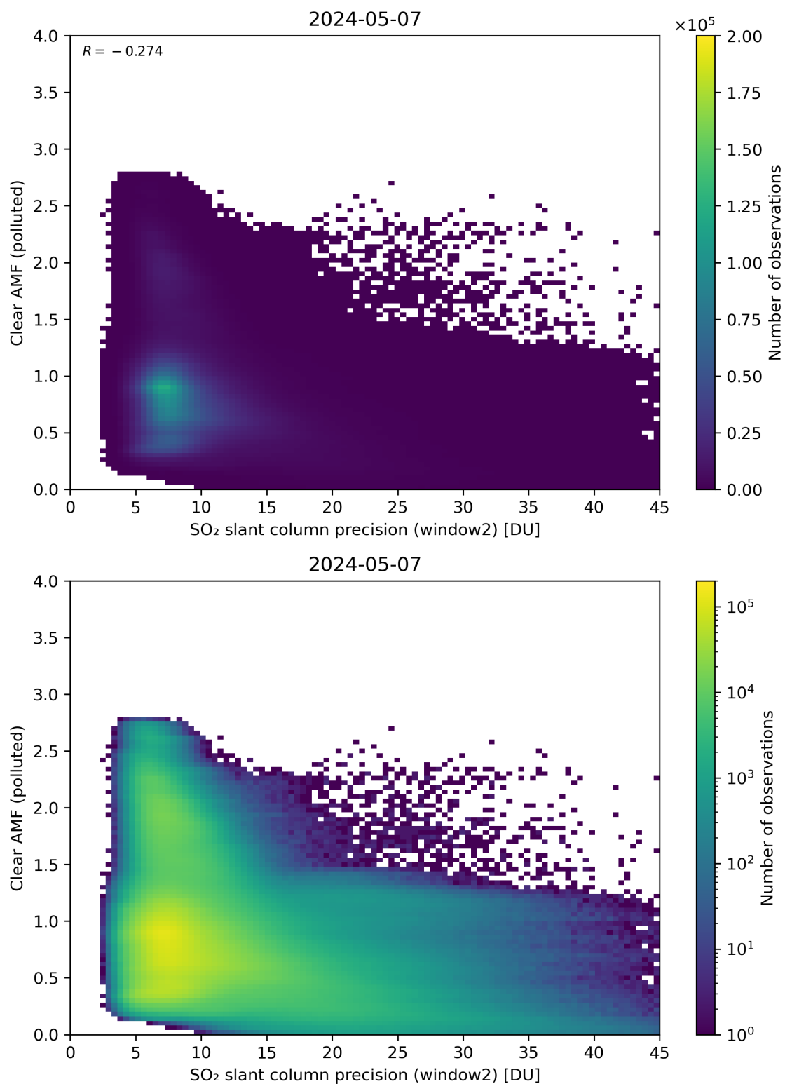
Figure 246: Scatter density plot of “SO 2 slant column precision (window2)” against “Clear AMF (polluted)” for 2024-05-07 to 2024-05-08.
