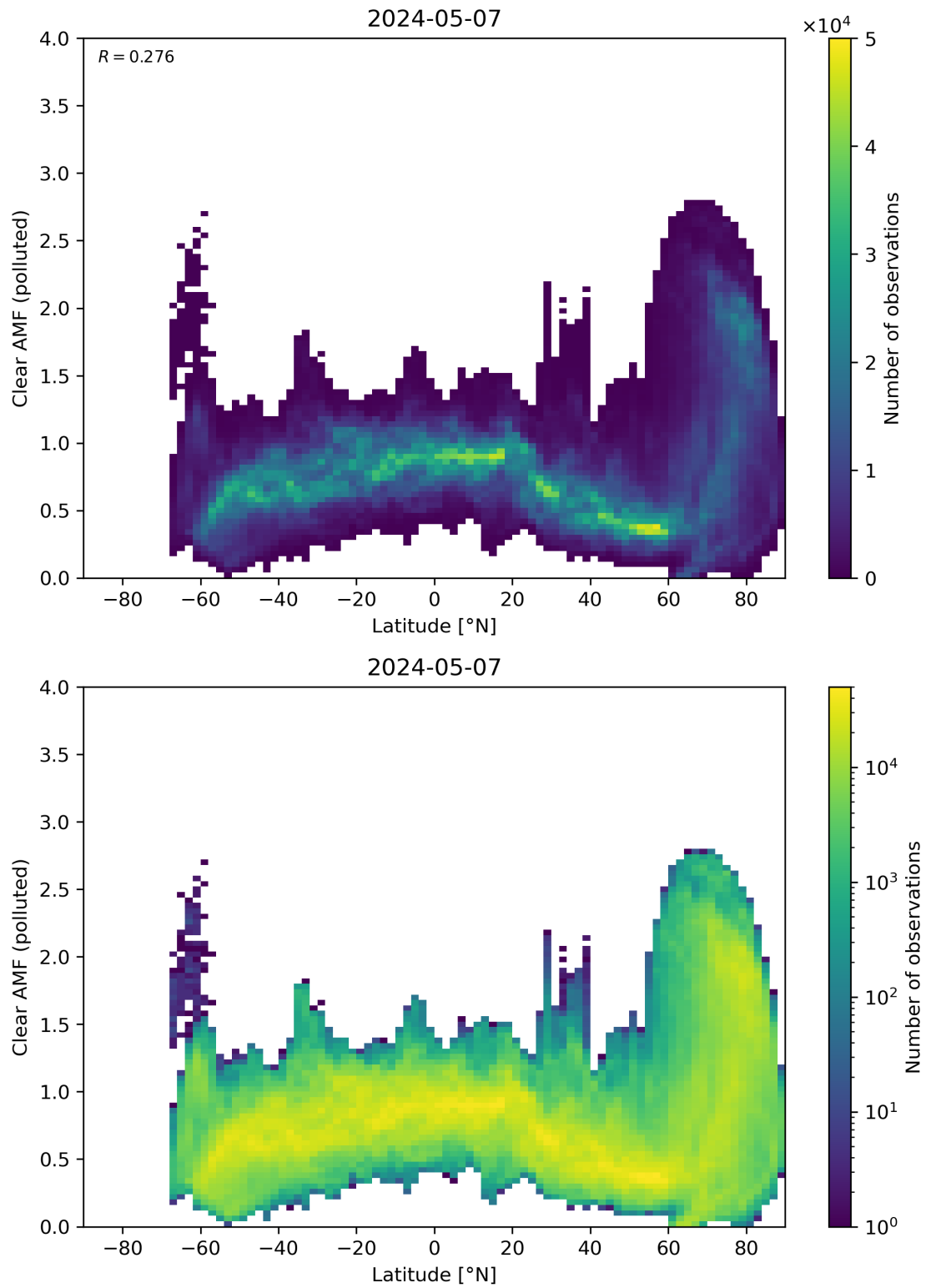
Figure 145: Scatter density plot of “Latitude” against “Clear AMF (polluted)” for 2024-05-07 to 2024-05-08.
