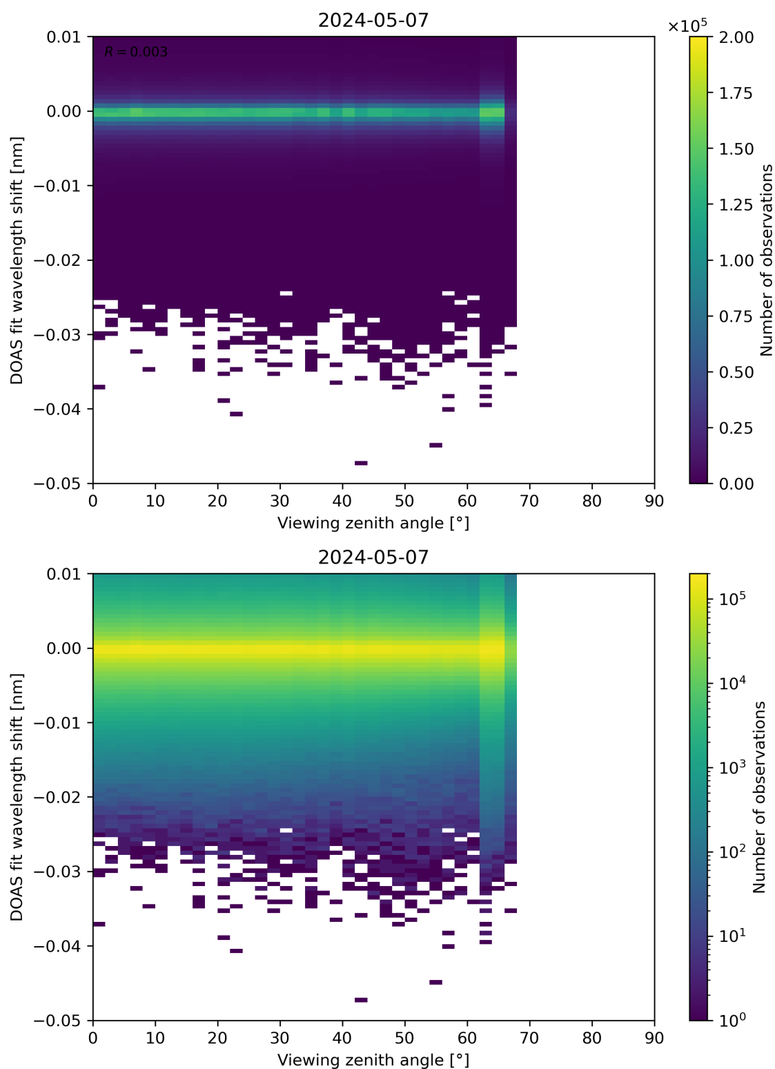
Figure 311: Scatter density plot of “Viewing zenith angle” against “DOAS fit wavelength shift” for 2024-05-07 to 2024-05-08.
