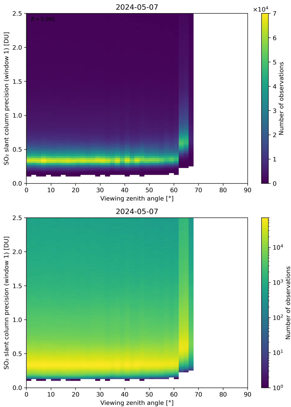
Figure 321: Scatter density plot of “Viewing zenith angle” against “SO 2 slant column precision (window 1)” for 2024-05-07 to 2024-05-08.
