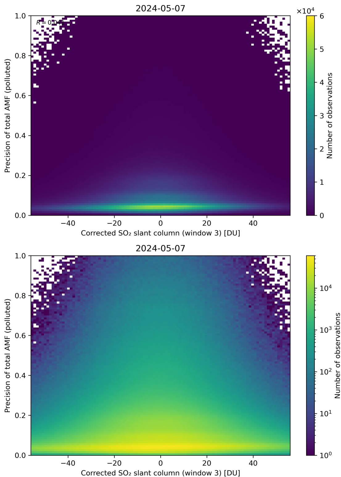
Figure 211: Scatter density plot of “Corrected SO 2 slant column (window 3)” against “Precision of total AMF (polluted)” for 2024-05-07 to 2024-05-08.
