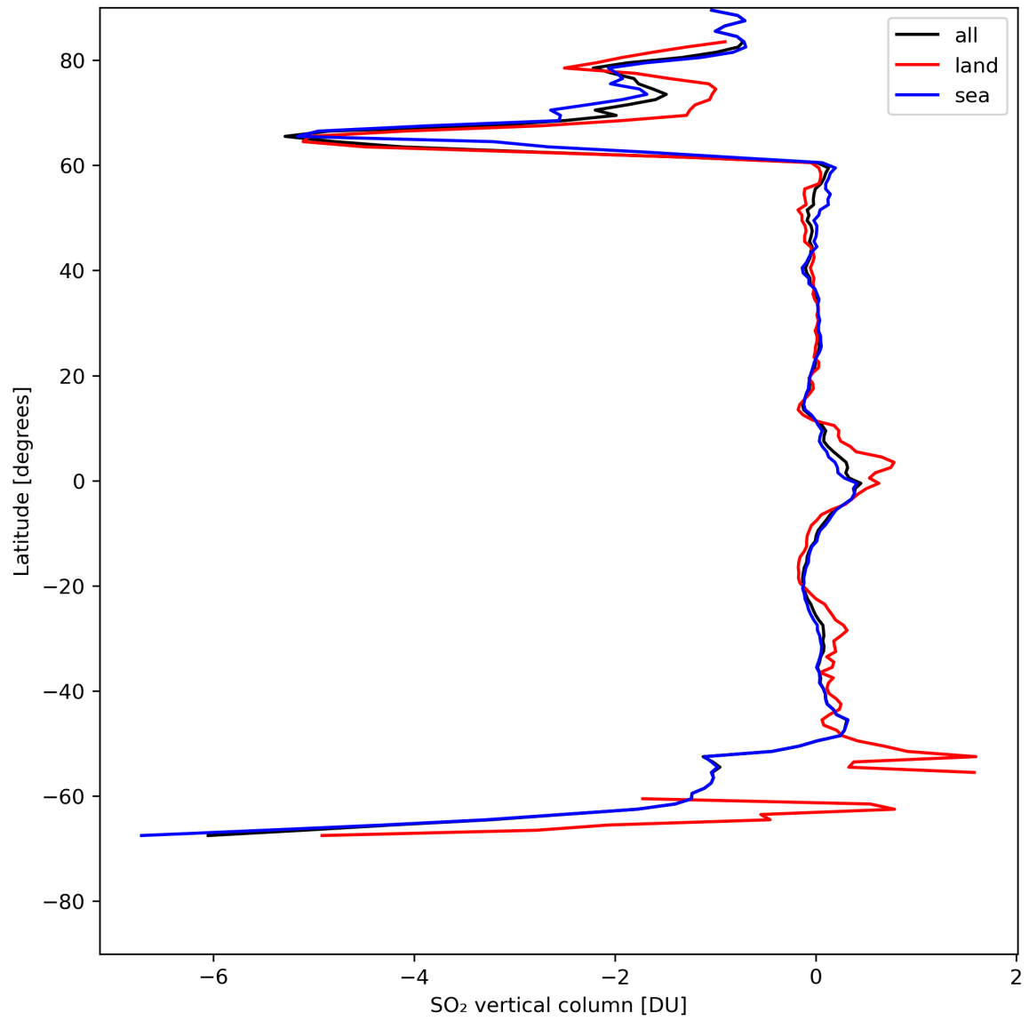
Figure 30: Zonal average of “SO 2 vertical column” for 2024-05-07 to 2024-05-08.
