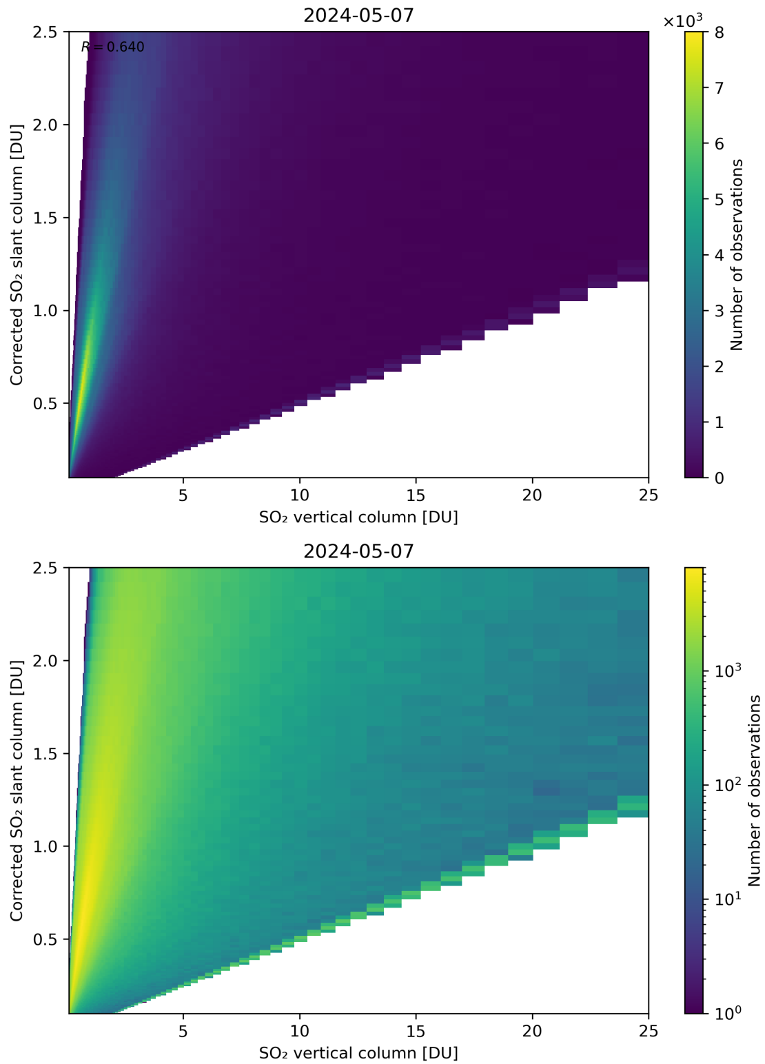
Figure 297: Scatter density plot of “SO 2 vertical column” against “Corrected SO 2 slant column” for 2024-05-07 to 2024-05-08.
