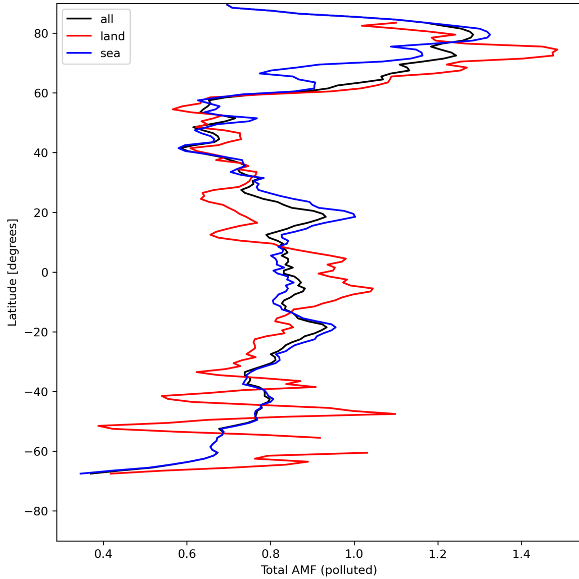
Figure 48: Zonal average of “Total AMF (polluted)” for 2024-05-07 to 2024-05-08.
