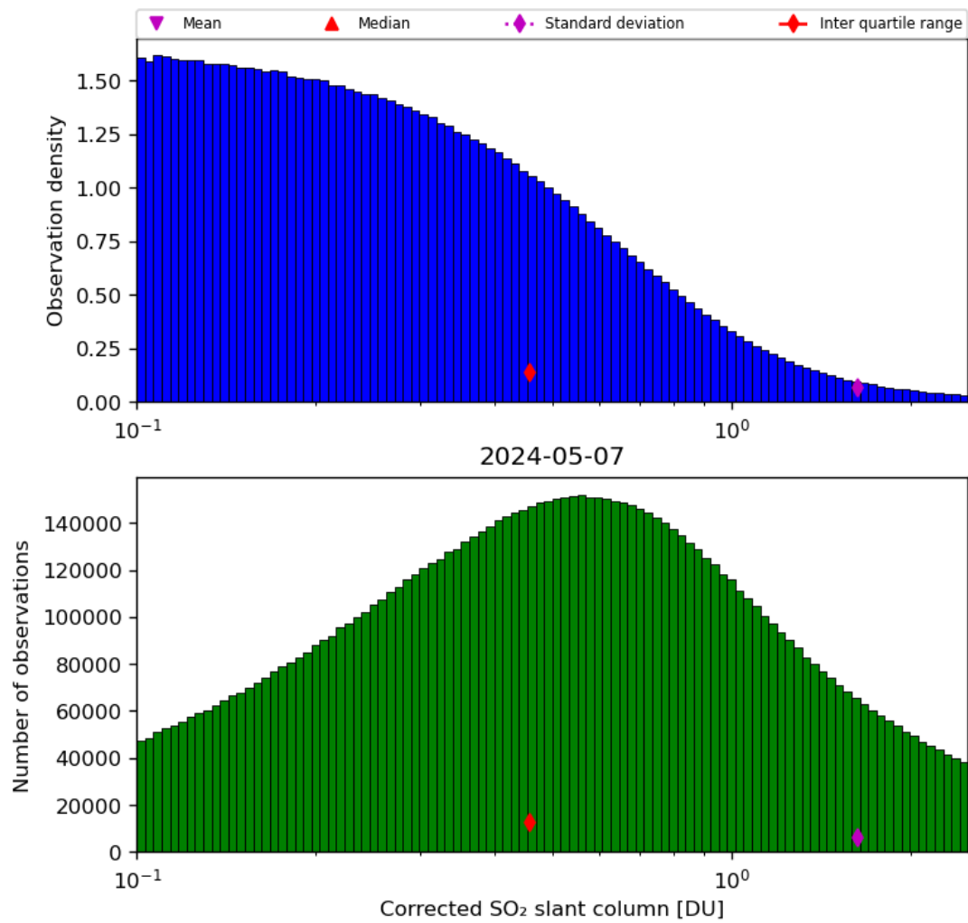
Figure 55: Histogram of “Corrected SO 2 slant column” for 2024-05-07 to 2024-05-08
