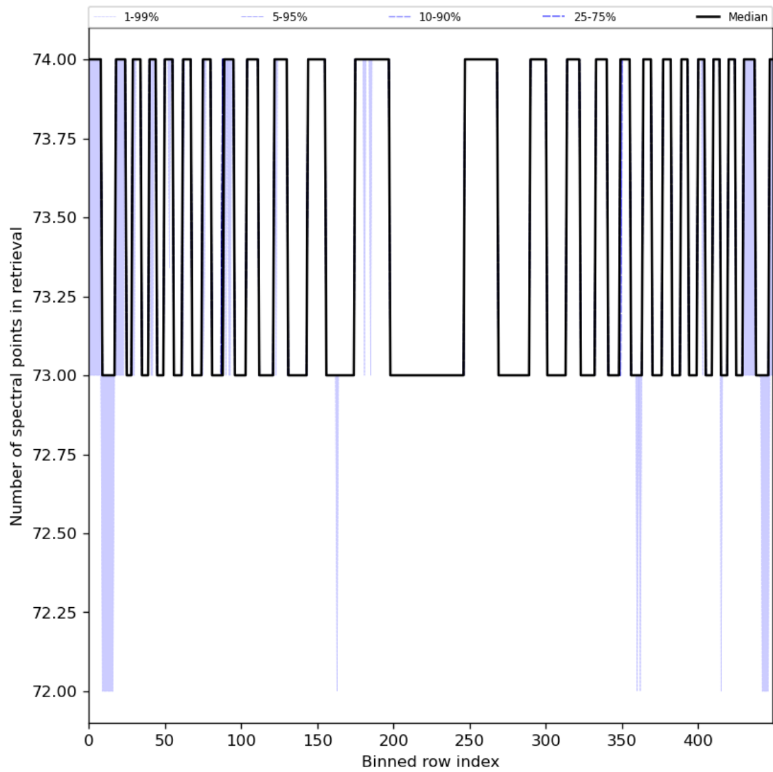
Figure 97: Along track statistics of “Number of spectral points in retrieval” for 2024-05-07 to 2024-05-08
