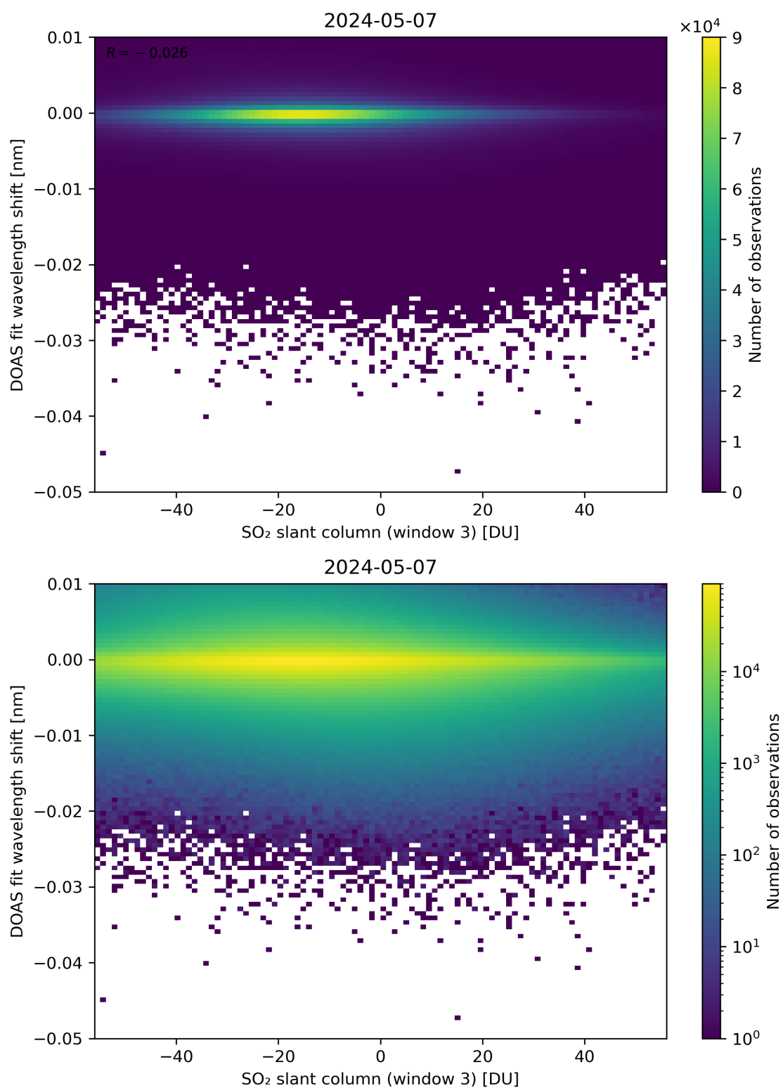
Figure 254: Scatter density plot of “SO 2 slant column (window 3)” against “DOAS fit wavelength shift” for 2024-05-07 to 2024-05-08.
