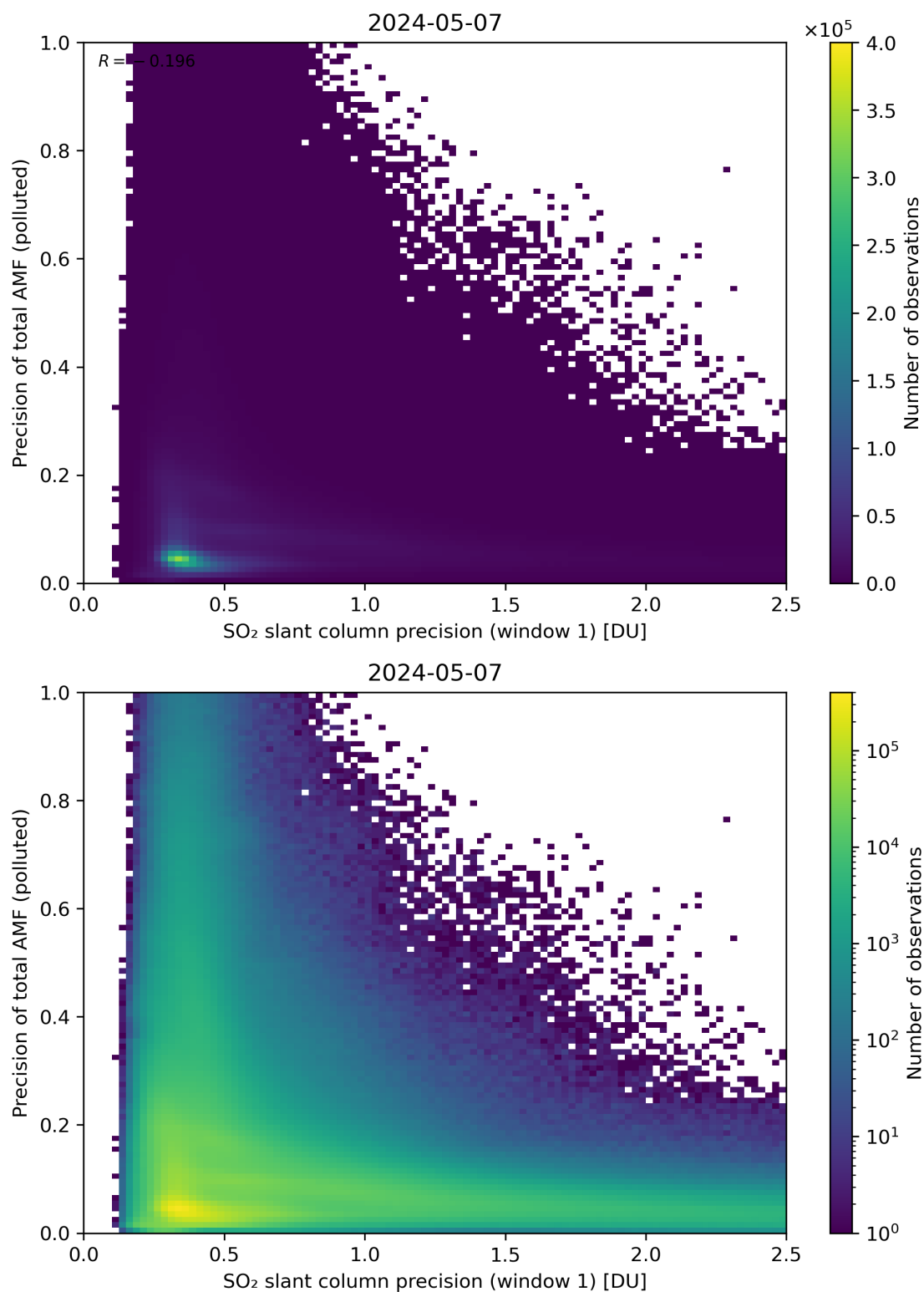
Figure 231: Scatter density plot of “SO 2 slant column precision (window 1)” against “Precision of total AMF (polluted)” for 2024-05-07 to 2024-05-08.
