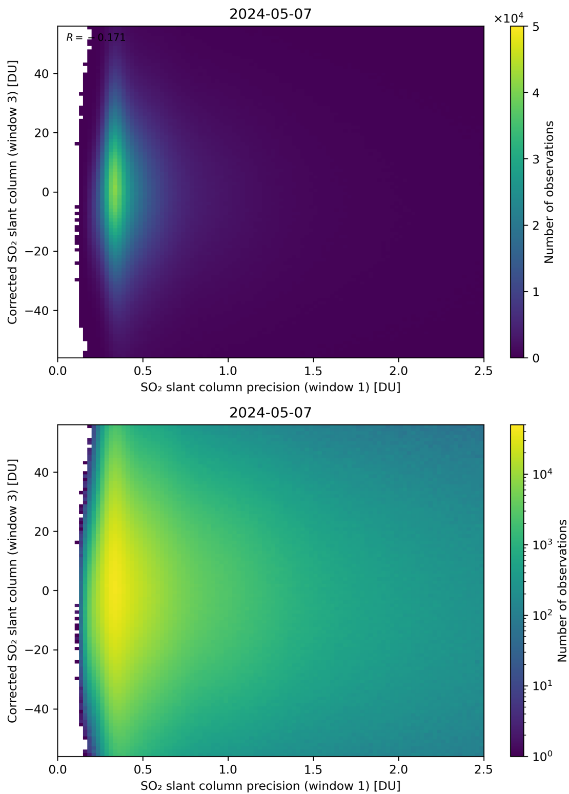
Figure 226: Scatter density plot of “SO 2 slant column precision (window 1)” against “Corrected SO 2 slant column (window 3)” for 2024-05-07 to 2024-05-08.
