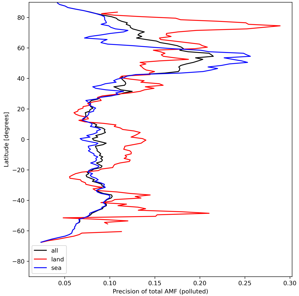
Figure 49: Zonal average of “Precision of total AMF (polluted)” for 2024-05-07 to 2024-05-08.
