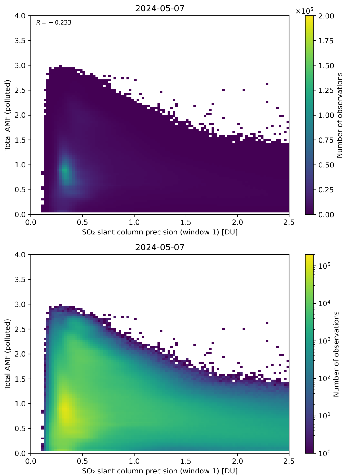
Figure 230: Scatter density plot of “SO 2 slant column precision (window 1)” against “Total AMF (polluted)” for 2024-05-07 to 2024-05-08.
