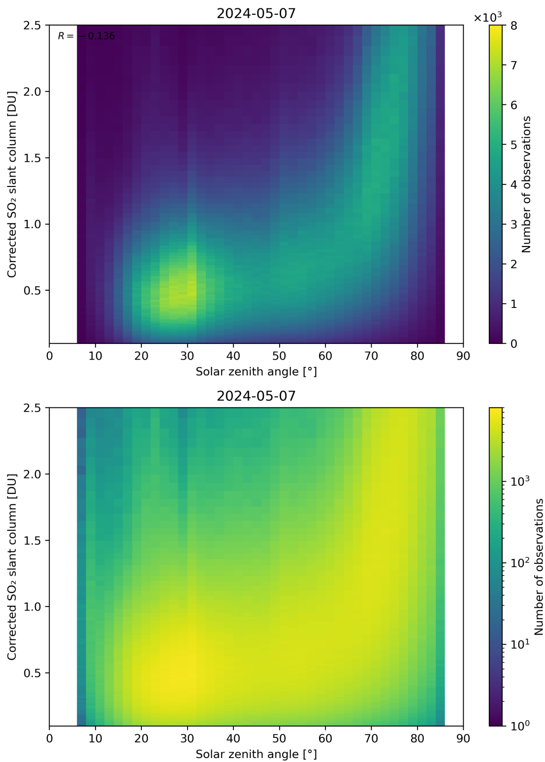
Figure 166: Scatter density plot of “Solar zenith angle” against “Corrected SO 2 slant column” for 2024-05-07 to 2024-05-08.
