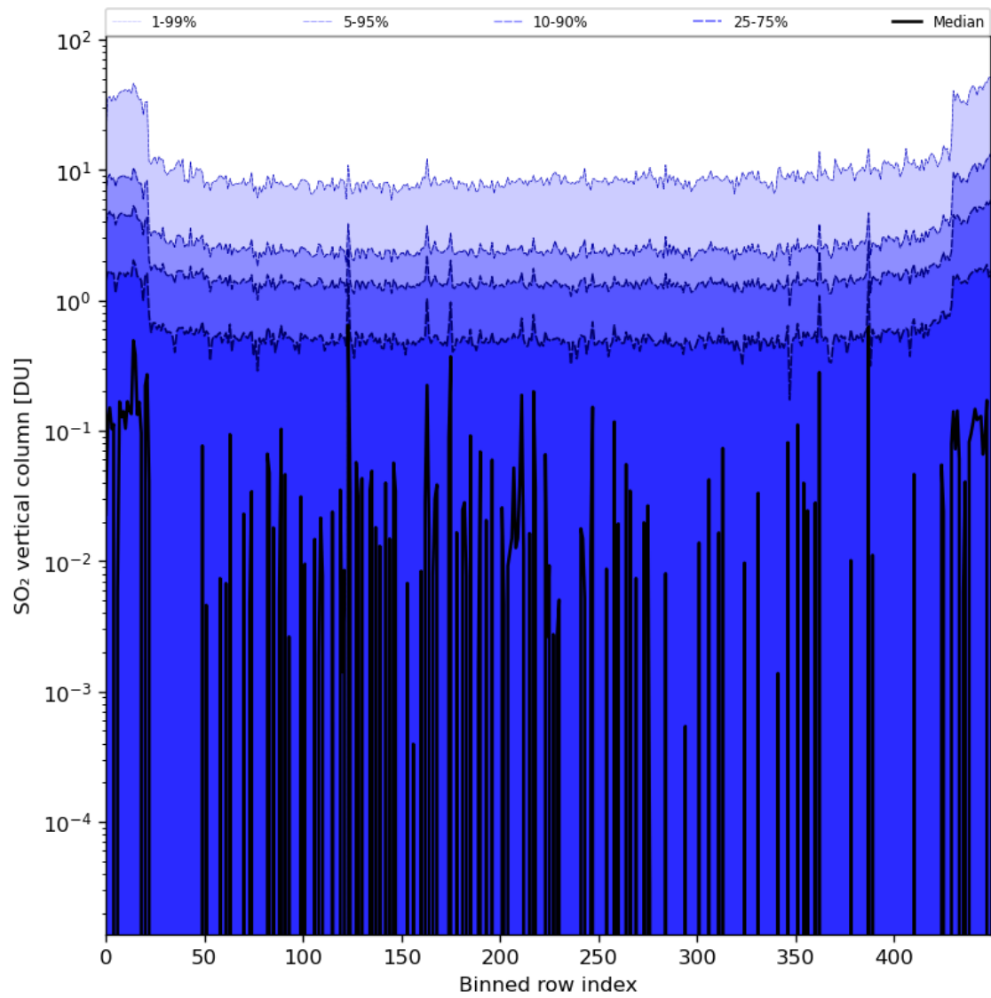
Figure 76: Along track statistics of “SO 2 vertical column” for 2024-05-07 to 2024-05-08
