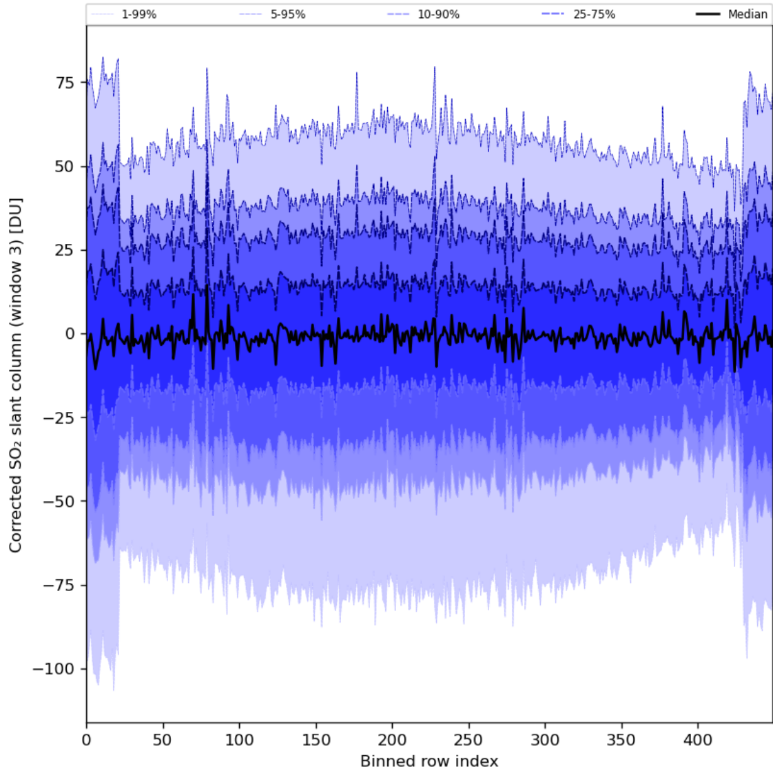
Figure 89: Along track statistics of “Corrected SO 2 slant column (window 3)” for 2024-05-07 to 2024-05-08
