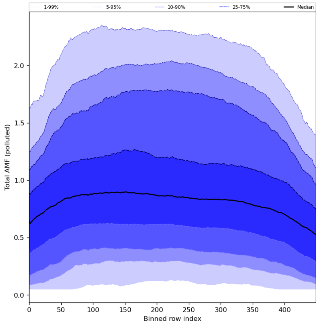
Figure 94: Along track statistics of “Total AMF (polluted)” for 2024-05-07 to 2024-05-08
