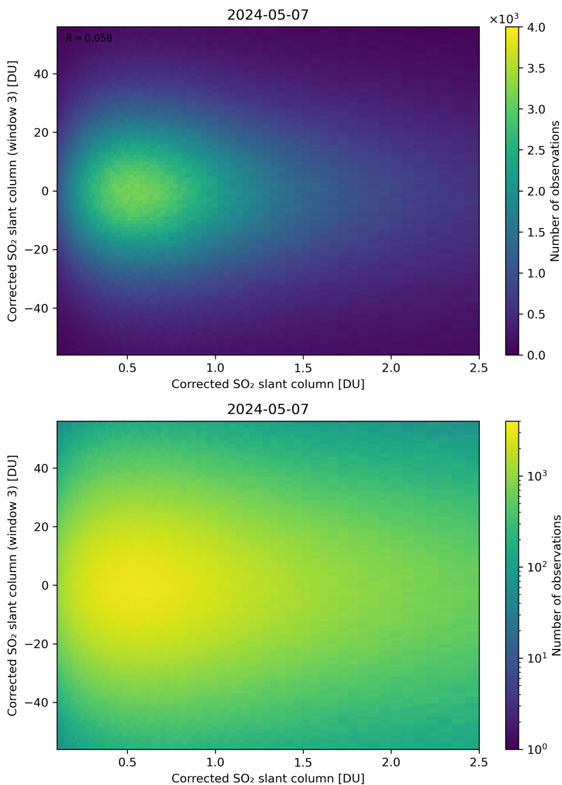
Figure 186: Scatter density plot of “Corrected SO 2 slant column” against “Corrected SO 2 slant column (window 3)” for 2024-05-07 to 2024-05-08.
