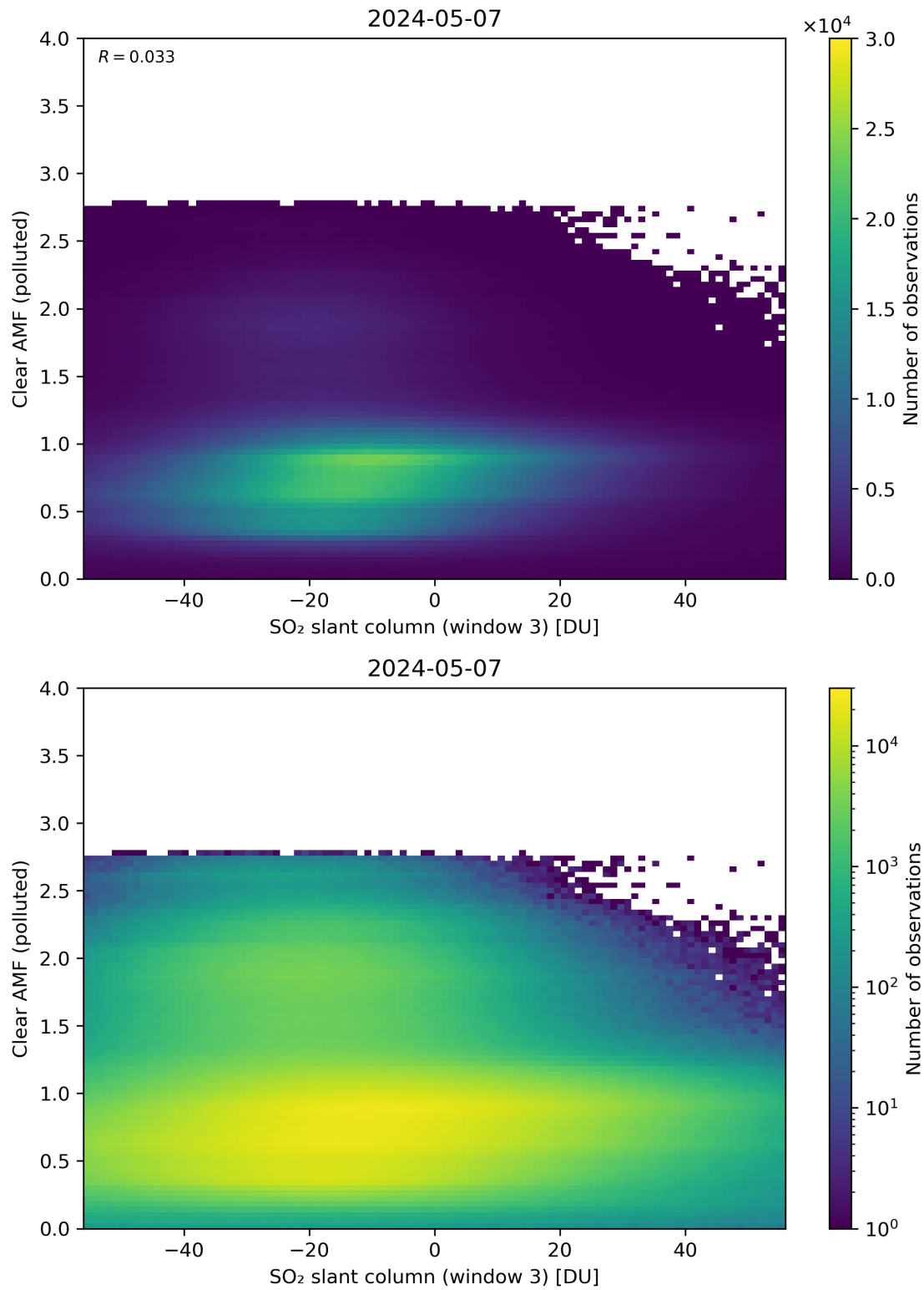
Figure 265: Scatter density plot of “SO 2 slant column (window 3)” against “Clear AMF (polluted)” for 2024-05-07 to 2024-05-08.
