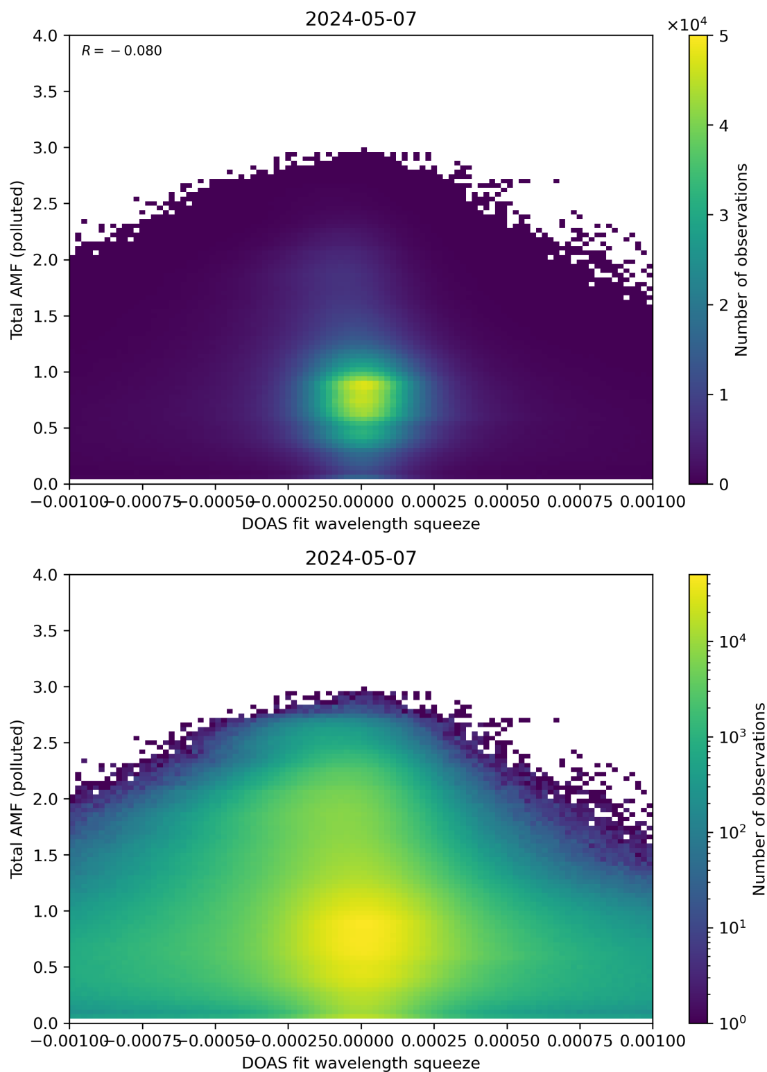
Figure 134: Scatter density plot of “DOAS fit wavelength squeeze” against “Total AMF (polluted)” for 2024-05-07 to 2024-05-08.
