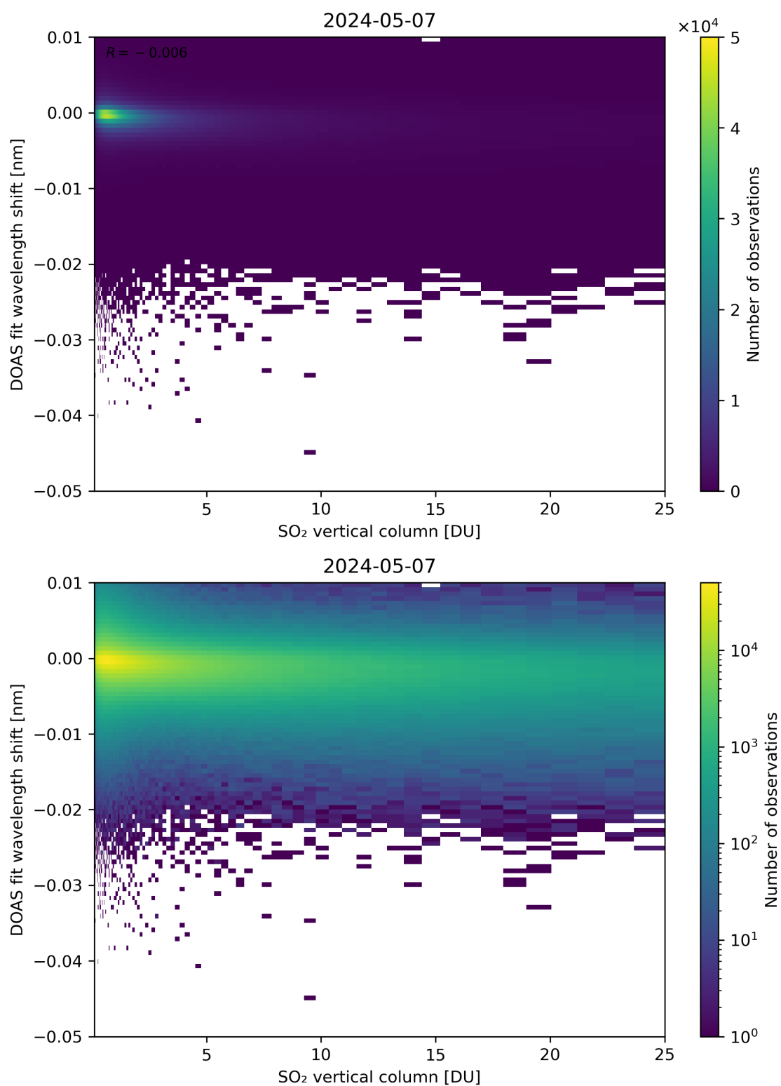
Figure 276: Scatter density plot of “SO 2 vertical column” against “DOAS fit wavelength shift” for 2024-05-07 to 2024-05-08.
