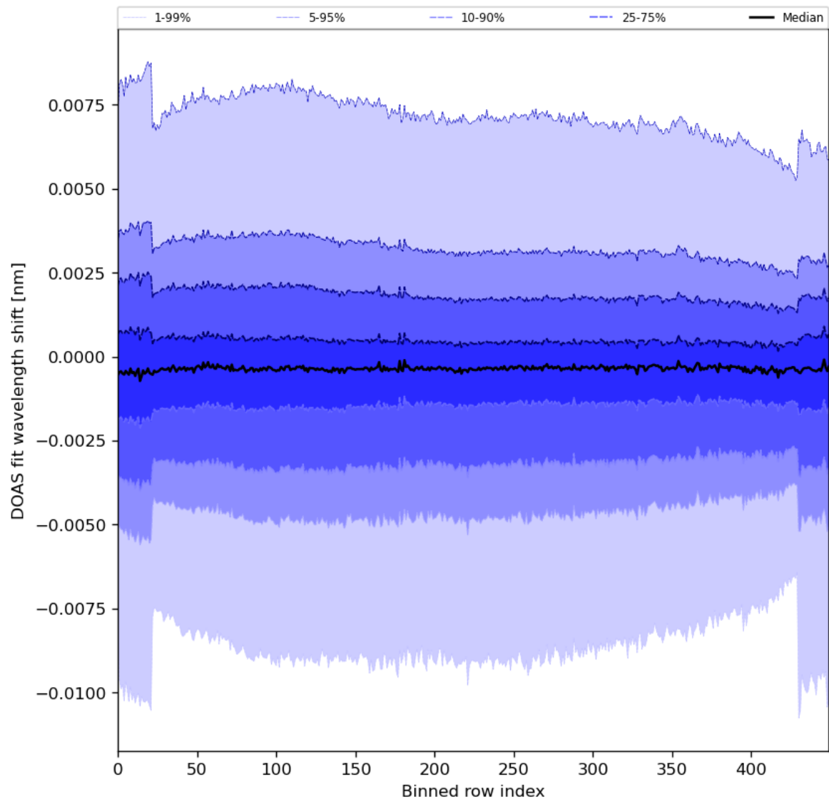
Figure 91: Along track statistics of “DOAS fit wavelength shift” for 2024-05-07 to 2024-05-09
