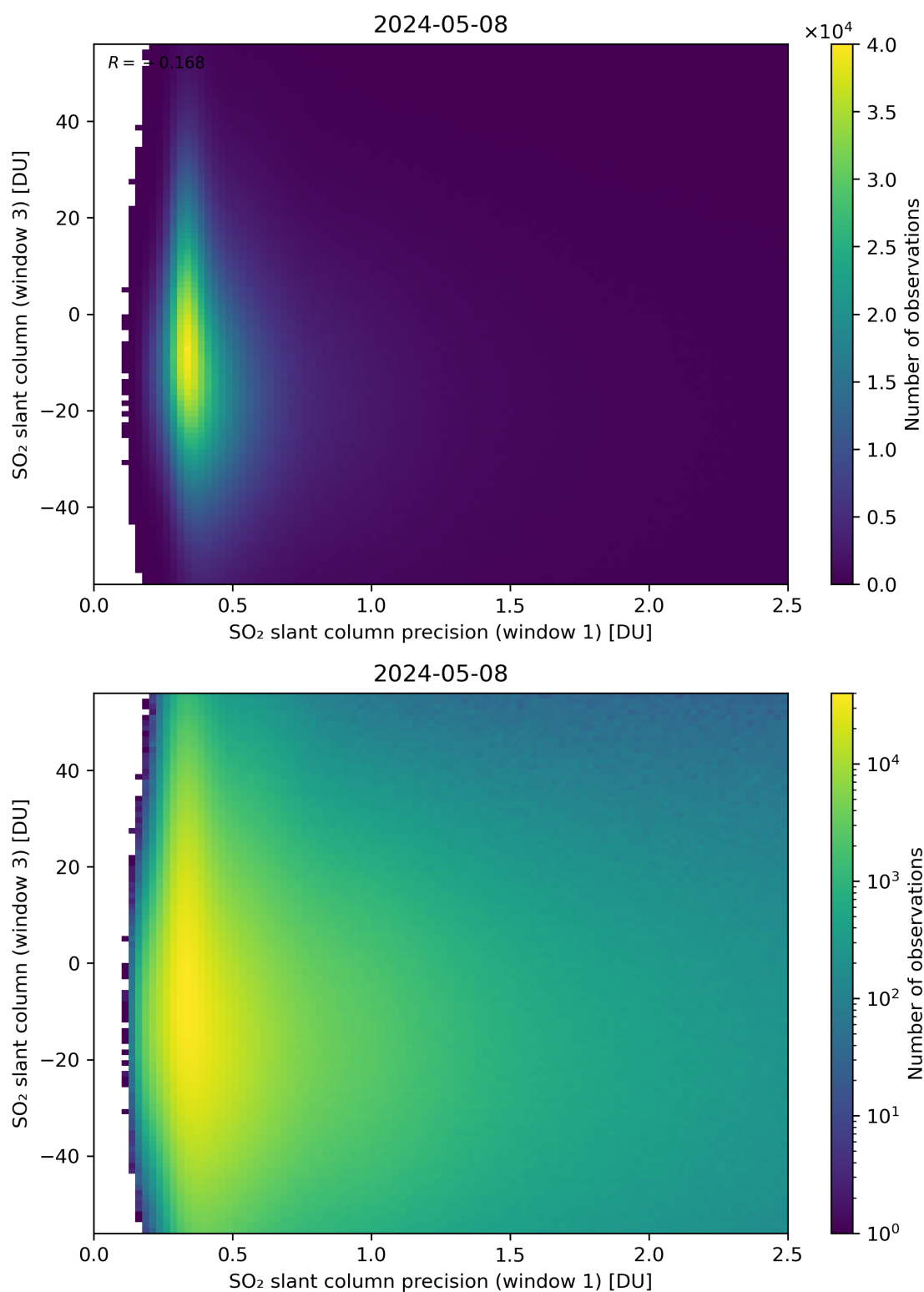
Figure 228: Scatter density plot of “SO 2 slant column precision (window 1)” against “SO 2 slant column (window 3)” for 2024-05-07 to 2024-05-09.
