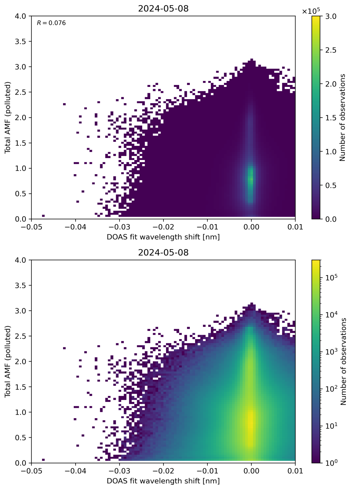
Figure 130: Scatter density plot of “DOAS fit wavelength shift” against “Total AMF (polluted)” for 2024-05-07 to 2024-05-09.
