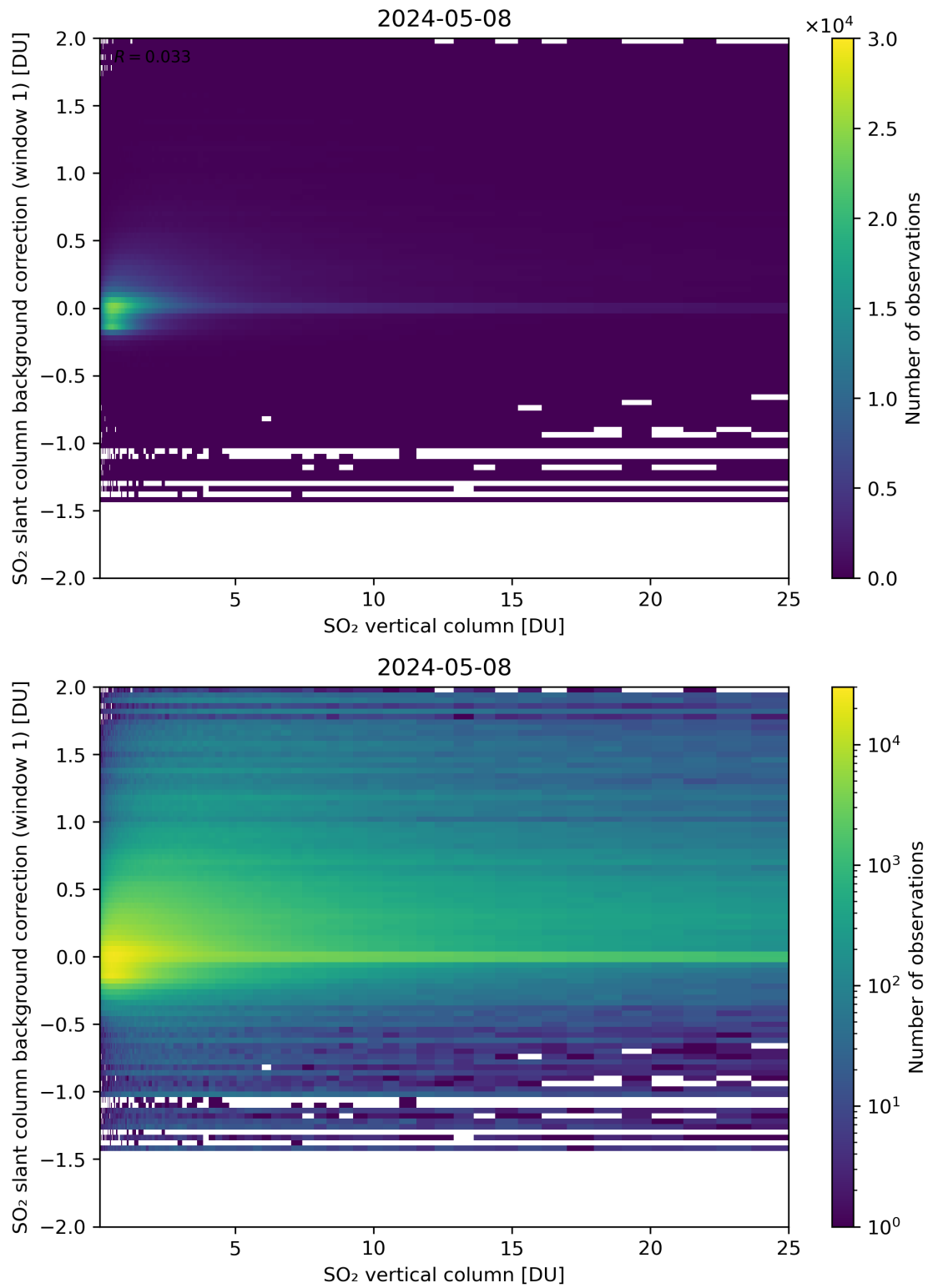
Figure 273: Scatter density plot of “SO 2 vertical column” against “SO 2 slant column background correction (window 1)” for 2024-05-07 to 2024-05-09.
