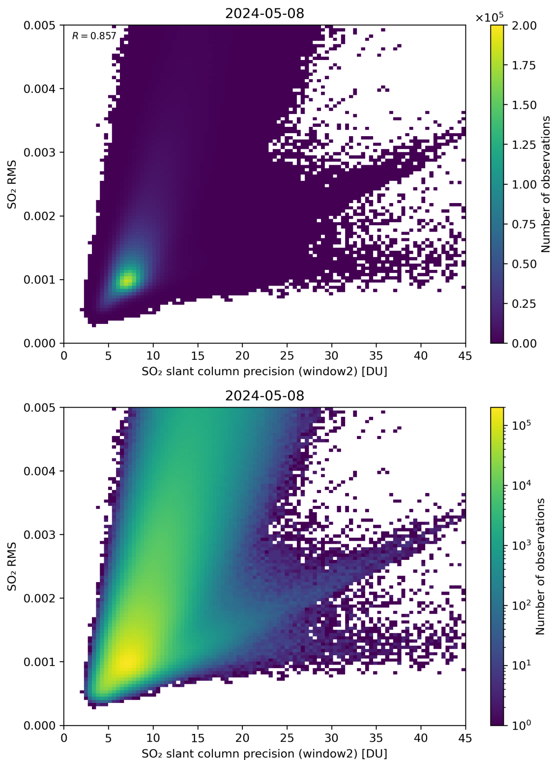
Figure 245: Scatter density plot of “SO 2 slant column precision (window2)” against “SO 2 RMS” for 2024-05-07 to 2024-05-09.
