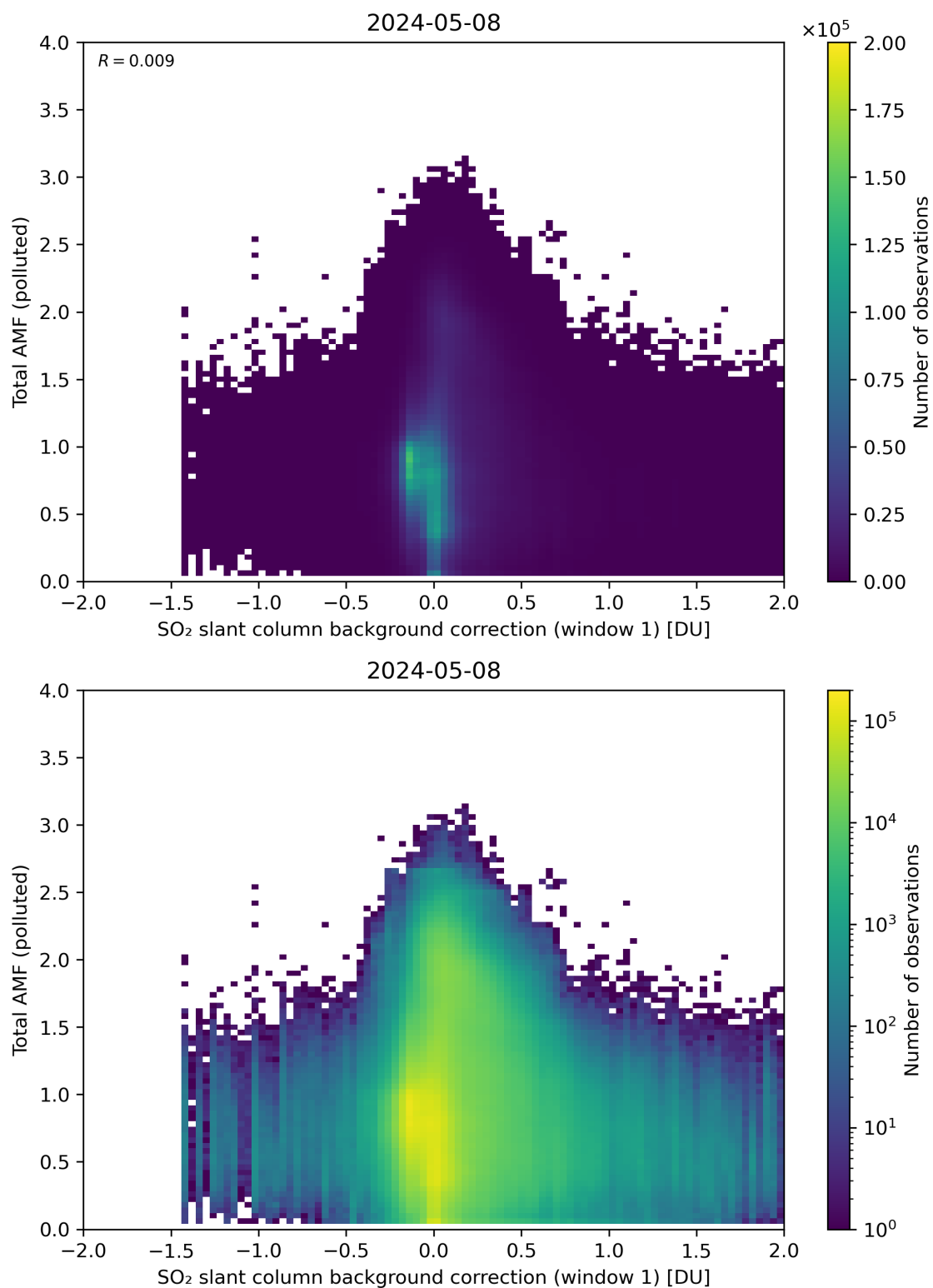
Figure 109: Scatter density plot of “SO 2 slant column background correction (window 1)” against “Total AMF (polluted)” for 2024-05-07 to 2024-05-09.
