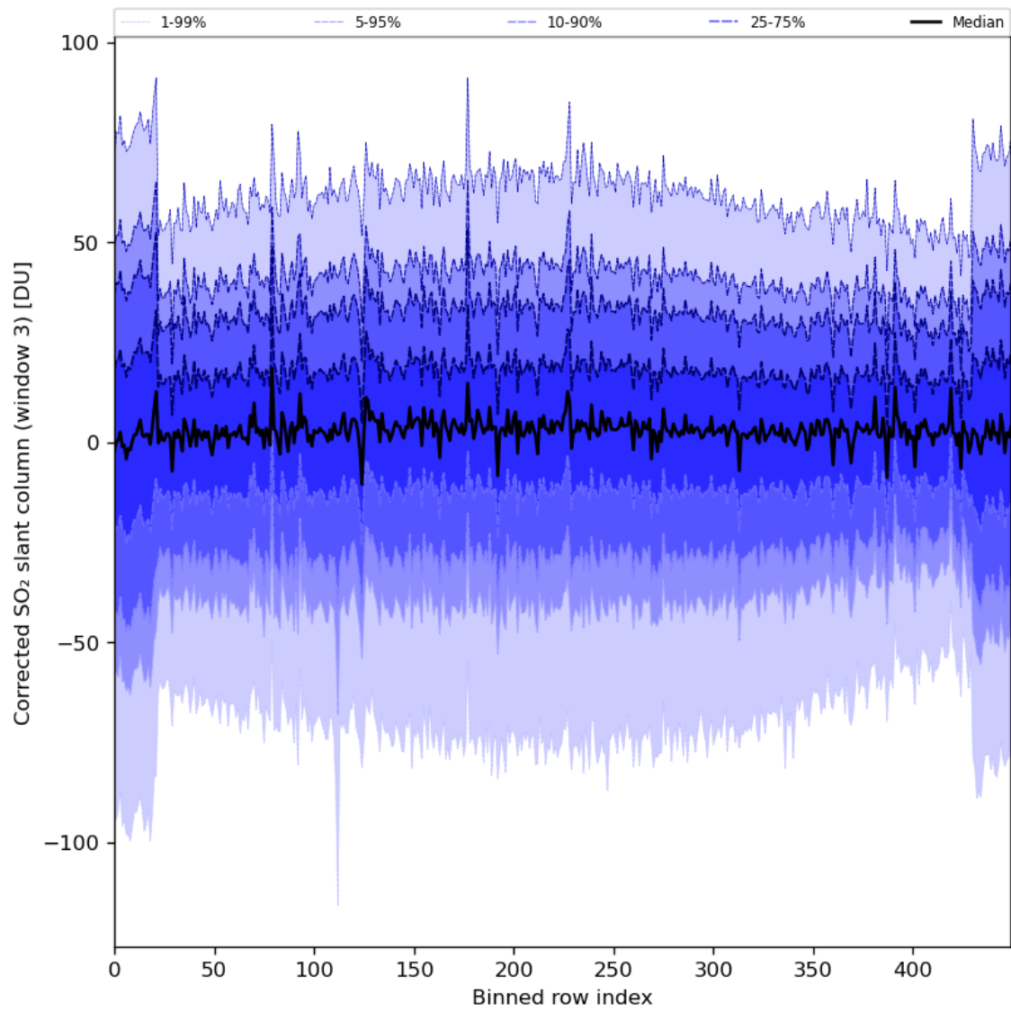
Figure 89: Along track statistics of “Corrected SO 2 slant column (window 3)” for 2024-05-07 to 2024-05-09
