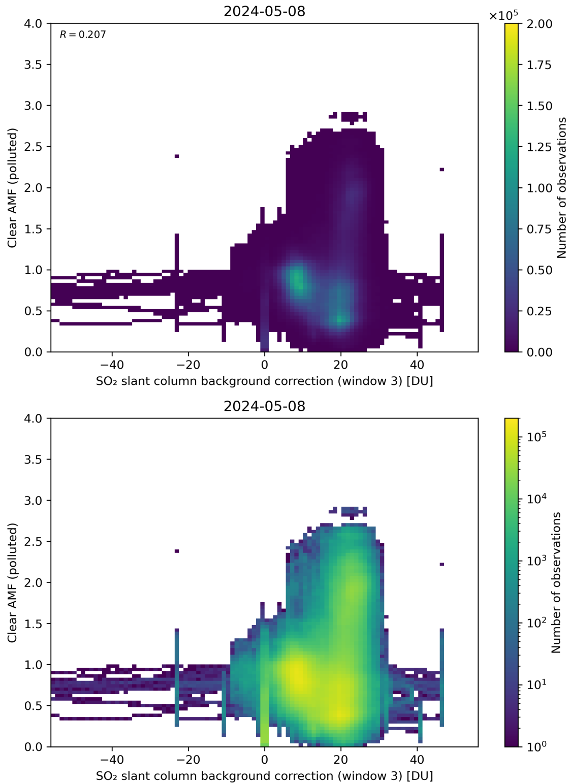
Figure 124: Scatter density plot of “SO 2 slant column background correction (window 3)” against “Clear AMF (polluted)” for 2024-05-07 to 2024-05-09.
