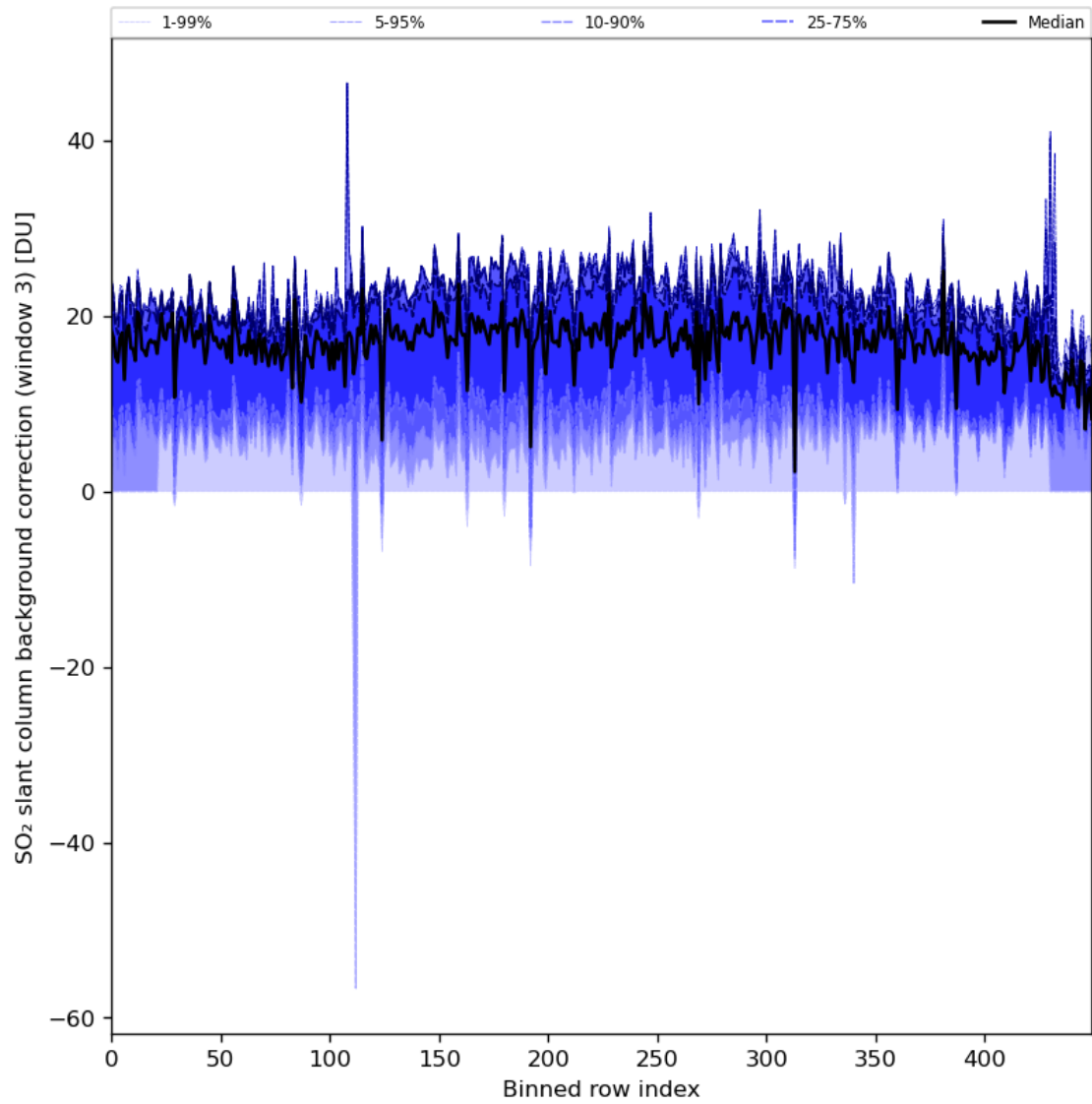
Figure 90: Along track statistics of “SO 2 slant column background correction (window 3)” for 2024-05-07 to 2024-05-09
