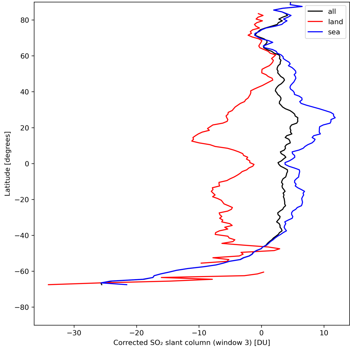
Figure 43: Zonal average of “Corrected SO 2 slant column (window 3)” for 2024-05-07 to 2024-05-09.
