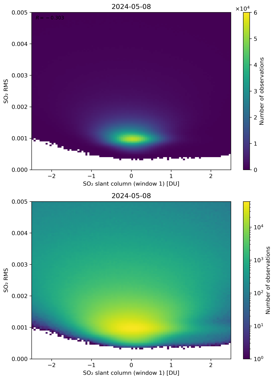
Figure 217: Scatter density plot of “SO 2 slant column (window 1)” against “SO 2 RMS” for 2024-05-07 to 2024-05-09.
