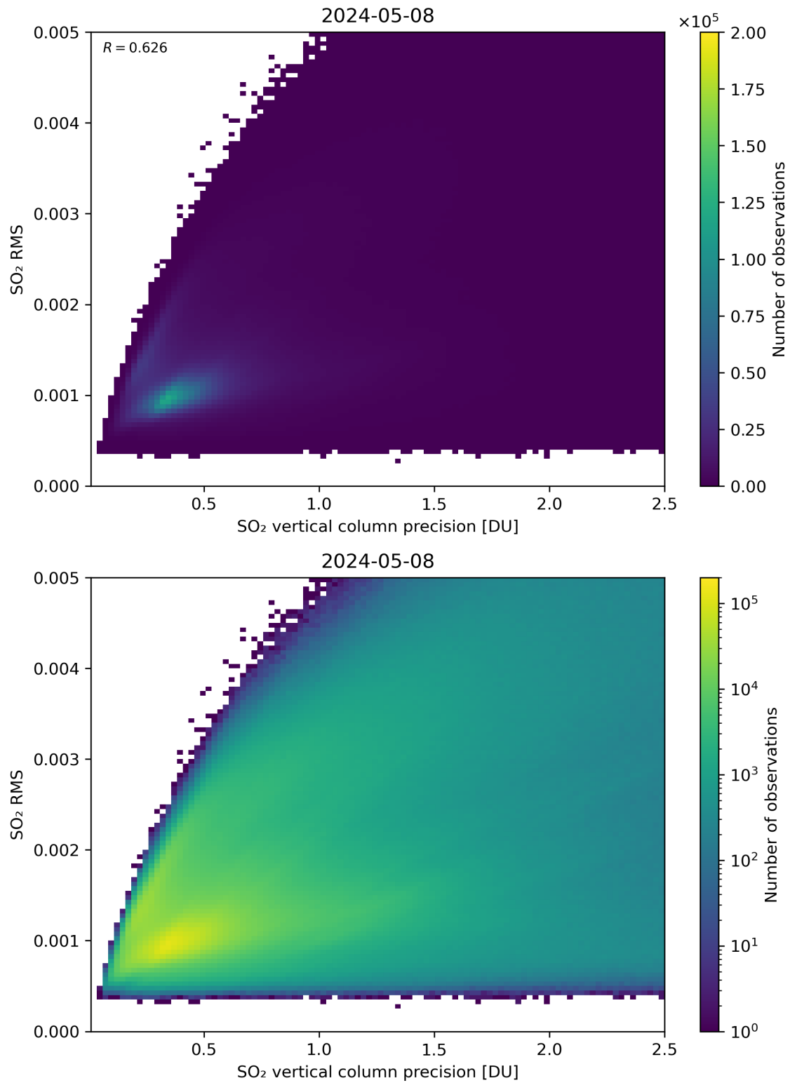
Figure 284: Scatter density plot of “SO 2 vertical column precision” against “SO 2 RMS” for 2024-05-07 to 2024-05-09.
