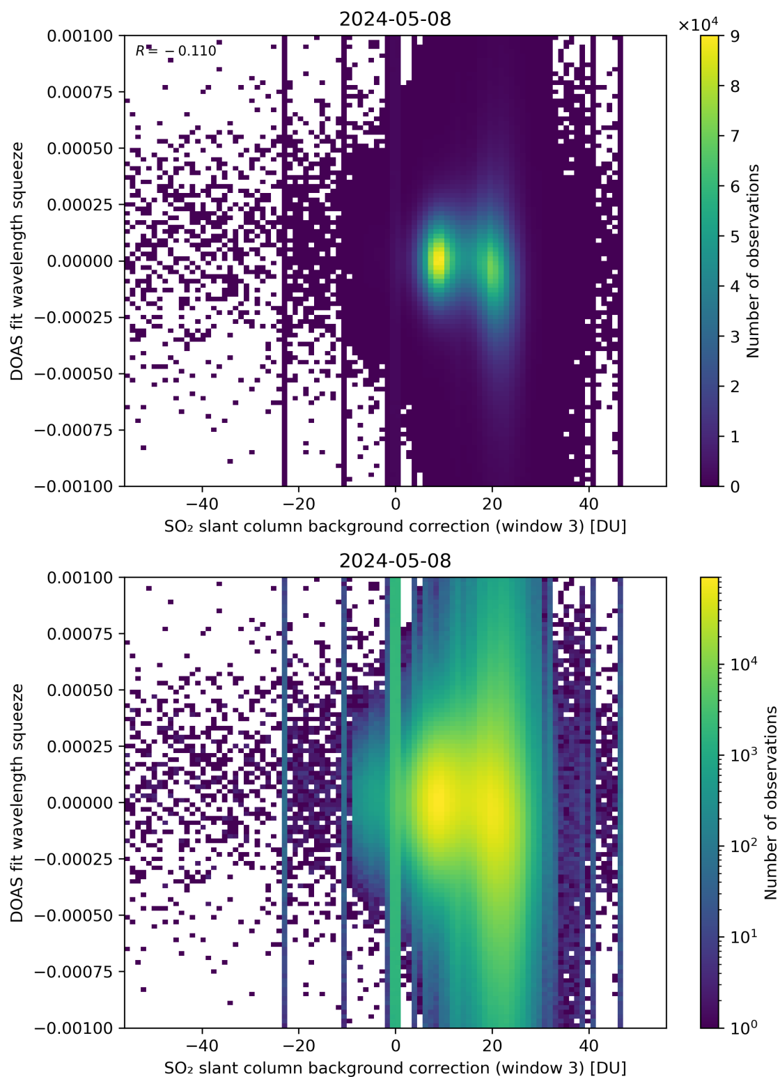
Figure 122: Scatter density plot of “SO 2 slant column background correction (window 3)” against “DOAS fit wavelength squeeze” for 2024-05-07 to 2024-05-09.
