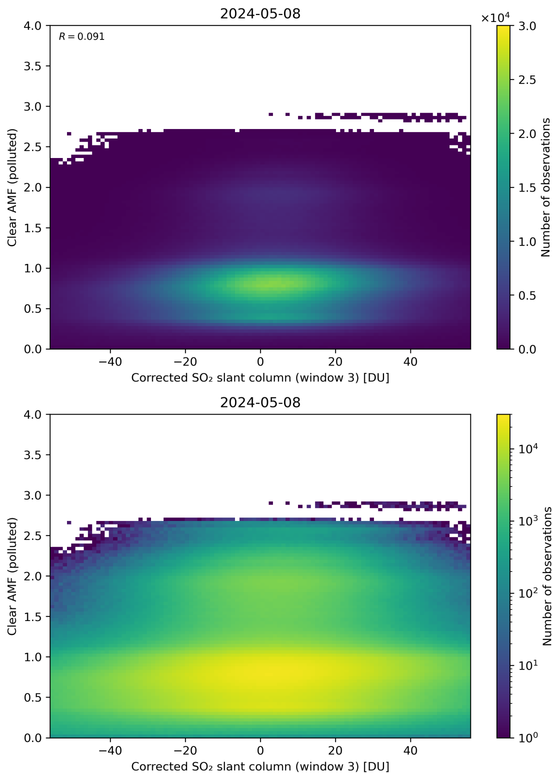
Figure 209: Scatter density plot of “Corrected SO 2 slant column (window 3)” against “Clear AMF (polluted)” for 2024-05-07 to 2024-05-09.
