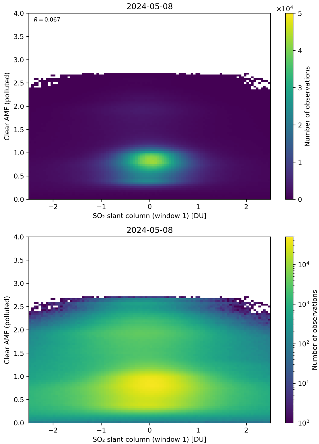
Figure 232: Scatter density plot of “SO 2 slant column (window 1)” against “Clear AMF (polluted)” for 2024-05-07 to 2024-05-09.
