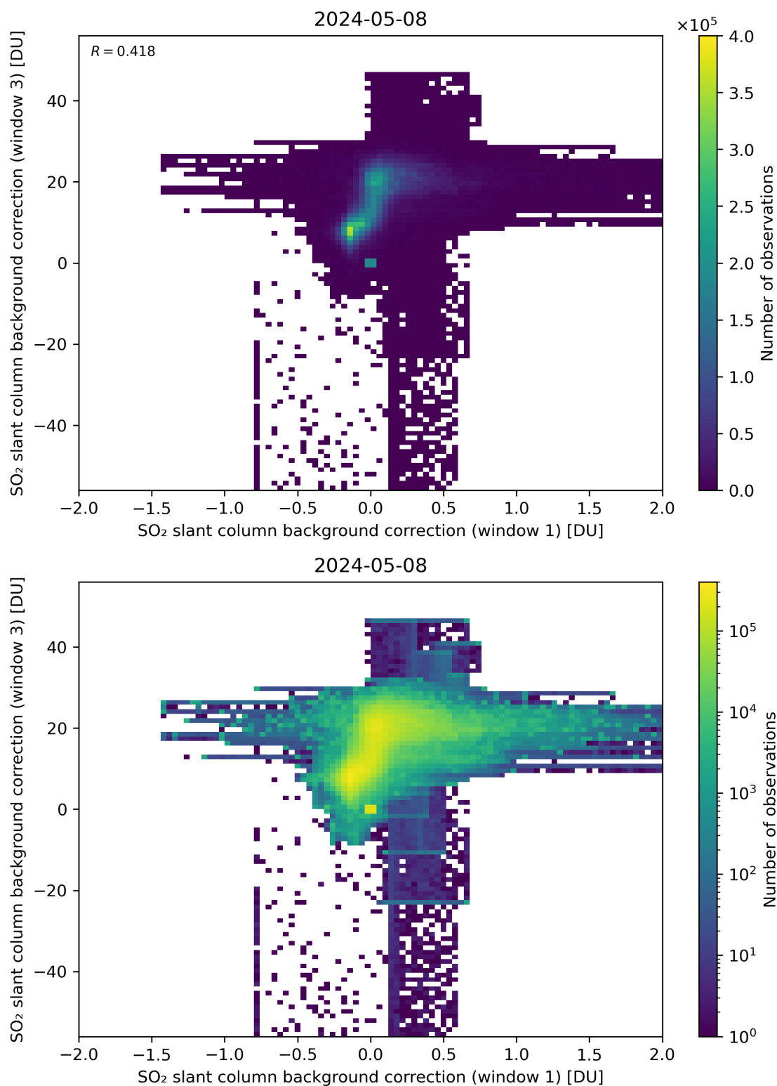
Figure 99: Scatter density plot of “SO 2 slant column background correction (window 1)” against “SO 2 slant column background correction (window 3)” for 2024-05-07 to 2024-05-09.
