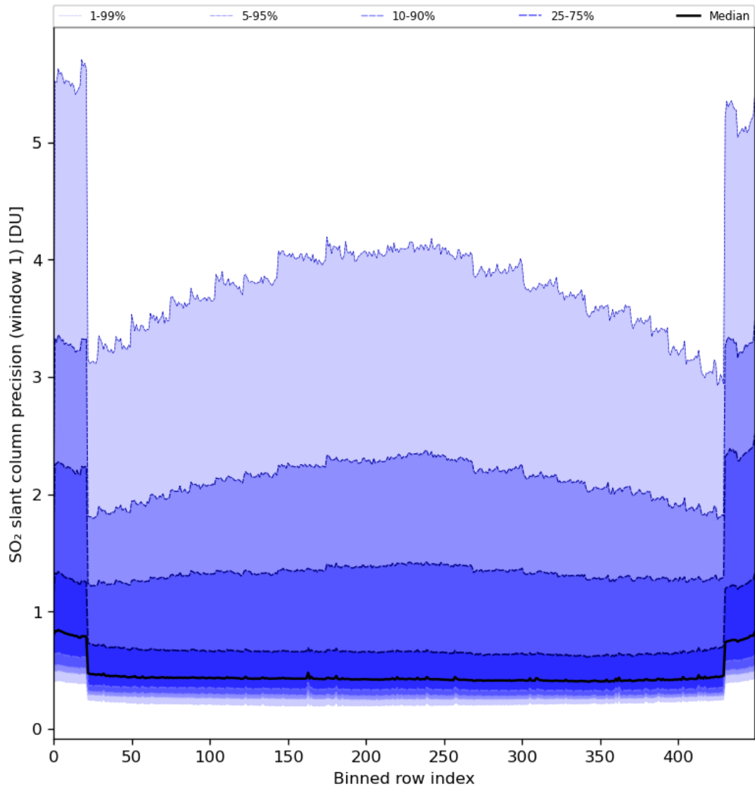
Figure 80: Along track statistics of “SO 2 slant column precision (window 1)” for 2024-05-07 to 2024-05-09
