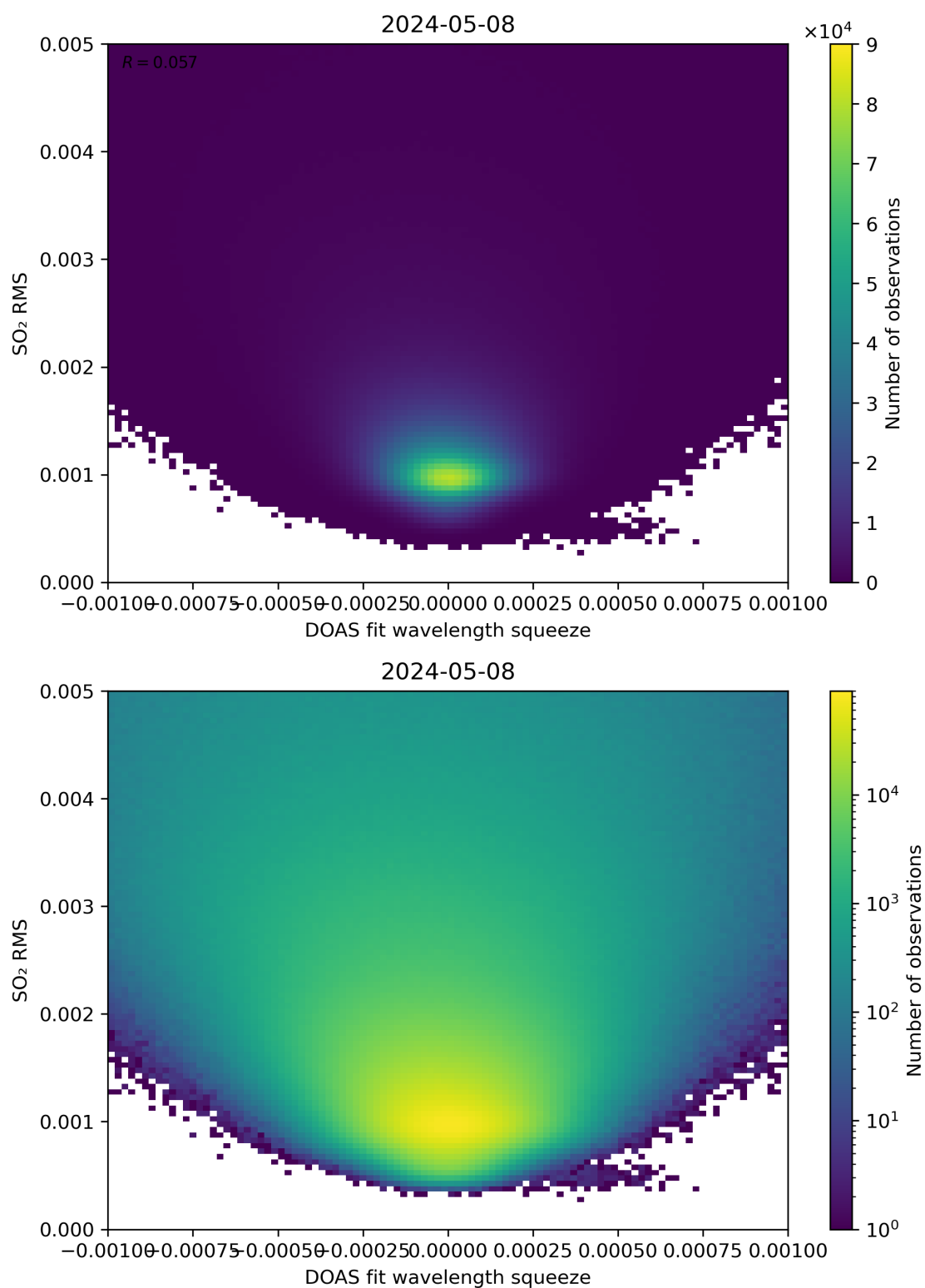
Figure 132: Scatter density plot of “DOAS fit wavelength squeeze” against “SO 2 RMS” for 2024-05-07 to 2024-05-09.
