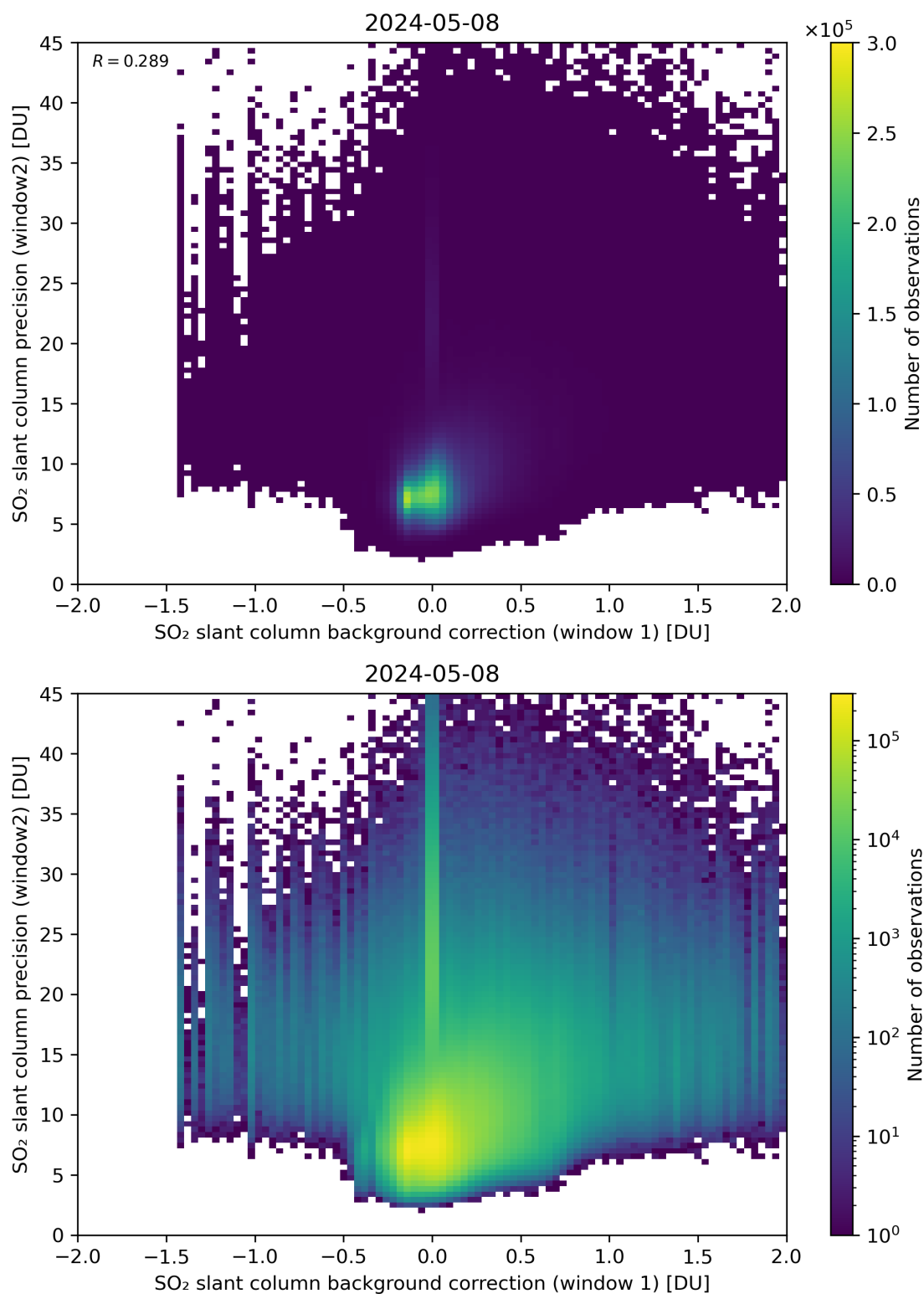
Figure 106: Scatter density plot of “SO 2 slant column background correction (window 1)” against “SO 2 slant column precision (window2)” for 2024-05-07 to 2024-05-09.
