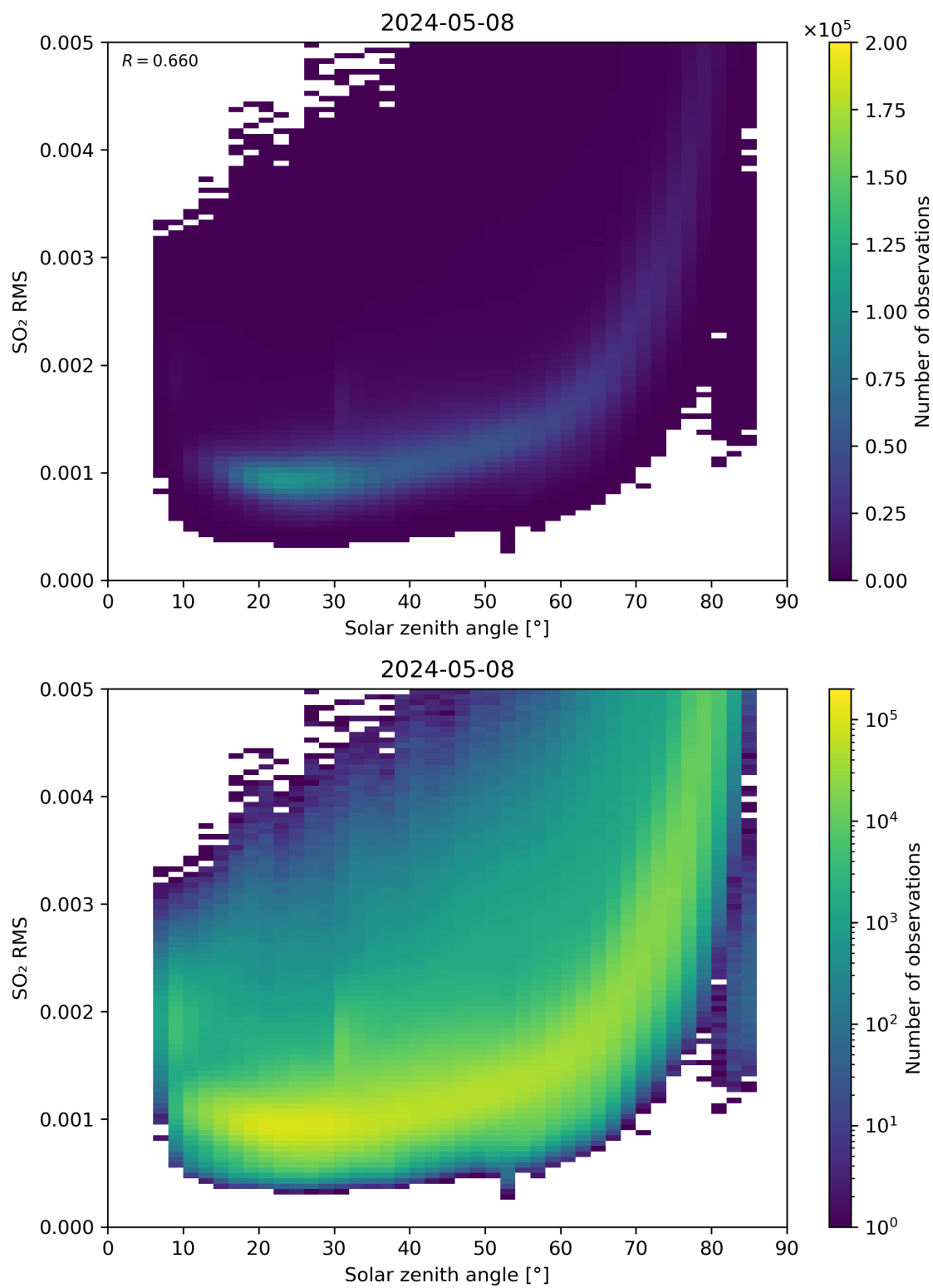
Figure 163: Scatter density plot of “Solar zenith angle” against “SO 2 RMS” for 2024-05-07 to 2024-05-09.
