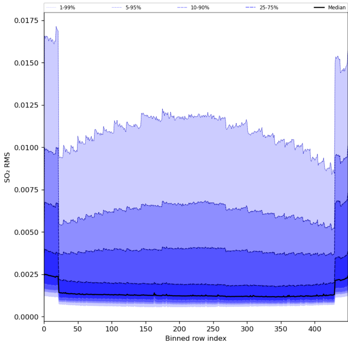
Figure 93: Along track statistics of “SO 2 RMS” for 2024-05-07 to 2024-05-09
