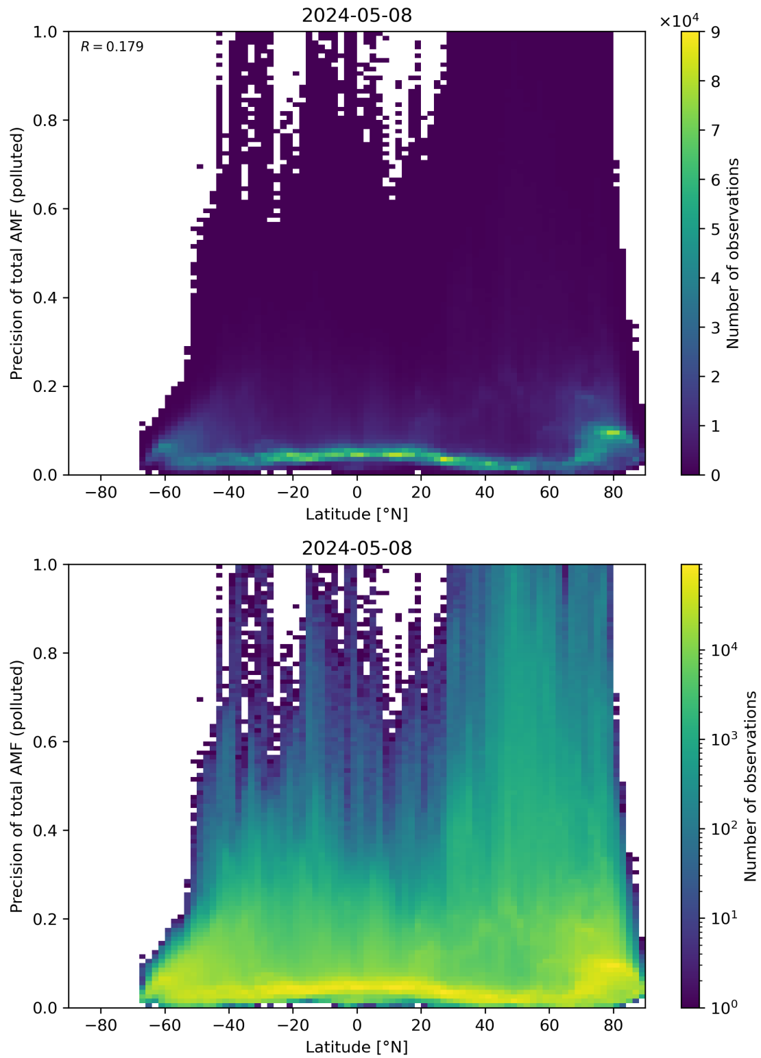
Figure 155: Scatter density plot of “Latitude” against “Precision of total AMF (polluted)” for 2024-05-07 to 2024-05-09.
