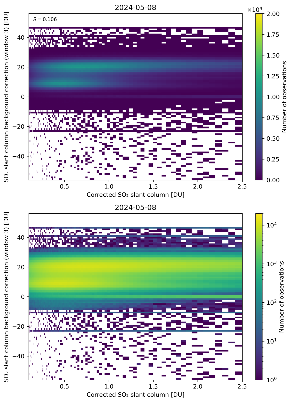
Figure 180: Scatter density plot of “Corrected SO 2 slant column” against “SO 2 slant column background correction (window 3)” for 2024-05-07 to 2024-05-09.
