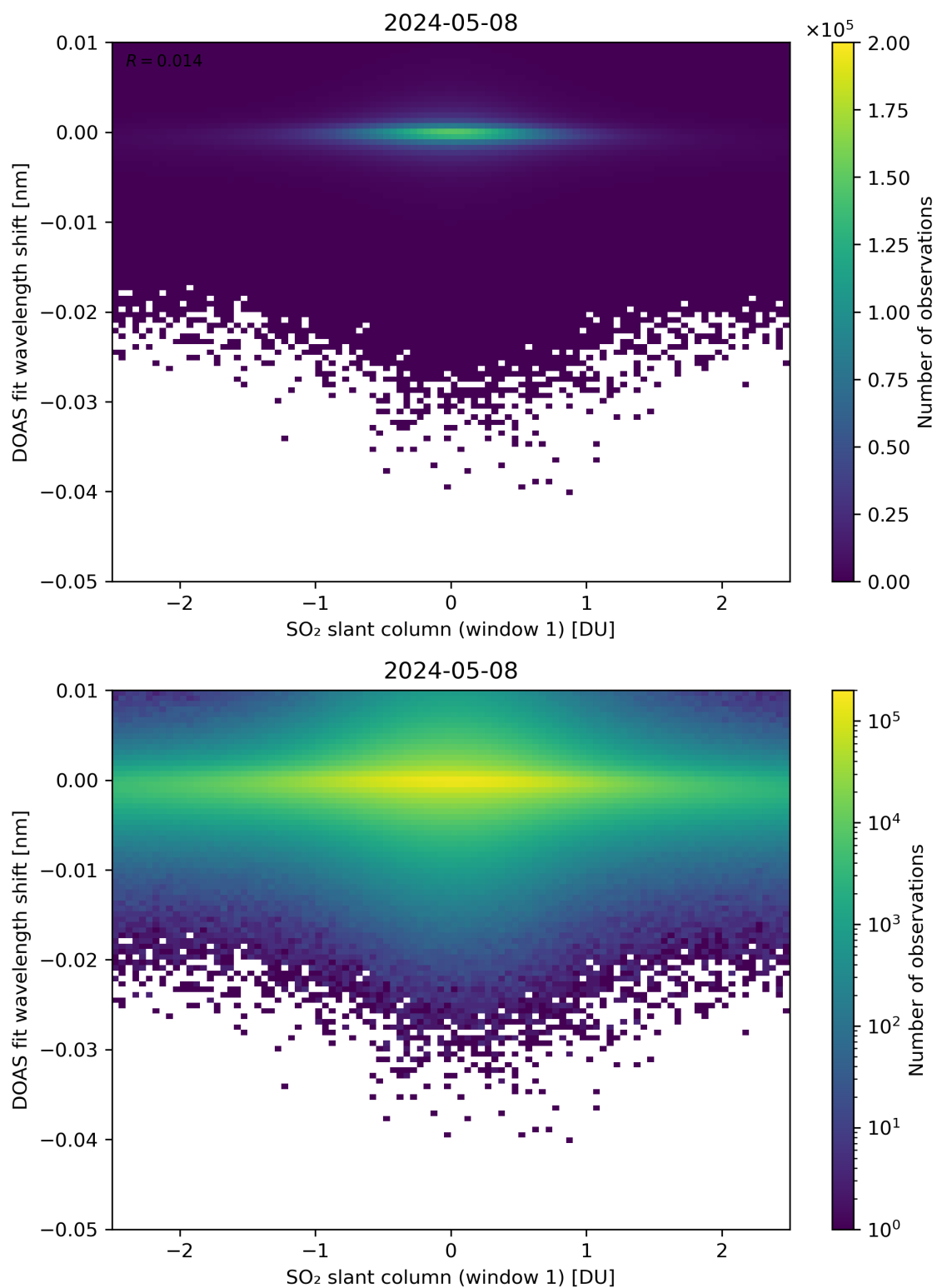
Figure 215: Scatter density plot of “SO 2 slant column (window 1)” against “DOAS fit wavelength shift” for 2024-05-07 to 2024-05-09.
