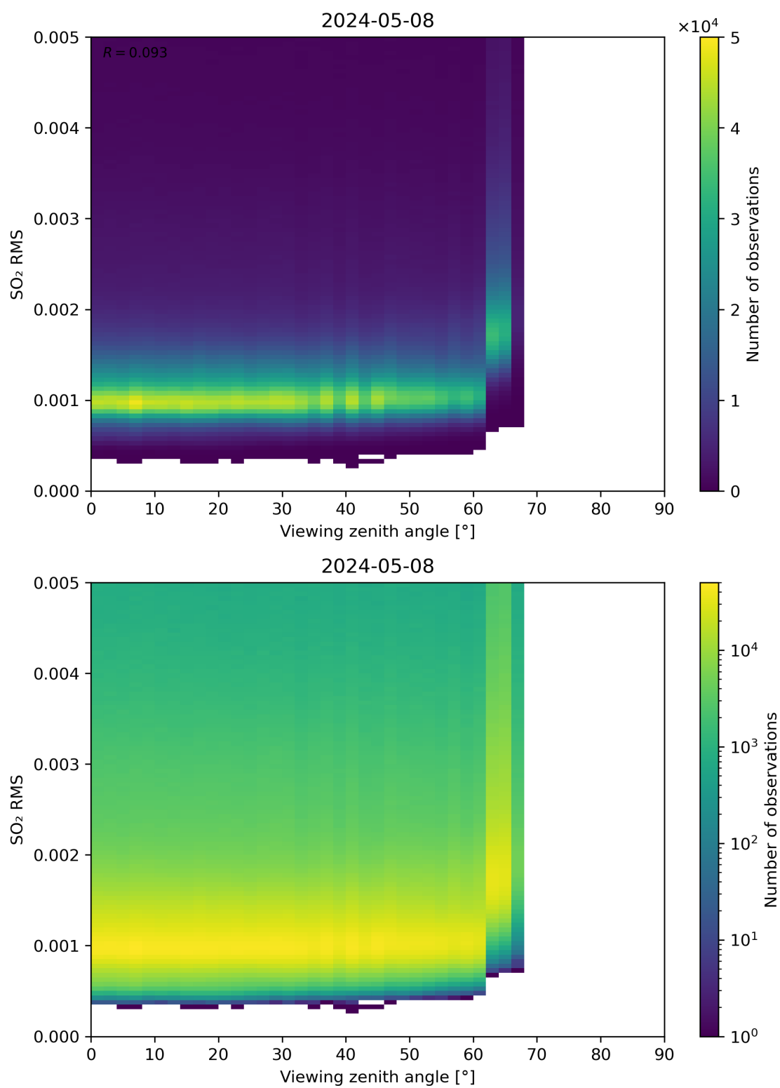
Figure 313: Scatter density plot of “Viewing zenith angle” against “SO 2 RMS” for 2024-05-07 to 2024-05-09.
