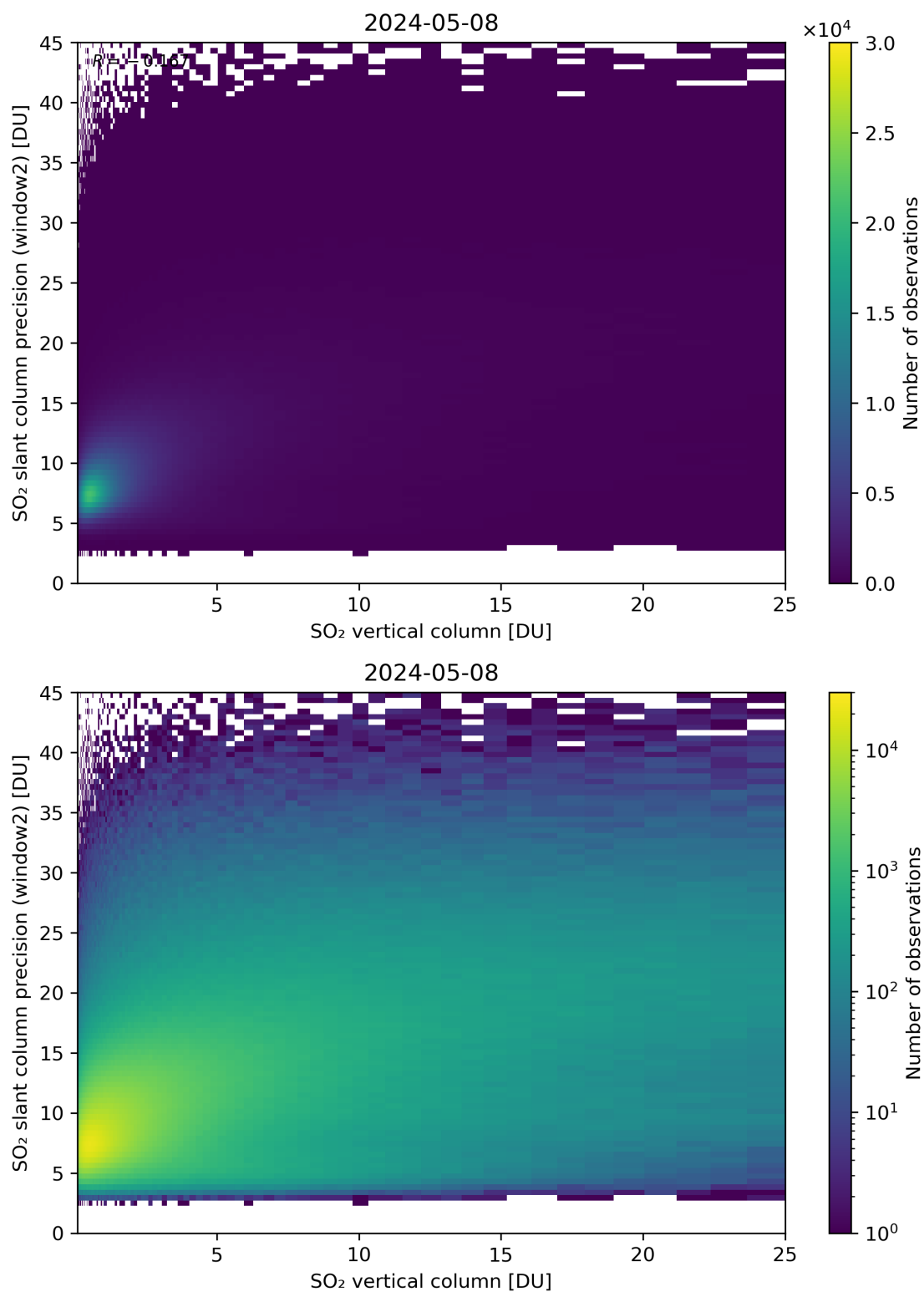
Figure 302: Scatter density plot of “SO 2 vertical column” against “SO 2 slant column precision (window2)” for 2024-05-07 to 2024-05-09.
