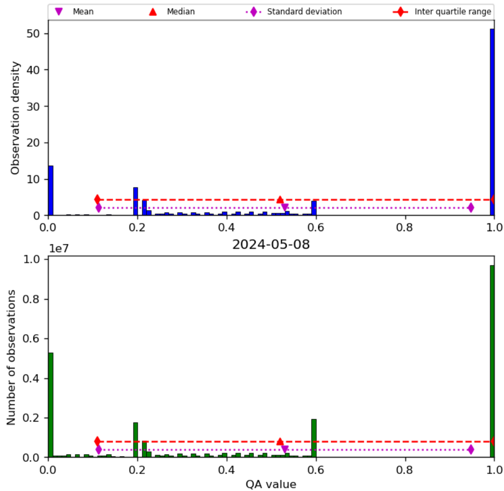
Figure 52: Histogram of “QA value” for 2024-05-07 to 2024-05-09
