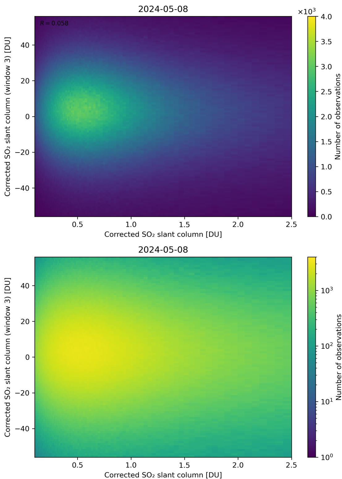
Figure 186: Scatter density plot of “Corrected SO 2 slant column” against “Corrected SO 2 slant column (window 3)” for 2024-05-07 to 2024-05-09.
