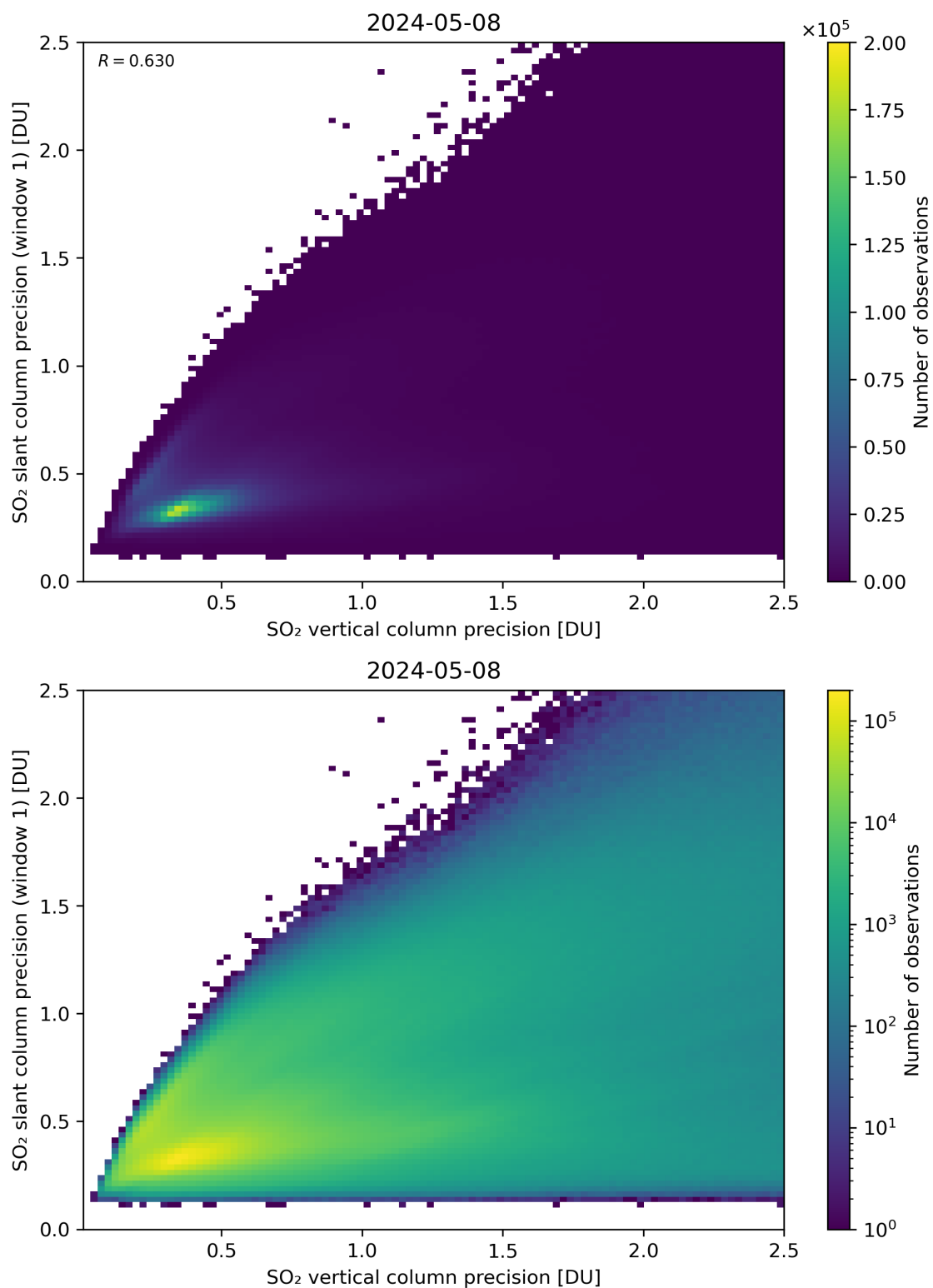
Figure 290: Scatter density plot of “SO 2 vertical column precision” against “SO 2 slant column precision (window 1)” for 2024-05-07 to 2024-05-09.
