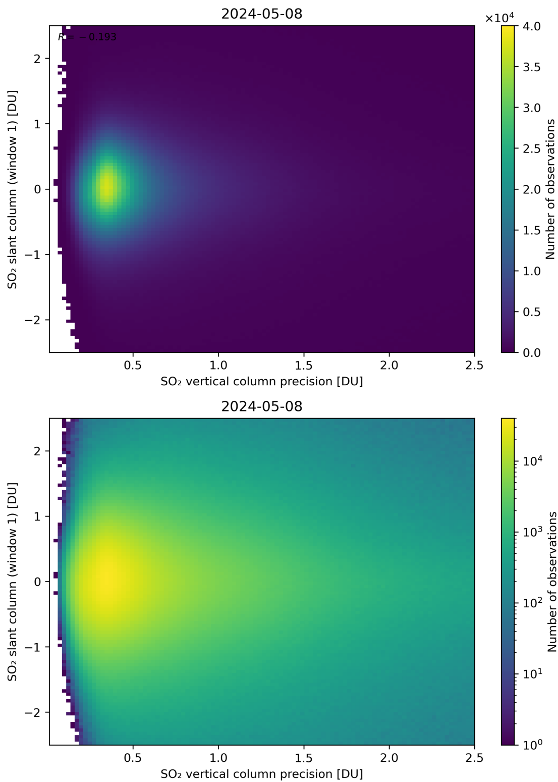
Figure 289: Scatter density plot of “SO 2 vertical column precision” against “SO 2 slant column (window 1)” for 2024-05-07 to 2024-05-09.
