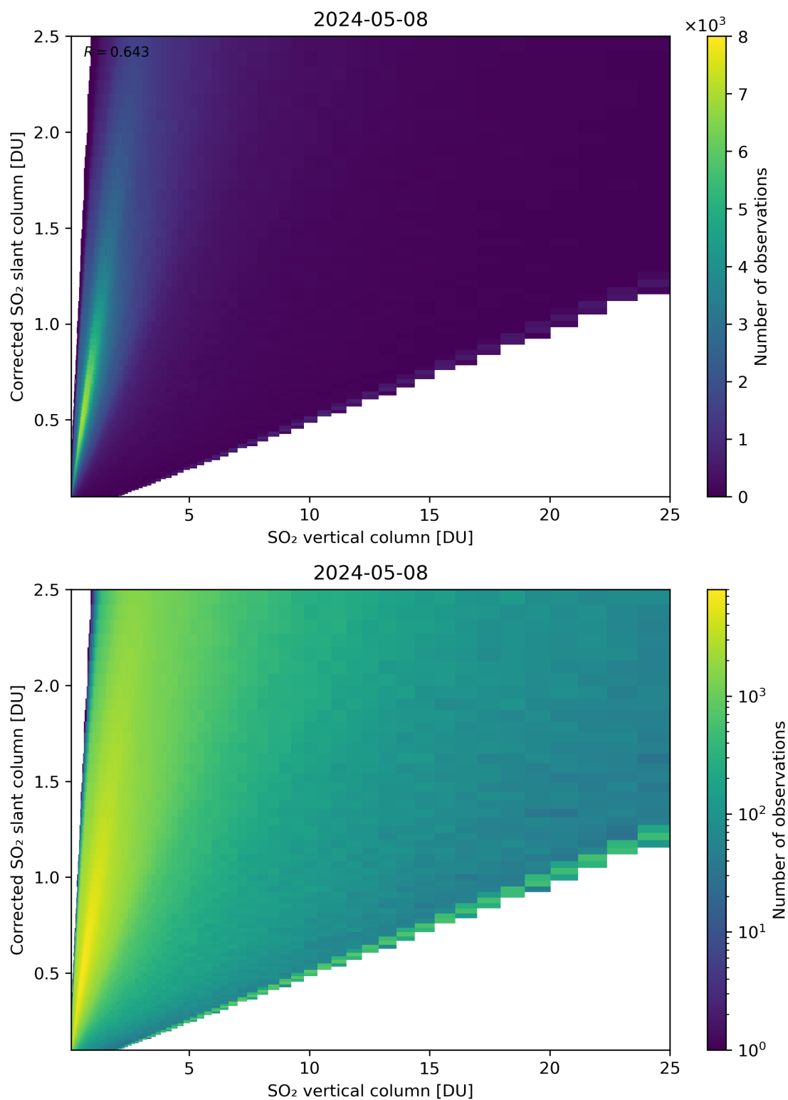
Figure 297: Scatter density plot of “SO 2 vertical column” against “Corrected SO 2 slant column” for 2024-05-07 to 2024-05-09.
