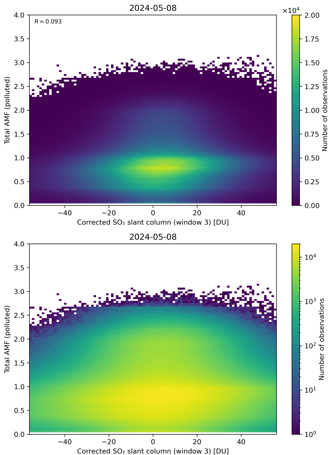
Figure 210: Scatter density plot of “Corrected SO 2 slant column (window 3)” against “Total AMF (polluted)” for 2024-05-07 to 2024-05-09.
