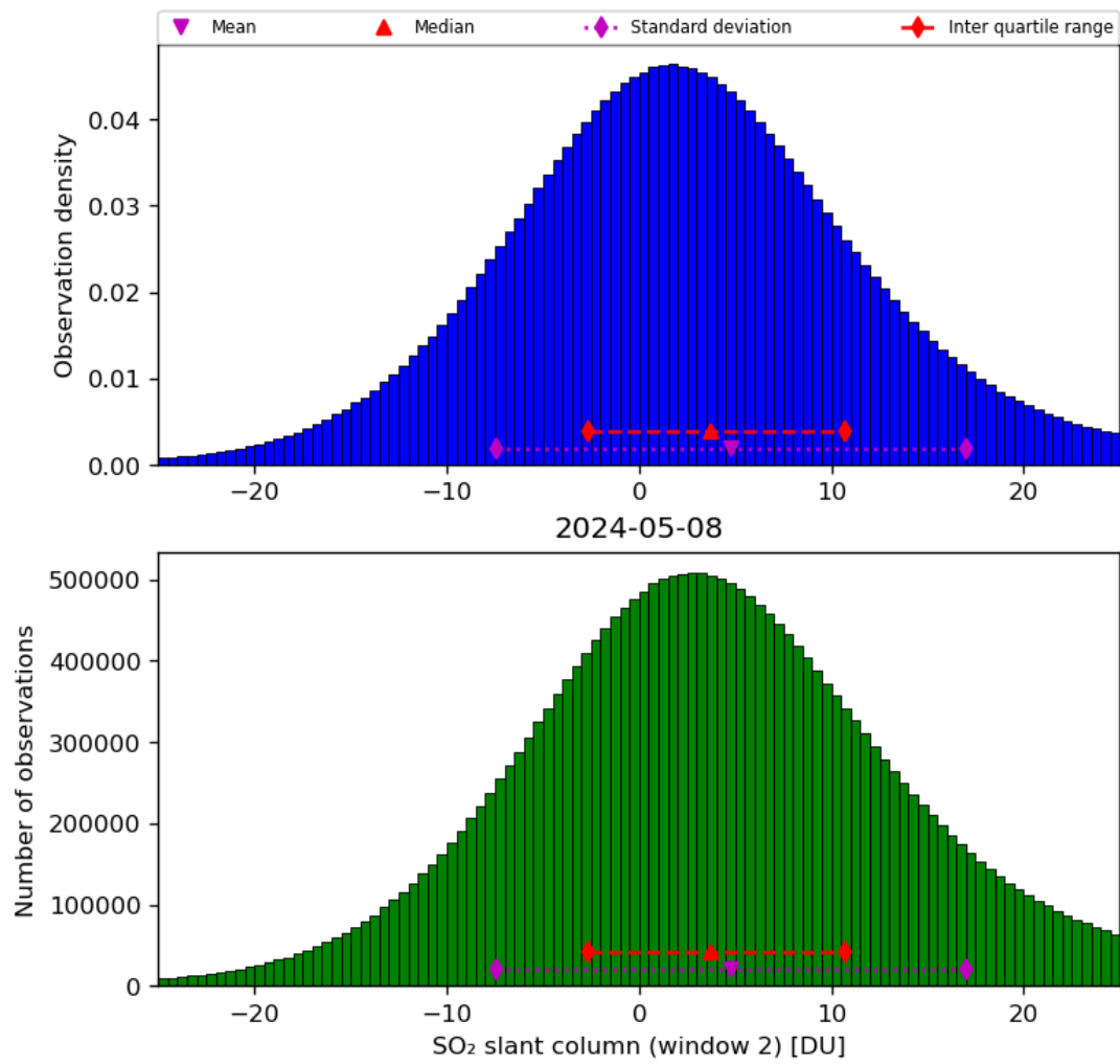
Figure 60: Histogram of “SO 2 slant column (window 2)” for 2024-05-07 to 2024-05-09
