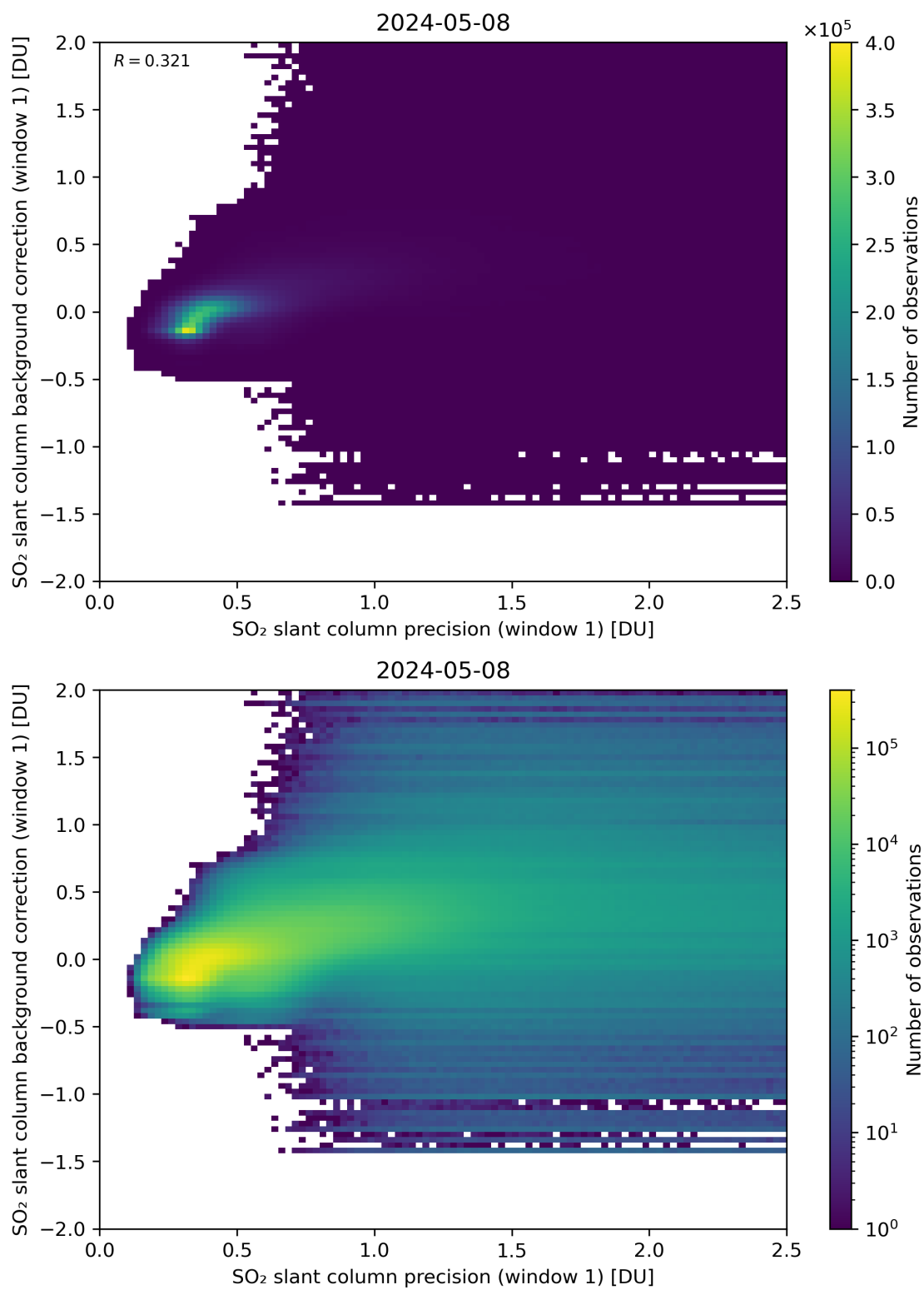
Figure 218: Scatter density plot of “SO 2 slant column precision (window 1)” against “SO 2 slant column background correction (window 1)” for 2024-05-07 to 2024-05-09.
