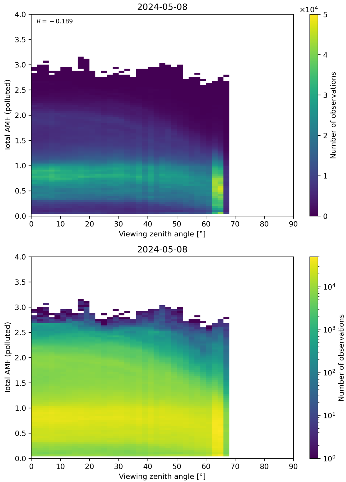
Figure 325: Scatter density plot of “Viewing zenith angle” against “Total AMF (polluted)” for 2024-05-07 to 2024-05-09.
