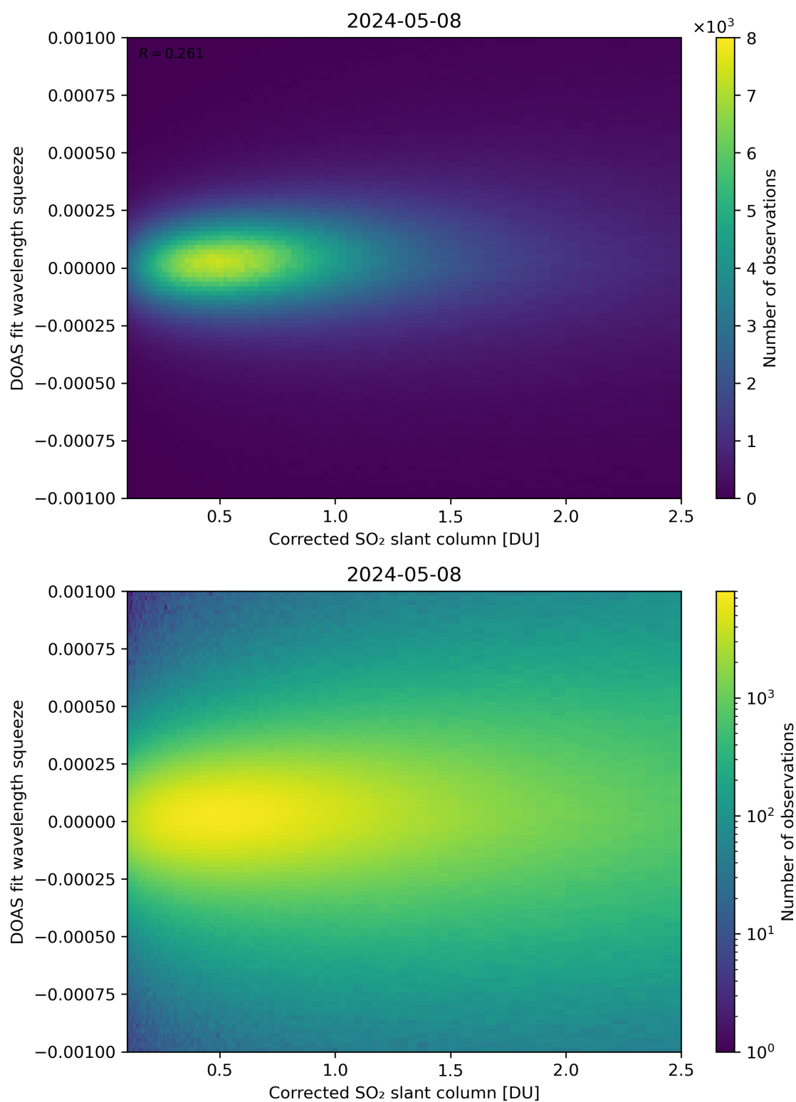
Figure 182: Scatter density plot of “Corrected SO 2 slant column” against “DOAS fit wavelength squeeze” for 2024-05-07 to 2024-05-09.
