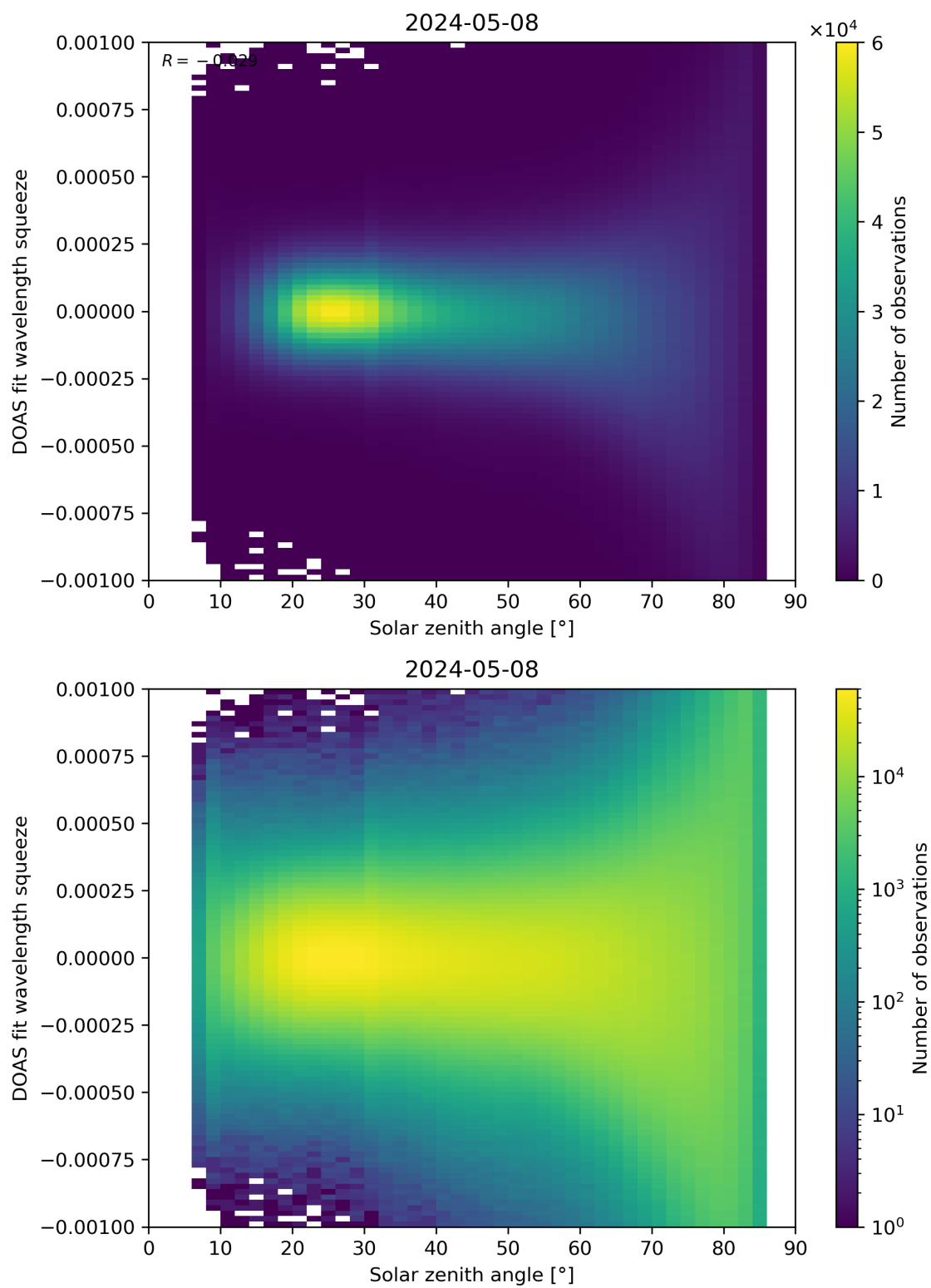
Figure 162: Scatter density plot of “Solar zenith angle” against “DOAS fit wavelength squeeze” for 2024-05-07 to 2024-05-09.
