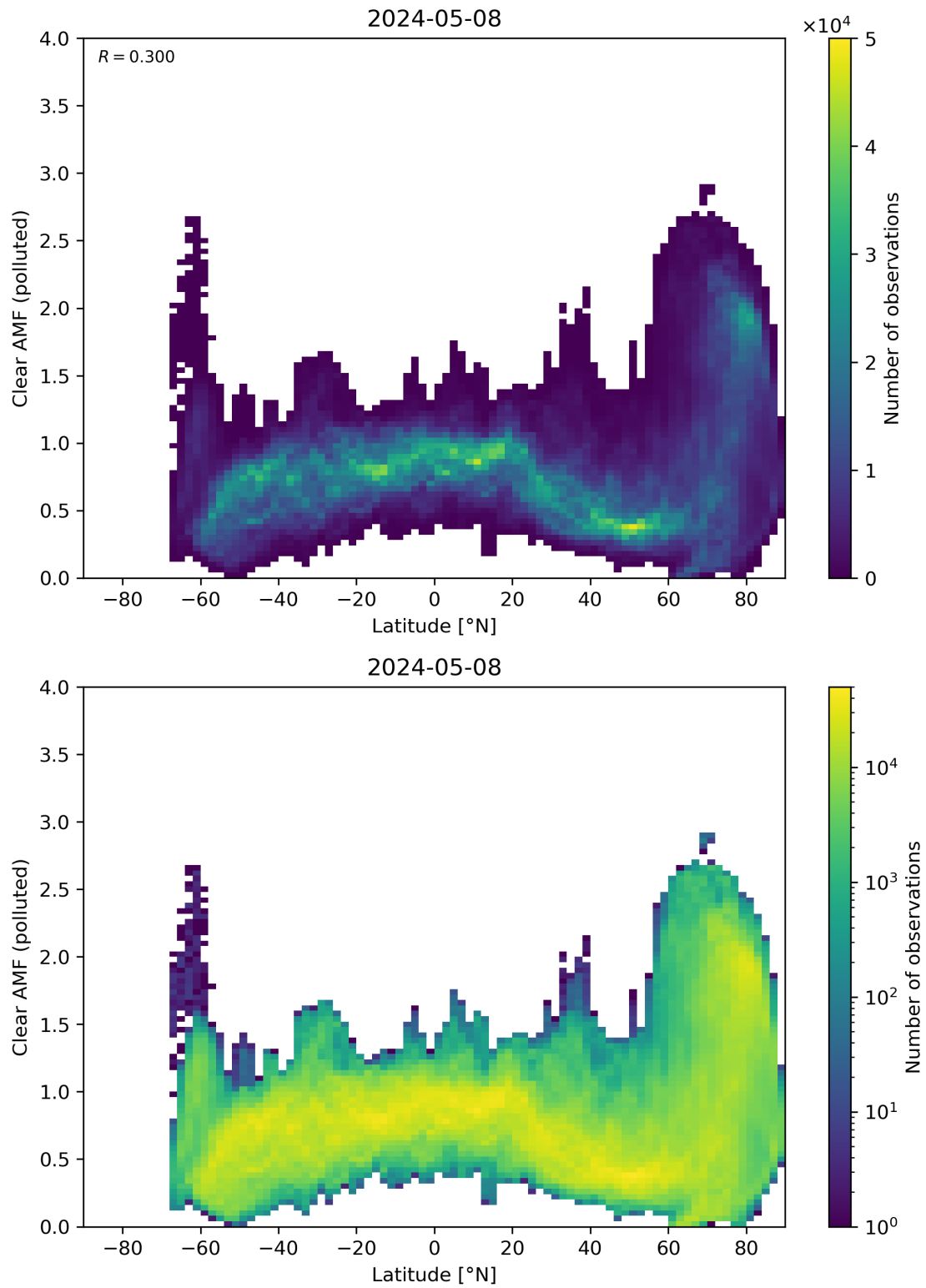
Figure 145: Scatter density plot of “Latitude” against “Clear AMF (polluted)” for 2024-05-07 to 2024-05-09.
