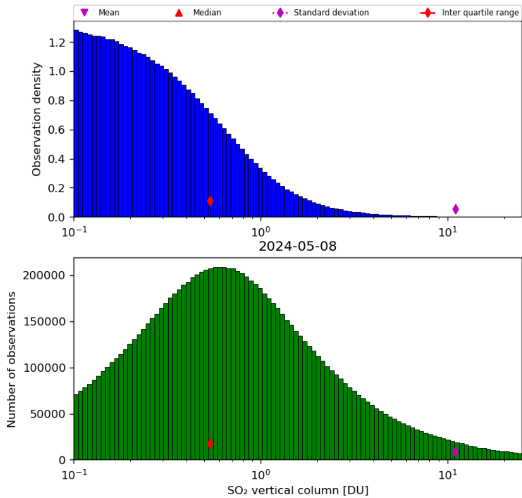
Figure 53: Histogram of “SO 2 vertical column” for 2024-05-07 to 2024-05-09
