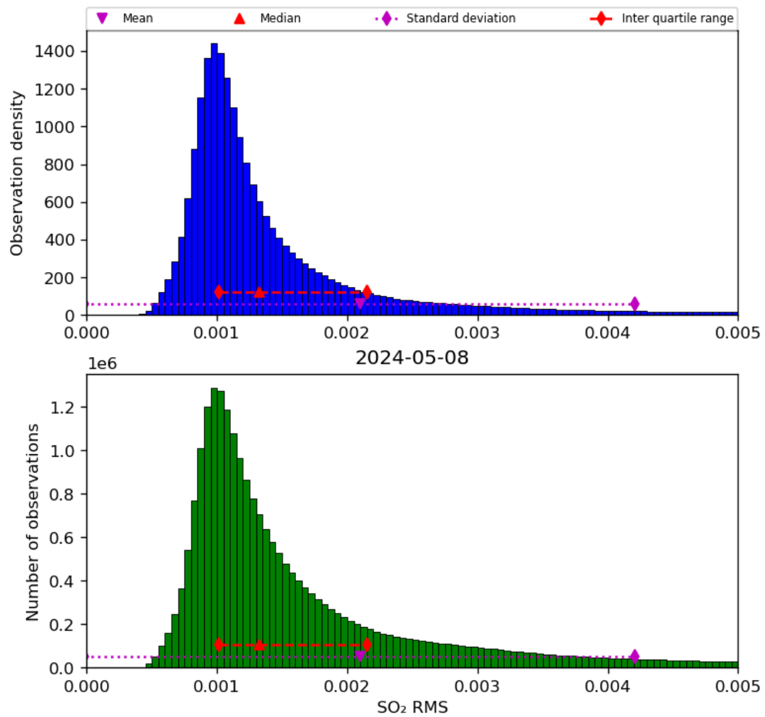
Figure 70: Histogram of “SO 2 RMS” for 2024-05-07 to 2024-05-09
