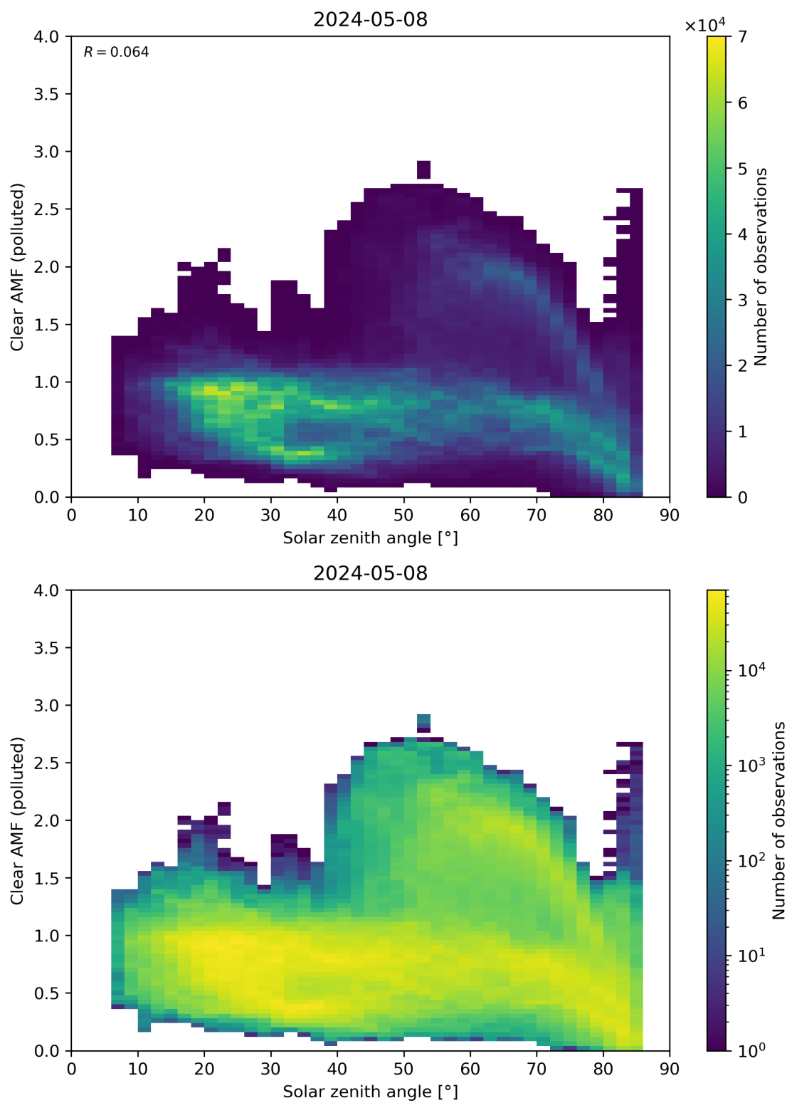
Figure 165: Scatter density plot of “Solar zenith angle” against “Clear AMF (polluted)” for 2024-05-07 to 2024-05-09.
