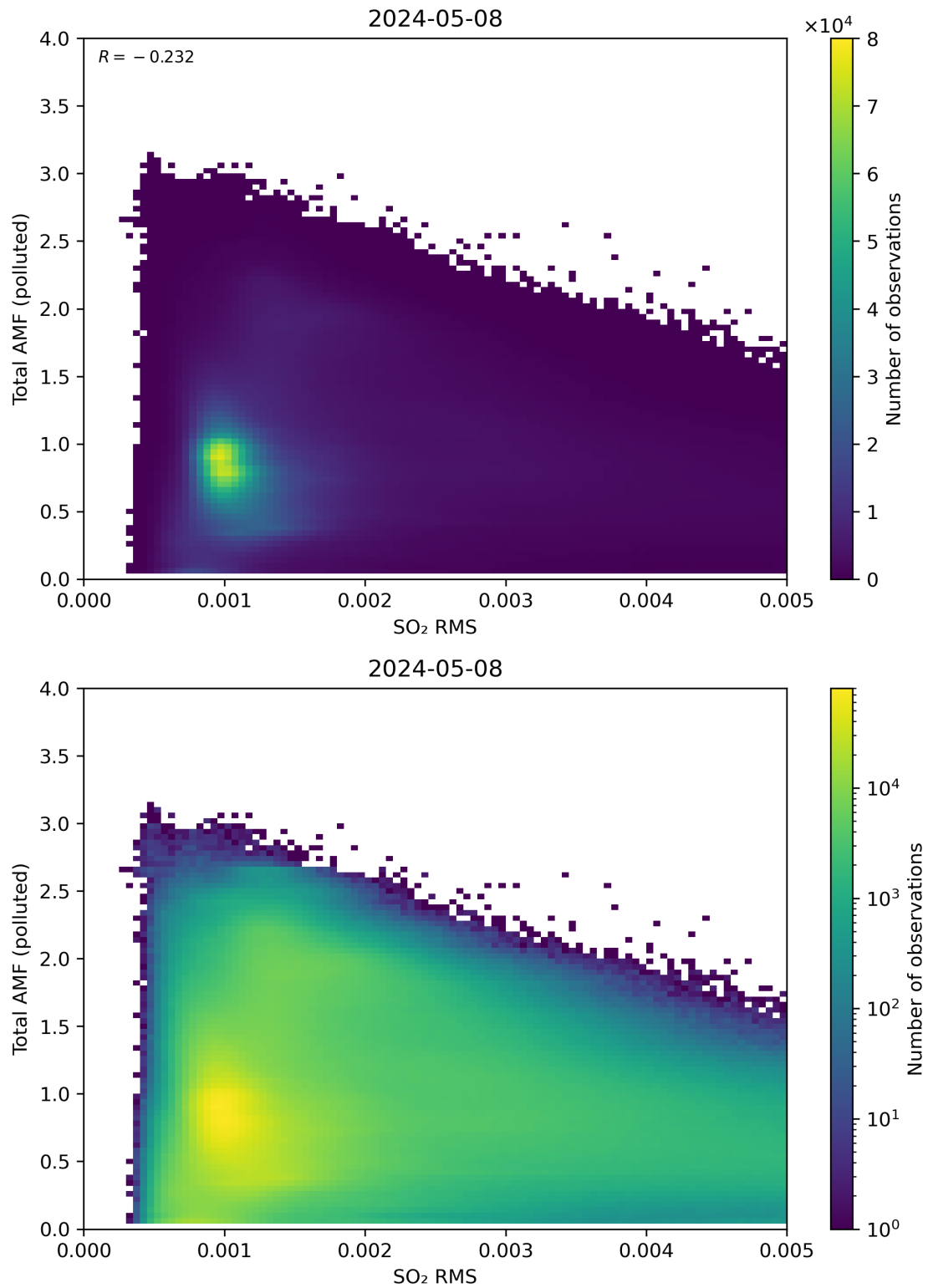
Figure 137: Scatter density plot of “SO 2 RMS” against “Total AMF (polluted)” for 2024-05-07 to 2024-05-09.
