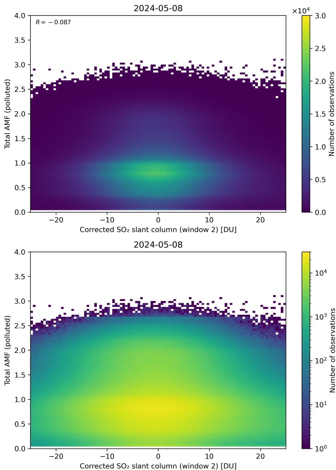
Figure 203: Scatter density plot of “Corrected SO 2 slant column (window 2)” against “Total AMF (polluted)” for 2024-05-07 to 2024-05-09.
