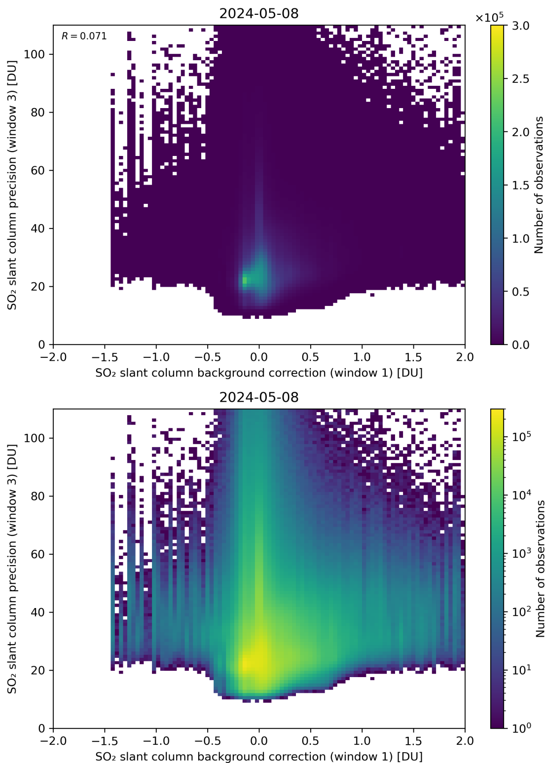
Figure 108: Scatter density plot of “SO 2 slant column background correction (window 1)” against “SO 2 slant column precision (window 3)” for 2024-05-07 to 2024-05-09.
