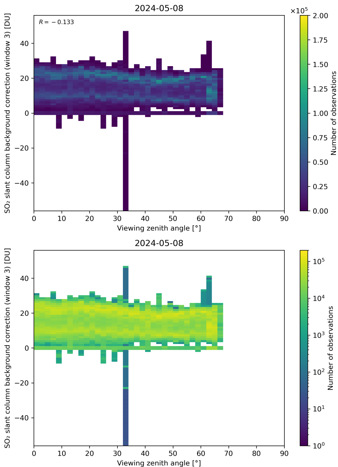
Figure 310: Scatter density plot of “Viewing zenith angle” against “SO 2 slant column background correction (window 3)” for 2024-05-07 to 2024-05-09.
