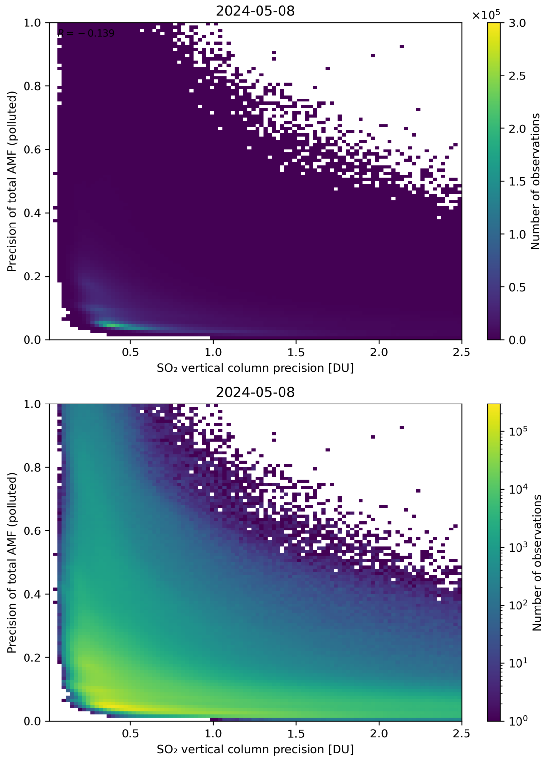
Figure 295: Scatter density plot of “SO 2 vertical column precision” against “Precision of total AMF (polluted)” for 2024-05-07 to 2024-05-09.
