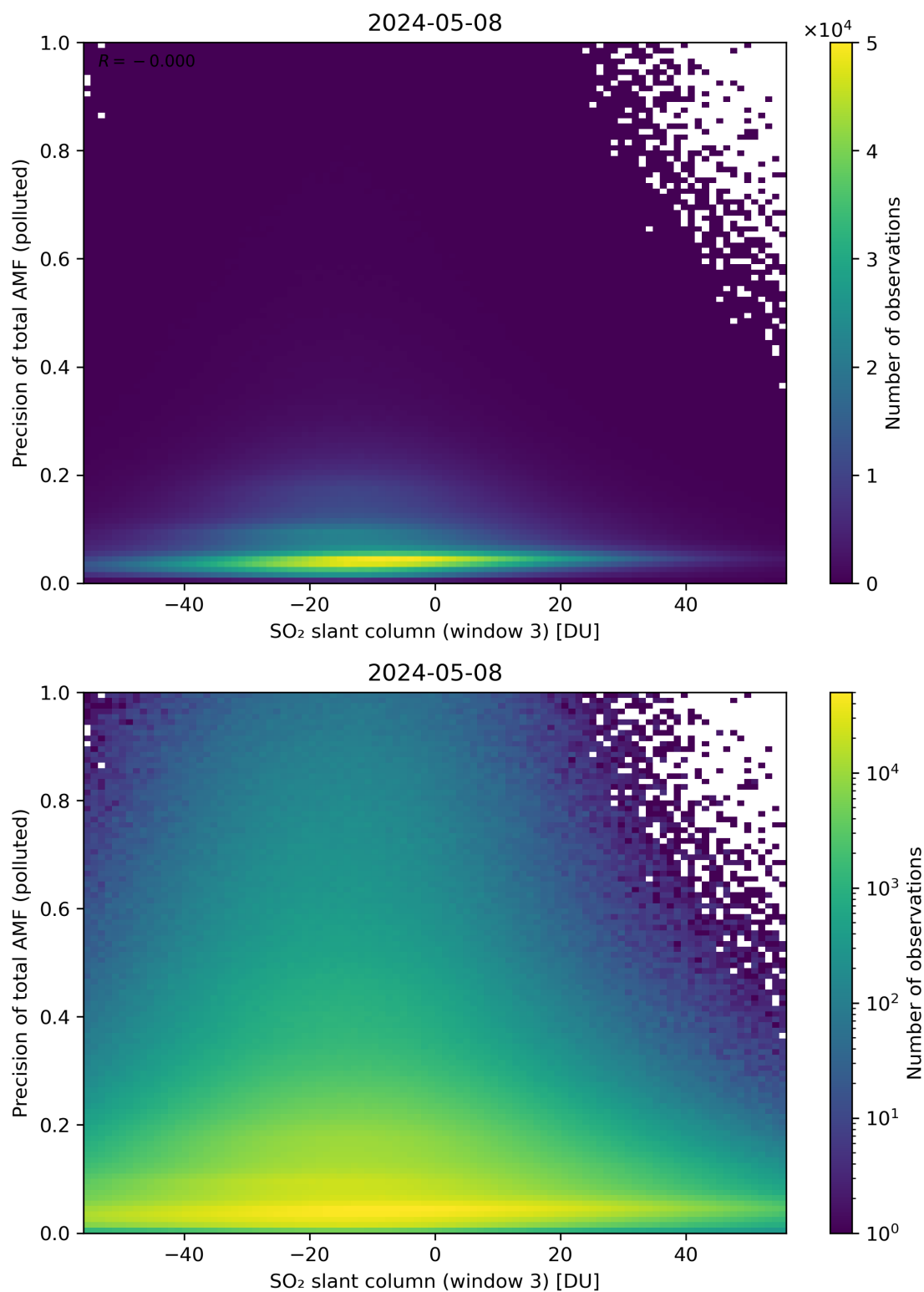
Figure 269: Scatter density plot of “SO 2 slant column (window 3)” against “Precision of total AMF (polluted)” for 2024-05-07 to 2024-05-09.
