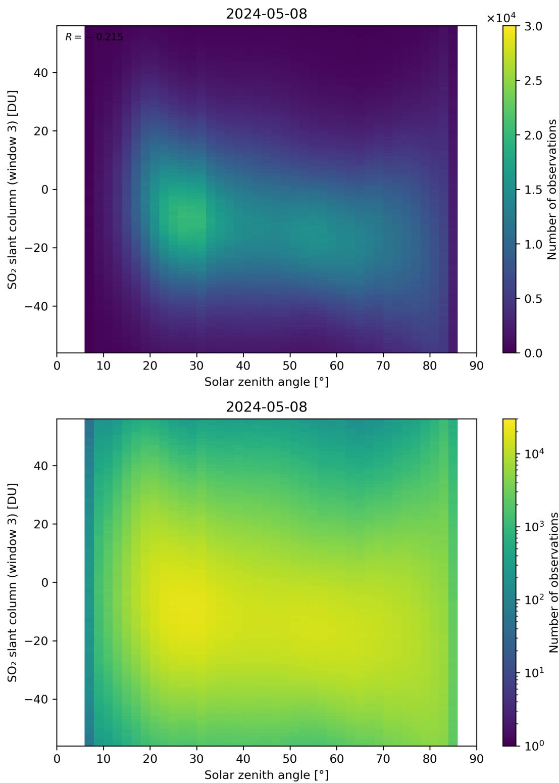
Figure 172: Scatter density plot of “Solar zenith angle” against “SO 2 slant column (window 3)” for 2024-05-07 to 2024-05-09.
