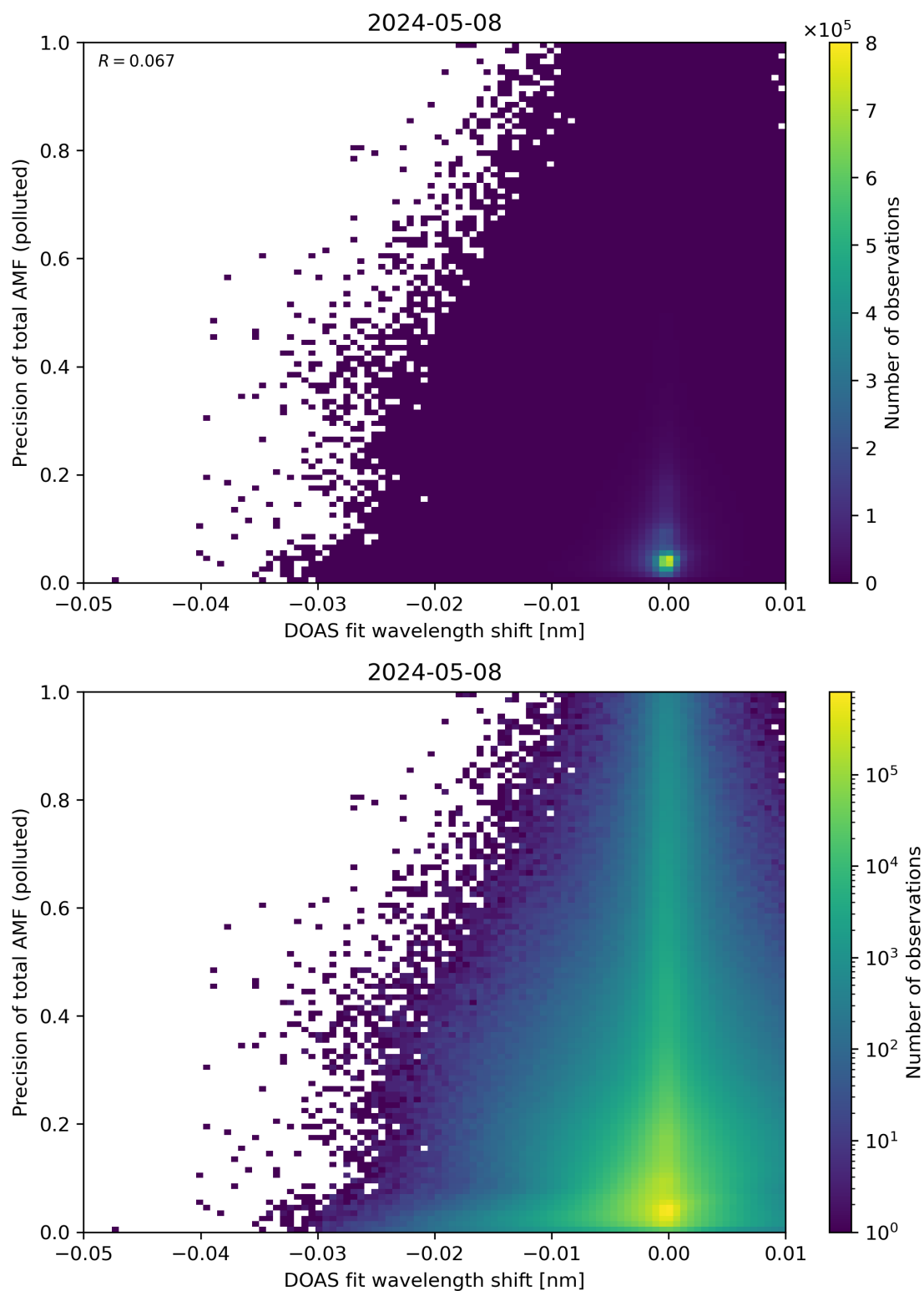
Figure 131: Scatter density plot of “DOAS fit wavelength shift” against “Precision of total AMF (polluted)” for 2024-05-07 to 2024-05-09.
