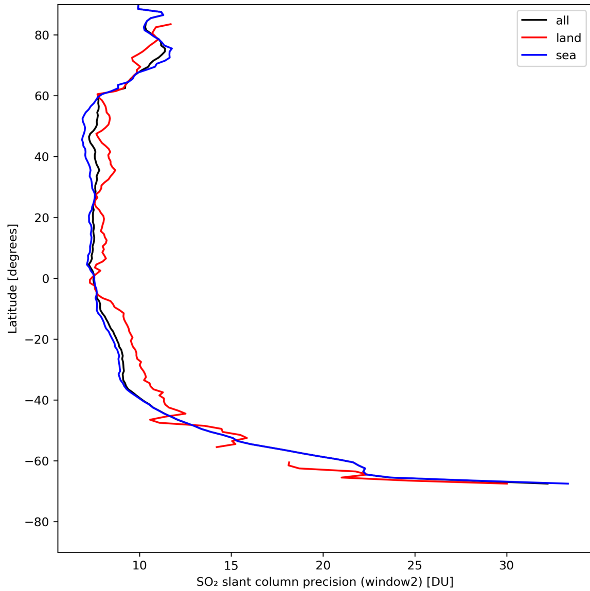
Figure 38: Zonal average of “SO 2 slant column precision (window2)” for 2024-05-07 to 2024-05-09.
