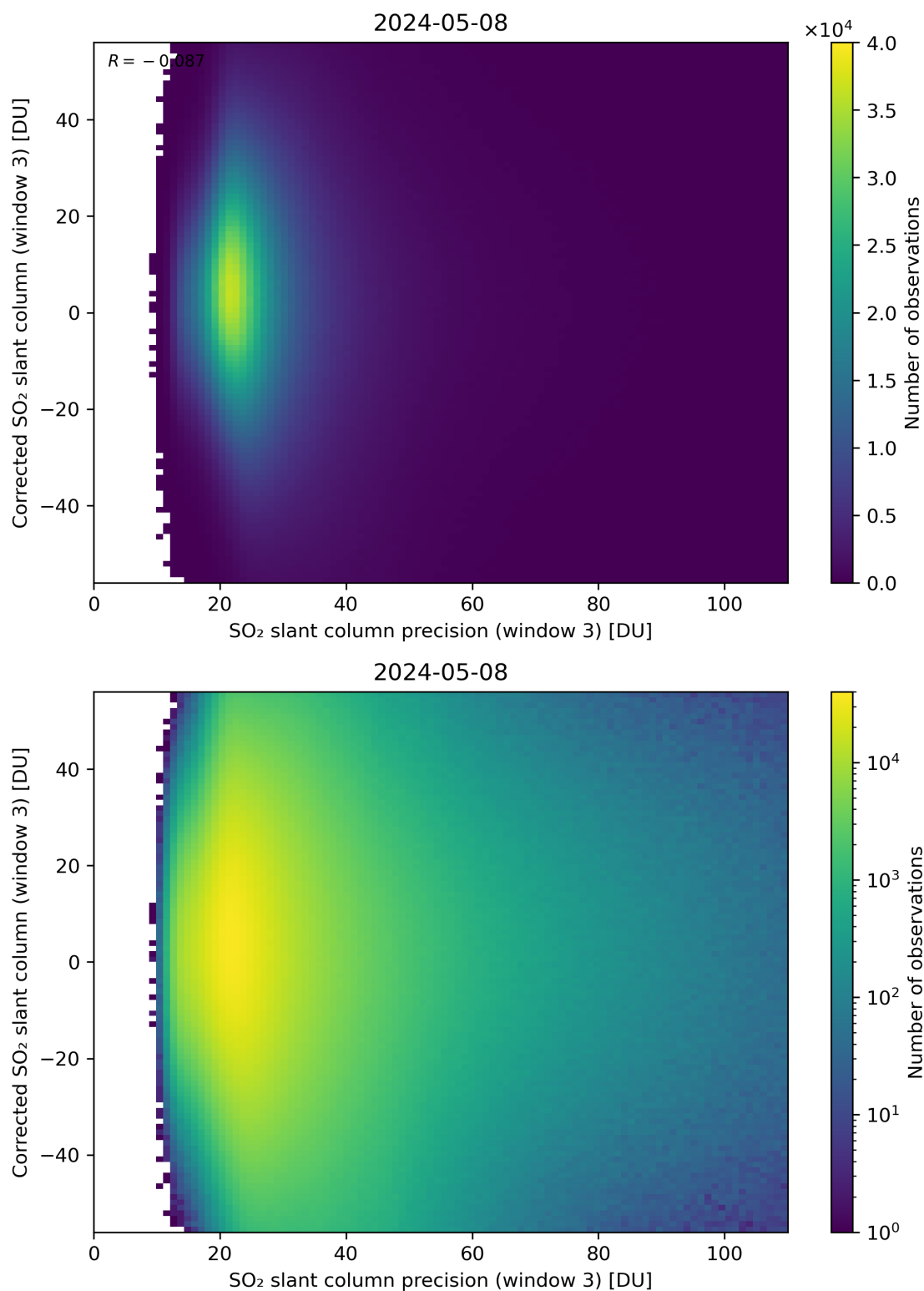
Figure 262: Scatter density plot of “SO 2 slant column precision (window 3)” against “Corrected SO 2 slant column (window 3)” for 2024-05-07 to 2024-05-09.
