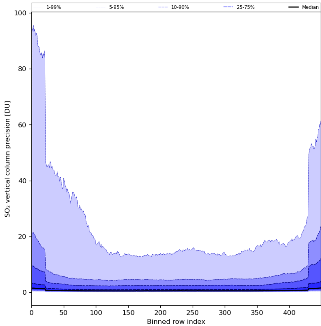
Figure 77: Along track statistics of “SO 2 vertical column precision” for 2024-05-07 to 2024-05-09
