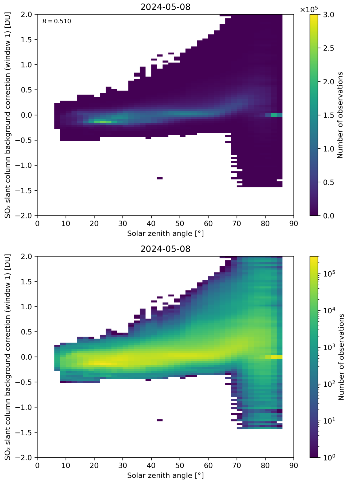
Figure 158: Scatter density plot of “Solar zenith angle” against “SO 2 slant column background correction (window 1)” for 2024-05-07 to 2024-05-09.
