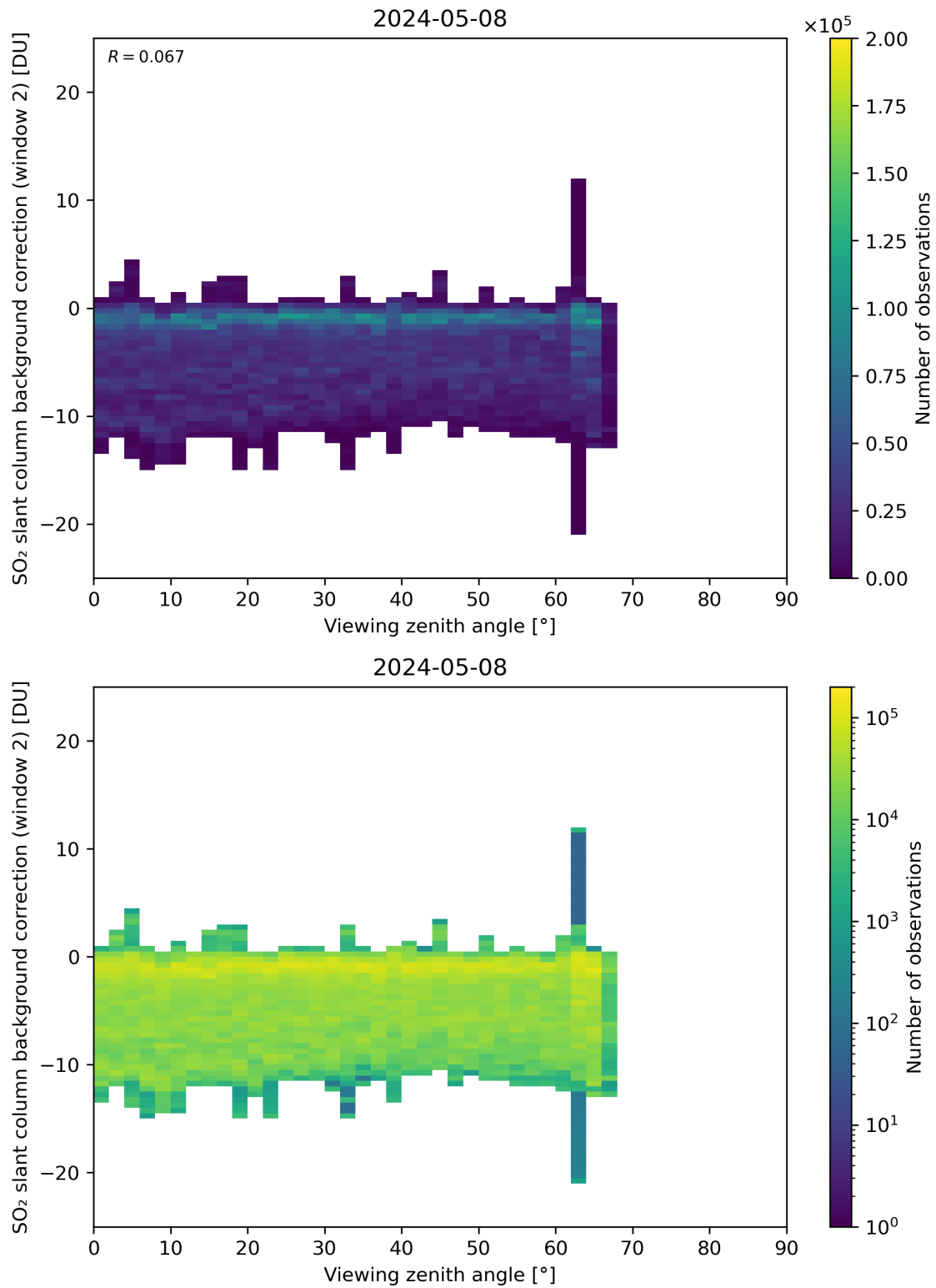
Figure 309: Scatter density plot of “Viewing zenith angle” against “SO 2 slant column background correction (window 2)” for 2024-05-07 to 2024-05-09.
