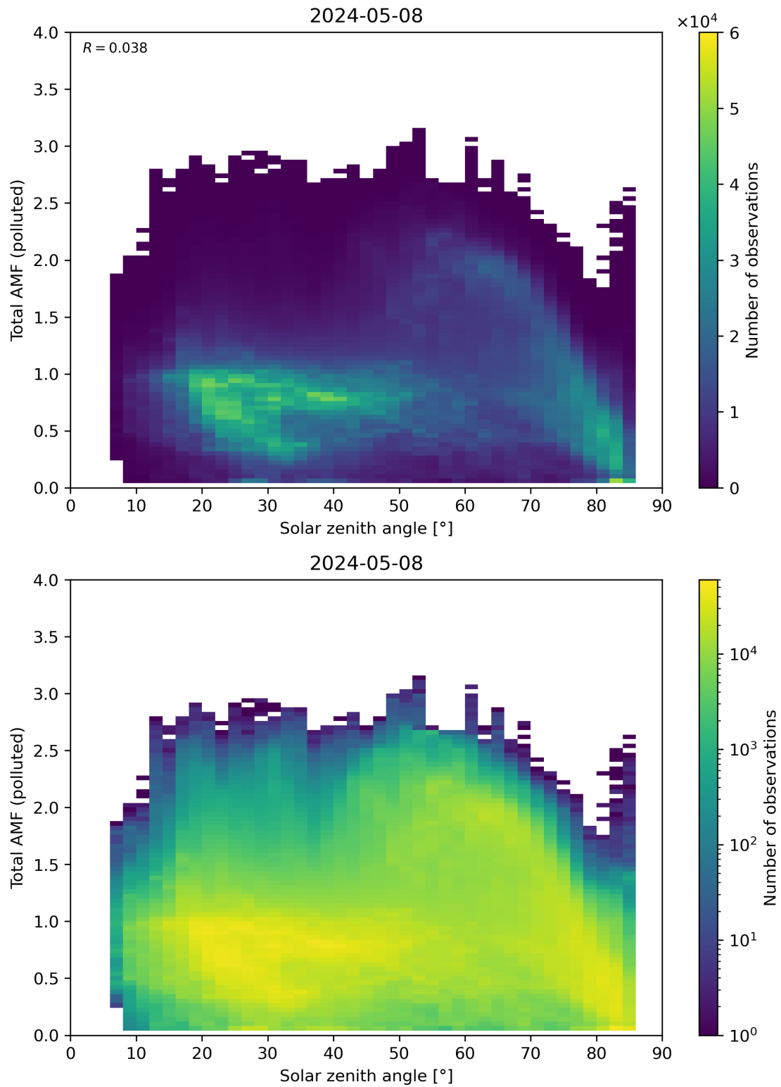
Figure 174: Scatter density plot of “Solar zenith angle” against “Total AMF (polluted)” for 2024-05-07 to 2024-05-09.
