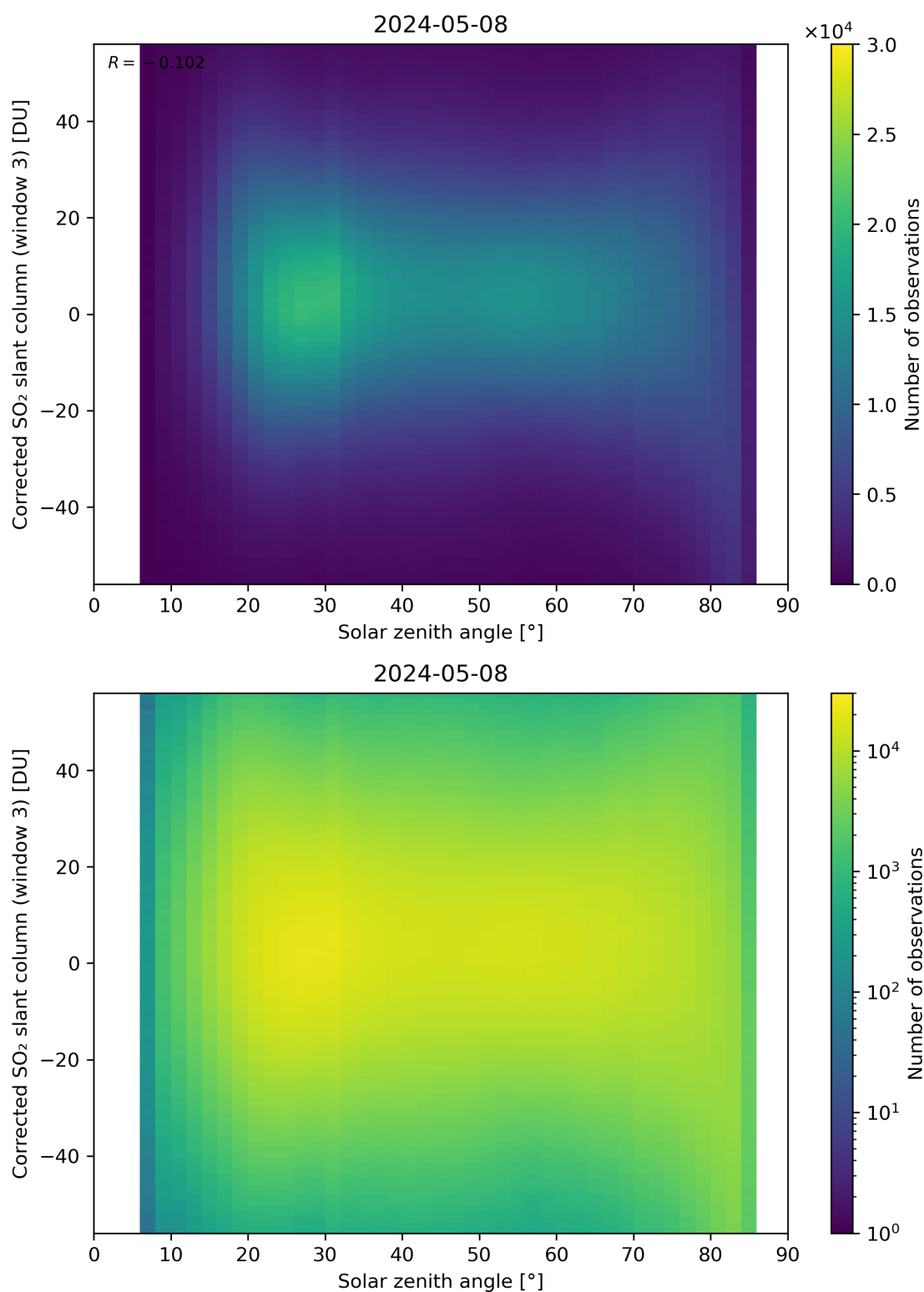
Figure 168: Scatter density plot of “Solar zenith angle” against “Corrected SO 2 slant column (window 3)” for 2024-05-07 to 2024-05-09.
