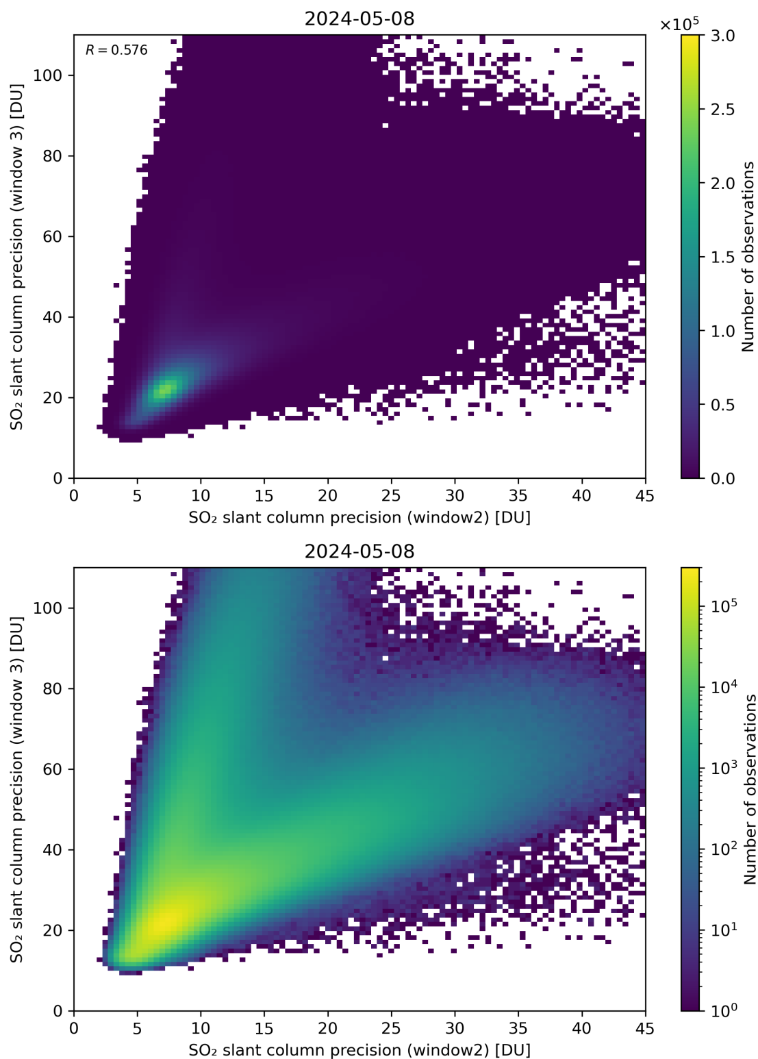
Figure 250: Scatter density plot of “SO 2 slant column precision (window2)” against “SO 2 slant column precision (window 3)” for 2024-05-07 to 2024-05-09.
