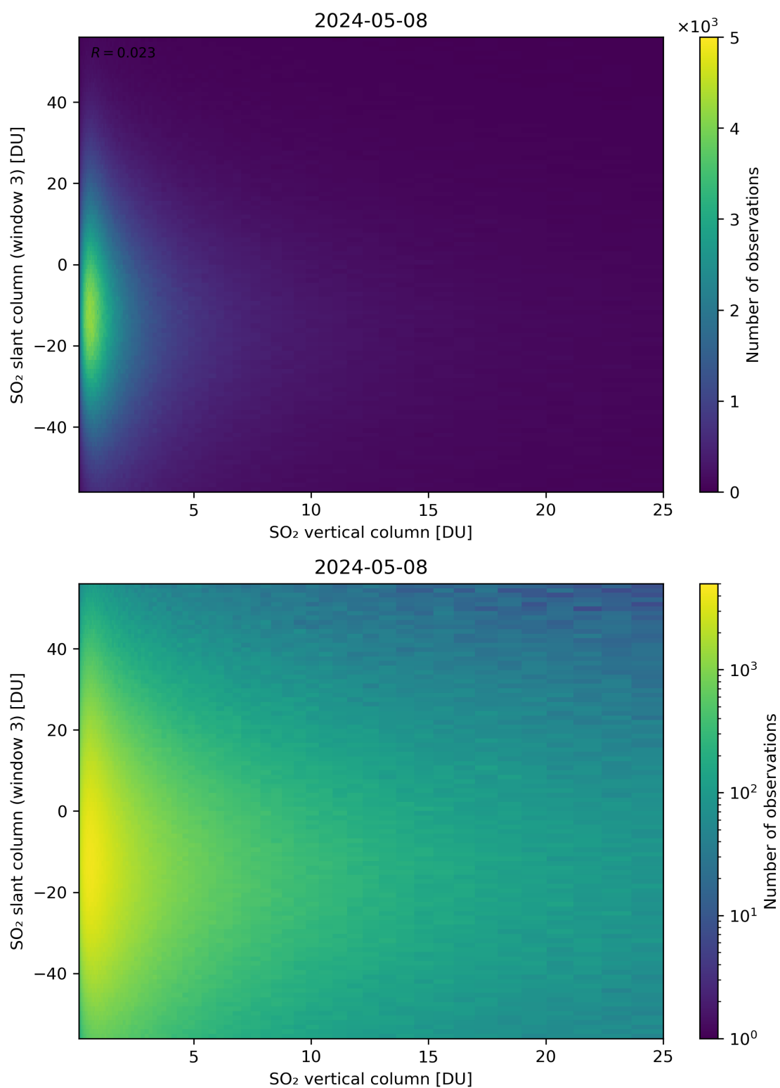
Figure 303: Scatter density plot of “SO 2 vertical column” against “SO 2 slant column (window 3)” for 2024-05-07 to 2024-05-09.
