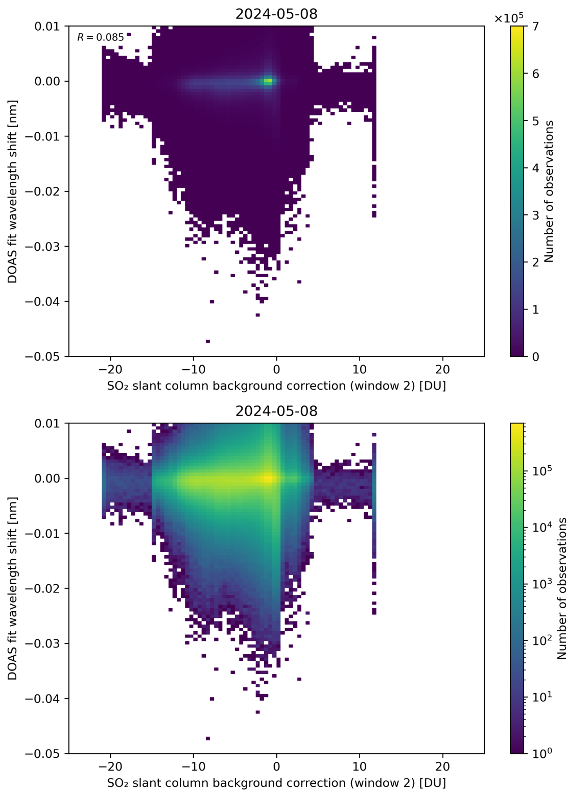
Figure 112: Scatter density plot of “SO 2 slant column background correction (window 2)” against “DOAS fit wavelength shift” for 2024-05-07 to 2024-05-09.
