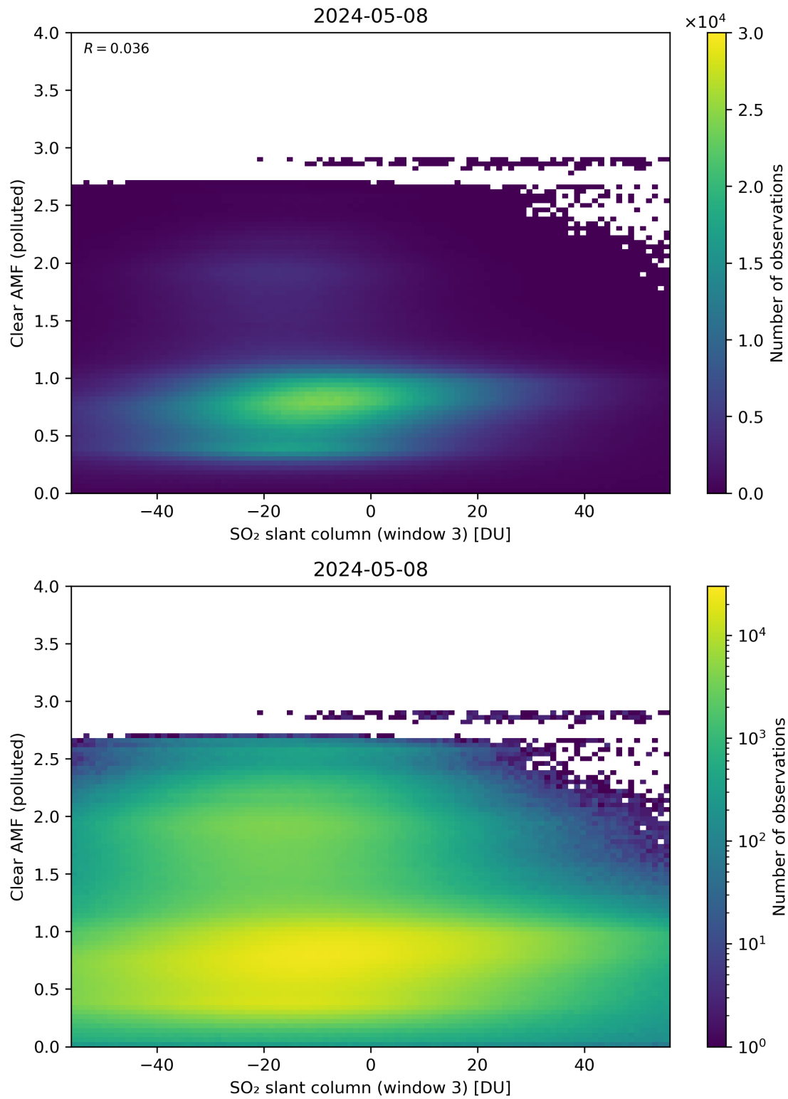
Figure 265: Scatter density plot of “SO 2 slant column (window 3)” against “Clear AMF (polluted)” for 2024-05-07 to 2024-05-09.
