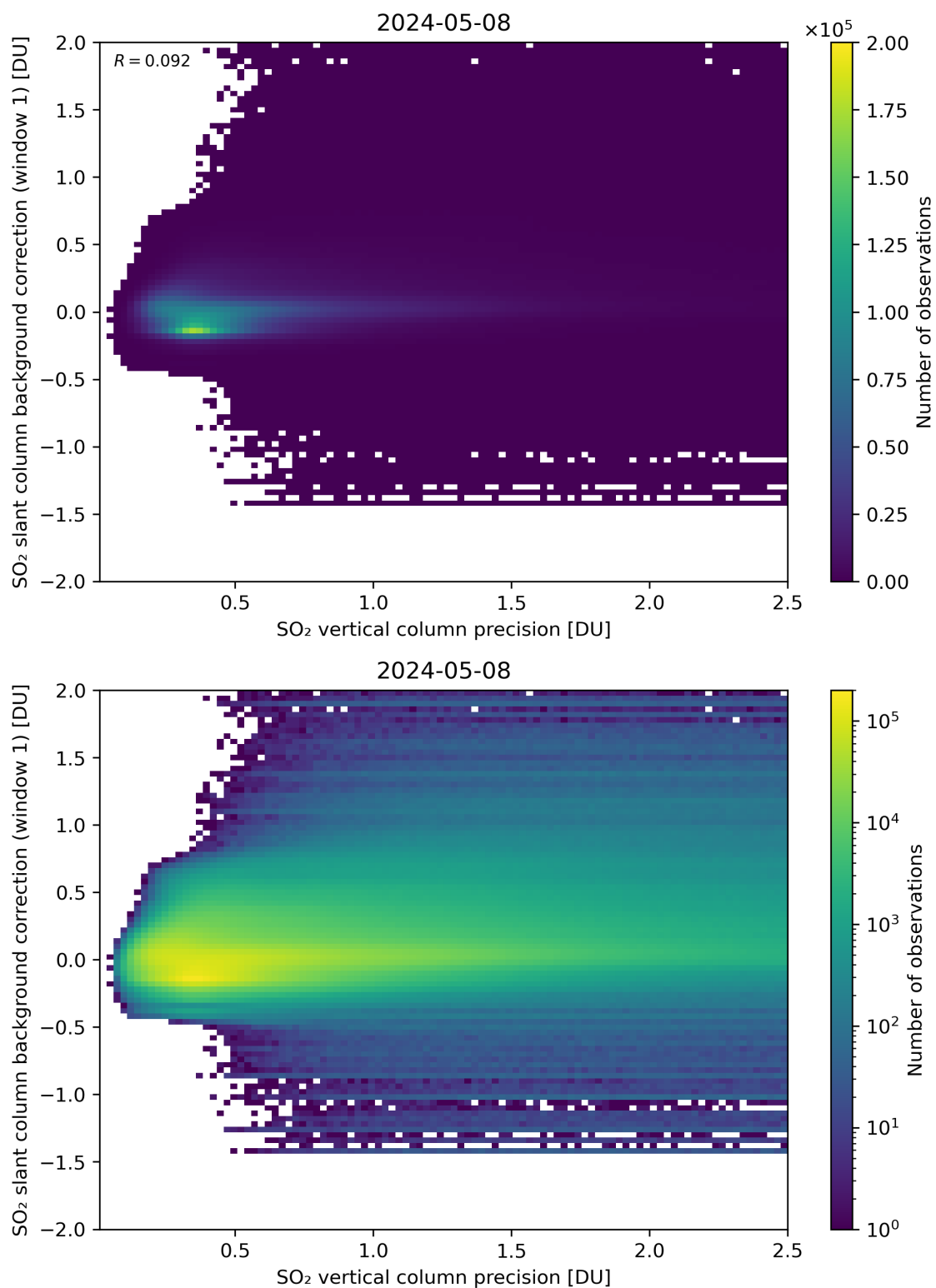
Figure 279: Scatter density plot of “SO 2 vertical column precision” against “SO 2 slant column background correction (window 1)” for 2024-05-07 to 2024-05-09.
