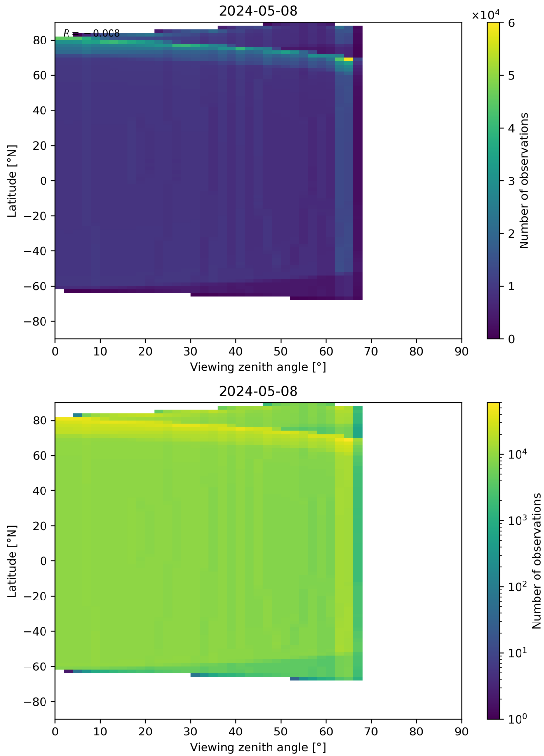
Figure 314: Scatter density plot of “Viewing zenith angle” against “Latitude” for 2024-05-07 to 2024-05-09.
