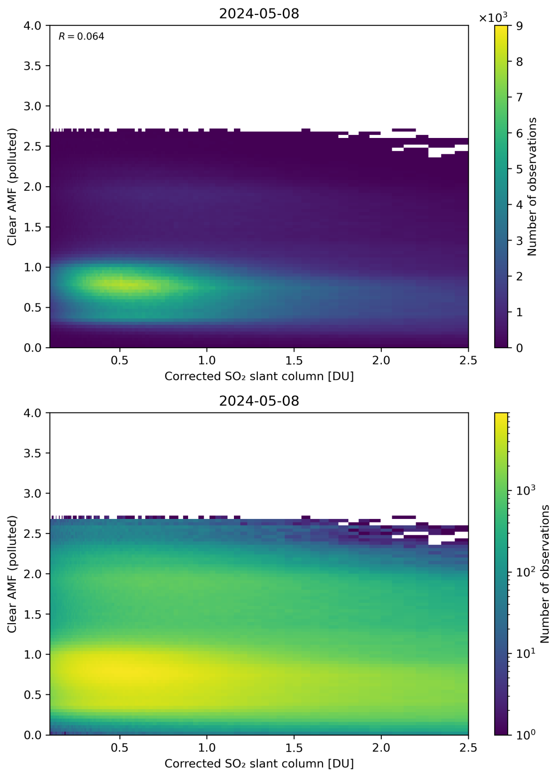
Figure 184: Scatter density plot of “Corrected SO 2 slant column” against “Clear AMF (polluted)” for 2024-05-07 to 2024-05-09.
