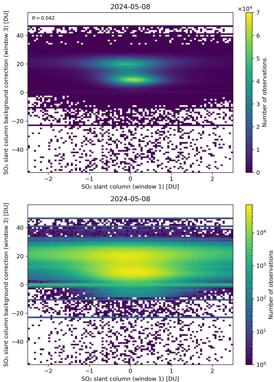
Figure 214: Scatter density plot of “SO 2 slant column (window 1)” against “SO 2 slant column background correction (window 3)” for 2024-05-07 to 2024-05-09.
