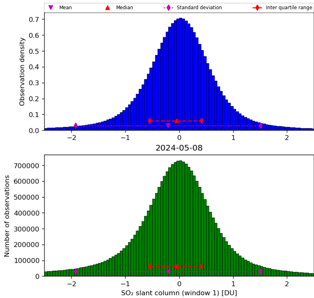
Figure 56: Histogram of “SO 2 slant column (window 1)” for 2024-05-07 to 2024-05-09
