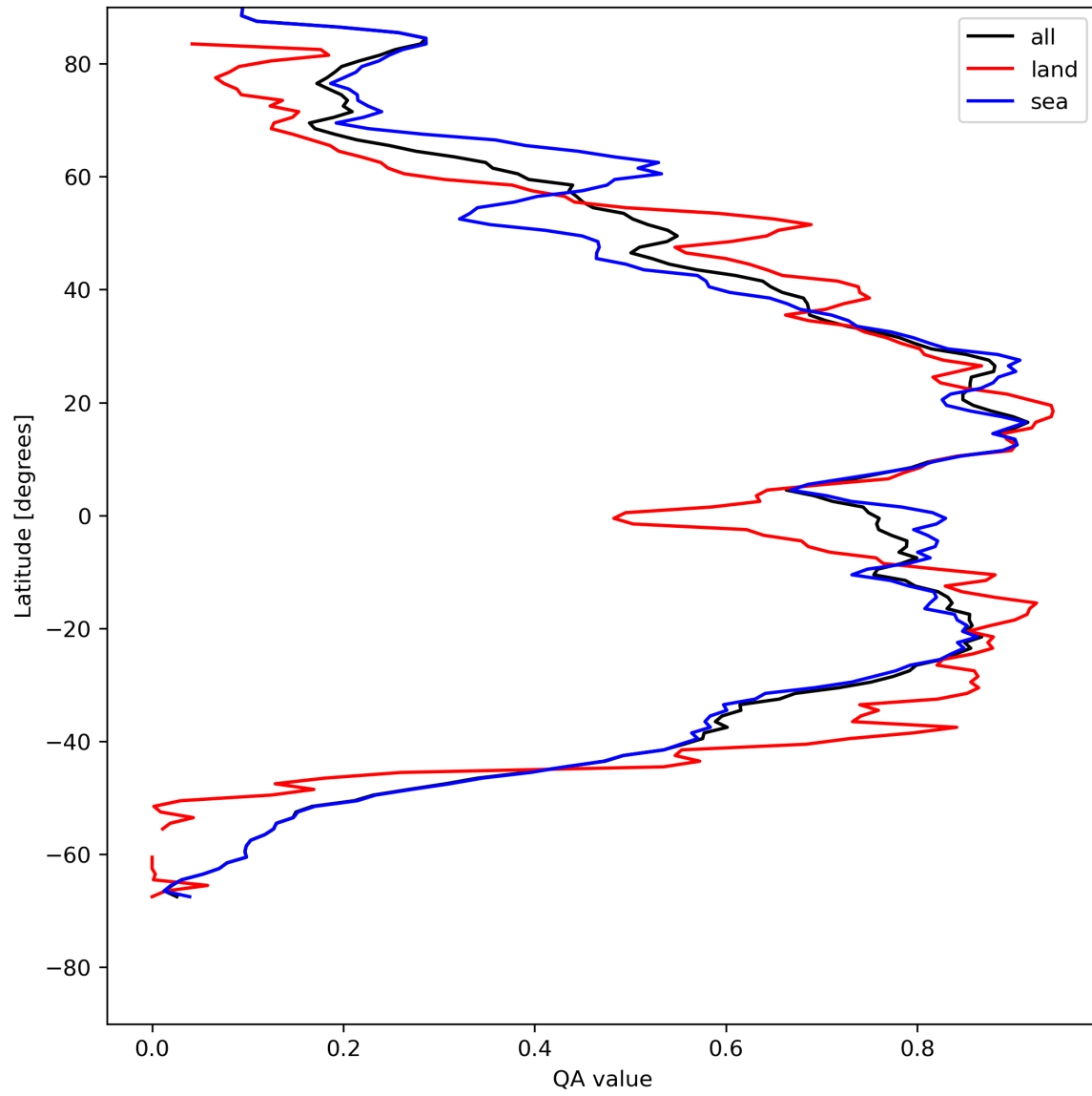
Figure 29: Zonal average of “QA value” for 2024-05-07 to 2024-05-09.
