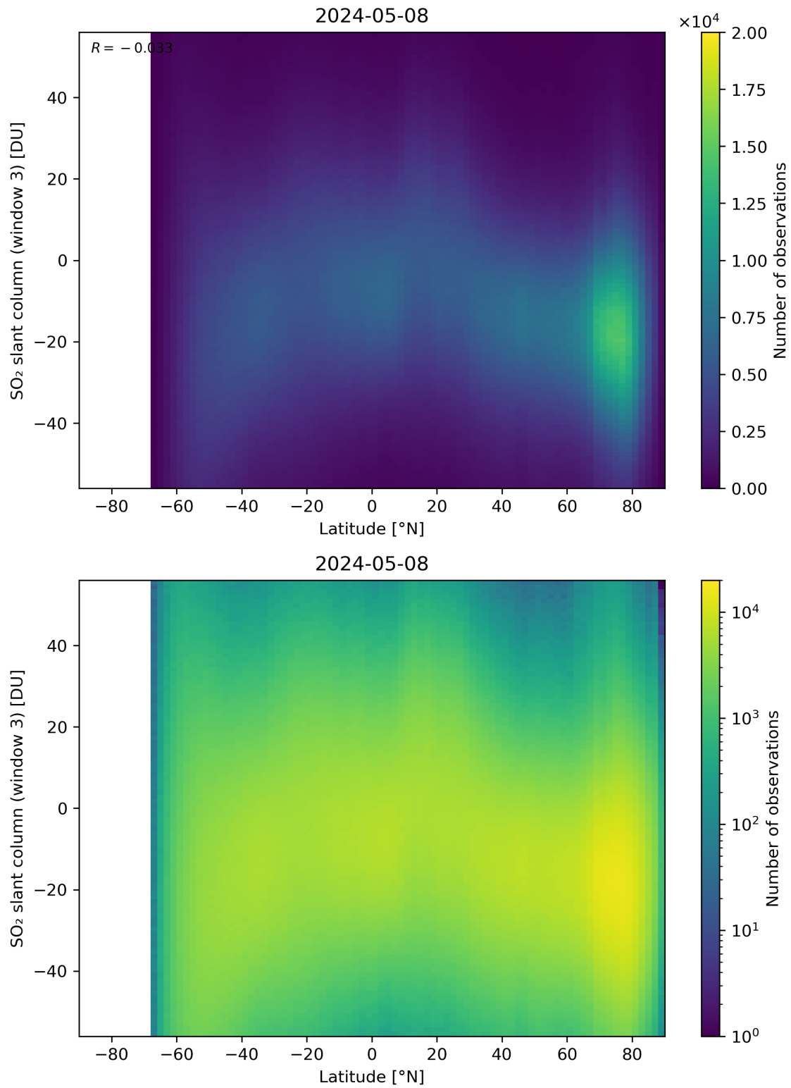
Figure 152: Scatter density plot of “Latitude” against “SO 2 slant column (window 3)” for 2024-05-07 to 2024-05-09.
