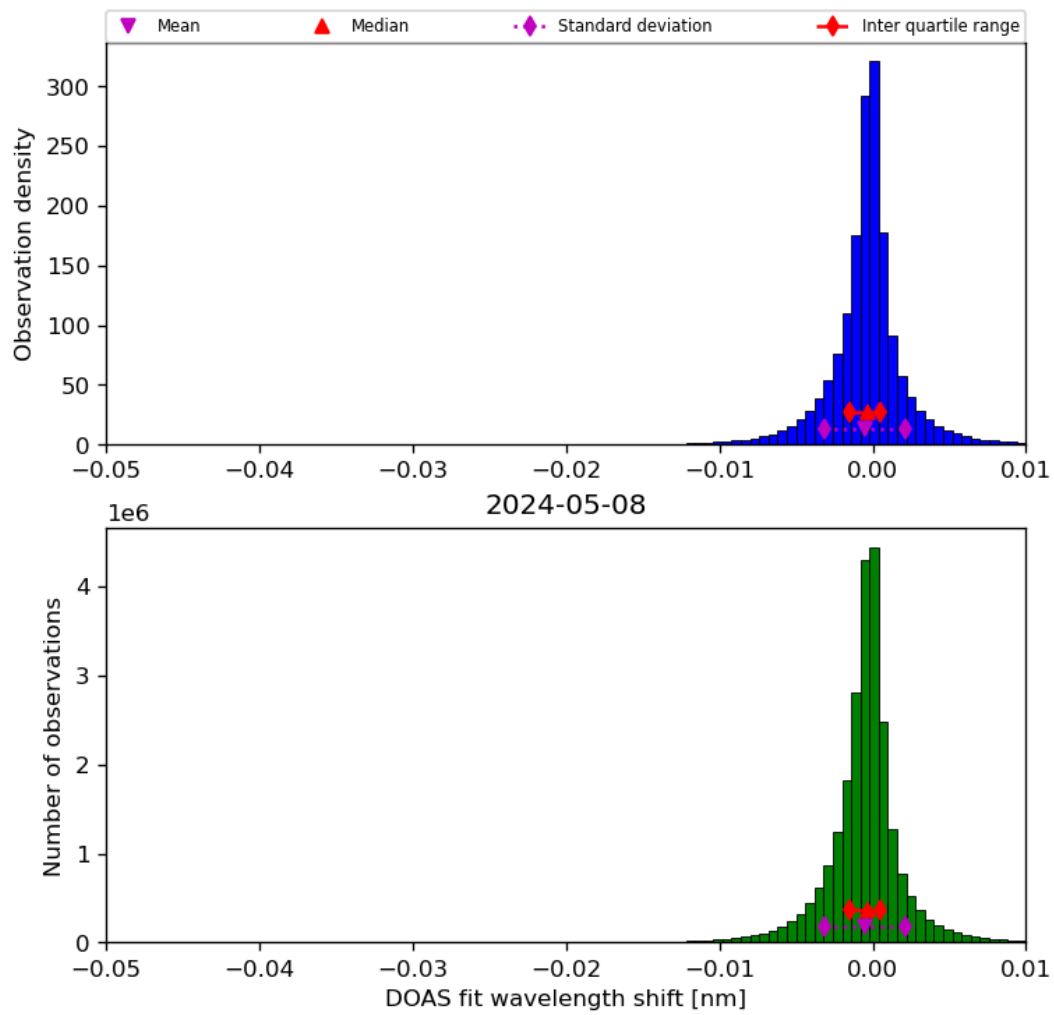
Figure 68: Histogram of “DOAS fit wavelength shift” for 2024-05-07 to 2024-05-09
