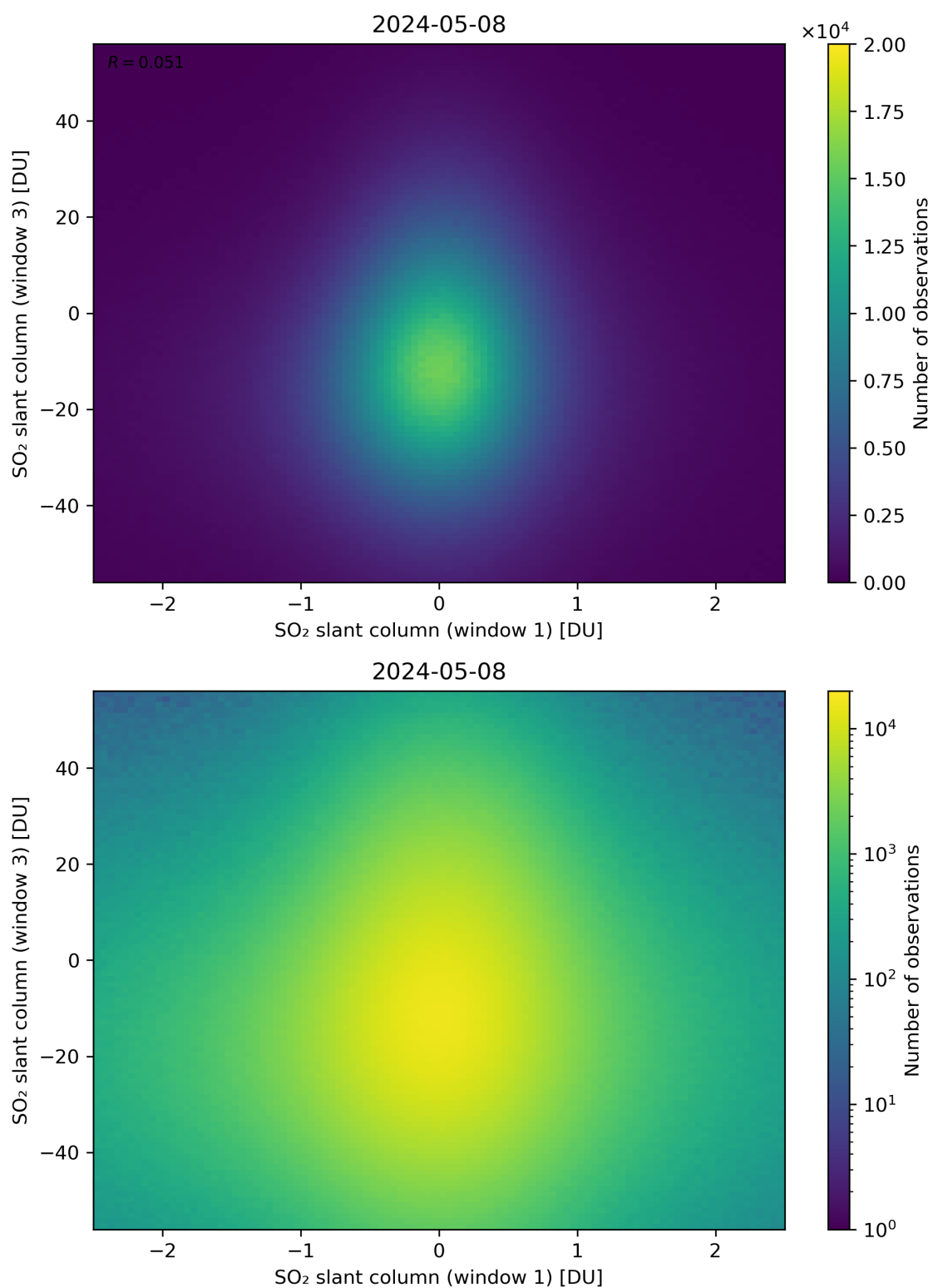
Figure 237: Scatter density plot of “SO 2 slant column (window 1)” against “SO 2 slant column (window 3)” for 2024-05-07 to 2024-05-09.
