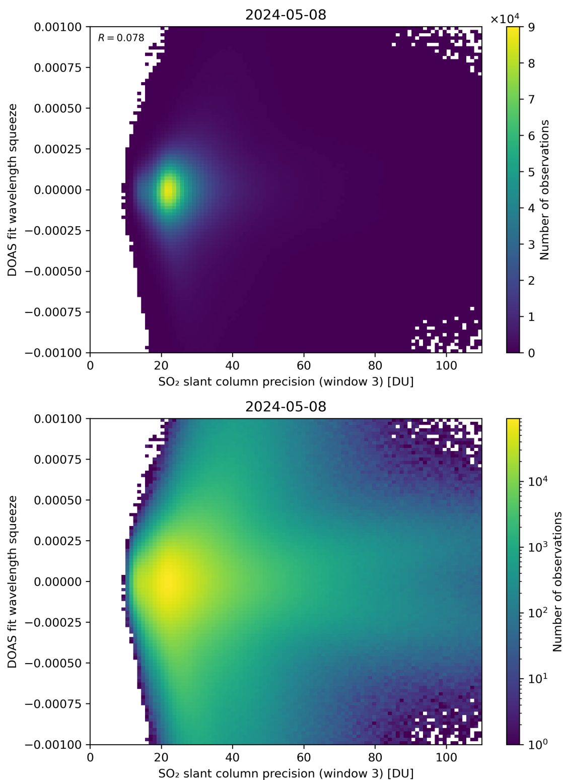
Figure 259: Scatter density plot of “SO 2 slant column precision (window 3)” against “DOAS fit wavelength squeeze” for 2024-05-07 to 2024-05-09.
