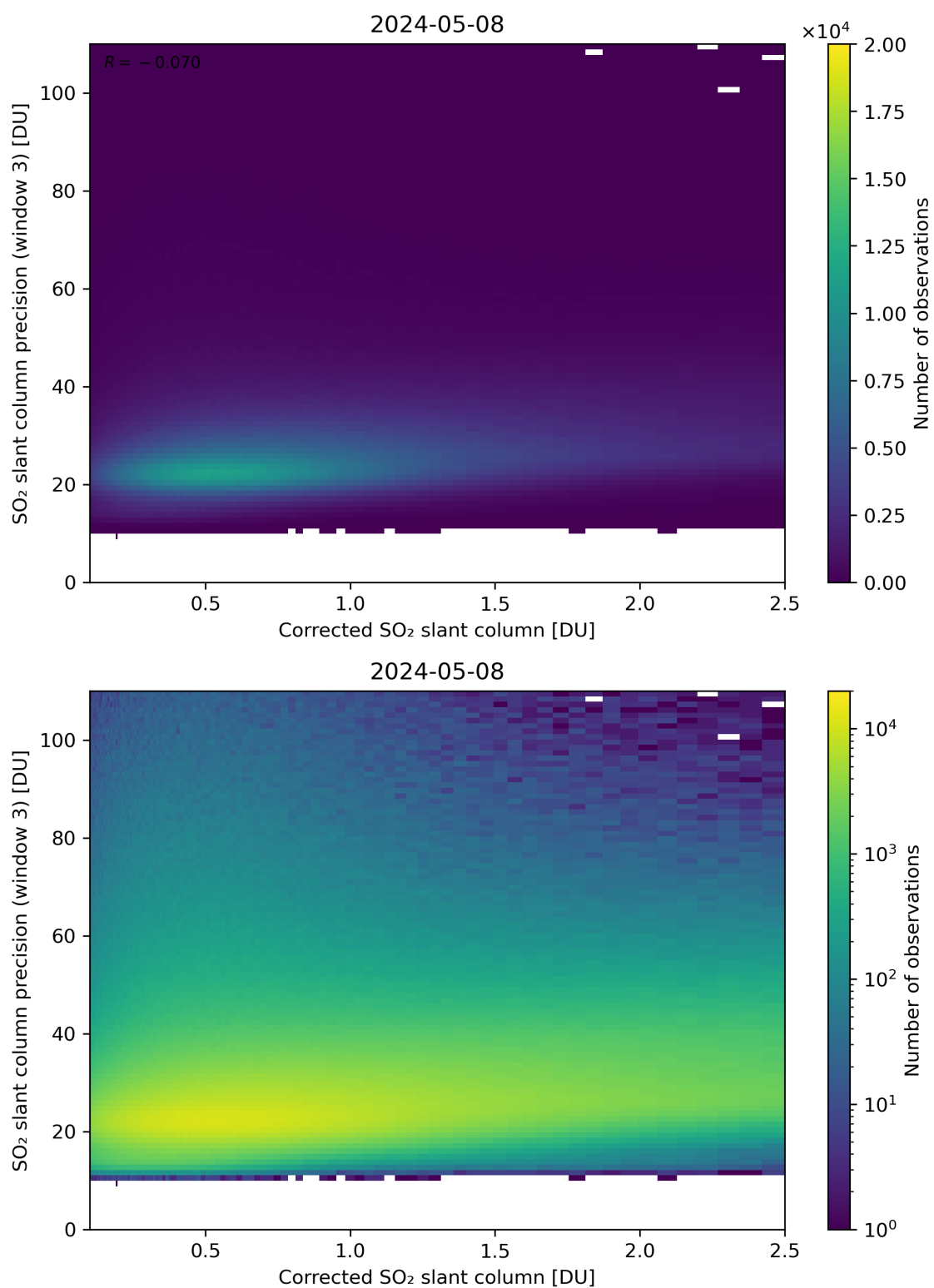
Figure 191: Scatter density plot of “Corrected SO 2 slant column” against “SO 2 slant column precision (window 3)” for 2024-05-07 to 2024-05-09.
