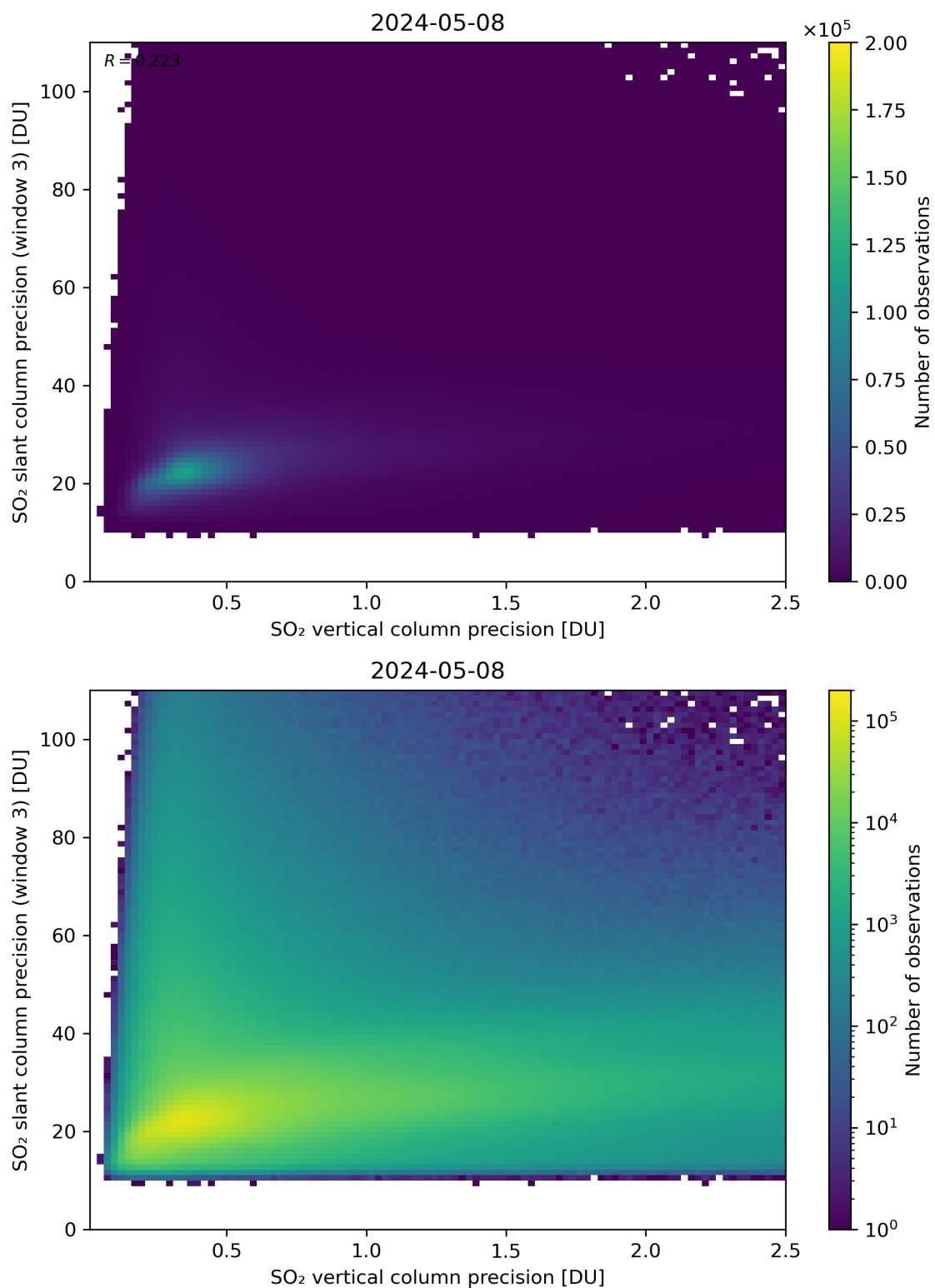
Figure 293: Scatter density plot of “SO 2 vertical column precision” against “SO 2 slant column precision (window 3)” for 2024-05-07 to 2024-05-09.
