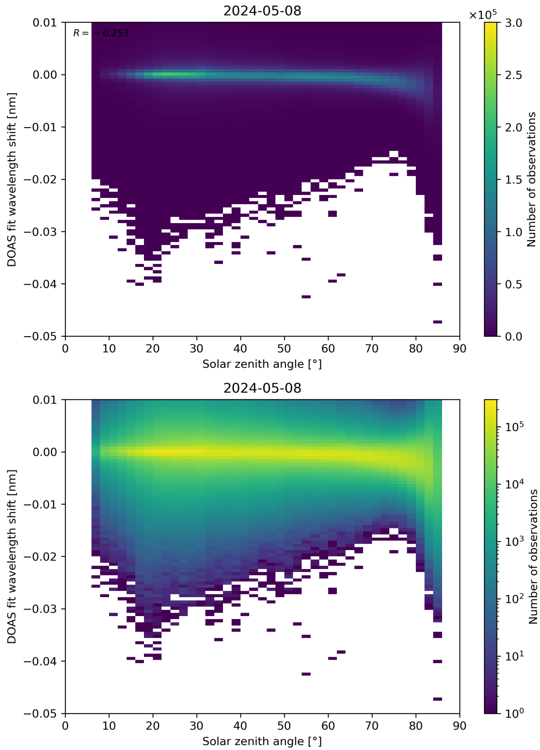
Figure 161: Scatter density plot of “Solar zenith angle” against “DOAS fit wavelength shift” for 2024-05-07 to 2024-05-09.
