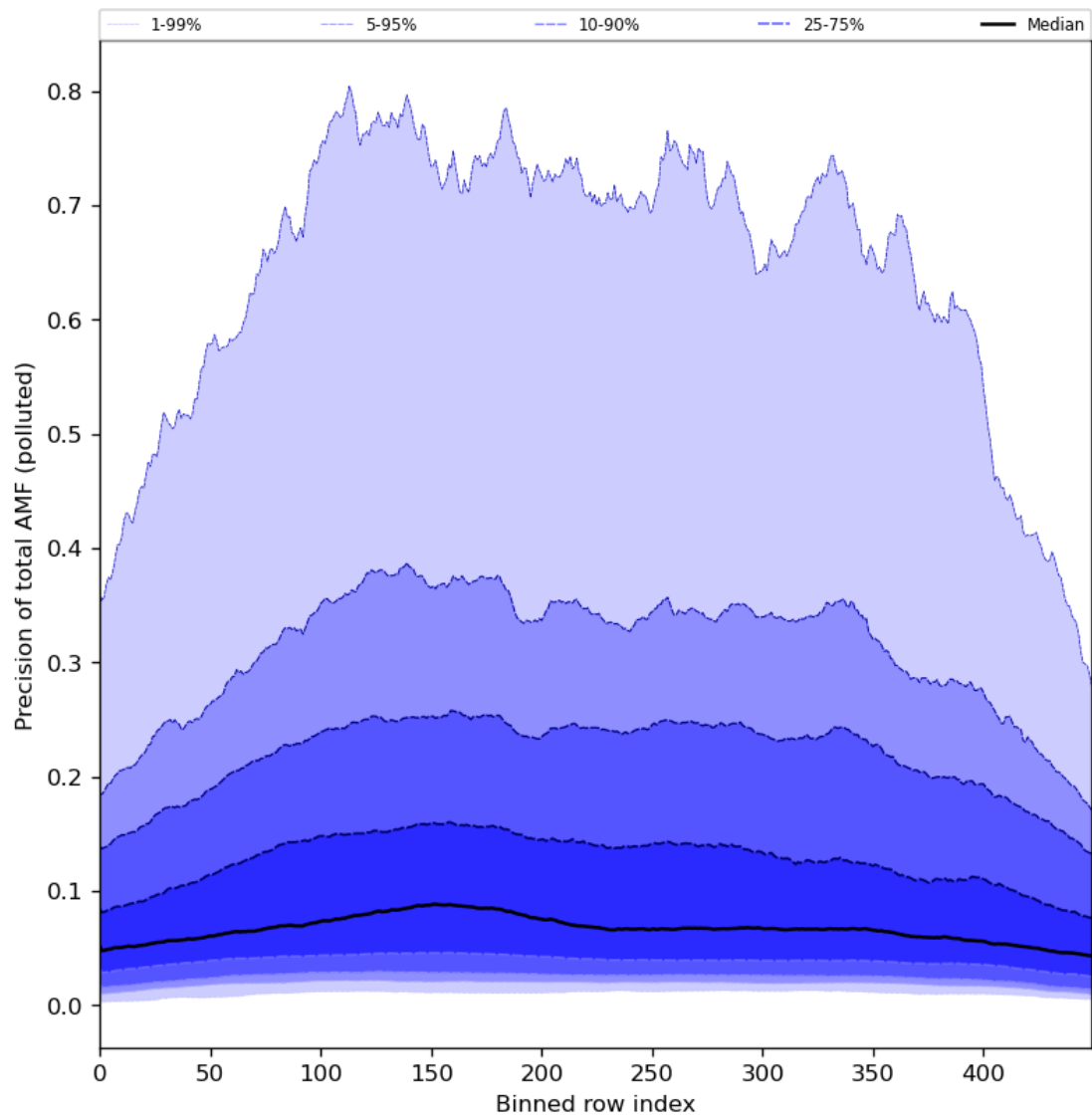
Figure 95: Along track statistics of “Precision of total AMF (polluted)” for 2024-05-07 to 2024-05-09
