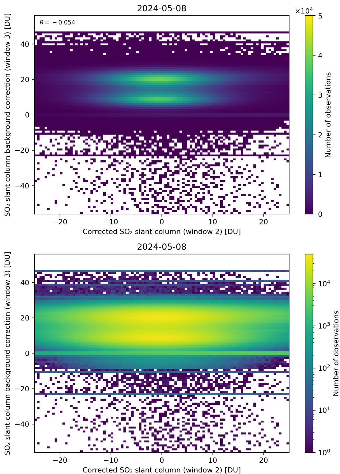
Figure 195: Scatter density plot of “Corrected SO 2 slant column (window 2)” against “SO 2 slant column background correction (window 3)” for 2024-05-07 to 2024-05-09.
