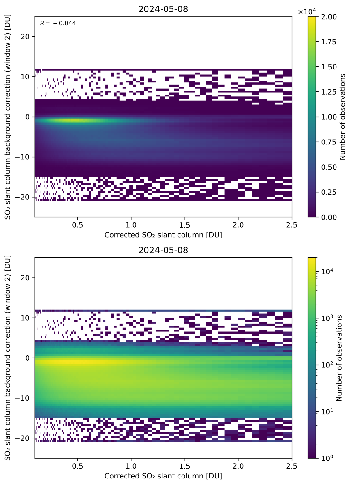
Figure 179: Scatter density plot of “Corrected SO 2 slant column” against “SO 2 slant column background correction (window 2)” for 2024-05-07 to 2024-05-09.
