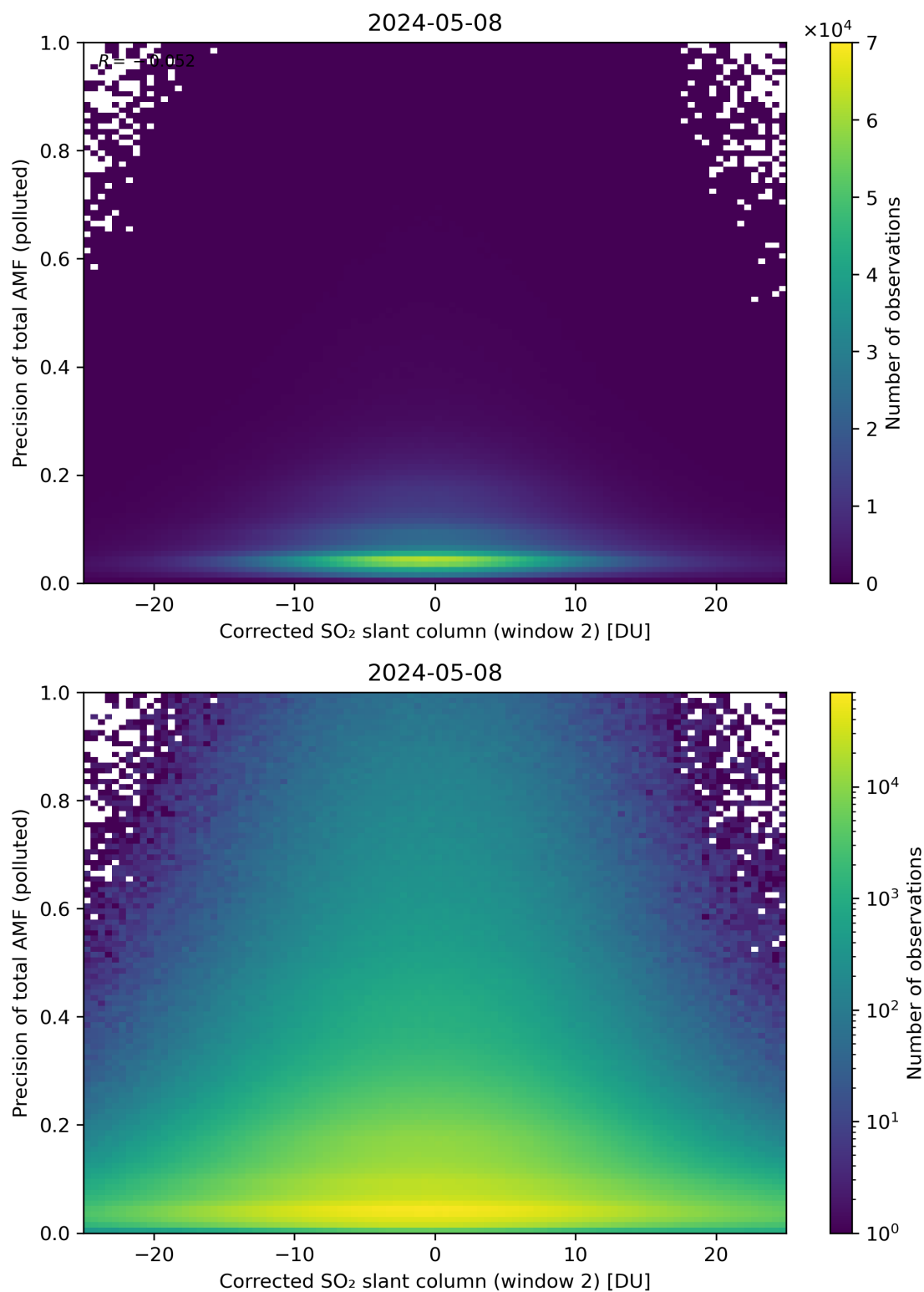
Figure 204: Scatter density plot of “Corrected SO 2 slant column (window 2)” against “Precision of total AMF (polluted)” for 2024-05-07 to 2024-05-09.
