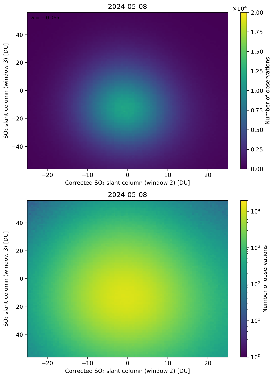
Figure 201: Scatter density plot of “Corrected SO 2 slant column (window 2)” against “SO 2 slant column (window 3)” for 2024-05-07 to 2024-05-09.
