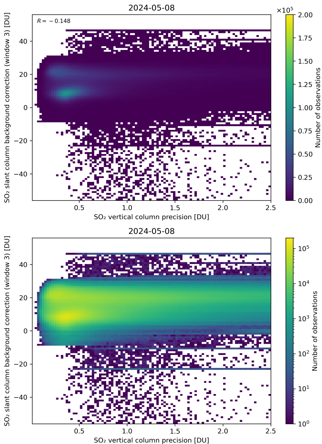
Figure 281: Scatter density plot of “SO 2 vertical column precision” against “SO 2 slant column background correction (window 3)” for 2024-05-07 to 2024-05-09.
