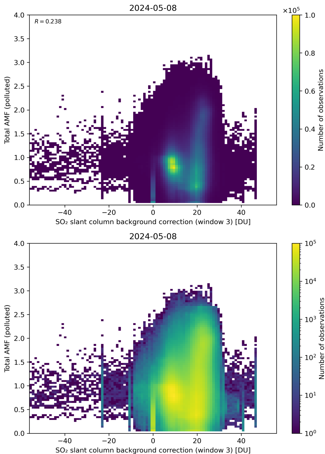
Figure 125: Scatter density plot of “SO 2 slant column background correction (window 3)” against “Total AMF (polluted)” for 2024-05-07 to 2024-05-09.
