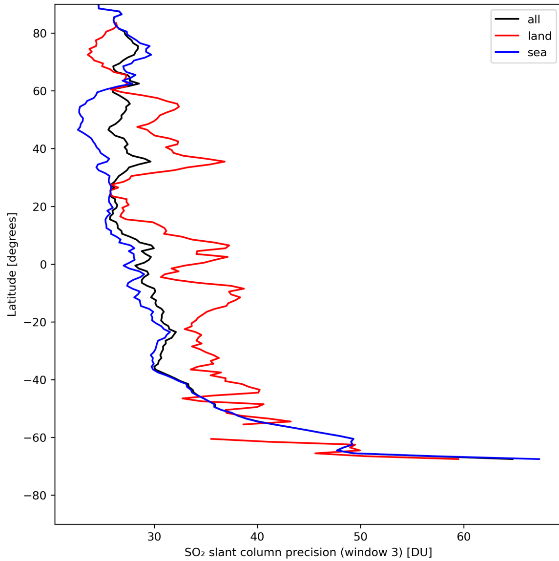
Figure 42: Zonal average of “SO 2 slant column precision (window 3)” for 2024-05-07 to 2024-05-09.
