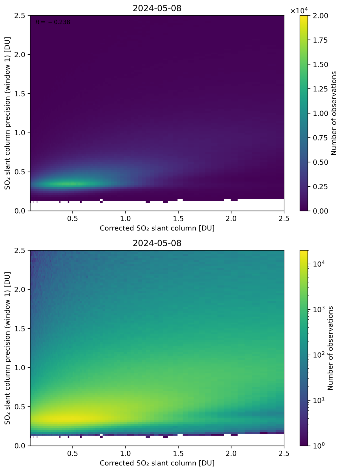
Figure 188: Scatter density plot of “Corrected SO 2 slant column” against “SO 2 slant column precision (window 1)” for 2024-05-07 to 2024-05-09.
