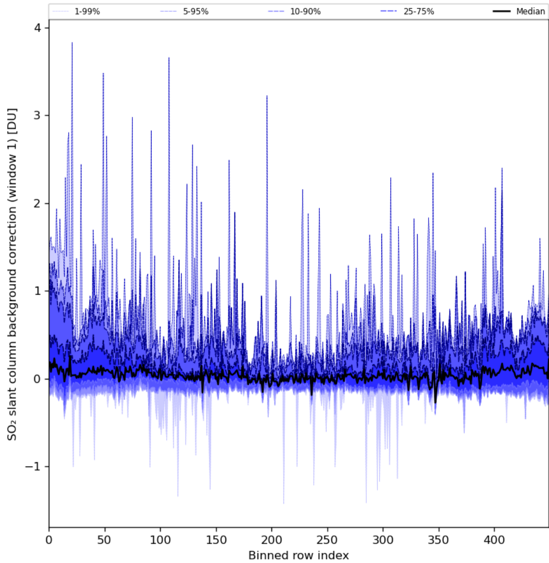
Figure 82: Along track statistics of “SO 2 slant column background correction (window 1)” for 2024-05-07 to 2024-05-09
