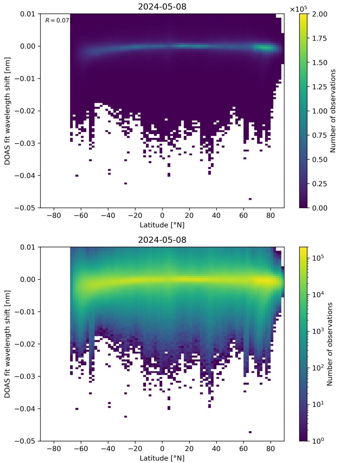
Figure 142: Scatter density plot of “Latitude” against “DOAS fit wavelength shift” for 2024-05-07 to 2024-05-09.
