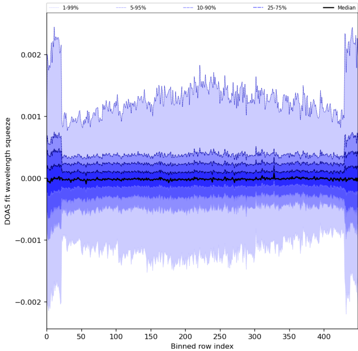
Figure 92: Along track statistics of “DOAS fit wavelength squeeze” for 2024-05-07 to 2024-05-09
