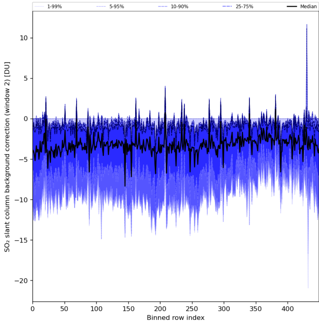
Figure 86: Along track statistics of “SO 2 slant column background correction (window 2)” for 2024-05-07 to 2024-05-09
