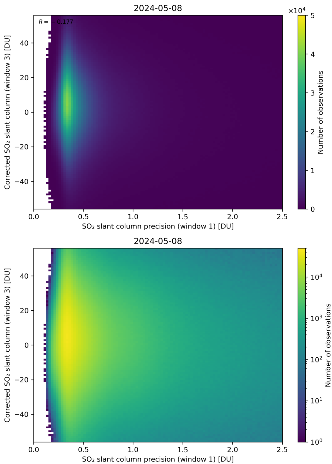
Figure 226: Scatter density plot of “SO 2 slant column precision (window 1)” against “Corrected SO 2 slant column (window 3)” for 2024-05-07 to 2024-05-09.
