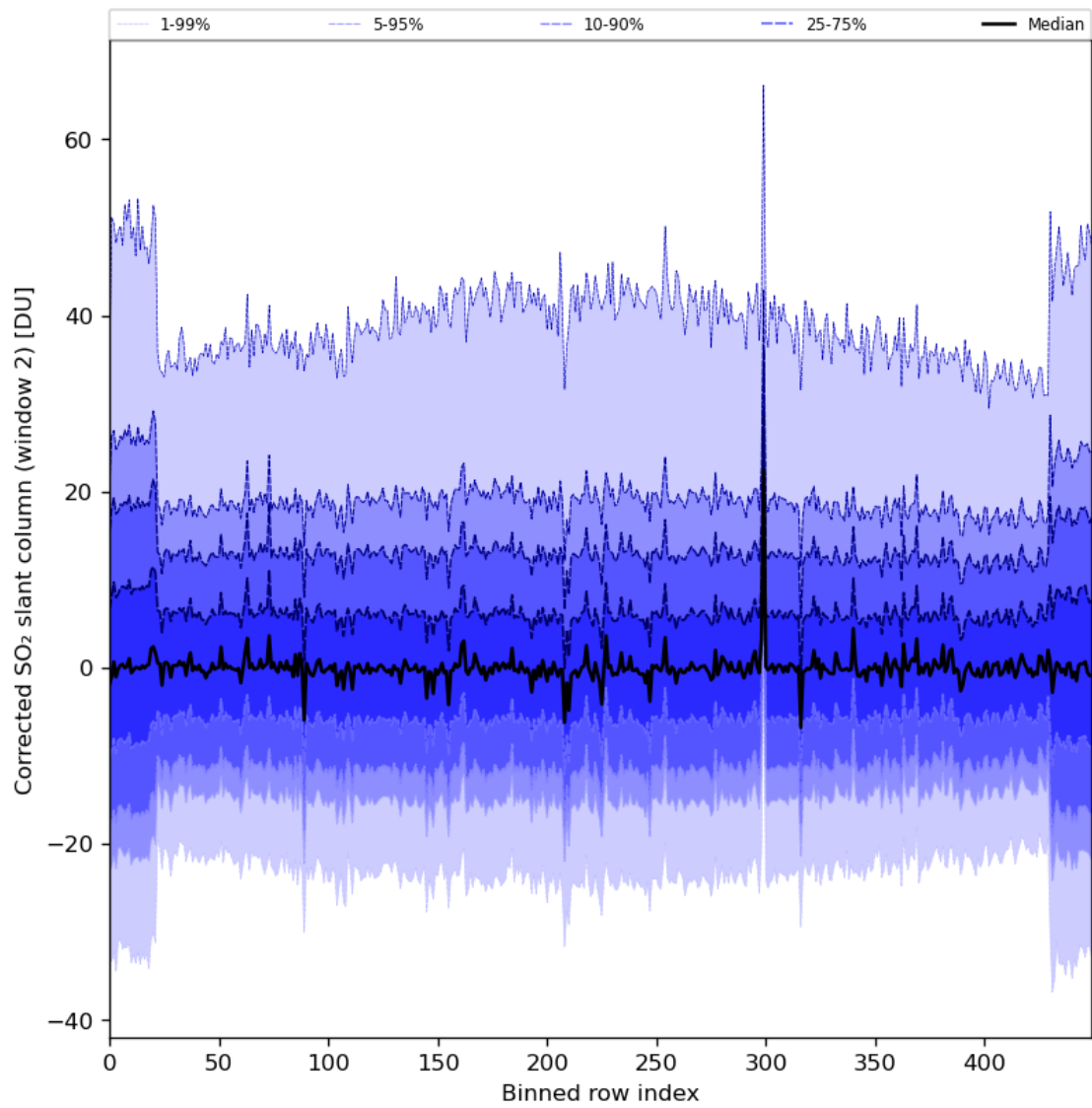
Figure 85: Along track statistics of “Corrected SO 2 slant column (window 2)” for 2024-05-07 to 2024-05-09
