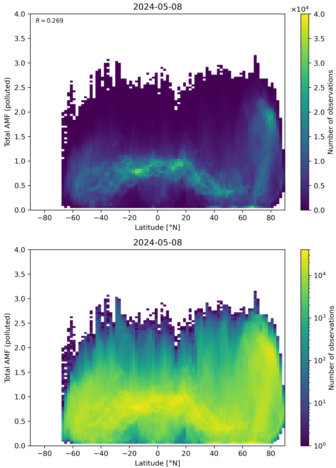
Figure 154: Scatter density plot of “Latitude” against “Total AMF (polluted)” for 2024-05-07 to 2024-05-09.
