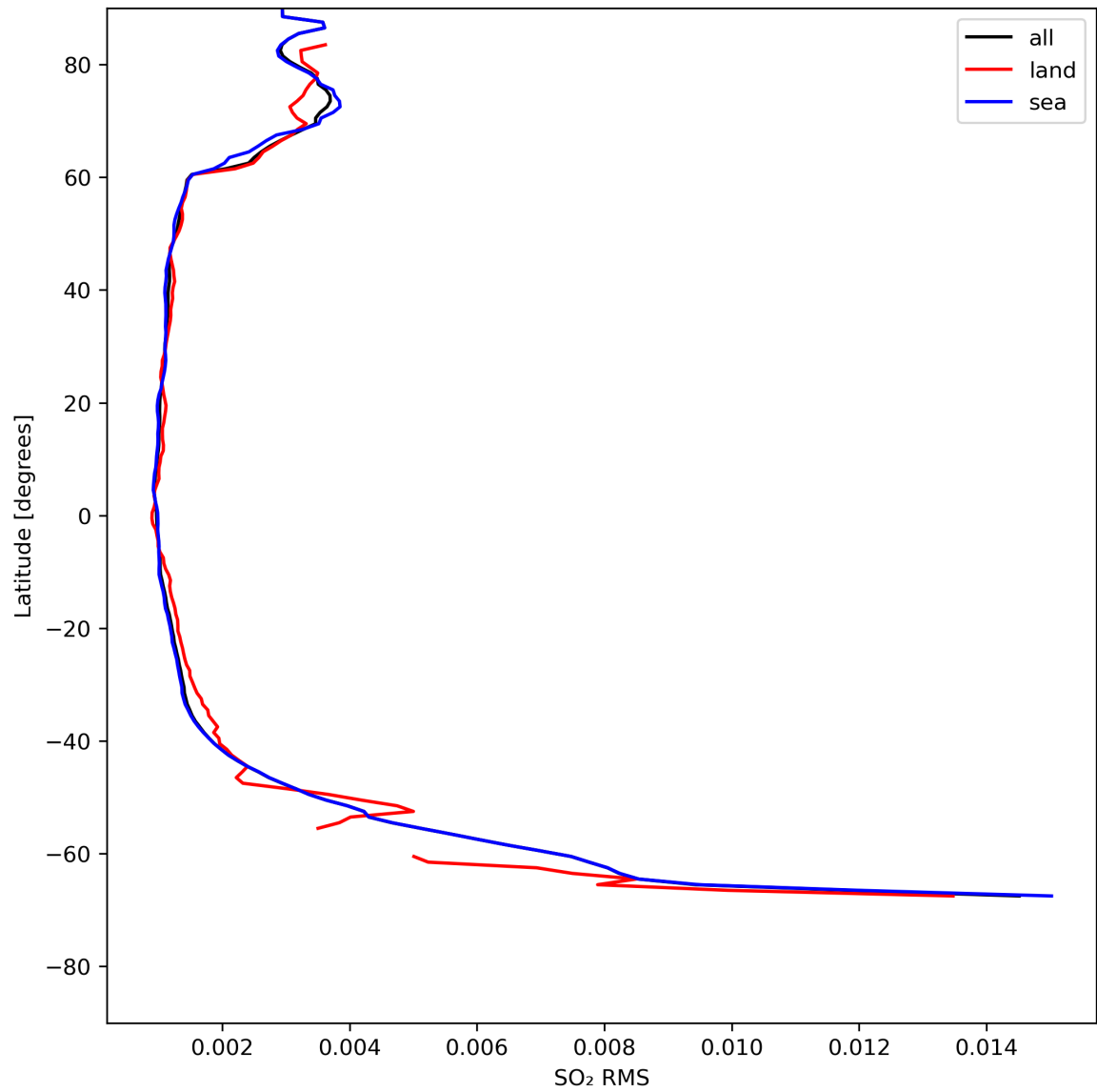
Figure 47: Zonal average of “SO 2 RMS” for 2024-05-07 to 2024-05-09.
