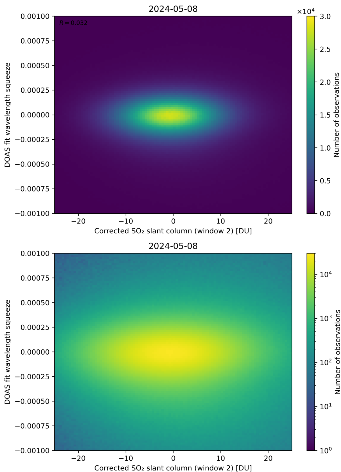
Figure 197: Scatter density plot of “Corrected SO 2 slant column (window 2)” against “DOAS fit wavelength squeeze” for 2024-05-07 to 2024-05-09.
