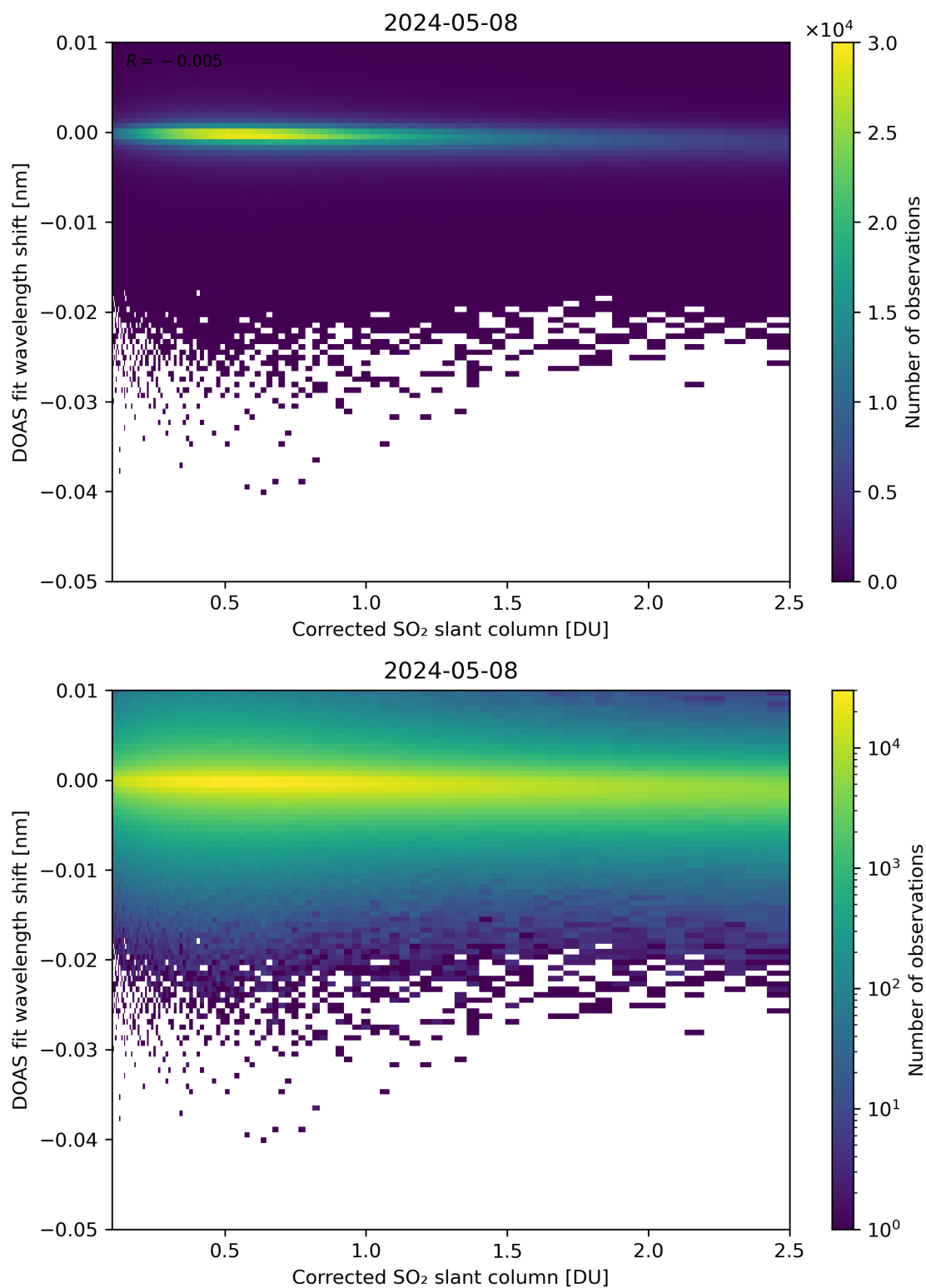
Figure 181: Scatter density plot of “Corrected SO 2 slant column” against “DOAS fit wavelength shift” for 2024-05-07 to 2024-05-09.
