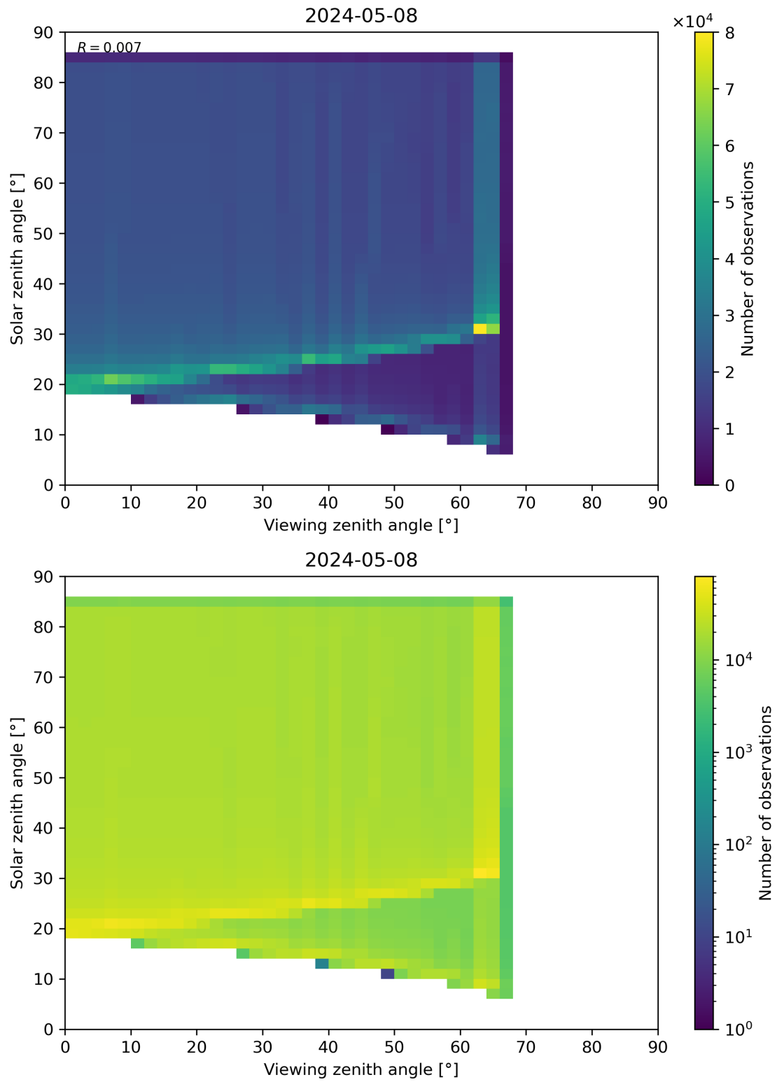
Figure 315: Scatter density plot of “Viewing zenith angle” against “Solar zenith angle” for 2024-05-07 to 2024-05-09.
