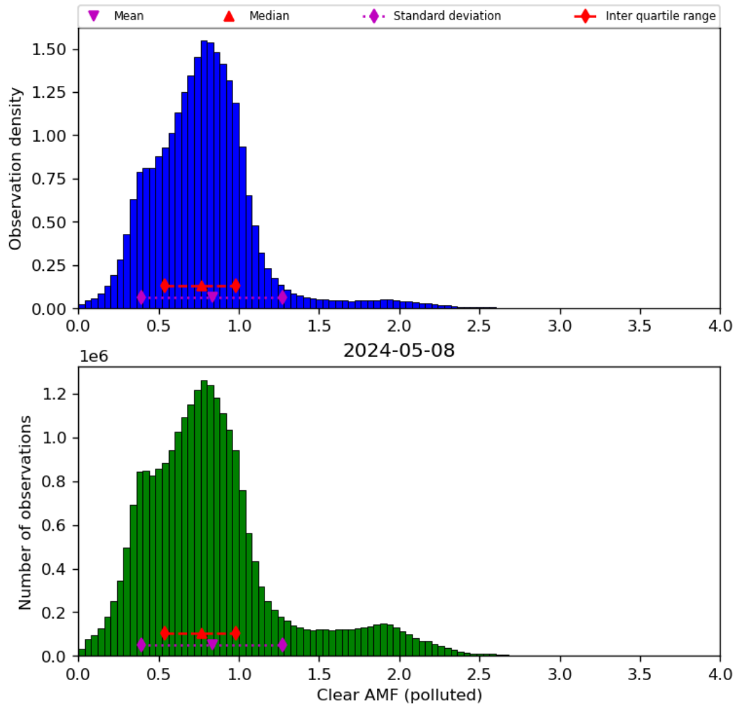
Figure 73: Histogram of “Clear AMF (polluted)” for 2024-05-07 to 2024-05-09
