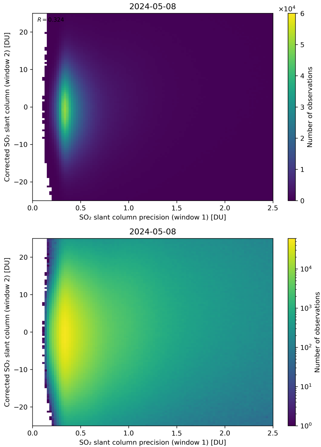
Figure 225: Scatter density plot of “SO 2 slant column precision (window 1)” against “Corrected SO 2 slant column (window 2)” for 2024-05-07 to 2024-05-09.
