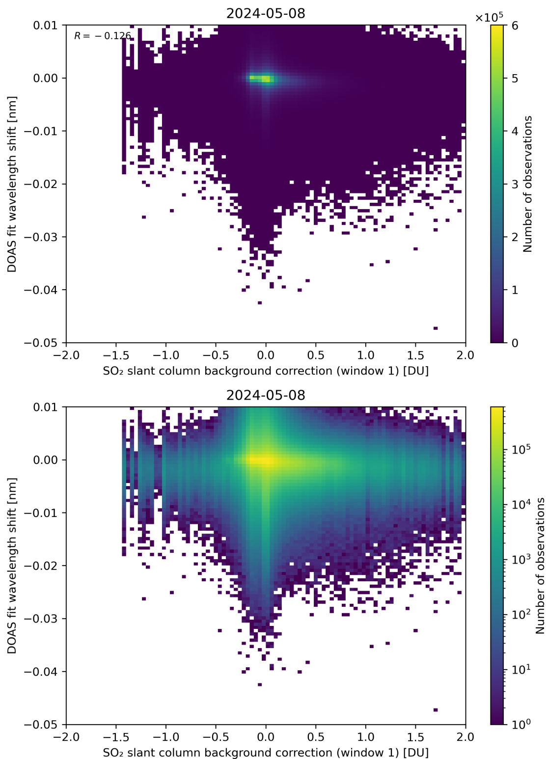
Figure 100: Scatter density plot of “SO 2 slant column background correction (window 1)” against “DOAS fit wavelength shift” for 2024-05-07 to 2024-05-09.
