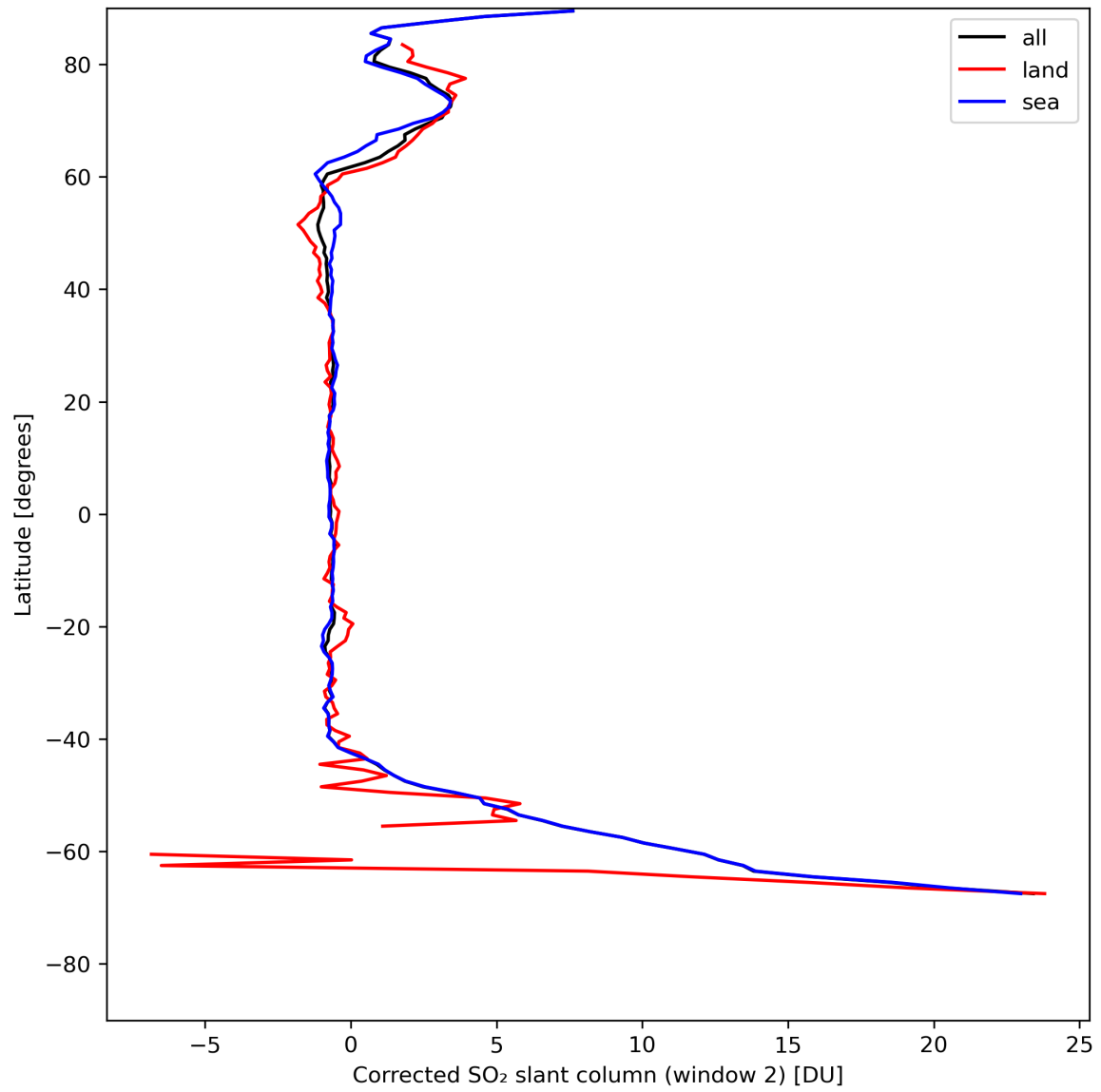
Figure 39: Zonal average of “Corrected SO 2 slant column (window 2)” for 2024-05-07 to 2024-05-09.
