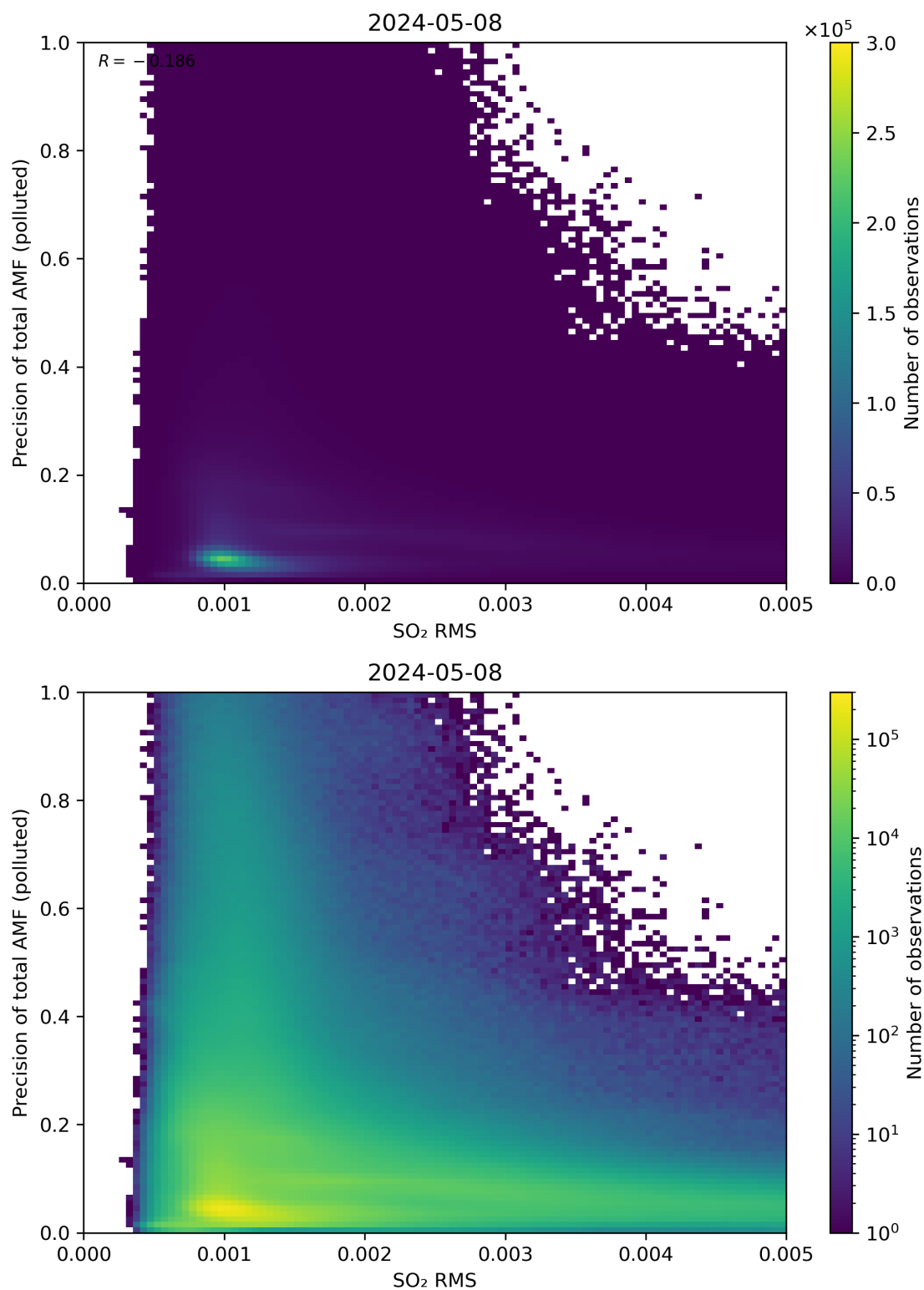
Figure 138: Scatter density plot of “SO 2 RMS” against “Precision of total AMF (polluted)” for 2024-05-07 to 2024-05-09.
