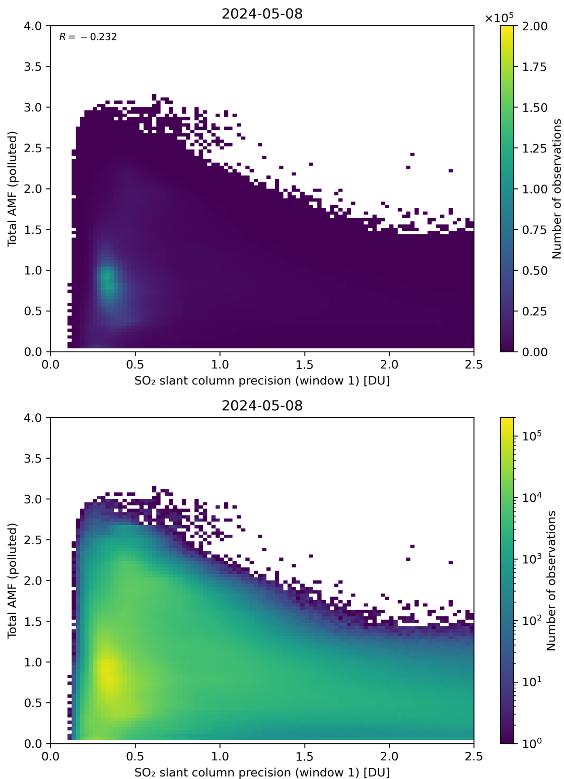
Figure 230: Scatter density plot of “SO 2 slant column precision (window 1)” against “Total AMF (polluted)” for 2024-05-07 to 2024-05-09.
