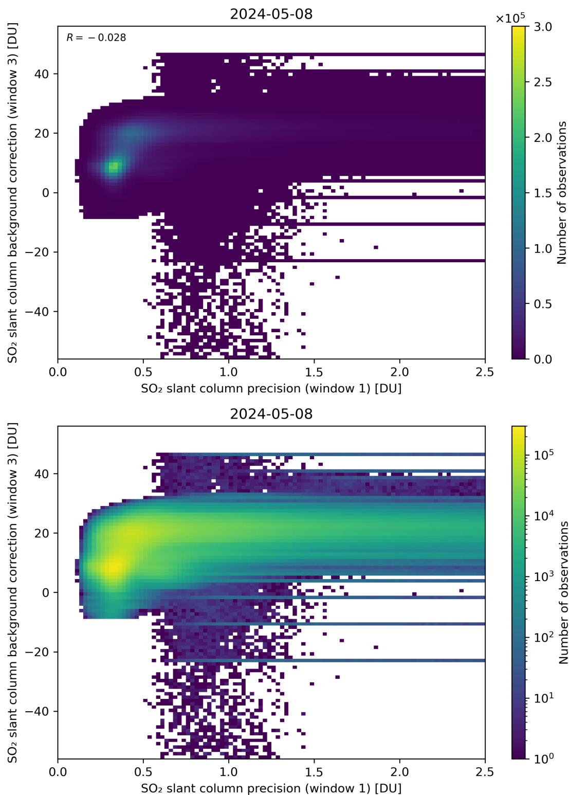
Figure 220: Scatter density plot of “SO 2 slant column precision (window 1)” against “SO 2 slant column background correction (window 3)” for 2024-05-07 to 2024-05-09.
