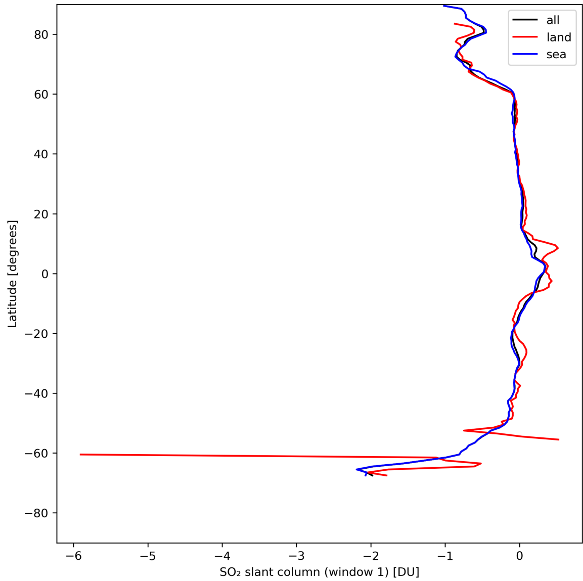
Figure 33: Zonal average of “SO 2 slant column (window 1)” for 2024-05-07 to 2024-05-09.
