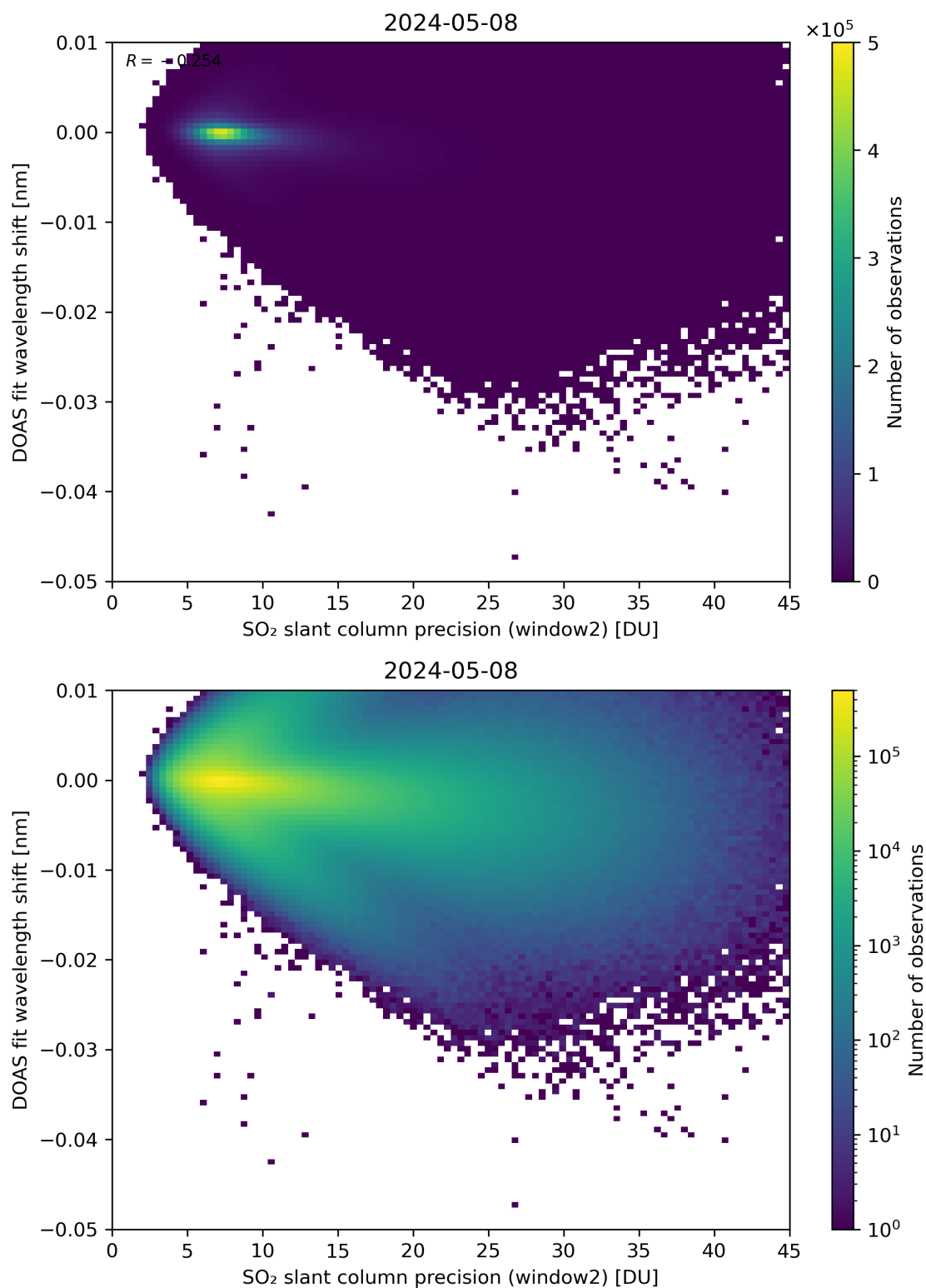
Figure 243: Scatter density plot of “SO 2 slant column precision (window2)” against “DOAS fit wavelength shift” for 2024-05-07 to 2024-05-09.
