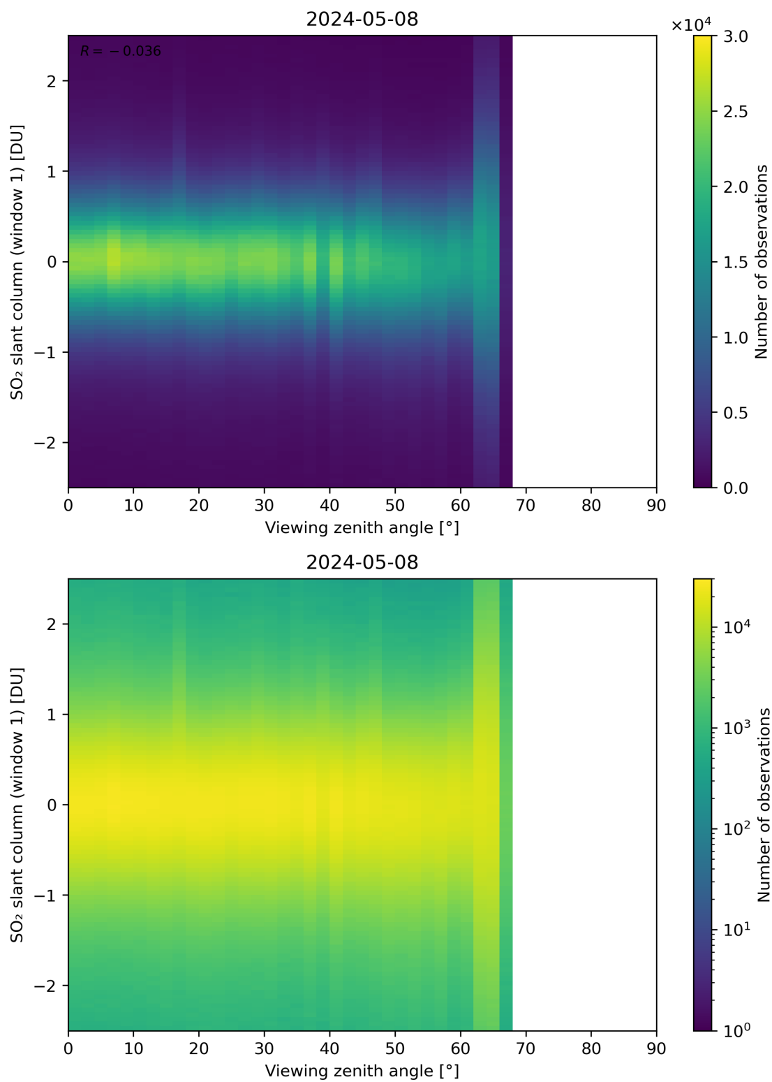
Figure 320: Scatter density plot of “Viewing zenith angle” against “SO 2 slant column (window 1)” for 2024-05-07 to 2024-05-09.
