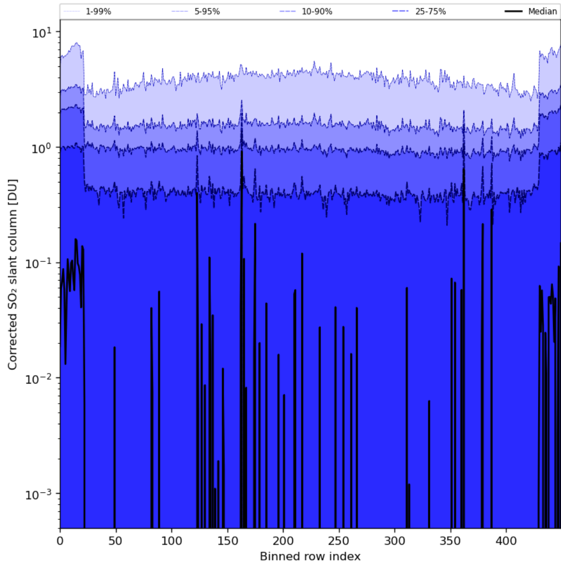
Figure 78: Along track statistics of “Corrected SO 2 slant column” for 2024-05-07 to 2024-05-09
