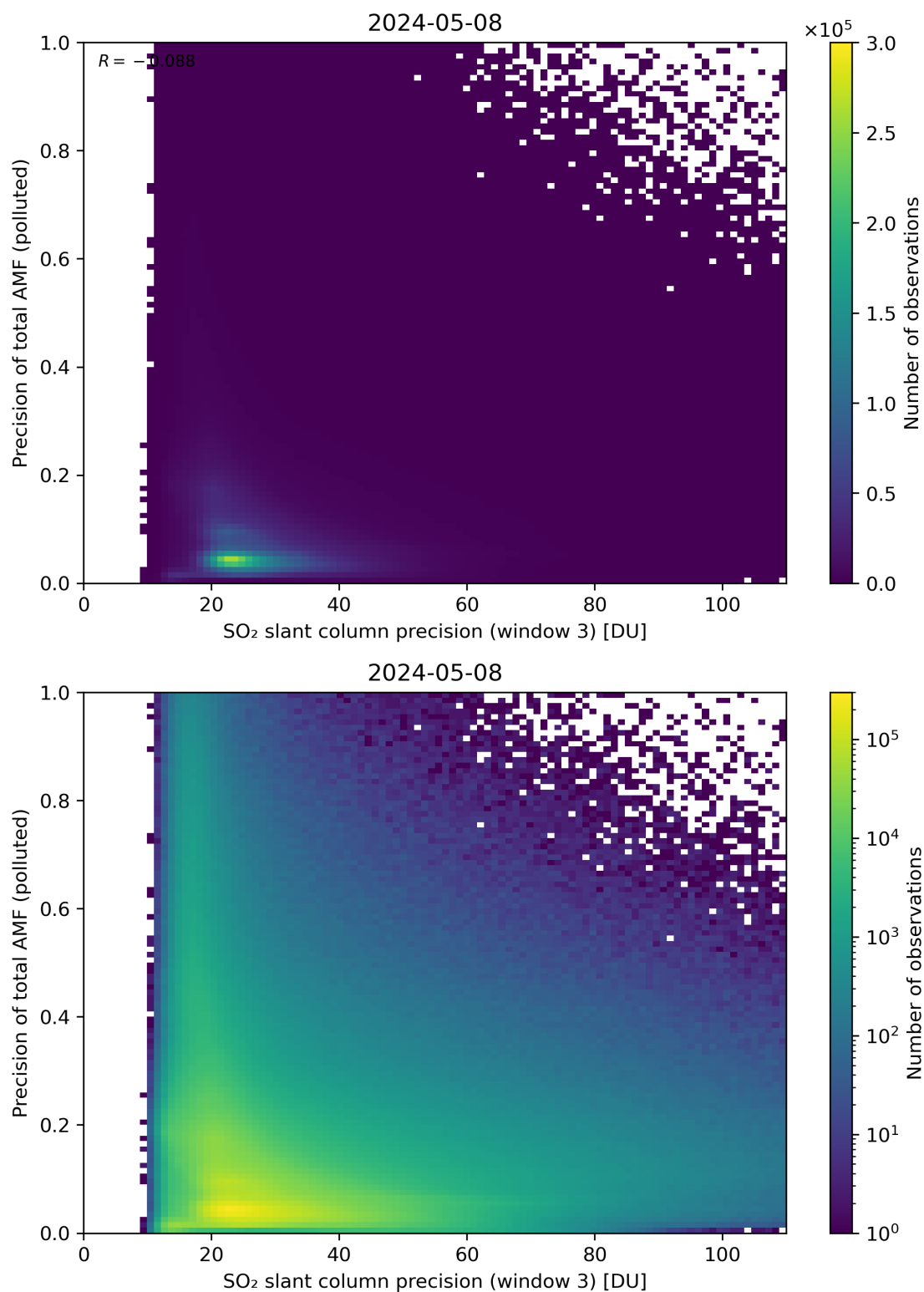
Figure 264: Scatter density plot of “SO 2 slant column precision (window 3)” against “Precision of total AMF (polluted)” for 2024-05-07 to 2024-05-09.
