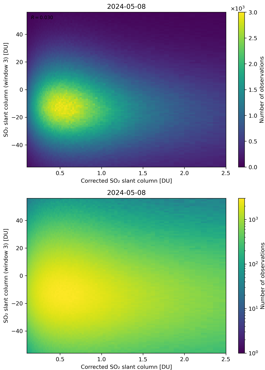
Figure 190: Scatter density plot of “Corrected SO 2 slant column” against “SO 2 slant column (window 3)” for 2024-05-07 to 2024-05-09.
