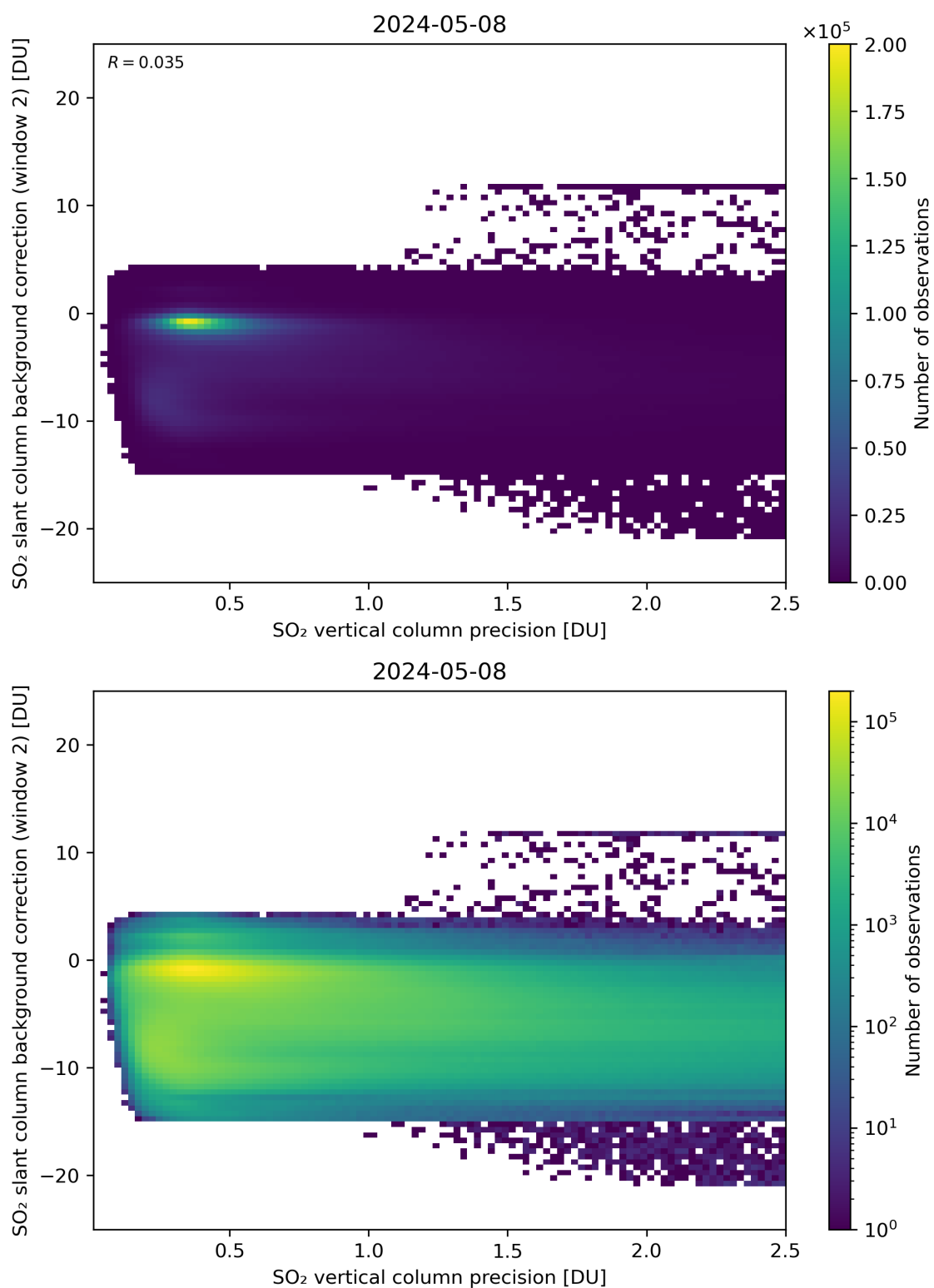
Figure 280: Scatter density plot of “SO 2 vertical column precision” against “SO 2 slant column background correction (window 2)” for 2024-05-07 to 2024-05-09.
