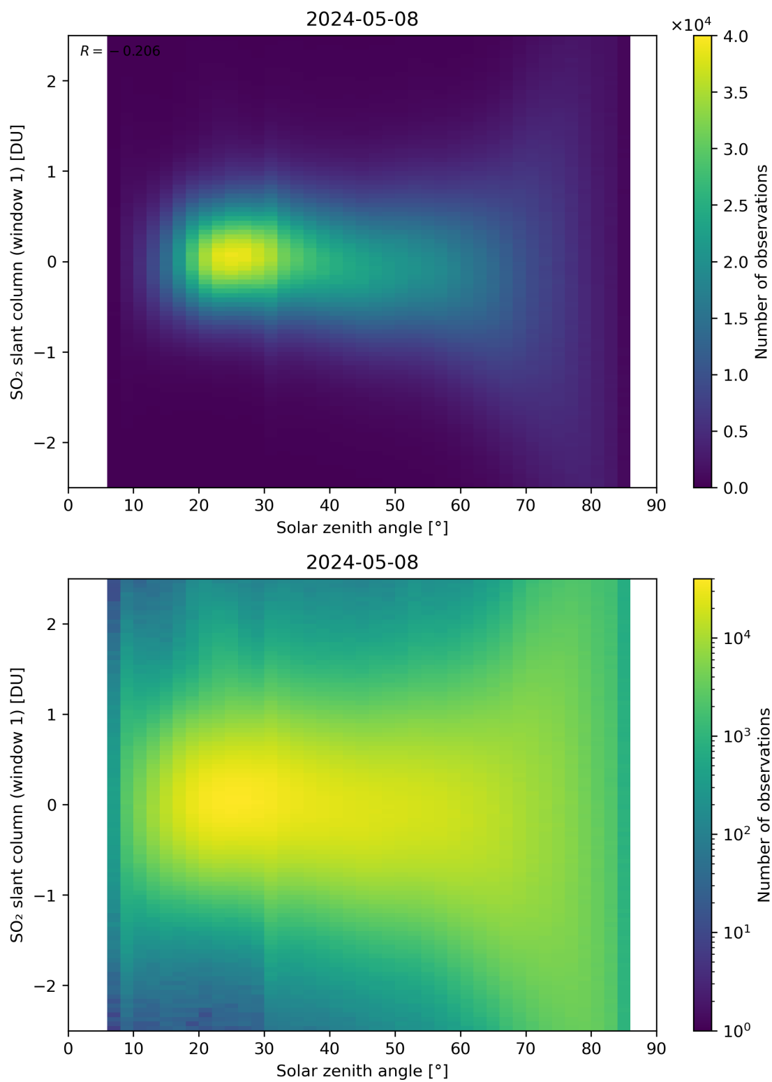
Figure 169: Scatter density plot of “Solar zenith angle” against “SO 2 slant column (window 1)” for 2024-05-07 to 2024-05-09.
