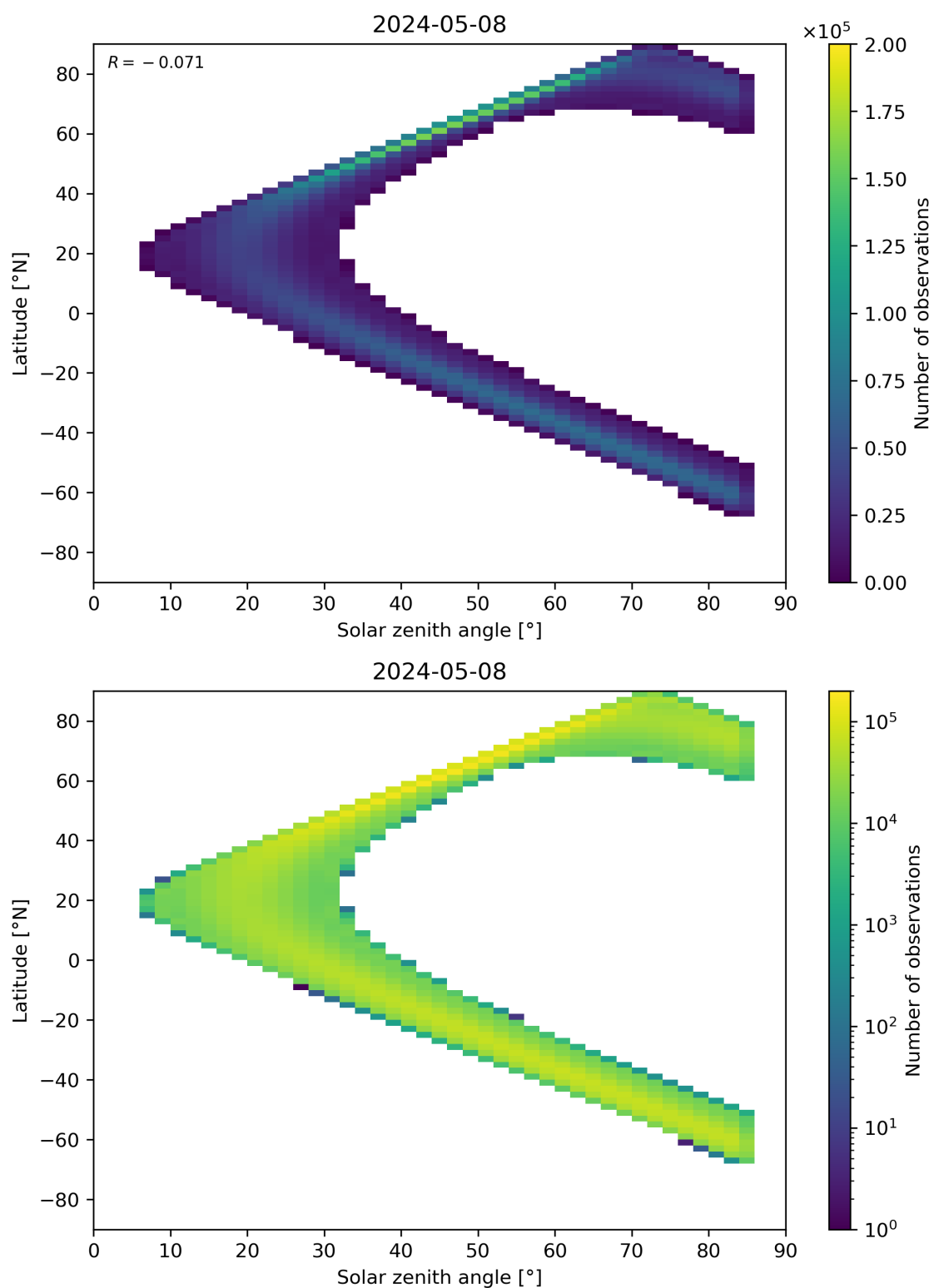
Figure 164: Scatter density plot of “Solar zenith angle” against “Latitude” for 2024-05-07 to 2024-05-09.
