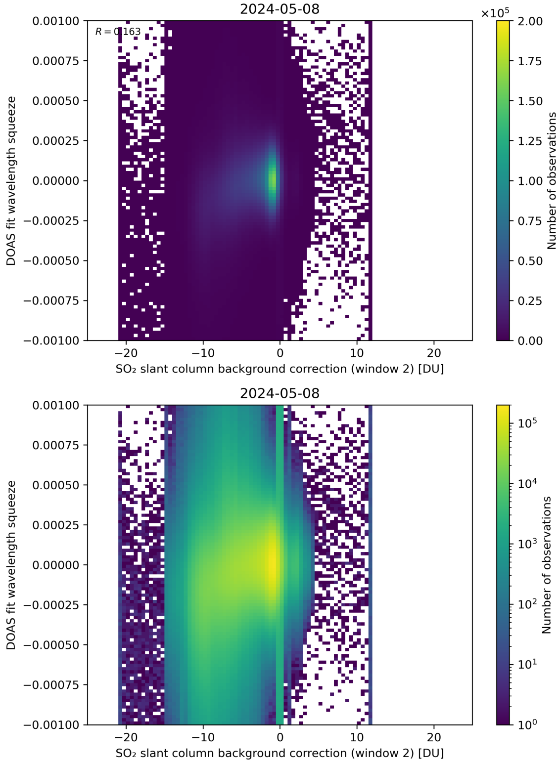
Figure 113: Scatter density plot of “SO 2 slant column background correction (window 2)” against “DOAS fit wavelength squeeze” for 2024-05-07 to 2024-05-09.
