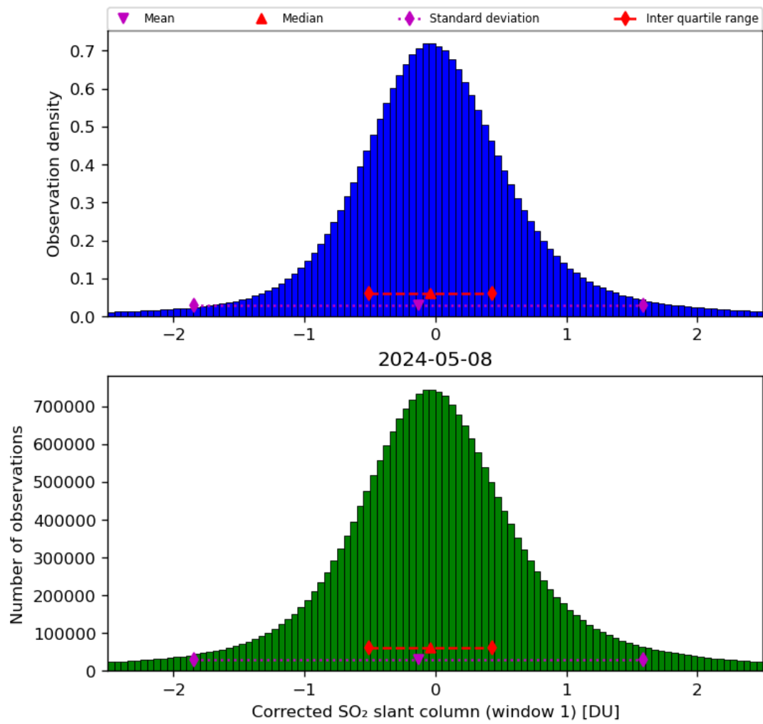
Figure 58: Histogram of “Corrected SO 2 slant column (window 1)” for 2024-05-07 to 2024-05-09
