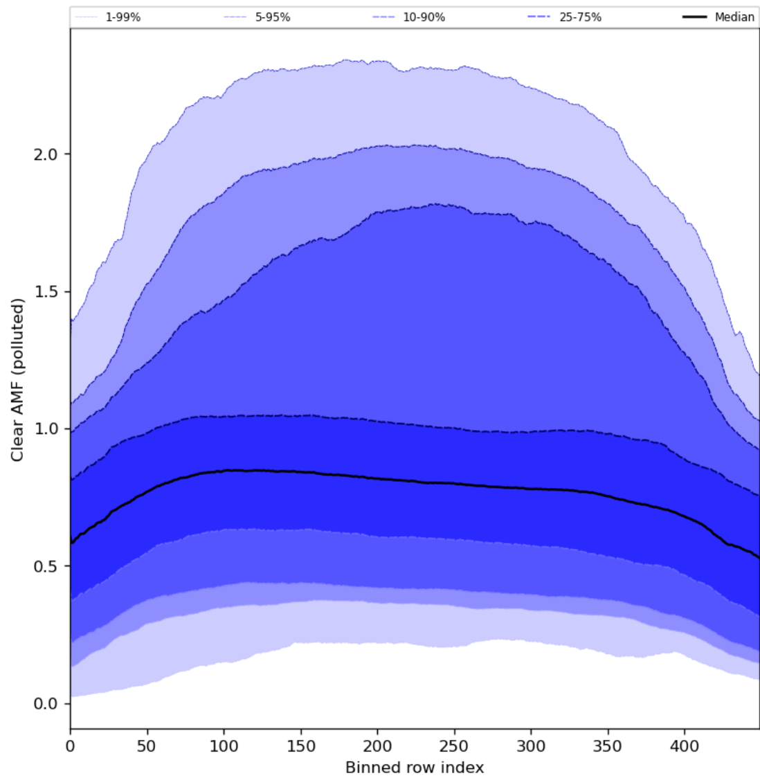
Figure 96: Along track statistics of “Clear AMF (polluted)” for 2024-05-07 to 2024-05-09
