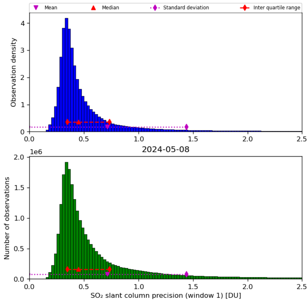
Figure 57: Histogram of “SO 2 slant column precision (window 1)” for 2024-05-07 to 2024-05-09
