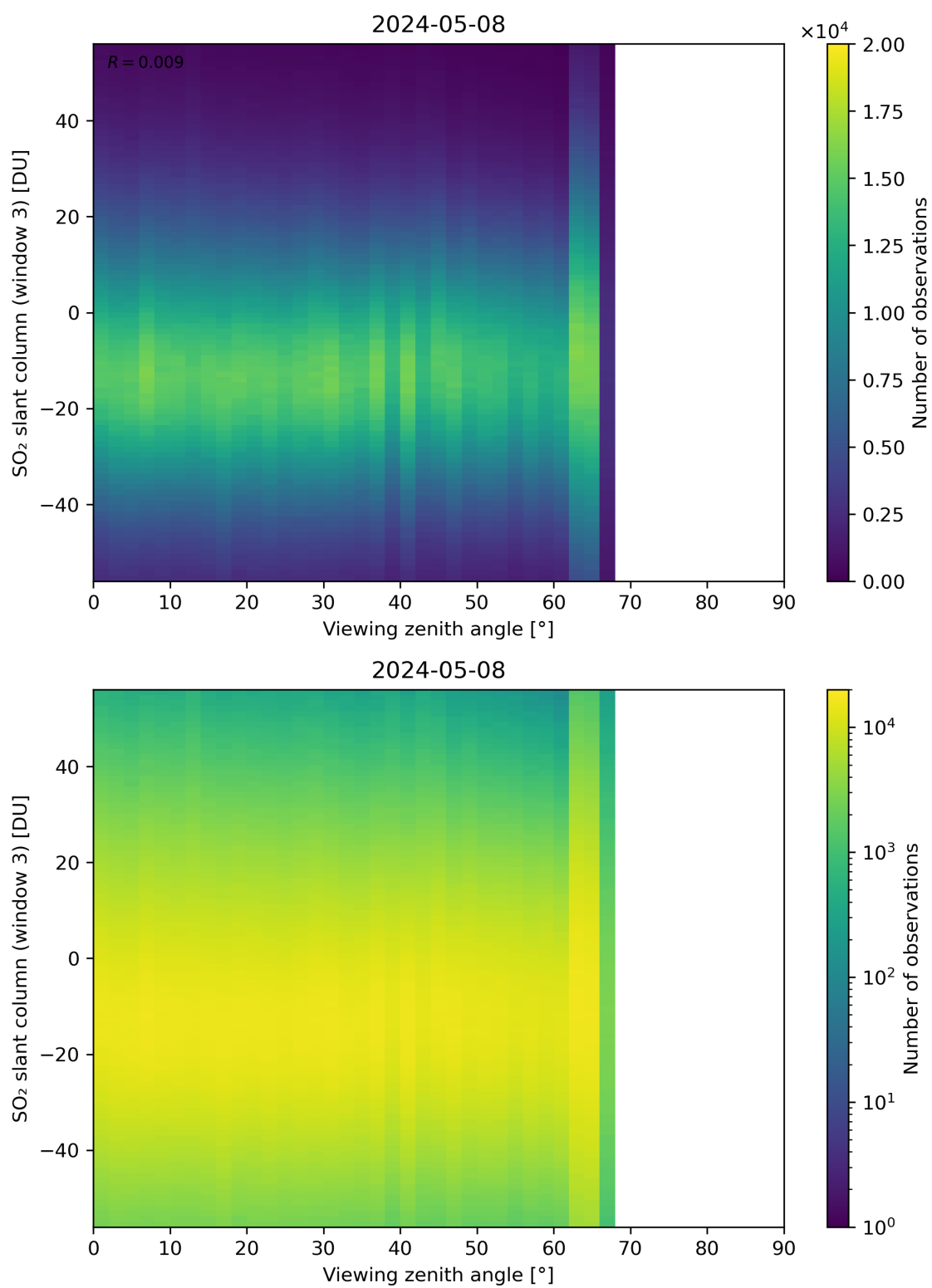
Figure 323: Scatter density plot of “Viewing zenith angle” against “SO 2 slant column (window 3)” for 2024-05-07 to 2024-05-09.
