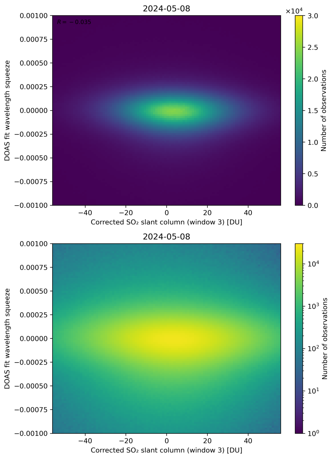
Figure 207: Scatter density plot of “Corrected SO 2 slant column (window 3)” against “DOAS fit wavelength squeeze” for 2024-05-07 to 2024-05-09.
