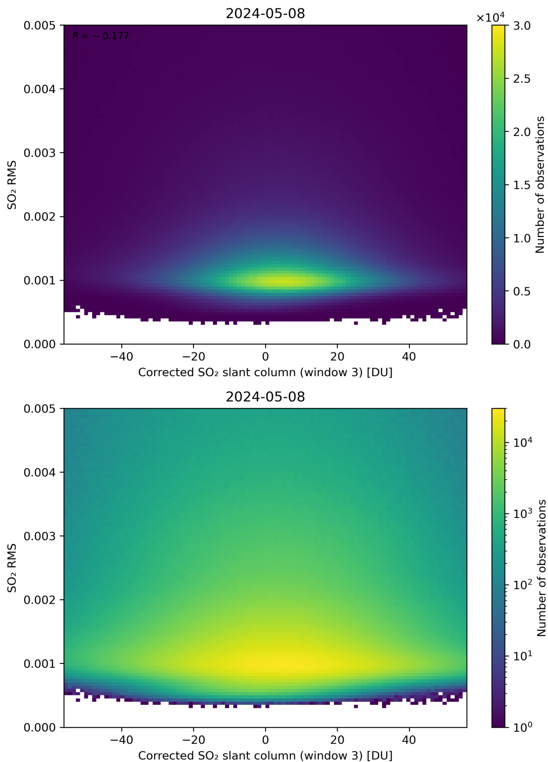
Figure 208: Scatter density plot of “Corrected SO 2 slant column (window 3)” against “SO 2 RMS” for 2024-05-07 to 2024-05-09.
