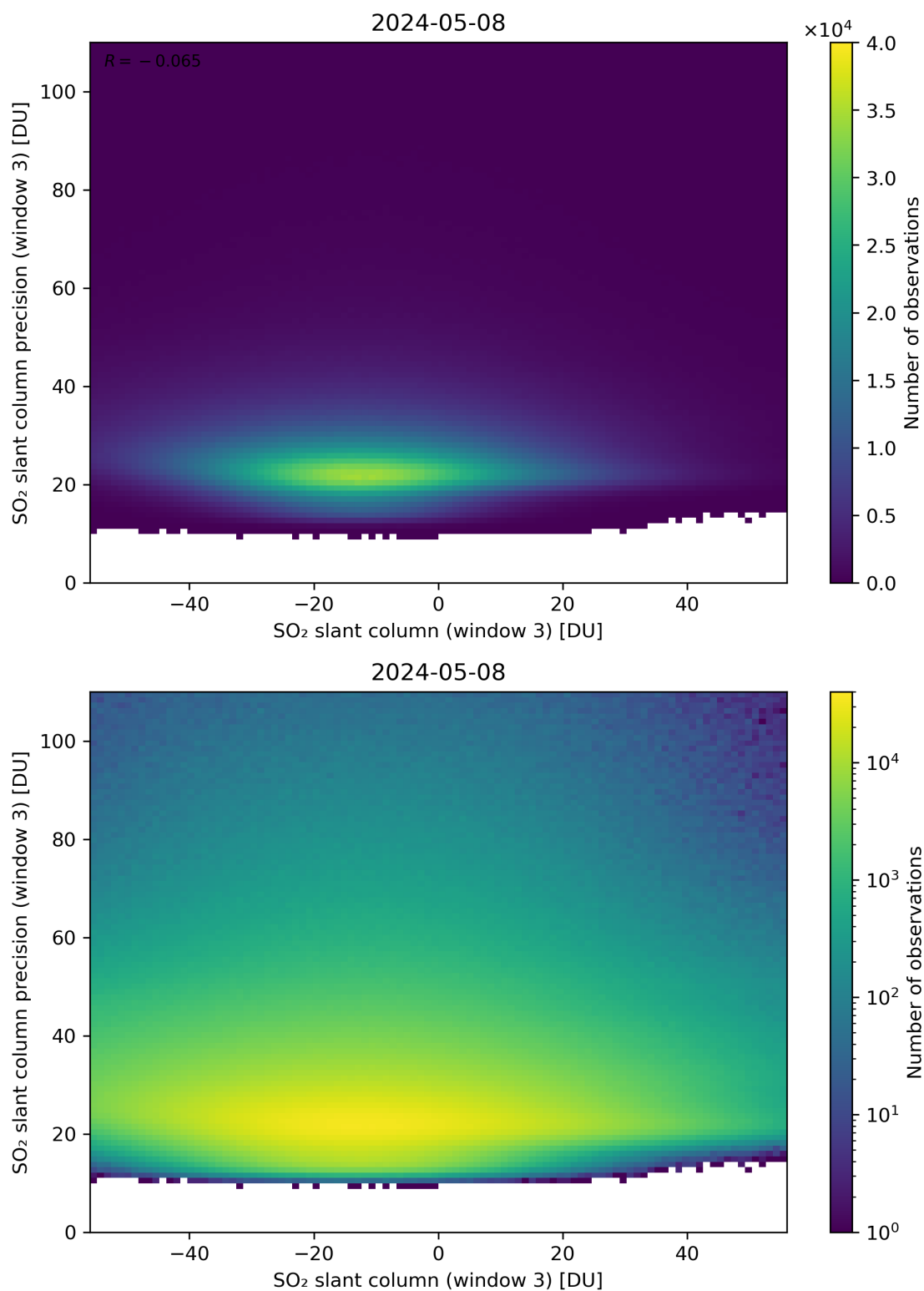
Figure 267: Scatter density plot of “SO 2 slant column (window 3)” against “SO 2 slant column precision (window 3)” for 2024-05-07 to 2024-05-09.
