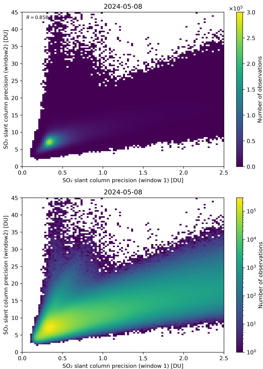
Figure 227: Scatter density plot of “SO 2 slant column precision (window 1)” against “SO 2 slant column precision (window2)” for 2024-05-07 to 2024-05-09.
