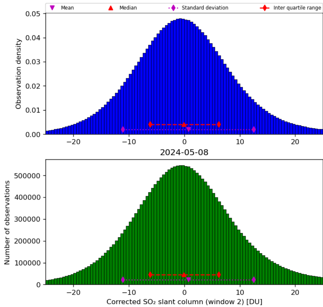
Figure 62: Histogram of “Corrected SO 2 slant column (window 2)” for 2024-05-07 to 2024-05-09
