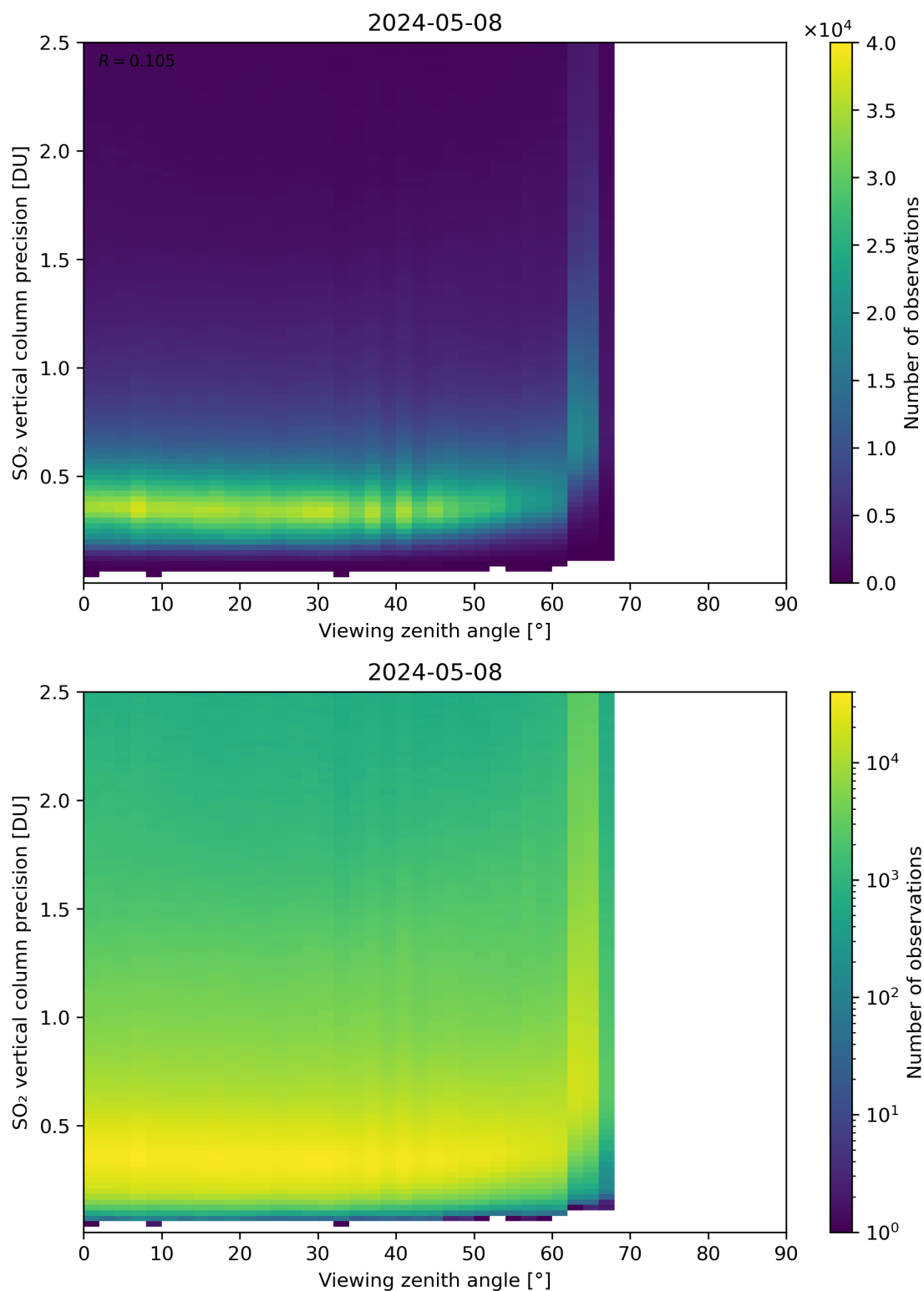
Figure 328: Scatter density plot of “Viewing zenith angle” against “SO 2 vertical column precision” for 2024-05-07 to 2024-05-09.
