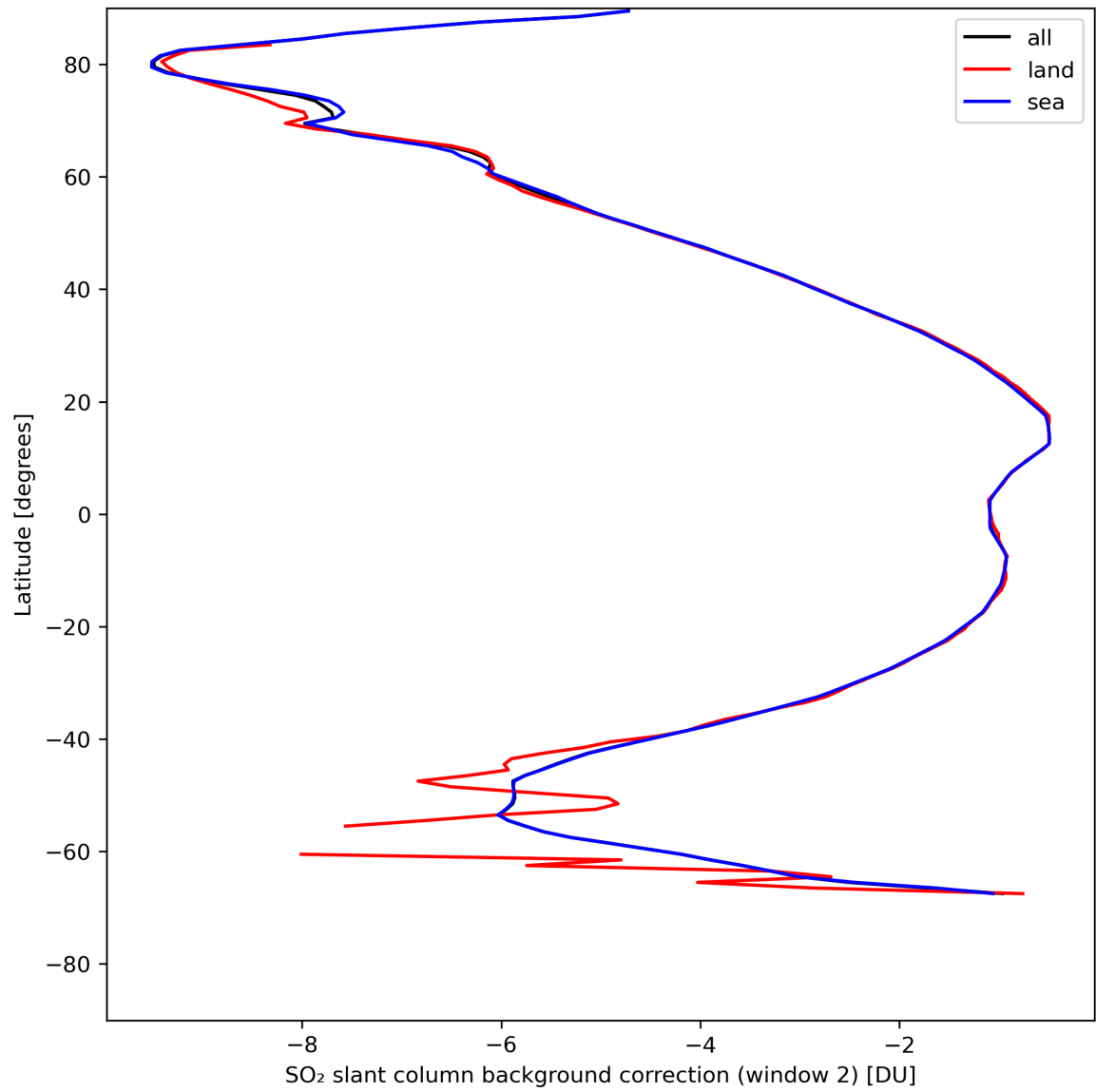
Figure 40: Zonal average of “SO 2 slant column background correction (window 2)” for 2024-05-07 to 2024-05-09.
