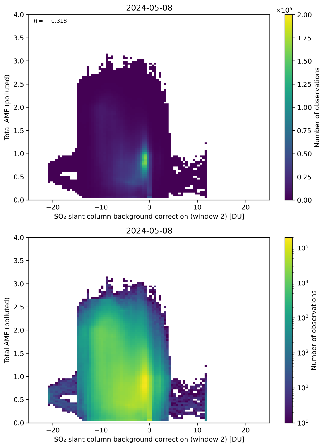
Figure 119: Scatter density plot of “SO 2 slant column background correction (window 2)” against “Total AMF (polluted)” for 2024-05-07 to 2024-05-09.
