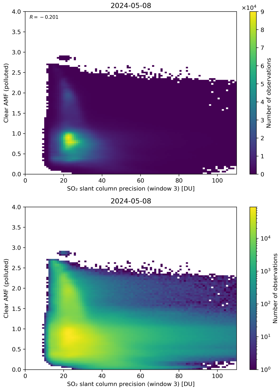
Figure 261: Scatter density plot of “SO 2 slant column precision (window 3)” against “Clear AMF (polluted)” for 2024-05-07 to 2024-05-09.
