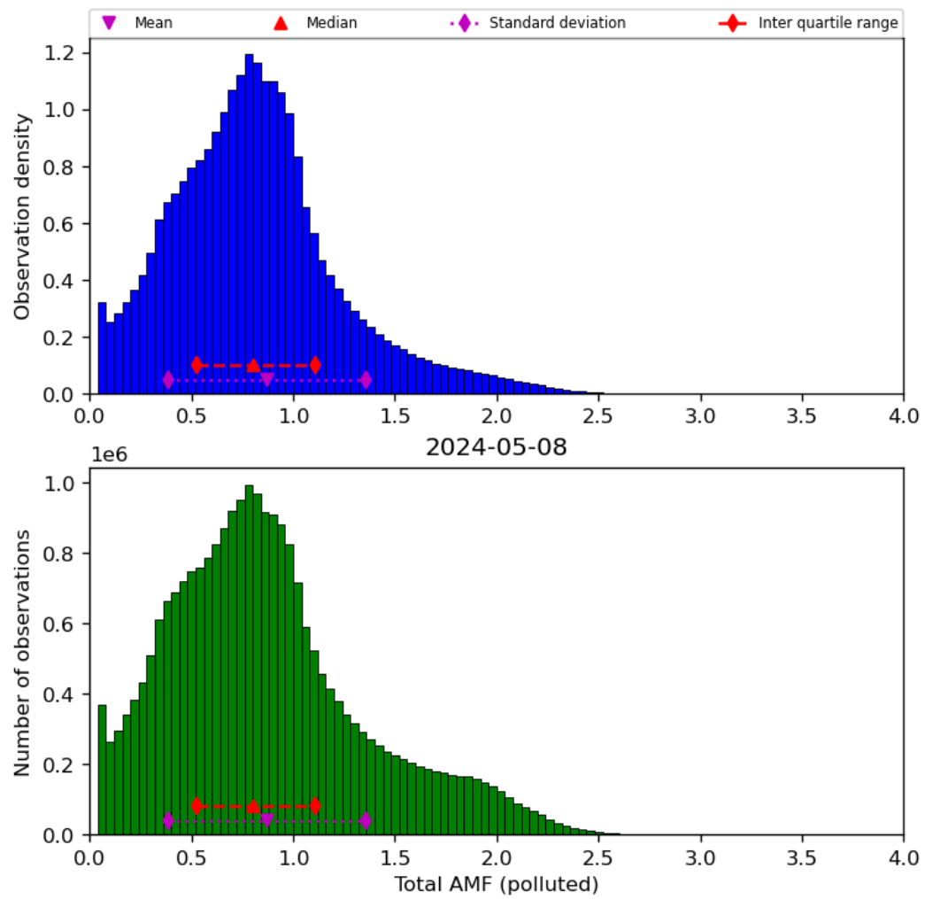
Figure 71: Histogram of “Total AMF (polluted)” for 2024-05-07 to 2024-05-09
