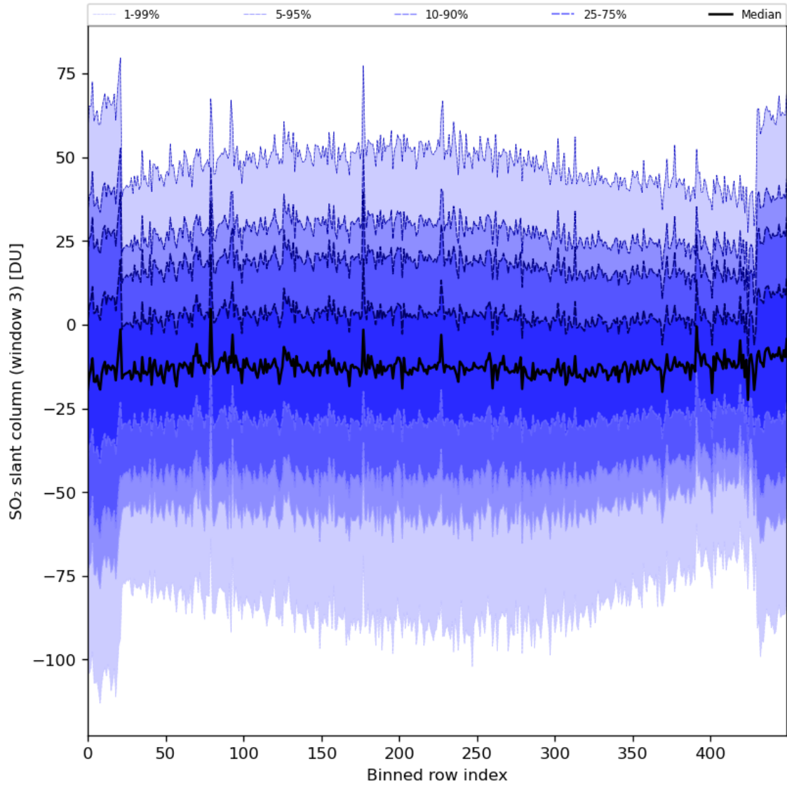
Figure 87: Along track statistics of "SO 2 slant column (window 3)" for 2024-05-07 to 2024-05-09
