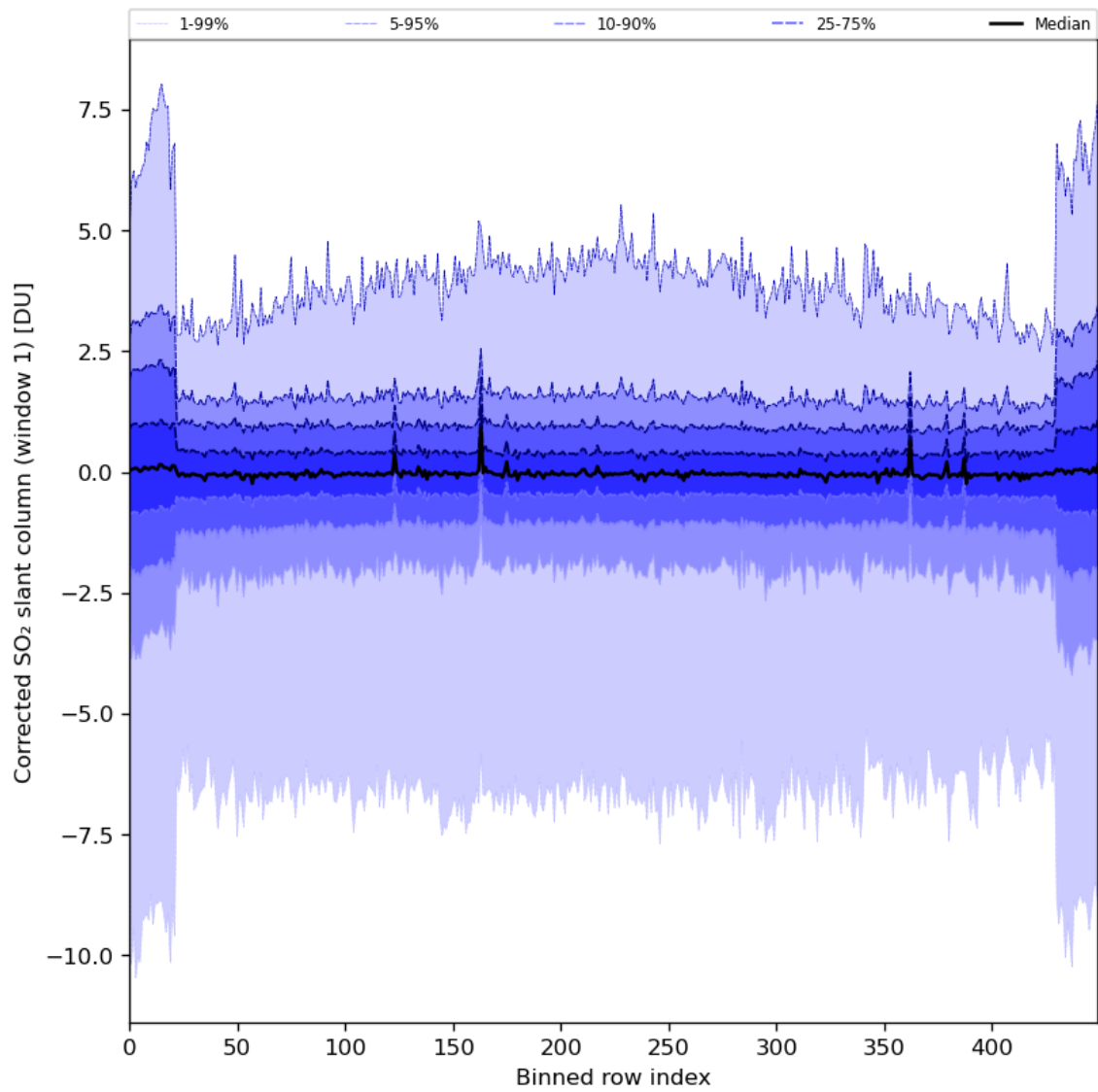
Figure 81: Along track statistics of “Corrected SO 2 slant column (window 1)” for 2024-05-07 to 2024-05-09
