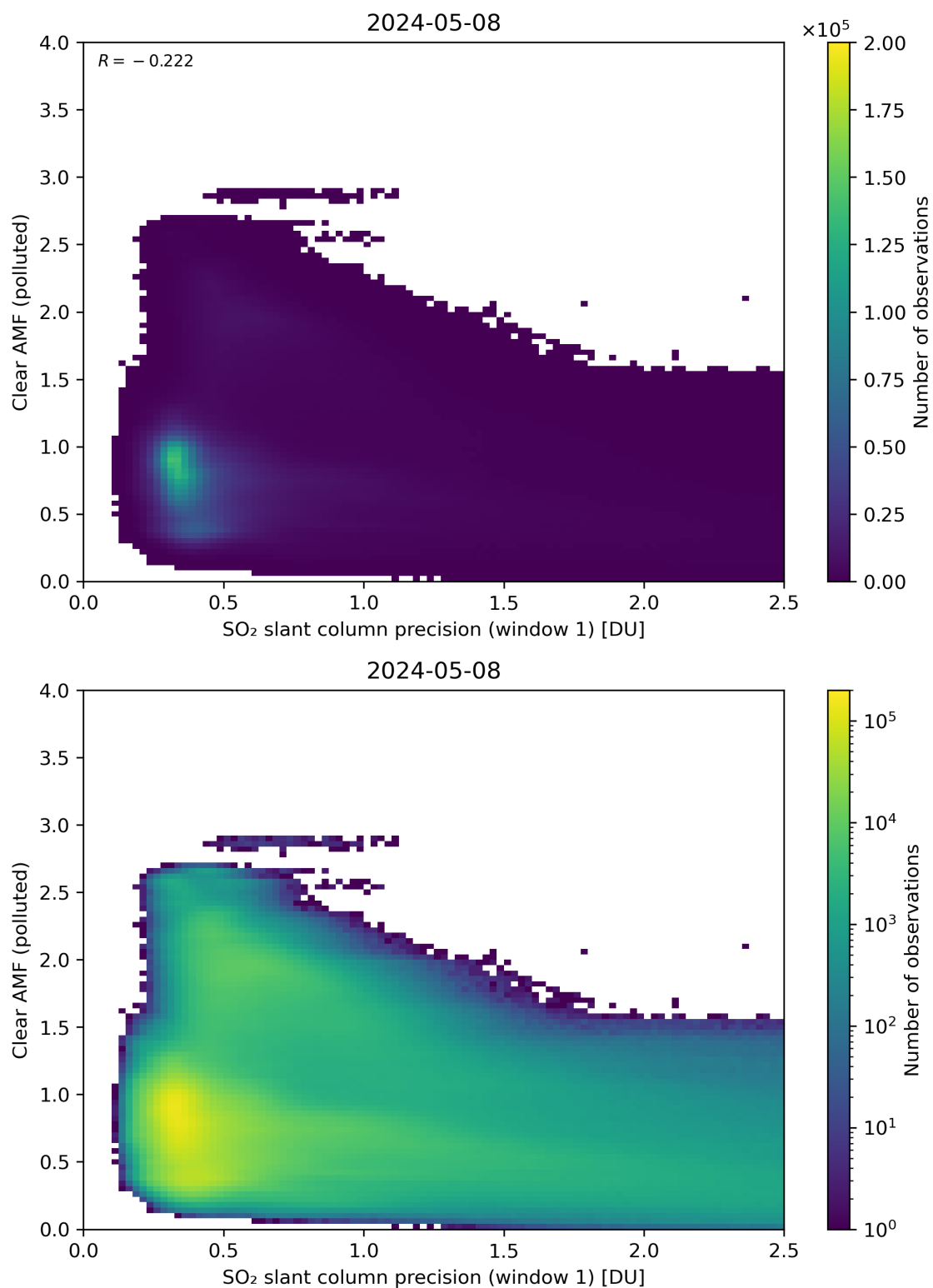
Figure 224: Scatter density plot of “SO 2 slant column precision (window 1)” against “Clear AMF (polluted)” for 2024-05-07 to 2024-05-09.
