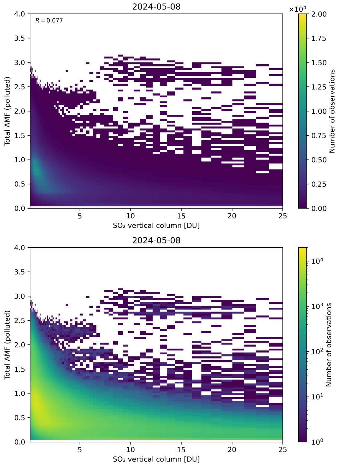
Figure 305: Scatter density plot of “SO 2 vertical column” against “Total AMF (polluted)” for 2024-05-07 to 2024-05-09.
