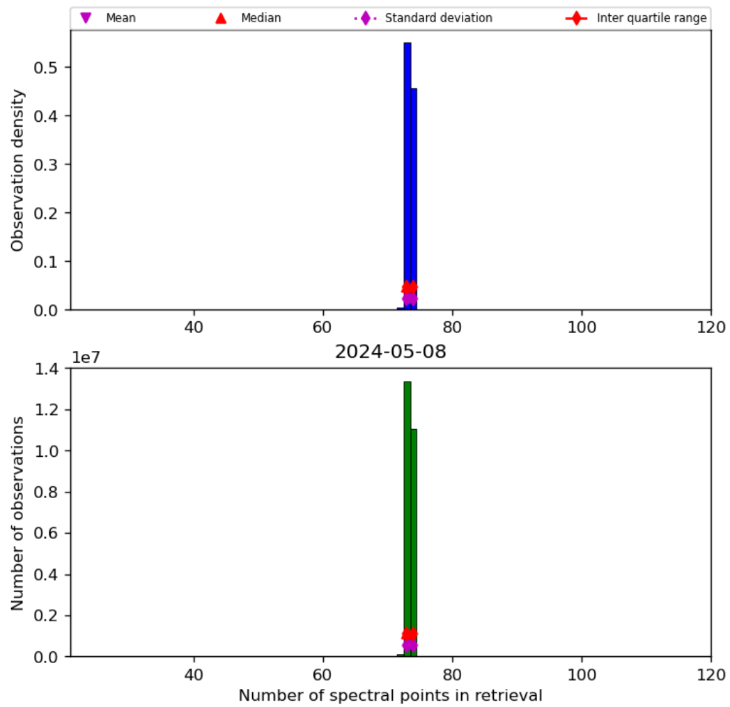
Figure 74: Histogram of “Number of spectral points in retrieval” for 2024-05-07 to 2024-05-09
