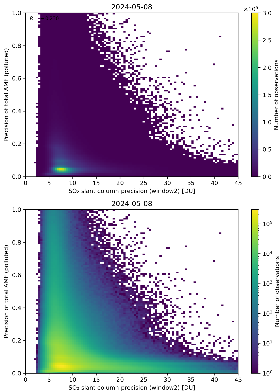
Figure 252: Scatter density plot of “SO 2 slant column precision (window2)” against “Precision of total AMF (polluted)” for 2024-05-07 to 2024-05-09.
