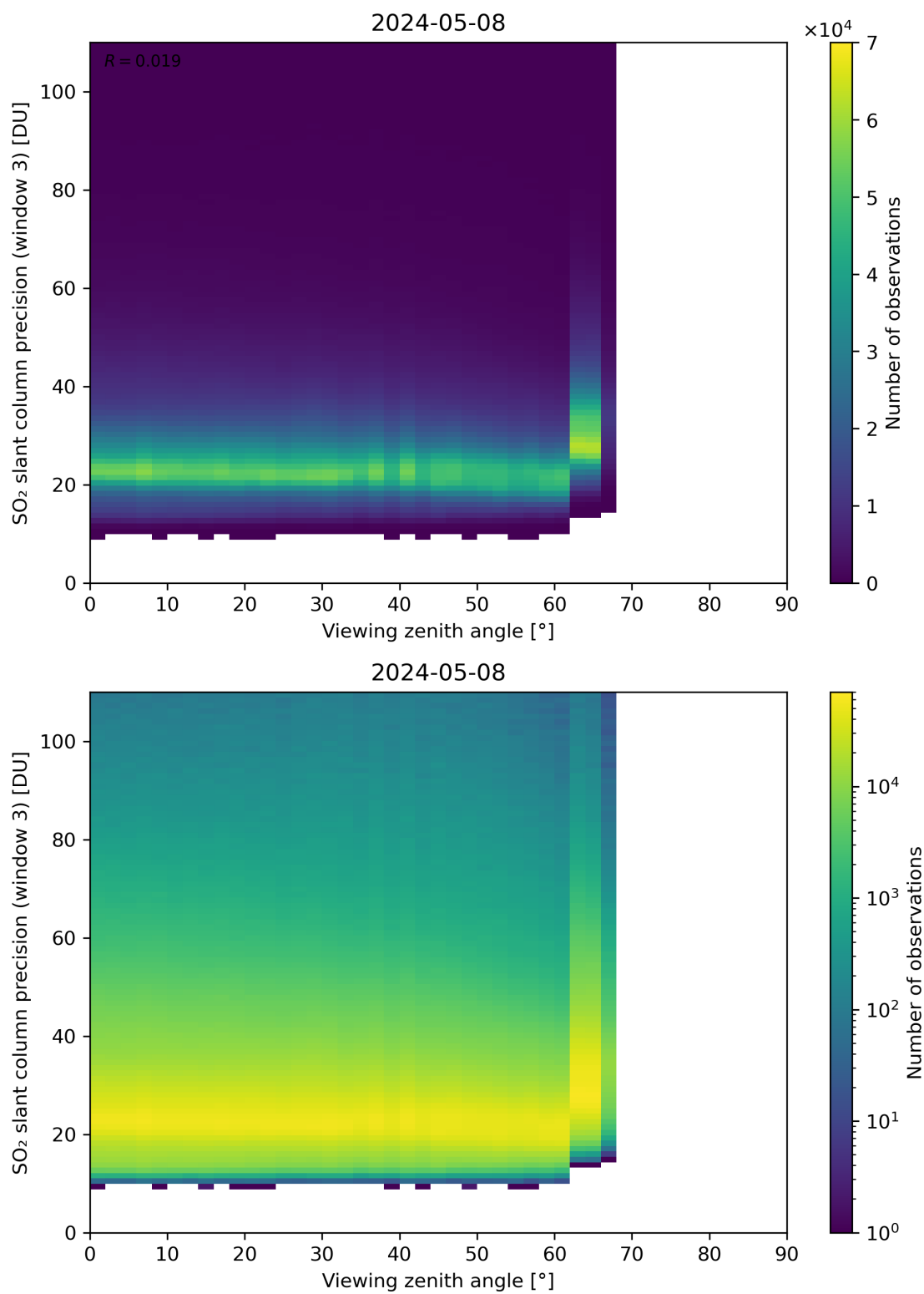
Figure 324: Scatter density plot of “Viewing zenith angle” against “SO 2 slant column precision (window 3)” for 2024-05-07 to 2024-05-09.
