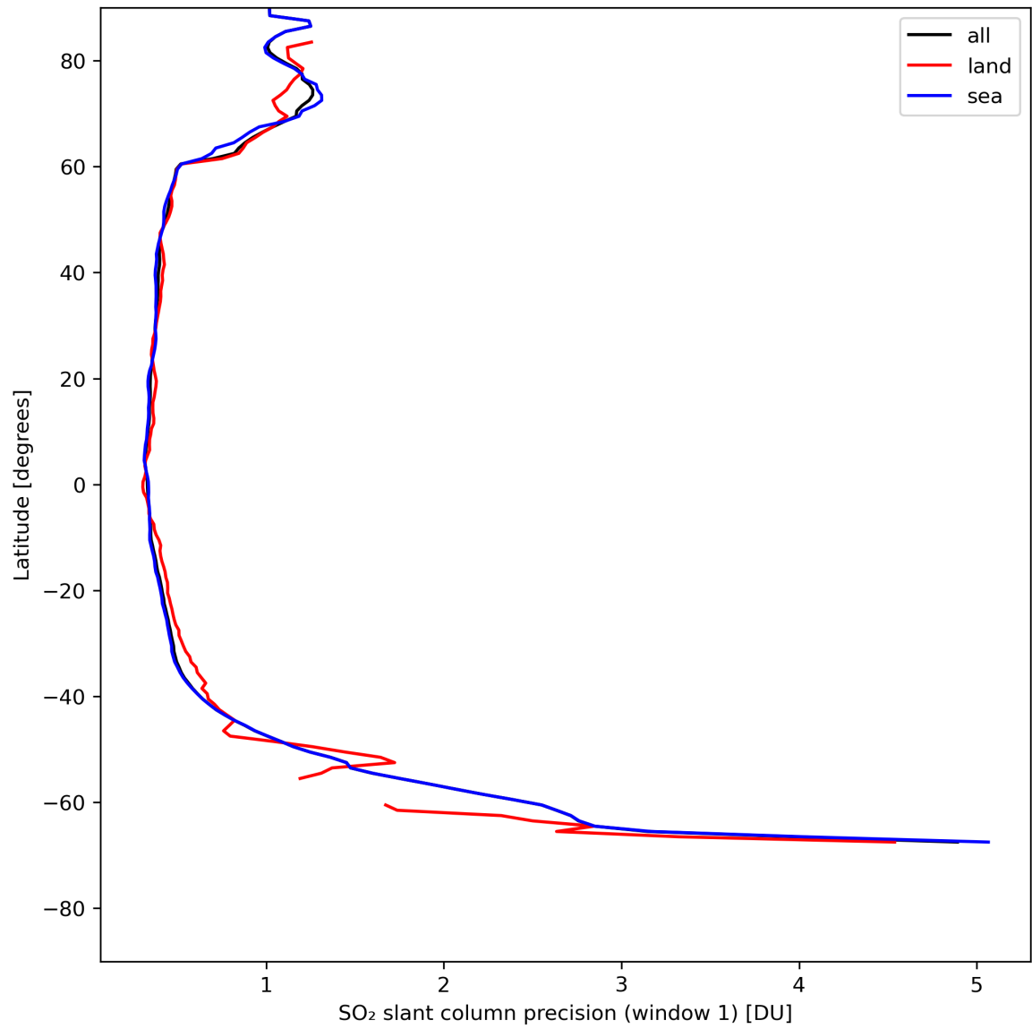
Figure 34: Zonal average of “SO 2 slant column precision (window 1)” for 2024-05-07 to 2024-05-09.
