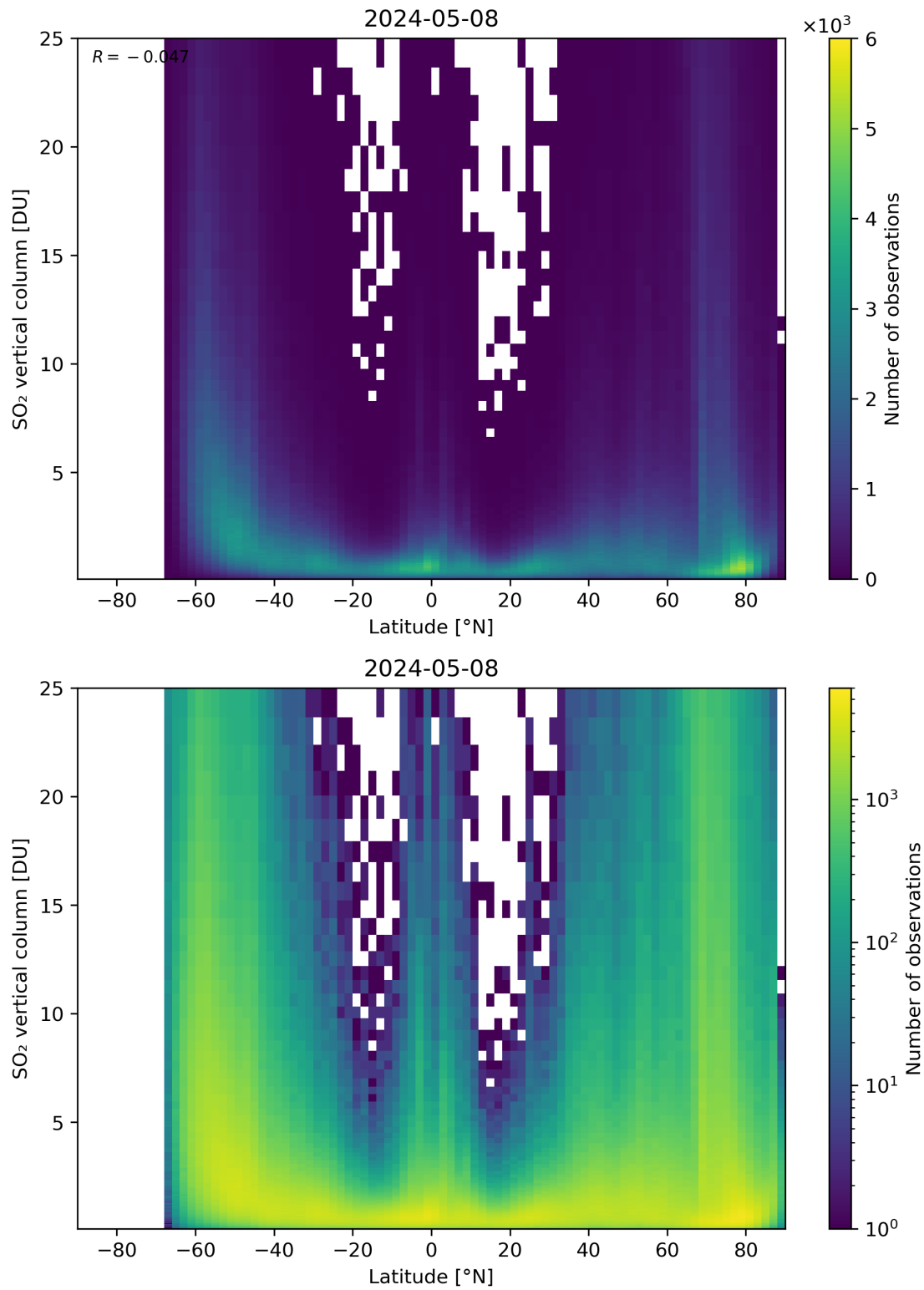
Figure 156: Scatter density plot of “Latitude” against “SO 2 vertical column” for 2024-05-07 to 2024-05-09.
