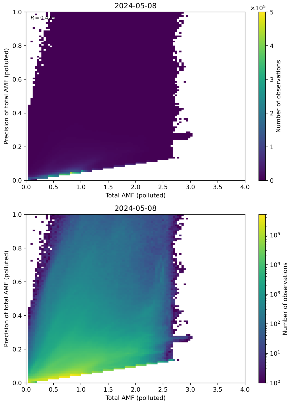
Figure 272: Scatter density plot of “Total AMF (polluted)” against “Precision of total AMF (polluted)” for 2024-05-07 to 2024-05-09.
