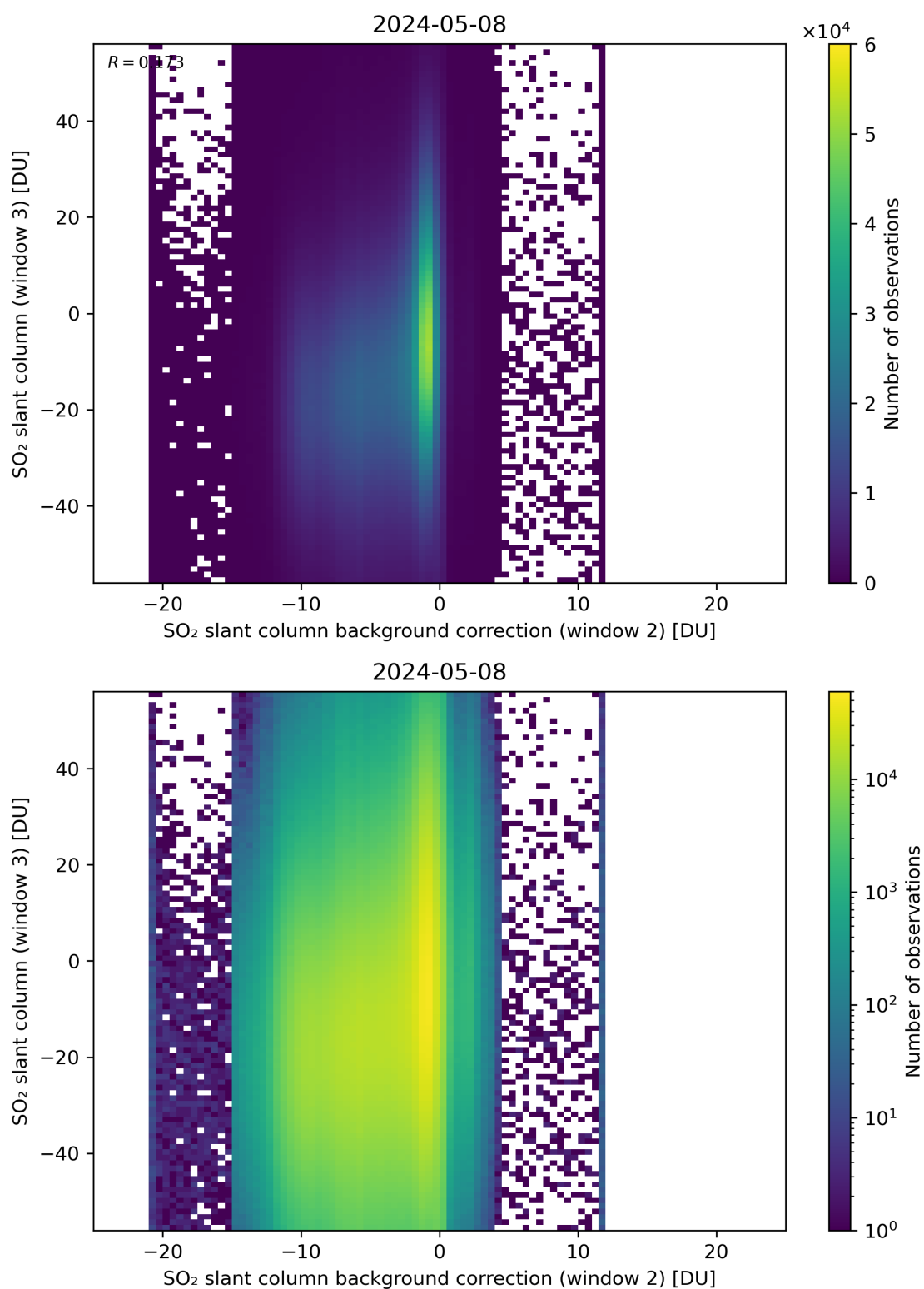
Figure 117: Scatter density plot of “SO 2 slant column background correction (window 2)” against “SO 2 slant column (window 3)” for 2024-05-07 to 2024-05-09.
