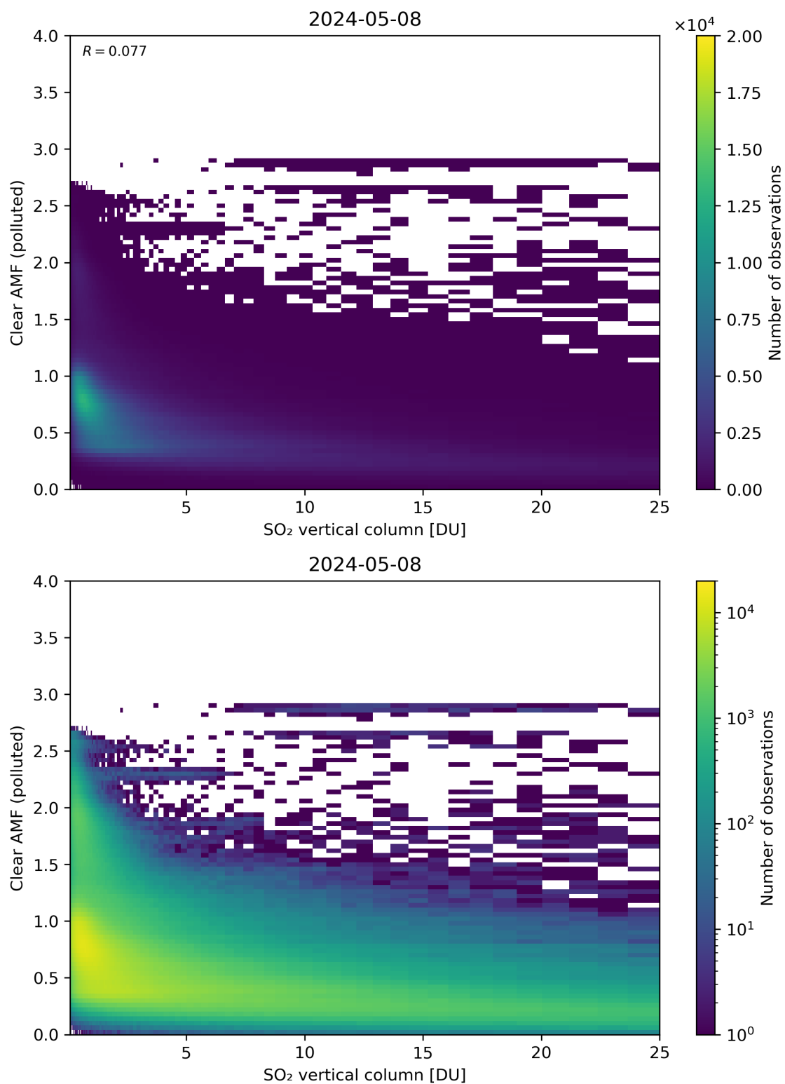
Figure 296: Scatter density plot of “SO 2 vertical column” against “Clear AMF (polluted)” for 2024-05-07 to 2024-05-09.
