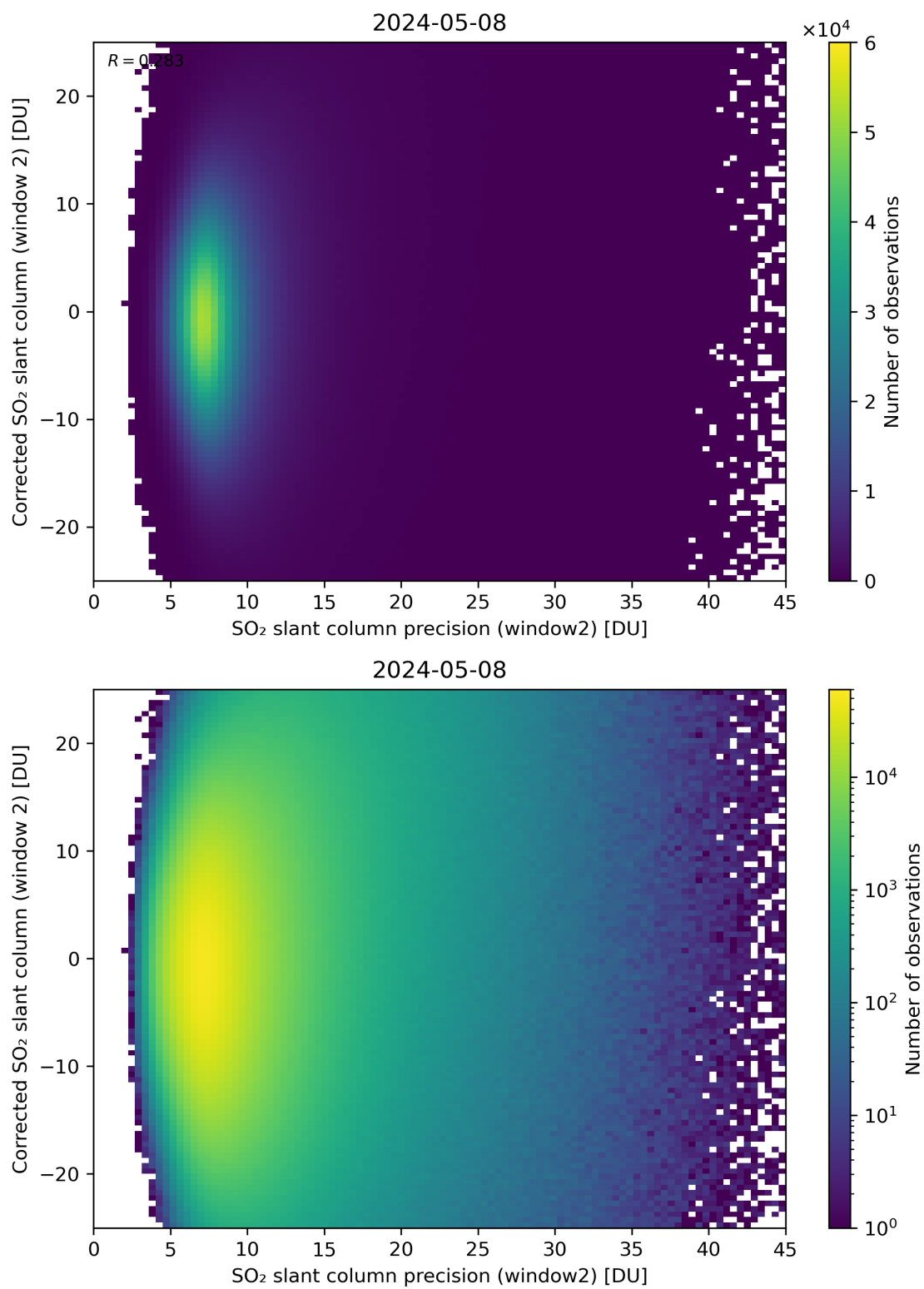
Figure 247: Scatter density plot of “SO 2 slant column precision (window2)” against “Corrected SO 2 slant column (window 2)” for 2024-05-07 to 2024-05-09.
