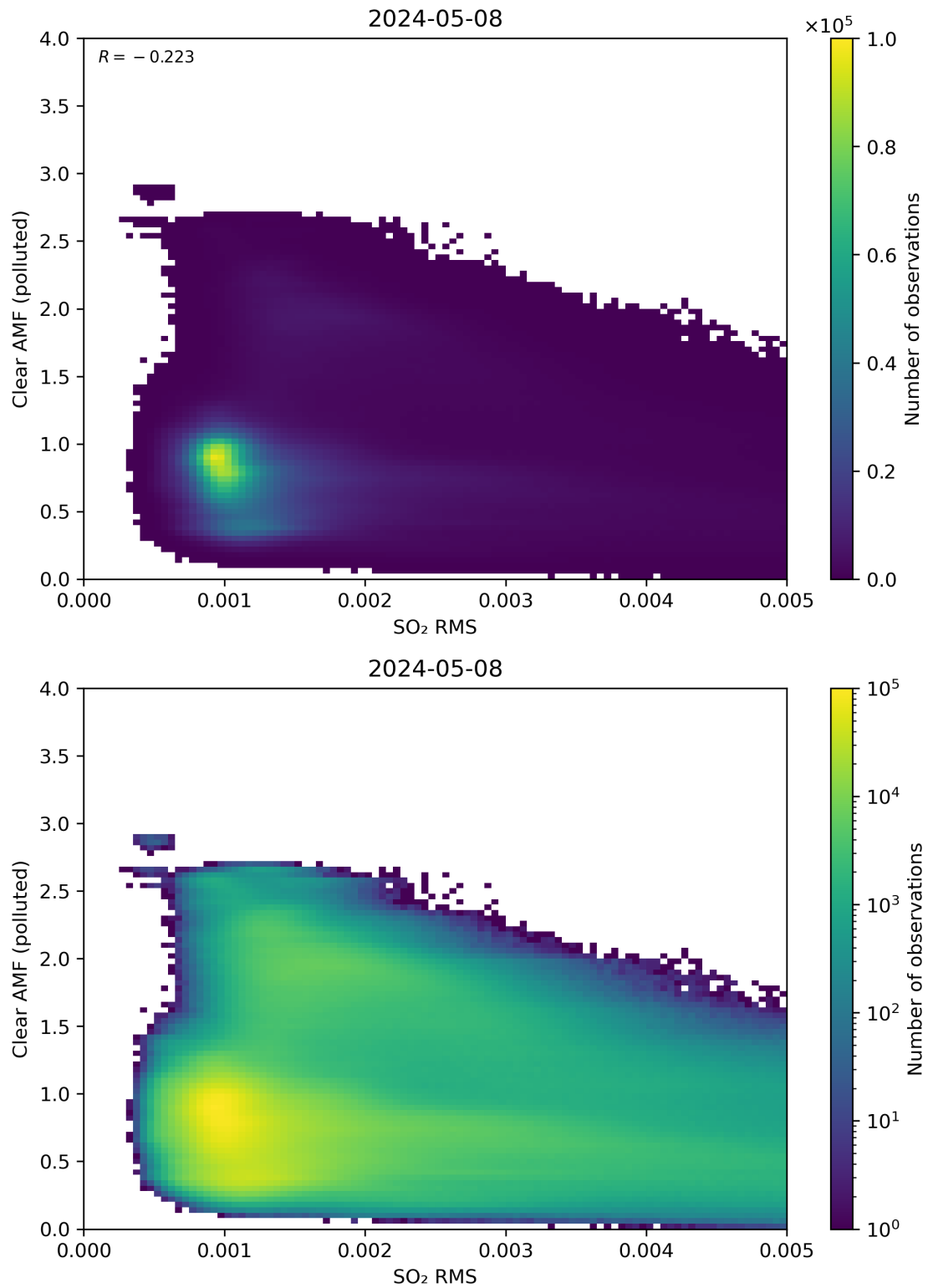
Figure 136: Scatter density plot of “SO 2 RMS” against “Clear AMF (polluted)” for 2024-05-07 to 2024-05-09.
