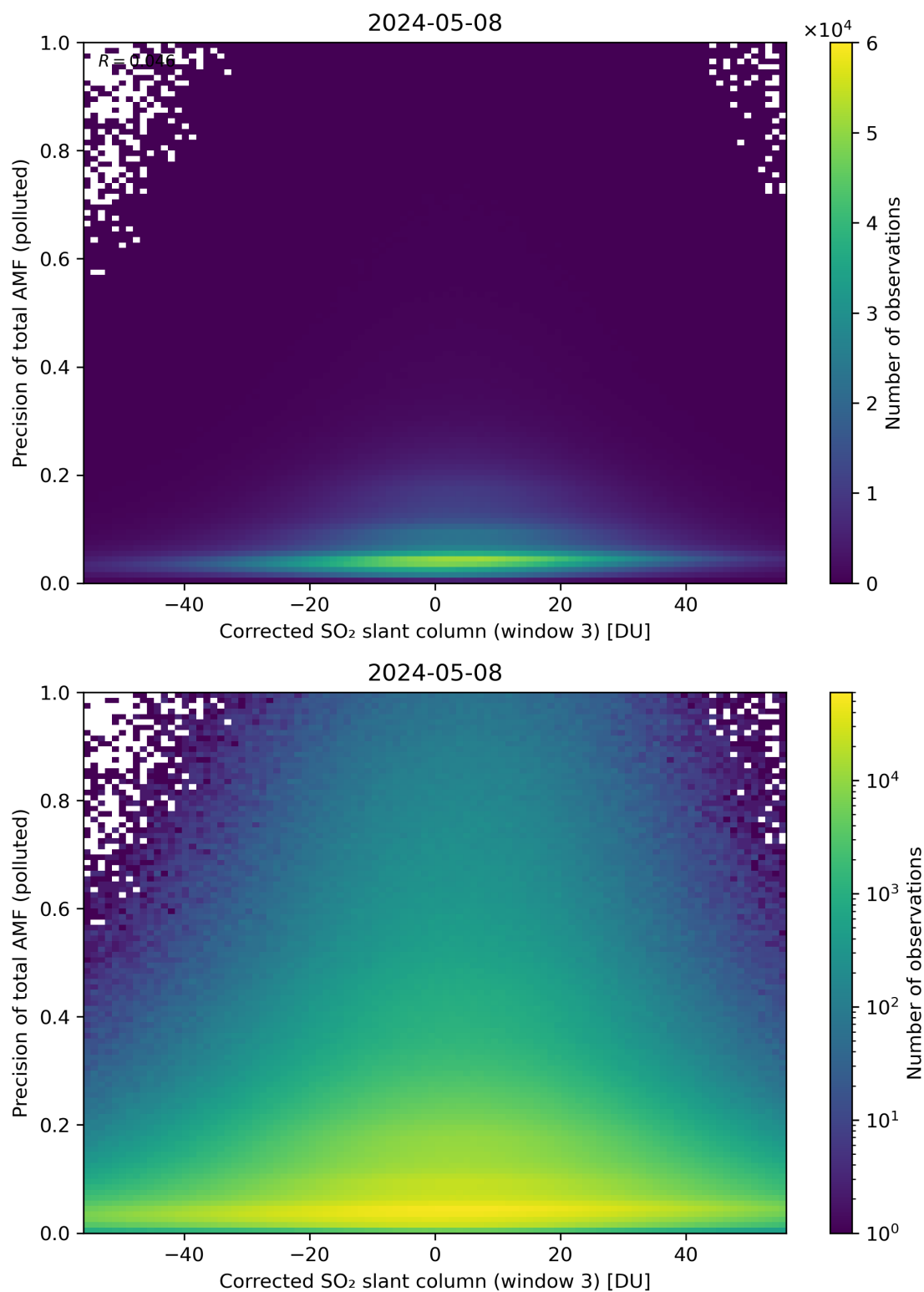
Figure 211: Scatter density plot of “Corrected SO 2 slant column (window 3)” against “Precision of total AMF (polluted)” for 2024-05-07 to 2024-05-09.
