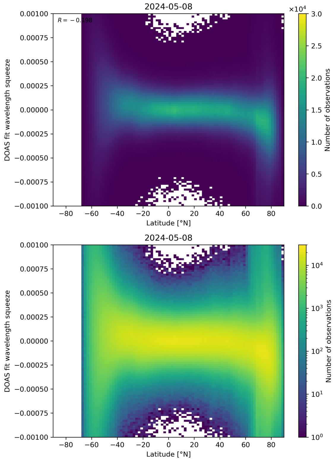
Figure 143: Scatter density plot of “Latitude” against “DOAS fit wavelength squeeze” for 2024-05-07 to 2024-05-09.
