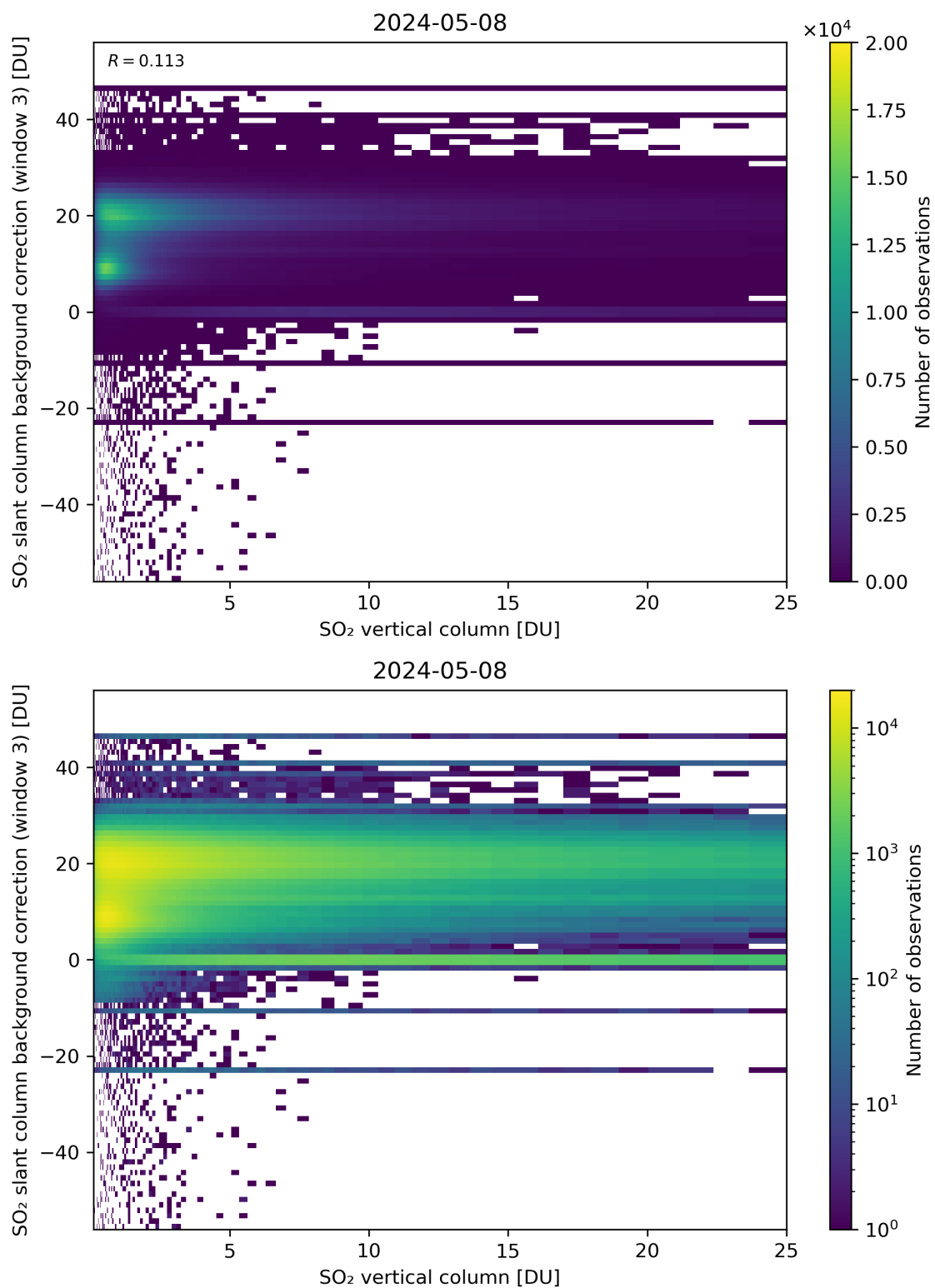
Figure 275: Scatter density plot of “SO 2 vertical column” against “SO 2 slant column background correction (window 3)” for 2024-05-07 to 2024-05-09.
