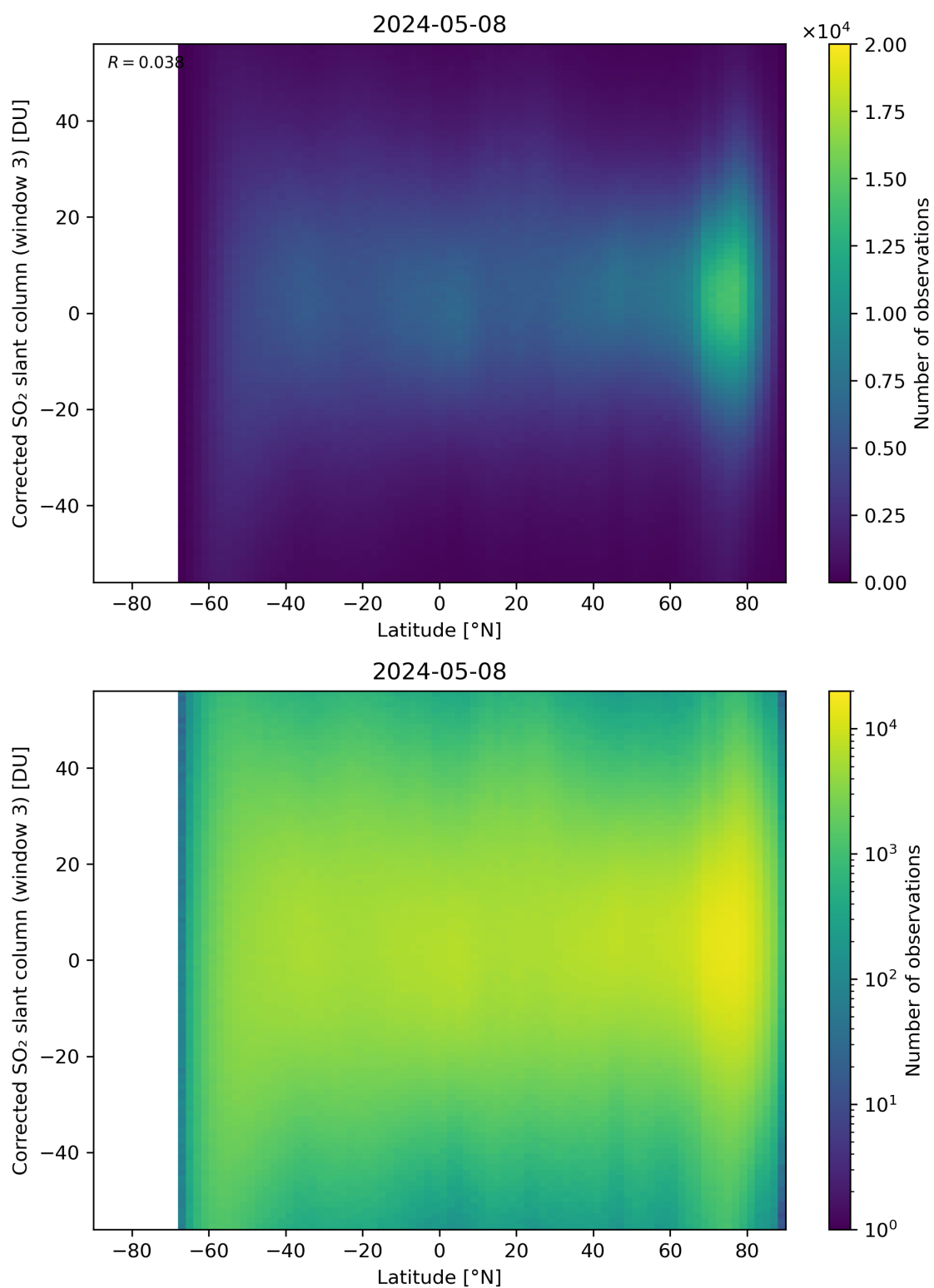
Figure 148: Scatter density plot of “Latitude” against “Corrected SO 2 slant column (window 3)” for 2024-05-07 to 2024-05-09.
