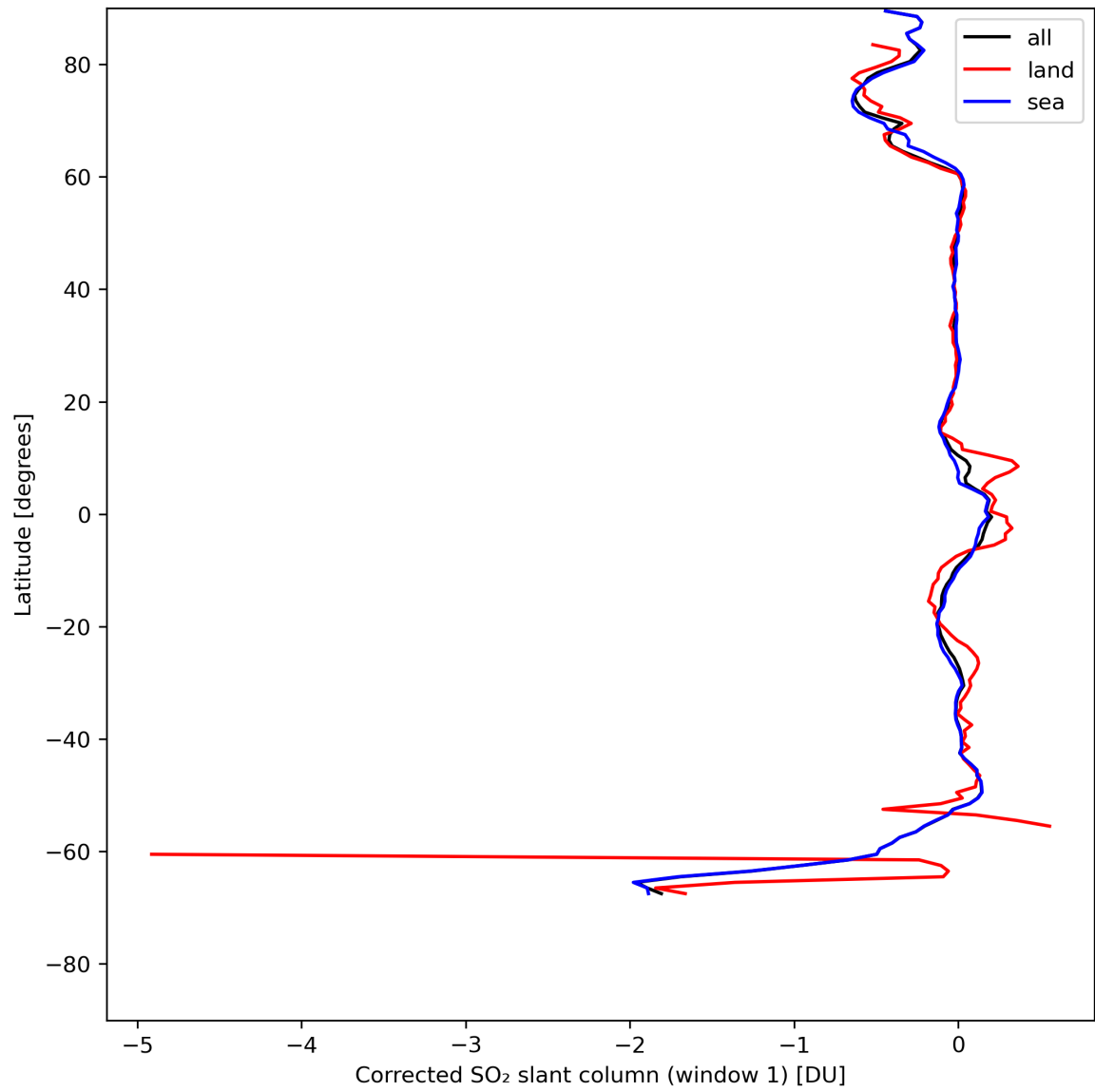
Figure 35: Zonal average of “Corrected SO 2 slant column (window 1)” for 2024-05-07 to 2024-05-09.
