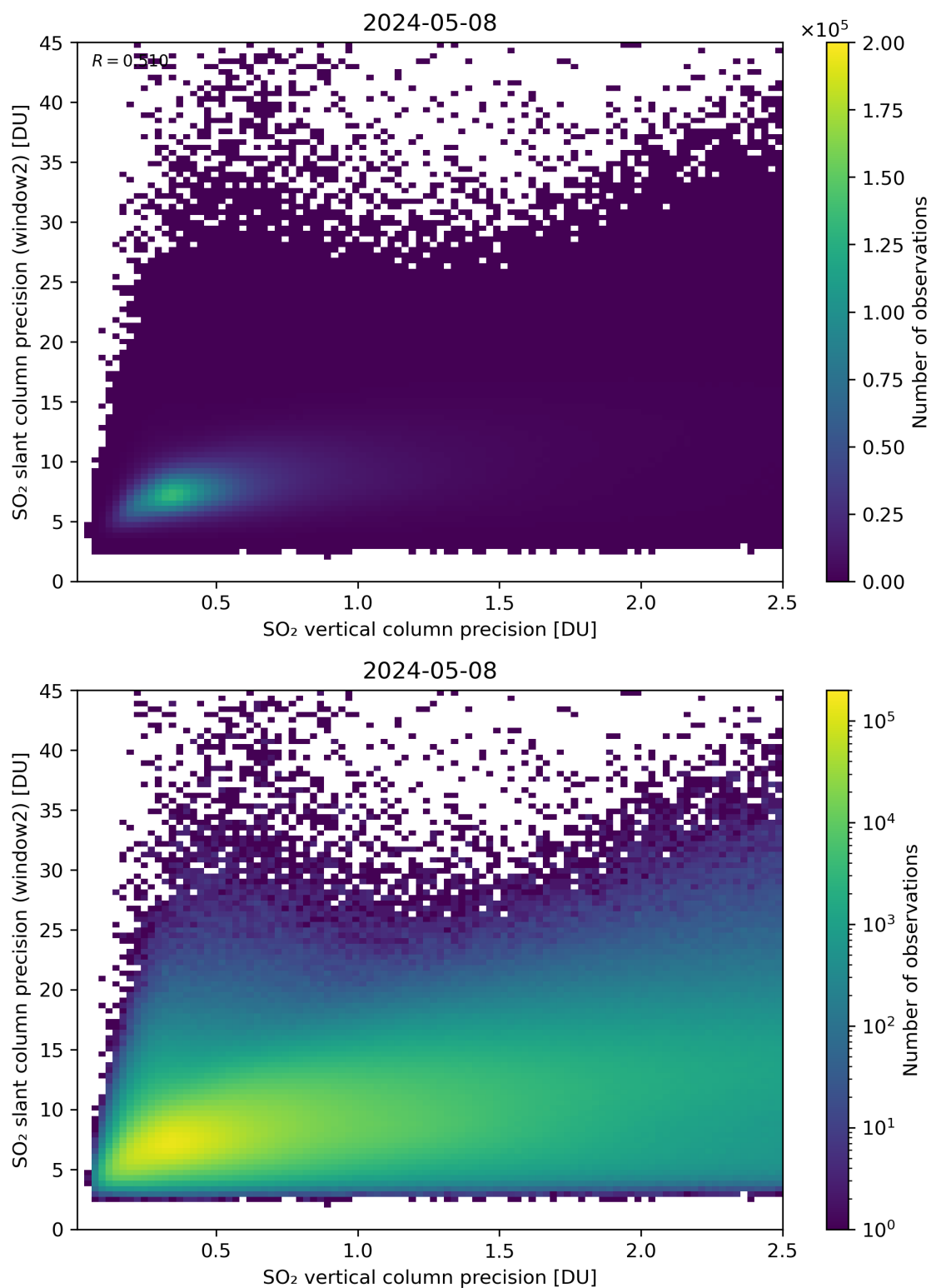
Figure 291: Scatter density plot of “SO 2 vertical column precision” against “SO 2 slant column precision (window2)” for 2024-05-07 to 2024-05-09.
