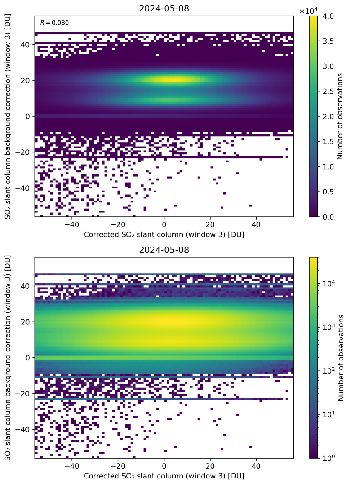
Figure 205: Scatter density plot of “Corrected SO 2 slant column (window 3)” against “SO 2 slant column background correction (window 3)” for 2024-05-07 to 2024-05-09.
