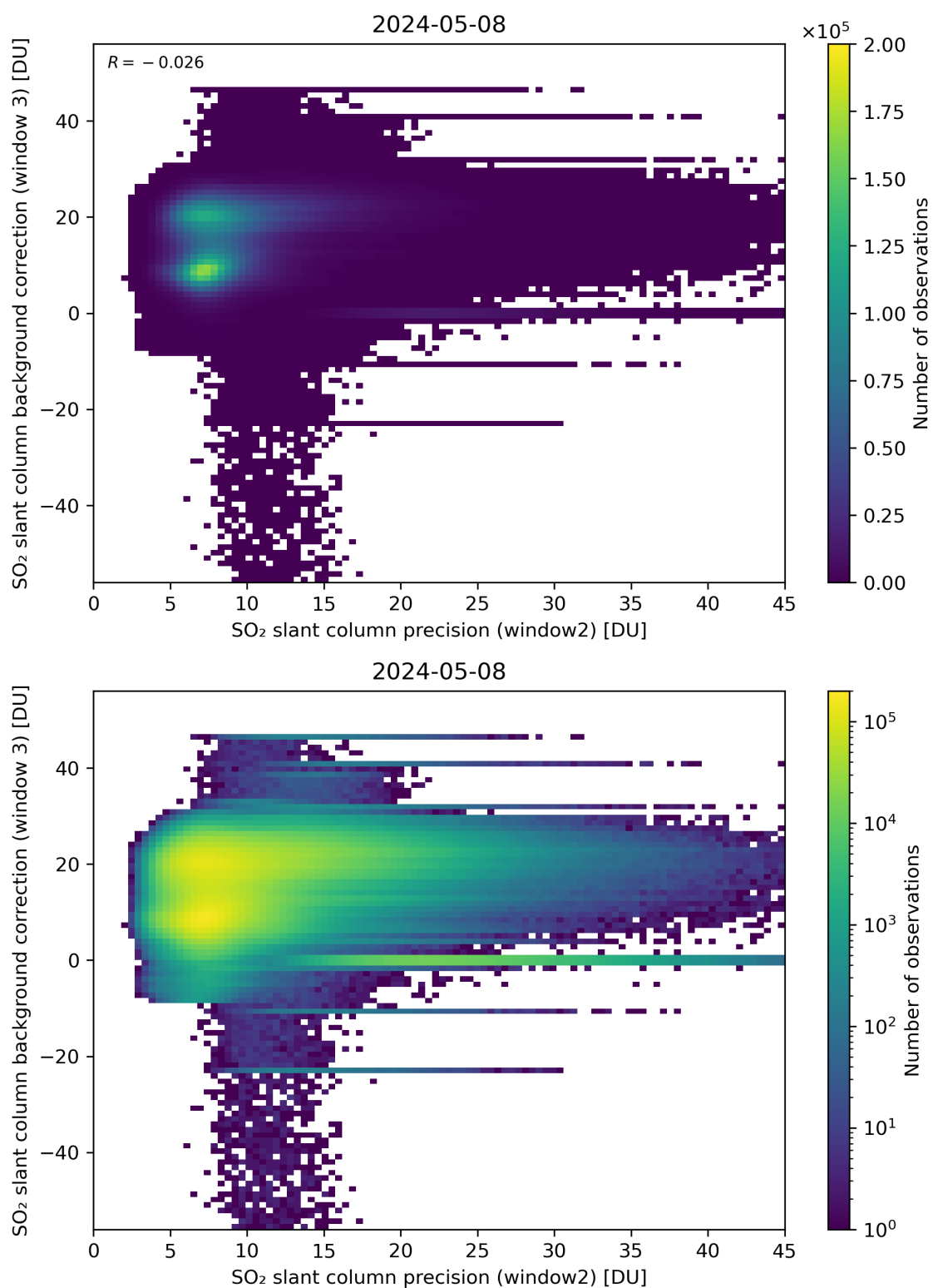
Figure 242: Scatter density plot of “SO 2 slant column precision (window2)” against “SO 2 slant column background correction (window 3)” for 2024-05-07 to 2024-05-09.
