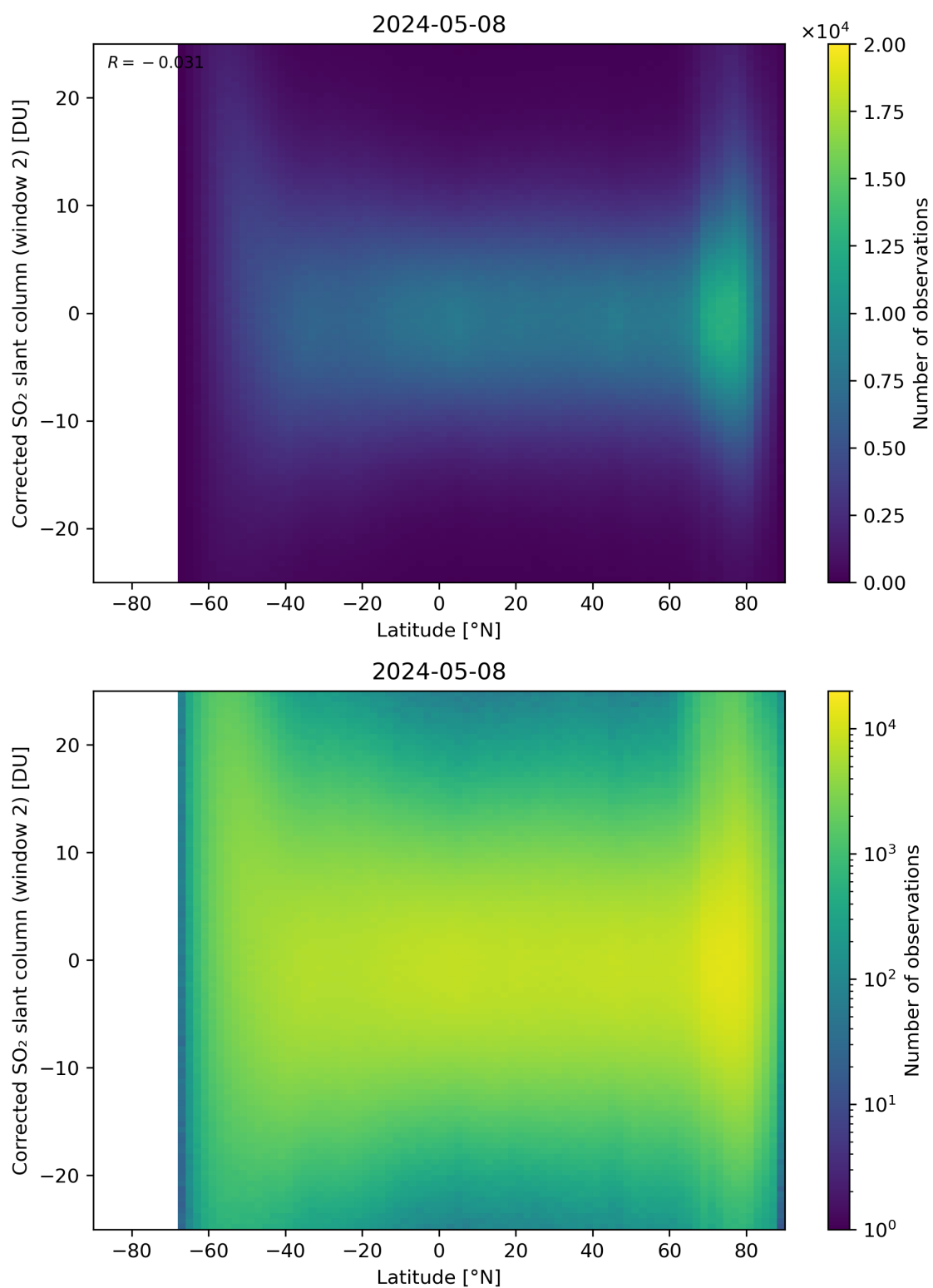
Figure 147: Scatter density plot of “Latitude” against “Corrected SO 2 slant column (window 2)” for 2024-05-07 to 2024-05-09.
