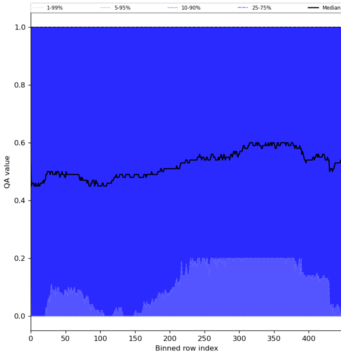
Figure 75: Along track statistics of “QA value” for 2024-05-07 to 2024-05-09
