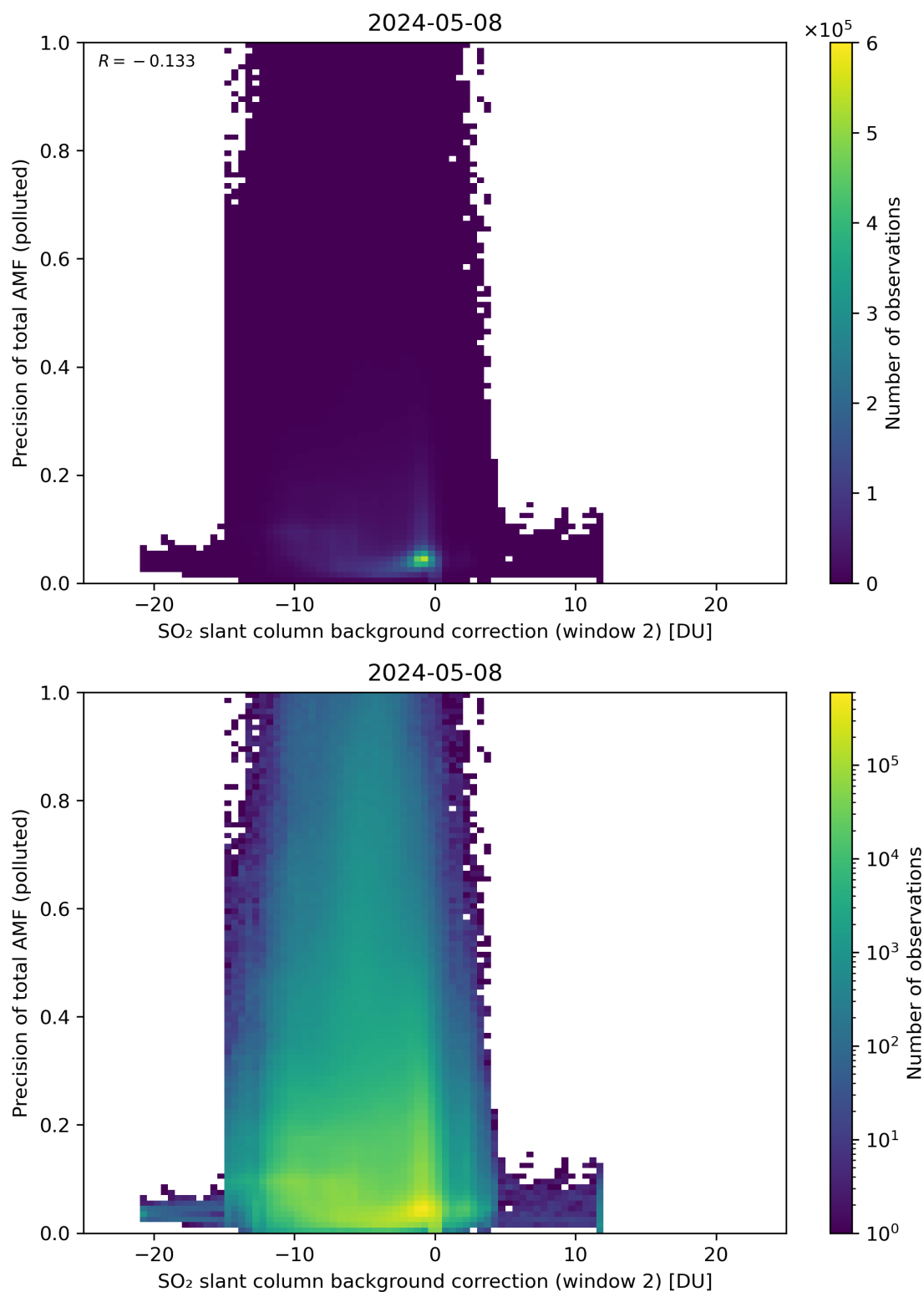
Figure 120: Scatter density plot of “SO 2 slant column background correction (window 2)” against “Precision of total AMF (polluted)” for 2024-05-07 to 2024-05-09.
