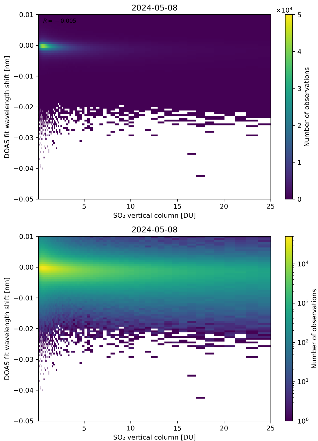
Figure 276: Scatter density plot of “SO 2 vertical column” against “DOAS fit wavelength shift” for 2024-05-07 to 2024-05-09.
