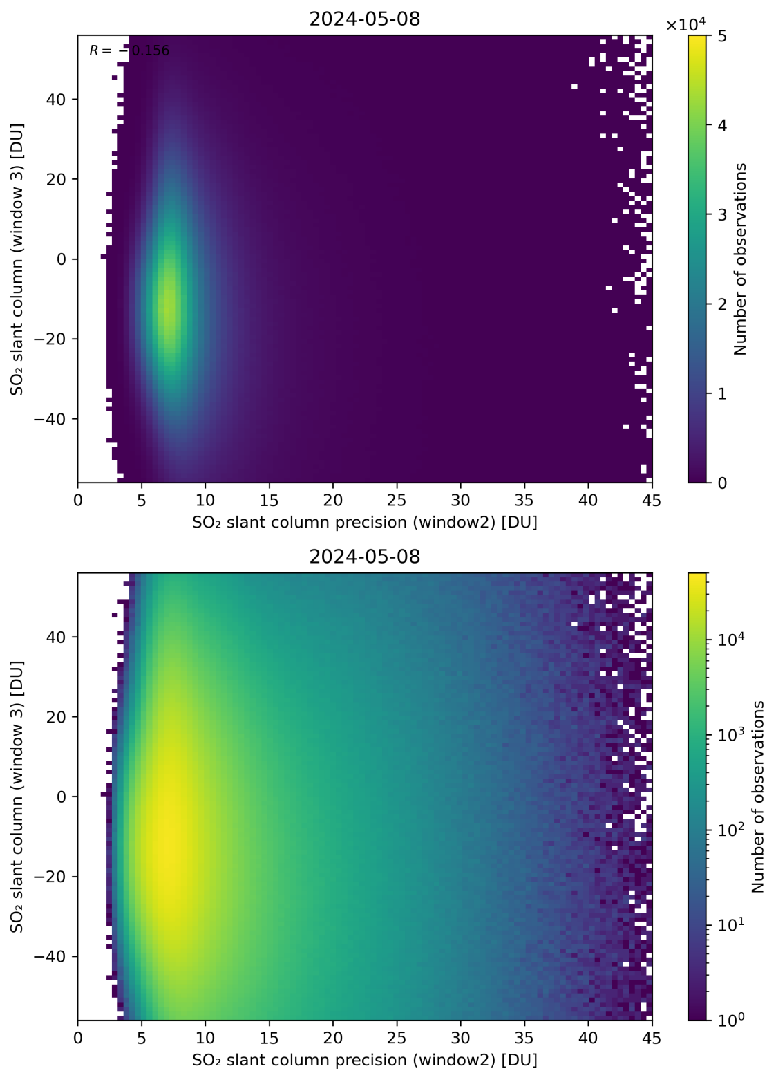
Figure 249: Scatter density plot of “SO 2 slant column precision (window2)” against “SO 2 slant column (window 3)” for 2024-05-07 to 2024-05-09.
