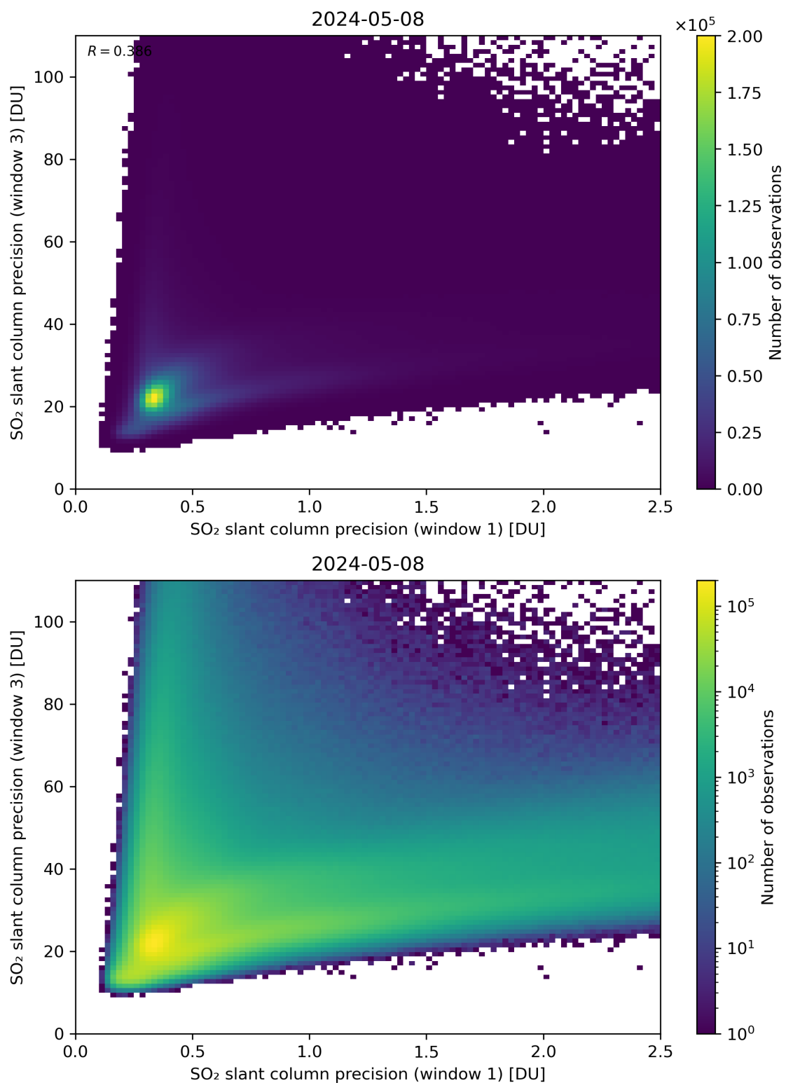
Figure 229: Scatter density plot of “SO 2 slant column precision (window 1)” against “SO 2 slant column precision (window 3)” for 2024-05-07 to 2024-05-09.
