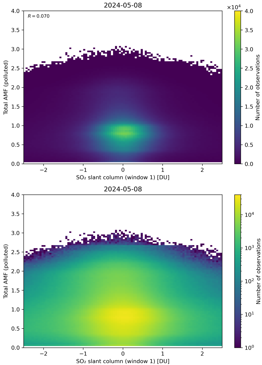
Figure 239: Scatter density plot of “SO 2 slant column (window 1)” against “Total AMF (polluted)” for 2024-05-07 to 2024-05-09.
