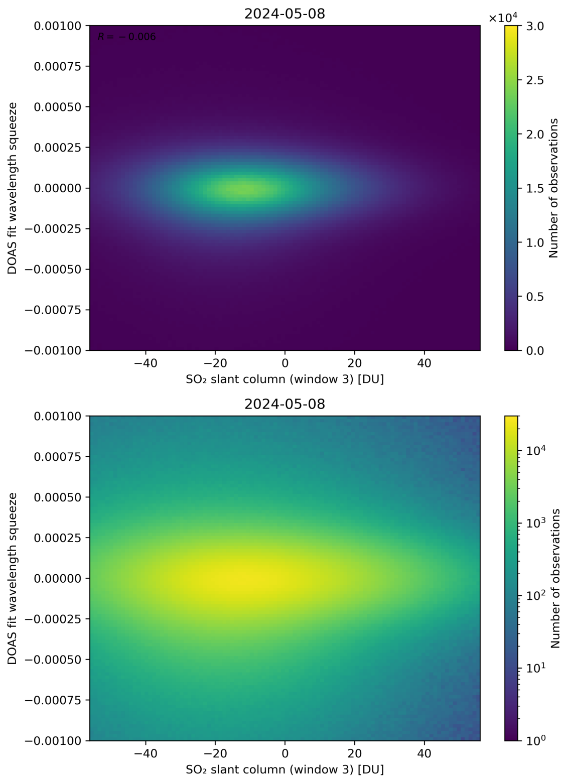
Figure 255: Scatter density plot of “SO 2 slant column (window 3)” against “DOAS fit wavelength squeeze” for 2024-05-07 to 2024-05-09.
