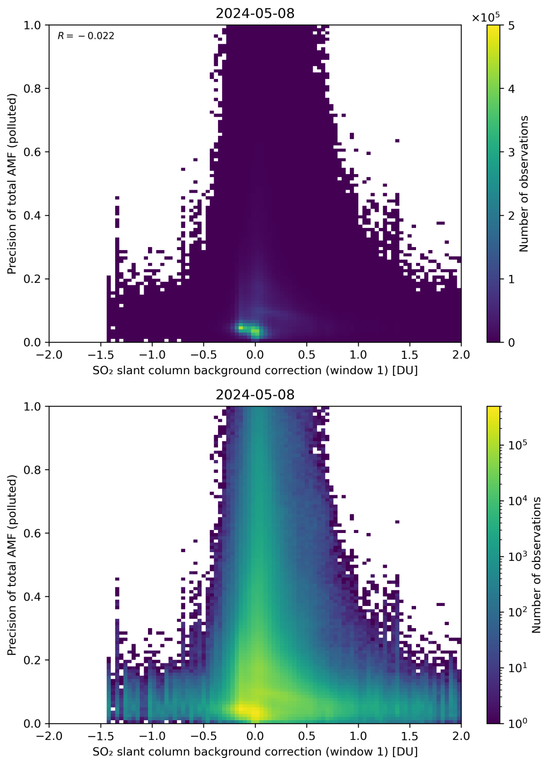
Figure 110: Scatter density plot of “SO 2 slant column background correction (window 1)” against “Precision of total AMF (polluted)” for 2024-05-07 to 2024-05-09.
