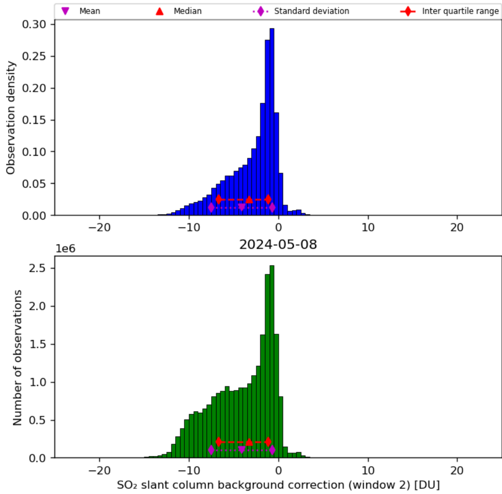
Figure 63: Histogram of “SO 2 slant column background correction (window 2)” for 2024-05-07 to 2024-05-09
