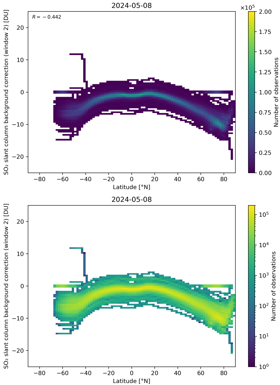
Figure 140: Scatter density plot of “Latitude” against “SO 2 slant column background correction (window 2)” for 2024-05-07 to 2024-05-09.
