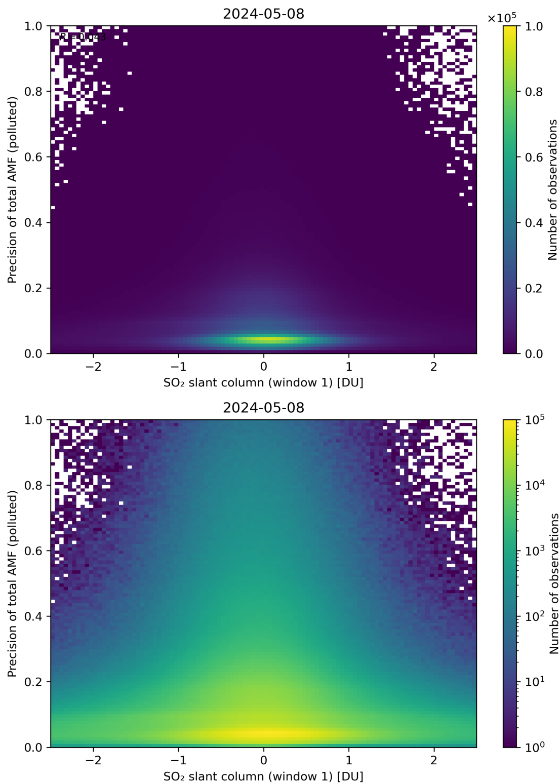
Figure 240: Scatter density plot of “SO 2 slant column (window 1)” against “Precision of total AMF (polluted)” for 2024-05-07 to 2024-05-09.
