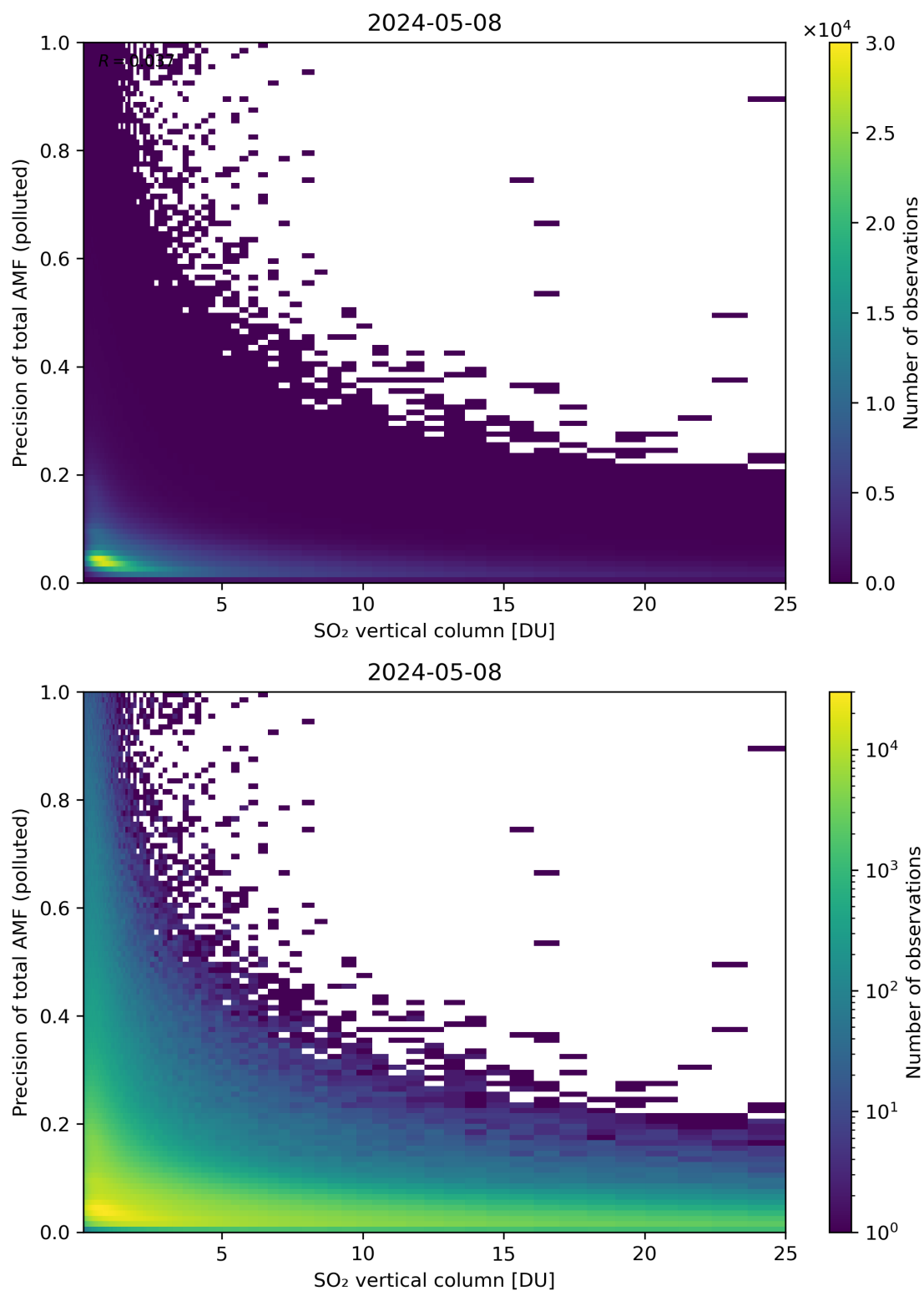
Figure 306: Scatter density plot of “SO 2 vertical column” against “Precision of total AMF (polluted)” for 2024-05-07 to 2024-05-09.
