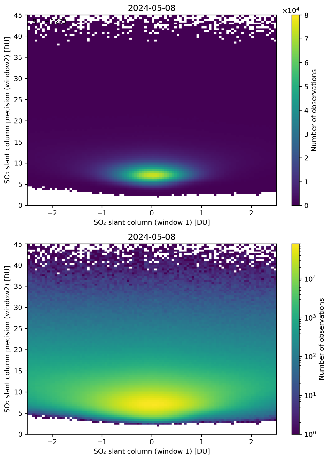
Figure 236: Scatter density plot of “SO 2 slant column (window 1)” against “SO 2 slant column precision (window2)” for 2024-05-07 to 2024-05-09.
