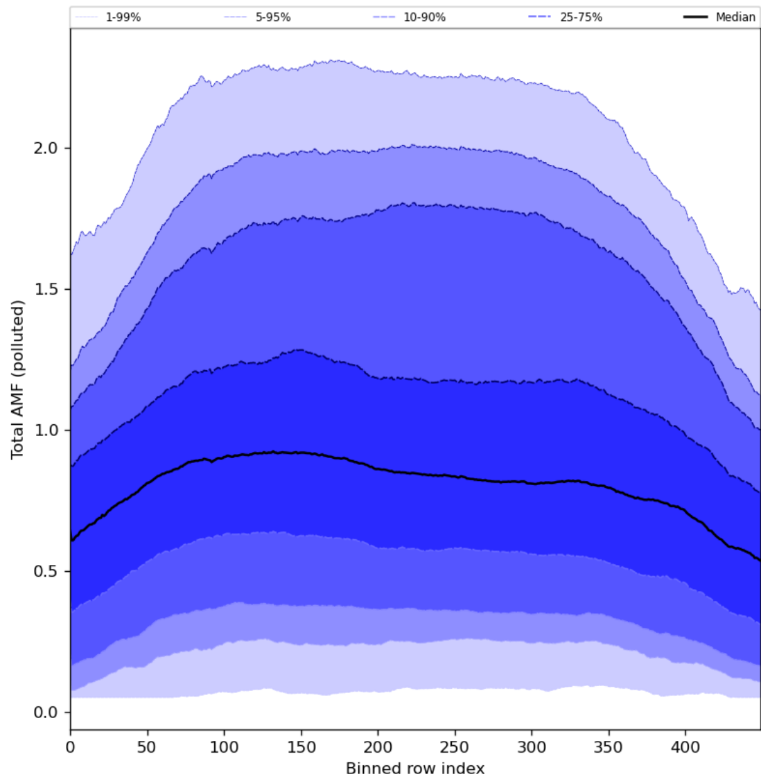
Figure 94: Along track statistics of “Total AMF (polluted)” for 2024-05-07 to 2024-05-09
