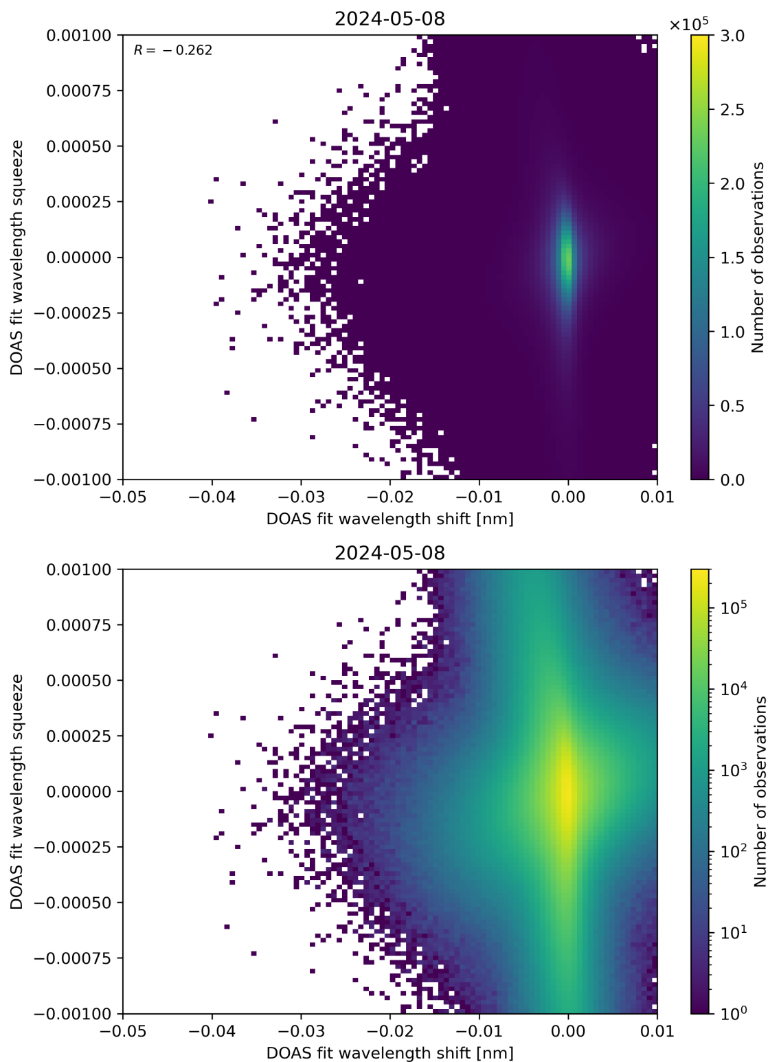
Figure 127: Scatter density plot of “DOAS fit wavelength shift” against “DOAS fit wavelength squeeze” for 2024-05-07 to 2024-05-09.
