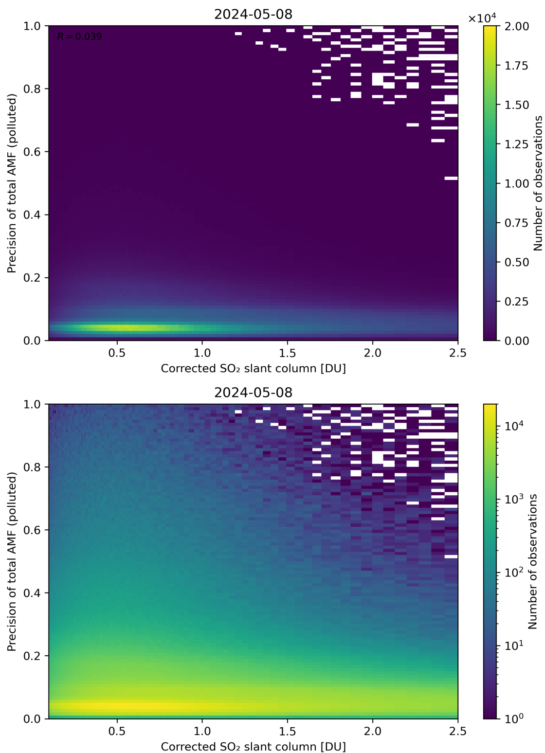
Figure 193: Scatter density plot of “Corrected SO 2 slant column” against “Precision of total AMF (polluted)” for 2024-05-07 to 2024-05-09.
