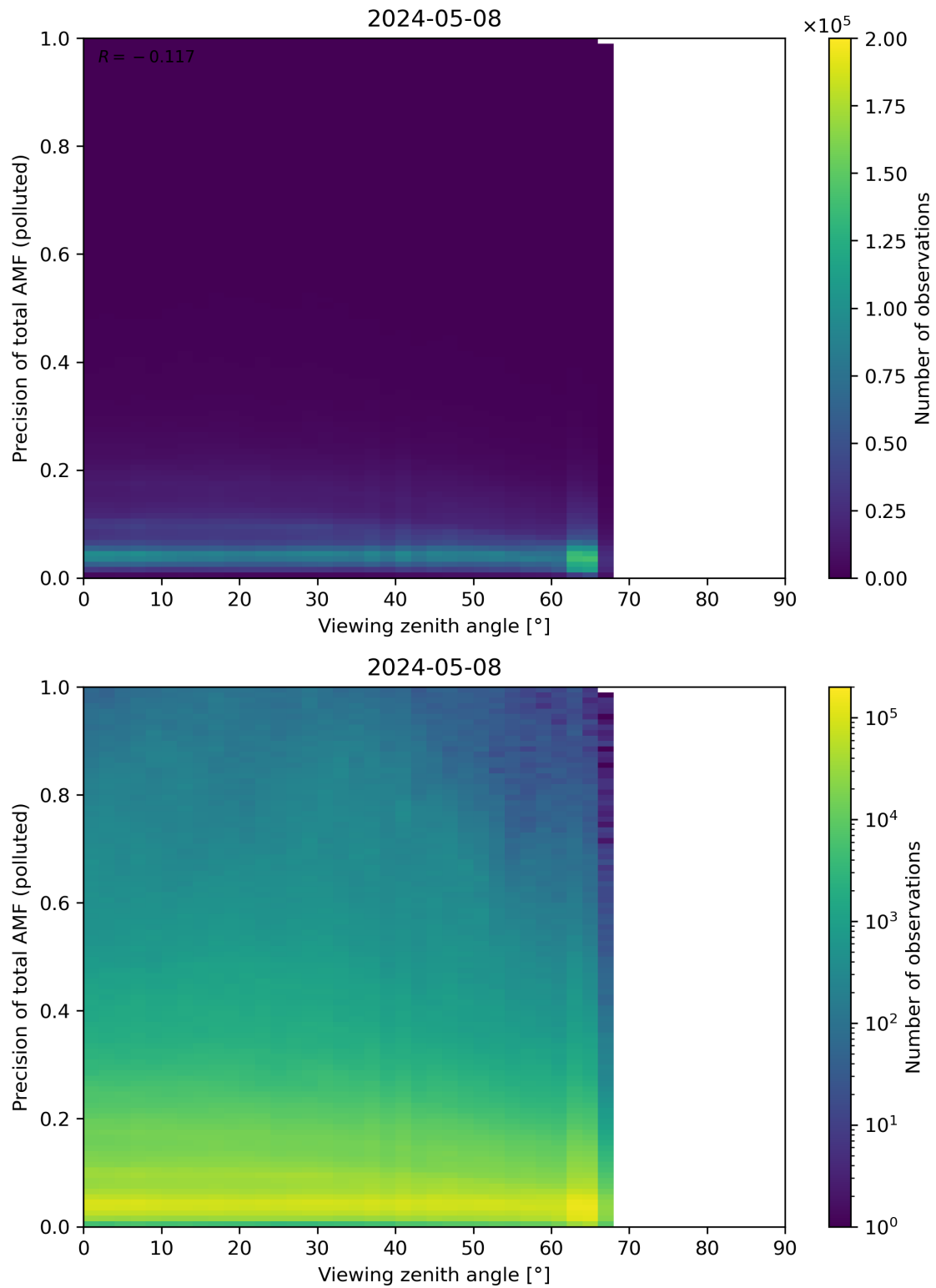
Figure 326: Scatter density plot of “Viewing zenith angle” against “Precision of total AMF (polluted)” for 2024-05-07 to 2024-05-09.
