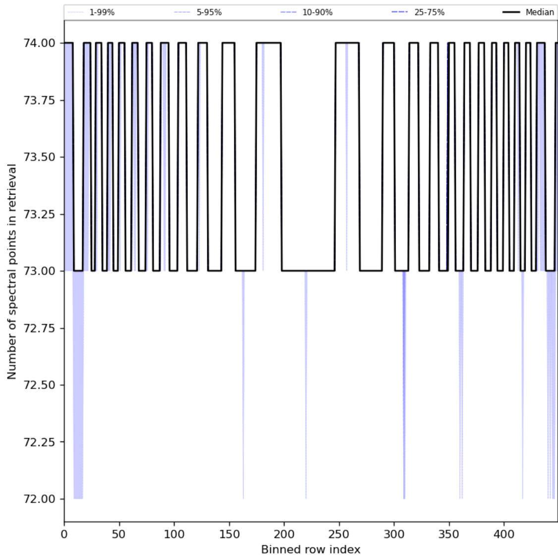
Figure 97: Along track statistics of “Number of spectral points in retrieval” for 2024-05-07 to 2024-05-09
