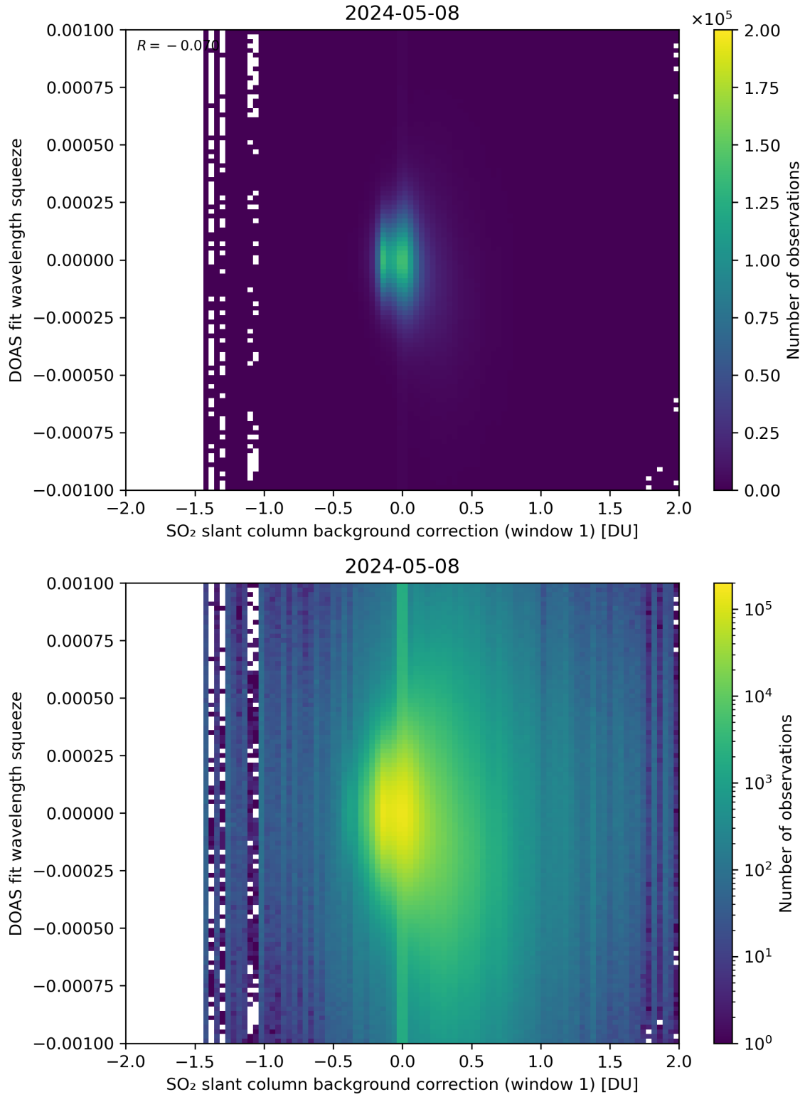
Figure 101: Scatter density plot of “SO 2 slant column background correction (window 1)” against “DOAS fit wavelength squeeze” for 2024-05-07 to 2024-05-09.
