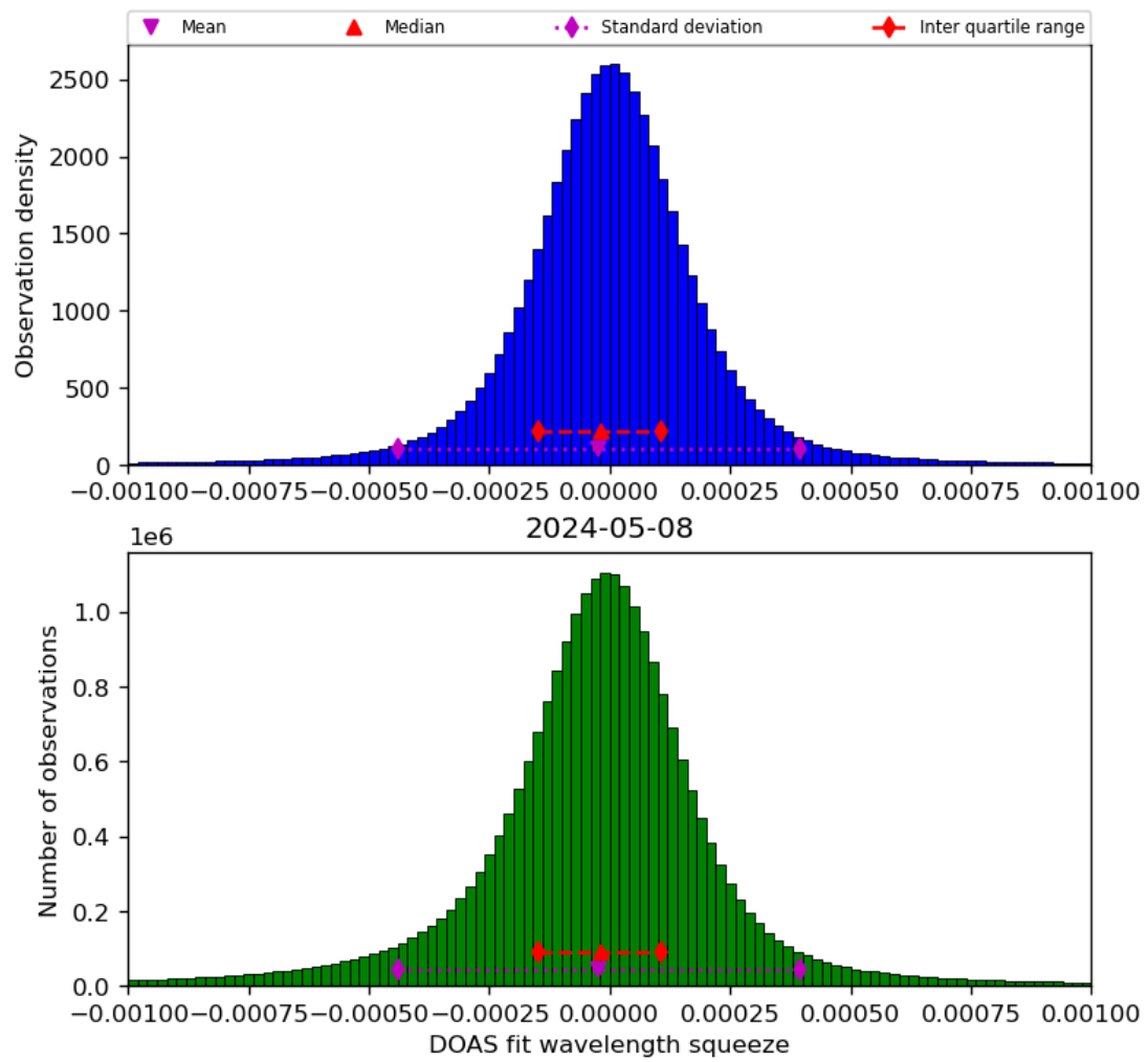
Figure 69: Histogram of “DOAS fit wavelength squeeze” for 2024-05-07 to 2024-05-09
