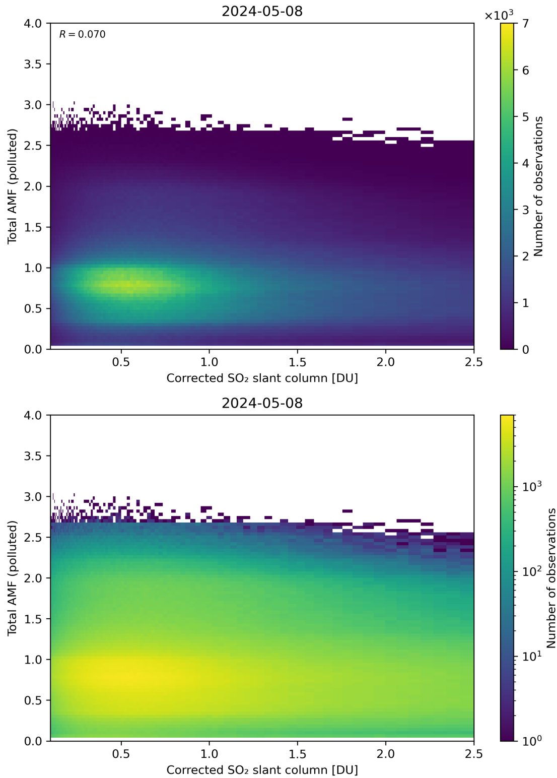
Figure 192: Scatter density plot of “Corrected SO 2 slant column” against “Total AMF (polluted)” for 2024-05-07 to 2024-05-09.
