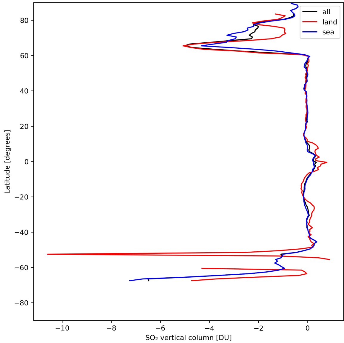
Figure 30: Zonal average of “SO 2 vertical column” for 2024-05-07 to 2024-05-09.
