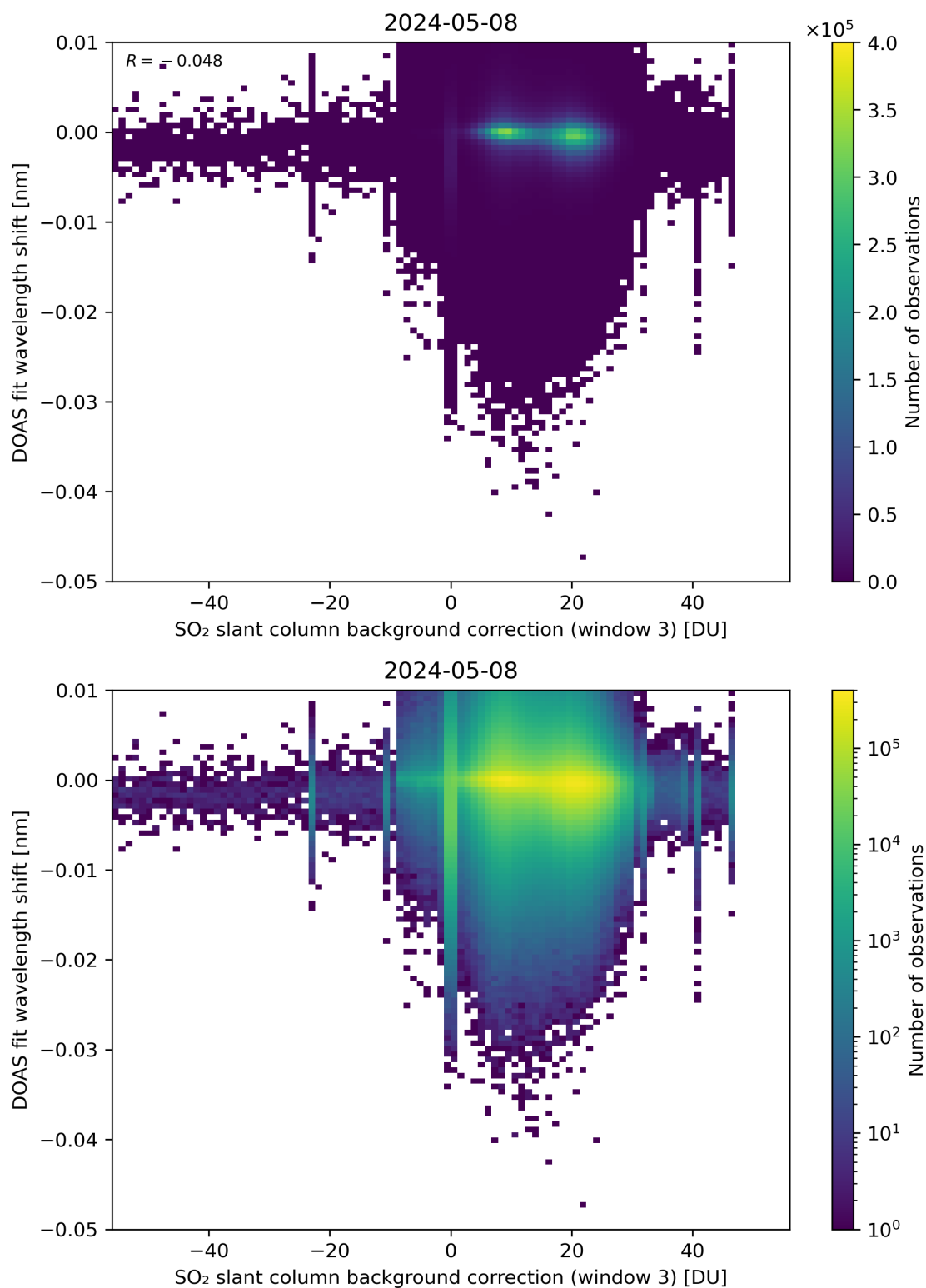
Figure 121: Scatter density plot of “SO 2 slant column background correction (window 3)” against “DOAS fit wavelength shift” for 2024-05-07 to 2024-05-09.
