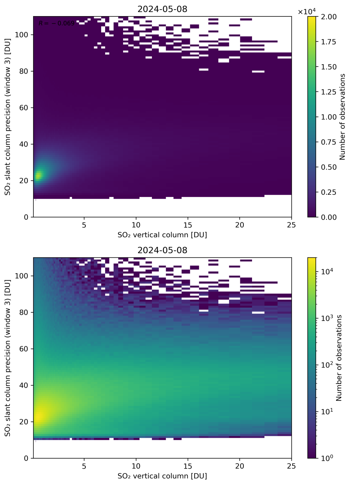
Figure 304: Scatter density plot of “SO 2 vertical column” against “SO 2 slant column precision (window 3)” for 2024-05-07 to 2024-05-09.
