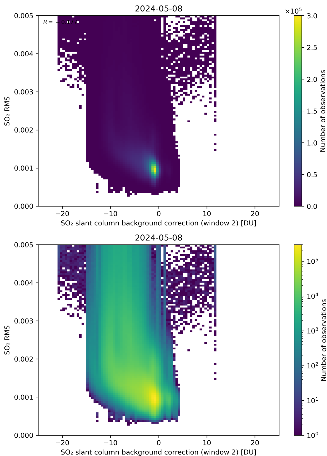
Figure 114: Scatter density plot of “SO 2 slant column background correction (window 2)” against “SO 2 RMS” for 2024-05-07 to 2024-05-09.
