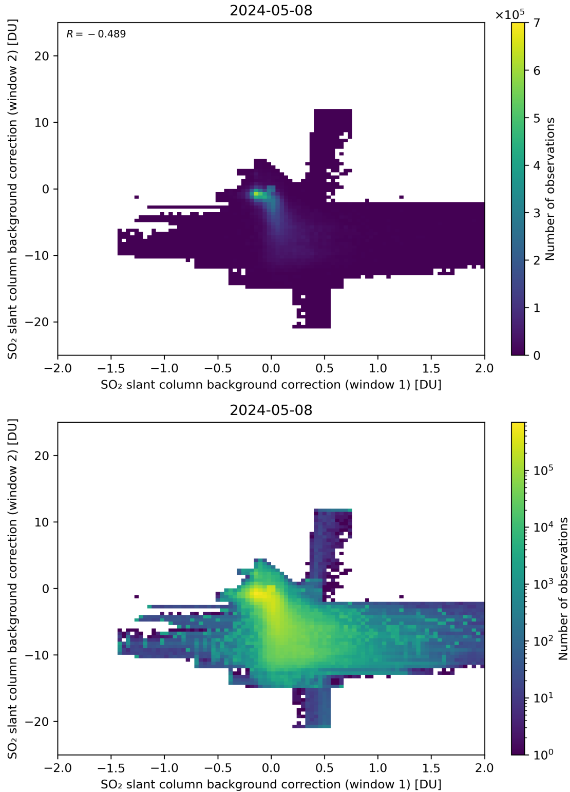
Figure 98: Scatter density plot of “SO 2 slant column background correction (window 1)” against “SO 2 slant column background correction (window 2)” for 2024-05-07 to 2024-05-09.
