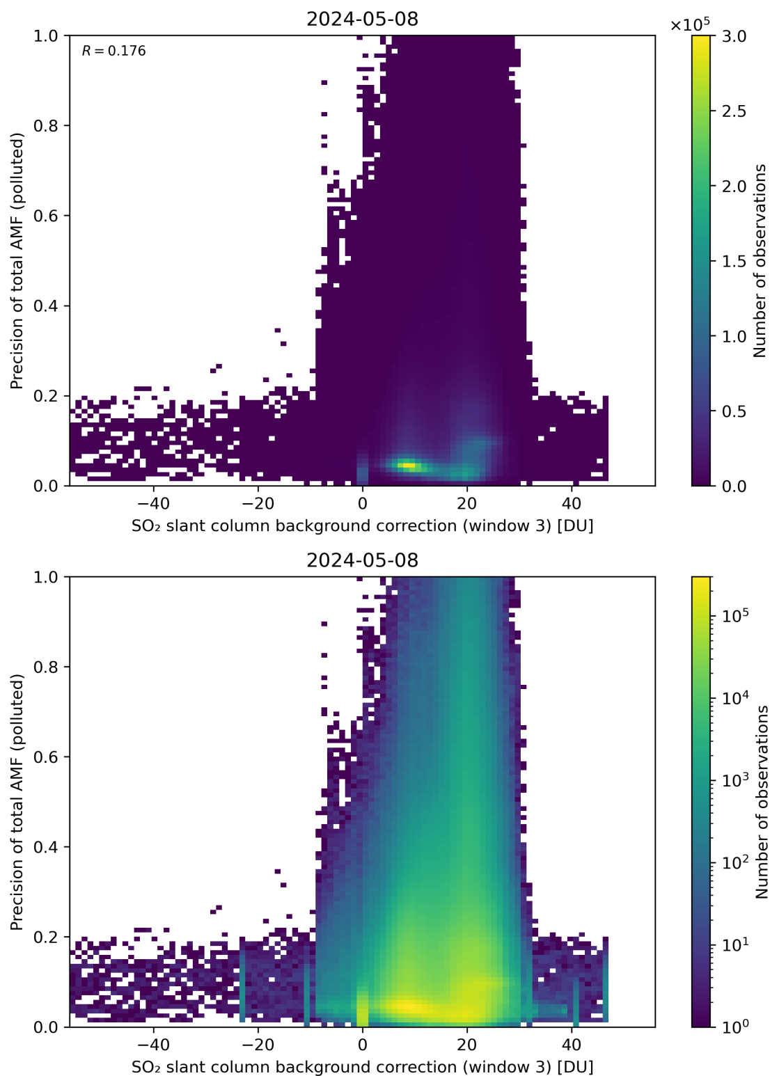
Figure 126: Scatter density plot of “SO 2 slant column background correction (window 3)” against “Precision of total AMF (polluted)” for 2024-05-07 to 2024-05-09.
