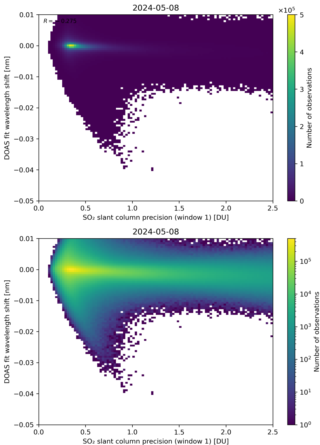
Figure 221: Scatter density plot of “SO 2 slant column precision (window 1)” against “DOAS fit wavelength shift” for 2024-05-07 to 2024-05-09.
