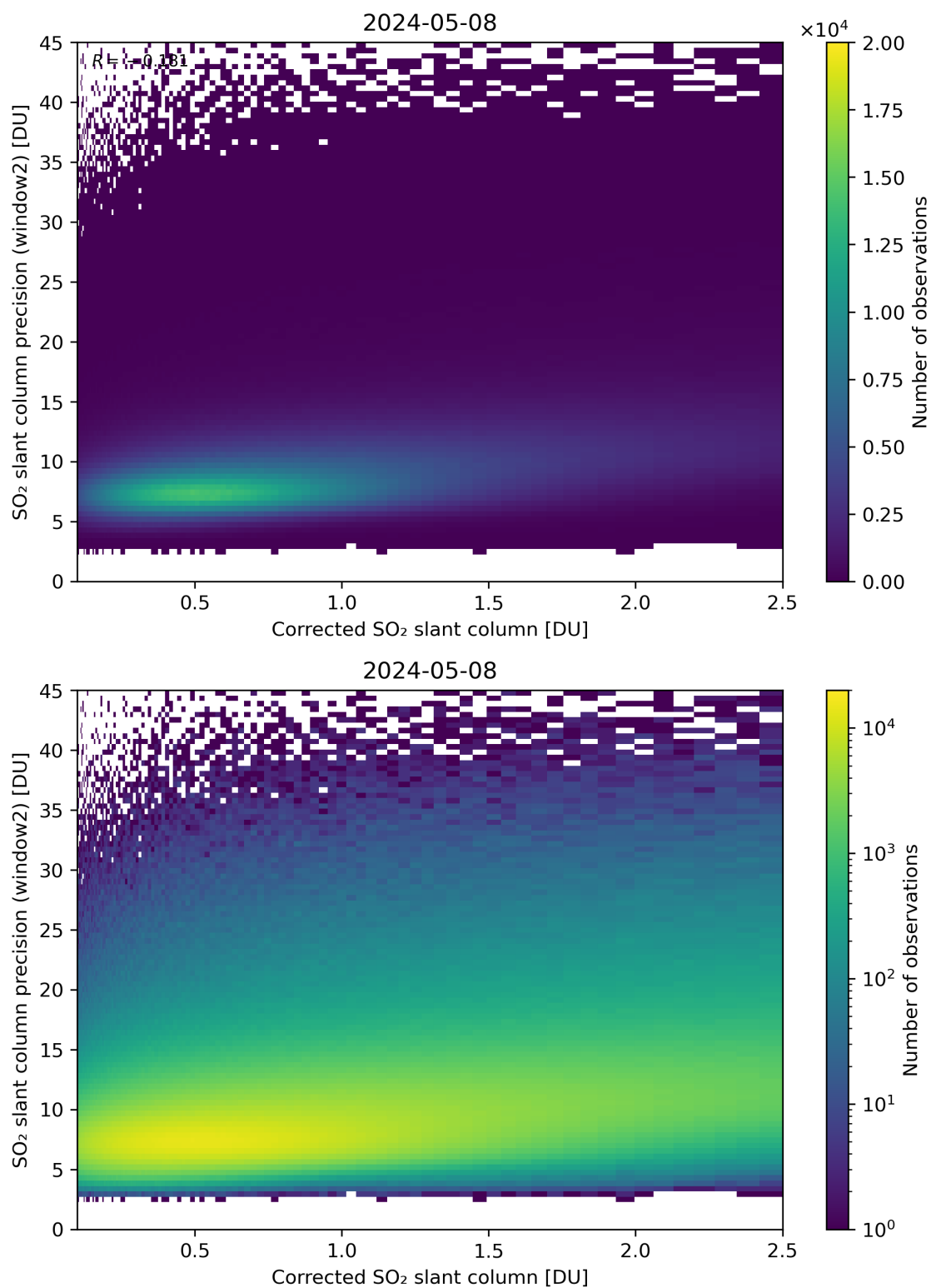
Figure 189: Scatter density plot of “Corrected SO 2 slant column” against “SO 2 slant column precision (window2)” for 2024-05-07 to 2024-05-09.
