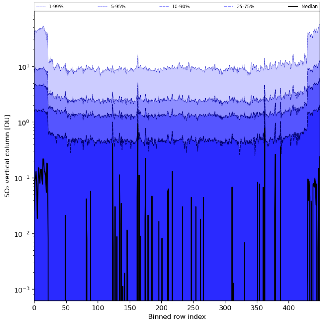
Figure 76: Along track statistics of “SO 2 vertical column” for 2024-05-07 to 2024-05-09
