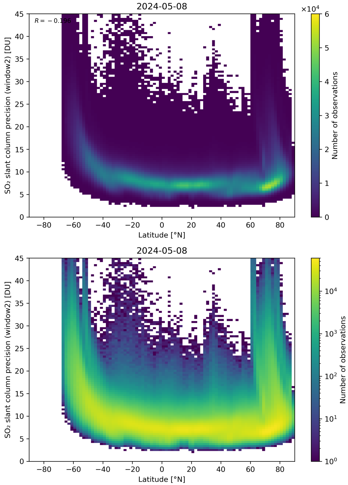
Figure 151: Scatter density plot of “Latitude” against “SO 2 slant column precision (window2)” for 2024-05-07 to 2024-05-09.
