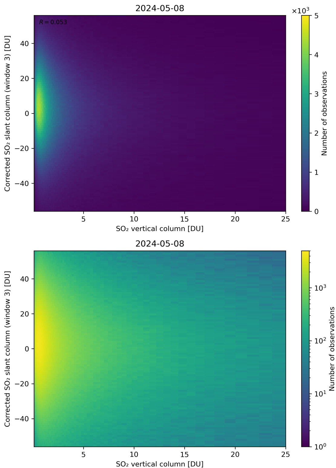
Figure 299: Scatter density plot of “SO 2 vertical column” against “Corrected SO 2 slant column (window 3)” for 2024-05-07 to 2024-05-09.
