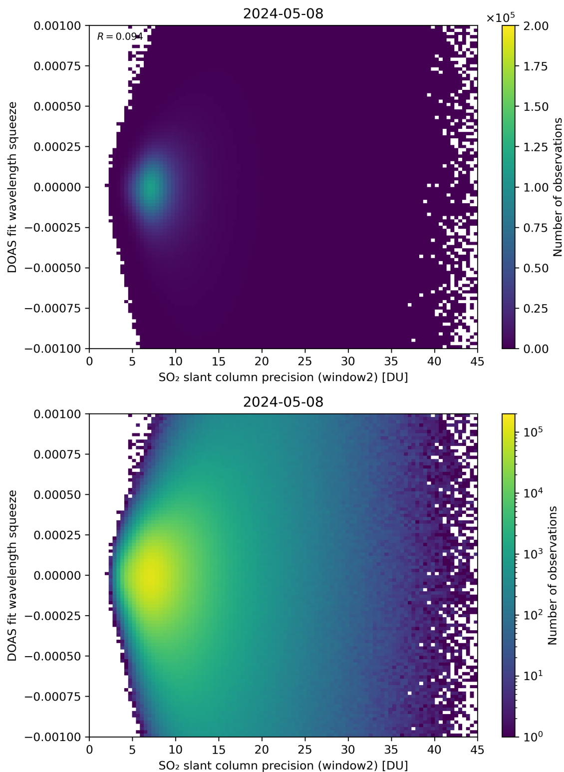
Figure 244: Scatter density plot of “SO 2 slant column precision (window2)” against “DOAS fit wavelength squeeze” for 2024-05-07 to 2024-05-09.
