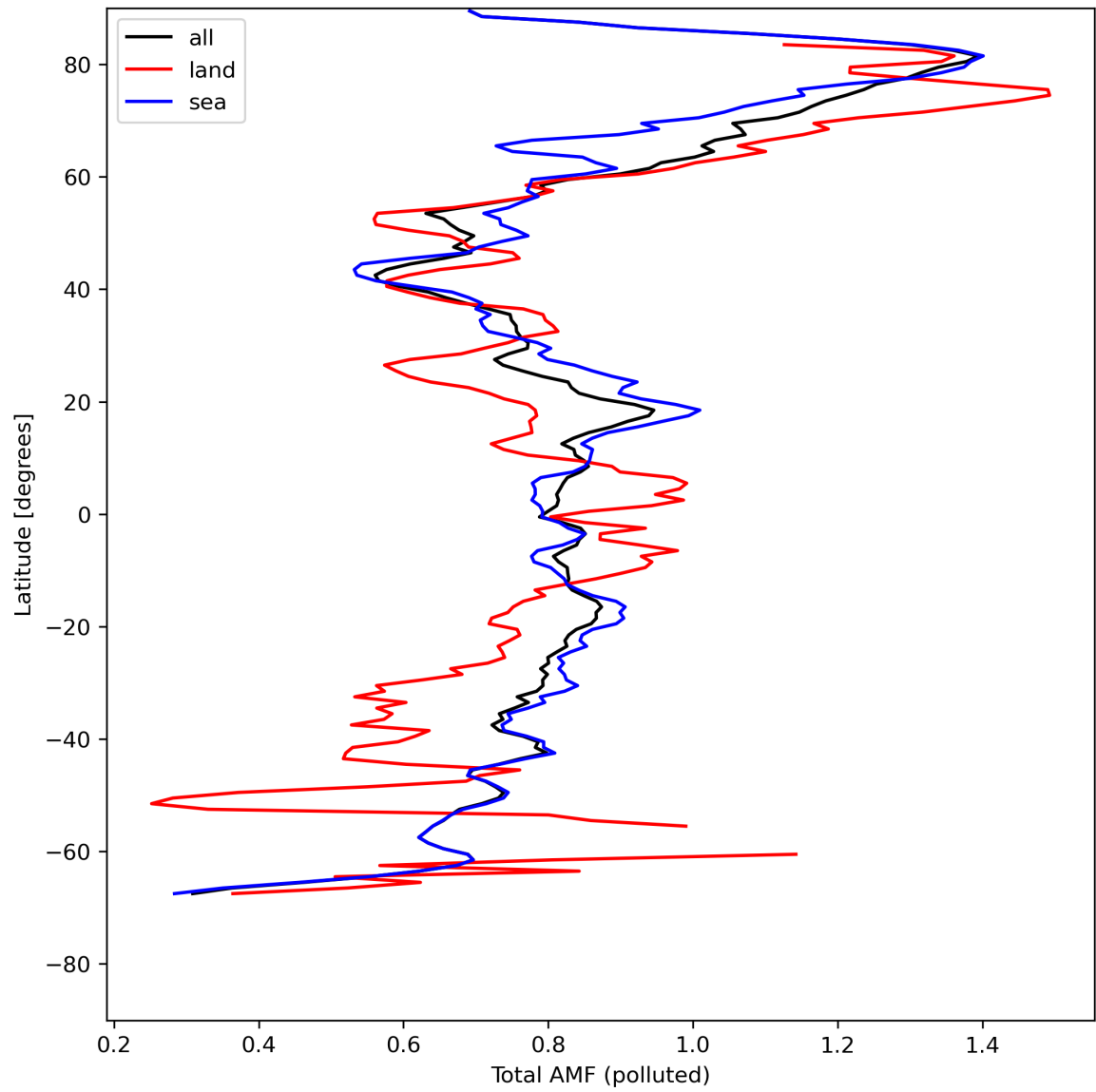
Figure 48: Zonal average of “Total AMF (polluted)” for 2024-05-07 to 2024-05-09.
