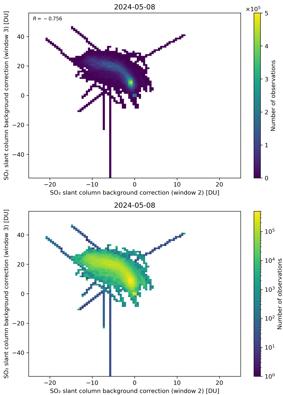
Figure 111: Scatter density plot of “SO 2 slant column background correction (window 2)” against “SO 2 slant column background correction (window 3)” for 2024-05-07 to 2024-05-09.
