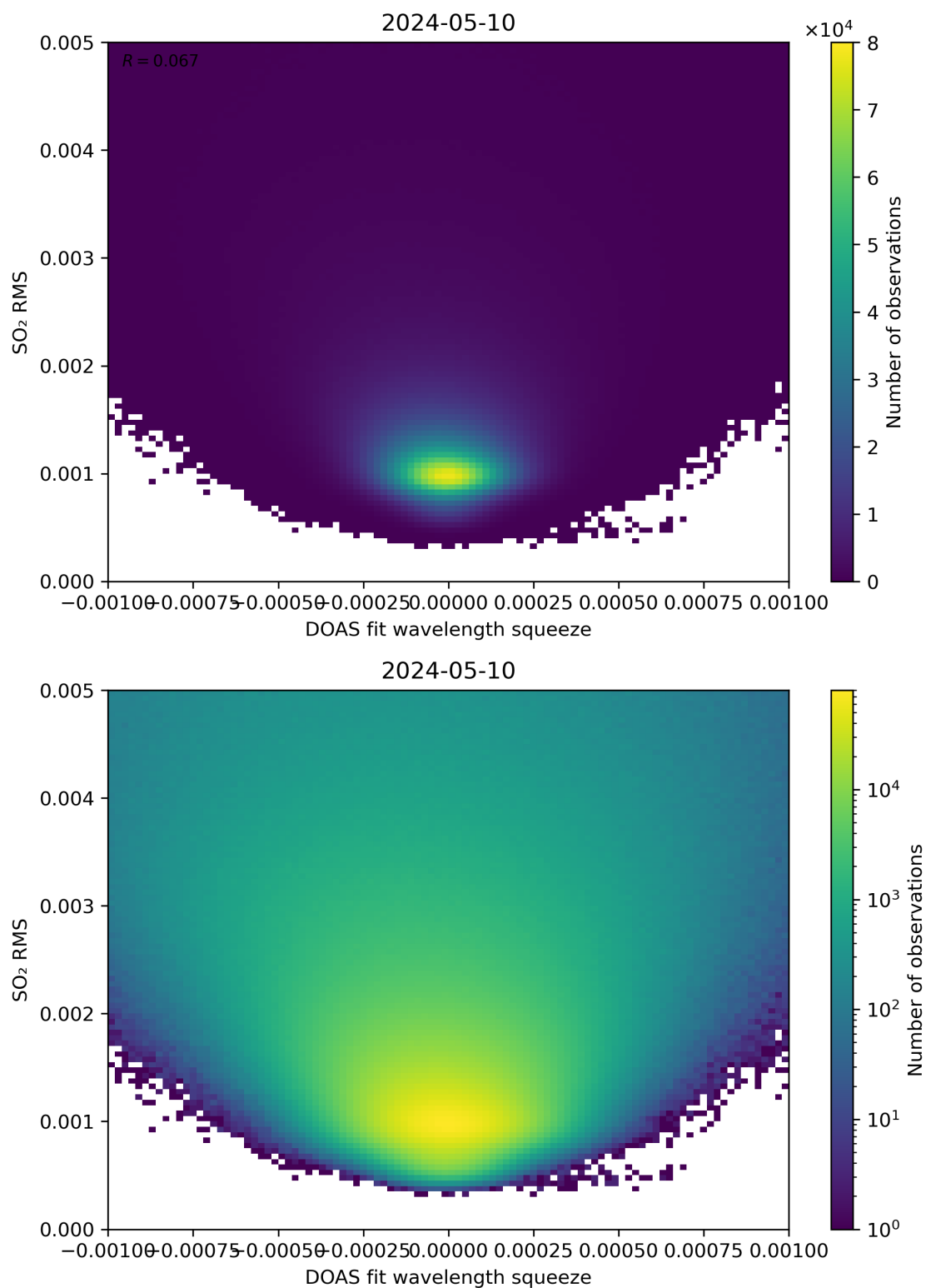
Figure 132: Scatter density plot of “DOAS fit wavelength squeeze” against “SO 2 RMS” for 2024-05-09 to 2024-05-11.
