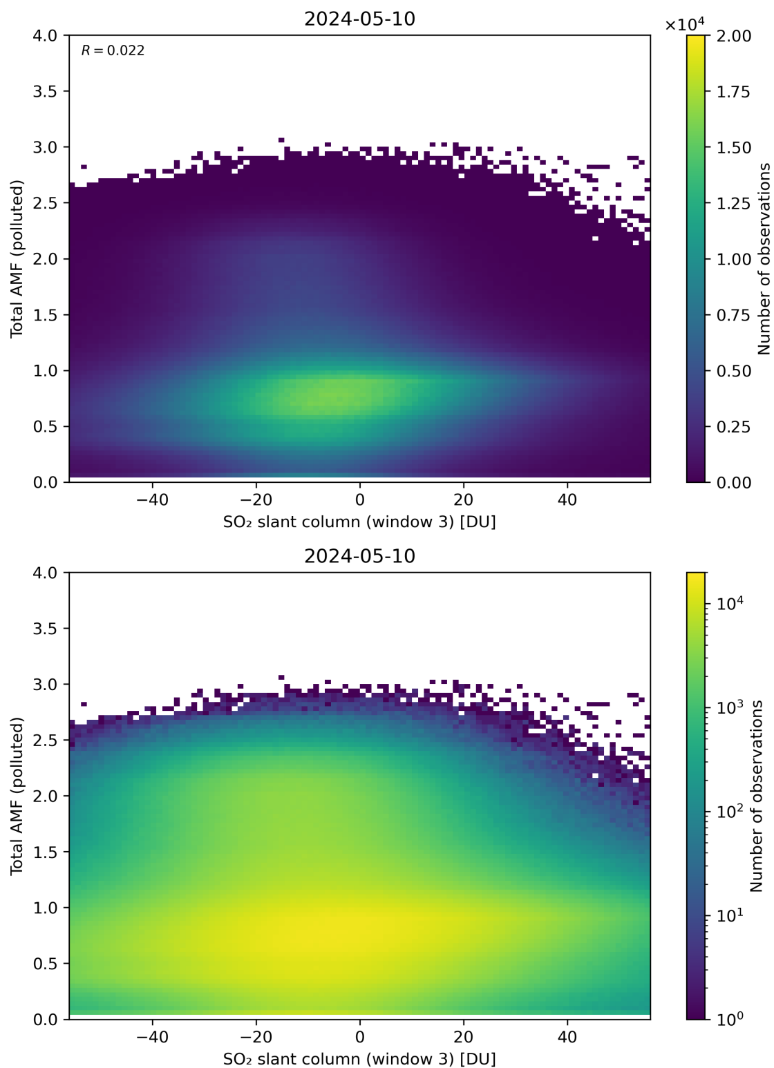
Figure 268: Scatter density plot of “SO 2 slant column (window 3)” against “Total AMF (polluted)” for 2024-05-09 to 2024-05-11.
