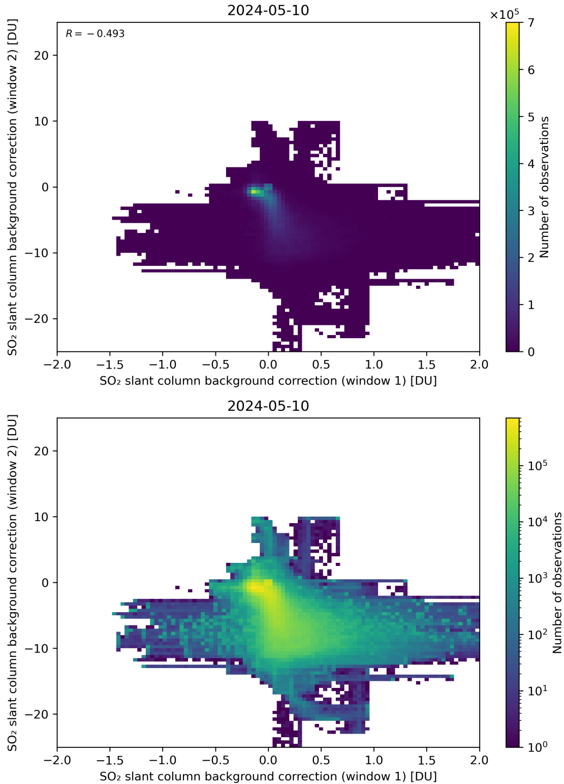
Figure 98: Scatter density plot of “SO 2 slant column background correction (window 1)” against “SO 2 slant column background correction (window 2)” for 2024-05-09 to 2024-05-11.
