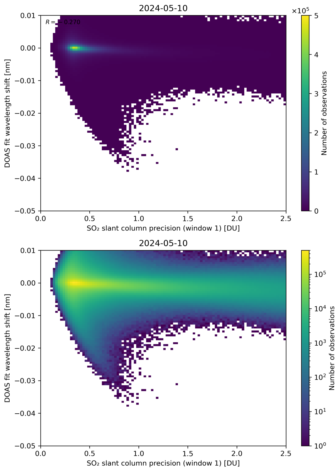
Figure 221: Scatter density plot of “SO 2 slant column precision (window 1)” against “DOAS fit wavelength shift” for 2024-05-09 to 2024-05-11.
