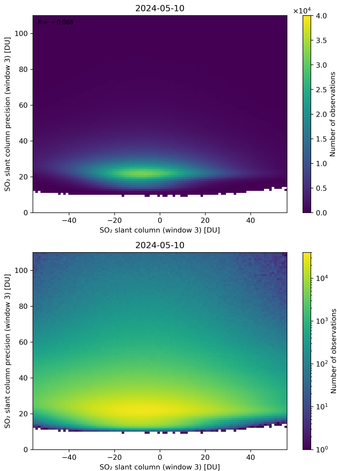
Figure 267: Scatter density plot of “SO 2 slant column (window 3)” against “SO 2 slant column precision (window 3)” for 2024-05-09 to 2024-05-11.
