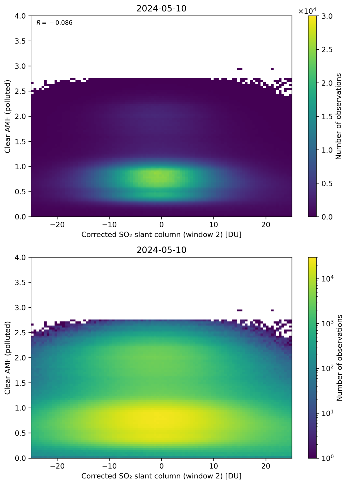
Figure 199: Scatter density plot of “Corrected SO 2 slant column (window 2)” against “Clear AMF (polluted)” for 2024-05-09 to 2024-05-11.
