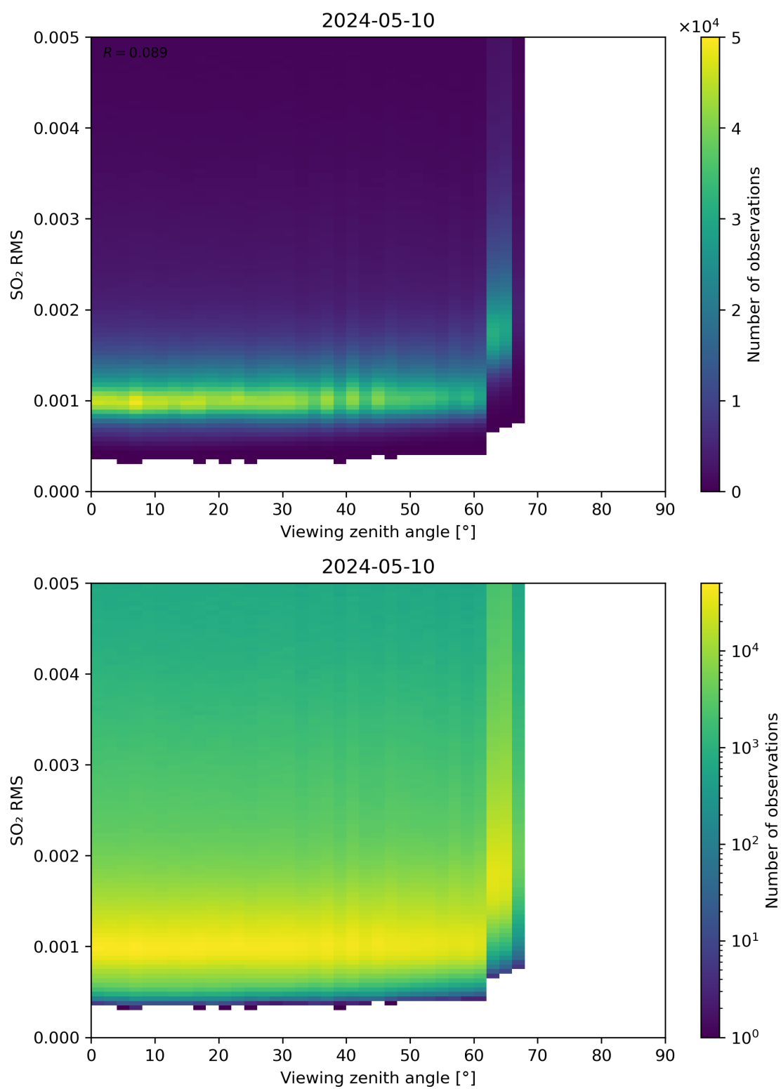
Figure 313: Scatter density plot of “Viewing zenith angle” against “SO 2 RMS” for 2024-05-09 to 2024-05-11.
