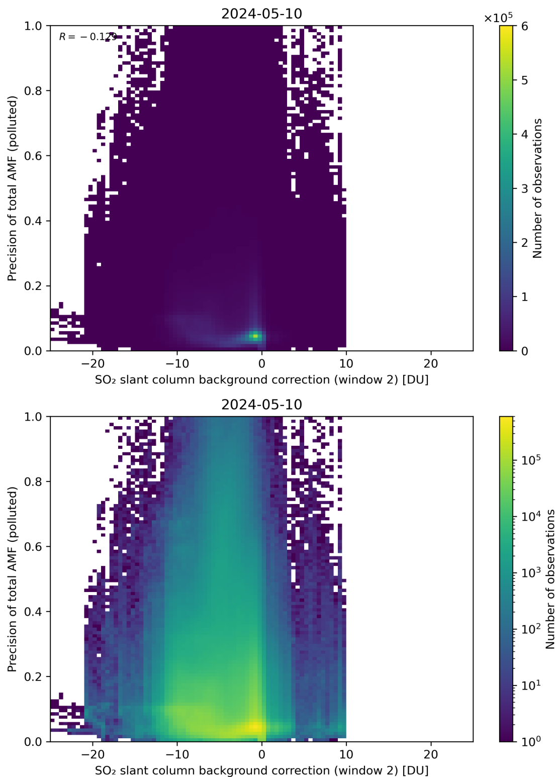
Figure 120: Scatter density plot of “SO 2 slant column background correction (window 2)” against “Precision of total AMF (polluted)” for 2024-05-09 to 2024-05-11.
