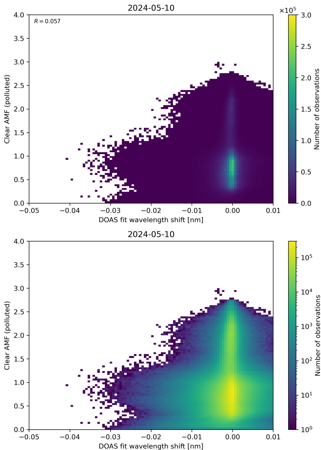
Figure 129: Scatter density plot of “DOAS fit wavelength shift” against “Clear AMF (polluted)” for 2024-05-09 to 2024-05-11.
