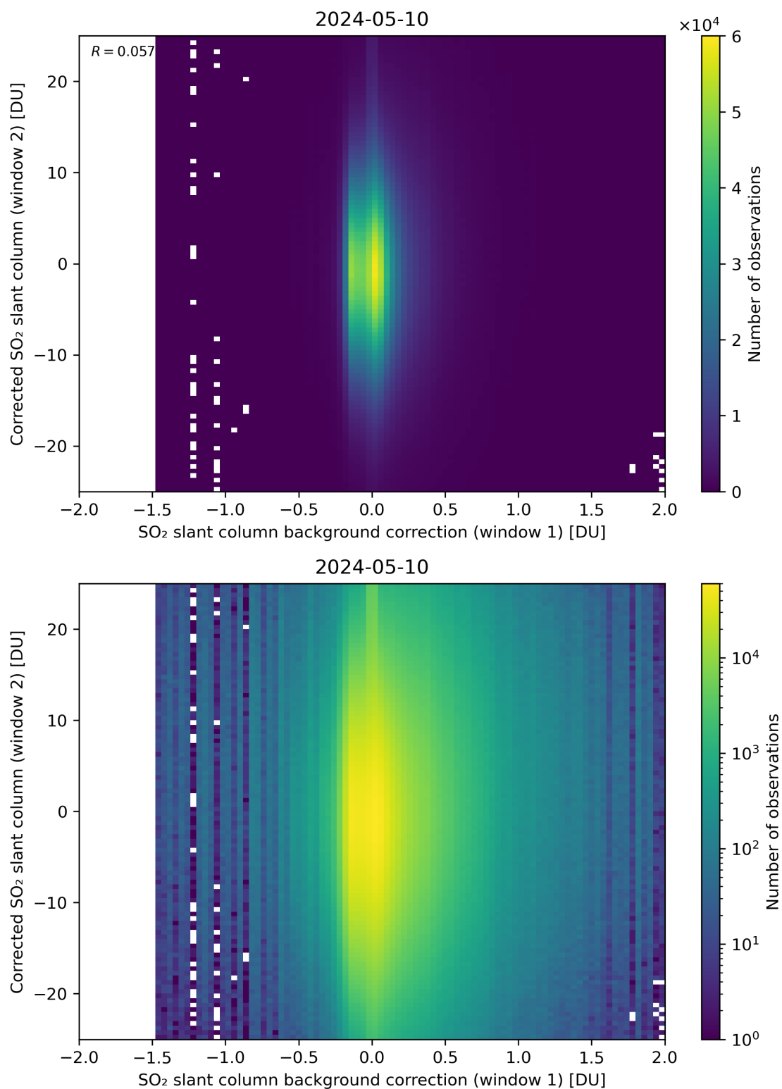
Figure 104: Scatter density plot of “SO 2 slant column background correction (window 1)” against “Corrected SO 2 slant column (window 2)” for 2024-05-09 to 2024-05-11.
