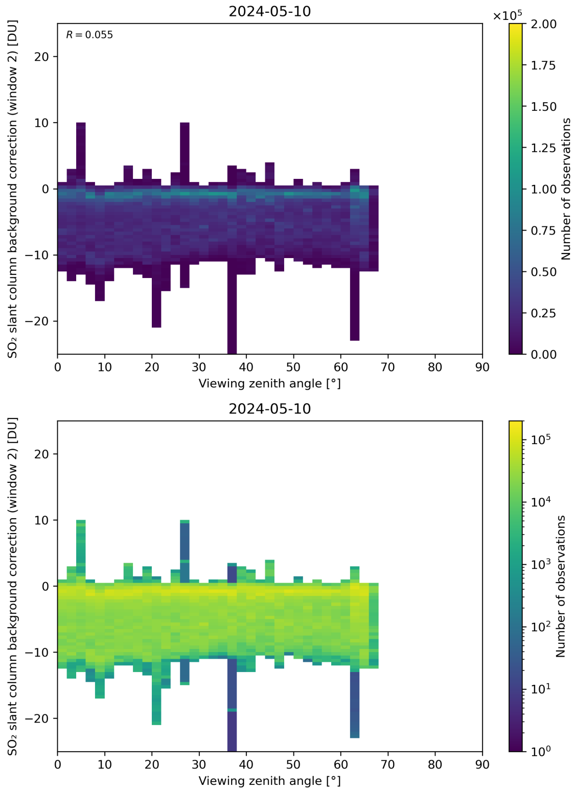
Figure 309: Scatter density plot of “Viewing zenith angle” against “SO 2 slant column background correction (window 2)” for 2024-05-09 to 2024-05-11.
