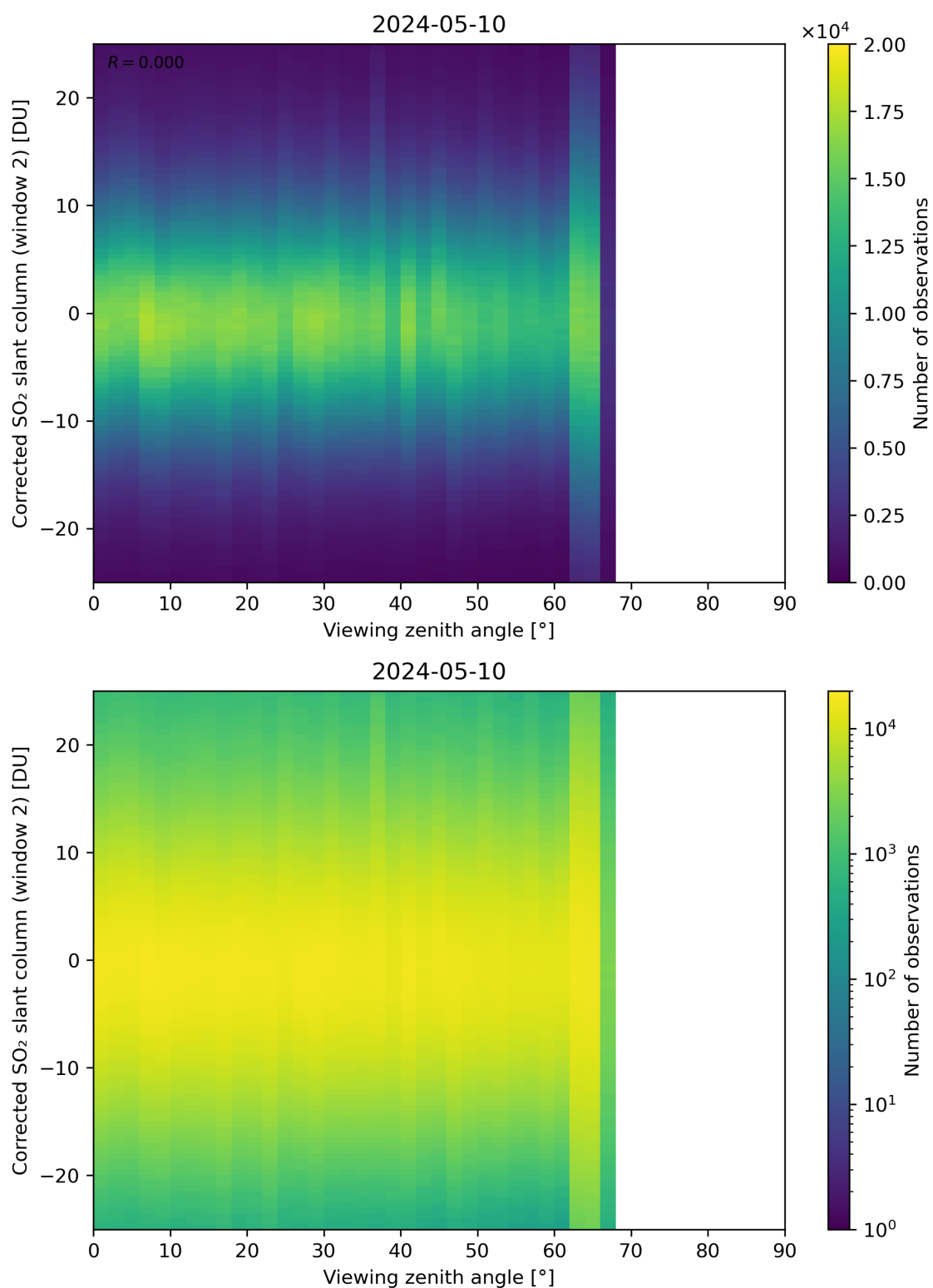
Figure 318: Scatter density plot of “Viewing zenith angle” against “Corrected SO 2 slant column (window 2)” for 2024-05-09 to 2024-05-11.
