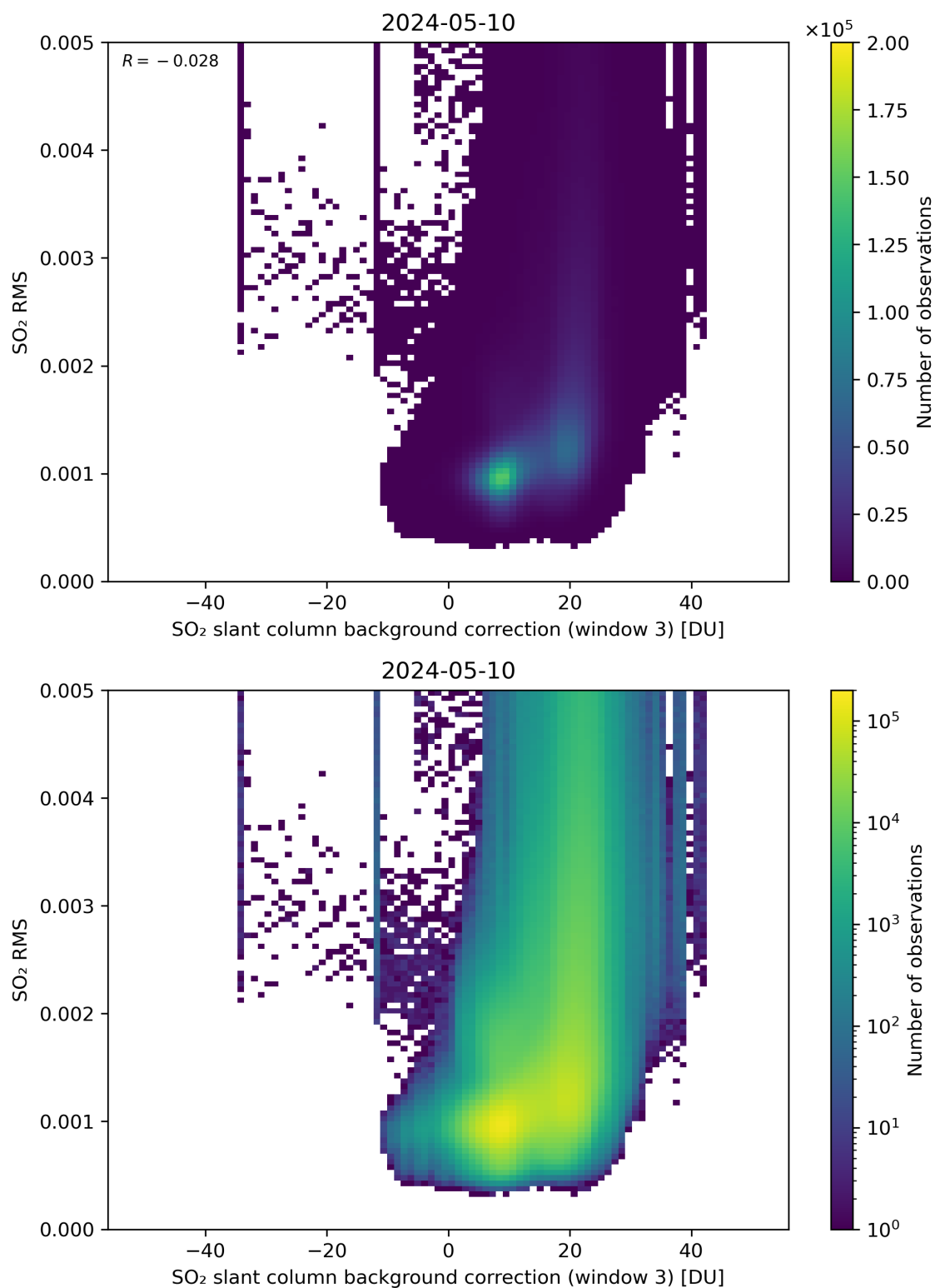
Figure 123: Scatter density plot of “SO 2 slant column background correction (window 3)” against “SO 2 RMS” for 2024-05-09 to 2024-05-11.
