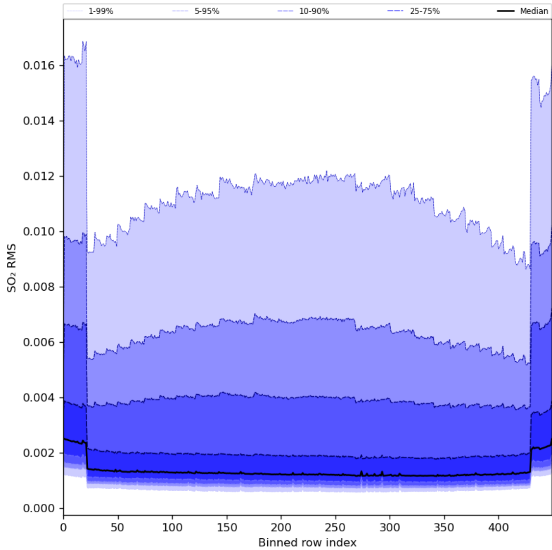
Figure 93: Along track statistics of “SO 2 RMS” for 2024-05-09 to 2024-05-11
