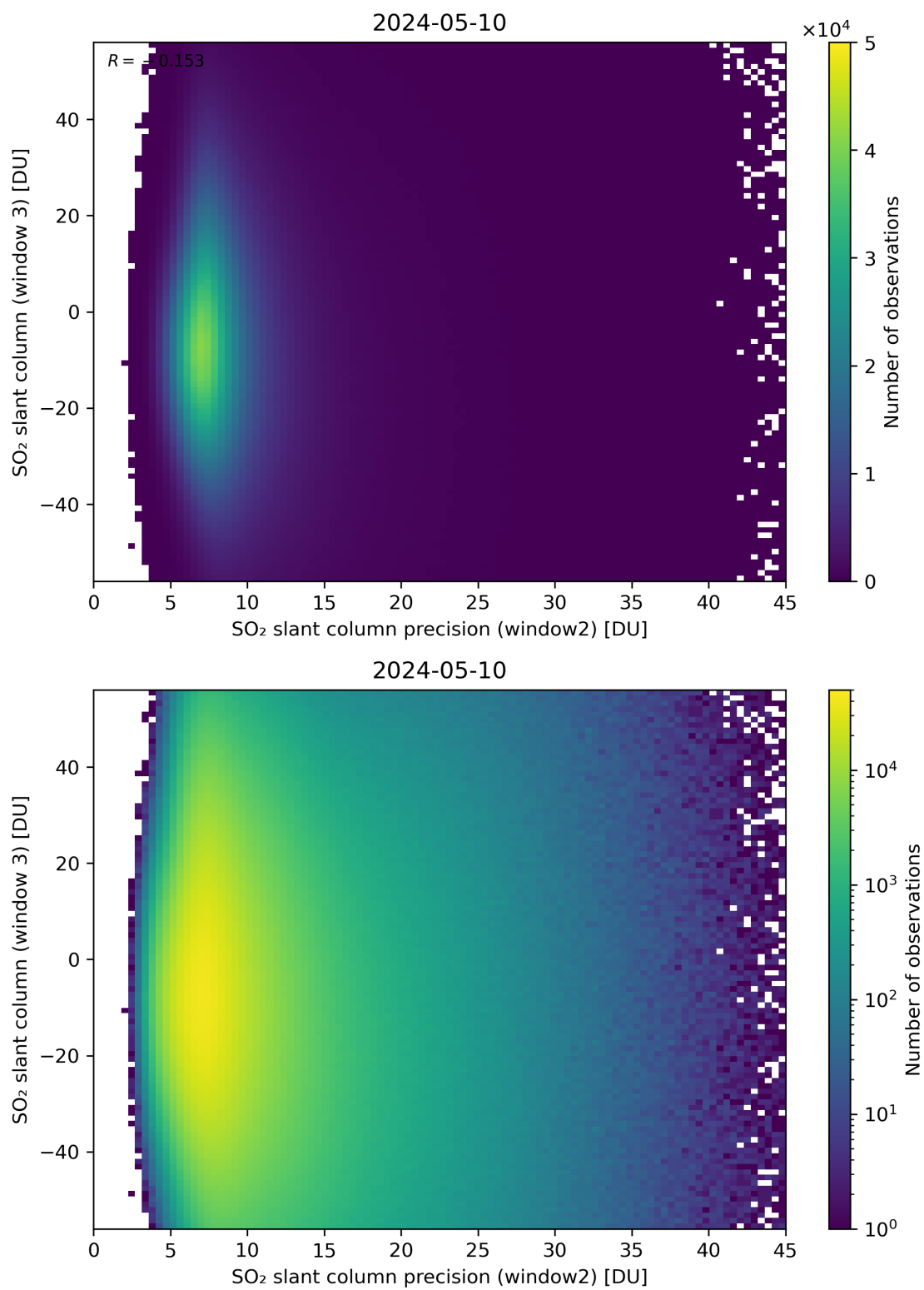
Figure 249: Scatter density plot of “SO 2 slant column precision (window2)” against “SO 2 slant column (window 3)” for 2024-05-09 to 2024-05-11.
