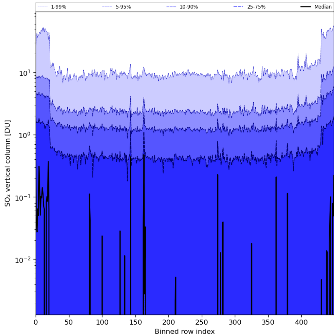
Figure 76: Along track statistics of “SO 2 vertical column” for 2024-05-09 to 2024-05-11
