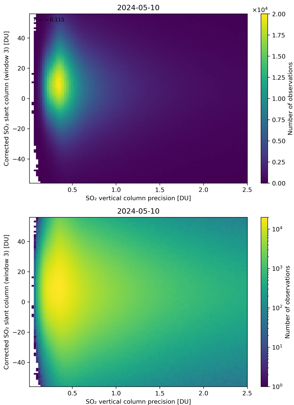
Figure 288: Scatter density plot of “SO 2 vertical column precision” against “Corrected SO 2 slant column (window 3)” for 2024-05-09 to 2024-05-11.
