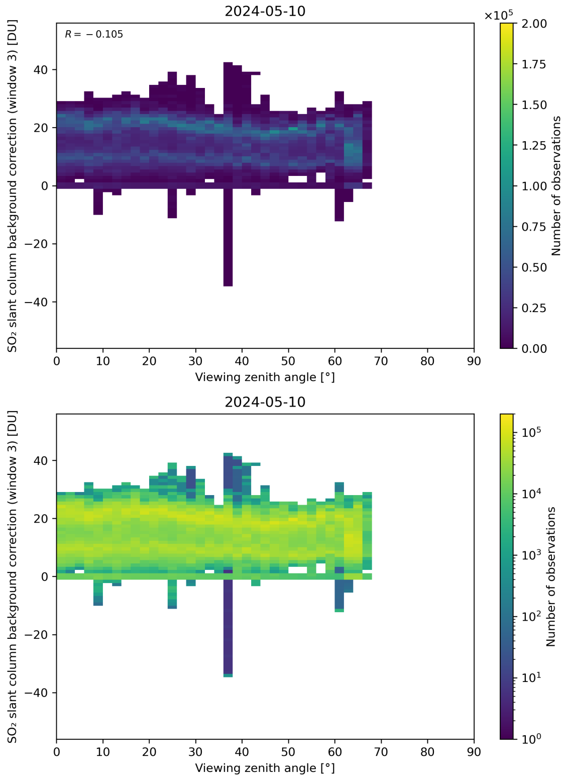
Figure 310: Scatter density plot of “Viewing zenith angle” against “SO 2 slant column background correction (window 3)” for 2024-05-09 to 2024-05-11.
