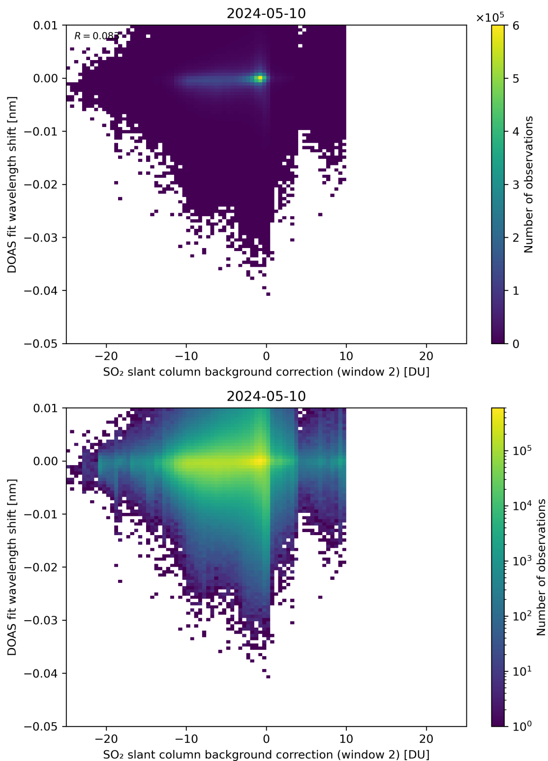
Figure 112: Scatter density plot of “SO 2 slant column background correction (window 2)” against “DOAS fit wavelength shift” for 2024-05-09 to 2024-05-11.
