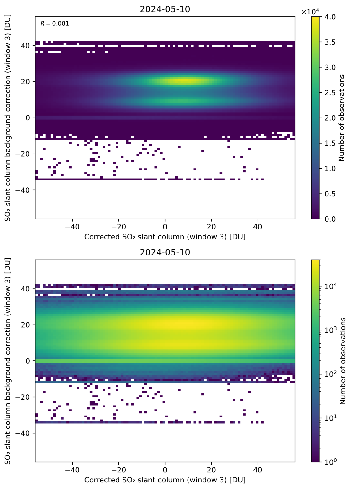
Figure 205: Scatter density plot of “Corrected SO 2 slant column (window 3)” against “SO 2 slant column background correction (window 3)” for 2024-05-09 to 2024-05-11.
