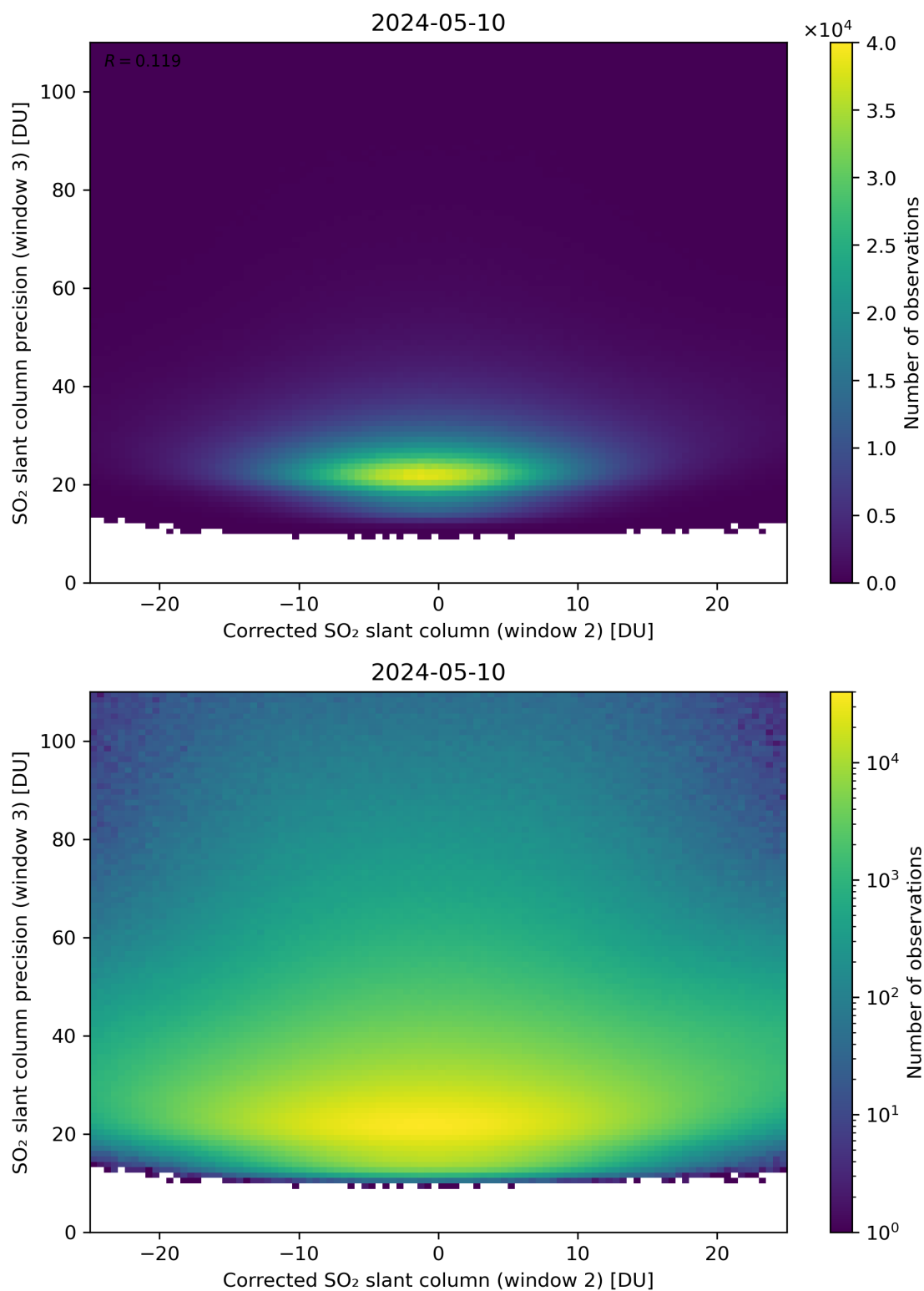
Figure 202: Scatter density plot of “Corrected SO 2 slant column (window 2)” against “SO 2 slant column precision (window 3)” for 2024-05-09 to 2024-05-11.
