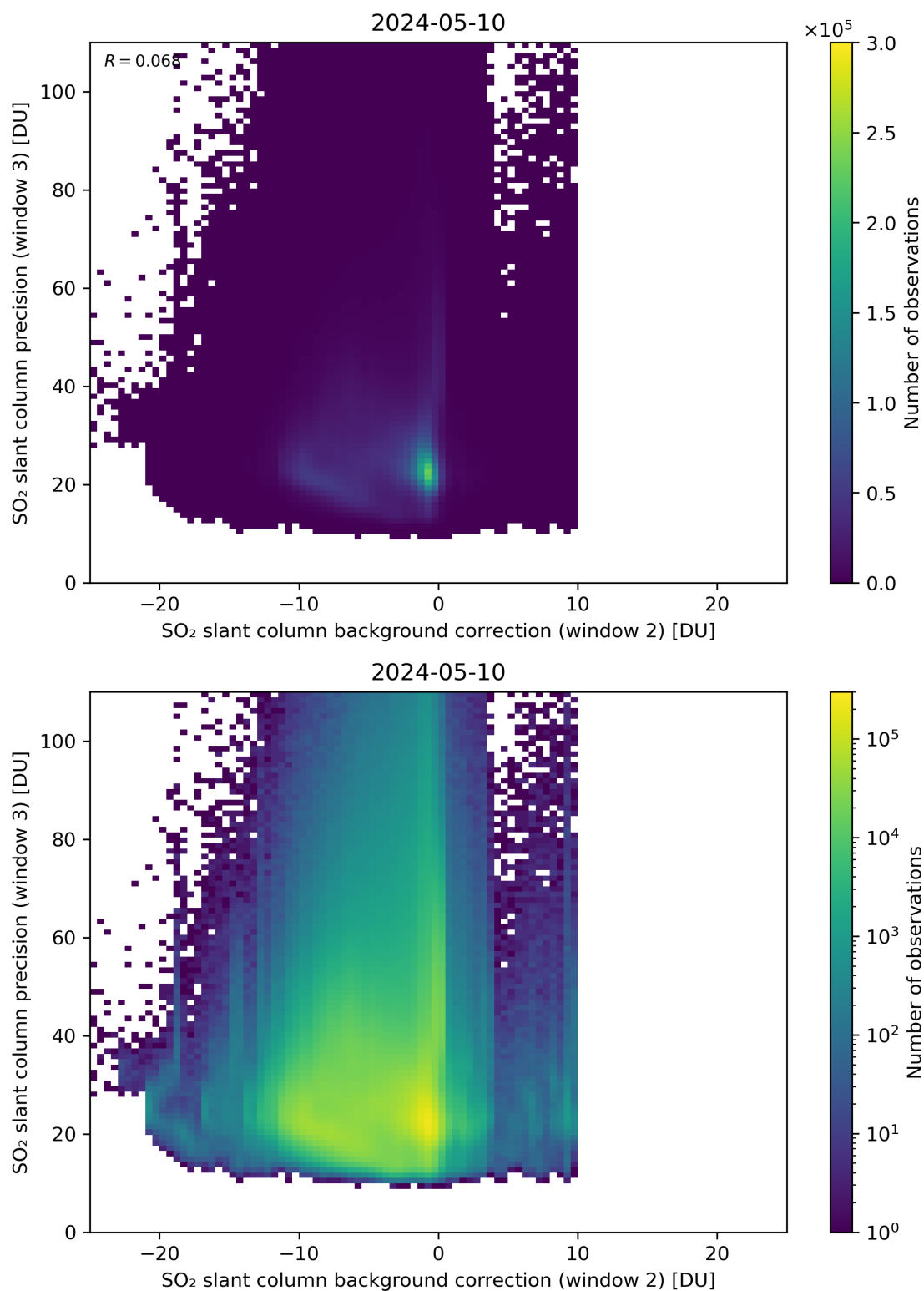
Figure 118: Scatter density plot of “SO 2 slant column background correction (window 2)” against “SO 2 slant column precision (window 3)” for 2024-05-09 to 2024-05-11.
