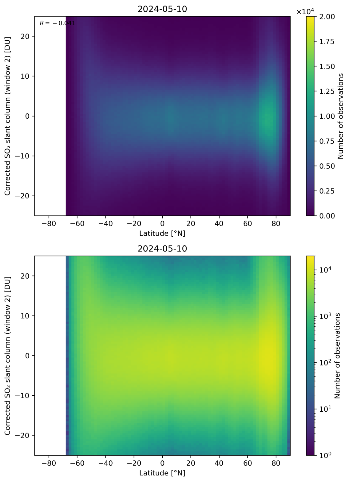
Figure 147: Scatter density plot of “Latitude” against “Corrected SO 2 slant column (window 2)” for 2024-05-09 to 2024-05-11.
