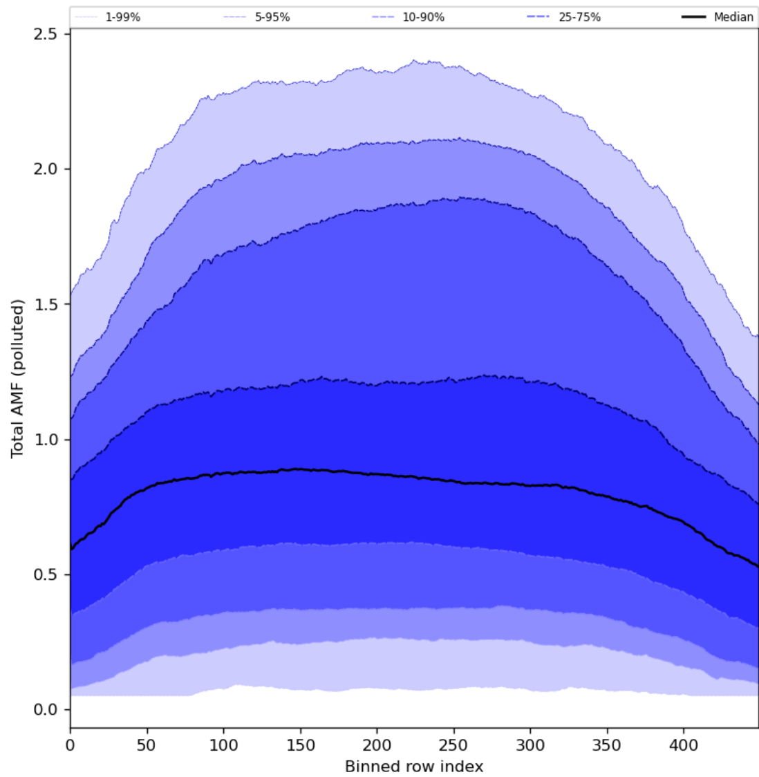
Figure 94: Along track statistics of “Total AMF (polluted)” for 2024-05-09 to 2024-05-11
