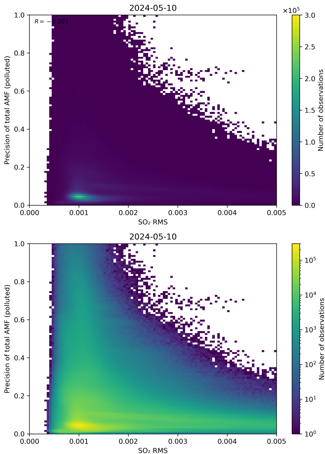
Figure 138: Scatter density plot of “SO 2 RMS” against “Precision of total AMF (polluted)” for 2024-05-09 to 2024-05-11.
