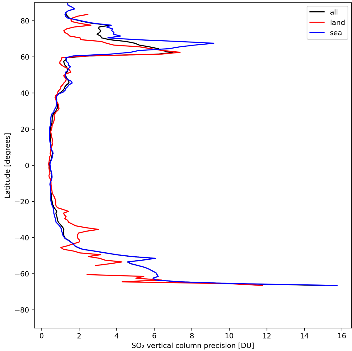
Figure 31: Zonal average of “SO 2 vertical column precision” for 2024-05-09 to 2024-05-11.
