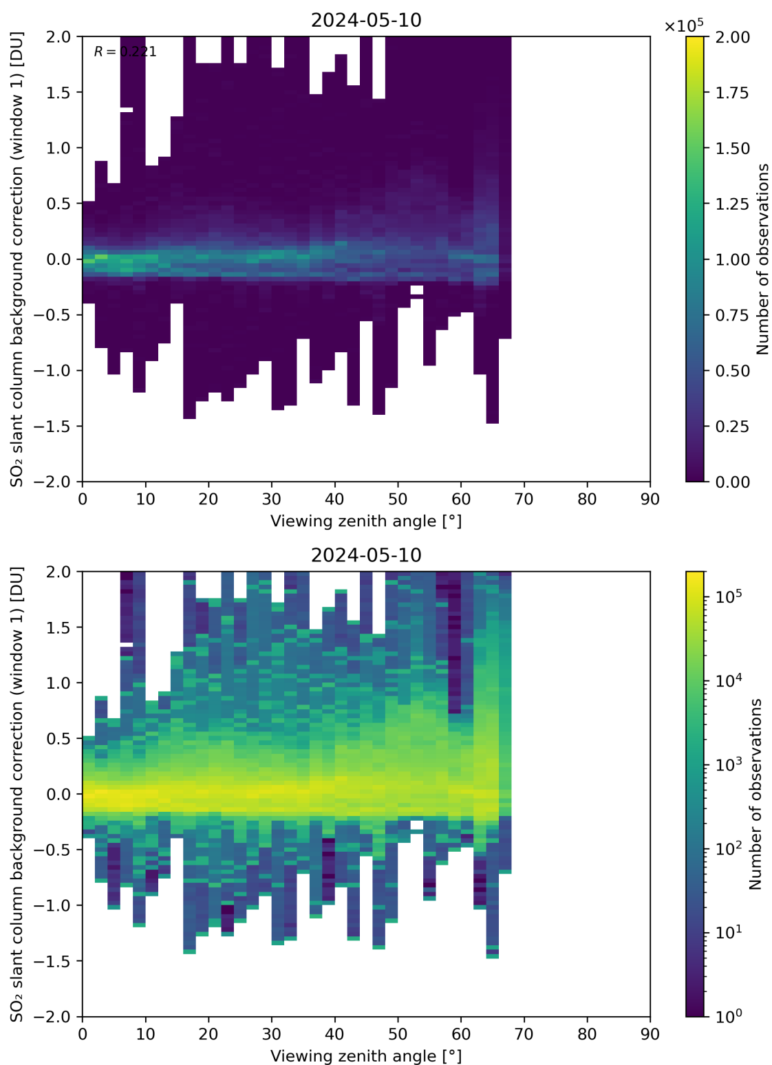
Figure 308: Scatter density plot of “Viewing zenith angle” against “SO 2 slant column background correction (window 1)” for 2024-05-09 to 2024-05-11.
