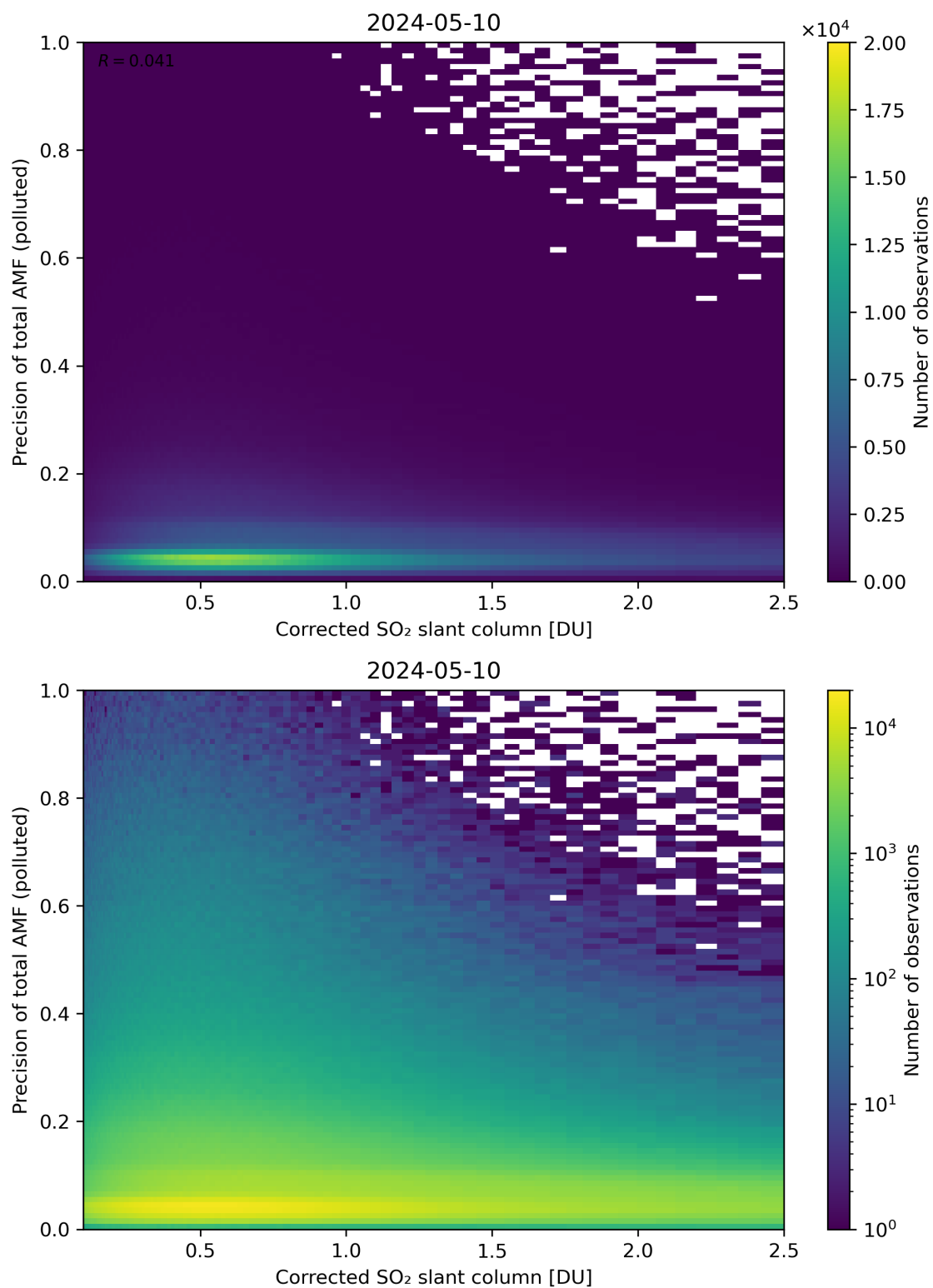
Figure 193: Scatter density plot of “Corrected SO 2 slant column” against “Precision of total AMF (polluted)” for 2024-05-09 to 2024-05-11.
