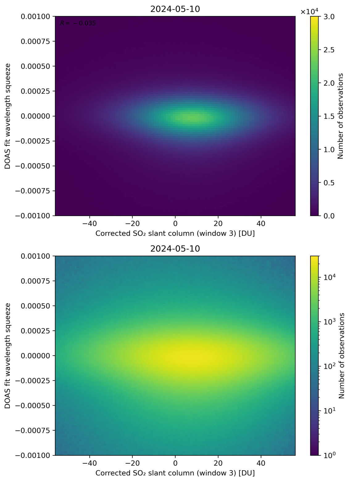
Figure 207: Scatter density plot of “Corrected SO 2 slant column (window 3)” against “DOAS fit wavelength squeeze” for 2024-05-09 to 2024-05-11.
