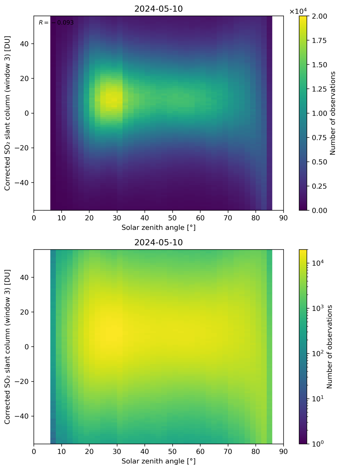
Figure 168: Scatter density plot of “Solar zenith angle” against “Corrected SO 2 slant column (window 3)” for 2024-05-09 to 2024-05-11.
