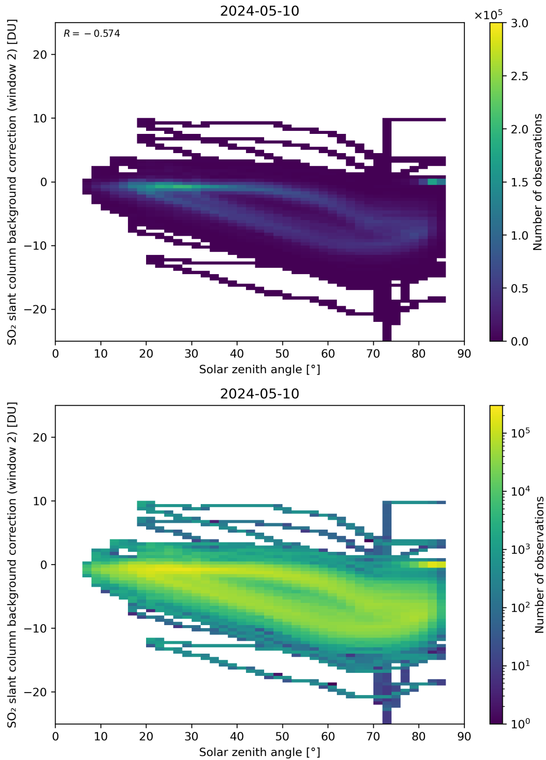
Figure 159: Scatter density plot of “Solar zenith angle” against “SO 2 slant column background correction (window 2)” for 2024-05-09 to 2024-05-11.
