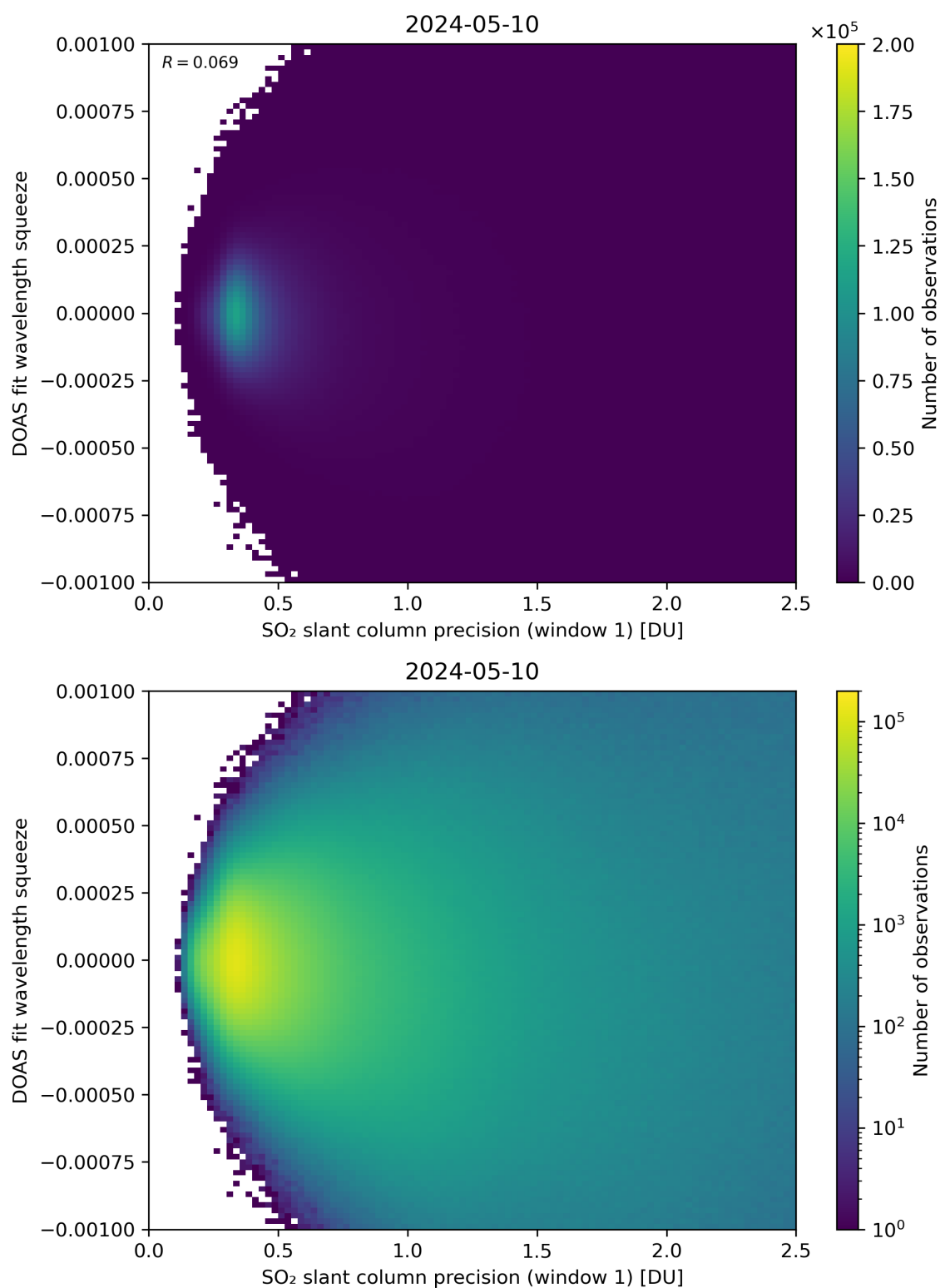
Figure 222: Scatter density plot of “SO 2 slant column precision (window 1)” against “DOAS fit wavelength squeeze” for 2024-05-09 to 2024-05-11.
