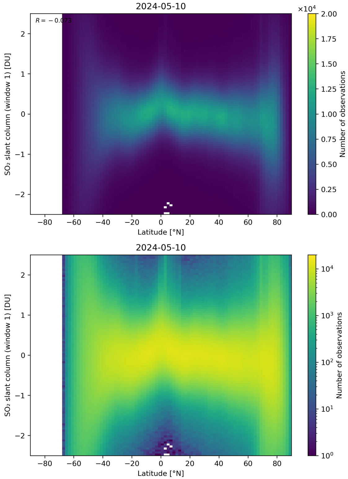
Figure 149: Scatter density plot of “Latitude” against “SO 2 slant column (window 1)” for 2024-05-09 to 2024-05-11.
