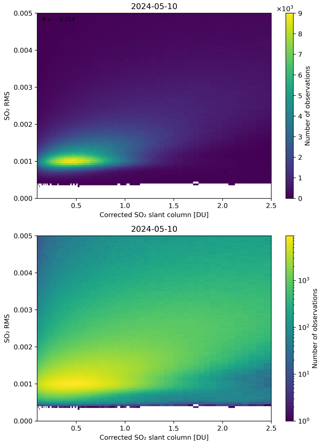
Figure 183: Scatter density plot of “Corrected SO 2 slant column” against “SO 2 RMS” for 2024-05-09 to 2024-05-11.
