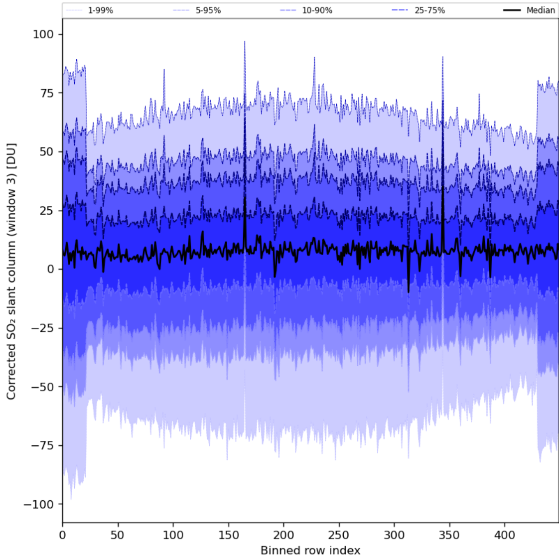
Figure 89: Along track statistics of “Corrected SO 2 slant column (window 3)” for 2024-05-09 to 2024-05-11
