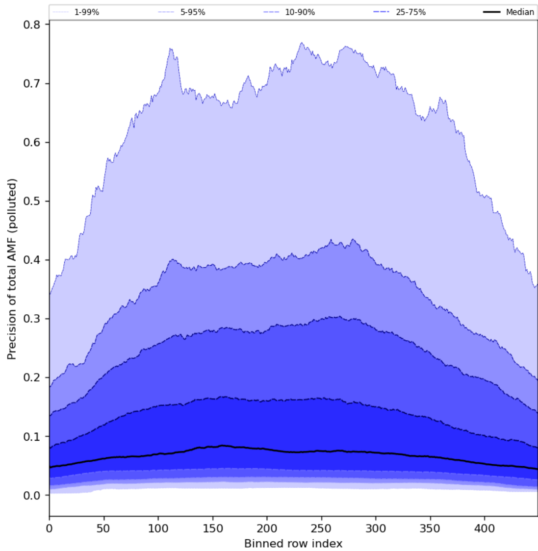
Figure 95: Along track statistics of “Precision of total AMF (polluted)” for 2024-05-09 to 2024-05-11
