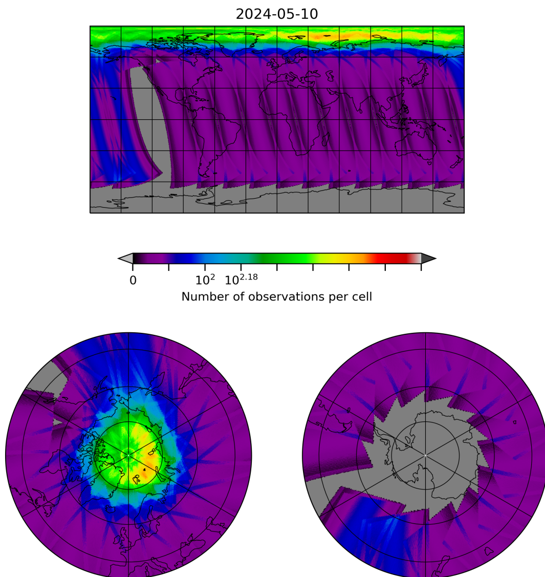
Figure 28: Map of the number of observations for 2024-05-09 to 2024-05-11
