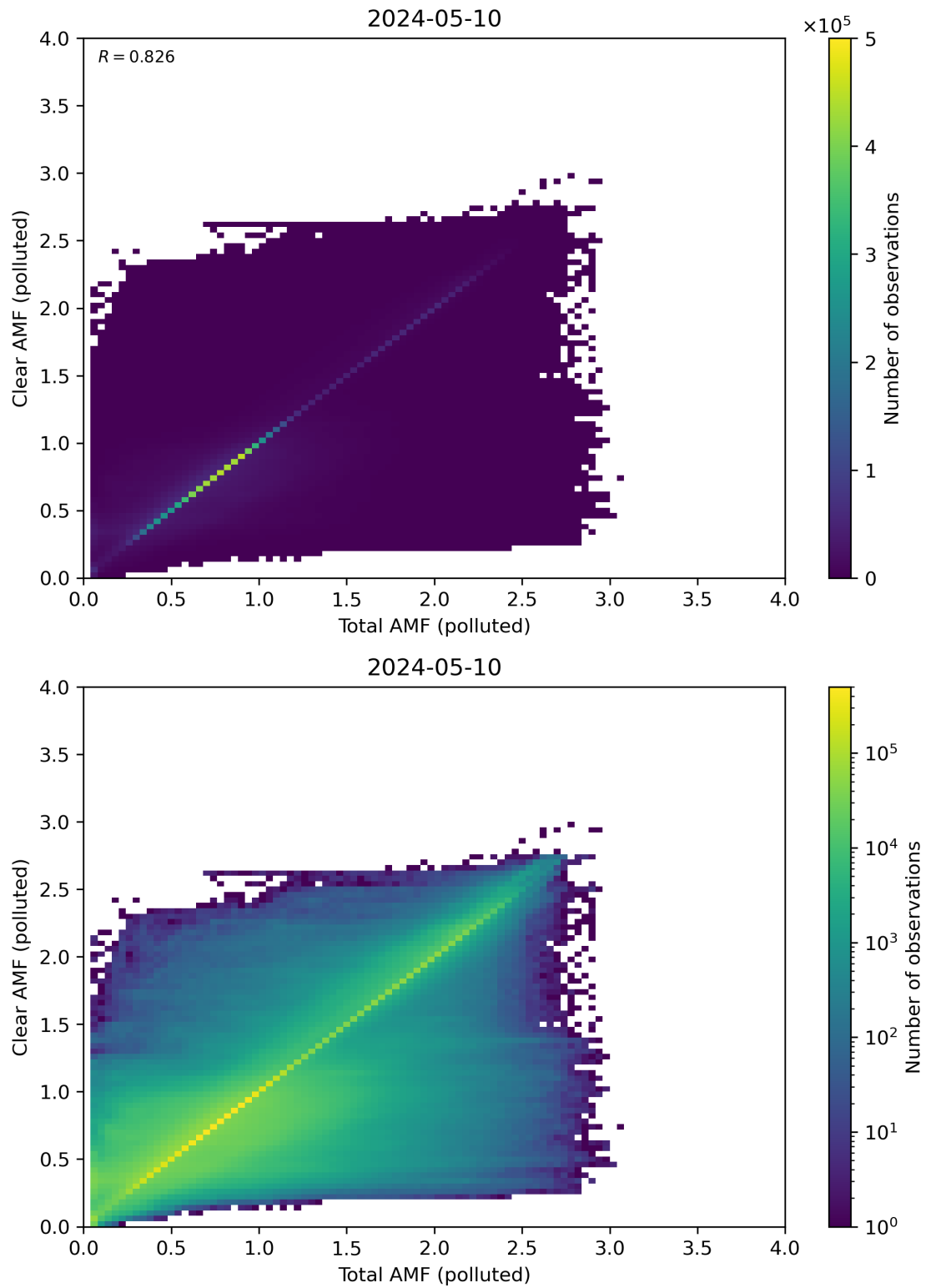
Figure 271: Scatter density plot of “Total AMF (polluted)” against “Clear AMF (polluted)” for 2024-05-09 to 2024-05-11.
