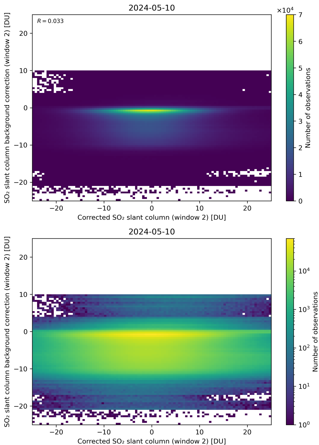
Figure 194: Scatter density plot of “Corrected SO 2 slant column (window 2)” against “SO 2 slant column background correction (window 2)” for 2024-05-09 to 2024-05-11.
