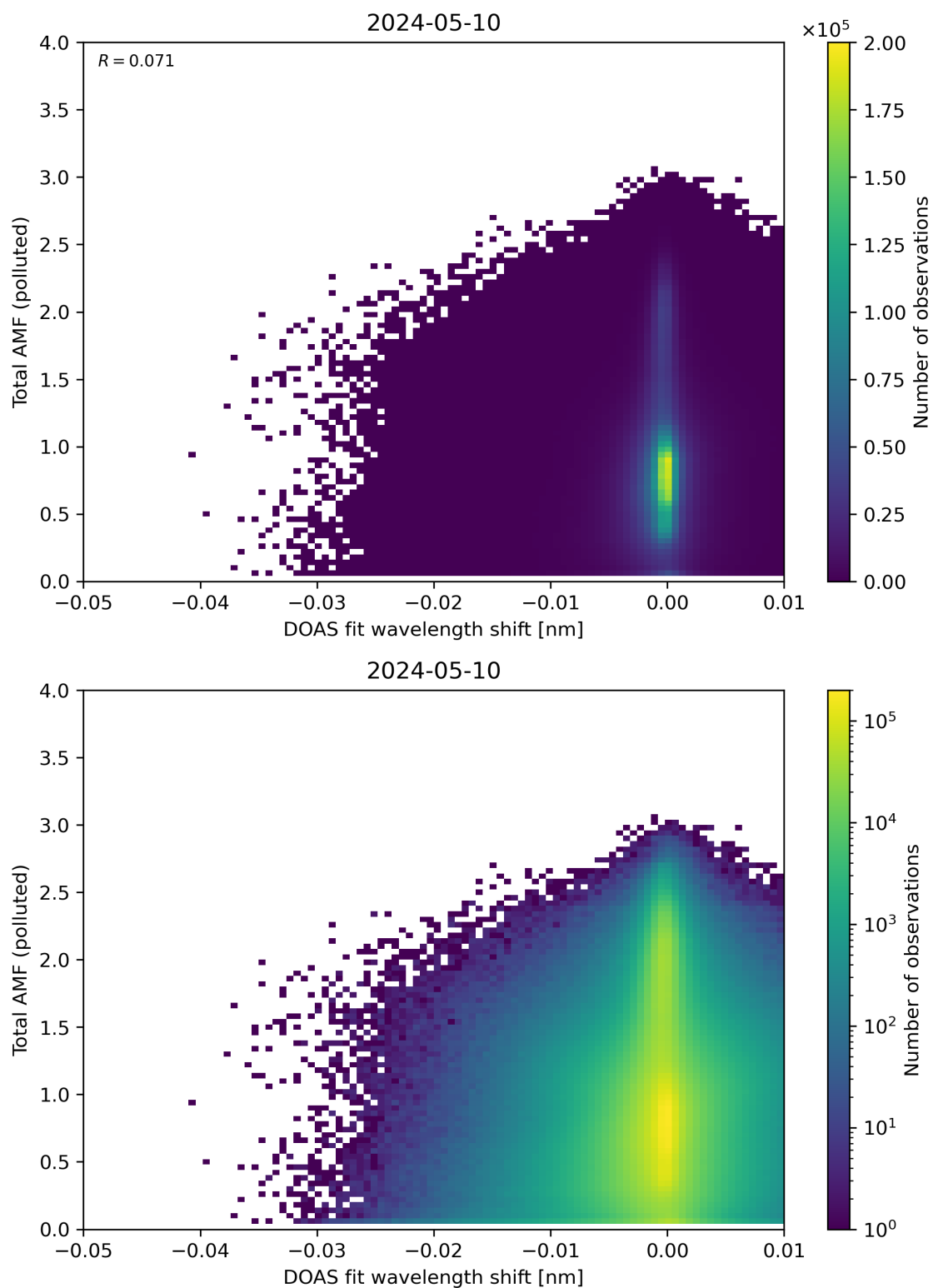
Figure 130: Scatter density plot of “DOAS fit wavelength shift” against “Total AMF (polluted)” for 2024-05-09 to 2024-05-11.
