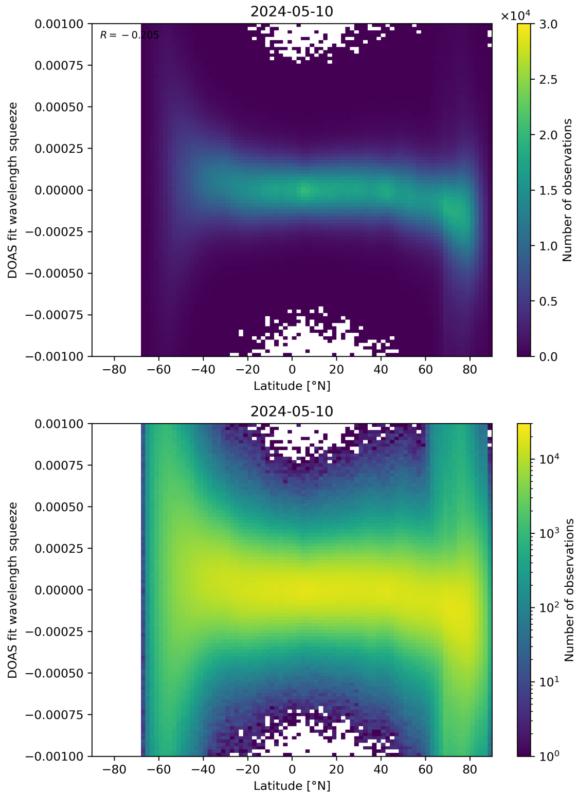
Figure 143: Scatter density plot of “Latitude” against “DOAS fit wavelength squeeze” for 2024-05-09 to 2024-05-11.
