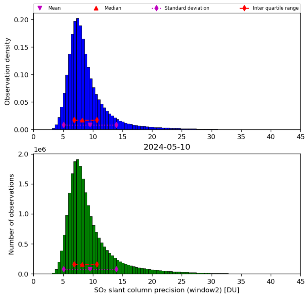
Figure 61: Histogram of “SO 2 slant column precision (window2)” for 2024-05-09 to 2024-05-11
