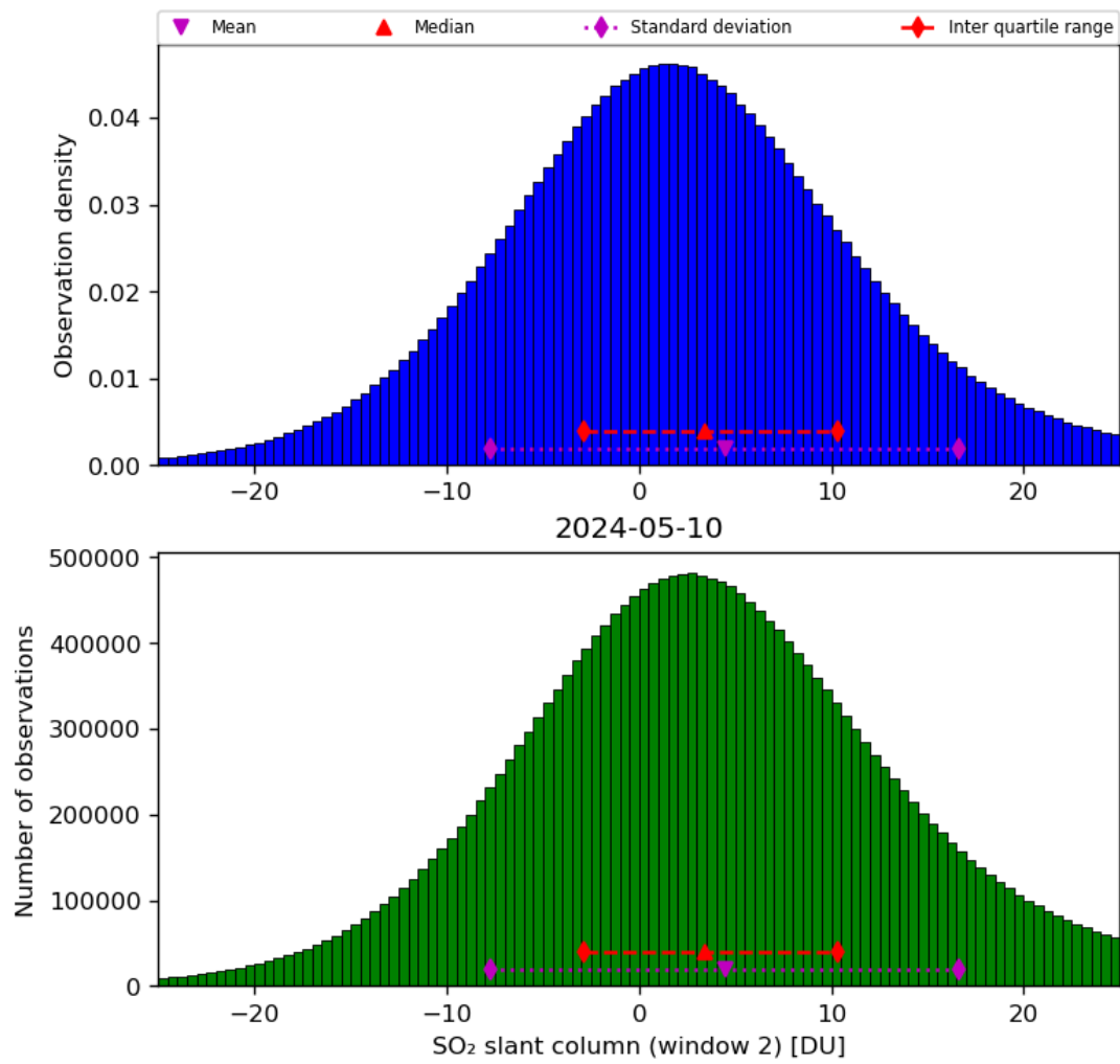
Figure 60: Histogram of “SO 2 slant column (window 2)” for 2024-05-09 to 2024-05-11
