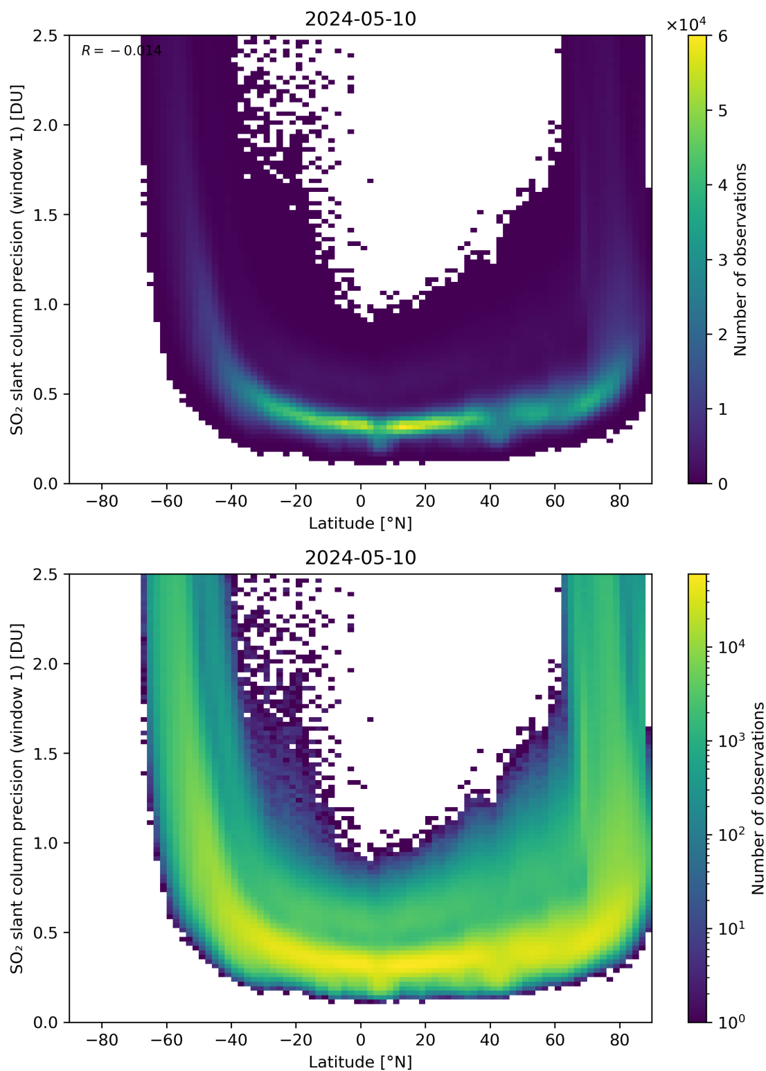
Figure 150: Scatter density plot of “Latitude” against “SO 2 slant column precision (window 1)” for 2024-05-09 to 2024-05-11.
