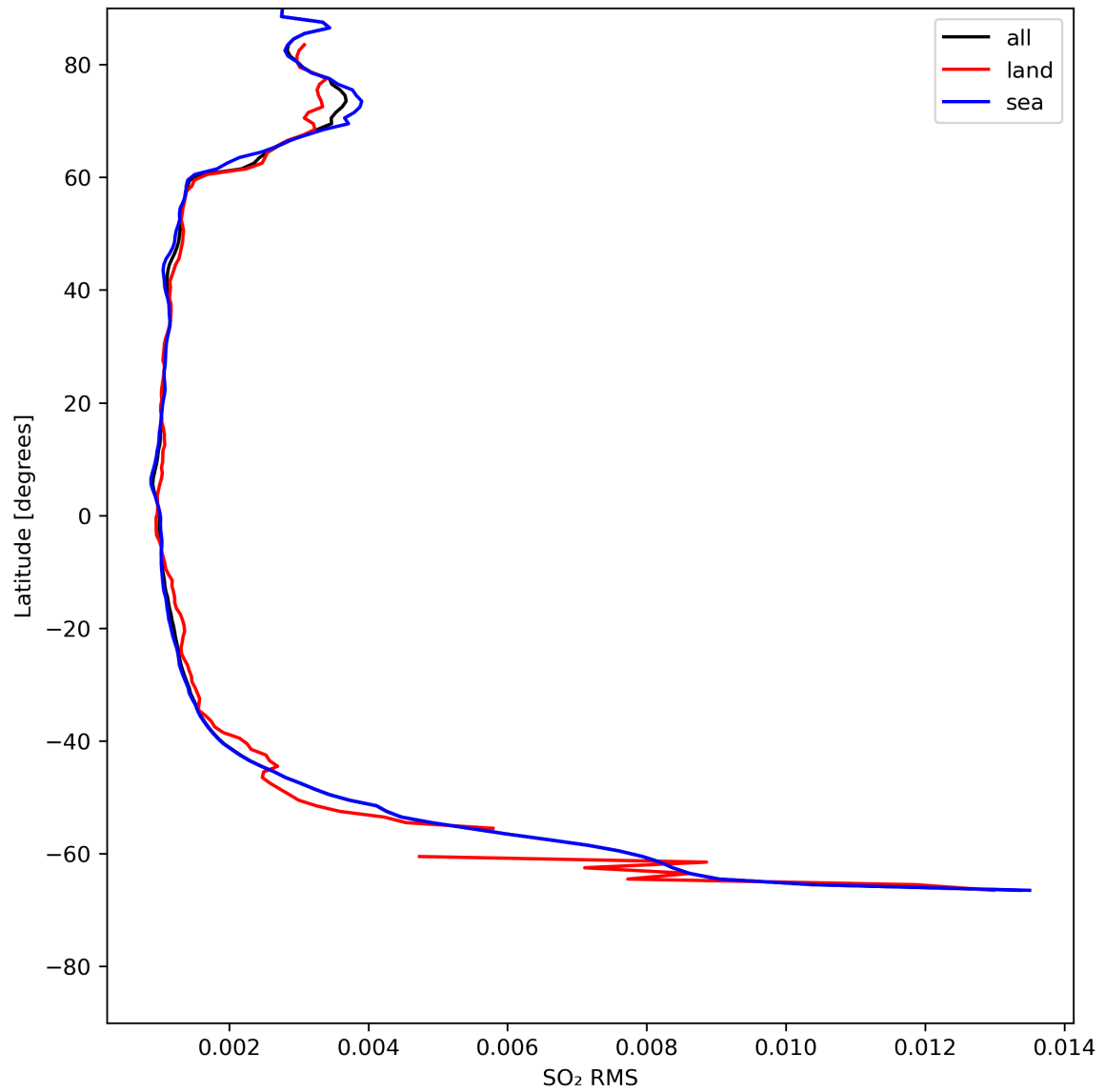
Figure 47: Zonal average of “SO 2 RMS” for 2024-05-09 to 2024-05-11.
