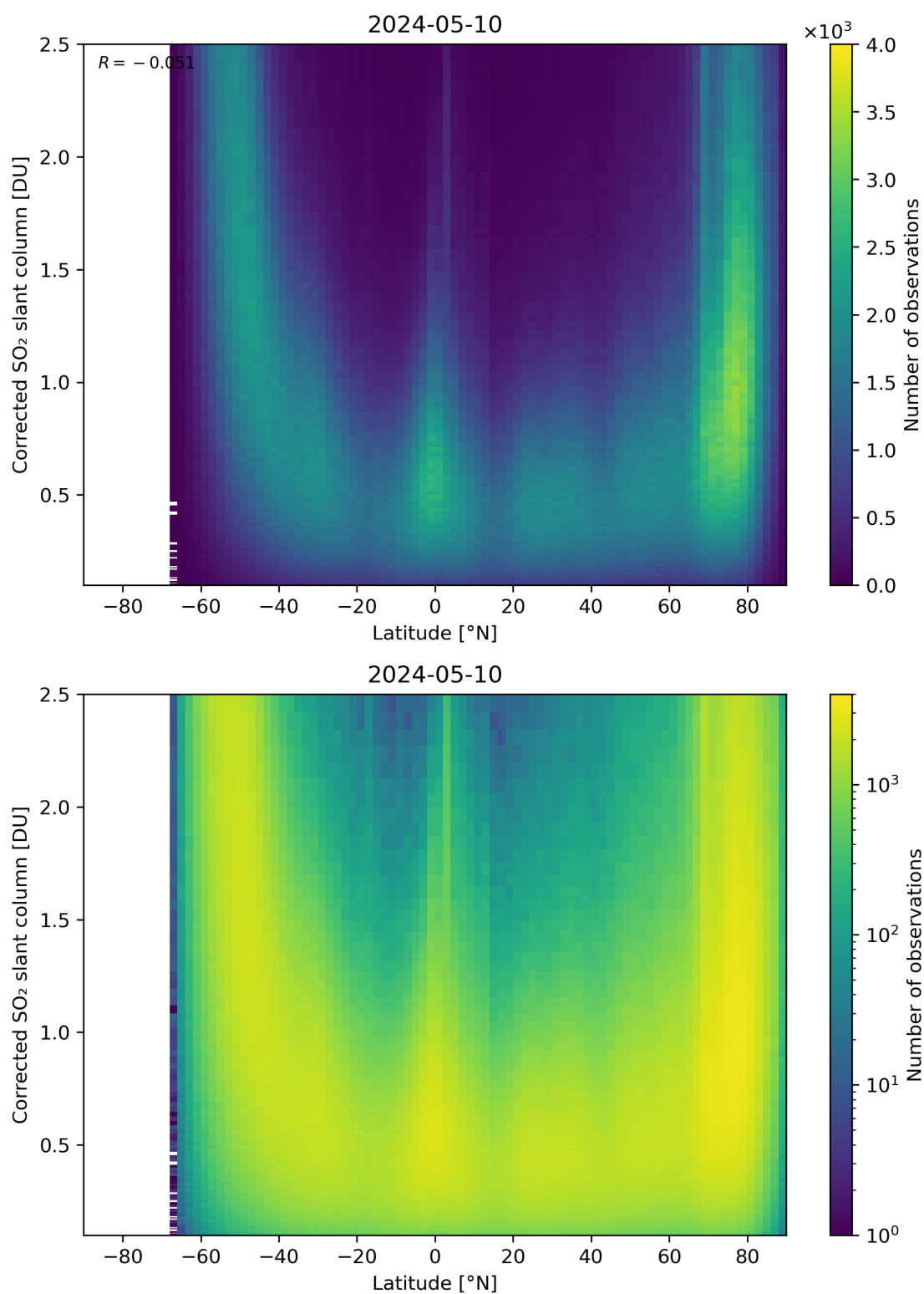
Figure 146: Scatter density plot of “Latitude” against “Corrected SO 2 slant column” for 2024-05-09 to 2024-05-11.
