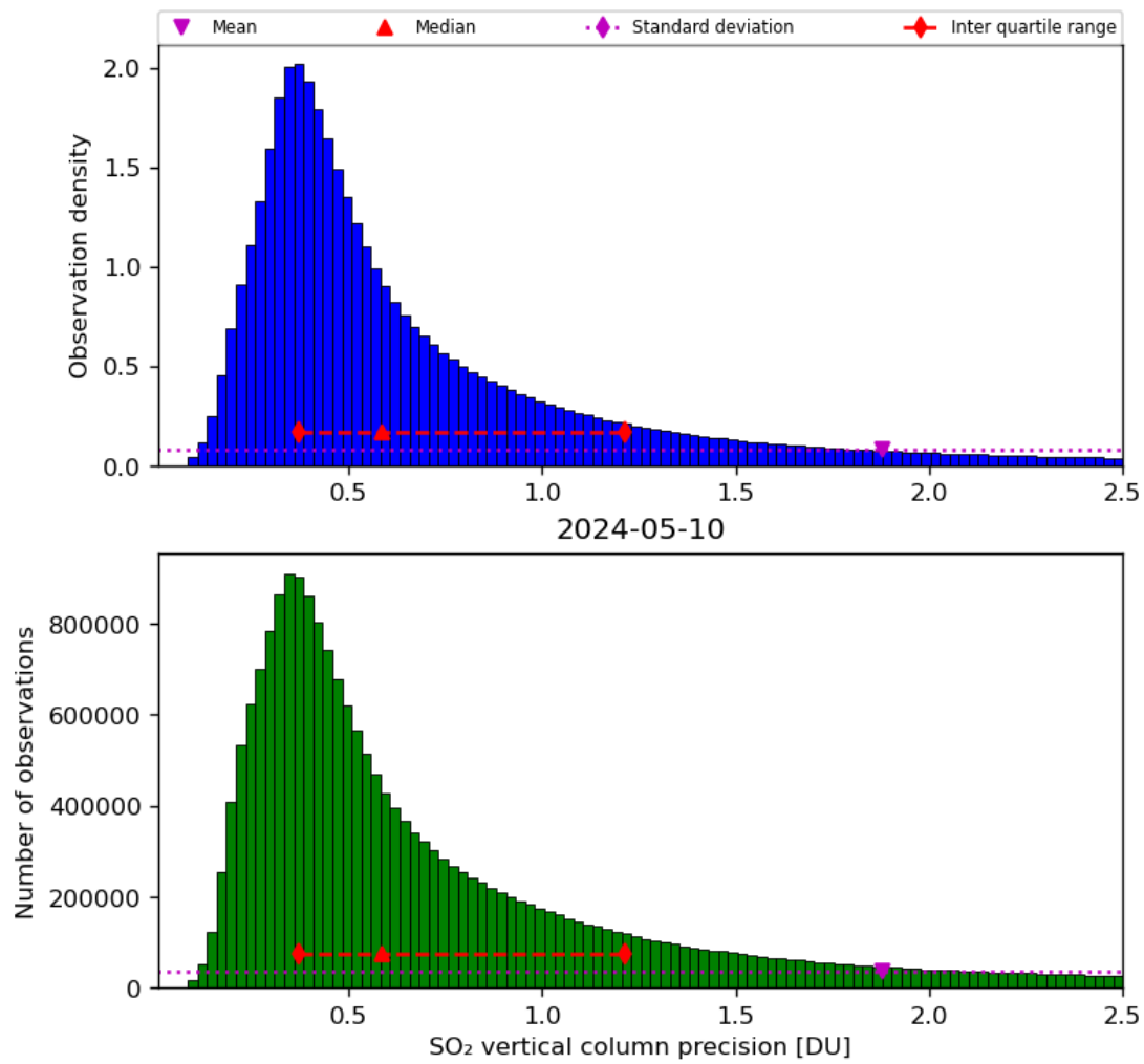
Figure 54: Histogram of “SO 2 vertical column precision” for 2024-05-09 to 2024-05-11
