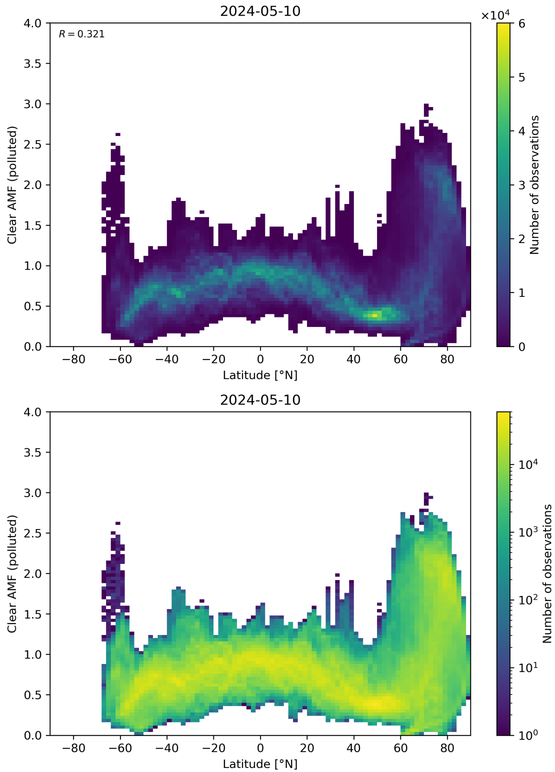
Figure 145: Scatter density plot of “Latitude” against “Clear AMF (polluted)” for 2024-05-09 to 2024-05-11.
