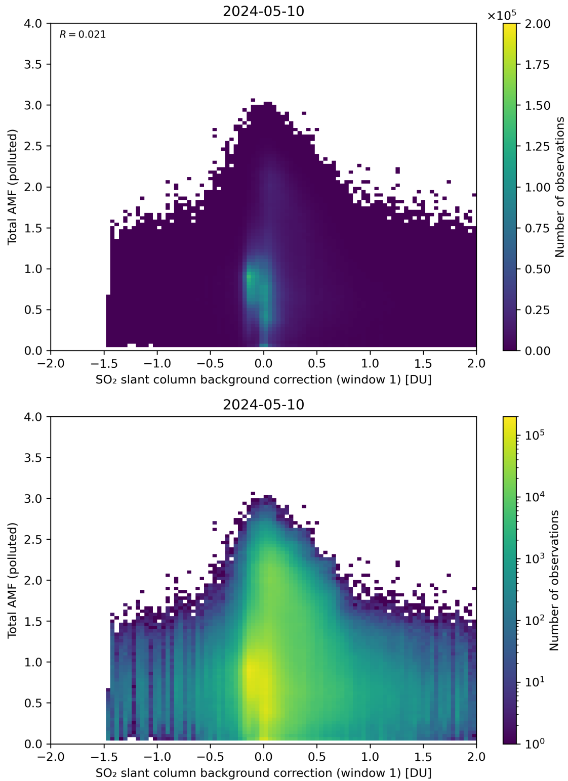
Figure 109: Scatter density plot of “SO 2 slant column background correction (window 1)” against “Total AMF (polluted)” for 2024-05-09 to 2024-05-11.
