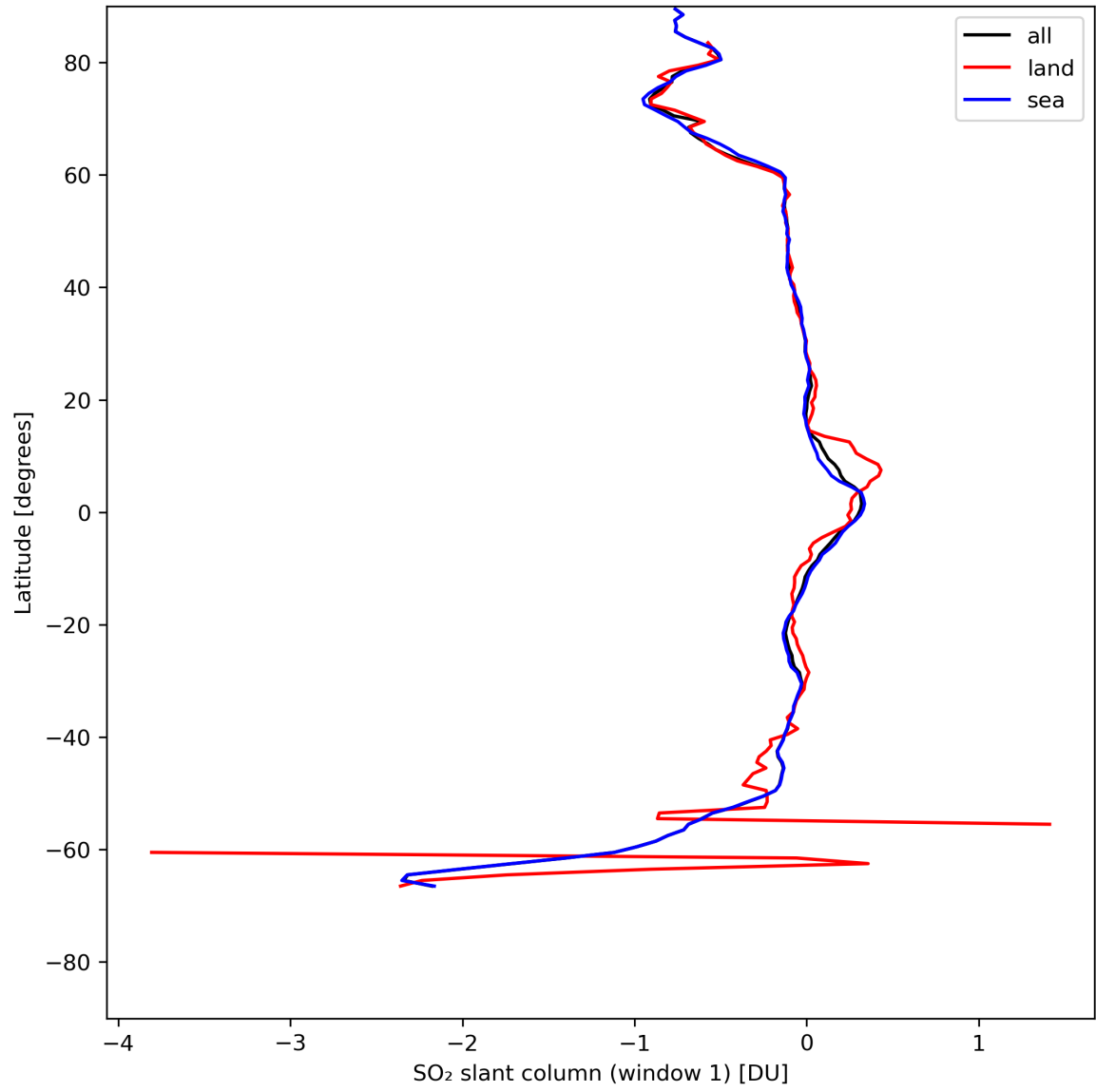
Figure 33: Zonal average of “SO 2 slant column (window 1)” for 2024-05-09 to 2024-05-11.
