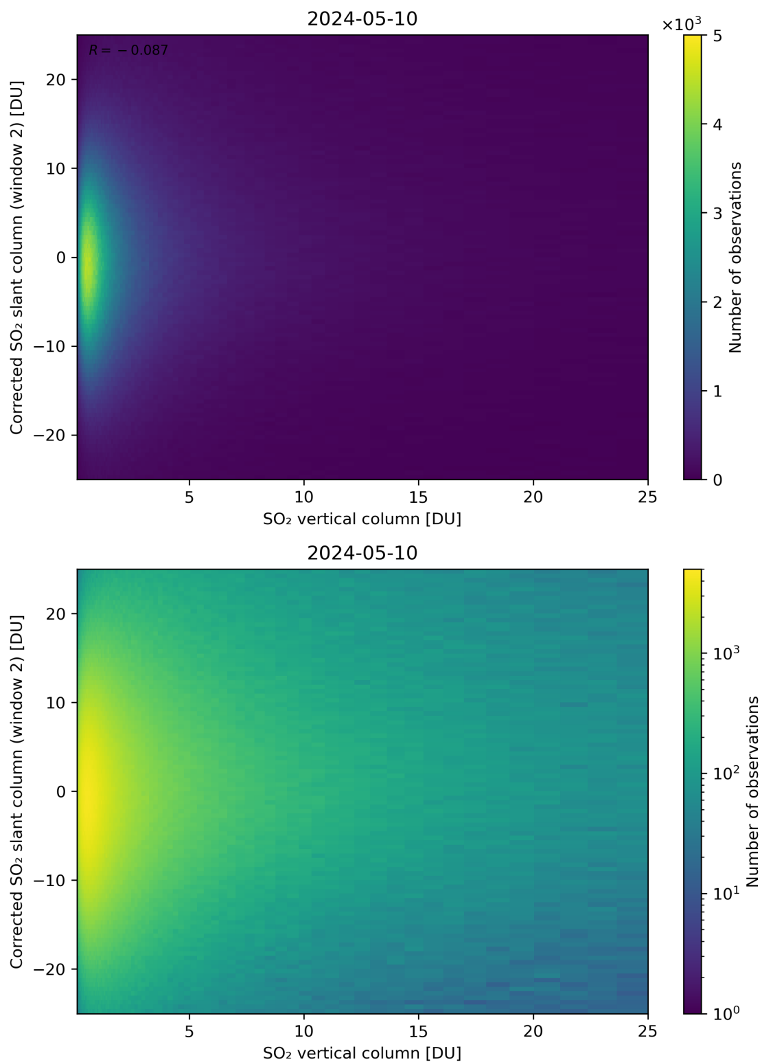
Figure 298: Scatter density plot of “SO 2 vertical column” against “Corrected SO 2 slant column (window 2)” for 2024-05-09 to 2024-05-11.
