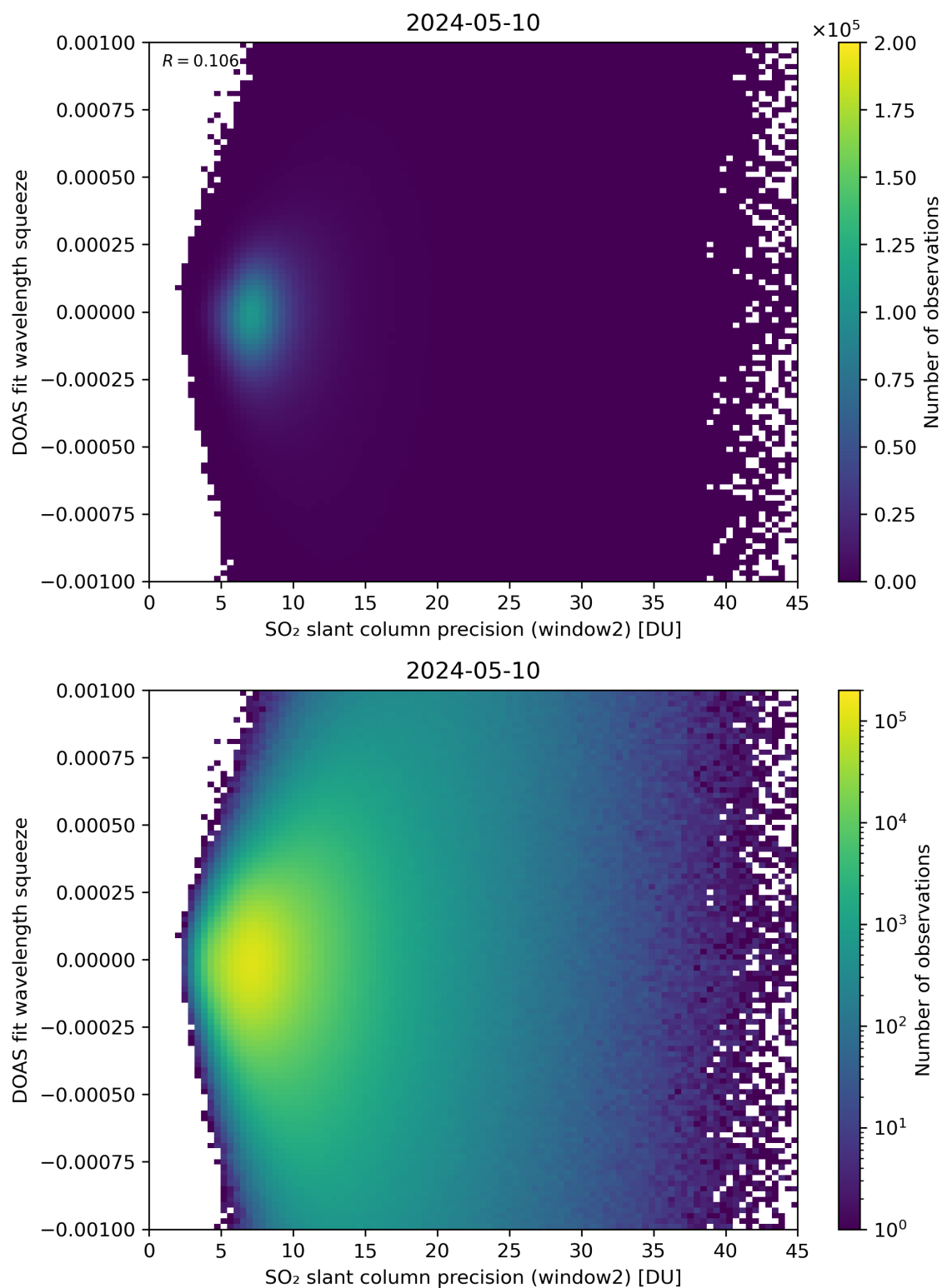
Figure 244: Scatter density plot of “SO 2 slant column precision (window2)” against “DOAS fit wavelength squeeze” for 2024-05-09 to 2024-05-11.
