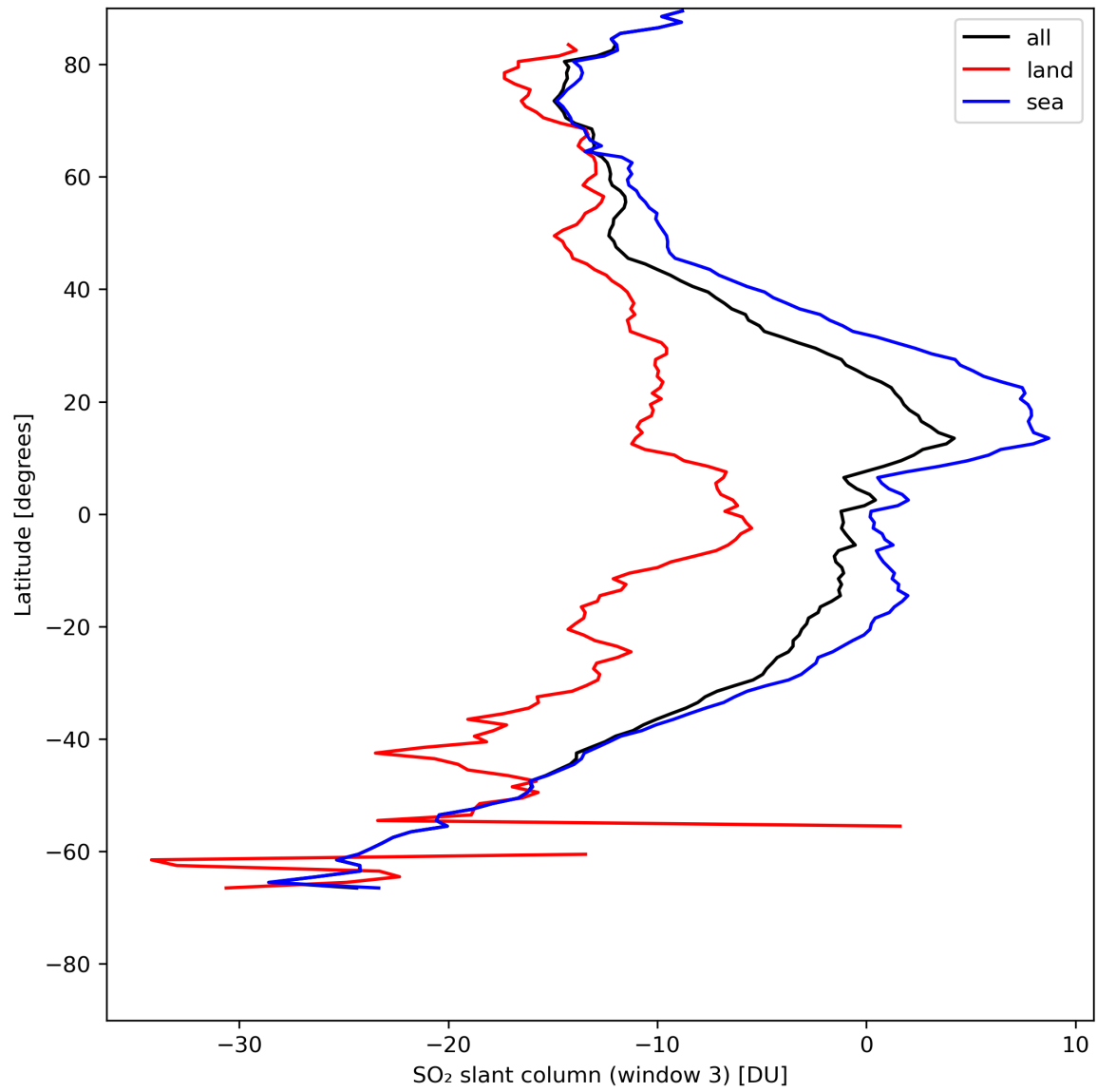
Figure 41: Zonal average of “SO 2 slant column (window 3)” for 2024-05-09 to 2024-05-11.
