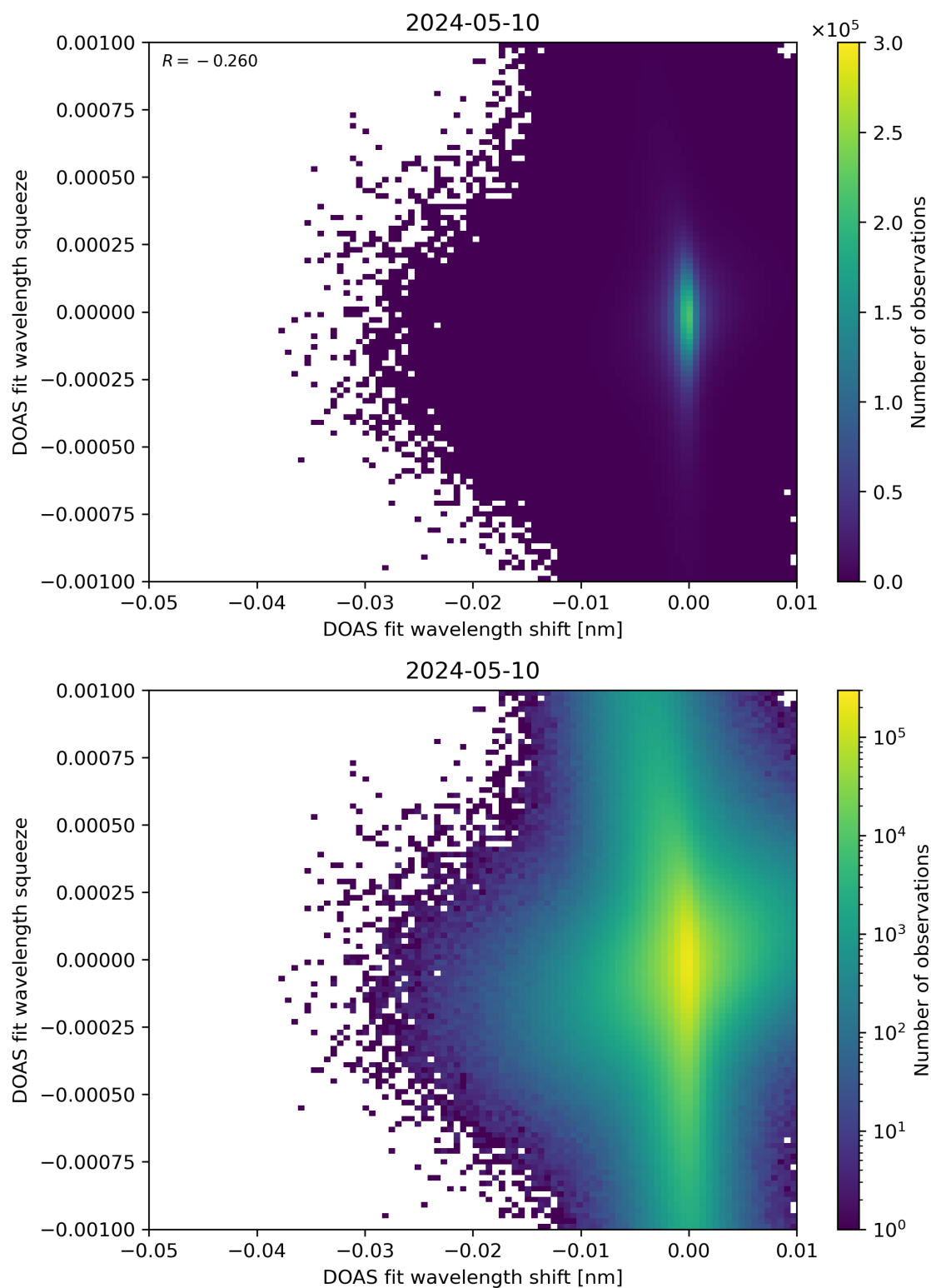
Figure 127: Scatter density plot of “DOAS fit wavelength shift” against “DOAS fit wavelength squeeze” for 2024-05-09 to 2024-05-11.
