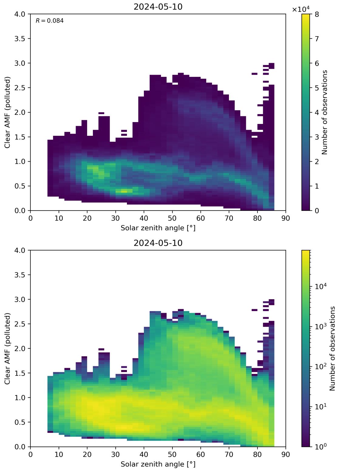
Figure 165: Scatter density plot of “Solar zenith angle” against “Clear AMF (polluted)” for 2024-05-09 to 2024-05-11.
