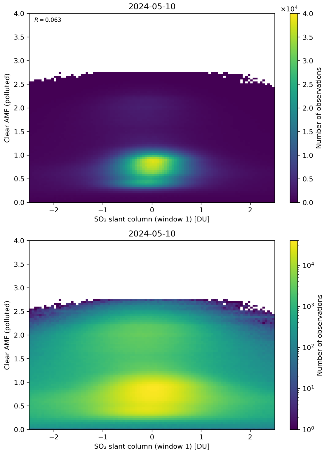
Figure 232: Scatter density plot of “SO 2 slant column (window 1)” against “Clear AMF (polluted)” for 2024-05-09 to 2024-05-11.
