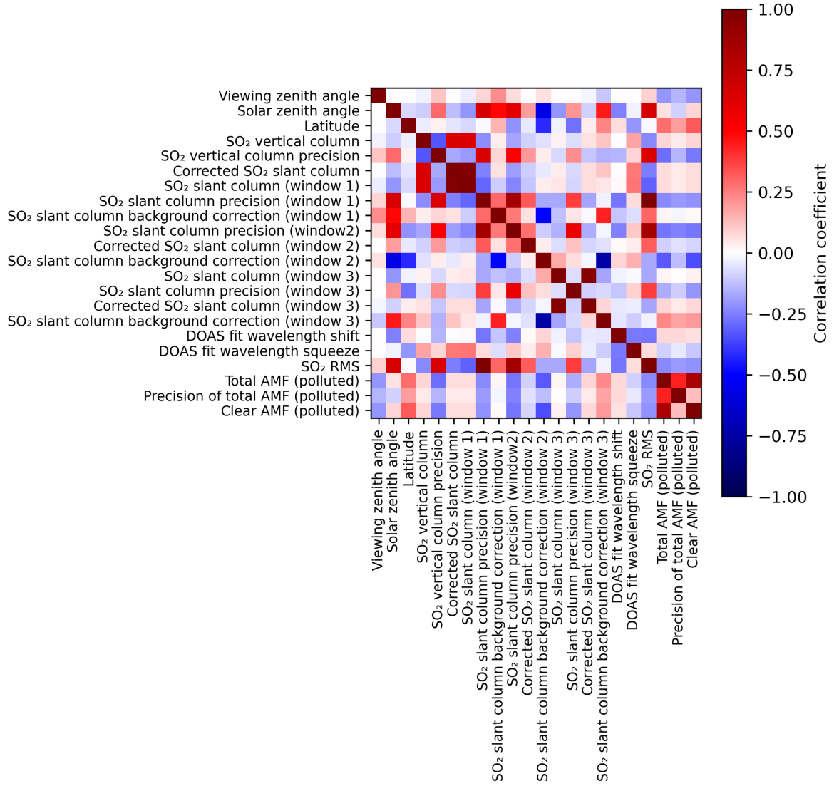
Figure 2: Map of correlation matrix for 2024-05-09 to 2024-05-11.
