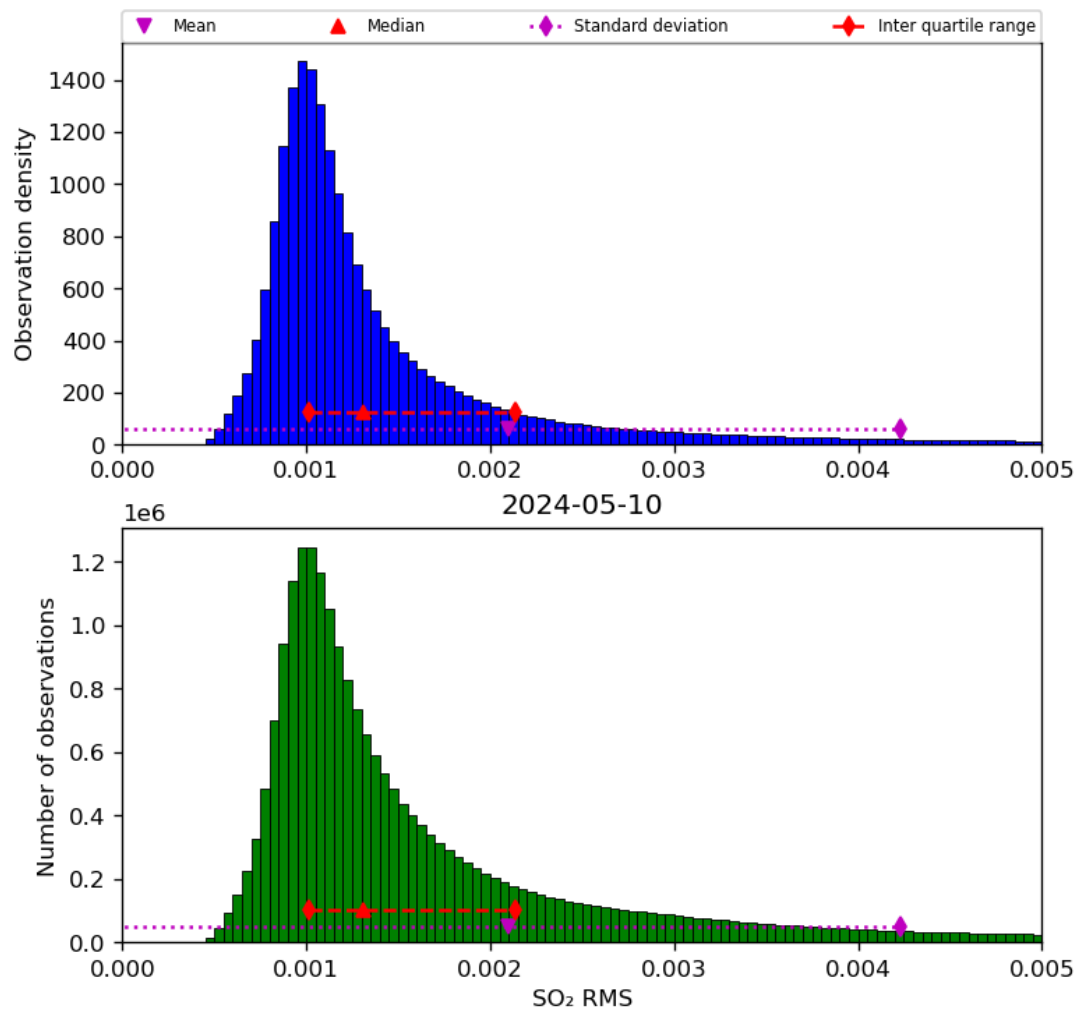
Figure 70: Histogram of “SO 2 RMS” for 2024-05-09 to 2024-05-11
