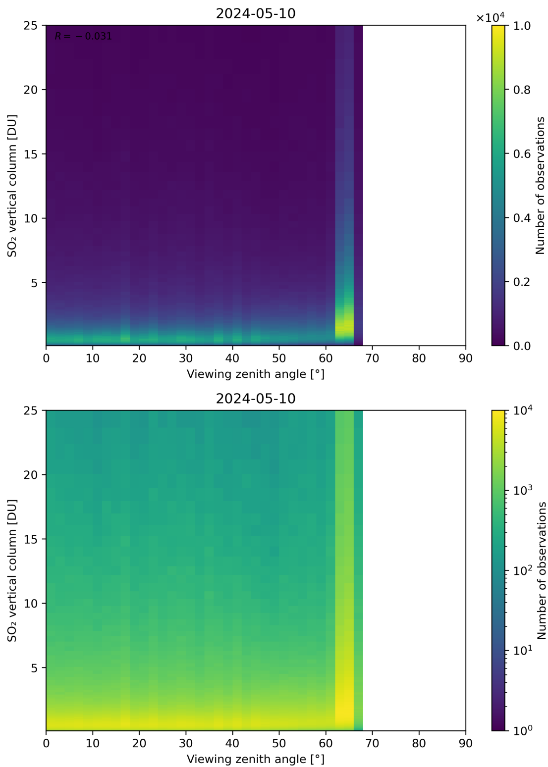
Figure 327: Scatter density plot of “Viewing zenith angle” against “SO 2 vertical column” for 2024-05-09 to 2024-05-11.
