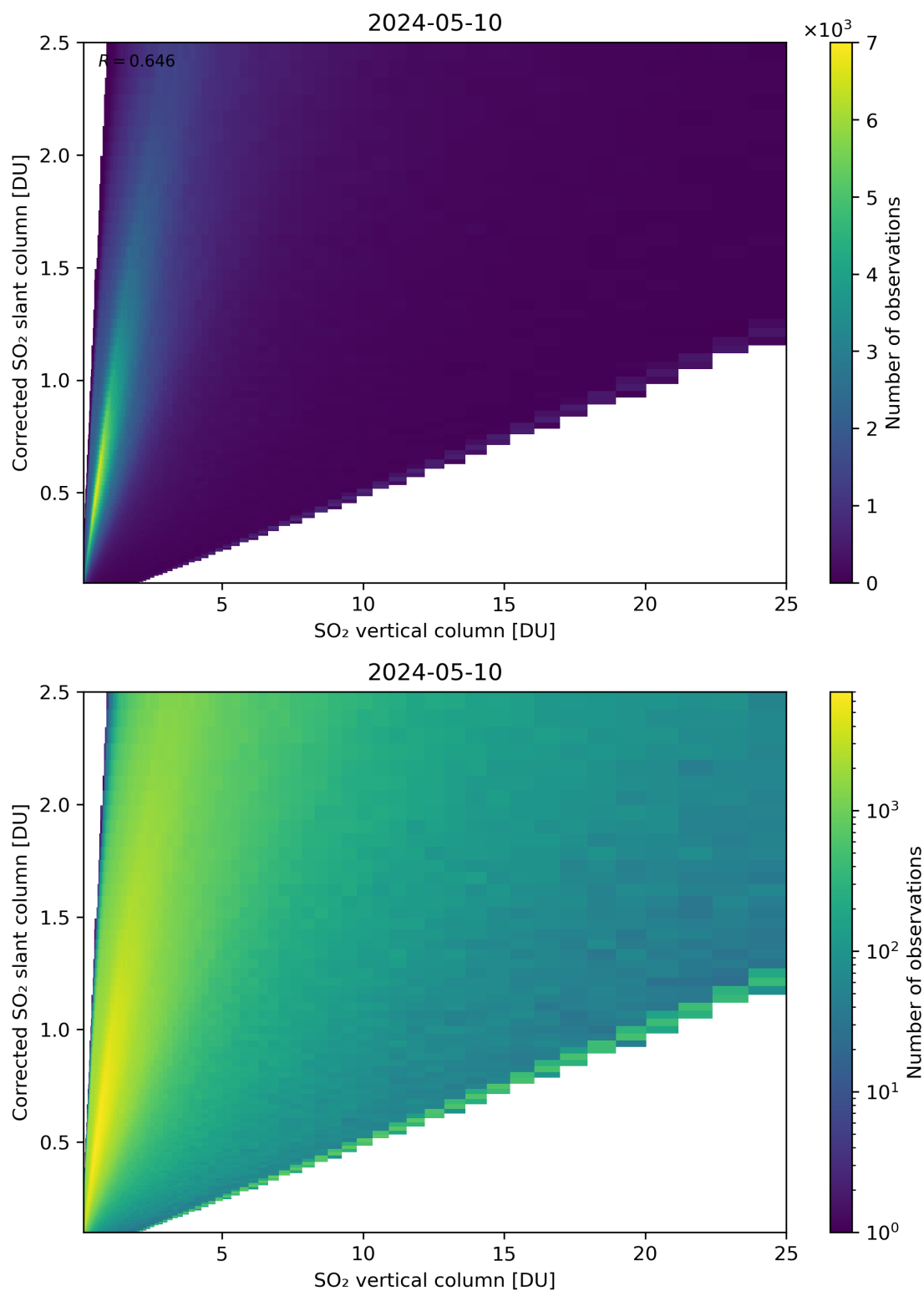
Figure 297: Scatter density plot of “SO 2 vertical column” against “Corrected SO 2 slant column” for 2024-05-09 to 2024-05-11.
