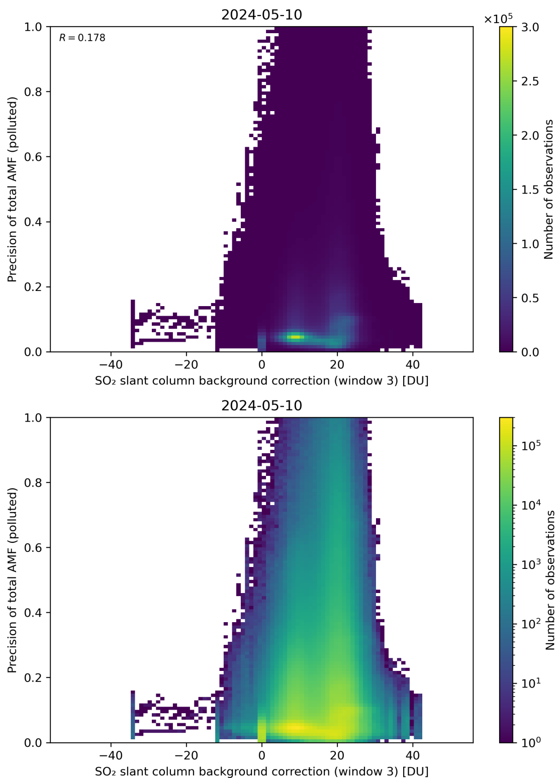
Figure 126: Scatter density plot of “SO 2 slant column background correction (window 3)” against “Precision of total AMF (polluted)” for 2024-05-09 to 2024-05-11.
