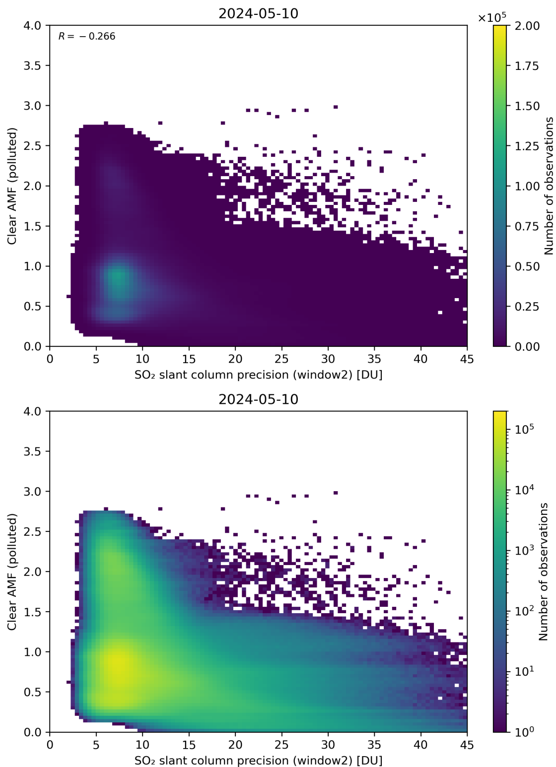
Figure 246: Scatter density plot of “SO 2 slant column precision (window2)” against “Clear AMF (polluted)” for 2024-05-09 to 2024-05-11.
