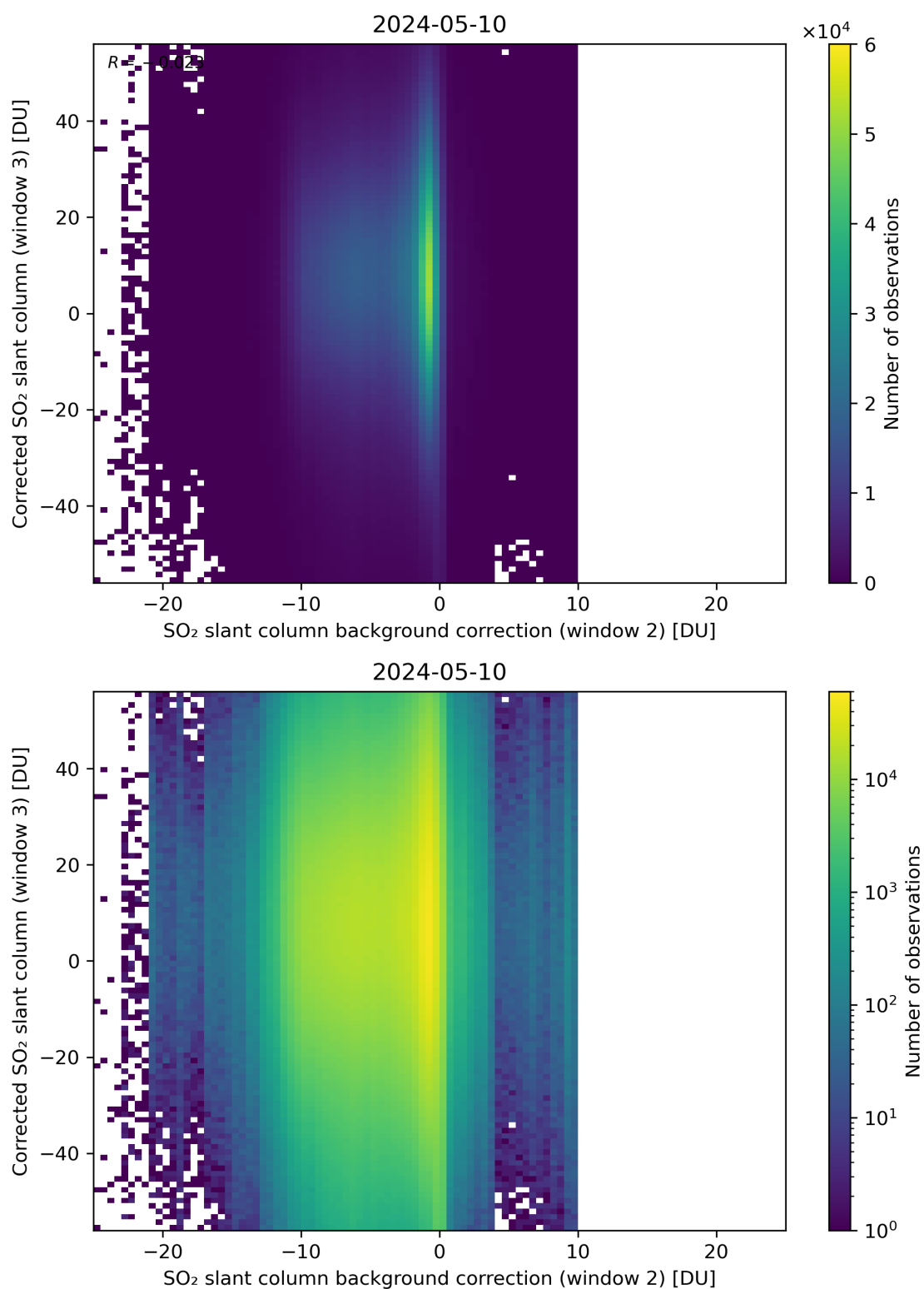
Figure 116: Scatter density plot of “SO 2 slant column background correction (window 2)” against “Corrected SO 2 slant column (window 3)” for 2024-05-09 to 2024-05-11.
