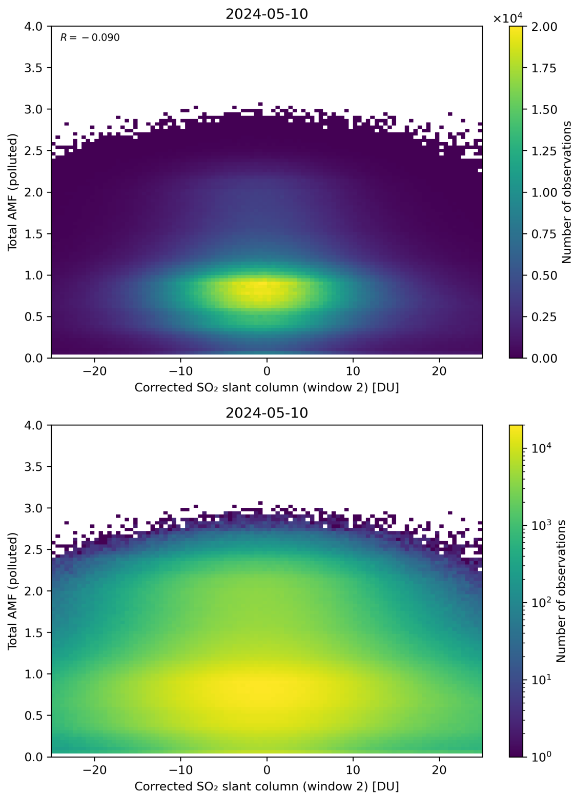
Figure 203: Scatter density plot of “Corrected SO 2 slant column (window 2)” against “Total AMF (polluted)” for 2024-05-09 to 2024-05-11.
