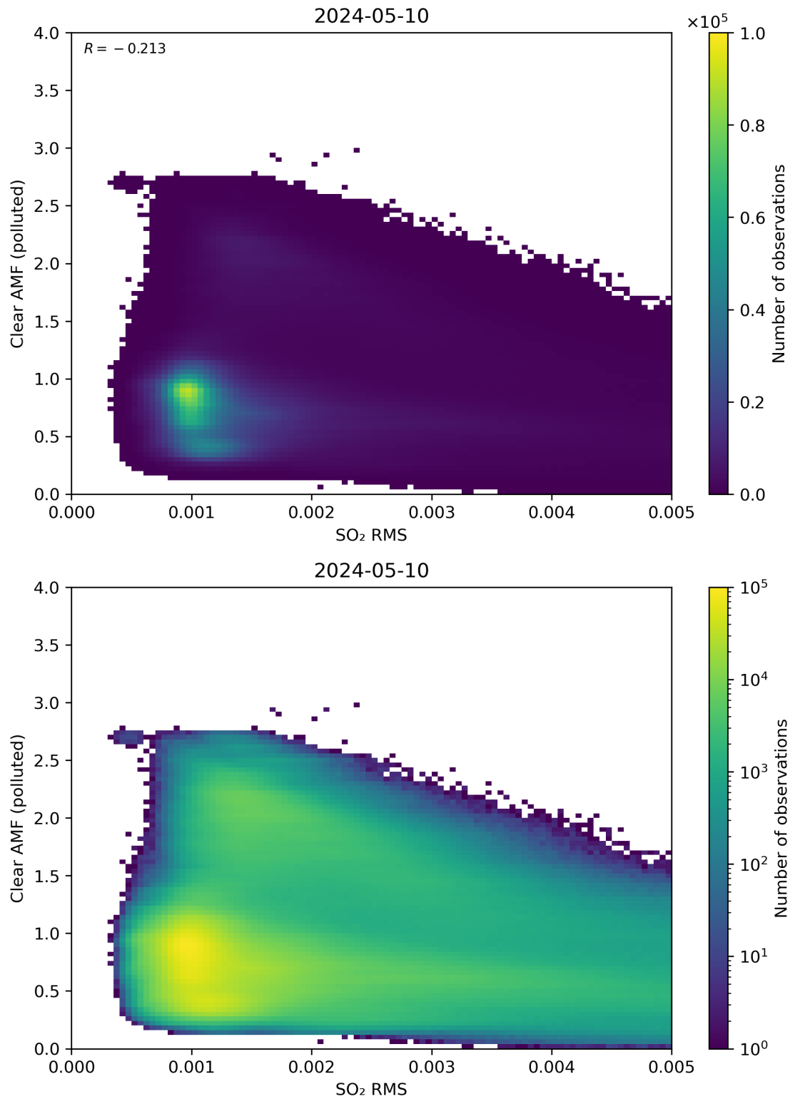
Figure 136: Scatter density plot of “SO 2 RMS” against “Clear AMF (polluted)” for 2024-05-09 to 2024-05-11.
