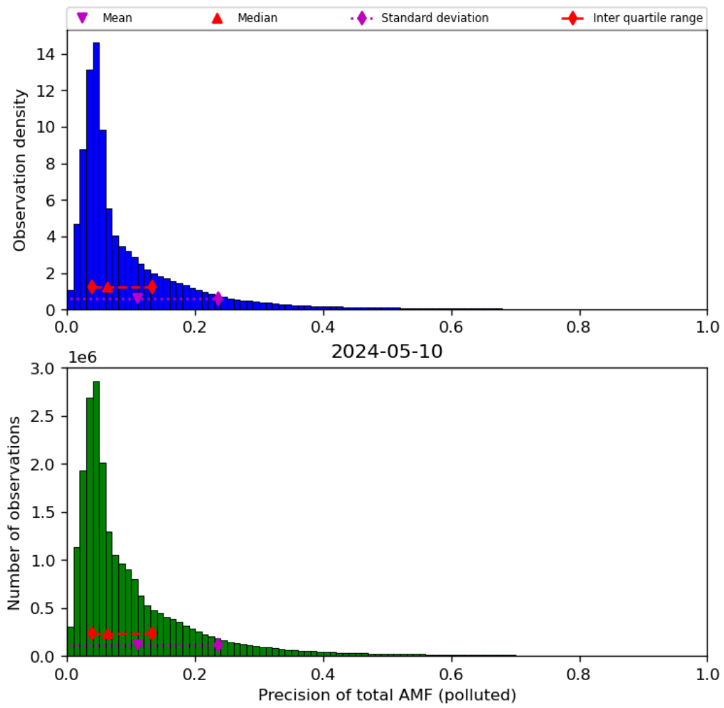
Figure 72: Histogram of “Precision of total AMF (polluted)” for 2024-05-09 to 2024-05-11
