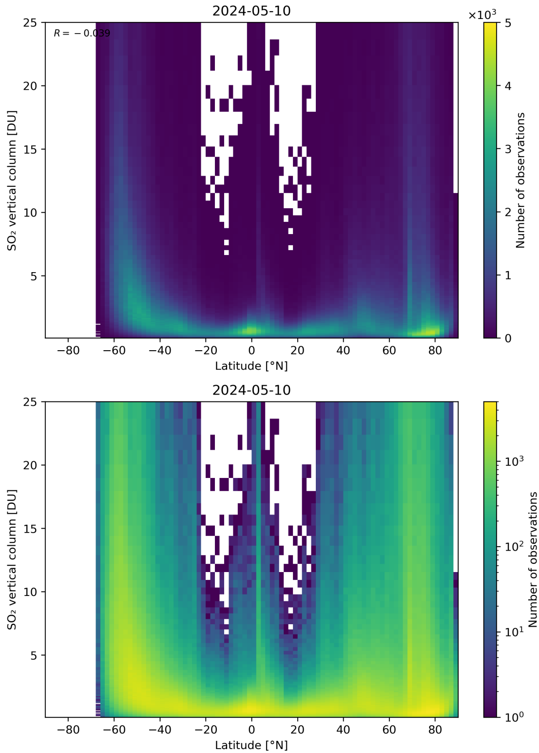
Figure 156: Scatter density plot of “Latitude” against “SO 2 vertical column” for 2024-05-09 to 2024-05-11.
