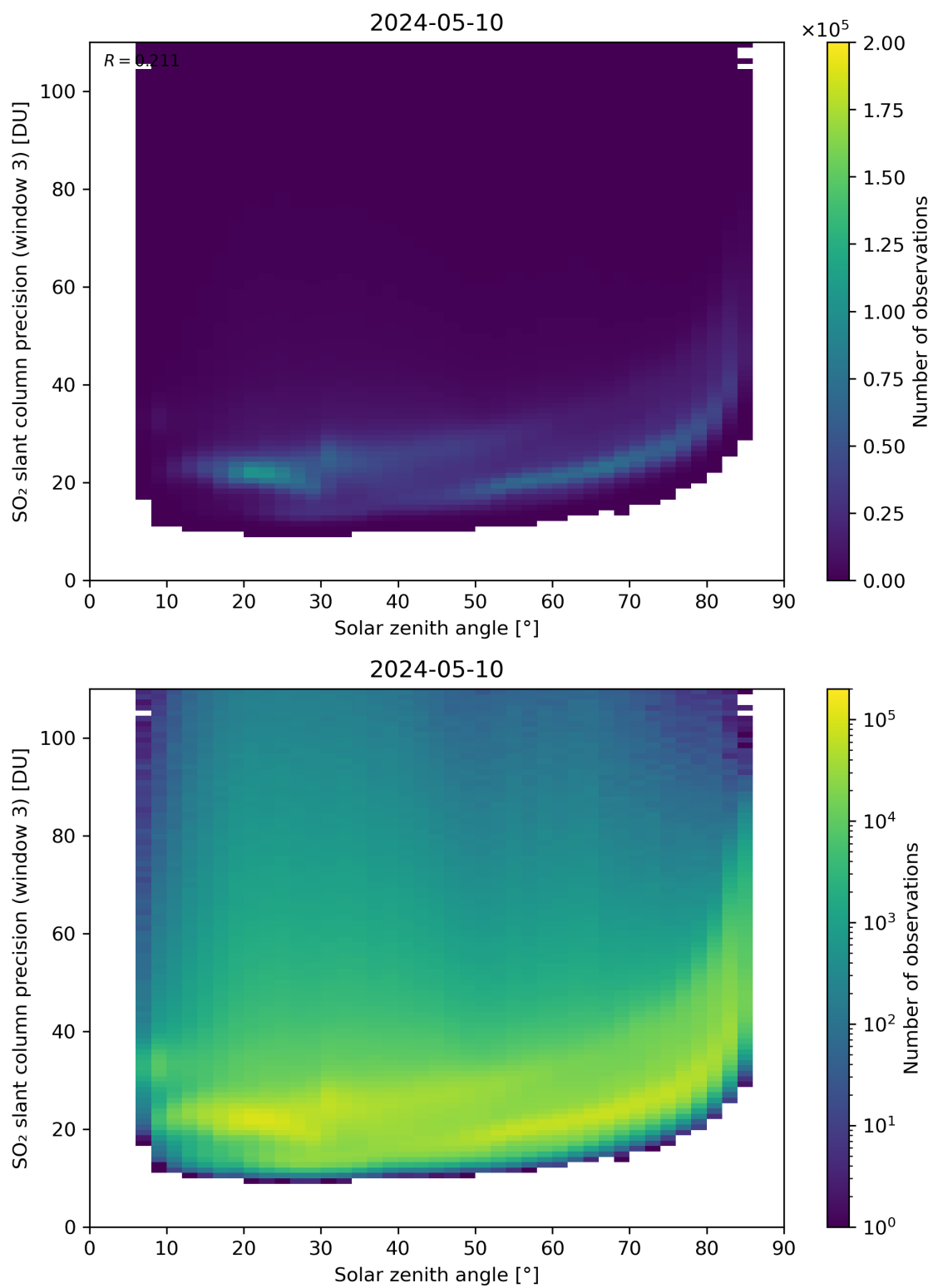
Figure 173: Scatter density plot of “Solar zenith angle” against “SO 2 slant column precision (window 3)” for 2024-05-09 to 2024-05-11.
