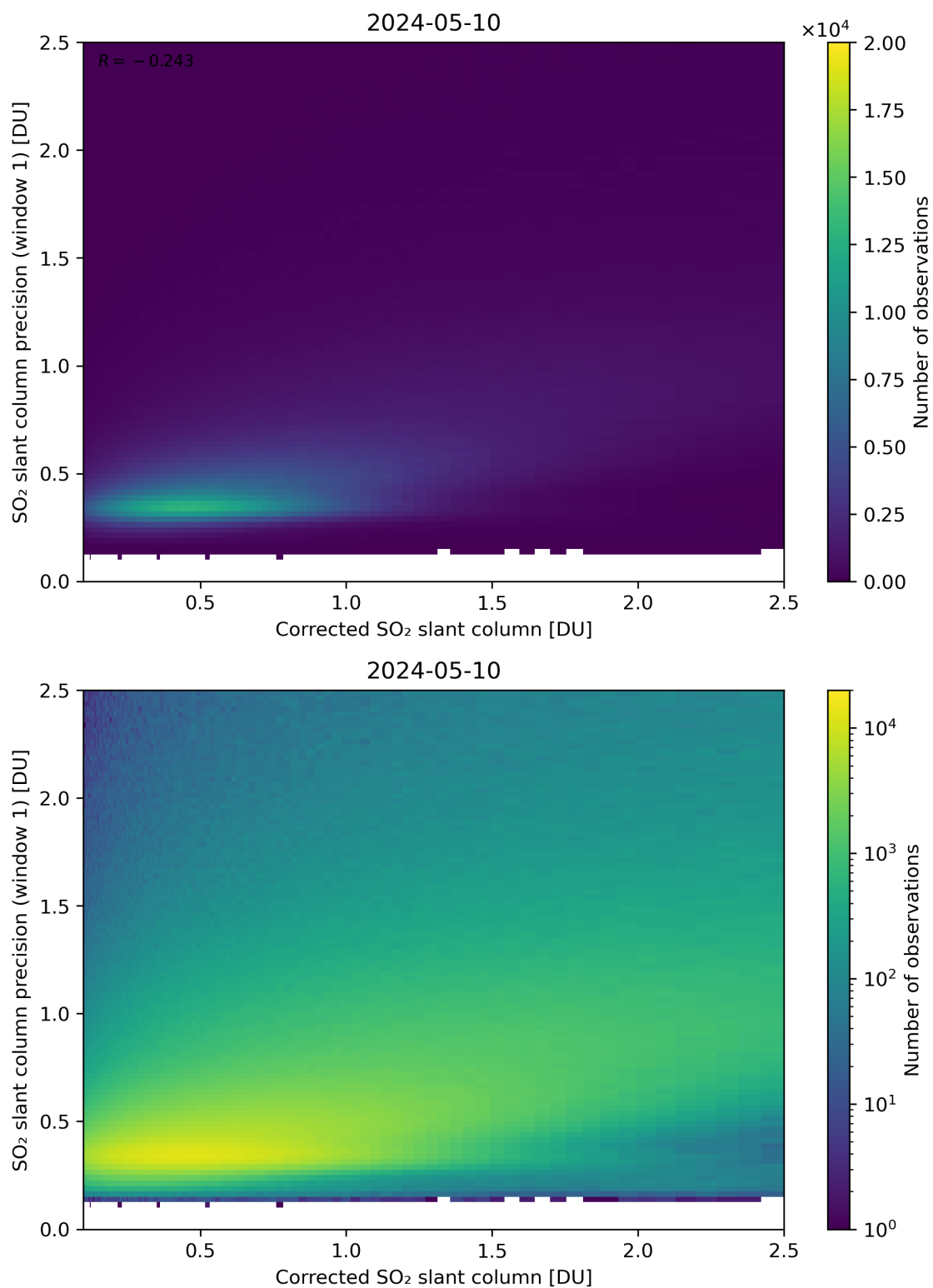
Figure 188: Scatter density plot of “Corrected SO 2 slant column” against “SO 2 slant column precision (window 1)” for 2024-05-09 to 2024-05-11.
