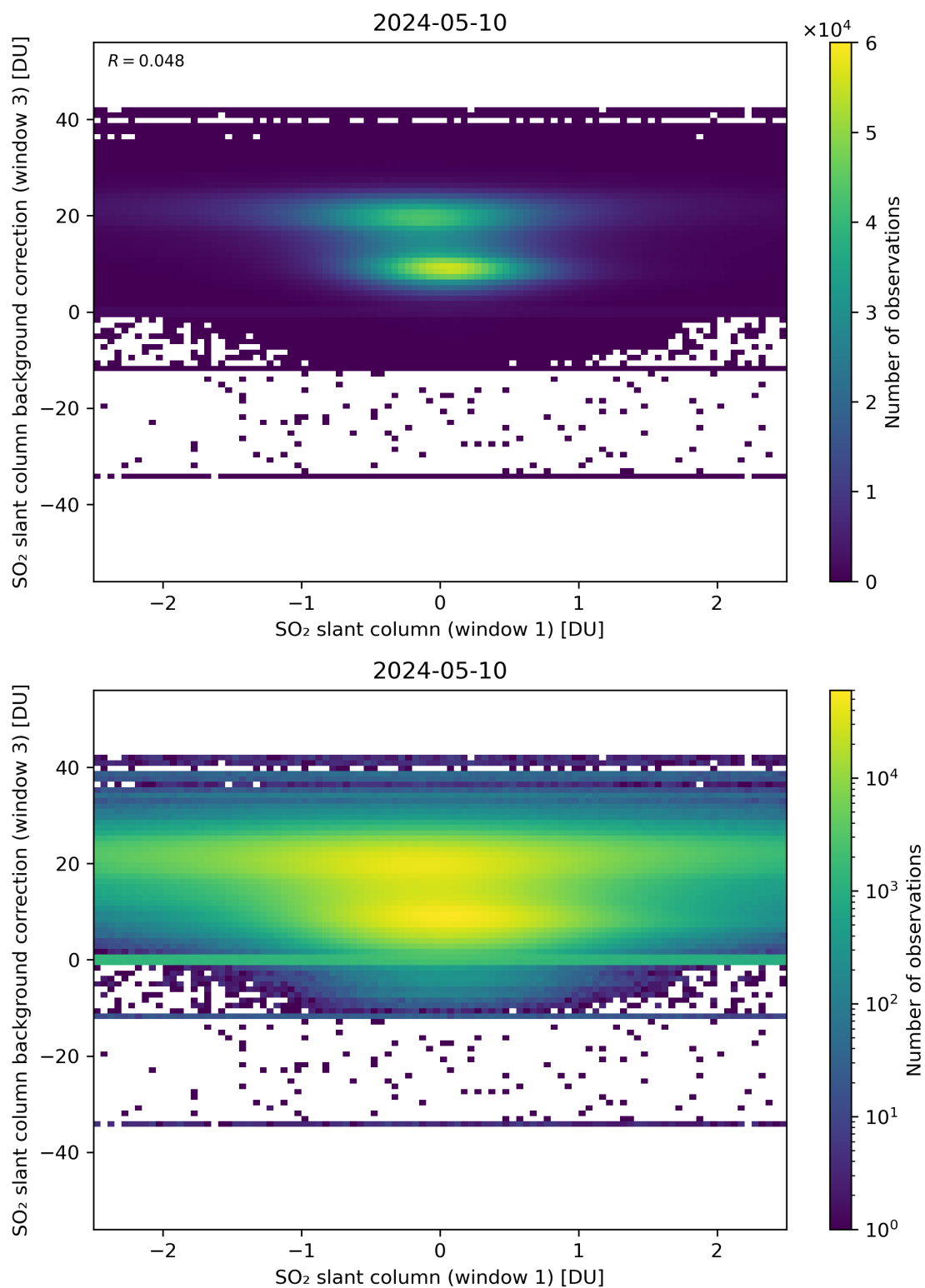
Figure 214: Scatter density plot of “SO 2 slant column (window 1)” against “SO 2 slant column background correction (window 3)” for 2024-05-09 to 2024-05-11.
