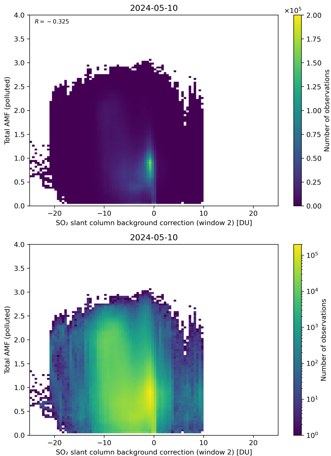
Figure 119: Scatter density plot of “SO 2 slant column background correction (window 2)” against “Total AMF (polluted)” for 2024-05-09 to 2024-05-11.
