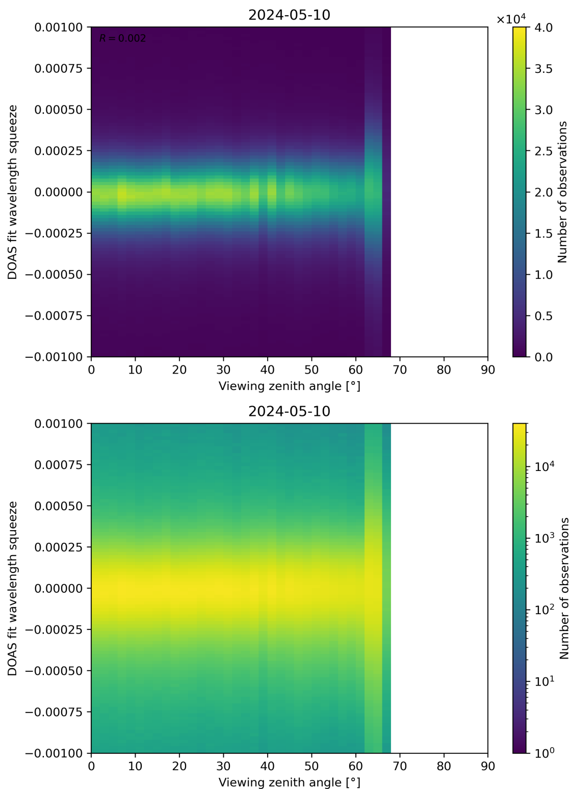
Figure 312: Scatter density plot of “Viewing zenith angle” against “DOAS fit wavelength squeeze” for 2024-05-09 to 2024-05-11.
