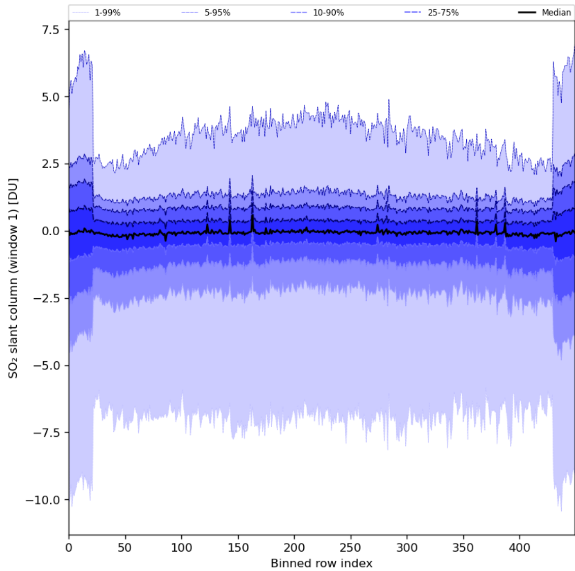
Figure 79: Along track statistics of "SO 2 slant column (window 1)" for 2024-05-09 to 2024-05-11
