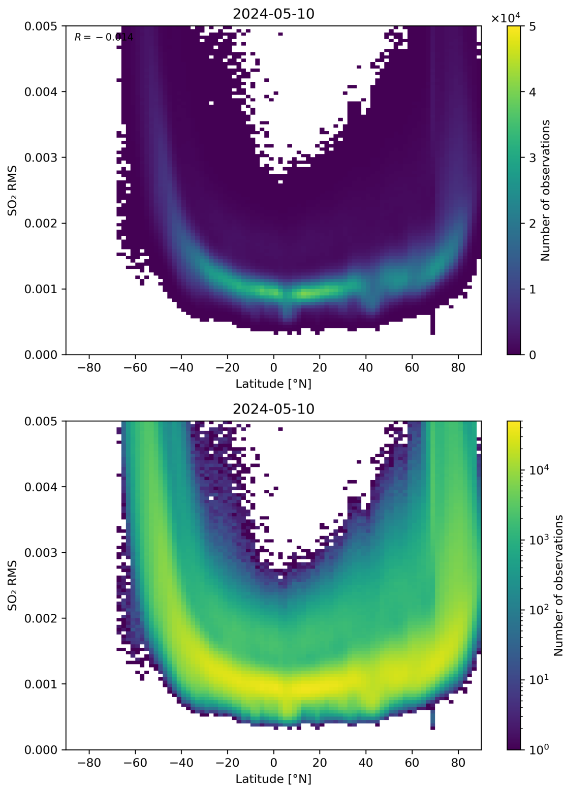
Figure 144: Scatter density plot of “Latitude” against “SO 2 RMS” for 2024-05-09 to 2024-05-11.
