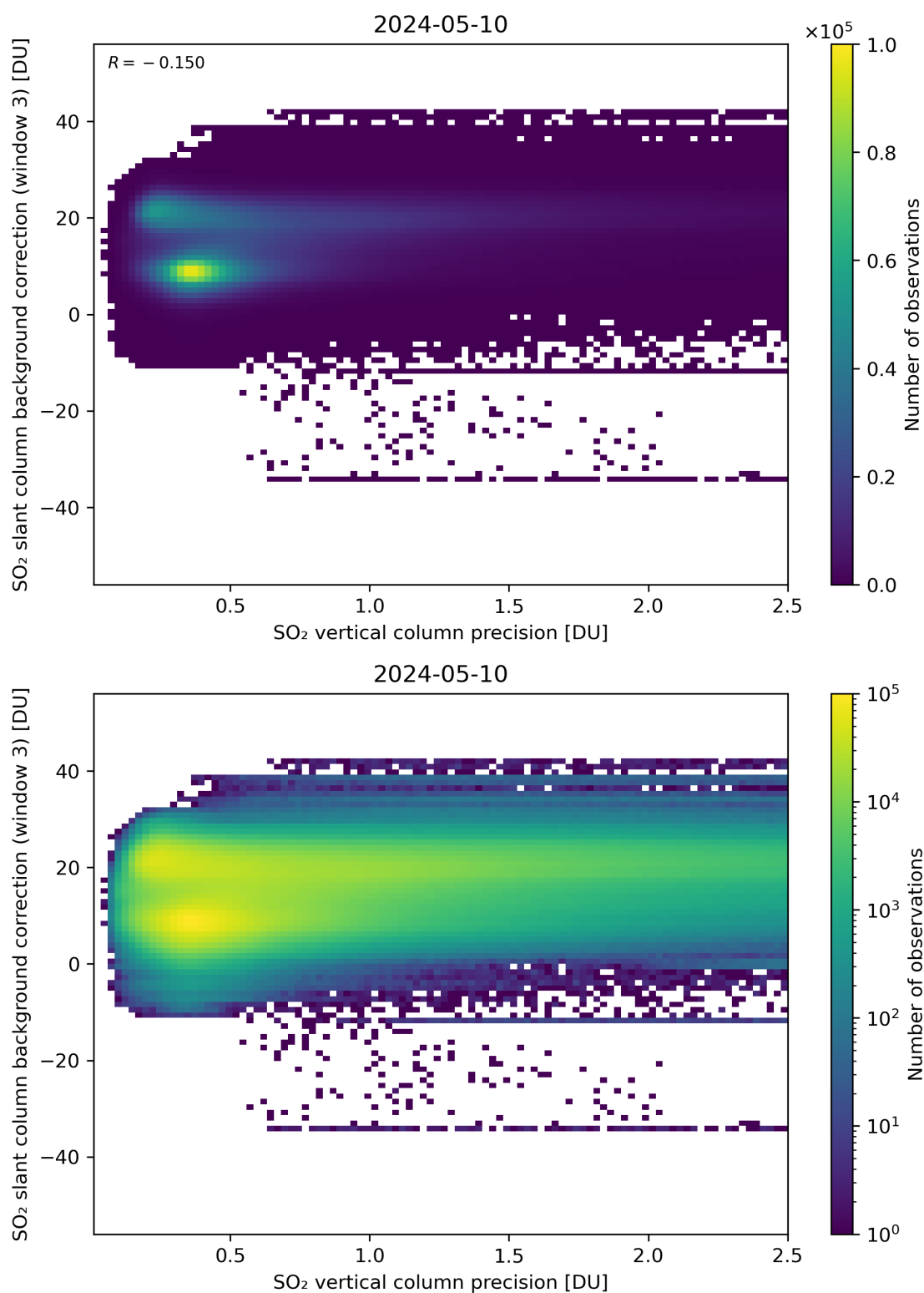
Figure 281: Scatter density plot of “SO 2 vertical column precision” against “SO 2 slant column background correction (window 3)” for 2024-05-09 to 2024-05-11.
