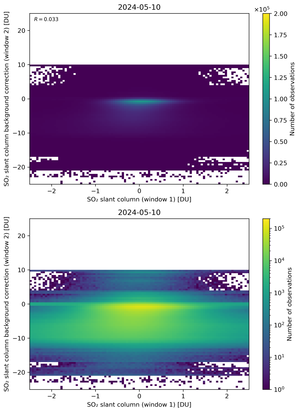
Figure 213: Scatter density plot of “SO 2 slant column (window 1)” against “SO 2 slant column background correction (window 2)” for 2024-05-09 to 2024-05-11.
