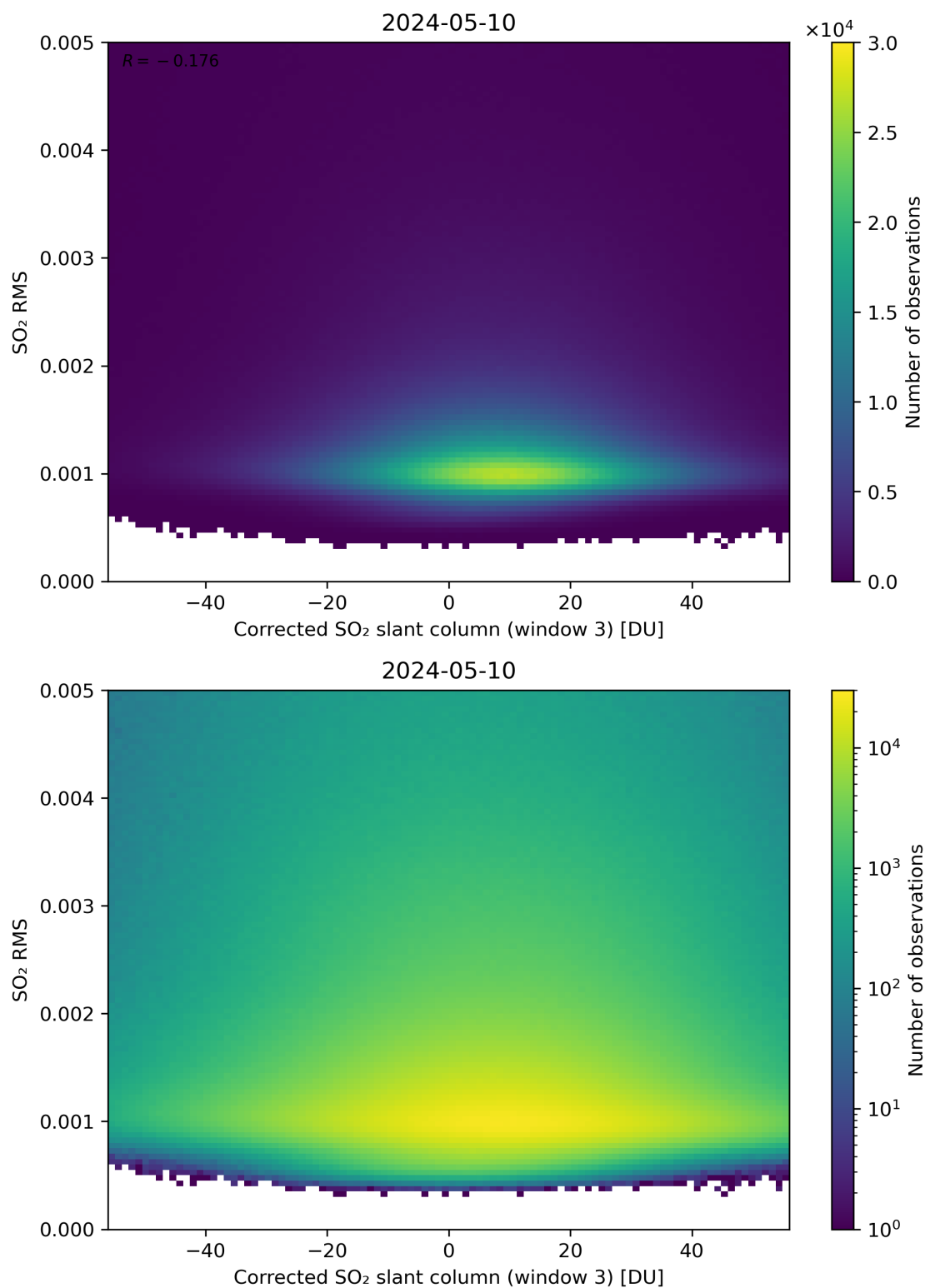
Figure 208: Scatter density plot of “Corrected SO 2 slant column (window 3)” against “SO 2 RMS” for 2024-05-09 to 2024-05-11.
