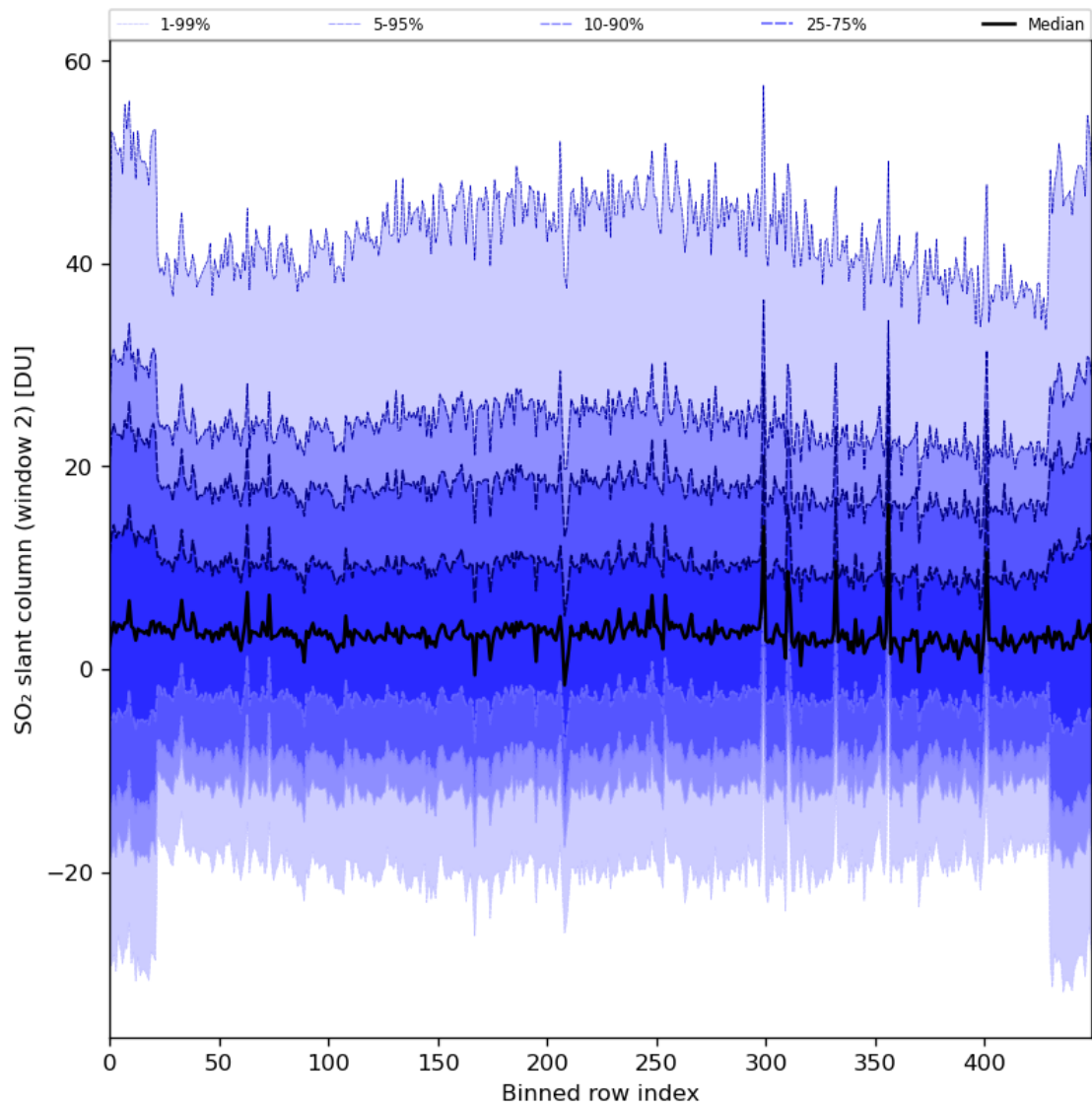
Figure 83: Along track statistics of “SO 2 slant column (window 2)” for 2024-05-09 to 2024-05-11
