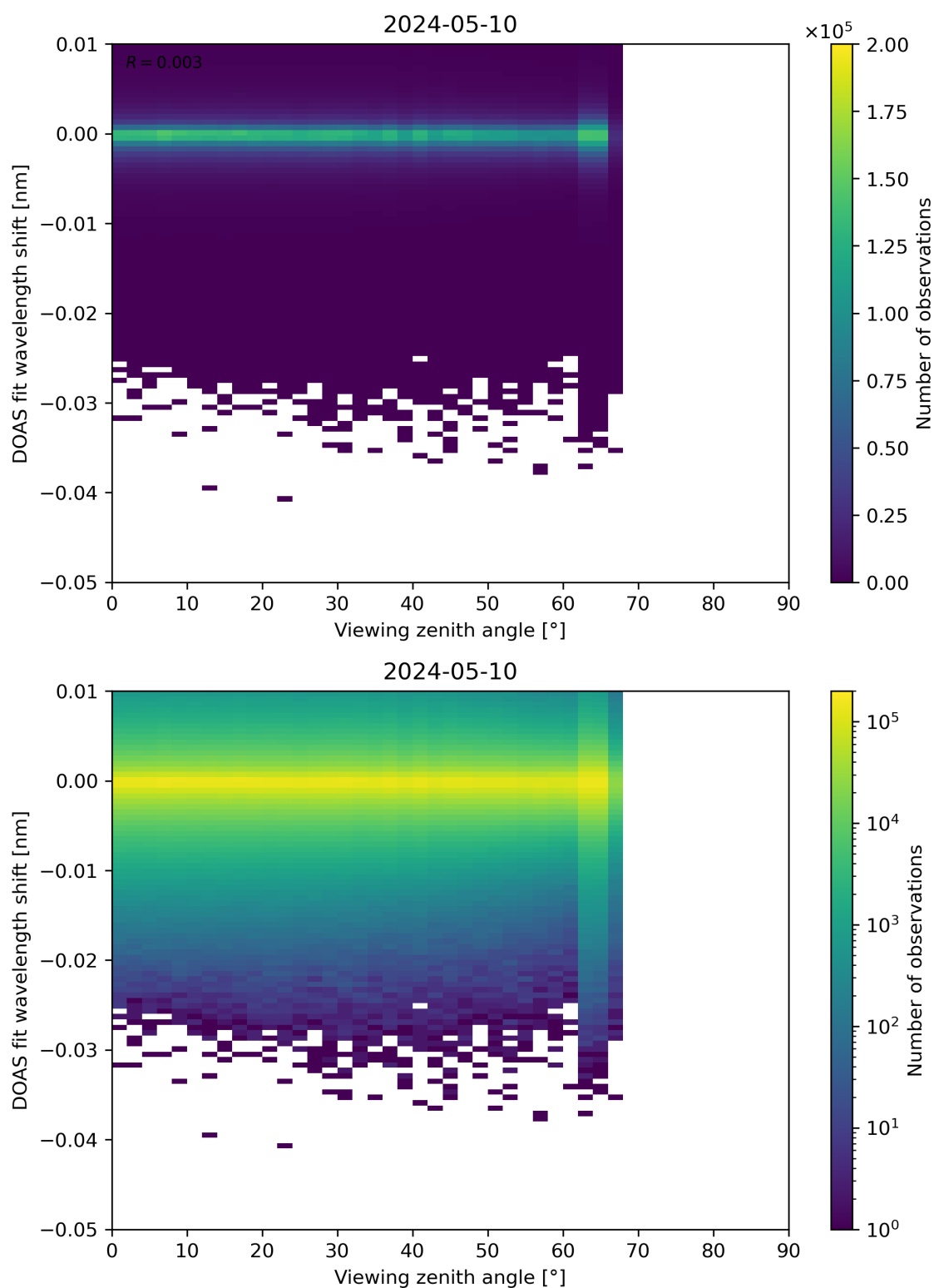
Figure 311: Scatter density plot of “Viewing zenith angle” against “DOAS fit wavelength shift” for 2024-05-09 to 2024-05-11.
