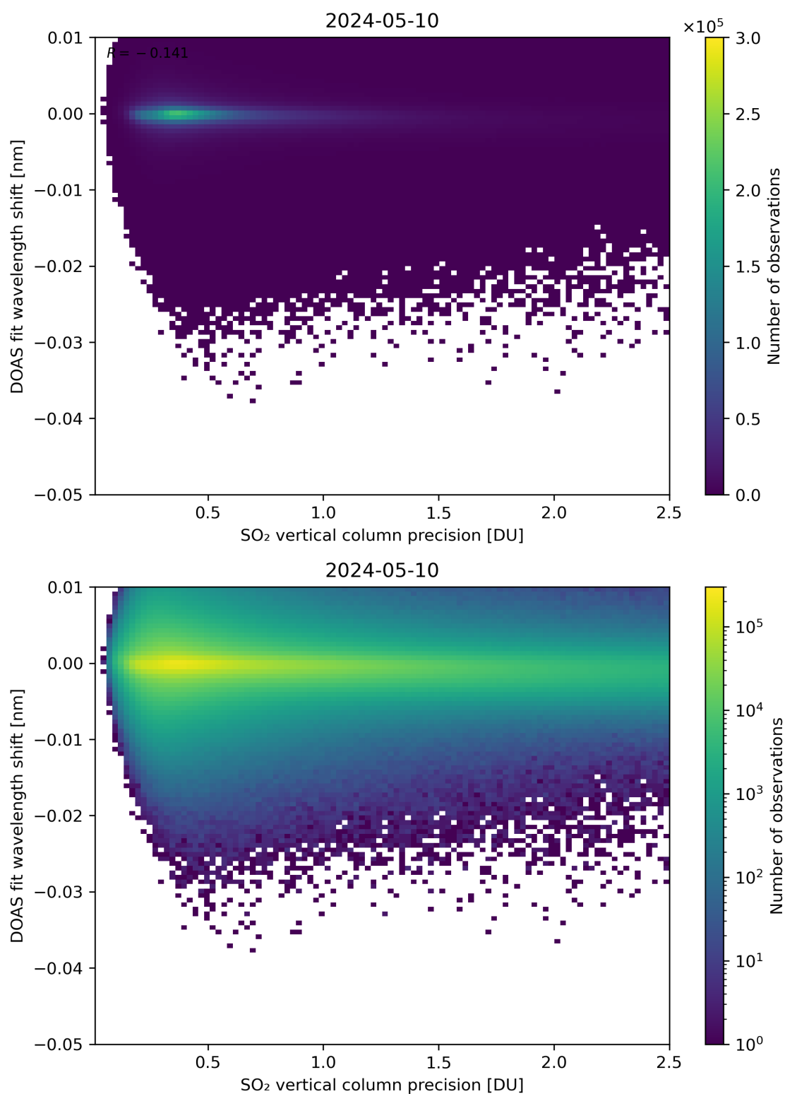
Figure 282: Scatter density plot of “SO 2 vertical column precision” against “DOAS fit wavelength shift” for 2024-05-09 to 2024-05-11.
