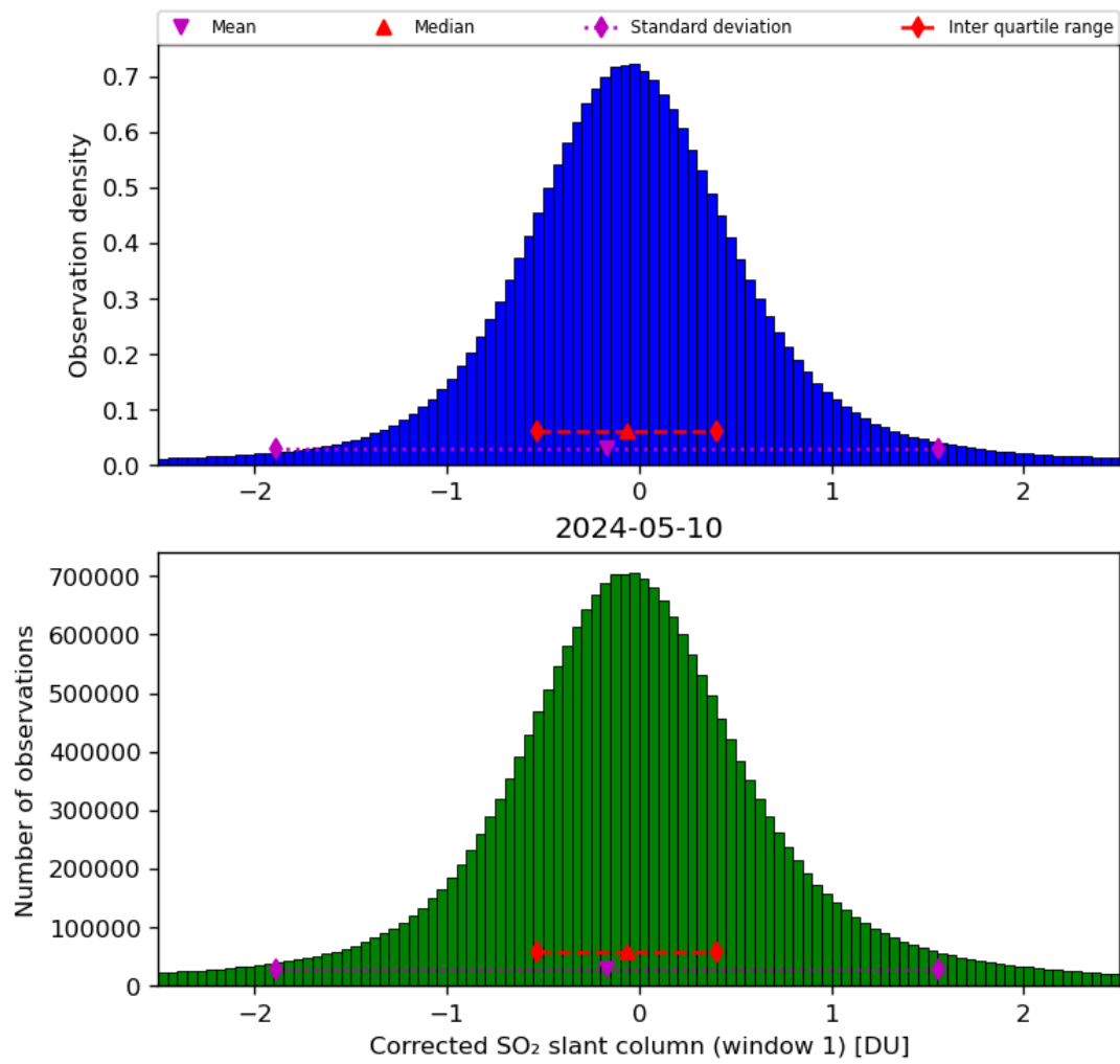
Figure 58: Histogram of “Corrected SO 2 slant column (window 1)” for 2024-05-09 to 2024-05-11
