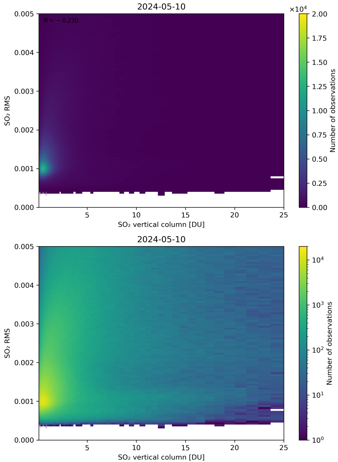
Figure 278: Scatter density plot of “SO 2 vertical column” against “SO 2 RMS” for 2024-05-09 to 2024-05-11.
