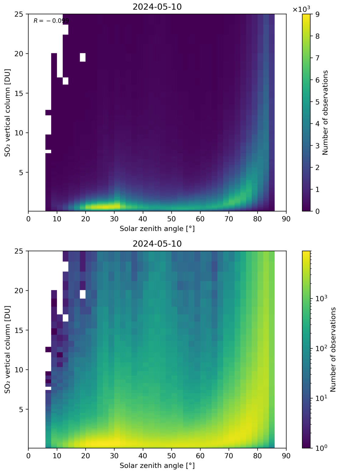
Figure 176: Scatter density plot of “Solar zenith angle” against “SO 2 vertical column” for 2024-05-09 to 2024-05-11.
