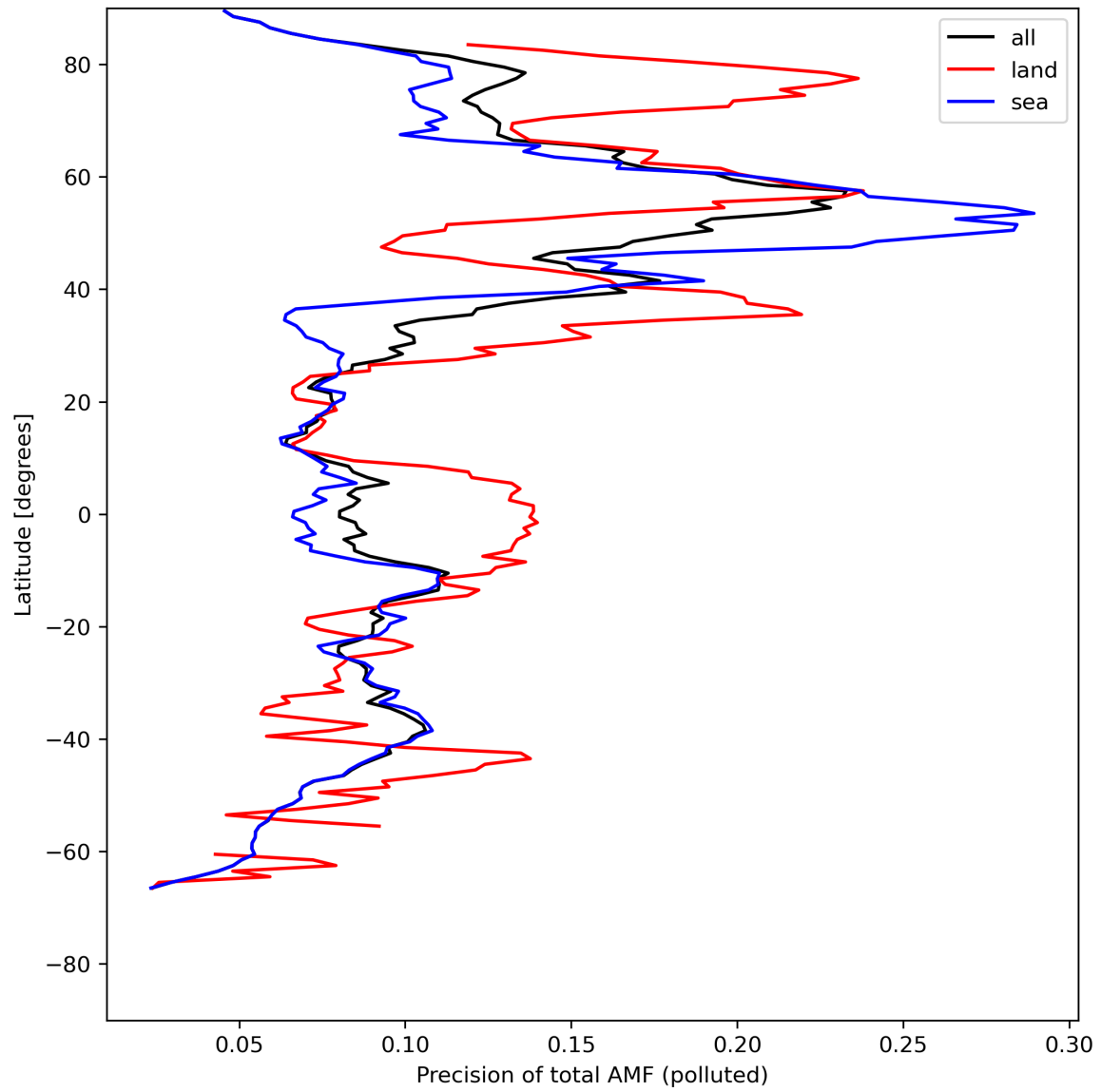
Figure 49: Zonal average of “Precision of total AMF (polluted)” for 2024-05-09 to 2024-05-11.
