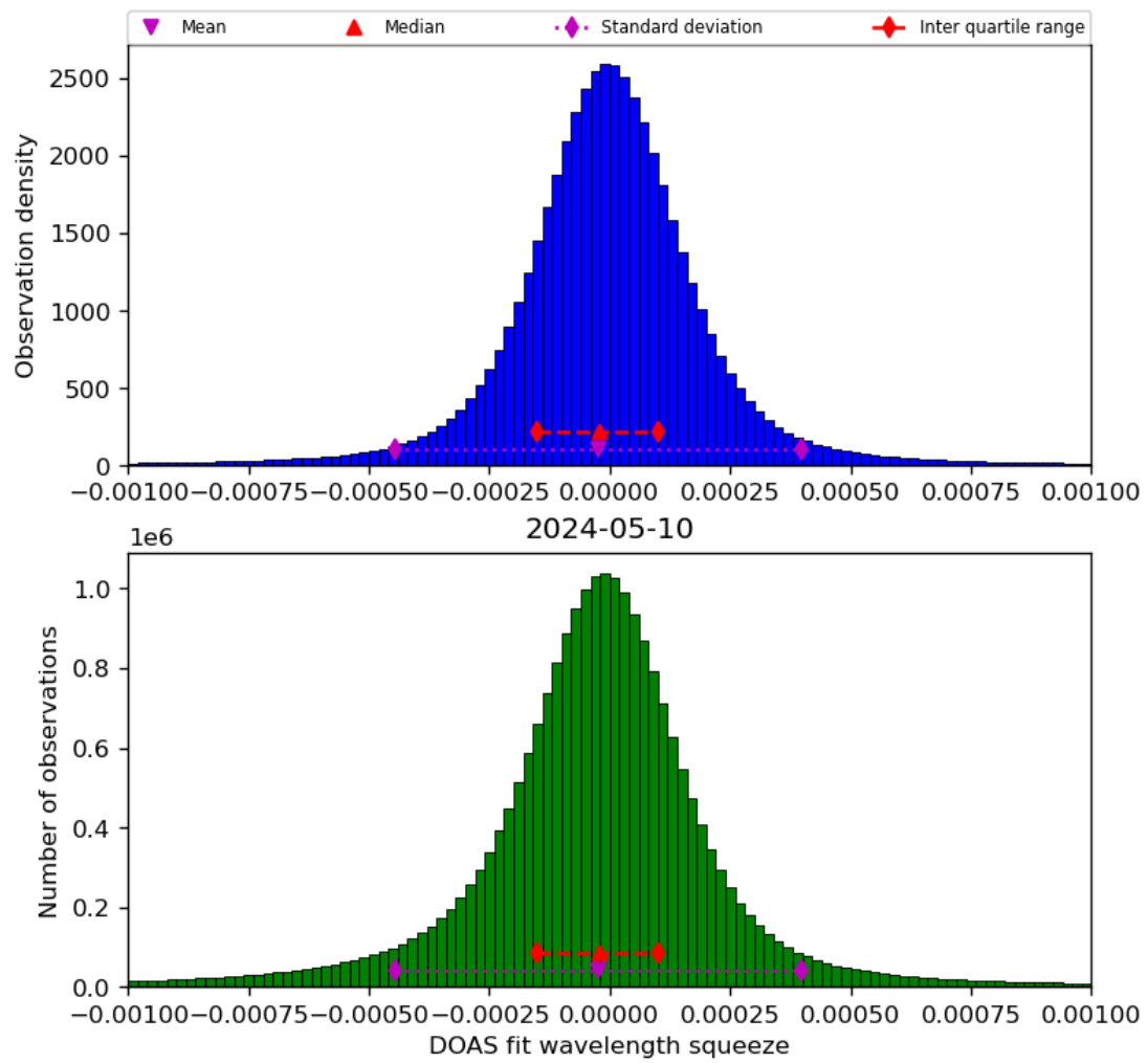
Figure 69: Histogram of “DOAS fit wavelength squeeze” for 2024-05-09 to 2024-05-11
