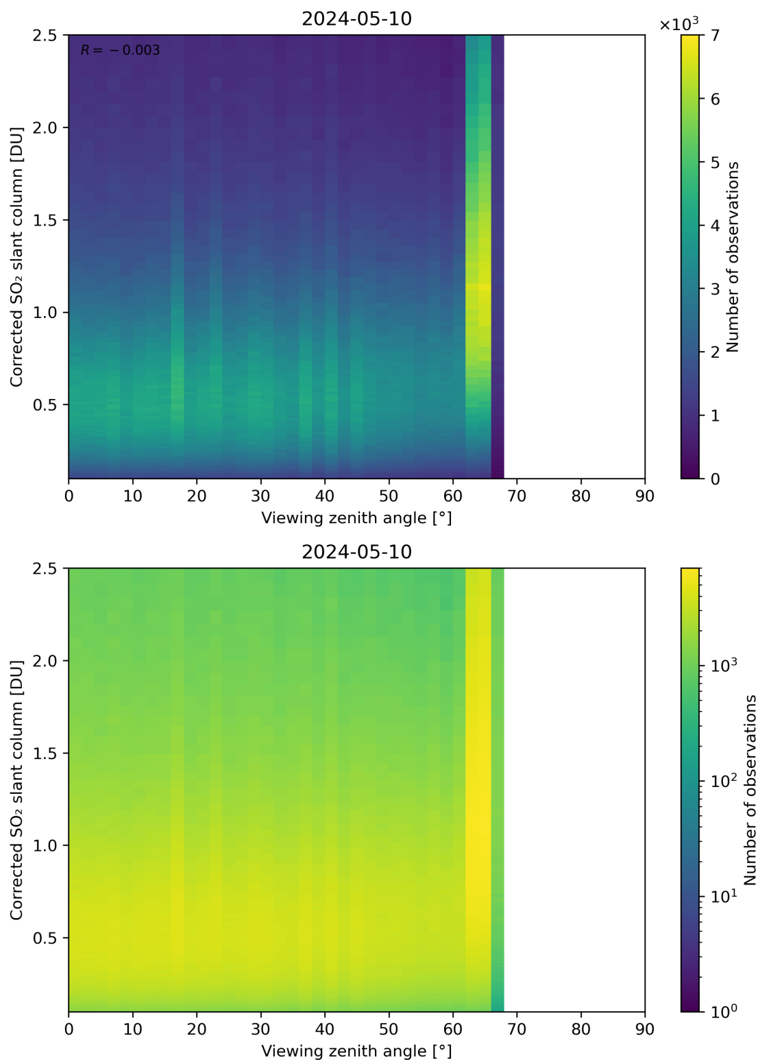
Figure 317: Scatter density plot of “Viewing zenith angle” against “Corrected SO 2 slant column” for 2024-05-09 to 2024-05-11.
