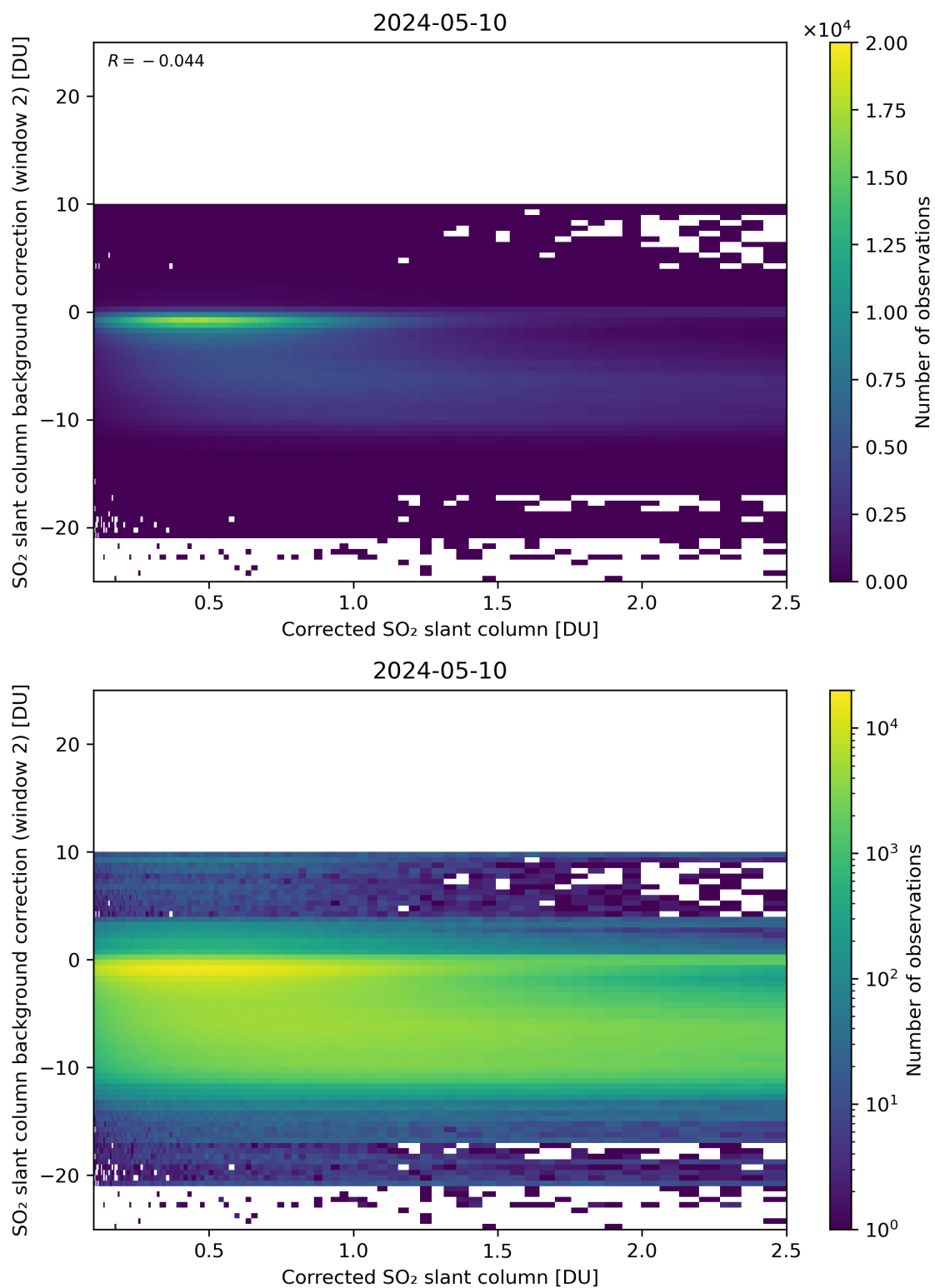
Figure 179: Scatter density plot of “Corrected SO 2 slant column” against “SO 2 slant column background correction (window 2)” for 2024-05-09 to 2024-05-11.
