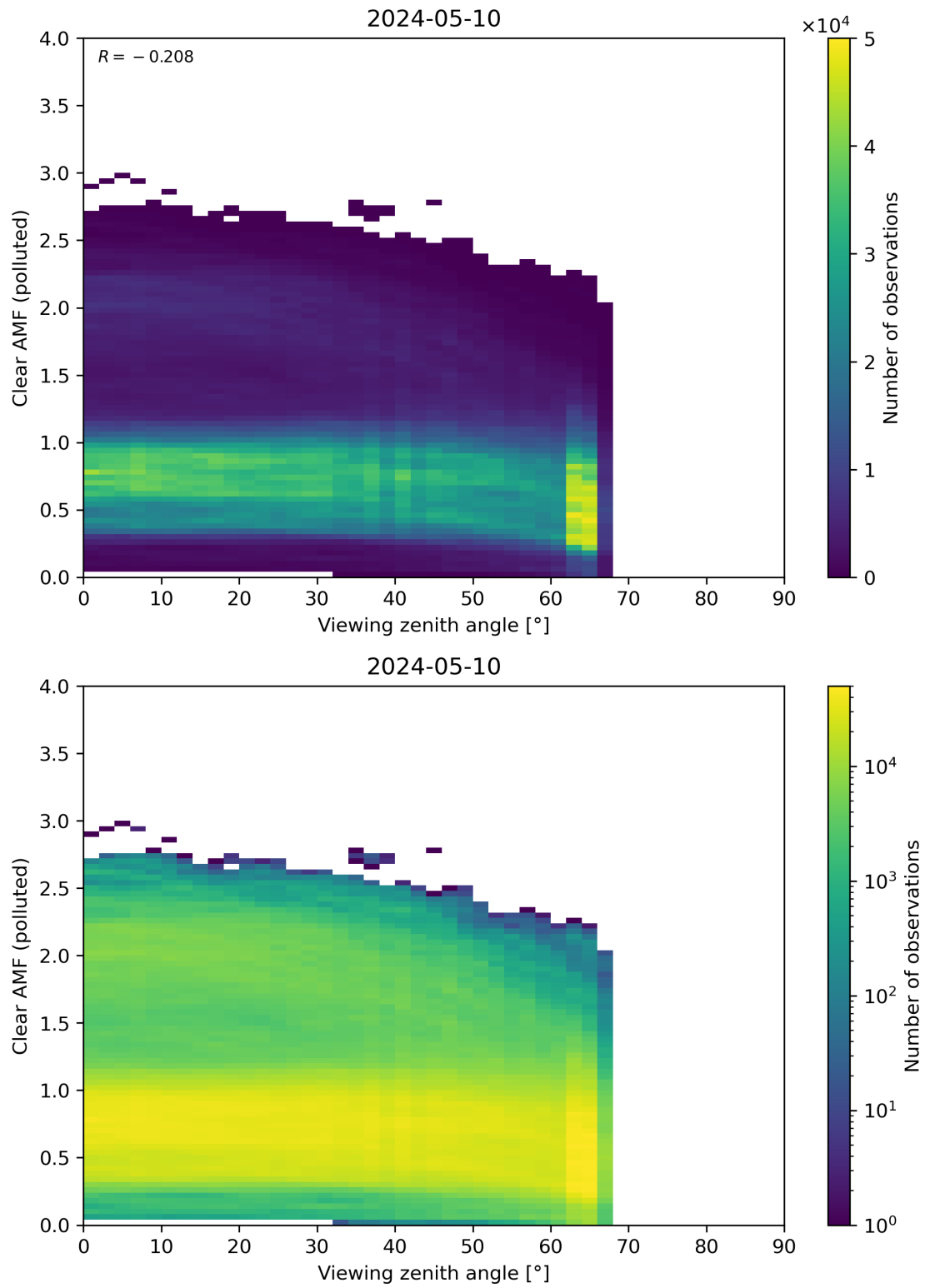
Figure 316: Scatter density plot of “Viewing zenith angle” against “Clear AMF (polluted)” for 2024-05-09 to 2024-05-11.
