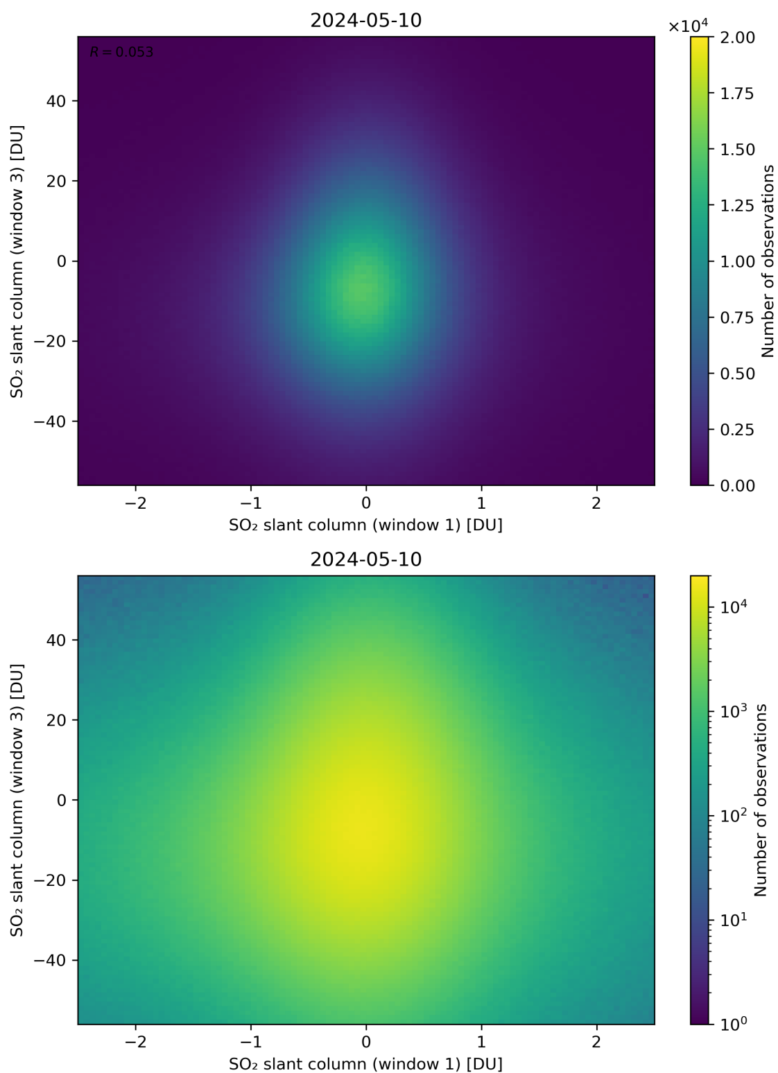
Figure 237: Scatter density plot of “SO 2 slant column (window 1)” against “SO 2 slant column (window 3)” for 2024-05-09 to 2024-05-11.
