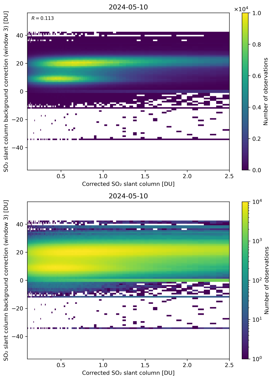
Figure 180: Scatter density plot of “Corrected SO 2 slant column” against “SO 2 slant column background correction (window 3)” for 2024-05-09 to 2024-05-11.
