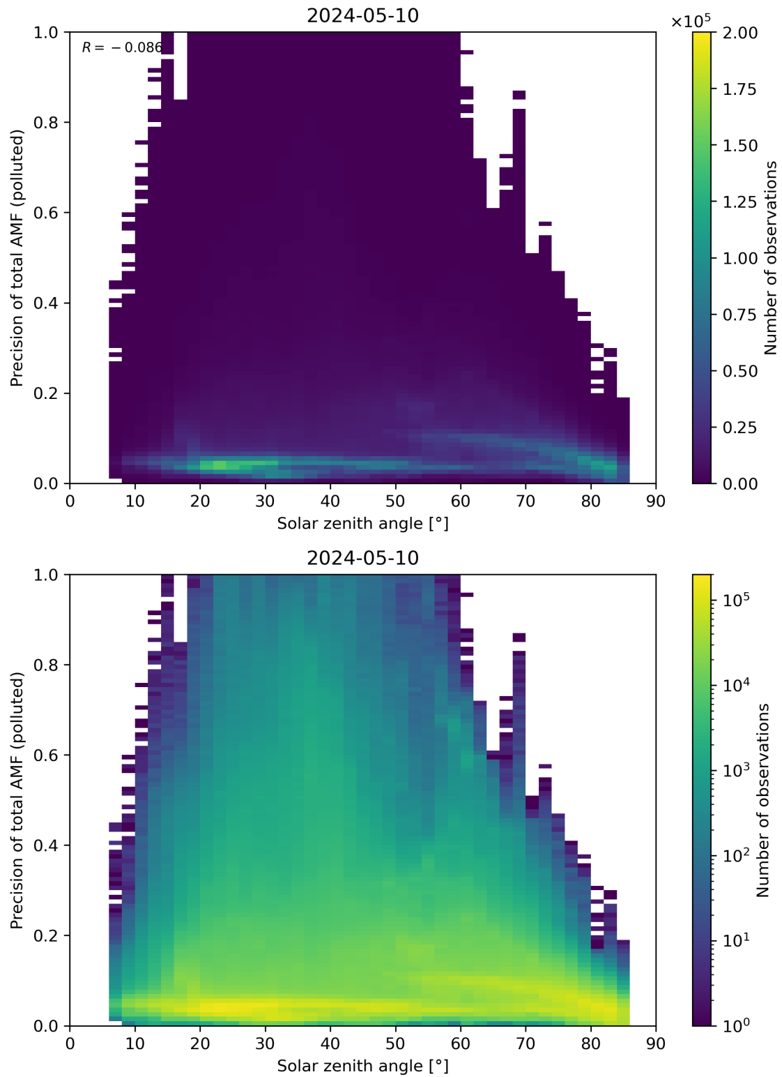
Figure 175: Scatter density plot of “Solar zenith angle” against “Precision of total AMF (polluted)” for 2024-05-09 to 2024-05-11.
