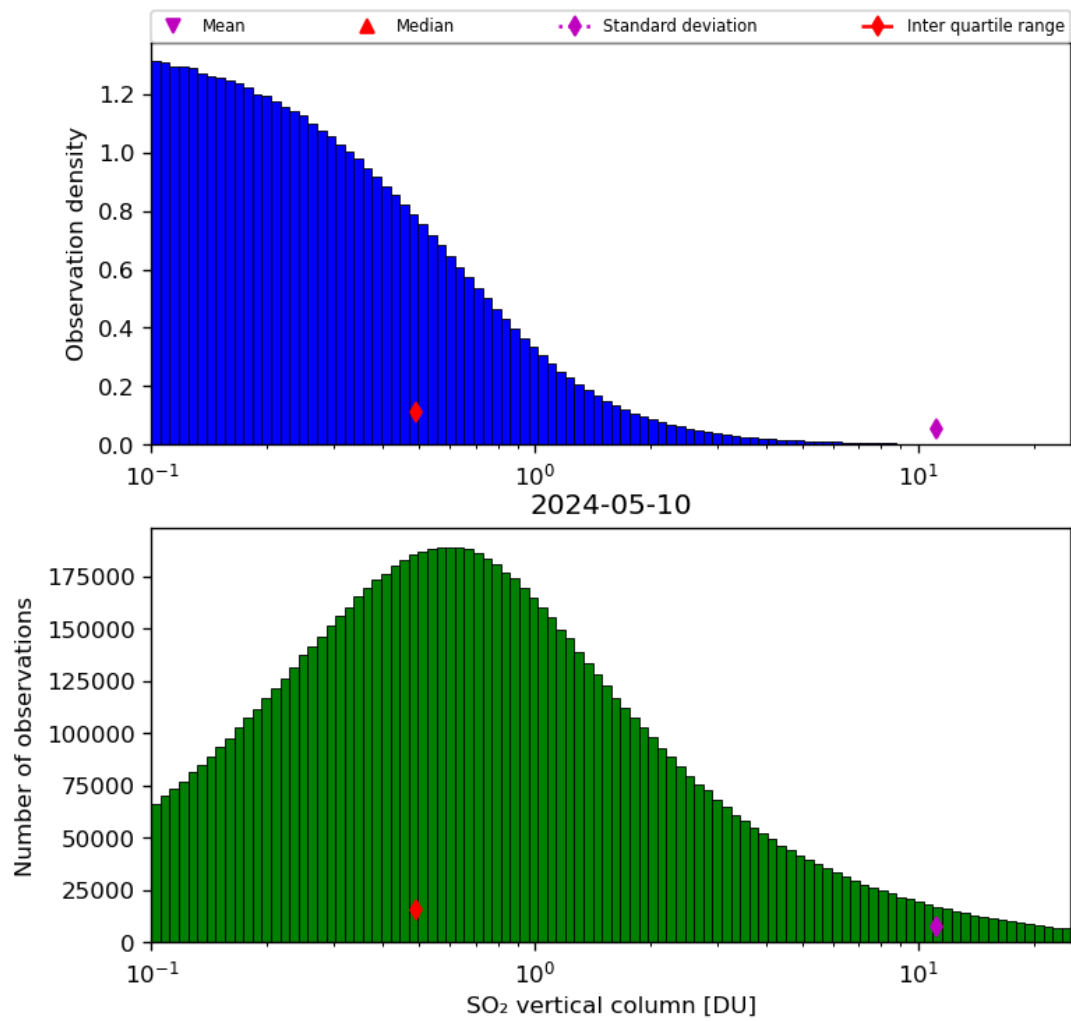
Figure 53: Histogram of “SO 2 vertical column” for 2024-05-09 to 2024-05-11
