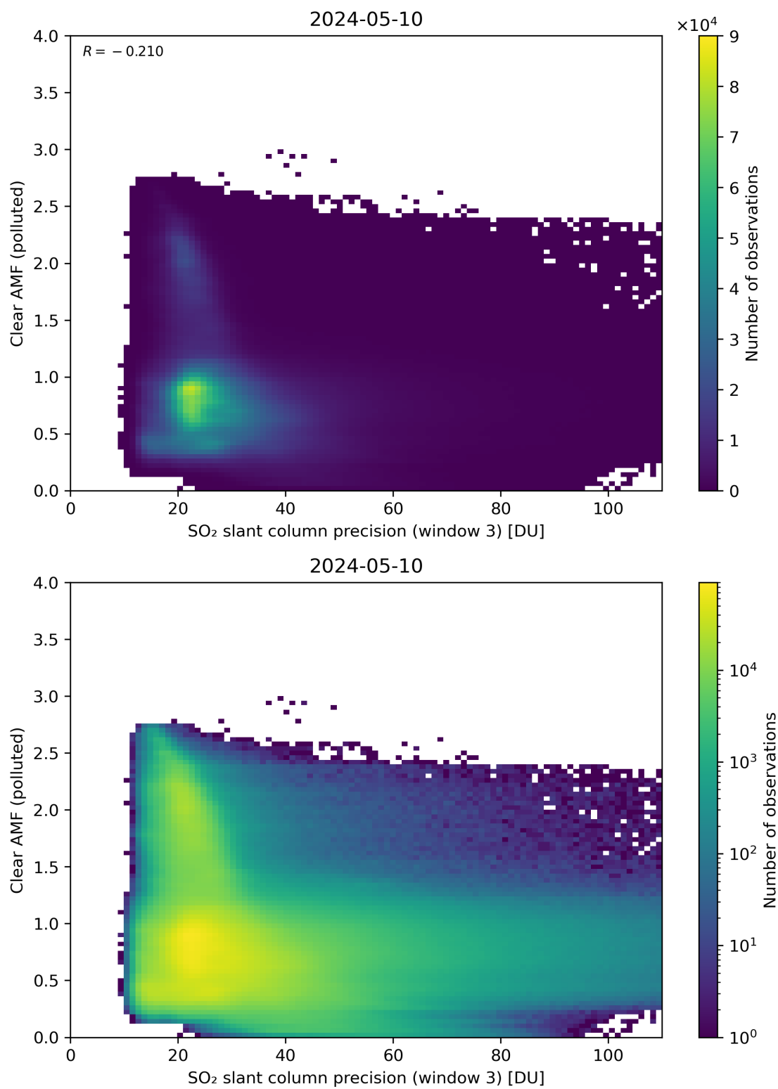
Figure 261: Scatter density plot of “SO 2 slant column precision (window 3)” against “Clear AMF (polluted)” for 2024-05-09 to 2024-05-11.
