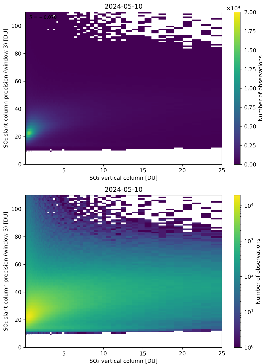
Figure 304: Scatter density plot of “SO 2 vertical column” against “SO 2 slant column precision (window 3)” for 2024-05-09 to 2024-05-11.
