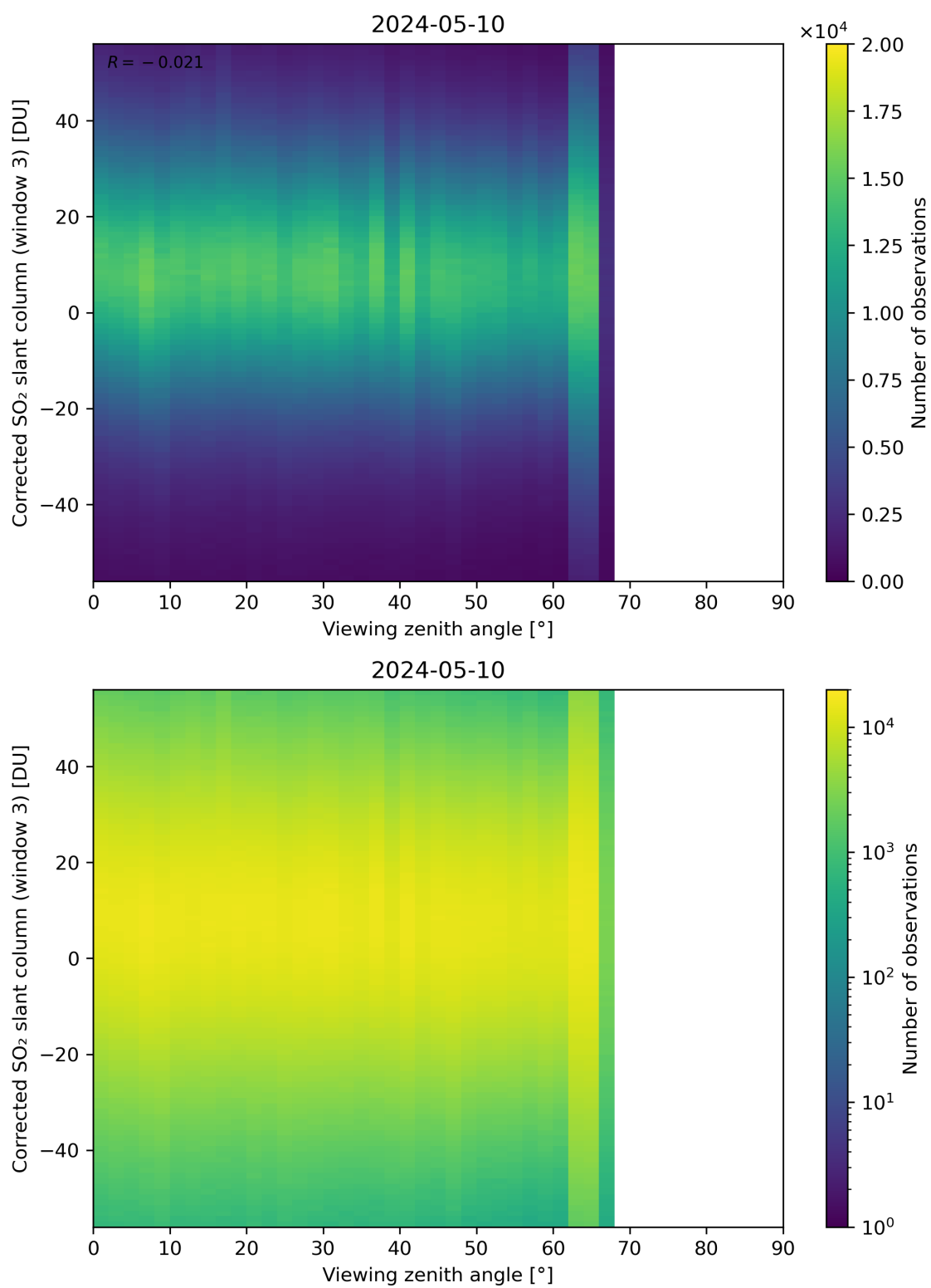
Figure 319: Scatter density plot of “Viewing zenith angle” against “Corrected SO 2 slant column (window 3)” for 2024-05-09 to 2024-05-11.
