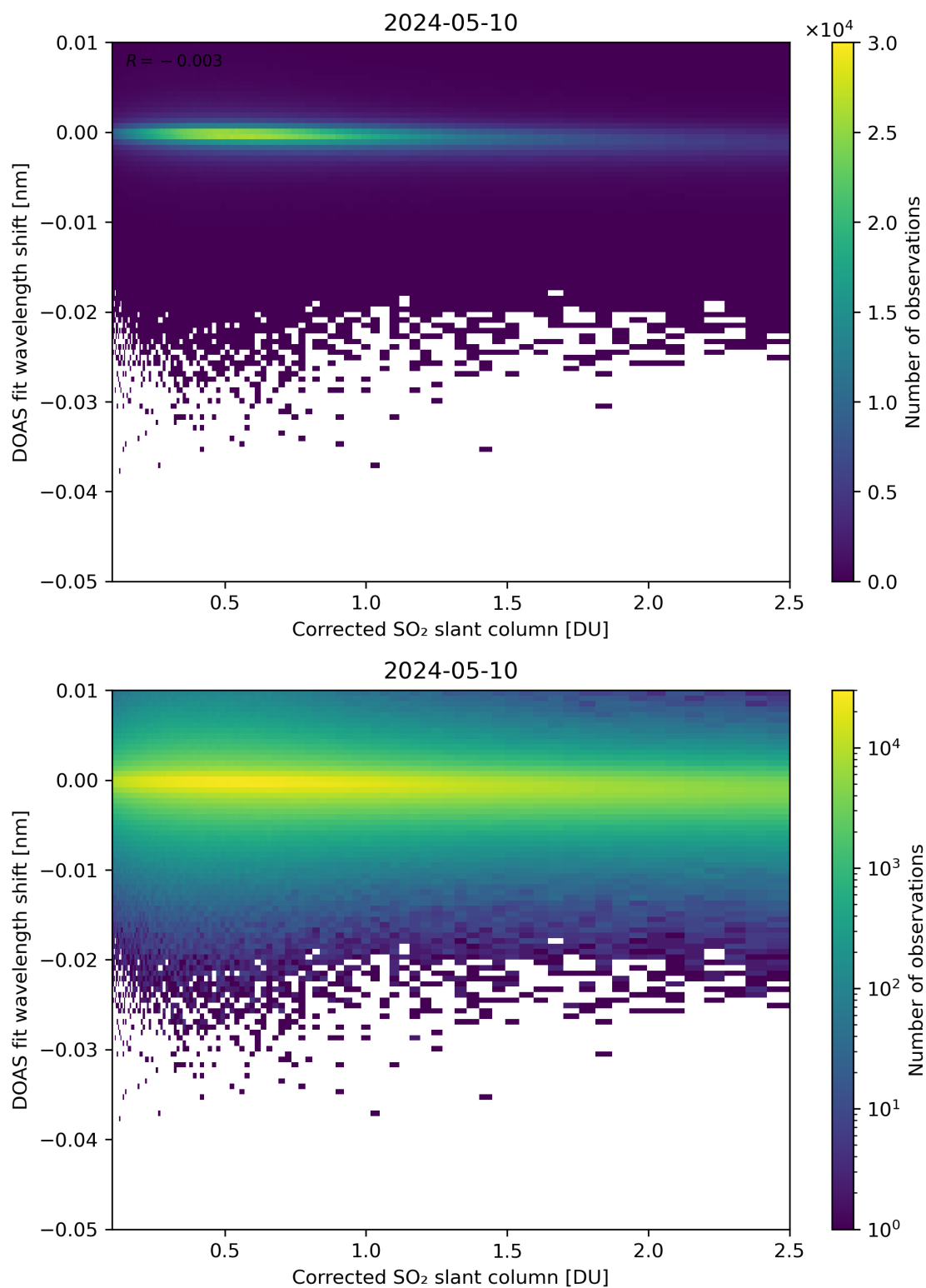
Figure 181: Scatter density plot of “Corrected SO 2 slant column” against “DOAS fit wavelength shift” for 2024-05-09 to 2024-05-11.
