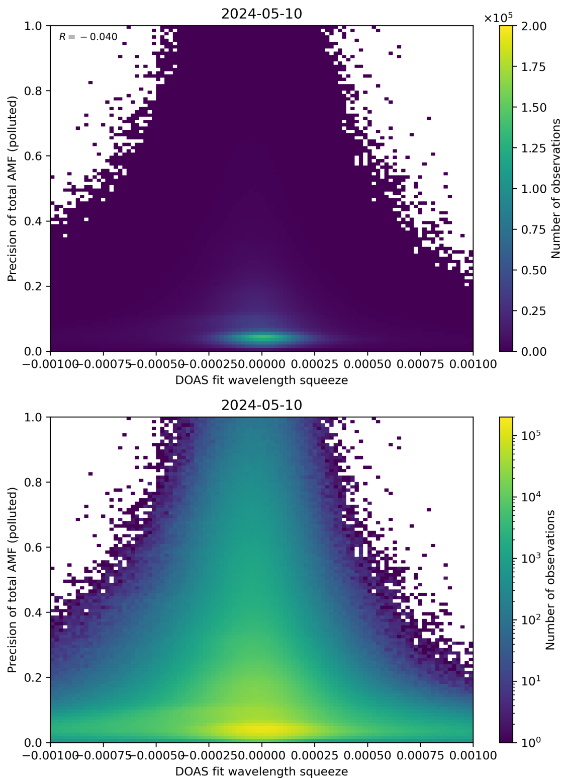
Figure 135: Scatter density plot of “DOAS fit wavelength squeeze” against “Precision of total AMF (polluted)” for 2024-05-09 to 2024-05-11.
