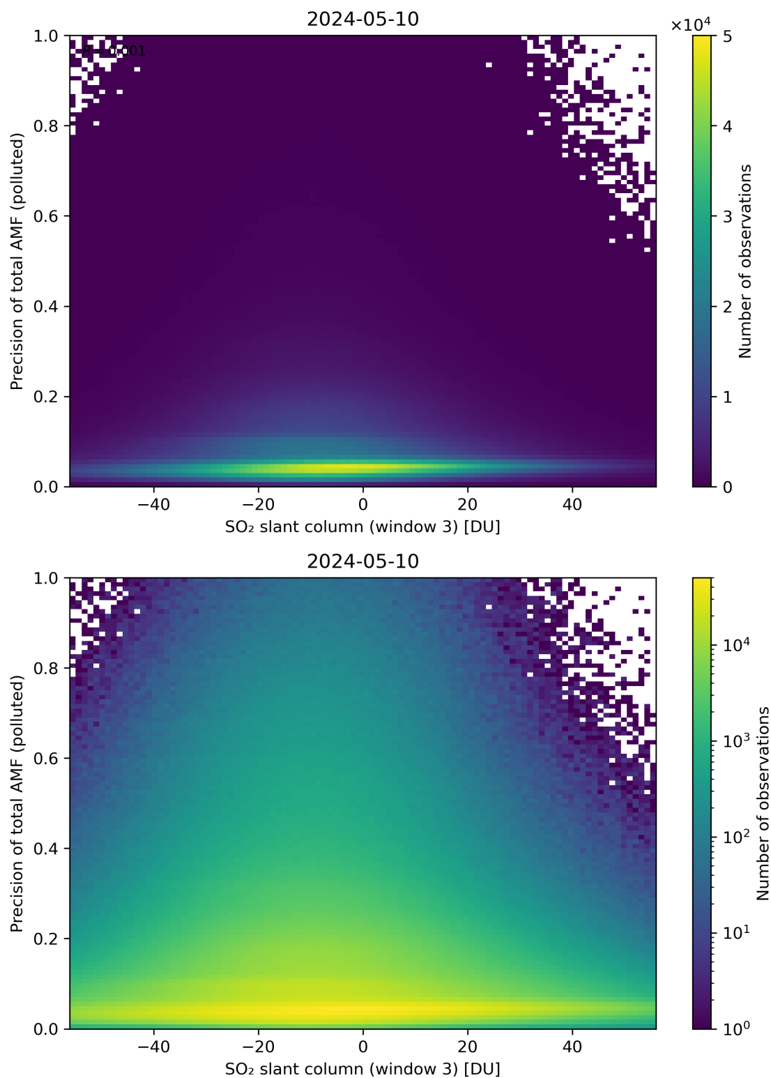
Figure 269: Scatter density plot of “SO 2 slant column (window 3)” against “Precision of total AMF (polluted)” for 2024-05-09 to 2024-05-11.
