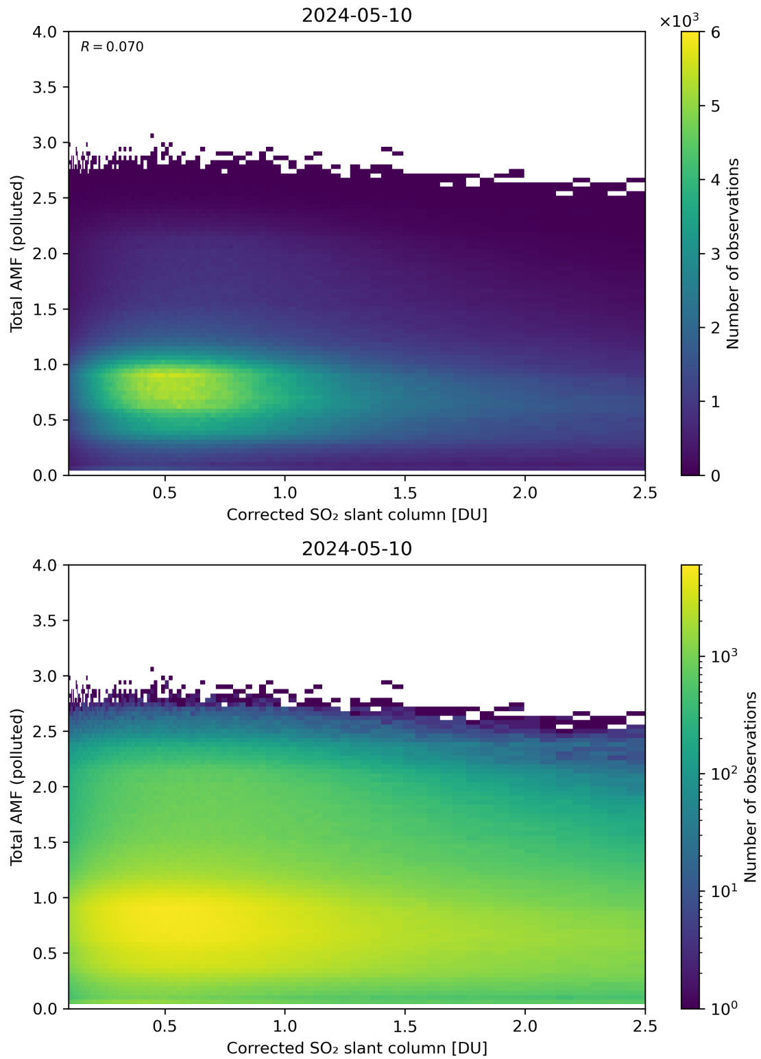
Figure 192: Scatter density plot of “Corrected SO 2 slant column” against “Total AMF (polluted)” for 2024-05-09 to 2024-05-11.
