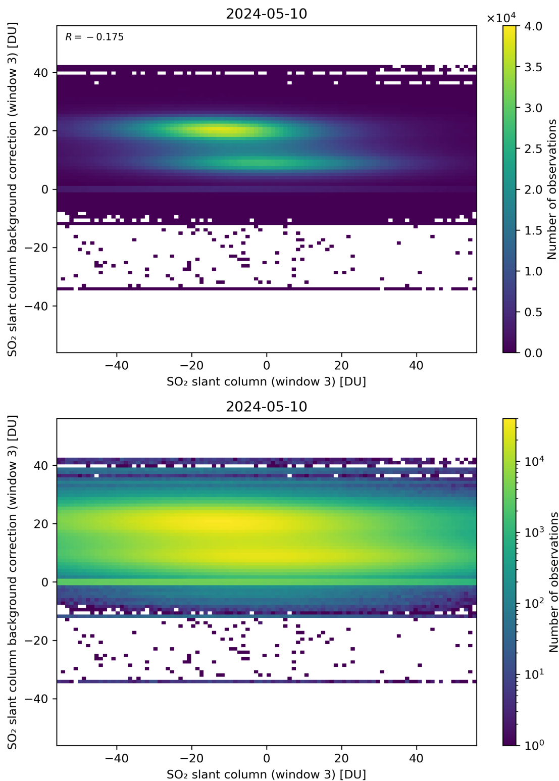
Figure 253: Scatter density plot of “SO 2 slant column (window 3)” against “SO 2 slant column background correction (window 3)” for 2024-05-09 to 2024-05-11.
