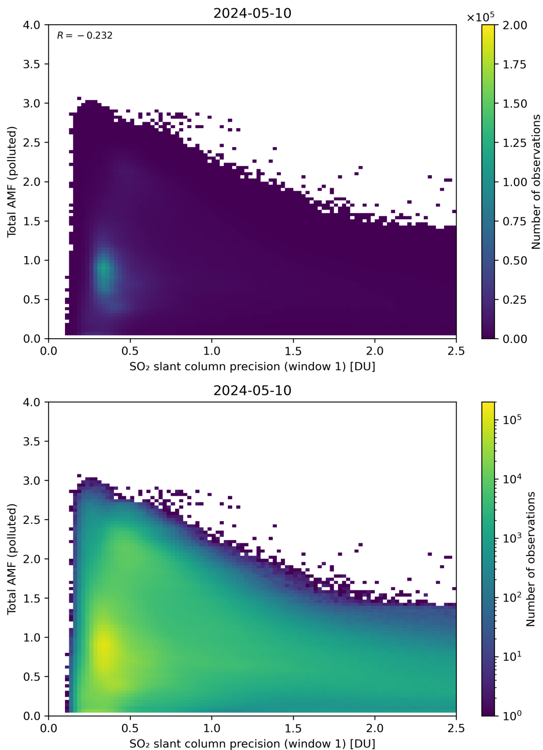
Figure 230: Scatter density plot of “SO 2 slant column precision (window 1)” against “Total AMF (polluted)” for 2024-05-09 to 2024-05-11.
