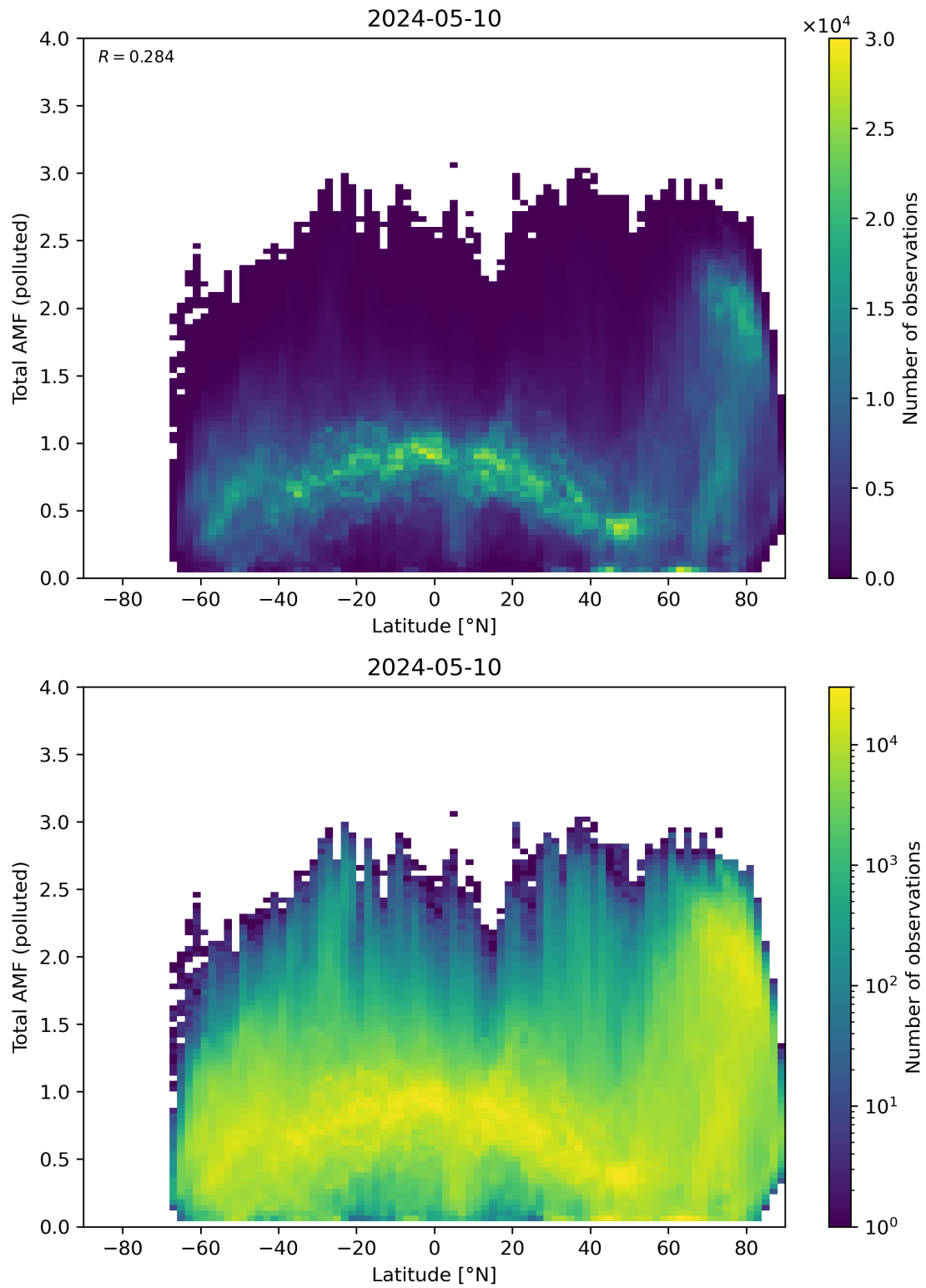
Figure 154: Scatter density plot of “Latitude” against “Total AMF (polluted)” for 2024-05-09 to 2024-05-11.
