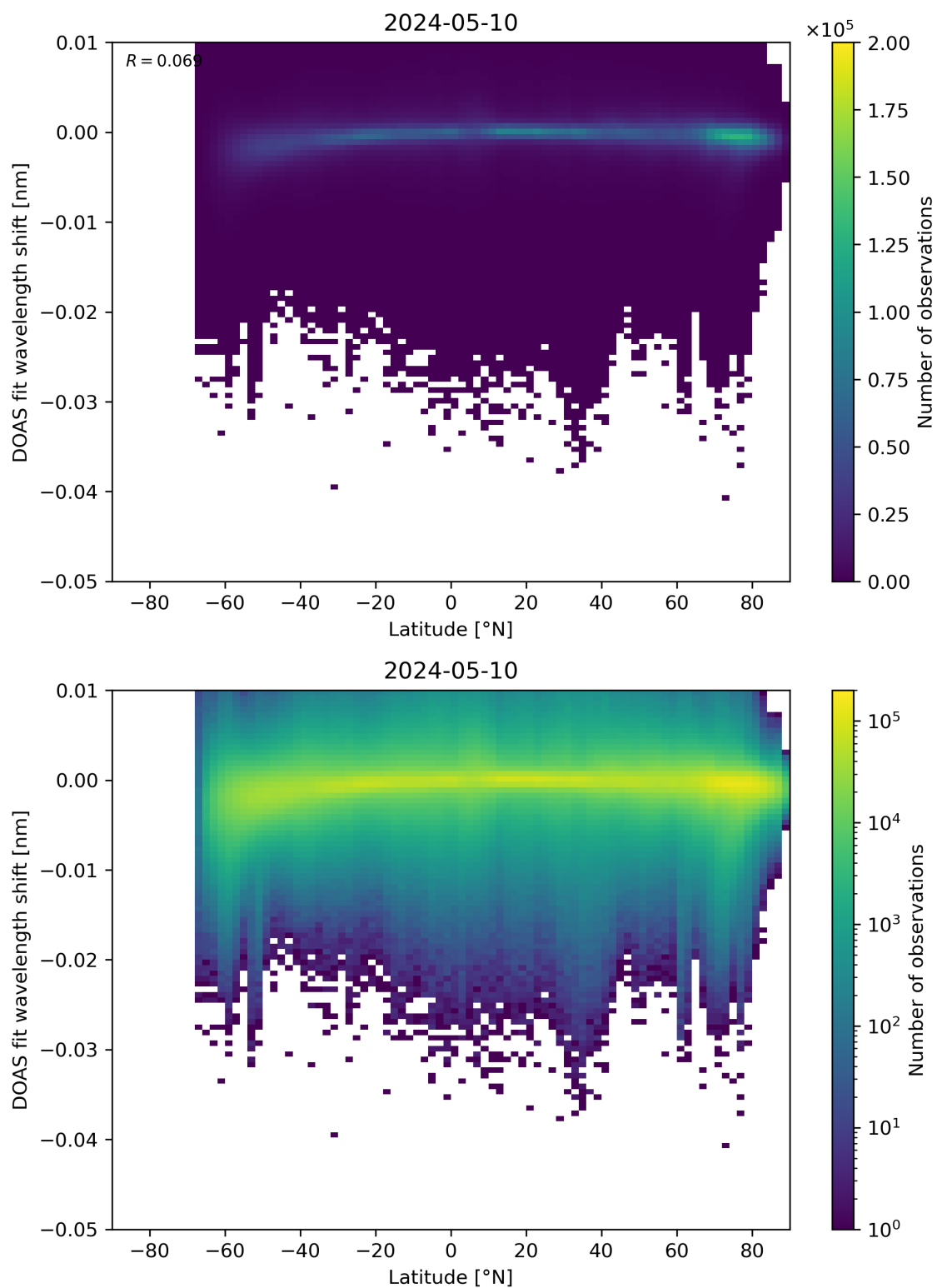
Figure 142: Scatter density plot of “Latitude” against “DOAS fit wavelength shift” for 2024-05-09 to 2024-05-11.
