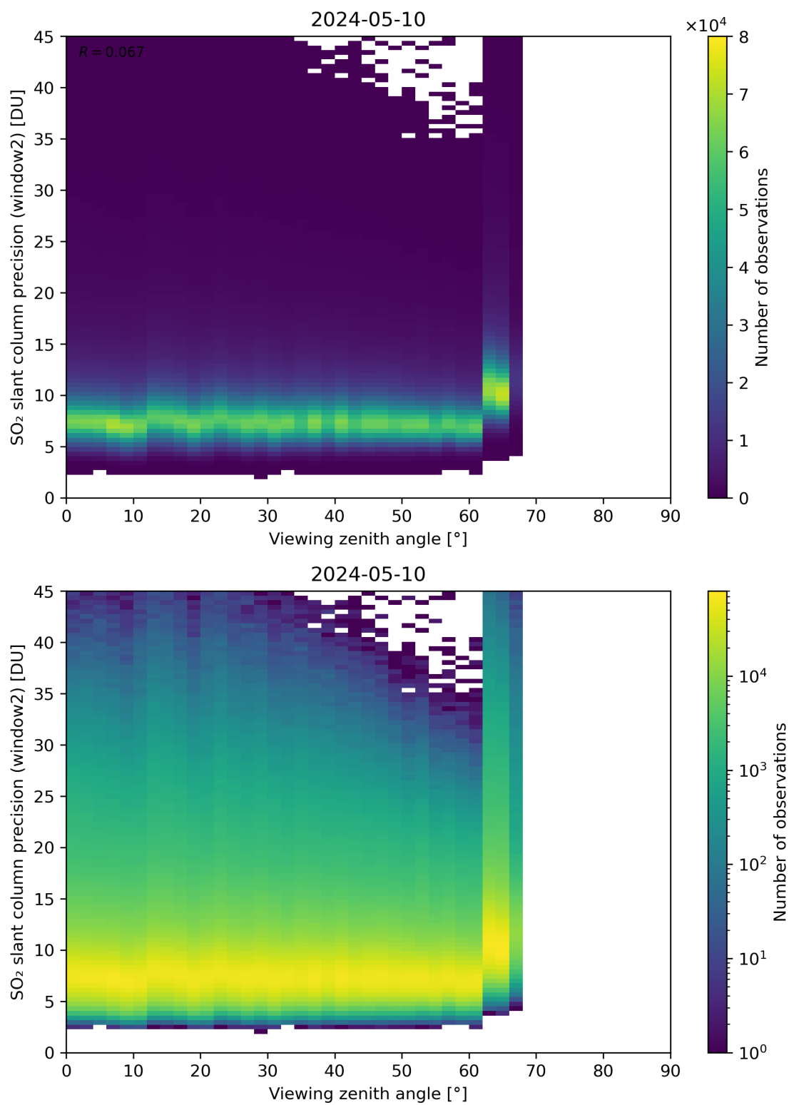
Figure 322: Scatter density plot of “Viewing zenith angle” against “SO 2 slant column precision (window2)” for 2024-05-09 to 2024-05-11.
