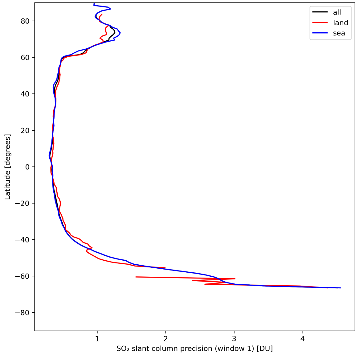
Figure 34: Zonal average of “SO 2 slant column precision (window 1)” for 2024-05-09 to 2024-05-11.
