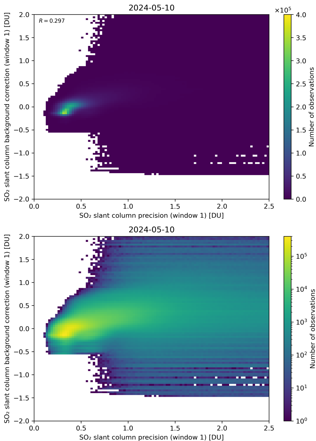
Figure 218: Scatter density plot of “SO 2 slant column precision (window 1)” against “SO 2 slant column background correction (window 1)” for 2024-05-09 to 2024-05-11.
