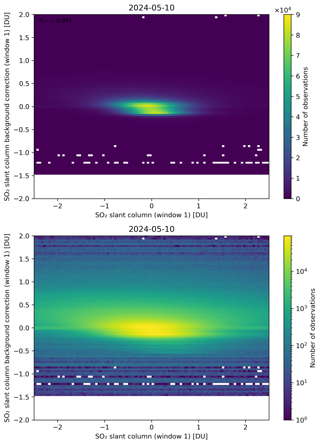
Figure 212: Scatter density plot of “SO 2 slant column (window 1)” against “SO 2 slant column background correction (window 1)” for 2024-05-09 to 2024-05-11.
