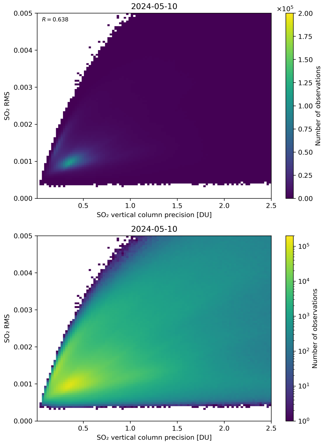
Figure 284: Scatter density plot of “SO 2 vertical column precision” against “SO 2 RMS” for 2024-05-09 to 2024-05-11.
