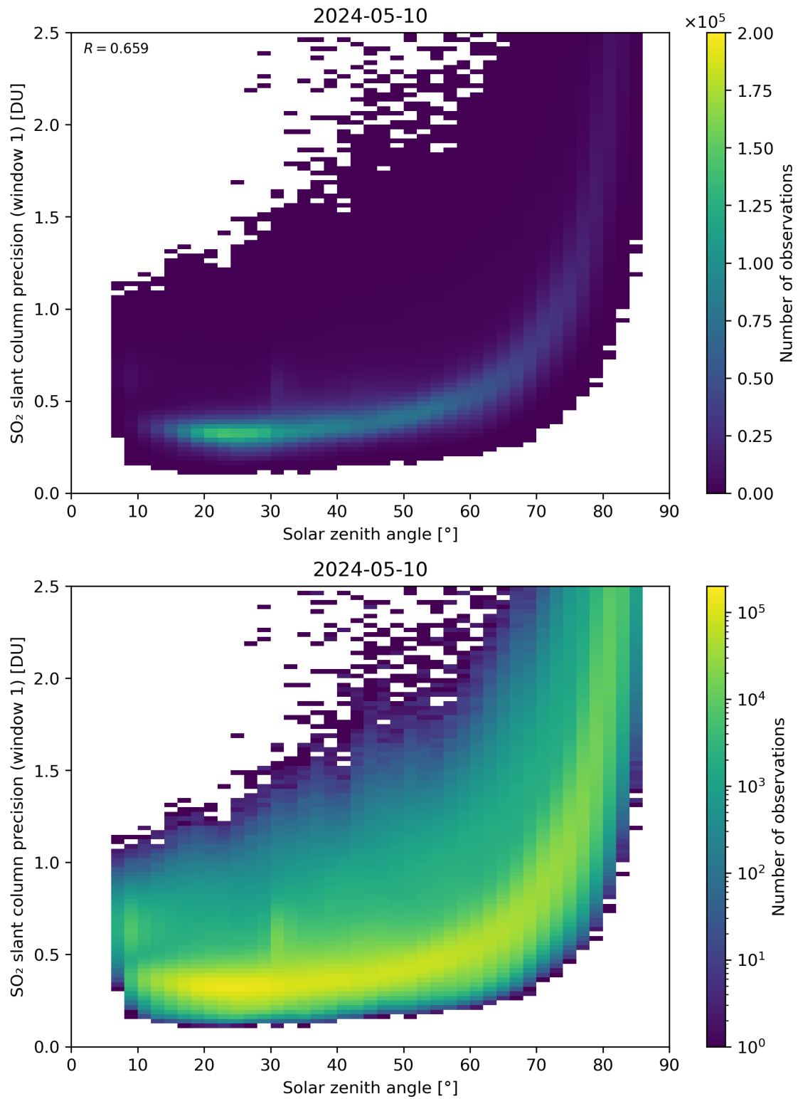
Figure 170: Scatter density plot of “Solar zenith angle” against “SO 2 slant column precision (window 1)” for 2024-05-09 to 2024-05-11.
