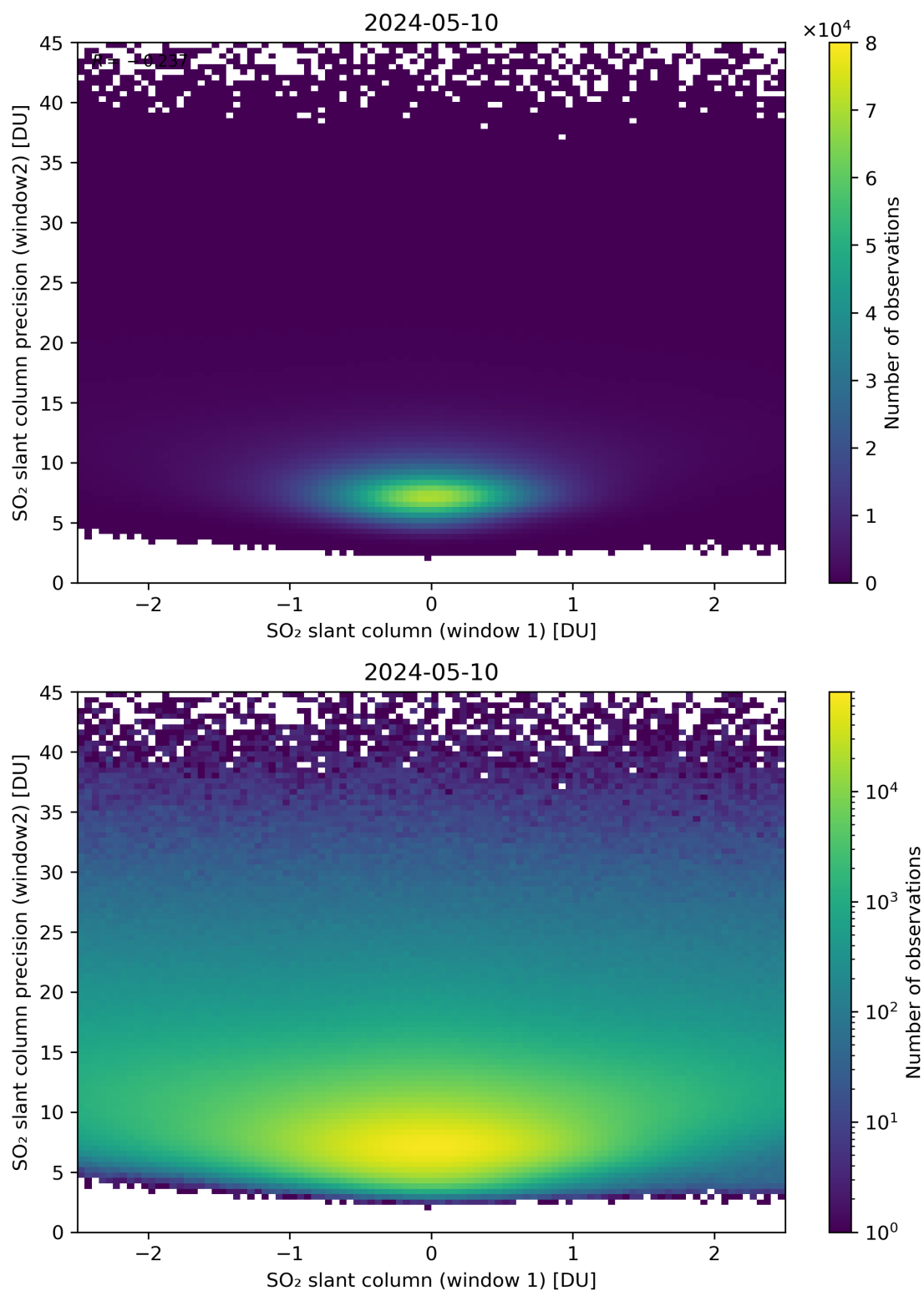
Figure 236: Scatter density plot of “SO 2 slant column (window 1)” against “SO 2 slant column precision (window2)” for 2024-05-09 to 2024-05-11.
