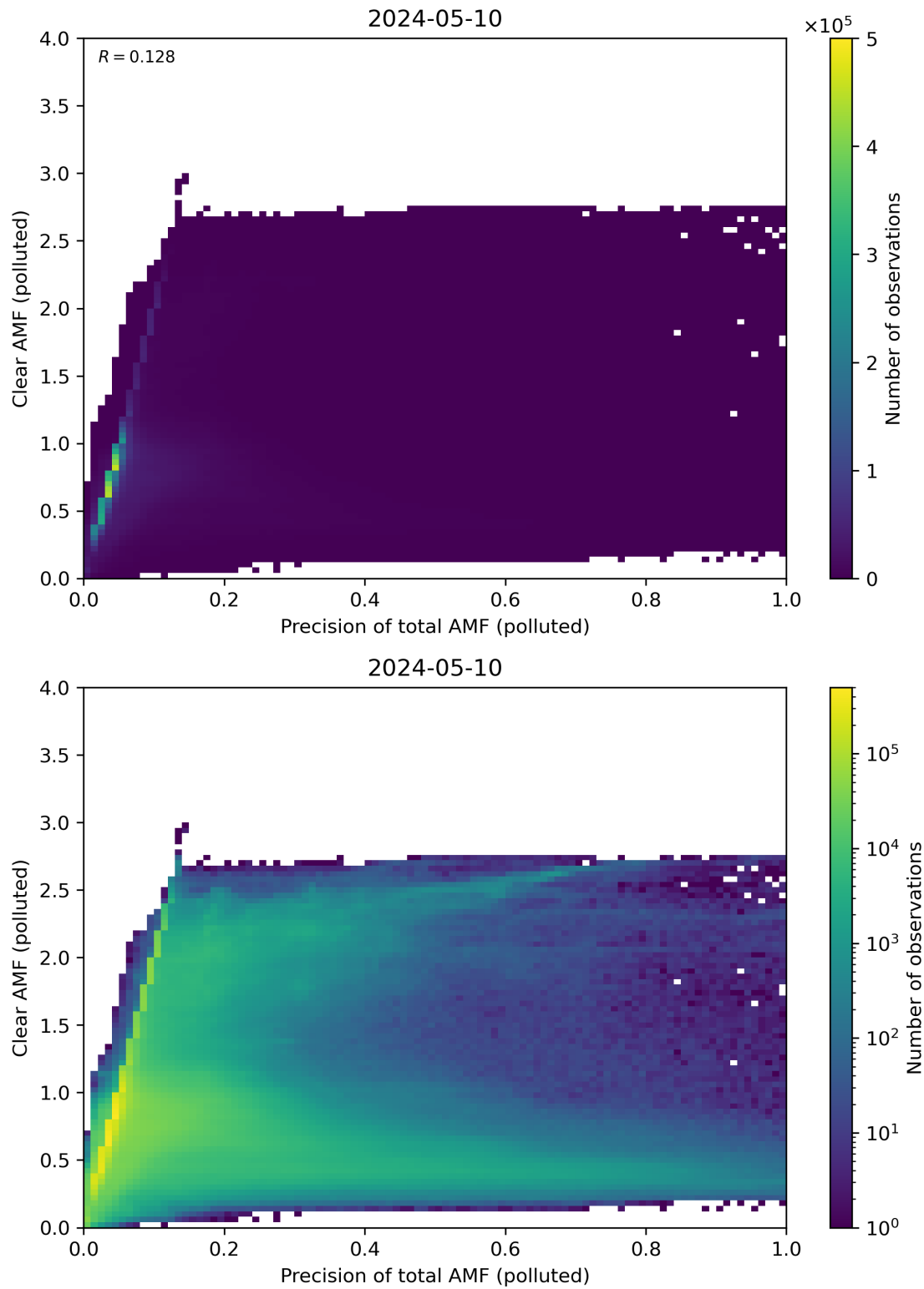
Figure 270: Scatter density plot of “Precision of total AMF (polluted)” against “Clear AMF (polluted)” for 2024-05-09 to 2024-05-11.
