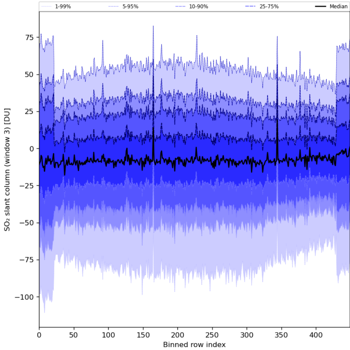
Figure 87: Along track statistics of "SO 2 slant column (window 3)" for 2024-05-09 to 2024-05-11
