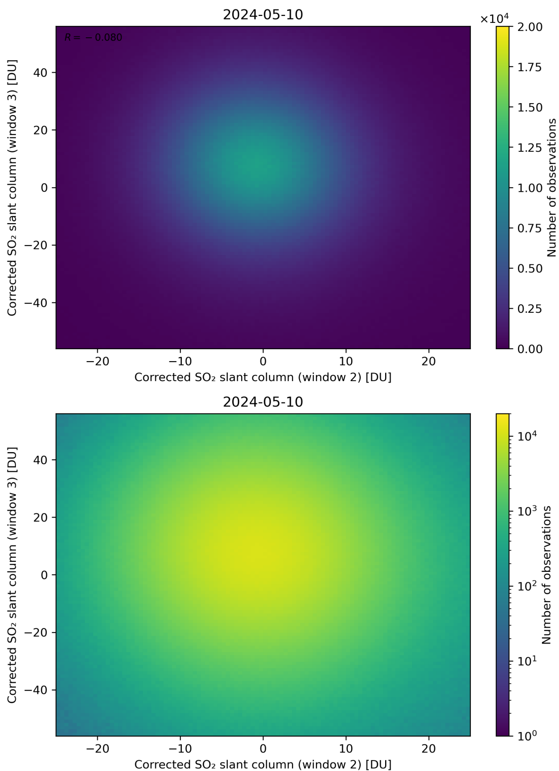
Figure 200: Scatter density plot of “Corrected SO 2 slant column (window 2)” against “Corrected SO 2 slant column (window 3)” for 2024-05-09 to 2024-05-11.
