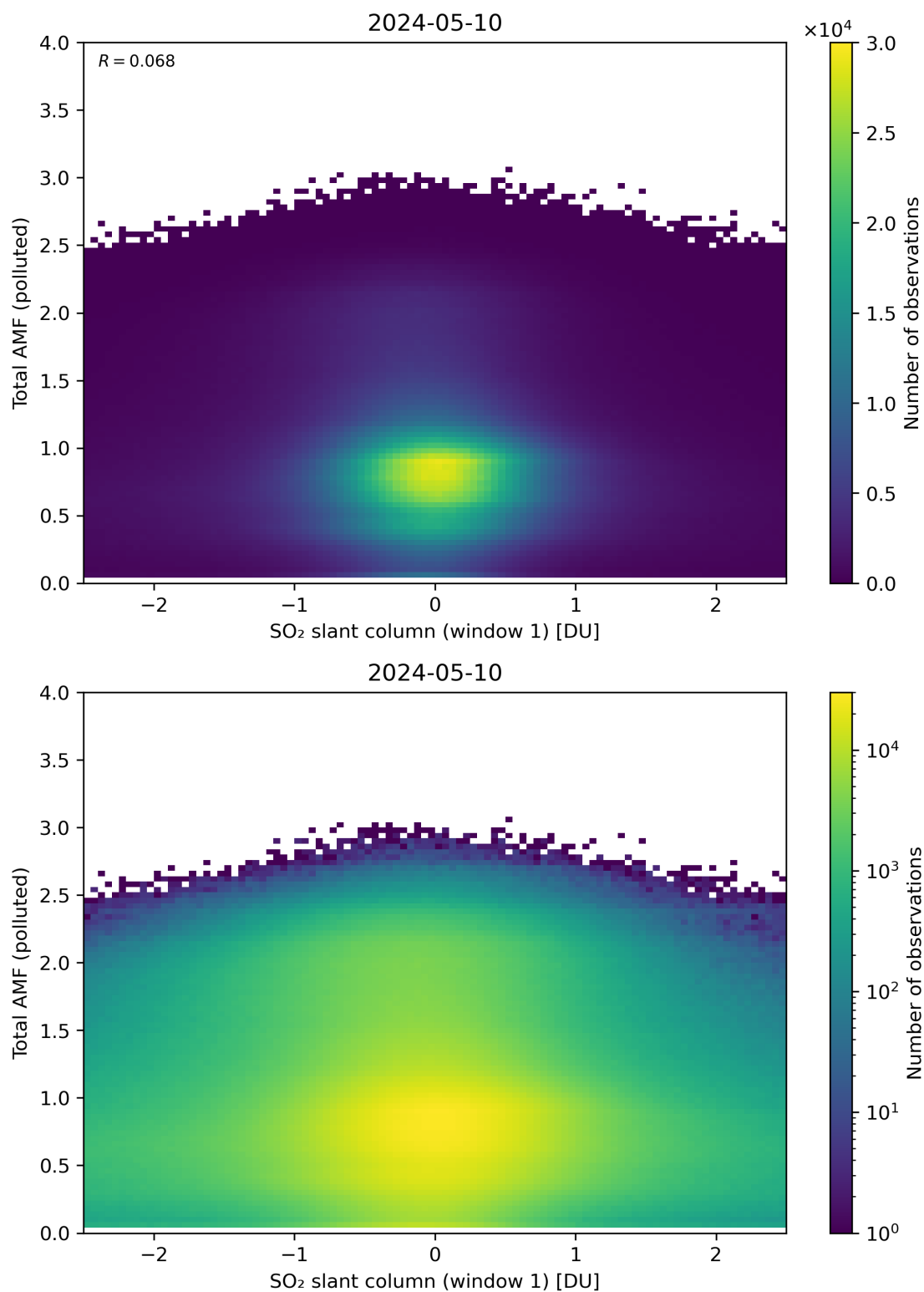
Figure 239: Scatter density plot of “SO 2 slant column (window 1)” against “Total AMF (polluted)” for 2024-05-09 to 2024-05-11.
