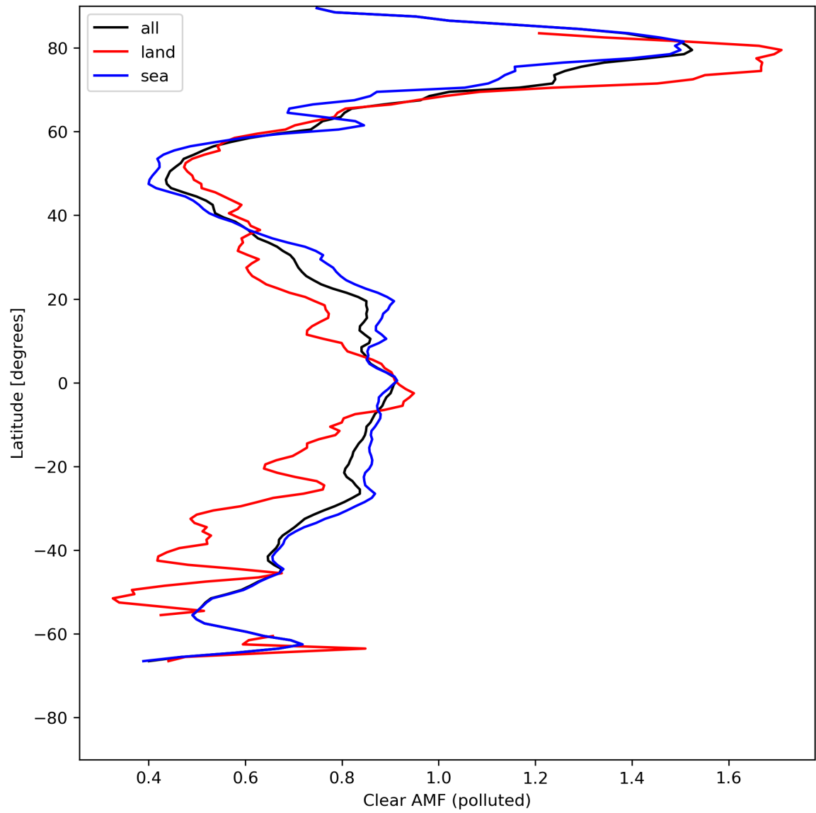
Figure 50: Zonal average of “Clear AMF (polluted)” for 2024-05-09 to 2024-05-11.
