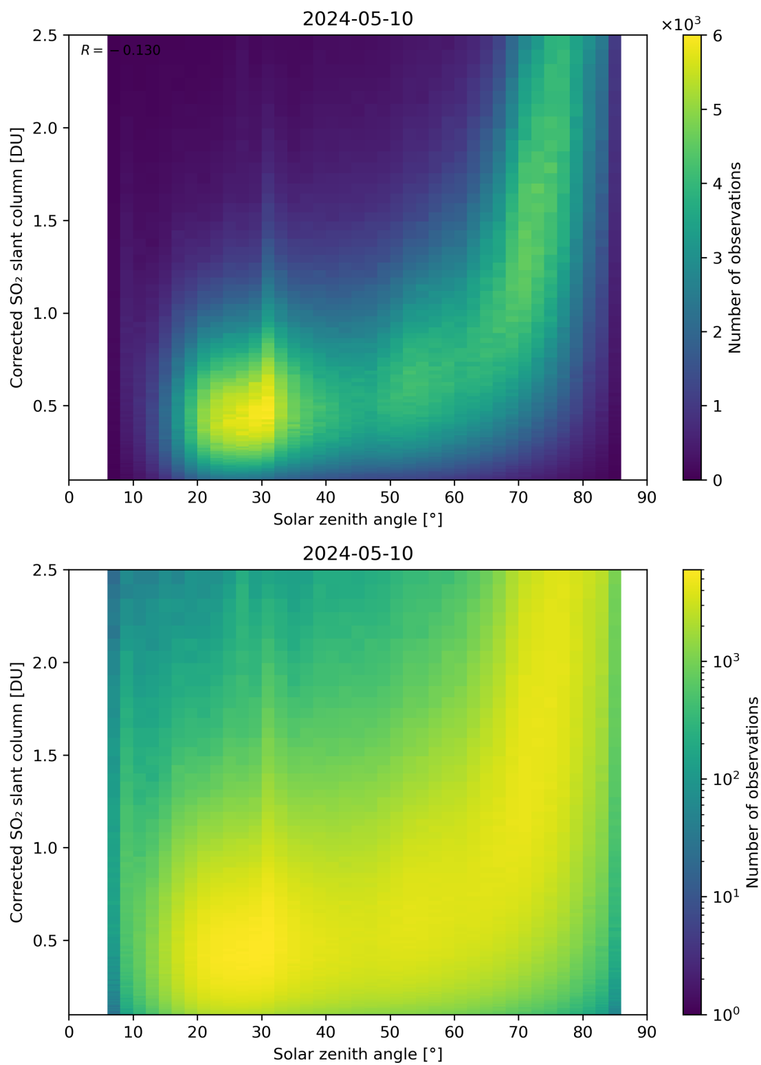
Figure 166: Scatter density plot of “Solar zenith angle” against “Corrected SO 2 slant column” for 2024-05-09 to 2024-05-11.
