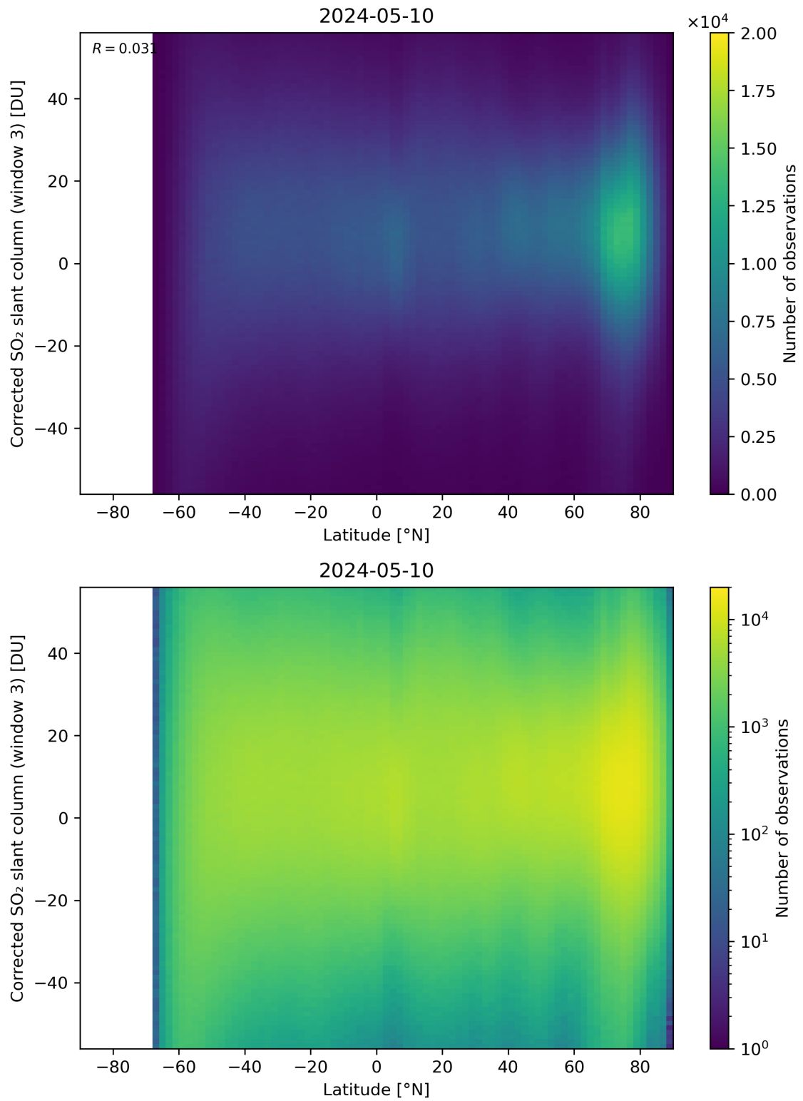
Figure 148: Scatter density plot of “Latitude” against “Corrected SO 2 slant column (window 3)” for 2024-05-09 to 2024-05-11.
