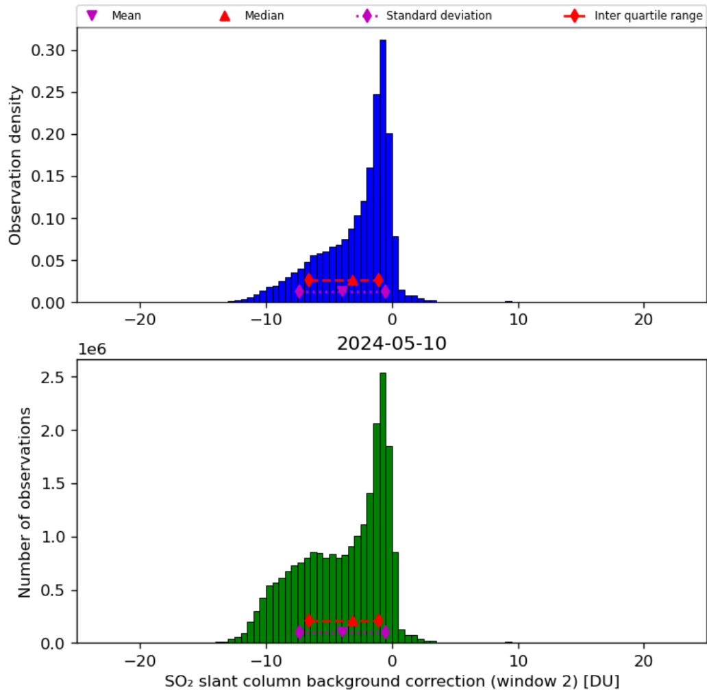
Figure 63: Histogram of “SO 2 slant column background correction (window 2)” for 2024-05-09 to 2024-05-11
