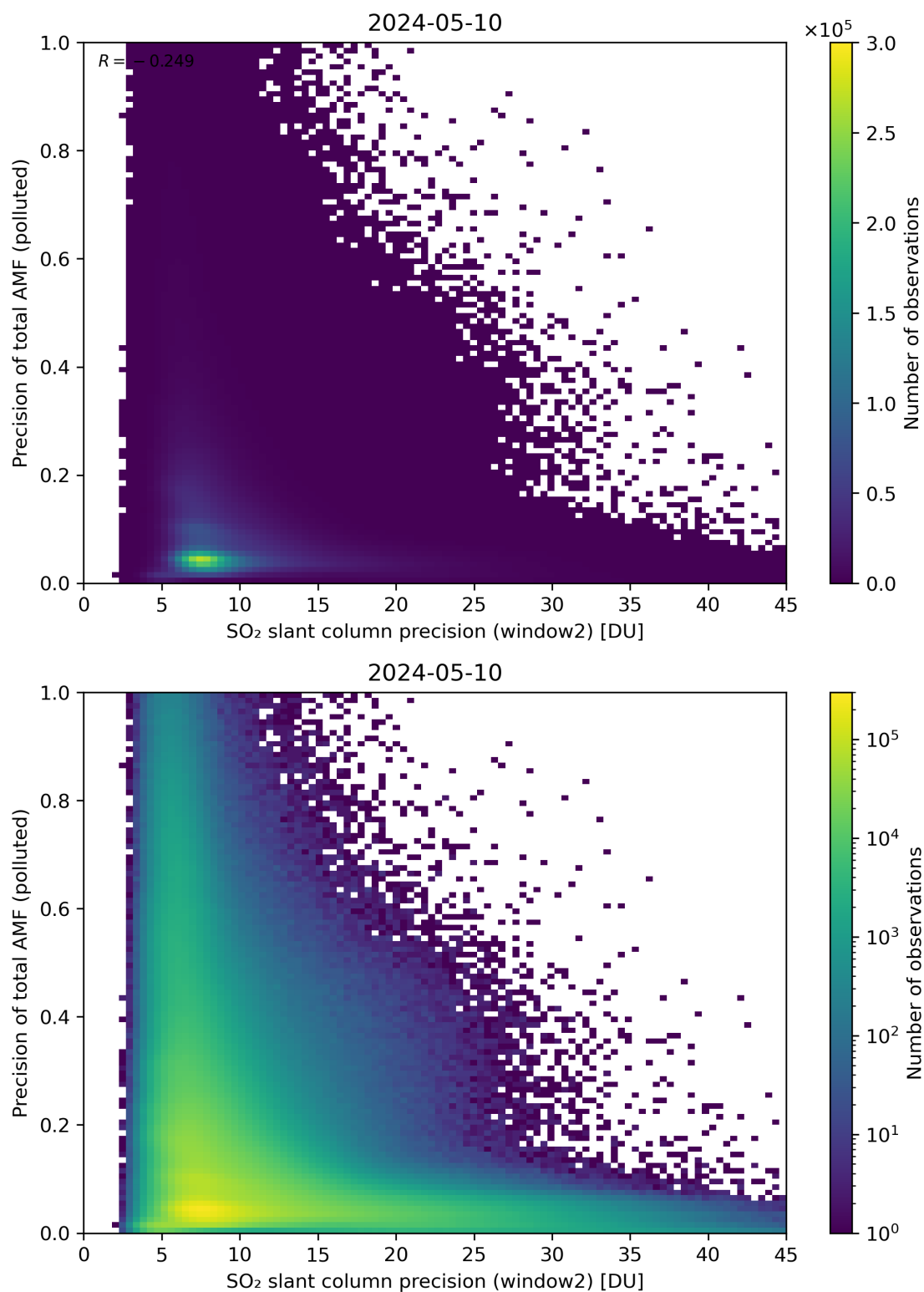
Figure 252: Scatter density plot of “SO 2 slant column precision (window2)” against “Precision of total AMF (polluted)” for 2024-05-09 to 2024-05-11.
