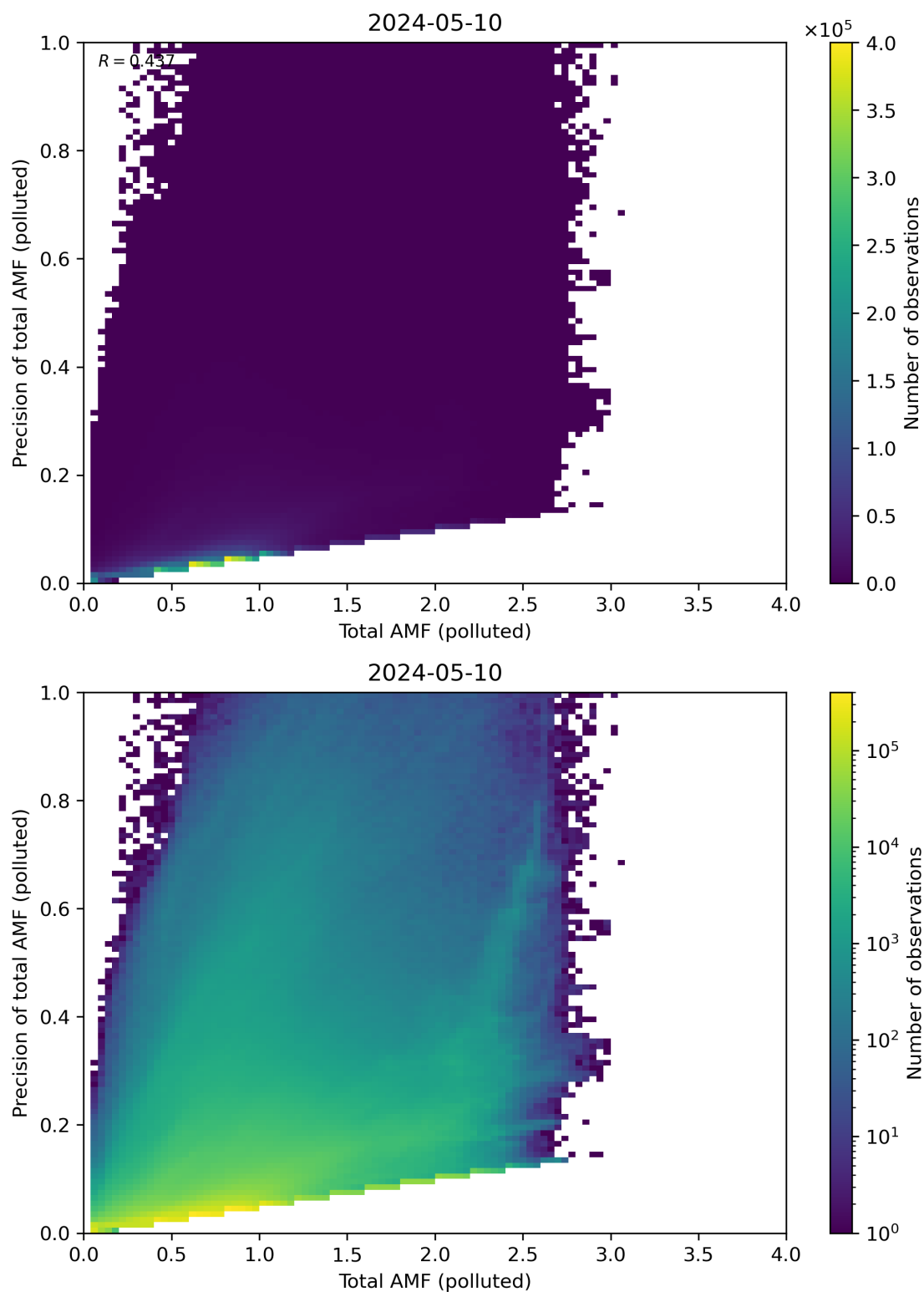
Figure 272: Scatter density plot of “Total AMF (polluted)” against “Precision of total AMF (polluted)” for 2024-05-09 to 2024-05-11.
