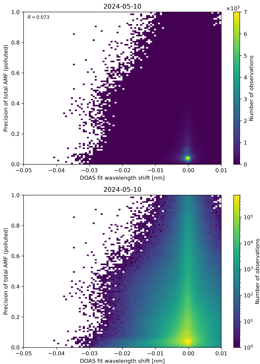
Figure 131: Scatter density plot of “DOAS fit wavelength shift” against “Precision of total AMF (polluted)” for 2024-05-09 to 2024-05-11.
