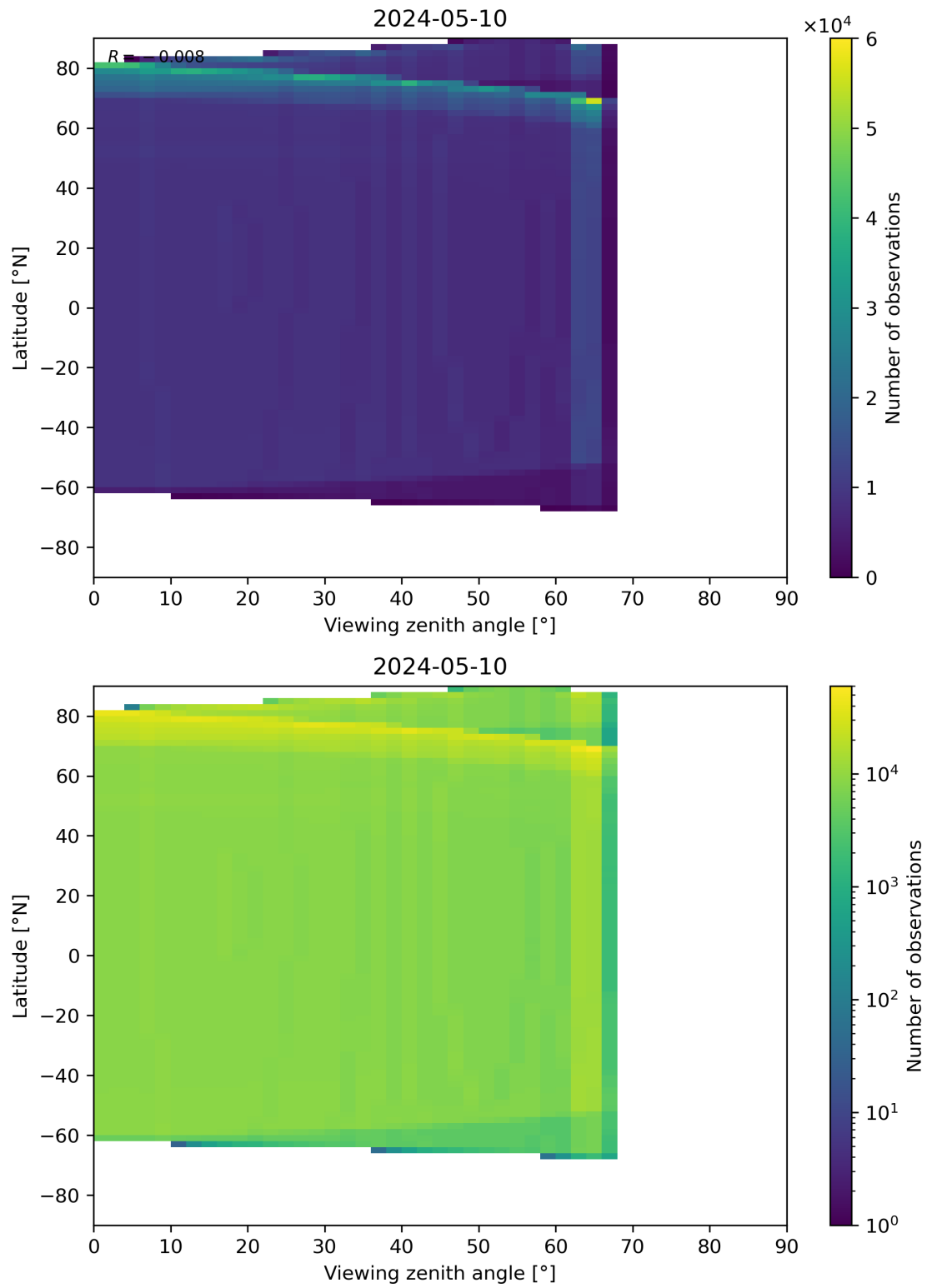
Figure 314: Scatter density plot of “Viewing zenith angle” against “Latitude” for 2024-05-09 to 2024-05-11.
