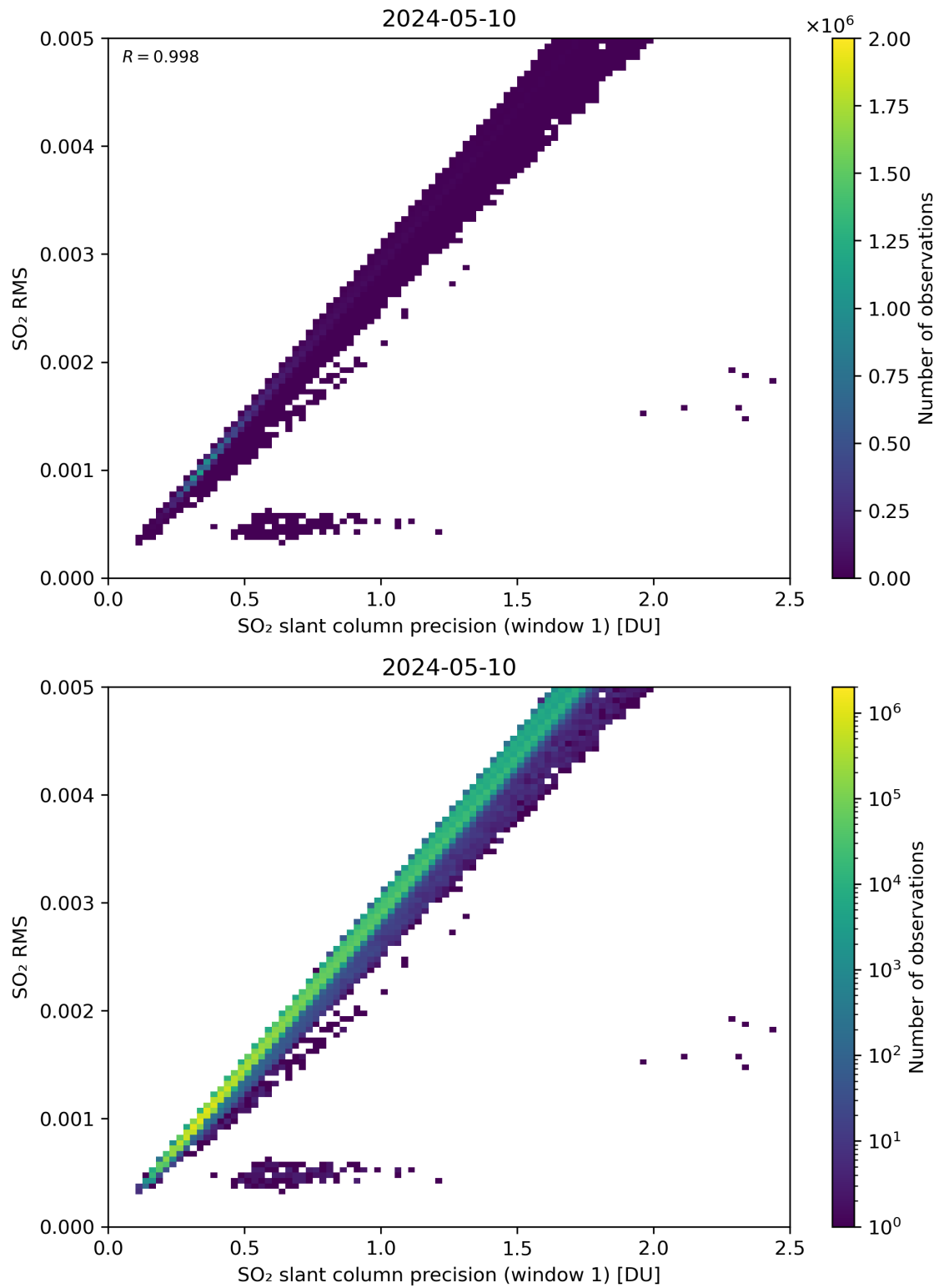
Figure 223: Scatter density plot of “SO 2 slant column precision (window 1)” against “SO 2 RMS” for 2024-05-09 to 2024-05-11.
