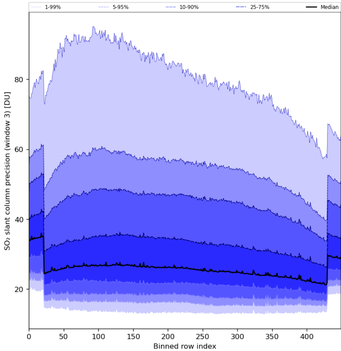
Figure 88: Along track statistics of “SO 2 slant column precision (window 3)” for 2024-05-09 to 2024-05-11
