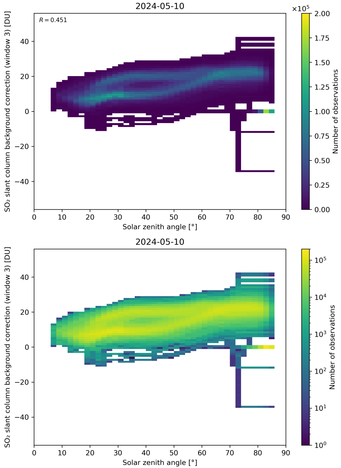
Figure 160: Scatter density plot of “Solar zenith angle” against “SO 2 slant column background correction (window 3)” for 2024-05-09 to 2024-05-11.
