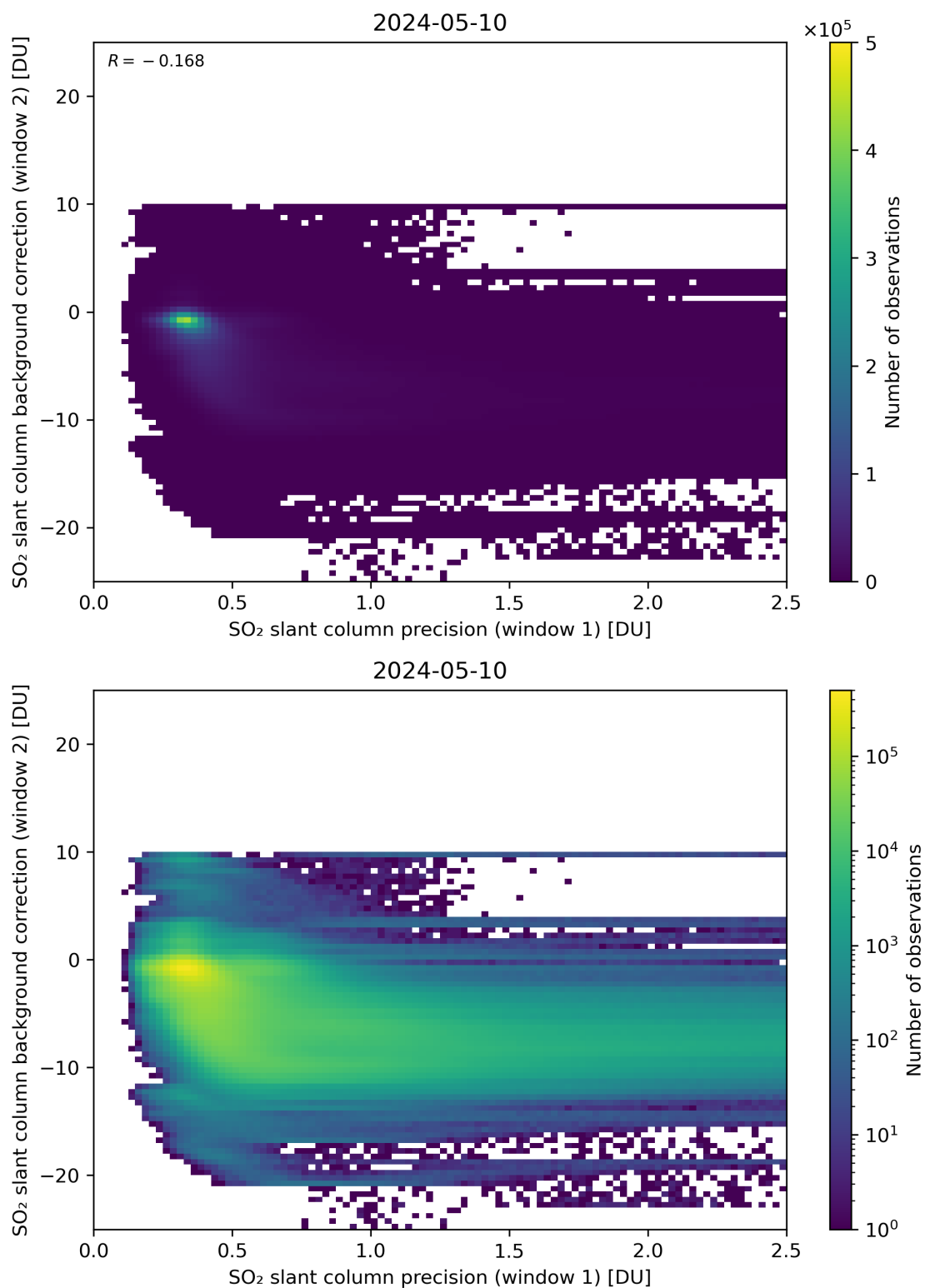
Figure 219: Scatter density plot of “SO 2 slant column precision (window 1)” against “SO 2 slant column background correction (window 2)” for 2024-05-09 to 2024-05-11.
