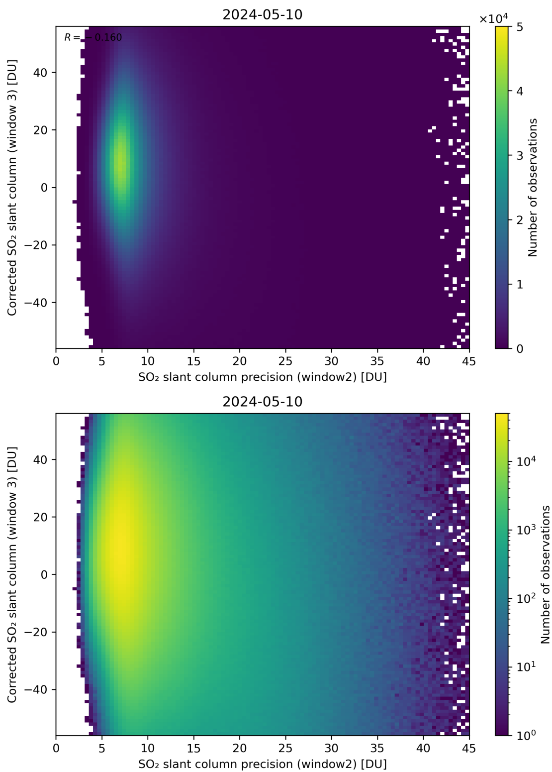
Figure 248: Scatter density plot of “SO 2 slant column precision (window2)” against “Corrected SO 2 slant column (window 3)” for 2024-05-09 to 2024-05-11.
