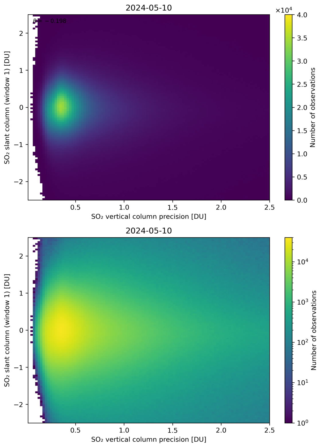
Figure 289: Scatter density plot of “SO 2 vertical column precision” against “SO 2 slant column (window 1)” for 2024-05-09 to 2024-05-11.
