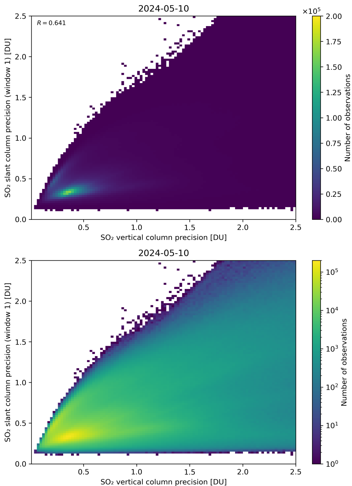
Figure 290: Scatter density plot of “SO 2 vertical column precision” against “SO 2 slant column precision (window 1)” for 2024-05-09 to 2024-05-11.
