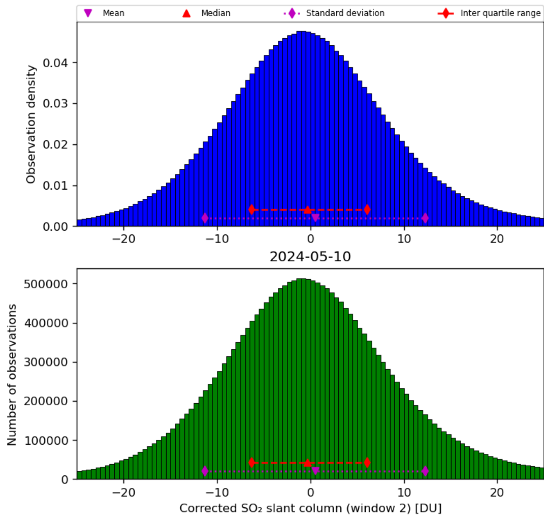
Figure 62: Histogram of “Corrected SO 2 slant column (window 2)” for 2024-05-09 to 2024-05-11
