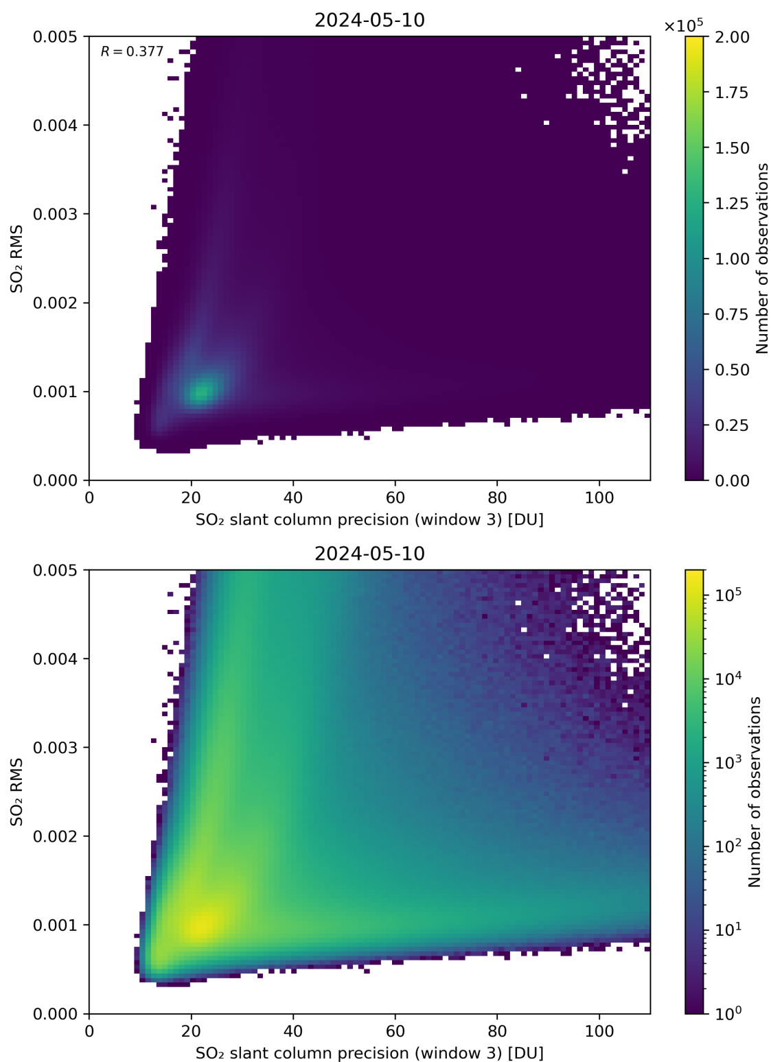
Figure 260: Scatter density plot of “SO 2 slant column precision (window 3)” against “SO 2 RMS” for 2024-05-09 to 2024-05-11.
