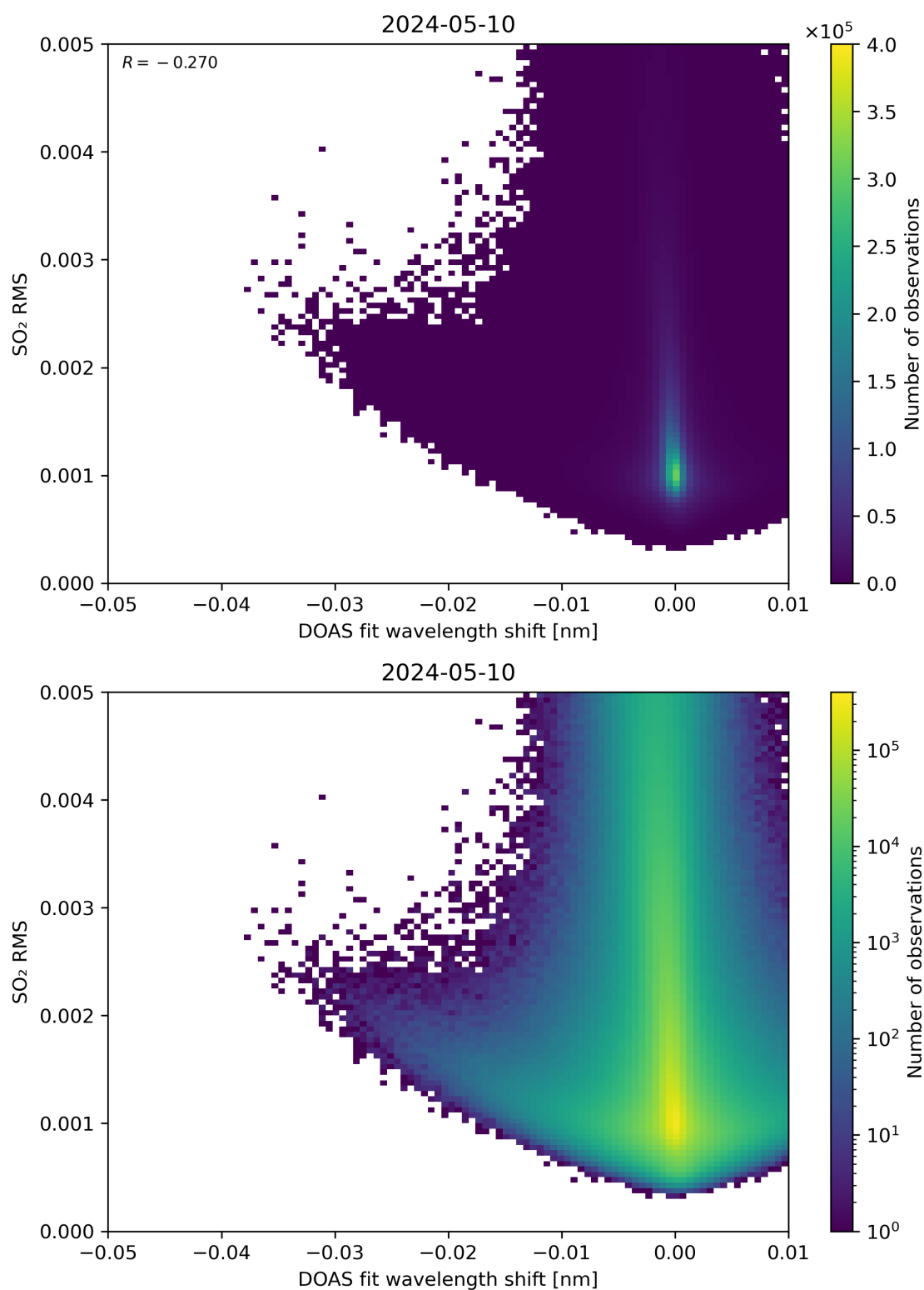
Figure 128: Scatter density plot of “DOAS fit wavelength shift” against “SO 2 RMS” for 2024-05-09 to 2024-05-11.
