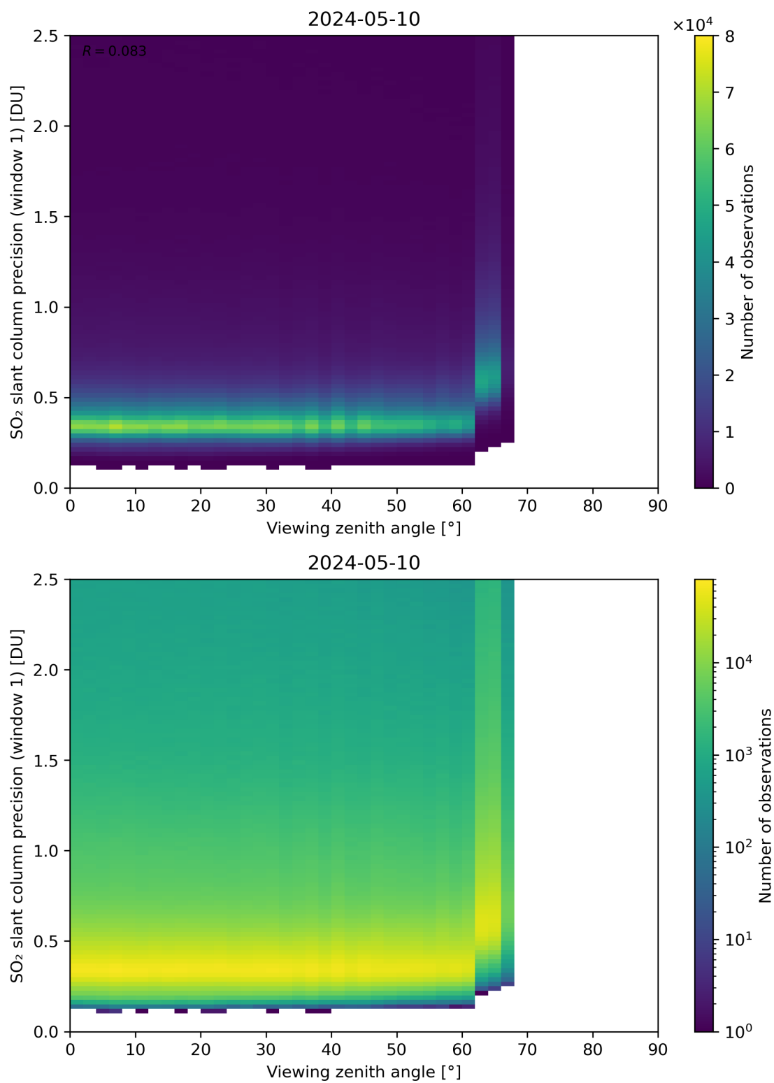
Figure 321: Scatter density plot of “Viewing zenith angle” against “SO 2 slant column precision (window 1)” for 2024-05-09 to 2024-05-11.
