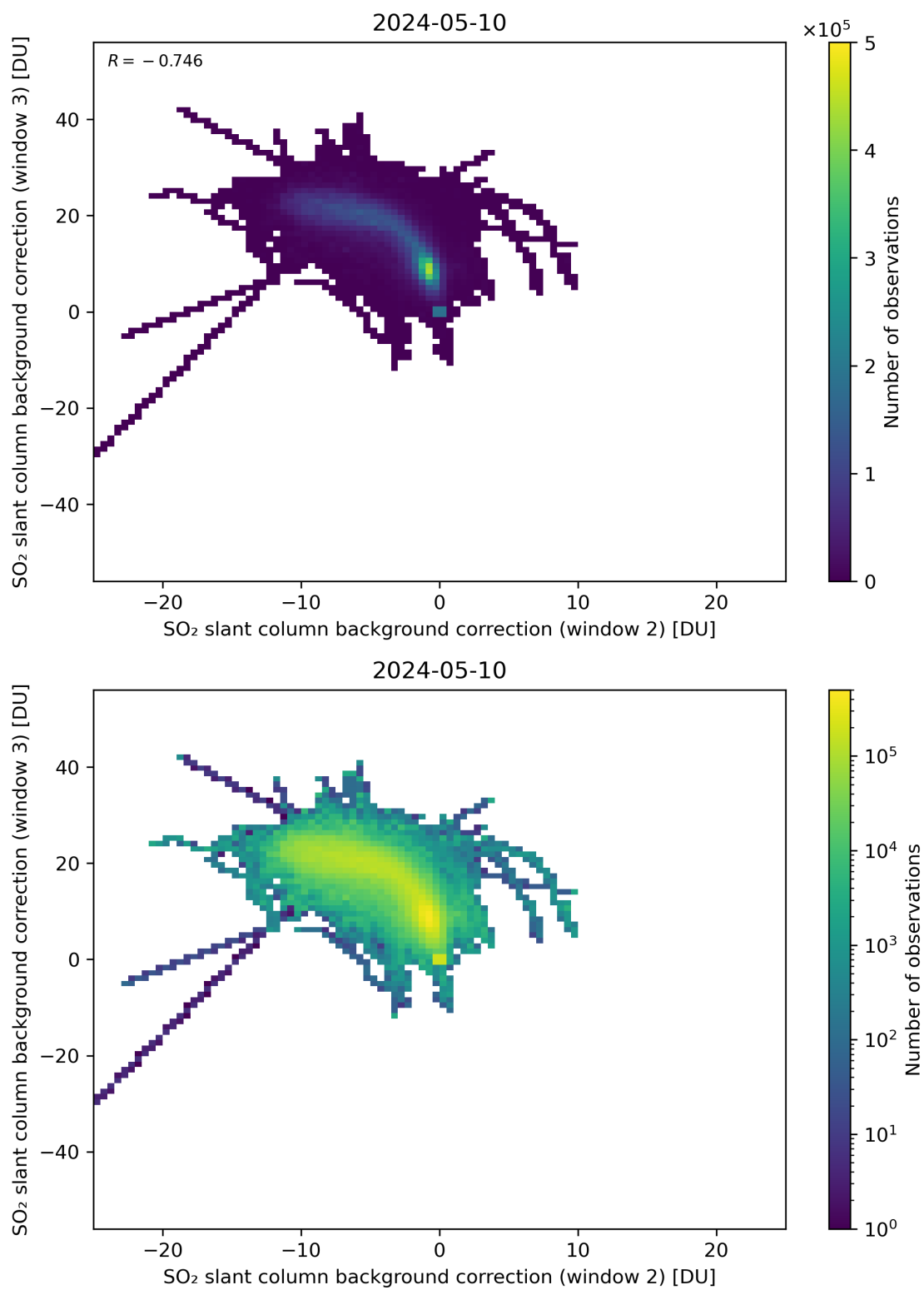
Figure 111: Scatter density plot of “SO 2 slant column background correction (window 2)” against “SO 2 slant column background correction (window 3)” for 2024-05-09 to 2024-05-11.
