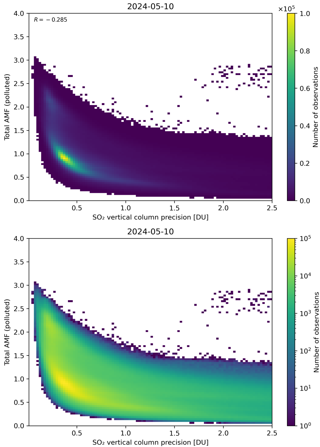
Figure 294: Scatter density plot of “SO 2 vertical column precision” against “Total AMF (polluted)” for 2024-05-09 to 2024-05-11.
