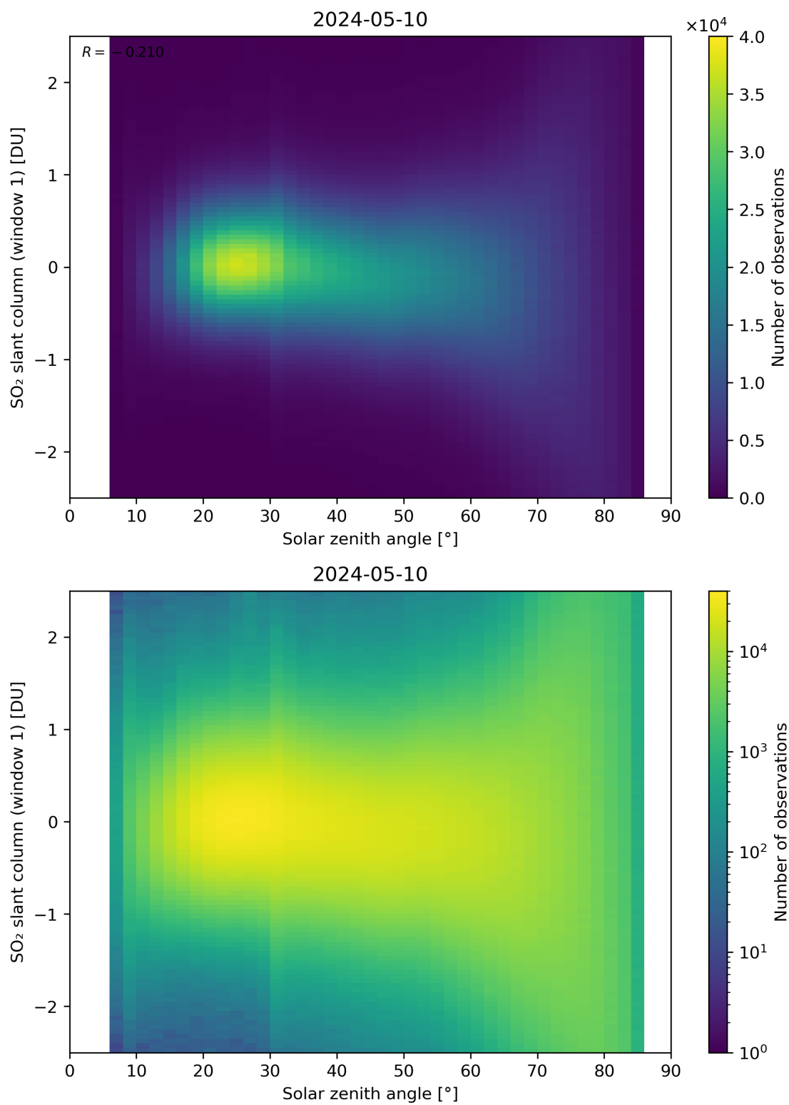
Figure 169: Scatter density plot of “Solar zenith angle” against “SO 2 slant column (window 1)” for 2024-05-09 to 2024-05-11.
