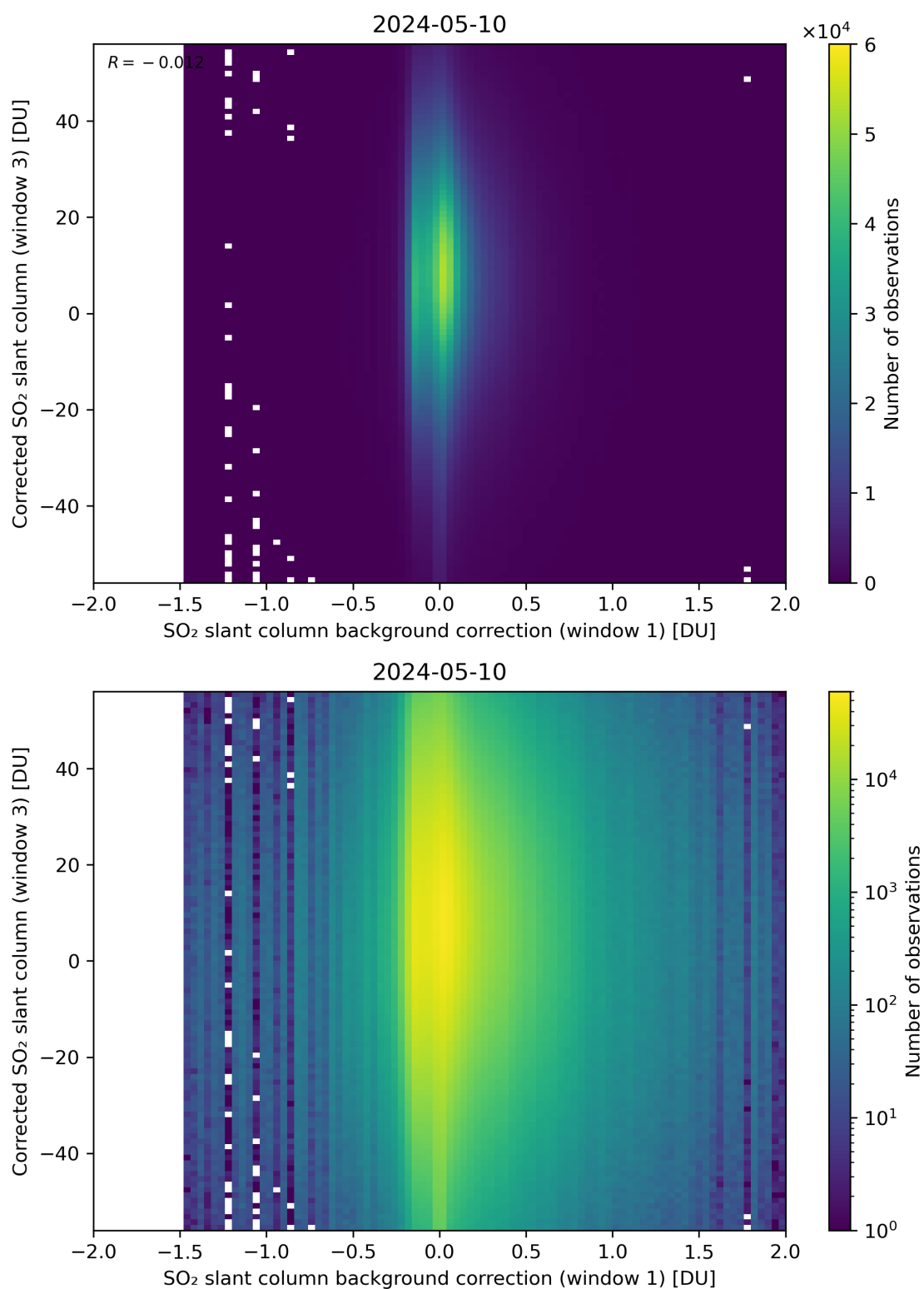
Figure 105: Scatter density plot of “SO 2 slant column background correction (window 1)” against “Corrected SO 2 slant column (window 3)” for 2024-05-09 to 2024-05-11.
