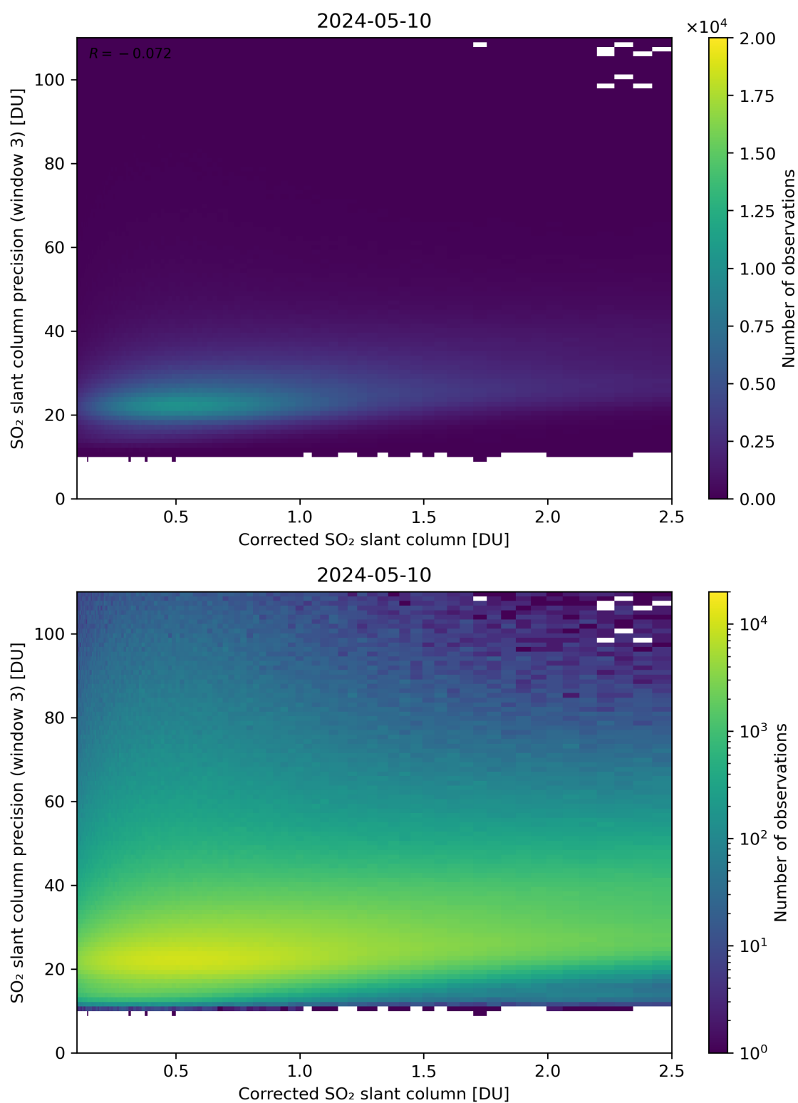
Figure 191: Scatter density plot of “Corrected SO 2 slant column” against “SO 2 slant column precision (window 3)” for 2024-05-09 to 2024-05-11.
