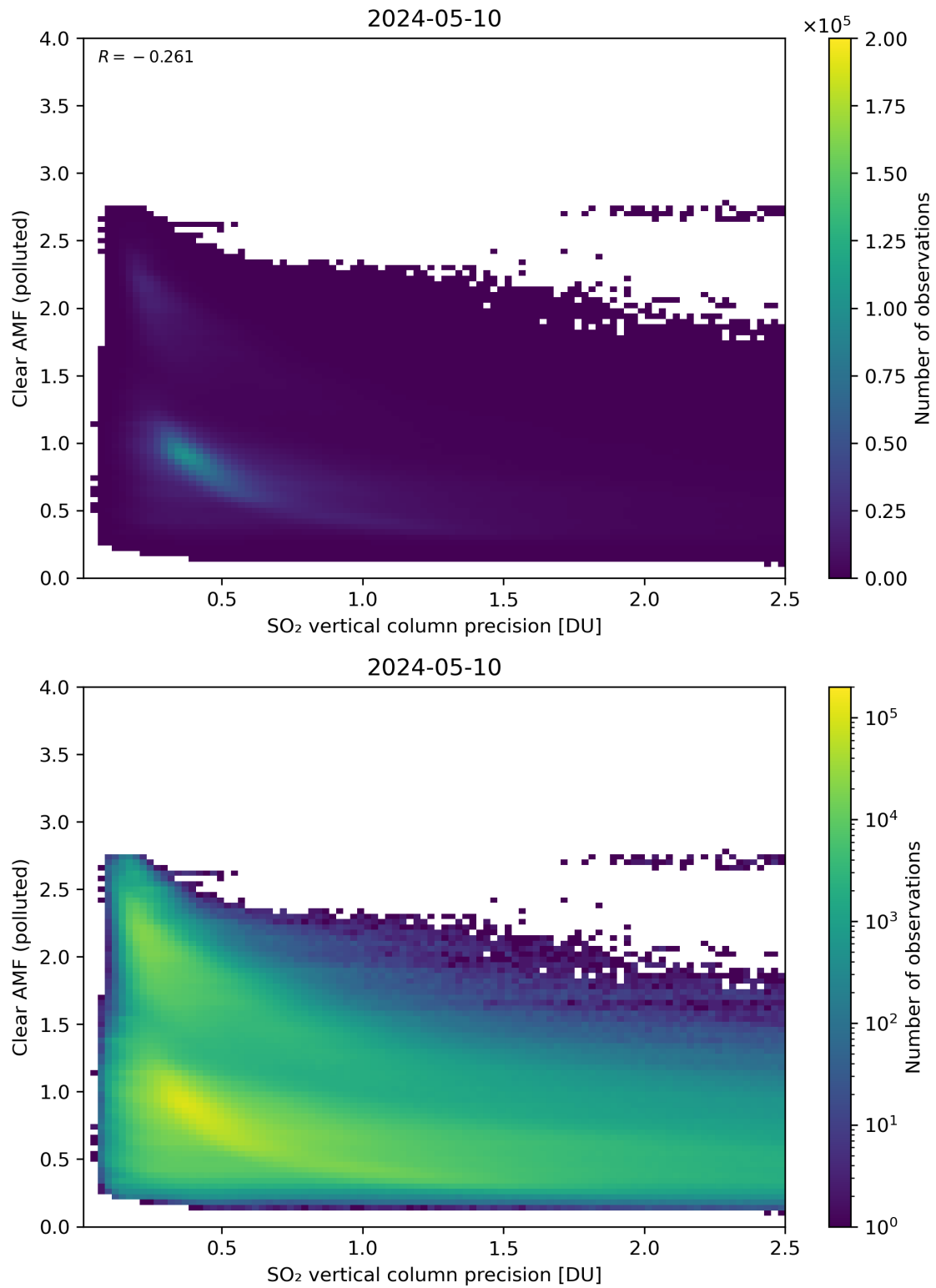
Figure 285: Scatter density plot of “SO 2 vertical column precision” against “Clear AMF (polluted)” for 2024-05-09 to 2024-05-11.
