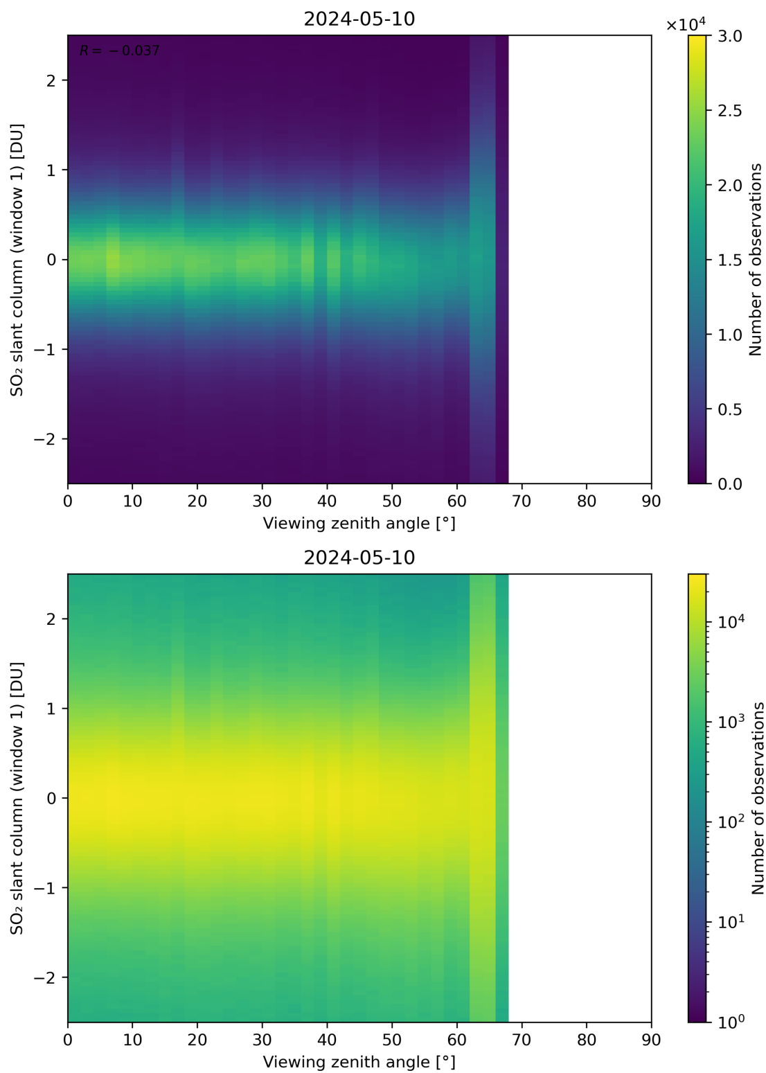
Figure 320: Scatter density plot of “Viewing zenith angle” against “SO 2 slant column (window 1)” for 2024-05-09 to 2024-05-11.
