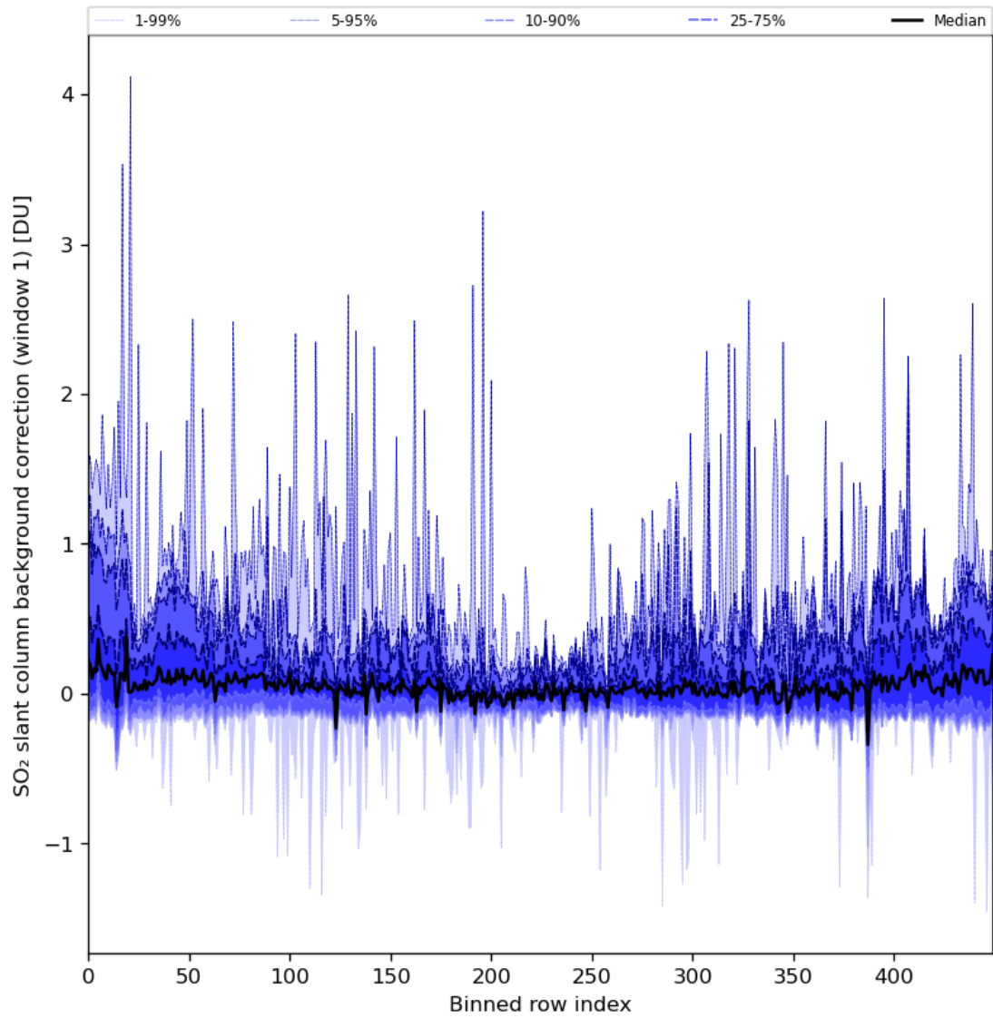
Figure 82: Along track statistics of “SO 2 slant column background correction (window 1)” for 2024-05-09 to 2024-05-11
