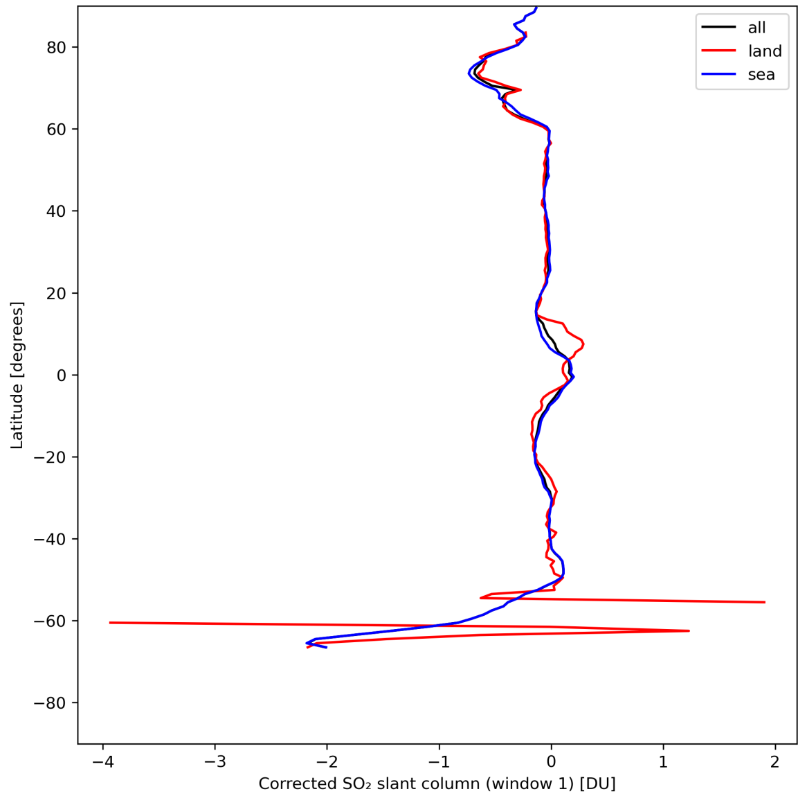
Figure 35: Zonal average of “Corrected SO 2 slant column (window 1)” for 2024-05-09 to 2024-05-11.
