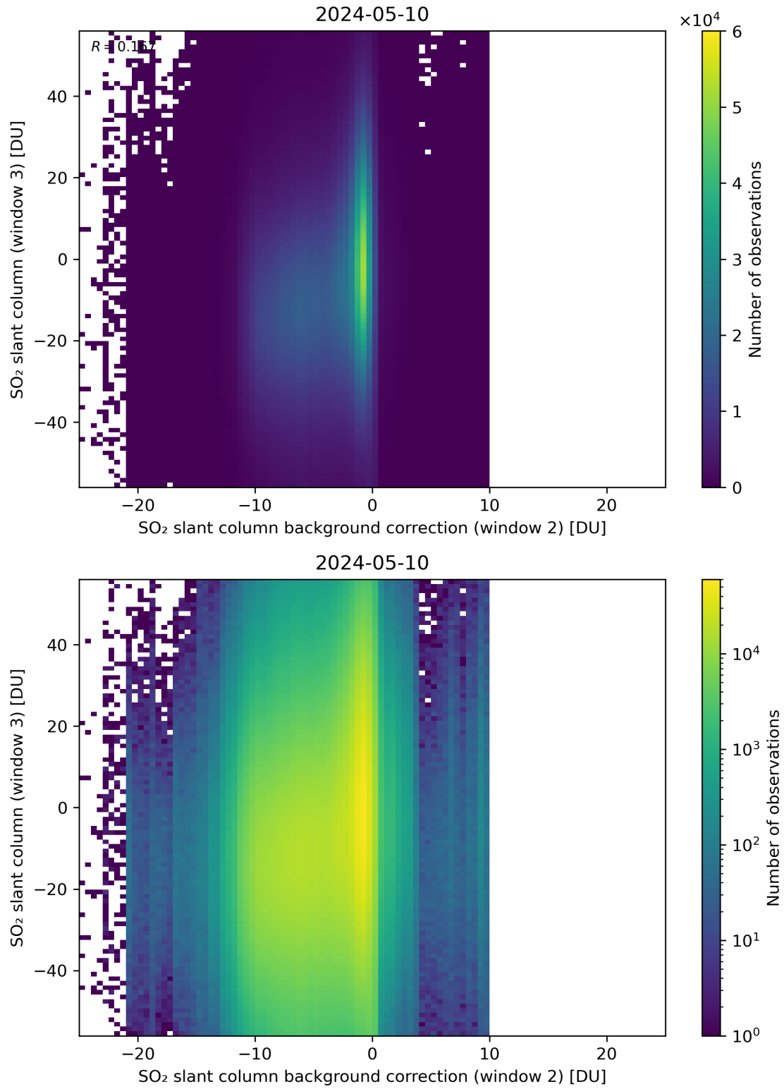
Figure 117: Scatter density plot of “SO 2 slant column background correction (window 2)” against “SO 2 slant column (window 3)” for 2024-05-09 to 2024-05-11.
