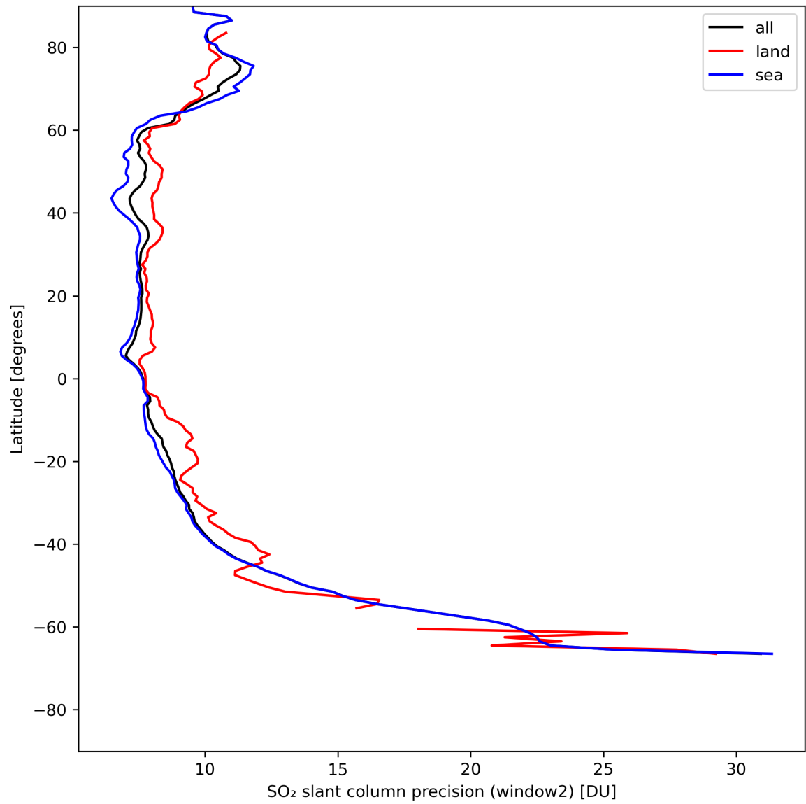
Figure 38: Zonal average of “SO 2 slant column precision (window2)” for 2024-05-09 to 2024-05-11.
