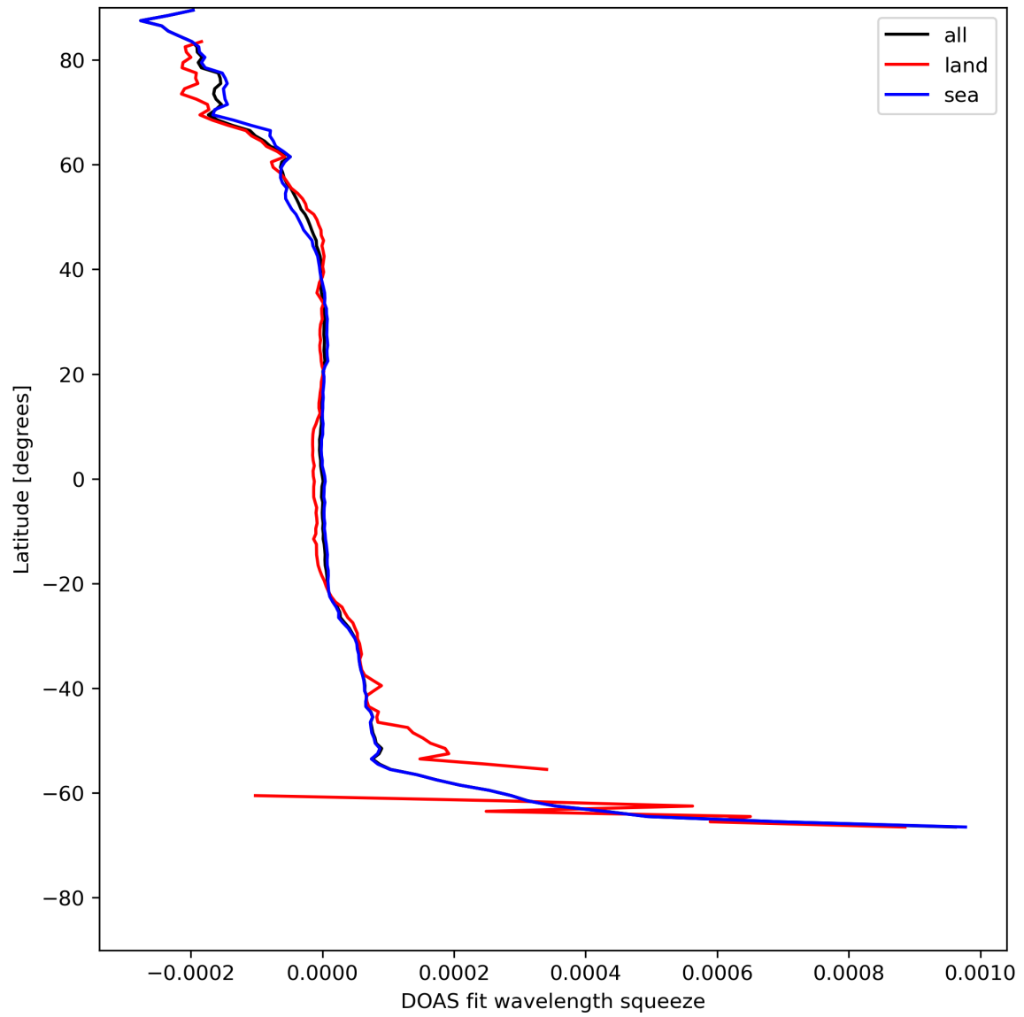
Figure 46: Zonal average of “DOAS fit wavelength squeeze” for 2024-05-09 to 2024-05-11.
