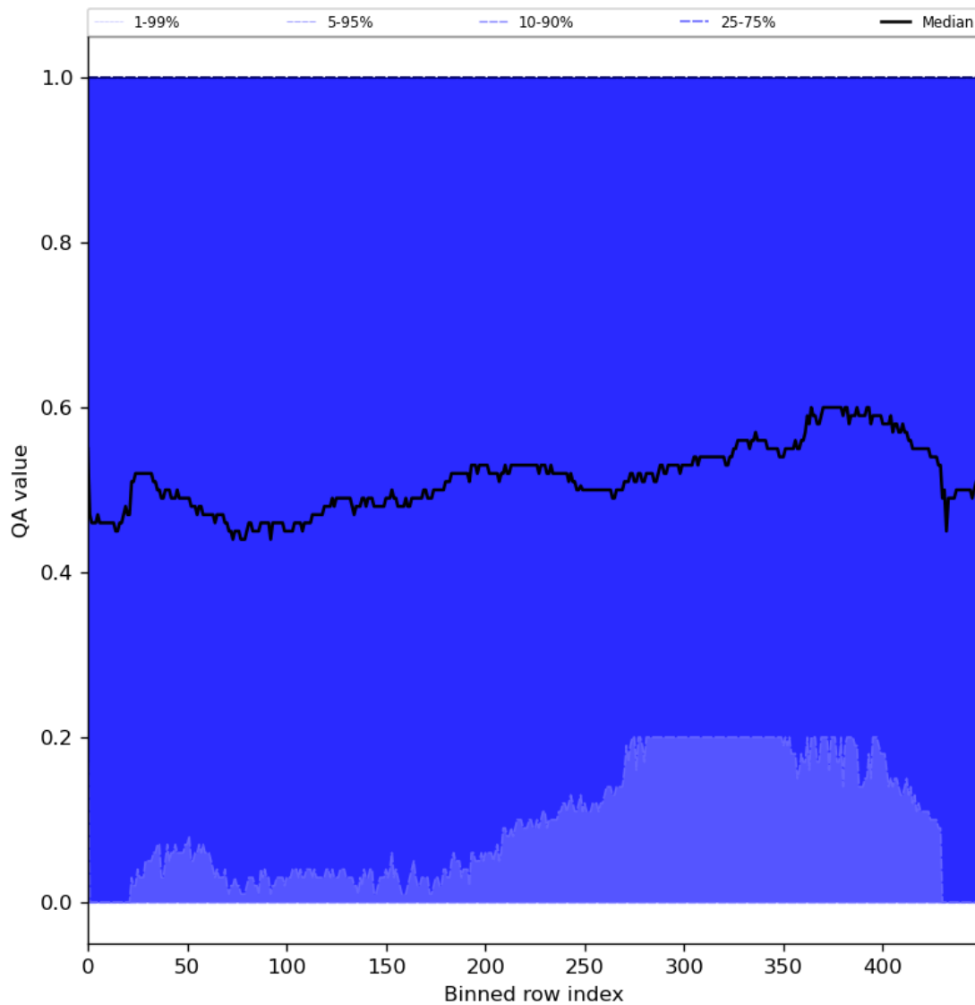
Figure 75: Along track statistics of “QA value” for 2024-05-09 to 2024-05-11
