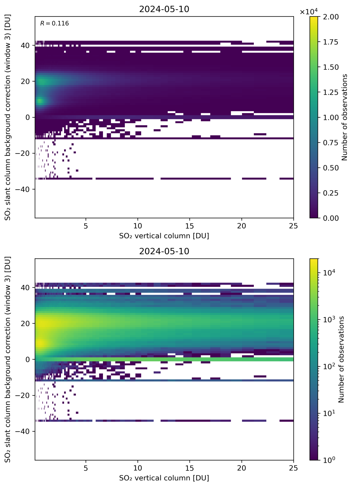
Figure 275: Scatter density plot of “SO 2 vertical column” against “SO 2 slant column background correction (window 3)” for 2024-05-09 to 2024-05-11.
