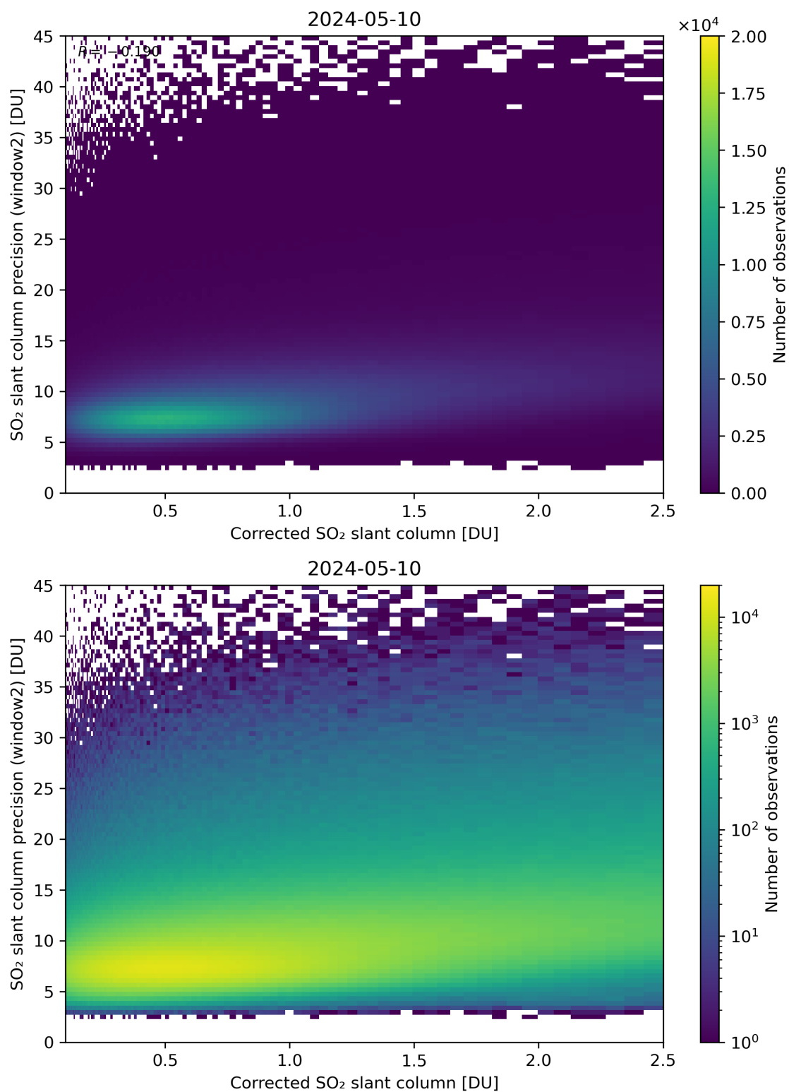
Figure 189: Scatter density plot of “Corrected SO 2 slant column” against “SO 2 slant column precision (window2)” for 2024-05-09 to 2024-05-11.
