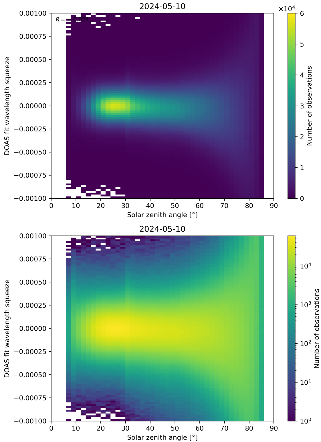
Figure 162: Scatter density plot of “Solar zenith angle” against “DOAS fit wavelength squeeze” for 2024-05-09 to 2024-05-11.
