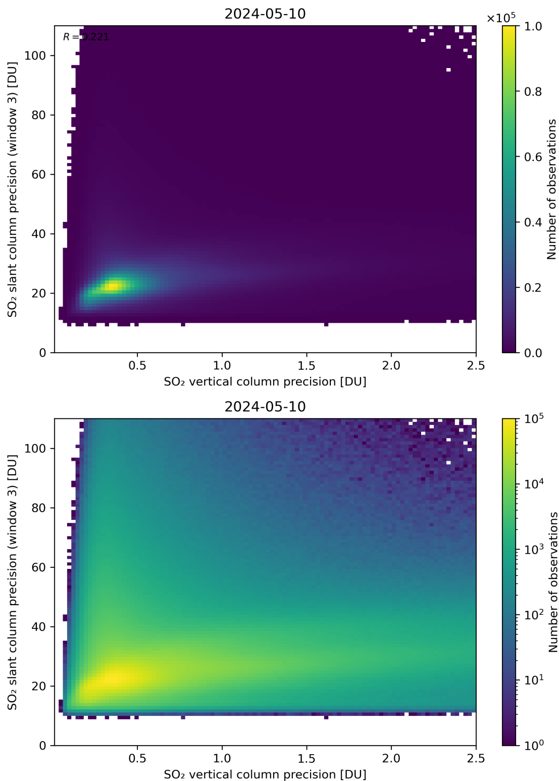
Figure 293: Scatter density plot of “SO 2 vertical column precision” against “SO 2 slant column precision (window 3)” for 2024-05-09 to 2024-05-11.
