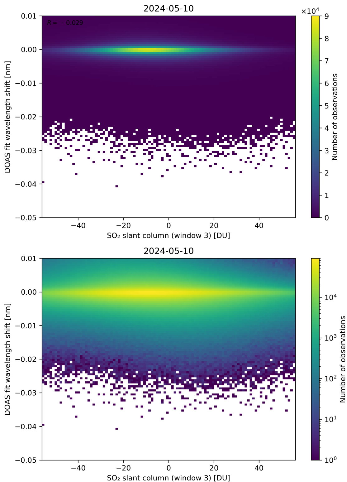
Figure 254: Scatter density plot of “SO 2 slant column (window 3)” against “DOAS fit wavelength shift” for 2024-05-09 to 2024-05-11.
