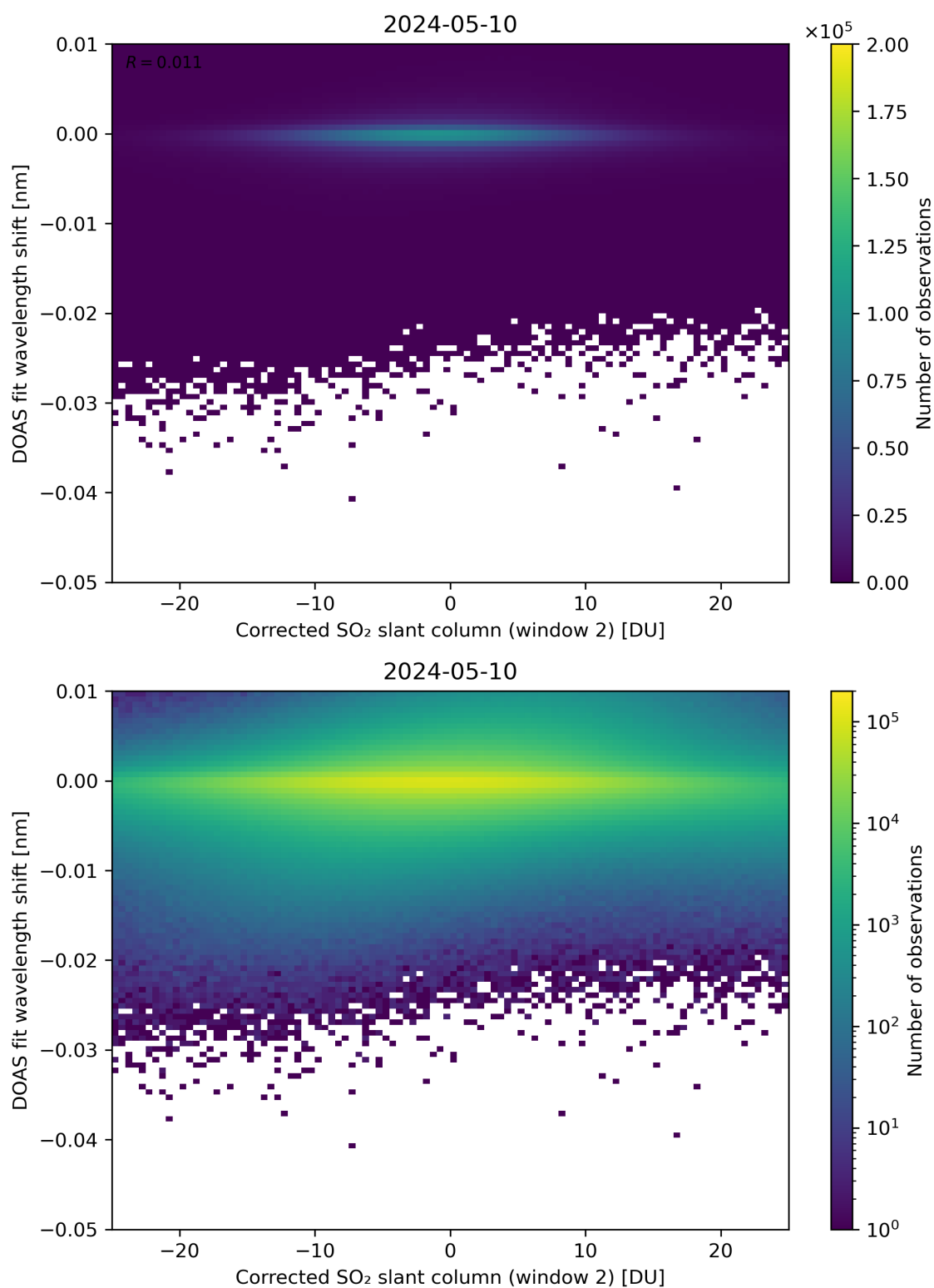
Figure 196: Scatter density plot of “Corrected SO 2 slant column (window 2)” against “DOAS fit wavelength shift” for 2024-05-09 to 2024-05-11.
