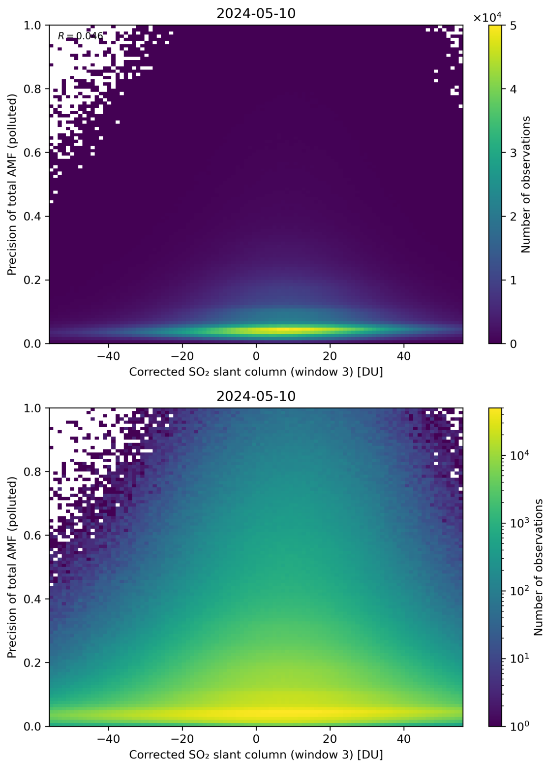
Figure 211: Scatter density plot of “Corrected SO 2 slant column (window 3)” against “Precision of total AMF (polluted)” for 2024-05-09 to 2024-05-11.
