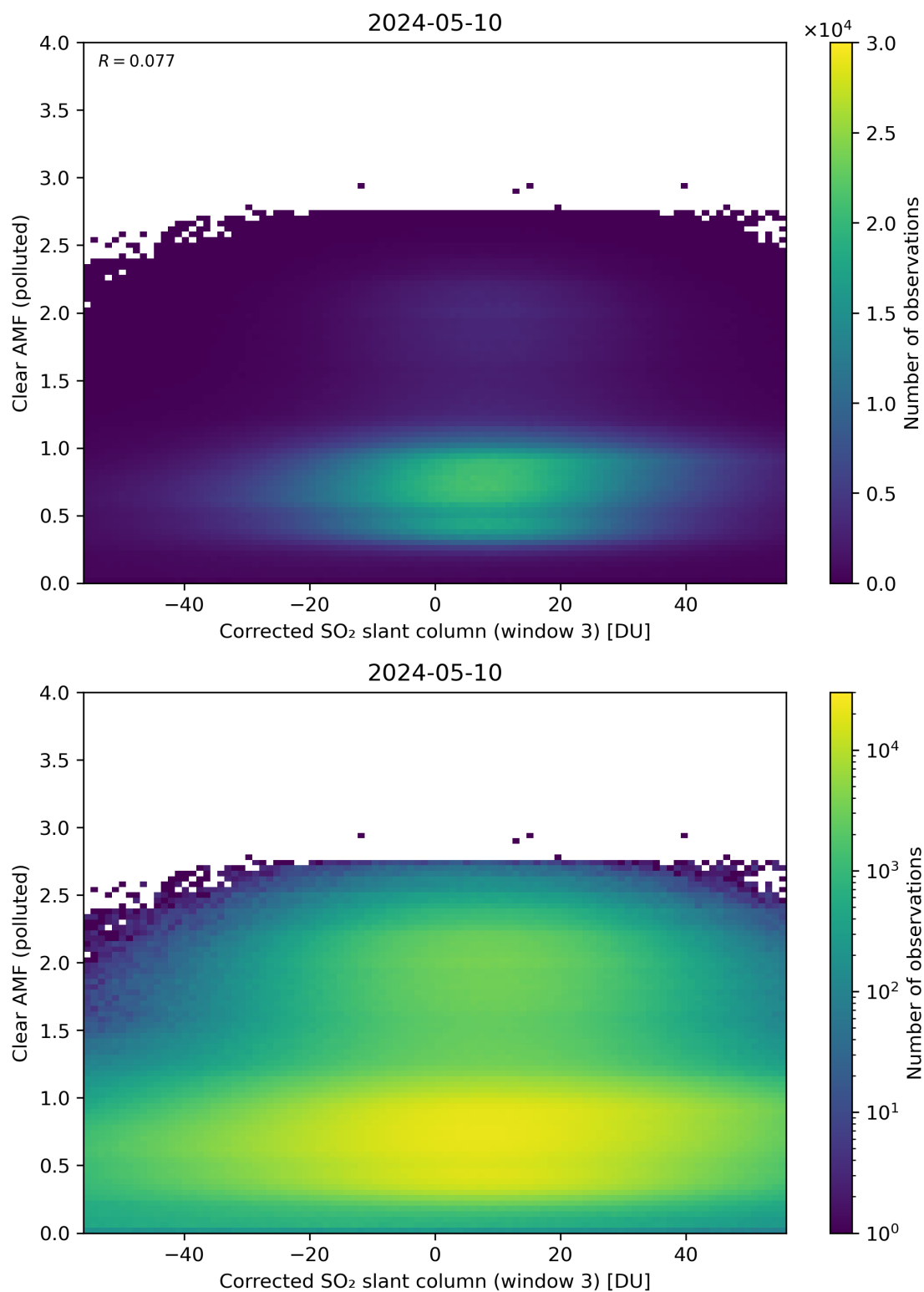
Figure 209: Scatter density plot of “Corrected SO 2 slant column (window 3)” against “Clear AMF (polluted)” for 2024-05-09 to 2024-05-11.
