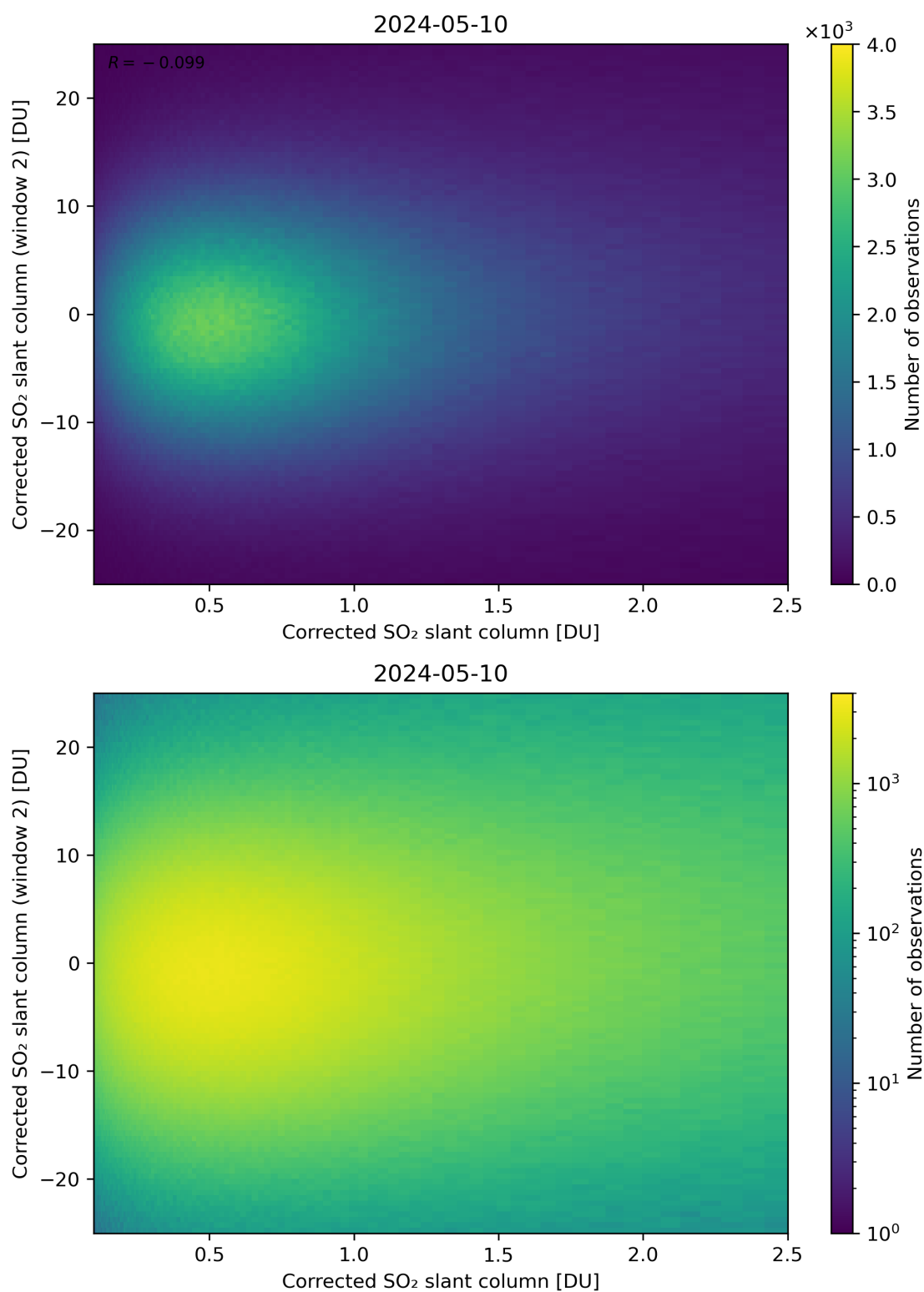
Figure 185: Scatter density plot of “Corrected SO 2 slant column” against “Corrected SO 2 slant column (window 2)” for 2024-05-09 to 2024-05-11.
