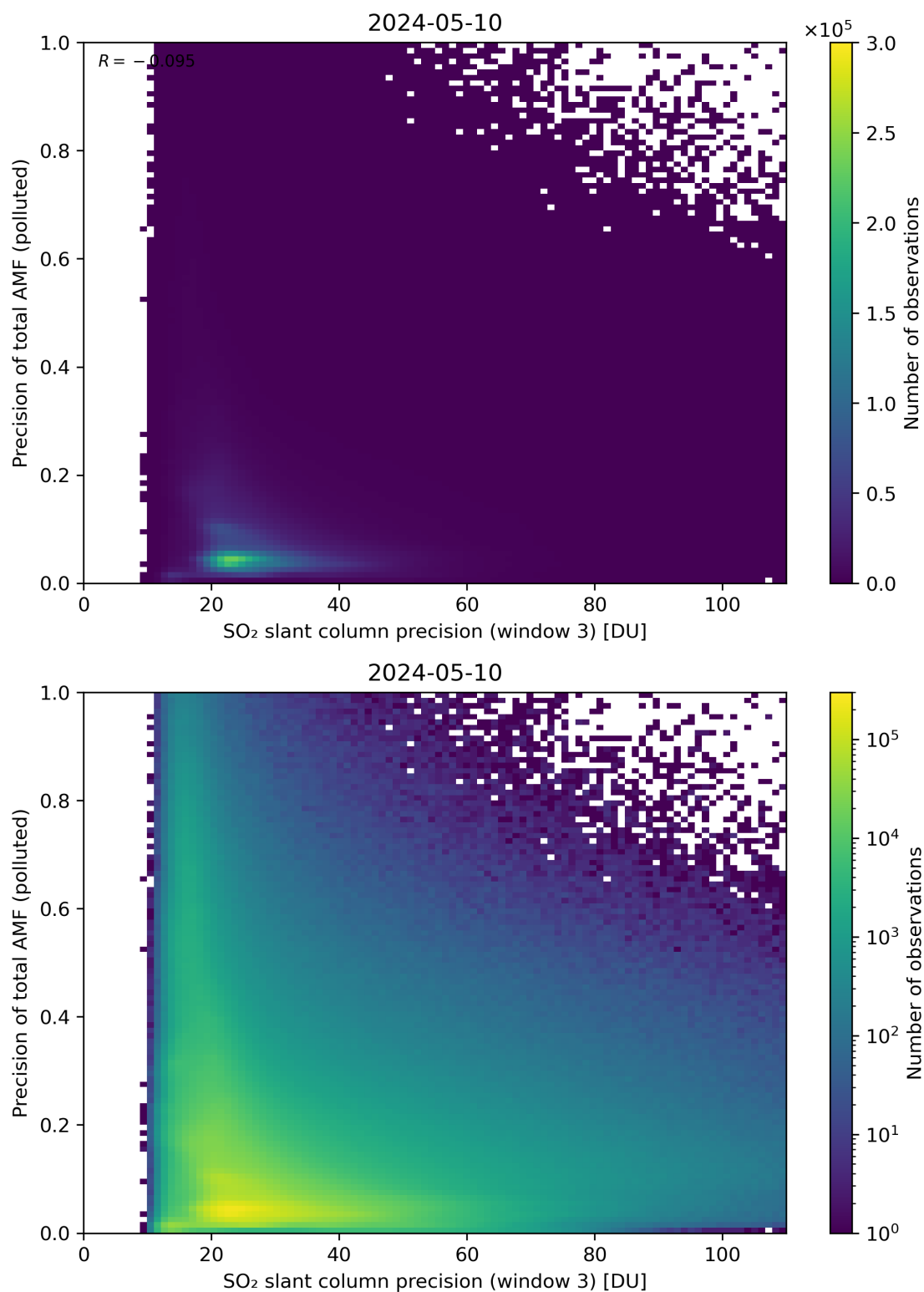
Figure 264: Scatter density plot of “SO 2 slant column precision (window 3)” against “Precision of total AMF (polluted)” for 2024-05-09 to 2024-05-11.
