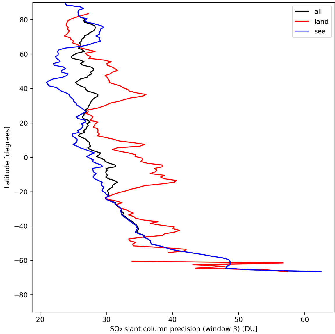
Figure 42: Zonal average of “SO 2 slant column precision (window 3)” for 2024-05-09 to 2024-05-11.
