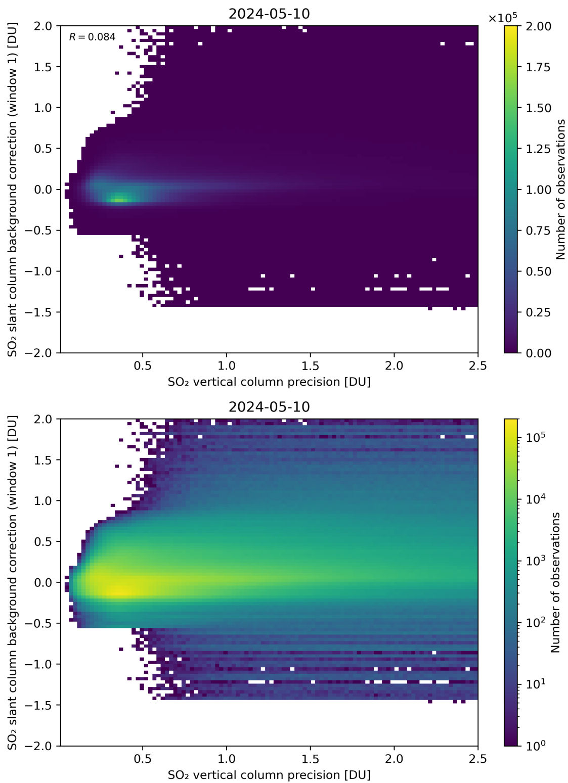
Figure 279: Scatter density plot of “SO 2 vertical column precision” against “SO 2 slant column background correction (window 1)” for 2024-05-09 to 2024-05-11.
