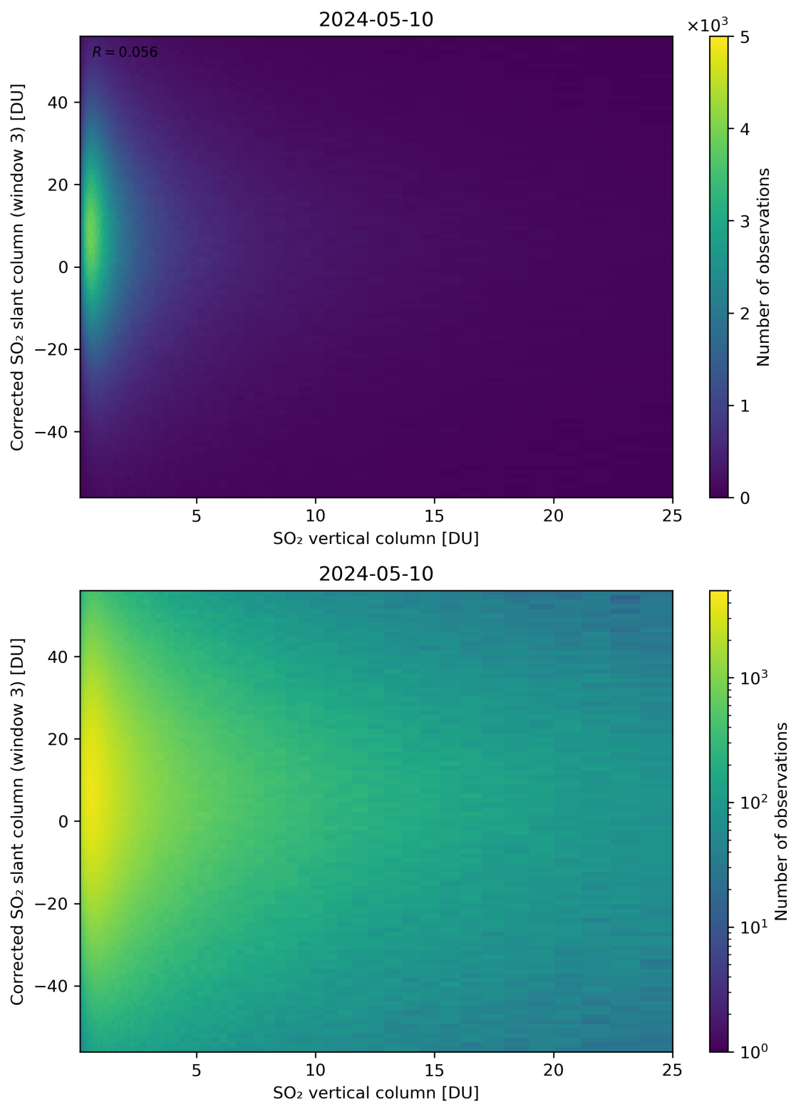
Figure 299: Scatter density plot of “SO 2 vertical column” against “Corrected SO 2 slant column (window 3)” for 2024-05-09 to 2024-05-11.
