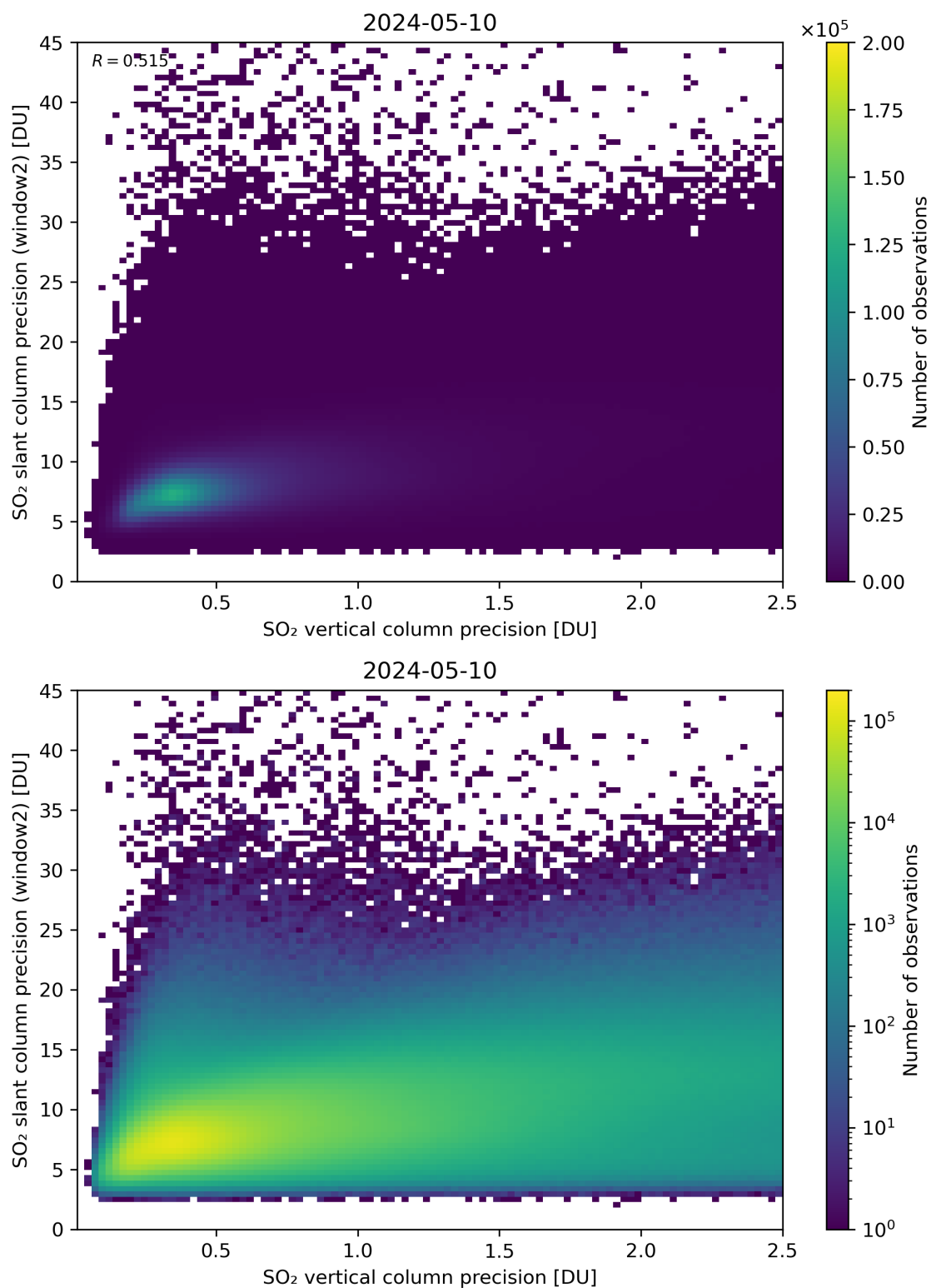
Figure 291: Scatter density plot of “SO 2 vertical column precision” against “SO 2 slant column precision (window2)” for 2024-05-09 to 2024-05-11.
