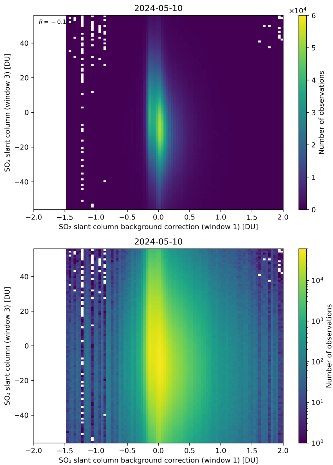
Figure 107: Scatter density plot of “SO 2 slant column background correction (window 1)” against “SO 2 slant column (window 3)” for 2024-05-09 to 2024-05-11.
