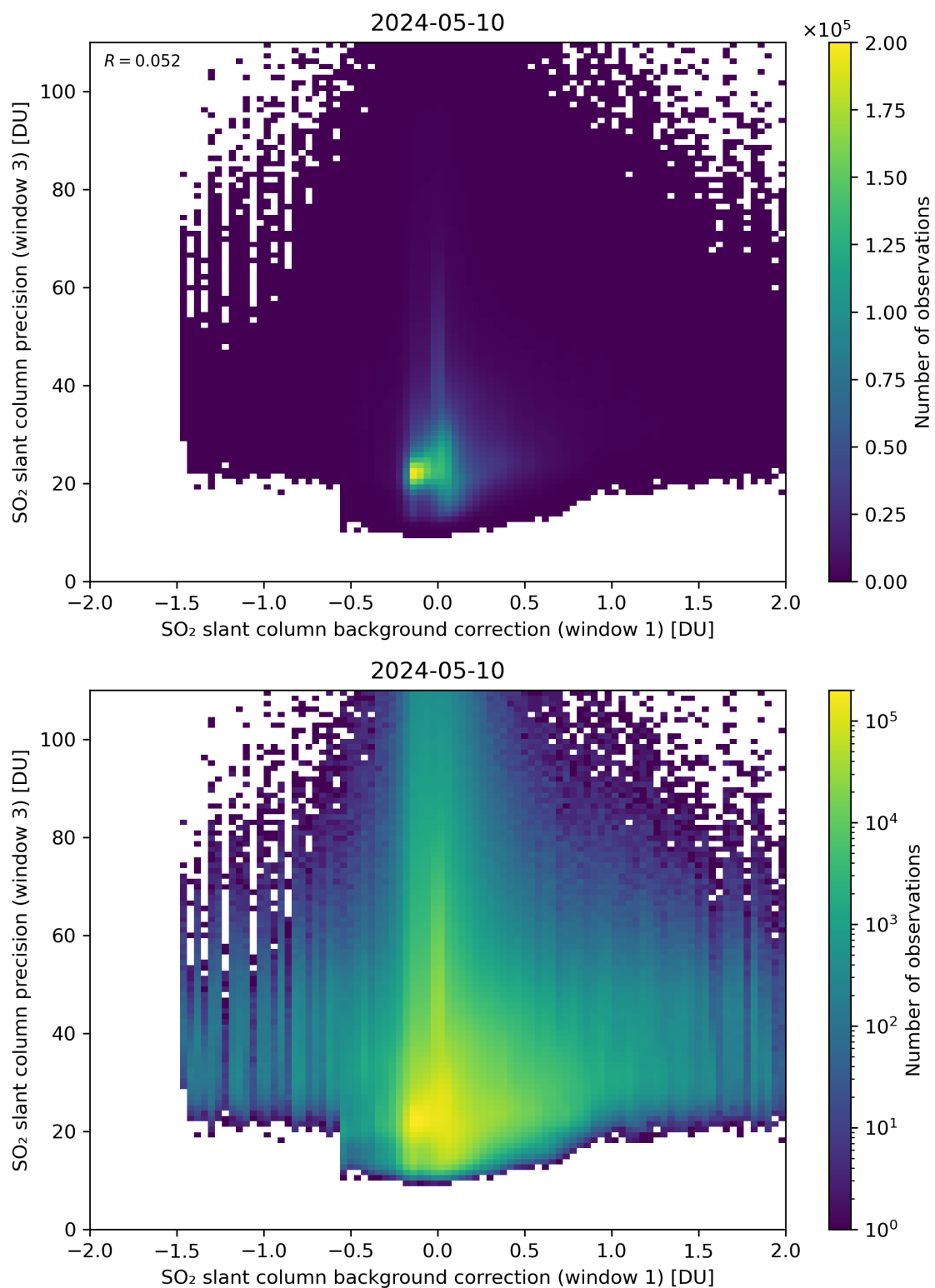
Figure 108: Scatter density plot of “SO 2 slant column background correction (window 1)” against “SO 2 slant column precision (window 3)” for 2024-05-09 to 2024-05-11.
