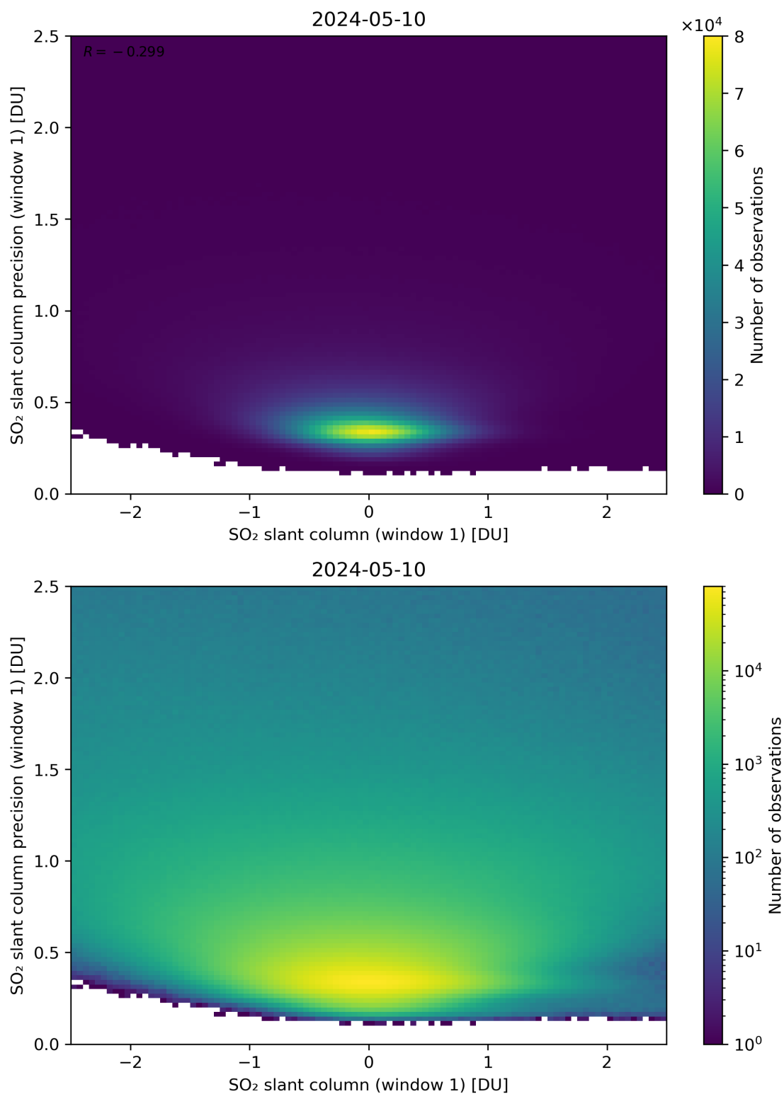
Figure 235: Scatter density plot of “SO 2 slant column (window 1)” against “SO 2 slant column precision (window 1)” for 2024-05-09 to 2024-05-11.
