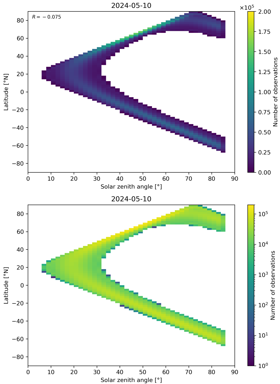
Figure 164: Scatter density plot of “Solar zenith angle” against “Latitude” for 2024-05-09 to 2024-05-11.
