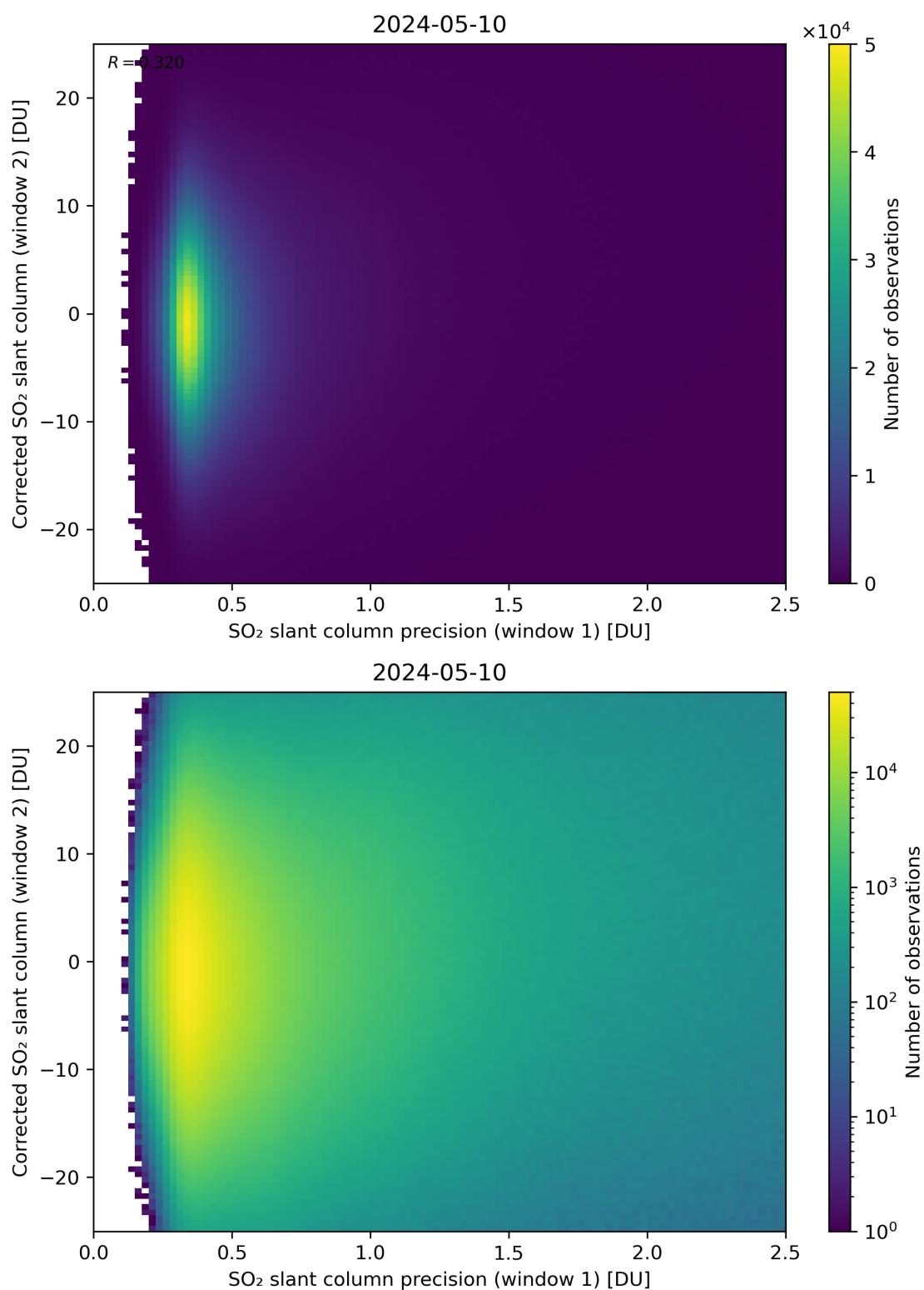
Figure 225: Scatter density plot of “SO 2 slant column precision (window 1)” against “Corrected SO 2 slant column (window 2)” for 2024-05-09 to 2024-05-11.
