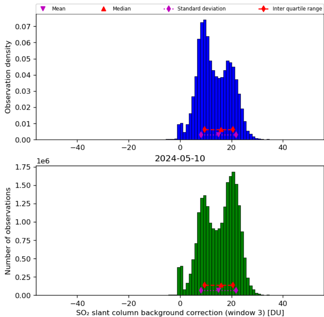
Figure 67: Histogram of “SO 2 slant column background correction (window 3)” for 2024-05-09 to 2024-05-11
