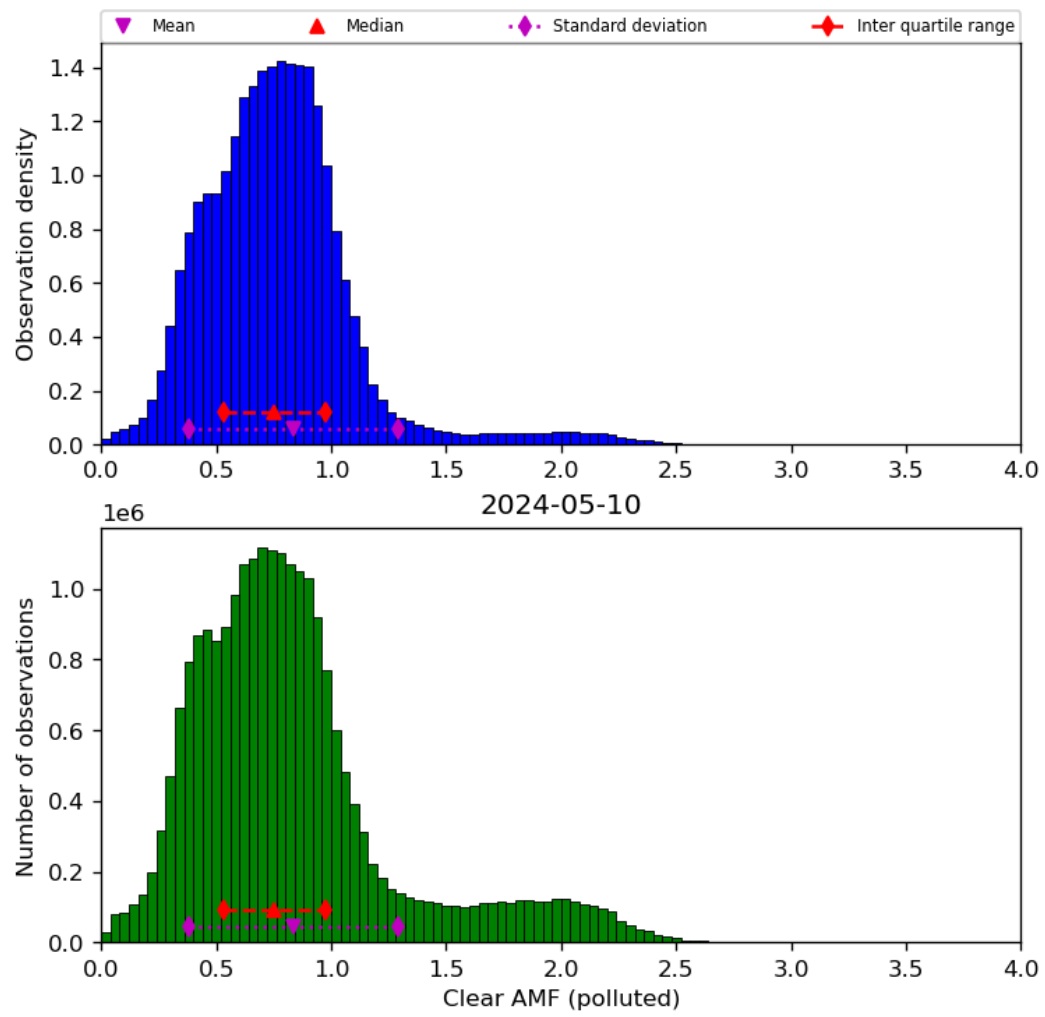
Figure 73: Histogram of “Clear AMF (polluted)” for 2024-05-09 to 2024-05-11
