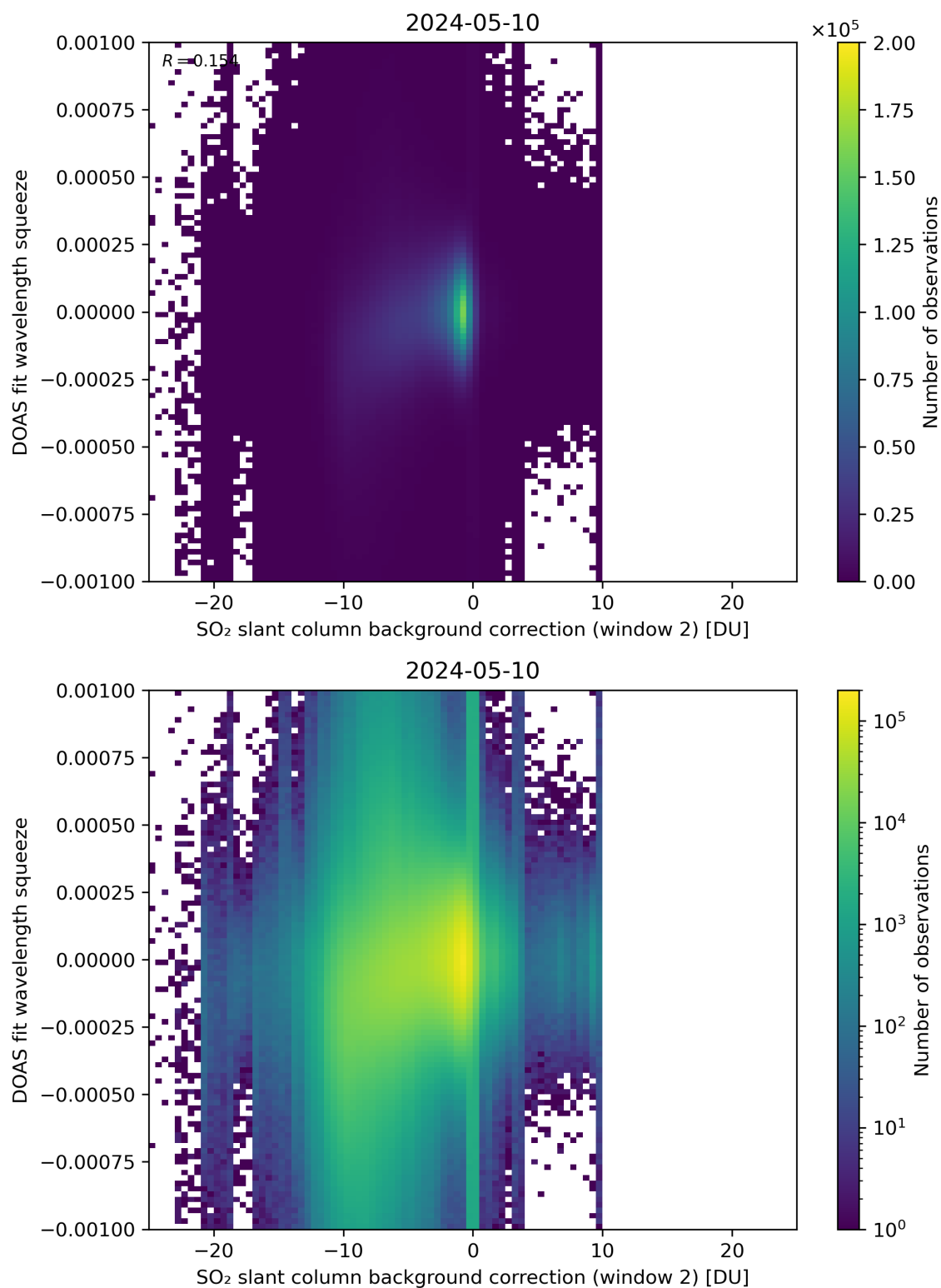
Figure 113: Scatter density plot of “SO 2 slant column background correction (window 2)” against “DOAS fit wavelength squeeze” for 2024-05-09 to 2024-05-11.
