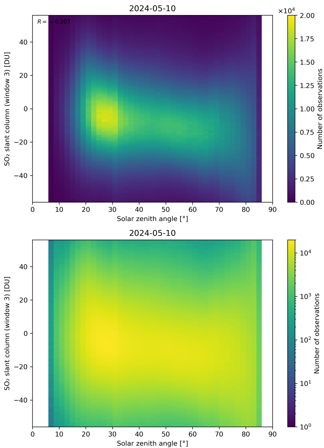
Figure 172: Scatter density plot of “Solar zenith angle” against “SO 2 slant column (window 3)” for 2024-05-09 to 2024-05-11.
