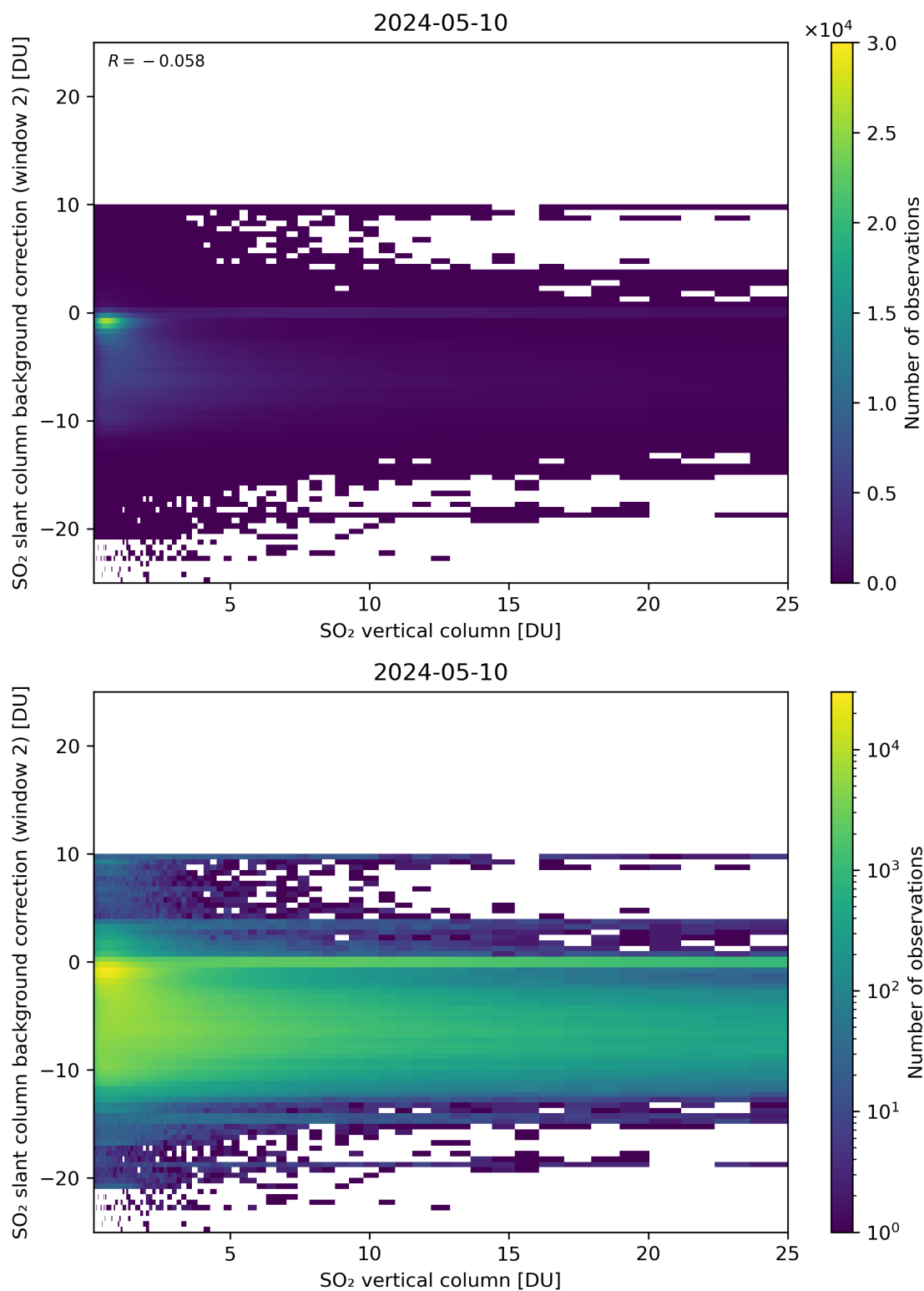
Figure 274: Scatter density plot of “SO 2 vertical column” against “SO 2 slant column background correction (window 2)” for 2024-05-09 to 2024-05-11.
