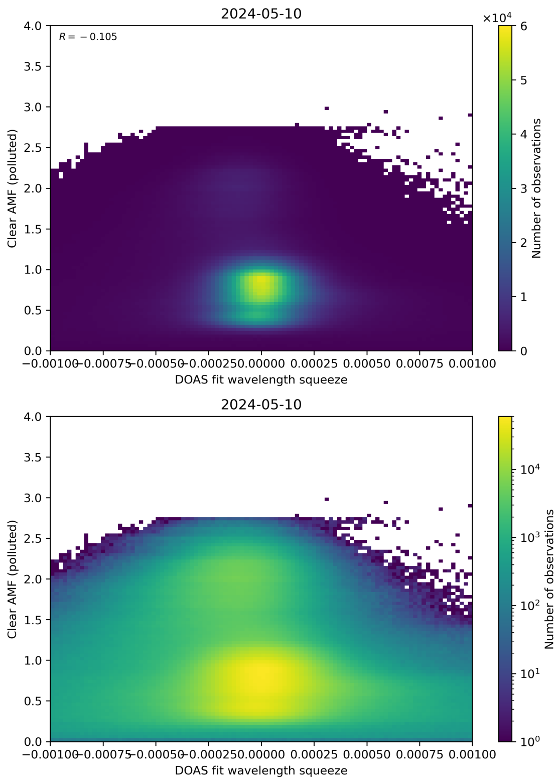
Figure 133: Scatter density plot of “DOAS fit wavelength squeeze” against “Clear AMF (polluted)” for 2024-05-09 to 2024-05-11.
