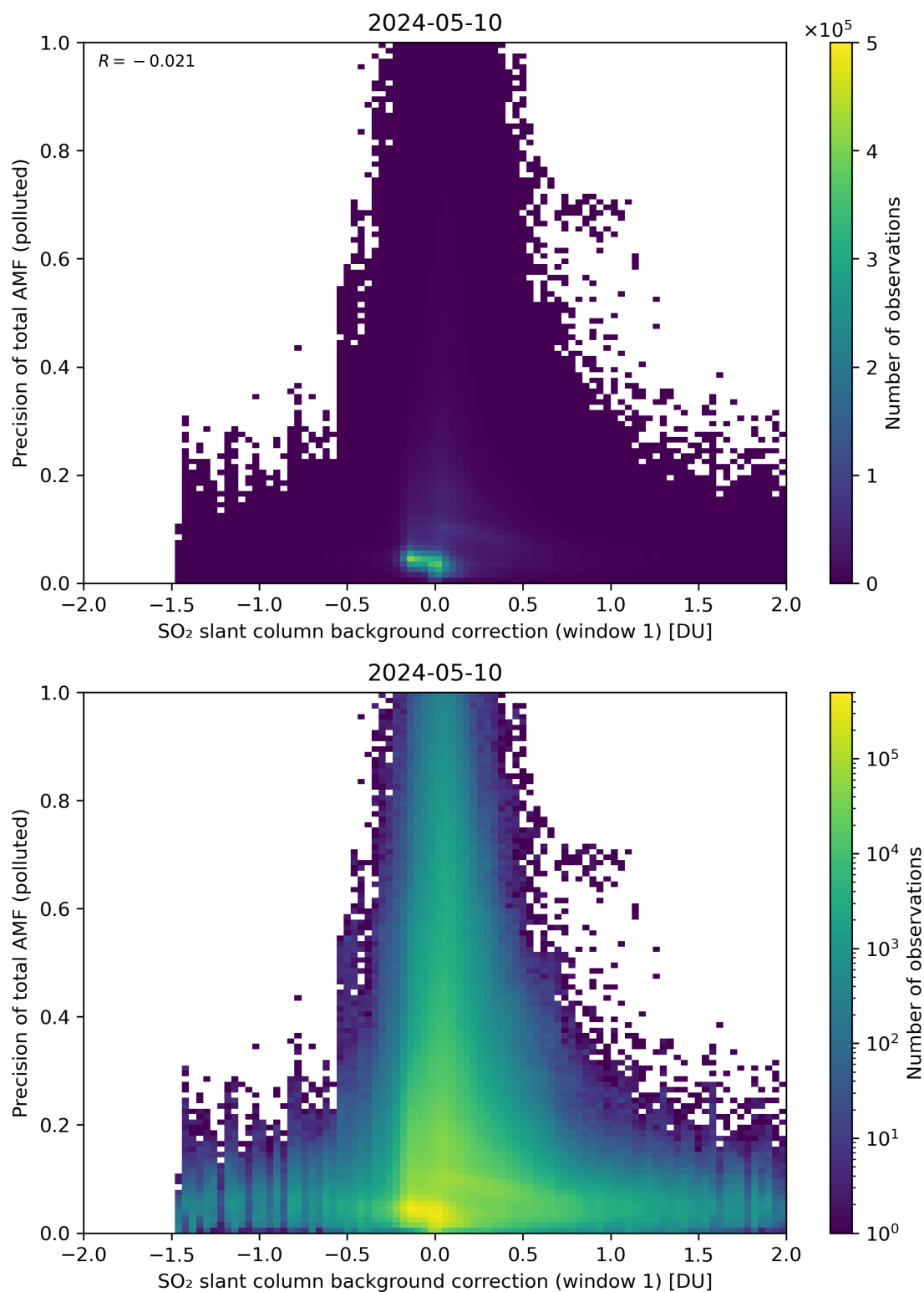
Figure 110: Scatter density plot of “SO 2 slant column background correction (window 1)” against “Precision of total AMF (polluted)” for 2024-05-09 to 2024-05-11.
