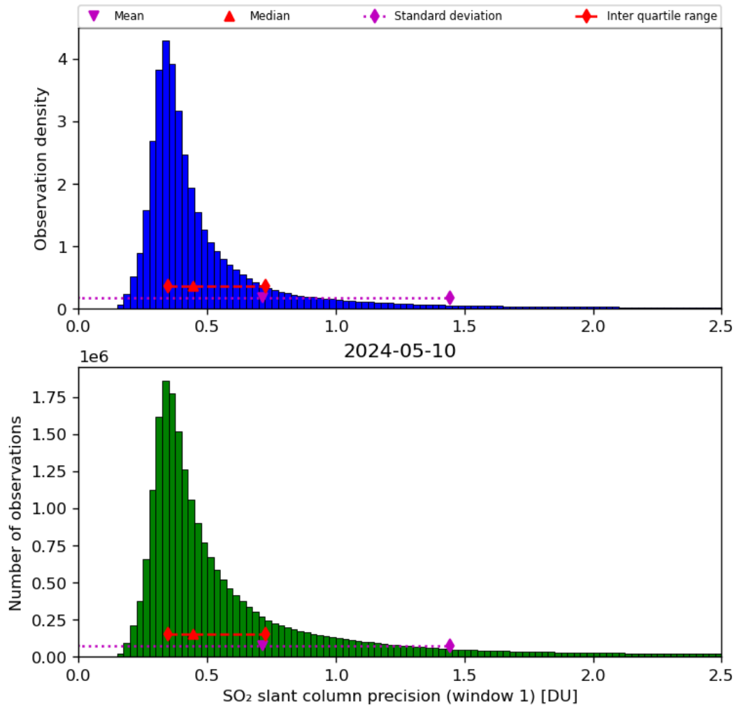
Figure 57: Histogram of “SO 2 slant column precision (window 1)” for 2024-05-09 to 2024-05-11
