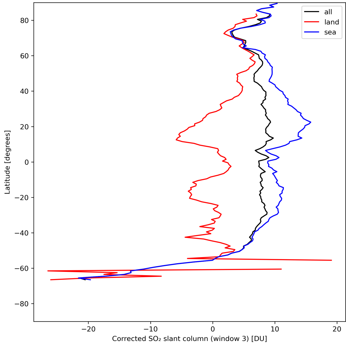
Figure 43: Zonal average of “Corrected SO 2 slant column (window 3)” for 2024-05-09 to 2024-05-11.
