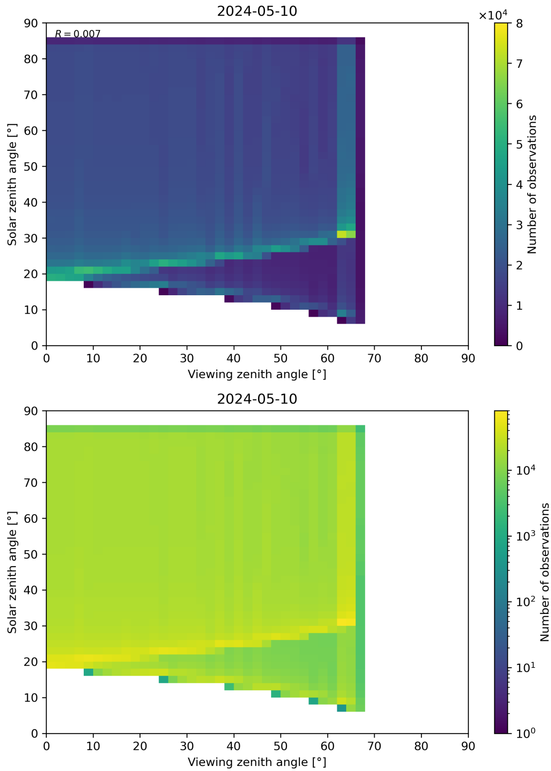
Figure 315: Scatter density plot of “Viewing zenith angle” against “Solar zenith angle” for 2024-05-09 to 2024-05-11.
