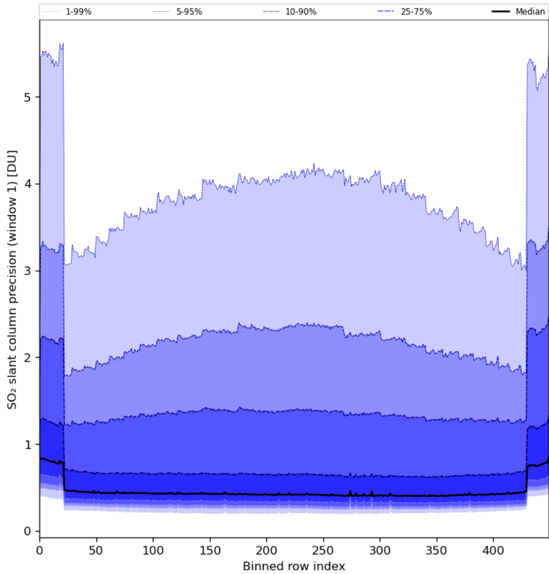
Figure 80: Along track statistics of “SO 2 slant column precision (window 1)” for 2024-05-09 to 2024-05-11
