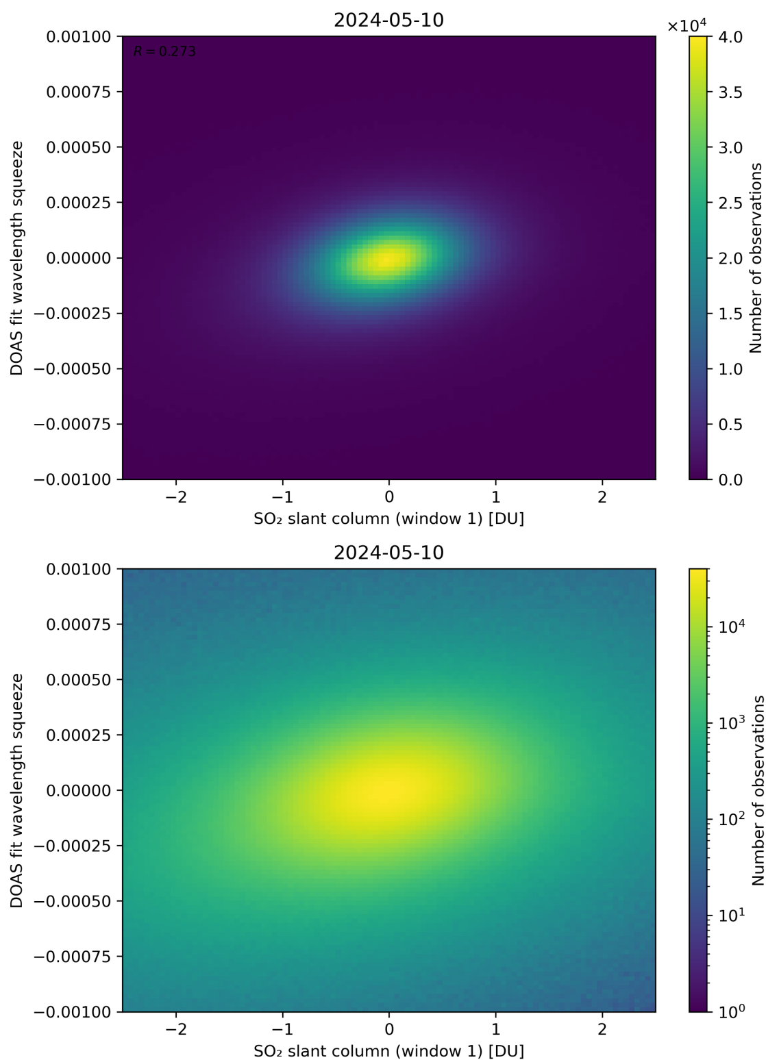
Figure 216: Scatter density plot of “SO 2 slant column (window 1)” against “DOAS fit wavelength squeeze” for 2024-05-09 to 2024-05-11.
