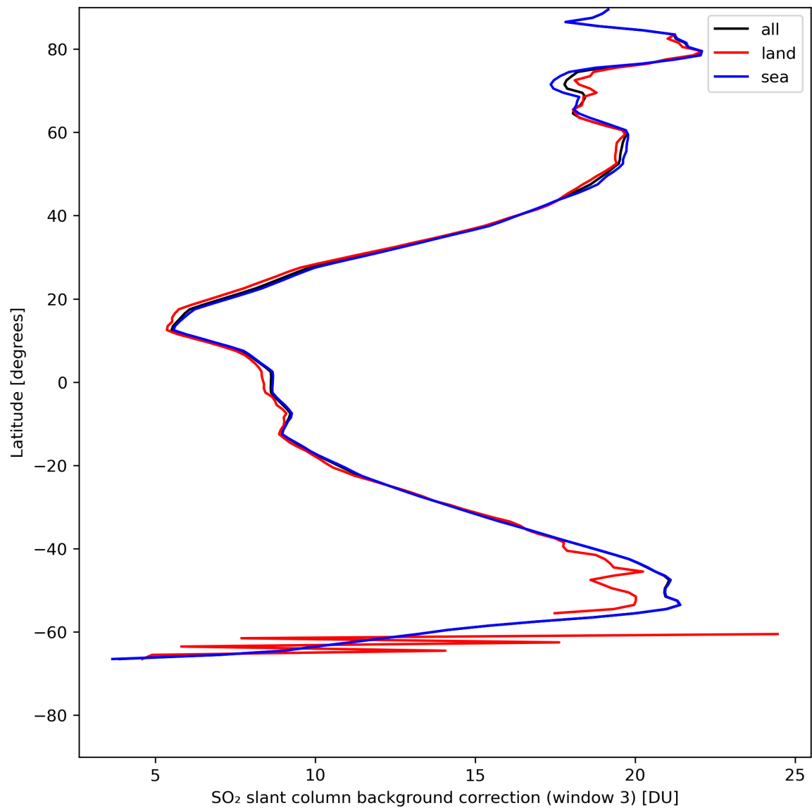
Figure 44: Zonal average of “SO 2 slant column background correction (window 3)” for 2024-05-09 to 2024-05-11.
