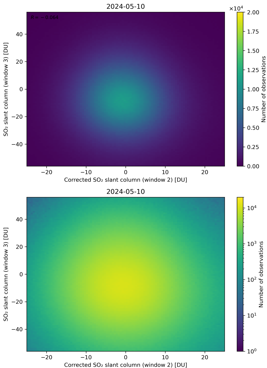
Figure 201: Scatter density plot of “Corrected SO 2 slant column (window 2)” against “SO 2 slant column (window 3)” for 2024-05-09 to 2024-05-11.
