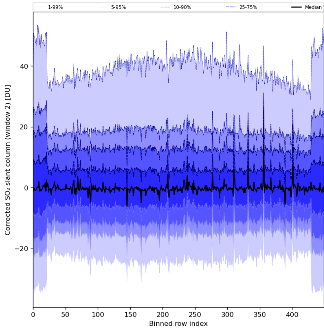
Figure 85: Along track statistics of “Corrected SO 2 slant column (window 2)” for 2024-05-09 to 2024-05-11
