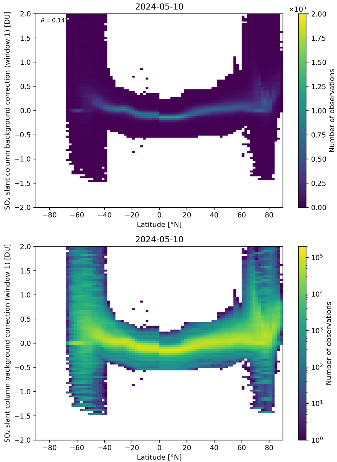
Figure 139: Scatter density plot of “Latitude” against “SO 2 slant column background correction (window 1)” for 2024-05-09 to 2024-05-11.
