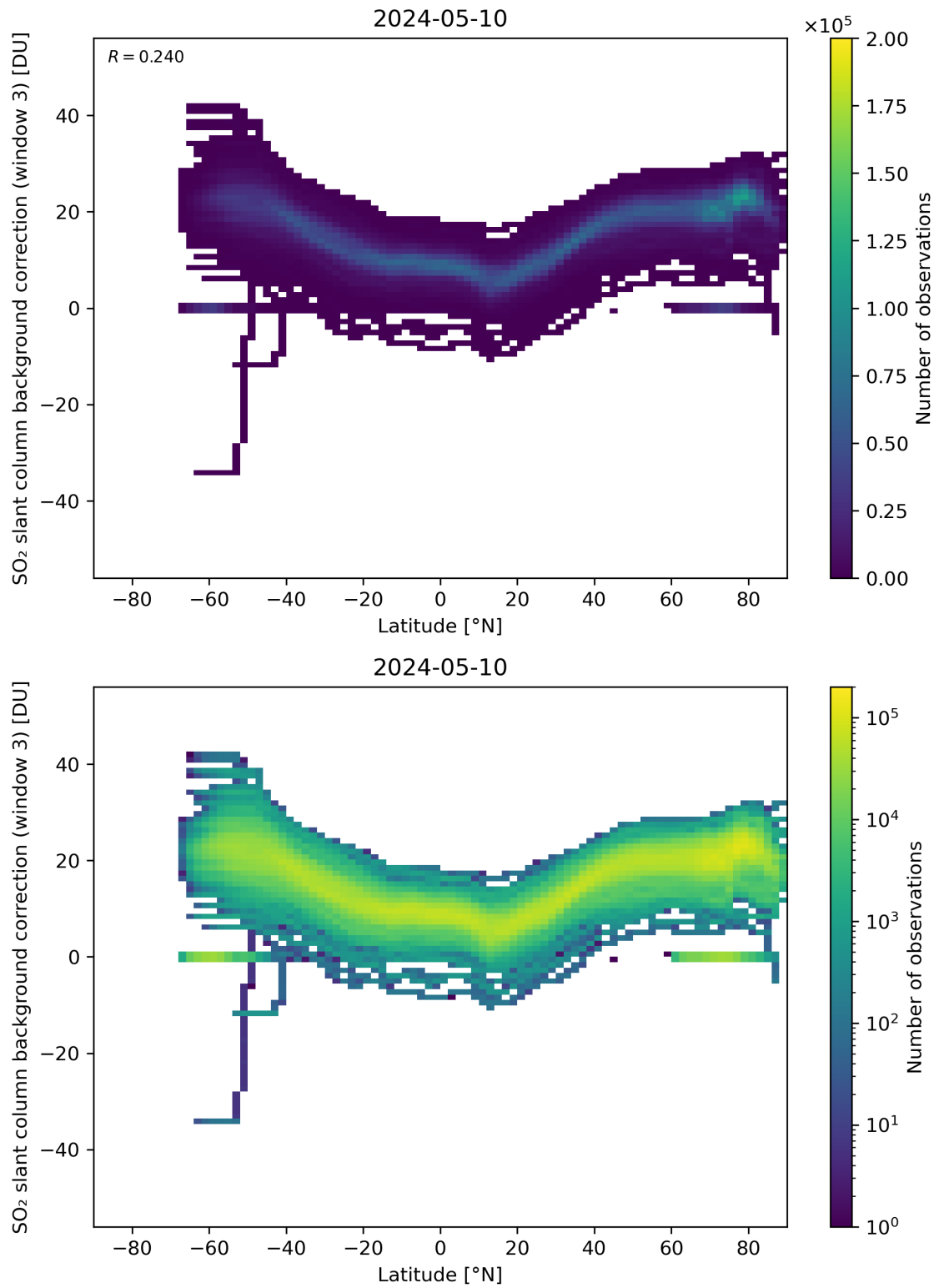
Figure 141: Scatter density plot of “Latitude” against “SO 2 slant column background correction (window 3)” for 2024-05-09 to 2024-05-11.
