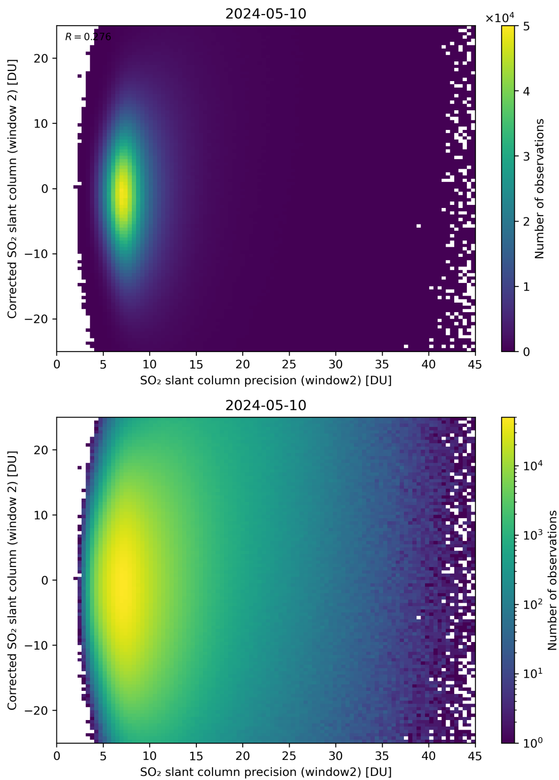
Figure 247: Scatter density plot of “SO 2 slant column precision (window2)” against “Corrected SO 2 slant column (window 2)” for 2024-05-09 to 2024-05-11.
