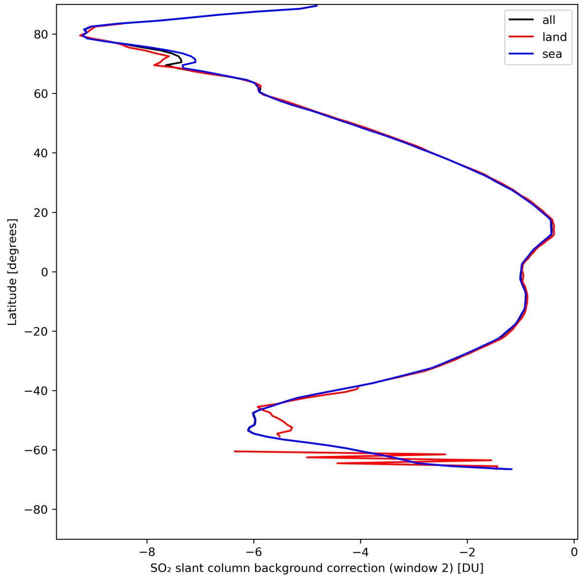
Figure 40: Zonal average of “SO 2 slant column background correction (window 2)” for 2024-05-09 to 2024-05-11.
