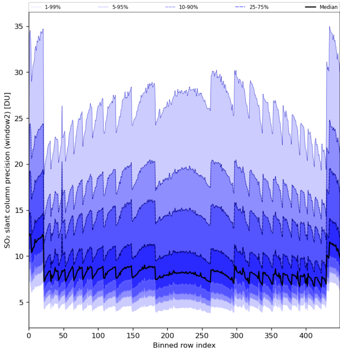
Figure 84: Along track statistics of “SO 2 slant column precision (window2)” for 2024-05-09 to 2024-05-11
