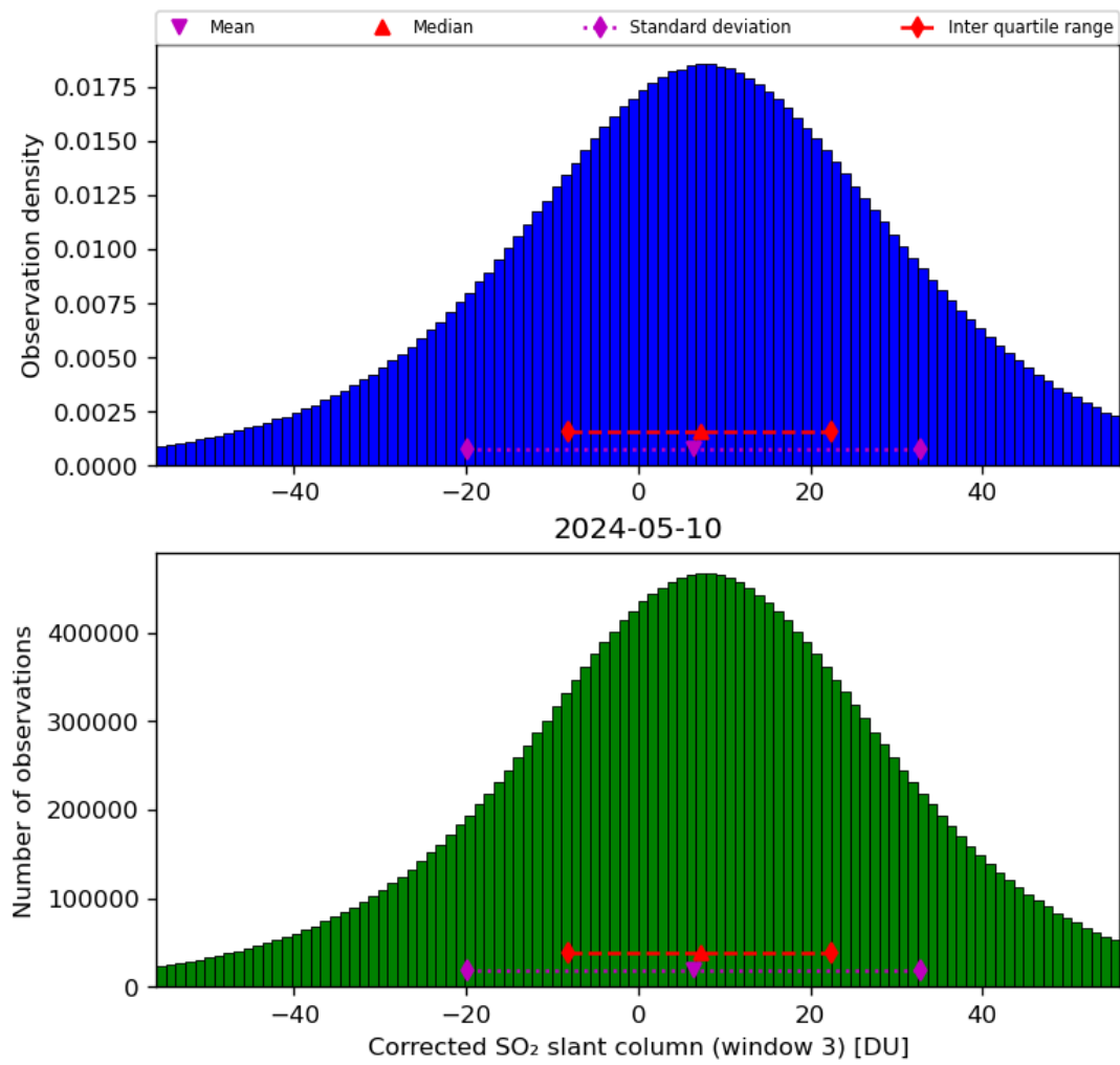
Figure 66: Histogram of “Corrected SO 2 slant column (window 3)” for 2024-05-09 to 2024-05-11
