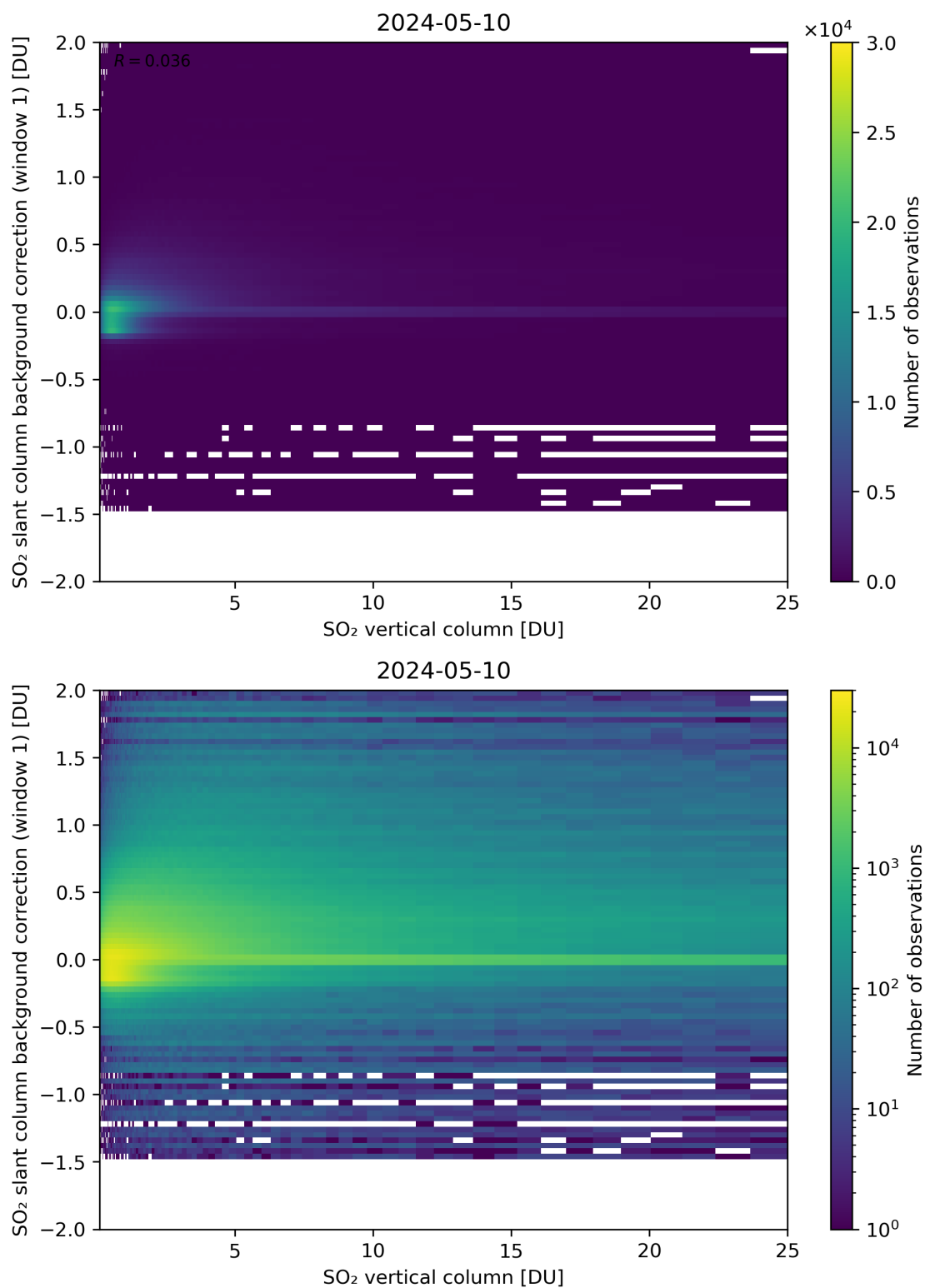
Figure 273: Scatter density plot of “SO 2 vertical column” against “SO 2 slant column background correction (window 1)” for 2024-05-09 to 2024-05-11.
