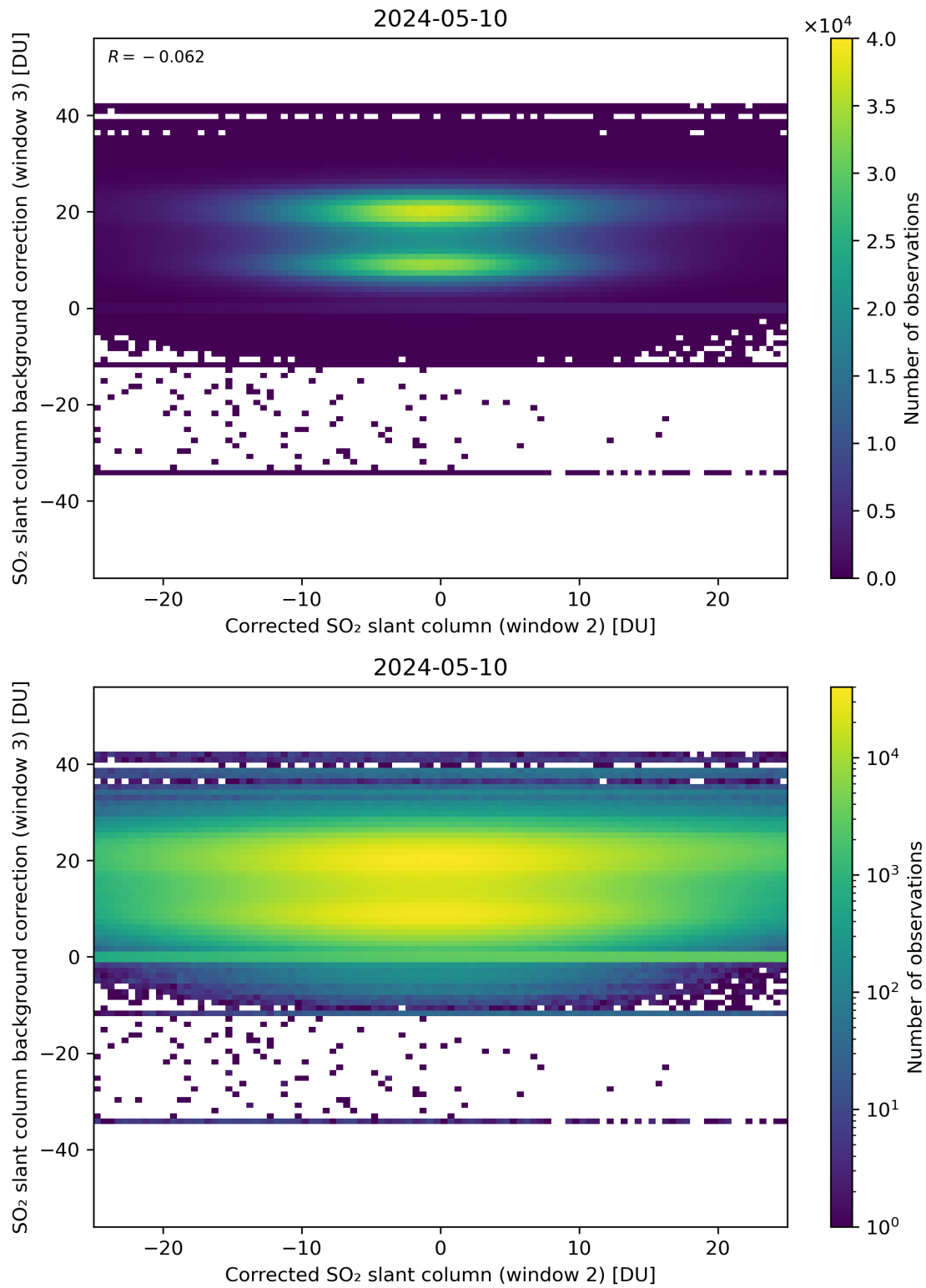
Figure 195: Scatter density plot of “Corrected SO 2 slant column (window 2)” against “SO 2 slant column background correction (window 3)” for 2024-05-09 to 2024-05-11.
