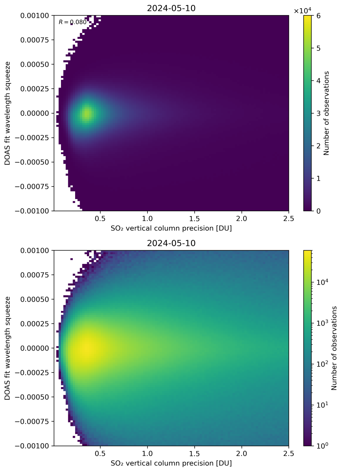
Figure 283: Scatter density plot of “SO 2 vertical column precision” against “DOAS fit wavelength squeeze” for 2024-05-09 to 2024-05-11.
