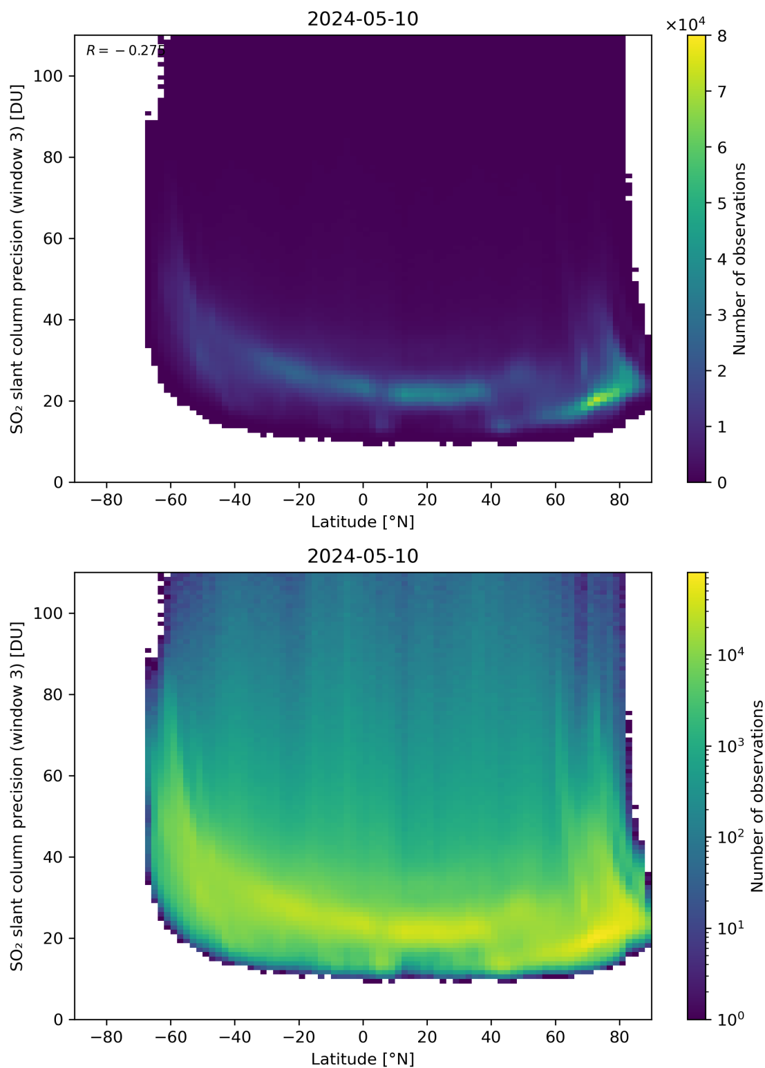
Figure 153: Scatter density plot of “Latitude” against “SO 2 slant column precision (window 3)” for 2024-05-09 to 2024-05-11.
