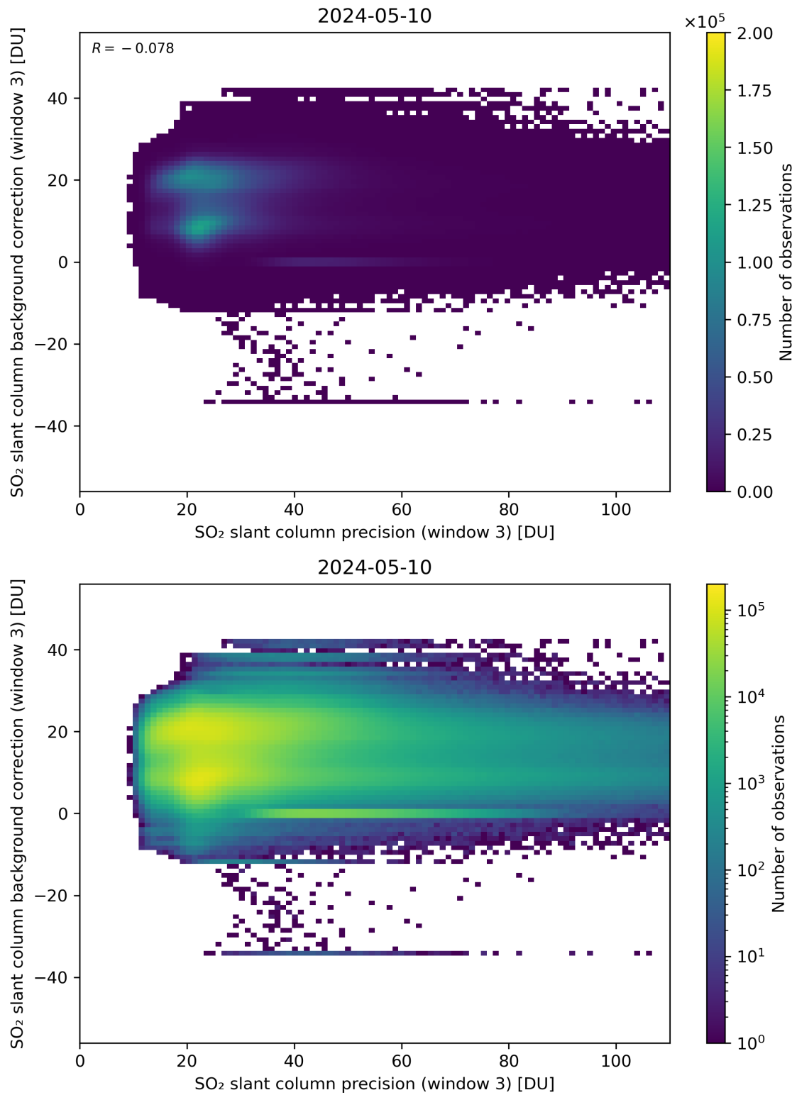
Figure 257: Scatter density plot of “SO 2 slant column precision (window 3)” against “SO 2 slant column background correction (window 3)” for 2024-05-09 to 2024-05-11.
