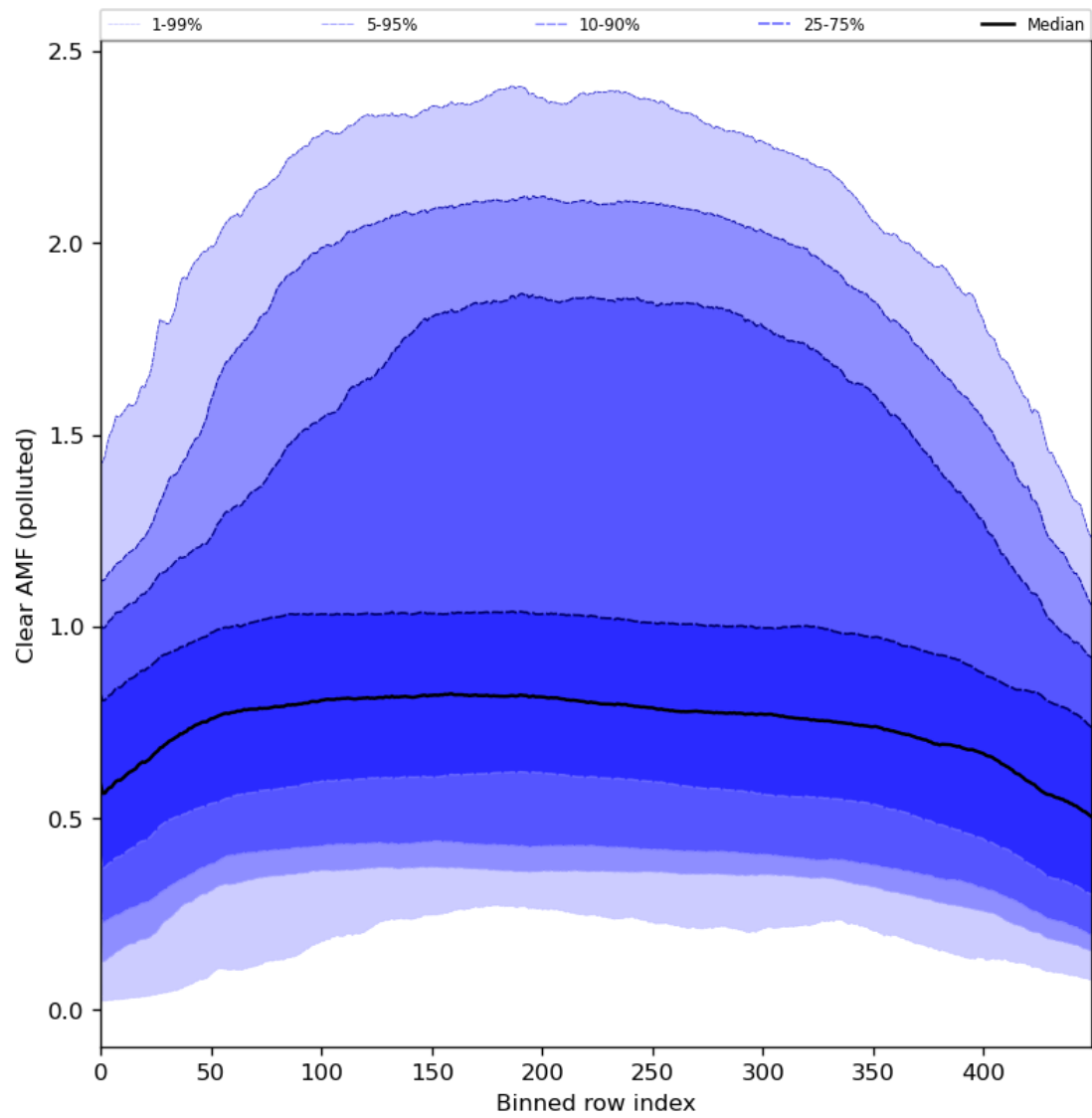
Figure 96: Along track statistics of “Clear AMF (polluted)” for 2024-05-09 to 2024-05-11
