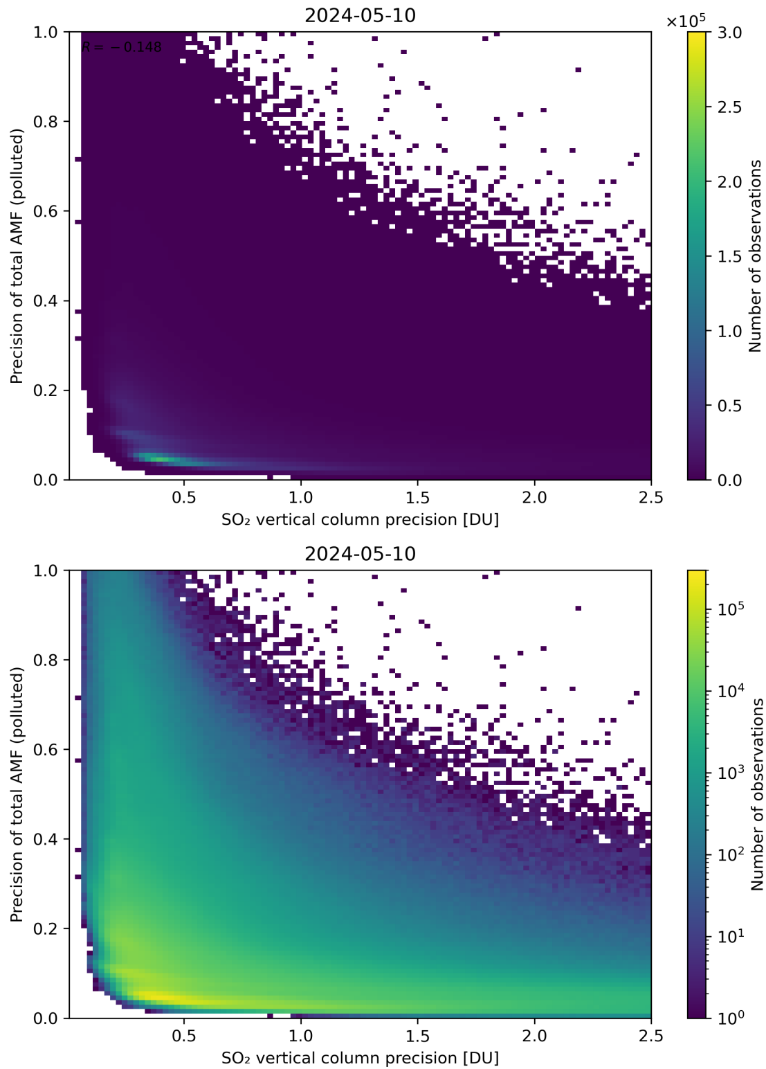
Figure 295: Scatter density plot of “SO 2 vertical column precision” against “Precision of total AMF (polluted)” for 2024-05-09 to 2024-05-11.
