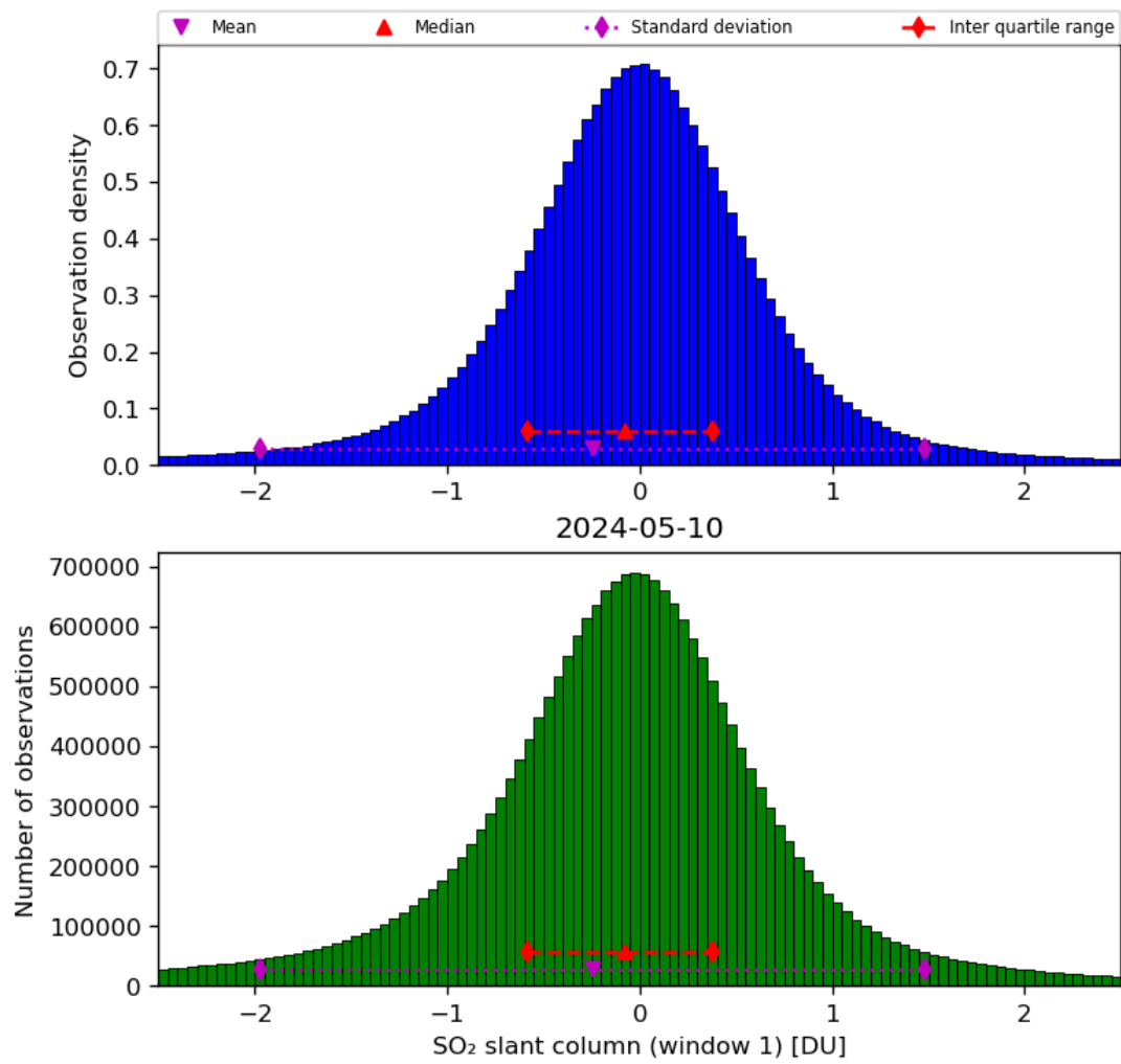
Figure 56: Histogram of “SO 2 slant column (window 1)” for 2024-05-09 to 2024-05-11
