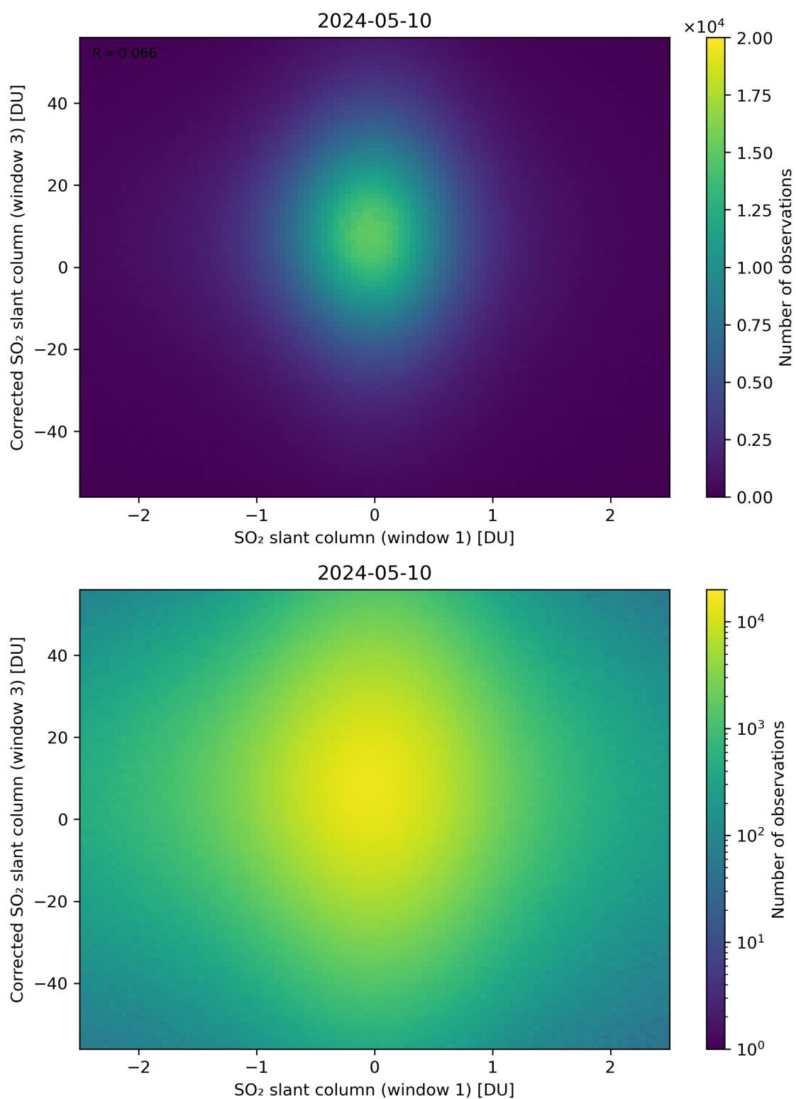
Figure 234: Scatter density plot of “SO 2 slant column (window 1)” against “Corrected SO 2 slant column (window 3)” for 2024-05-09 to 2024-05-11.
