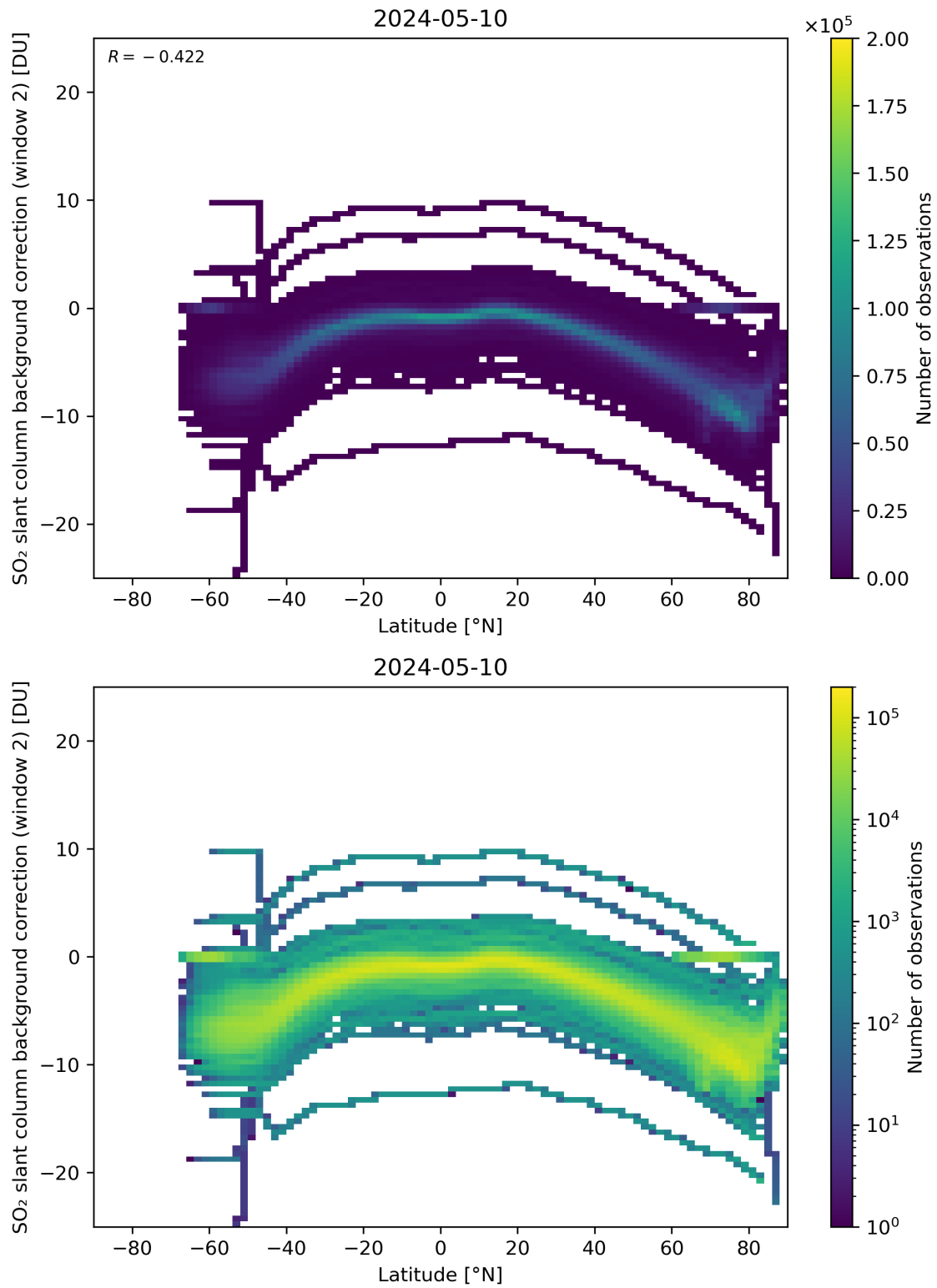
Figure 140: Scatter density plot of “Latitude” against “SO 2 slant column background correction (window 2)” for 2024-05-09 to 2024-05-11.
