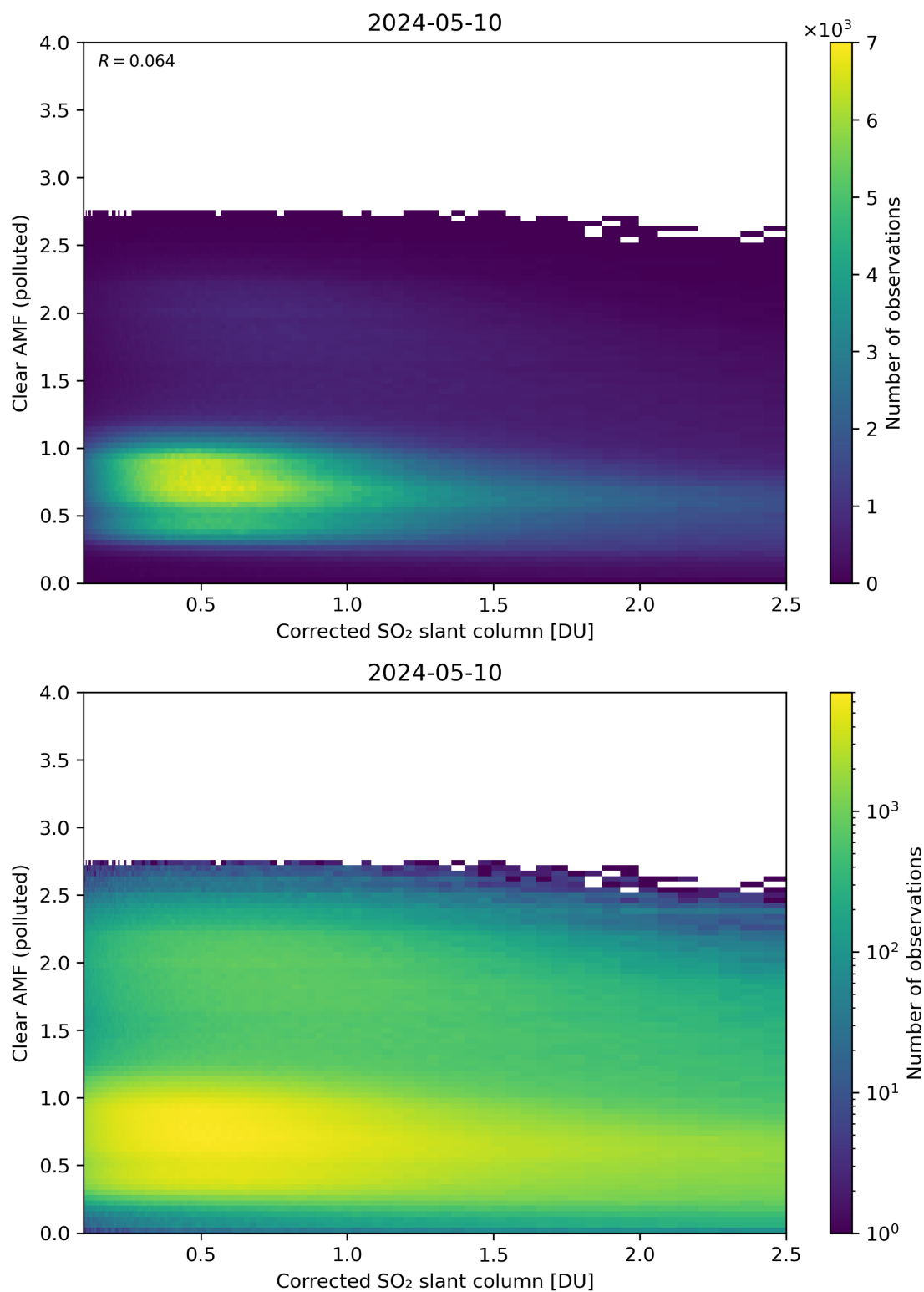
Figure 184: Scatter density plot of “Corrected SO 2 slant column” against “Clear AMF (polluted)” for 2024-05-09 to 2024-05-11.
