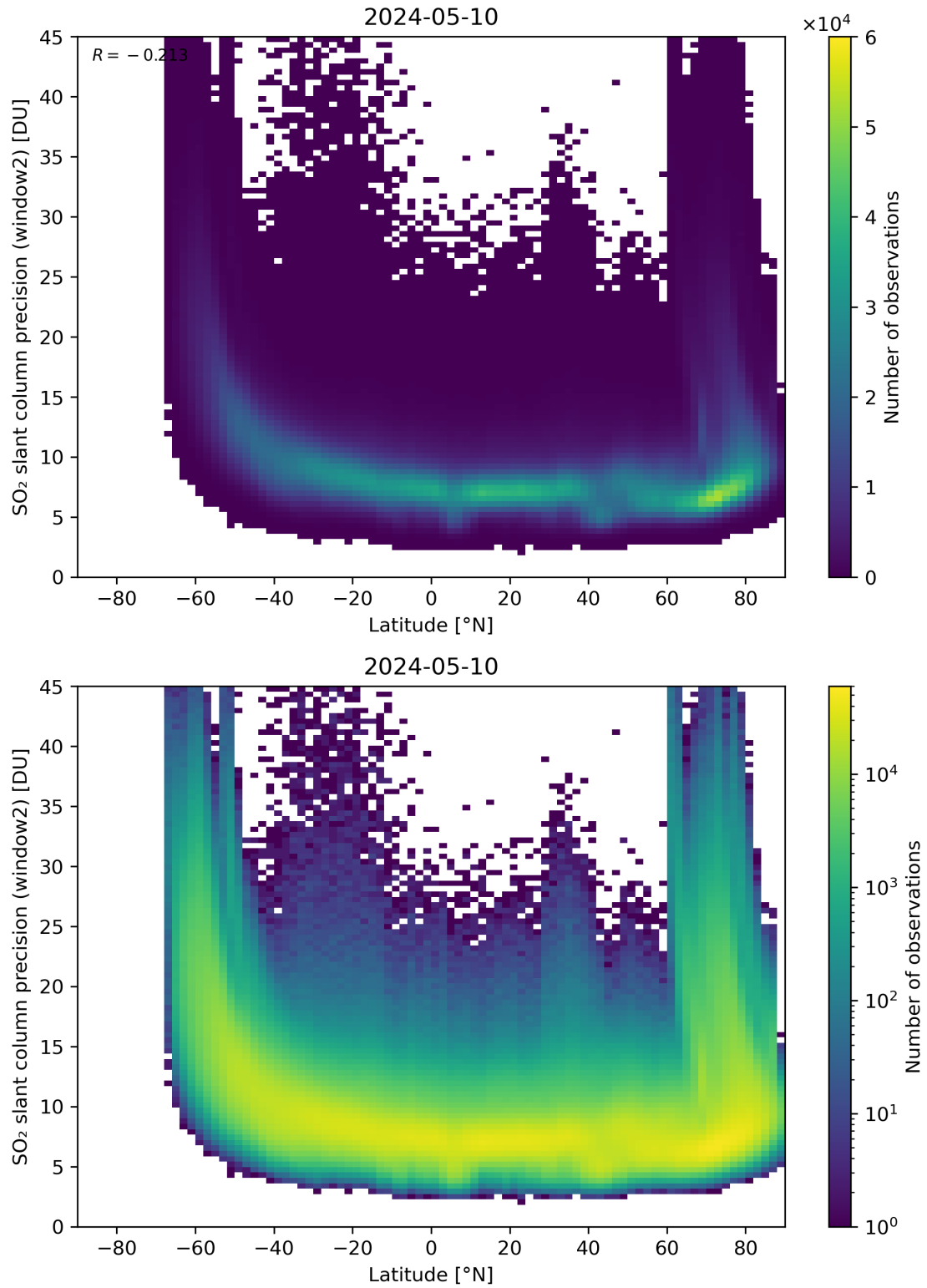
Figure 151: Scatter density plot of “Latitude” against “SO 2 slant column precision (window2)” for 2024-05-09 to 2024-05-11.
