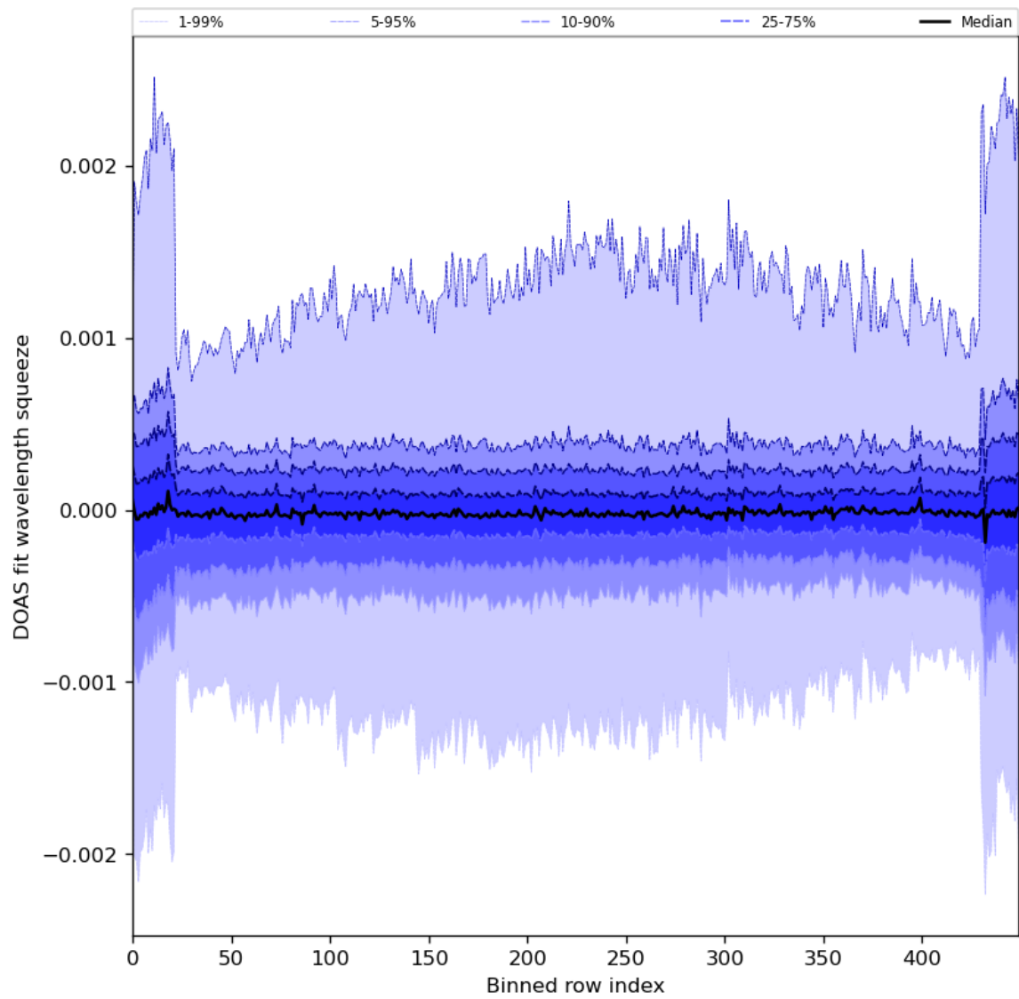
Figure 92: Along track statistics of “DOAS fit wavelength squeeze” for 2024-05-09 to 2024-05-11
