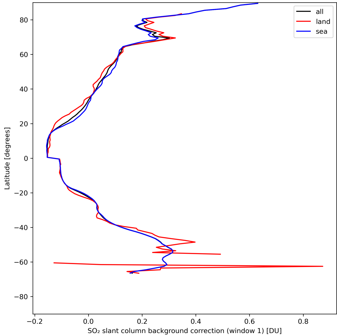
Figure 36: Zonal average of “SO 2 slant column background correction (window 1)” for 2024-05-09 to 2024-05-11.
