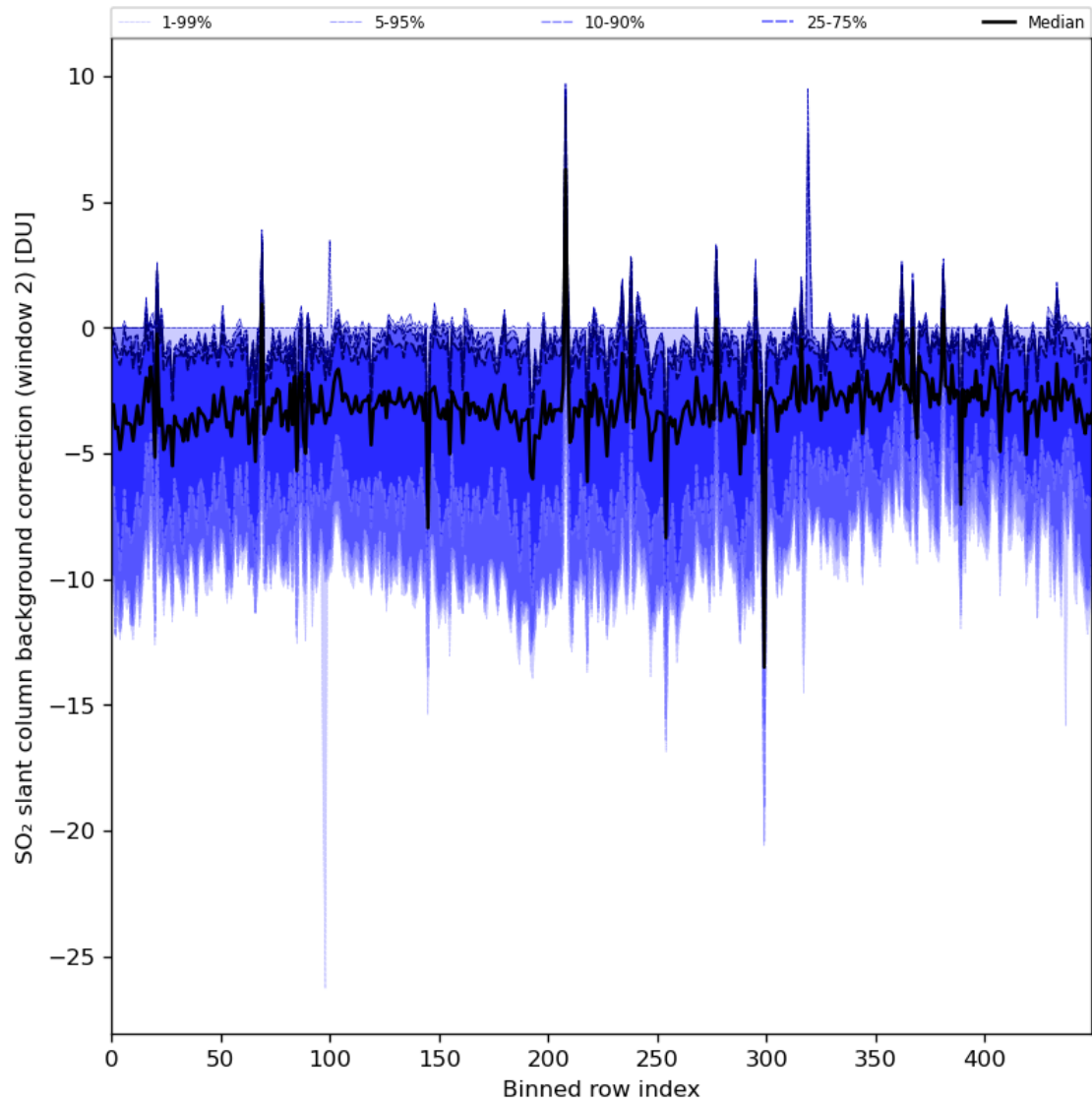
Figure 86: Along track statistics of “SO 2 slant column background correction (window 2)” for 2024-05-09 to 2024-05-11
