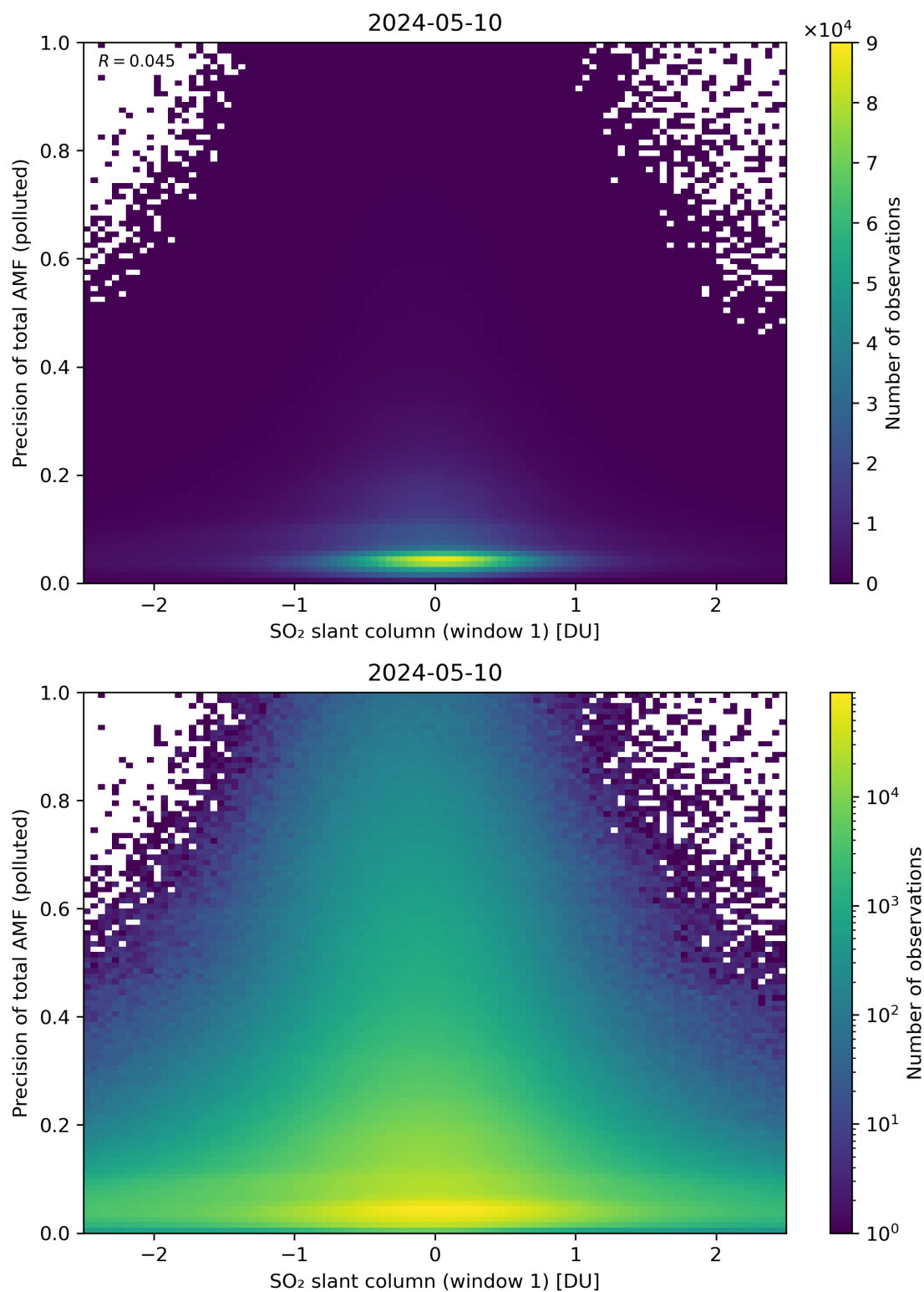
Figure 240: Scatter density plot of “SO 2 slant column (window 1)” against “Precision of total AMF (polluted)” for 2024-05-09 to 2024-05-11.
