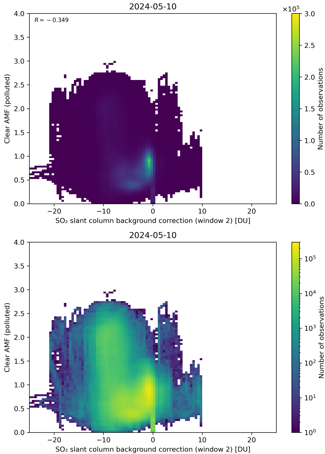
Figure 115: Scatter density plot of “SO 2 slant column background correction (window 2)” against “Clear AMF (polluted)” for 2024-05-09 to 2024-05-11.
