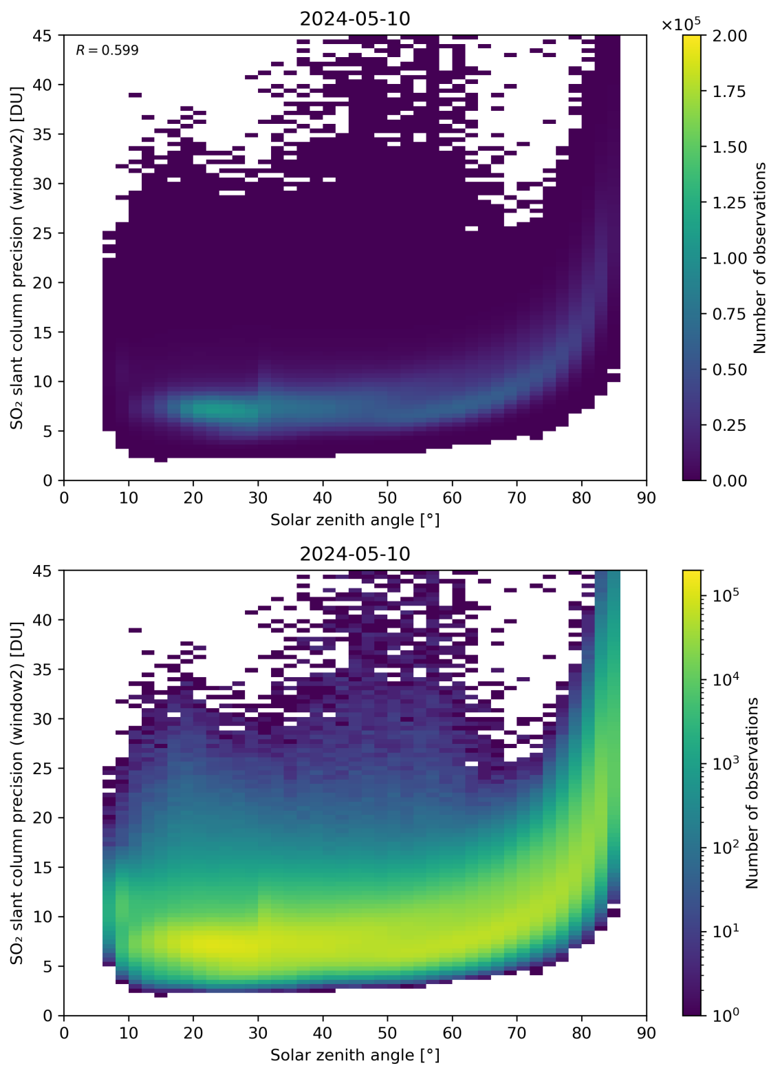
Figure 171: Scatter density plot of “Solar zenith angle” against “SO 2 slant column precision (window2)” for 2024-05-09 to 2024-05-11.
