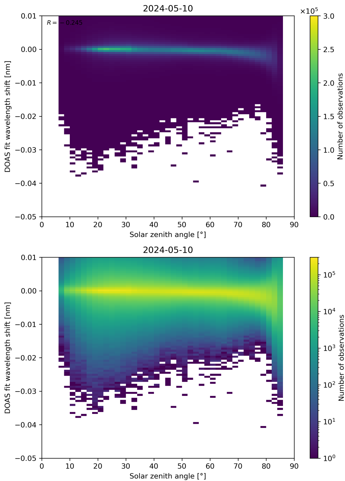
Figure 161: Scatter density plot of “Solar zenith angle” against “DOAS fit wavelength shift” for 2024-05-09 to 2024-05-11.
