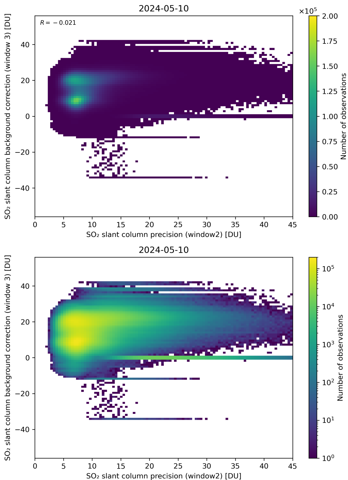
Figure 242: Scatter density plot of “SO 2 slant column precision (window2)” against “SO 2 slant column background correction (window 3)” for 2024-05-09 to 2024-05-11.
