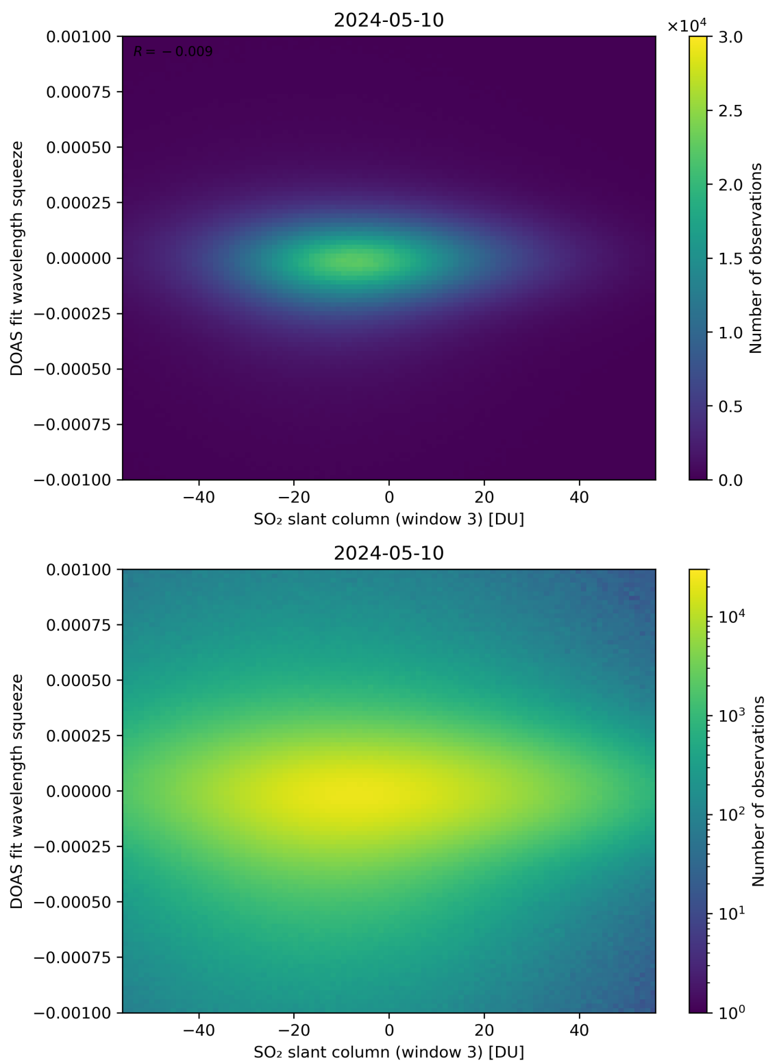
Figure 255: Scatter density plot of “SO 2 slant column (window 3)” against “DOAS fit wavelength squeeze” for 2024-05-09 to 2024-05-11.
