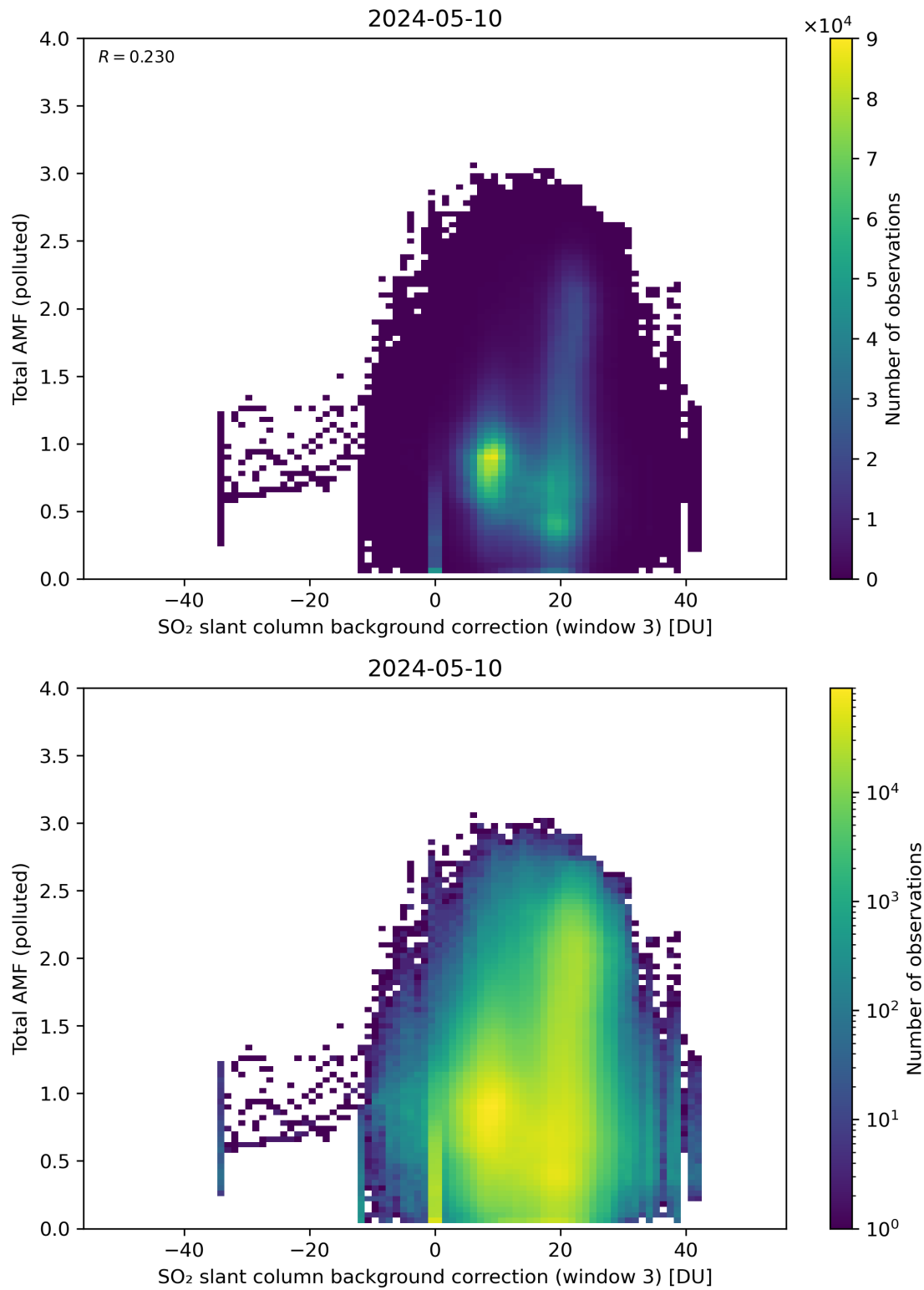
Figure 125: Scatter density plot of “SO 2 slant column background correction (window 3)” against “Total AMF (polluted)” for 2024-05-09 to 2024-05-11.
