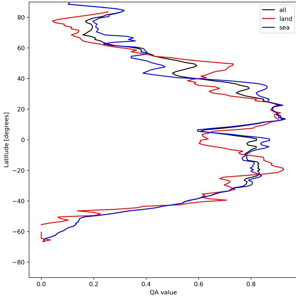
Figure 29: Zonal average of “QA value” for 2024-05-09 to 2024-05-11.
