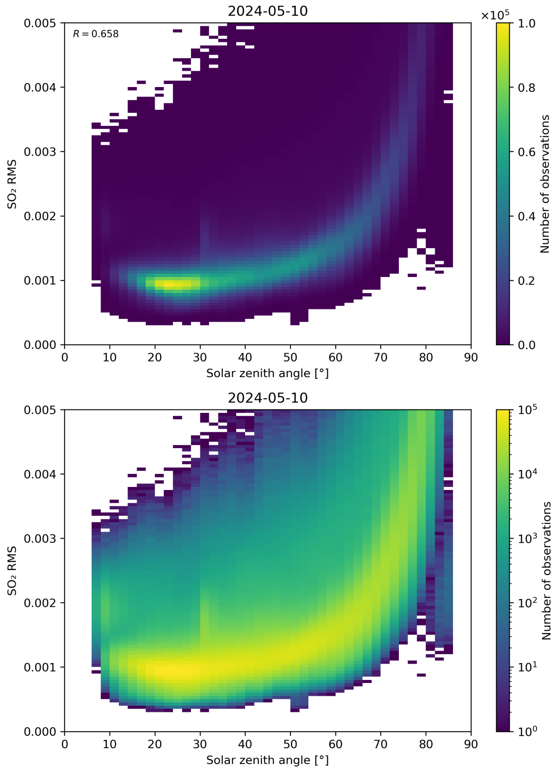
Figure 163: Scatter density plot of “Solar zenith angle” against “SO 2 RMS” for 2024-05-09 to 2024-05-11.
