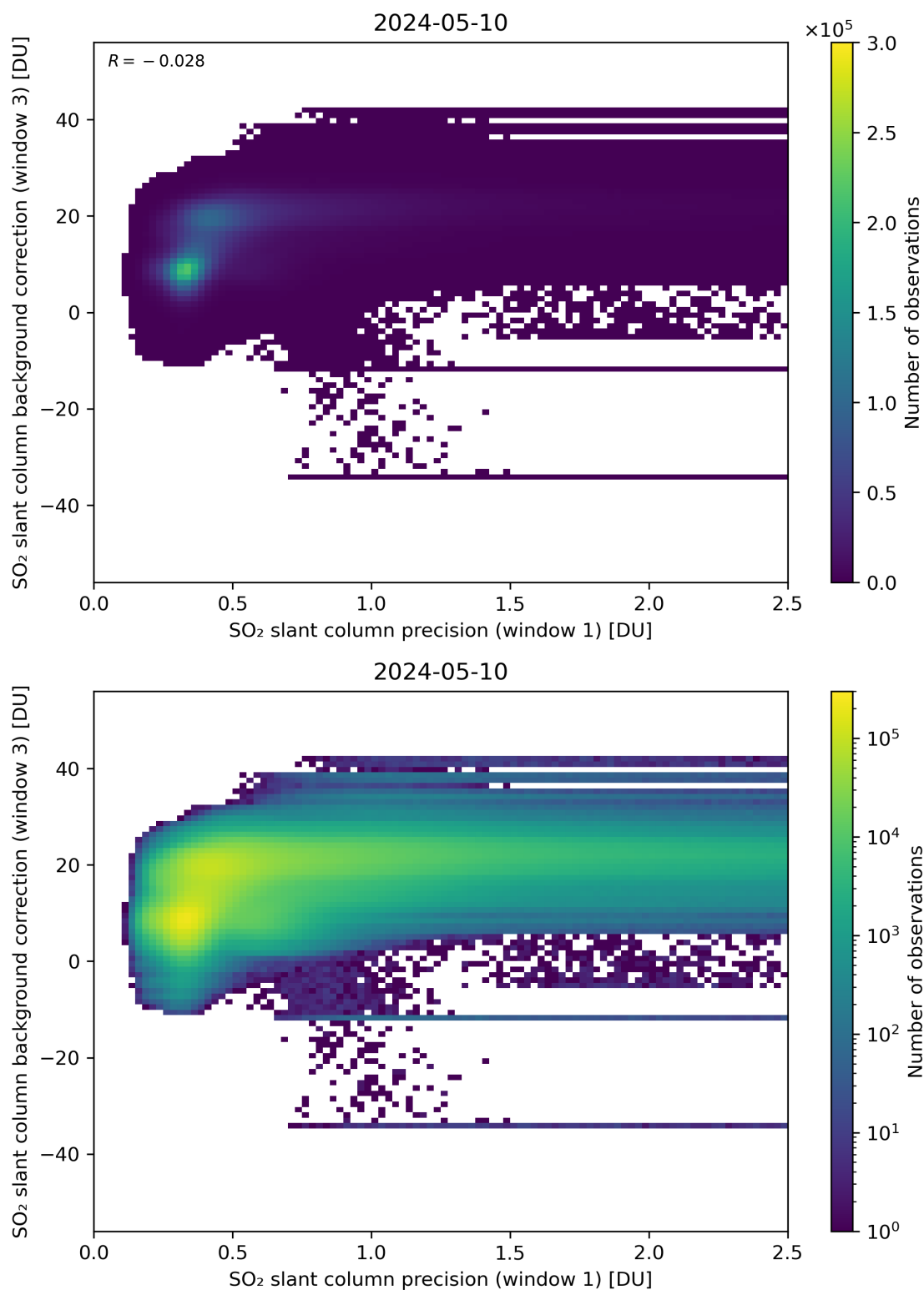
Figure 220: Scatter density plot of “SO 2 slant column precision (window 1)” against “SO 2 slant column background correction (window 3)” for 2024-05-09 to 2024-05-11.
