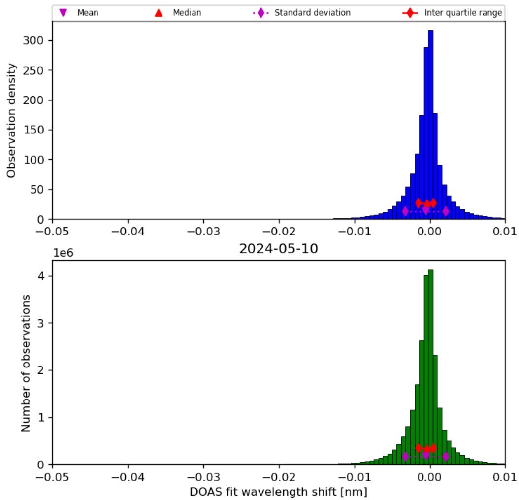
Figure 68: Histogram of “DOAS fit wavelength shift” for 2024-05-09 to 2024-05-11
