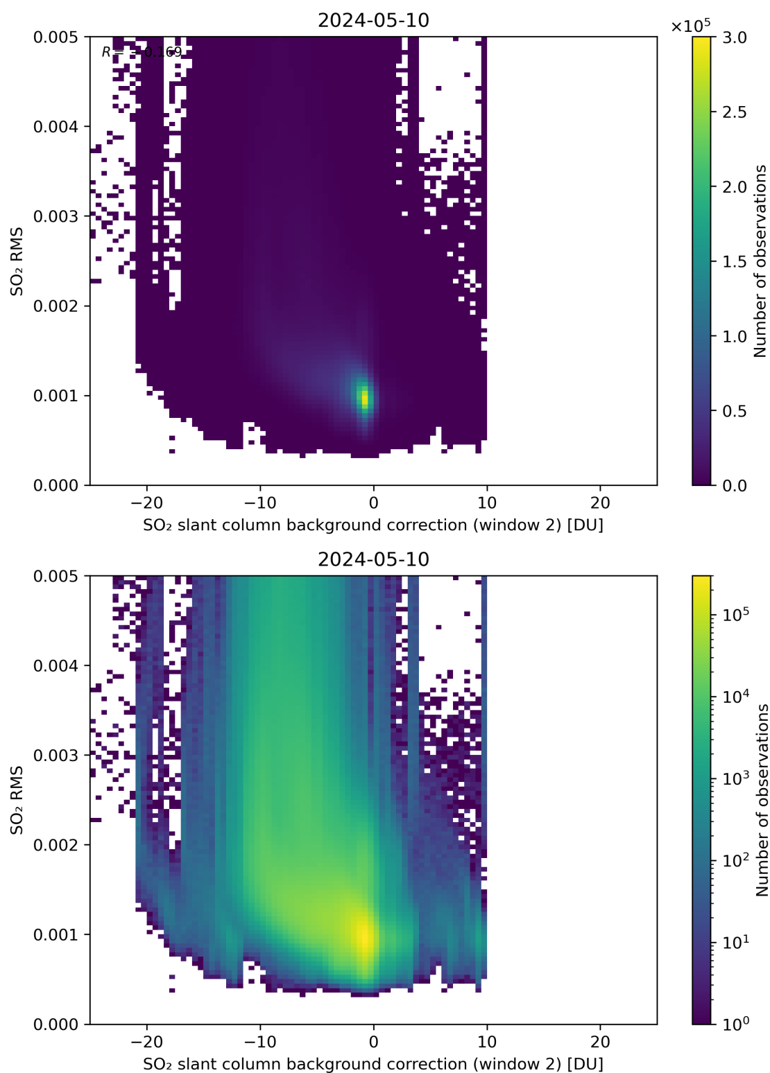
Figure 114: Scatter density plot of “SO 2 slant column background correction (window 2)” against “SO 2 RMS” for 2024-05-09 to 2024-05-11.
