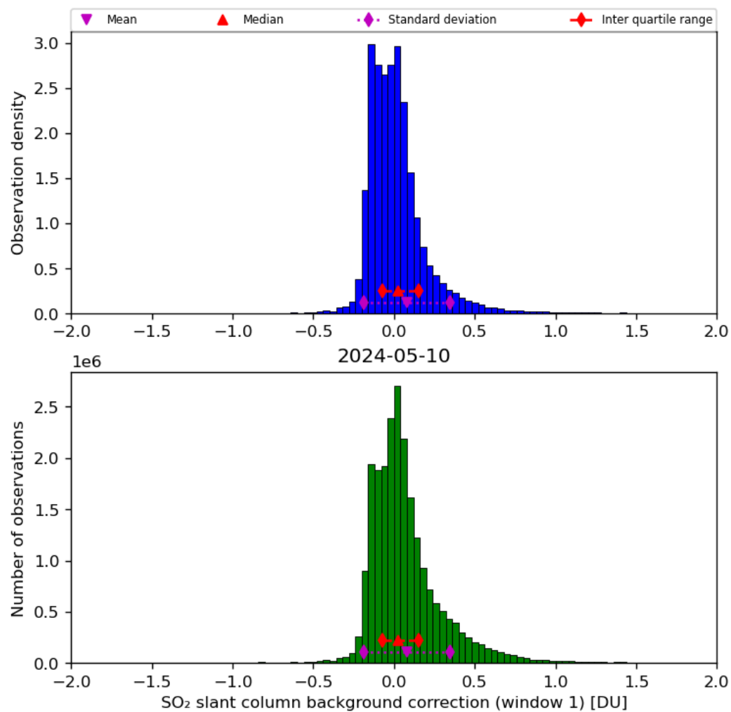
Figure 59: Histogram of “SO 2 slant column background correction (window 1)” for 2024-05-09 to 2024-05-11
