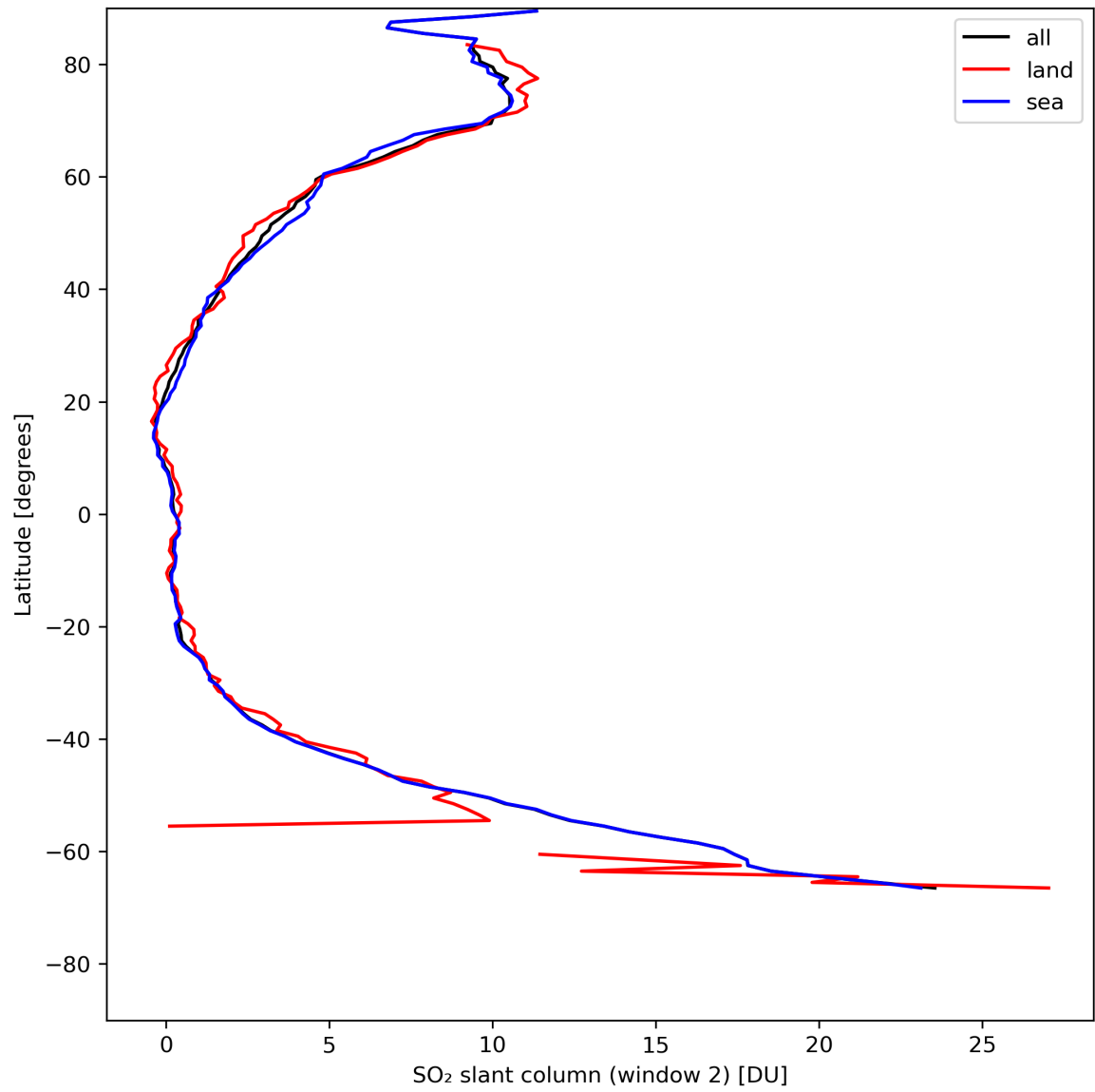
Figure 37: Zonal average of “SO 2 slant column (window 2)” for 2024-05-09 to 2024-05-11.
