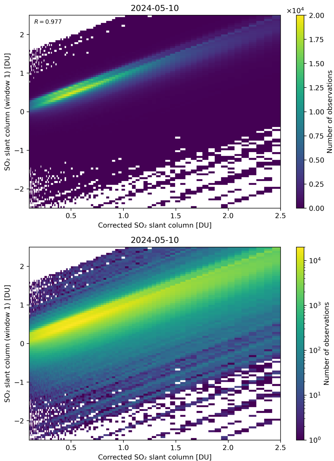
Figure 187: Scatter density plot of “Corrected SO 2 slant column” against “SO 2 slant column (window 1)” for 2024-05-09 to 2024-05-11.
