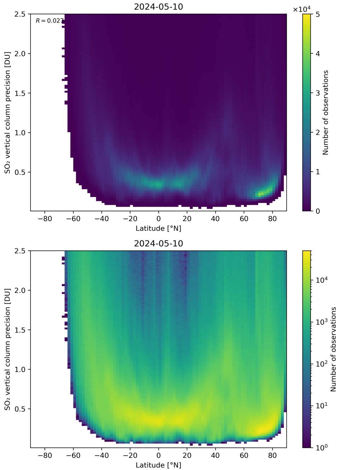
Figure 157: Scatter density plot of “Latitude” against “SO 2 vertical column precision” for 2024-05-09 to 2024-05-11.
