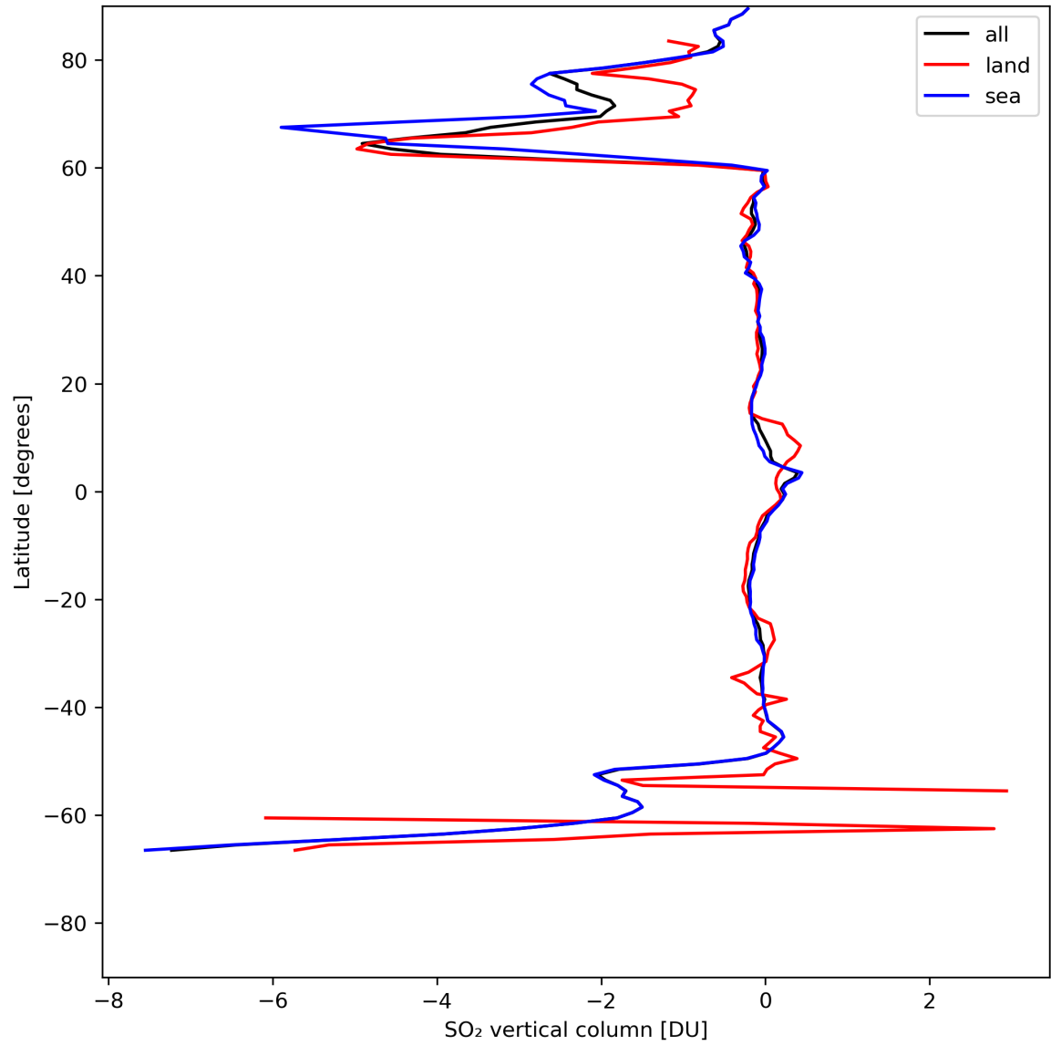
Figure 30: Zonal average of “SO 2 vertical column” for 2024-05-09 to 2024-05-11.
