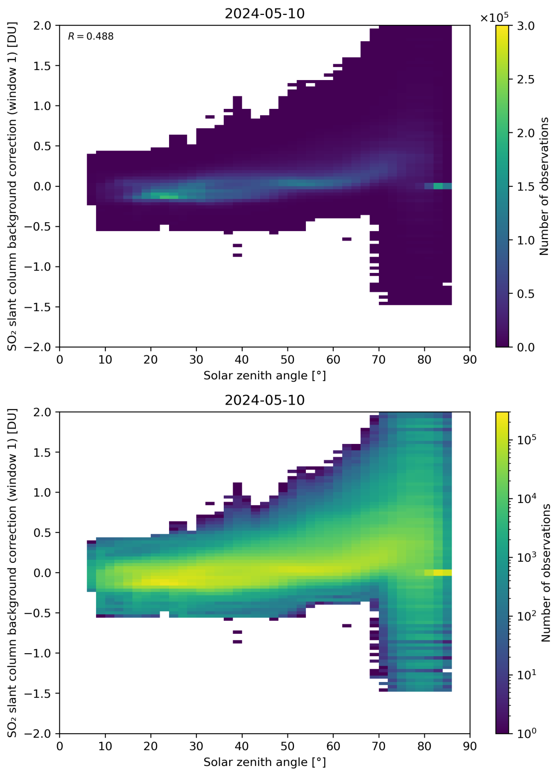
Figure 158: Scatter density plot of “Solar zenith angle” against “SO 2 slant column background correction (window 1)” for 2024-05-09 to 2024-05-11.
