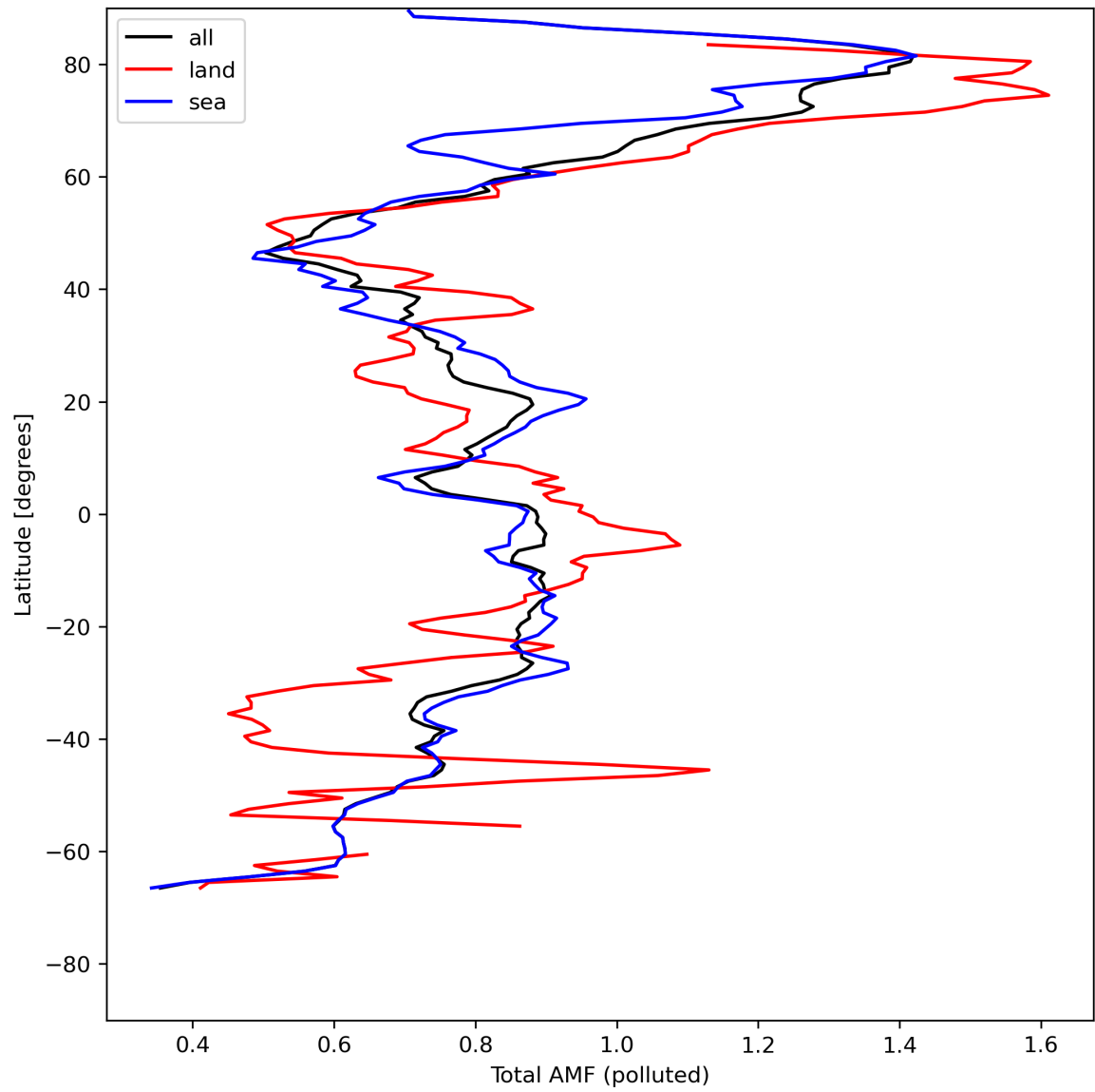
Figure 48: Zonal average of “Total AMF (polluted)” for 2024-05-09 to 2024-05-11.
