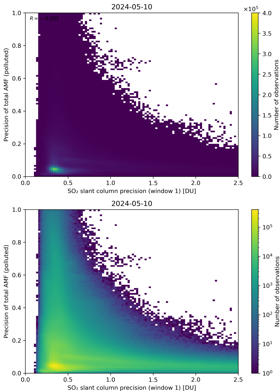
Figure 231: Scatter density plot of “SO 2 slant column precision (window 1)” against “Precision of total AMF (polluted)” for 2024-05-09 to 2024-05-11.
