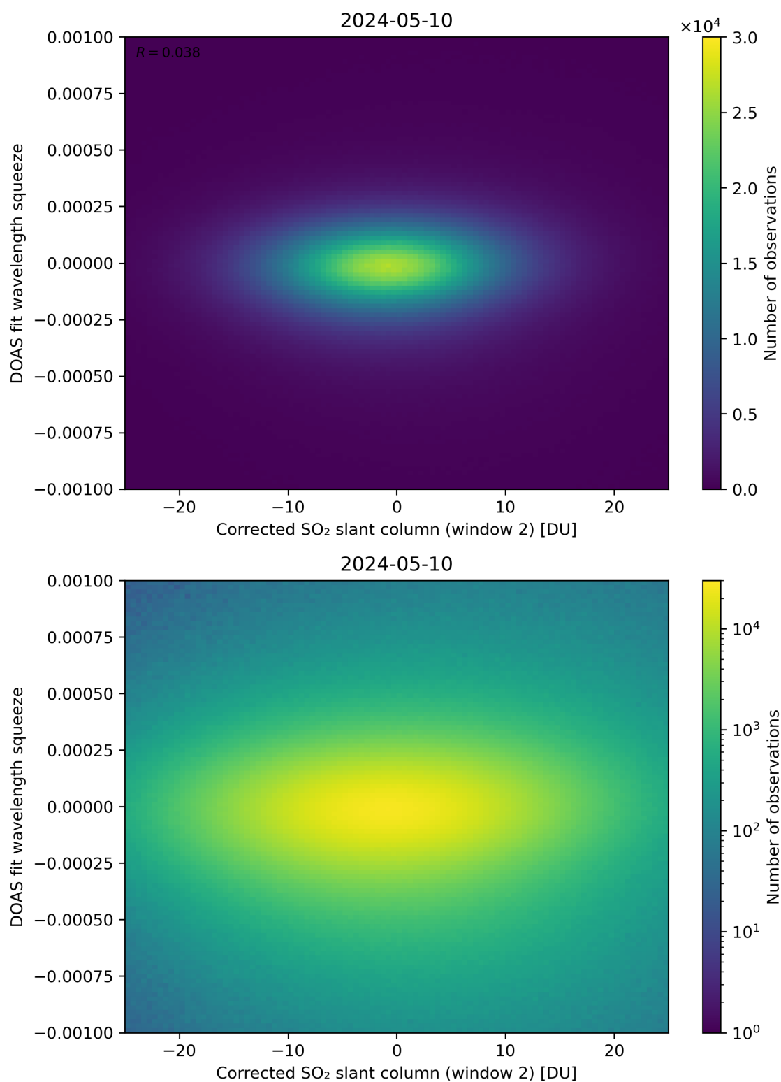
Figure 197: Scatter density plot of “Corrected SO 2 slant column (window 2)” against “DOAS fit wavelength squeeze” for 2024-05-09 to 2024-05-11.
