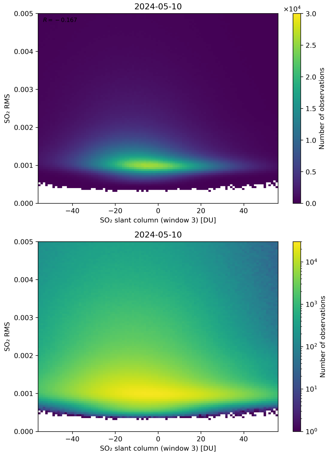
Figure 256: Scatter density plot of “SO 2 slant column (window 3)” against “SO 2 RMS” for 2024-05-09 to 2024-05-11.
