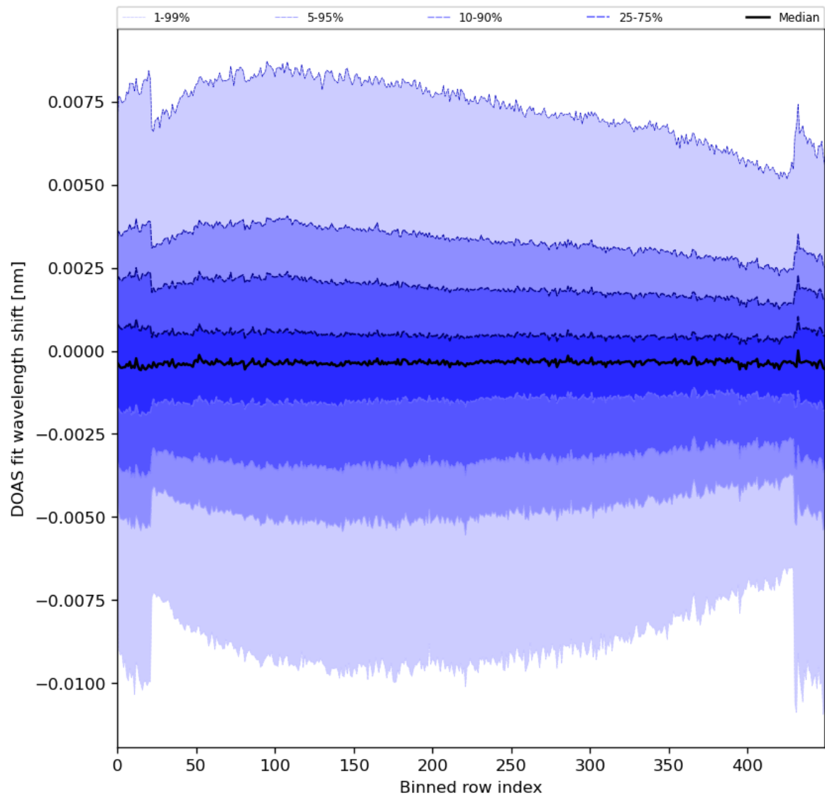
Figure 91: Along track statistics of “DOAS fit wavelength shift” for 2024-05-09 to 2024-05-11
