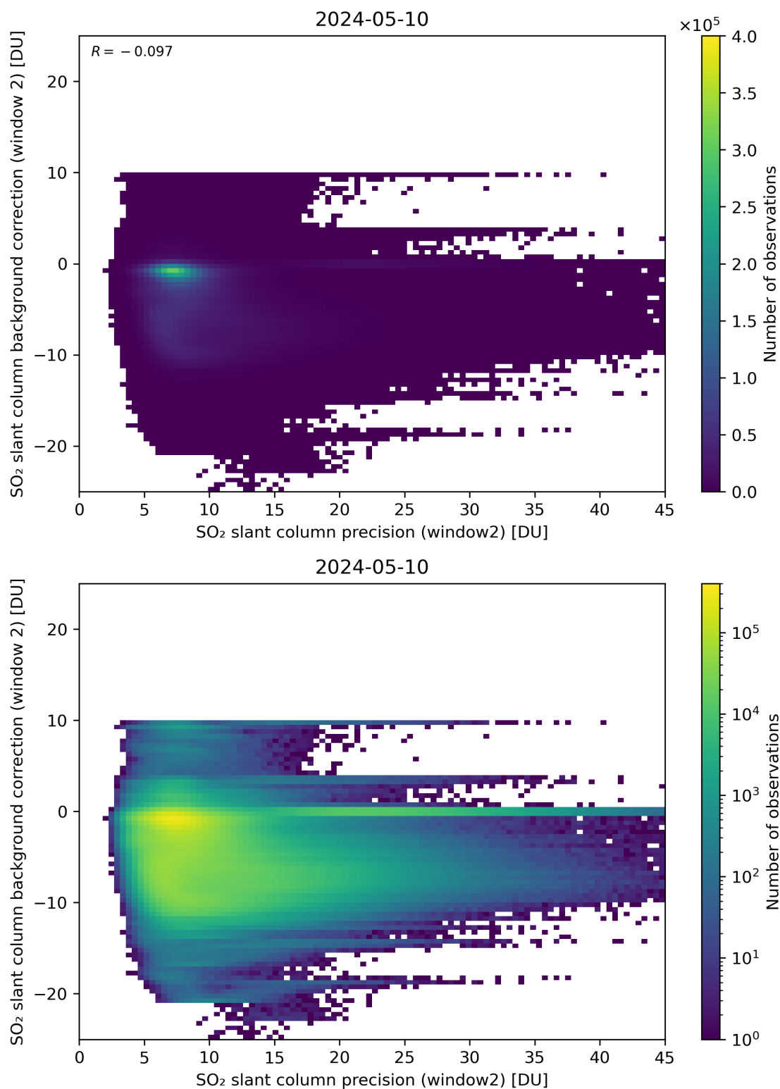
Figure 241: Scatter density plot of “SO 2 slant column precision (window2)” against “SO 2 slant column background correction (window 2)” for 2024-05-09 to 2024-05-11.
