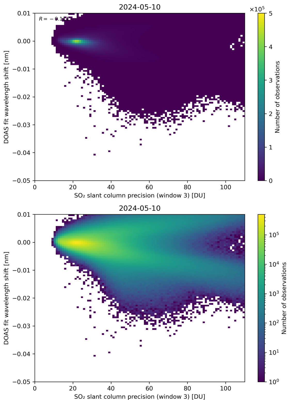
Figure 258: Scatter density plot of “SO 2 slant column precision (window 3)” against “DOAS fit wavelength shift” for 2024-05-09 to 2024-05-11.
