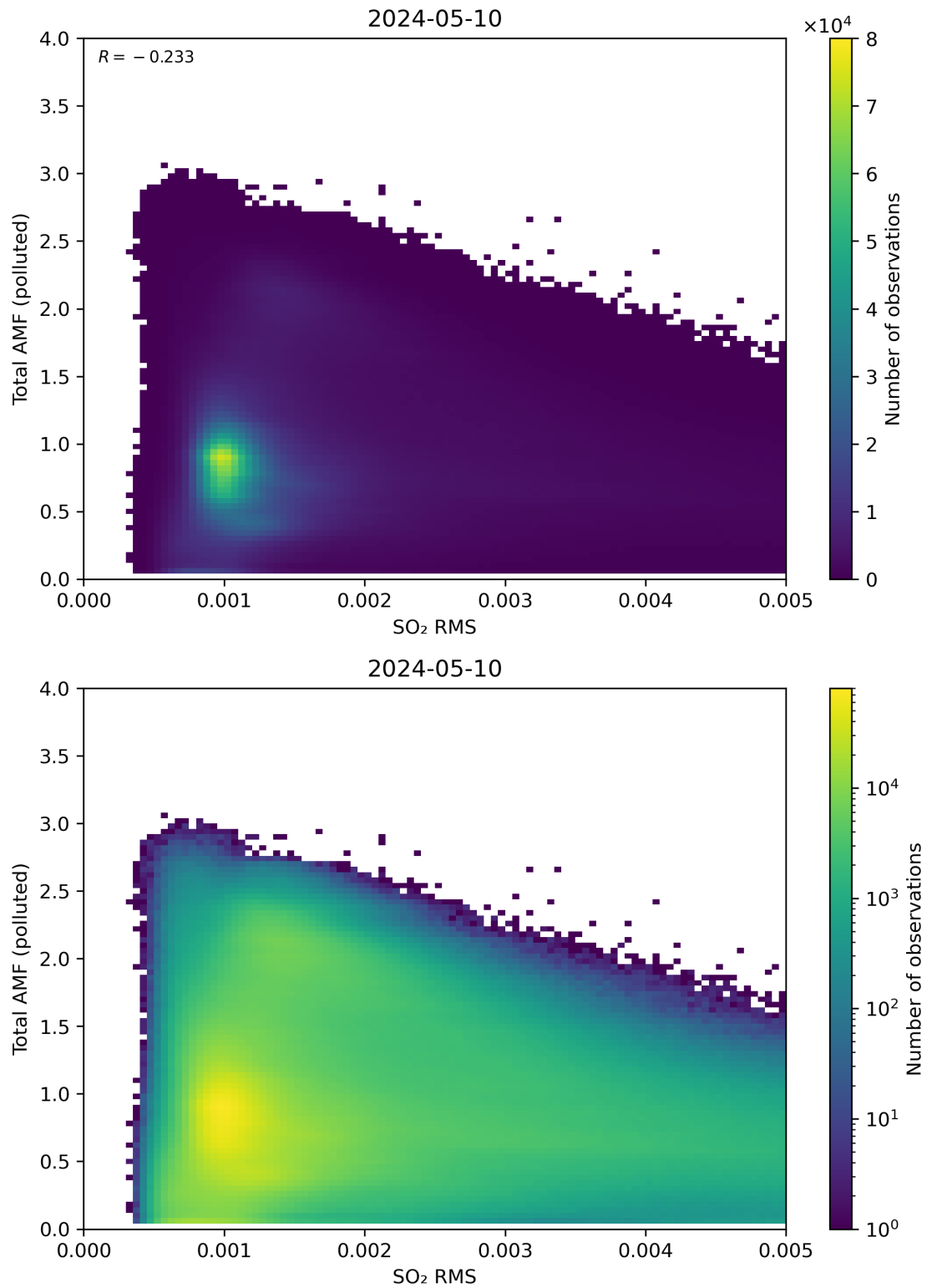
Figure 137: Scatter density plot of “SO 2 RMS” against “Total AMF (polluted)” for 2024-05-09 to 2024-05-11.
