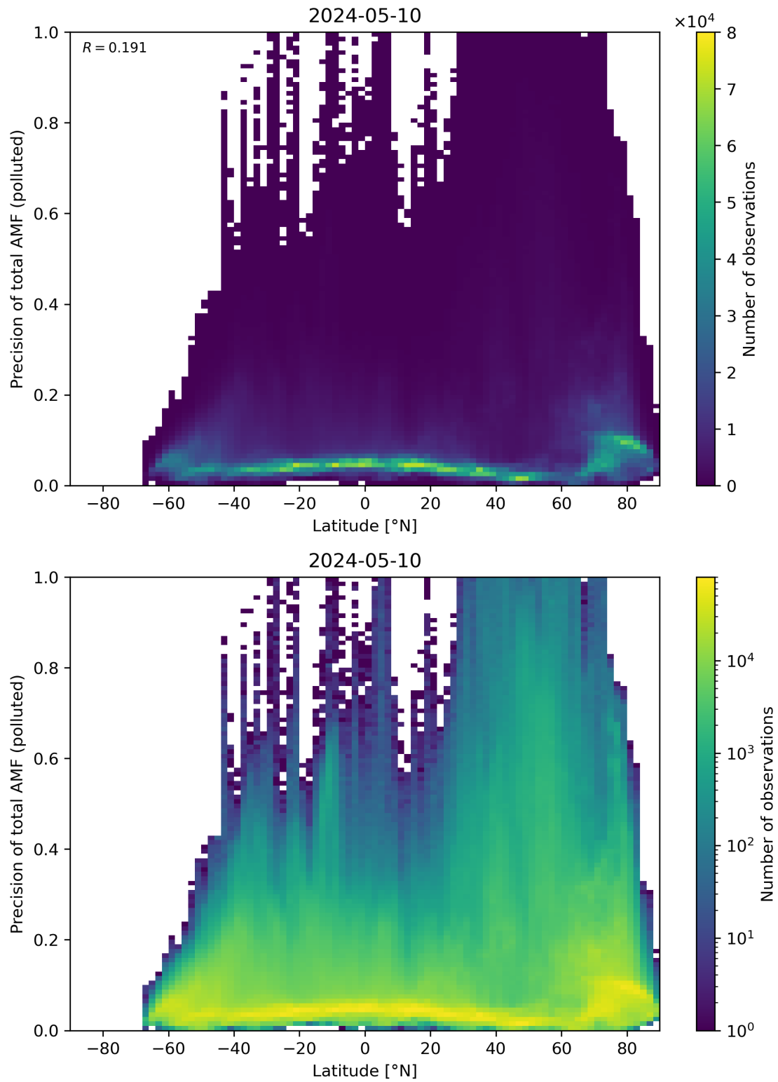
Figure 155: Scatter density plot of “Latitude” against “Precision of total AMF (polluted)” for 2024-05-09 to 2024-05-11.
