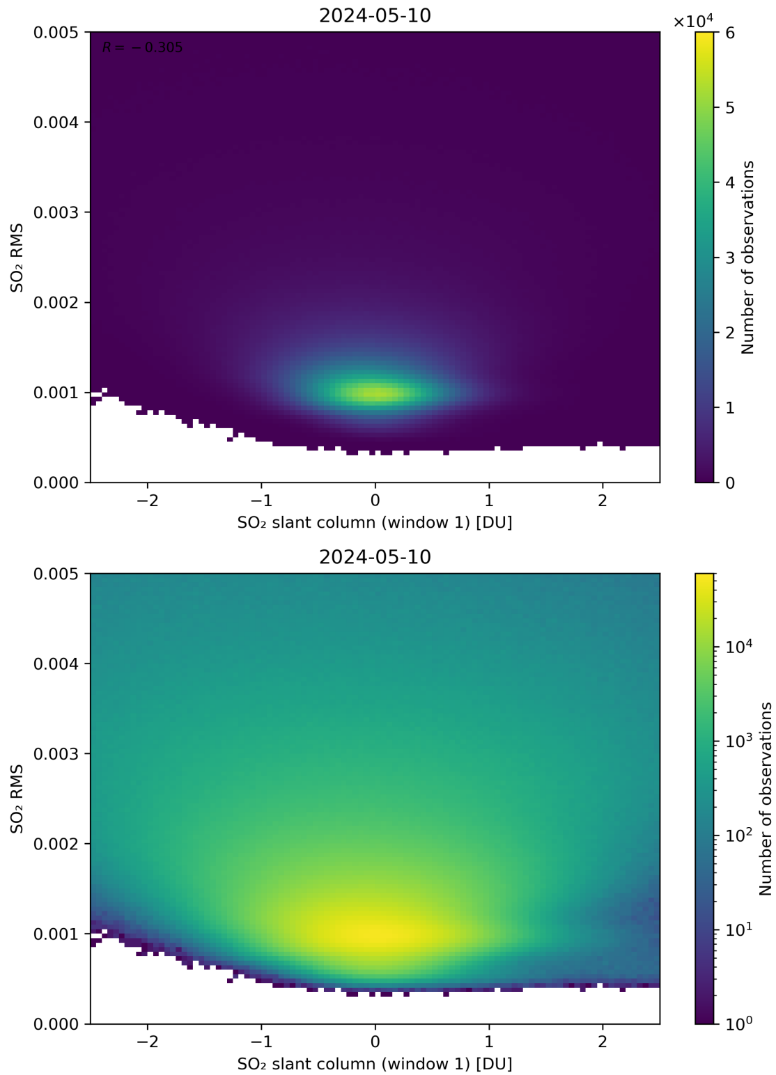
Figure 217: Scatter density plot of “SO 2 slant column (window 1)” against “SO 2 RMS” for 2024-05-09 to 2024-05-11.
