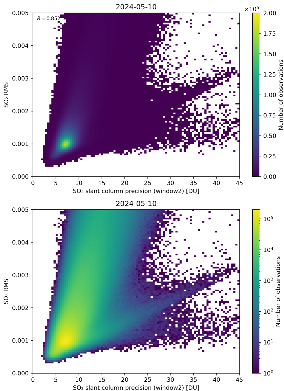
Figure 245: Scatter density plot of “SO 2 slant column precision (window2)” against “SO 2 RMS” for 2024-05-09 to 2024-05-11.
