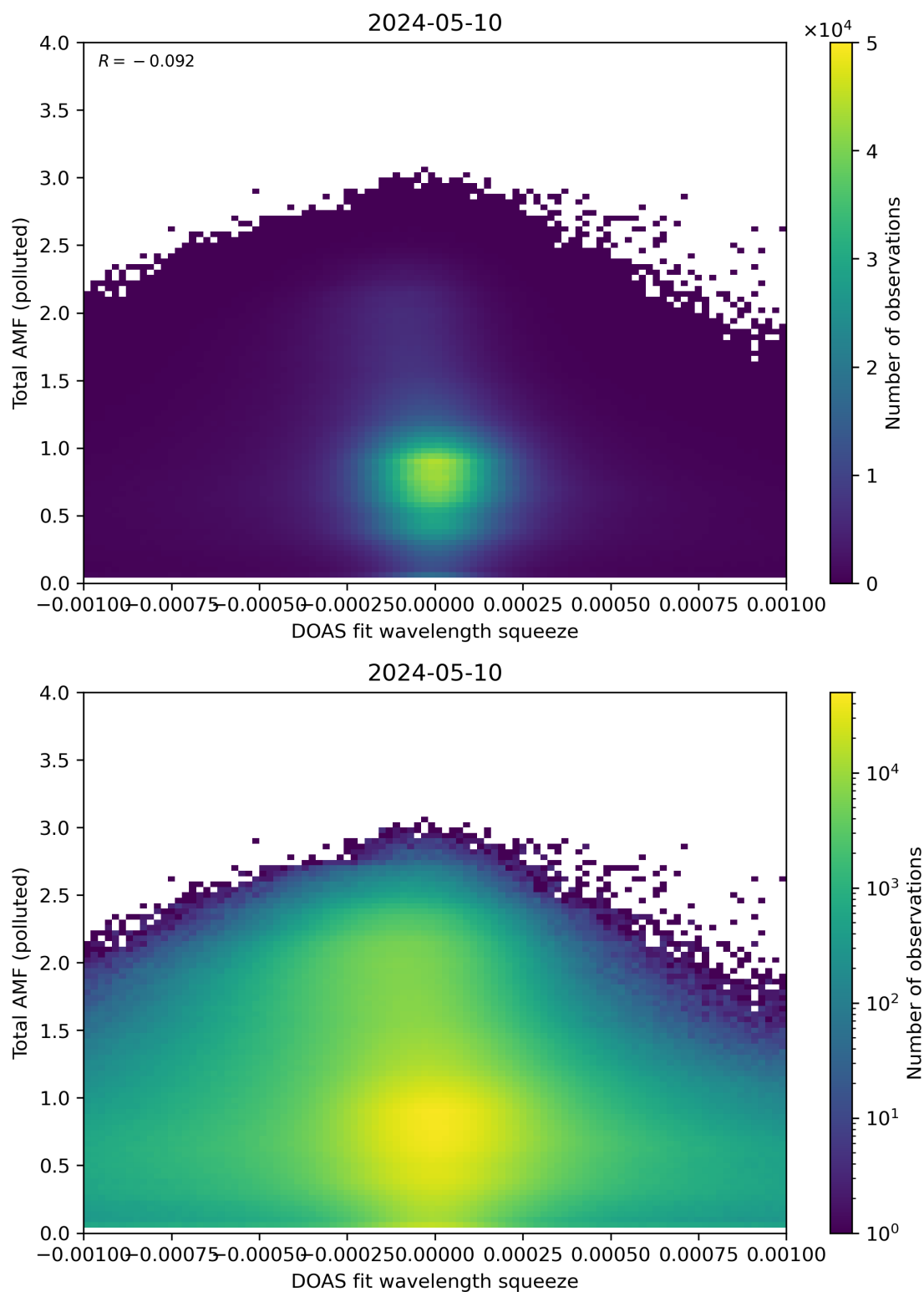
Figure 134: Scatter density plot of “DOAS fit wavelength squeeze” against “Total AMF (polluted)” for 2024-05-09 to 2024-05-11.
