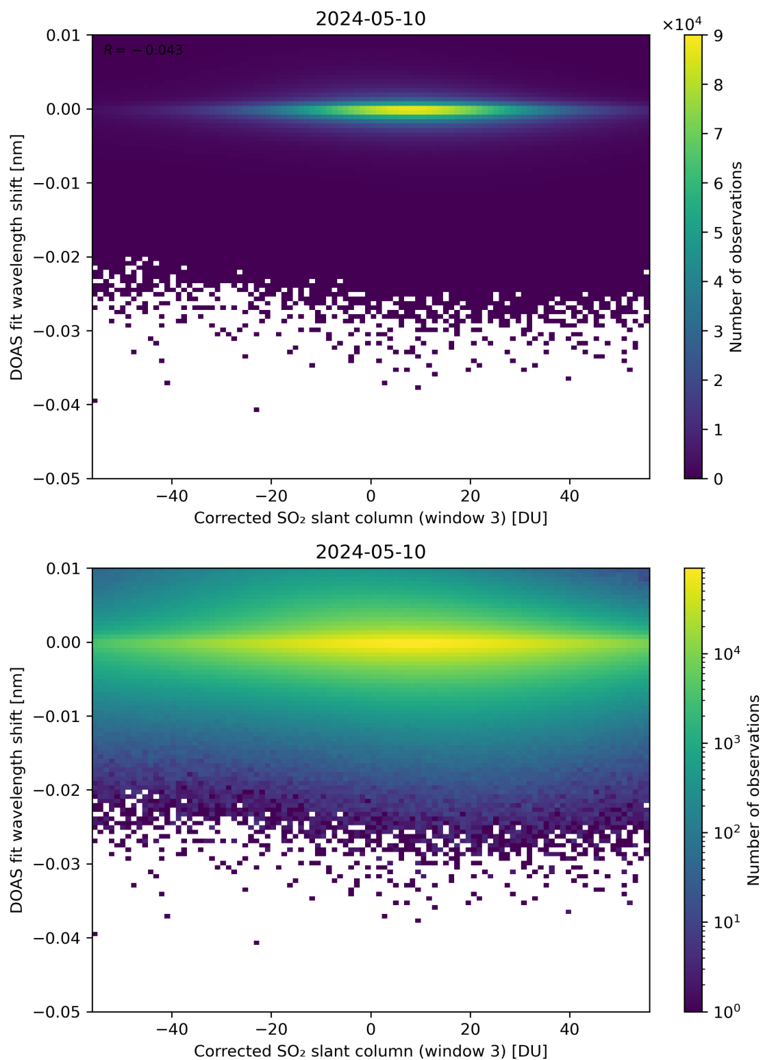
Figure 206: Scatter density plot of “Corrected SO 2 slant column (window 3)” against “DOAS fit wavelength shift” for 2024-05-09 to 2024-05-11.
