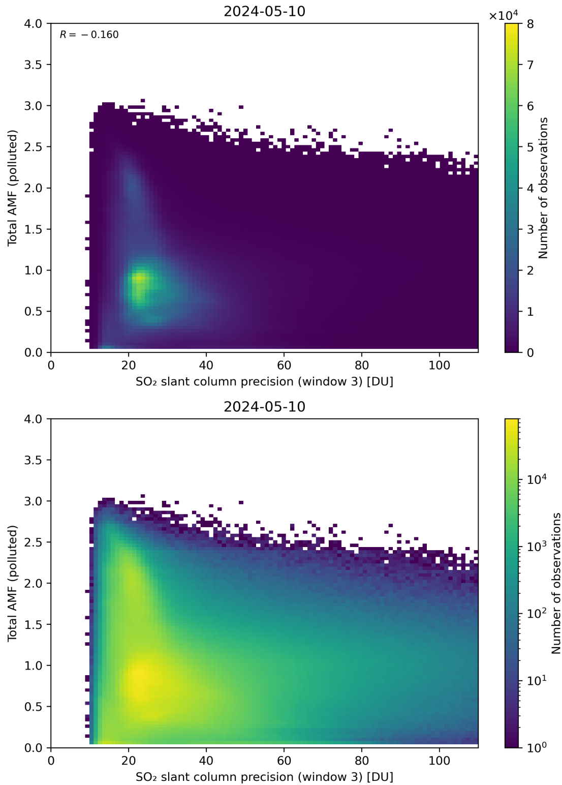
Figure 263: Scatter density plot of “SO 2 slant column precision (window 3)” against “Total AMF (polluted)” for 2024-05-09 to 2024-05-11.
