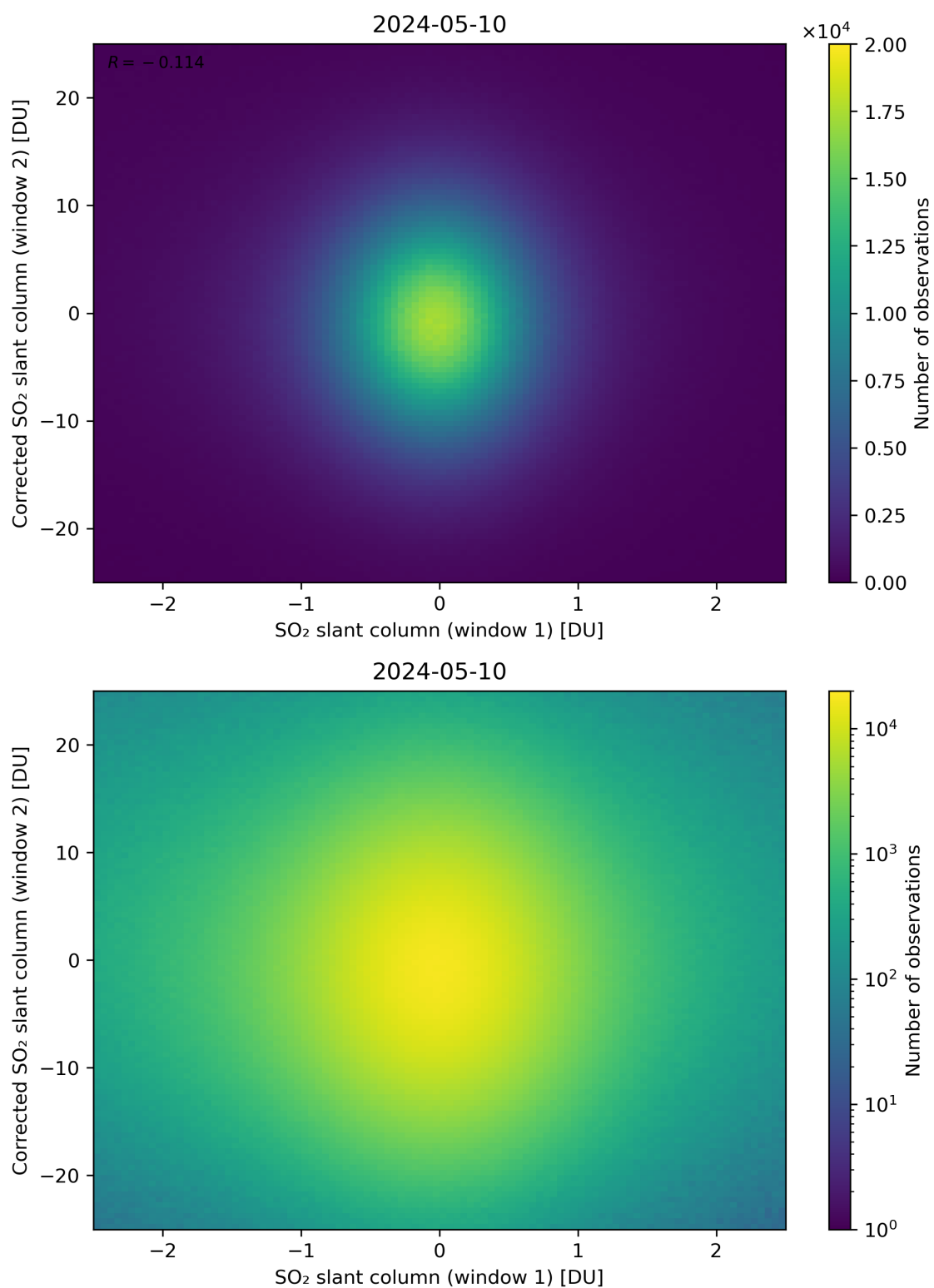
Figure 233: Scatter density plot of “SO 2 slant column (window 1)” against “Corrected SO 2 slant column (window 2)” for 2024-05-09 to 2024-05-11.
