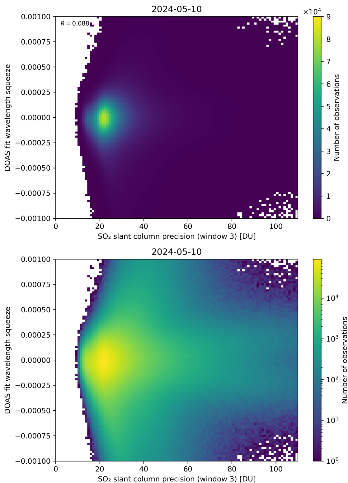
Figure 259: Scatter density plot of “SO 2 slant column precision (window 3)” against “DOAS fit wavelength squeeze” for 2024-05-09 to 2024-05-11.
