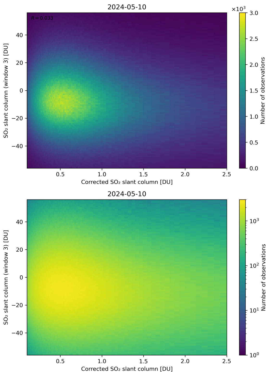
Figure 190: Scatter density plot of “Corrected SO 2 slant column” against “SO 2 slant column (window 3)” for 2024-05-09 to 2024-05-11.
