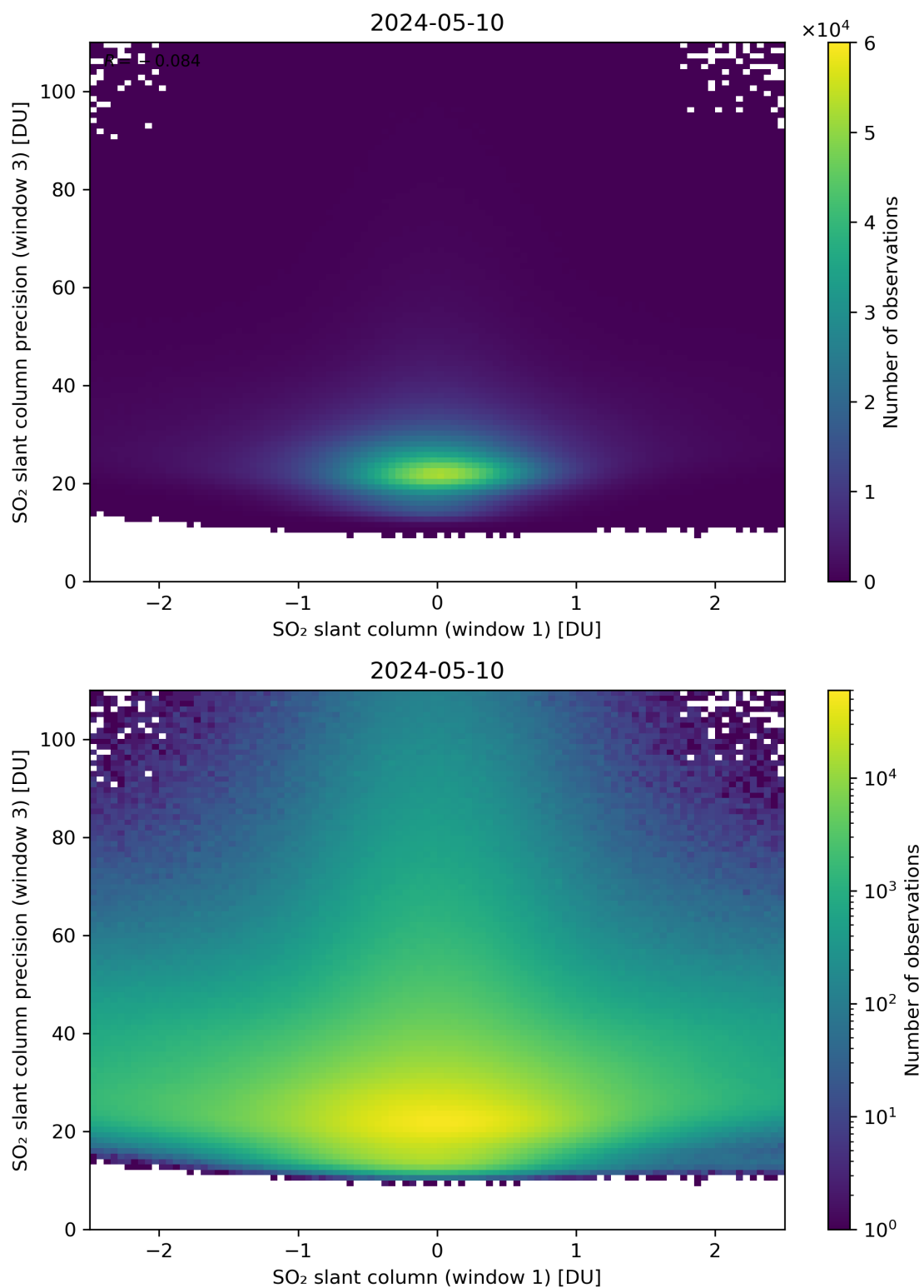
Figure 238: Scatter density plot of “SO 2 slant column (window 1)” against “SO 2 slant column precision (window 3)” for 2024-05-09 to 2024-05-11.
