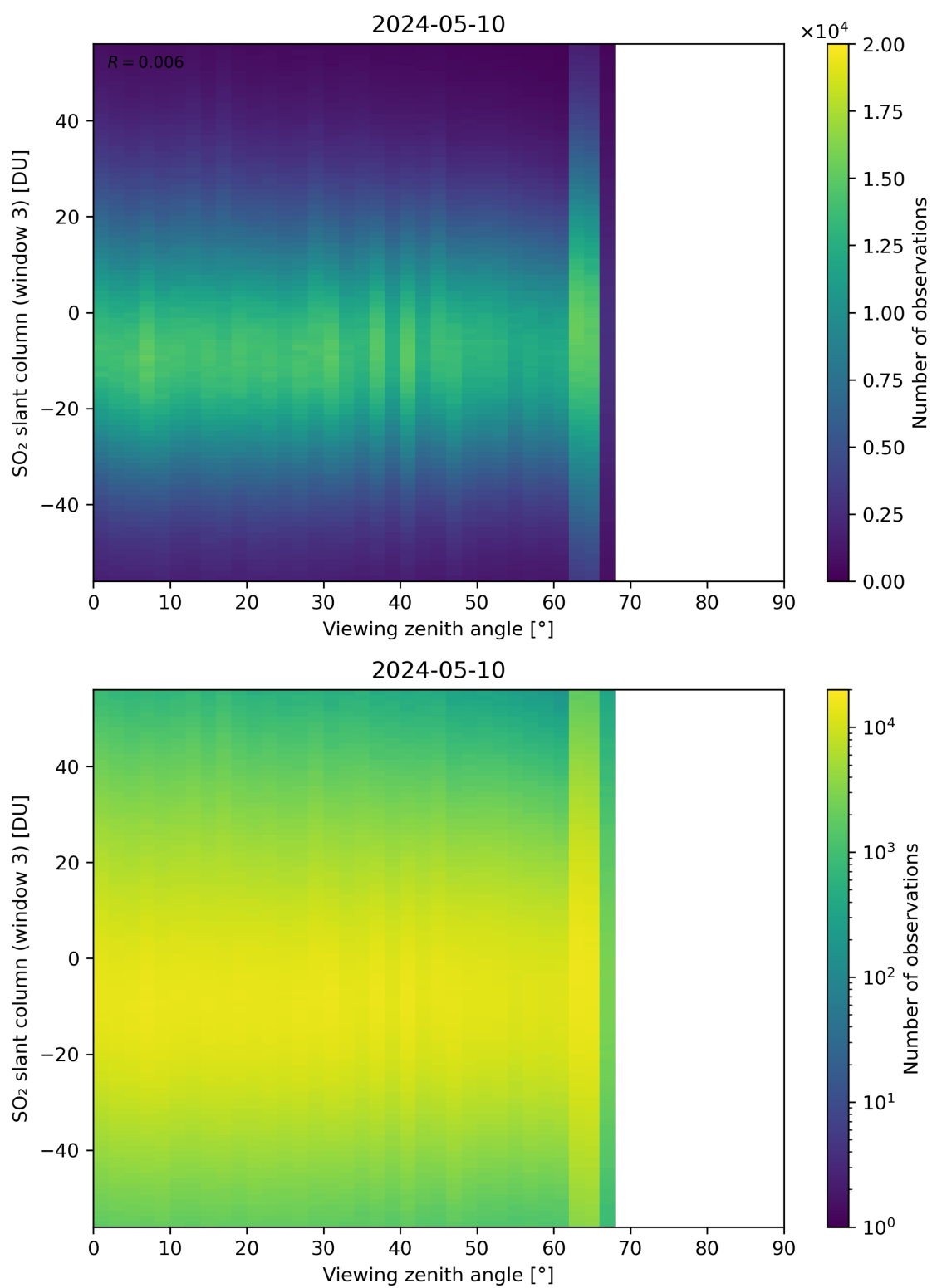
Figure 323: Scatter density plot of “Viewing zenith angle” against “SO 2 slant column (window 3)” for 2024-05-09 to 2024-05-11.
