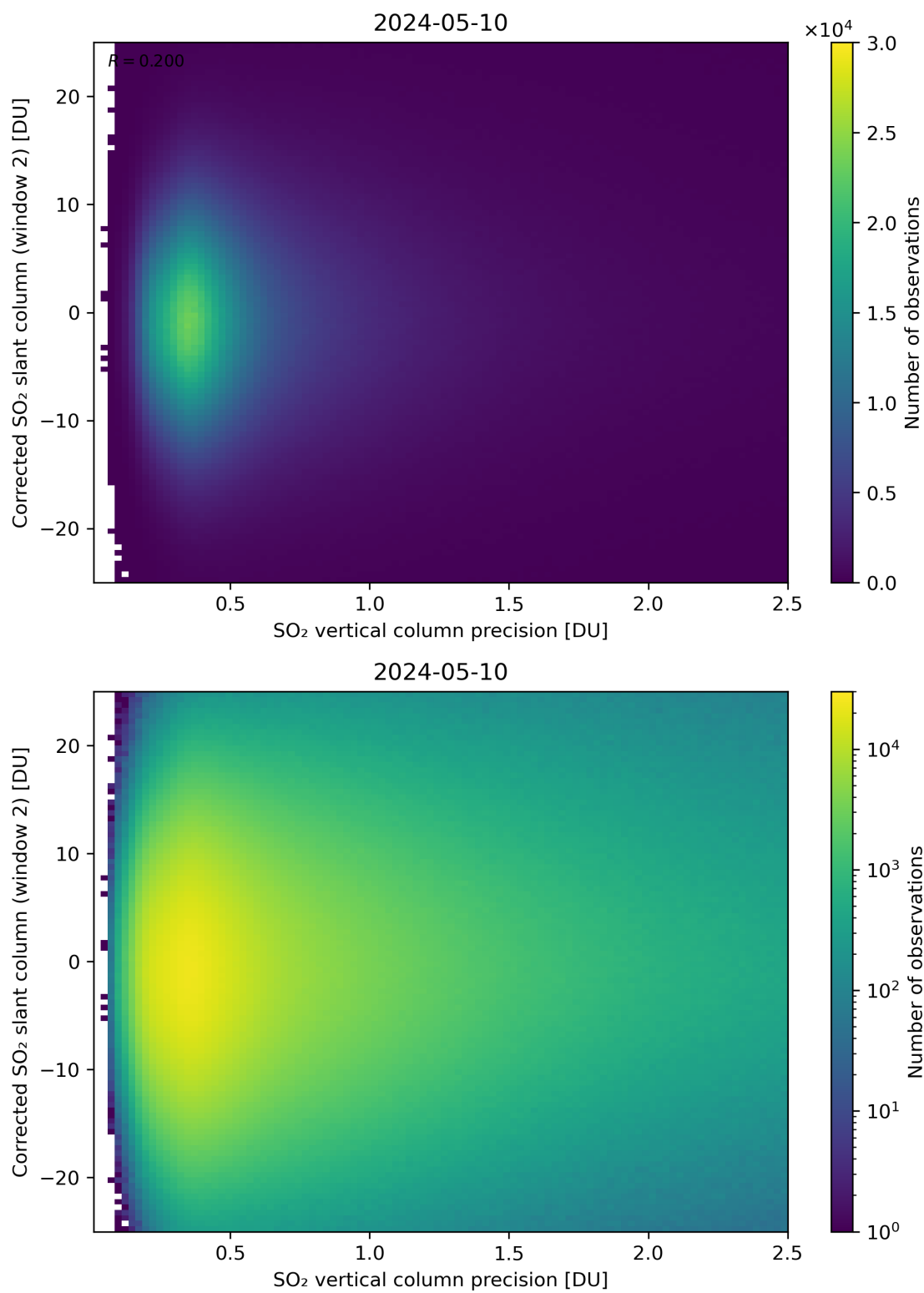
Figure 287: Scatter density plot of “SO 2 vertical column precision” against “Corrected SO 2 slant column (window 2)” for 2024-05-09 to 2024-05-11.
