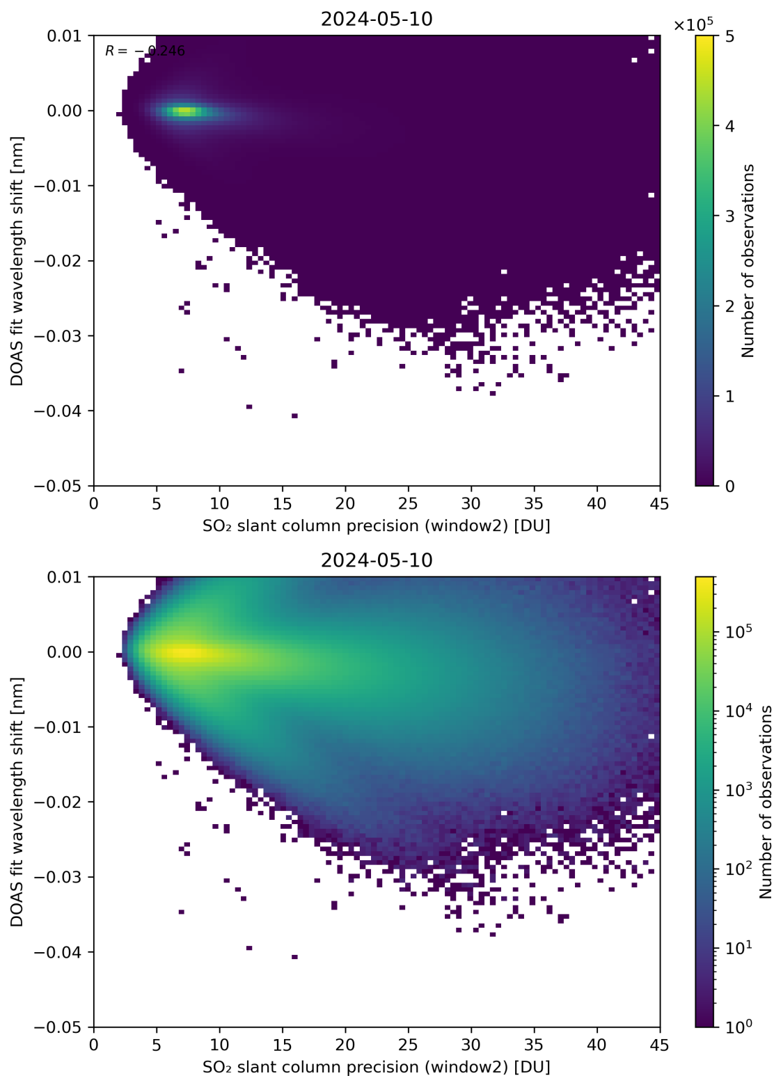
Figure 243: Scatter density plot of “SO 2 slant column precision (window2)” against “DOAS fit wavelength shift” for 2024-05-09 to 2024-05-11.
