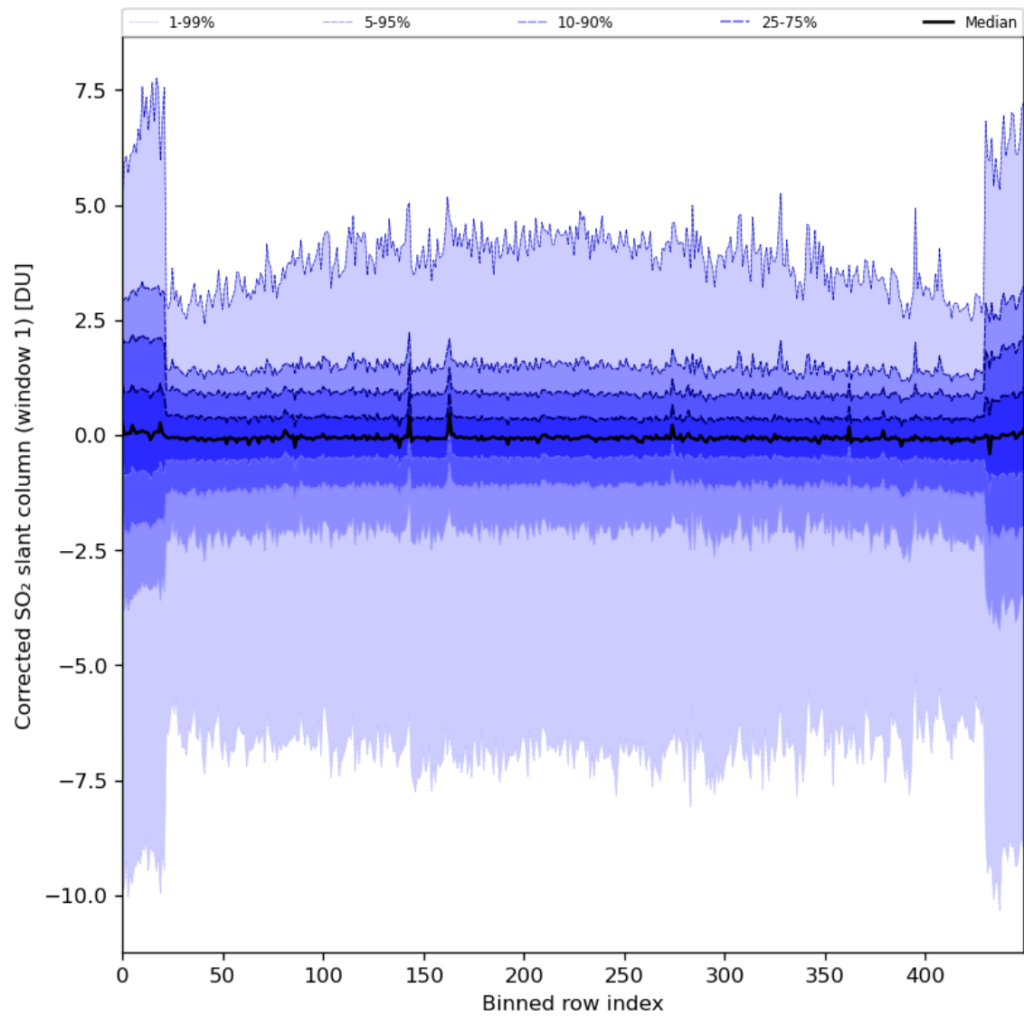
Figure 81: Along track statistics of “Corrected SO 2 slant column (window 1)” for 2024-05-09 to 2024-05-11
