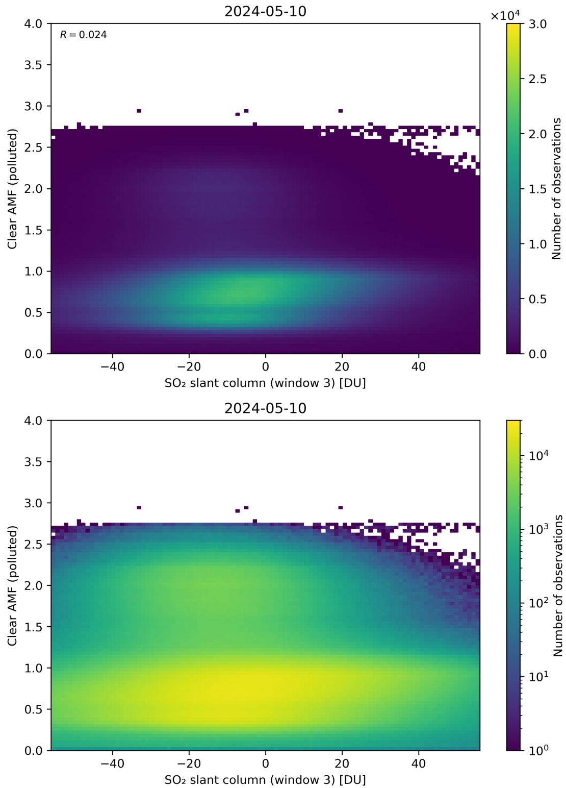
Figure 265: Scatter density plot of “SO 2 slant column (window 3)” against “Clear AMF (polluted)” for 2024-05-09 to 2024-05-11.
