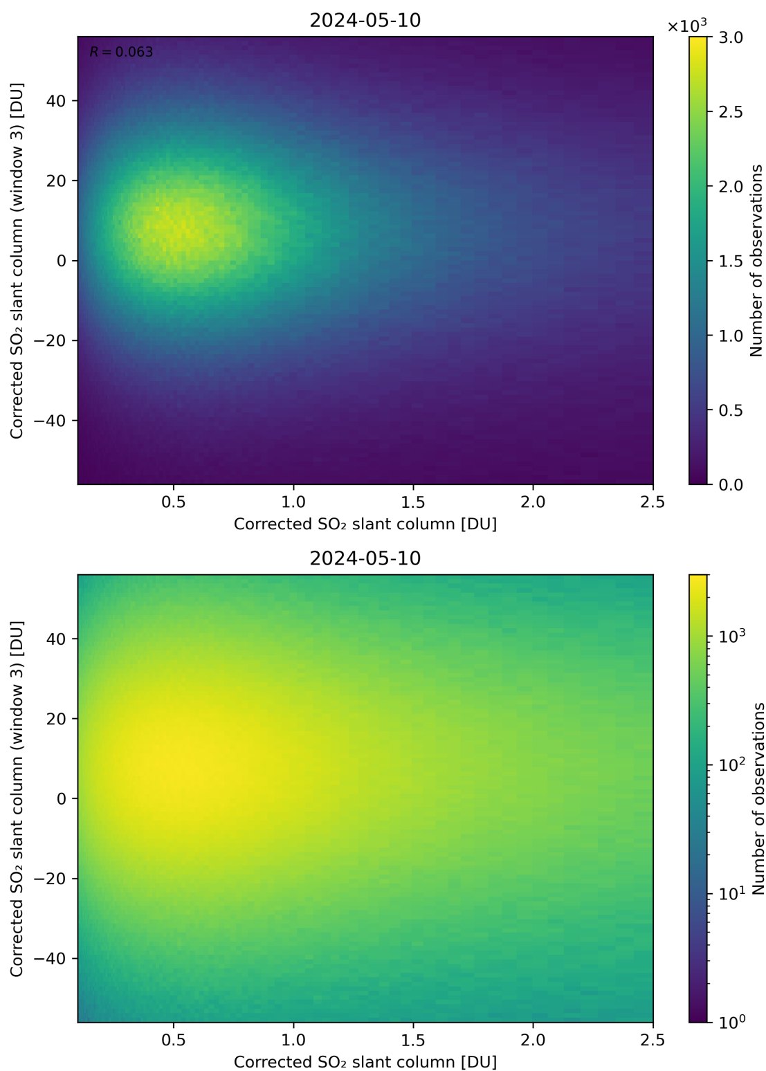
Figure 186: Scatter density plot of “Corrected SO 2 slant column” against “Corrected SO 2 slant column (window 3)” for 2024-05-09 to 2024-05-11.
