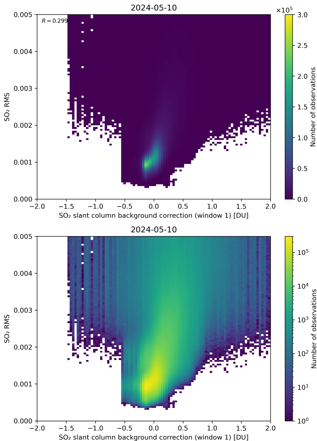
Figure 102: Scatter density plot of “SO 2 slant column background correction (window 1)” against “SO 2 RMS” for 2024-05-09 to 2024-05-11.
