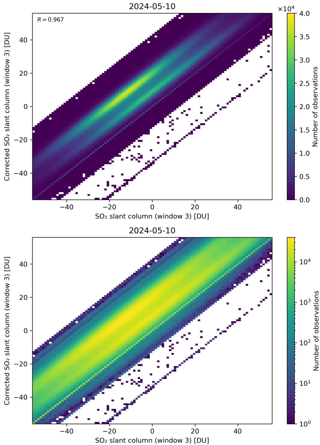
Figure 266: Scatter density plot of “SO 2 slant column (window 3)” against “Corrected SO 2 slant column (window 3)” for 2024-05-09 to 2024-05-11.
