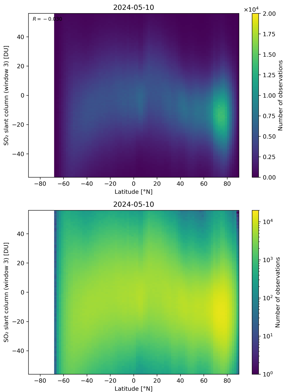
Figure 152: Scatter density plot of “Latitude” against “SO 2 slant column (window 3)” for 2024-05-09 to 2024-05-11.
