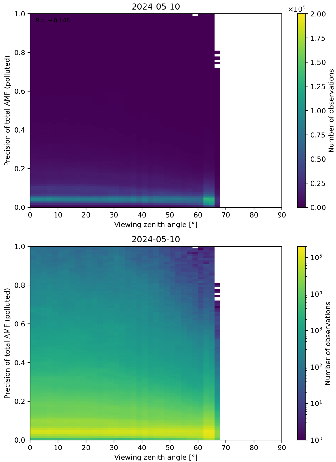
Figure 326: Scatter density plot of “Viewing zenith angle” against “Precision of total AMF (polluted)” for 2024-05-09 to 2024-05-11.
