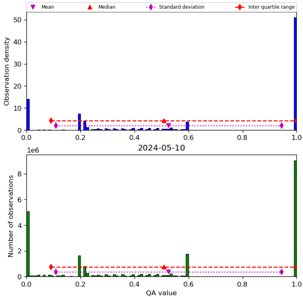
Figure 52: Histogram of “QA value” for 2024-05-09 to 2024-05-11
