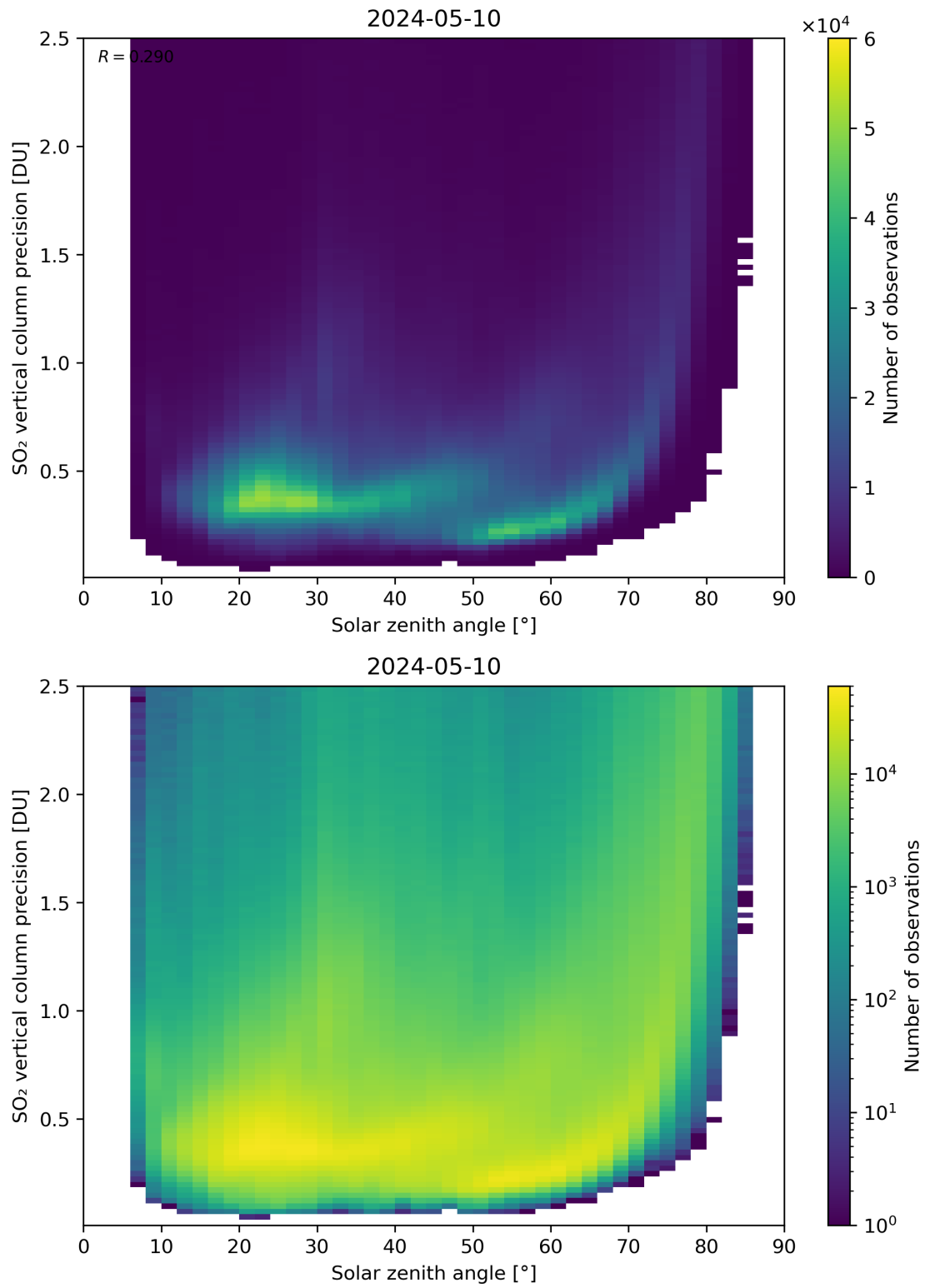
Figure 177: Scatter density plot of “Solar zenith angle” against “SO 2 vertical column precision” for 2024-05-09 to 2024-05-11.
