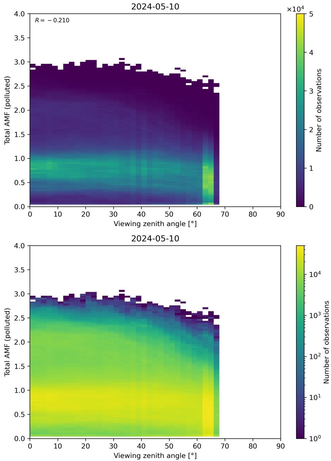
Figure 325: Scatter density plot of “Viewing zenith angle” against “Total AMF (polluted)” for 2024-05-09 to 2024-05-11.
