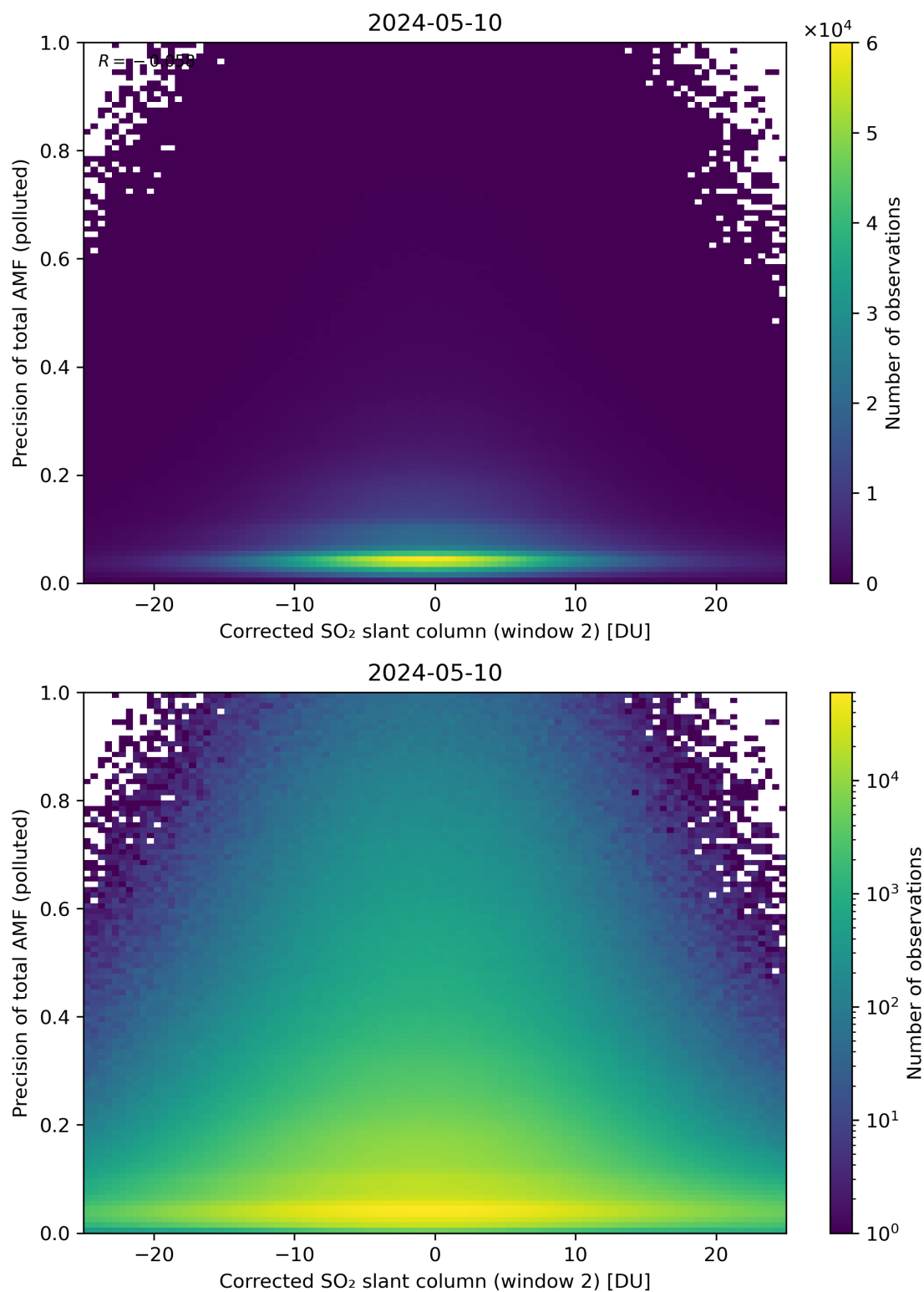
Figure 204: Scatter density plot of “Corrected SO 2 slant column (window 2)” against “Precision of total AMF (polluted)” for 2024-05-09 to 2024-05-11.
