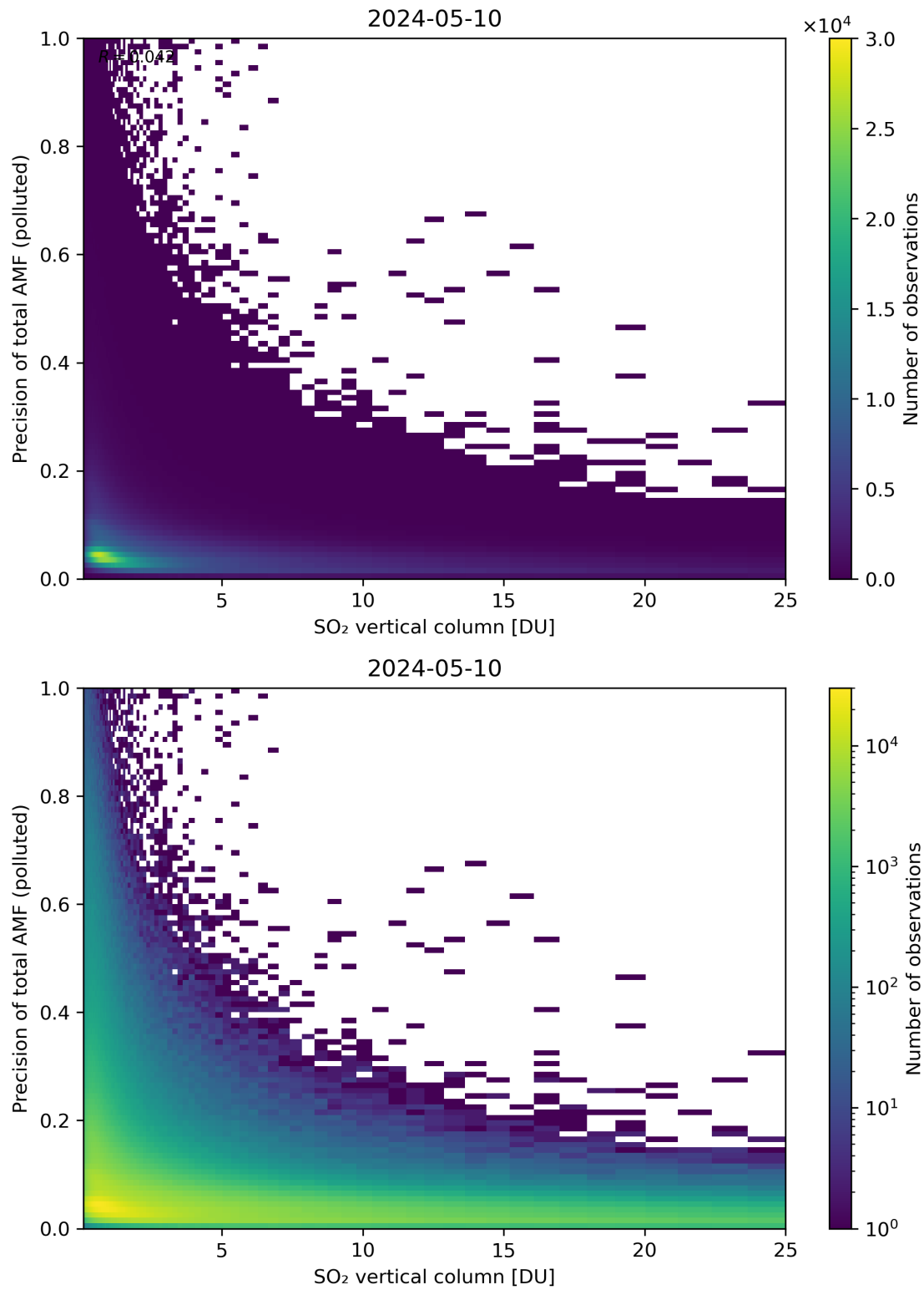
Figure 306: Scatter density plot of “SO 2 vertical column” against “Precision of total AMF (polluted)” for 2024-05-09 to 2024-05-11.
