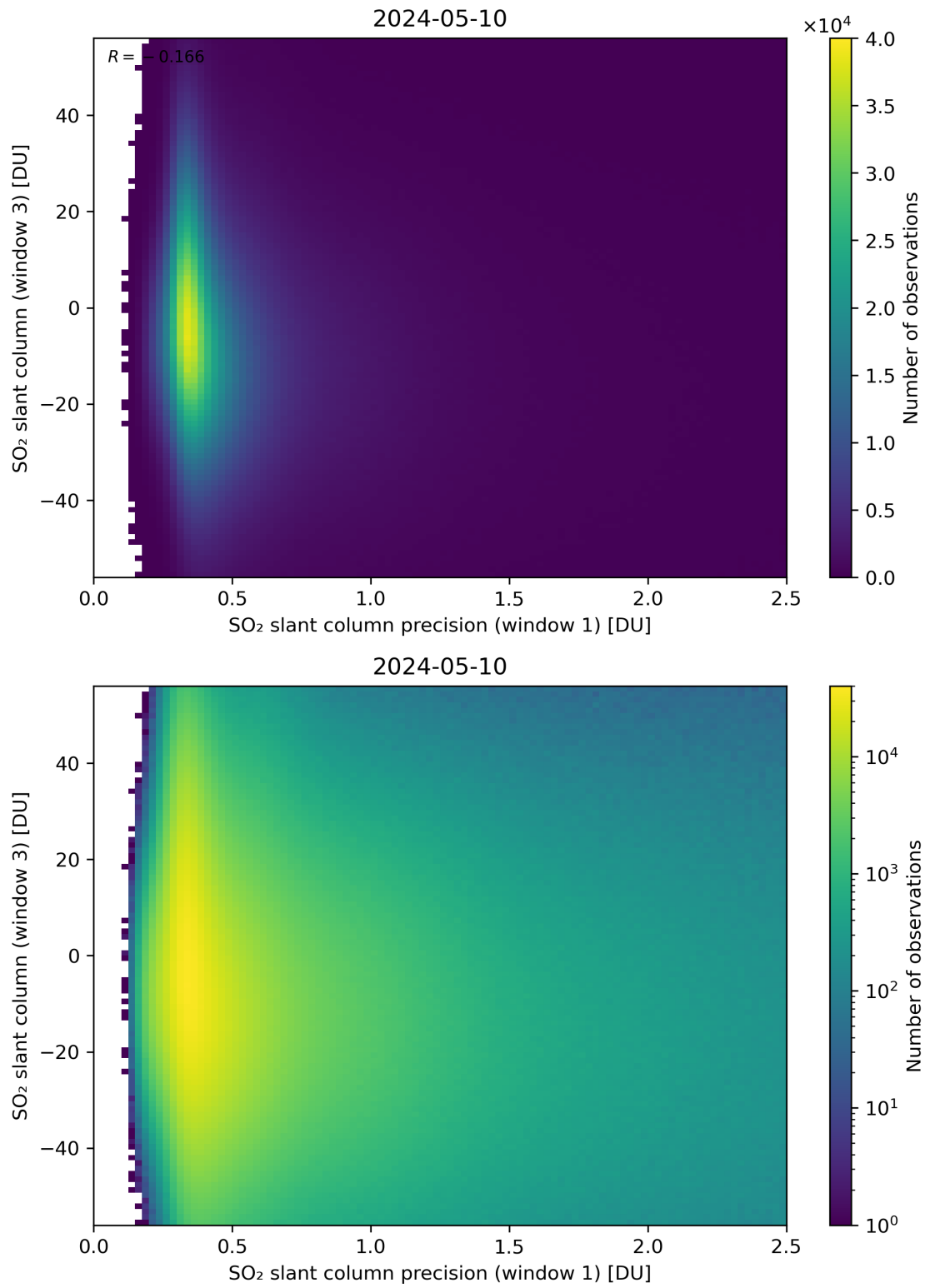
Figure 228: Scatter density plot of “SO 2 slant column precision (window 1)” against “SO 2 slant column (window 3)” for 2024-05-09 to 2024-05-11.
