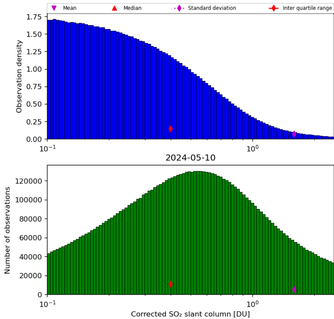
Figure 55: Histogram of “Corrected SO 2 slant column” for 2024-05-09 to 2024-05-11
