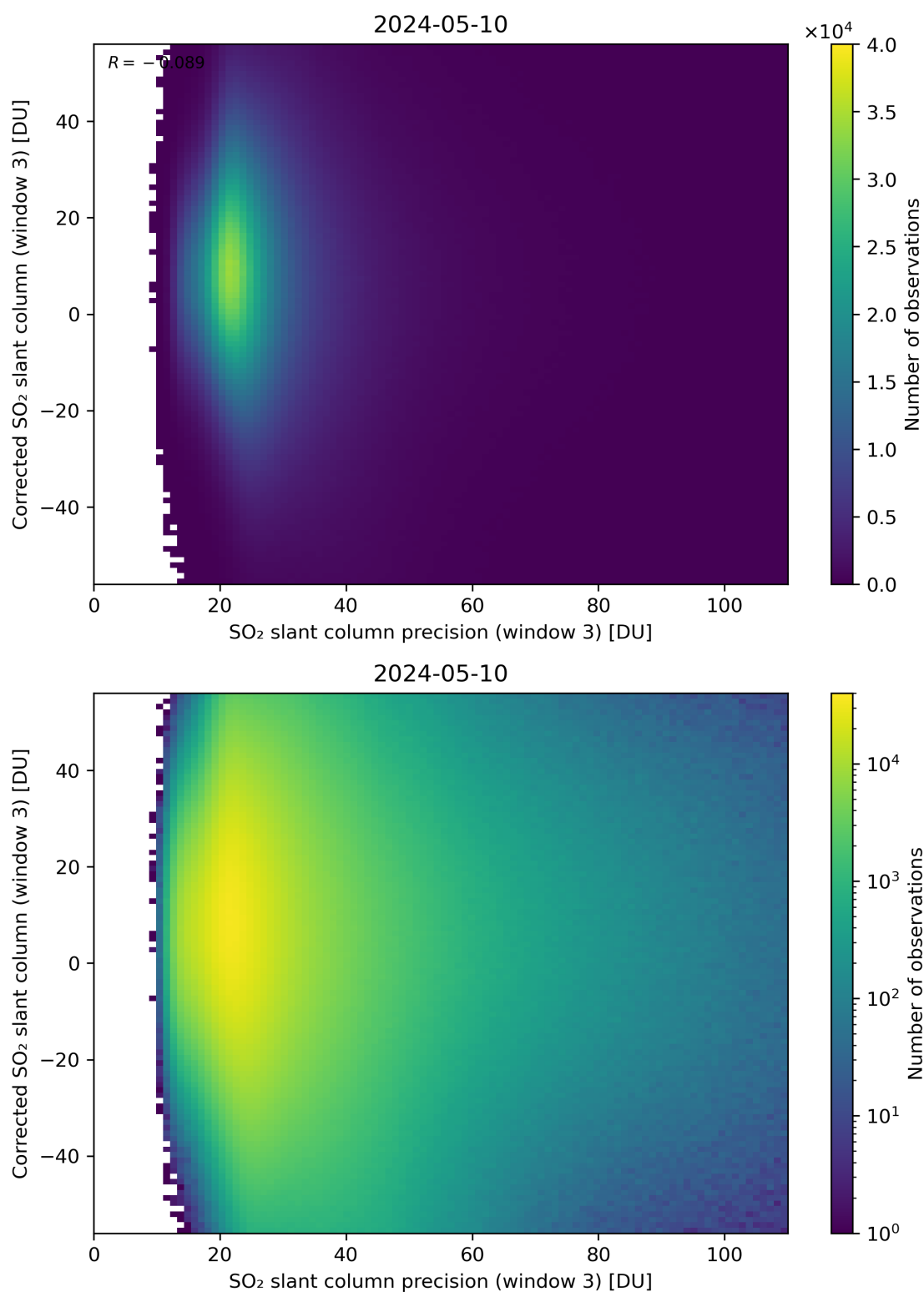
Figure 262: Scatter density plot of “SO 2 slant column precision (window 3)” against “Corrected SO 2 slant column (window 3)” for 2024-05-09 to 2024-05-11.
