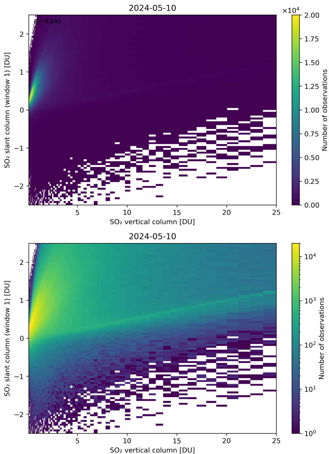
Figure 300: Scatter density plot of “SO 2 vertical column” against “SO 2 slant column (window 1)” for 2024-05-09 to 2024-05-11.
