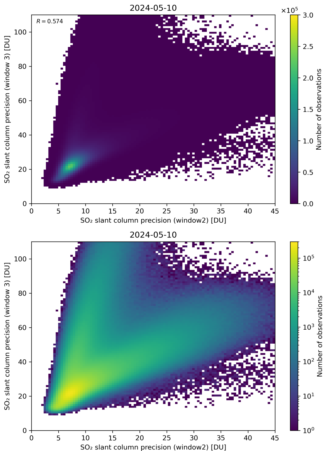
Figure 250: Scatter density plot of “SO 2 slant column precision (window2)” against “SO 2 slant column precision (window 3)” for 2024-05-09 to 2024-05-11.
