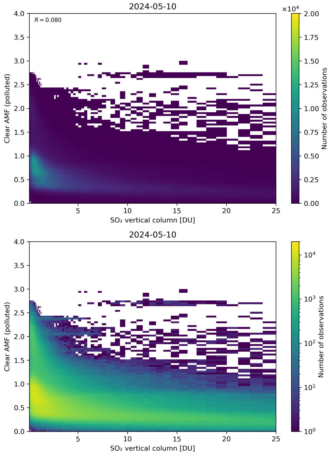
Figure 296: Scatter density plot of “SO 2 vertical column” against “Clear AMF (polluted)” for 2024-05-09 to 2024-05-11.
