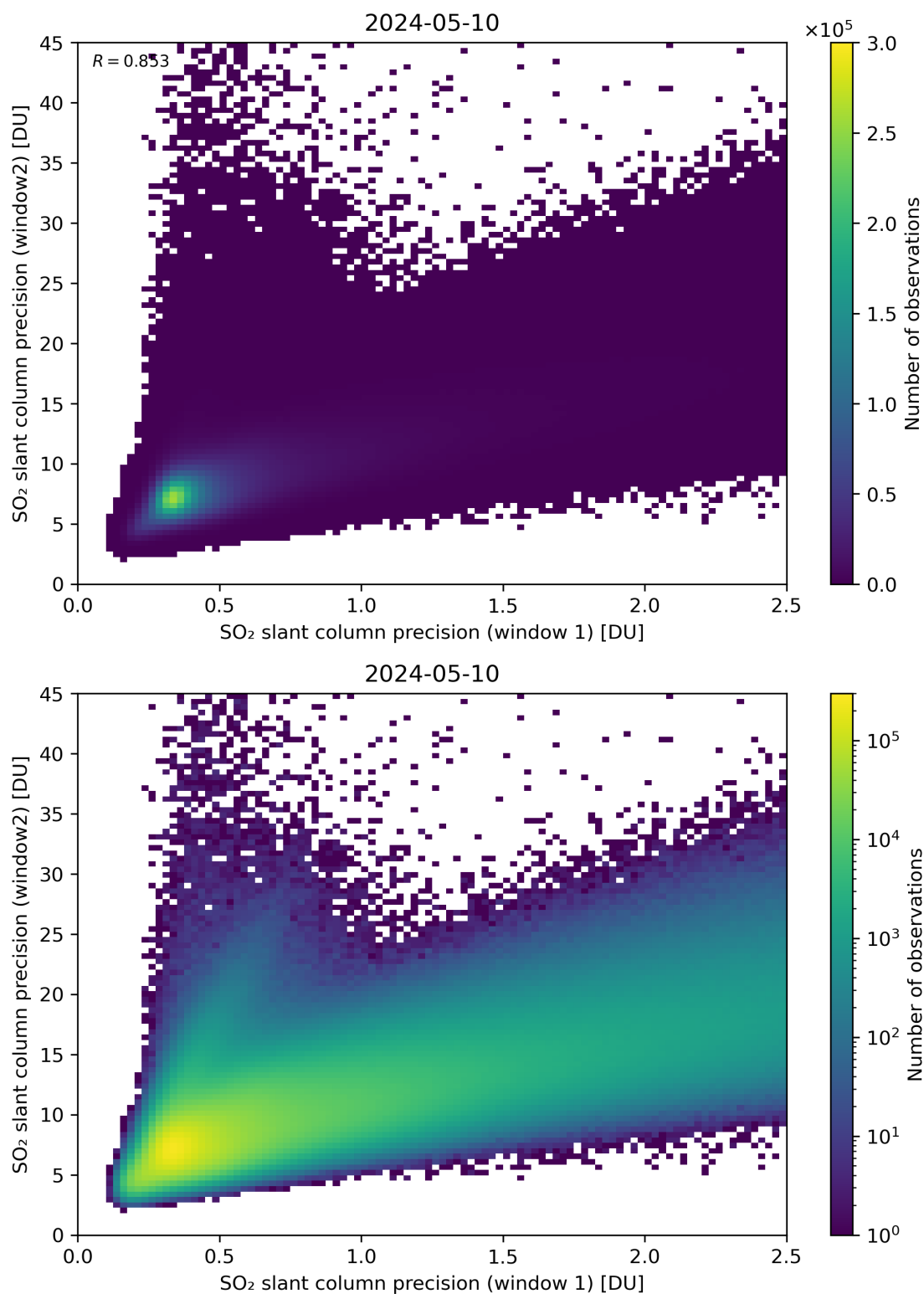
Figure 227: Scatter density plot of “SO 2 slant column precision (window 1)” against “SO 2 slant column precision (window2)” for 2024-05-09 to 2024-05-11.
