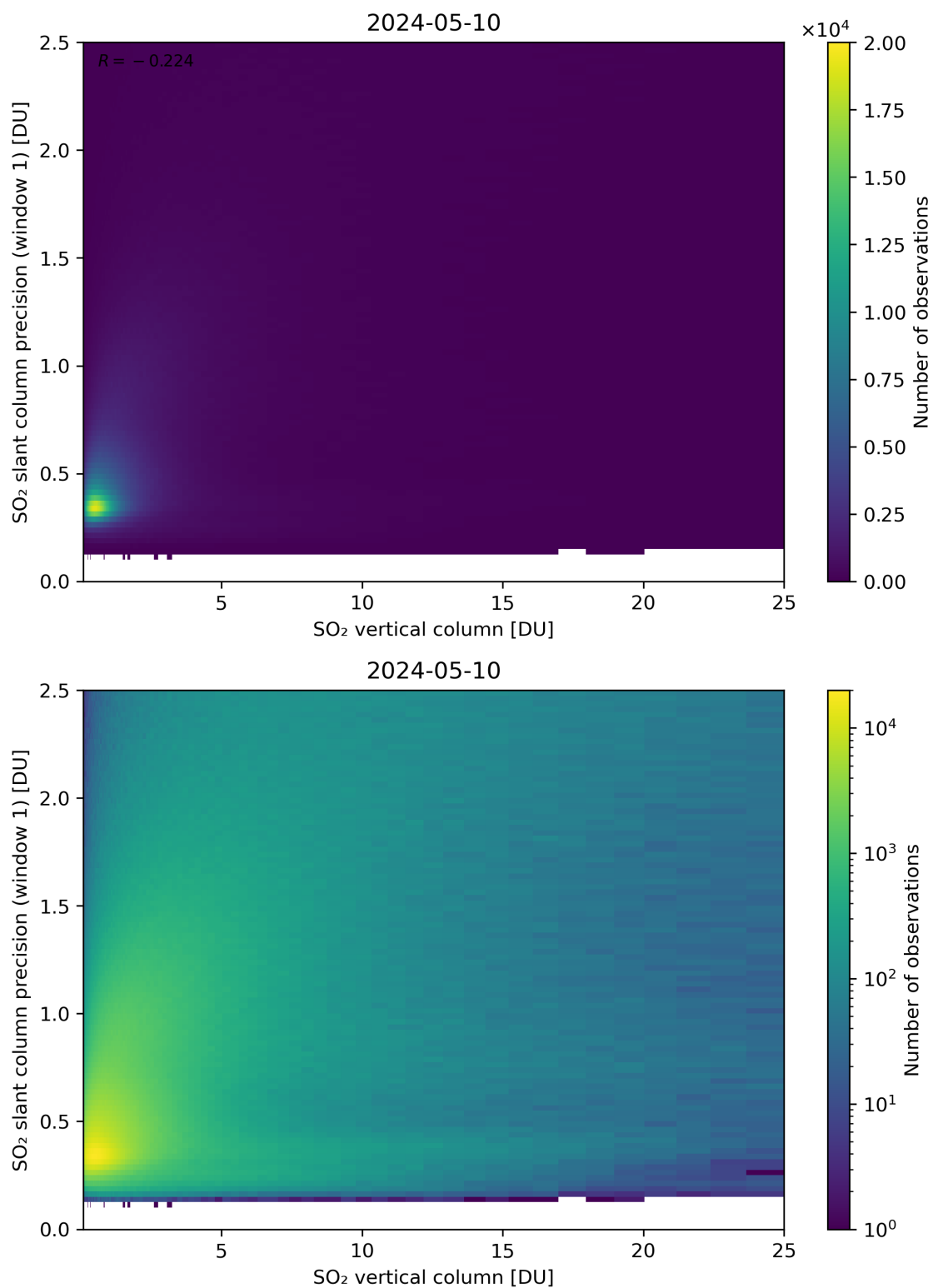
Figure 301: Scatter density plot of “SO 2 vertical column” against “SO 2 slant column precision (window 1)” for 2024-05-09 to 2024-05-11.
