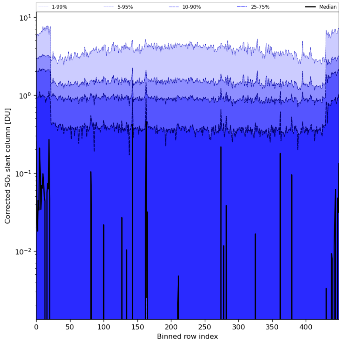
Figure 78: Along track statistics of “Corrected SO 2 slant column” for 2024-05-09 to 2024-05-11
