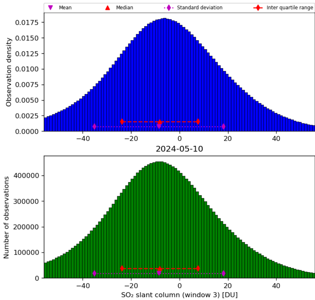
Figure 64: Histogram of “SO 2 slant column (window 3)” for 2024-05-09 to 2024-05-11
