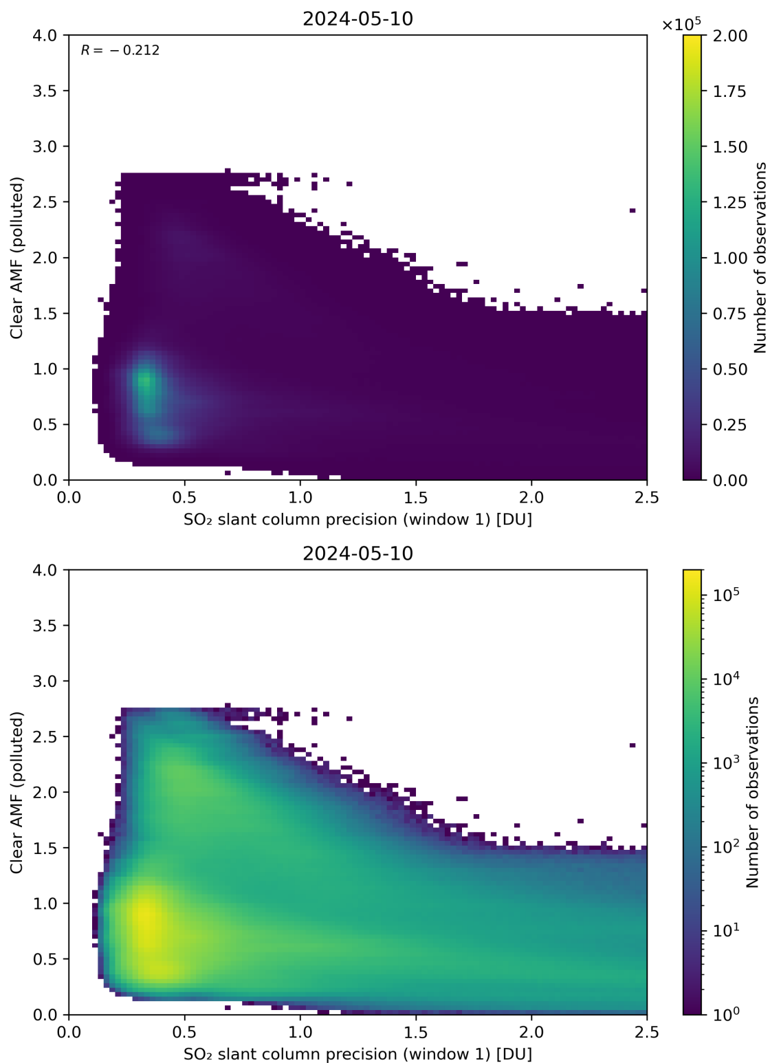
Figure 224: Scatter density plot of “SO 2 slant column precision (window 1)” against “Clear AMF (polluted)” for 2024-05-09 to 2024-05-11.
