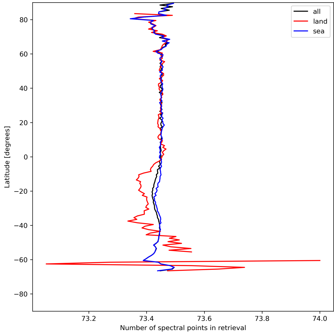
Figure 51: Zonal average of “Number of spectral points in retrieval” for 2024-05-09 to 2024-05-11.
