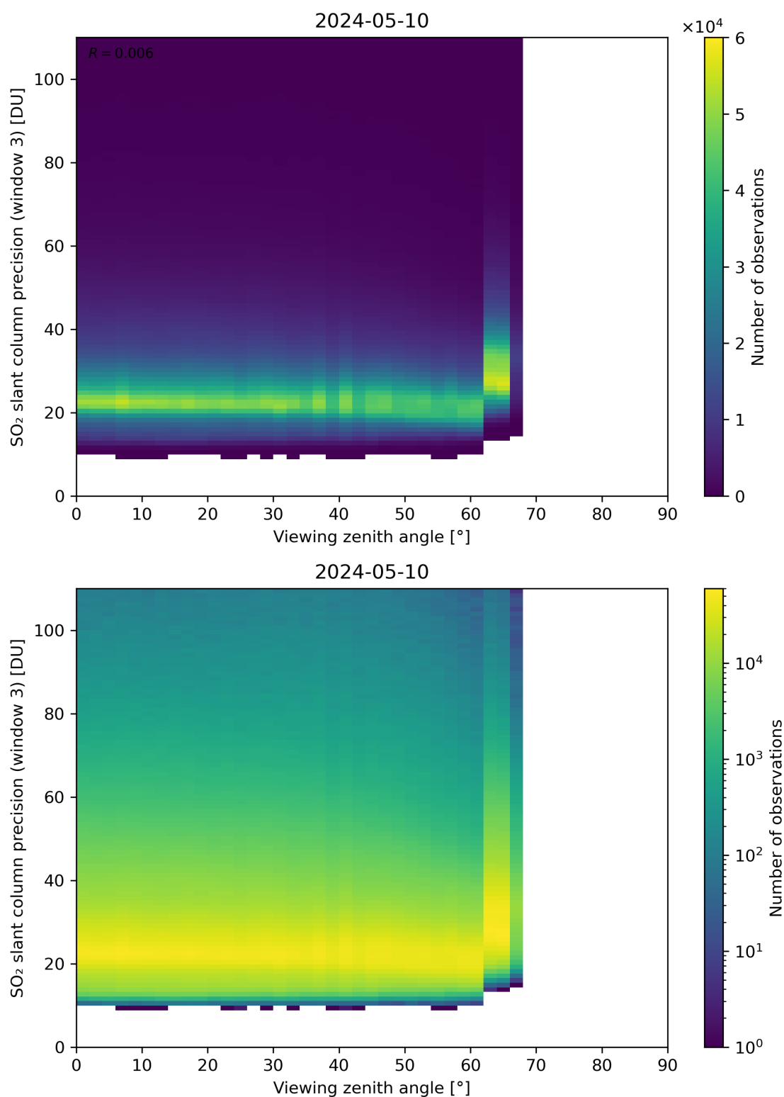
Figure 324: Scatter density plot of “Viewing zenith angle” against “SO 2 slant column precision (window 3)” for 2024-05-09 to 2024-05-11.
