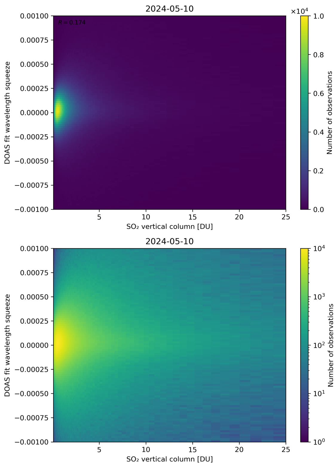
Figure 277: Scatter density plot of “SO 2 vertical column” against “DOAS fit wavelength squeeze” for 2024-05-09 to 2024-05-11.
