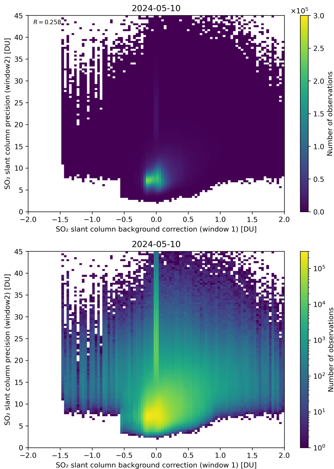
Figure 106: Scatter density plot of “SO 2 slant column background correction (window 1)” against “SO 2 slant column precision (window2)” for 2024-05-09 to 2024-05-11.
