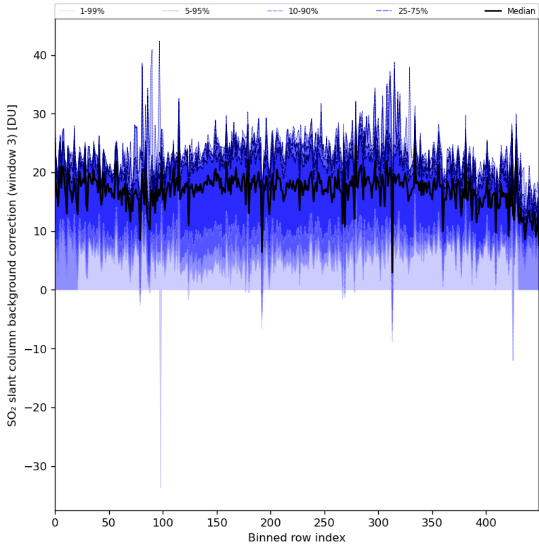
Figure 90: Along track statistics of “SO 2 slant column background correction (window 3)” for 2024-05-09 to 2024-05-11
