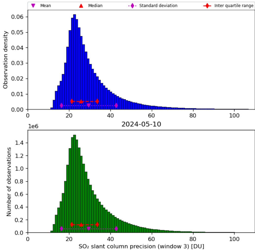
Figure 65: Histogram of “SO 2 slant column precision (window 3)” for 2024-05-09 to 2024-05-11
