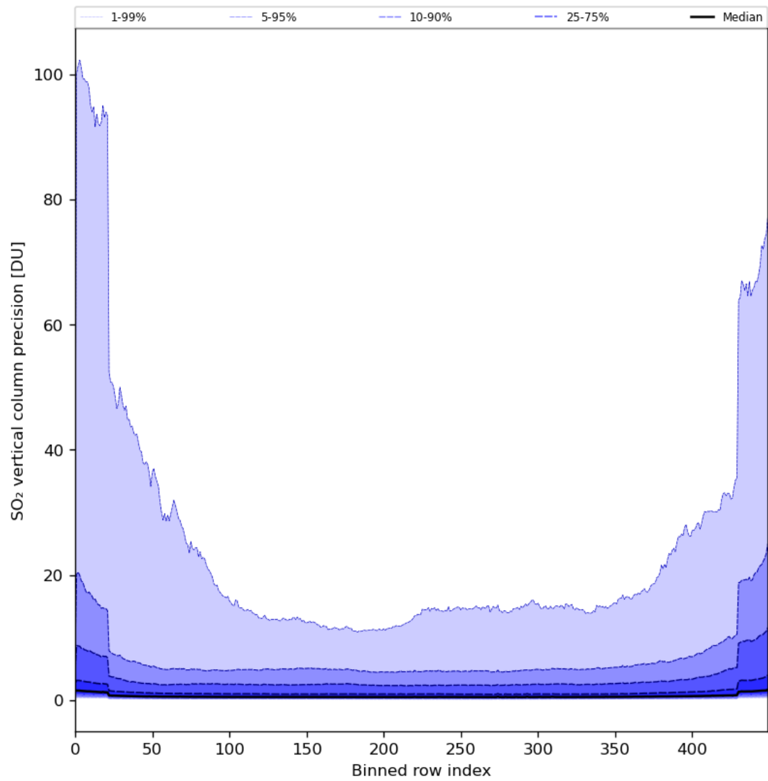
Figure 77: Along track statistics of “SO 2 vertical column precision” for 2024-05-09 to 2024-05-11
