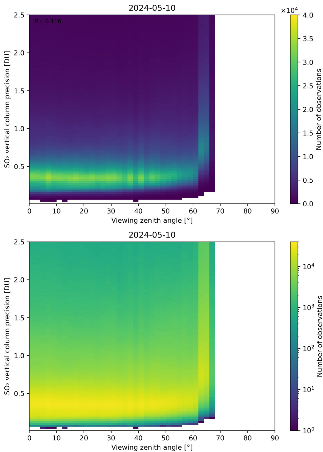
Figure 328: Scatter density plot of “Viewing zenith angle” against “SO 2 vertical column precision” for 2024-05-09 to 2024-05-11.
