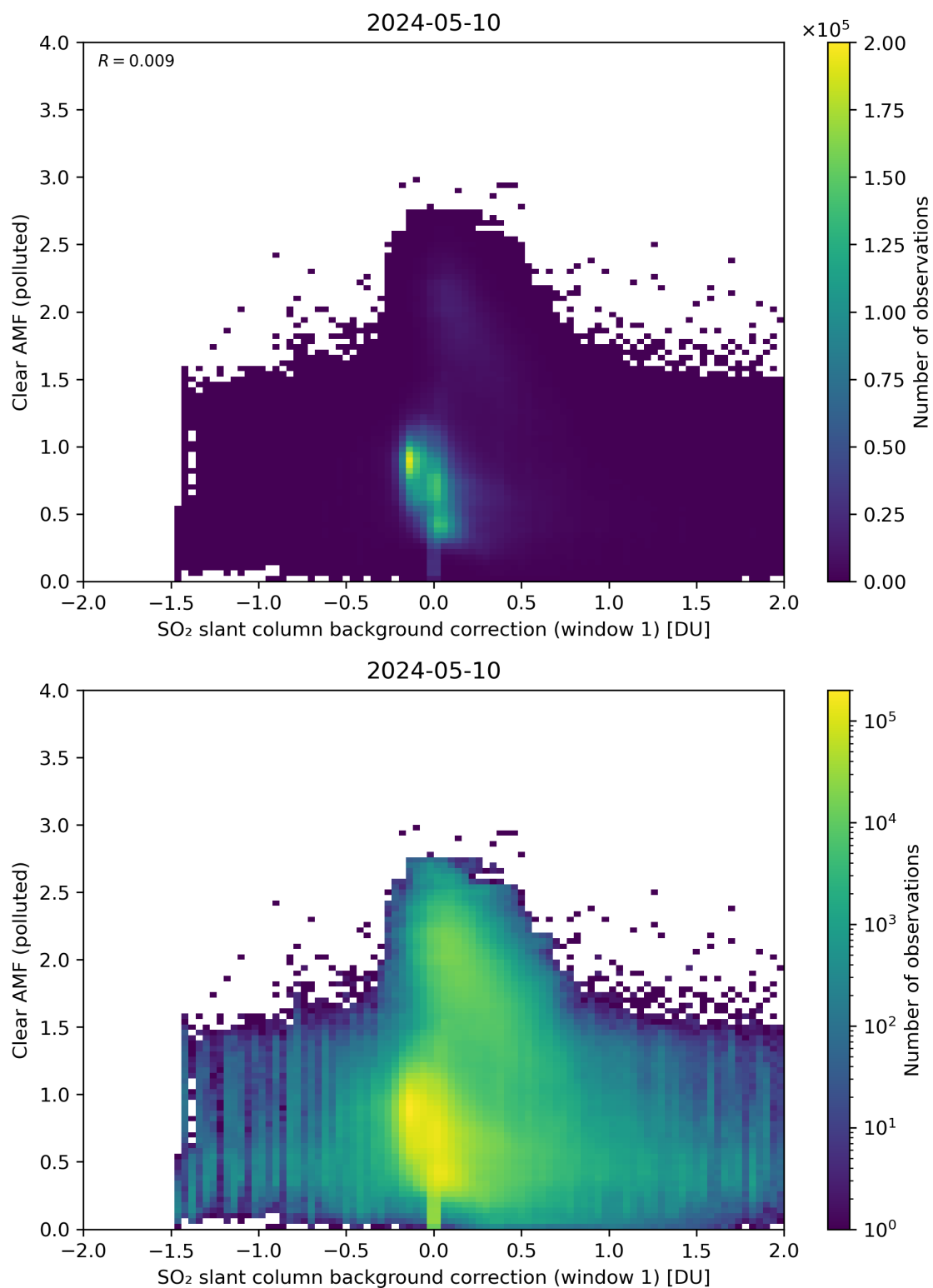
Figure 103: Scatter density plot of “SO 2 slant column background correction (window 1)” against “Clear AMF (polluted)” for 2024-05-09 to 2024-05-11.
