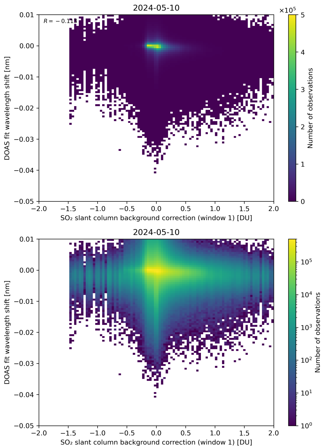
Figure 100: Scatter density plot of “SO 2 slant column background correction (window 1)” against “DOAS fit wavelength shift” for 2024-05-09 to 2024-05-11.
