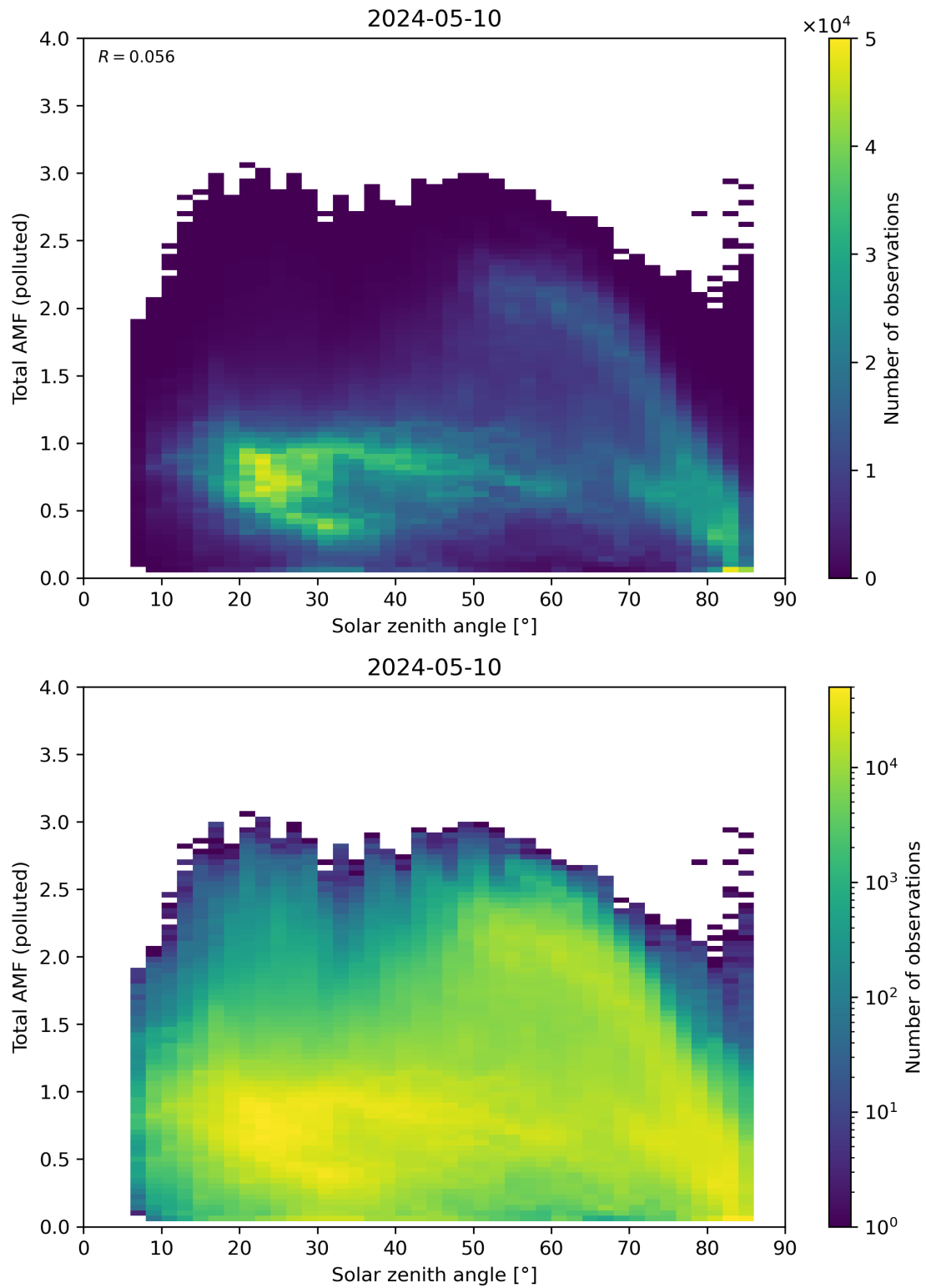
Figure 174: Scatter density plot of “Solar zenith angle” against “Total AMF (polluted)” for 2024-05-09 to 2024-05-11.
