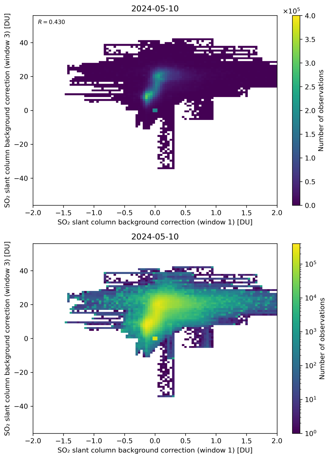
Figure 99: Scatter density plot of “SO 2 slant column background correction (window 1)” against “SO 2 slant column background correction (window 3)” for 2024-05-09 to 2024-05-11.
