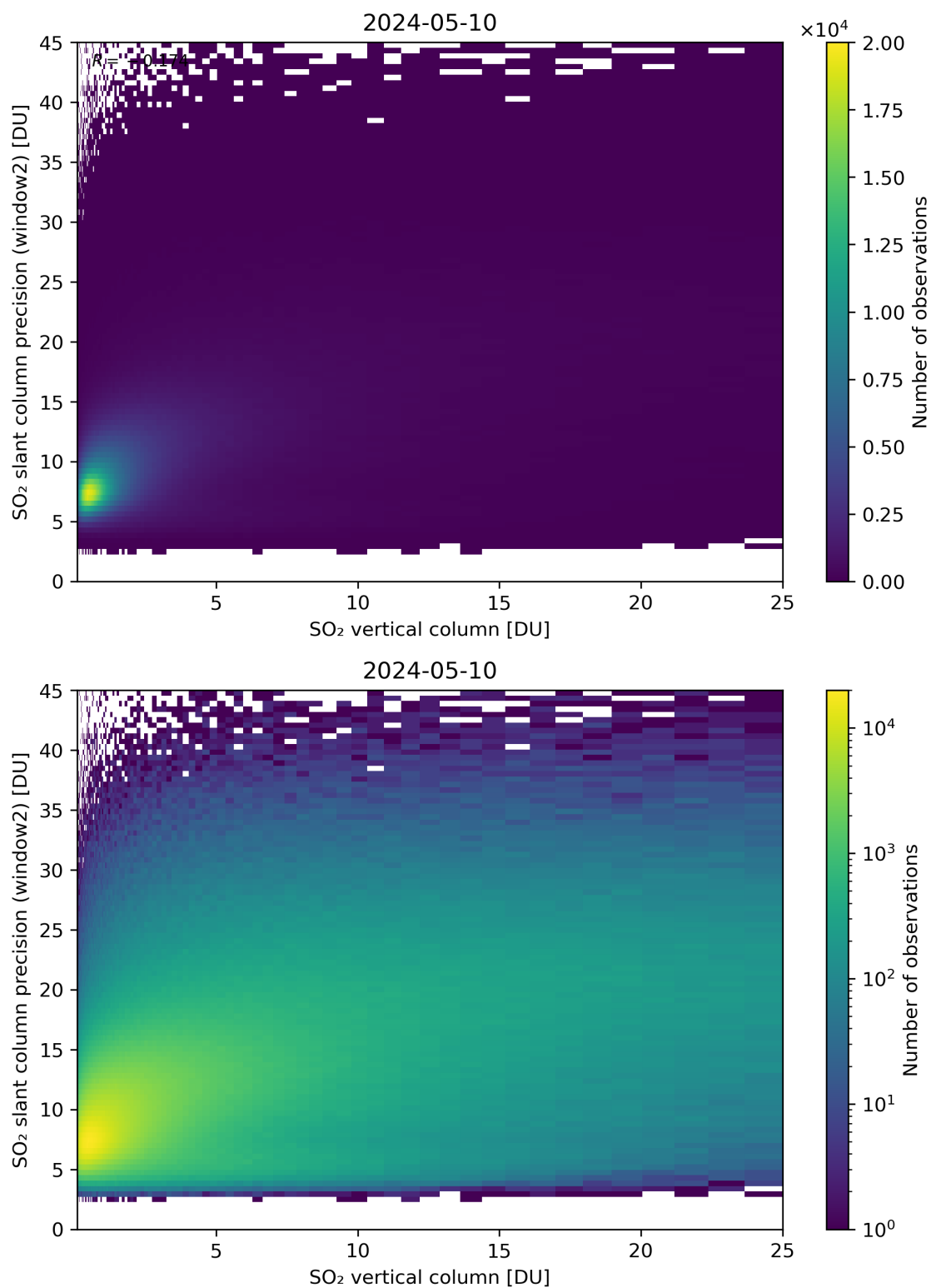
Figure 302: Scatter density plot of “SO 2 vertical column” against “SO 2 slant column precision (window2)” for 2024-05-09 to 2024-05-11.
