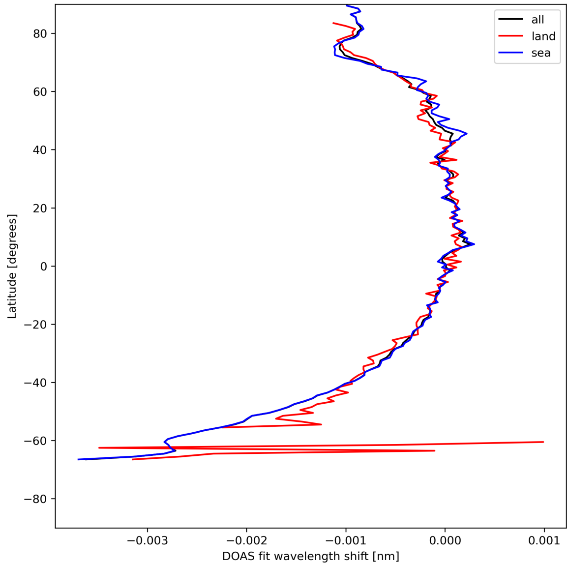
Figure 45: Zonal average of “DOAS fit wavelength shift” for 2024-05-09 to 2024-05-11.
