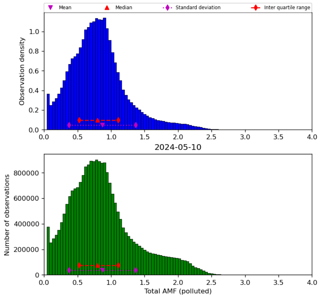
Figure 71: Histogram of “Total AMF (polluted)” for 2024-05-09 to 2024-05-11
