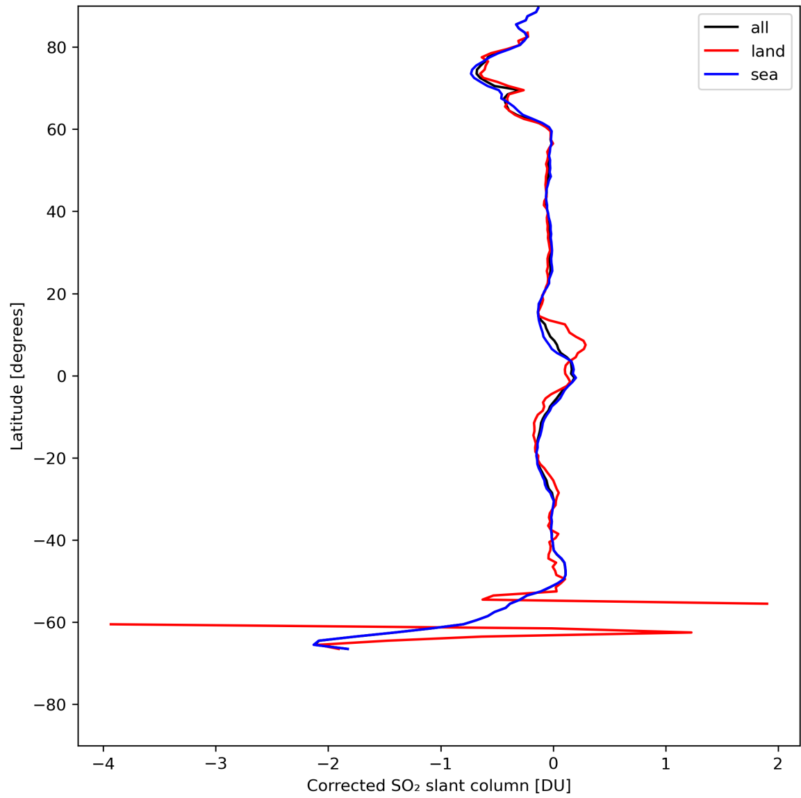
Figure 32: Zonal average of "Corrected SO 2 slant column" for 2024-05-09 to 2024-05-11.
