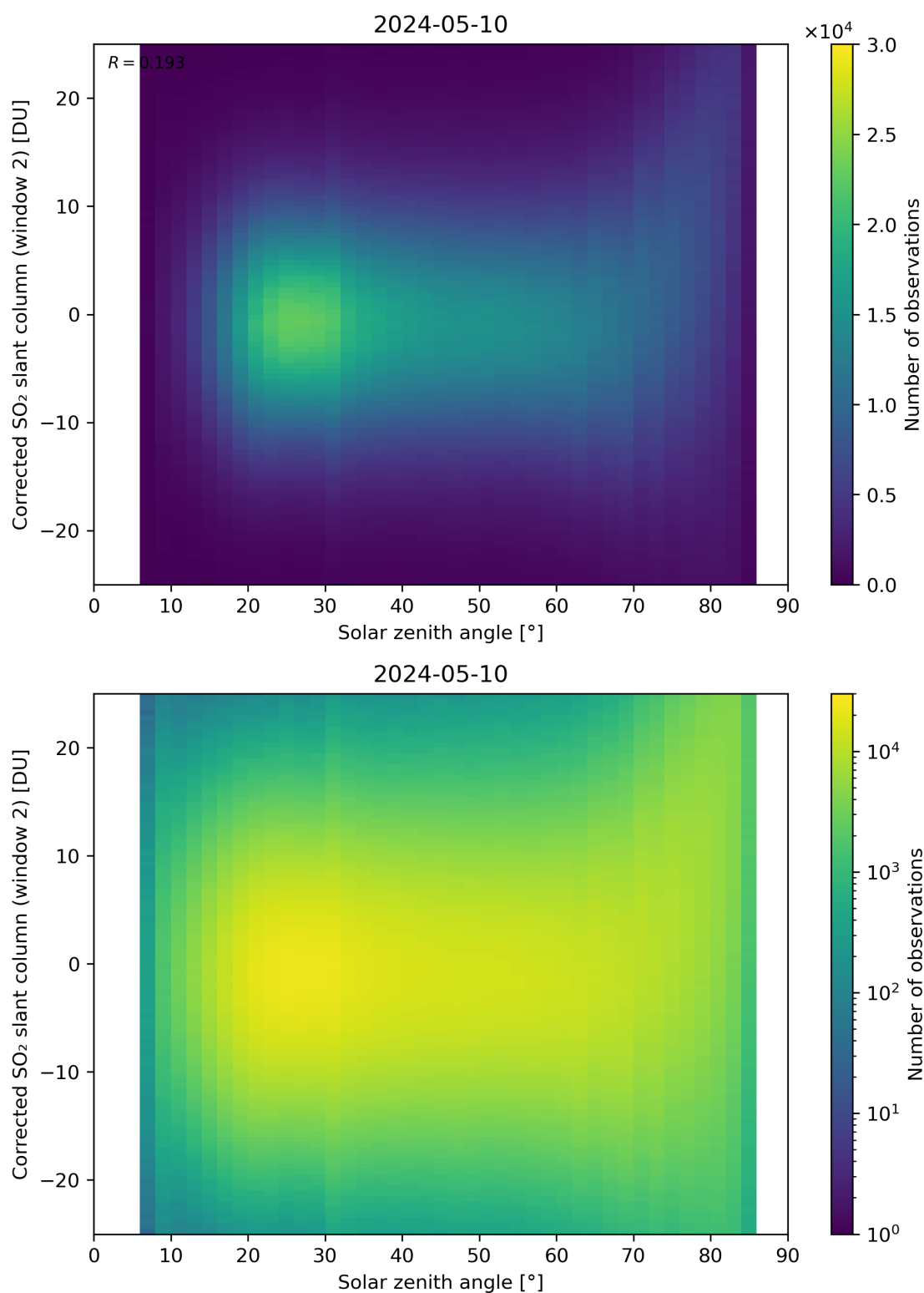
Figure 167: Scatter density plot of “Solar zenith angle” against “Corrected SO 2 slant column (window 2)” for 2024-05-09 to 2024-05-11.
