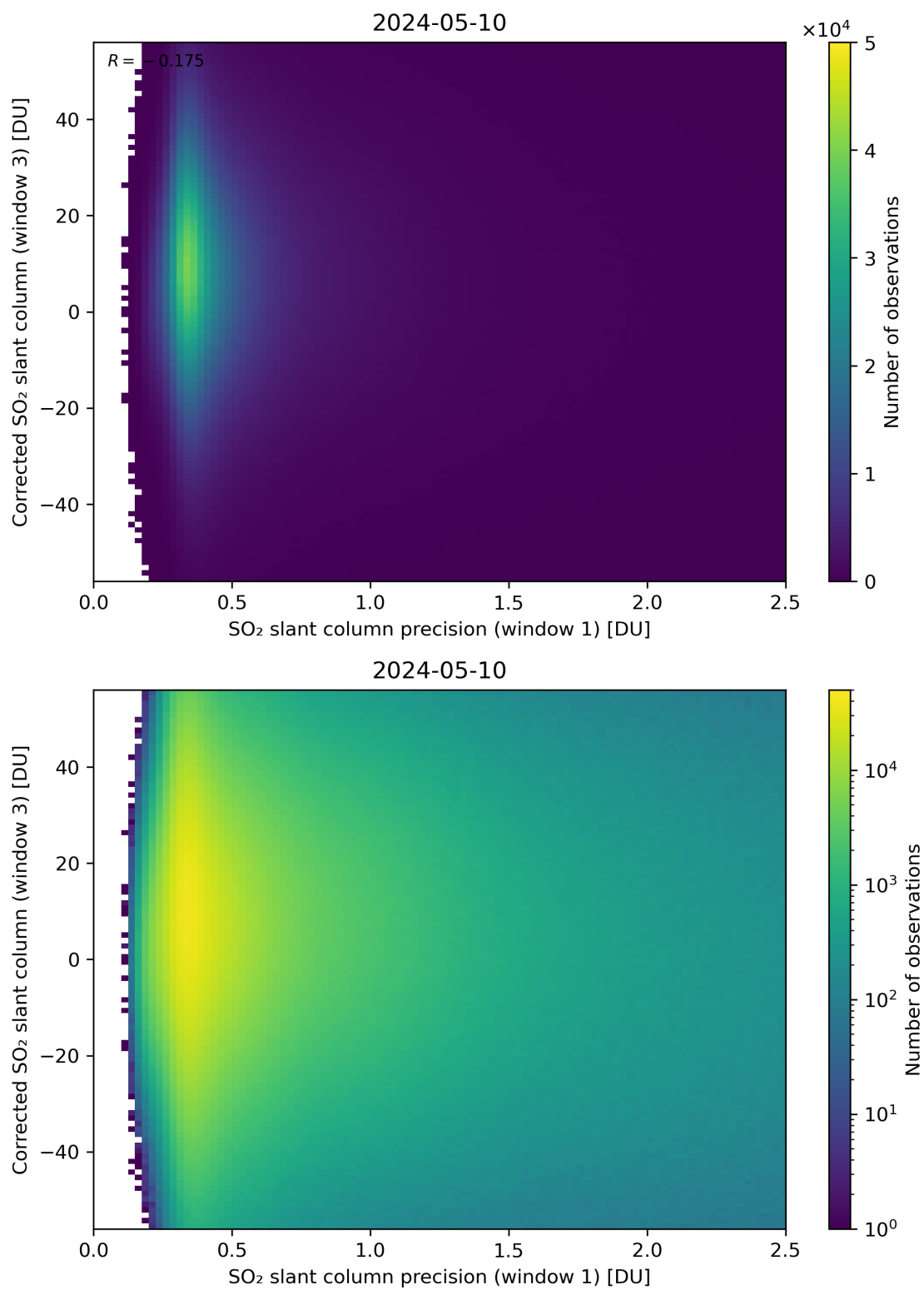
Figure 226: Scatter density plot of “SO 2 slant column precision (window 1)” against “Corrected SO 2 slant column (window 3)” for 2024-05-09 to 2024-05-11.
