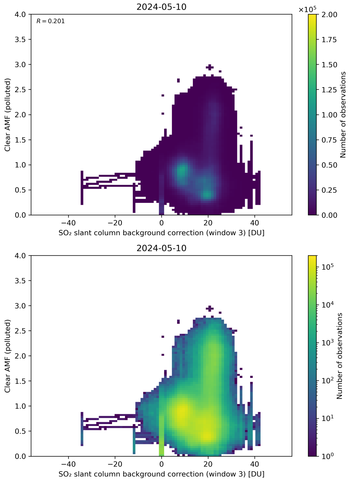
Figure 124: Scatter density plot of “SO 2 slant column background correction (window 3)” against “Clear AMF (polluted)” for 2024-05-09 to 2024-05-11.
