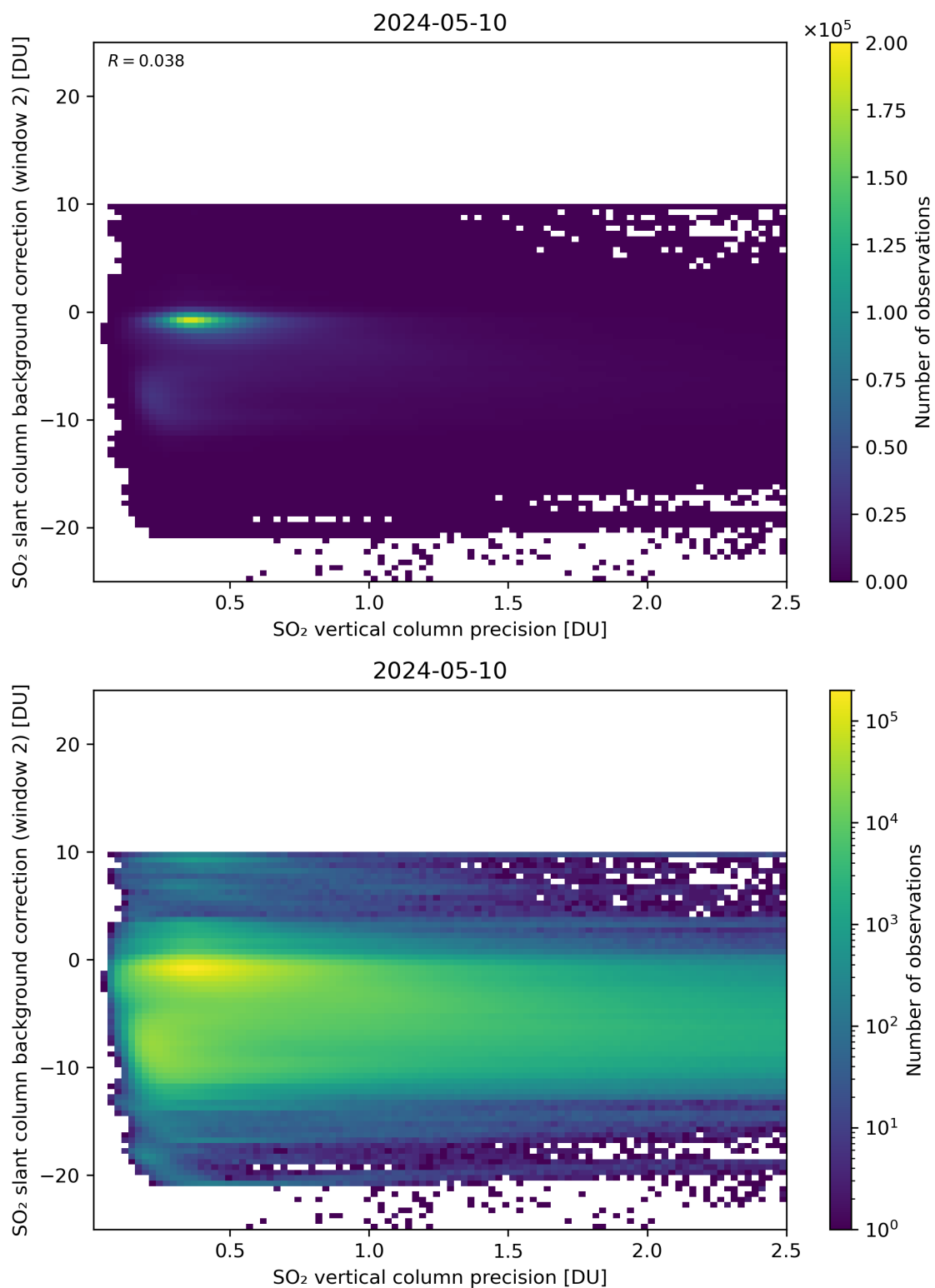
Figure 280: Scatter density plot of “SO 2 vertical column precision” against “SO 2 slant column background correction (window 2)” for 2024-05-09 to 2024-05-11.
