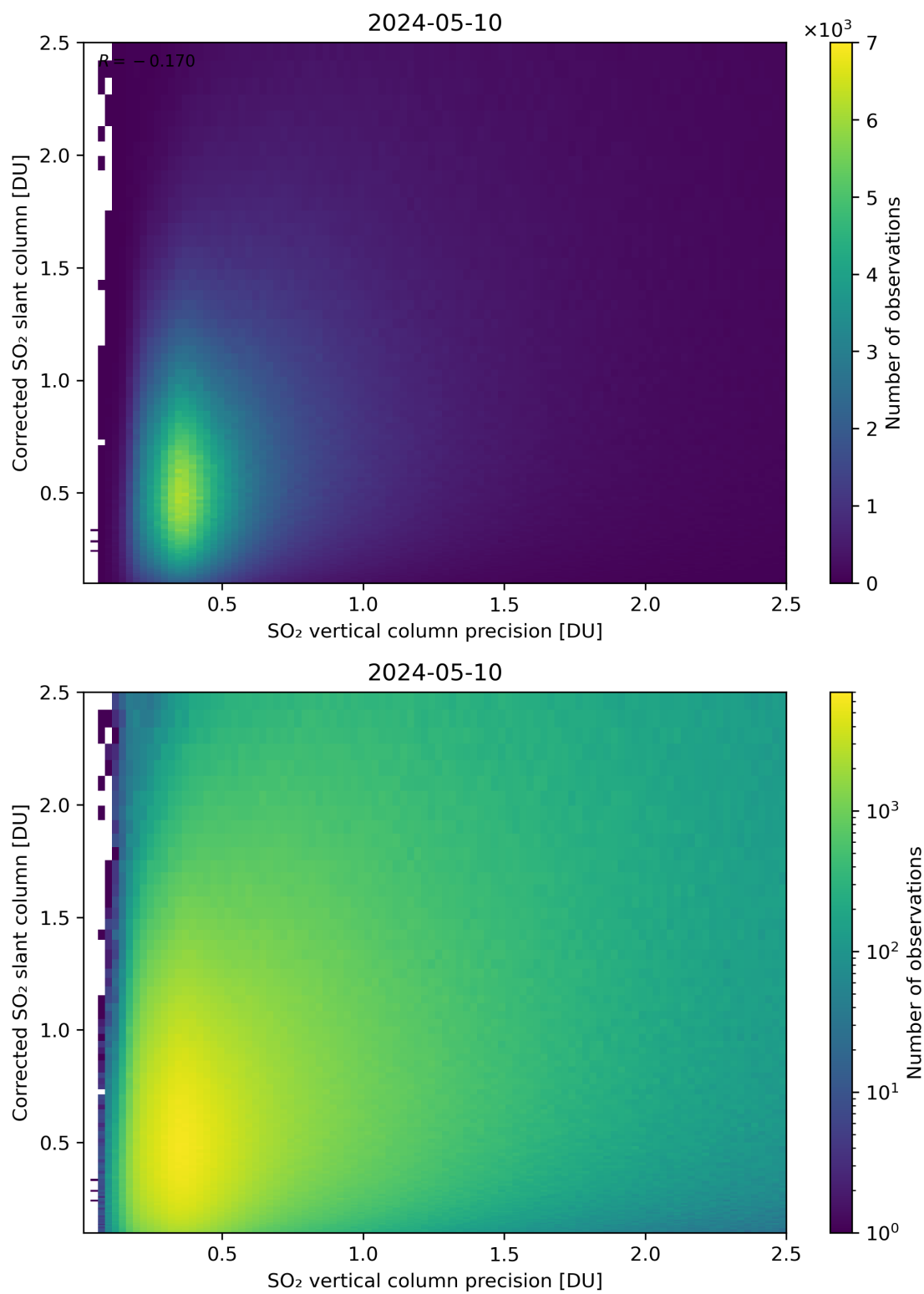
Figure 286: Scatter density plot of “SO 2 vertical column precision” against “Corrected SO 2 slant column” for 2024-05-09 to 2024-05-11.
