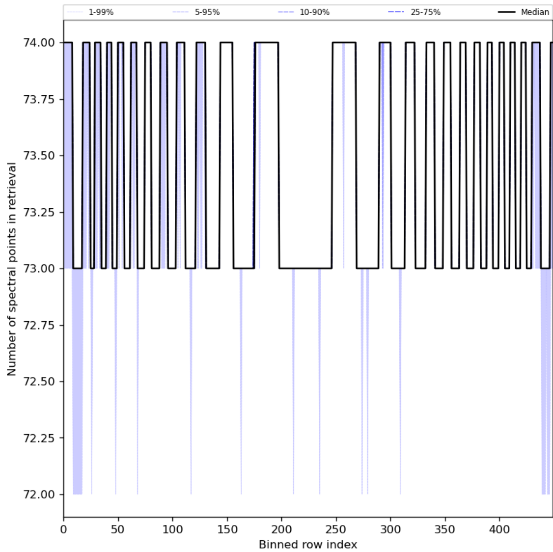
Figure 97: Along track statistics of “Number of spectral points in retrieval” for 2024-05-09 to 2024-05-11
