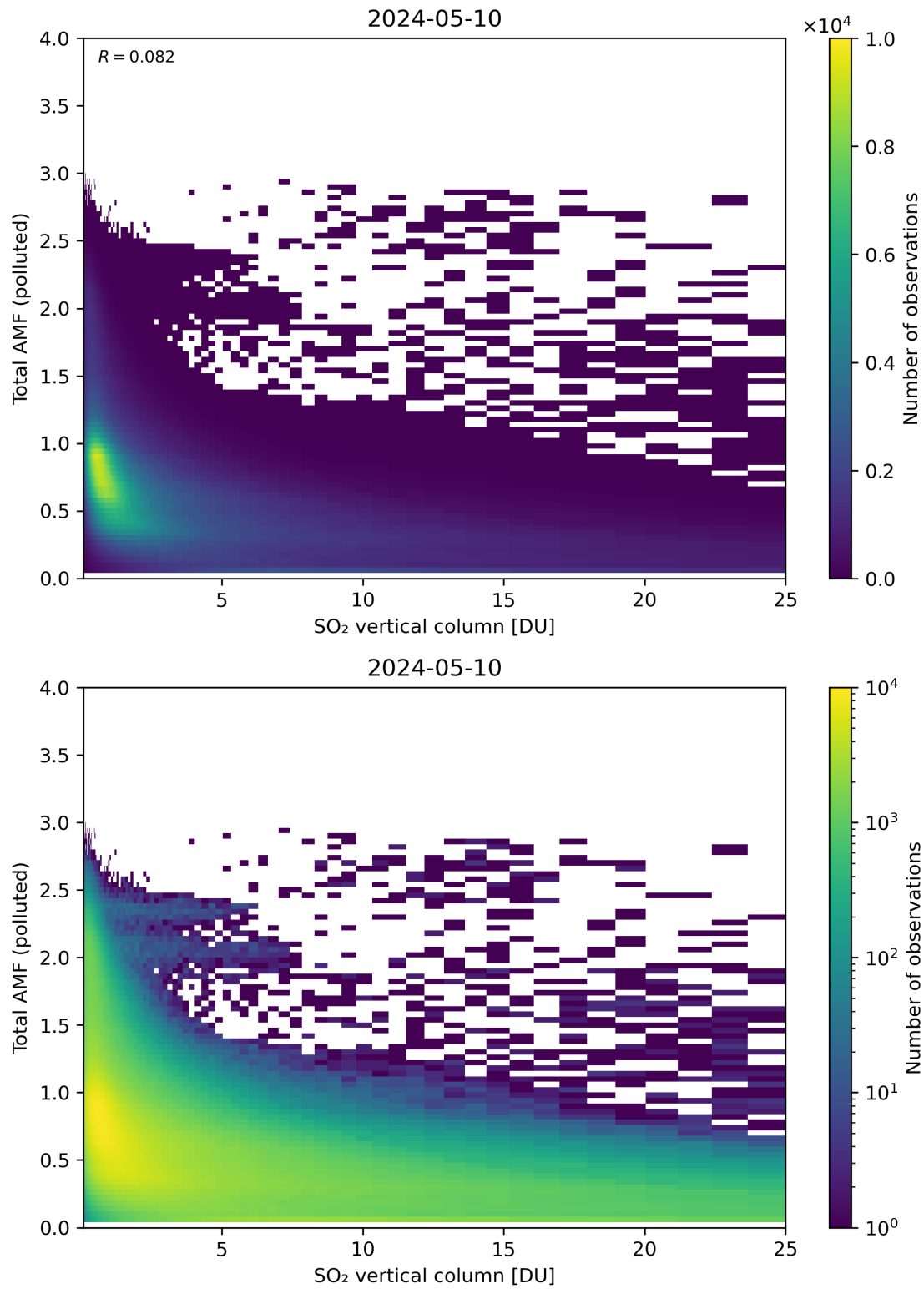
Figure 305: Scatter density plot of “SO 2 vertical column” against “Total AMF (polluted)” for 2024-05-09 to 2024-05-11.
