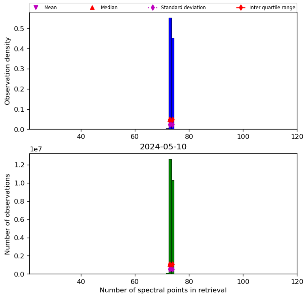
Figure 74: Histogram of “Number of spectral points in retrieval” for 2024-05-09 to 2024-05-11
