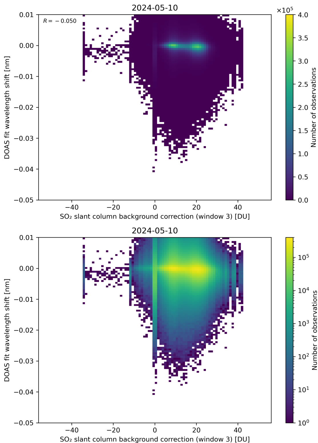
Figure 121: Scatter density plot of “SO 2 slant column background correction (window 3)” against “DOAS fit wavelength shift” for 2024-05-09 to 2024-05-11.
