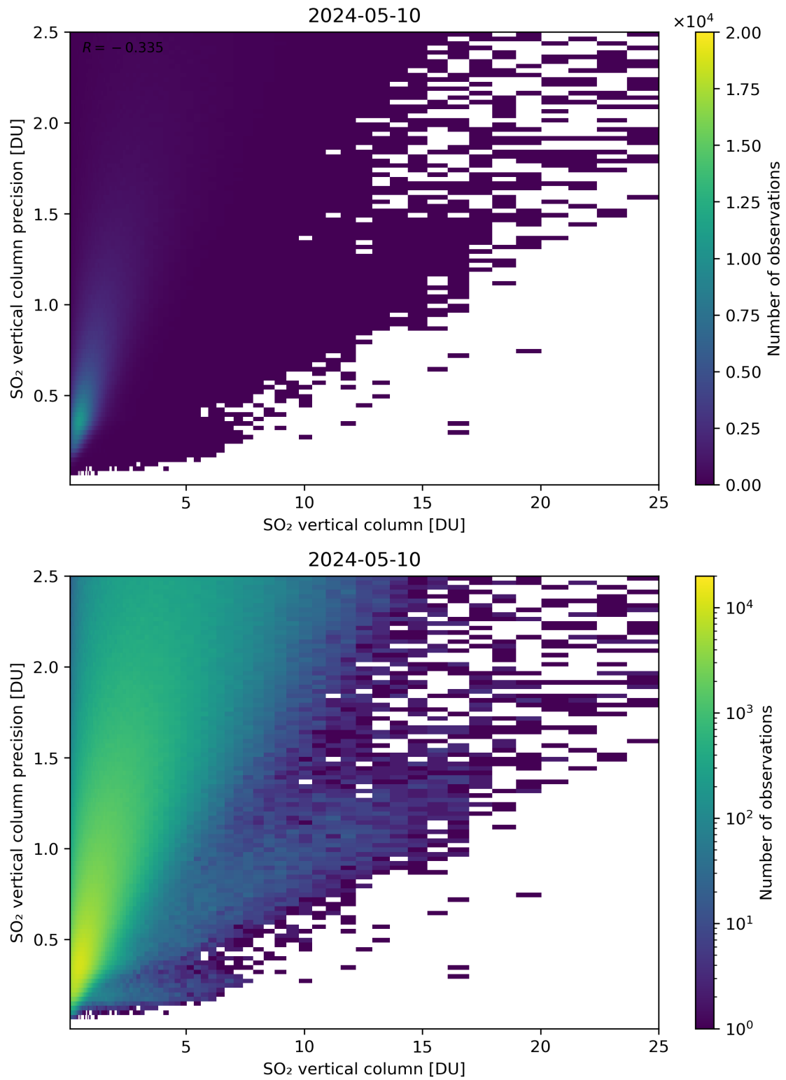
Figure 307: Scatter density plot of “SO 2 vertical column” against “SO 2 vertical column precision” for 2024-05-09 to 2024-05-11.
