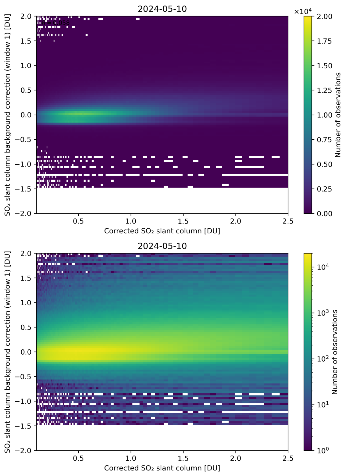
Figure 178: Scatter density plot of “Corrected SO 2 slant column” against “SO 2 slant column background correction (window 1)” for 2024-05-09 to 2024-05-11.
