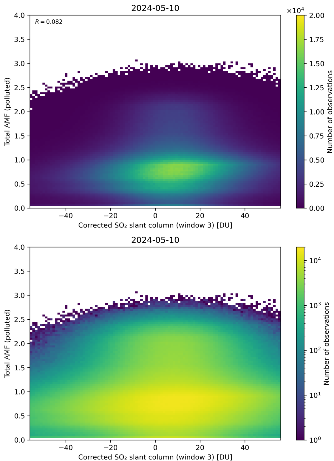
Figure 210: Scatter density plot of “Corrected SO 2 slant column (window 3)” against “Total AMF (polluted)” for 2024-05-09 to 2024-05-11.
