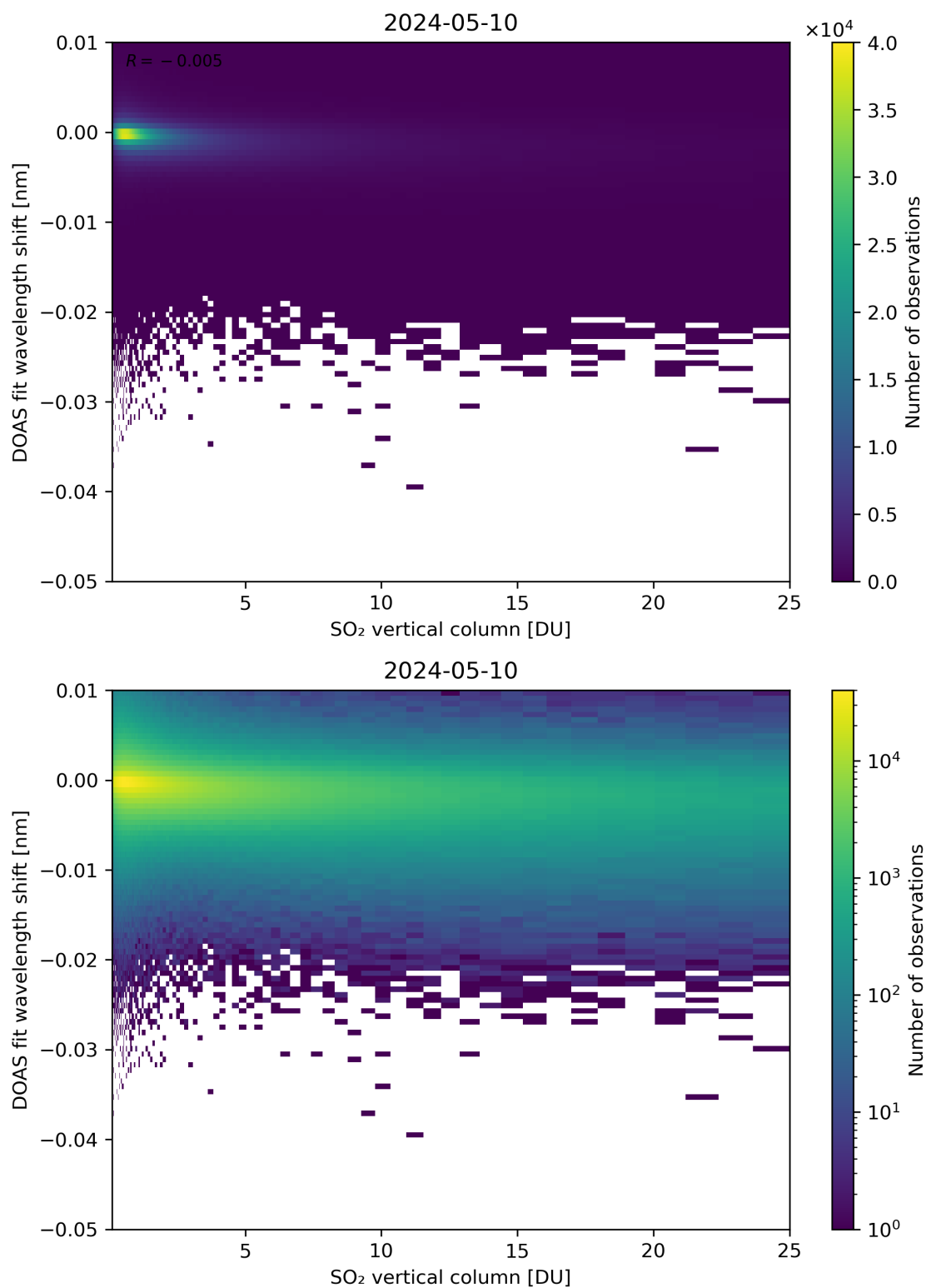
Figure 276: Scatter density plot of “SO 2 vertical column” against “DOAS fit wavelength shift” for 2024-05-09 to 2024-05-11.
