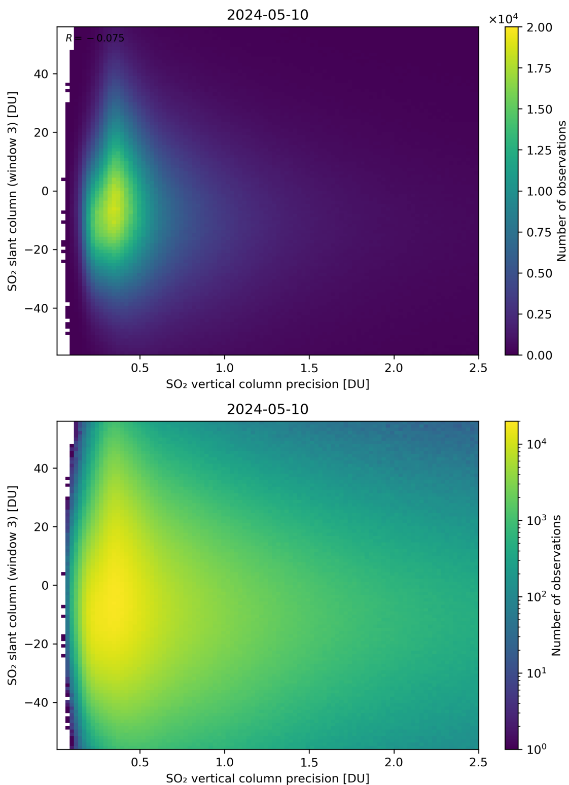
Figure 292: Scatter density plot of “SO 2 vertical column precision” against “SO 2 slant column (window 3)” for 2024-05-09 to 2024-05-11.
