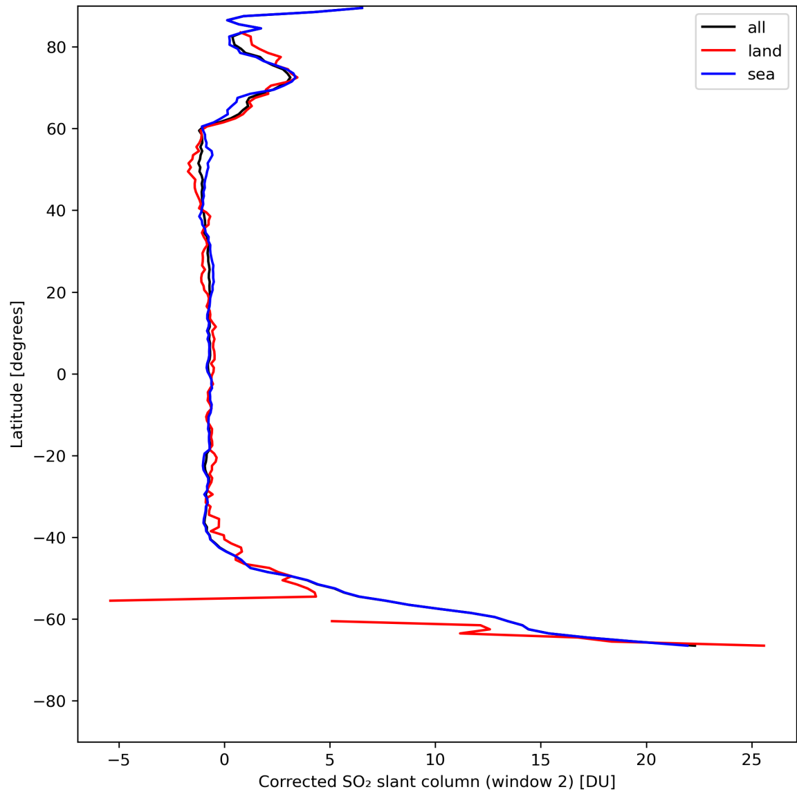
Figure 39: Zonal average of “Corrected SO 2 slant column (window 2)” for 2024-05-09 to 2024-05-11.
