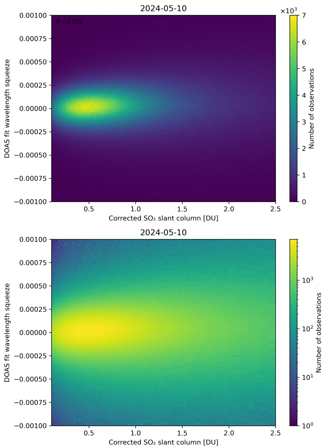
Figure 182: Scatter density plot of “Corrected SO 2 slant column” against “DOAS fit wavelength squeeze” for 2024-05-09 to 2024-05-11.
