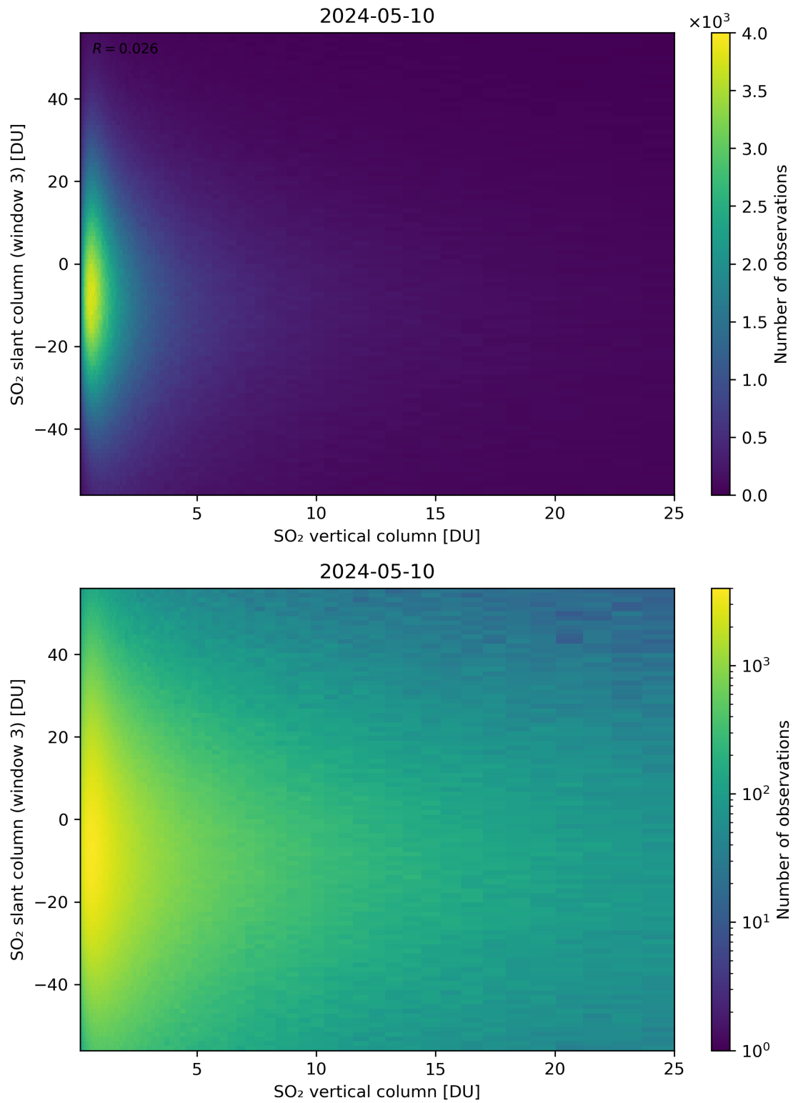
Figure 303: Scatter density plot of “SO 2 vertical column” against “SO 2 slant column (window 3)” for 2024-05-09 to 2024-05-11.
