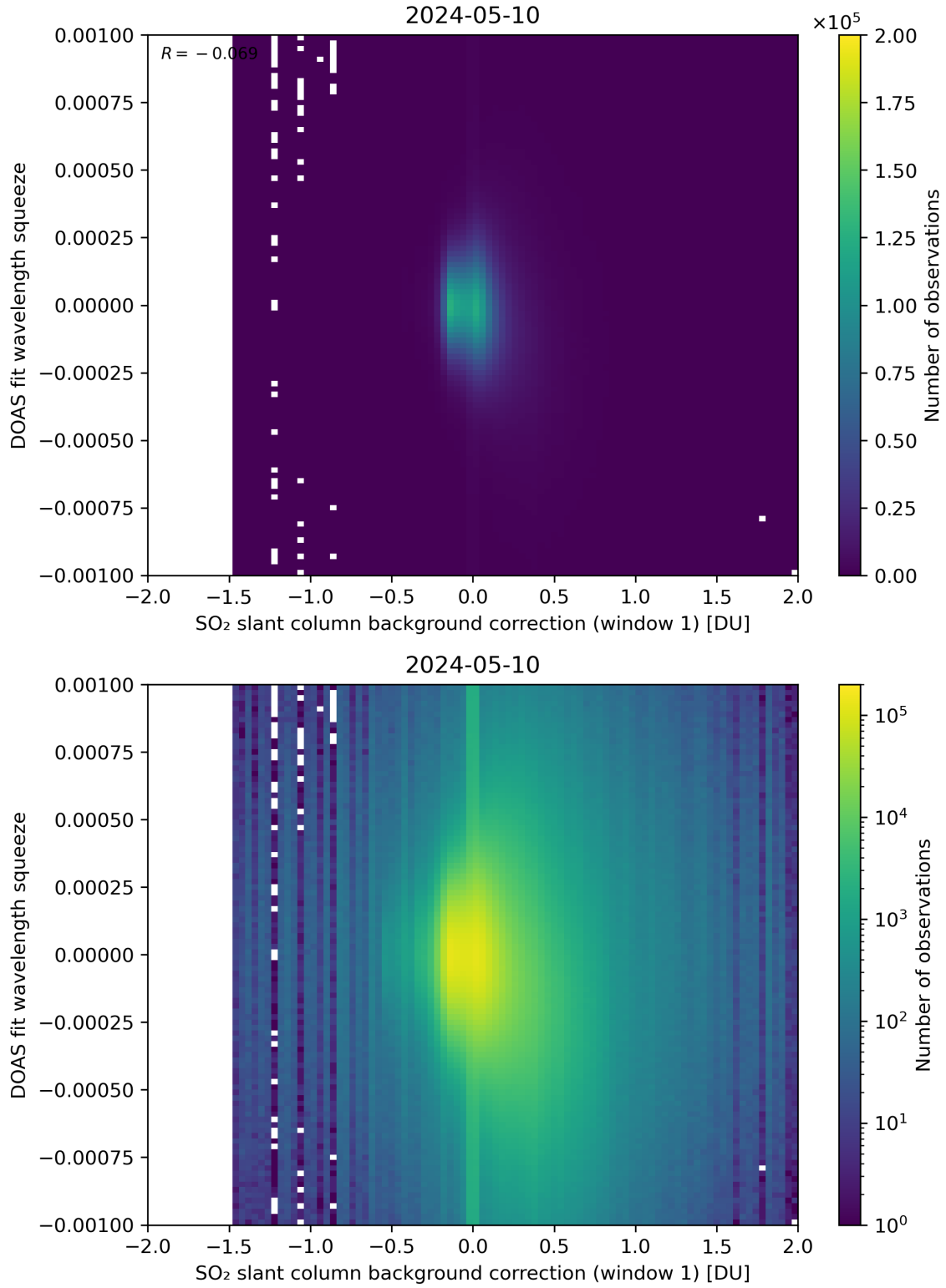
Figure 101: Scatter density plot of “SO 2 slant column background correction (window 1)” against “DOAS fit wavelength squeeze” for 2024-05-09 to 2024-05-11.
