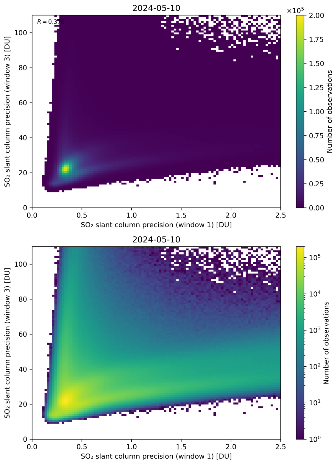
Figure 229: Scatter density plot of “SO 2 slant column precision (window 1)” against “SO 2 slant column precision (window 3)” for 2024-05-09 to 2024-05-11.
