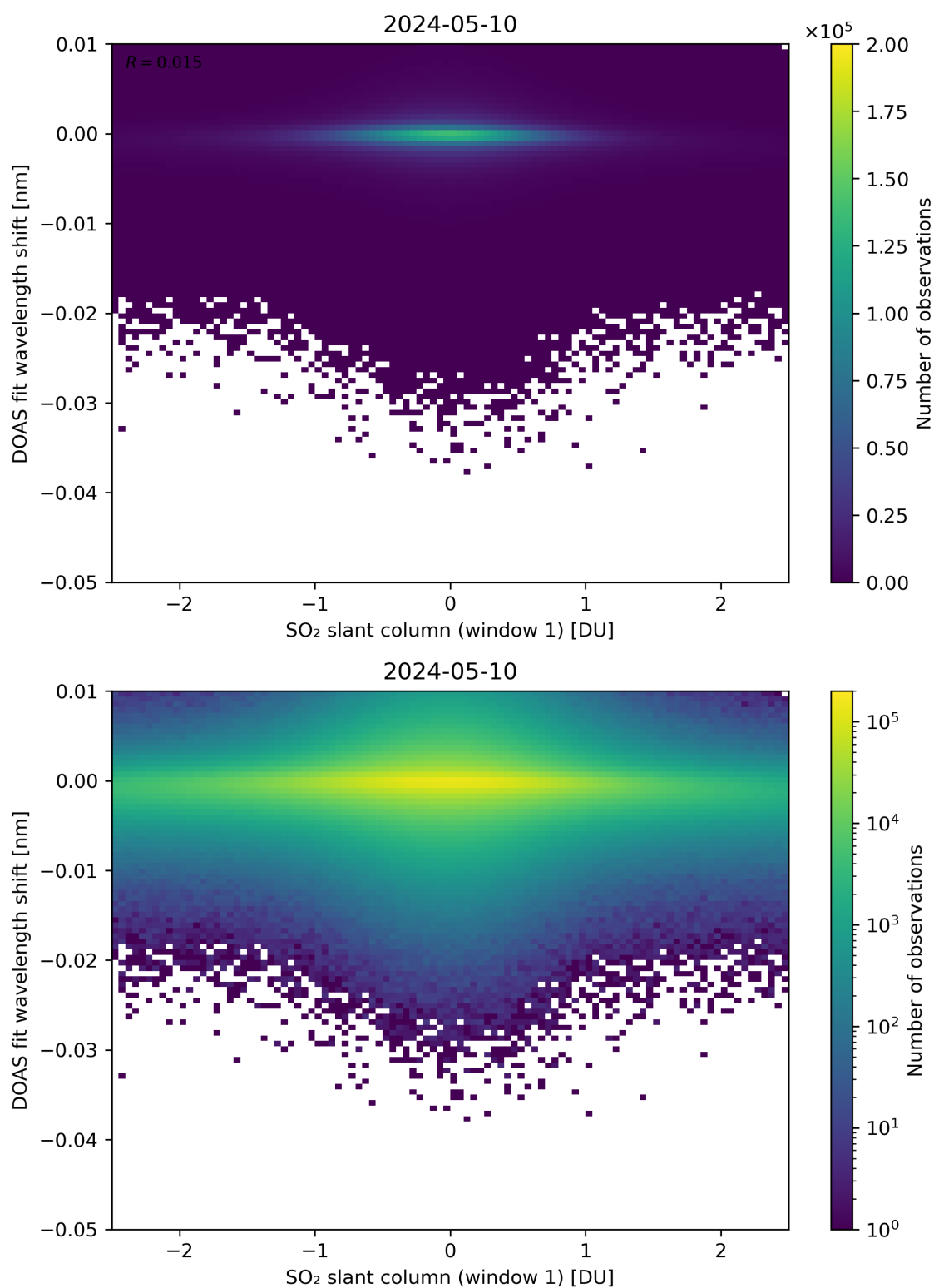
Figure 215: Scatter density plot of “SO 2 slant column (window 1)” against “DOAS fit wavelength shift” for 2024-05-09 to 2024-05-11.
