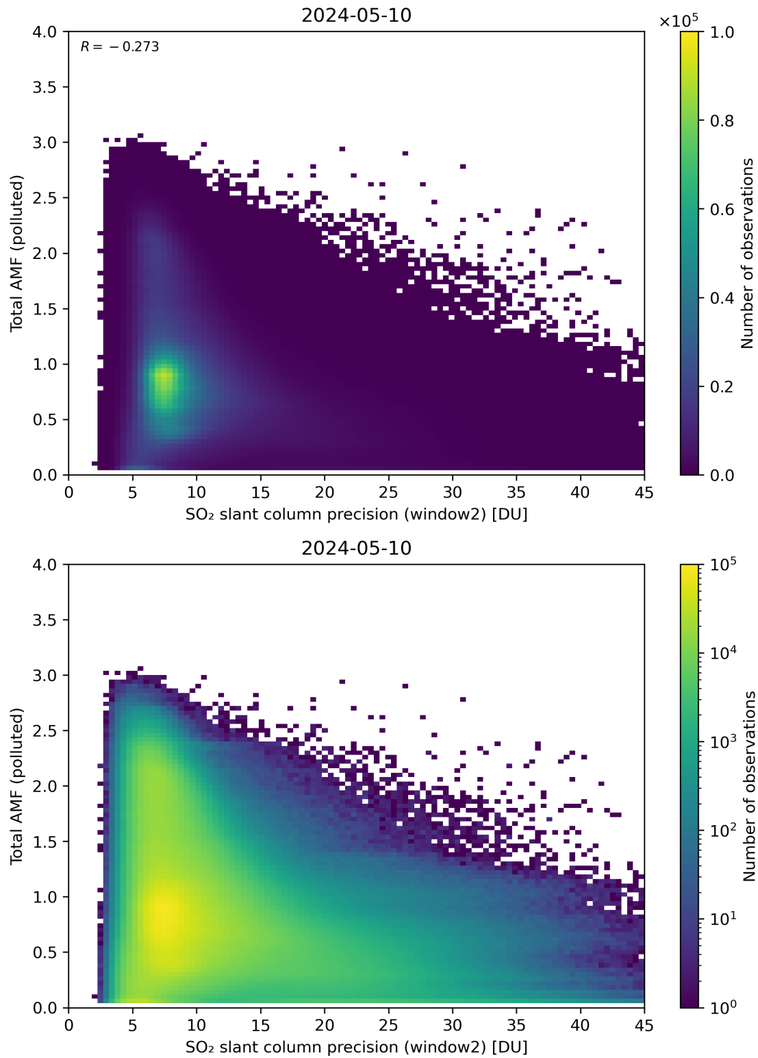
Figure 251: Scatter density plot of “SO 2 slant column precision (window2)” against “Total AMF (polluted)” for 2024-05-09 to 2024-05-11.
