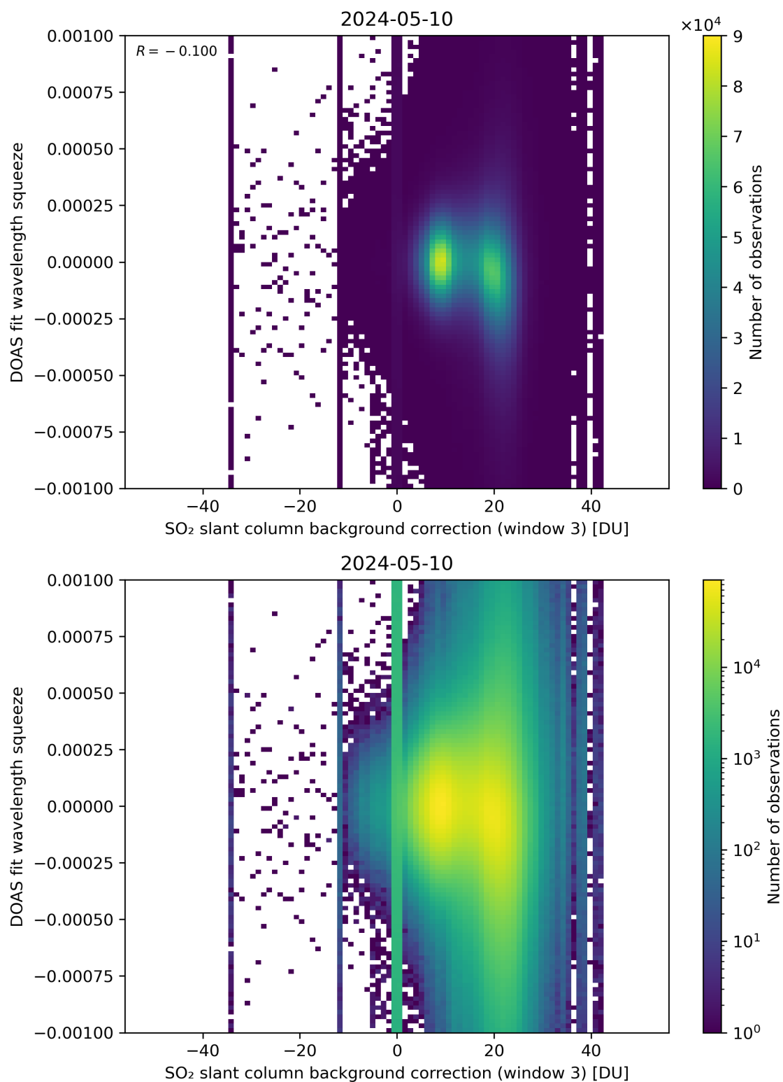
Figure 122: Scatter density plot of “SO 2 slant column background correction (window 3)” against “DOAS fit wavelength squeeze” for 2024-05-09 to 2024-05-11.
