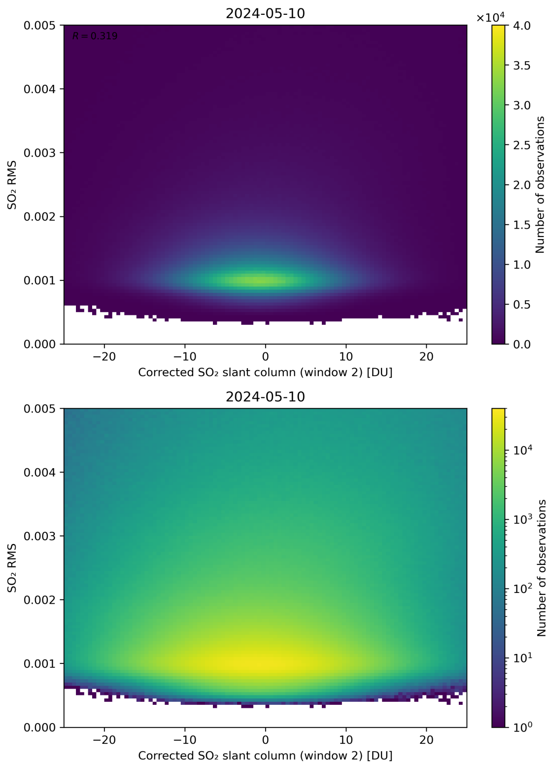
Figure 198: Scatter density plot of “Corrected SO 2 slant column (window 2)” against “SO 2 RMS” for 2024-05-09 to 2024-05-11.
