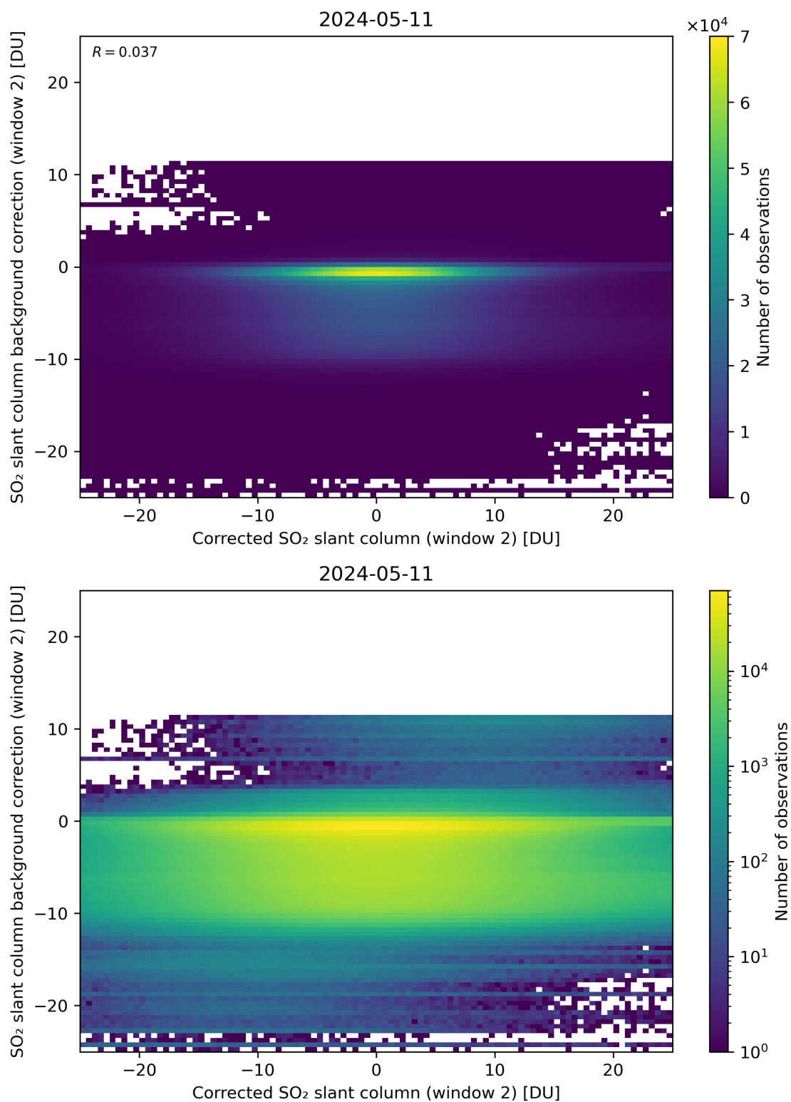
Figure 194: Scatter density plot of “Corrected SO 2 slant column (window 2)” against “SO 2 slant column background correction (window 2)” for 2024-05-10 to 2024-05-12.
