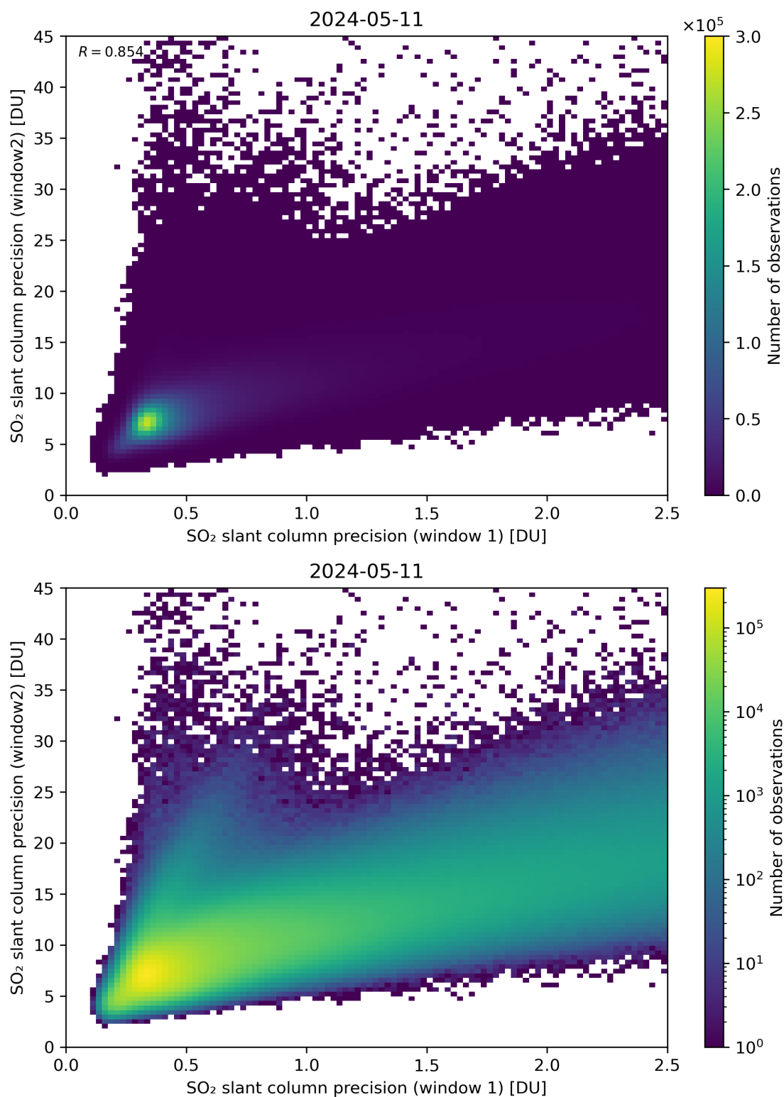
Figure 227: Scatter density plot of “SO 2 slant column precision (window 1)” against “SO 2 slant column precision (window2)” for 2024-05-10 to 2024-05-12.
