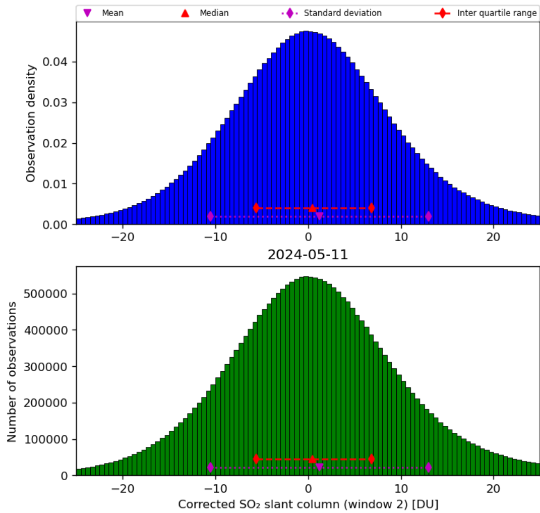
Figure 62: Histogram of “Corrected SO 2 slant column (window 2)” for 2024-05-10 to 2024-05-12
