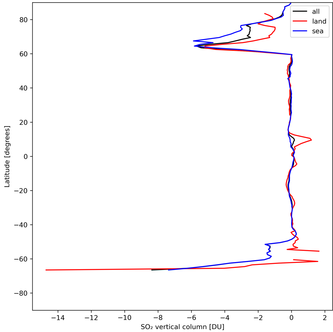
Figure 30: Zonal average of “SO 2 vertical column” for 2024-05-10 to 2024-05-12.
