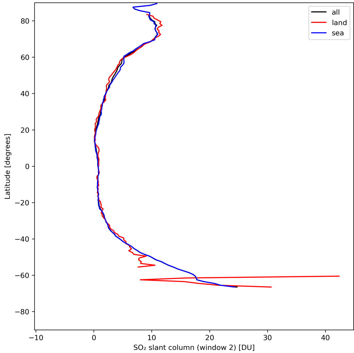
Figure 37: Zonal average of “SO 2 slant column (window 2)” for 2024-05-10 to 2024-05-12.
