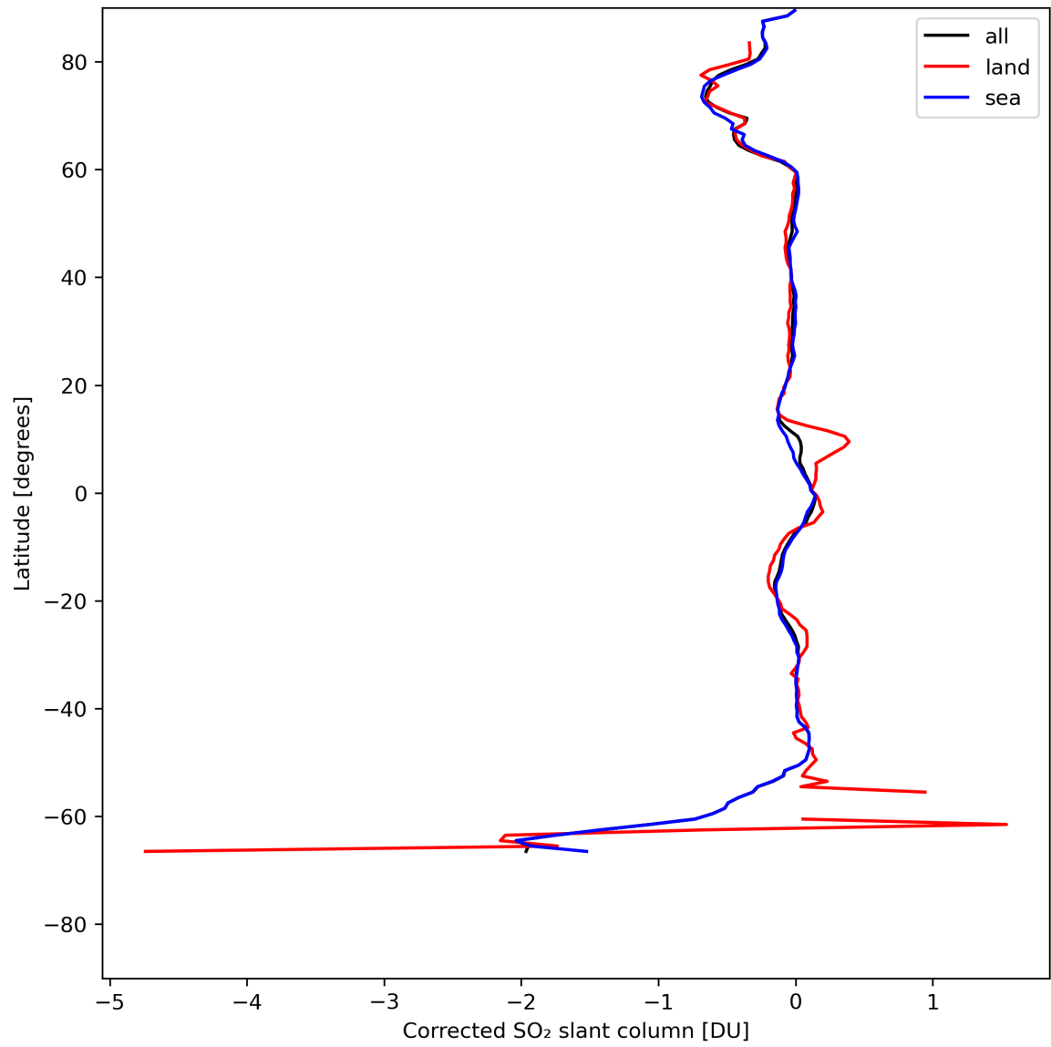
Figure 32: Zonal average of “Corrected SO 2 slant column” for 2024-05-10 to 2024-05-12.
