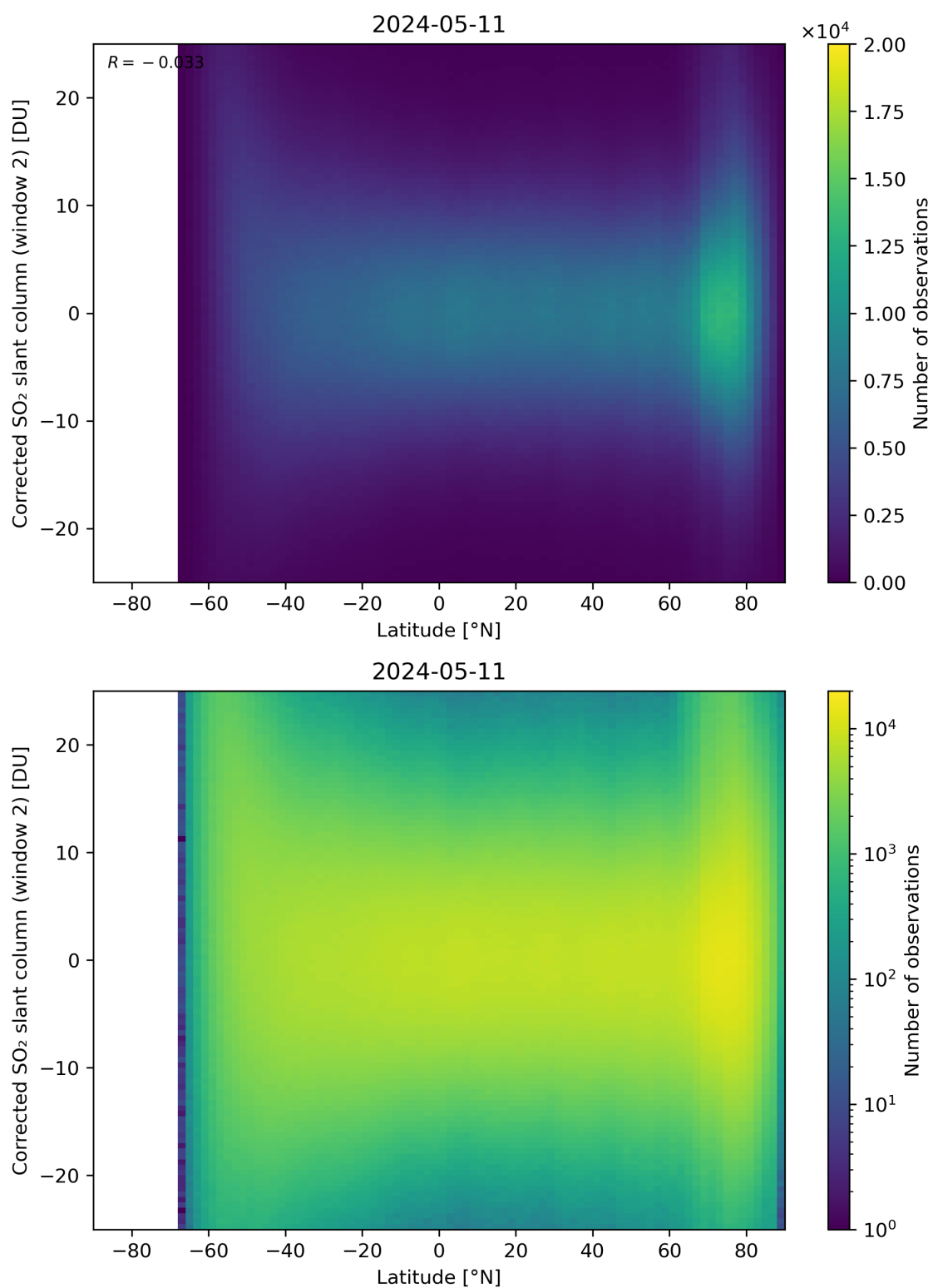
Figure 147: Scatter density plot of “Latitude” against “Corrected SO 2 slant column (window 2)” for 2024-05-10 to 2024-05-12.
