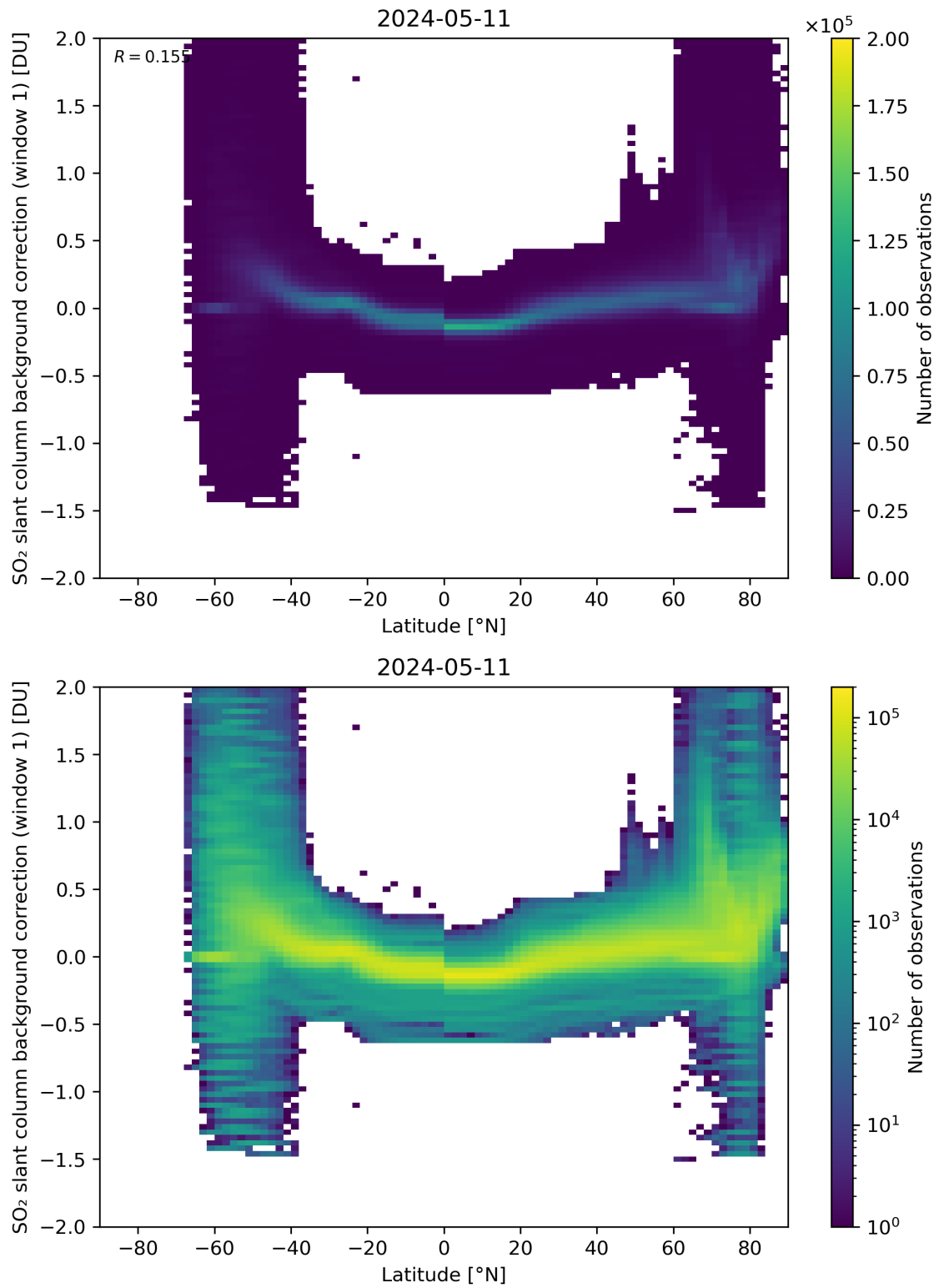
Figure 139: Scatter density plot of “Latitude” against “SO 2 slant column background correction (window 1)” for 2024-05-10 to 2024-05-12.
