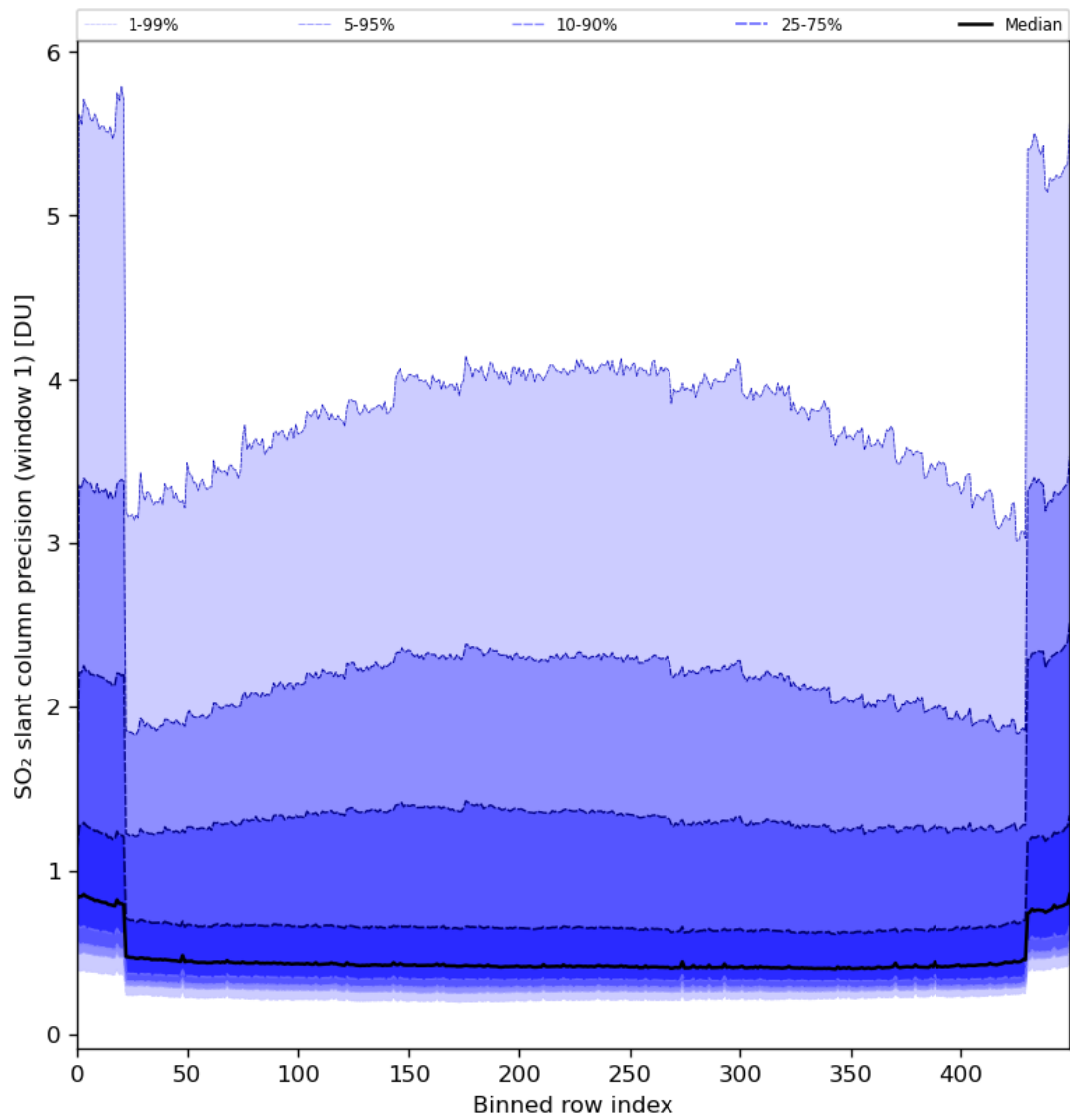
Figure 80: Along track statistics of “SO 2 slant column precision (window 1)” for 2024-05-10 to 2024-05-12
