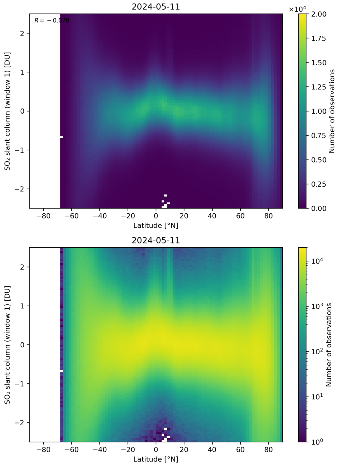
Figure 149: Scatter density plot of “Latitude” against “SO 2 slant column (window 1)” for 2024-05-10 to 2024-05-12.
