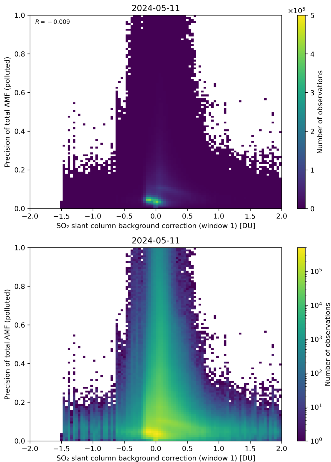
Figure 110: Scatter density plot of “SO 2 slant column background correction (window 1)” against “Precision of total AMF (polluted)” for 2024-05-10 to 2024-05-12.
