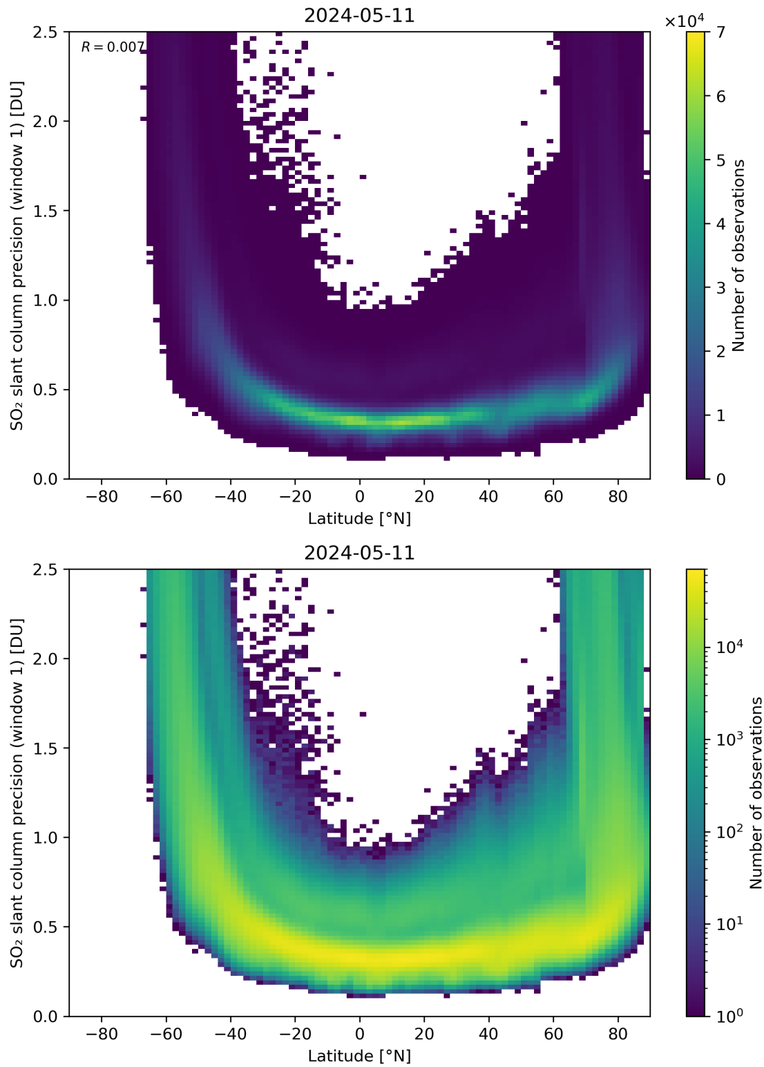
Figure 150: Scatter density plot of “Latitude” against “SO 2 slant column precision (window 1)” for 2024-05-10 to 2024-05-12.
