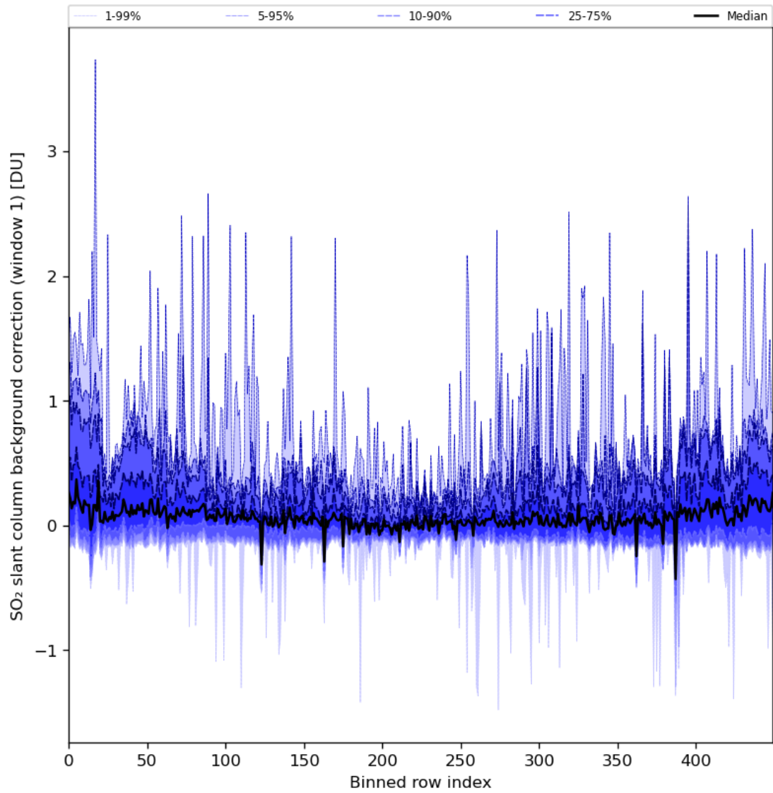
Figure 82: Along track statistics of “SO 2 slant column background correction (window 1)” for 2024-05-10 to 2024-05-12
