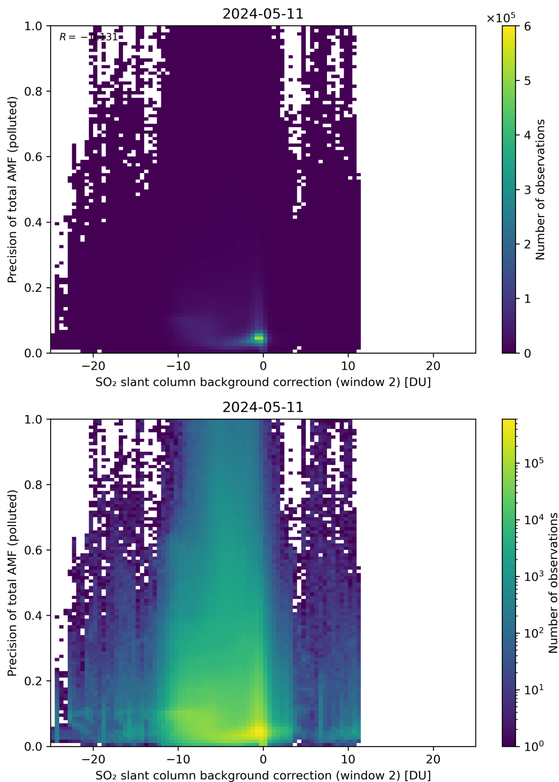
Figure 120: Scatter density plot of “SO 2 slant column background correction (window 2)” against “Precision of total AMF (polluted)” for 2024-05-10 to 2024-05-12.
