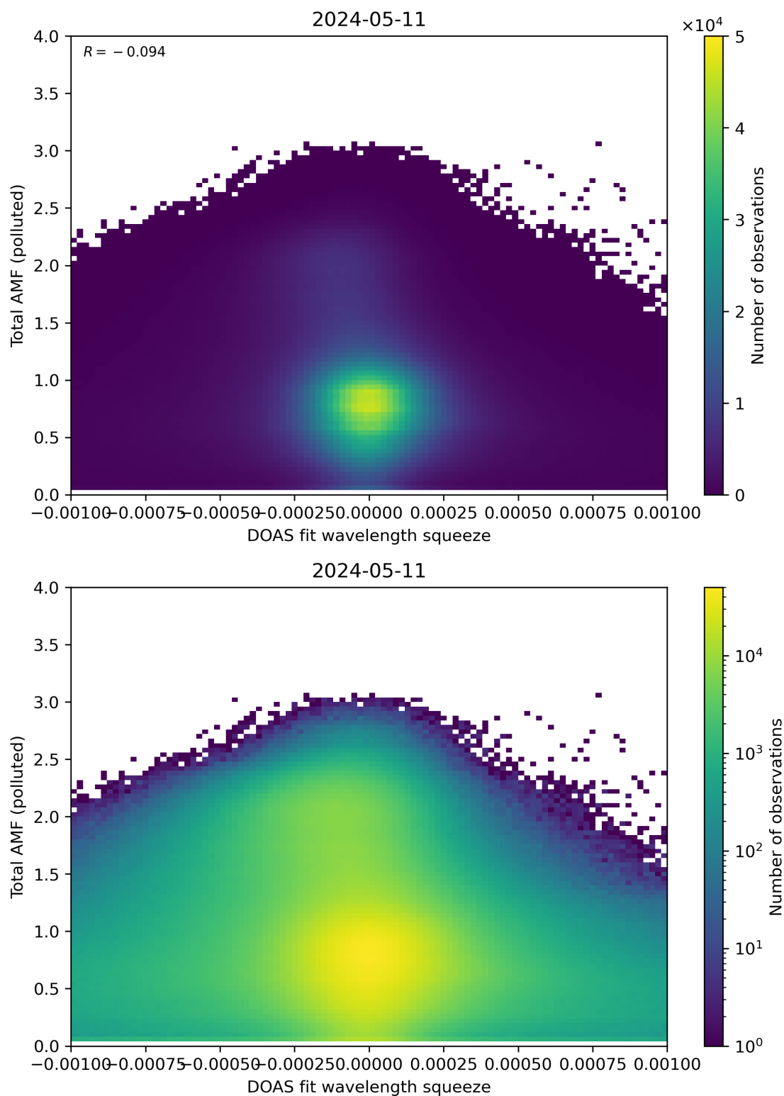
Figure 134: Scatter density plot of “DOAS fit wavelength squeeze” against “Total AMF (polluted)” for 2024-05-10 to 2024-05-12.
