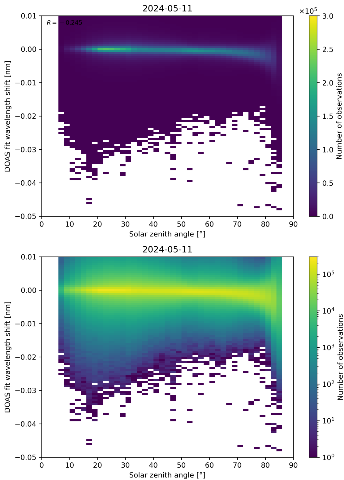
Figure 161: Scatter density plot of “Solar zenith angle” against “DOAS fit wavelength shift” for 2024-05-10 to 2024-05-12.
