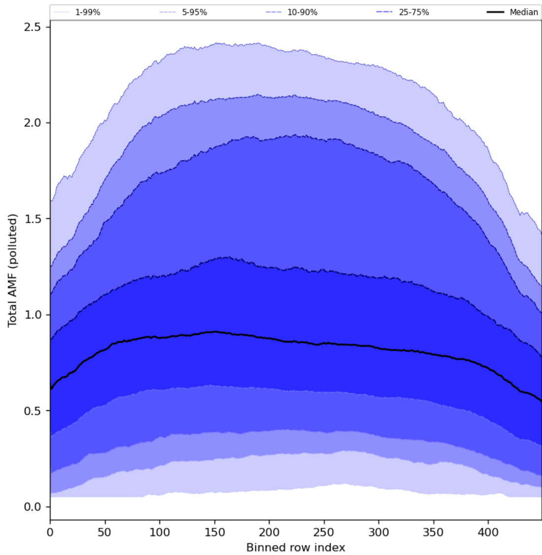
Figure 94: Along track statistics of “Total AMF (polluted)” for 2024-05-10 to 2024-05-12
