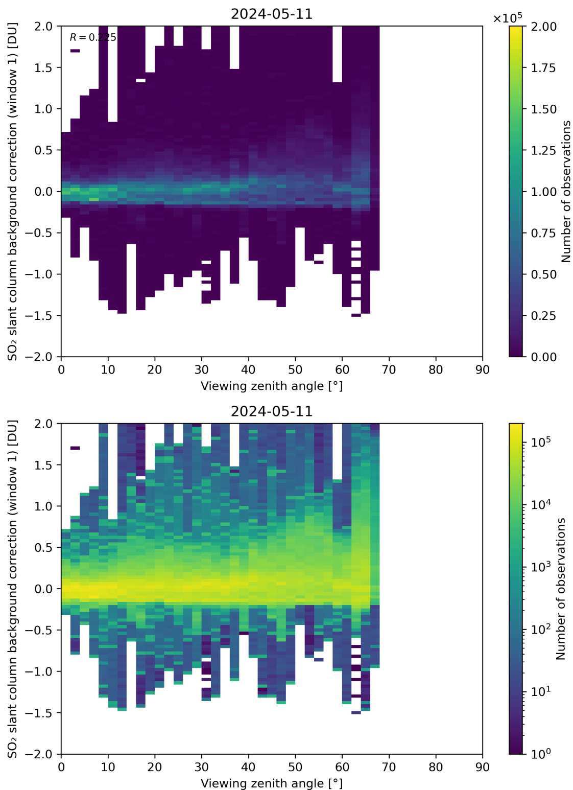
Figure 308: Scatter density plot of “Viewing zenith angle” against “SO 2 slant column background correction (window 1)” for 2024-05-10 to 2024-05-12.
