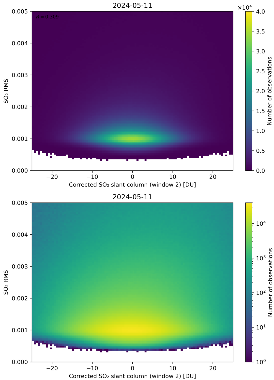
Figure 198: Scatter density plot of “Corrected SO 2 slant column (window 2)” against “SO 2 RMS” for 2024-05-10 to 2024-05-12.
