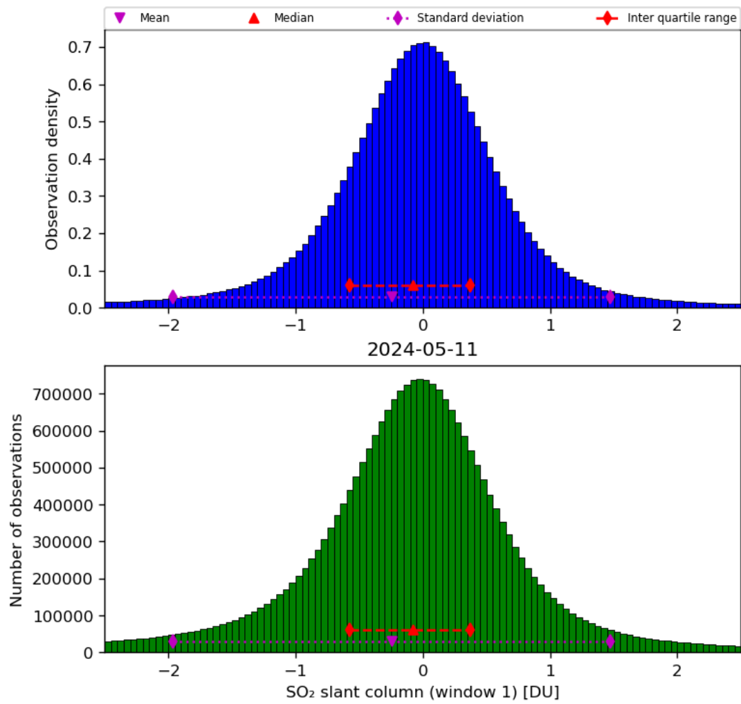
Figure 56: Histogram of “SO 2 slant column (window 1)” for 2024-05-10 to 2024-05-12
