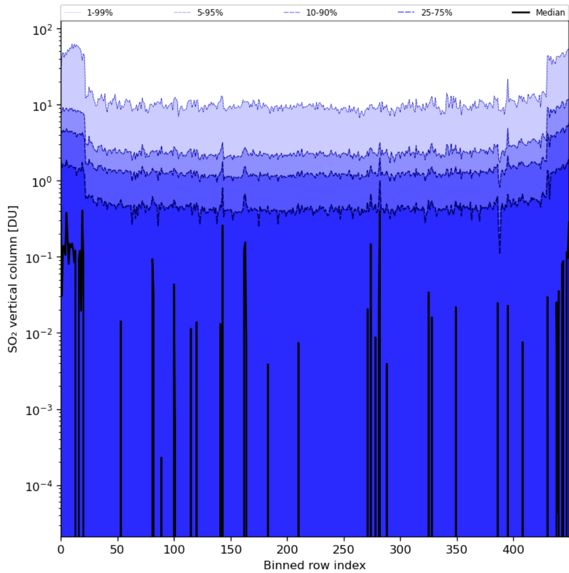
Figure 76: Along track statistics of “SO 2 vertical column” for 2024-05-10 to 2024-05-12
