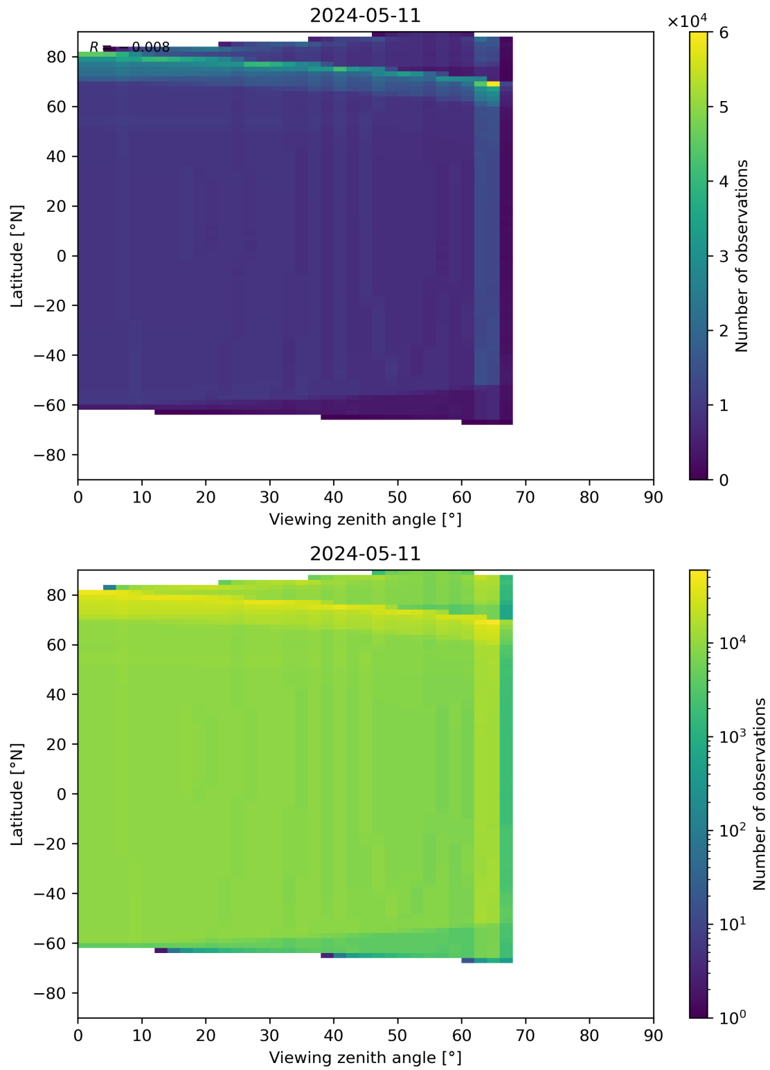
Figure 314: Scatter density plot of “Viewing zenith angle” against “Latitude” for 2024-05-10 to 2024-05-12.
