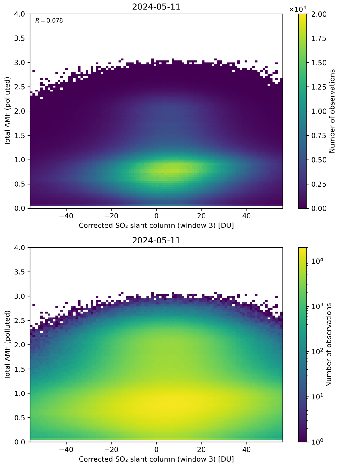
Figure 210: Scatter density plot of “Corrected SO 2 slant column (window 3)” against “Total AMF (polluted)” for 2024-05-10 to 2024-05-12.
