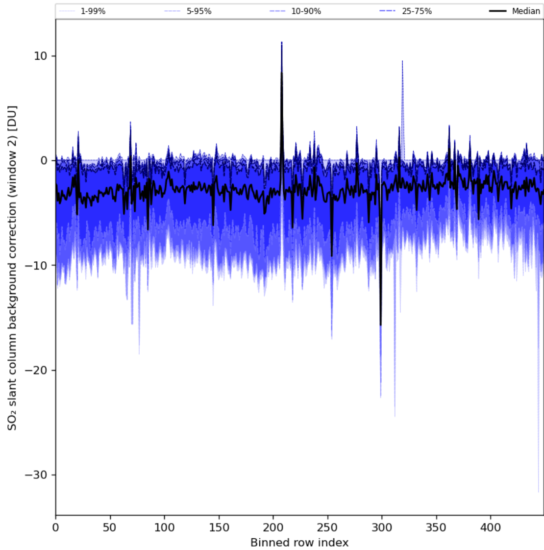
Figure 86: Along track statistics of “SO 2 slant column background correction (window 2)” for 2024-05-10 to 2024-05-12
