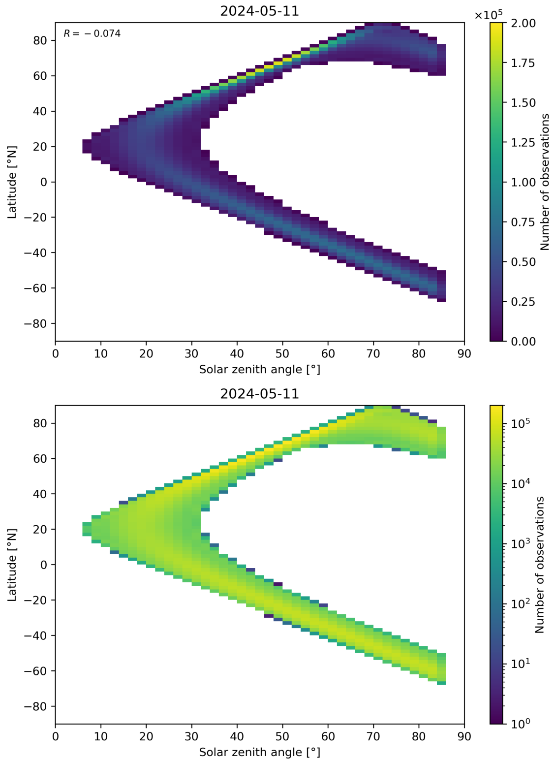
Figure 164: Scatter density plot of “Solar zenith angle” against “Latitude” for 2024-05-10 to 2024-05-12.
