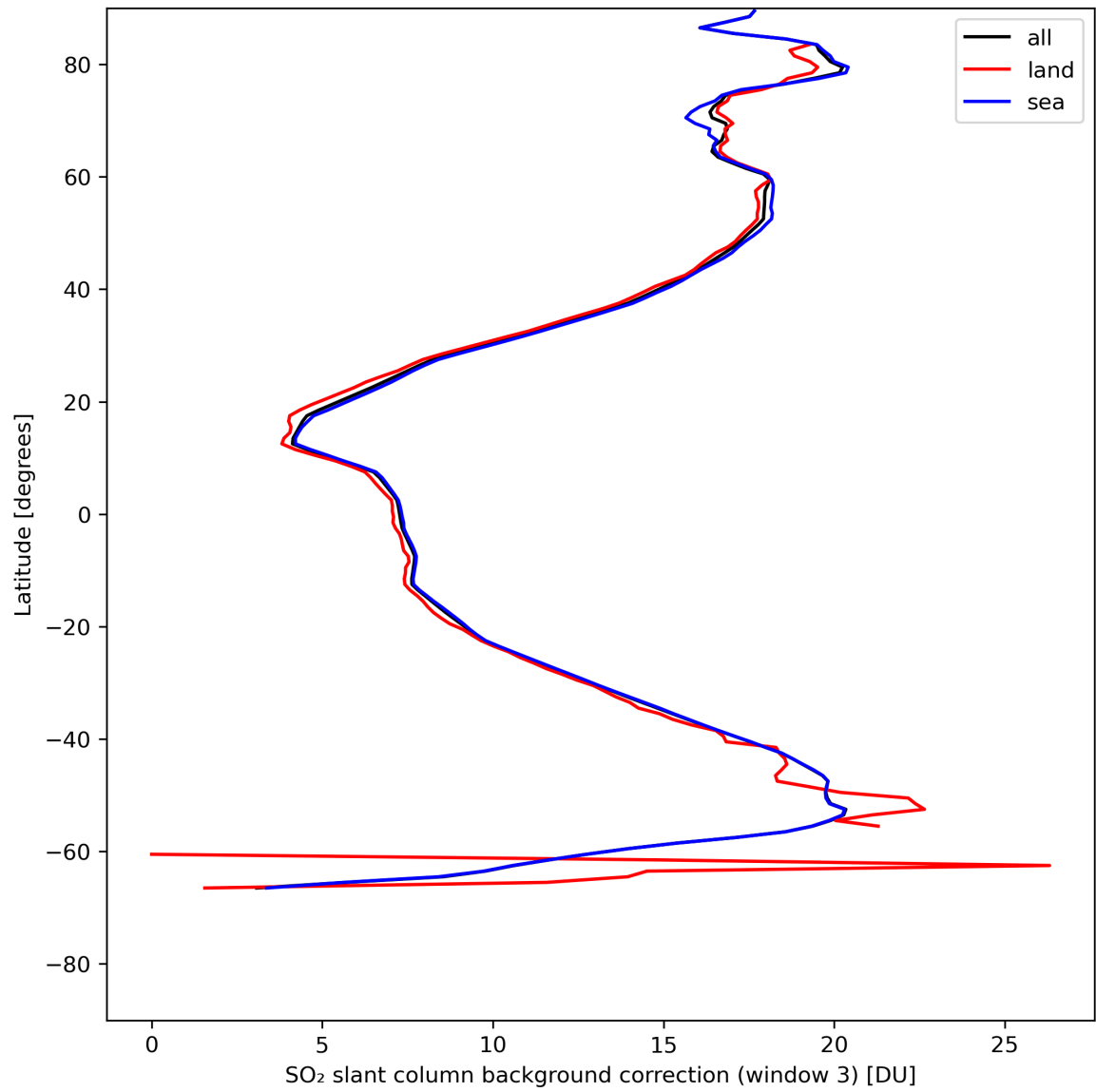
Figure 44: Zonal average of “SO 2 slant column background correction (window 3)” for 2024-05-10 to 2024-05-12.
