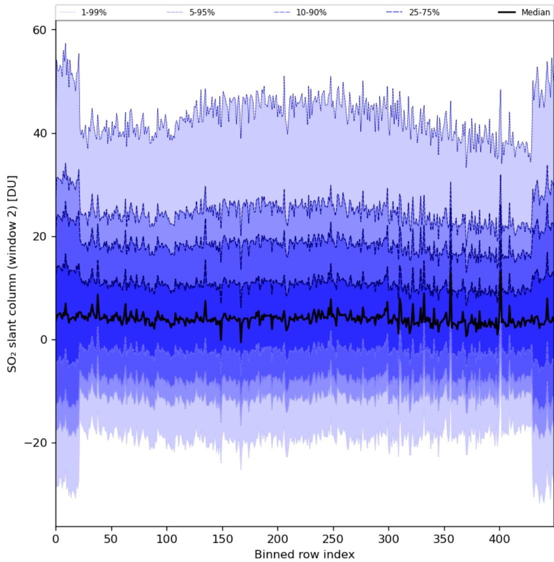
Figure 83: Along track statistics of “SO 2 slant column (window 2)” for 2024-05-10 to 2024-05-12
