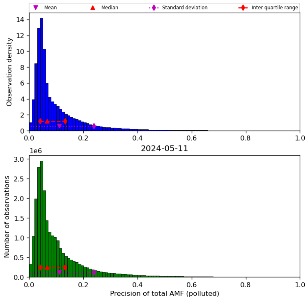
Figure 72: Histogram of “Precision of total AMF (polluted)” for 2024-05-10 to 2024-05-12
