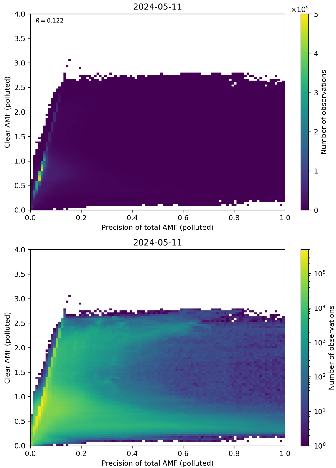
Figure 270: Scatter density plot of “Precision of total AMF (polluted)” against “Clear AMF (polluted)” for 2024-05-10 to 2024-05-12.
