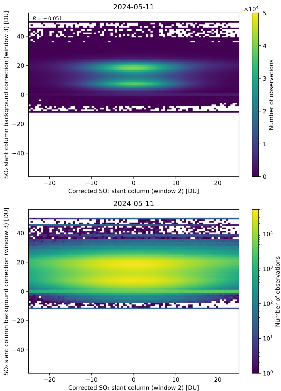
Figure 195: Scatter density plot of “Corrected SO 2 slant column (window 2)” against “SO 2 slant column background correction (window 3)” for 2024-05-10 to 2024-05-12.
