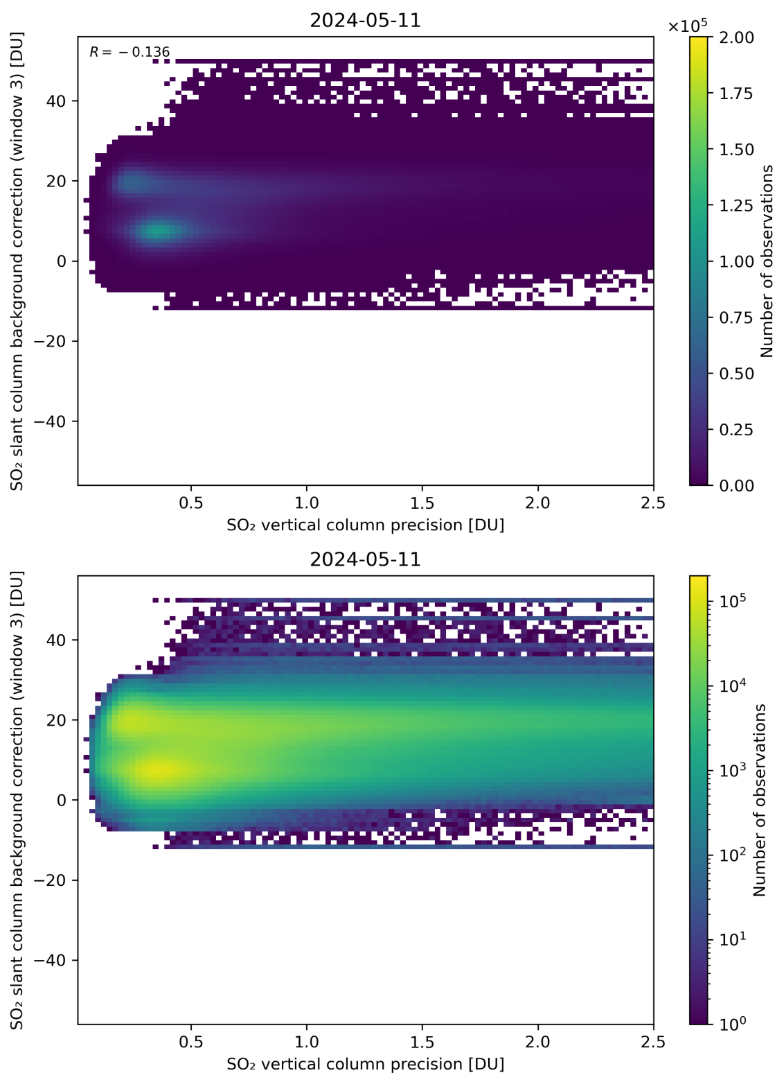
Figure 281: Scatter density plot of “SO 2 vertical column precision” against “SO 2 slant column background correction (window 3)” for 2024-05-10 to 2024-05-12.
