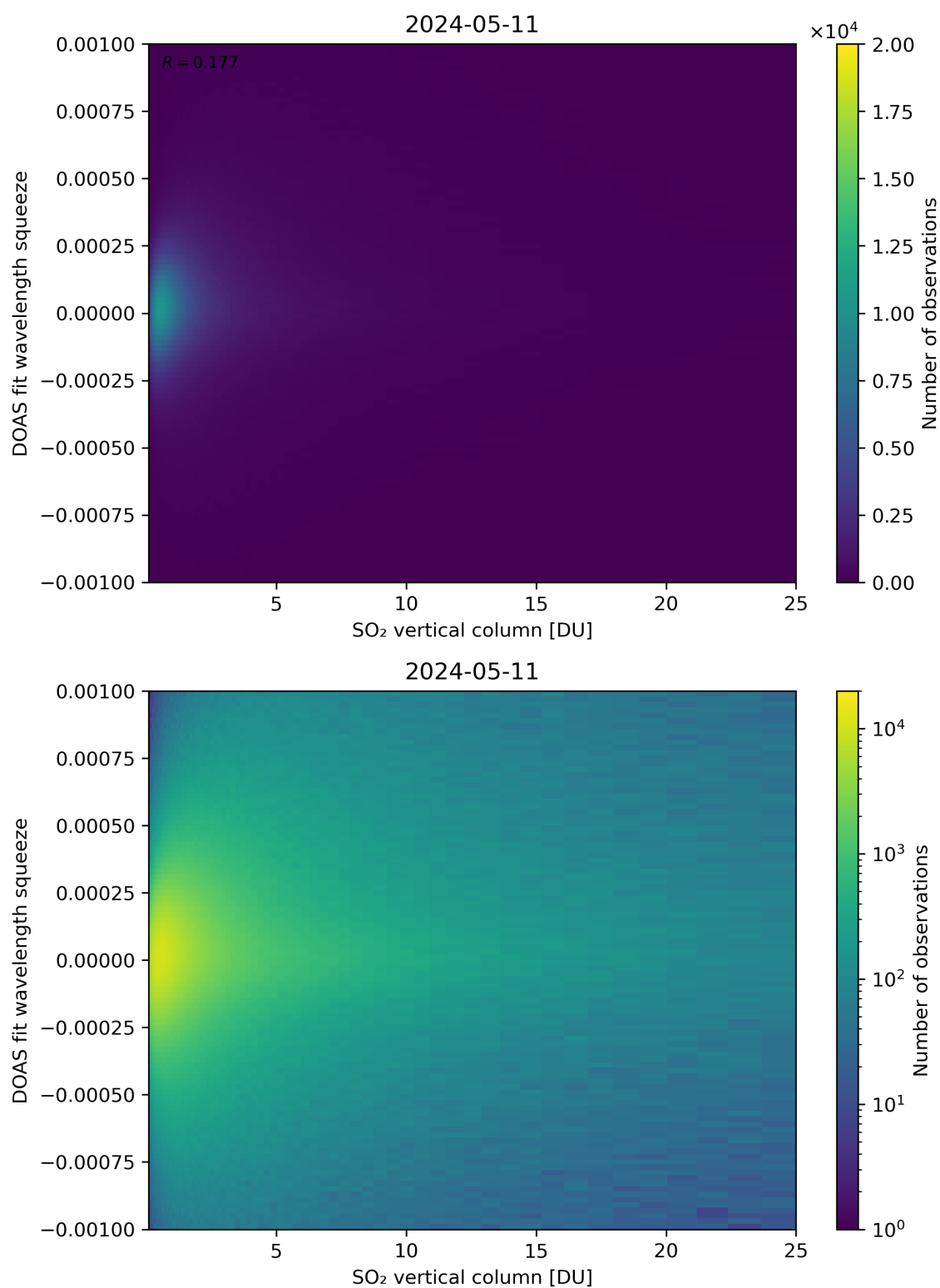
Figure 277: Scatter density plot of “SO 2 vertical column” against “DOAS fit wavelength squeeze” for 2024-05-10 to 2024-05-12.
