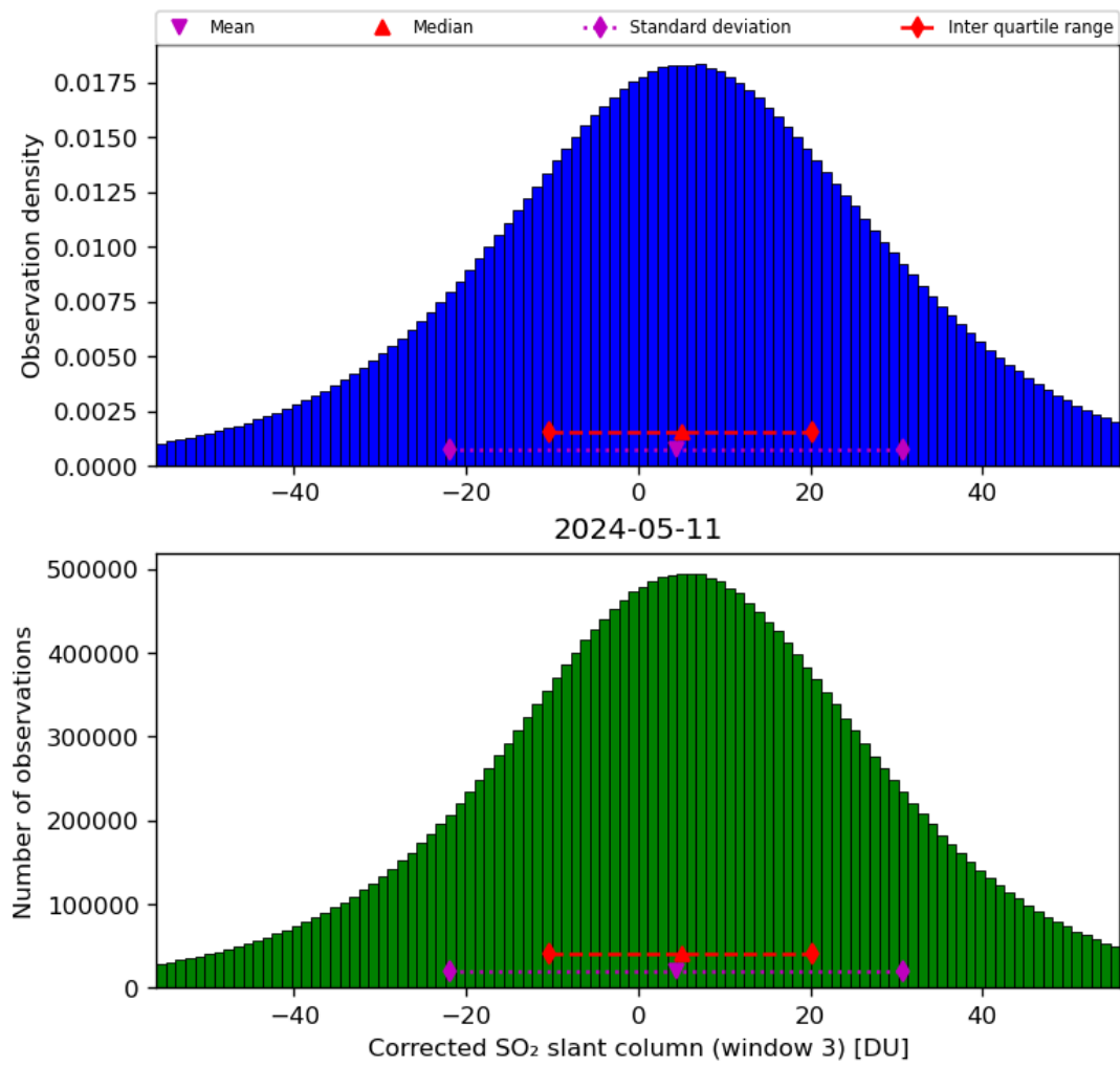
Figure 66: Histogram of “Corrected SO 2 slant column (window 3)” for 2024-05-10 to 2024-05-12
