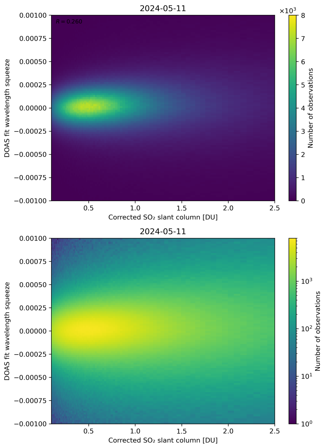
Figure 182: Scatter density plot of “Corrected SO 2 slant column” against “DOAS fit wavelength squeeze” for 2024-05-10 to 2024-05-12.
