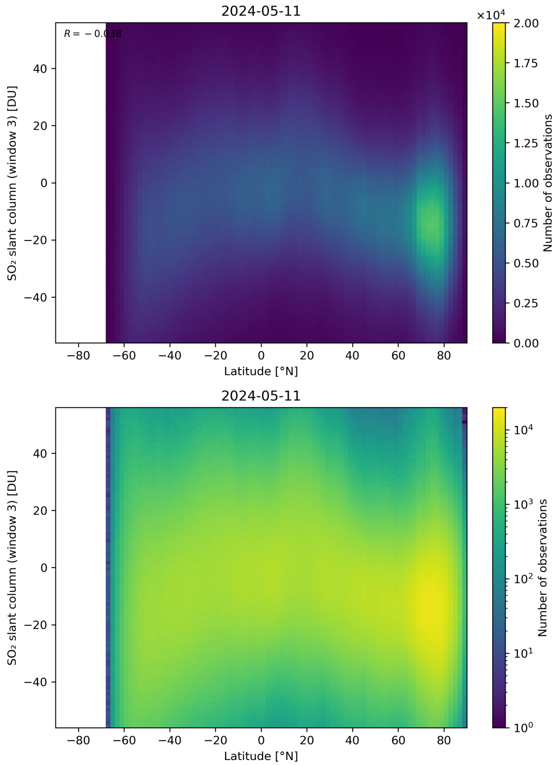
Figure 152: Scatter density plot of “Latitude” against “SO 2 slant column (window 3)” for 2024-05-10 to 2024-05-12.
