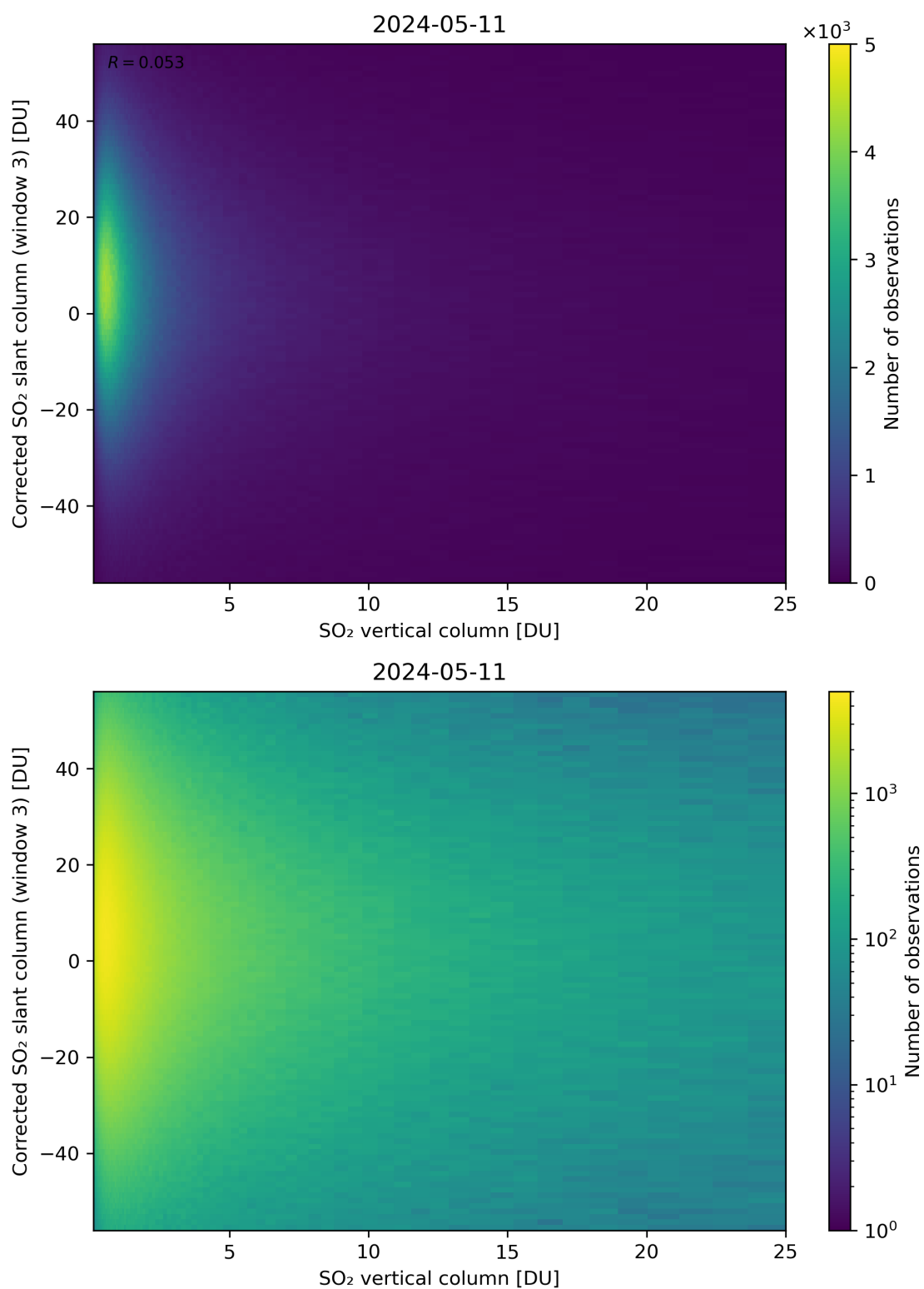
Figure 299: Scatter density plot of “SO 2 vertical column” against “Corrected SO 2 slant column (window 3)” for 2024-05-10 to 2024-05-12.
