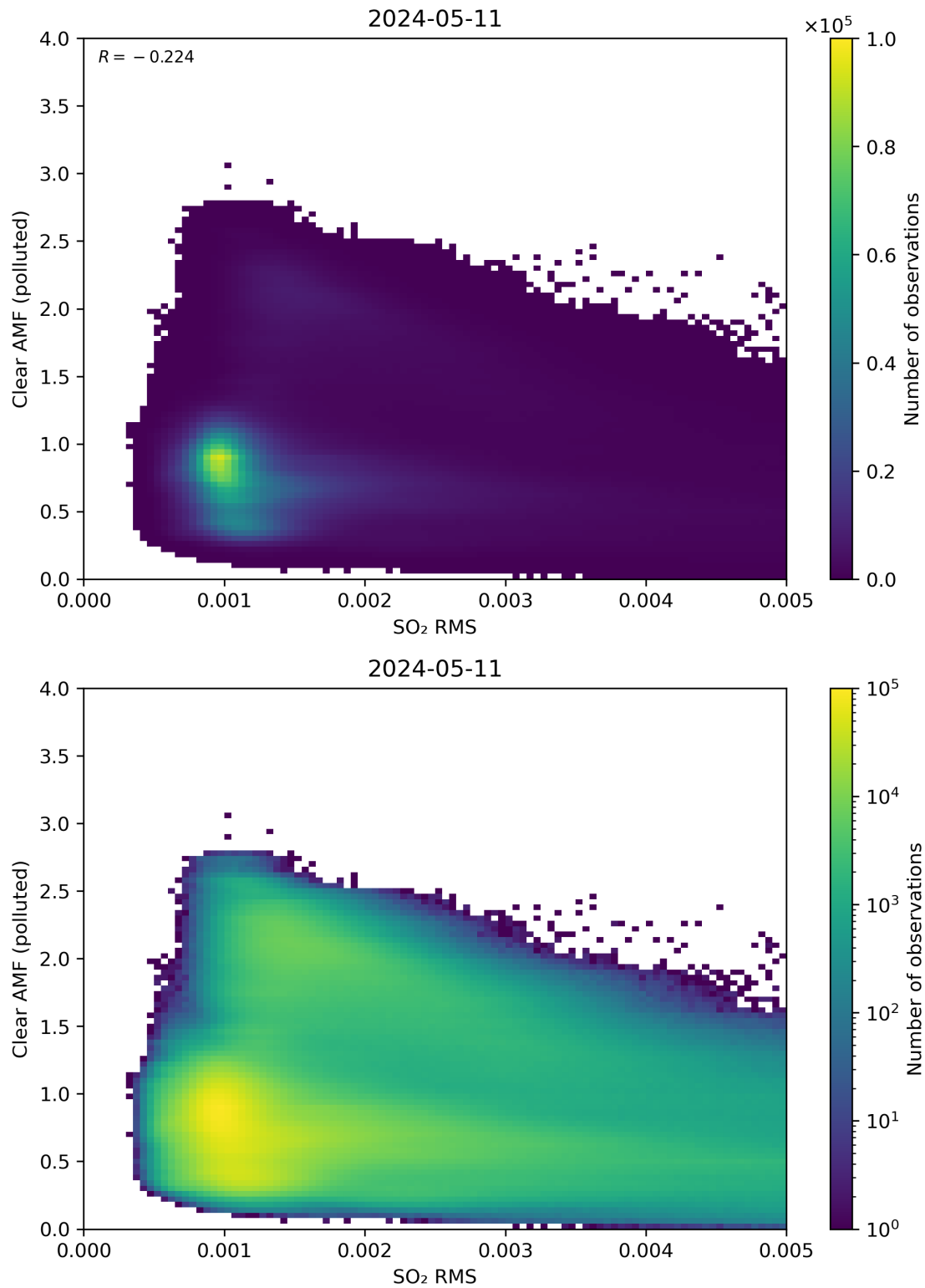
Figure 136: Scatter density plot of “SO 2 RMS” against “Clear AMF (polluted)” for 2024-05-10 to 2024-05-12.
