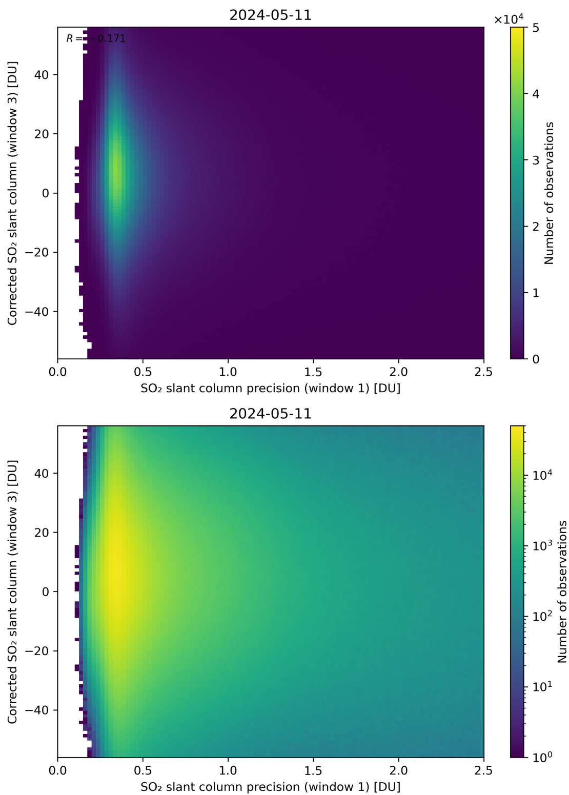
Figure 226: Scatter density plot of “SO 2 slant column precision (window 1)” against “Corrected SO 2 slant column (window 3)” for 2024-05-10 to 2024-05-12.
