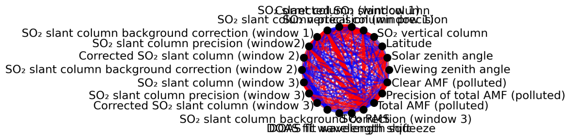
Figure 1: Map of correlation graph for 2024-05-10 to 2024-05-12.
