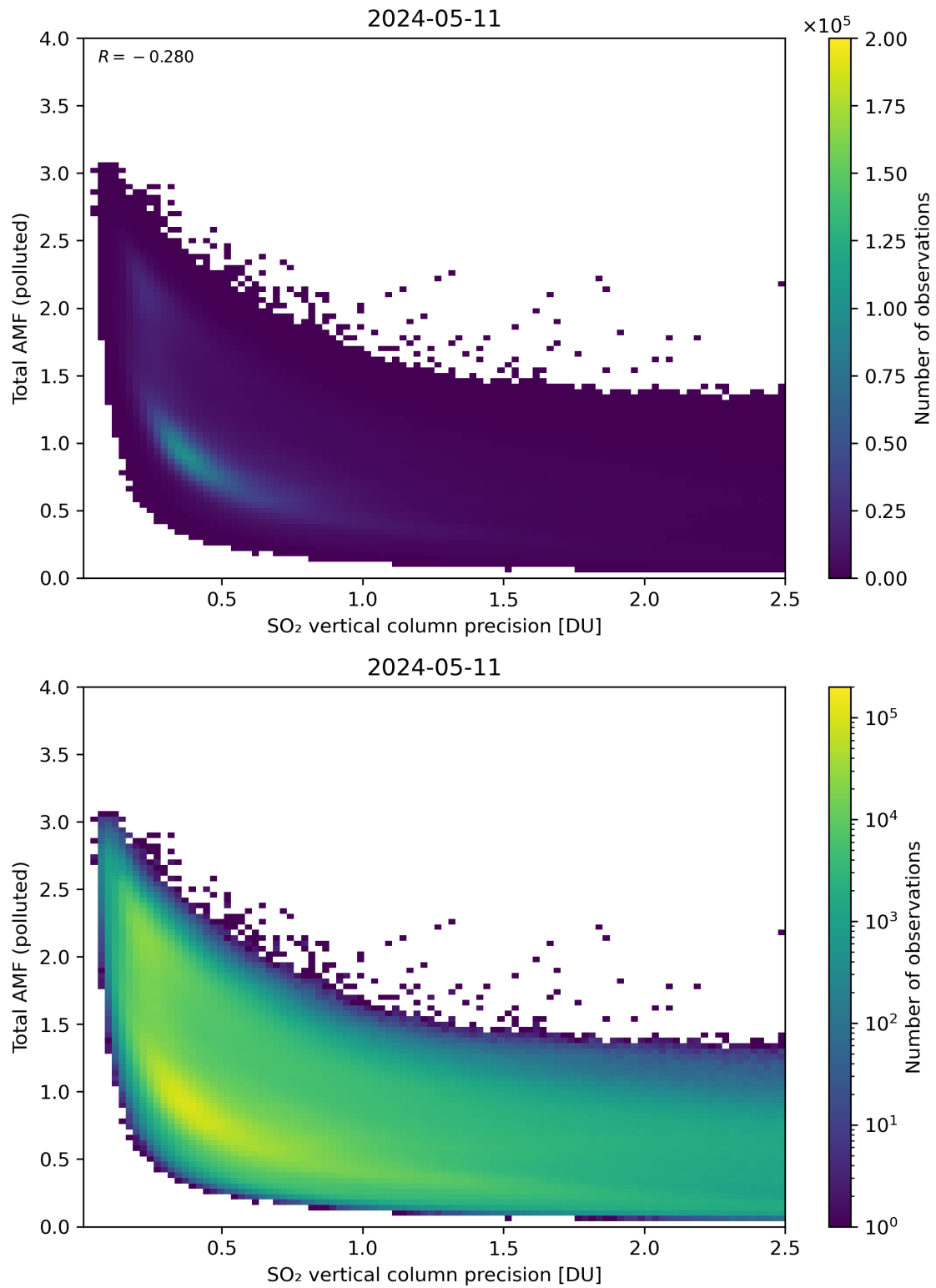
Figure 294: Scatter density plot of “SO 2 vertical column precision” against “Total AMF (polluted)” for 2024-05-10 to 2024-05-12.
