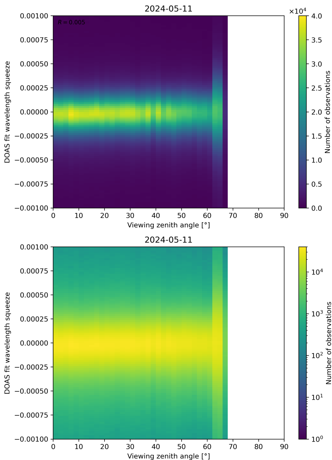
Figure 312: Scatter density plot of “Viewing zenith angle” against “DOAS fit wavelength squeeze” for 2024-05-10 to 2024-05-12.
