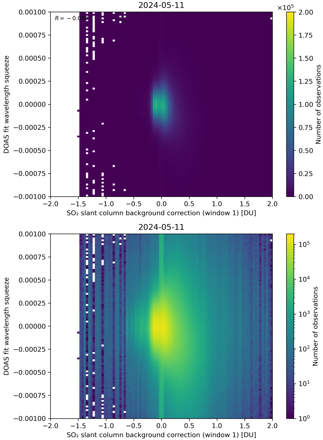
Figure 101: Scatter density plot of “SO 2 slant column background correction (window 1)” against “DOAS fit wavelength squeeze” for 2024-05-10 to 2024-05-12.
