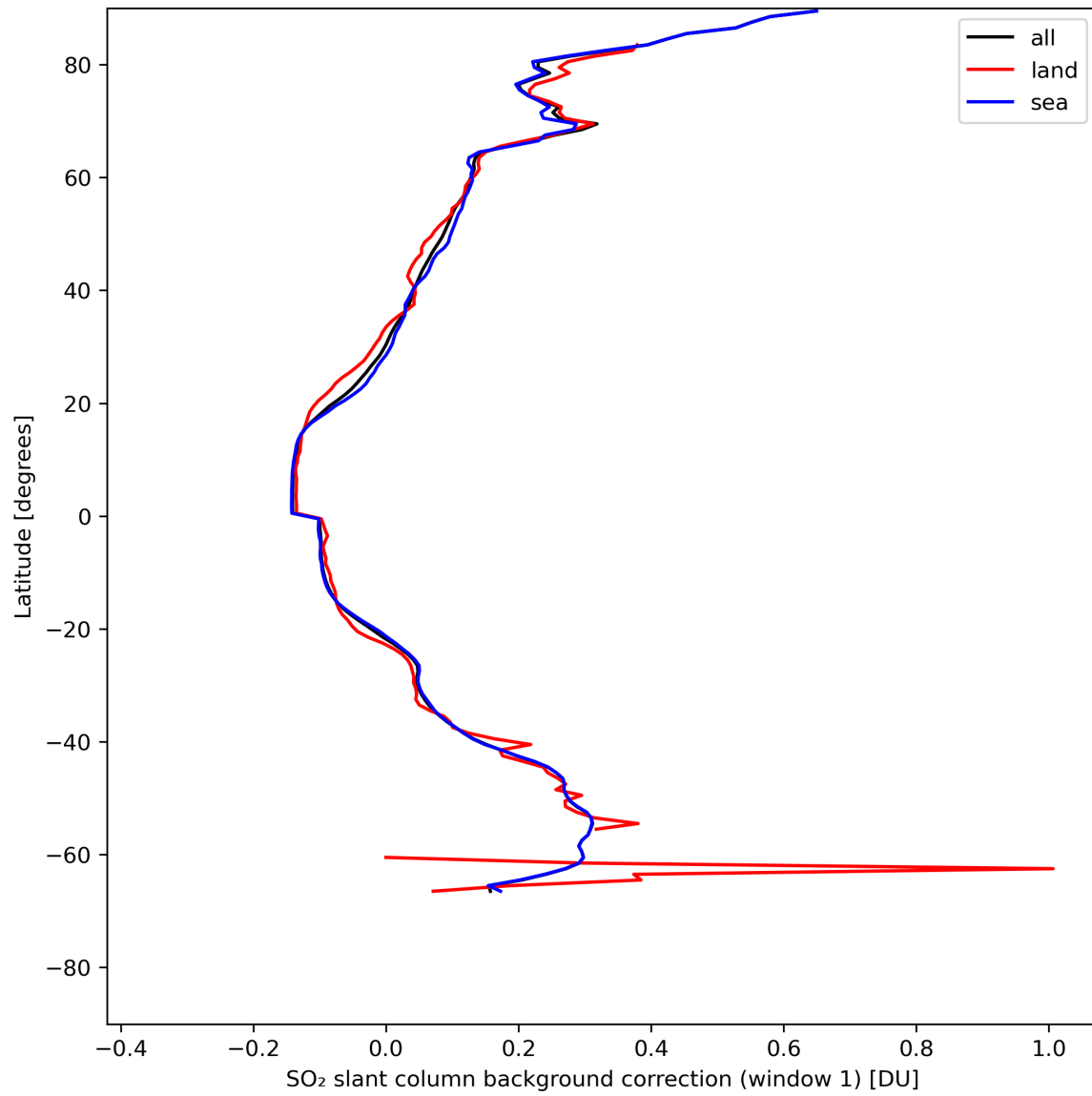
Figure 36: Zonal average of “SO 2 slant column background correction (window 1)” for 2024-05-10 to 2024-05-12.
