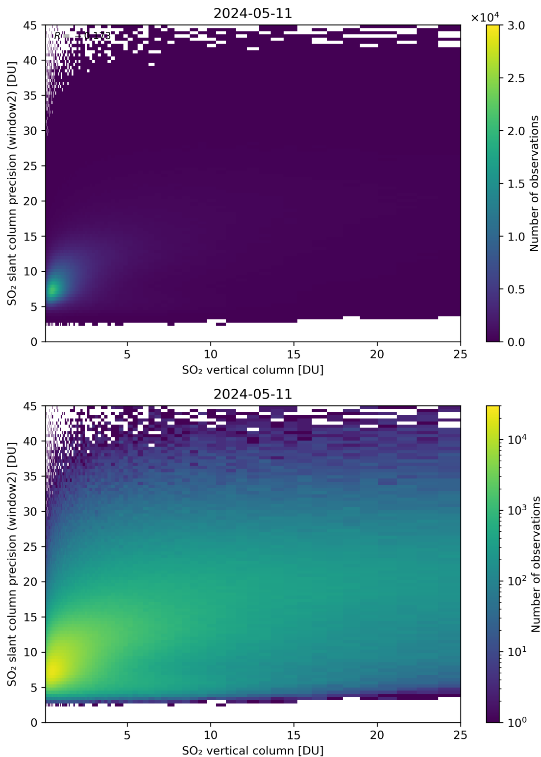
Figure 302: Scatter density plot of “SO 2 vertical column” against “SO 2 slant column precision (window2)” for 2024-05-10 to 2024-05-12.
