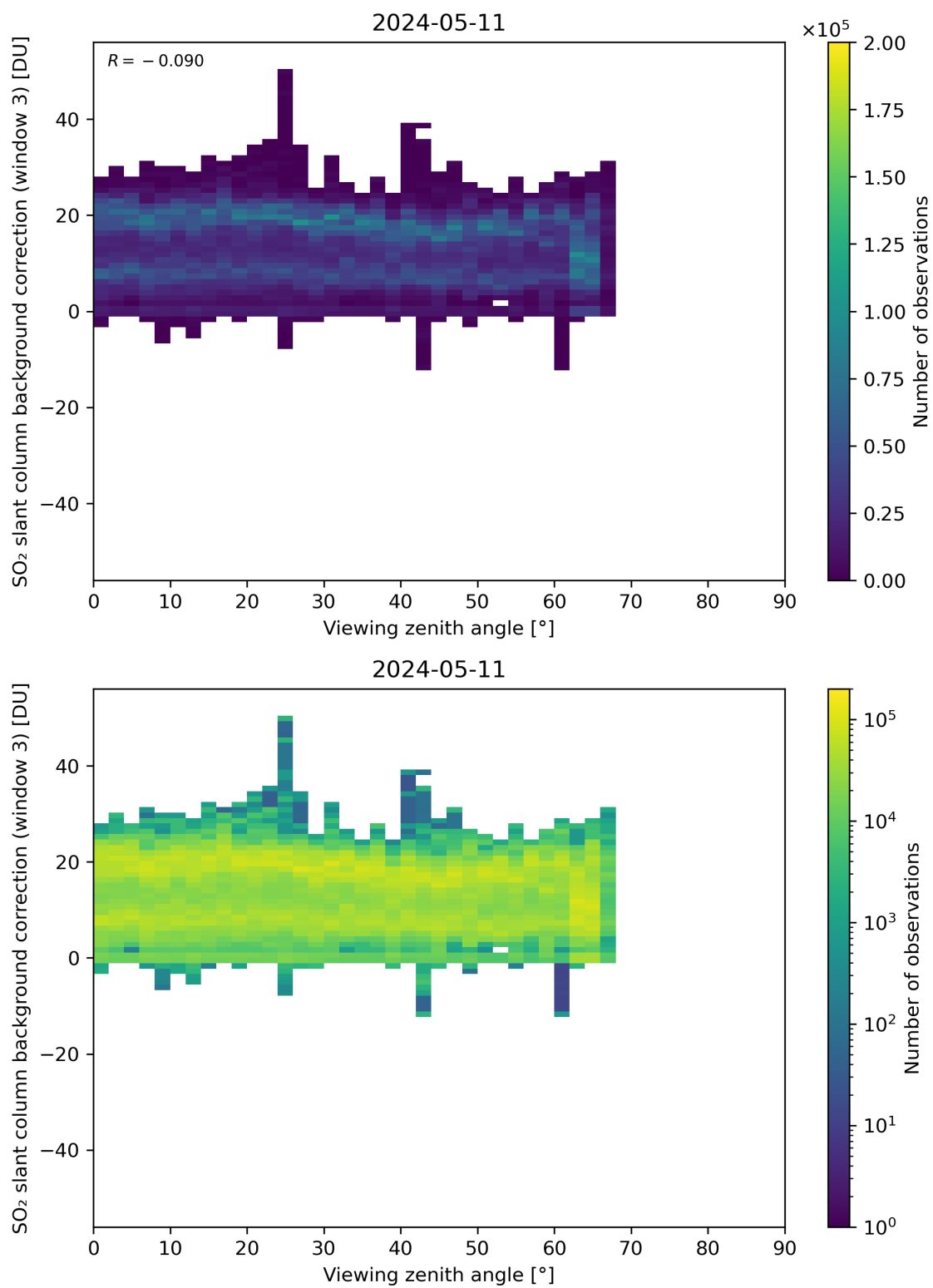
Figure 310: Scatter density plot of “Viewing zenith angle” against “SO 2 slant column background correction (window 3)” for 2024-05-10 to 2024-05-12.
