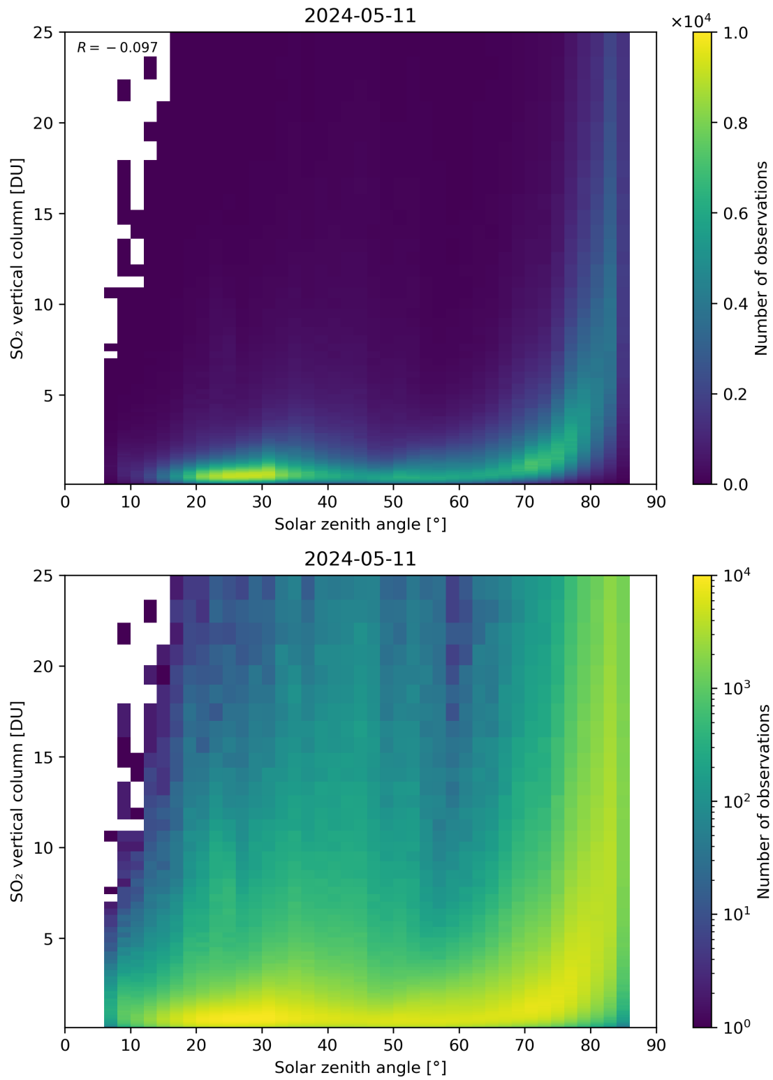
Figure 176: Scatter density plot of “Solar zenith angle” against “SO 2 vertical column” for 2024-05-10 to 2024-05-12.
