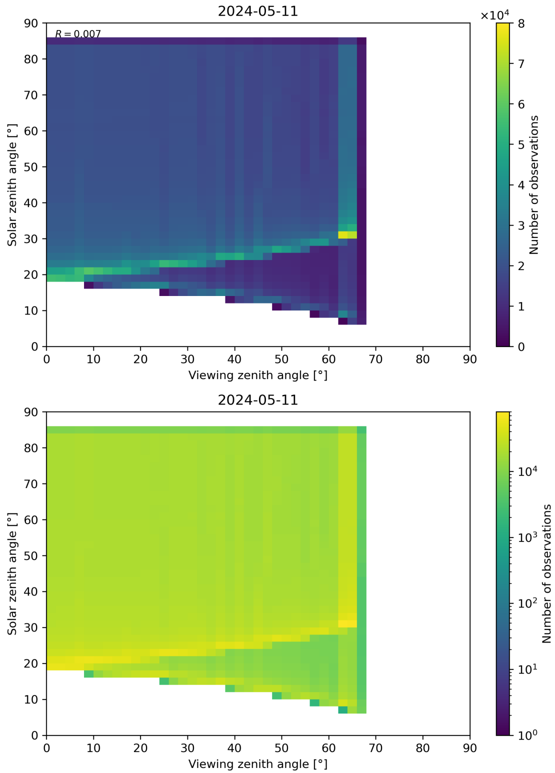
Figure 315: Scatter density plot of “Viewing zenith angle” against “Solar zenith angle” for 2024-05-10 to 2024-05-12.
