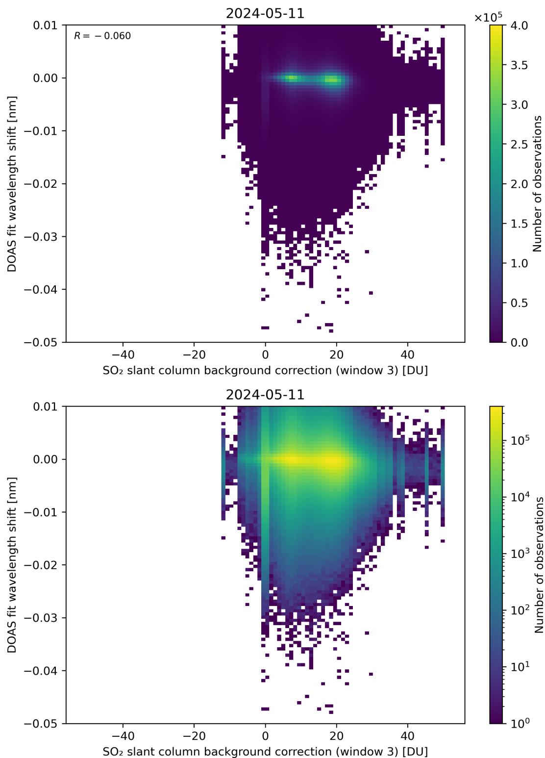
Figure 121: Scatter density plot of “SO 2 slant column background correction (window 3)” against “DOAS fit wavelength shift” for 2024-05-10 to 2024-05-12.
