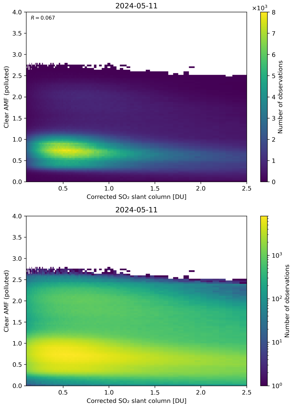
Figure 184: Scatter density plot of “Corrected SO 2 slant column” against “Clear AMF (polluted)” for 2024-05-10 to 2024-05-12.
