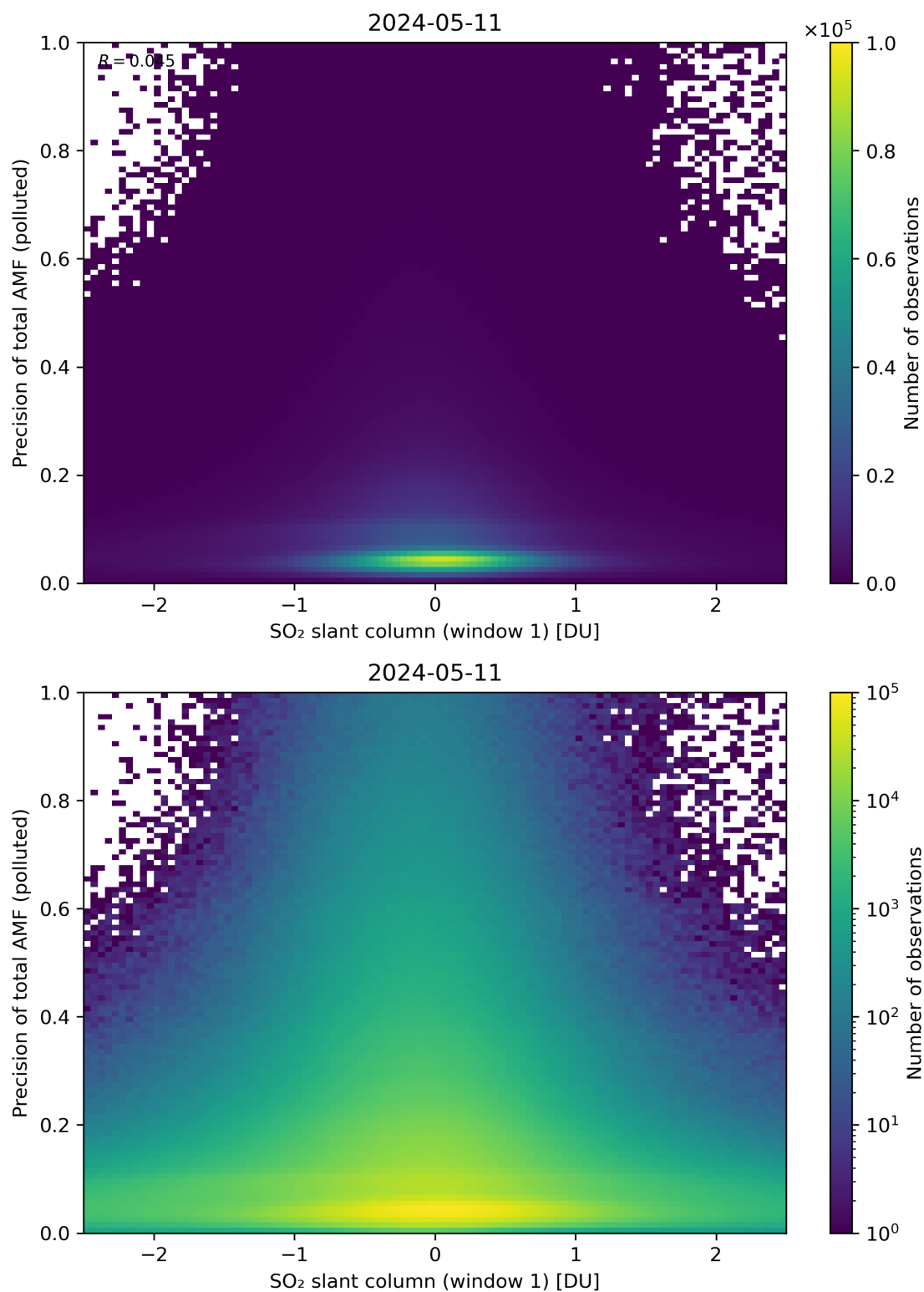
Figure 240: Scatter density plot of “SO 2 slant column (window 1)” against “Precision of total AMF (polluted)” for 2024-05-10 to 2024-05-12.
