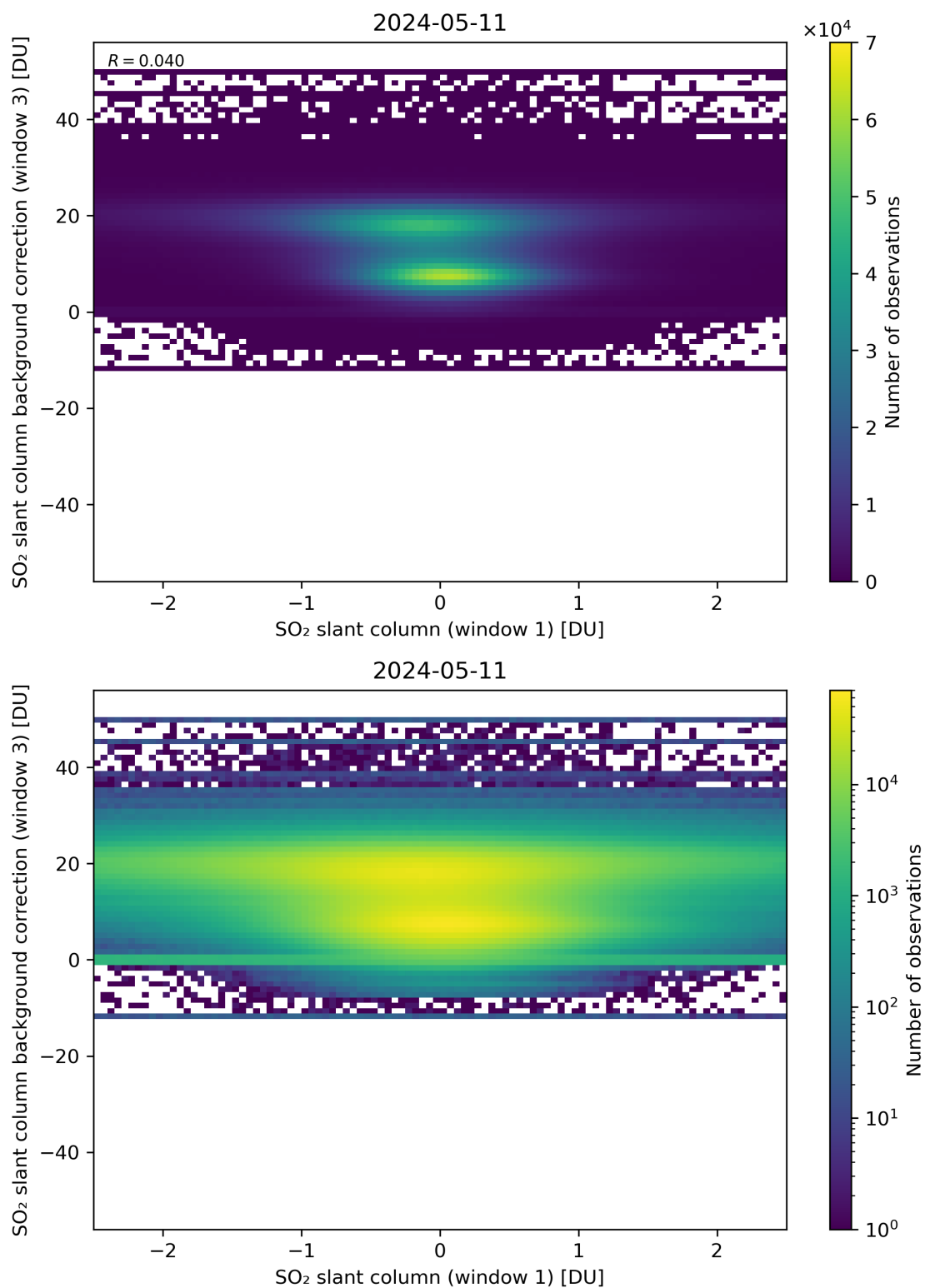
Figure 214: Scatter density plot of “SO 2 slant column (window 1)” against “SO 2 slant column background correction (window 3)” for 2024-05-10 to 2024-05-12.
