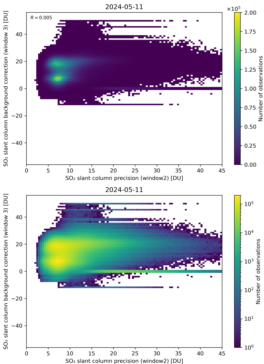
Figure 242: Scatter density plot of “SO 2 slant column precision (window2)” against “SO 2 slant column background correction (window 3)” for 2024-05-10 to 2024-05-12.
