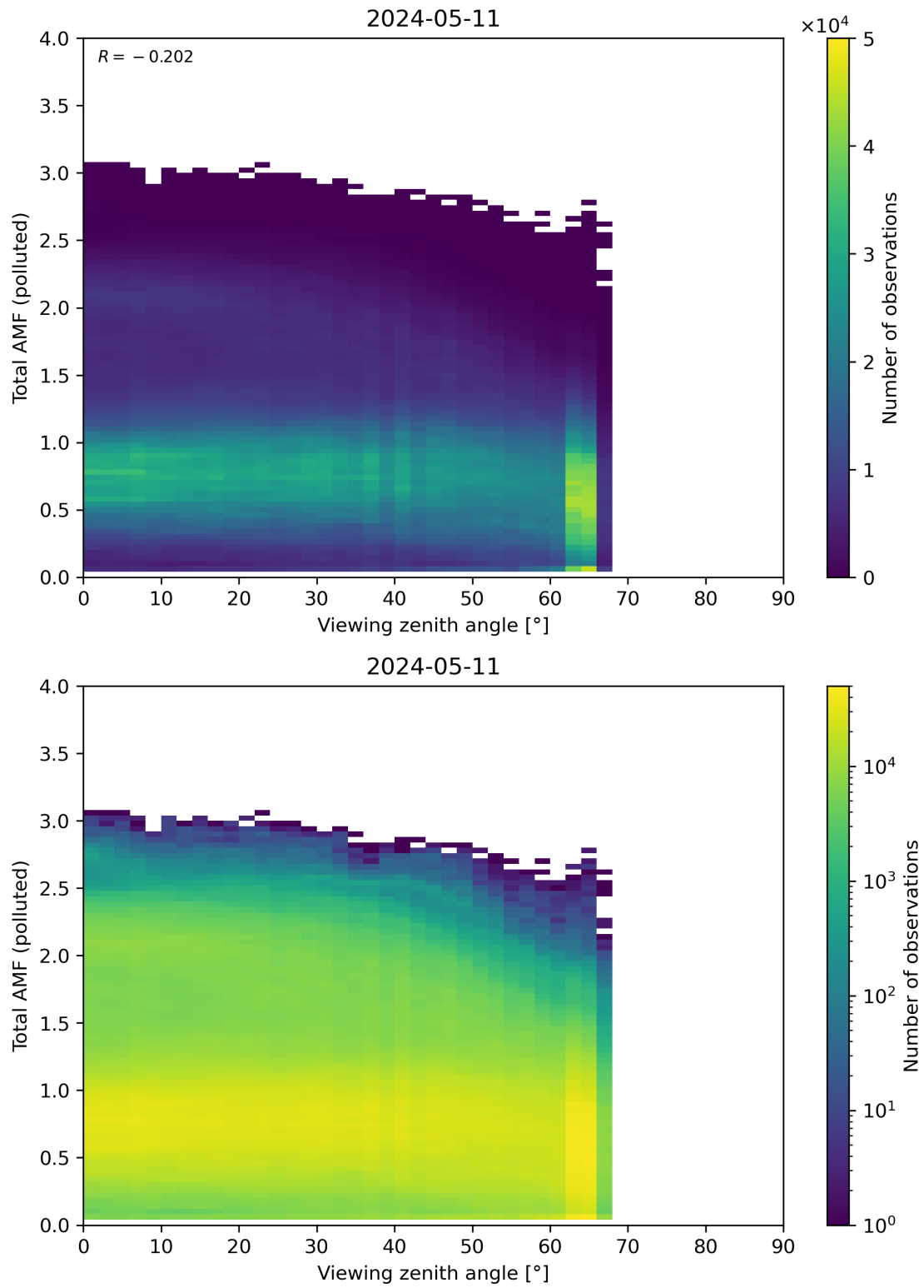
Figure 325: Scatter density plot of “Viewing zenith angle” against “Total AMF (polluted)” for 2024-05-10 to 2024-05-12.
