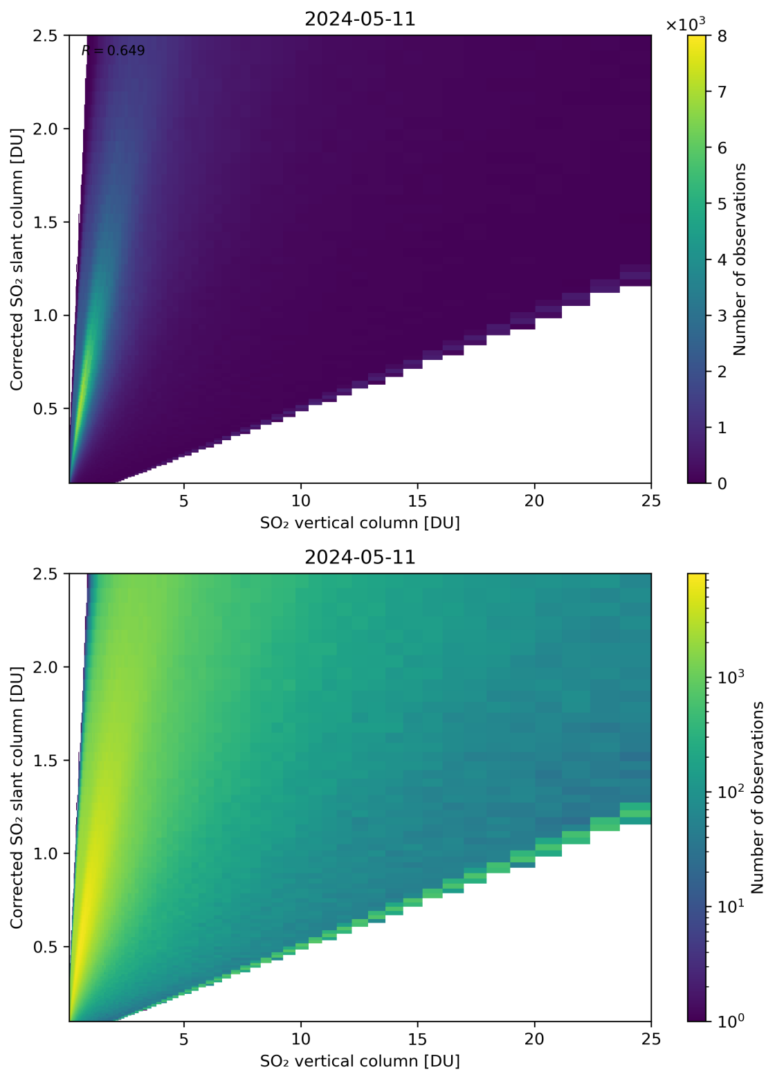
Figure 297: Scatter density plot of “SO 2 vertical column” against “Corrected SO 2 slant column” for 2024-05-10 to 2024-05-12.
