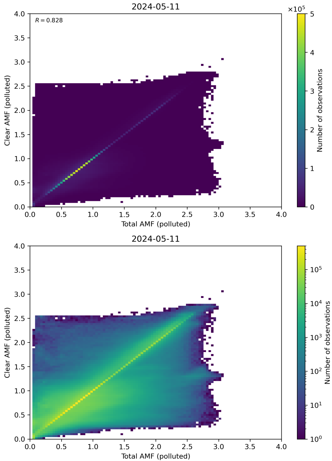
Figure 271: Scatter density plot of “Total AMF (polluted)” against “Clear AMF (polluted)” for 2024-05-10 to 2024-05-12.
