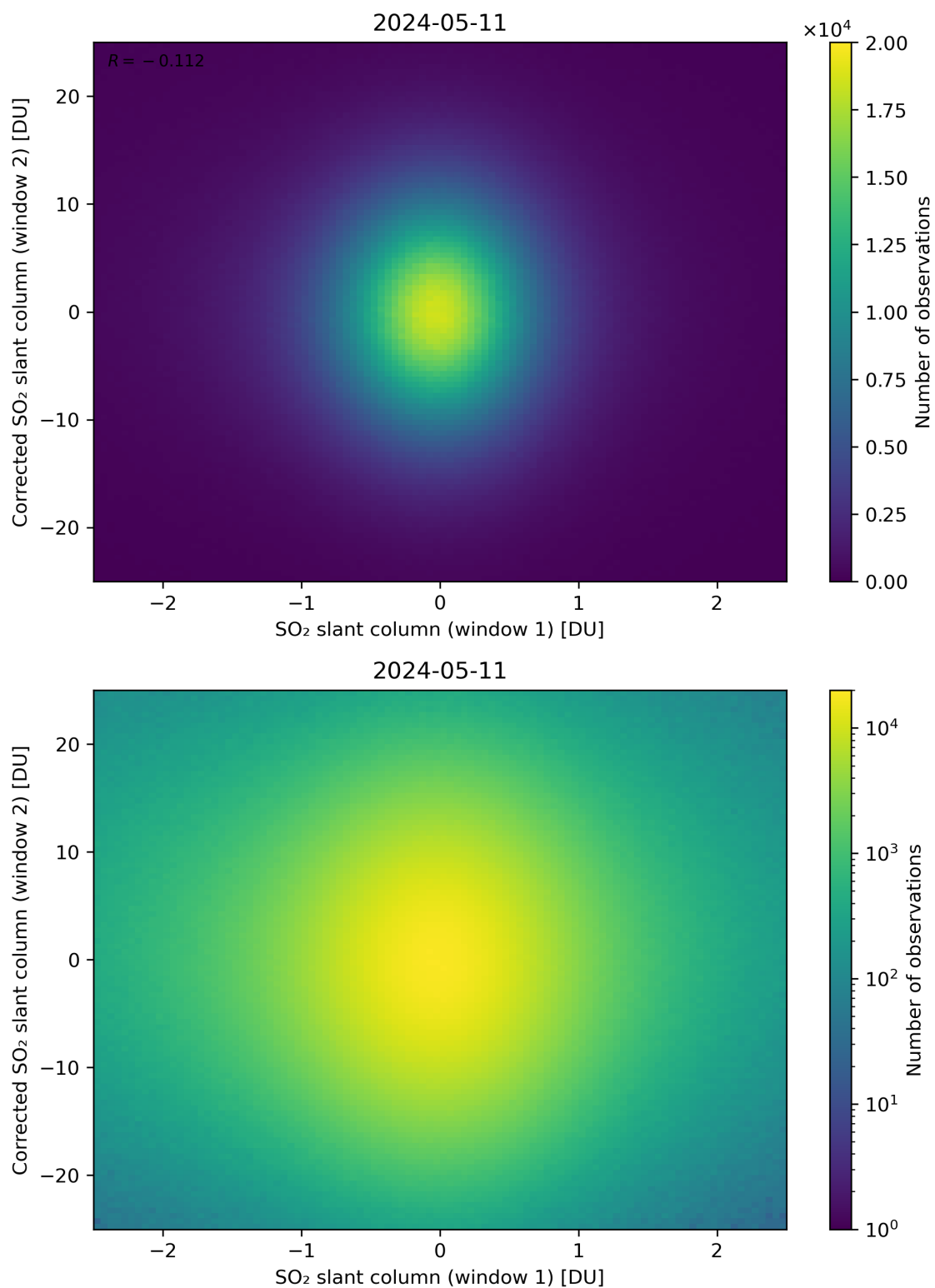
Figure 233: Scatter density plot of “SO 2 slant column (window 1)” against “Corrected SO 2 slant column (window 2)” for 2024-05-10 to 2024-05-12.
