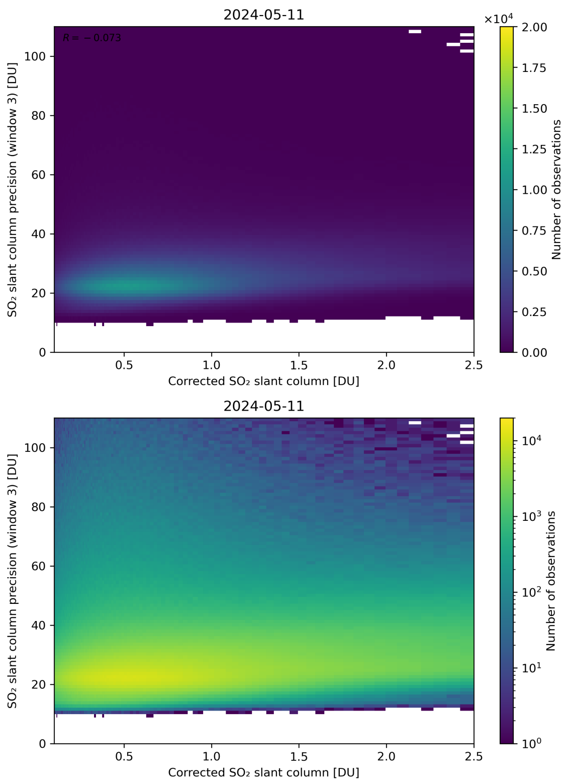
Figure 191: Scatter density plot of “Corrected SO 2 slant column” against “SO 2 slant column precision (window 3)” for 2024-05-10 to 2024-05-12.
