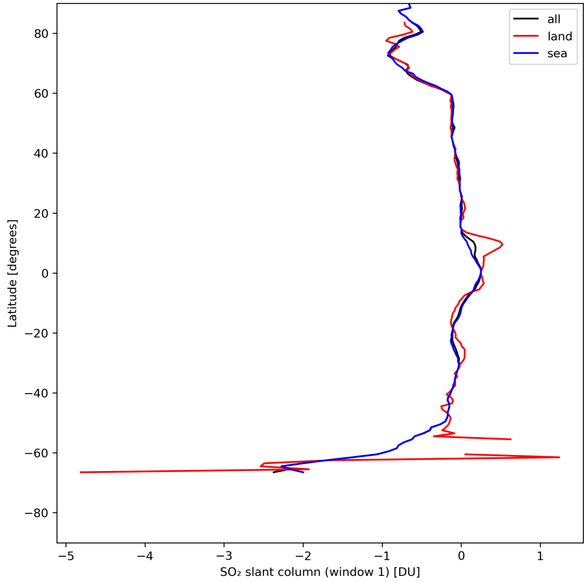
Figure 33: Zonal average of “SO 2 slant column (window 1)” for 2024-05-10 to 2024-05-12.
