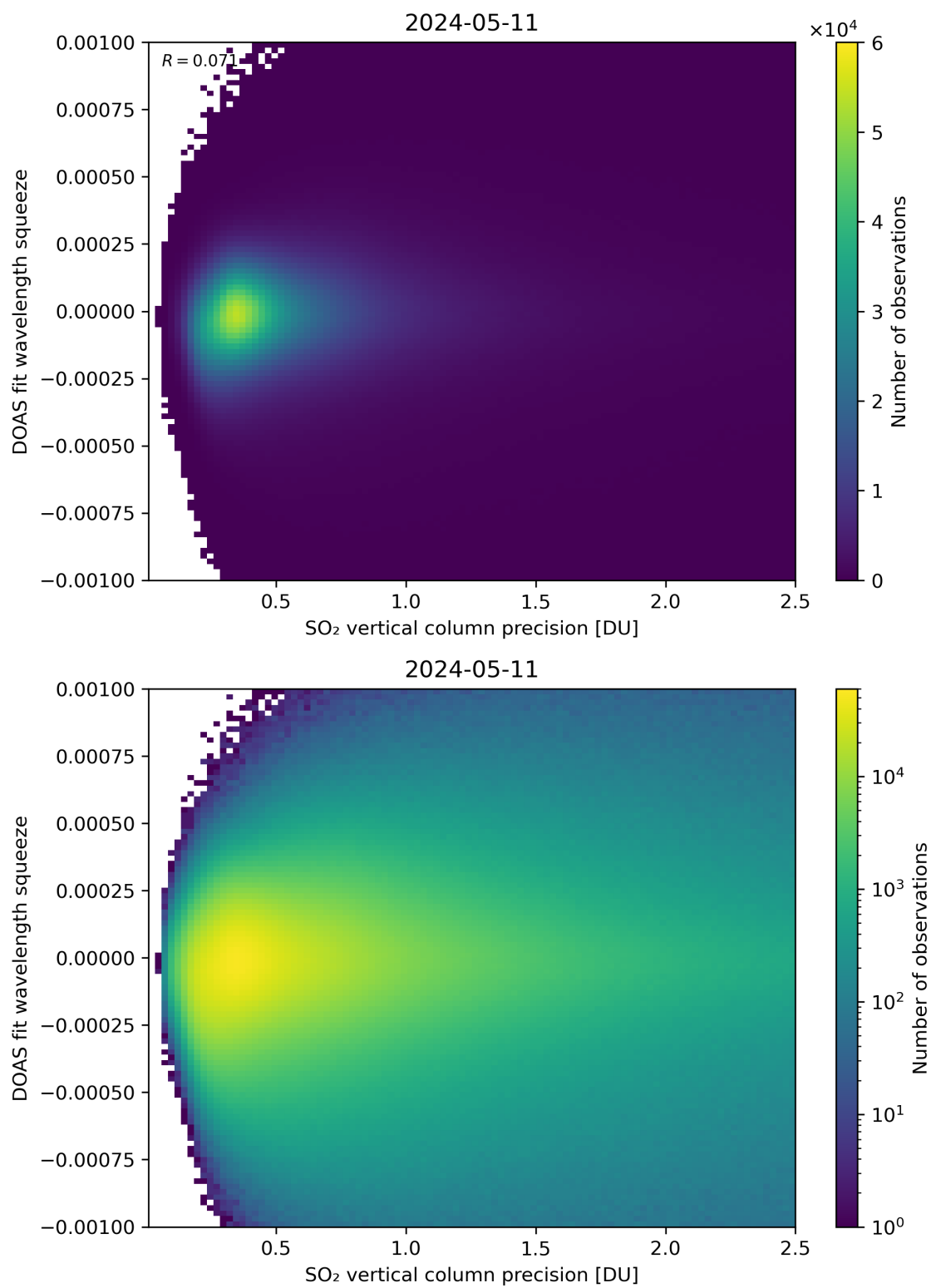
Figure 283: Scatter density plot of “SO 2 vertical column precision” against “DOAS fit wavelength squeeze” for 2024-05-10 to 2024-05-12.
