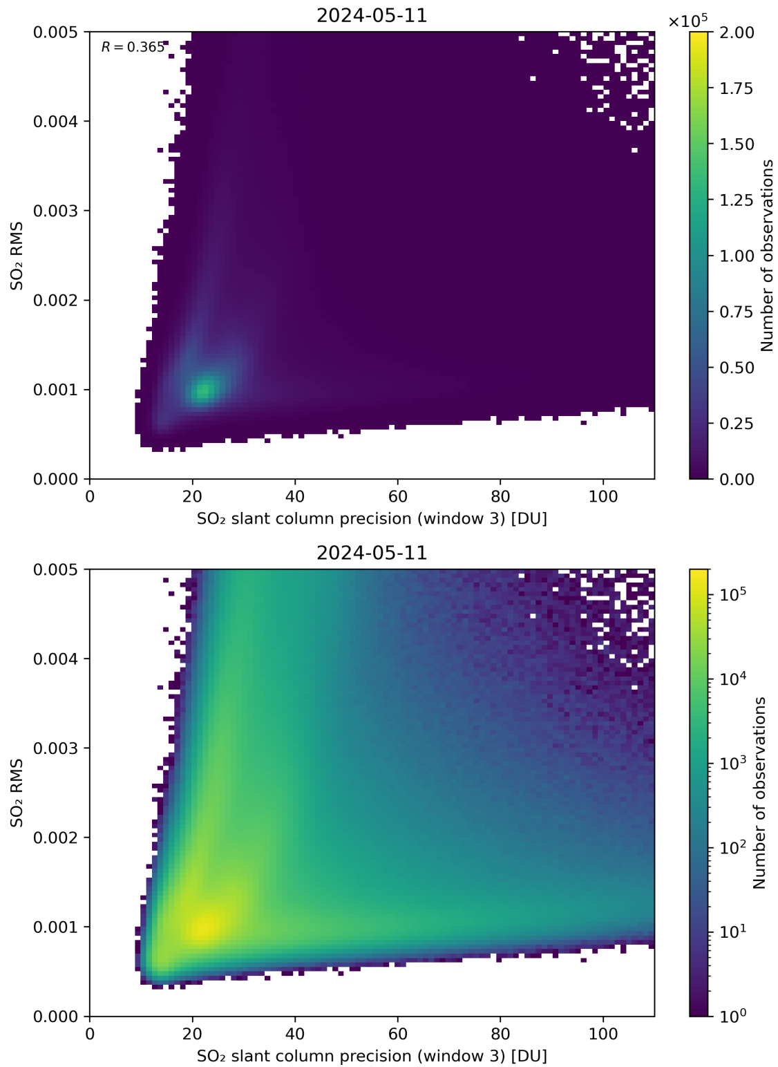
Figure 260: Scatter density plot of “SO 2 slant column precision (window 3)” against “SO 2 RMS” for 2024-05-10 to 2024-05-12.
