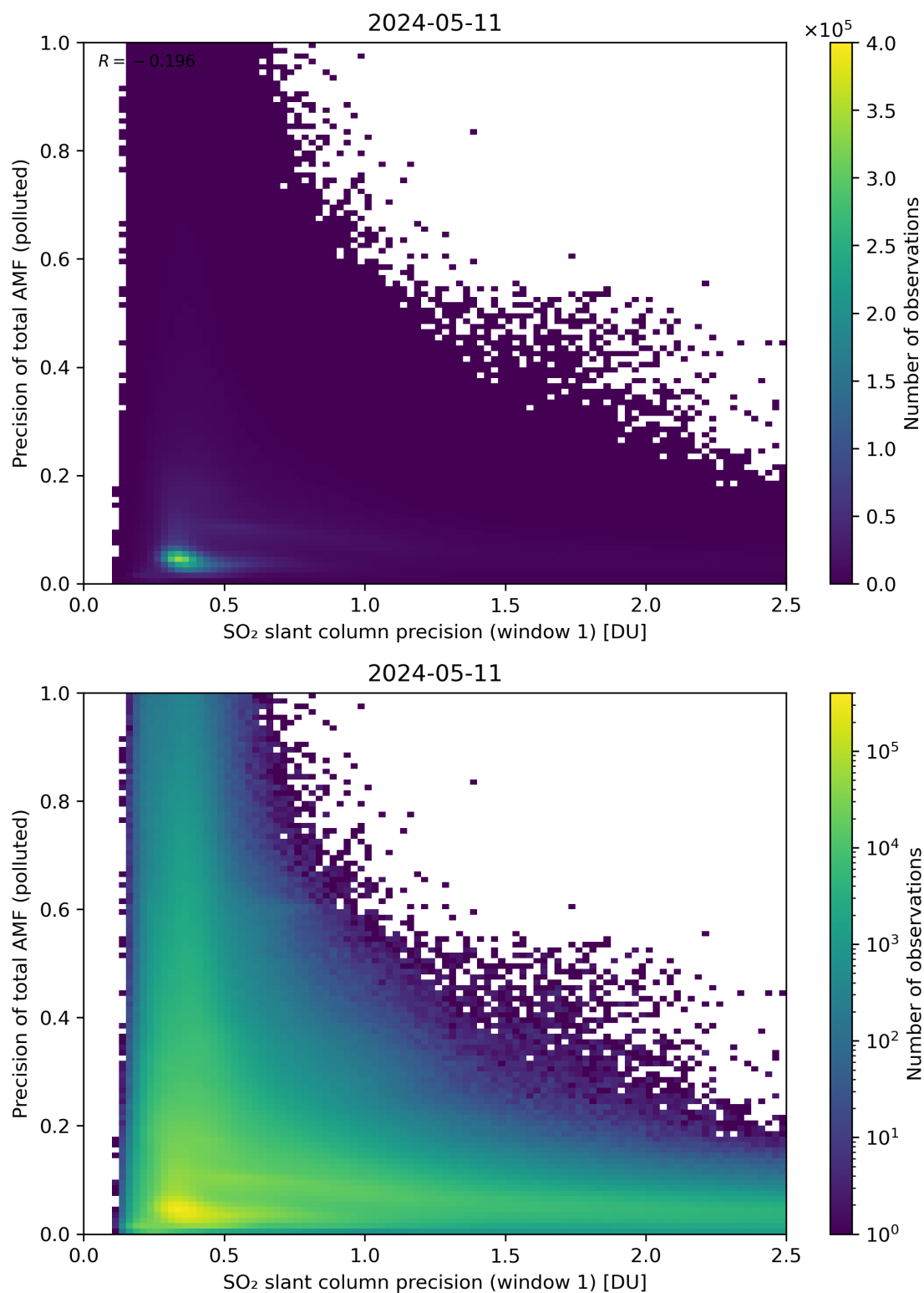
Figure 231: Scatter density plot of “SO 2 slant column precision (window 1)” against “Precision of total AMF (polluted)” for 2024-05-10 to 2024-05-12.
