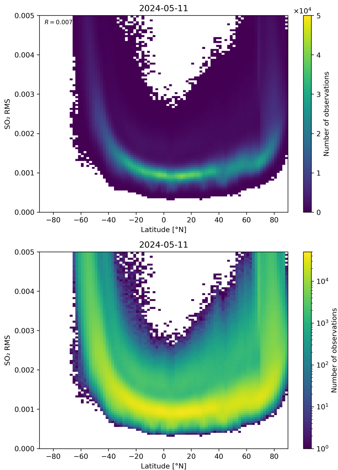
Figure 144: Scatter density plot of “Latitude” against “SO 2 RMS” for 2024-05-10 to 2024-05-12.
