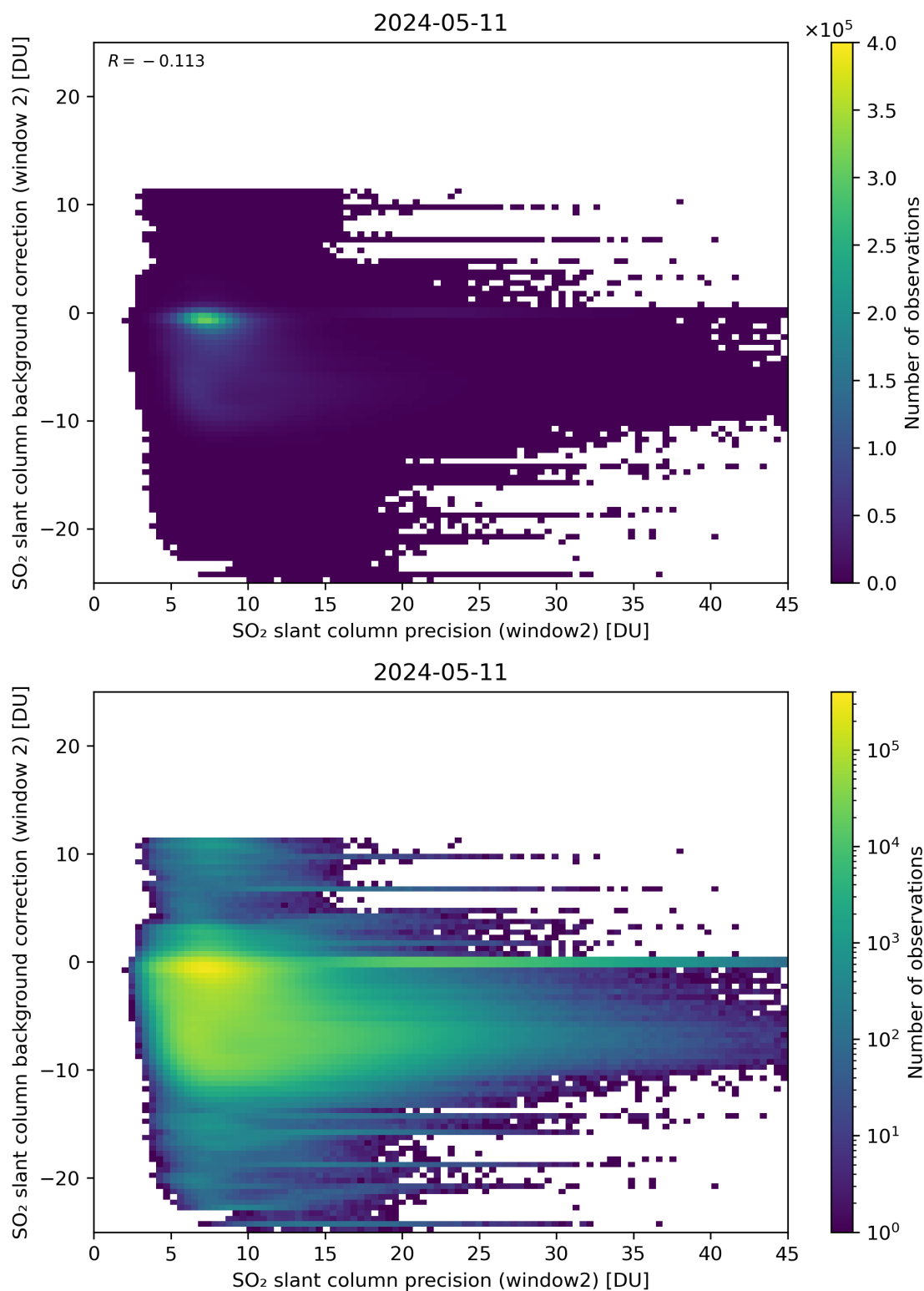
Figure 241: Scatter density plot of “SO 2 slant column precision (window2)” against “SO 2 slant column background correction (window 2)” for 2024-05-10 to 2024-05-12.
