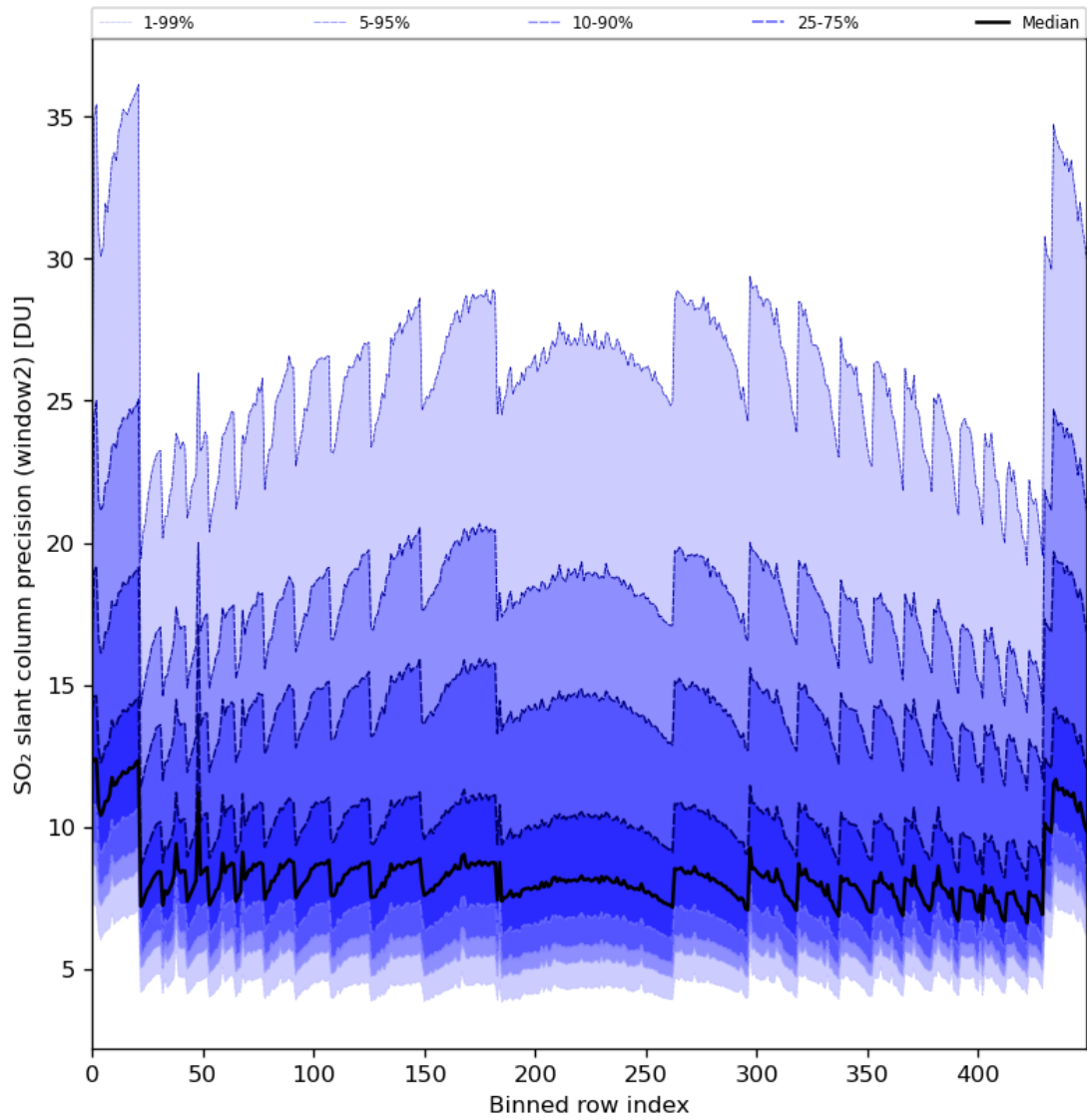
Figure 84: Along track statistics of “SO 2 slant column precision (window2)” for 2024-05-10 to 2024-05-12
