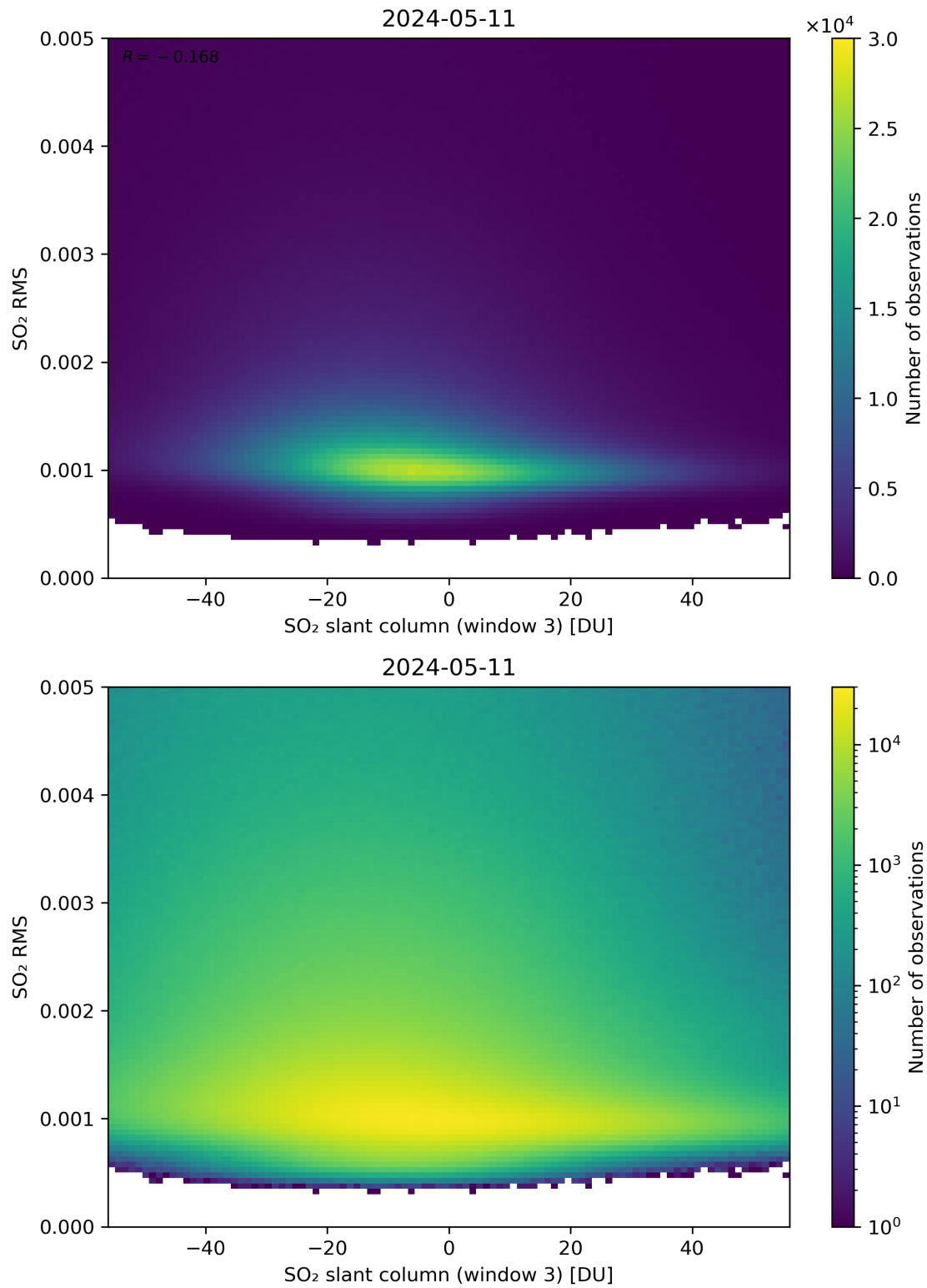
Figure 256: Scatter density plot of “SO 2 slant column (window 3)” against “SO 2 RMS” for 2024-05-10 to 2024-05-12.
