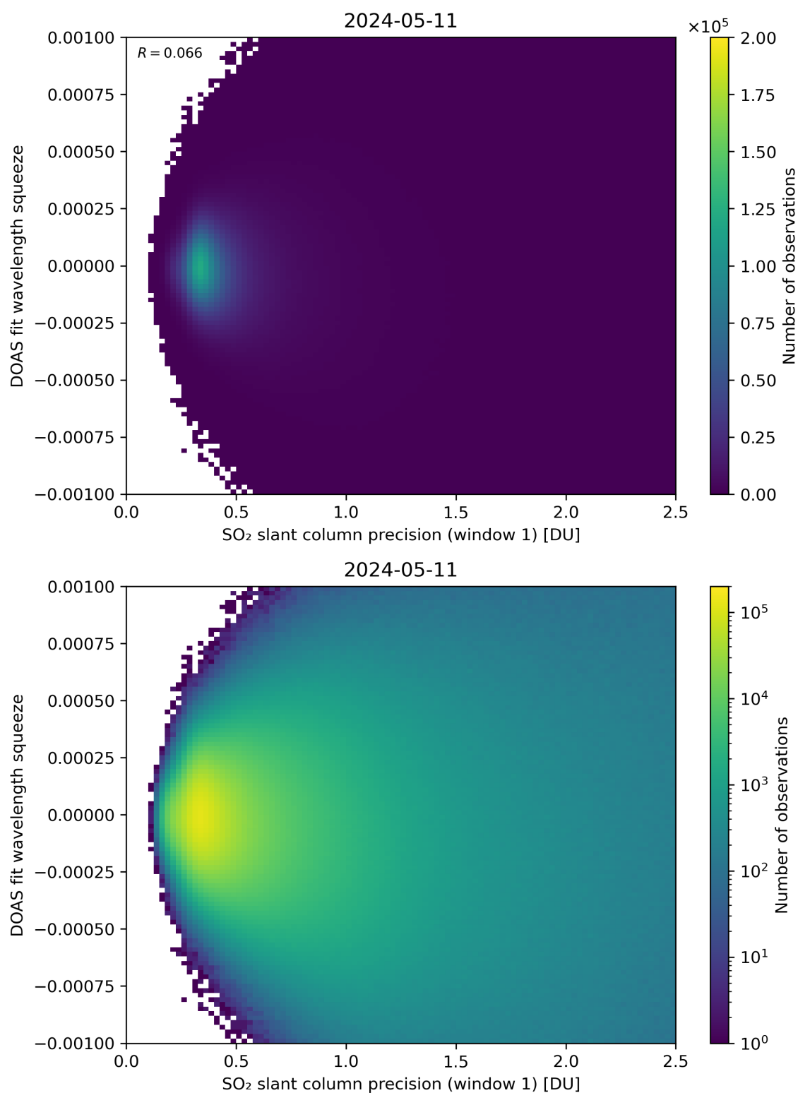
Figure 222: Scatter density plot of “SO 2 slant column precision (window 1)” against “DOAS fit wavelength squeeze” for 2024-05-10 to 2024-05-12.
