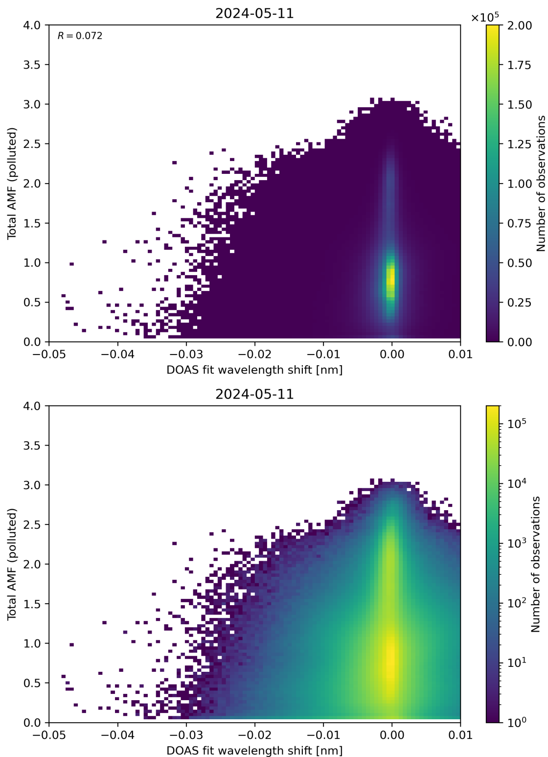
Figure 130: Scatter density plot of “DOAS fit wavelength shift” against “Total AMF (polluted)” for 2024-05-10 to 2024-05-12.
