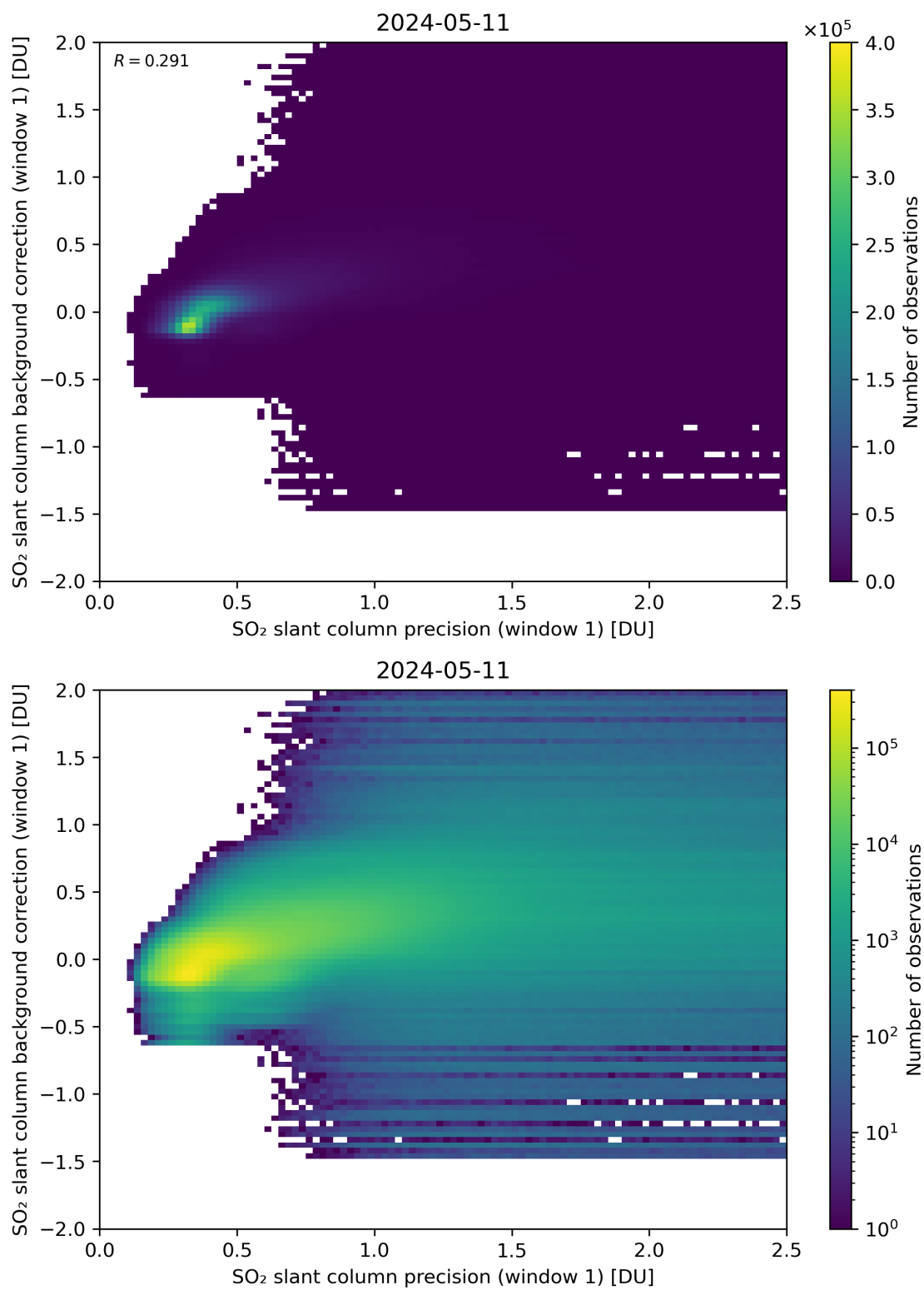
Figure 218: Scatter density plot of “SO 2 slant column precision (window 1)” against “SO 2 slant column background correction (window 1)” for 2024-05-10 to 2024-05-12.
