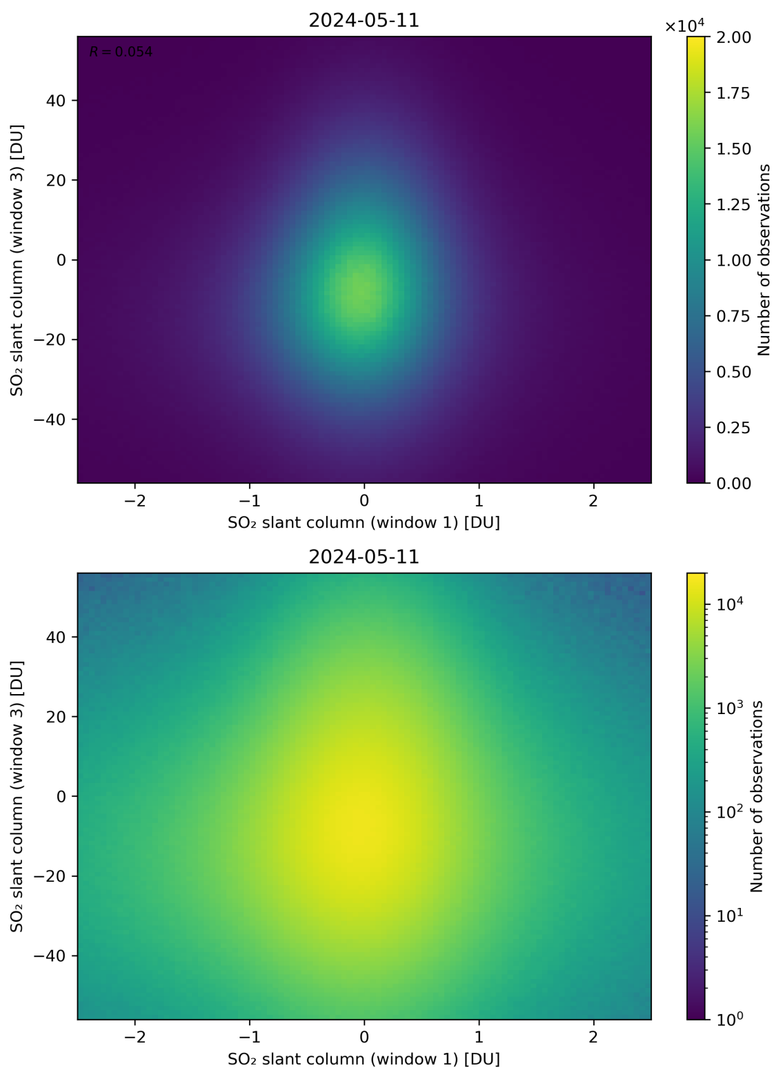
Figure 237: Scatter density plot of “SO 2 slant column (window 1)” against “SO 2 slant column (window 3)” for 2024-05-10 to 2024-05-12.
