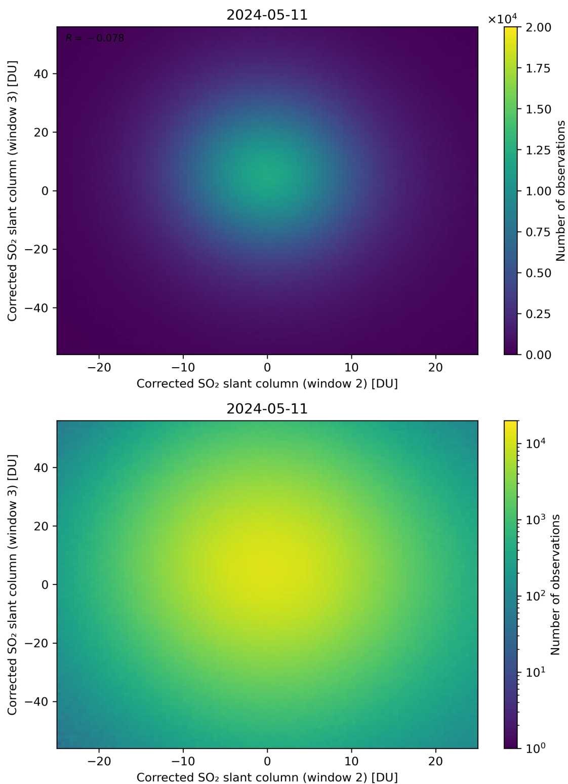
Figure 200: Scatter density plot of “Corrected SO 2 slant column (window 2)” against “Corrected SO 2 slant column (window 3)” for 2024-05-10 to 2024-05-12.
