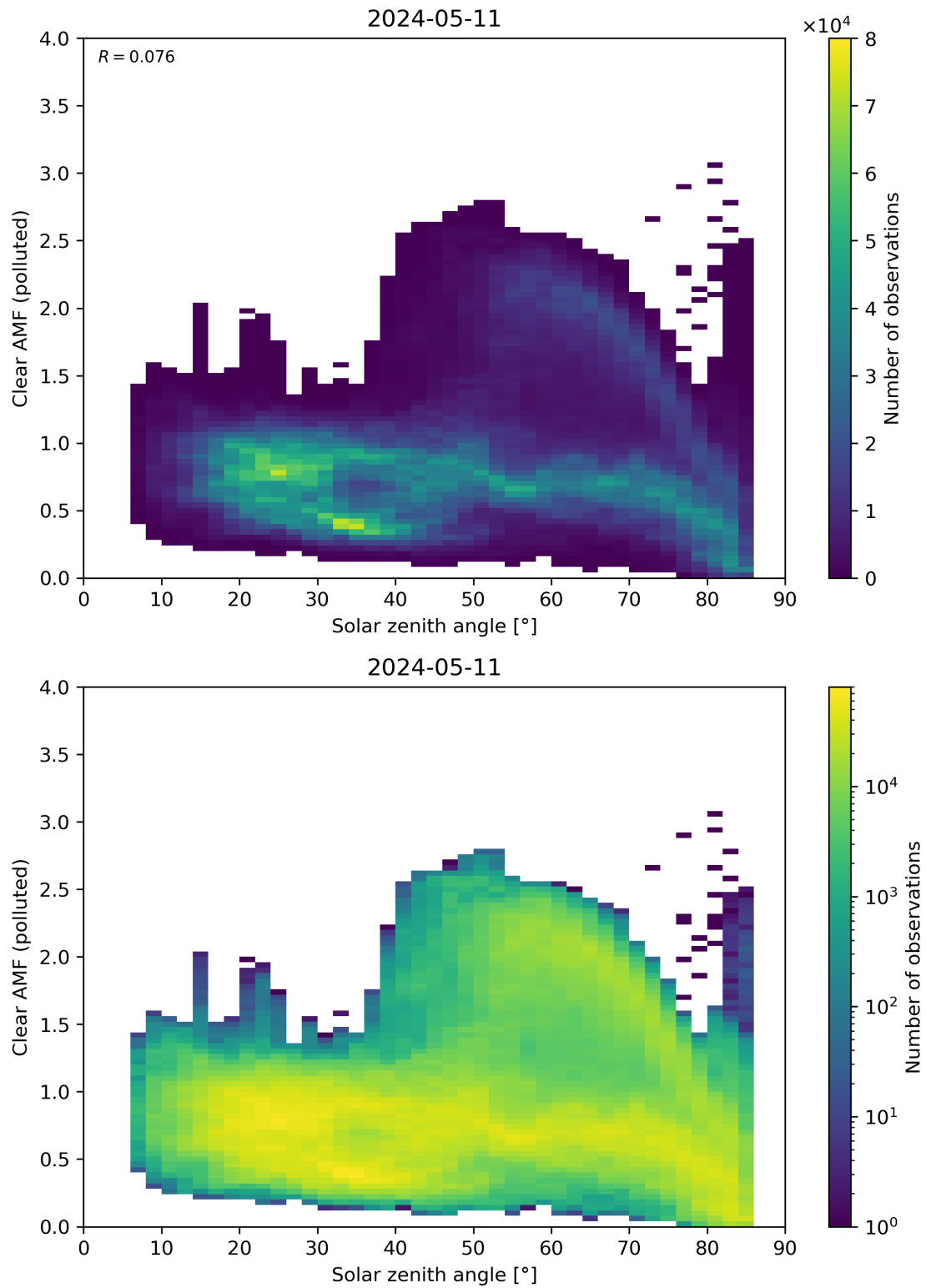
Figure 165: Scatter density plot of “Solar zenith angle” against “Clear AMF (polluted)” for 2024-05-10 to 2024-05-12.
