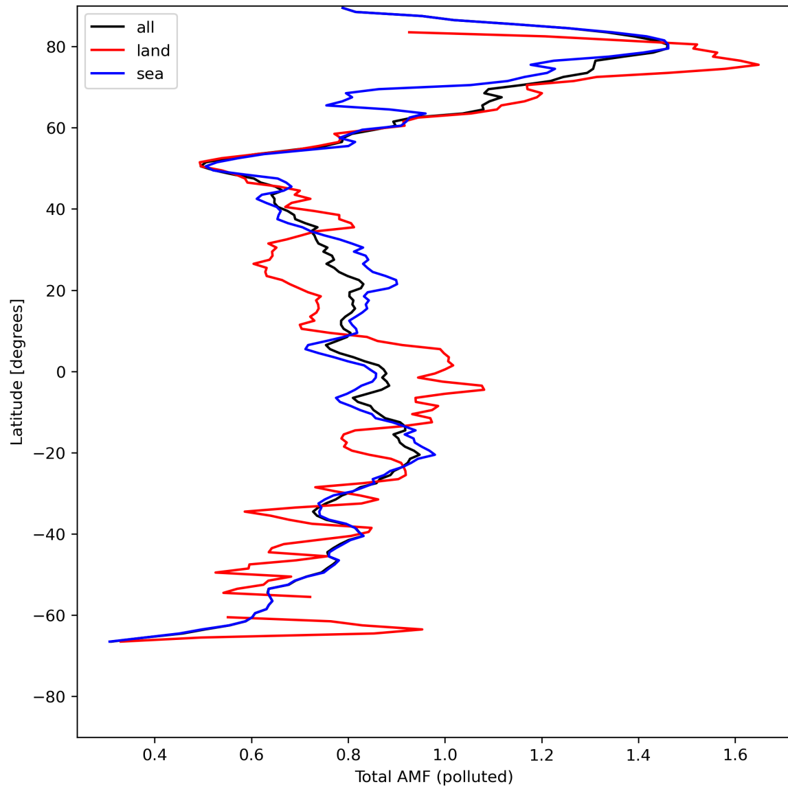
Figure 48: Zonal average of “Total AMF (polluted)” for 2024-05-10 to 2024-05-12.
