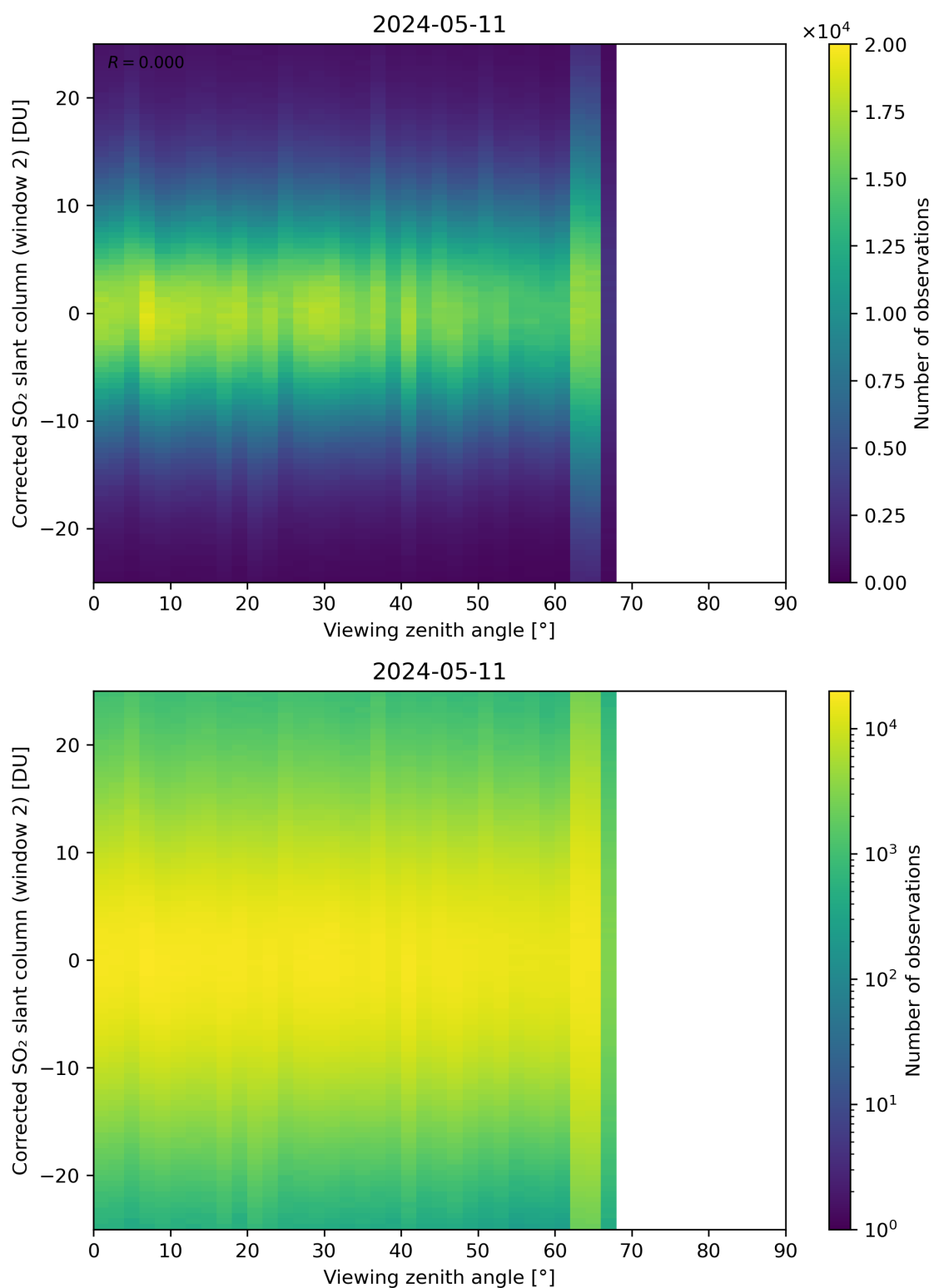
Figure 318: Scatter density plot of “Viewing zenith angle” against “Corrected SO 2 slant column (window 2)” for 2024-05-10 to 2024-05-12.
