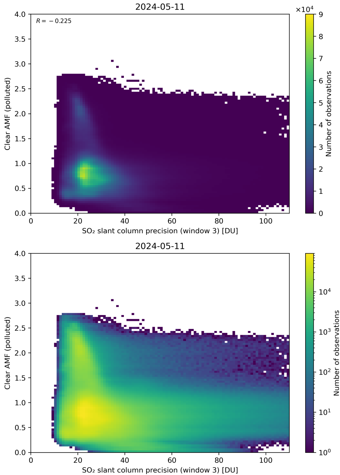
Figure 261: Scatter density plot of “SO 2 slant column precision (window 3)” against “Clear AMF (polluted)” for 2024-05-10 to 2024-05-12.
