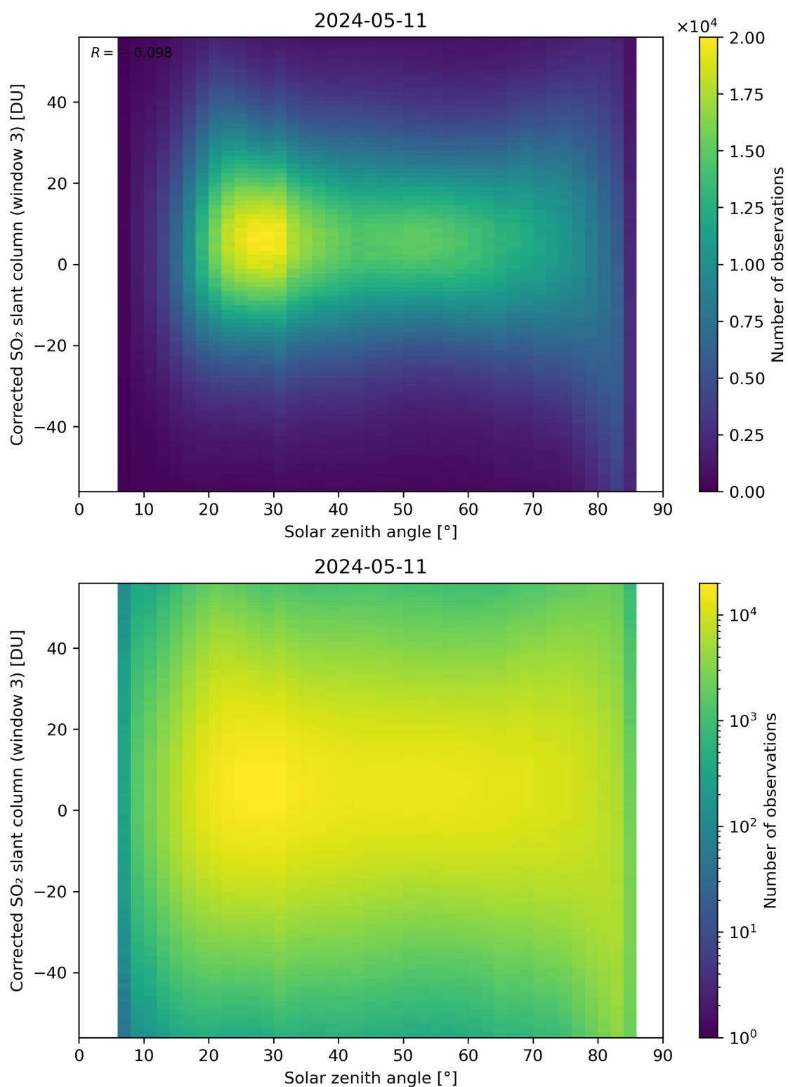
Figure 168: Scatter density plot of “Solar zenith angle” against “Corrected SO 2 slant column (window 3)” for 2024-05-10 to 2024-05-12.
