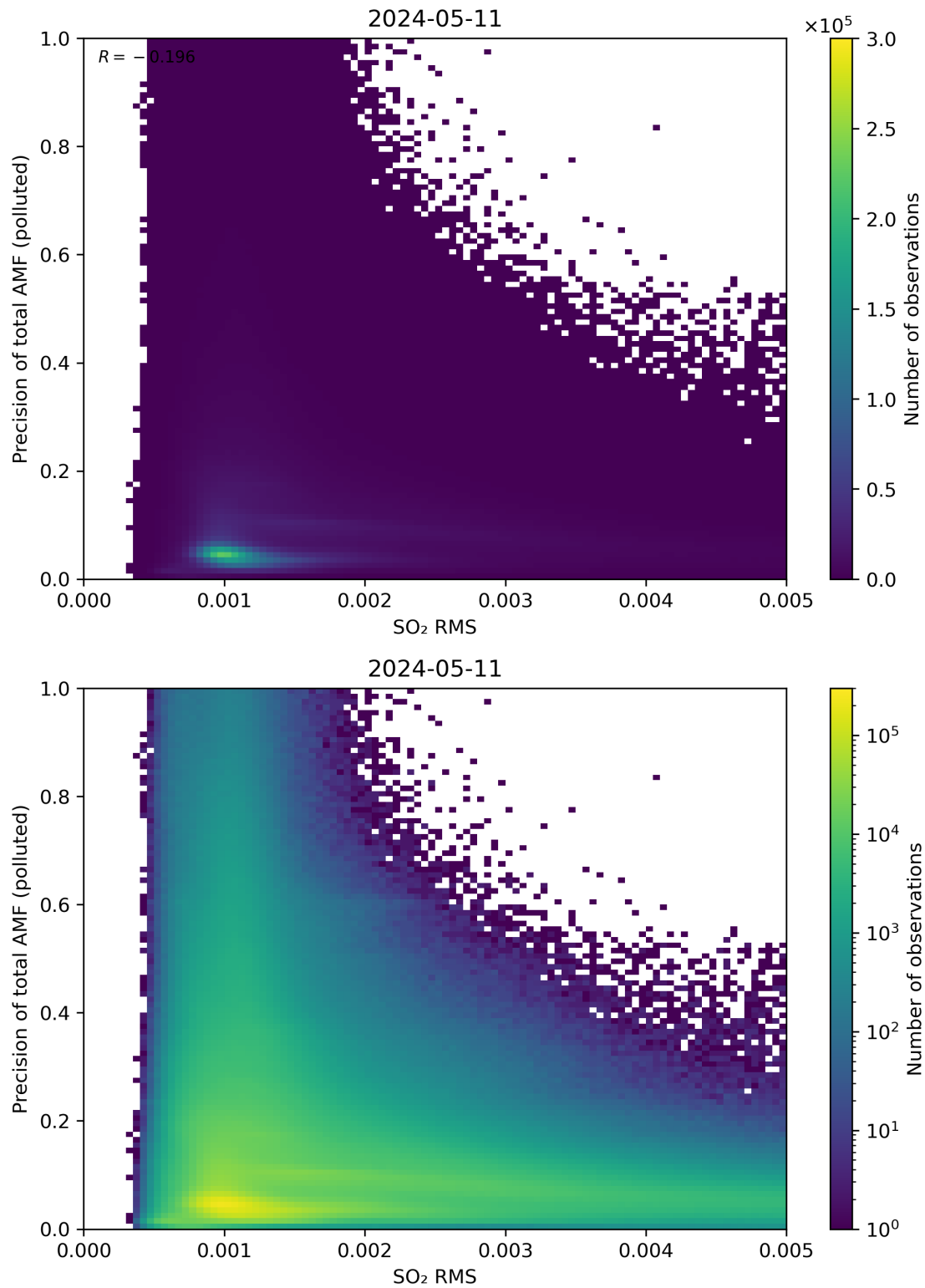
Figure 138: Scatter density plot of “SO 2 RMS” against “Precision of total AMF (polluted)” for 2024-05-10 to 2024-05-12.
