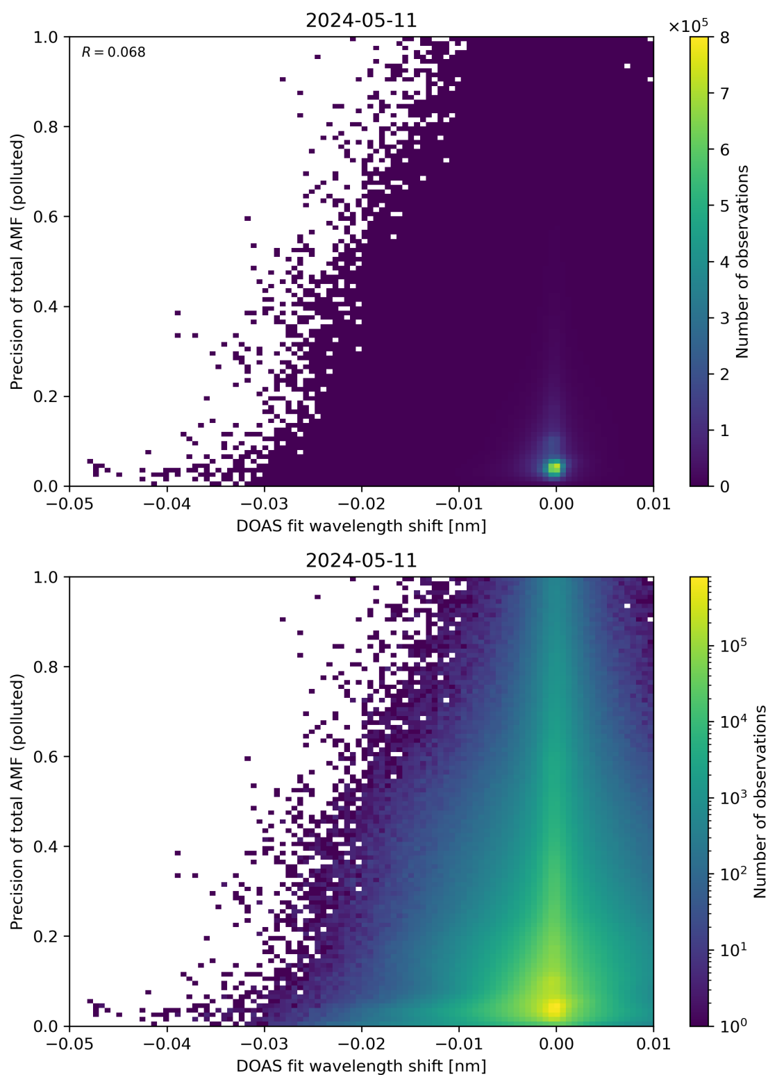
Figure 131: Scatter density plot of “DOAS fit wavelength shift” against “Precision of total AMF (polluted)” for 2024-05-10 to 2024-05-12.
