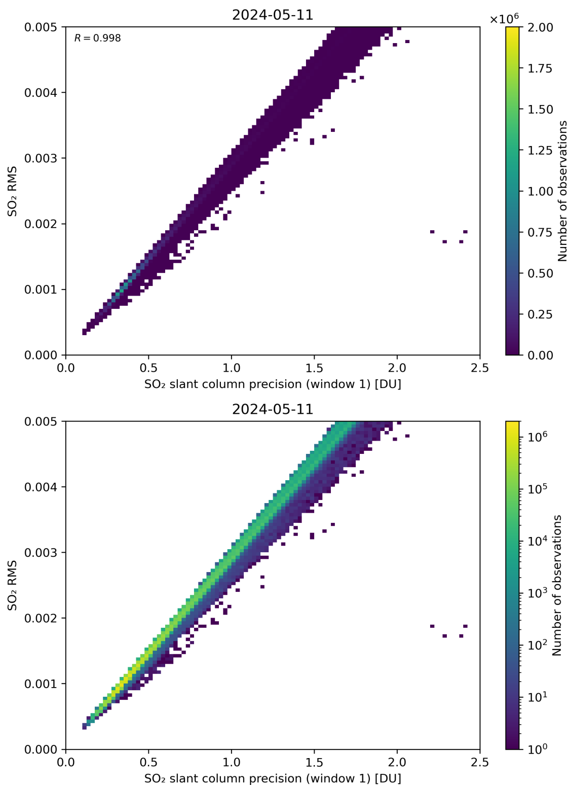
Figure 223: Scatter density plot of “SO 2 slant column precision (window 1)” against “SO 2 RMS” for 2024-05-10 to 2024-05-12.
