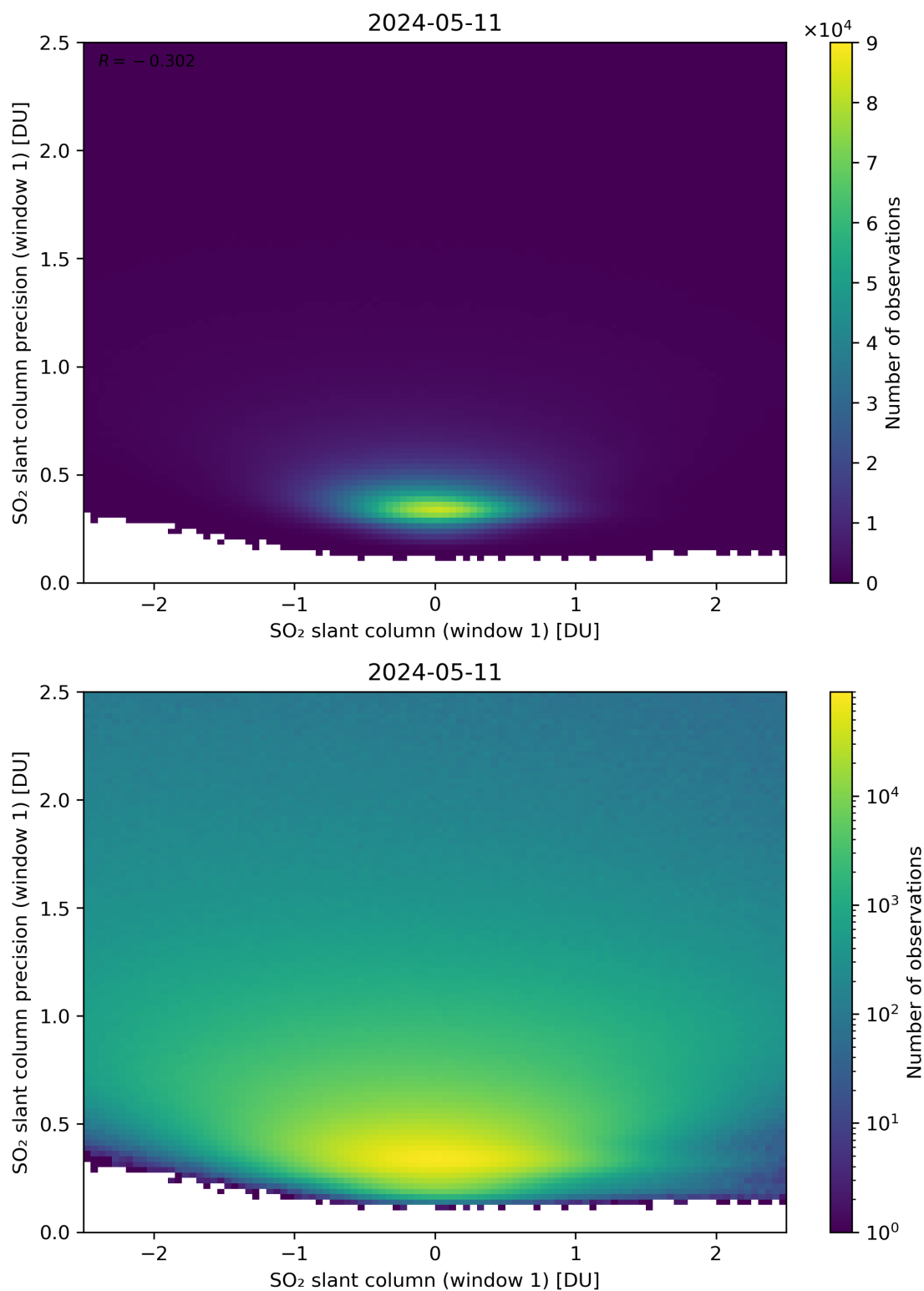
Figure 235: Scatter density plot of “SO 2 slant column (window 1)” against “SO 2 slant column precision (window 1)” for 2024-05-10 to 2024-05-12.
