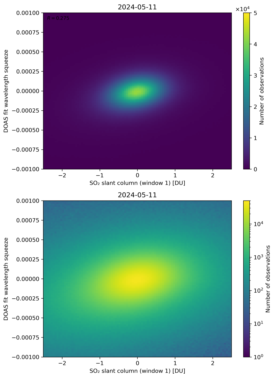
Figure 216: Scatter density plot of “SO 2 slant column (window 1)” against “DOAS fit wavelength squeeze” for 2024-05-10 to 2024-05-12.
