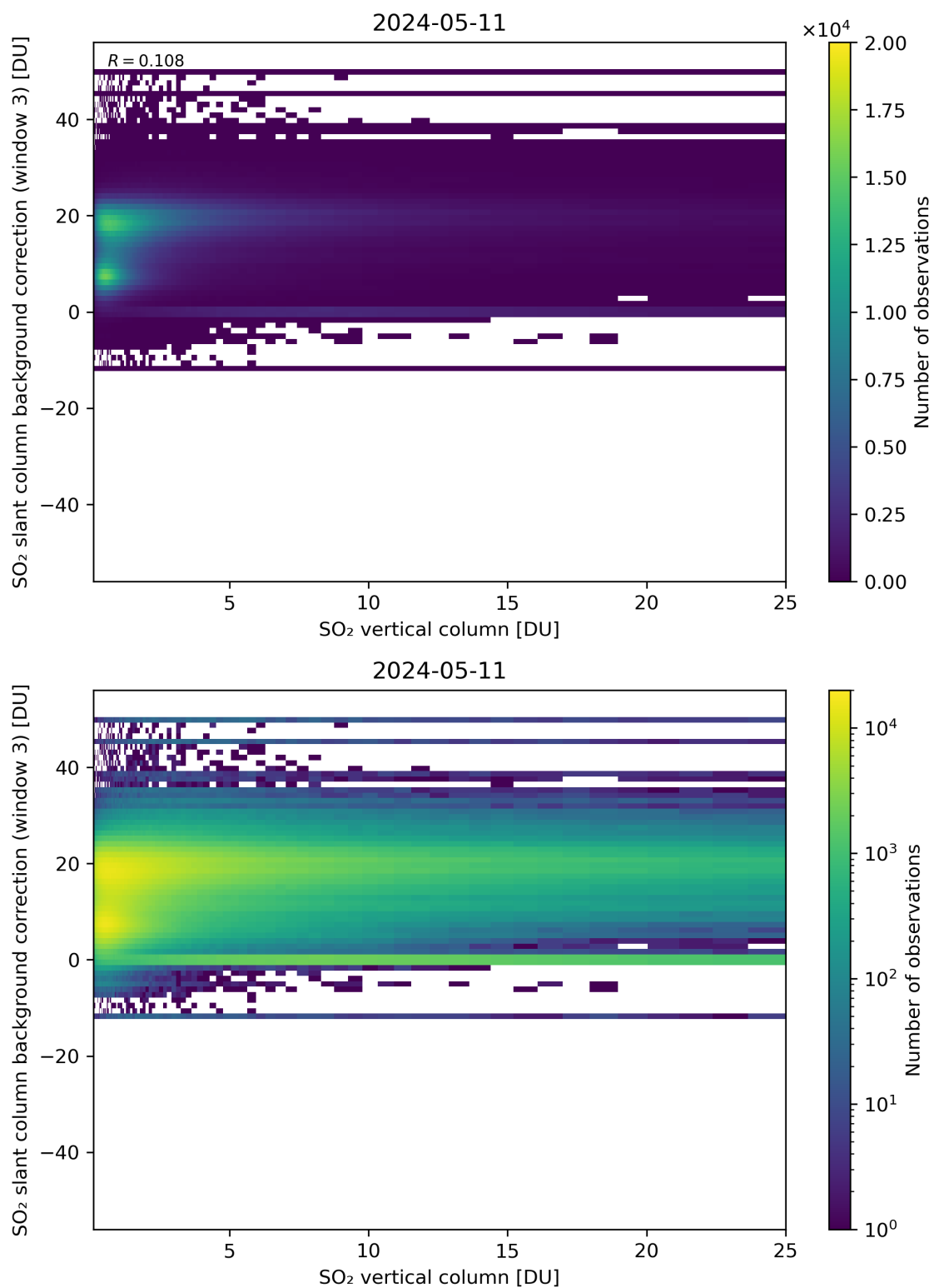
Figure 275: Scatter density plot of “SO 2 vertical column” against “SO 2 slant column background correction (window 3)” for 2024-05-10 to 2024-05-12.
