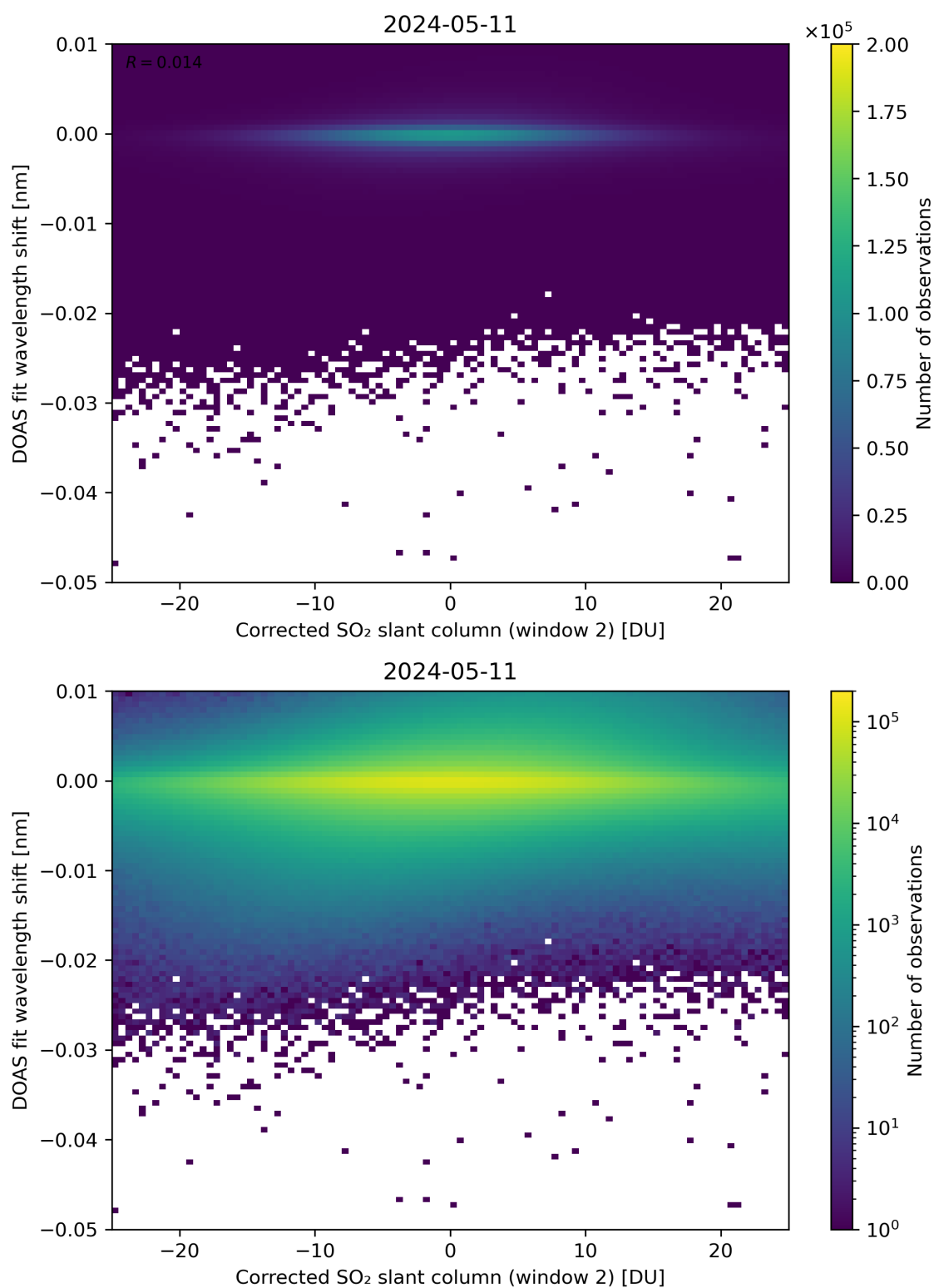
Figure 196: Scatter density plot of “Corrected SO 2 slant column (window 2)” against “DOAS fit wavelength shift” for 2024-05-10 to 2024-05-12.
