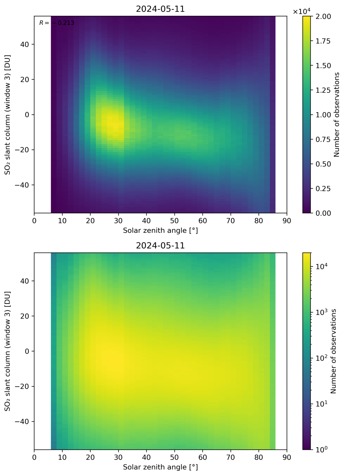
Figure 172: Scatter density plot of “Solar zenith angle” against “SO 2 slant column (window 3)” for 2024-05-10 to 2024-05-12.
