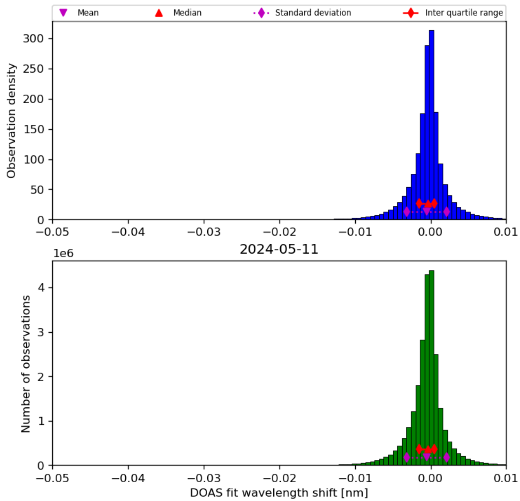
Figure 68: Histogram of “DOAS fit wavelength shift” for 2024-05-10 to 2024-05-12
