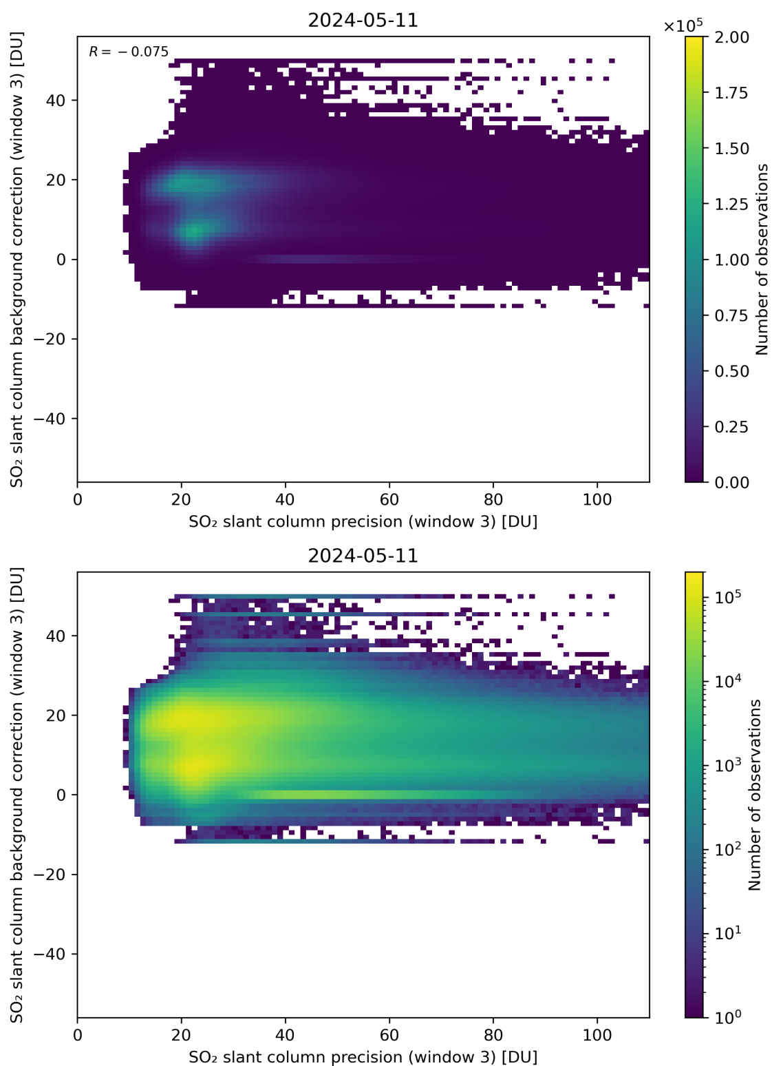
Figure 257: Scatter density plot of “SO 2 slant column precision (window 3)” against “SO 2 slant column background correction (window 3)” for 2024-05-10 to 2024-05-12.
