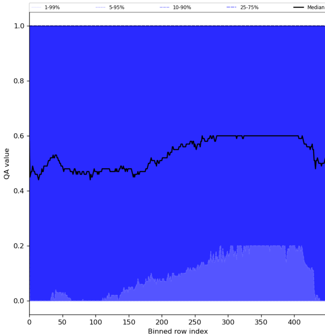
Figure 75: Along track statistics of “QA value” for 2024-05-10 to 2024-05-12
