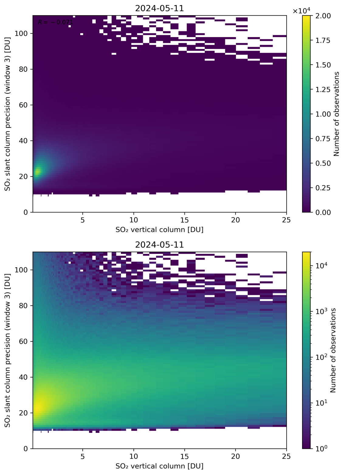
Figure 304: Scatter density plot of “SO 2 vertical column” against “SO 2 slant column precision (window 3)” for 2024-05-10 to 2024-05-12.
