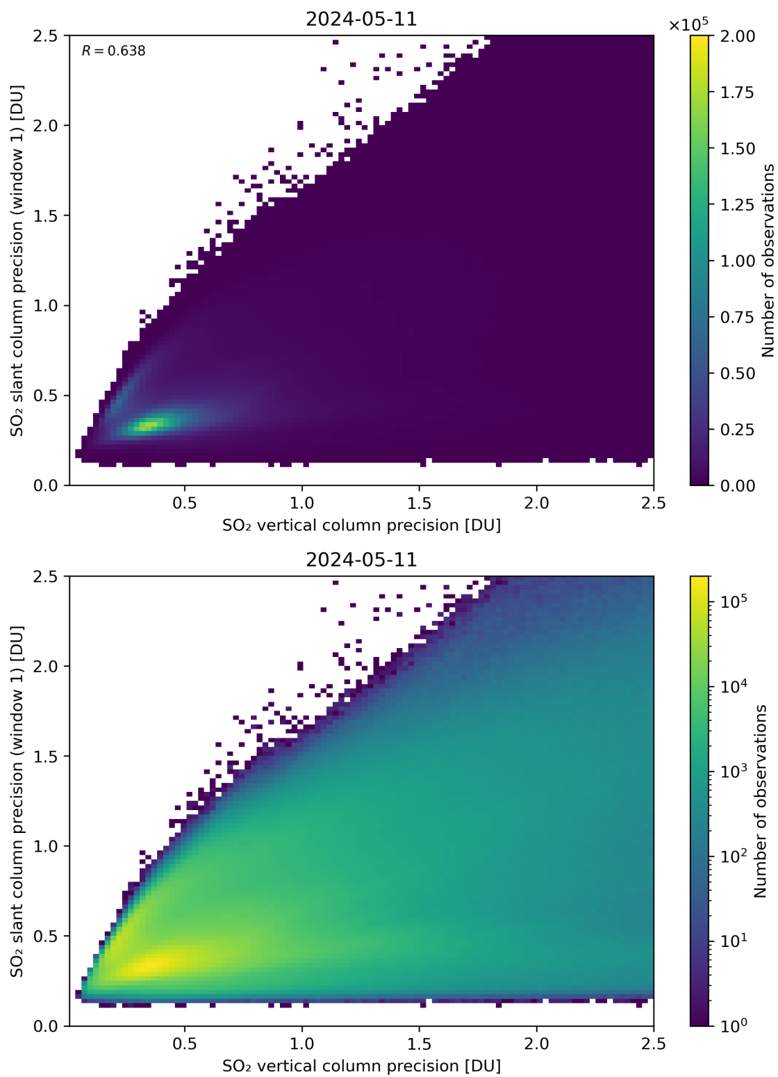
Figure 290: Scatter density plot of “SO 2 vertical column precision” against “SO 2 slant column precision (window 1)” for 2024-05-10 to 2024-05-12.
