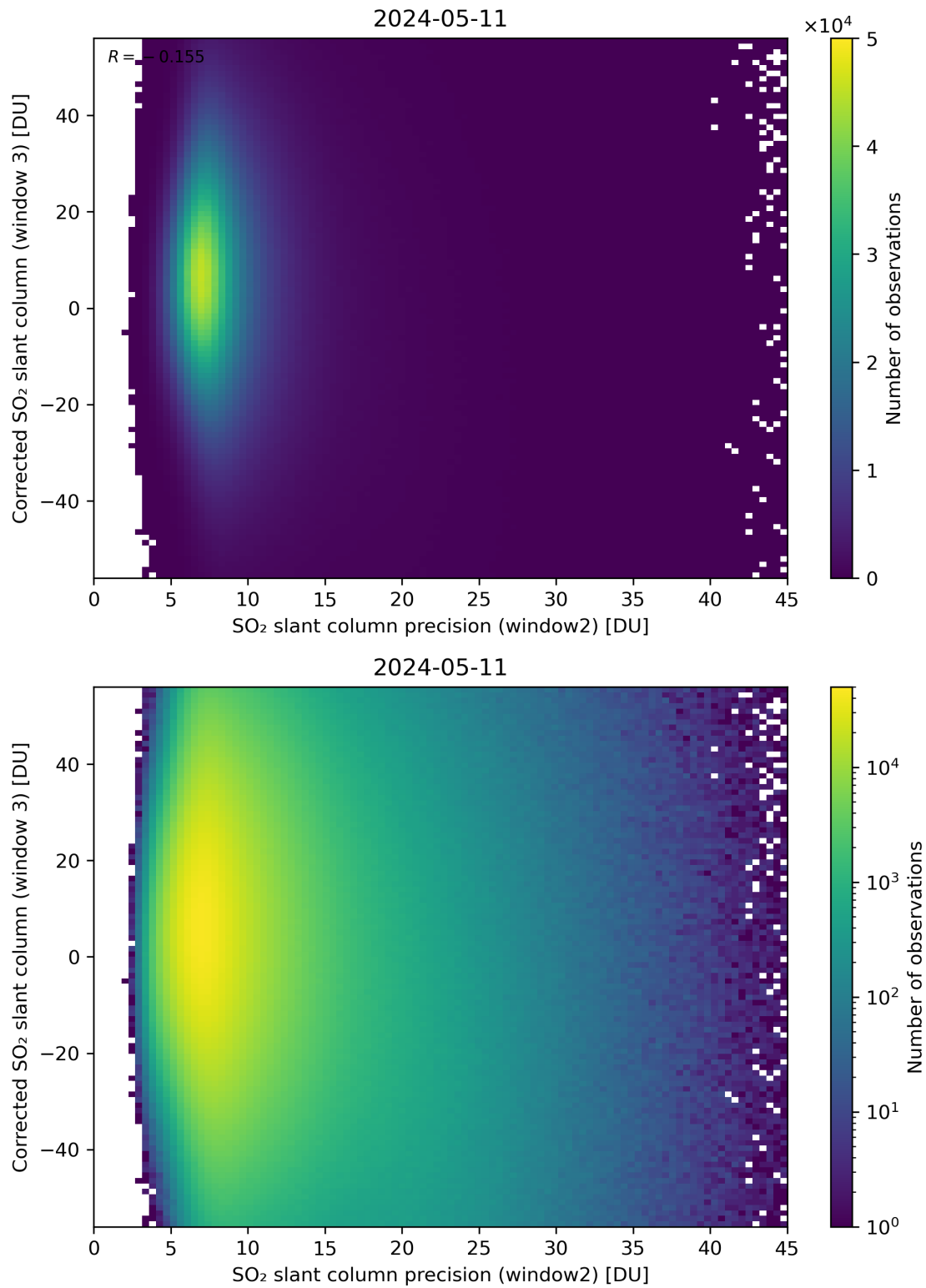
Figure 248: Scatter density plot of “SO 2 slant column precision (window2)” against “Corrected SO 2 slant column (window 3)” for 2024-05-10 to 2024-05-12.
