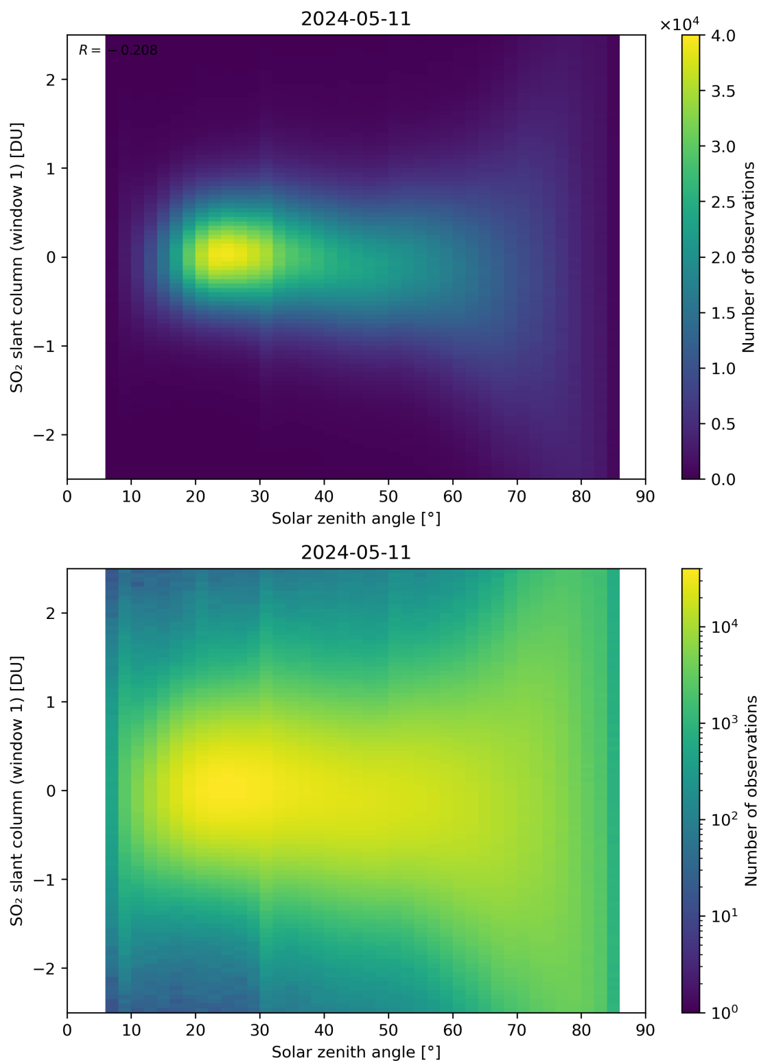
Figure 169: Scatter density plot of “Solar zenith angle” against “SO 2 slant column (window 1)” for 2024-05-10 to 2024-05-12.
