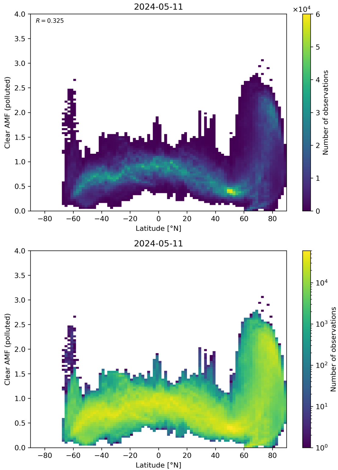
Figure 145: Scatter density plot of “Latitude” against “Clear AMF (polluted)” for 2024-05-10 to 2024-05-12.
