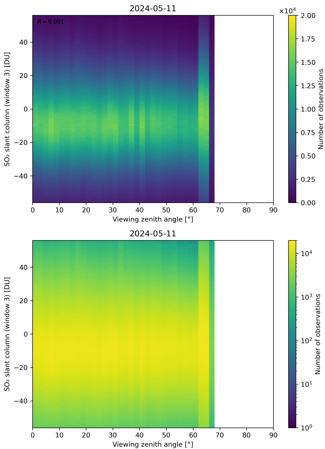
Figure 323: Scatter density plot of “Viewing zenith angle” against “SO 2 slant column (window 3)” for 2024-05-10 to 2024-05-12.
