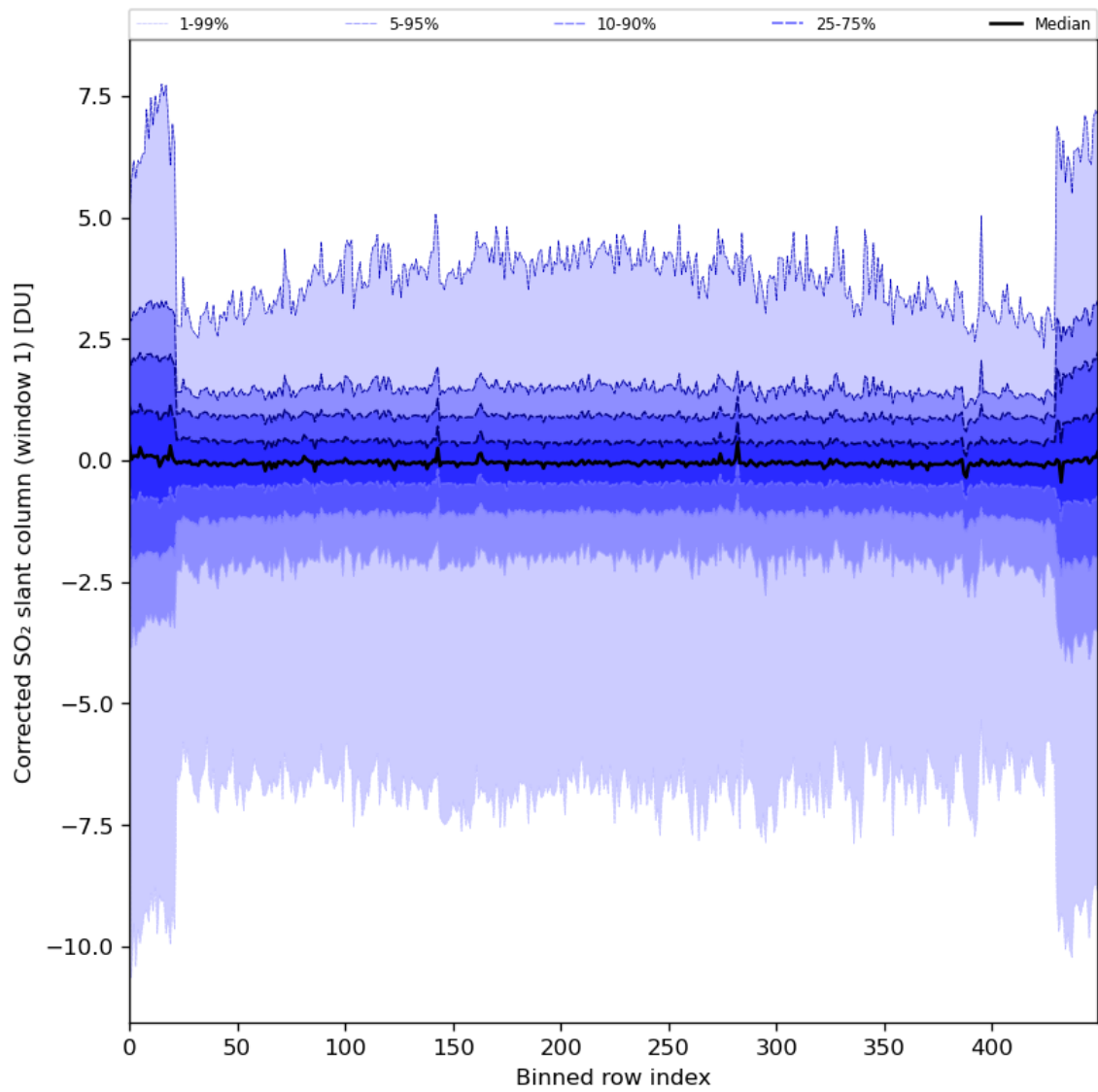
Figure 81: Along track statistics of “Corrected SO 2 slant column (window 1)” for 2024-05-10 to 2024-05-12
