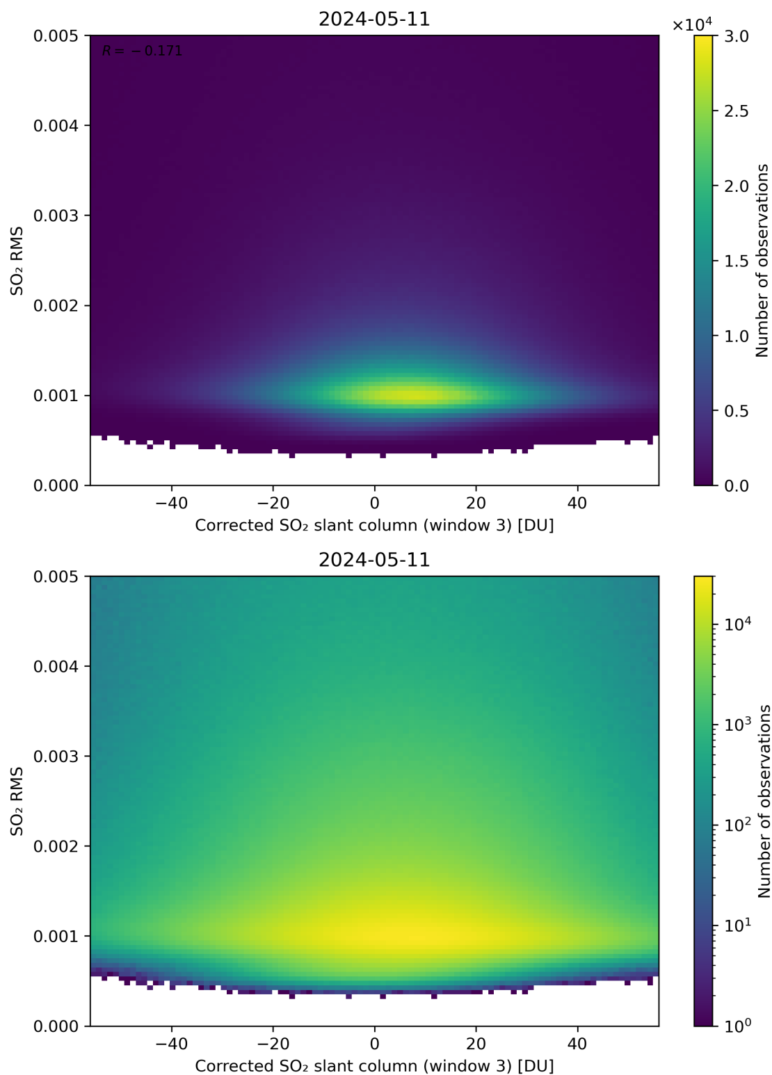
Figure 208: Scatter density plot of “Corrected SO 2 slant column (window 3)” against “SO 2 RMS” for 2024-05-10 to 2024-05-12.
