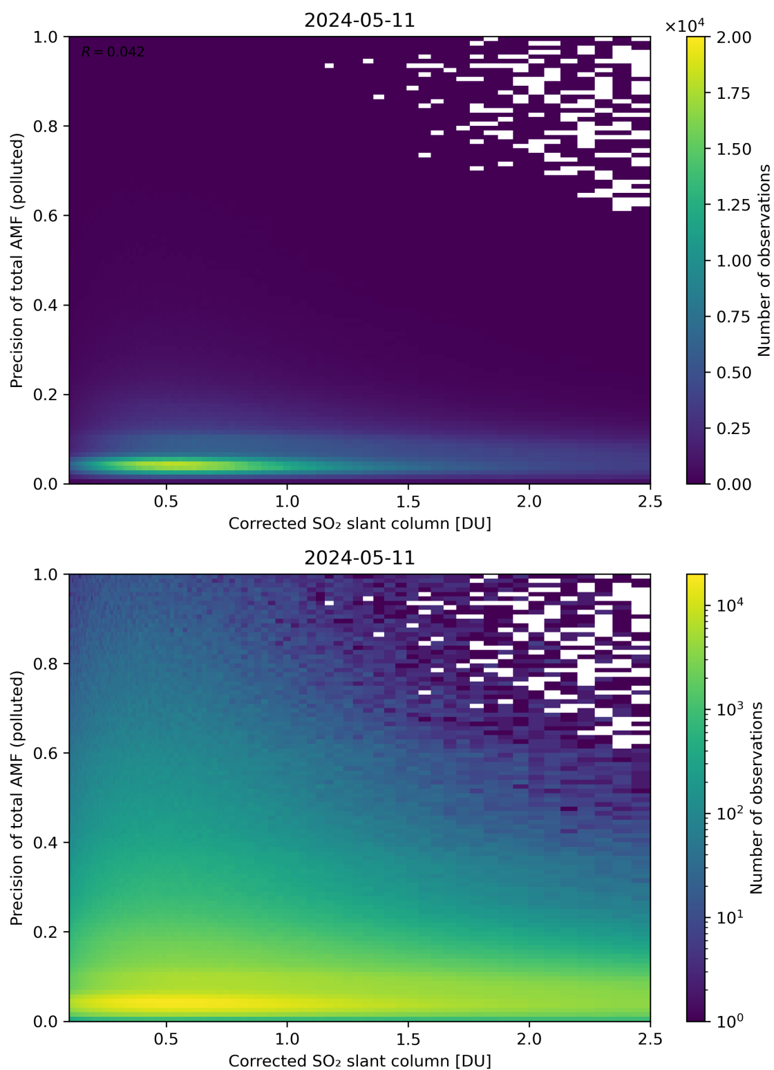
Figure 193: Scatter density plot of “Corrected SO 2 slant column” against “Precision of total AMF (polluted)” for 2024-05-10 to 2024-05-12.
