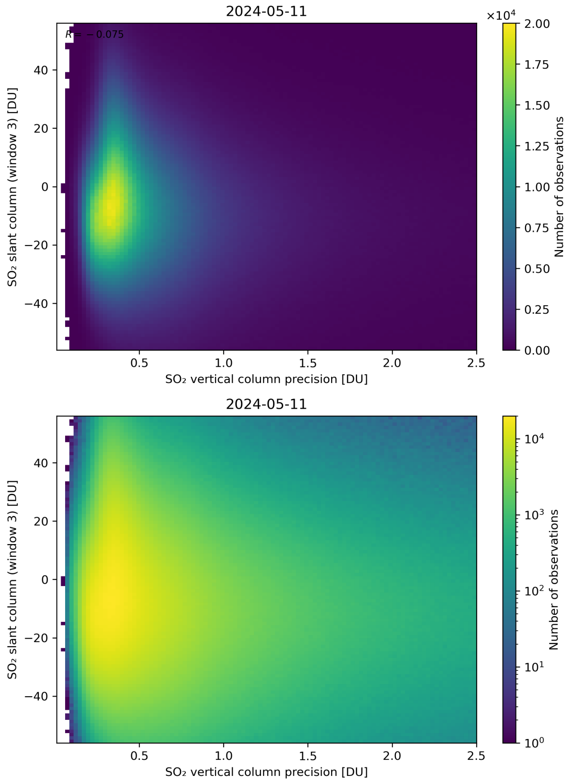
Figure 292: Scatter density plot of “SO 2 vertical column precision” against “SO 2 slant column (window 3)” for 2024-05-10 to 2024-05-12.
