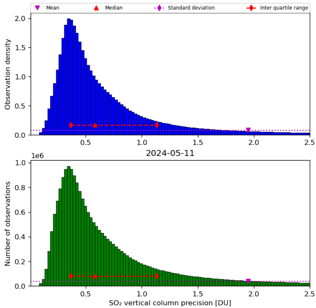
Figure 54: Histogram of “SO 2 vertical column precision” for 2024-05-10 to 2024-05-12
