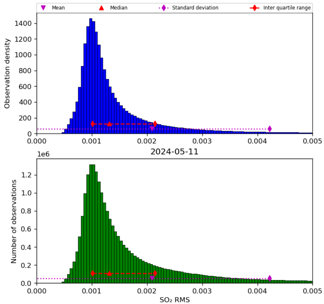
Figure 70: Histogram of “SO 2 RMS” for 2024-05-10 to 2024-05-12
