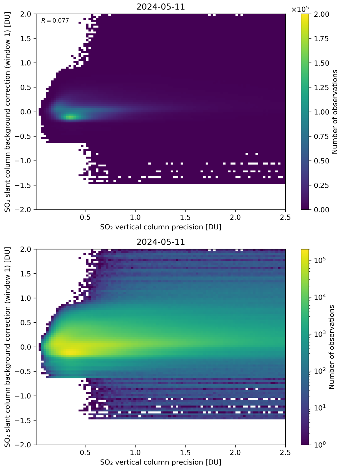
Figure 279: Scatter density plot of “SO 2 vertical column precision” against “SO 2 slant column background correction (window 1)” for 2024-05-10 to 2024-05-12.
