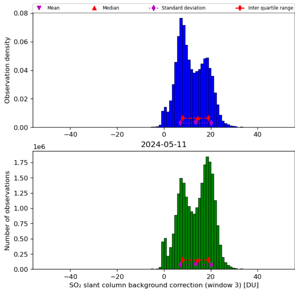
Figure 67: Histogram of “SO 2 slant column background correction (window 3)” for 2024-05-10 to 2024-05-12
