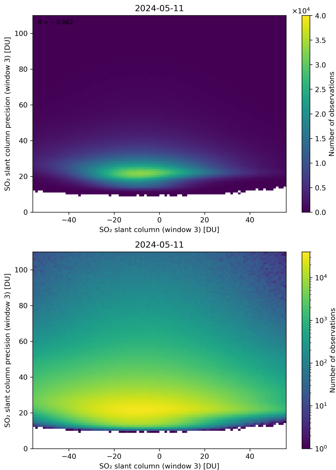
Figure 267: Scatter density plot of “SO 2 slant column (window 3)” against “SO 2 slant column precision (window 3)” for 2024-05-10 to 2024-05-12.
