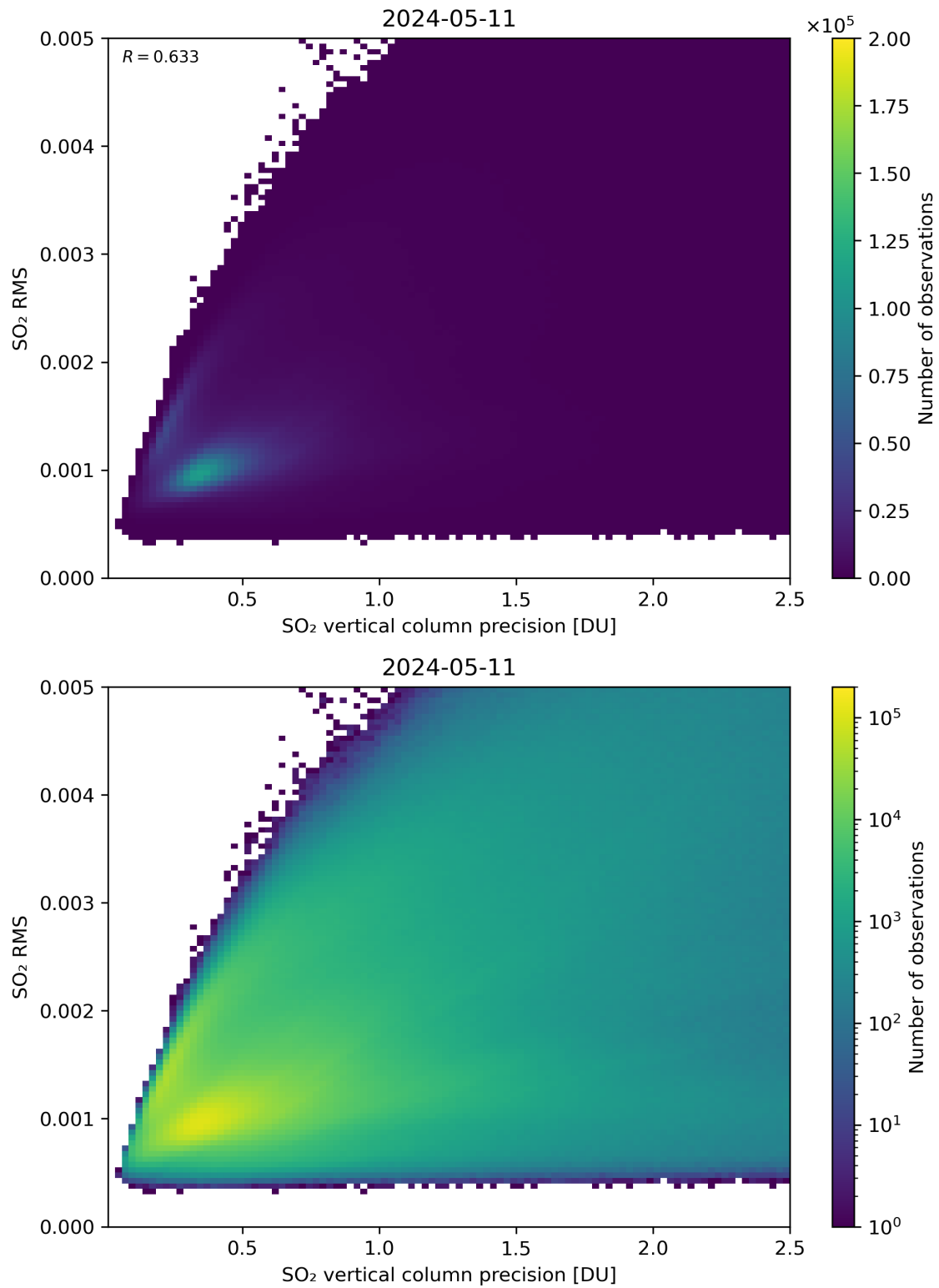
Figure 284: Scatter density plot of “SO 2 vertical column precision” against “SO 2 RMS” for 2024-05-10 to 2024-05-12.
