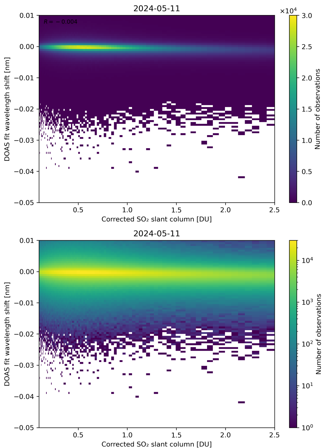
Figure 181: Scatter density plot of “Corrected SO 2 slant column” against “DOAS fit wavelength shift” for 2024-05-10 to 2024-05-12.
