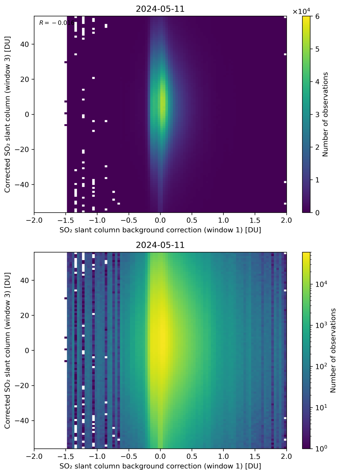
Figure 105: Scatter density plot of “SO 2 slant column background correction (window 1)” against “Corrected SO 2 slant column (window 3)” for 2024-05-10 to 2024-05-12.
