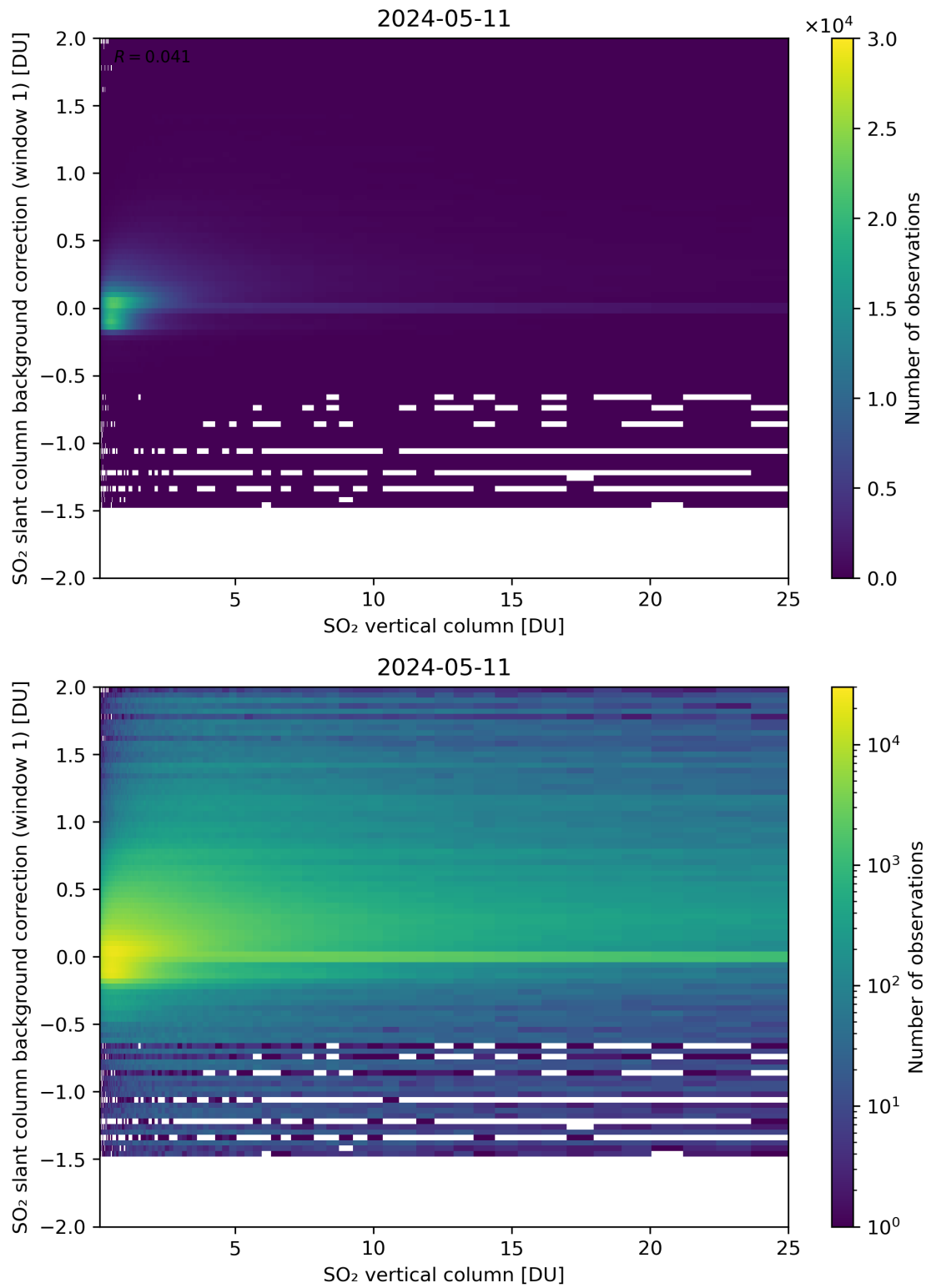
Figure 273: Scatter density plot of “SO 2 vertical column” against “SO 2 slant column background correction (window 1)” for 2024-05-10 to 2024-05-12.
