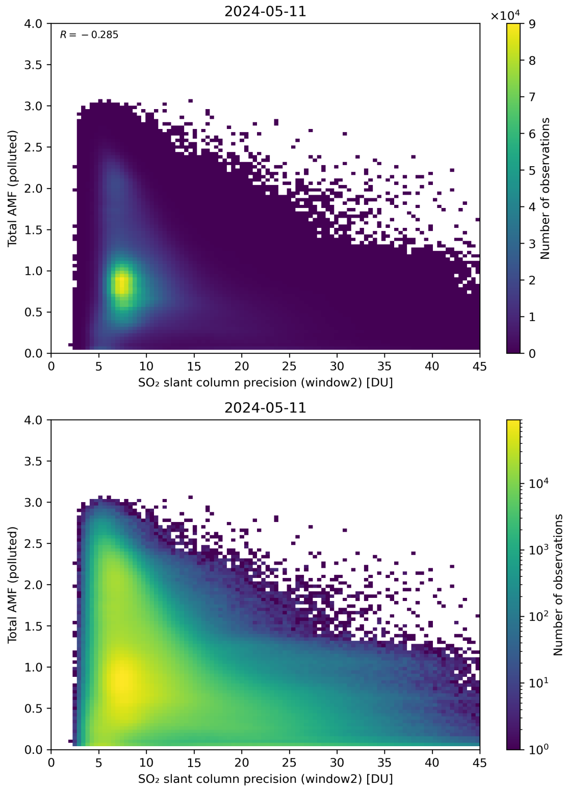
Figure 251: Scatter density plot of “SO 2 slant column precision (window2)” against “Total AMF (polluted)” for 2024-05-10 to 2024-05-12.
