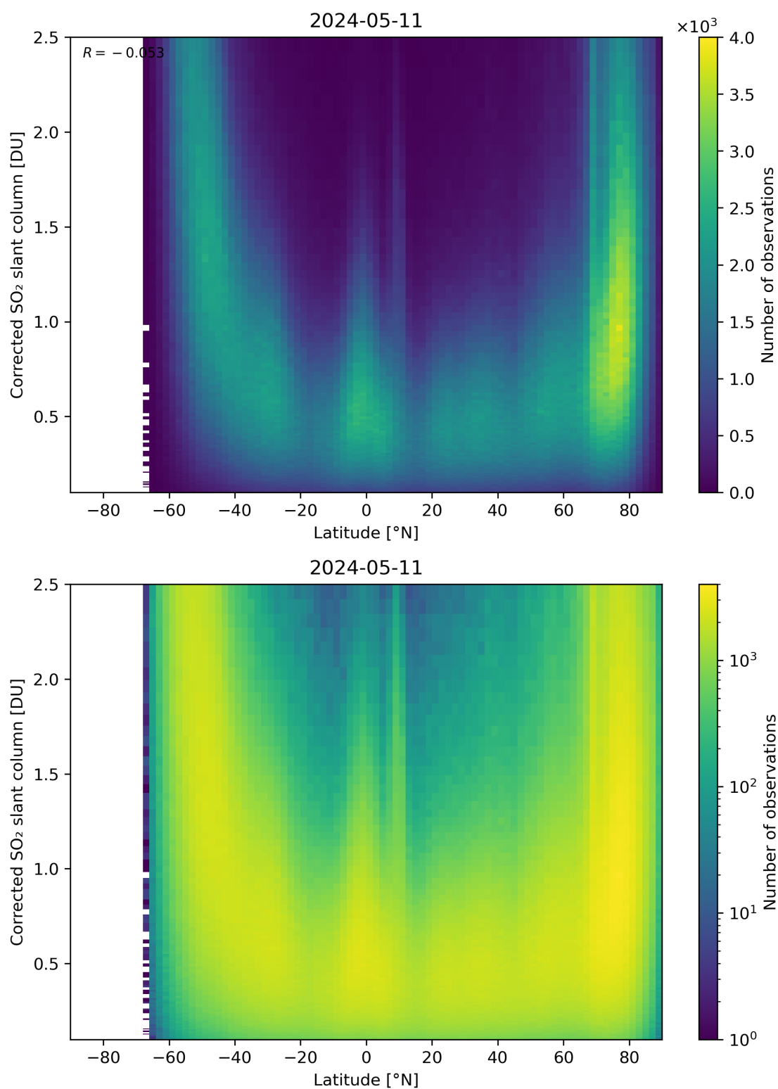
Figure 146: Scatter density plot of “Latitude” against “Corrected SO 2 slant column” for 2024-05-10 to 2024-05-12.
