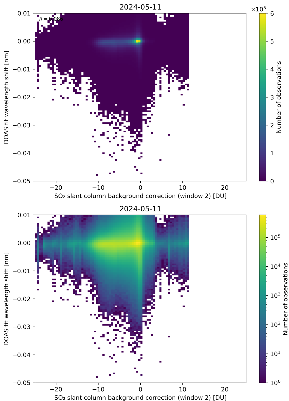
Figure 112: Scatter density plot of “SO 2 slant column background correction (window 2)” against “DOAS fit wavelength shift” for 2024-05-10 to 2024-05-12.
