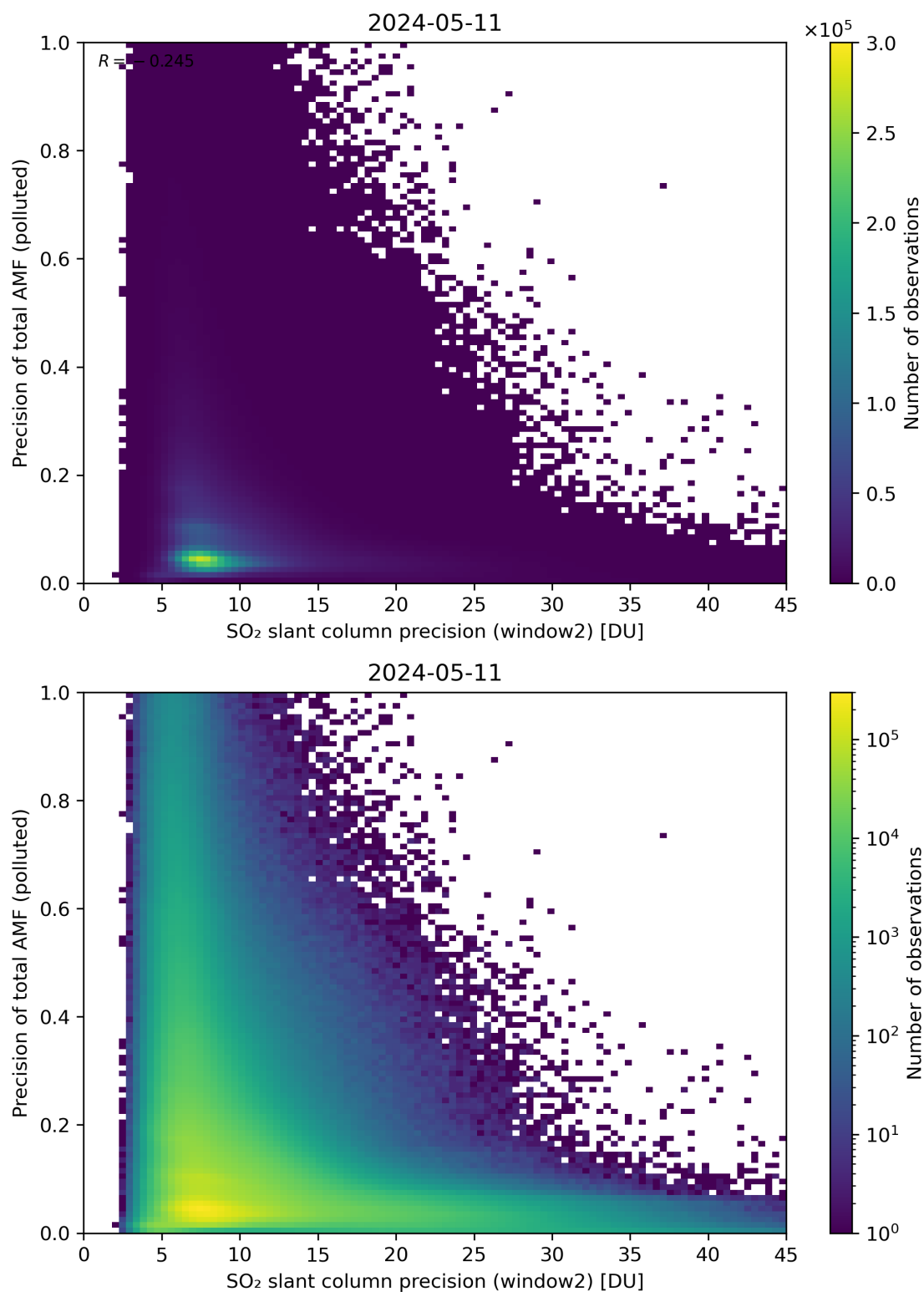
Figure 252: Scatter density plot of “SO 2 slant column precision (window2)” against “Precision of total AMF (polluted)” for 2024-05-10 to 2024-05-12.
