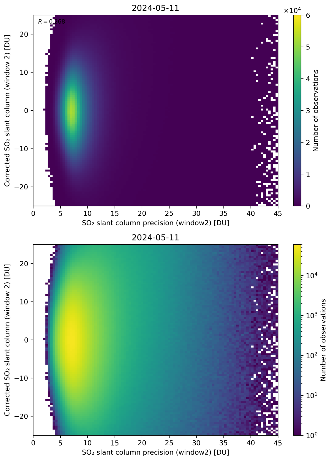
Figure 247: Scatter density plot of “SO 2 slant column precision (window2)” against “Corrected SO 2 slant column (window 2)” for 2024-05-10 to 2024-05-12.
