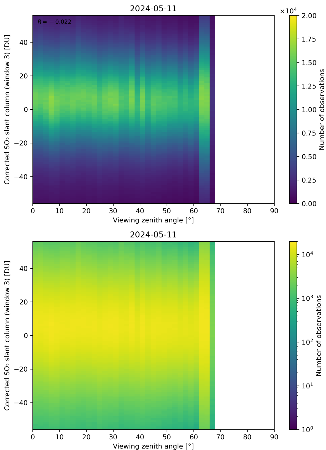
Figure 319: Scatter density plot of “Viewing zenith angle” against “Corrected SO 2 slant column (window 3)” for 2024-05-10 to 2024-05-12.
