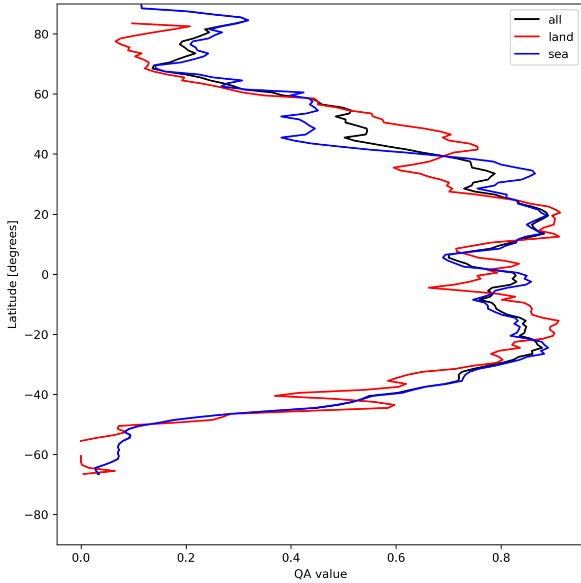
Figure 29: Zonal average of “QA value” for 2024-05-10 to 2024-05-12.
