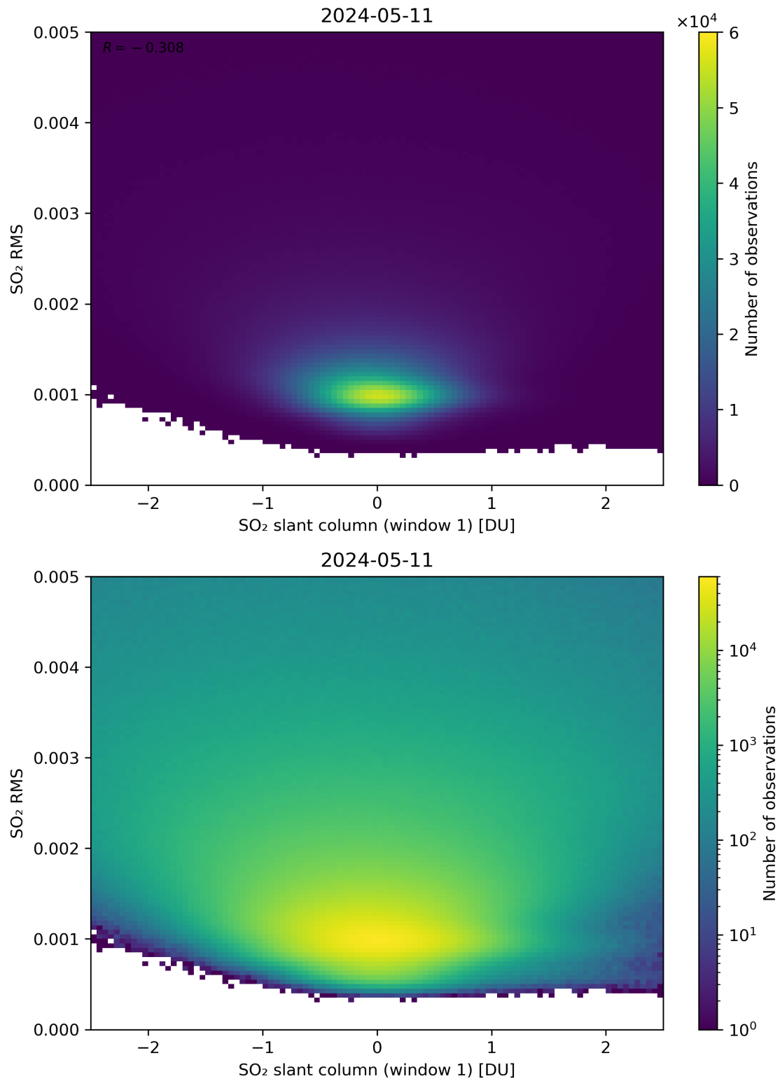
Figure 217: Scatter density plot of “SO 2 slant column (window 1)” against “SO 2 RMS” for 2024-05-10 to 2024-05-12.
