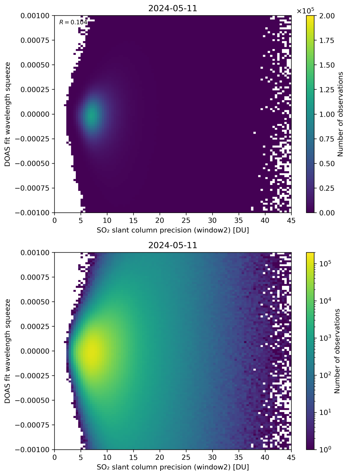
Figure 244: Scatter density plot of “SO 2 slant column precision (window2)” against “DOAS fit wavelength squeeze” for 2024-05-10 to 2024-05-12.
