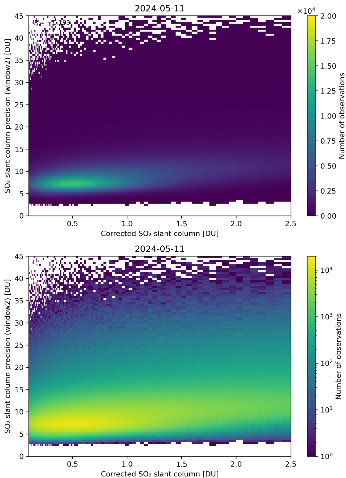
Figure 189: Scatter density plot of “Corrected SO 2 slant column” against “SO 2 slant column precision (window2)” for 2024-05-10 to 2024-05-12.
