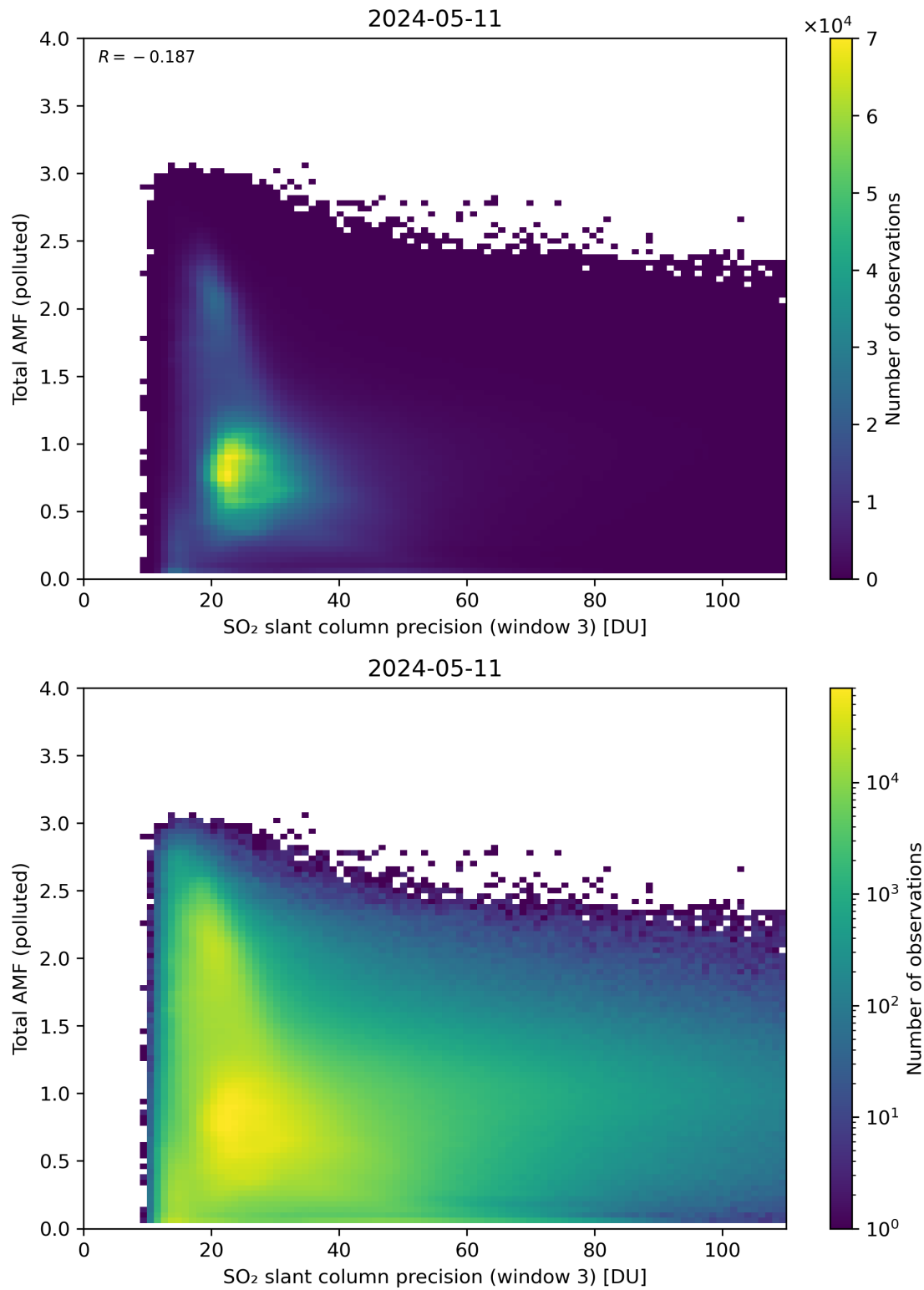
Figure 263: Scatter density plot of “SO 2 slant column precision (window 3)” against “Total AMF (polluted)” for 2024-05-10 to 2024-05-12.
