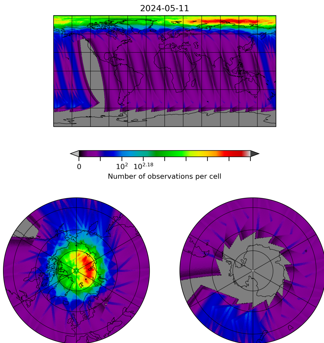
Figure 28: Map of the number of observations for 2024-05-10 to 2024-05-12
