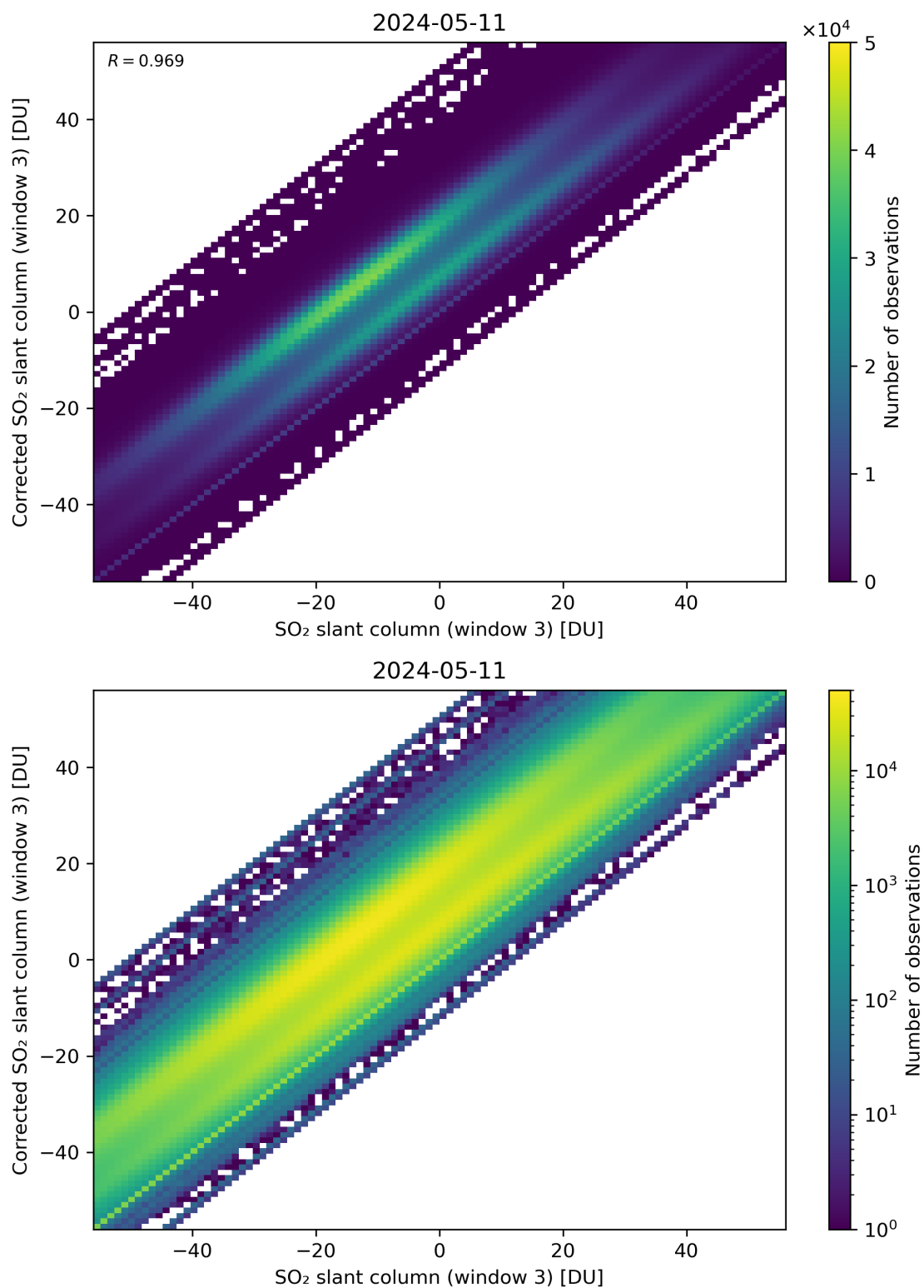
Figure 266: Scatter density plot of “SO 2 slant column (window 3)” against “Corrected SO 2 slant column (window 3)” for 2024-05-10 to 2024-05-12.
