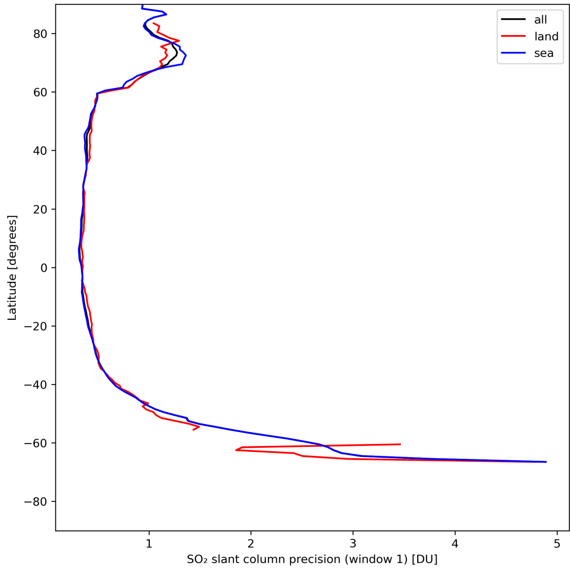
Figure 34: Zonal average of “SO 2 slant column precision (window 1)” for 2024-05-10 to 2024-05-12.
