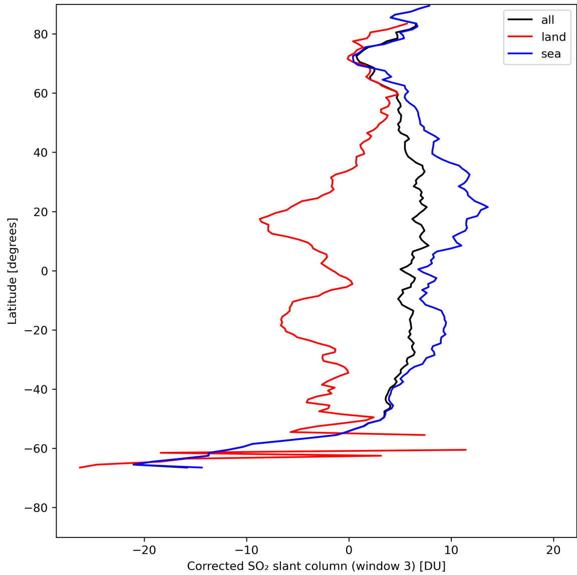
Figure 43: Zonal average of “Corrected SO 2 slant column (window 3)” for 2024-05-10 to 2024-05-12.
