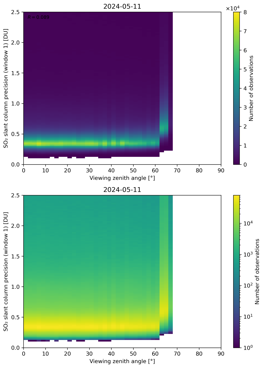
Figure 321: Scatter density plot of “Viewing zenith angle” against “SO 2 slant column precision (window 1)” for 2024-05-10 to 2024-05-12.
