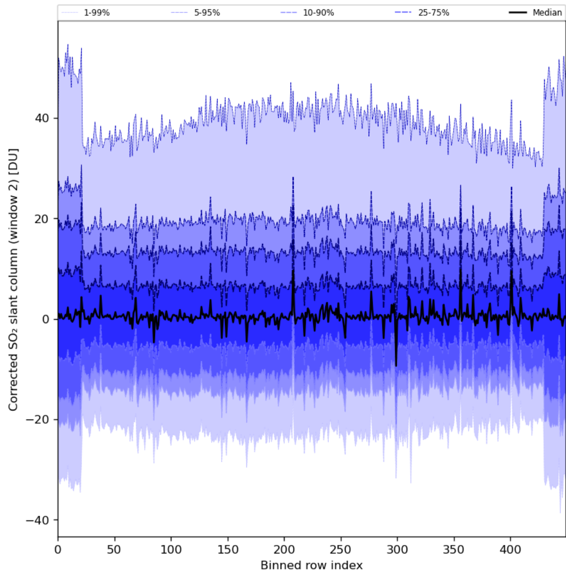
Figure 85: Along track statistics of “Corrected SO 2 slant column (window 2)” for 2024-05-10 to 2024-05-12
