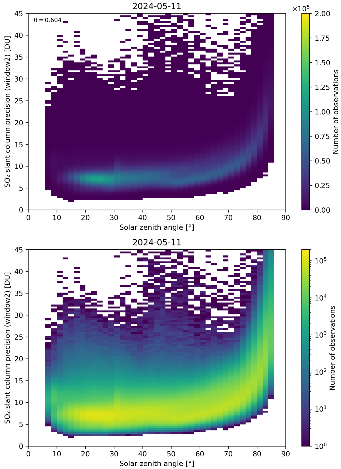
Figure 171: Scatter density plot of “Solar zenith angle” against “SO 2 slant column precision (window2)” for 2024-05-10 to 2024-05-12.
