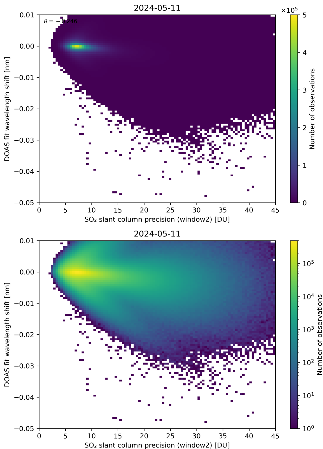
Figure 243: Scatter density plot of “SO 2 slant column precision (window2)” against “DOAS fit wavelength shift” for 2024-05-10 to 2024-05-12.
