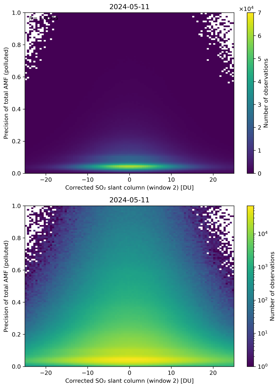
Figure 204: Scatter density plot of “Corrected SO 2 slant column (window 2)” against “Precision of total AMF (polluted)” for 2024-05-10 to 2024-05-12.
