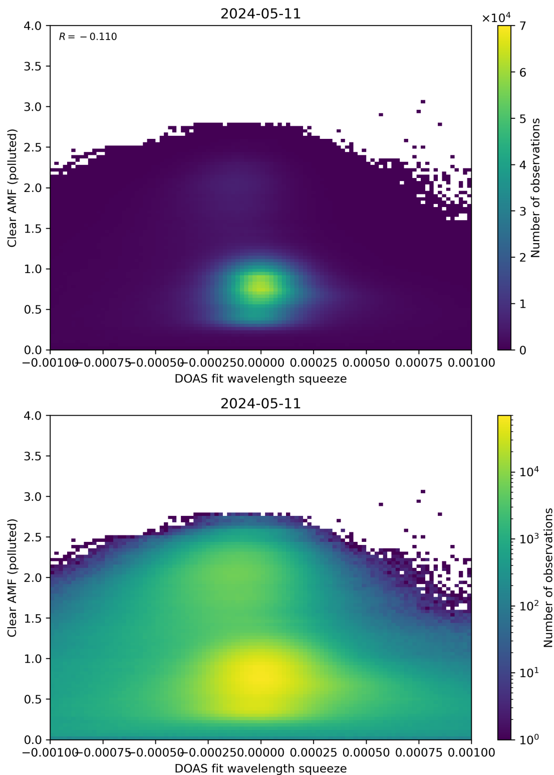
Figure 133: Scatter density plot of “DOAS fit wavelength squeeze” against “Clear AMF (polluted)” for 2024-05-10 to 2024-05-12.
