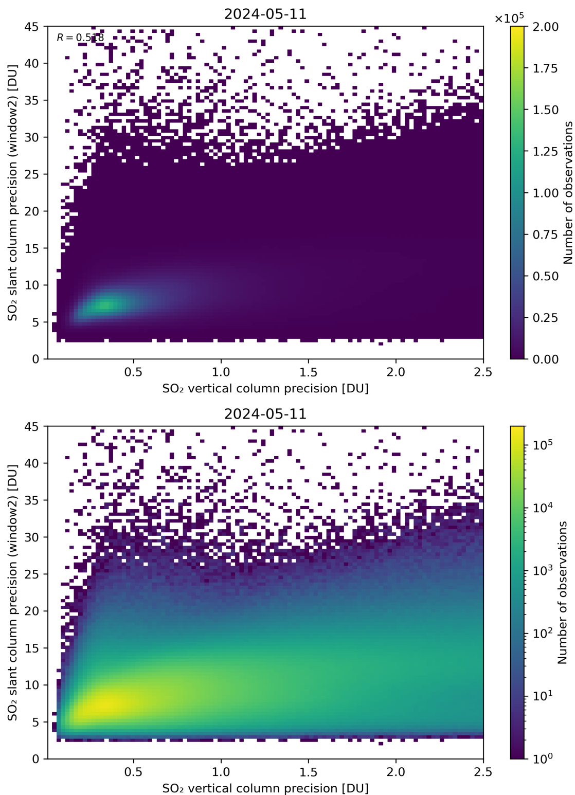
Figure 291: Scatter density plot of “SO 2 vertical column precision” against “SO 2 slant column precision (window2)” for 2024-05-10 to 2024-05-12.
