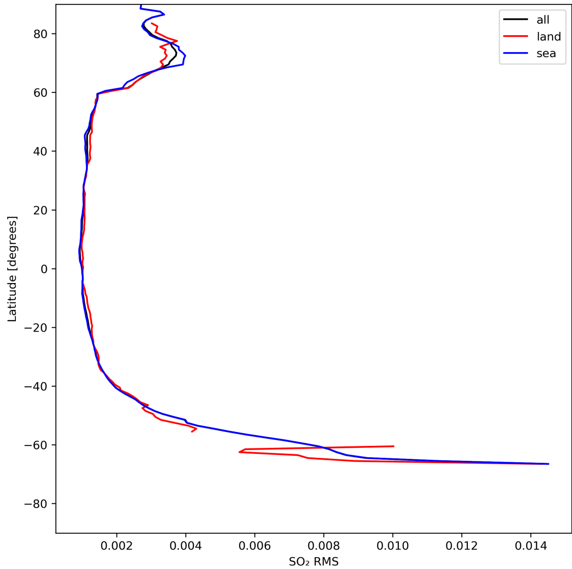
Figure 47: Zonal average of “SO 2 RMS” for 2024-05-10 to 2024-05-12.
