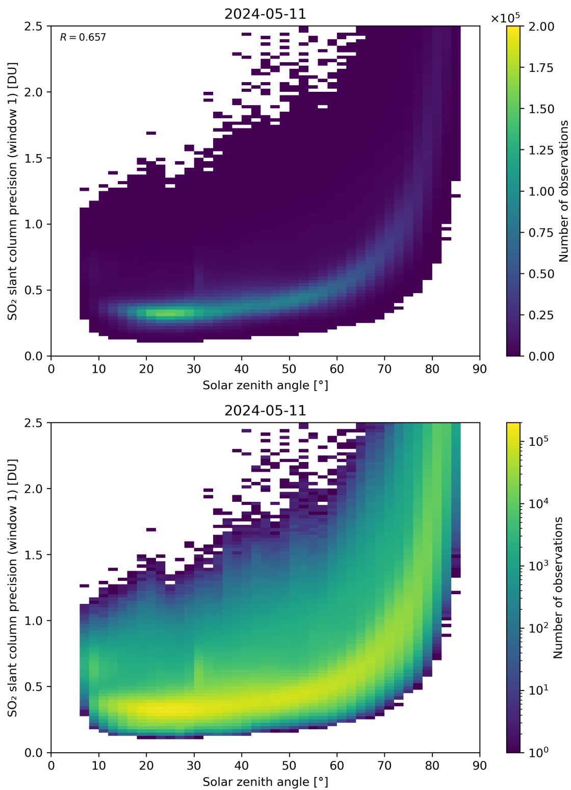
Figure 170: Scatter density plot of “Solar zenith angle” against “SO 2 slant column precision (window 1)” for 2024-05-10 to 2024-05-12.
