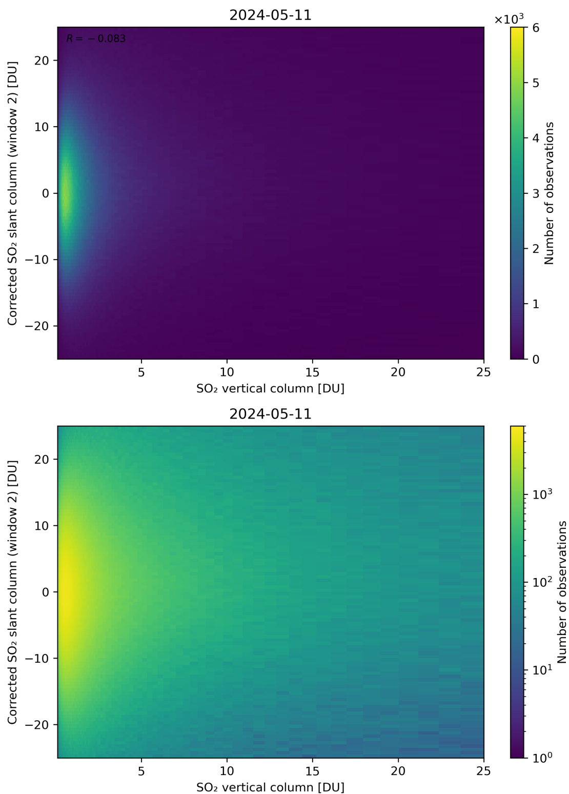
Figure 298: Scatter density plot of “SO 2 vertical column” against “Corrected SO 2 slant column (window 2)” for 2024-05-10 to 2024-05-12.
