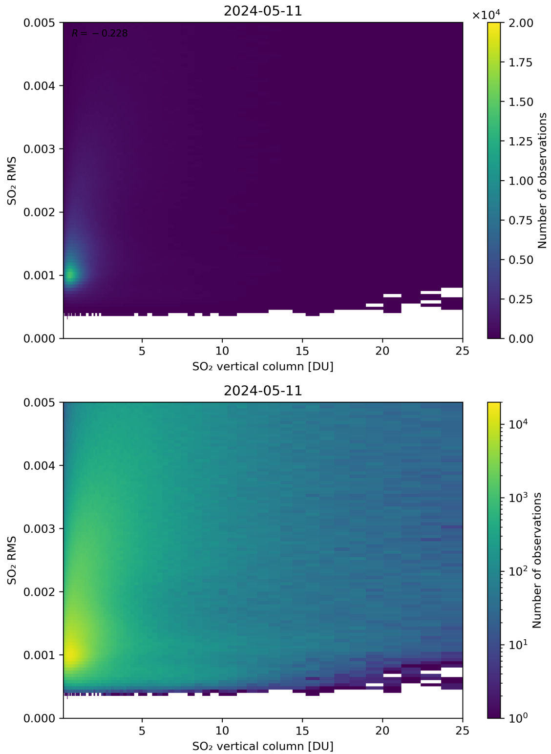
Figure 278: Scatter density plot of “SO 2 vertical column” against “SO 2 RMS” for 2024-05-10 to 2024-05-12.
