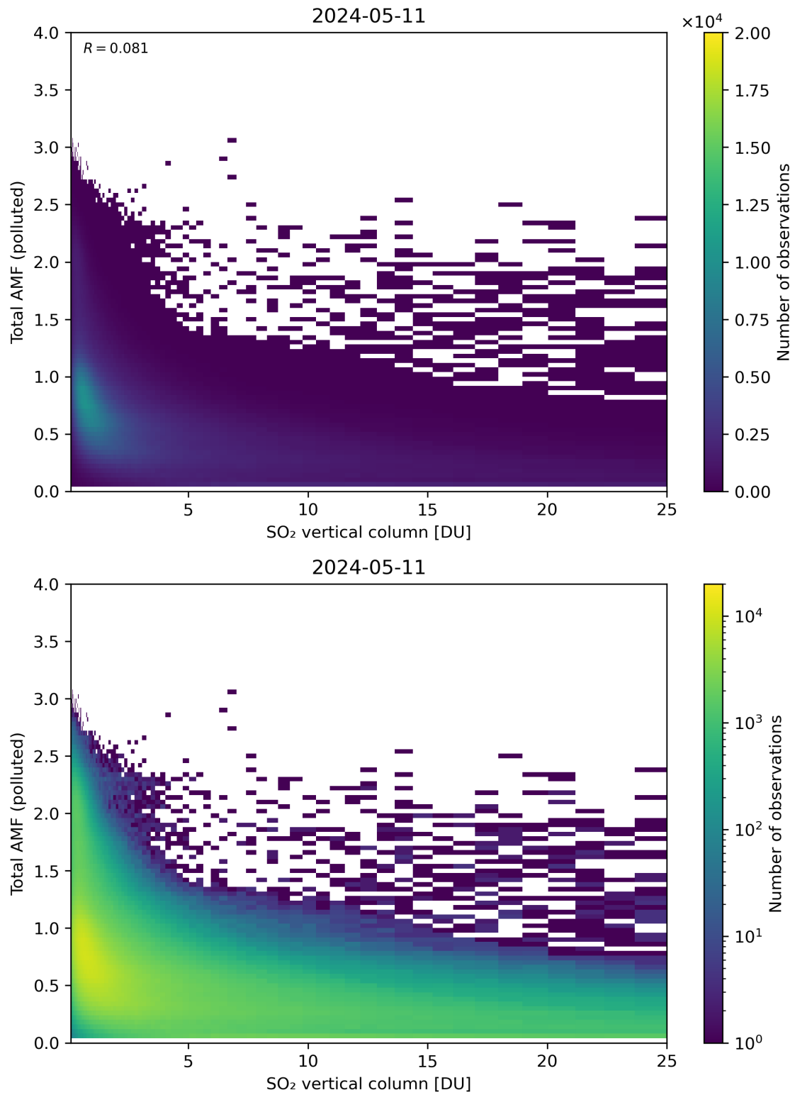
Figure 305: Scatter density plot of “SO 2 vertical column” against “Total AMF (polluted)” for 2024-05-10 to 2024-05-12.
