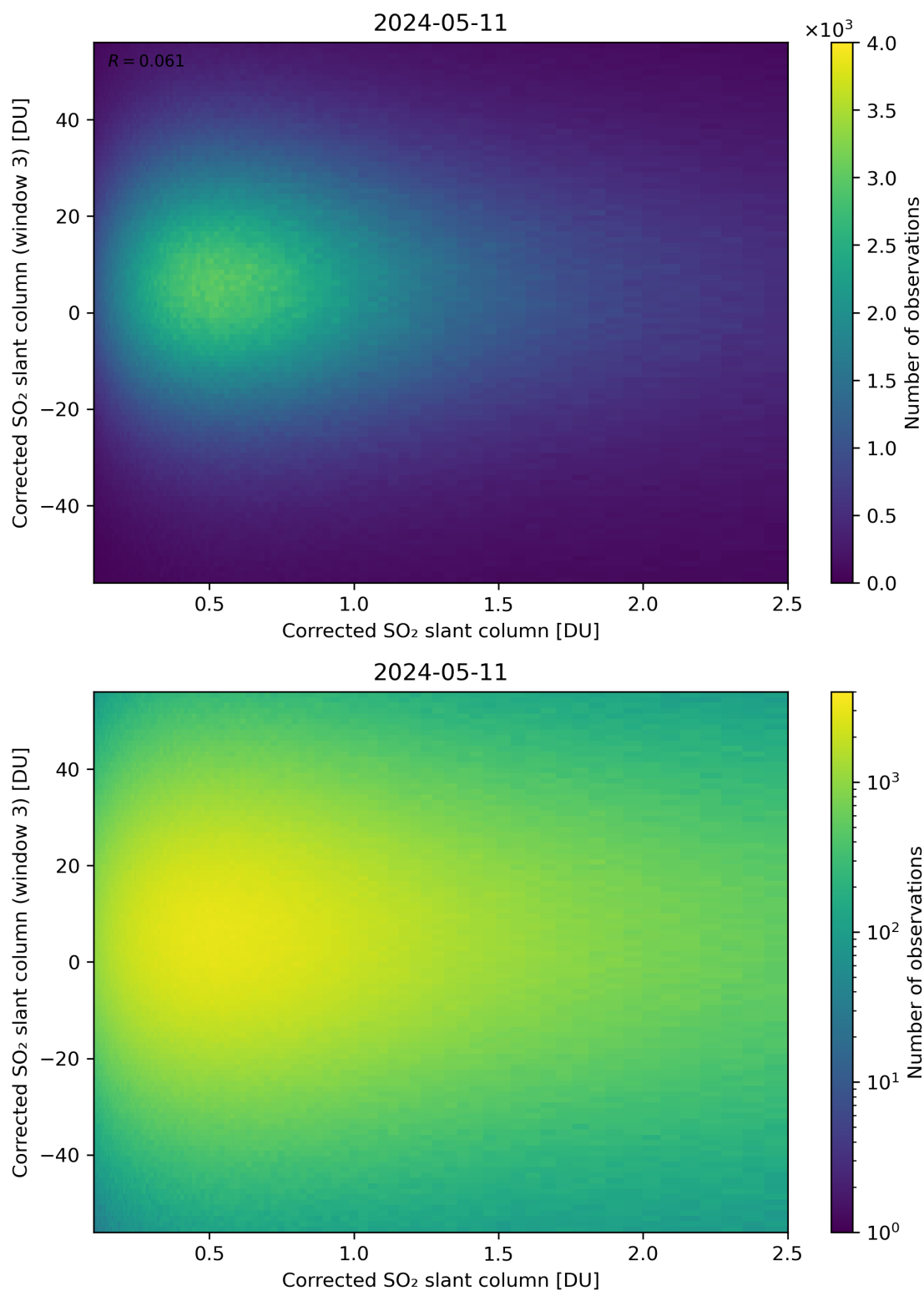
Figure 186: Scatter density plot of “Corrected SO 2 slant column” against “Corrected SO 2 slant column (window 3)” for 2024-05-10 to 2024-05-12.
