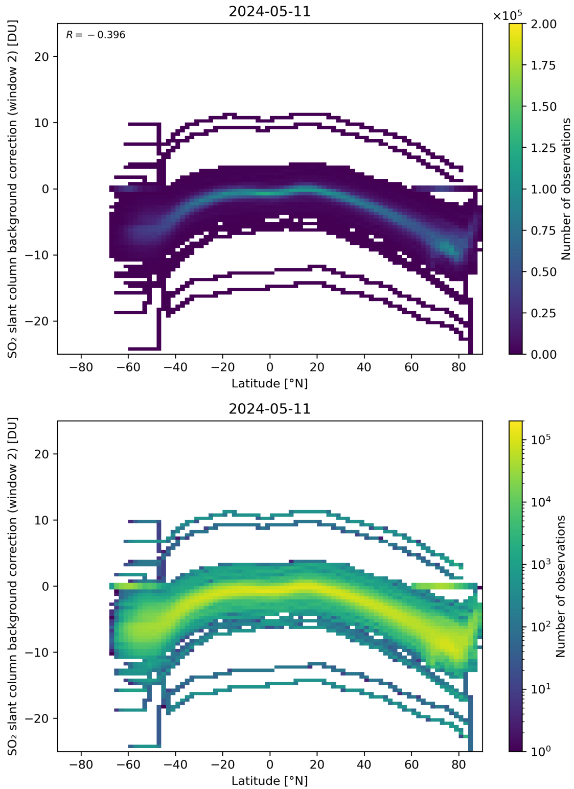
Figure 140: Scatter density plot of “Latitude” against “SO 2 slant column background correction (window 2)” for 2024-05-10 to 2024-05-12.
