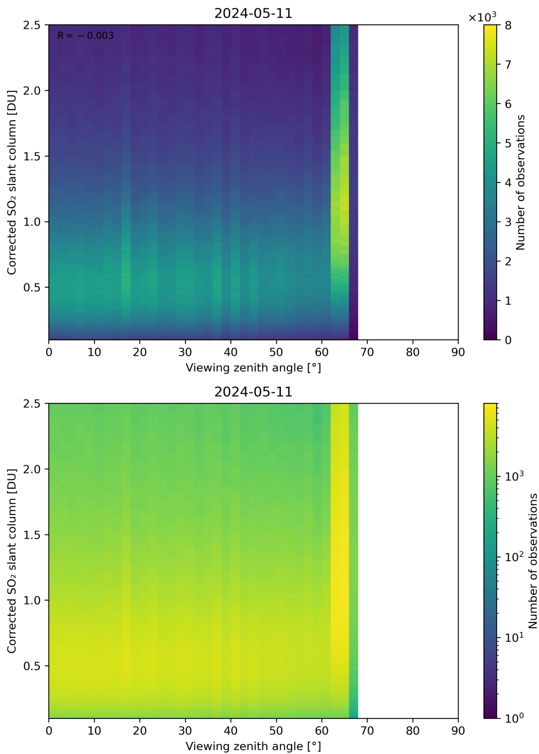
Figure 317: Scatter density plot of “Viewing zenith angle” against “Corrected SO 2 slant column” for 2024-05-10 to 2024-05-12.
