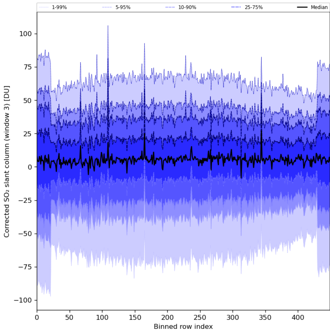
Figure 89: Along track statistics of “Corrected SO 2 slant column (window 3)” for 2024-05-10 to 2024-05-12
