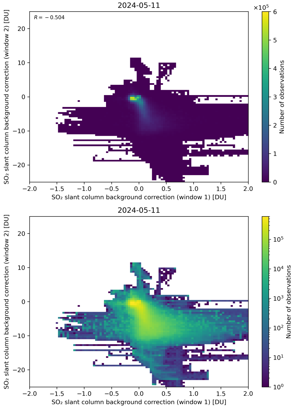
Figure 98: Scatter density plot of “SO 2 slant column background correction (window 1)” against “SO 2 slant column background correction (window 2)” for 2024-05-10 to 2024-05-12.
