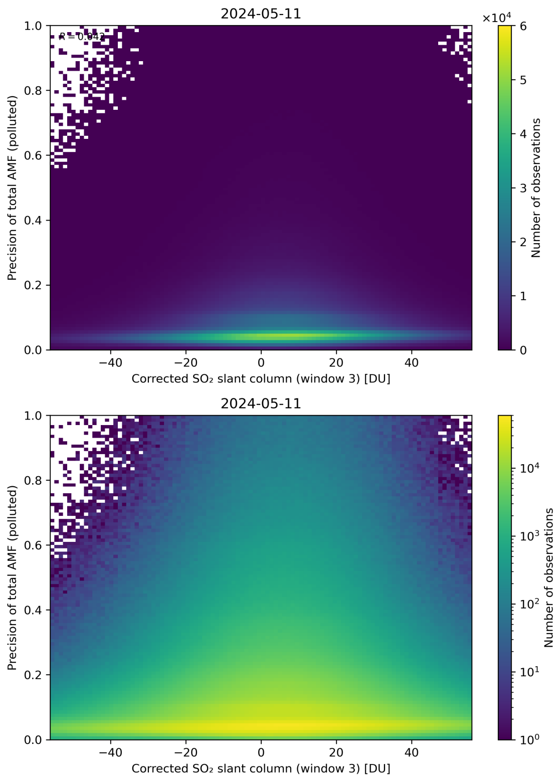
Figure 211: Scatter density plot of “Corrected SO 2 slant column (window 3)” against “Precision of total AMF (polluted)” for 2024-05-10 to 2024-05-12.
