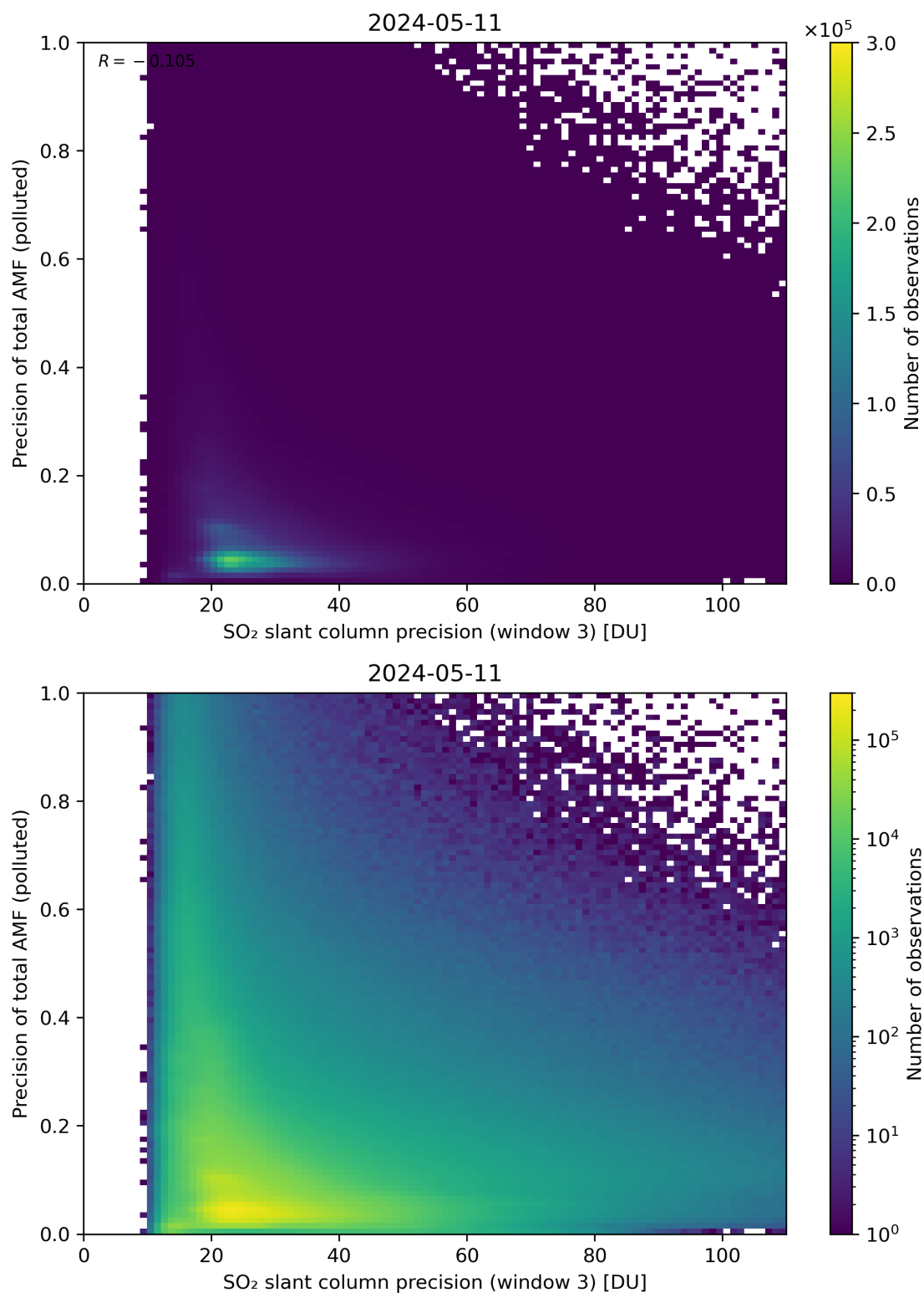
Figure 264: Scatter density plot of “SO 2 slant column precision (window 3)” against “Precision of total AMF (polluted)” for 2024-05-10 to 2024-05-12.
