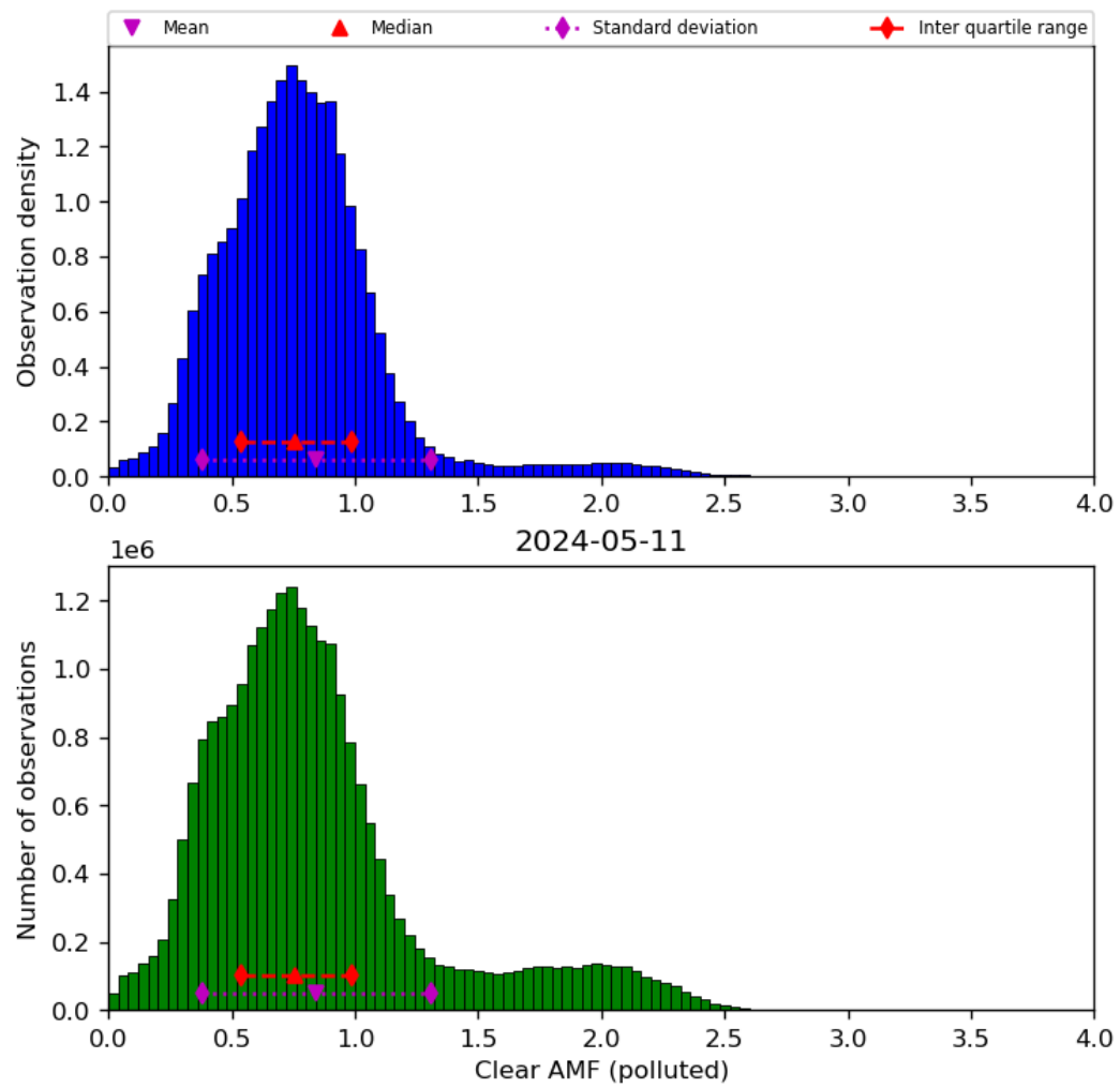
Figure 73: Histogram of “Clear AMF (polluted)” for 2024-05-10 to 2024-05-12
