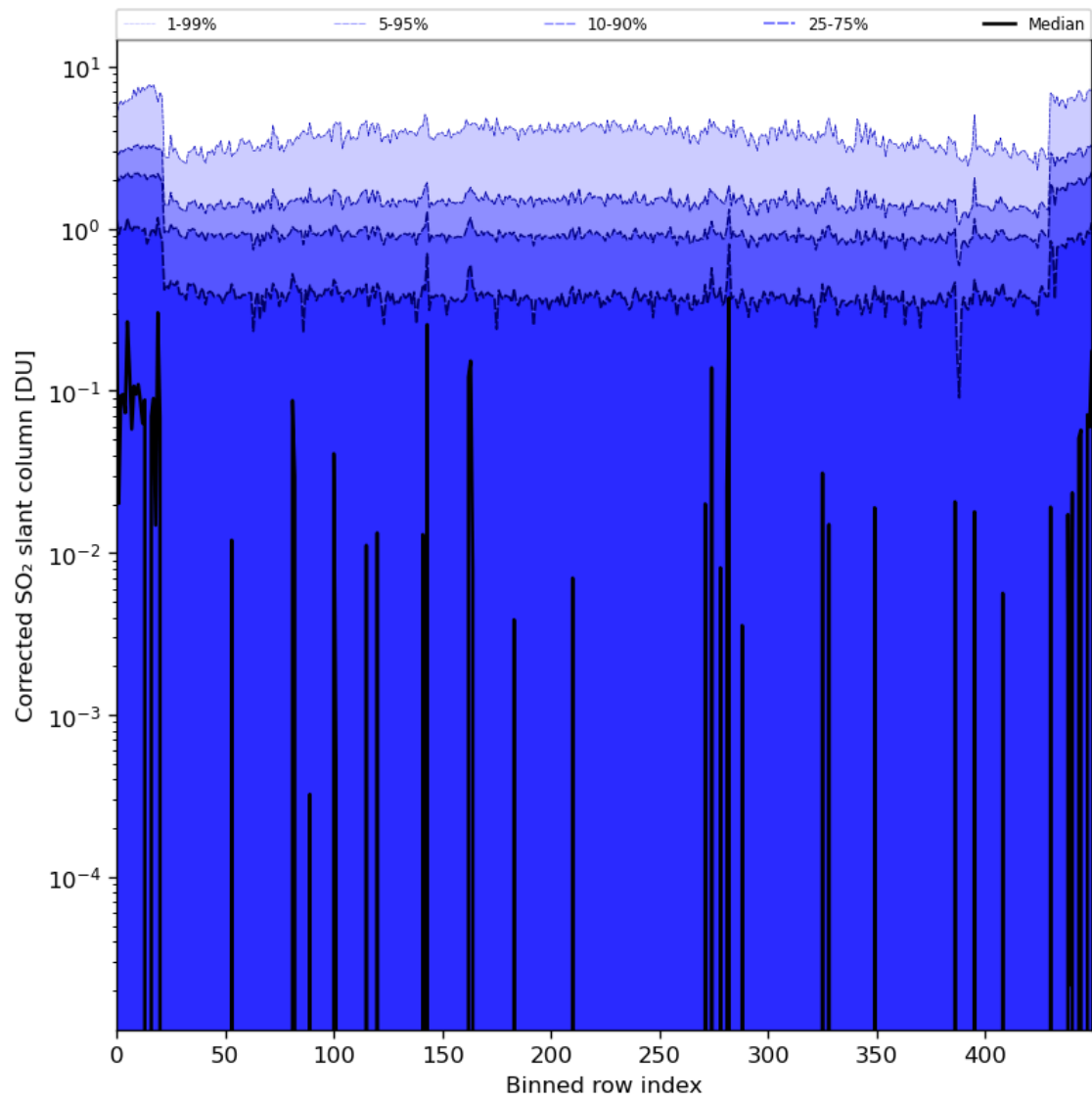
Figure 78: Along track statistics of “Corrected SO 2 slant column” for 2024-05-10 to 2024-05-12
