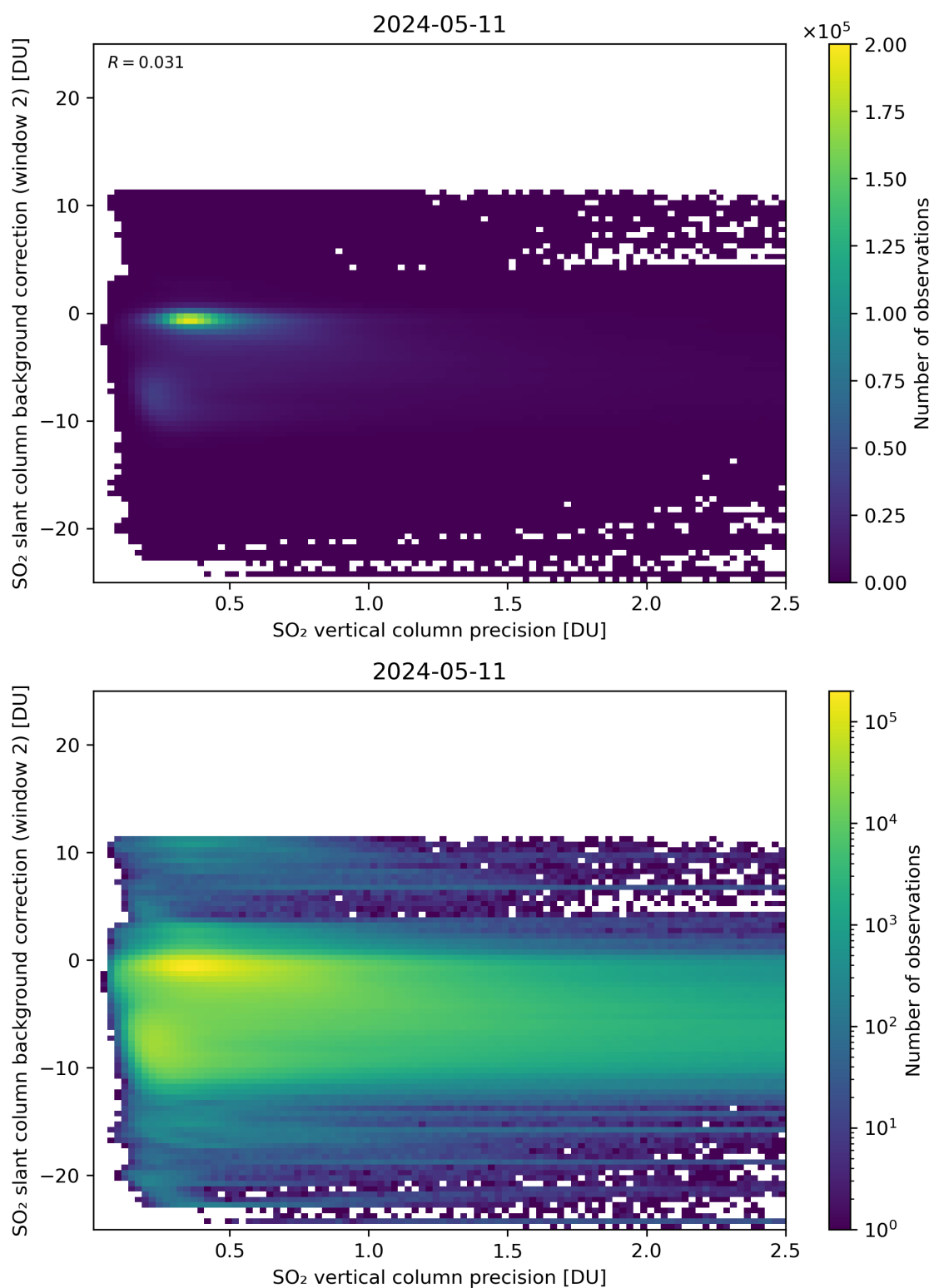
Figure 280: Scatter density plot of “SO 2 vertical column precision” against “SO 2 slant column background correction (window 2)” for 2024-05-10 to 2024-05-12.
