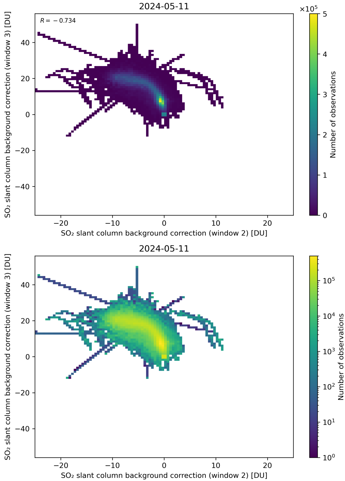
Figure 111: Scatter density plot of “SO 2 slant column background correction (window 2)” against “SO 2 slant column background correction (window 3)” for 2024-05-10 to 2024-05-12.
