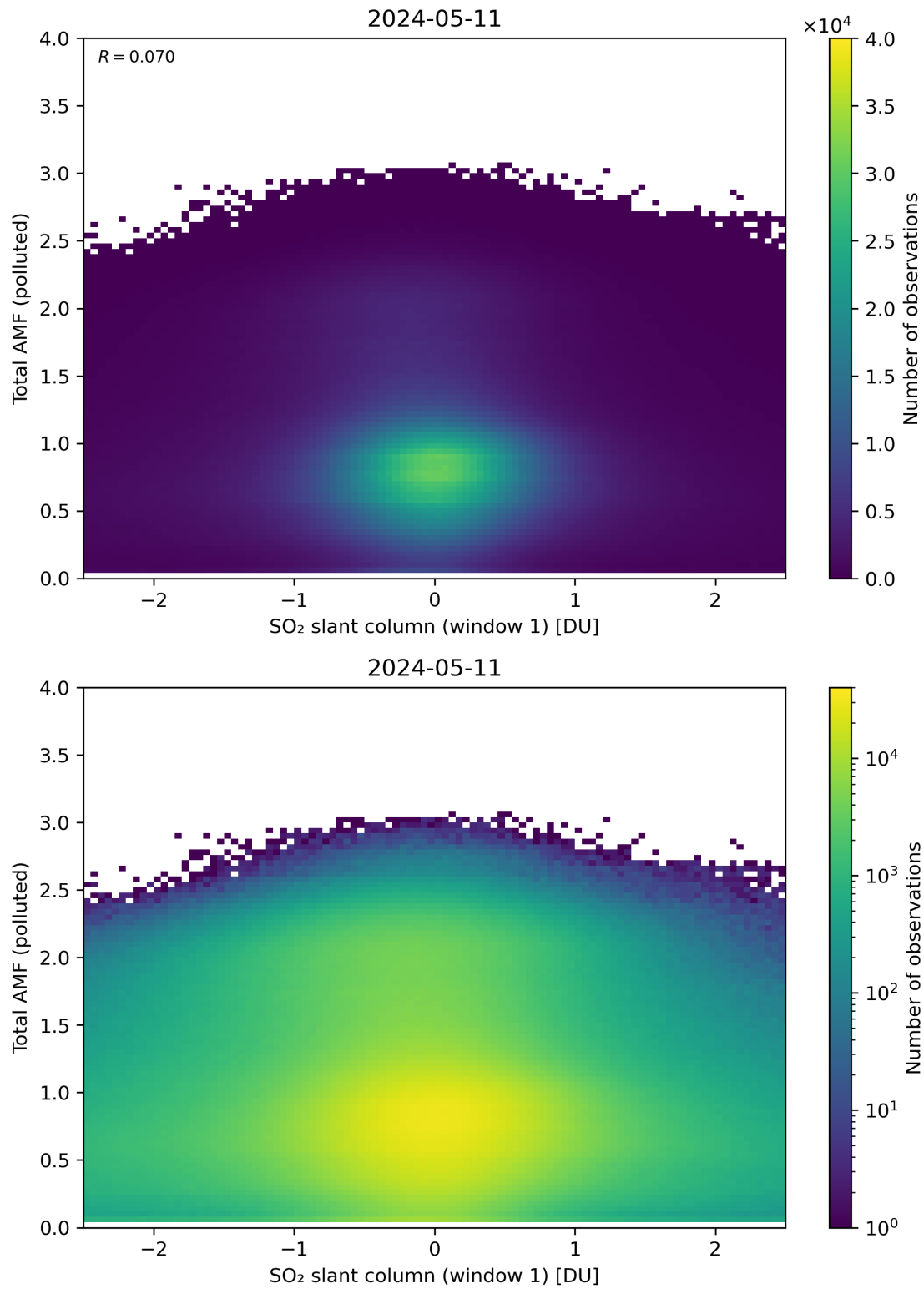
Figure 239: Scatter density plot of “SO 2 slant column (window 1)” against “Total AMF (polluted)” for 2024-05-10 to 2024-05-12.
