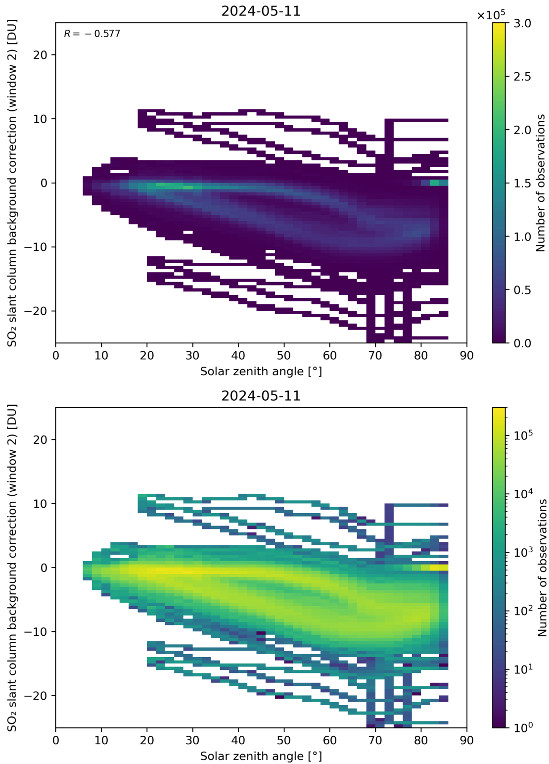
Figure 159: Scatter density plot of “Solar zenith angle” against “SO 2 slant column background correction (window 2)” for 2024-05-10 to 2024-05-12.
