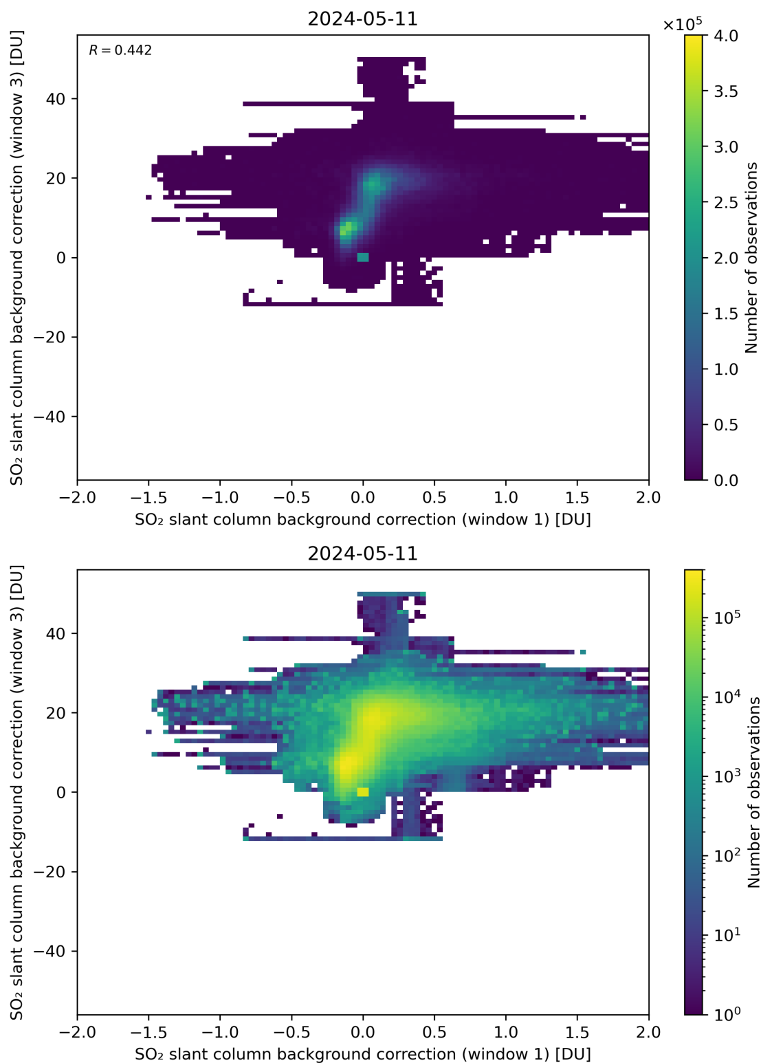
Figure 99: Scatter density plot of “SO 2 slant column background correction (window 1)” against “SO 2 slant column background correction (window 3)” for 2024-05-10 to 2024-05-12.
