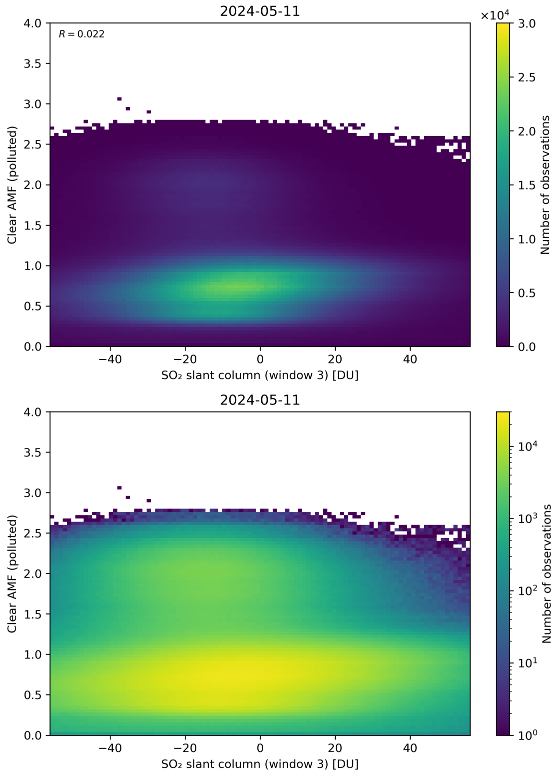
Figure 265: Scatter density plot of “SO 2 slant column (window 3)” against “Clear AMF (polluted)” for 2024-05-10 to 2024-05-12.
