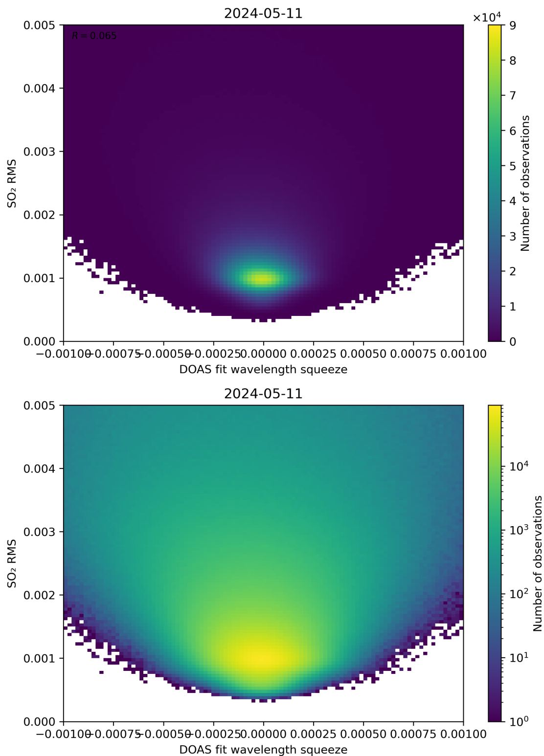
Figure 132: Scatter density plot of “DOAS fit wavelength squeeze” against “SO 2 RMS” for 2024-05-10 to 2024-05-12.
