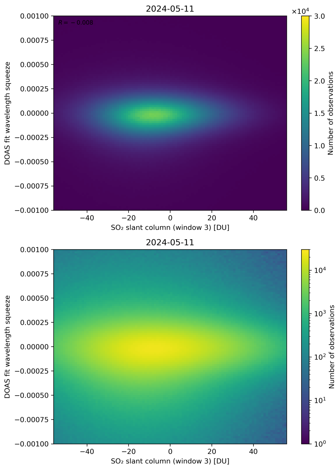
Figure 255: Scatter density plot of “SO 2 slant column (window 3)” against “DOAS fit wavelength squeeze” for 2024-05-10 to 2024-05-12.
