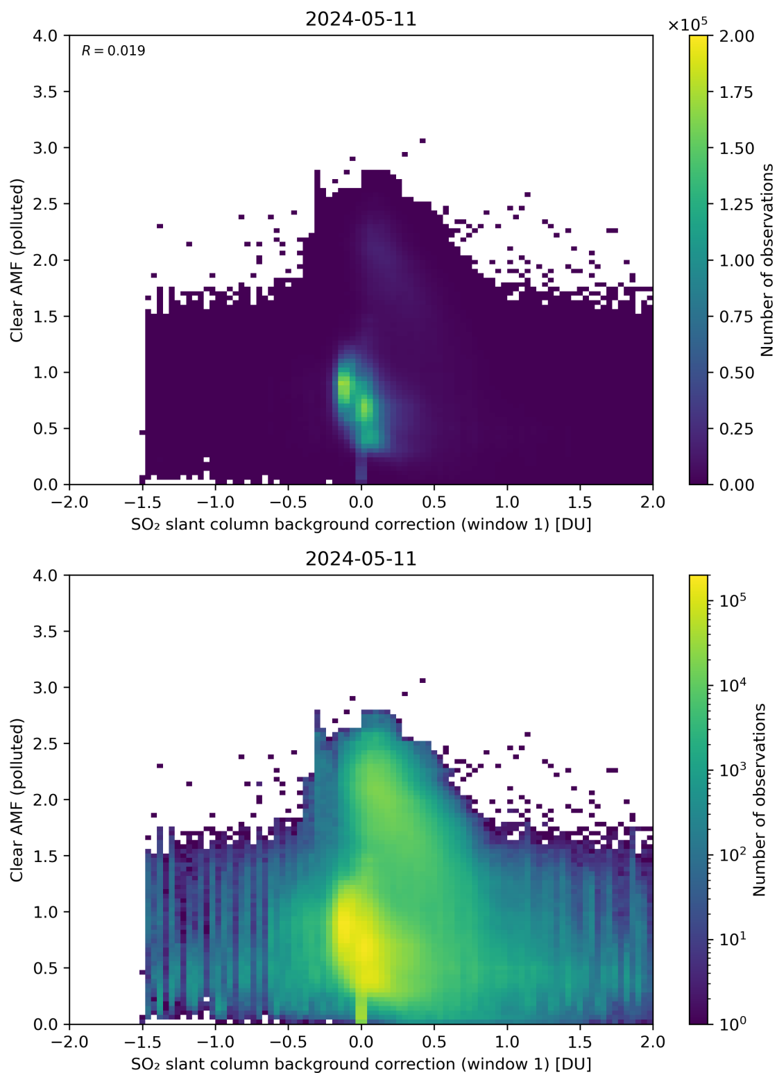
Figure 103: Scatter density plot of “SO 2 slant column background correction (window 1)” against “Clear AMF (polluted)” for 2024-05-10 to 2024-05-12.
