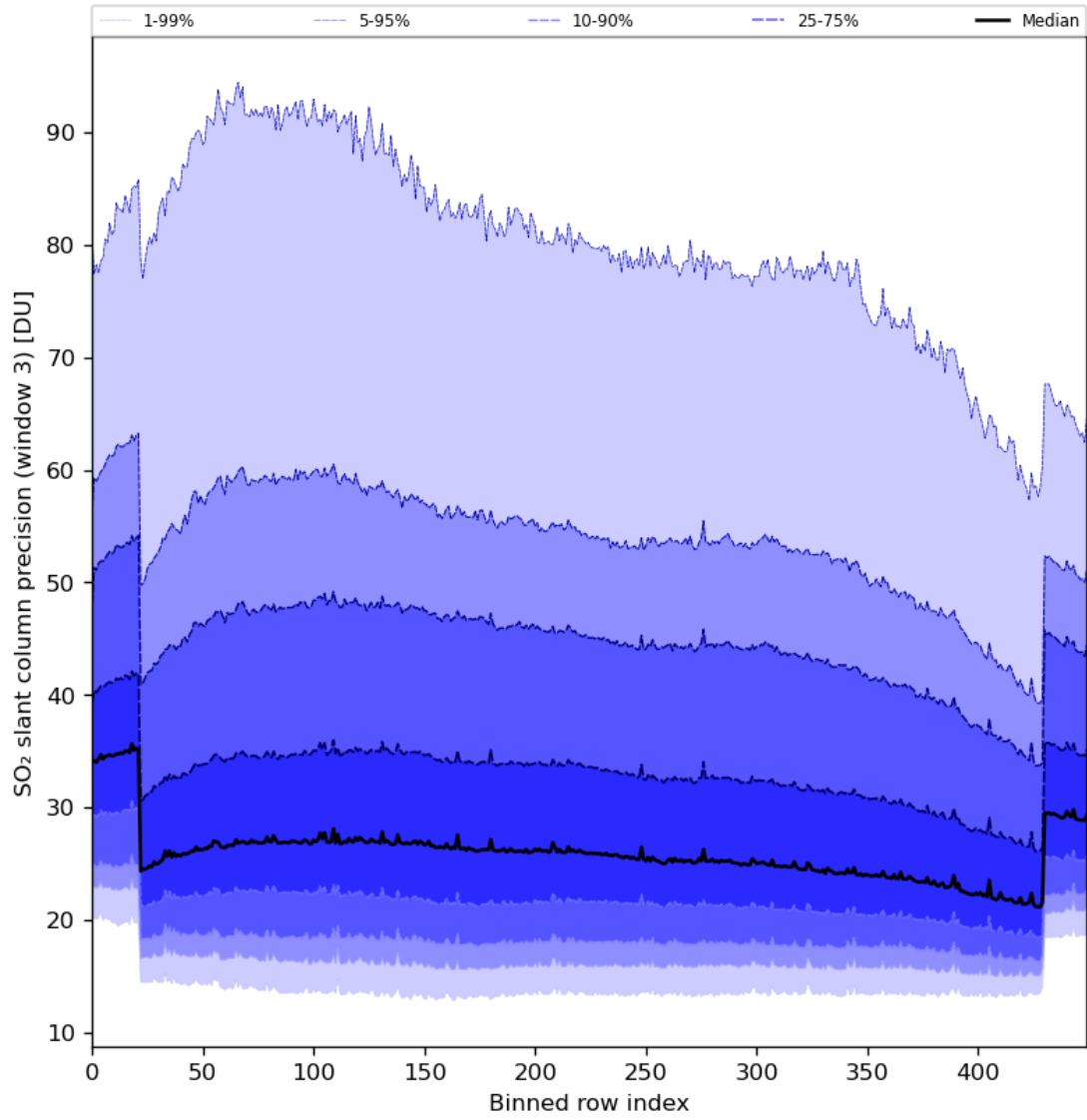
Figure 88: Along track statistics of “SO 2 slant column precision (window 3)” for 2024-05-10 to 2024-05-12
