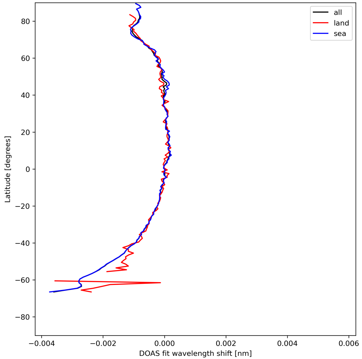
Figure 45: Zonal average of “DOAS fit wavelength shift” for 2024-05-10 to 2024-05-12.
