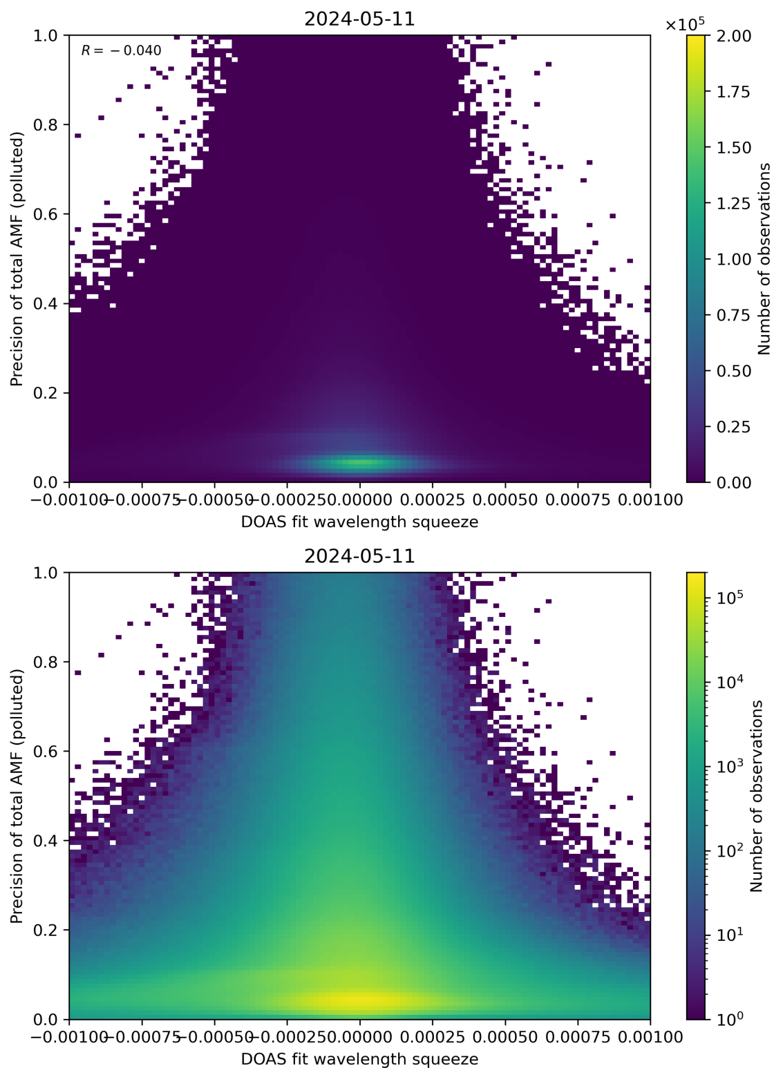
Figure 135: Scatter density plot of “DOAS fit wavelength squeeze” against “Precision of total AMF (polluted)” for 2024-05-10 to 2024-05-12.
