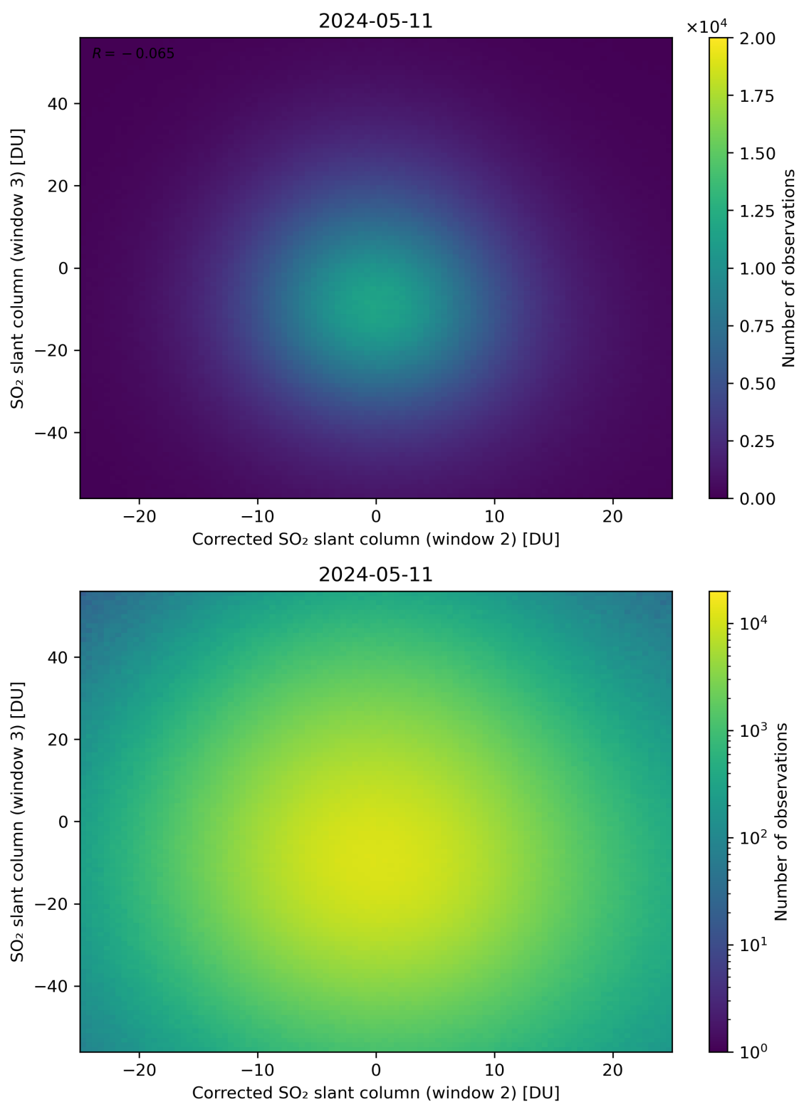
Figure 201: Scatter density plot of “Corrected SO 2 slant column (window 2)” against “SO 2 slant column (window 3)” for 2024-05-10 to 2024-05-12.
