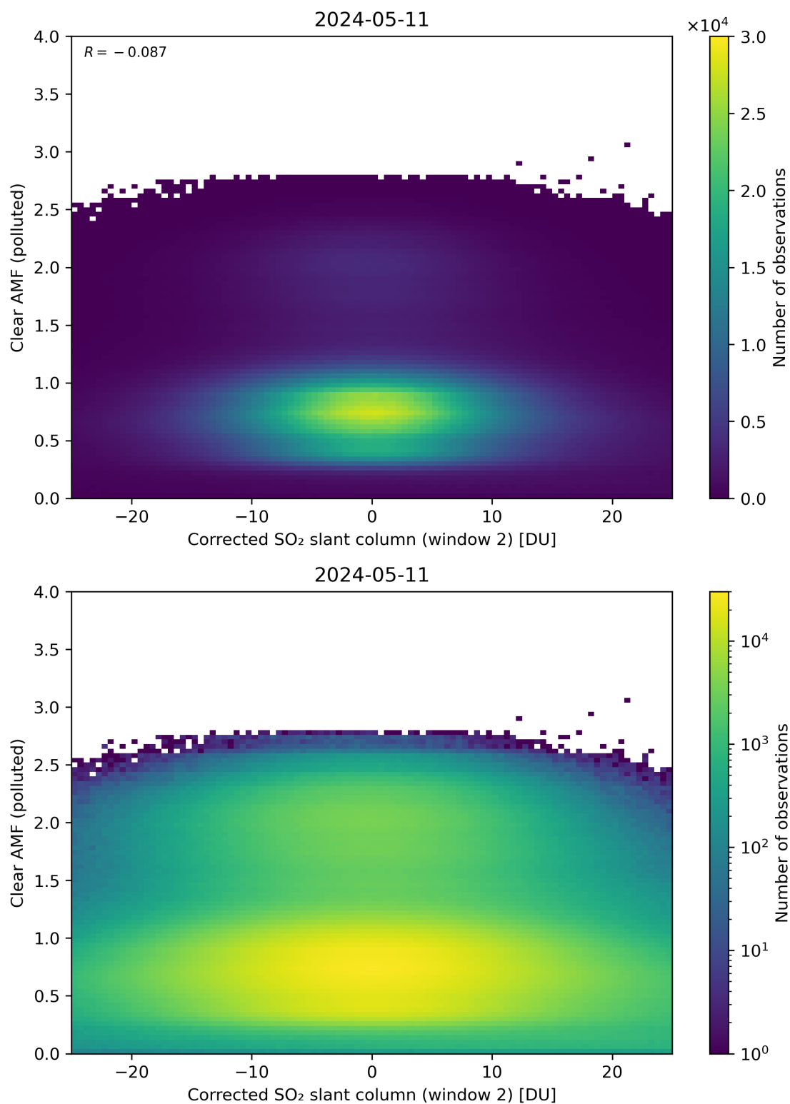
Figure 199: Scatter density plot of “Corrected SO 2 slant column (window 2)” against “Clear AMF (polluted)” for 2024-05-10 to 2024-05-12.
