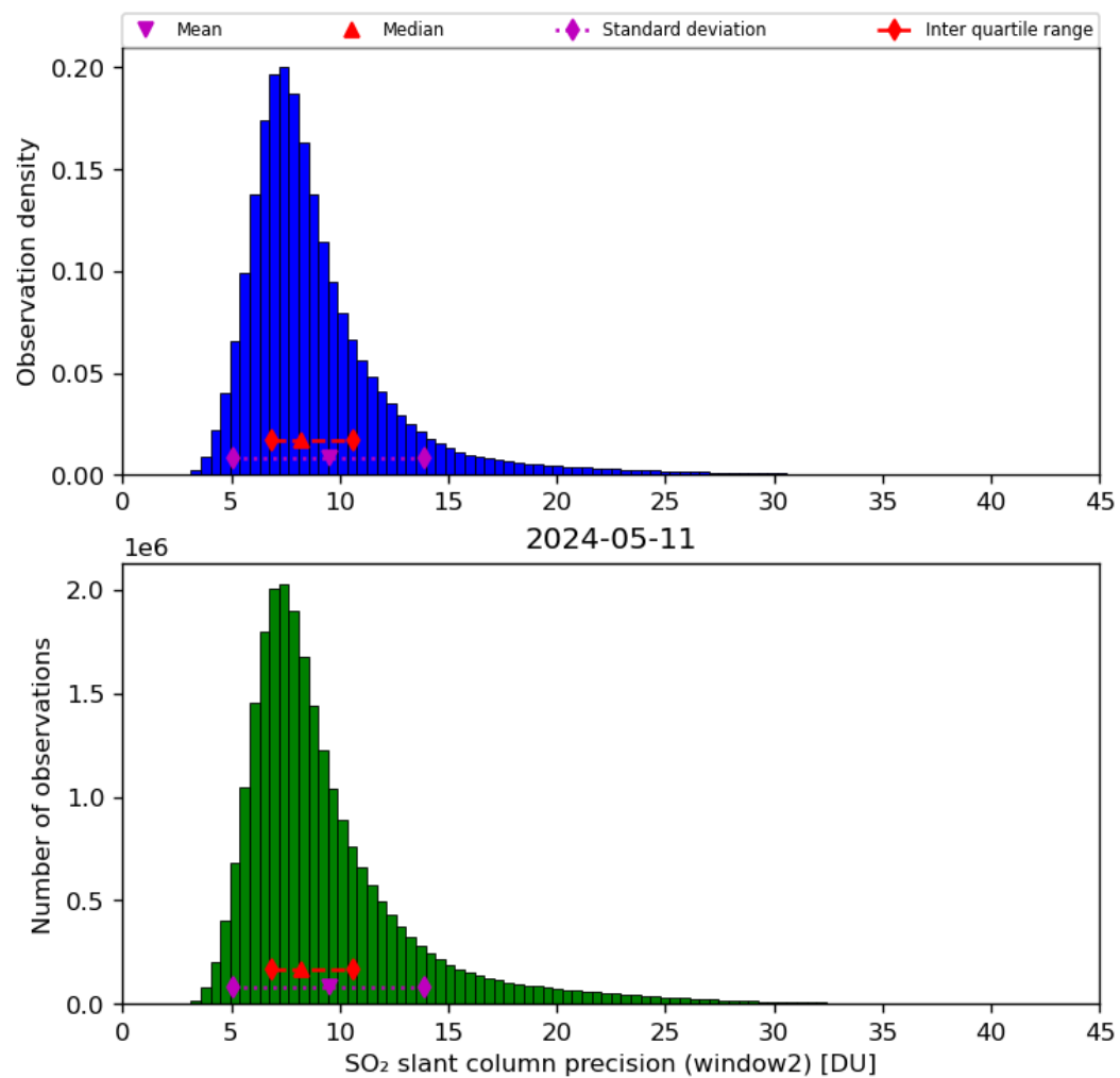
Figure 61: Histogram of “SO 2 slant column precision (window2)” for 2024-05-10 to 2024-05-12
