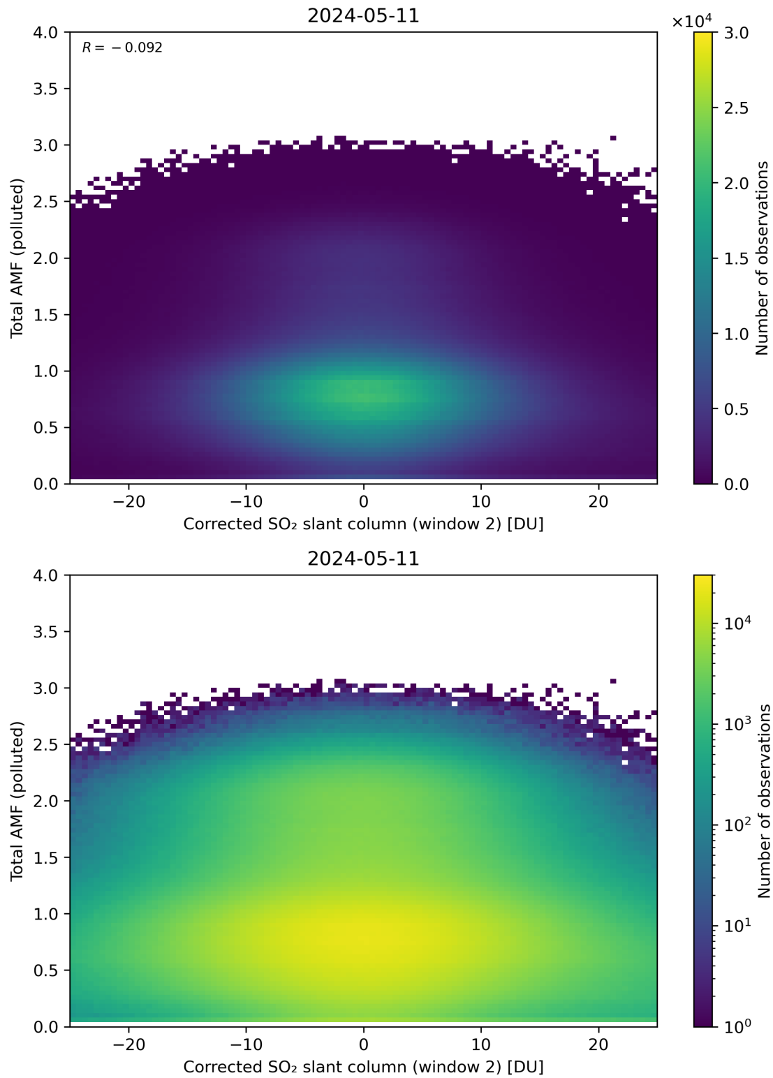
Figure 203: Scatter density plot of “Corrected SO 2 slant column (window 2)” against “Total AMF (polluted)” for 2024-05-10 to 2024-05-12.
