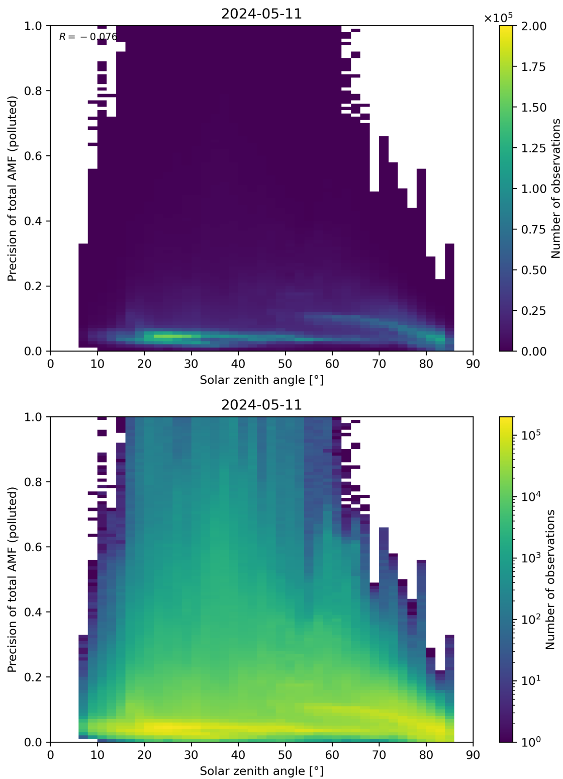
Figure 175: Scatter density plot of “Solar zenith angle” against “Precision of total AMF (polluted)” for 2024-05-10 to 2024-05-12.
