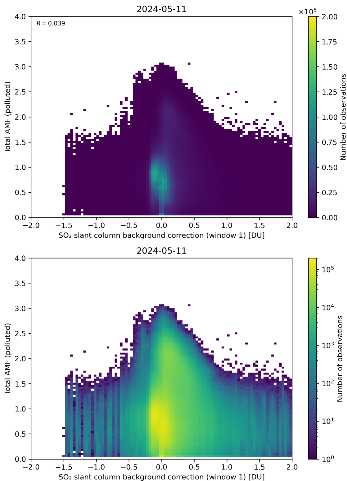
Figure 109: Scatter density plot of “SO 2 slant column background correction (window 1)” against “Total AMF (polluted)” for 2024-05-10 to 2024-05-12.
