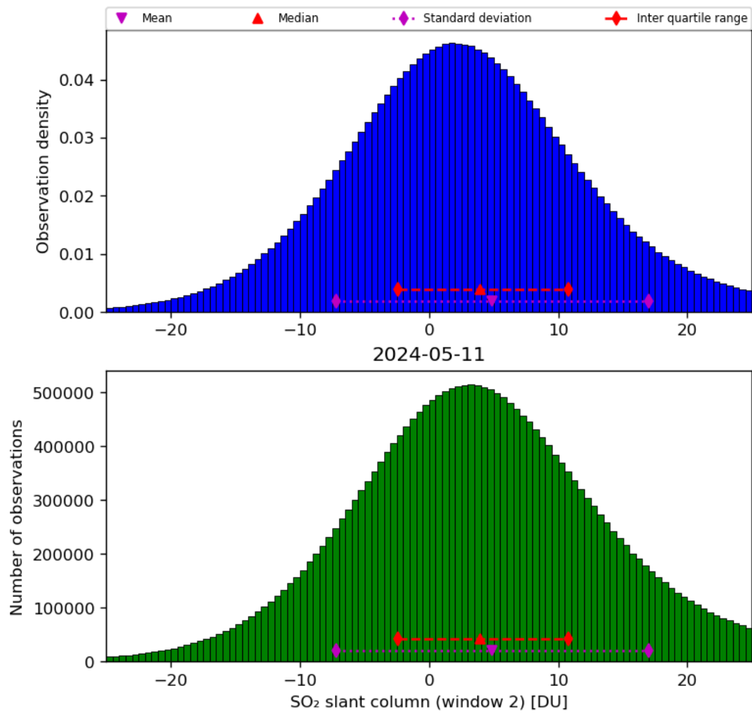
Figure 60: Histogram of “SO 2 slant column (window 2)” for 2024-05-10 to 2024-05-12
