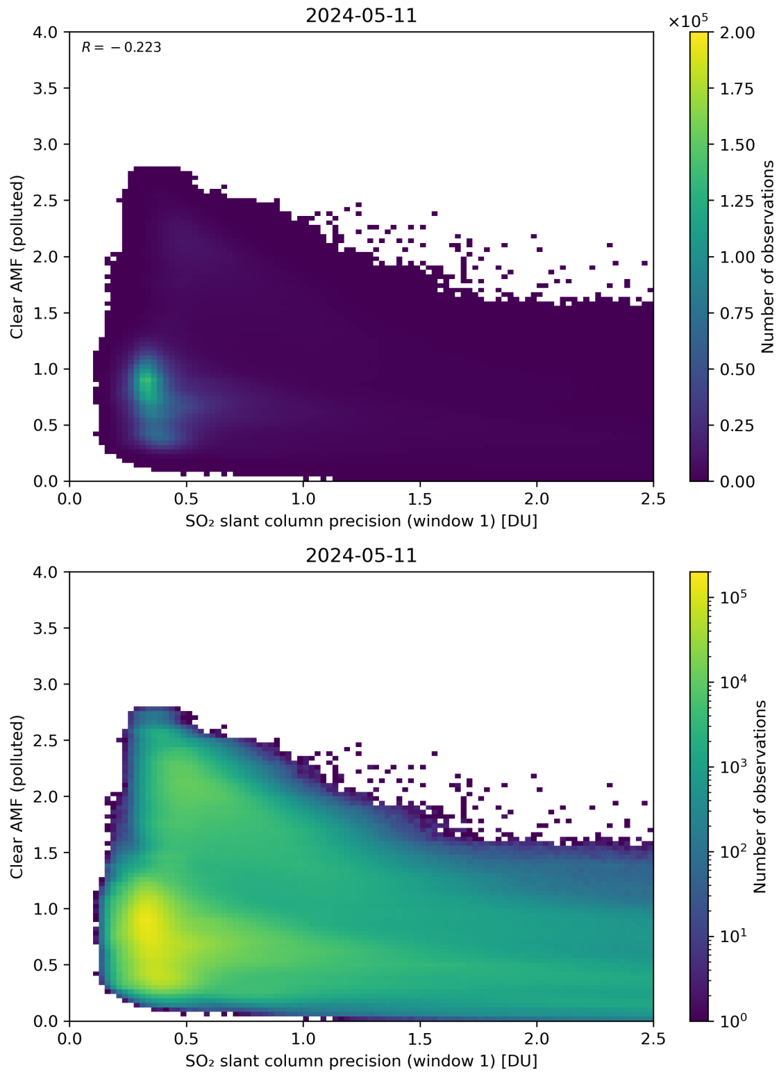
Figure 224: Scatter density plot of “SO 2 slant column precision (window 1)” against “Clear AMF (polluted)” for 2024-05-10 to 2024-05-12.
