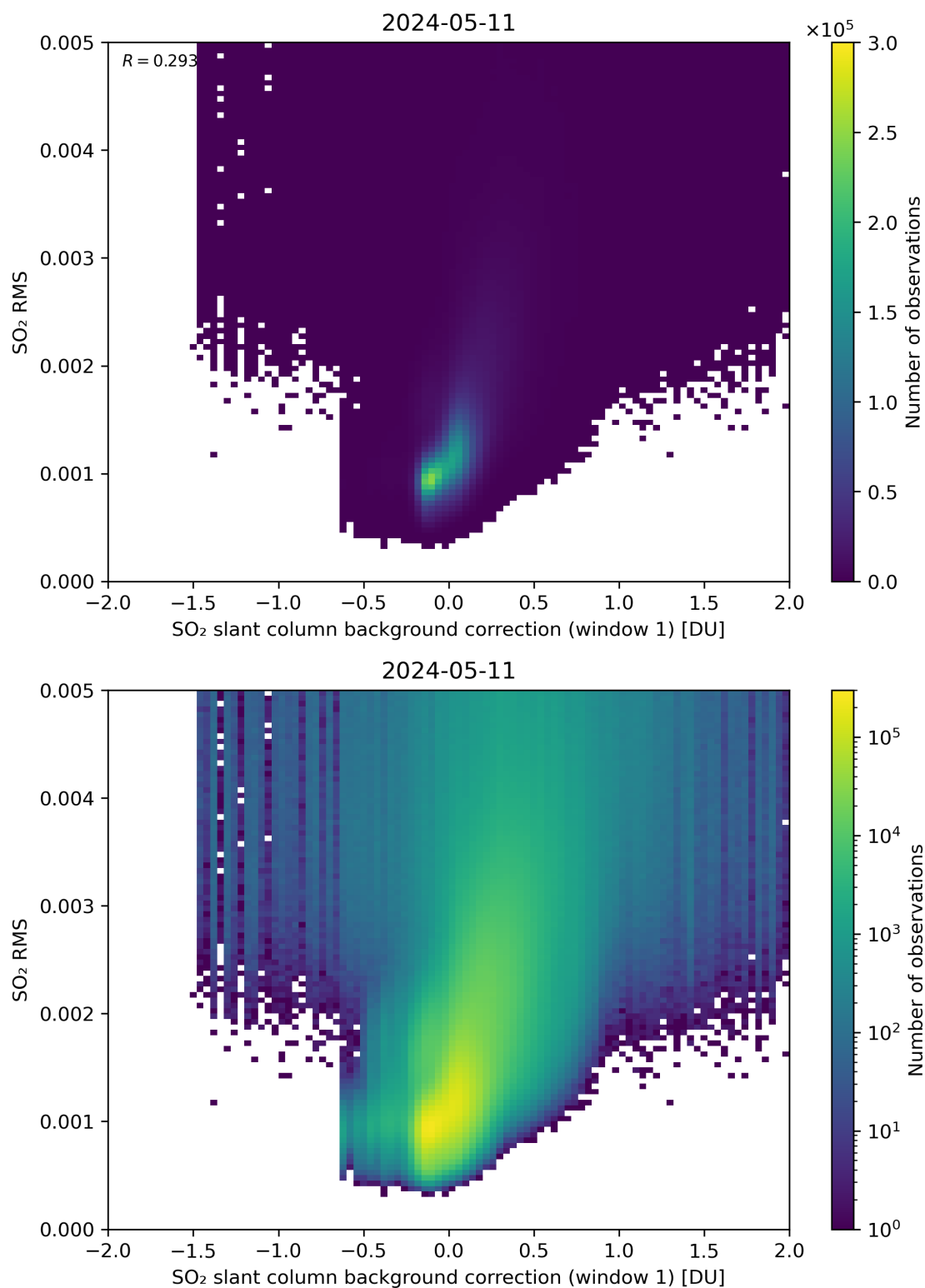
Figure 102: Scatter density plot of “SO 2 slant column background correction (window 1)” against “SO 2 RMS” for 2024-05-10 to 2024-05-12.
