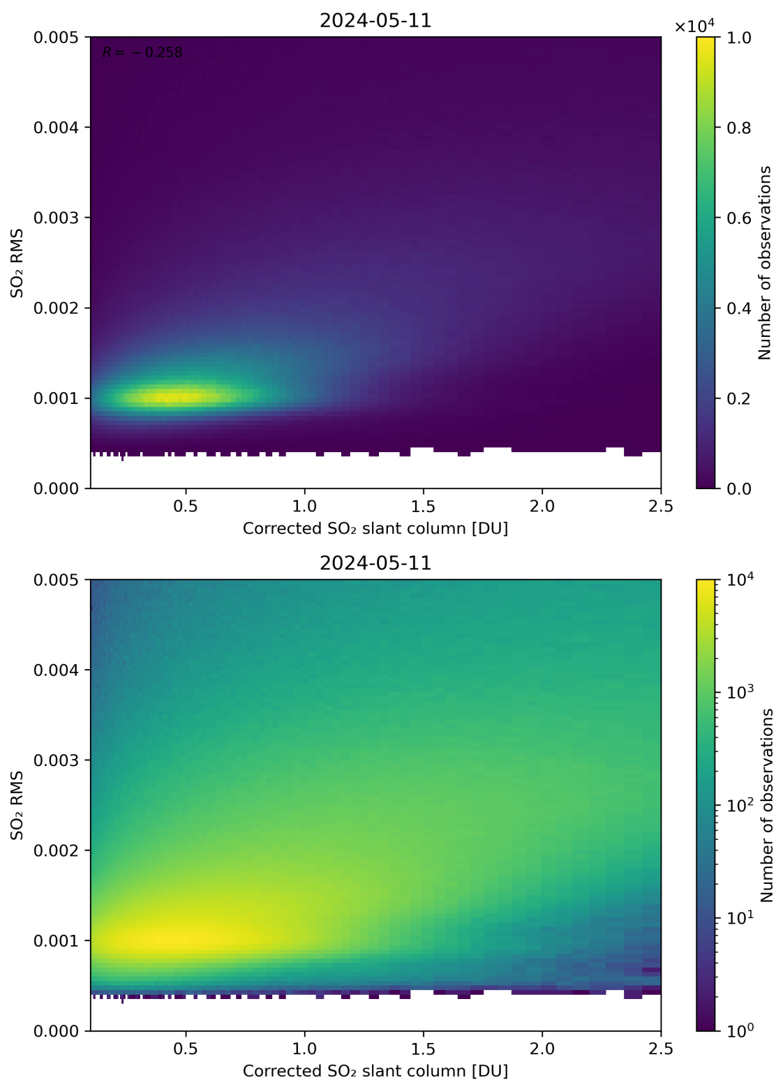
Figure 183: Scatter density plot of “Corrected SO 2 slant column” against “SO 2 RMS” for 2024-05-10 to 2024-05-12.
