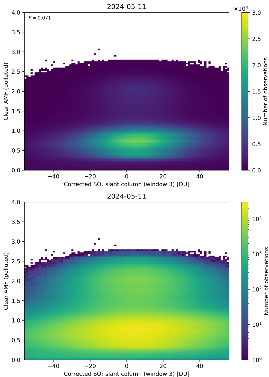
Figure 209: Scatter density plot of “Corrected SO 2 slant column (window 3)” against “Clear AMF (polluted)” for 2024-05-10 to 2024-05-12.
