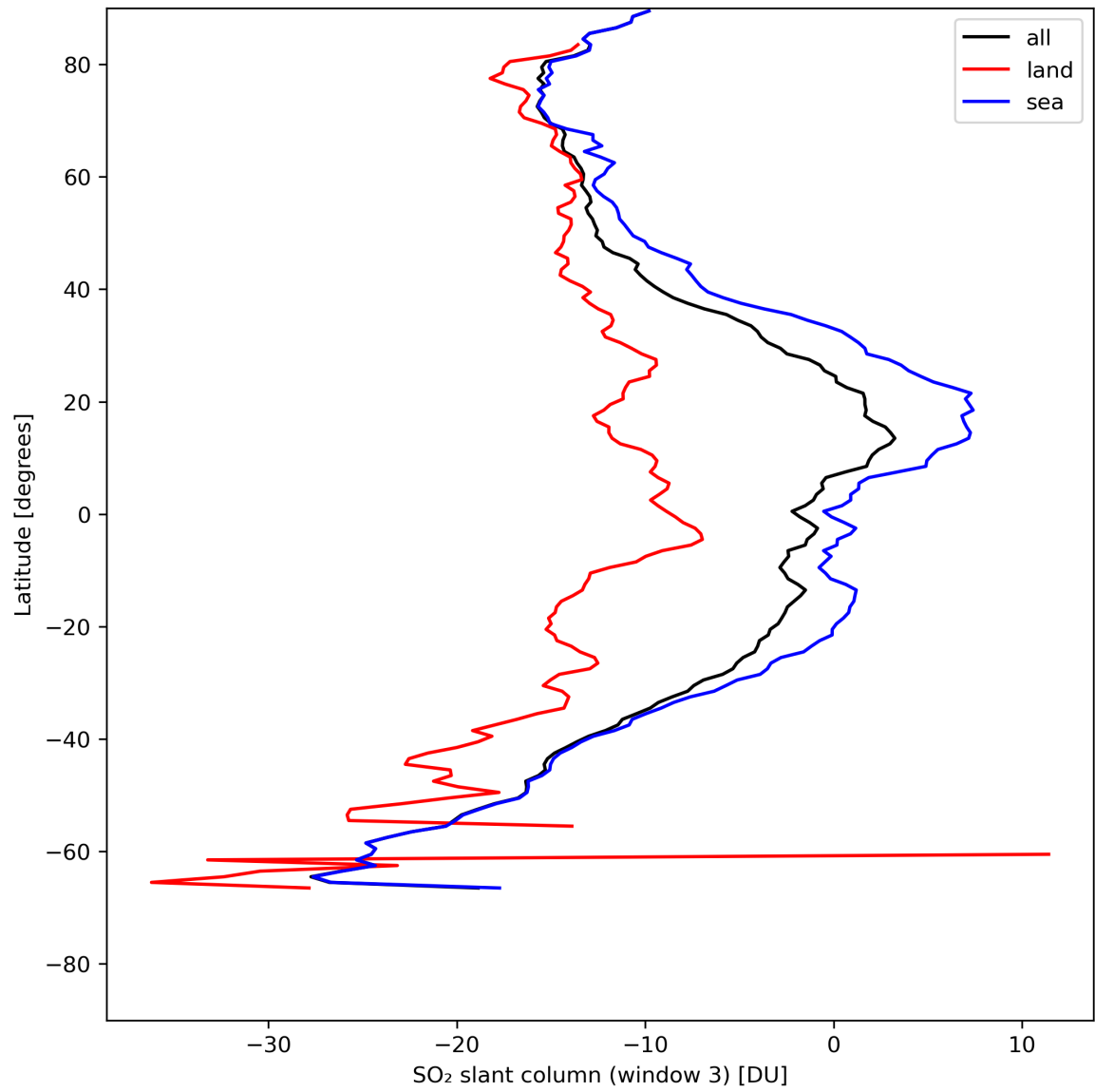
Figure 41: Zonal average of “SO 2 slant column (window 3)” for 2024-05-10 to 2024-05-12.
