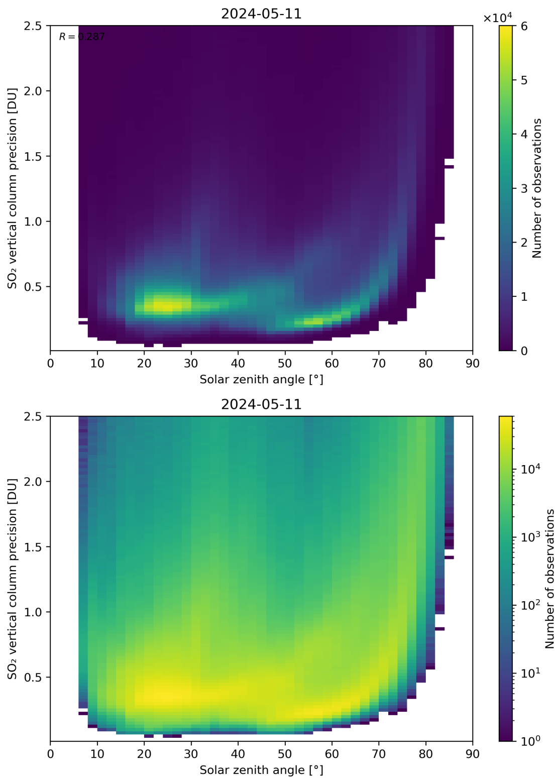
Figure 177: Scatter density plot of “Solar zenith angle” against “SO 2 vertical column precision” for 2024-05-10 to 2024-05-12.
