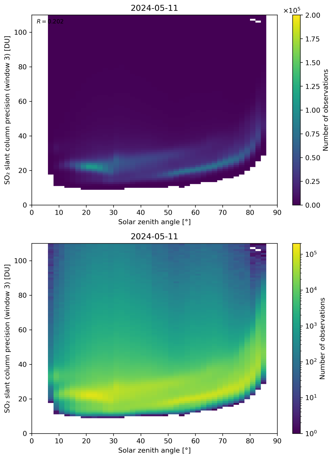
Figure 173: Scatter density plot of “Solar zenith angle” against “SO 2 slant column precision (window 3)” for 2024-05-10 to 2024-05-12.
