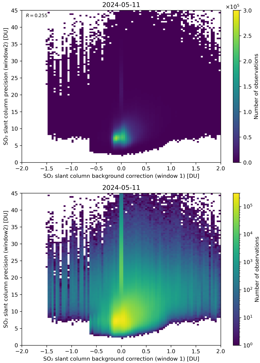
Figure 106: Scatter density plot of “SO 2 slant column background correction (window 1)” against “SO 2 slant column precision (window2)” for 2024-05-10 to 2024-05-12.
