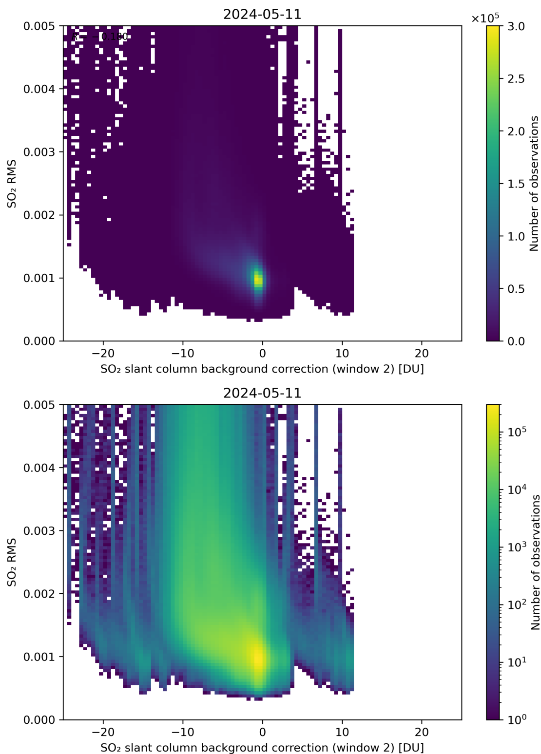
Figure 114: Scatter density plot of “SO 2 slant column background correction (window 2)” against “SO 2 RMS” for 2024-05-10 to 2024-05-12.
