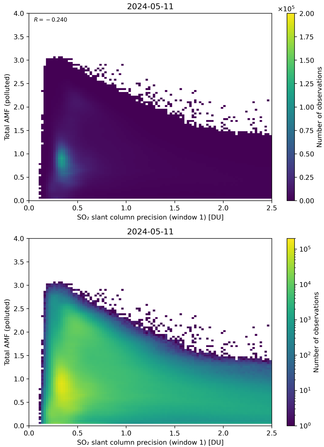
Figure 230: Scatter density plot of “SO 2 slant column precision (window 1)” against “Total AMF (polluted)” for 2024-05-10 to 2024-05-12.
