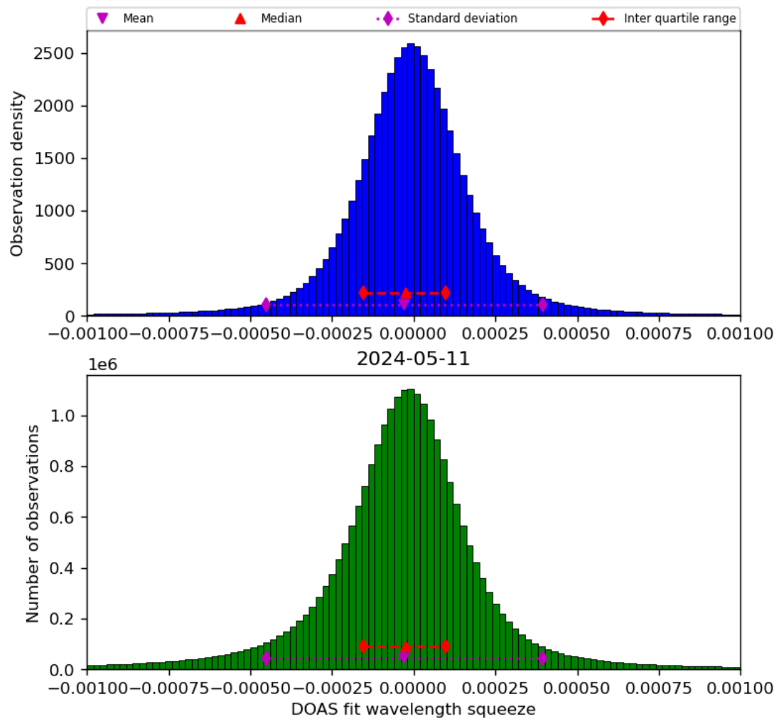
Figure 69: Histogram of “DOAS fit wavelength squeeze” for 2024-05-10 to 2024-05-12
