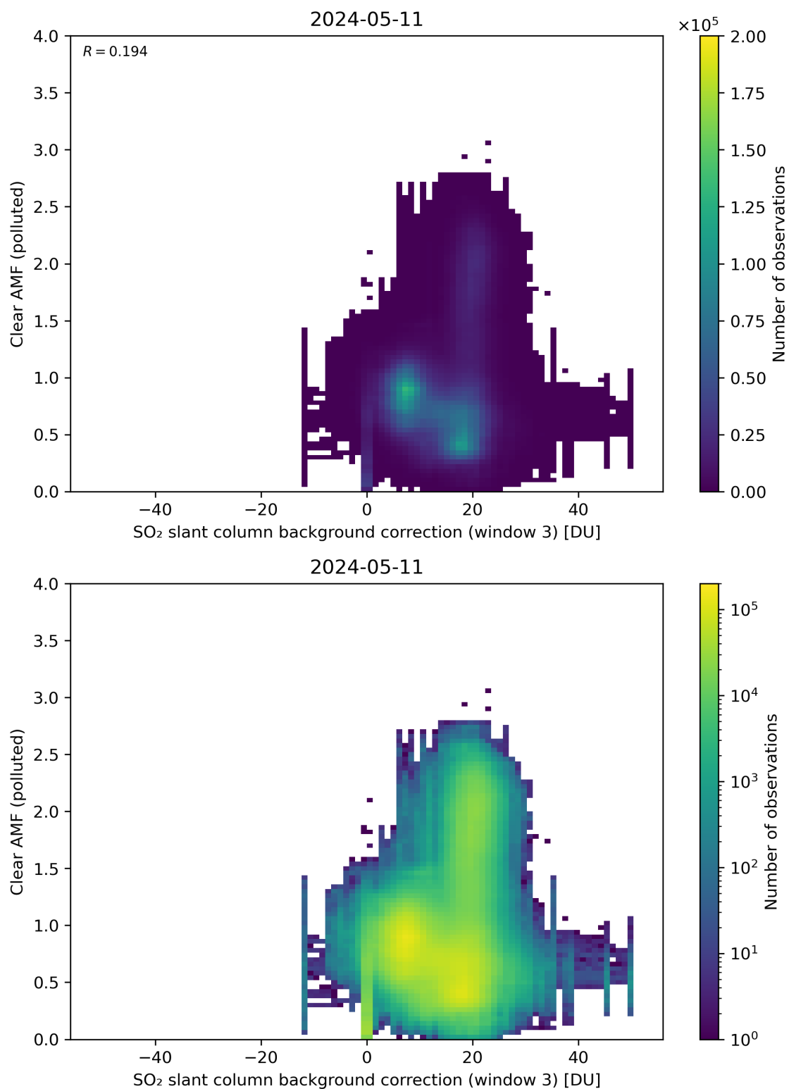
Figure 124: Scatter density plot of “SO 2 slant column background correction (window 3)” against “Clear AMF (polluted)” for 2024-05-10 to 2024-05-12.
