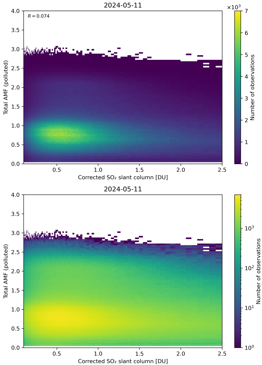
Figure 192: Scatter density plot of “Corrected SO 2 slant column” against “Total AMF (polluted)” for 2024-05-10 to 2024-05-12.
