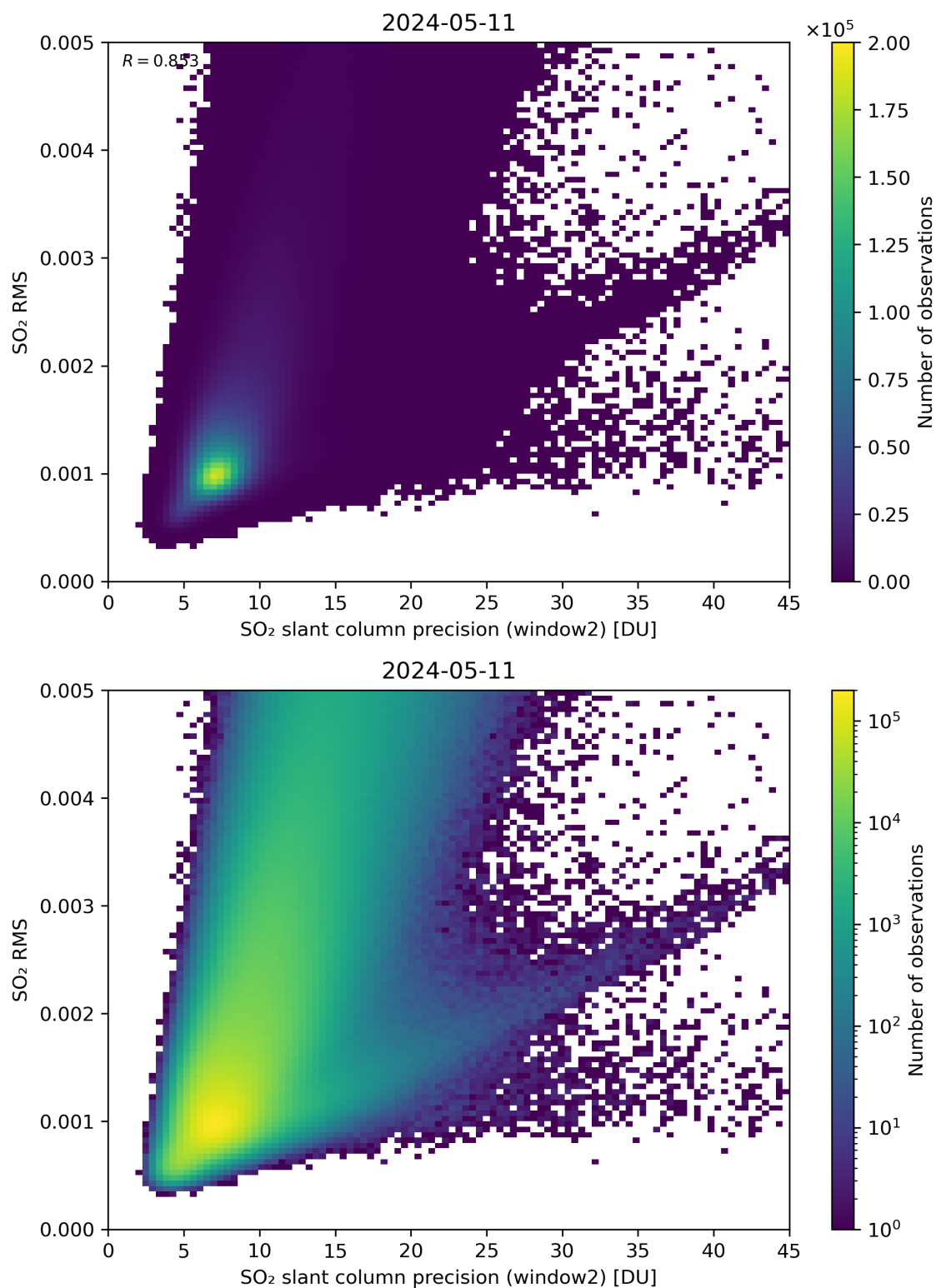
Figure 245: Scatter density plot of “SO 2 slant column precision (window2)” against “SO 2 RMS” for 2024-05-10 to 2024-05-12.
