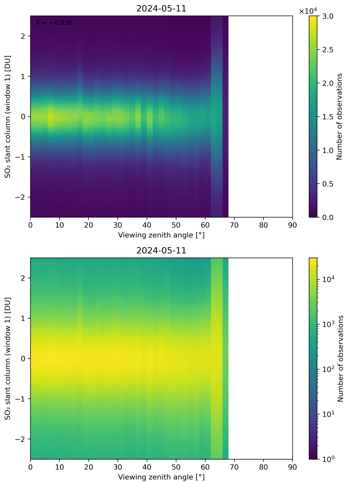
Figure 320: Scatter density plot of “Viewing zenith angle” against “SO 2 slant column (window 1)” for 2024-05-10 to 2024-05-12.
