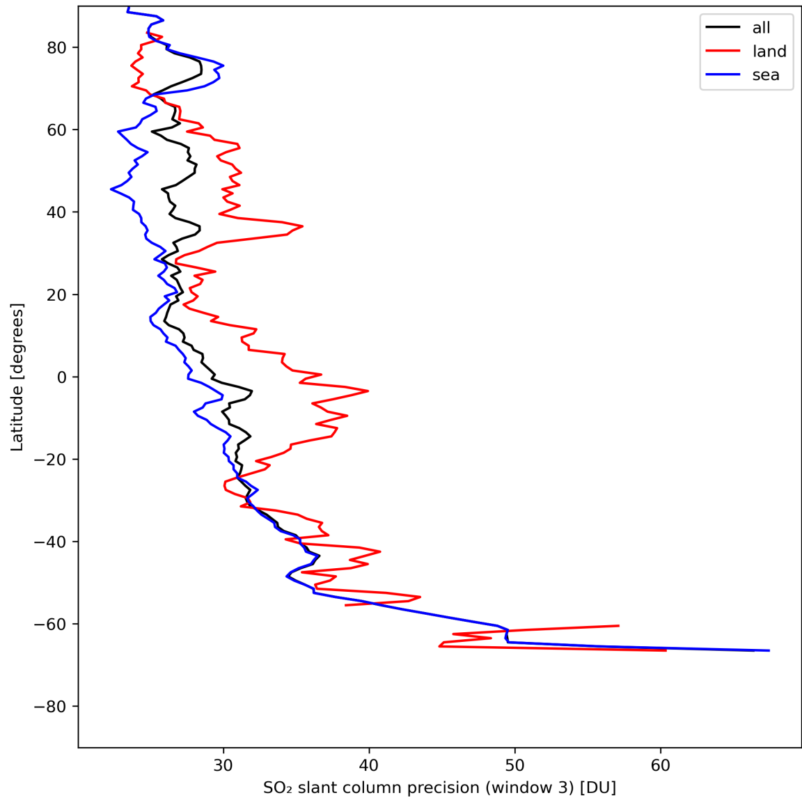
Figure 42: Zonal average of “SO 2 slant column precision (window 3)” for 2024-05-10 to 2024-05-12.
