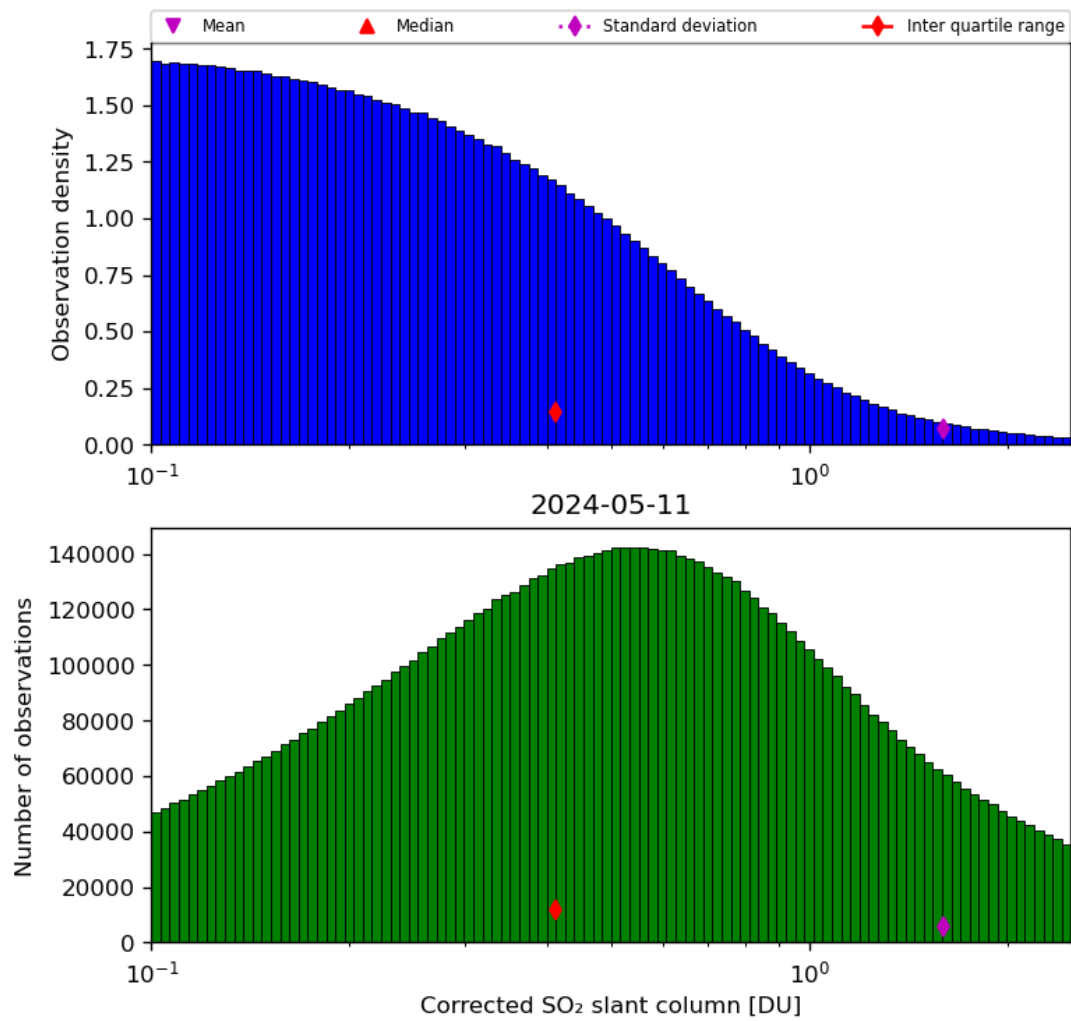
Figure 55: Histogram of “Corrected SO 2 slant column” for 2024-05-10 to 2024-05-12
