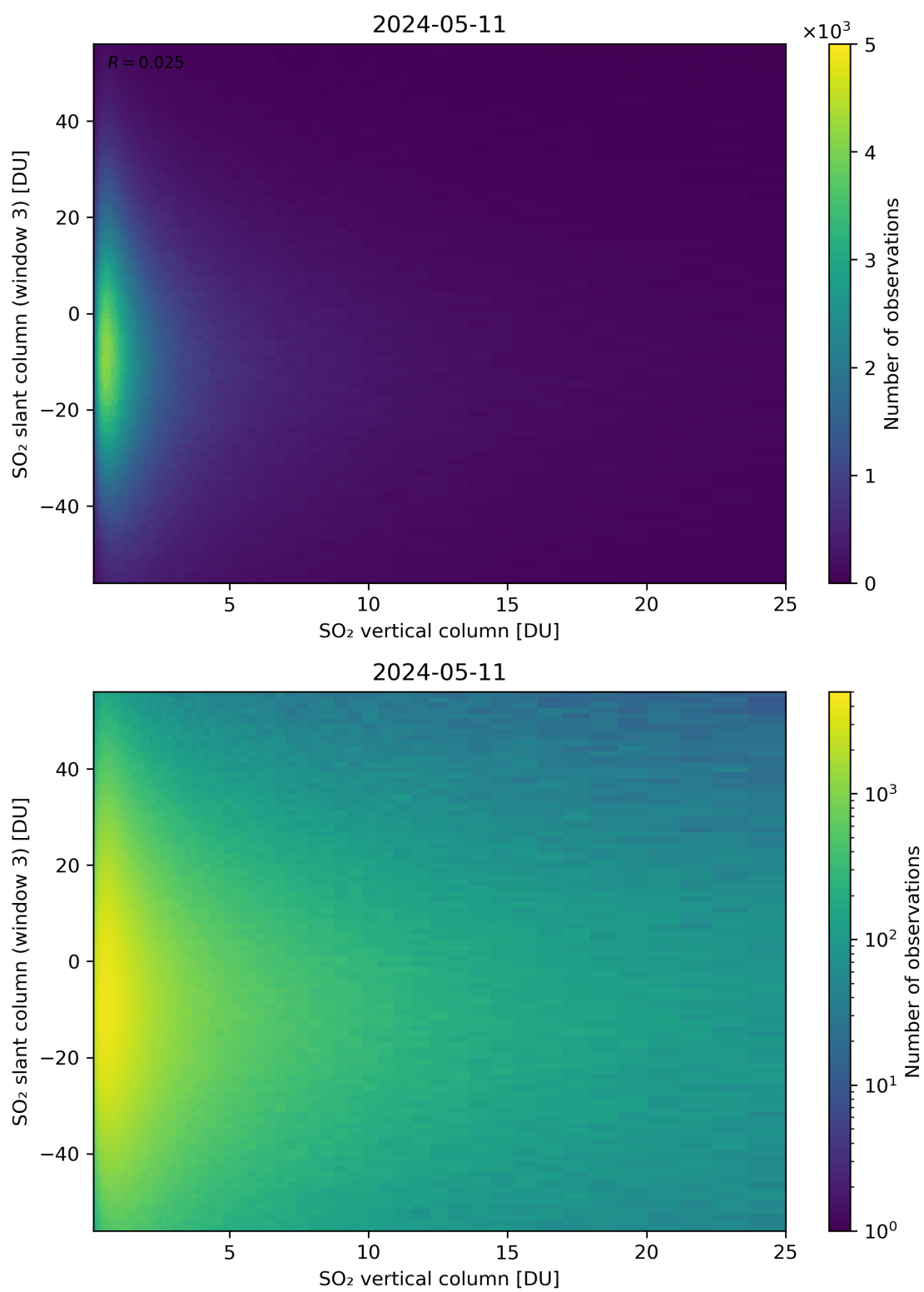
Figure 303: Scatter density plot of “SO 2 vertical column” against “SO 2 slant column (window 3)” for 2024-05-10 to 2024-05-12.
