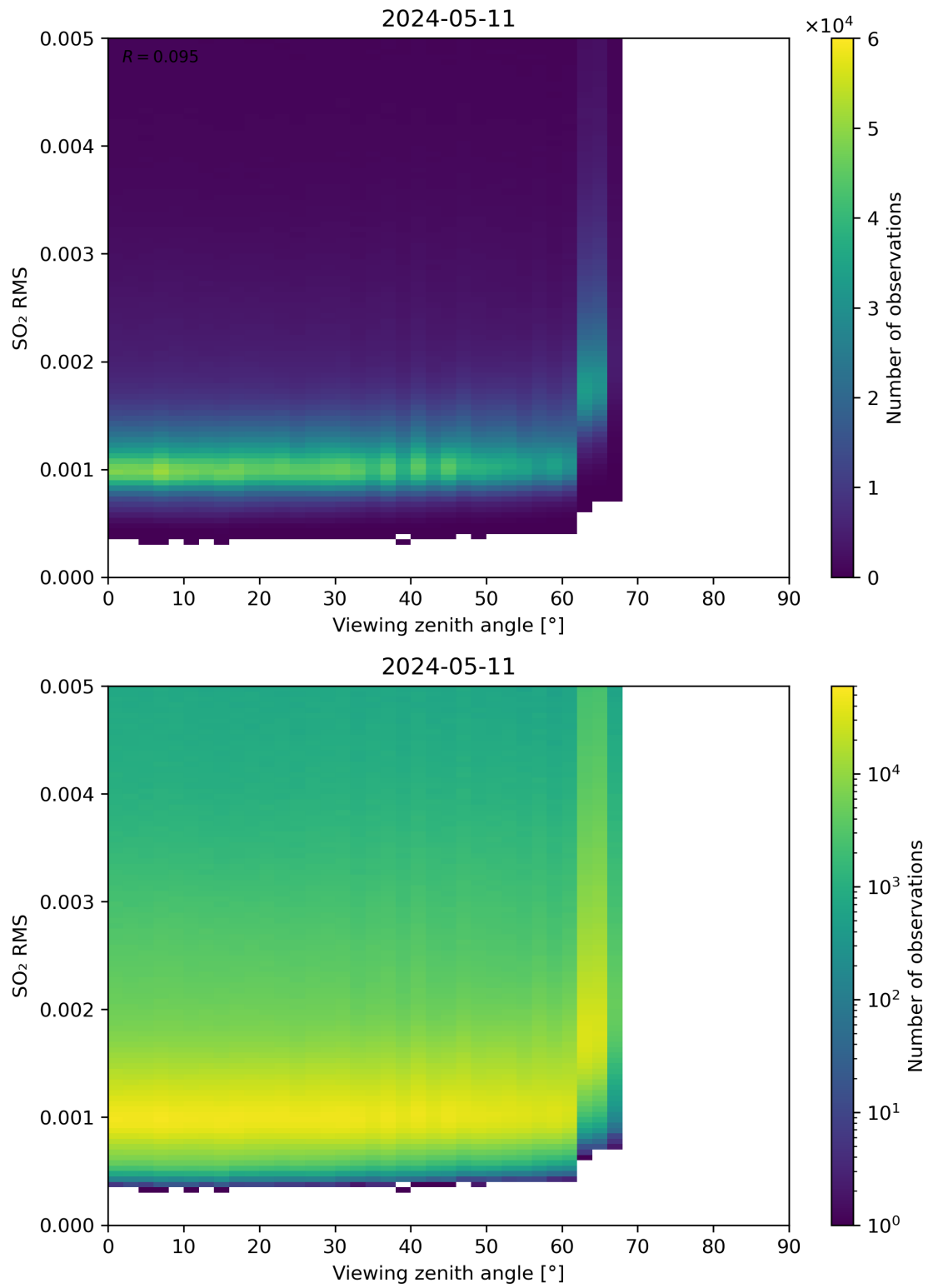
Figure 313: Scatter density plot of “Viewing zenith angle” against “SO 2 RMS” for 2024-05-10 to 2024-05-12.
