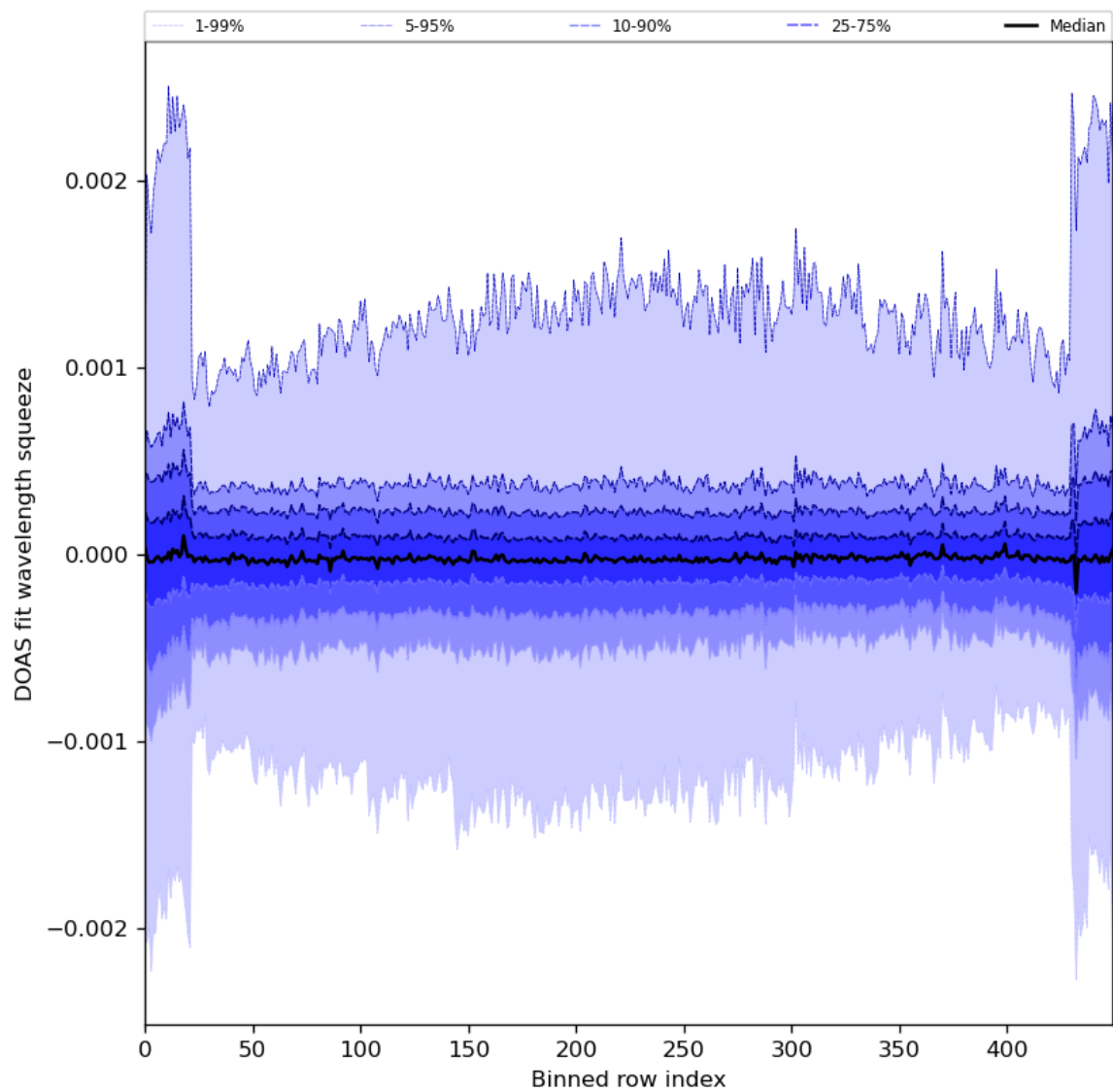
Figure 92: Along track statistics of “DOAS fit wavelength squeeze” for 2024-05-10 to 2024-05-12
