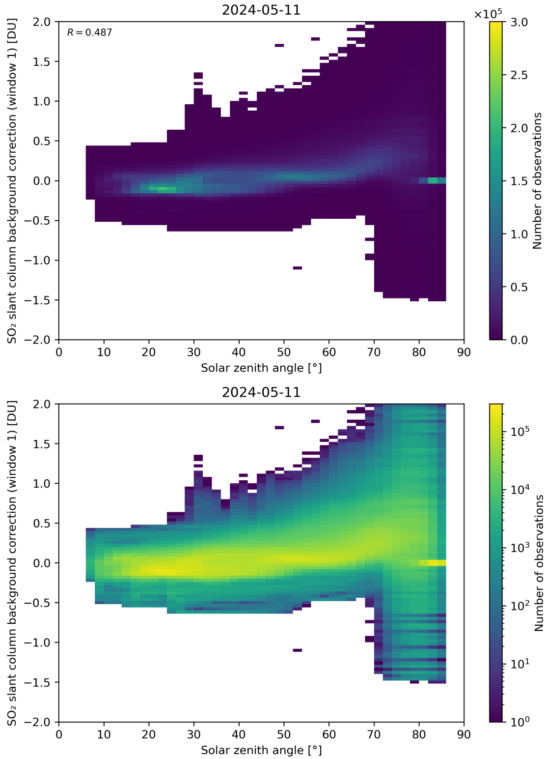
Figure 158: Scatter density plot of “Solar zenith angle” against “SO 2 slant column background correction (window 1)” for 2024-05-10 to 2024-05-12.
