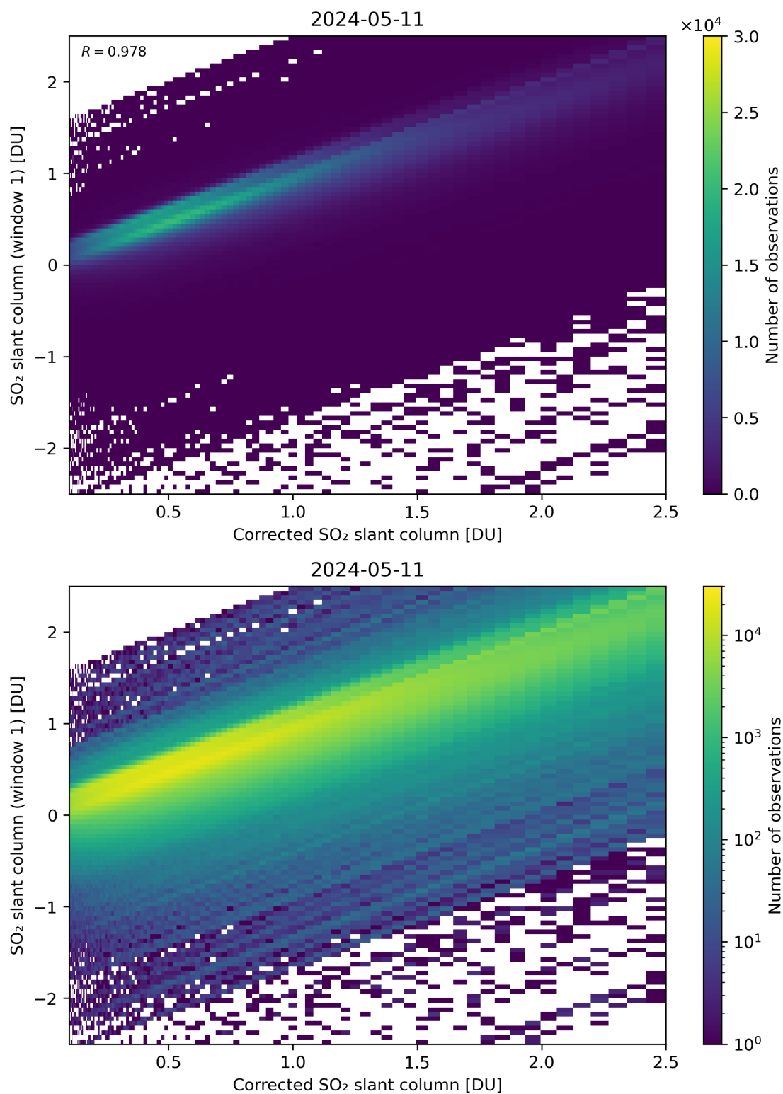
Figure 187: Scatter density plot of “Corrected SO 2 slant column” against “SO 2 slant column (window 1)” for 2024-05-10 to 2024-05-12.
