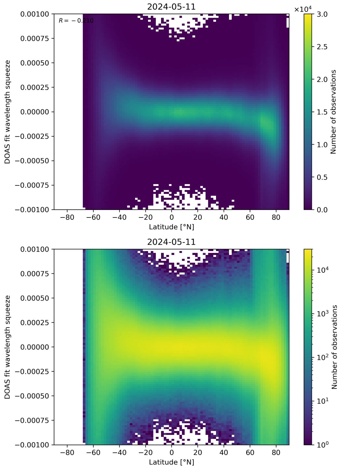
Figure 143: Scatter density plot of “Latitude” against “DOAS fit wavelength squeeze” for 2024-05-10 to 2024-05-12.
