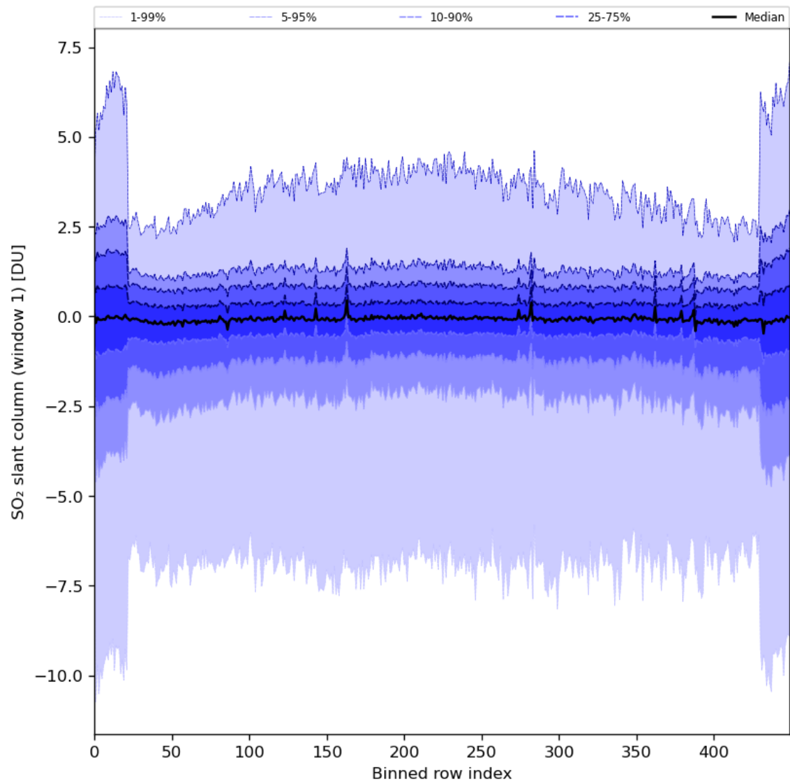
Figure 79: Along track statistics of “SO 2 slant column (window 1)” for 2024-05-10 to 2024-05-12
