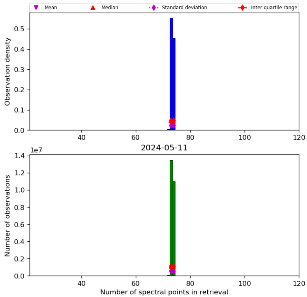
Figure 74: Histogram of “Number of spectral points in retrieval” for 2024-05-10 to 2024-05-12
