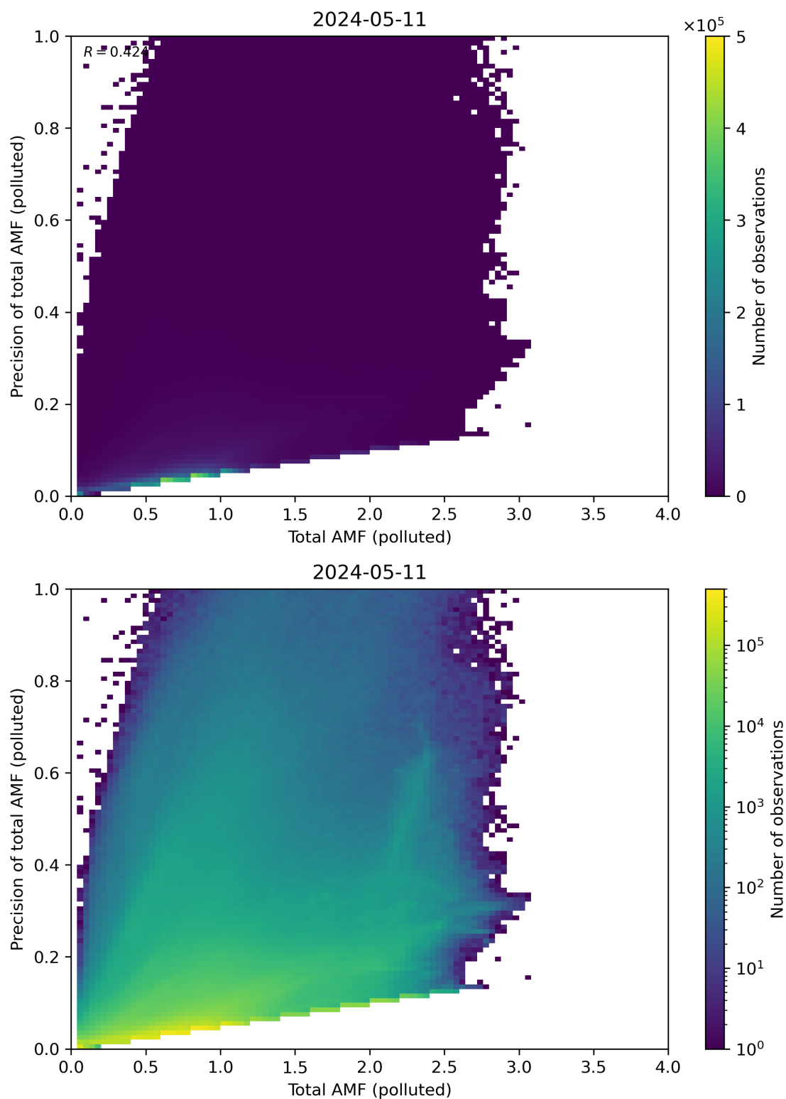
Figure 272: Scatter density plot of “Total AMF (polluted)” against “Precision of total AMF (polluted)” for 2024-05-10 to 2024-05-12.
