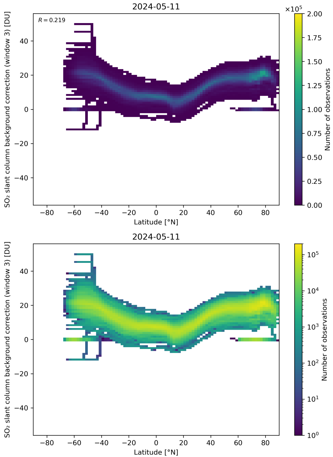
Figure 141: Scatter density plot of “Latitude” against “SO 2 slant column background correction (window 3)” for 2024-05-10 to 2024-05-12.
