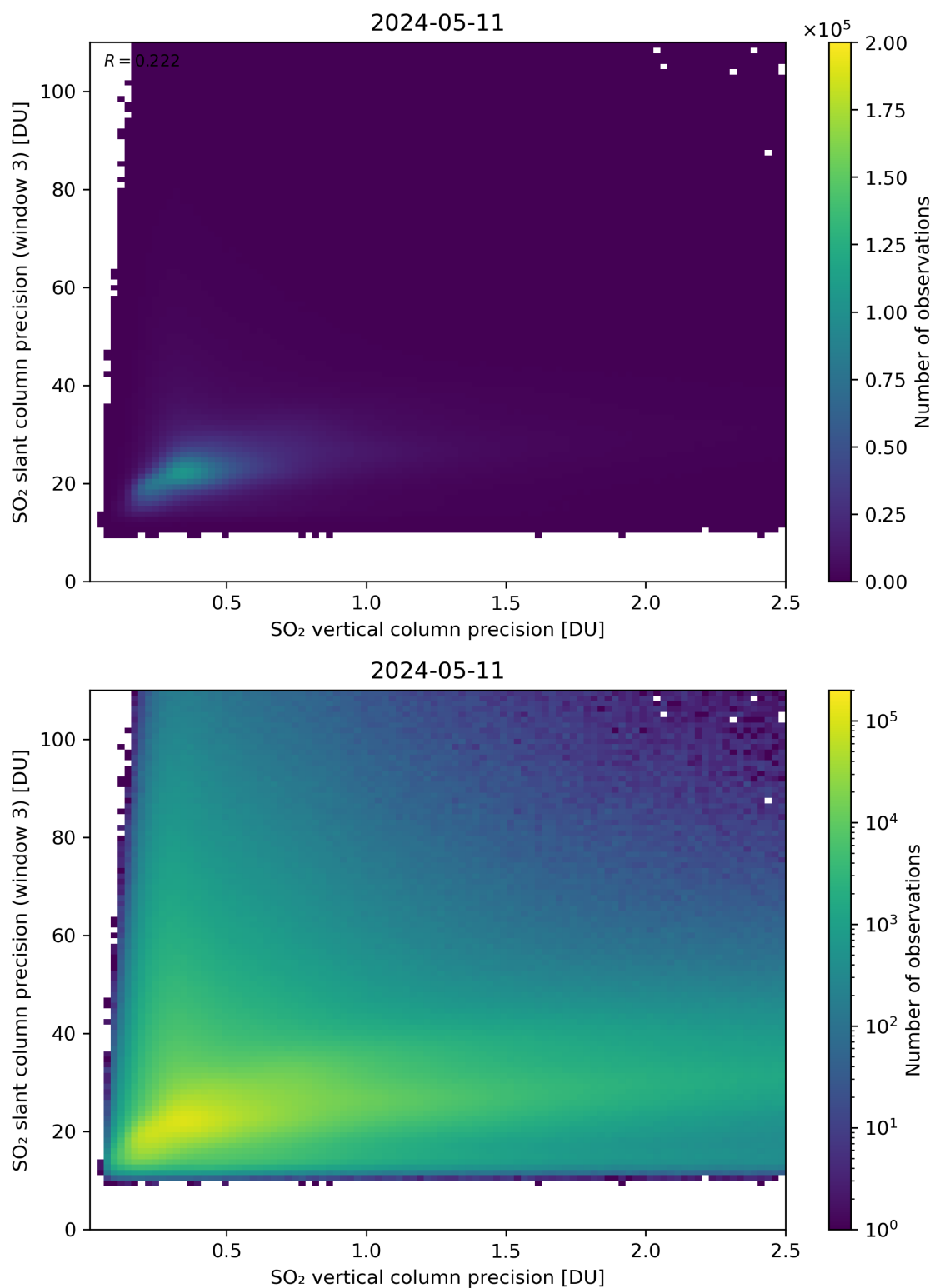
Figure 293: Scatter density plot of “SO 2 vertical column precision” against “SO 2 slant column precision (window 3)” for 2024-05-10 to 2024-05-12.
