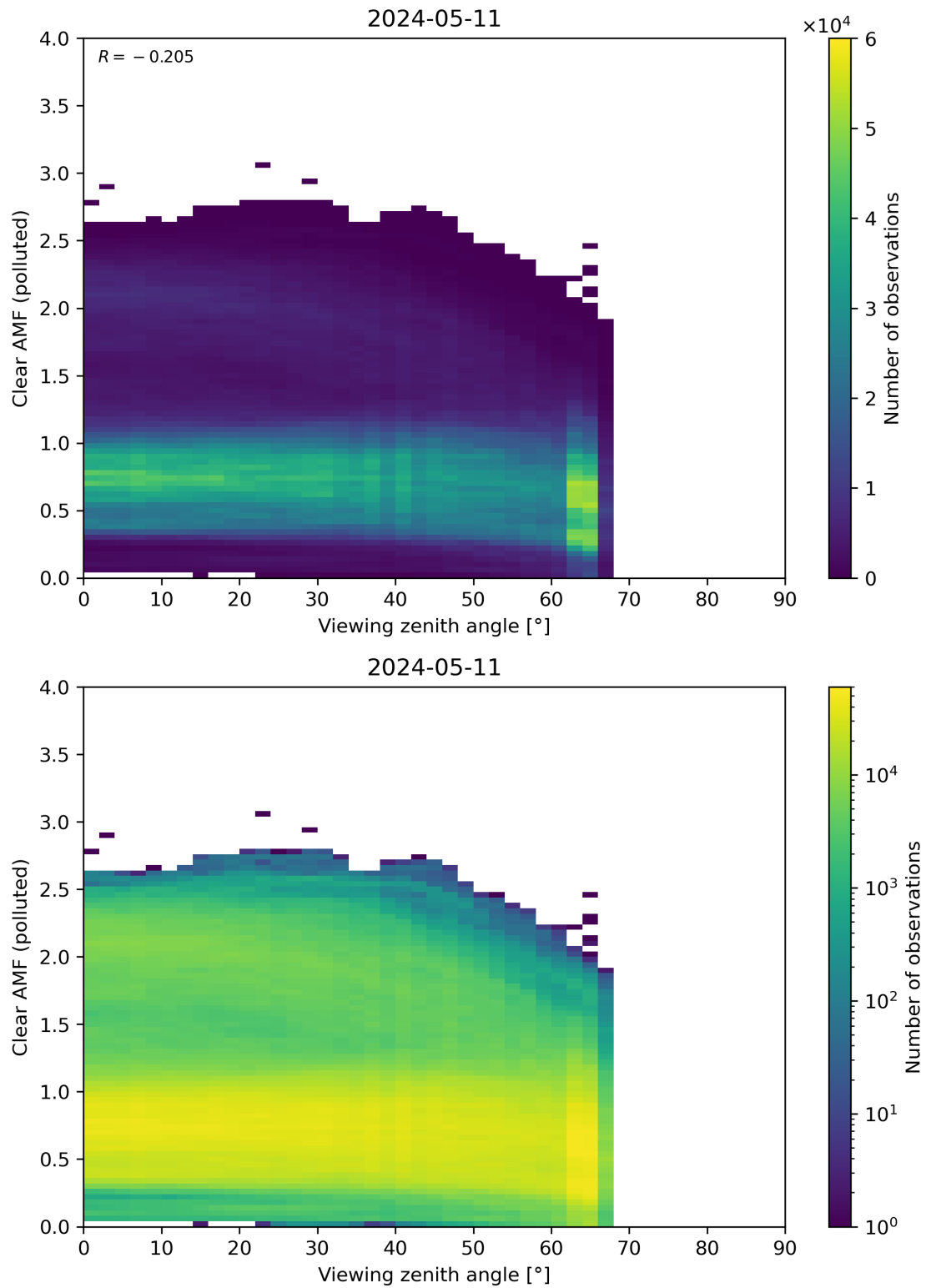
Figure 316: Scatter density plot of “Viewing zenith angle” against “Clear AMF (polluted)” for 2024-05-10 to 2024-05-12.
