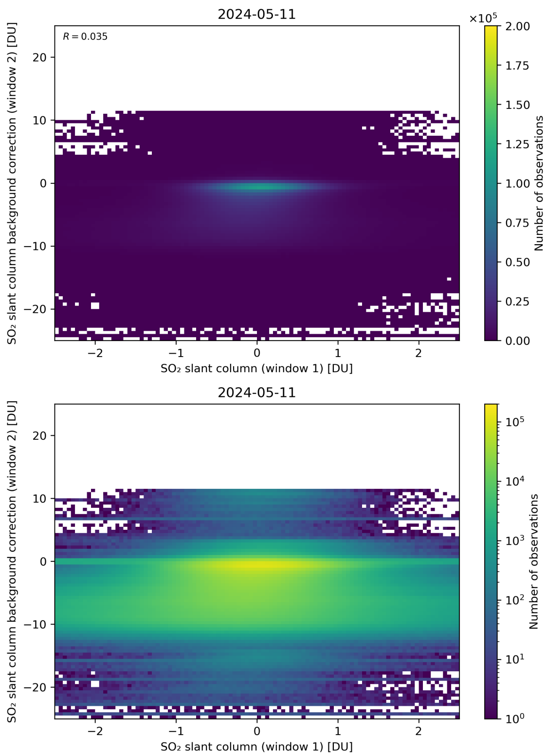
Figure 213: Scatter density plot of “SO 2 slant column (window 1)” against “SO 2 slant column background correction (window 2)” for 2024-05-10 to 2024-05-12.
