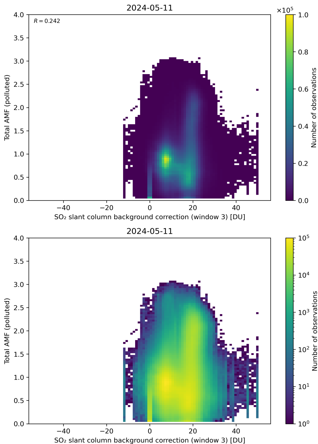
Figure 125: Scatter density plot of “SO 2 slant column background correction (window 3)” against “Total AMF (polluted)” for 2024-05-10 to 2024-05-12.
