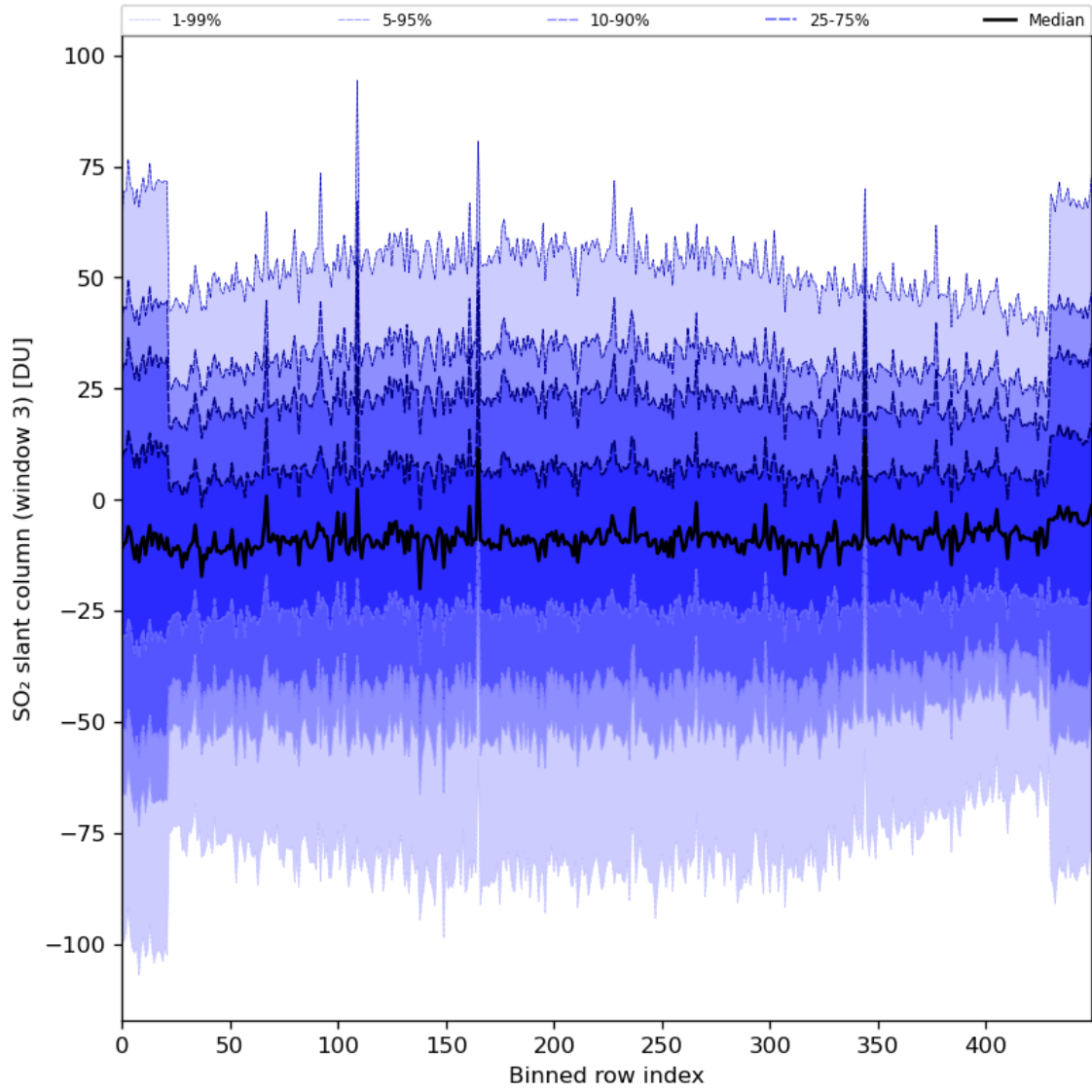
Figure 87: Along track statistics of “SO 2 slant column (window 3)” for 2024-05-10 to 2024-05-12
