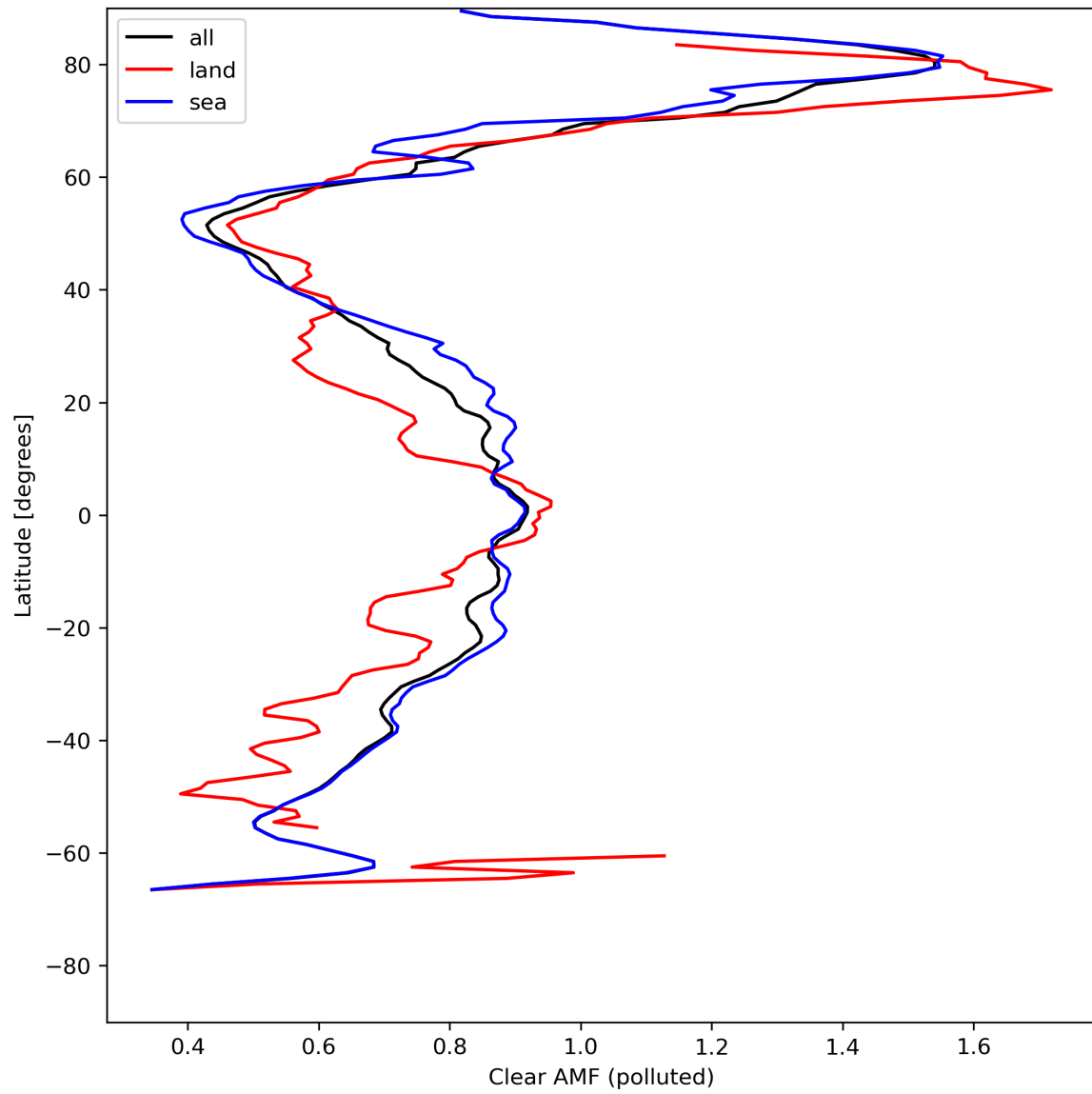
Figure 50: Zonal average of “Clear AMF (polluted)” for 2024-05-10 to 2024-05-12.
