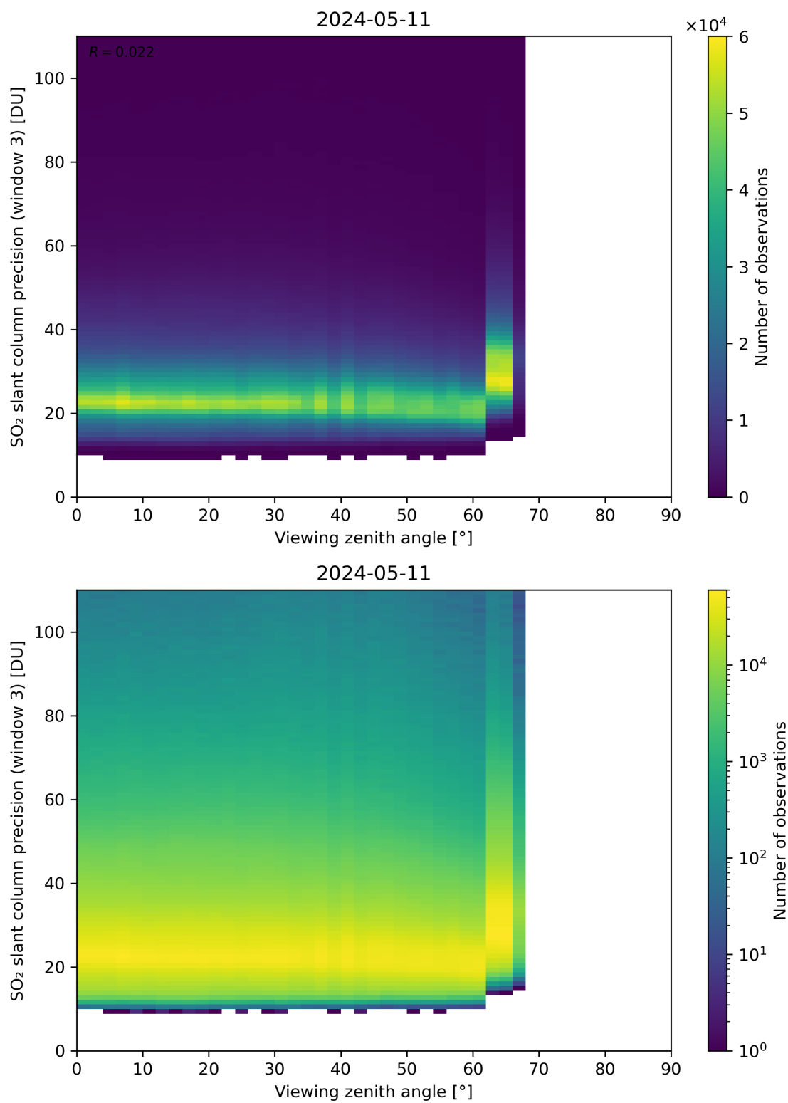
Figure 324: Scatter density plot of “Viewing zenith angle” against “SO 2 slant column precision (window 3)” for 2024-05-10 to 2024-05-12.
