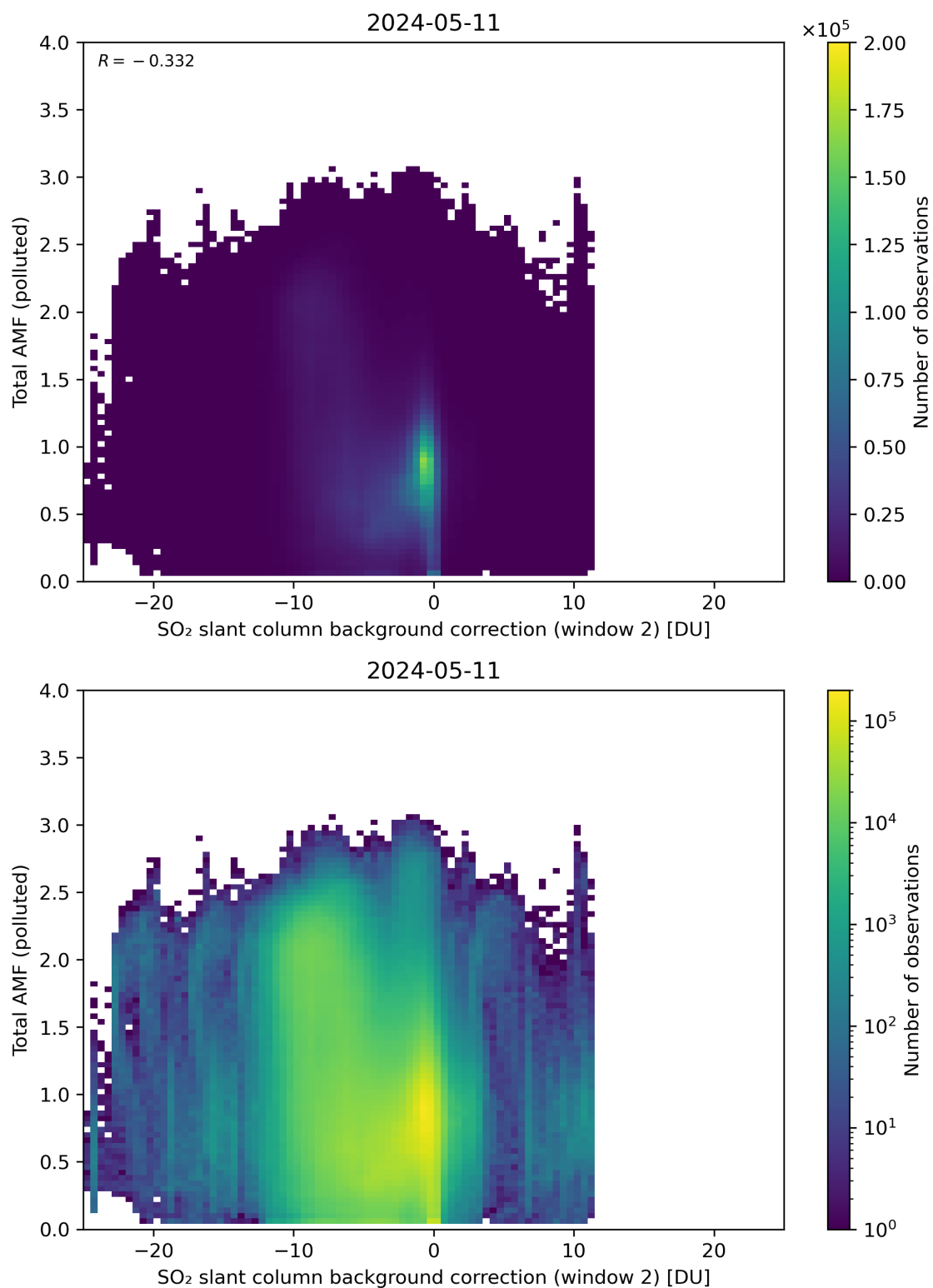
Figure 119: Scatter density plot of “SO 2 slant column background correction (window 2)” against “Total AMF (polluted)” for 2024-05-10 to 2024-05-12.
