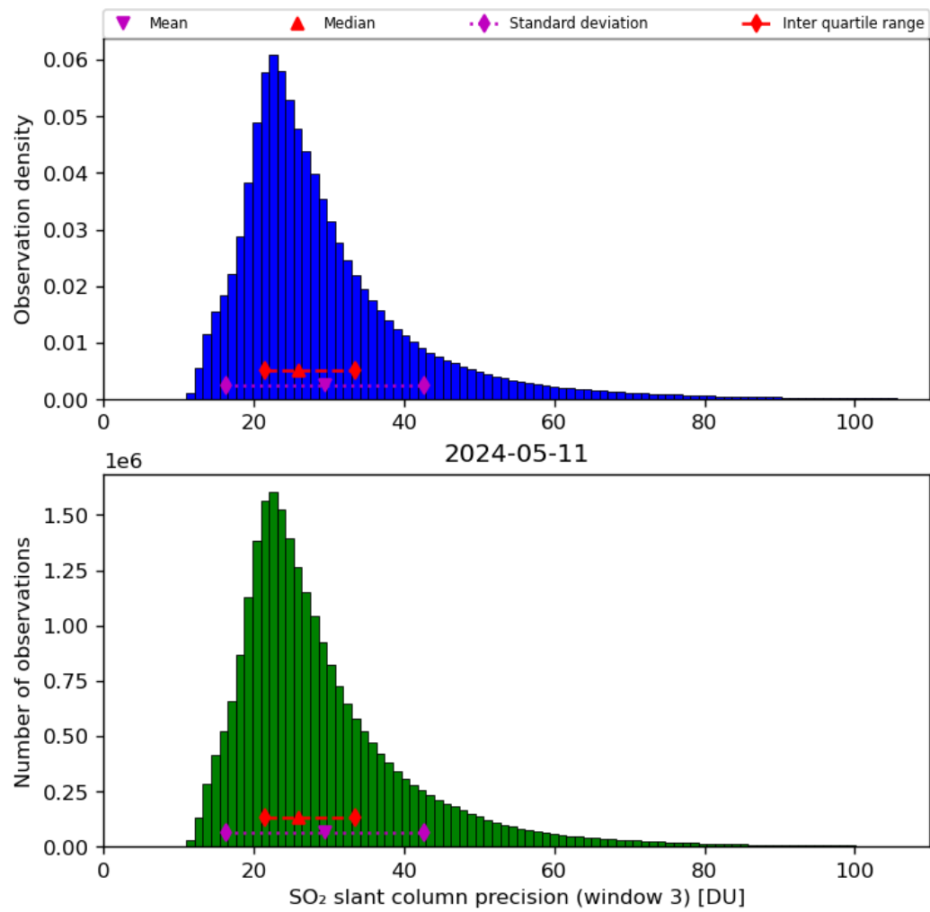
Figure 65: Histogram of “SO 2 slant column precision (window 3)” for 2024-05-10 to 2024-05-12
