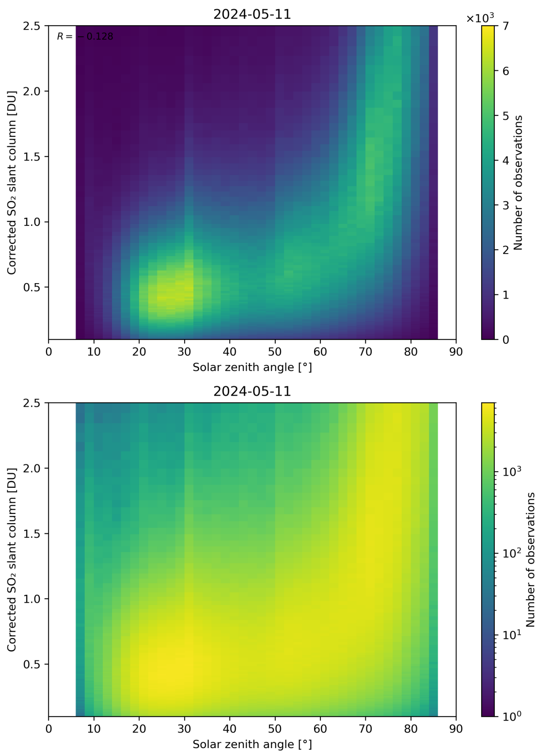
Figure 166: Scatter density plot of “Solar zenith angle” against “Corrected SO 2 slant column” for 2024-05-10 to 2024-05-12.
