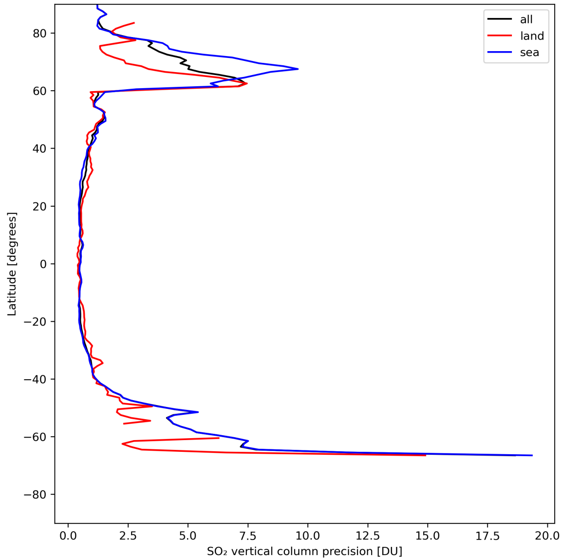
Figure 31: Zonal average of “SO 2 vertical column precision” for 2024-05-10 to 2024-05-12.
