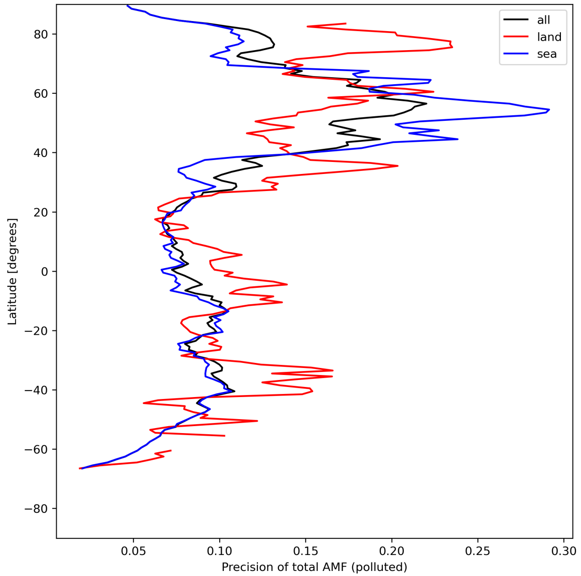
Figure 49: Zonal average of “Precision of total AMF (polluted)” for 2024-05-10 to 2024-05-12.
