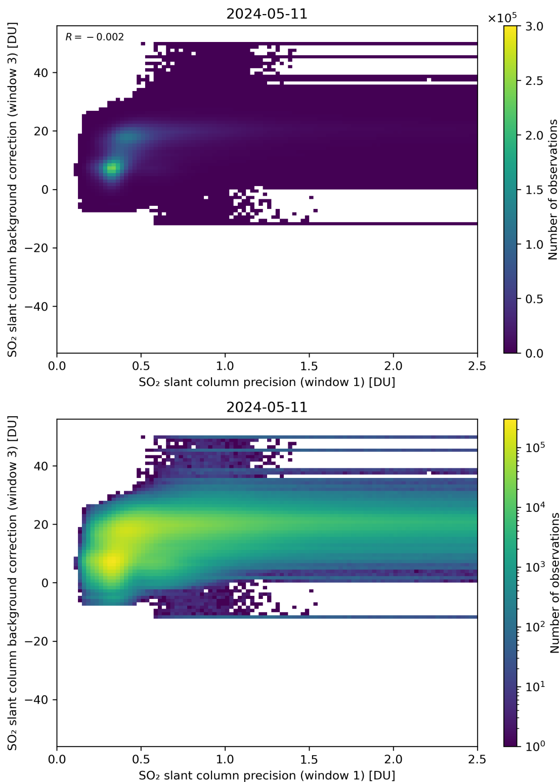
Figure 220: Scatter density plot of “SO 2 slant column precision (window 1)” against “SO 2 slant column background correction (window 3)” for 2024-05-10 to 2024-05-12.
