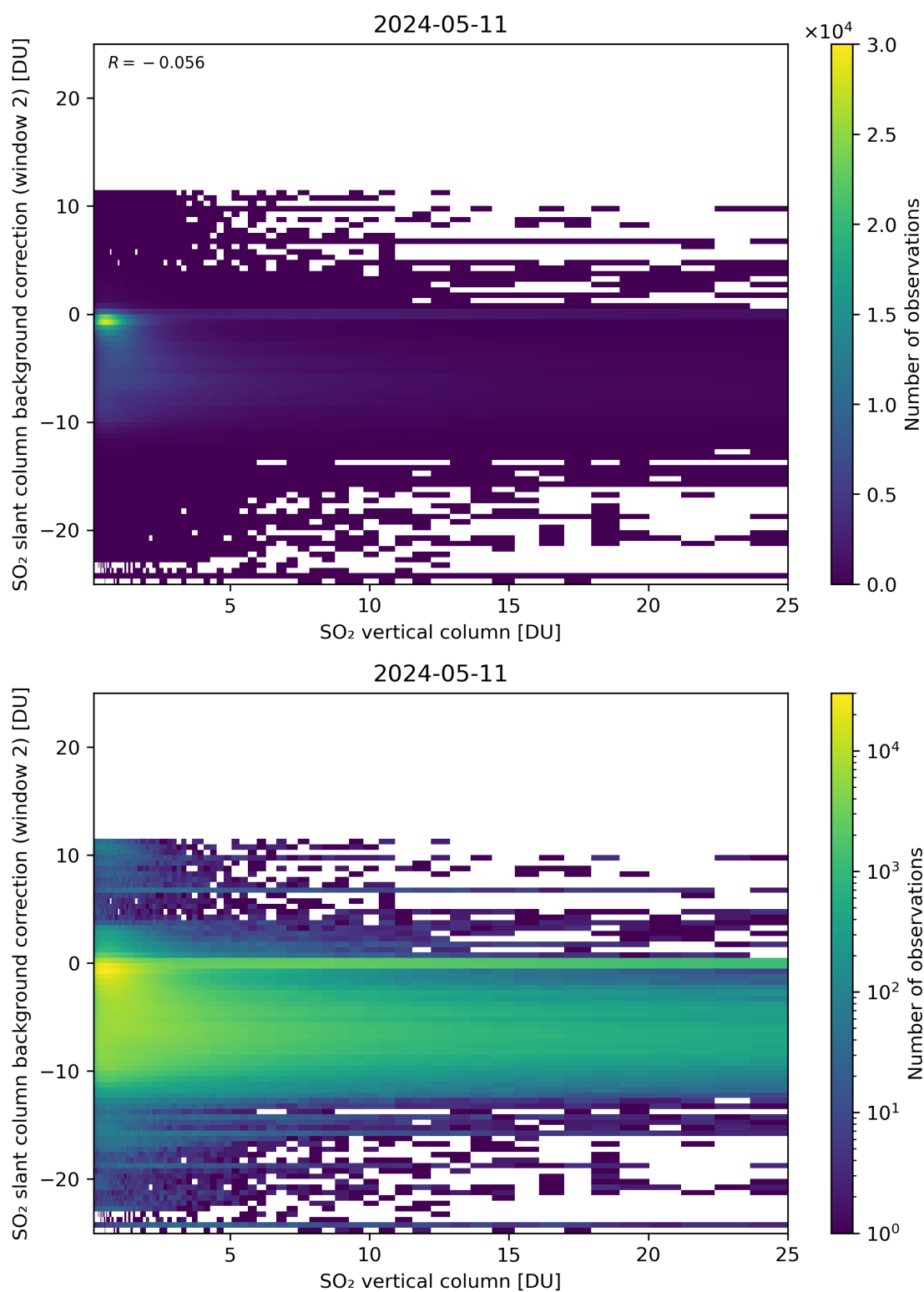
Figure 274: Scatter density plot of “SO 2 vertical column” against “SO 2 slant column background correction (window 2)” for 2024-05-10 to 2024-05-12.
