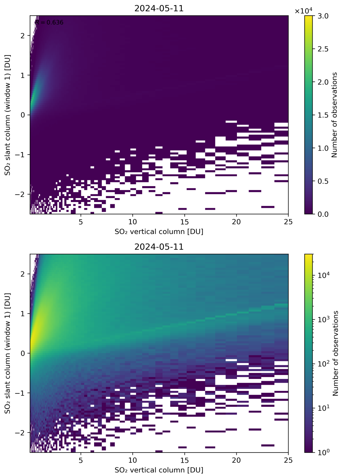
Figure 300: Scatter density plot of “SO 2 vertical column” against “SO 2 slant column (window 1)” for 2024-05-10 to 2024-05-12.
