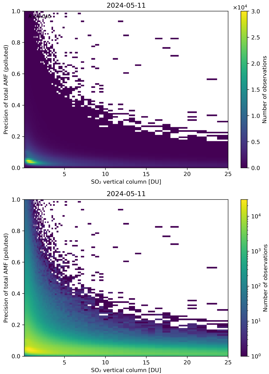
Figure 306: Scatter density plot of “SO 2 vertical column” against “Precision of total AMF (polluted)” for 2024-05-10 to 2024-05-12.
