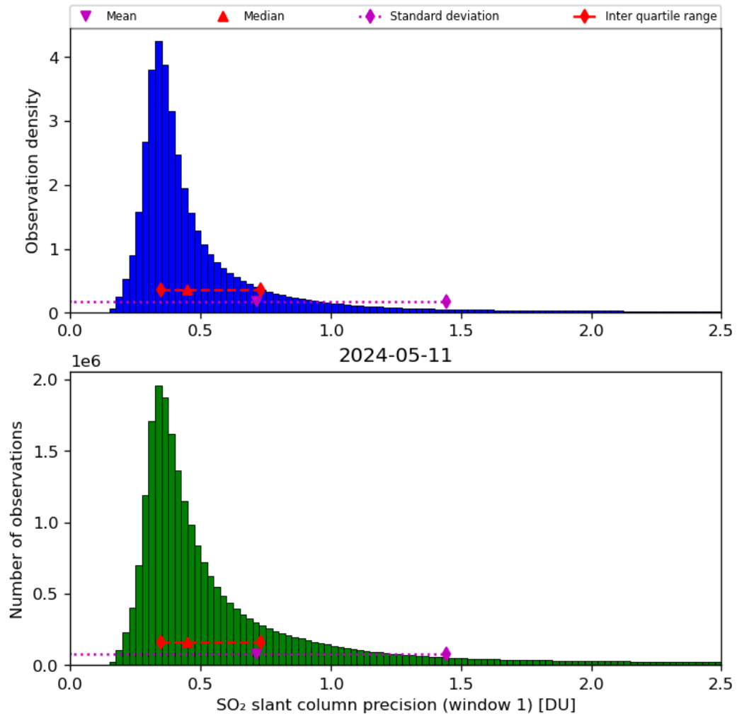
Figure 57: Histogram of “SO 2 slant column precision (window 1)” for 2024-05-10 to 2024-05-12
