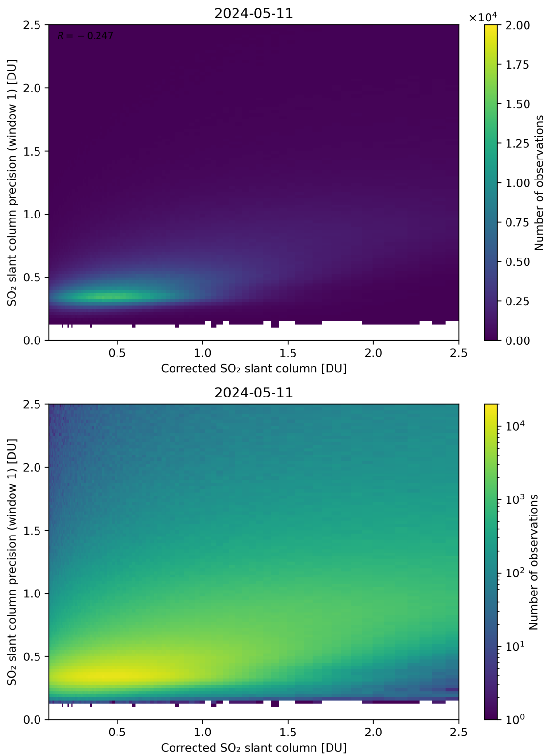
Figure 188: Scatter density plot of “Corrected SO 2 slant column” against “SO 2 slant column precision (window 1)” for 2024-05-10 to 2024-05-12.
