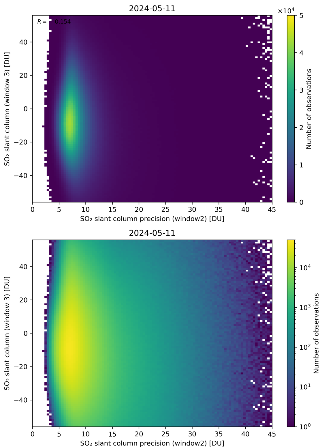
Figure 249: Scatter density plot of “SO 2 slant column precision (window2)” against “SO 2 slant column (window 3)” for 2024-05-10 to 2024-05-12.
