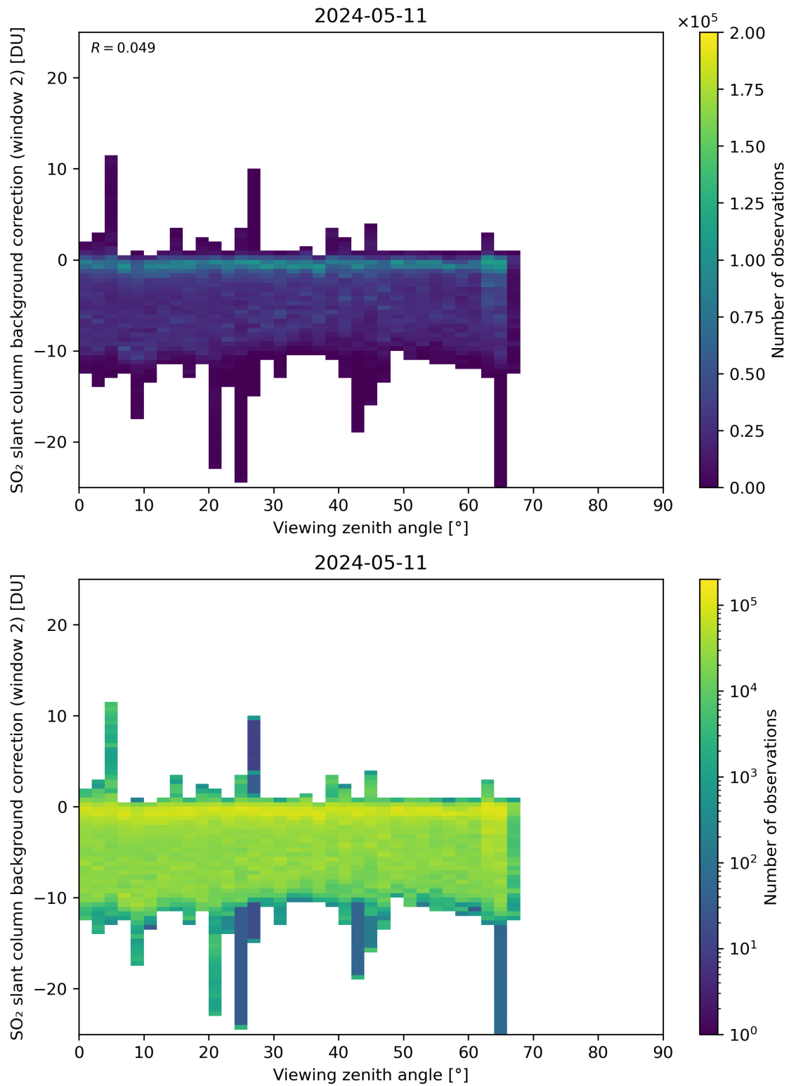
Figure 309: Scatter density plot of “Viewing zenith angle” against “SO 2 slant column background correction (window 2)” for 2024-05-10 to 2024-05-12.
