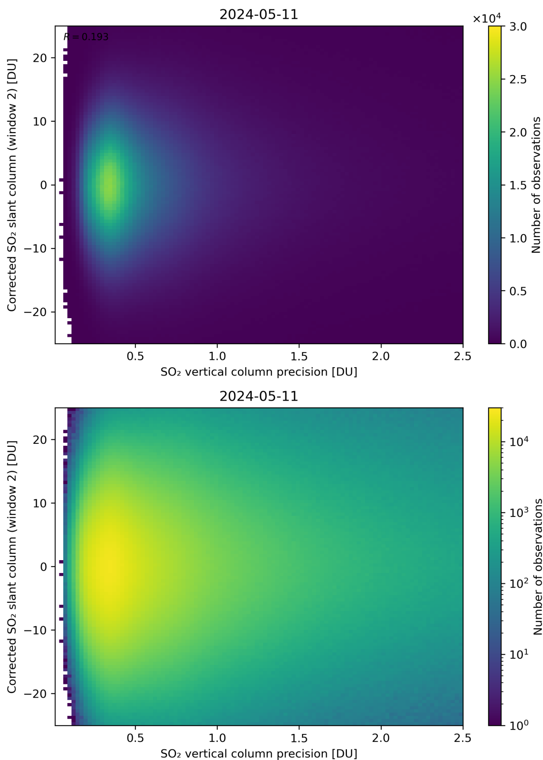
Figure 287: Scatter density plot of “SO 2 vertical column precision” against “Corrected SO 2 slant column (window 2)” for 2024-05-10 to 2024-05-12.
