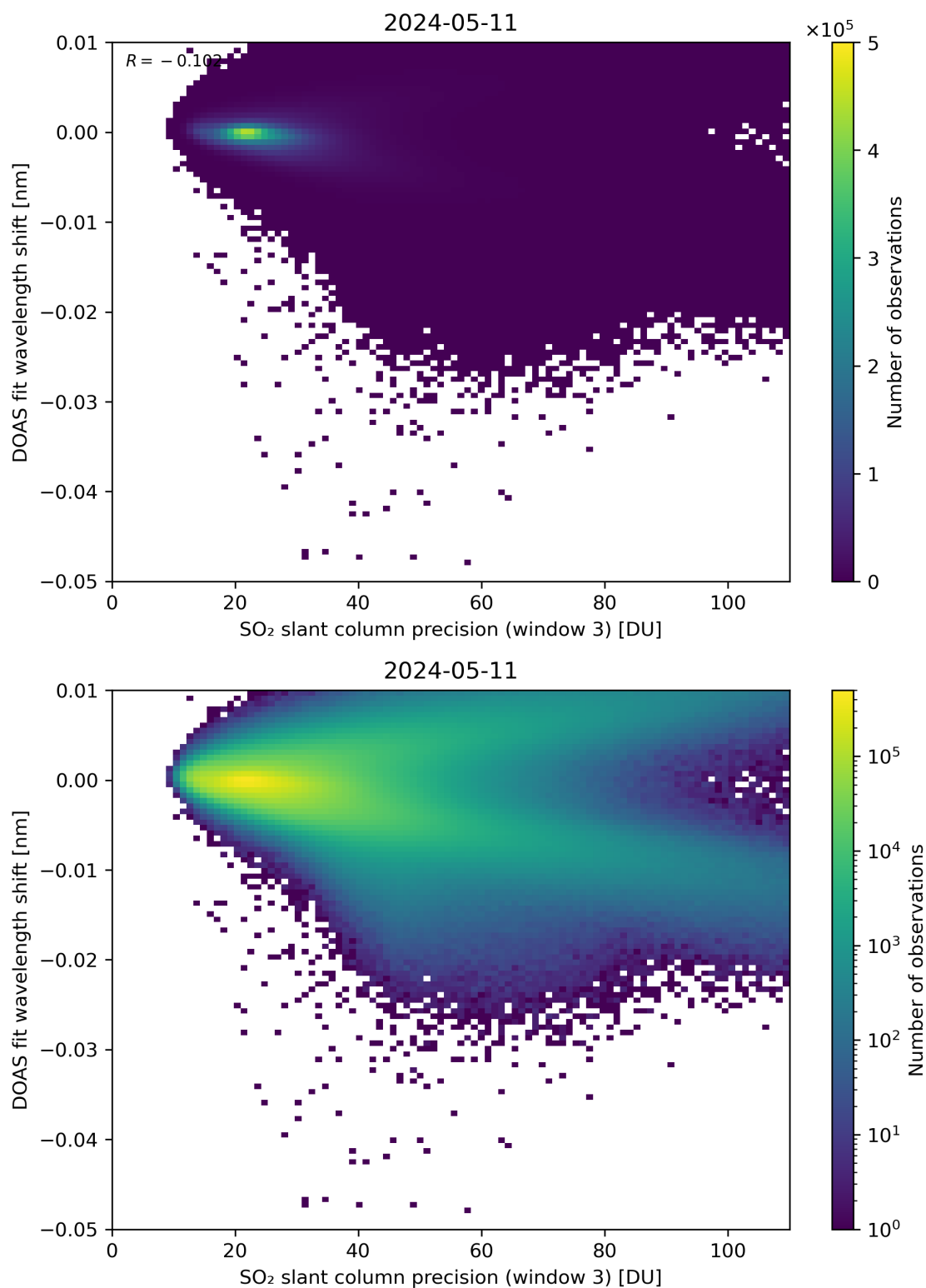
Figure 258: Scatter density plot of “SO 2 slant column precision (window 3)” against “DOAS fit wavelength shift” for 2024-05-10 to 2024-05-12.
