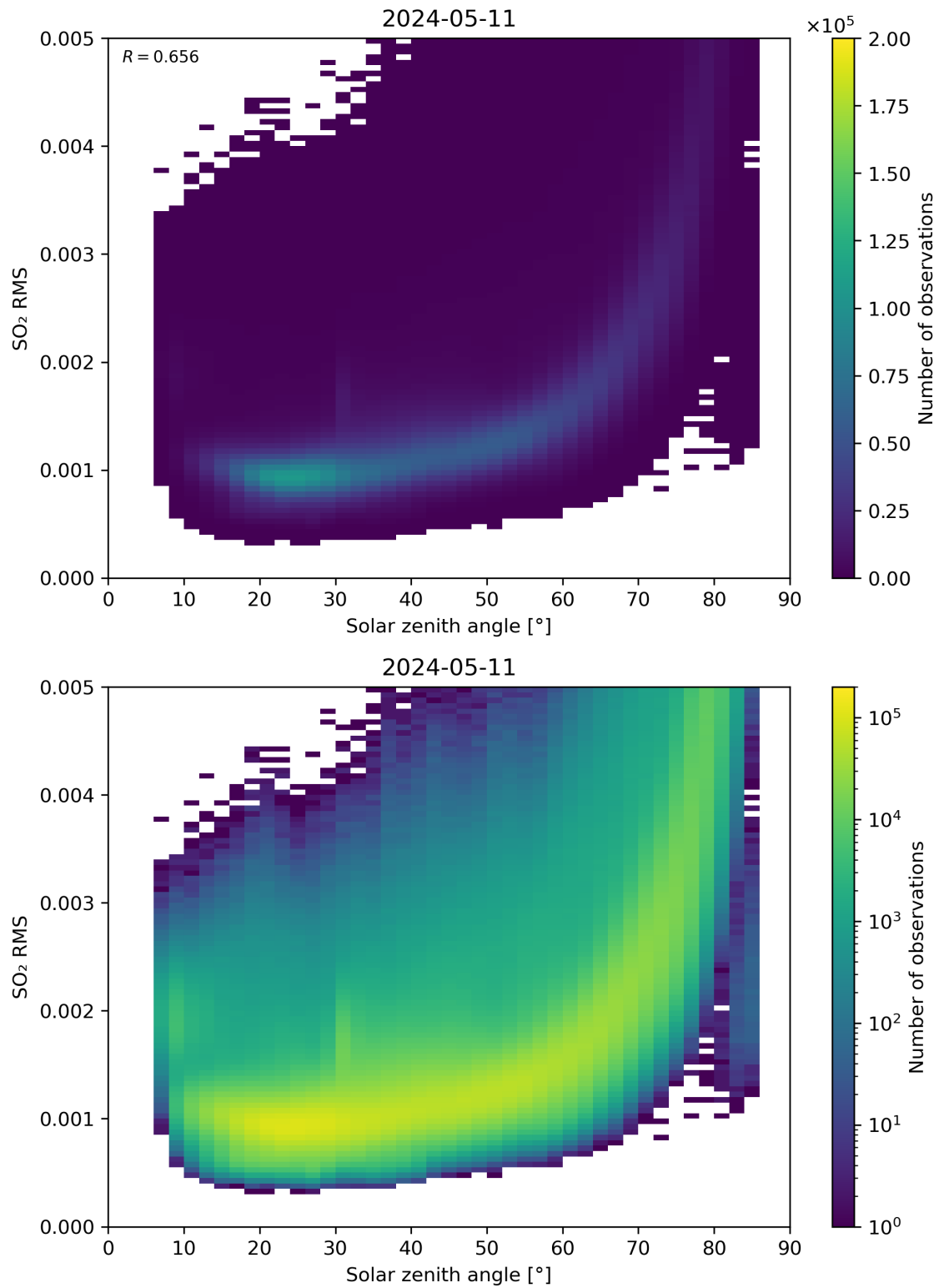
Figure 163: Scatter density plot of “Solar zenith angle” against “SO 2 RMS” for 2024-05-10 to 2024-05-12.
