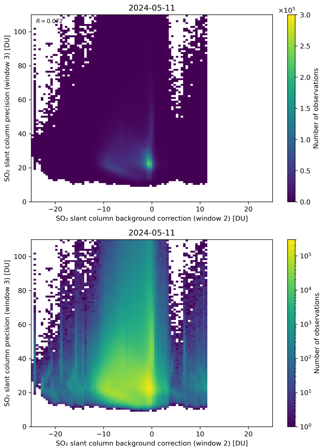
Figure 118: Scatter density plot of “SO 2 slant column background correction (window 2)” against “SO 2 slant column precision (window 3)” for 2024-05-10 to 2024-05-12.
