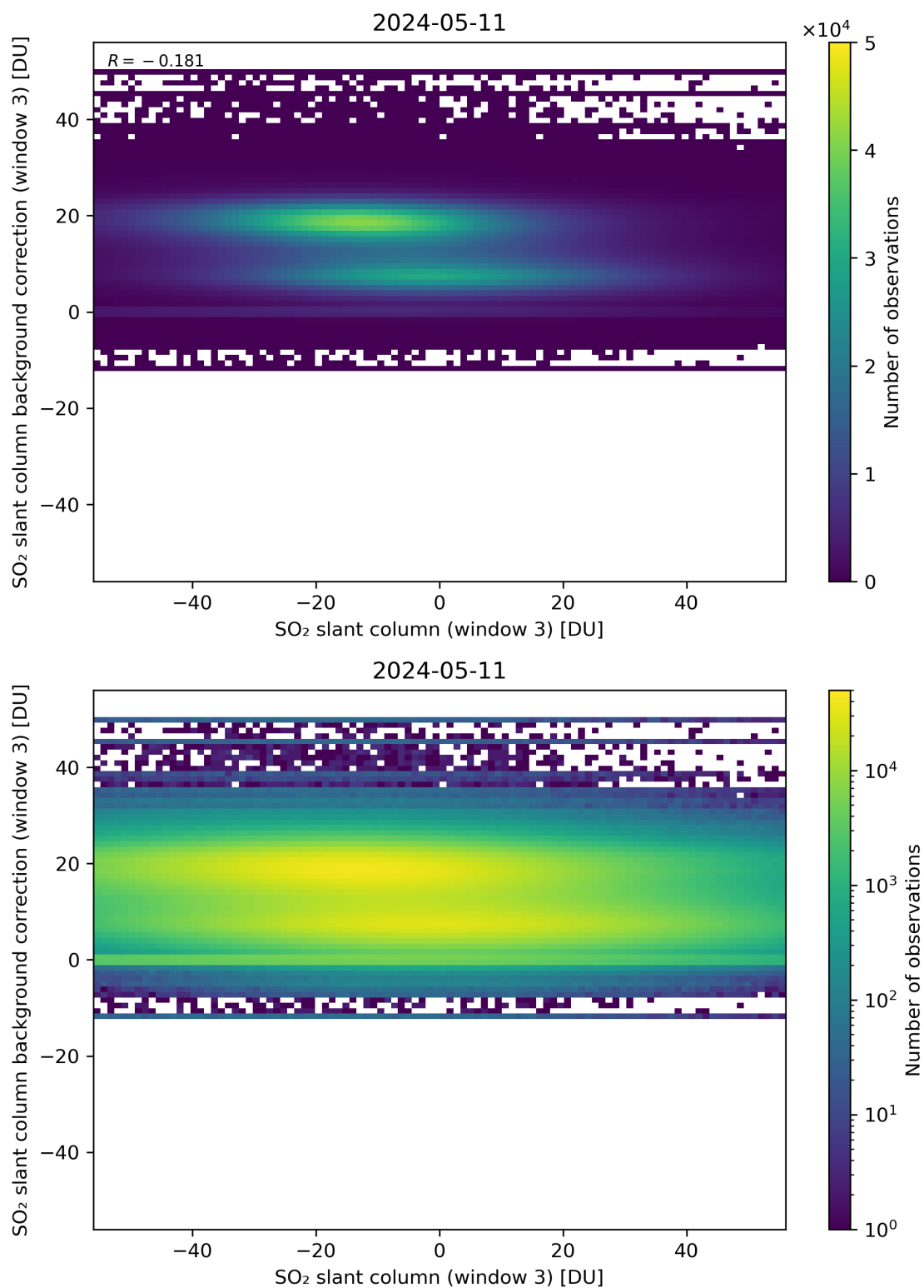
Figure 253: Scatter density plot of “SO 2 slant column (window 3)” against “SO 2 slant column background correction (window 3)” for 2024-05-10 to 2024-05-12.
