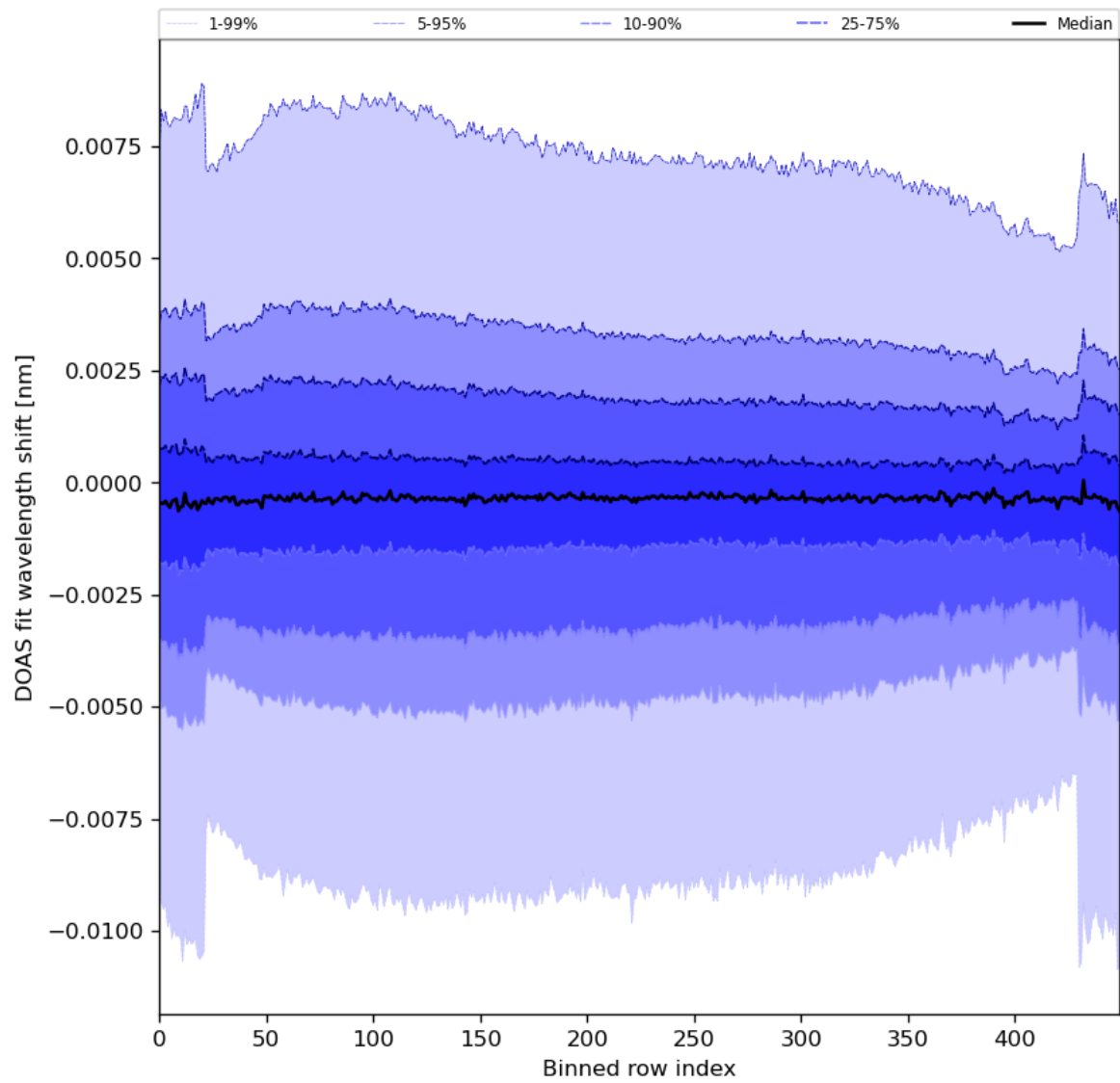
Figure 91: Along track statistics of “DOAS fit wavelength shift” for 2024-05-10 to 2024-05-12
