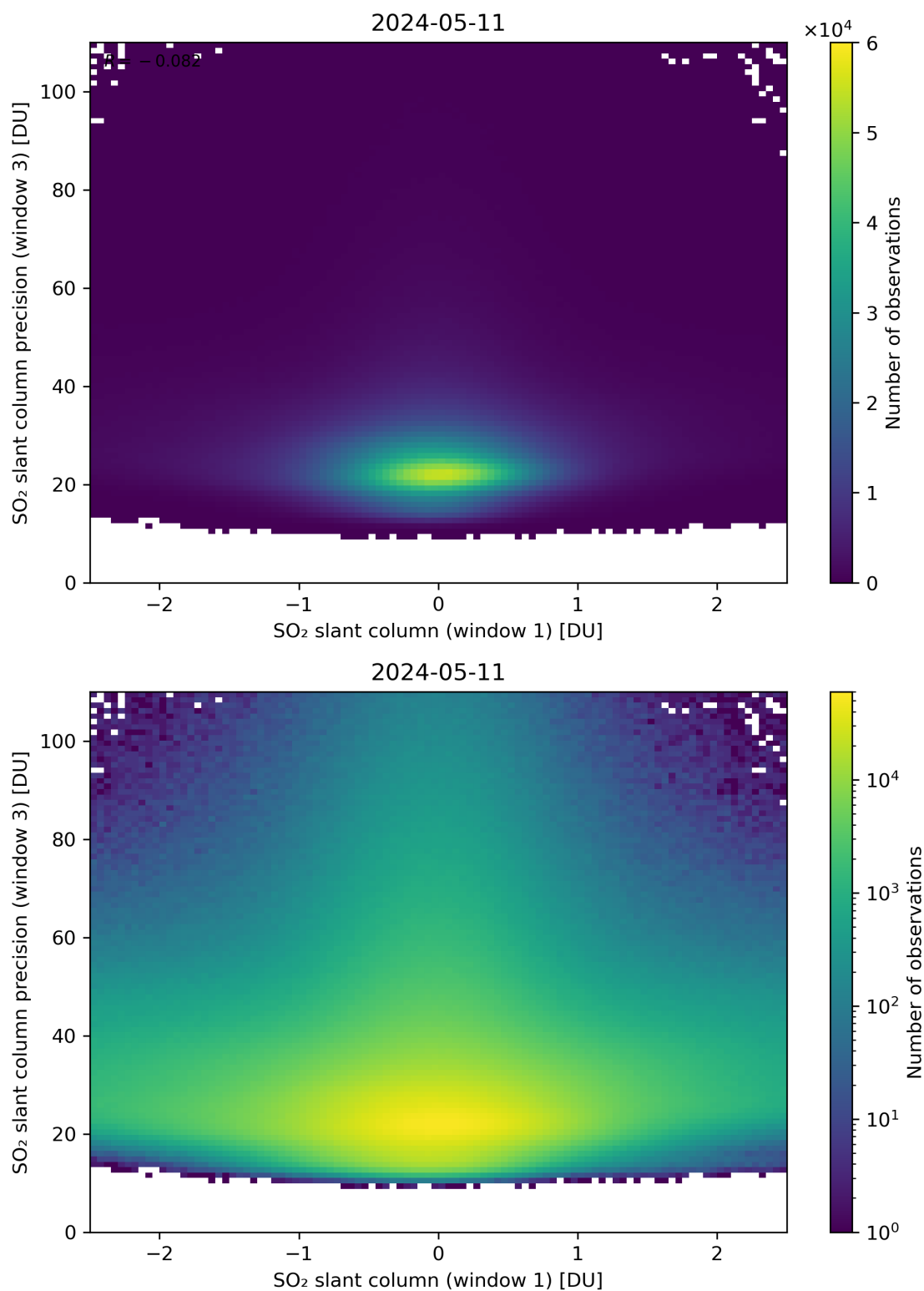
Figure 238: Scatter density plot of “SO 2 slant column (window 1)” against “SO 2 slant column precision (window 3)” for 2024-05-10 to 2024-05-12.
