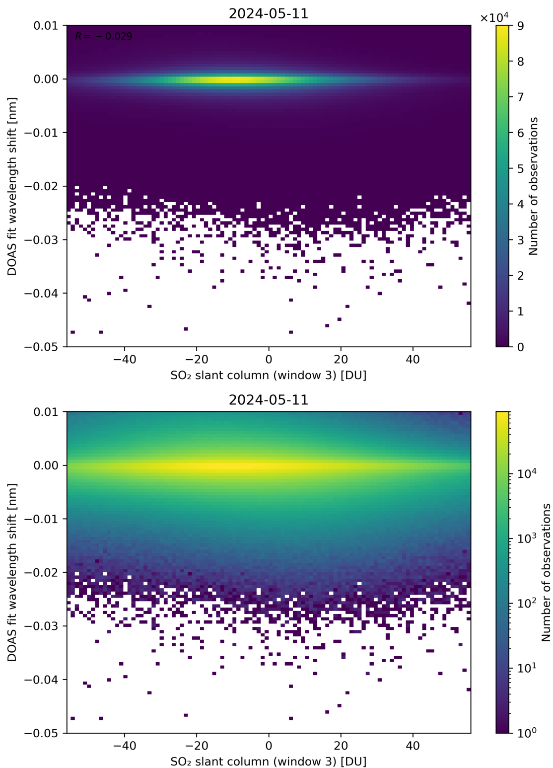
Figure 254: Scatter density plot of “SO 2 slant column (window 3)” against “DOAS fit wavelength shift” for 2024-05-10 to 2024-05-12.
