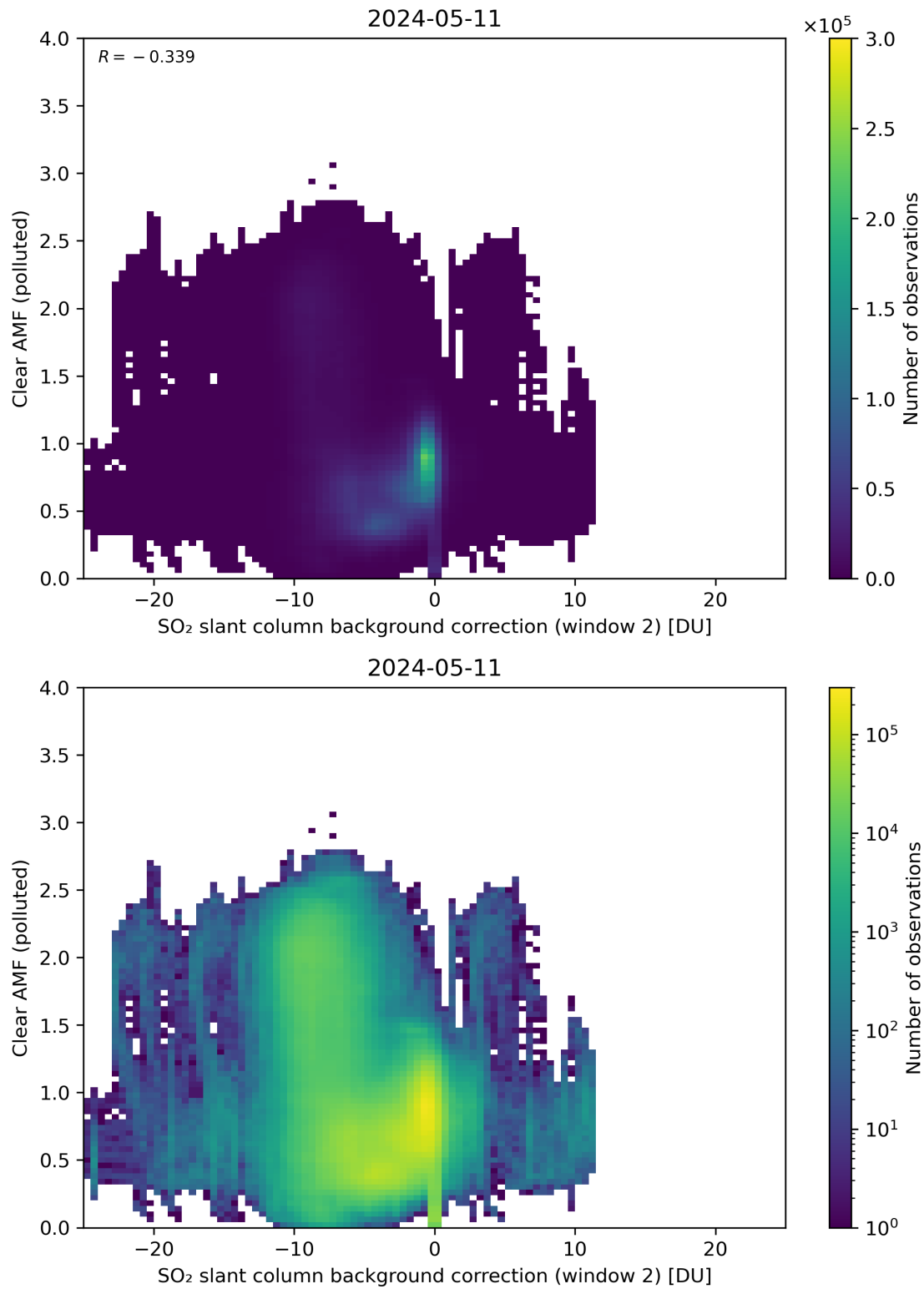
Figure 115: Scatter density plot of “SO 2 slant column background correction (window 2)” against “Clear AMF (polluted)” for 2024-05-10 to 2024-05-12.
