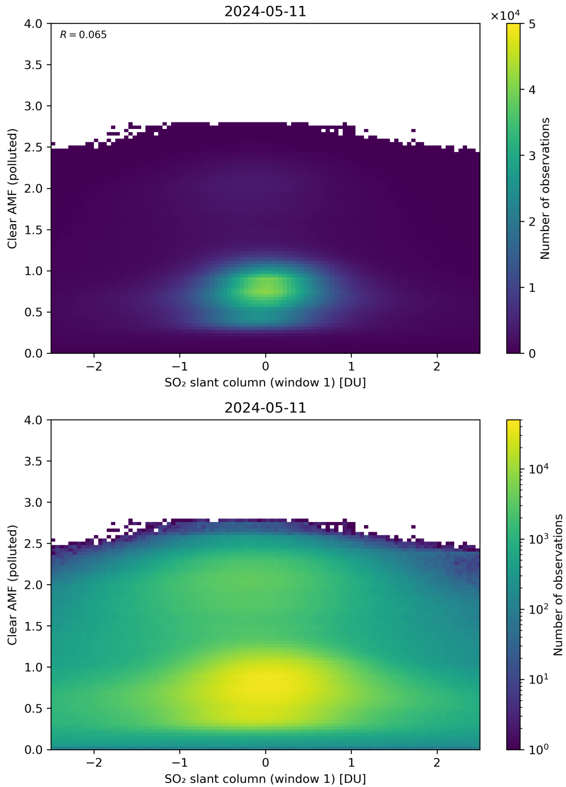
Figure 232: Scatter density plot of “SO 2 slant column (window 1)” against “Clear AMF (polluted)” for 2024-05-10 to 2024-05-12.
