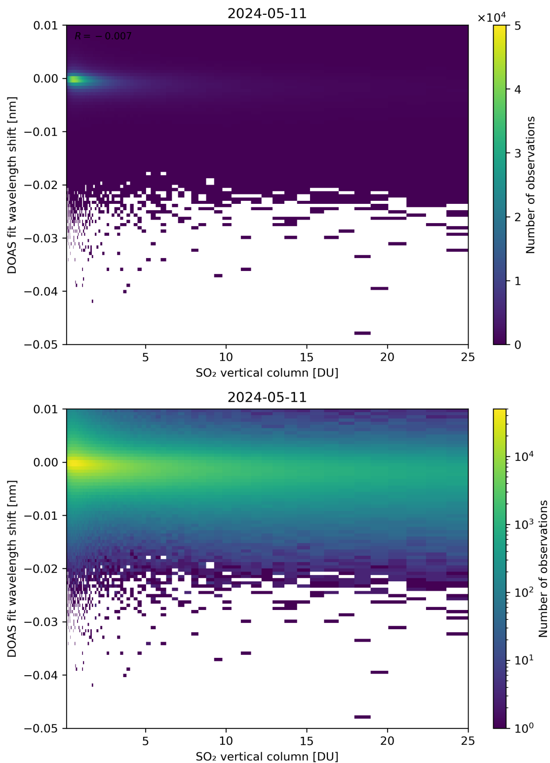
Figure 276: Scatter density plot of “SO 2 vertical column” against “DOAS fit wavelength shift” for 2024-05-10 to 2024-05-12.
