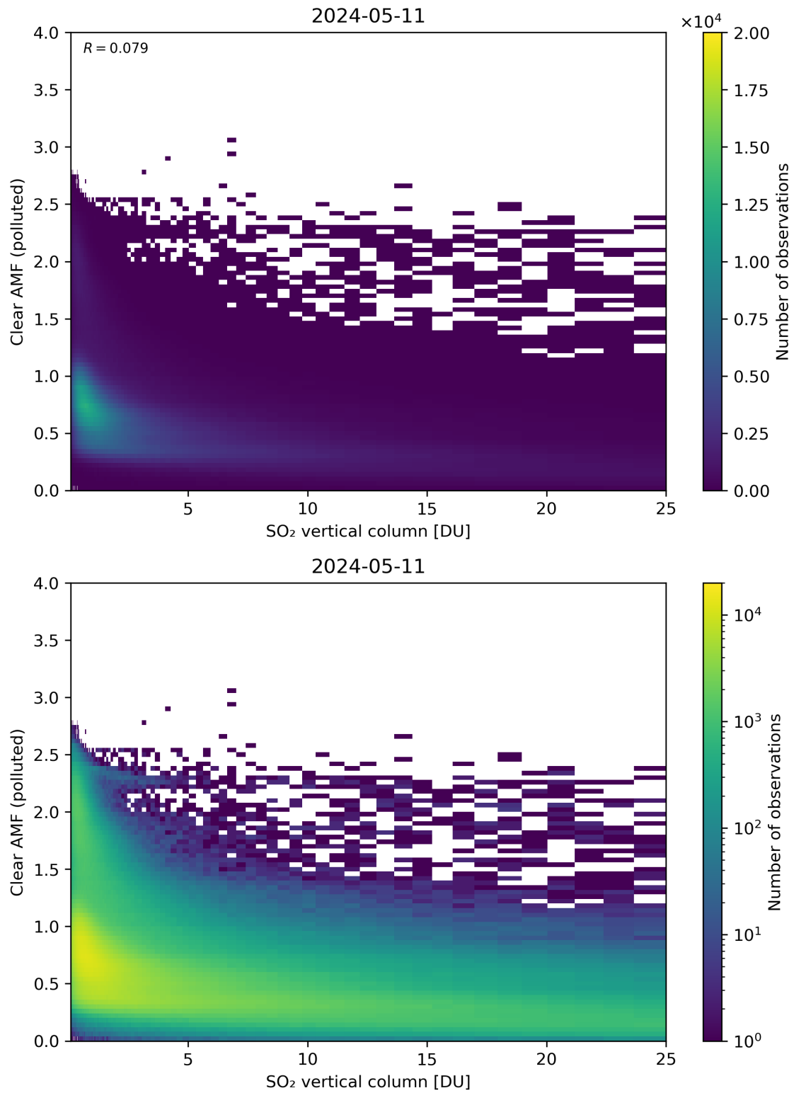
Figure 296: Scatter density plot of “SO 2 vertical column” against “Clear AMF (polluted)” for 2024-05-10 to 2024-05-12.
