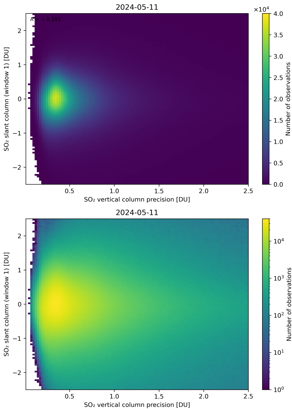
Figure 289: Scatter density plot of “SO 2 vertical column precision” against “SO 2 slant column (window 1)” for 2024-05-10 to 2024-05-12.
