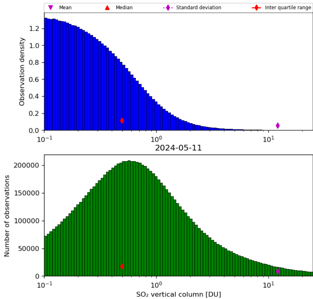
Figure 53: Histogram of “SO 2 vertical column” for 2024-05-10 to 2024-05-12
