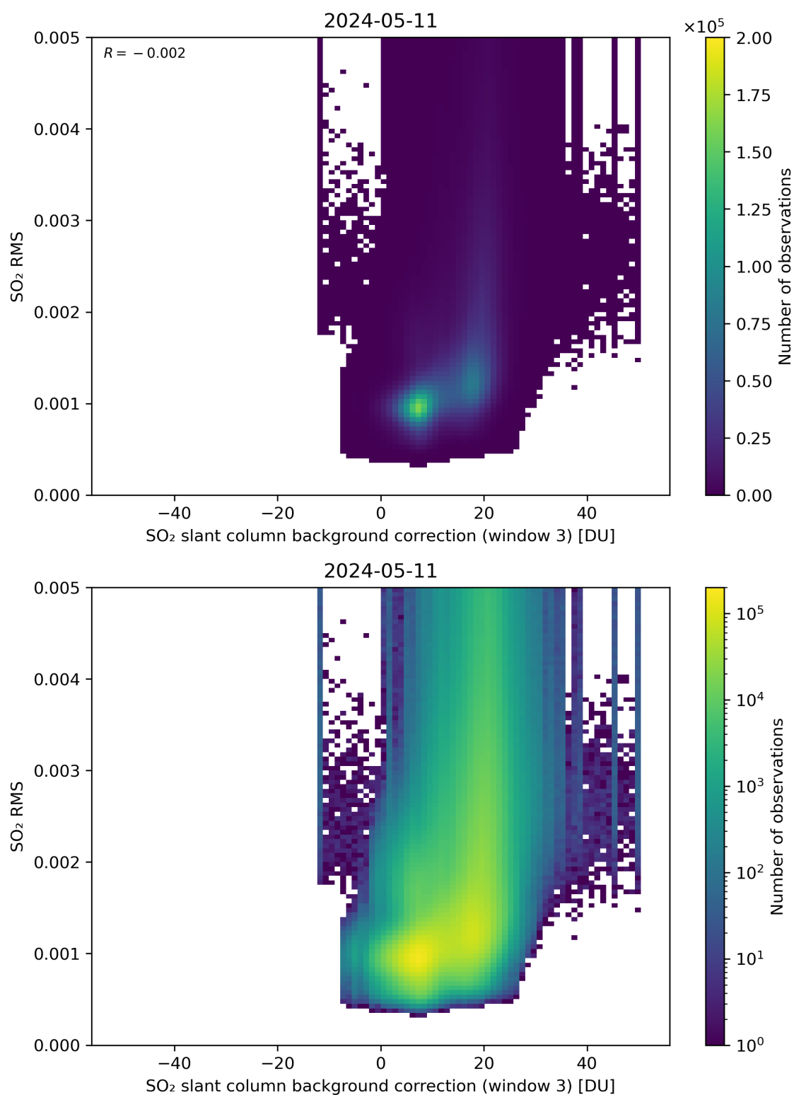
Figure 123: Scatter density plot of “SO 2 slant column background correction (window 3)” against “SO 2 RMS” for 2024-05-10 to 2024-05-12.
