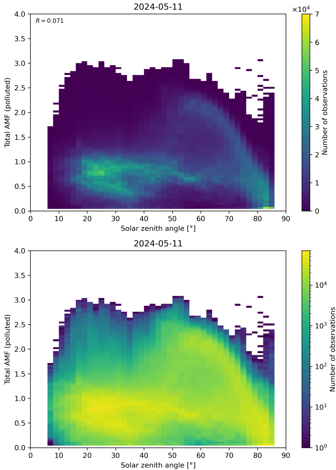
Figure 174: Scatter density plot of “Solar zenith angle” against “Total AMF (polluted)” for 2024-05-10 to 2024-05-12.
