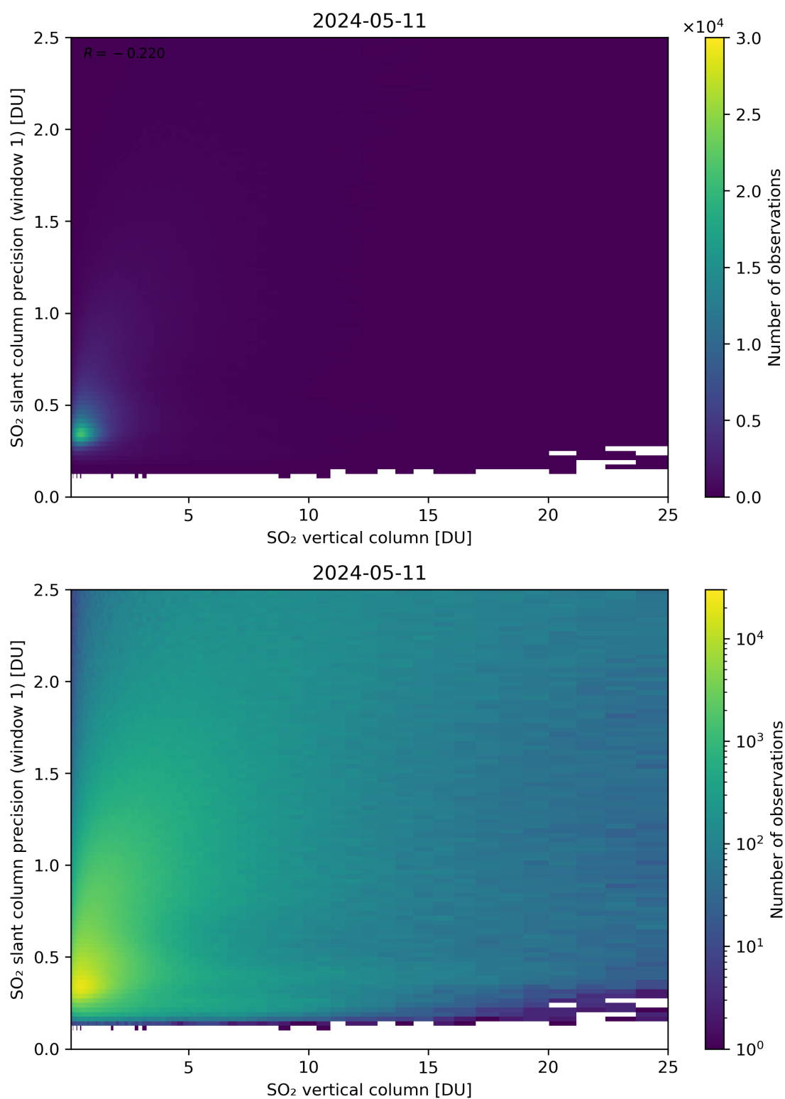
Figure 301: Scatter density plot of “SO 2 vertical column” against “SO 2 slant column precision (window 1)” for 2024-05-10 to 2024-05-12.
