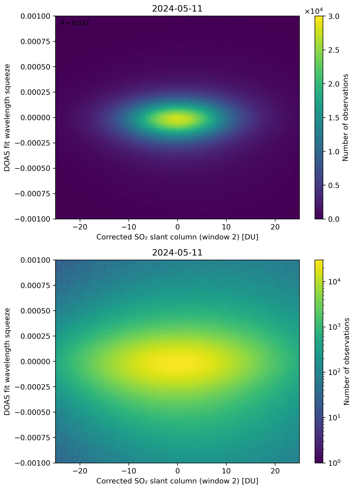
Figure 197: Scatter density plot of “Corrected SO 2 slant column (window 2)” against “DOAS fit wavelength squeeze” for 2024-05-10 to 2024-05-12.
