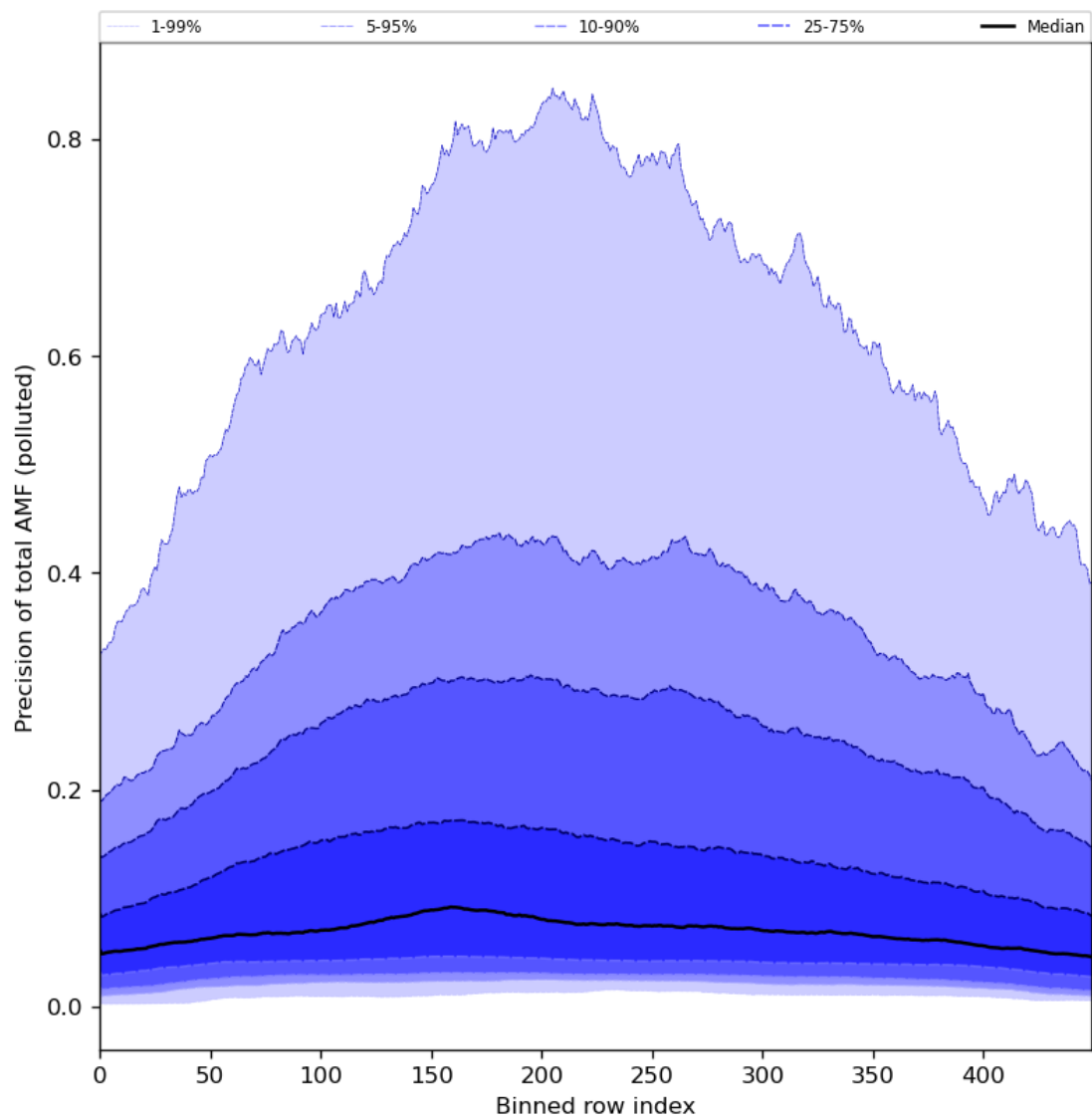
Figure 95: Along track statistics of “Precision of total AMF (polluted)” for 2024-05-10 to 2024-05-12
