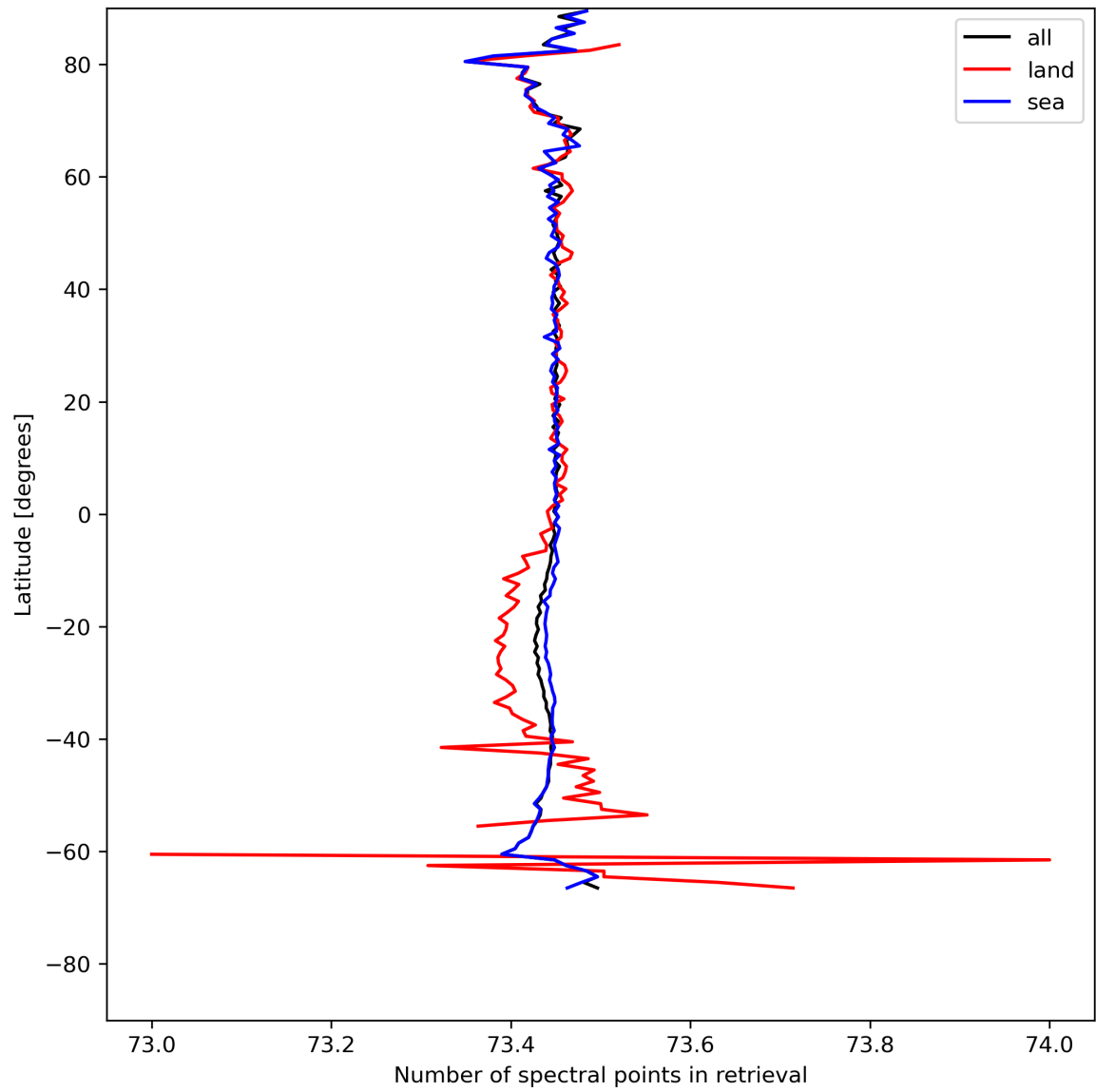
Figure 51: Zonal average of “Number of spectral points in retrieval” for 2024-05-10 to 2024-05-12.
