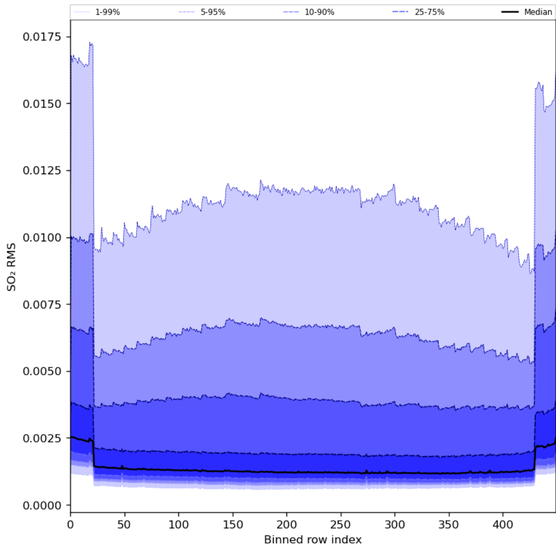
Figure 93: Along track statistics of "SO 2 RMS" for 2024-05-10 to 2024-05-12
