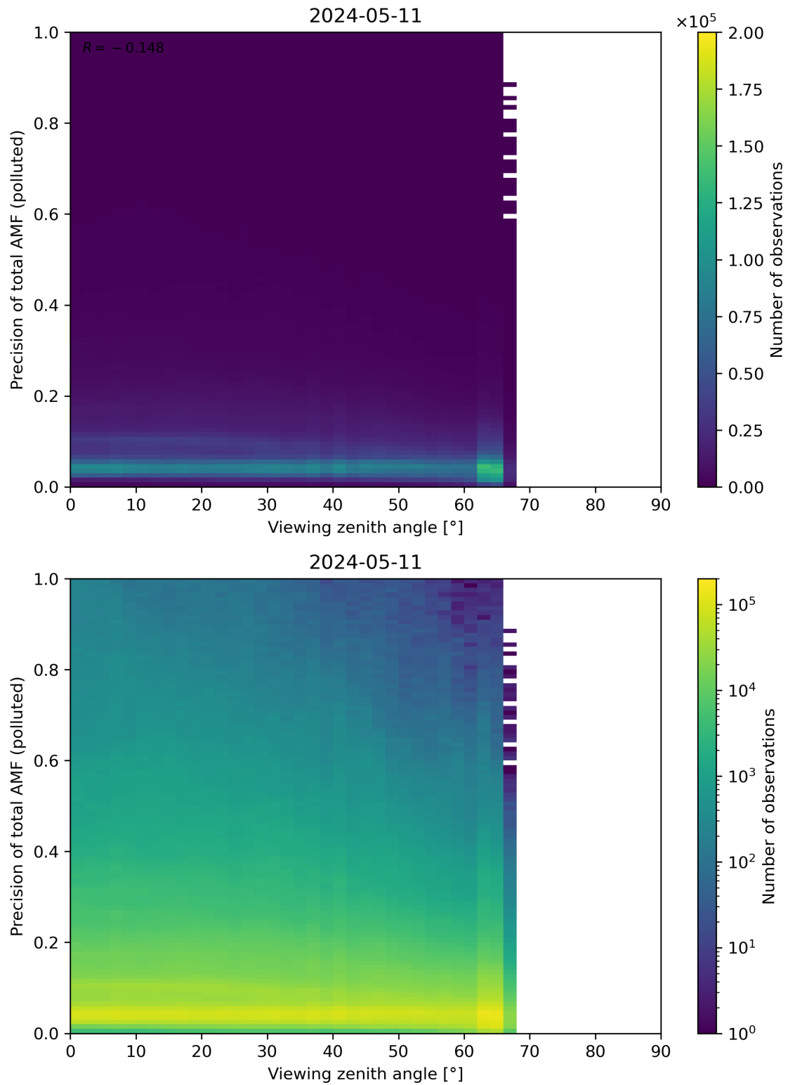
Figure 326: Scatter density plot of “Viewing zenith angle” against “Precision of total AMF (polluted)” for 2024-05-10 to 2024-05-12.
