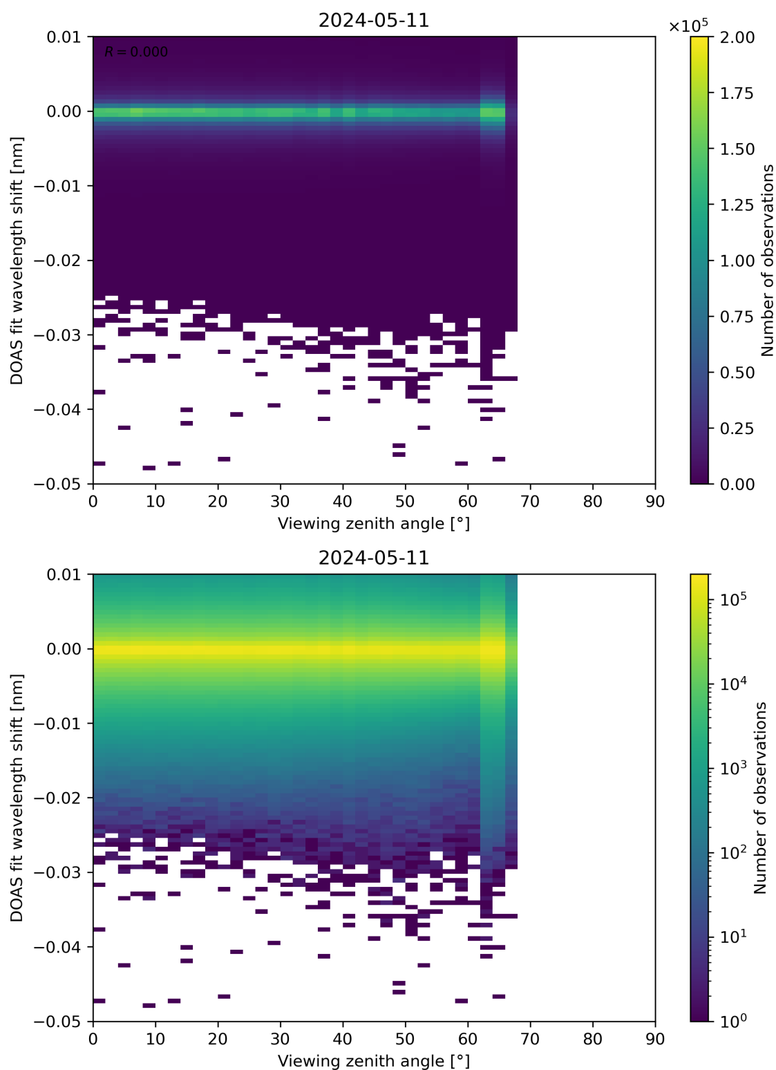
Figure 311: Scatter density plot of “Viewing zenith angle” against “DOAS fit wavelength shift” for 2024-05-10 to 2024-05-12.
