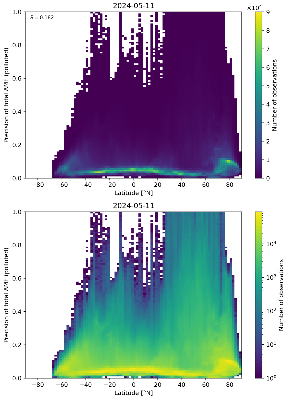
Figure 155: Scatter density plot of “Latitude” against “Precision of total AMF (polluted)” for 2024-05-10 to 2024-05-12.
