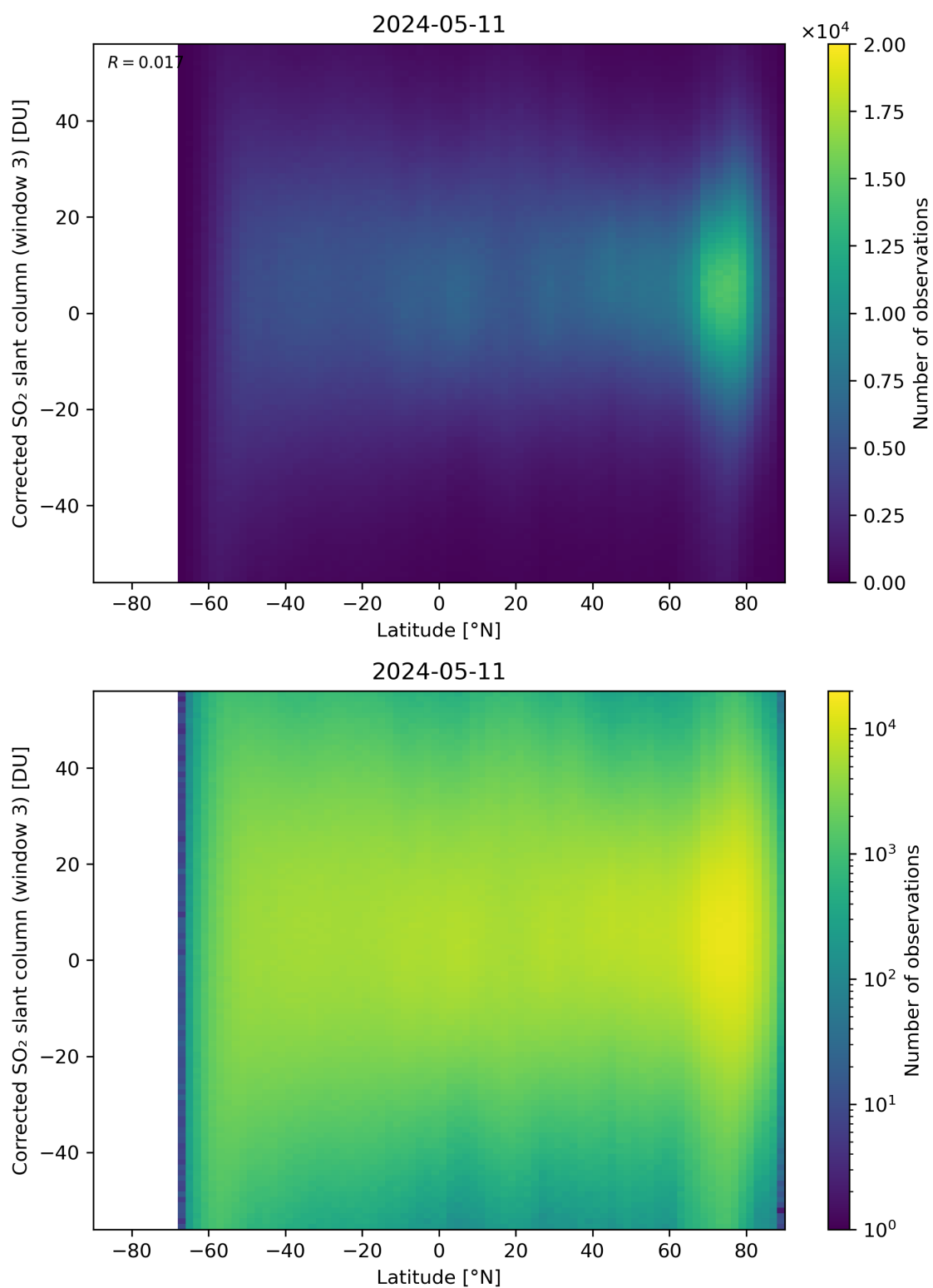
Figure 148: Scatter density plot of “Latitude” against “Corrected SO 2 slant column (window 3)” for 2024-05-10 to 2024-05-12.
