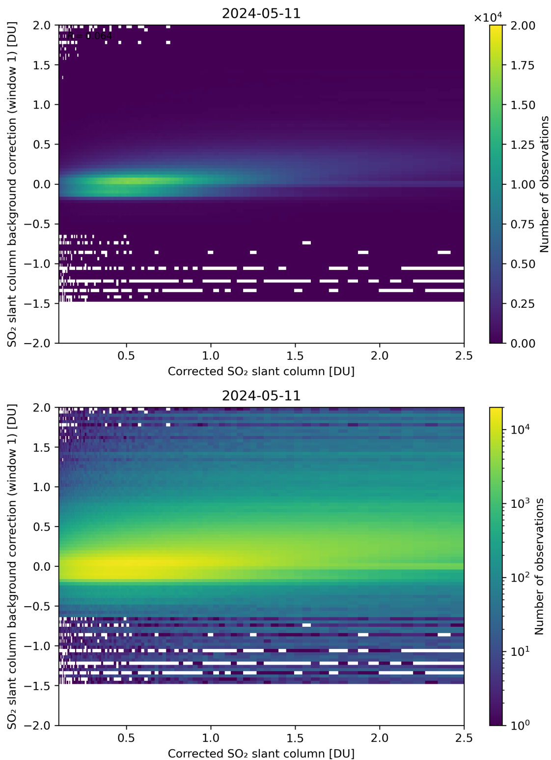
Figure 178: Scatter density plot of “Corrected SO 2 slant column” against “SO 2 slant column background correction (window 1)” for 2024-05-10 to 2024-05-12.
