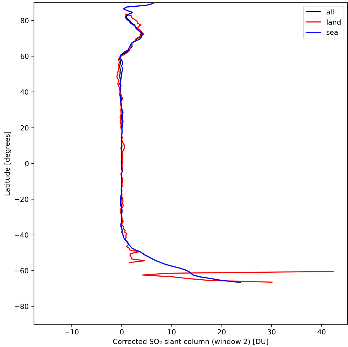
Figure 39: Zonal average of “Corrected SO 2 slant column (window 2)” for 2024-05-10 to 2024-05-12.
