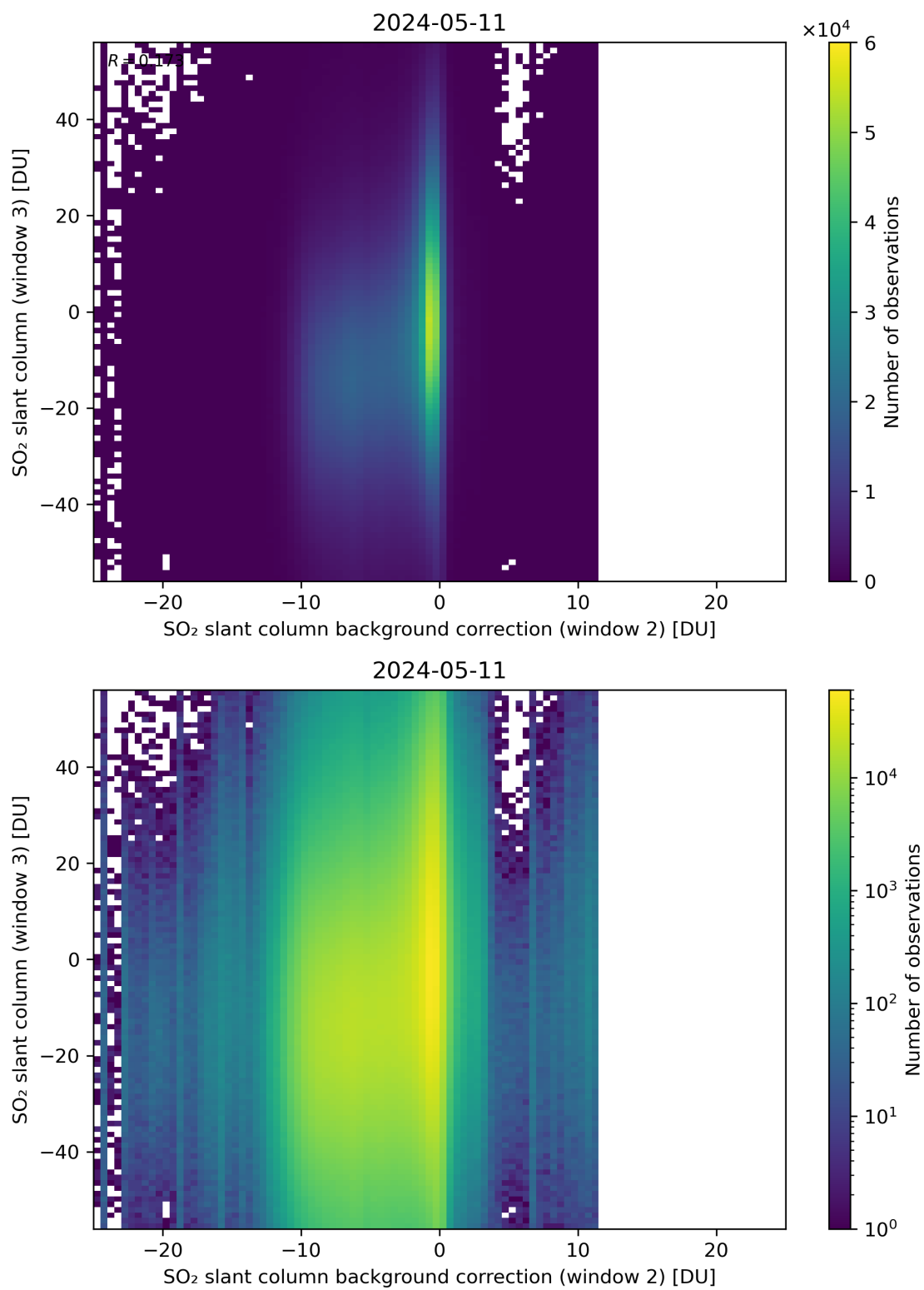
Figure 117: Scatter density plot of “SO 2 slant column background correction (window 2)” against “SO 2 slant column (window 3)” for 2024-05-10 to 2024-05-12.
