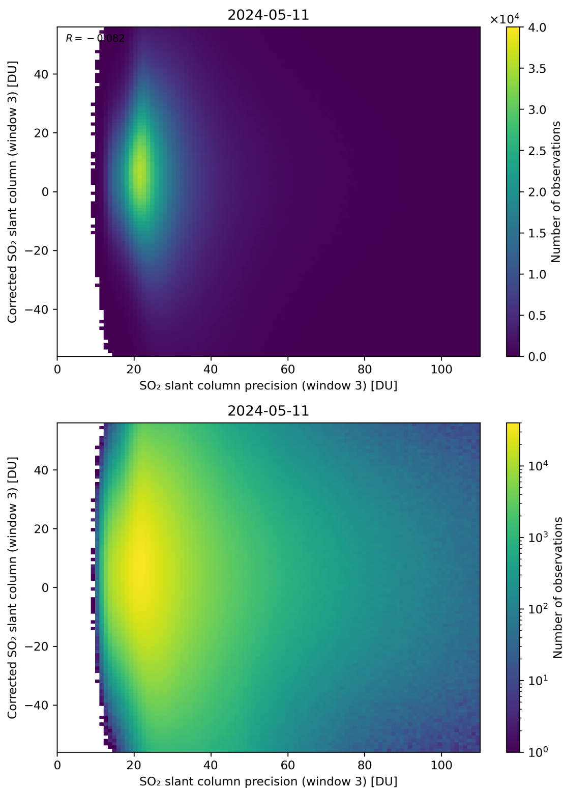
Figure 262: Scatter density plot of “SO 2 slant column precision (window 3)” against “Corrected SO 2 slant column (window 3)” for 2024-05-10 to 2024-05-12.
