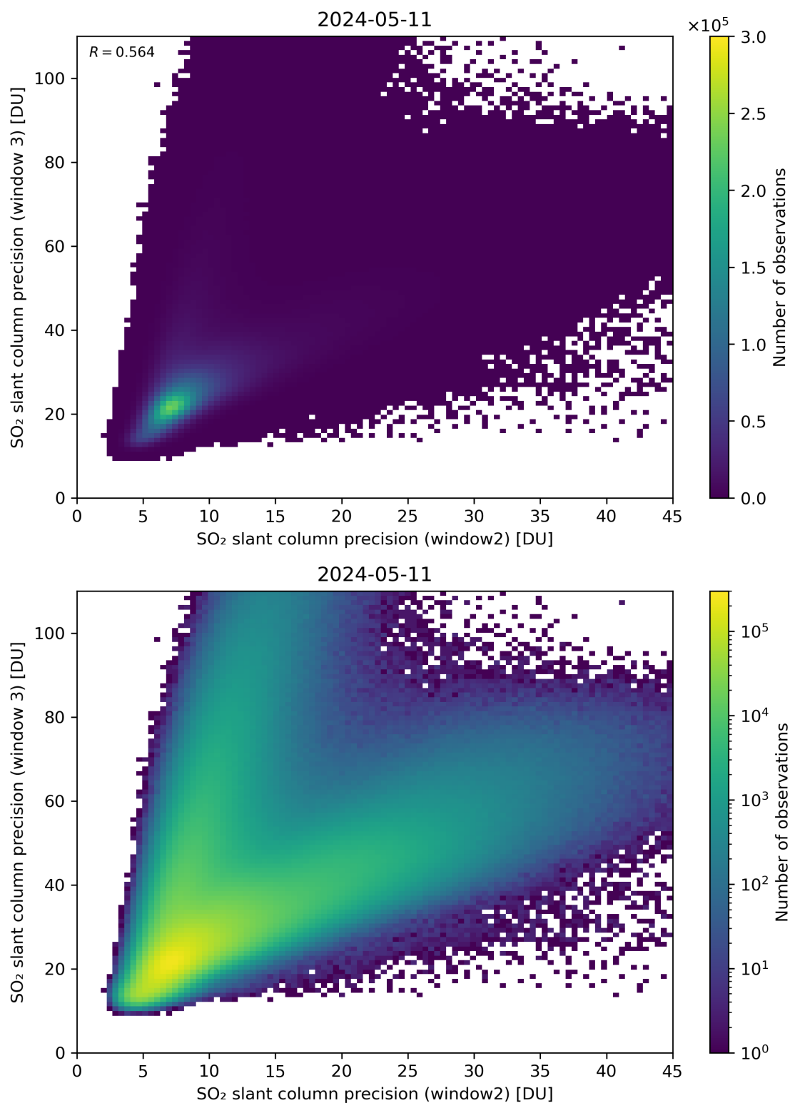
Figure 250: Scatter density plot of “SO 2 slant column precision (window2)” against “SO 2 slant column precision (window 3)” for 2024-05-10 to 2024-05-12.
