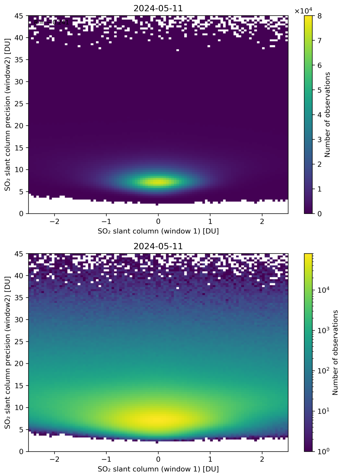
Figure 236: Scatter density plot of “SO 2 slant column (window 1)” against “SO 2 slant column precision (window2)” for 2024-05-10 to 2024-05-12.
