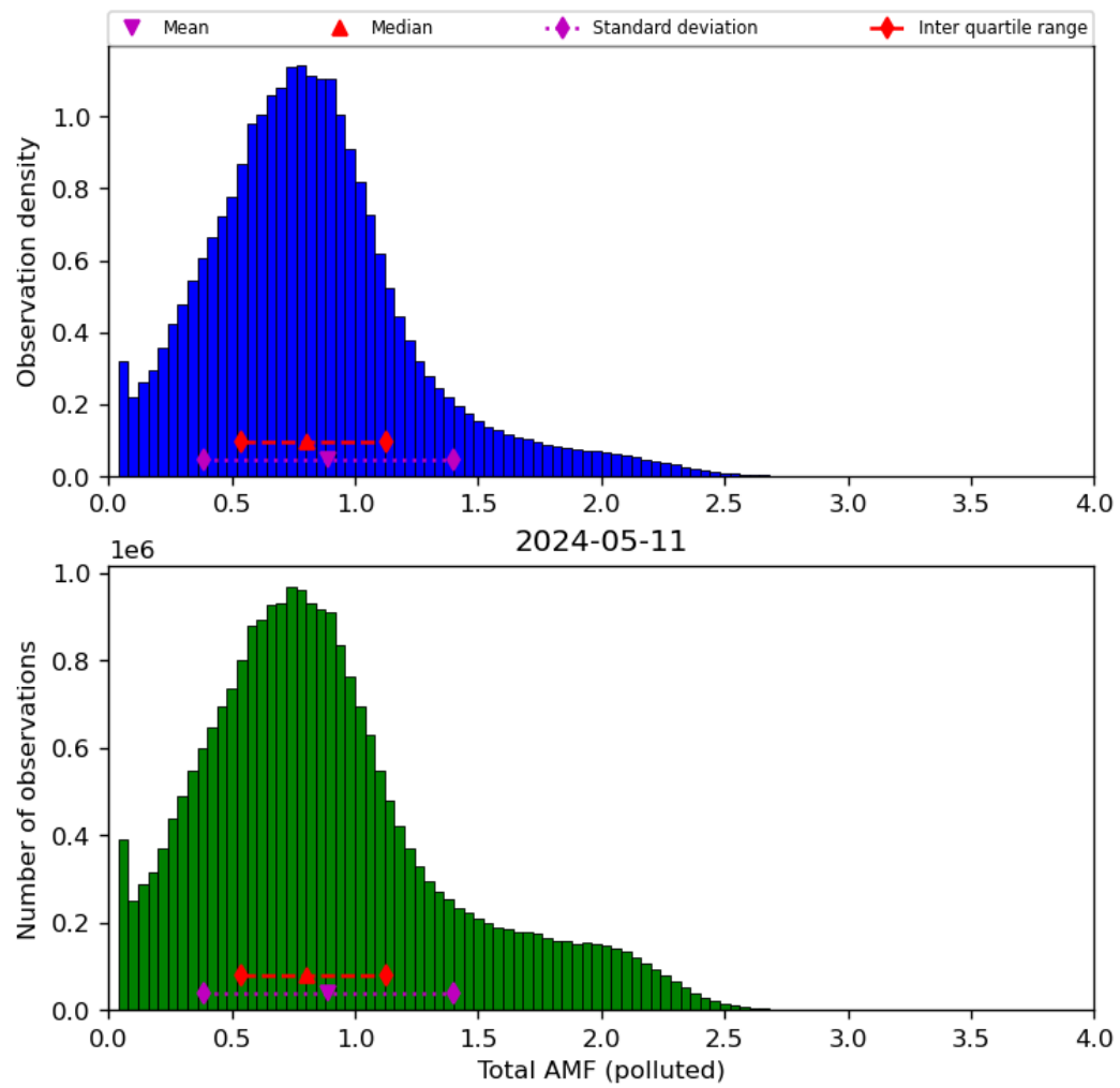
Figure 71: Histogram of “Total AMF (polluted)” for 2024-05-10 to 2024-05-12
