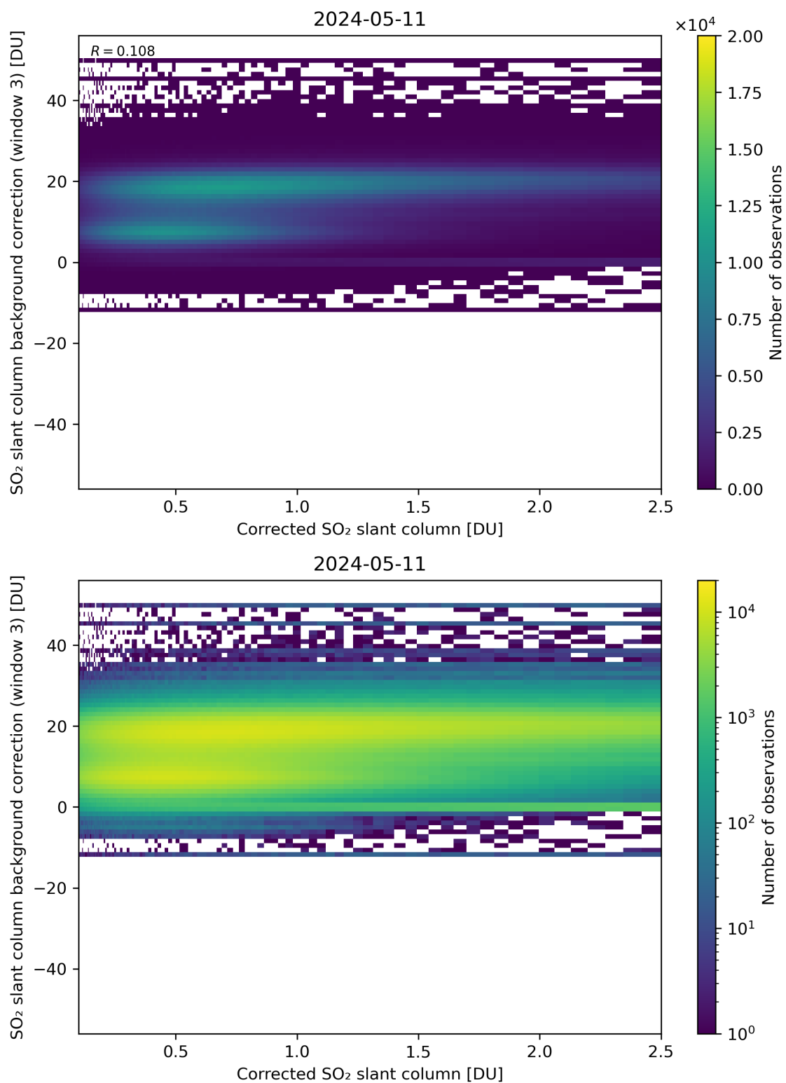
Figure 180: Scatter density plot of “Corrected SO 2 slant column” against “SO 2 slant column background correction (window 3)” for 2024-05-10 to 2024-05-12.
