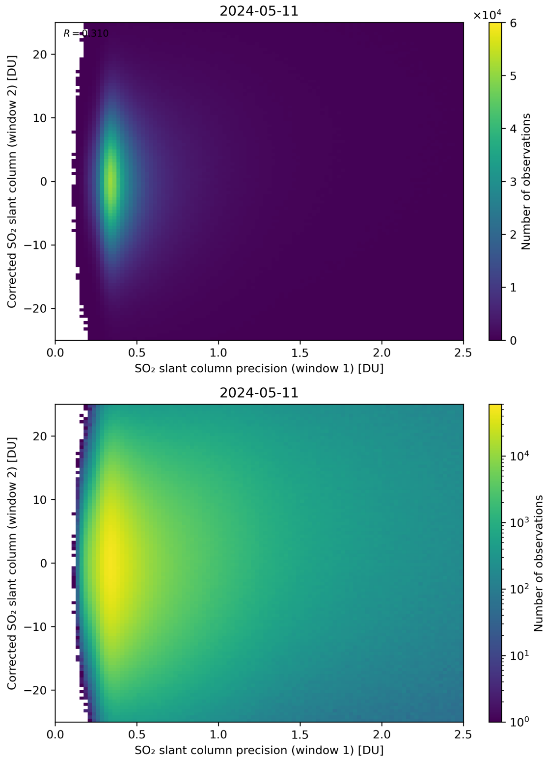
Figure 225: Scatter density plot of “SO 2 slant column precision (window 1)” against “Corrected SO 2 slant column (window 2)” for 2024-05-10 to 2024-05-12.
