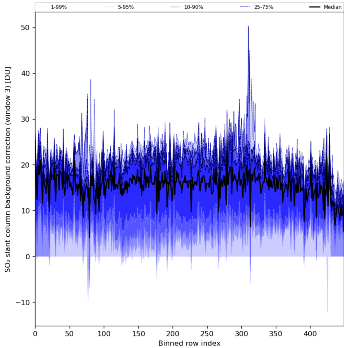
Figure 90: Along track statistics of “SO 2 slant column background correction (window 3)” for 2024-05-10 to 2024-05-12
