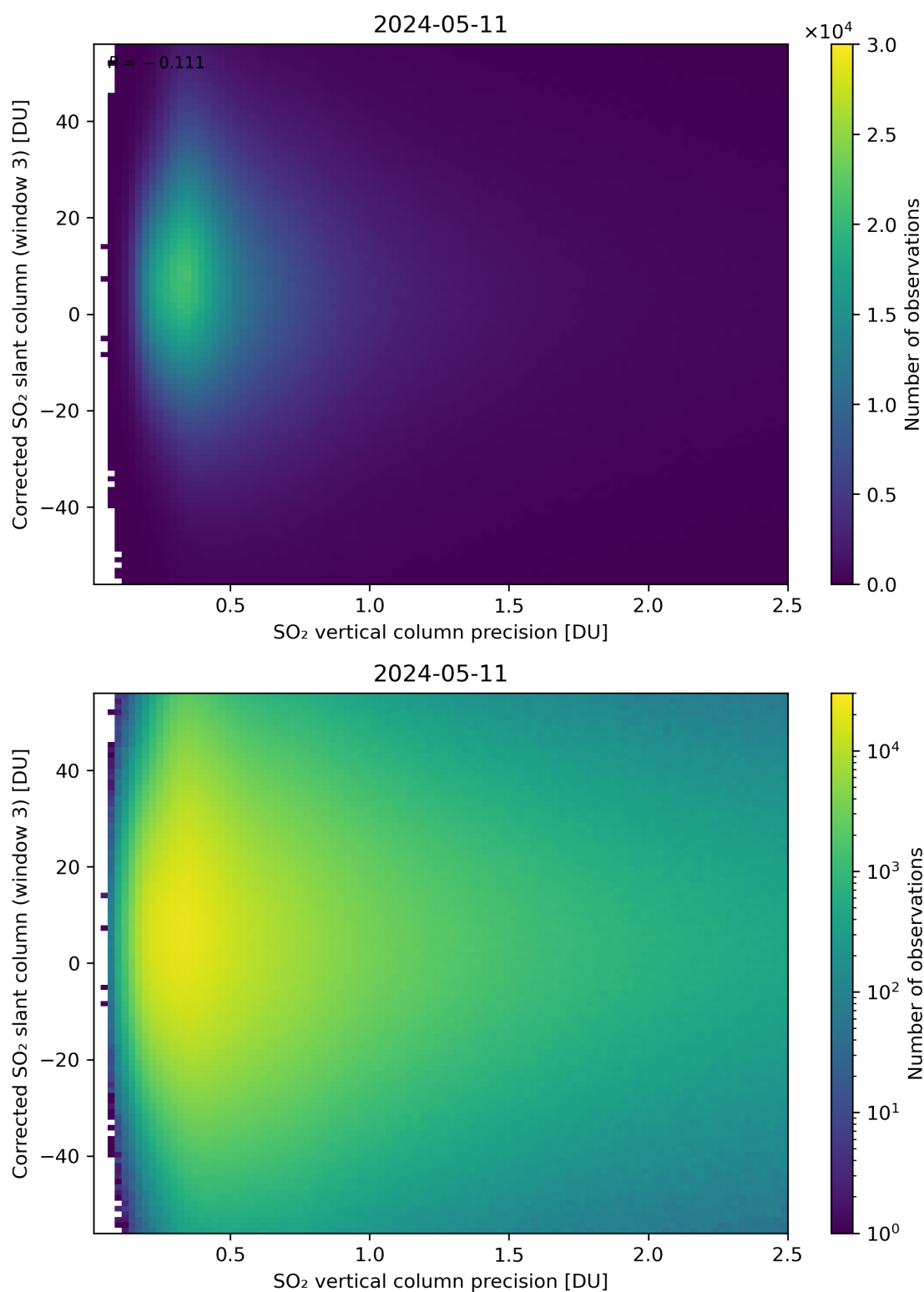
Figure 288: Scatter density plot of “SO 2 vertical column precision” against “Corrected SO 2 slant column (window 3)” for 2024-05-10 to 2024-05-12.
