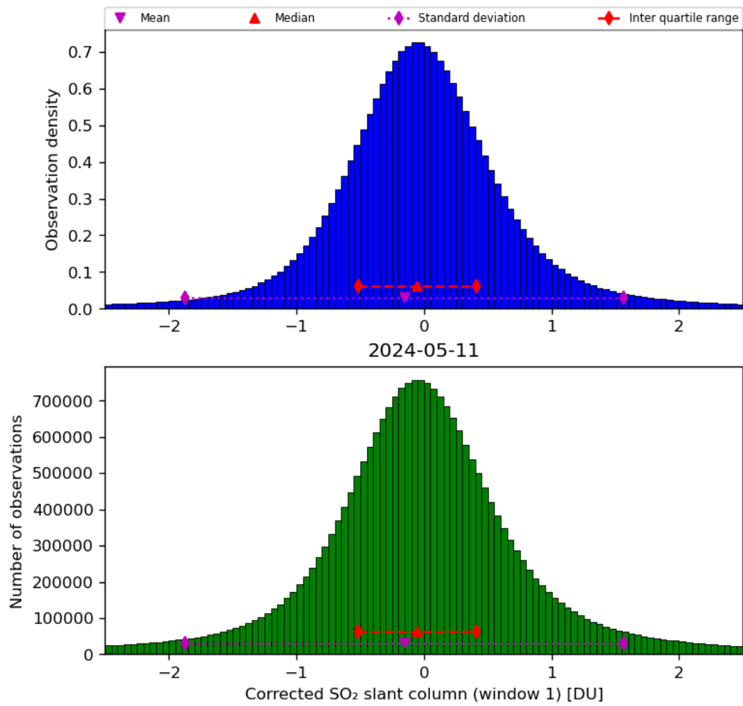
Figure 58: Histogram of “Corrected SO 2 slant column (window 1)” for 2024-05-10 to 2024-05-12
