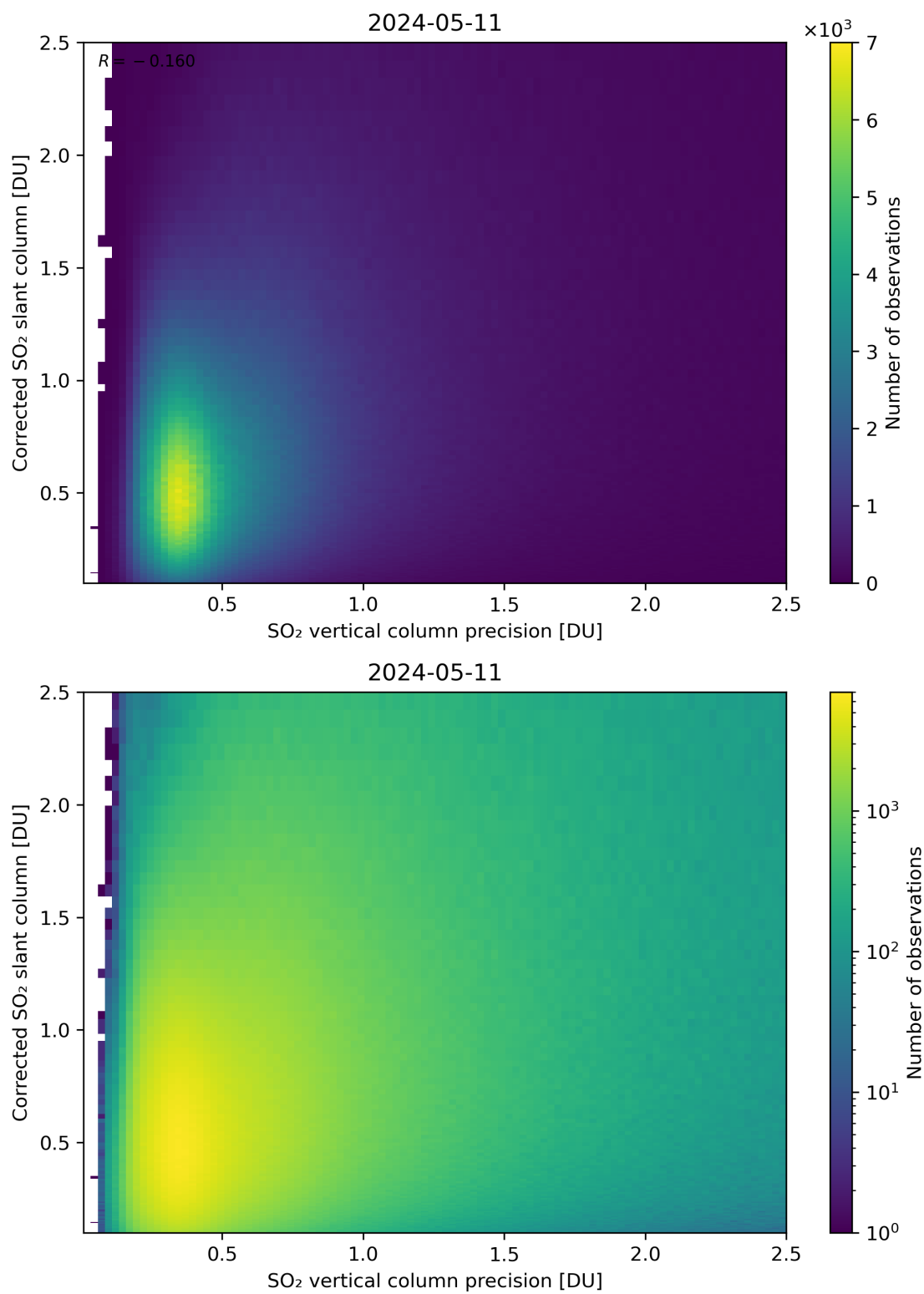
Figure 286: Scatter density plot of “SO 2 vertical column precision” against “Corrected SO 2 slant column” for 2024-05-10 to 2024-05-12.
