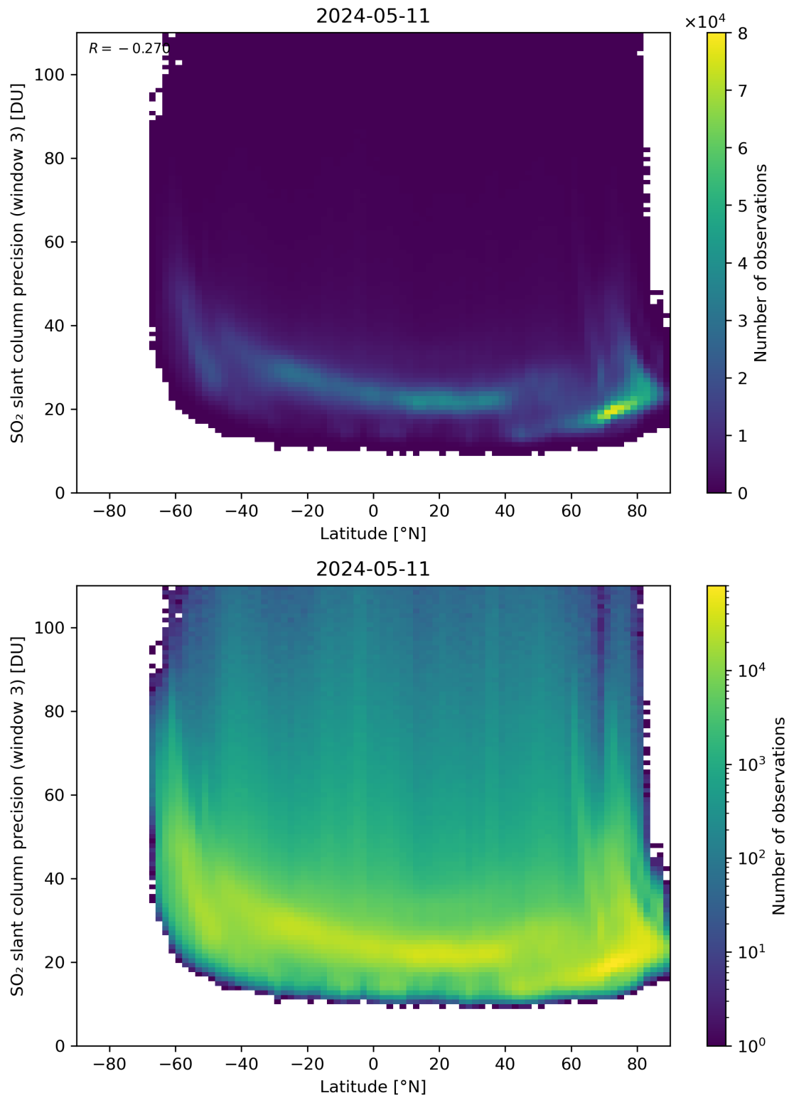
Figure 153: Scatter density plot of “Latitude” against “SO 2 slant column precision (window 3)” for 2024-05-10 to 2024-05-12.
