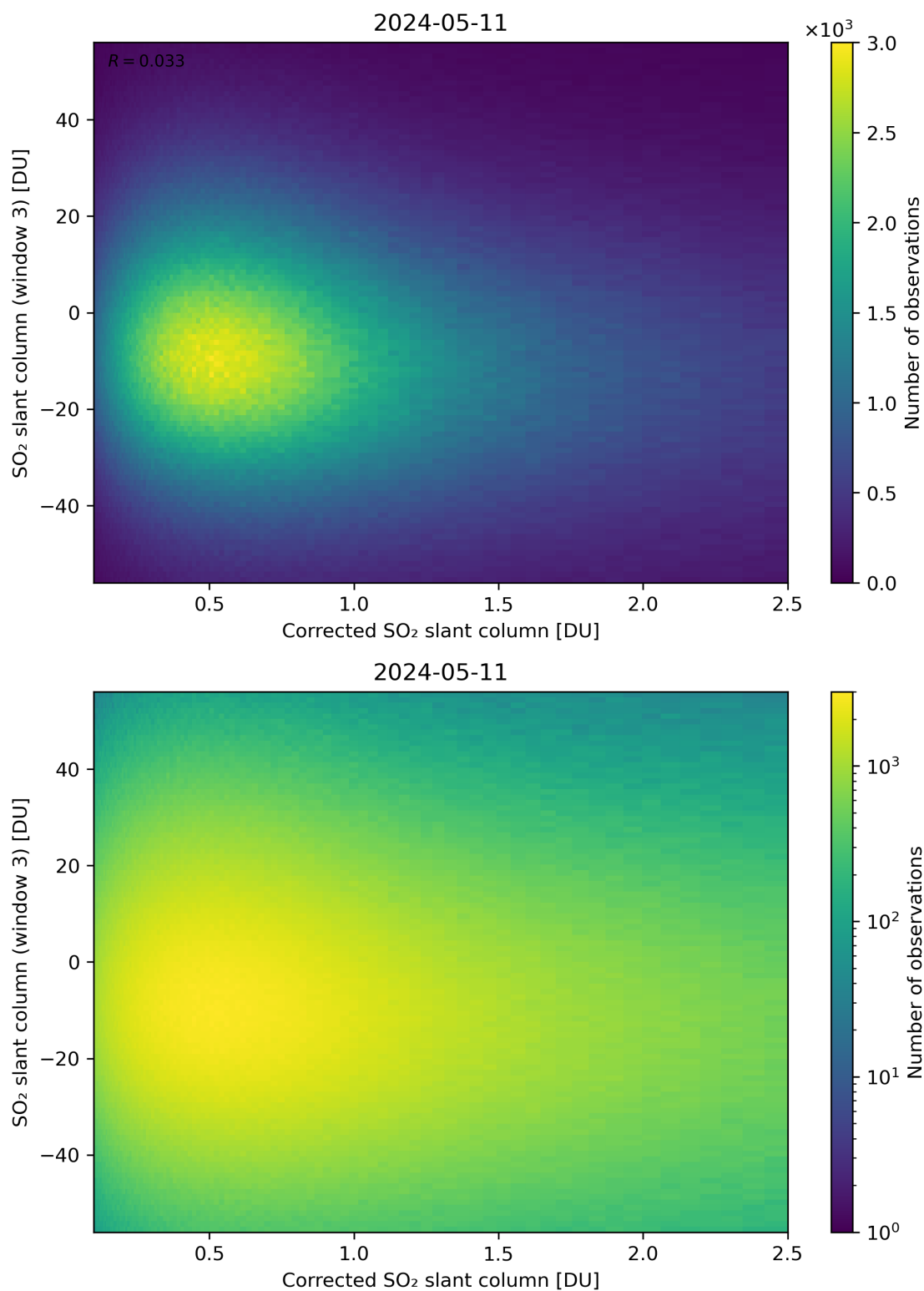
Figure 190: Scatter density plot of “Corrected SO 2 slant column” against “SO 2 slant column (window 3)” for 2024-05-10 to 2024-05-12.
