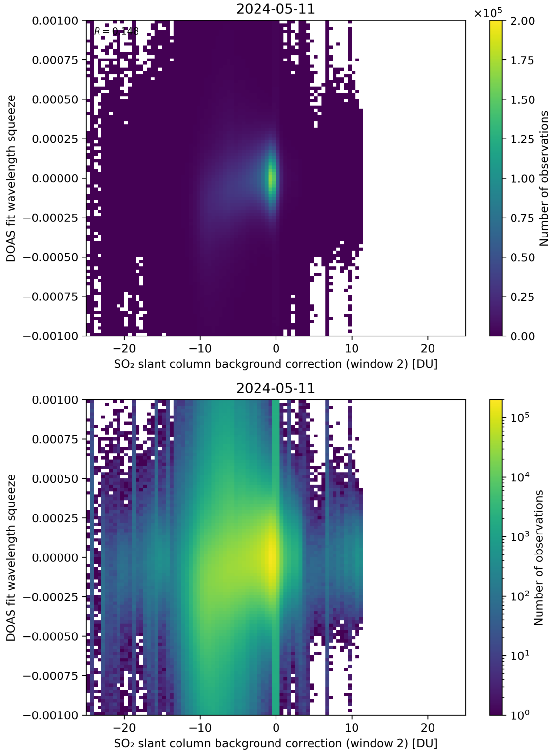
Figure 113: Scatter density plot of “SO 2 slant column background correction (window 2)” against “DOAS fit wavelength squeeze” for 2024-05-10 to 2024-05-12.
