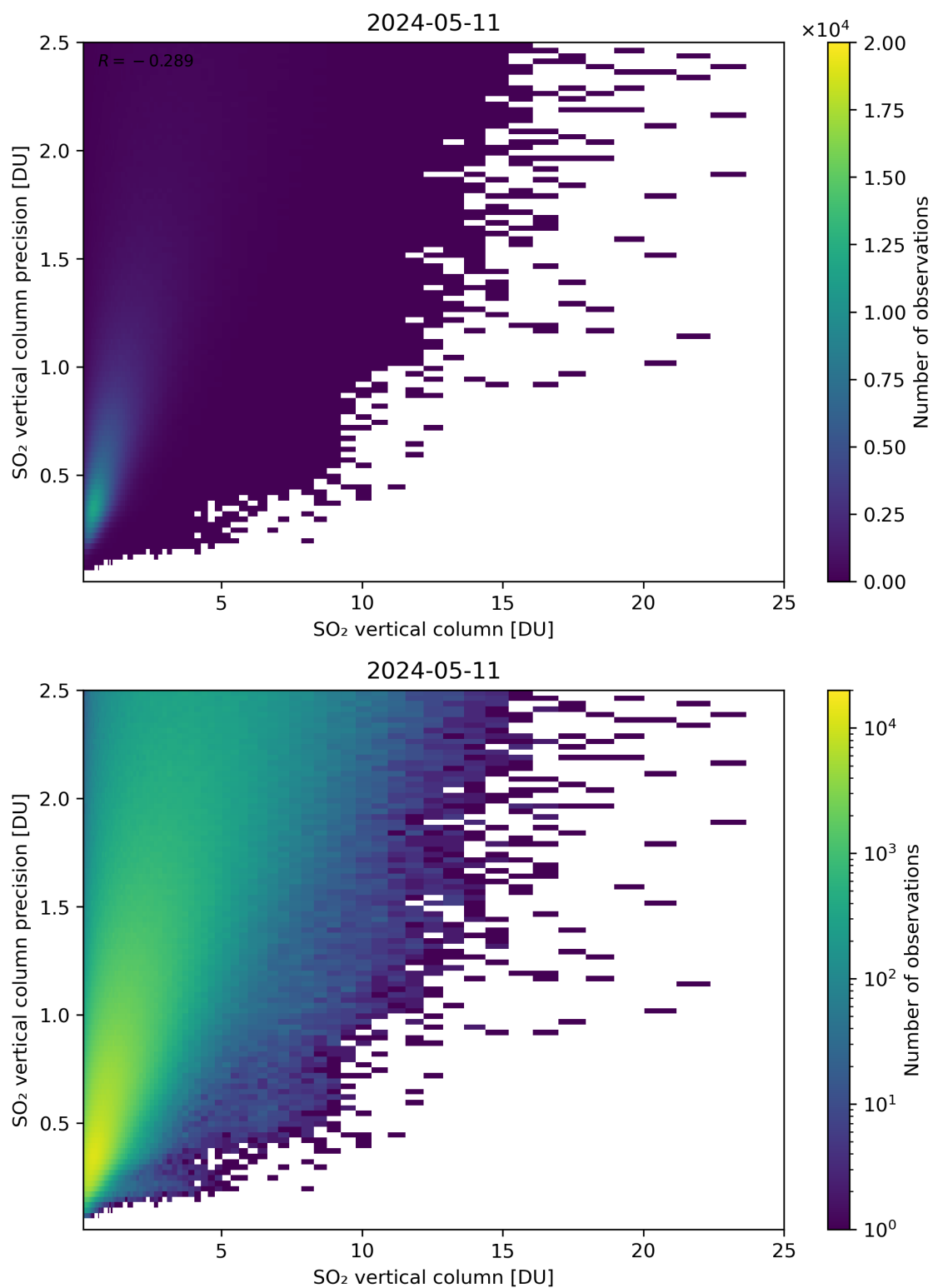
Figure 307: Scatter density plot of “SO 2 vertical column” against “SO 2 vertical column precision” for 2024-05-10 to 2024-05-12.
