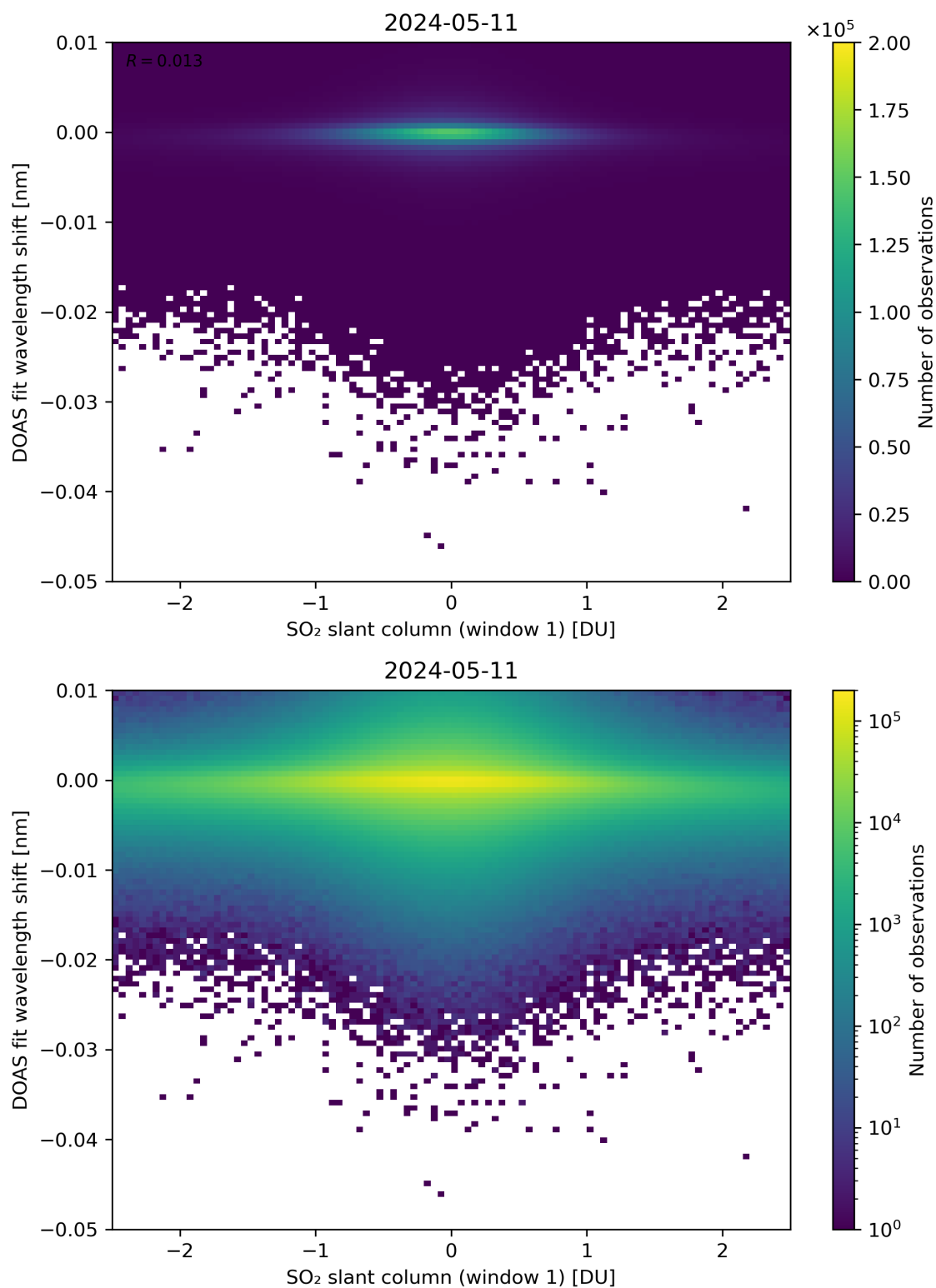
Figure 215: Scatter density plot of “SO 2 slant column (window 1)” against “DOAS fit wavelength shift” for 2024-05-10 to 2024-05-12.
