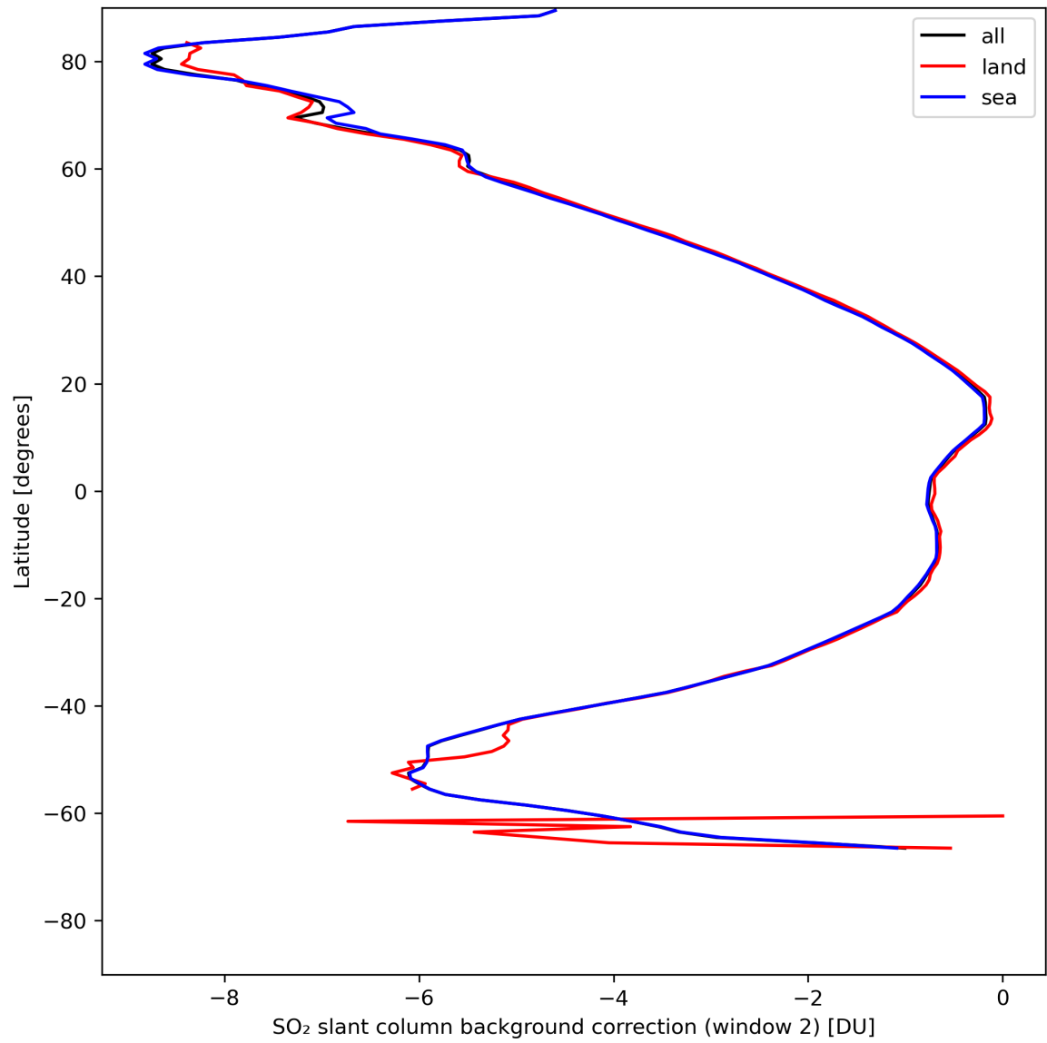
Figure 40: Zonal average of “SO 2 slant column background correction (window 2)” for 2024-05-10 to 2024-05-12.
