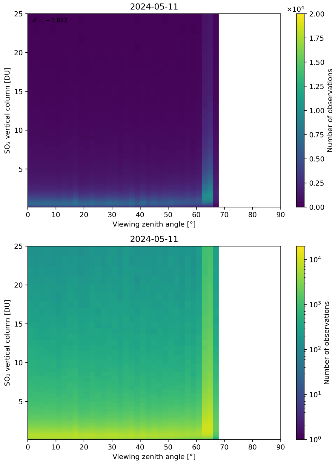
Figure 327: Scatter density plot of “Viewing zenith angle” against “SO 2 vertical column” for 2024-05-10 to 2024-05-12.
