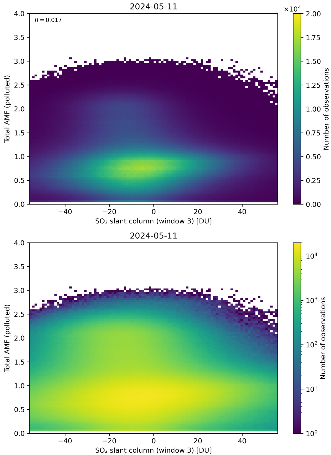
Figure 268: Scatter density plot of “SO 2 slant column (window 3)” against “Total AMF (polluted)” for 2024-05-10 to 2024-05-12.
