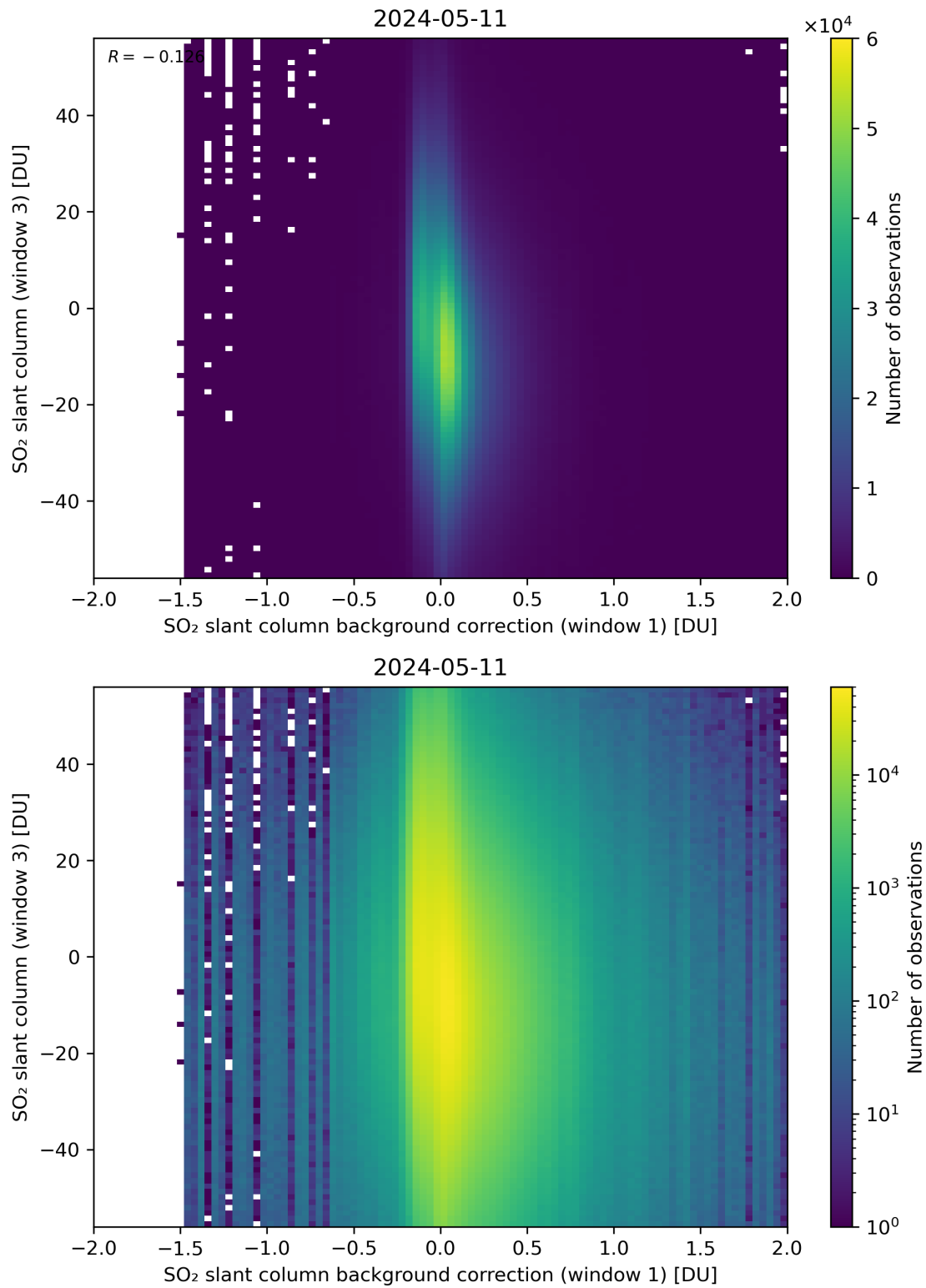
Figure 107: Scatter density plot of “SO 2 slant column background correction (window 1)” against “SO 2 slant column (window 3)” for 2024-05-10 to 2024-05-12.
