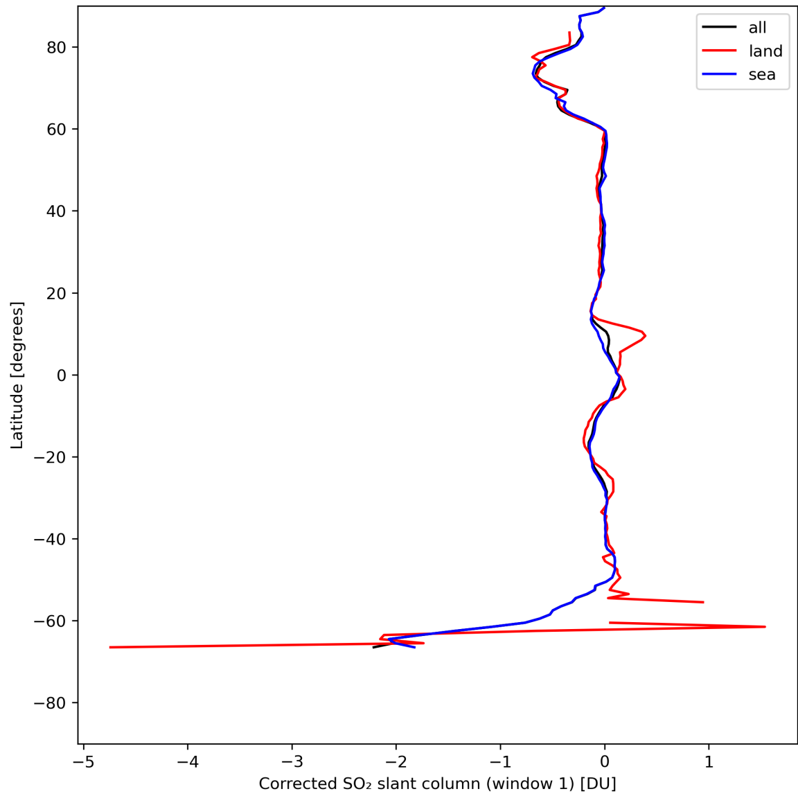
Figure 35: Zonal average of “Corrected SO 2 slant column (window 1)” for 2024-05-10 to 2024-05-12.
