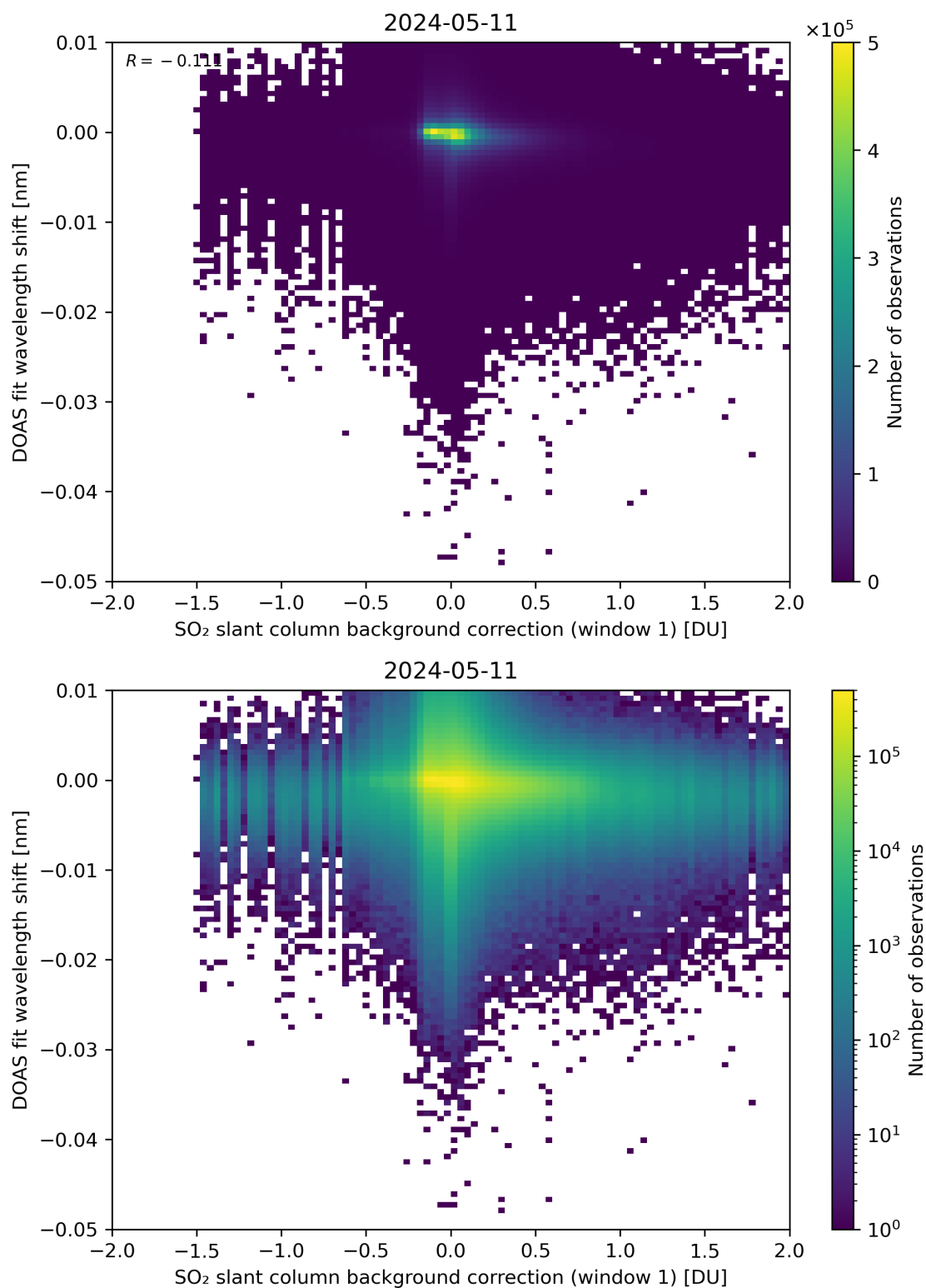
Figure 100: Scatter density plot of “SO 2 slant column background correction (window 1)” against “DOAS fit wavelength shift” for 2024-05-10 to 2024-05-12.
