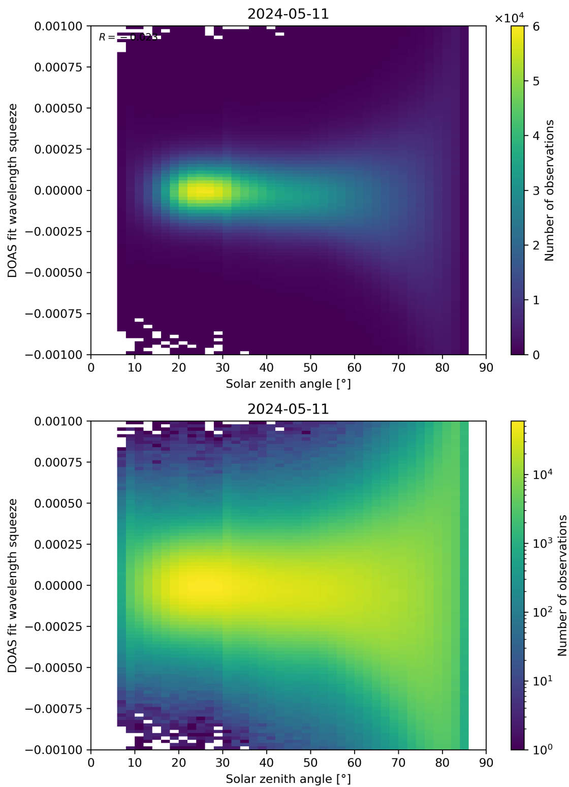
Figure 162: Scatter density plot of “Solar zenith angle” against “DOAS fit wavelength squeeze” for 2024-05-10 to 2024-05-12.
