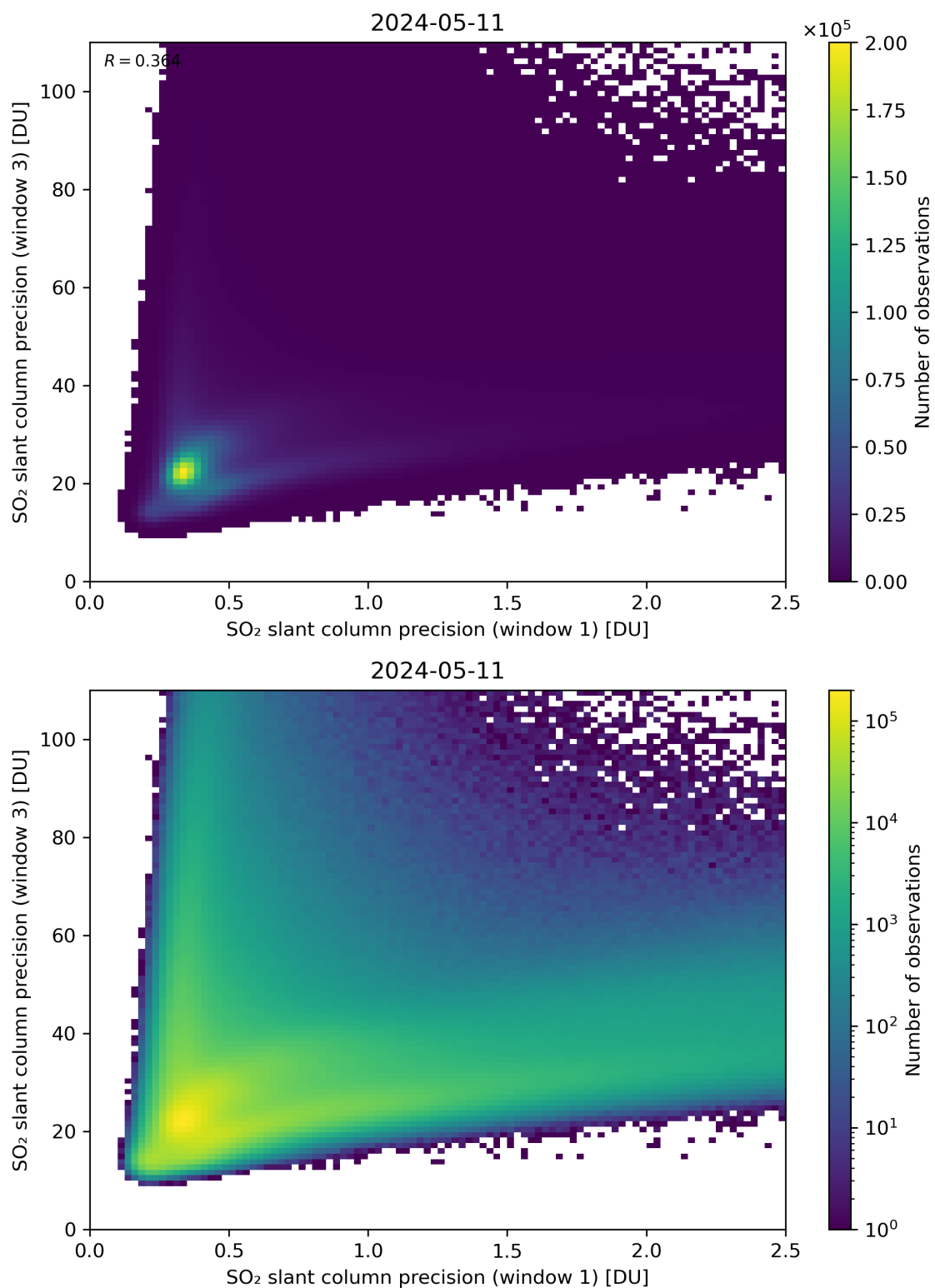
Figure 229: Scatter density plot of “SO 2 slant column precision (window 1)” against “SO 2 slant column precision (window 3)” for 2024-05-10 to 2024-05-12.
