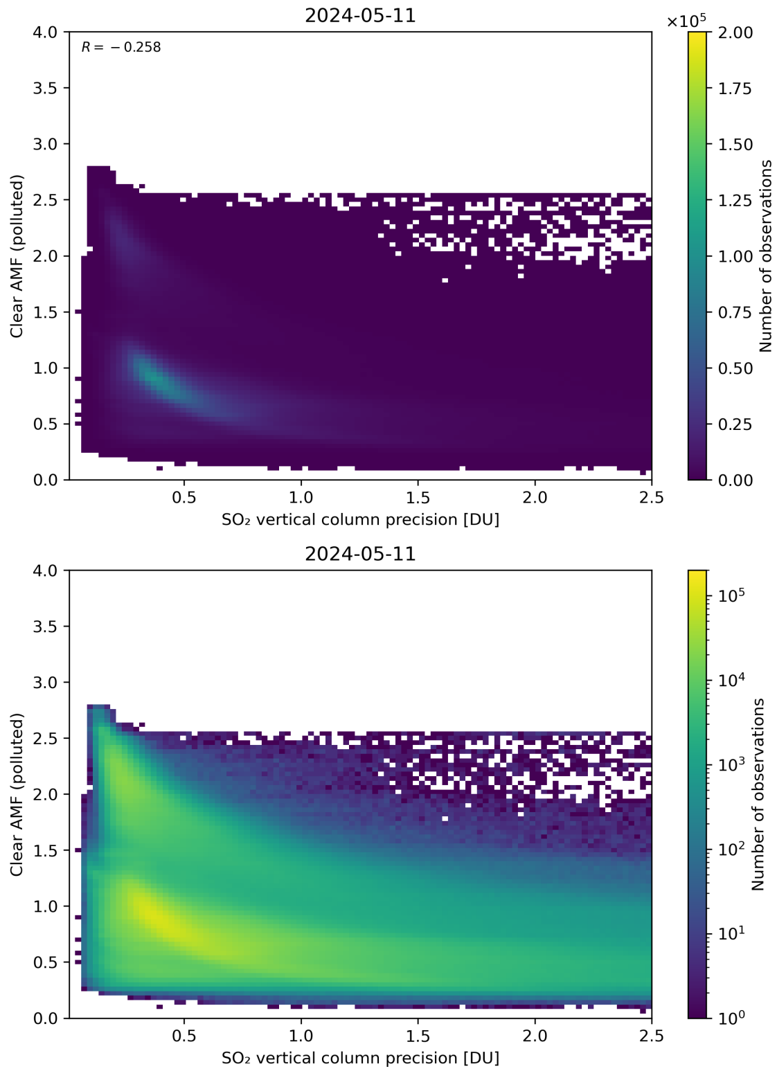
Figure 285: Scatter density plot of “SO 2 vertical column precision” against “Clear AMF (polluted)” for 2024-05-10 to 2024-05-12.
