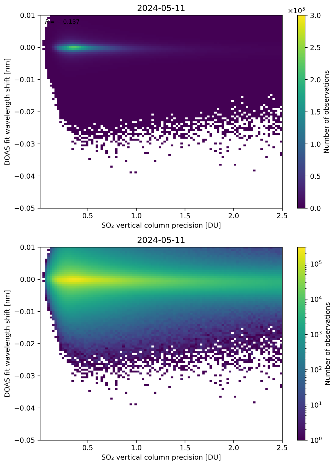
Figure 282: Scatter density plot of “SO 2 vertical column precision” against “DOAS fit wavelength shift” for 2024-05-10 to 2024-05-12.
