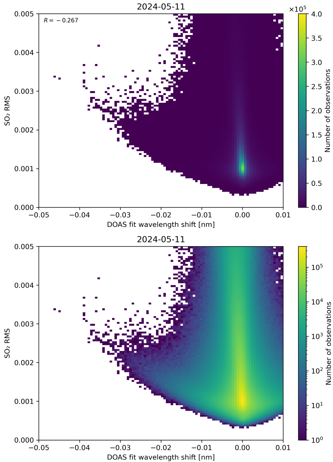
Figure 128: Scatter density plot of “DOAS fit wavelength shift” against “SO 2 RMS” for 2024-05-10 to 2024-05-12.
