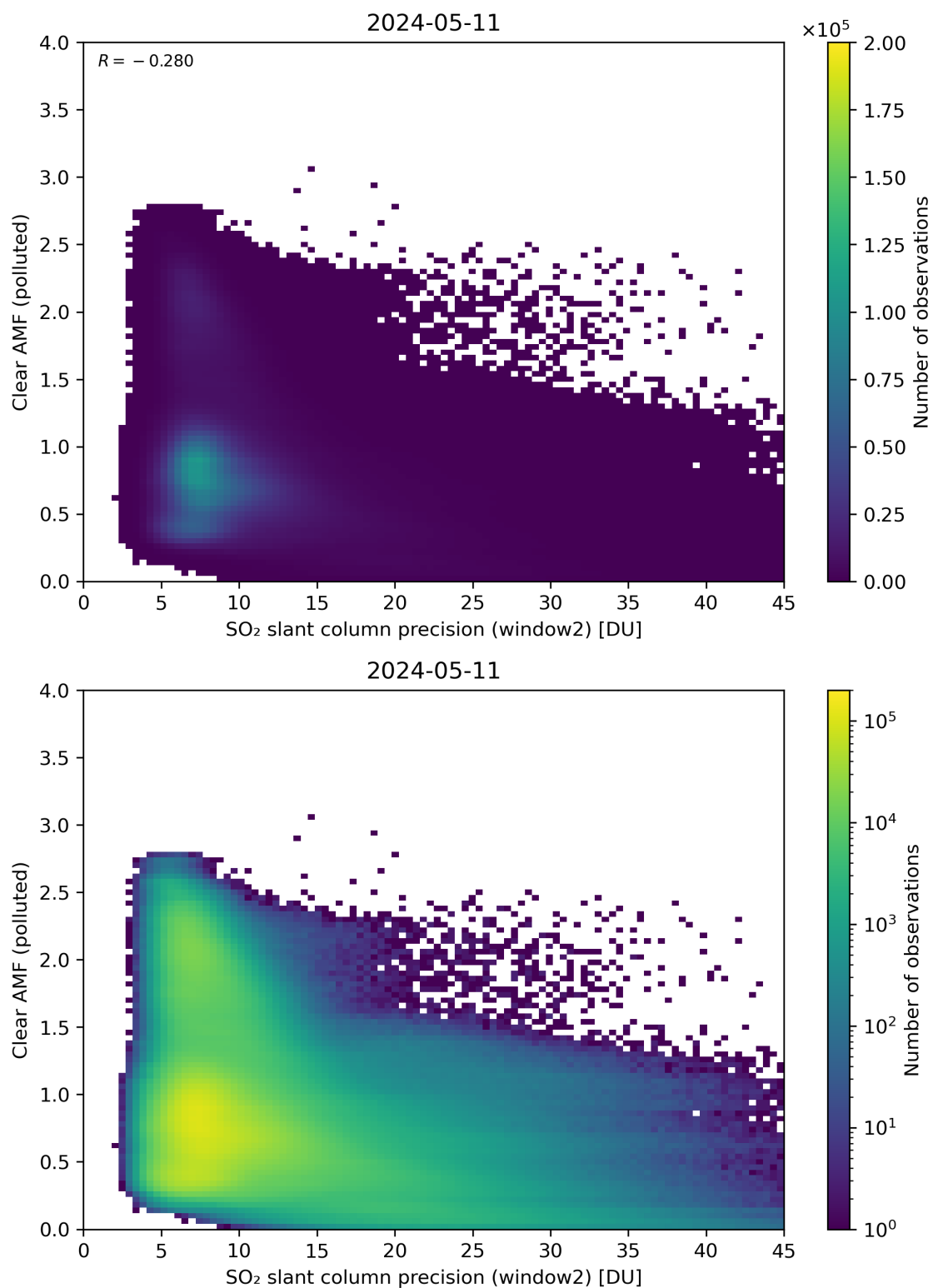
Figure 246: Scatter density plot of “SO 2 slant column precision (window2)” against “Clear AMF (polluted)” for 2024-05-10 to 2024-05-12.
