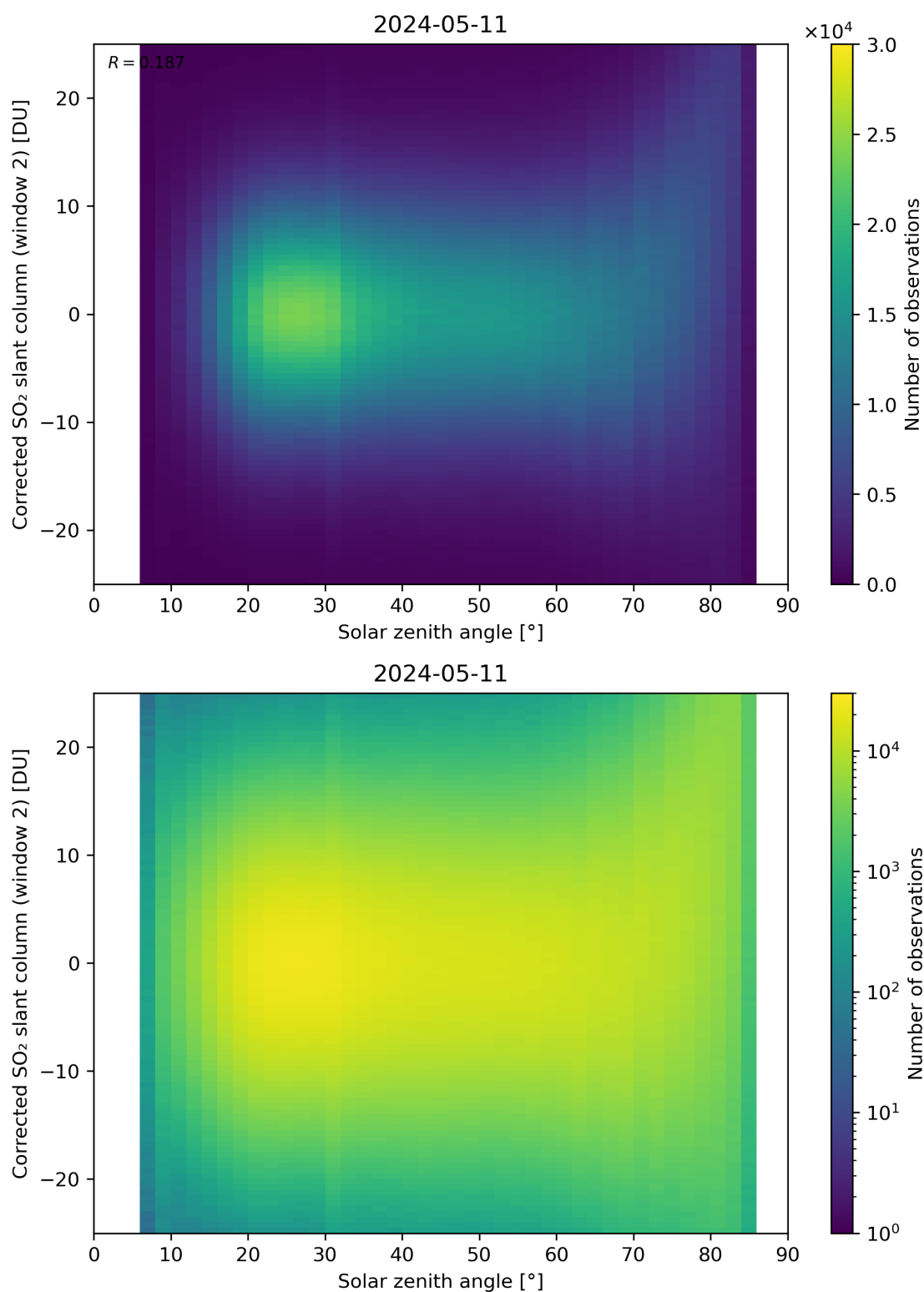
Figure 167: Scatter density plot of “Solar zenith angle” against “Corrected SO 2 slant column (window 2)” for 2024-05-10 to 2024-05-12.
