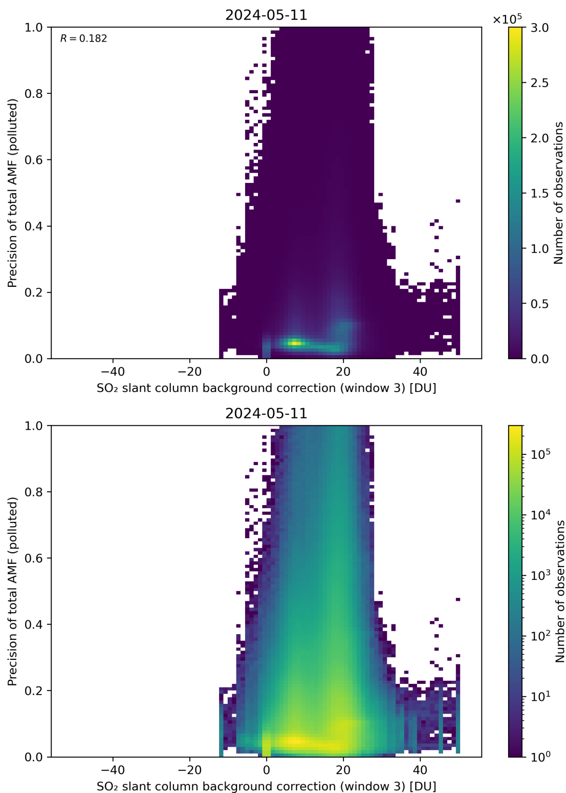
Figure 126: Scatter density plot of “SO 2 slant column background correction (window 3)” against “Precision of total AMF (polluted)” for 2024-05-10 to 2024-05-12.
