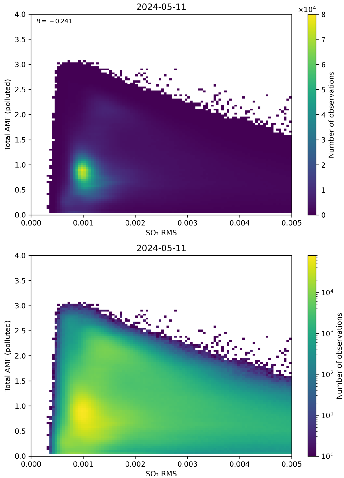
Figure 137: Scatter density plot of “SO 2 RMS” against “Total AMF (polluted)” for 2024-05-10 to 2024-05-12.
