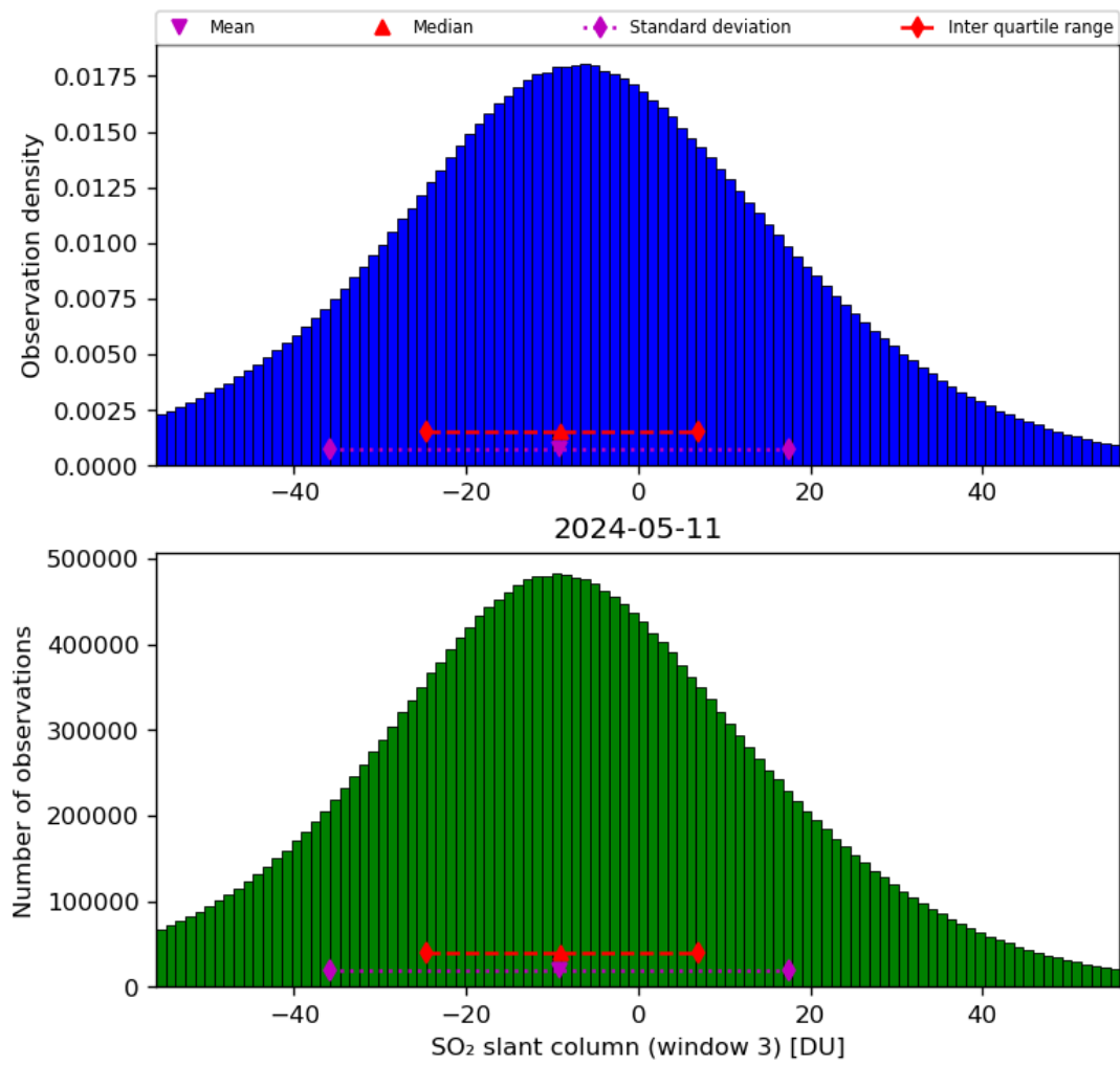
Figure 64: Histogram of “SO 2 slant column (window 3)” for 2024-05-10 to 2024-05-12
