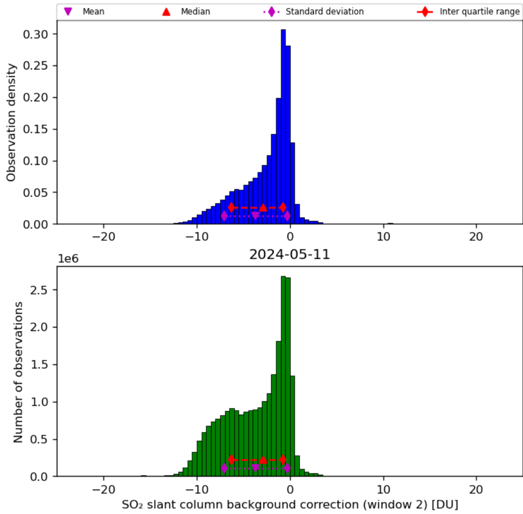
Figure 63: Histogram of “SO 2 slant column background correction (window 2)” for 2024-05-10 to 2024-05-12
