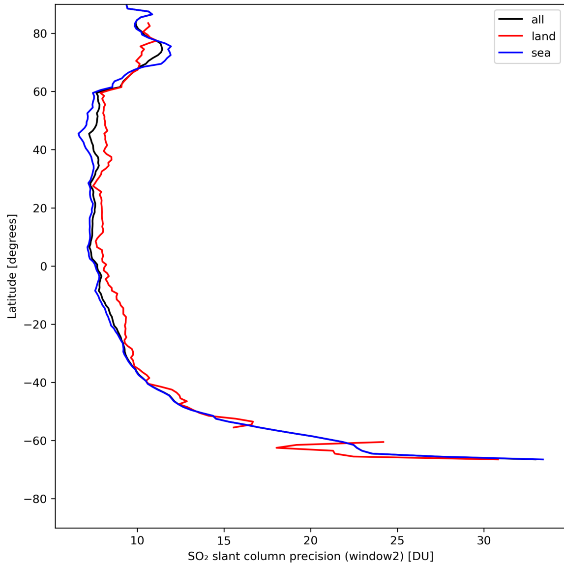
Figure 38: Zonal average of “SO 2 slant column precision (window2)” for 2024-05-10 to 2024-05-12.
