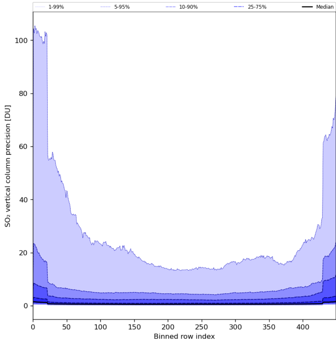
Figure 77: Along track statistics of “SO 2 vertical column precision” for 2024-05-10 to 2024-05-12
