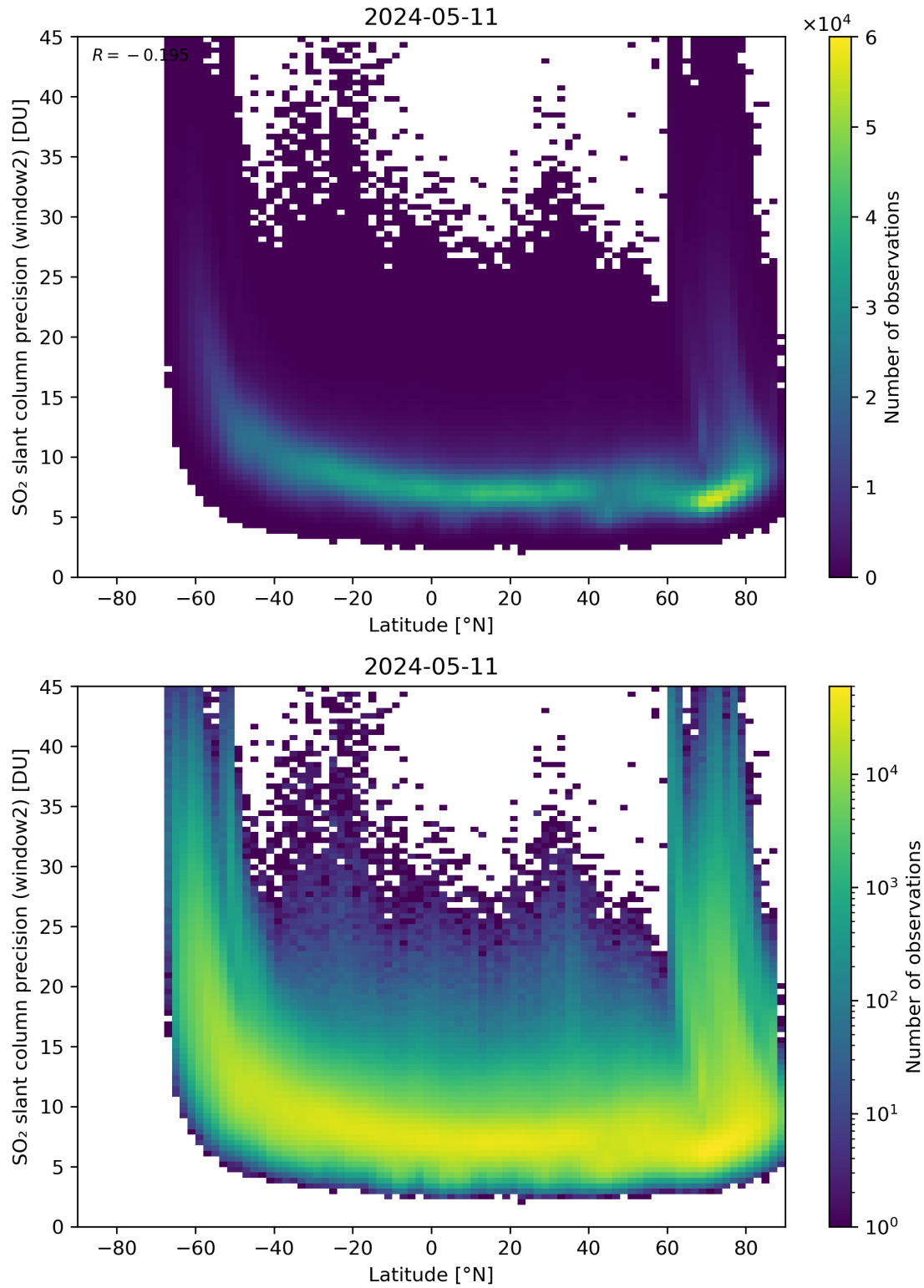
Figure 151: Scatter density plot of “Latitude” against “SO 2 slant column precision (window2)” for 2024-05-10 to 2024-05-12.
