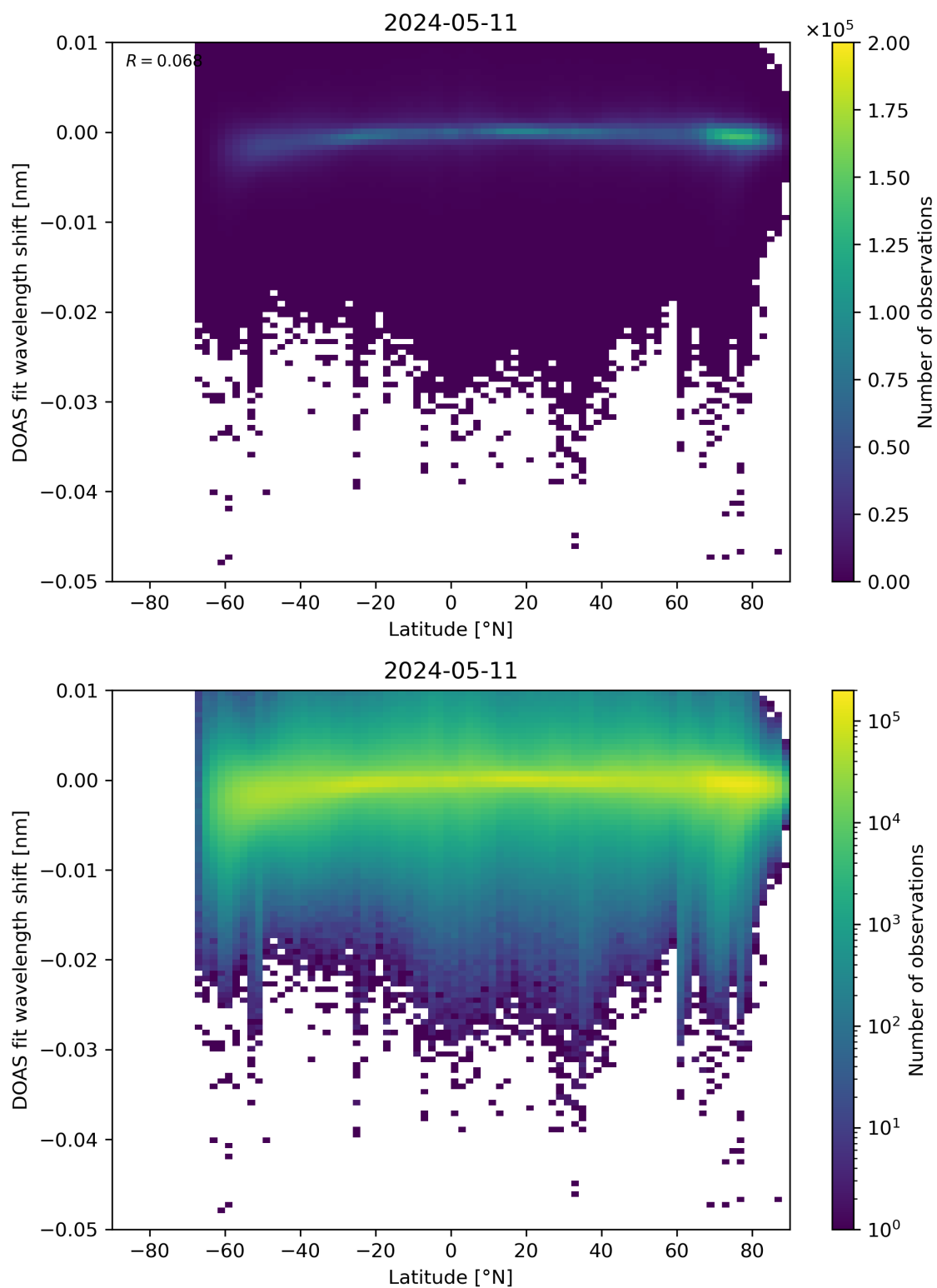
Figure 142: Scatter density plot of “Latitude” against “DOAS fit wavelength shift” for 2024-05-10 to 2024-05-12.
