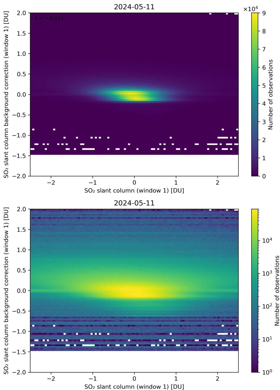
Figure 212: Scatter density plot of “SO 2 slant column (window 1)” against “SO 2 slant column background correction (window 1)” for 2024-05-10 to 2024-05-12.
