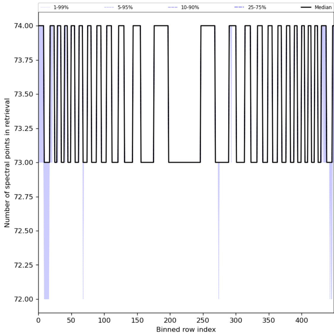
Figure 97: Along track statistics of “Number of spectral points in retrieval” for 2024-05-10 to 2024-05-12
