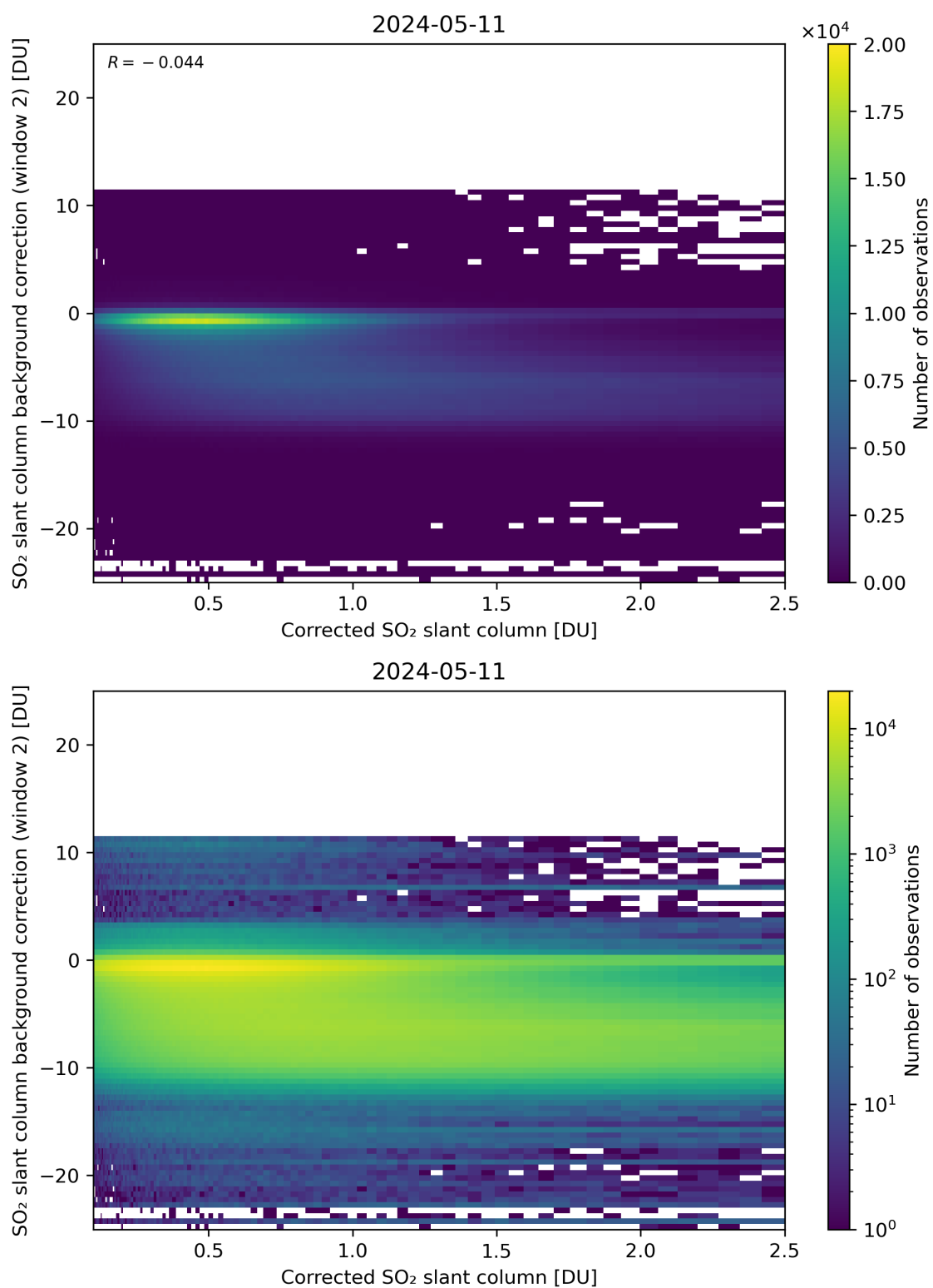
Figure 179: Scatter density plot of “Corrected SO 2 slant column” against “SO 2 slant column background correction (window 2)” for 2024-05-10 to 2024-05-12.
