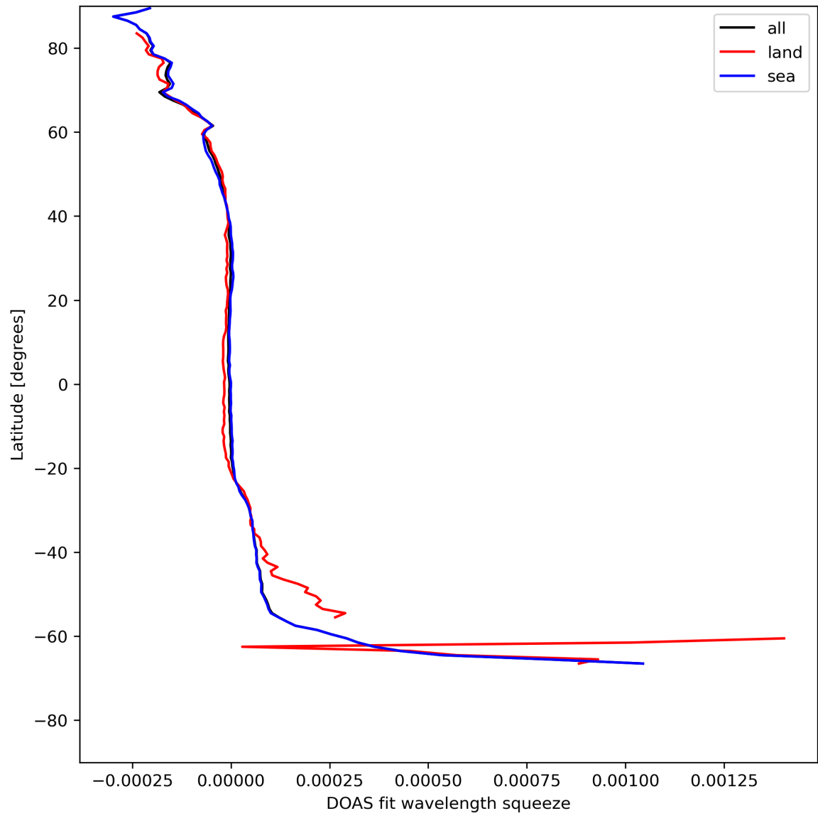
Figure 46: Zonal average of “DOAS fit wavelength squeeze” for 2024-05-10 to 2024-05-12.
