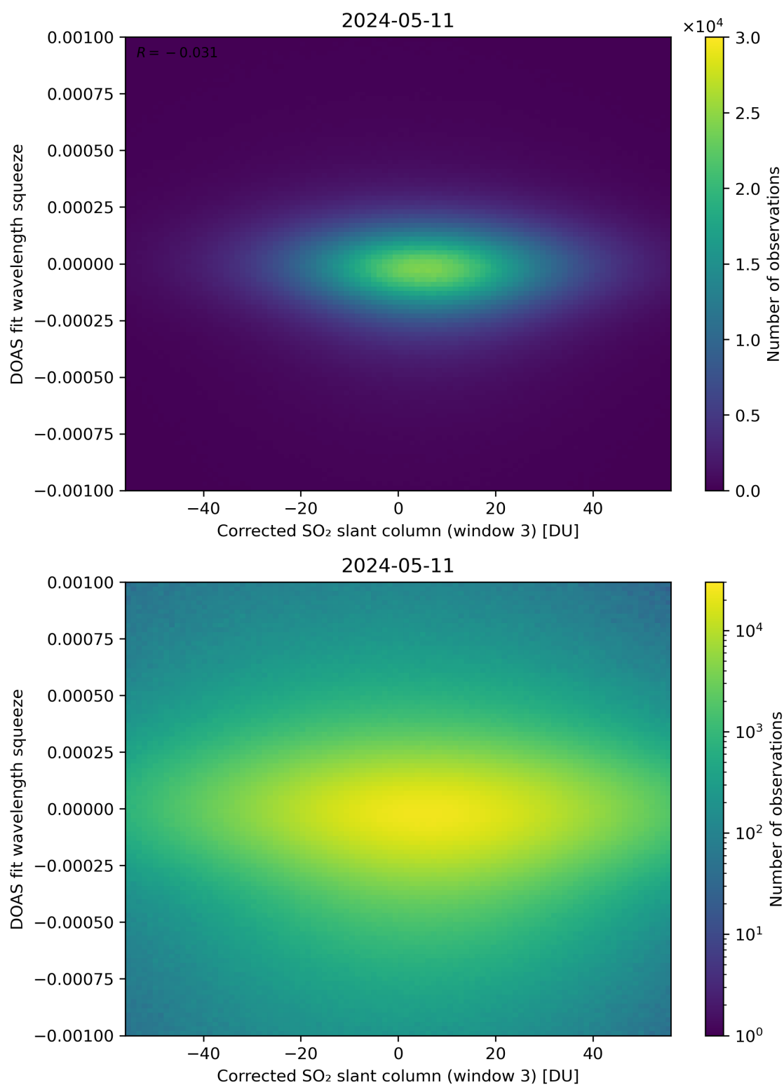
Figure 207: Scatter density plot of “Corrected SO 2 slant column (window 3)” against “DOAS fit wavelength squeeze” for 2024-05-10 to 2024-05-12.
