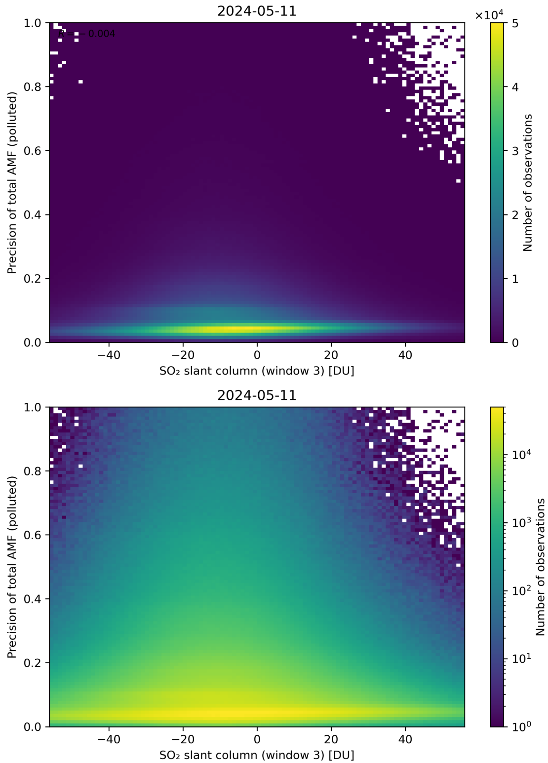
Figure 269: Scatter density plot of “SO 2 slant column (window 3)” against “Precision of total AMF (polluted)” for 2024-05-10 to 2024-05-12.
