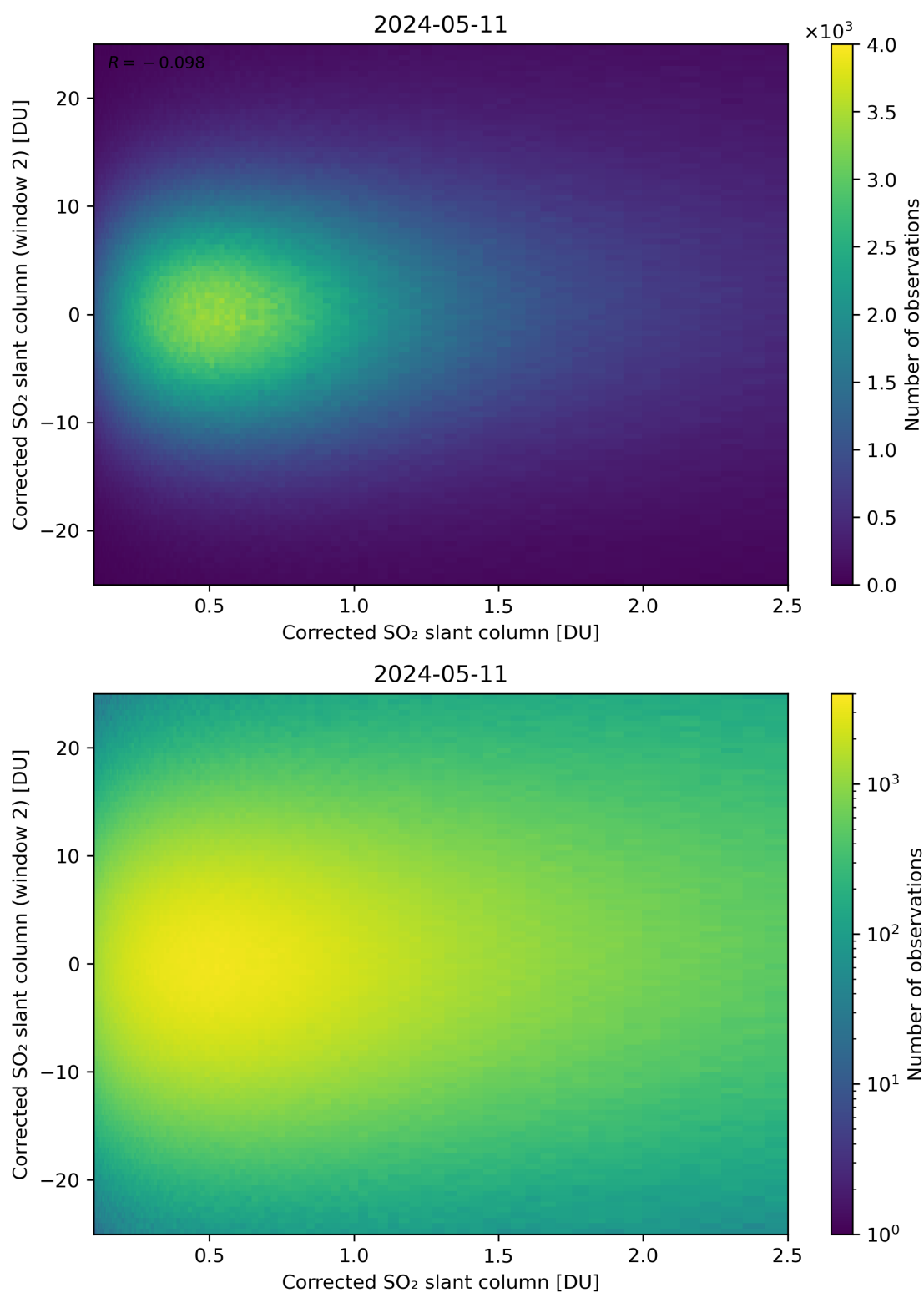
Figure 185: Scatter density plot of “Corrected SO 2 slant column” against “Corrected SO 2 slant column (window 2)” for 2024-05-10 to 2024-05-12.
