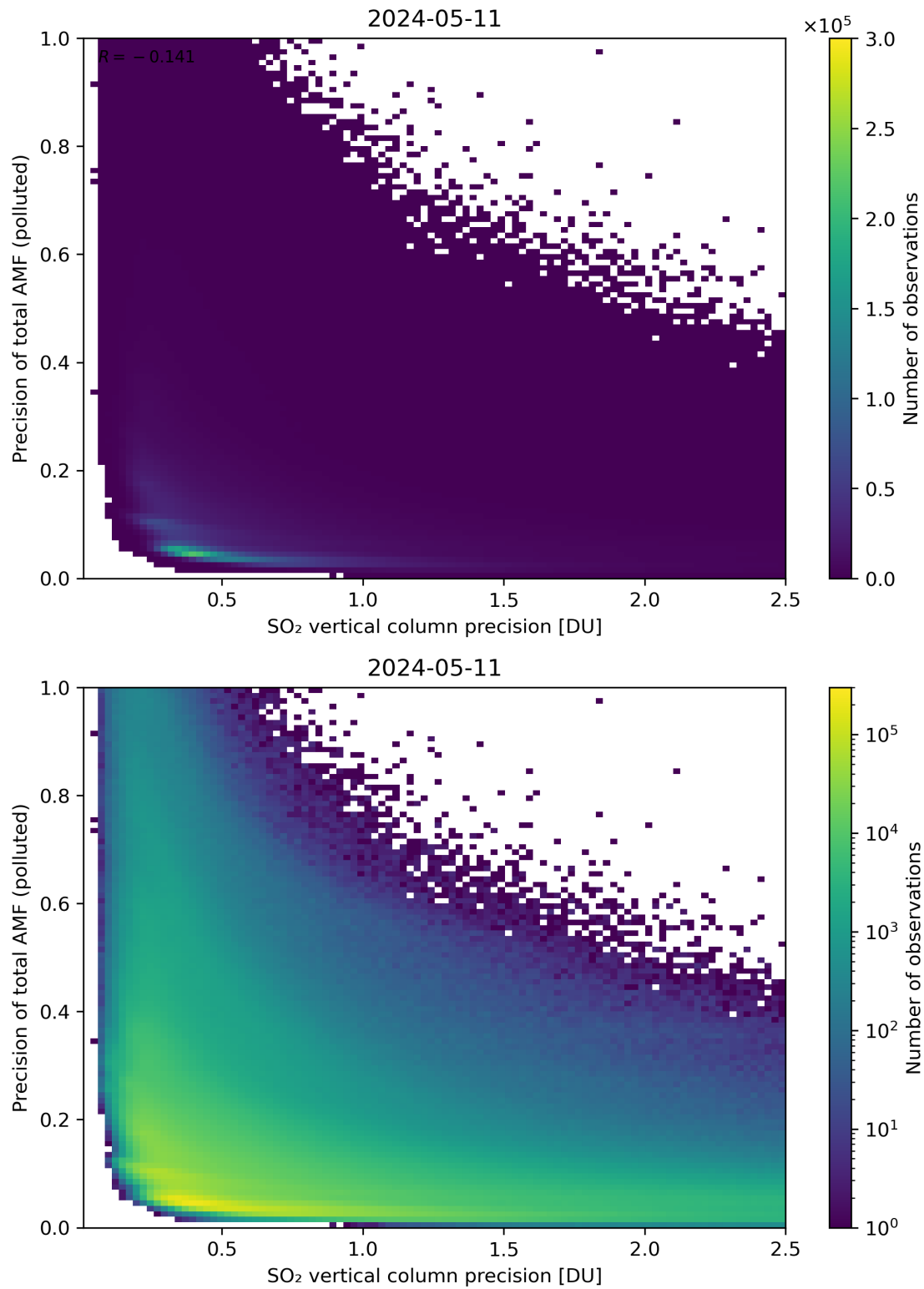
Figure 295: Scatter density plot of “SO 2 vertical column precision” against “Precision of total AMF (polluted)” for 2024-05-10 to 2024-05-12.
