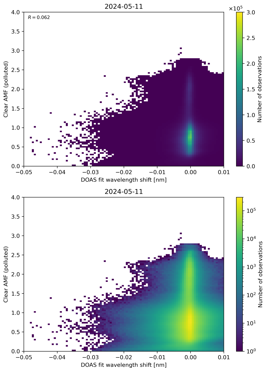
Figure 129: Scatter density plot of “DOAS fit wavelength shift” against “Clear AMF (polluted)” for 2024-05-10 to 2024-05-12.
