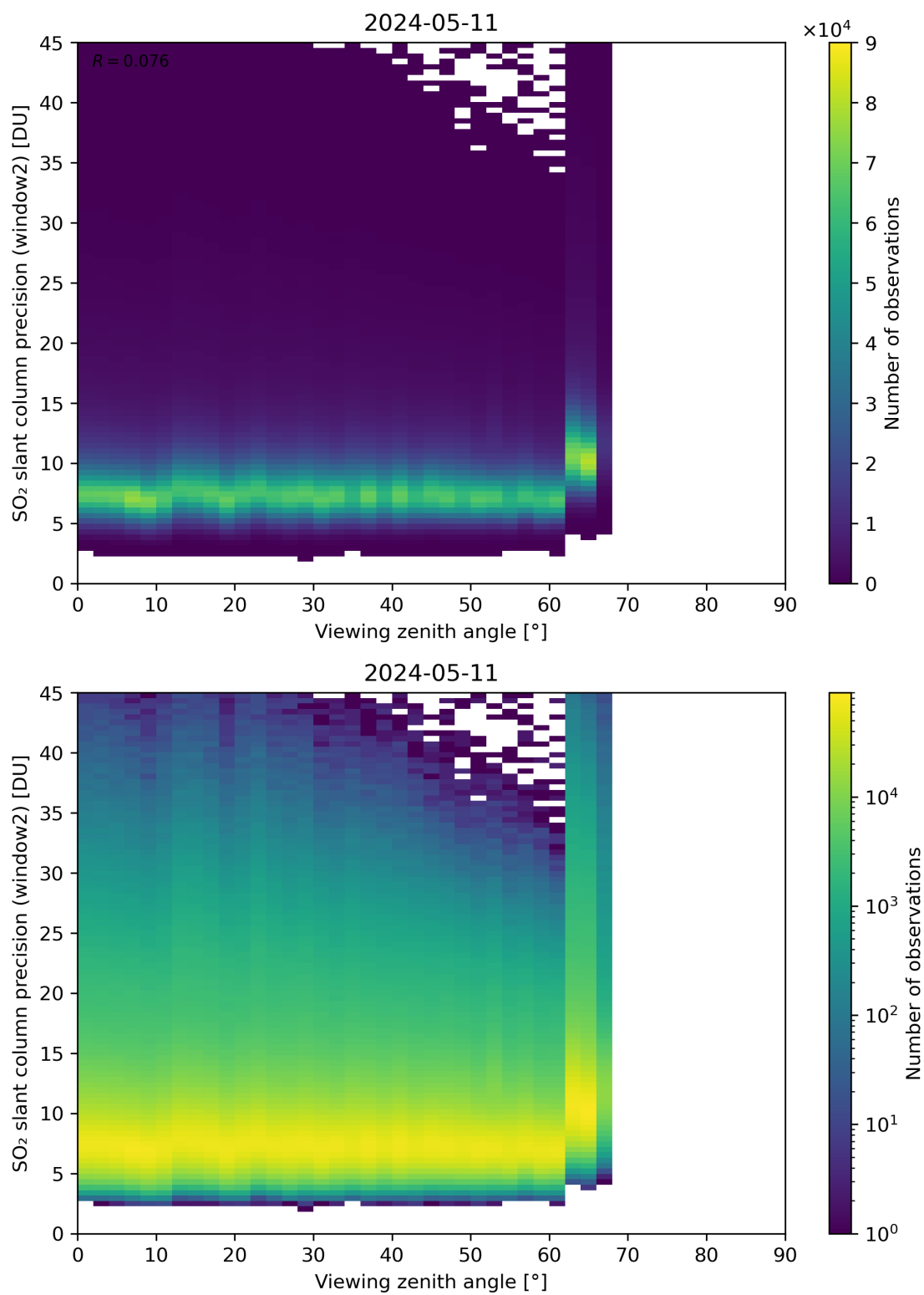
Figure 322: Scatter density plot of “Viewing zenith angle” against “SO 2 slant column precision (window2)” for 2024-05-10 to 2024-05-12.
