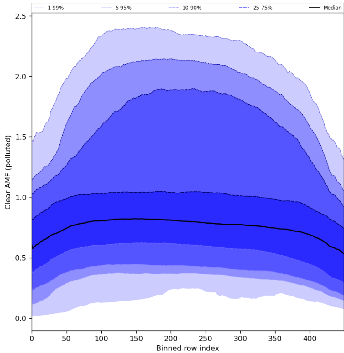
Figure 96: Along track statistics of “Clear AMF (polluted)” for 2024-05-10 to 2024-05-12
