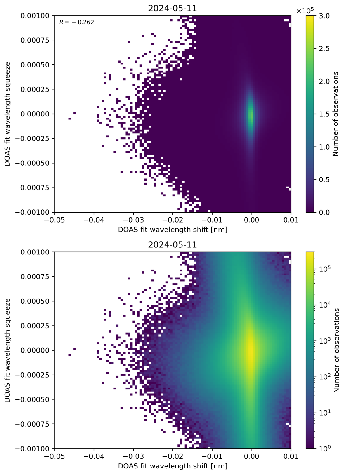
Figure 127: Scatter density plot of “DOAS fit wavelength shift” against “DOAS fit wavelength squeeze” for 2024-05-10 to 2024-05-12.
