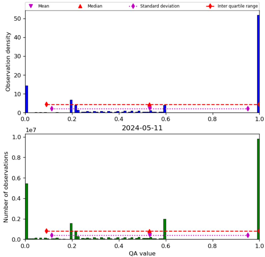
Figure 52: Histogram of “QA value” for 2024-05-10 to 2024-05-12
