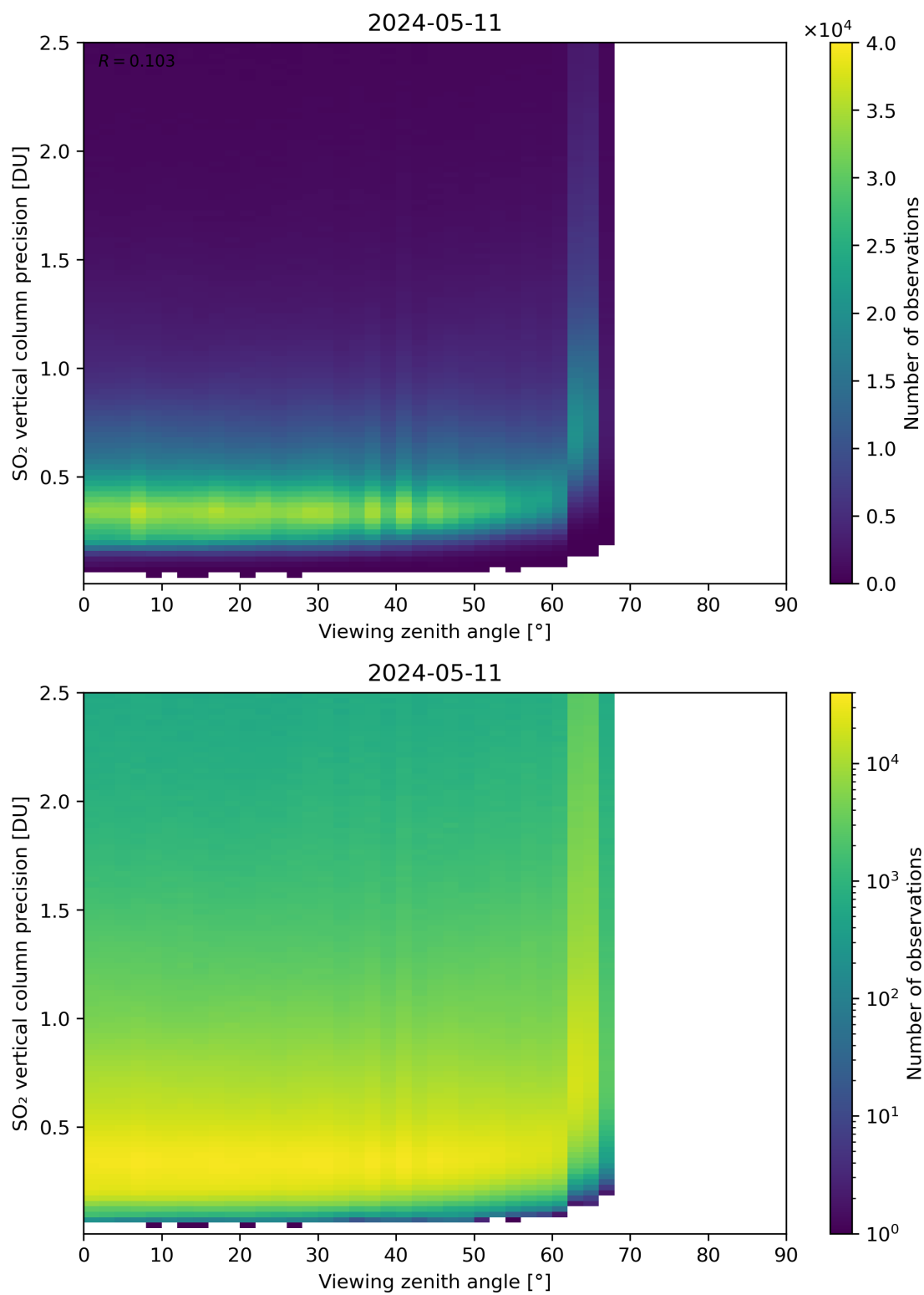
Figure 328: Scatter density plot of “Viewing zenith angle” against “SO 2 vertical column precision” for 2024-05-10 to 2024-05-12.
