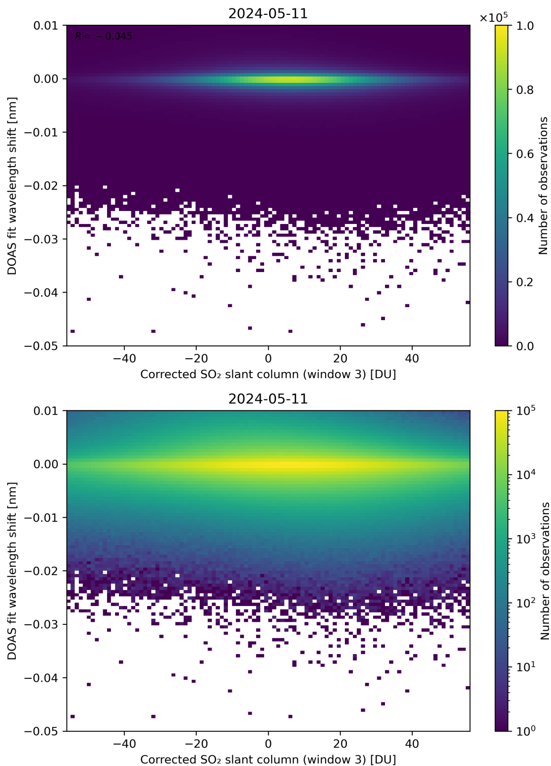
Figure 206: Scatter density plot of “Corrected SO 2 slant column (window 3)” against “DOAS fit wavelength shift” for 2024-05-10 to 2024-05-12.
