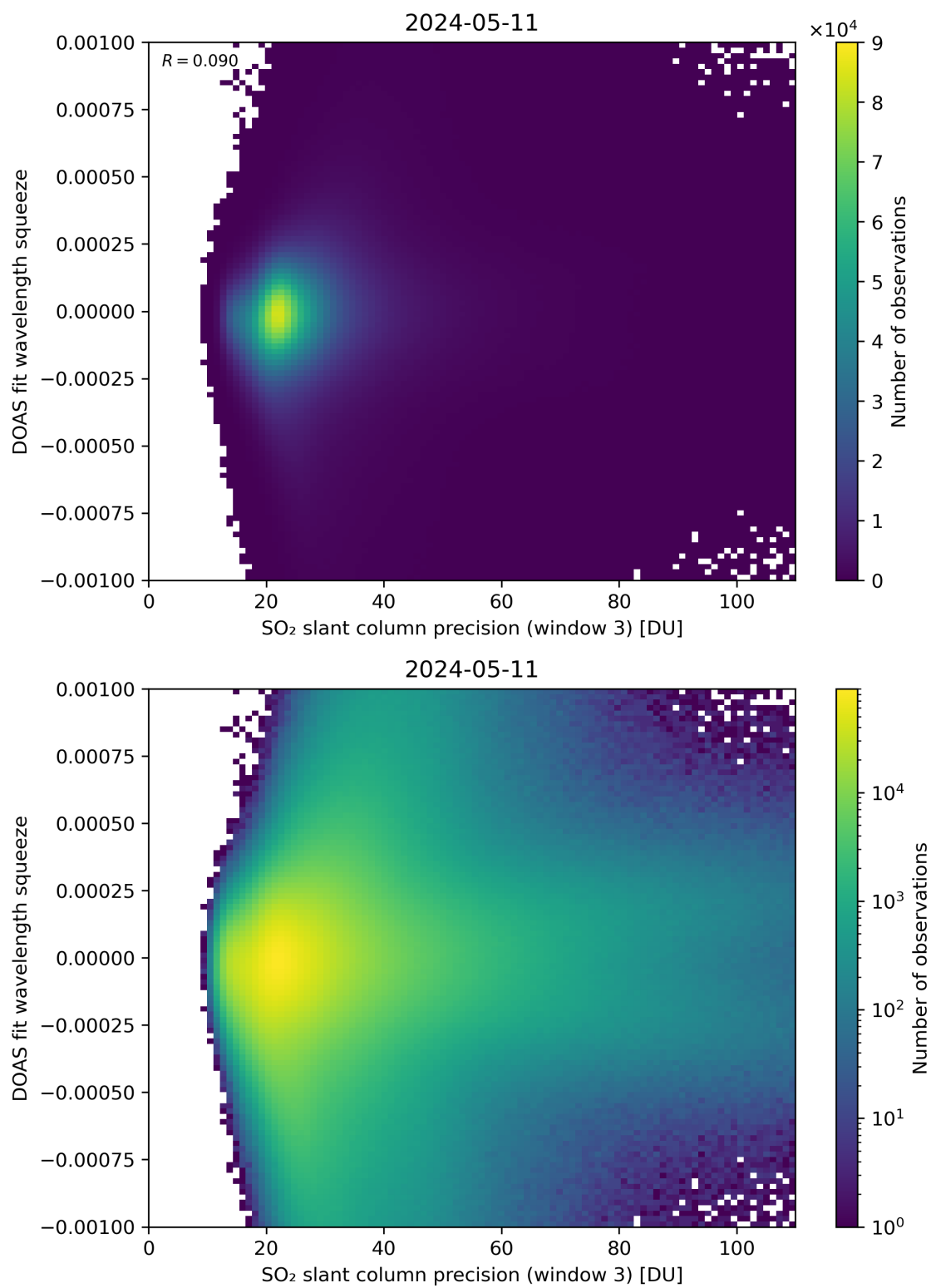
Figure 259: Scatter density plot of “SO 2 slant column precision (window 3)” against “DOAS fit wavelength squeeze” for 2024-05-10 to 2024-05-12.
