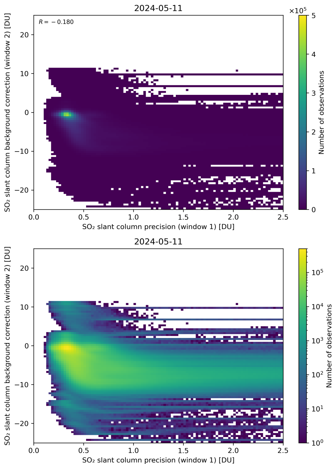
Figure 219: Scatter density plot of “SO 2 slant column precision (window 1)” against “SO 2 slant column background correction (window 2)” for 2024-05-10 to 2024-05-12.
