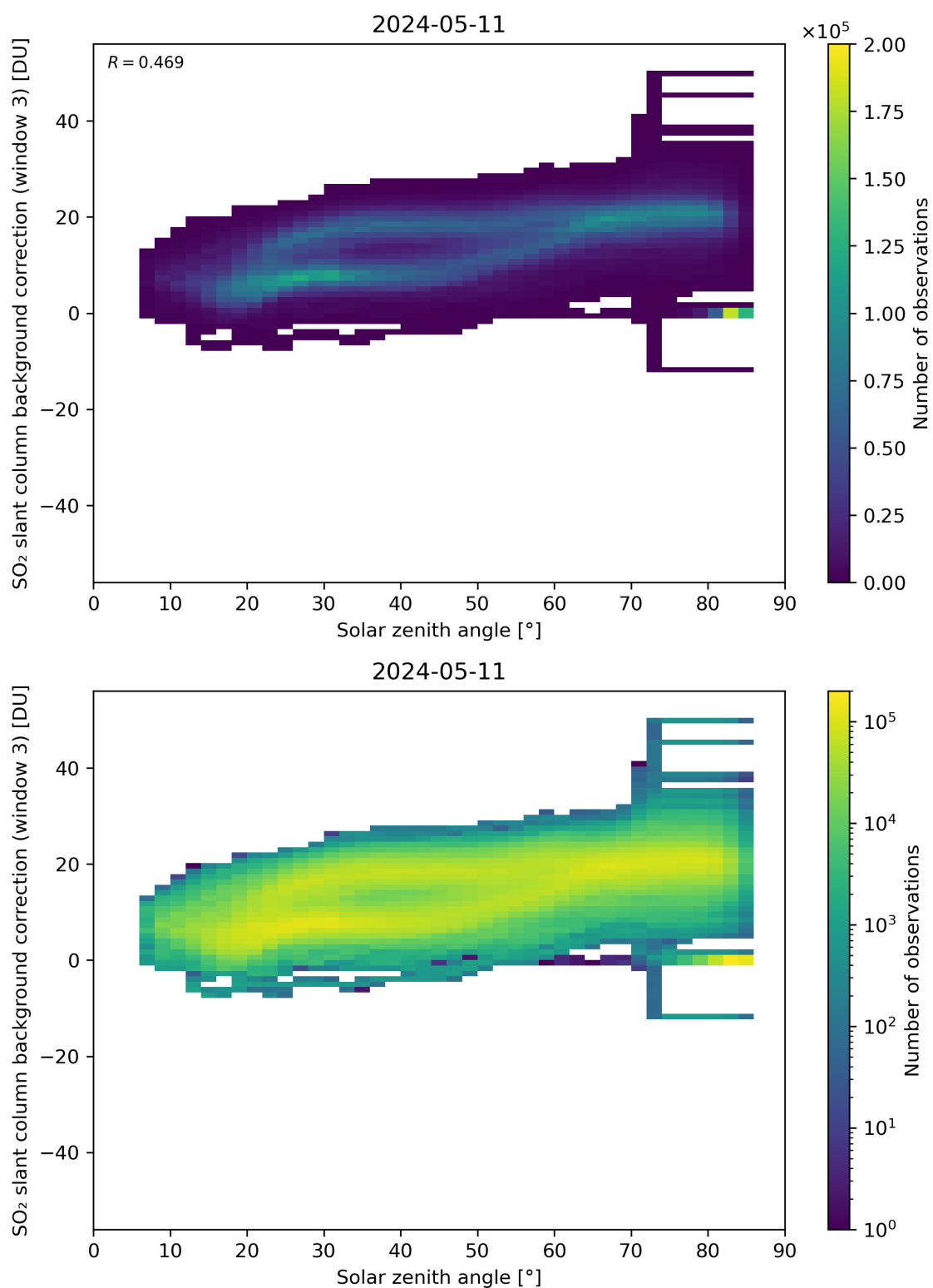
Figure 160: Scatter density plot of “Solar zenith angle” against “SO 2 slant column background correction (window 3)” for 2024-05-10 to 2024-05-12.
