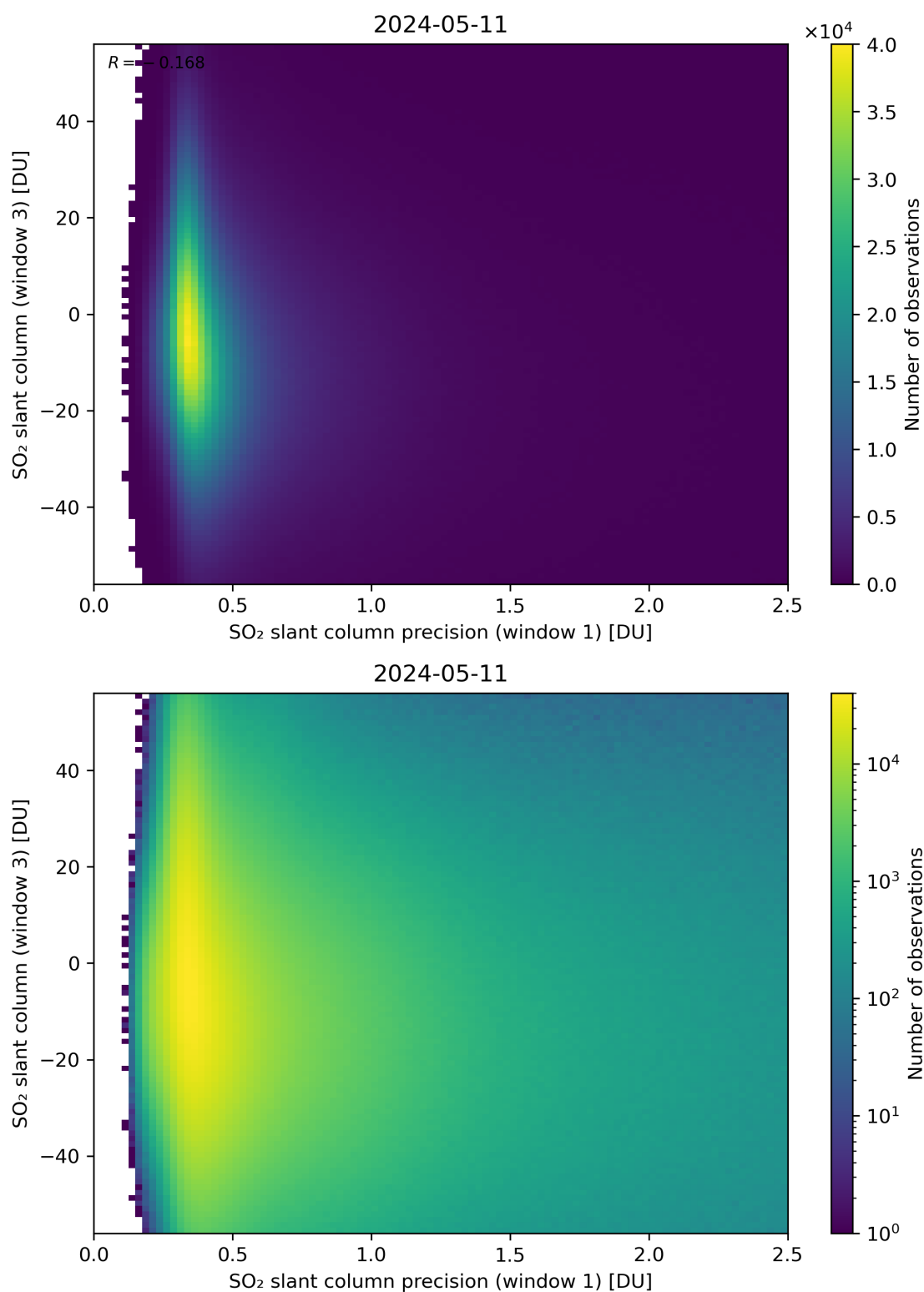
Figure 228: Scatter density plot of “SO 2 slant column precision (window 1)” against “SO 2 slant column (window 3)” for 2024-05-10 to 2024-05-12.
