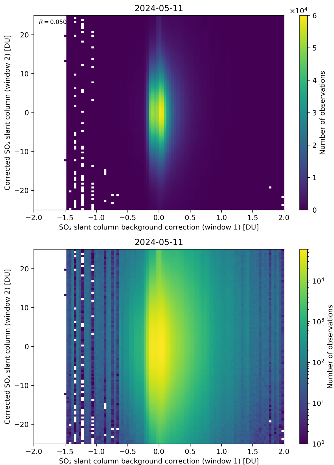
Figure 104: Scatter density plot of “SO 2 slant column background correction (window 1)” against “Corrected SO 2 slant column (window 2)” for 2024-05-10 to 2024-05-12.
