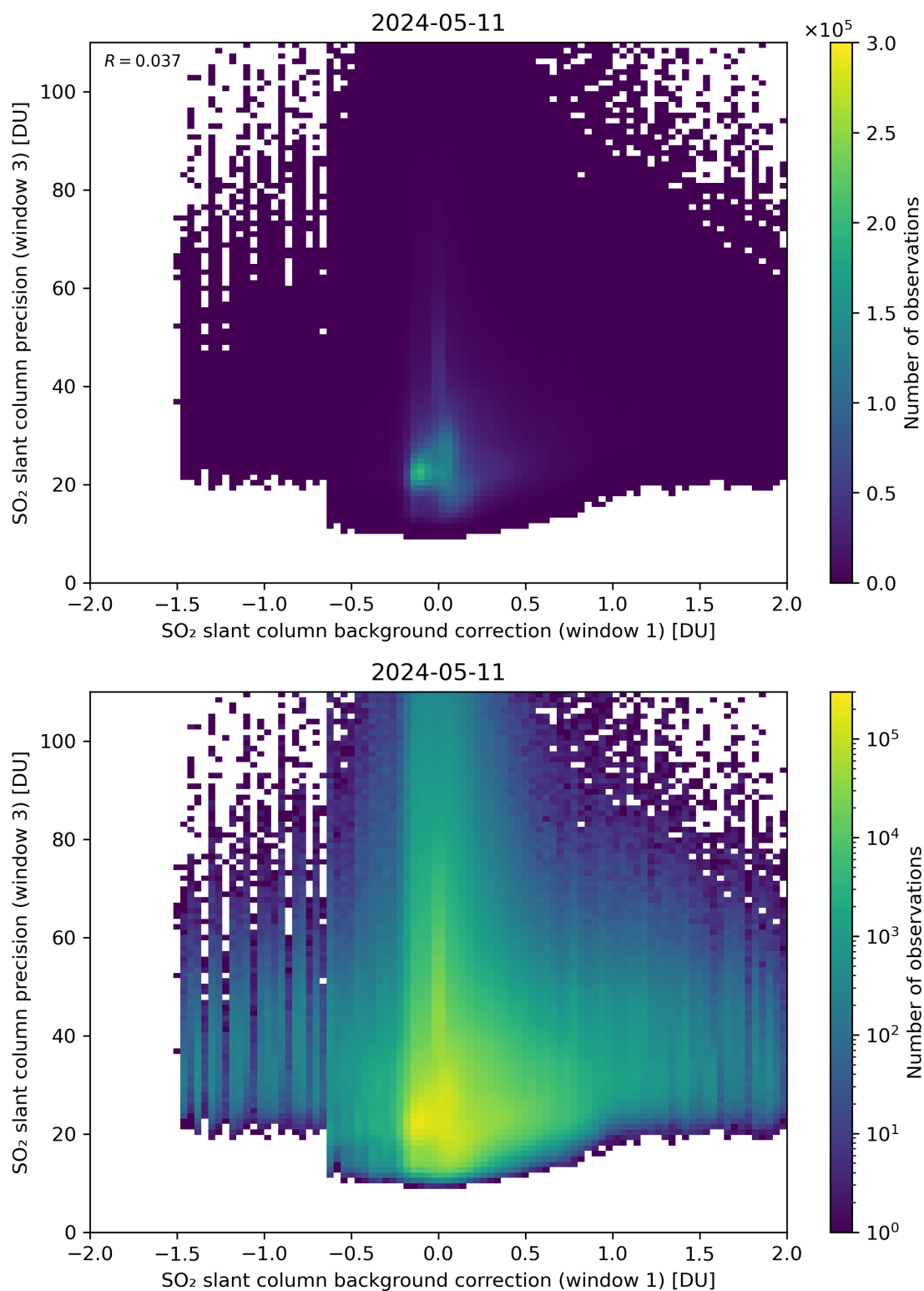
Figure 108: Scatter density plot of “SO 2 slant column background correction (window 1)” against “SO 2 slant column precision (window 3)” for 2024-05-10 to 2024-05-12.
