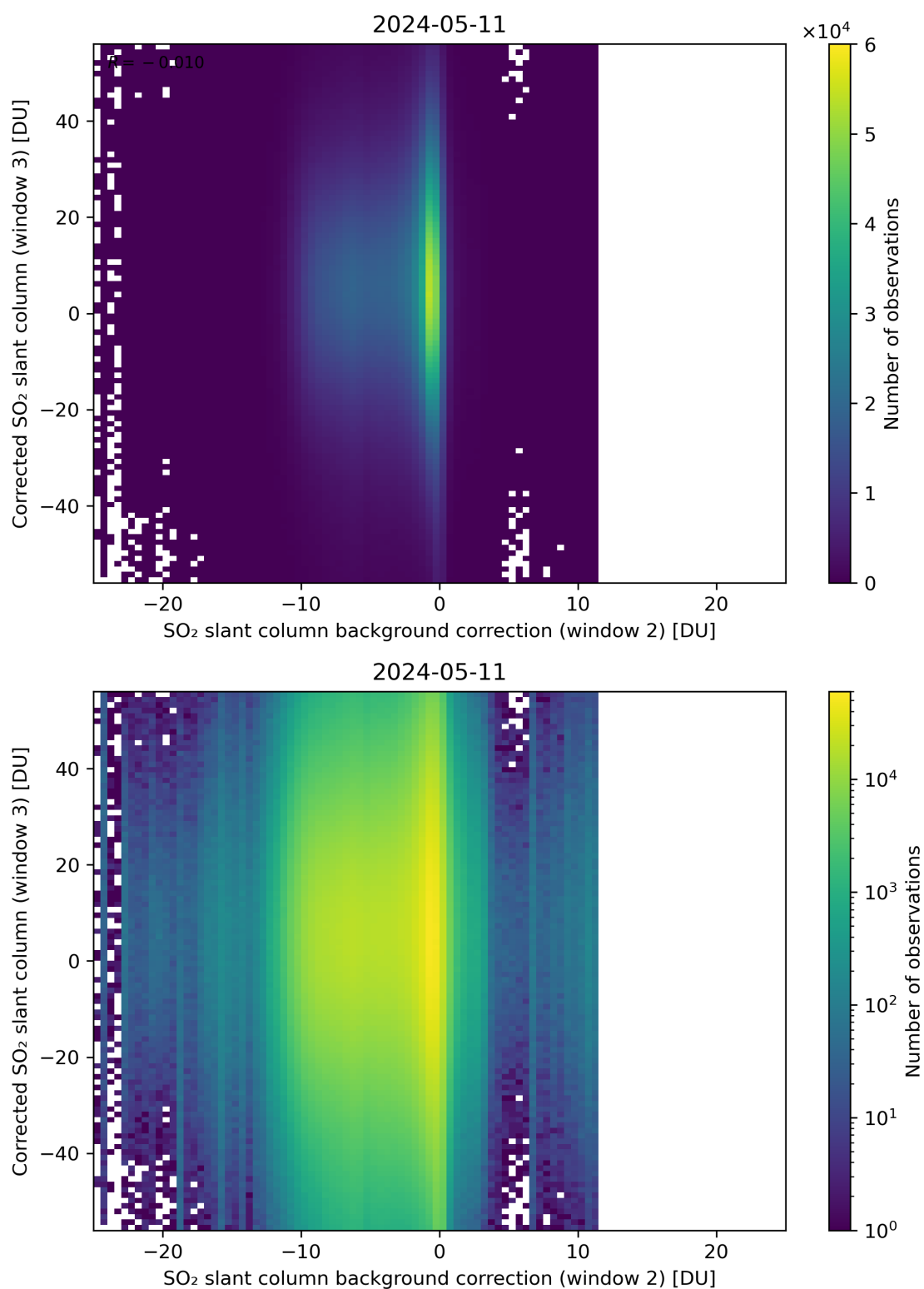
Figure 116: Scatter density plot of “SO 2 slant column background correction (window 2)” against “Corrected SO 2 slant column (window 3)” for 2024-05-10 to 2024-05-12.
