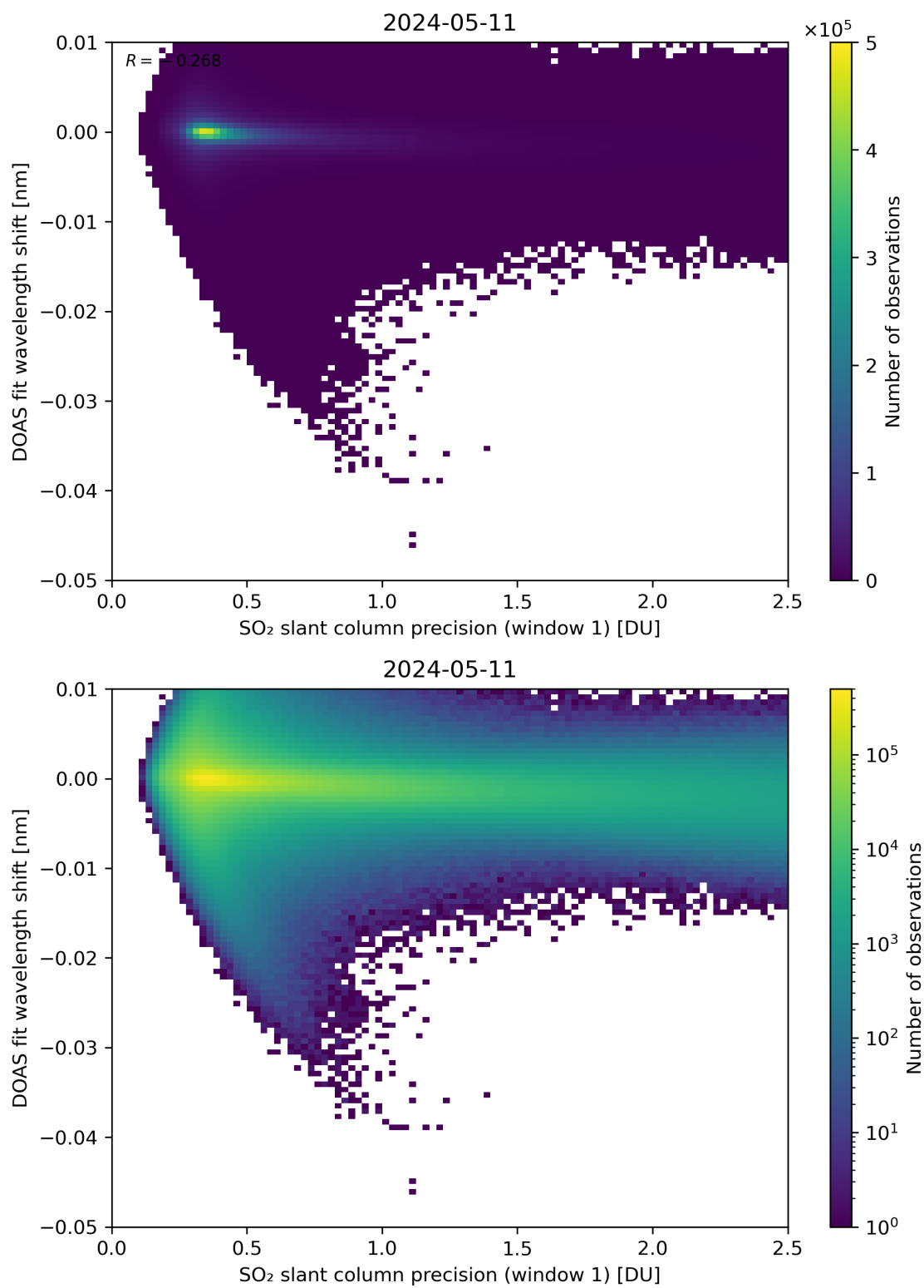
Figure 221: Scatter density plot of “SO 2 slant column precision (window 1)” against “DOAS fit wavelength shift” for 2024-05-10 to 2024-05-12.
