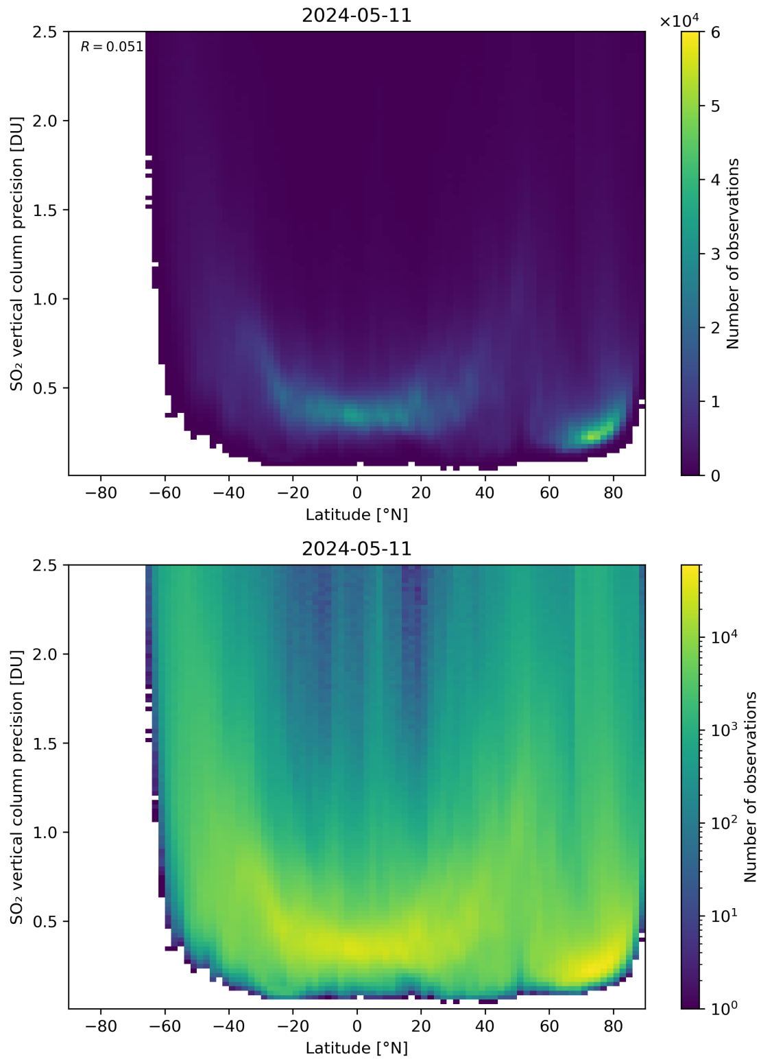
Figure 157: Scatter density plot of “Latitude” against “SO 2 vertical column precision” for 2024-05-10 to 2024-05-12.
