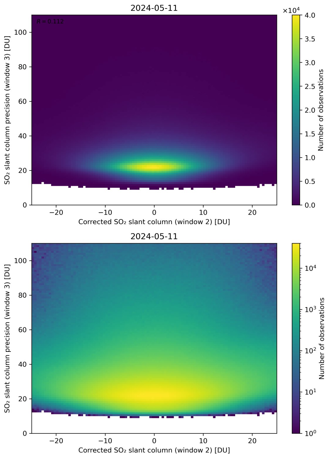
Figure 202: Scatter density plot of “Corrected SO 2 slant column (window 2)” against “SO 2 slant column precision (window 3)” for 2024-05-10 to 2024-05-12.
