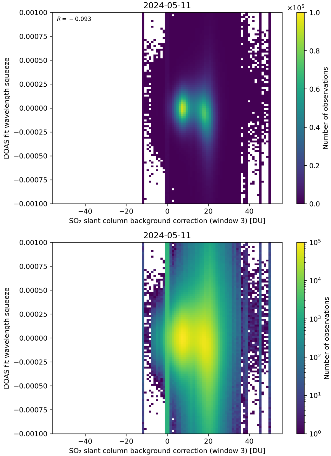
Figure 122: Scatter density plot of “SO 2 slant column background correction (window 3)” against “DOAS fit wavelength squeeze” for 2024-05-10 to 2024-05-12.
