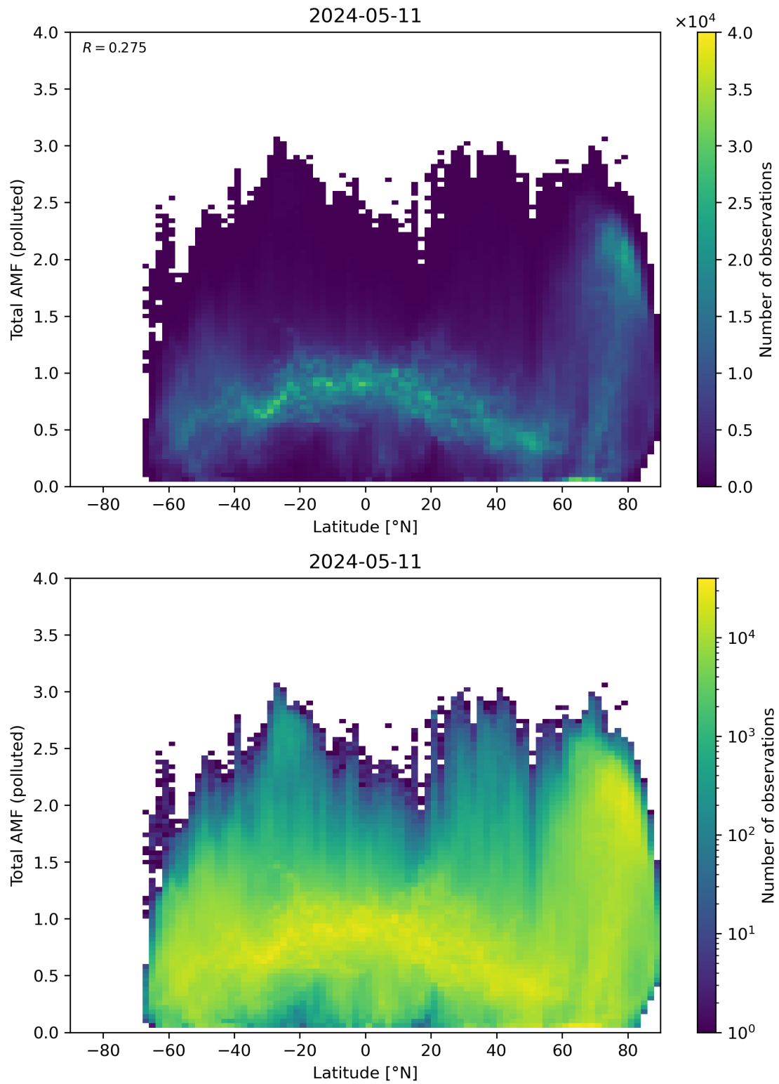
Figure 154: Scatter density plot of “Latitude” against “Total AMF (polluted)” for 2024-05-10 to 2024-05-12.
