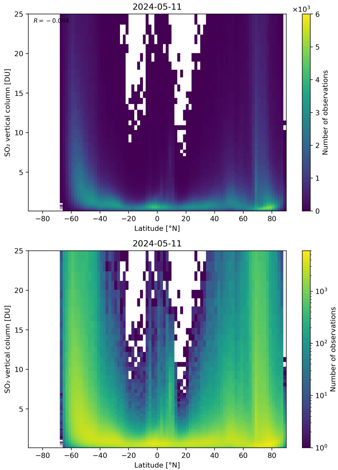
Figure 156: Scatter density plot of “Latitude” against “SO 2 vertical column” for 2024-05-10 to 2024-05-12.
