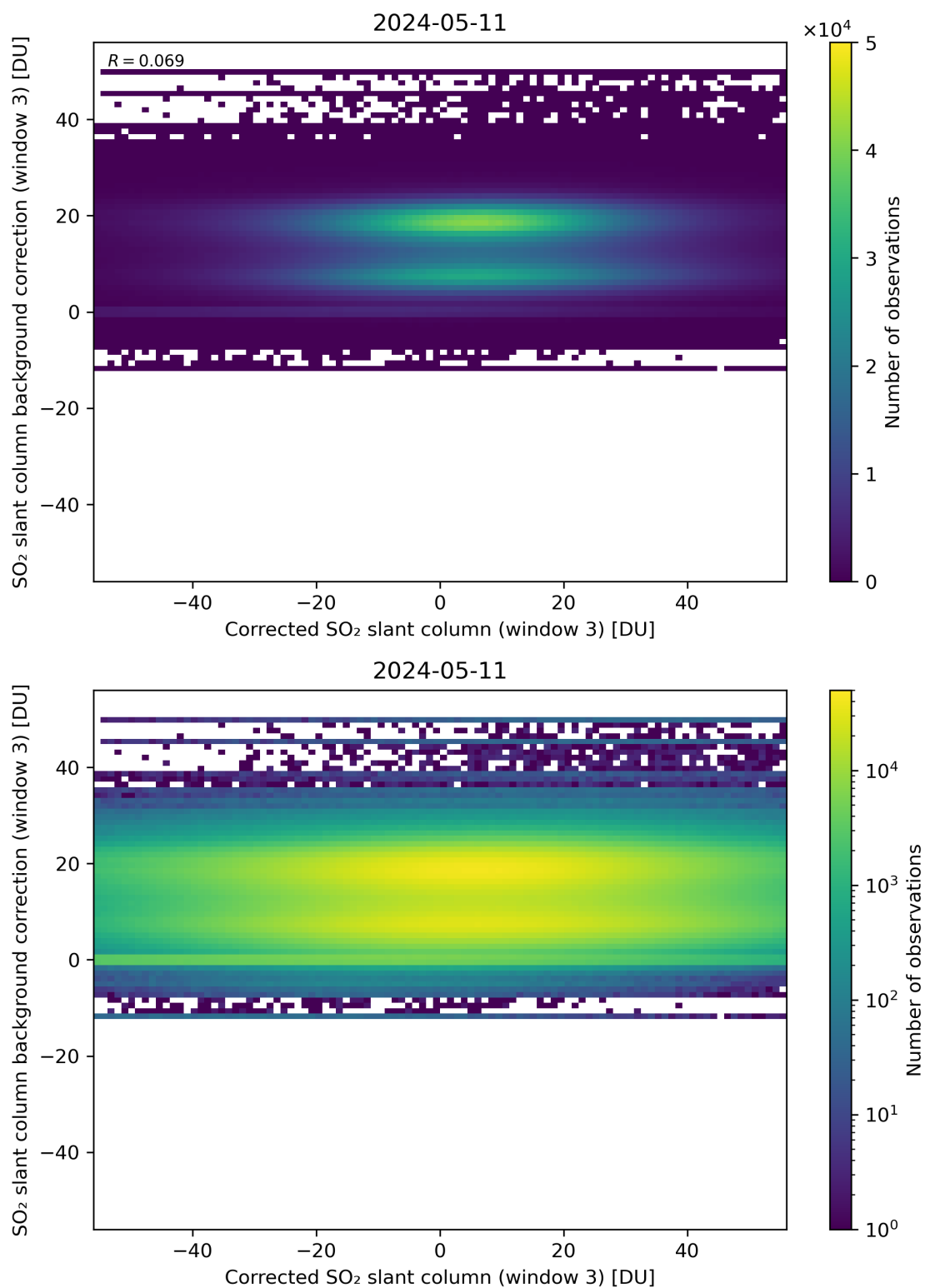
Figure 205: Scatter density plot of “Corrected SO 2 slant column (window 3)” against “SO 2 slant column background correction (window 3)” for 2024-05-10 to 2024-05-12.
