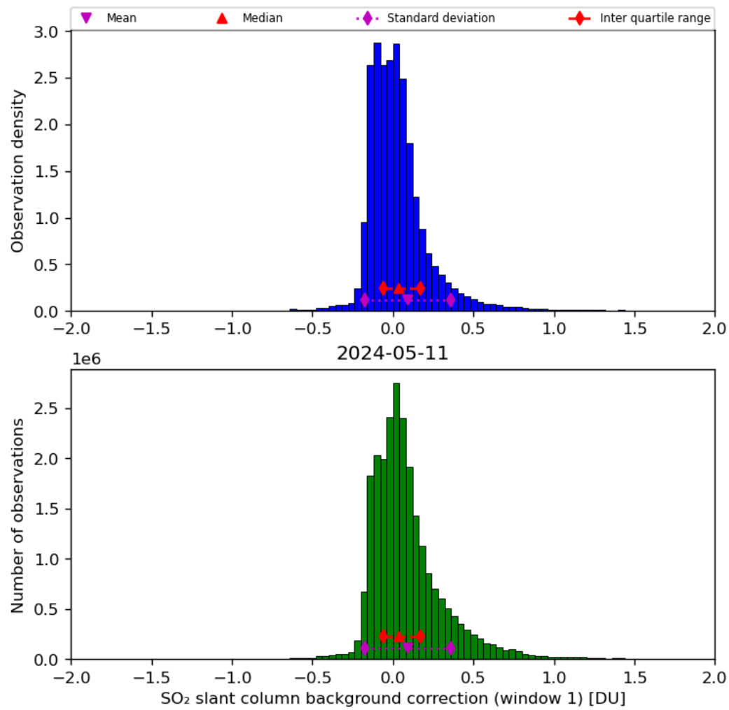
Figure 59: Histogram of “SO 2 slant column background correction (window 1)” for 2024-05-10 to 2024-05-12
