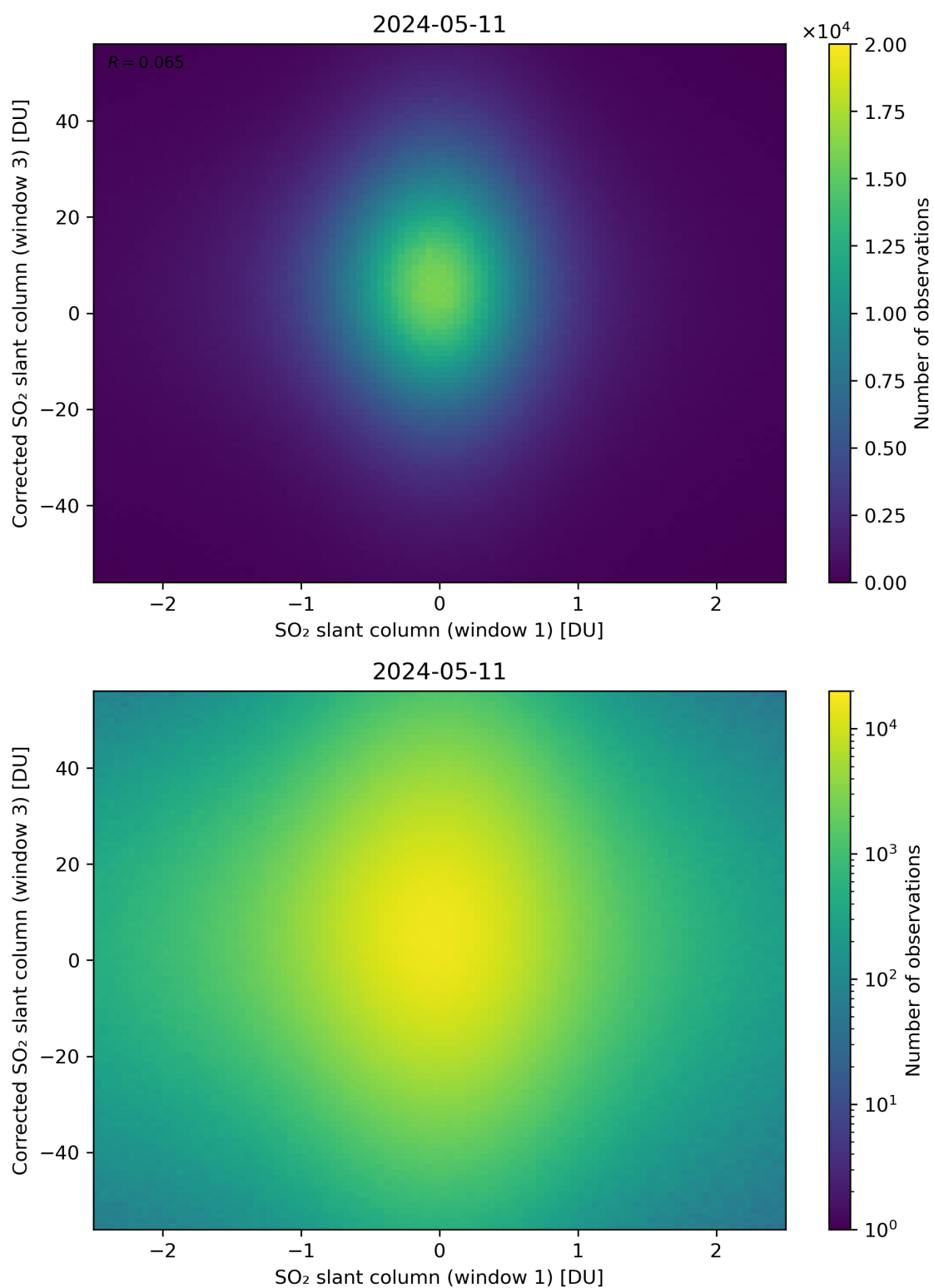
Figure 234: Scatter density plot of “SO 2 slant column (window 1)” against “Corrected SO 2 slant column (window 3)” for 2024-05-10 to 2024-05-12.
