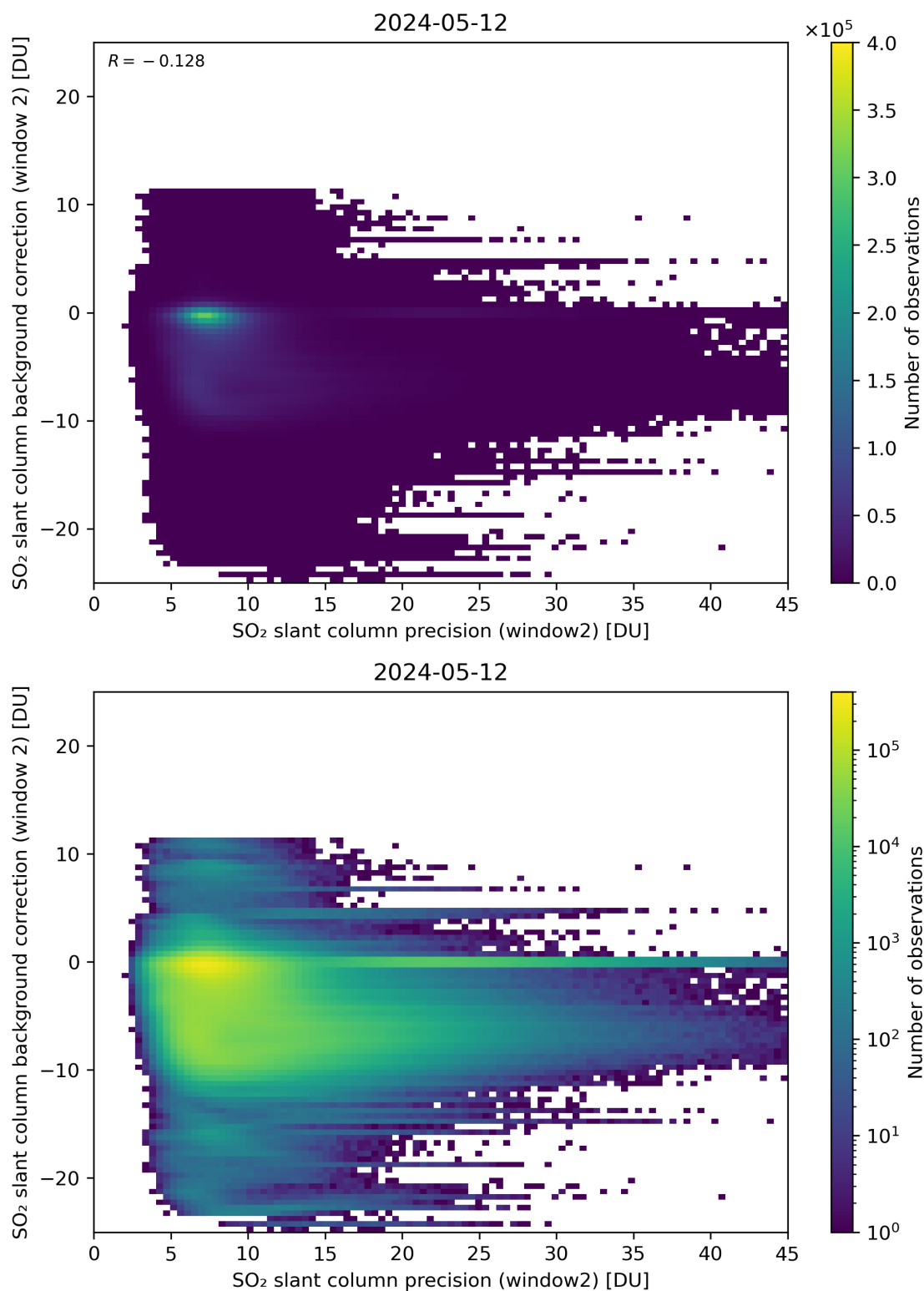
Figure 241: Scatter density plot of “SO 2 slant column precision (window2)” against “SO 2 slant column background correction (window 2)” for 2024-05-12 to 2024-05-13.
