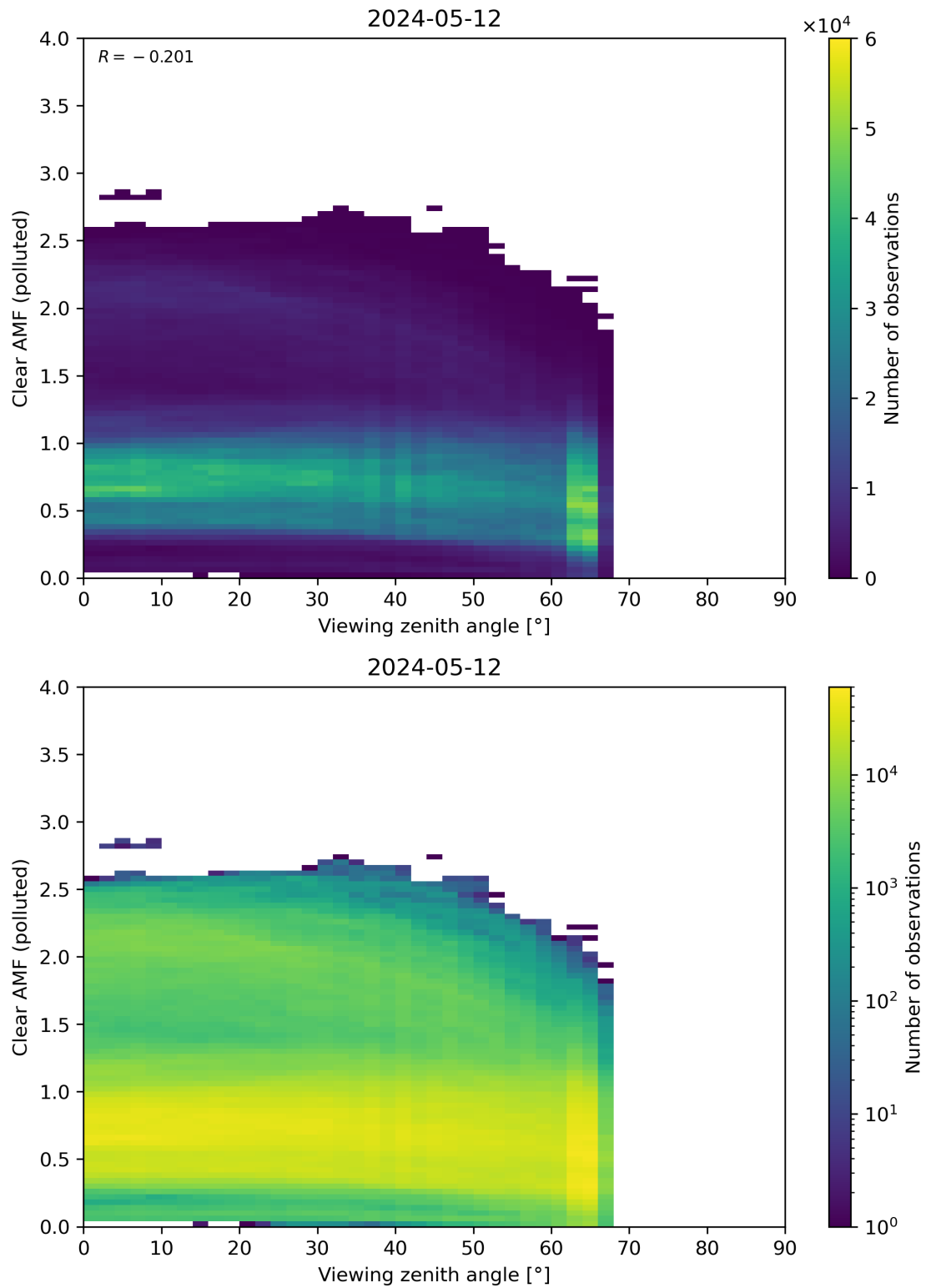
Figure 316: Scatter density plot of “Viewing zenith angle” against “Clear AMF (polluted)” for 2024-05-12 to 2024-05-13.
