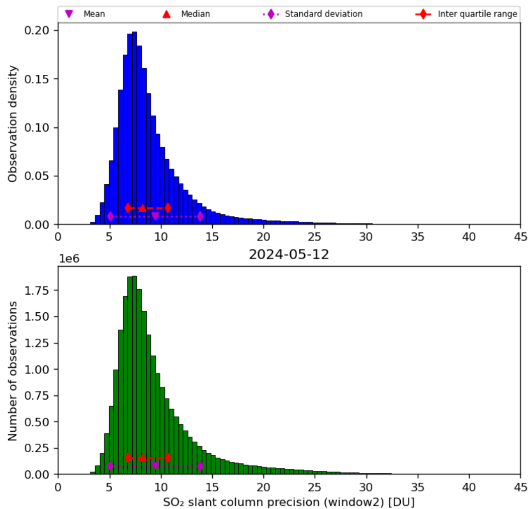
Figure 61: Histogram of “SO 2 slant column precision (window2)” for 2024-05-12 to 2024-05-13
