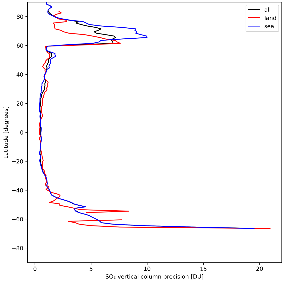
Figure 31: Zonal average of “SO 2 vertical column precision” for 2024-05-12 to 2024-05-13.
