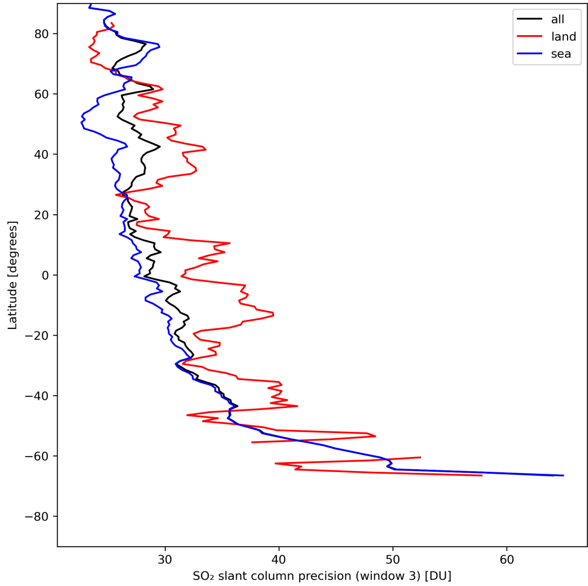
Figure 42: Zonal average of “SO 2 slant column precision (window 3)” for 2024-05-12 to 2024-05-13.
