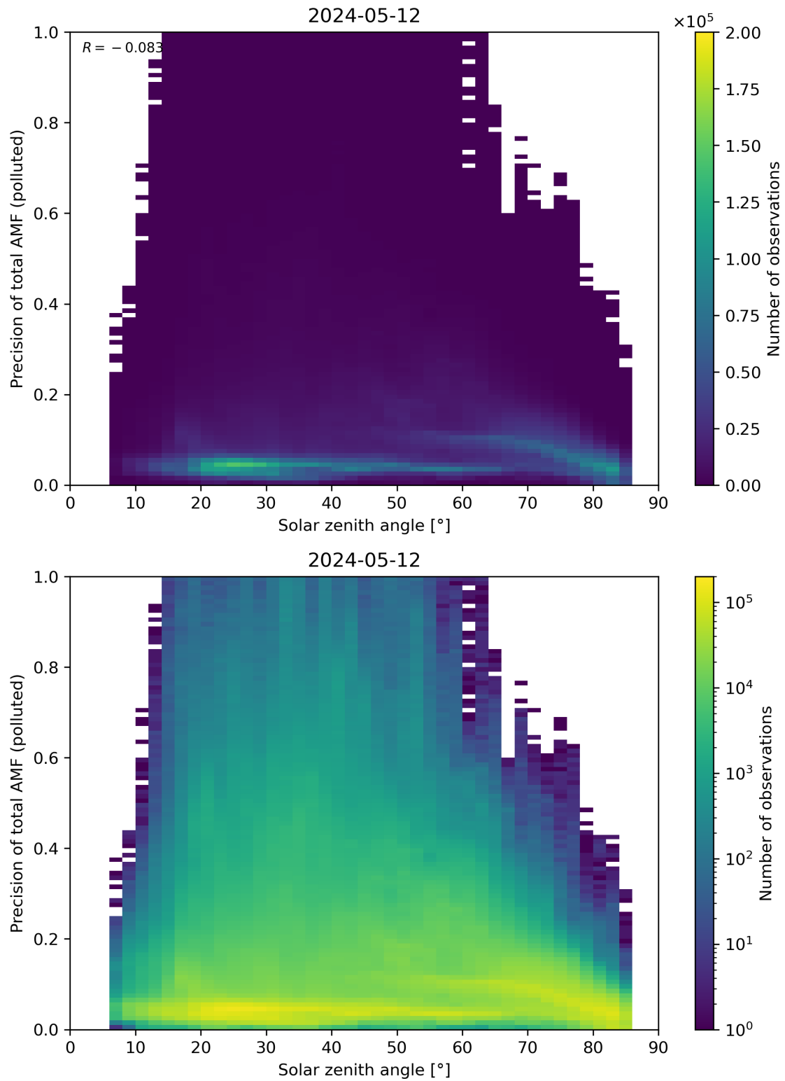
Figure 175: Scatter density plot of “Solar zenith angle” against “Precision of total AMF (polluted)” for 2024-05-12 to 2024-05-13.
