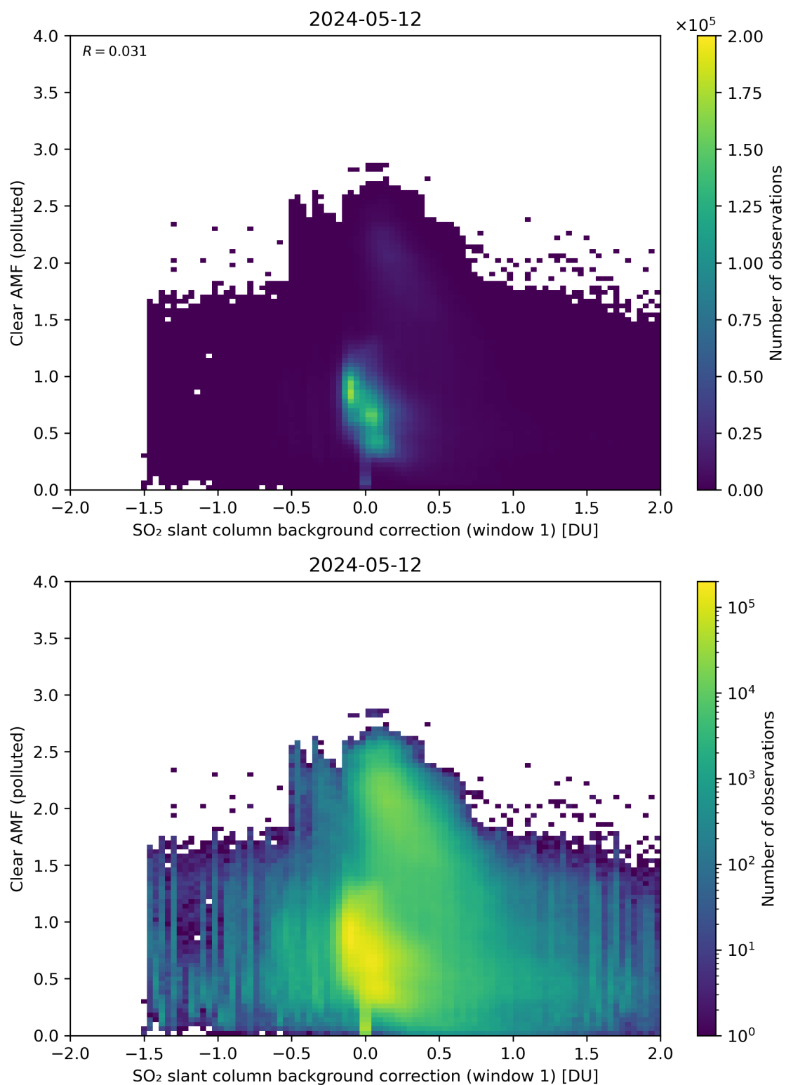
Figure 103: Scatter density plot of “SO 2 slant column background correction (window 1)” against “Clear AMF (polluted)” for 2024-05-12 to 2024-05-13.
