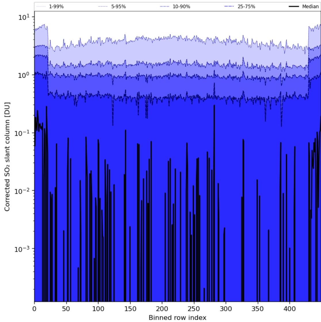
Figure 78: Along track statistics of “Corrected SO 2 slant column” for 2024-05-12 to 2024-05-13
