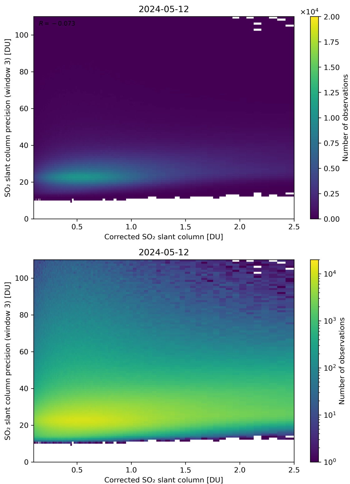
Figure 191: Scatter density plot of “Corrected SO 2 slant column” against “SO 2 slant column precision (window 3)” for 2024-05-12 to 2024-05-13.
