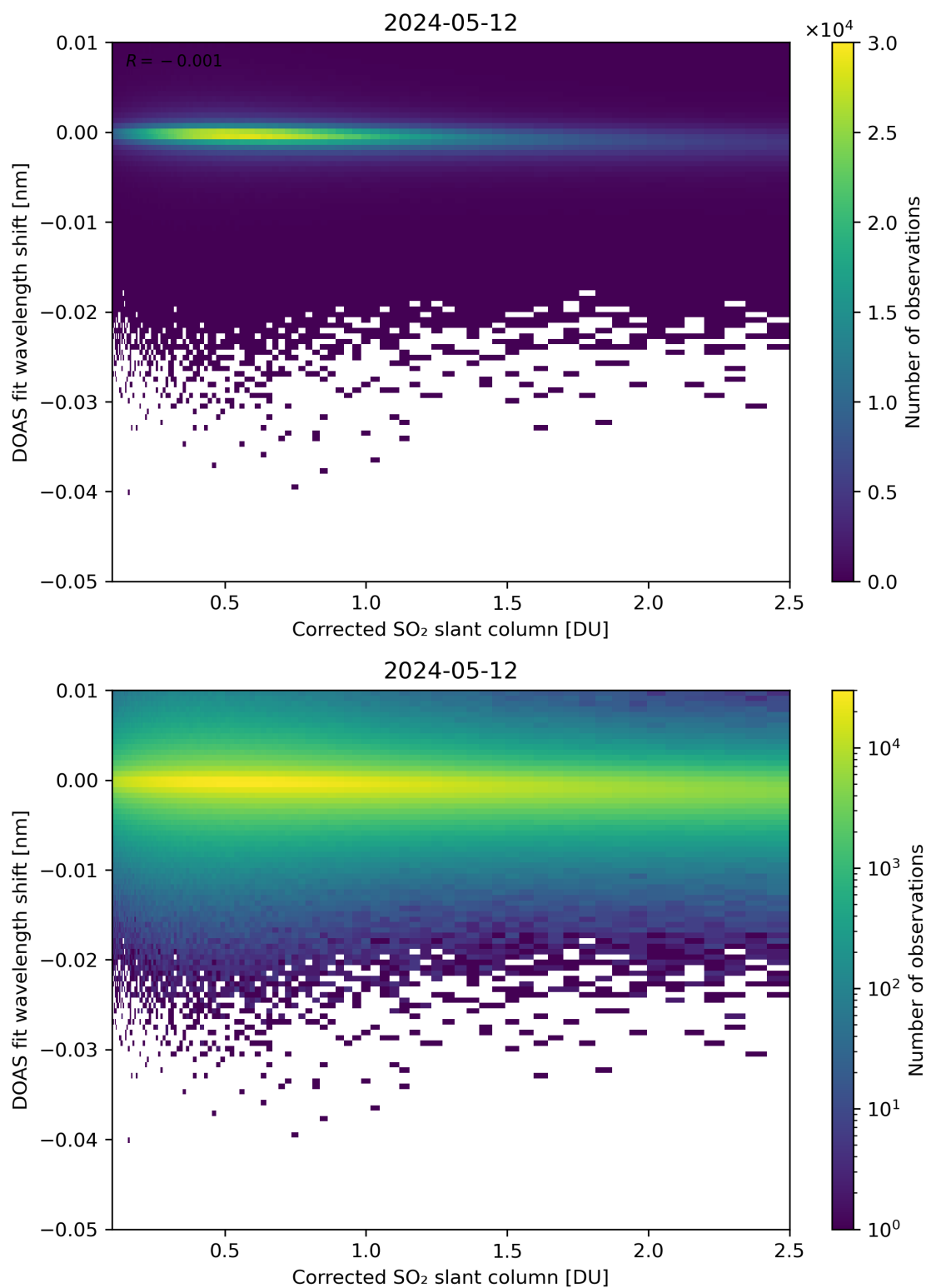
Figure 181: Scatter density plot of “Corrected SO 2 slant column” against “DOAS fit wavelength shift” for 2024-05-12 to 2024-05-13.
