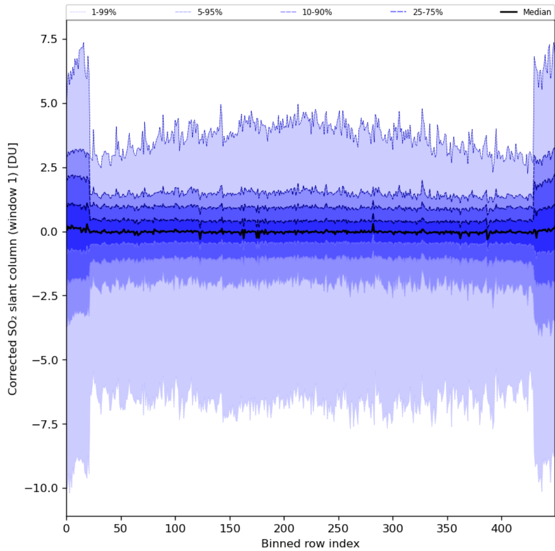
Figure 81: Along track statistics of “Corrected SO 2 slant column (window 1)” for 2024-05-12 to 2024-05-13
