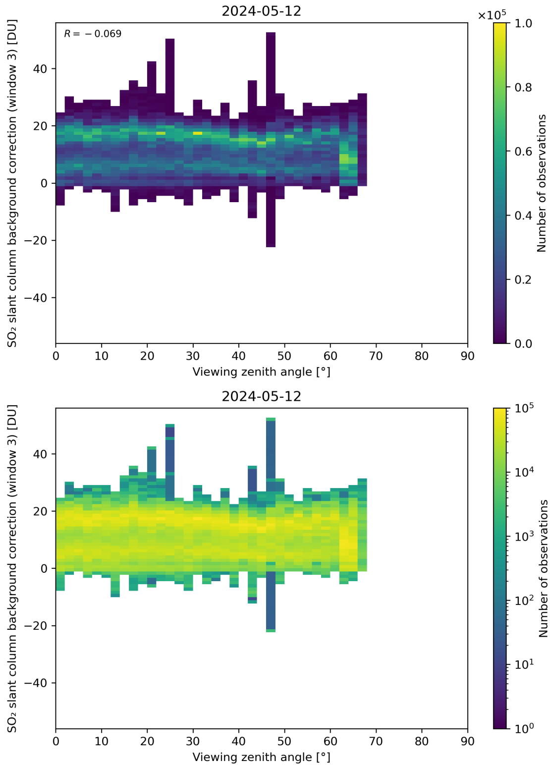
Figure 310: Scatter density plot of “Viewing zenith angle” against “SO 2 slant column background correction (window 3)” for 2024-05-12 to 2024-05-13.
