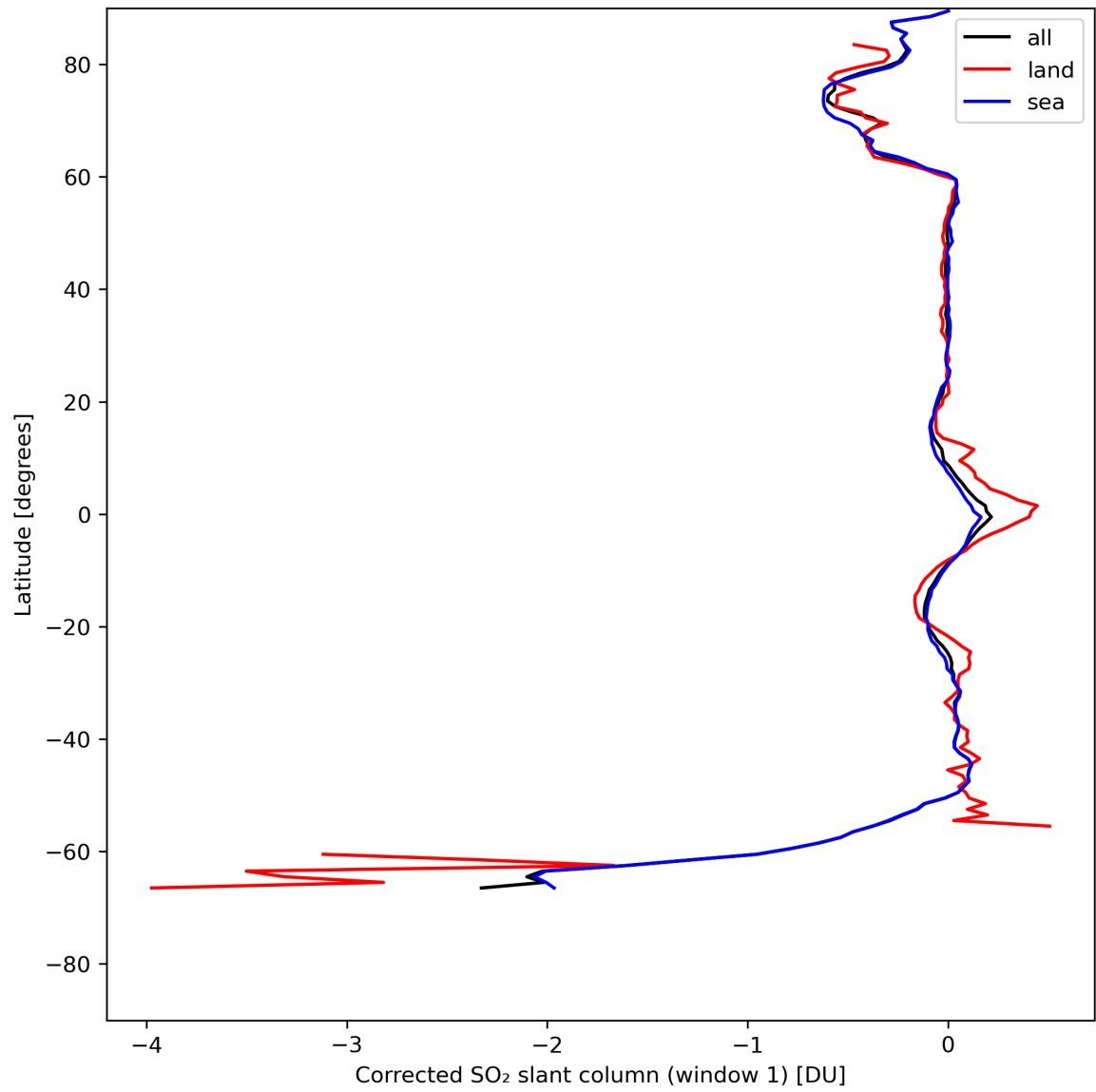
Figure 35: Zonal average of “Corrected SO 2 slant column (window 1)” for 2024-05-12 to 2024-05-13.
