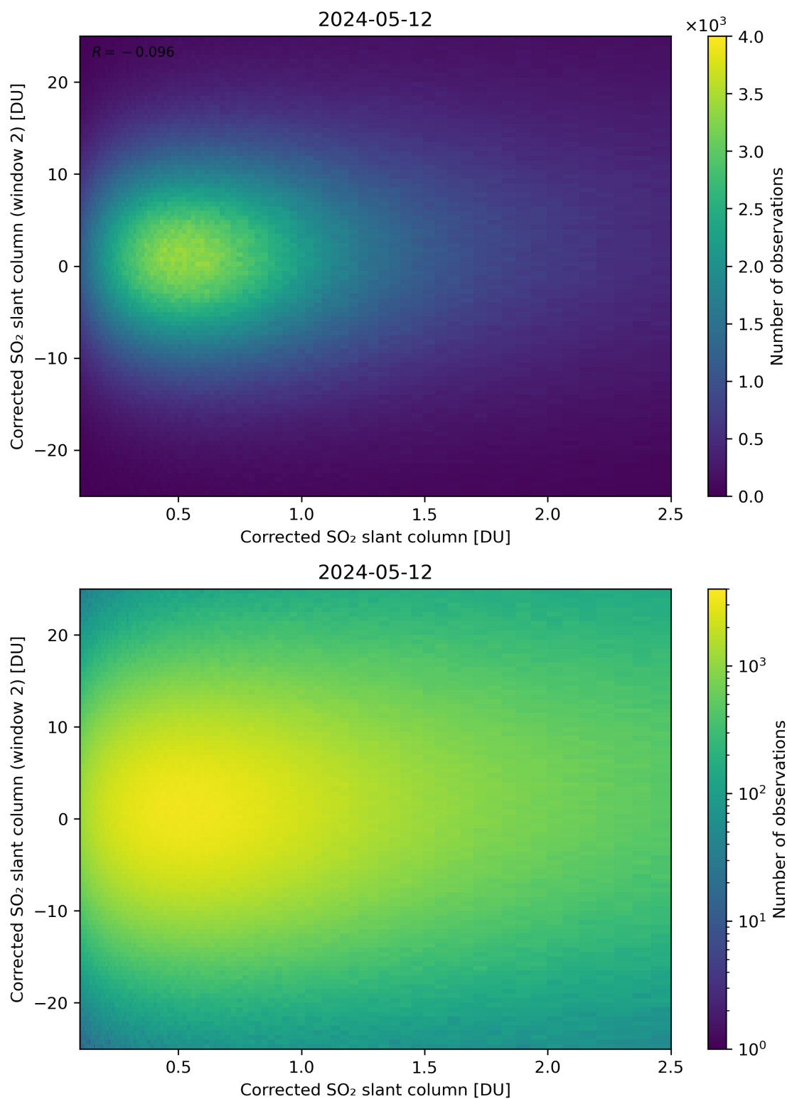
Figure 185: Scatter density plot of “Corrected SO 2 slant column” against “Corrected SO 2 slant column (window 2)” for 2024-05-12 to 2024-05-13.
