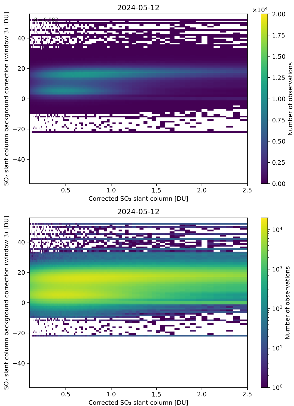
Figure 180: Scatter density plot of “Corrected SO 2 slant column” against “SO 2 slant column background correction (window 3)” for 2024-05-12 to 2024-05-13.
