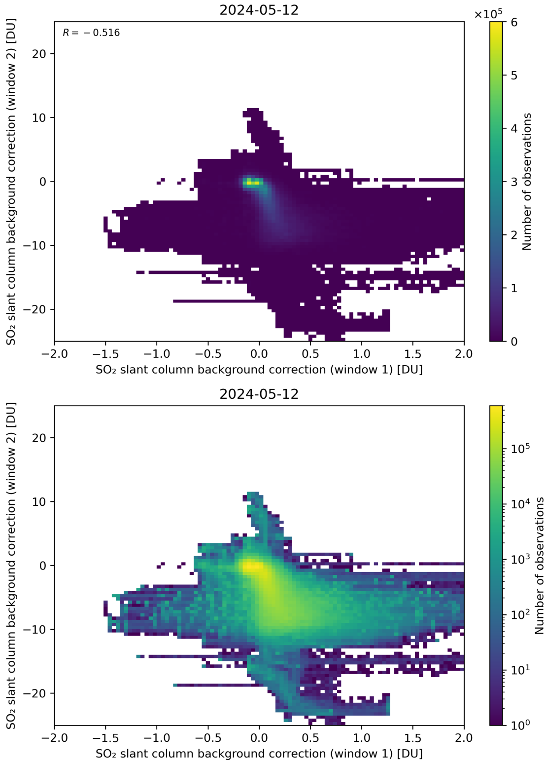
Figure 98: Scatter density plot of “SO 2 slant column background correction (window 1)” against “SO 2 slant column background correction (window 2)” for 2024-05-12 to 2024-05-13.
