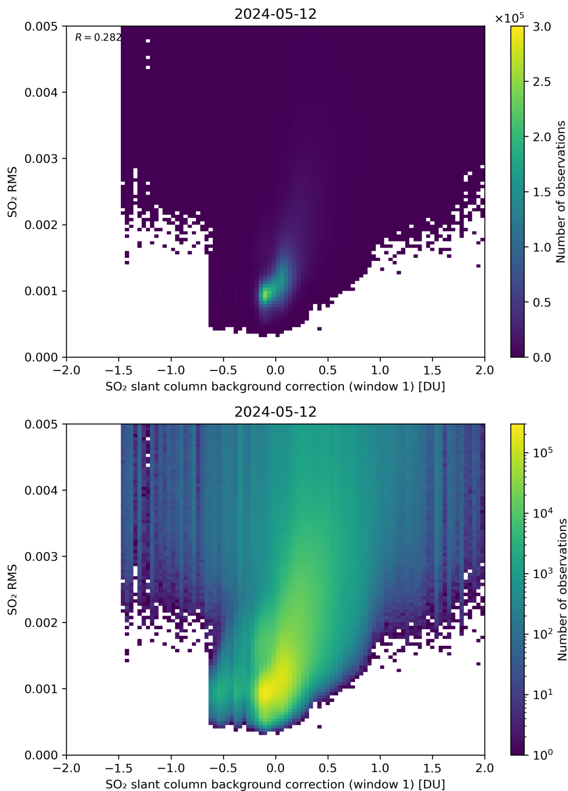
Figure 102: Scatter density plot of “SO 2 slant column background correction (window 1)” against “SO 2 RMS” for 2024-05-12 to 2024-05-13.
