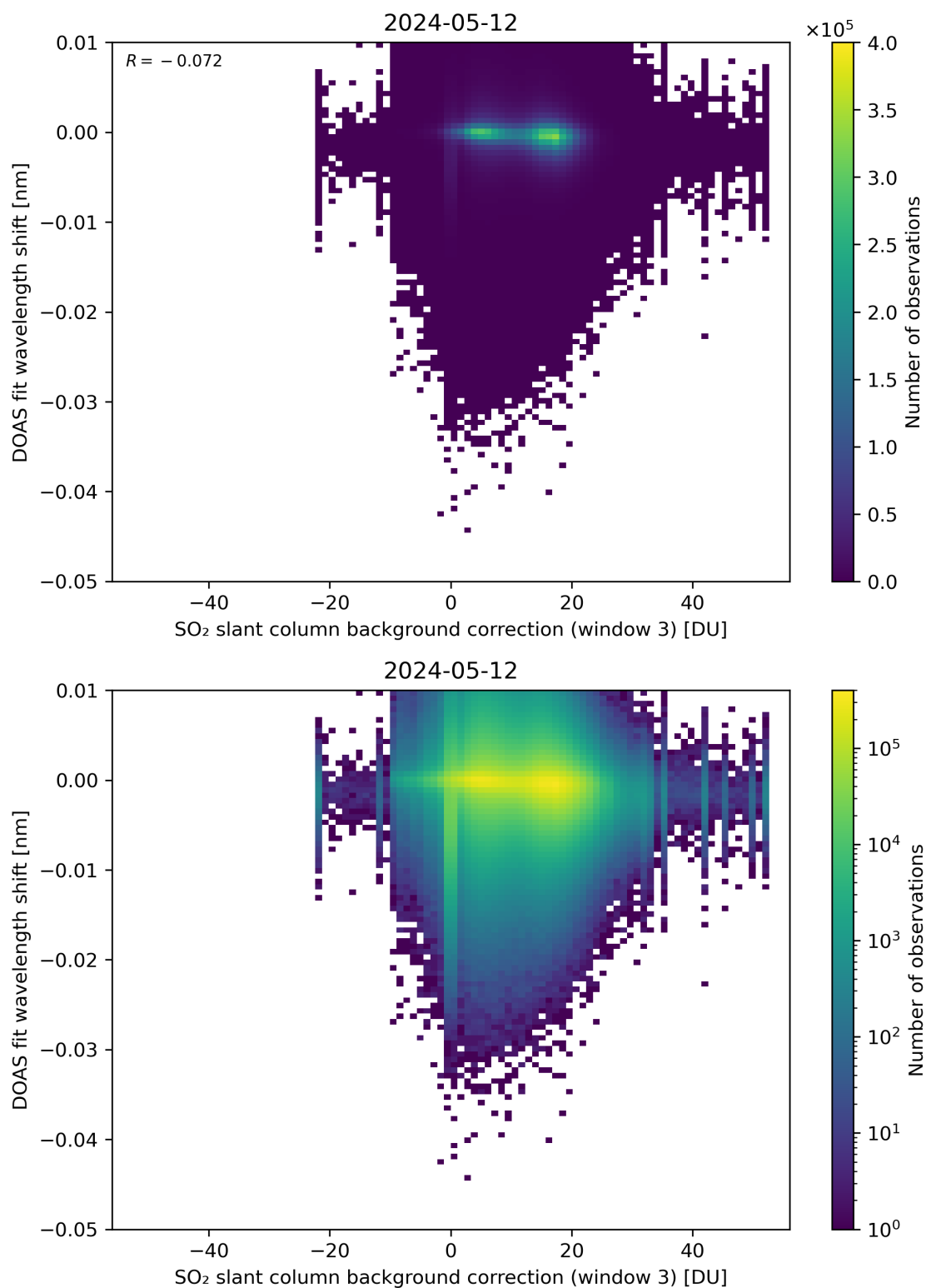
Figure 121: Scatter density plot of “SO 2 slant column background correction (window 3)” against “DOAS fit wavelength shift” for 2024-05-12 to 2024-05-13.
