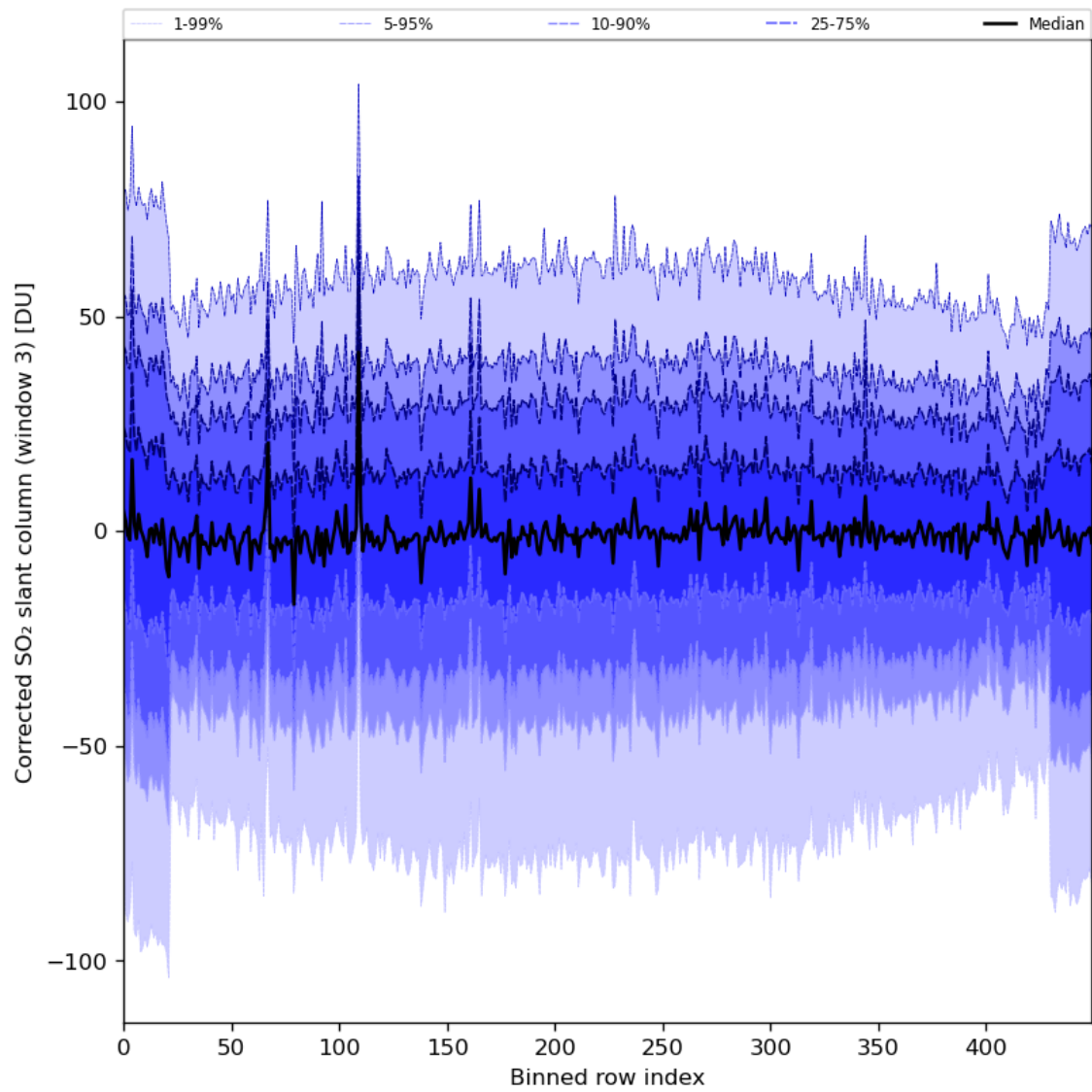
Figure 89: Along track statistics of “Corrected SO 2 slant column (window 3)” for 2024-05-12 to 2024-05-13
