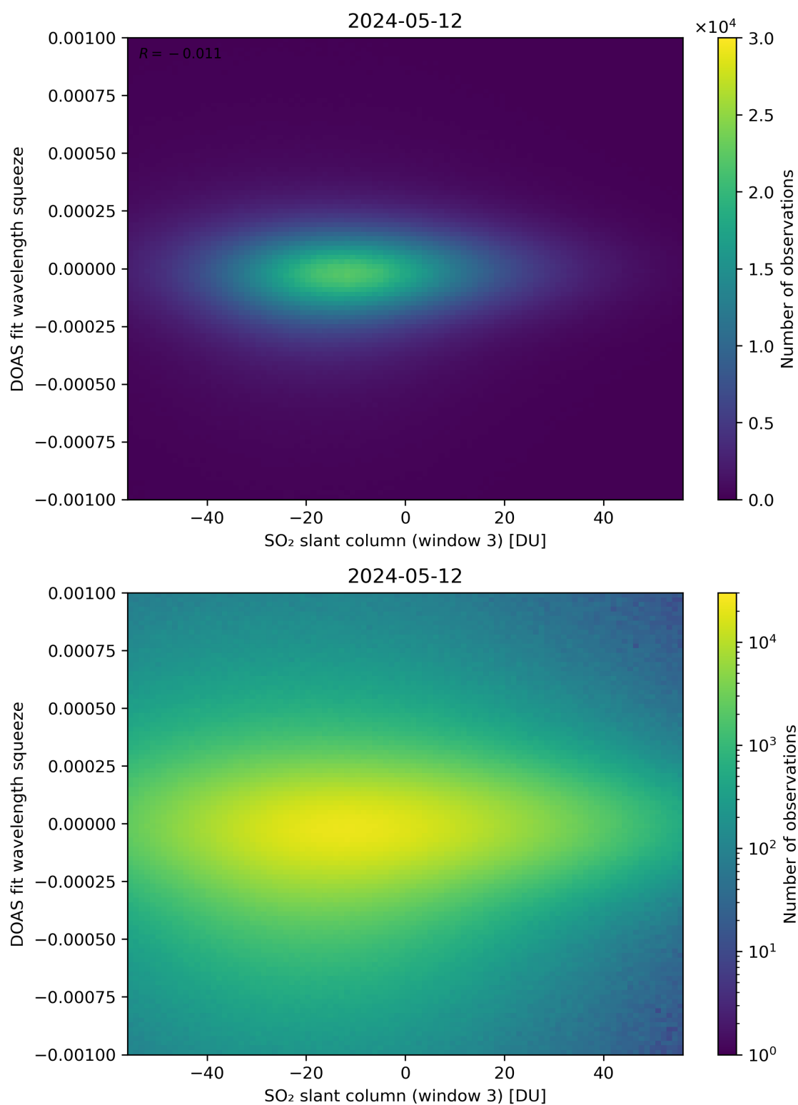
Figure 255: Scatter density plot of “SO 2 slant column (window 3)” against “DOAS fit wavelength squeeze” for 2024-05-12 to 2024-05-13.
