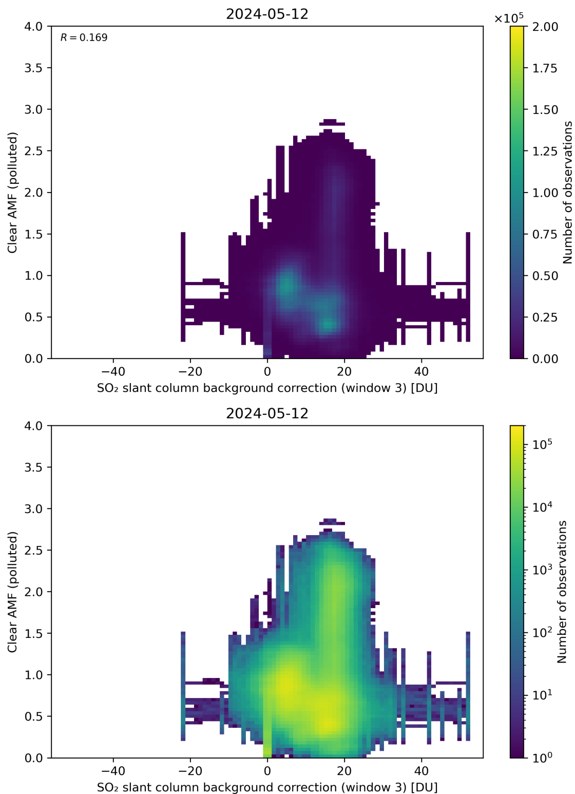
Figure 124: Scatter density plot of “SO 2 slant column background correction (window 3)” against “Clear AMF (polluted)” for 2024-05-12 to 2024-05-13.
