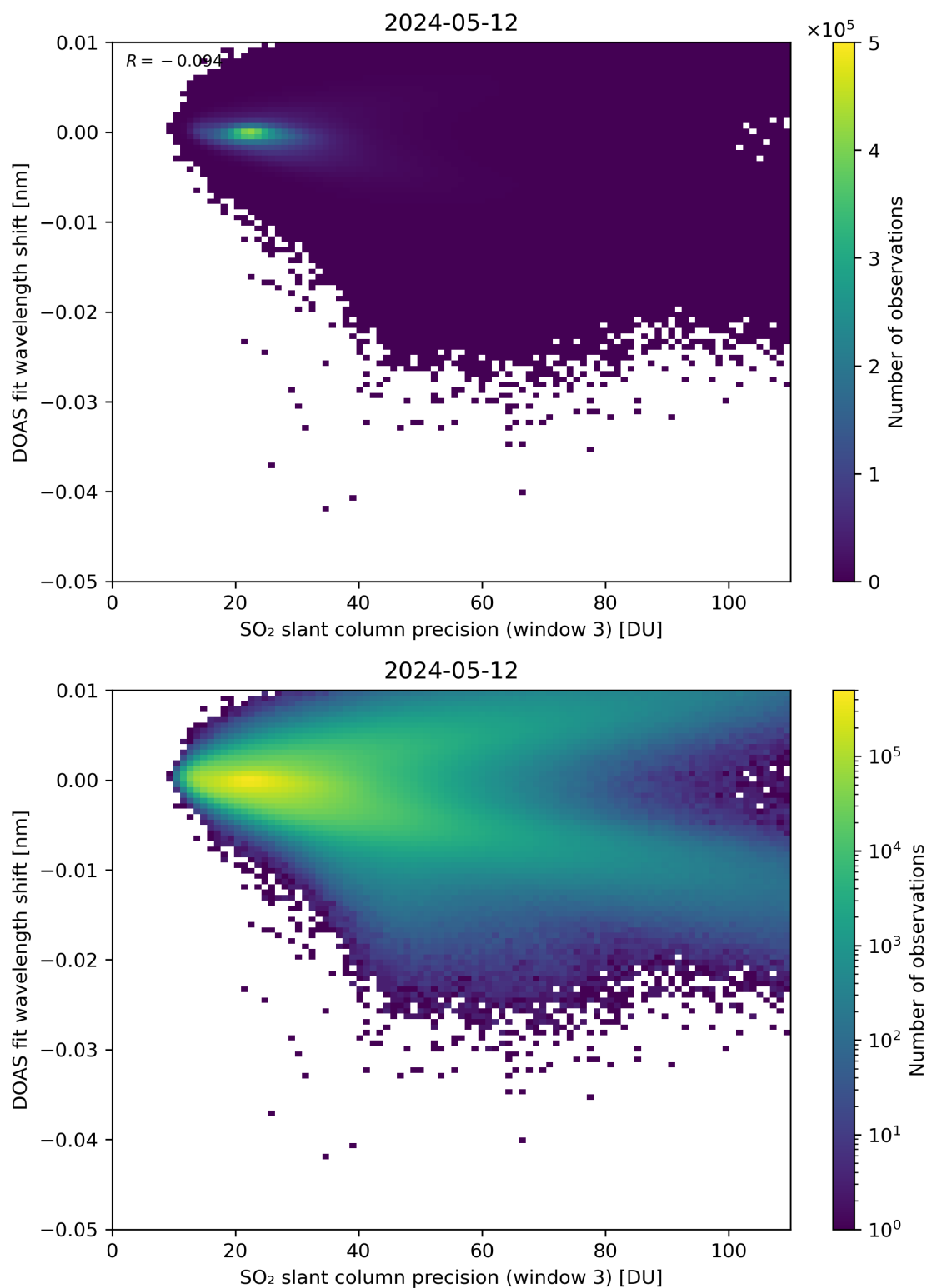
Figure 258: Scatter density plot of “SO 2 slant column precision (window 3)” against “DOAS fit wavelength shift” for 2024-05-12 to 2024-05-13.
