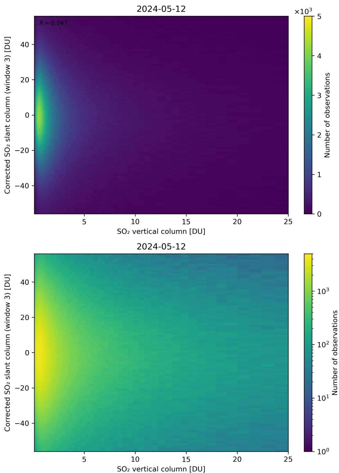
Figure 299: Scatter density plot of “SO 2 vertical column” against “Corrected SO 2 slant column (window 3)” for 2024-05-12 to 2024-05-13.
