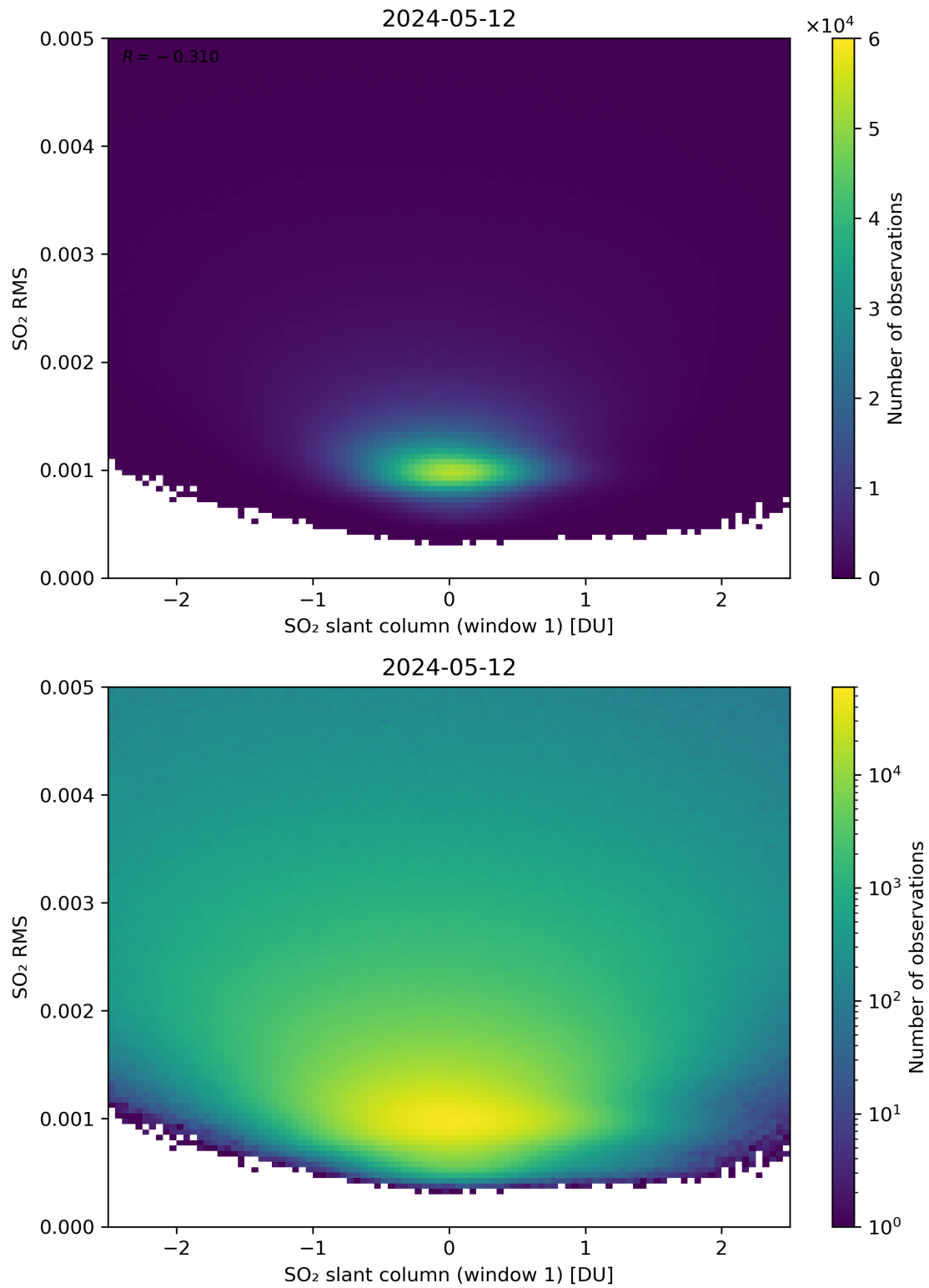
Figure 217: Scatter density plot of “SO 2 slant column (window 1)” against “SO 2 RMS” for 2024-05-12 to 2024-05-13.
