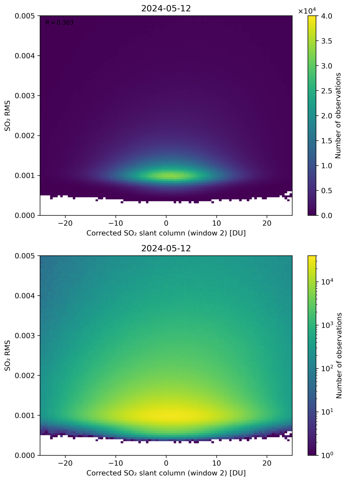
Figure 198: Scatter density plot of “Corrected SO 2 slant column (window 2)” against “SO 2 RMS” for 2024-05-12 to 2024-05-13.
