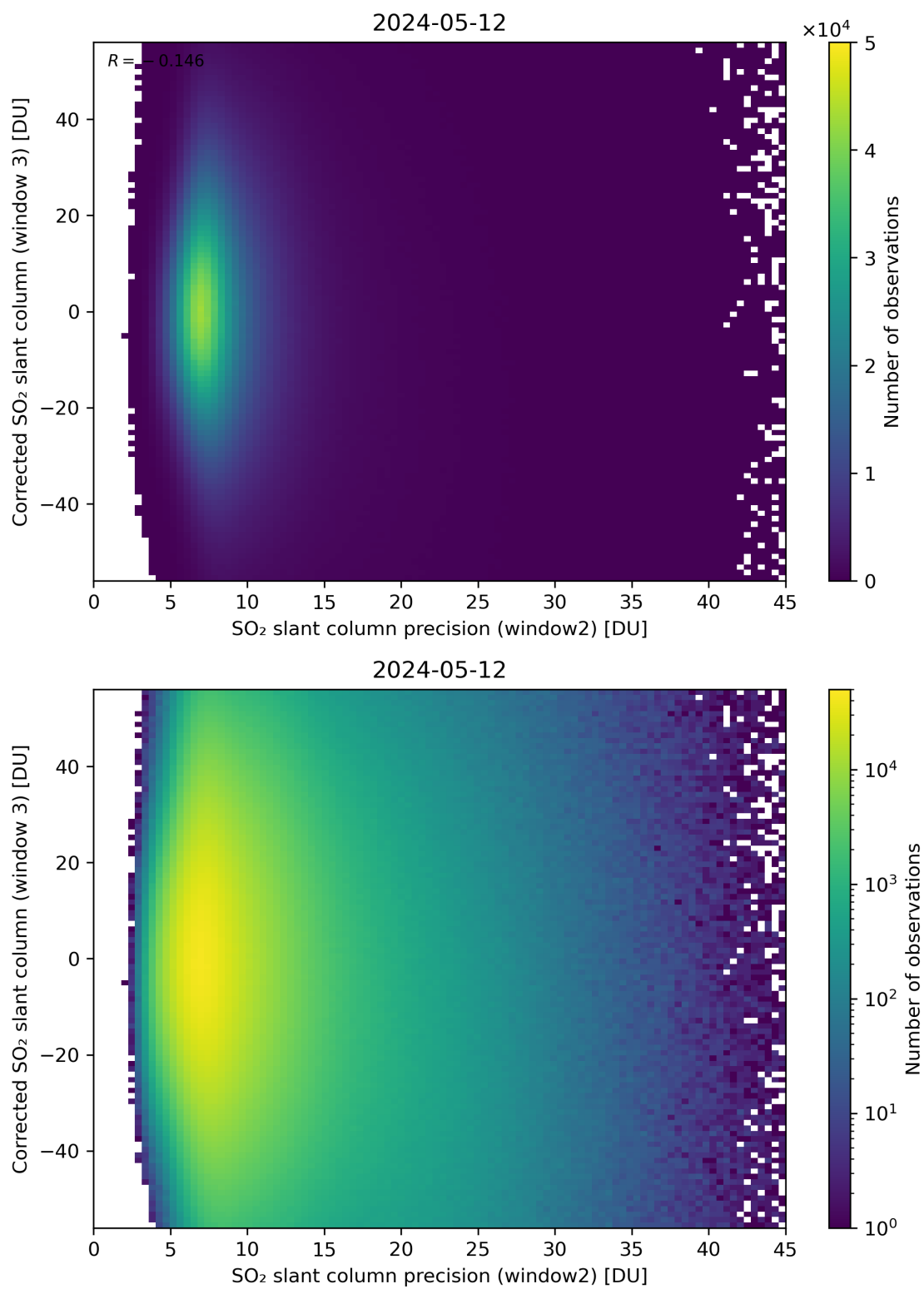
Figure 248: Scatter density plot of “SO 2 slant column precision (window2)” against “Corrected SO 2 slant column (window 3)” for 2024-05-12 to 2024-05-13.
