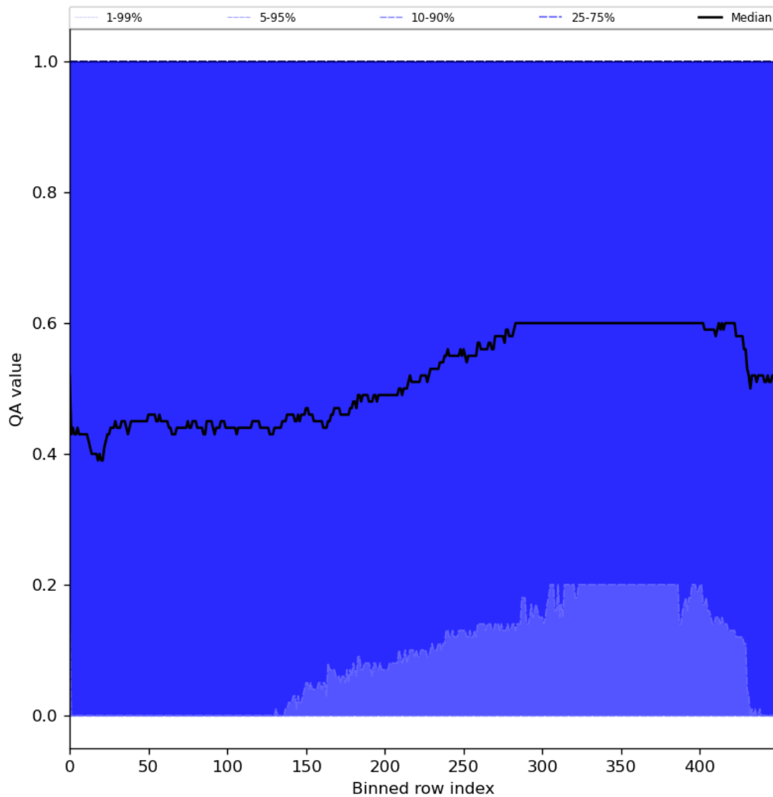
Figure 75: Along track statistics of “QA value” for 2024-05-12 to 2024-05-13
