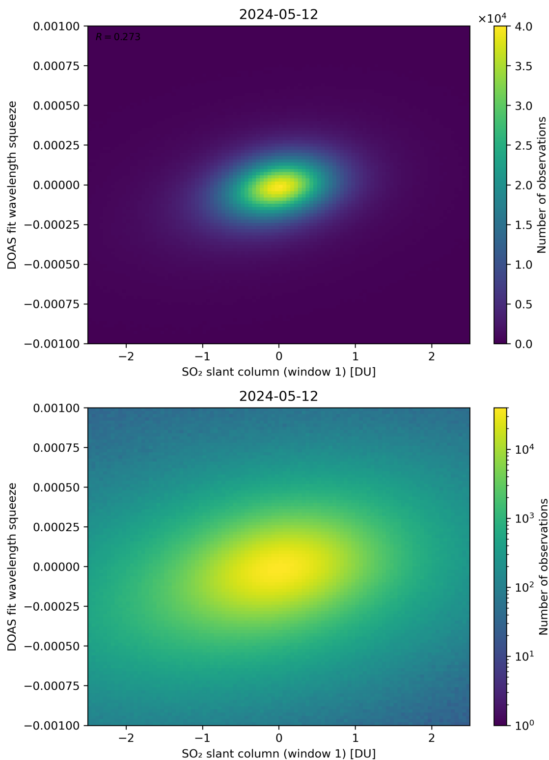
Figure 216: Scatter density plot of “SO 2 slant column (window 1)” against “DOAS fit wavelength squeeze” for 2024-05-12 to 2024-05-13.
