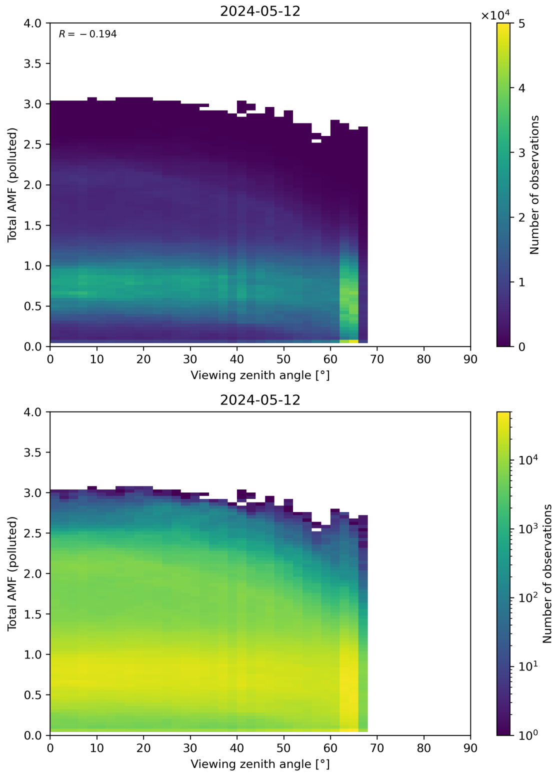
Figure 325: Scatter density plot of “Viewing zenith angle” against “Total AMF (polluted)” for 2024-05-12 to 2024-05-13.
