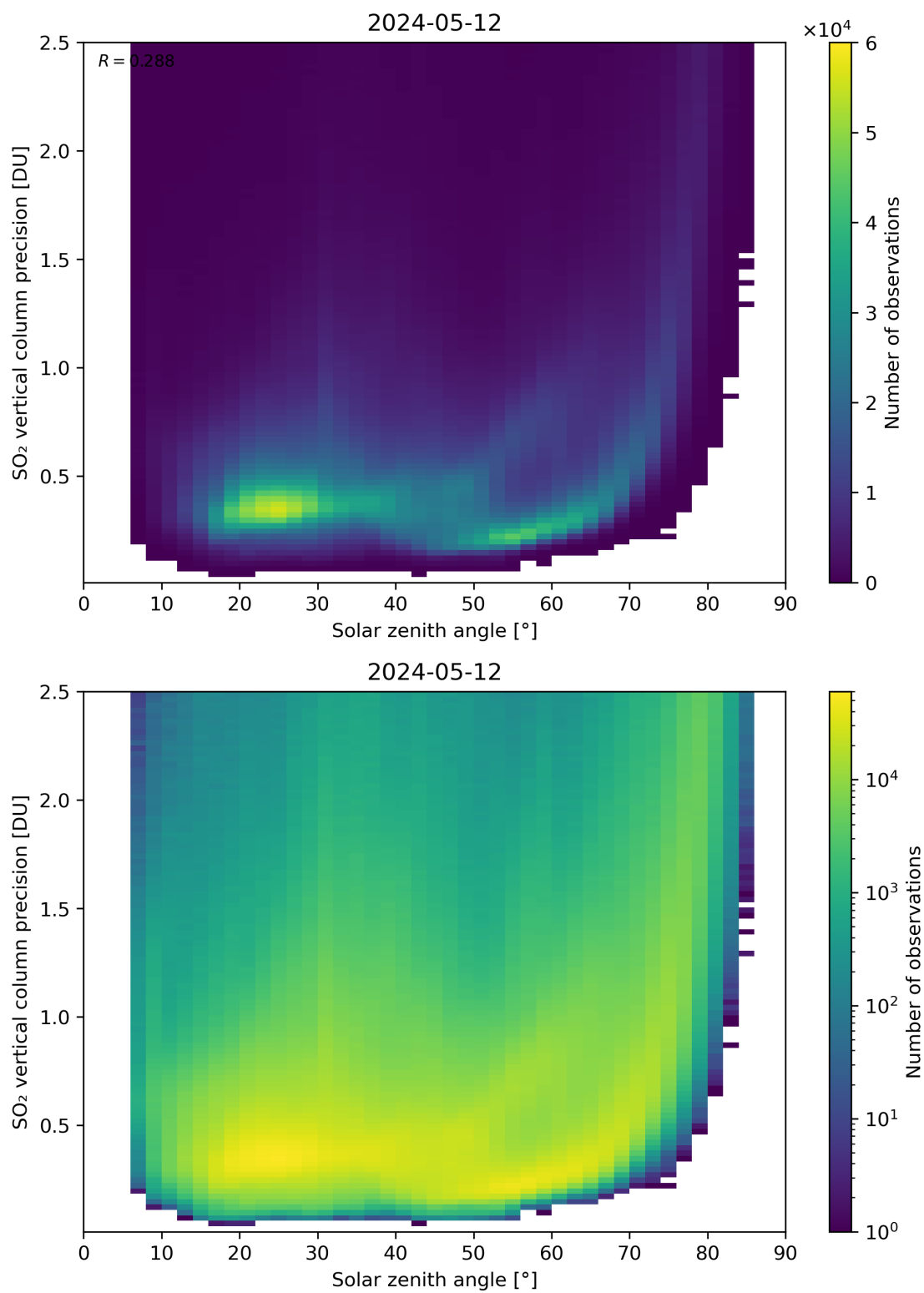
Figure 177: Scatter density plot of “Solar zenith angle” against “SO 2 vertical column precision” for 2024-05-12 to 2024-05-13.
