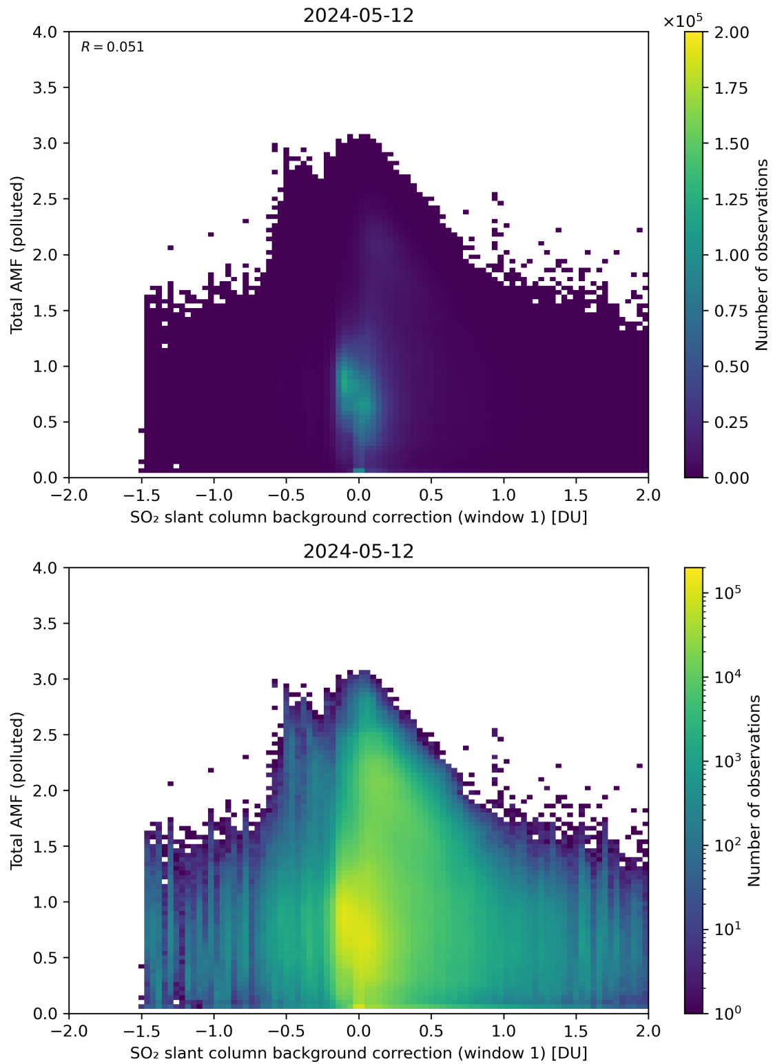
Figure 109: Scatter density plot of “SO 2 slant column background correction (window 1)” against “Total AMF (polluted)” for 2024-05-12 to 2024-05-13.
