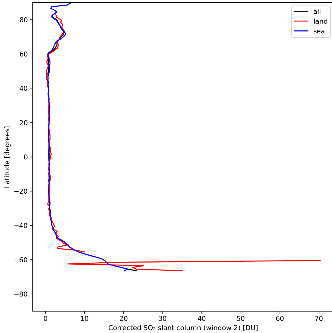
Figure 39: Zonal average of “Corrected SO 2 slant column (window 2)” for 2024-05-12 to 2024-05-13.
