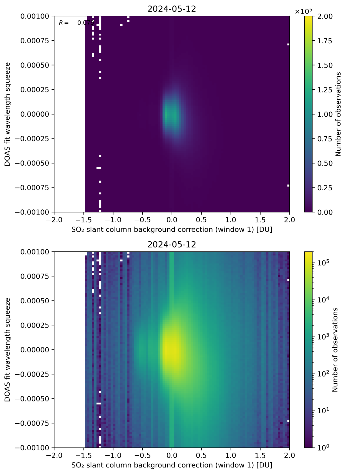
Figure 101: Scatter density plot of “SO 2 slant column background correction (window 1)” against “DOAS fit wavelength squeeze” for 2024-05-12 to 2024-05-13.
