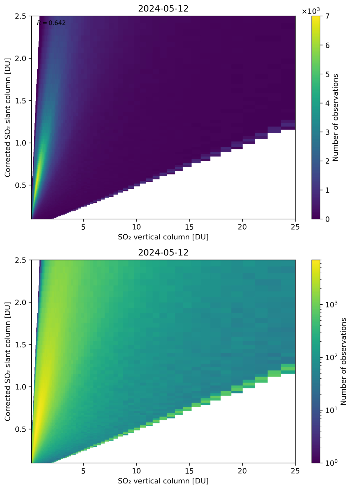
Figure 297: Scatter density plot of “SO 2 vertical column” against “Corrected SO 2 slant column” for 2024-05-12 to 2024-05-13.
