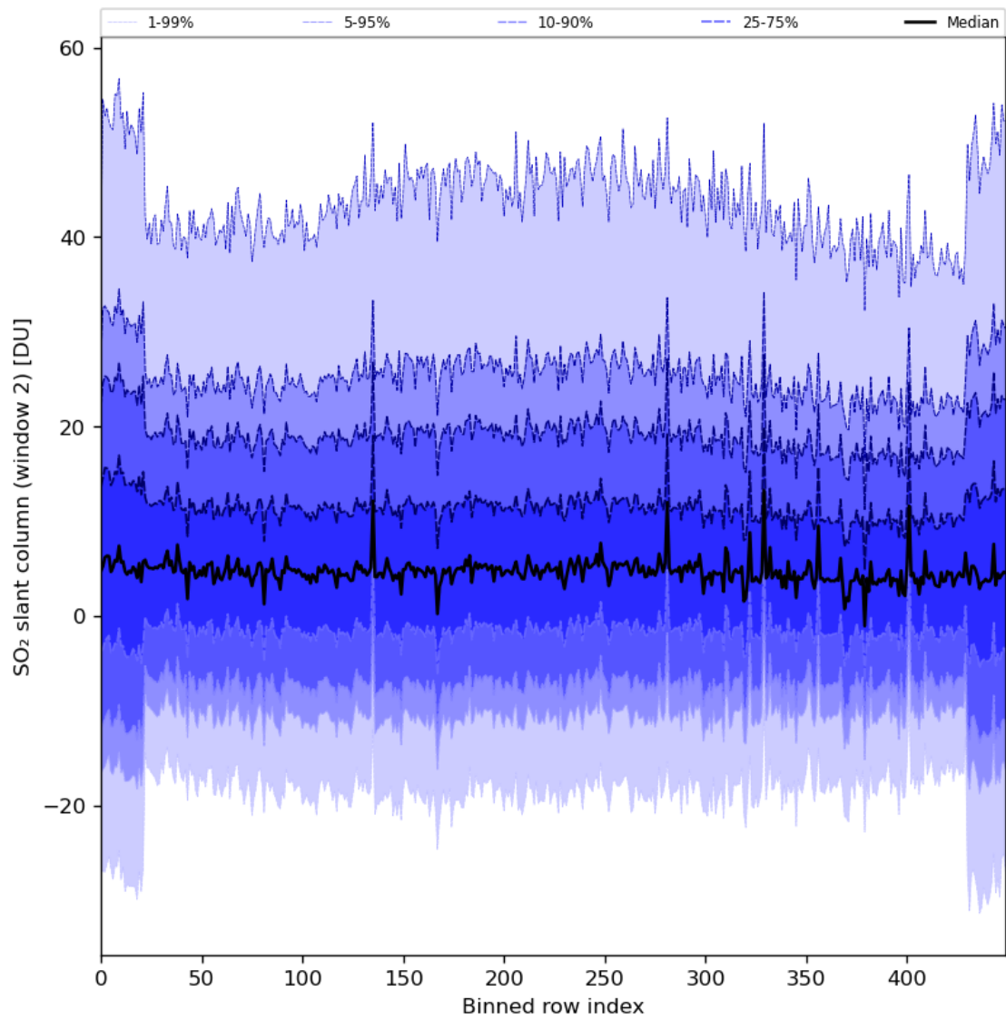
Figure 83: Along track statistics of “SO 2 slant column (window 2)” for 2024-05-12 to 2024-05-13
