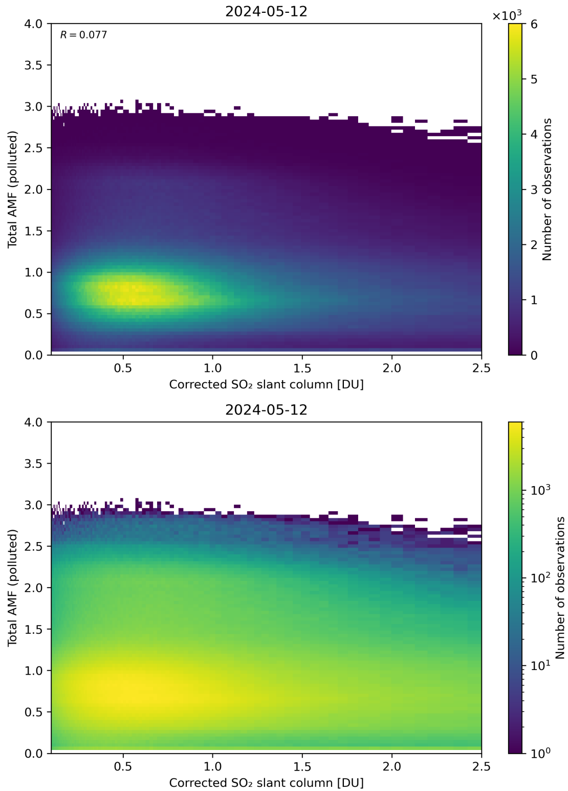
Figure 192: Scatter density plot of “Corrected SO 2 slant column” against “Total AMF (polluted)” for 2024-05-12 to 2024-05-13.
