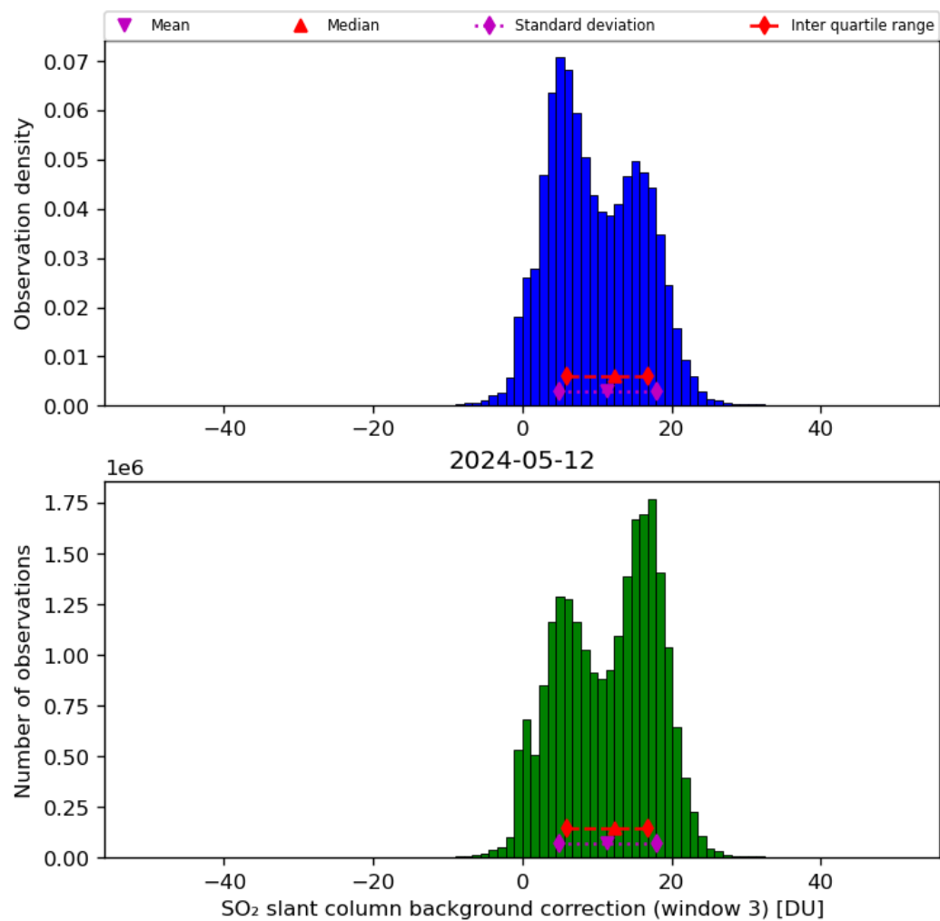
Figure 67: Histogram of “SO 2 slant column background correction (window 3)” for 2024-05-12 to 2024-05-13
