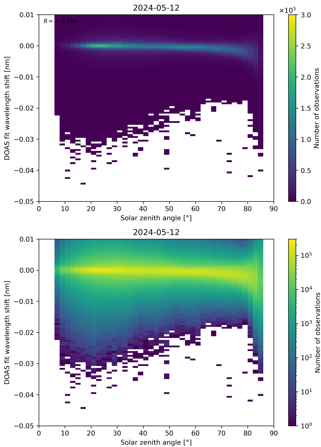
Figure 161: Scatter density plot of “Solar zenith angle” against “DOAS fit wavelength shift” for 2024-05-12 to 2024-05-13.
