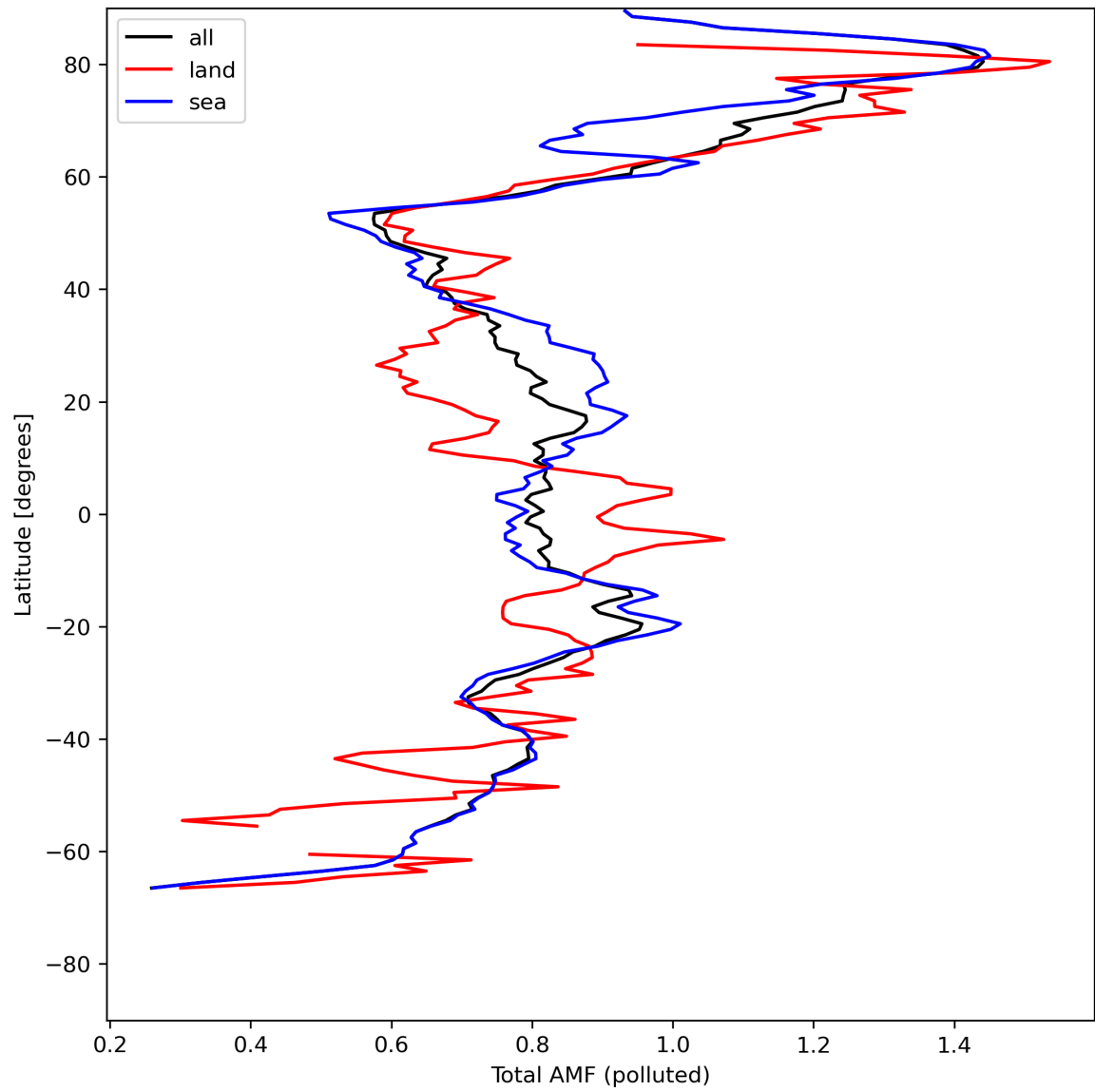
Figure 48: Zonal average of “Total AMF (polluted)” for 2024-05-12 to 2024-05-13.
