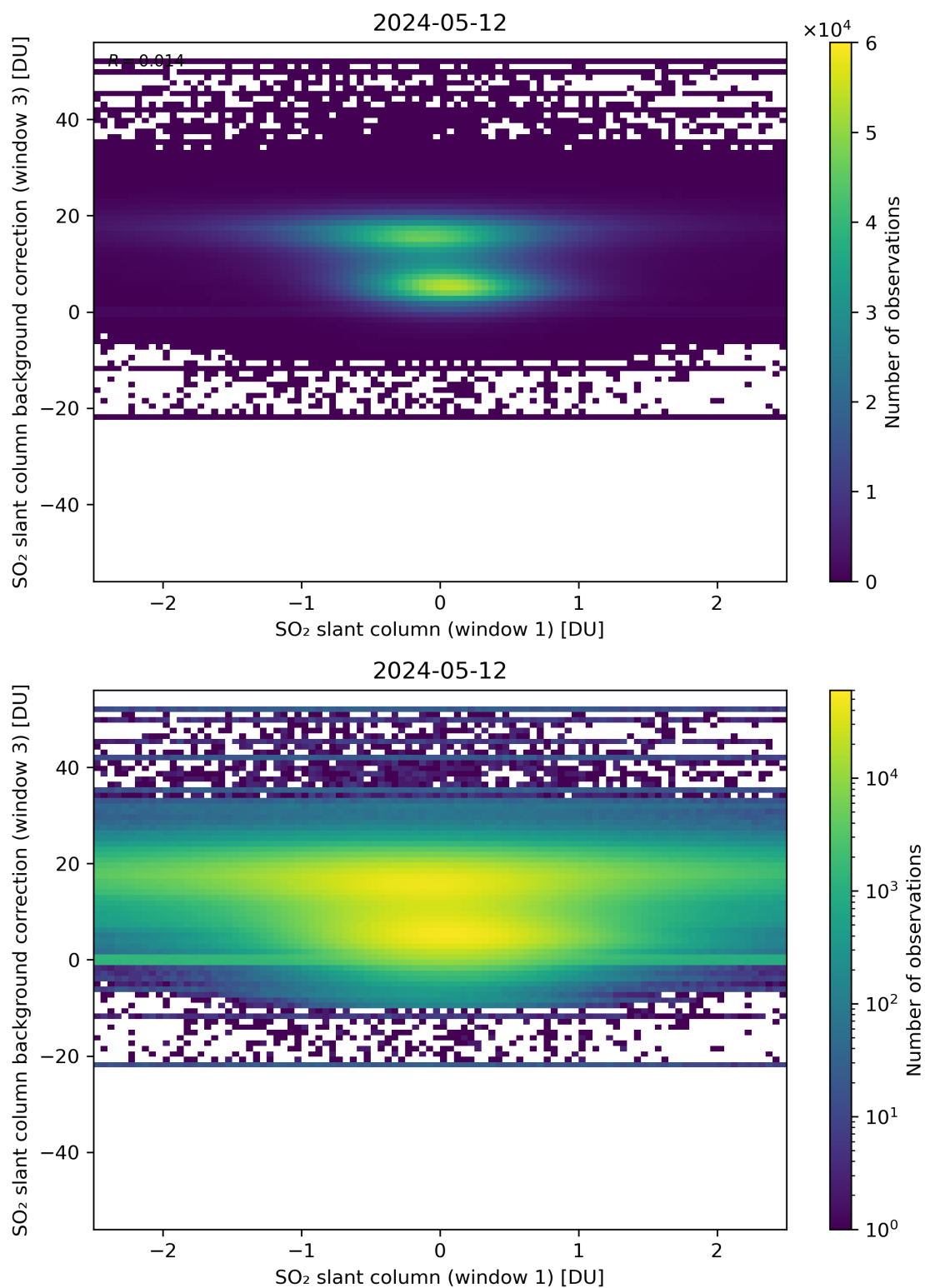
Figure 214: Scatter density plot of “SO 2 slant column (window 1)” against “SO 2 slant column background correction (window 3)” for 2024-05-12 to 2024-05-13.
