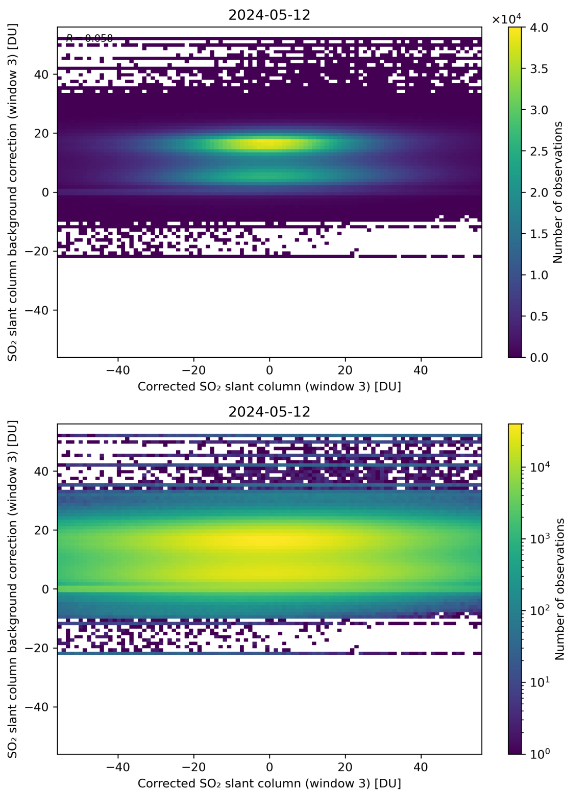
Figure 205: Scatter density plot of “Corrected SO 2 slant column (window 3)” against “SO 2 slant column background correction (window 3)” for 2024-05-12 to 2024-05-13.
