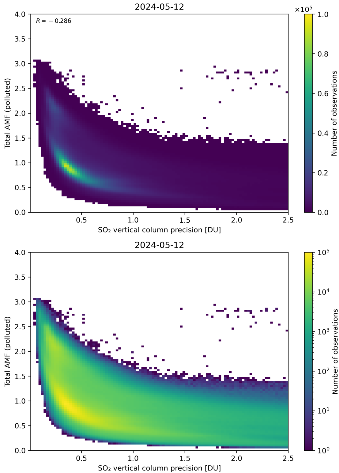
Figure 294: Scatter density plot of “SO 2 vertical column precision” against “Total AMF (polluted)” for 2024-05-12 to 2024-05-13.
