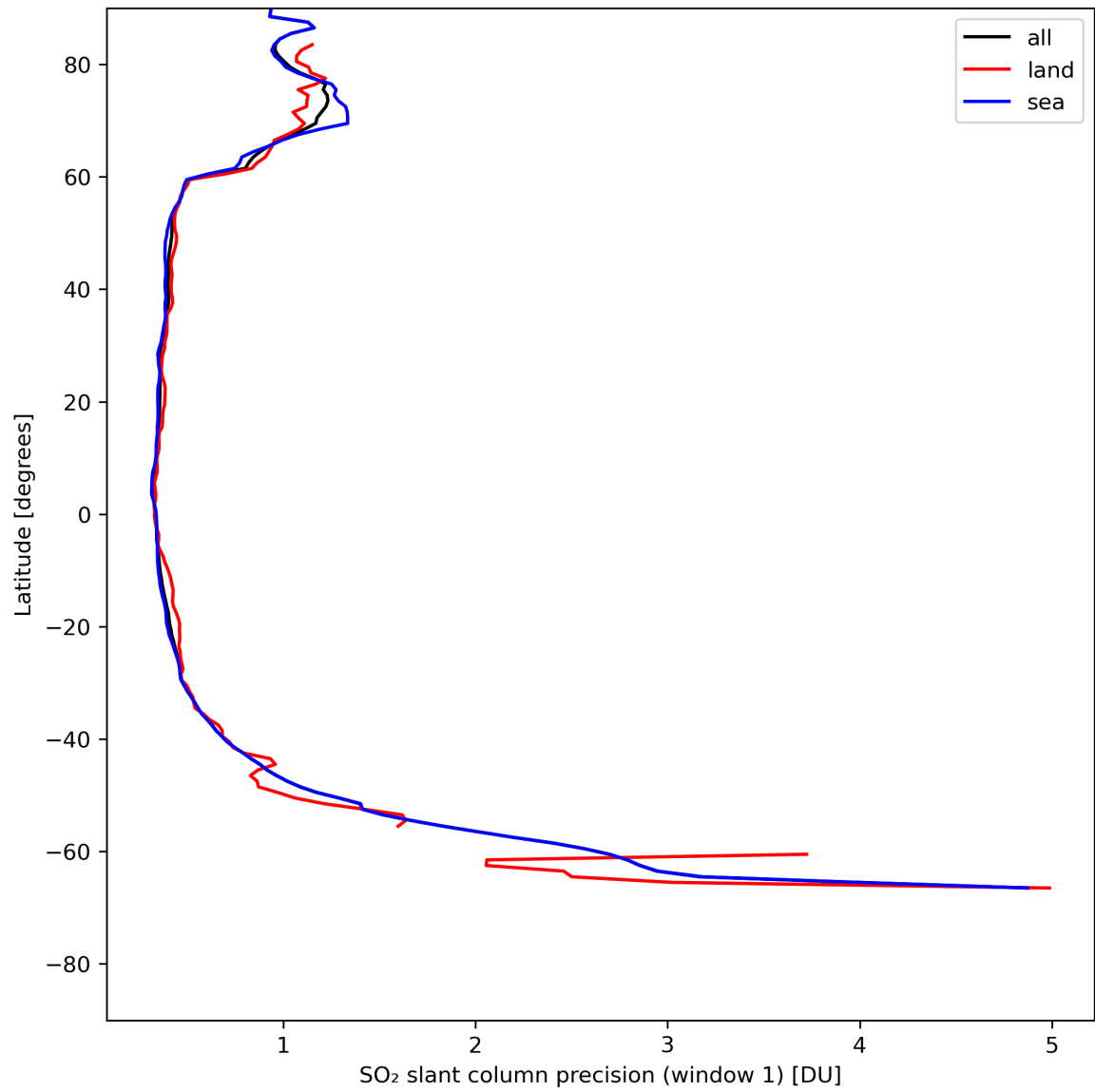
Figure 34: Zonal average of “SO 2 slant column precision (window 1)” for 2024-05-12 to 2024-05-13.
