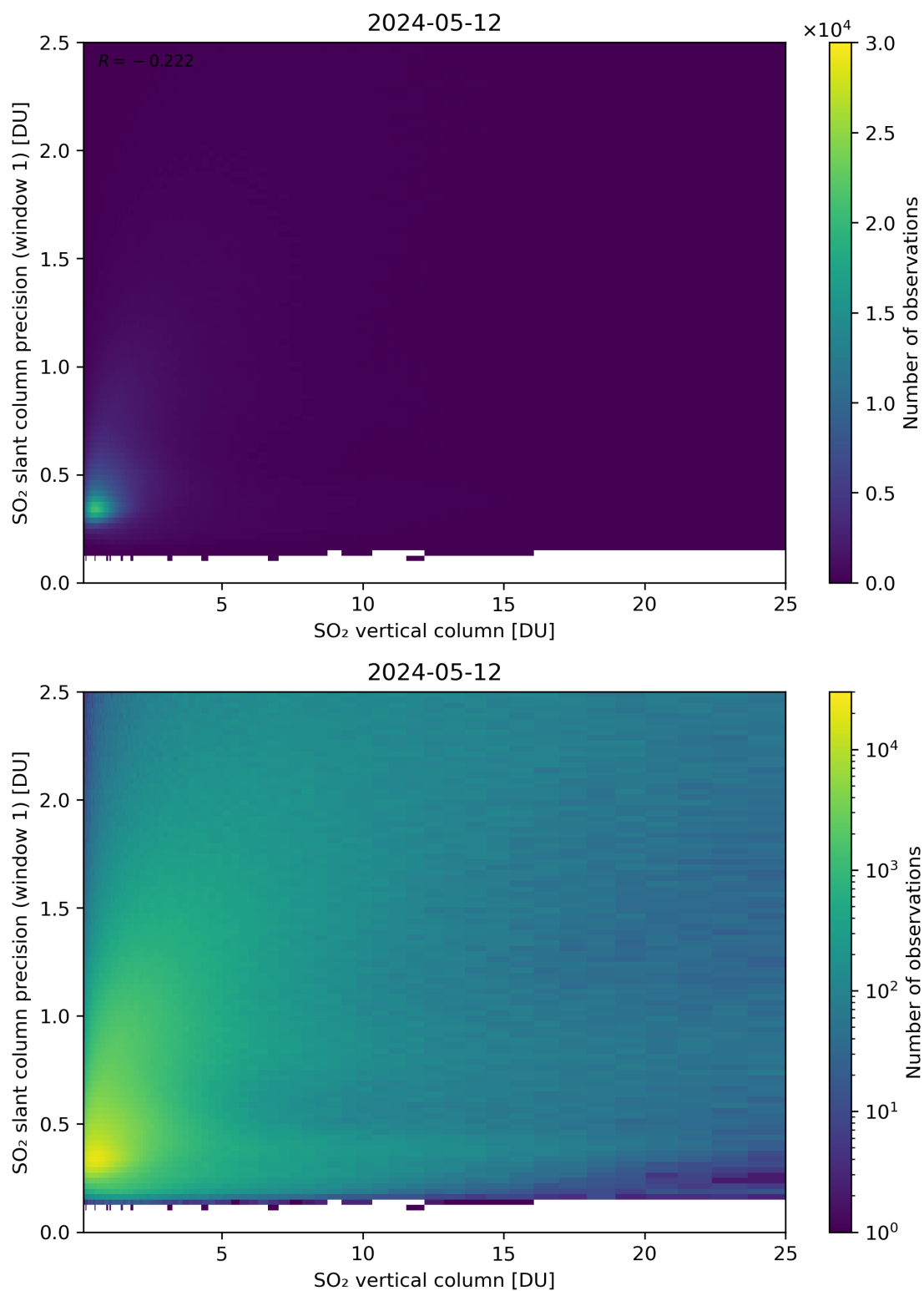
Figure 301: Scatter density plot of “SO 2 vertical column” against “SO 2 slant column precision (window 1)” for 2024-05-12 to 2024-05-13.
