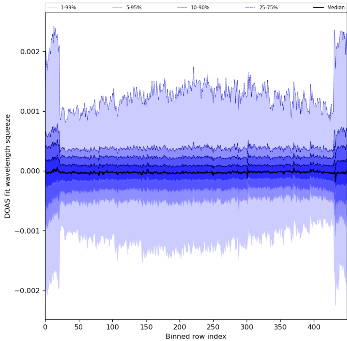
Figure 92: Along track statistics of “DOAS fit wavelength squeeze” for 2024-05-12 to 2024-05-13
