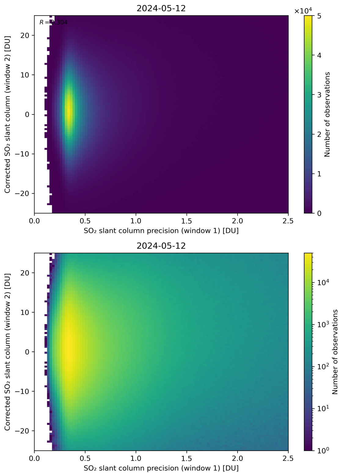
Figure 225: Scatter density plot of “SO 2 slant column precision (window 1)” against “Corrected SO 2 slant column (window 2)” for 2024-05-12 to 2024-05-13.
