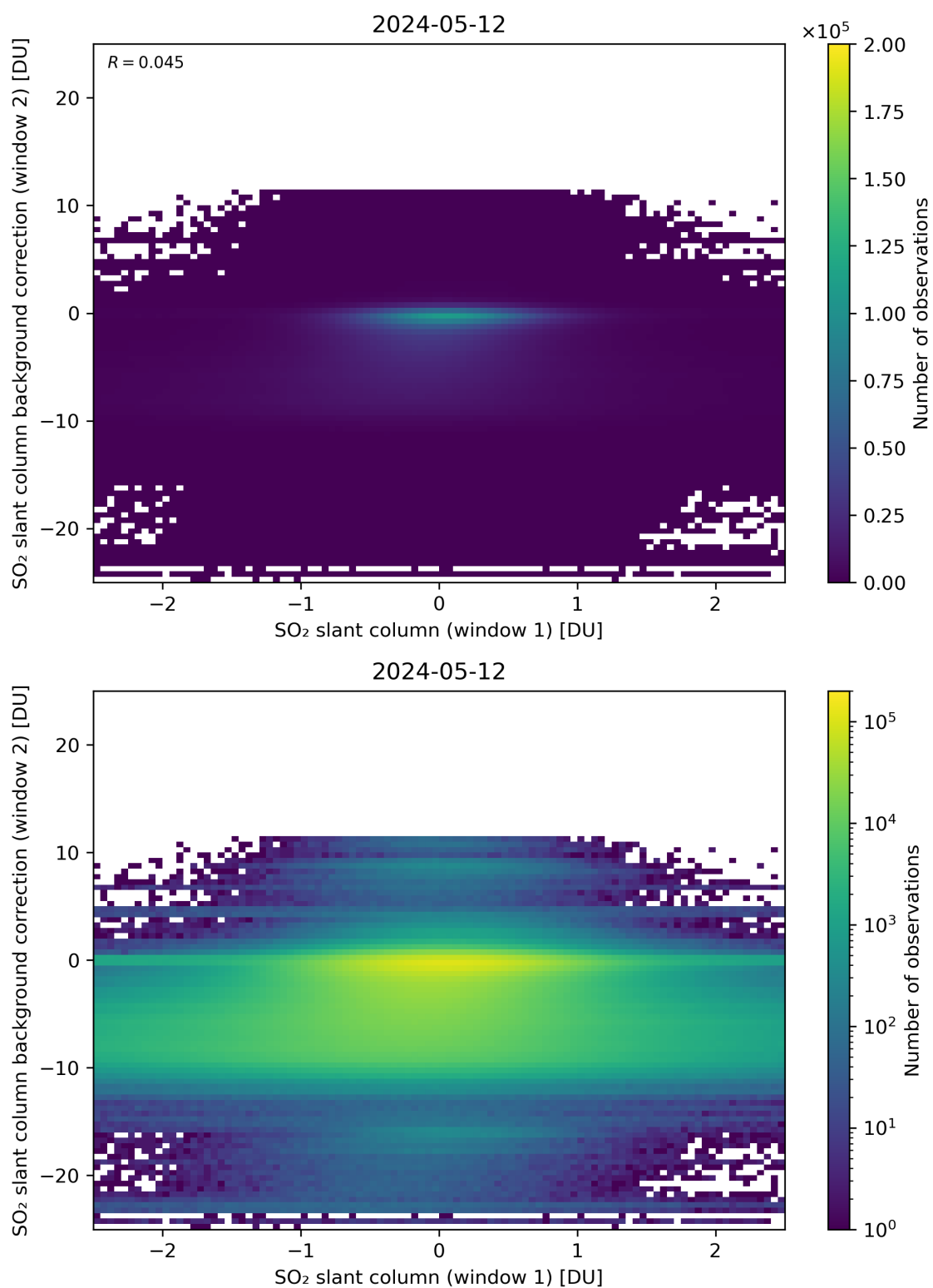
Figure 213: Scatter density plot of “SO 2 slant column (window 1)” against “SO 2 slant column background correction (window 2)” for 2024-05-12 to 2024-05-13.
