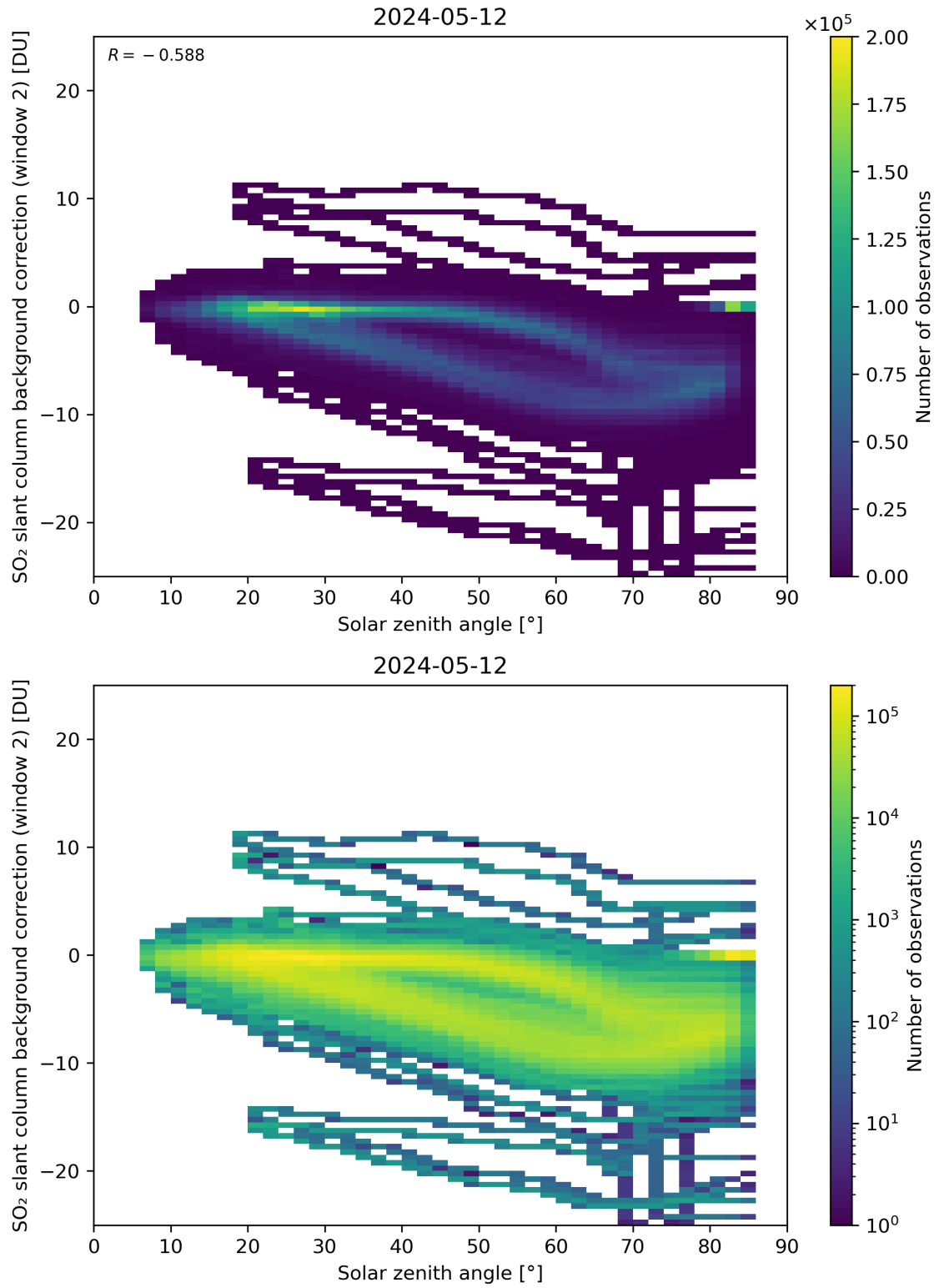
Figure 159: Scatter density plot of “Solar zenith angle” against “SO 2 slant column background correction (window 2)” for 2024-05-12 to 2024-05-13.
