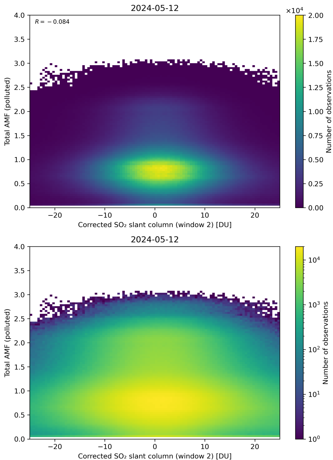
Figure 203: Scatter density plot of “Corrected SO 2 slant column (window 2)” against “Total AMF (polluted)” for 2024-05-12 to 2024-05-13.
