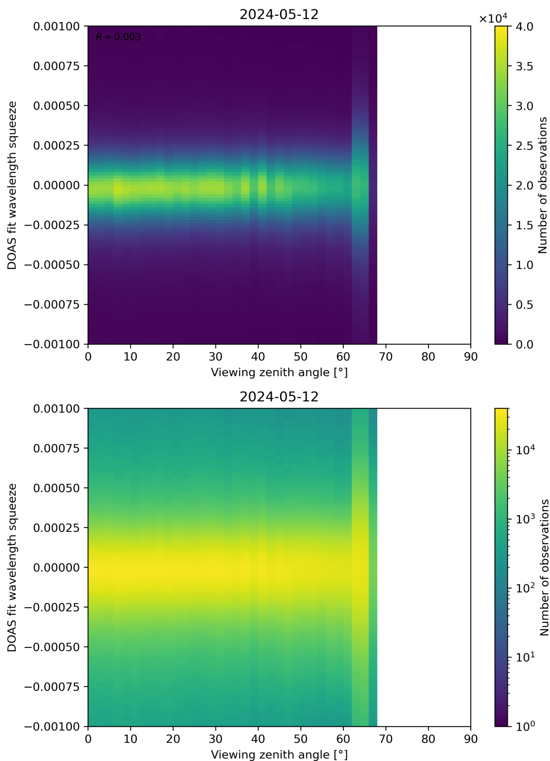
Figure 312: Scatter density plot of “Viewing zenith angle” against “DOAS fit wavelength squeeze” for 2024-05-12 to 2024-05-13.
