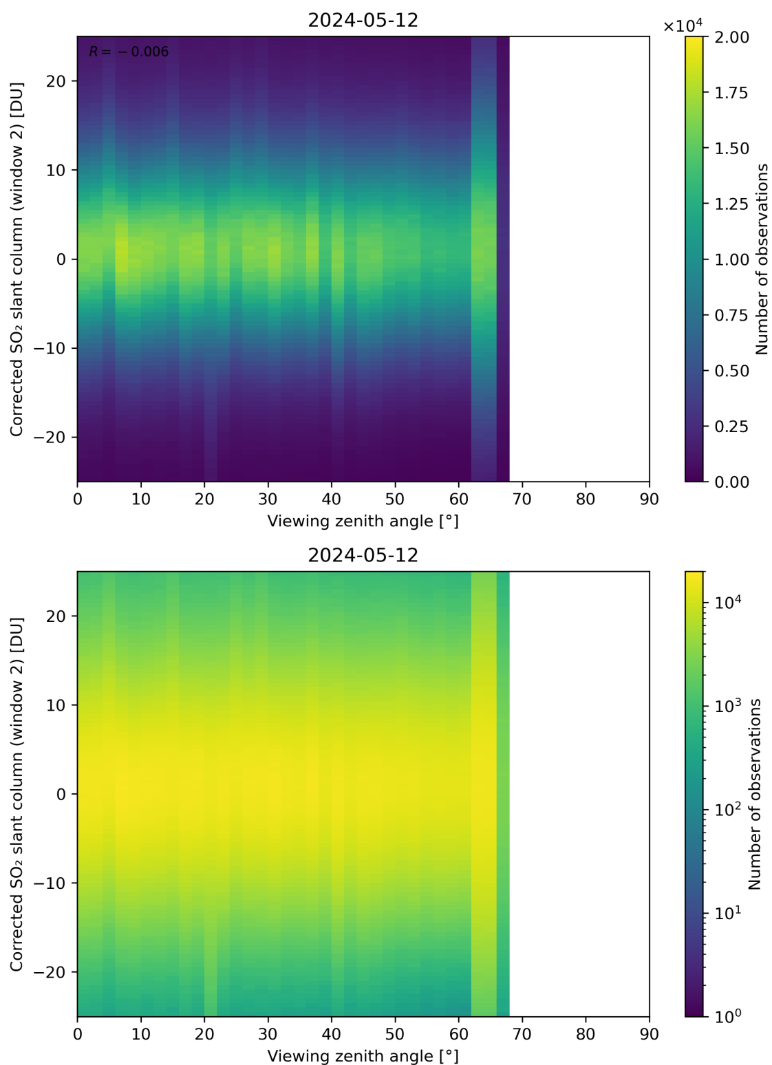
Figure 318: Scatter density plot of “Viewing zenith angle” against “Corrected SO 2 slant column (window 2)” for 2024-05-12 to 2024-05-13.
