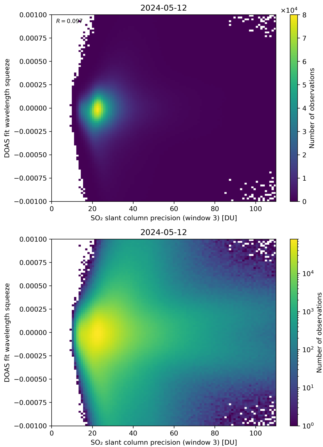
Figure 259: Scatter density plot of “SO 2 slant column precision (window 3)” against “DOAS fit wavelength squeeze” for 2024-05-12 to 2024-05-13.
