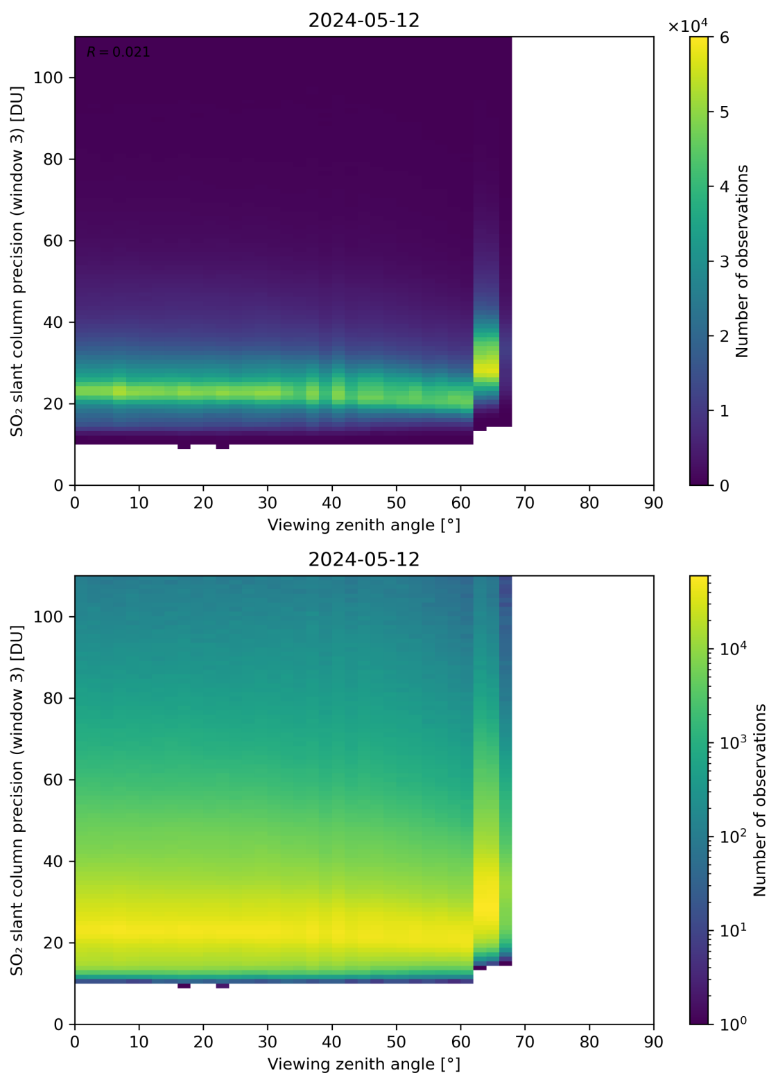
Figure 324: Scatter density plot of “Viewing zenith angle” against “SO 2 slant column precision (window 3)” for 2024-05-12 to 2024-05-13.
