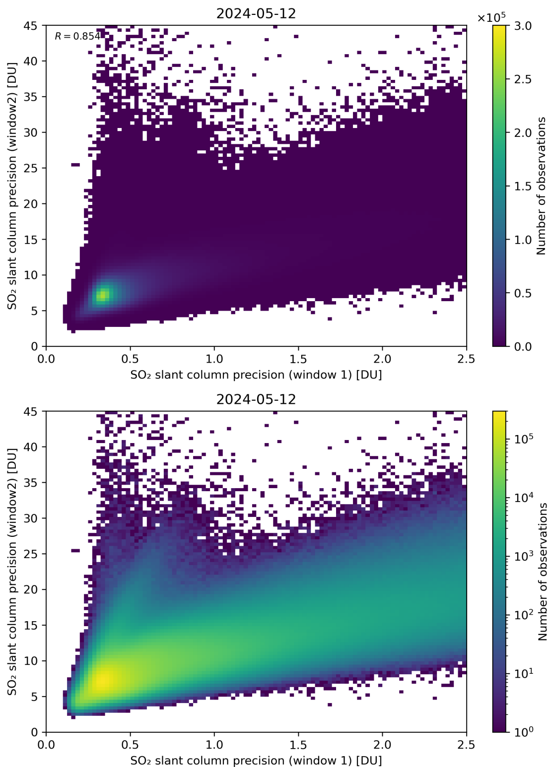
Figure 227: Scatter density plot of “SO 2 slant column precision (window 1)” against “SO 2 slant column precision (window 2)” for 2024-05-12 to 2024-05-13.
