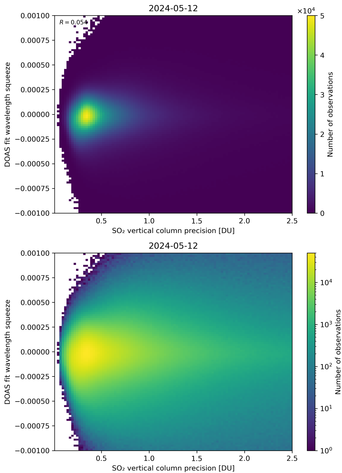
Figure 283: Scatter density plot of “SO 2 vertical column precision” against “DOAS fit wavelength squeeze” for 2024-05-12 to 2024-05-13.
