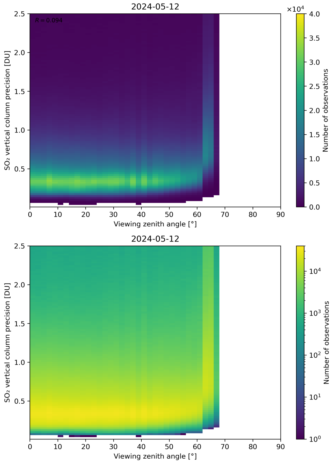
Figure 328: Scatter density plot of “Viewing zenith angle” against “SO 2 vertical column precision” for 2024-05-12 to 2024-05-13.
