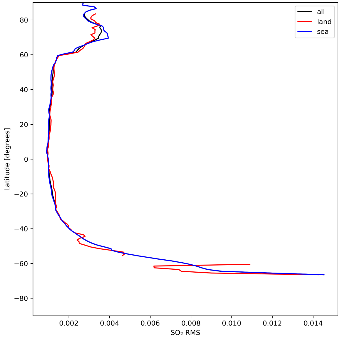
Figure 47: Zonal average of “SO 2 RMS” for 2024-05-12 to 2024-05-13.
