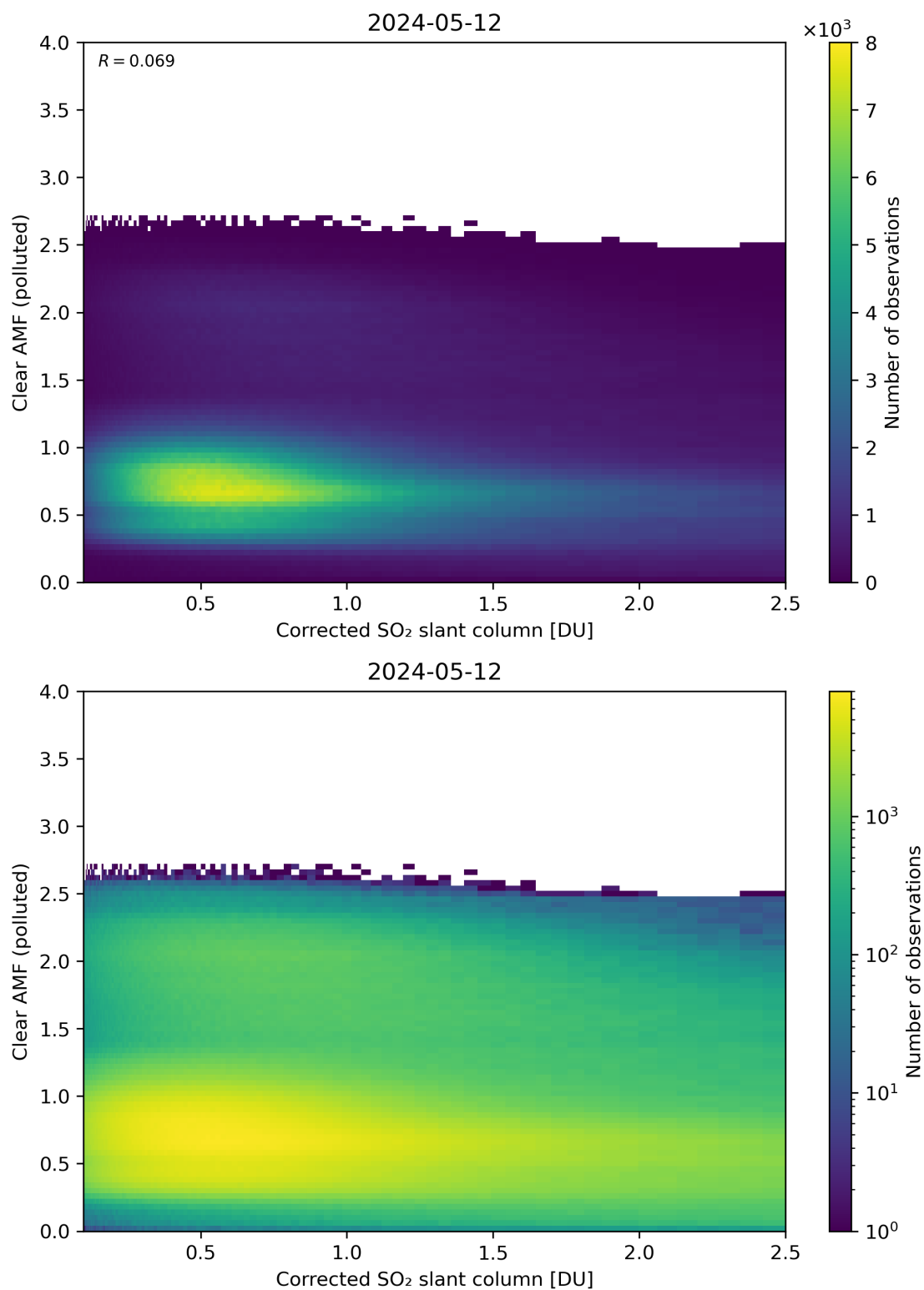
Figure 184: Scatter density plot of “Corrected SO 2 slant column” against “Clear AMF (polluted)” for 2024-05-12 to 2024-05-13.
