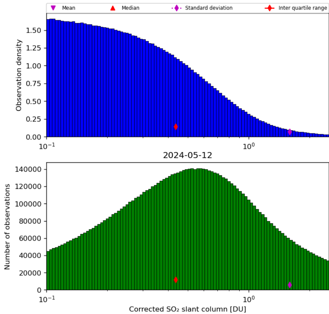
Figure 55: Histogram of “Corrected SO 2 slant column” for 2024-05-12 to 2024-05-13
