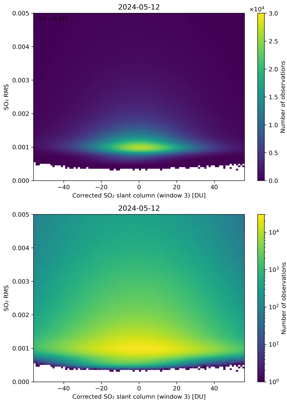
Figure 208: Scatter density plot of “Corrected SO 2 slant column (window 3)” against “SO 2 RMS” for 2024-05-12 to 2024-05-13.
