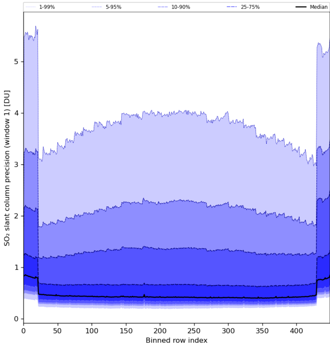
Figure 80: Along track statistics of “SO 2 slant column precision (window 1)” for 2024-05-12 to 2024-05-13
