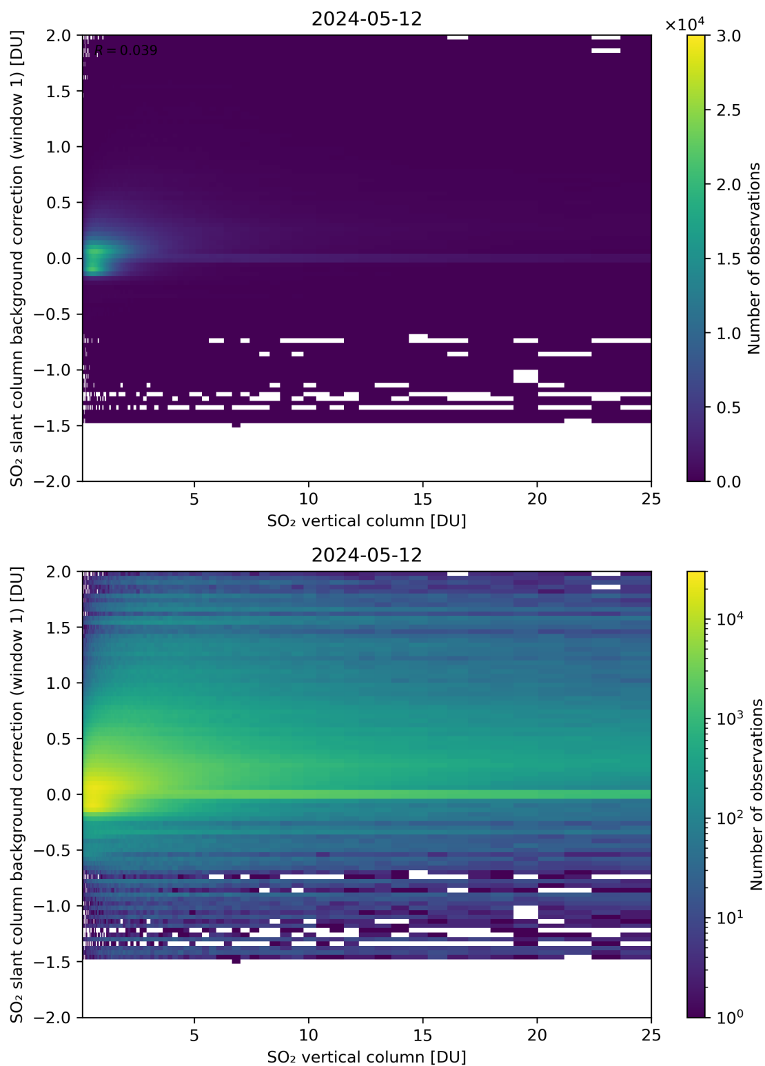
Figure 273: Scatter density plot of “SO 2 vertical column” against “SO 2 slant column background correction (window 1)” for 2024-05-12 to 2024-05-13.
