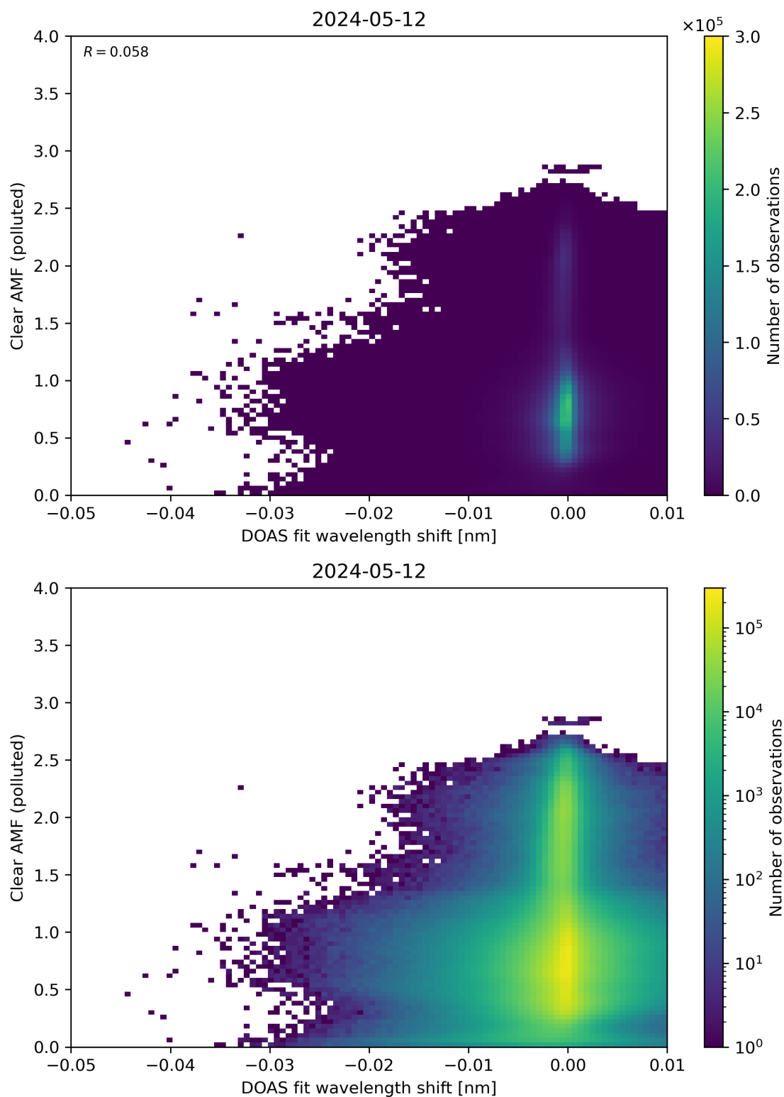
Figure 129: Scatter density plot of “DOAS fit wavelength shift” against “Clear AMF (polluted)” for 2024-05-12 to 2024-05-13.
