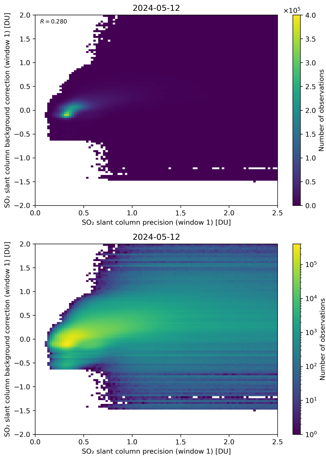
Figure 218: Scatter density plot of “SO 2 slant column precision (window 1)” against “SO 2 slant column background correction (window 1)” for 2024-05-12 to 2024-05-13.
