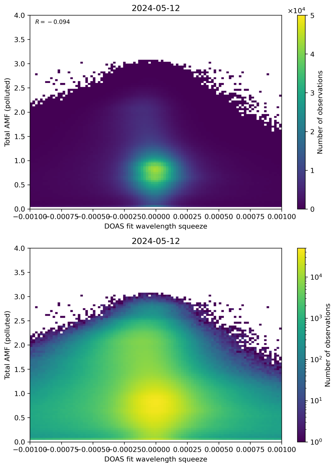
Figure 134: Scatter density plot of “DOAS fit wavelength squeeze” against “Total AMF (polluted)” for 2024-05-12 to 2024-05-13.
