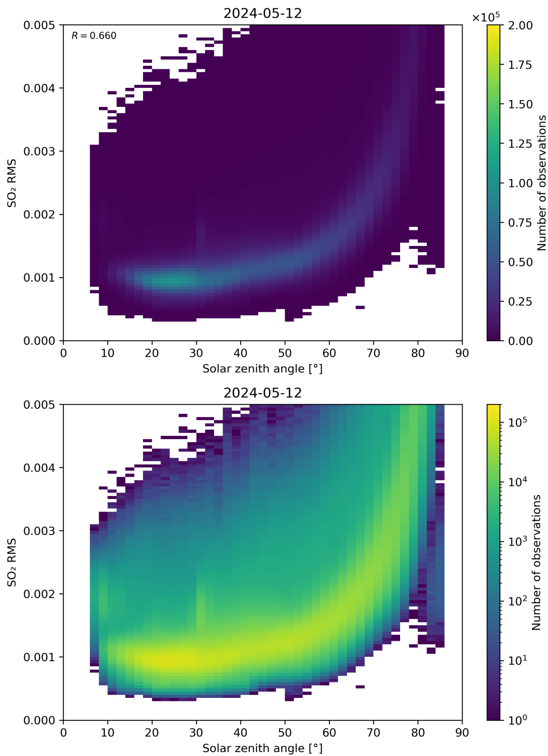
Figure 163: Scatter density plot of “Solar zenith angle” against “SO 2 RMS” for 2024-05-12 to 2024-05-13.
