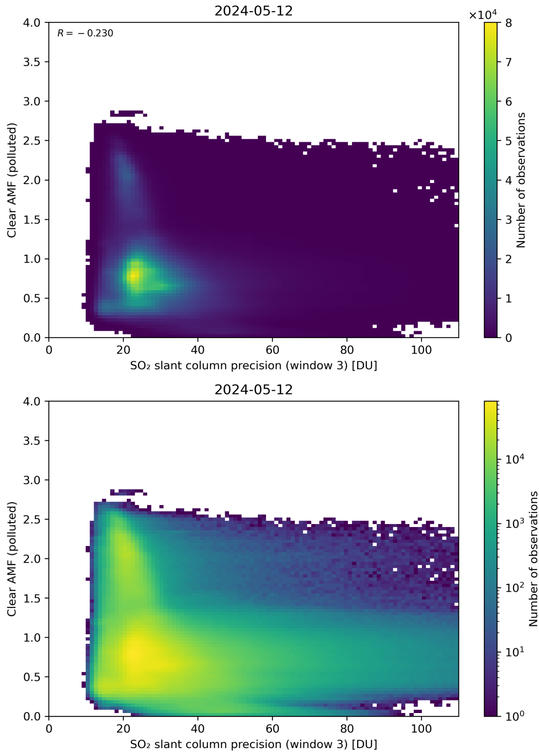
Figure 261: Scatter density plot of “SO 2 slant column precision (window 3)” against “Clear AMF (polluted)” for 2024-05-12 to 2024-05-13.
