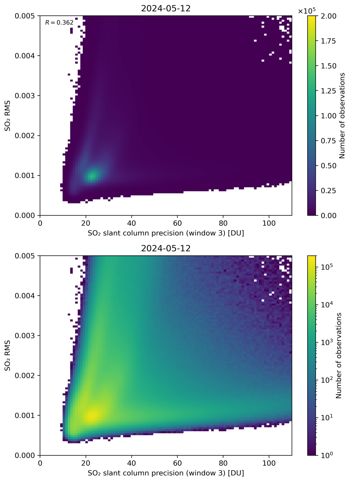
Figure 260: Scatter density plot of “SO 2 slant column precision (window 3)” against “SO 2 RMS” for 2024-05-12 to 2024-05-13.
