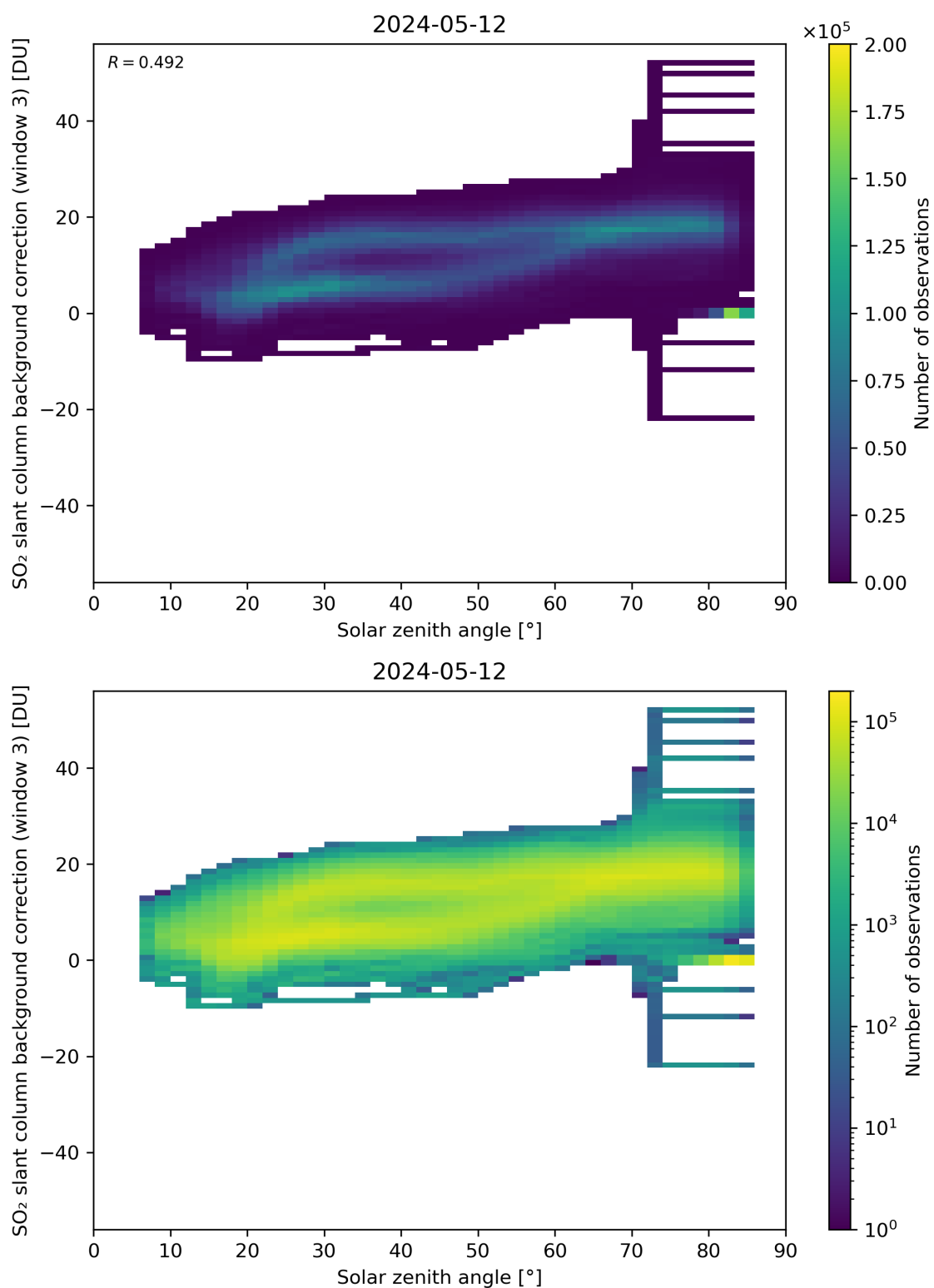
Figure 160: Scatter density plot of “Solar zenith angle” against “SO 2 slant column background correction (window 3)” for 2024-05-12 to 2024-05-13.
