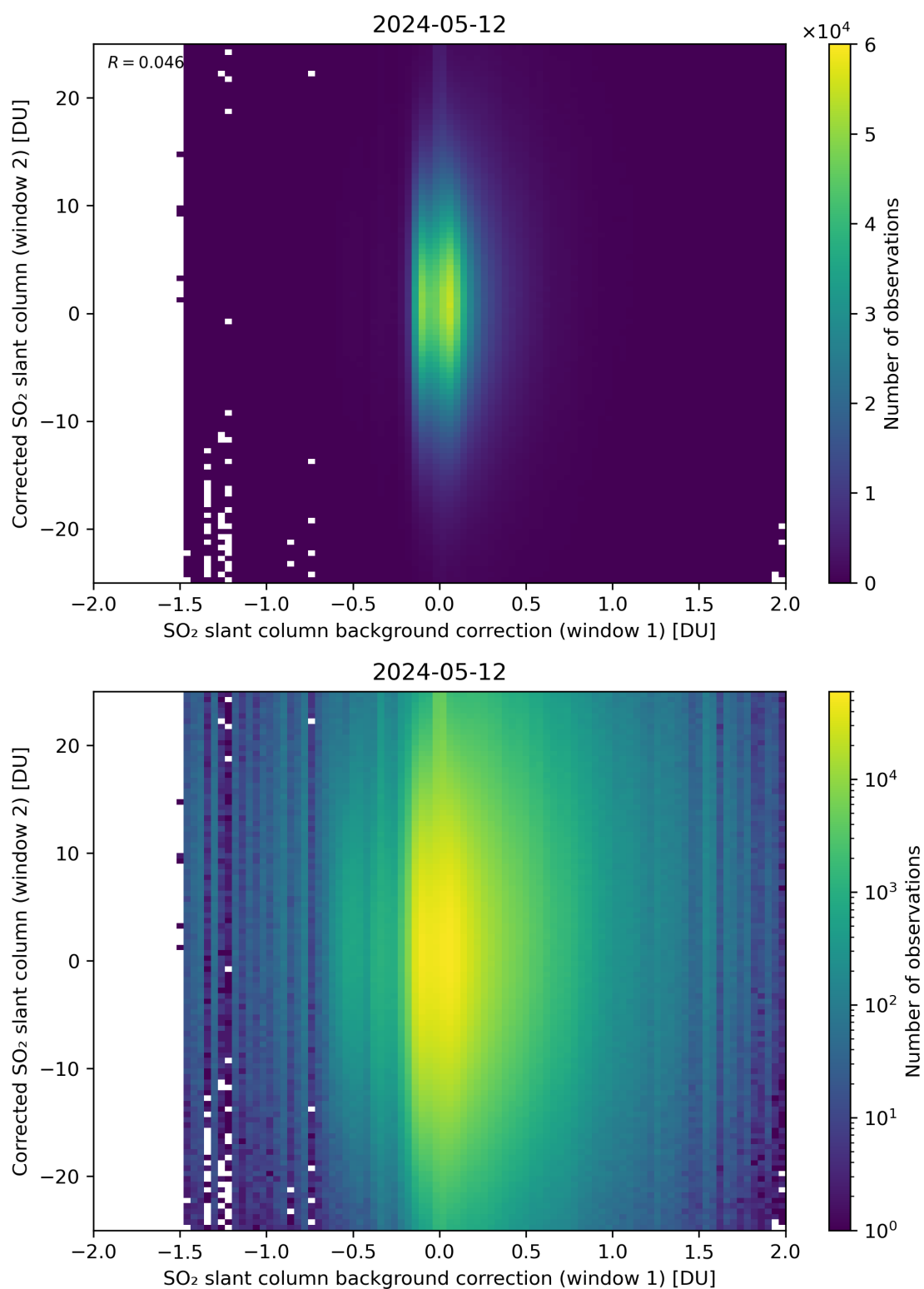
Figure 104: Scatter density plot of “SO 2 slant column background correction (window 1)” against “Corrected SO 2 slant column (window 2)” for 2024-05-12 to 2024-05-13.
