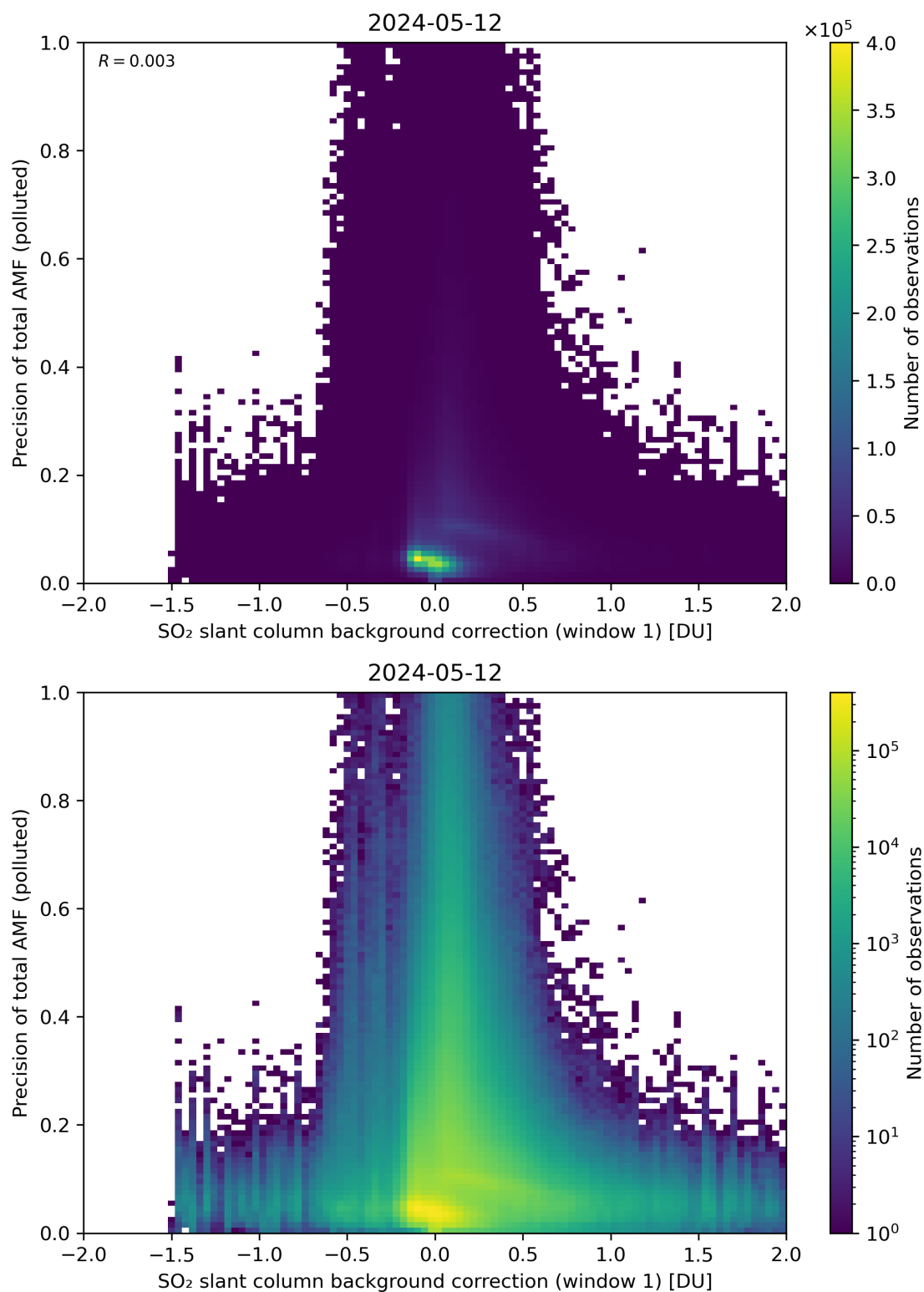
Figure 110: Scatter density plot of “SO 2 slant column background correction (window 1)” against “Precision of total AMF (polluted)” for 2024-05-12 to 2024-05-13.
