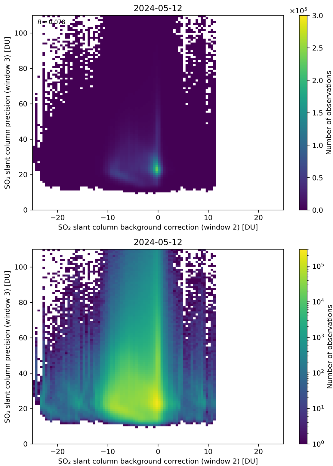
Figure 118: Scatter density plot of “SO 2 slant column background correction (window 2)” against “SO 2 slant column precision (window 3)” for 2024-05-12 to 2024-05-13.
