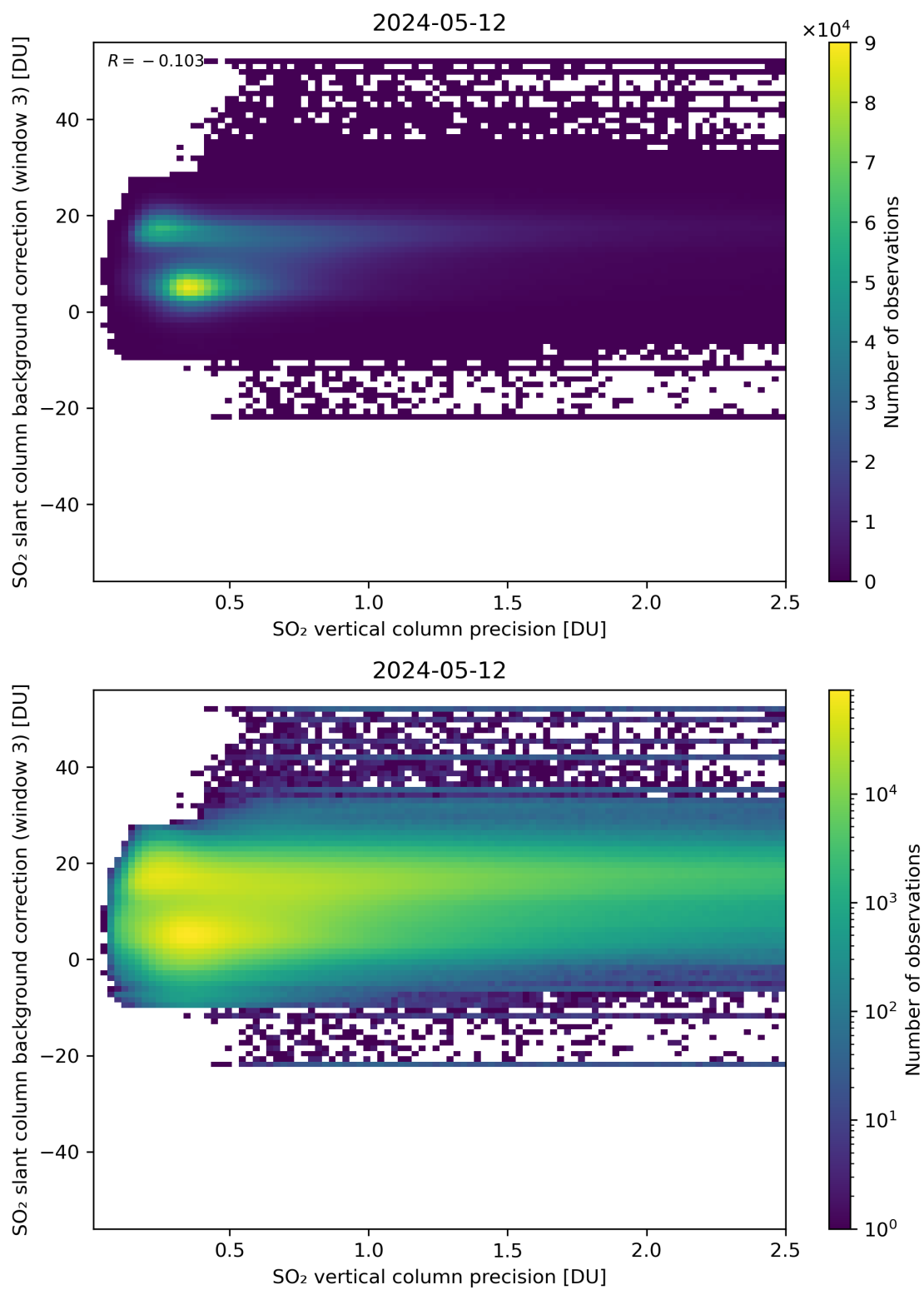
Figure 281: Scatter density plot of “SO 2 vertical column precision” against “SO 2 slant column background correction (window 3)” for 2024-05-12 to 2024-05-13.
