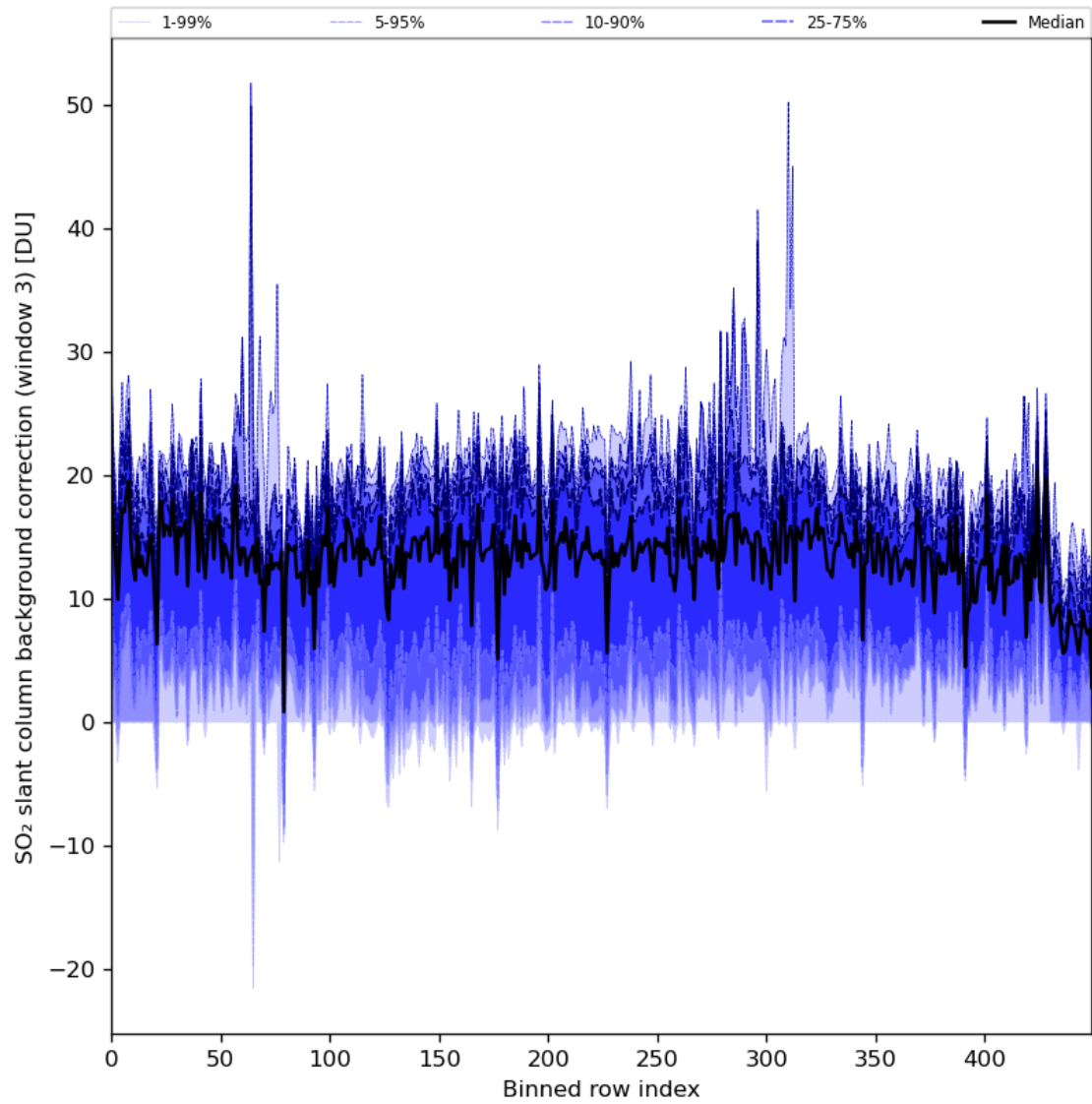
Figure 90: Along track statistics of “SO 2 slant column background correction (window 3)” for 2024-05-12 to 2024-05-13
