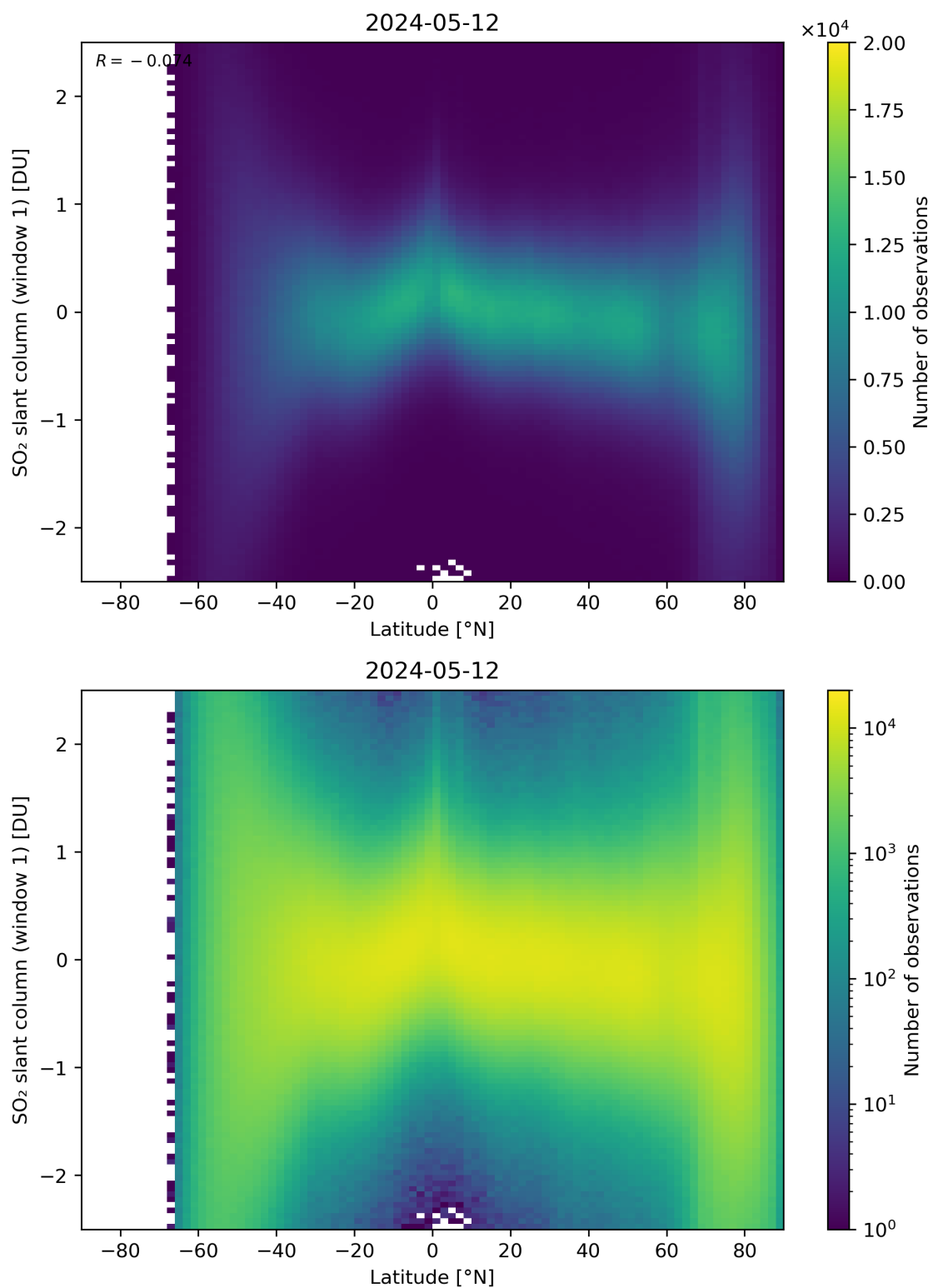
Figure 149: Scatter density plot of “Latitude” against “SO 2 slant column (window 1)” for 2024-05-12 to 2024-05-13.
