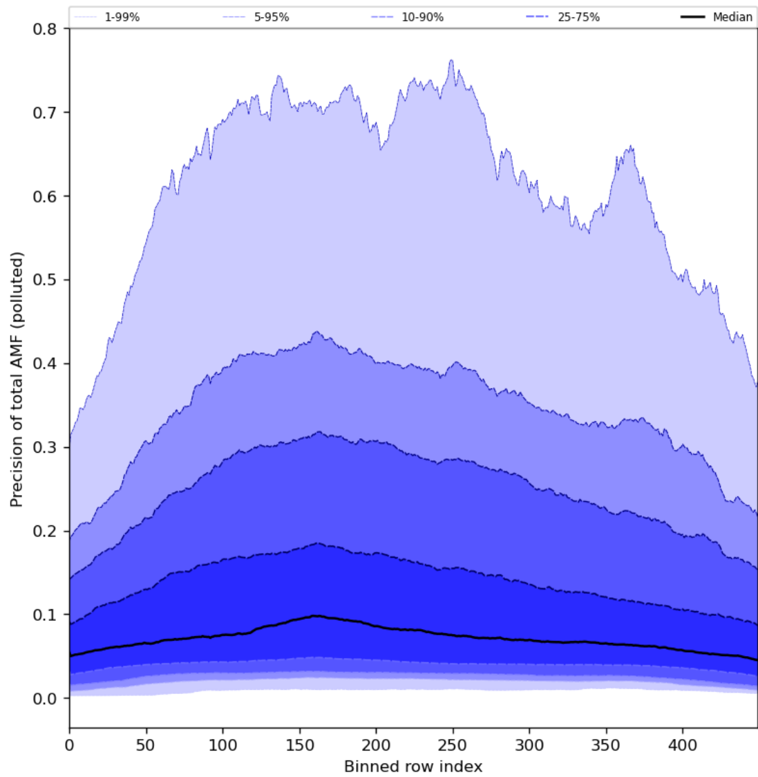
Figure 95: Along track statistics of “Precision of total AMF (polluted)” for 2024-05-12 to 2024-05-13
