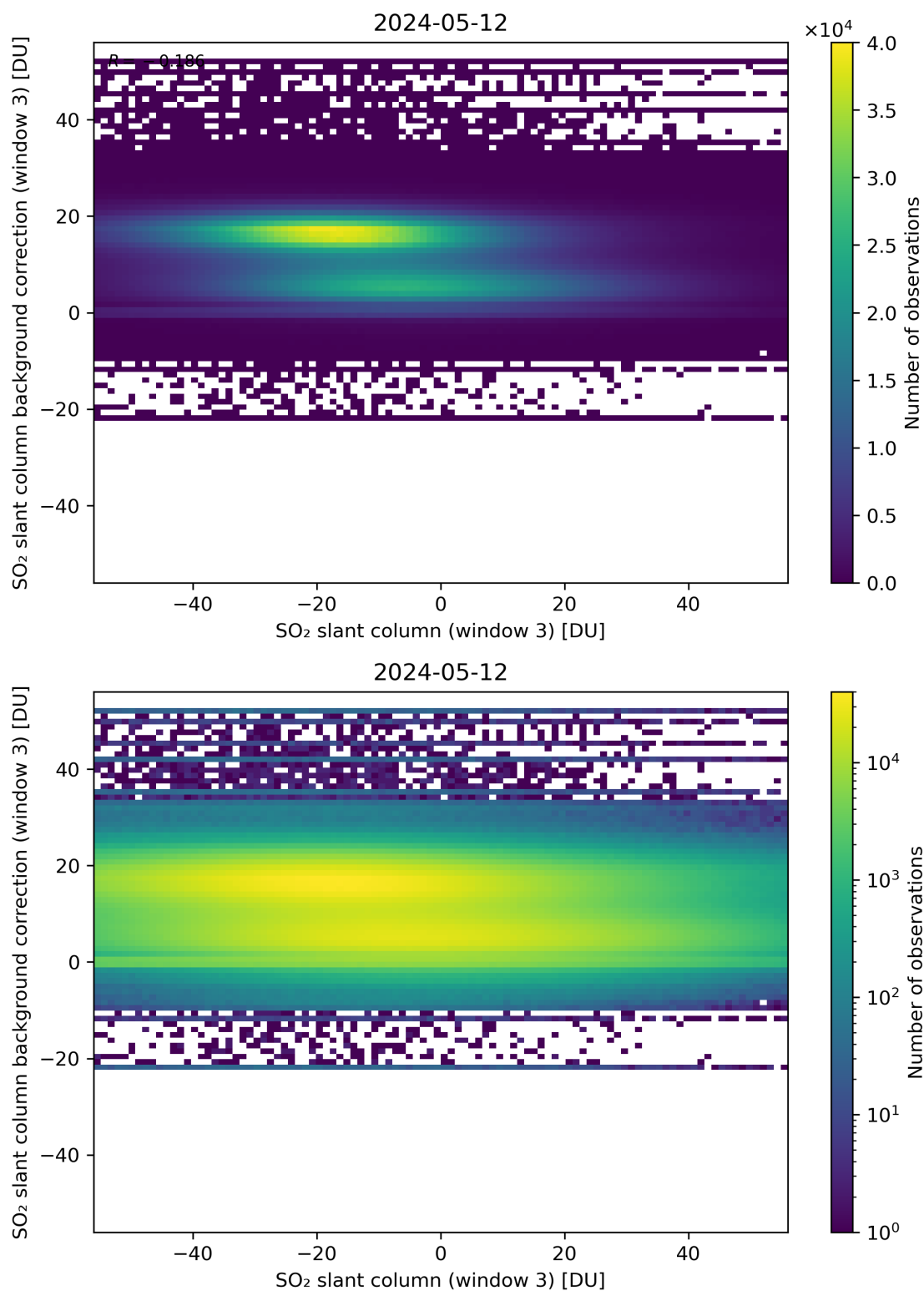
Figure 253: Scatter density plot of “SO 2 slant column (window 3)” against “SO 2 slant column background correction (window 3)” for 2024-05-12 to 2024-05-13.
