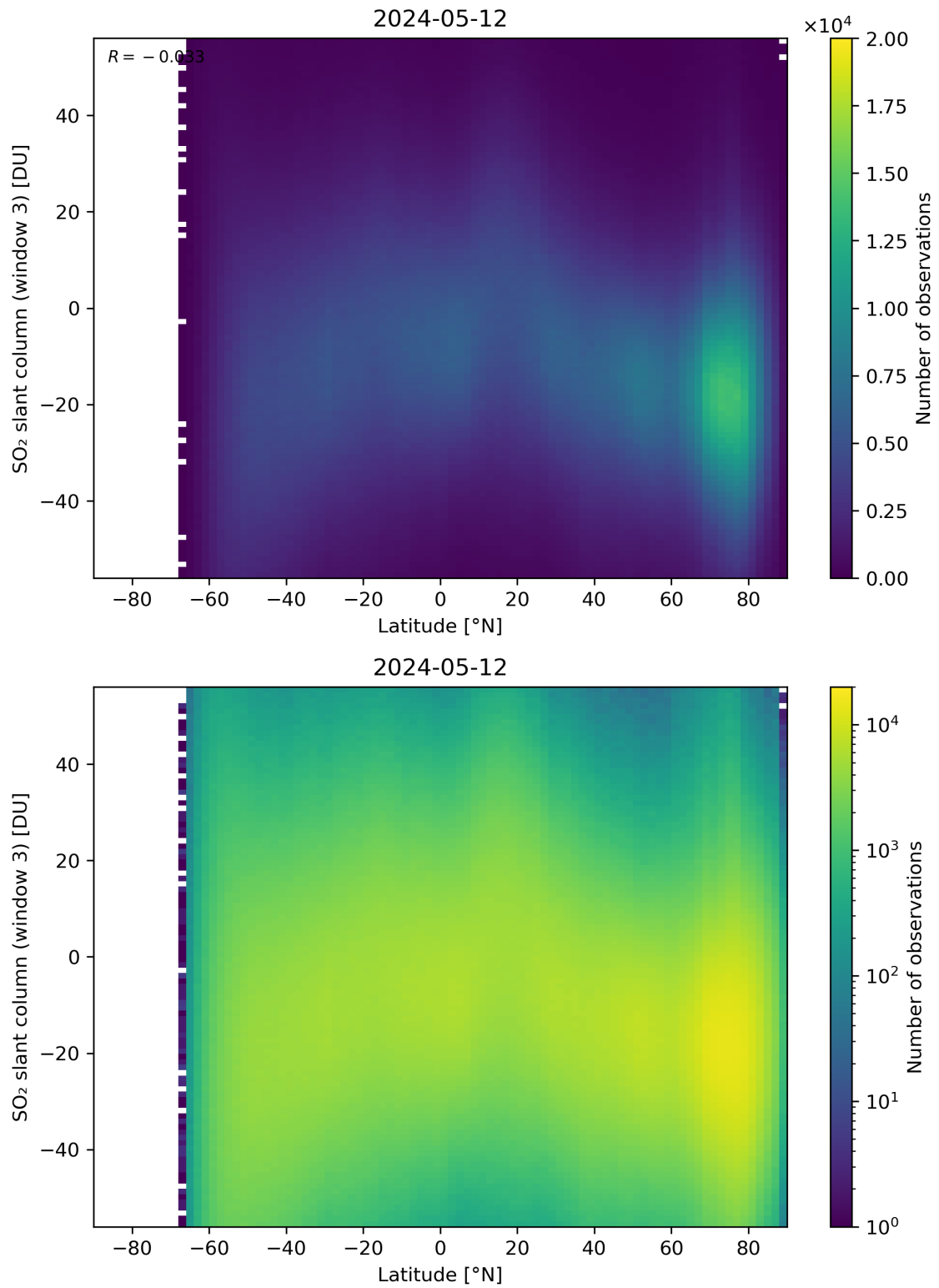
Figure 152: Scatter density plot of “Latitude” against “SO 2 slant column (window 3)” for 2024-05-12 to 2024-05-13.
