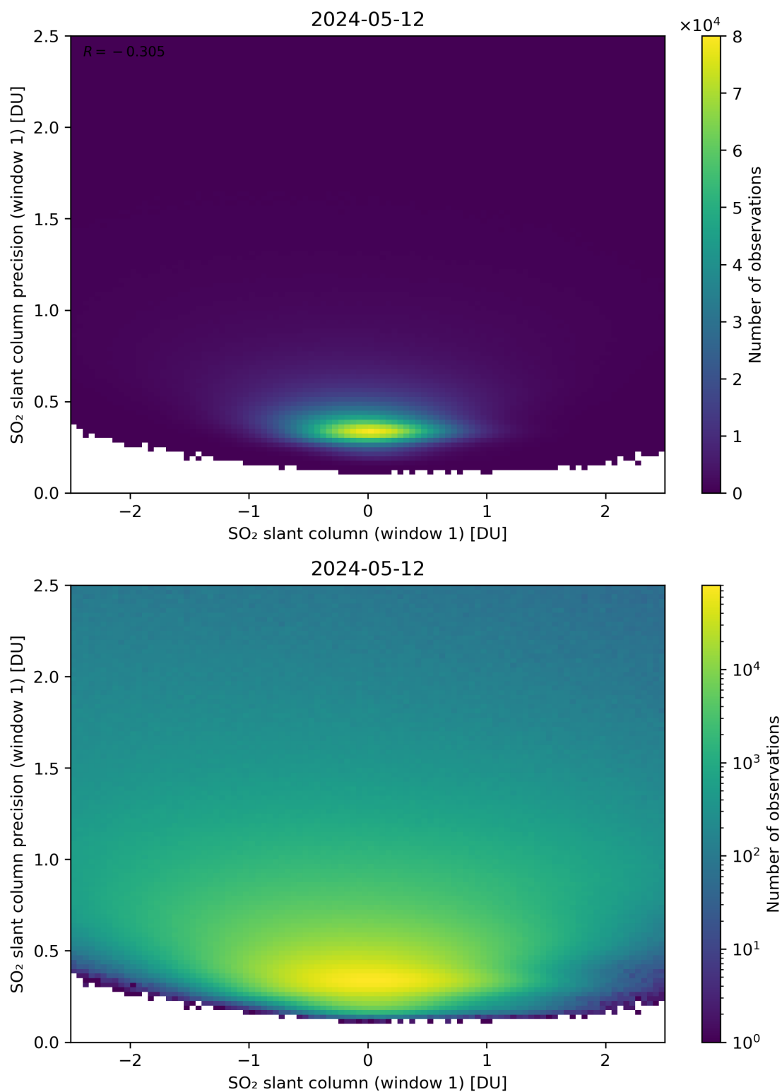
Figure 235: Scatter density plot of “SO 2 slant column (window 1)” against “SO 2 slant column precision (window 1)” for 2024-05-12 to 2024-05-13.
