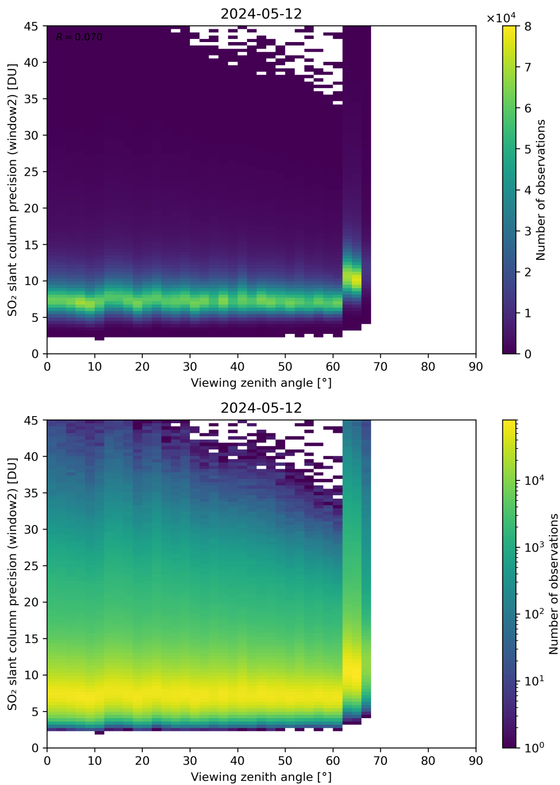
Figure 322: Scatter density plot of “Viewing zenith angle” against “SO 2 slant column precision (window2)” for 2024-05-12 to 2024-05-13.
