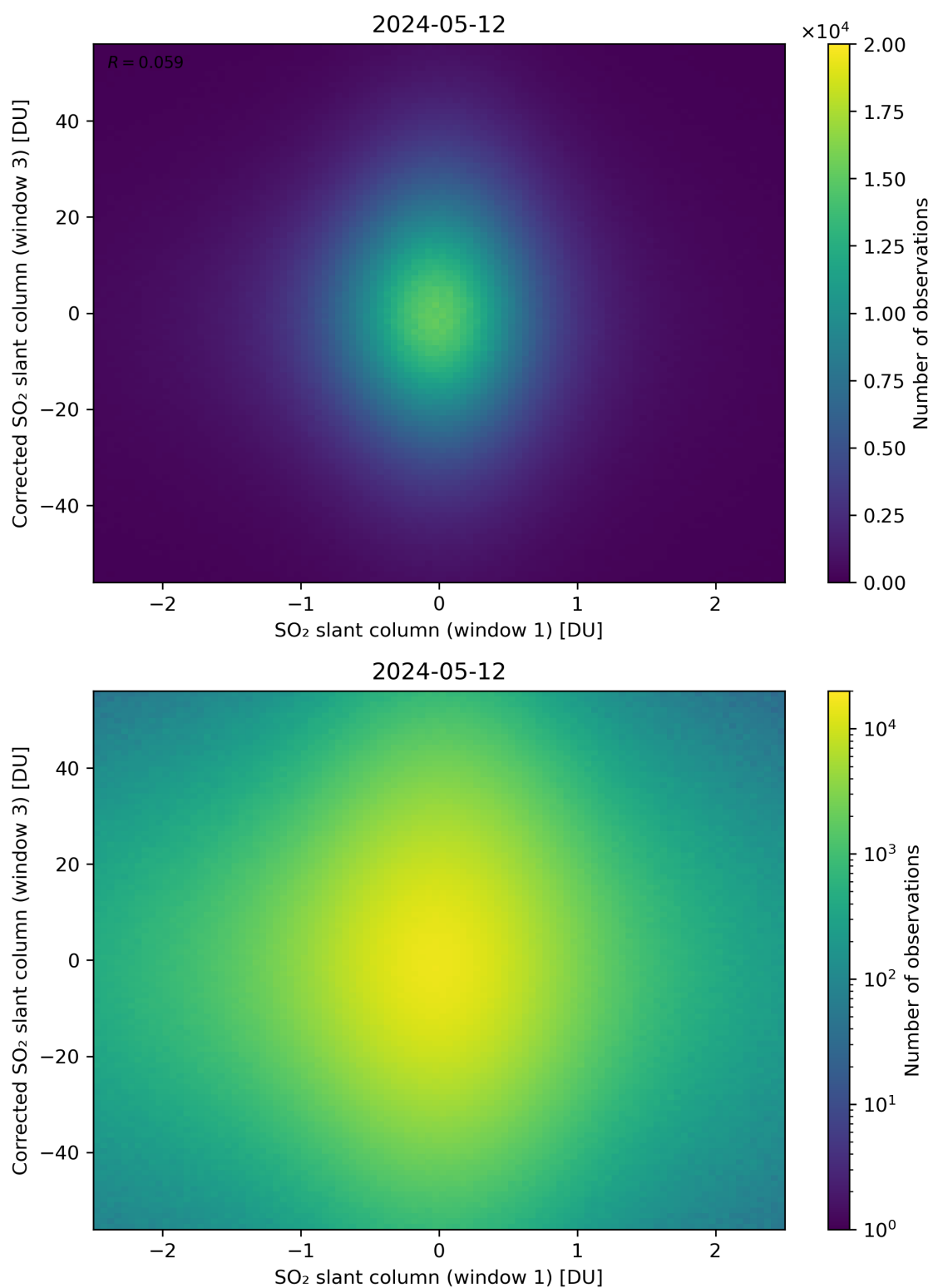
Figure 234: Scatter density plot of “SO 2 slant column (window 1)” against “Corrected SO 2 slant column (window 3)” for 2024-05-12 to 2024-05-13.
