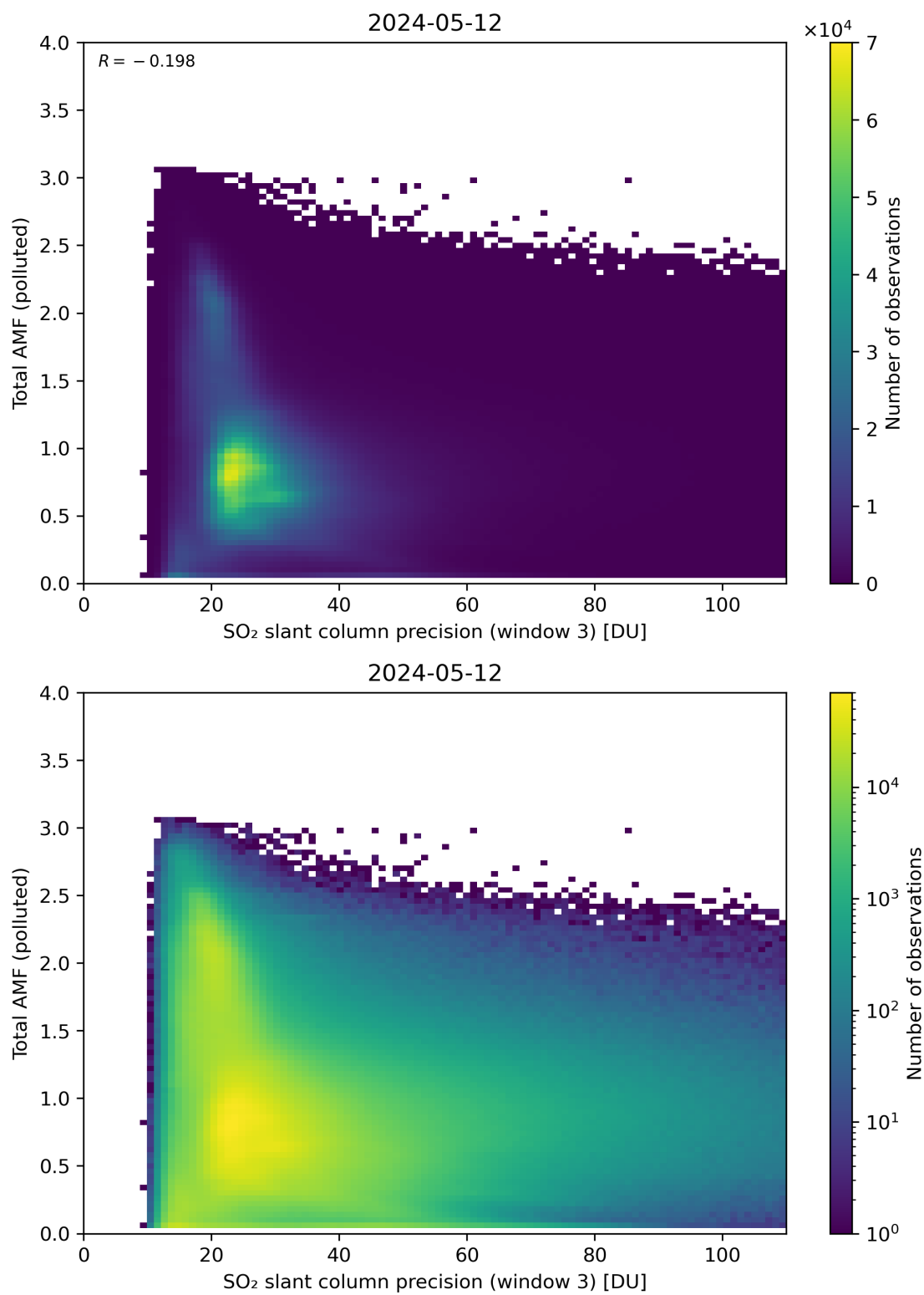
Figure 263: Scatter density plot of “SO 2 slant column precision (window 3)” against “Total AMF (polluted)” for 2024-05-12 to 2024-05-13.
