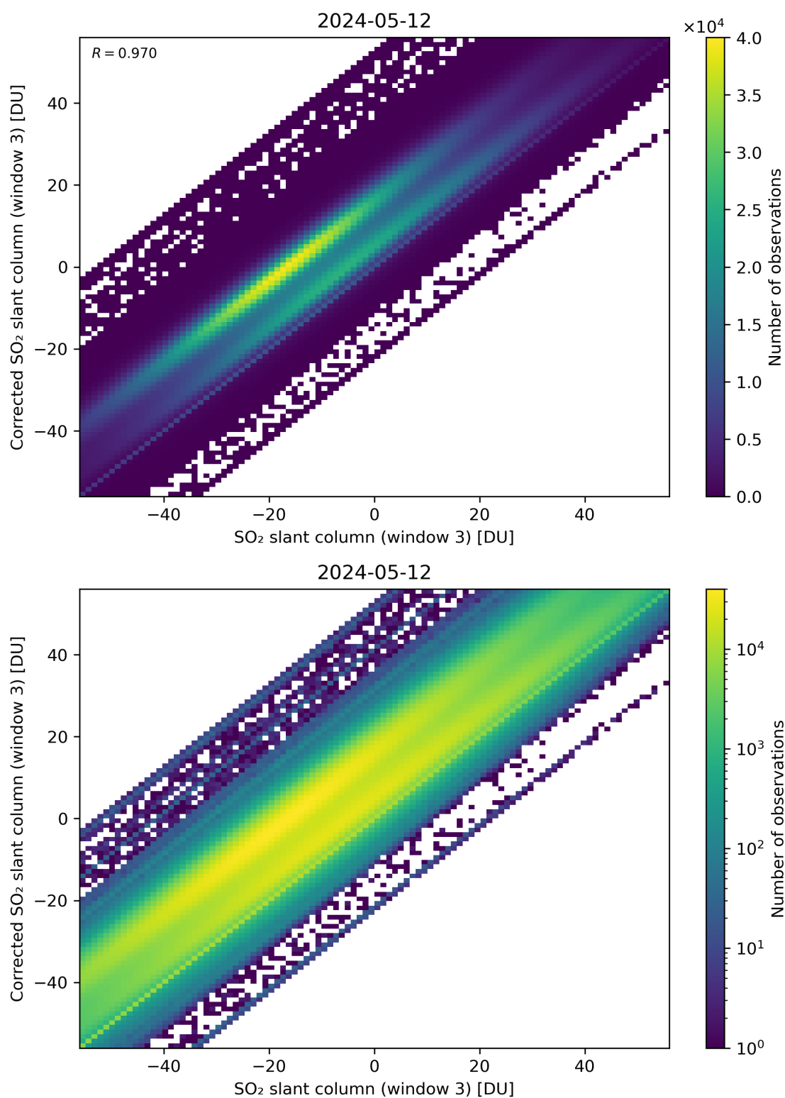
Figure 266: Scatter density plot of “SO 2 slant column (window 3)” against “Corrected SO 2 slant column (window 3)” for 2024-05-12 to 2024-05-13.
