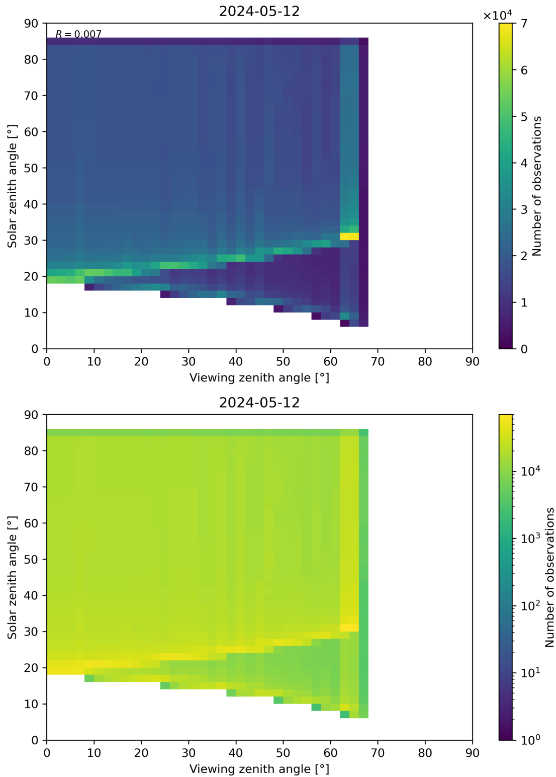
Figure 315: Scatter density plot of “Viewing zenith angle” against “Solar zenith angle” for 2024-05-12 to 2024-05-13.
