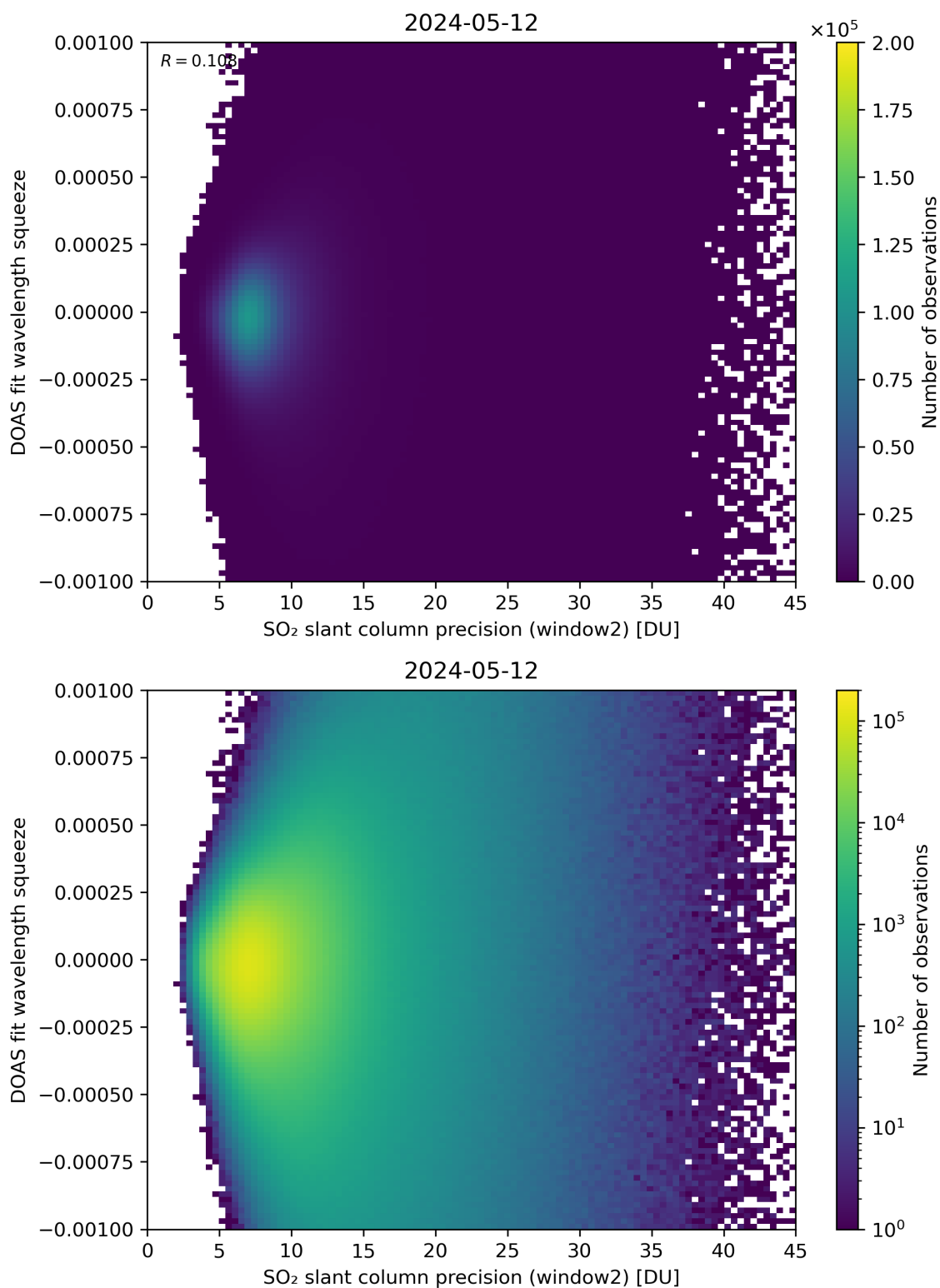
Figure 244: Scatter density plot of “SO 2 slant column precision (window2)” against “DOAS fit wavelength squeeze” for 2024-05-12 to 2024-05-13.
