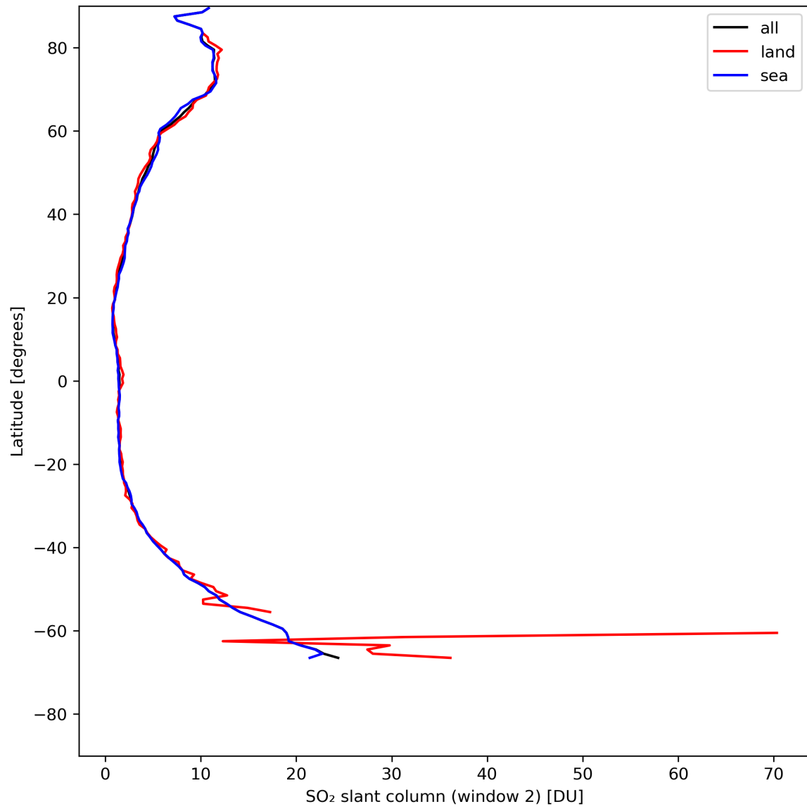
Figure 37: Zonal average of “SO 2 slant column (window 2)” for 2024-05-12 to 2024-05-13.
