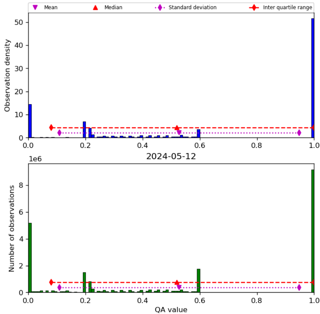
Figure 52: Histogram of “QA value” for 2024-05-12 to 2024-05-13
