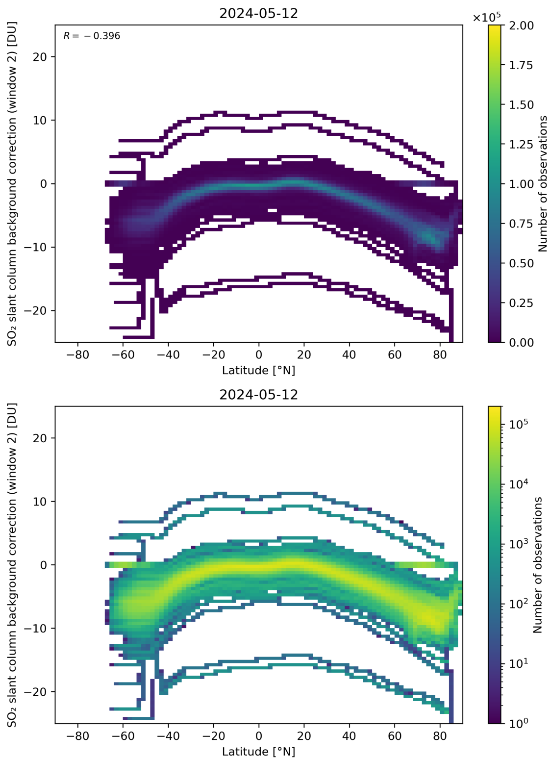
Figure 140: Scatter density plot of “Latitude” against “SO 2 slant column background correction (window 2)” for 2024-05-12 to 2024-05-13.
