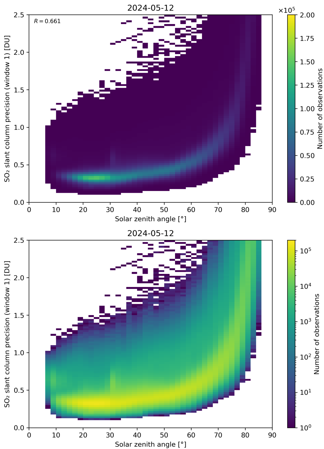
Figure 170: Scatter density plot of “Solar zenith angle” against “SO 2 slant column precision (window 1)” for 2024-05-12 to 2024-05-13.
