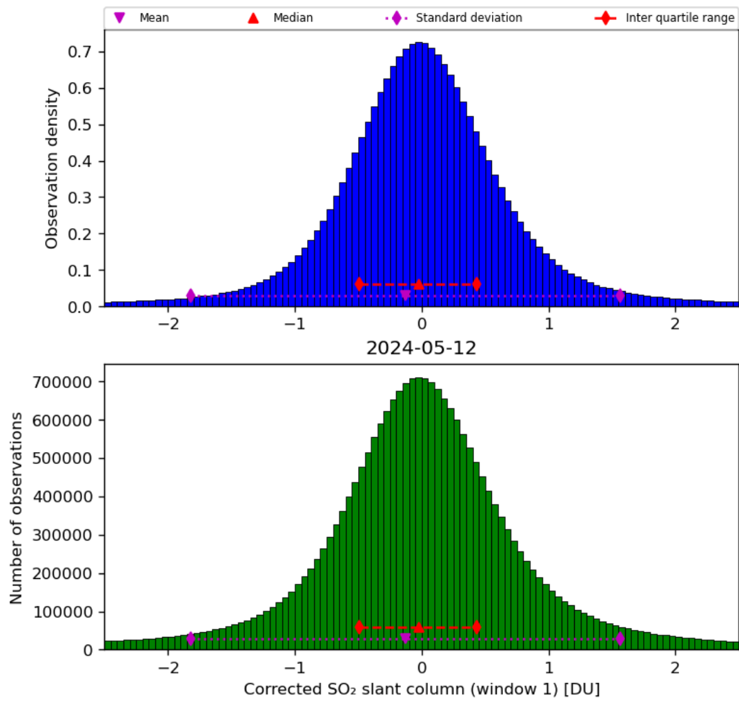
Figure 58: Histogram of “Corrected SO 2 slant column (window 1)” for 2024-05-12 to 2024-05-13
