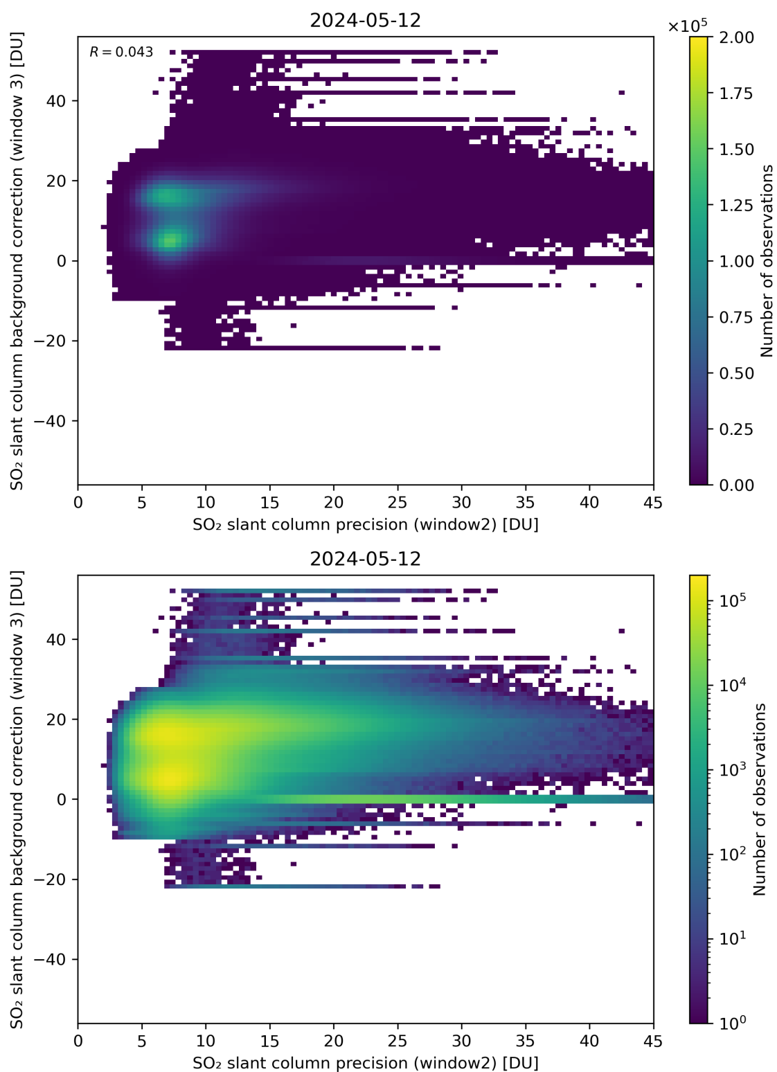
Figure 242: Scatter density plot of “SO 2 slant column precision (window2)” against “SO 2 slant column background correction (window 3)” for 2024-05-12 to 2024-05-13.
