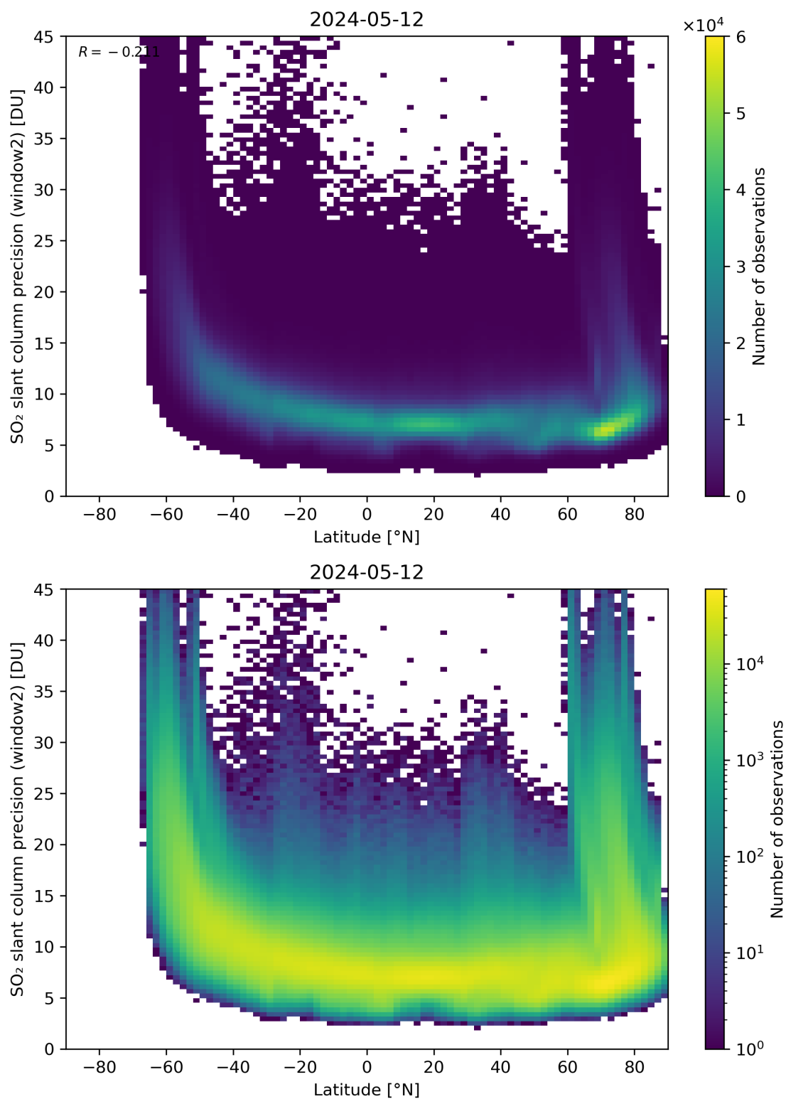
Figure 151: Scatter density plot of “Latitude” against “SO 2 slant column precision (window2)” for 2024-05-12 to 2024-05-13.
