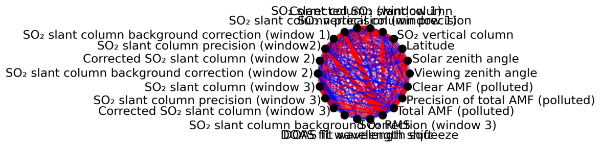
Figure 1: Map of correlation graph for 2024-05-12 to 2024-05-13.
