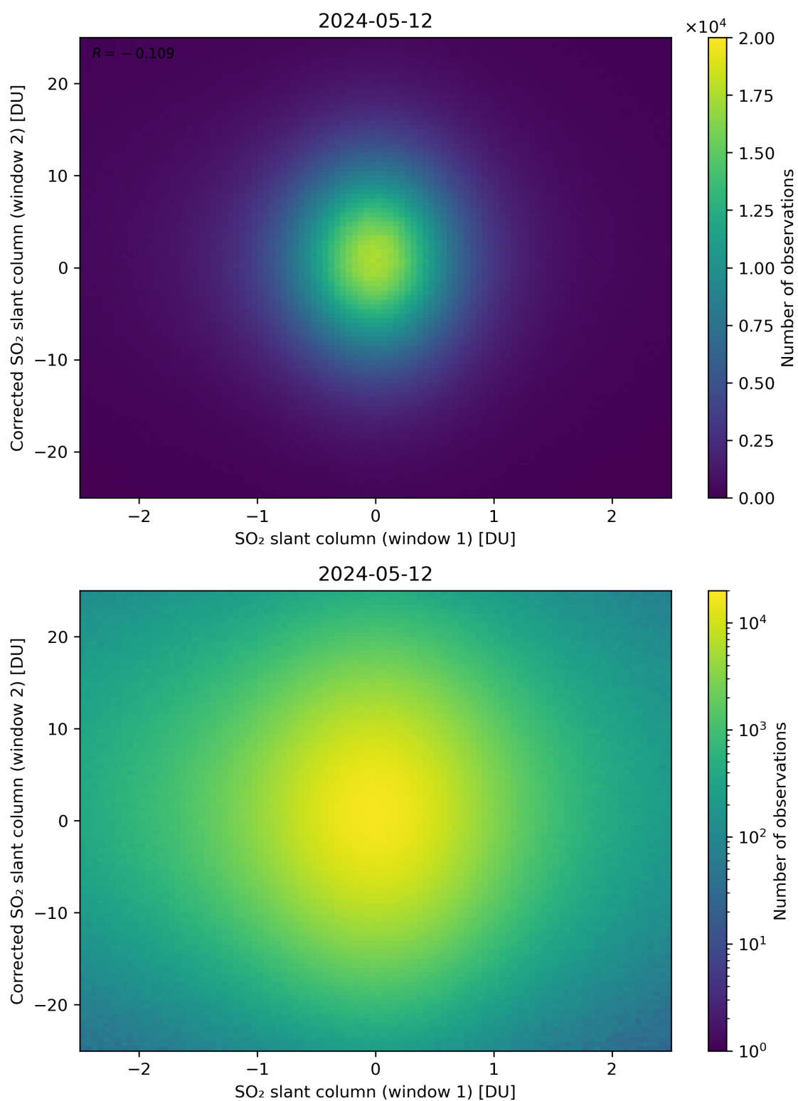
Figure 233: Scatter density plot of “SO 2 slant column (window 1)” against “Corrected SO 2 slant column (window 2)” for 2024-05-12 to 2024-05-13.
