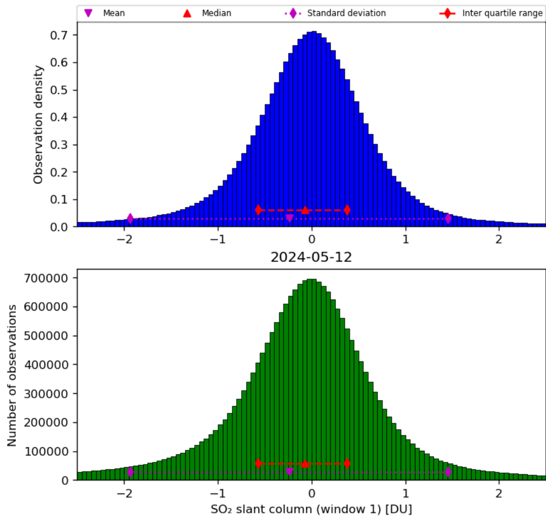
Figure 56: Histogram of “SO 2 slant column (window 1)” for 2024-05-12 to 2024-05-13
