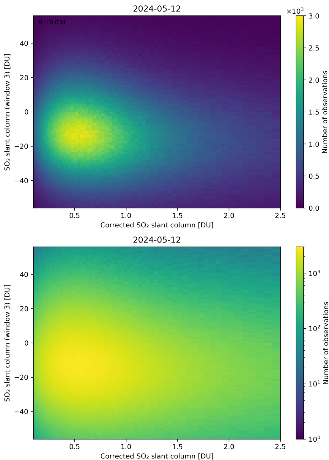
Figure 190: Scatter density plot of “Corrected SO 2 slant column” against “SO 2 slant column (window 3)” for 2024-05-12 to 2024-05-13.
