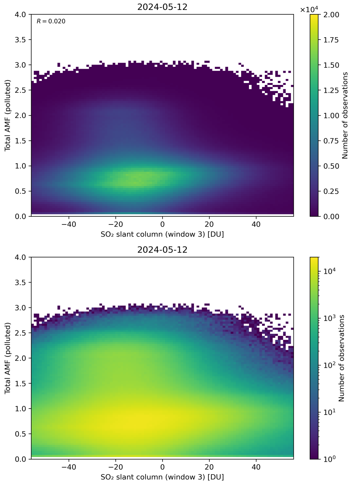
Figure 268: Scatter density plot of “SO 2 slant column (window 3)” against “Total AMF (polluted)” for 2024-05-12 to 2024-05-13.
