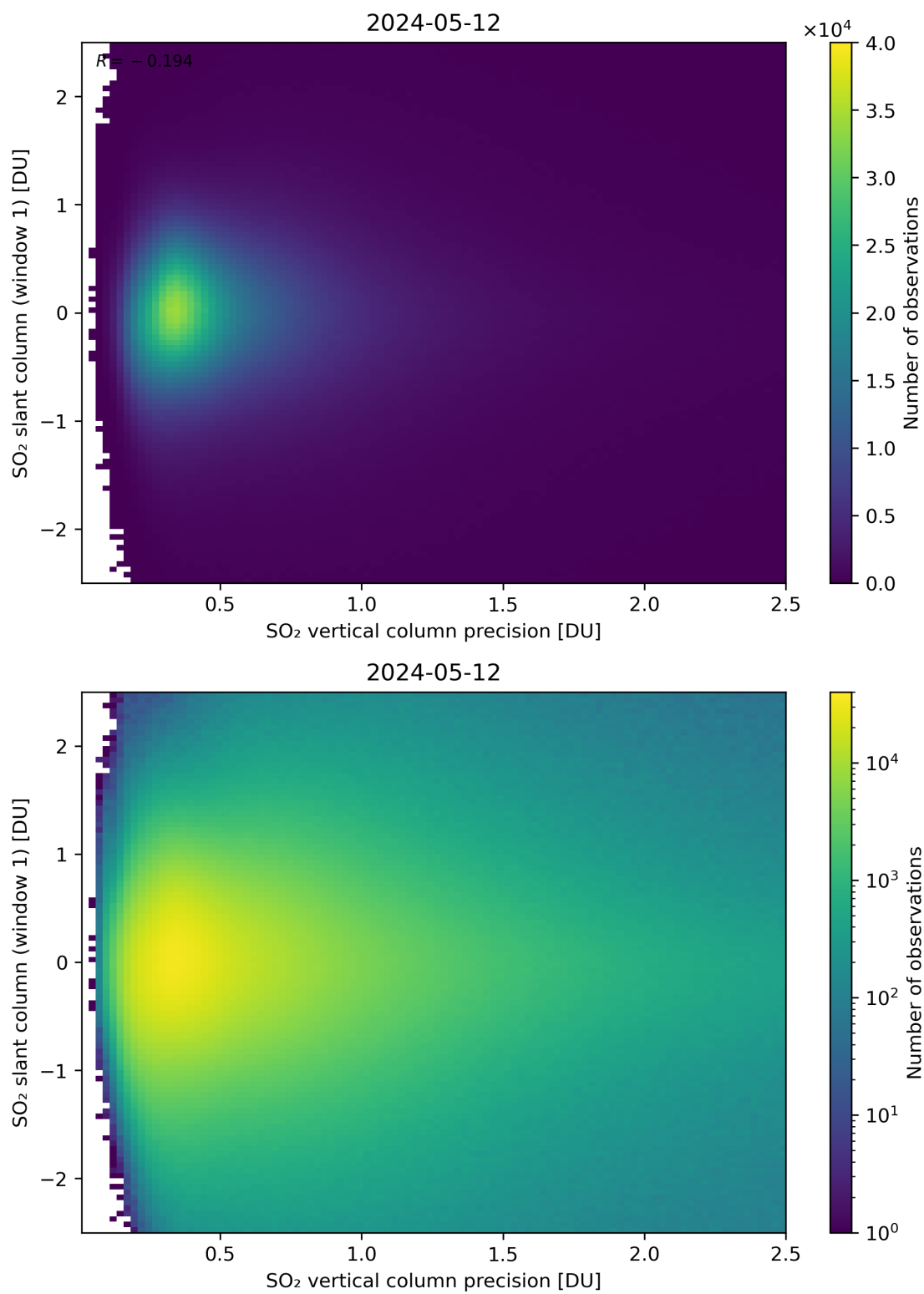
Figure 289: Scatter density plot of “SO 2 vertical column precision” against “SO 2 slant column (window 1)” for 2024-05-12 to 2024-05-13.
