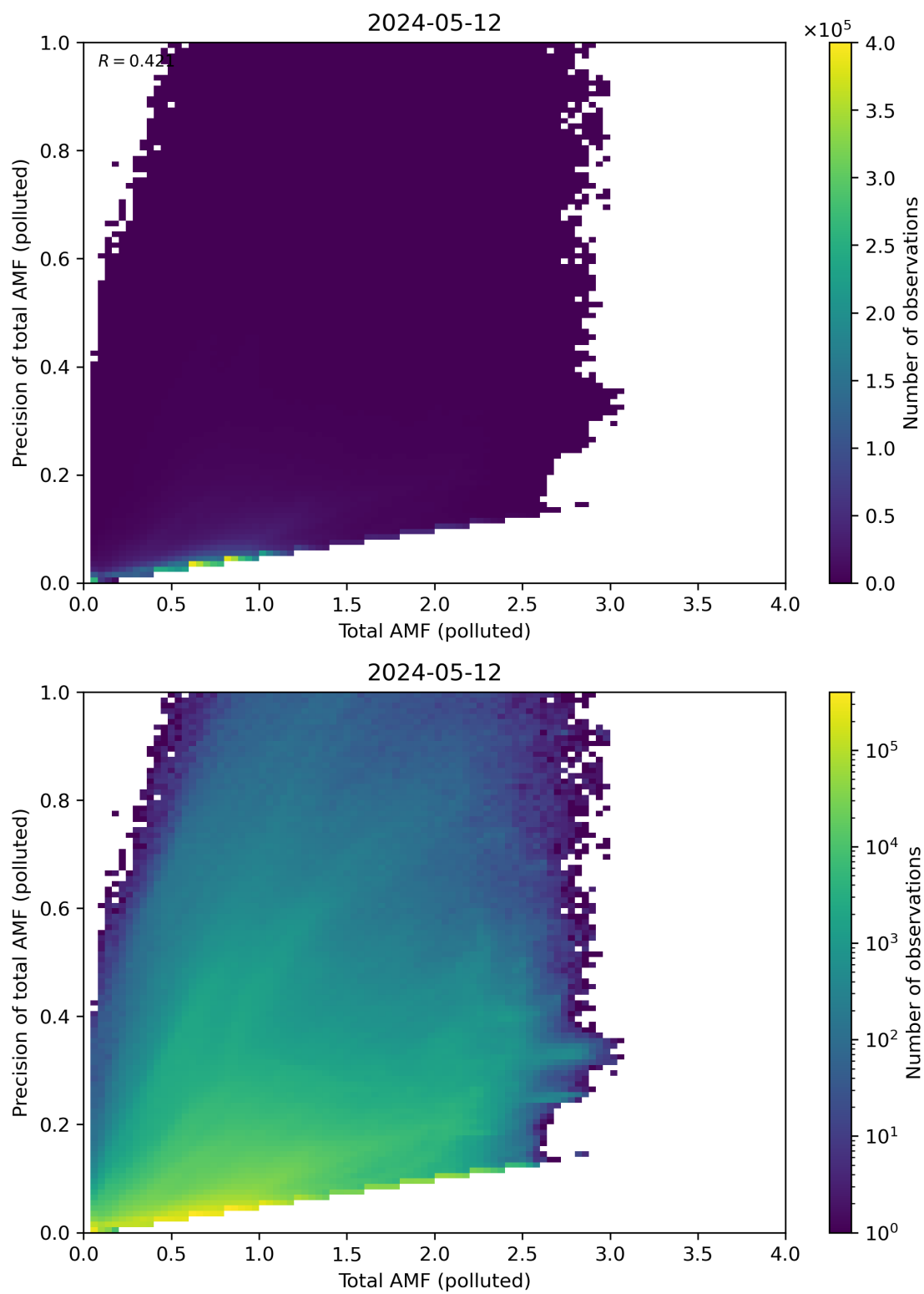
Figure 272: Scatter density plot of “Total AMF (polluted)” against “Precision of total AMF (polluted)” for 2024-05-12 to 2024-05-13.
