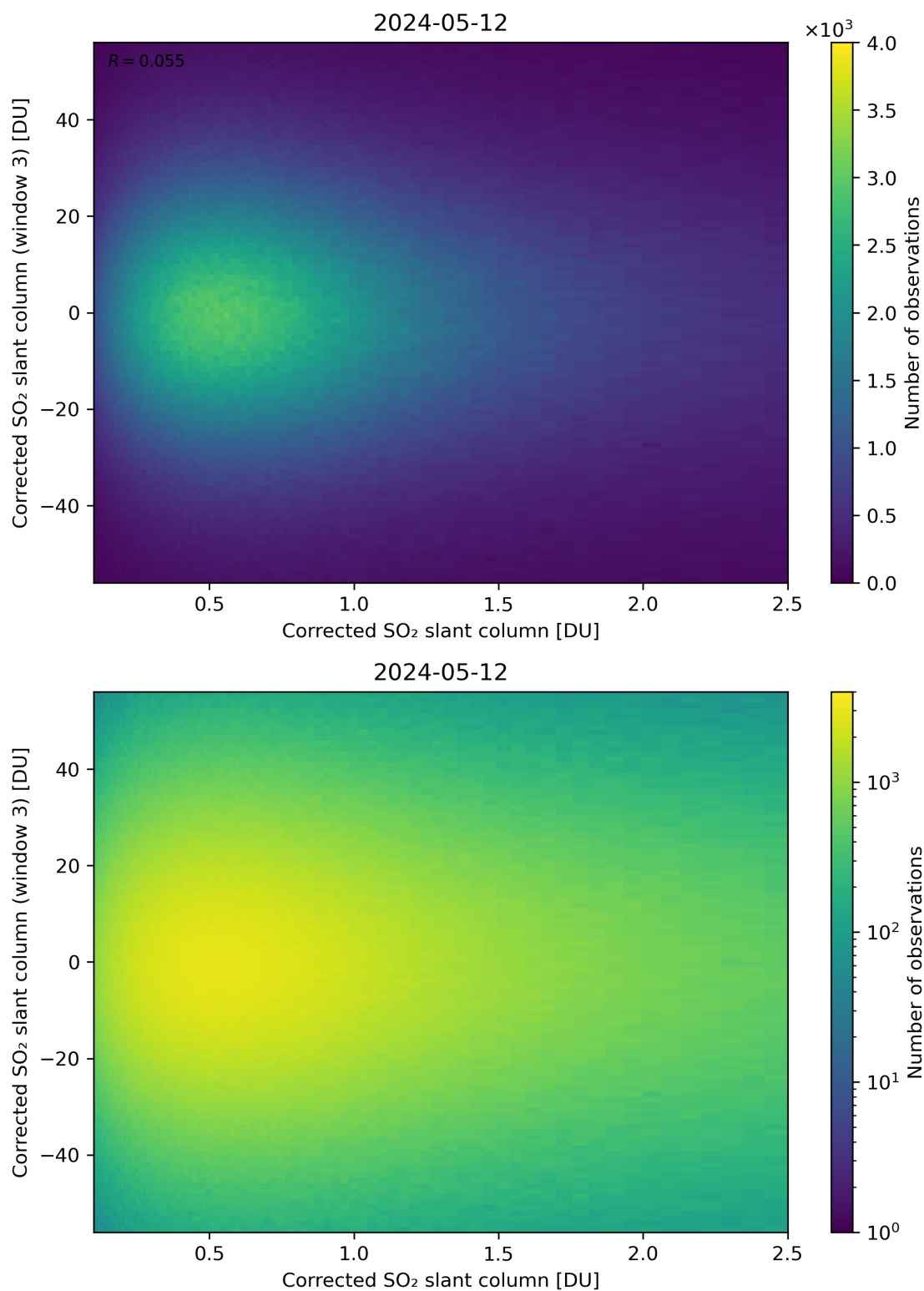
Figure 186: Scatter density plot of “Corrected SO 2 slant column” against “Corrected SO 2 slant column (window 3)” for 2024-05-12 to 2024-05-13.
