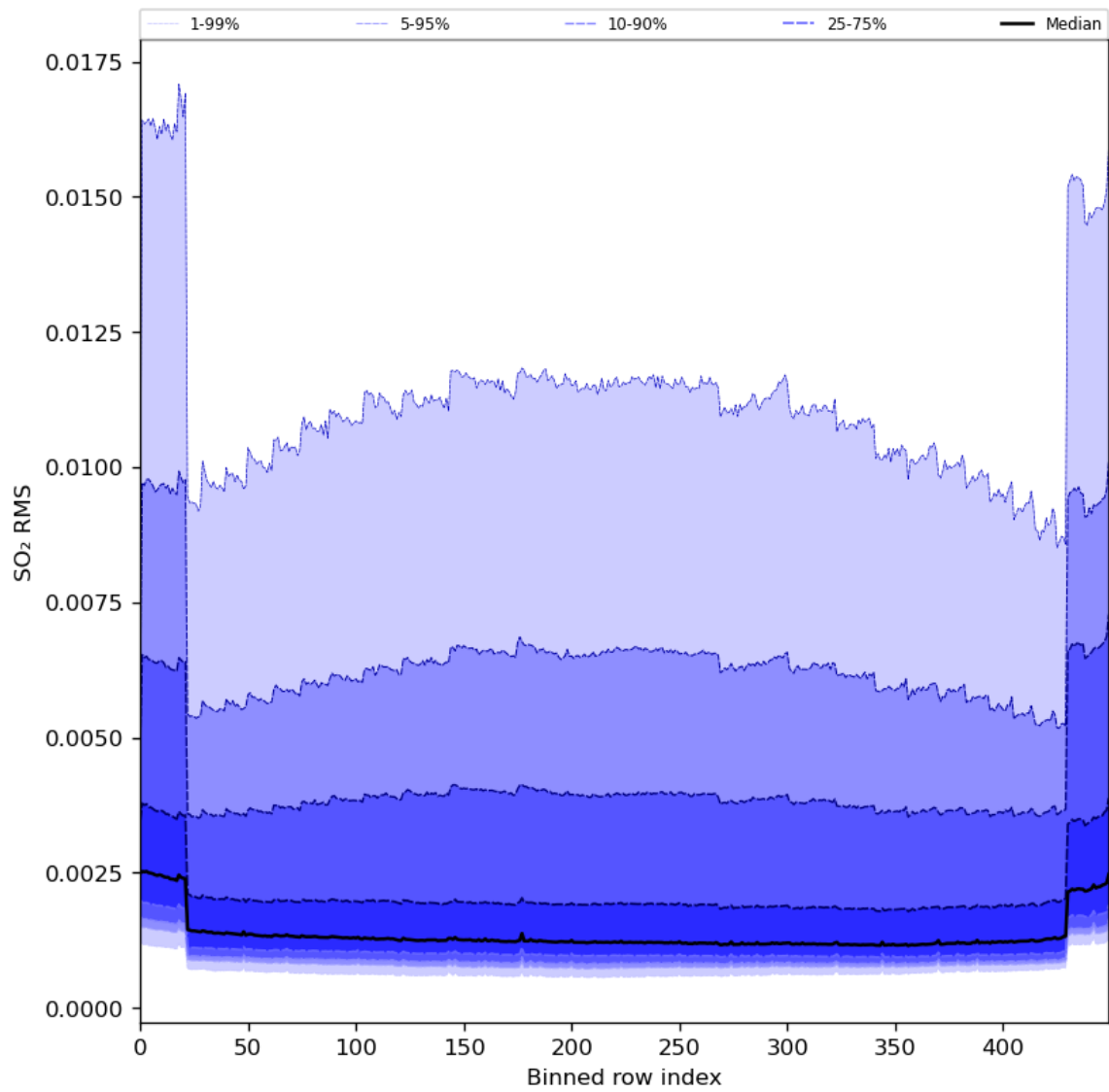
Figure 93: Along track statistics of “SO 2 RMS” for 2024-05-12 to 2024-05-13
