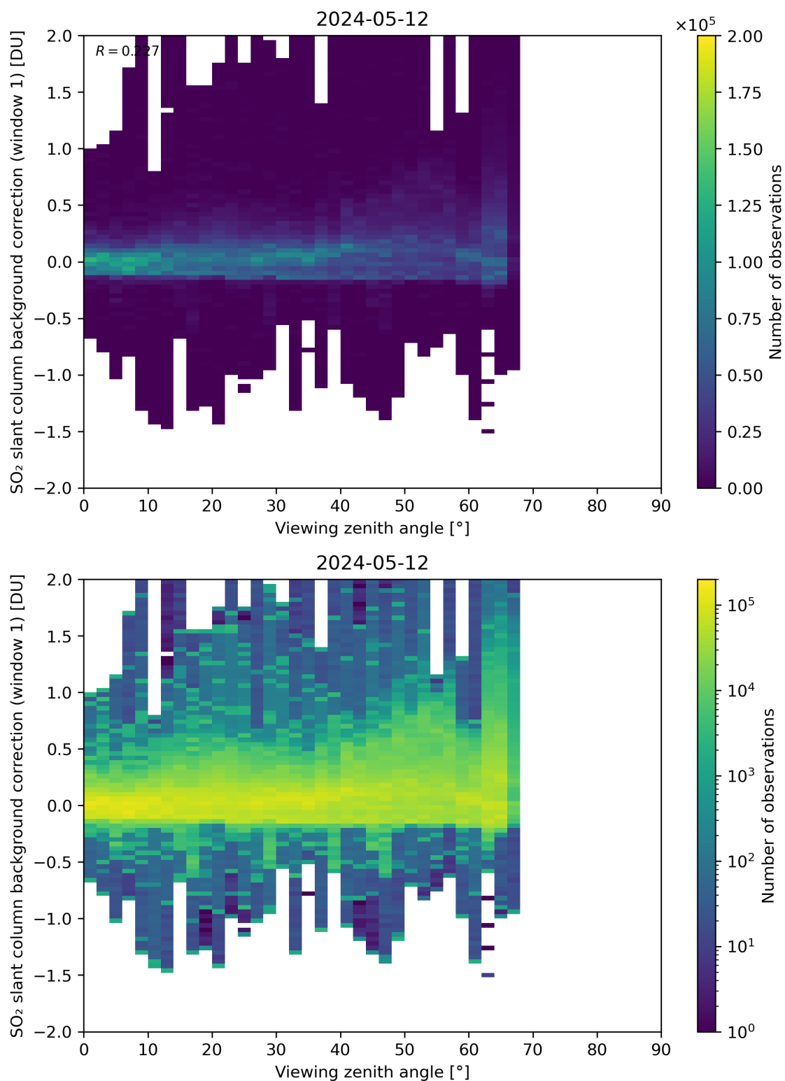
Figure 308: Scatter density plot of “Viewing zenith angle” against “SO 2 slant column background correction (window 1)” for 2024-05-12 to 2024-05-13.
