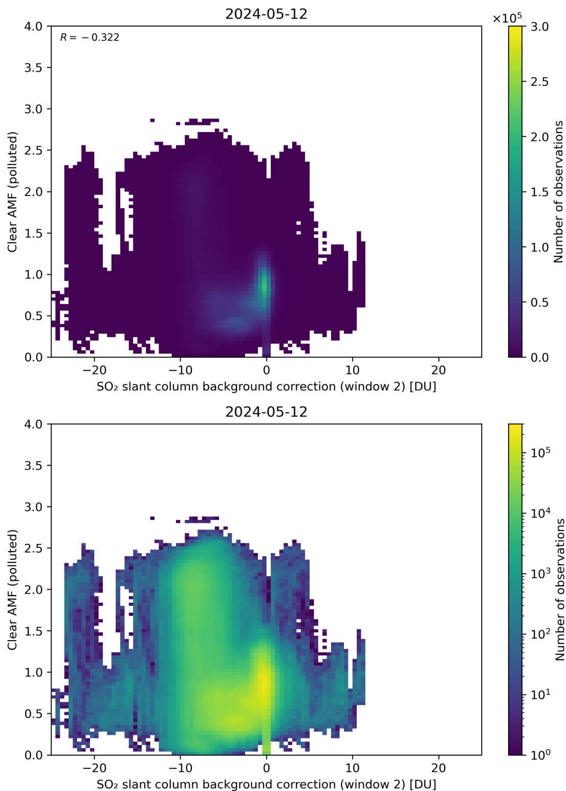
Figure 115: Scatter density plot of “SO 2 slant column background correction (window 2)” against “Clear AMF (polluted)” for 2024-05-12 to 2024-05-13.
