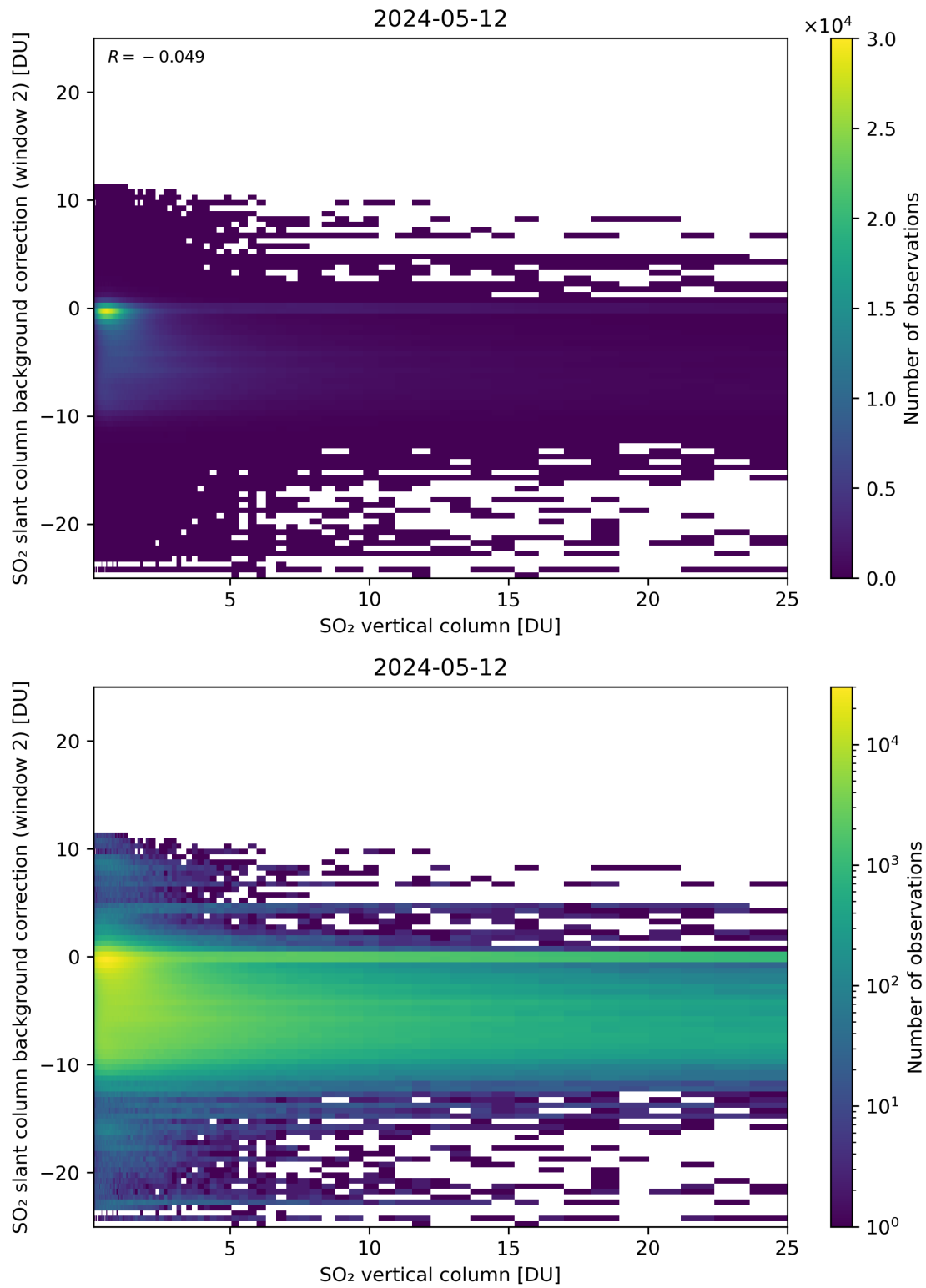
Figure 274: Scatter density plot of “SO 2 vertical column” against “SO 2 slant column background correction (window 2)” for 2024-05-12 to 2024-05-13.
