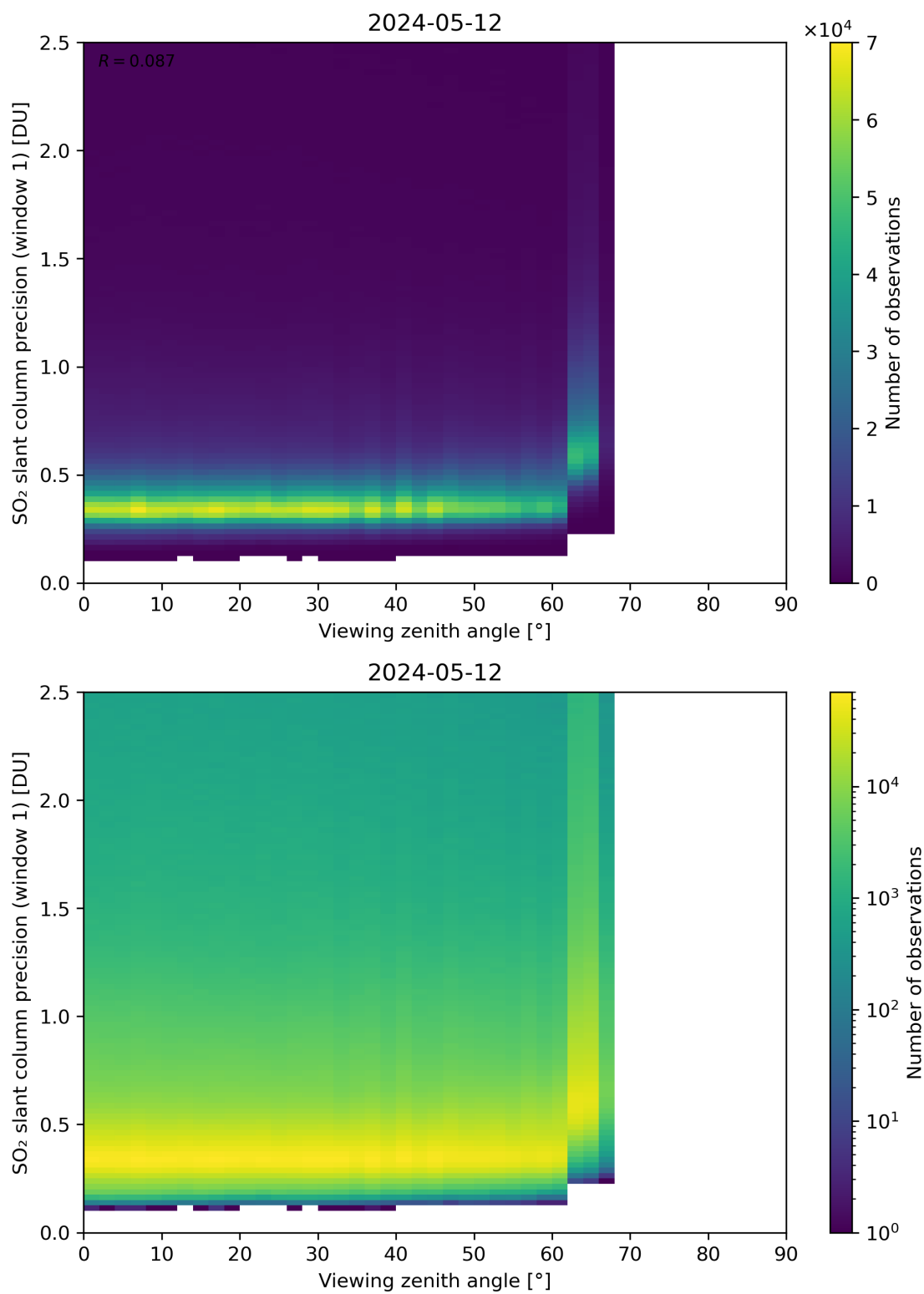
Figure 321: Scatter density plot of “Viewing zenith angle” against “SO 2 slant column precision (window 1)” for 2024-05-12 to 2024-05-13.
