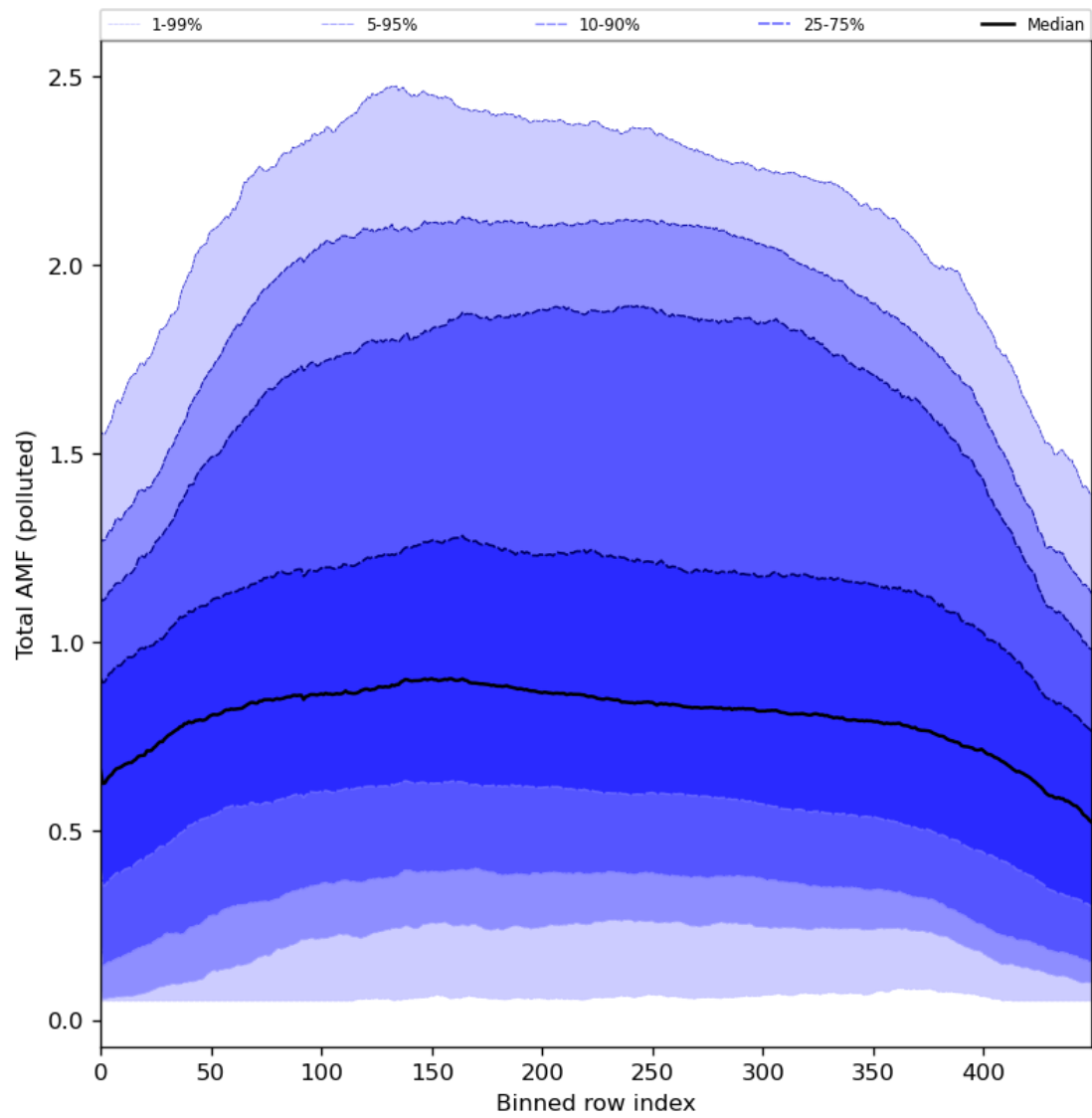
Figure 94: Along track statistics of “Total AMF (polluted)” for 2024-05-12 to 2024-05-13
