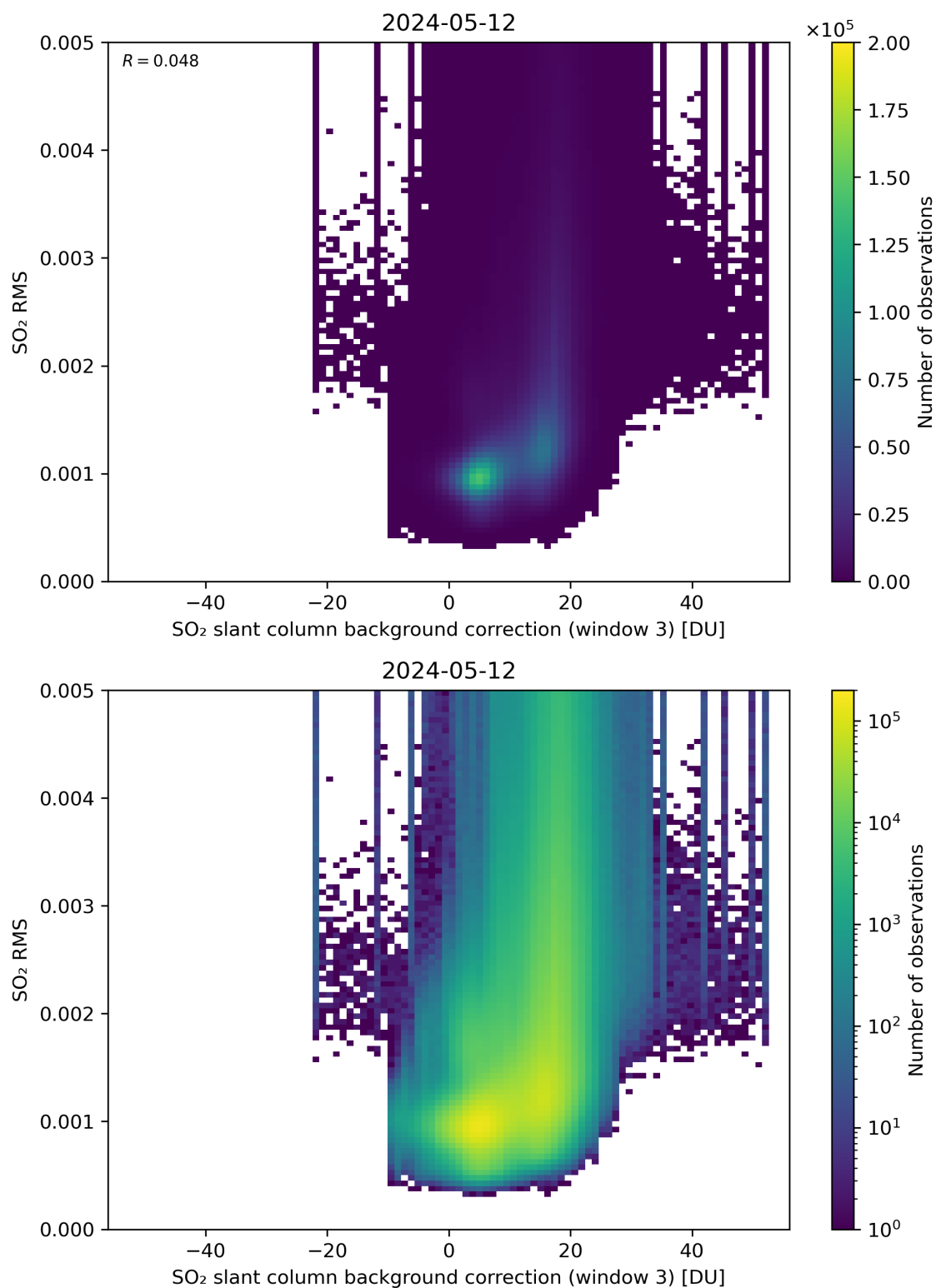
Figure 123: Scatter density plot of “SO 2 slant column background correction (window 3)” against “SO 2 RMS” for 2024-05-12 to 2024-05-13.
