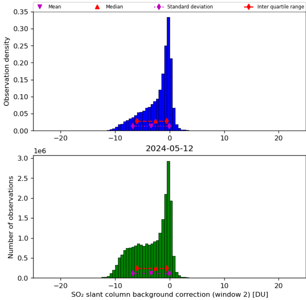
Figure 63: Histogram of “SO 2 slant column background correction (window 2)” for 2024-05-12 to 2024-05-13
