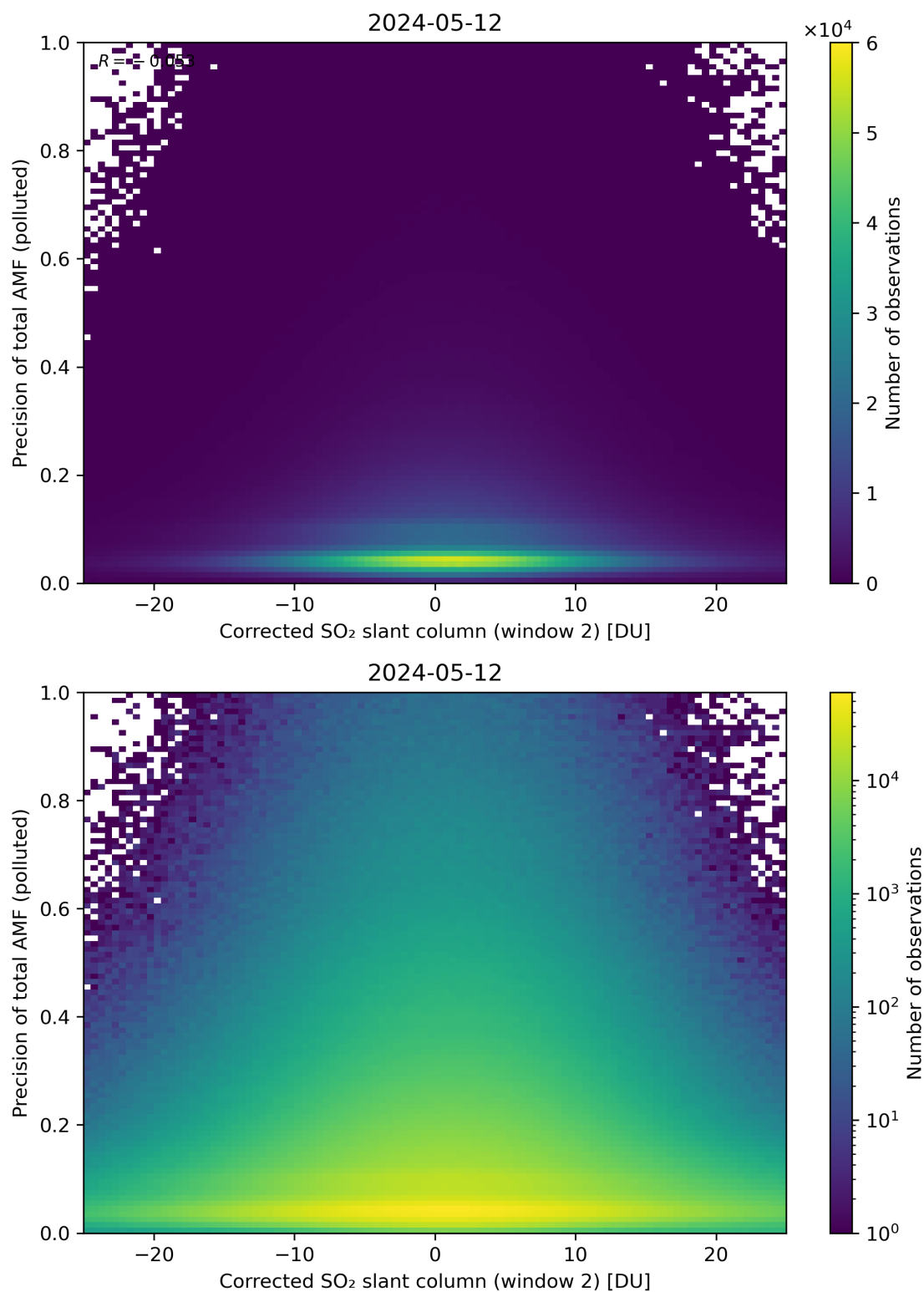
Figure 204: Scatter density plot of “Corrected SO 2 slant column (window 2)” against “Precision of total AMF (polluted)” for 2024-05-12 to 2024-05-13.
