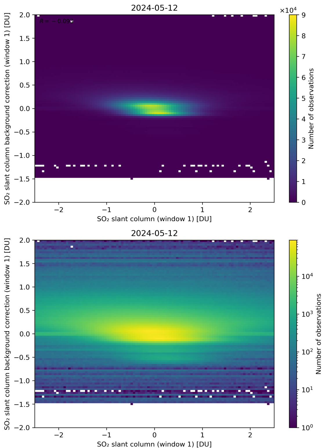
Figure 212: Scatter density plot of “SO 2 slant column (window 1)” against “SO 2 slant column background correction (window 1)” for 2024-05-12 to 2024-05-13.
