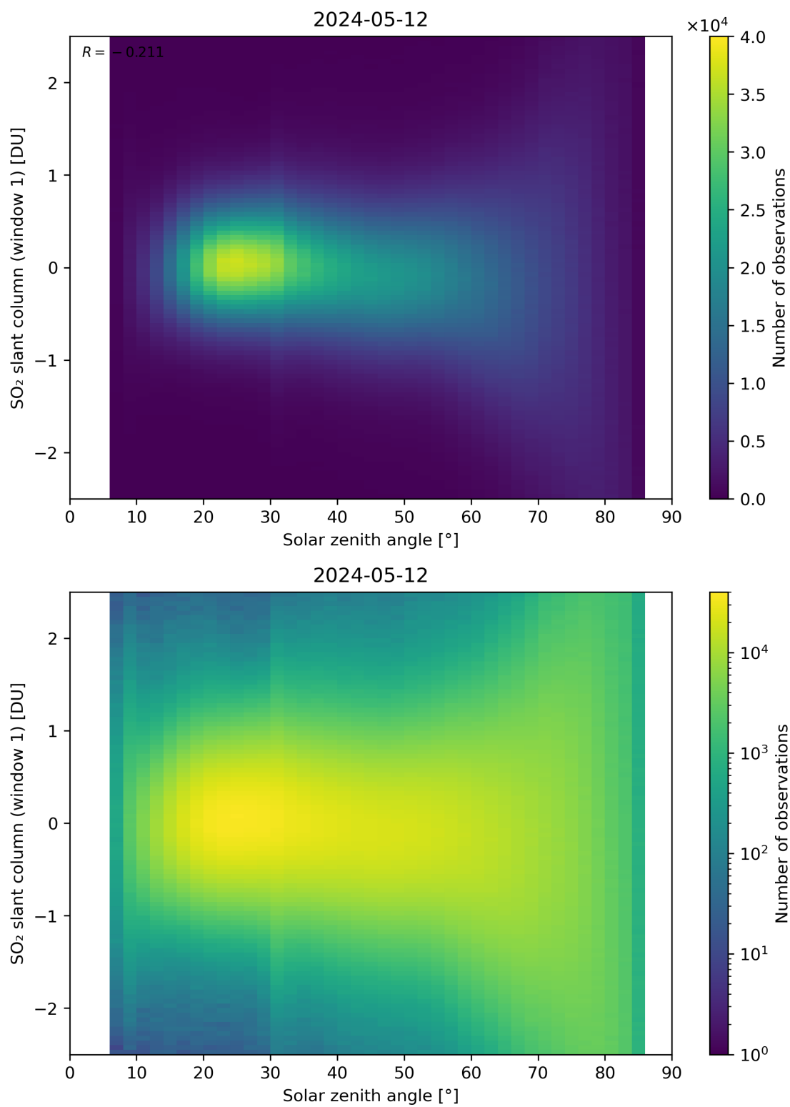
Figure 169: Scatter density plot of “Solar zenith angle” against “SO 2 slant column (window 1)” for 2024-05-12 to 2024-05-13.
