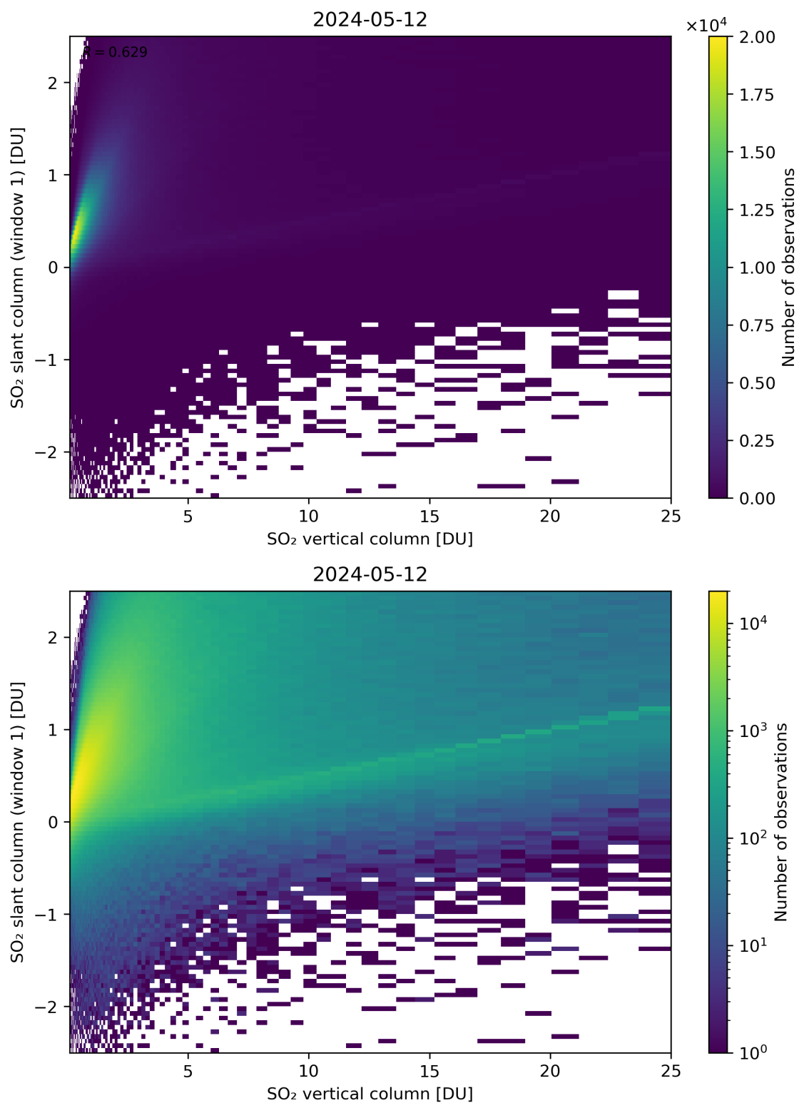
Figure 300: Scatter density plot of “SO 2 vertical column” against “SO 2 slant column (window 1)” for 2024-05-12 to 2024-05-13.
