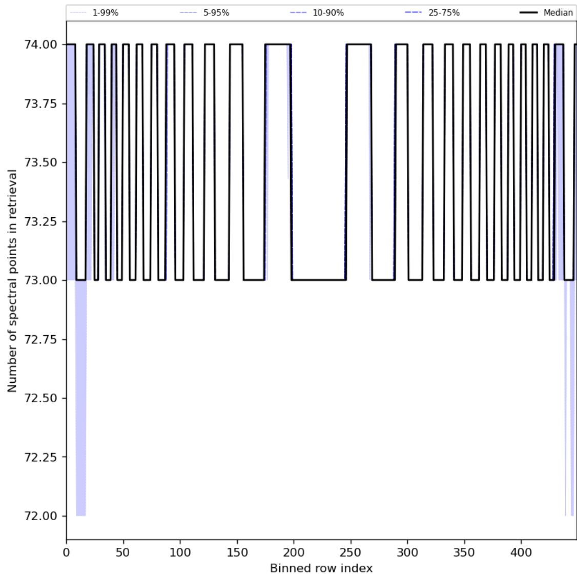
Figure 97: Along track statistics of “Number of spectral points in retrieval” for 2024-05-12 to 2024-05-13
