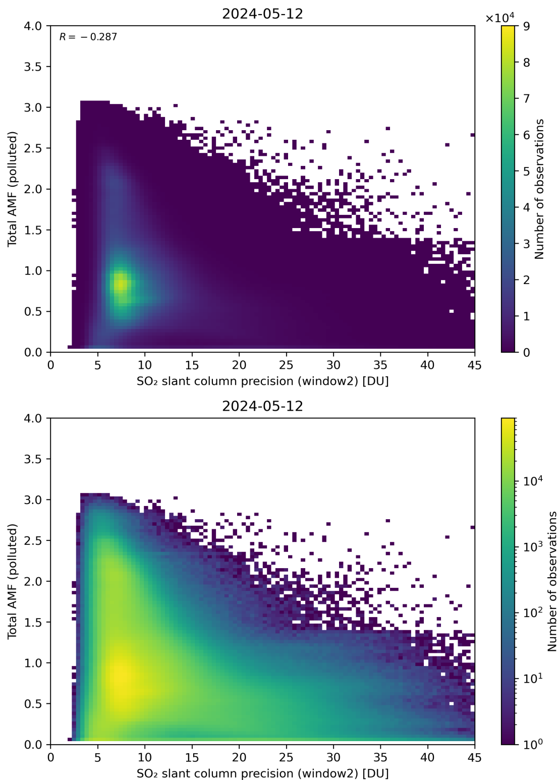
Figure 251: Scatter density plot of “SO 2 slant column precision (window2)” against “Total AMF (polluted)” for 2024-05-12 to 2024-05-13.
