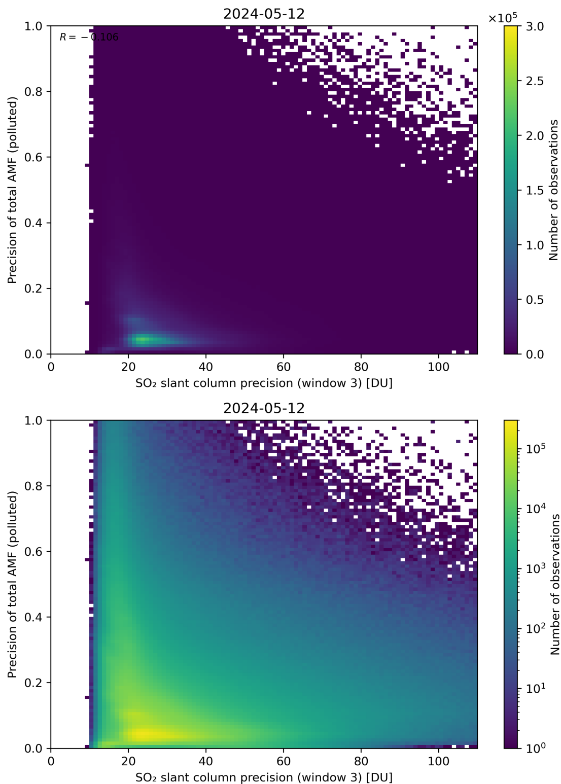
Figure 264: Scatter density plot of “SO 2 slant column precision (window 3)” against “Precision of total AMF (polluted)” for 2024-05-12 to 2024-05-13.
