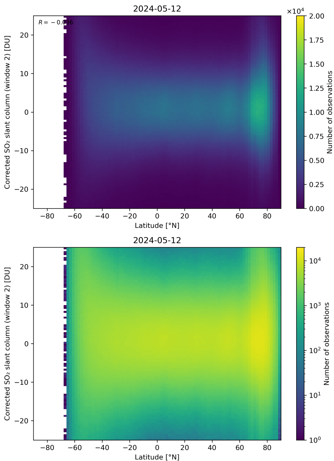
Figure 147: Scatter density plot of “Latitude” against “Corrected SO 2 slant column (window 2)” for 2024-05-12 to 2024-05-13.
