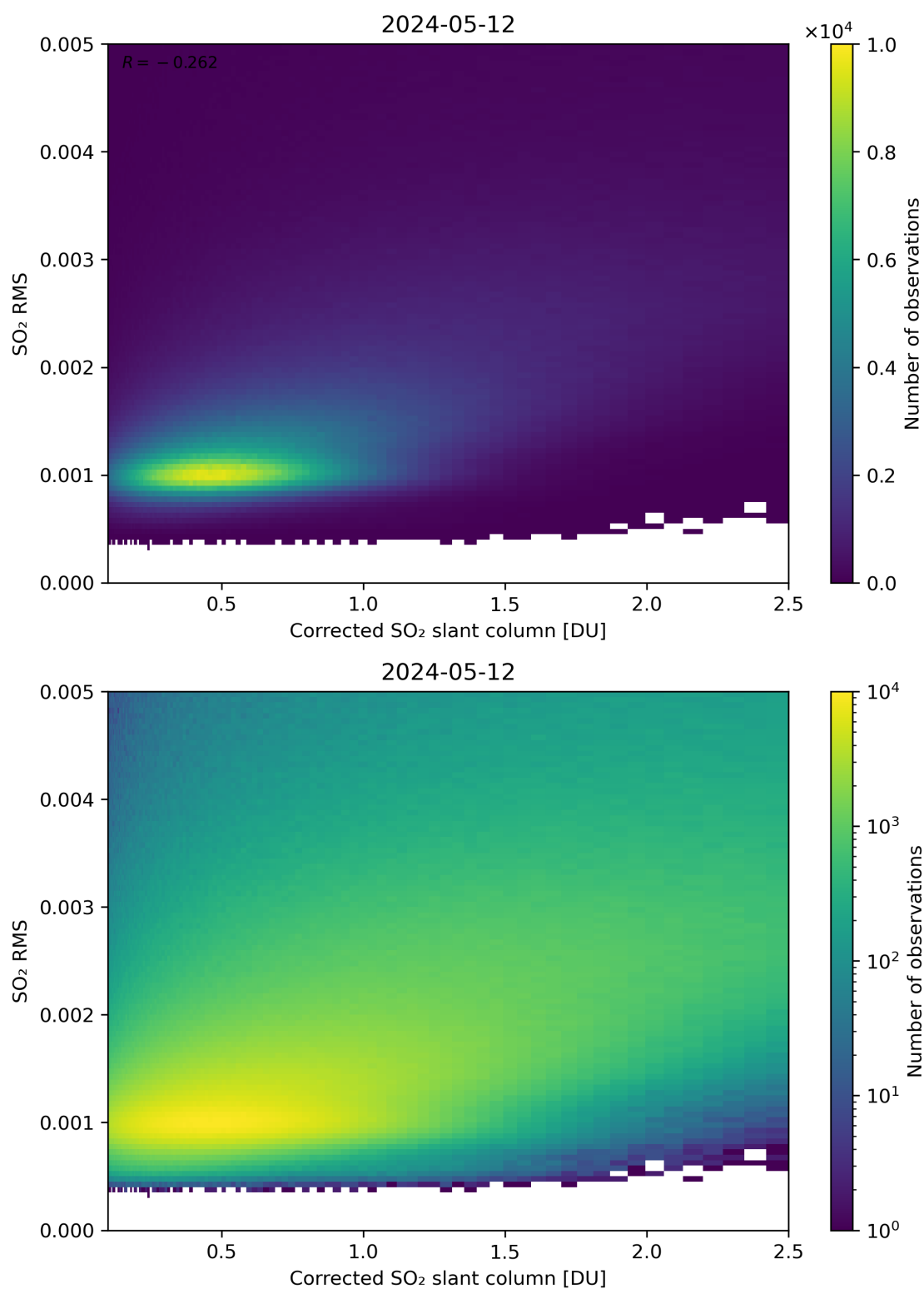
Figure 183: Scatter density plot of “Corrected SO 2 slant column” against “SO 2 RMS” for 2024-05-12 to 2024-05-13.
