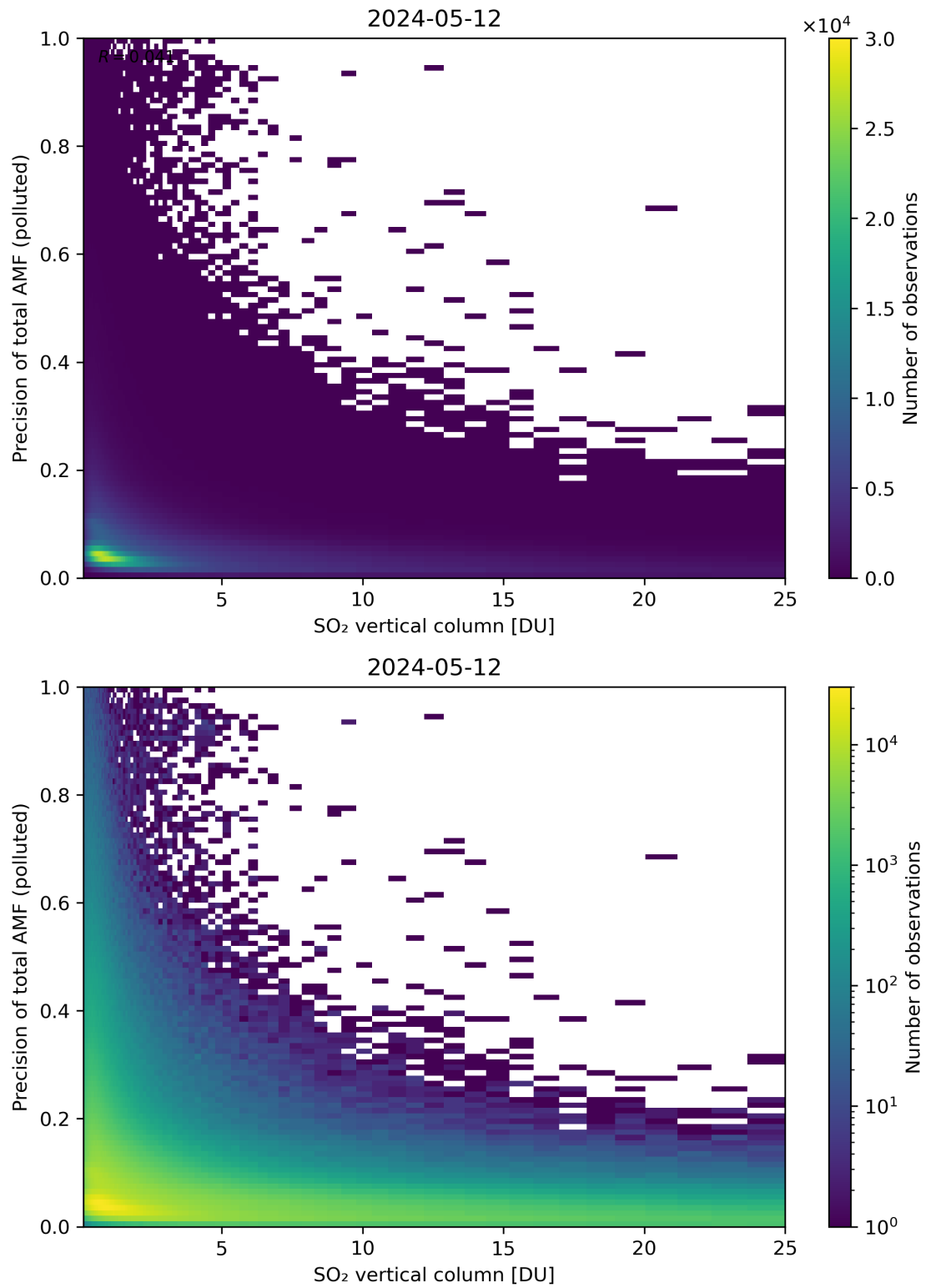
Figure 306: Scatter density plot of “SO 2 vertical column” against “Precision of total AMF (polluted)” for 2024-05-12 to 2024-05-13.
