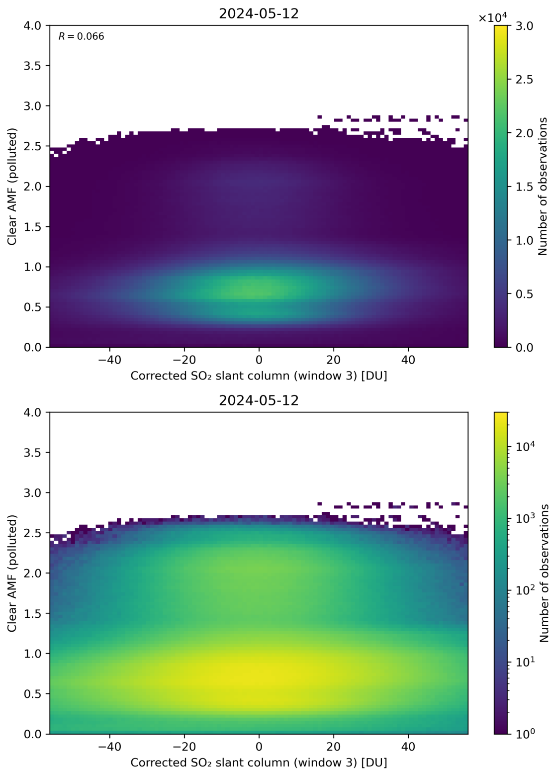
Figure 209: Scatter density plot of “Corrected SO 2 slant column (window 3)” against “Clear AMF (polluted)” for 2024-05-12 to 2024-05-13.
