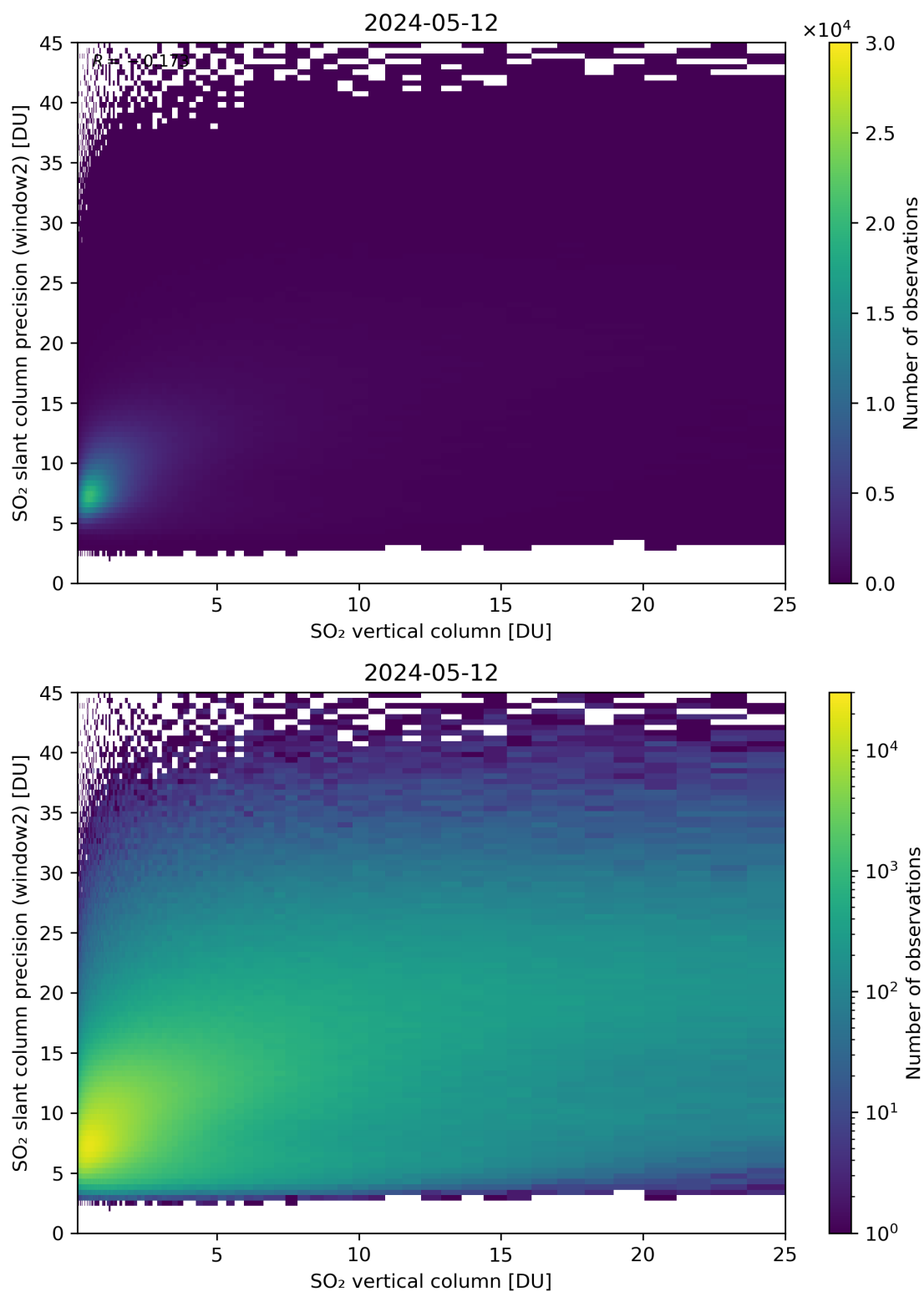
Figure 302: Scatter density plot of “SO 2 vertical column” against “SO 2 slant column precision (window2)” for 2024-05-12 to 2024-05-13.
