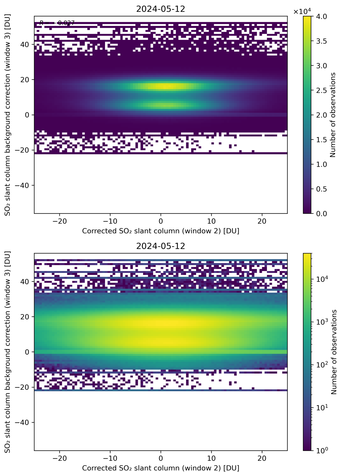
Figure 195: Scatter density plot of “Corrected SO 2 slant column (window 2)” against “SO 2 slant column background correction (window 3)” for 2024-05-12 to 2024-05-13.
