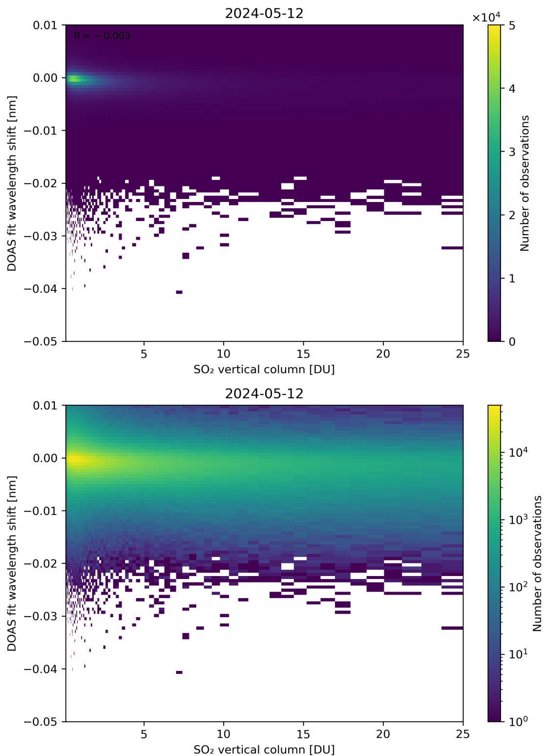
Figure 276: Scatter density plot of “SO 2 vertical column” against “DOAS fit wavelength shift” for 2024-05-12 to 2024-05-13.
