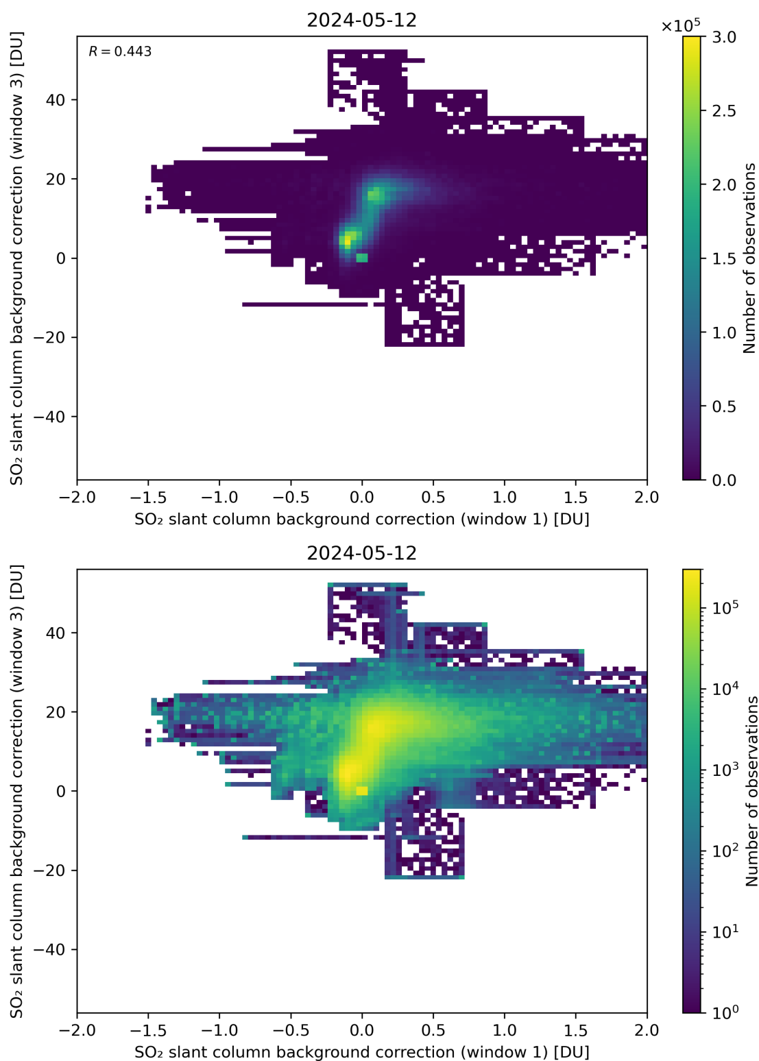
Figure 99: Scatter density plot of “SO 2 slant column background correction (window 1)” against “SO 2 slant column background correction (window 3)” for 2024-05-12 to 2024-05-13.
