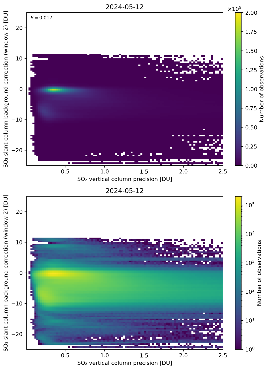
Figure 280: Scatter density plot of “SO 2 vertical column precision” against “SO 2 slant column background correction (window 2)” for 2024-05-12 to 2024-05-13.
