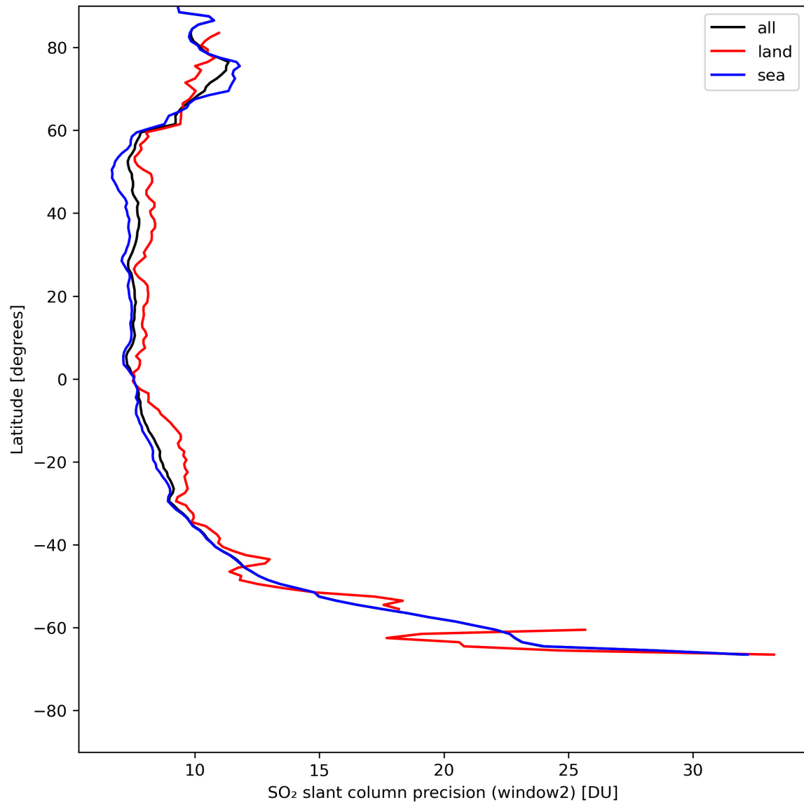
Figure 38: Zonal average of “SO 2 slant column precision (window2)” for 2024-05-12 to 2024-05-13.
