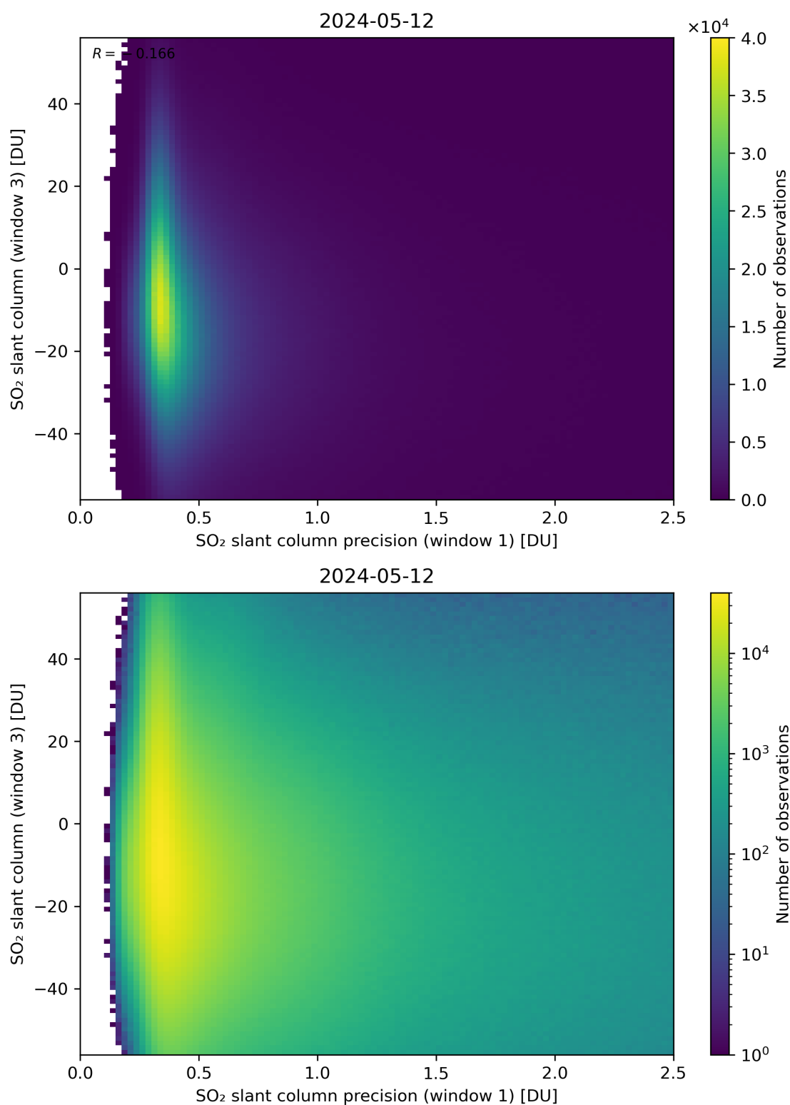
Figure 228: Scatter density plot of “SO 2 slant column precision (window 1)” against “SO 2 slant column (window 3)” for 2024-05-12 to 2024-05-13.
