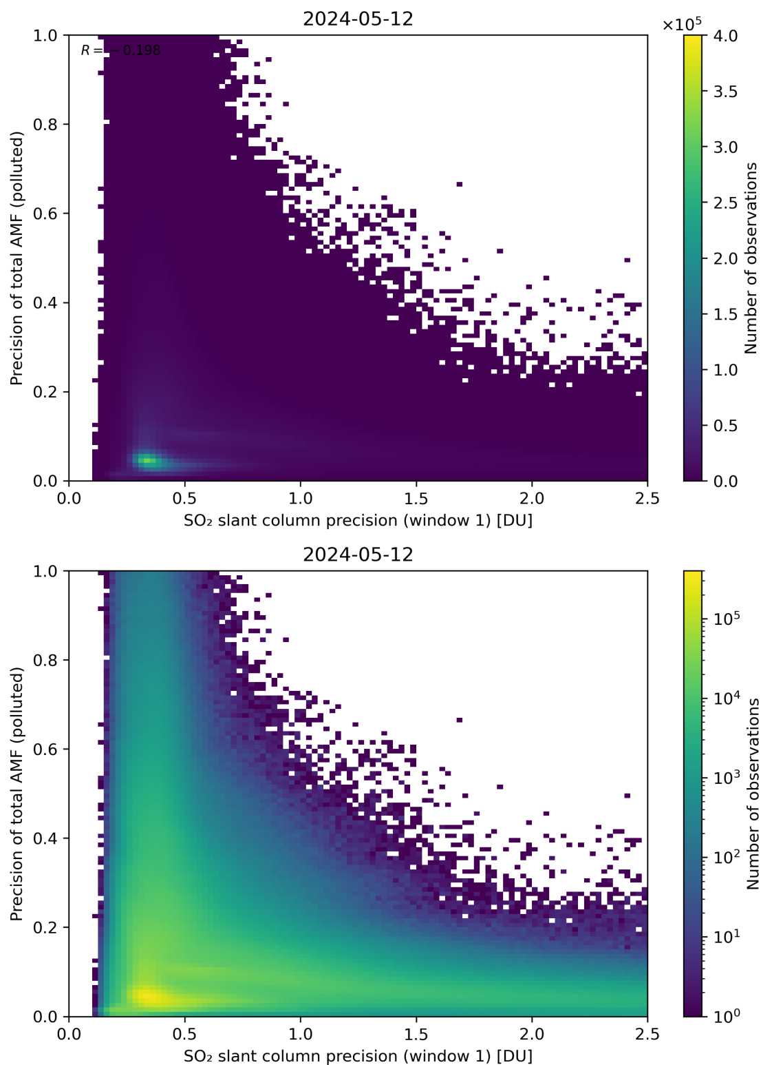
Figure 231: Scatter density plot of “SO 2 slant column precision (window 1)” against “Precision of total AMF (polluted)” for 2024-05-12 to 2024-05-13.
