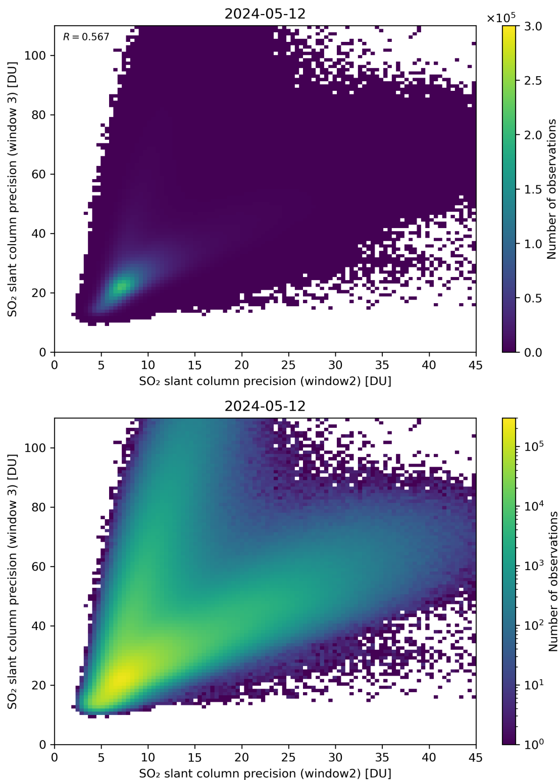
Figure 250: Scatter density plot of “SO 2 slant column precision (window2)” against “SO 2 slant column precision (window 3)” for 2024-05-12 to 2024-05-13.
