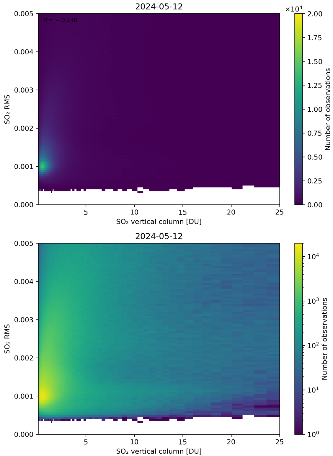
Figure 278: Scatter density plot of “SO 2 vertical column” against “SO 2 RMS” for 2024-05-12 to 2024-05-13.
