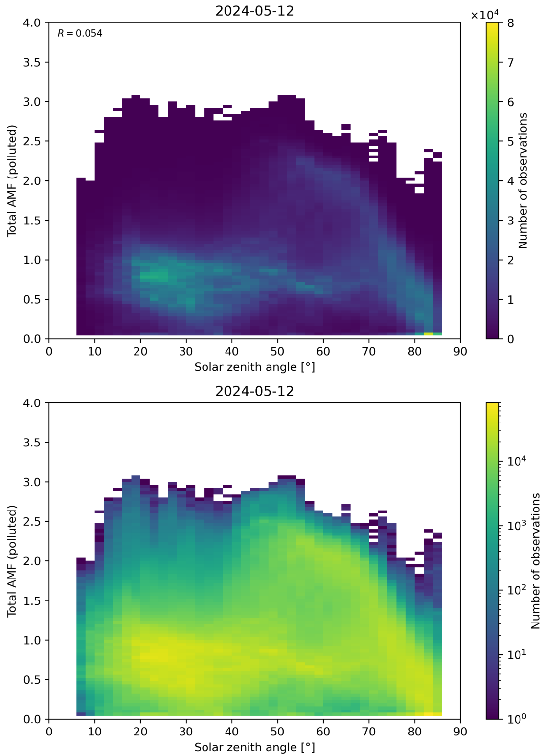
Figure 174: Scatter density plot of “Solar zenith angle” against “Total AMF (polluted)” for 2024-05-12 to 2024-05-13.
