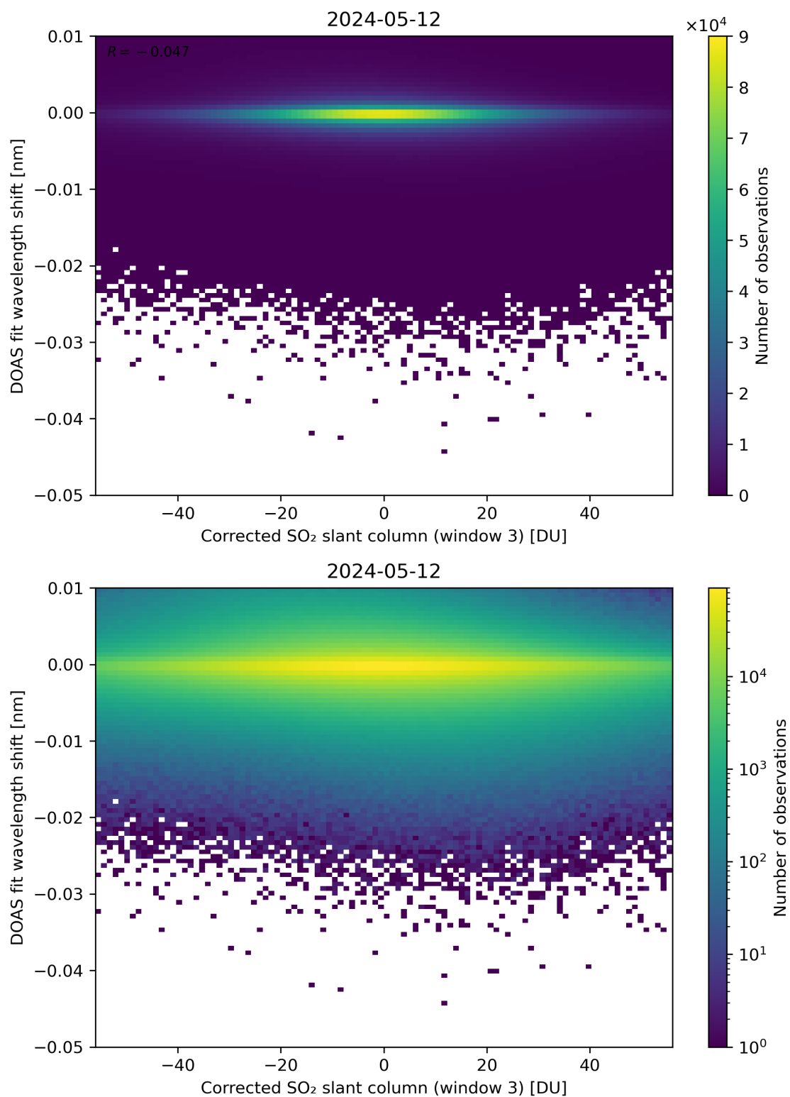
Figure 206: Scatter density plot of “Corrected SO 2 slant column (window 3)” against “DOAS fit wavelength shift” for 2024-05-12 to 2024-05-13.
