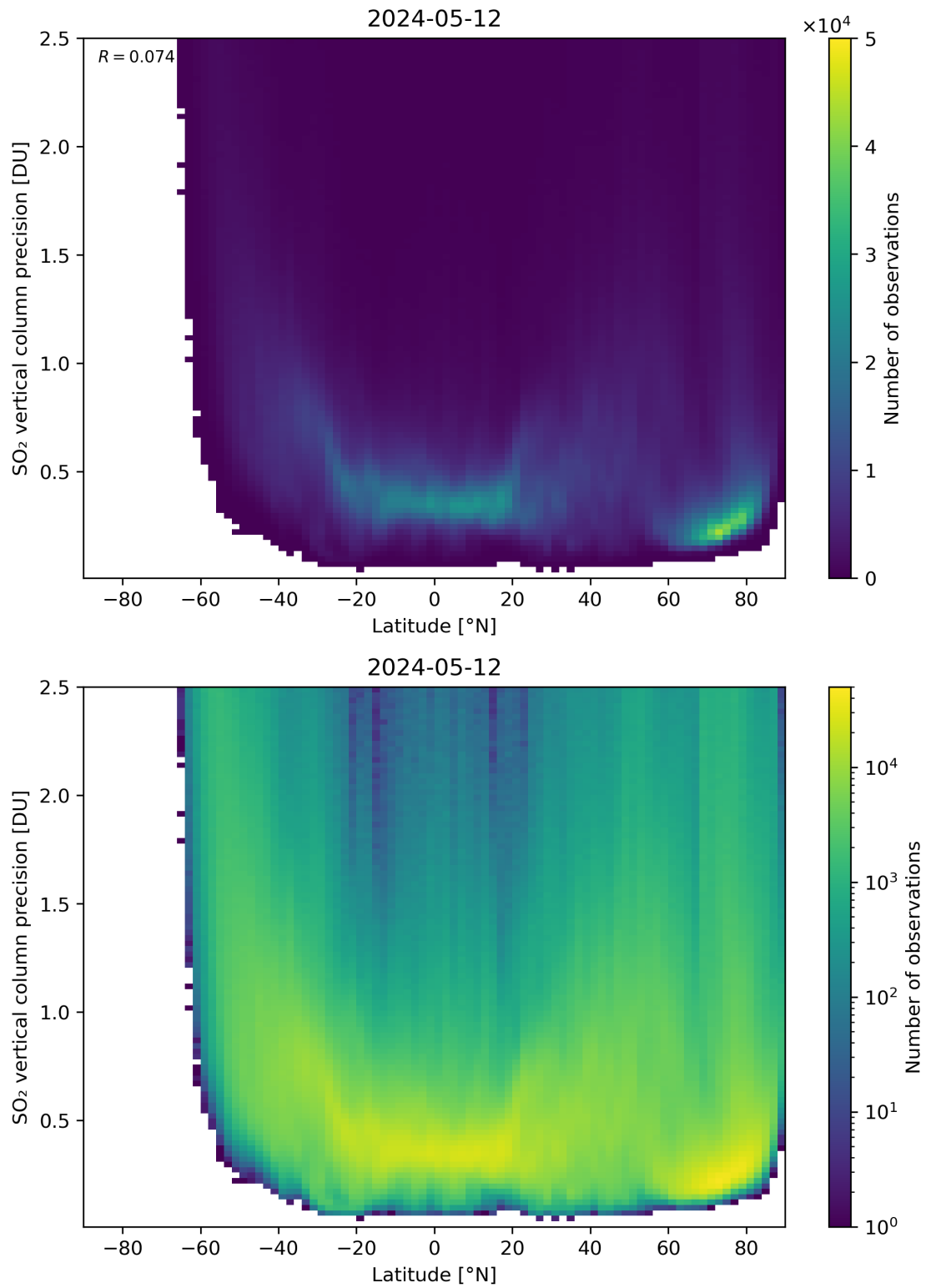
Figure 157: Scatter density plot of “Latitude” against “SO 2 vertical column precision” for 2024-05-12 to 2024-05-13.
