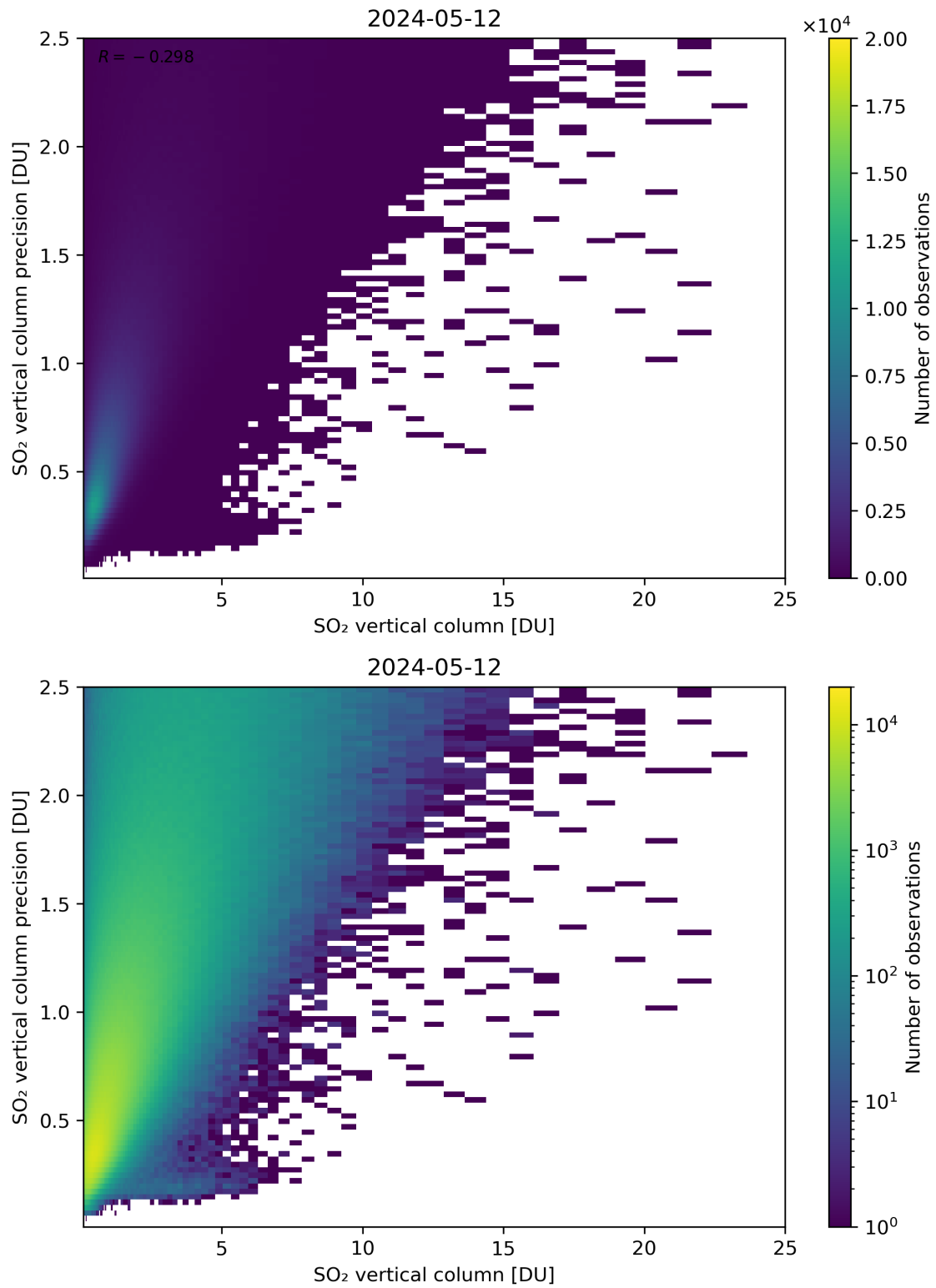
Figure 307: Scatter density plot of “SO 2 vertical column” against “SO 2 vertical column precision” for 2024-05-12 to 2024-05-13.
