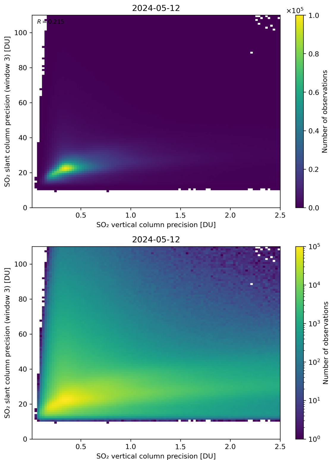
Figure 293: Scatter density plot of “SO 2 vertical column precision” against “SO 2 slant column precision (window 3)” for 2024-05-12 to 2024-05-13.
