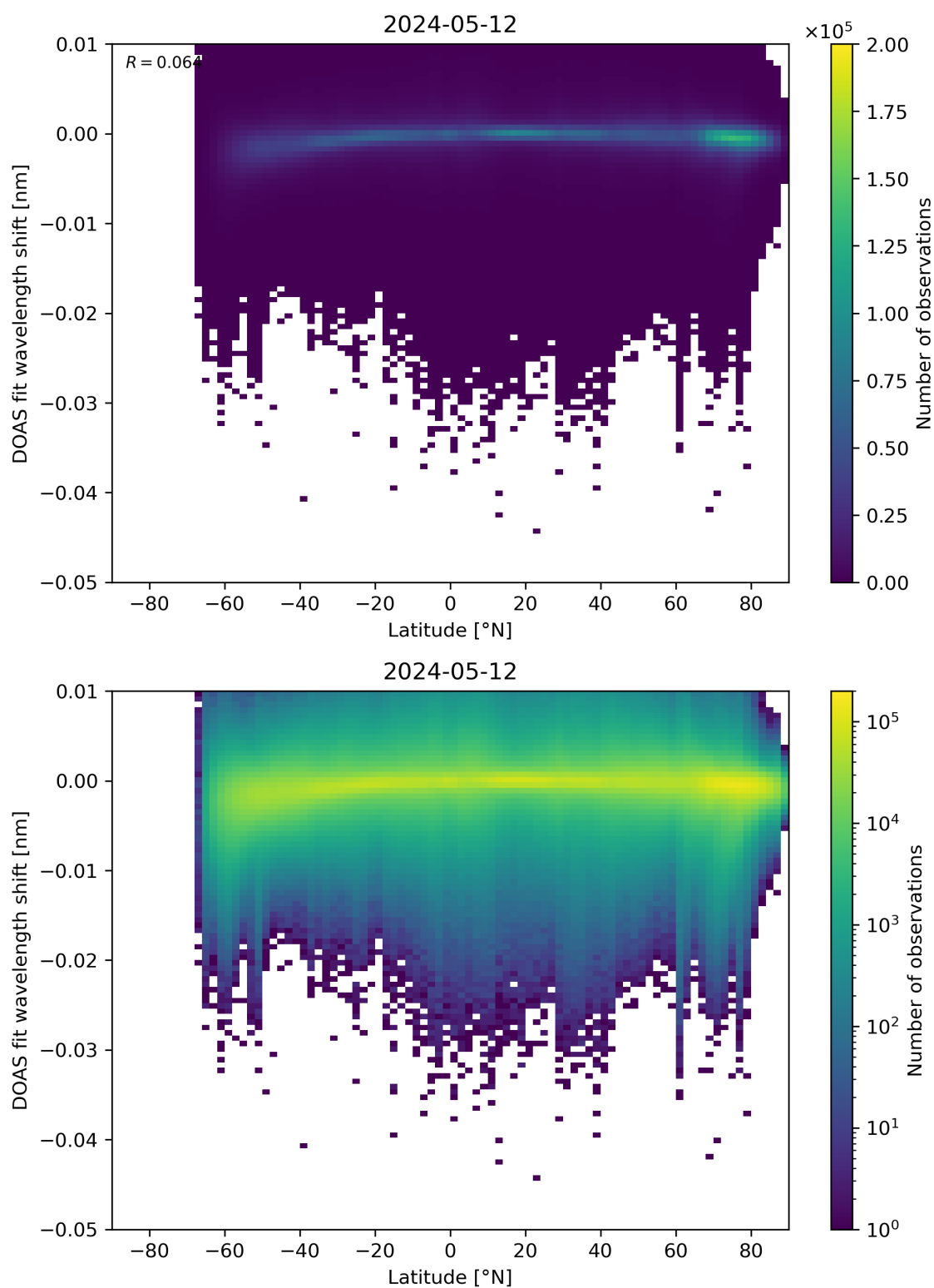
Figure 142: Scatter density plot of “Latitude” against “DOAS fit wavelength shift” for 2024-05-12 to 2024-05-13.
