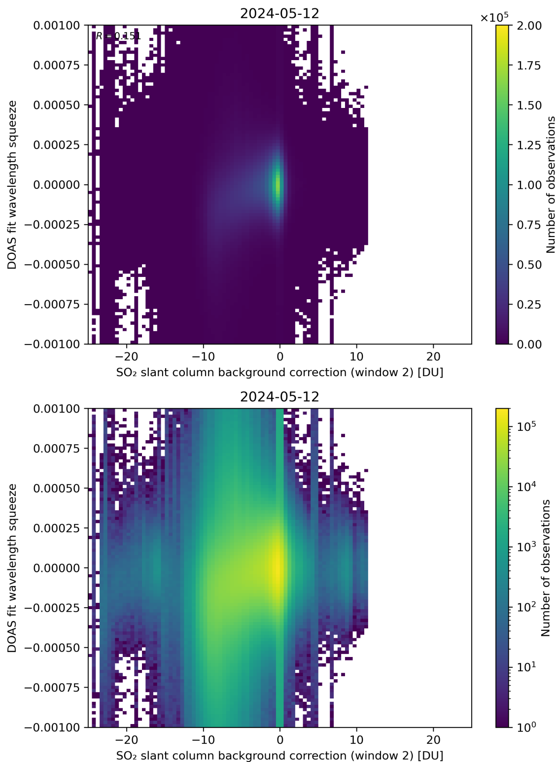
Figure 113: Scatter density plot of “SO 2 slant column background correction (window 2)” against “DOAS fit wavelength squeeze” for 2024-05-12 to 2024-05-13.
