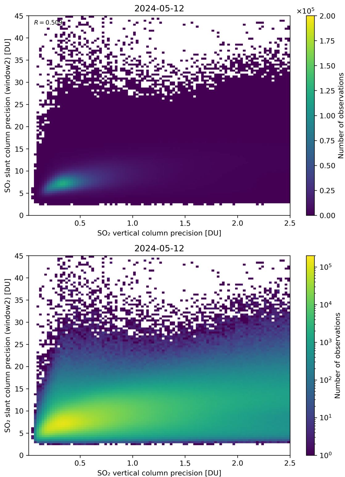
Figure 291: Scatter density plot of “SO 2 vertical column precision” against “SO 2 slant column precision (window2)” for 2024-05-12 to 2024-05-13.
