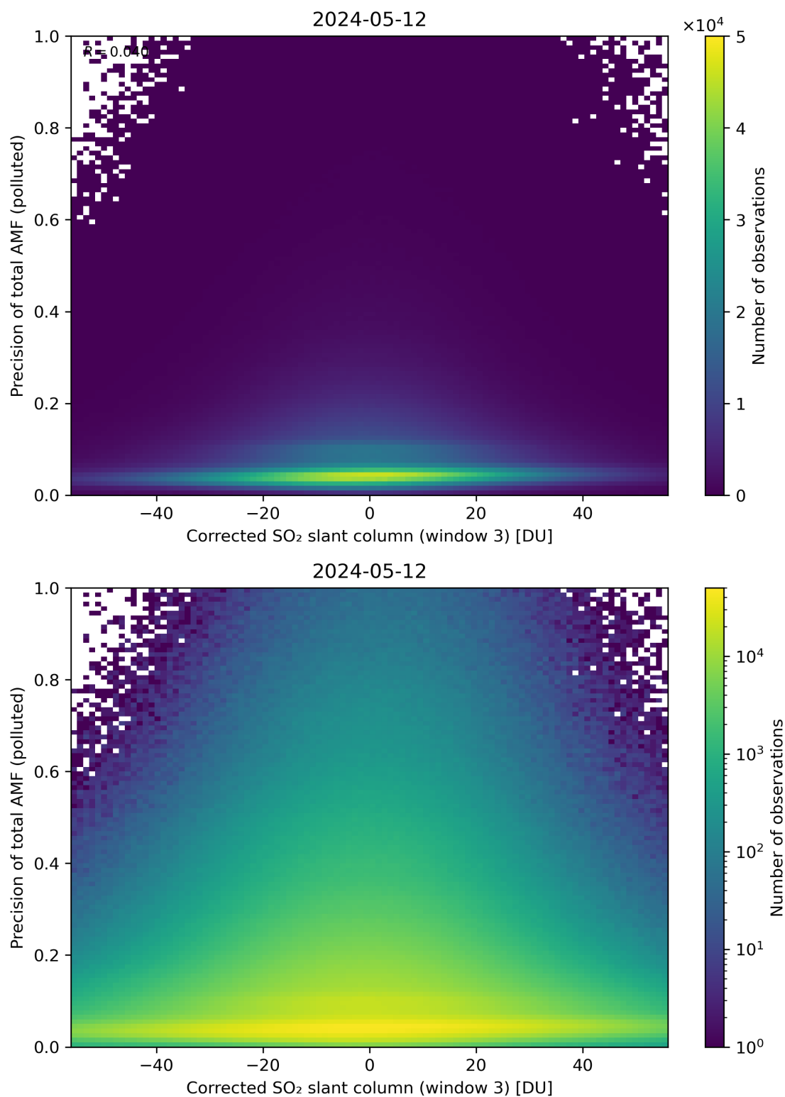
Figure 211: Scatter density plot of “Corrected SO 2 slant column (window 3)” against “Precision of total AMF (polluted)” for 2024-05-12 to 2024-05-13.
