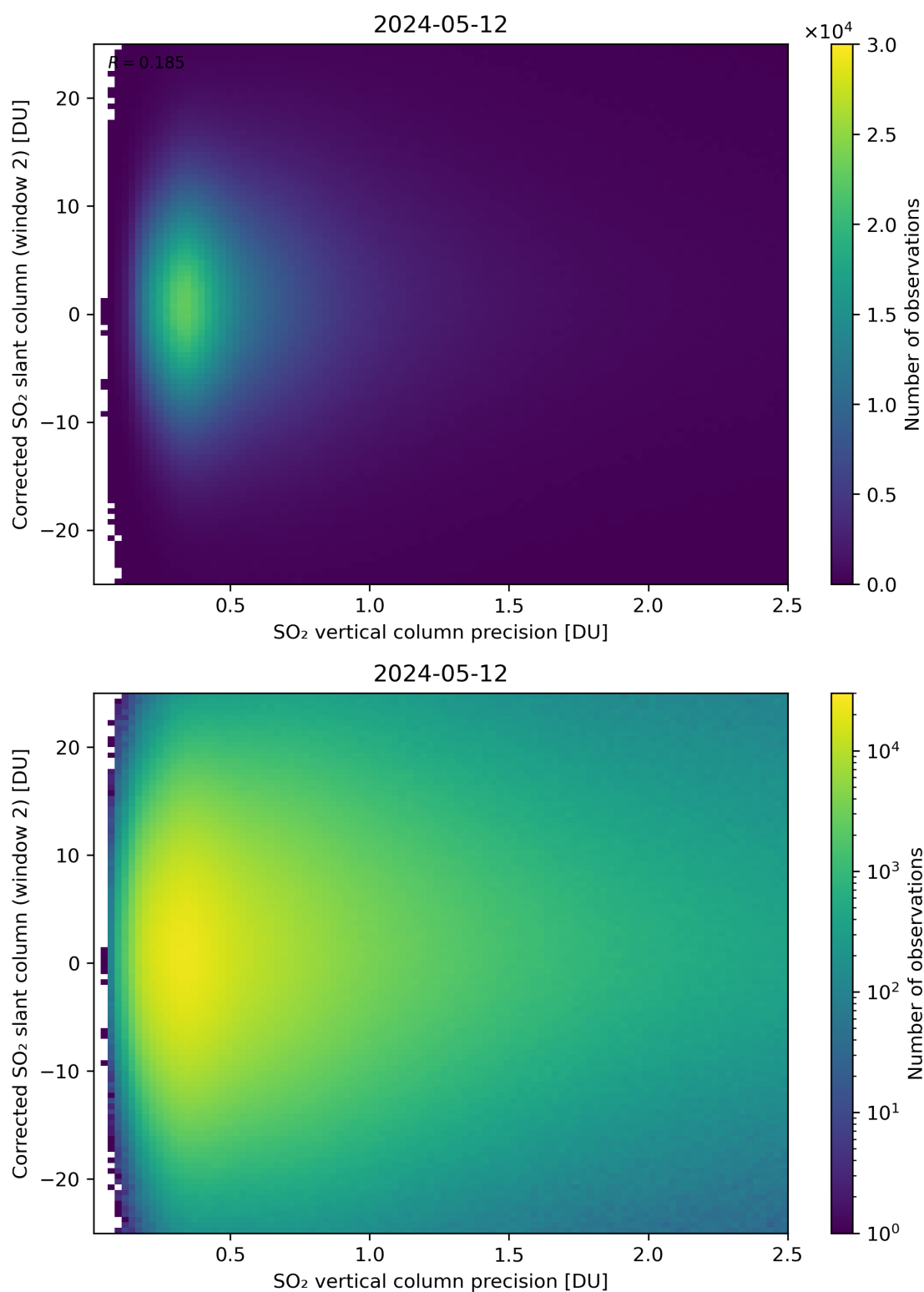
Figure 287: Scatter density plot of “SO 2 vertical column precision” against “Corrected SO 2 slant column (window 2)” for 2024-05-12 to 2024-05-13.
