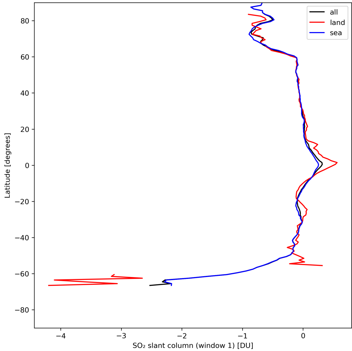
Figure 33: Zonal average of “SO 2 slant column (window 1)” for 2024-05-12 to 2024-05-13.
