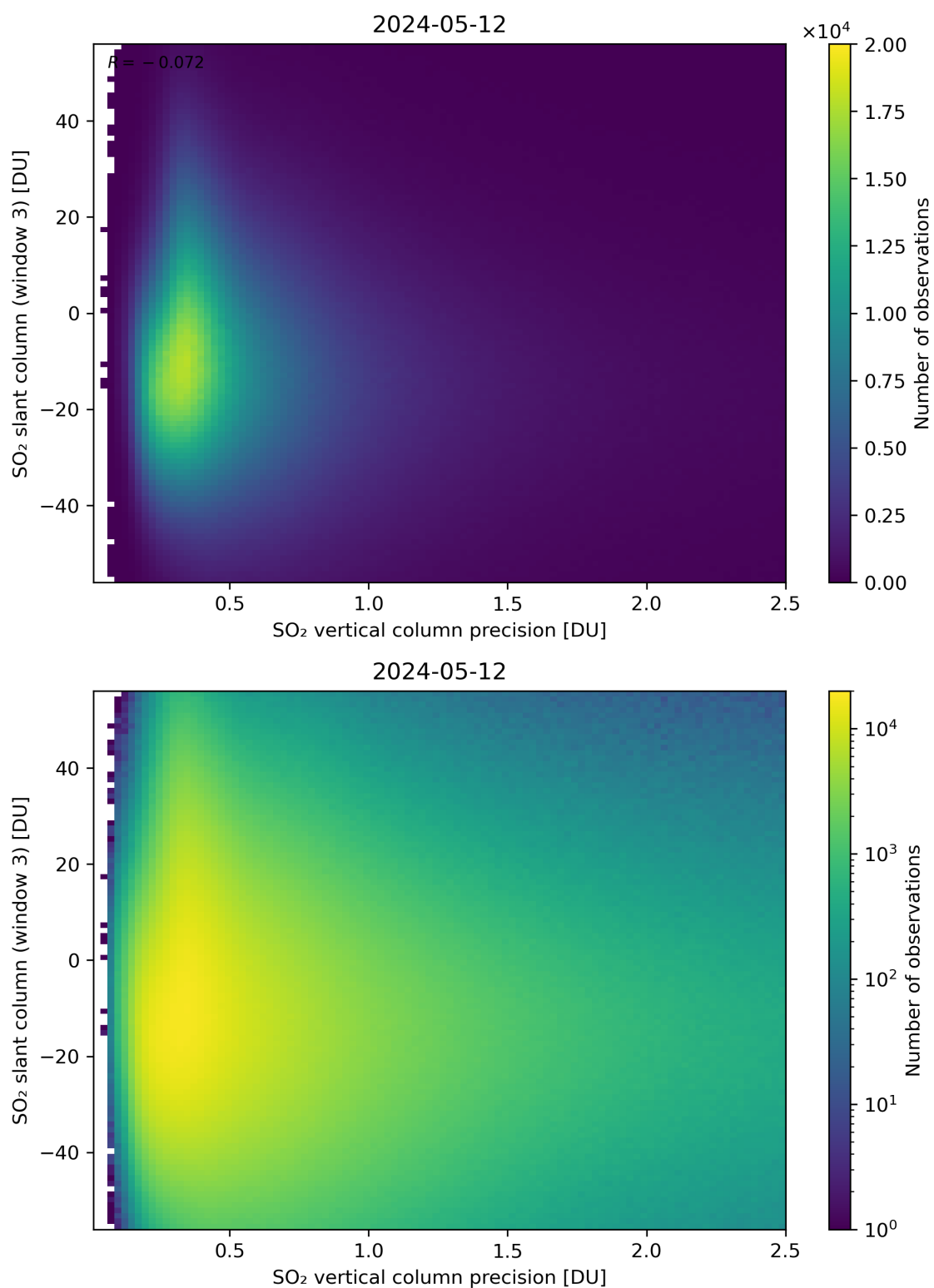
Figure 292: Scatter density plot of “SO 2 vertical column precision” against “SO 2 slant column (window 3)” for 2024-05-12 to 2024-05-13.
