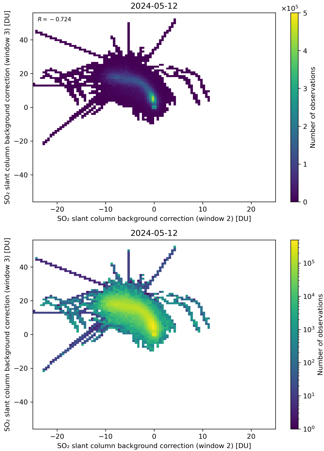
Figure 111: Scatter density plot of “SO 2 slant column background correction (window 2)” against “SO 2 slant column background correction (window 3)” for 2024-05-12 to 2024-05-13.
