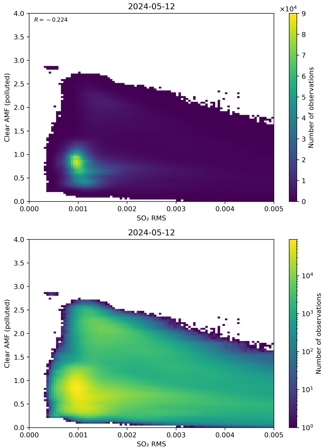
Figure 136: Scatter density plot of “SO 2 RMS” against “Clear AMF (polluted)” for 2024-05-12 to 2024-05-13.
