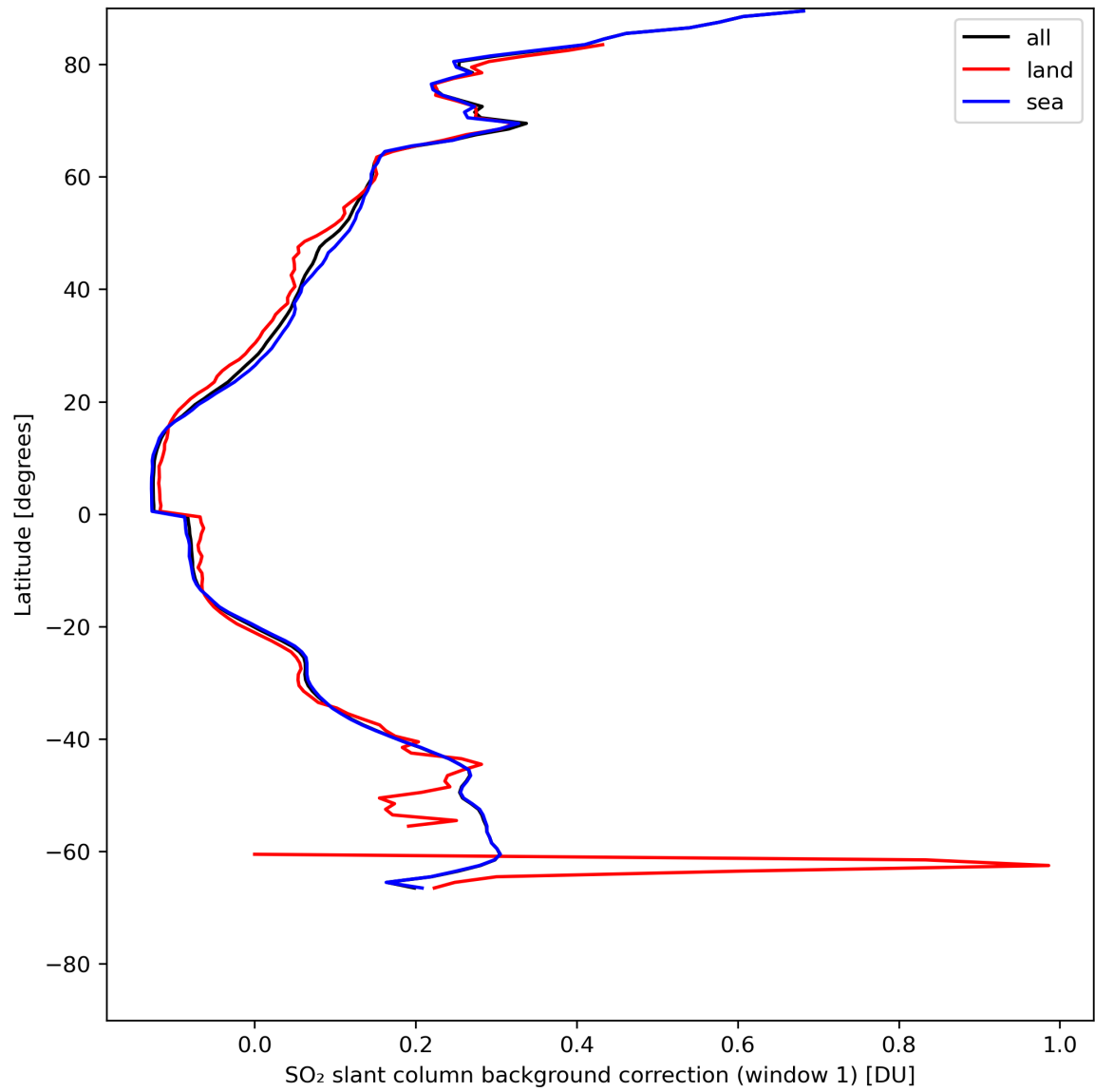
Figure 36: Zonal average of “SO 2 slant column background correction (window 1)” for 2024-05-12 to 2024-05-13.
