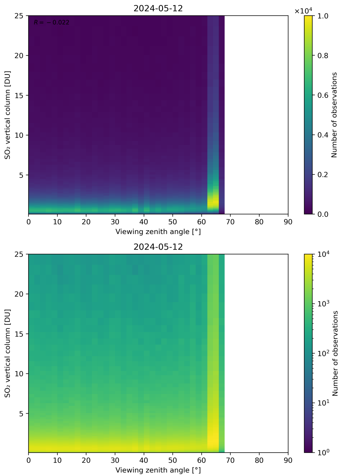
Figure 327: Scatter density plot of “Viewing zenith angle” against “SO 2 vertical column” for 2024-05-12 to 2024-05-13.
