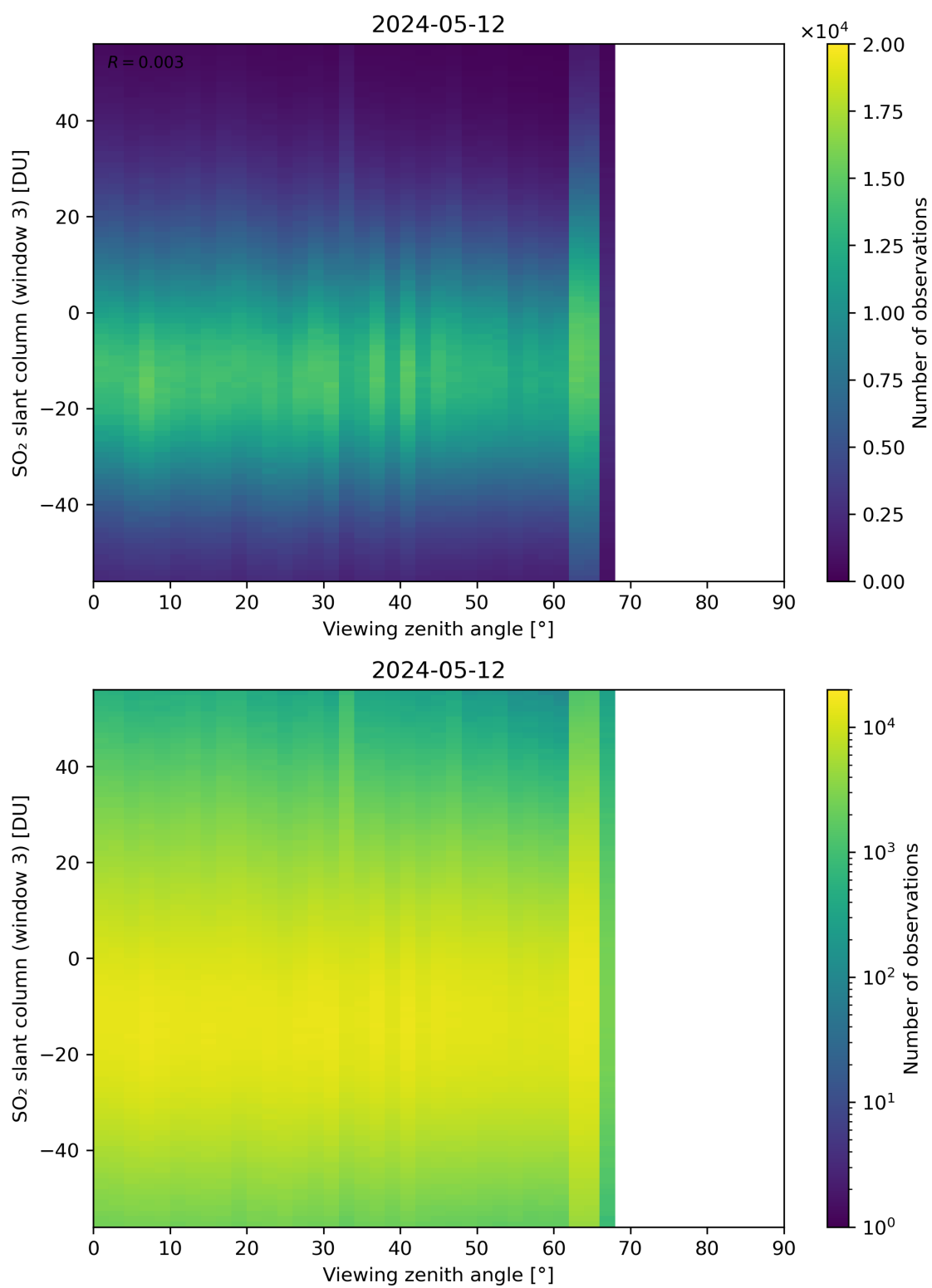
Figure 323: Scatter density plot of “Viewing zenith angle” against “SO 2 slant column (window 3)” for 2024-05-12 to 2024-05-13.
