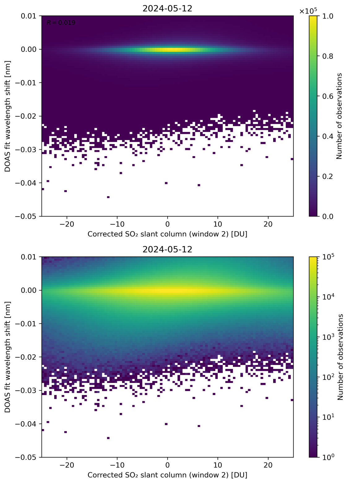
Figure 196: Scatter density plot of “Corrected SO 2 slant column (window 2)” against “DOAS fit wavelength shift” for 2024-05-12 to 2024-05-13.
