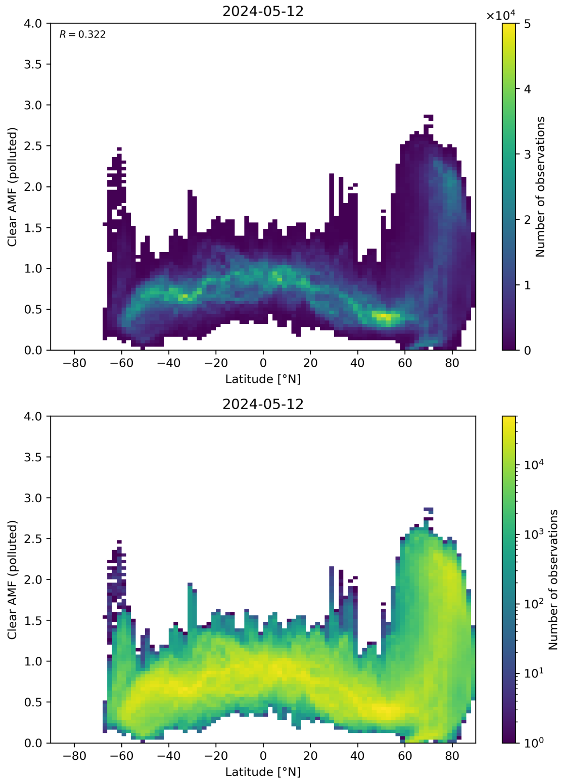
Figure 145: Scatter density plot of “Latitude” against “Clear AMF (polluted)” for 2024-05-12 to 2024-05-13.
