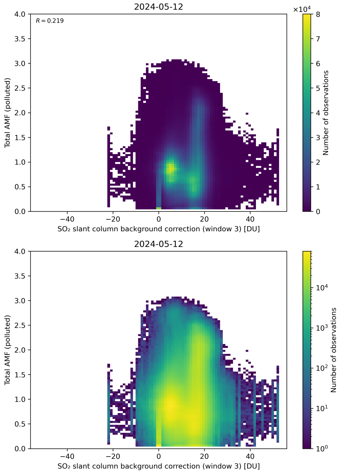
Figure 125: Scatter density plot of “SO 2 slant column background correction (window 3)” against “Total AMF (polluted)” for 2024-05-12 to 2024-05-13.
