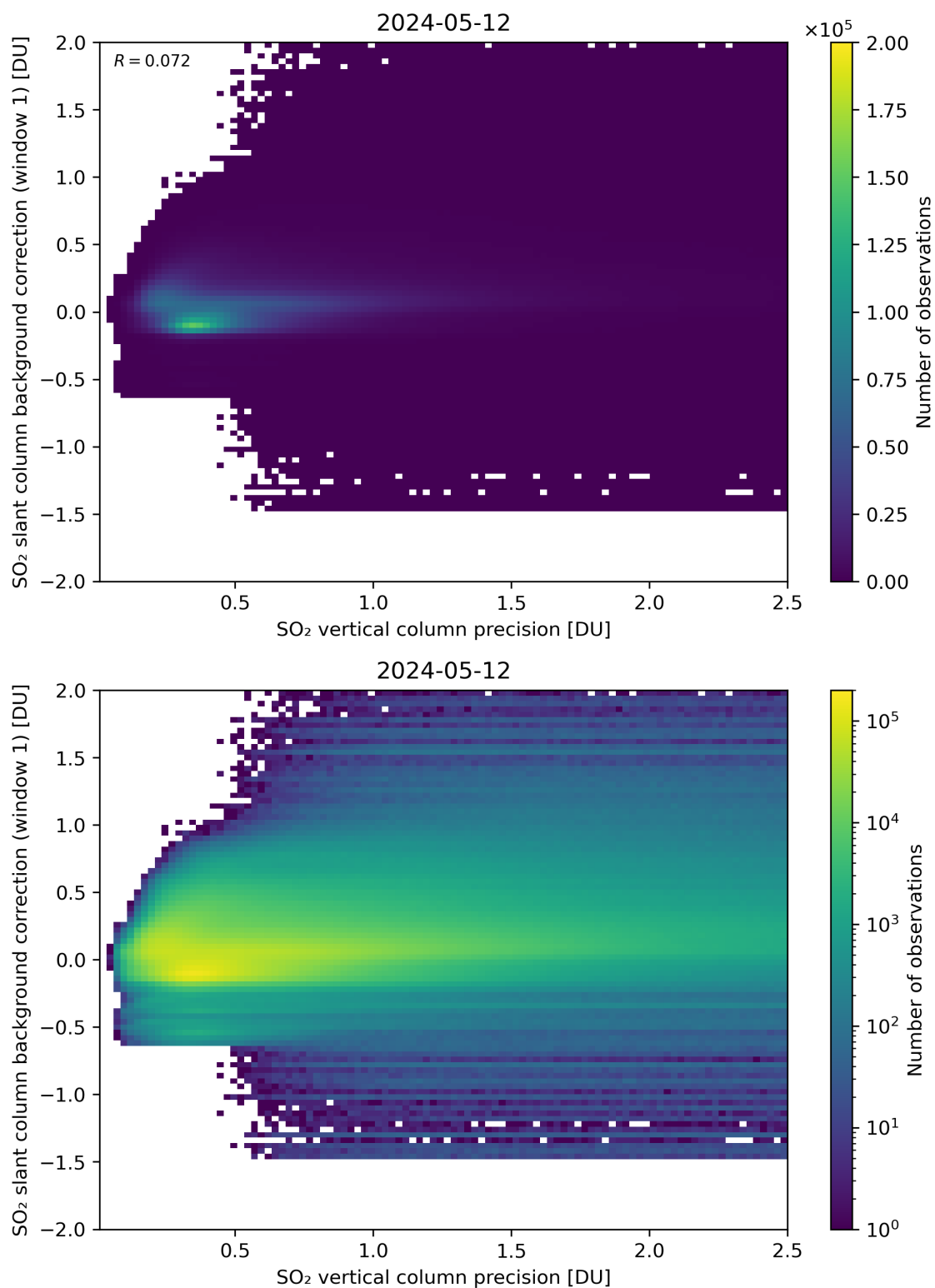
Figure 279: Scatter density plot of “SO 2 vertical column precision” against “SO 2 slant column background correction (window 1)” for 2024-05-12 to 2024-05-13.
