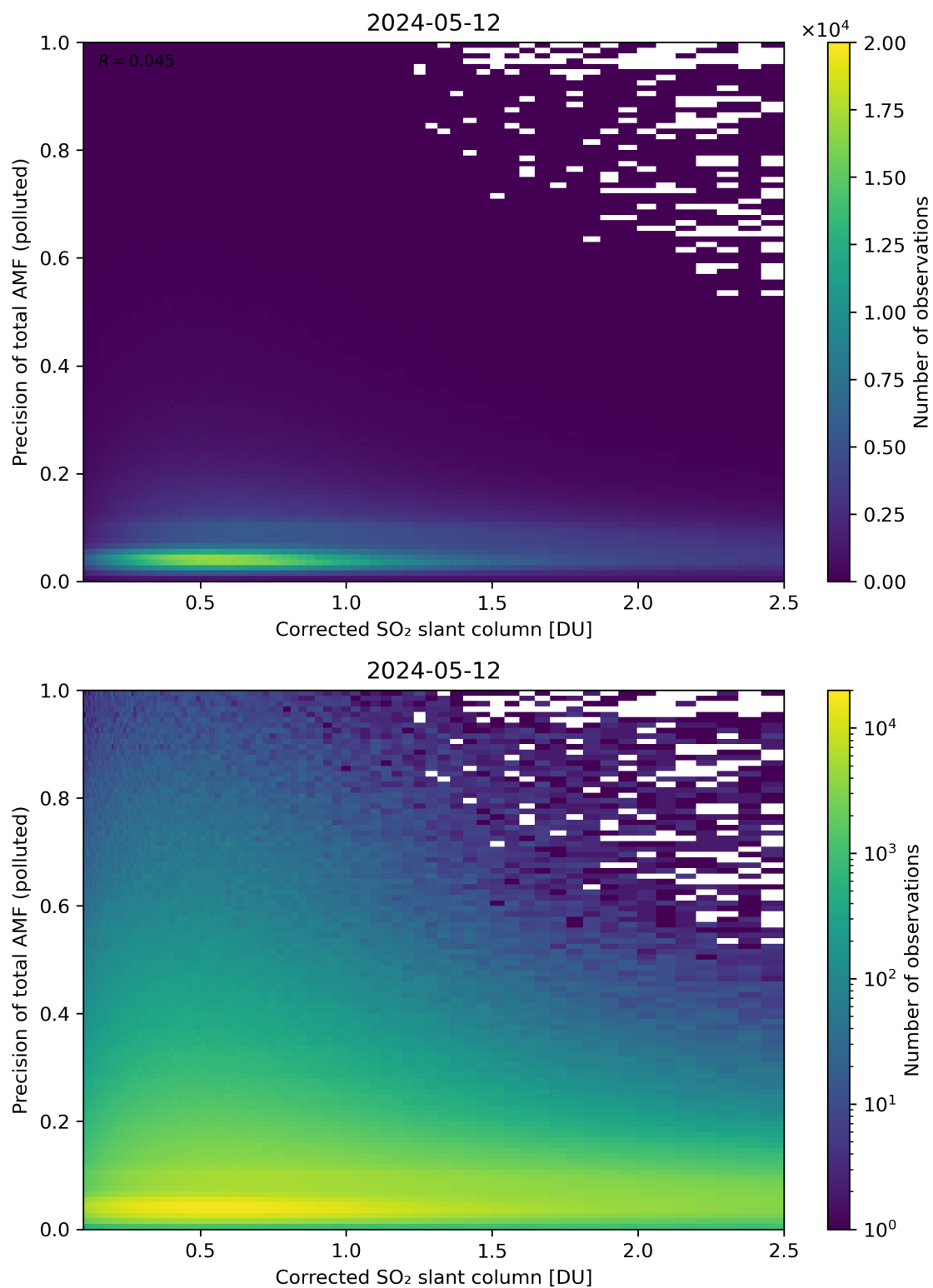
Figure 193: Scatter density plot of “Corrected SO 2 slant column” against “Precision of total AMF (polluted)” for 2024-05-12 to 2024-05-13.
