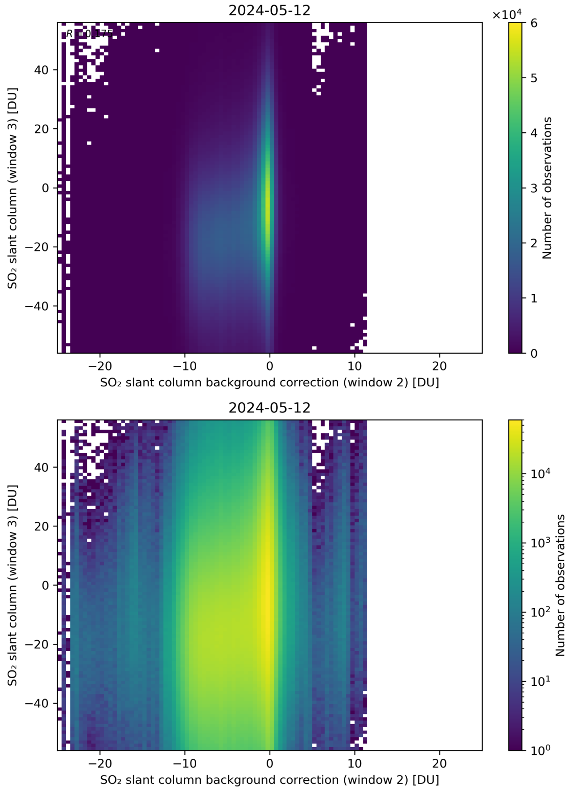
Figure 117: Scatter density plot of “SO 2 slant column background correction (window 2)” against “SO 2 slant column (window 3)” for 2024-05-12 to 2024-05-13.
