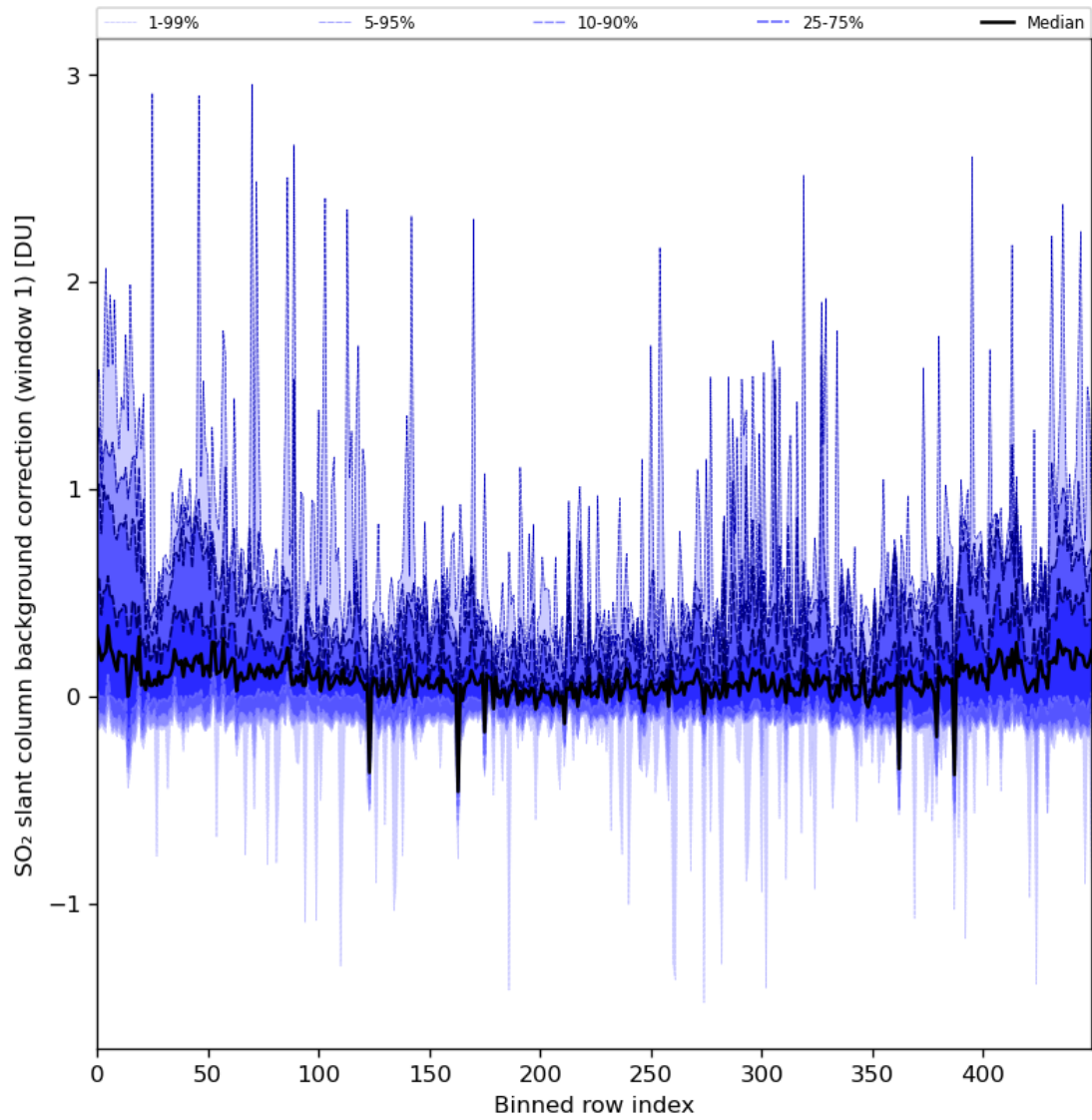
Figure 82: Along track statistics of “SO 2 slant column background correction (window 1)” for 2024-05-12 to 2024-05-13
