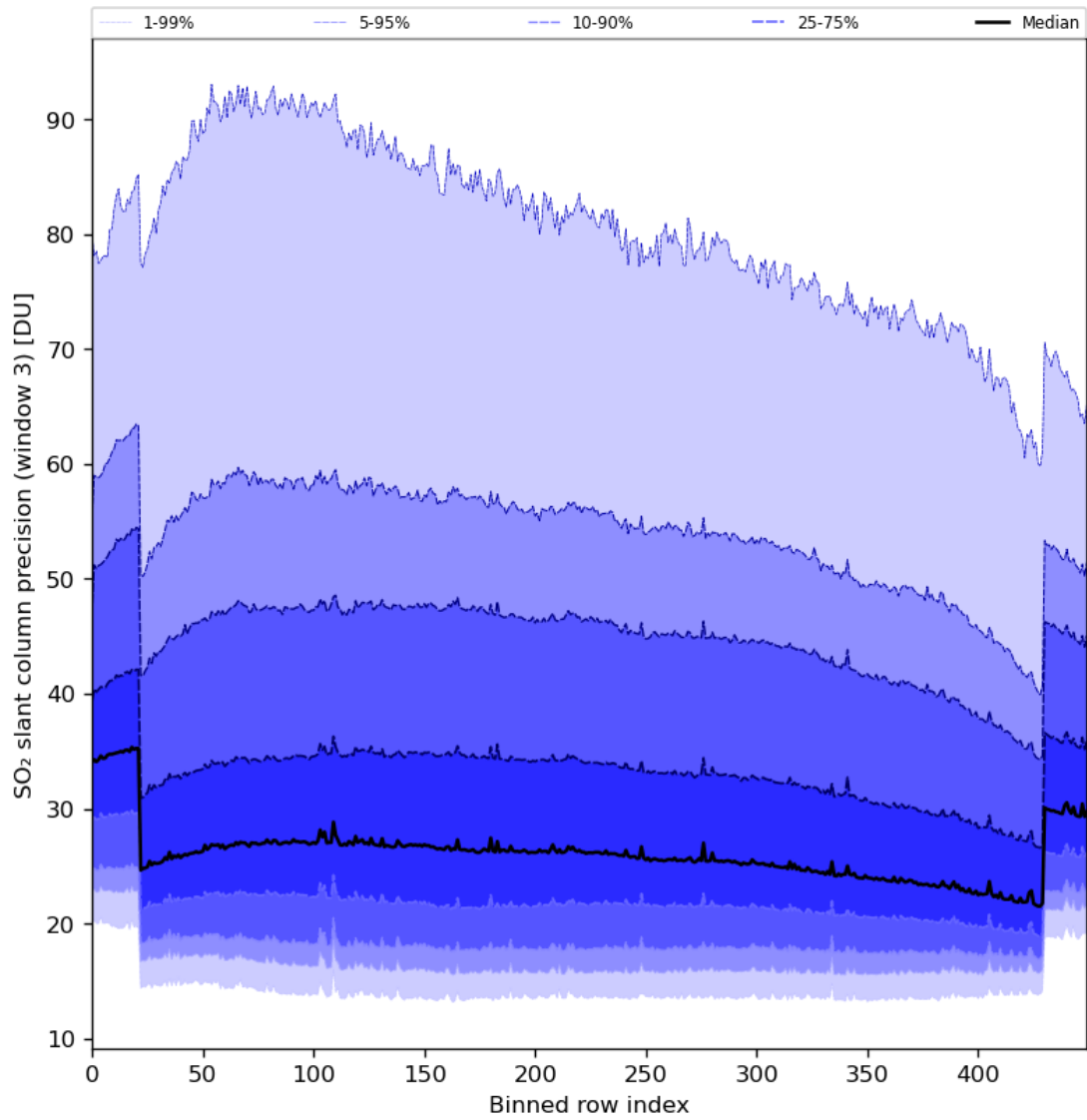
Figure 88: Along track statistics of “SO 2 slant column precision (window 3)” for 2024-05-12 to 2024-05-13
