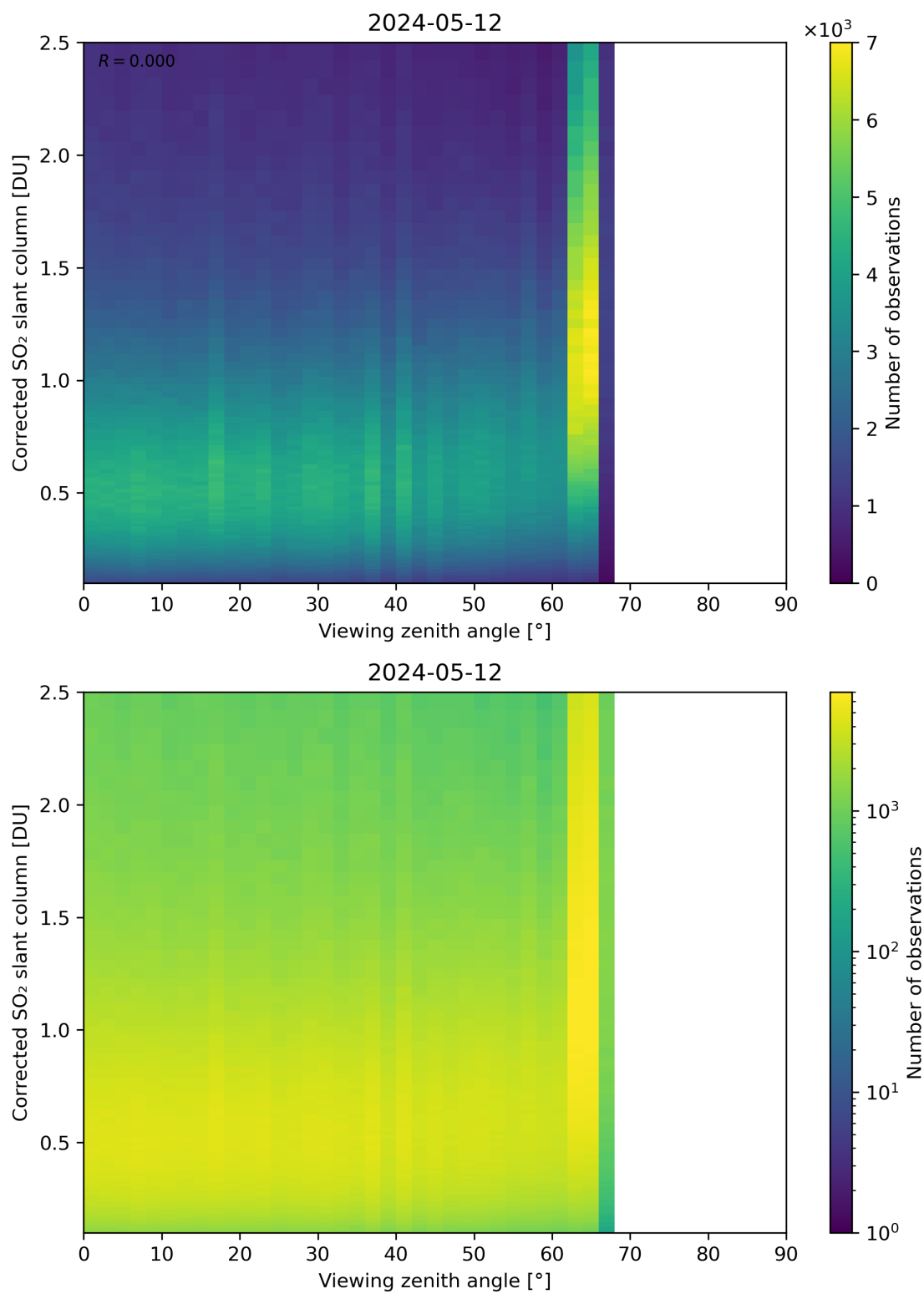
Figure 317: Scatter density plot of “Viewing zenith angle” against “Corrected SO 2 slant column” for 2024-05-12 to 2024-05-13.
