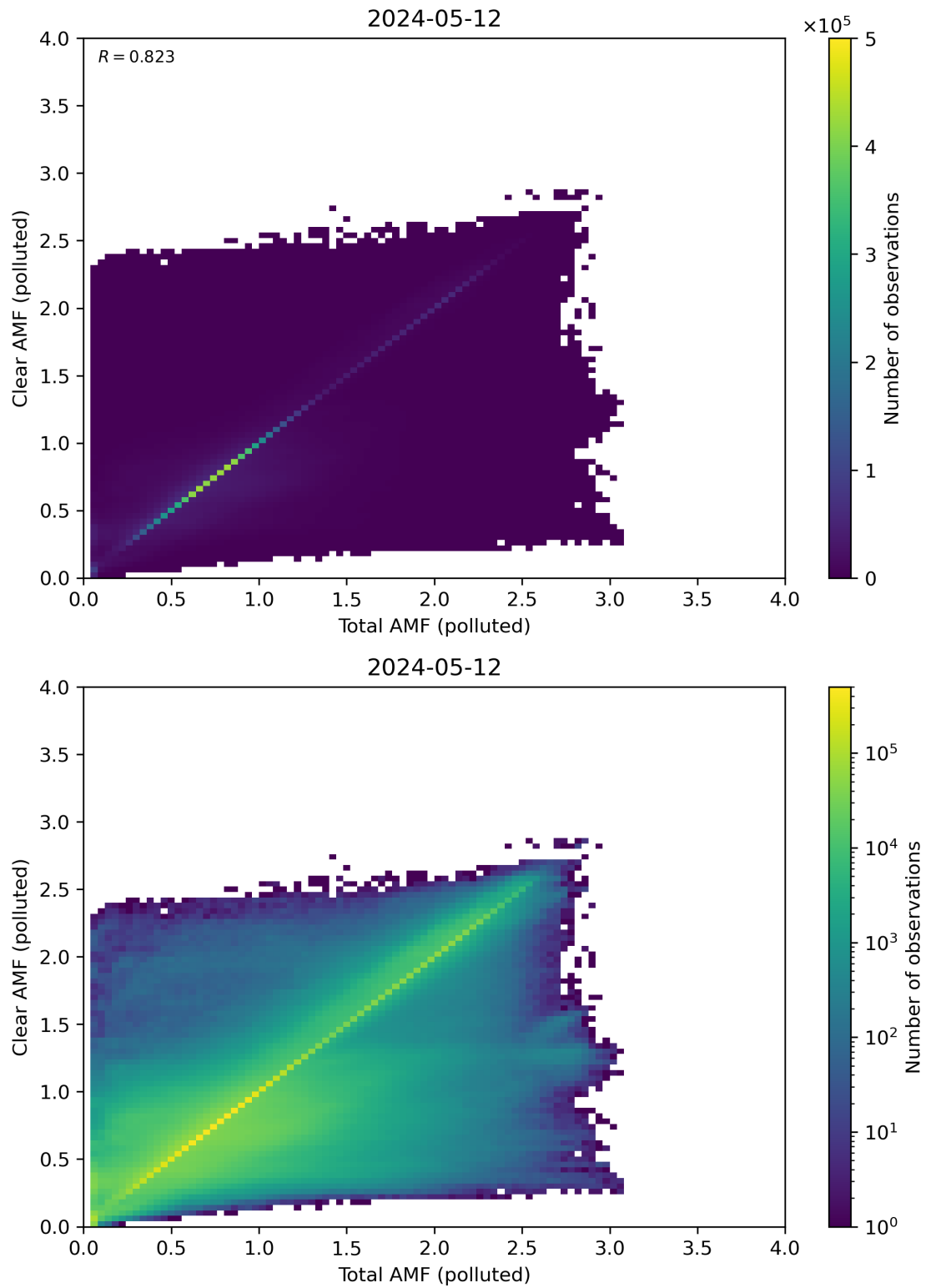
Figure 271: Scatter density plot of “Total AMF (polluted)” against “Clear AMF (polluted)” for 2024-05-12 to 2024-05-13.
