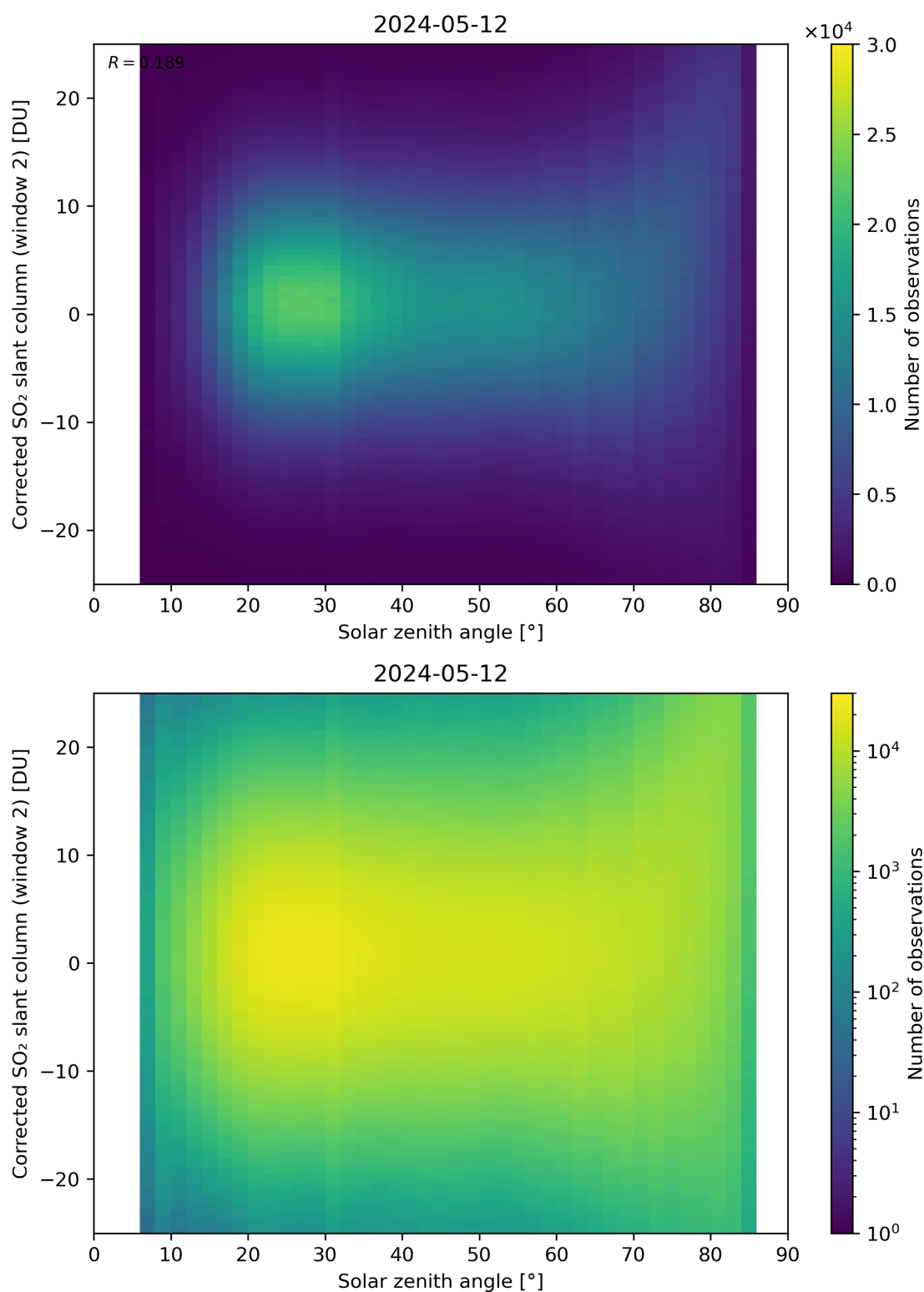
Figure 167: Scatter density plot of “Solar zenith angle” against “Corrected SO 2 slant column (window 2)” for 2024-05-12 to 2024-05-13.
