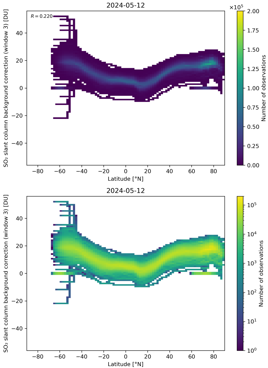
Figure 141: Scatter density plot of “Latitude” against “SO 2 slant column background correction (window 3)” for 2024-05-12 to 2024-05-13.
