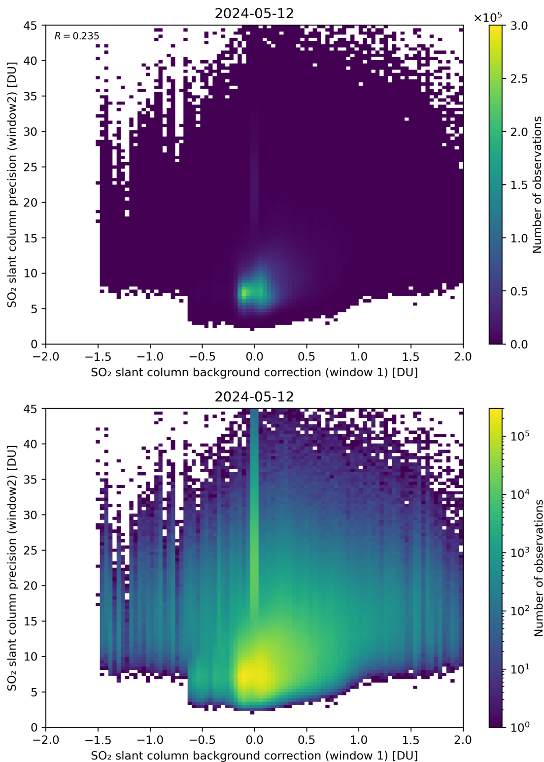
Figure 106: Scatter density plot of “SO 2 slant column background correction (window 1)” against “SO 2 slant column precision (window2)” for 2024-05-12 to 2024-05-13.
