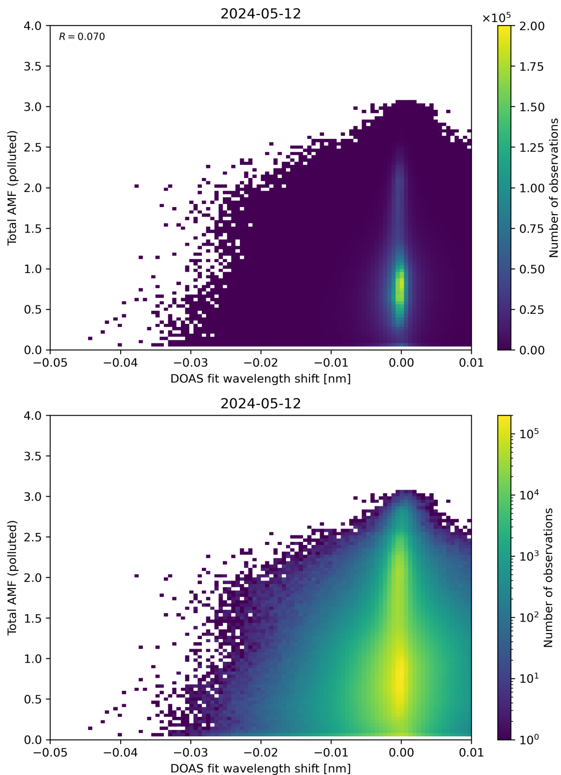
Figure 130: Scatter density plot of “DOAS fit wavelength shift” against “Total AMF (polluted)” for 2024-05-12 to 2024-05-13.
