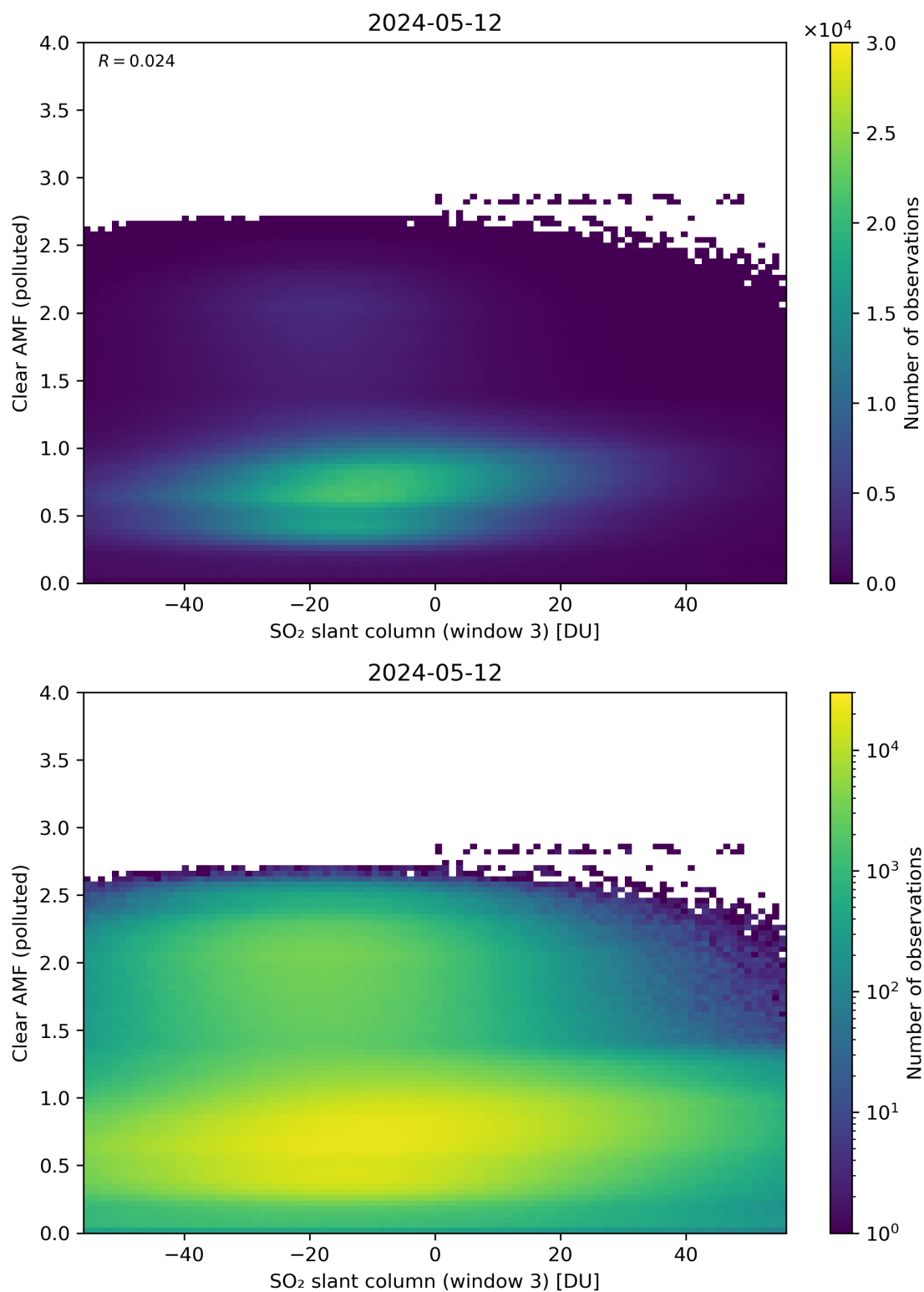
Figure 265: Scatter density plot of “SO 2 slant column (window 3)” against “Clear AMF (polluted)” for 2024-05-12 to 2024-05-13.
