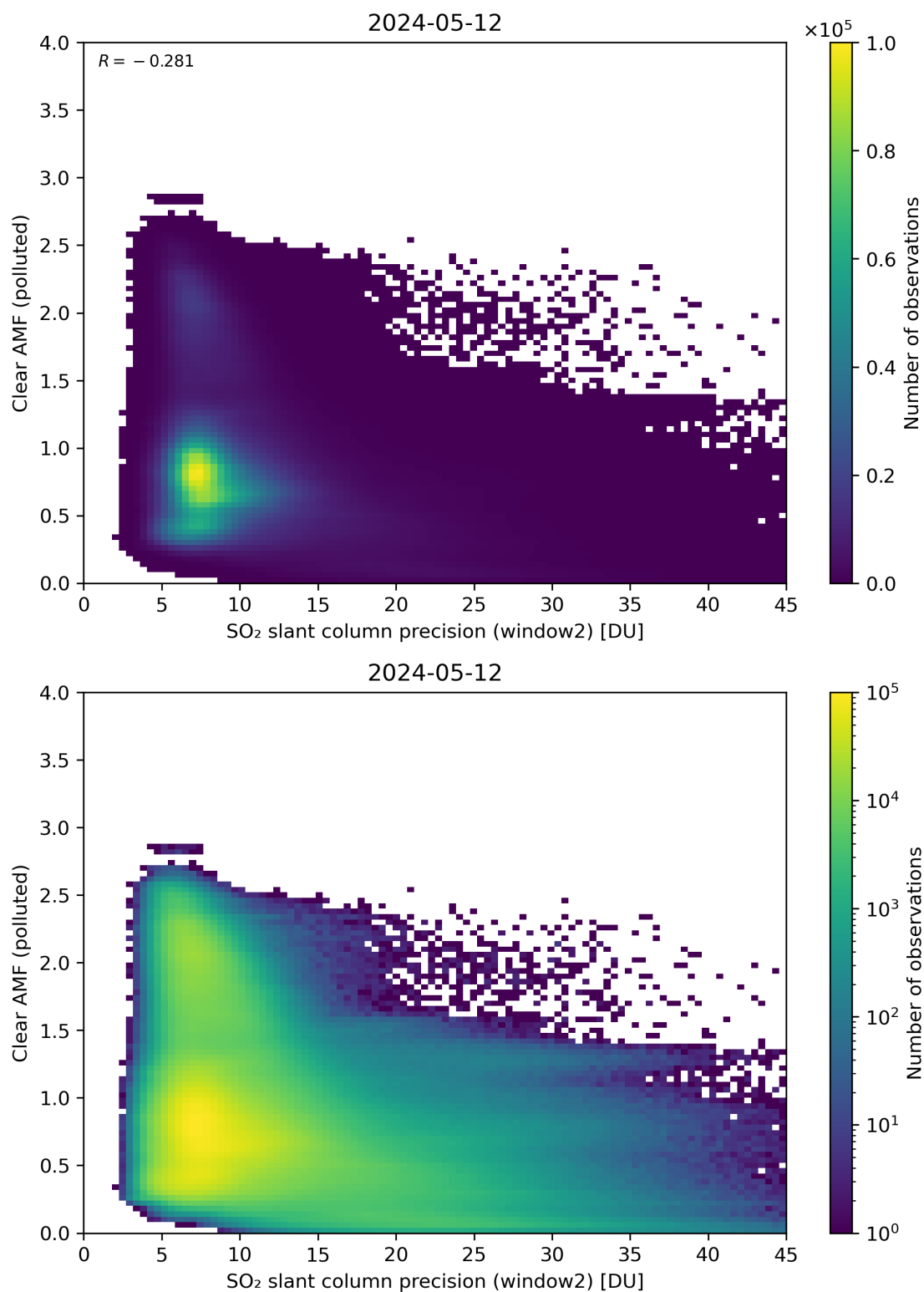
Figure 246: Scatter density plot of “SO 2 slant column precision (window2)” against “Clear AMF (polluted)” for 2024-05-12 to 2024-05-13.
