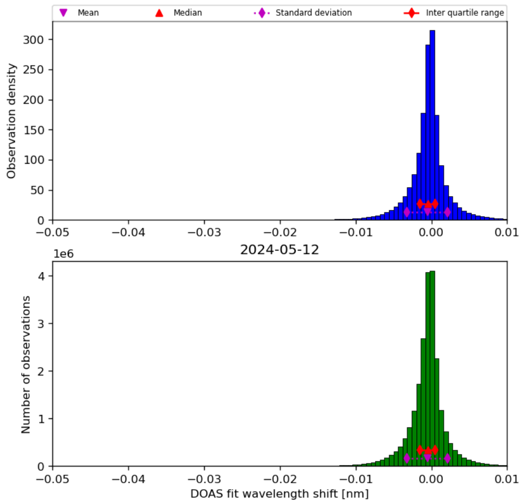
Figure 68: Histogram of “DOAS fit wavelength shift” for 2024-05-12 to 2024-05-13
