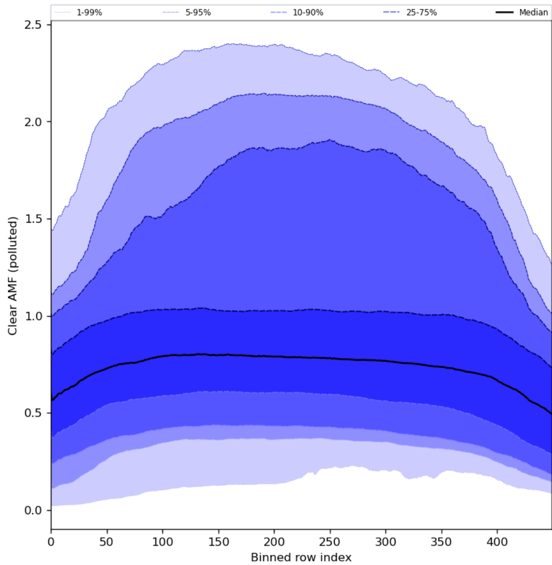
Figure 96: Along track statistics of “Clear AMF (polluted)” for 2024-05-12 to 2024-05-13
