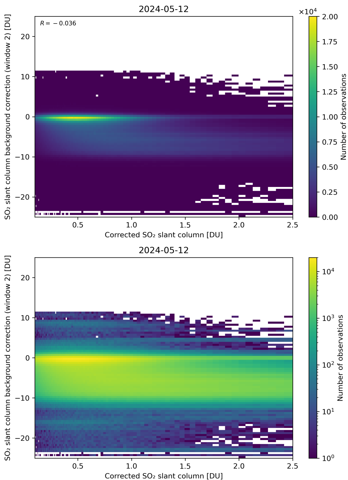
Figure 179: Scatter density plot of “Corrected SO 2 slant column” against “SO 2 slant column background correction (window 2)” for 2024-05-12 to 2024-05-13.
