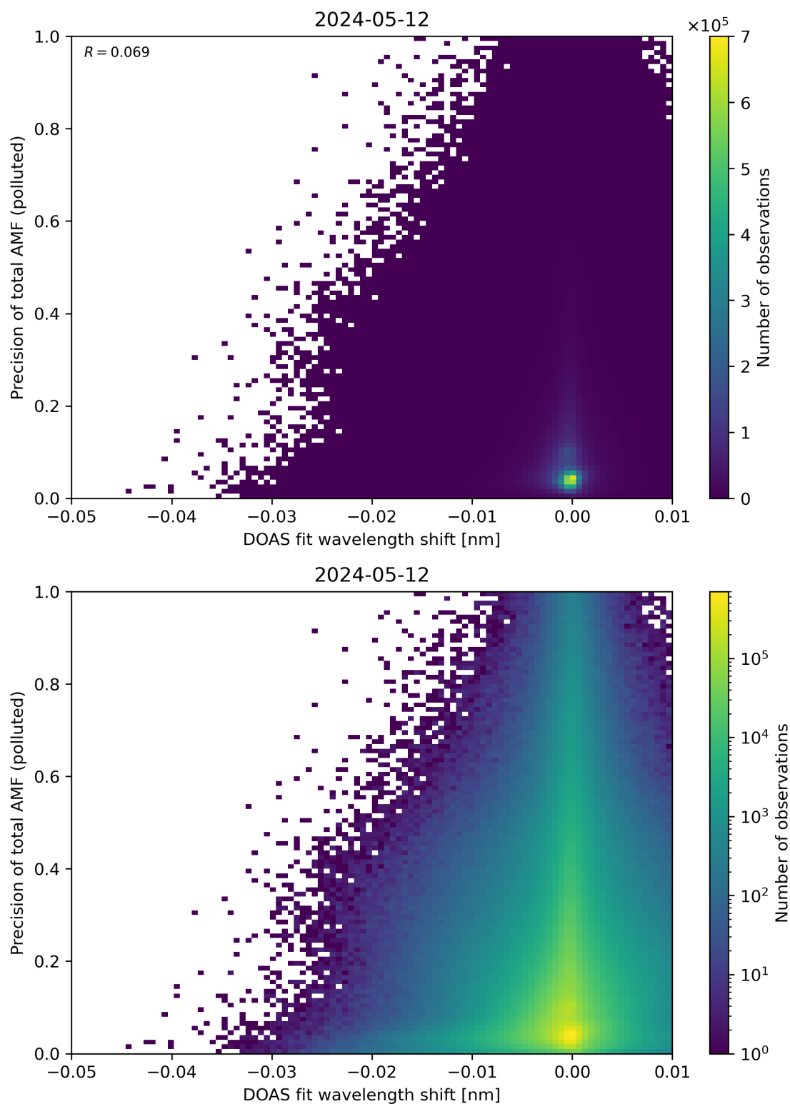
Figure 131: Scatter density plot of “DOAS fit wavelength shift” against “Precision of total AMF (polluted)” for 2024-05-12 to 2024-05-13.
