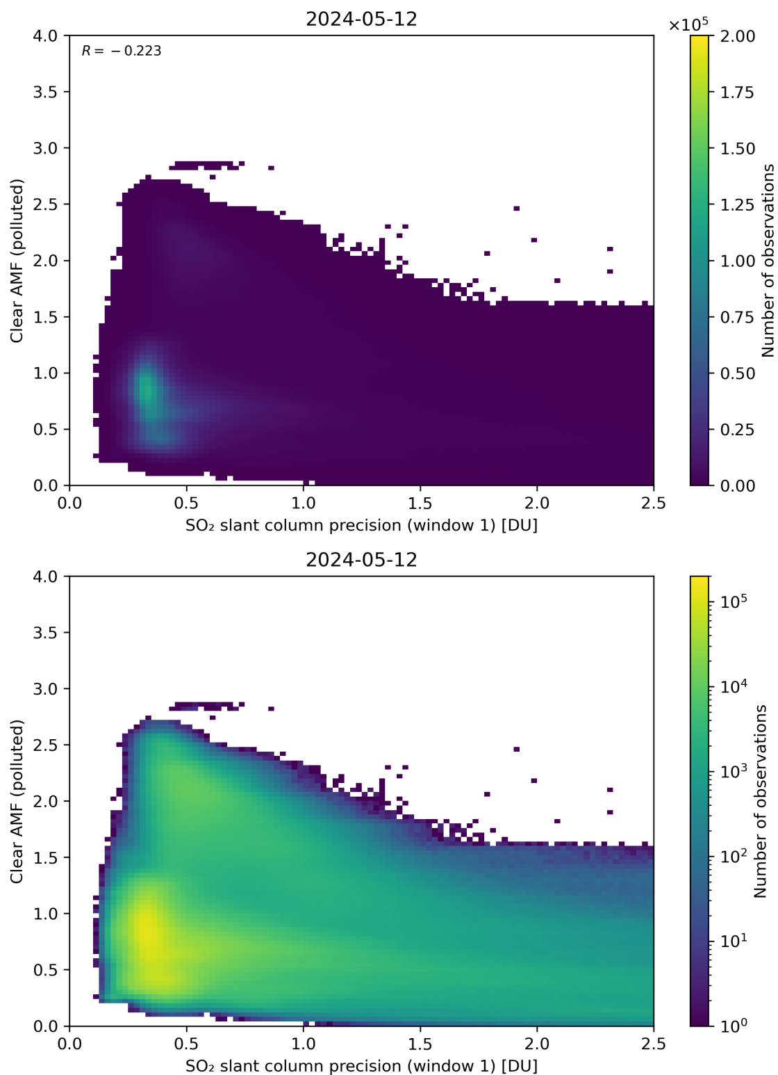
Figure 224: Scatter density plot of “SO 2 slant column precision (window 1)” against “Clear AMF (polluted)” for 2024-05-12 to 2024-05-13.
