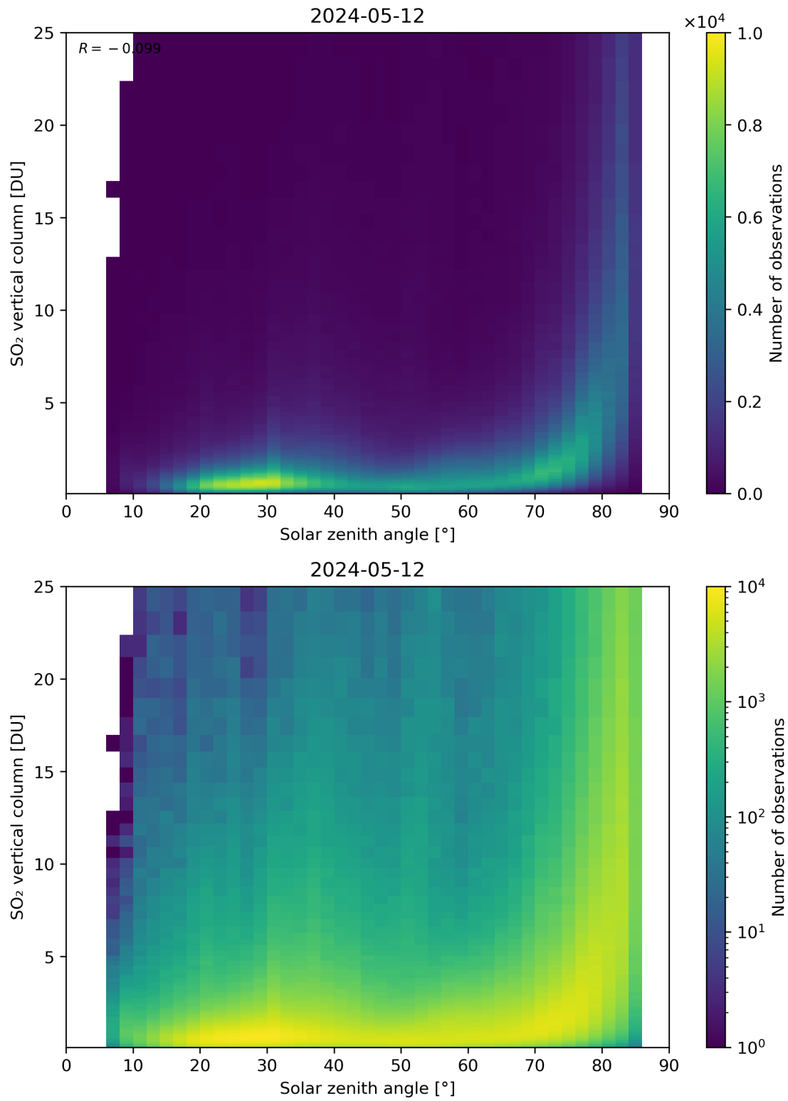
Figure 176: Scatter density plot of “Solar zenith angle” against “SO 2 vertical column” for 2024-05-12 to 2024-05-13.
