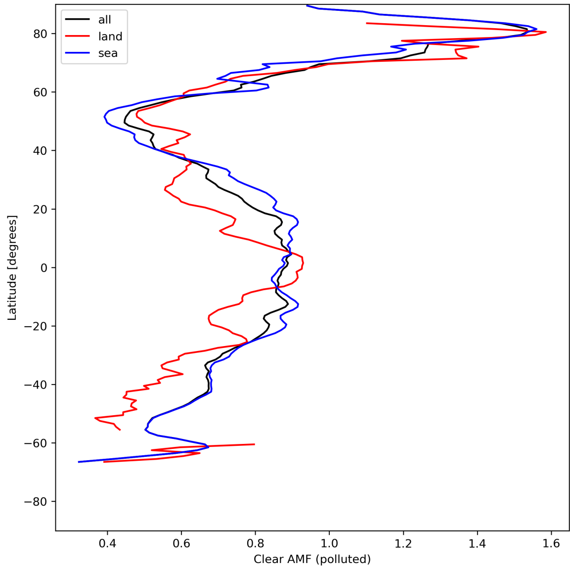
Figure 50: Zonal average of “Clear AMF (polluted)” for 2024-05-12 to 2024-05-13.
