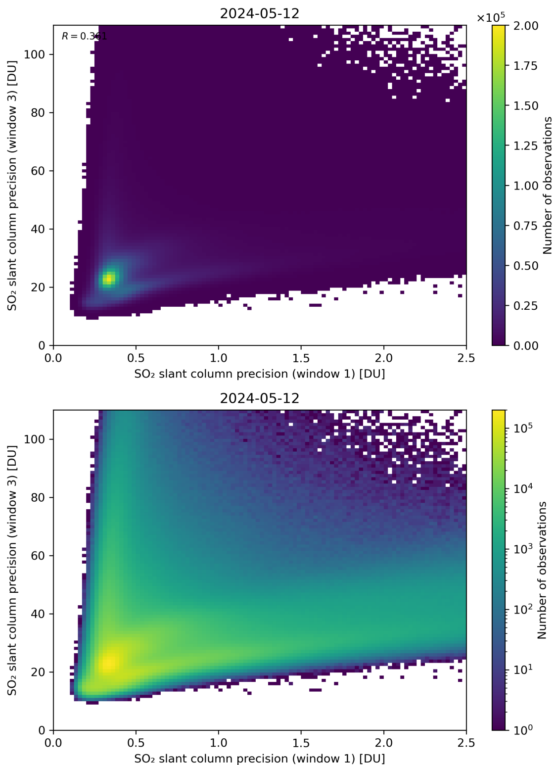
Figure 229: Scatter density plot of “SO 2 slant column precision (window 1)” against “SO 2 slant column precision (window 3)” for 2024-05-12 to 2024-05-13.
