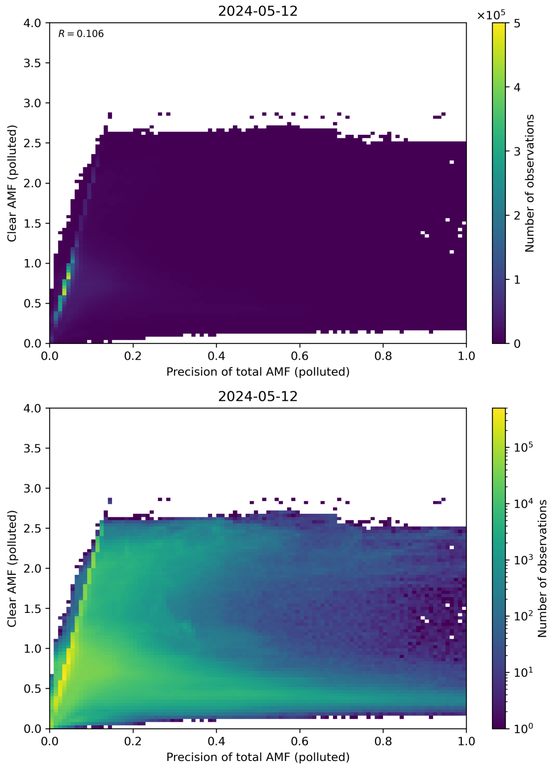
Figure 270: Scatter density plot of “Precision of total AMF (polluted)” against “Clear AMF (polluted)” for 2024-05-12 to 2024-05-13.
