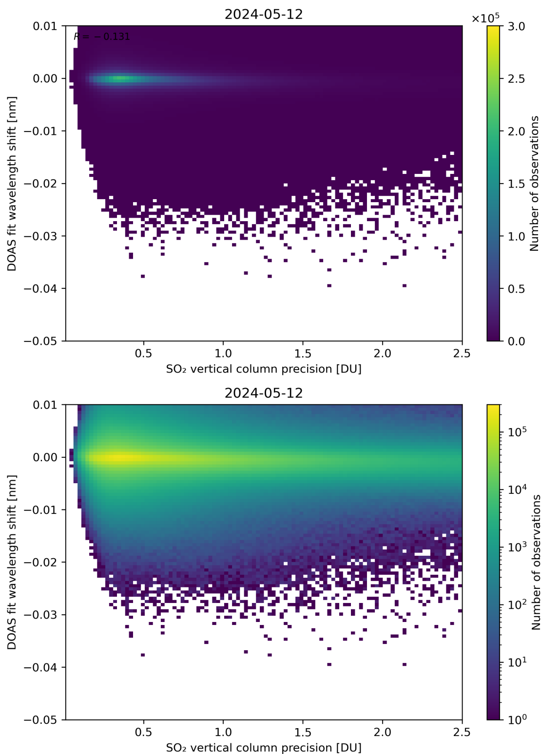
Figure 282: Scatter density plot of “SO 2 vertical column precision” against “DOAS fit wavelength shift” for 2024-05-12 to 2024-05-13.
