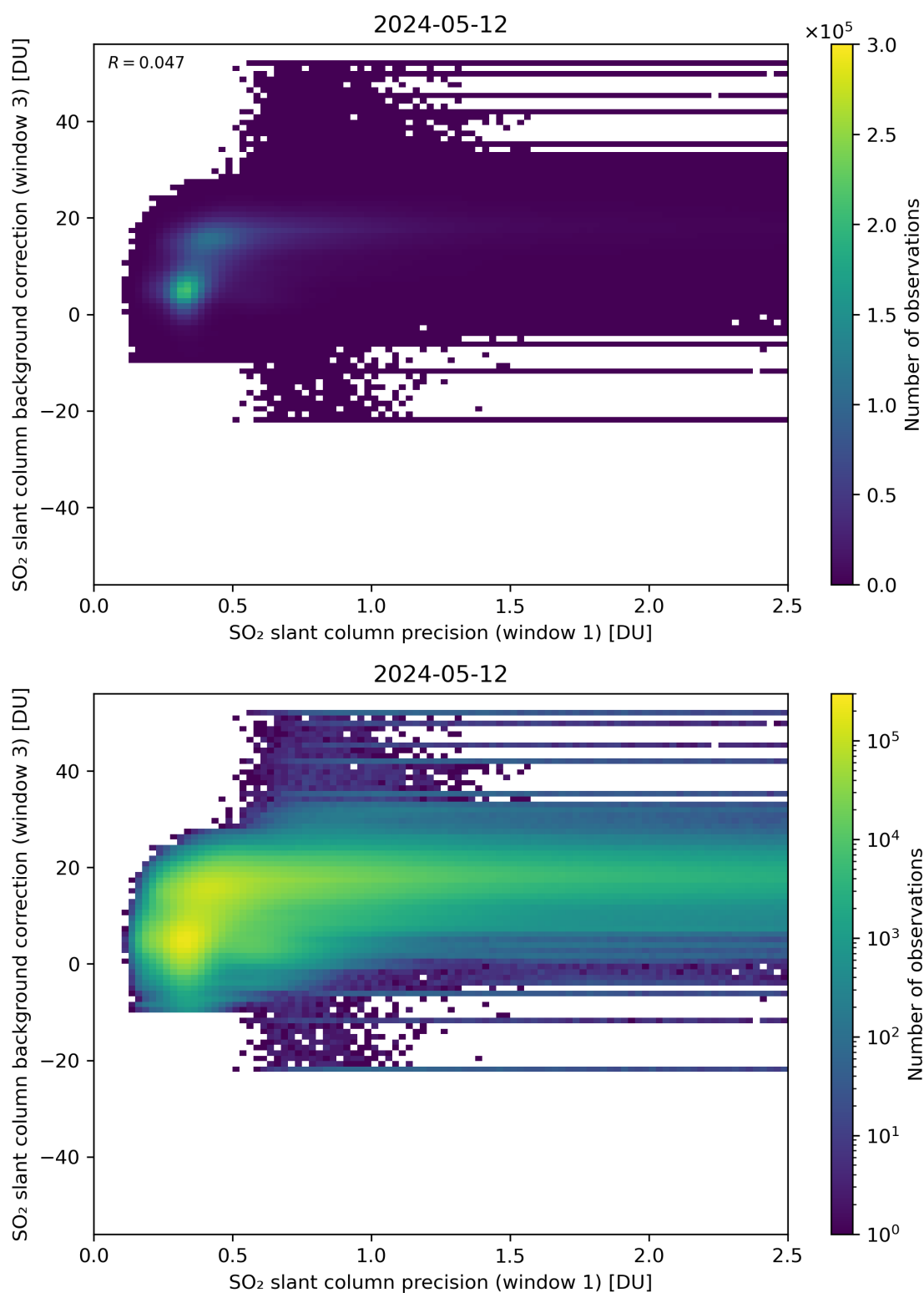
Figure 220: Scatter density plot of “SO 2 slant column precision (window 1)” against “SO 2 slant column background correction (window 3)” for 2024-05-12 to 2024-05-13.
