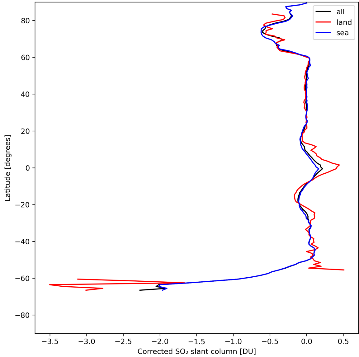
Figure 32: Zonal average of “Corrected SO 2 slant column” for 2024-05-12 to 2024-05-13.
