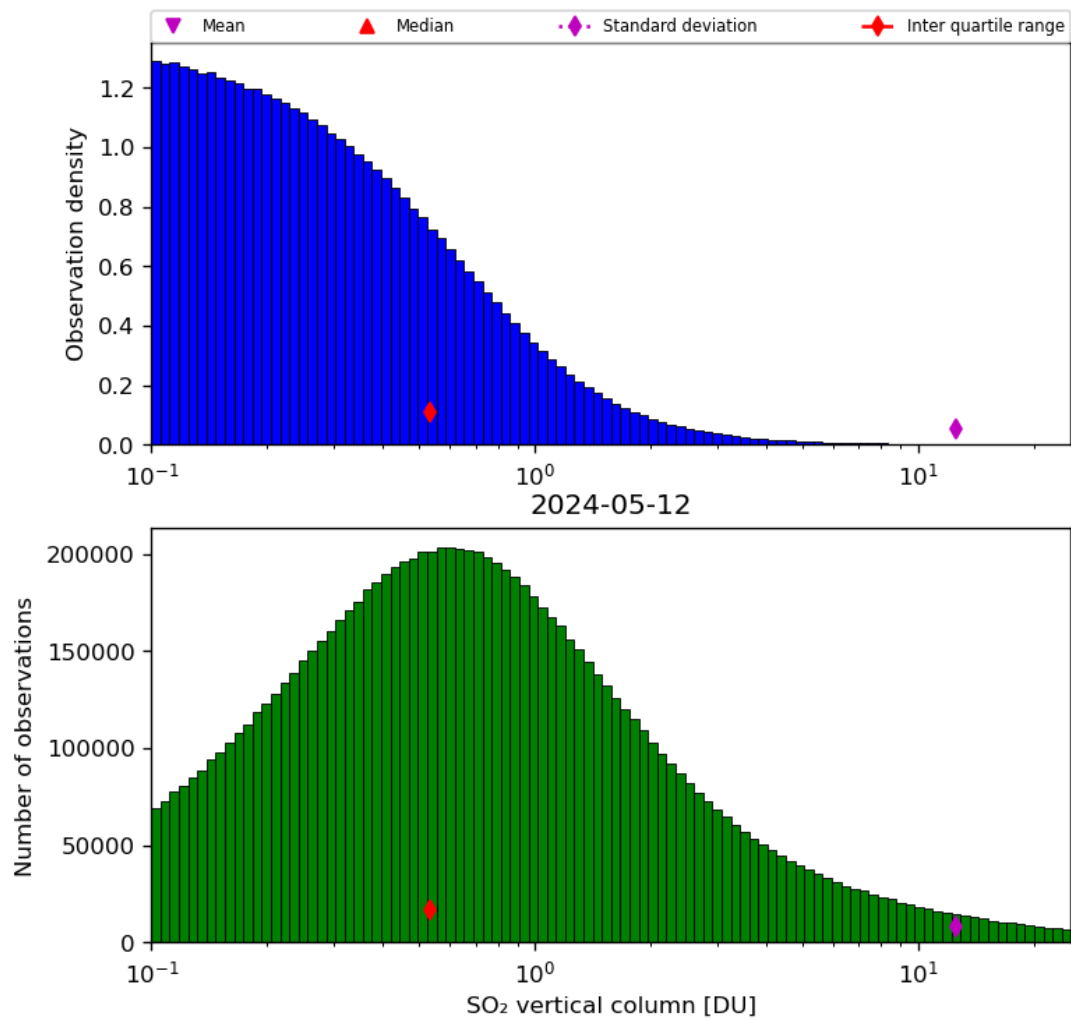
Figure 53: Histogram of “SO 2 vertical column” for 2024-05-12 to 2024-05-13
