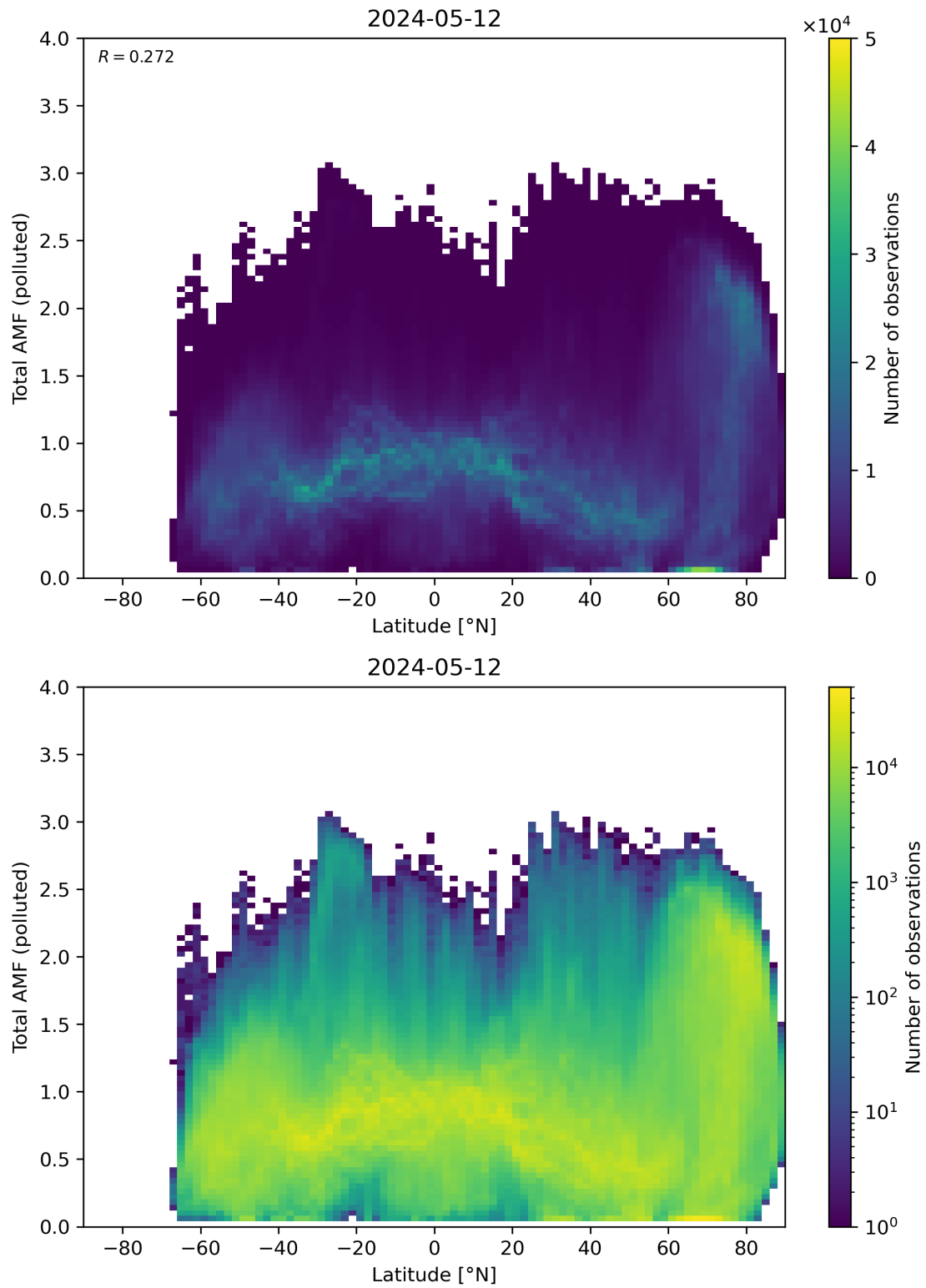
Figure 154: Scatter density plot of “Latitude” against “Total AMF (polluted)” for 2024-05-12 to 2024-05-13.
