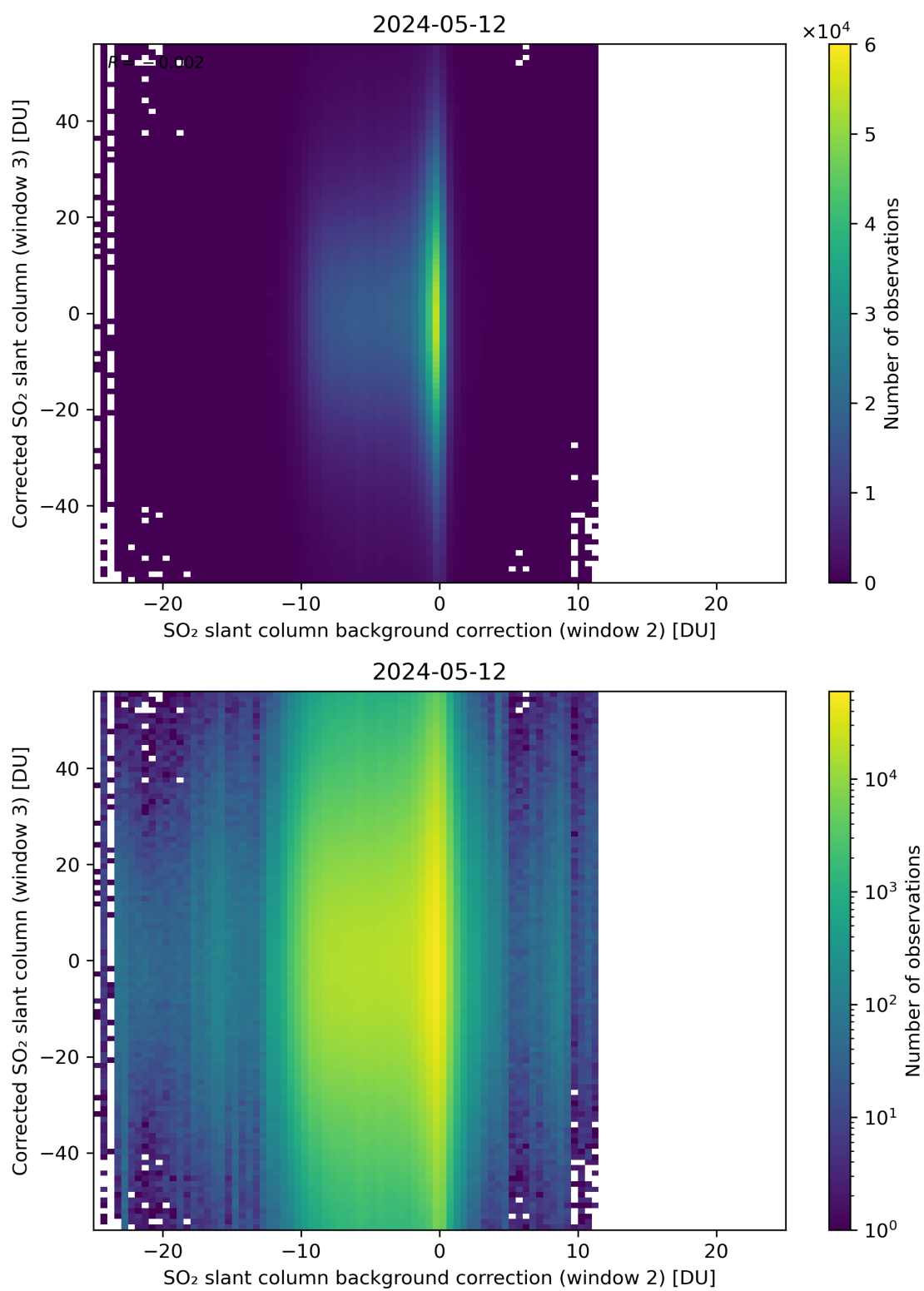
Figure 116: Scatter density plot of “SO 2 slant column background correction (window 2)” against “Corrected SO 2 slant column (window 3)” for 2024-05-12 to 2024-05-13.
