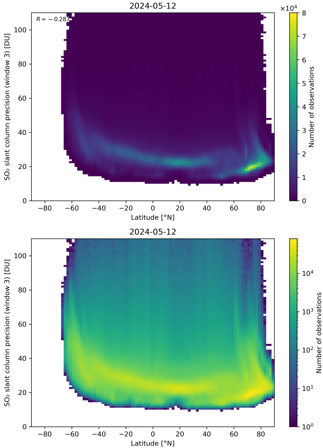
Figure 153: Scatter density plot of “Latitude” against “SO 2 slant column precision (window 3)” for 2024-05-12 to 2024-05-13.
