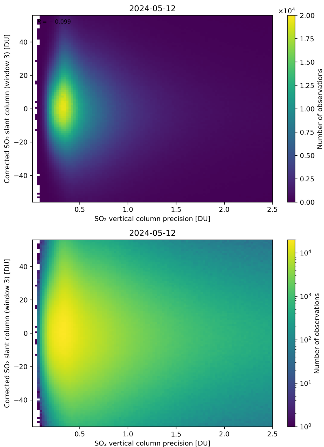
Figure 288: Scatter density plot of “SO 2 vertical column precision” against “Corrected SO 2 slant column (window 3)” for 2024-05-12 to 2024-05-13.
