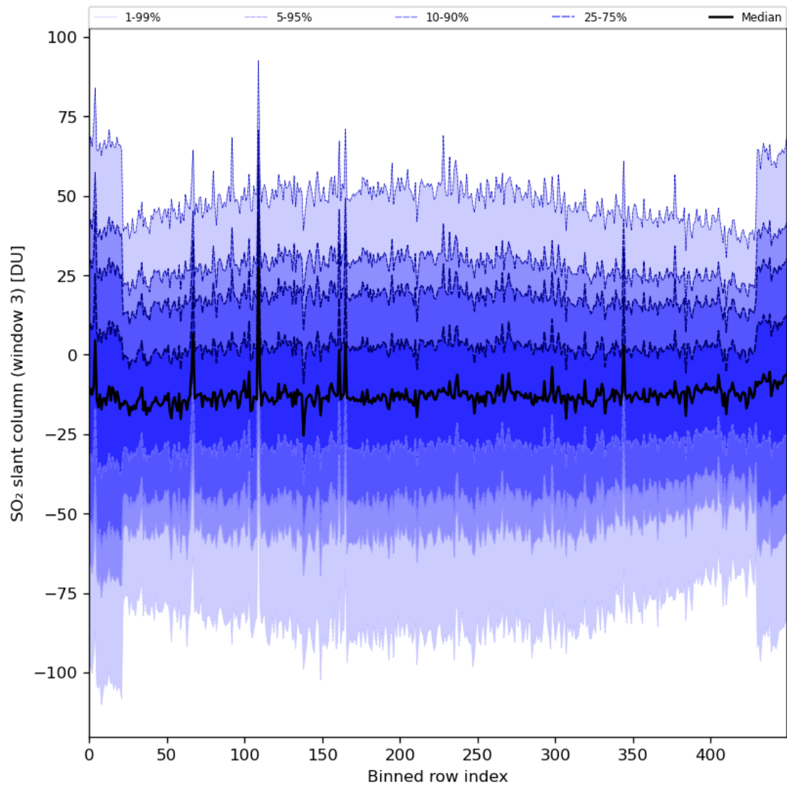
Figure 87: Along track statistics of “SO 2 slant column (window 3)” for 2024-05-12 to 2024-05-13
