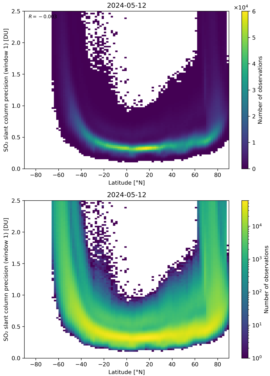
Figure 150: Scatter density plot of “Latitude” against “SO 2 slant column precision (window 1)” for 2024-05-12 to 2024-05-13.
