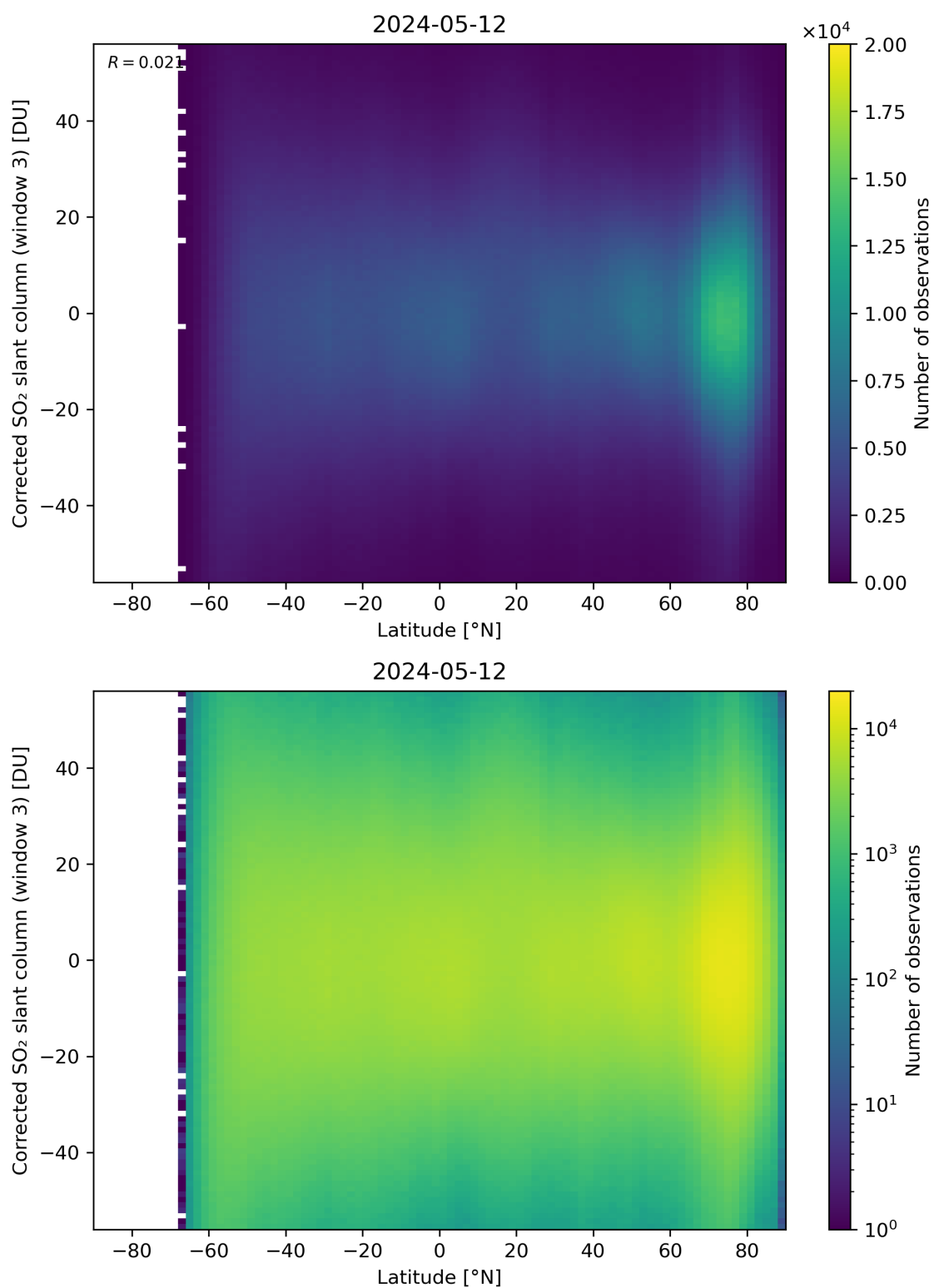
Figure 148: Scatter density plot of “Latitude” against “Corrected SO 2 slant column (window 3)” for 2024-05-12 to 2024-05-13.
