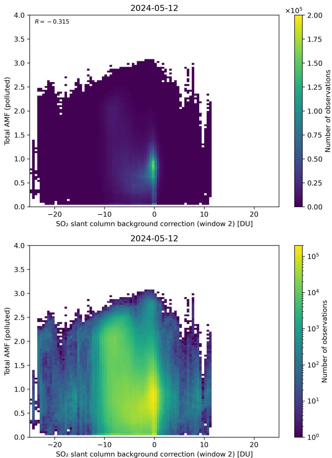
Figure 119: Scatter density plot of “SO 2 slant column background correction (window 2)” against “Total AMF (polluted)” for 2024-05-12 to 2024-05-13.
