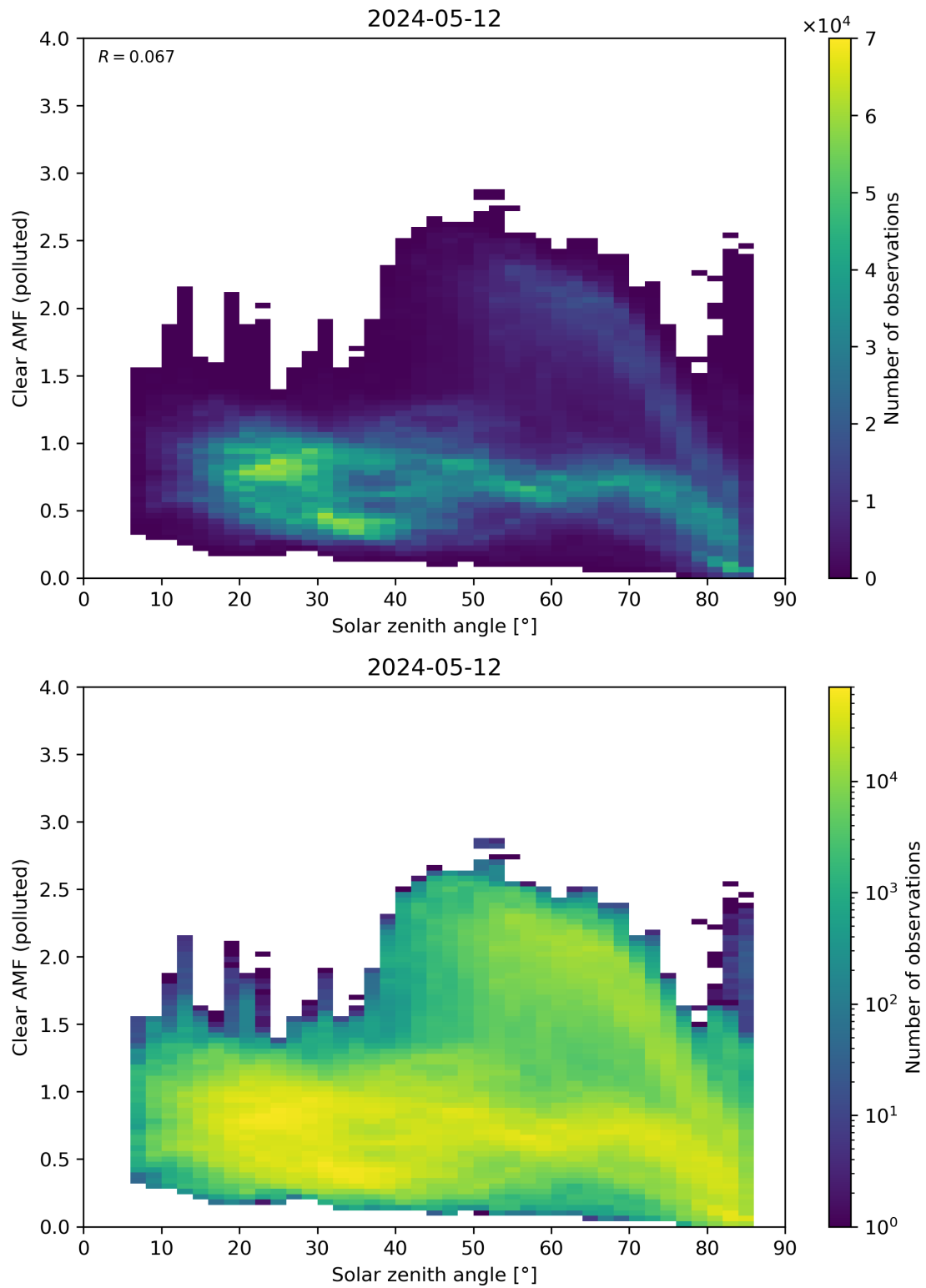
Figure 165: Scatter density plot of “Solar zenith angle” against “Clear AMF (polluted)” for 2024-05-12 to 2024-05-13.
