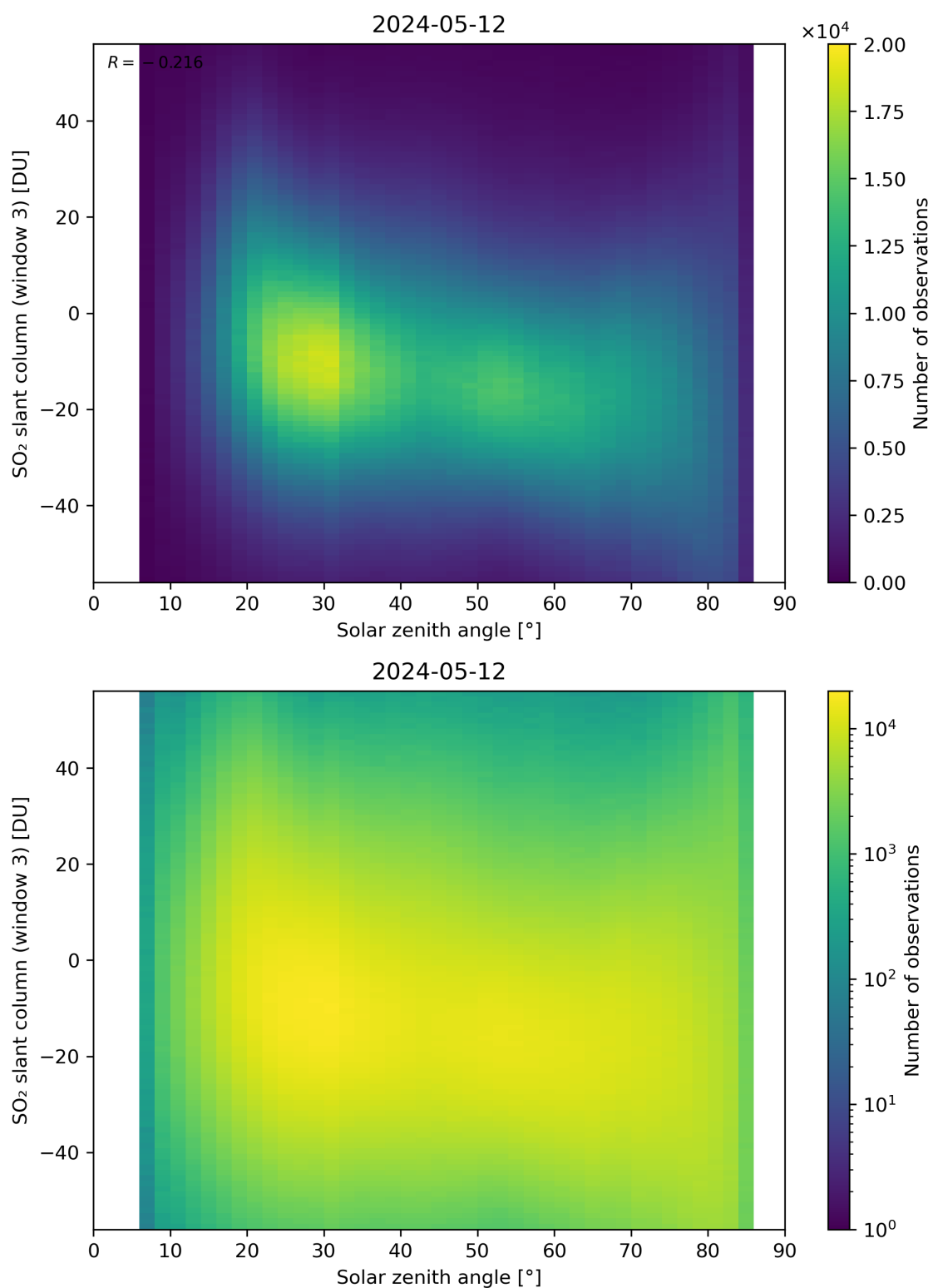
Figure 172: Scatter density plot of “Solar zenith angle” against “SO 2 slant column (window 3)” for 2024-05-12 to 2024-05-13.
