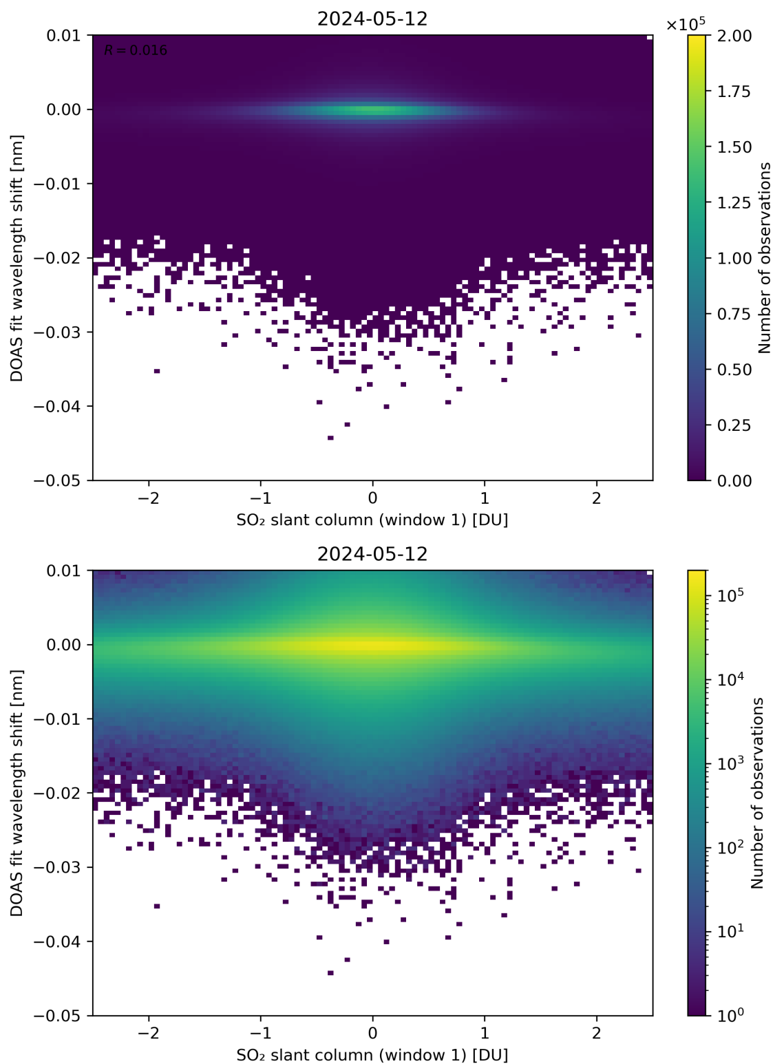
Figure 215: Scatter density plot of “SO 2 slant column (window 1)” against “DOAS fit wavelength shift” for 2024-05-12 to 2024-05-13.
