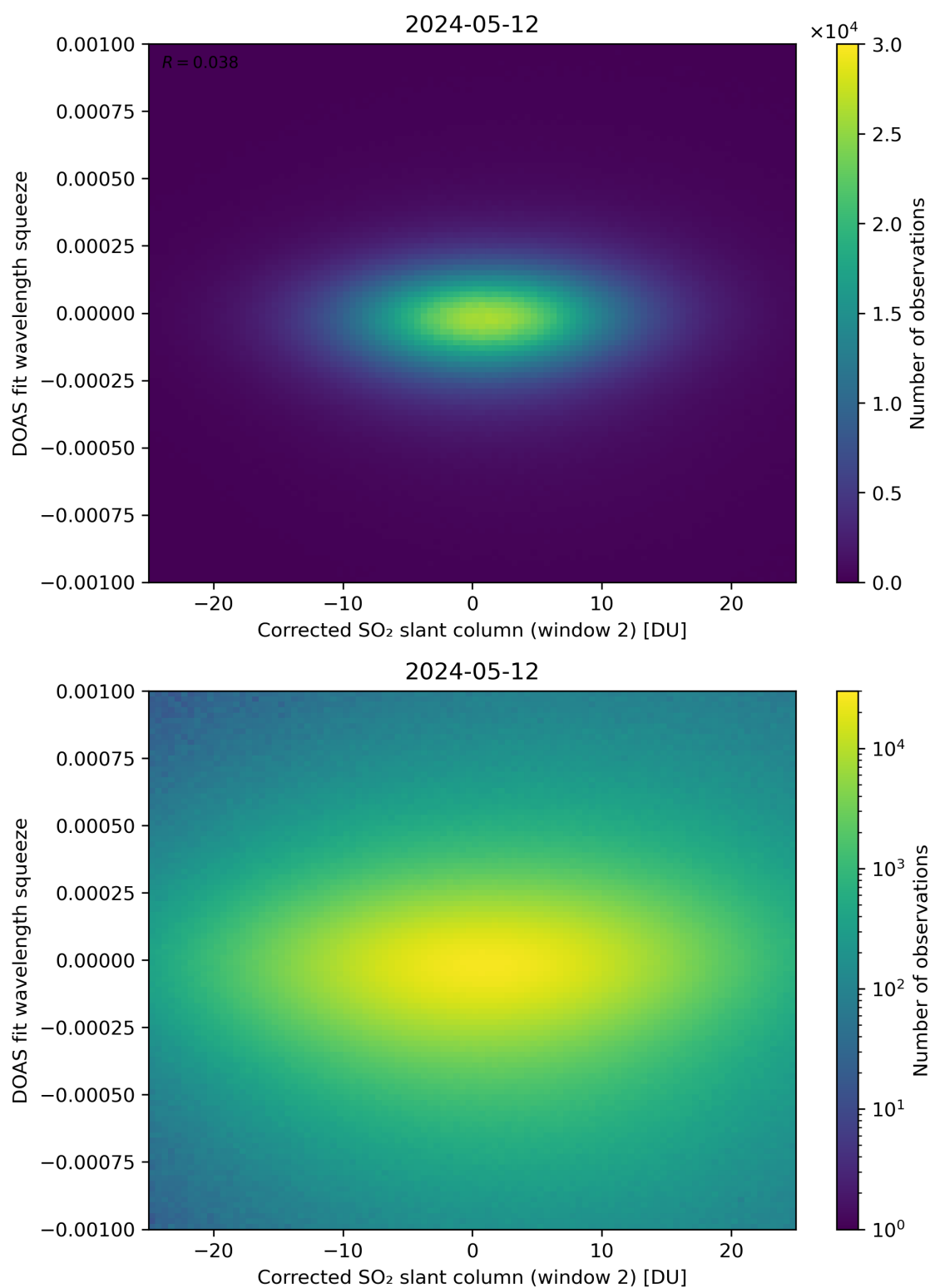
Figure 197: Scatter density plot of “Corrected SO 2 slant column (window 2)” against “DOAS fit wavelength squeeze” for 2024-05-12 to 2024-05-13.
