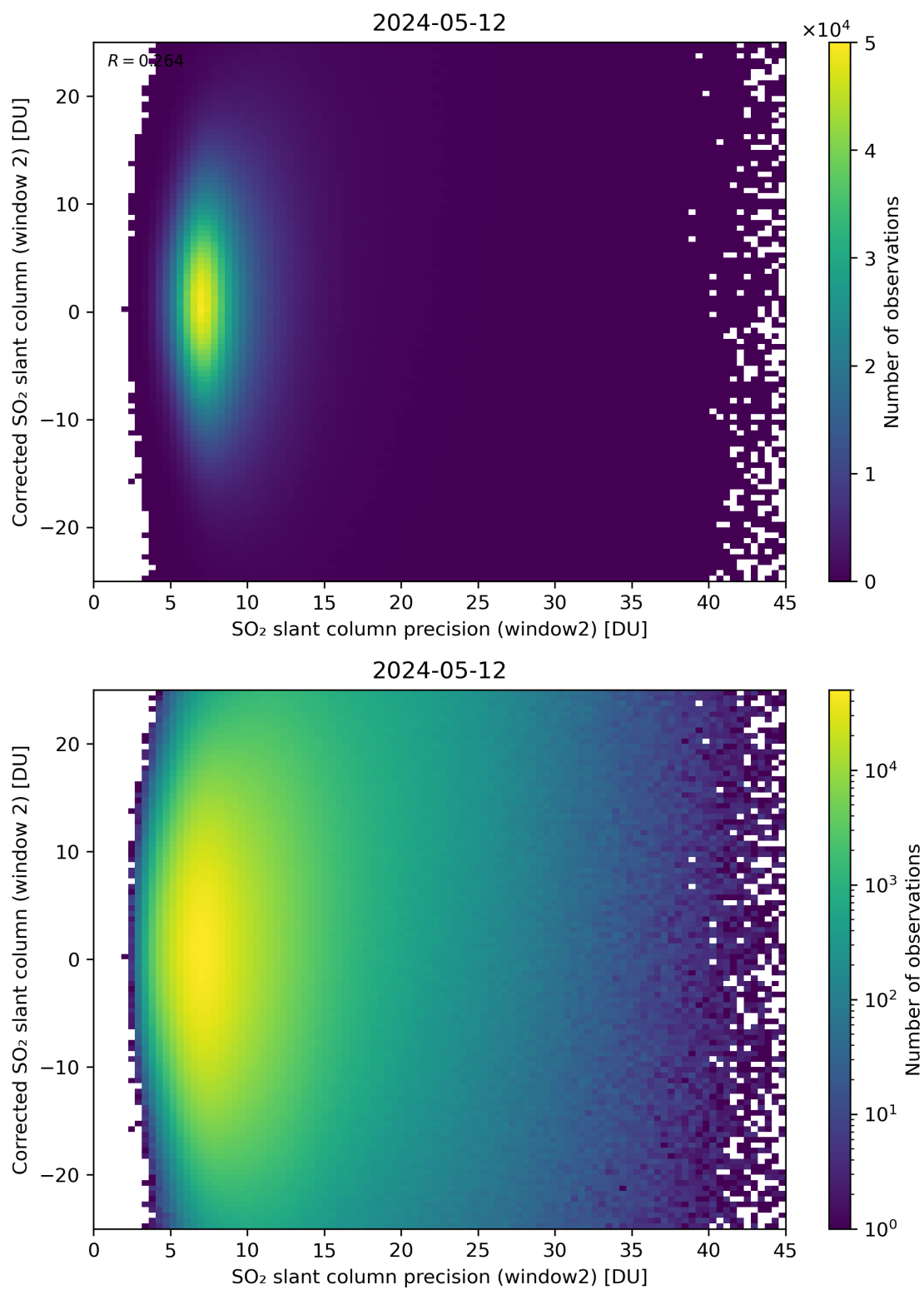
Figure 247: Scatter density plot of “SO 2 slant column precision (window2)” against “Corrected SO 2 slant column (window 2)” for 2024-05-12 to 2024-05-13.
