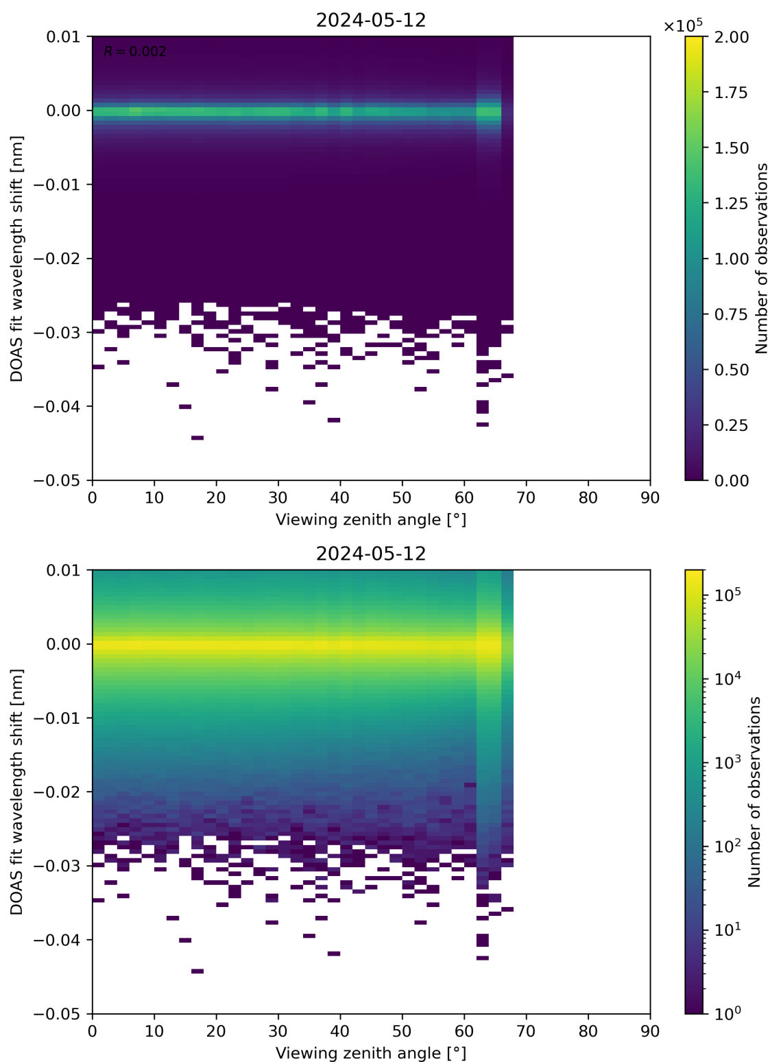
Figure 311: Scatter density plot of “Viewing zenith angle” against “DOAS fit wavelength shift” for 2024-05-12 to 2024-05-13.
