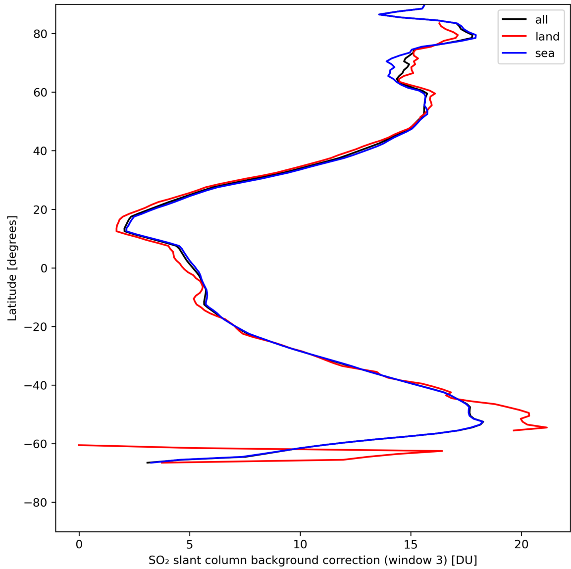
Figure 44: Zonal average of “SO 2 slant column background correction (window 3)” for 2024-05-12 to 2024-05-13.
