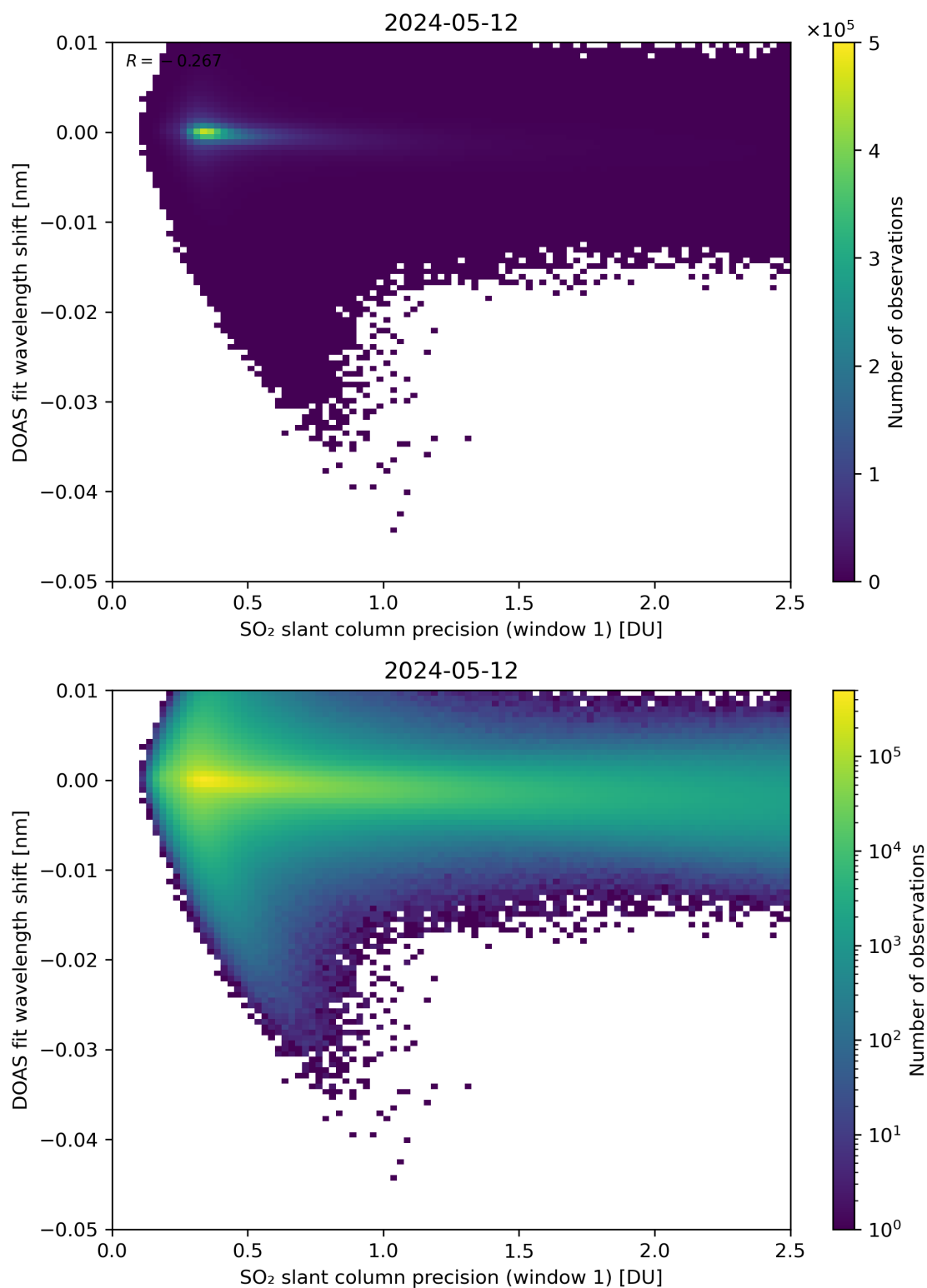
Figure 221: Scatter density plot of “SO 2 slant column precision (window 1)” against “DOAS fit wavelength shift” for 2024-05-12 to 2024-05-13.
