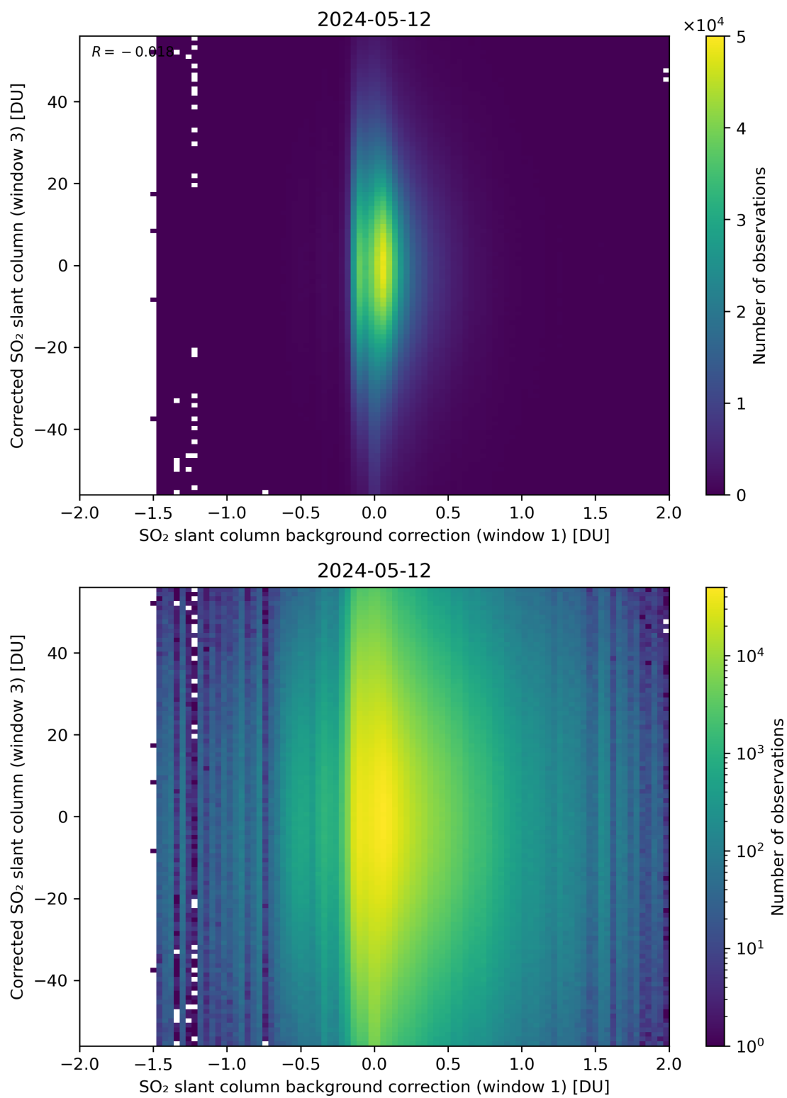
Figure 105: Scatter density plot of “SO 2 slant column background correction (window 1)” against “Corrected SO 2 slant column (window 3)” for 2024-05-12 to 2024-05-13.
