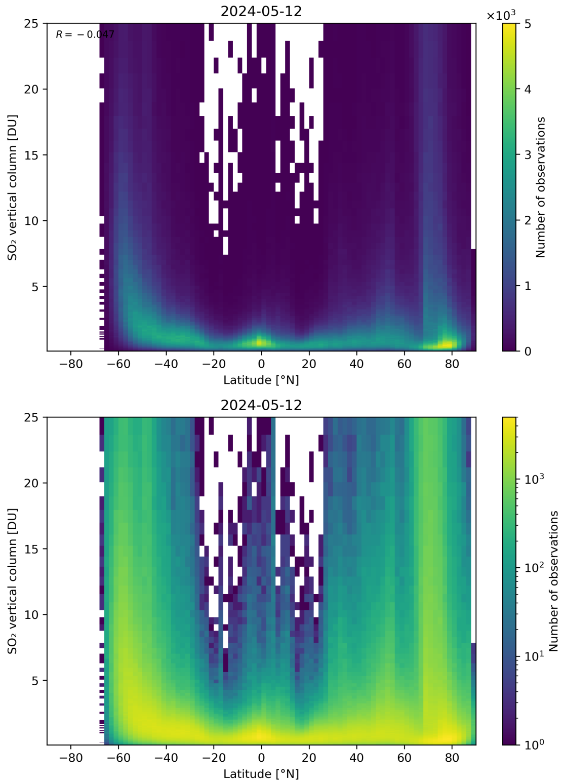
Figure 156: Scatter density plot of “Latitude” against “SO 2 vertical column” for 2024-05-12 to 2024-05-13.
