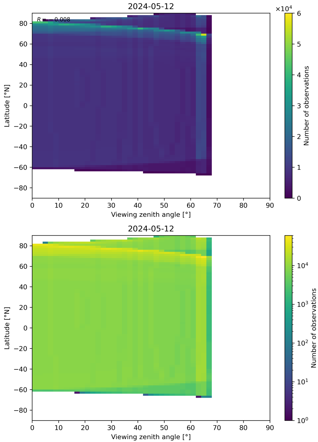
Figure 314: Scatter density plot of “Viewing zenith angle” against “Latitude” for 2024-05-12 to 2024-05-13.
