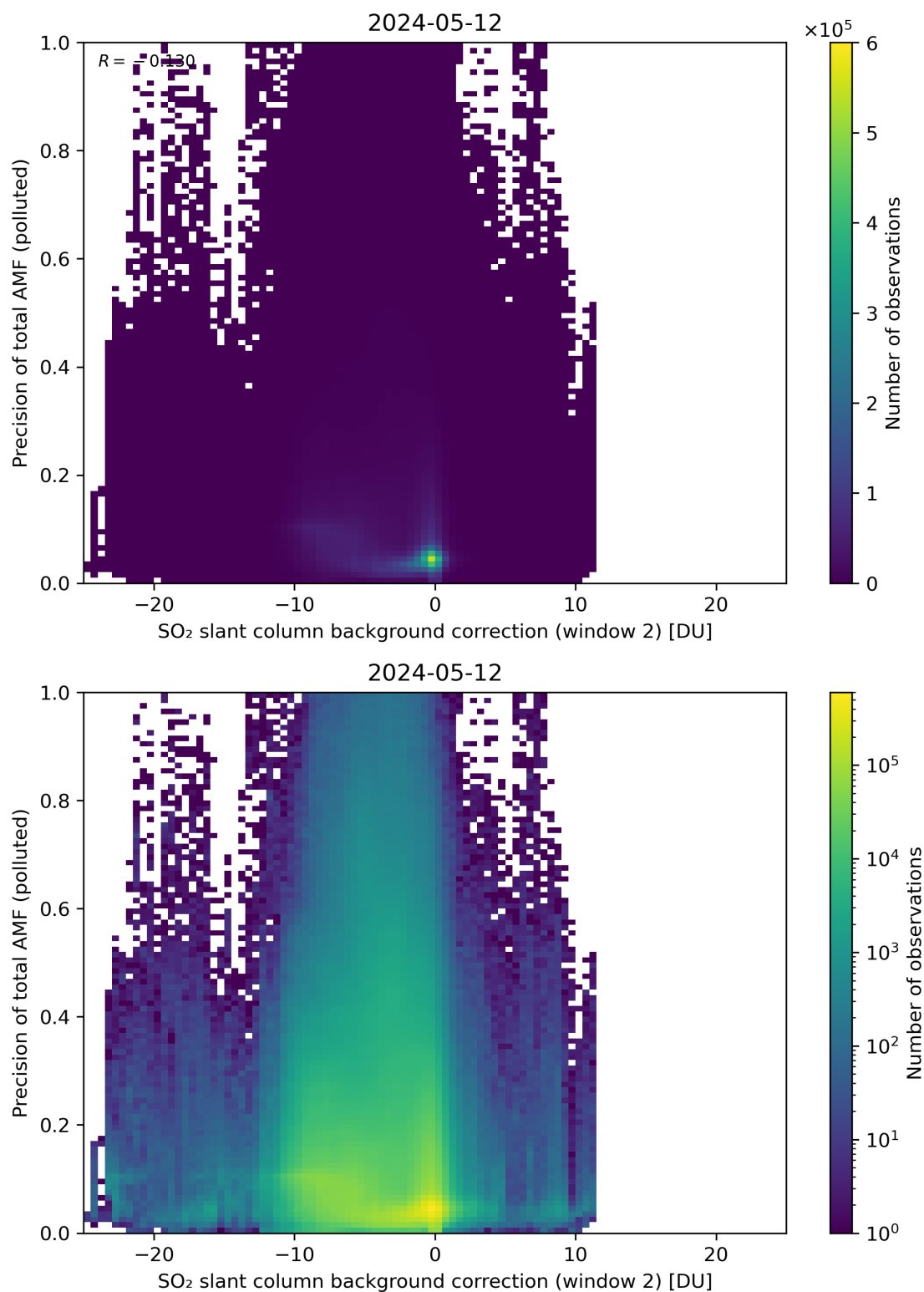
Figure 120: Scatter density plot of “SO 2 slant column background correction (window 2)” against “Precision of total AMF (polluted)” for 2024-05-12 to 2024-05-13.
