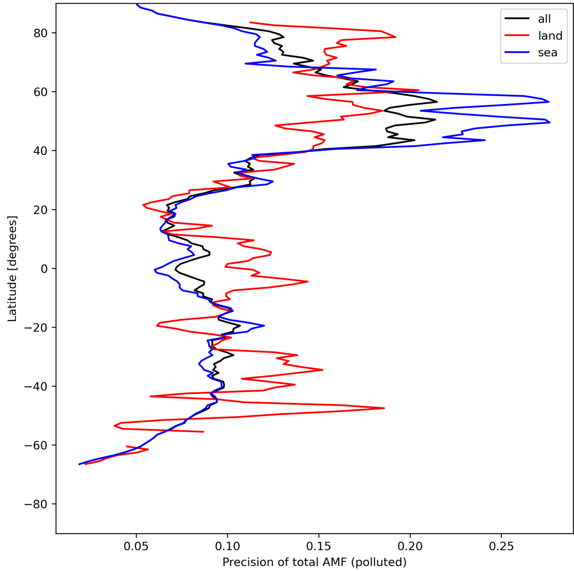
Figure 49: Zonal average of “Precision of total AMF (polluted)” for 2024-05-12 to 2024-05-13.
