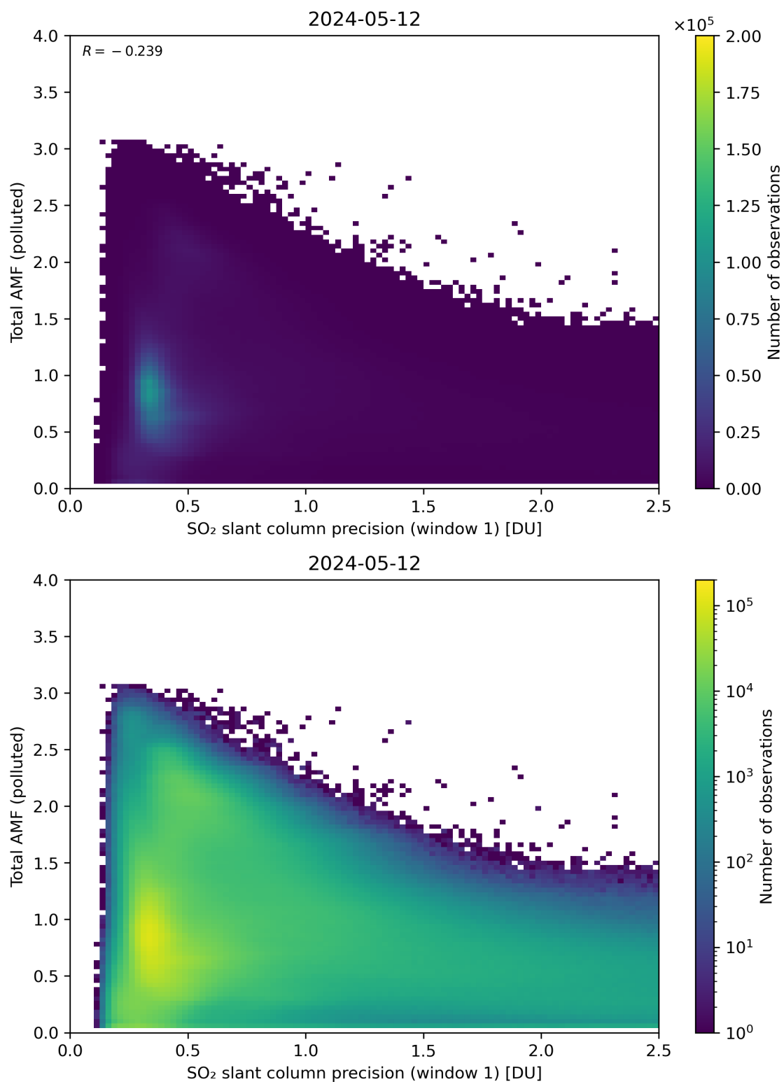
Figure 230: Scatter density plot of “SO 2 slant column precision (window 1)” against “Total AMF (polluted)” for 2024-05-12 to 2024-05-13.
