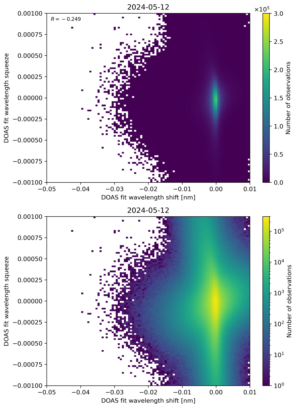
Figure 127: Scatter density plot of “DOAS fit wavelength shift” against “DOAS fit wavelength squeeze” for 2024-05-12 to 2024-05-13.
