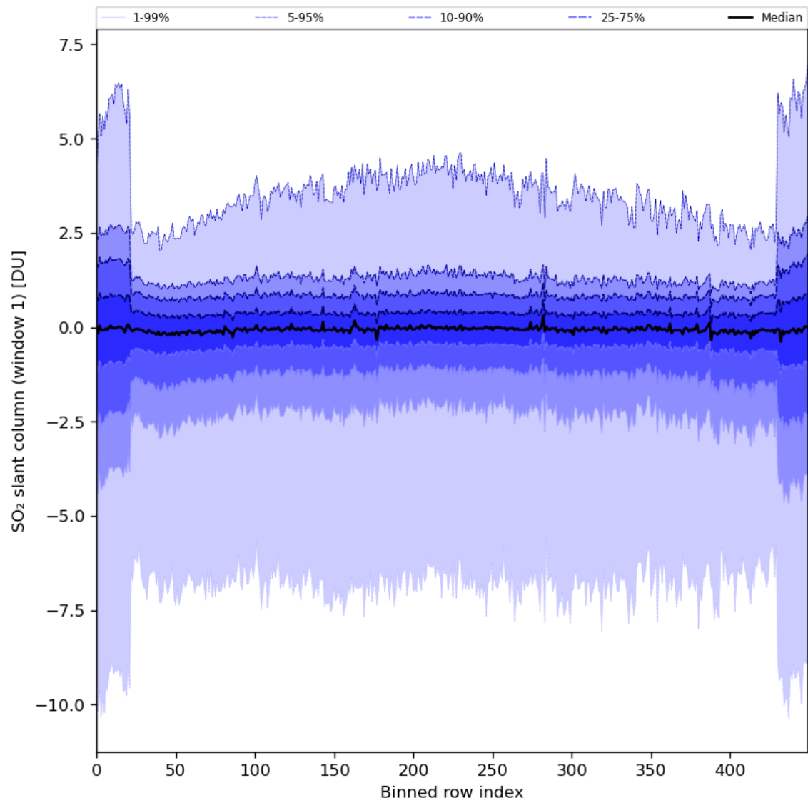
Figure 79: Along track statistics of “SO 2 slant column (window 1)” for 2024-05-12 to 2024-05-13
