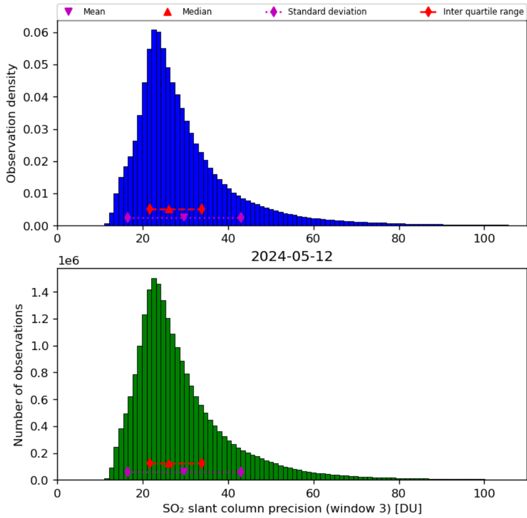
Figure 65: Histogram of “SO 2 slant column precision (window 3)” for 2024-05-12 to 2024-05-13
