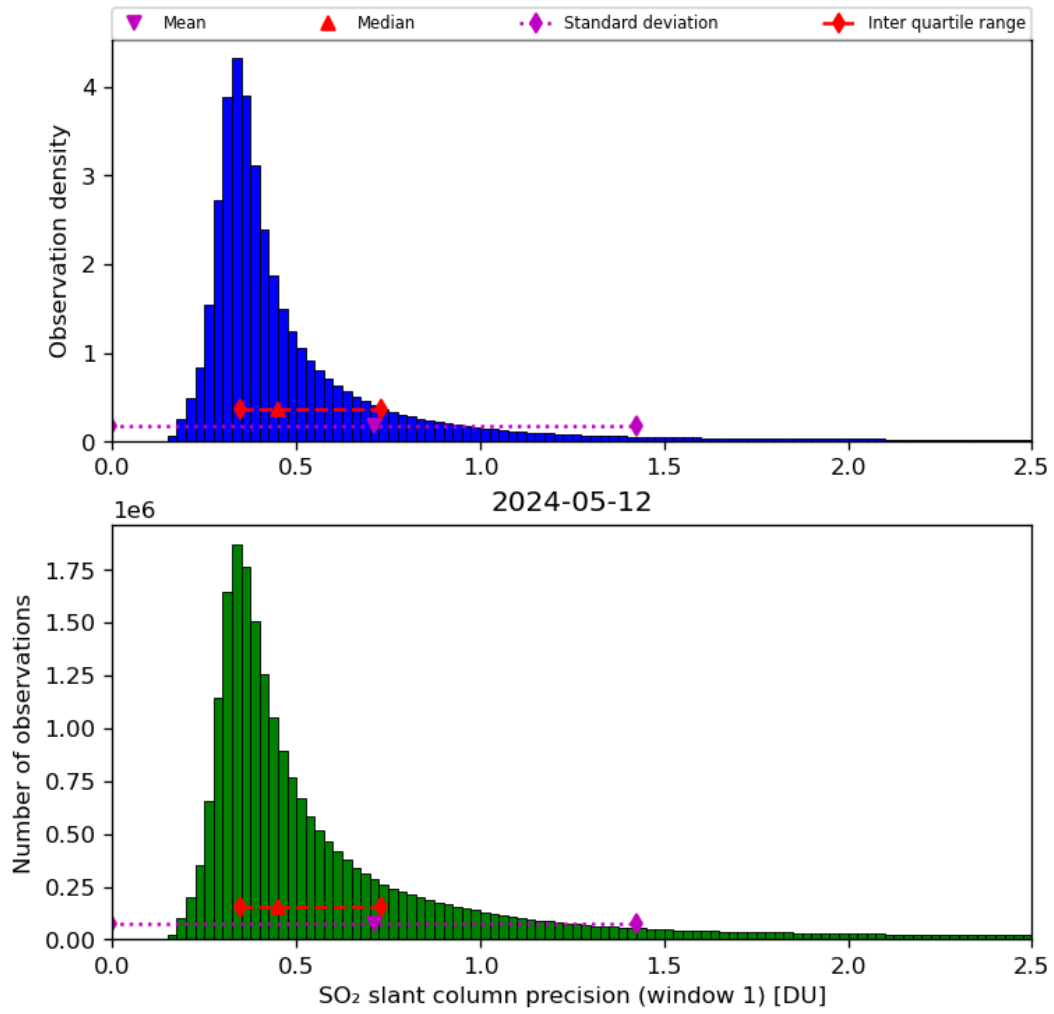
Figure 57: Histogram of “SO 2 slant column precision (window 1)” for 2024-05-12 to 2024-05-13
