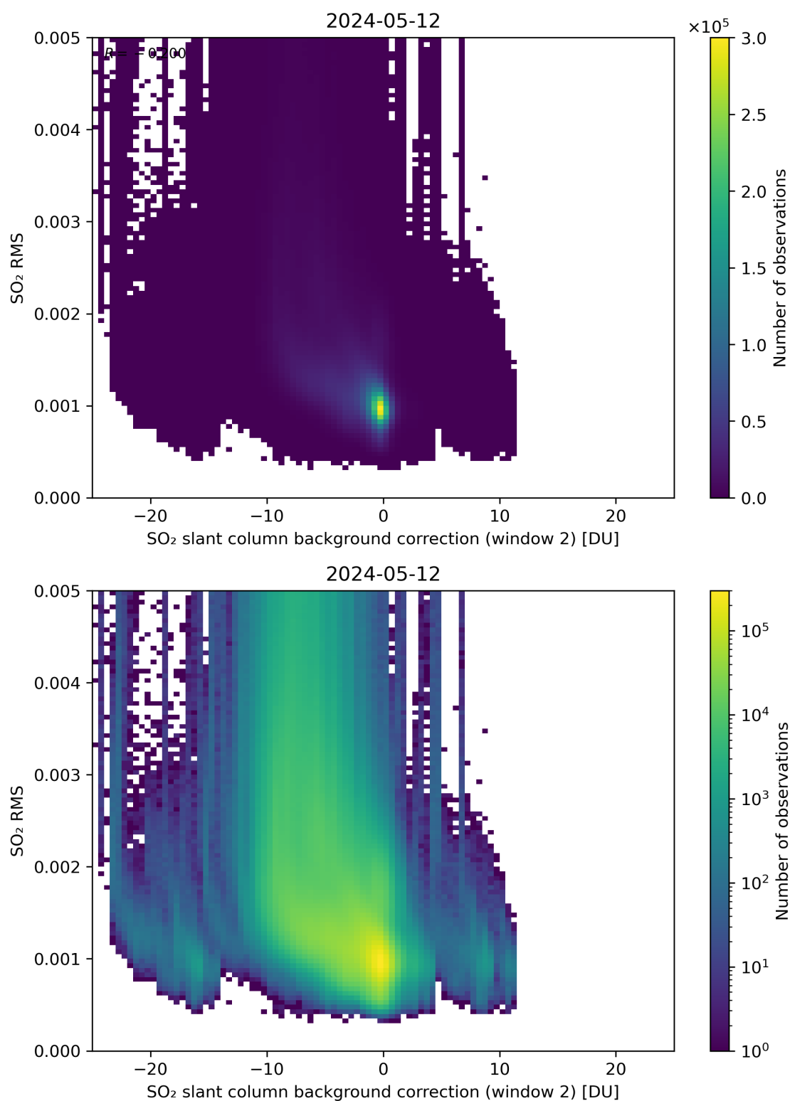
Figure 114: Scatter density plot of “SO 2 slant column background correction (window 2)” against “SO 2 RMS” for 2024-05-12 to 2024-05-13.
