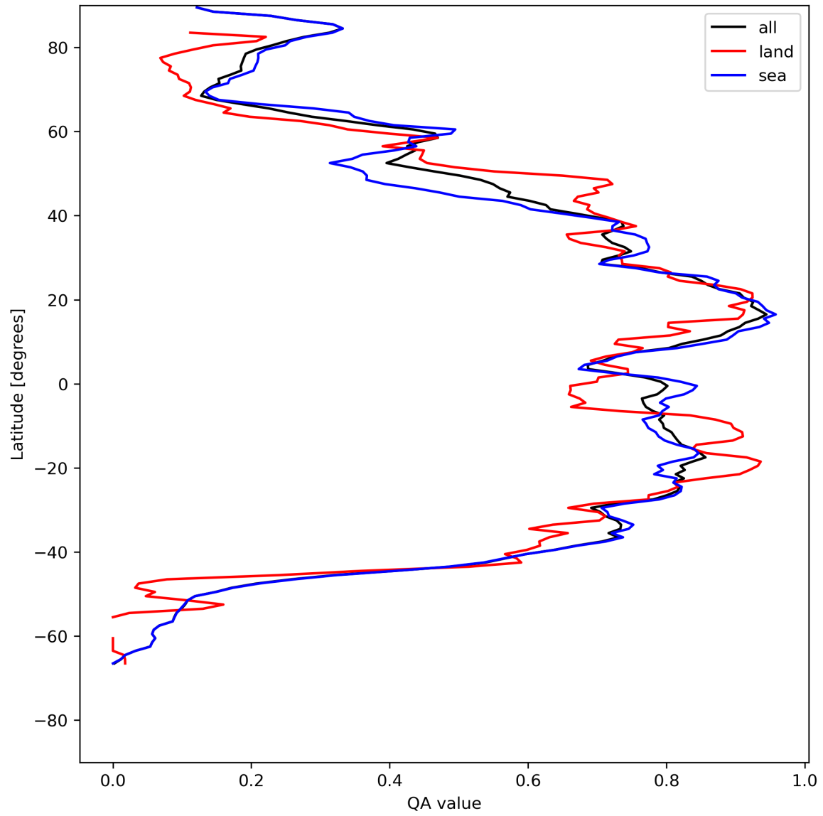
Figure 29: Zonal average of “QA value” for 2024-05-12 to 2024-05-13.
