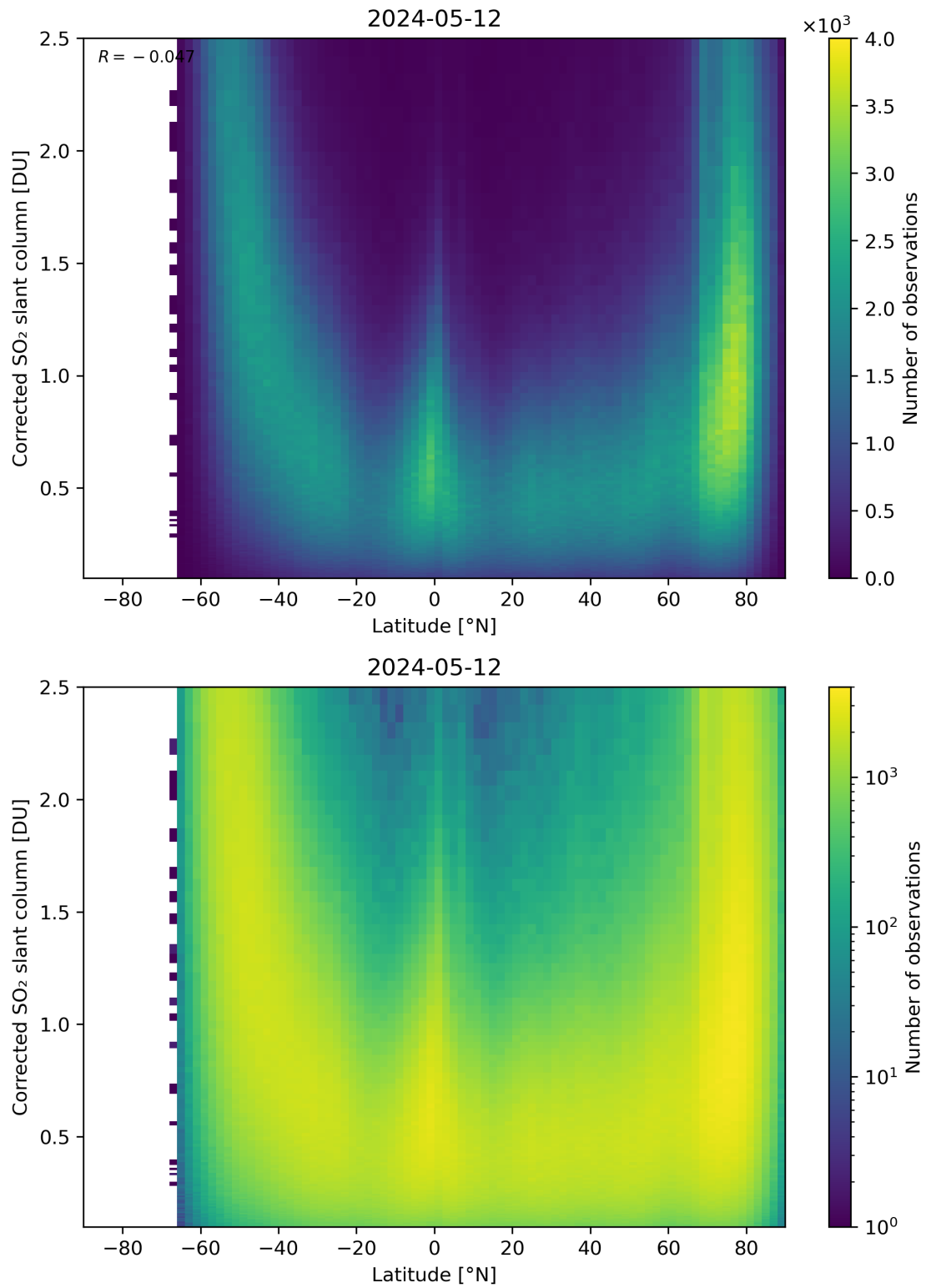
Figure 146: Scatter density plot of “Latitude” against “Corrected SO 2 slant column” for 2024-05-12 to 2024-05-13.
