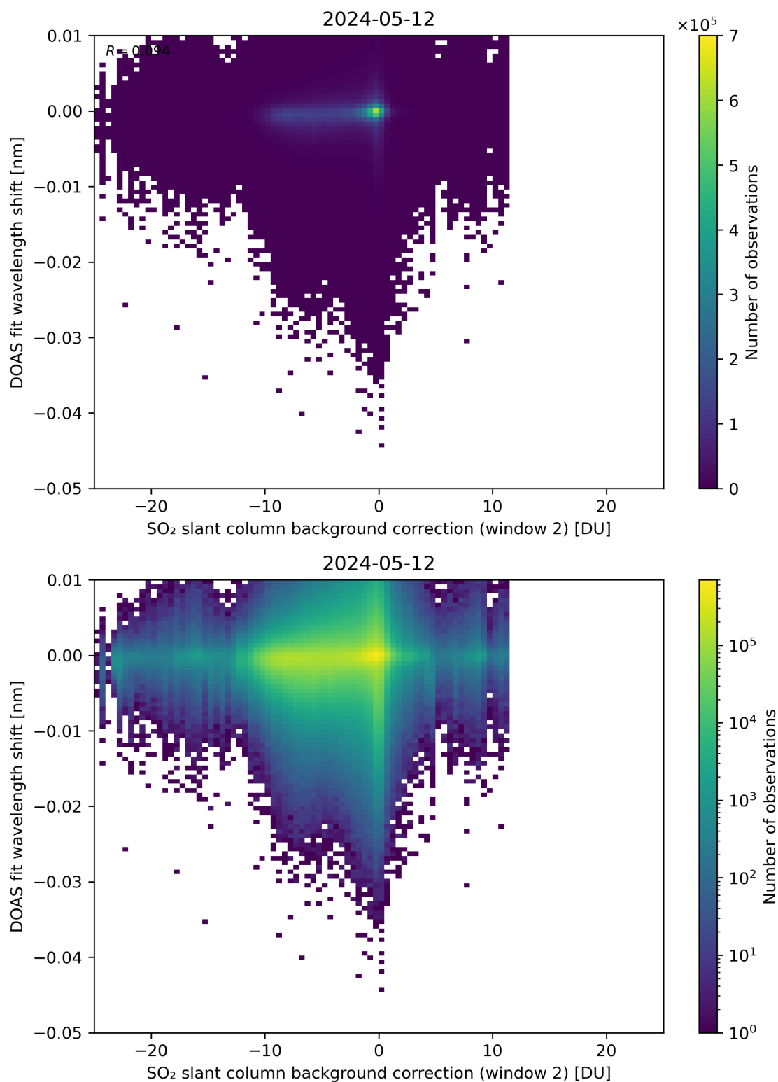
Figure 112: Scatter density plot of “SO 2 slant column background correction (window 2)” against “DOAS fit wavelength shift” for 2024-05-12 to 2024-05-13.
