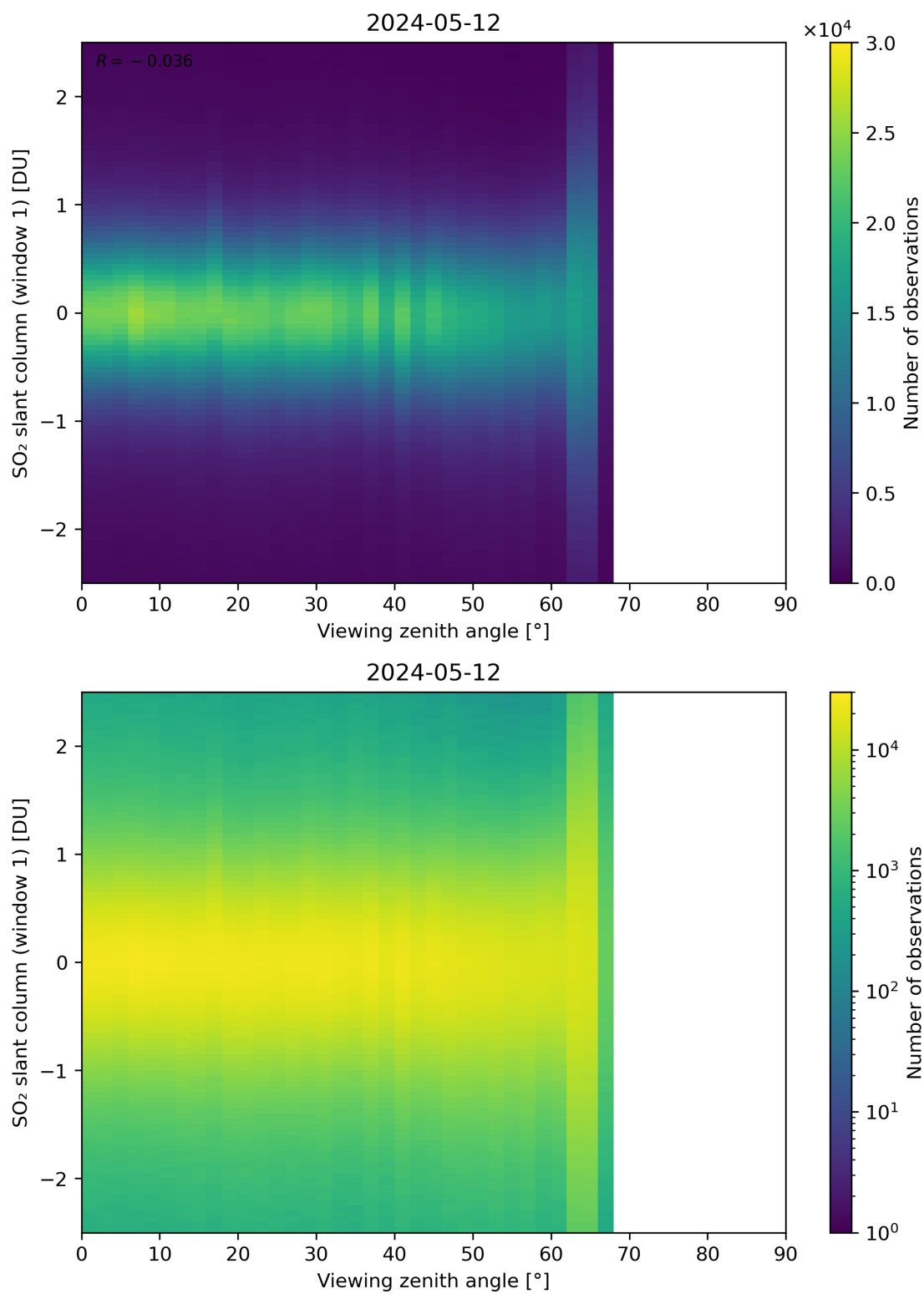
Figure 320: Scatter density plot of “Viewing zenith angle” against “SO 2 slant column (window 1)” for 2024-05-12 to 2024-05-13.
