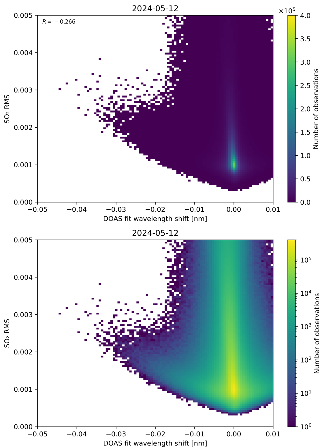
Figure 128: Scatter density plot of “DOAS fit wavelength shift” against “SO 2 RMS” for 2024-05-12 to 2024-05-13.
