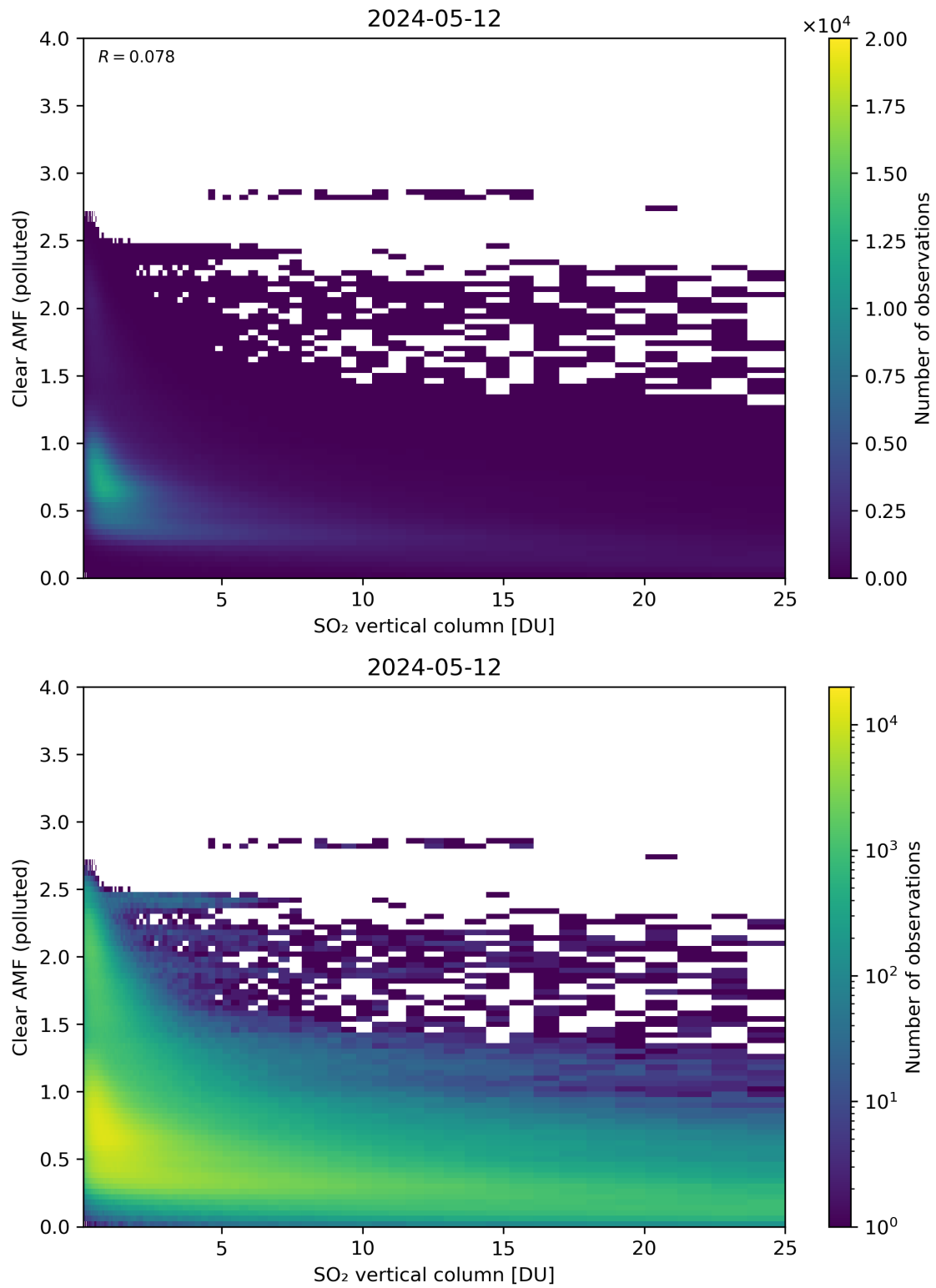
Figure 296: Scatter density plot of “SO 2 vertical column” against “Clear AMF (polluted)” for 2024-05-12 to 2024-05-13.
