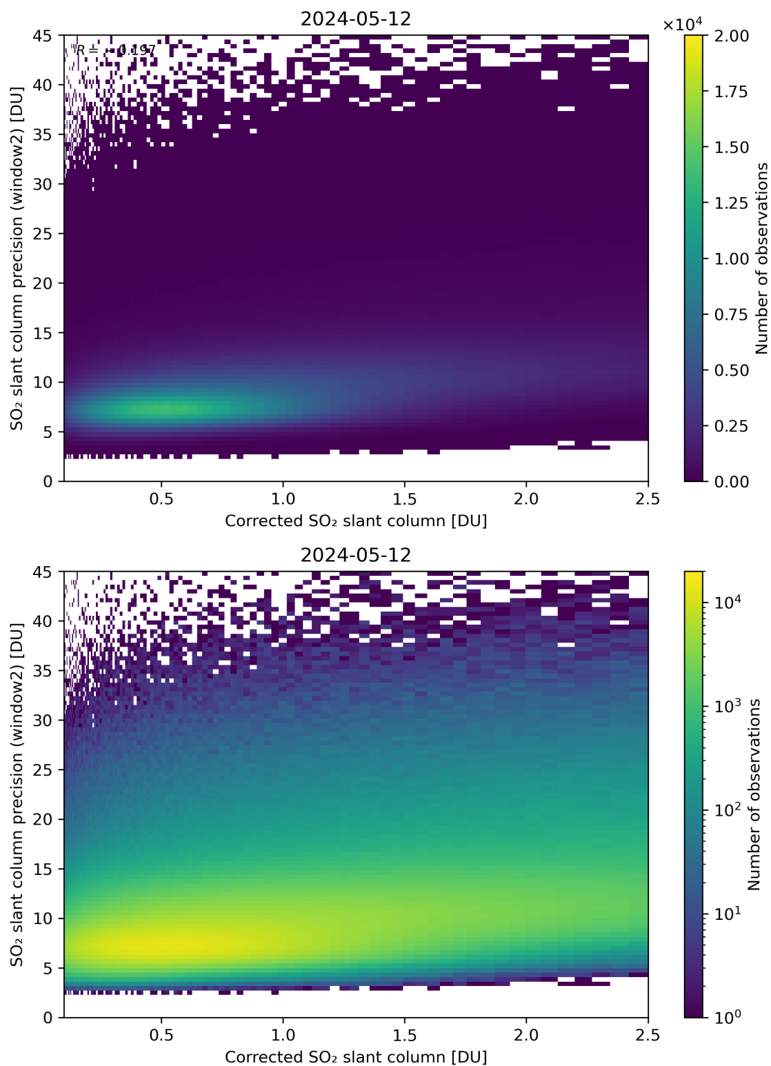
Figure 189: Scatter density plot of “Corrected SO 2 slant column” against “SO 2 slant column precision (window2)” for 2024-05-12 to 2024-05-13.
