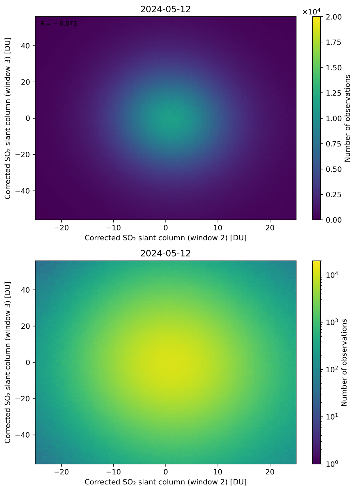
Figure 200: Scatter density plot of “Corrected SO 2 slant column (window 2)” against “Corrected SO 2 slant column (window 3)” for 2024-05-12 to 2024-05-13.
