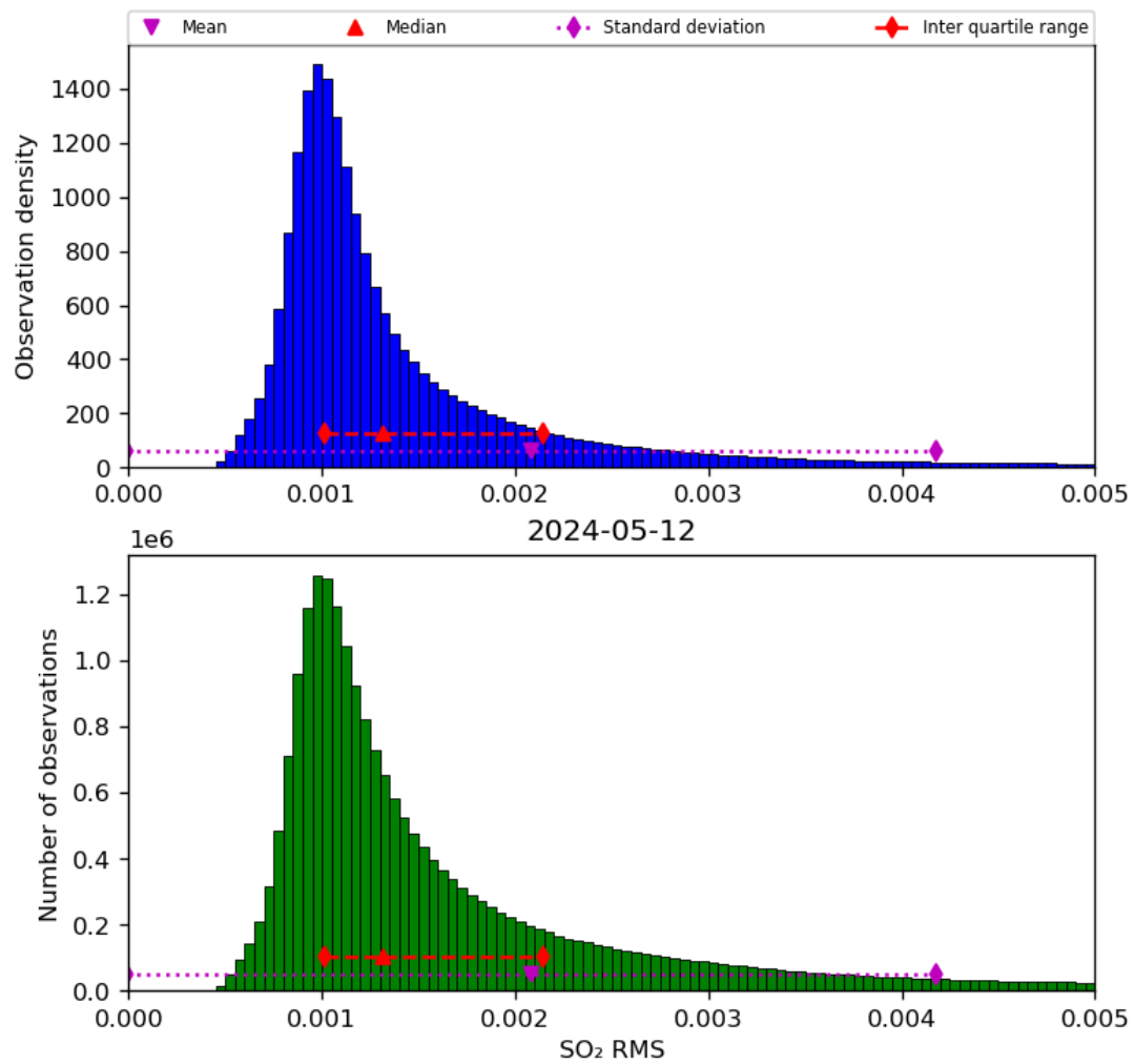
Figure 70: Histogram of “SO 2 RMS” for 2024-05-12 to 2024-05-13
