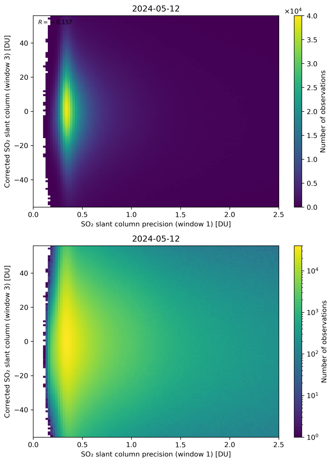
Figure 226: Scatter density plot of “SO 2 slant column precision (window 1)” against “Corrected SO 2 slant column (window 3)” for 2024-05-12 to 2024-05-13.
