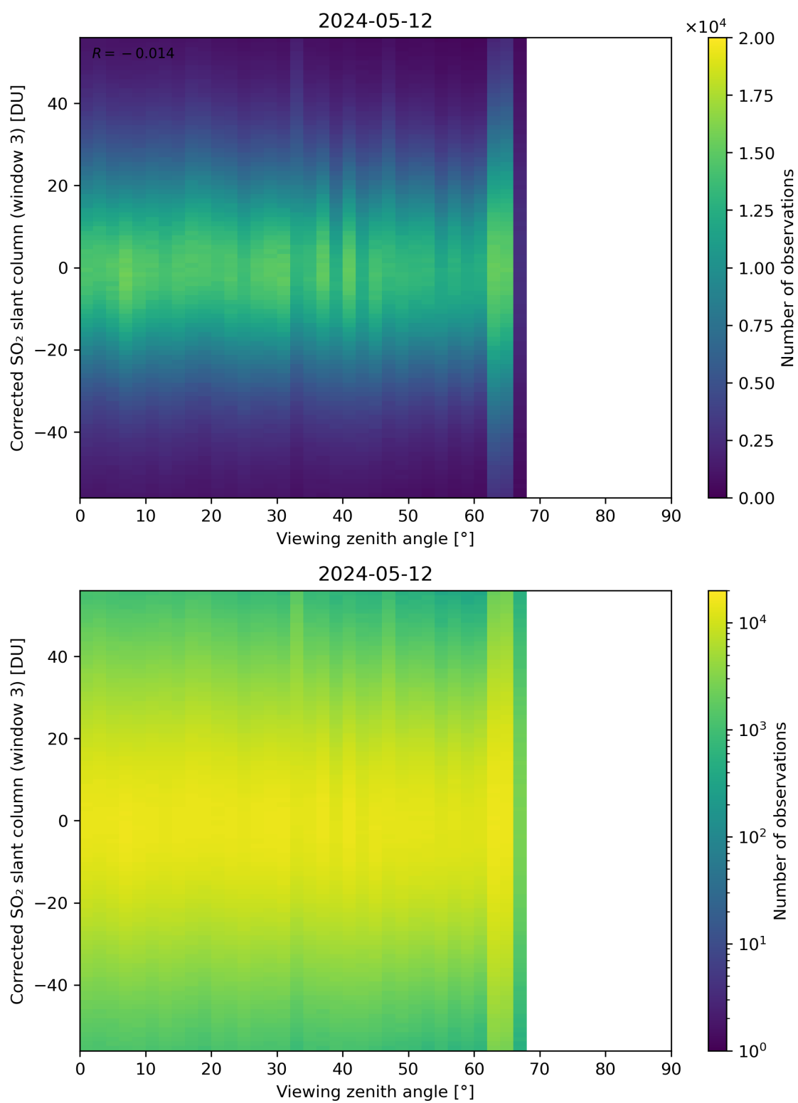
Figure 319: Scatter density plot of “Viewing zenith angle” against “Corrected SO 2 slant column (window 3)” for 2024-05-12 to 2024-05-13.
