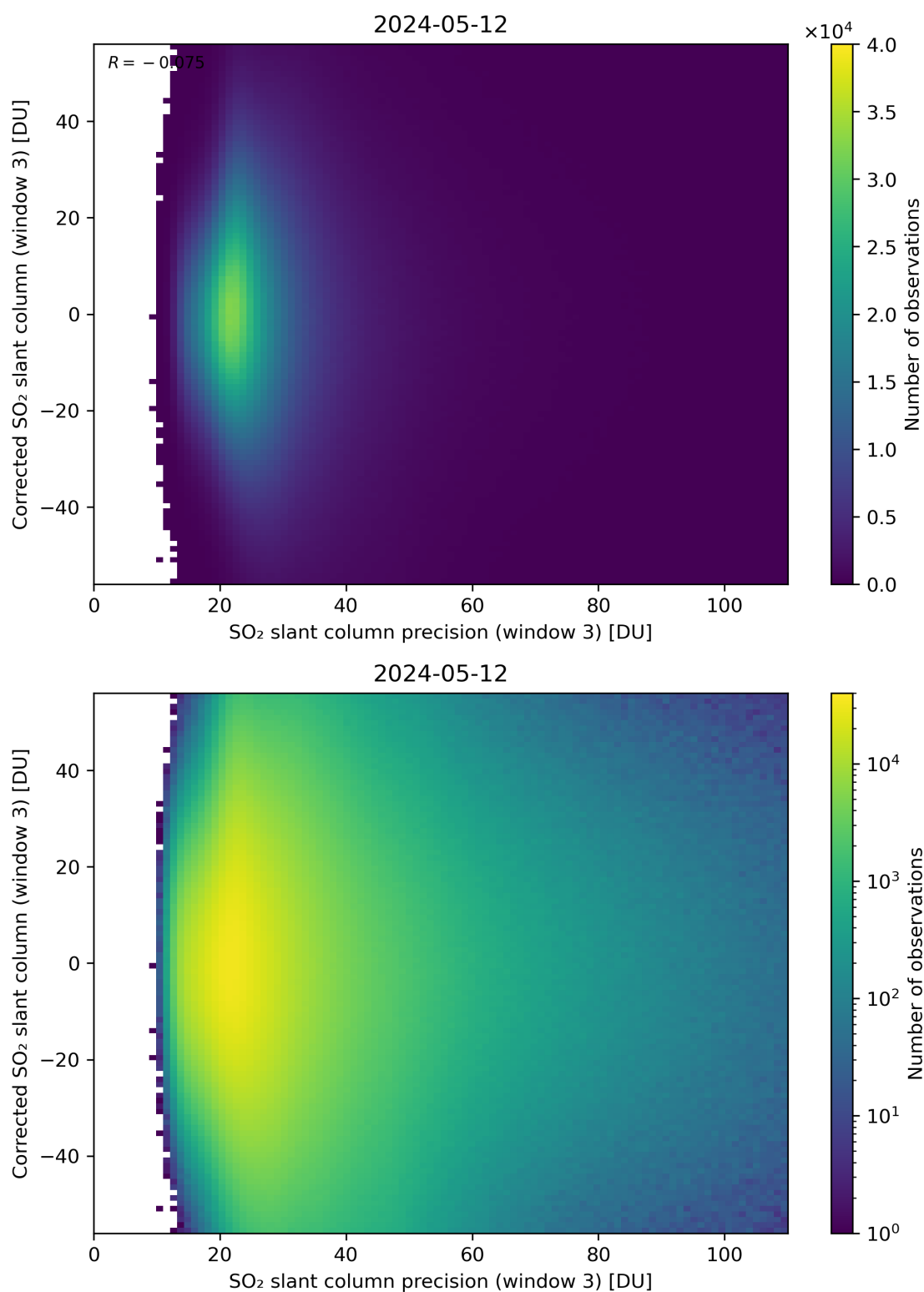
Figure 262: Scatter density plot of “SO 2 slant column precision (window 3)” against “Corrected SO 2 slant column (window 3)” for 2024-05-12 to 2024-05-13.
