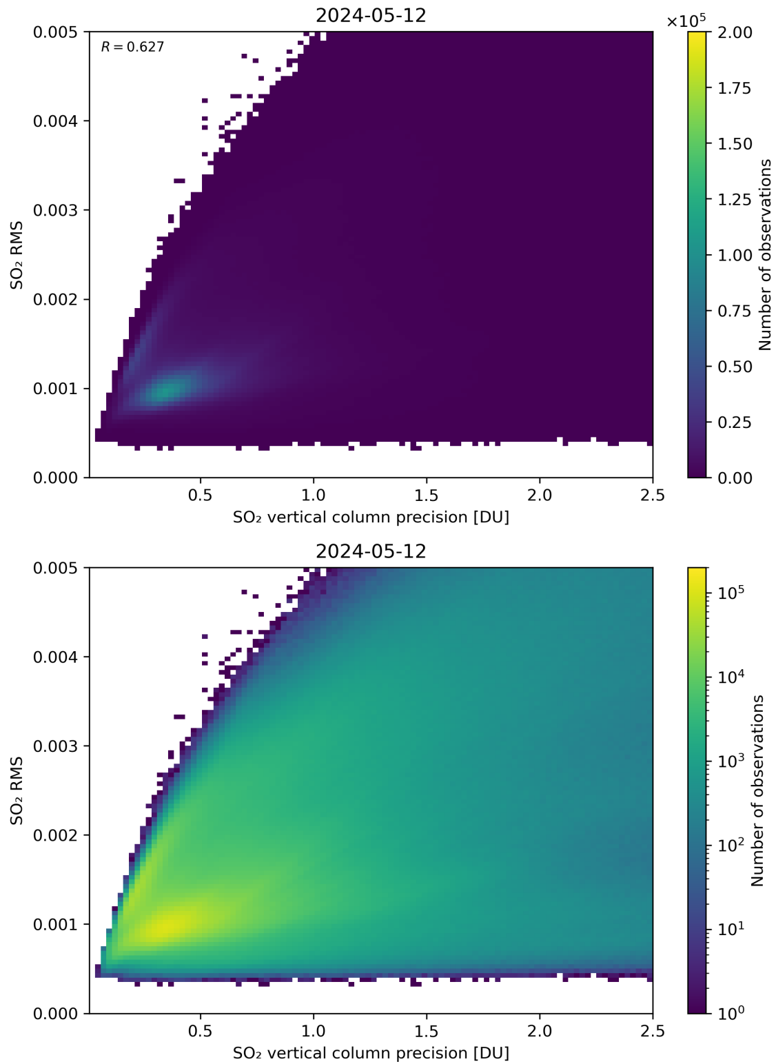
Figure 284: Scatter density plot of “SO 2 vertical column precision” against “SO 2 RMS” for 2024-05-12 to 2024-05-13.
