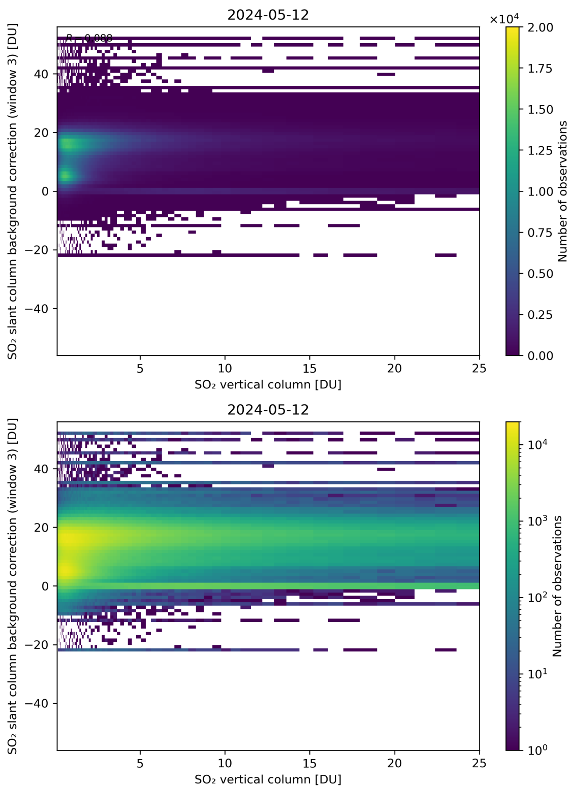
Figure 275: Scatter density plot of “SO 2 vertical column” against “SO 2 slant column background correction (window 3)” for 2024-05-12 to 2024-05-13.
