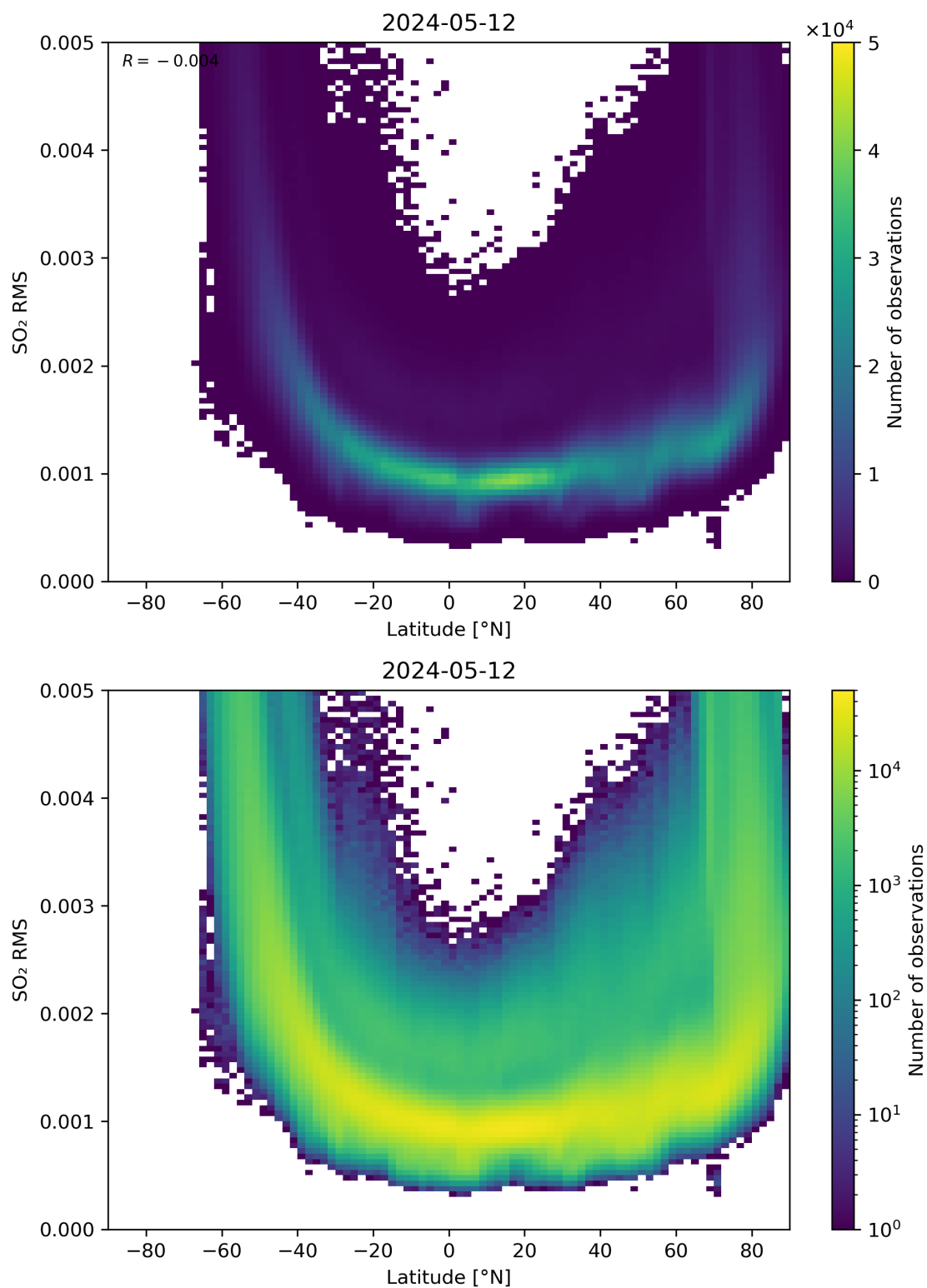
Figure 144: Scatter density plot of “Latitude” against “SO 2 RMS” for 2024-05-12 to 2024-05-13.
