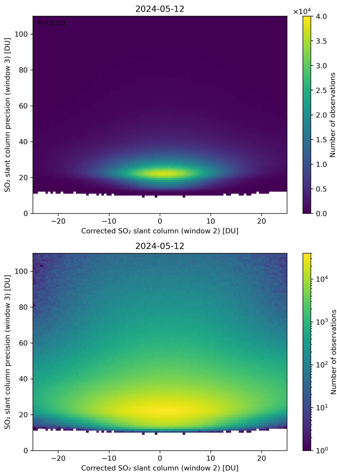
Figure 202: Scatter density plot of “Corrected SO 2 slant column (window 2)” against “SO 2 slant column precision (window 3)” for 2024-05-12 to 2024-05-13.
