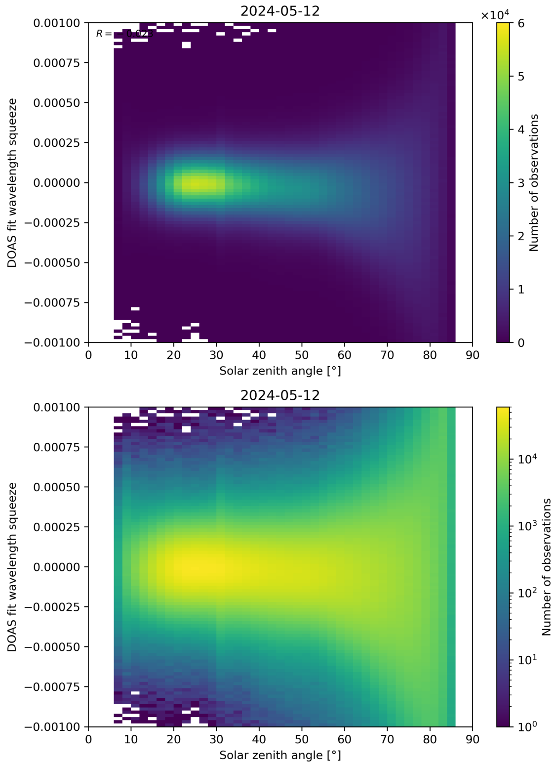
Figure 162: Scatter density plot of “Solar zenith angle” against “DOAS fit wavelength squeeze” for 2024-05-12 to 2024-05-13.
