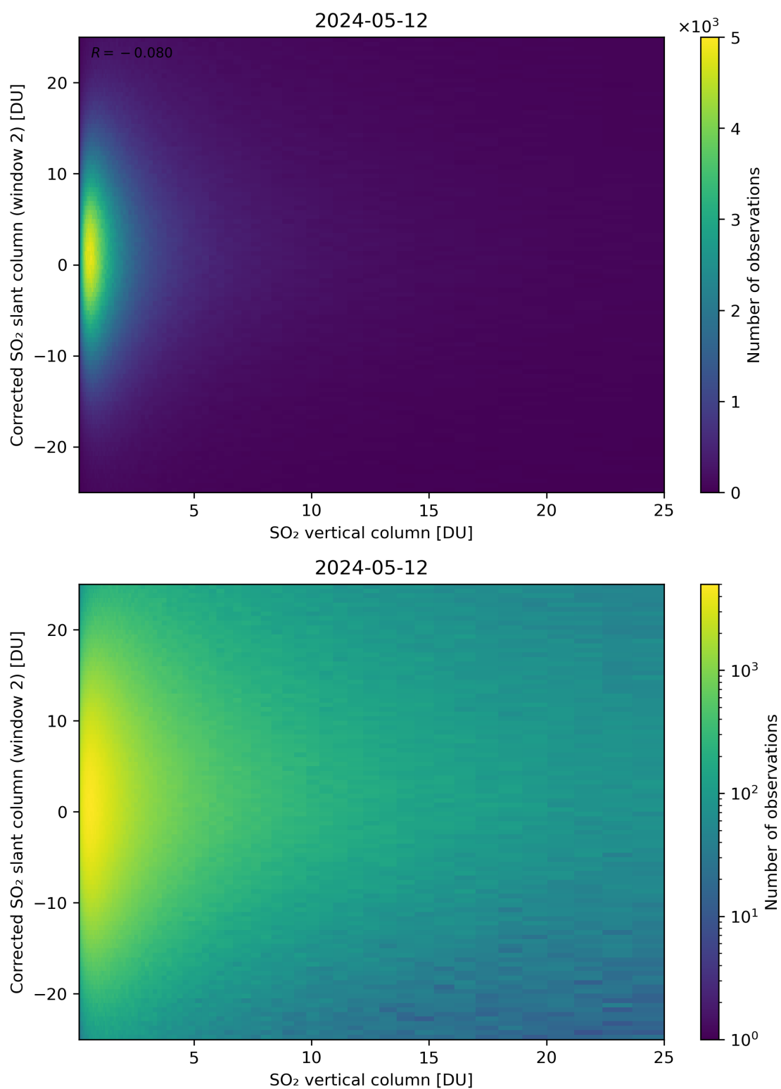
Figure 298: Scatter density plot of “SO 2 vertical column” against “Corrected SO 2 slant column (window 2)” for 2024-05-12 to 2024-05-13.
