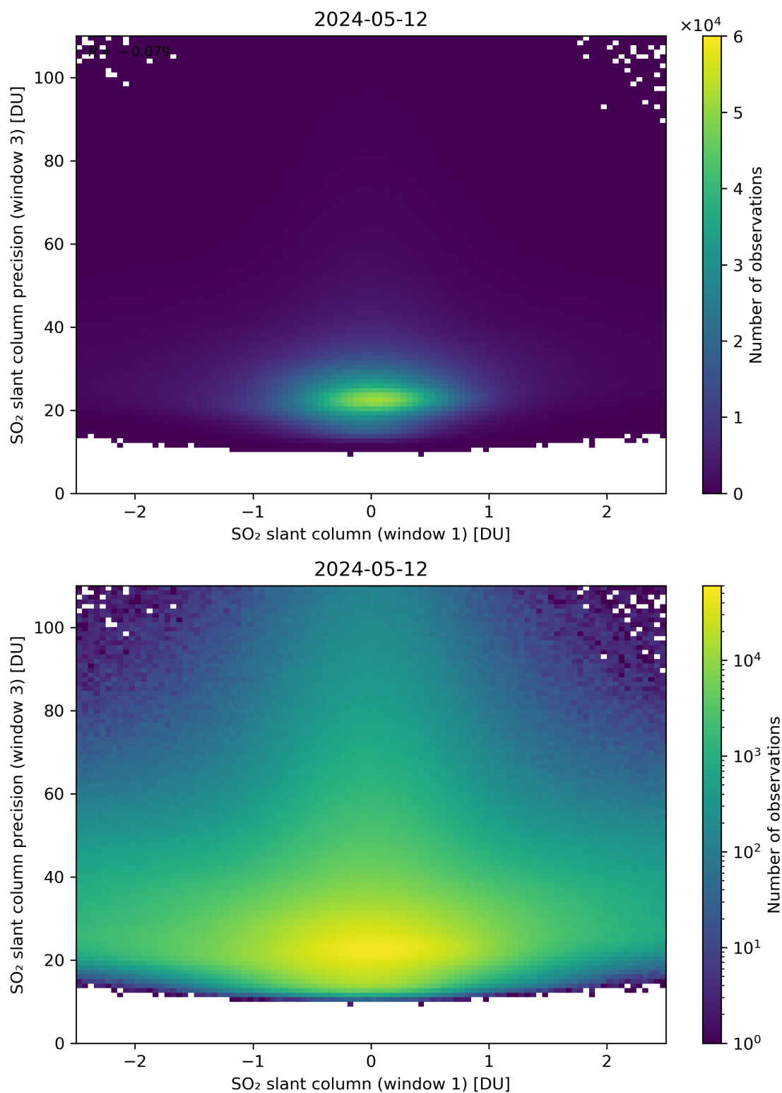
Figure 238: Scatter density plot of “SO 2 slant column (window 1)” against “SO 2 slant column precision (window 3)” for 2024-05-12 to 2024-05-13.
