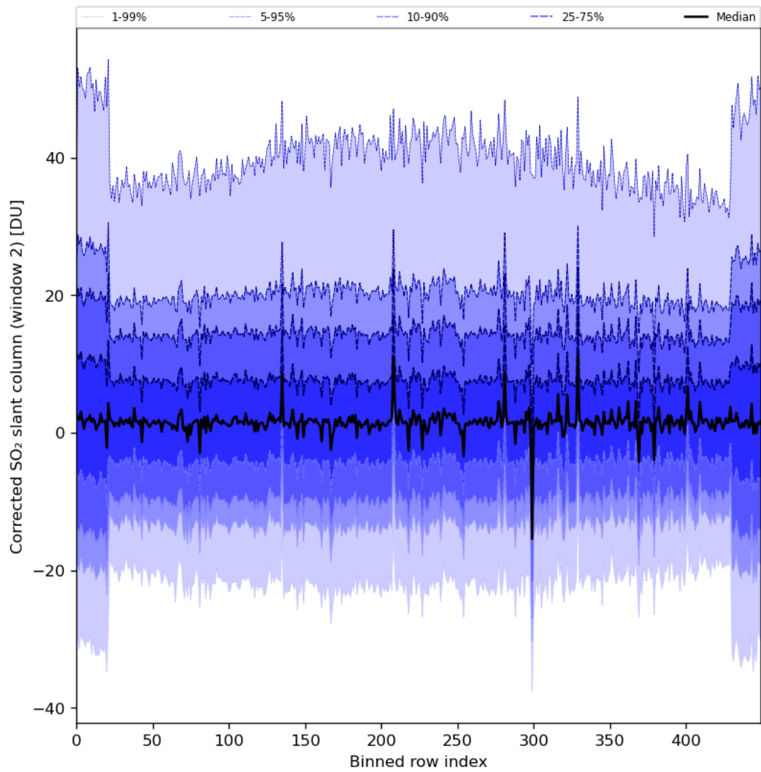
Figure 85: Along track statistics of “Corrected SO 2 slant column (window 2)” for 2024-05-12 to 2024-05-13
