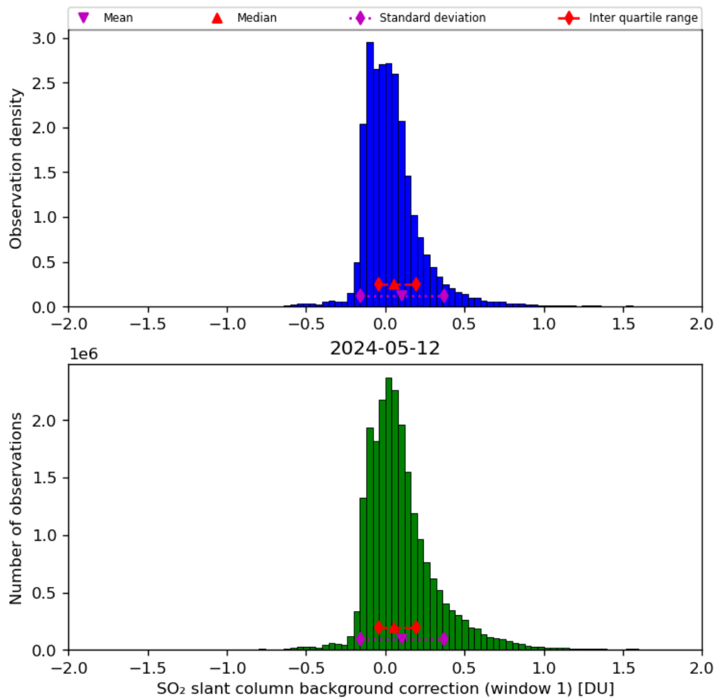
Figure 59: Histogram of “SO 2 slant column background correction (window 1)” for 2024-05-12 to 2024-05-13
