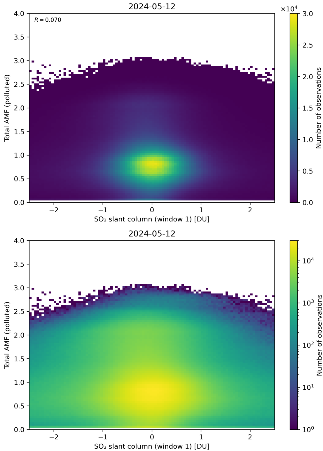
Figure 239: Scatter density plot of “SO 2 slant column (window 1)” against “Total AMF (polluted)” for 2024-05-12 to 2024-05-13.
