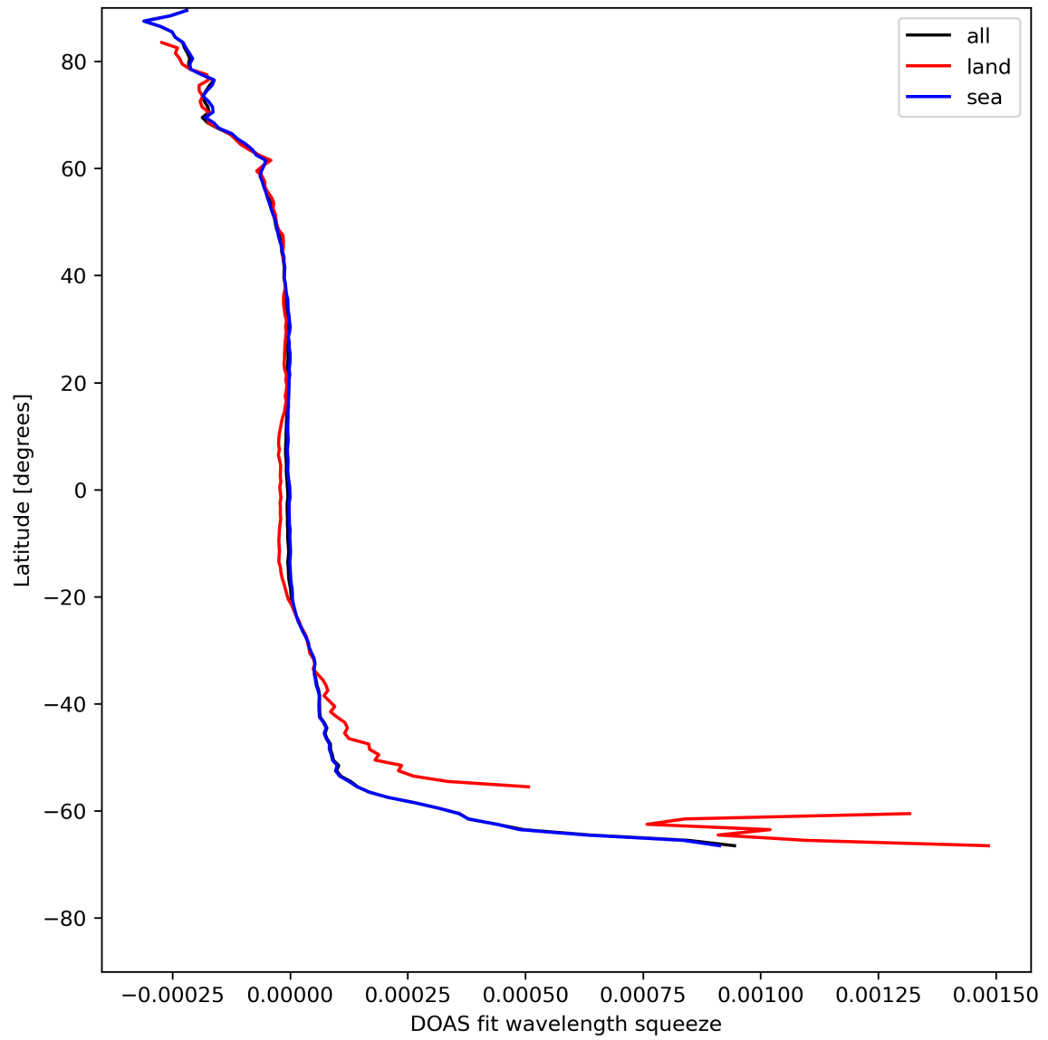
Figure 46: Zonal average of “DOAS fit wavelength squeeze” for 2024-05-12 to 2024-05-13.
