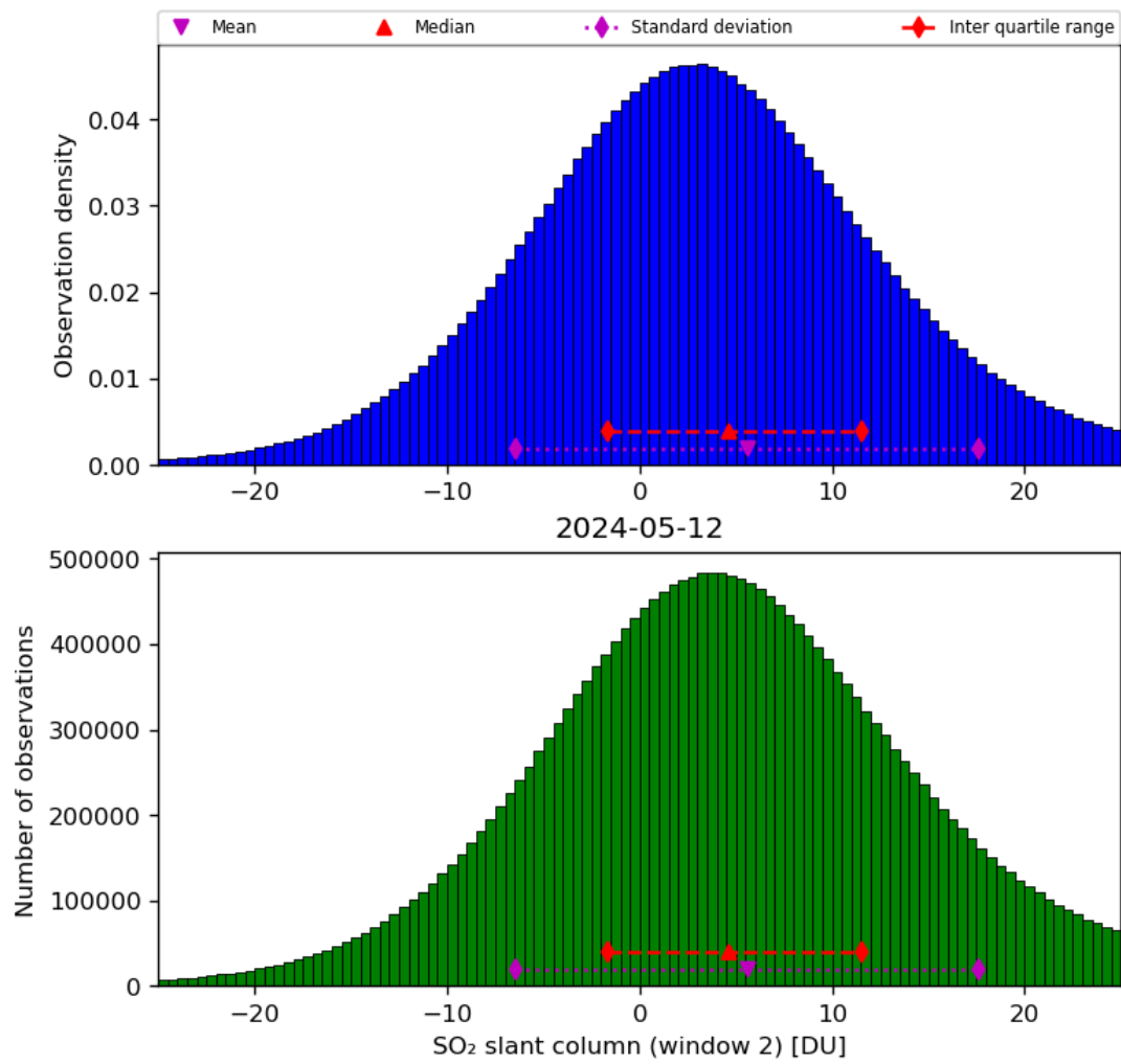
Figure 60: Histogram of “SO 2 slant column (window 2)” for 2024-05-12 to 2024-05-13
