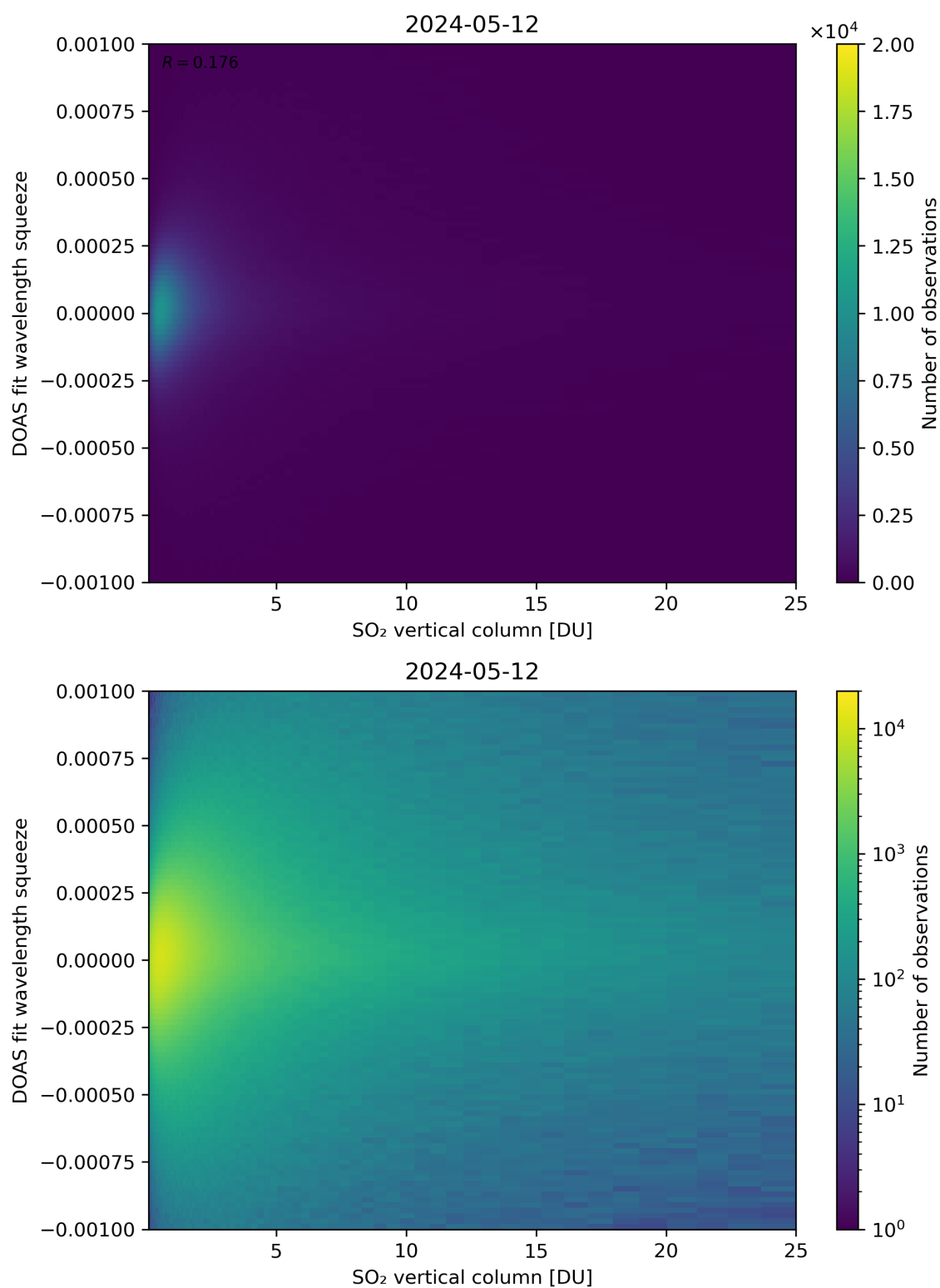
Figure 277: Scatter density plot of “SO 2 vertical column” against “DOAS fit wavelength squeeze” for 2024-05-12 to 2024-05-13.
