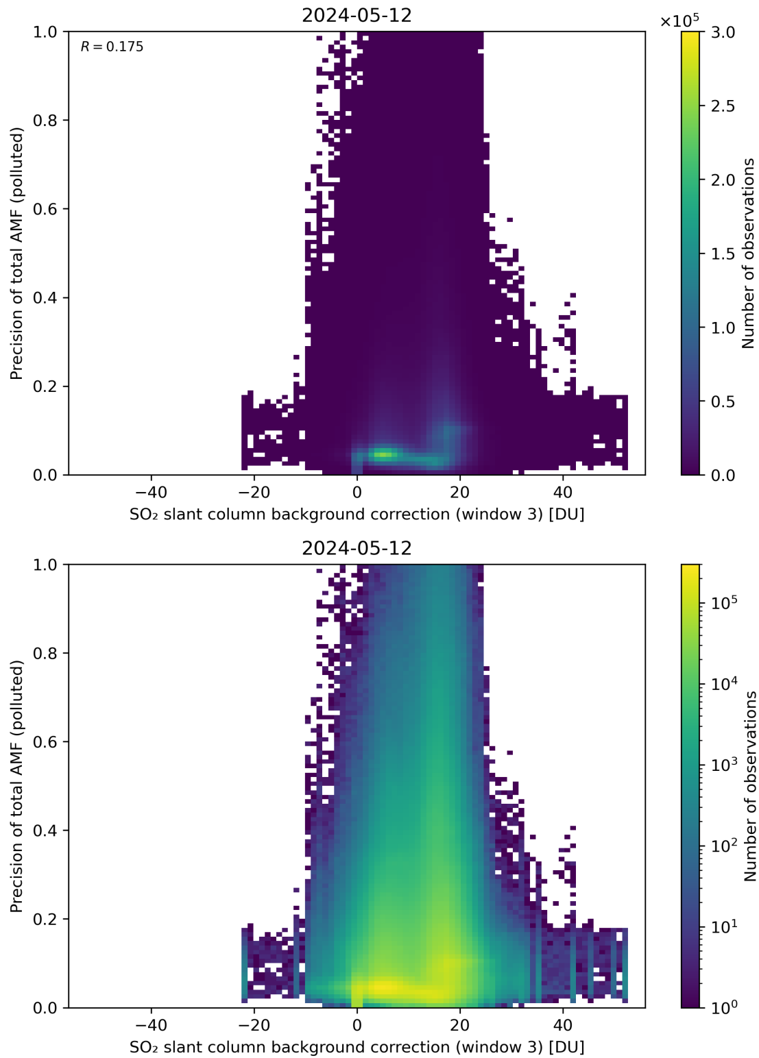
Figure 126: Scatter density plot of “SO 2 slant column background correction (window 3)” against “Precision of total AMF (polluted)” for 2024-05-12 to 2024-05-13.
