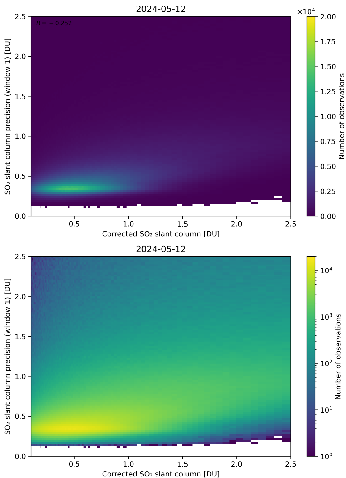
Figure 188: Scatter density plot of “Corrected SO 2 slant column” against “SO 2 slant column precision (window 1)” for 2024-05-12 to 2024-05-13.
