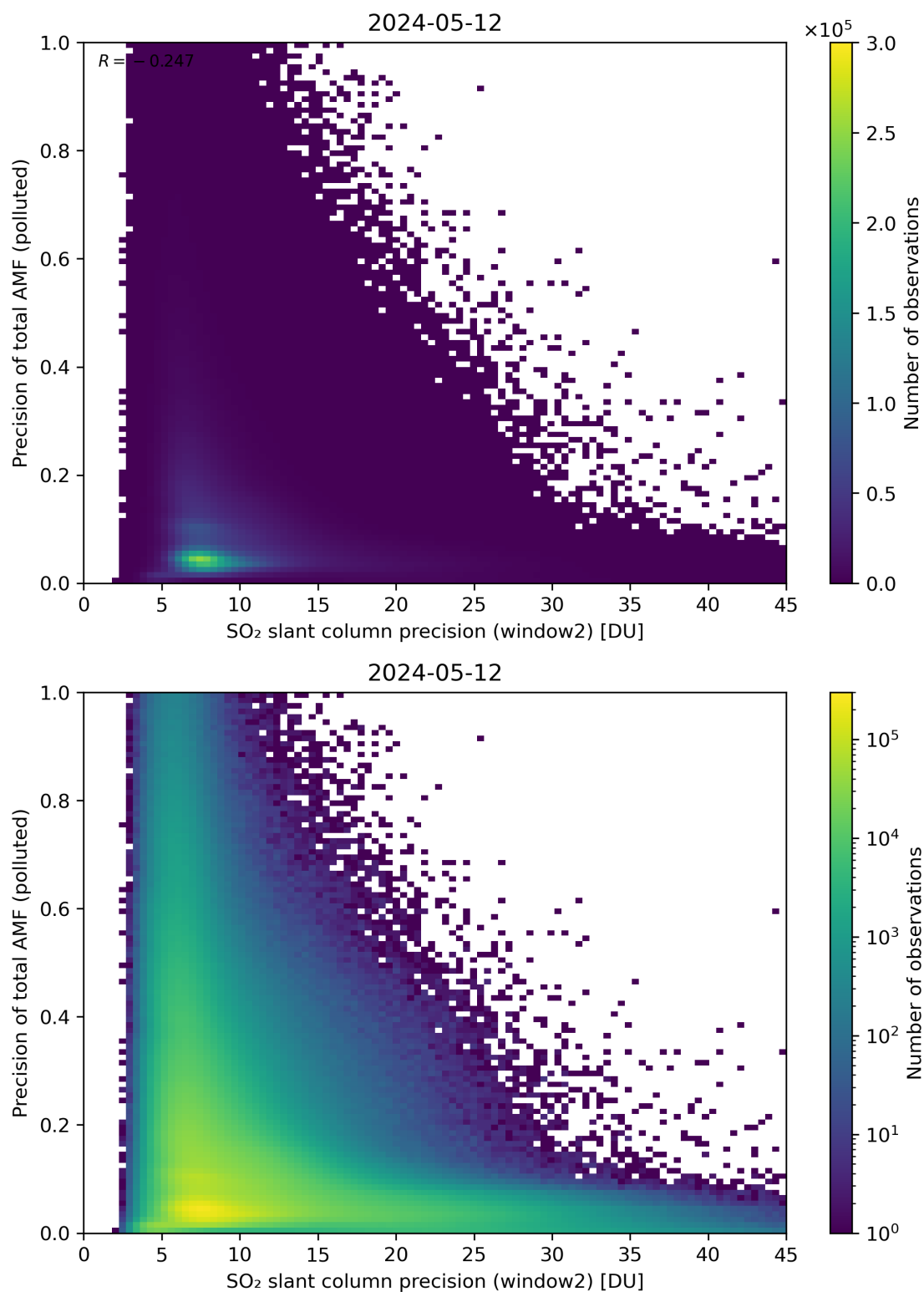
Figure 252: Scatter density plot of “SO 2 slant column precision (window2)” against “Precision of total AMF (polluted)” for 2024-05-12 to 2024-05-13.
