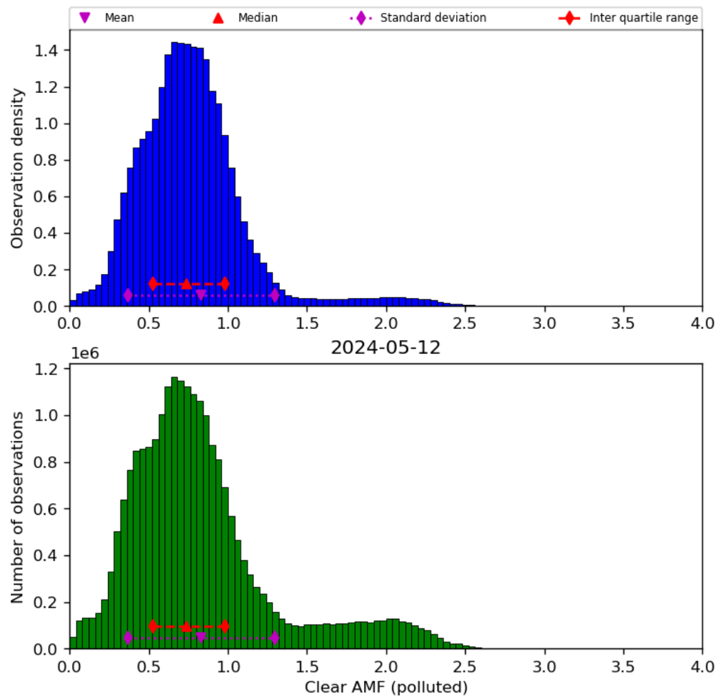
Figure 73: Histogram of “Clear AMF (polluted)” for 2024-05-12 to 2024-05-13
