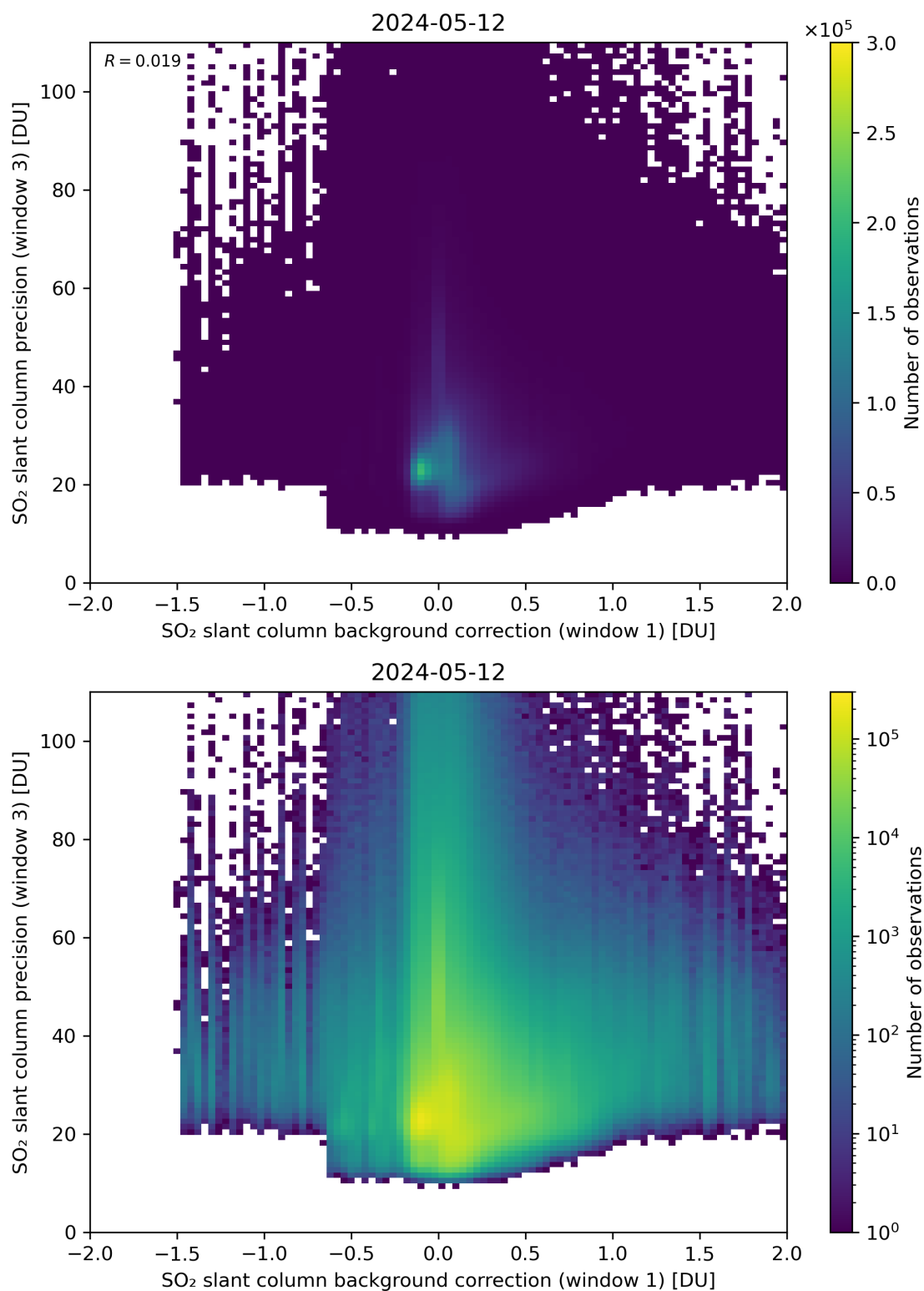
Figure 108: Scatter density plot of “SO 2 slant column background correction (window 1)” against “SO 2 slant column precision (window 3)” for 2024-05-12 to 2024-05-13.
