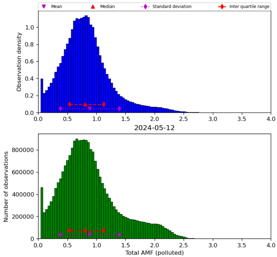
Figure 71: Histogram of “Total AMF (polluted)” for 2024-05-12 to 2024-05-13
