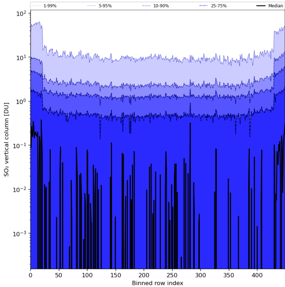
Figure 76: Along track statistics of “SO 2 vertical column” for 2024-05-12 to 2024-05-13
