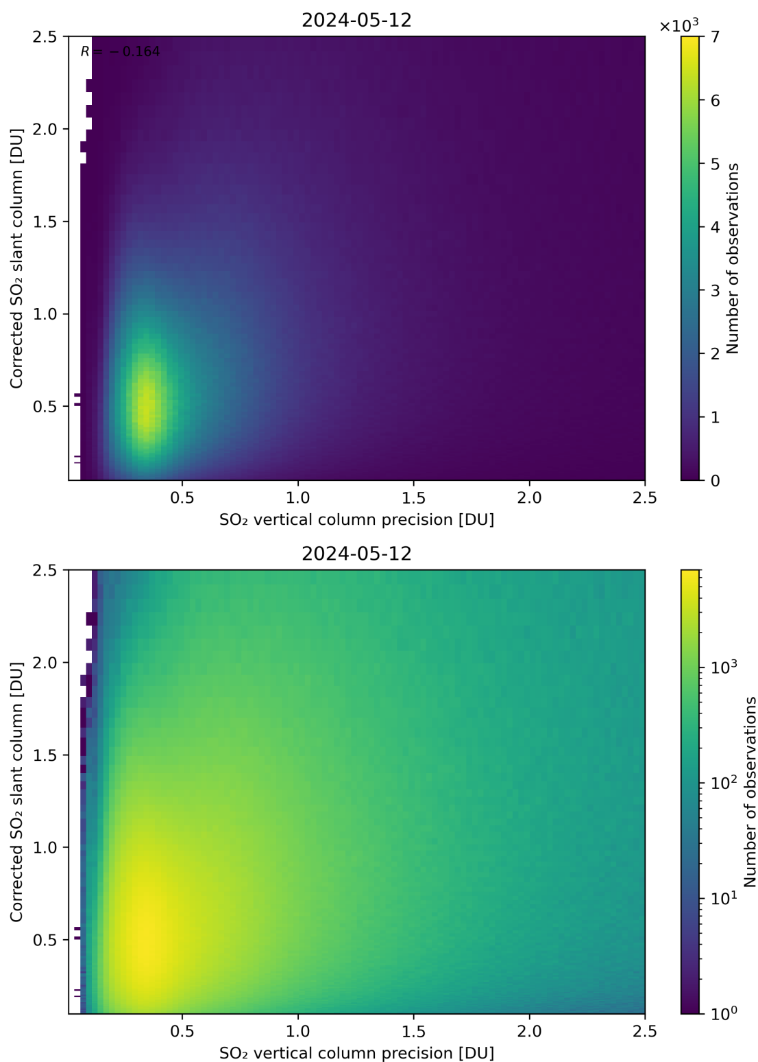
Figure 286: Scatter density plot of “SO 2 vertical column precision” against “Corrected SO 2 slant column” for 2024-05-12 to 2024-05-13.
