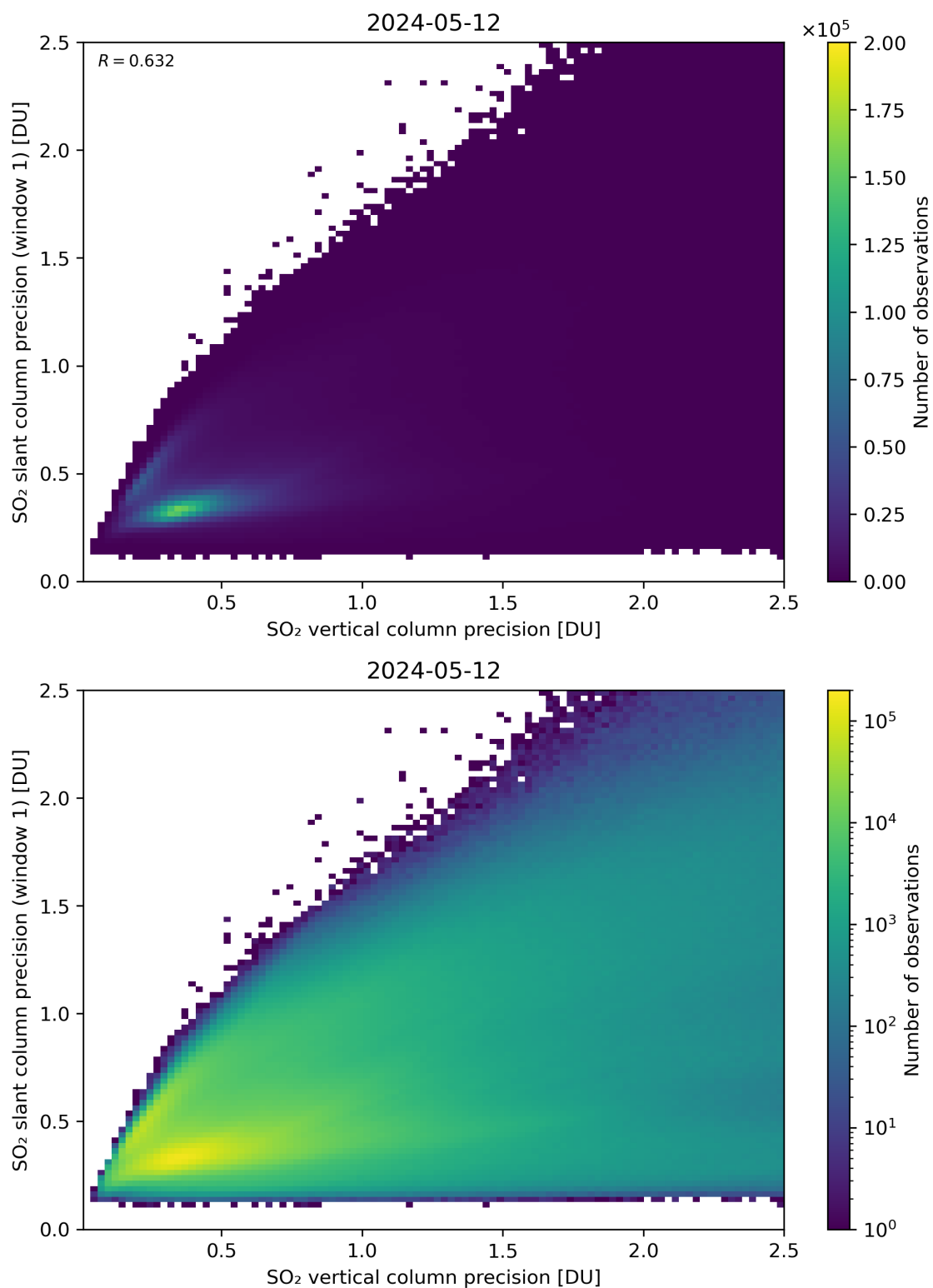
Figure 290: Scatter density plot of “SO 2 vertical column precision” against “SO 2 slant column precision (window 1)” for 2024-05-12 to 2024-05-13.
