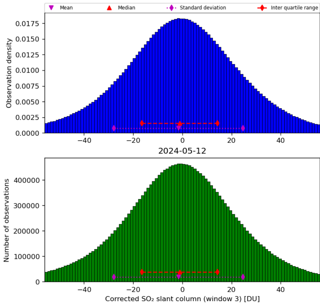
Figure 66: Histogram of “Corrected SO 2 slant column (window 3)” for 2024-05-12 to 2024-05-13
