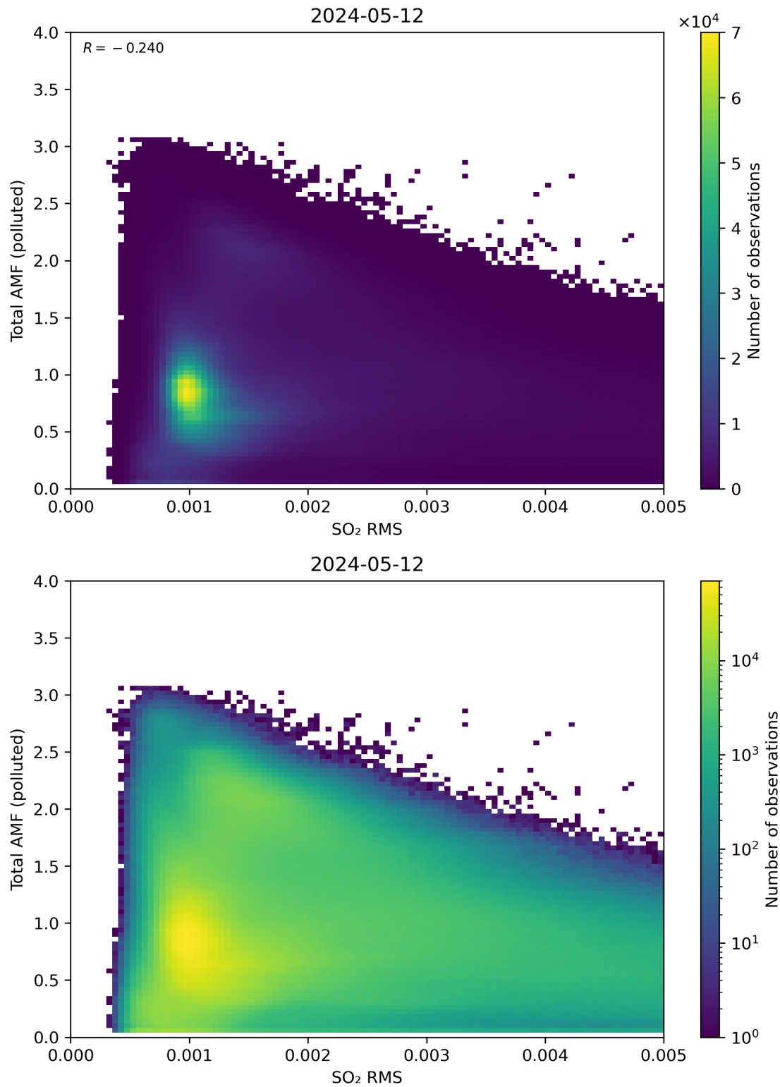
Figure 137: Scatter density plot of “SO 2 RMS” against “Total AMF (polluted)” for 2024-05-12 to 2024-05-13.
