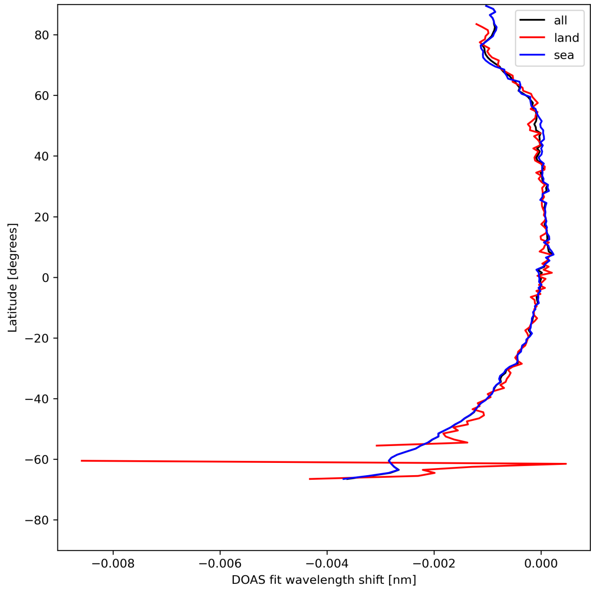
Figure 45: Zonal average of “DOAS fit wavelength shift” for 2024-05-12 to 2024-05-13.
