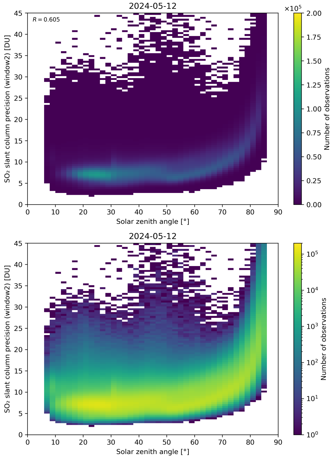
Figure 171: Scatter density plot of “Solar zenith angle” against “SO 2 slant column precision (window2)” for 2024-05-12 to 2024-05-13.
