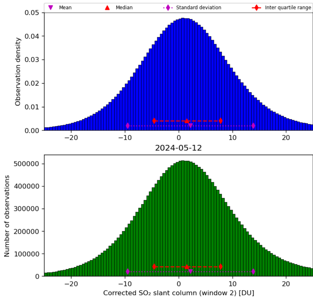
Figure 62: Histogram of “Corrected SO 2 slant column (window 2)” for 2024-05-12 to 2024-05-13
