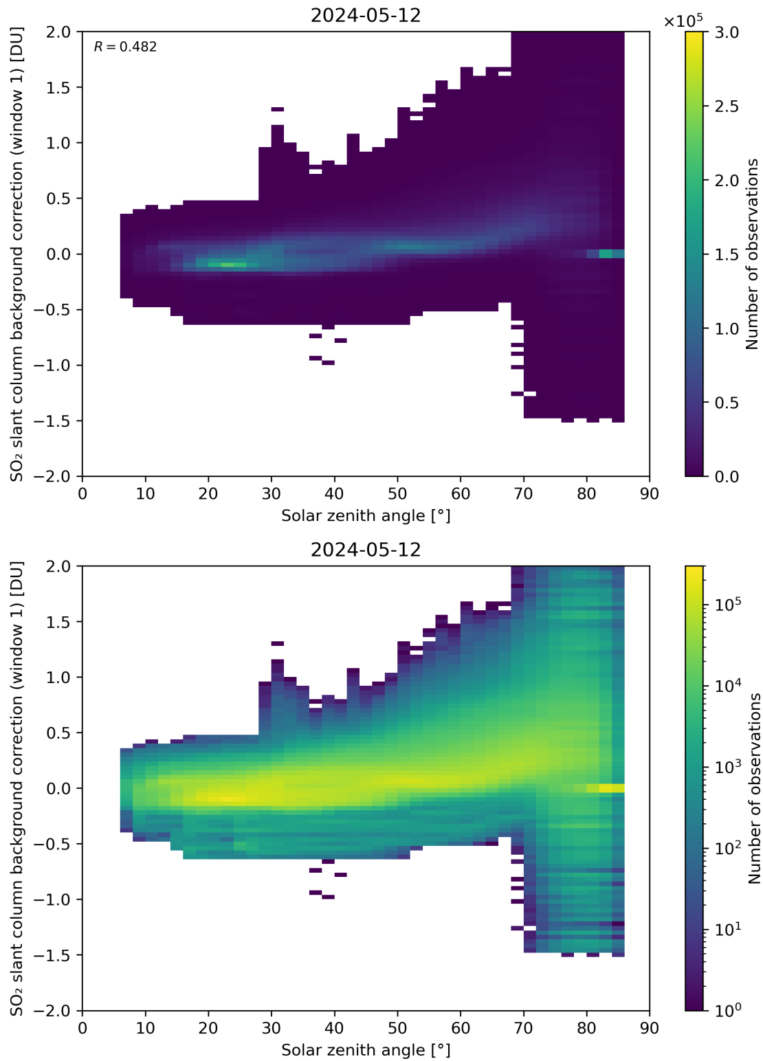
Figure 158: Scatter density plot of “Solar zenith angle” against “SO 2 slant column background correction (window 1)” for 2024-05-12 to 2024-05-13.
