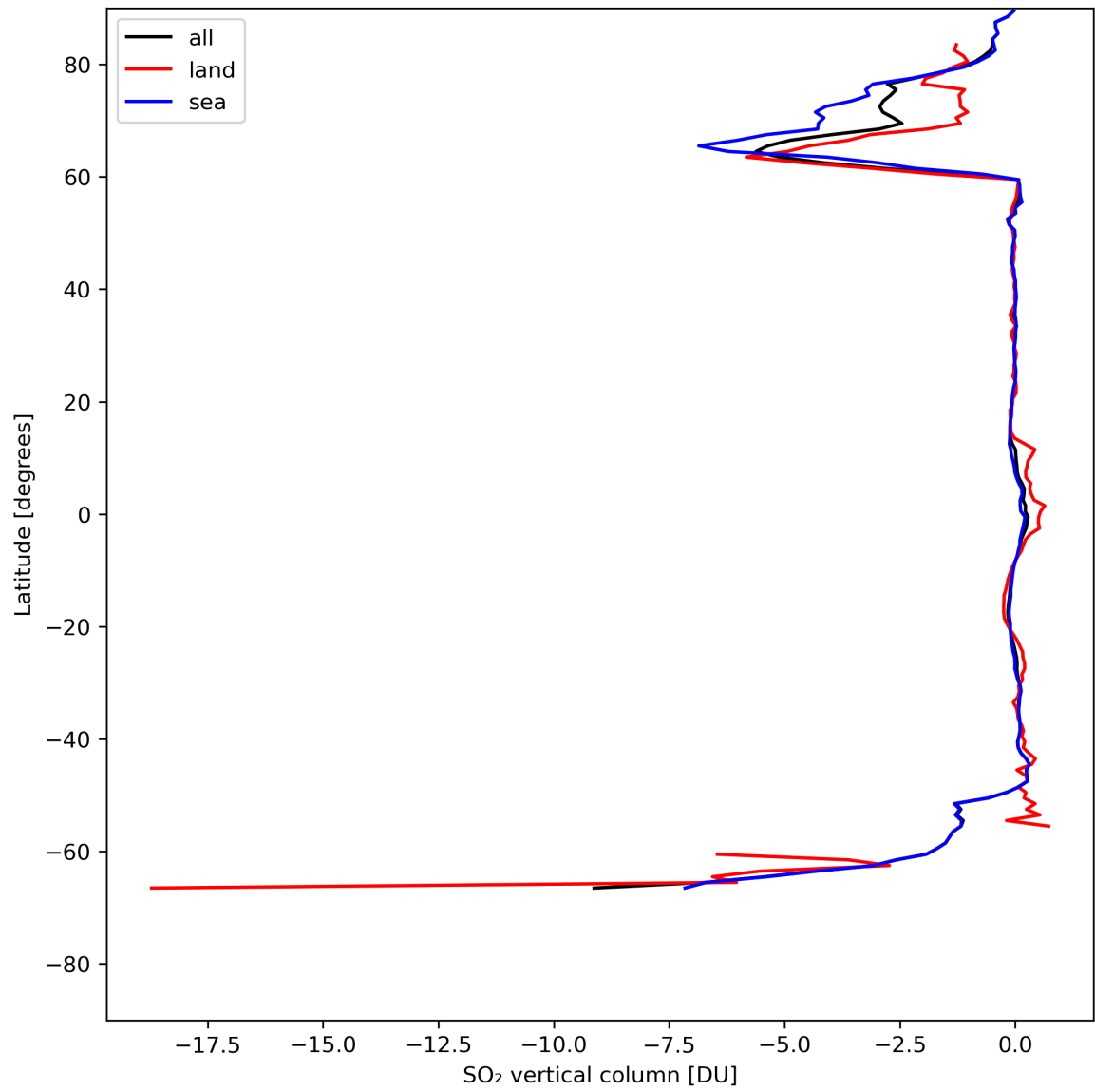
Figure 30: Zonal average of “SO 2 vertical column” for 2024-05-12 to 2024-05-13.
