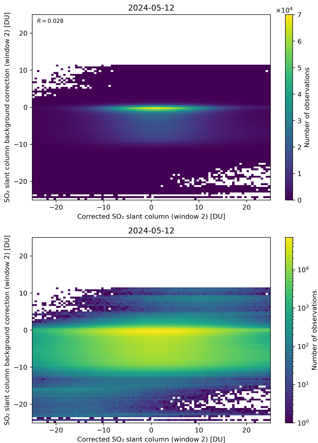
Figure 194: Scatter density plot of “Corrected SO 2 slant column (window 2)” against “SO 2 slant column background correction (window 2)” for 2024-05-12 to 2024-05-13.
