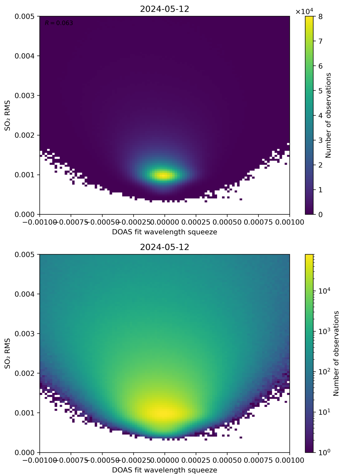
Figure 132: Scatter density plot of “DOAS fit wavelength squeeze” against “SO 2 RMS” for 2024-05-12 to 2024-05-13.
