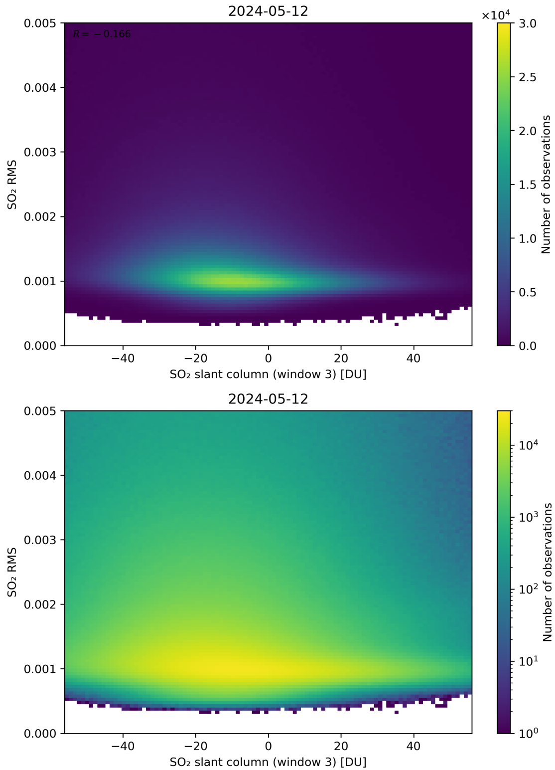
Figure 256: Scatter density plot of “SO 2 slant column (window 3)” against “SO 2 RMS” for 2024-05-12 to 2024-05-13.
