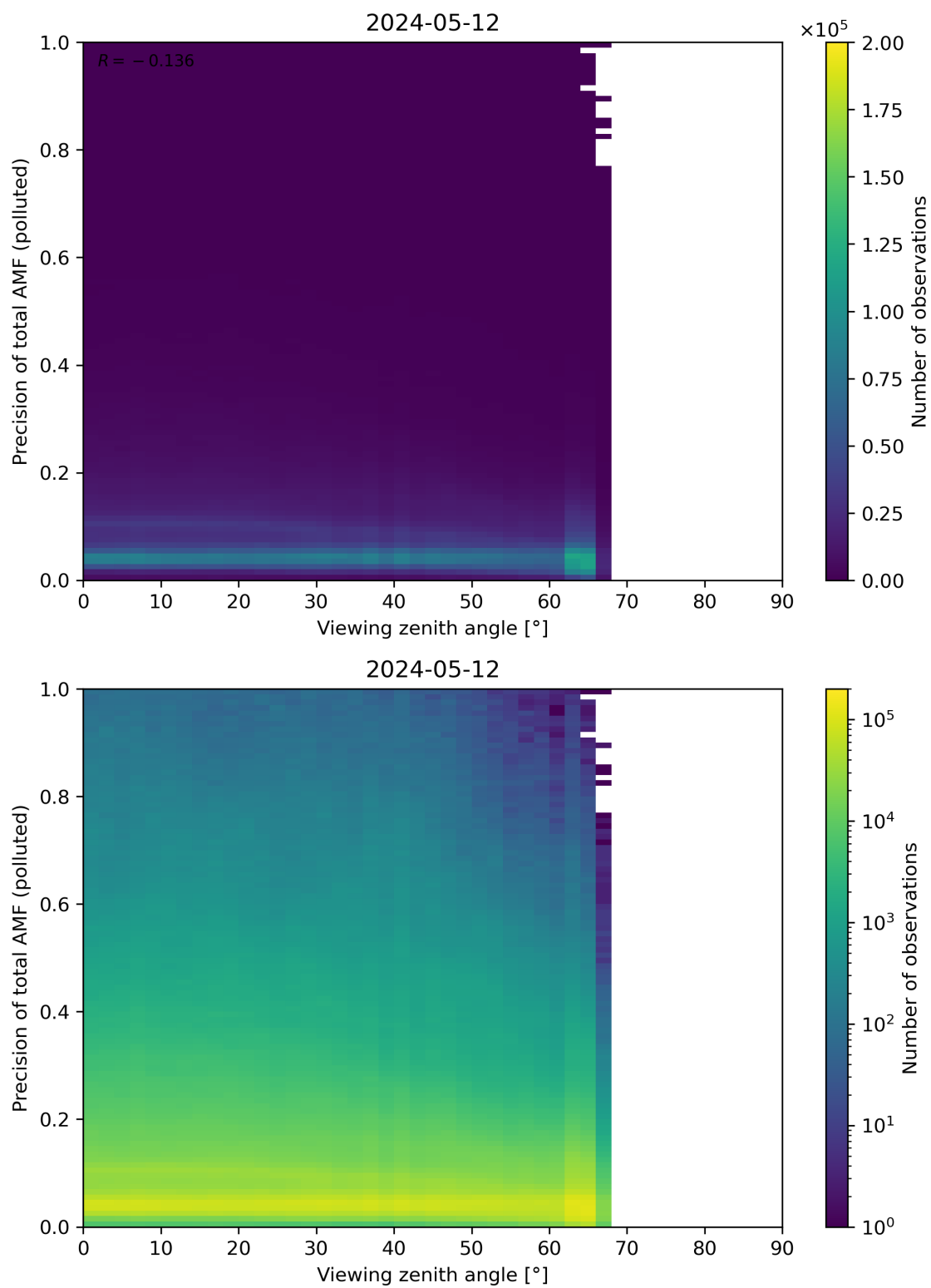
Figure 326: Scatter density plot of “Viewing zenith angle” against “Precision of total AMF (polluted)” for 2024-05-12 to 2024-05-13.
