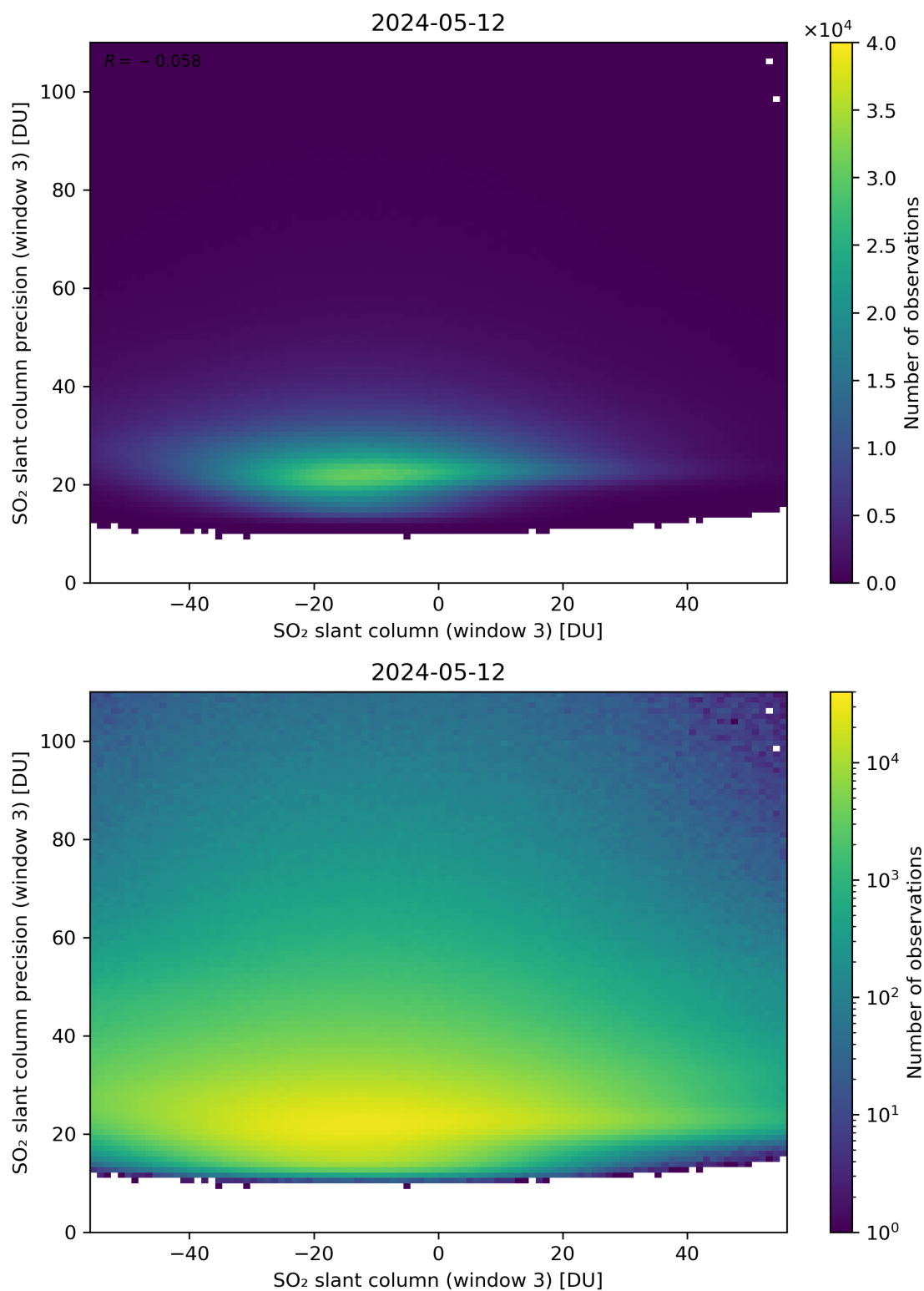
Figure 267: Scatter density plot of “SO 2 slant column (window 3)” against “SO 2 slant column precision (window 3)” for 2024-05-12 to 2024-05-13.
