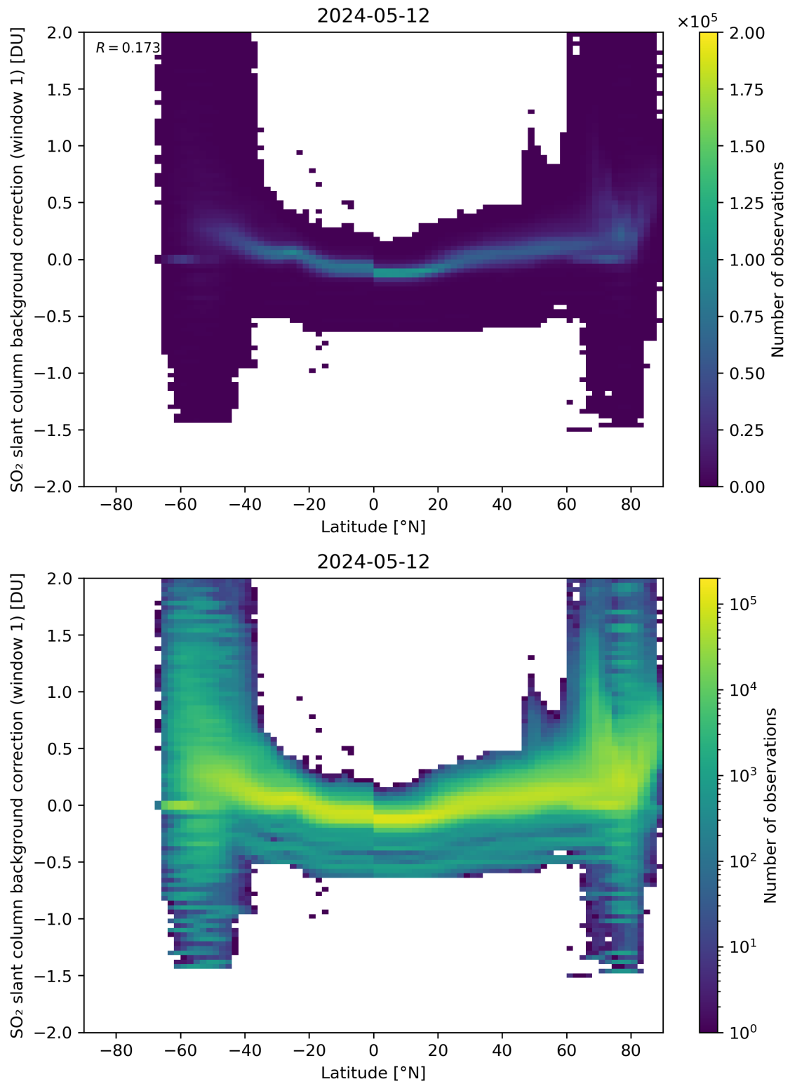
Figure 139: Scatter density plot of “Latitude” against “SO 2 slant column background correction (window 1)” for 2024-05-12 to 2024-05-13.
