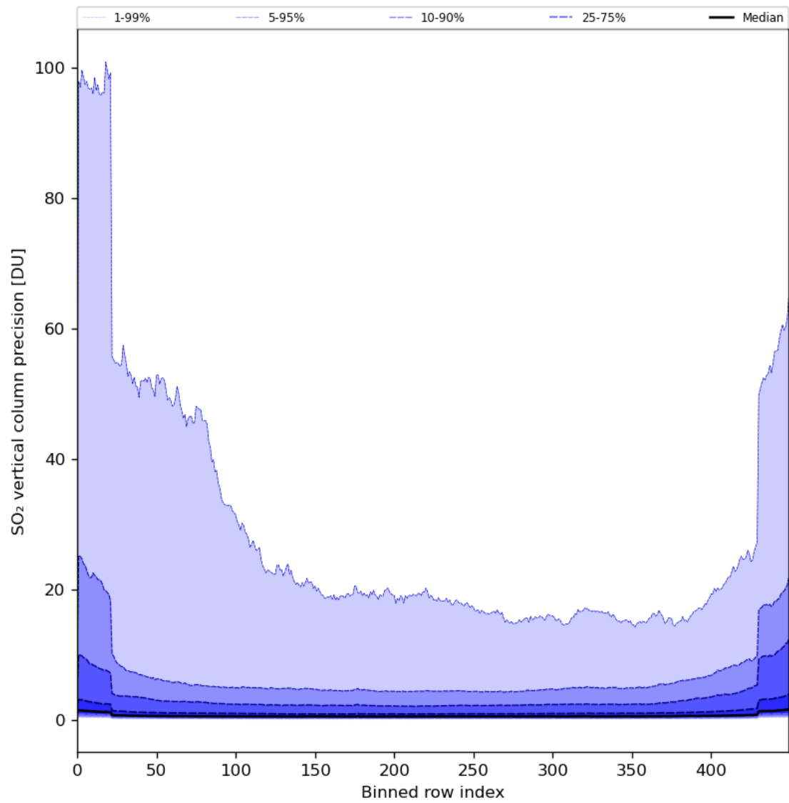
Figure 77: Along track statistics of “SO 2 vertical column precision” for 2024-05-12 to 2024-05-13
