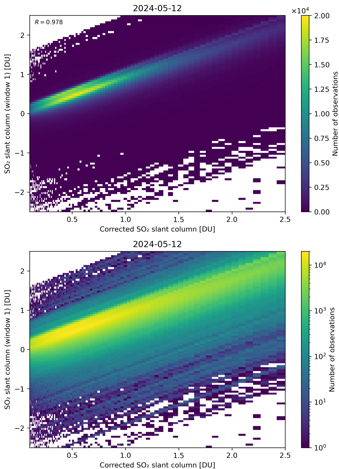
Figure 187: Scatter density plot of “Corrected SO 2 slant column” against “SO 2 slant column (window 1)” for 2024-05-12 to 2024-05-13.
