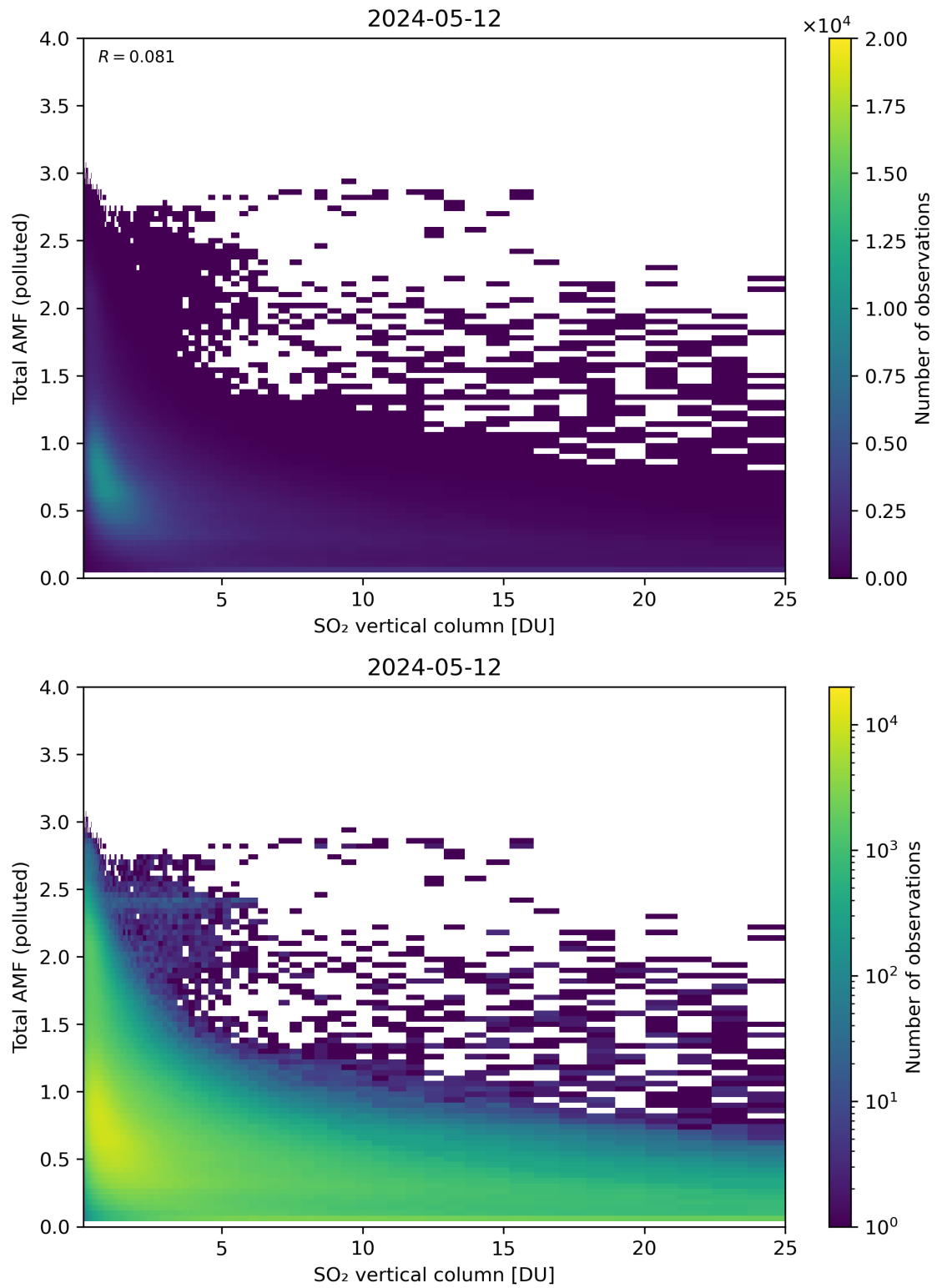
Figure 305: Scatter density plot of “SO 2 vertical column” against “Total AMF (polluted)” for 2024-05-12 to 2024-05-13.
