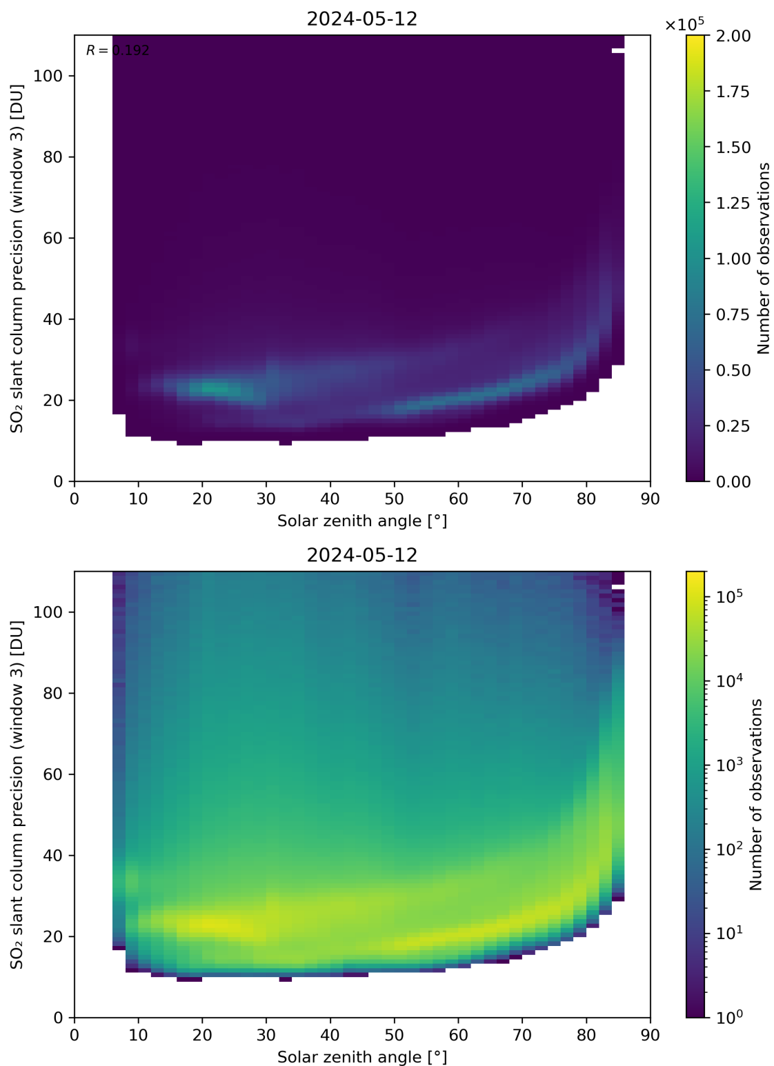
Figure 173: Scatter density plot of “Solar zenith angle” against “SO 2 slant column precision (window 3)” for 2024-05-12 to 2024-05-13.
