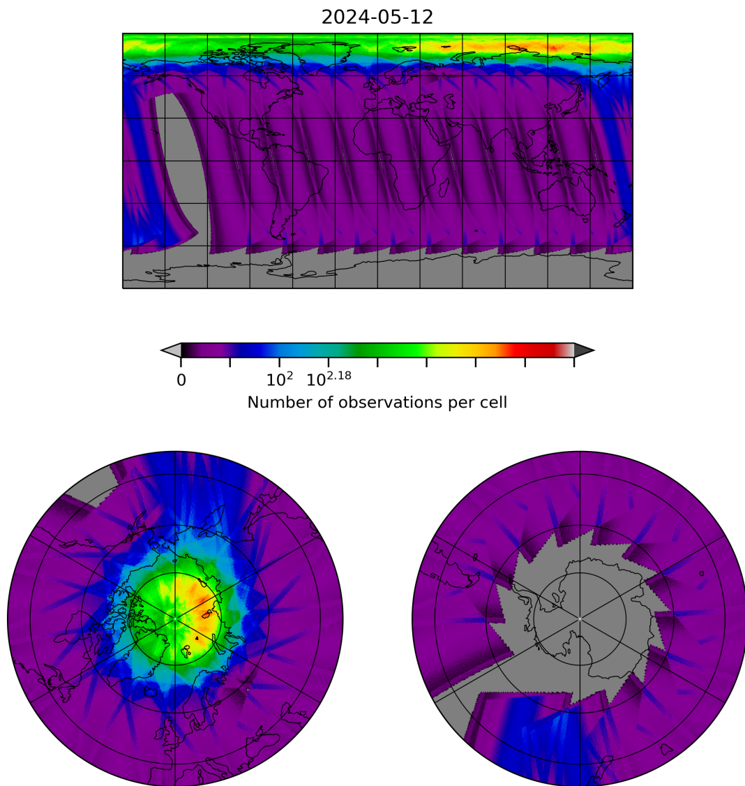
Figure 28: Map of the number of observations for 2024-05-12 to 2024-05-13
