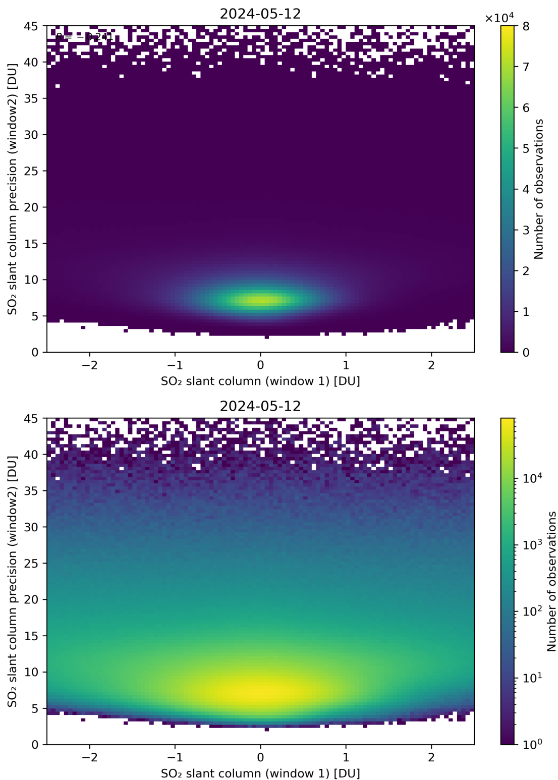
Figure 236: Scatter density plot of “SO 2 slant column (window 1)” against “SO 2 slant column precision (window2)” for 2024-05-12 to 2024-05-13.
