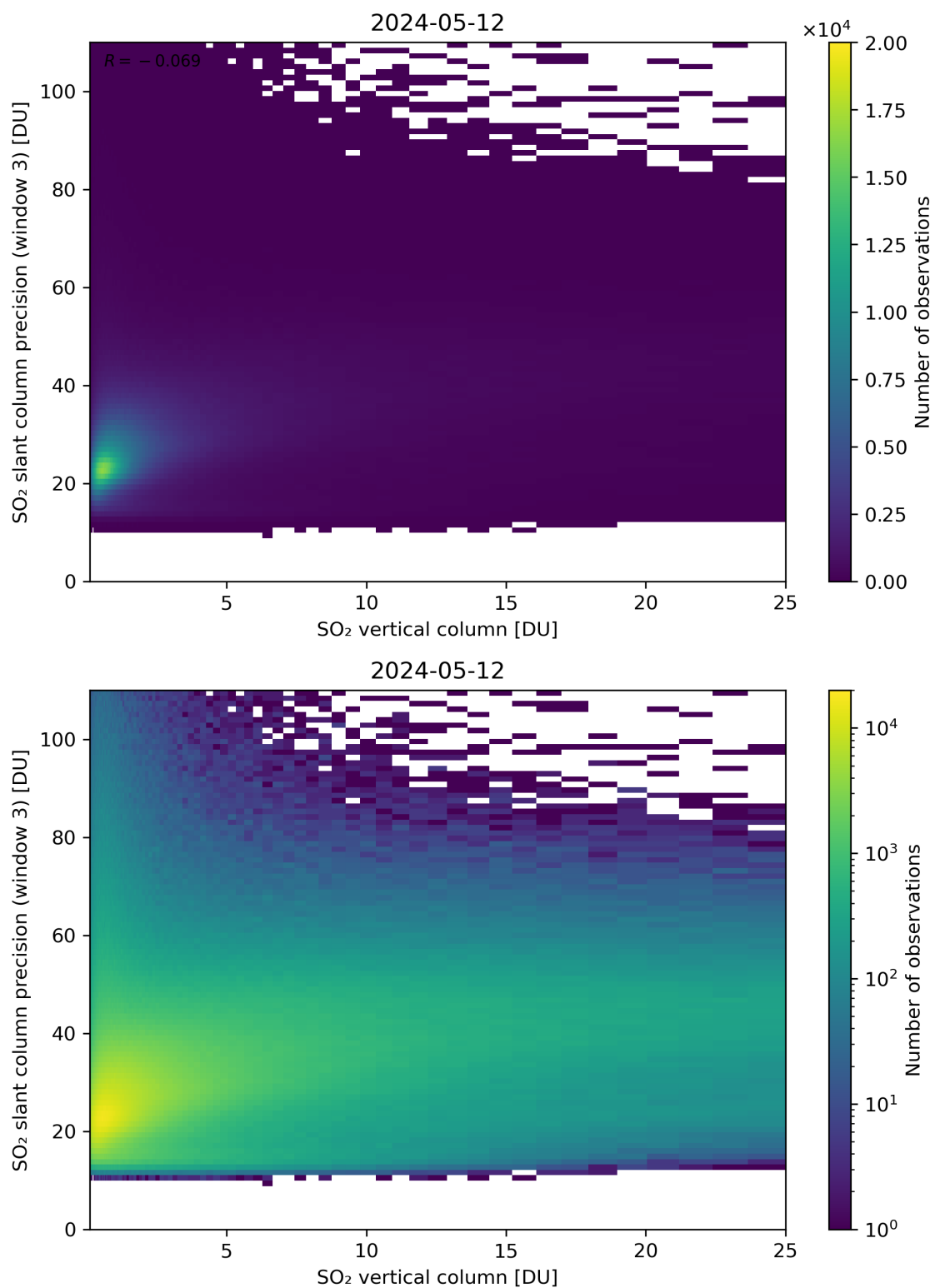
Figure 304: Scatter density plot of “SO 2 vertical column” against “SO 2 slant column precision (window 3)” for 2024-05-12 to 2024-05-13.
