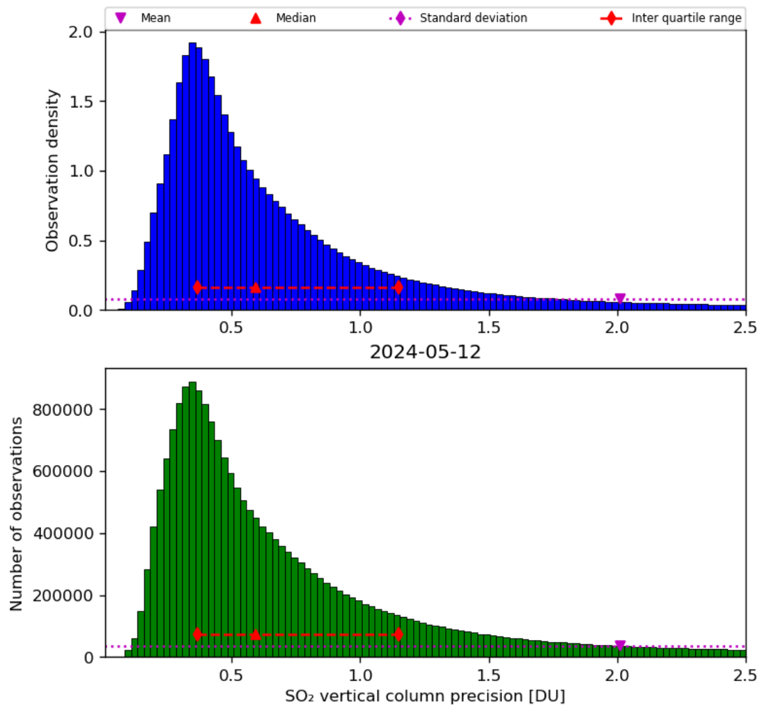
Figure 54: Histogram of “SO 2 vertical column precision” for 2024-05-12 to 2024-05-13
