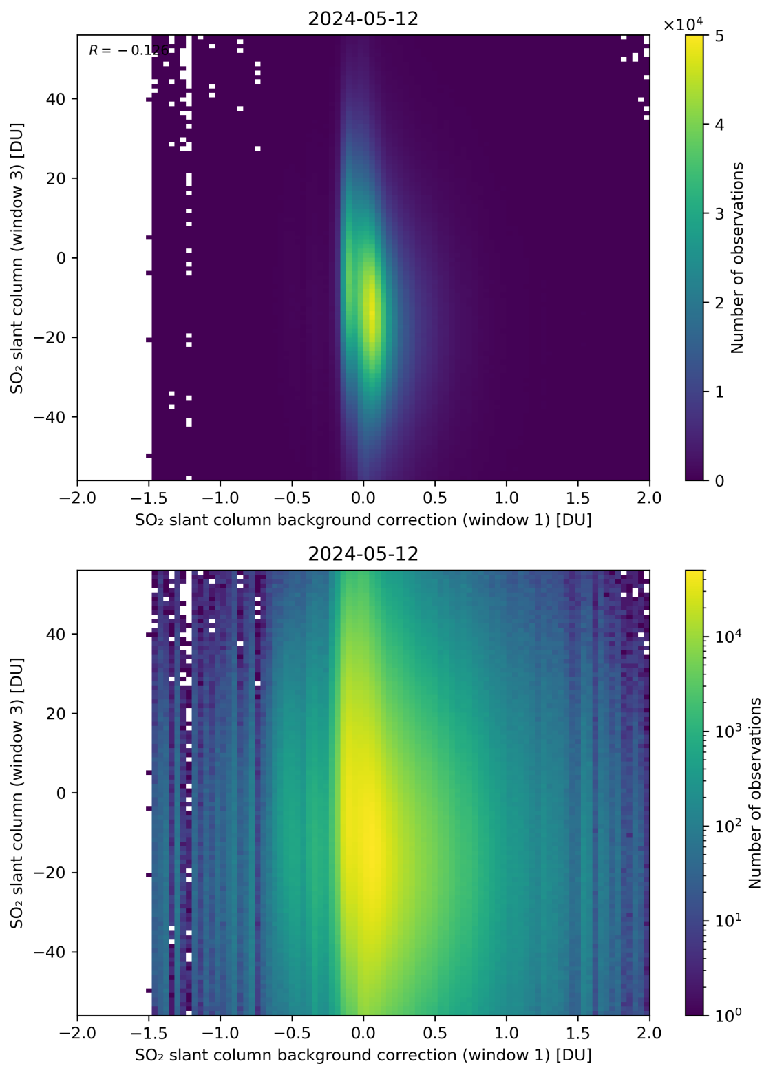
Figure 107: Scatter density plot of “SO 2 slant column background correction (window 1)” against “SO 2 slant column (window 3)” for 2024-05-12 to 2024-05-13.
