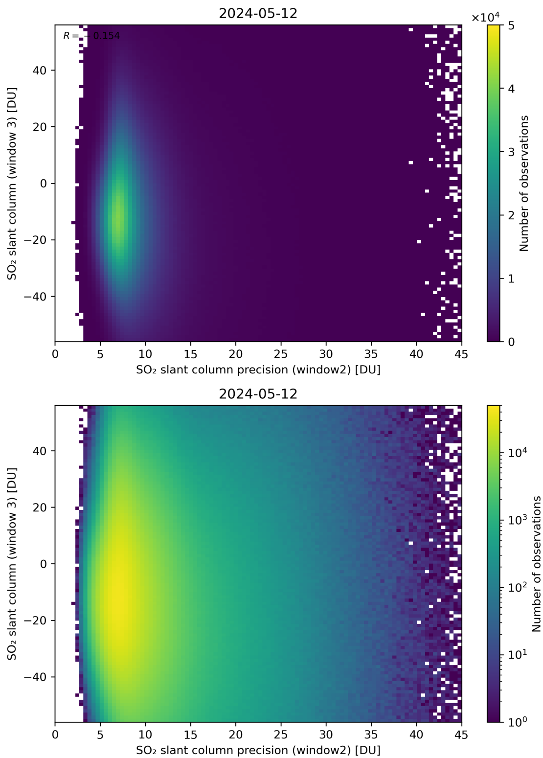
Figure 249: Scatter density plot of “SO 2 slant column precision (window2)” against “SO 2 slant column (window 3)” for 2024-05-12 to 2024-05-13.
