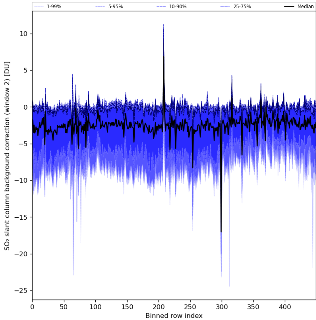
Figure 86: Along track statistics of “SO 2 slant column background correction (window 2)” for 2024-05-12 to 2024-05-13
