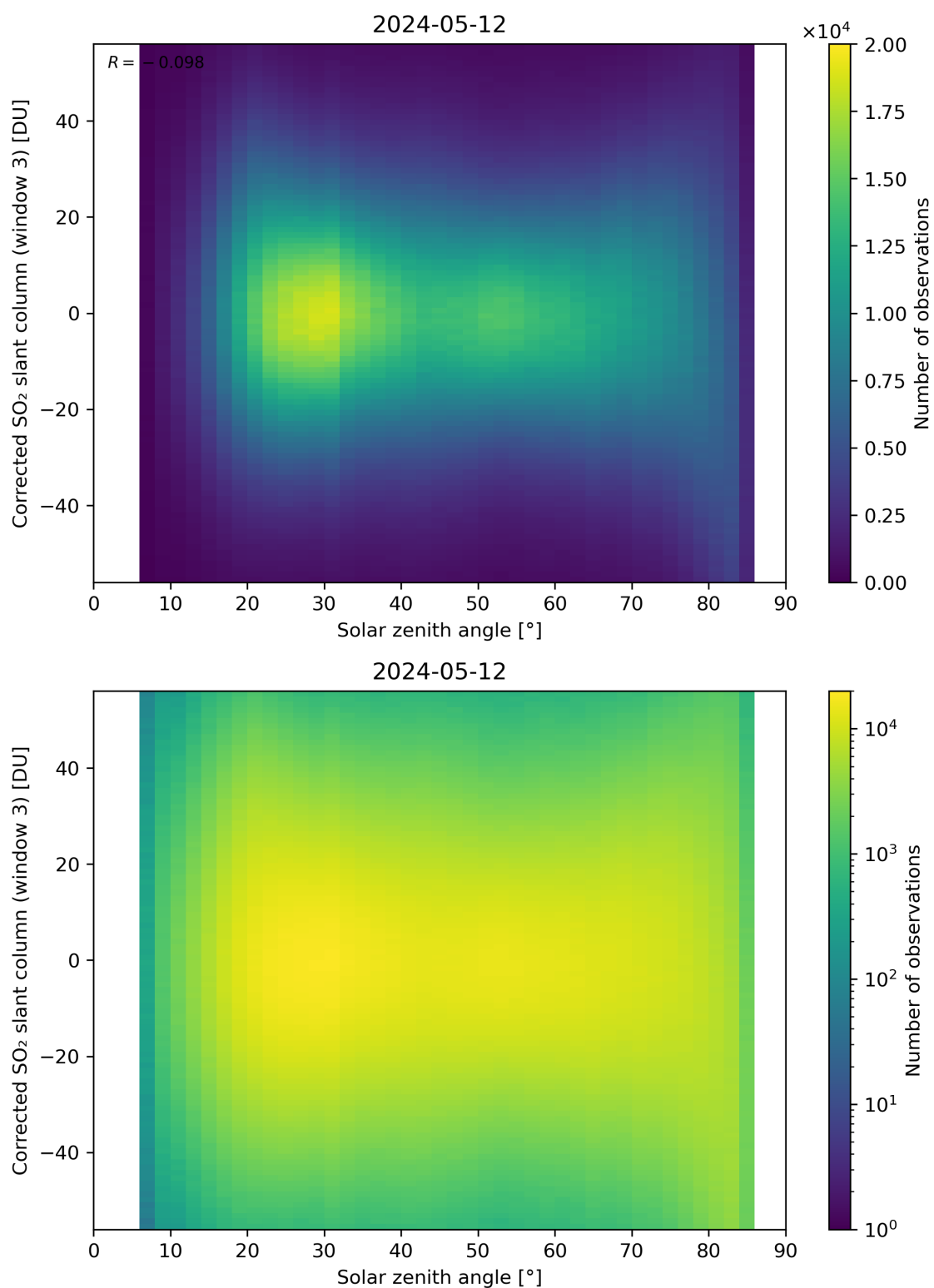
Figure 168: Scatter density plot of “Solar zenith angle” against “Corrected SO 2 slant column (window 3)” for 2024-05-12 to 2024-05-13.
