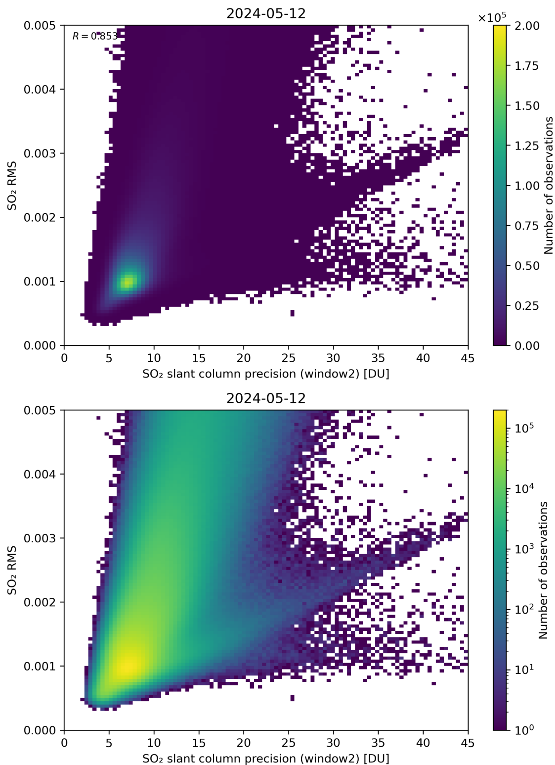
Figure 245: Scatter density plot of “SO 2 slant column precision (window2)” against “SO 2 RMS” for 2024-05-12 to 2024-05-13.
