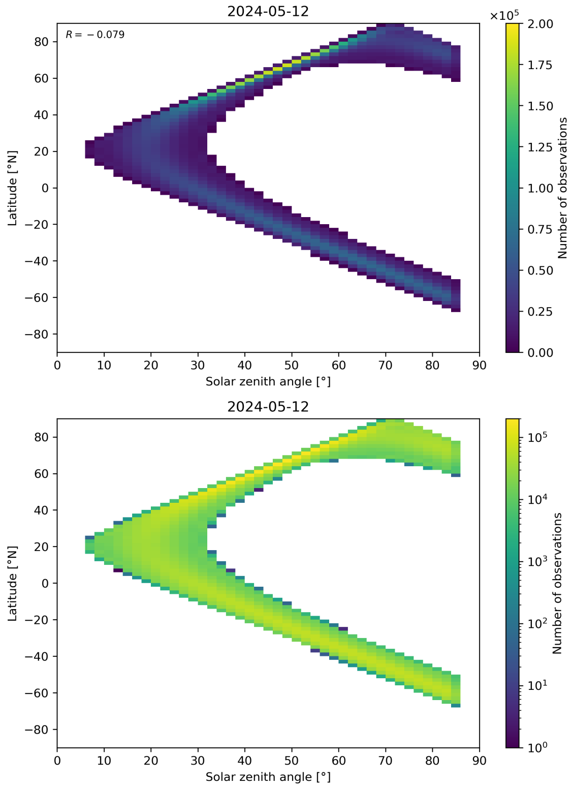
Figure 164: Scatter density plot of “Solar zenith angle” against “Latitude” for 2024-05-12 to 2024-05-13.
