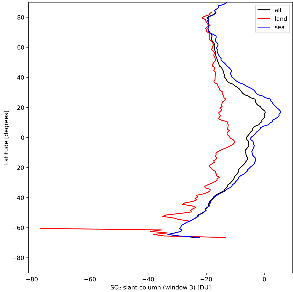
Figure 41: Zonal average of “SO 2 slant column (window 3)” for 2024-05-12 to 2024-05-13.
