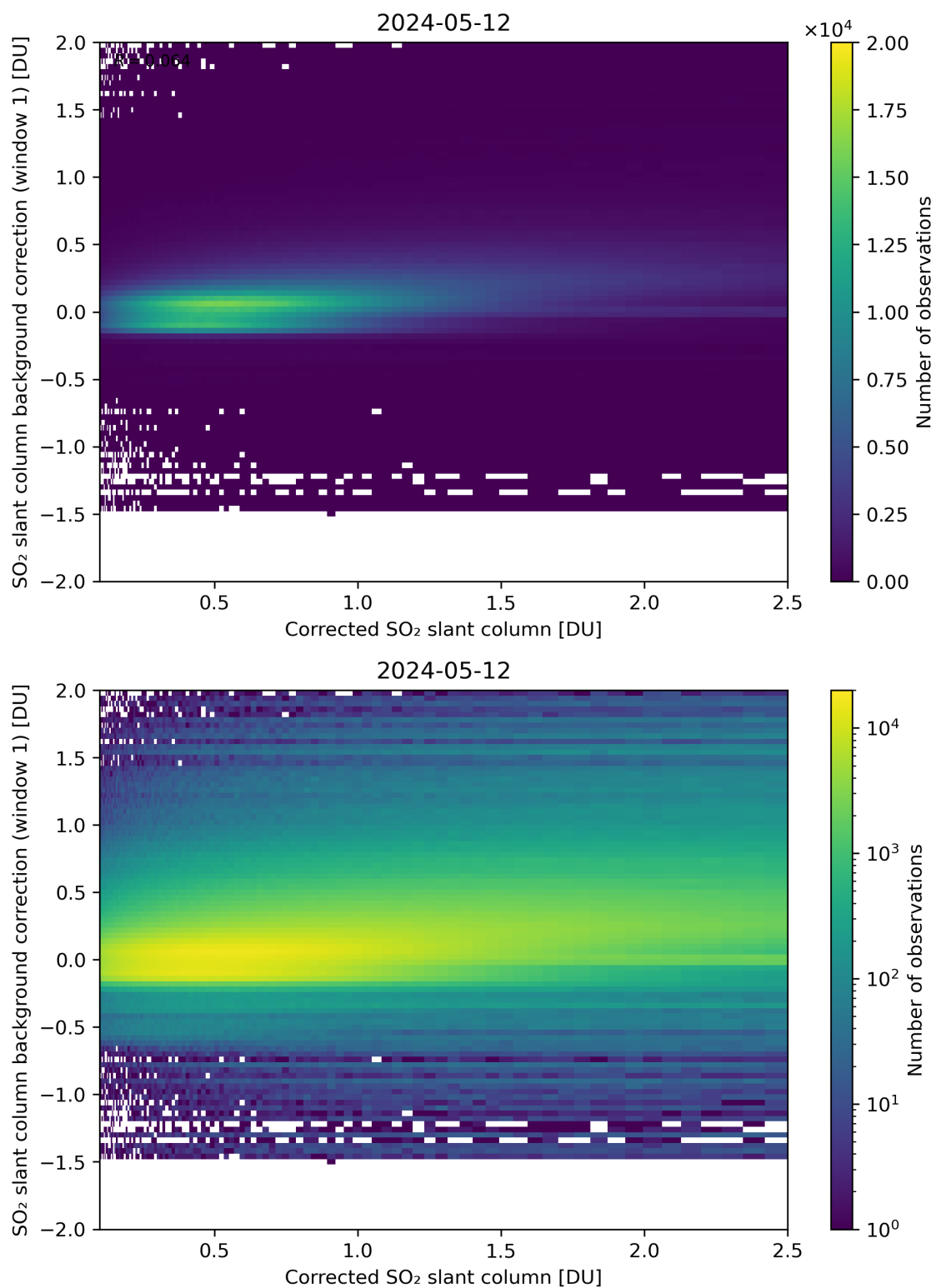
Figure 178: Scatter density plot of “Corrected SO 2 slant column” against “SO 2 slant column background correction (window 1)” for 2024-05-12 to 2024-05-13.
