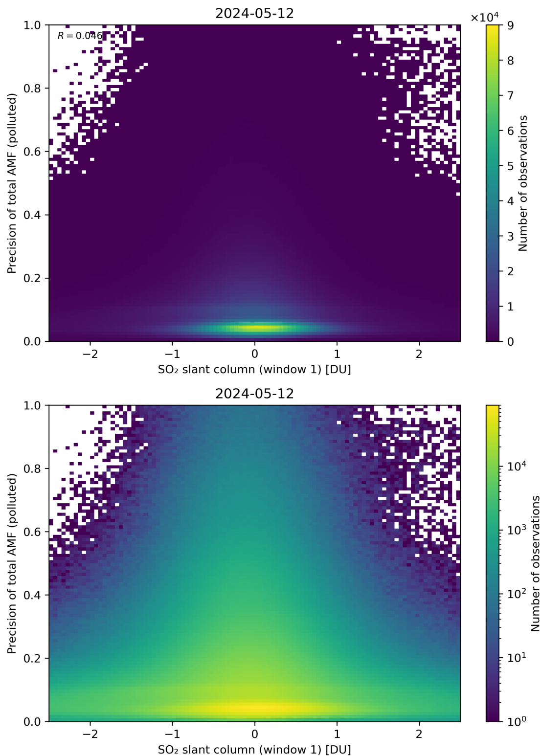
Figure 240: Scatter density plot of “SO 2 slant column (window 1)” against “Precision of total AMF (polluted)” for 2024-05-12 to 2024-05-13.
