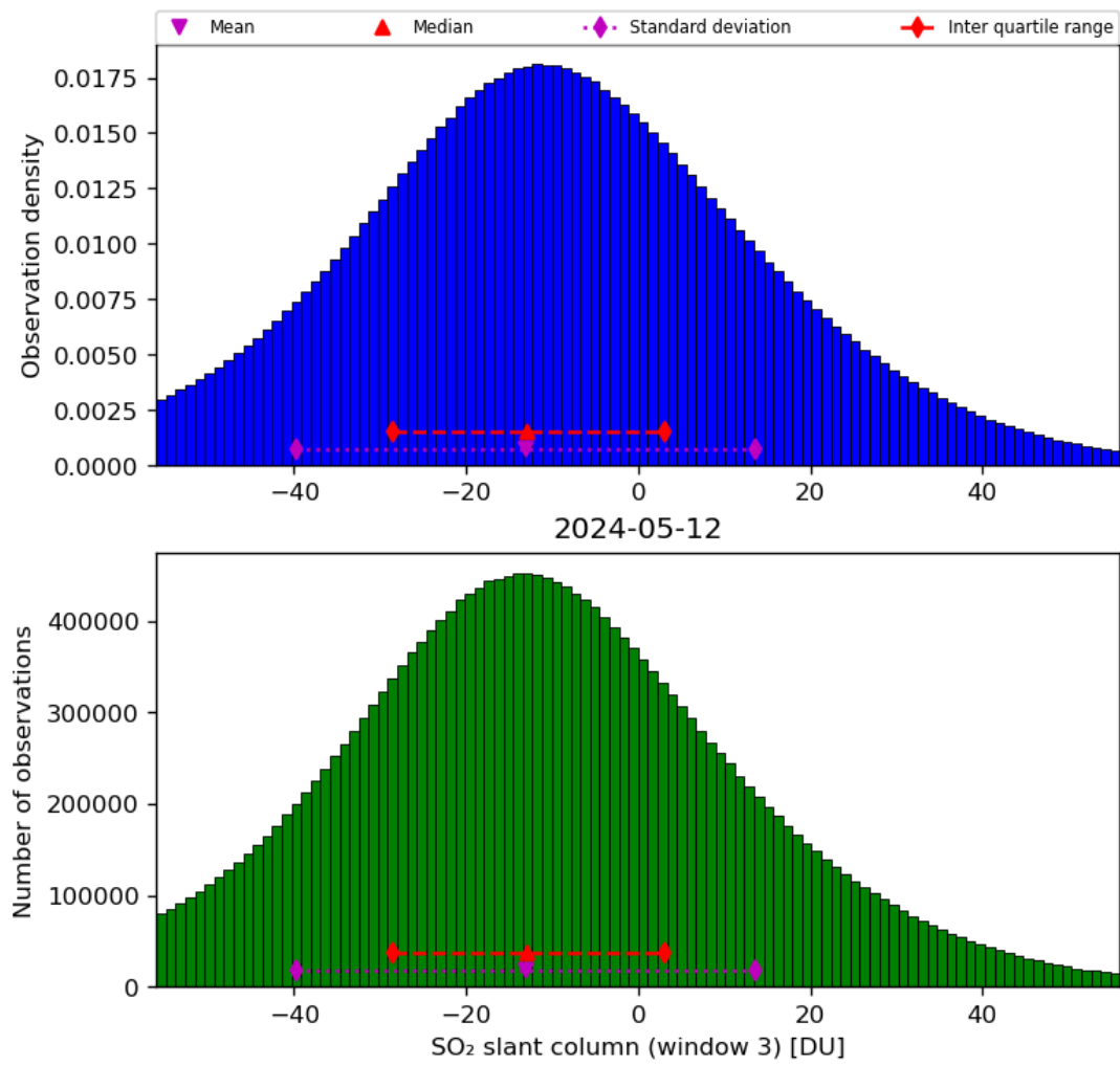
Figure 64: Histogram of “SO 2 slant column (window 3)” for 2024-05-12 to 2024-05-13
