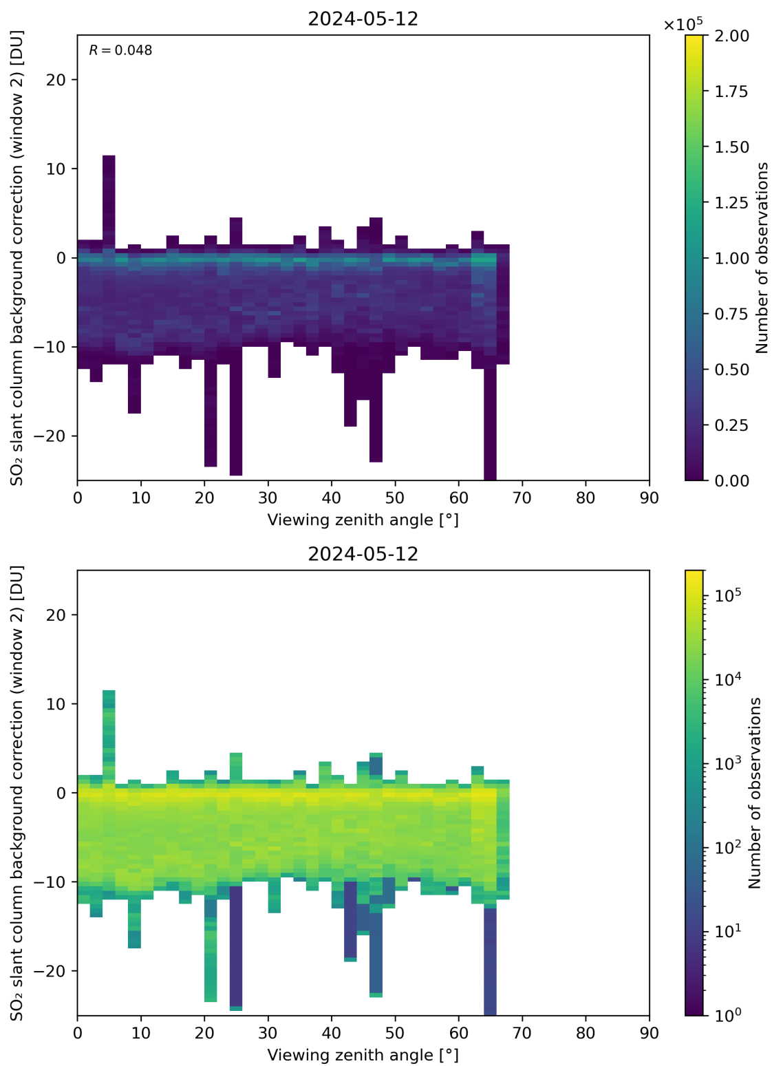
Figure 309: Scatter density plot of “Viewing zenith angle” against “SO 2 slant column background correction (window 2)” for 2024-05-12 to 2024-05-13.
