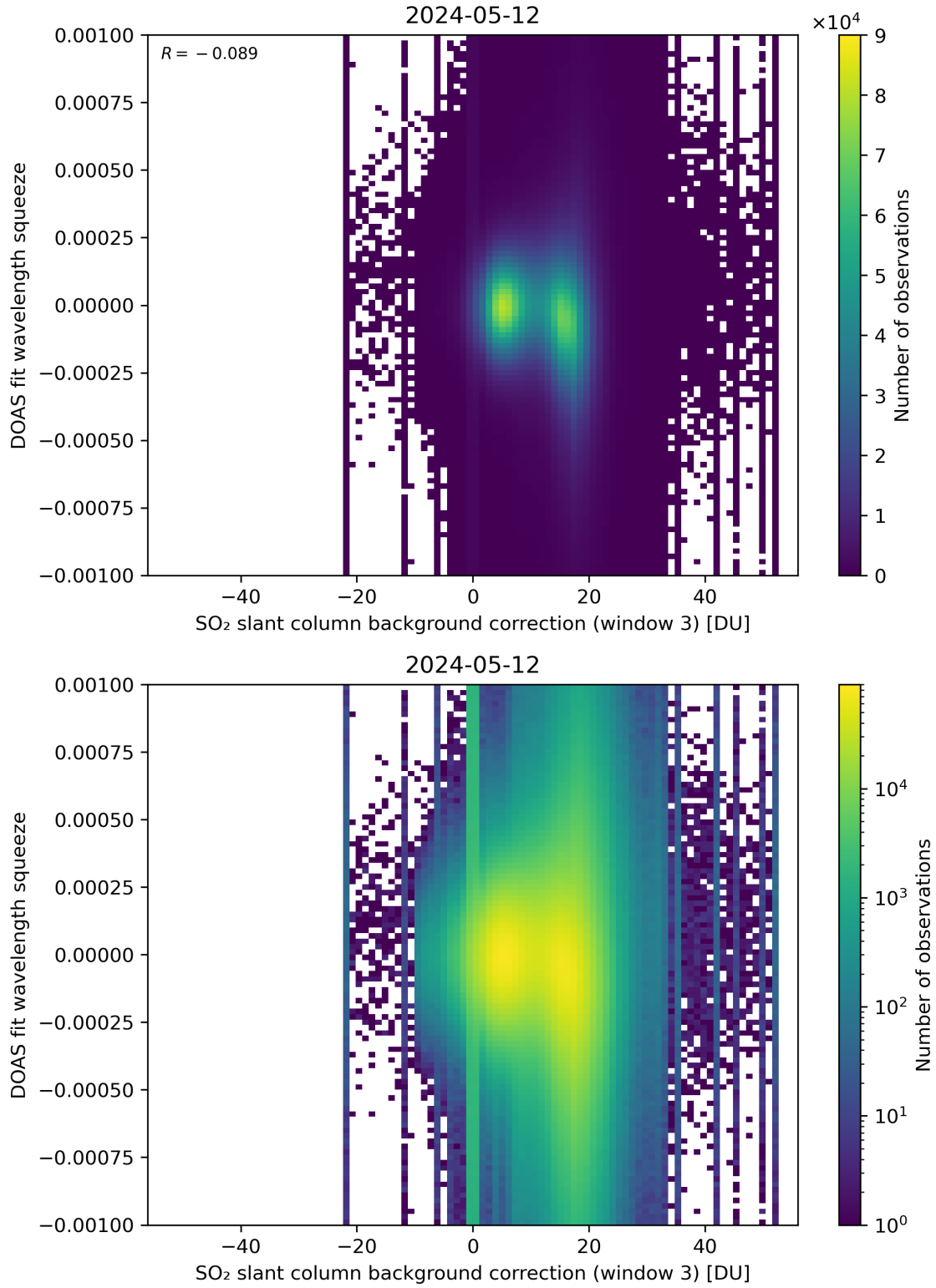
Figure 122: Scatter density plot of “SO 2 slant column background correction (window 3)” against “DOAS fit wavelength squeeze” for 2024-05-12 to 2024-05-13.
