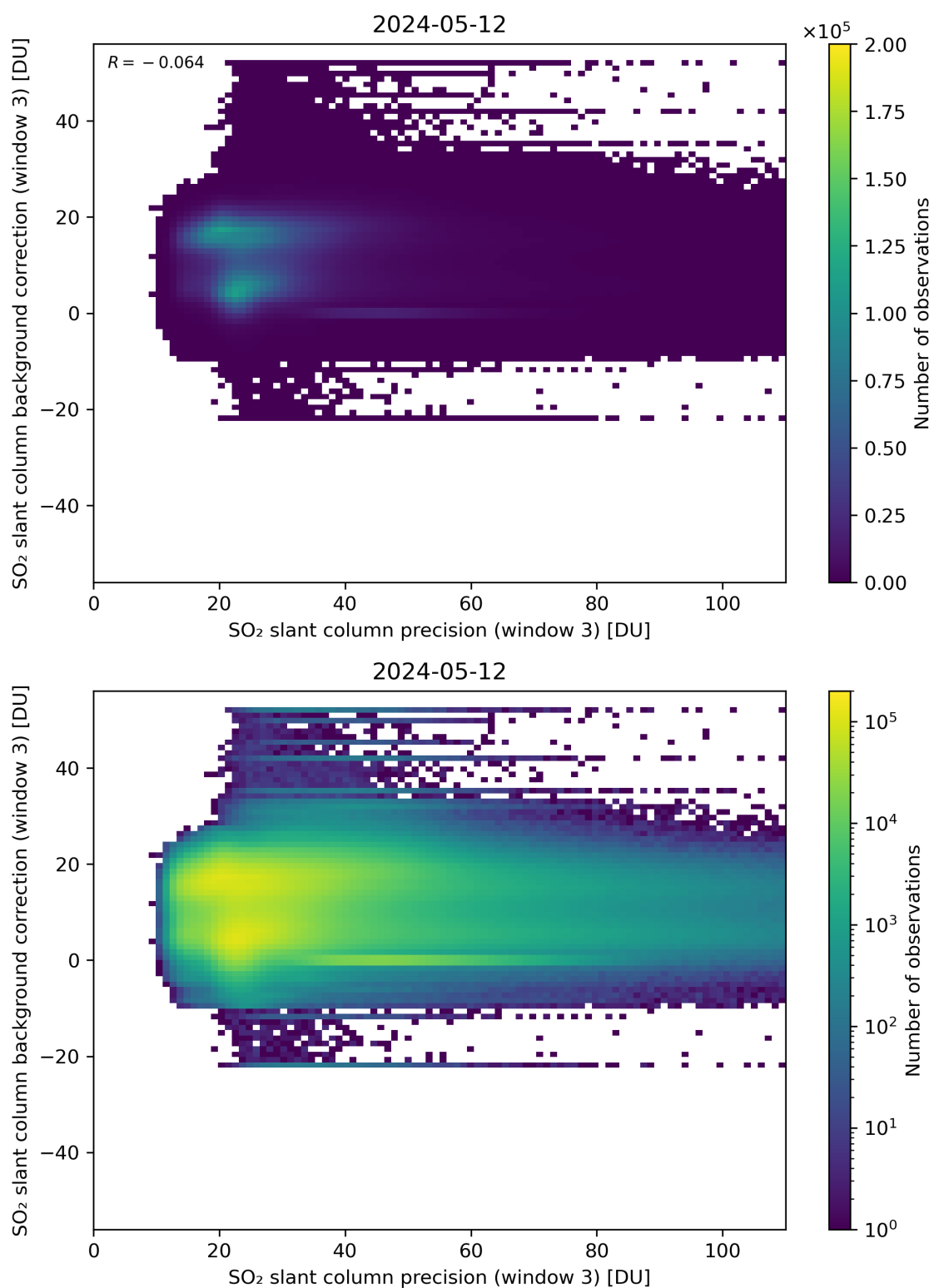
Figure 257: Scatter density plot of “SO 2 slant column precision (window 3)” against “SO 2 slant column background correction (window 3)” for 2024-05-12 to 2024-05-13.
