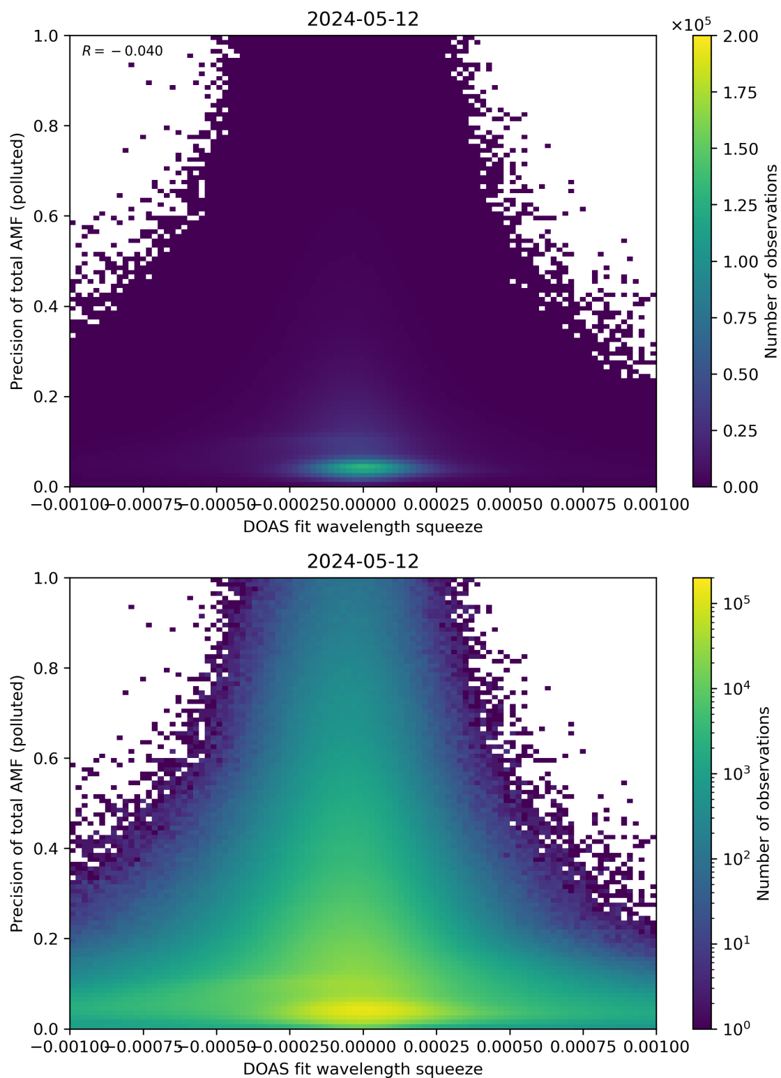
Figure 135: Scatter density plot of “DOAS fit wavelength squeeze” against “Precision of total AMF (polluted)” for 2024-05-12 to 2024-05-13.
