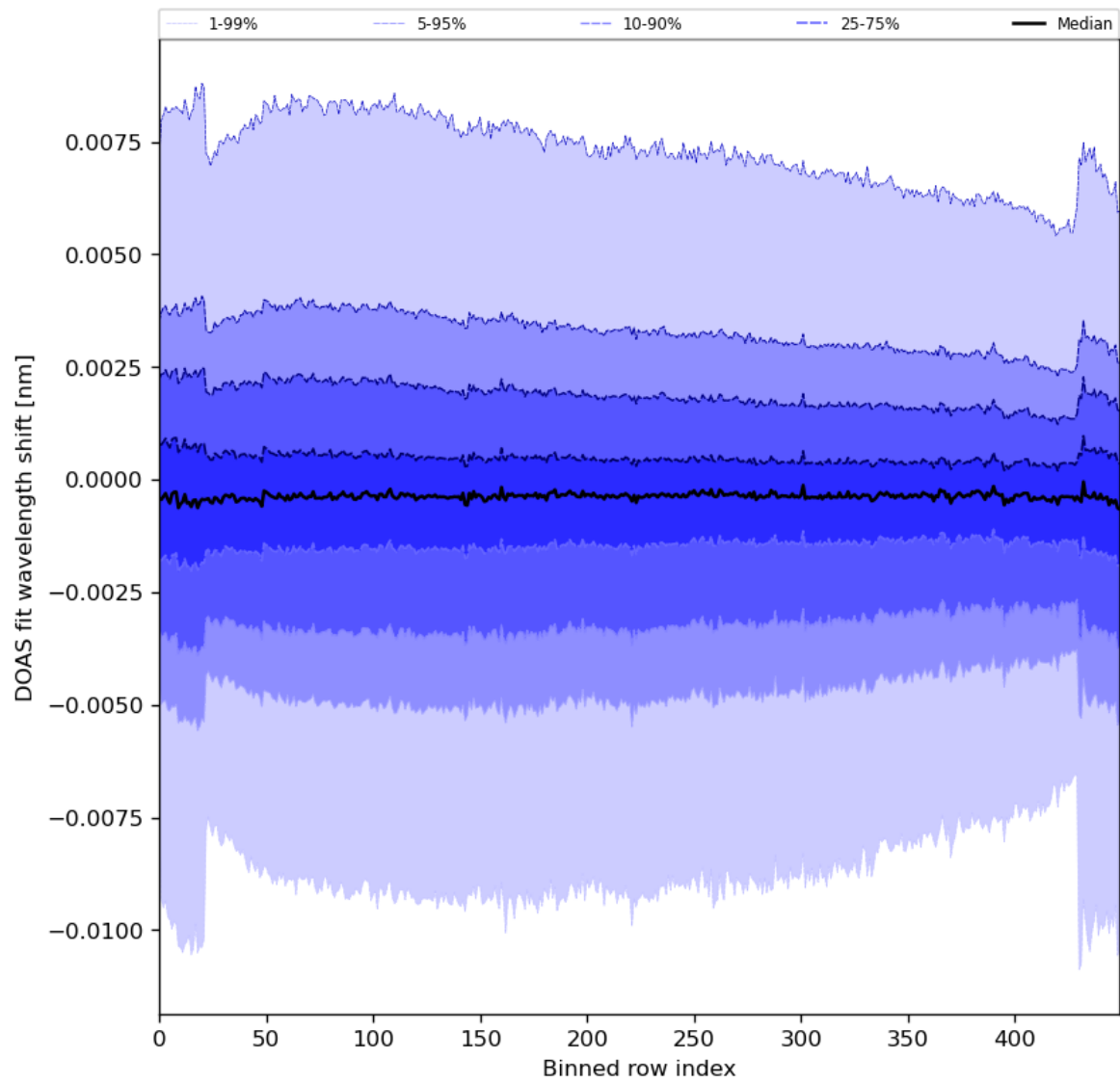
Figure 91: Along track statistics of “DOAS fit wavelength shift” for 2024-05-12 to 2024-05-13
