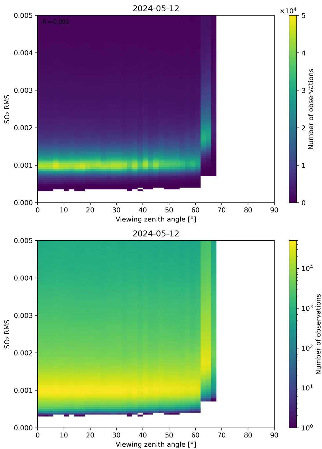
Figure 313: Scatter density plot of “Viewing zenith angle” against “SO 2 RMS” for 2024-05-12 to 2024-05-13.
