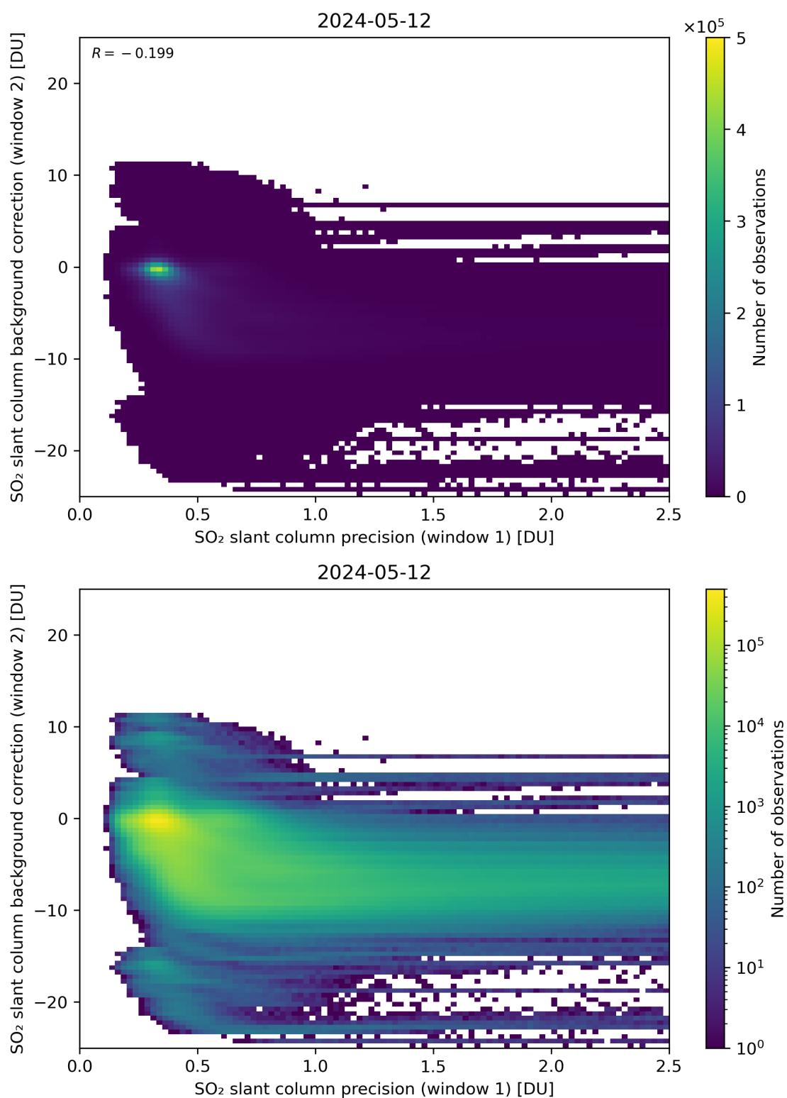
Figure 219: Scatter density plot of “SO 2 slant column precision (window 1)” against “SO 2 slant column background correction (window 2)” for 2024-05-12 to 2024-05-13.
