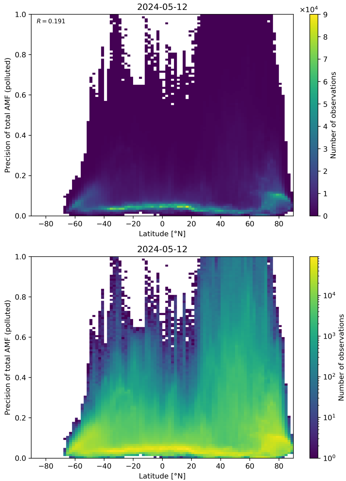
Figure 155: Scatter density plot of “Latitude” against “Precision of total AMF (polluted)” for 2024-05-12 to 2024-05-13.
