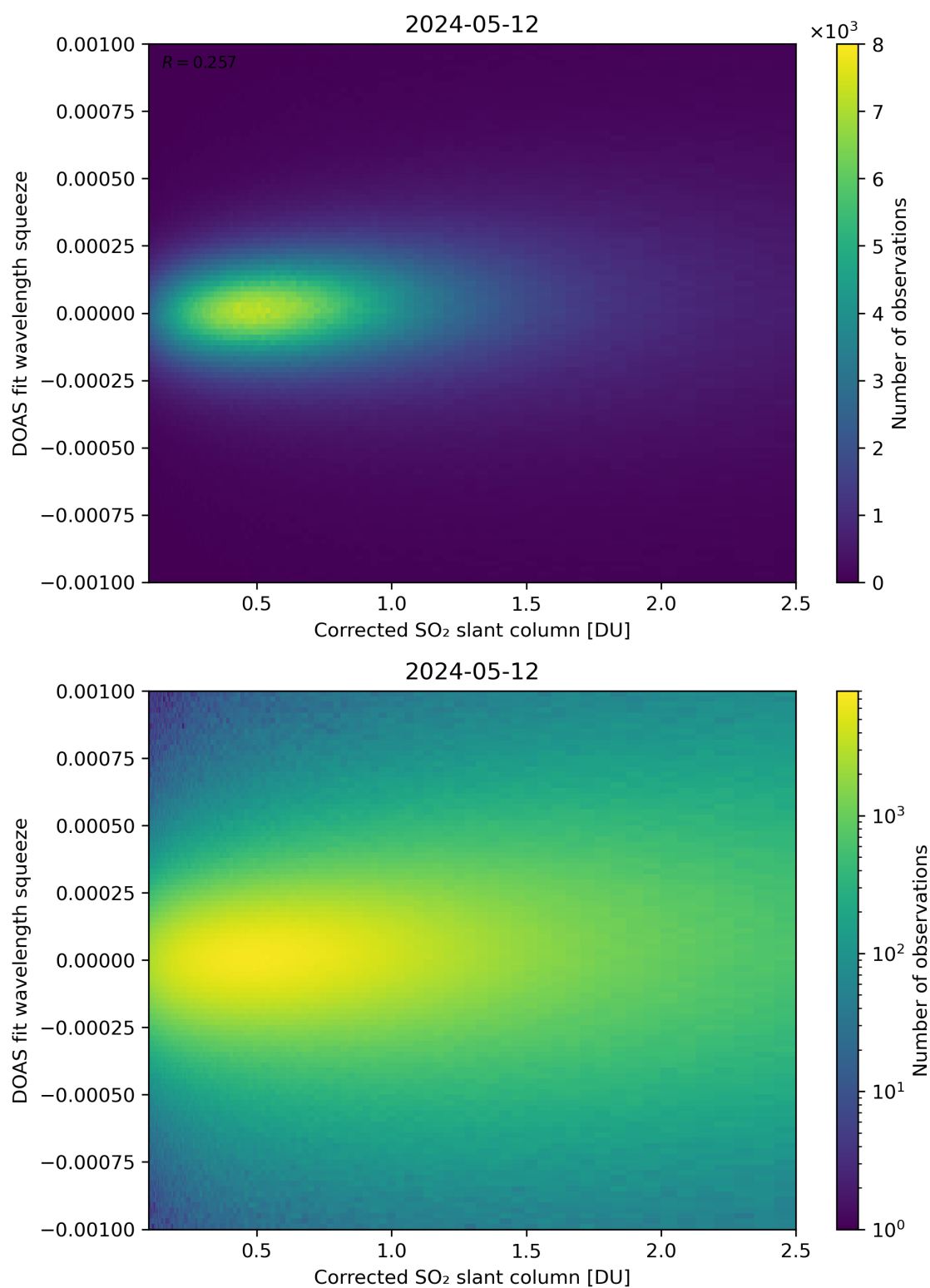
Figure 182: Scatter density plot of “Corrected SO 2 slant column” against “DOAS fit wavelength squeeze” for 2024-05-12 to 2024-05-13.
