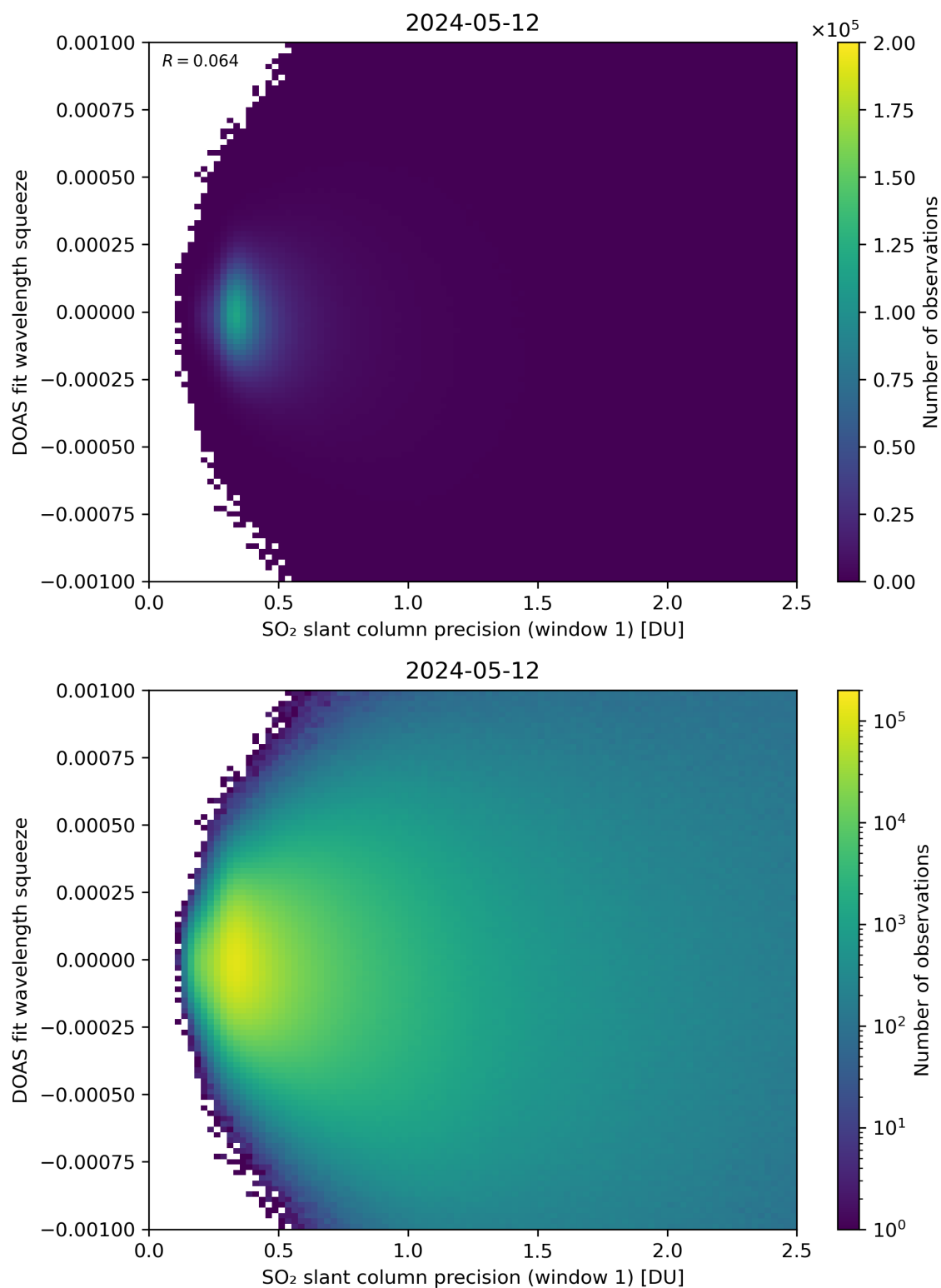
Figure 222: Scatter density plot of “SO 2 slant column precision (window 1)” against “DOAS fit wavelength squeeze” for 2024-05-12 to 2024-05-13.
