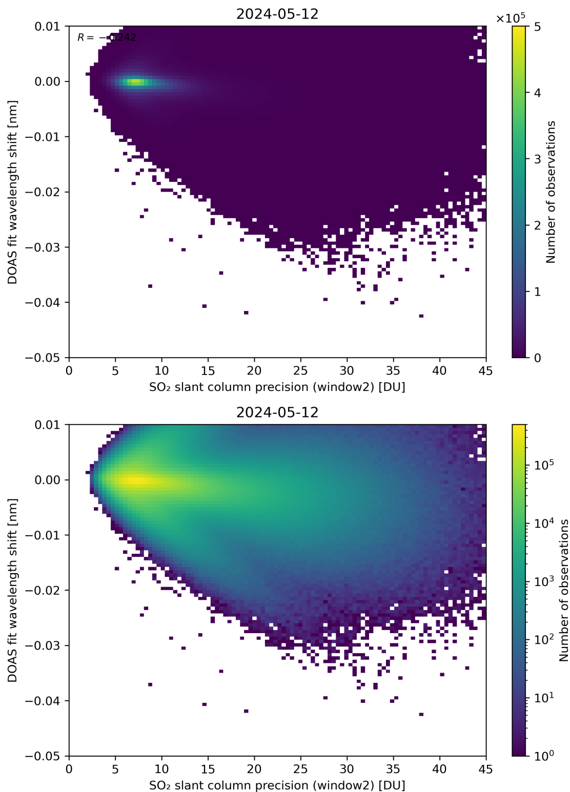
Figure 243: Scatter density plot of “SO 2 slant column precision (window2)” against “DOAS fit wavelength shift” for 2024-05-12 to 2024-05-13.
