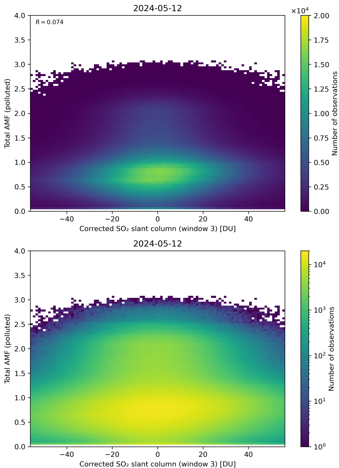
Figure 210: Scatter density plot of “Corrected SO 2 slant column (window 3)” against “Total AMF (polluted)” for 2024-05-12 to 2024-05-13.
