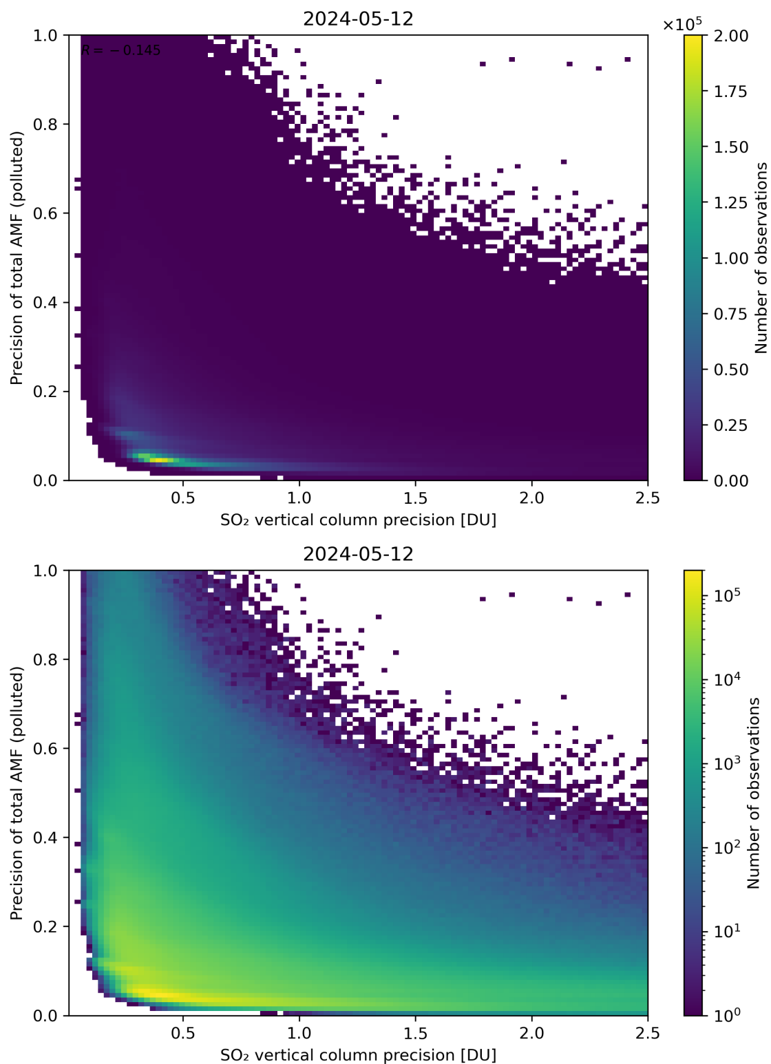
Figure 295: Scatter density plot of “SO 2 vertical column precision” against “Precision of total AMF (polluted)” for 2024-05-12 to 2024-05-13.
