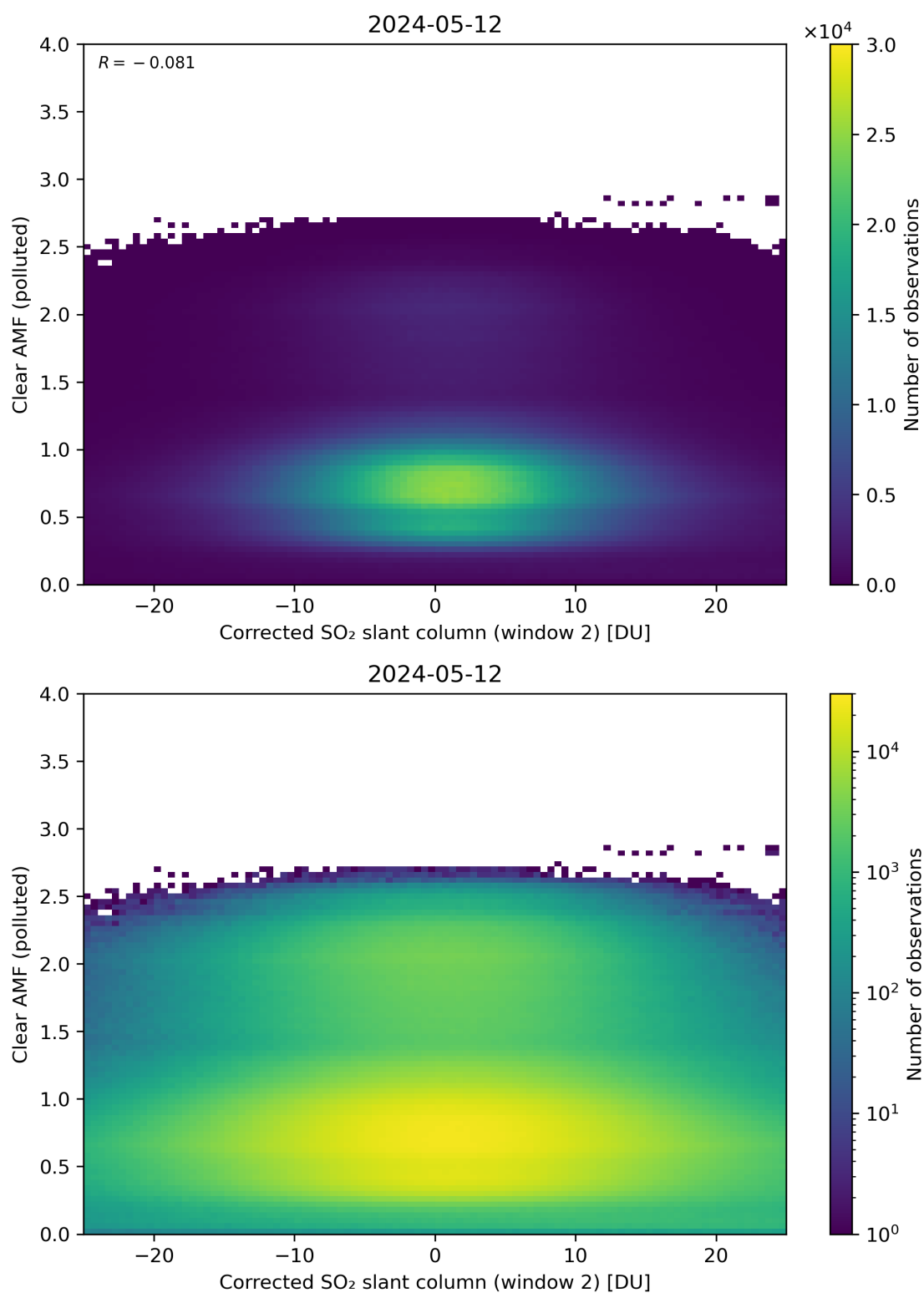
Figure 199: Scatter density plot of “Corrected SO 2 slant column (window 2)” against “Clear AMF (polluted)” for 2024-05-12 to 2024-05-13.
