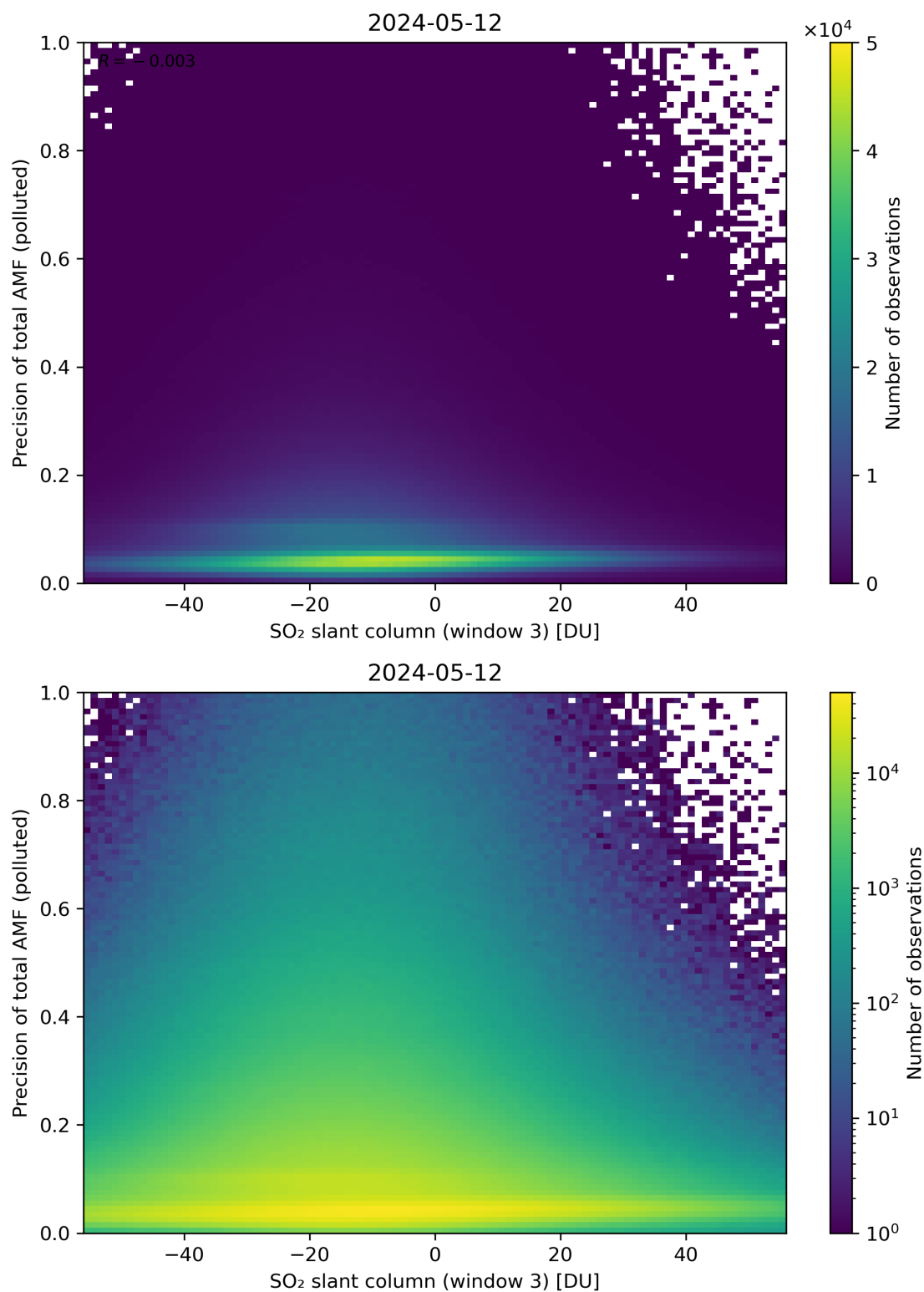
Figure 269: Scatter density plot of “SO 2 slant column (window 3)” against “Precision of total AMF (polluted)” for 2024-05-12 to 2024-05-13.
