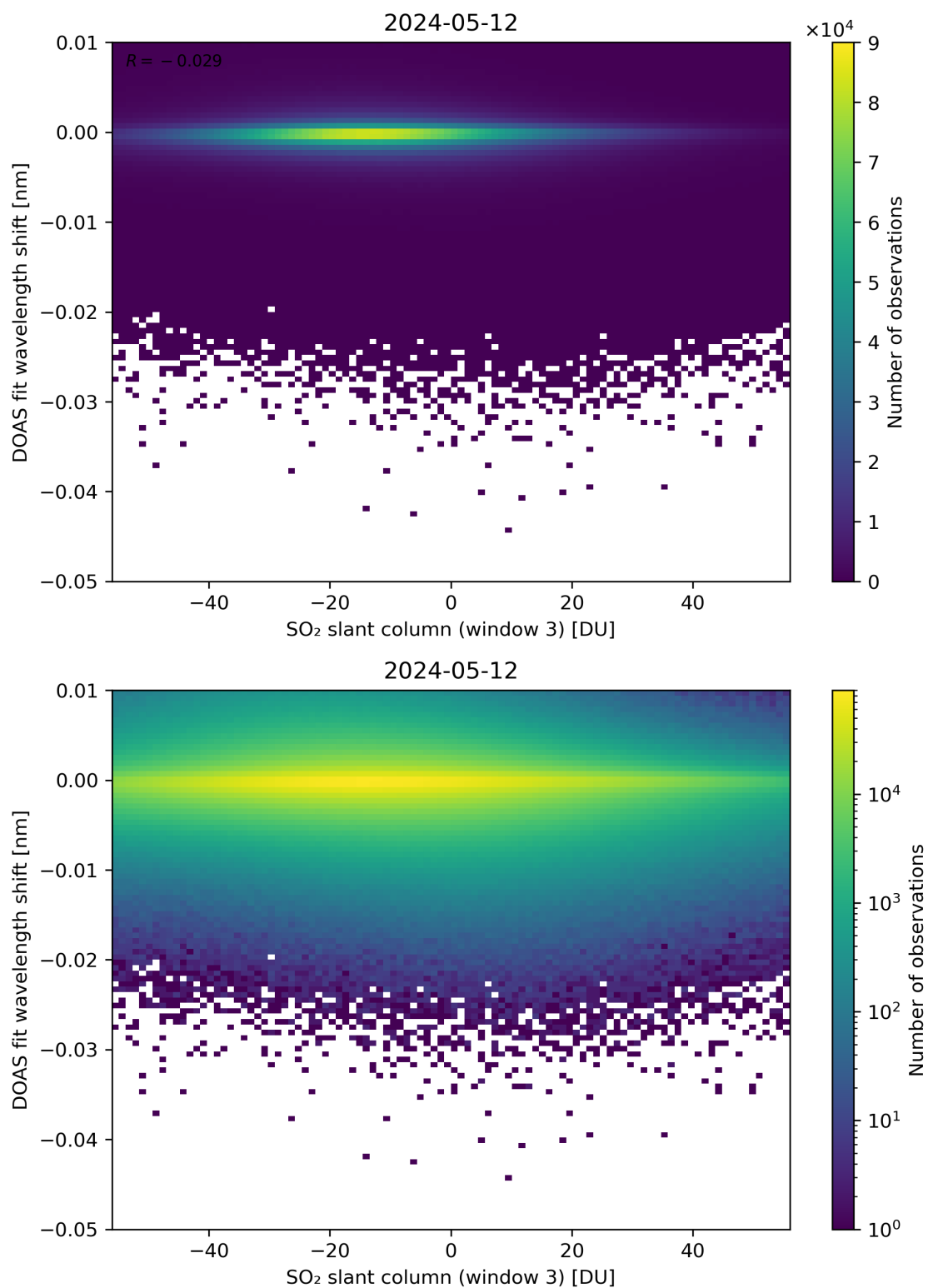
Figure 254: Scatter density plot of “SO 2 slant column (window 3)” against “DOAS fit wavelength shift” for 2024-05-12 to 2024-05-13.
