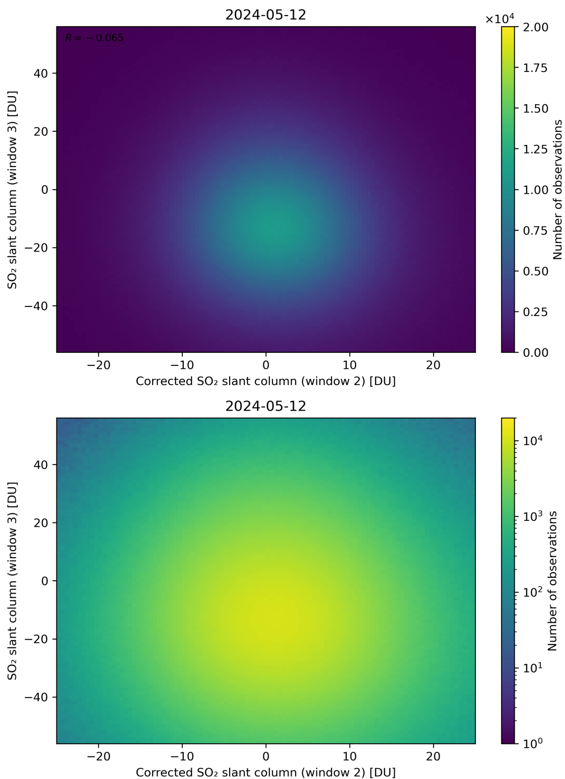
Figure 201: Scatter density plot of “Corrected SO 2 slant column (window 2)” against “SO 2 slant column (window 3)” for 2024-05-12 to 2024-05-13.
