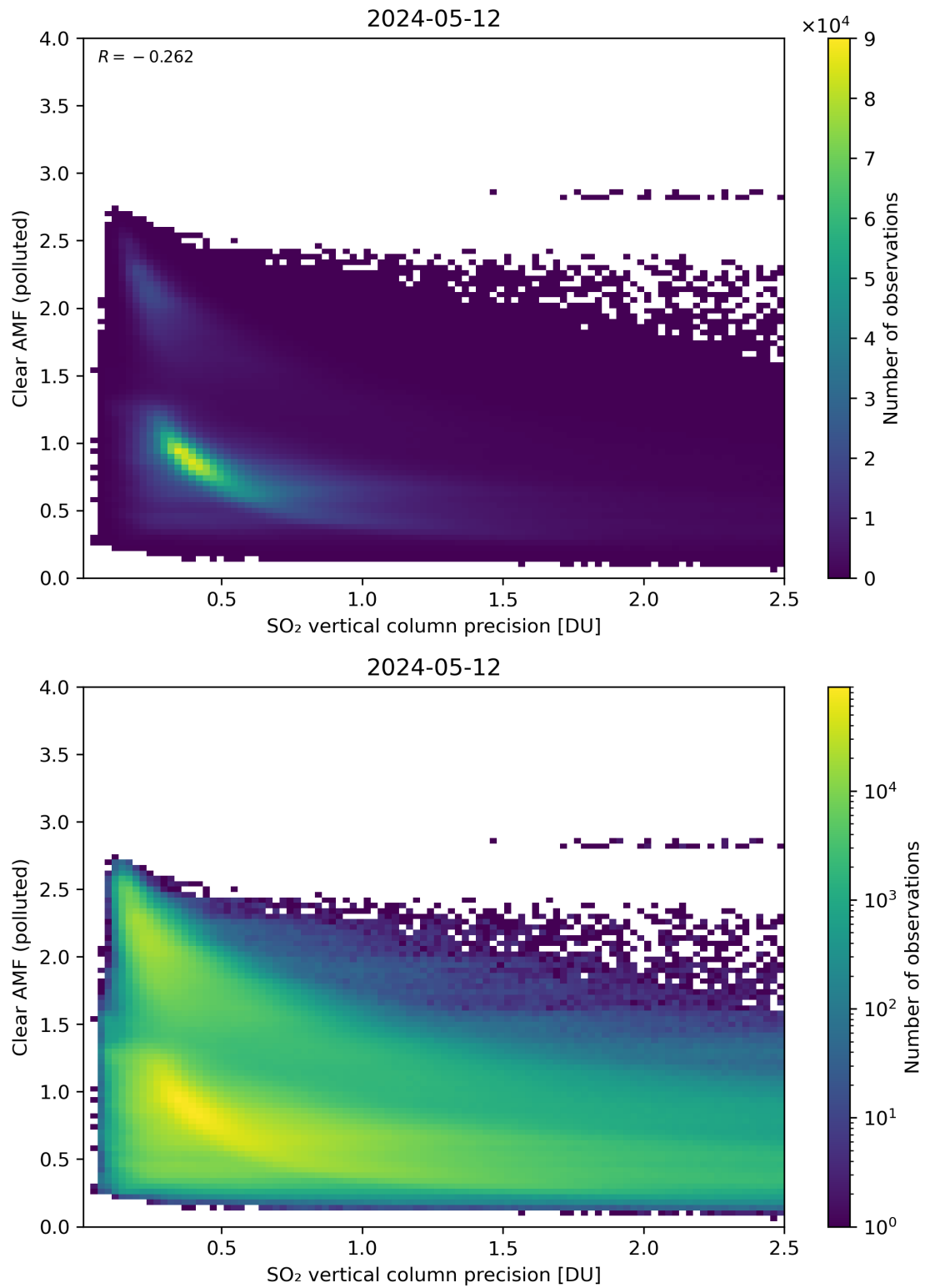
Figure 285: Scatter density plot of “SO 2 vertical column precision” against “Clear AMF (polluted)” for 2024-05-12 to 2024-05-13.
