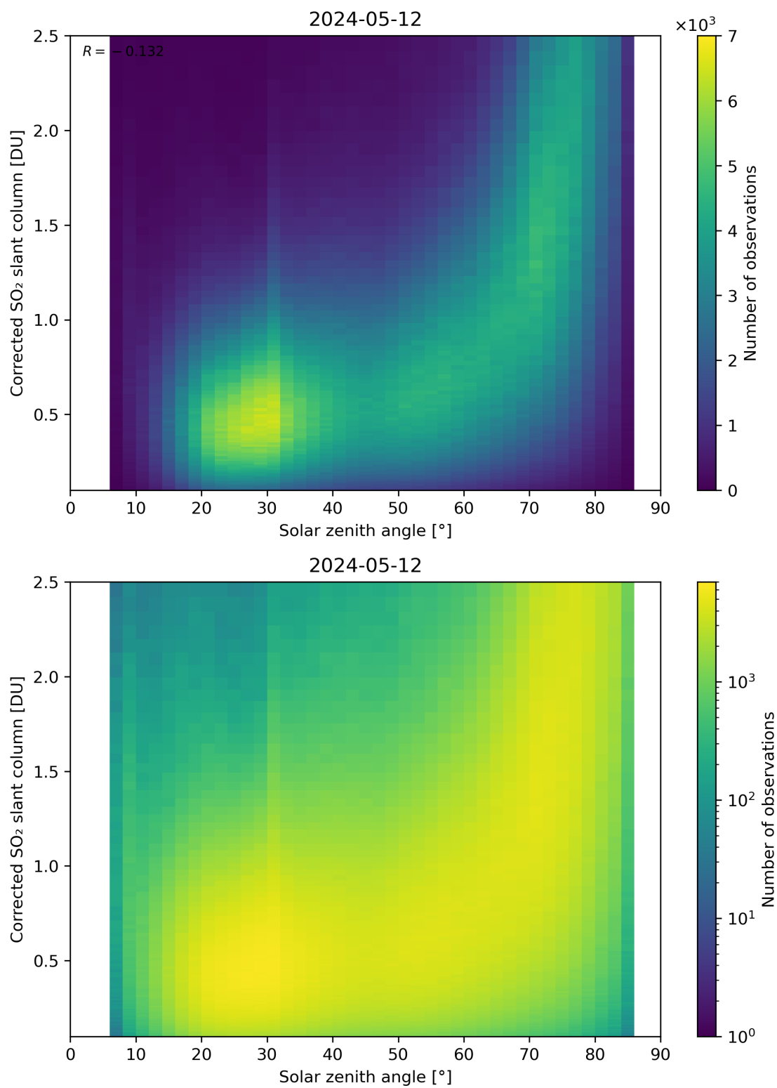
Figure 166: Scatter density plot of “Solar zenith angle” against “Corrected SO 2 slant column” for 2024-05-12 to 2024-05-13.
