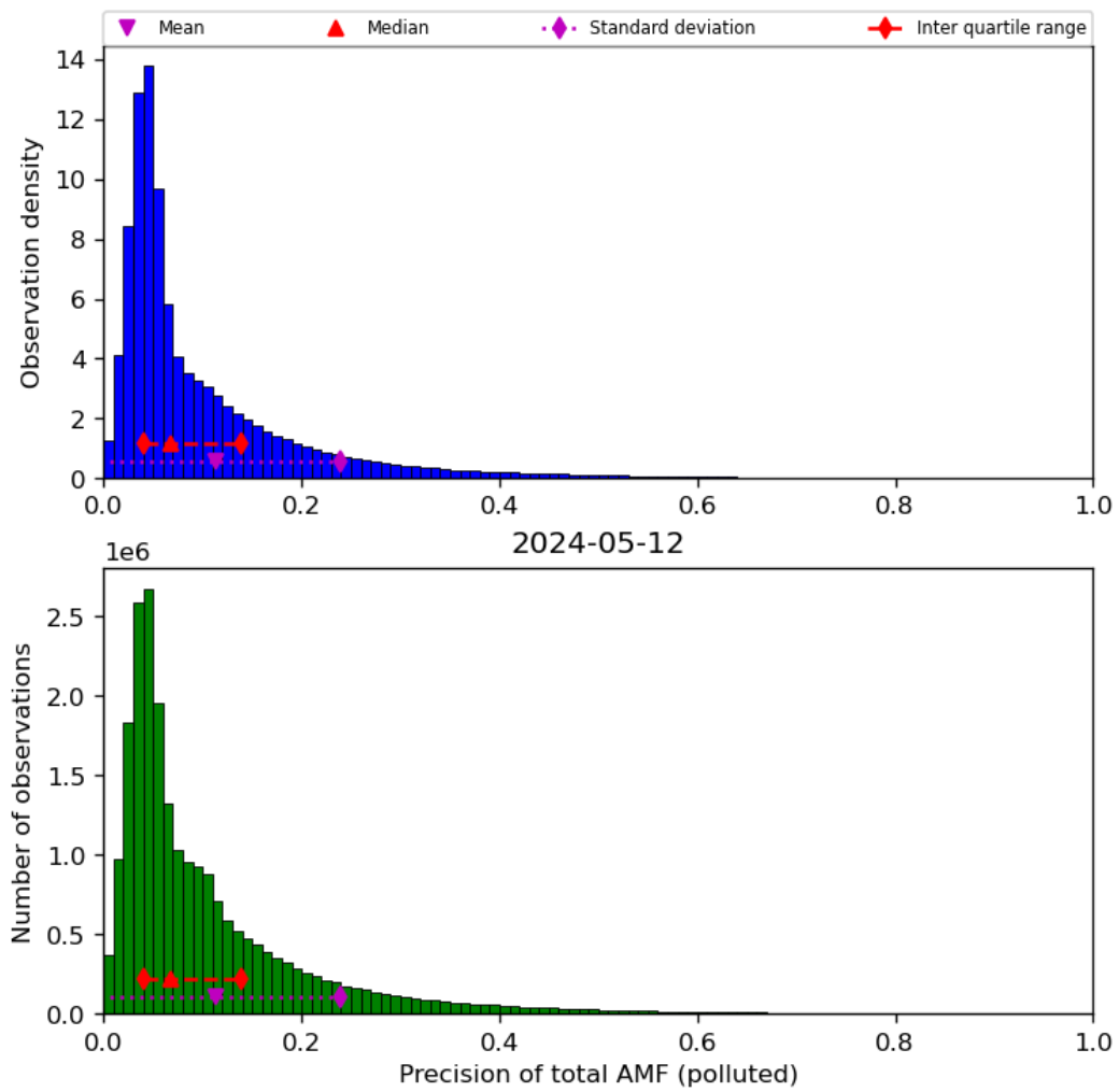
Figure 72: Histogram of “Precision of total AMF (polluted)” for 2024-05-12 to 2024-05-13
