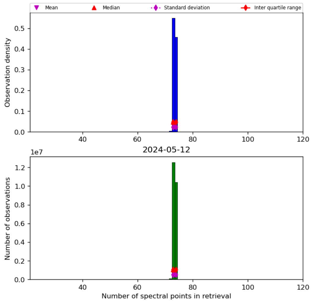
Figure 74: Histogram of “Number of spectral points in retrieval” for 2024-05-12 to 2024-05-13
