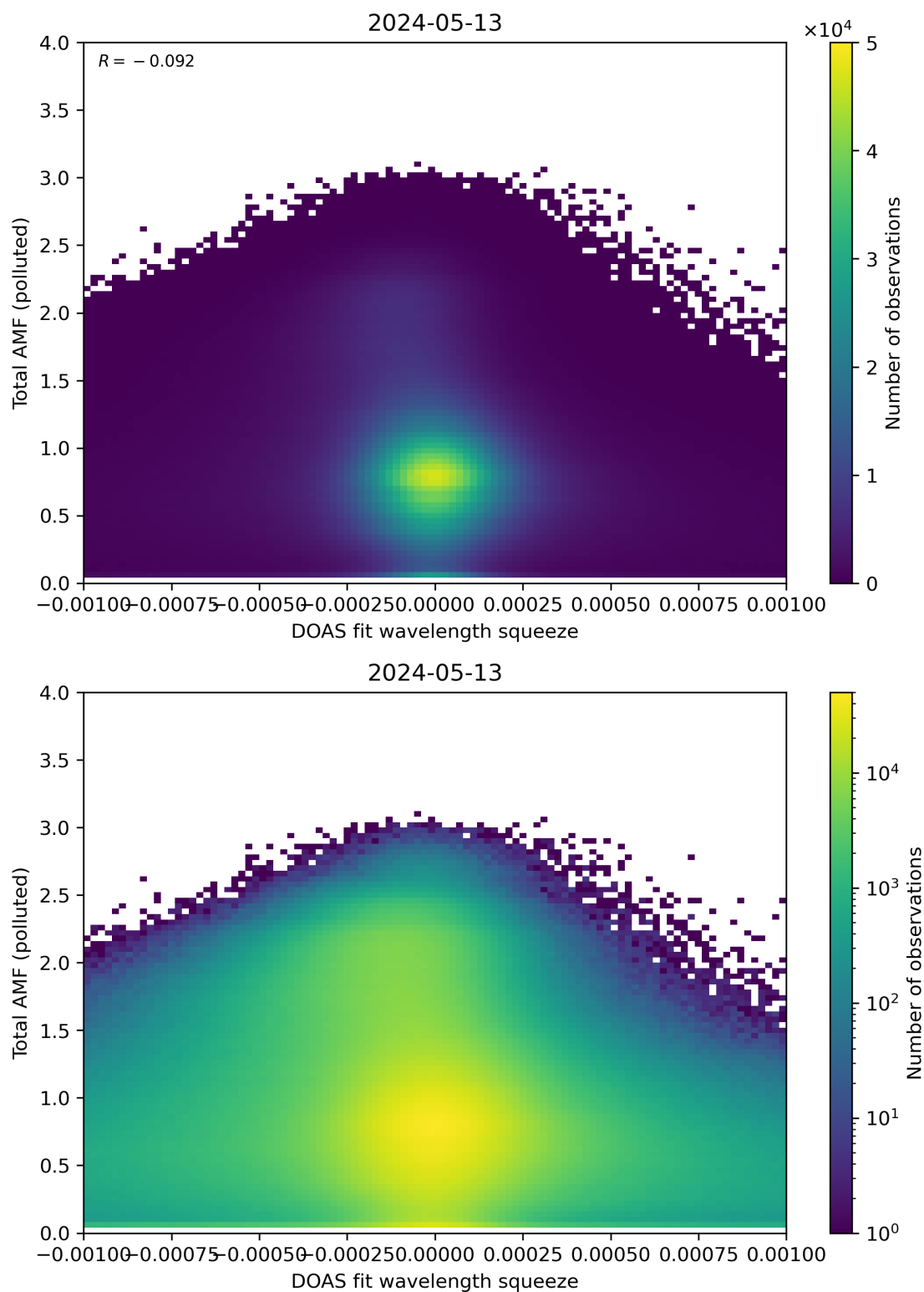
Figure 134: Scatter density plot of “DOAS fit wavelength squeeze” against “Total AMF (polluted)” for 2024-05-12 to 2024-05-14.
