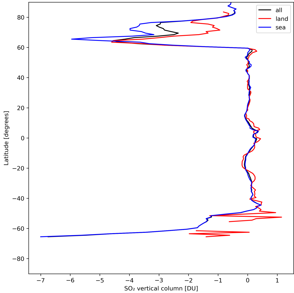
Figure 30: Zonal average of “SO 2 vertical column” for 2024-05-12 to 2024-05-14.
