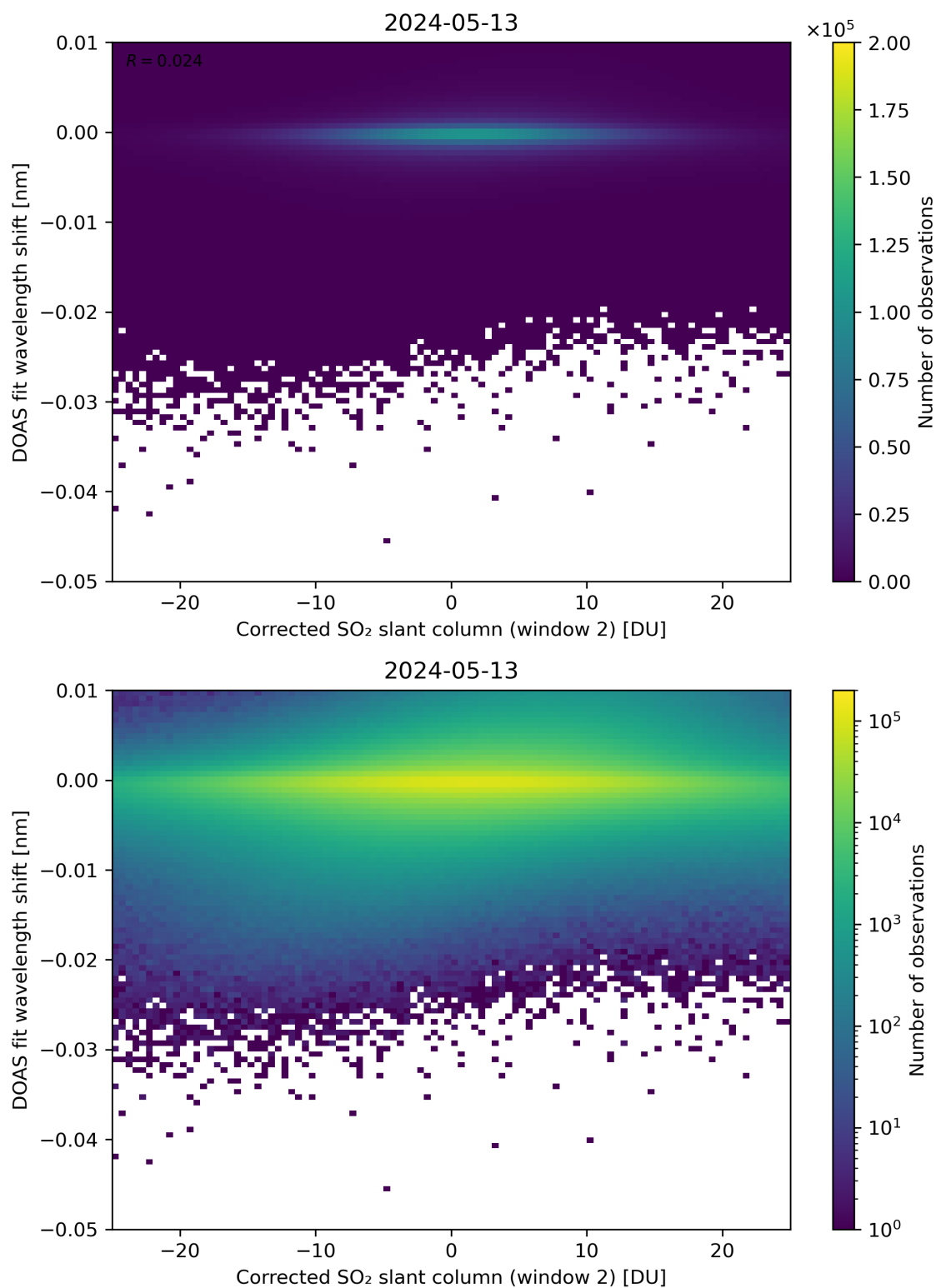
Figure 196: Scatter density plot of “Corrected SO 2 slant column (window 2)” against “DOAS fit wavelength shift” for 2024-05-12 to 2024-05-14.
