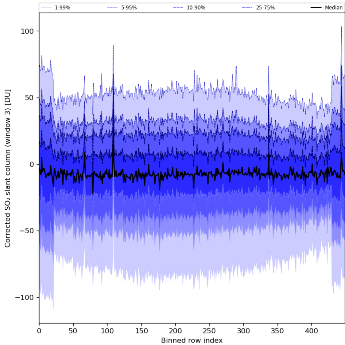
Figure 89: Along track statistics of “Corrected SO 2 slant column (window 3)” for 2024-05-12 to 2024-05-14
