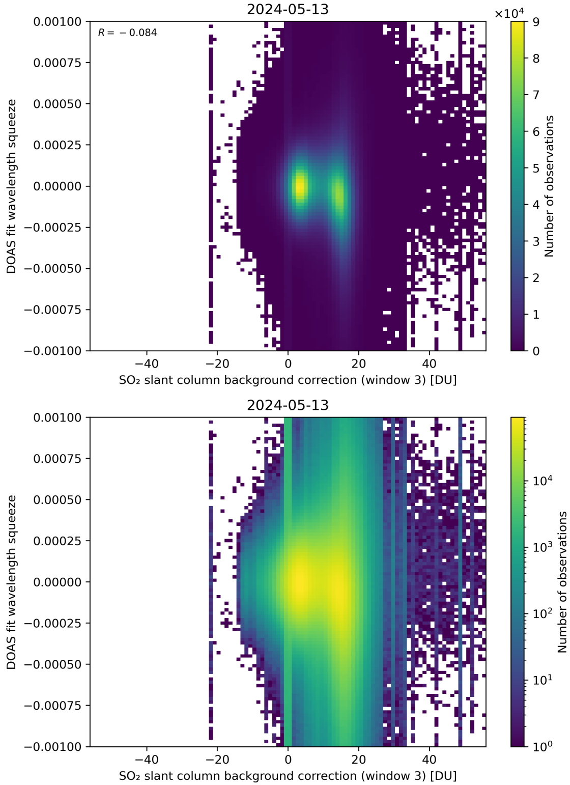
Figure 122: Scatter density plot of “SO 2 slant column background correction (window 3)” against “DOAS fit wavelength squeeze” for 2024-05-12 to 2024-05-14.
