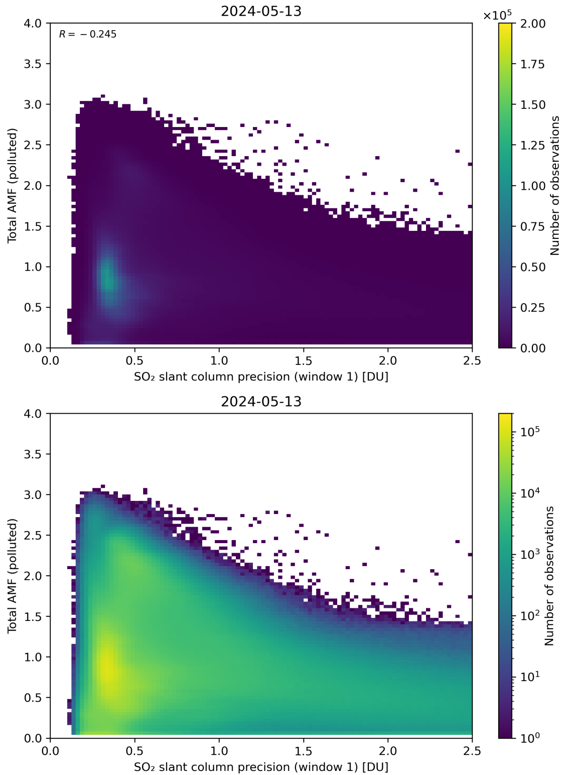
Figure 230: Scatter density plot of “SO 2 slant column precision (window 1)” against “Total AMF (polluted)” for 2024-05-12 to 2024-05-14.
