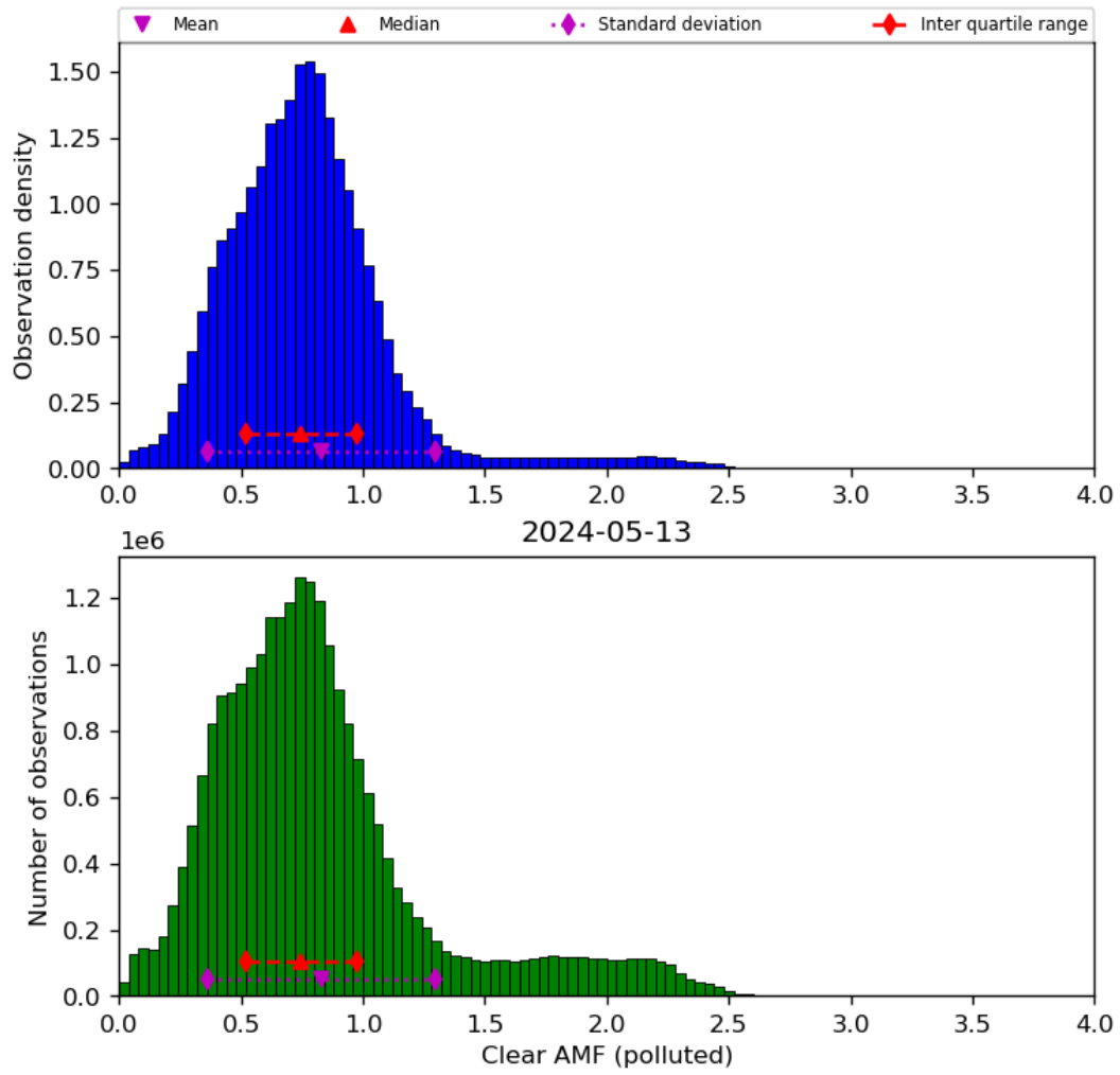
Figure 73: Histogram of “Clear AMF (polluted)” for 2024-05-12 to 2024-05-14
