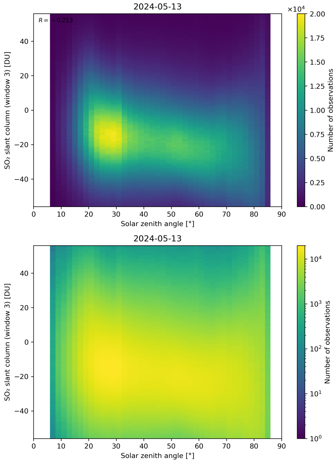
Figure 172: Scatter density plot of “Solar zenith angle” against “SO 2 slant column (window 3)” for 2024-05-12 to 2024-05-14.
