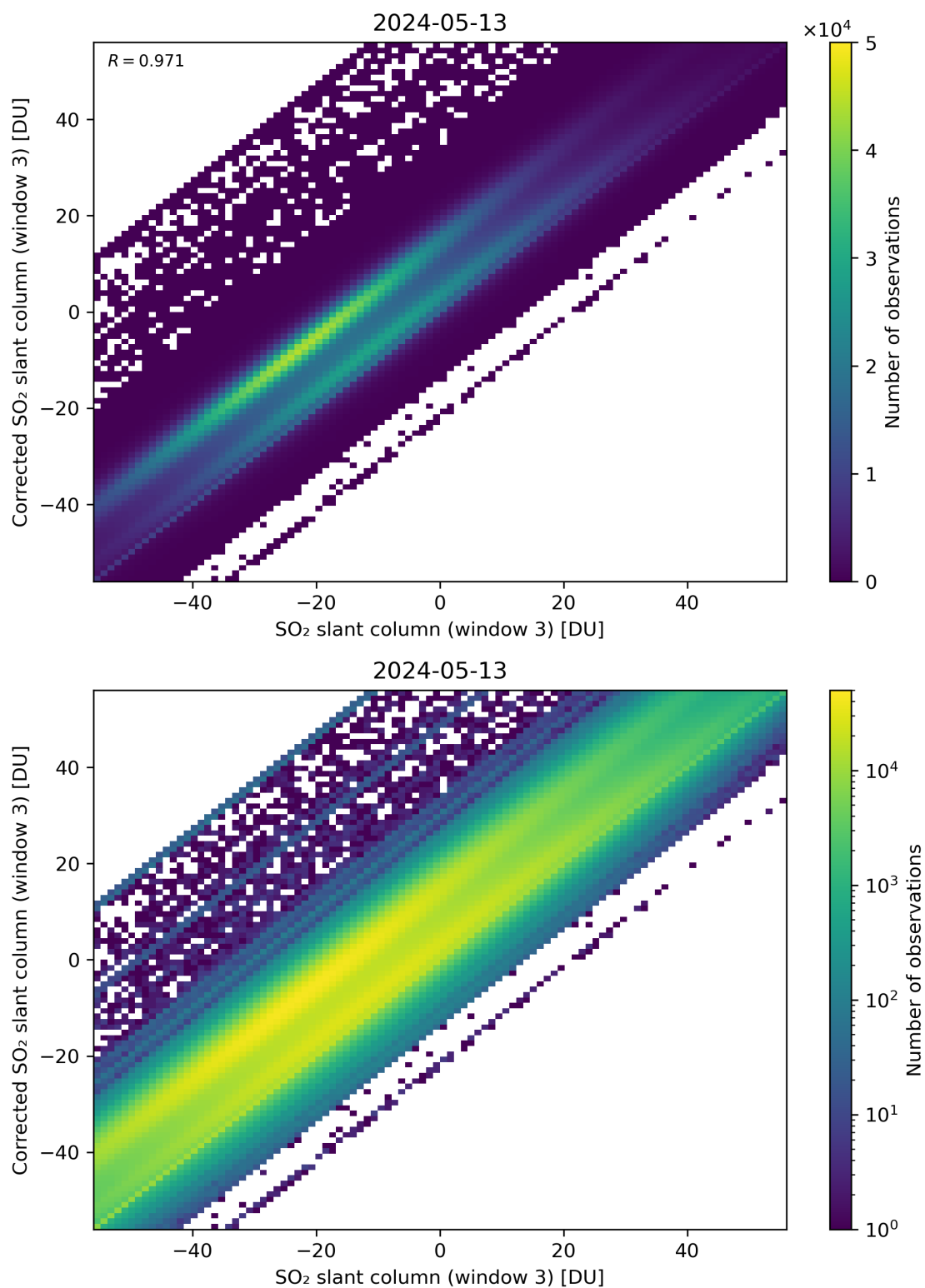
Figure 266: Scatter density plot of “SO 2 slant column (window 3)” against “Corrected SO 2 slant column (window 3)” for 2024-05-12 to 2024-05-14.
