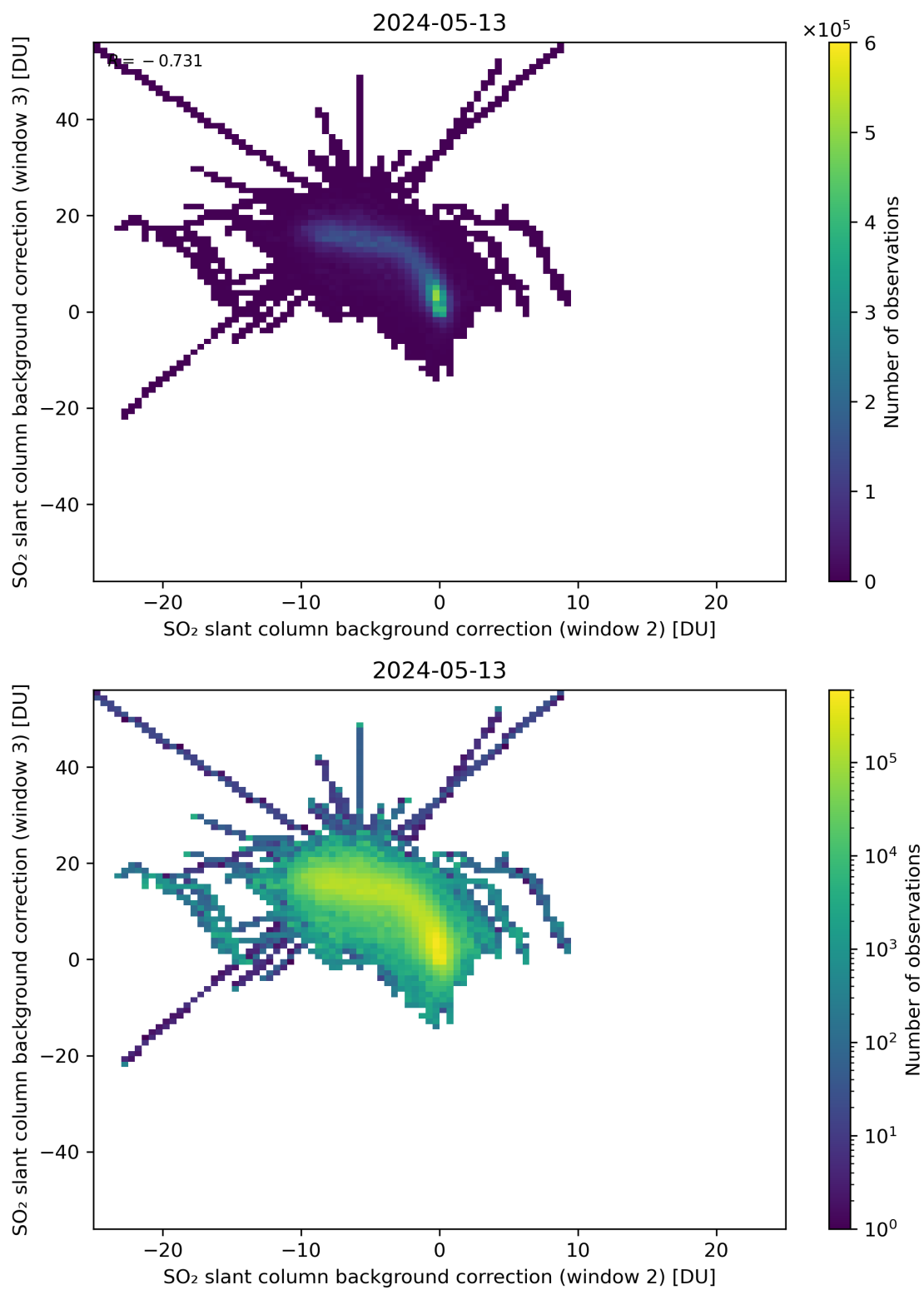
Figure 111: Scatter density plot of “SO 2 slant column background correction (window 2)” against “SO 2 slant column background correction (window 3)” for 2024-05-12 to 2024-05-14.
