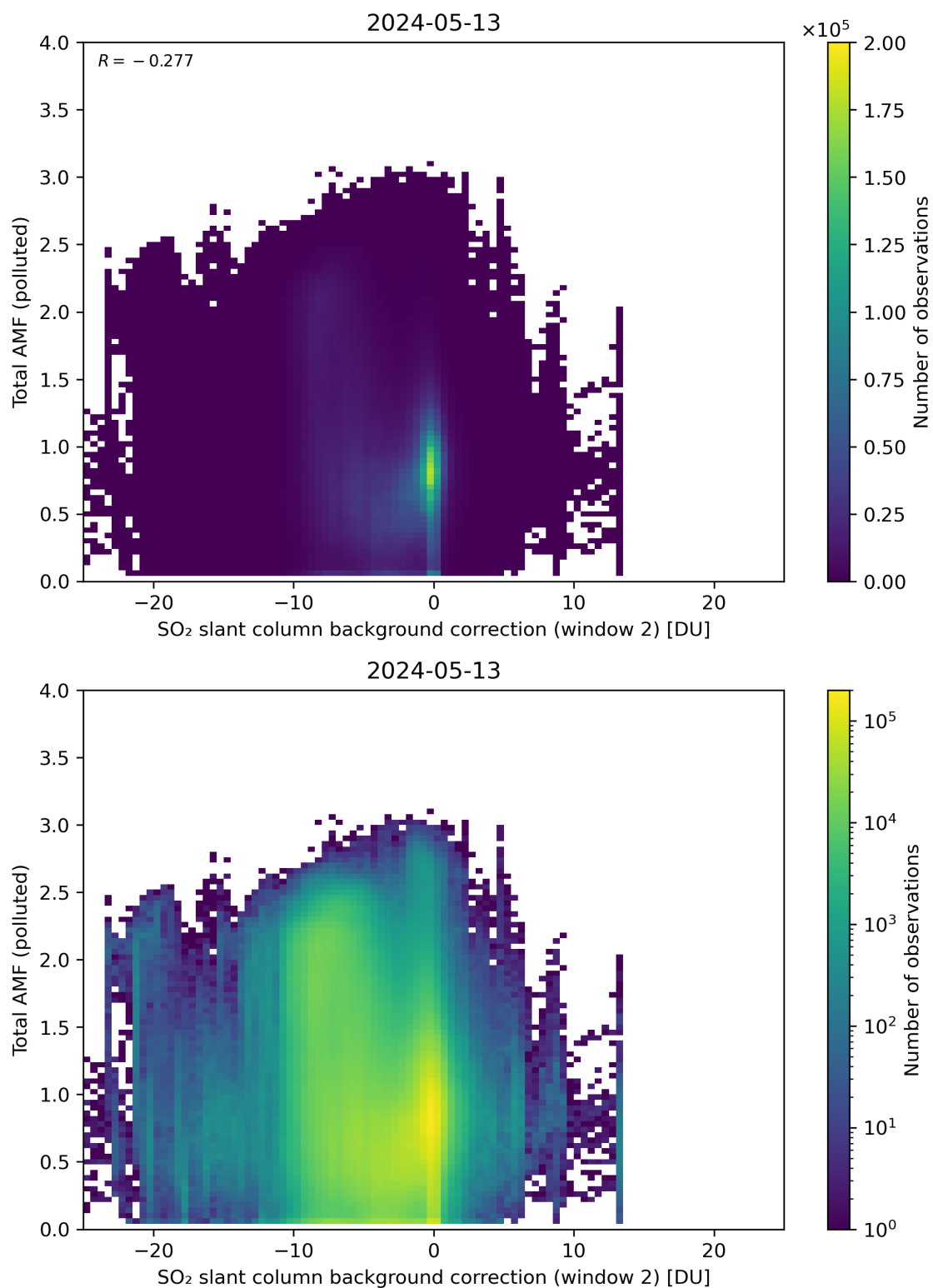
Figure 119: Scatter density plot of “SO 2 slant column background correction (window 2)” against “Total AMF (polluted)” for 2024-05-12 to 2024-05-14.
