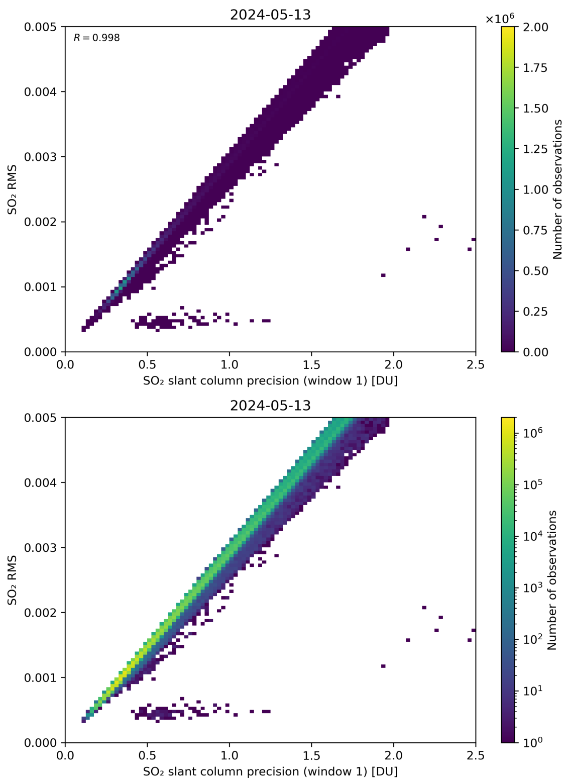
Figure 223: Scatter density plot of “SO 2 slant column precision (window 1)” against “SO 2 RMS” for 2024-05-12 to 2024-05-14.
