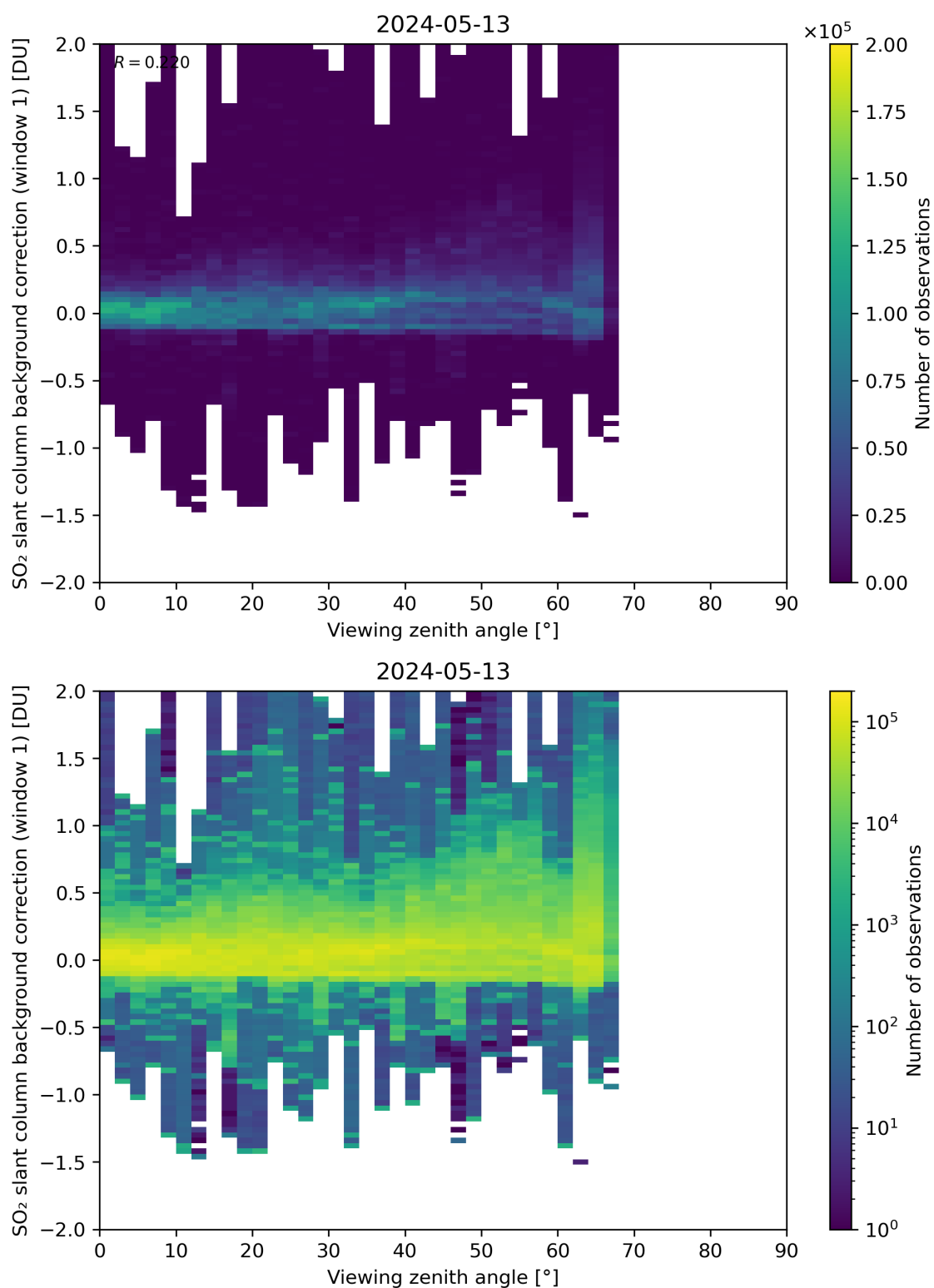
Figure 308: Scatter density plot of “Viewing zenith angle” against “SO 2 slant column background correction (window 1)” for 2024-05-12 to 2024-05-14.
