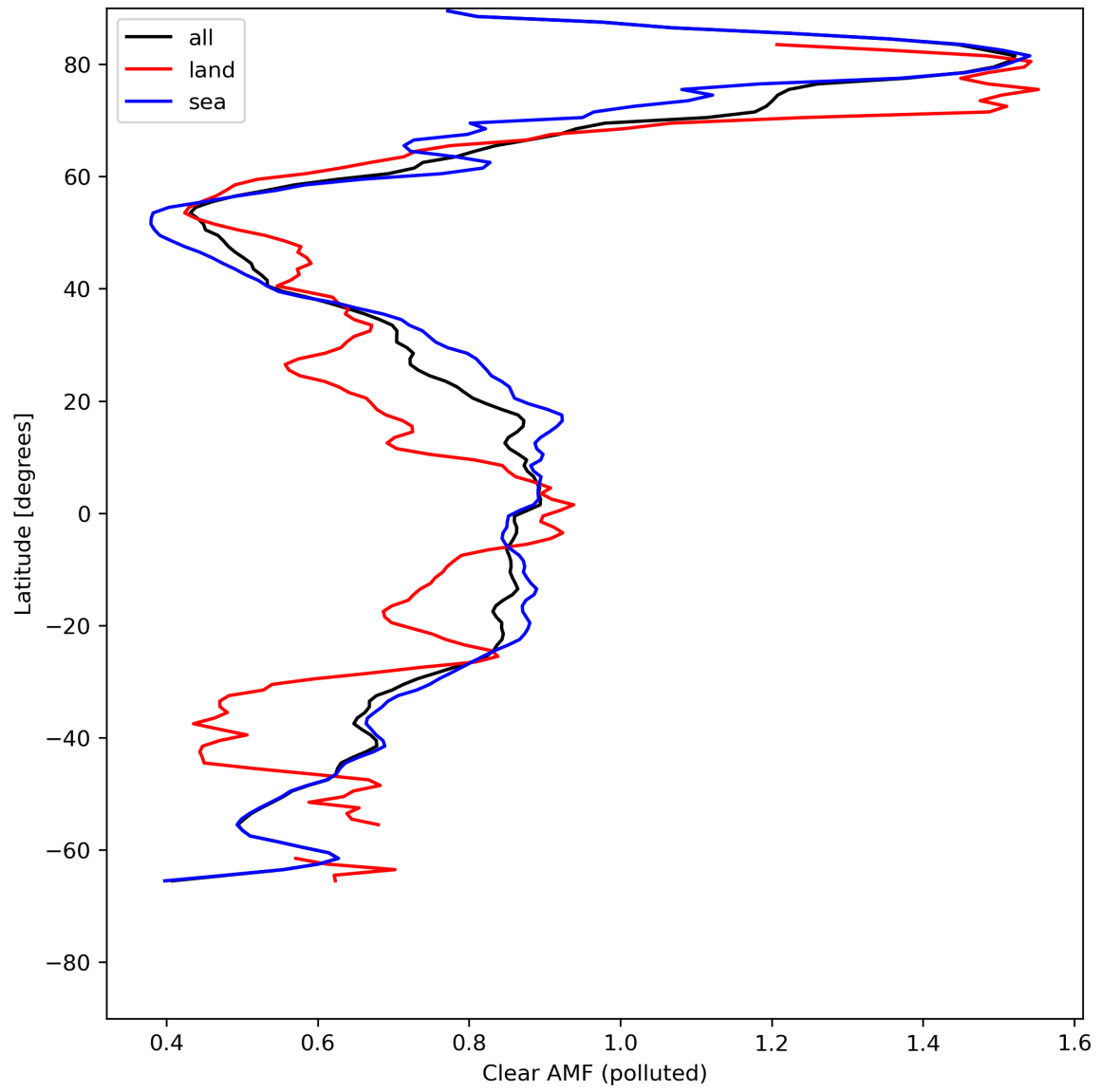
Figure 50: Zonal average of “Clear AMF (polluted)” for 2024-05-12 to 2024-05-14.
