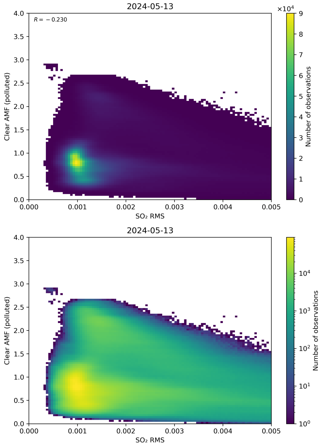
Figure 136: Scatter density plot of “SO 2 RMS” against “Clear AMF (polluted)” for 2024-05-12 to 2024-05-14.
