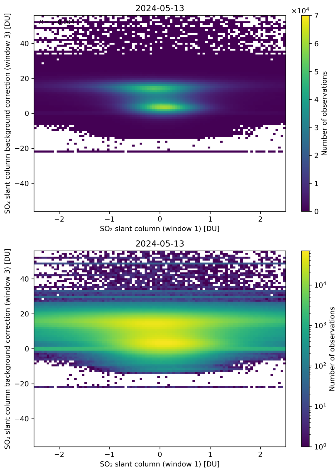
Figure 214: Scatter density plot of “SO 2 slant column (window 1)” against “SO 2 slant column background correction (window 3)” for 2024-05-12 to 2024-05-14.
