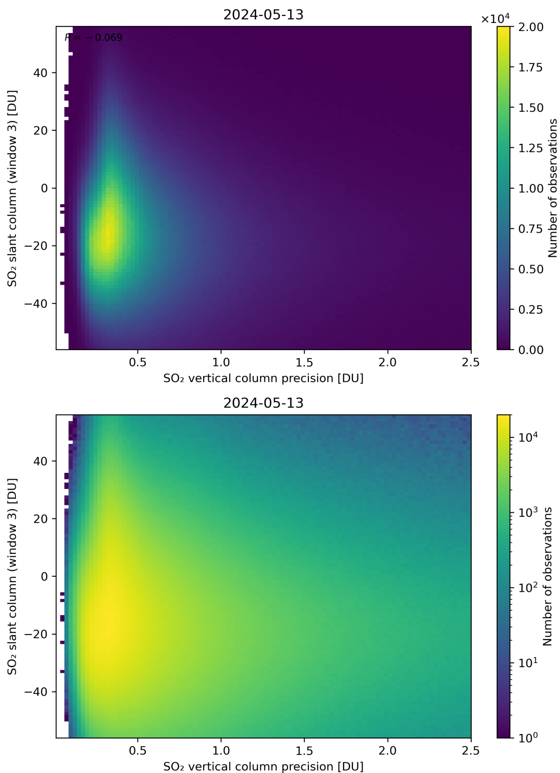
Figure 292: Scatter density plot of “SO 2 vertical column precision” against “SO 2 slant column (window 3)” for 2024-05-12 to 2024-05-14.
