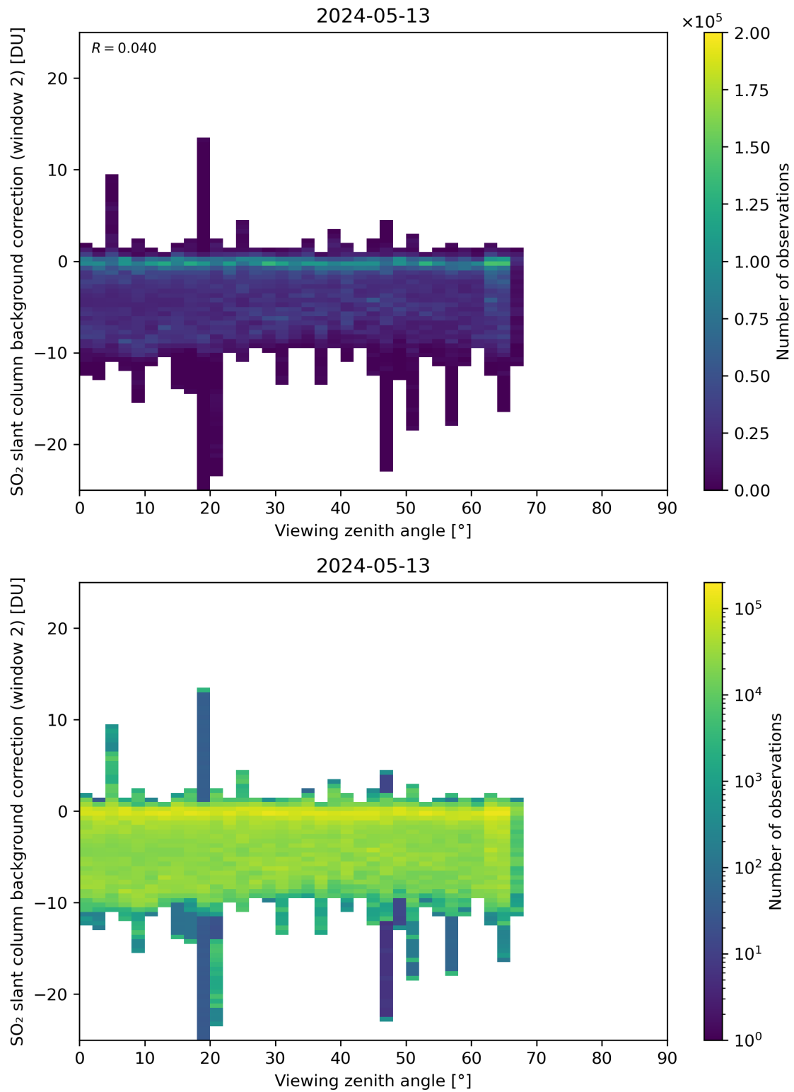
Figure 309: Scatter density plot of “Viewing zenith angle” against “SO 2 slant column background correction (window 2)” for 2024-05-12 to 2024-05-14.
