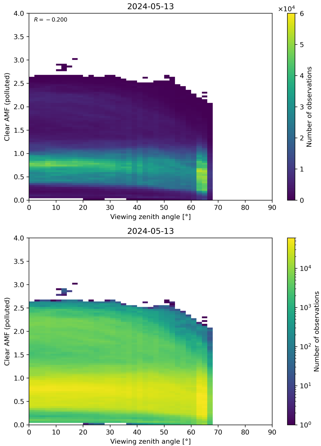
Figure 316: Scatter density plot of “Viewing zenith angle” against “Clear AMF (polluted)” for 2024-05-12 to 2024-05-14.
