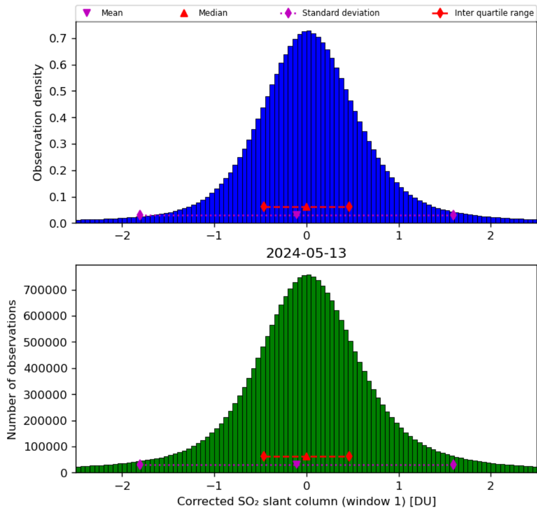
Figure 58: Histogram of “Corrected SO 2 slant column (window 1)” for 2024-05-12 to 2024-05-14
