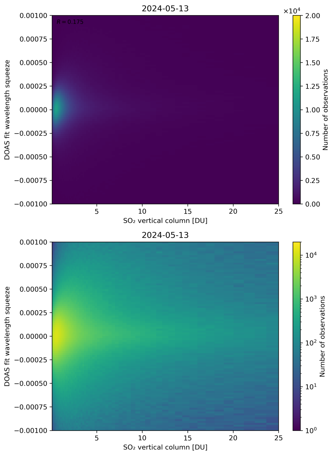
Figure 277: Scatter density plot of “SO 2 vertical column” against “DOAS fit wavelength squeeze” for 2024-05-12 to 2024-05-14.
