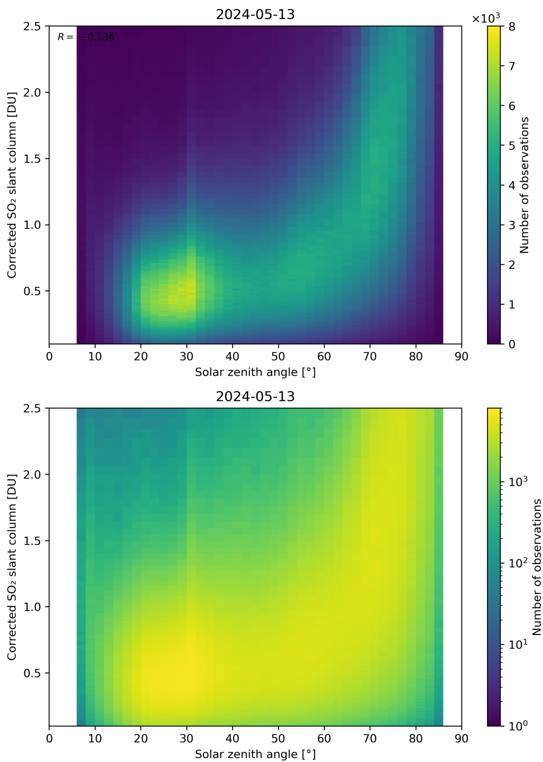
Figure 166: Scatter density plot of “Solar zenith angle” against “Corrected SO 2 slant column” for 2024-05-12 to 2024-05-14.
