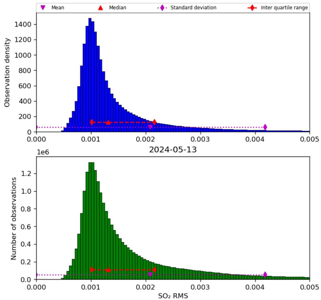
Figure 70: Histogram of “SO 2 RMS” for 2024-05-12 to 2024-05-14
