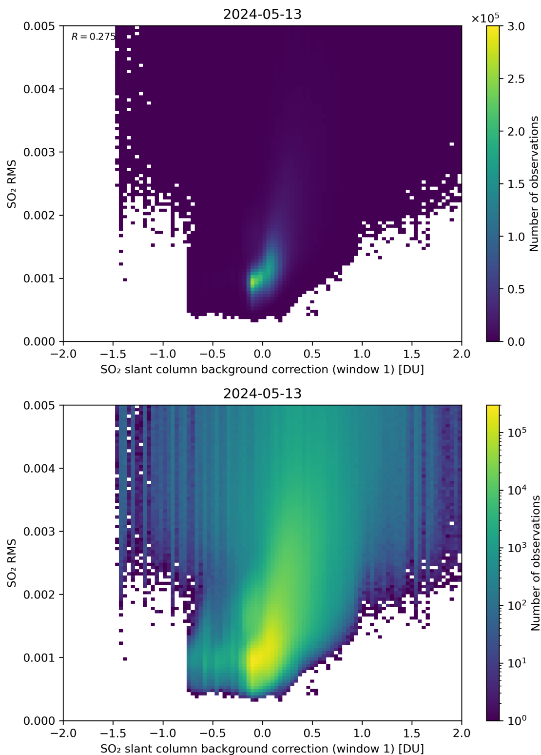
Figure 102: Scatter density plot of “SO 2 slant column background correction (window 1)” against “SO 2 RMS” for 2024-05-12 to 2024-05-14.
