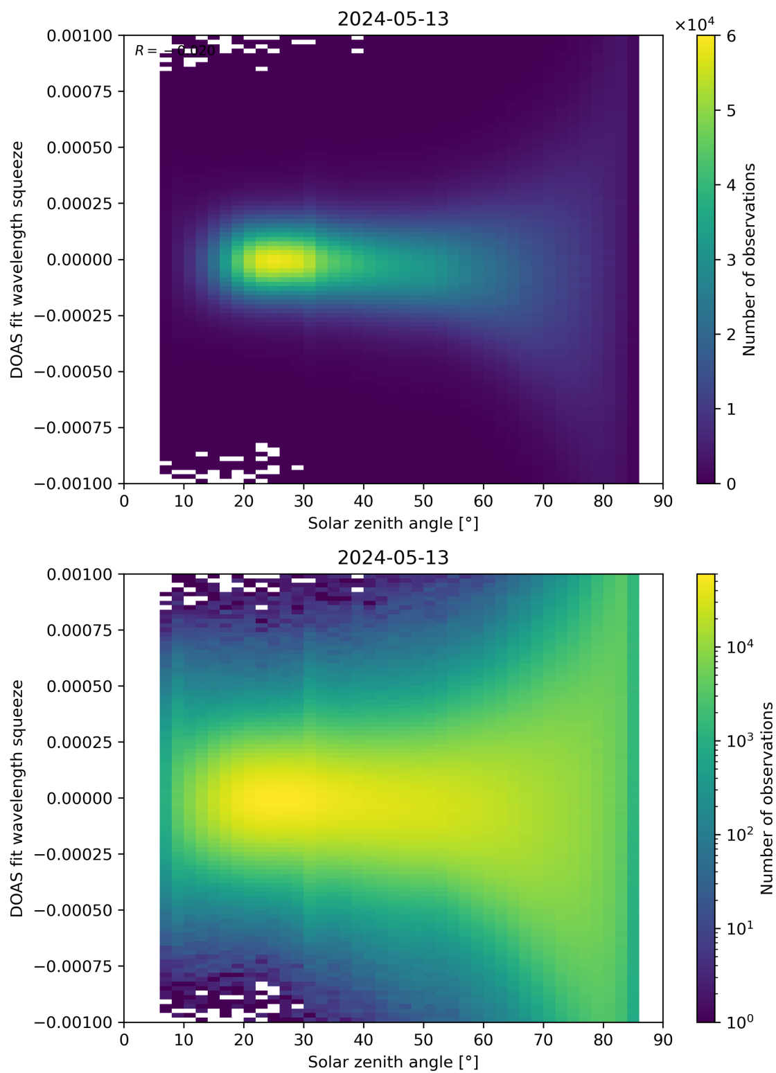
Figure 162: Scatter density plot of “Solar zenith angle” against “DOAS fit wavelength squeeze” for 2024-05-12 to 2024-05-14.
