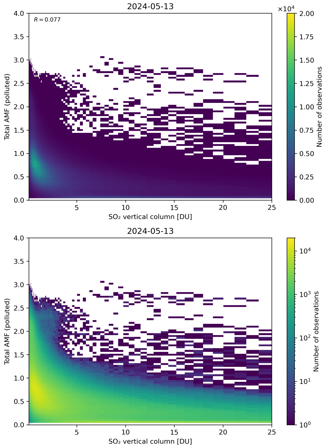
Figure 305: Scatter density plot of “SO 2 vertical column” against “Total AMF (polluted)” for 2024-05-12 to 2024-05-14.
