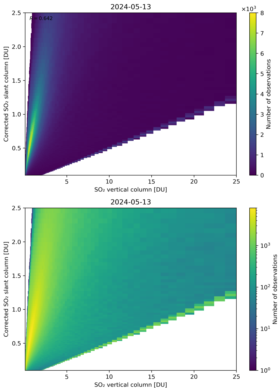
Figure 297: Scatter density plot of “SO 2 vertical column” against “Corrected SO 2 slant column” for 2024-05-12 to 2024-05-14.
