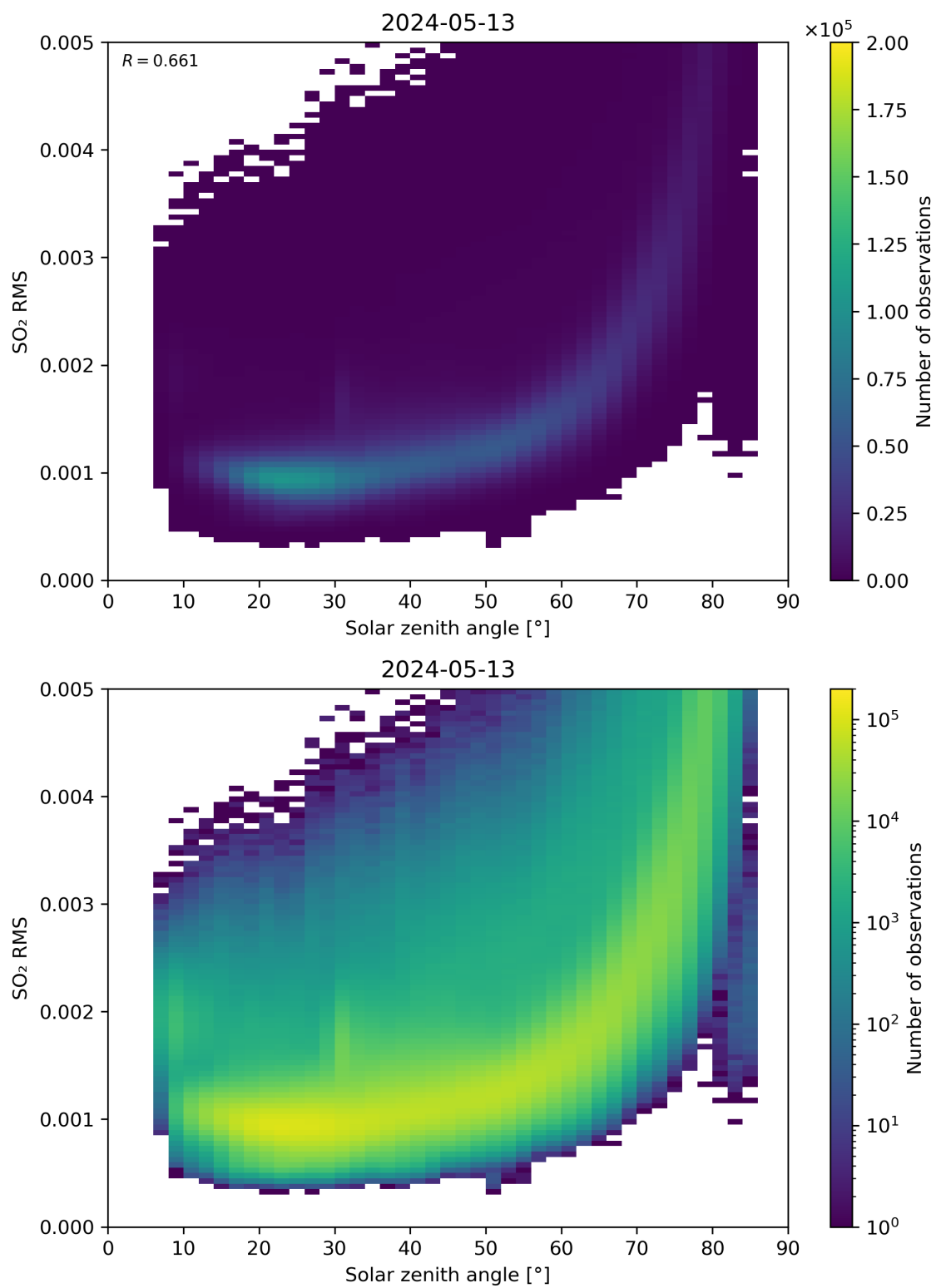
Figure 163: Scatter density plot of “Solar zenith angle” against “SO 2 RMS” for 2024-05-12 to 2024-05-14.
