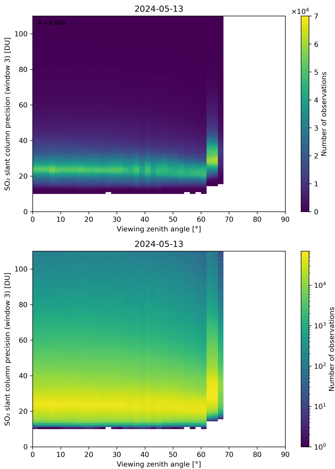
Figure 324: Scatter density plot of “Viewing zenith angle” against “SO 2 slant column precision (window 3)” for 2024-05-12 to 2024-05-14.
