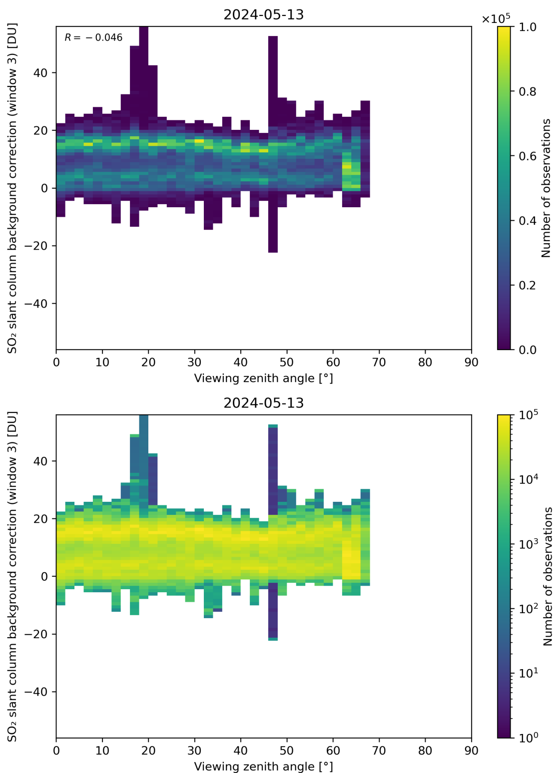
Figure 310: Scatter density plot of “Viewing zenith angle” against “SO 2 slant column background correction (window 3)” for 2024-05-12 to 2024-05-14.
