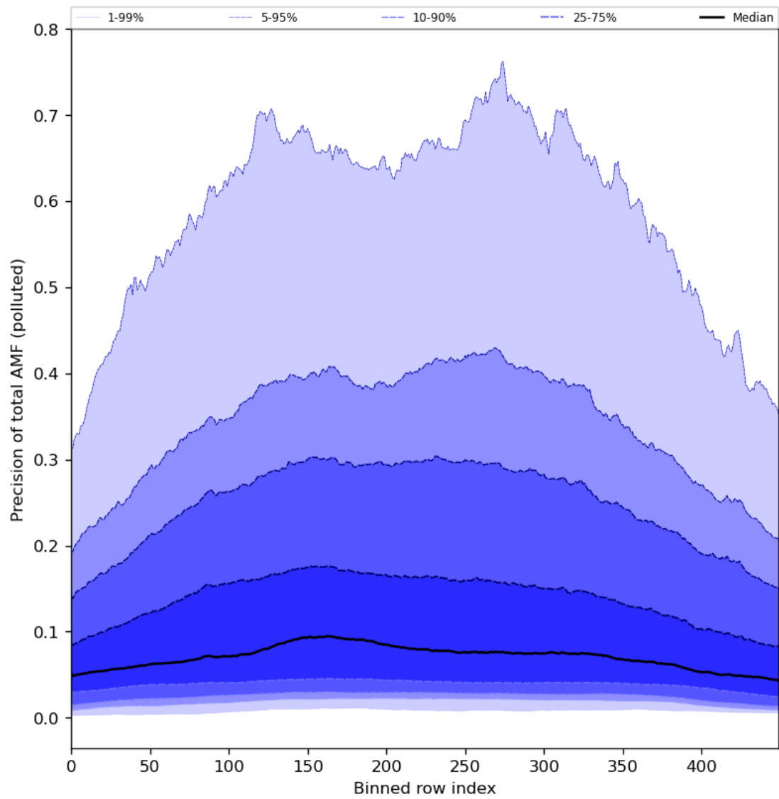
Figure 95: Along track statistics of “Precision of total AMF (polluted)” for 2024-05-12 to 2024-05-14
