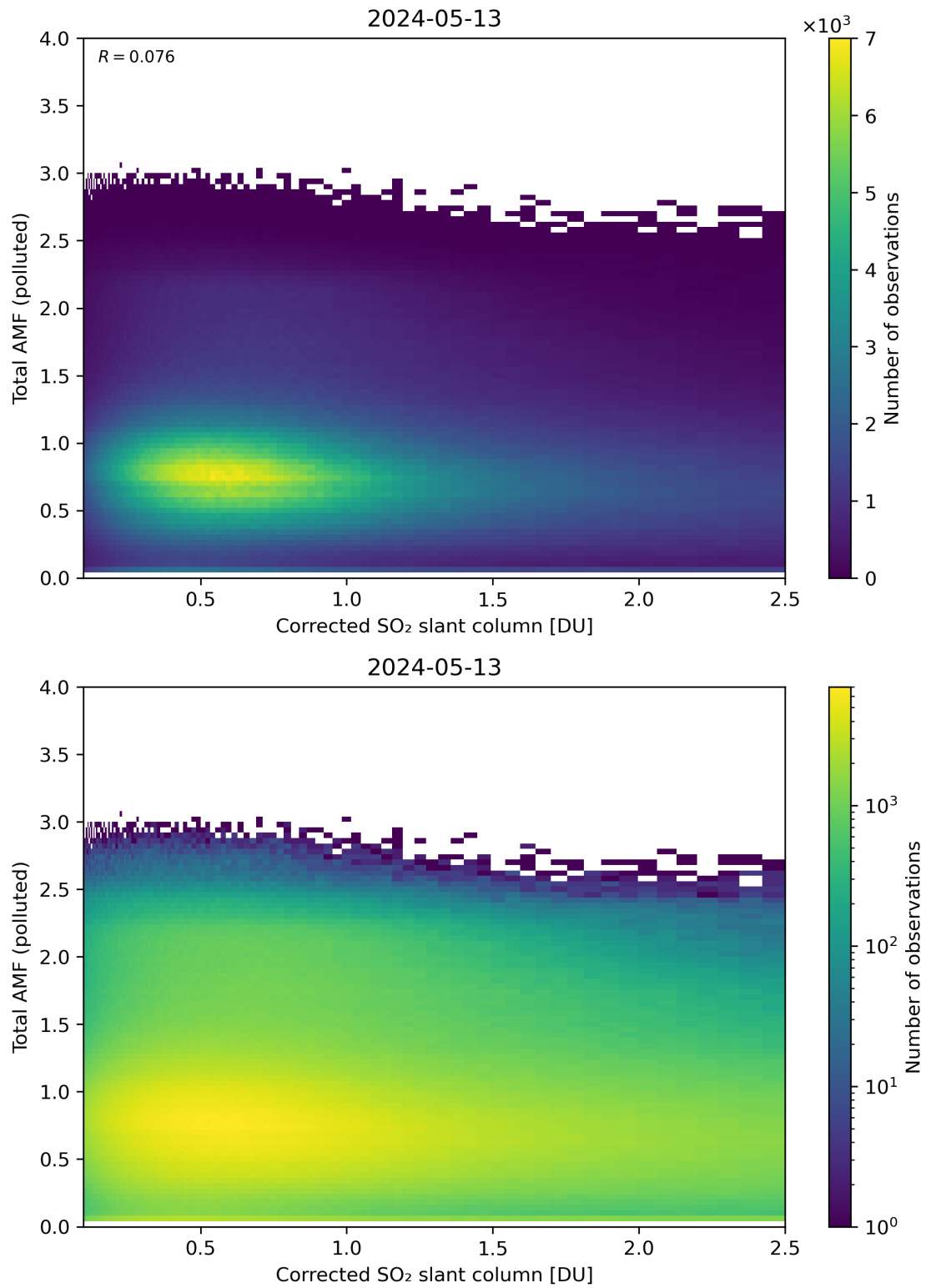
Figure 192: Scatter density plot of “Corrected SO 2 slant column” against “Total AMF (polluted)” for 2024-05-12 to 2024-05-14.
