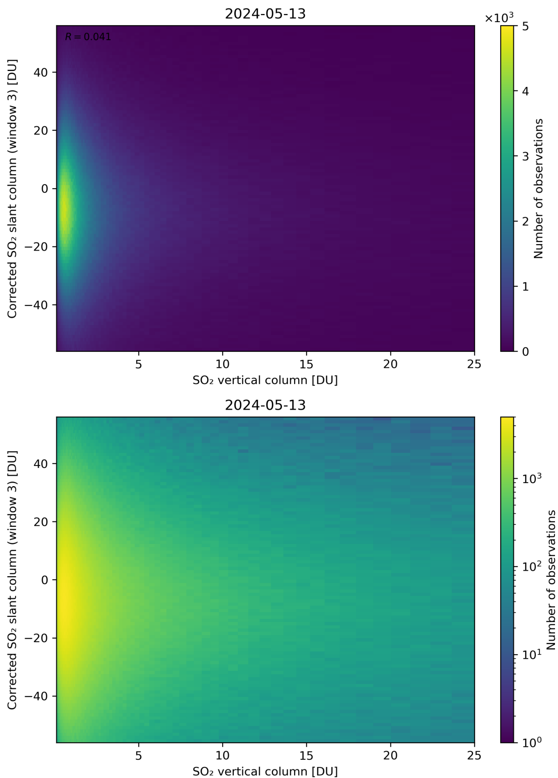
Figure 299: Scatter density plot of “SO 2 vertical column” against “Corrected SO 2 slant column (window 3)” for 2024-05-12 to 2024-05-14.
