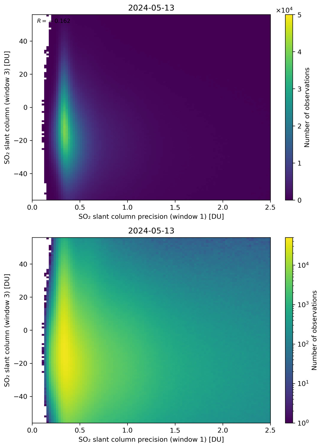
Figure 228: Scatter density plot of “SO 2 slant column precision (window 1)” against “SO 2 slant column (window 3)” for 2024-05-12 to 2024-05-14.
