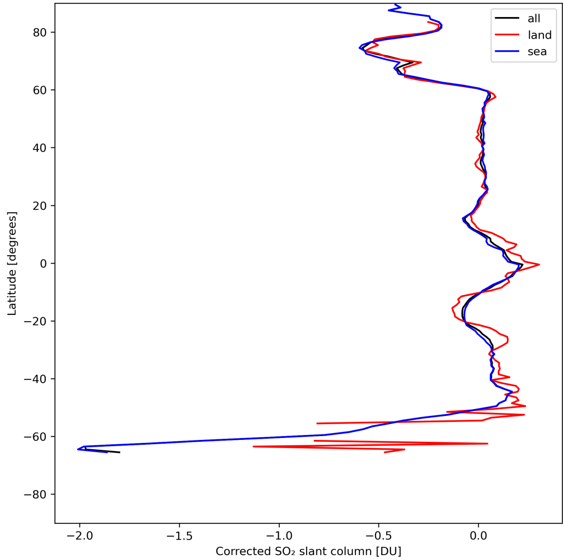
Figure 32: Zonal average of “Corrected SO 2 slant column” for 2024-05-12 to 2024-05-14.
