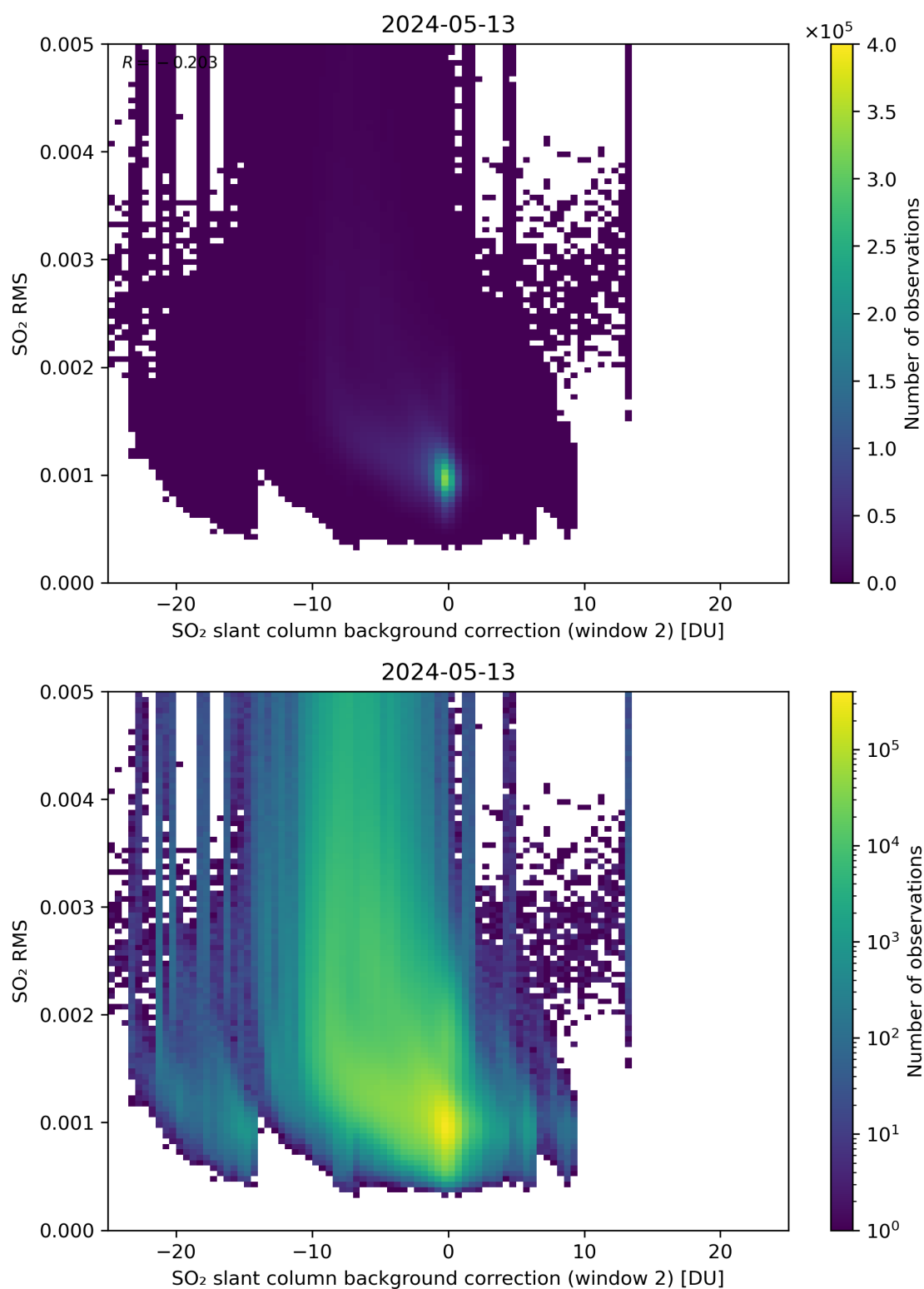
Figure 114: Scatter density plot of “SO 2 slant column background correction (window 2)” against “SO 2 RMS” for 2024-05-12 to 2024-05-14.
