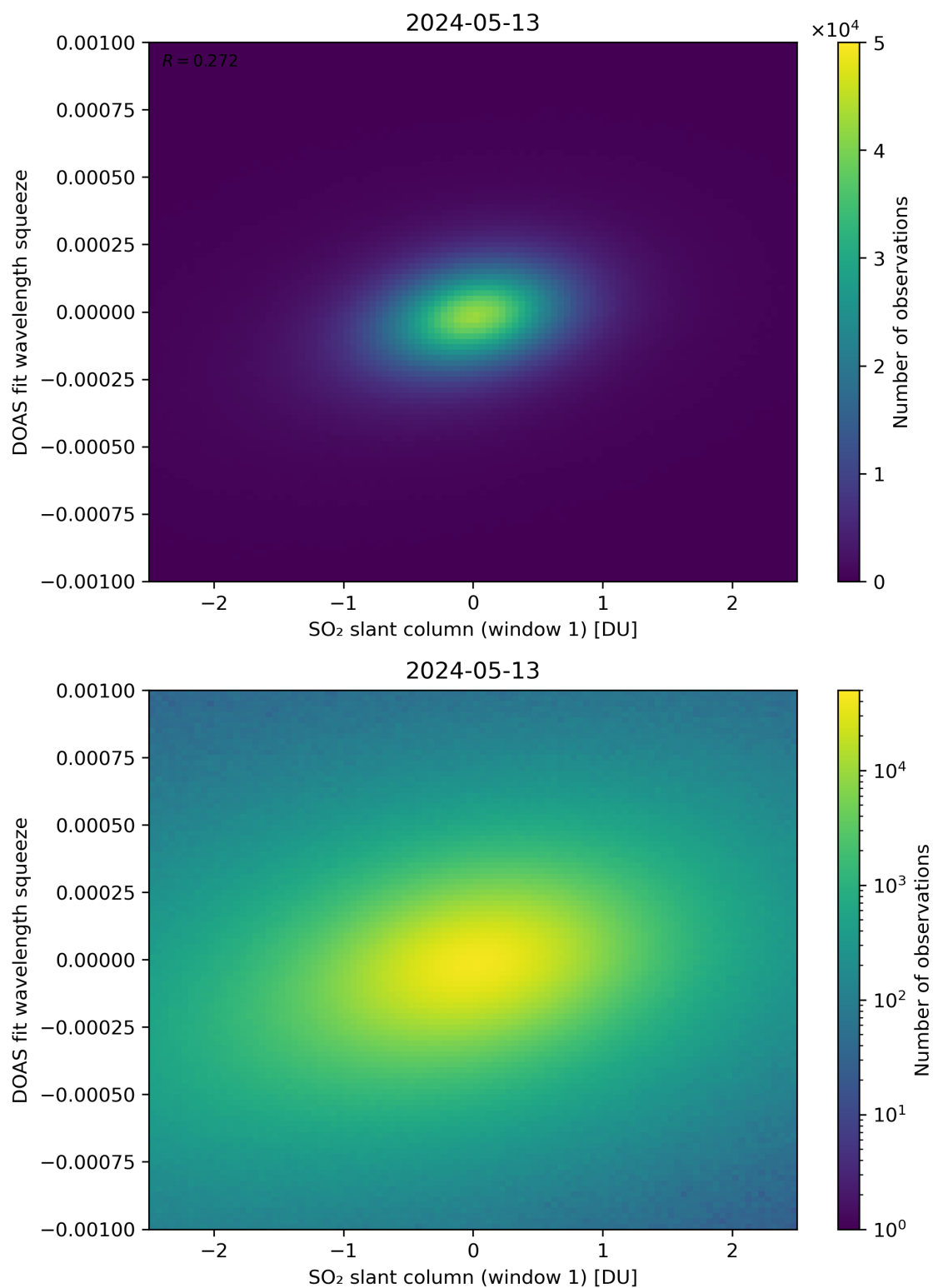
Figure 216: Scatter density plot of “SO 2 slant column (window 1)” against “DOAS fit wavelength squeeze” for 2024-05-12 to 2024-05-14.
