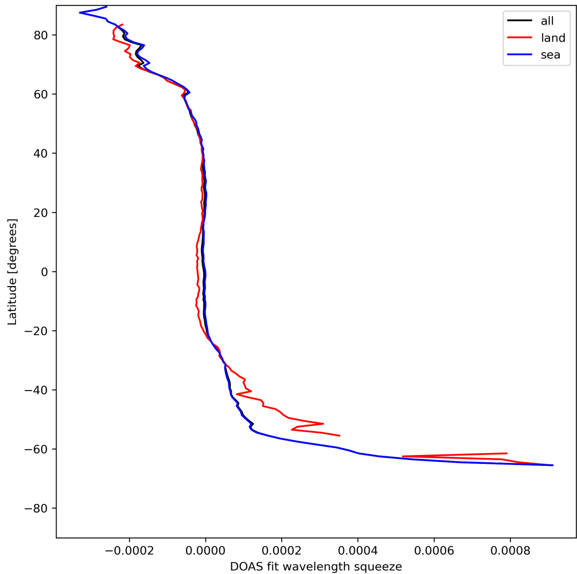
Figure 46: Zonal average of “DOAS fit wavelength squeeze” for 2024-05-12 to 2024-05-14.
