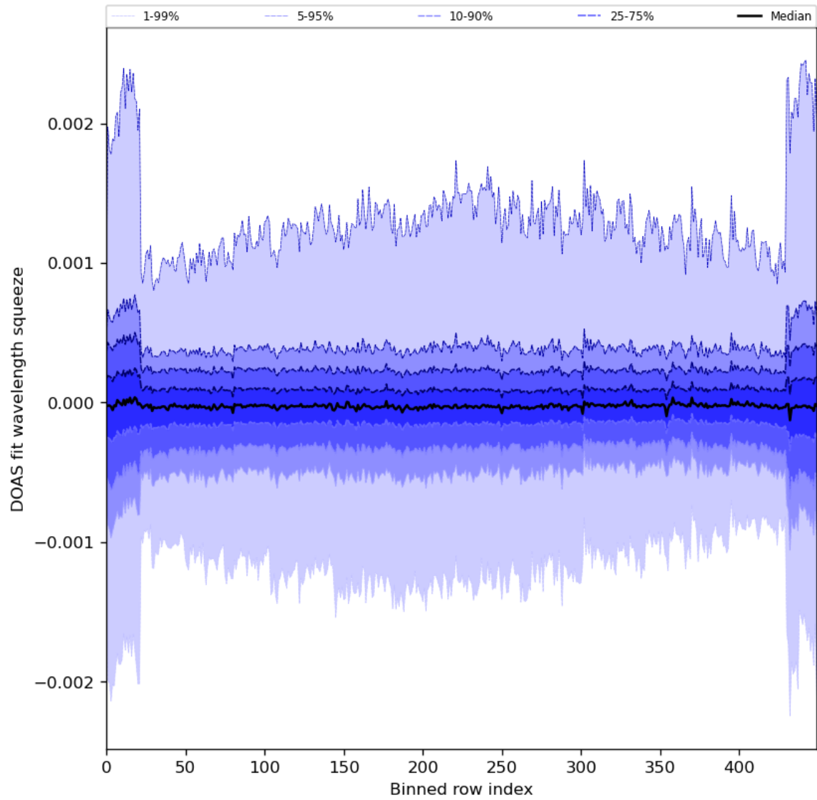
Figure 92: Along track statistics of “DOAS fit wavelength squeeze” for 2024-05-12 to 2024-05-14
