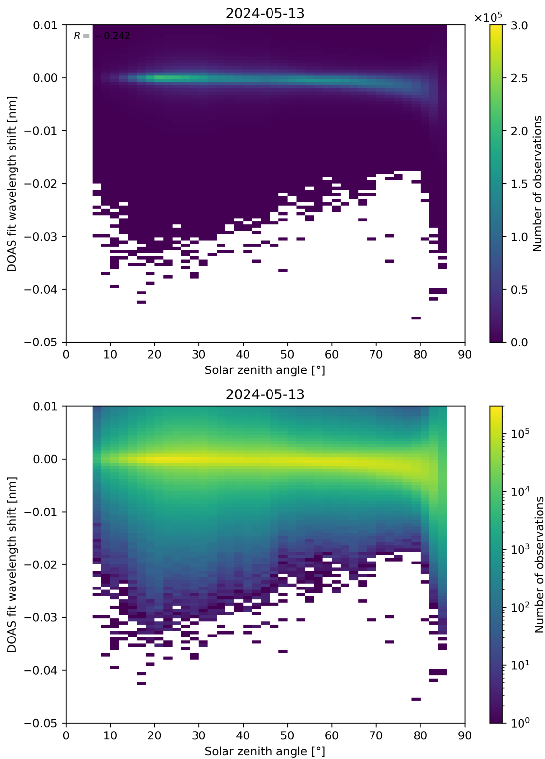
Figure 161: Scatter density plot of “Solar zenith angle” against “DOAS fit wavelength shift” for 2024-05-12 to 2024-05-14.
