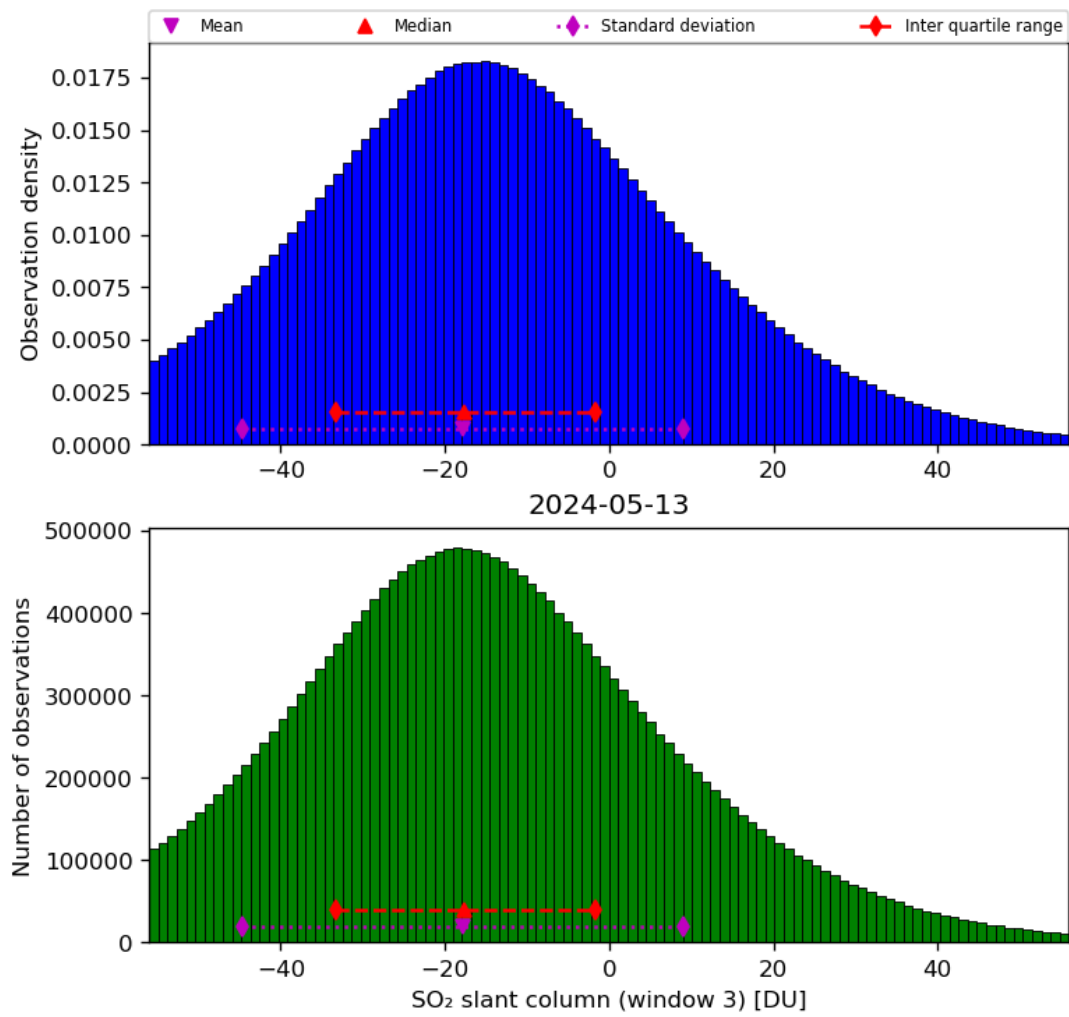
Figure 64: Histogram of “SO 2 slant column (window 3)” for 2024-05-12 to 2024-05-14
