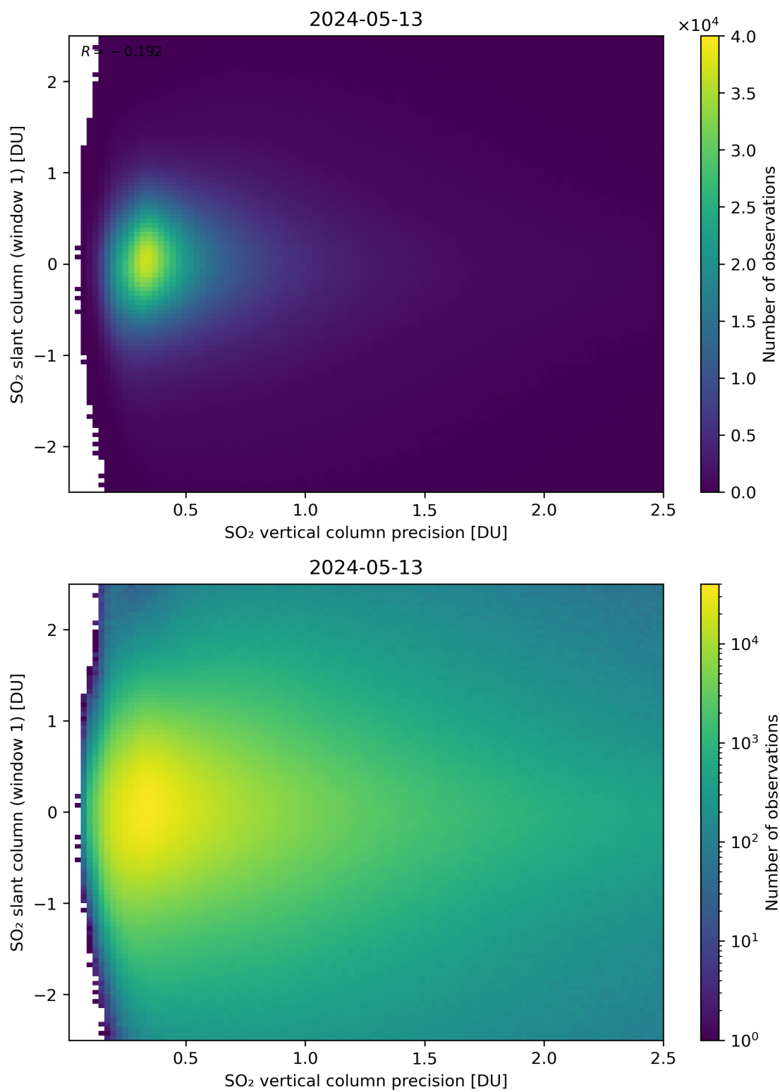
Figure 289: Scatter density plot of “SO 2 vertical column precision” against “SO 2 slant column (window 1)” for 2024-05-12 to 2024-05-14.
