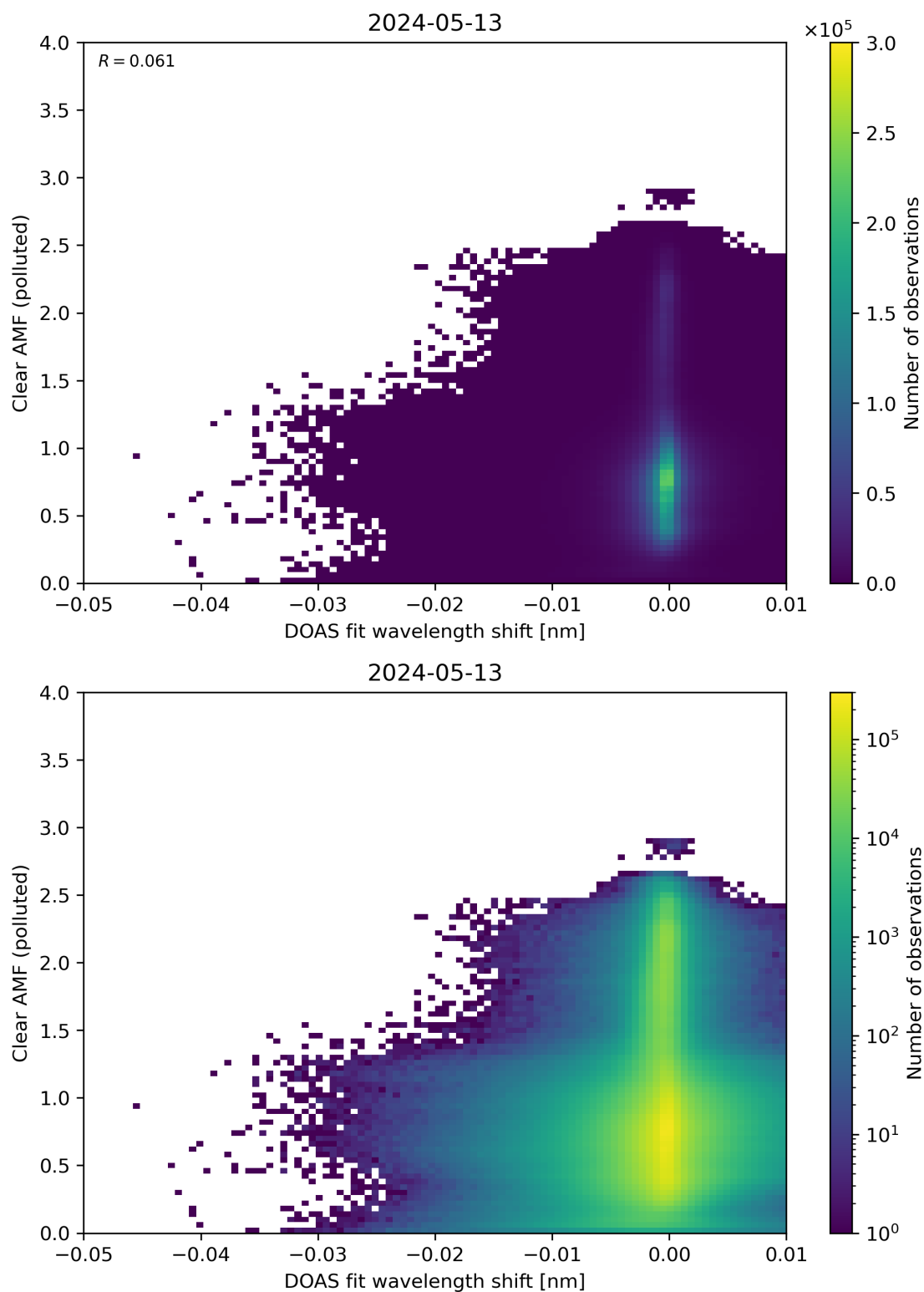
Figure 129: Scatter density plot of “DOAS fit wavelength shift” against “Clear AMF (polluted)” for 2024-05-12 to 2024-05-14.
