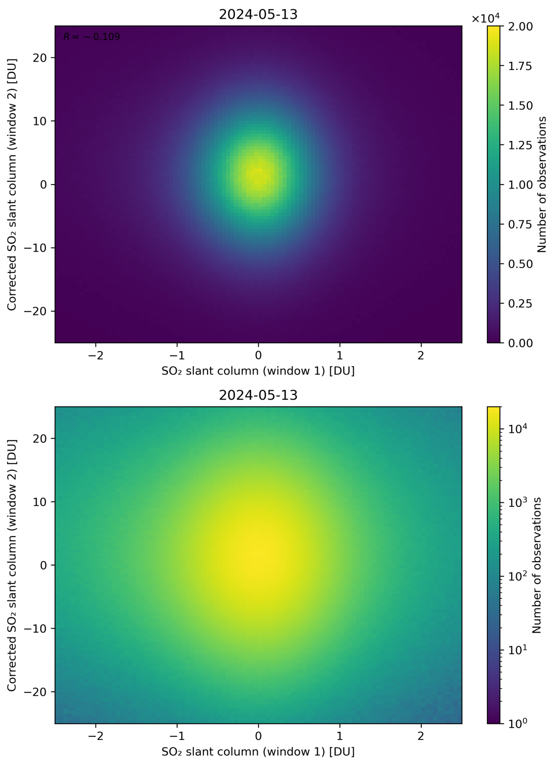
Figure 233: Scatter density plot of “SO 2 slant column (window 1)” against “Corrected SO 2 slant column (window 2)” for 2024-05-12 to 2024-05-14.
