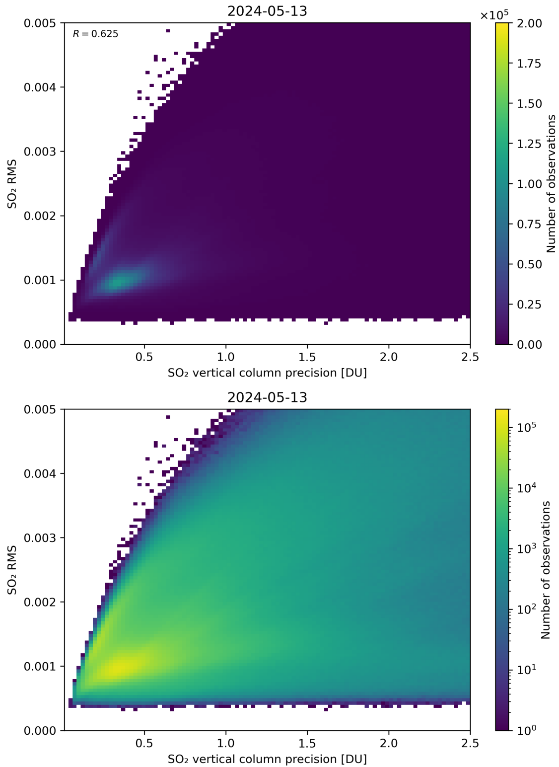
Figure 284: Scatter density plot of “SO 2 vertical column precision” against “SO 2 RMS” for 2024-05-12 to 2024-05-14.
