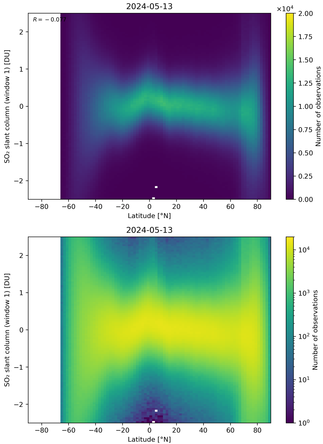
Figure 149: Scatter density plot of “Latitude” against “SO 2 slant column (window 1)” for 2024-05-12 to 2024-05-14.
