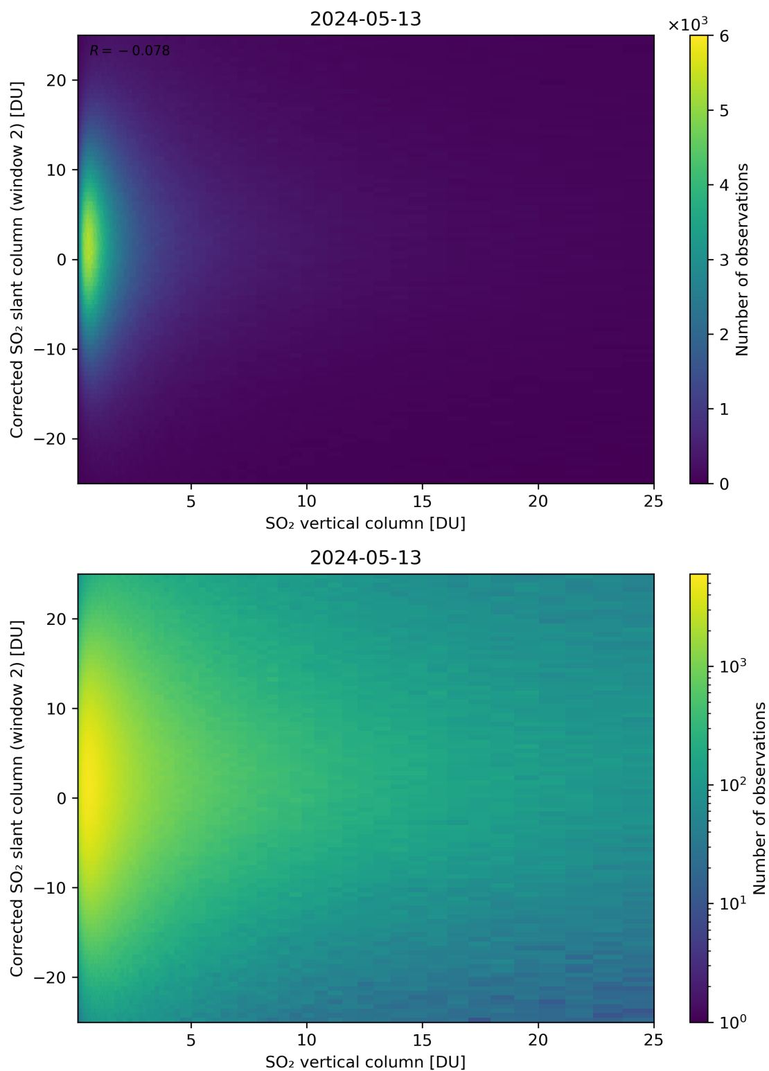
Figure 298: Scatter density plot of “SO 2 vertical column” against “Corrected SO 2 slant column (window 2)” for 2024-05-12 to 2024-05-14.
