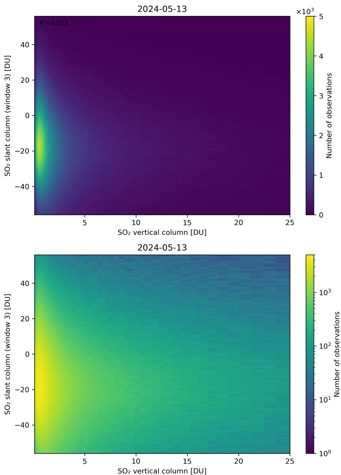
Figure 303: Scatter density plot of “SO 2 vertical column” against “SO 2 slant column (window 3)” for 2024-05-12 to 2024-05-14.
