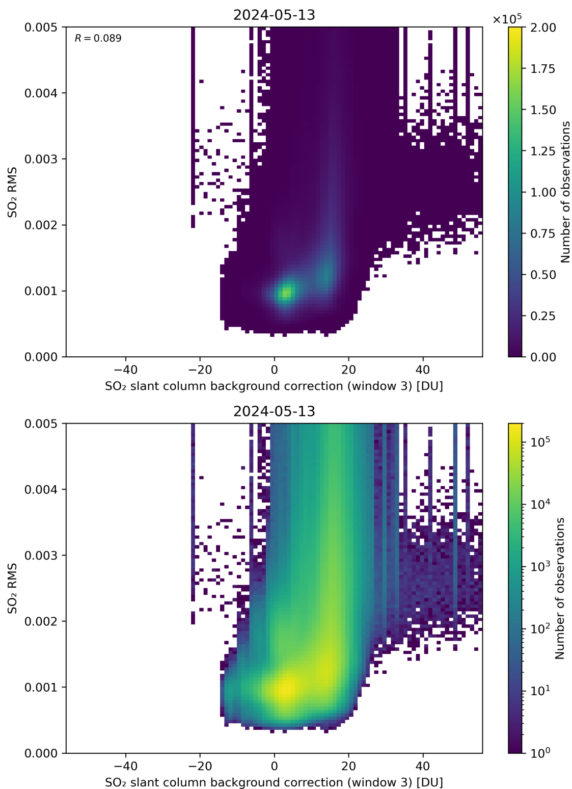
Figure 123: Scatter density plot of “SO 2 slant column background correction (window 3)” against “SO 2 RMS” for 2024-05-12 to 2024-05-14.
