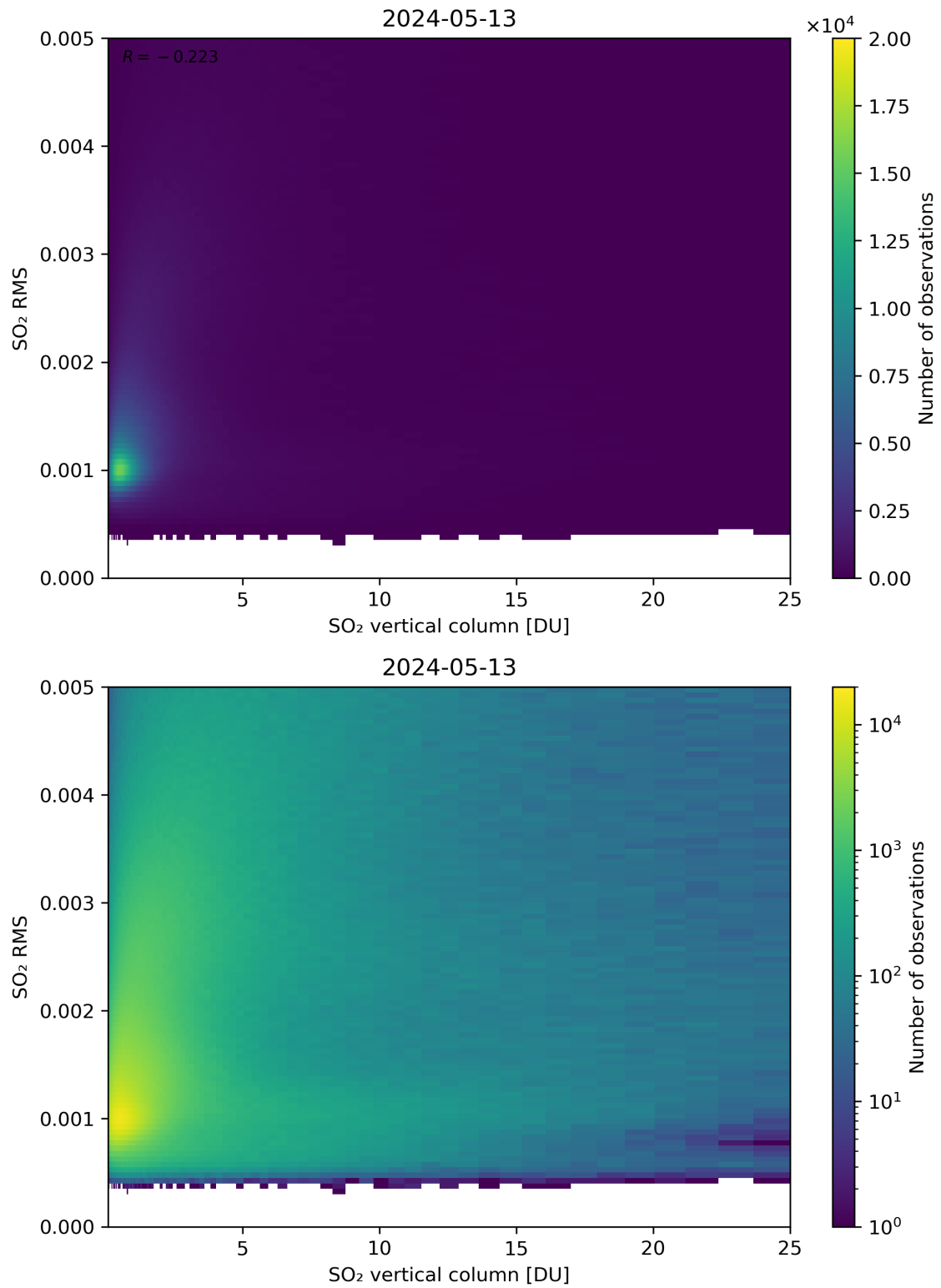
Figure 278: Scatter density plot of “SO 2 vertical column” against “SO 2 RMS” for 2024-05-12 to 2024-05-14.
