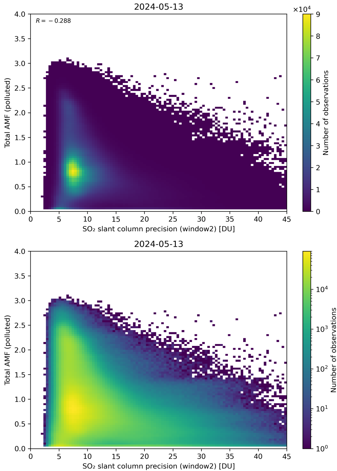
Figure 251: Scatter density plot of “SO 2 slant column precision (window2)” against “Total AMF (polluted)” for 2024-05-12 to 2024-05-14.
