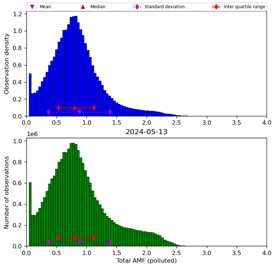
Figure 71: Histogram of “Total AMF (polluted)” for 2024-05-12 to 2024-05-14
