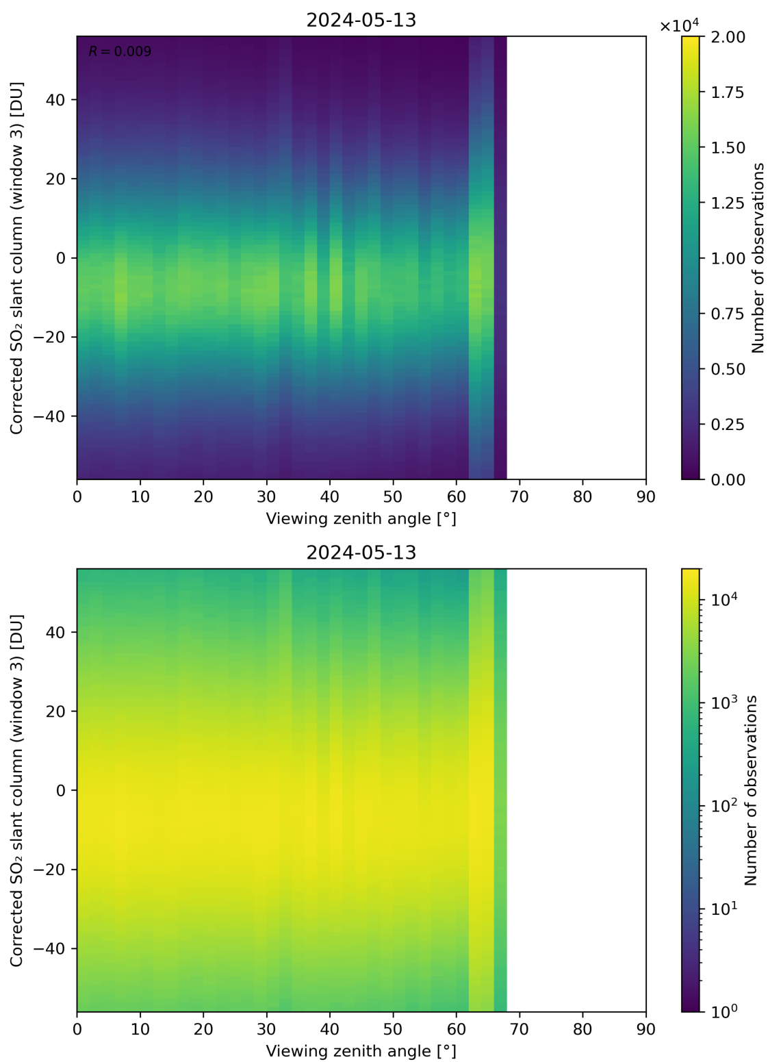
Figure 319: Scatter density plot of “Viewing zenith angle” against “Corrected SO 2 slant column (window 3)” for 2024-05-12 to 2024-05-14.
