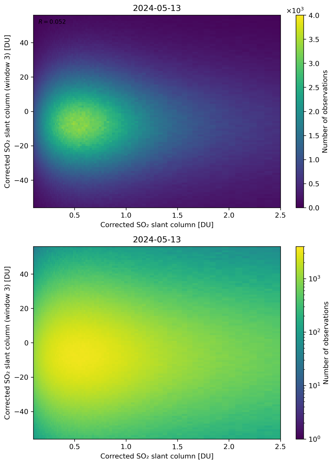
Figure 186: Scatter density plot of “Corrected SO 2 slant column” against “Corrected SO 2 slant column (window 3)” for 2024-05-12 to 2024-05-14.
