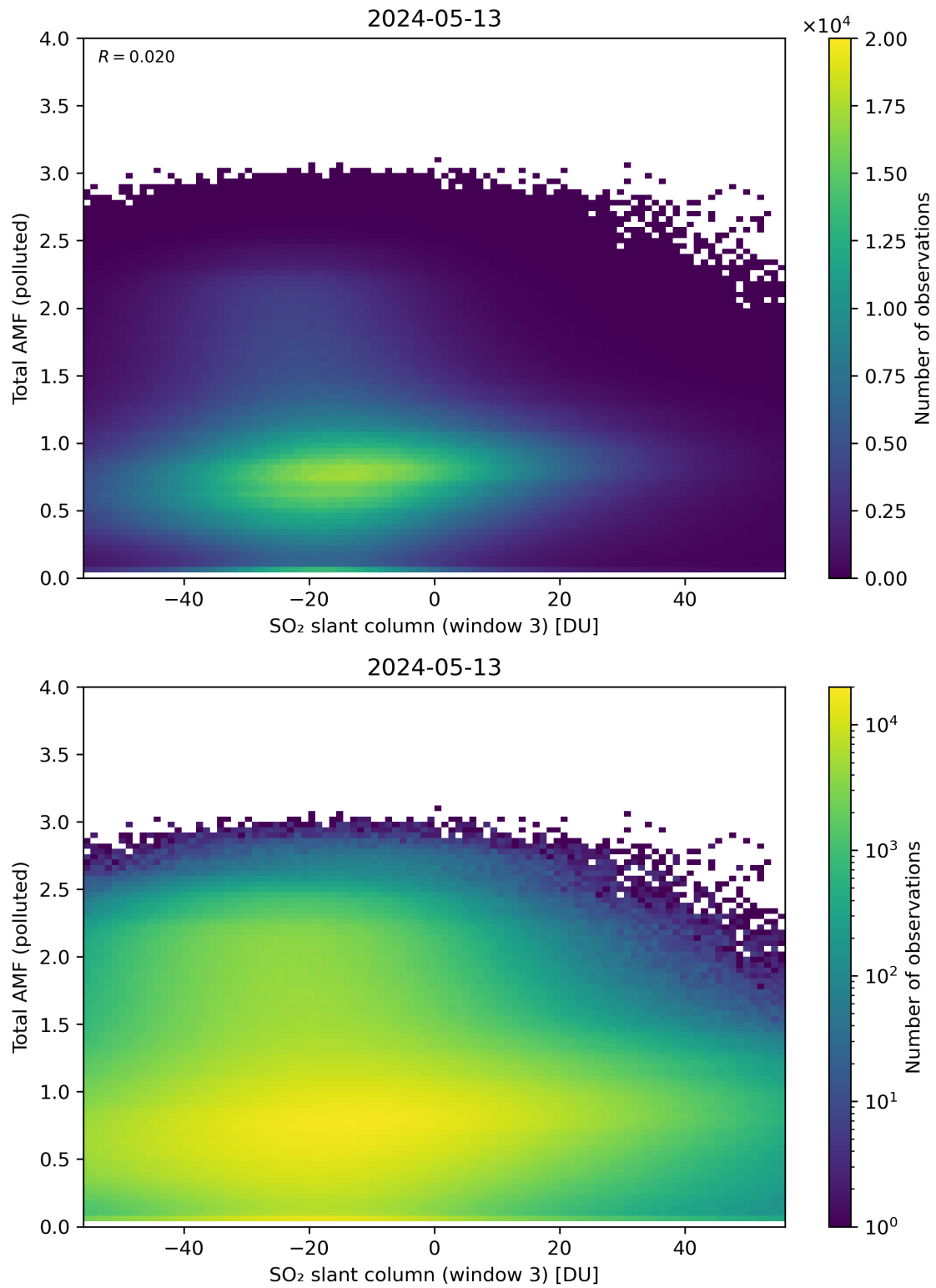
Figure 268: Scatter density plot of “SO 2 slant column (window 3)” against “Total AMF (polluted)” for 2024-05-12 to 2024-05-14.
