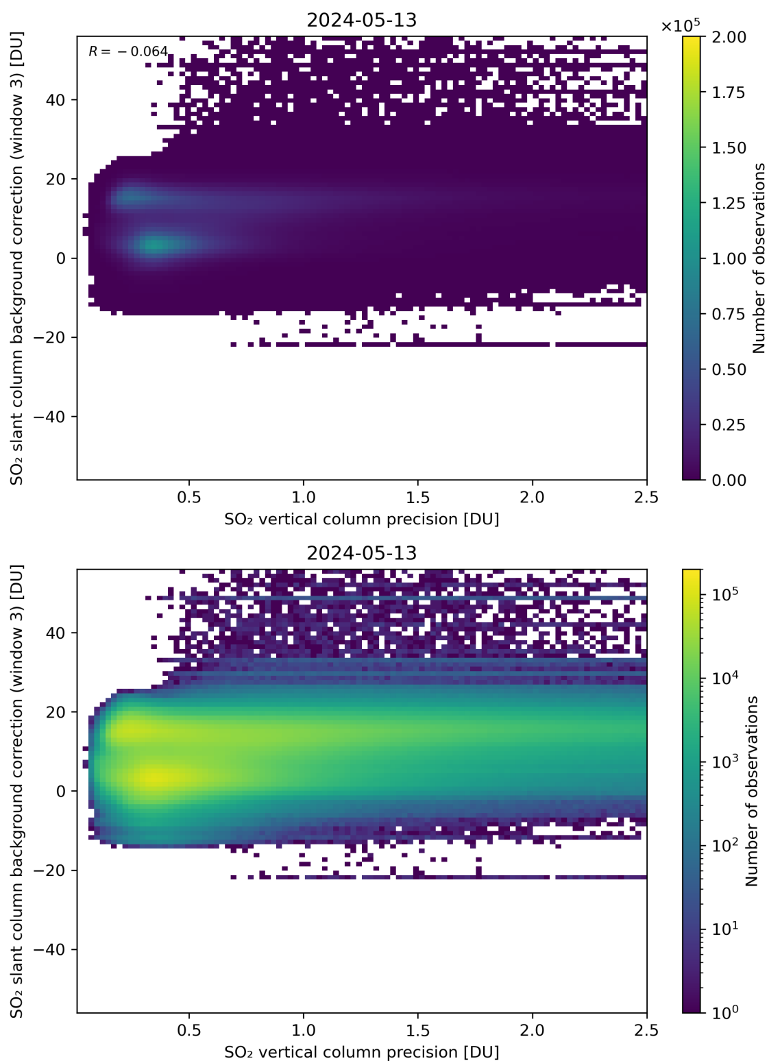
Figure 281: Scatter density plot of “SO 2 vertical column precision” against “SO 2 slant column background correction (window 3)” for 2024-05-12 to 2024-05-14.
