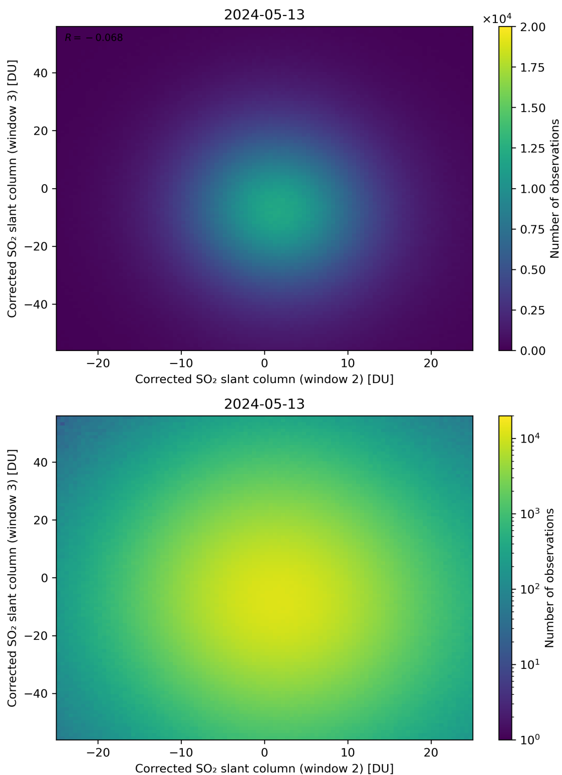
Figure 200: Scatter density plot of “Corrected SO 2 slant column (window 2)” against “Corrected SO 2 slant column (window 3)” for 2024-05-12 to 2024-05-14.
