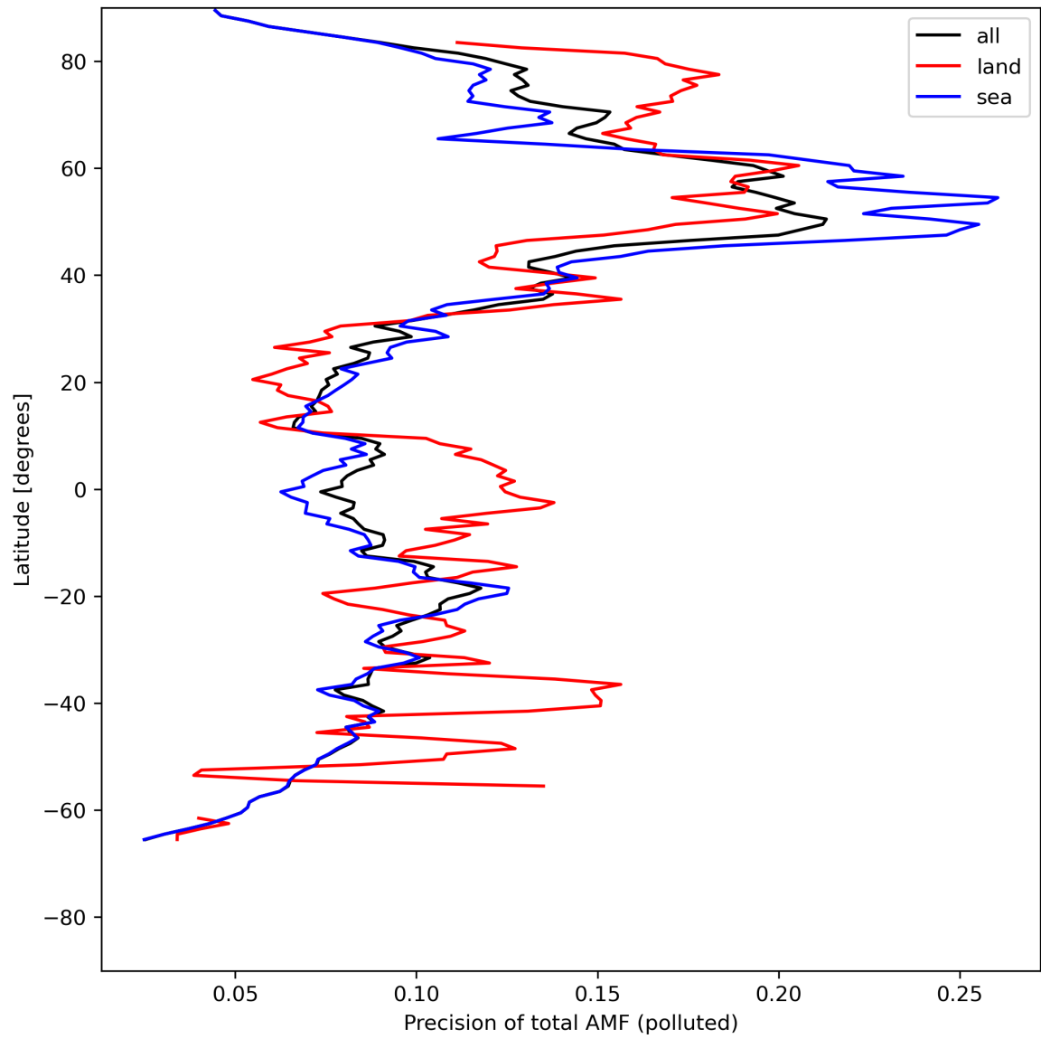
Figure 49: Zonal average of “Precision of total AMF (polluted)” for 2024-05-12 to 2024-05-14.
