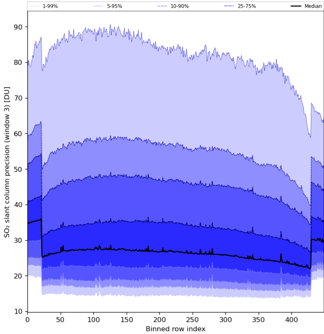
Figure 88: Along track statistics of “SO 2 slant column precision (window 3)” for 2024-05-12 to 2024-05-14
