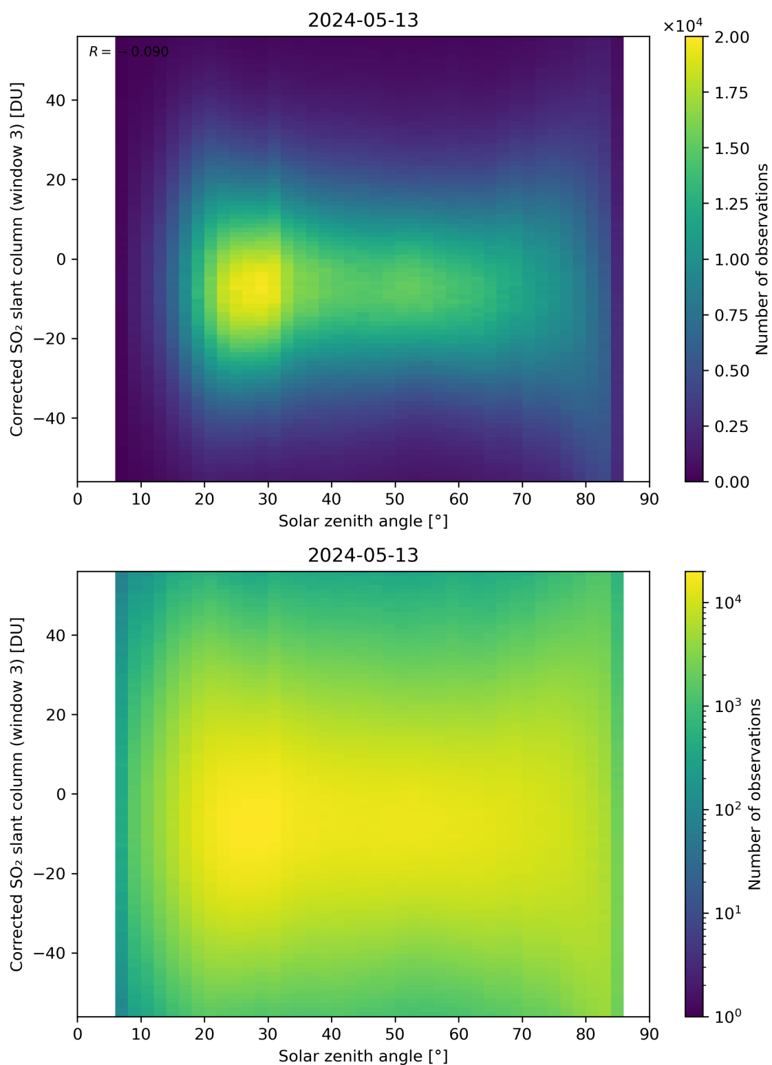
Figure 168: Scatter density plot of “Solar zenith angle” against “Corrected SO 2 slant column (window 3)” for 2024-05-12 to 2024-05-14.
