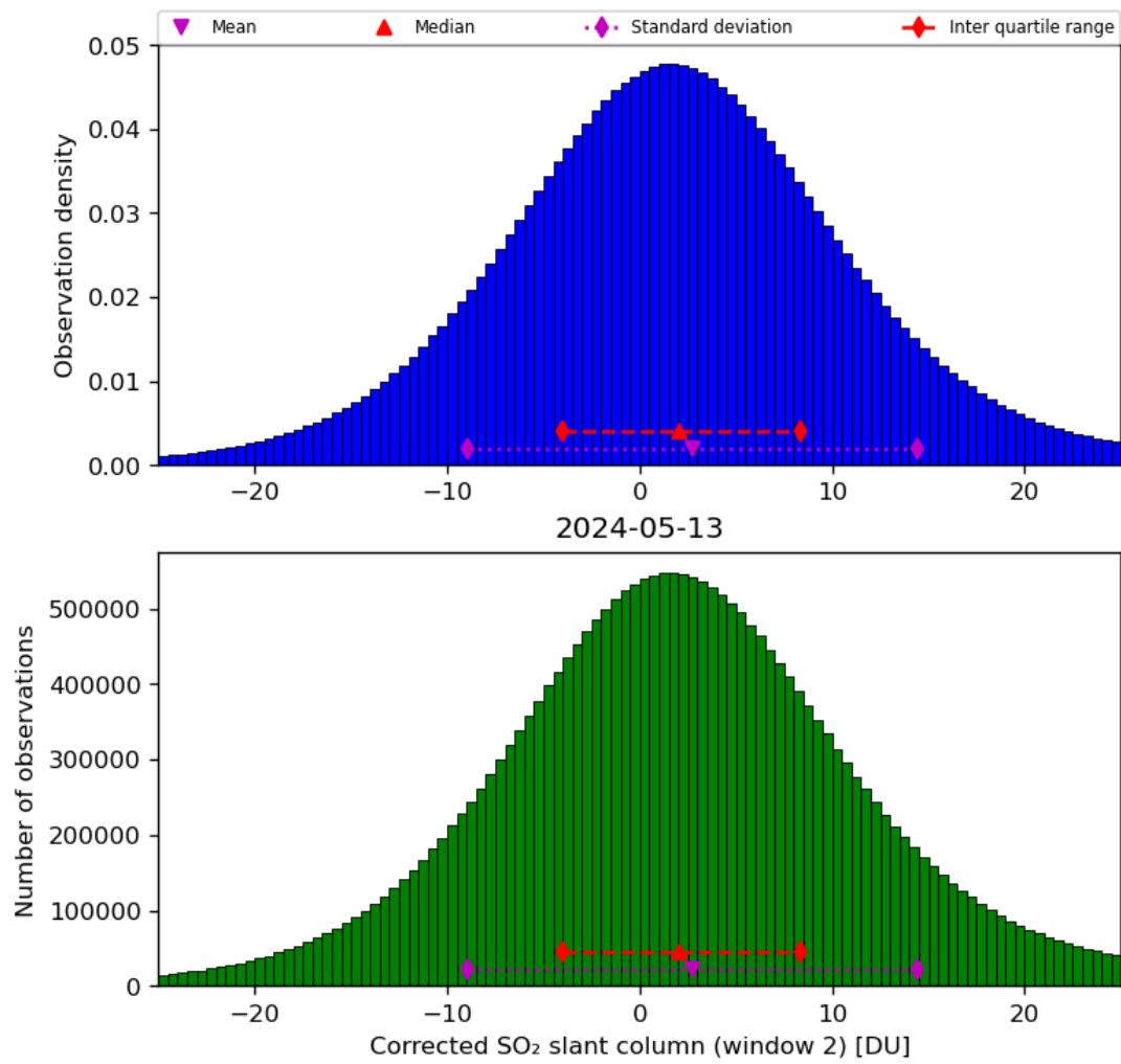
Figure 62: Histogram of “Corrected SO 2 slant column (window 2)” for 2024-05-12 to 2024-05-14
