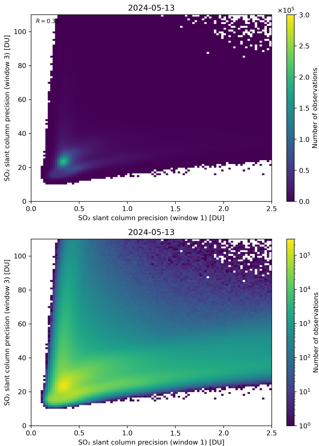
Figure 229: Scatter density plot of “SO 2 slant column precision (window 1)” against “SO 2 slant column precision (window 3)” for 2024-05-12 to 2024-05-14.
