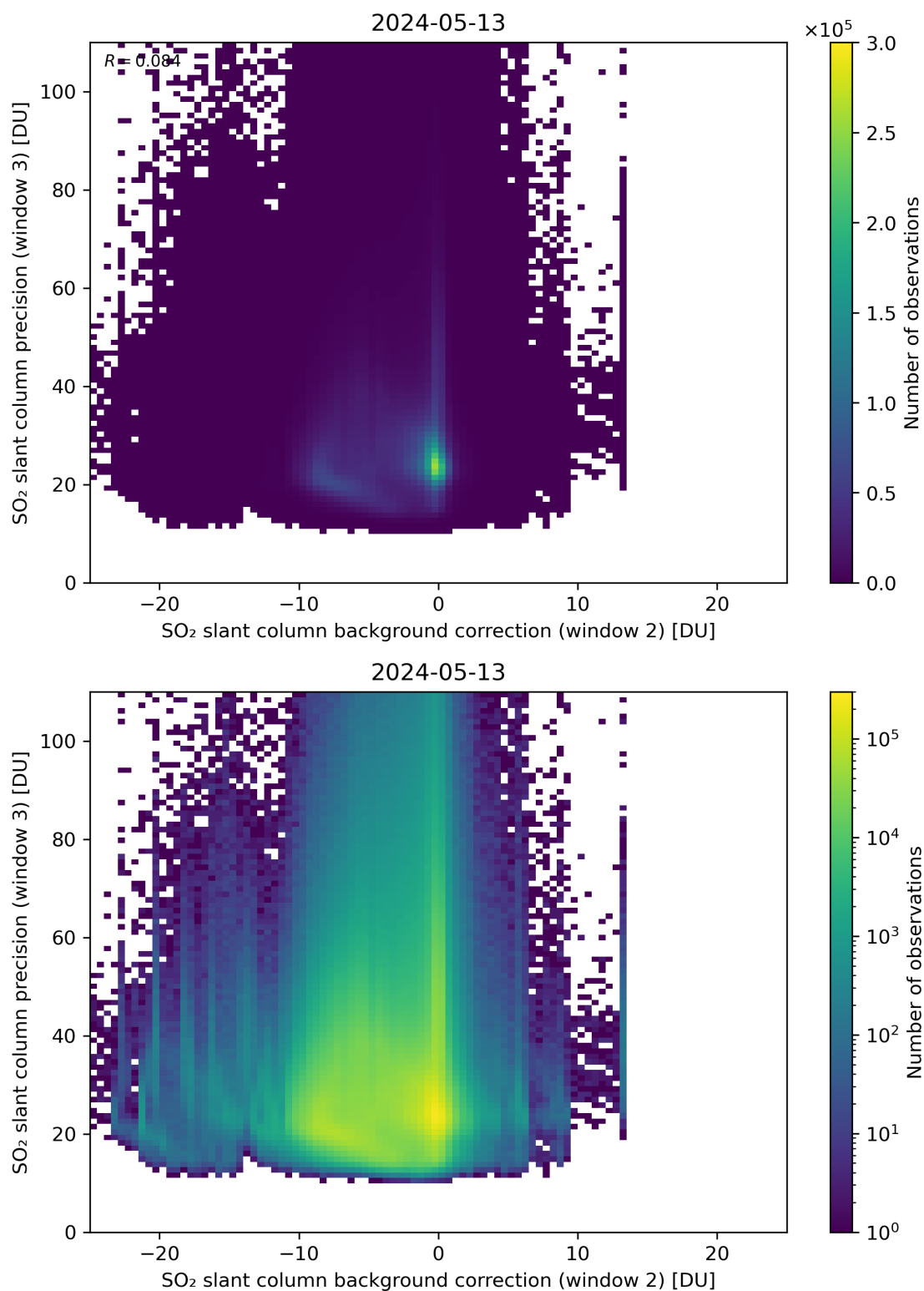
Figure 118: Scatter density plot of “SO 2 slant column background correction (window 2)” against “SO 2 slant column precision (window 3)” for 2024-05-12 to 2024-05-14.
