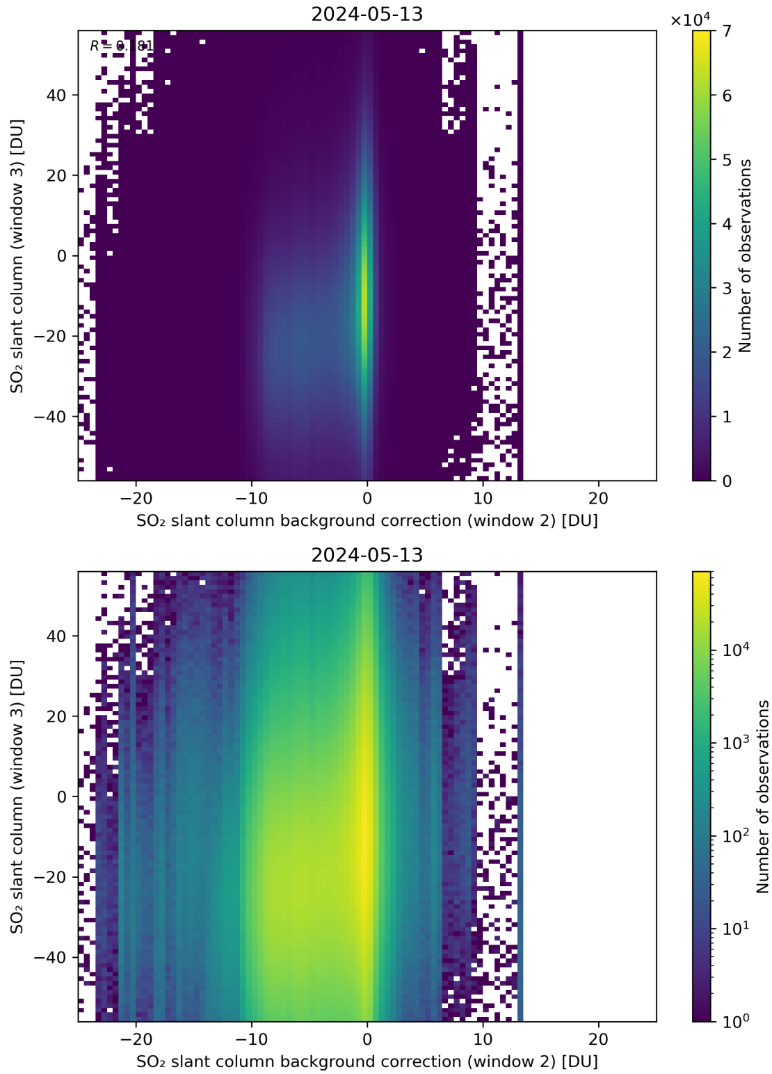
Figure 117: Scatter density plot of “SO 2 slant column background correction (window 2)” against “SO 2 slant column (window 3)” for 2024-05-12 to 2024-05-14.
