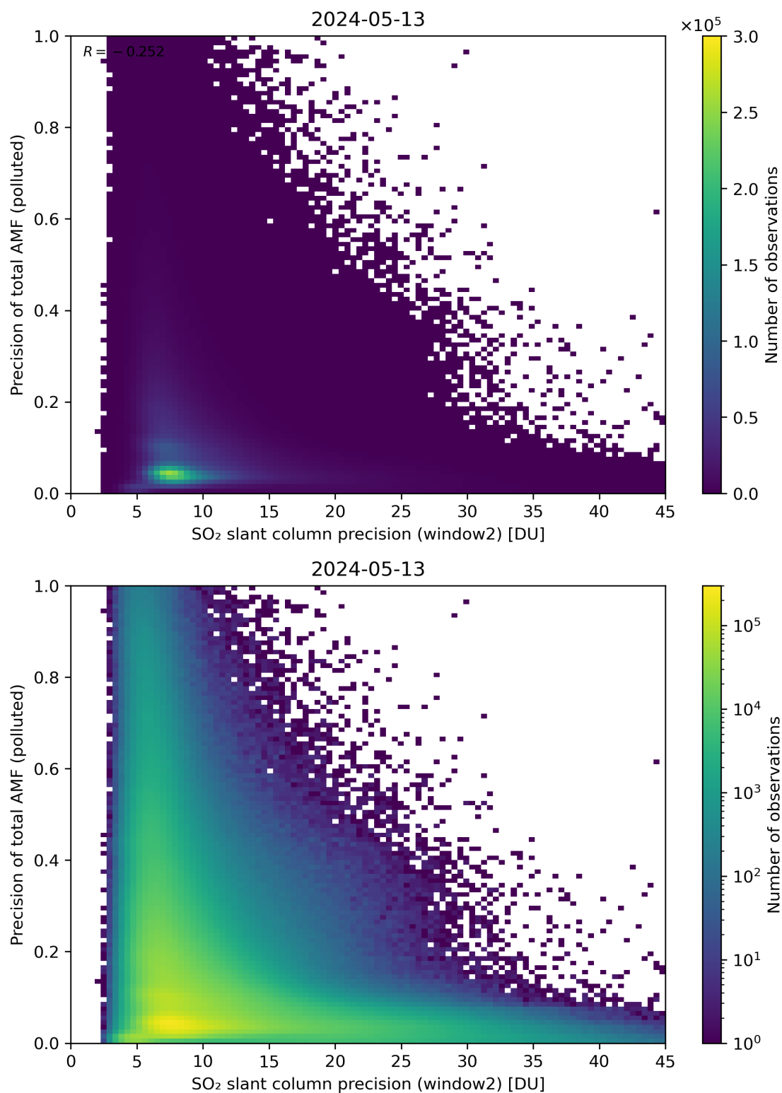
Figure 252: Scatter density plot of “SO 2 slant column precision (window2)” against “Precision of total AMF (polluted)” for 2024-05-12 to 2024-05-14.
