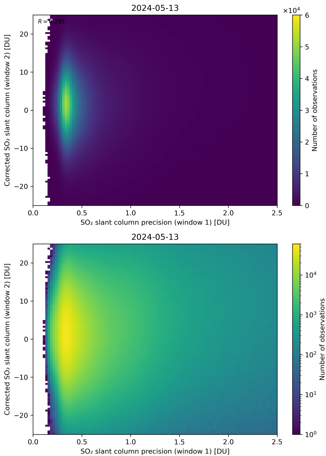
Figure 225: Scatter density plot of “SO 2 slant column precision (window 1)” against “Corrected SO 2 slant column (window 2)” for 2024-05-12 to 2024-05-14.
