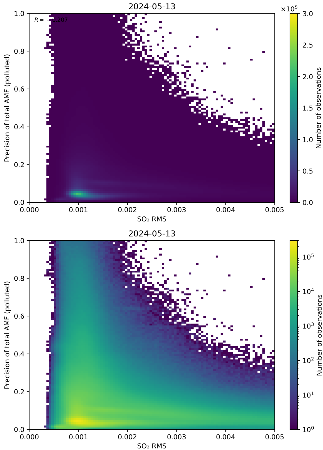
Figure 138: Scatter density plot of “SO 2 RMS” against “Precision of total AMF (polluted)” for 2024-05-12 to 2024-05-14.
