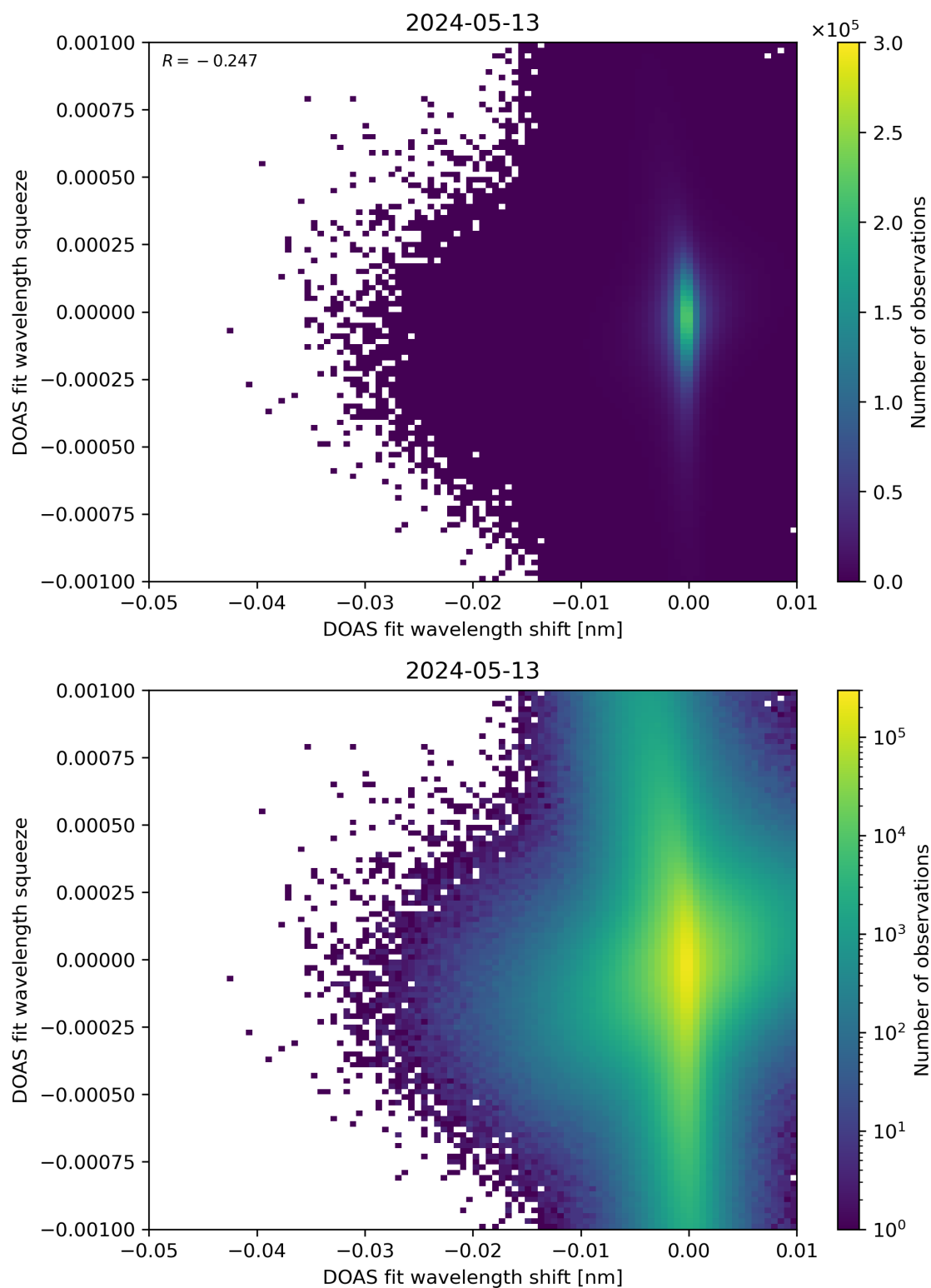
Figure 127: Scatter density plot of “DOAS fit wavelength shift” against “DOAS fit wavelength squeeze” for 2024-05-12 to 2024-05-14.
