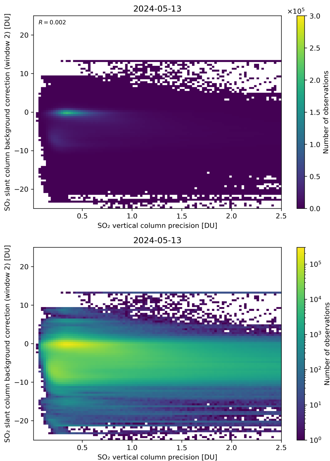
Figure 280: Scatter density plot of “SO 2 vertical column precision” against “SO 2 slant column background correction (window 2)” for 2024-05-12 to 2024-05-14.
