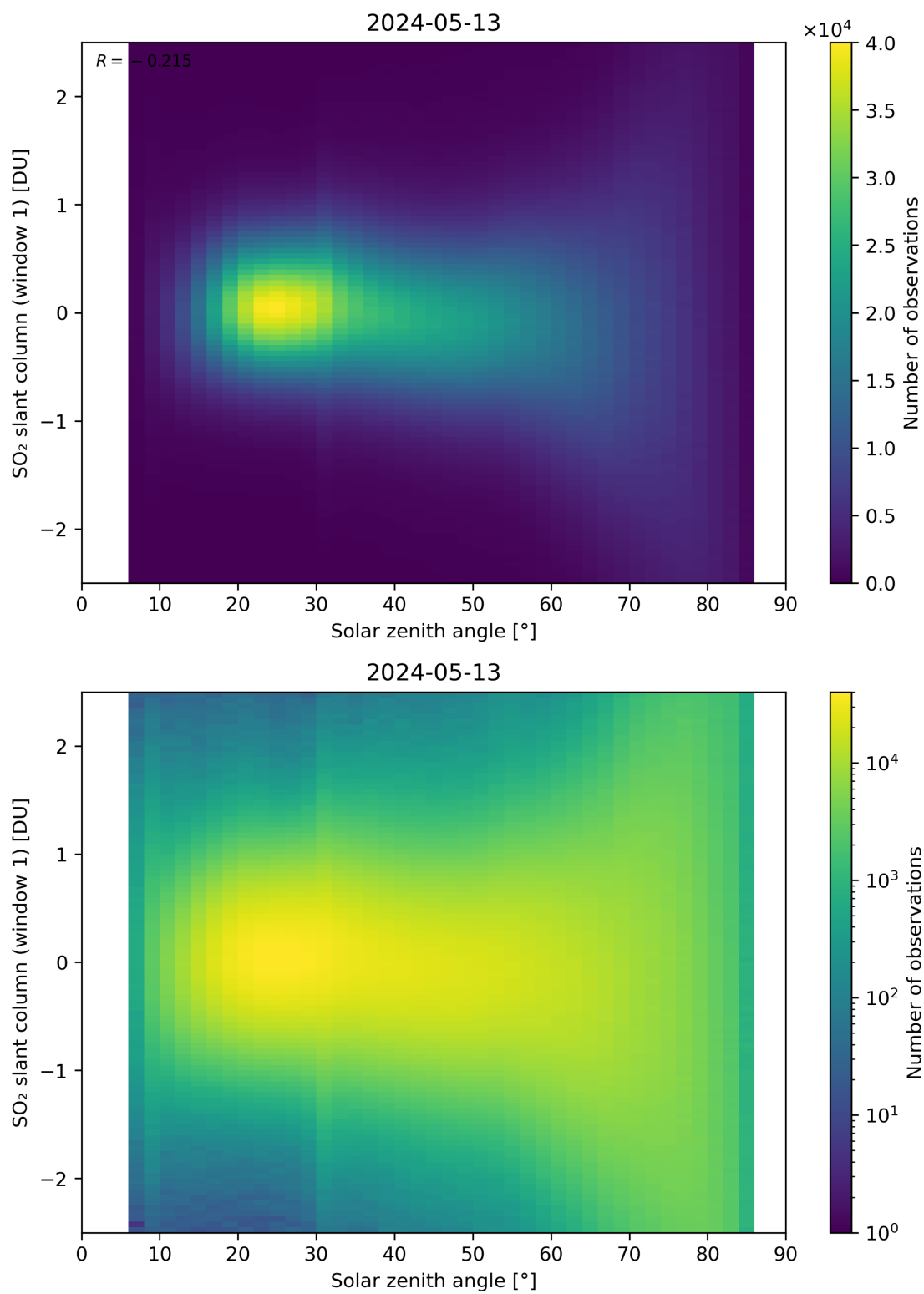
Figure 169: Scatter density plot of “Solar zenith angle” against “SO 2 slant column (window 1)” for 2024-05-12 to 2024-05-14.
