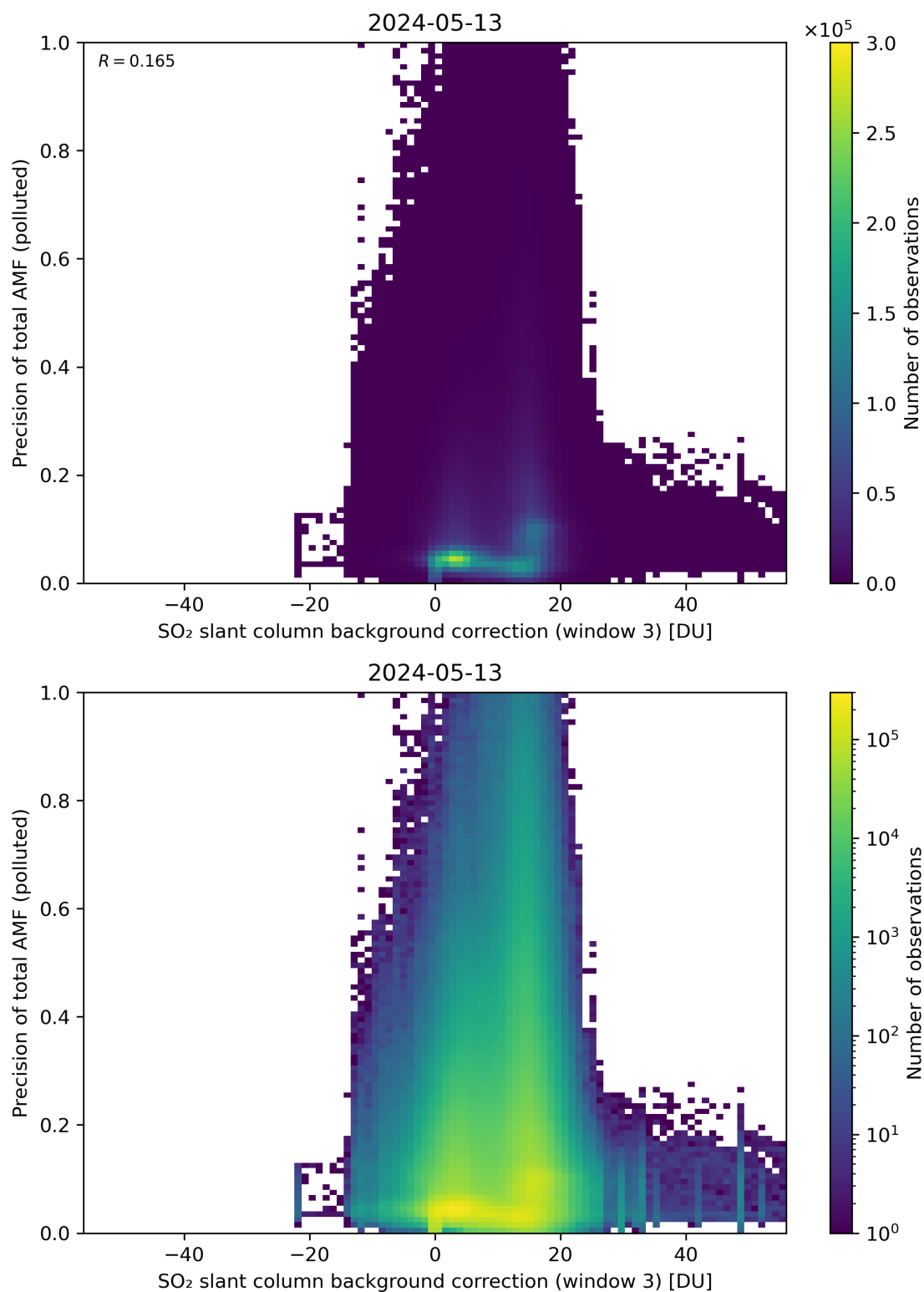
Figure 126: Scatter density plot of “SO 2 slant column background correction (window 3)” against “Precision of total AMF (polluted)” for 2024-05-12 to 2024-05-14.
