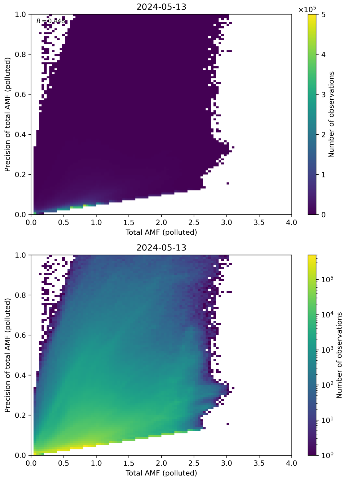
Figure 272: Scatter density plot of “Total AMF (polluted)” against “Precision of total AMF (polluted)” for 2024-05-12 to 2024-05-14.
