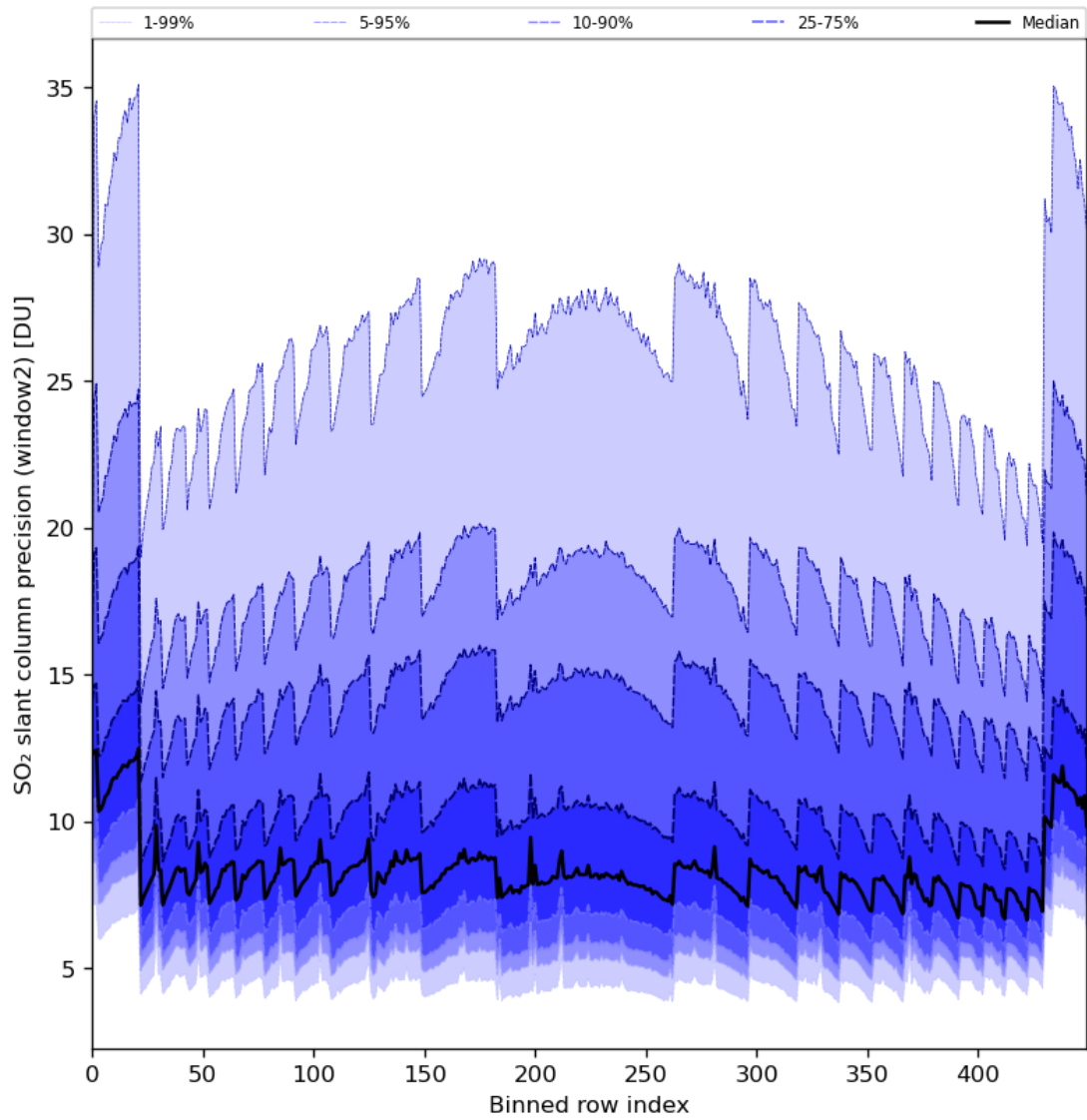
Figure 84: Along track statistics of “SO 2 slant column precision (window2)” for 2024-05-12 to 2024-05-14
