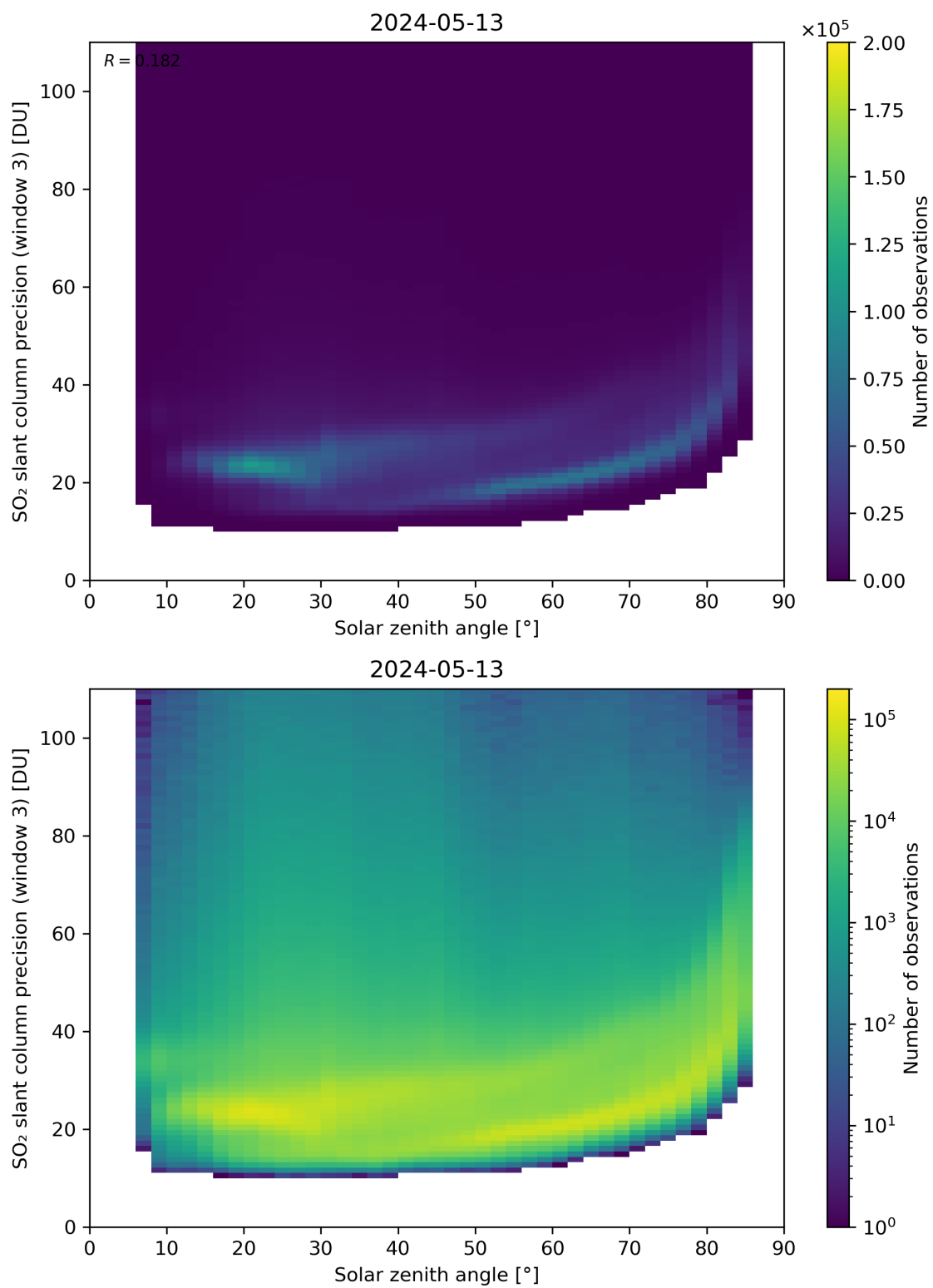
Figure 173: Scatter density plot of “Solar zenith angle” against “SO 2 slant column precision (window 3)” for 2024-05-12 to 2024-05-14.
