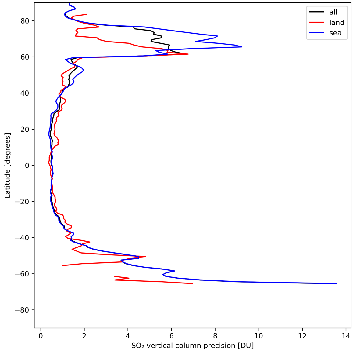
Figure 31: Zonal average of “SO 2 vertical column precision” for 2024-05-12 to 2024-05-14.
