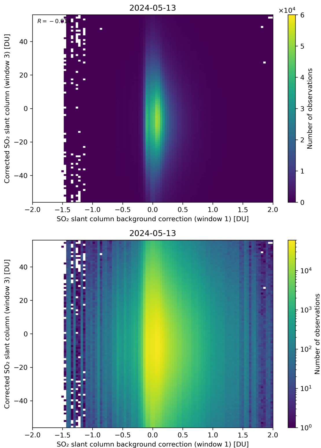
Figure 105: Scatter density plot of “SO 2 slant column background correction (window 1)” against “Corrected SO 2 slant column (window 3)” for 2024-05-12 to 2024-05-14.
