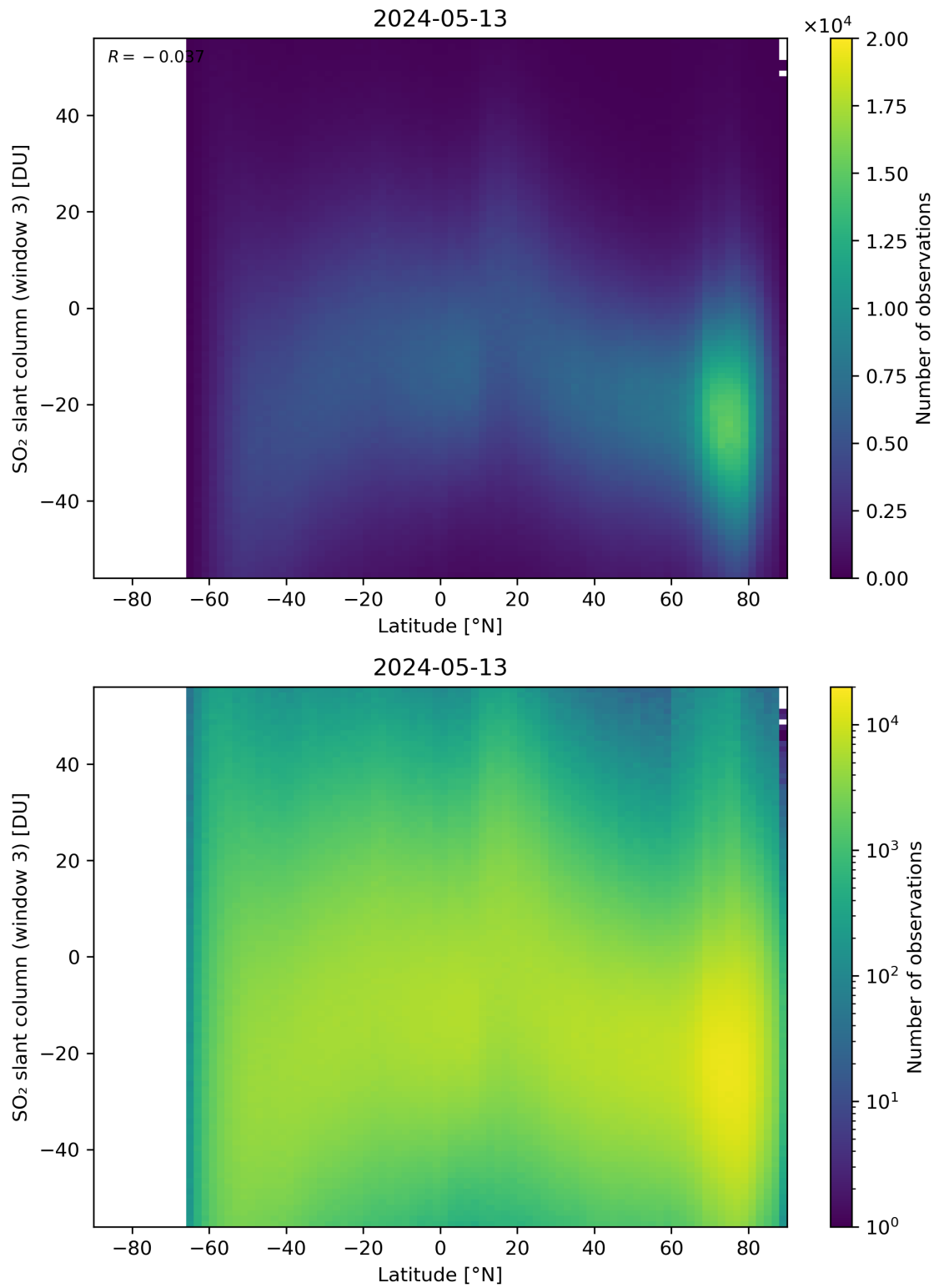
Figure 152: Scatter density plot of “Latitude” against “SO 2 slant column (window 3)” for 2024-05-12 to 2024-05-14.
