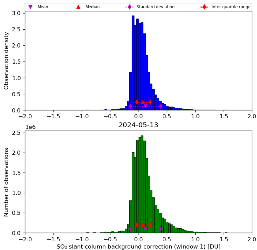
Figure 59: Histogram of “SO 2 slant column background correction (window 1)” for 2024-05-12 to 2024-05-14
