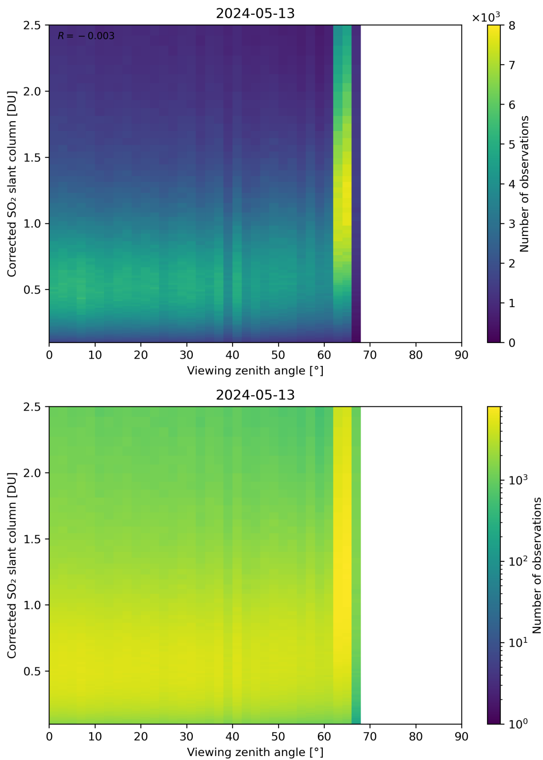
Figure 317: Scatter density plot of “Viewing zenith angle” against “Corrected SO 2 slant column” for 2024-05-12 to 2024-05-14.
