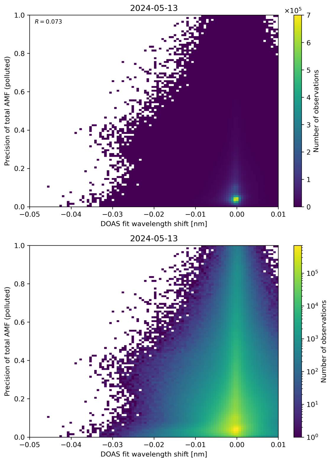
Figure 131: Scatter density plot of “DOAS fit wavelength shift” against “Precision of total AMF (polluted)” for 2024-05-12 to 2024-05-14.
