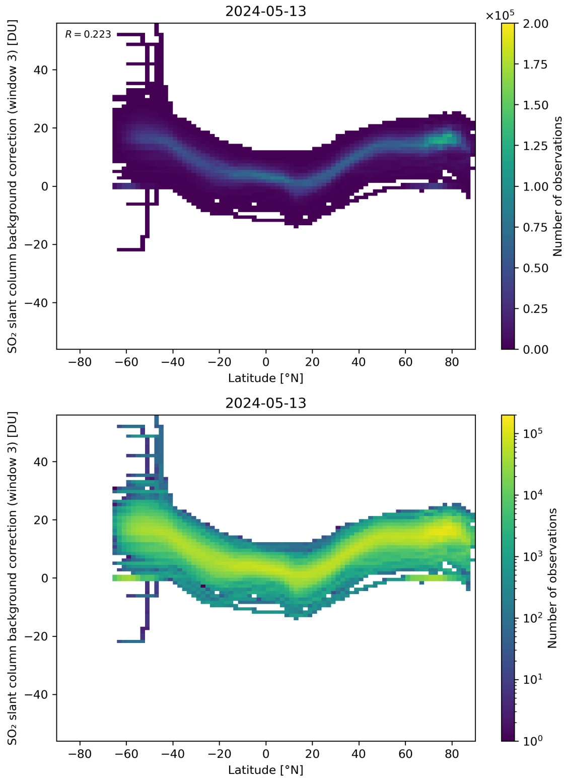
Figure 141: Scatter density plot of “Latitude” against “SO 2 slant column background correction (window 3)” for 2024-05-12 to 2024-05-14.
