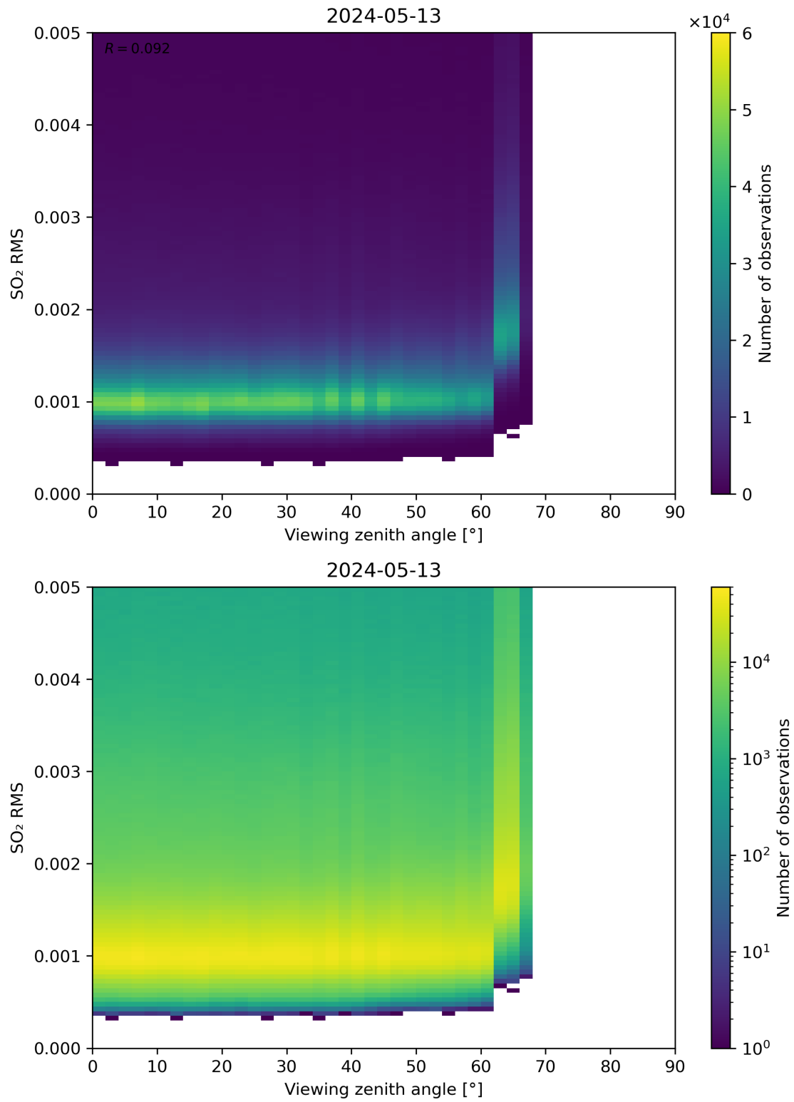
Figure 313: Scatter density plot of “Viewing zenith angle” against “SO 2 RMS” for 2024-05-12 to 2024-05-14.
