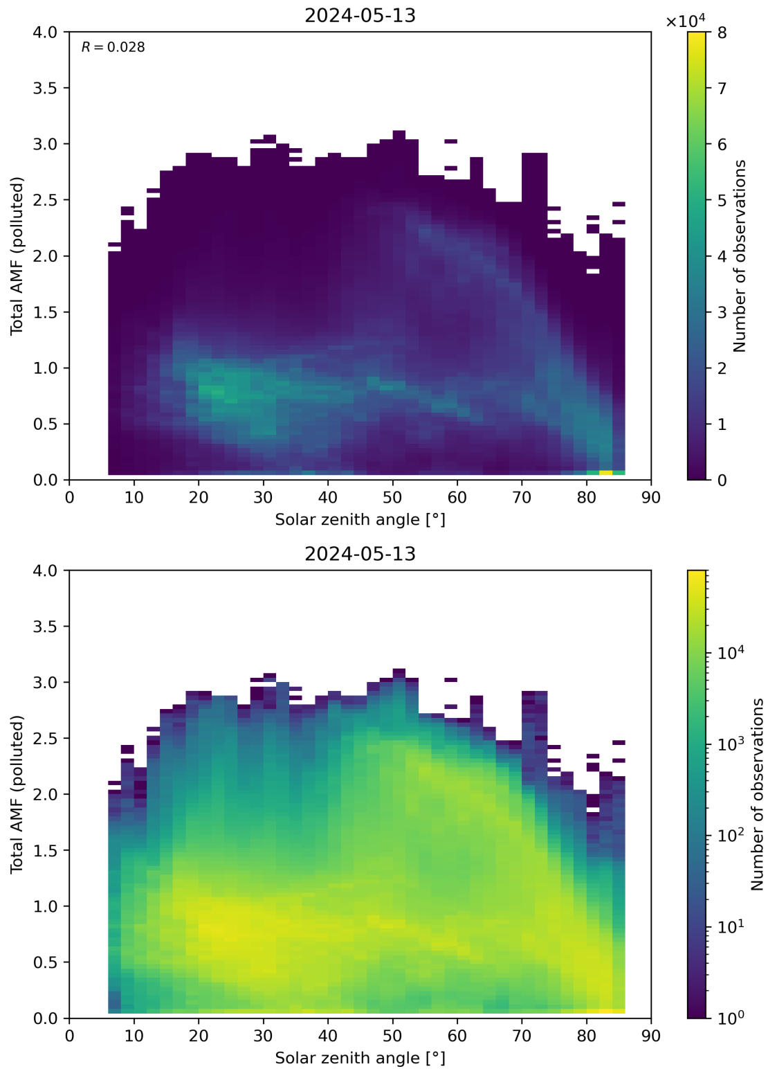
Figure 174: Scatter density plot of “Solar zenith angle” against “Total AMF (polluted)” for 2024-05-12 to 2024-05-14.
