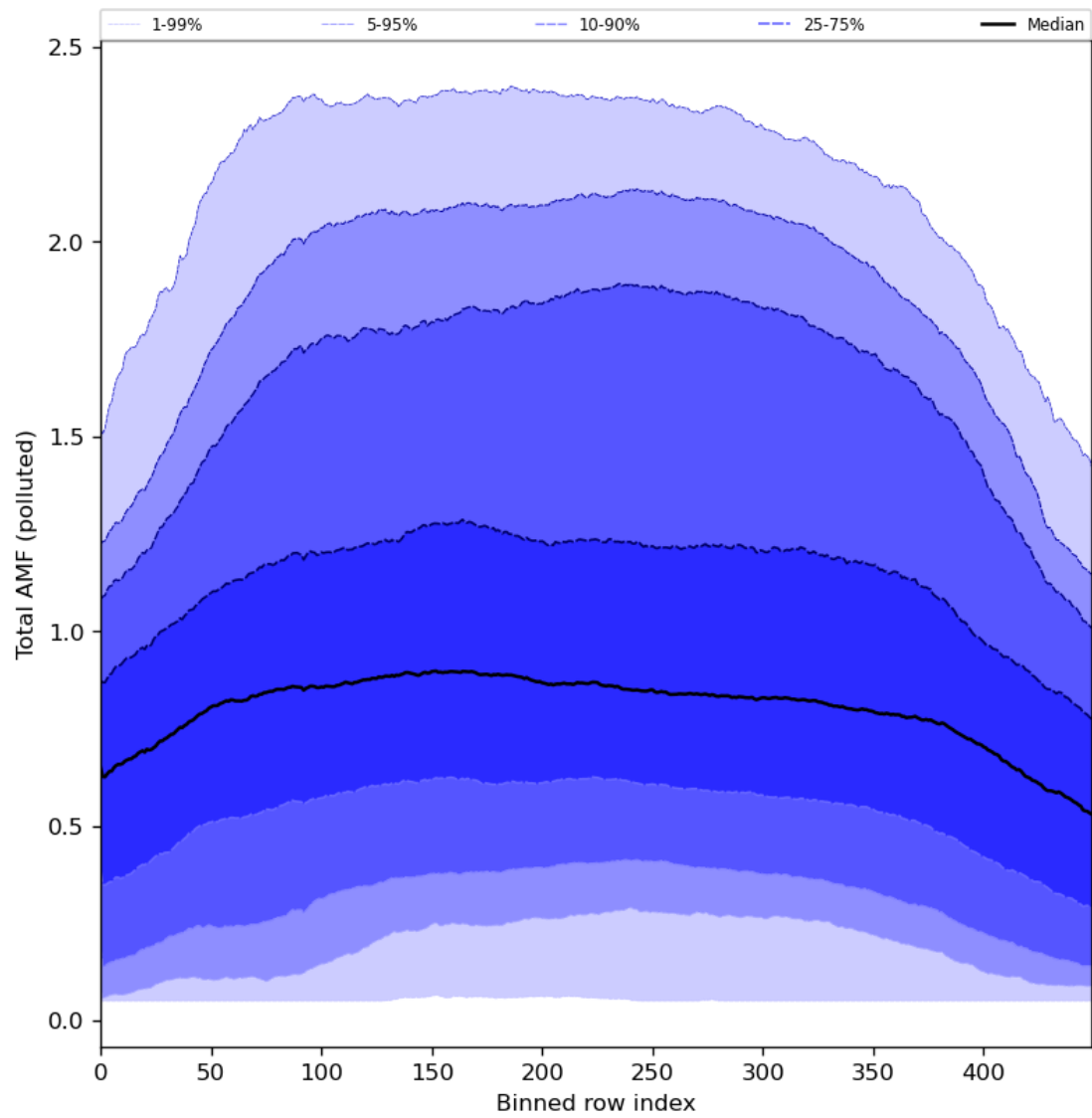
Figure 94: Along track statistics of “Total AMF (polluted)” for 2024-05-12 to 2024-05-14
