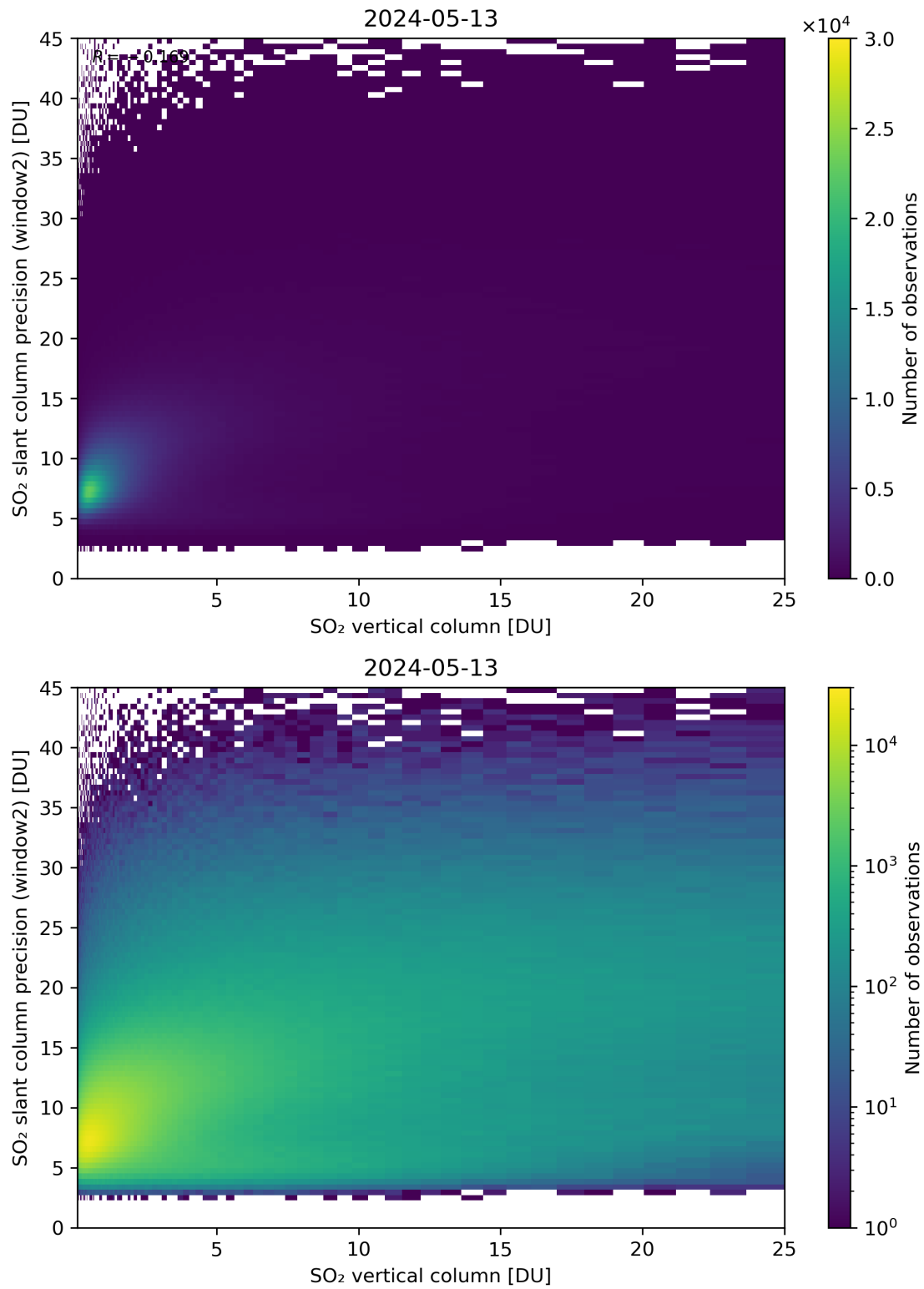
Figure 302: Scatter density plot of “SO 2 vertical column” against “SO 2 slant column precision (window2)” for 2024-05-12 to 2024-05-14.
