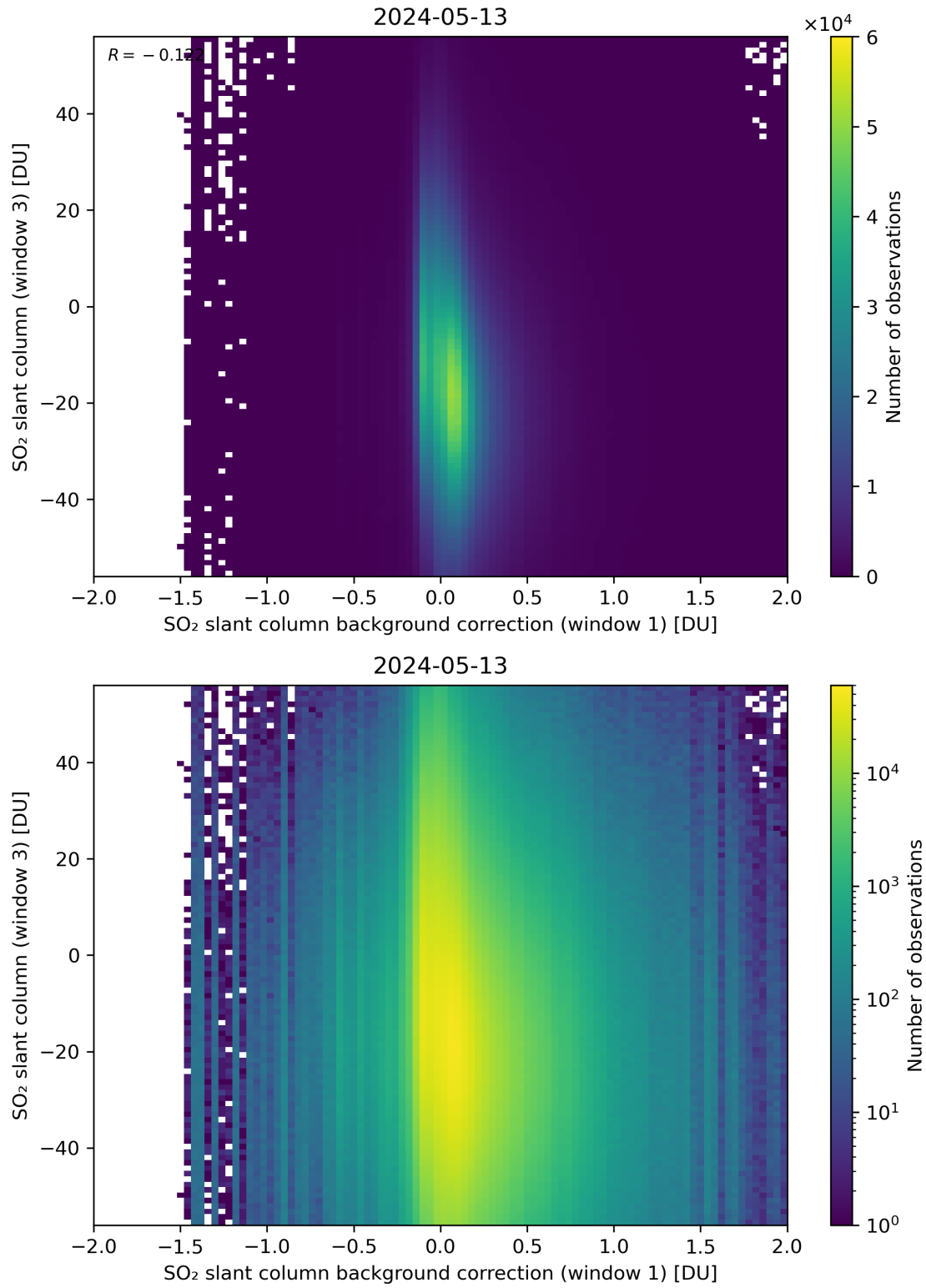
Figure 107: Scatter density plot of “SO 2 slant column background correction (window 1)” against “SO 2 slant column (window 3)” for 2024-05-12 to 2024-05-14.
