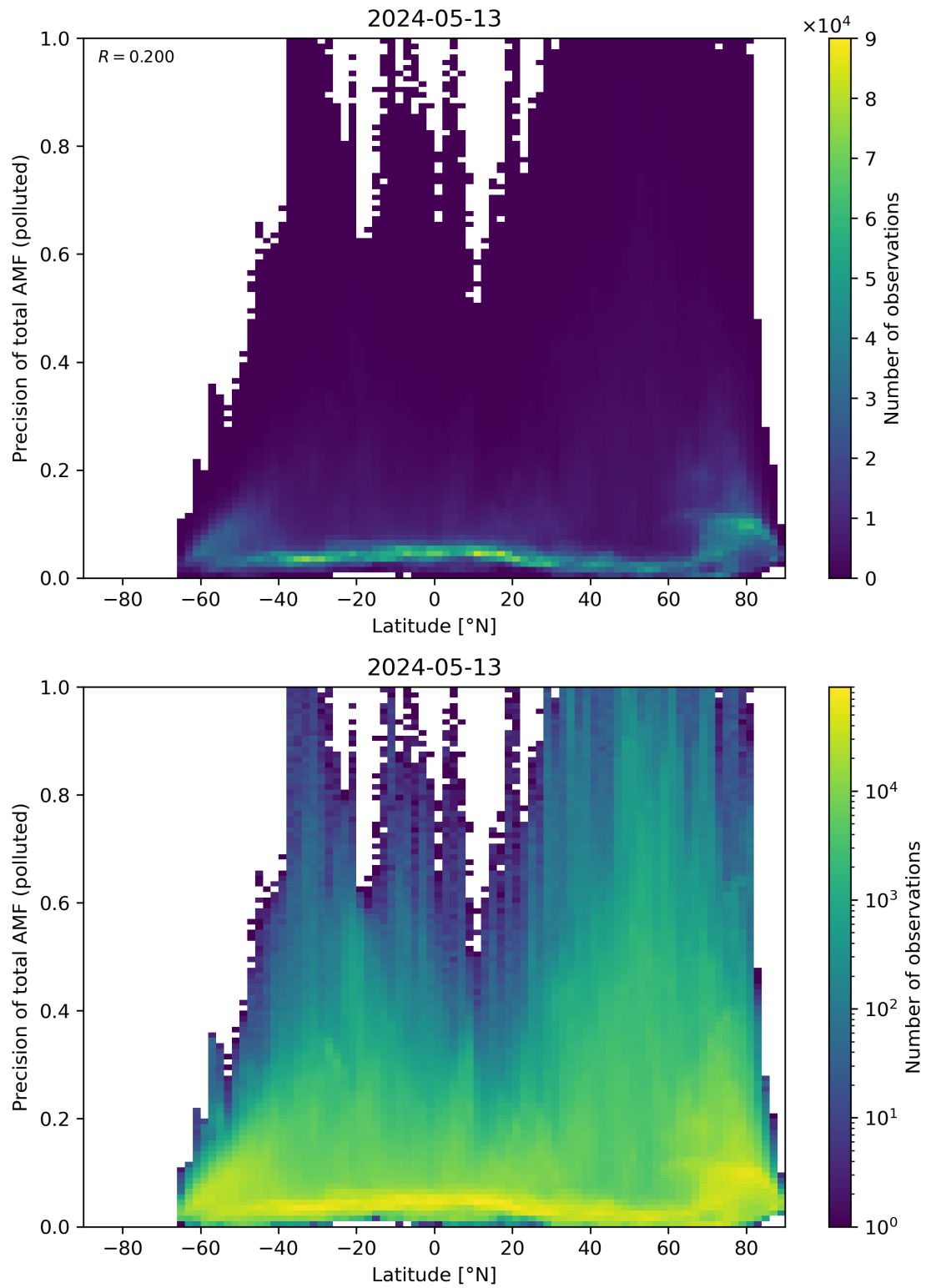
Figure 155: Scatter density plot of “Latitude” against “Precision of total AMF (polluted)” for 2024-05-12 to 2024-05-14.
