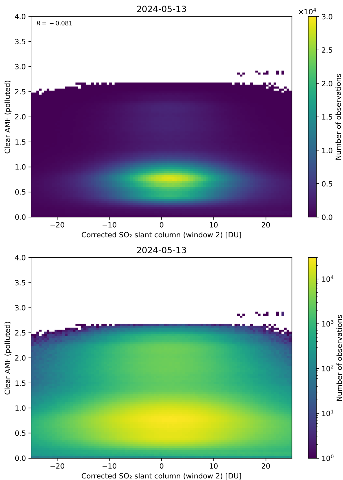
Figure 199: Scatter density plot of “Corrected SO 2 slant column (window 2)” against “Clear AMF (polluted)” for 2024-05-12 to 2024-05-14.
