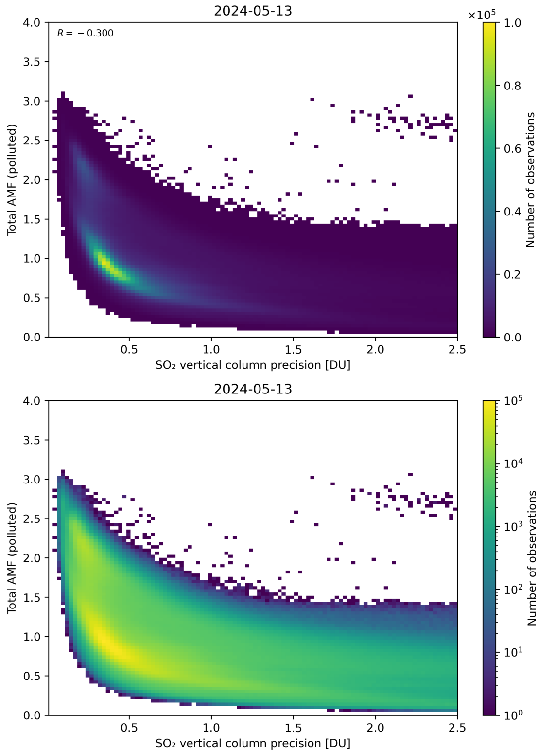
Figure 294: Scatter density plot of “SO 2 vertical column precision” against “Total AMF (polluted)” for 2024-05-12 to 2024-05-14.
