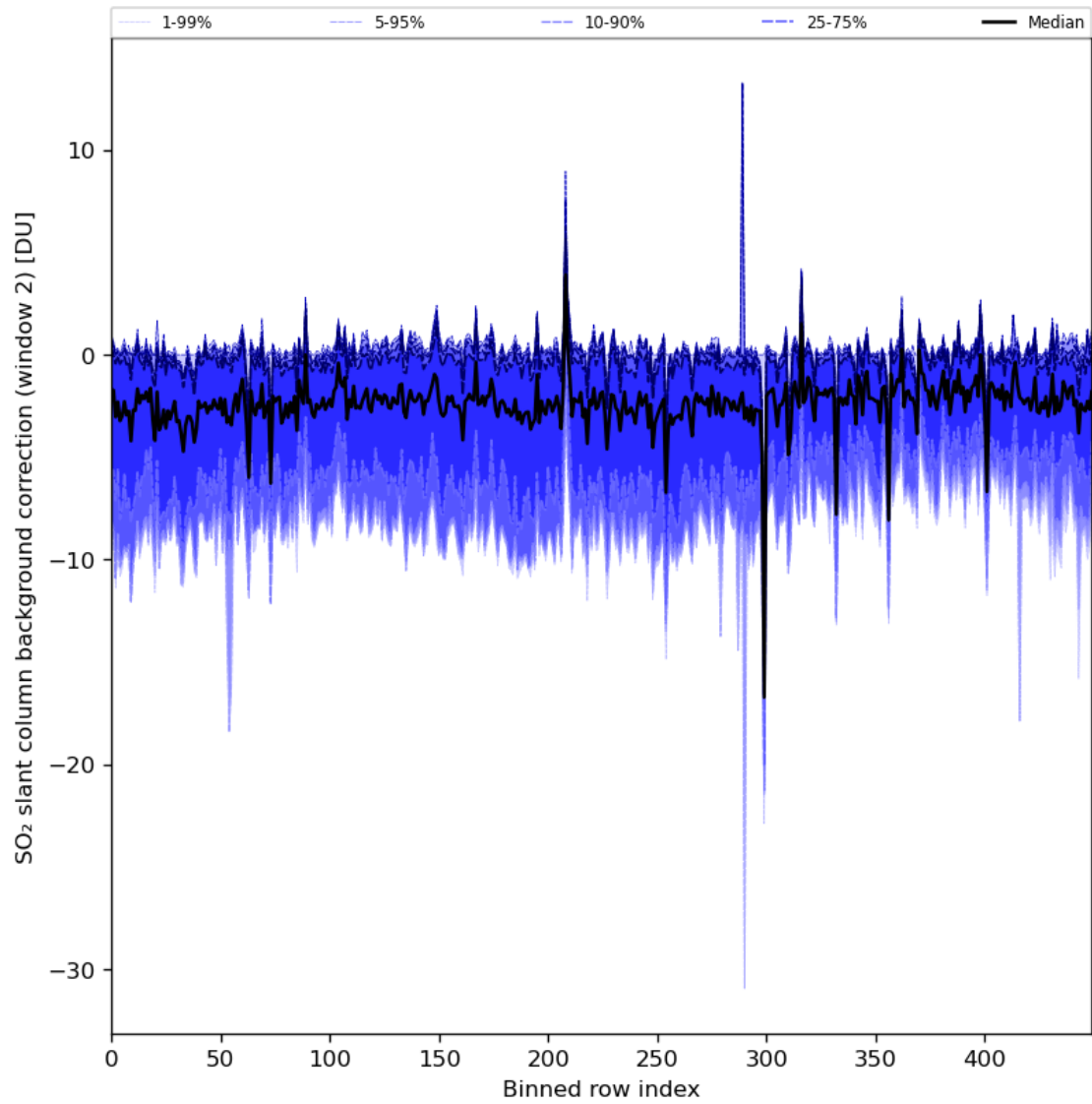
Figure 86: Along track statistics of “SO 2 slant column background correction (window 2)” for 2024-05-12 to 2024-05-14
