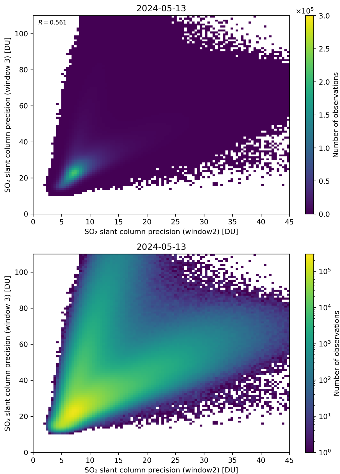
Figure 250: Scatter density plot of “SO 2 slant column precision (window2)” against “SO 2 slant column precision (window 3)” for 2024-05-12 to 2024-05-14.
