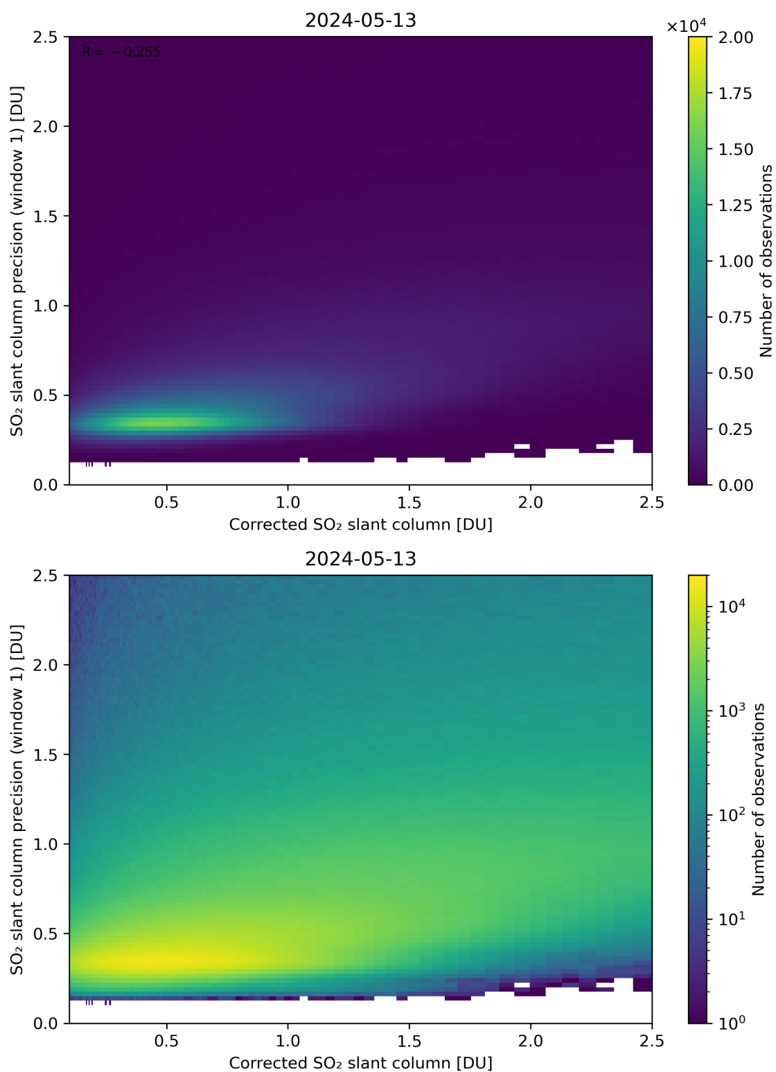
Figure 188: Scatter density plot of “Corrected SO 2 slant column” against “SO 2 slant column precision (window 1)” for 2024-05-12 to 2024-05-14.
