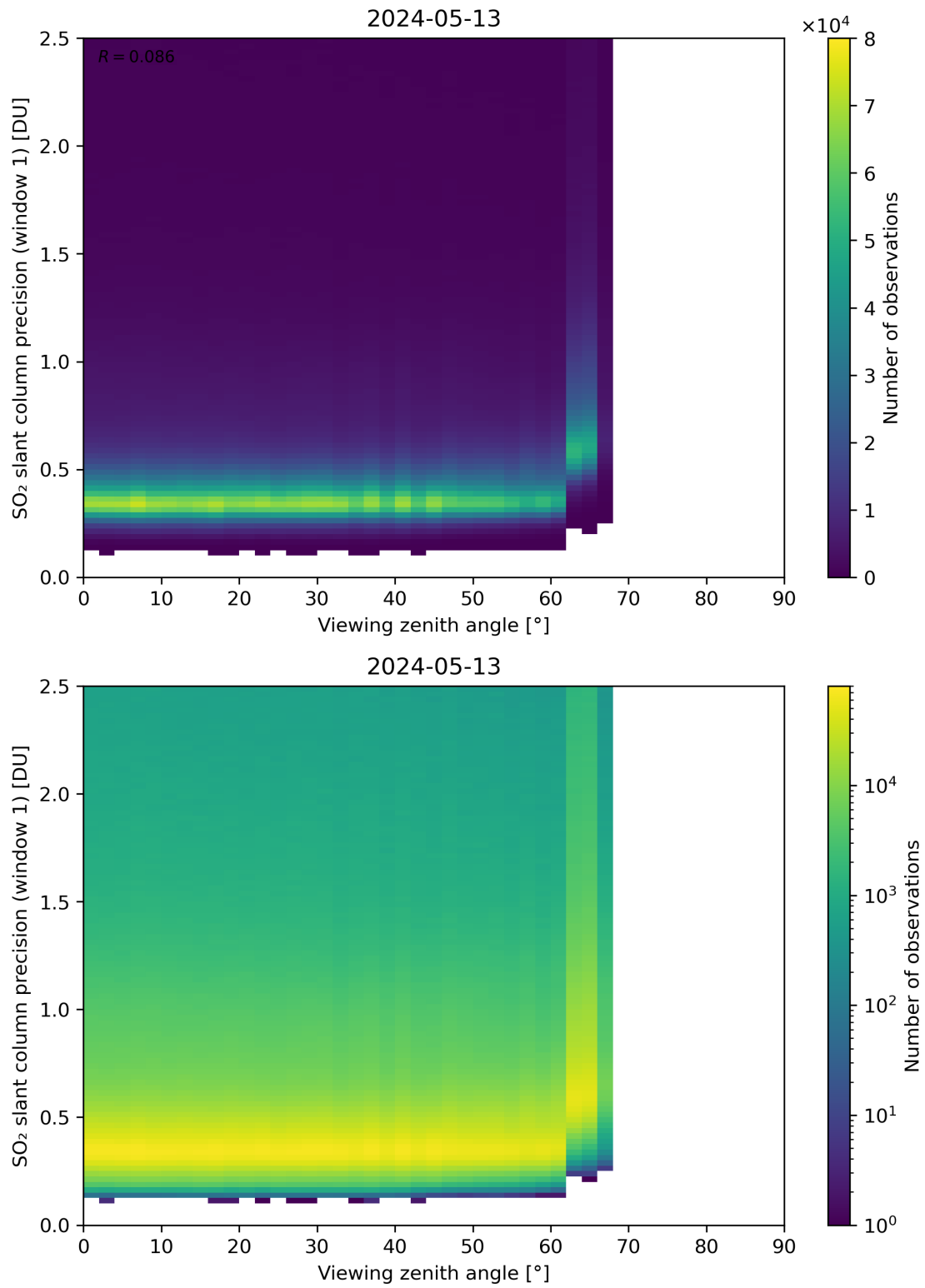
Figure 321: Scatter density plot of “Viewing zenith angle” against “SO 2 slant column precision (window 1)” for 2024-05-12 to 2024-05-14.
