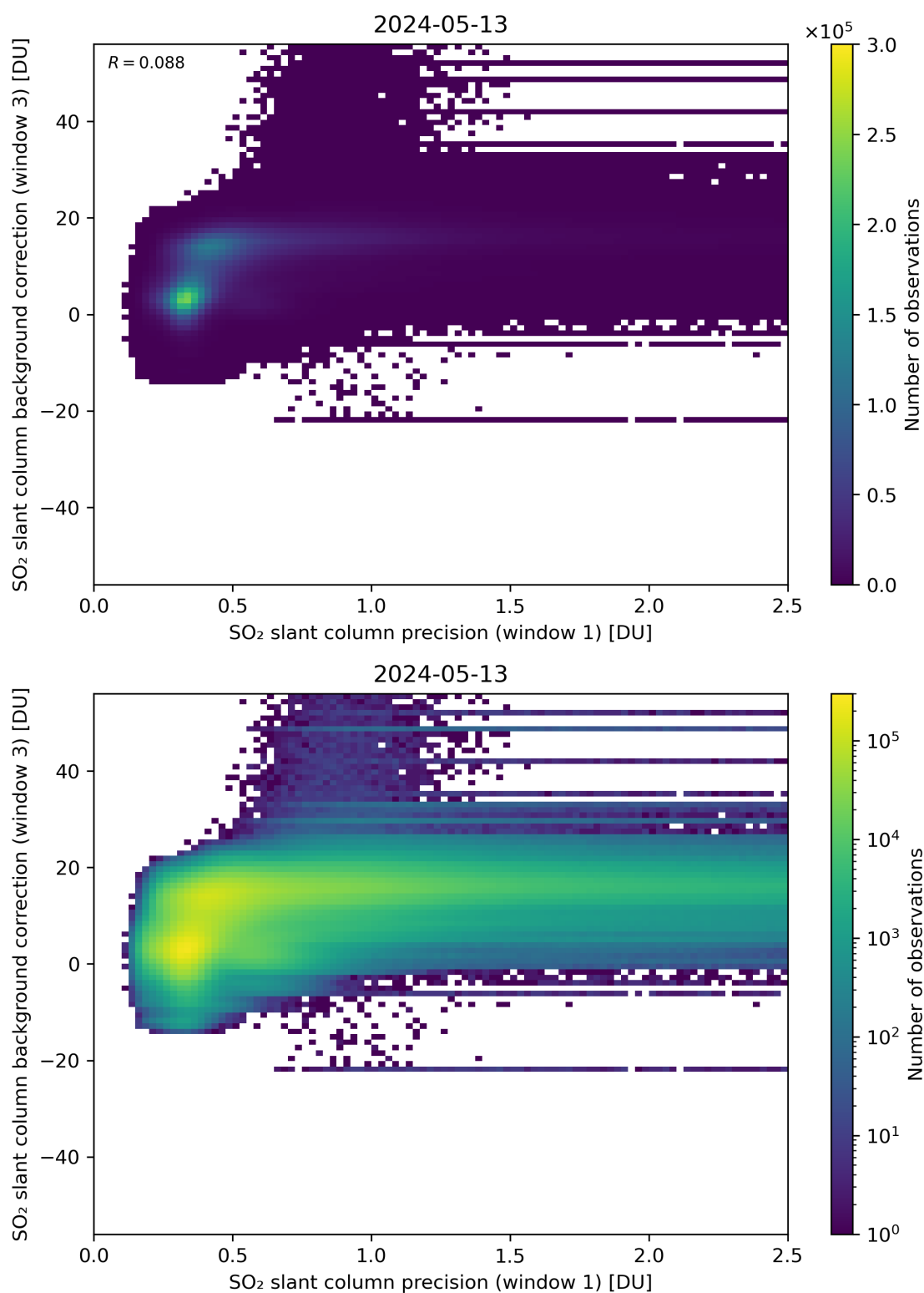
Figure 220: Scatter density plot of “SO 2 slant column precision (window 1)” against “SO 2 slant column background correction (window 3)” for 2024-05-12 to 2024-05-14.
