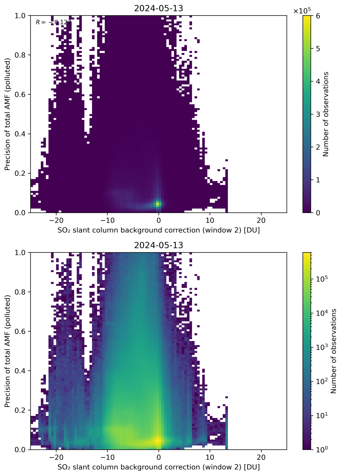
Figure 120: Scatter density plot of “SO 2 slant column background correction (window 2)” against “Precision of total AMF (polluted)” for 2024-05-12 to 2024-05-14.
