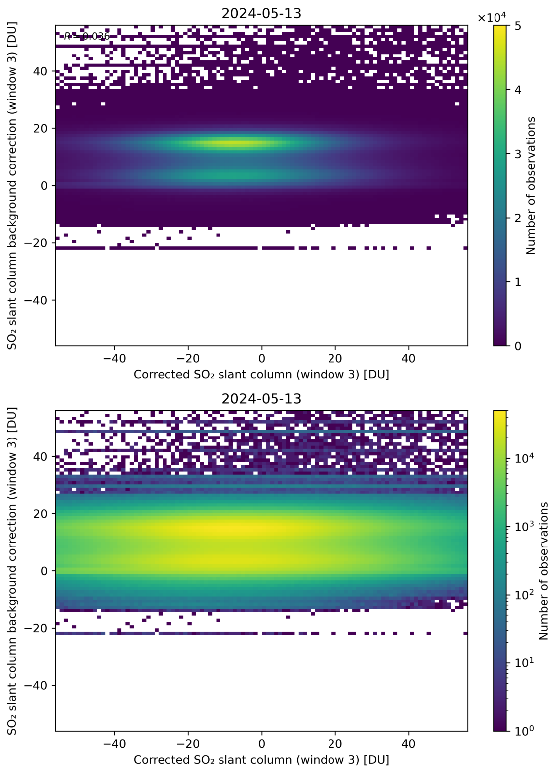
Figure 205: Scatter density plot of “Corrected SO 2 slant column (window 3)” against “SO 2 slant column background correction (window 3)” for 2024-05-12 to 2024-05-14.
