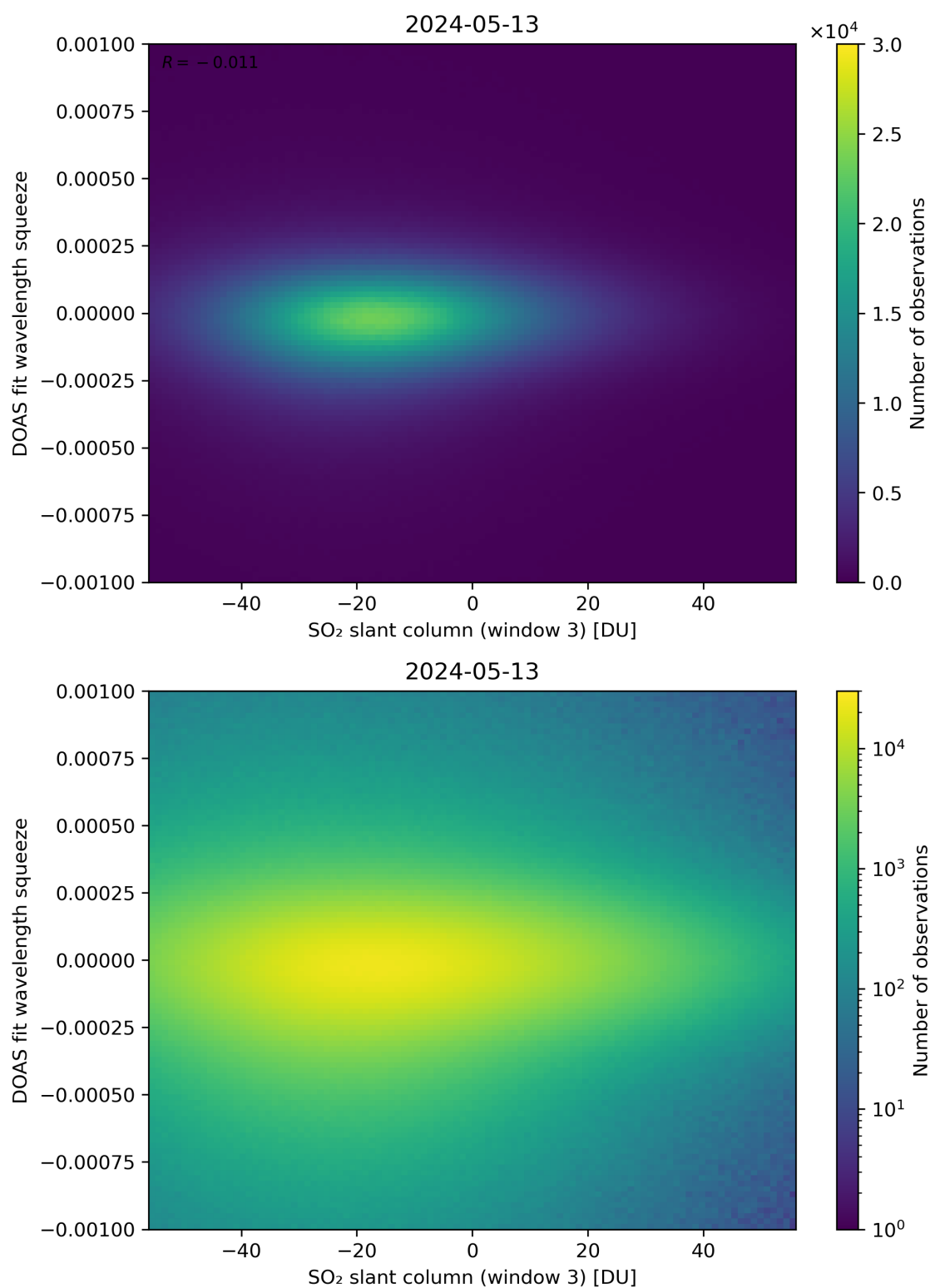
Figure 255: Scatter density plot of “SO 2 slant column (window 3)” against “DOAS fit wavelength squeeze” for 2024-05-12 to 2024-05-14.
