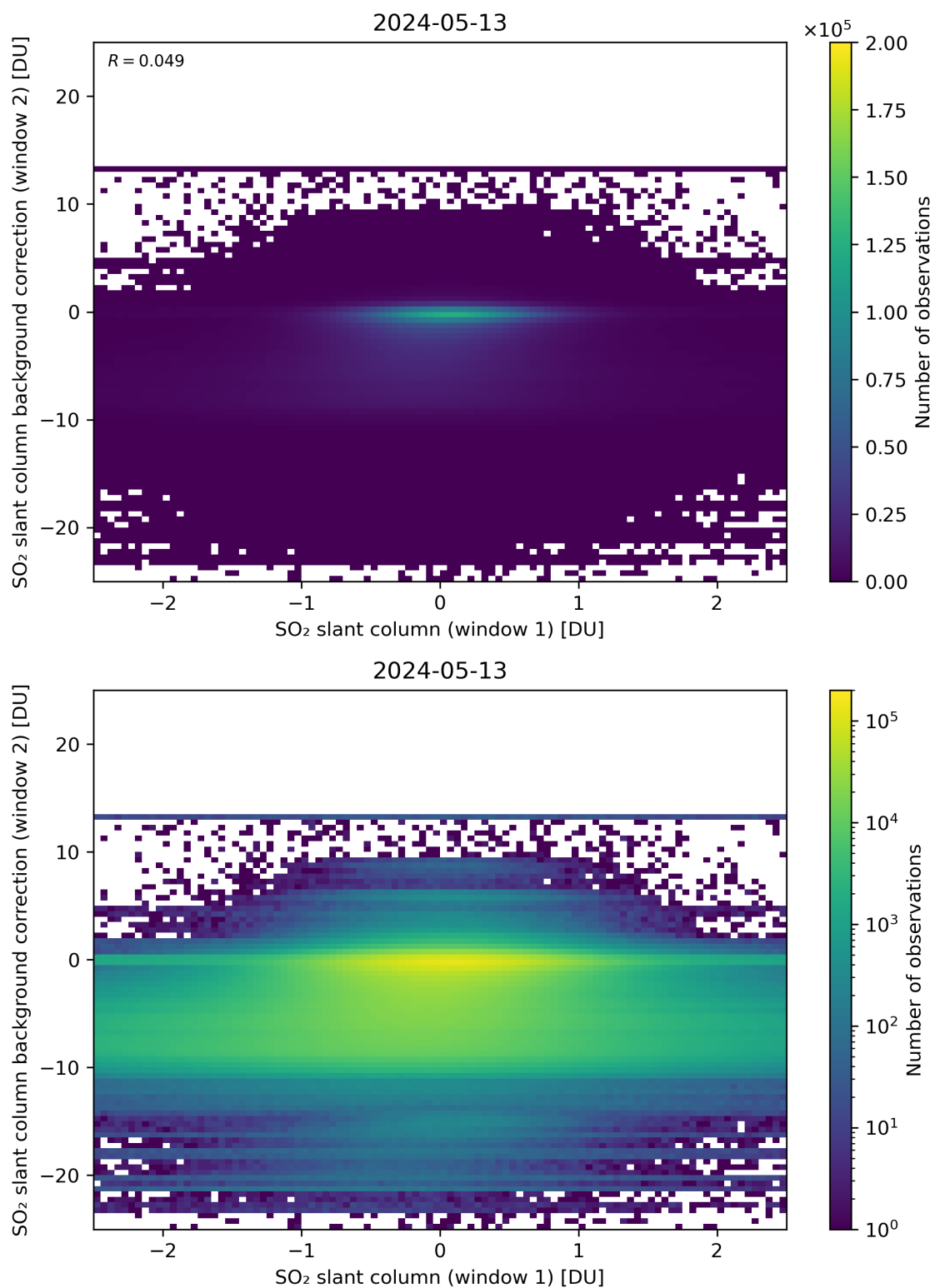
Figure 213: Scatter density plot of “SO 2 slant column (window 1)” against “SO 2 slant column background correction (window 2)” for 2024-05-12 to 2024-05-14.
