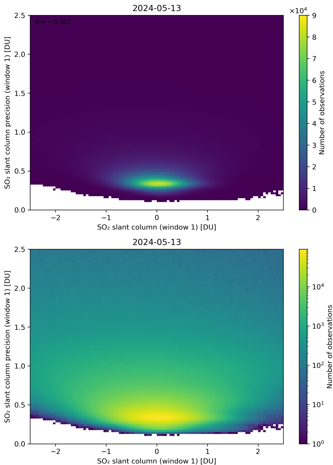
Figure 235: Scatter density plot of “SO 2 slant column (window 1)” against “SO 2 slant column precision (window 1)” for 2024-05-12 to 2024-05-14.
