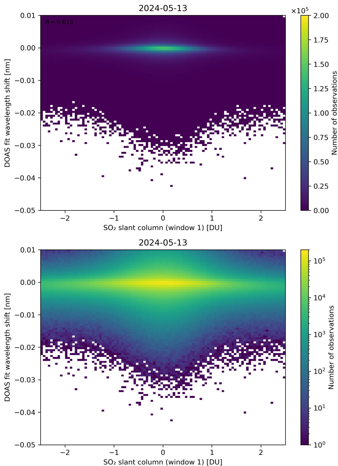
Figure 215: Scatter density plot of “SO 2 slant column (window 1)” against “DOAS fit wavelength shift” for 2024-05-12 to 2024-05-14.
