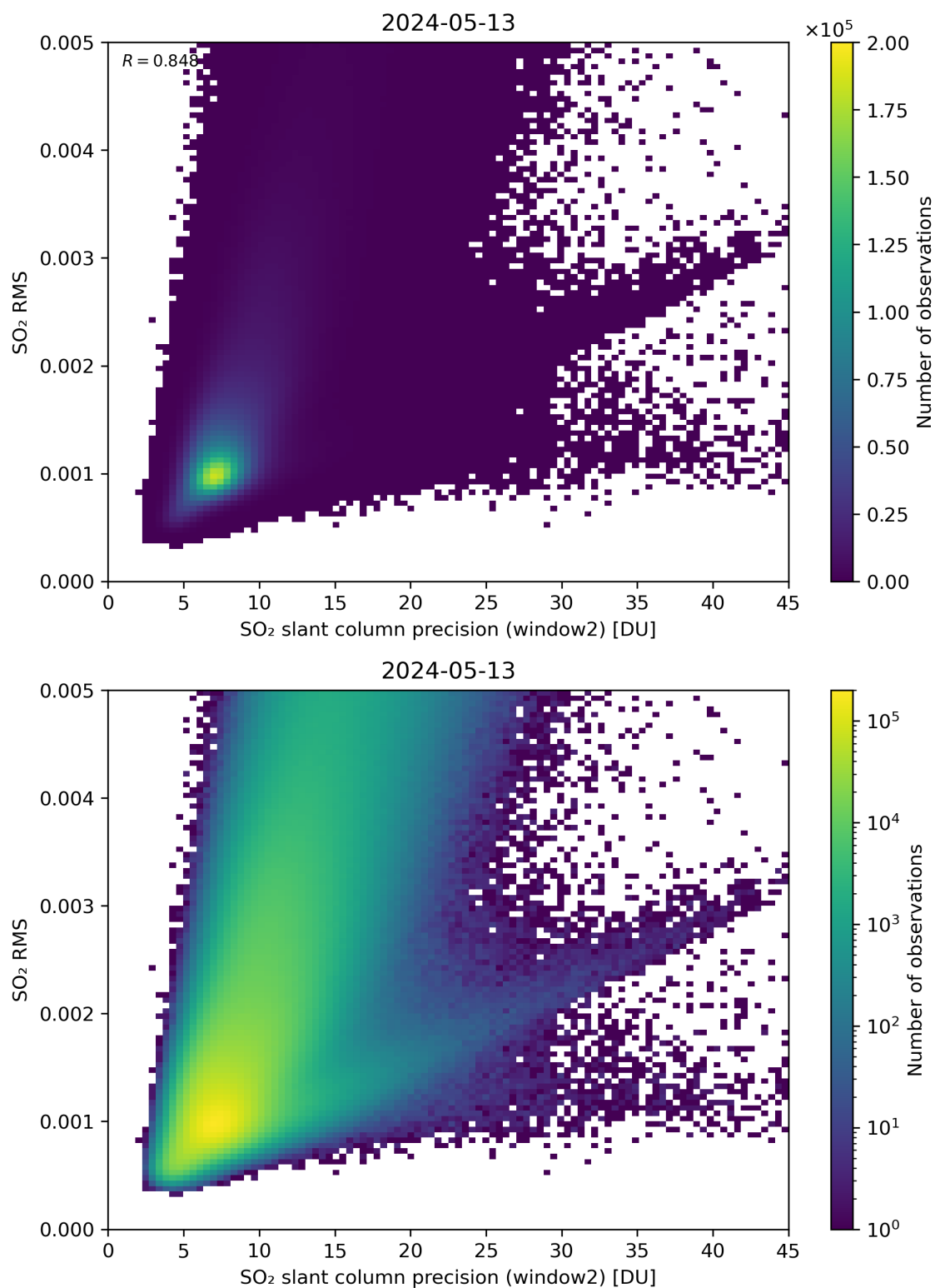
Figure 245: Scatter density plot of “SO 2 slant column precision (window2)” against “SO 2 RMS” for 2024-05-12 to 2024-05-14.
