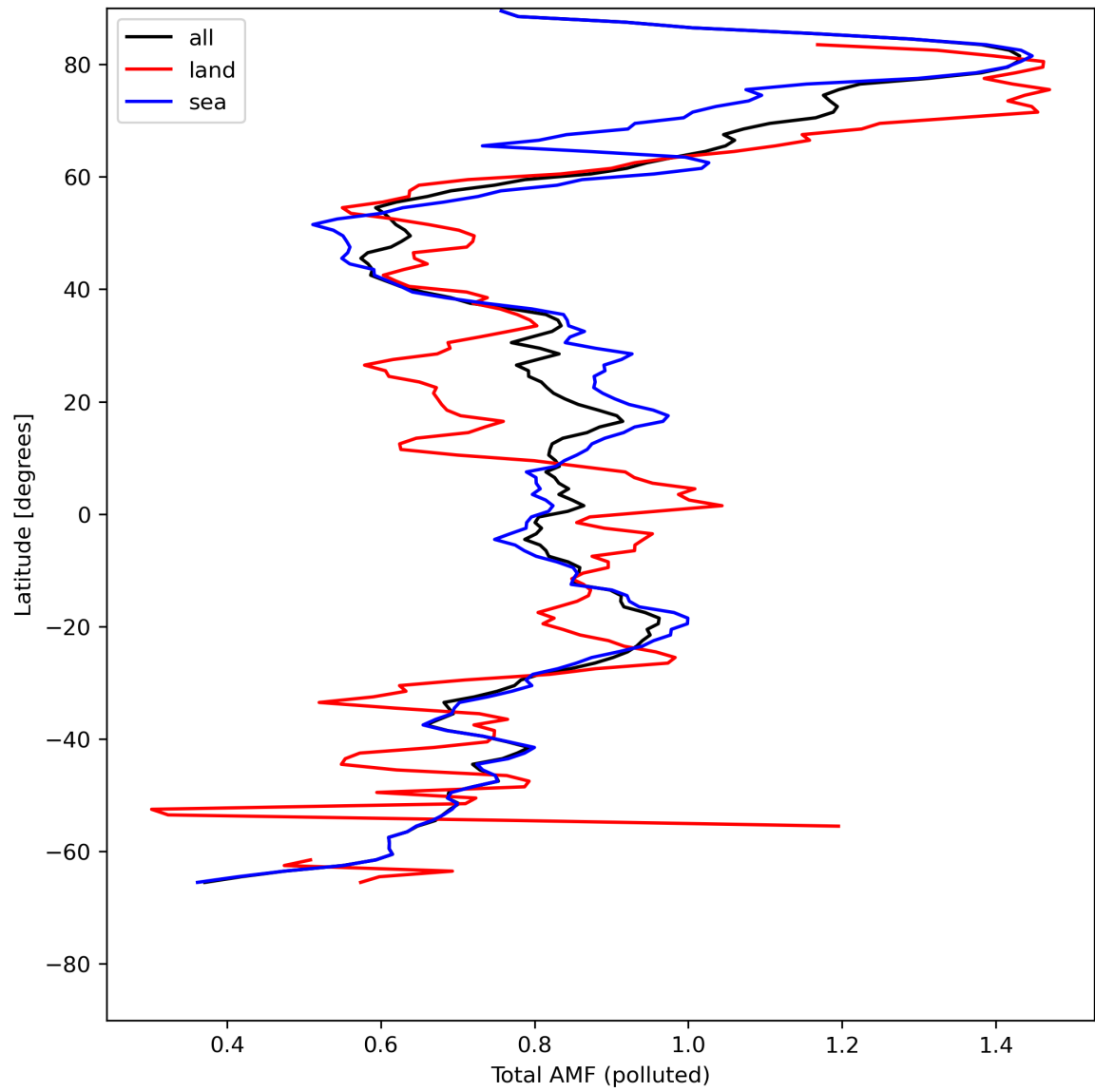
Figure 48: Zonal average of “Total AMF (polluted)” for 2024-05-12 to 2024-05-14.
