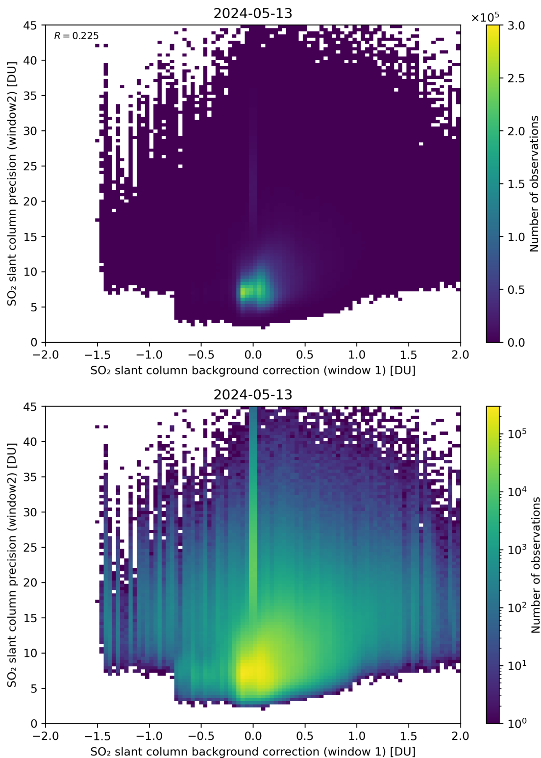
Figure 106: Scatter density plot of “SO 2 slant column background correction (window 1)” against “SO 2 slant column precision (window2)” for 2024-05-12 to 2024-05-14.
