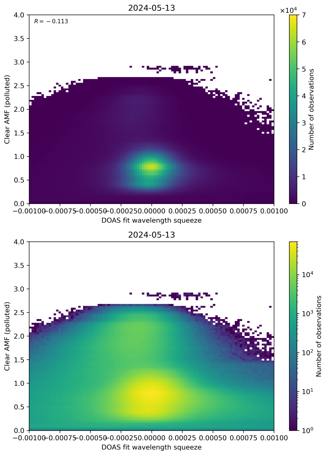
Figure 133: Scatter density plot of “DOAS fit wavelength squeeze” against “Clear AMF (polluted)” for 2024-05-12 to 2024-05-14.
