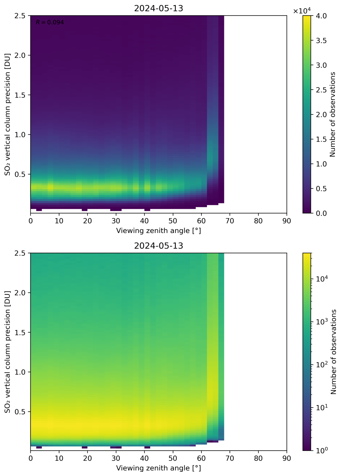
Figure 328: Scatter density plot of “Viewing zenith angle” against “SO 2 vertical column precision” for 2024-05-12 to 2024-05-14.
