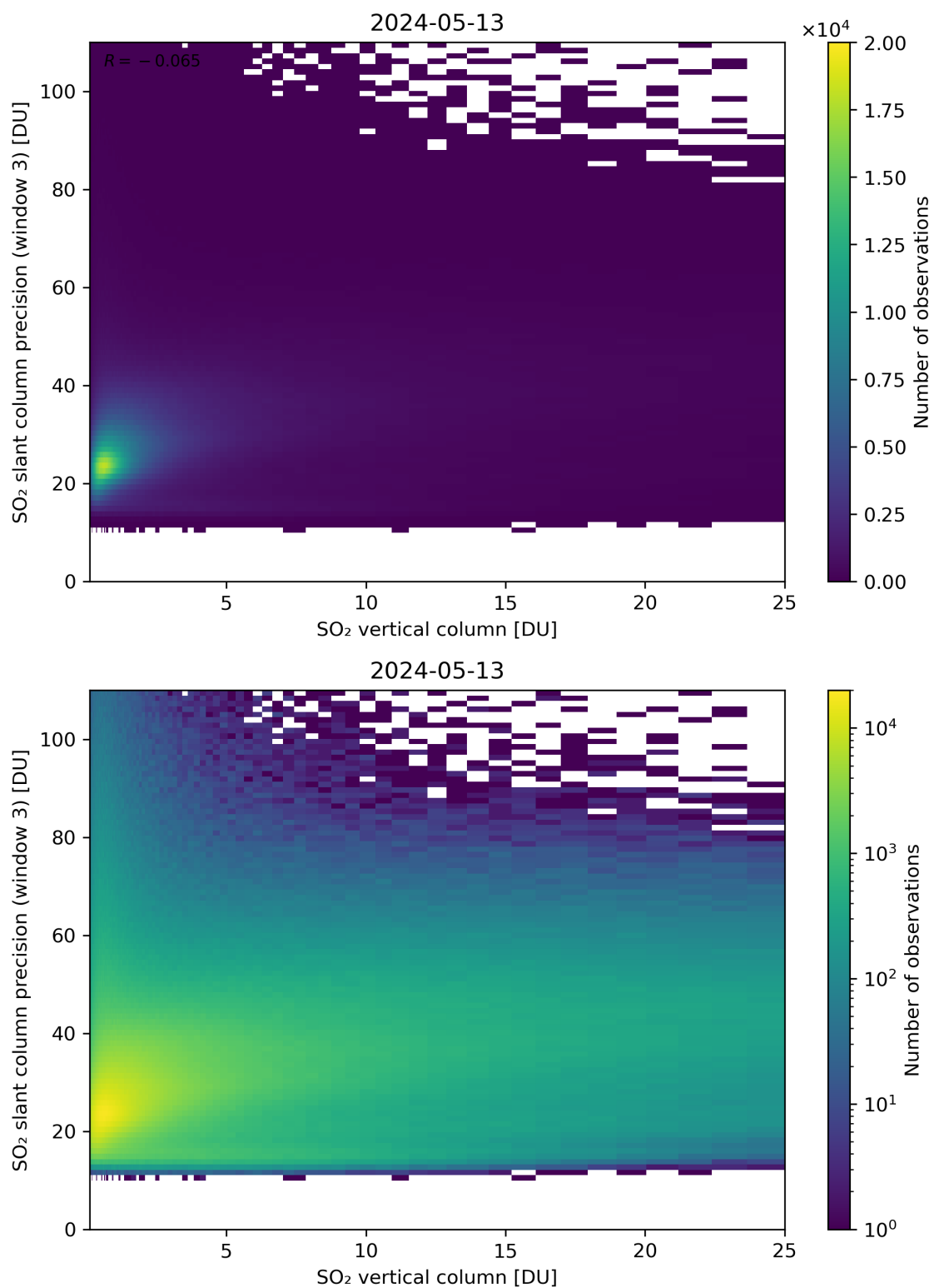
Figure 304: Scatter density plot of “SO 2 vertical column” against “SO 2 slant column precision (window 3)” for 2024-05-12 to 2024-05-14.
