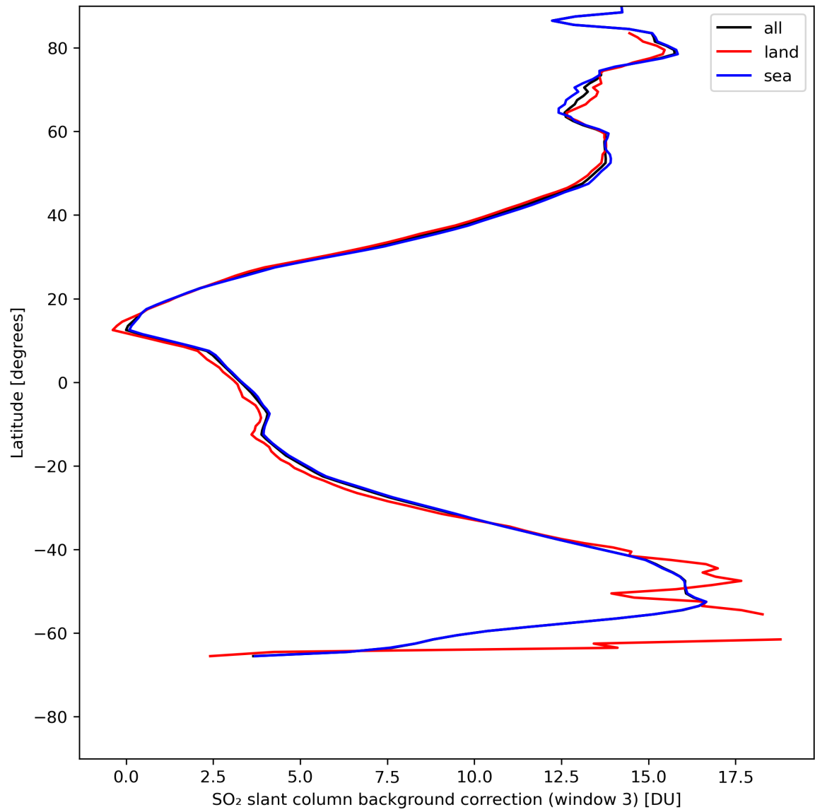
Figure 44: Zonal average of “SO 2 slant column background correction (window 3)” for 2024-05-12 to 2024-05-14.
