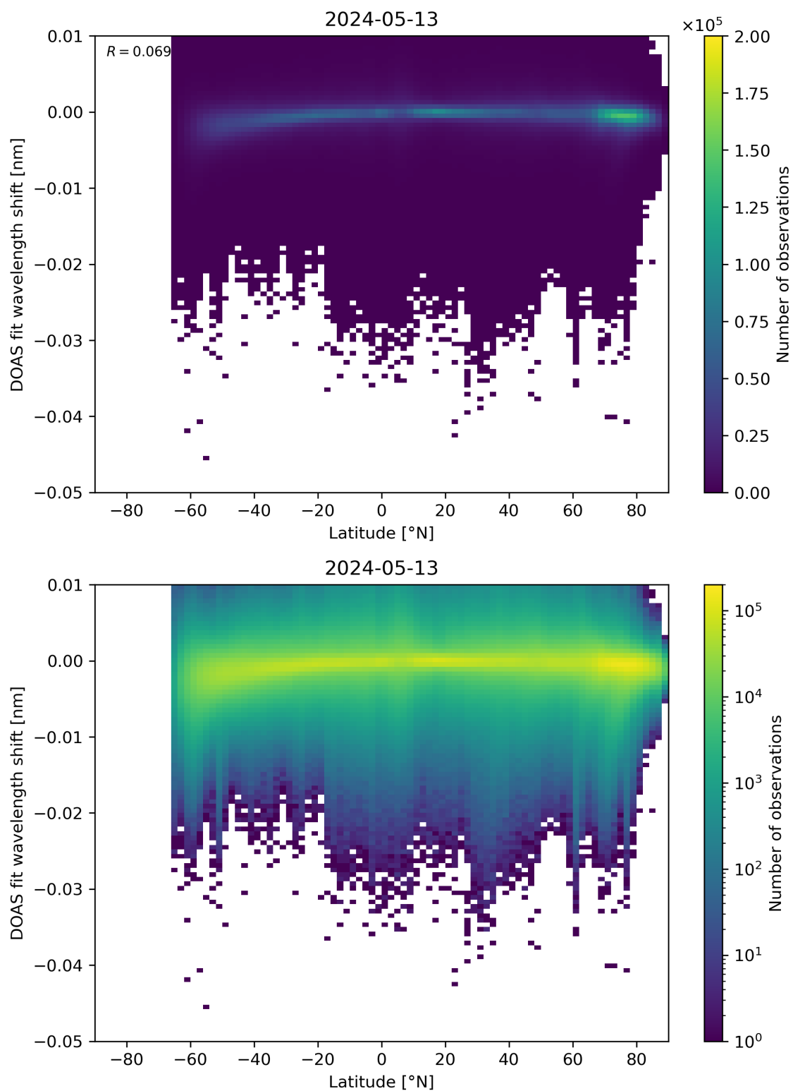
Figure 142: Scatter density plot of “Latitude” against “DOAS fit wavelength shift” for 2024-05-12 to 2024-05-14.
