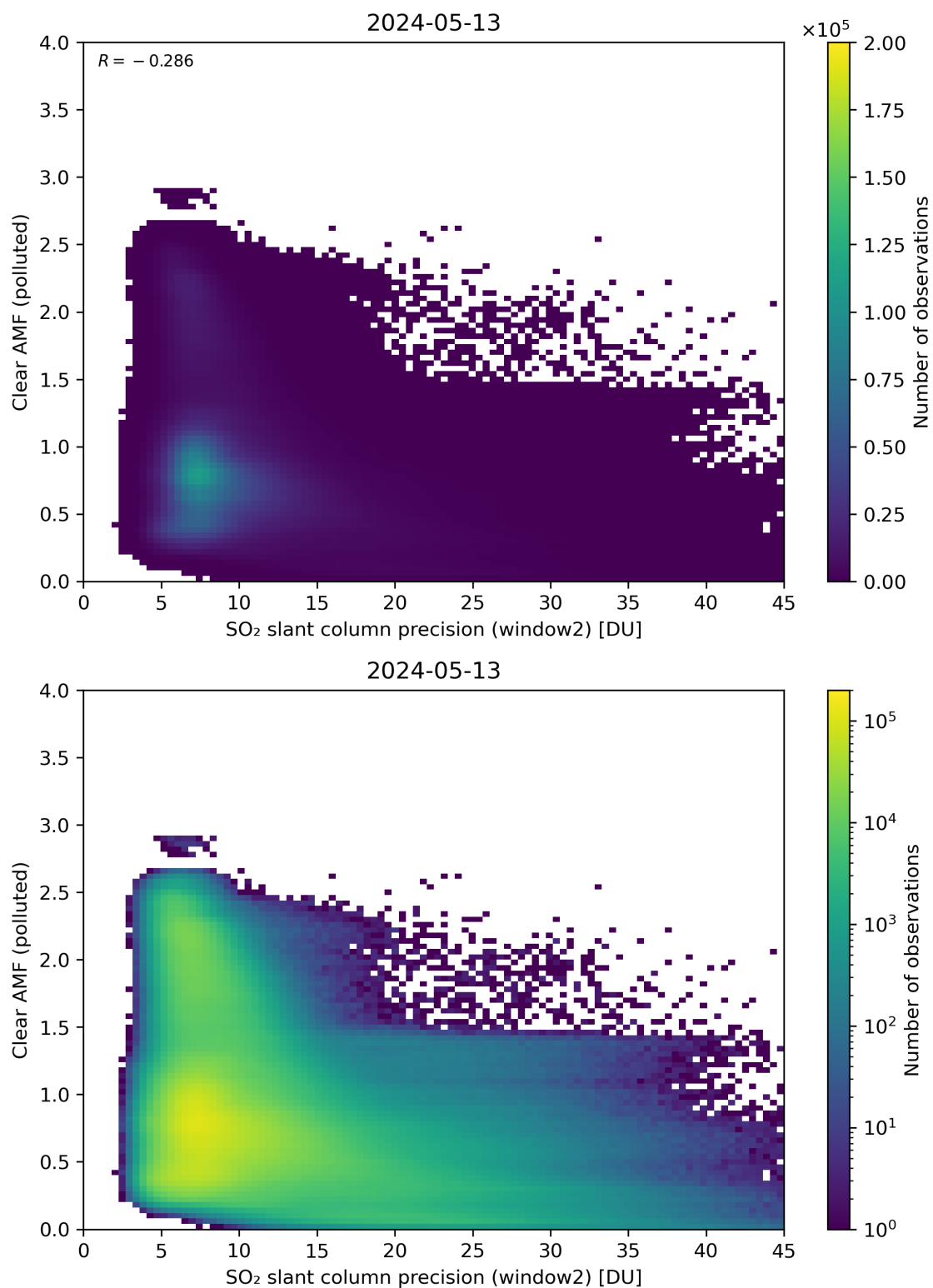
Figure 246: Scatter density plot of “SO 2 slant column precision (window2)” against “Clear AMF (polluted)” for 2024-05-12 to 2024-05-14.
