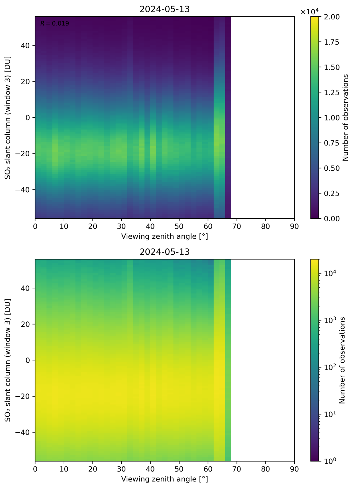
Figure 323: Scatter density plot of “Viewing zenith angle” against “SO 2 slant column (window 3)” for 2024-05-12 to 2024-05-14.
