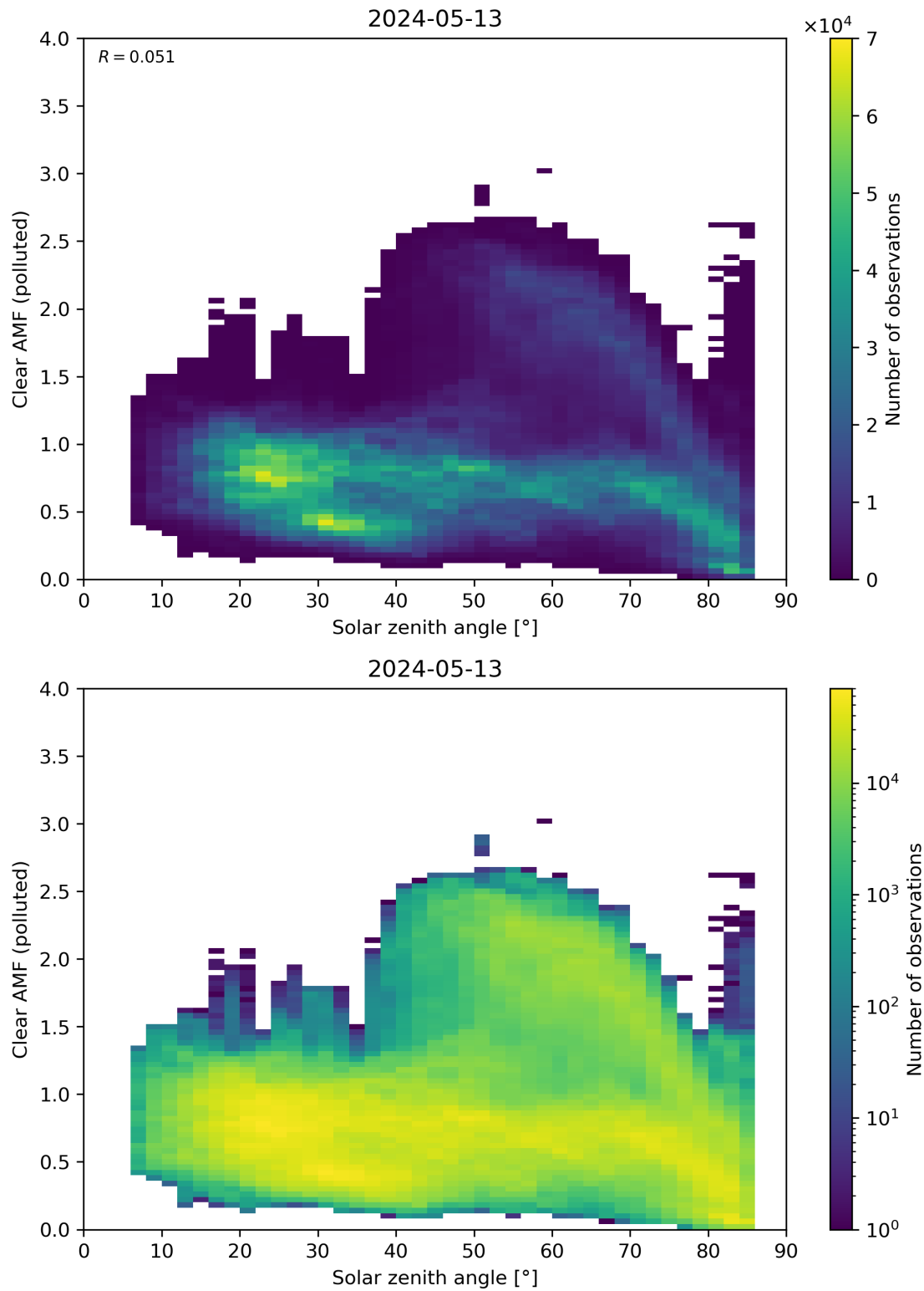
Figure 165: Scatter density plot of “Solar zenith angle” against “Clear AMF (polluted)” for 2024-05-12 to 2024-05-14.
