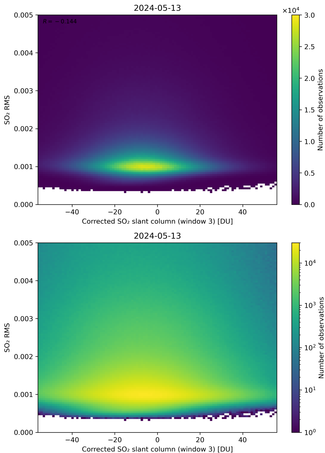
Figure 208: Scatter density plot of “Corrected SO 2 slant column (window 3)” against “SO 2 RMS” for 2024-05-12 to 2024-05-14.
