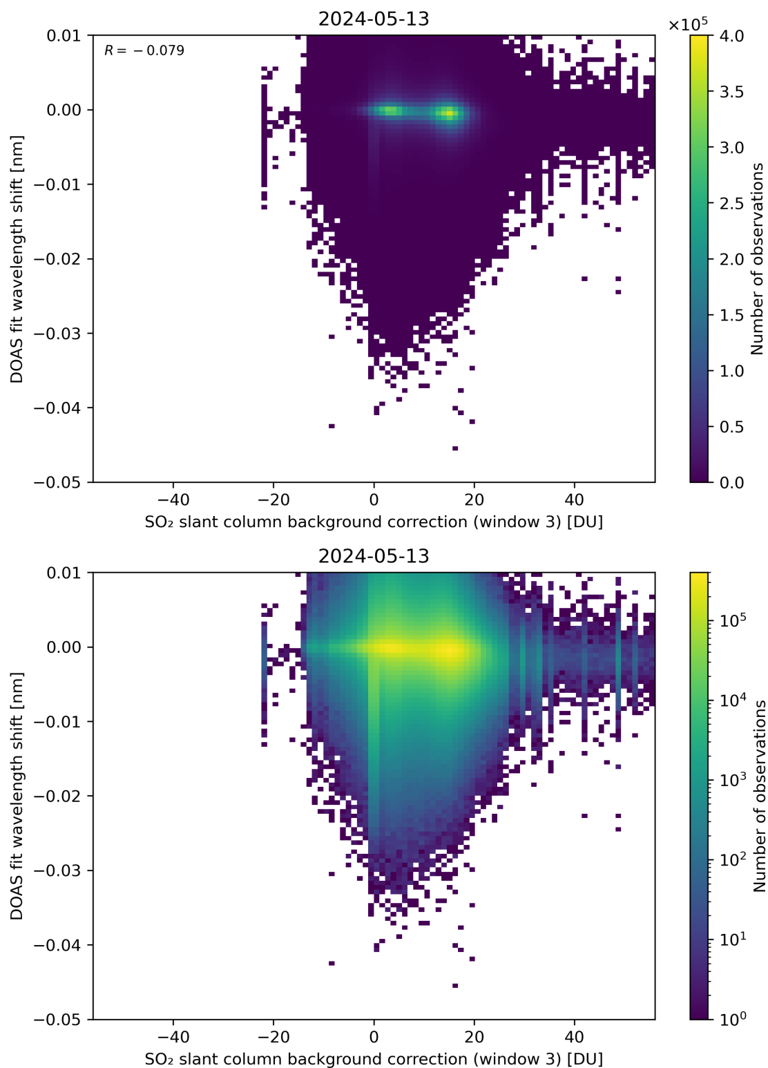
Figure 121: Scatter density plot of “SO 2 slant column background correction (window 3)” against “DOAS fit wavelength shift” for 2024-05-12 to 2024-05-14.
