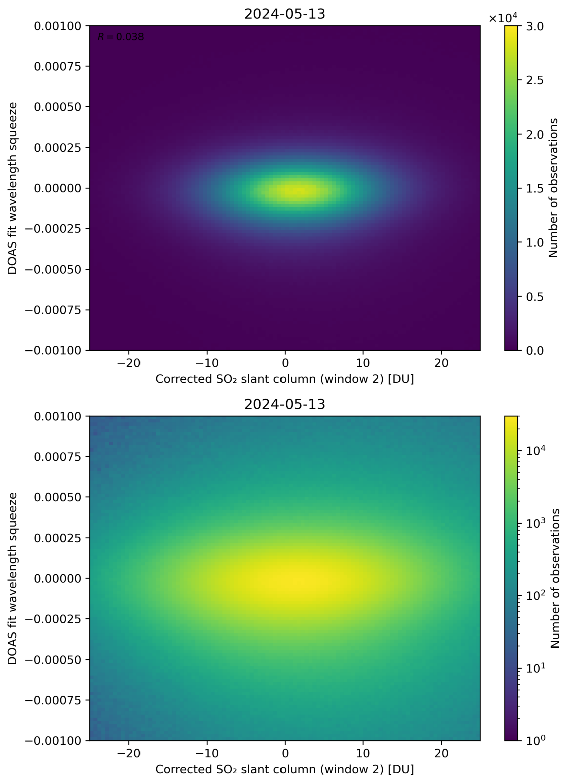
Figure 197: Scatter density plot of “Corrected SO 2 slant column (window 2)” against “DOAS fit wavelength squeeze” for 2024-05-12 to 2024-05-14.
