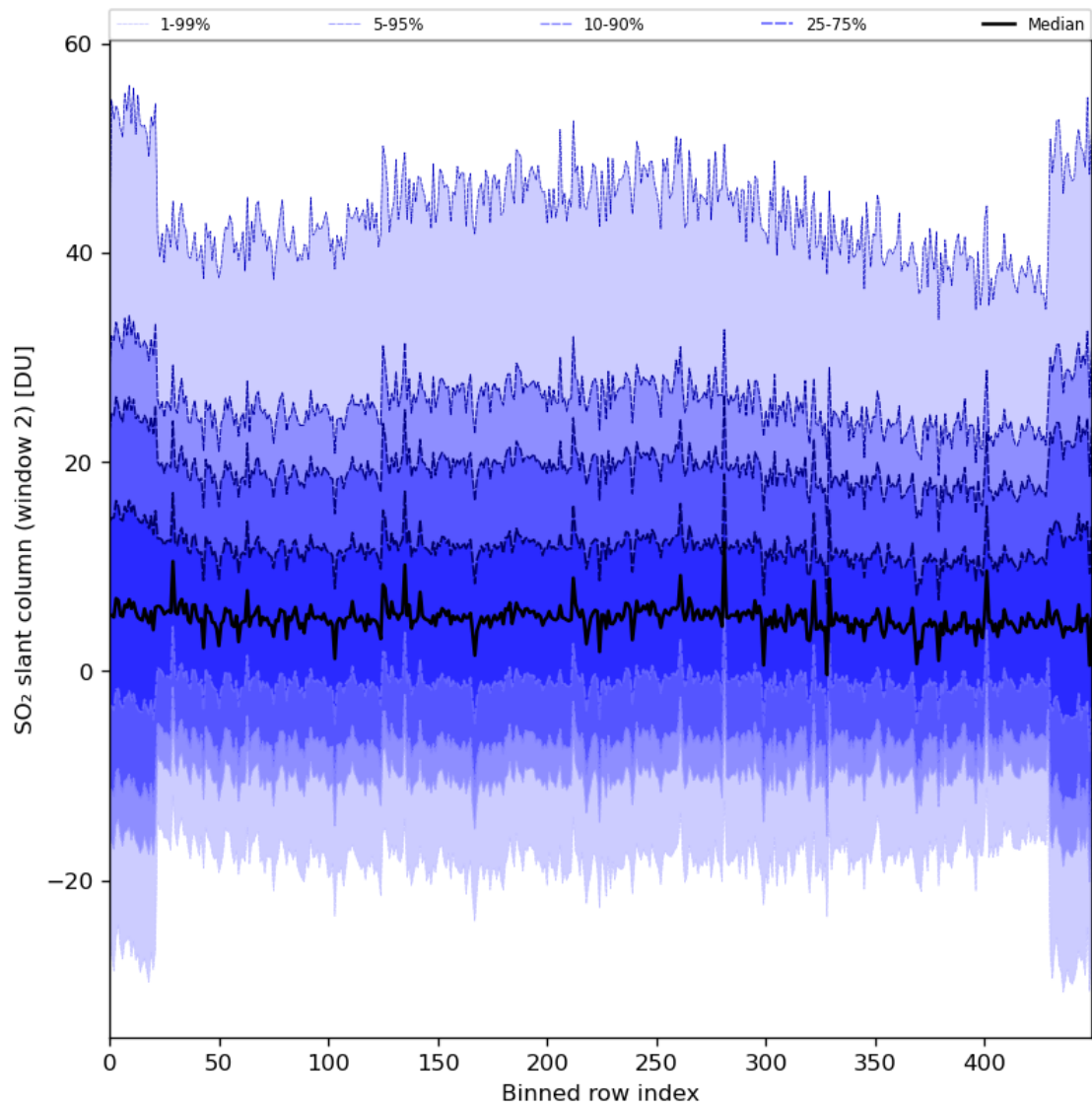
Figure 83: Along track statistics of “SO 2 slant column (window 2)” for 2024-05-12 to 2024-05-14
