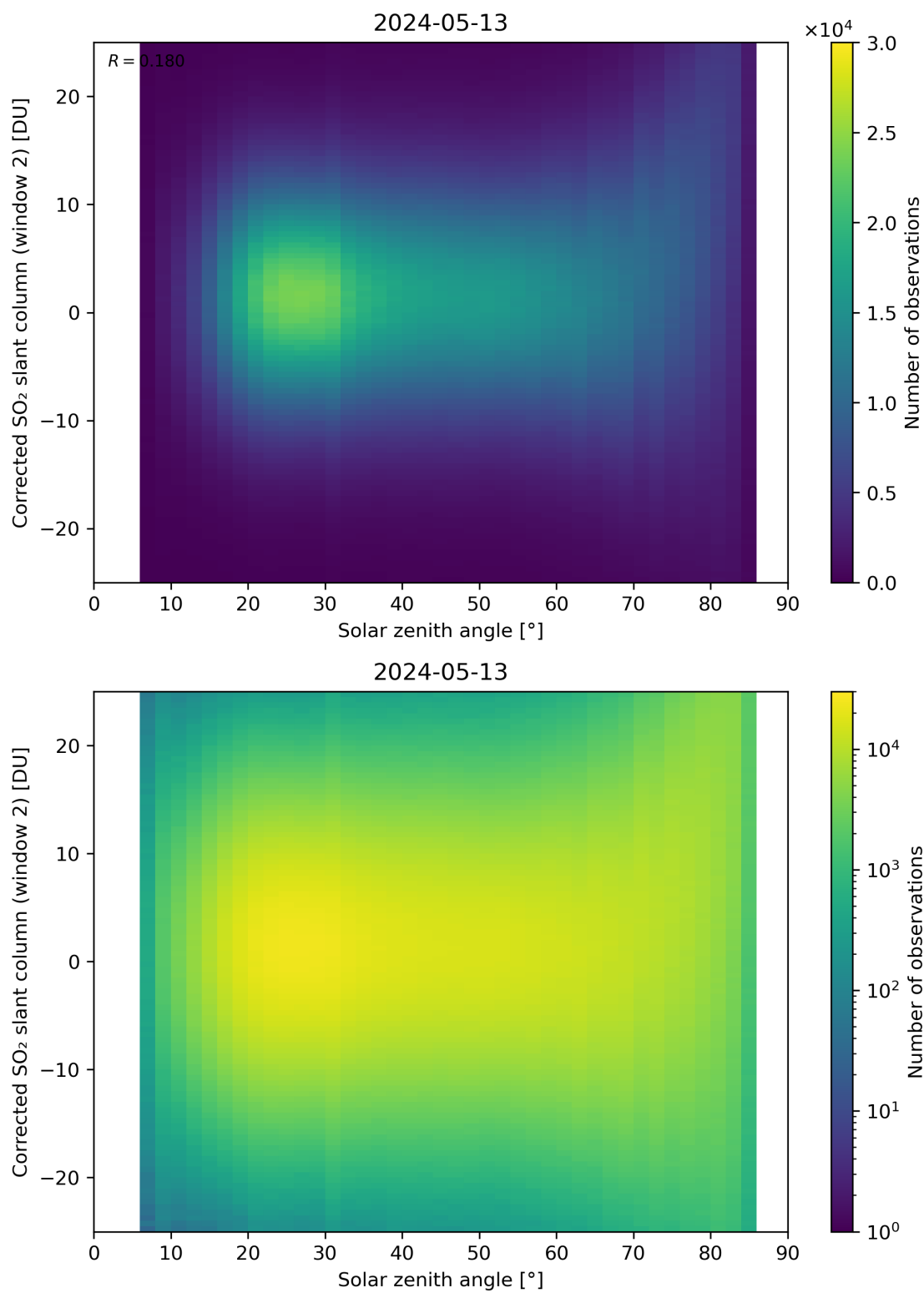
Figure 167: Scatter density plot of “Solar zenith angle” against “Corrected SO 2 slant column (window 2)” for 2024-05-12 to 2024-05-14.
