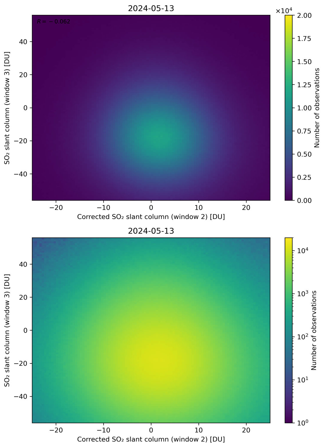
Figure 201: Scatter density plot of “Corrected SO 2 slant column (window 2)” against “SO 2 slant column (window 3)” for 2024-05-12 to 2024-05-14.
