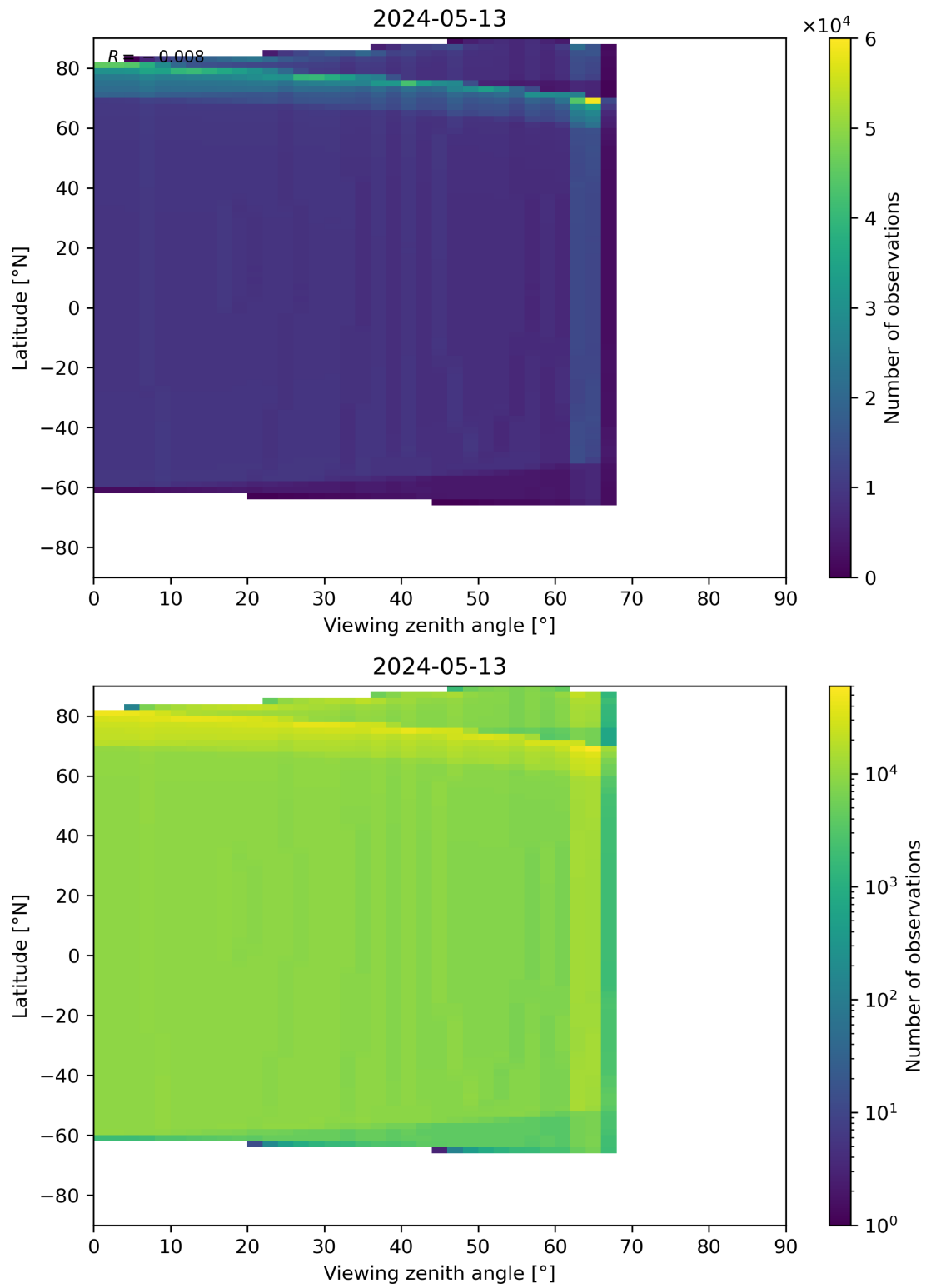
Figure 314: Scatter density plot of “Viewing zenith angle” against “Latitude” for 2024-05-12 to 2024-05-14.
