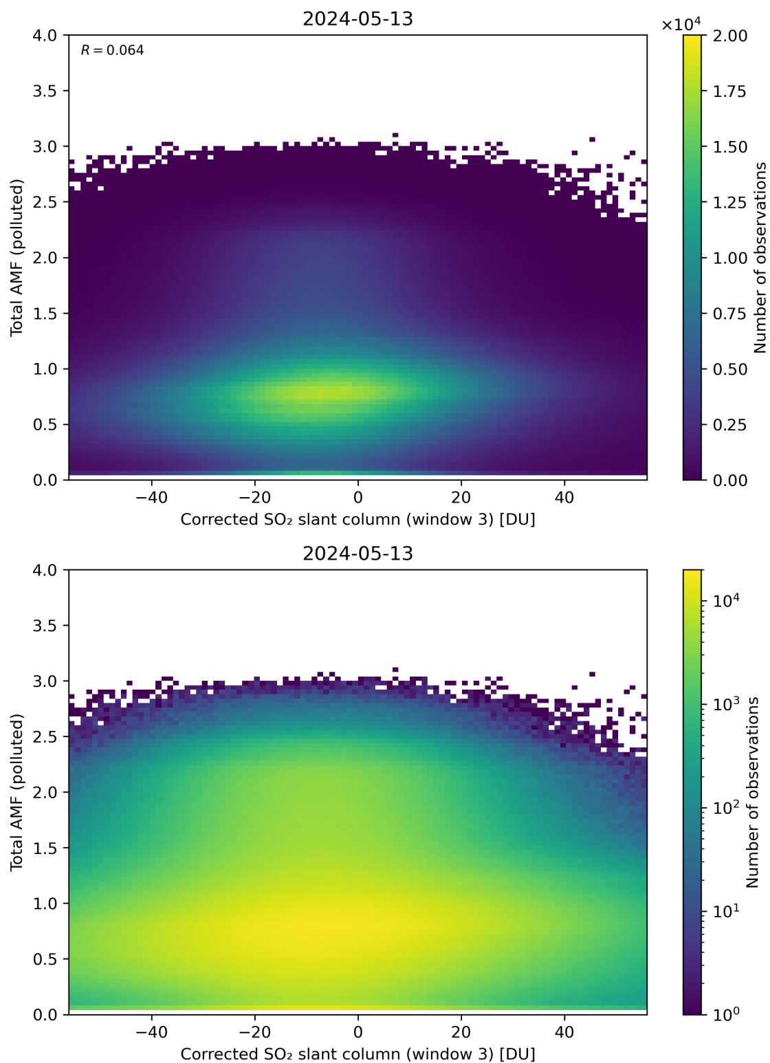
Figure 210: Scatter density plot of “Corrected SO 2 slant column (window 3)” against “Total AMF (polluted)” for 2024-05-12 to 2024-05-14.
