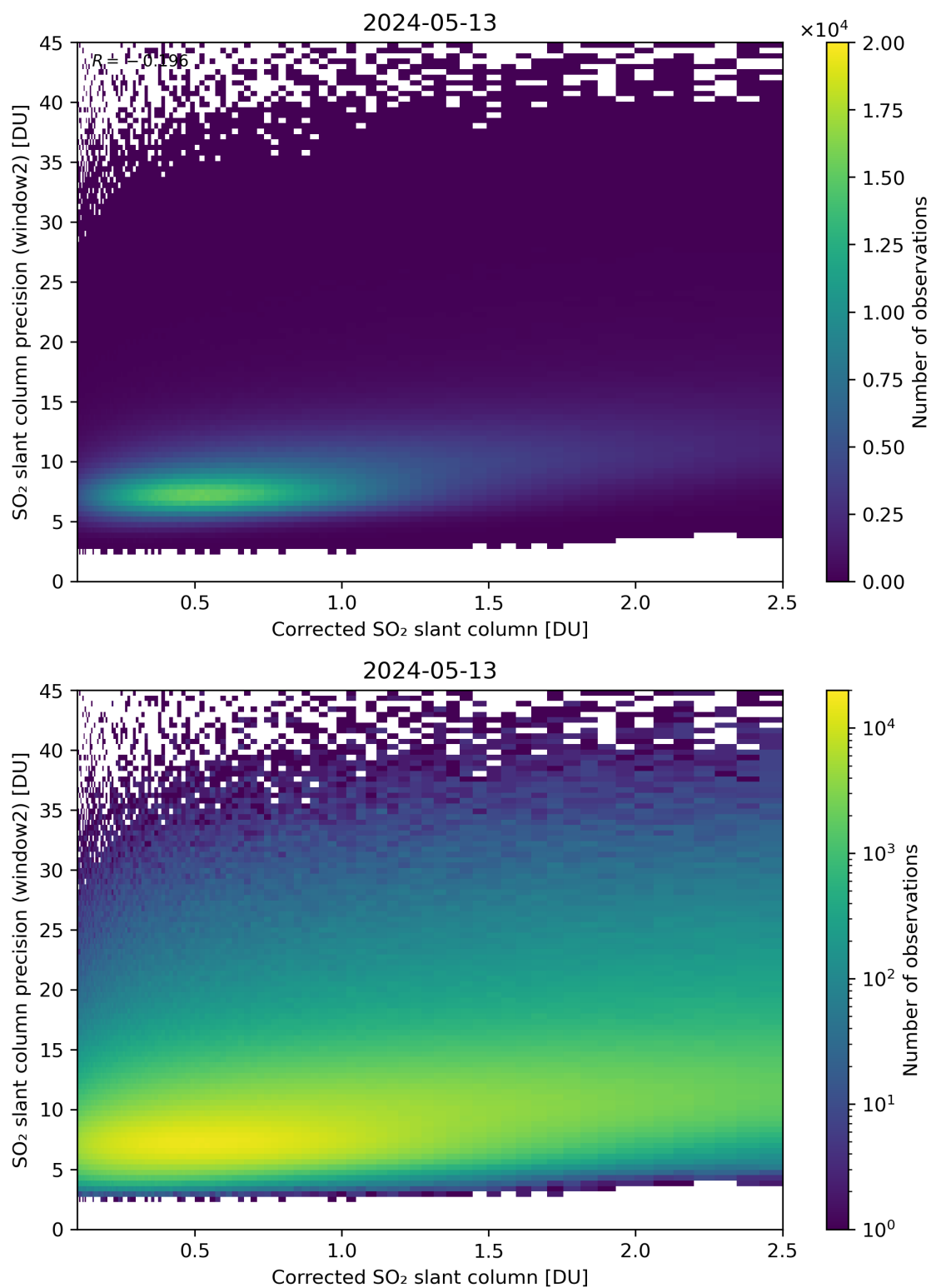
Figure 189: Scatter density plot of “Corrected SO 2 slant column” against “SO 2 slant column precision (window2)” for 2024-05-12 to 2024-05-14.
