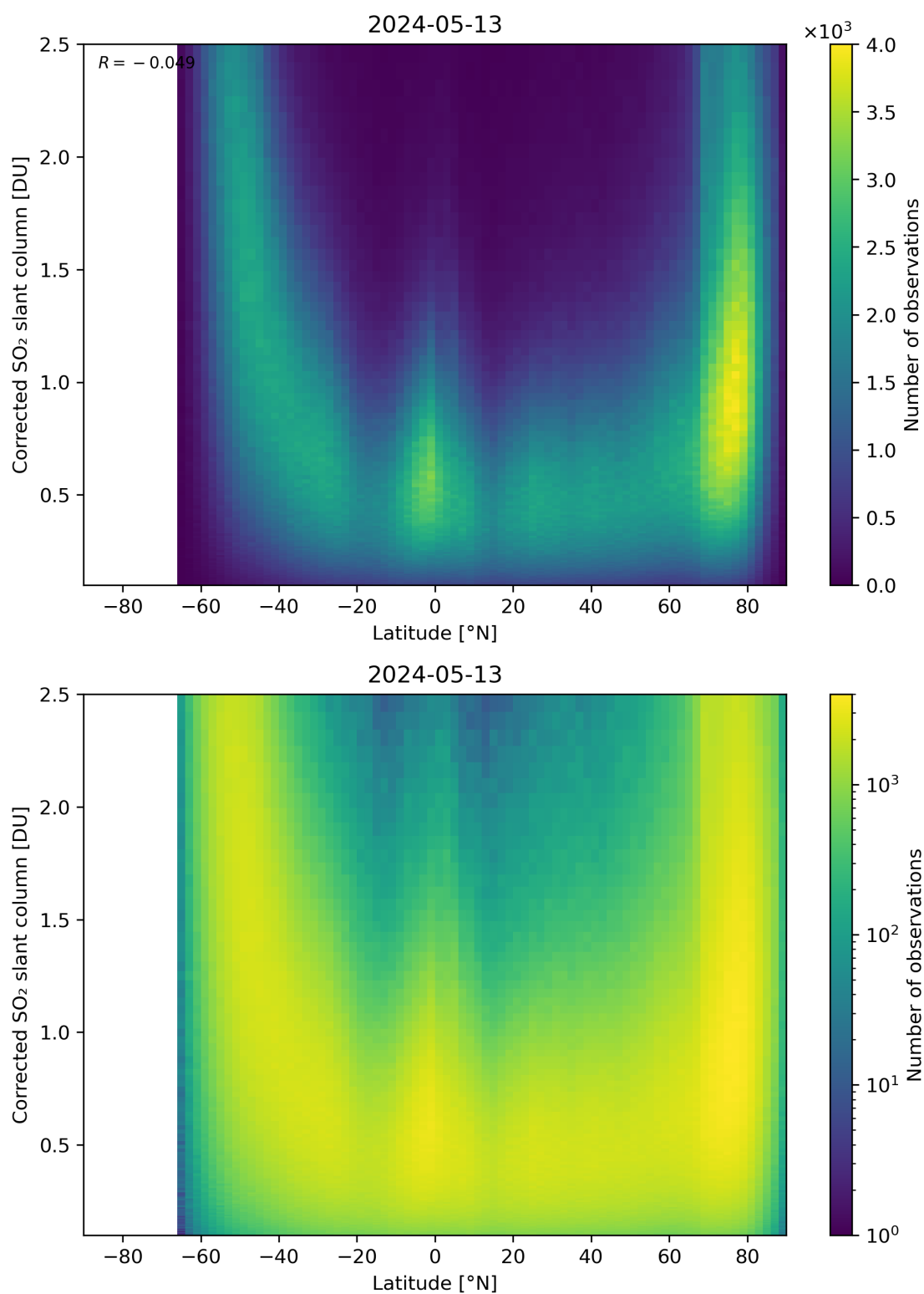
Figure 146: Scatter density plot of “Latitude” against “Corrected SO 2 slant column” for 2024-05-12 to 2024-05-14.
