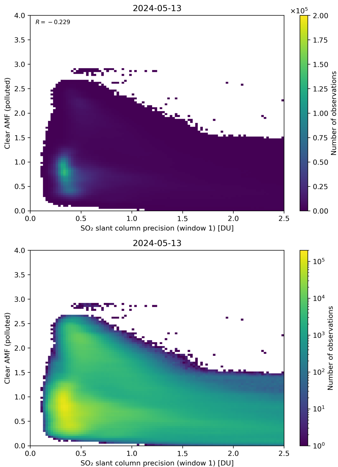
Figure 224: Scatter density plot of “SO 2 slant column precision (window 1)” against “Clear AMF (polluted)” for 2024-05-12 to 2024-05-14.
