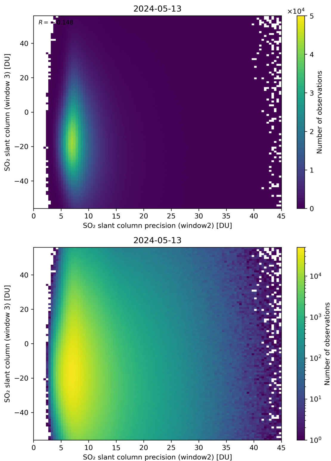
Figure 249: Scatter density plot of “SO 2 slant column precision (window2)” against “SO 2 slant column (window 3)” for 2024-05-12 to 2024-05-14.
