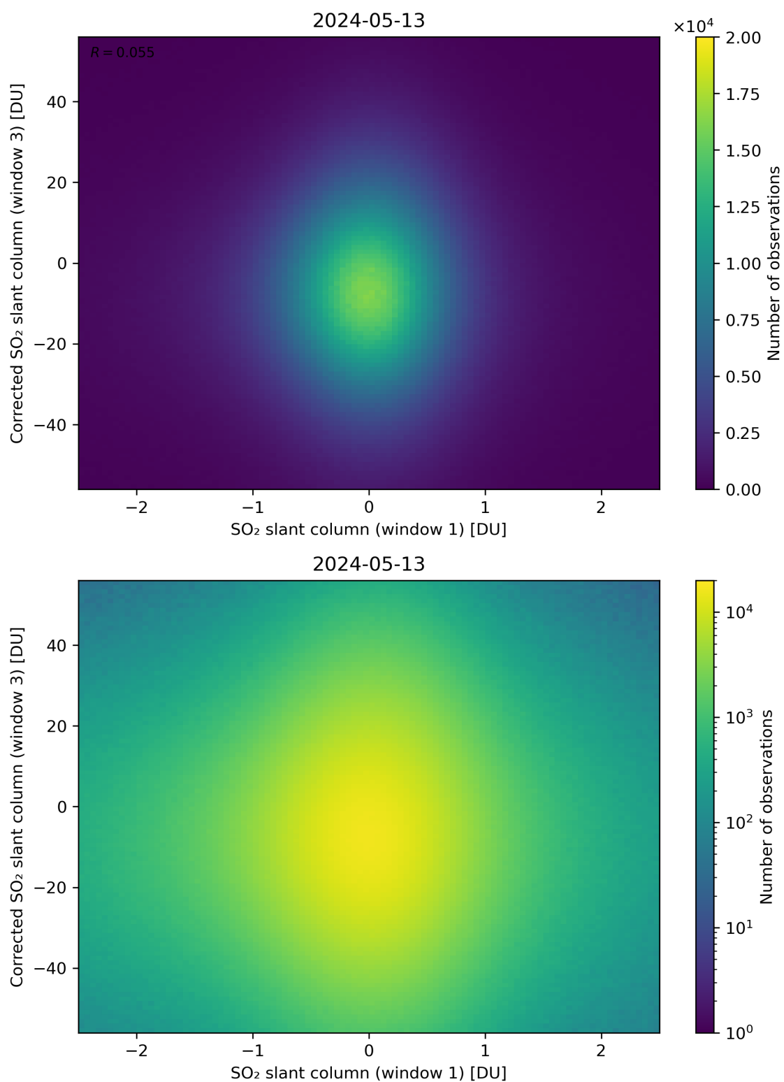
Figure 234: Scatter density plot of “SO 2 slant column (window 1)” against “Corrected SO 2 slant column (window 3)” for 2024-05-12 to 2024-05-14.
