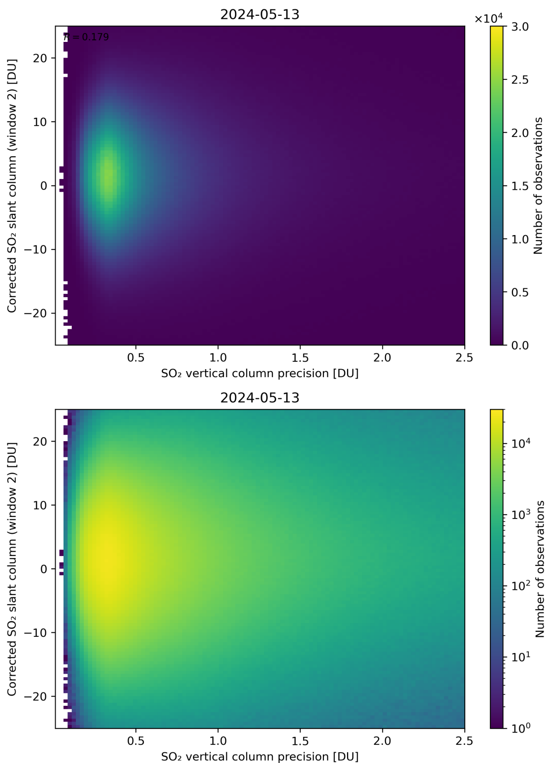
Figure 287: Scatter density plot of “SO 2 vertical column precision” against “Corrected SO 2 slant column (window 2)” for 2024-05-12 to 2024-05-14.
