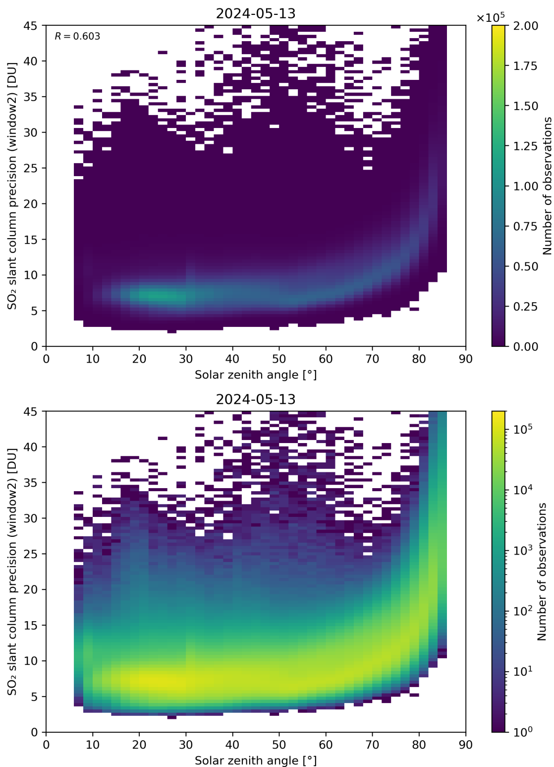
Figure 171: Scatter density plot of “Solar zenith angle” against “SO 2 slant column precision (window2)” for 2024-05-12 to 2024-05-14.
