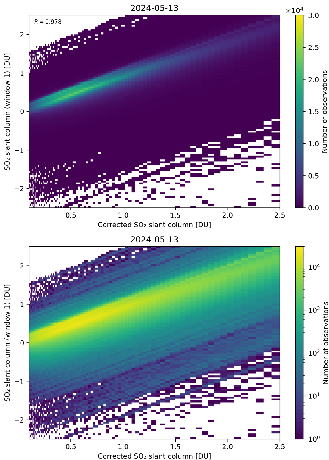
Figure 187: Scatter density plot of “Corrected SO 2 slant column” against “SO 2 slant column (window 1)” for 2024-05-12 to 2024-05-14.
