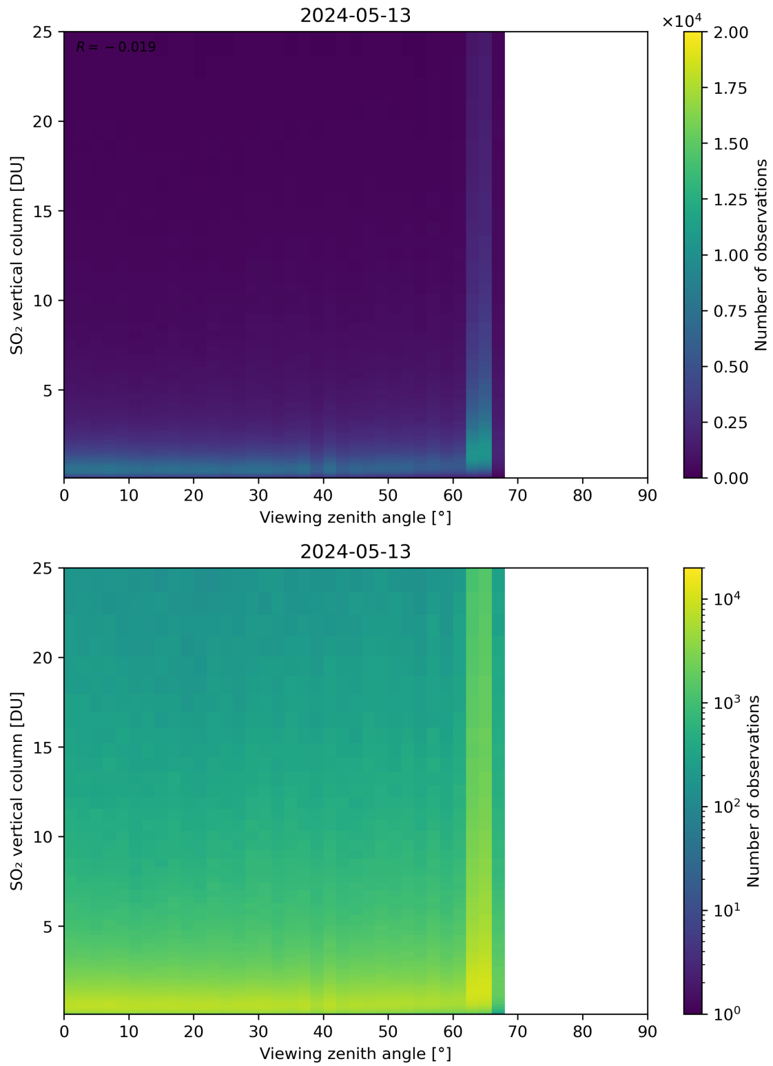
Figure 327: Scatter density plot of “Viewing zenith angle” against “SO 2 vertical column” for 2024-05-12 to 2024-05-14.
