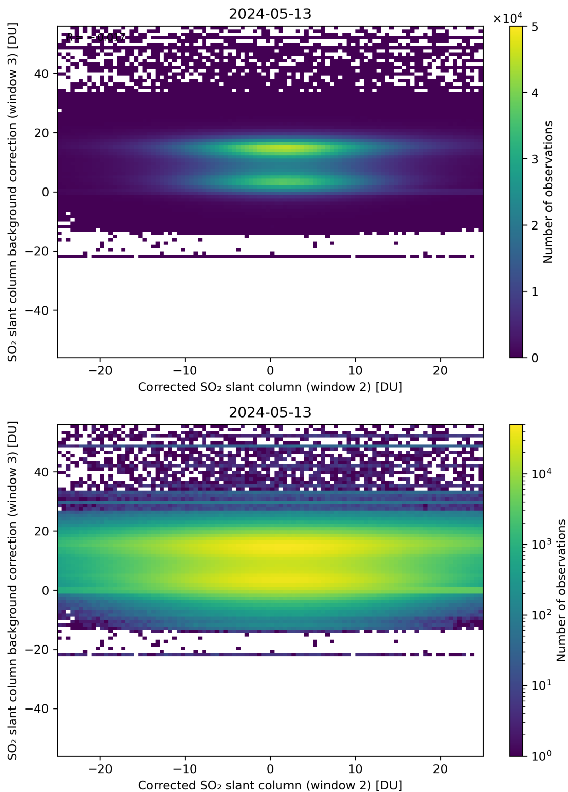
Figure 195: Scatter density plot of “Corrected SO 2 slant column (window 2)” against “SO 2 slant column background correction (window 3)” for 2024-05-12 to 2024-05-14.
