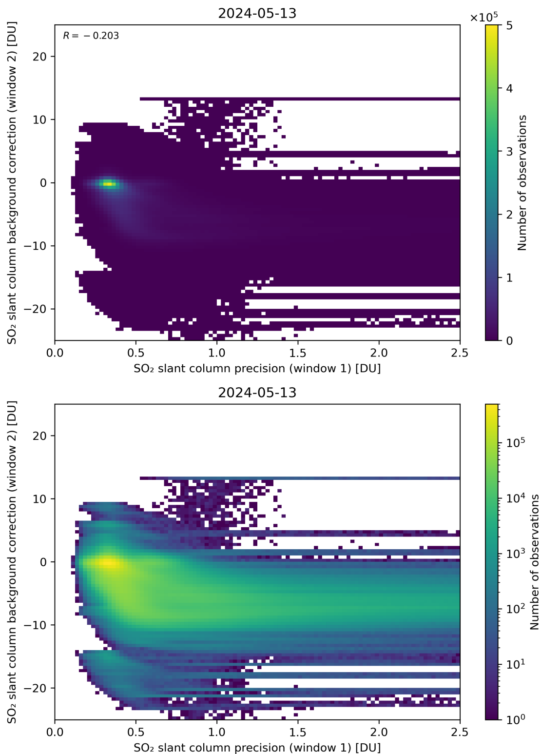
Figure 219: Scatter density plot of “SO 2 slant column precision (window 1)” against “SO 2 slant column background correction (window 2)” for 2024-05-12 to 2024-05-14.
