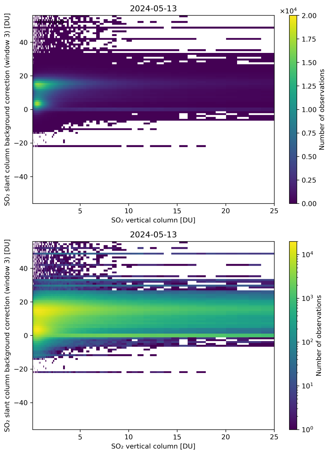
Figure 275: Scatter density plot of “SO 2 vertical column” against “SO 2 slant column background correction (window 3)” for 2024-05-12 to 2024-05-14.
