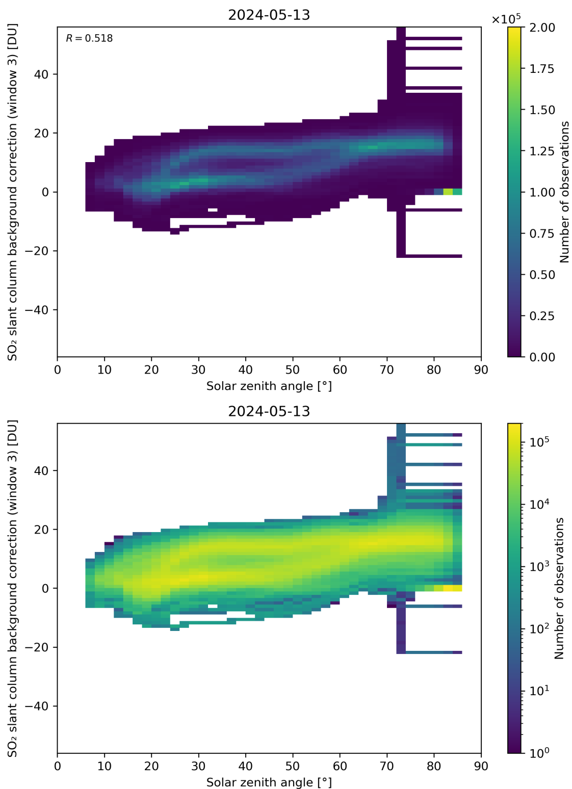
Figure 160: Scatter density plot of “Solar zenith angle” against “SO 2 slant column background correction (window 3)” for 2024-05-12 to 2024-05-14.
