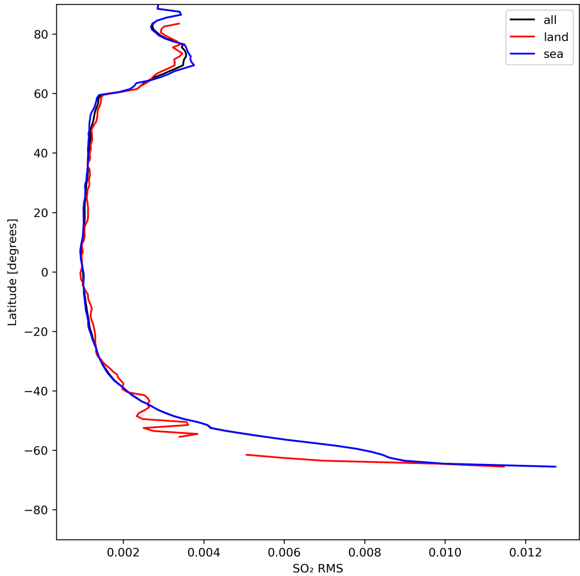
Figure 47: Zonal average of “SO 2 RMS” for 2024-05-12 to 2024-05-14.
