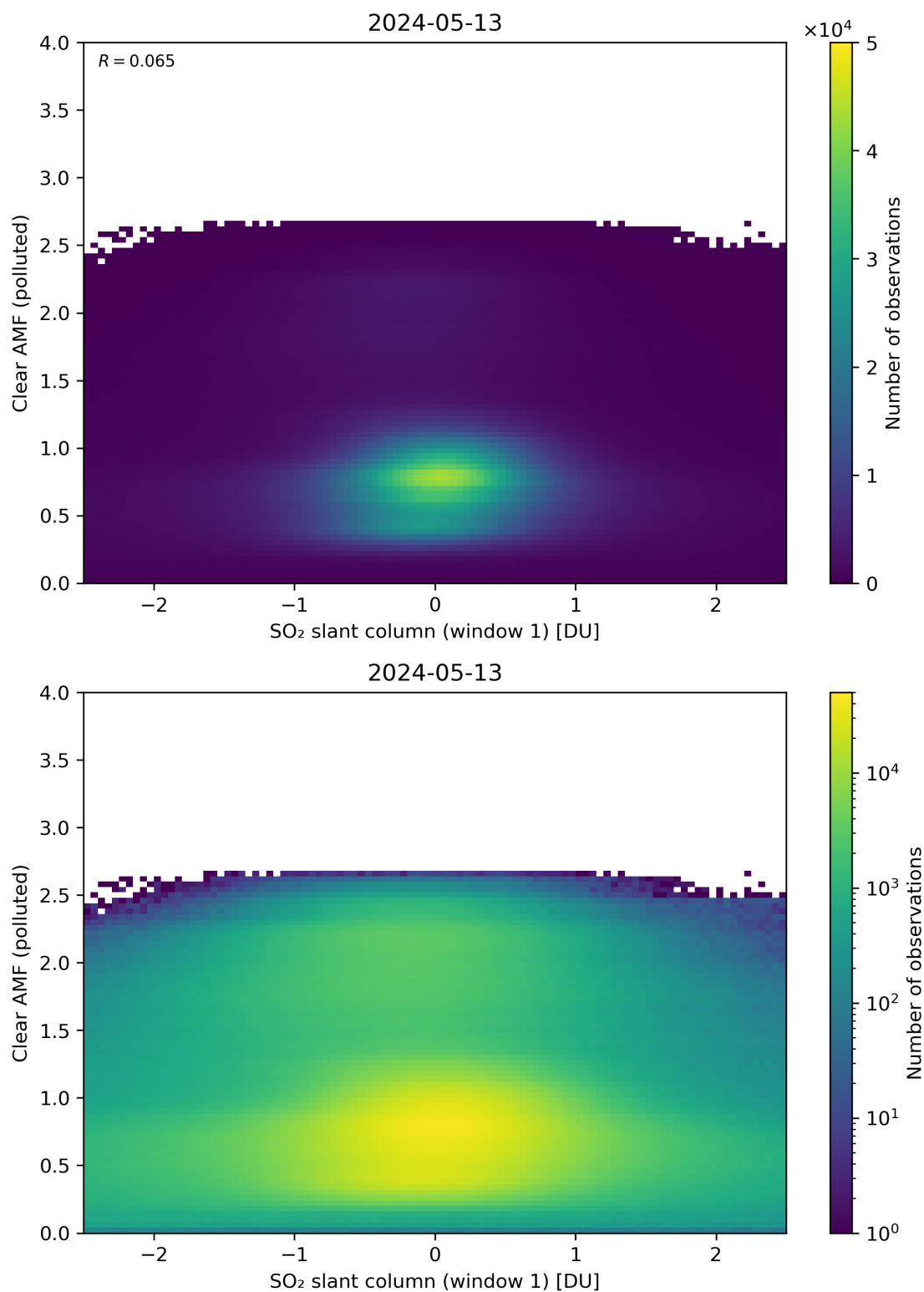
Figure 232: Scatter density plot of “SO 2 slant column (window 1)” against “Clear AMF (polluted)” for 2024-05-12 to 2024-05-14.
