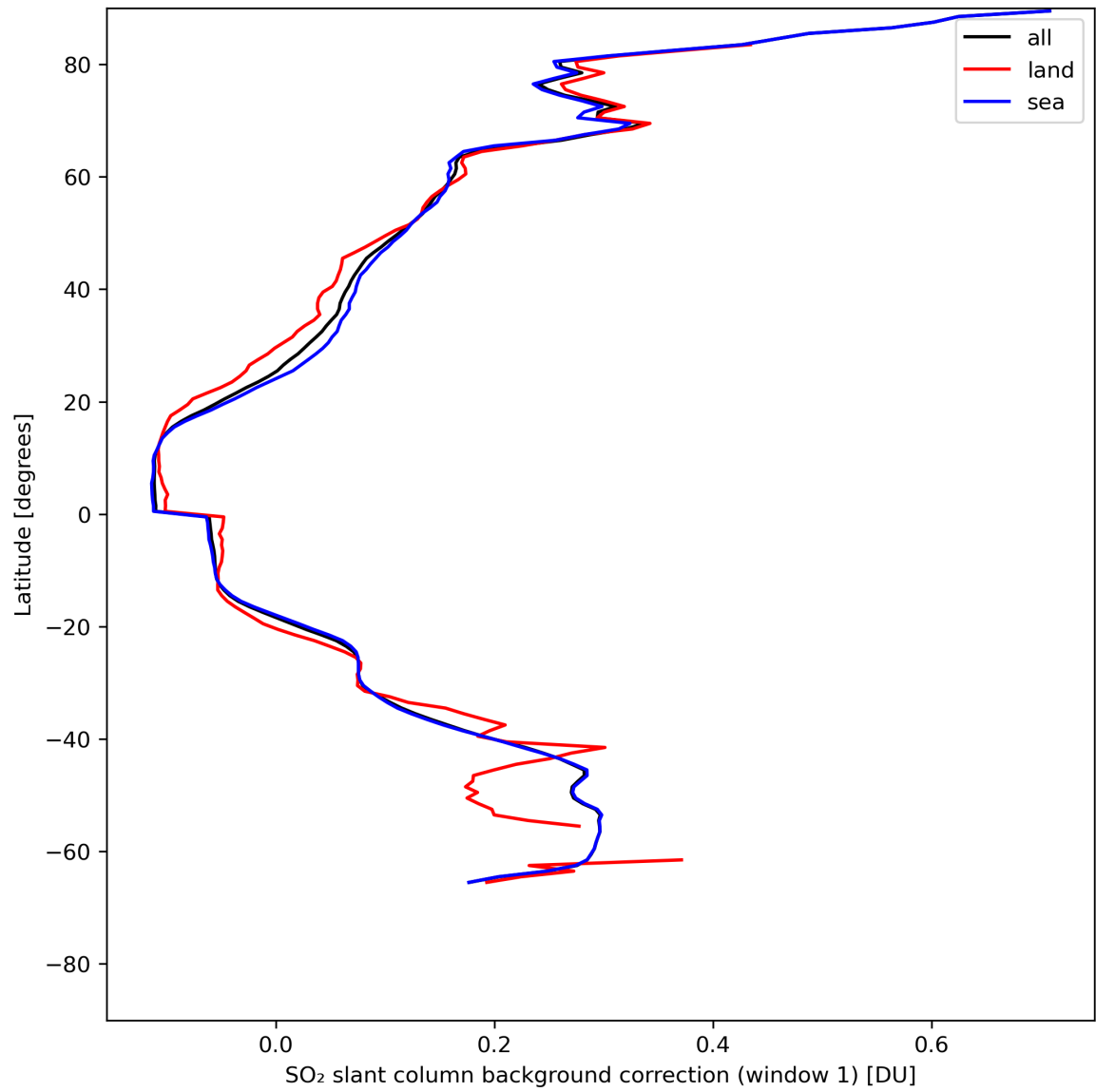
Figure 36: Zonal average of “SO 2 slant column background correction (window 1)” for 2024-05-12 to 2024-05-14.
