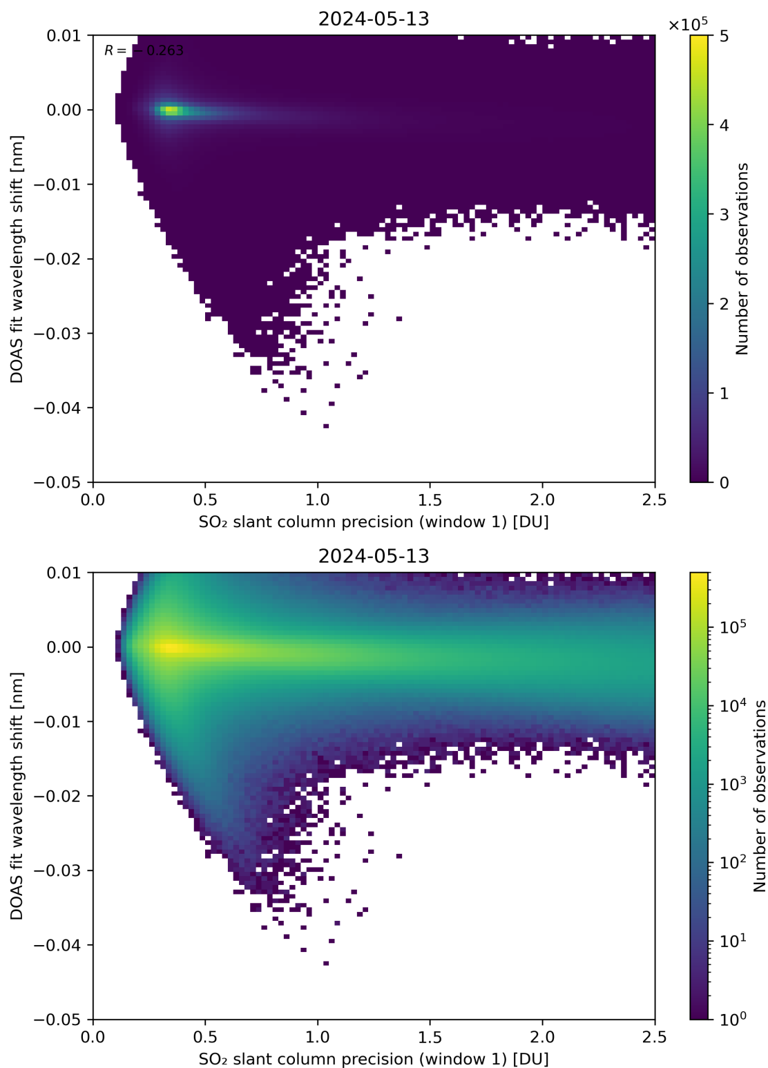
Figure 221: Scatter density plot of “SO 2 slant column precision (window 1)” against “DOAS fit wavelength shift” for 2024-05-12 to 2024-05-14.
