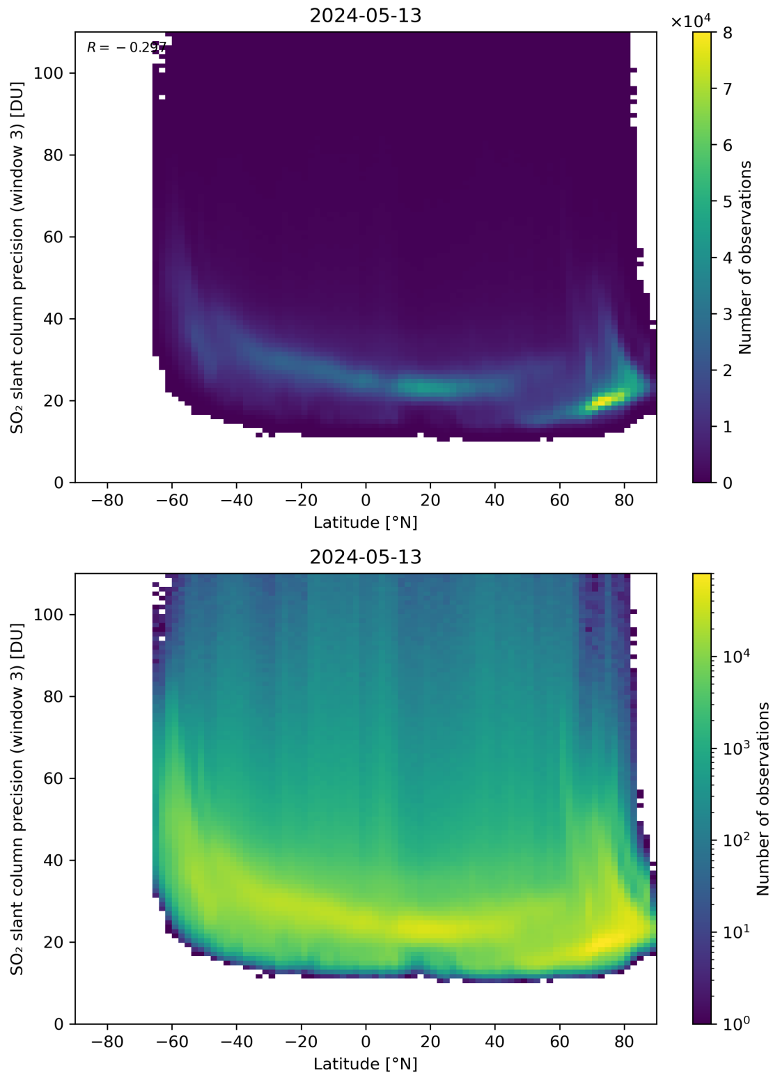
Figure 153: Scatter density plot of “Latitude” against “SO 2 slant column precision (window 3)” for 2024-05-12 to 2024-05-14.
