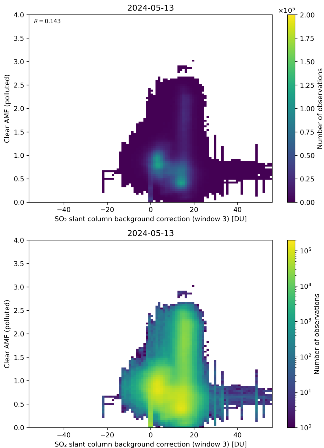
Figure 124: Scatter density plot of “SO 2 slant column background correction (window 3)” against “Clear AMF (polluted)” for 2024-05-12 to 2024-05-14.
