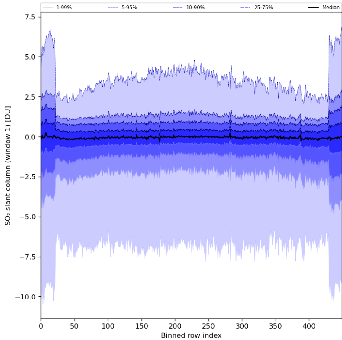
Figure 79: Along track statistics of “SO 2 slant column (window 1)” for 2024-05-12 to 2024-05-14
