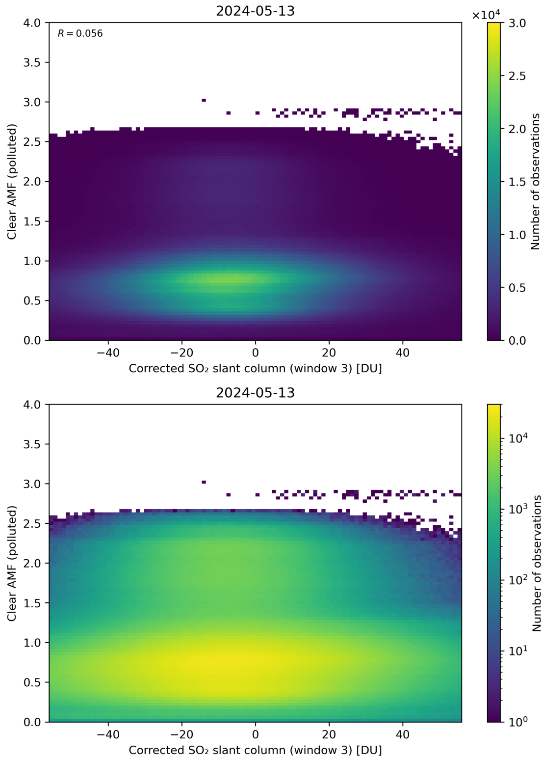
Figure 209: Scatter density plot of “Corrected SO 2 slant column (window 3)” against “Clear AMF (polluted)” for 2024-05-12 to 2024-05-14.
