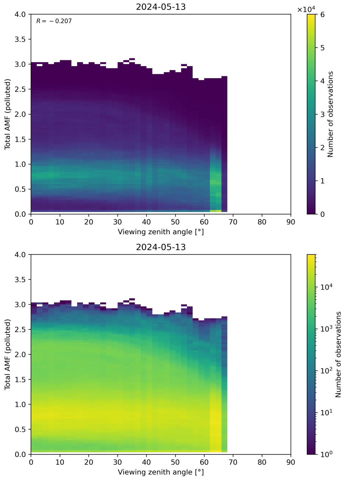
Figure 325: Scatter density plot of “Viewing zenith angle” against “Total AMF (polluted)” for 2024-05-12 to 2024-05-14.
