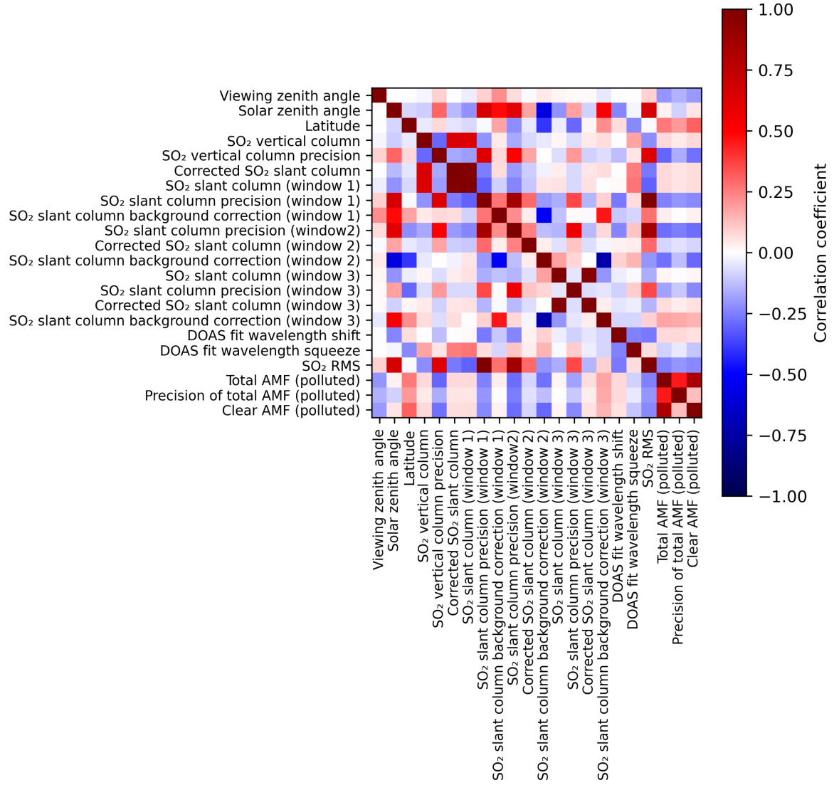
Figure 2: Map of correlation matrix for 2024-05-12 to 2024-05-14.
