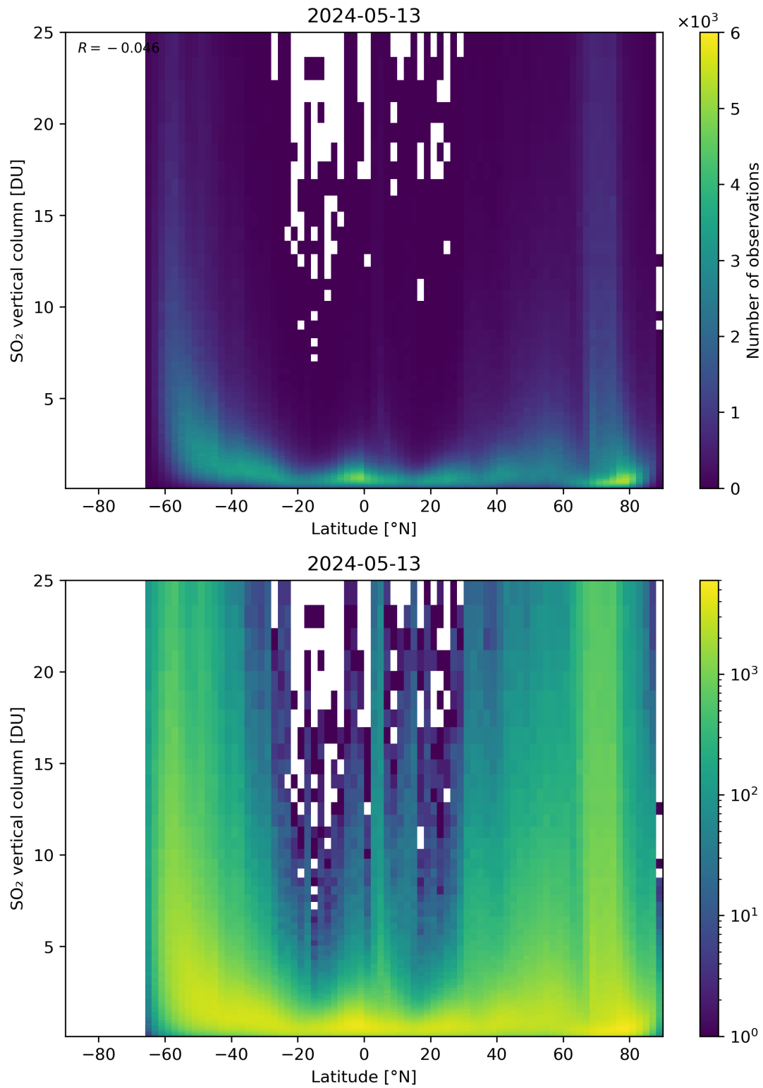
Figure 156: Scatter density plot of “Latitude” against “SO 2 vertical column” for 2024-05-12 to 2024-05-14.
