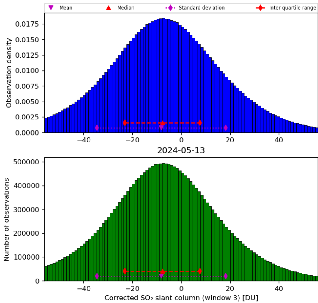
Figure 66: Histogram of “Corrected SO 2 slant column (window 3)” for 2024-05-12 to 2024-05-14
