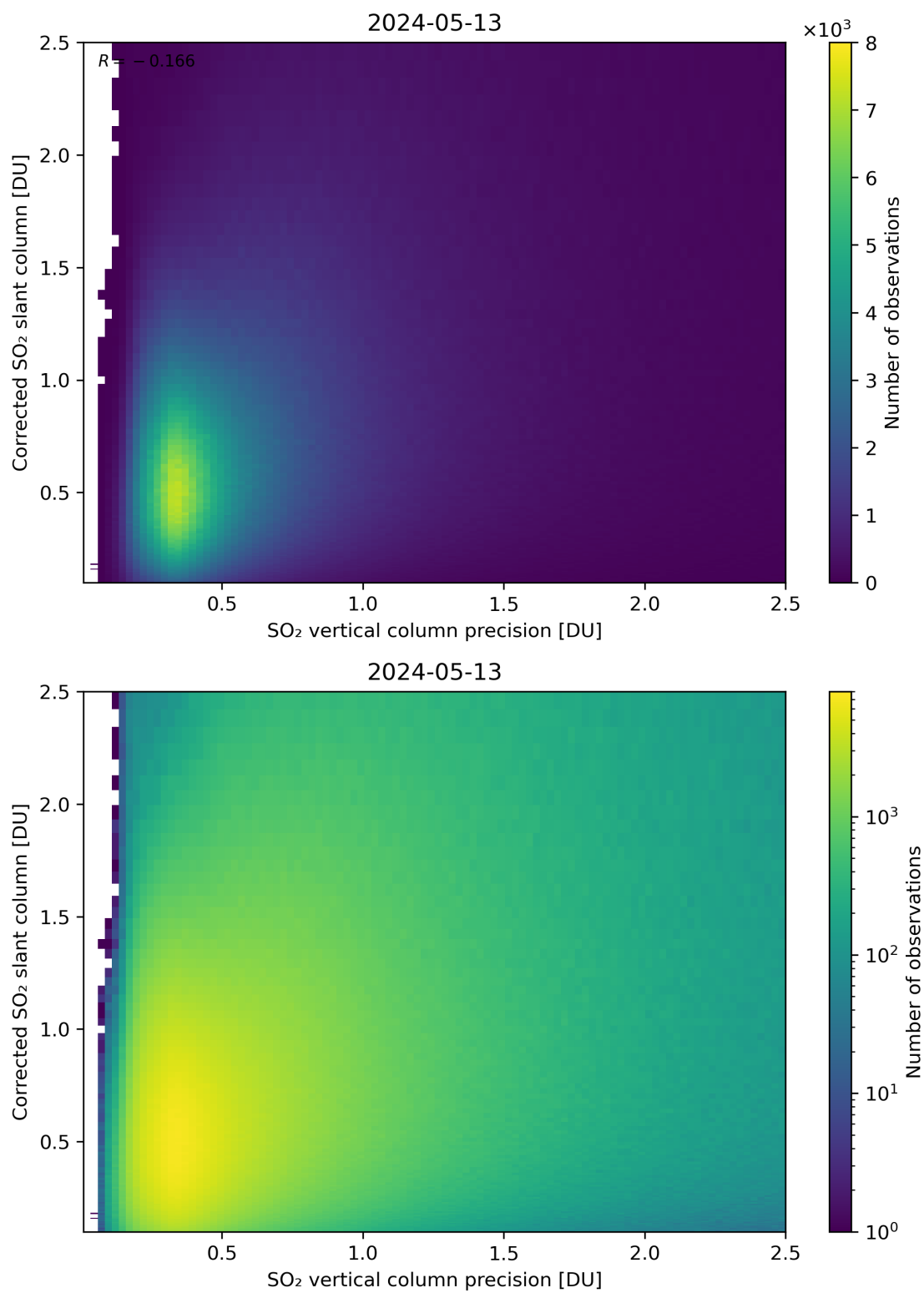
Figure 286: Scatter density plot of “SO 2 vertical column precision” against “Corrected SO 2 slant column” for 2024-05-12 to 2024-05-14.
