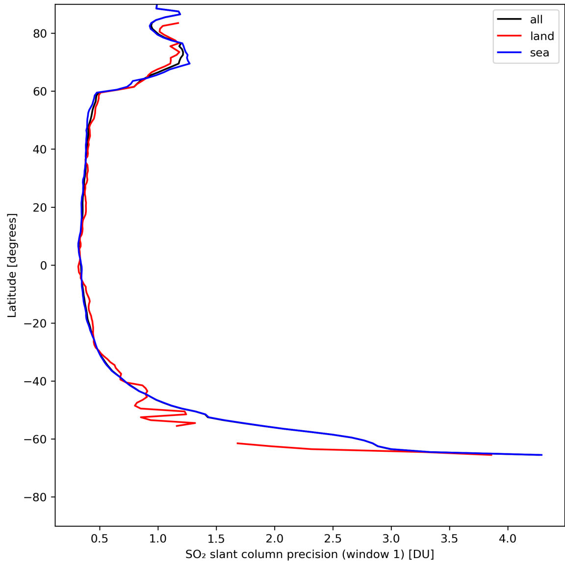
Figure 34: Zonal average of “SO 2 slant column precision (window 1)” for 2024-05-12 to 2024-05-14.
