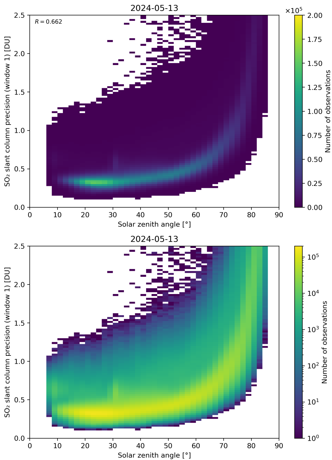
Figure 170: Scatter density plot of “Solar zenith angle” against “SO 2 slant column precision (window 1)” for 2024-05-12 to 2024-05-14.
