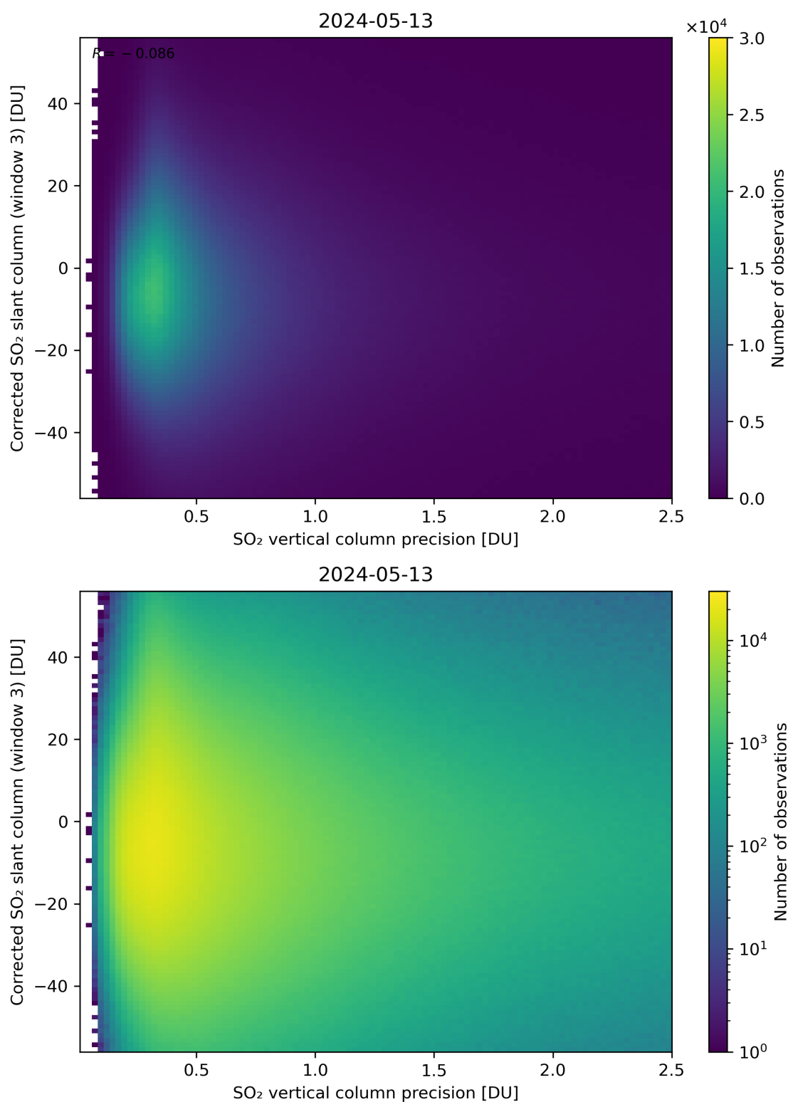
Figure 288: Scatter density plot of “SO 2 vertical column precision” against “Corrected SO 2 slant column (window 3)” for 2024-05-12 to 2024-05-14.
