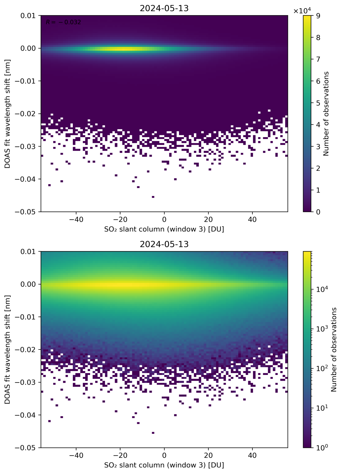
Figure 254: Scatter density plot of “SO 2 slant column (window 3)” against “DOAS fit wavelength shift” for 2024-05-12 to 2024-05-14.
