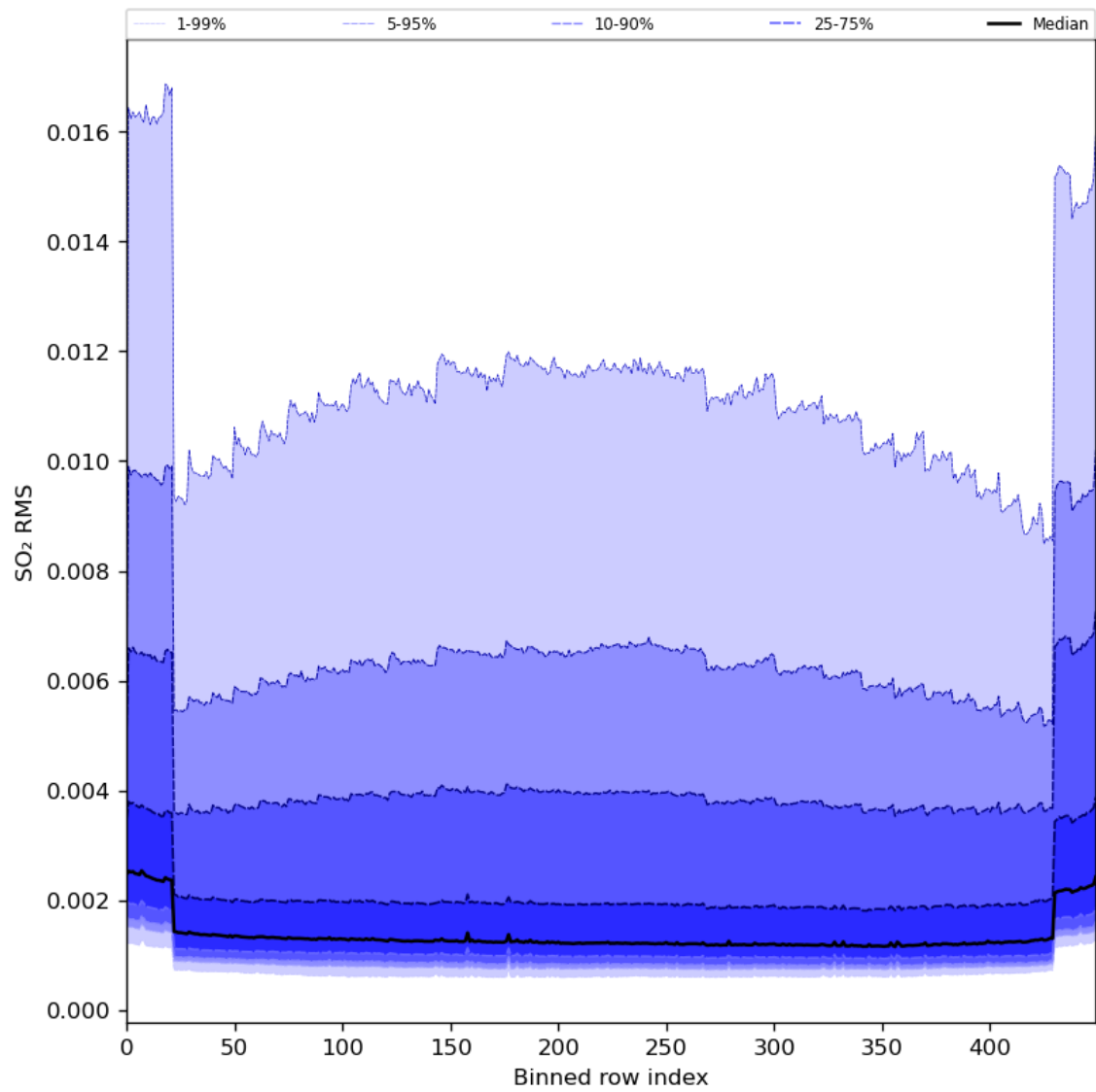
Figure 93: Along track statistics of “SO 2 RMS” for 2024-05-12 to 2024-05-14
