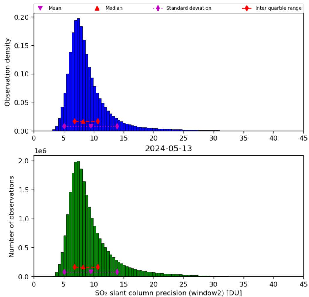
Figure 61: Histogram of “SO 2 slant column precision (window2)” for 2024-05-12 to 2024-05-14
