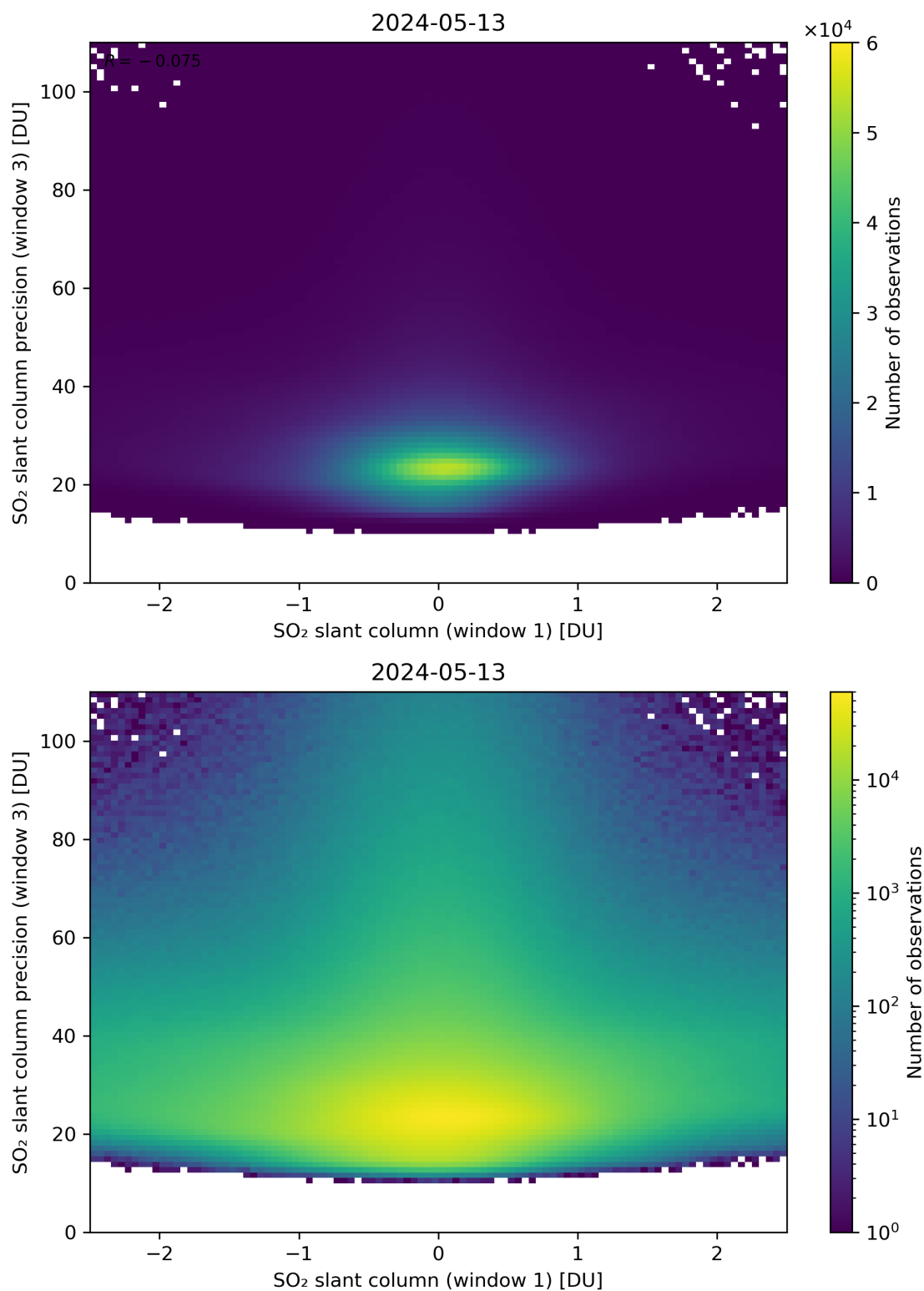
Figure 238: Scatter density plot of “SO 2 slant column (window 1)” against “SO 2 slant column precision (window 3)” for 2024-05-12 to 2024-05-14.
