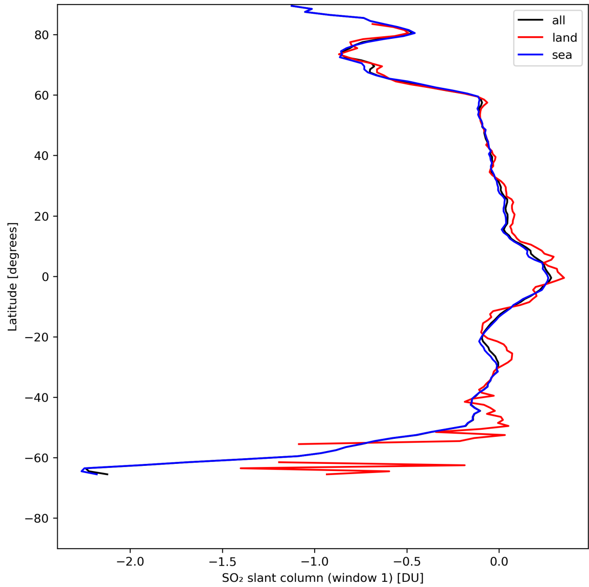
Figure 33: Zonal average of “SO 2 slant column (window 1)” for 2024-05-12 to 2024-05-14.
