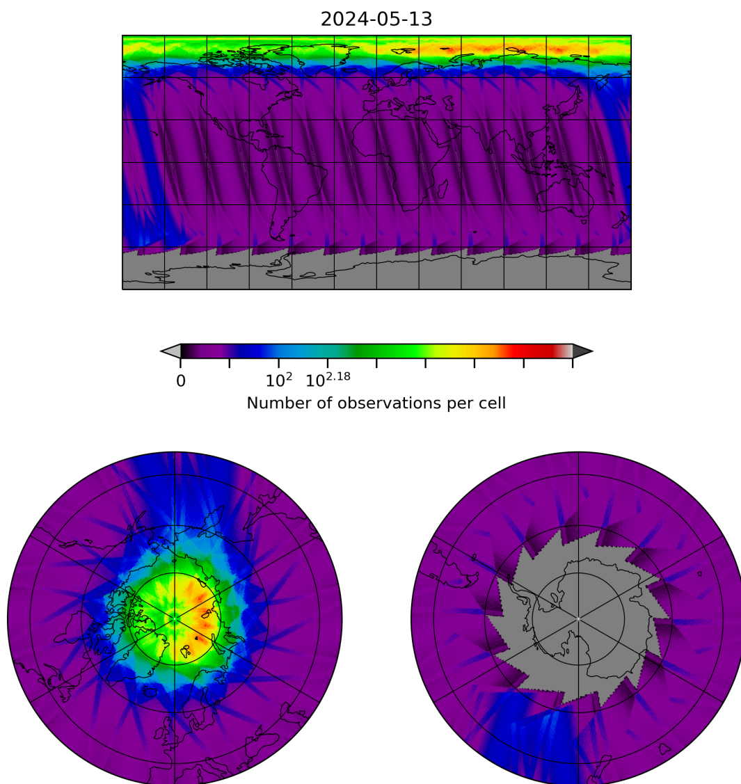
Figure 28: Map of the number of observations for 2024-05-12 to 2024-05-14
