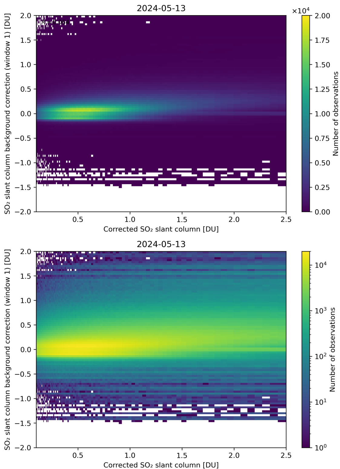
Figure 178: Scatter density plot of “Corrected SO 2 slant column” against “SO 2 slant column background correction (window 1)” for 2024-05-12 to 2024-05-14.
