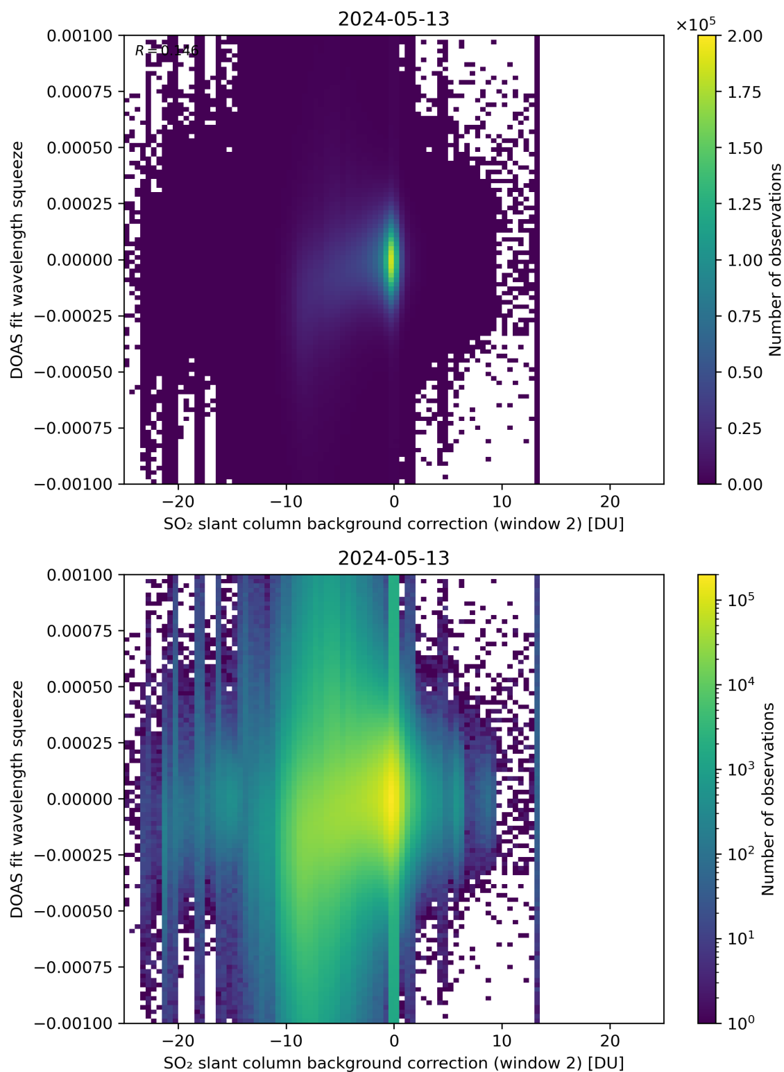
Figure 113: Scatter density plot of “SO 2 slant column background correction (window 2)” against “DOAS fit wavelength squeeze” for 2024-05-12 to 2024-05-14.
