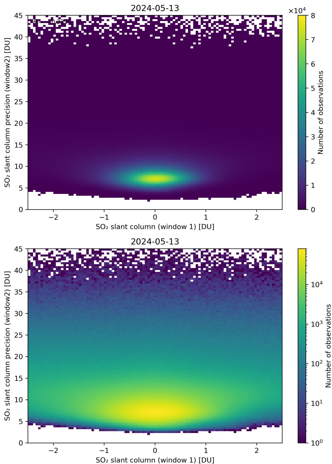
Figure 236: Scatter density plot of “SO 2 slant column (window 1)” against “SO 2 slant column precision (window2)” for 2024-05-12 to 2024-05-14.
