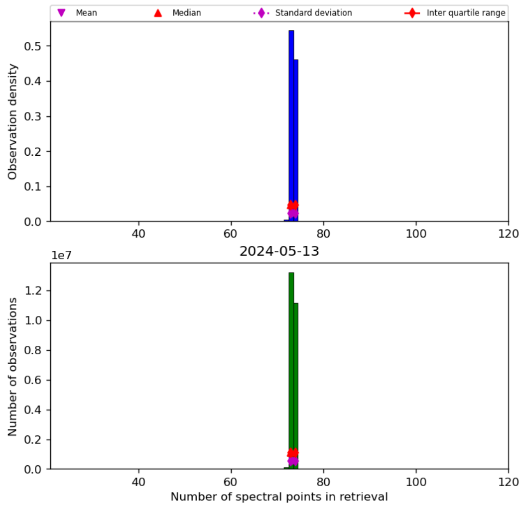
Figure 74: Histogram of “Number of spectral points in retrieval” for 2024-05-12 to 2024-05-14
