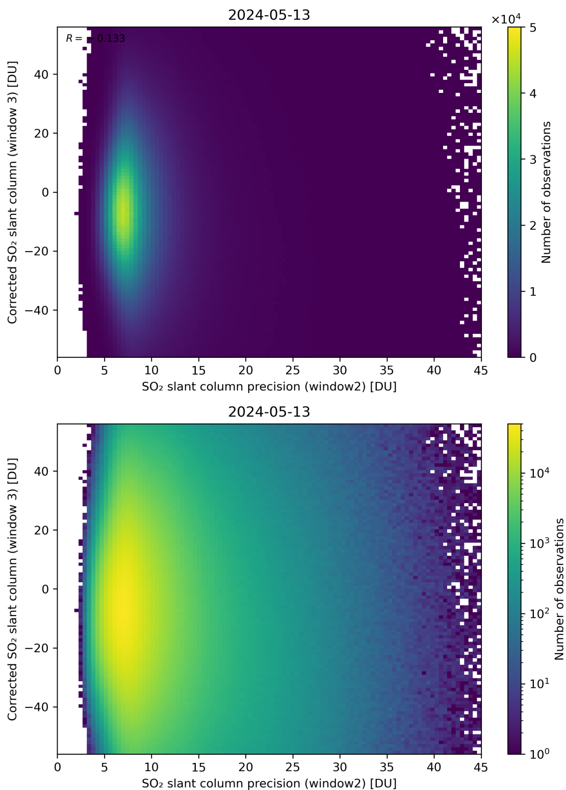
Figure 248: Scatter density plot of “SO 2 slant column precision (window2)” against “Corrected SO 2 slant column (window 3)” for 2024-05-12 to 2024-05-14.
