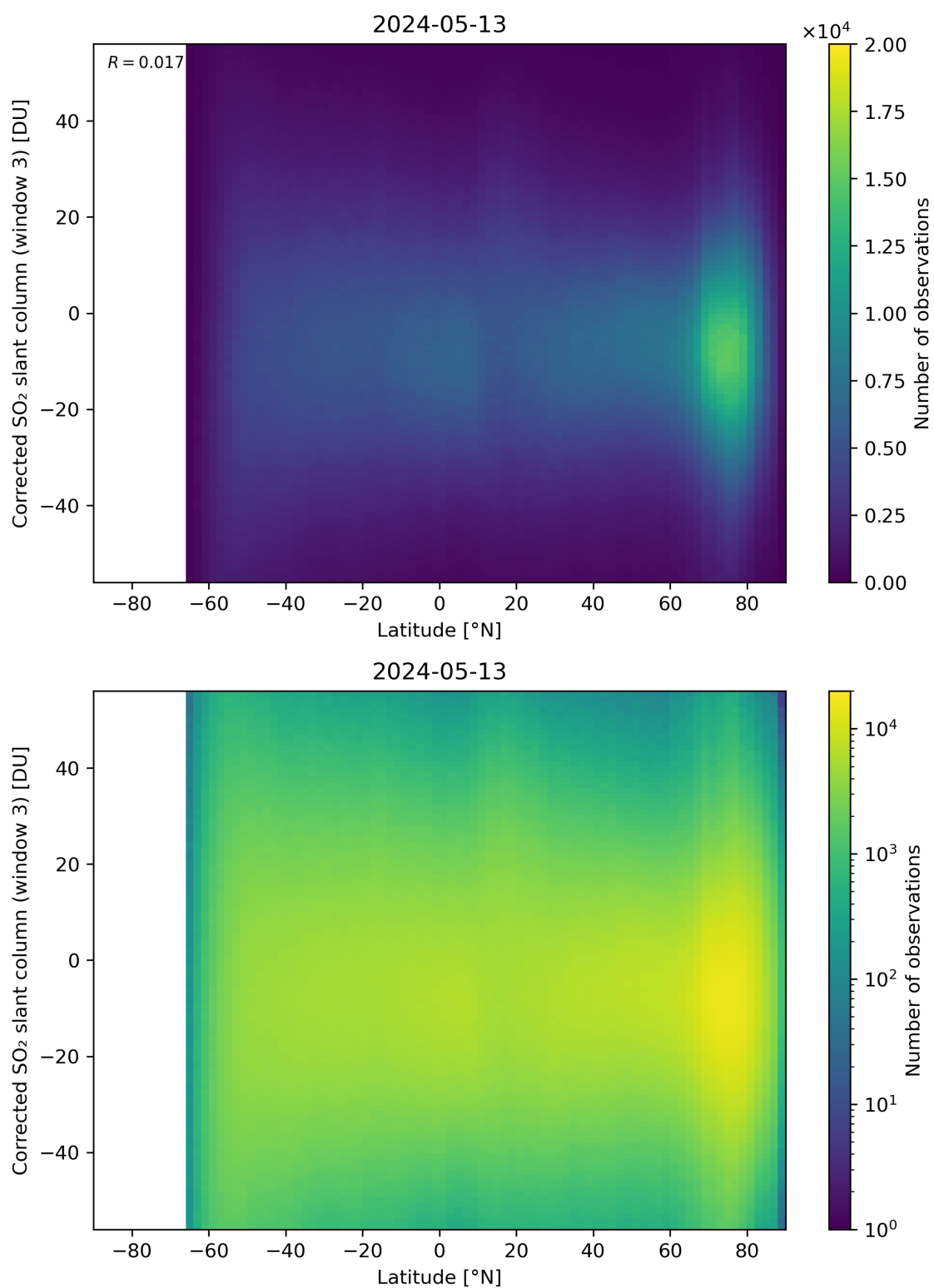
Figure 148: Scatter density plot of “Latitude” against “Corrected SO 2 slant column (window 3)” for 2024-05-12 to 2024-05-14.
