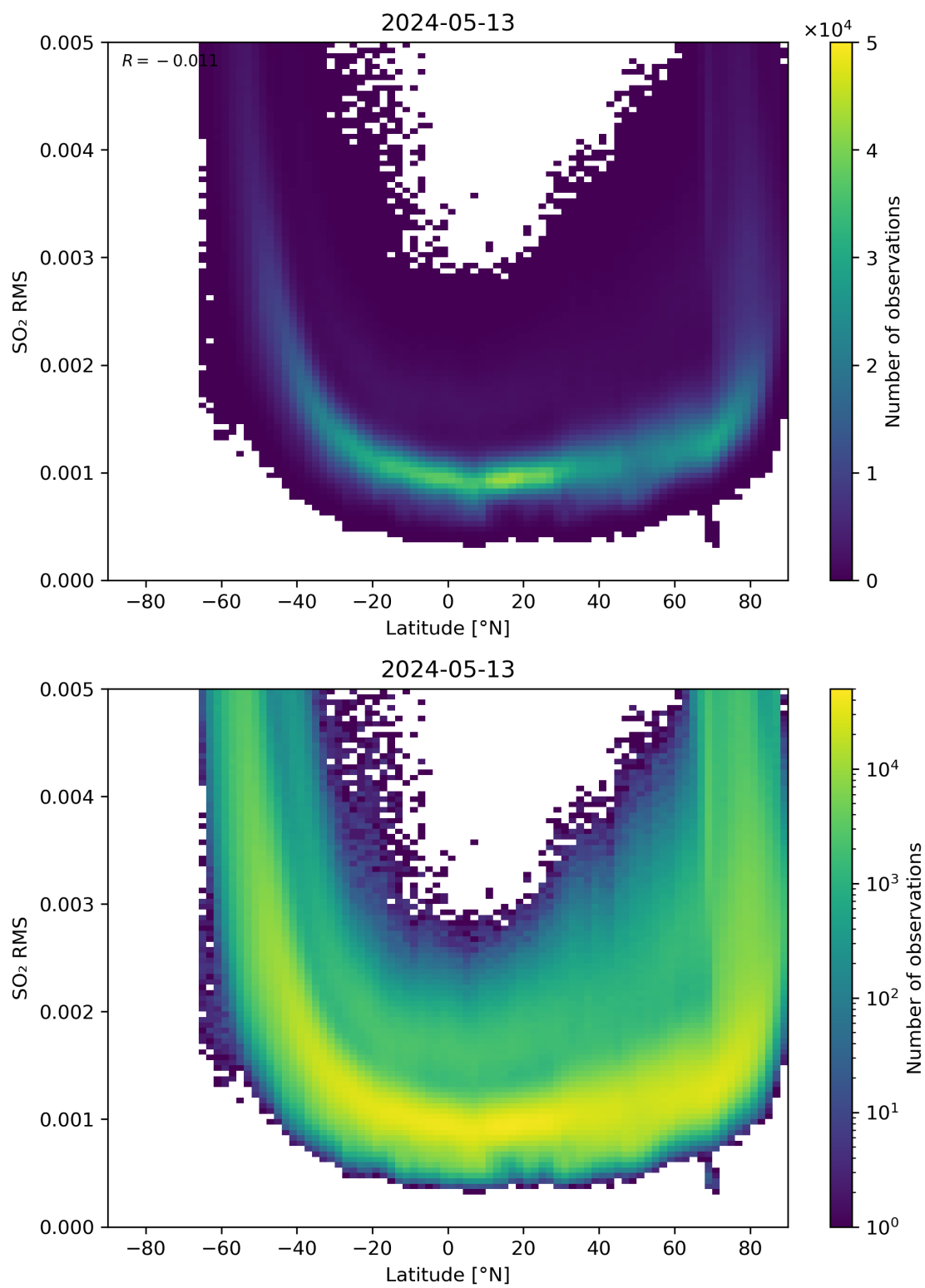
Figure 144: Scatter density plot of “Latitude” against “SO 2 RMS” for 2024-05-12 to 2024-05-14.
