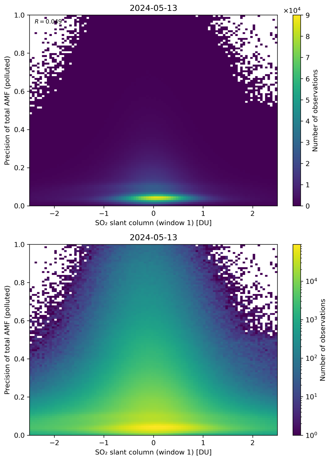
Figure 240: Scatter density plot of “SO 2 slant column (window 1)” against “Precision of total AMF (polluted)” for 2024-05-12 to 2024-05-14.
