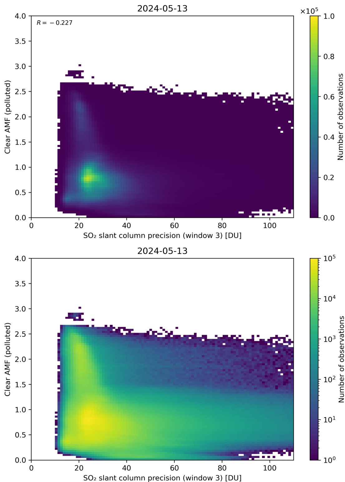
Figure 261: Scatter density plot of “SO 2 slant column precision (window 3)” against “Clear AMF (polluted)” for 2024-05-12 to 2024-05-14.
