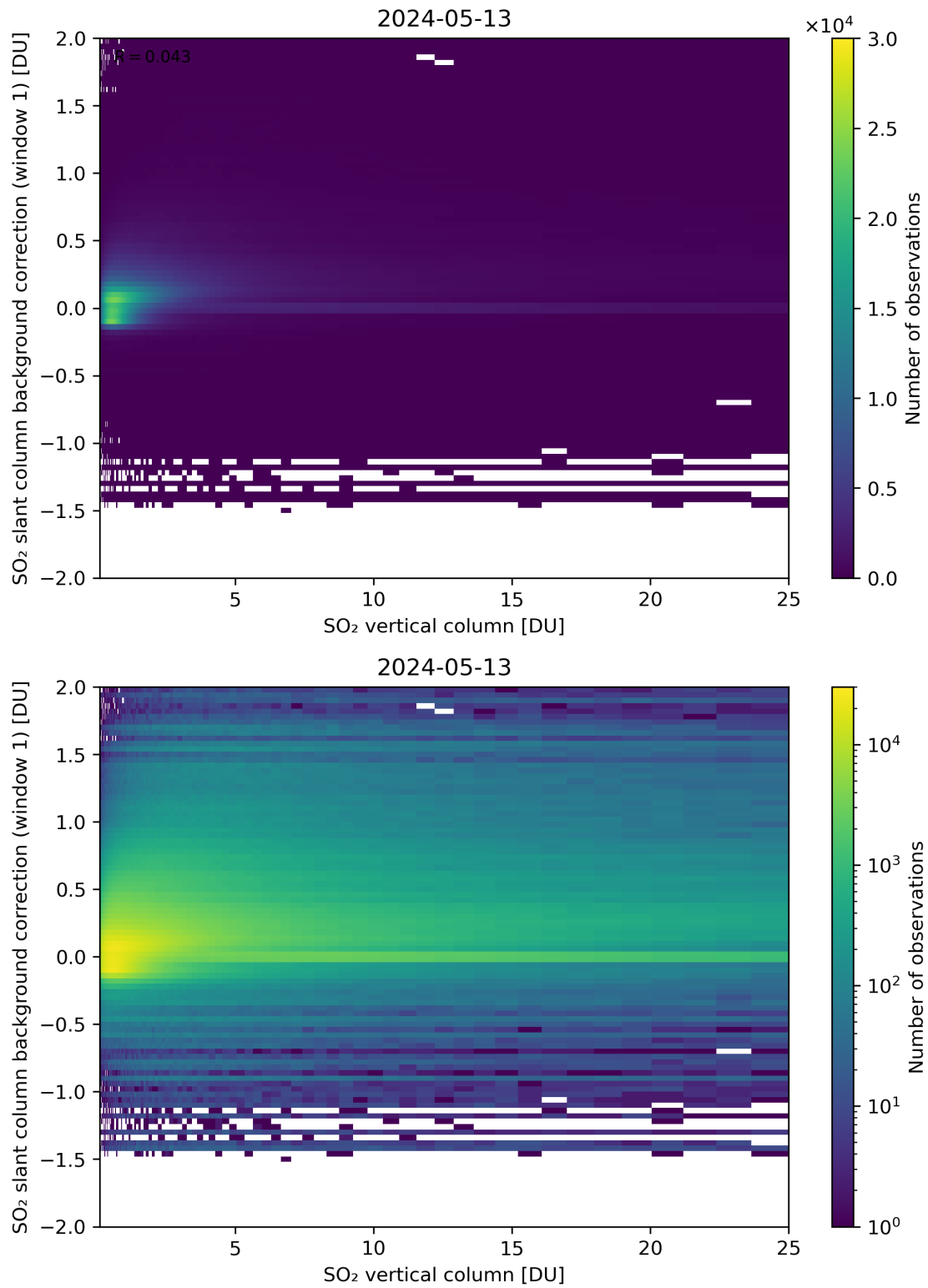
Figure 273: Scatter density plot of “SO 2 vertical column” against “SO 2 slant column background correction (window 1)” for 2024-05-12 to 2024-05-14.
