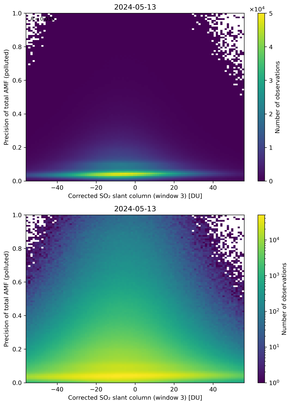
Figure 211: Scatter density plot of “Corrected SO 2 slant column (window 3)” against “Precision of total AMF (polluted)” for 2024-05-12 to 2024-05-14.
