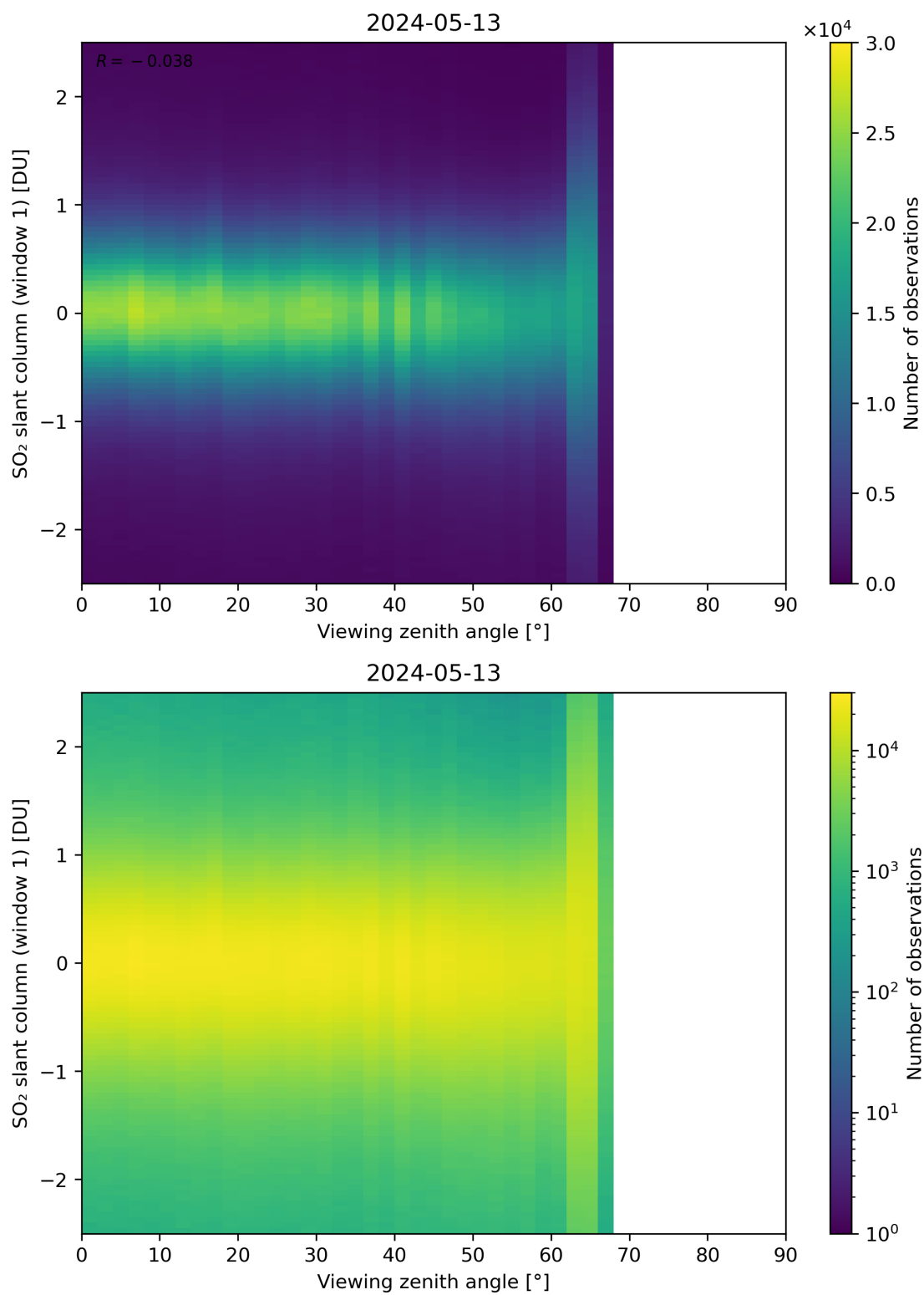
Figure 320: Scatter density plot of “Viewing zenith angle” against “SO 2 slant column (window 1)” for 2024-05-12 to 2024-05-14.
