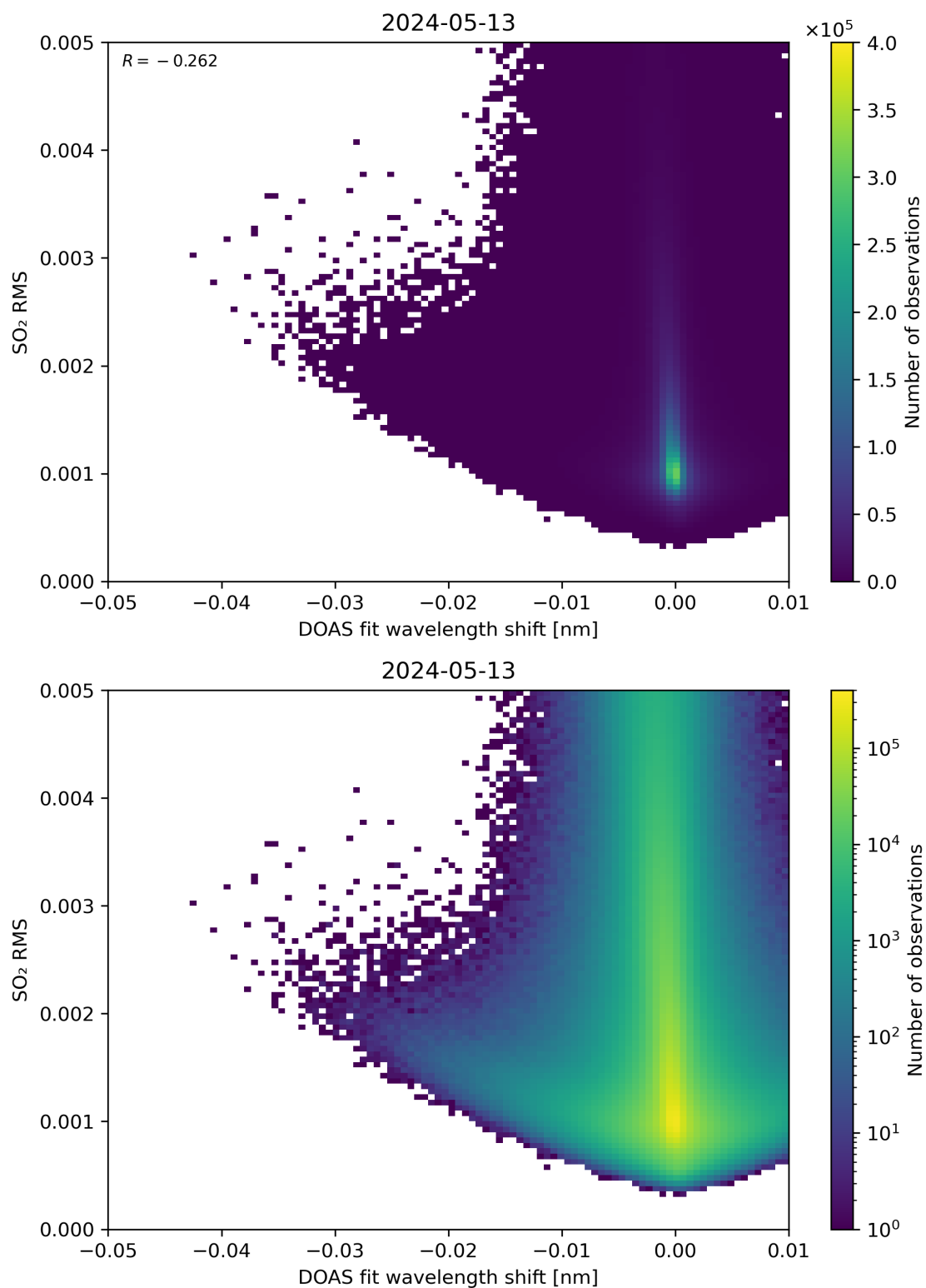
Figure 128: Scatter density plot of “DOAS fit wavelength shift” against “SO 2 RMS” for 2024-05-12 to 2024-05-14.
