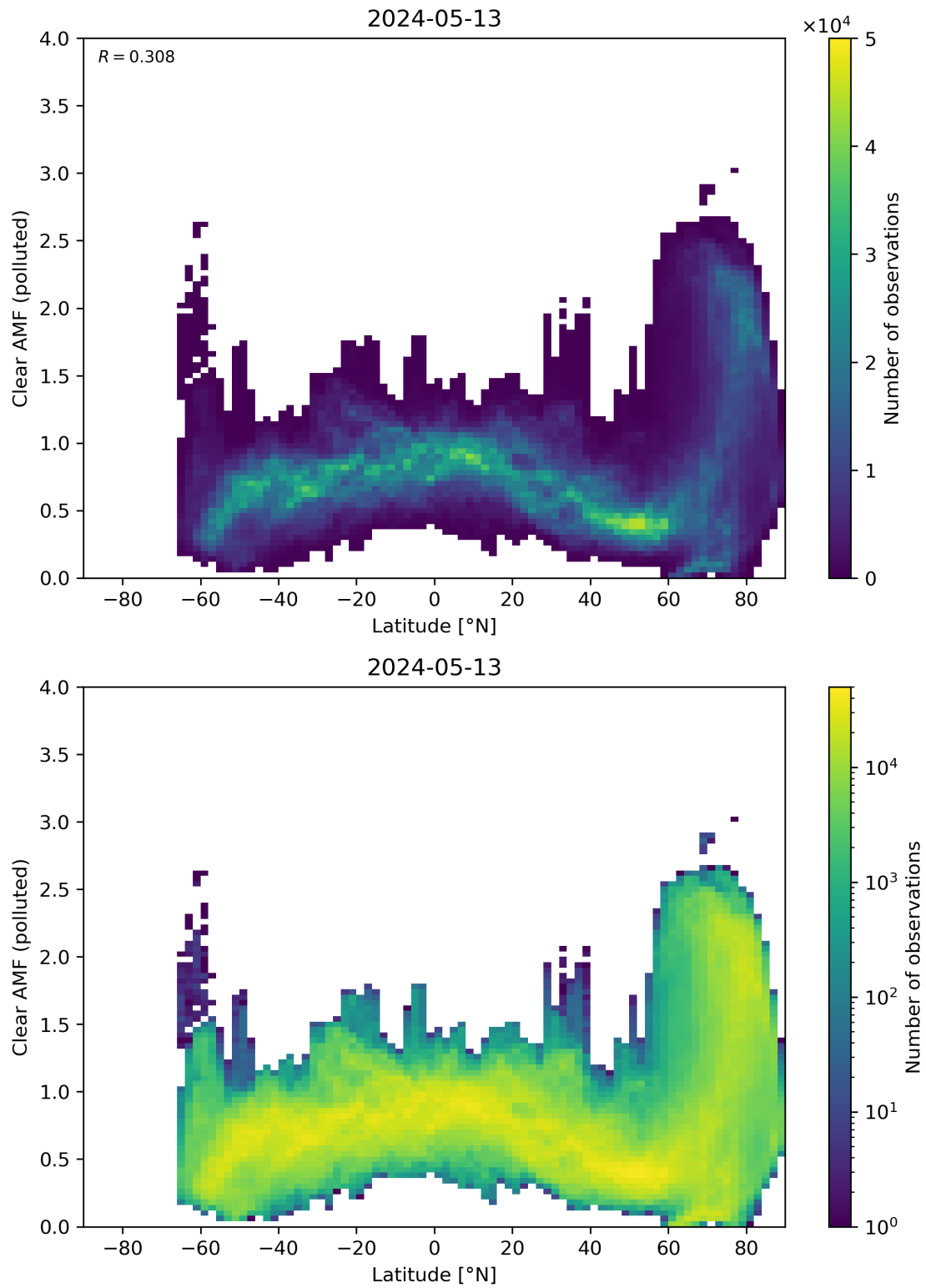
Figure 145: Scatter density plot of “Latitude” against “Clear AMF (polluted)” for 2024-05-12 to 2024-05-14.
