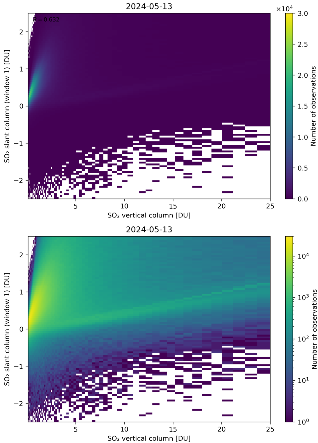
Figure 300: Scatter density plot of “SO 2 vertical column” against “SO 2 slant column (window 1)” for 2024-05-12 to 2024-05-14.
