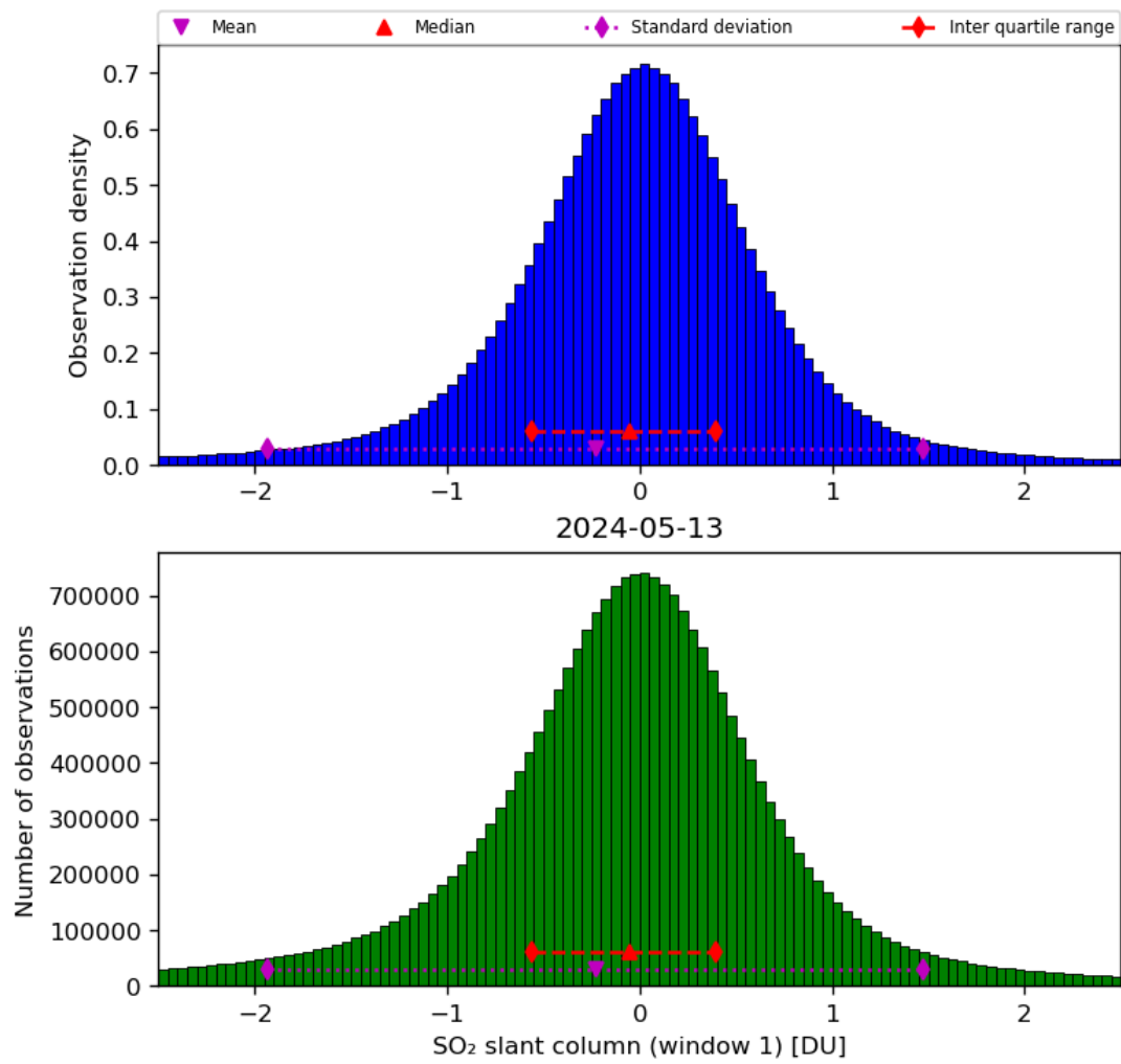
Figure 56: Histogram of “SO 2 slant column (window 1)” for 2024-05-12 to 2024-05-14
