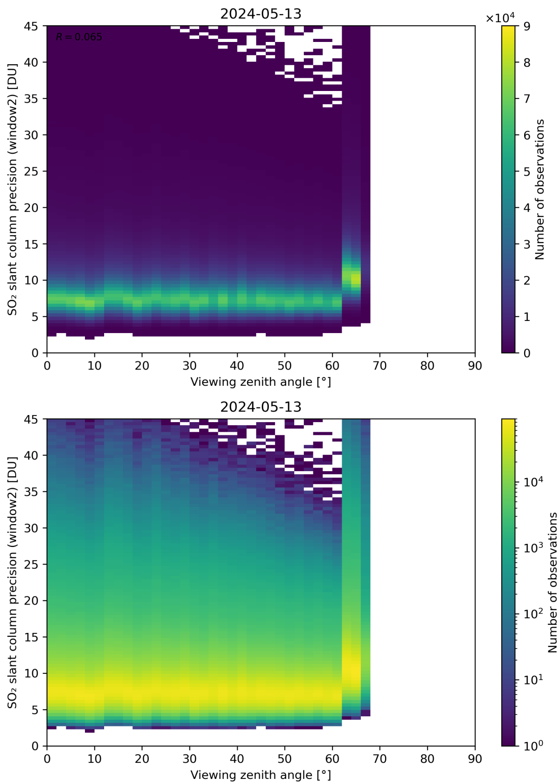
Figure 322: Scatter density plot of “Viewing zenith angle” against “SO 2 slant column precision (window2)” for 2024-05-12 to 2024-05-14.
