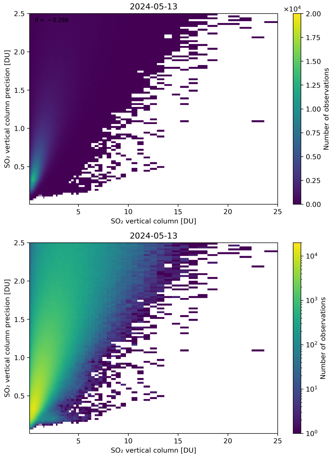
Figure 307: Scatter density plot of “SO 2 vertical column” against “SO 2 vertical column precision” for 2024-05-12 to 2024-05-14.
