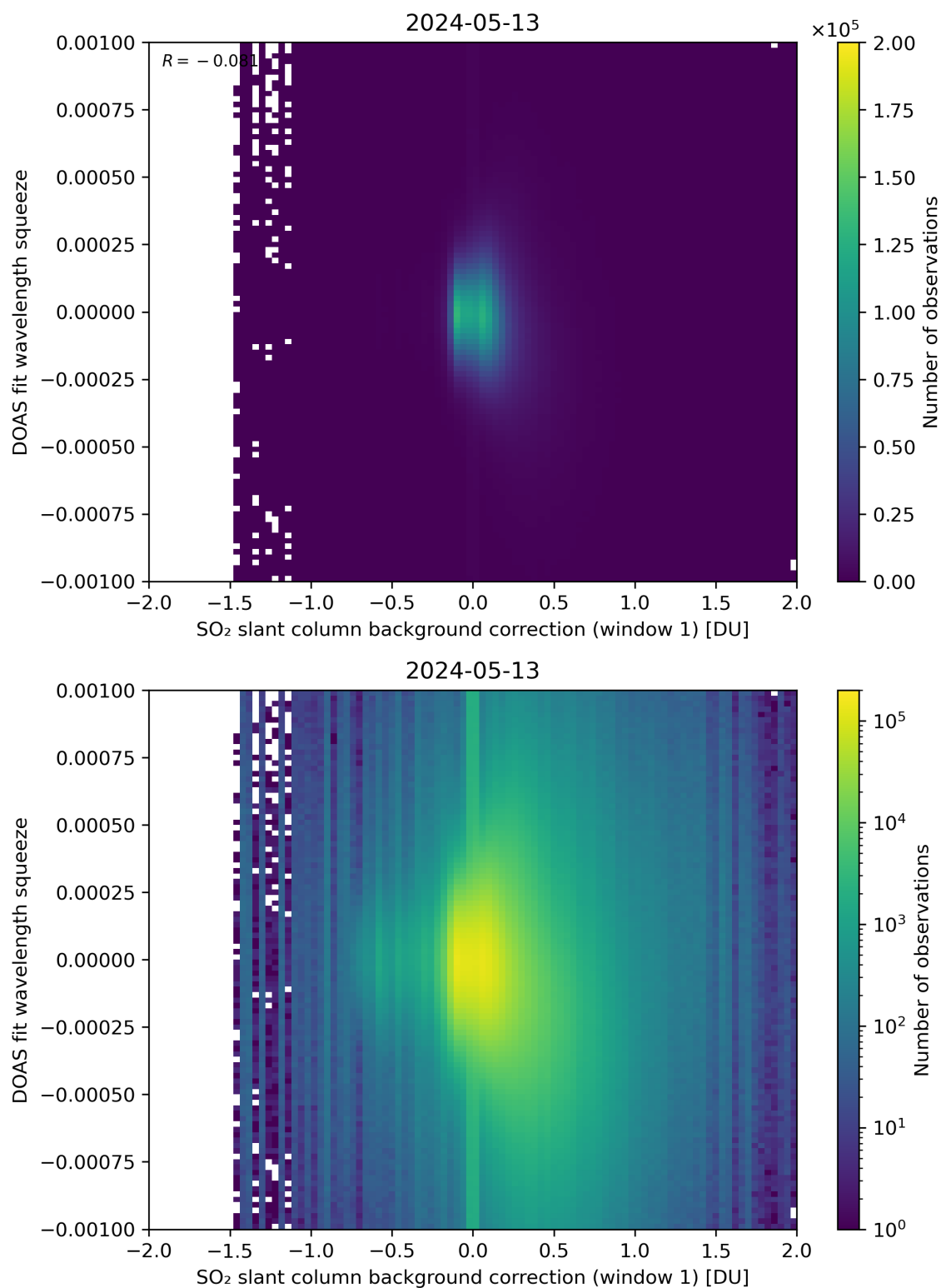
Figure 101: Scatter density plot of “SO 2 slant column background correction (window 1)” against “DOAS fit wavelength squeeze” for 2024-05-12 to 2024-05-14.
