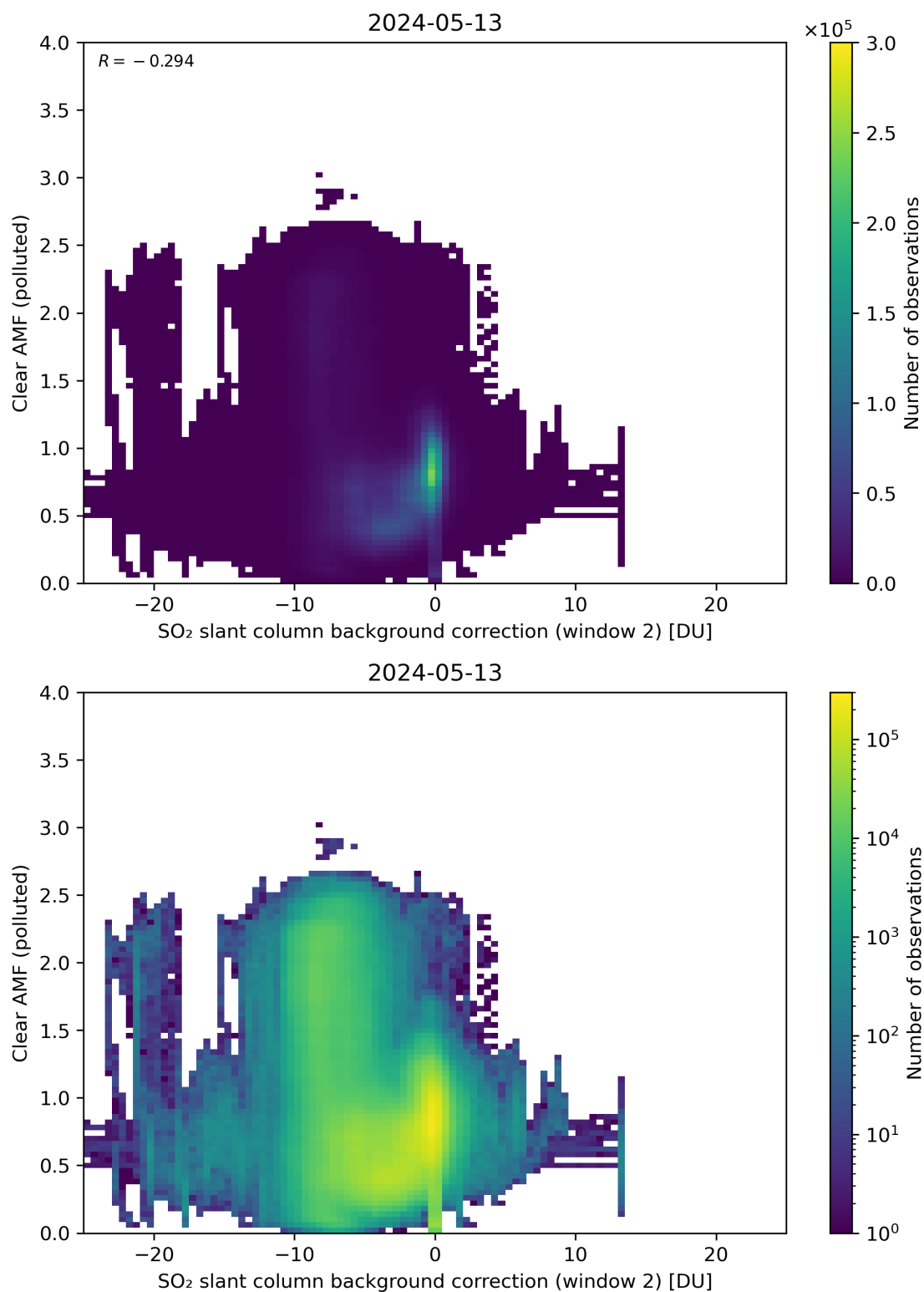
Figure 115: Scatter density plot of “SO 2 slant column background correction (window 2)” against “Clear AMF (polluted)” for 2024-05-12 to 2024-05-14.
