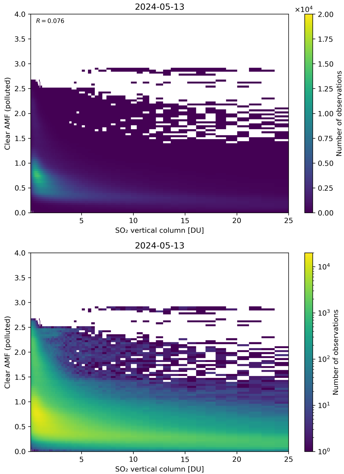
Figure 296: Scatter density plot of “SO 2 vertical column” against “Clear AMF (polluted)” for 2024-05-12 to 2024-05-14.
