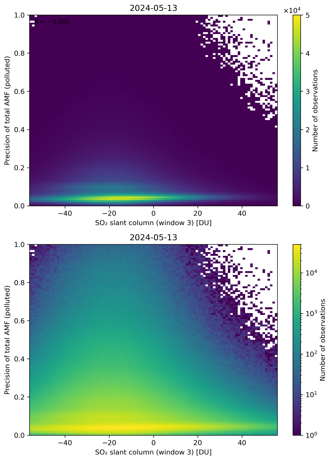
Figure 269: Scatter density plot of “SO 2 slant column (window 3)” against “Precision of total AMF (polluted)” for 2024-05-12 to 2024-05-14.
