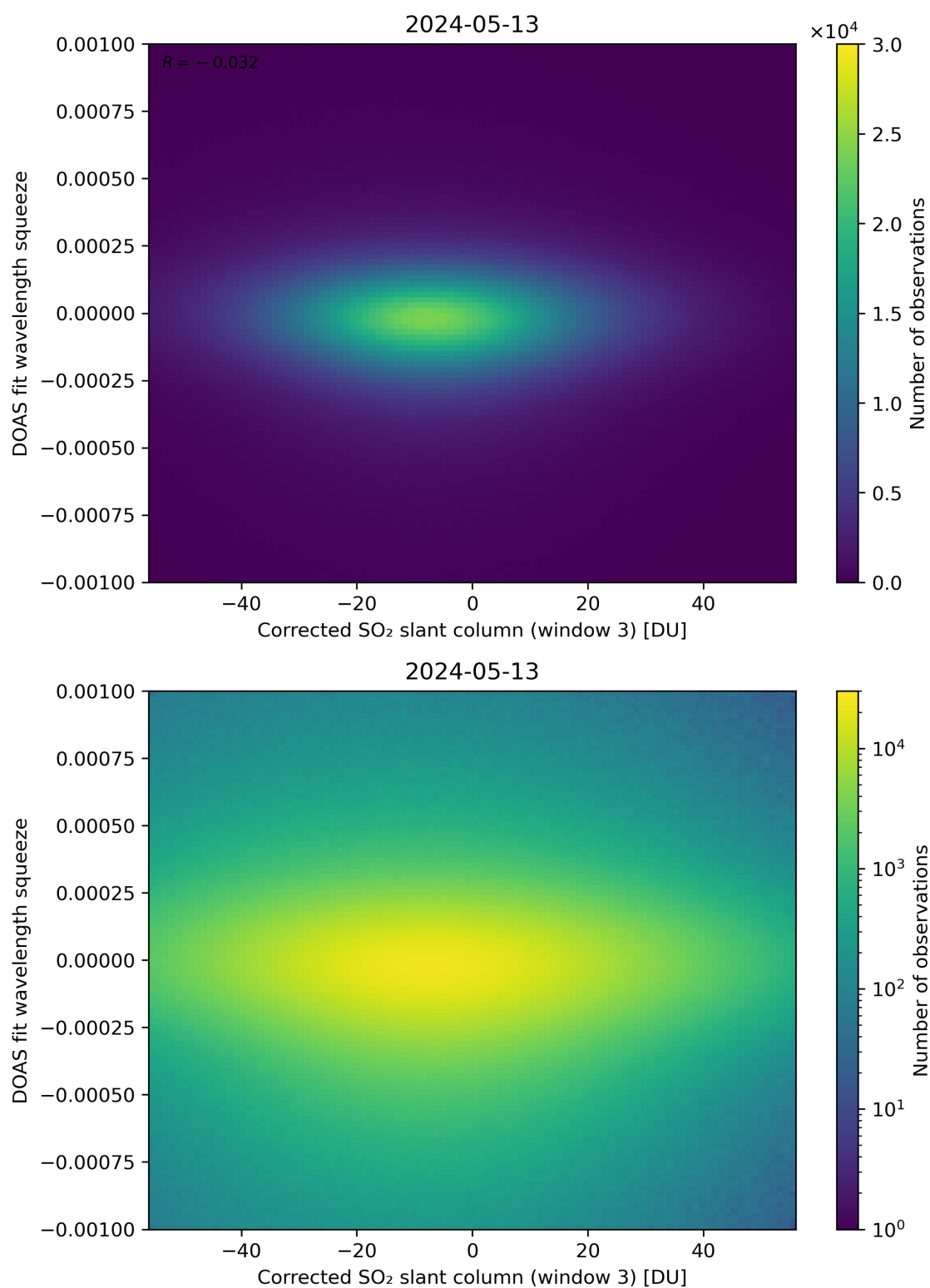
Figure 207: Scatter density plot of “Corrected SO 2 slant column (window 3)” against “DOAS fit wavelength squeeze” for 2024-05-12 to 2024-05-14.
