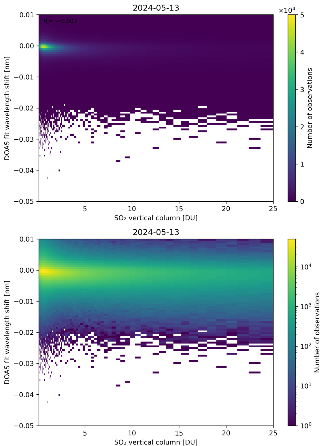
Figure 276: Scatter density plot of “SO 2 vertical column” against “DOAS fit wavelength shift” for 2024-05-12 to 2024-05-14.
