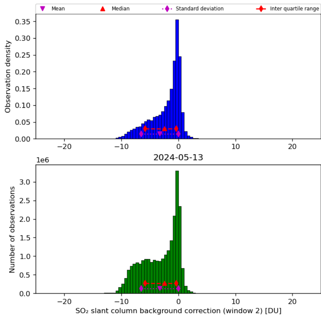
Figure 63: Histogram of “SO 2 slant column background correction (window 2)” for 2024-05-12 to 2024-05-14
