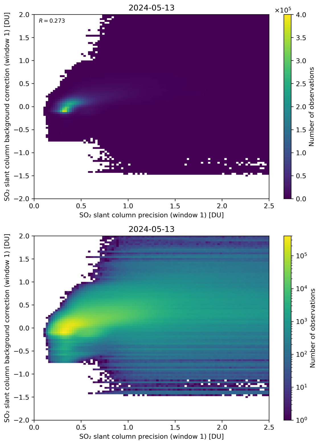
Figure 218: Scatter density plot of “SO 2 slant column precision (window 1)” against “SO 2 slant column background correction (window 1)” for 2024-05-12 to 2024-05-14.
