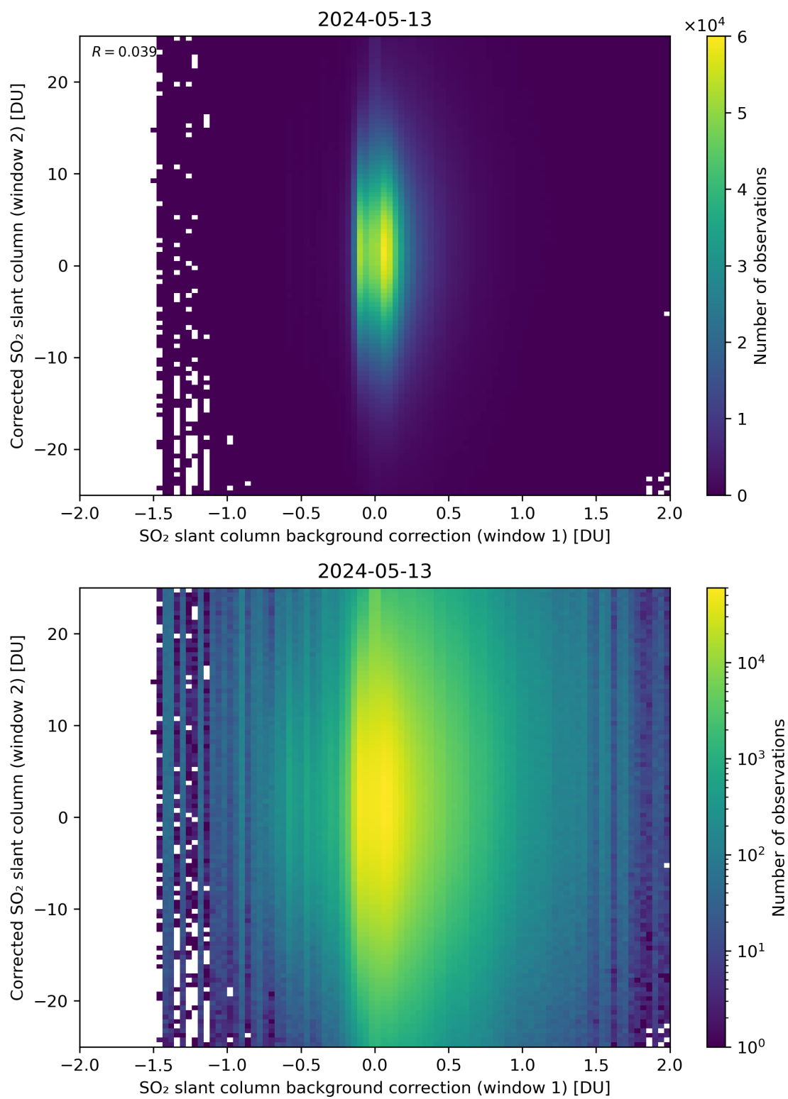
Figure 104: Scatter density plot of “SO 2 slant column background correction (window 1)” against “Corrected SO 2 slant column (window 2)” for 2024-05-12 to 2024-05-14.
