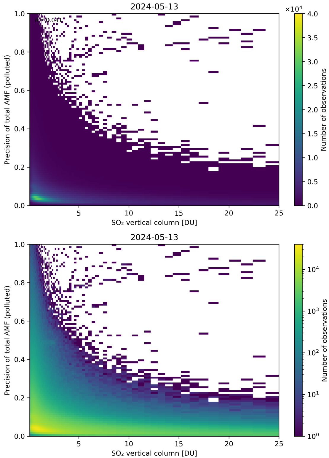
Figure 306: Scatter density plot of “SO 2 vertical column” against “Precision of total AMF (polluted)” for 2024-05-12 to 2024-05-14.
