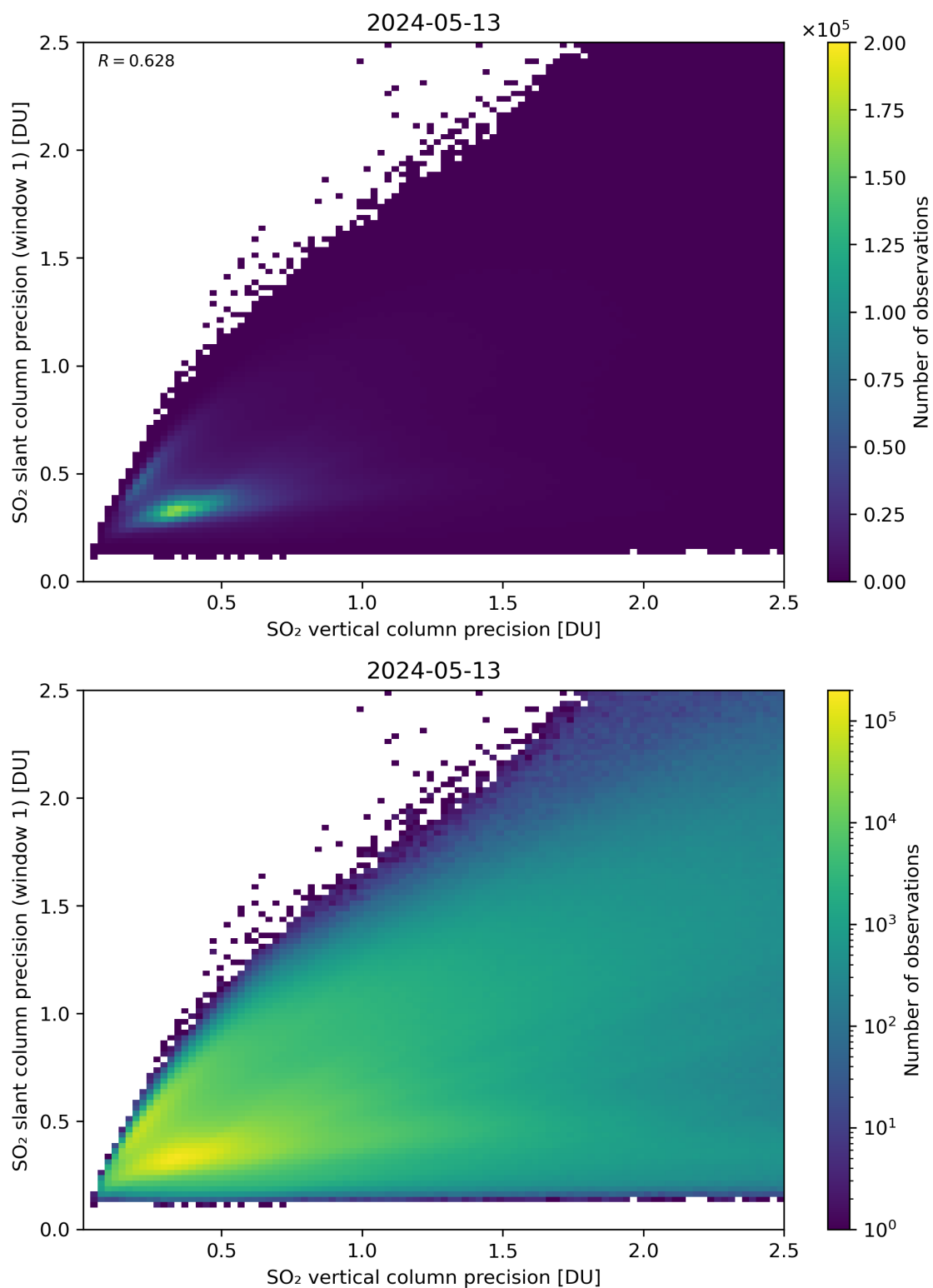
Figure 290: Scatter density plot of “SO 2 vertical column precision” against “SO 2 slant column precision (window 1)” for 2024-05-12 to 2024-05-14.
