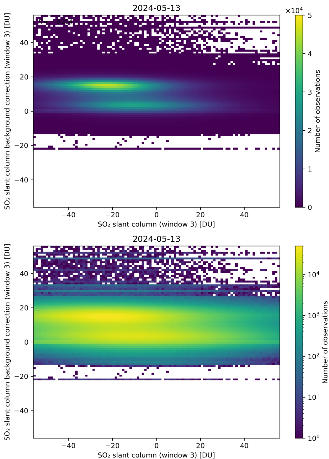
Figure 253: Scatter density plot of “SO 2 slant column (window 3)” against “SO 2 slant column background correction (window 3)” for 2024-05-12 to 2024-05-14.
