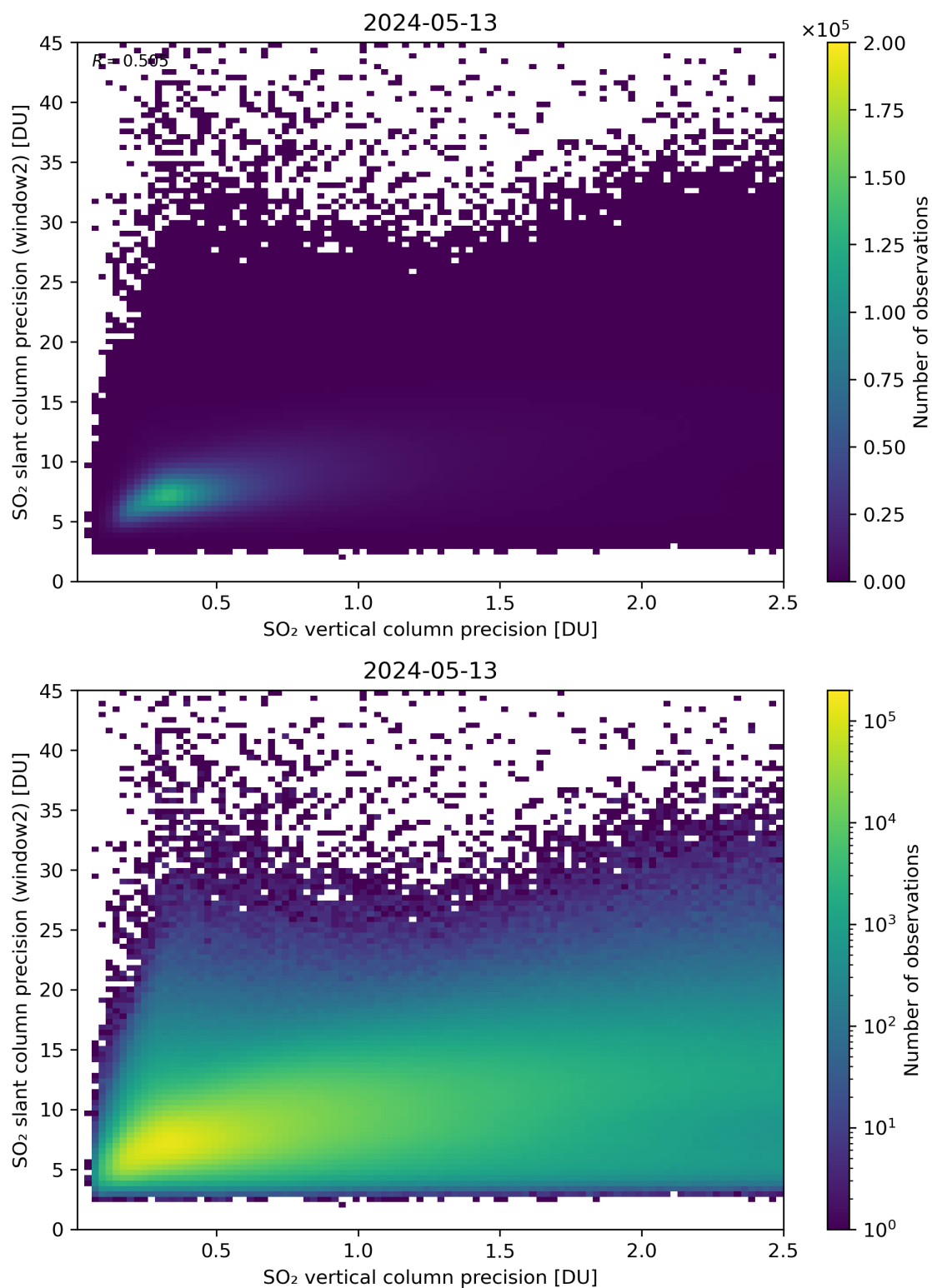
Figure 291: Scatter density plot of “SO 2 vertical column precision” against “SO 2 slant column precision (window2)” for 2024-05-12 to 2024-05-14.
