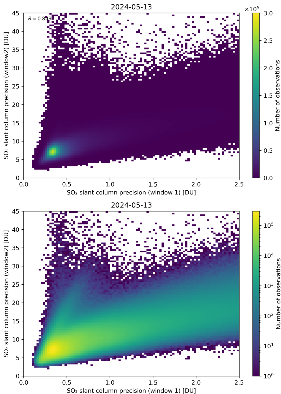
Figure 227: Scatter density plot of “SO 2 slant column precision (window 1)” against “SO 2 slant column precision (window 2)” for 2024-05-12 to 2024-05-14.
