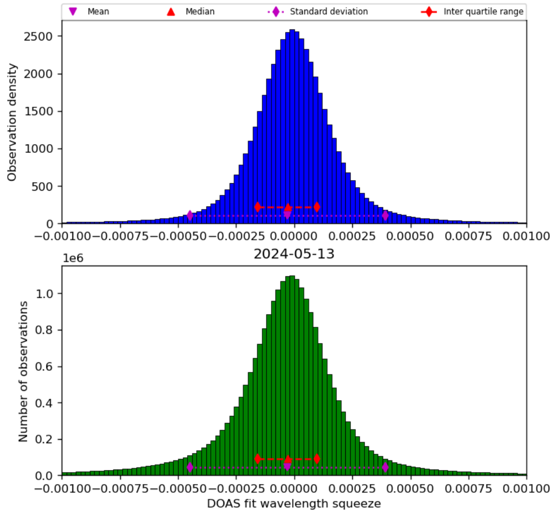
Figure 69: Histogram of “DOAS fit wavelength squeeze” for 2024-05-12 to 2024-05-14
