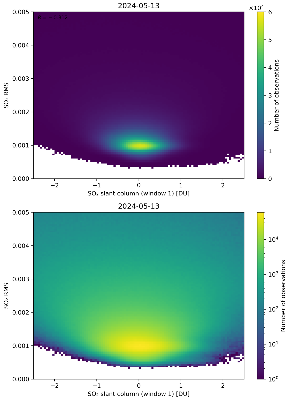
Figure 217: Scatter density plot of “SO 2 slant column (window 1)” against “SO 2 RMS” for 2024-05-12 to 2024-05-14.
