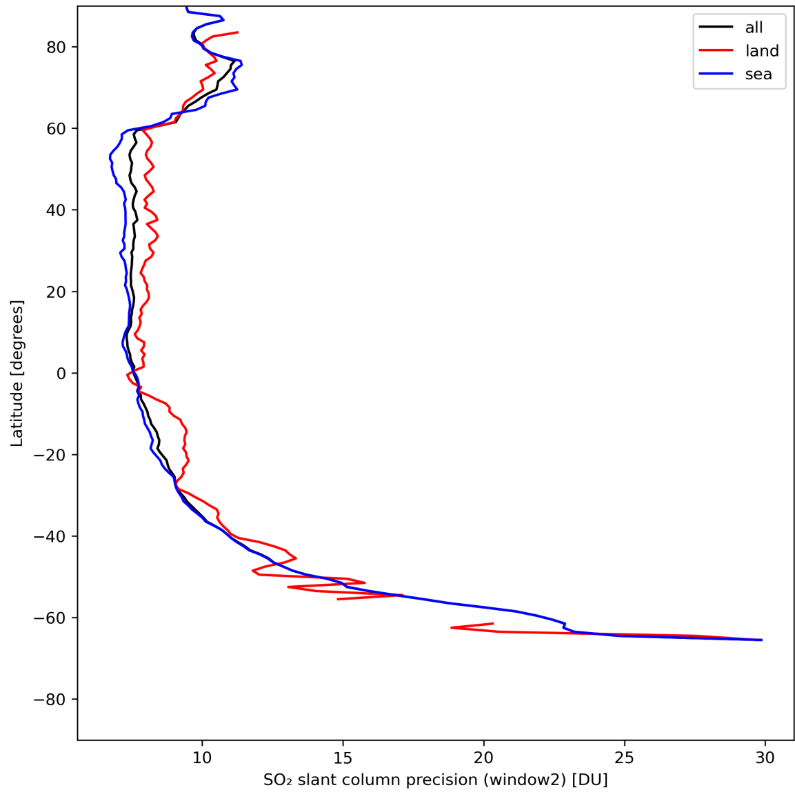
Figure 38: Zonal average of “SO 2 slant column precision (window2)” for 2024-05-12 to 2024-05-14.
