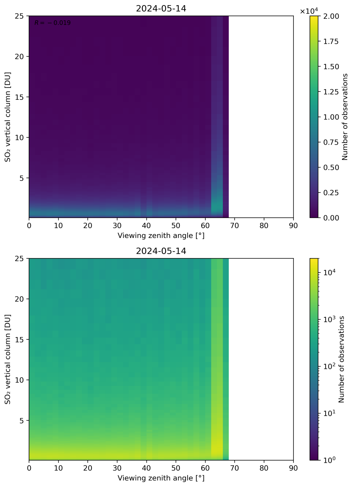
Figure 327: Scatter density plot of “Viewing zenith angle” against “SO 2 vertical column” for 2024-05-13 to 2024-05-15.
