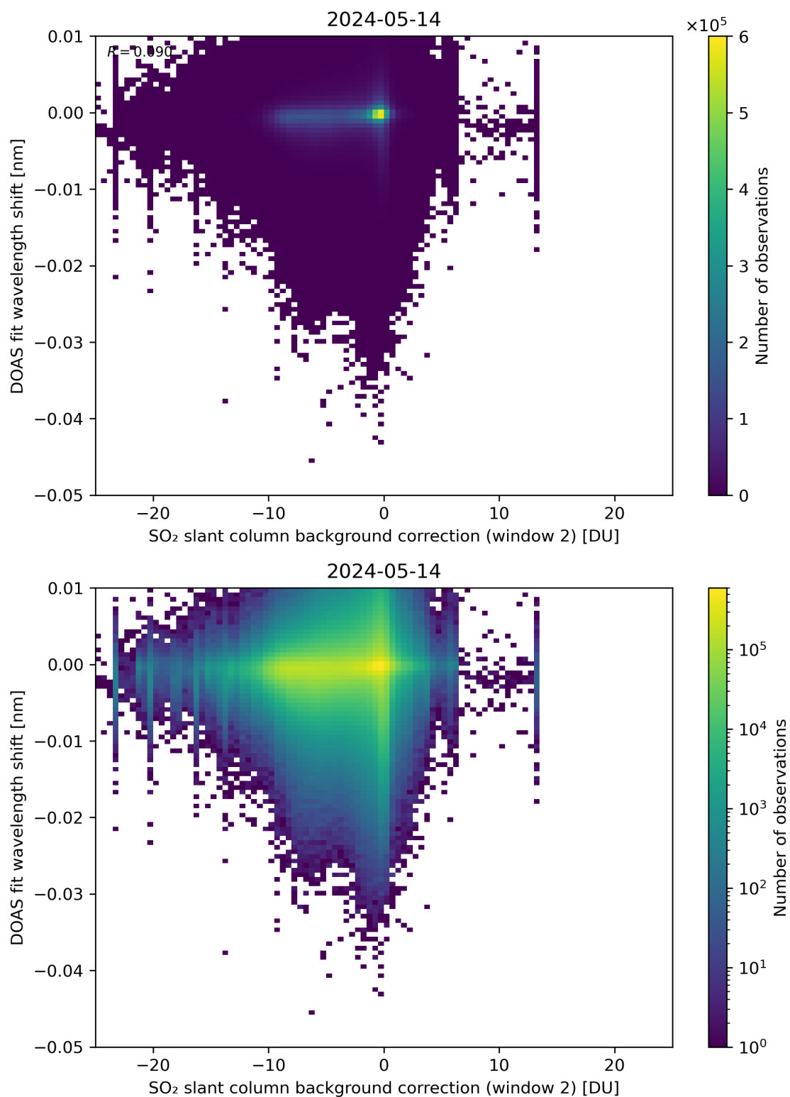
Figure 112: Scatter density plot of “SO 2 slant column background correction (window 2)” against “DOAS fit wavelength shift” for 2024-05-13 to 2024-05-15.
