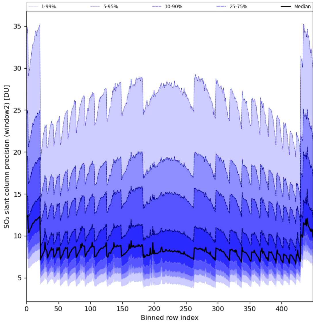
Figure 84: Along track statistics of “SO 2 slant column precision (window2)” for 2024-05-13 to 2024-05-15
