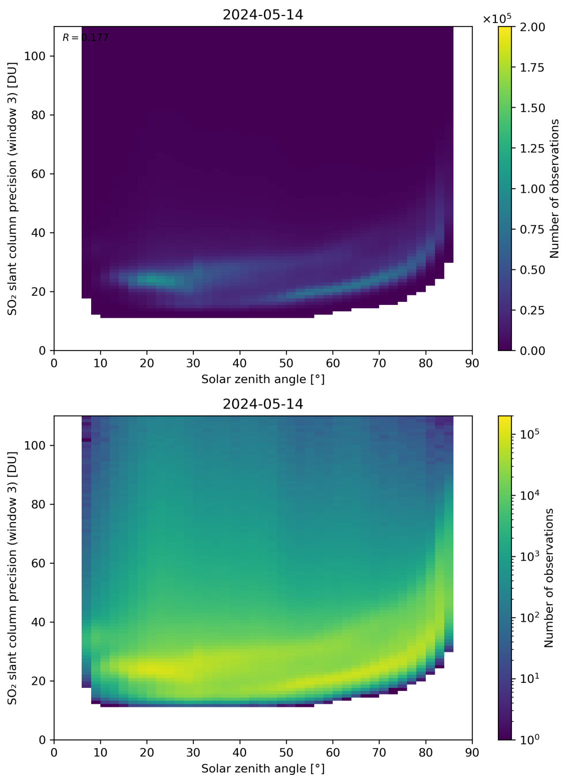
Figure 173: Scatter density plot of “Solar zenith angle” against “SO 2 slant column precision (window 3)” for 2024-05-13 to 2024-05-15.
