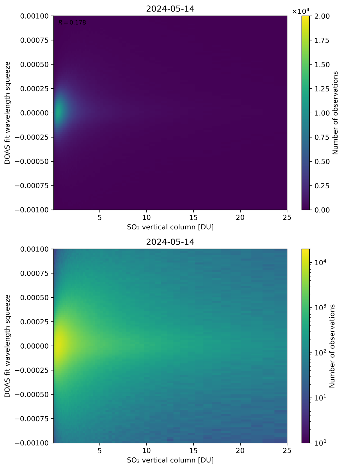
Figure 277: Scatter density plot of “SO 2 vertical column” against “DOAS fit wavelength squeeze” for 2024-05-13 to 2024-05-15.
