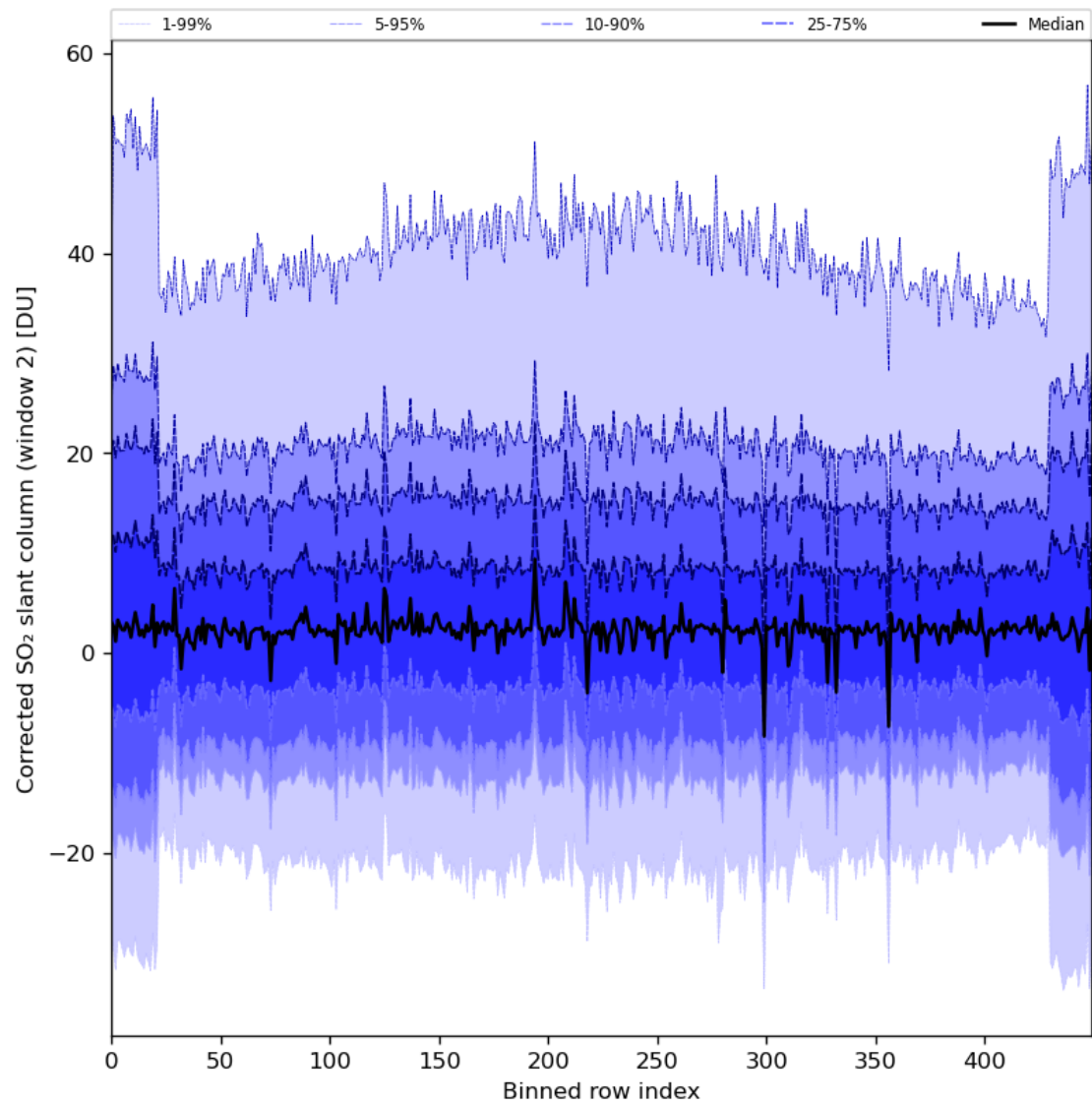
Figure 85: Along track statistics of “Corrected SO 2 slant column (window 2)” for 2024-05-13 to 2024-05-15
