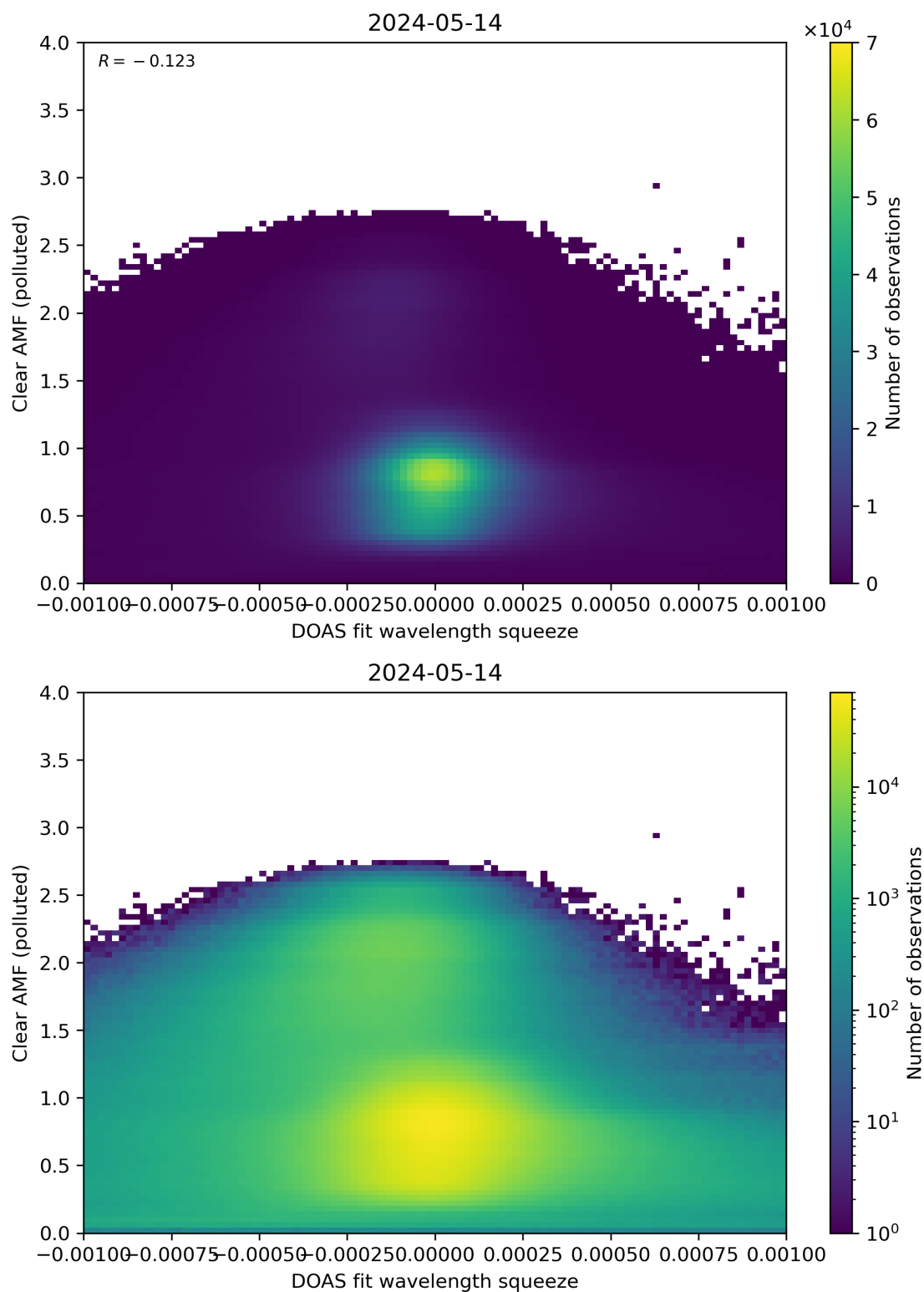
Figure 133: Scatter density plot of “DOAS fit wavelength squeeze” against “Clear AMF (polluted)” for 2024-05-13 to 2024-05-15.
