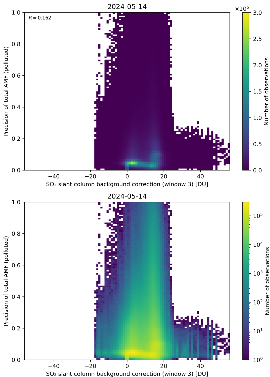
Figure 126: Scatter density plot of “SO 2 slant column background correction (window 3)” against “Precision of total AMF (polluted)” for 2024-05-13 to 2024-05-15.
