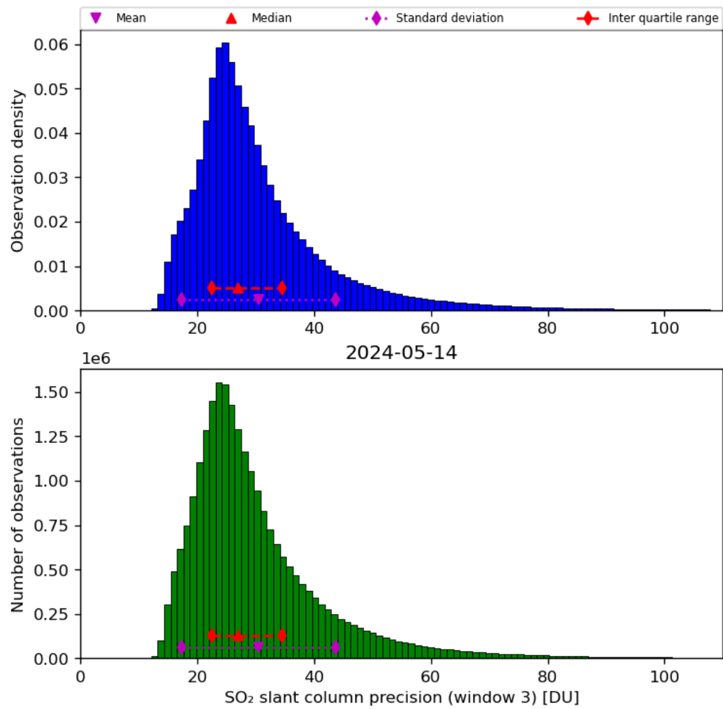
Figure 65: Histogram of “SO 2 slant column precision (window 3)” for 2024-05-13 to 2024-05-15
