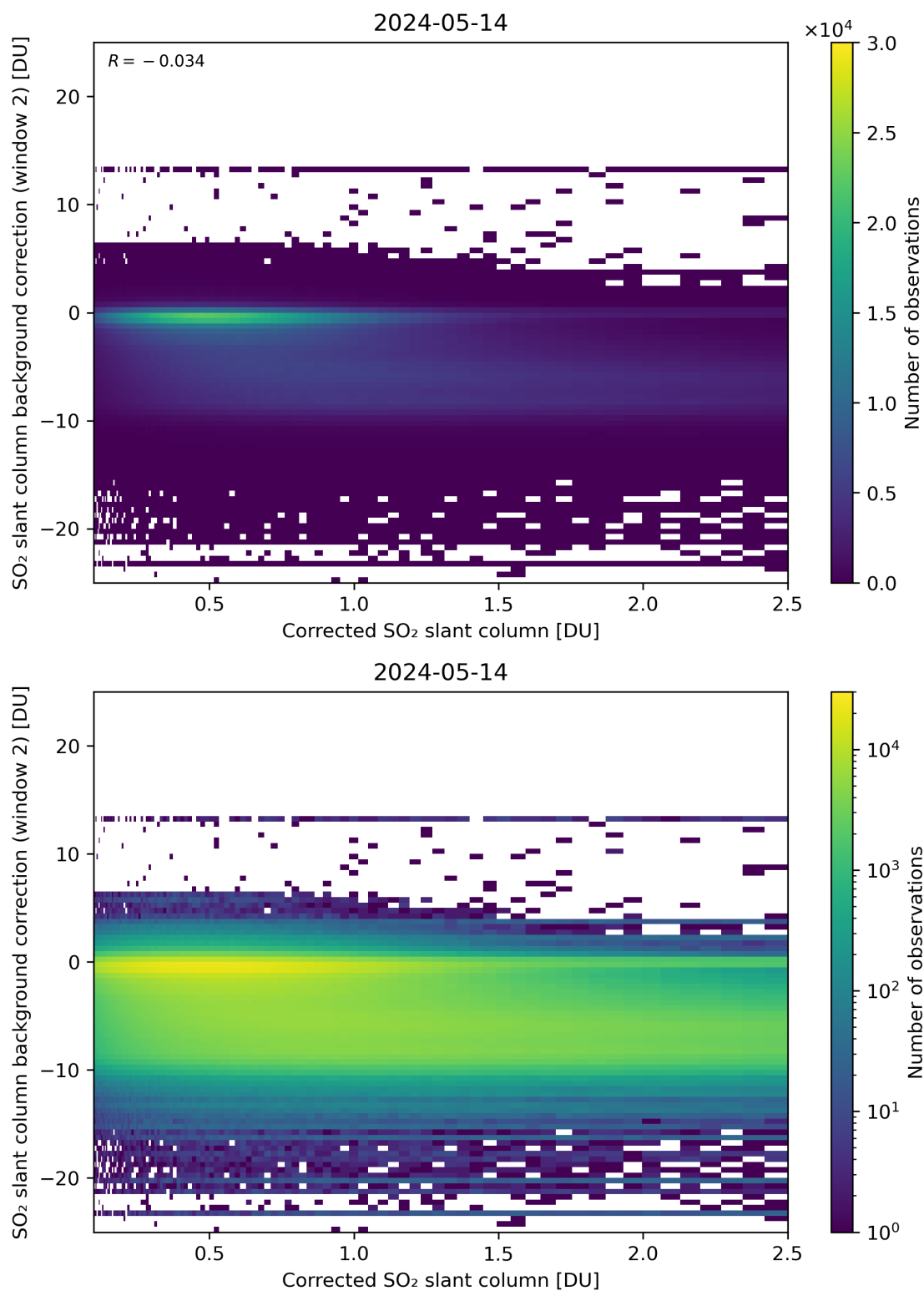
Figure 179: Scatter density plot of “Corrected SO 2 slant column” against “SO 2 slant column background correction (window 2)” for 2024-05-13 to 2024-05-15.
