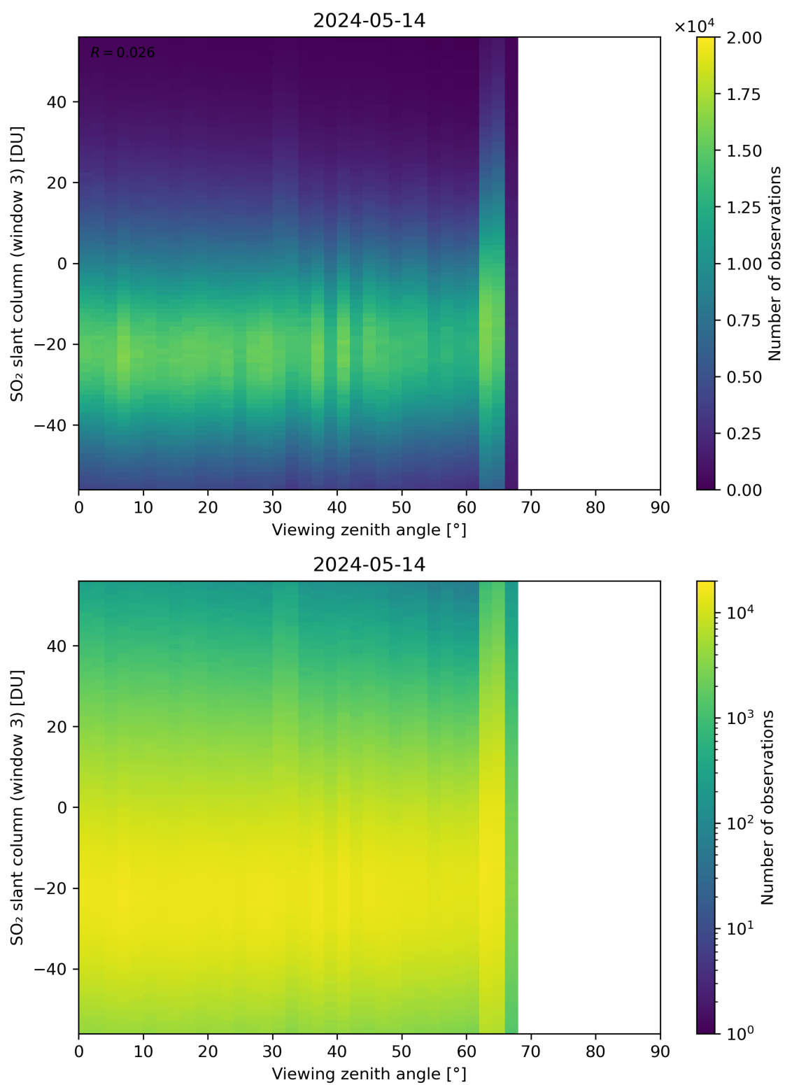
Figure 323: Scatter density plot of “Viewing zenith angle” against “SO 2 slant column (window 3)” for 2024-05-13 to 2024-05-15.
