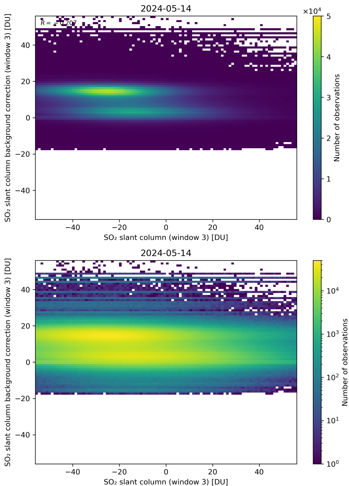
Figure 253: Scatter density plot of “SO 2 slant column (window 3)” against “SO 2 slant column background correction (window 3)” for 2024-05-13 to 2024-05-15.
