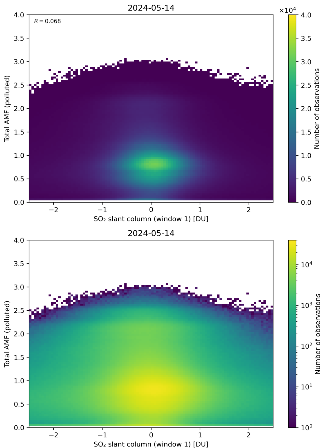
Figure 239: Scatter density plot of “SO 2 slant column (window 1)” against “Total AMF (polluted)” for 2024-05-13 to 2024-05-15.
