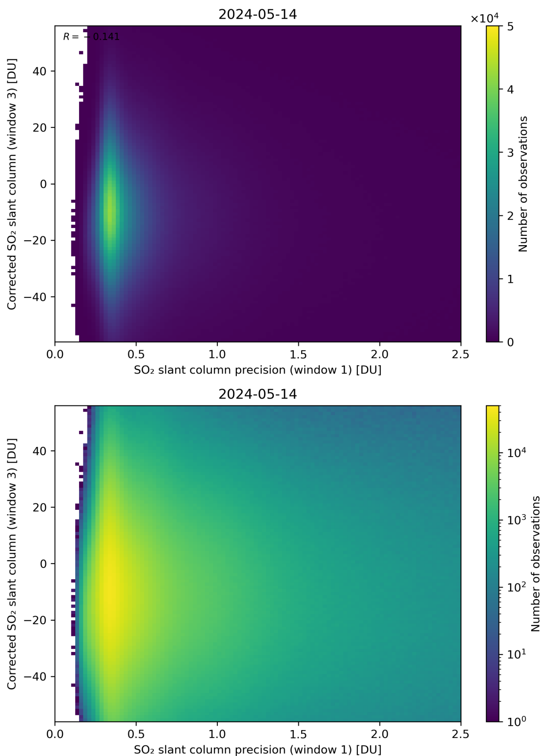
Figure 226: Scatter density plot of “SO 2 slant column precision (window 1)” against “Corrected SO 2 slant column (window 3)” for 2024-05-13 to 2024-05-15.
