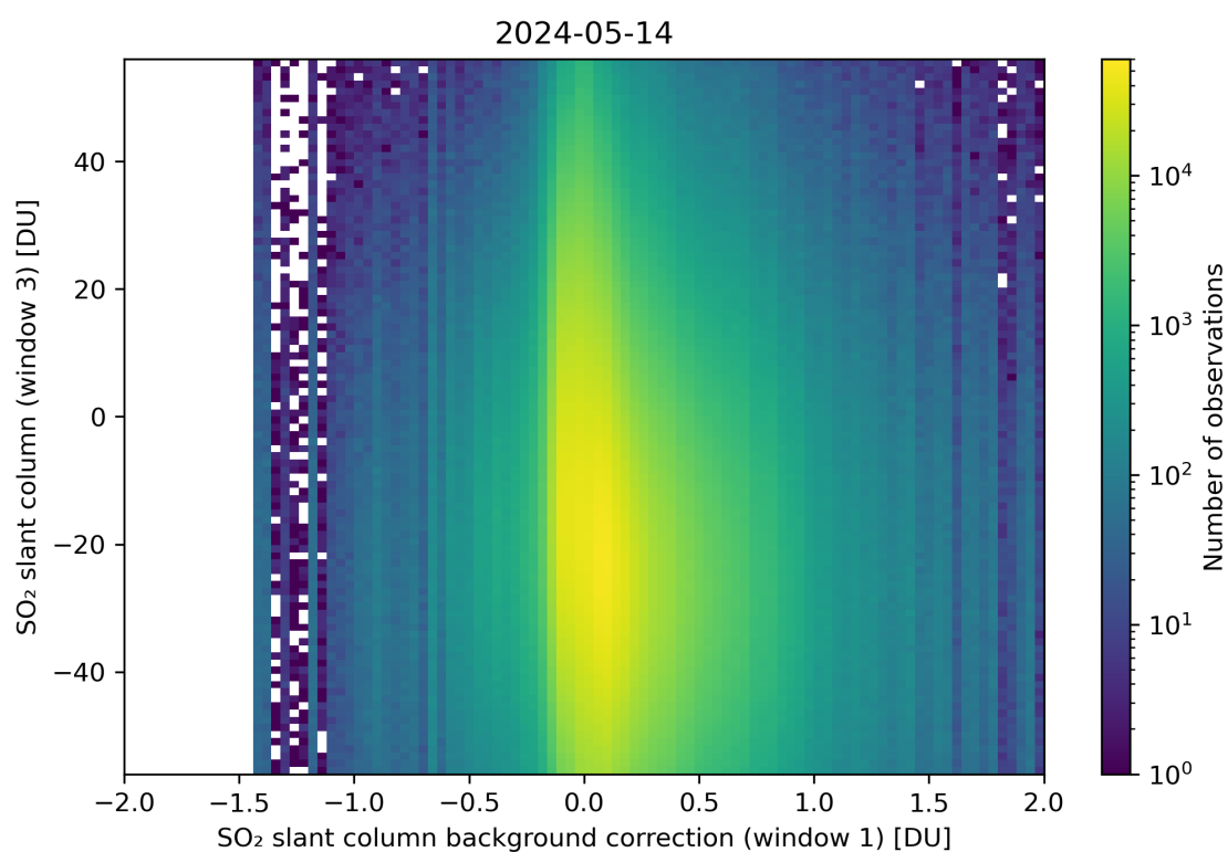
Figure 107: Scatter density plot of “SO 2 slant column background correction (window 1)” against “SO 2 slant column (window 3)” for 2024-05-13 to 2024-05-15.
