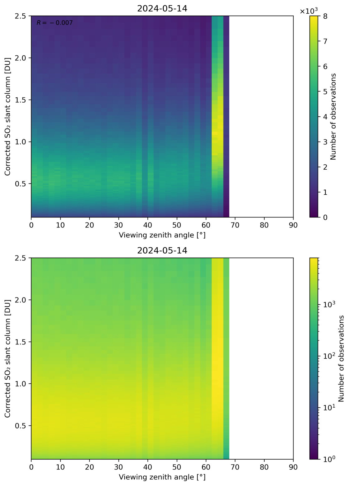
Figure 317: Scatter density plot of “Viewing zenith angle” against “Corrected SO 2 slant column” for 2024-05-13 to 2024-05-15.
