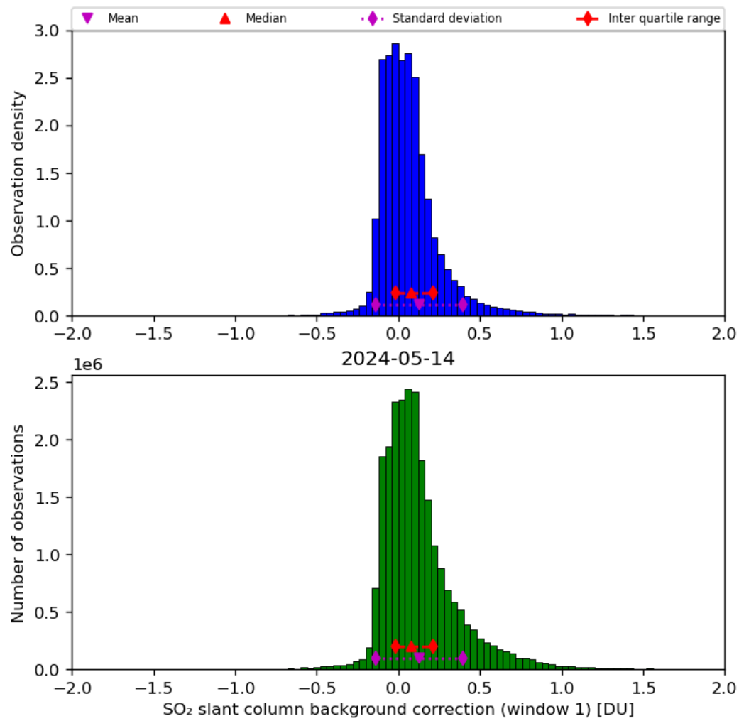
Figure 59: Histogram of “SO 2 slant column background correction (window 1)” for 2024-05-13 to 2024-05-15
