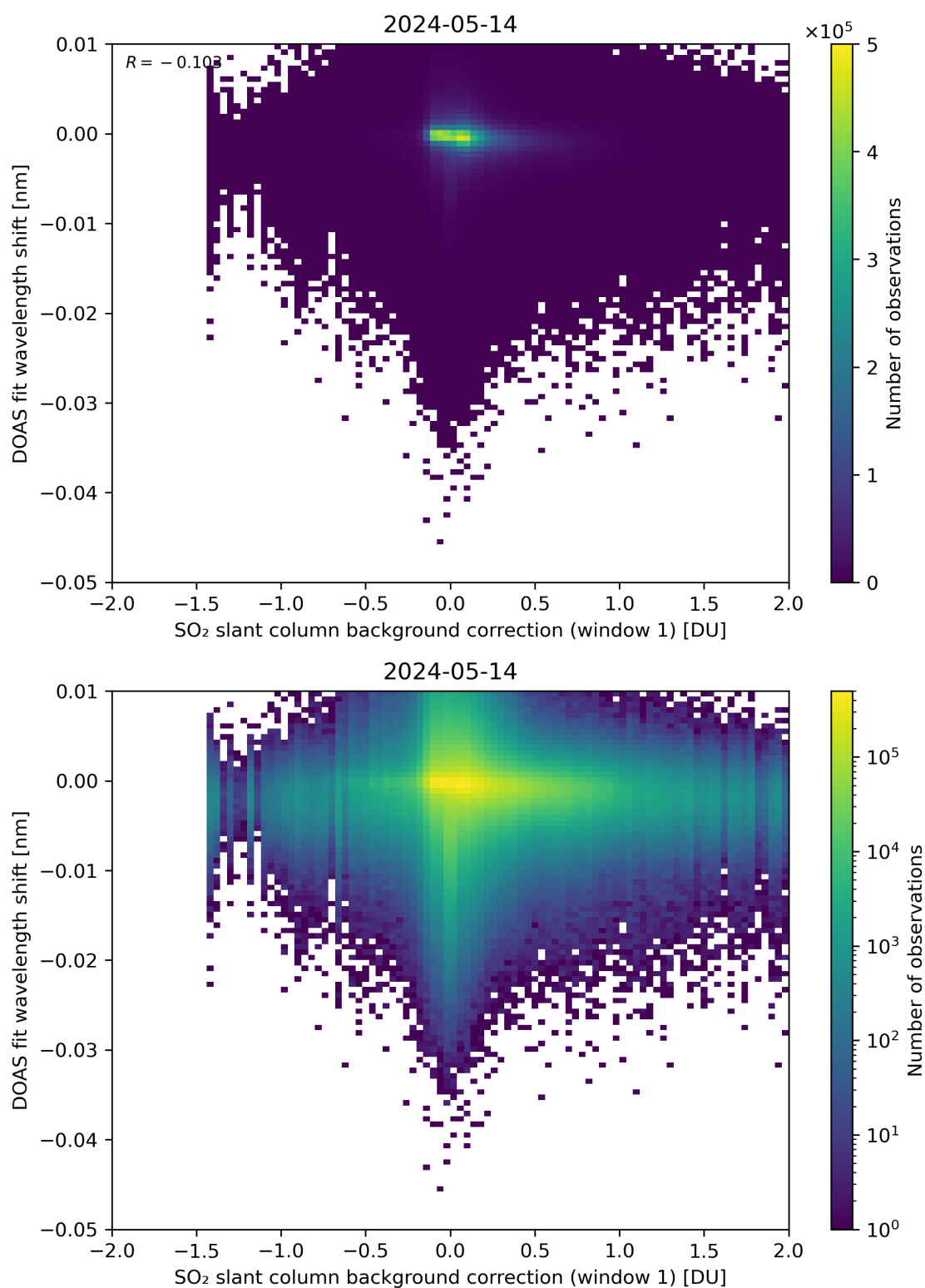
Figure 100: Scatter density plot of “SO 2 slant column background correction (window 1)” against “DOAS fit wavelength shift” for 2024-05-13 to 2024-05-15.
