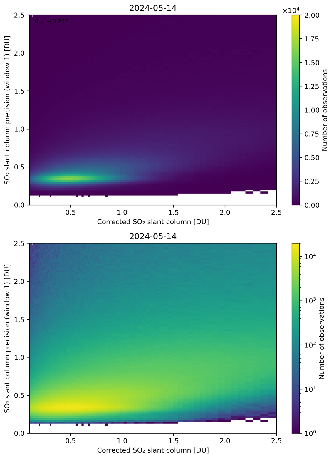
Figure 188: Scatter density plot of “Corrected SO 2 slant column” against “SO 2 slant column precision (window 1)” for 2024-05-13 to 2024-05-15.
