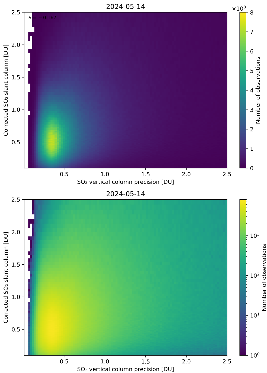
Figure 286: Scatter density plot of “SO 2 vertical column precision” against “Corrected SO 2 slant column” for 2024-05-13 to 2024-05-15.
