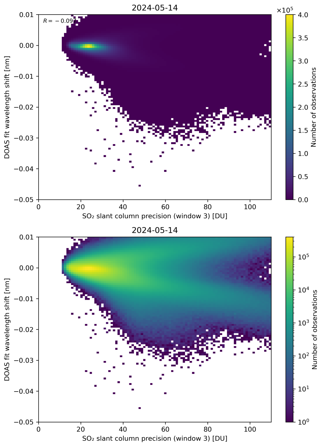
Figure 258: Scatter density plot of “SO 2 slant column precision (window 3)” against “DOAS fit wavelength shift” for 2024-05-13 to 2024-05-15.
