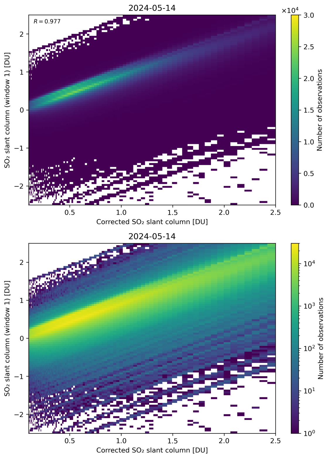
Figure 187: Scatter density plot of “Corrected SO 2 slant column” against “SO 2 slant column (window 1)” for 2024-05-13 to 2024-05-15.
