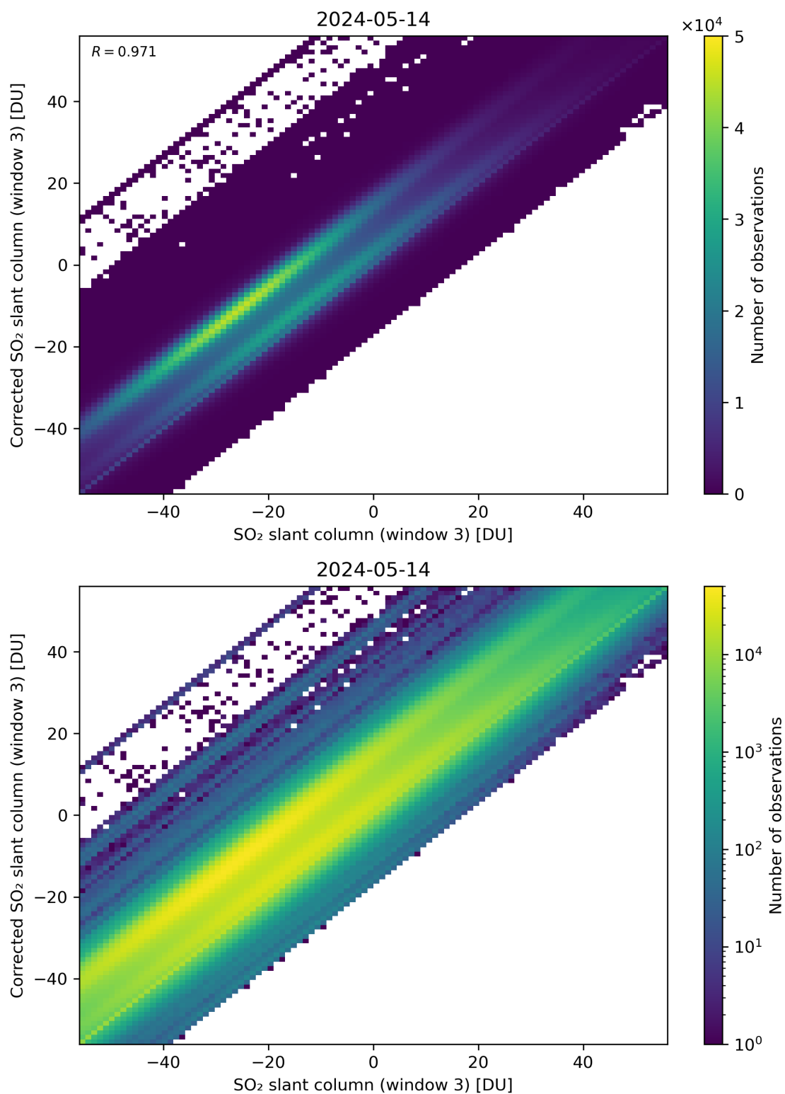
Figure 266: Scatter density plot of “SO 2 slant column (window 3)” against “Corrected SO 2 slant column (window 3)” for 2024-05-13 to 2024-05-15.
