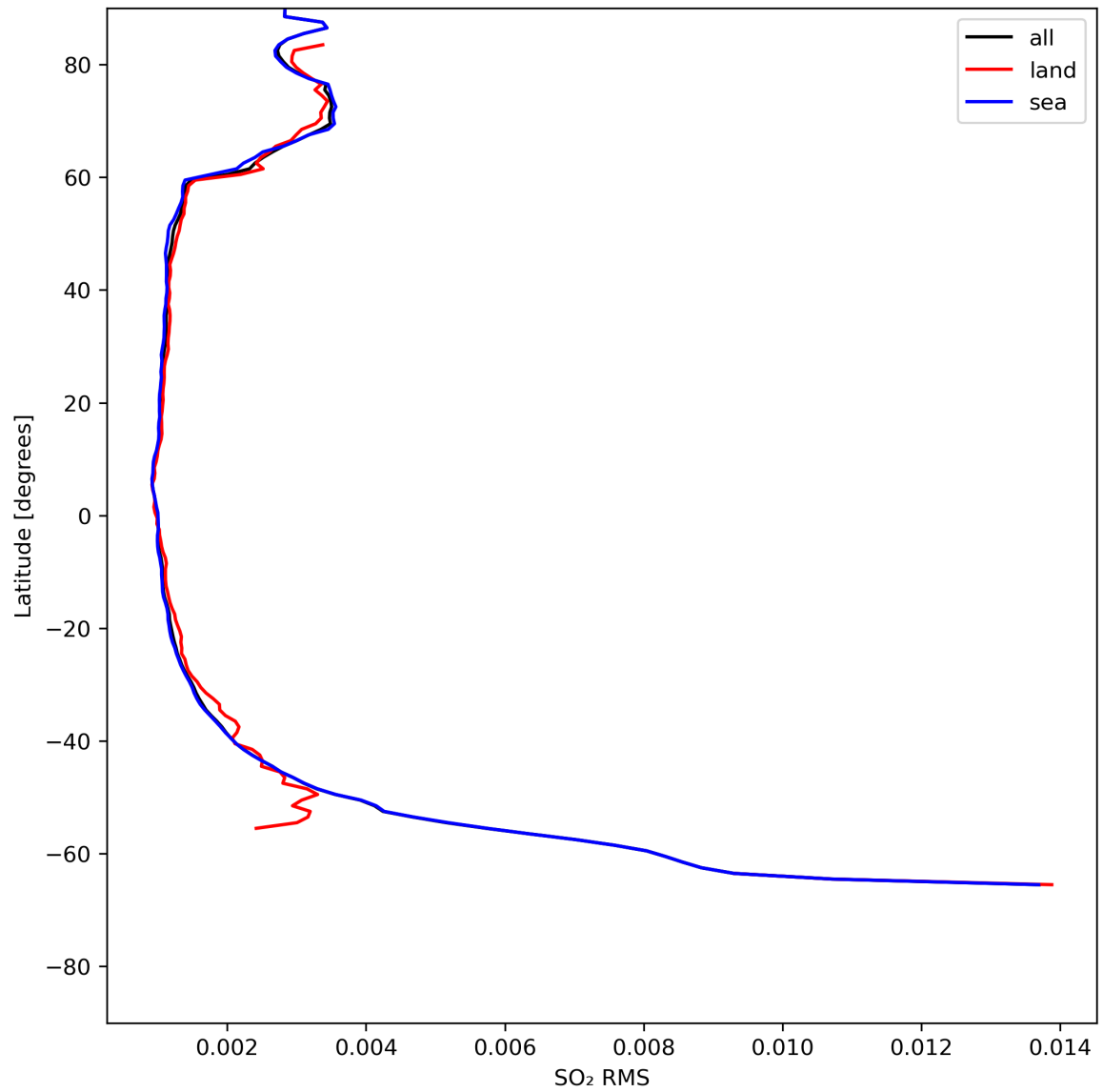
Figure 47: Zonal average of “SO 2 RMS” for 2024-05-13 to 2024-05-15.
