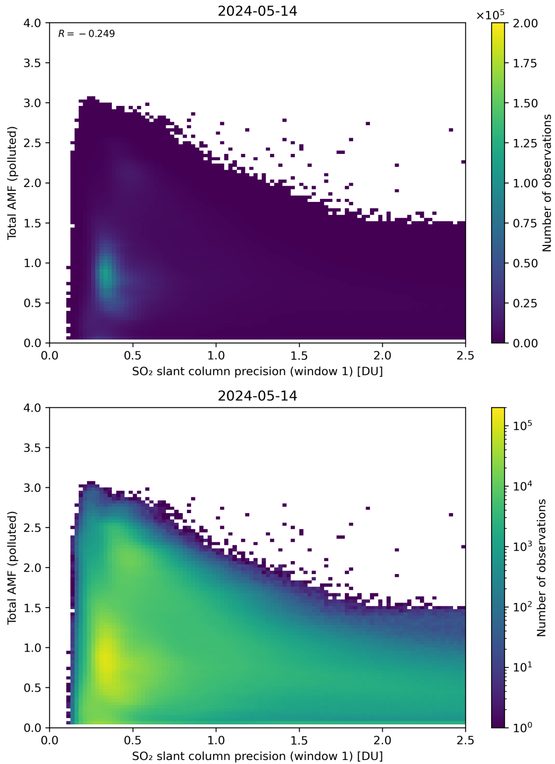
Figure 230: Scatter density plot of “SO 2 slant column precision (window 1)” against “Total AMF (polluted)” for 2024-05-13 to 2024-05-15.
