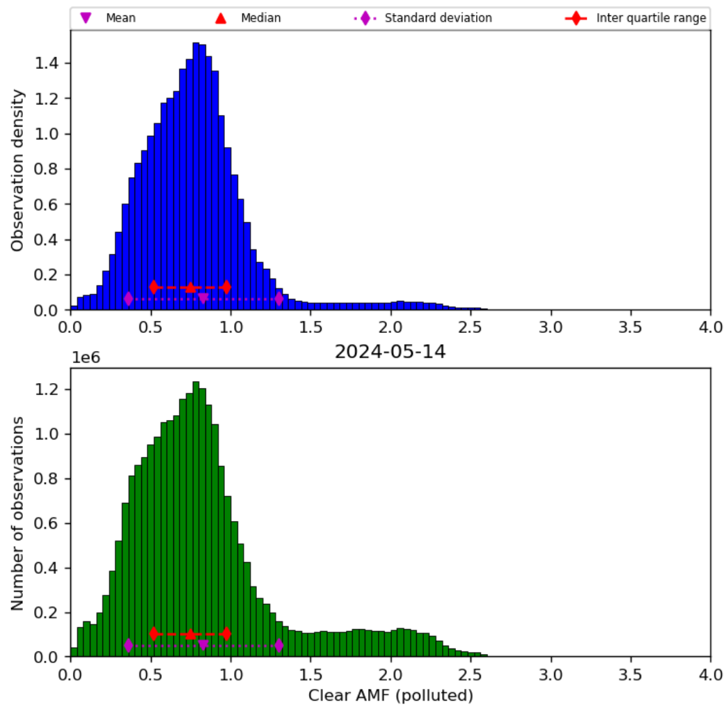
Figure 73: Histogram of “Clear AMF (polluted)” for 2024-05-13 to 2024-05-15
