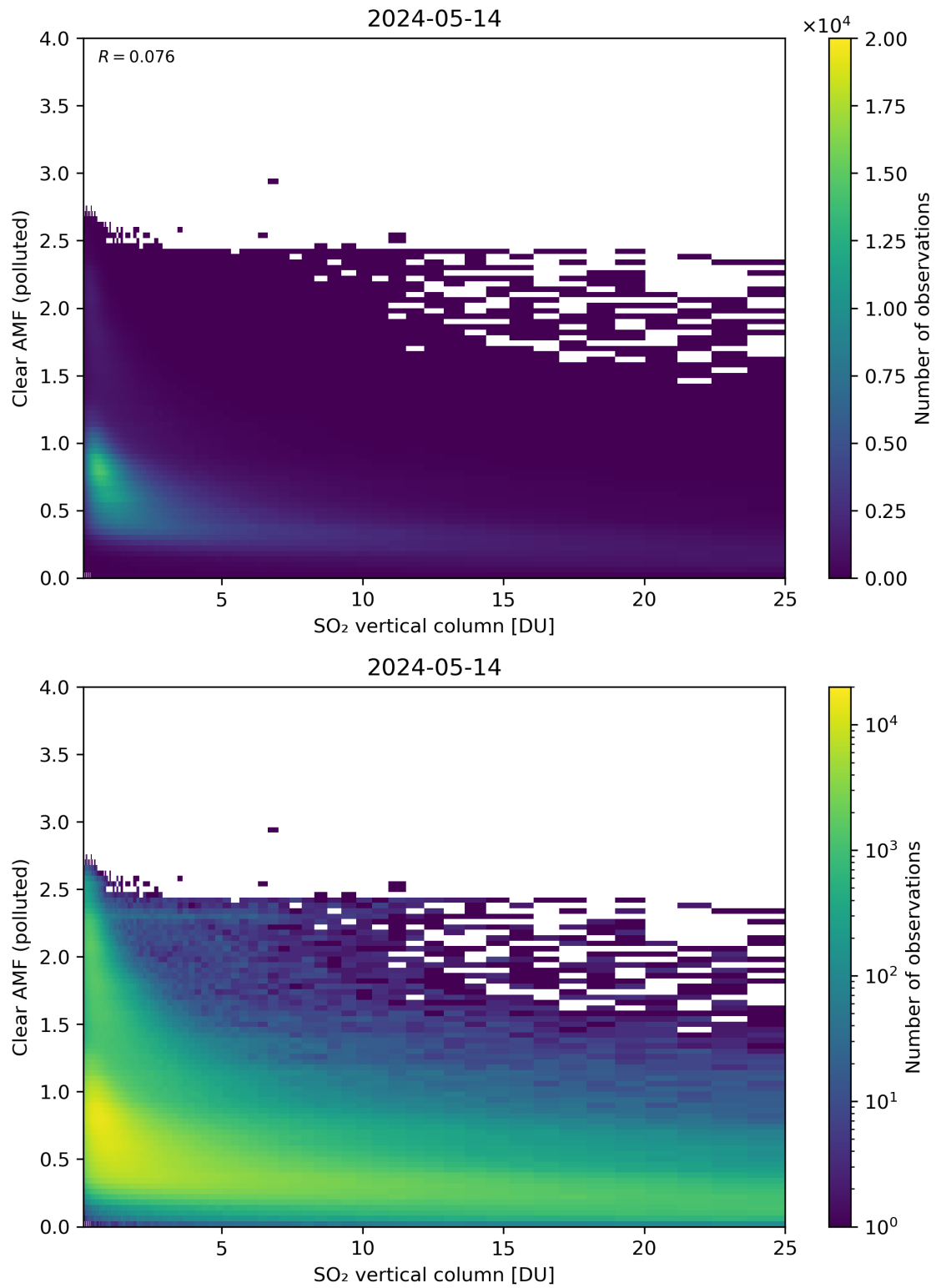
Figure 296: Scatter density plot of “SO 2 vertical column” against “Clear AMF (polluted)” for 2024-05-13 to 2024-05-15.
