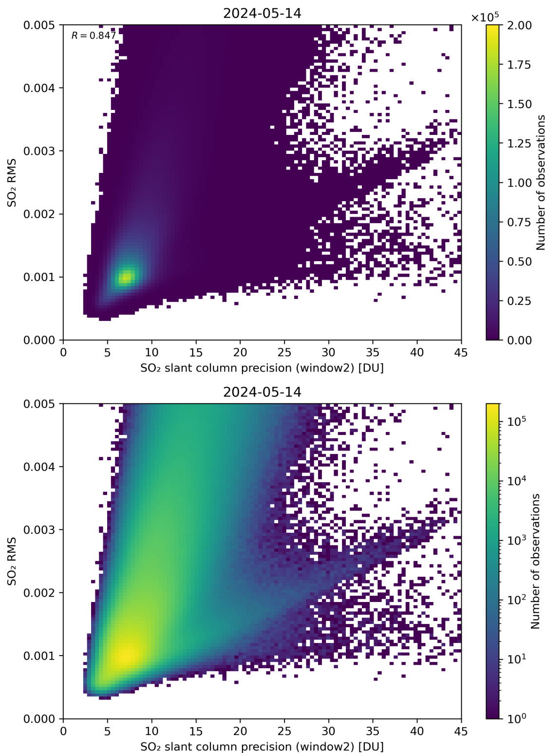
Figure 245: Scatter density plot of “SO 2 slant column precision (window2)” against “SO 2 RMS” for 2024-05-13 to 2024-05-15.
