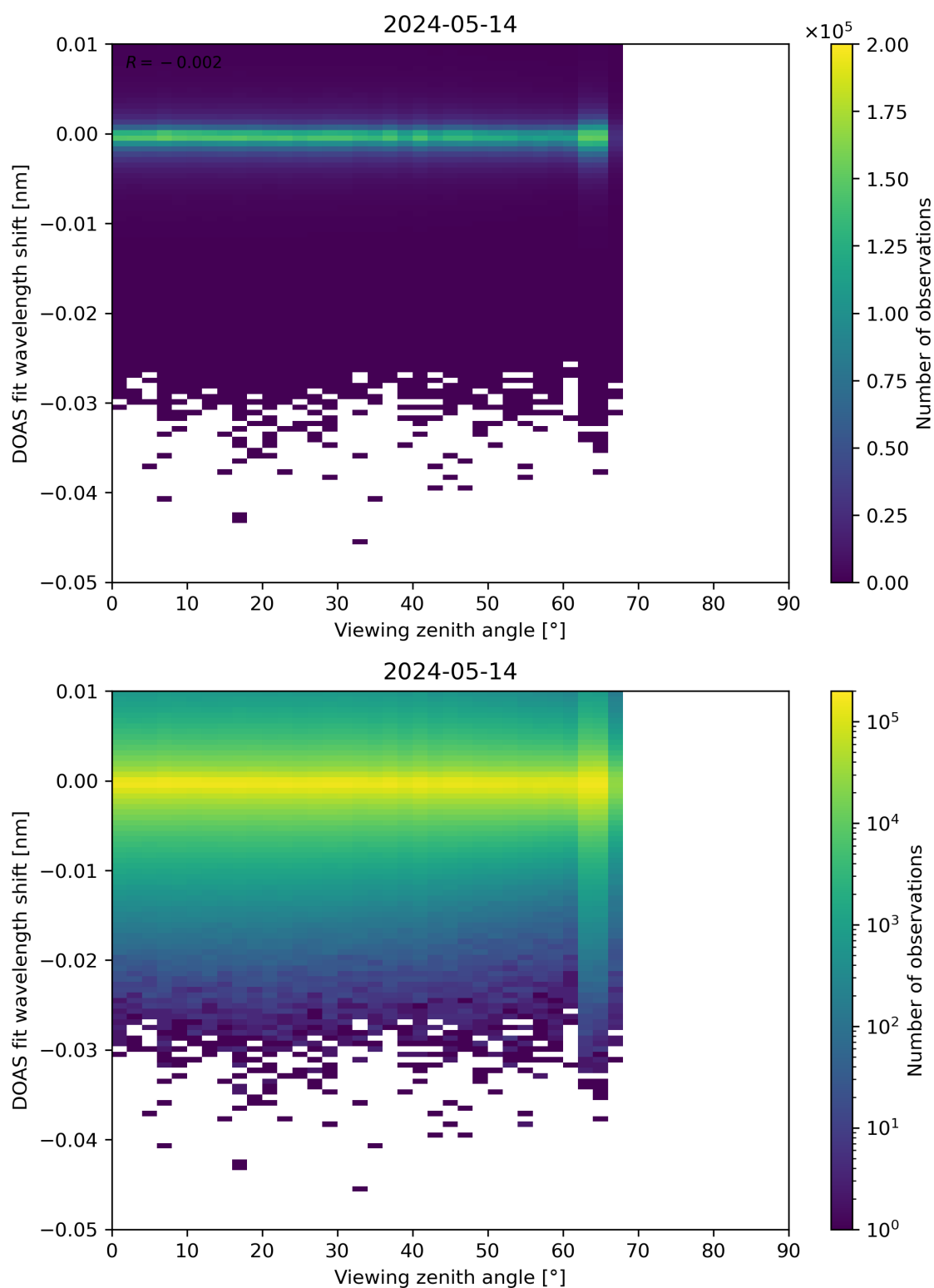
Figure 311: Scatter density plot of “Viewing zenith angle” against “DOAS fit wavelength shift” for 2024-05-13 to 2024-05-15.
