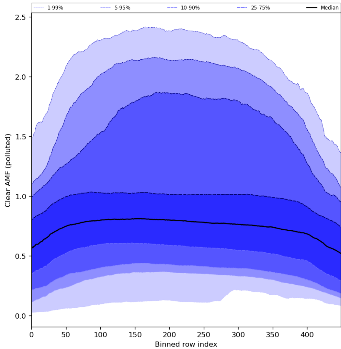
Figure 96: Along track statistics of “Clear AMF (polluted)” for 2024-05-13 to 2024-05-15
