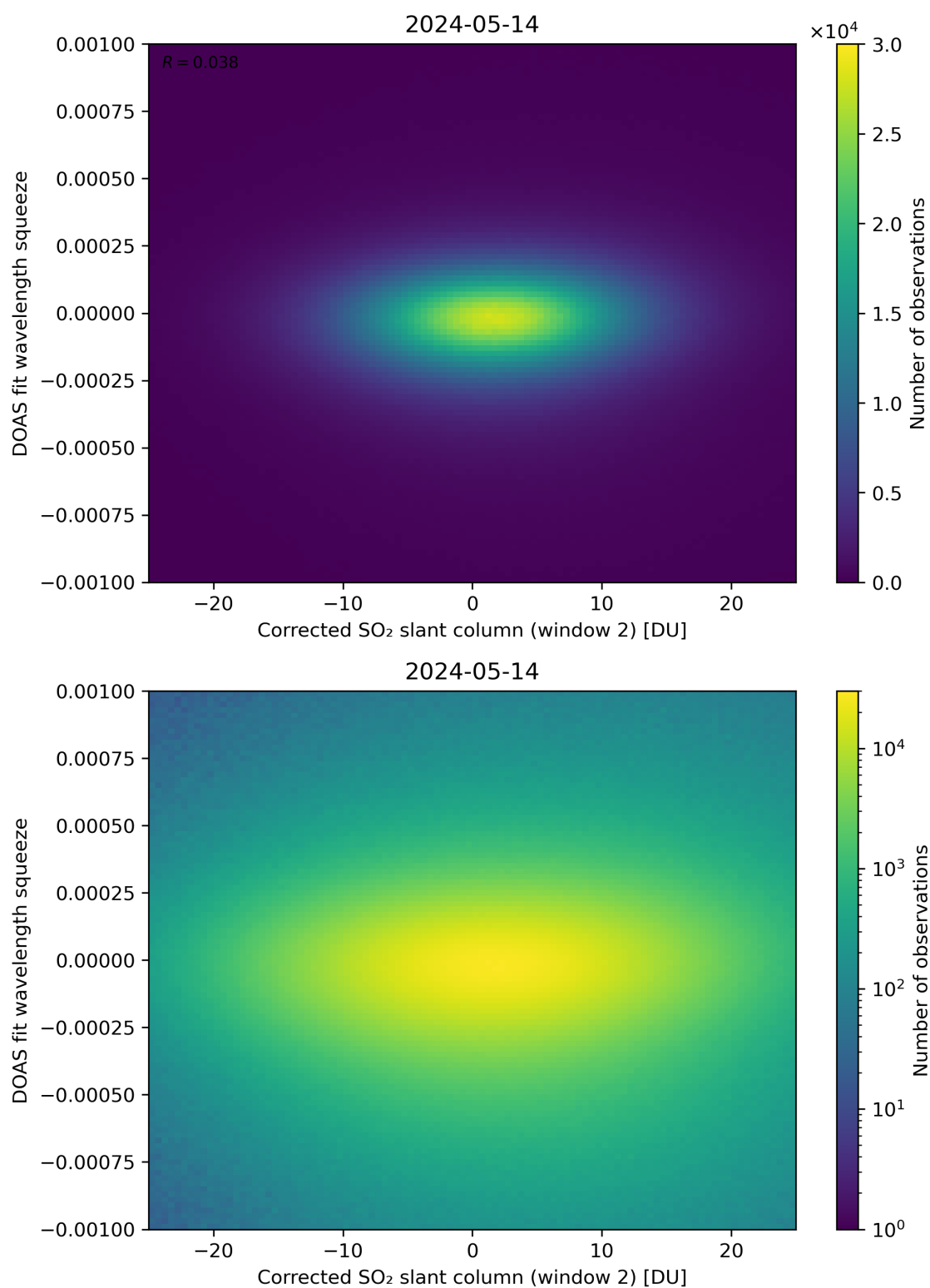
Figure 197: Scatter density plot of “Corrected SO 2 slant column (window 2)” against “DOAS fit wavelength squeeze” for 2024-05-13 to 2024-05-15.
