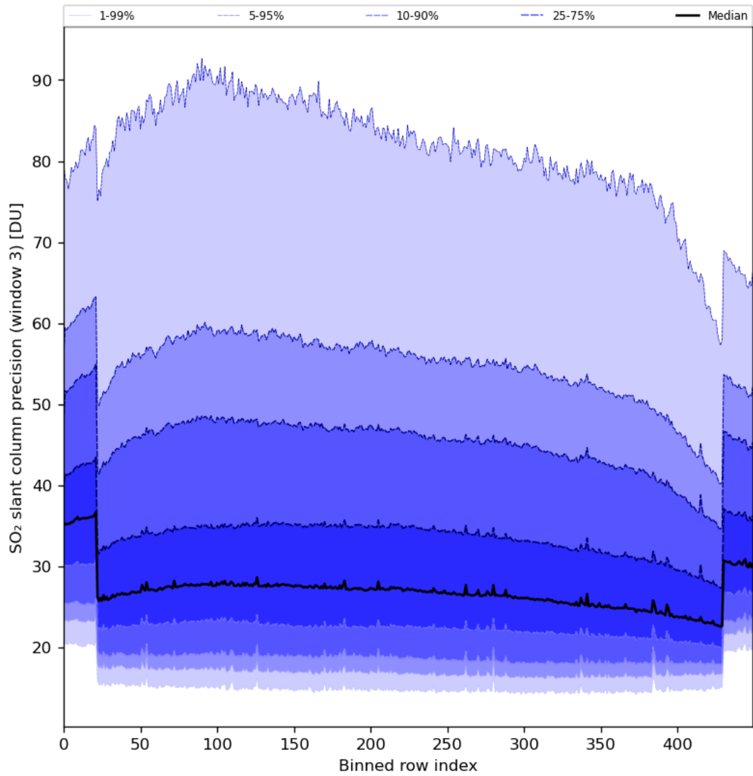
Figure 88: Along track statistics of “SO 2 slant column precision (window 3)” for 2024-05-13 to 2024-05-15
