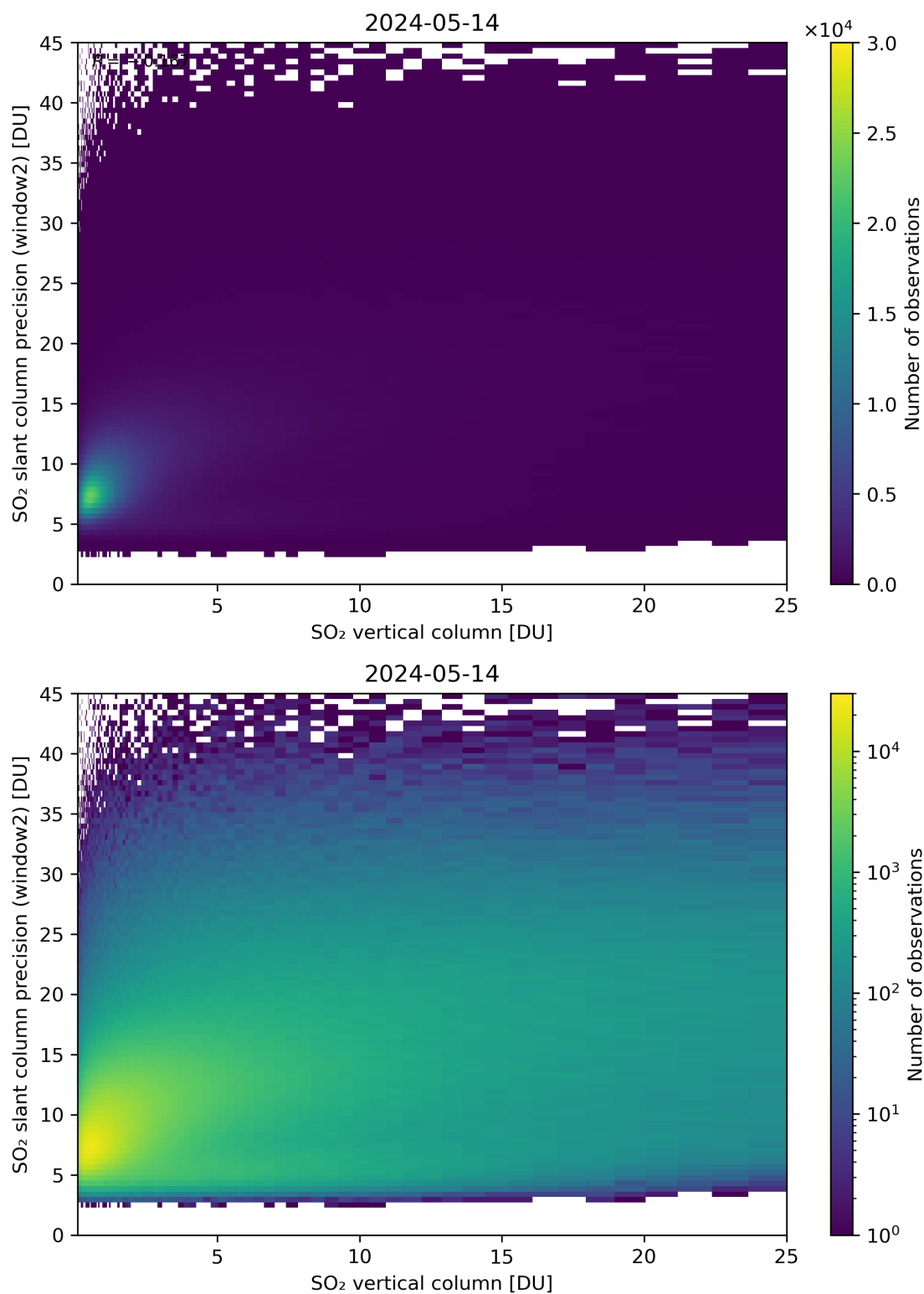
Figure 302: Scatter density plot of “SO 2 vertical column” against “SO 2 slant column precision (window2)” for 2024-05-13 to 2024-05-15.
