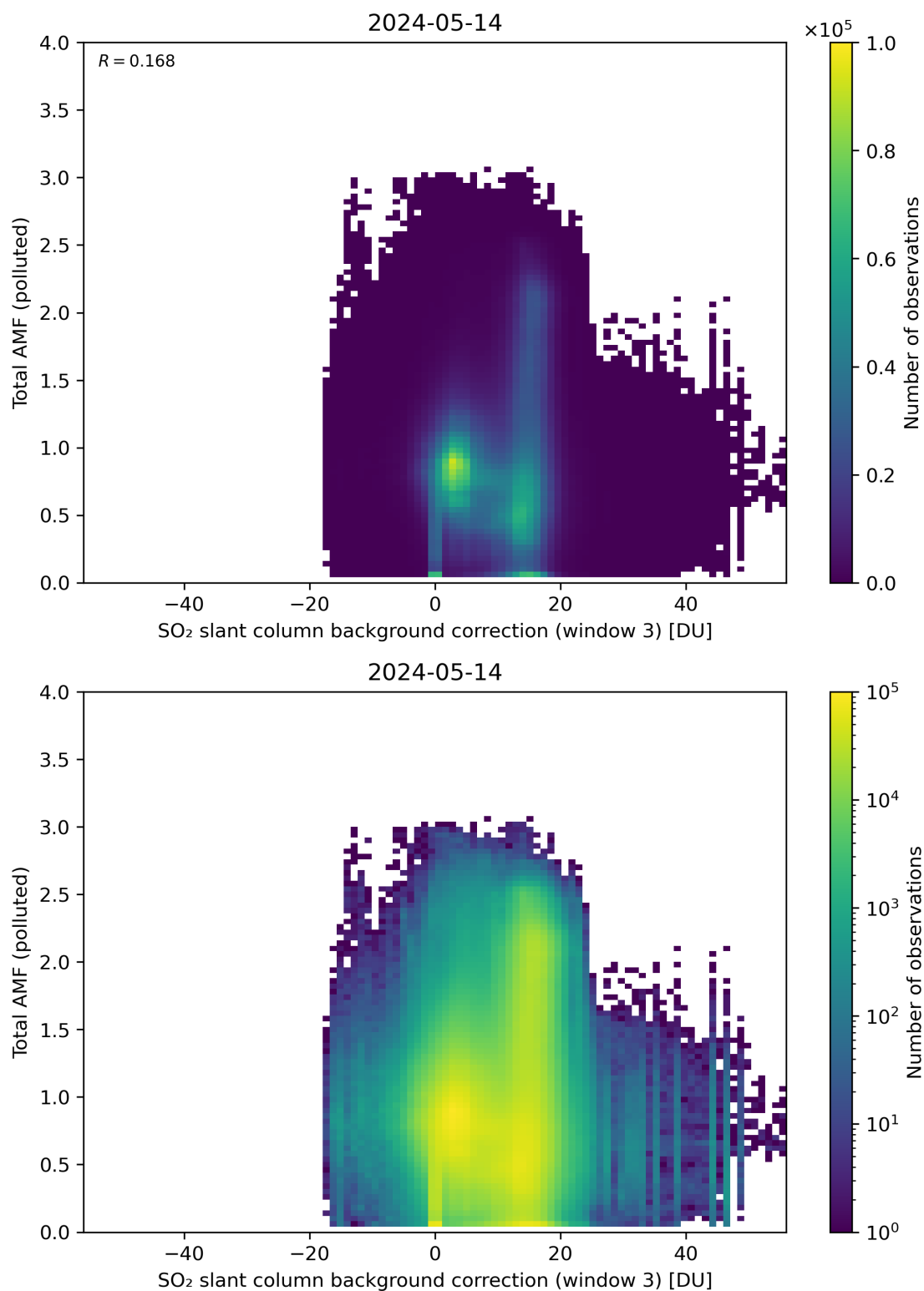
Figure 125: Scatter density plot of “SO 2 slant column background correction (window 3)” against “Total AMF (polluted)” for 2024-05-13 to 2024-05-15.
