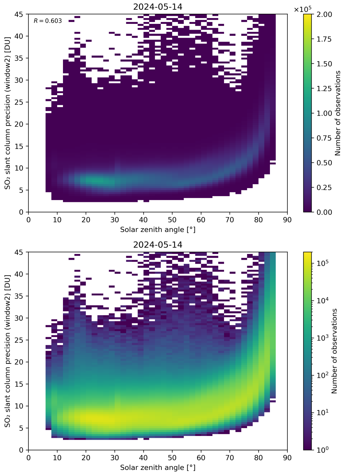
Figure 171: Scatter density plot of “Solar zenith angle” against “SO 2 slant column precision (window2)” for 2024-05-13 to 2024-05-15.
