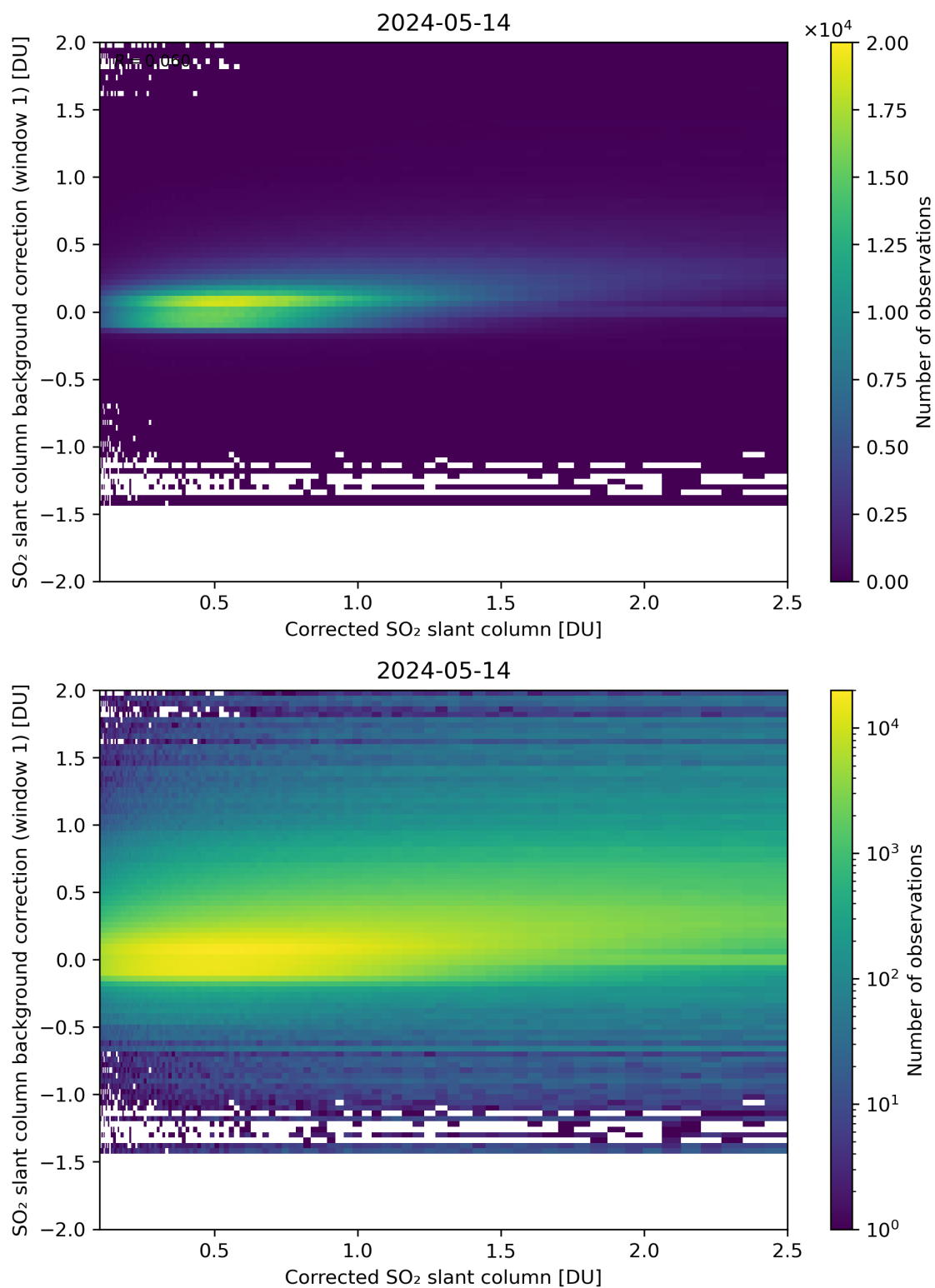
Figure 178: Scatter density plot of “Corrected SO 2 slant column” against “SO 2 slant column background correction (window 1)” for 2024-05-13 to 2024-05-15.
