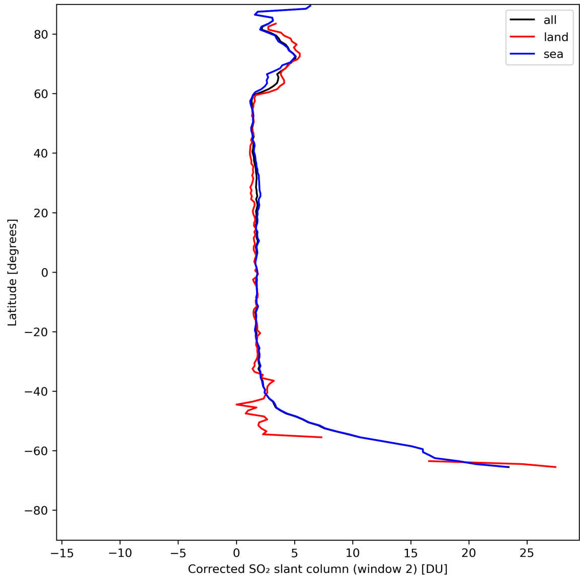
Figure 39: Zonal average of “Corrected SO 2 slant column (window 2)” for 2024-05-13 to 2024-05-15.
