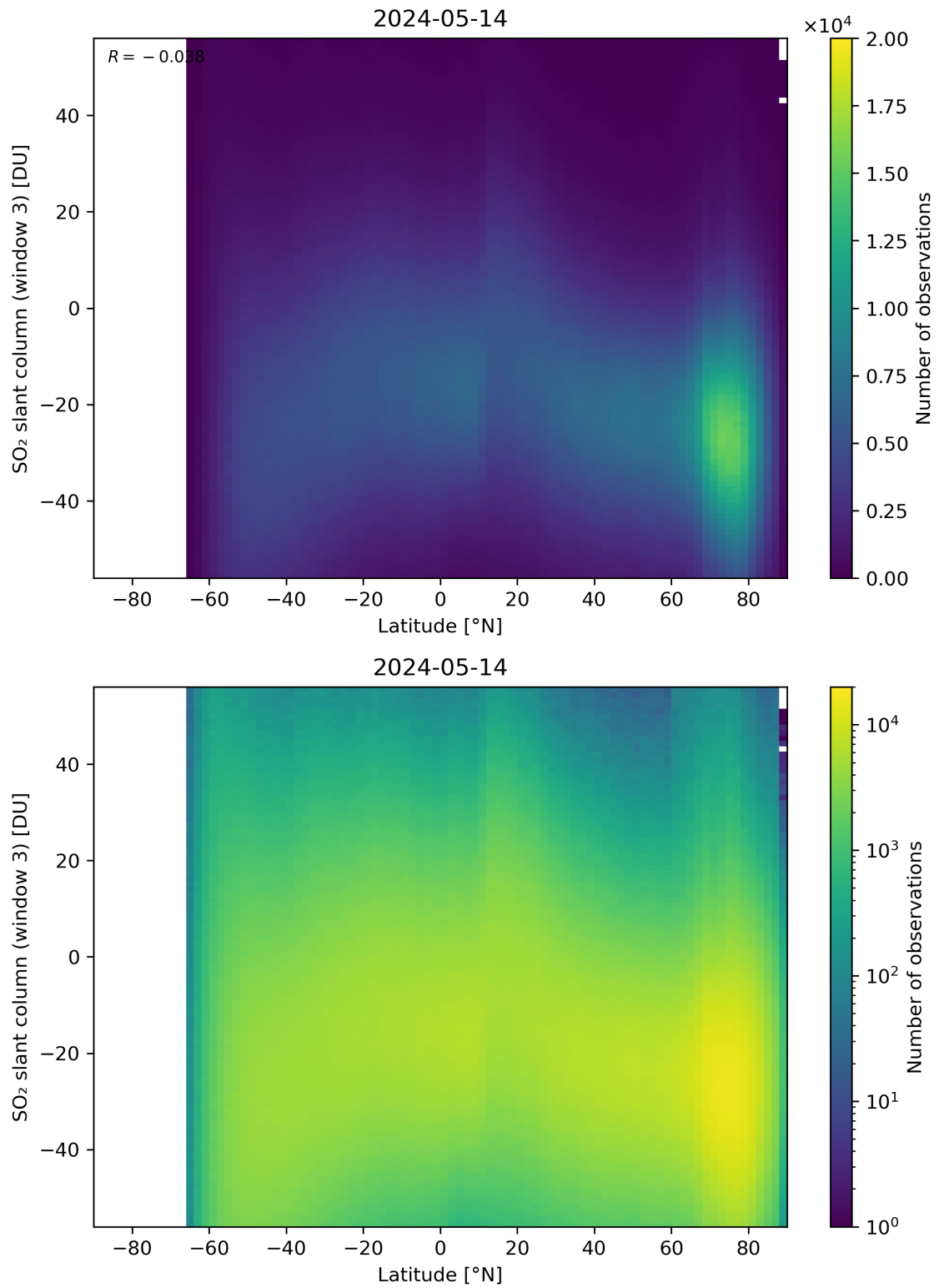
Figure 152: Scatter density plot of “Latitude” against “SO 2 slant column (window 3)” for 2024-05-13 to 2024-05-15.
