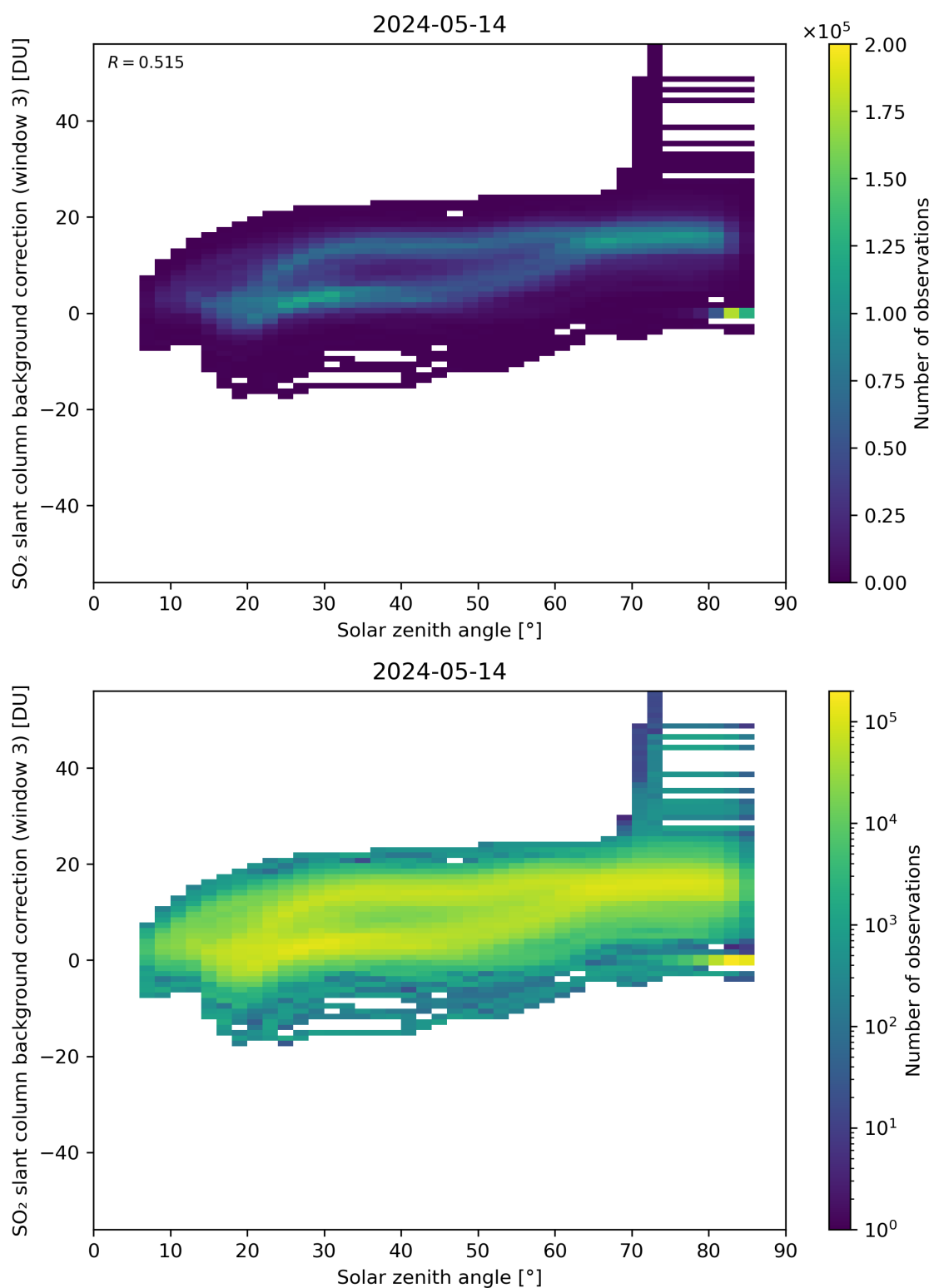
Figure 160: Scatter density plot of “Solar zenith angle” against “SO 2 slant column background correction (window 3)” for 2024-05-13 to 2024-05-15.
