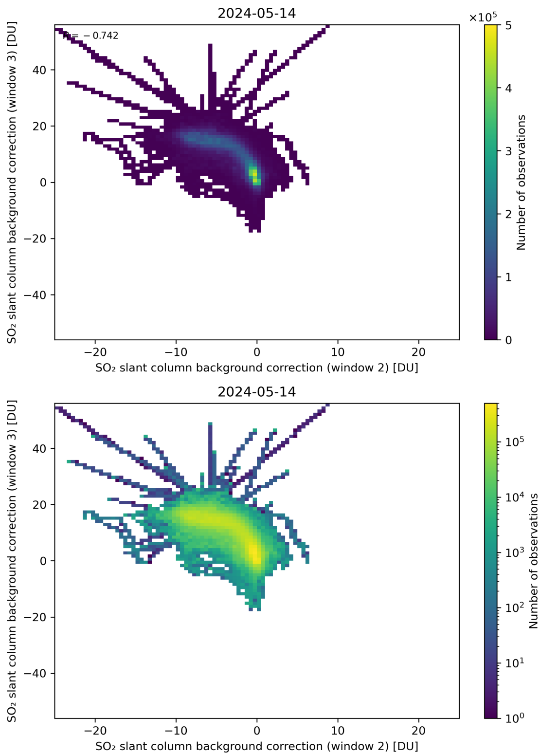
Figure 111: Scatter density plot of “SO 2 slant column background correction (window 2)” against “SO 2 slant column background correction (window 3)” for 2024-05-13 to 2024-05-15.
