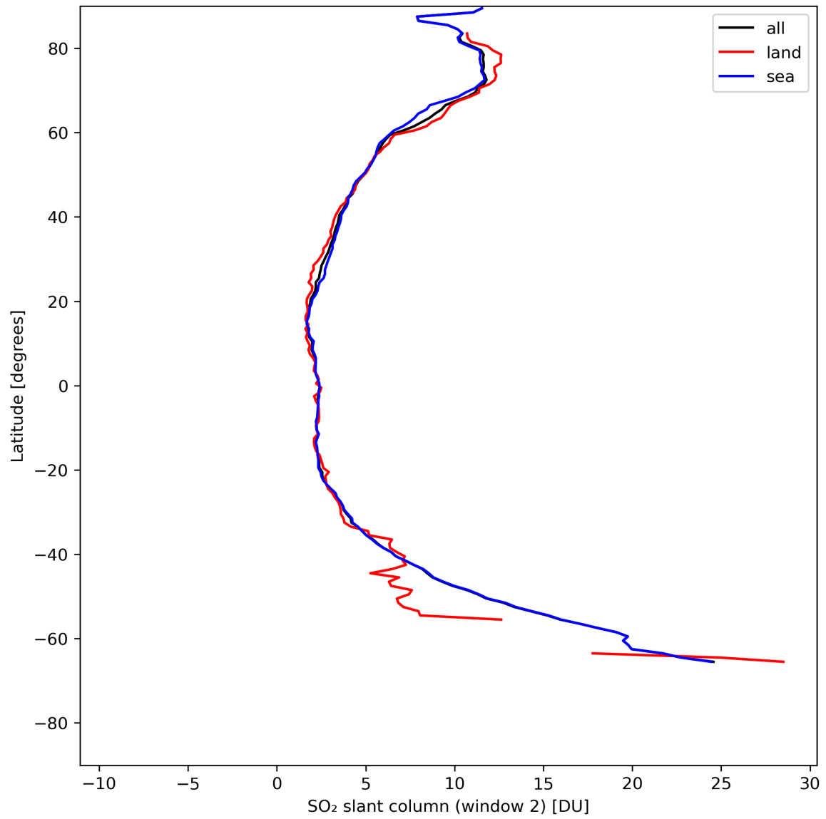
Figure 37: Zonal average of “SO 2 slant column (window 2)” for 2024-05-13 to 2024-05-15.
