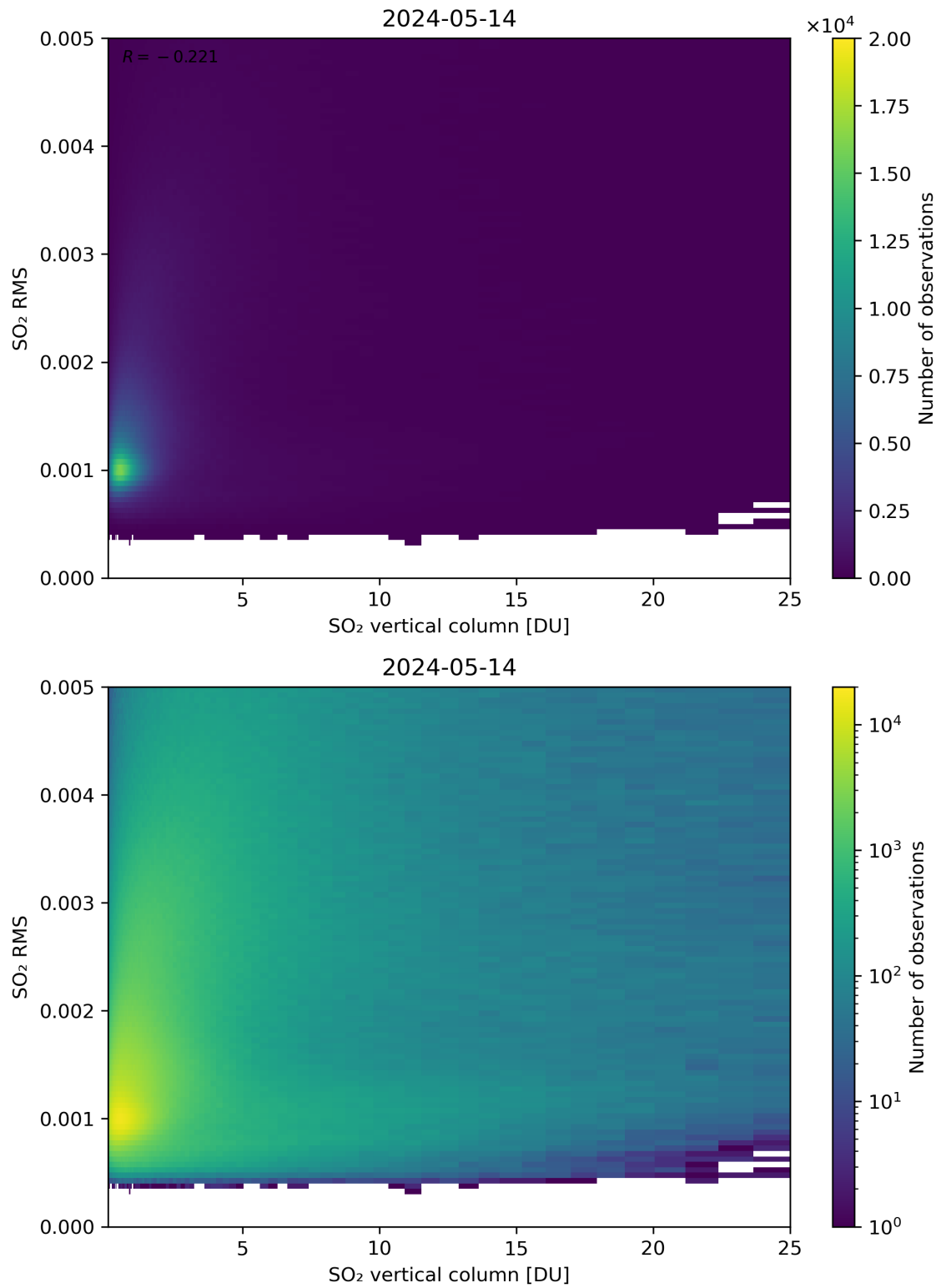
Figure 278: Scatter density plot of “SO 2 vertical column” against “SO 2 RMS” for 2024-05-13 to 2024-05-15.
