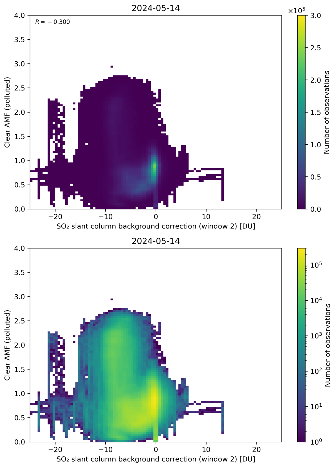
Figure 115: Scatter density plot of “SO 2 slant column background correction (window 2)” against “Clear AMF (polluted)” for 2024-05-13 to 2024-05-15.
