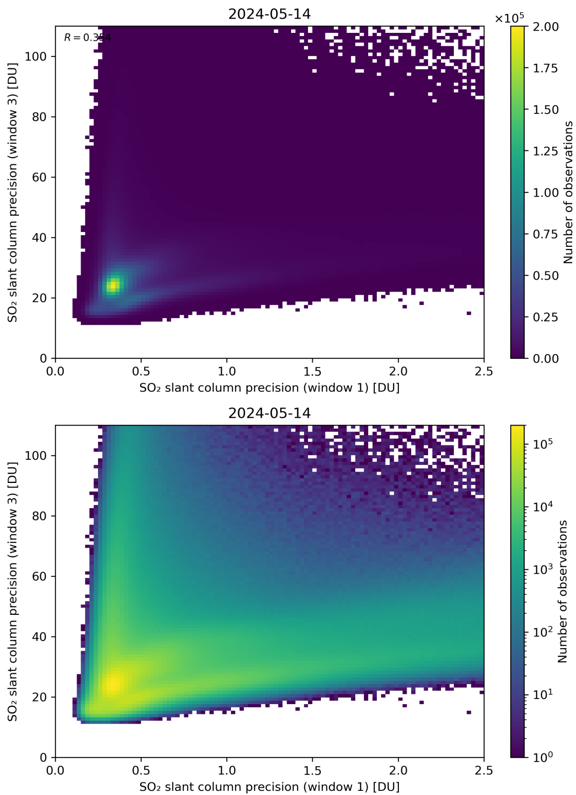
Figure 229: Scatter density plot of “SO 2 slant column precision (window 1)” against “SO 2 slant column precision (window 3)” for 2024-05-13 to 2024-05-15.
