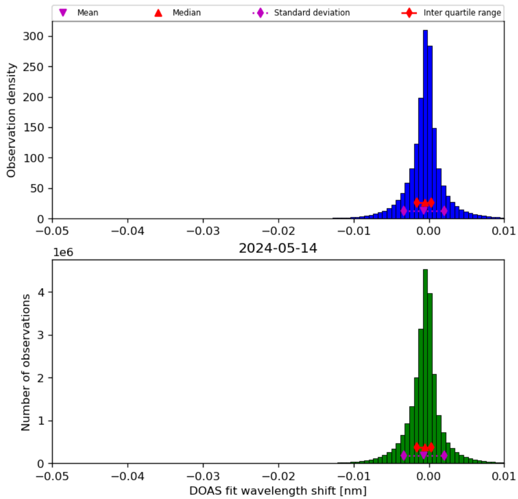
Figure 68: Histogram of “DOAS fit wavelength shift” for 2024-05-13 to 2024-05-15
