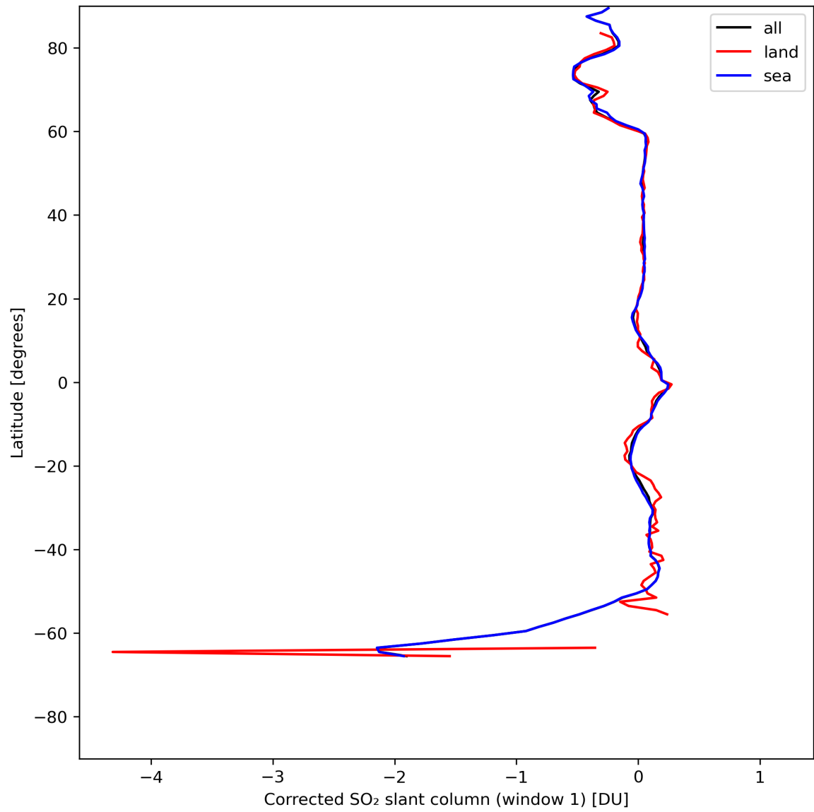
Figure 35: Zonal average of “Corrected SO 2 slant column (window 1)” for 2024-05-13 to 2024-05-15.
