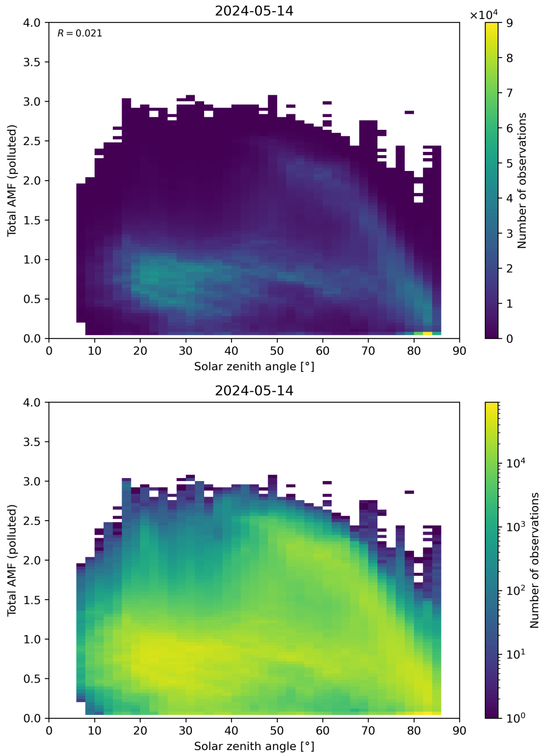
Figure 174: Scatter density plot of “Solar zenith angle” against “Total AMF (polluted)” for 2024-05-13 to 2024-05-15.
