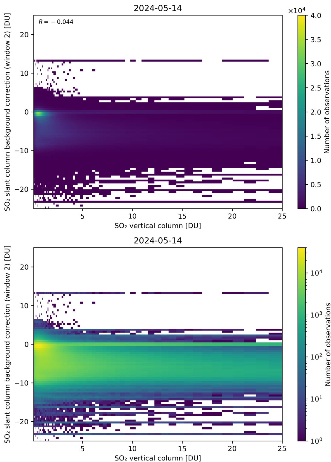
Figure 274: Scatter density plot of “SO 2 vertical column” against “SO 2 slant column background correction (window 2)” for 2024-05-13 to 2024-05-15.
