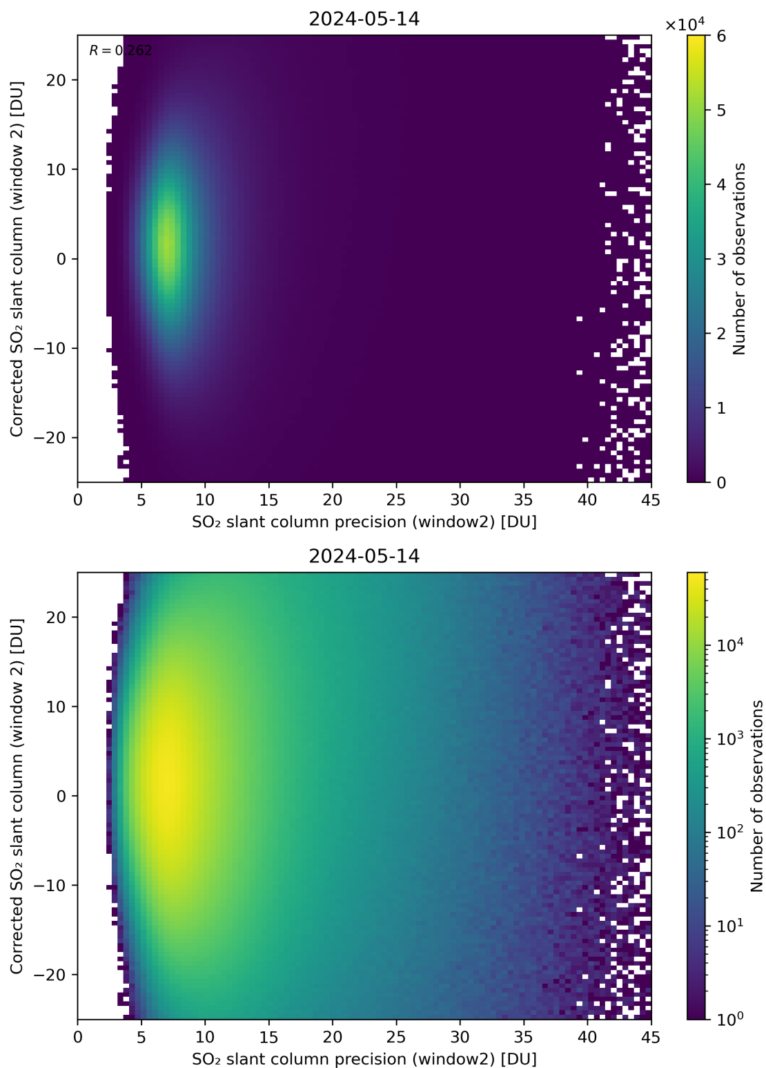
Figure 247: Scatter density plot of “SO 2 slant column precision (window2)” against “Corrected SO 2 slant column (window 2)” for 2024-05-13 to 2024-05-15.
