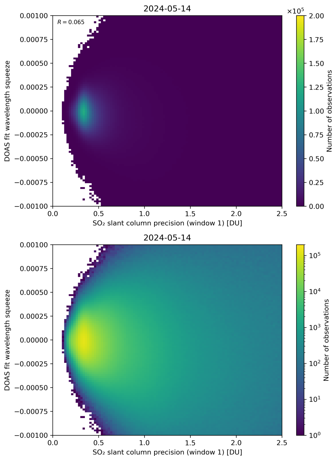
Figure 222: Scatter density plot of “SO 2 slant column precision (window 1)” against “DOAS fit wavelength squeeze” for 2024-05-13 to 2024-05-15.
