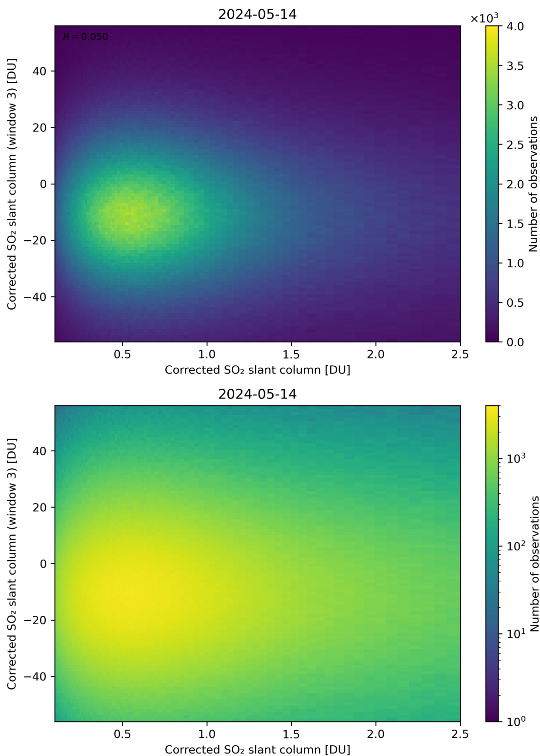
Figure 186: Scatter density plot of “Corrected SO 2 slant column” against “Corrected SO 2 slant column (window 3)” for 2024-05-13 to 2024-05-15.
