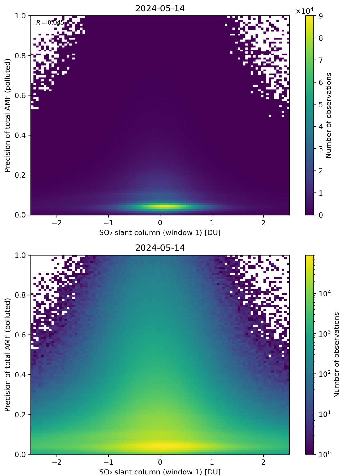
Figure 240: Scatter density plot of “SO 2 slant column (window 1)” against “Precision of total AMF (polluted)” for 2024-05-13 to 2024-05-15.
