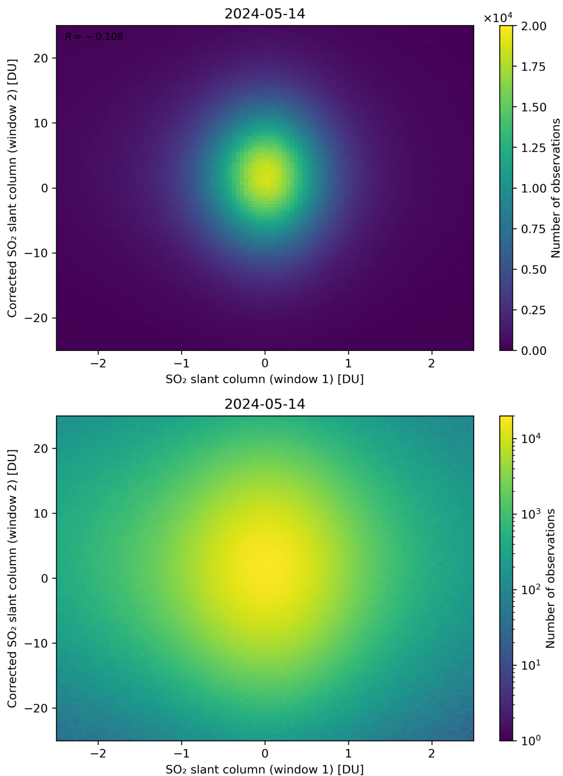
Figure 233: Scatter density plot of “SO 2 slant column (window 1)” against “Corrected SO 2 slant column (window 2)” for 2024-05-13 to 2024-05-15.
