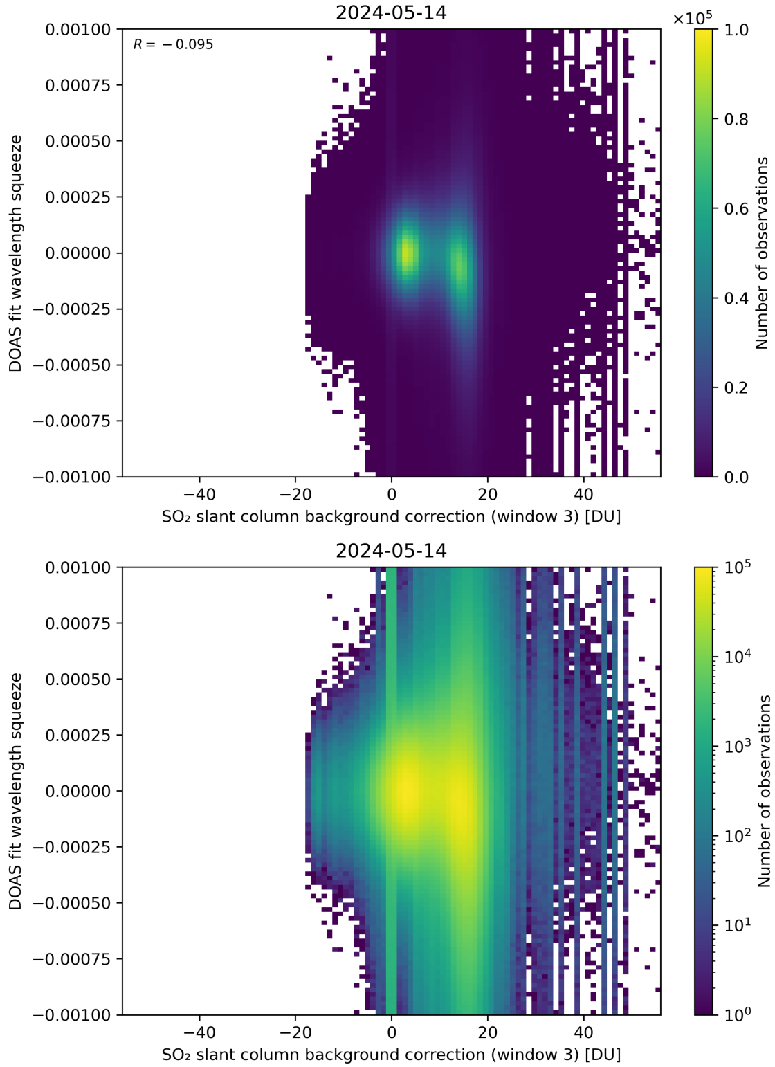
Figure 122: Scatter density plot of “SO 2 slant column background correction (window 3)” against “DOAS fit wavelength squeeze” for 2024-05-13 to 2024-05-15.
