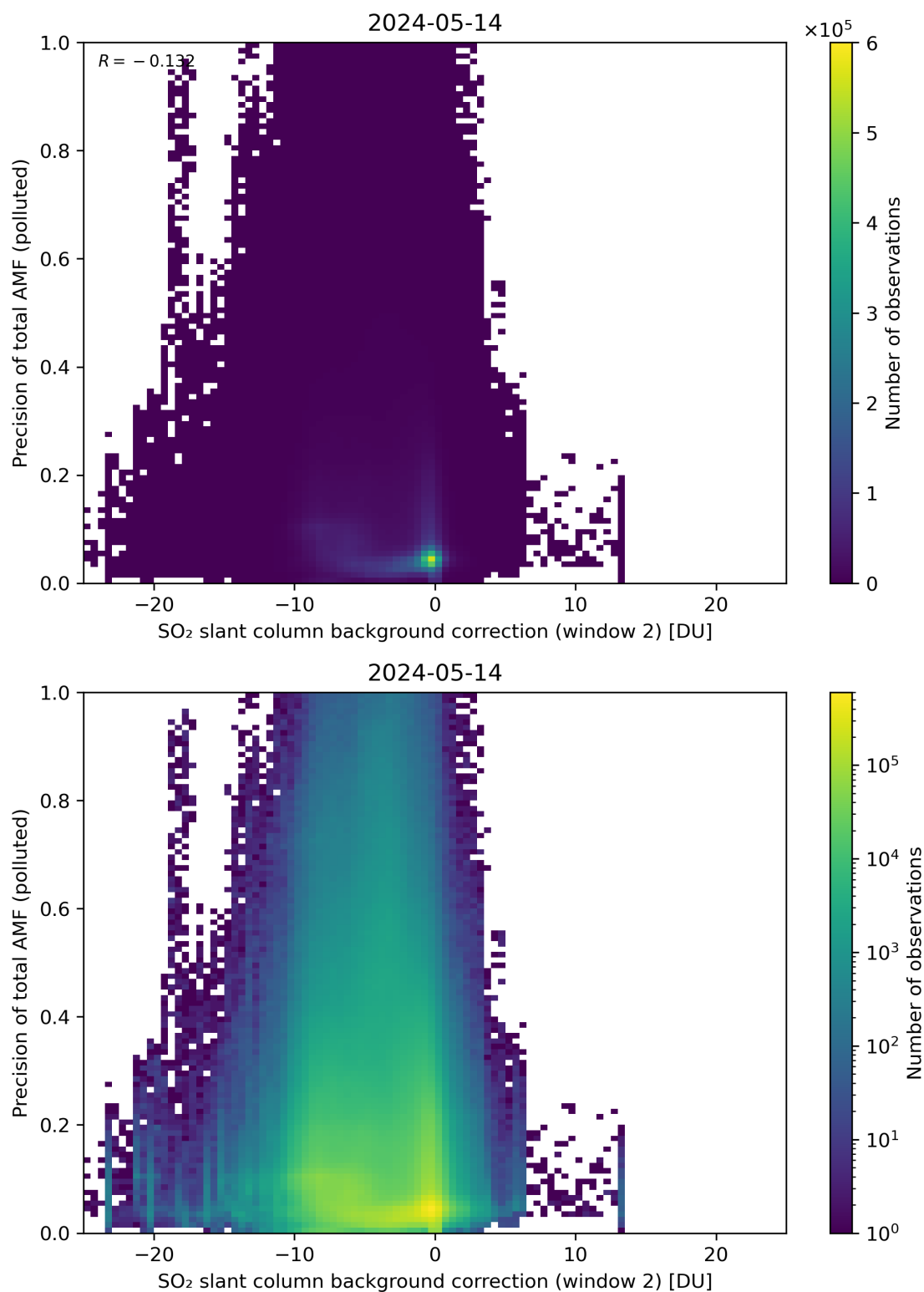
Figure 120: Scatter density plot of “SO 2 slant column background correction (window 2)” against “Precision of total AMF (polluted)” for 2024-05-13 to 2024-05-15.
