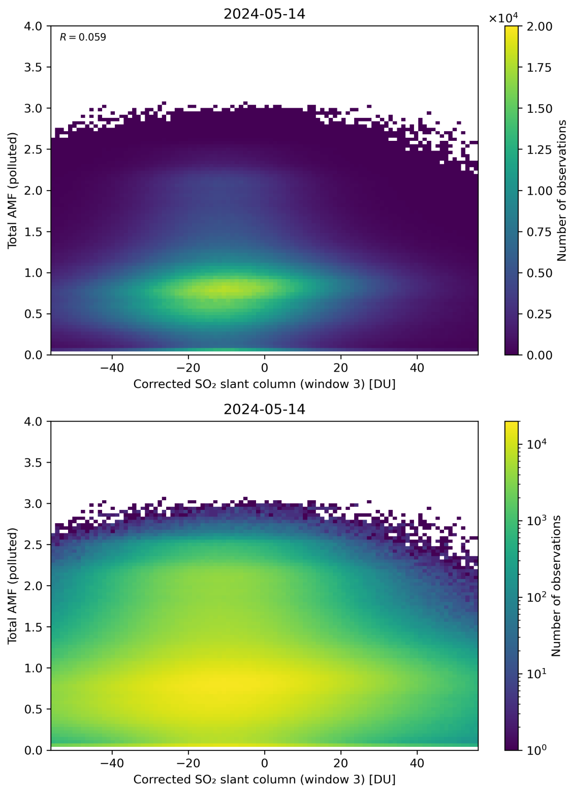
Figure 210: Scatter density plot of “Corrected SO 2 slant column (window 3)” against “Total AMF (polluted)” for 2024-05-13 to 2024-05-15.
