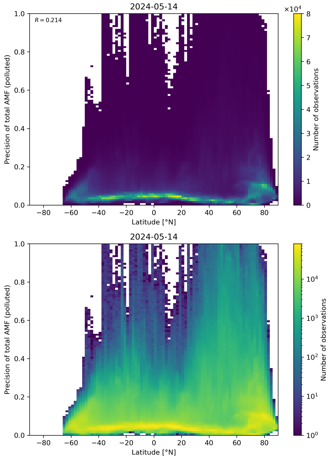
Figure 155: Scatter density plot of “Latitude” against “Precision of total AMF (polluted)” for 2024-05-13 to 2024-05-15.
