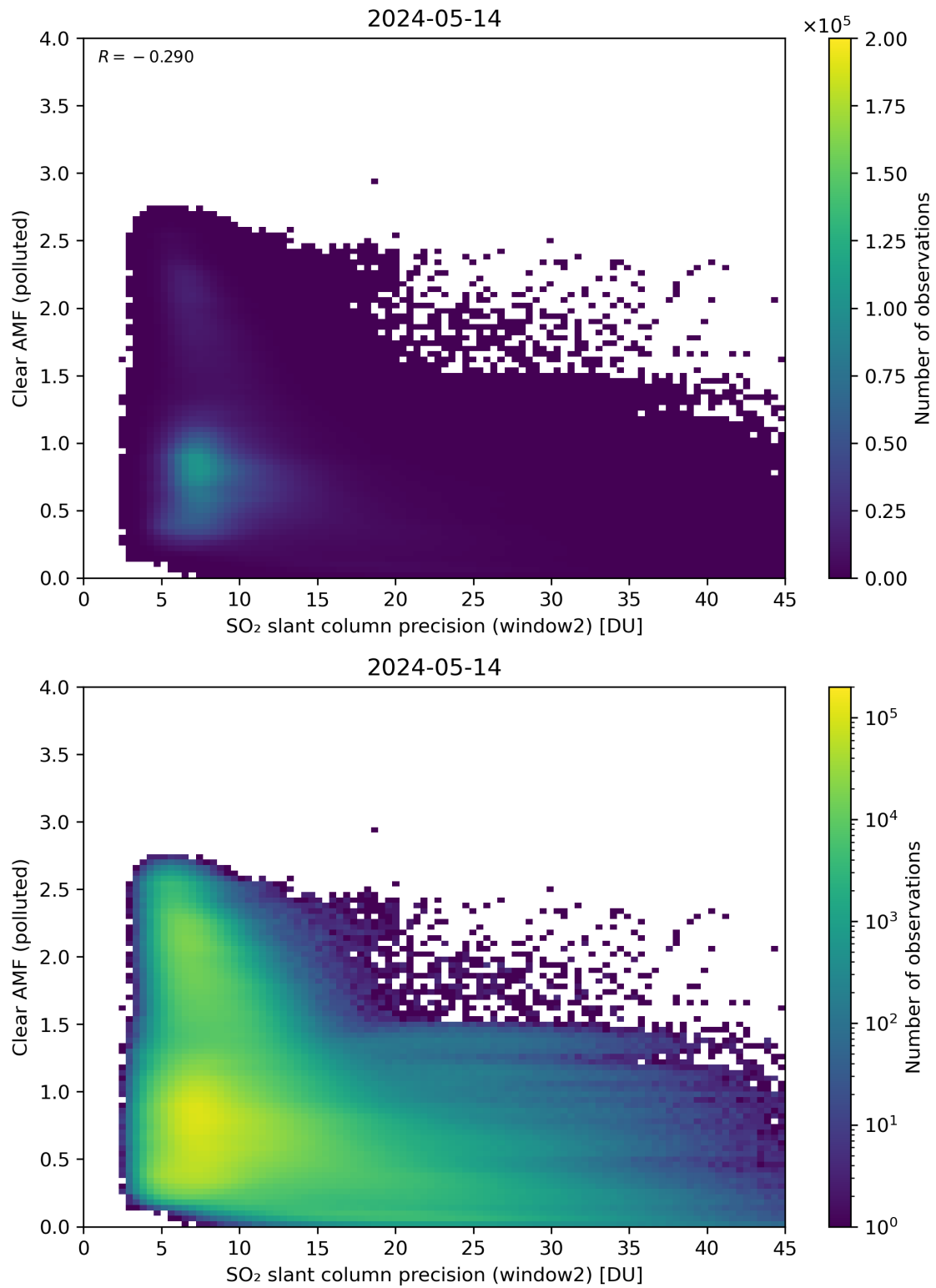
Figure 246: Scatter density plot of “SO 2 slant column precision (window2)” against “Clear AMF (polluted)” for 2024-05-13 to 2024-05-15.
