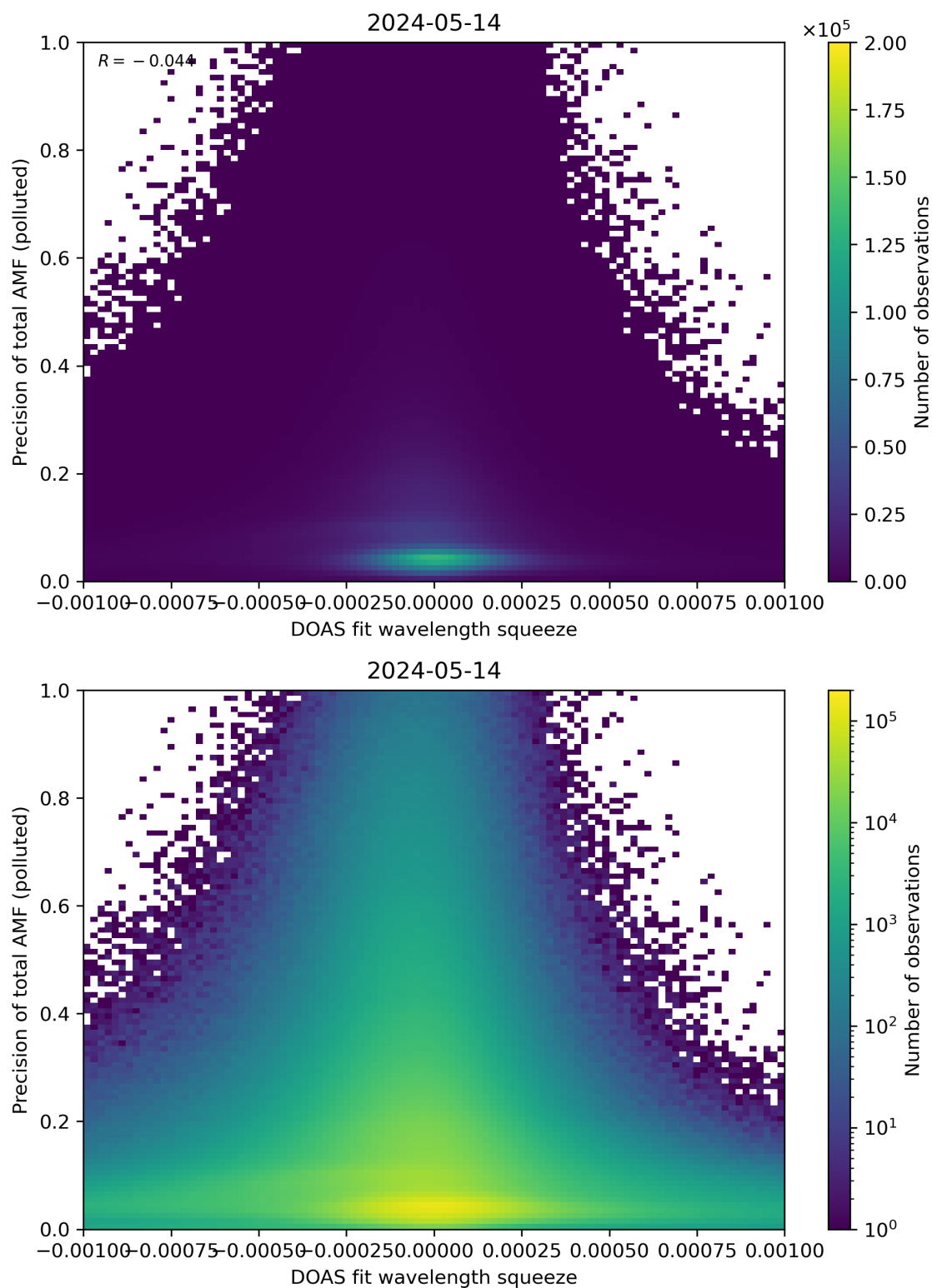
Figure 135: Scatter density plot of “DOAS fit wavelength squeeze” against “Precision of total AMF (polluted)” for 2024-05-13 to 2024-05-15.
