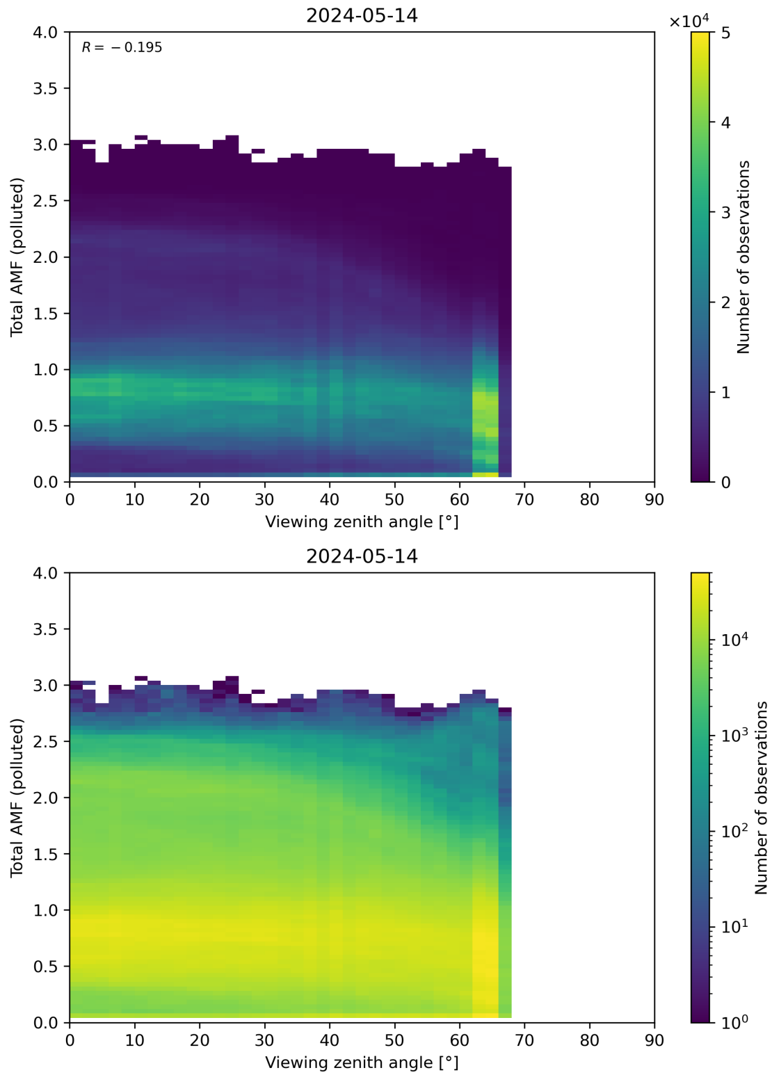
Figure 325: Scatter density plot of “Viewing zenith angle” against “Total AMF (polluted)” for 2024-05-13 to 2024-05-15.
