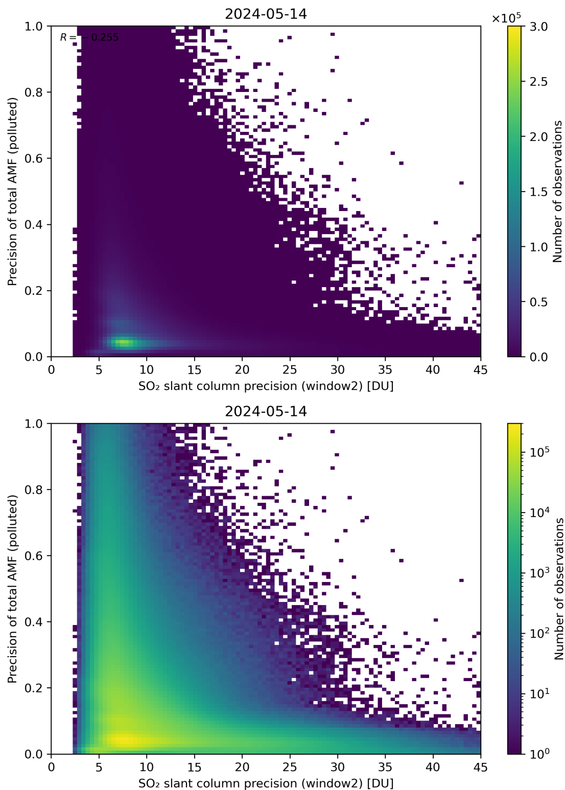
Figure 252: Scatter density plot of “SO 2 slant column precision (window2)” against “Precision of total AMF (polluted)” for 2024-05-13 to 2024-05-15.
