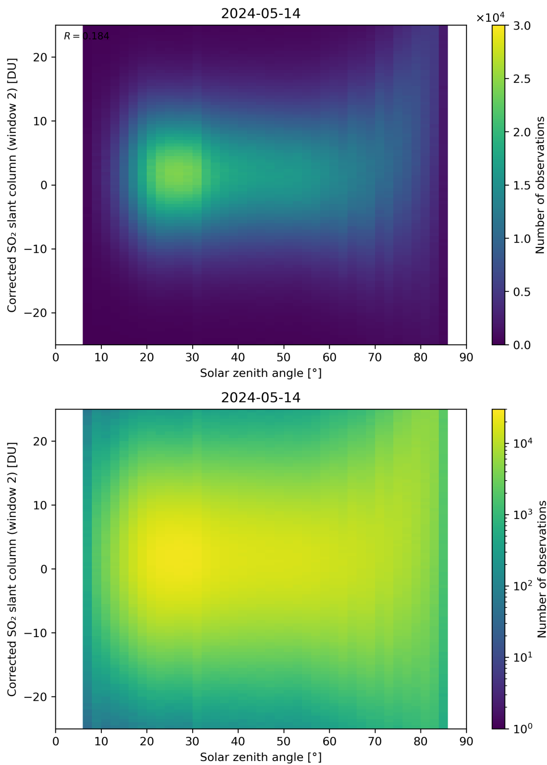
Figure 167: Scatter density plot of “Solar zenith angle” against “Corrected SO 2 slant column (window 2)” for 2024-05-13 to 2024-05-15.
