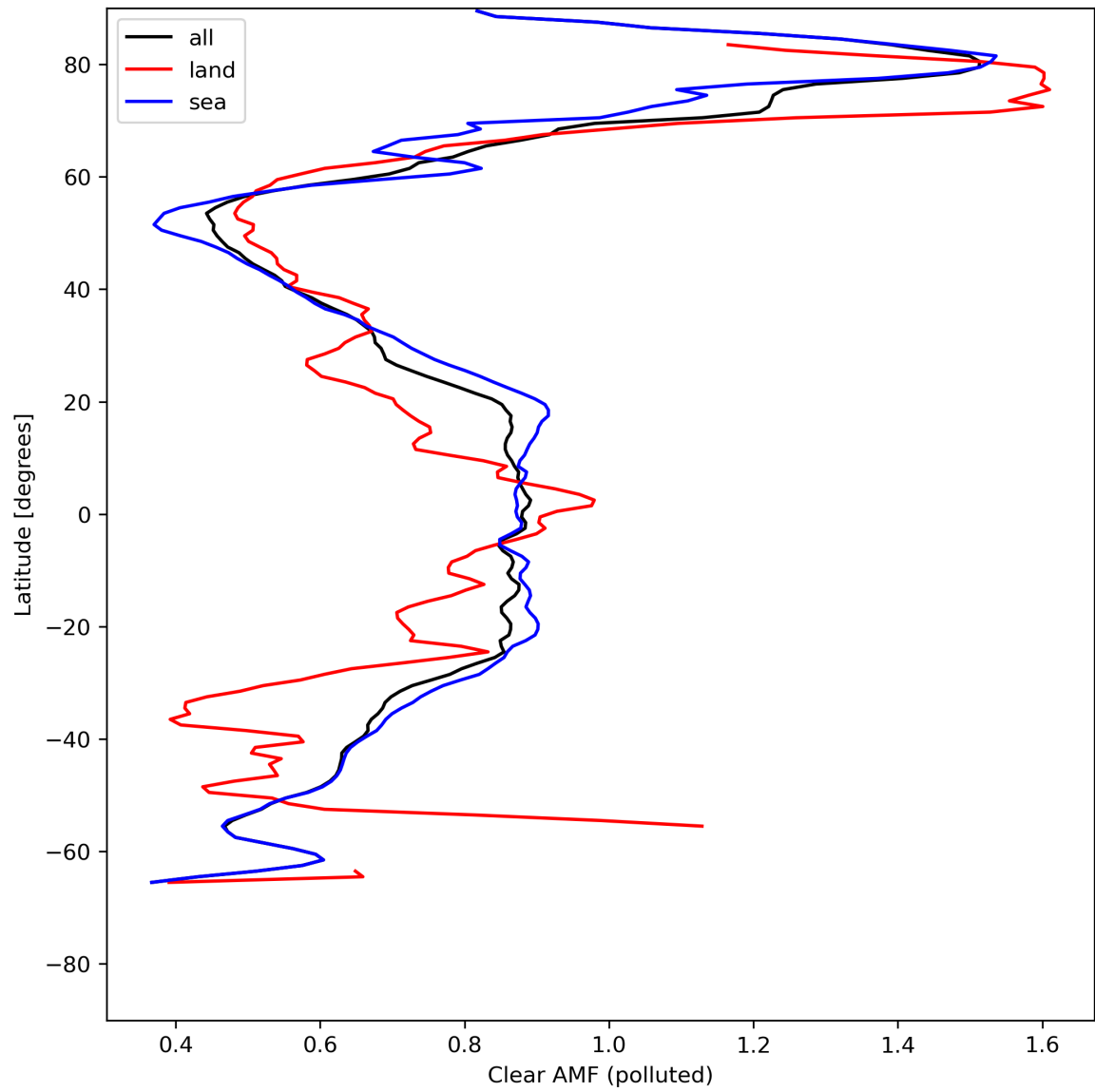
Figure 50: Zonal average of “Clear AMF (polluted)” for 2024-05-13 to 2024-05-15.
