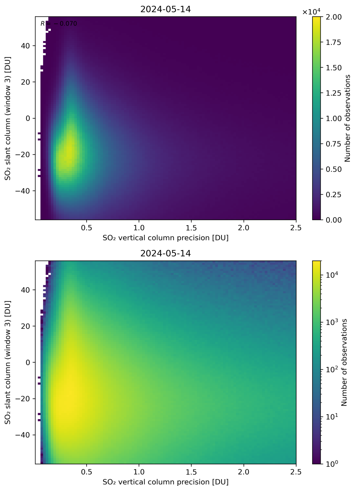
Figure 292: Scatter density plot of “SO 2 vertical column precision” against “SO 2 slant column (window 3)” for 2024-05-13 to 2024-05-15.
