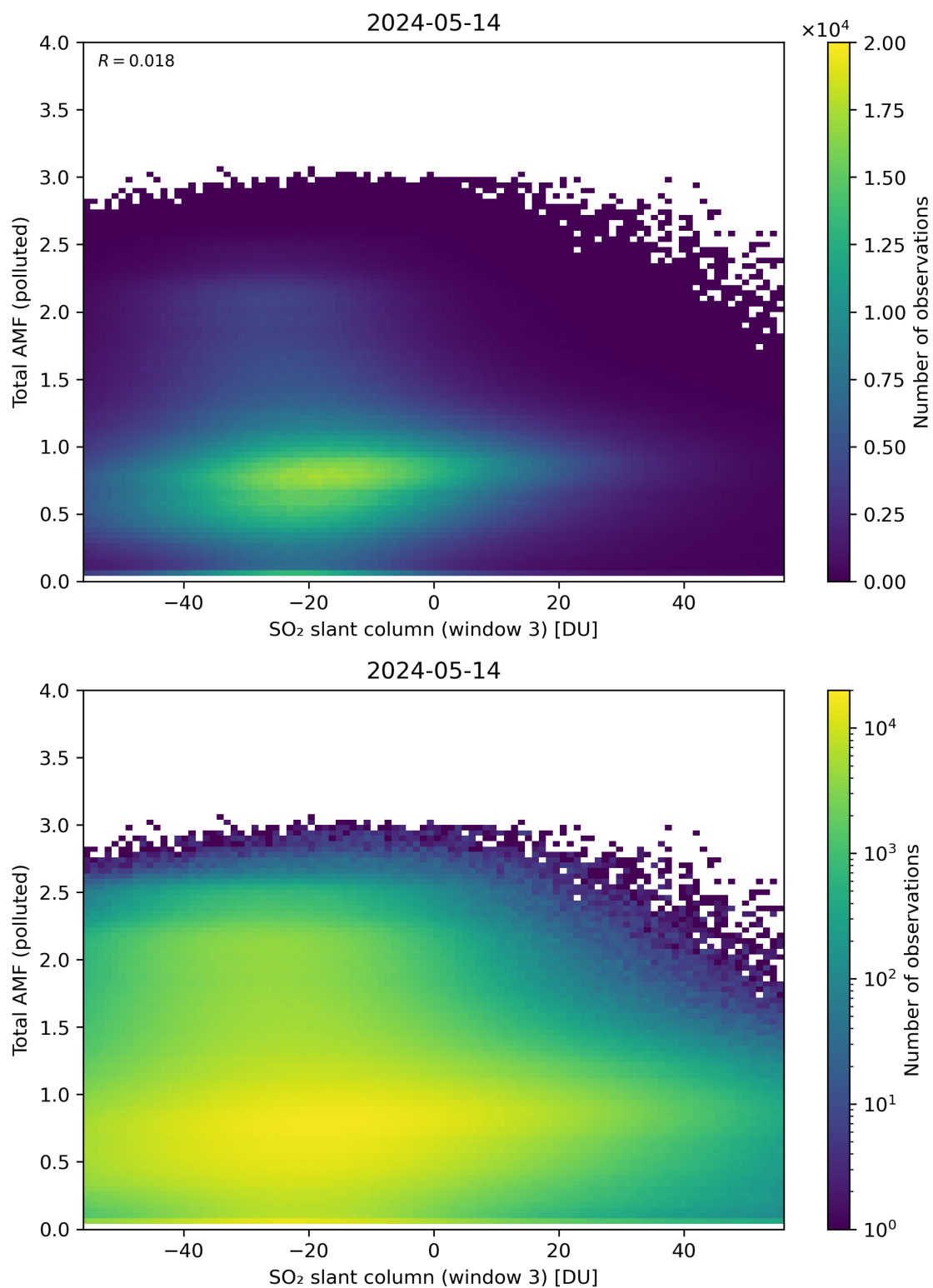
Figure 268: Scatter density plot of “SO 2 slant column (window 3)” against “Total AMF (polluted)” for 2024-05-13 to 2024-05-15.
