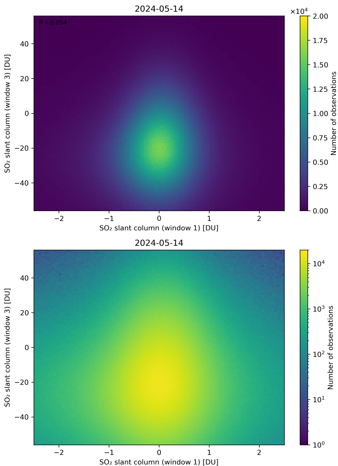
Figure 237: Scatter density plot of “SO 2 slant column (window 1)” against “SO 2 slant column (window 3)” for 2024-05-13 to 2024-05-15.
