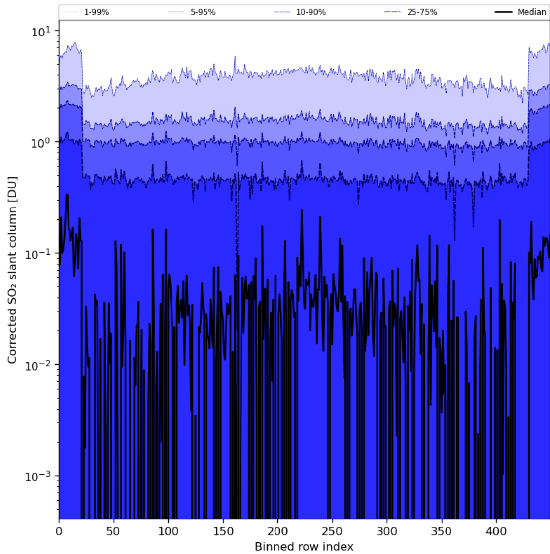
Figure 78: Along track statistics of “Corrected SO 2 slant column” for 2024-05-13 to 2024-05-15
