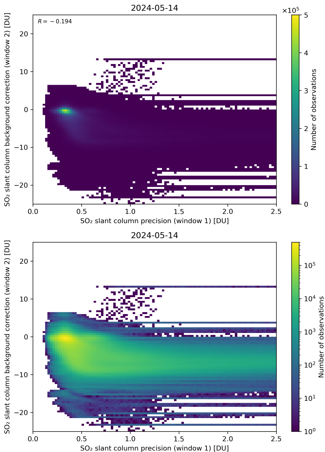
Figure 219: Scatter density plot of “SO 2 slant column precision (window 1)” against “SO 2 slant column background correction (window 2)” for 2024-05-13 to 2024-05-15.
