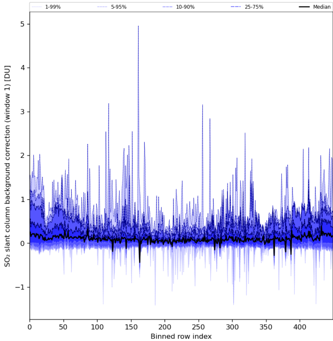
Figure 82: Along track statistics of “SO 2 slant column background correction (window 1)” for 2024-05-13 to 2024-05-15
