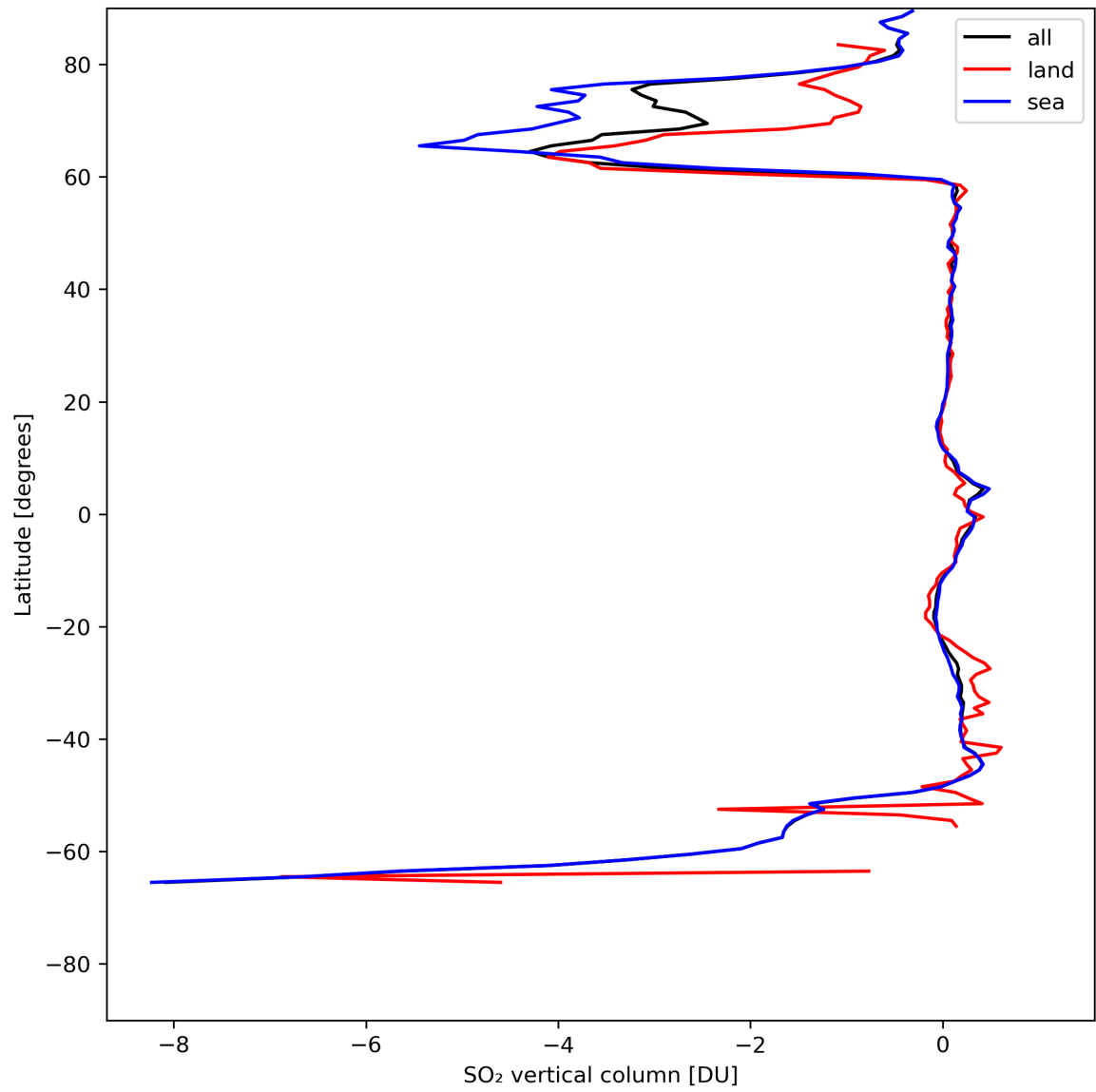
Figure 30: Zonal average of “SO 2 vertical column” for 2024-05-13 to 2024-05-15.
