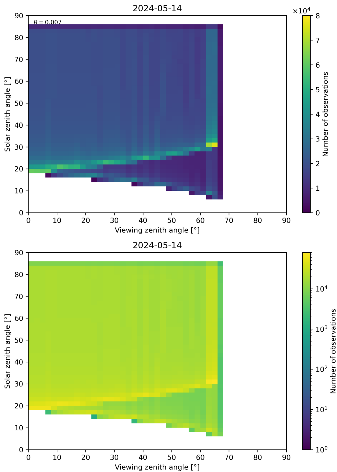
Figure 315: Scatter density plot of “Viewing zenith angle” against “Solar zenith angle” for 2024-05-13 to 2024-05-15.
