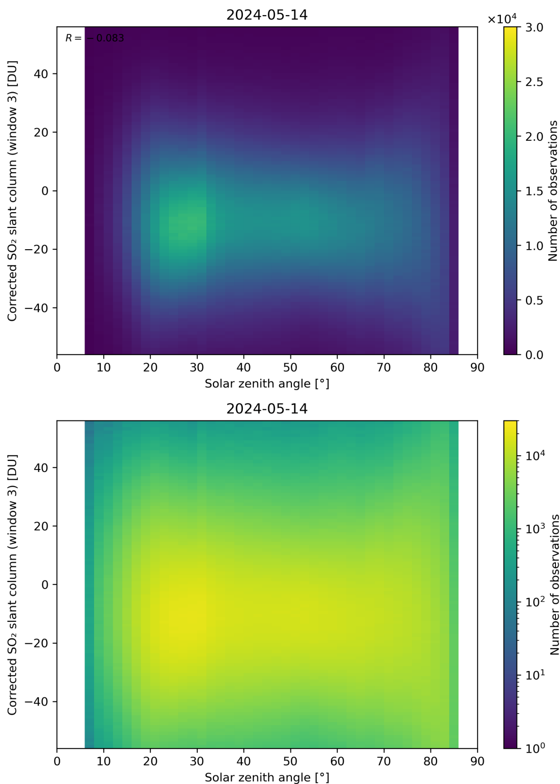
Figure 168: Scatter density plot of “Solar zenith angle” against “Corrected SO 2 slant column (window 3)” for 2024-05-13 to 2024-05-15.
