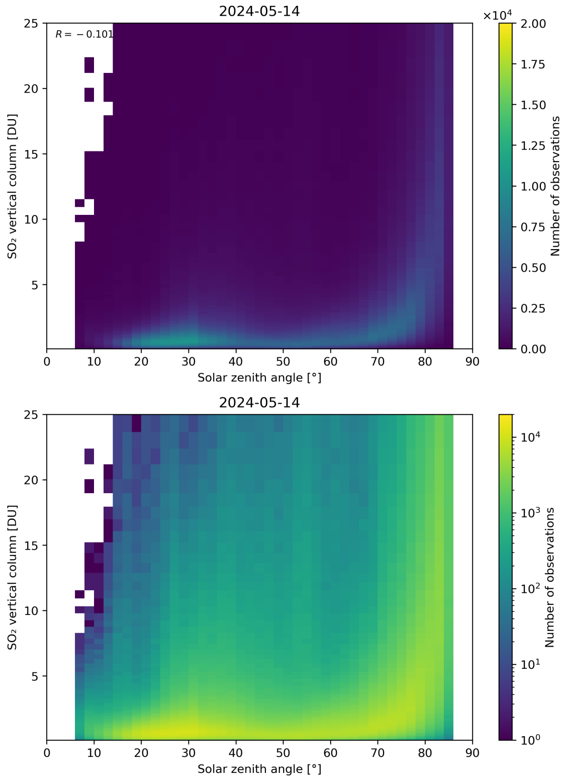
Figure 176: Scatter density plot of “Solar zenith angle” against “SO 2 vertical column” for 2024-05-13 to 2024-05-15.
