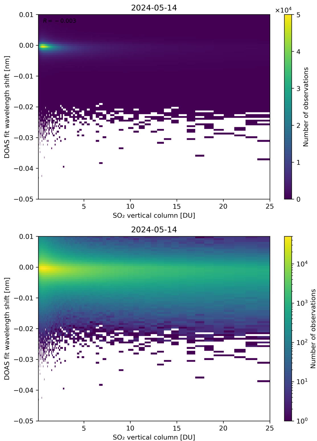
Figure 276: Scatter density plot of “SO 2 vertical column” against “DOAS fit wavelength shift” for 2024-05-13 to 2024-05-15.
