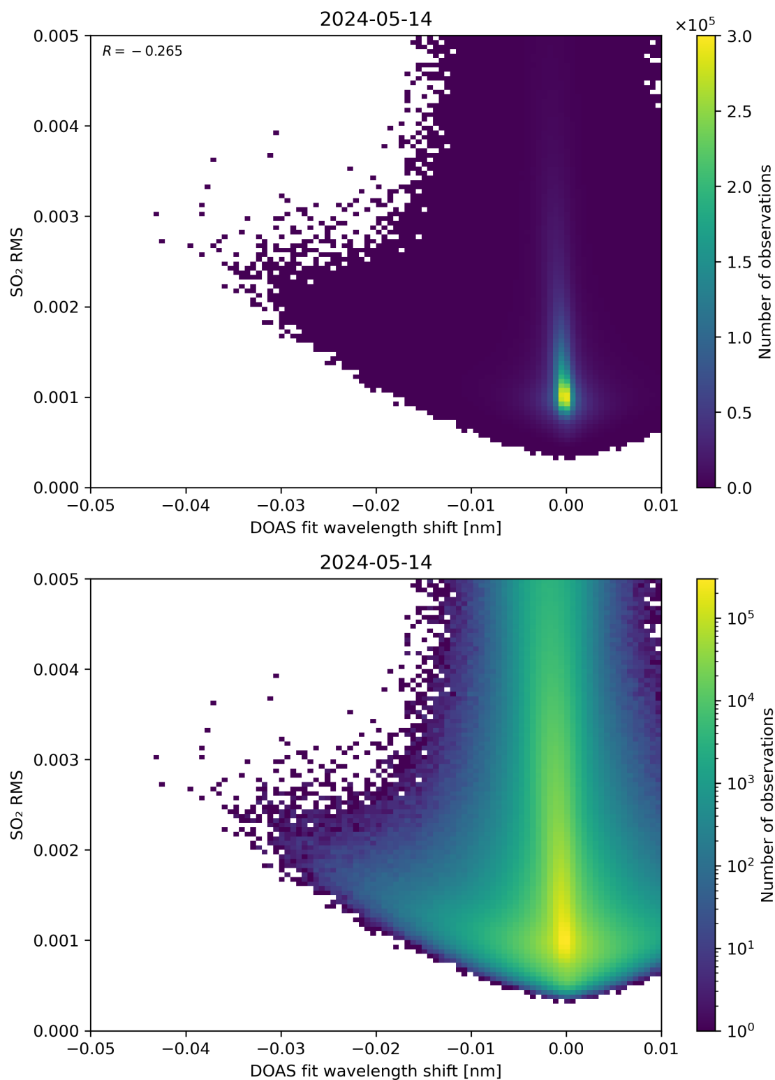
Figure 128: Scatter density plot of “DOAS fit wavelength shift” against “SO 2 RMS” for 2024-05-13 to 2024-05-15.
