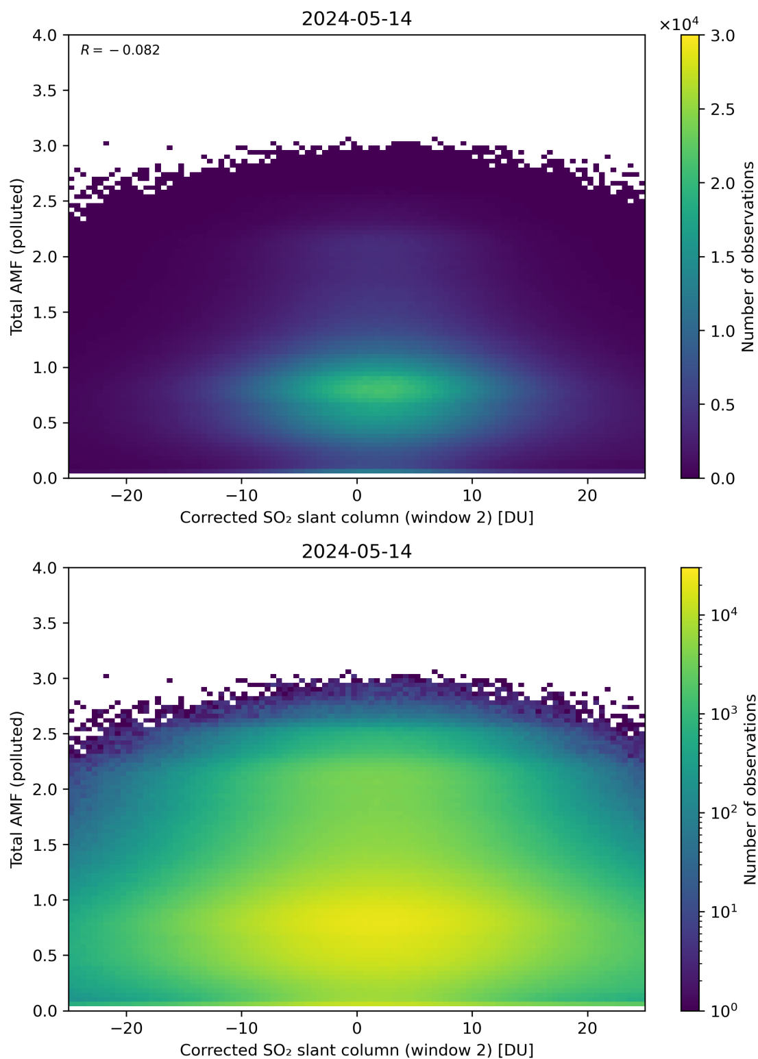
Figure 203: Scatter density plot of “Corrected SO 2 slant column (window 2)” against “Total AMF (polluted)” for 2024-05-13 to 2024-05-15.
