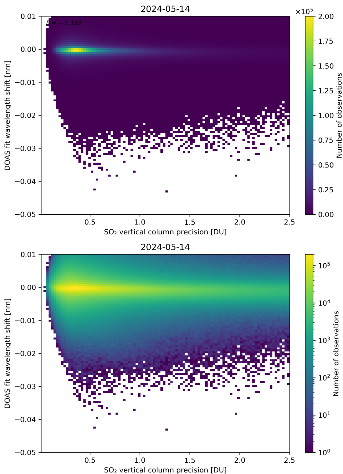
Figure 282: Scatter density plot of “SO 2 vertical column precision” against “DOAS fit wavelength shift” for 2024-05-13 to 2024-05-15.
