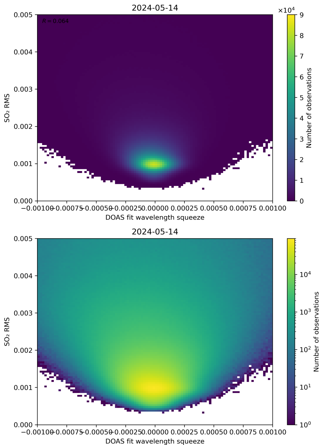
Figure 132: Scatter density plot of “DOAS fit wavelength squeeze” against “SO 2 RMS” for 2024-05-13 to 2024-05-15.
