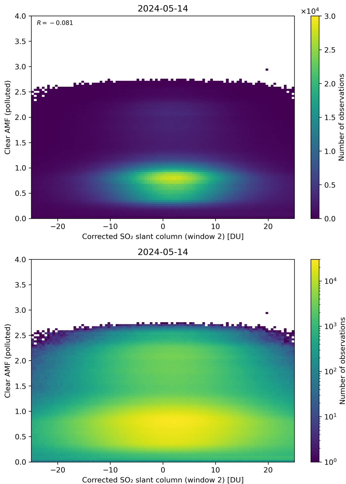
Figure 199: Scatter density plot of “Corrected SO 2 slant column (window 2)” against “Clear AMF (polluted)” for 2024-05-13 to 2024-05-15.
