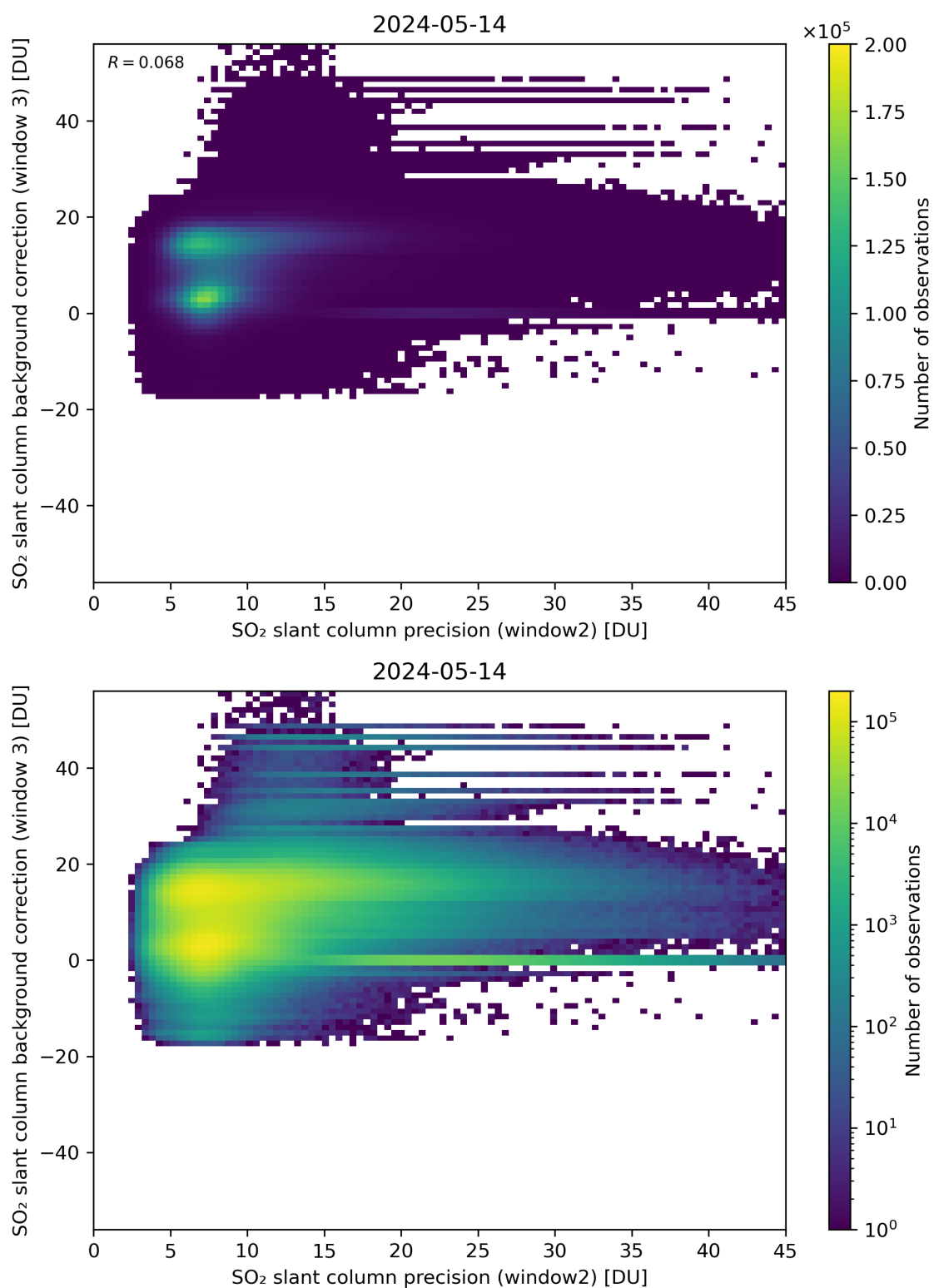
Figure 242: Scatter density plot of “SO 2 slant column precision (window2)” against “SO 2 slant column background correction (window 3)” for 2024-05-13 to 2024-05-15.
