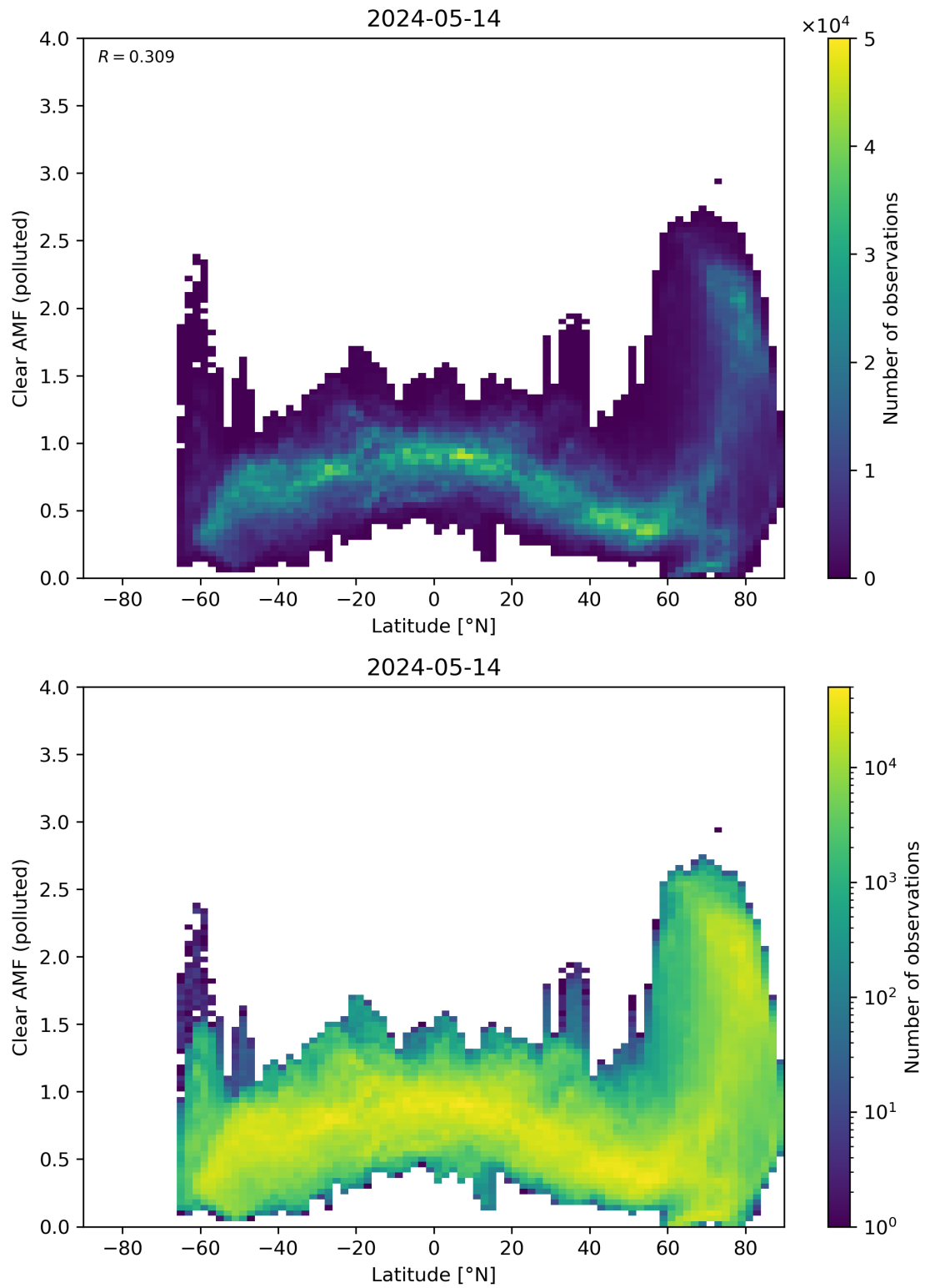
Figure 145: Scatter density plot of “Latitude” against “Clear AMF (polluted)” for 2024-05-13 to 2024-05-15.
