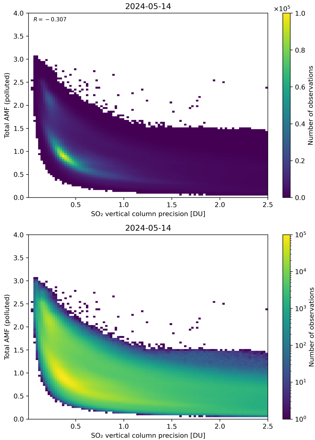
Figure 294: Scatter density plot of “SO 2 vertical column precision” against “Total AMF (polluted)” for 2024-05-13 to 2024-05-15.
