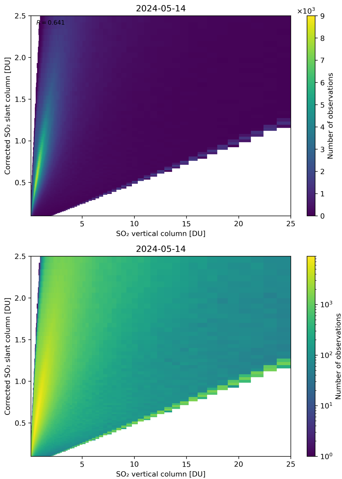
Figure 297: Scatter density plot of “SO 2 vertical column” against “Corrected SO 2 slant column” for 2024-05-13 to 2024-05-15.
