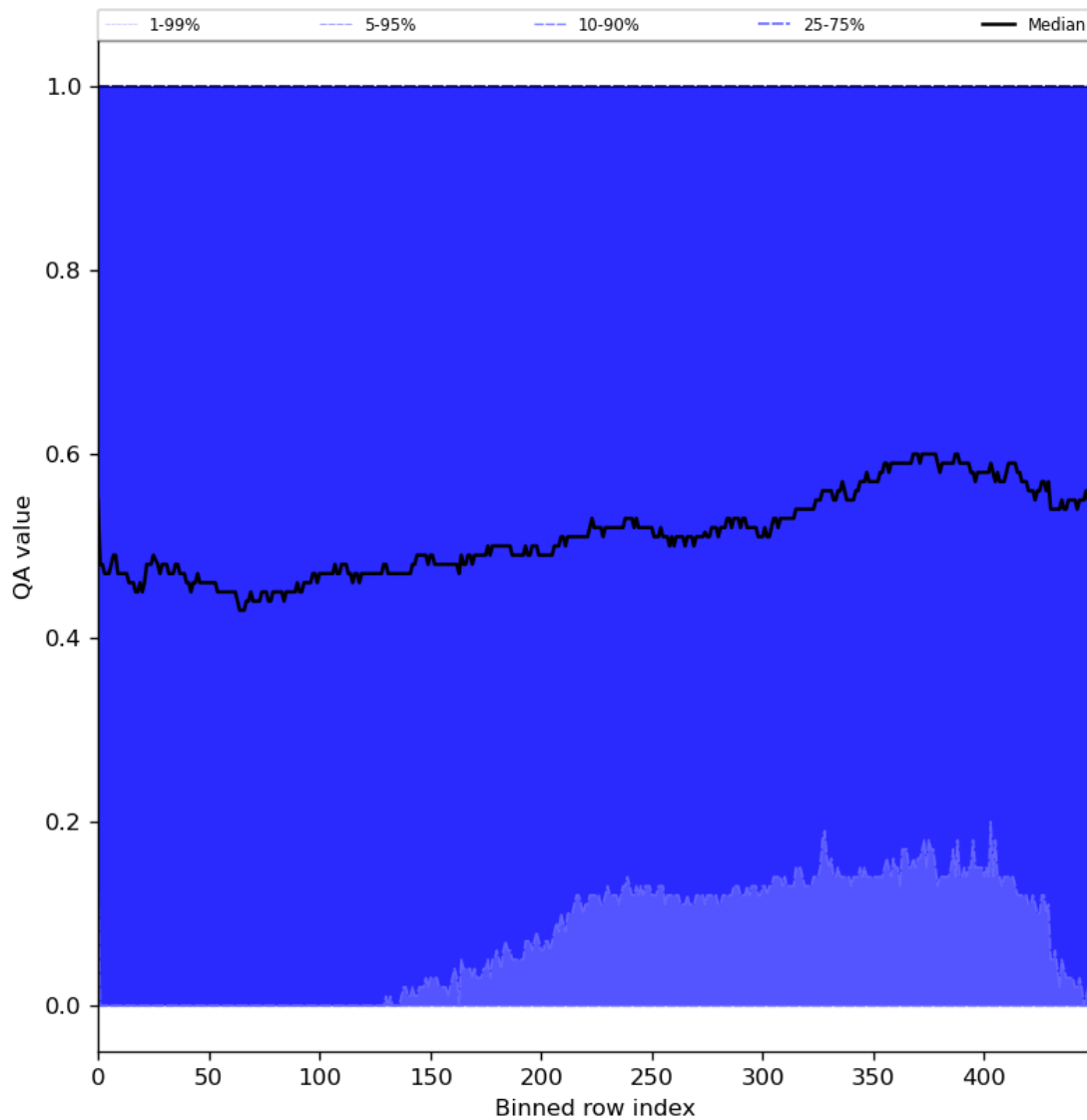
Figure 75: Along track statistics of “QA value” for 2024-05-13 to 2024-05-15
