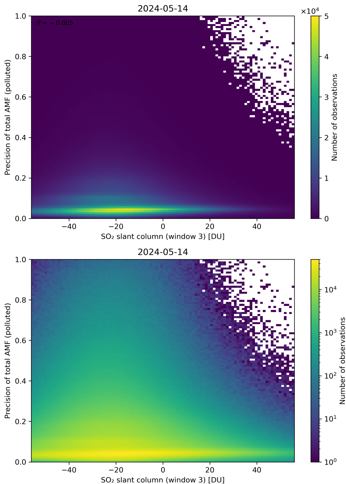
Figure 269: Scatter density plot of “SO 2 slant column (window 3)” against “Precision of total AMF (polluted)” for 2024-05-13 to 2024-05-15.
