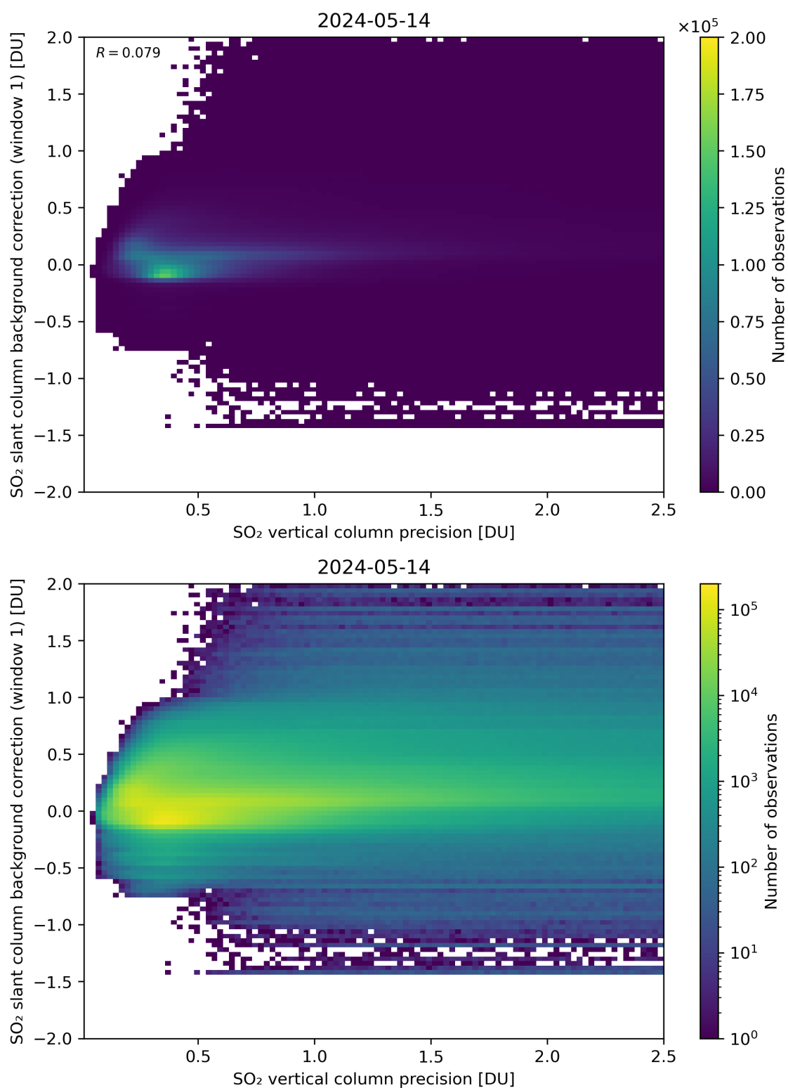
Figure 279: Scatter density plot of “SO 2 vertical column precision” against “SO 2 slant column background correction (window 1)” for 2024-05-13 to 2024-05-15.
