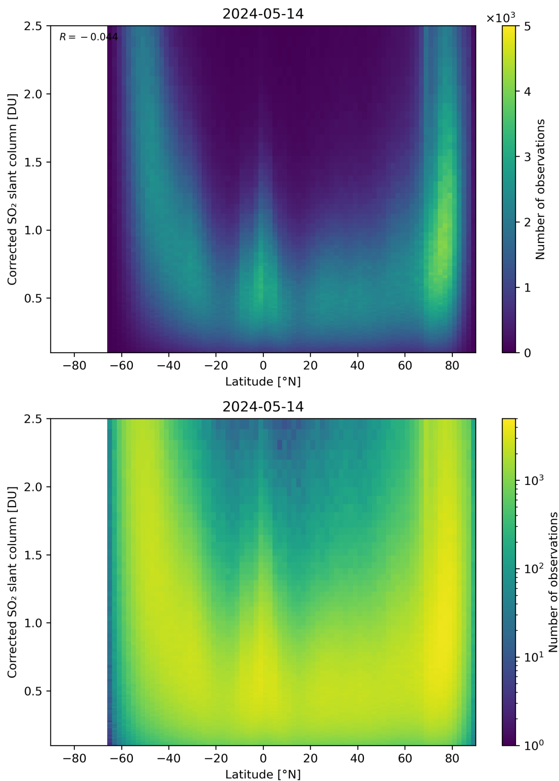
Figure 146: Scatter density plot of “Latitude” against “Corrected SO 2 slant column” for 2024-05-13 to 2024-05-15.
