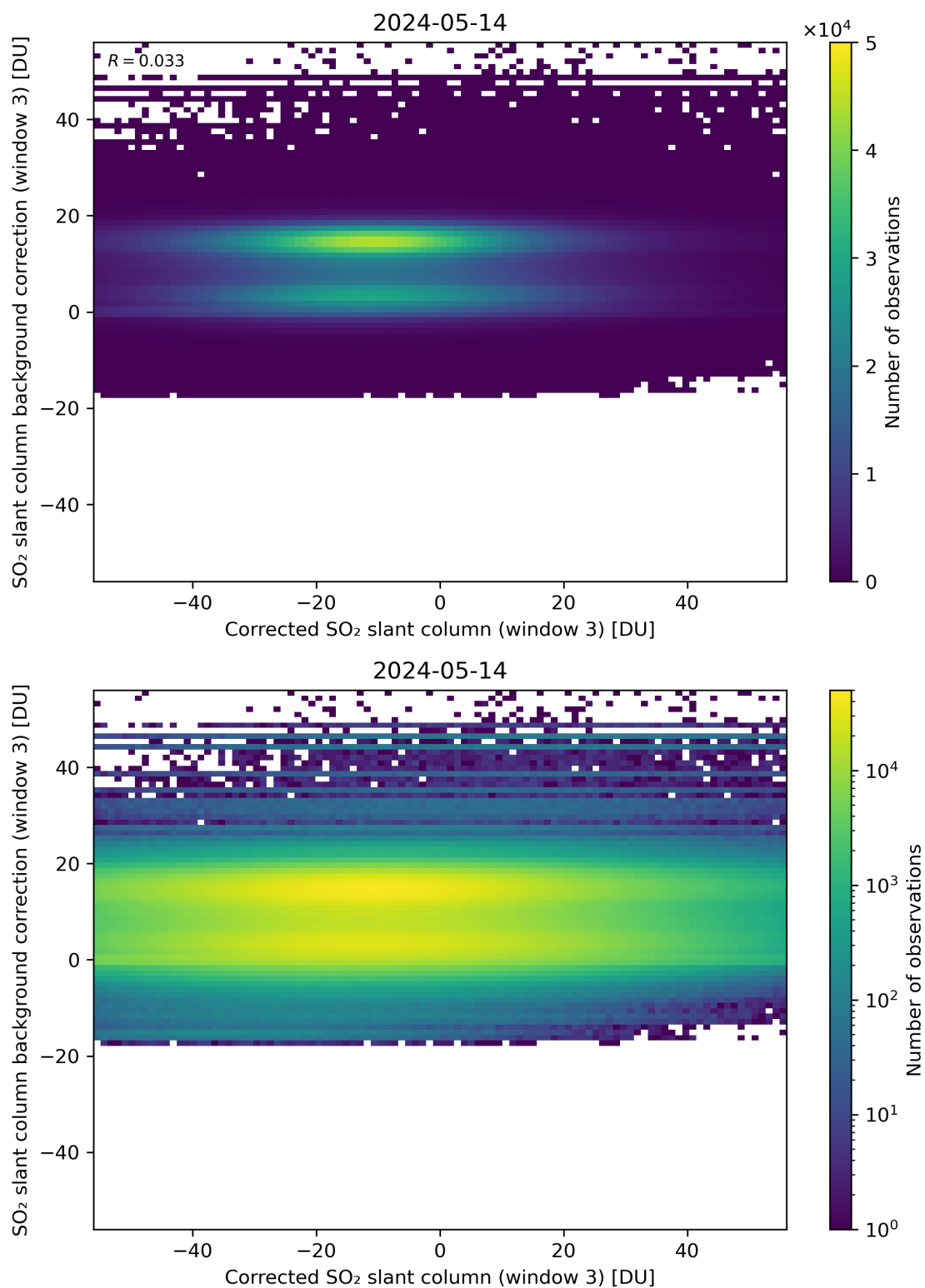
Figure 205: Scatter density plot of “Corrected SO 2 slant column (window 3)” against “SO 2 slant column background correction (window 3)” for 2024-05-13 to 2024-05-15.
