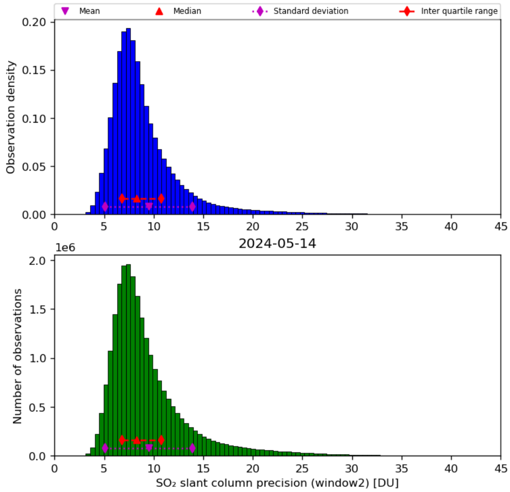
Figure 61: Histogram of “SO 2 slant column precision (window2)” for 2024-05-13 to 2024-05-15
