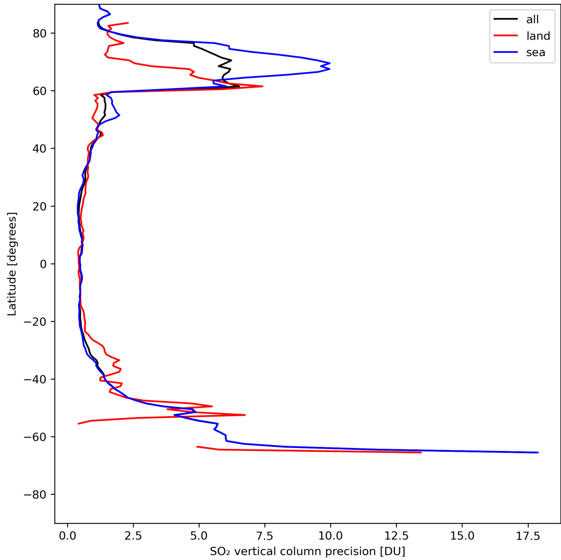
Figure 31: Zonal average of “SO 2 vertical column precision” for 2024-05-13 to 2024-05-15.
