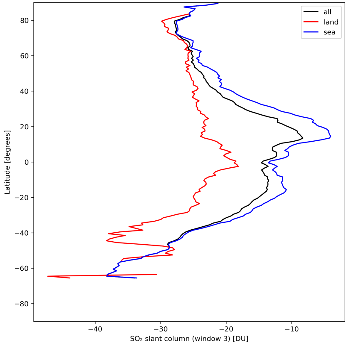
Figure 41: Zonal average of “SO 2 slant column (window 3)” for 2024-05-13 to 2024-05-15.
