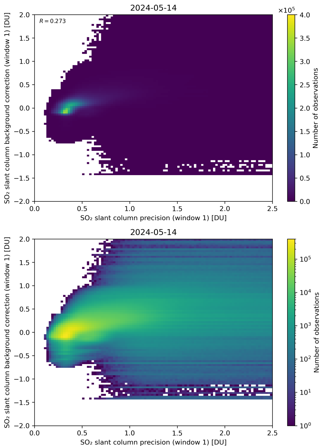
Figure 218: Scatter density plot of “SO 2 slant column precision (window 1)” against “SO 2 slant column background correction (window 1)” for 2024-05-13 to 2024-05-15.
