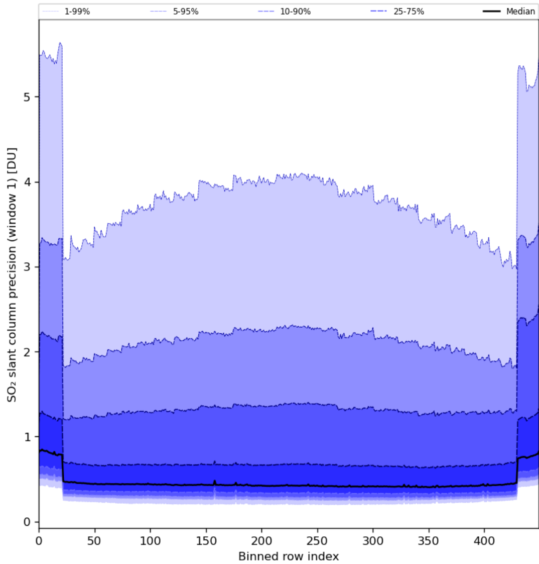
Figure 80: Along track statistics of “SO 2 slant column precision (window 1)” for 2024-05-13 to 2024-05-15
