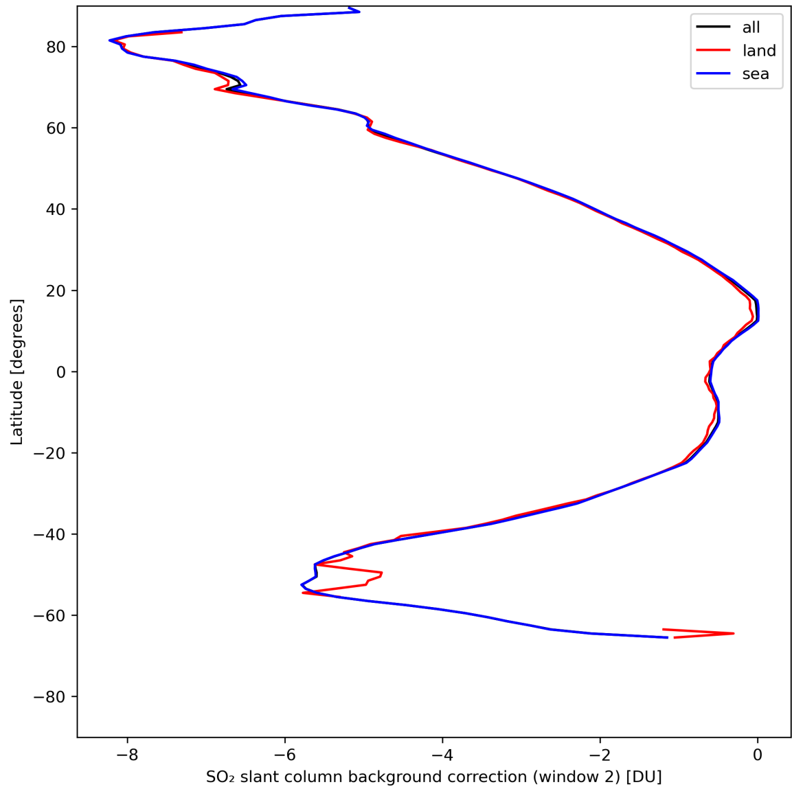
Figure 40: Zonal average of “SO 2 slant column background correction (window 2)” for 2024-05-13 to 2024-05-15.
