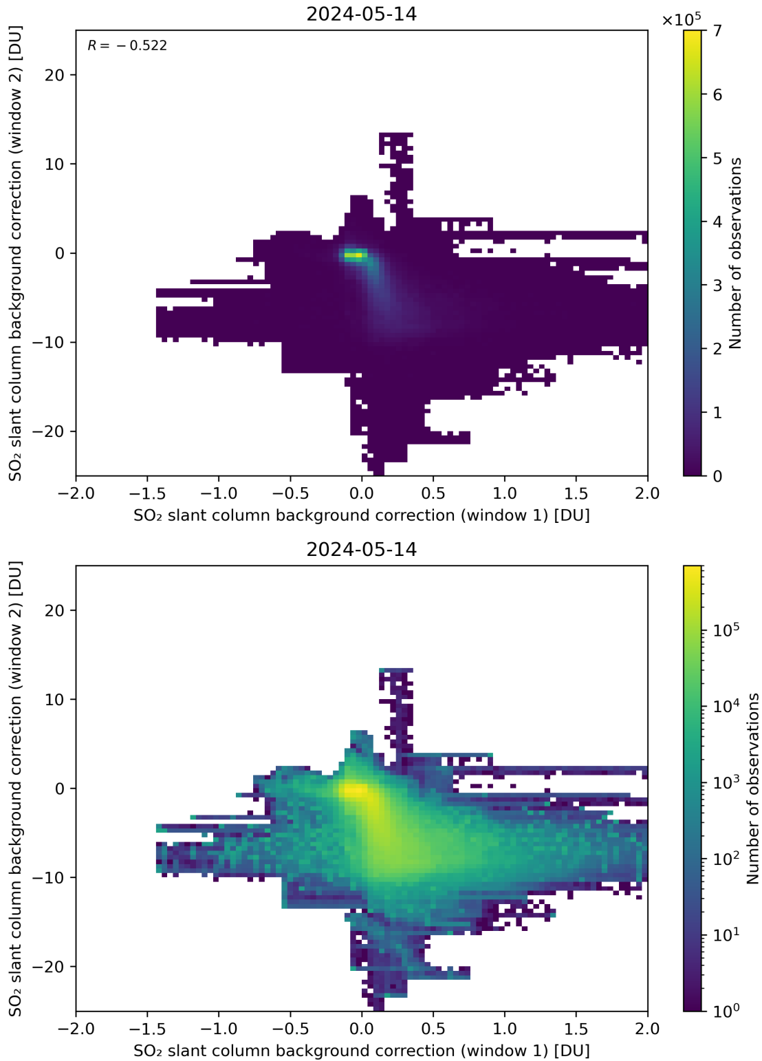
Figure 98: Scatter density plot of “SO 2 slant column background correction (window 1)” against “SO 2 slant column background correction (window 2)” for 2024-05-13 to 2024-05-15.
