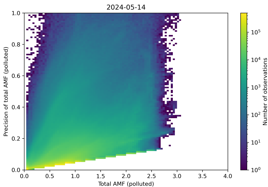
Figure 272: Scatter density plot of “Total AMF (polluted)” against “Precision of total AMF (polluted)” for 2024-05-13 to 2024-05-15.
