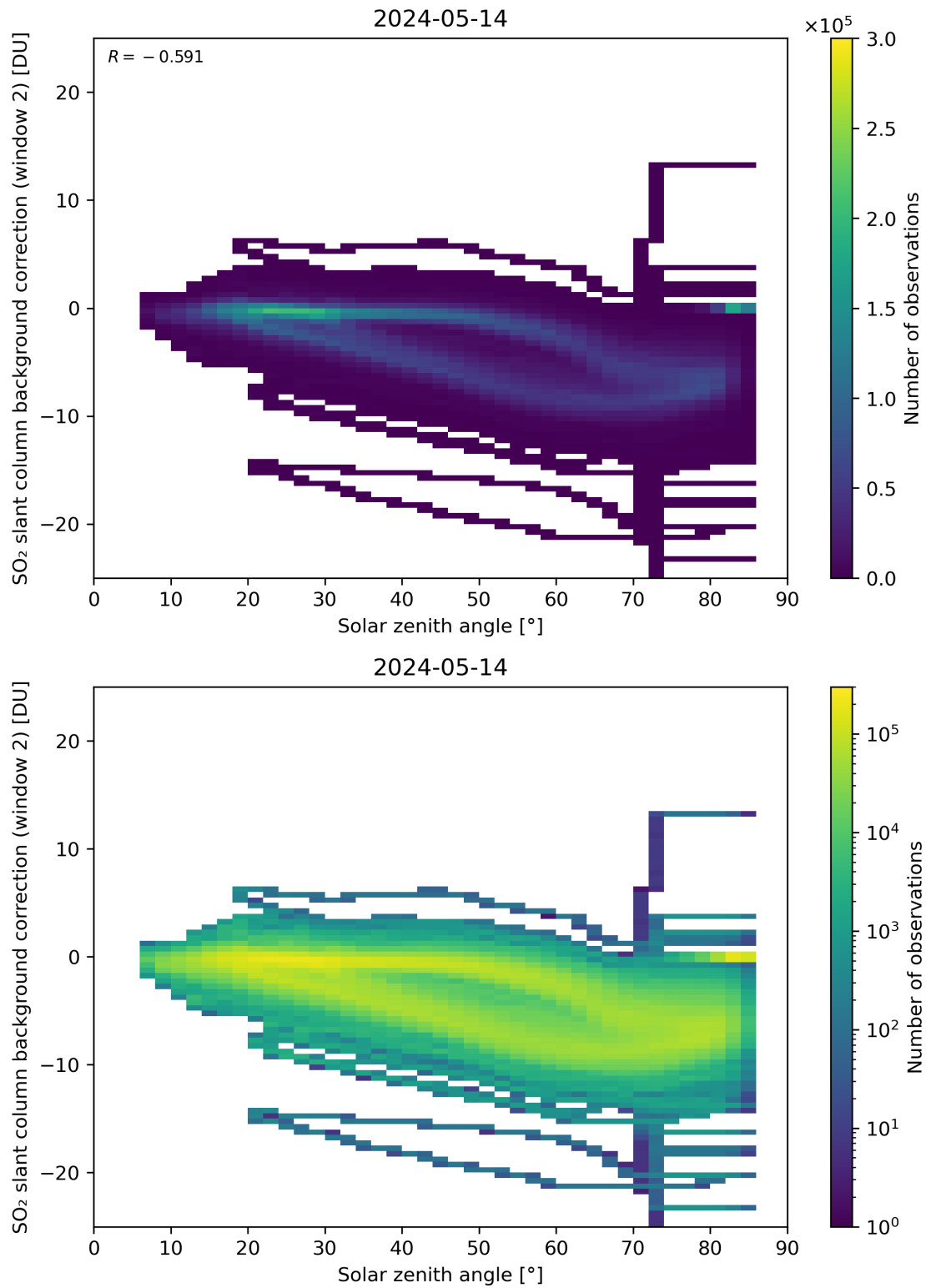
Figure 159: Scatter density plot of “Solar zenith angle” against “SO 2 slant column background correction (window 2)” for 2024-05-13 to 2024-05-15.
