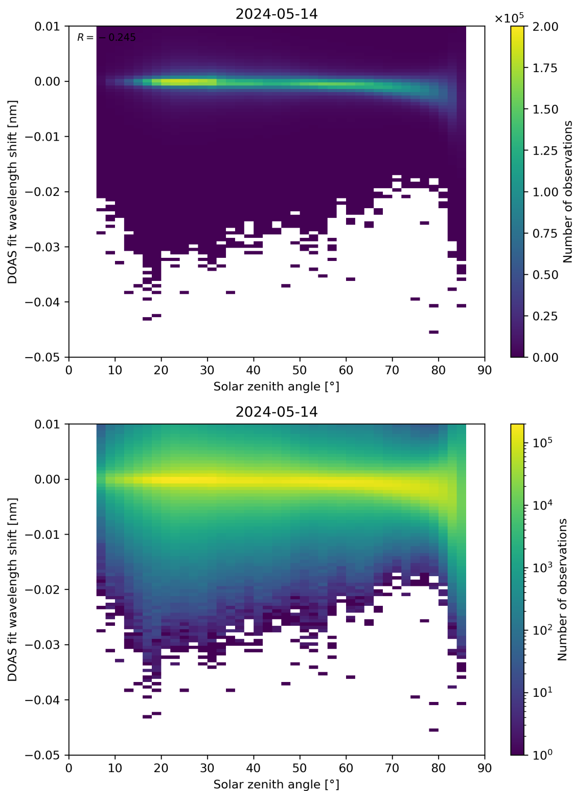
Figure 161: Scatter density plot of “Solar zenith angle” against “DOAS fit wavelength shift” for 2024-05-13 to 2024-05-15.
