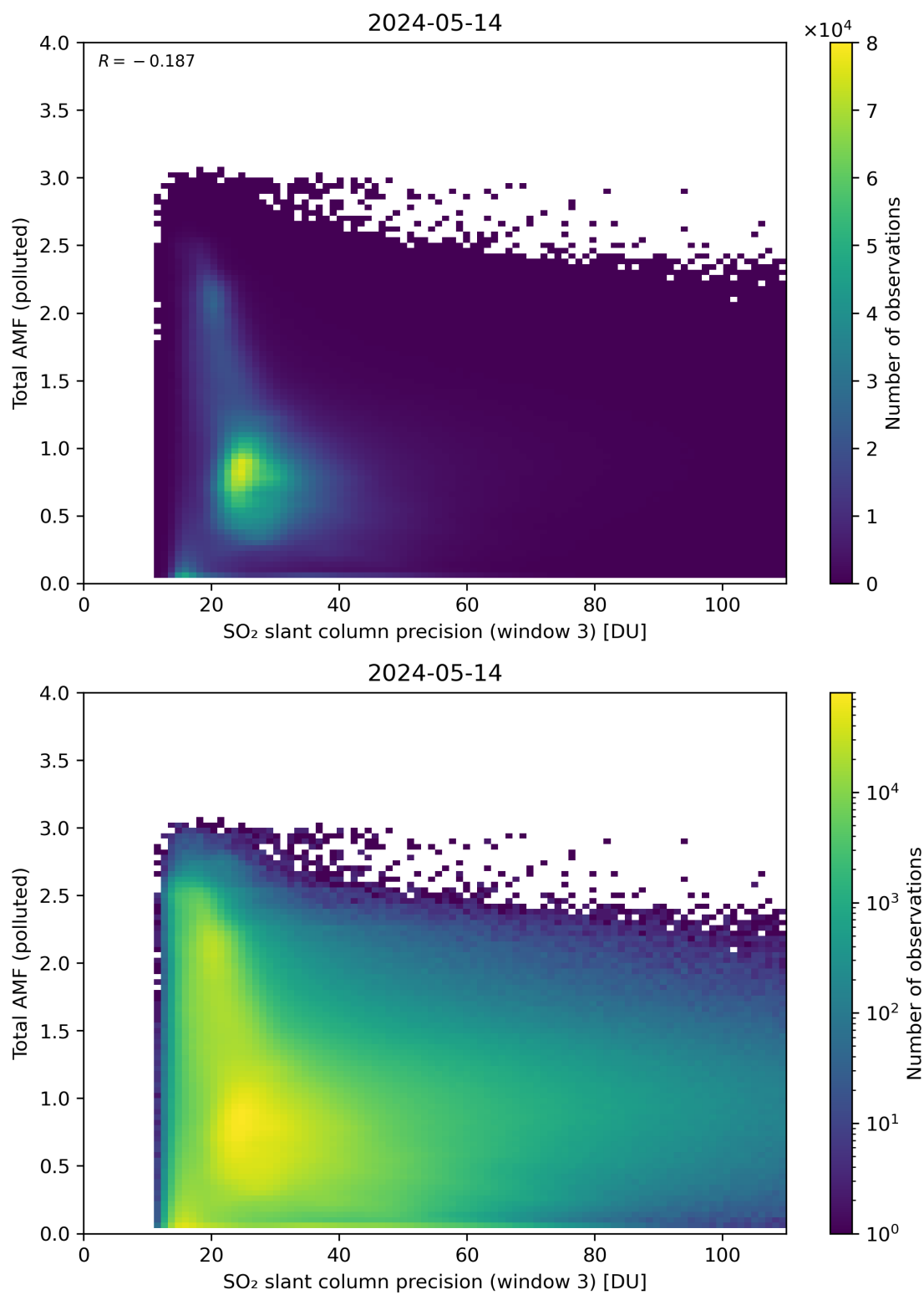
Figure 263: Scatter density plot of “SO 2 slant column precision (window 3)” against “Total AMF (polluted)” for 2024-05-13 to 2024-05-15.
