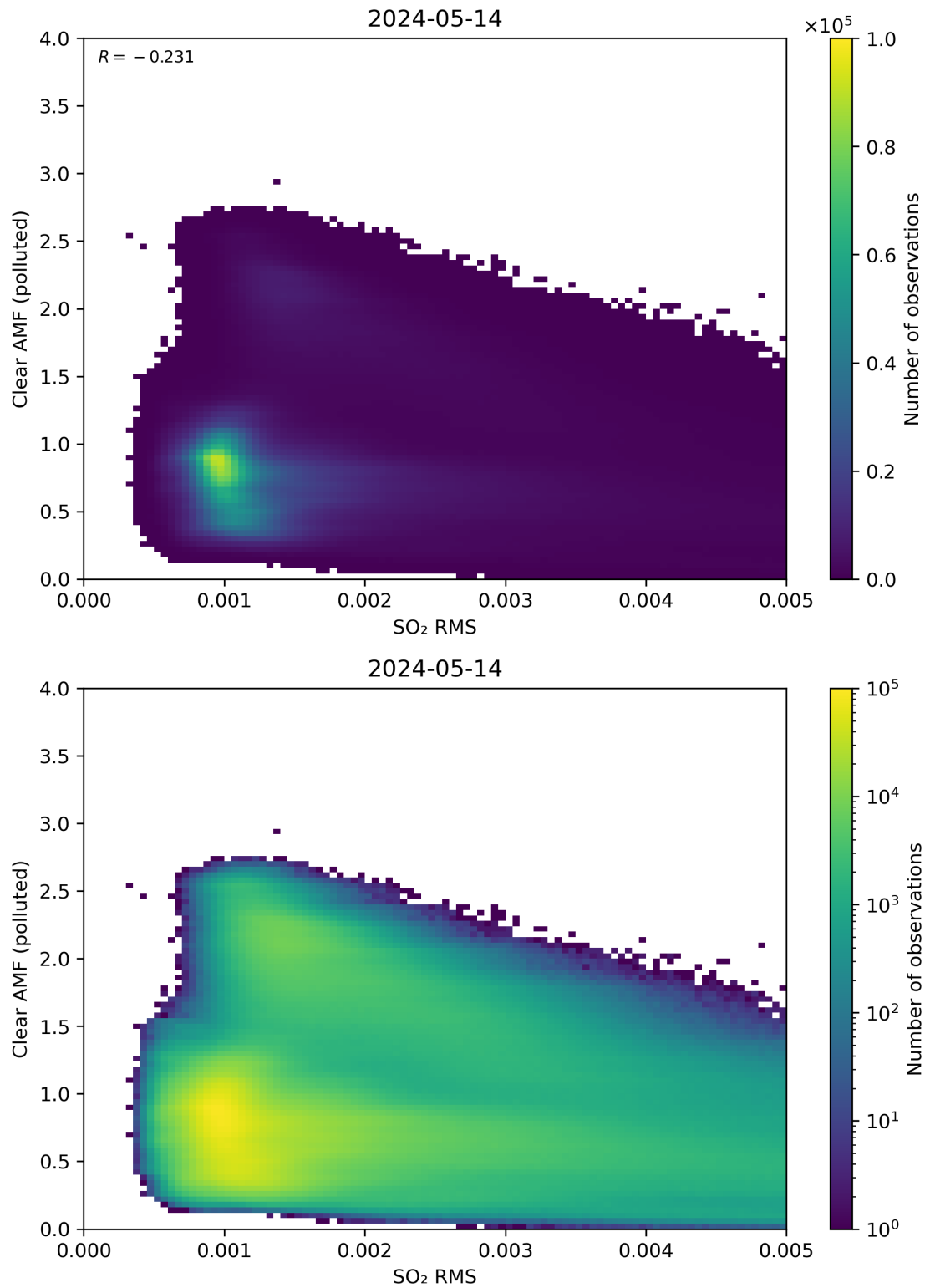
Figure 136: Scatter density plot of “SO 2 RMS” against “Clear AMF (polluted)” for 2024-05-13 to 2024-05-15.
