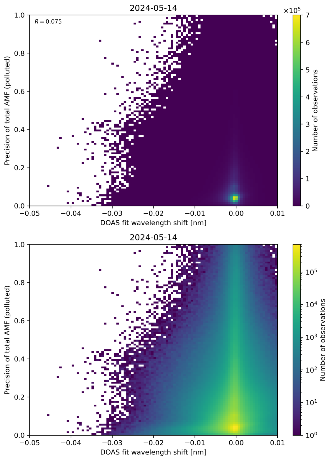
Figure 131: Scatter density plot of “DOAS fit wavelength shift” against “Precision of total AMF (polluted)” for 2024-05-13 to 2024-05-15.
