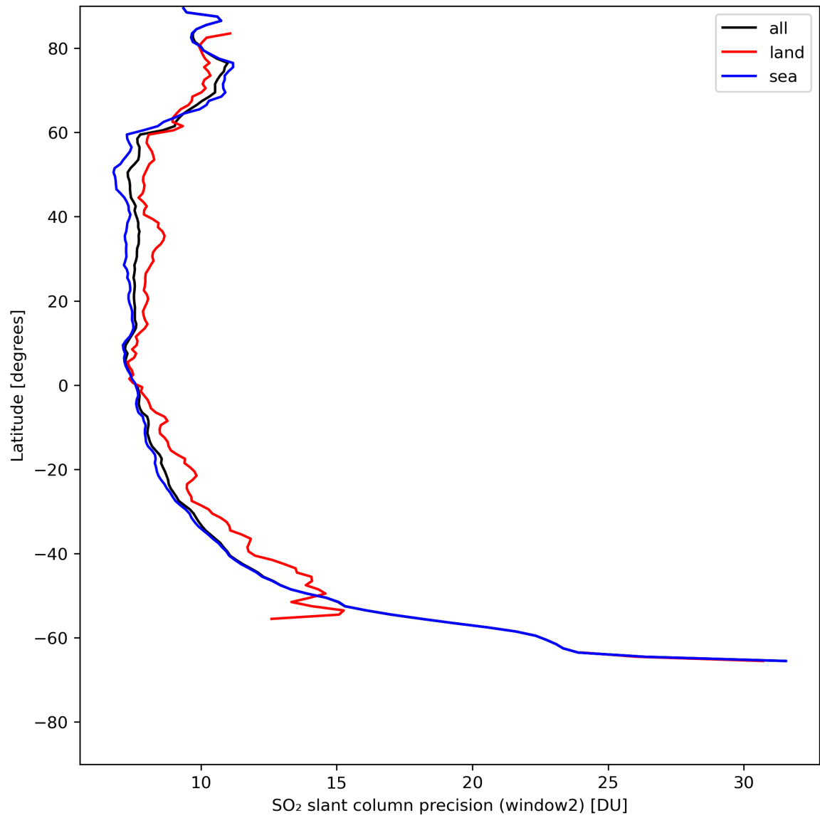
Figure 38: Zonal average of "SO 2 slant column precision (window2)" for 2024-05-13 to 2024-05-15.
