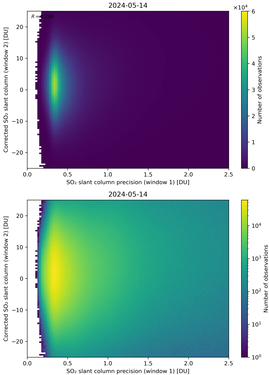
Figure 225: Scatter density plot of “SO 2 slant column precision (window 1)” against “Corrected SO 2 slant column (window 2)” for 2024-05-13 to 2024-05-15.
