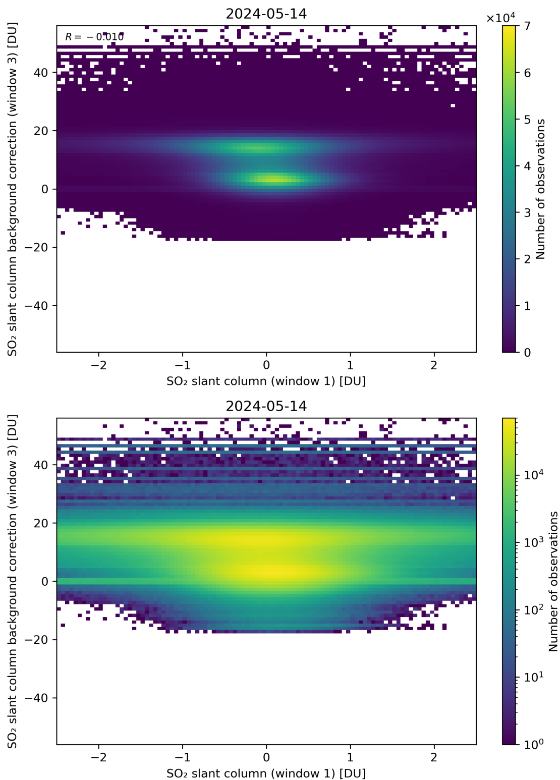
Figure 214: Scatter density plot of “SO 2 slant column (window 1)” against “SO 2 slant column background correction (window 3)” for 2024-05-13 to 2024-05-15.
