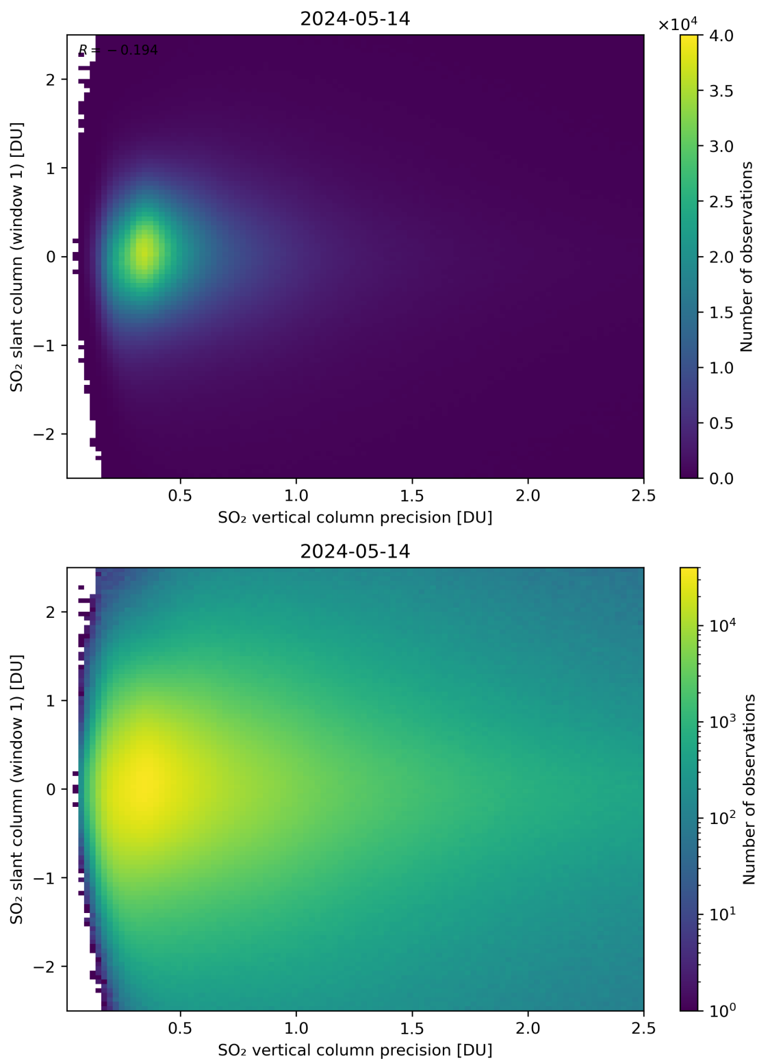
Figure 289: Scatter density plot of “SO 2 vertical column precision” against “SO 2 slant column (window 1)” for 2024-05-13 to 2024-05-15.
