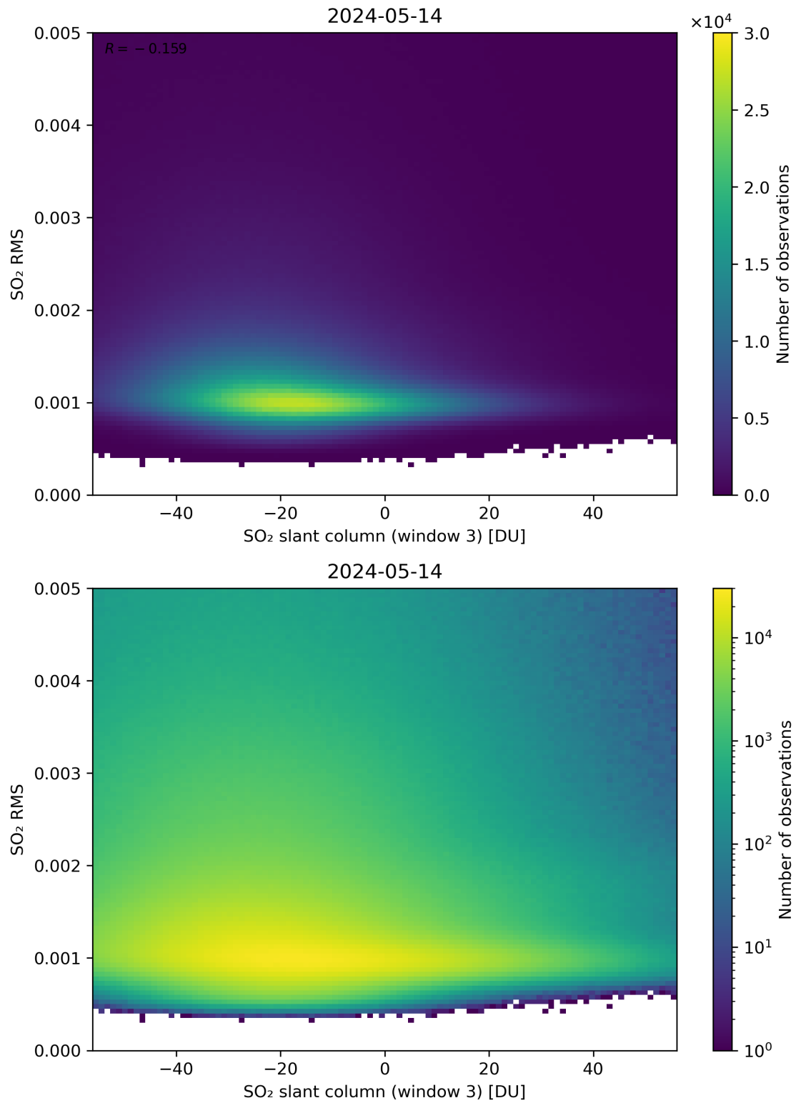
Figure 256: Scatter density plot of “SO 2 slant column (window 3)” against “SO 2 RMS” for 2024-05-13 to 2024-05-15.
