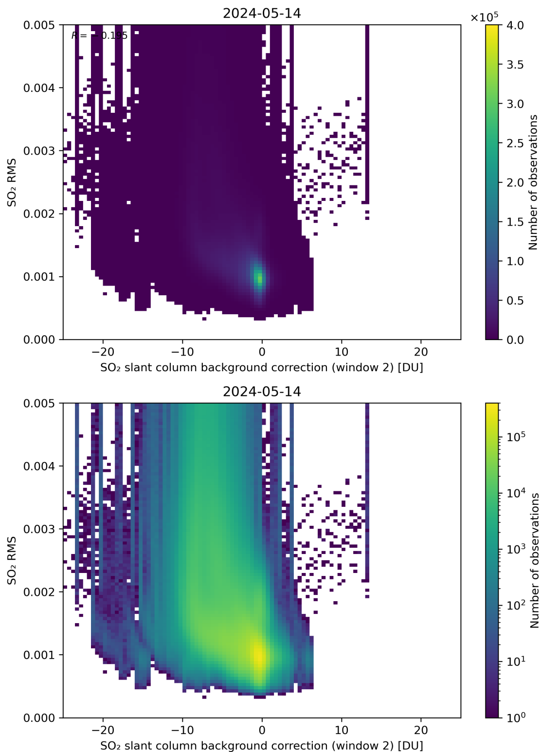
Figure 114: Scatter density plot of “SO 2 slant column background correction (window 2)” against “SO 2 RMS” for 2024-05-13 to 2024-05-15.
