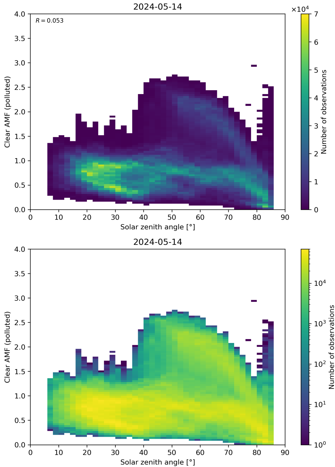
Figure 165: Scatter density plot of “Solar zenith angle” against “Clear AMF (polluted)” for 2024-05-13 to 2024-05-15.
