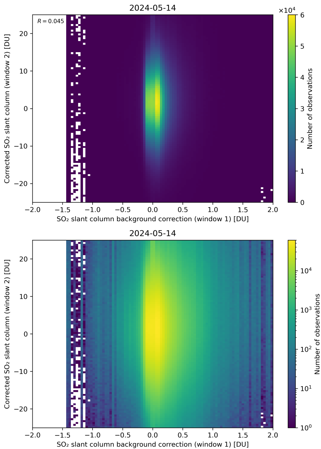
Figure 104: Scatter density plot of “SO 2 slant column background correction (window 1)” against “Corrected SO 2 slant column (window 2)” for 2024-05-13 to 2024-05-15.
