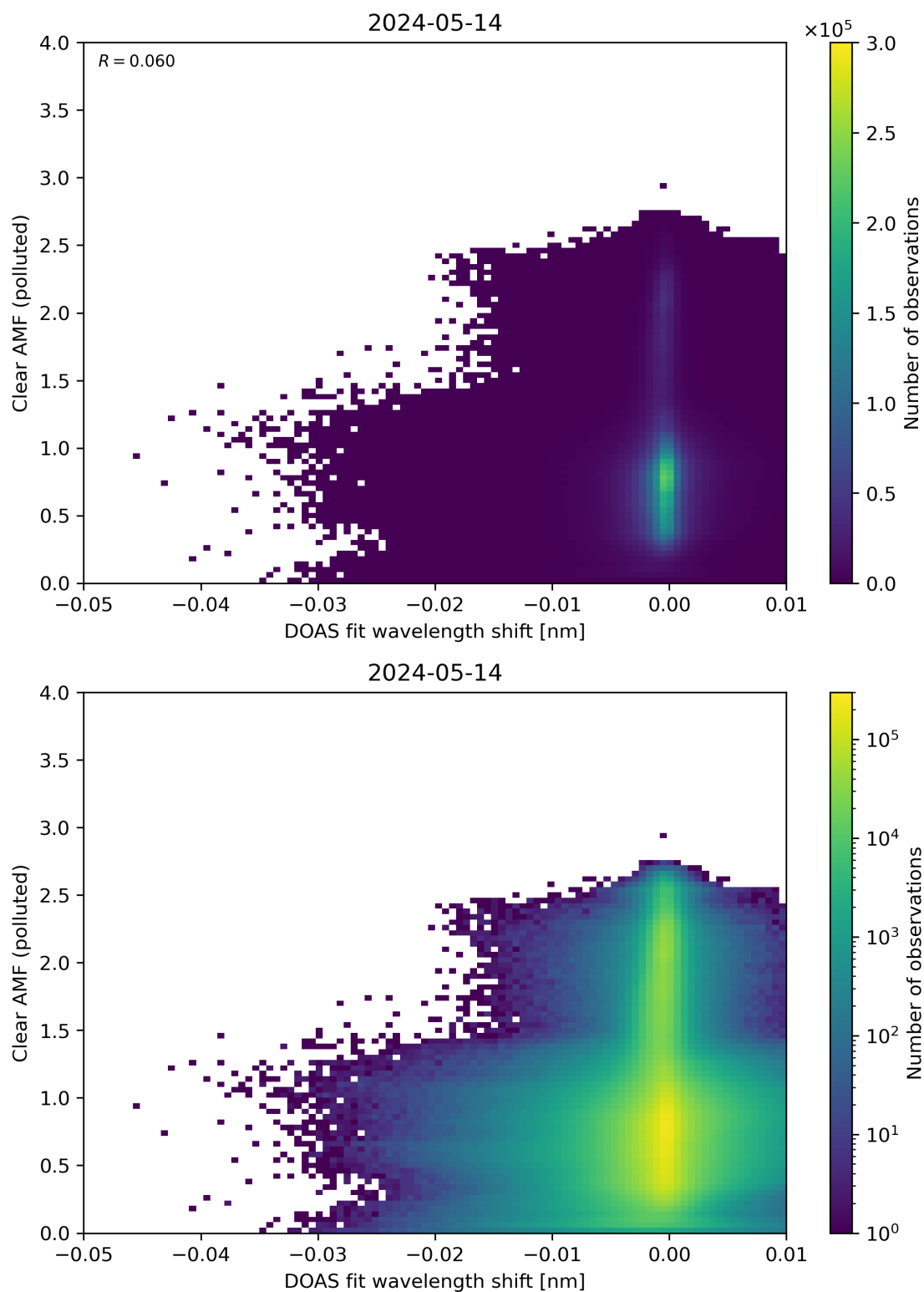
Figure 129: Scatter density plot of “DOAS fit wavelength shift” against “Clear AMF (polluted)” for 2024-05-13 to 2024-05-15.
