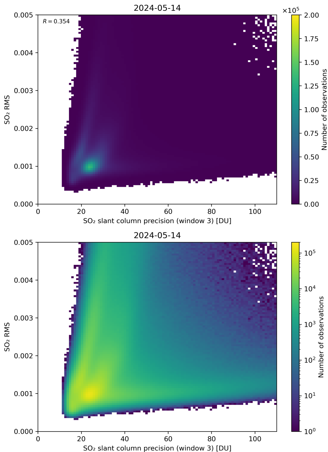
Figure 260: Scatter density plot of “SO 2 slant column precision (window 3)” against “SO 2 RMS” for 2024-05-13 to 2024-05-15.
