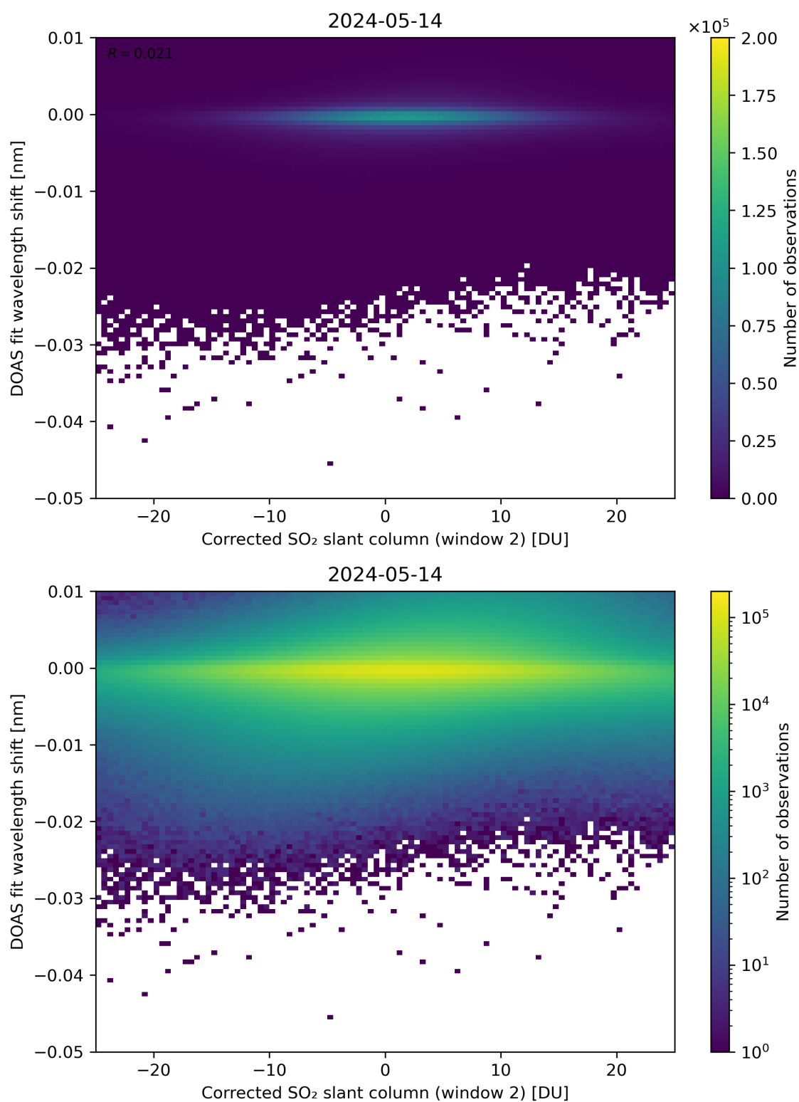
Figure 196: Scatter density plot of “Corrected SO 2 slant column (window 2)” against “DOAS fit wavelength shift” for 2024-05-13 to 2024-05-15.
