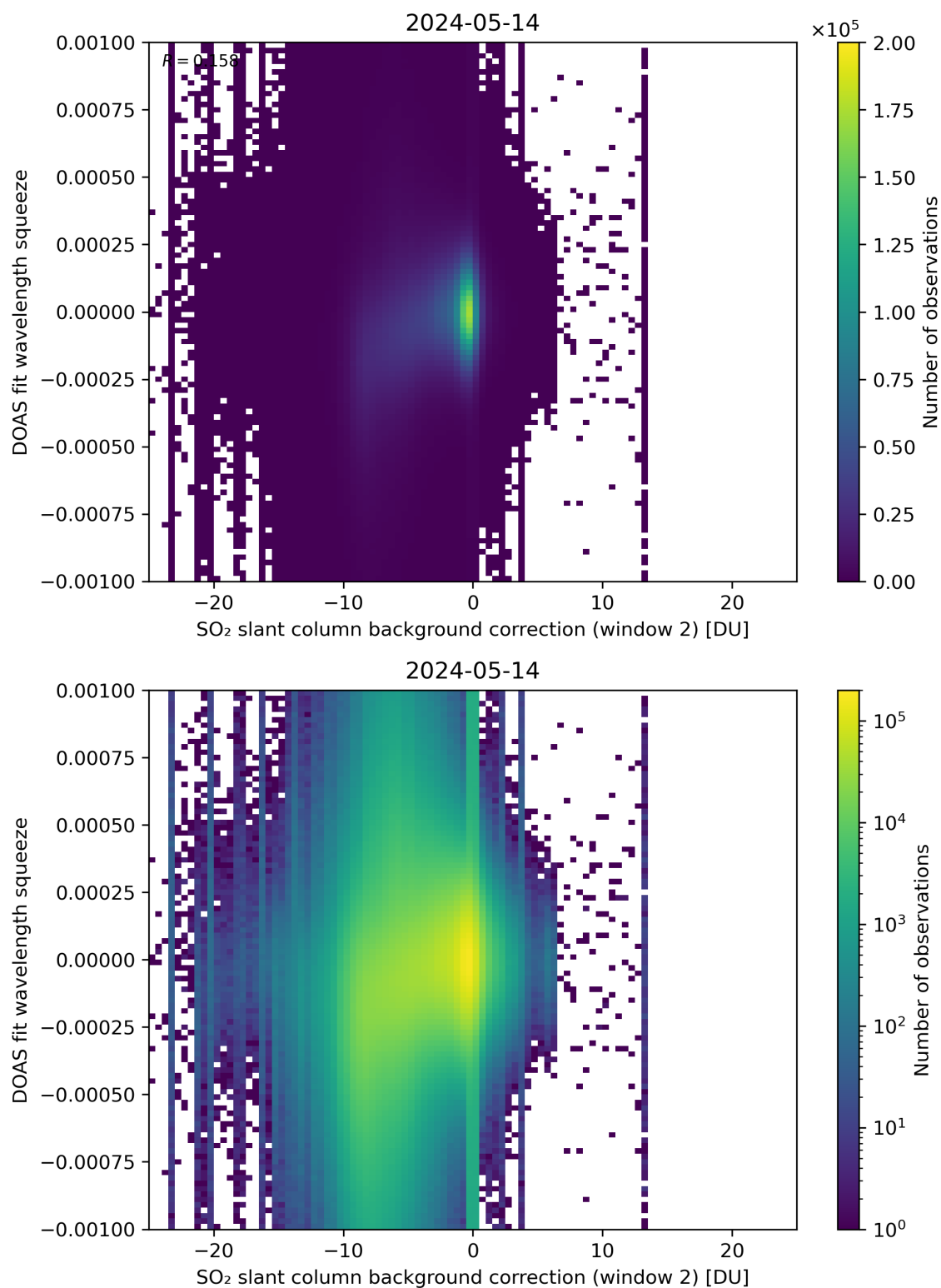
Figure 113: Scatter density plot of "SO 2 slant column background correction (window 2)" against "DOAS fit wavelength squeeze" for 2024-05-13 to 2024-05-15.
