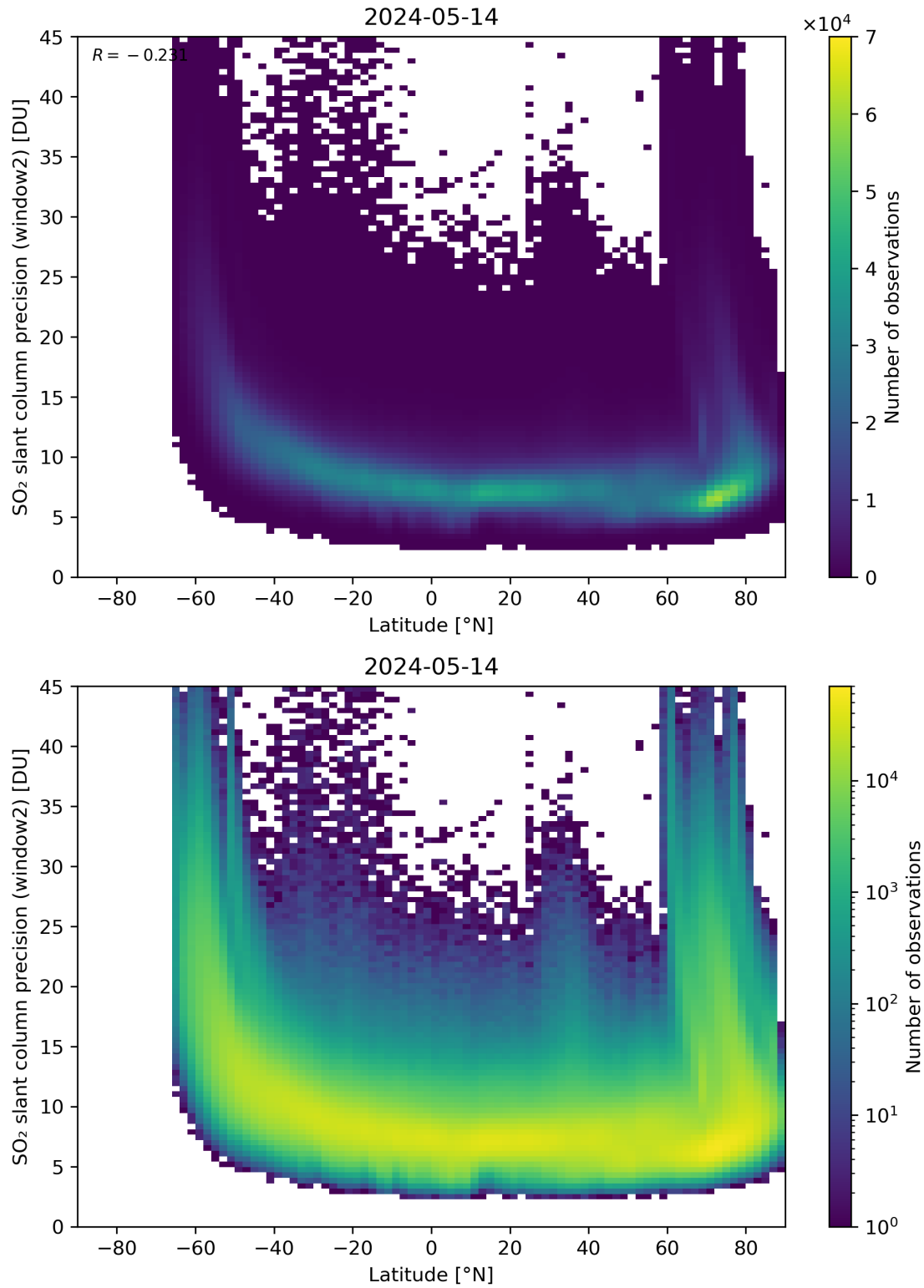
Figure 151: Scatter density plot of “Latitude” against “SO 2 slant column precision (window2)” for 2024-05-13 to 2024-05-15.
