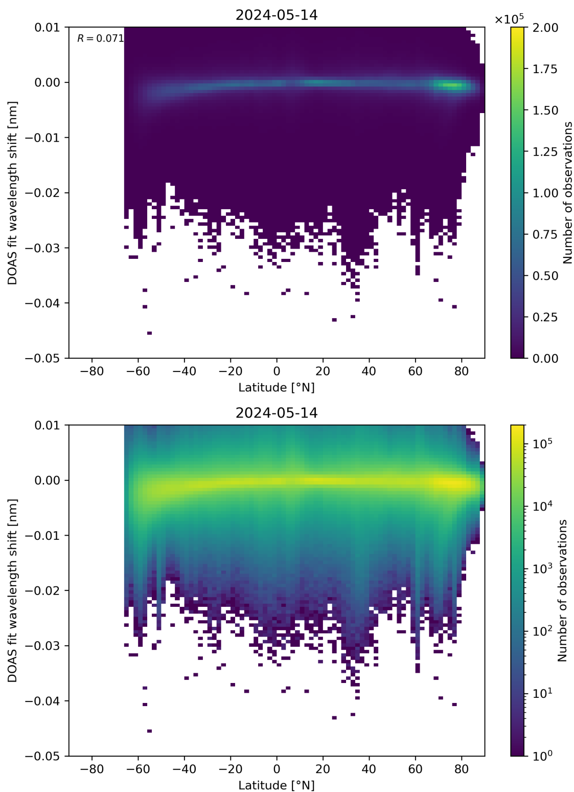
Figure 142: Scatter density plot of “Latitude” against “DOAS fit wavelength shift” for 2024-05-13 to 2024-05-15.
