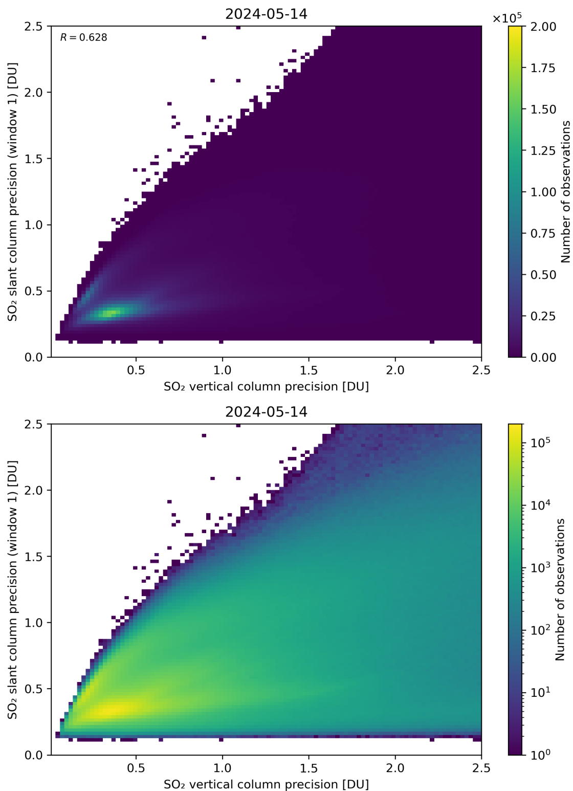
Figure 290: Scatter density plot of “SO 2 vertical column precision” against “SO 2 slant column precision (window 1)” for 2024-05-13 to 2024-05-15.
