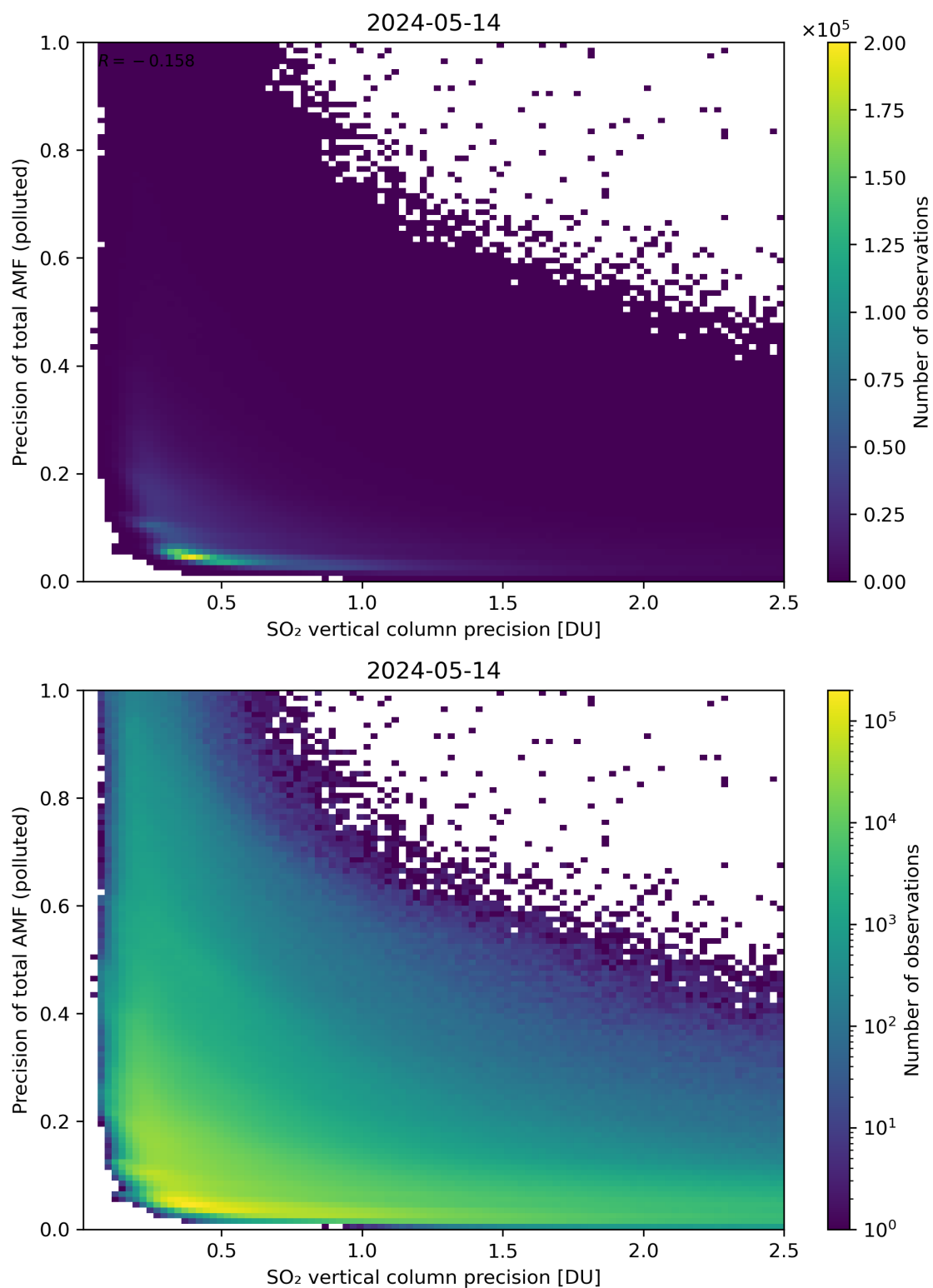
Figure 295: Scatter density plot of “SO 2 vertical column precision” against “Precision of total AMF (polluted)” for 2024-05-13 to 2024-05-15.
