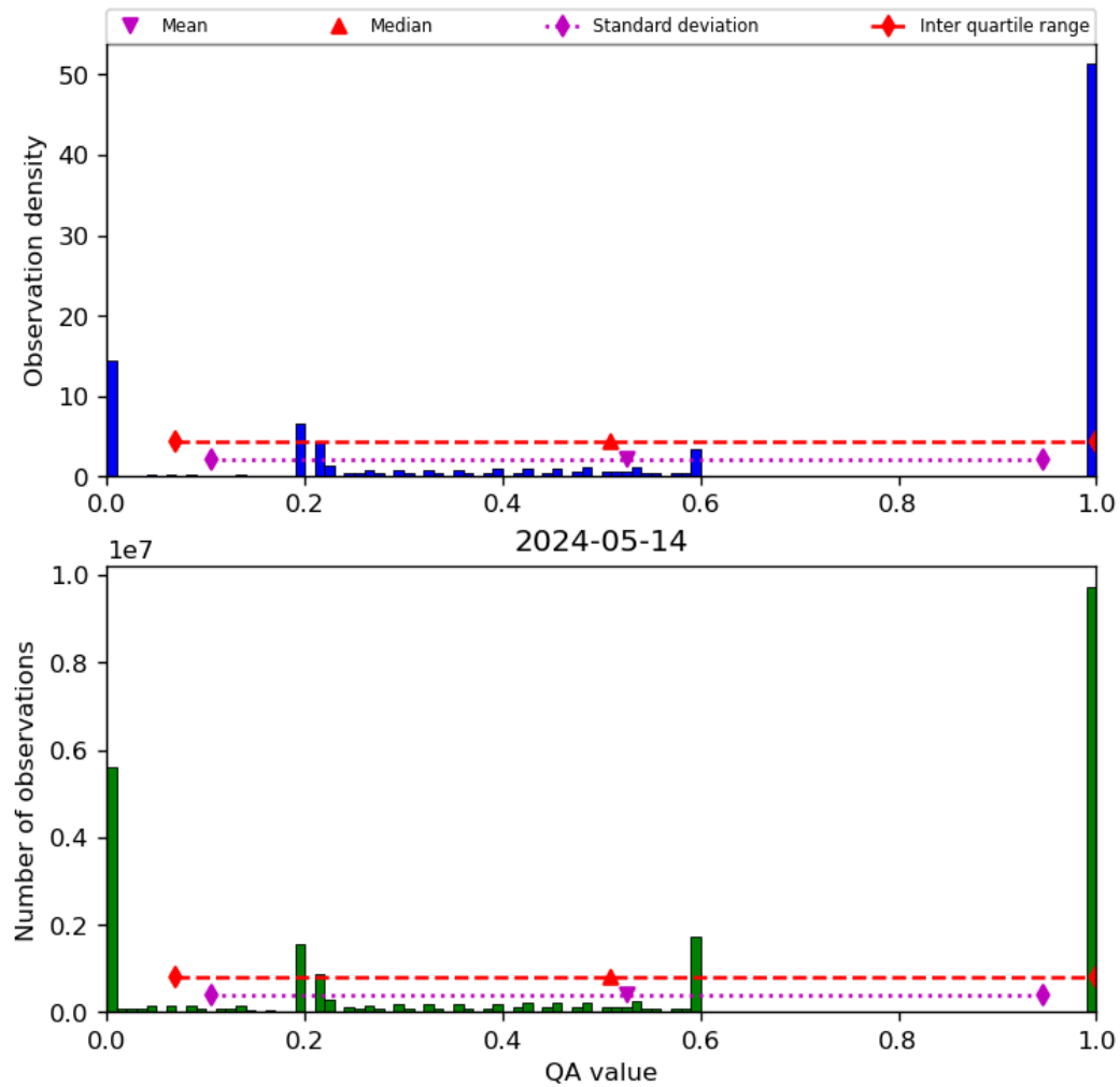
Figure 52: Histogram of “QA value” for 2024-05-13 to 2024-05-15
