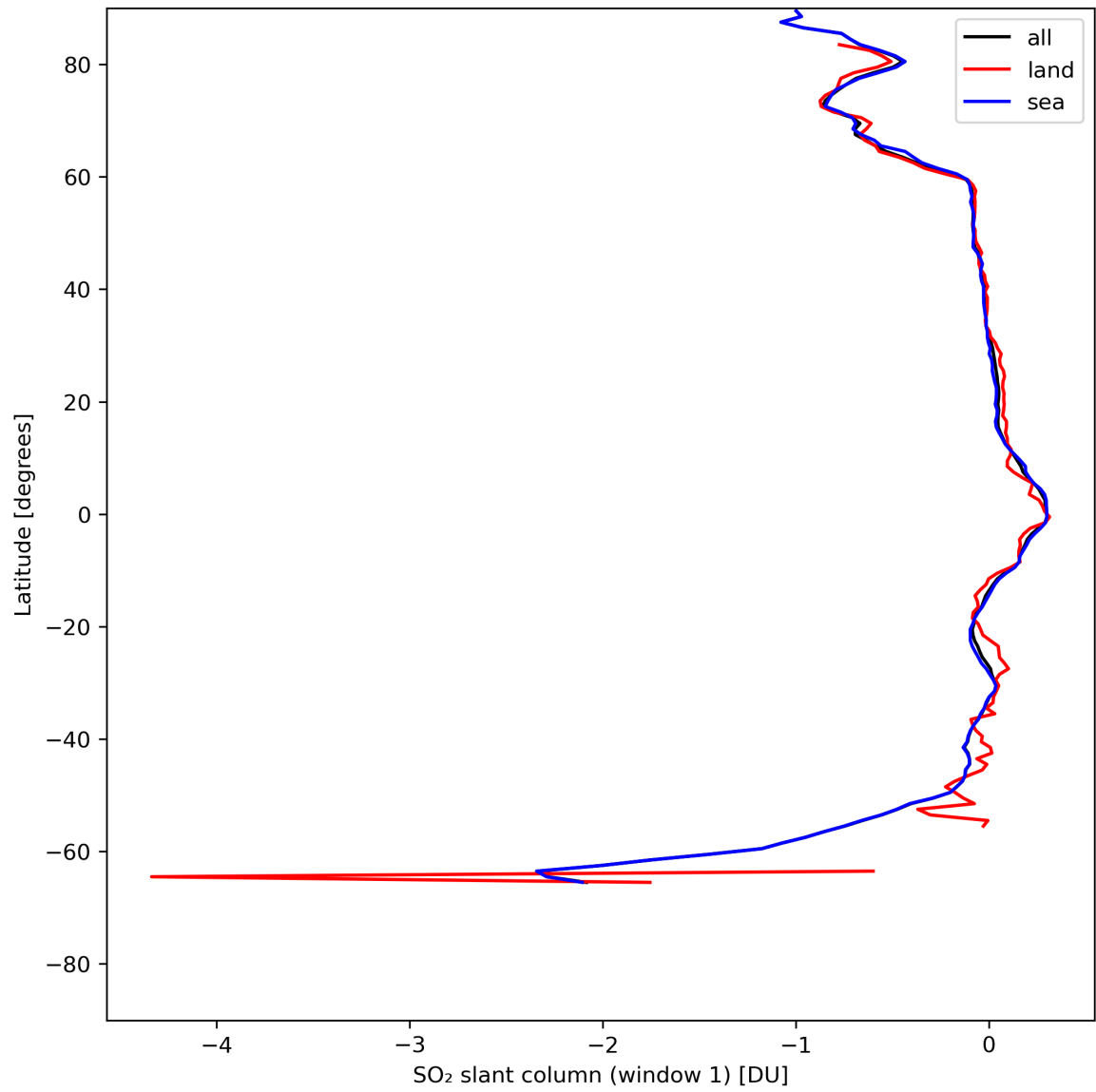
Figure 33: Zonal average of “SO 2 slant column (window 1)” for 2024-05-13 to 2024-05-15.
