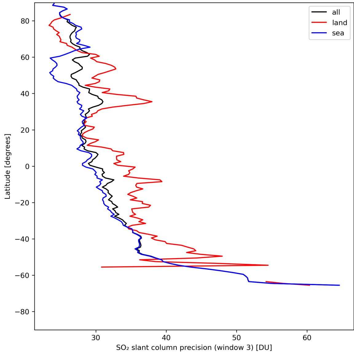
Figure 42: Zonal average of “SO 2 slant column precision (window 3)” for 2024-05-13 to 2024-05-15.
