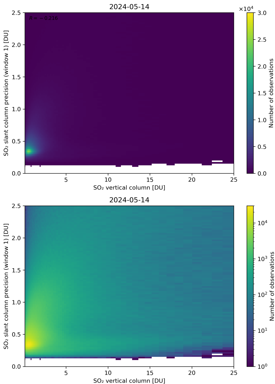
Figure 301: Scatter density plot of “SO 2 vertical column” against “SO 2 slant column precision (window 1)” for 2024-05-13 to 2024-05-15.
