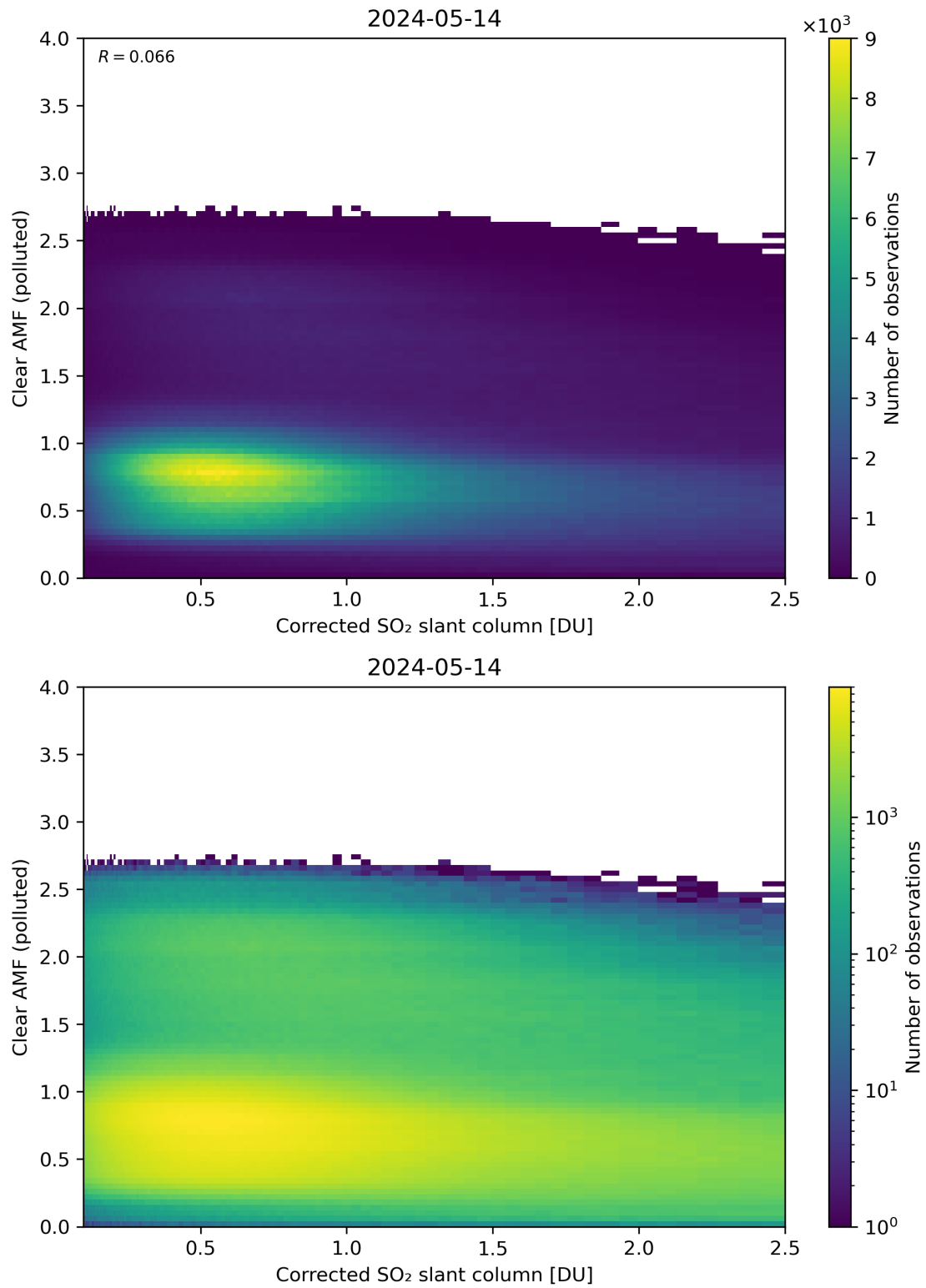
Figure 184: Scatter density plot of “Corrected SO 2 slant column” against “Clear AMF (polluted)” for 2024-05-13 to 2024-05-15.
