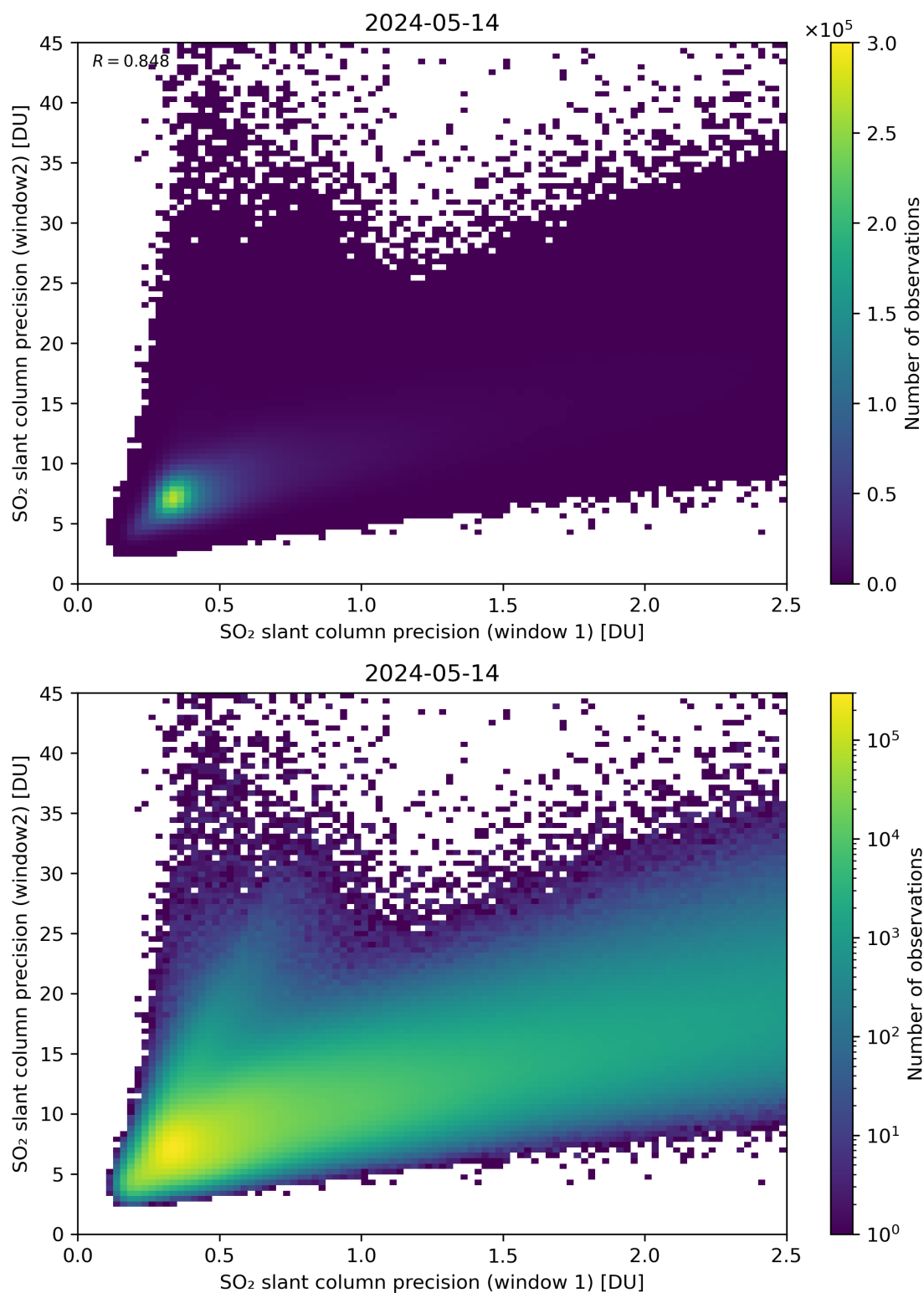
Figure 227: Scatter density plot of “SO 2 slant column precision (window 1)” against “SO 2 slant column precision (window2)” for 2024-05-13 to 2024-05-15.
