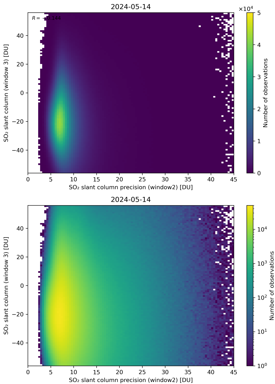
Figure 249: Scatter density plot of “SO 2 slant column precision (window2)” against “SO 2 slant column (window 3)” for 2024-05-13 to 2024-05-15.
