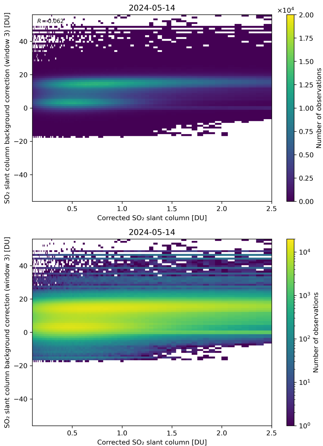
Figure 180: Scatter density plot of “Corrected SO 2 slant column” against “SO 2 slant column background correction (window 3)” for 2024-05-13 to 2024-05-15.
