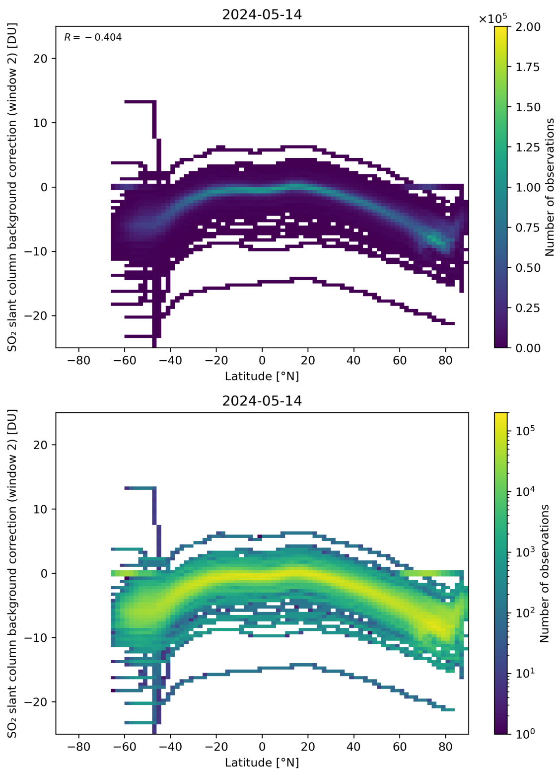
Figure 140: Scatter density plot of “Latitude” against “SO 2 slant column background correction (window 2)” for 2024-05-13 to 2024-05-15.
