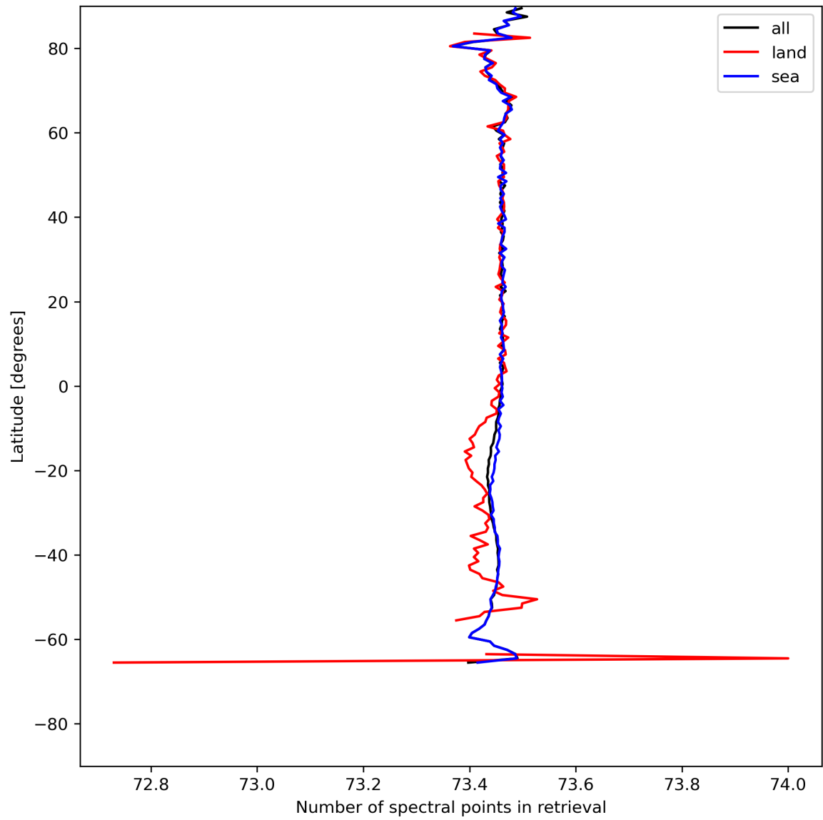
Figure 51: Zonal average of “Number of spectral points in retrieval” for 2024-05-13 to 2024-05-15.
