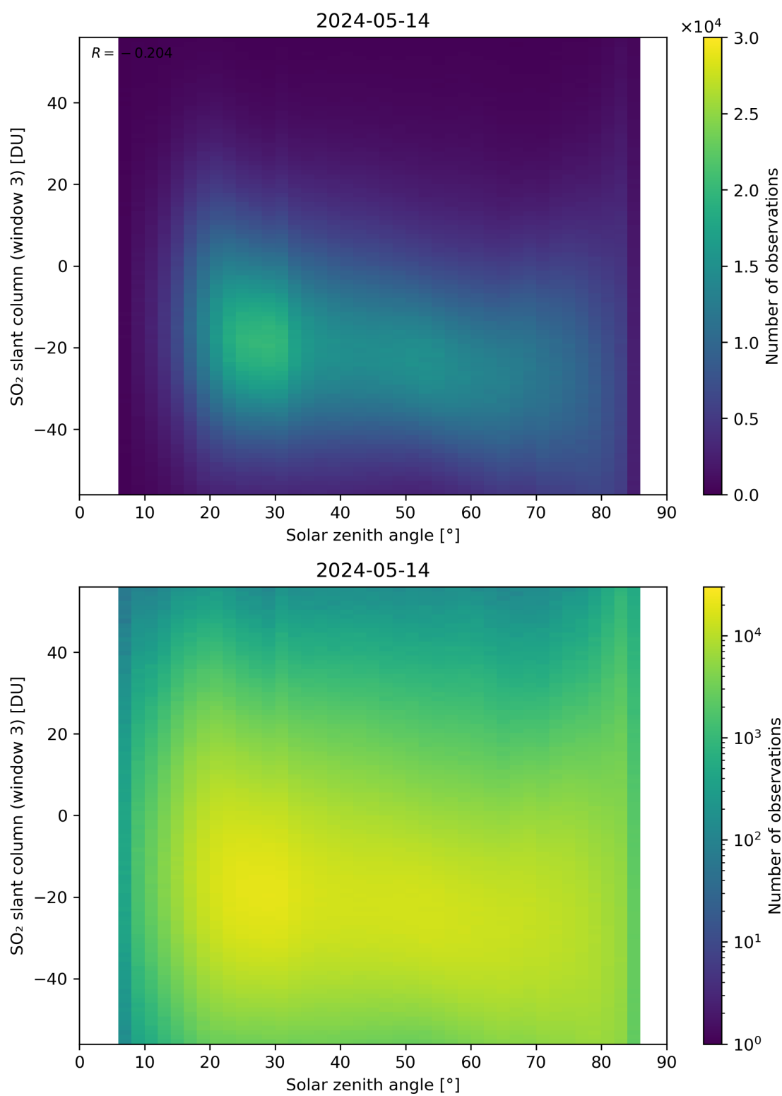
Figure 172: Scatter density plot of “Solar zenith angle” against “SO 2 slant column (window 3)” for 2024-05-13 to 2024-05-15.
