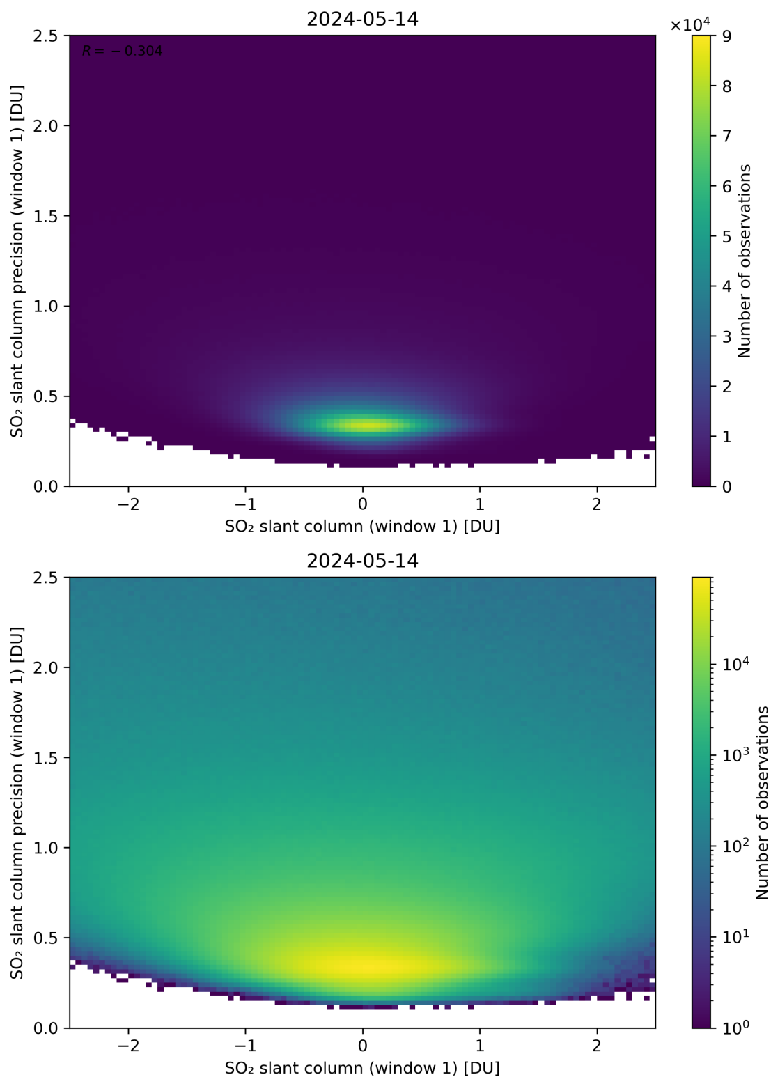
Figure 235: Scatter density plot of “SO 2 slant column (window 1)” against “SO 2 slant column precision (window 1)” for 2024-05-13 to 2024-05-15.
