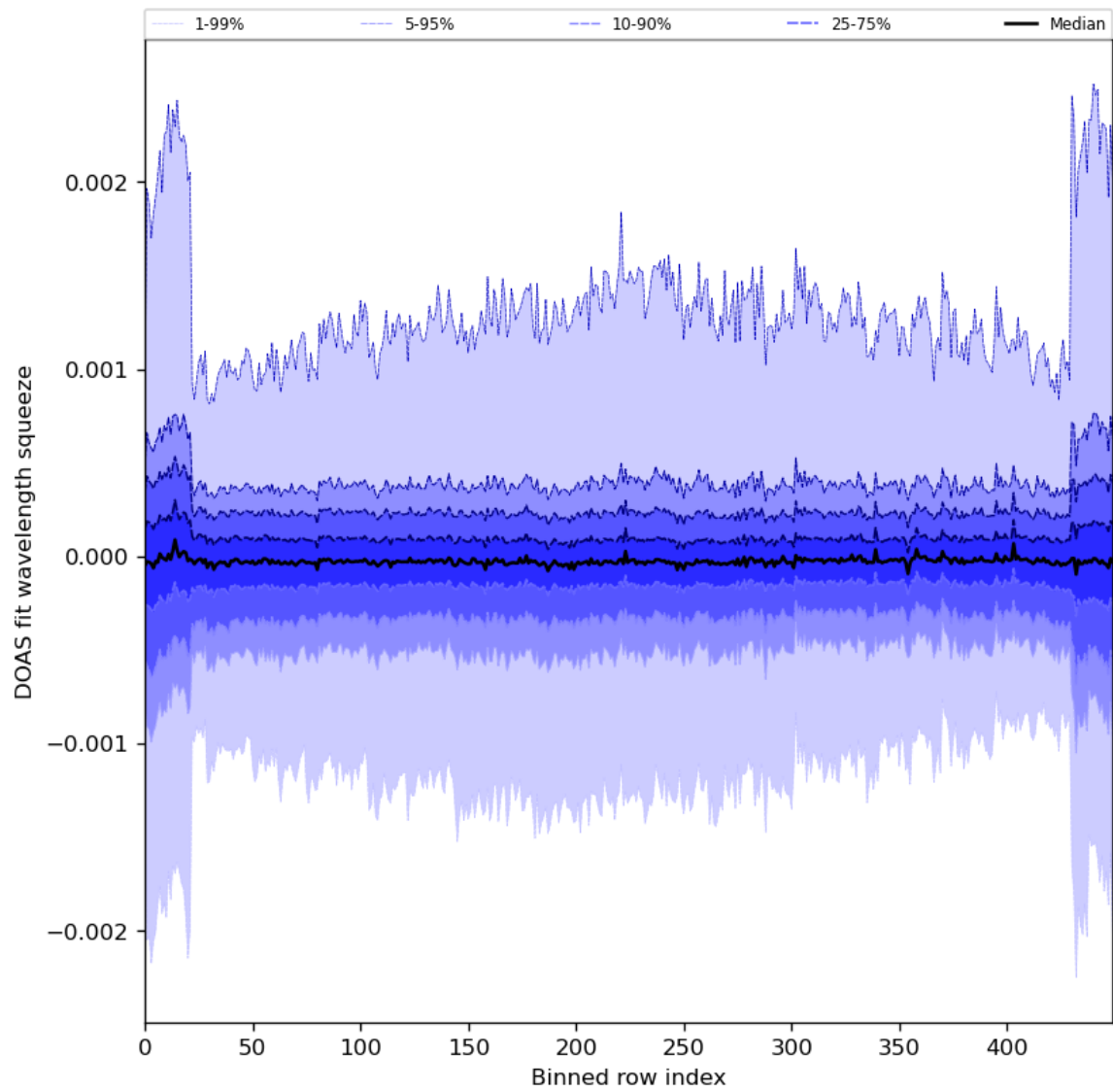
Figure 92: Along track statistics of “DOAS fit wavelength squeeze” for 2024-05-13 to 2024-05-15
