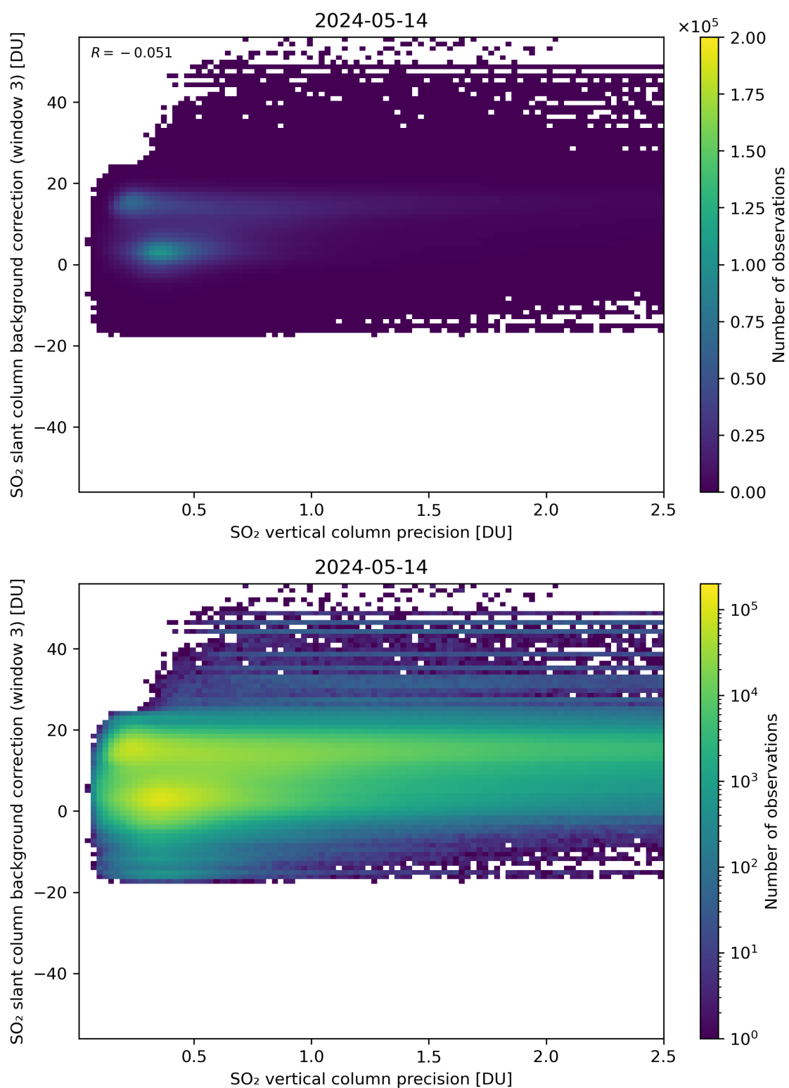
Figure 281: Scatter density plot of “SO 2 vertical column precision” against “SO 2 slant column background correction (window 3)” for 2024-05-13 to 2024-05-15.
