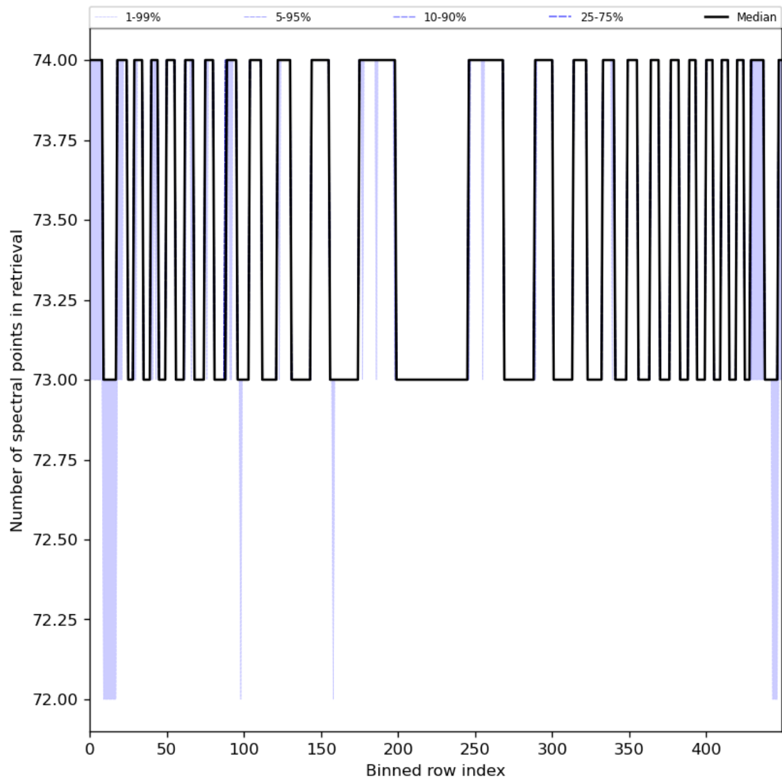
Figure 97: Along track statistics of “Number of spectral points in retrieval” for 2024-05-13 to 2024-05-15
