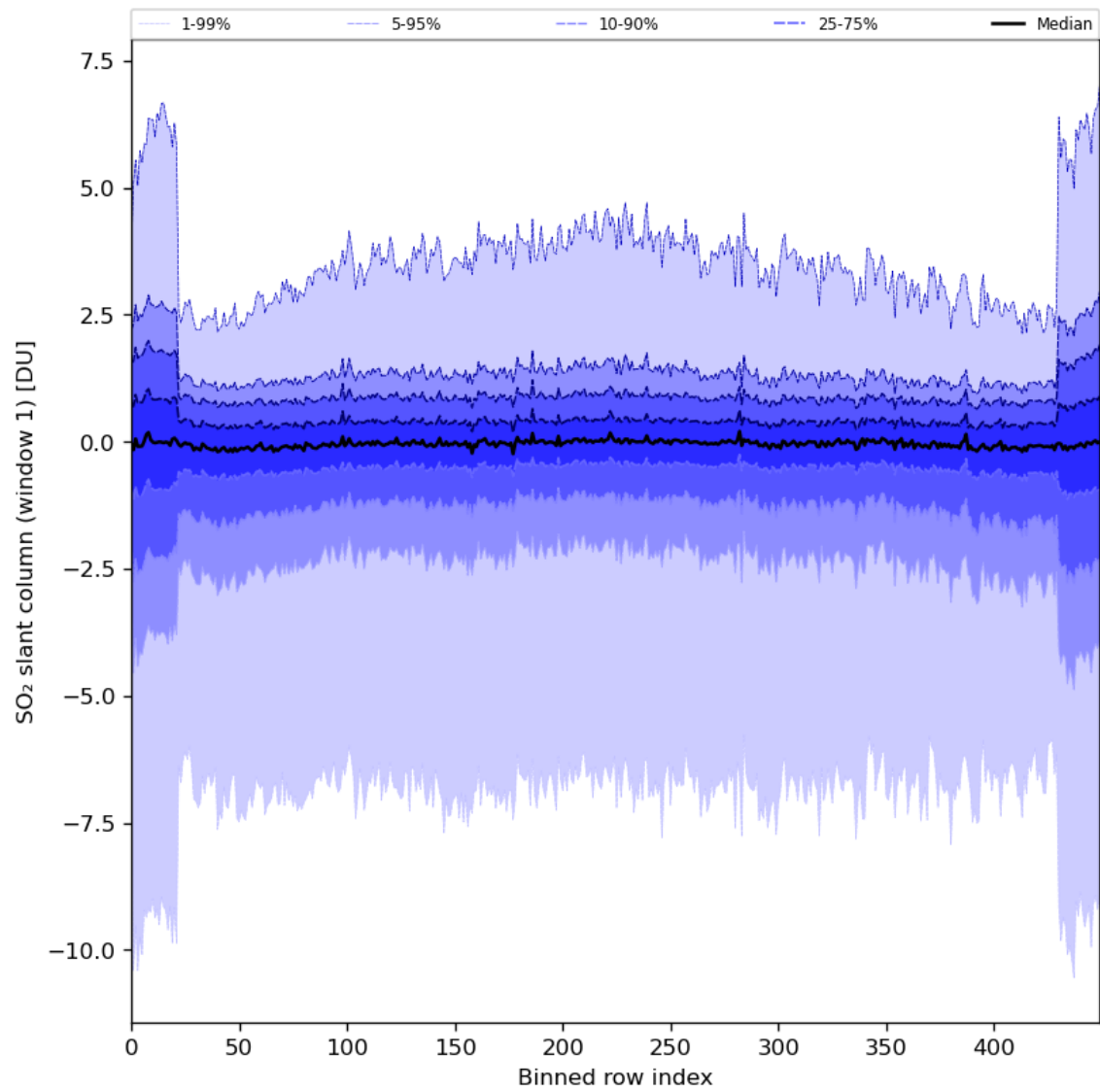
Figure 79: Along track statistics of “SO 2 slant column (window 1)” for 2024-05-13 to 2024-05-15
