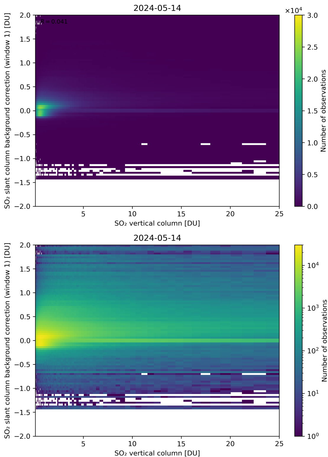
Figure 273: Scatter density plot of “SO 2 vertical column” against “SO 2 slant column background correction (window 1)” for 2024-05-13 to 2024-05-15.
