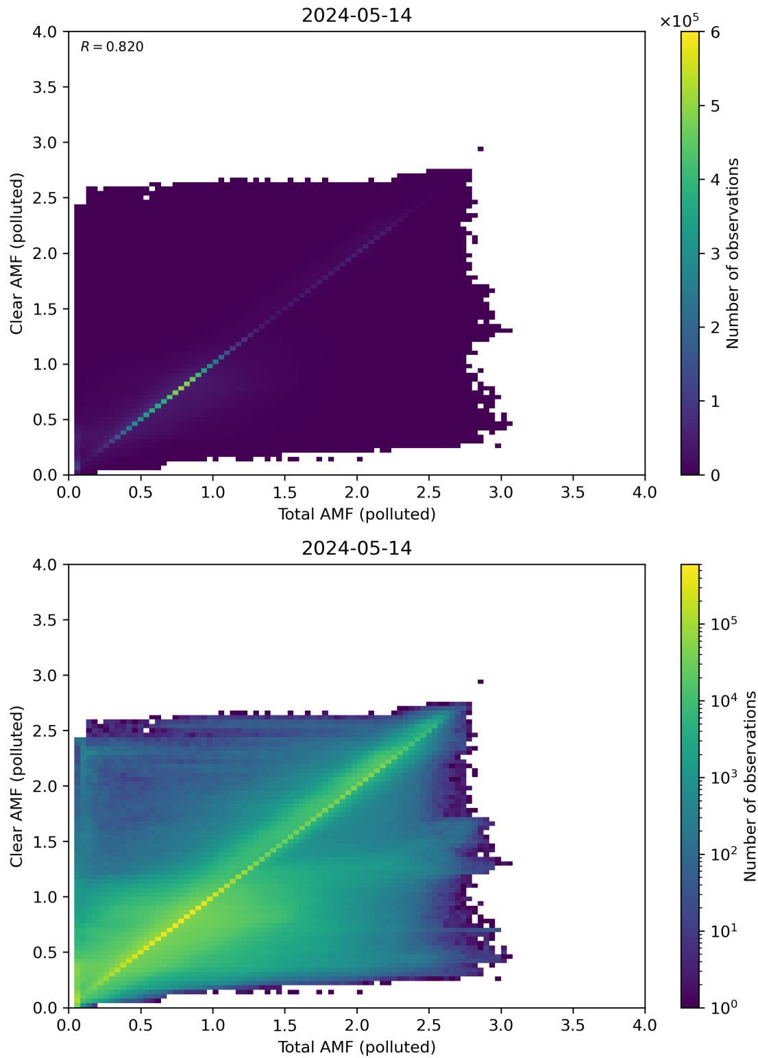
Figure 271: Scatter density plot of “Total AMF (polluted)” against “Clear AMF (polluted)” for 2024-05-13 to 2024-05-15.
