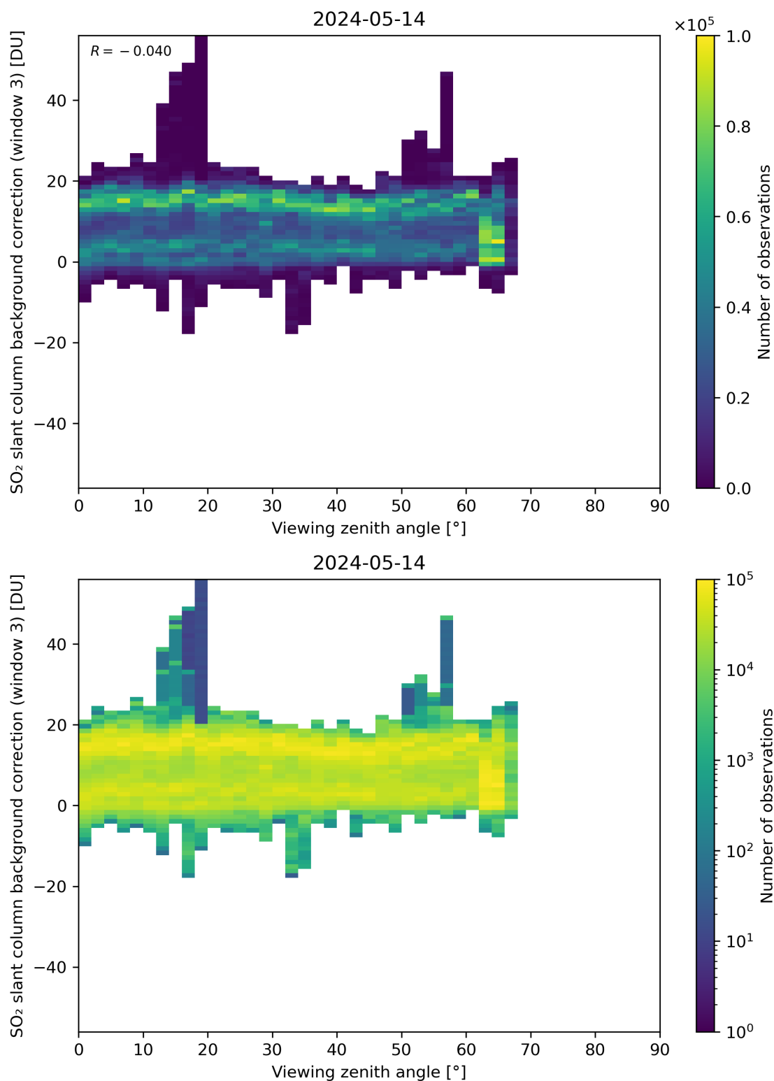
Figure 310: Scatter density plot of “Viewing zenith angle” against “SO 2 slant column background correction (window 3)” for 2024-05-13 to 2024-05-15.
