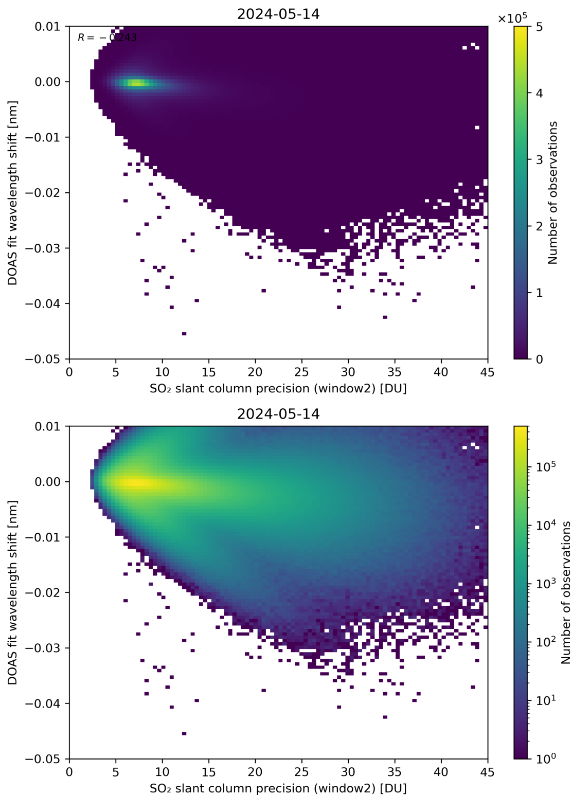
Figure 243: Scatter density plot of “SO 2 slant column precision (window2)” against “DOAS fit wavelength shift” for 2024-05-13 to 2024-05-15.
