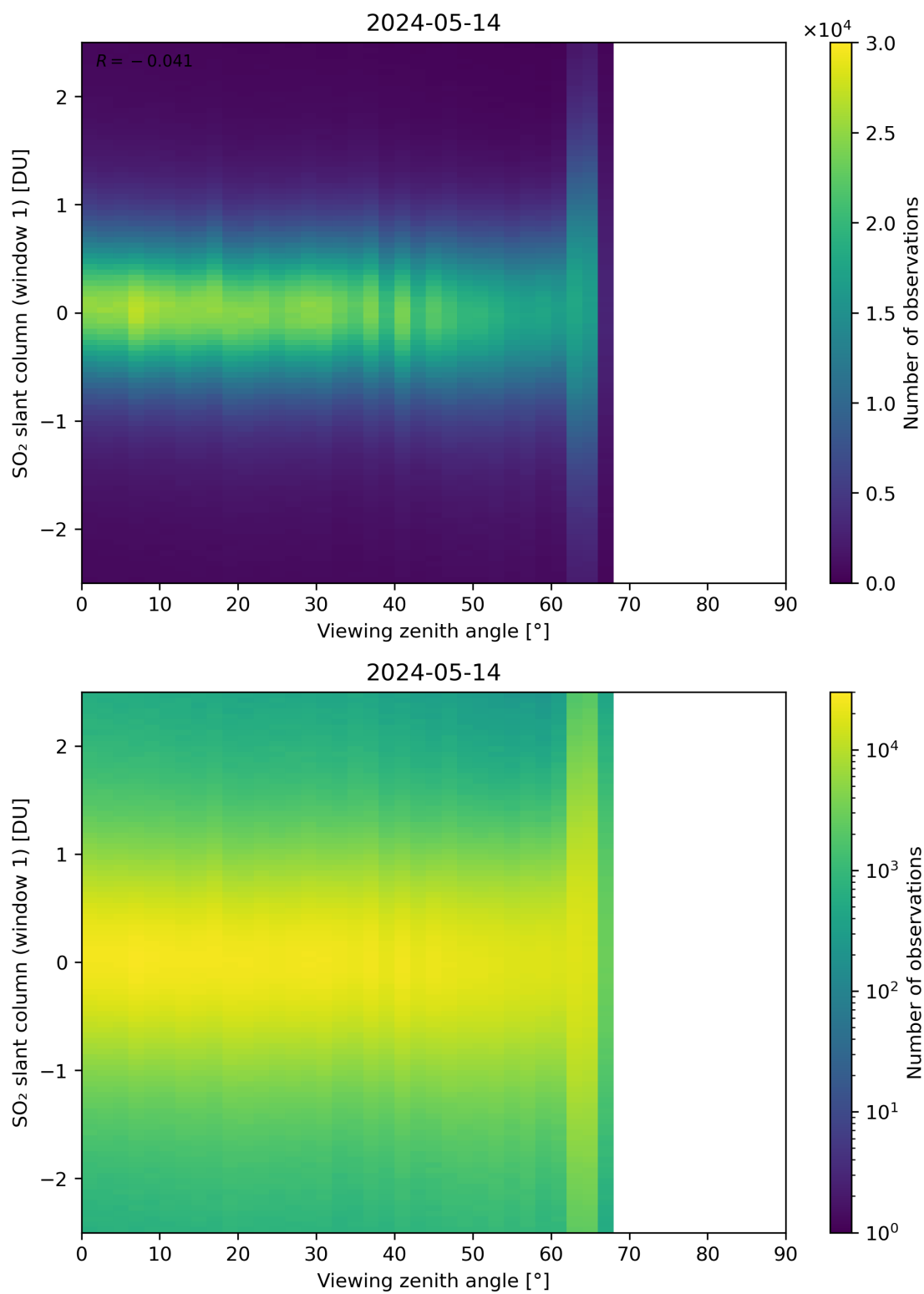
Figure 320: Scatter density plot of “Viewing zenith angle” against “SO 2 slant column (window 1)” for 2024-05-13 to 2024-05-15.
