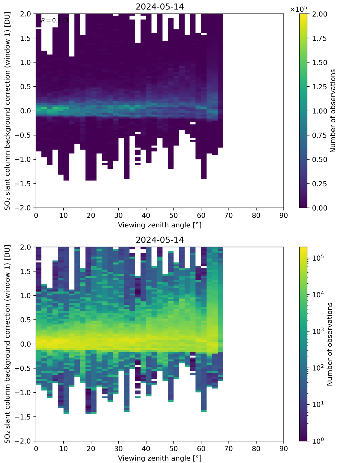
Figure 308: Scatter density plot of “Viewing zenith angle” against “SO 2 slant column background correction (window 1)” for 2024-05-13 to 2024-05-15.
