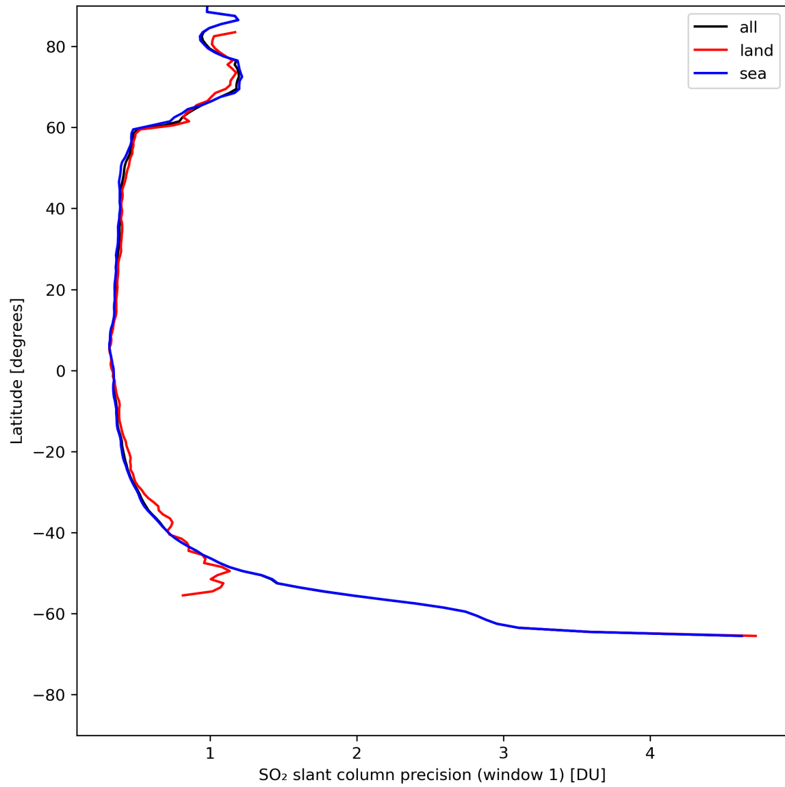
Figure 34: Zonal average of “SO 2 slant column precision (window 1)” for 2024-05-13 to 2024-05-15.
