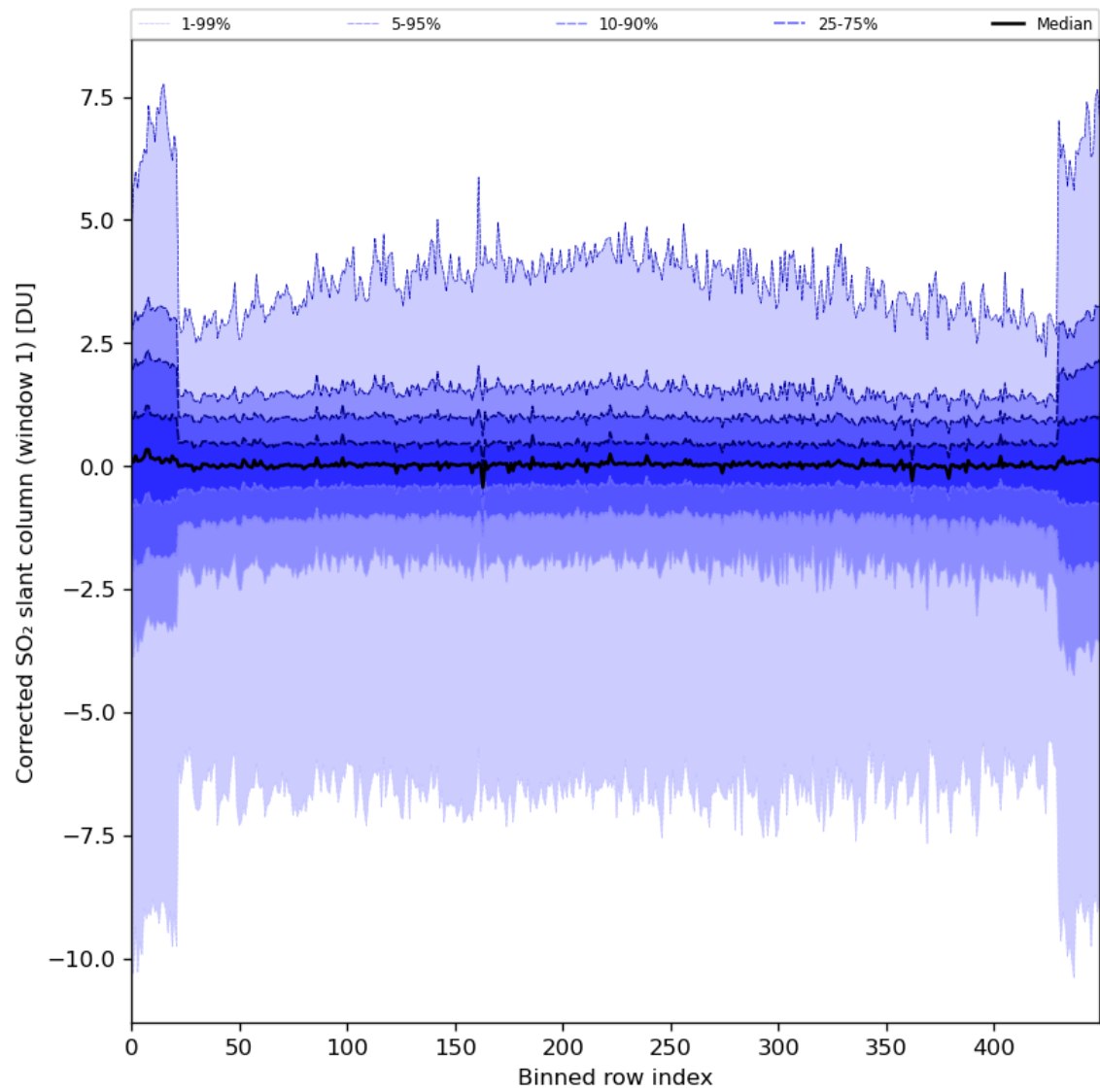
Figure 81: Along track statistics of “Corrected SO 2 slant column (window 1)” for 2024-05-13 to 2024-05-15
