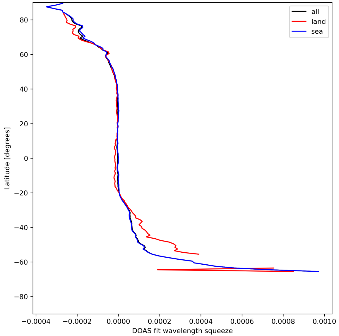
Figure 46: Zonal average of “DOAS fit wavelength squeeze” for 2024-05-13 to 2024-05-15.
