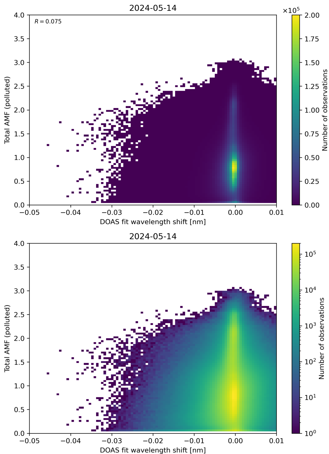
Figure 130: Scatter density plot of “DOAS fit wavelength shift” against “Total AMF (polluted)” for 2024-05-13 to 2024-05-15.
