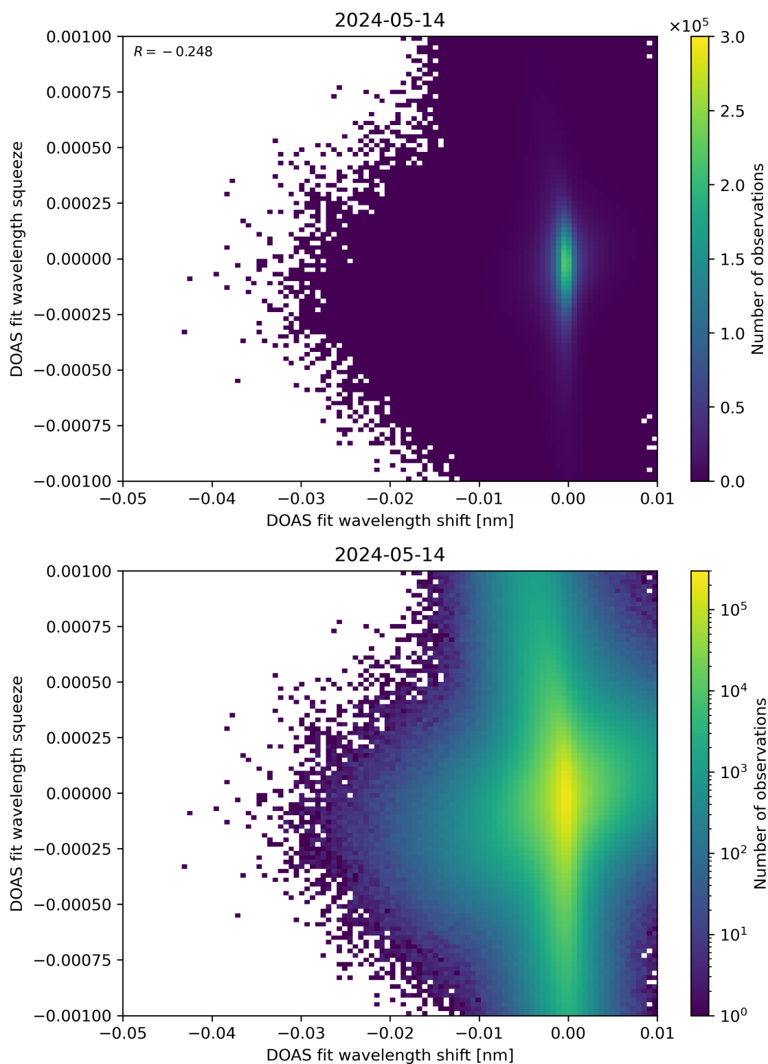
Figure 127: Scatter density plot of “DOAS fit wavelength shift” against “DOAS fit wavelength squeeze” for 2024-05-13 to 2024-05-15.
