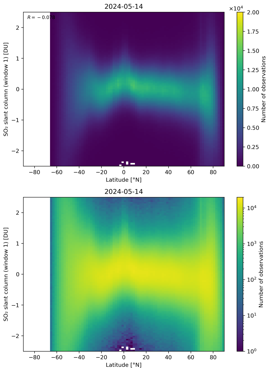
Figure 149: Scatter density plot of “Latitude” against “SO 2 slant column (window 1)” for 2024-05-13 to 2024-05-15.
