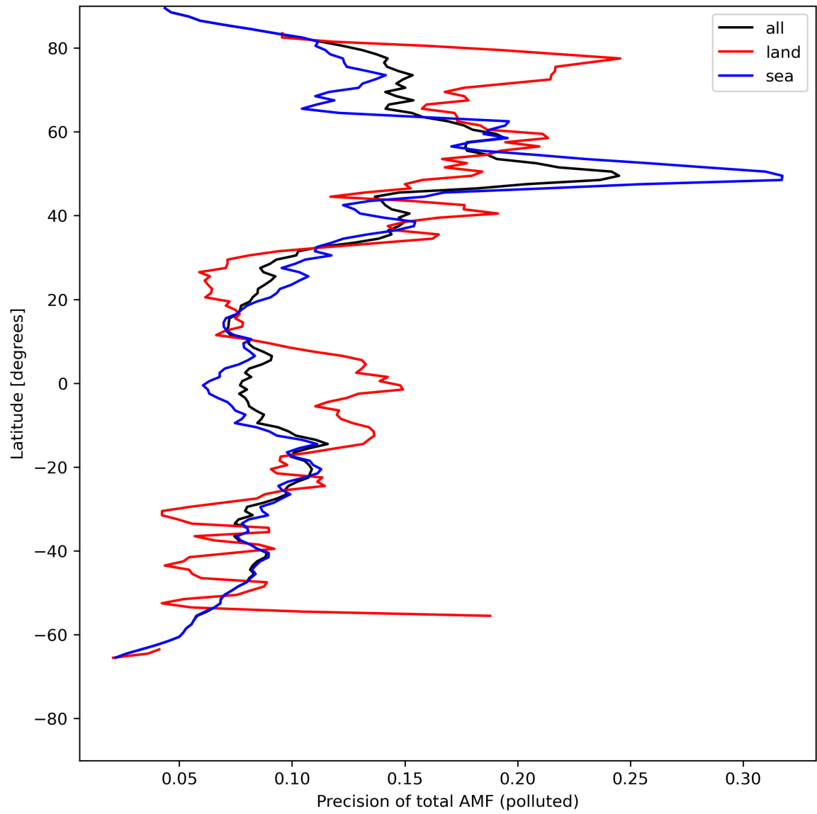
Figure 49: Zonal average of “Precision of total AMF (polluted)” for 2024-05-13 to 2024-05-15.
