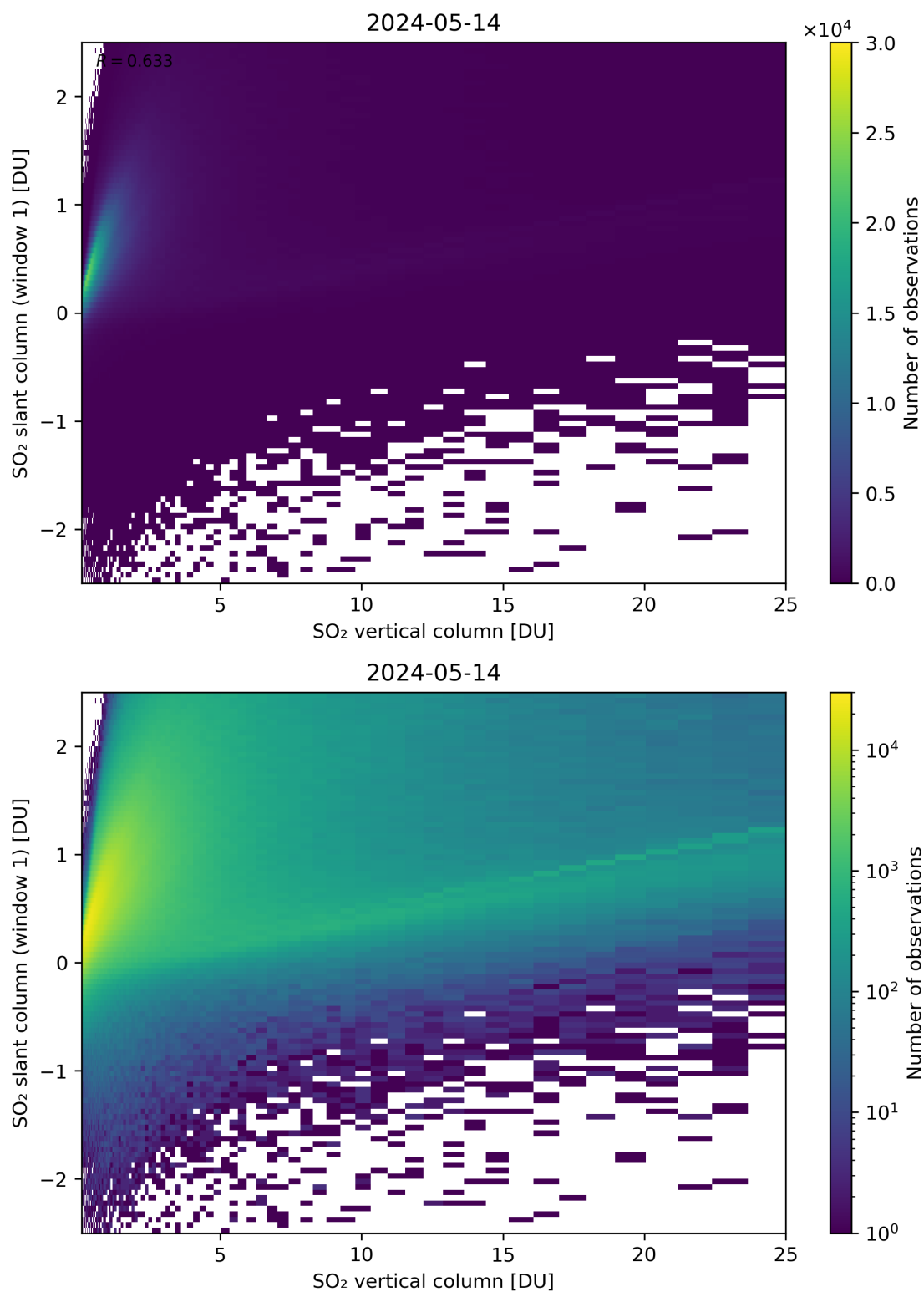
Figure 300: Scatter density plot of “SO 2 vertical column” against “SO 2 slant column (window 1)” for 2024-05-13 to 2024-05-15.
