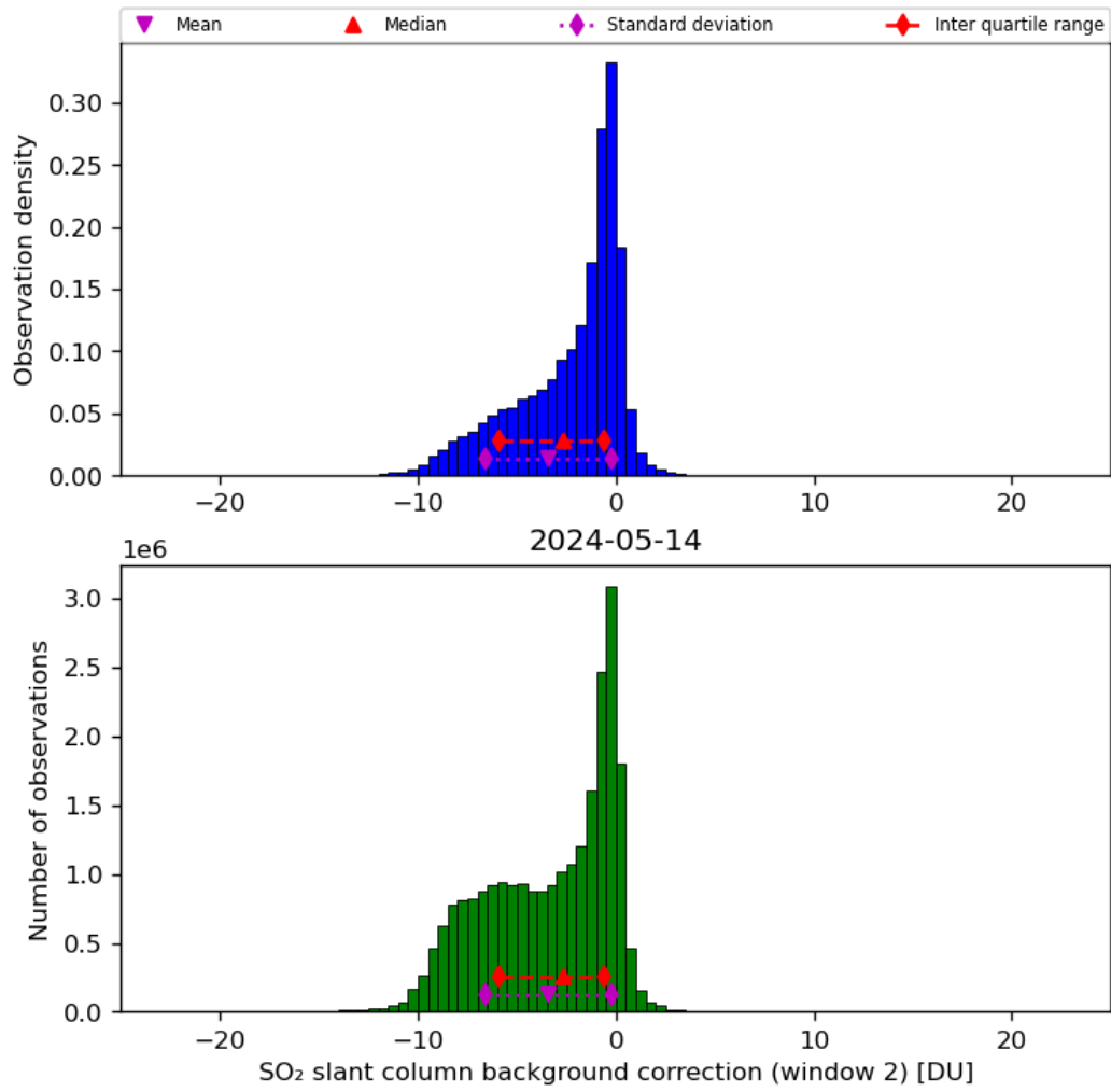
Figure 63: Histogram of “SO 2 slant column background correction (window 2)” for 2024-05-13 to 2024-05-15
