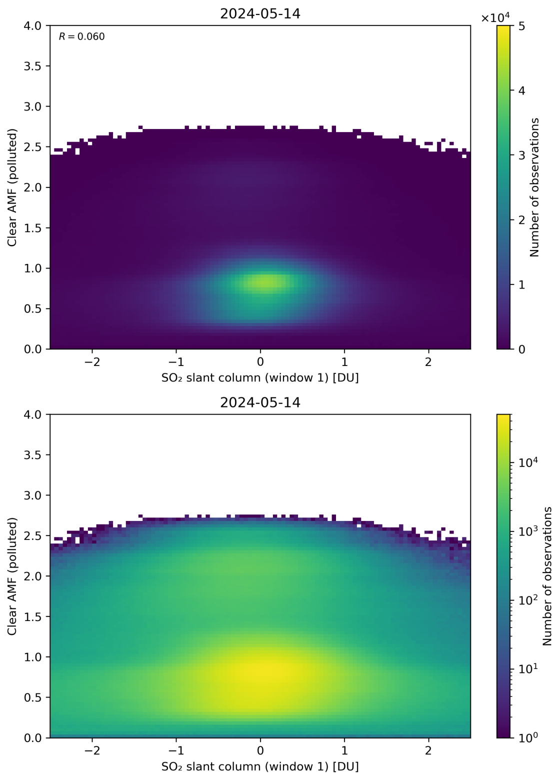
Figure 232: Scatter density plot of “SO 2 slant column (window 1)” against “Clear AMF (polluted)” for 2024-05-13 to 2024-05-15.
