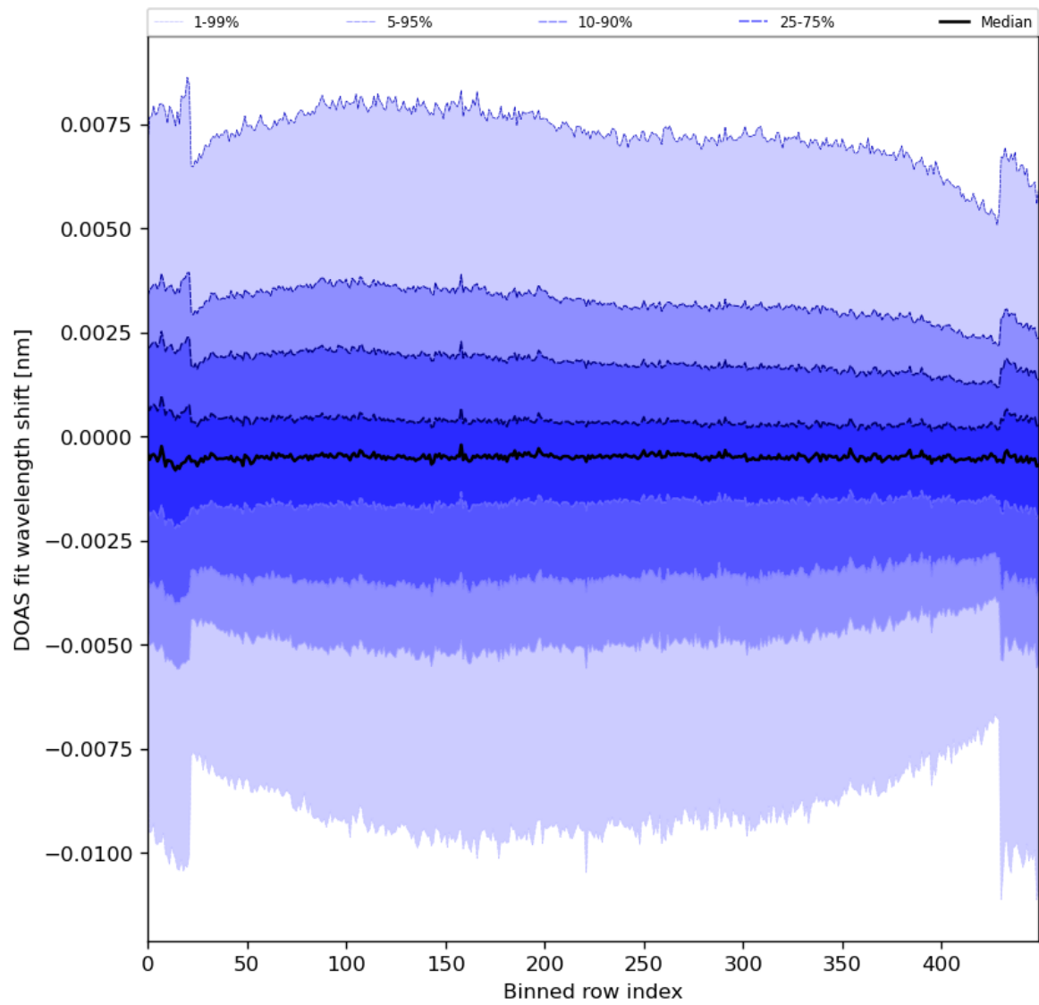
Figure 91: Along track statistics of “DOAS fit wavelength shift” for 2024-05-13 to 2024-05-15
