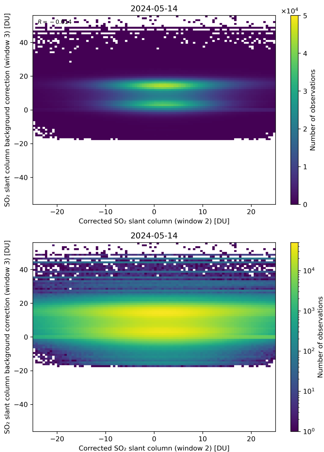
Figure 195: Scatter density plot of “Corrected SO 2 slant column (window 2)” against “SO 2 slant column background correction (window 3)” for 2024-05-13 to 2024-05-15.
