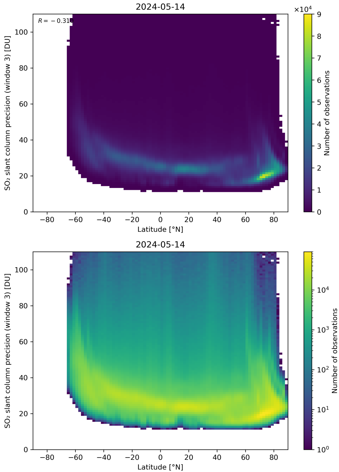
Figure 153: Scatter density plot of “Latitude” against “SO 2 slant column precision (window 3)” for 2024-05-13 to 2024-05-15.
