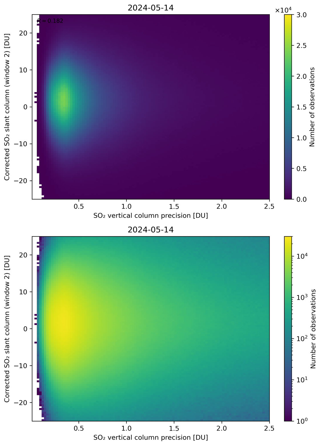
Figure 287: Scatter density plot of “SO 2 vertical column precision” against “Corrected SO 2 slant column (window 2)” for 2024-05-13 to 2024-05-15.
