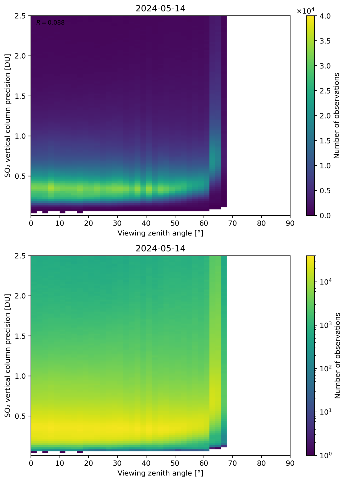
Figure 328: Scatter density plot of “Viewing zenith angle” against “SO 2 vertical column precision” for 2024-05-13 to 2024-05-15.
