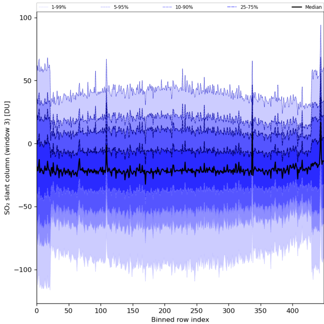
Figure 87: Along track statistics of “SO 2 slant column (window 3)” for 2024-05-13 to 2024-05-15
