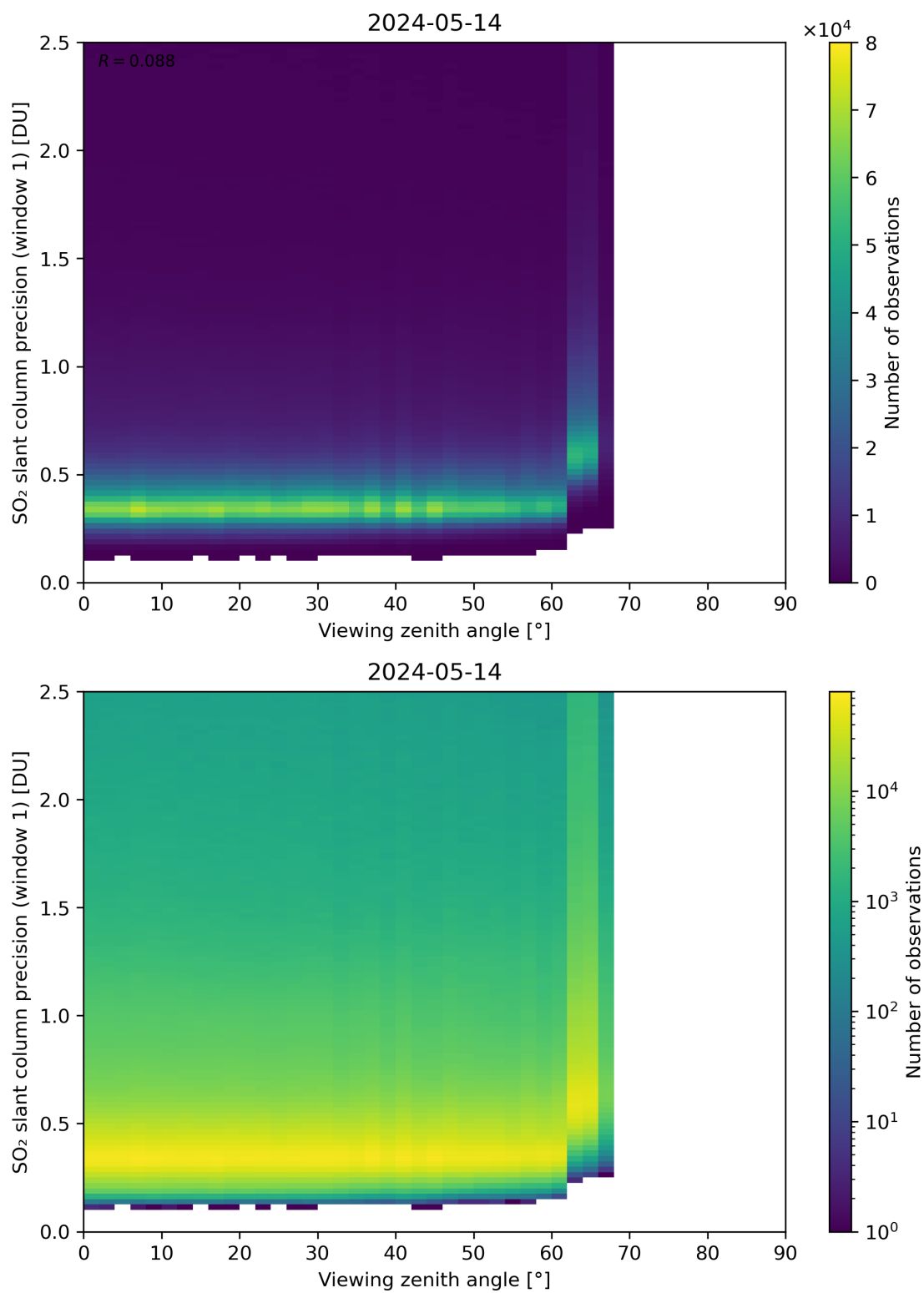
Figure 321: Scatter density plot of “Viewing zenith angle” against “SO 2 slant column precision (window 1)” for 2024-05-13 to 2024-05-15.
