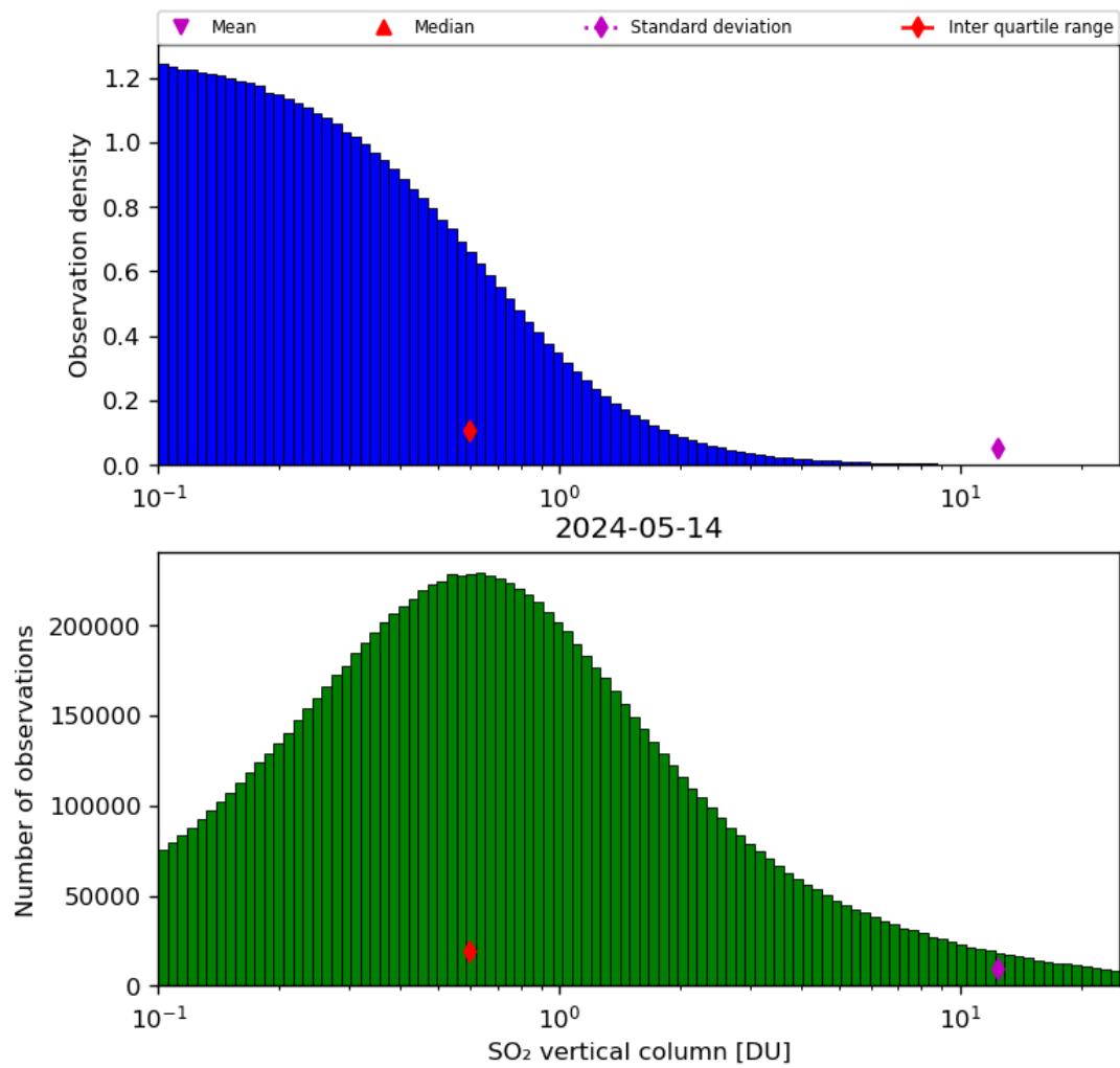
Figure 53: Histogram of “SO 2 vertical column” for 2024-05-13 to 2024-05-15
