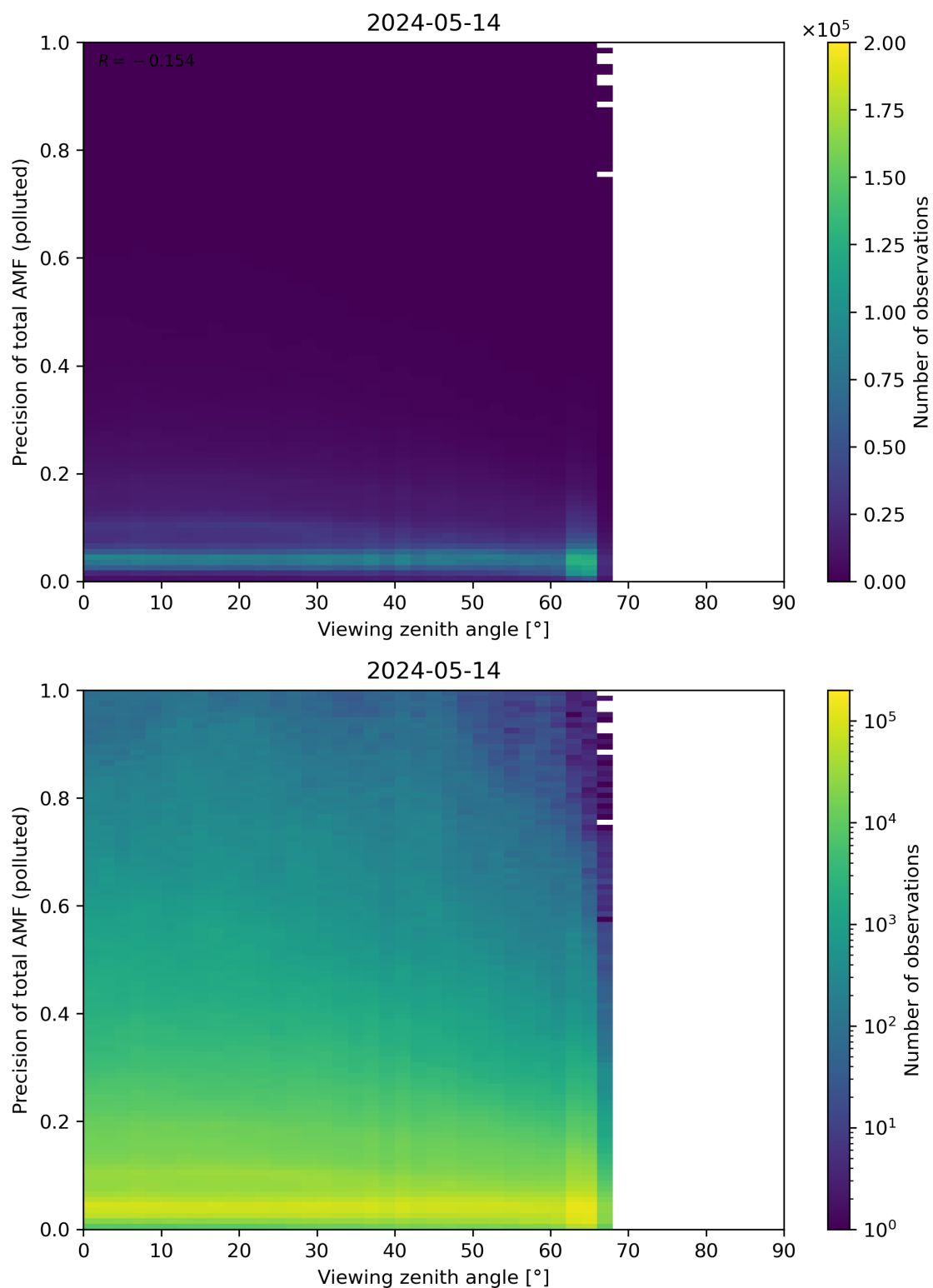
Figure 326: Scatter density plot of “Viewing zenith angle” against “Precision of total AMF (polluted)” for 2024-05-13 to 2024-05-15.
