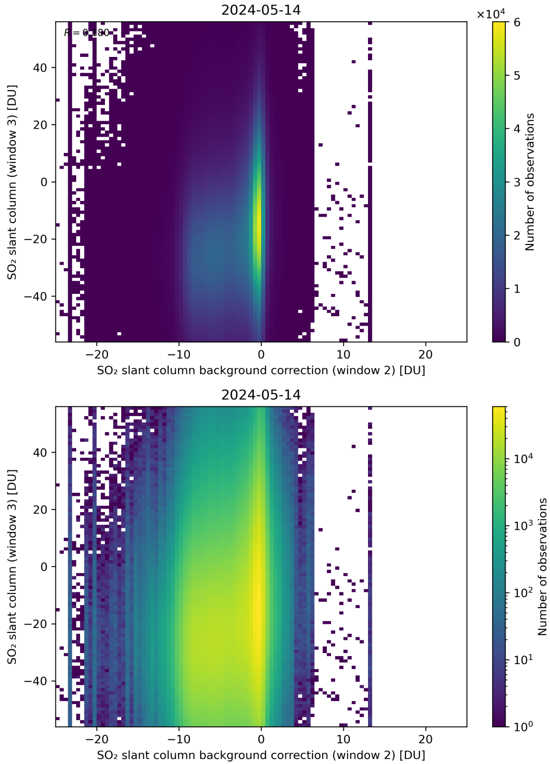
Figure 117: Scatter density plot of “SO 2 slant column background correction (window 2)” against “SO 2 slant column (window 3)” for 2024-05-13 to 2024-05-15.
