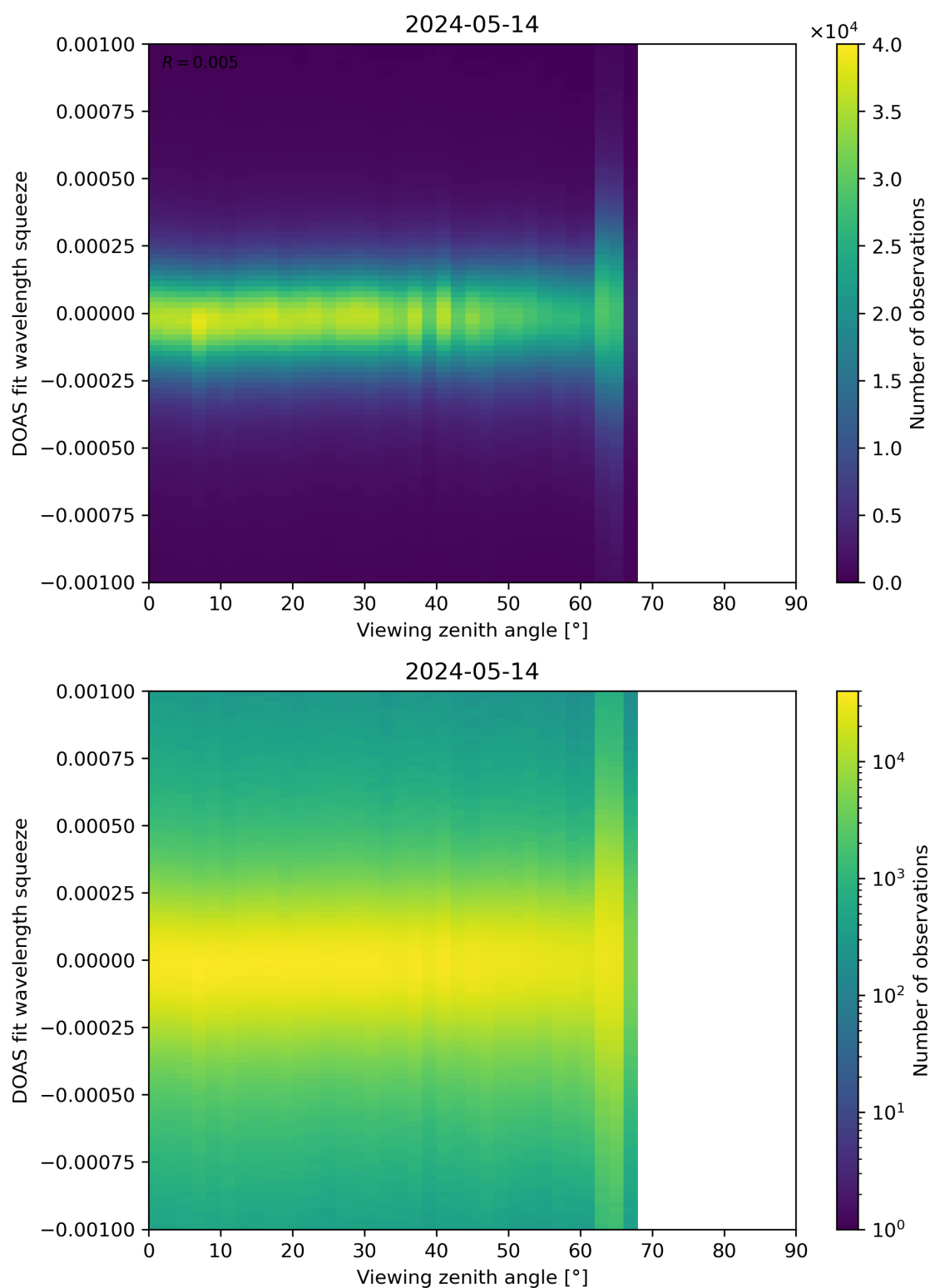
Figure 312: Scatter density plot of “Viewing zenith angle” against “DOAS fit wavelength squeeze” for 2024-05-13 to 2024-05-15.
