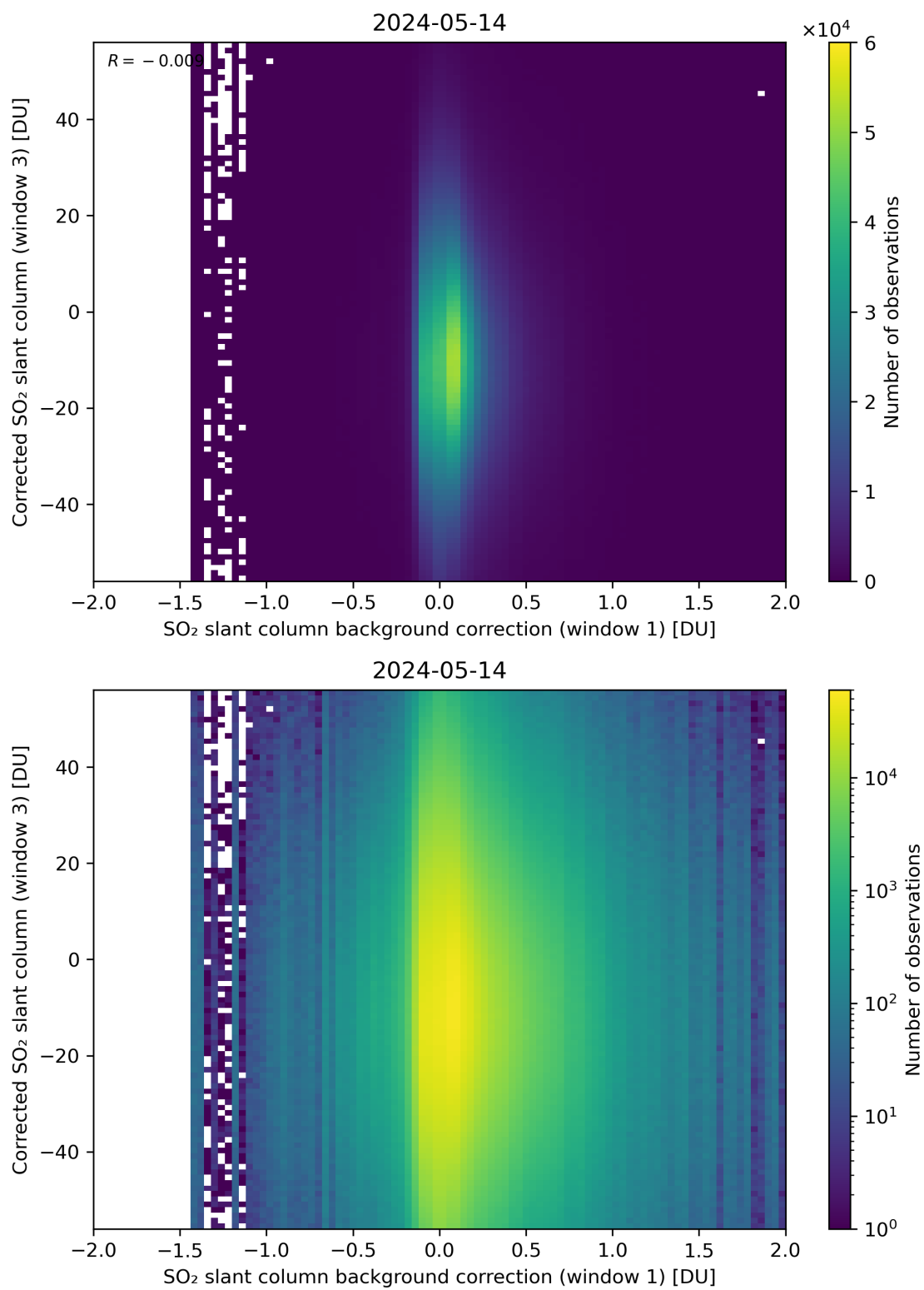
Figure 105: Scatter density plot of “SO 2 slant column background correction (window 1)” against “Corrected SO 2 slant column (window 3)” for 2024-05-13 to 2024-05-15.
