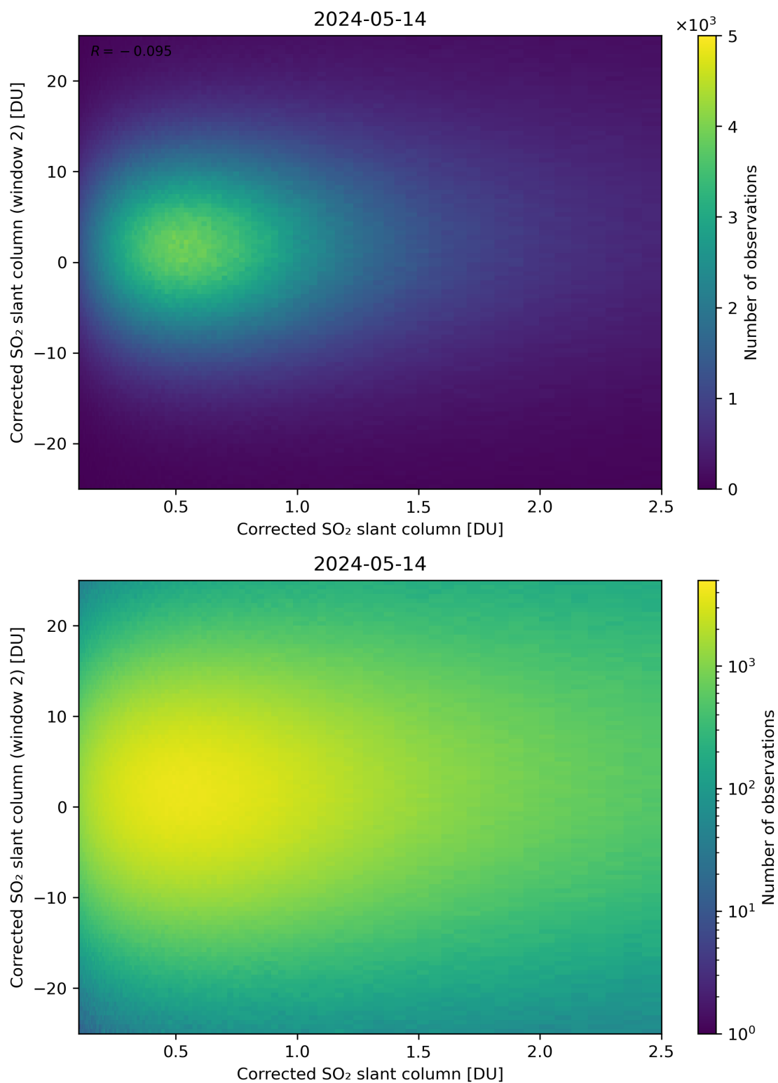
Figure 185: Scatter density plot of “Corrected SO 2 slant column” against “Corrected SO 2 slant column (window 2)” for 2024-05-13 to 2024-05-15.
