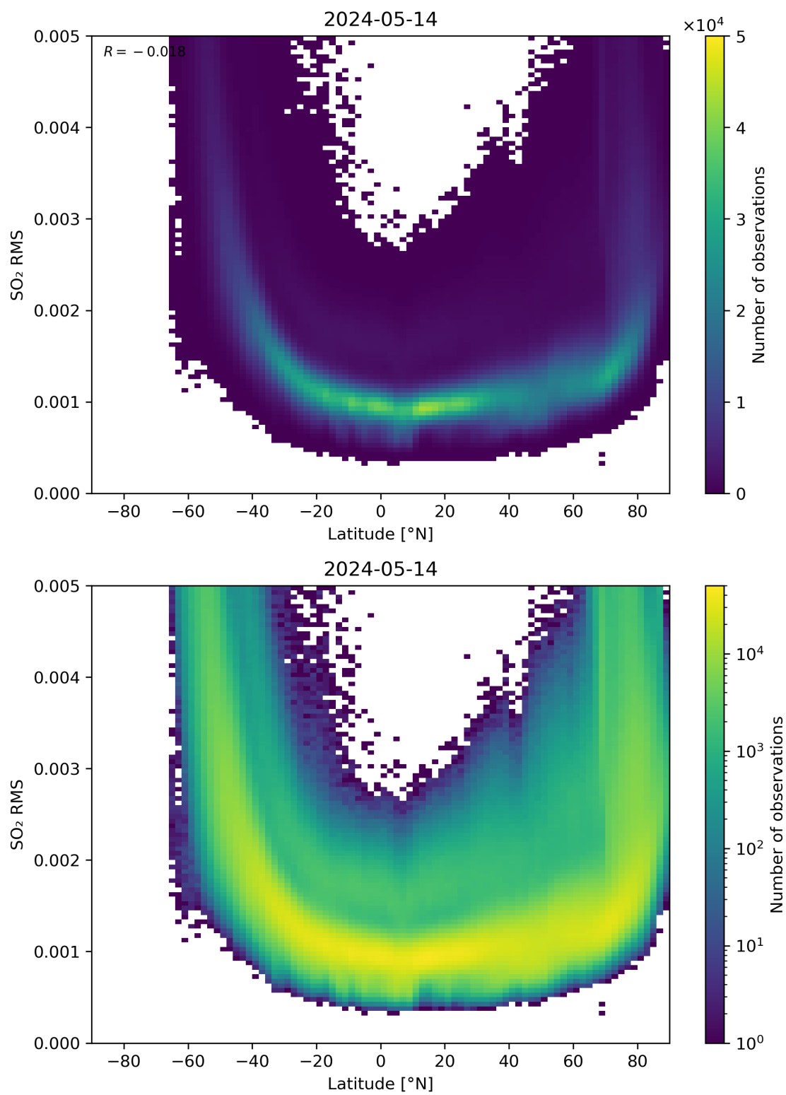
Figure 144: Scatter density plot of “Latitude” against “SO 2 RMS” for 2024-05-13 to 2024-05-15.
