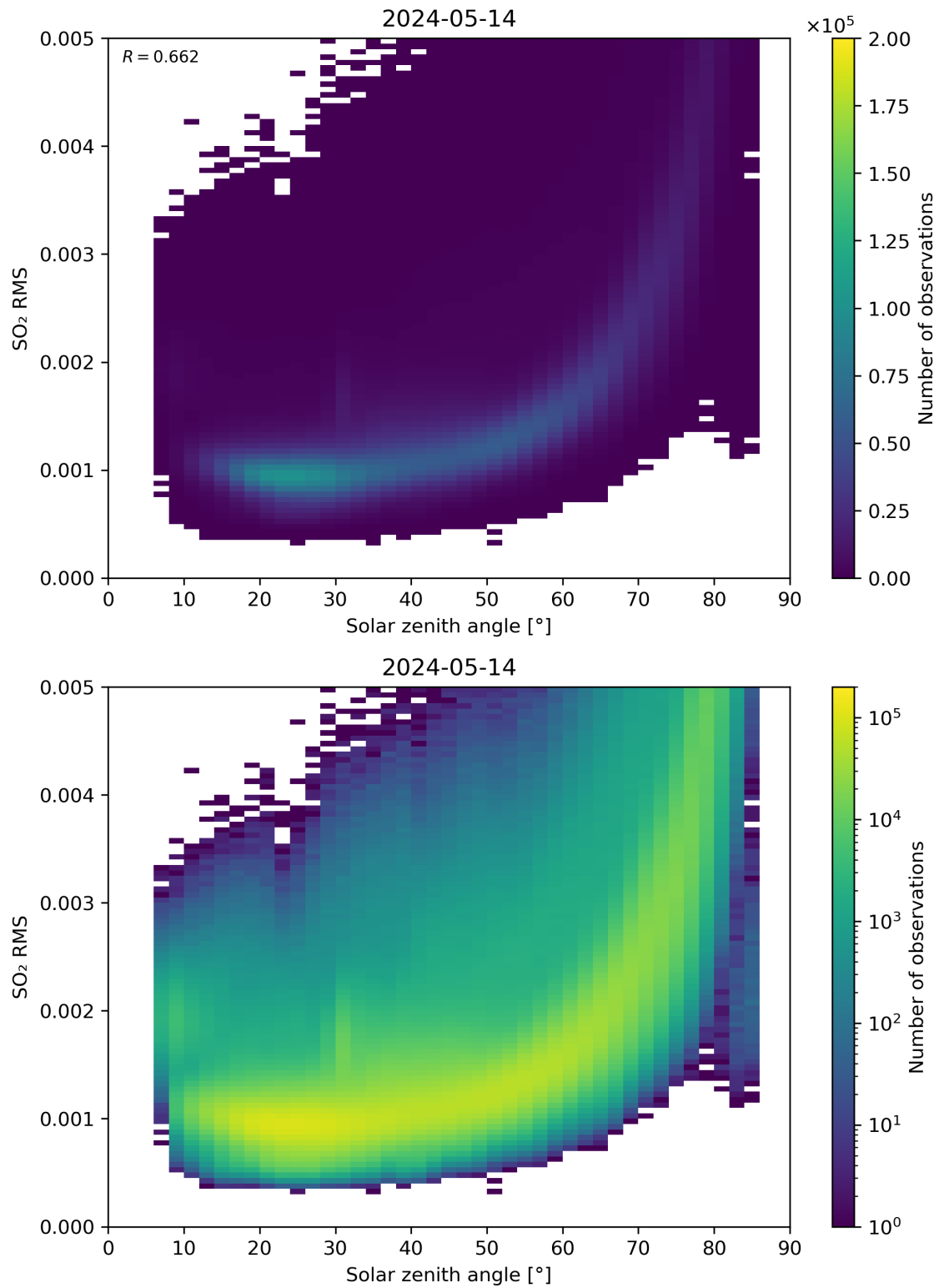
Figure 163: Scatter density plot of “Solar zenith angle” against “SO 2 RMS” for 2024-05-13 to 2024-05-15.
