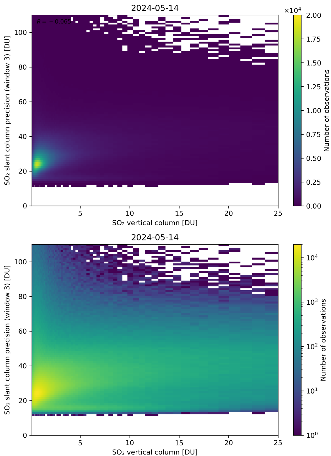
Figure 304: Scatter density plot of “SO 2 vertical column” against “SO 2 slant column precision (window 3)” for 2024-05-13 to 2024-05-15.
