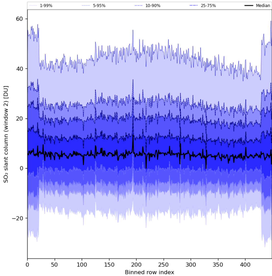
Figure 83: Along track statistics of “SO 2 slant column (window 2)” for 2024-05-13 to 2024-05-15
