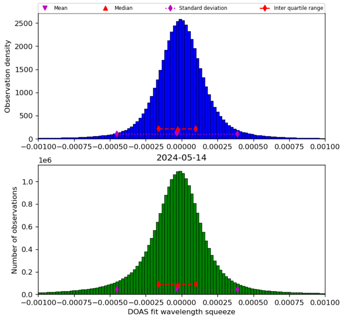
Figure 69: Histogram of “DOAS fit wavelength squeeze” for 2024-05-13 to 2024-05-15
