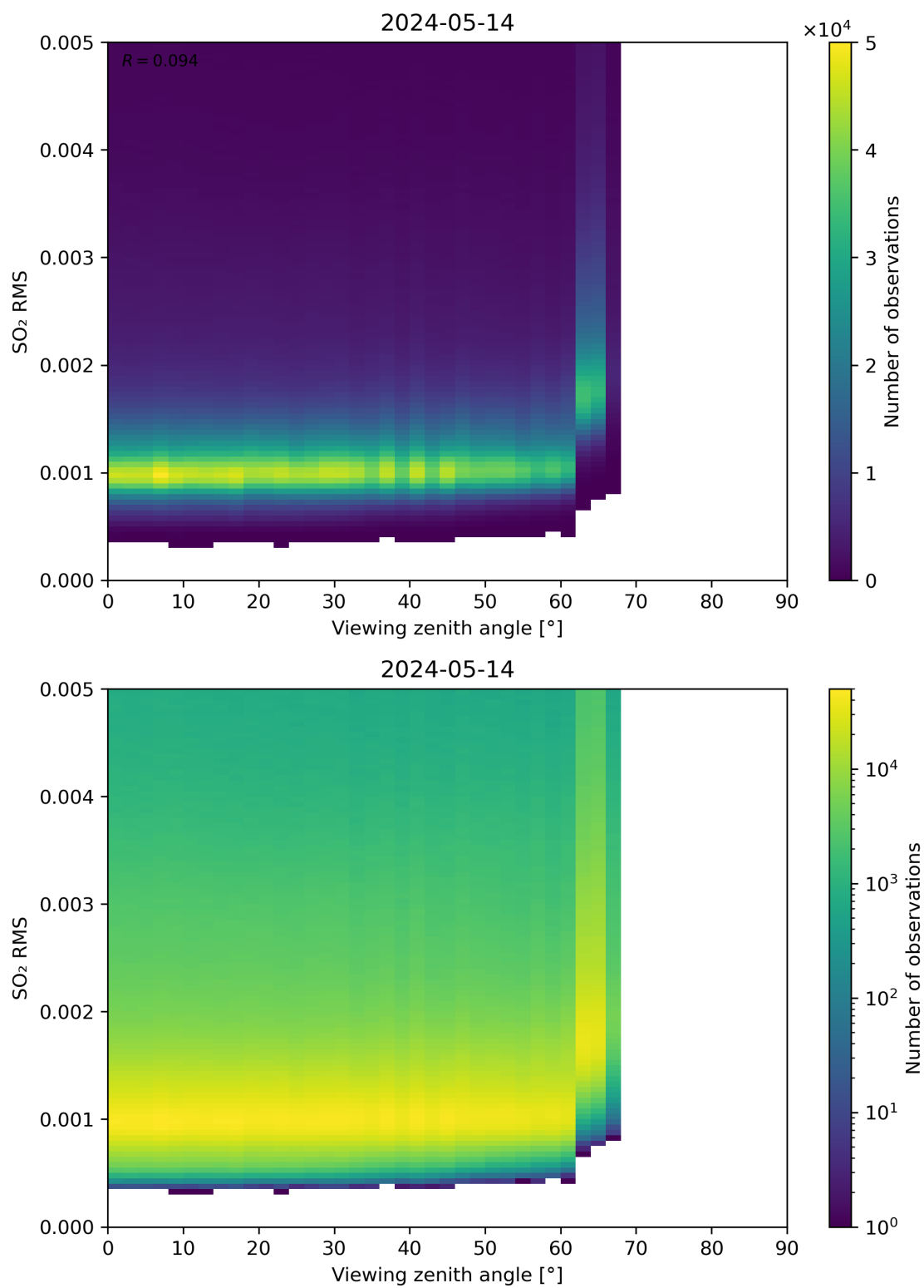
Figure 313: Scatter density plot of “Viewing zenith angle” against “SO 2 RMS” for 2024-05-13 to 2024-05-15.
