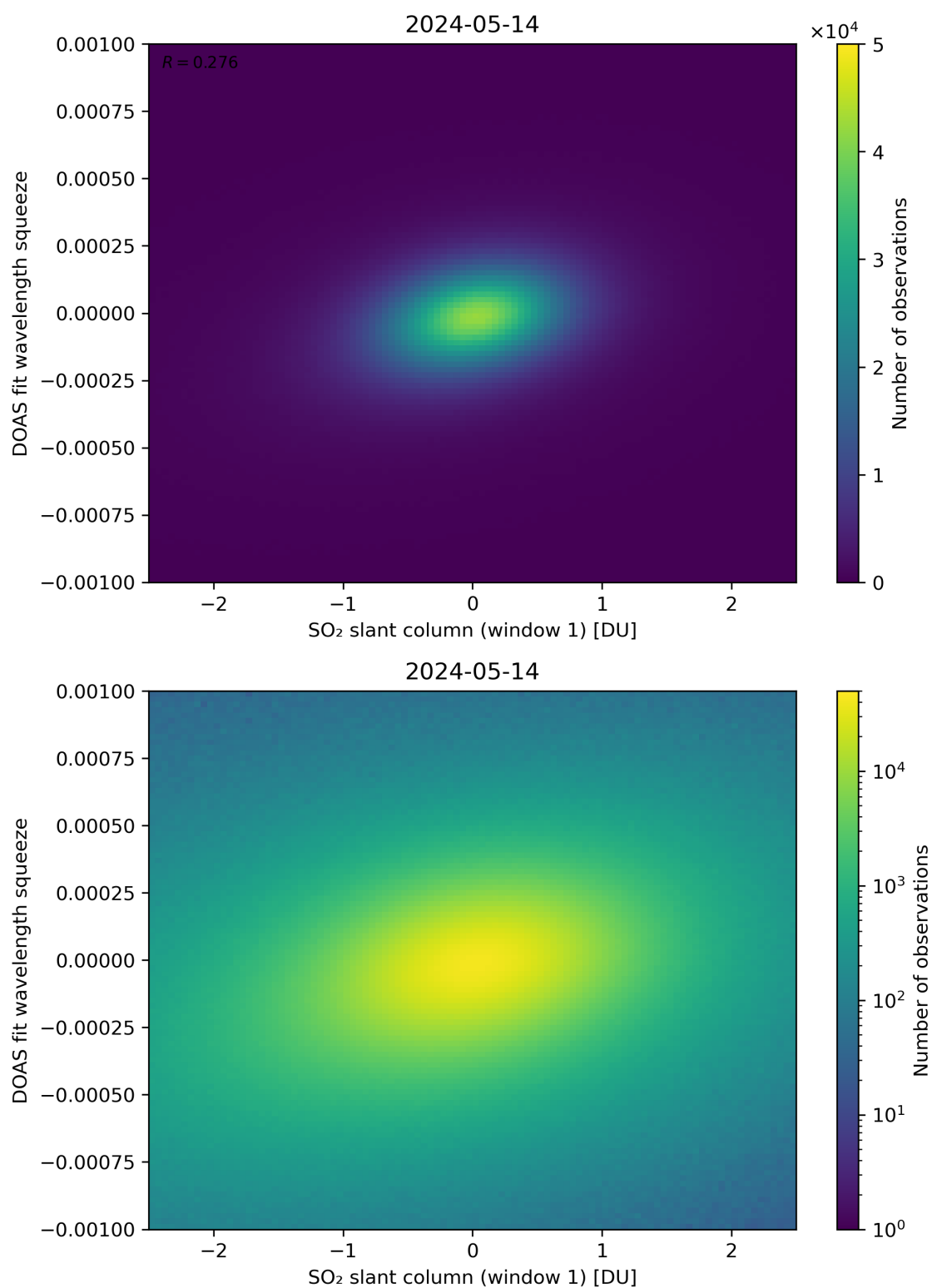
Figure 216: Scatter density plot of “SO 2 slant column (window 1)” against “DOAS fit wavelength squeeze” for 2024-05-13 to 2024-05-15.
