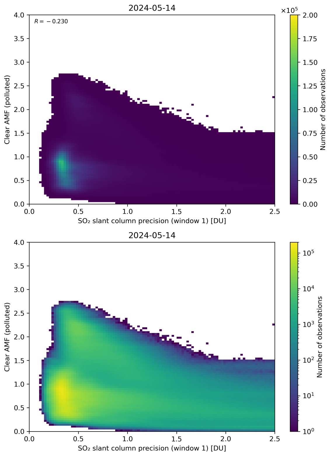
Figure 224: Scatter density plot of “SO 2 slant column precision (window 1)” against “Clear AMF (polluted)” for 2024-05-13 to 2024-05-15.
