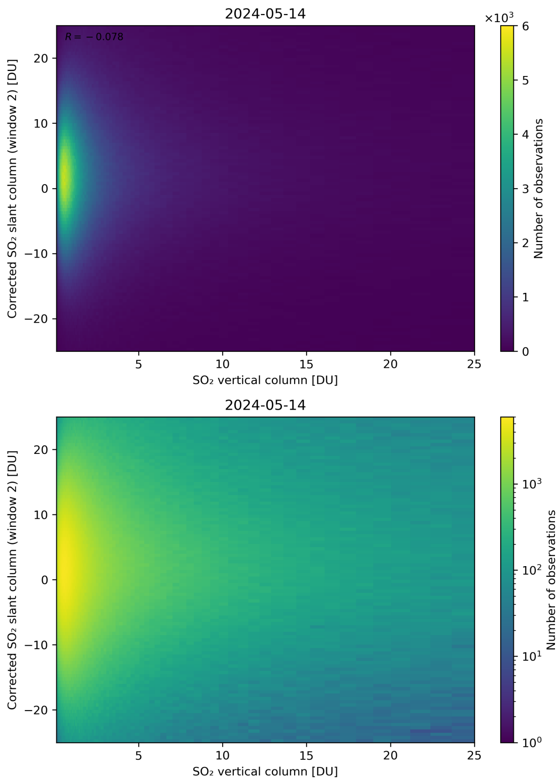
Figure 298: Scatter density plot of “SO 2 vertical column” against “Corrected SO 2 slant column (window 2)” for 2024-05-13 to 2024-05-15.
