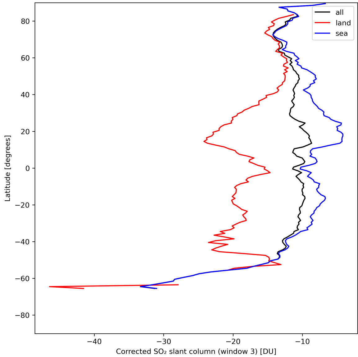
Figure 43: Zonal average of “Corrected SO 2 slant column (window 3)” for 2024-05-13 to 2024-05-15.
