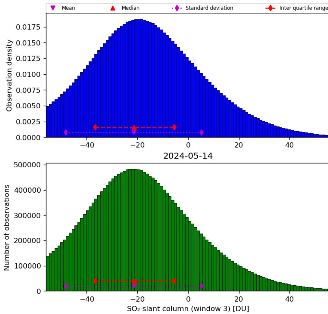
Figure 64: Histogram of “SO 2 slant column (window 3)” for 2024-05-13 to 2024-05-15
