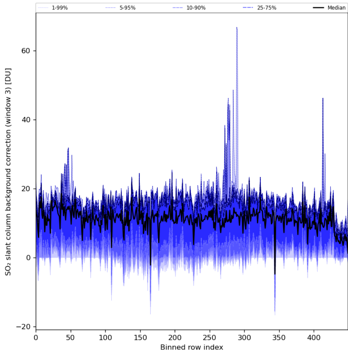
Figure 90: Along track statistics of “SO 2 slant column background correction (window 3)” for 2024-05-13 to 2024-05-15
