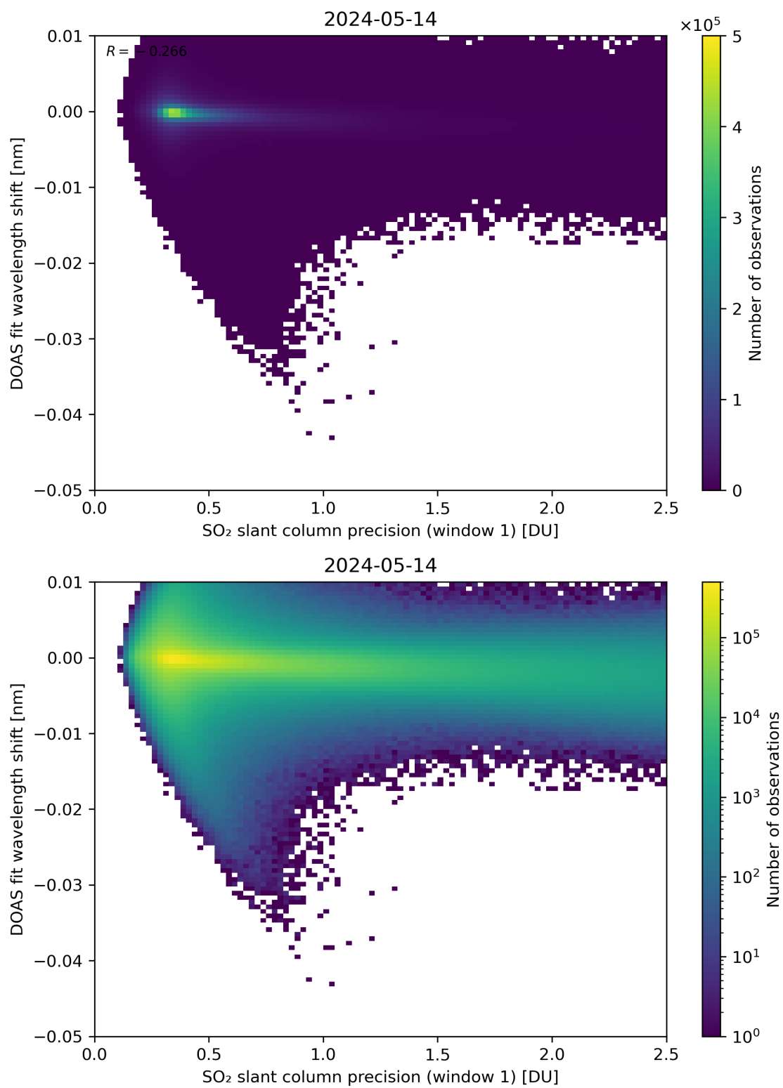
Figure 221: Scatter density plot of “SO 2 slant column precision (window 1)” against “DOAS fit wavelength shift” for 2024-05-13 to 2024-05-15.
