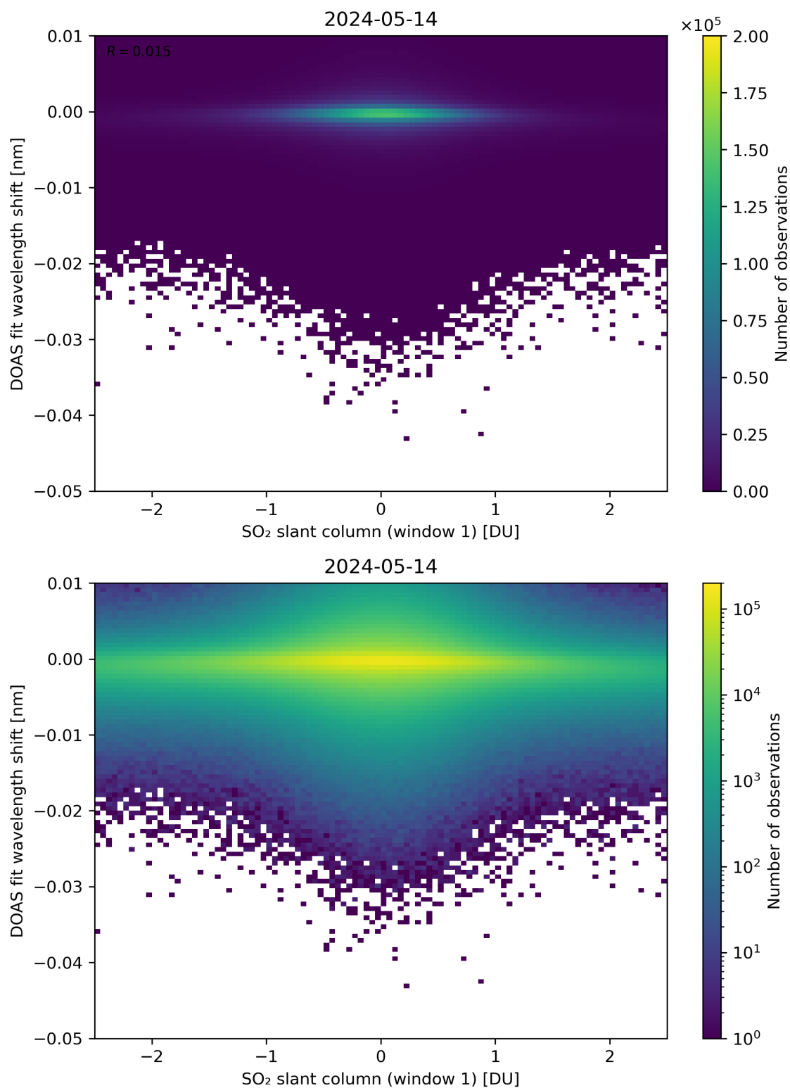
Figure 215: Scatter density plot of “SO 2 slant column (window 1)” against “DOAS fit wavelength shift” for 2024-05-13 to 2024-05-15.
