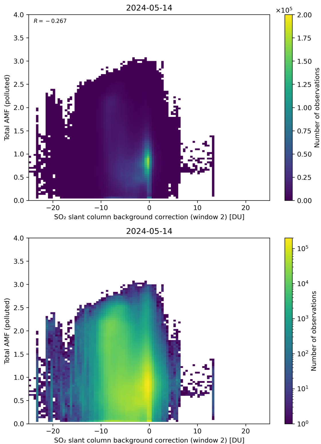
Figure 119: Scatter density plot of “SO 2 slant column background correction (window 2)” against “Total AMF (polluted)” for 2024-05-13 to 2024-05-15.
