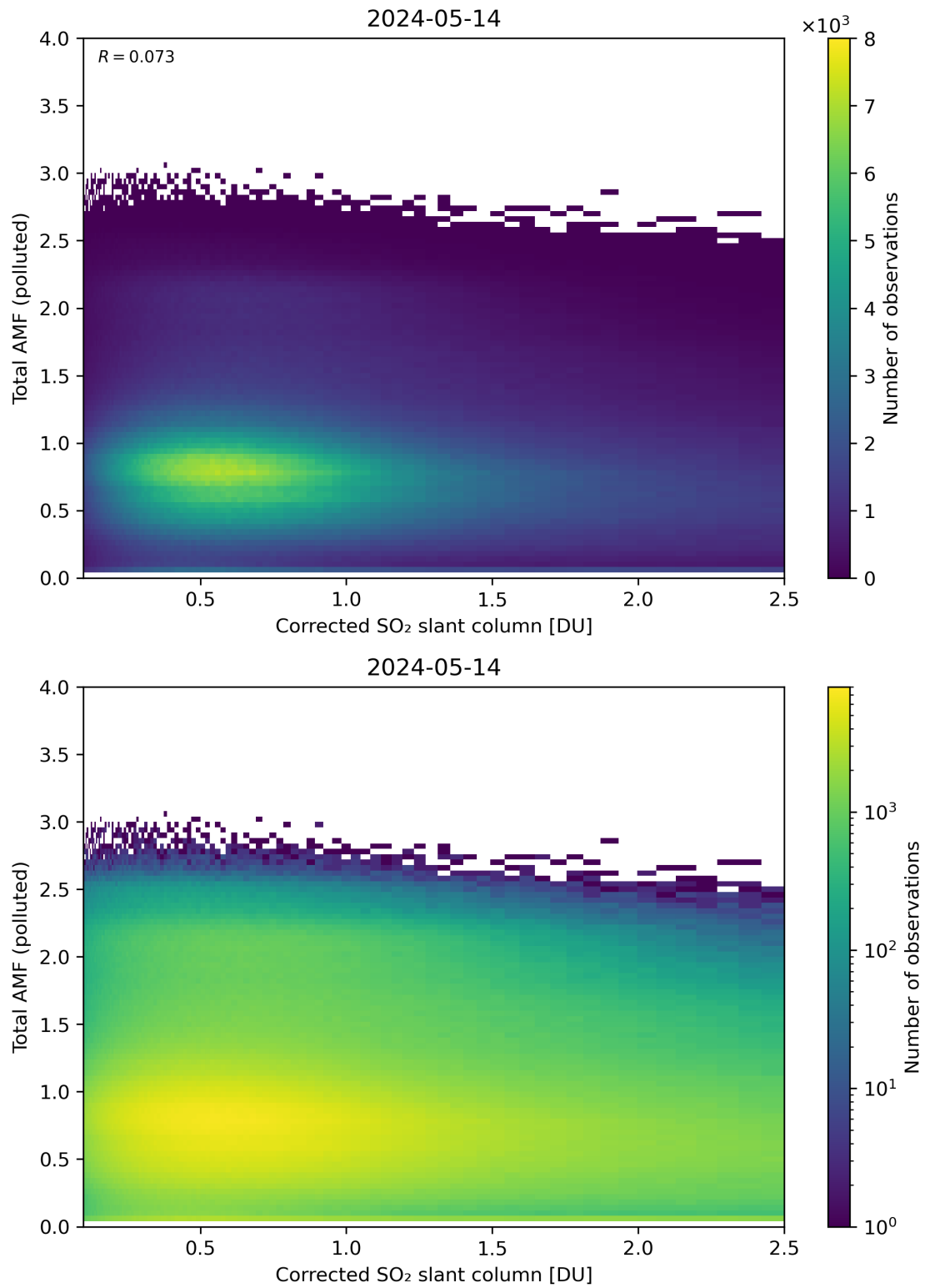
Figure 192: Scatter density plot of “Corrected SO 2 slant column” against “Total AMF (polluted)” for 2024-05-13 to 2024-05-15.
