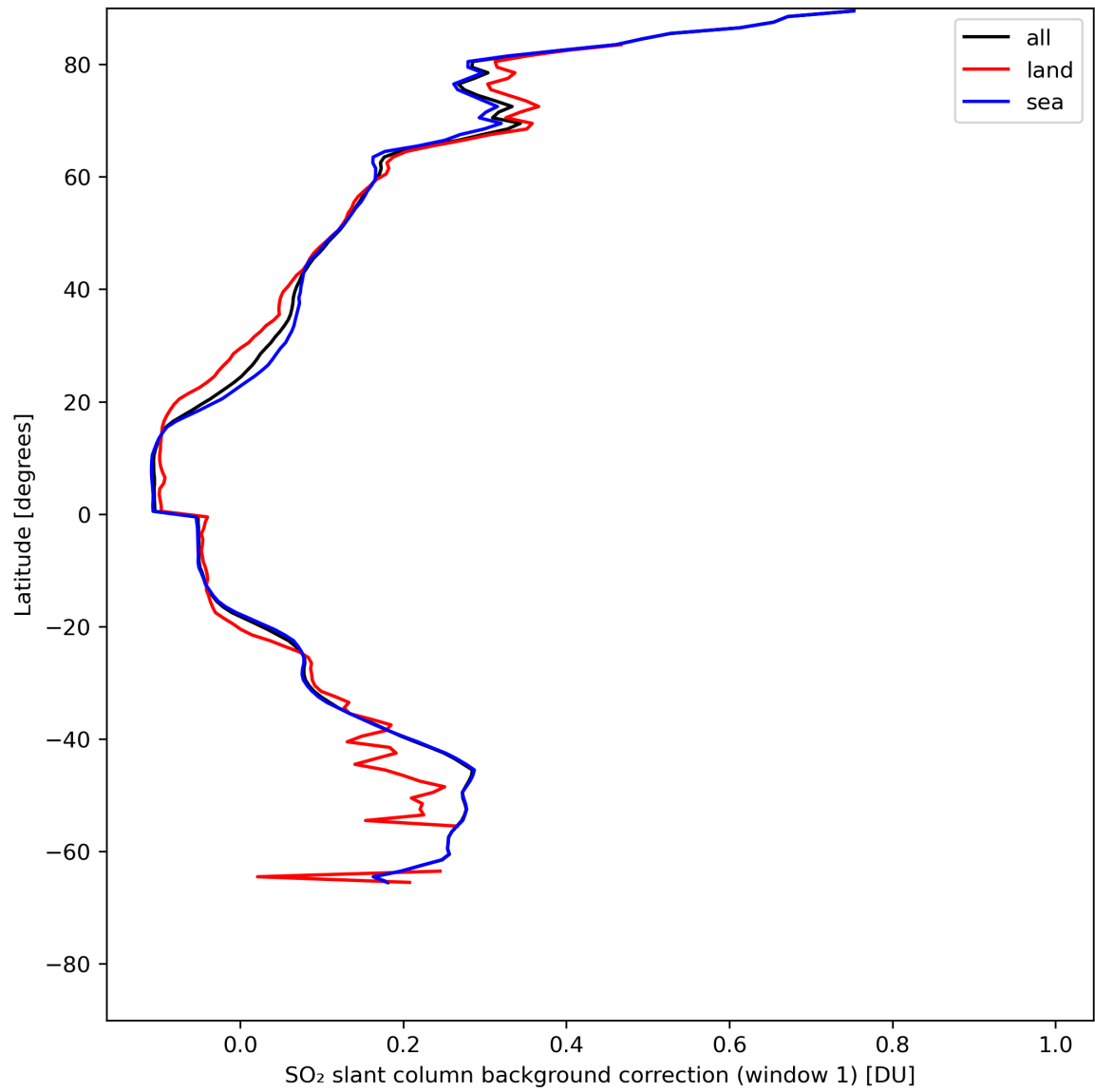
Figure 36: Zonal average of “SO 2 slant column background correction (window 1)” for 2024-05-13 to 2024-05-15.
