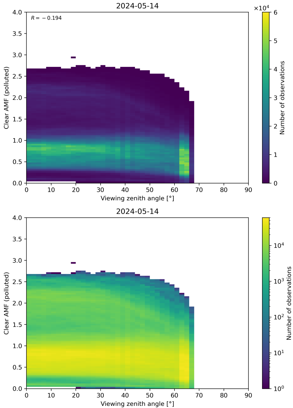
Figure 316: Scatter density plot of “Viewing zenith angle” against “Clear AMF (polluted)” for 2024-05-13 to 2024-05-15.
