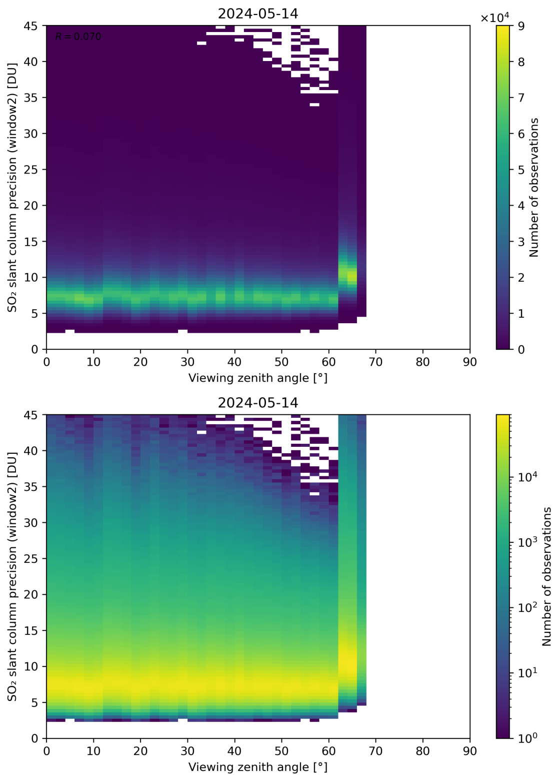
Figure 322: Scatter density plot of “Viewing zenith angle” against “SO 2 slant column precision (window2)” for 2024-05-13 to 2024-05-15.
