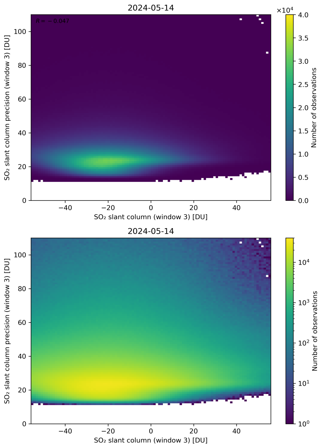
Figure 267: Scatter density plot of “SO 2 slant column (window 3)” against “SO 2 slant column precision (window 3)” for 2024-05-13 to 2024-05-15.
