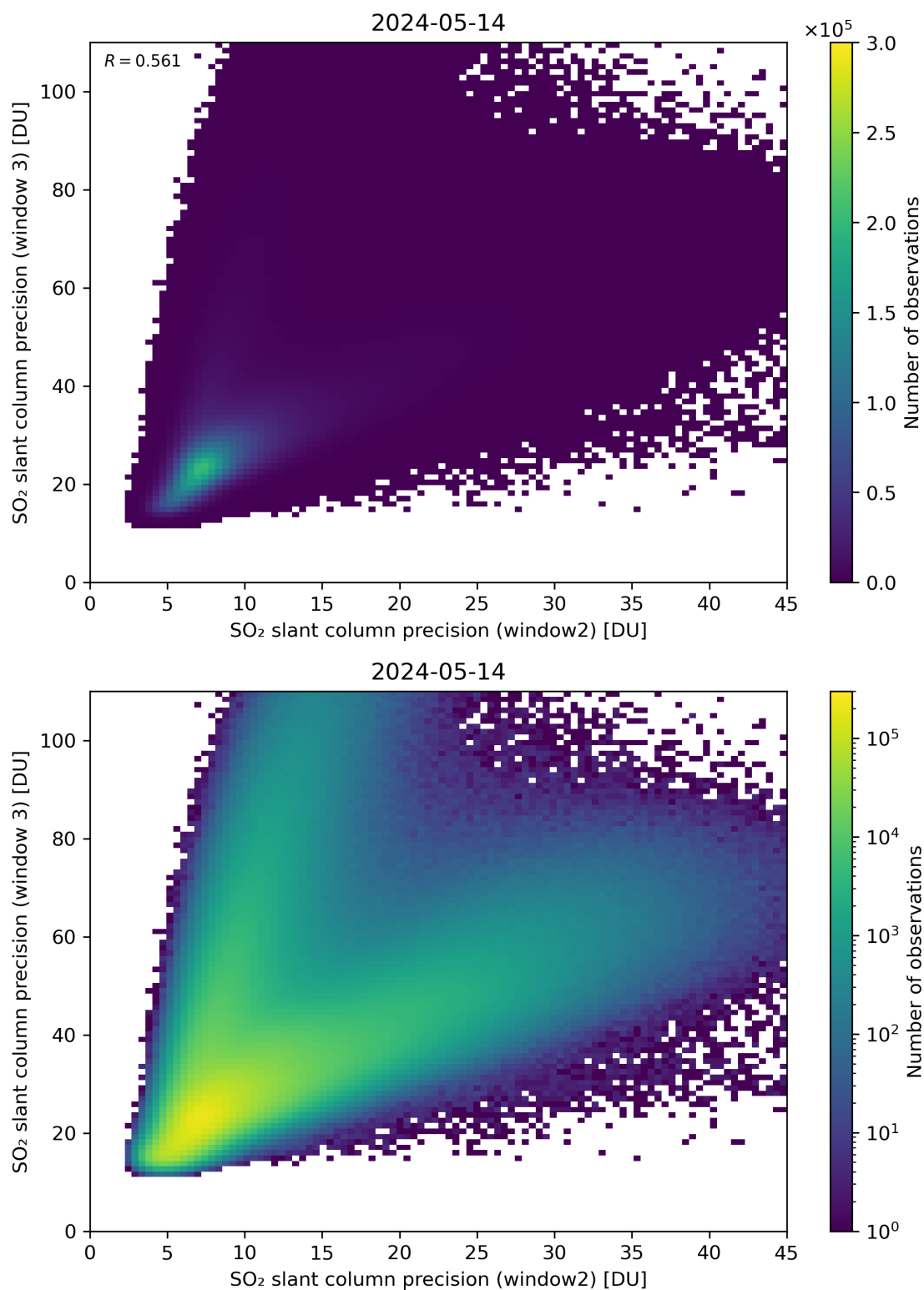
Figure 250: Scatter density plot of “SO 2 slant column precision (window2)” against “SO 2 slant column precision (window 3)” for 2024-05-13 to 2024-05-15.
