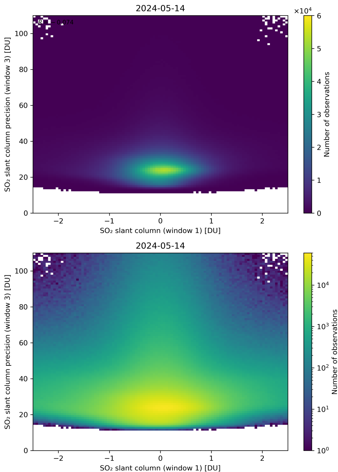
Figure 238: Scatter density plot of “SO 2 slant column (window 1)” against “SO 2 slant column precision (window 3)” for 2024-05-13 to 2024-05-15.
