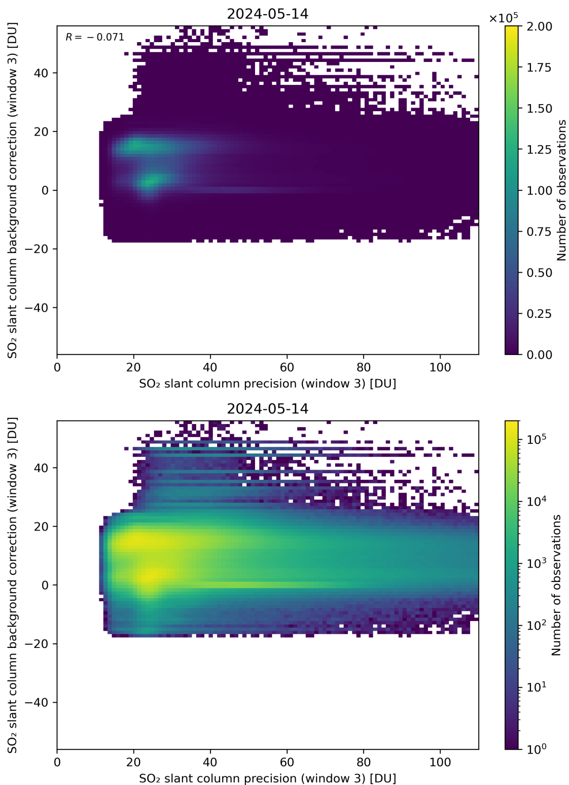
Figure 257: Scatter density plot of “SO 2 slant column precision (window 3)” against “SO 2 slant column background correction (window 3)” for 2024-05-13 to 2024-05-15.
