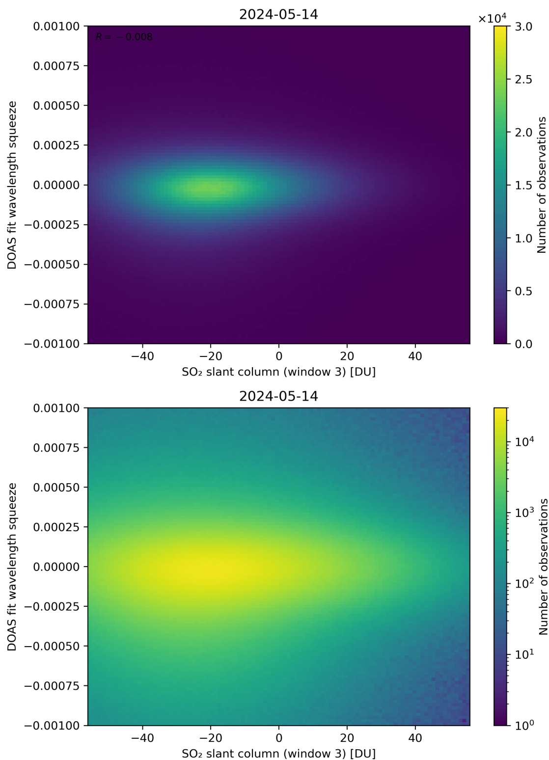
Figure 255: Scatter density plot of “SO 2 slant column (window 3)” against “DOAS fit wavelength squeeze” for 2024-05-13 to 2024-05-15.
