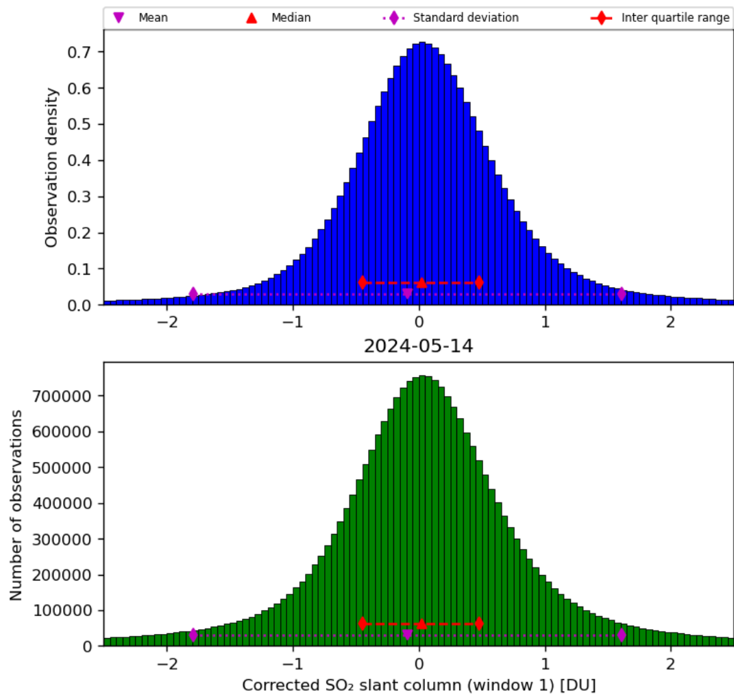
Figure 58: Histogram of “Corrected SO 2 slant column (window 1)” for 2024-05-13 to 2024-05-15
