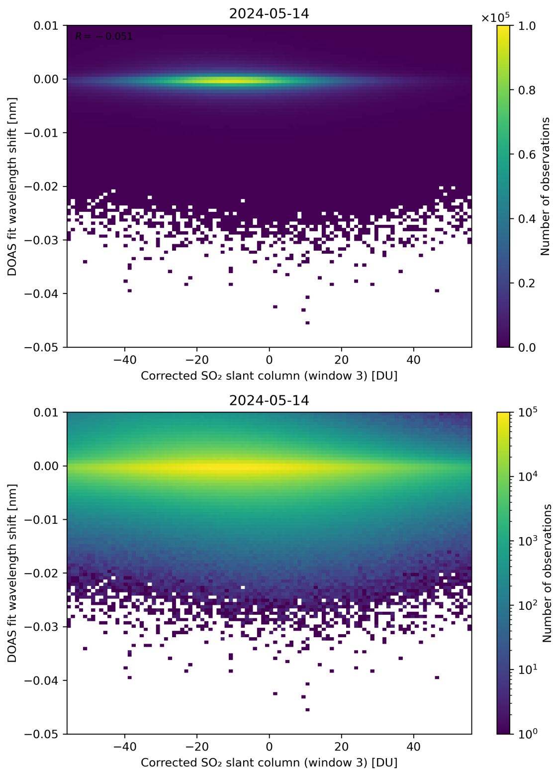
Figure 206: Scatter density plot of “Corrected SO 2 slant column (window 3)” against “DOAS fit wavelength shift” for 2024-05-13 to 2024-05-15.
