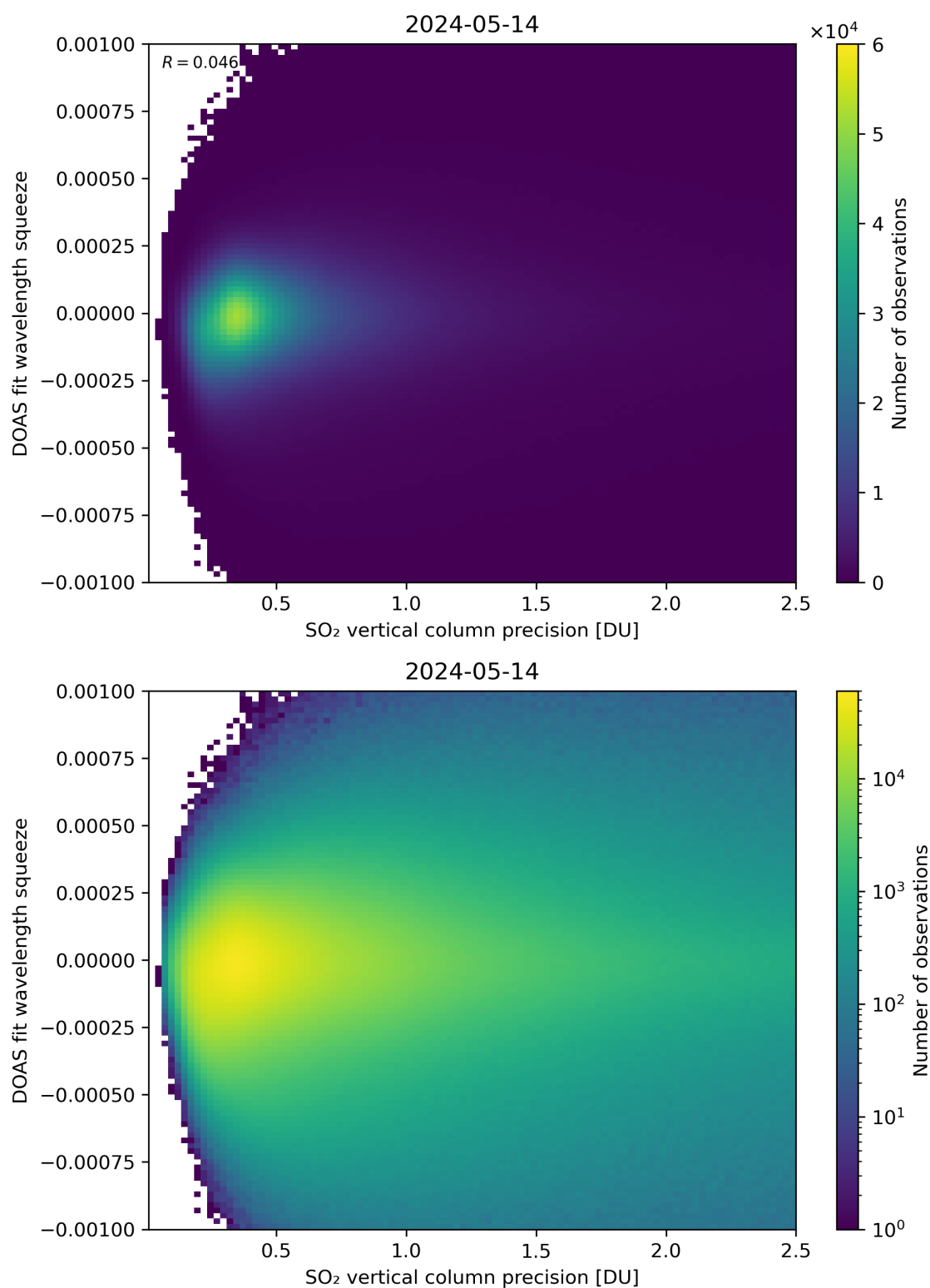
Figure 283: Scatter density plot of “SO 2 vertical column precision” against “DOAS fit wavelength squeeze” for 2024-05-13 to 2024-05-15.
