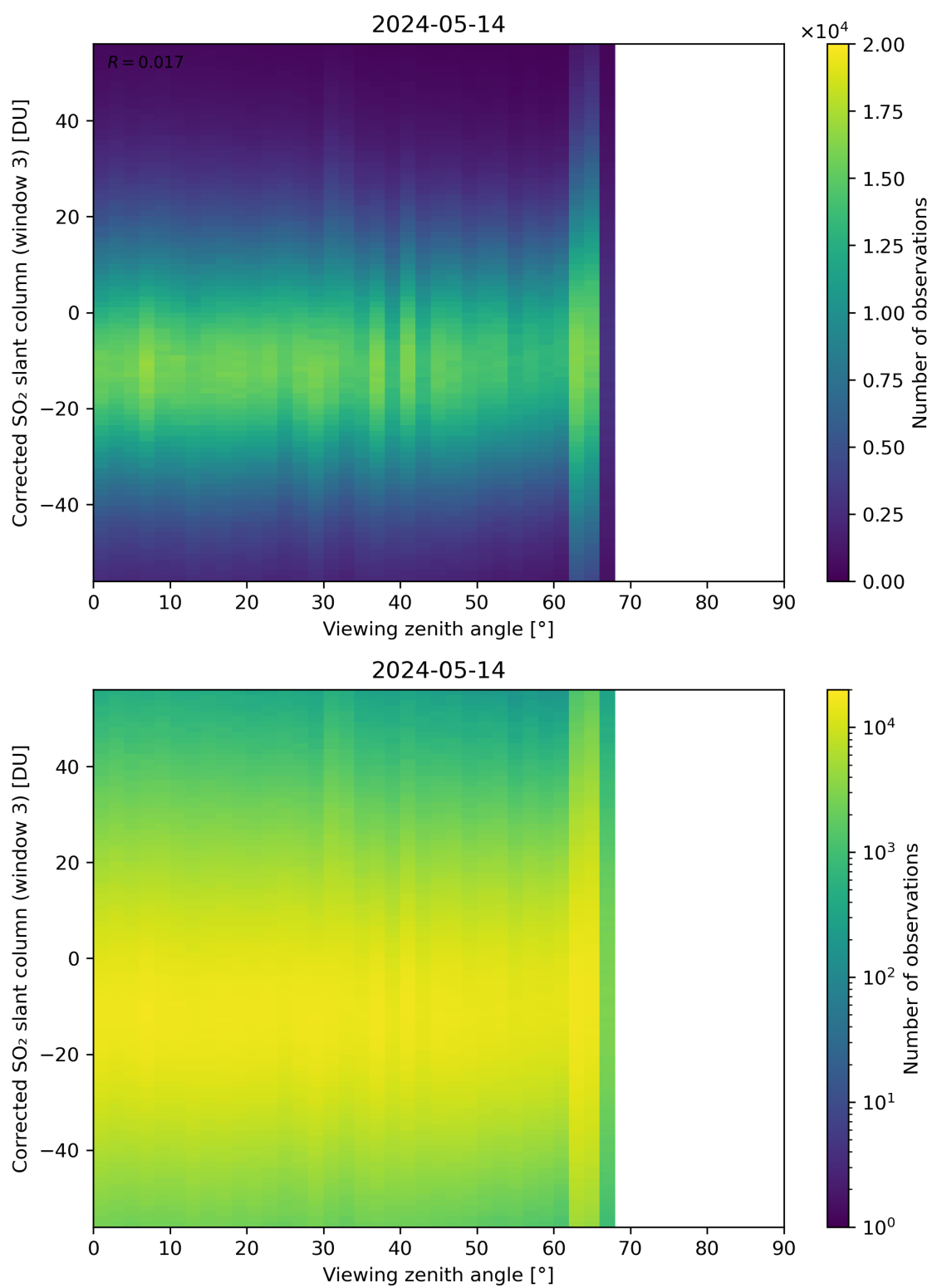
Figure 319: Scatter density plot of “Viewing zenith angle” against “Corrected SO 2 slant column (window 3)” for 2024-05-13 to 2024-05-15.
