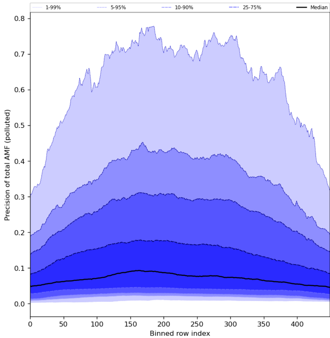
Figure 95: Along track statistics of “Precision of total AMF (polluted)” for 2024-05-13 to 2024-05-15
