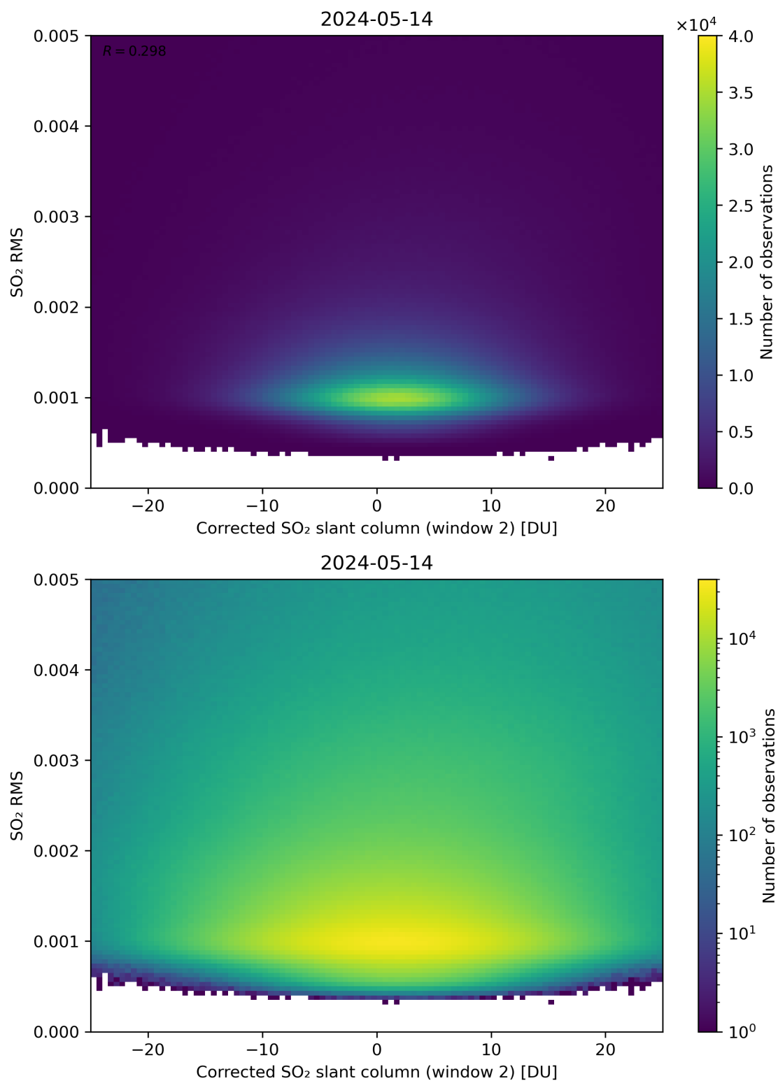
Figure 198: Scatter density plot of “Corrected SO 2 slant column (window 2)” against “SO 2 RMS” for 2024-05-13 to 2024-05-15.
