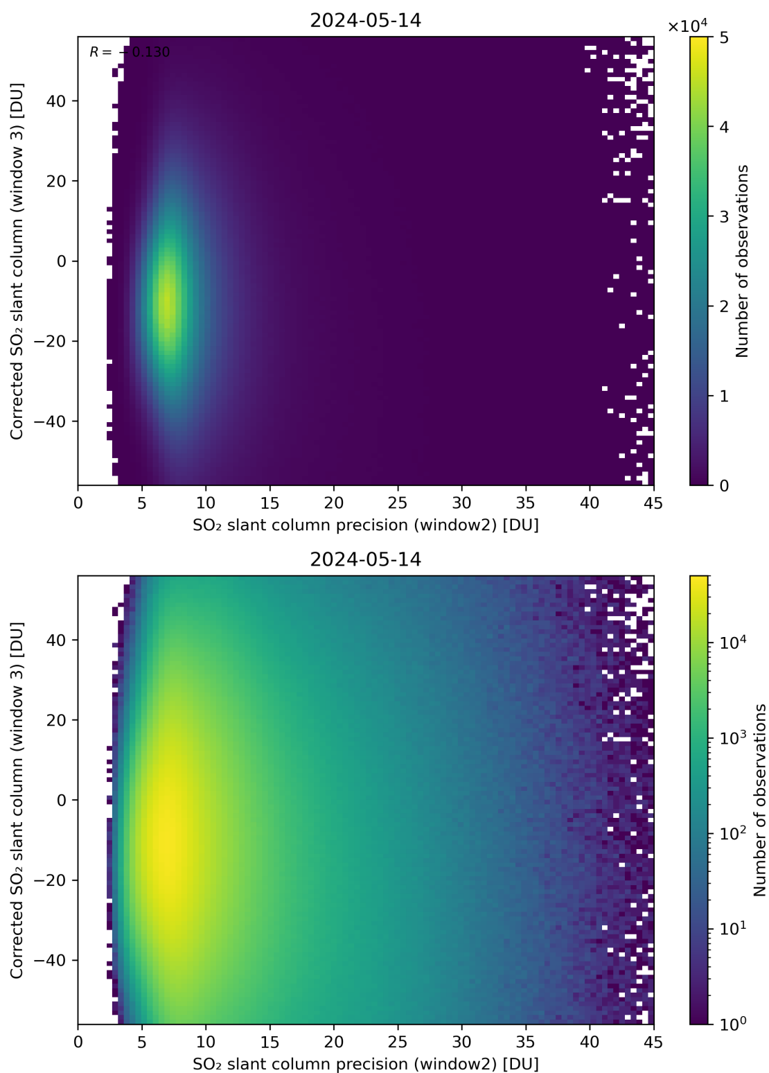
Figure 248: Scatter density plot of “SO 2 slant column precision (window2)” against “Corrected SO 2 slant column (window 3)” for 2024-05-13 to 2024-05-15.
