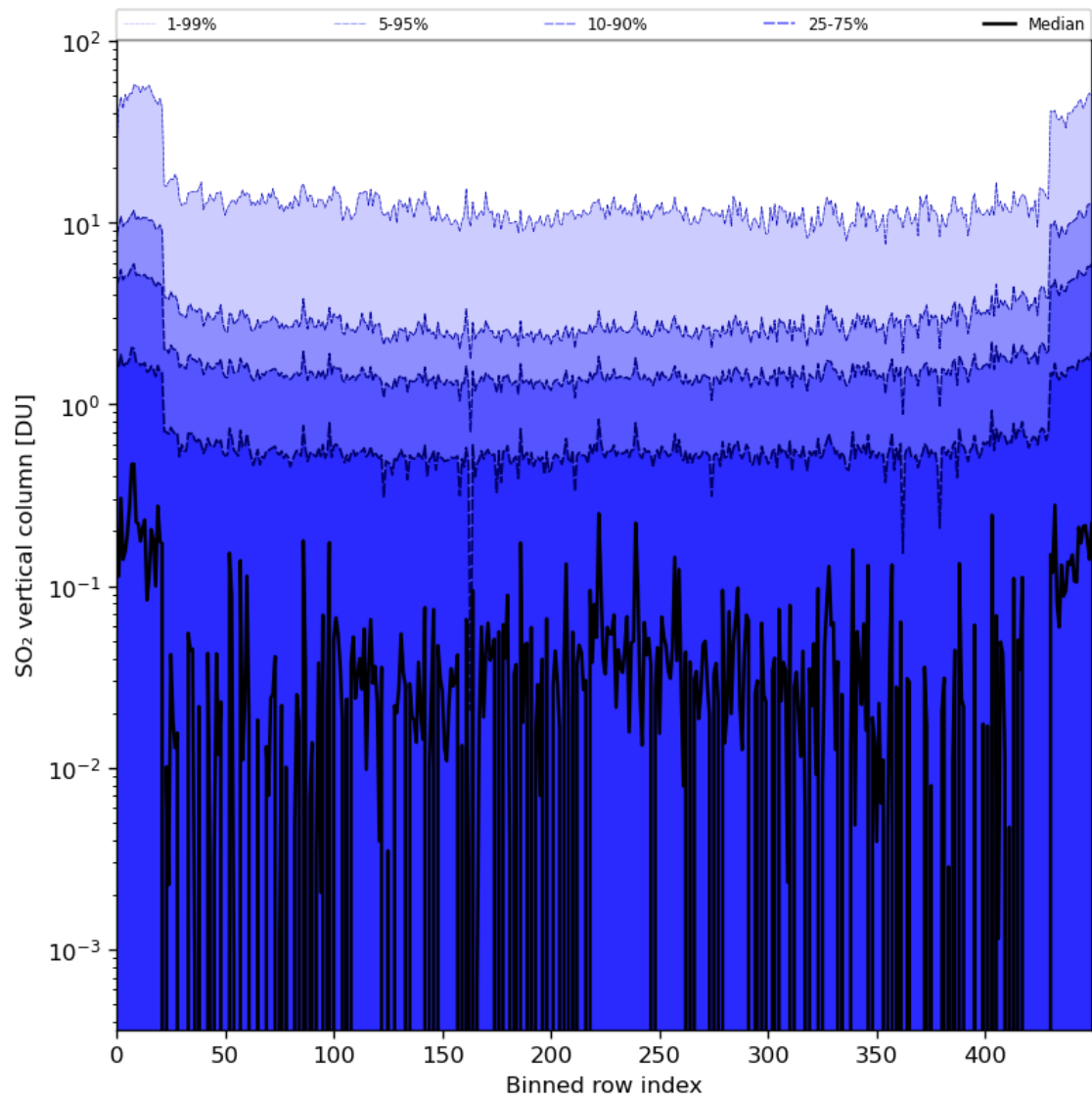
Figure 76: Along track statistics of “SO 2 vertical column” for 2024-05-13 to 2024-05-15
