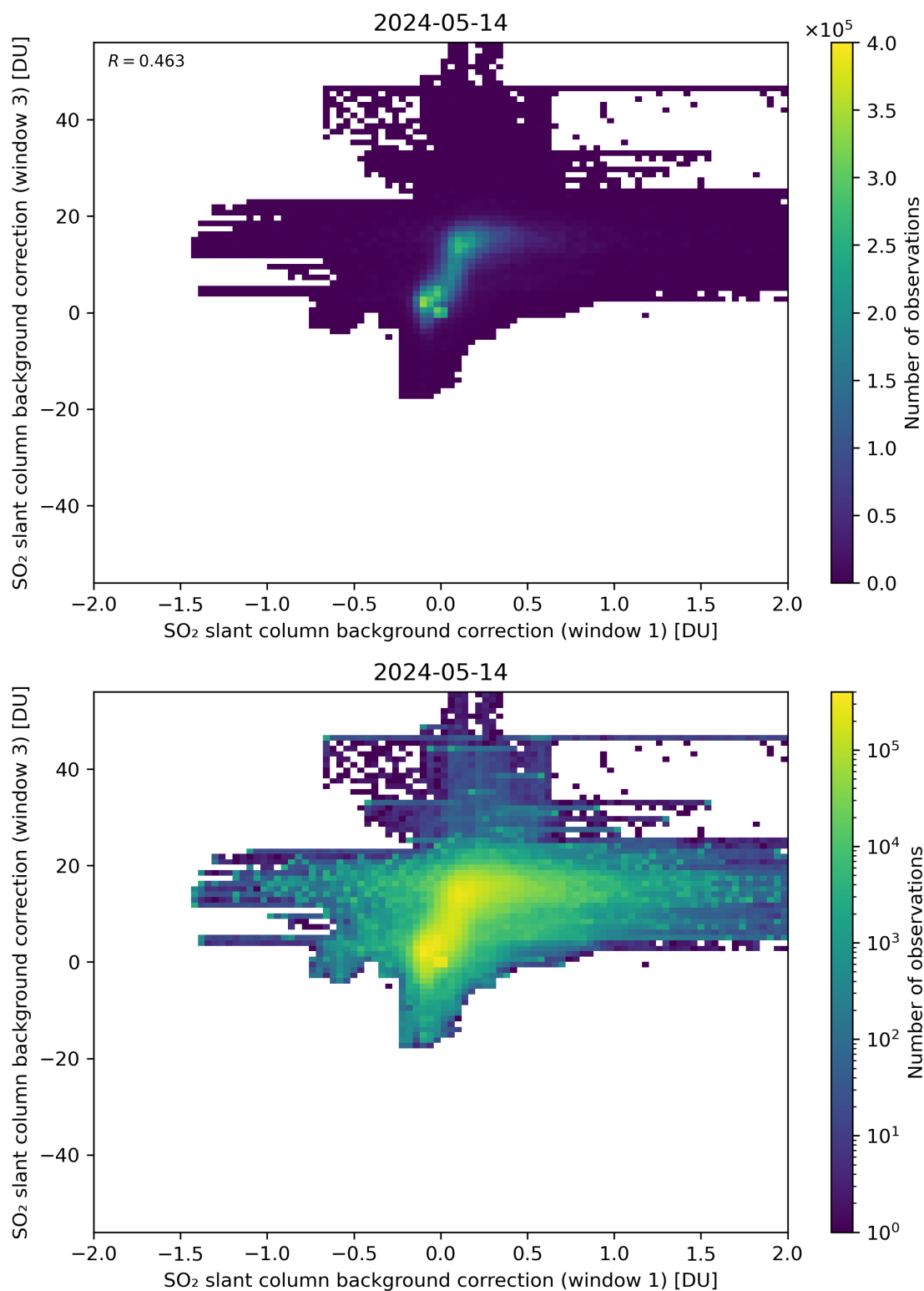
Figure 99: Scatter density plot of “SO 2 slant column background correction (window 1)” against “SO 2 slant column background correction (window 3)” for 2024-05-13 to 2024-05-15.
