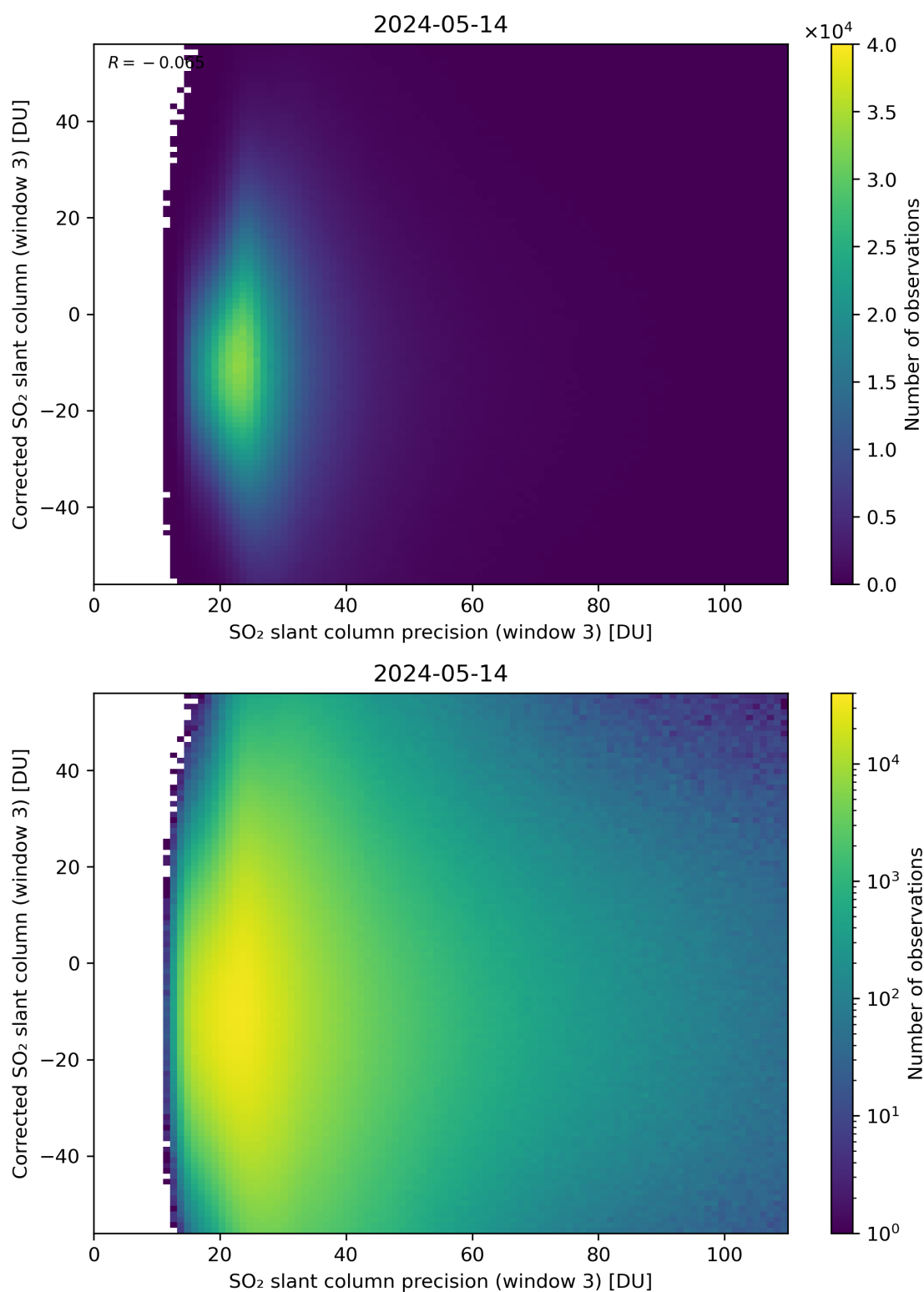
Figure 262: Scatter density plot of “SO 2 slant column precision (window 3)” against “Corrected SO 2 slant column (window 3)” for 2024-05-13 to 2024-05-15.
