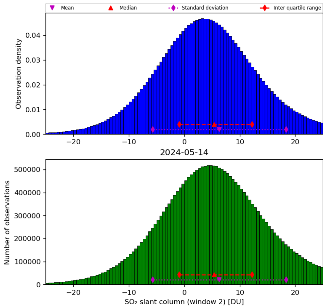
Figure 60: Histogram of “SO 2 slant column (window 2)” for 2024-05-13 to 2024-05-15
