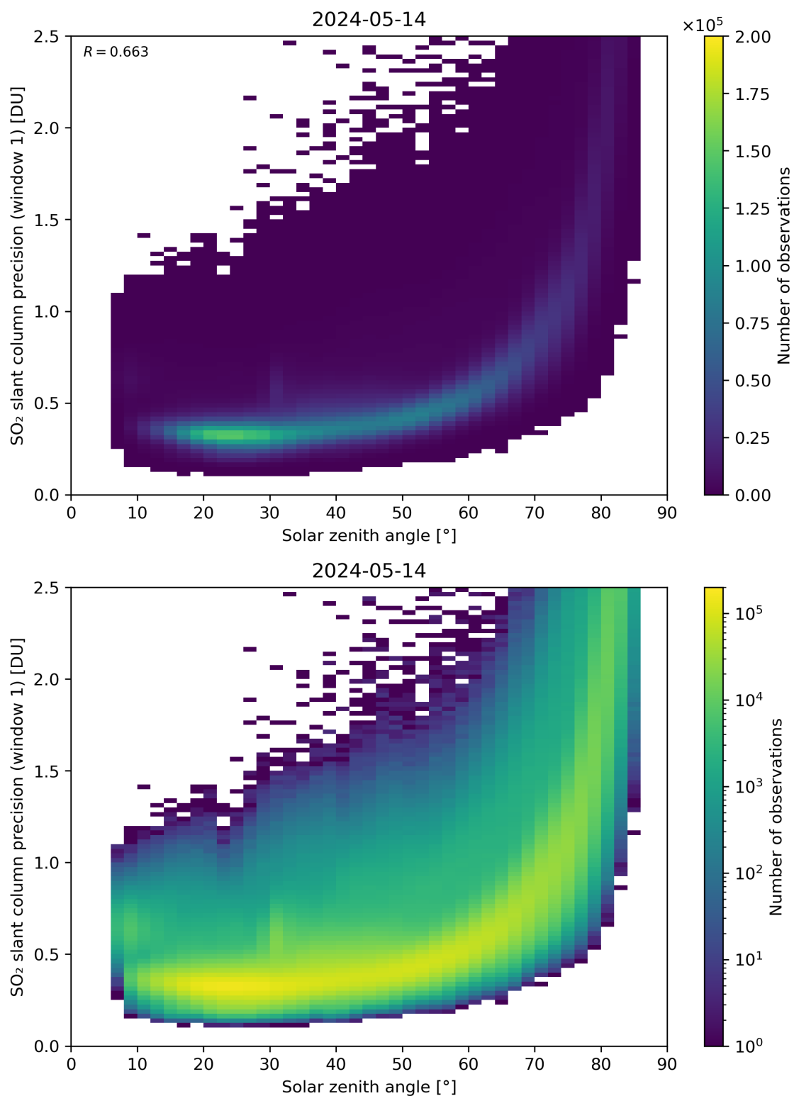
Figure 170: Scatter density plot of “Solar zenith angle” against “SO 2 slant column precision (window 1)” for 2024-05-13 to 2024-05-15.
