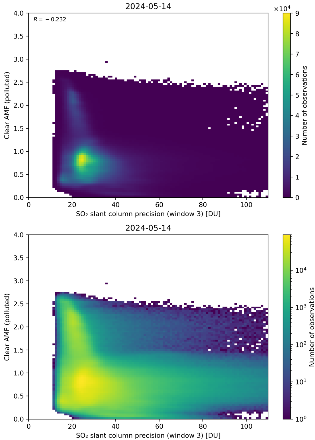
Figure 261: Scatter density plot of “SO 2 slant column precision (window 3)” against “Clear AMF (polluted)” for 2024-05-13 to 2024-05-15.
