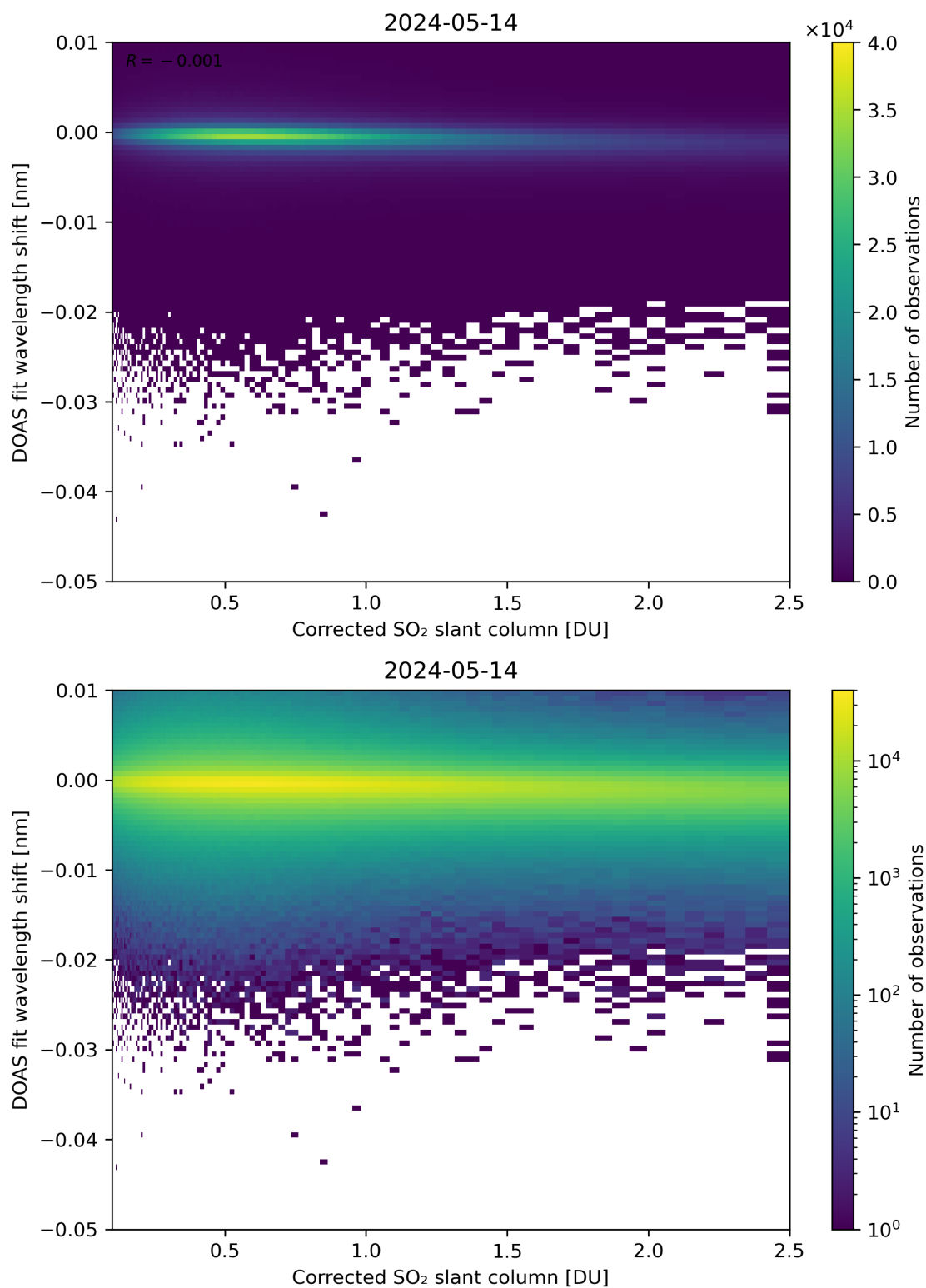
Figure 181: Scatter density plot of “Corrected SO 2 slant column” against “DOAS fit wavelength shift” for 2024-05-13 to 2024-05-15.
