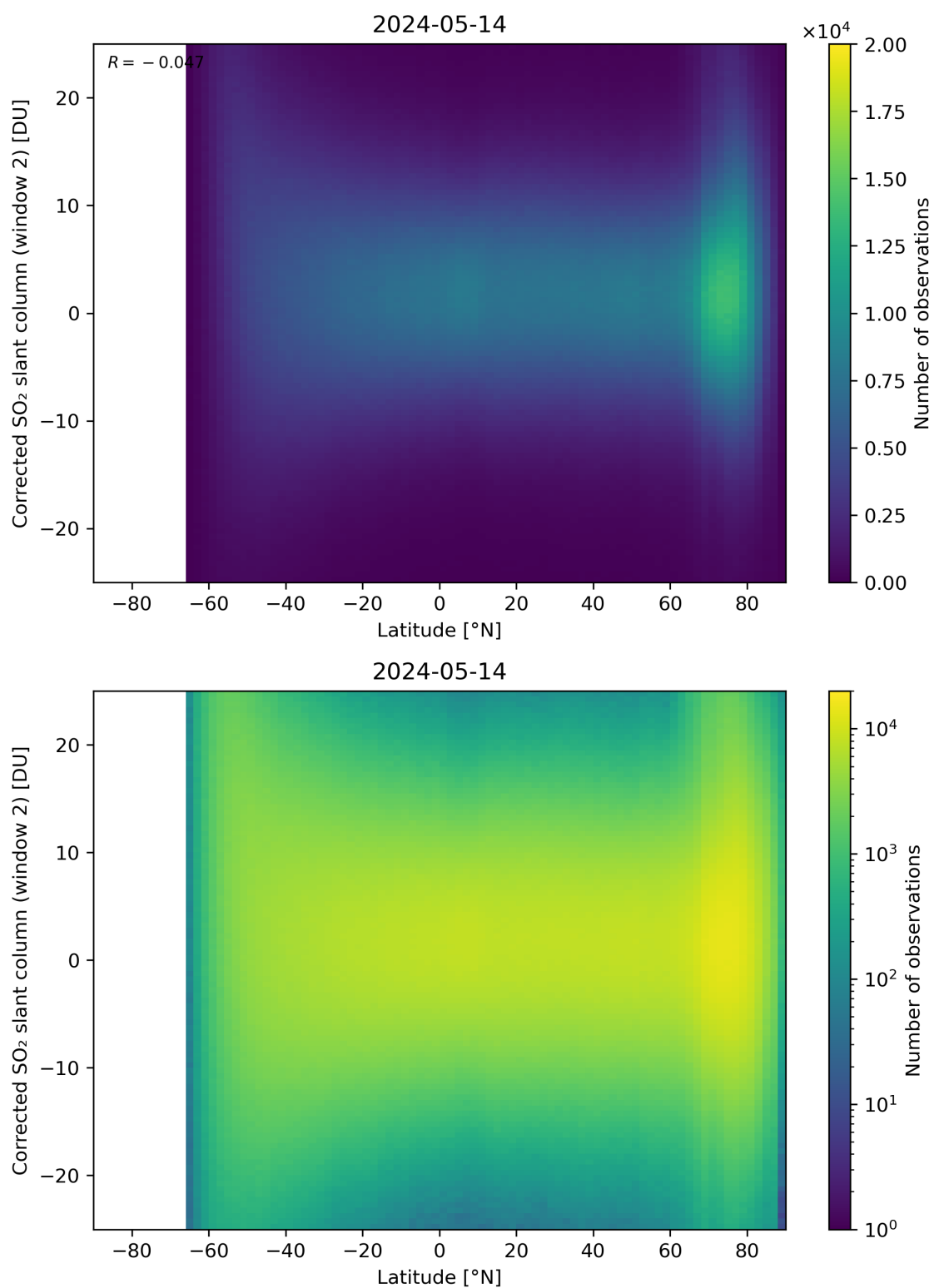
Figure 147: Scatter density plot of “Latitude” against “Corrected SO 2 slant column (window 2)” for 2024-05-13 to 2024-05-15.
