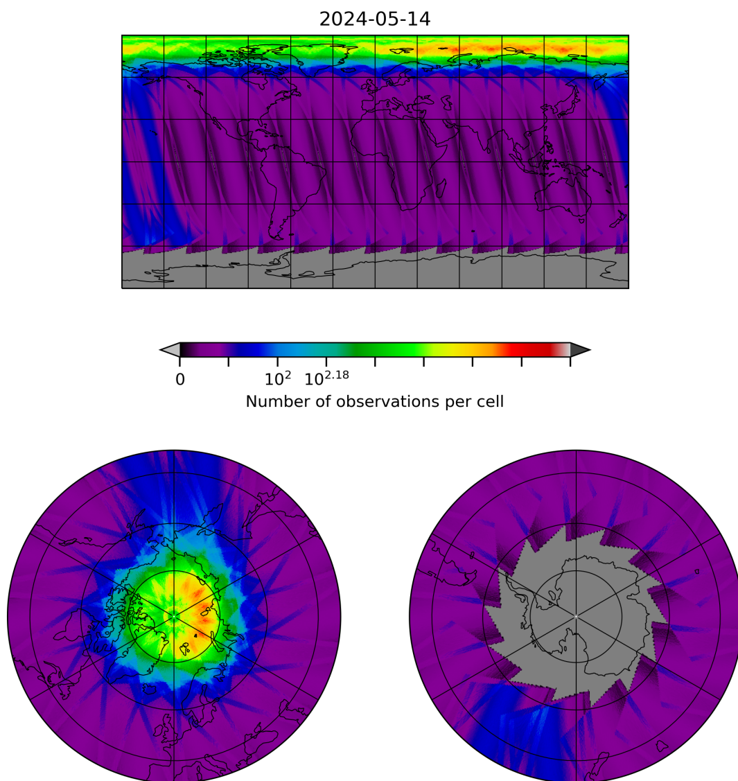
Figure 28: Map of the number of observations for 2024-05-13 to 2024-05-15
