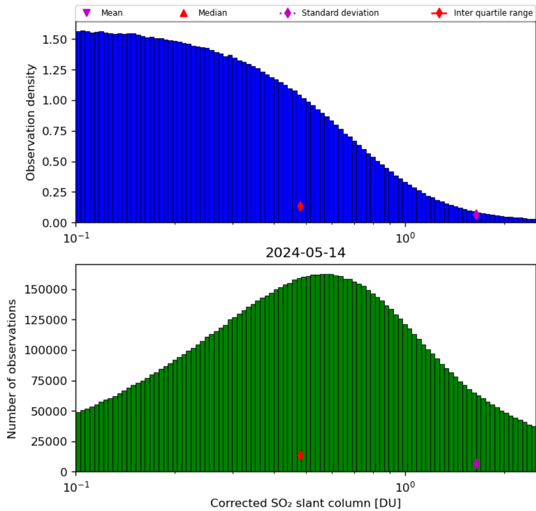
Figure 55: Histogram of “Corrected SO 2 slant column” for 2024-05-13 to 2024-05-15
