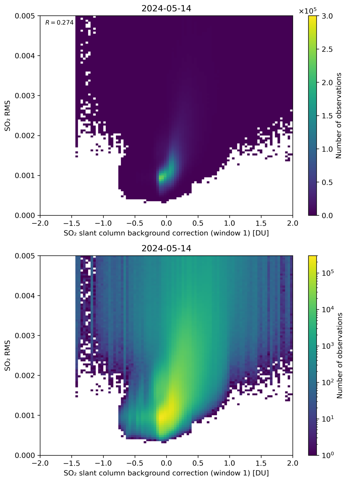
Figure 102: Scatter density plot of “SO 2 slant column background correction (window 1)” against “SO 2 RMS” for 2024-05-13 to 2024-05-15.
