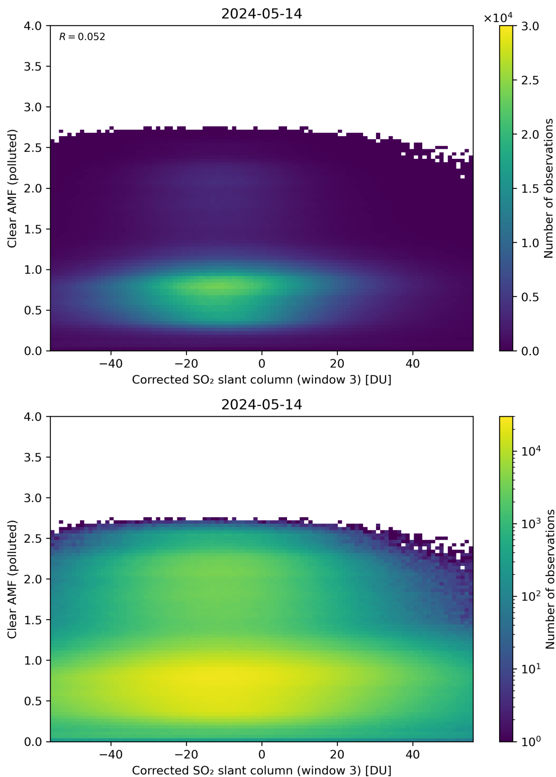
Figure 209: Scatter density plot of “Corrected SO 2 slant column (window 3)” against “Clear AMF (polluted)” for 2024-05-13 to 2024-05-15.
