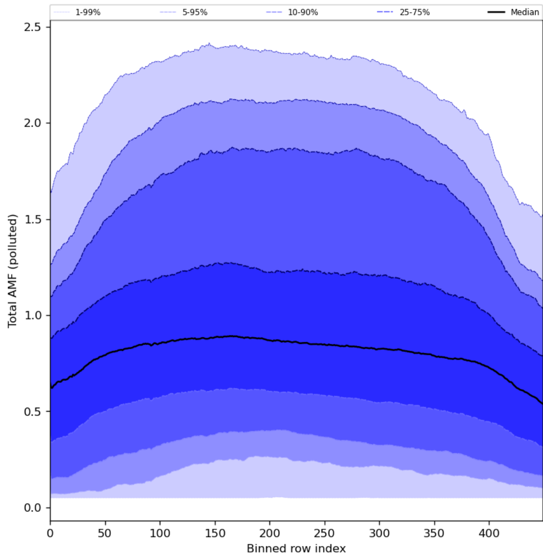
Figure 94: Along track statistics of “Total AMF (polluted)” for 2024-05-13 to 2024-05-15
