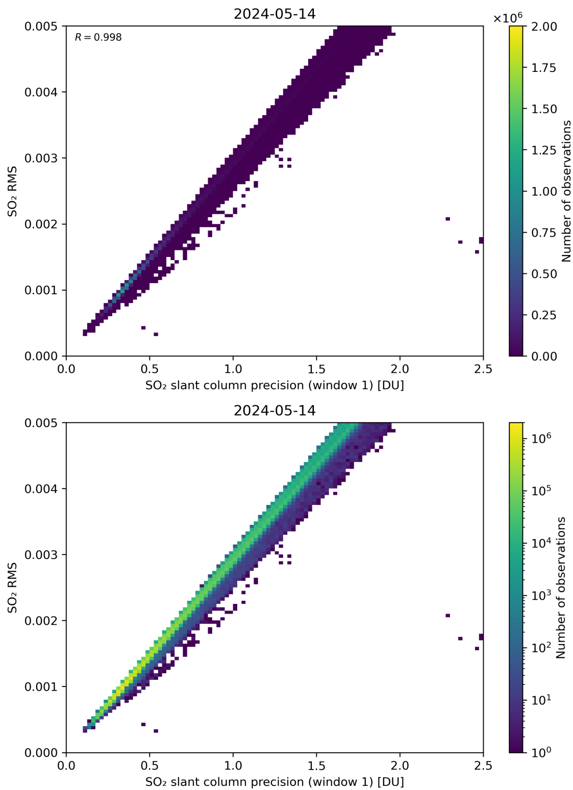
Figure 223: Scatter density plot of “SO 2 slant column precision (window 1)” against “SO 2 RMS” for 2024-05-13 to 2024-05-15.
