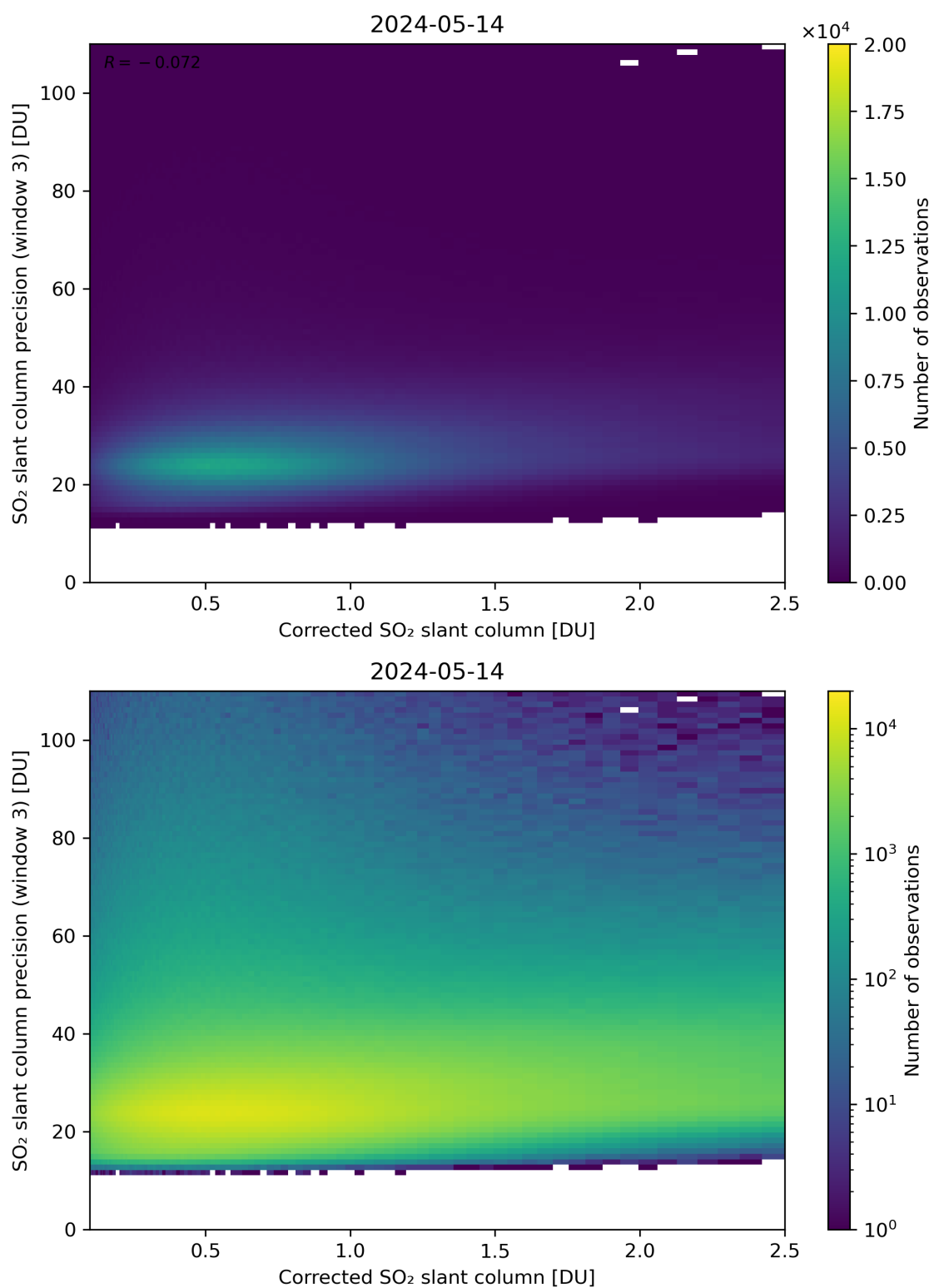
Figure 191: Scatter density plot of “Corrected SO 2 slant column” against “SO 2 slant column precision (window 3)” for 2024-05-13 to 2024-05-15.
