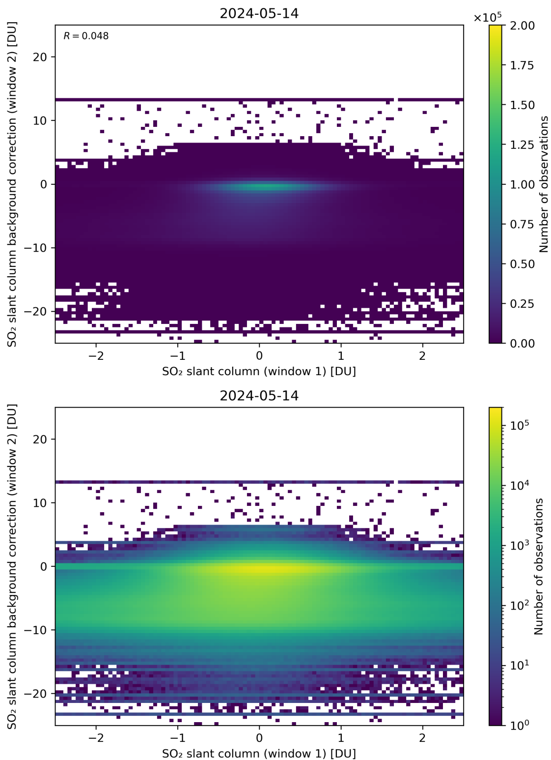
Figure 213: Scatter density plot of “SO 2 slant column (window 1)” against “SO 2 slant column background correction (window 2)” for 2024-05-13 to 2024-05-15.
