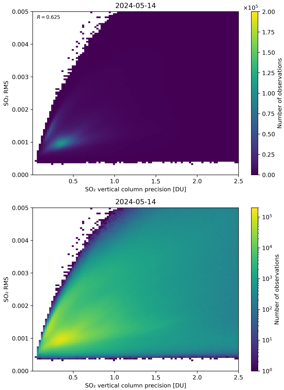
Figure 284: Scatter density plot of “SO 2 vertical column precision” against “SO 2 RMS” for 2024-05-13 to 2024-05-15.
