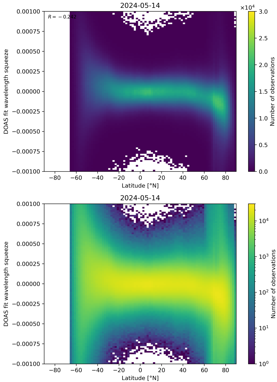
Figure 143: Scatter density plot of “Latitude” against “DOAS fit wavelength squeeze” for 2024-05-13 to 2024-05-15.
