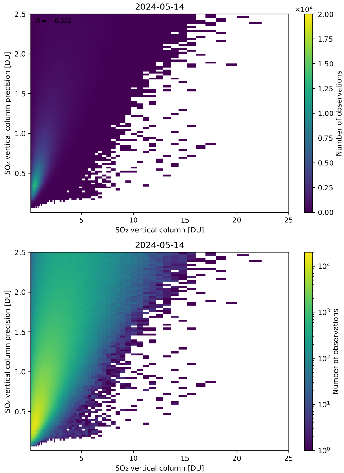
Figure 307: Scatter density plot of “SO 2 vertical column” against “SO 2 vertical column precision” for 2024-05-13 to 2024-05-15.
