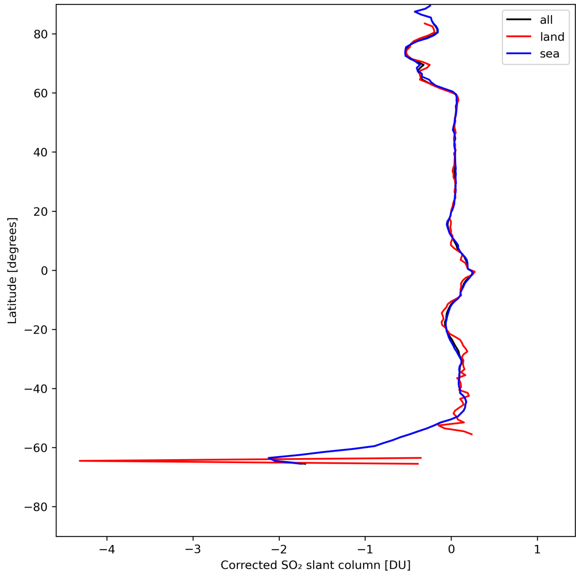
Figure 32: Zonal average of “Corrected SO 2 slant column” for 2024-05-13 to 2024-05-15.
