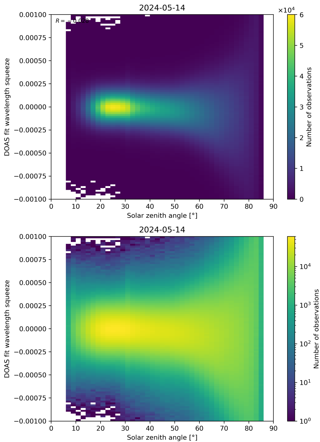
Figure 162: Scatter density plot of “Solar zenith angle” against “DOAS fit wavelength squeeze” for 2024-05-13 to 2024-05-15.
