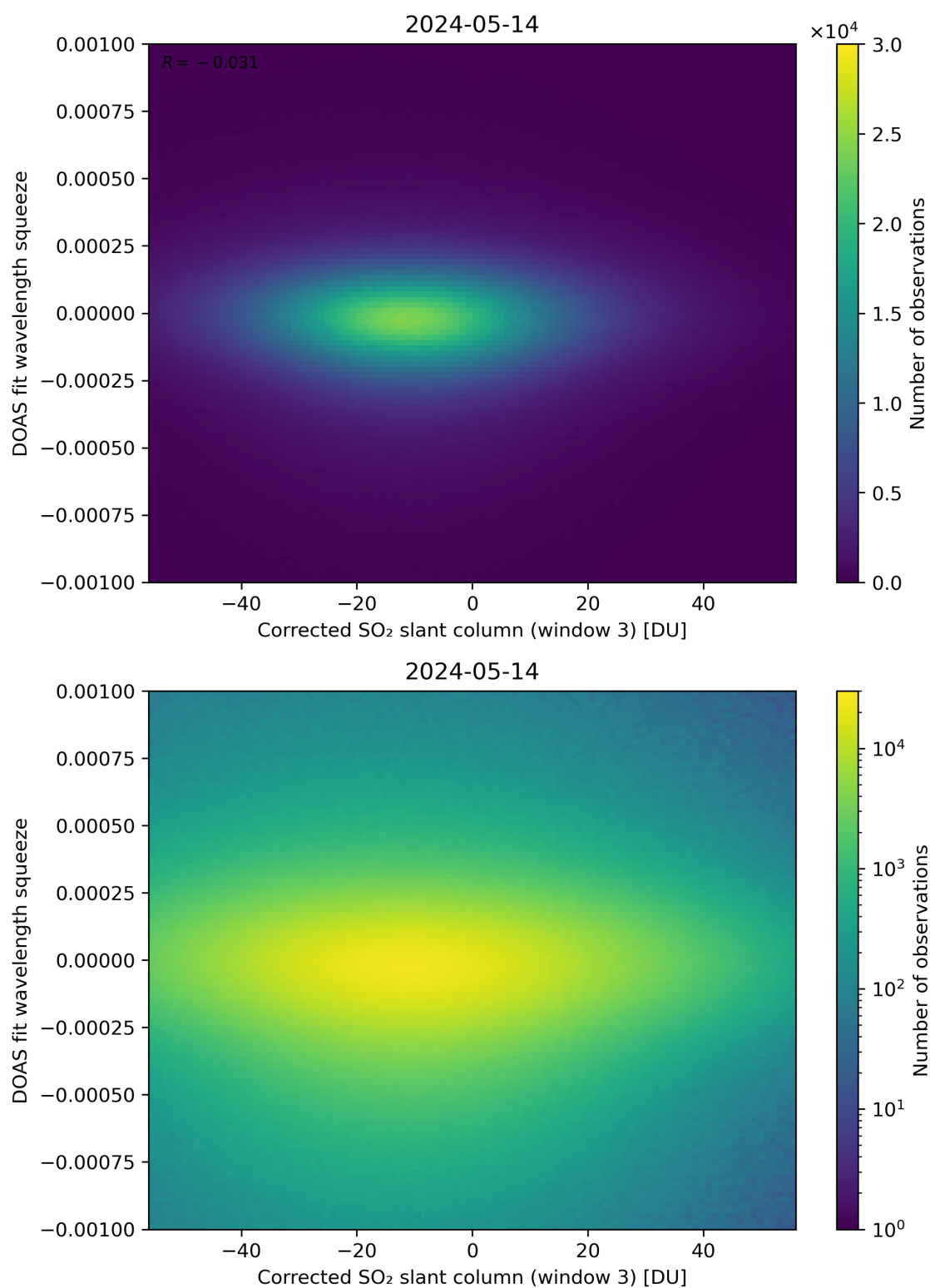
Figure 207: Scatter density plot of “Corrected SO 2 slant column (window 3)” against “DOAS fit wavelength squeeze” for 2024-05-13 to 2024-05-15.
