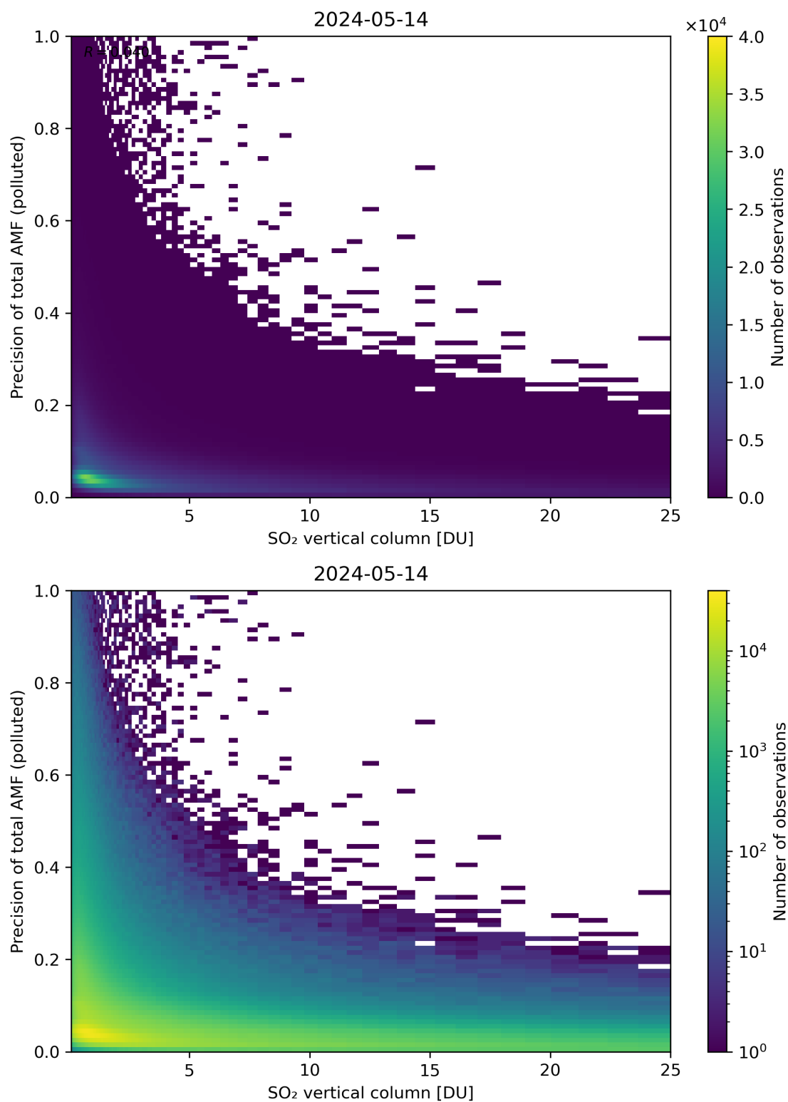
Figure 306: Scatter density plot of “SO 2 vertical column” against “Precision of total AMF (polluted)” for 2024-05-13 to 2024-05-15.
