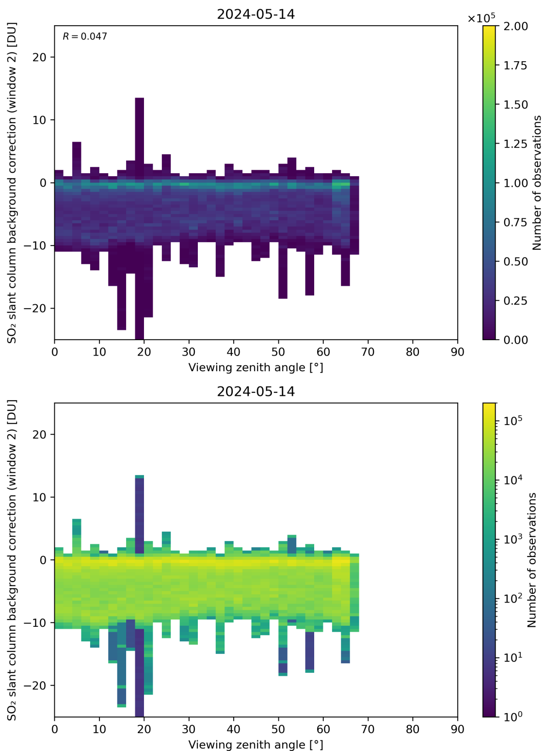
Figure 309: Scatter density plot of “Viewing zenith angle” against “SO 2 slant column background correction (window 2)” for 2024-05-13 to 2024-05-15.
