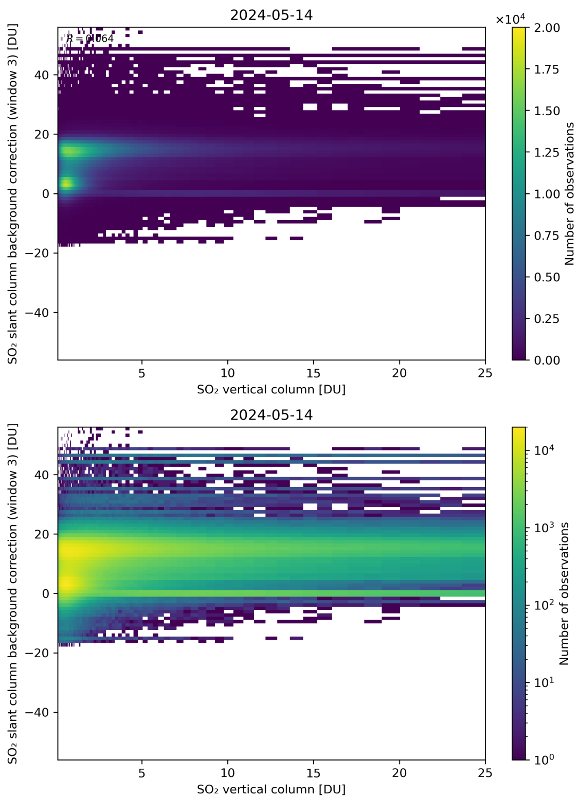
Figure 275: Scatter density plot of “SO 2 vertical column” against “SO 2 slant column background correction (window 3)” for 2024-05-13 to 2024-05-15.
