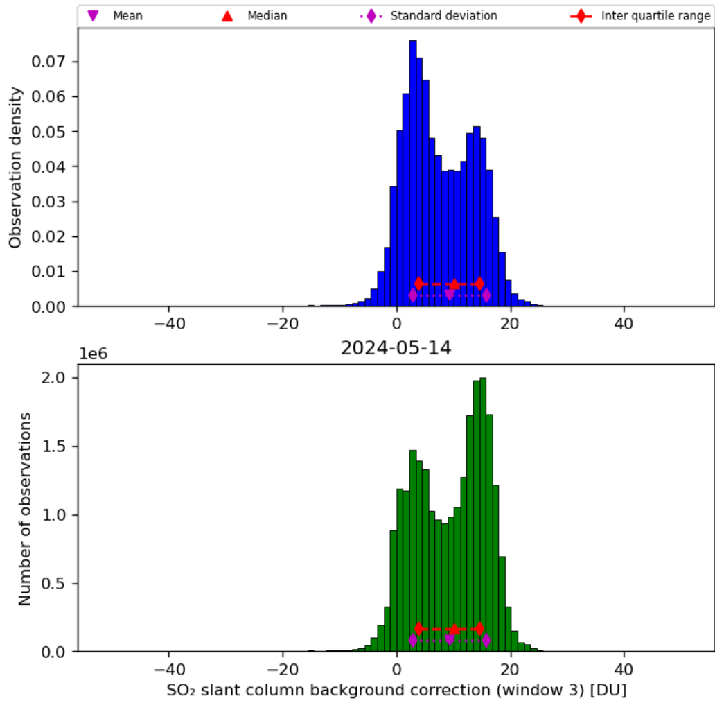
Figure 67: Histogram of “SO 2 slant column background correction (window 3)” for 2024-05-13 to 2024-05-15
