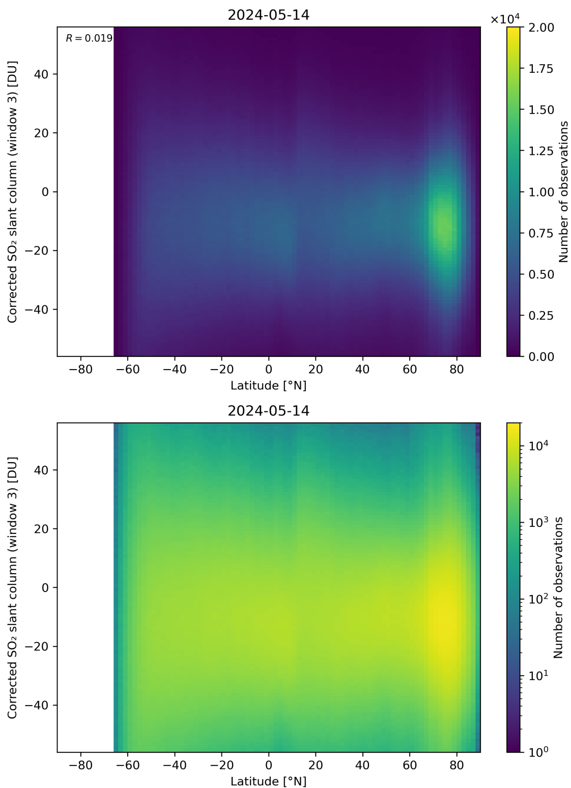
Figure 148: Scatter density plot of “Latitude” against “Corrected SO 2 slant column (window 3)” for 2024-05-13 to 2024-05-15.
