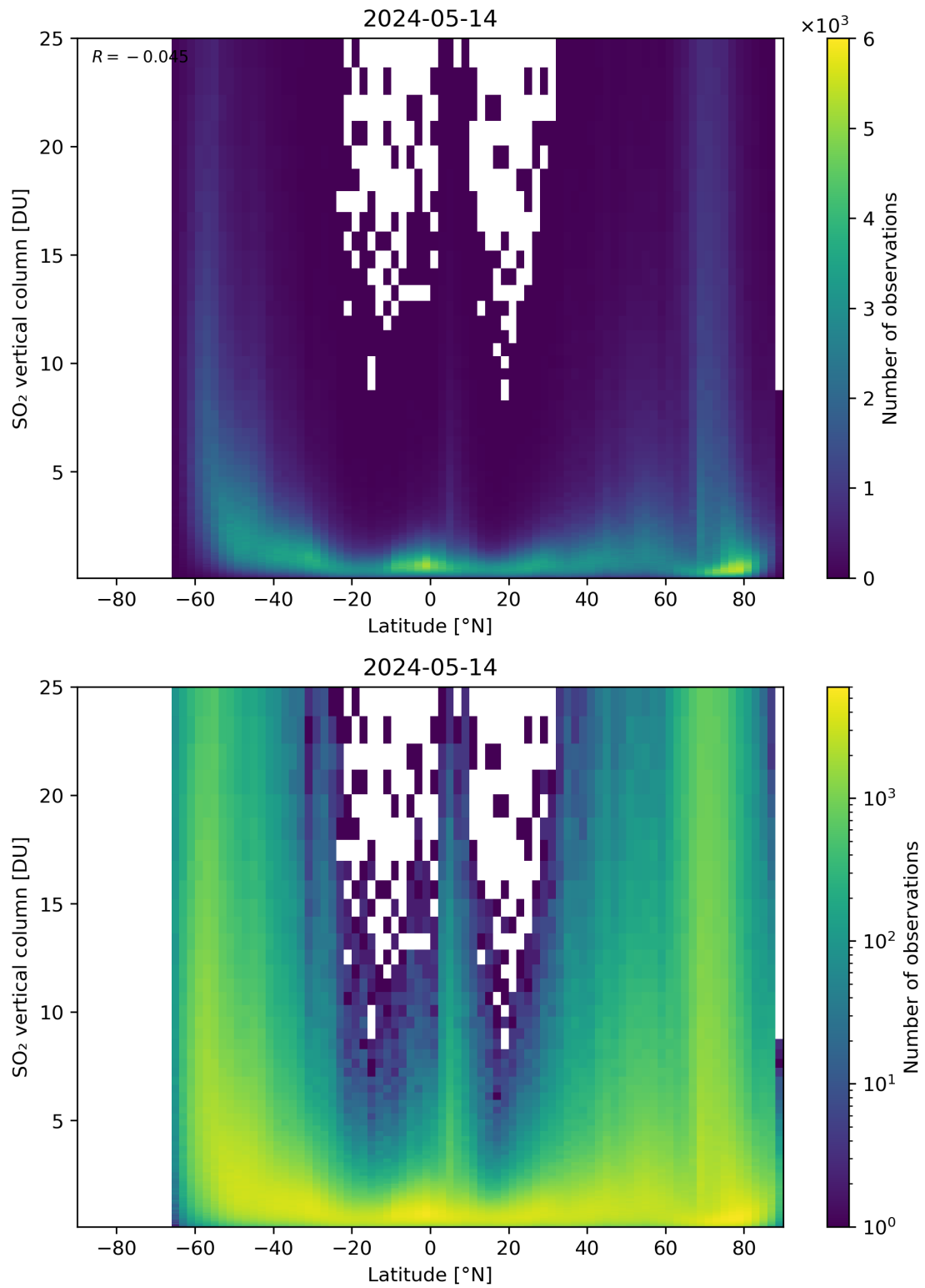
Figure 156: Scatter density plot of “Latitude” against “SO 2 vertical column” for 2024-05-13 to 2024-05-15.
