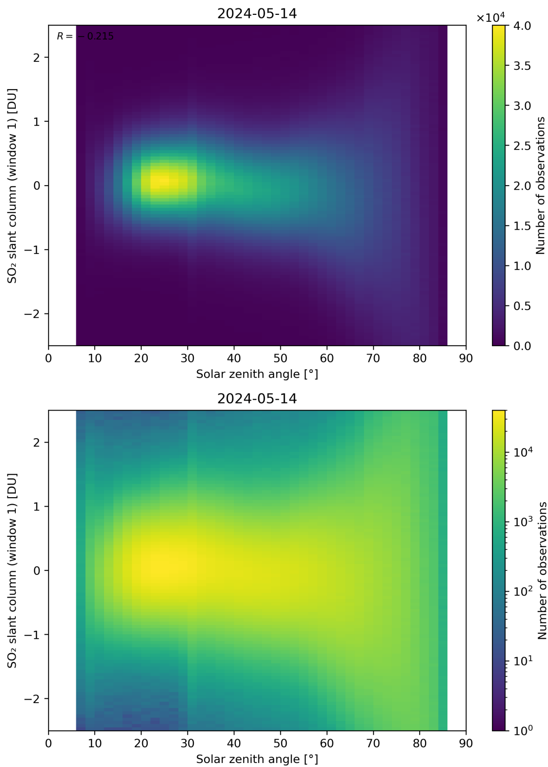
Figure 169: Scatter density plot of “Solar zenith angle” against “SO 2 slant column (window 1)” for 2024-05-13 to 2024-05-15.
