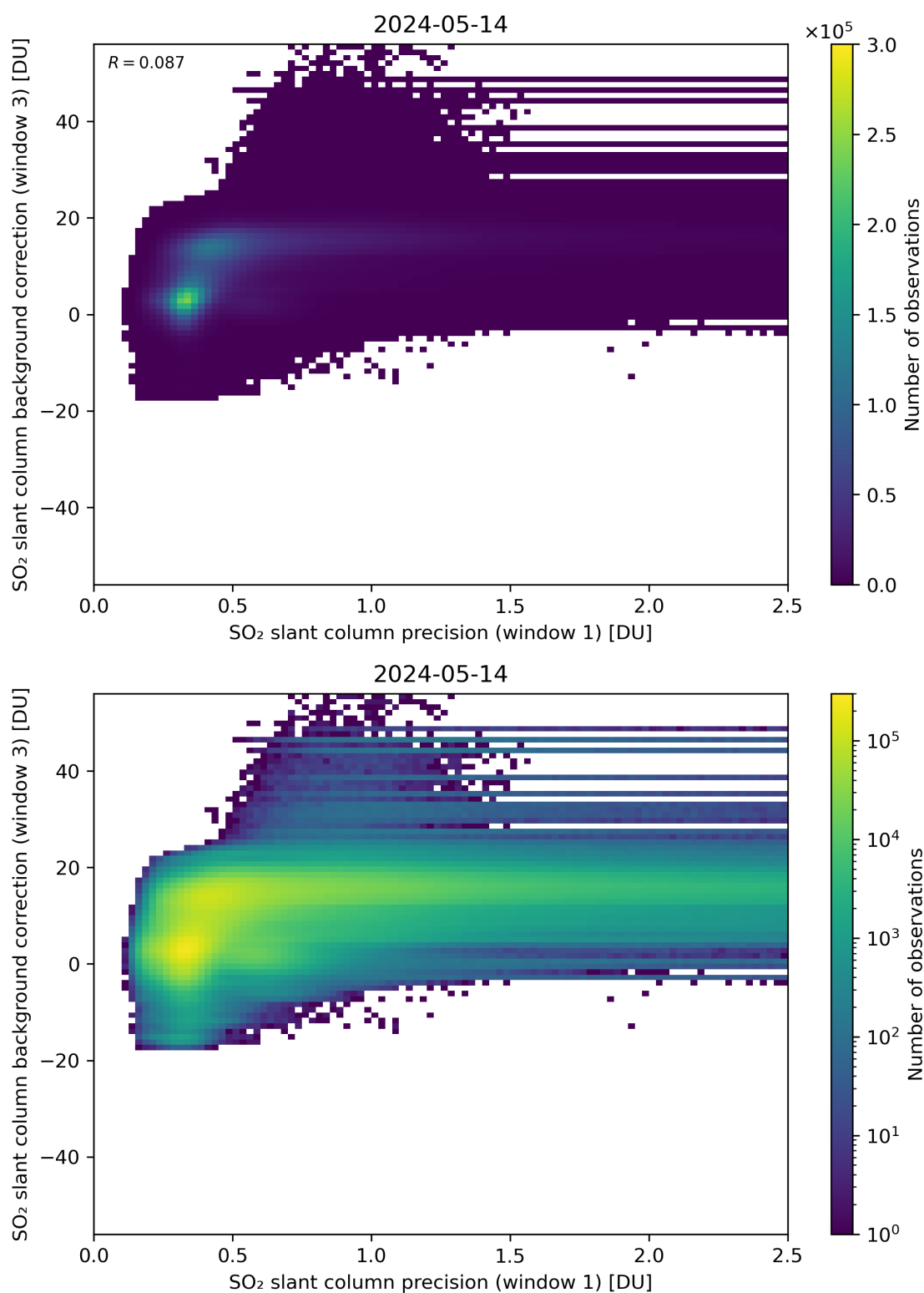
Figure 220: Scatter density plot of “SO 2 slant column precision (window 1)” against “SO 2 slant column background correction (window 3)” for 2024-05-13 to 2024-05-15.
