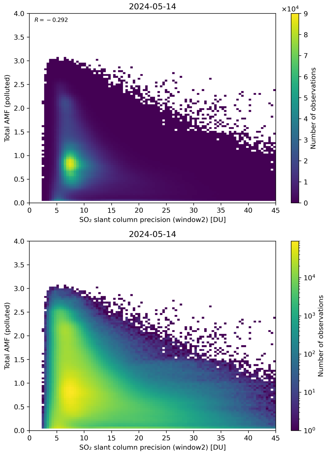
Figure 251: Scatter density plot of “SO 2 slant column precision (window2)” against “Total AMF (polluted)” for 2024-05-13 to 2024-05-15.
