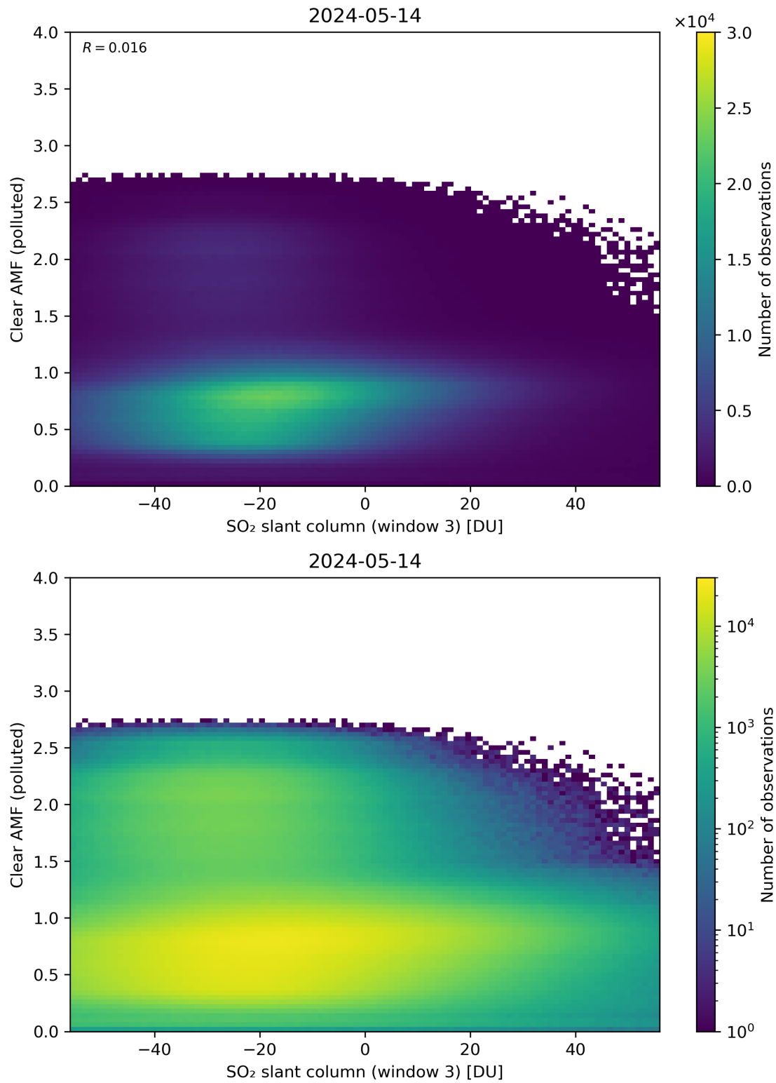
Figure 265: Scatter density plot of “SO 2 slant column (window 3)” against “Clear AMF (polluted)” for 2024-05-13 to 2024-05-15.
