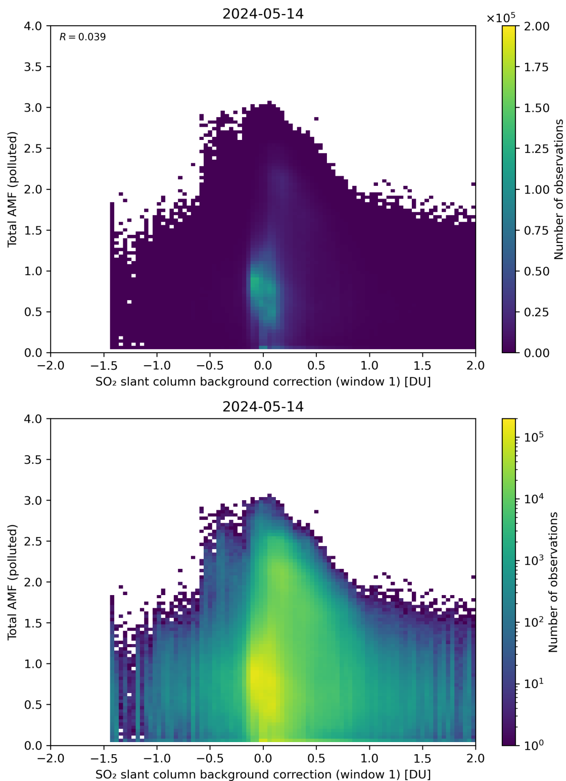
Figure 109: Scatter density plot of “SO 2 slant column background correction (window 1)” against “Total AMF (polluted)” for 2024-05-13 to 2024-05-15.
