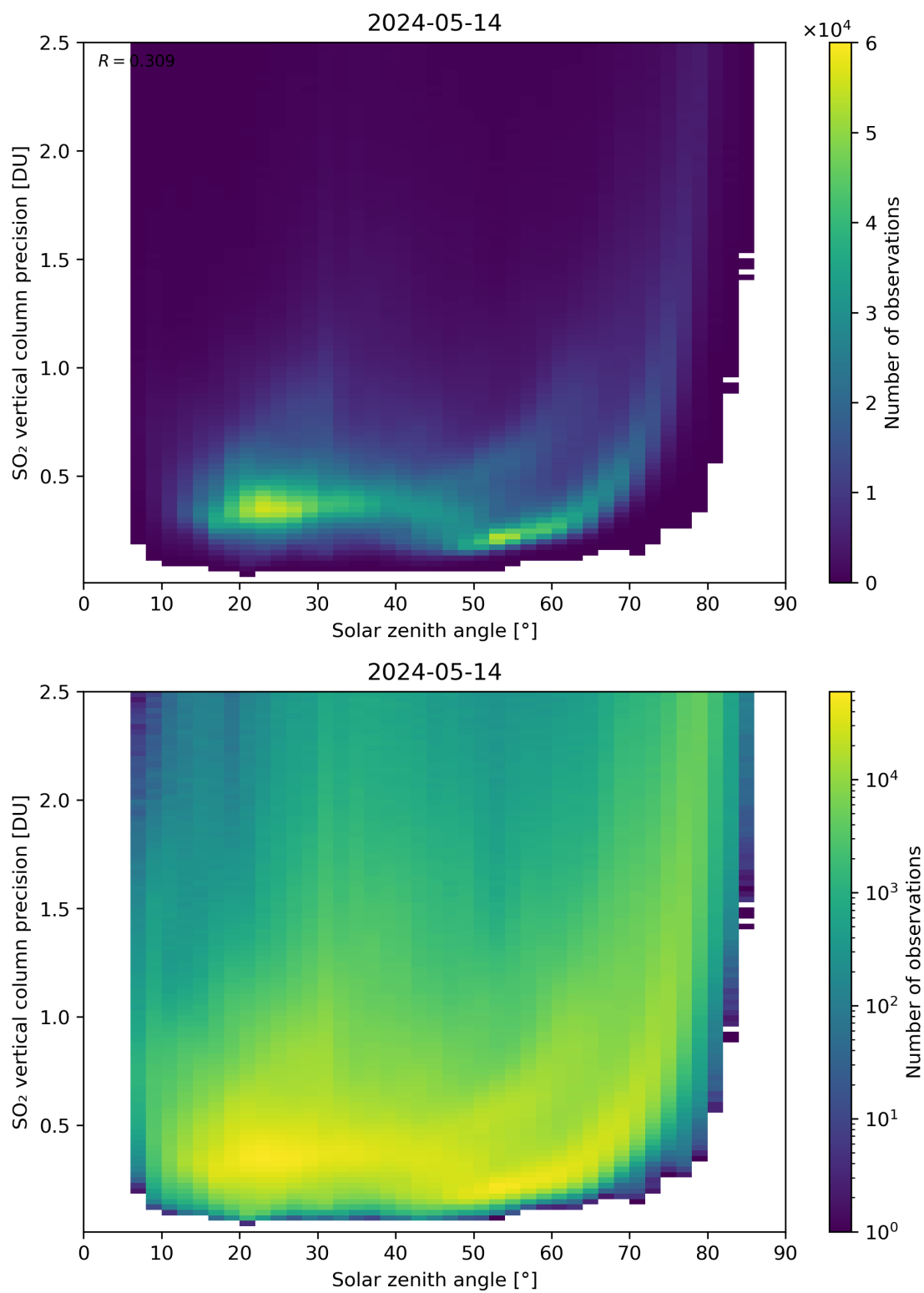
Figure 177: Scatter density plot of “Solar zenith angle” against “SO 2 vertical column precision” for 2024-05-13 to 2024-05-15.
