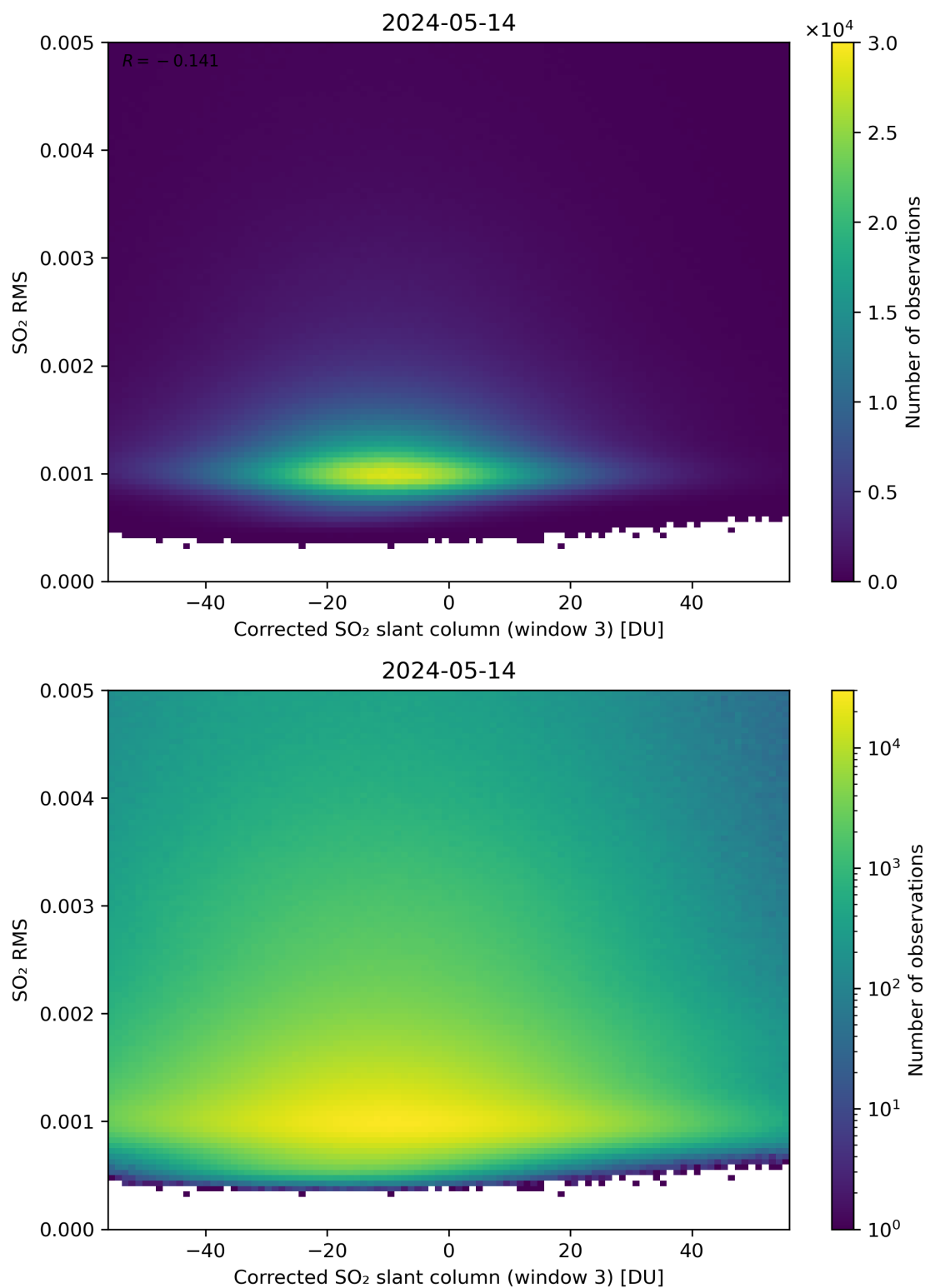
Figure 208: Scatter density plot of “Corrected SO 2 slant column (window 3)” against “SO 2 RMS” for 2024-05-13 to 2024-05-15.
