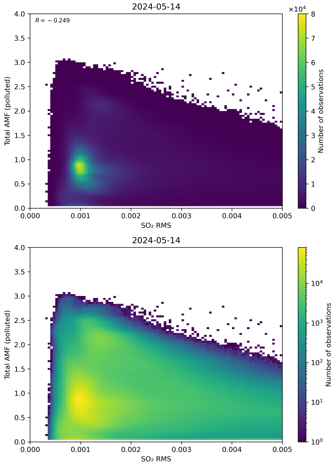
Figure 137: Scatter density plot of “SO 2 RMS” against “Total AMF (polluted)” for 2024-05-13 to 2024-05-15.
