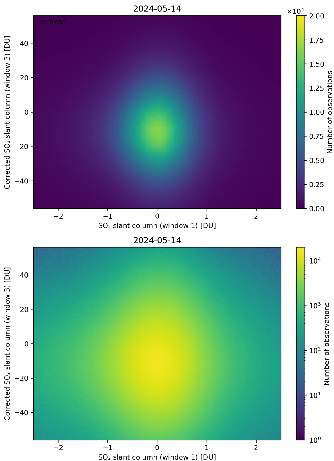
Figure 234: Scatter density plot of “SO 2 slant column (window 1)” against “Corrected SO 2 slant column (window 3)” for 2024-05-13 to 2024-05-15.
