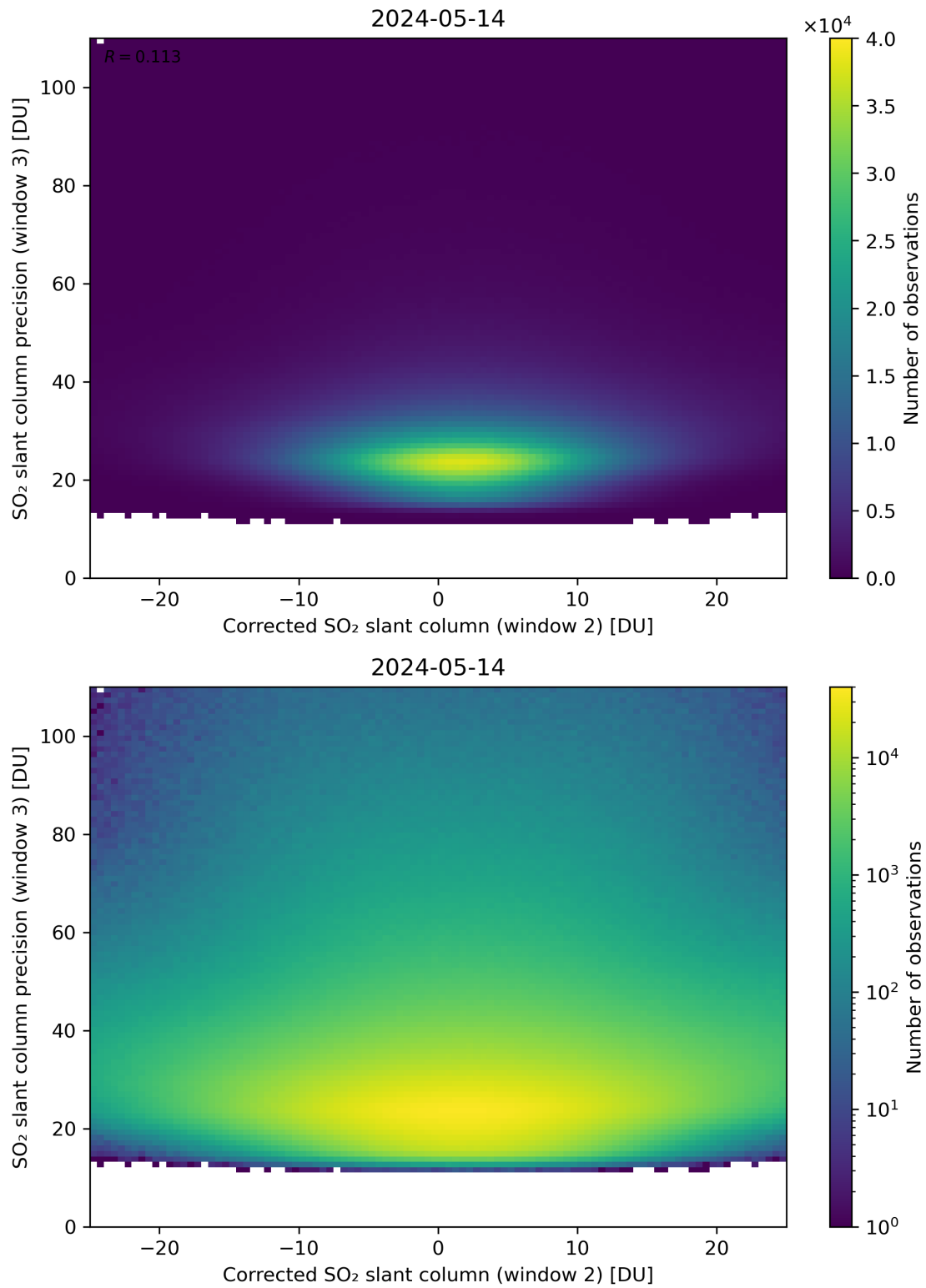
Figure 202: Scatter density plot of “Corrected SO 2 slant column (window 2)” against “SO 2 slant column precision (window 3)” for 2024-05-13 to 2024-05-15.
