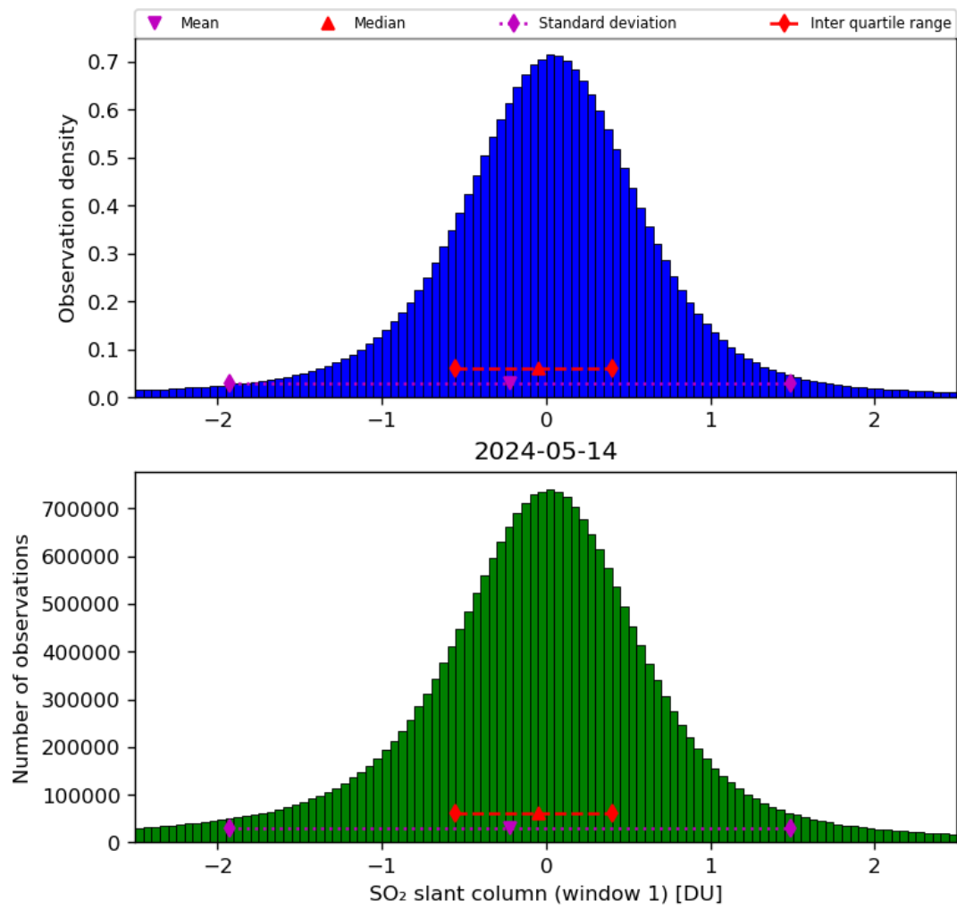
Figure 56: Histogram of “SO 2 slant column (window 1)” for 2024-05-13 to 2024-05-15
