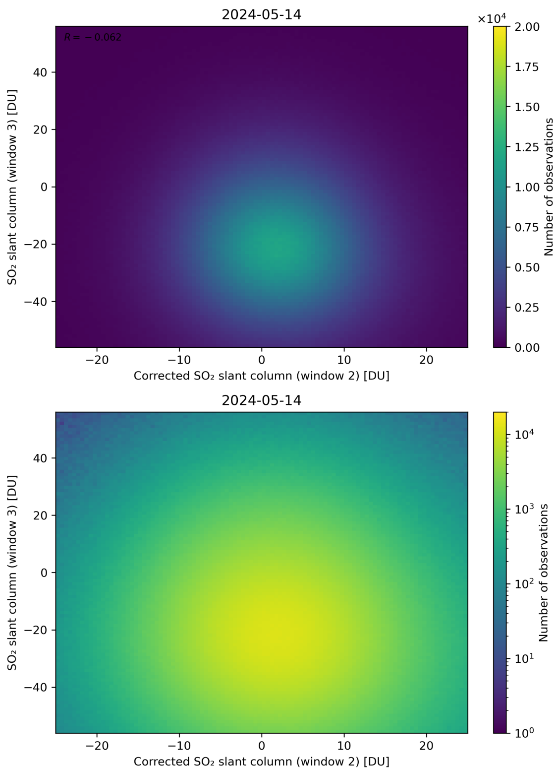
Figure 201: Scatter density plot of “Corrected SO 2 slant column (window 2)” against “SO 2 slant column (window 3)” for 2024-05-13 to 2024-05-15.
