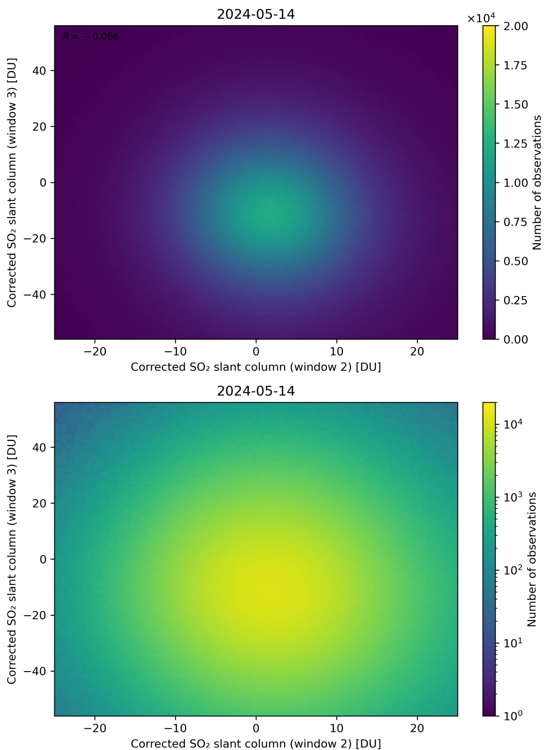
Figure 200: Scatter density plot of “Corrected SO 2 slant column (window 2)” against “Corrected SO 2 slant column (window 3)” for 2024-05-13 to 2024-05-15.
