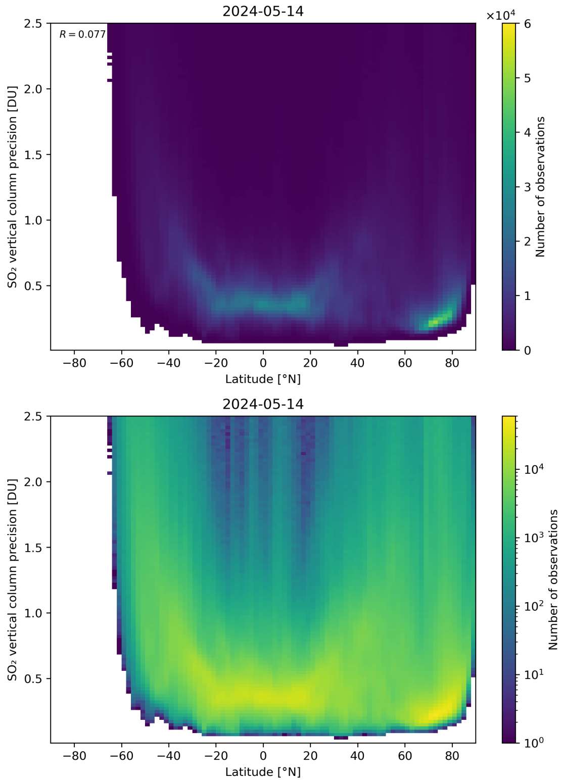
Figure 157: Scatter density plot of “Latitude” against “SO 2 vertical column precision” for 2024-05-13 to 2024-05-15.
