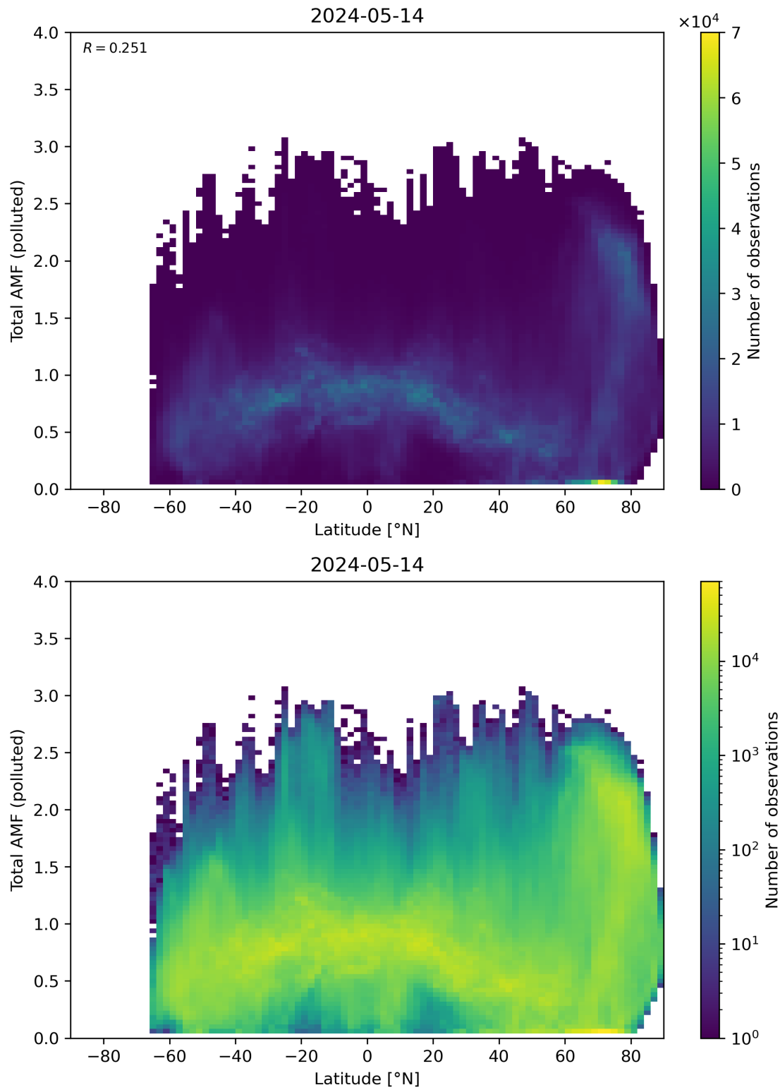
Figure 154: Scatter density plot of “Latitude” against “Total AMF (polluted)” for 2024-05-13 to 2024-05-15.
