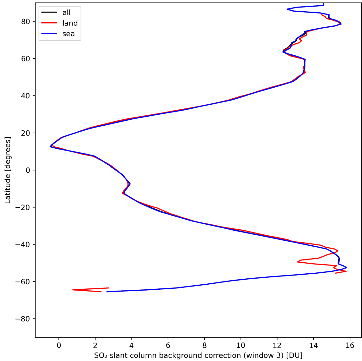
Figure 44: Zonal average of “SO 2 slant column background correction (window 3)” for 2024-05-13 to 2024-05-15.
