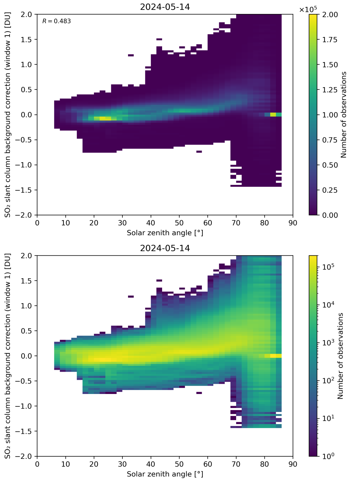
Figure 158: Scatter density plot of “Solar zenith angle” against “SO 2 slant column background correction (window 1)” for 2024-05-13 to 2024-05-15.
