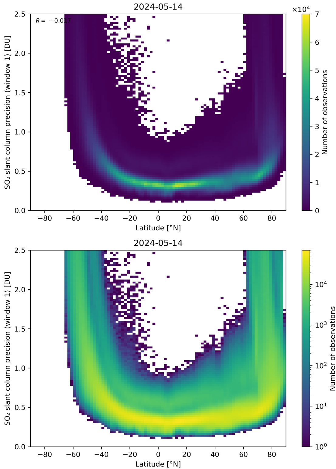
Figure 150: Scatter density plot of “Latitude” against “SO 2 slant column precision (window 1)” for 2024-05-13 to 2024-05-15.
