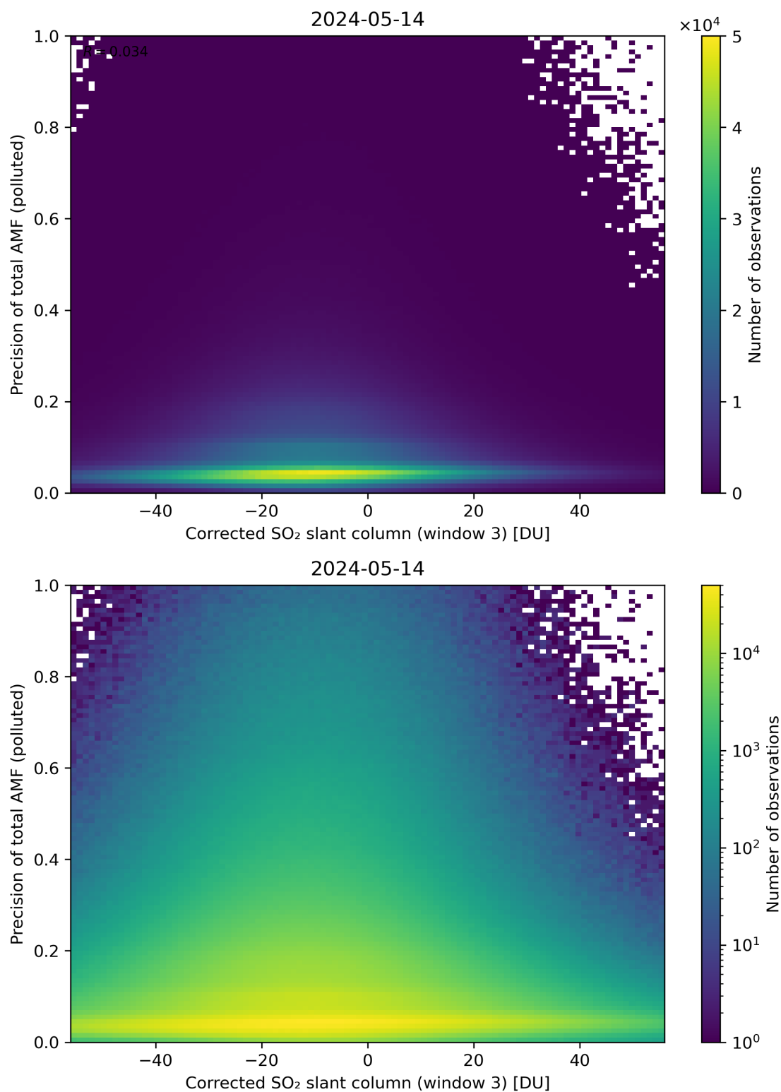
Figure 211: Scatter density plot of “Corrected SO 2 slant column (window 3)” against “Precision of total AMF (polluted)” for 2024-05-13 to 2024-05-15.
