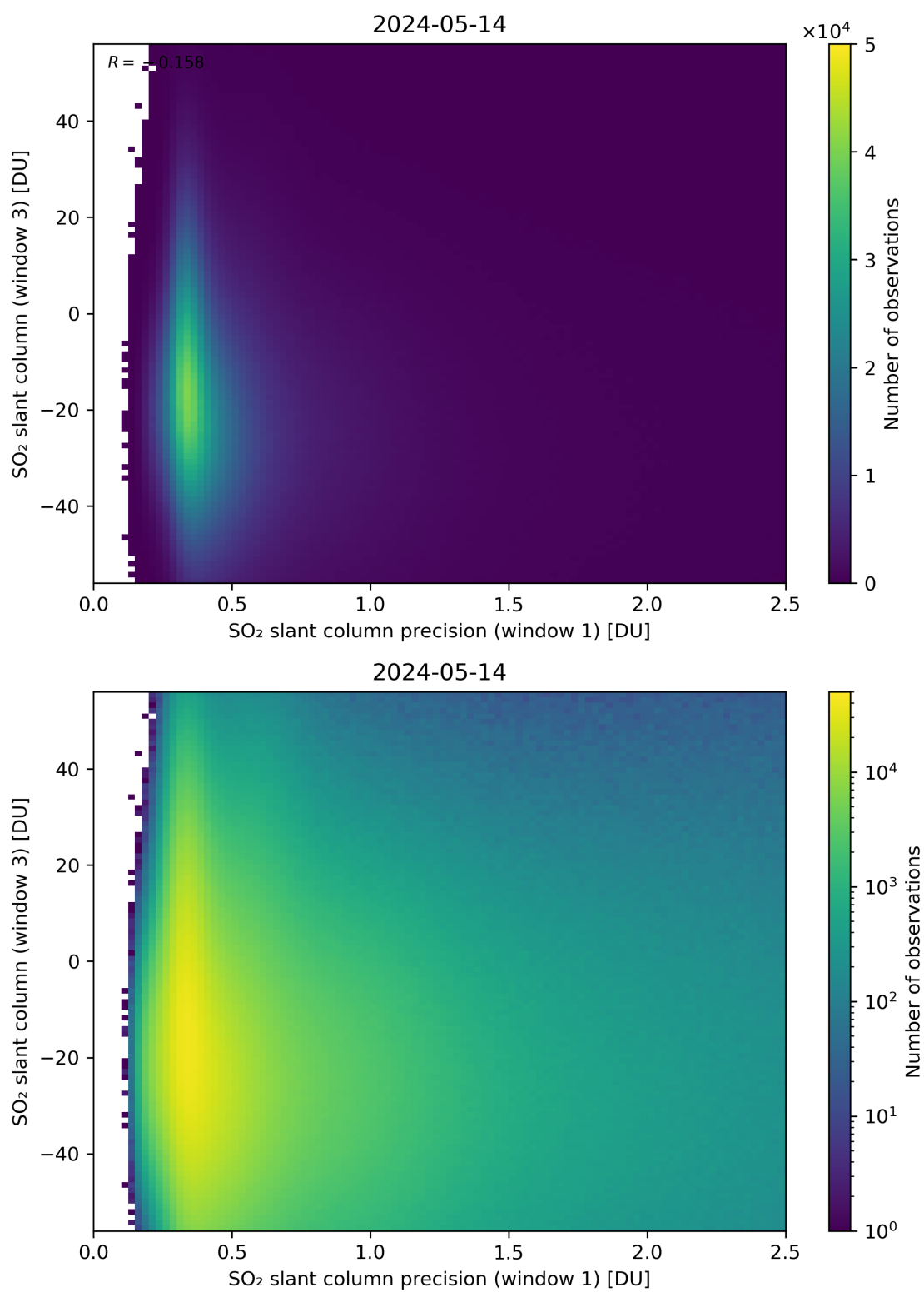
Figure 228: Scatter density plot of “SO 2 slant column precision (window 1)” against “SO 2 slant column (window 3)” for 2024-05-13 to 2024-05-15.
