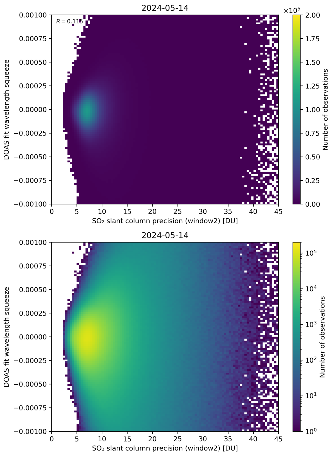
Figure 244: Scatter density plot of “SO 2 slant column precision (window2)” against “DOAS fit wavelength squeeze” for 2024-05-13 to 2024-05-15.
