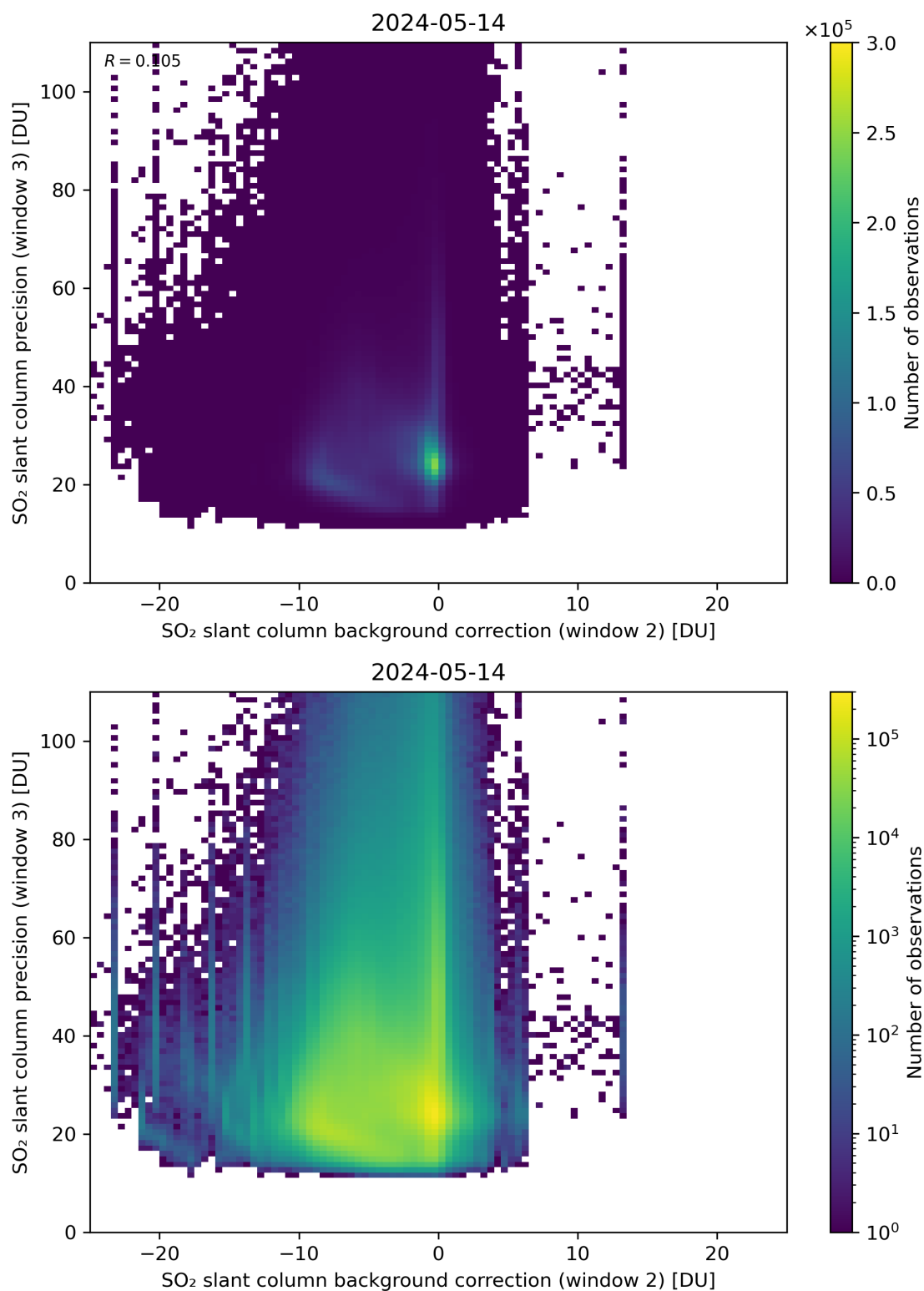
Figure 118: Scatter density plot of “SO 2 slant column background correction (window 2)” against “SO 2 slant column precision (window 3)” for 2024-05-13 to 2024-05-15.
