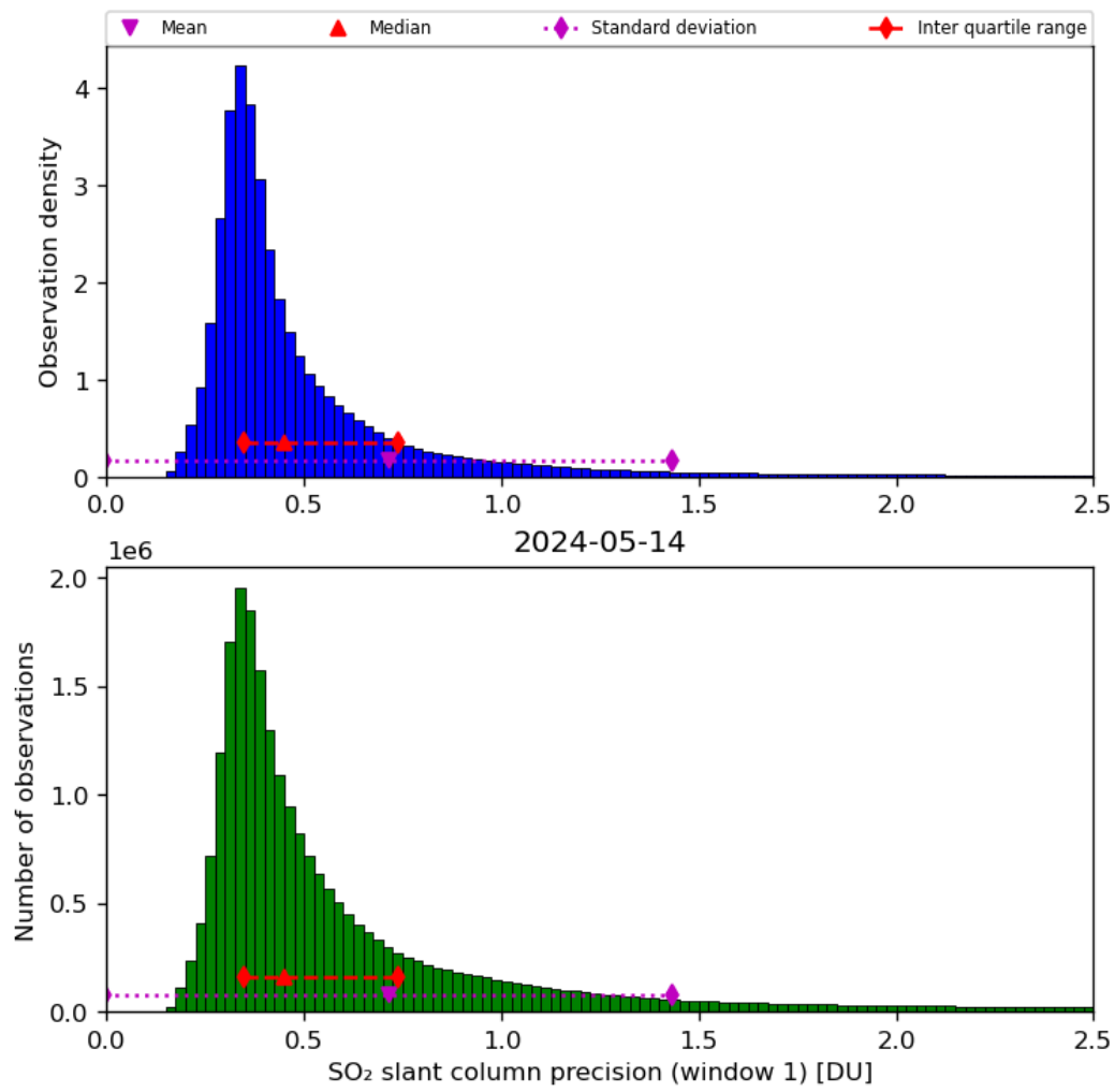
Figure 57: Histogram of “SO 2 slant column precision (window 1)” for 2024-05-13 to 2024-05-15
