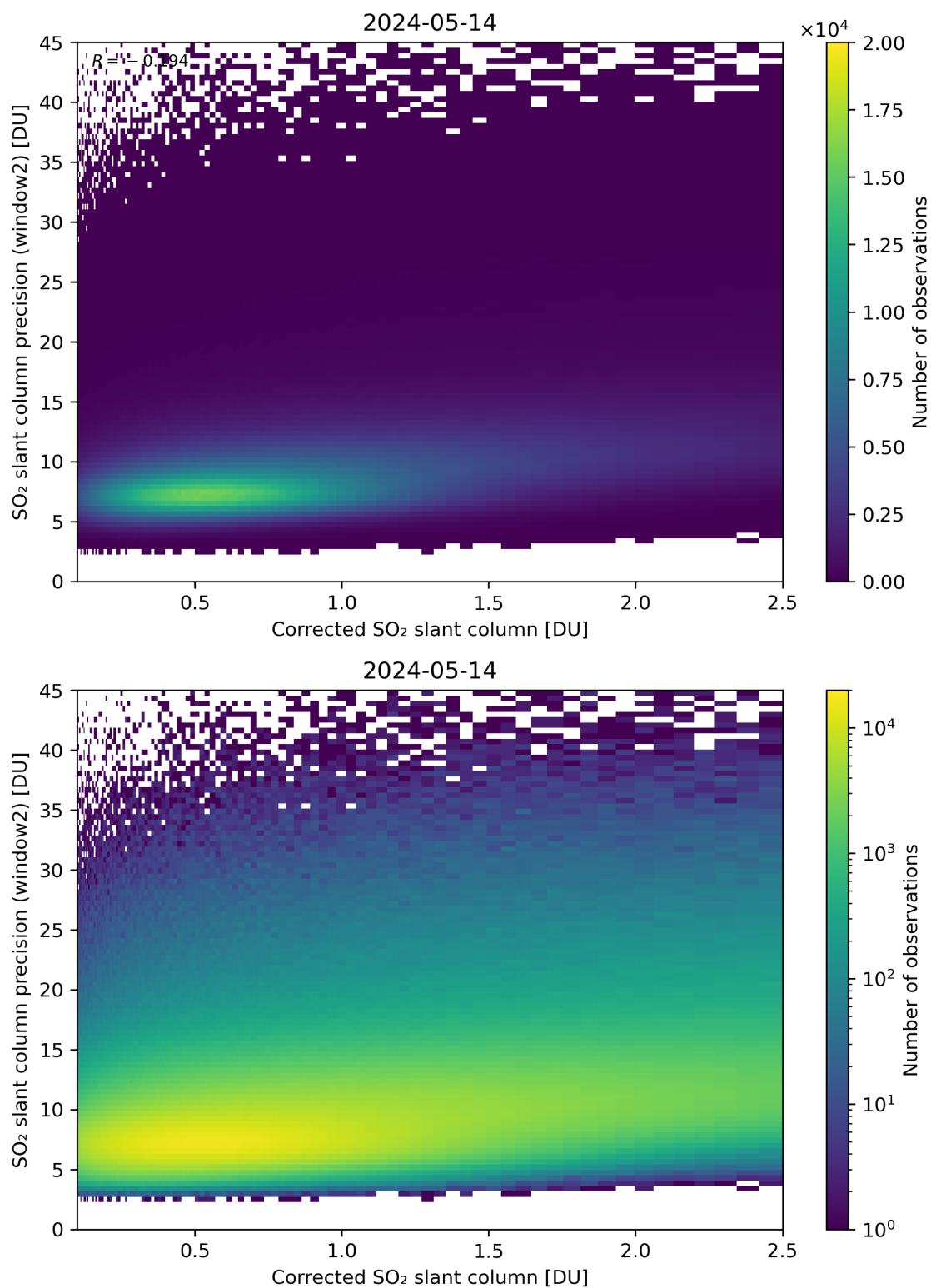
Figure 189: Scatter density plot of “Corrected SO 2 slant column” against “SO 2 slant column precision (window2)” for 2024-05-13 to 2024-05-15.
