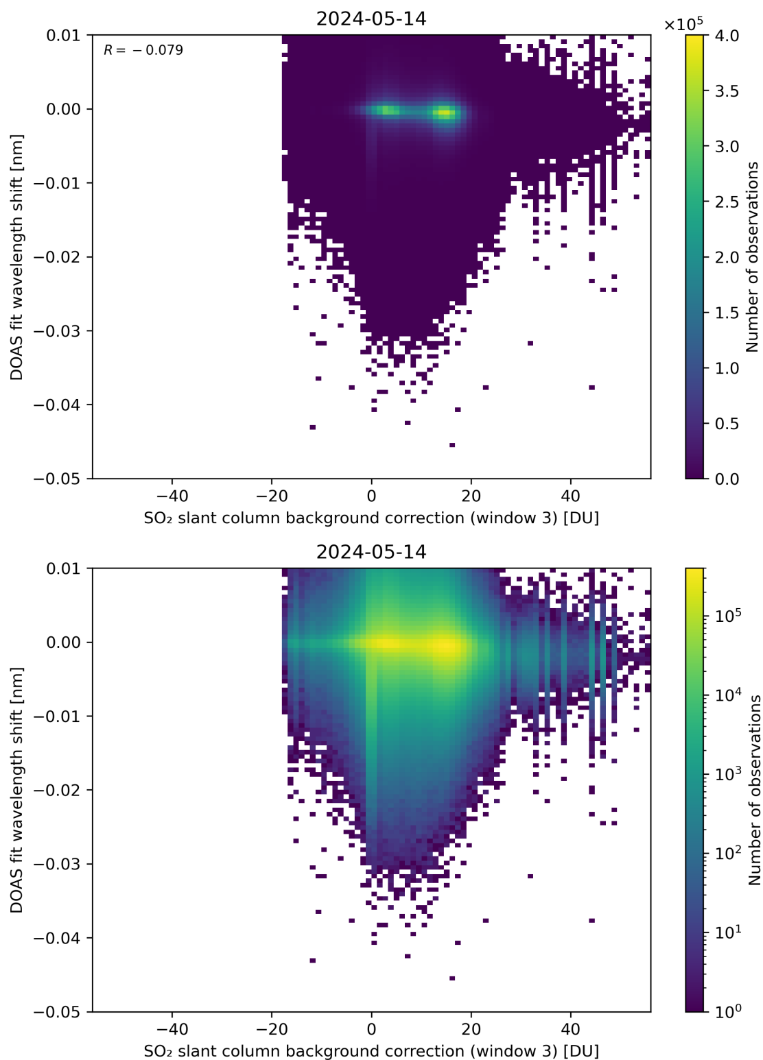
Figure 121: Scatter density plot of “SO 2 slant column background correction (window 3)” against “DOAS fit wavelength shift” for 2024-05-13 to 2024-05-15.
