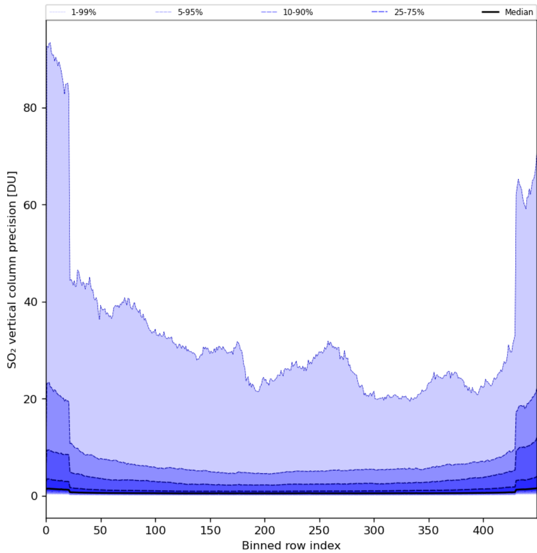
Figure 77: Along track statistics of “SO 2 vertical column precision” for 2024-05-13 to 2024-05-15
