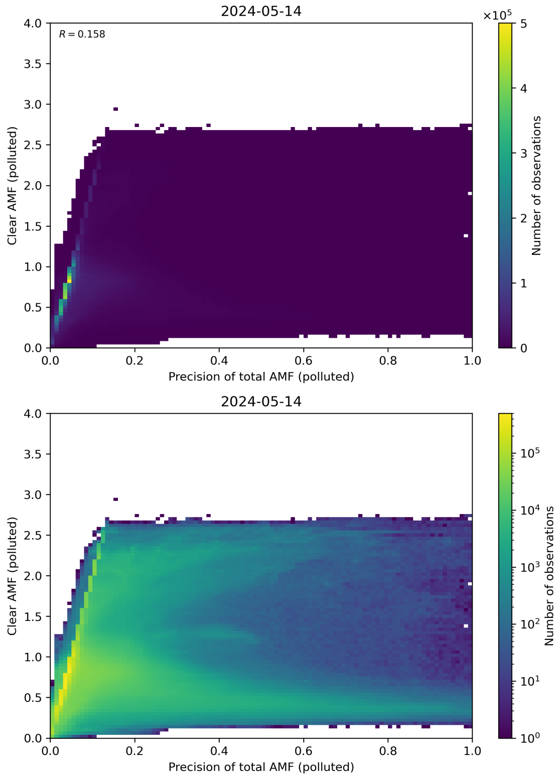
Figure 270: Scatter density plot of “Precision of total AMF (polluted)” against “Clear AMF (polluted)” for 2024-05-13 to 2024-05-15.
