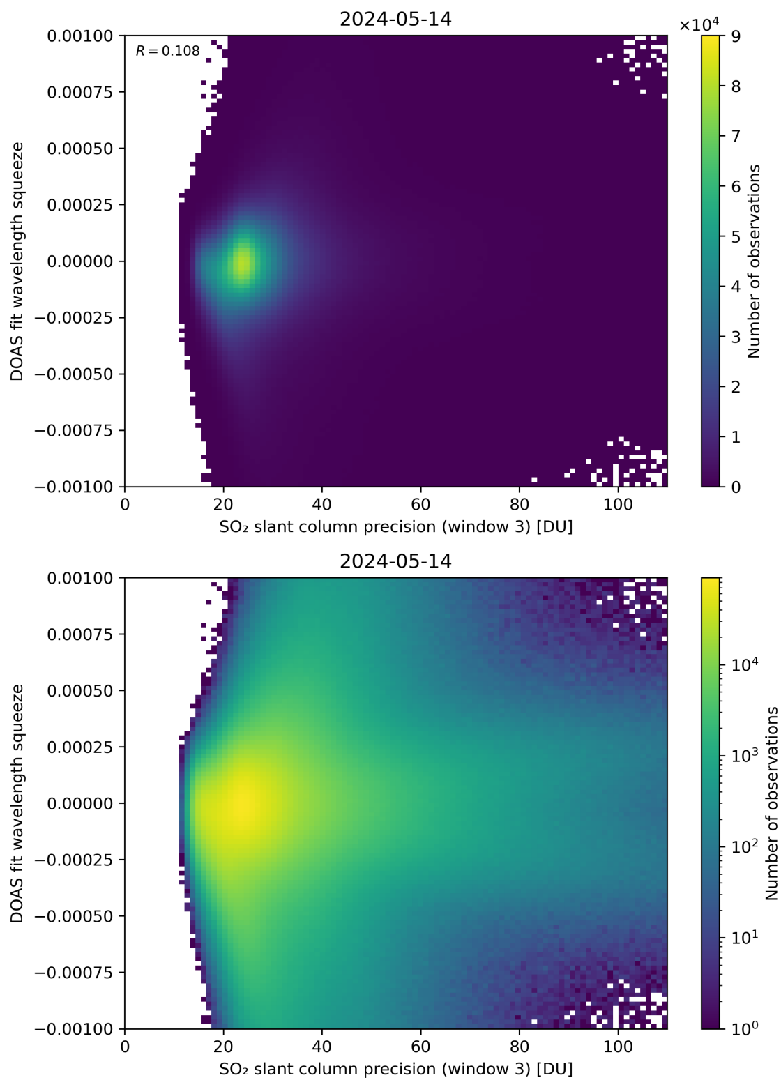
Figure 259: Scatter density plot of “SO 2 slant column precision (window 3)” against “DOAS fit wavelength squeeze” for 2024-05-13 to 2024-05-15.
