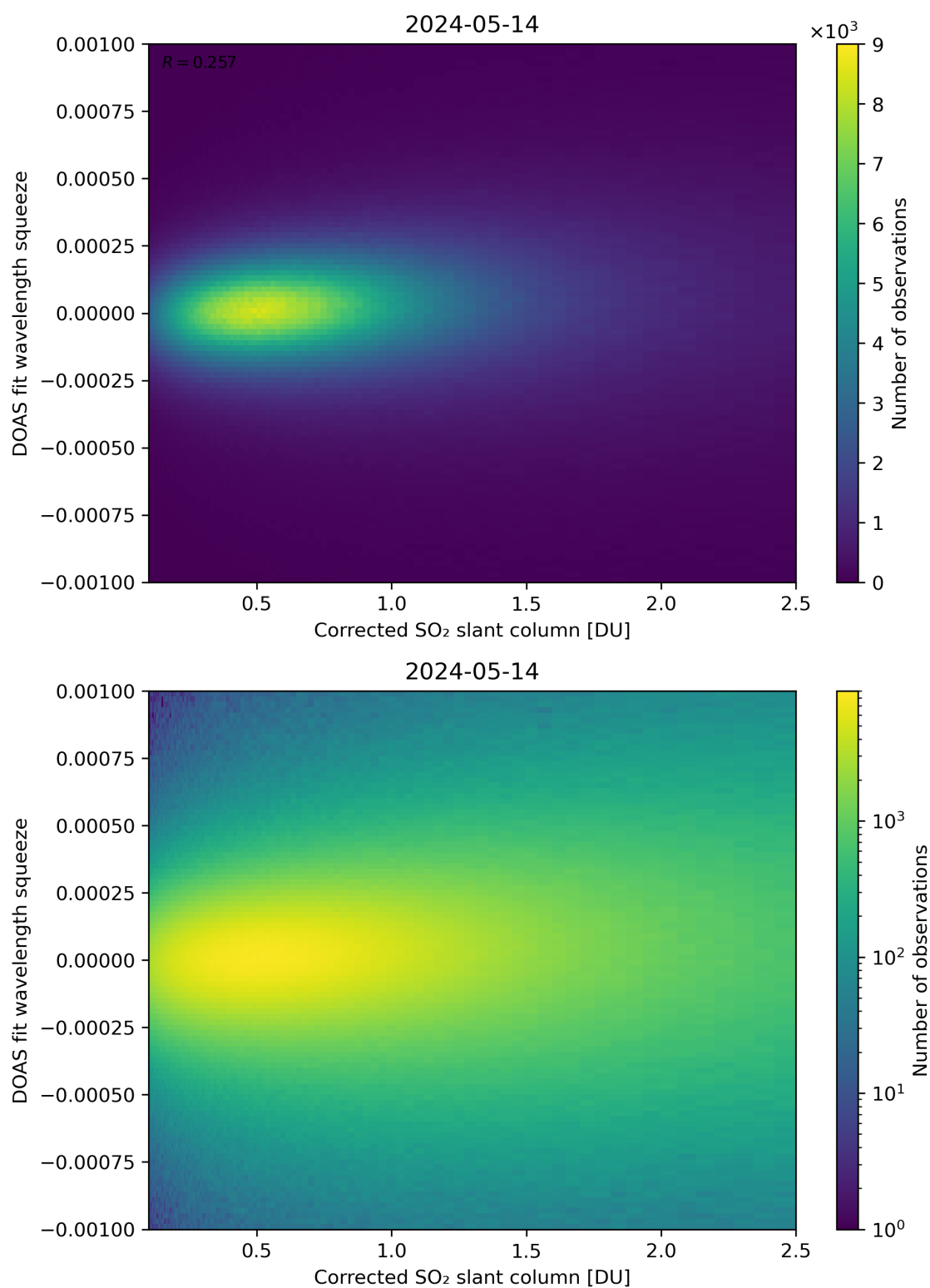
Figure 182: Scatter density plot of “Corrected SO 2 slant column” against “DOAS fit wavelength squeeze” for 2024-05-13 to 2024-05-15.
