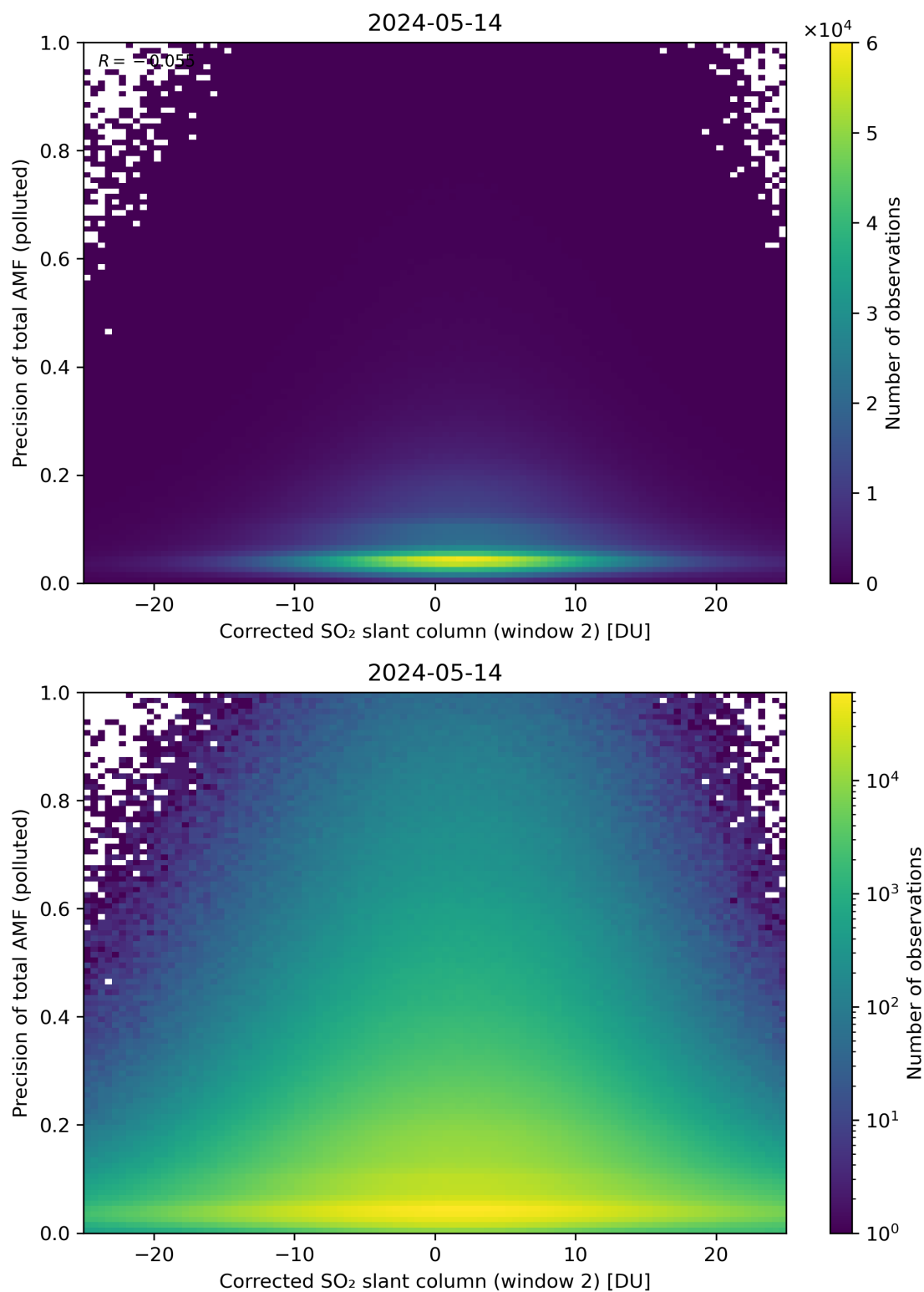
Figure 204: Scatter density plot of “Corrected SO 2 slant column (window 2)” against “Precision of total AMF (polluted)” for 2024-05-13 to 2024-05-15.
