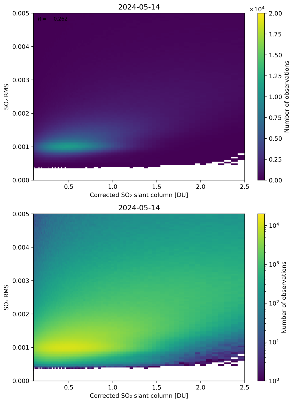
Figure 183: Scatter density plot of “Corrected SO 2 slant column” against “SO 2 RMS” for 2024-05-13 to 2024-05-15.
