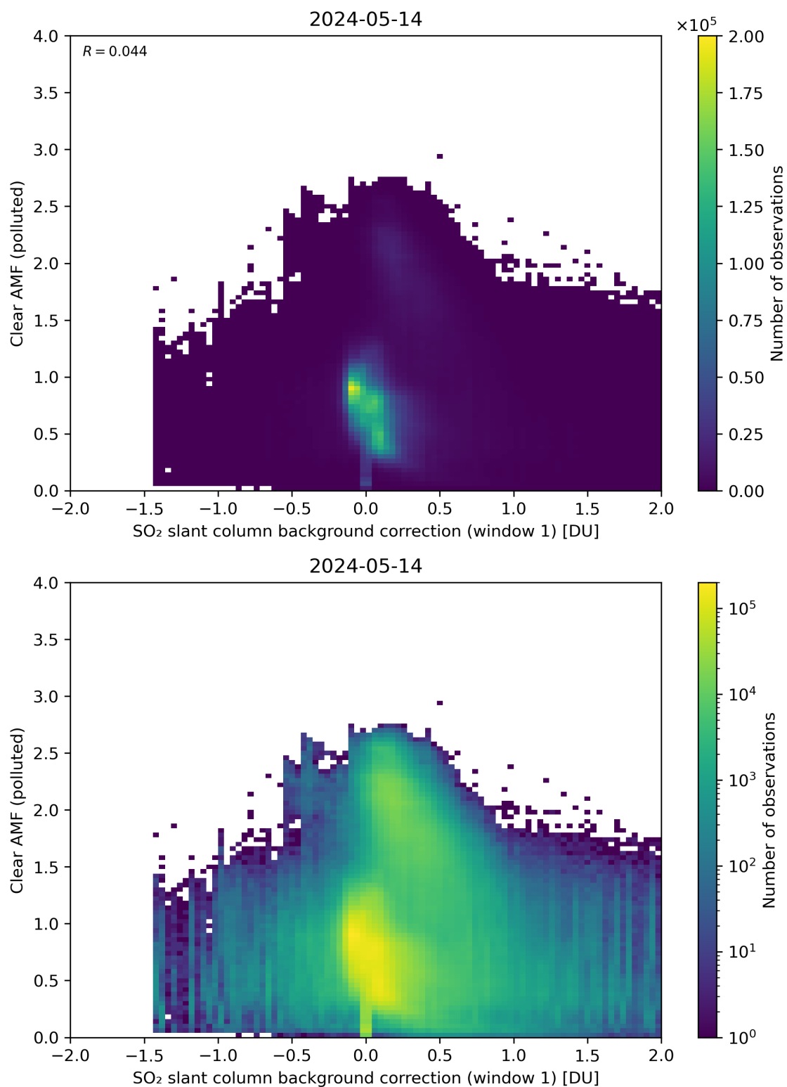
Figure 103: Scatter density plot of “SO 2 slant column background correction (window 1)” against “Clear AMF (polluted)” for 2024-05-13 to 2024-05-15.
