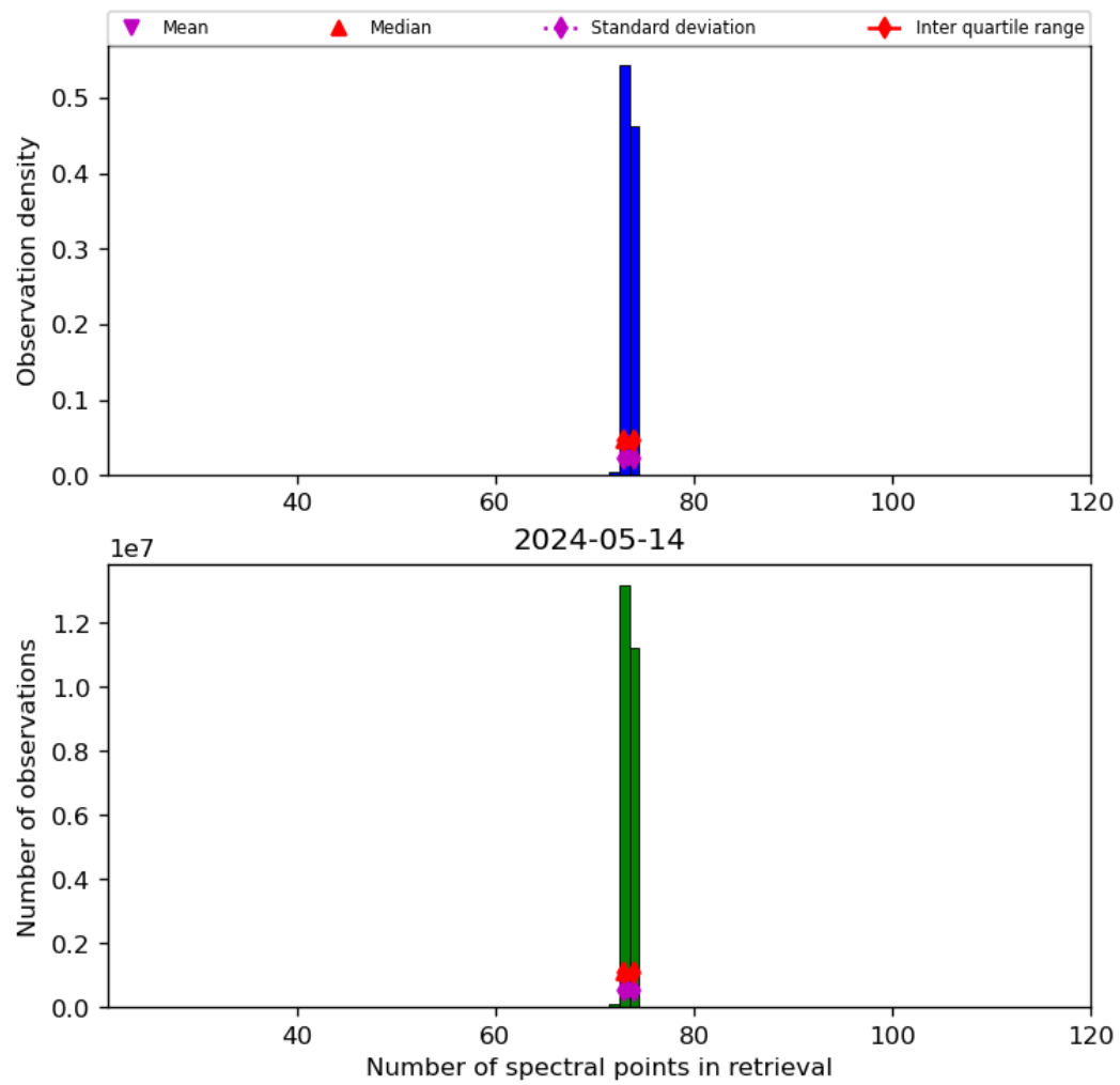
Figure 74: Histogram of “Number of spectral points in retrieval” for 2024-05-13 to 2024-05-15
