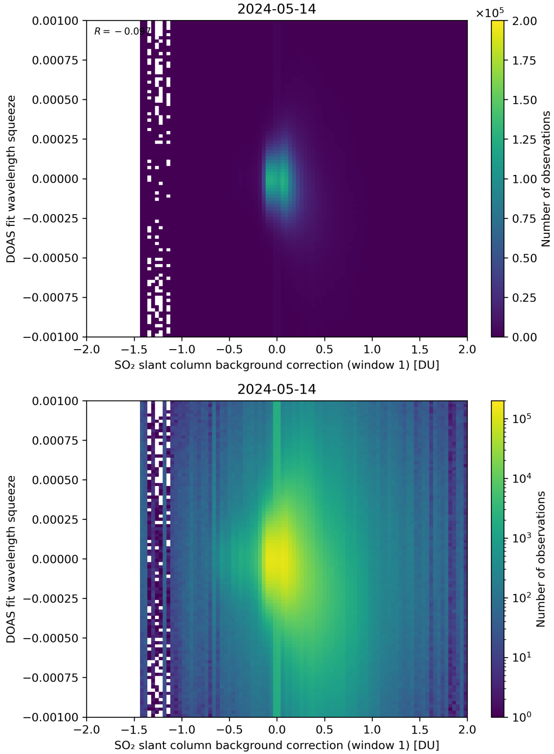
Figure 101: Scatter density plot of “SO 2 slant column background correction (window 1)” against “DOAS fit wavelength squeeze” for 2024-05-13 to 2024-05-15.
