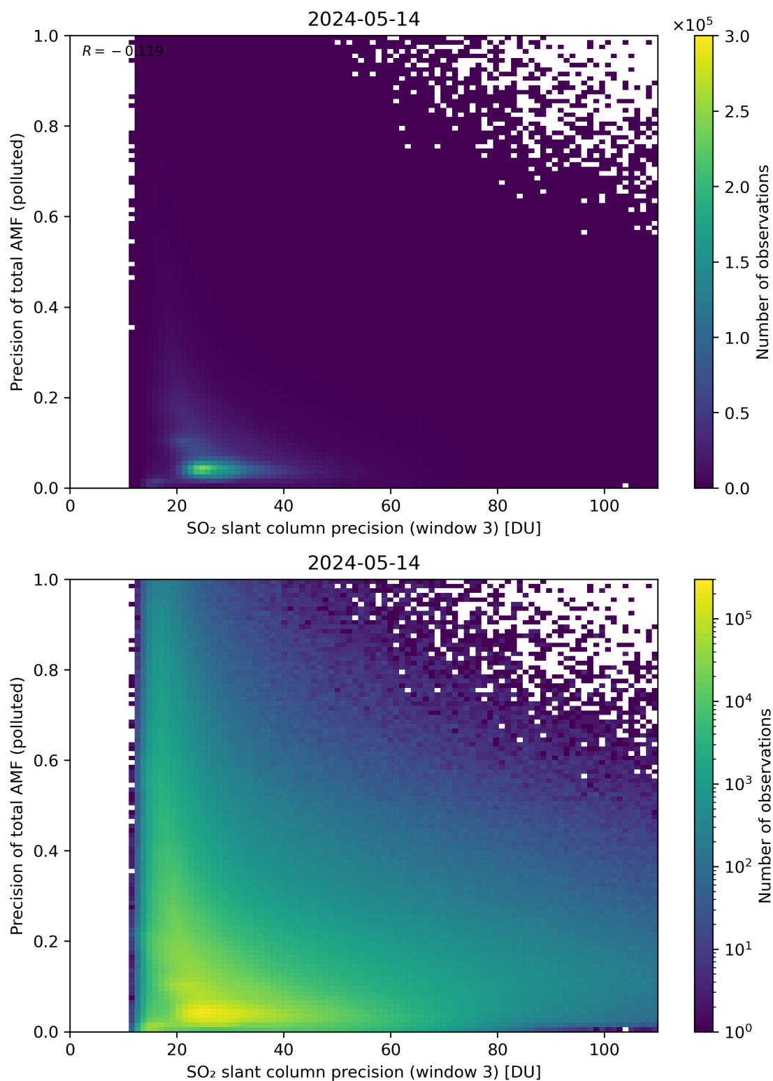
Figure 264: Scatter density plot of “SO 2 slant column precision (window 3)” against “Precision of total AMF (polluted)” for 2024-05-13 to 2024-05-15.
