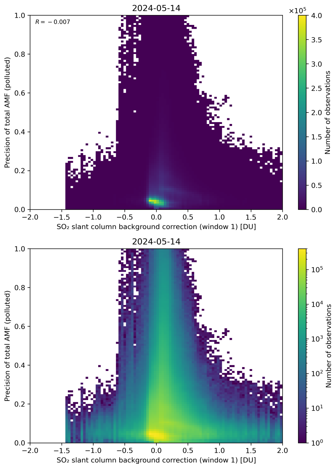
Figure 110: Scatter density plot of “SO 2 slant column background correction (window 1)” against “Precision of total AMF (polluted)” for 2024-05-13 to 2024-05-15.
