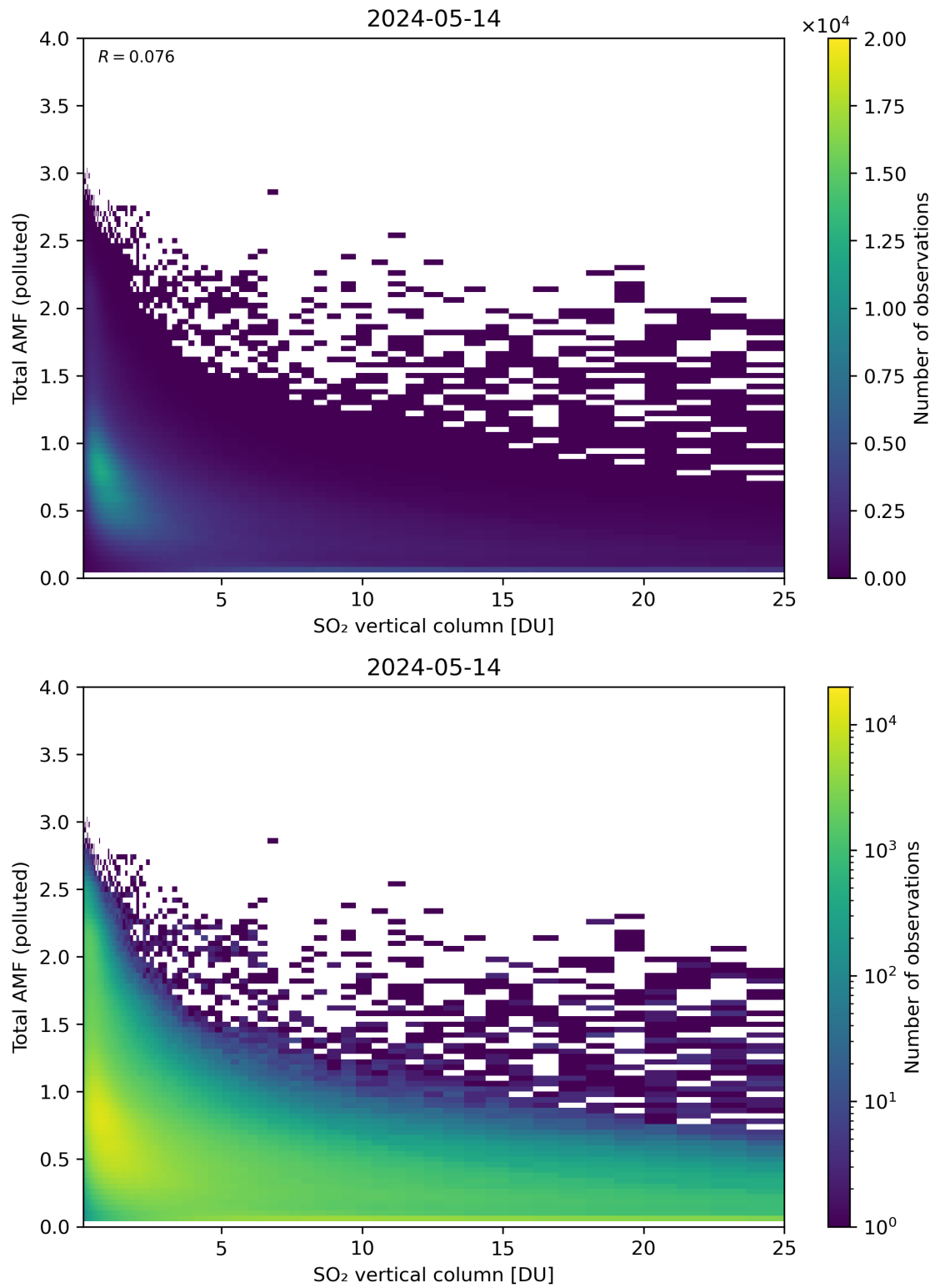
Figure 305: Scatter density plot of “SO 2 vertical column” against “Total AMF (polluted)” for 2024-05-13 to 2024-05-15.
