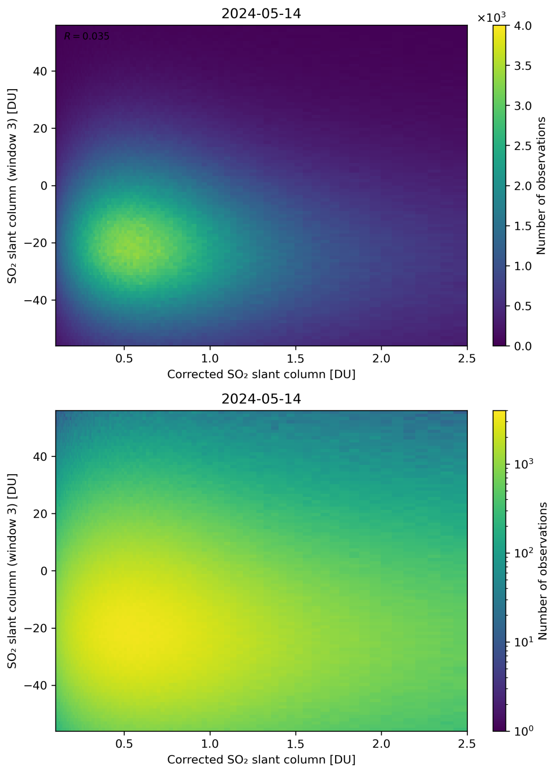
Figure 190: Scatter density plot of “Corrected SO 2 slant column” against “SO 2 slant column (window 3)” for 2024-05-13 to 2024-05-15.
