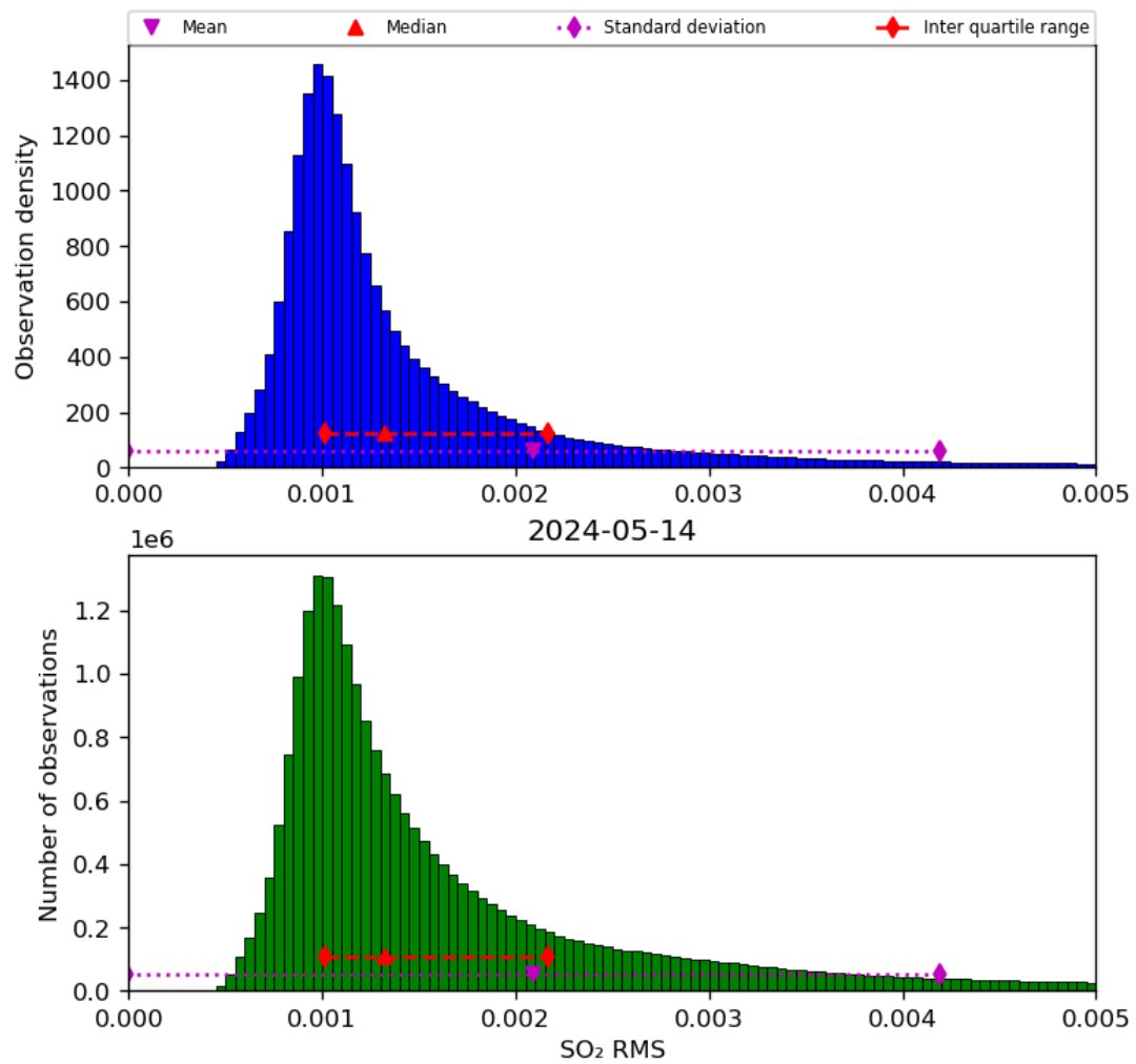
Figure 70: Histogram of “SO 2 RMS” for 2024-05-13 to 2024-05-15
