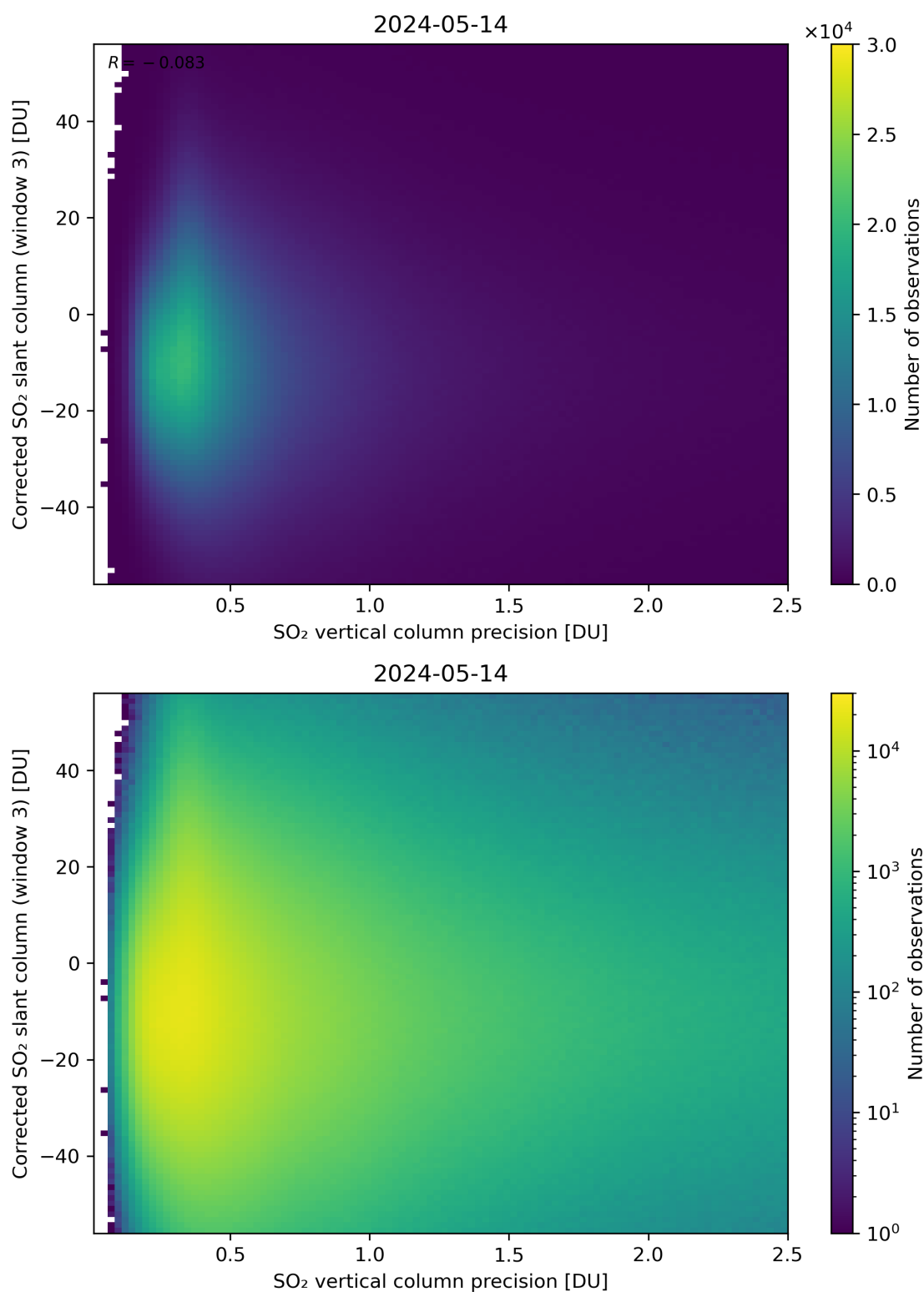
Figure 288: Scatter density plot of “SO 2 vertical column precision” against “Corrected SO 2 slant column (window 3)” for 2024-05-13 to 2024-05-15.
