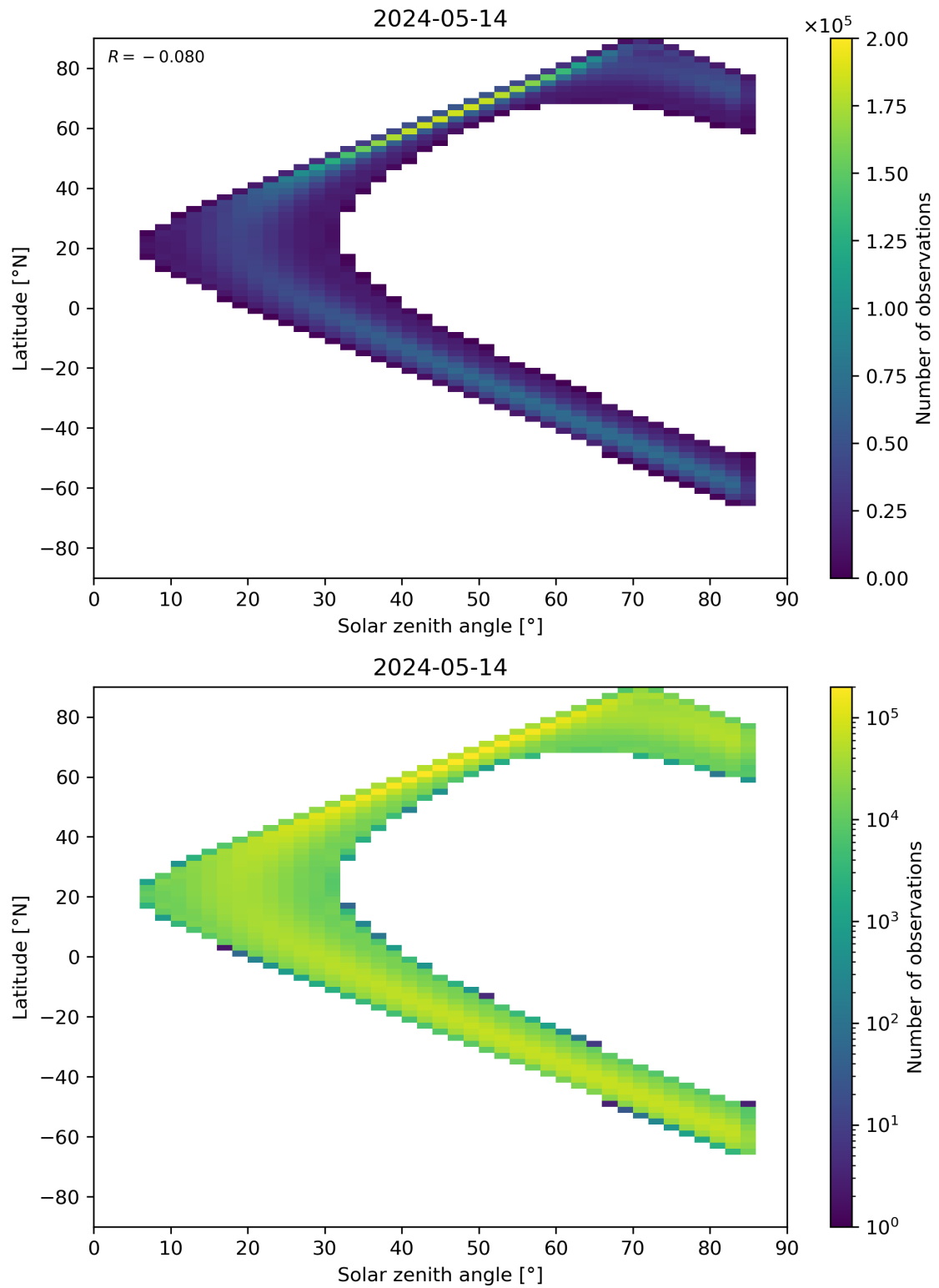
Figure 164: Scatter density plot of “Solar zenith angle” against “Latitude” for 2024-05-13 to 2024-05-15.
