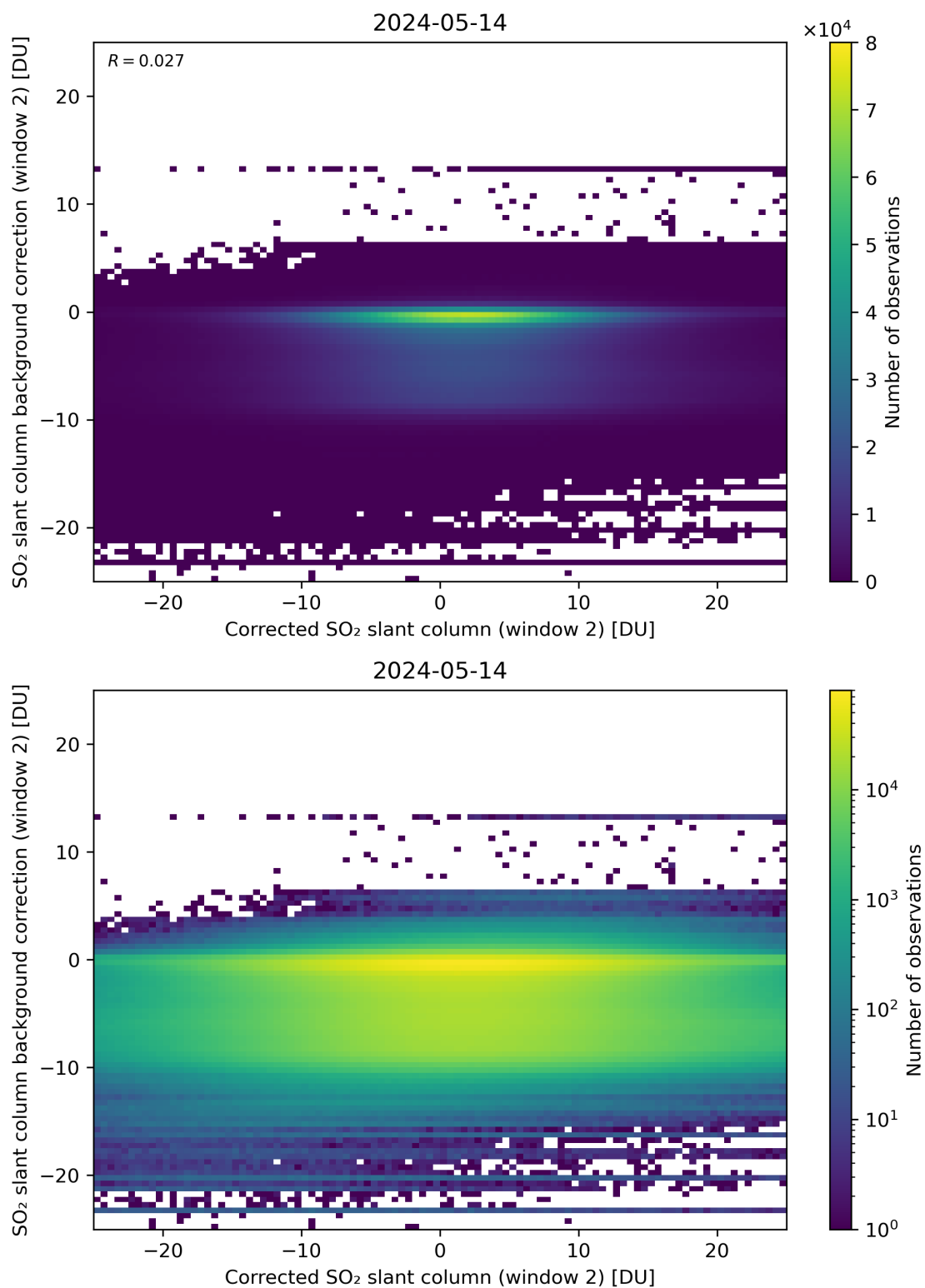
Figure 194: Scatter density plot of “Corrected SO 2 slant column (window 2)” against “SO 2 slant column background correction (window 2)” for 2024-05-13 to 2024-05-15.
