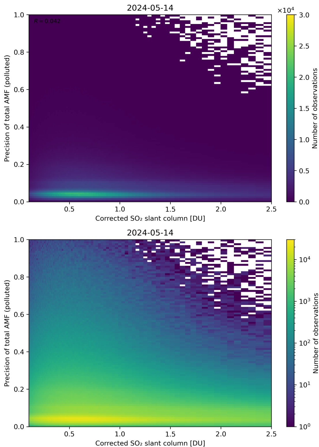
Figure 193: Scatter density plot of “Corrected SO 2 slant column” against “Precision of total AMF (polluted)” for 2024-05-13 to 2024-05-15.
