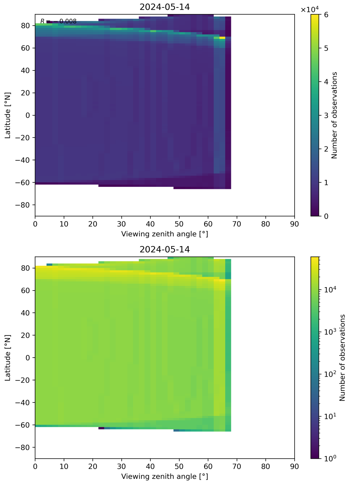
Figure 314: Scatter density plot of “Viewing zenith angle” against “Latitude” for 2024-05-13 to 2024-05-15.
