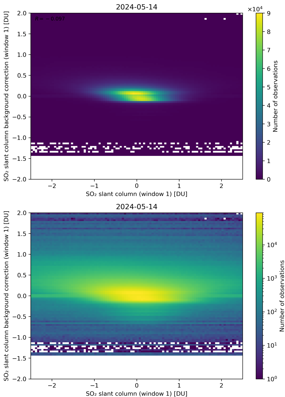
Figure 212: Scatter density plot of “SO 2 slant column (window 1)” against “SO 2 slant column background correction (window 1)” for 2024-05-13 to 2024-05-15.
