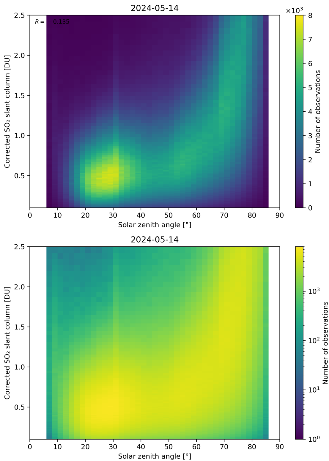
Figure 166: Scatter density plot of “Solar zenith angle” against “Corrected SO 2 slant column” for 2024-05-13 to 2024-05-15.
