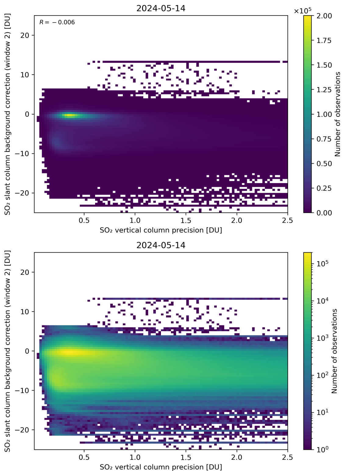
Figure 280: Scatter density plot of “SO 2 vertical column precision” against “SO 2 slant column background correction (window 2)” for 2024-05-13 to 2024-05-15.
