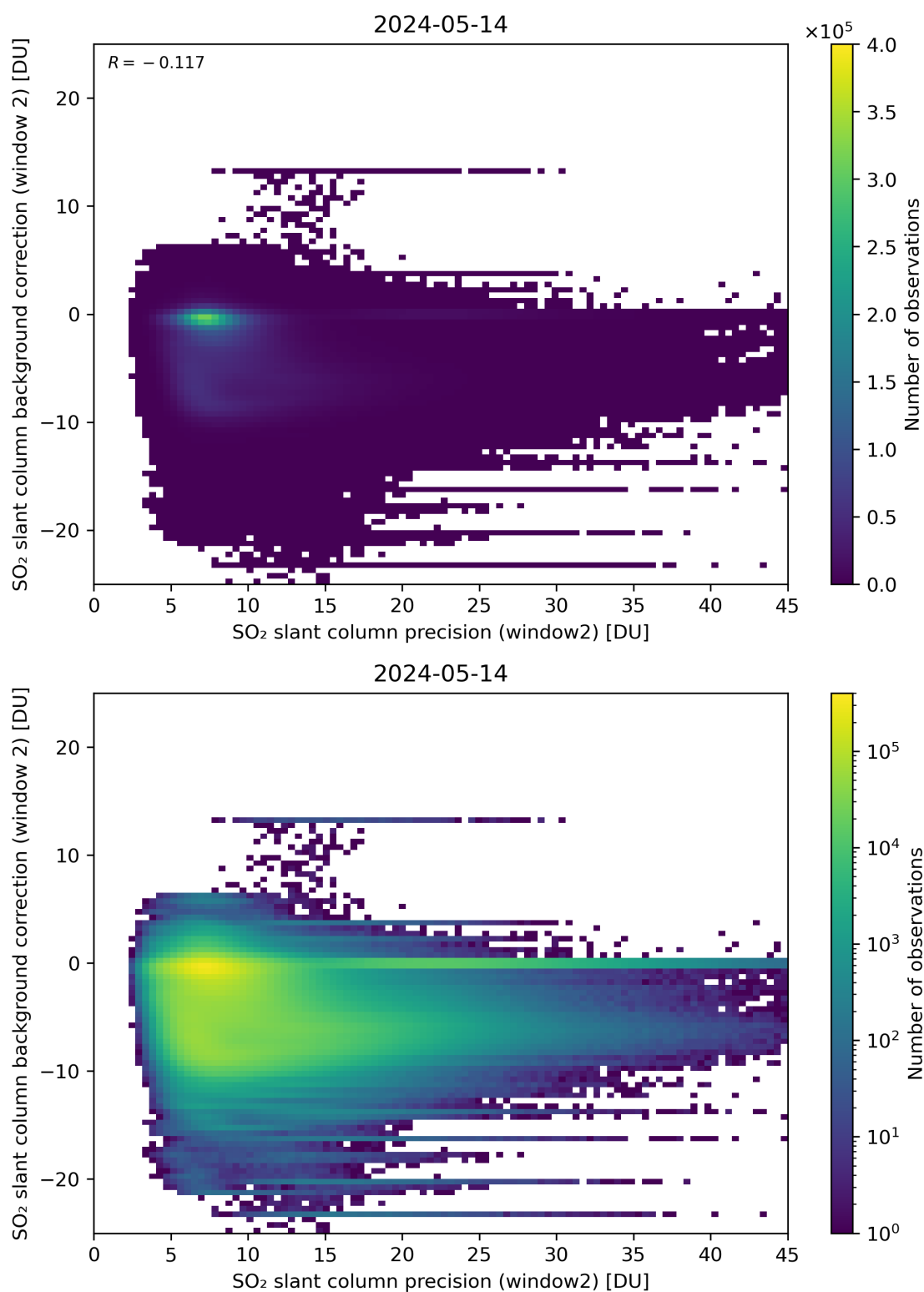
Figure 241: Scatter density plot of “SO 2 slant column precision (window2)” against “SO 2 slant column background correction (window 2)” for 2024-05-13 to 2024-05-15.
