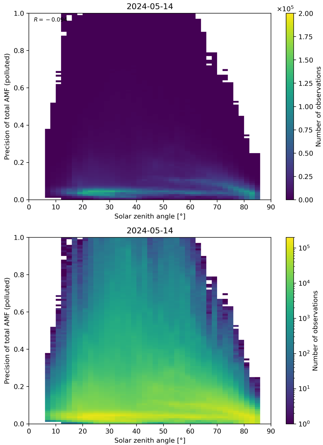
Figure 175: Scatter density plot of “Solar zenith angle” against “Precision of total AMF (polluted)” for 2024-05-13 to 2024-05-15.
