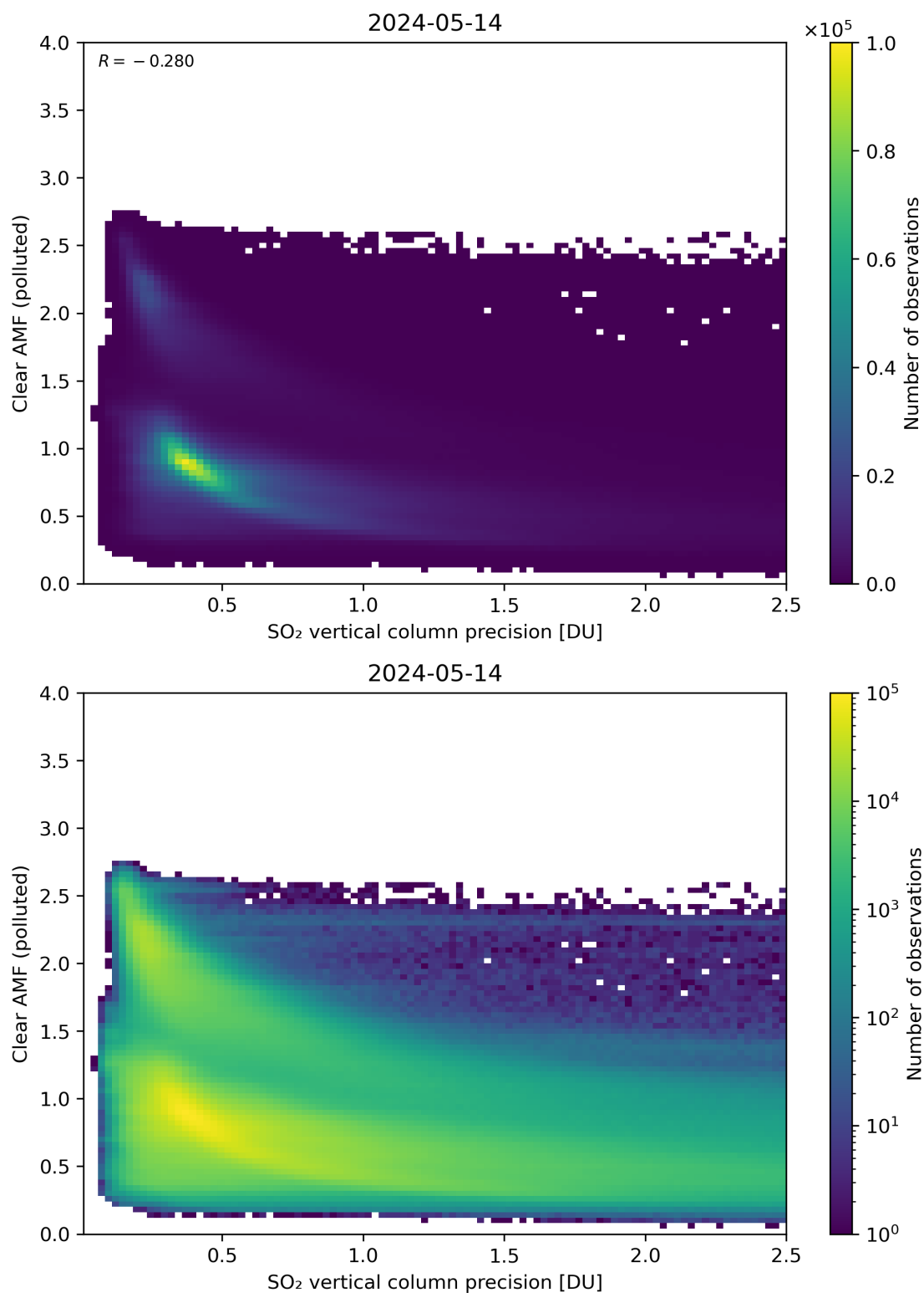
Figure 285: Scatter density plot of “SO 2 vertical column precision” against “Clear AMF (polluted)” for 2024-05-13 to 2024-05-15.
