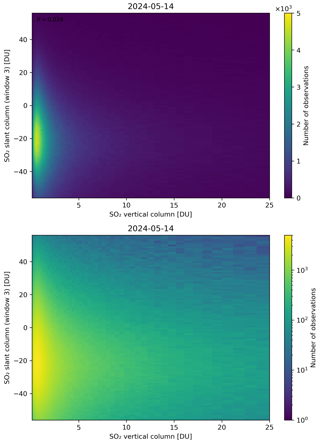
Figure 303: Scatter density plot of “SO 2 vertical column” against “SO 2 slant column (window 3)” for 2024-05-13 to 2024-05-15.
