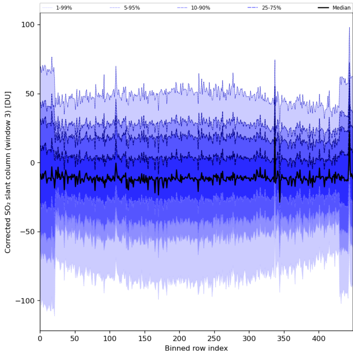
Figure 89: Along track statistics of “Corrected SO 2 slant column (window 3)” for 2024-05-13 to 2024-05-15
