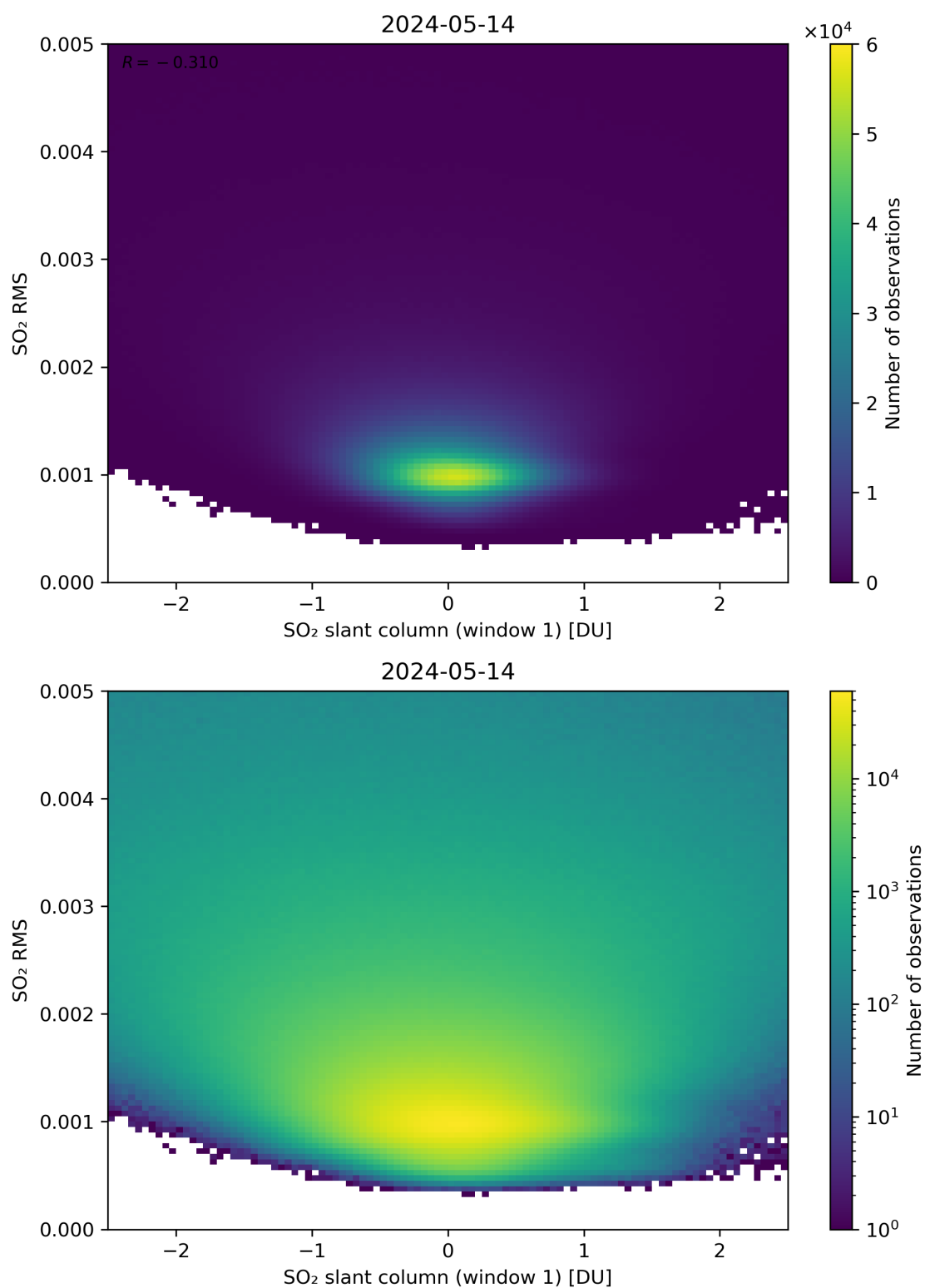
Figure 217: Scatter density plot of “SO 2 slant column (window 1)” against “SO 2 RMS” for 2024-05-13 to 2024-05-15.
