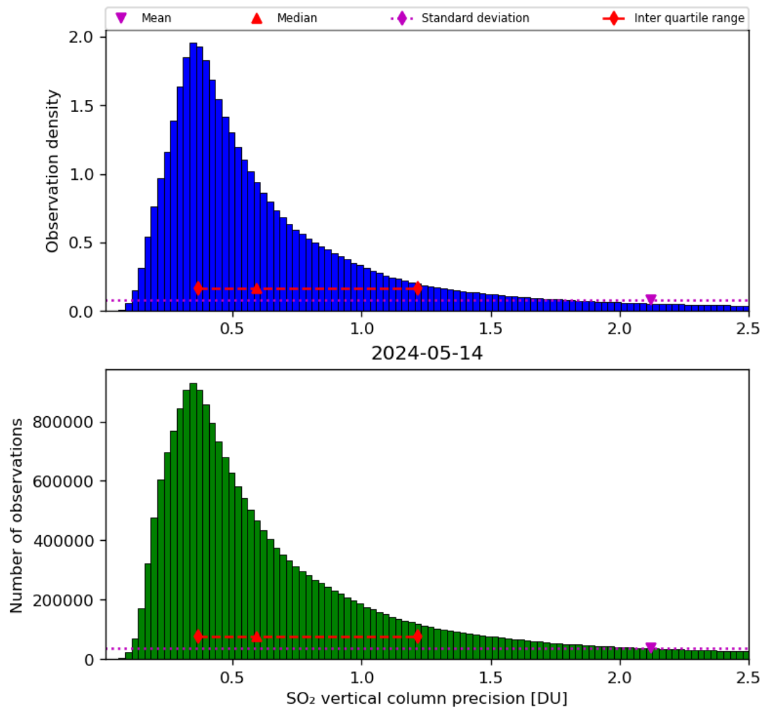
Figure 54: Histogram of “SO 2 vertical column precision” for 2024-05-13 to 2024-05-15
