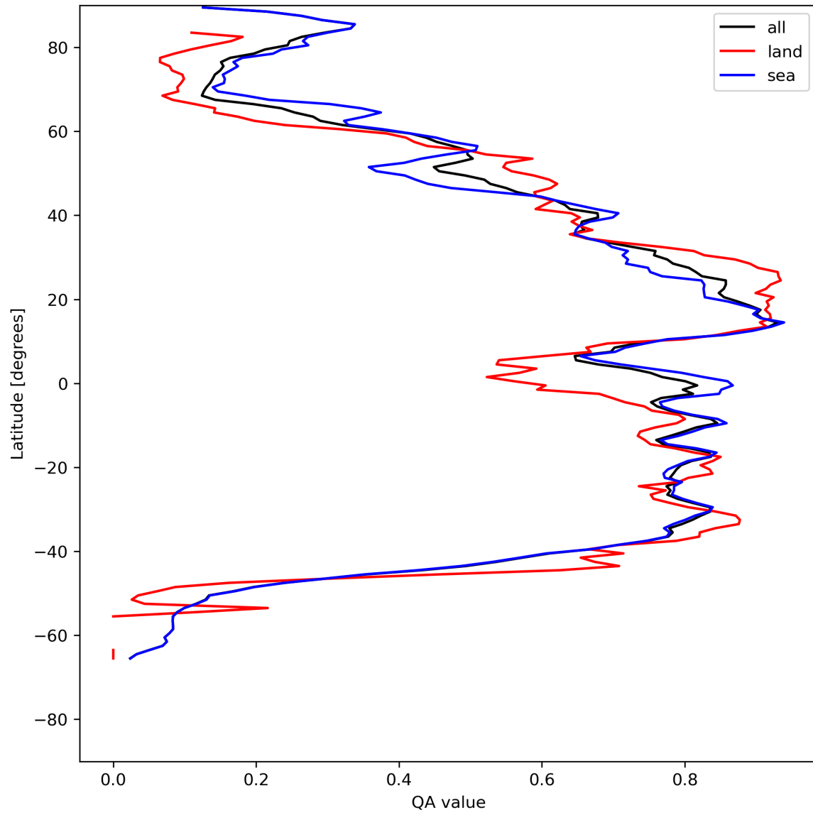
Figure 29: Zonal average of “QA value” for 2024-05-13 to 2024-05-15.
