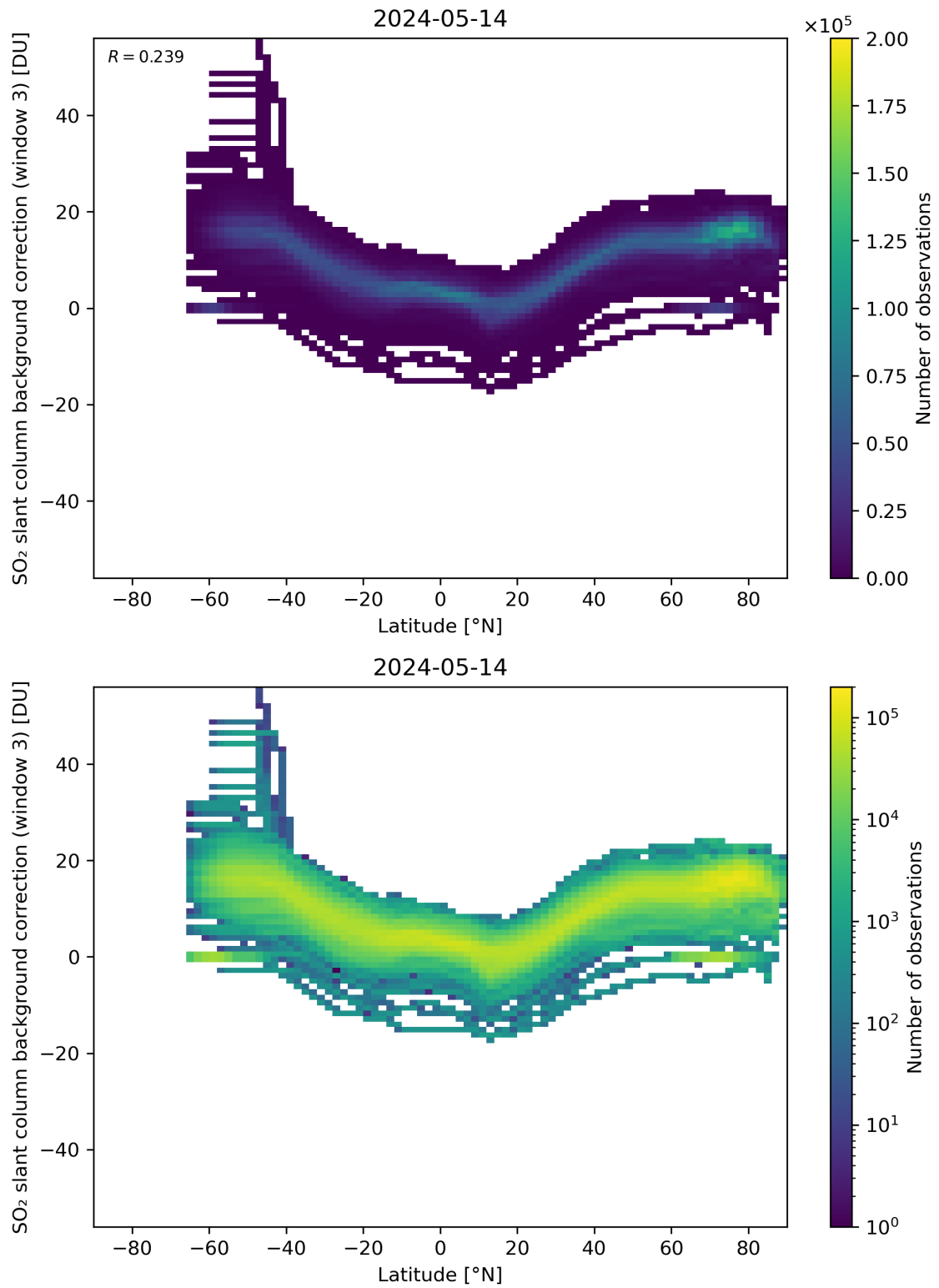
Figure 141: Scatter density plot of “Latitude” against “SO 2 slant column background correction (window 3)” for 2024-05-13 to 2024-05-15.
