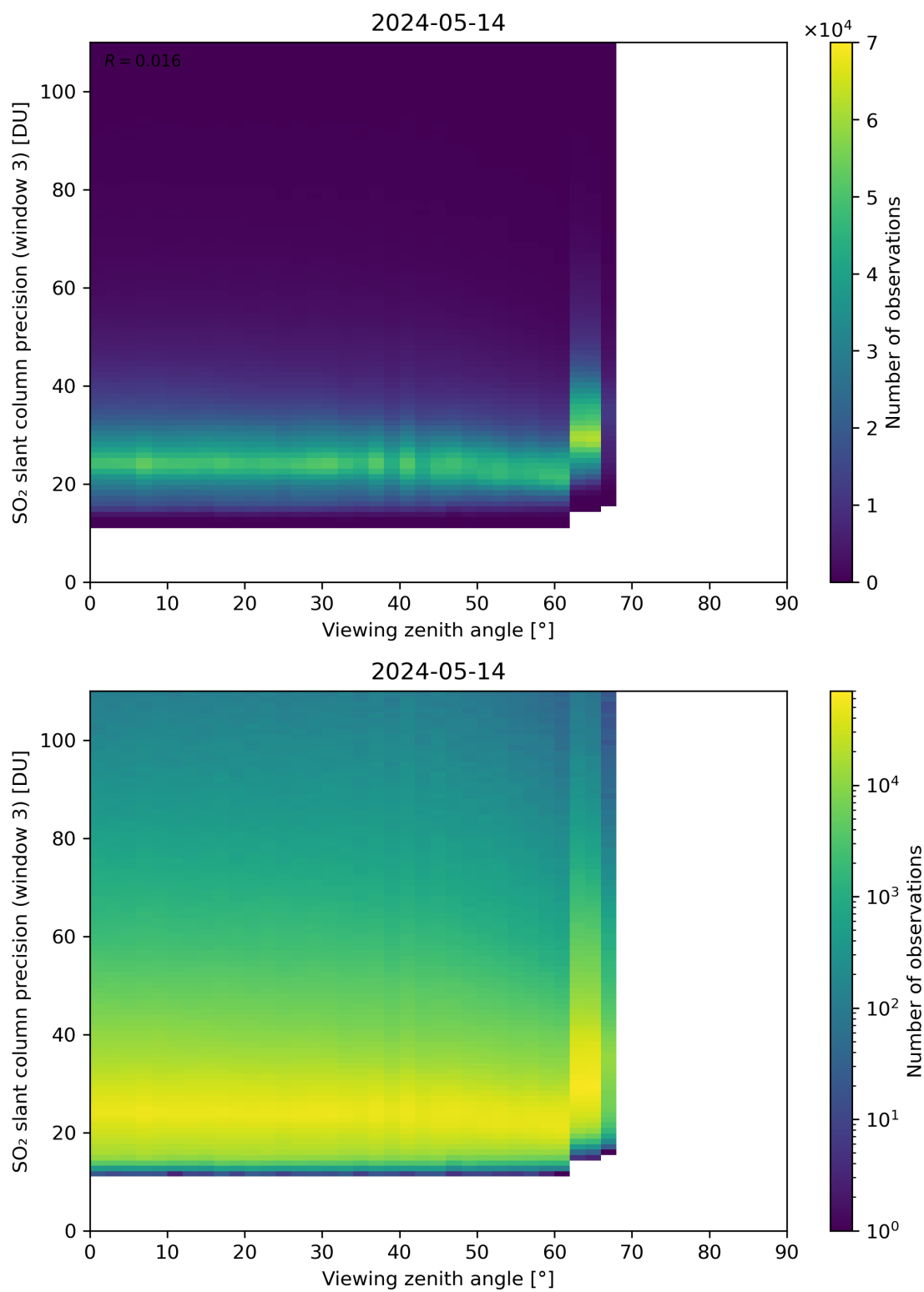
Figure 324: Scatter density plot of “Viewing zenith angle” against “SO 2 slant column precision (window 3)” for 2024-05-13 to 2024-05-15.
