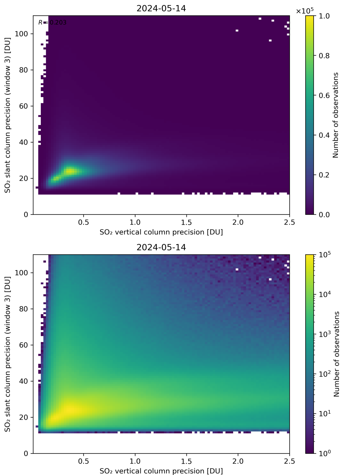
Figure 293: Scatter density plot of “SO 2 vertical column precision” against “SO 2 slant column precision (window 3)” for 2024-05-13 to 2024-05-15.
