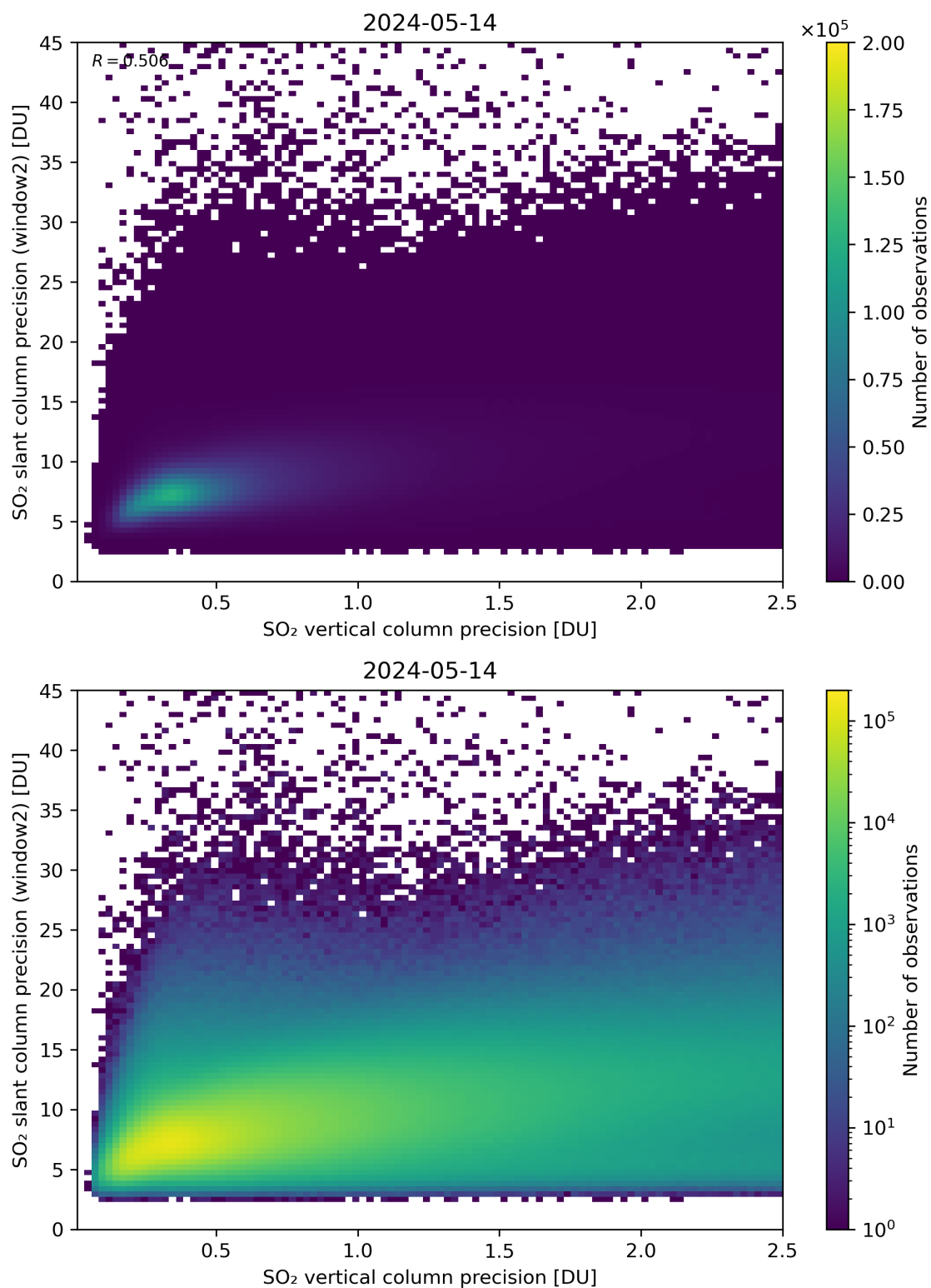
Figure 291: Scatter density plot of “SO 2 vertical column precision” against “SO 2 slant column precision (window2)” for 2024-05-13 to 2024-05-15.
