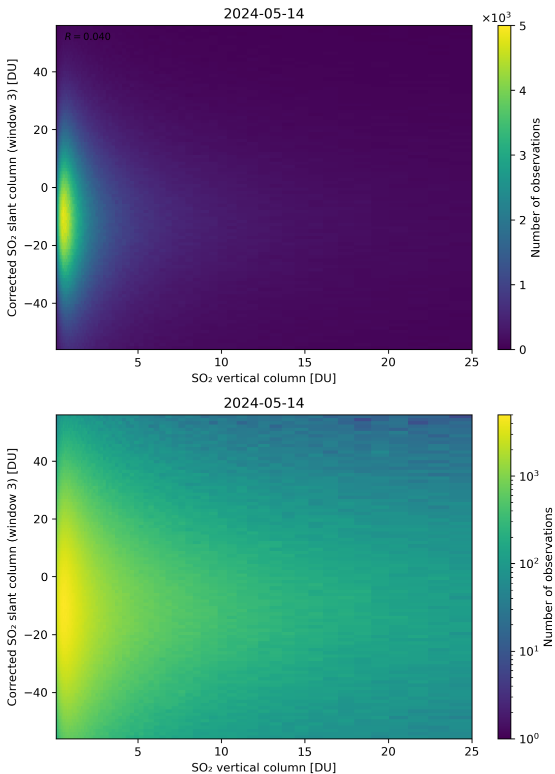
Figure 299: Scatter density plot of “SO 2 vertical column” against “Corrected SO 2 slant column (window 3)” for 2024-05-13 to 2024-05-15.
