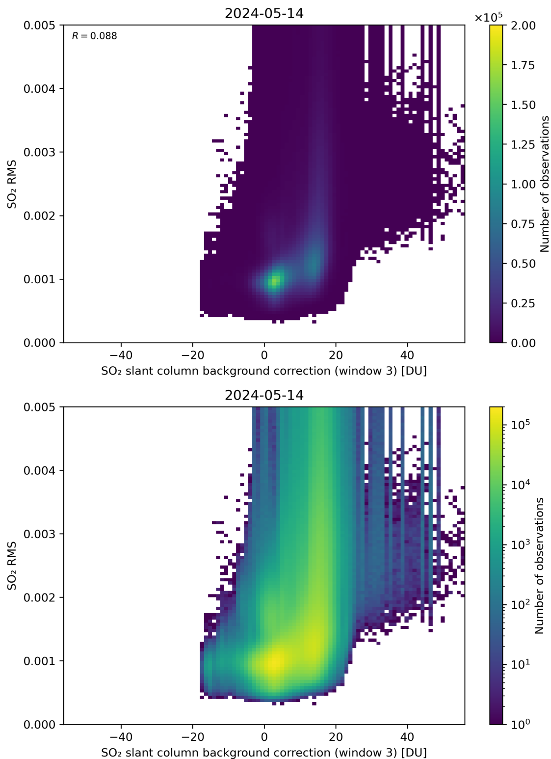
Figure 123: Scatter density plot of “SO 2 slant column background correction (window 3)” against “SO 2 RMS” for 2024-05-13 to 2024-05-15.
