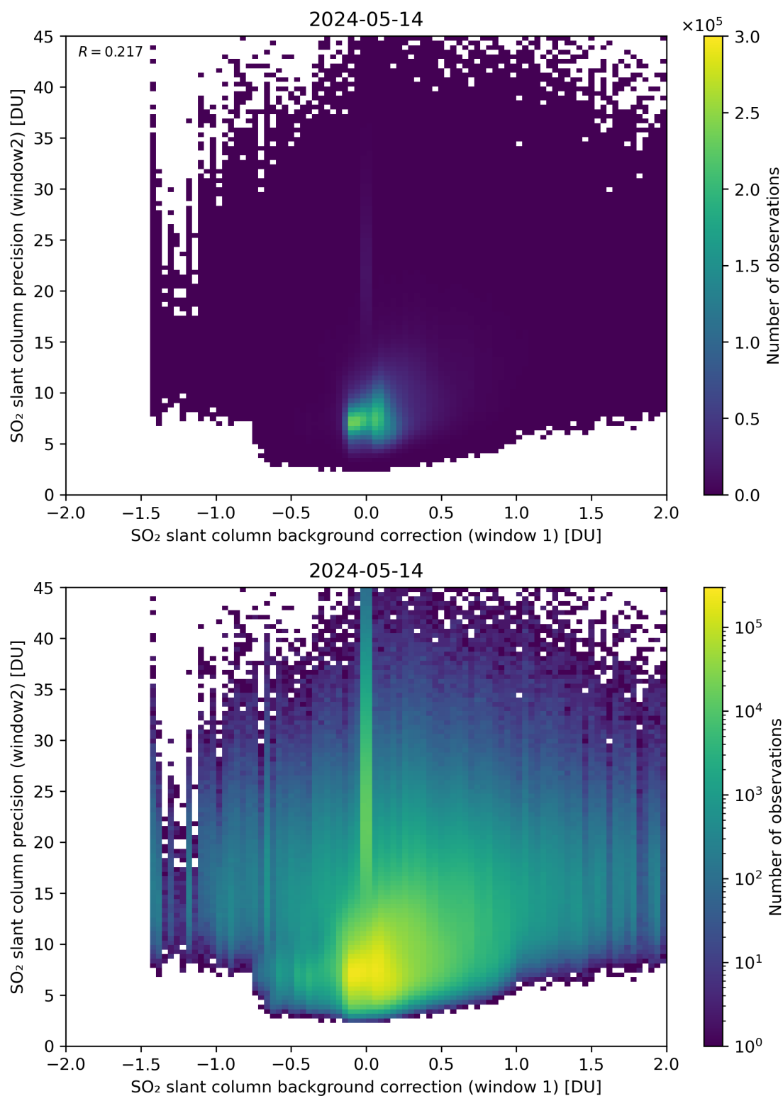
Figure 106: Scatter density plot of “SO 2 slant column background correction (window 1)” against “SO 2 slant column precision (window2)” for 2024-05-13 to 2024-05-15.
