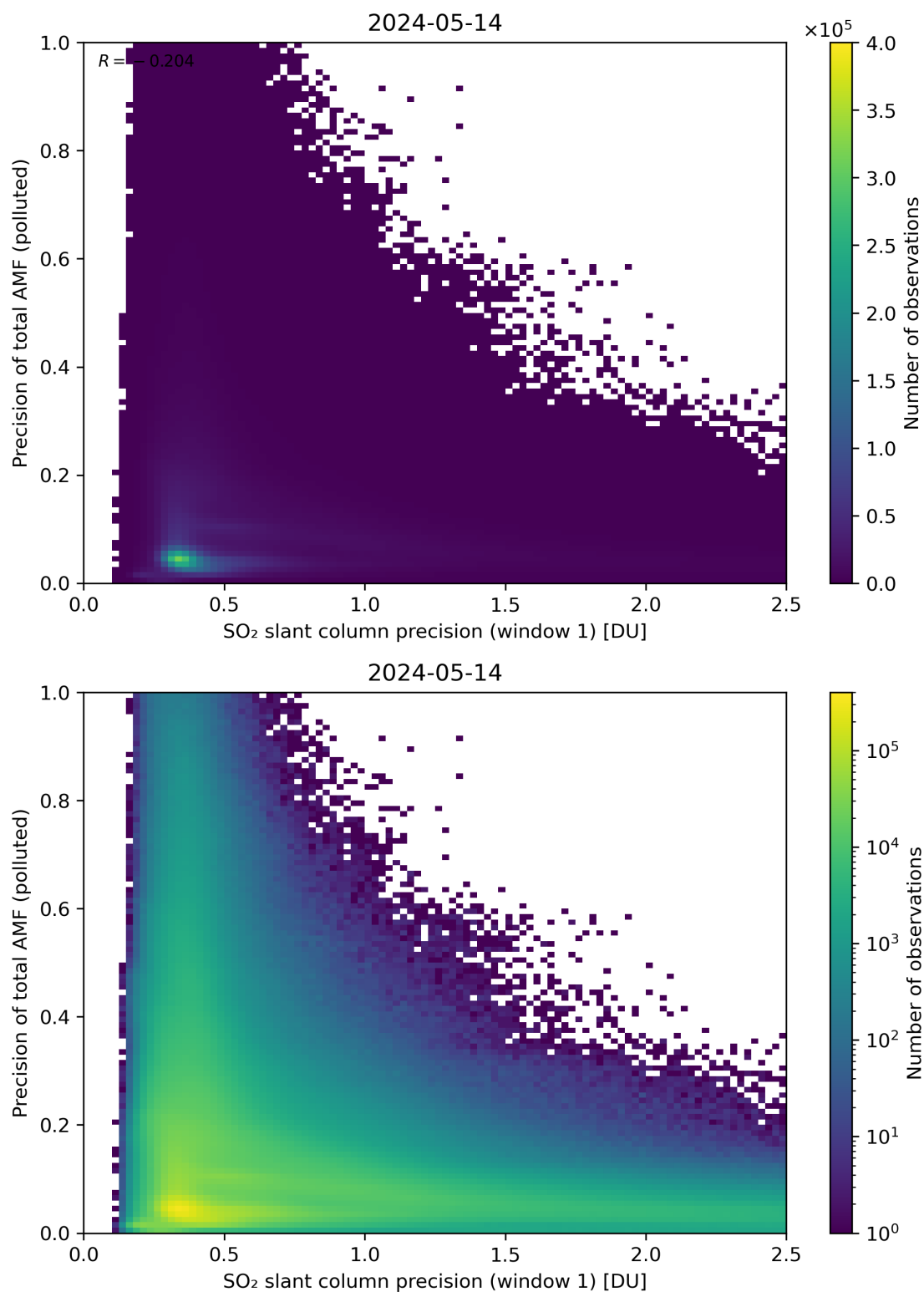
Figure 231: Scatter density plot of “SO 2 slant column precision (window 1)” against “Precision of total AMF (polluted)” for 2024-05-13 to 2024-05-15.
