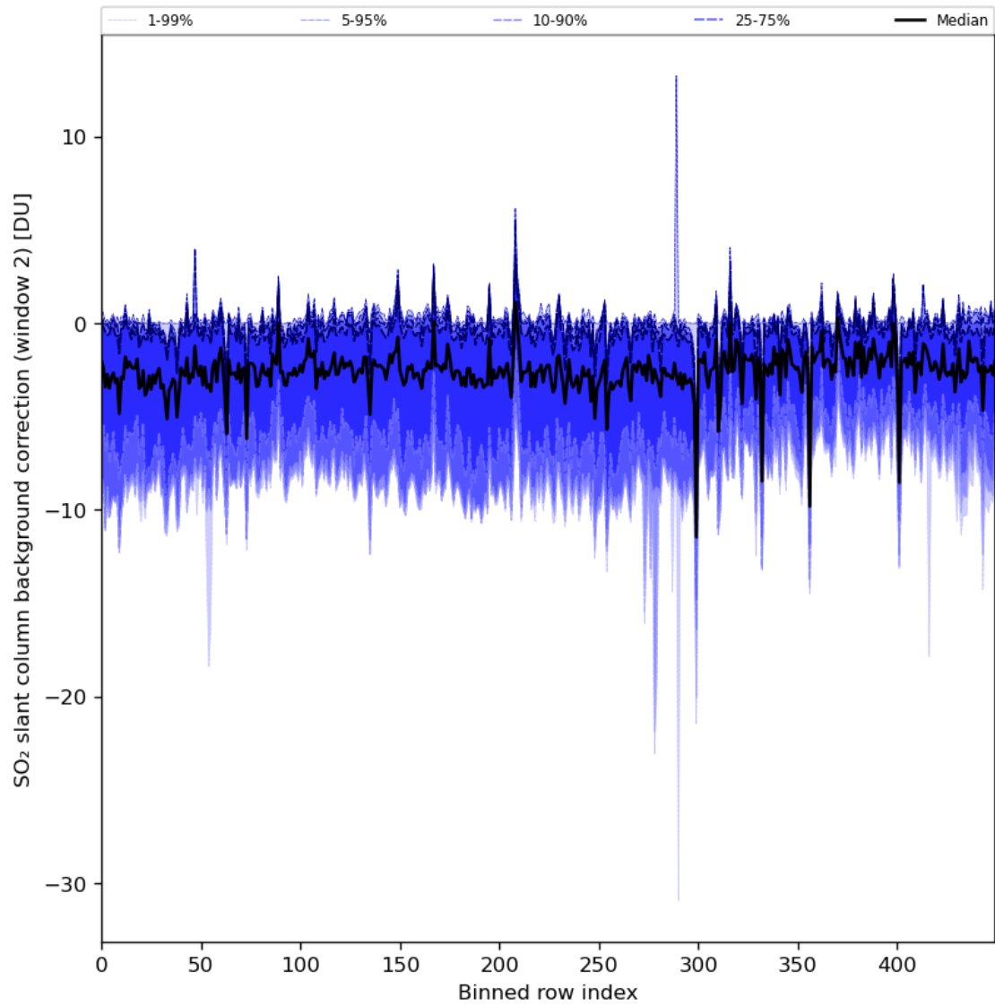
Figure 86: Along track statistics of “SO 2 slant column background correction (window 2)” for 2024-05-13 to 2024-05-15
