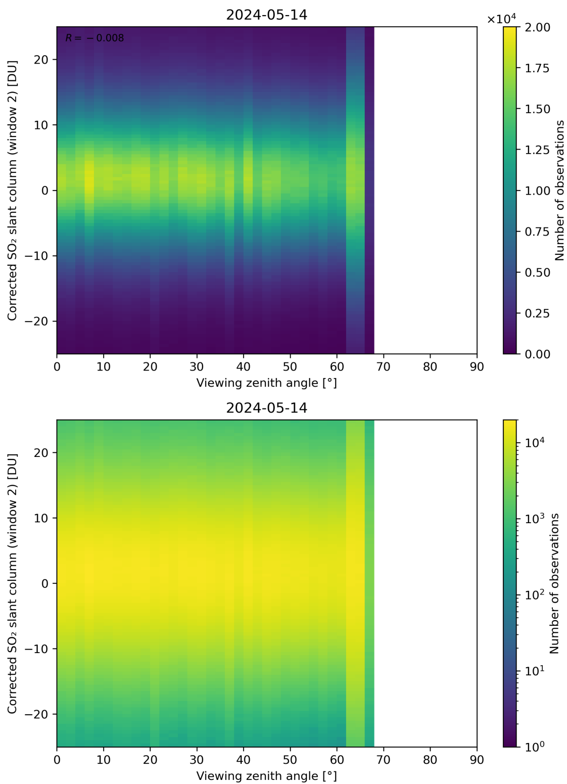
Figure 318: Scatter density plot of “Viewing zenith angle” against “Corrected SO 2 slant column (window 2)” for 2024-05-13 to 2024-05-15.
