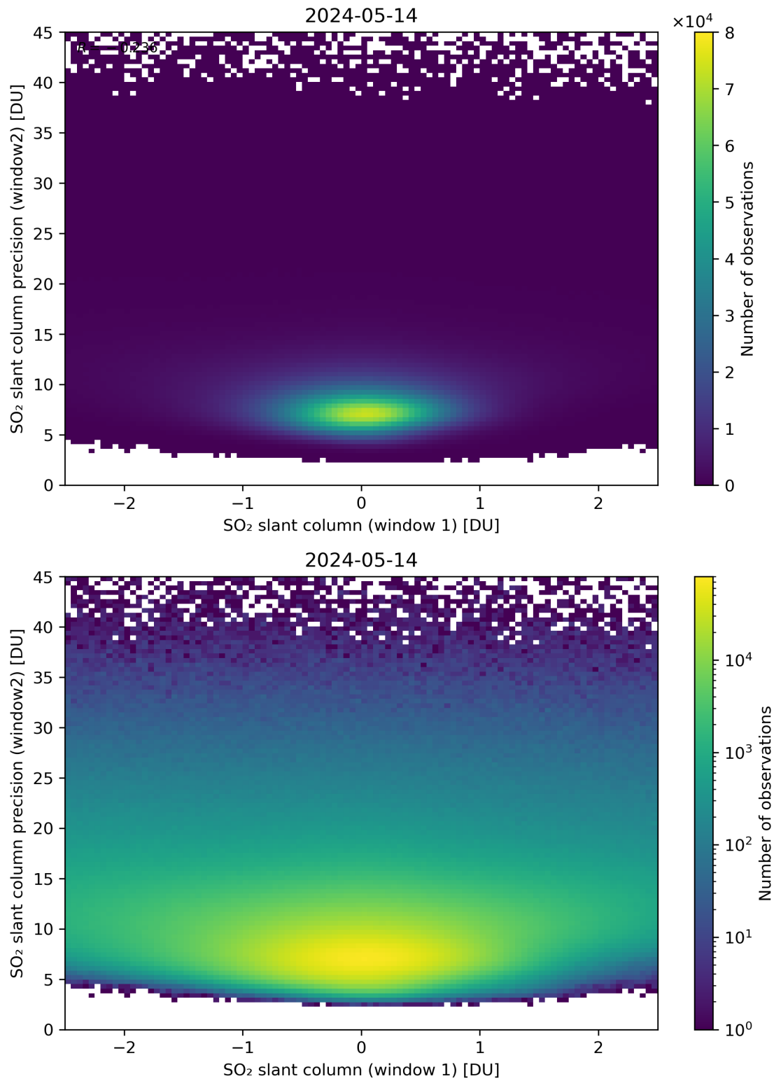
Figure 236: Scatter density plot of “SO 2 slant column (window 1)” against “SO 2 slant column precision (window2)” for 2024-05-13 to 2024-05-15.
