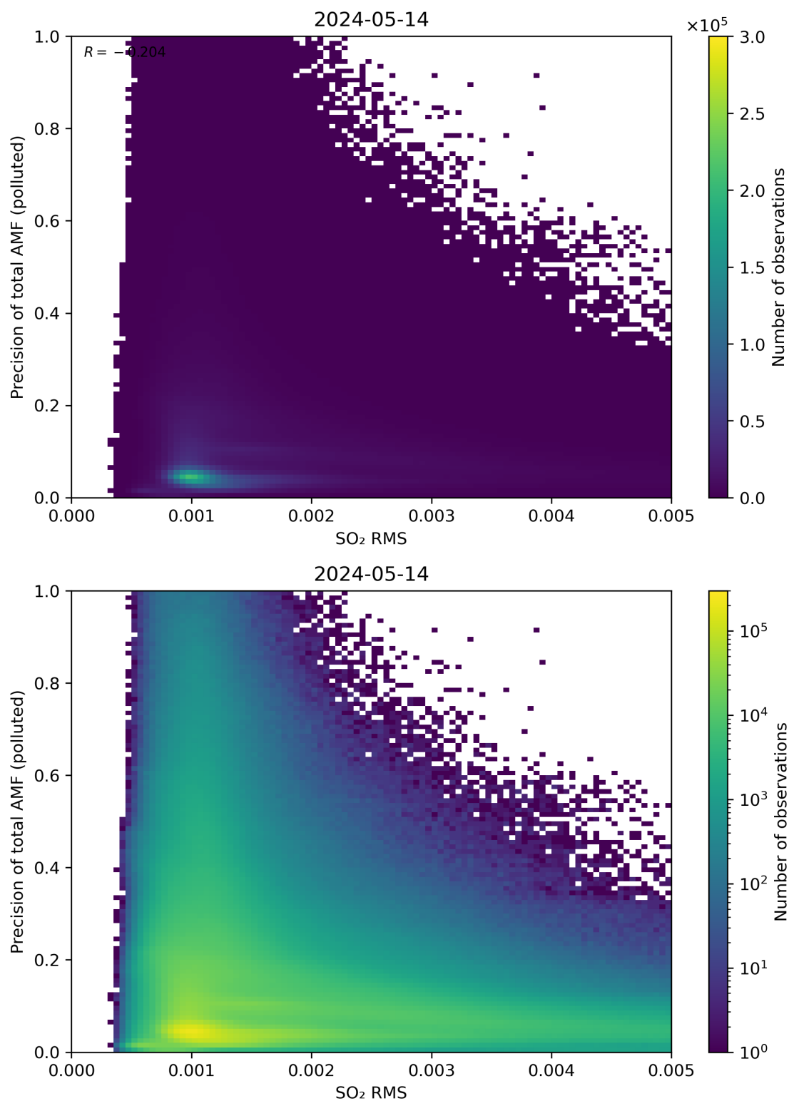
Figure 138: Scatter density plot of “SO 2 RMS” against “Precision of total AMF (polluted)” for 2024-05-13 to 2024-05-15.
