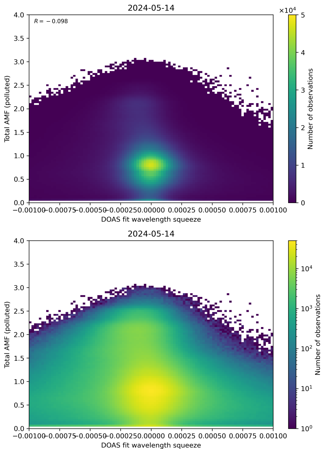
Figure 134: Scatter density plot of “DOAS fit wavelength squeeze” against “Total AMF (polluted)” for 2024-05-13 to 2024-05-15.
