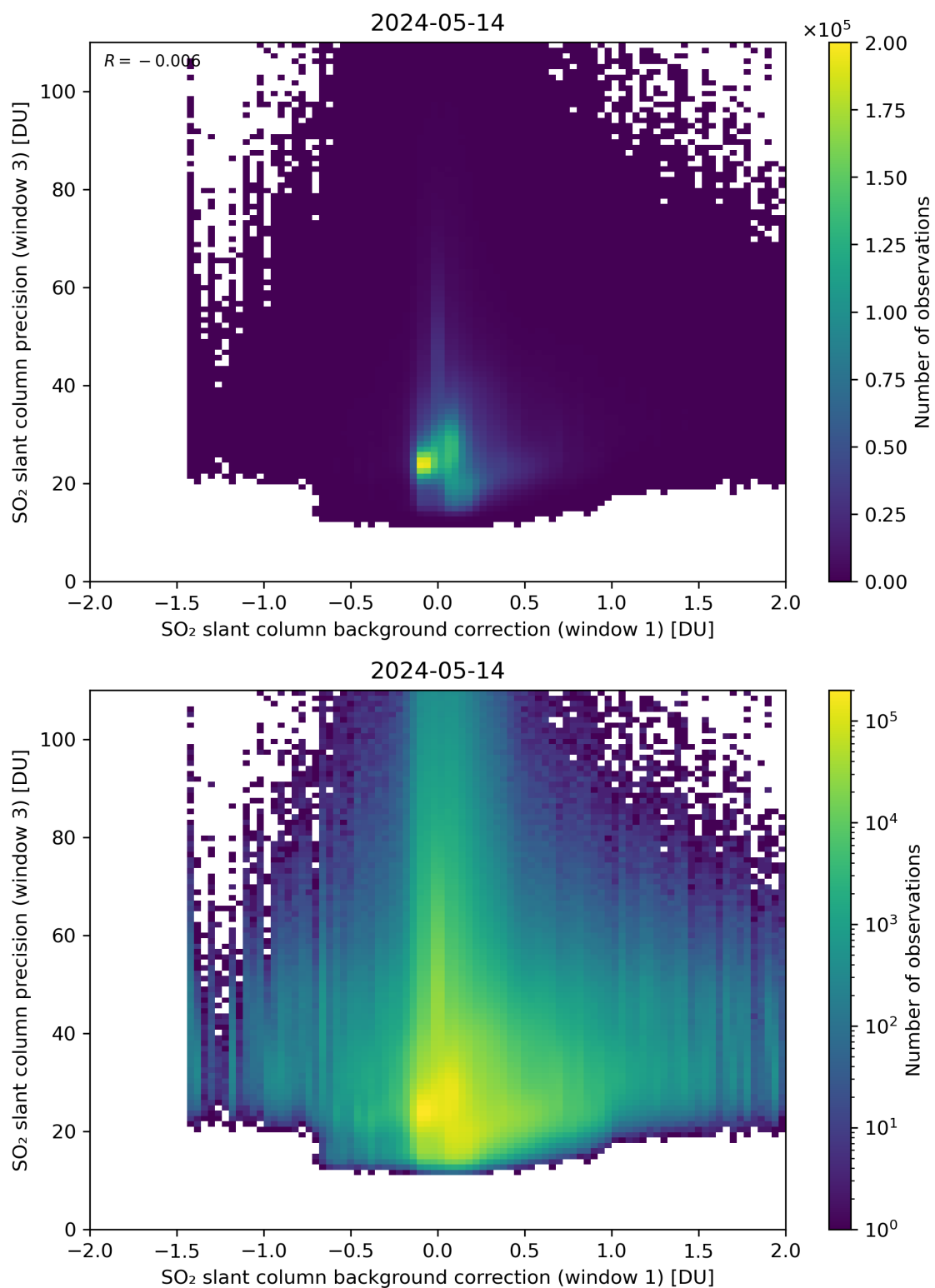
Figure 108: Scatter density plot of “SO 2 slant column background correction (window 1)” against “SO 2 slant column precision (window 3)” for 2024-05-13 to 2024-05-15.
