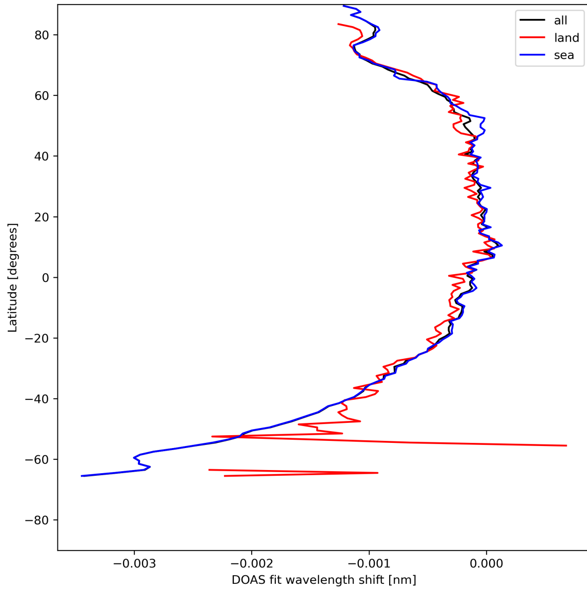
Figure 45: Zonal average of “DOAS fit wavelength shift” for 2024-05-13 to 2024-05-15.
