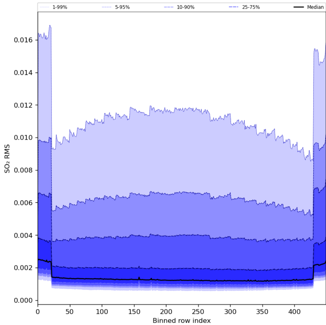
Figure 93: Along track statistics of “SO 2 RMS” for 2024-05-13 to 2024-05-15
