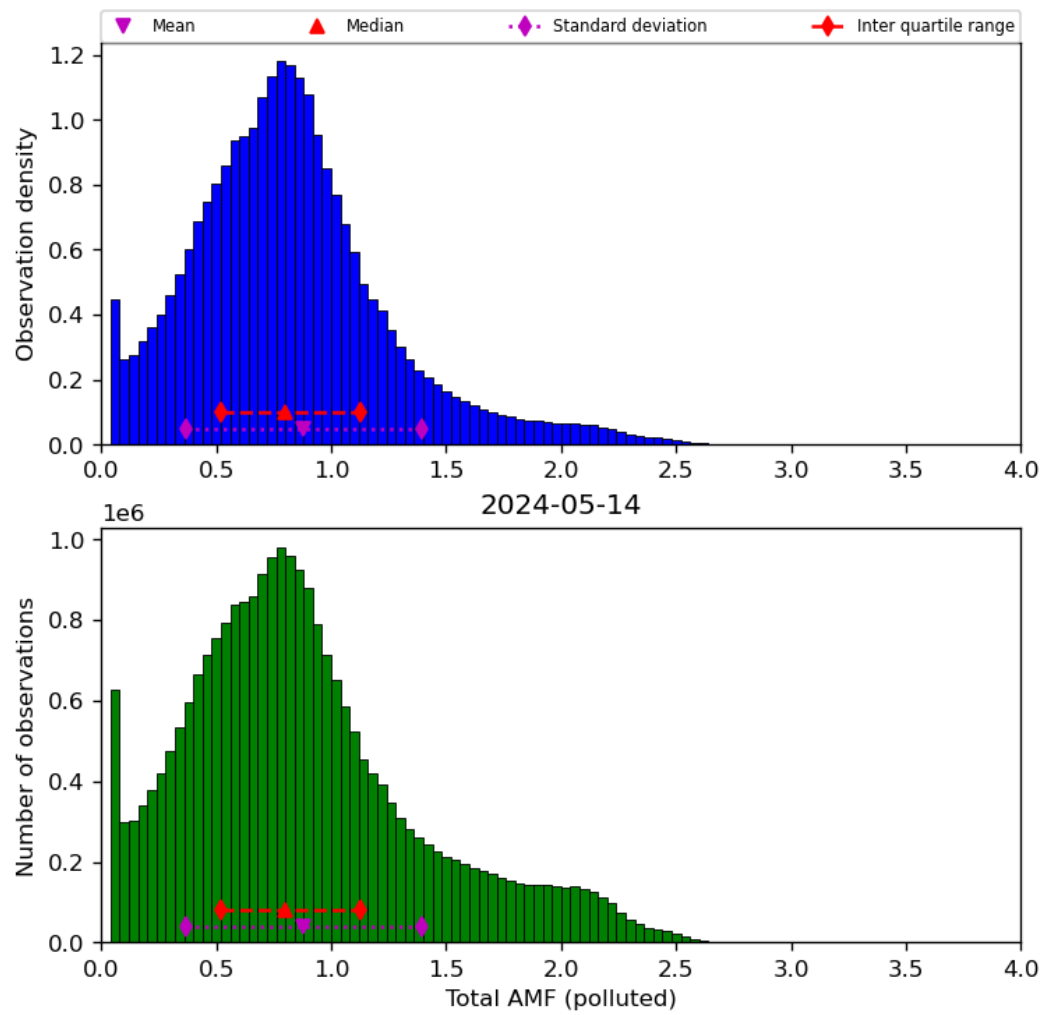
Figure 71: Histogram of “Total AMF (polluted)” for 2024-05-13 to 2024-05-15
