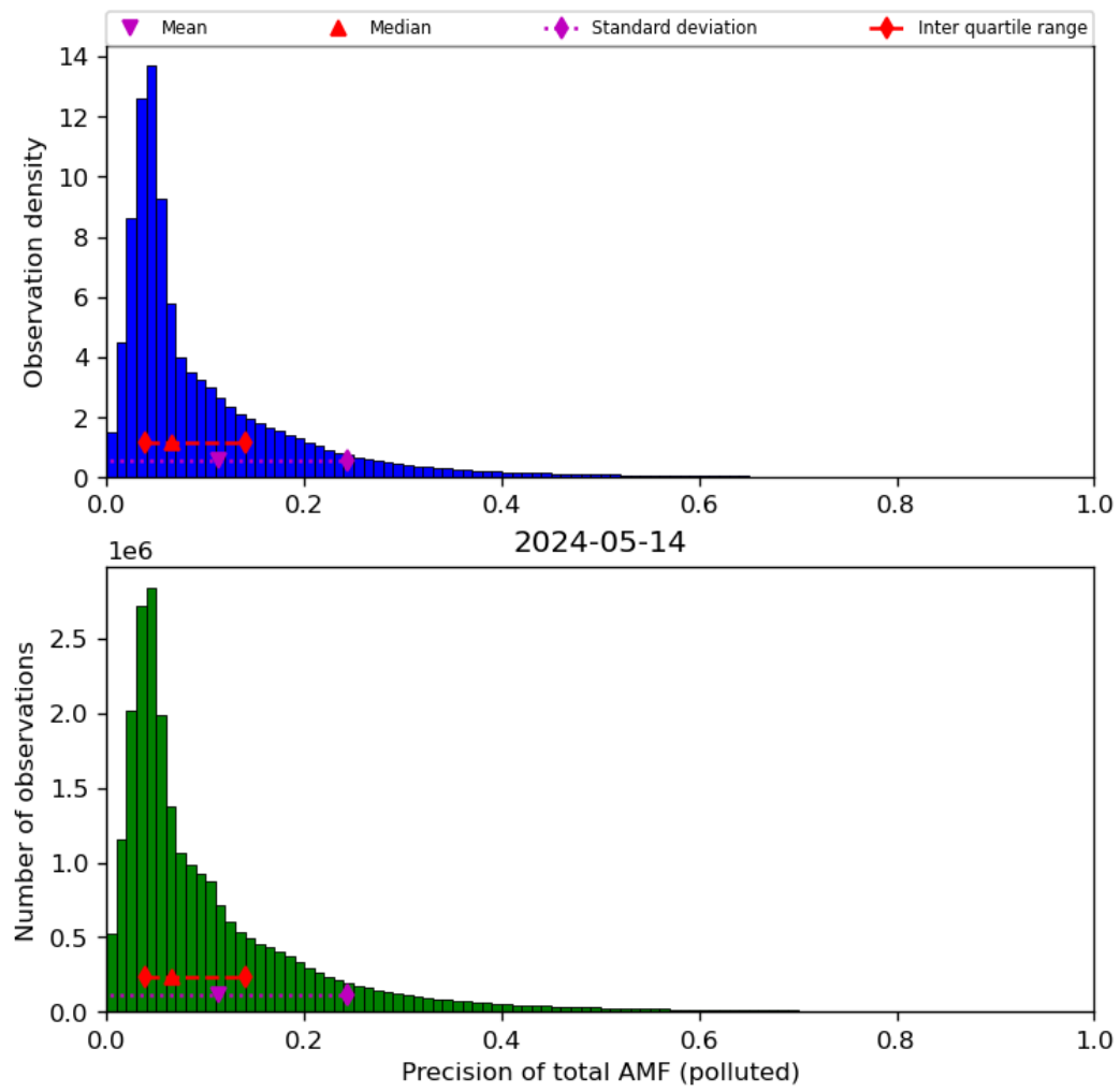
Figure 72: Histogram of “Precision of total AMF (polluted)” for 2024-05-13 to 2024-05-15
