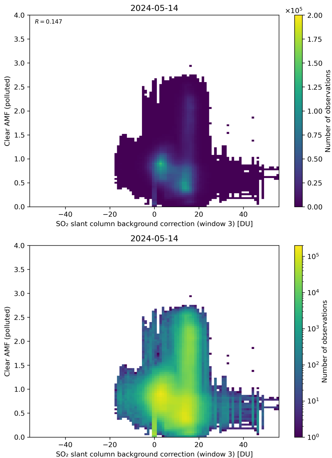
Figure 124: Scatter density plot of “SO 2 slant column background correction (window 3)” against “Clear AMF (polluted)” for 2024-05-13 to 2024-05-15.
