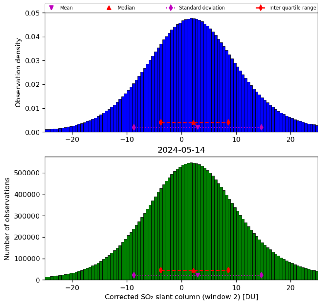
Figure 62: Histogram of “Corrected SO 2 slant column (window 2)” for 2024-05-13 to 2024-05-15
