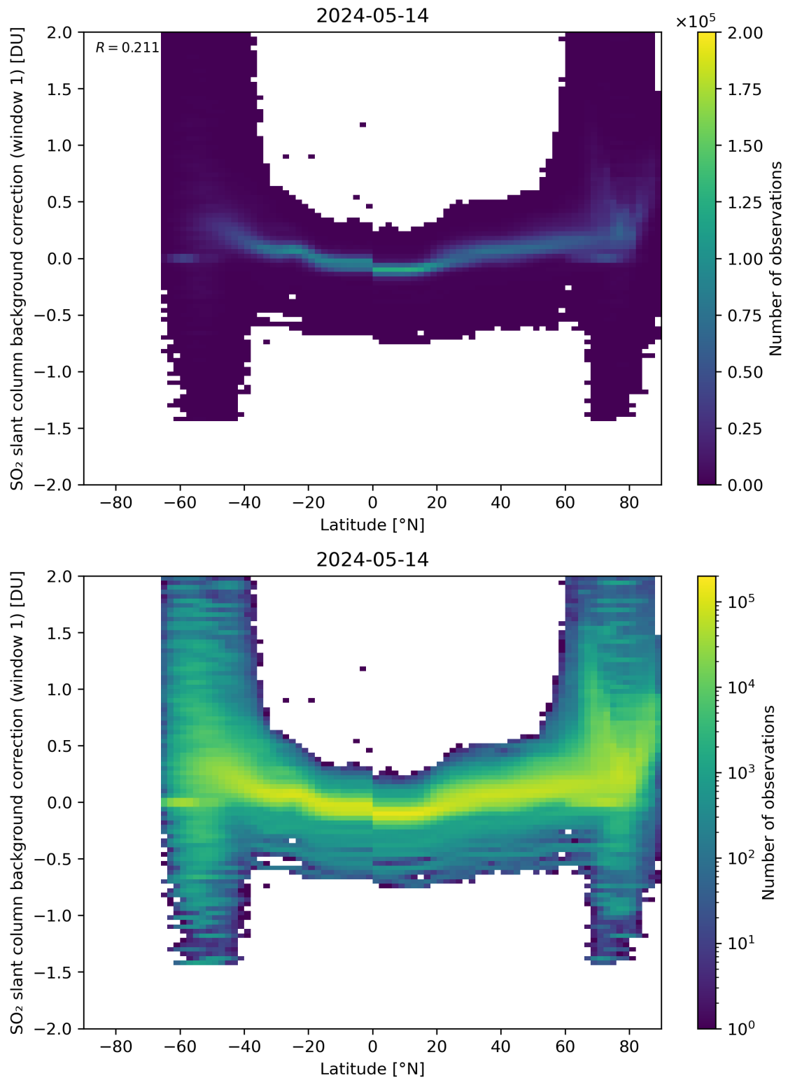
Figure 139: Scatter density plot of “Latitude” against “SO 2 slant column background correction (window 1)” for 2024-05-13 to 2024-05-15.
