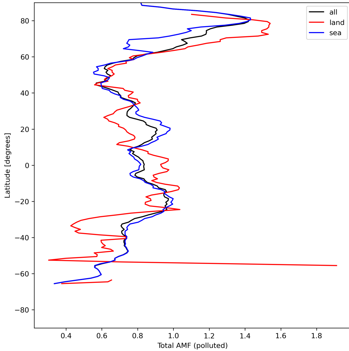
Figure 48: Zonal average of “Total AMF (polluted)” for 2024-05-13 to 2024-05-15.
