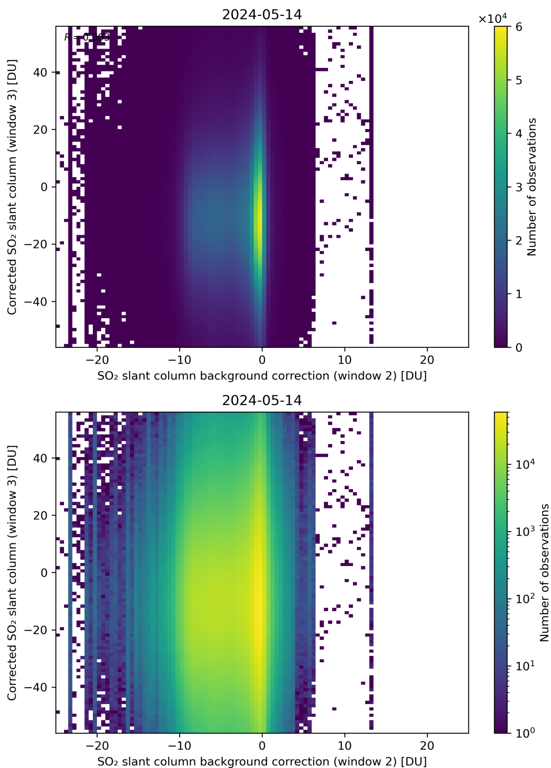
Figure 116: Scatter density plot of “SO 2 slant column background correction (window 2)” against “Corrected SO 2 slant column (window 3)” for 2024-05-13 to 2024-05-15.
