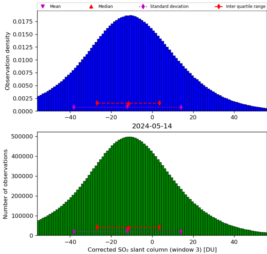
Figure 66: Histogram of “Corrected SO 2 slant column (window 3)” for 2024-05-13 to 2024-05-15
